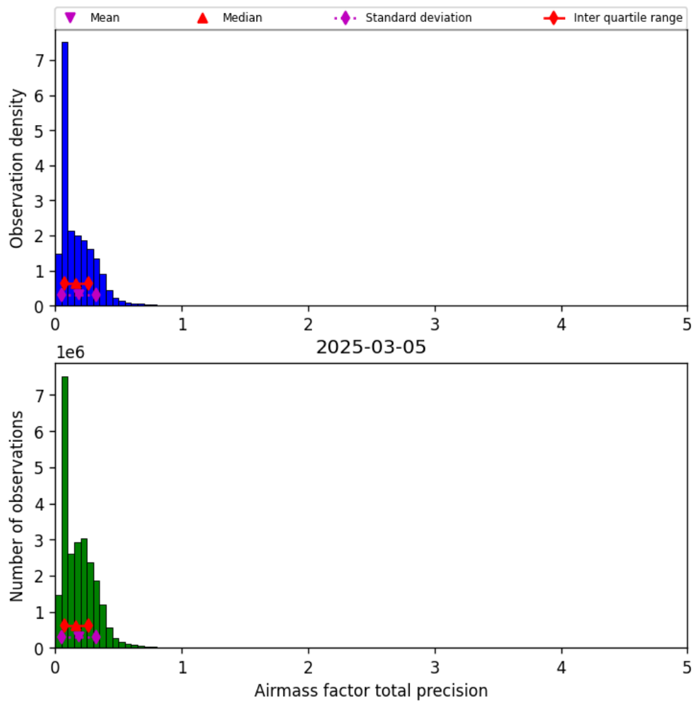
Figure 41: Histogram of “Airmass factor total precision” for 2025-03-04 to 2025-03-06
