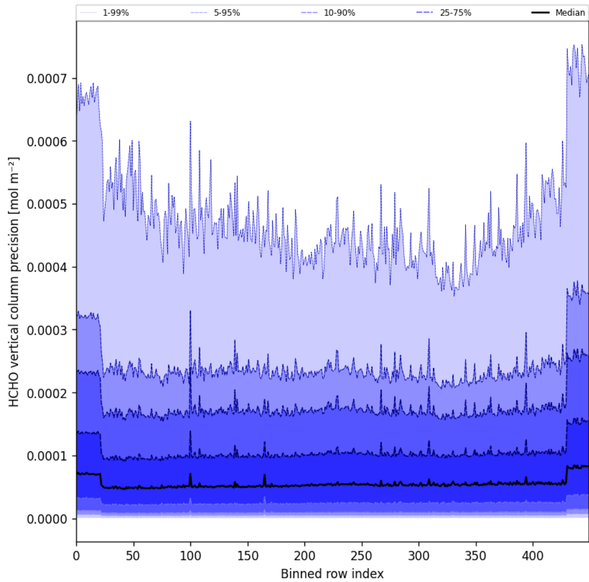
Figure 50: Along track statistics of “HCHO vertical column precision” for 2025-03-04 to 2025-03-06
