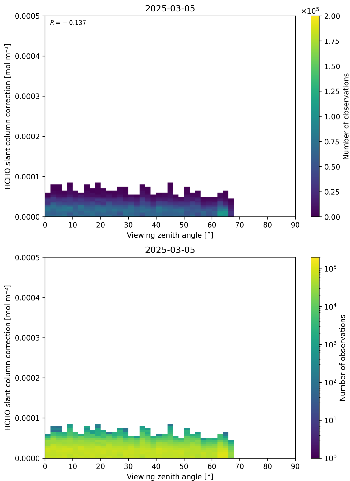
Figure 187: Scatter density plot of “Viewing zenith angle” against “HCHO slant column correction” for 2025-03-04 to 2025-03-06.
