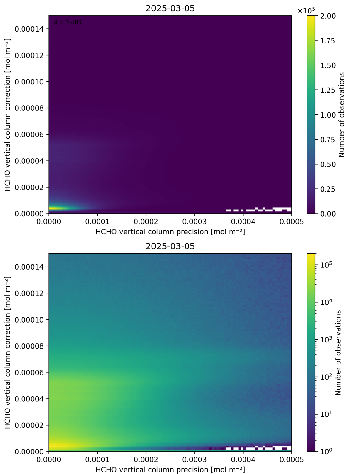
Figure 146: Scatter density plot of “HCHO vertical column precision” against “HCHO vertical column correction” for 2025-03-04 to 2025-03-06.
