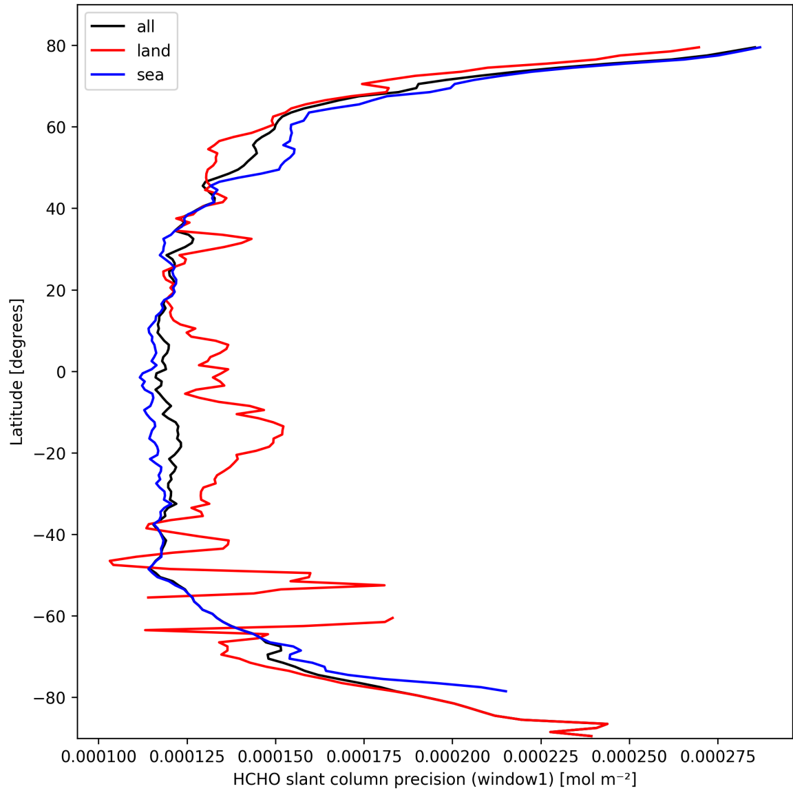
Figure 25: Zonal average of “HCHO slant column precision (window1)” for 2025-03-04 to 2025-03-06.
