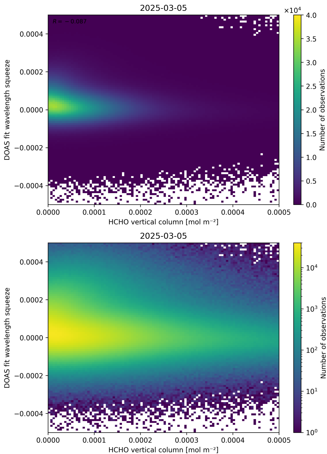
Figure 125: Scatter density plot of “HCHO vertical column” against “DOAS fit wavelength squeeze” for 2025-03-04 to 2025-03-06.
