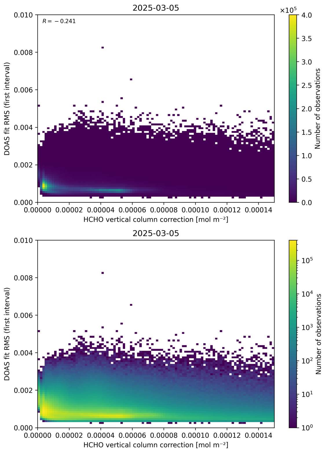
Figure 112: Scatter density plot of “HCHO vertical column correction” against “DOAS fit RMS (first interval)” for 2025-03-04 to 2025-03-06.
