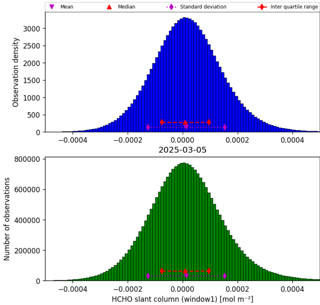
Figure 38: Histogram of “HCHO slant column (window1)” for 2025-03-04 to 2025-03-06
