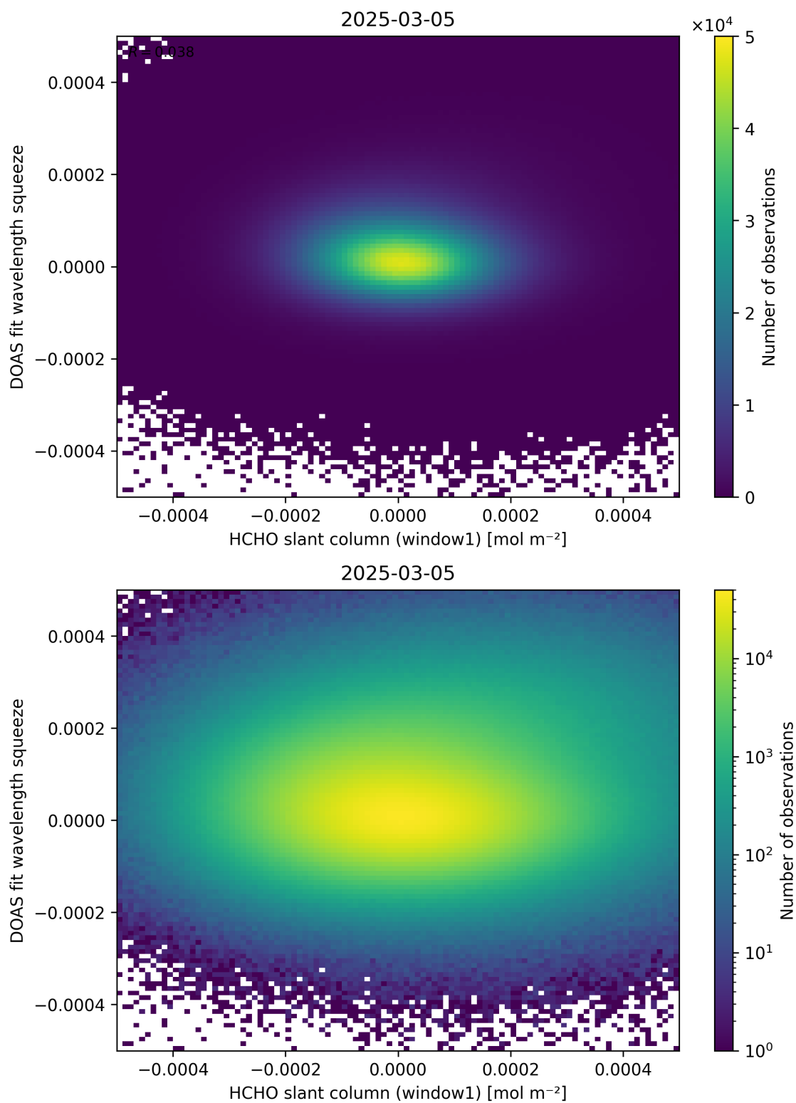
Figure 80: Scatter density plot of “HCHO slant column (window1)” against “DOAS fit wavelength squeeze” for 2025-03-04 to 2025-03-06.
