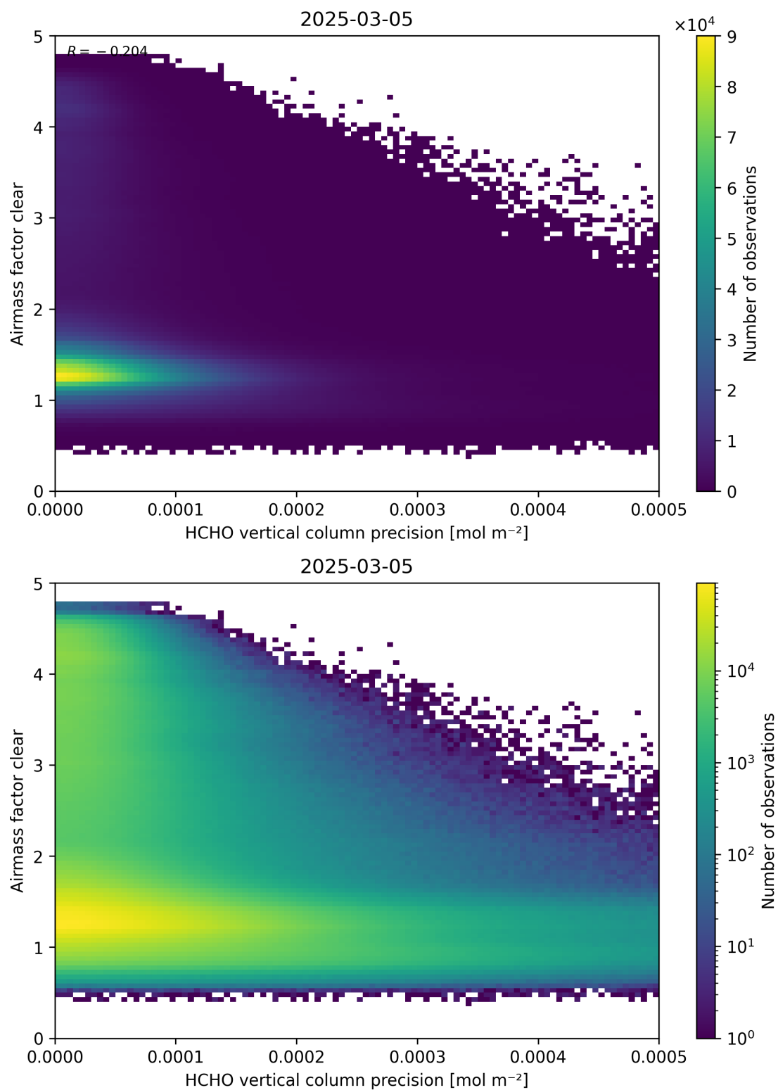
Figure 139: Scatter density plot of “HCHO vertical column precision” against “Airmass factor clear” for 2025-03-04 to 2025-03-06.
