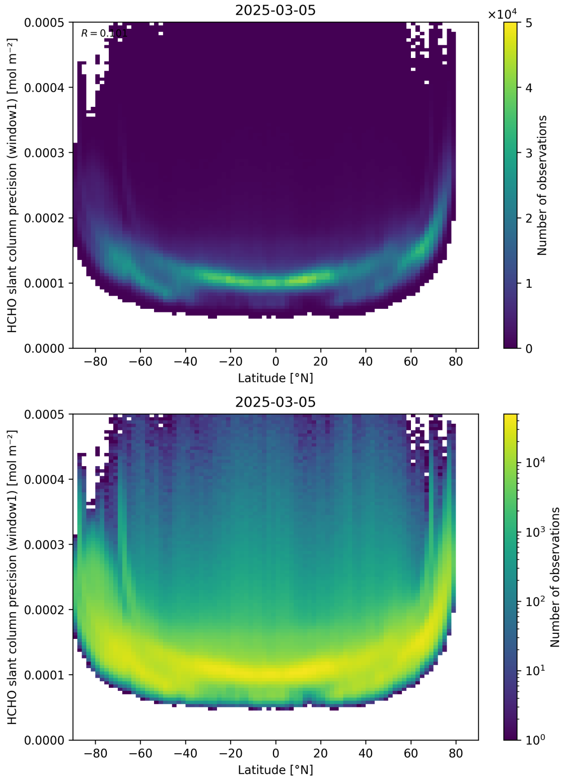
Figure 160: Scatter density plot of “Latitude” against “HCHO slant column precision (window1)” for 2025-03-04 to 2025-03-06.
