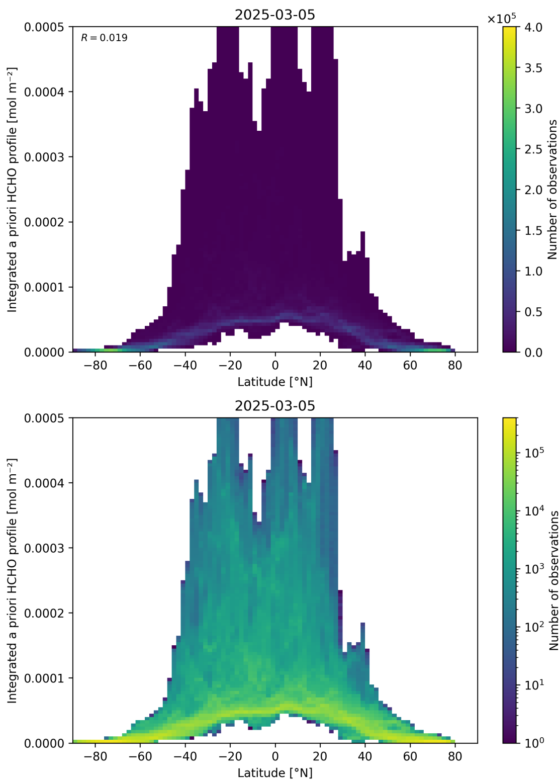
Figure 166: Scatter density plot of “Latitude” against “Integrated a priori HCHO profile” for 2025-03-04 to 2025-03-06.
