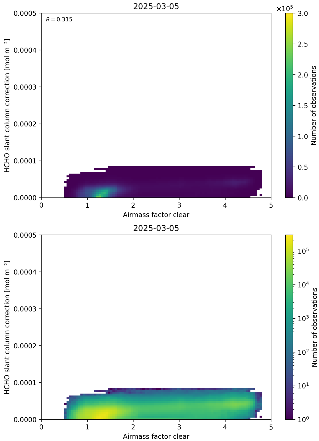
Figure 75: Scatter density plot of “Airmass factor clear” against “HCHO slant column correction” for 2025-03-04 to 2025-03-06.
