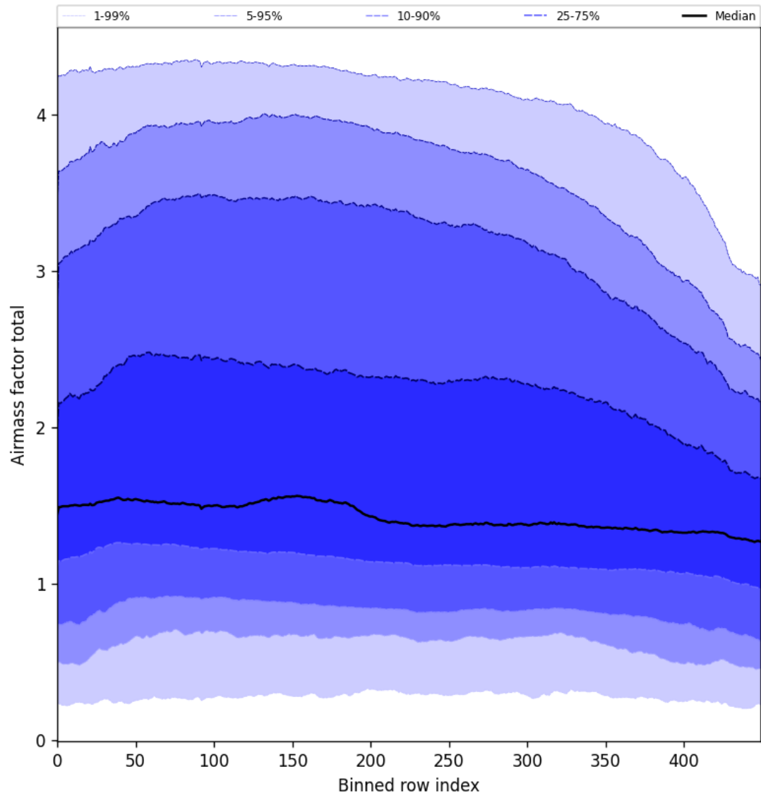
Figure 54: Along track statistics of “Airmass factor total” for 2025-03-04 to 2025-03-06
