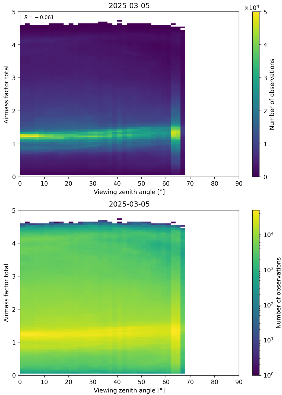
Figure 190: Scatter density plot of “Viewing zenith angle” against “Airmass factor total” for 2025-03-04 to 2025-03-06.
