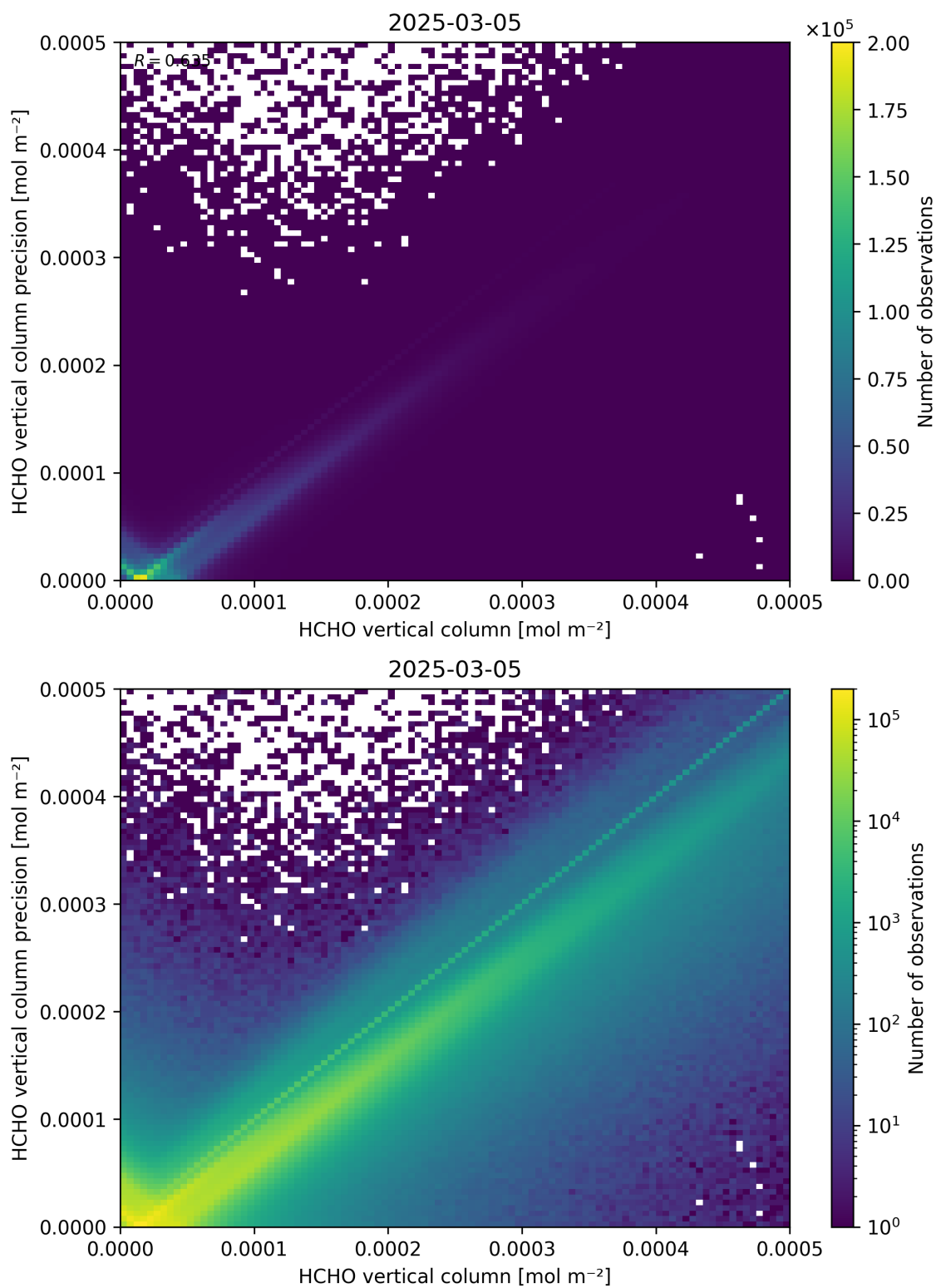
Figure 134: Scatter density plot of “HCHO vertical column” against “HCHO vertical column precision” for 2025-03-04 to 2025-03-06.
