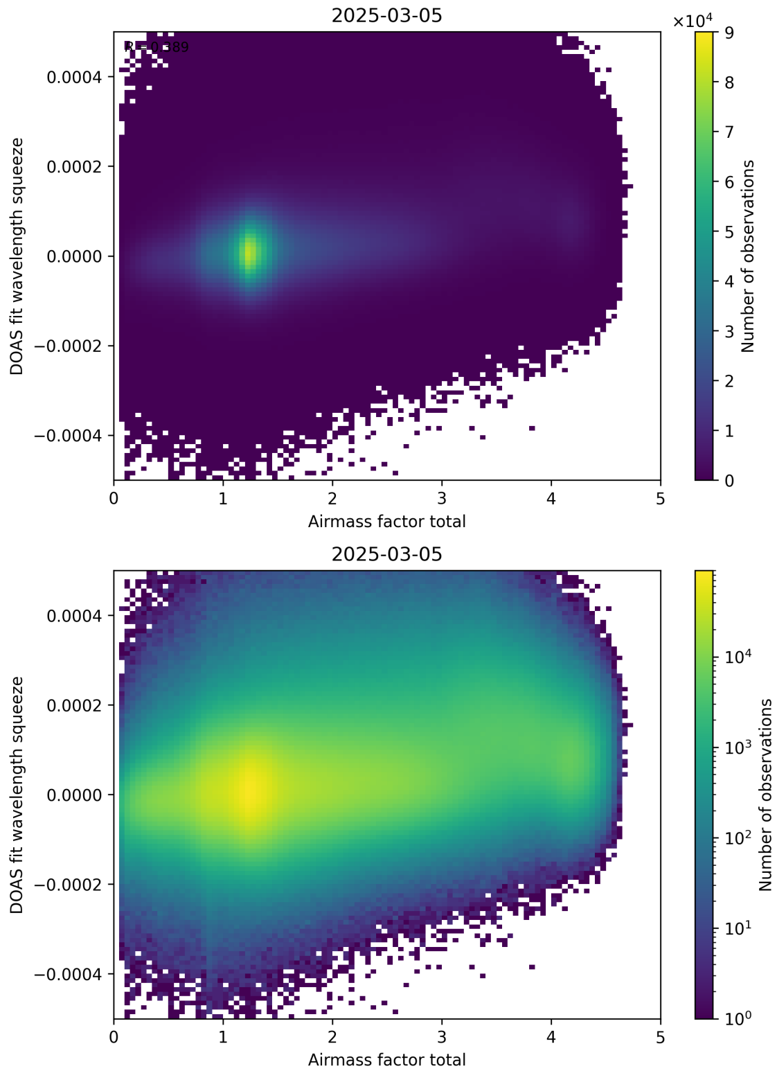
Figure 99: Scatter density plot of “Airmass factor total” against “DOAS fit wavelength squeeze” for 2025-03-04 to 2025-03-06.
