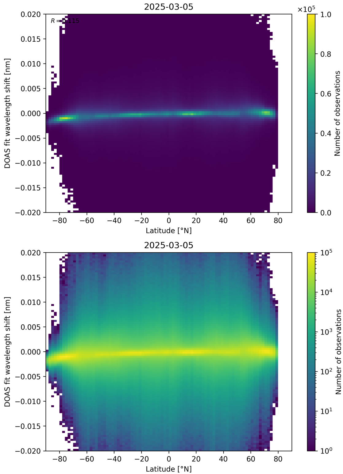
Figure 154: Scatter density plot of “Latitude” against “DOAS fit wavelength shift” for 2025-03-04 to 2025-03-06.
