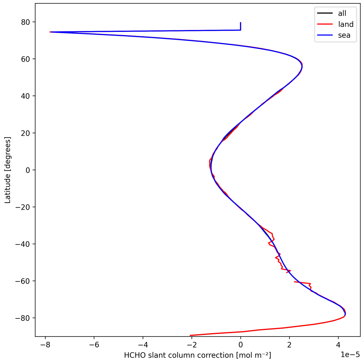
Figure 33: Zonal average of “HCHO slant column correction” for 2025-03-04 to 2025-03-06.
