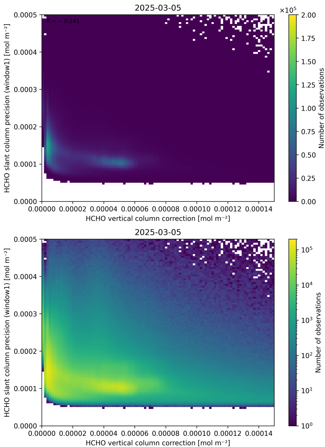
Figure 119: Scatter density plot of “HCHO vertical column correction” against “HCHO slant column precision (window1)” for 2025-03-04 to 2025-03-06.
