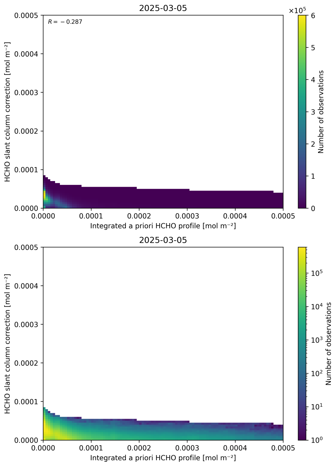
Figure 152: Scatter density plot of “Integrated a priori HCHO profile” against “HCHO slant column correction” for 2025-03-04 to 2025-03-06.
