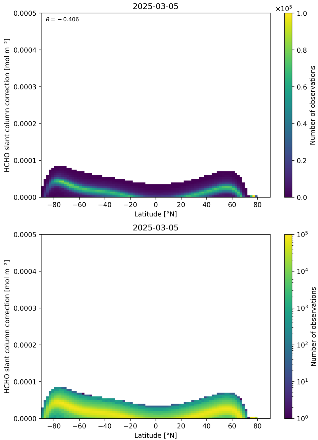
Figure 158: Scatter density plot of “Latitude” against “HCHO slant column correction” for 2025-03-04 to 2025-03-06.
