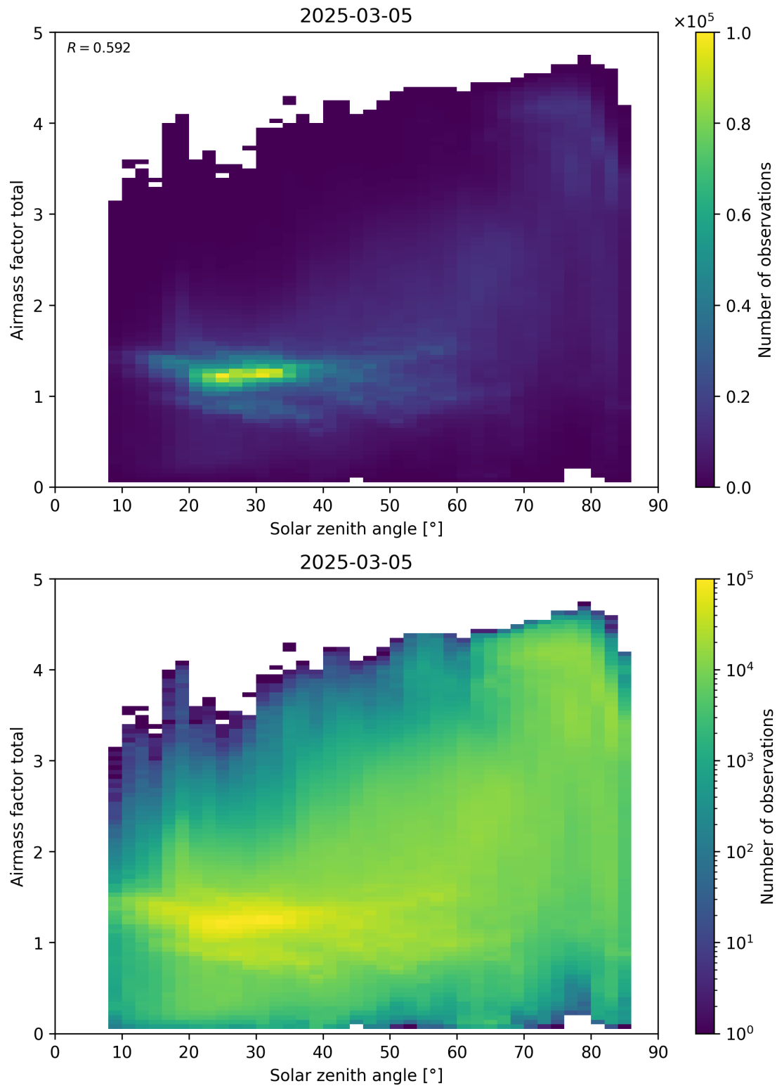
Figure 175: Scatter density plot of “Solar zenith angle” against “Airmass factor total” for 2025-03-04 to 2025-03-06.
