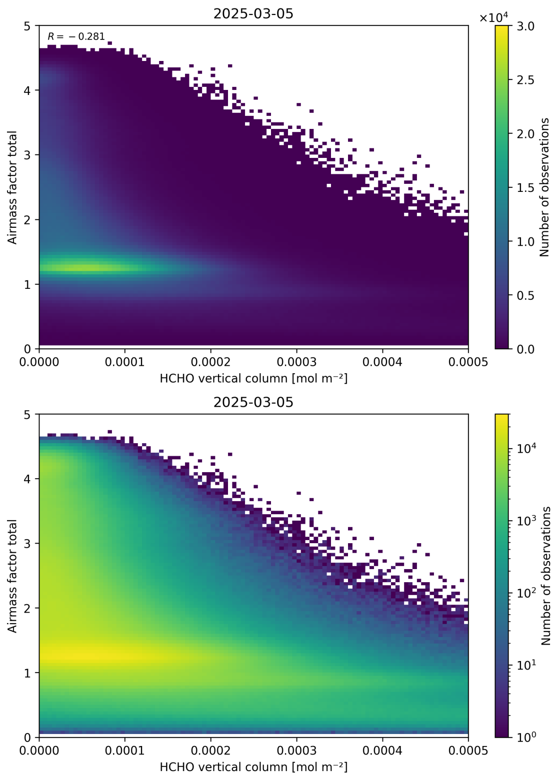
Figure 131: Scatter density plot of “HCHO vertical column” against “Airmass factor total” for 2025-03-04 to 2025-03-06.
