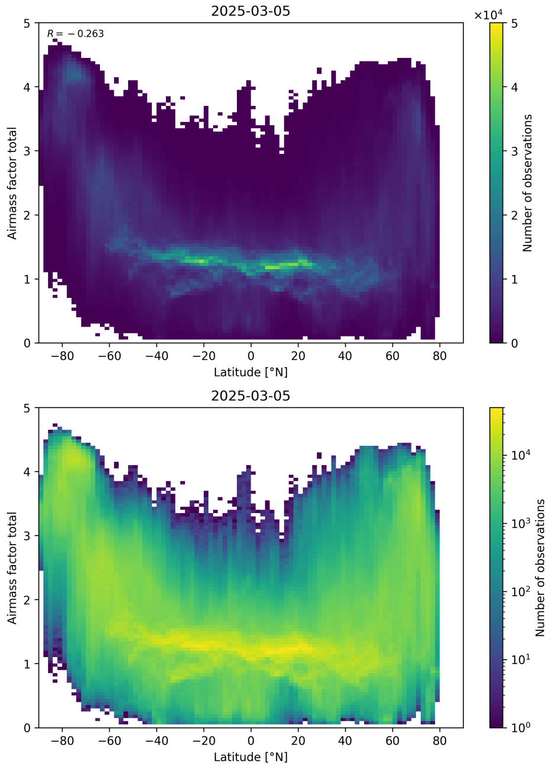
Figure 161: Scatter density plot of “Latitude” against “Airmass factor total” for 2025-03-04 to 2025-03-06.
