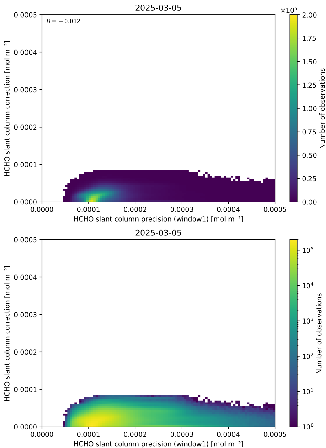
Figure 93: Scatter density plot of “HCHO slant column precision (window1)” against “HCHO slant column correction” for 2025-03-04 to 2025-03-06.
