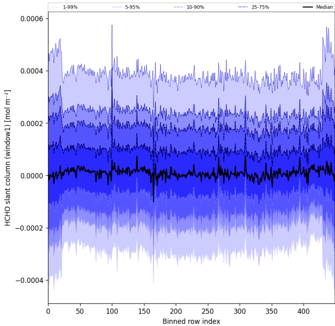
Figure 52: Along track statistics of “HCHO slant column (window1)” for 2025-03-04 to 2025-03-06
