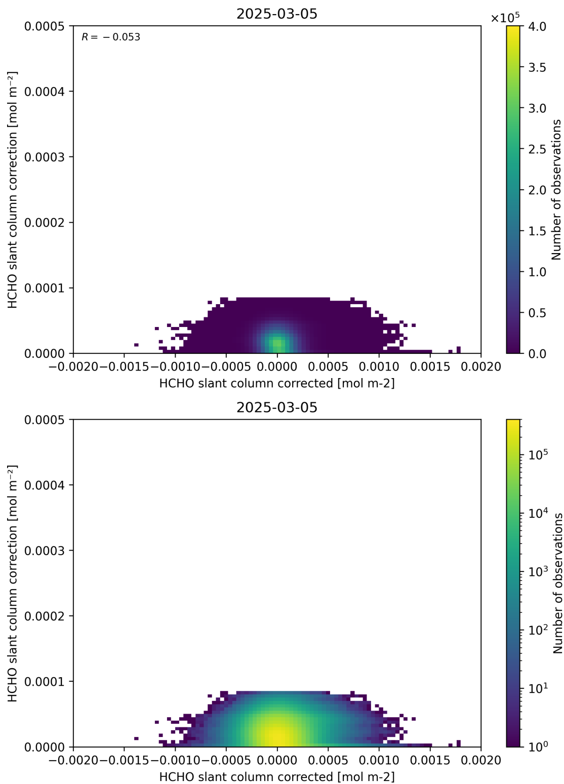
Figure 77: Scatter density plot of “HCHO slant column corrected” against “HCHO slant column correction” for 2025-03-04 to 2025-03-06.
