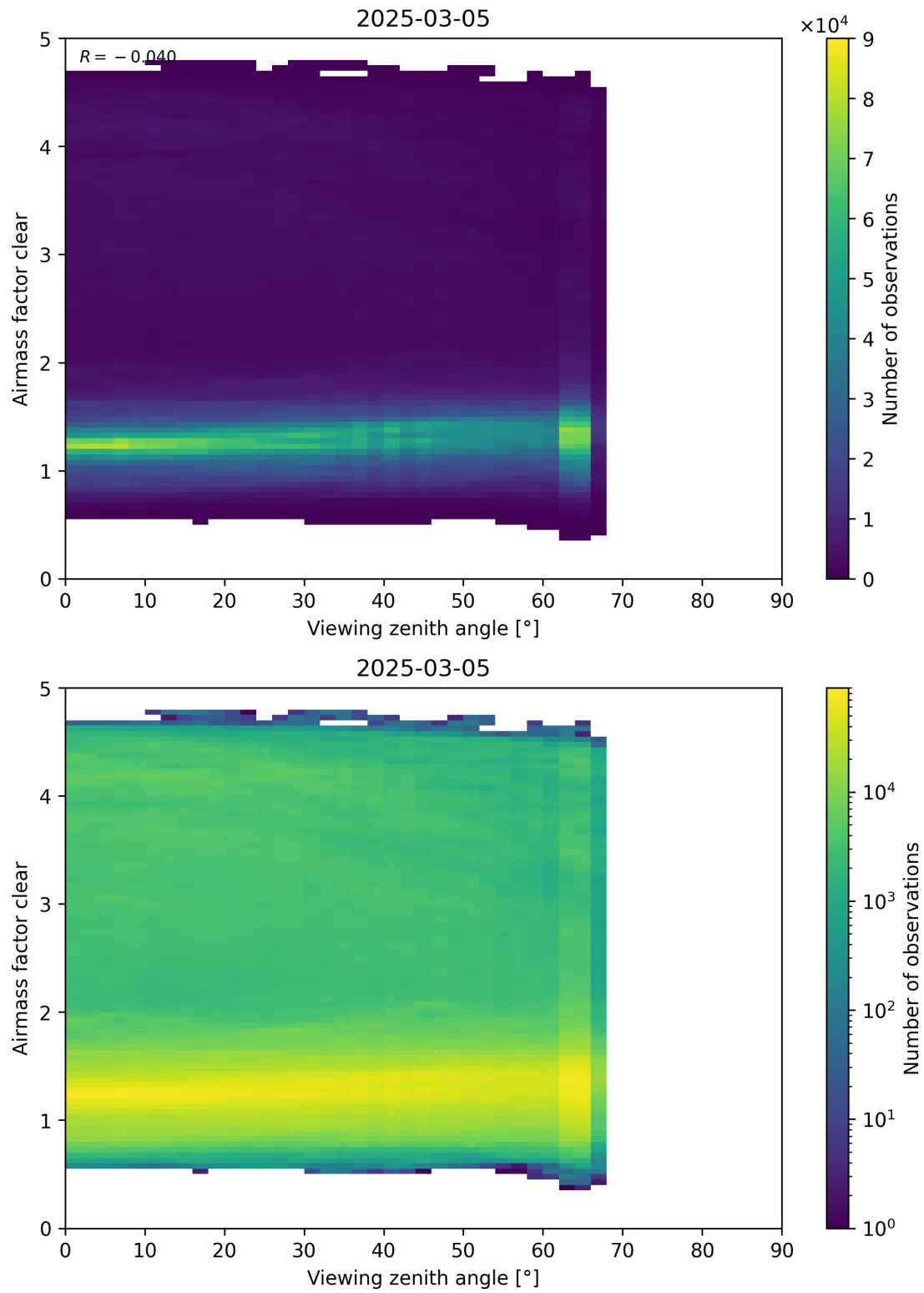
Figure 185: Scatter density plot of “Viewing zenith angle” against “Airmass factor clear” for 2025-03-04 to 2025-03-06.
