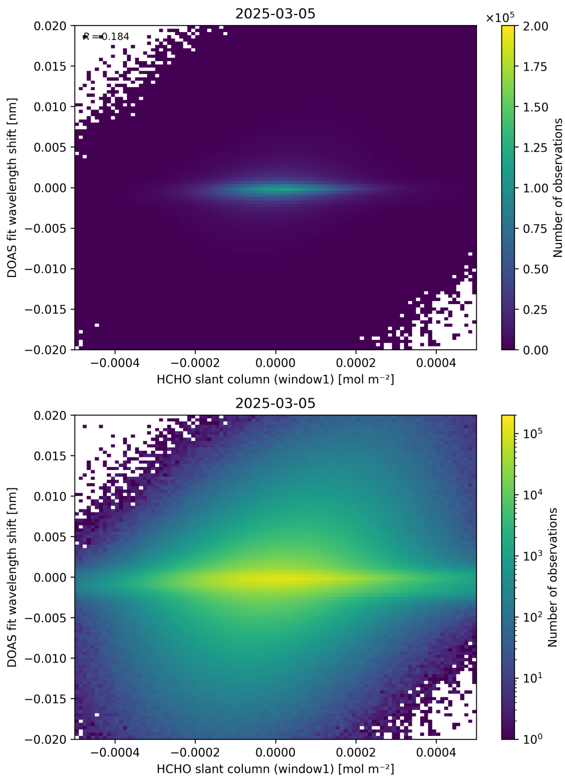
Figure 79: Scatter density plot of “HCHO slant column (window1)” against “DOAS fit wavelength shift” for 2025-03-04 to 2025-03-06.
