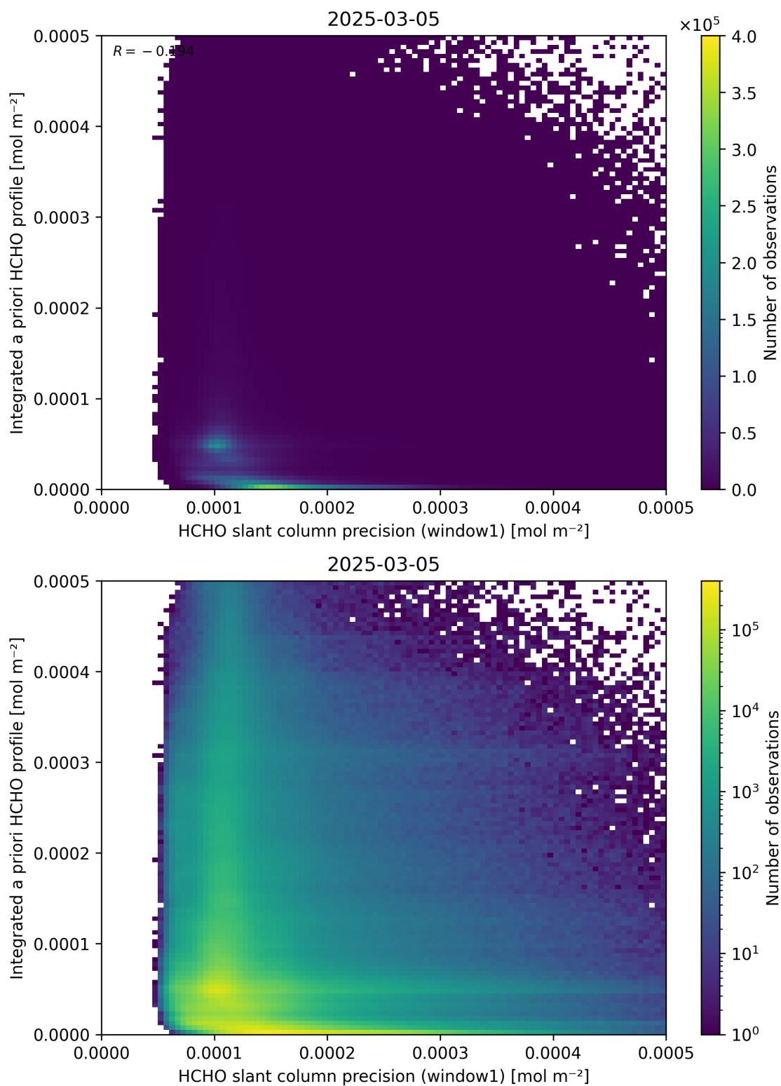
Figure 96: Scatter density plot of “HCHO slant column precision (window1)” against “Integrated a priori HCHO profile” for 2025-03-04 to 2025-03-06.
