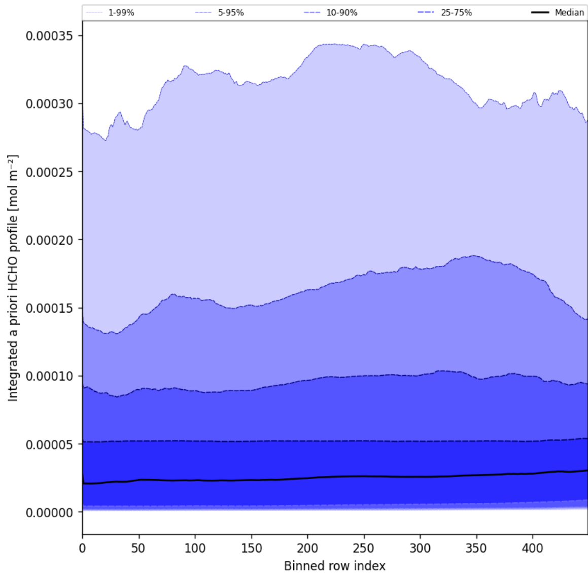
Figure 57: Along track statistics of "Integrated a priori HCHO profile" for 2025-03-04 to 2025-03-06
