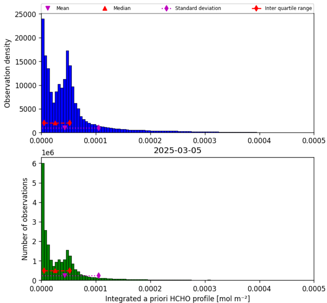
Figure 43: Histogram of “Integrated a priori HCHO profile” for 2025-03-04 to 2025-03-06
