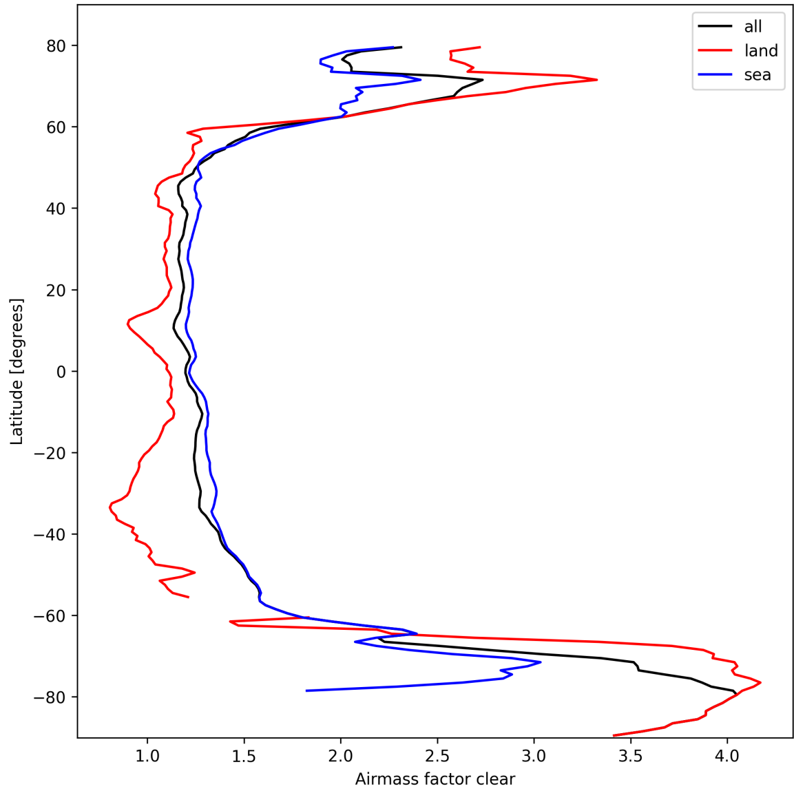
Figure 28: Zonal average of “Airmass factor clear” for 2025-03-04 to 2025-03-06.
