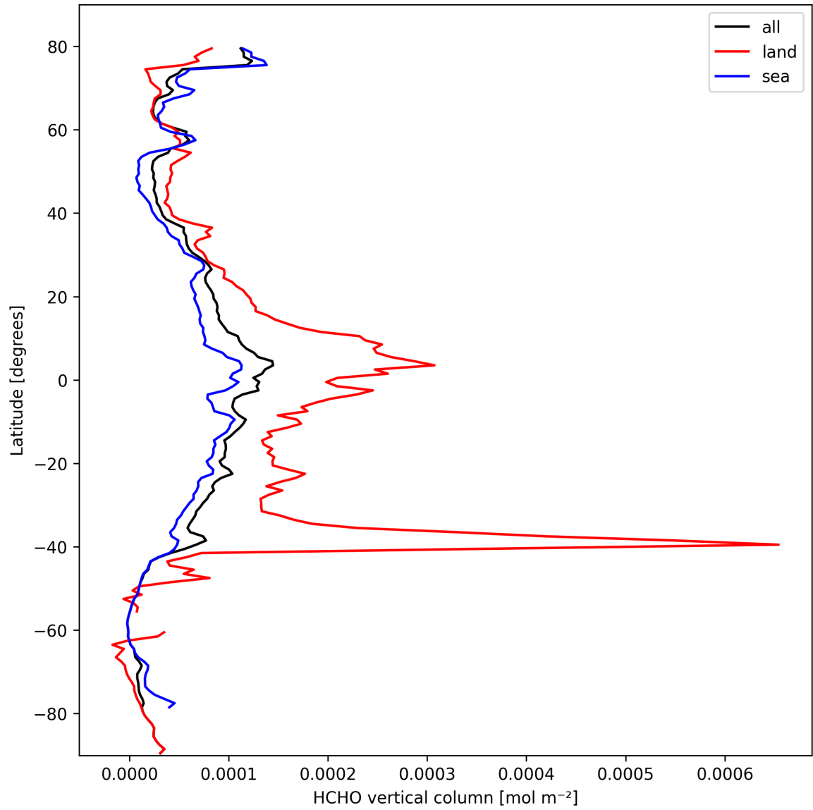
Figure 21: Zonal average of “HCHO vertical column” for 2025-03-04 to 2025-03-06.
