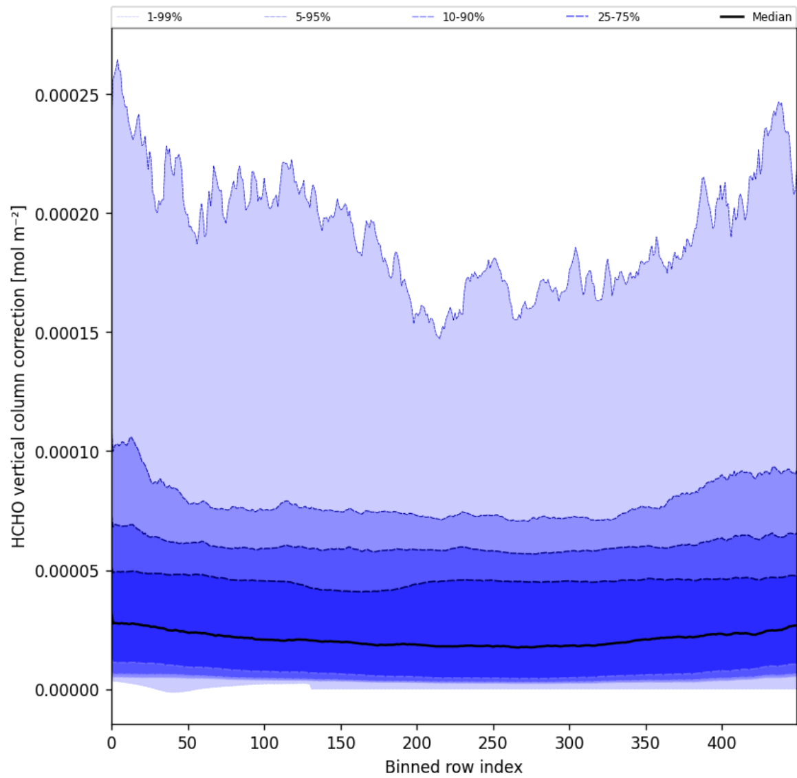
Figure 51: Along track statistics of “HCHO vertical column correction” for 2025-03-04 to 2025-03-06
