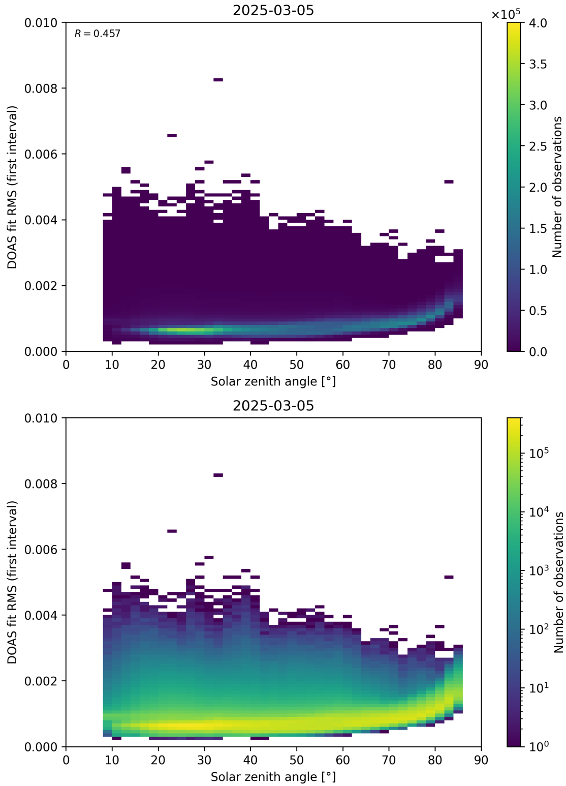
Figure 167: Scatter density plot of “Solar zenith angle” against “DOAS fit RMS (first interval)” for 2025-03-04 to 2025-03-06.
