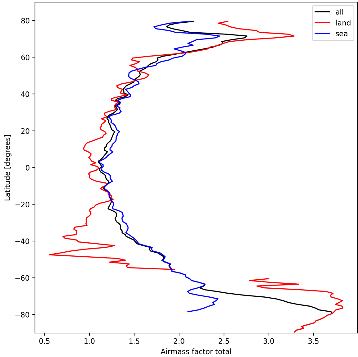
Figure 26: Zonal average of “Airmass factor total” for 2025-03-04 to 2025-03-06.
