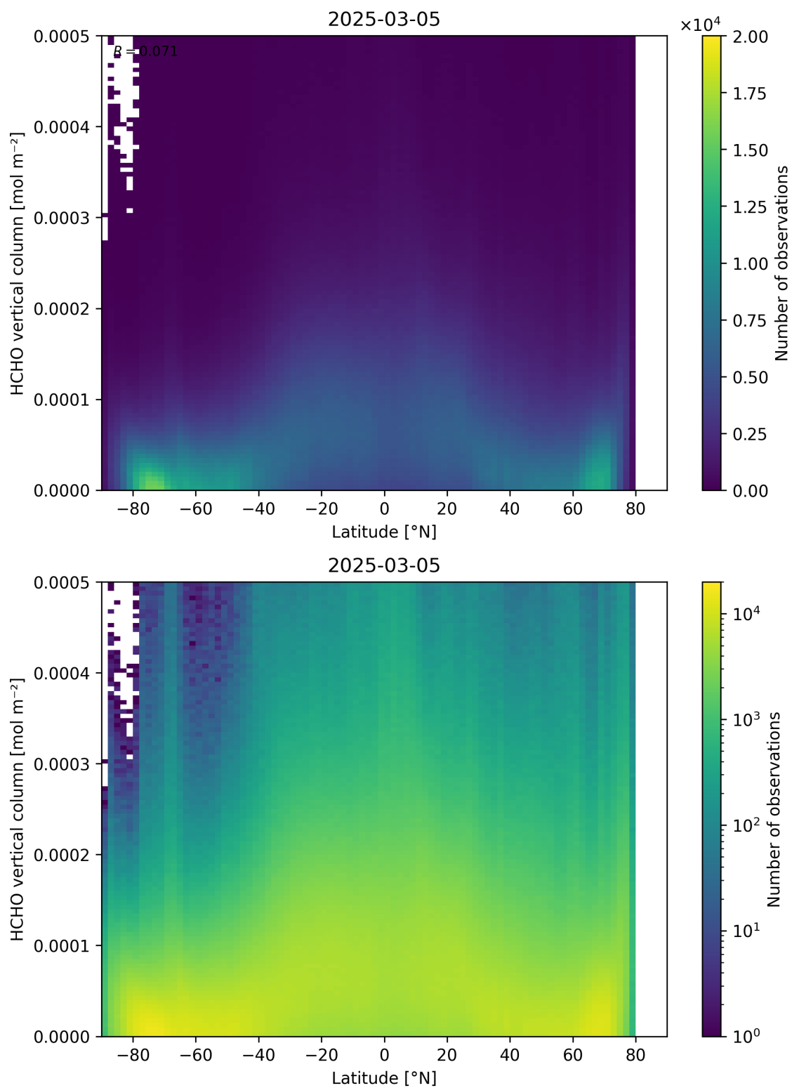
Figure 163: Scatter density plot of “Latitude” against “HCHO vertical column” for 2025-03-04 to 2025-03-06.
