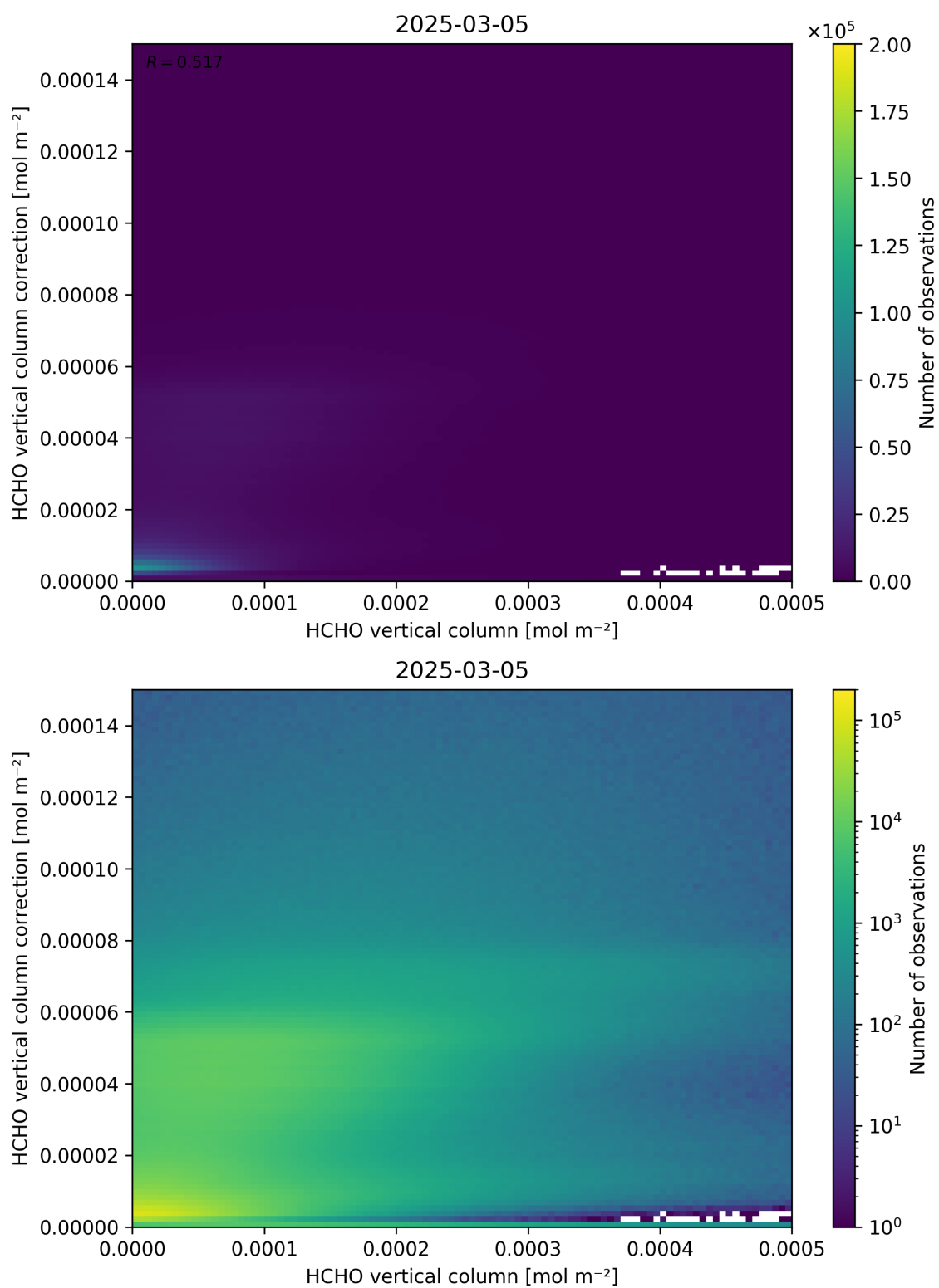
Figure 133: Scatter density plot of “HCHO vertical column” against “HCHO vertical column correction” for 2025-03-04 to 2025-03-06.
