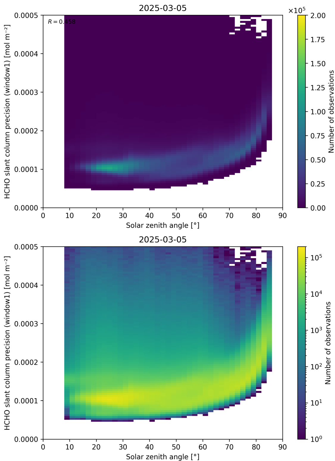
Figure 174: Scatter density plot of “Solar zenith angle” against “HCHO slant column precision (window1)” for 2025-03-04 to 2025-03-06.
