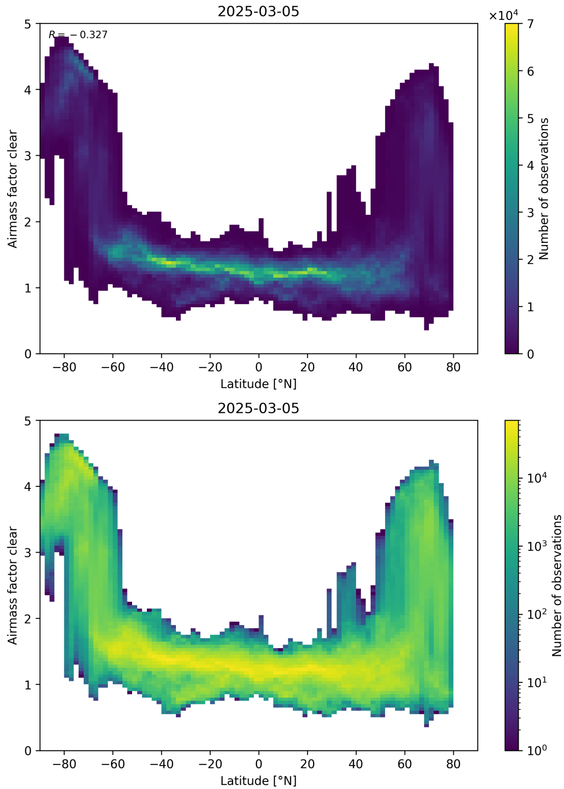
Figure 156: Scatter density plot of “Latitude” against “Airmass factor clear” for 2025-03-04 to 2025-03-06.
