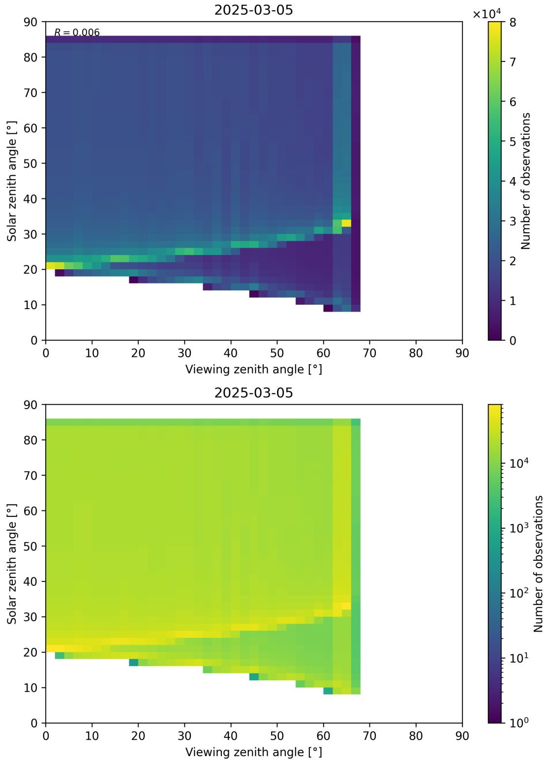
Figure 197: Scatter density plot of “Viewing zenith angle” against “Solar zenith angle” for 2025-03-04 to 2025-03-06.
