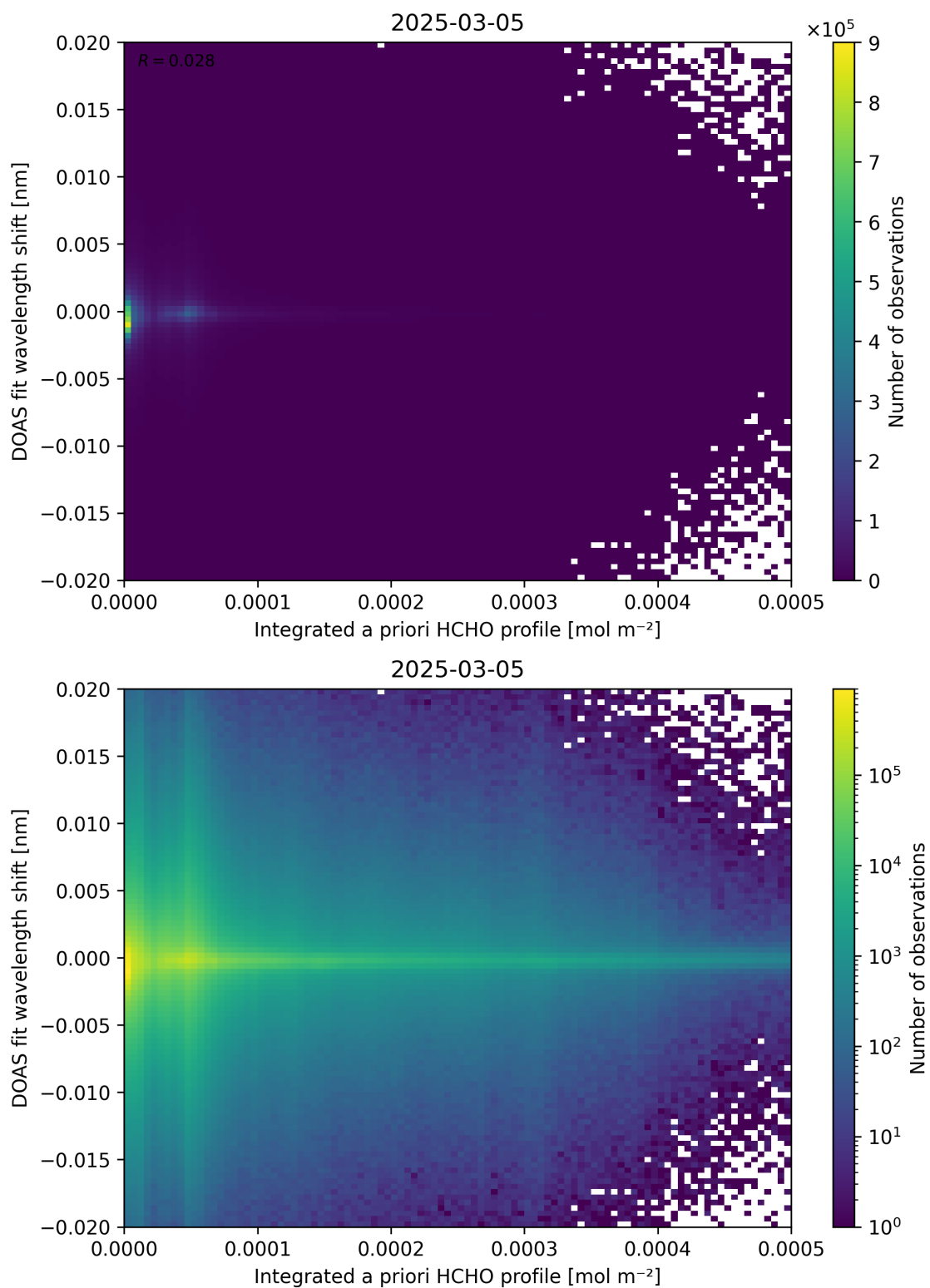
Figure 149: Scatter density plot of “Integrated a priori HCHO profile” against “DOAS fit wavelength shift” for 2025-03-04 to 2025-03-06.
