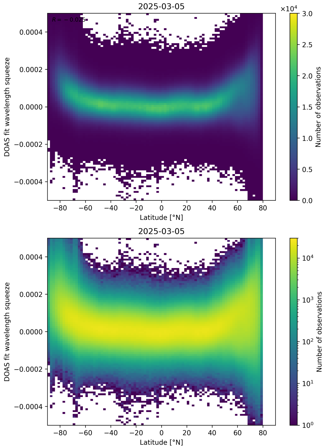
Figure 155: Scatter density plot of “Latitude” against “DOAS fit wavelength squeeze” for 2025-03-04 to 2025-03-06.
