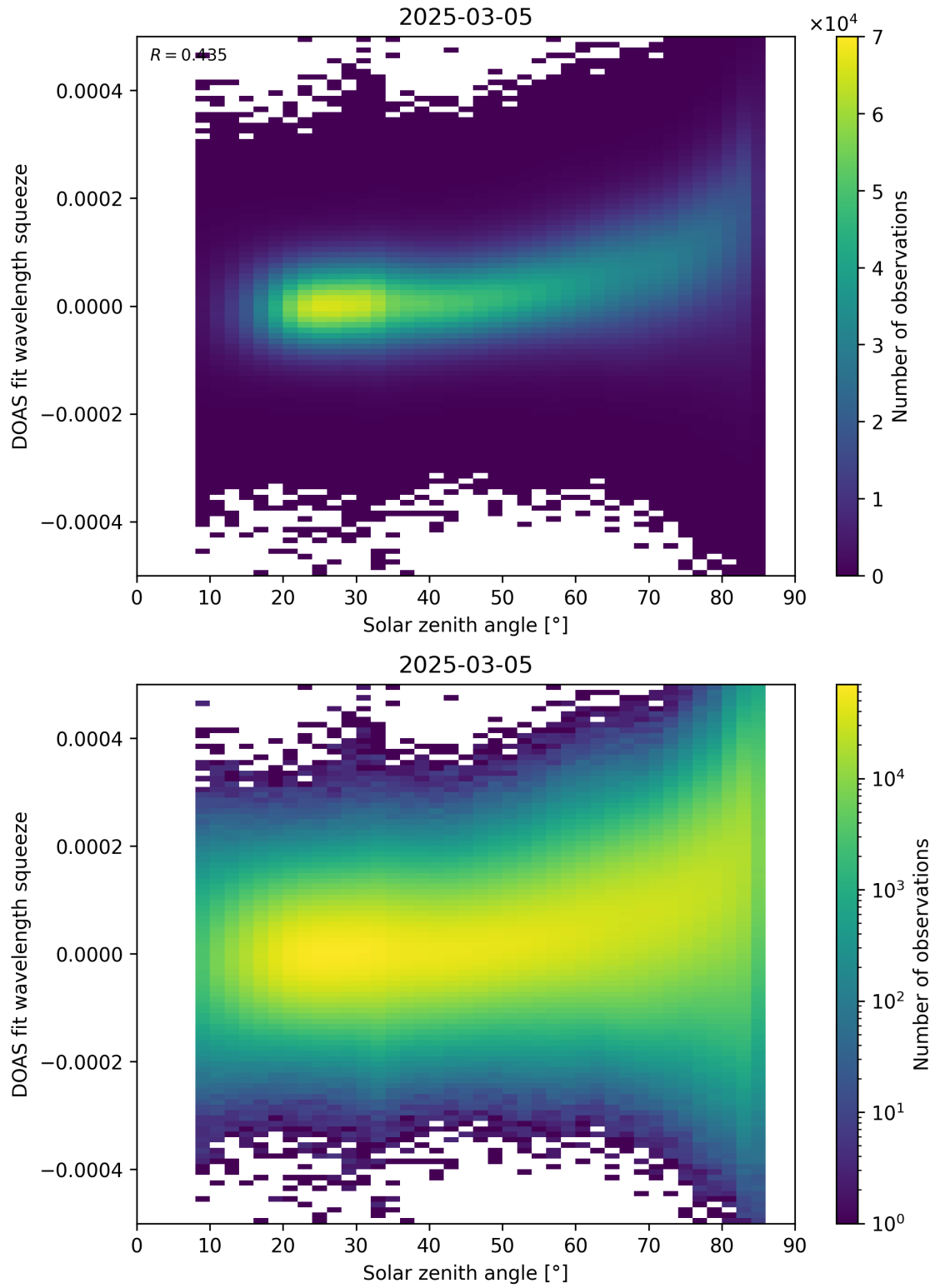
Figure 169: Scatter density plot of “Solar zenith angle” against “DOAS fit wavelength squeeze” for 2025-03-04 to 2025-03-06.
