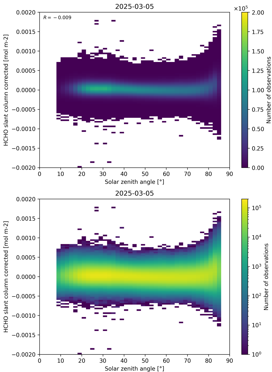
Figure 171: Scatter density plot of “Solar zenith angle” against “HCHO slant column corrected” for 2025-03-04 to 2025-03-06.
