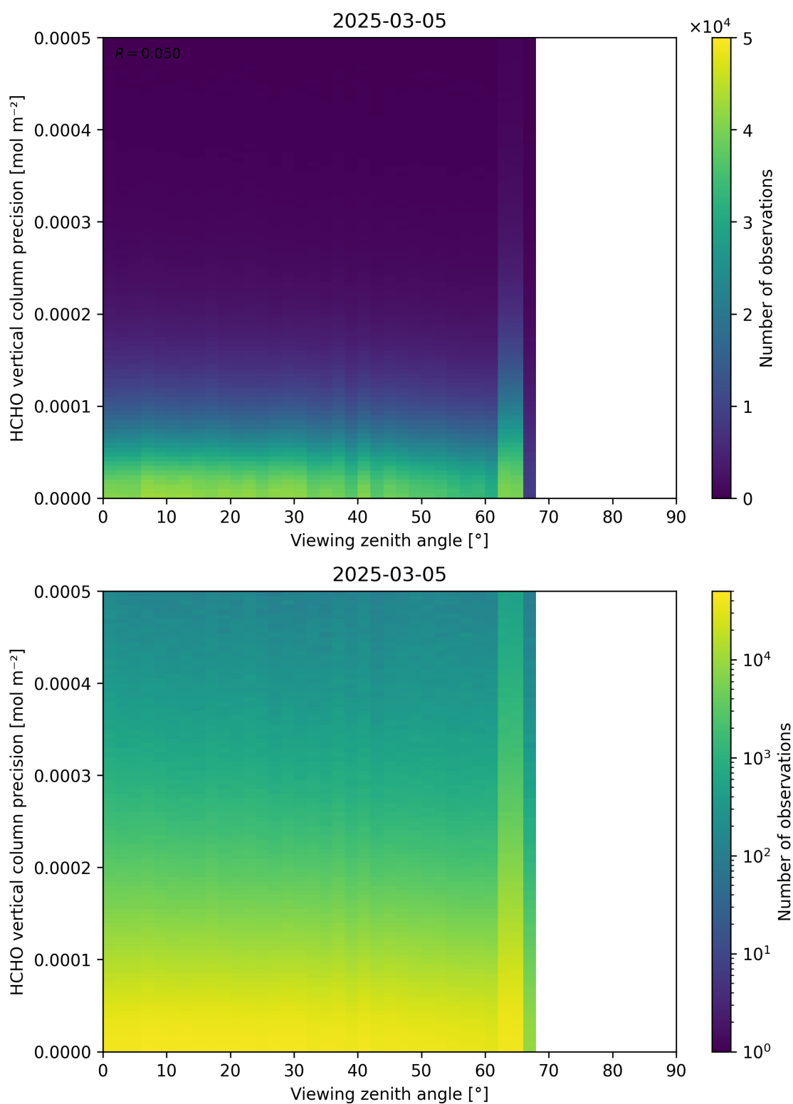
Figure 194: Scatter density plot of “Viewing zenith angle” against “HCHO vertical column precision” for 2025-03-04 to 2025-03-06.
