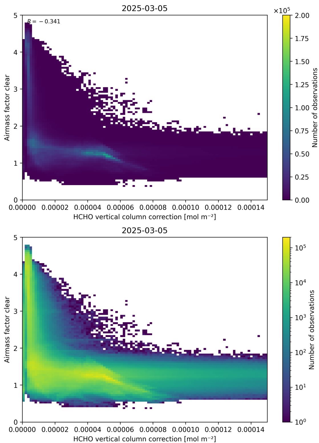
Figure 115: Scatter density plot of “HCHO vertical column correction” against “Airmass factor clear” for 2025-03-04 to 2025-03-06.
