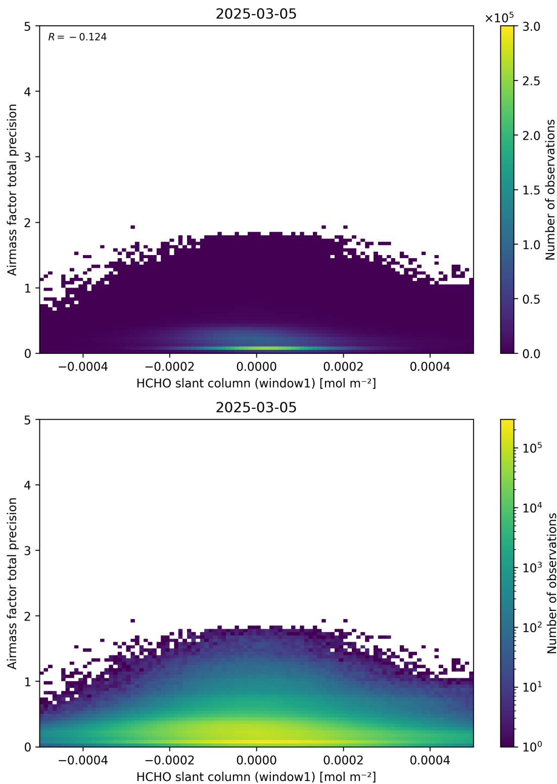
Figure 86: Scatter density plot of “HCHO slant column (window1)” against “Airmass factor total precision” for 2025-03-04 to 2025-03-06.
