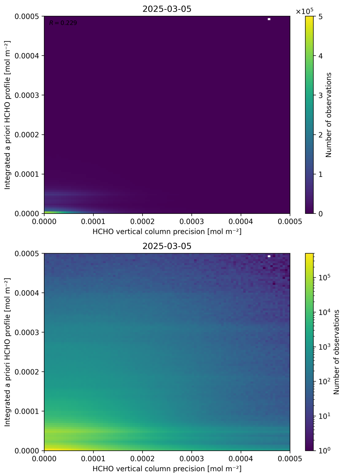
Figure 147: Scatter density plot of “HCHO vertical column precision” against “Integrated a priori HCHO profile” for 2025-03-04 to 2025-03-06.
