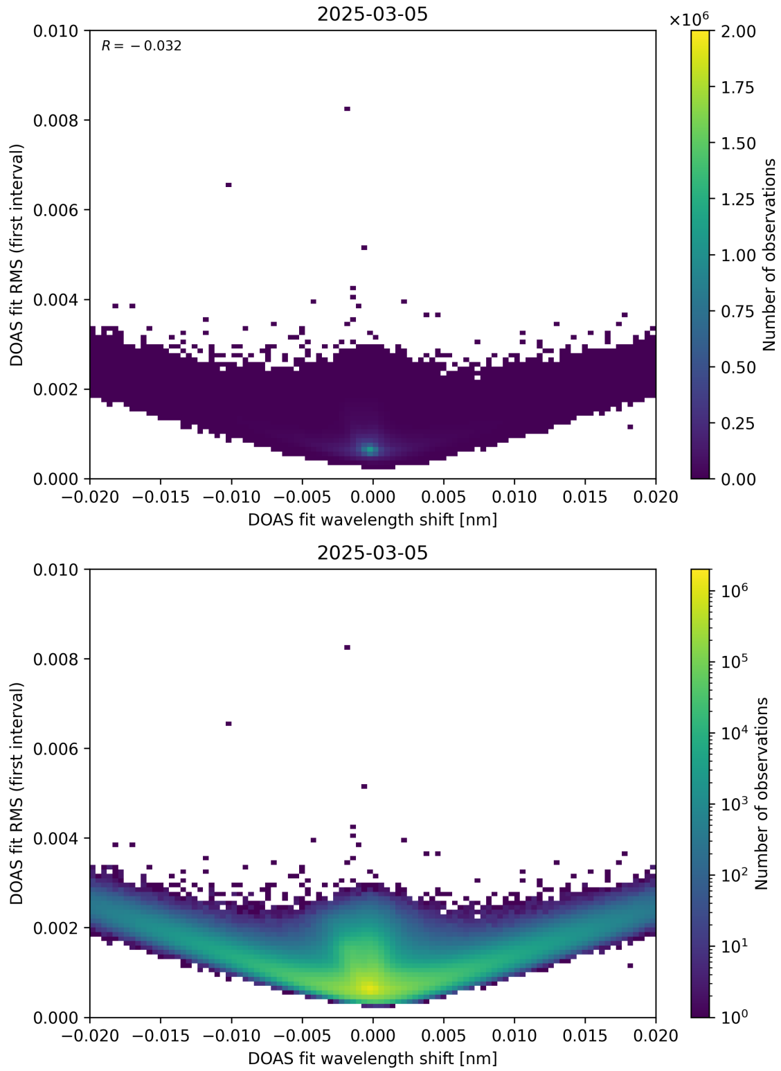
Figure 64: Scatter density plot of “DOAS fit wavelength shift” against “DOAS fit RMS (first interval)” for 2025-03-04 to 2025-03-06.
