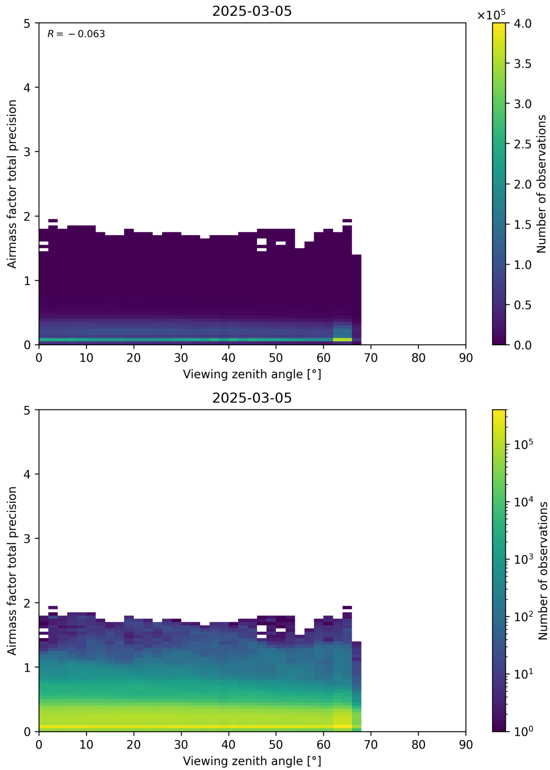
Figure 191: Scatter density plot of “Viewing zenith angle” against “Airmass factor total precision” for 2025-03-04 to 2025-03-06.
