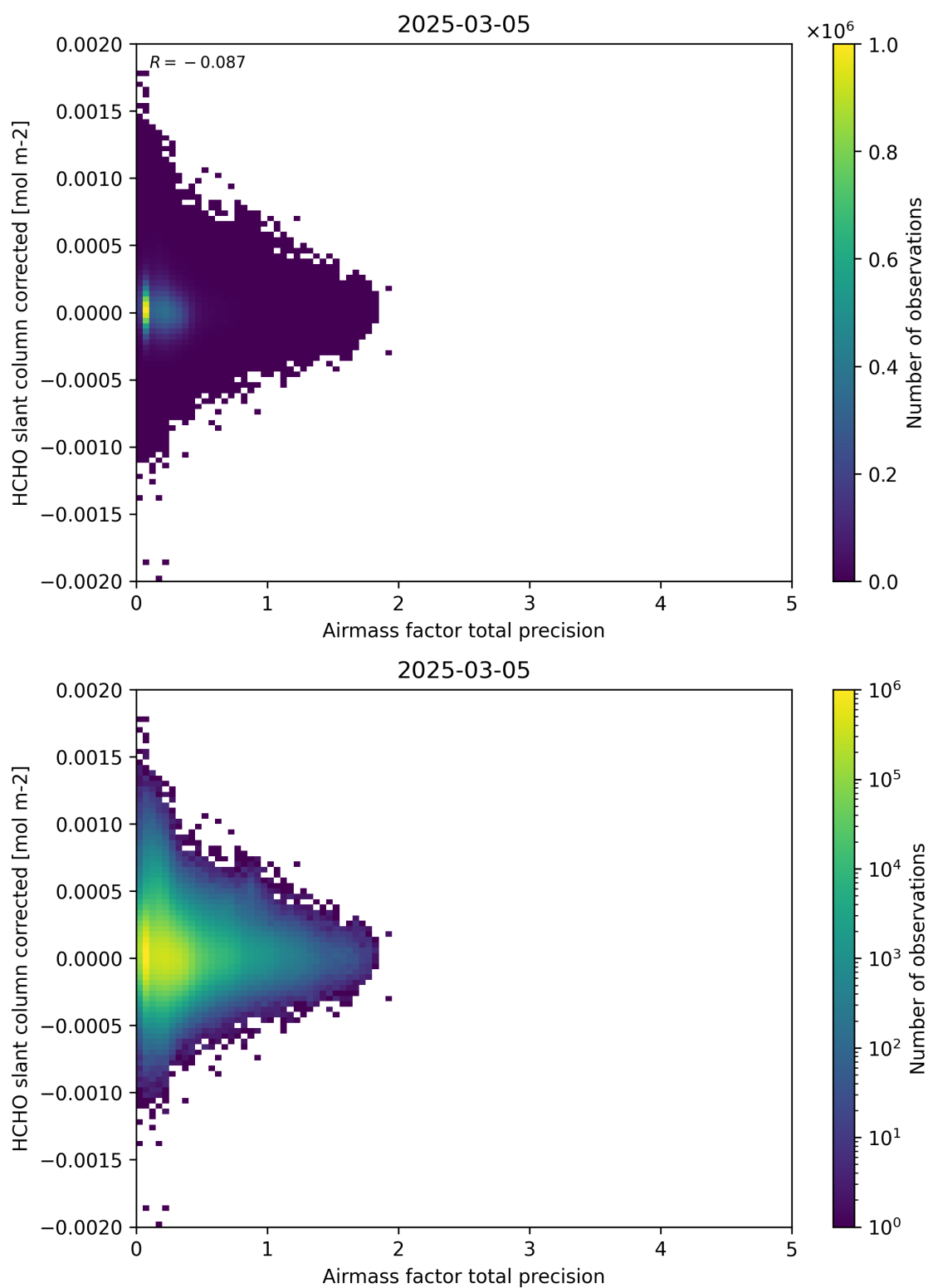
Figure 109: Scatter density plot of “Airmass factor total precision” against “HCHO slant column corrected” for 2025-03-04 to 2025-03-06.
