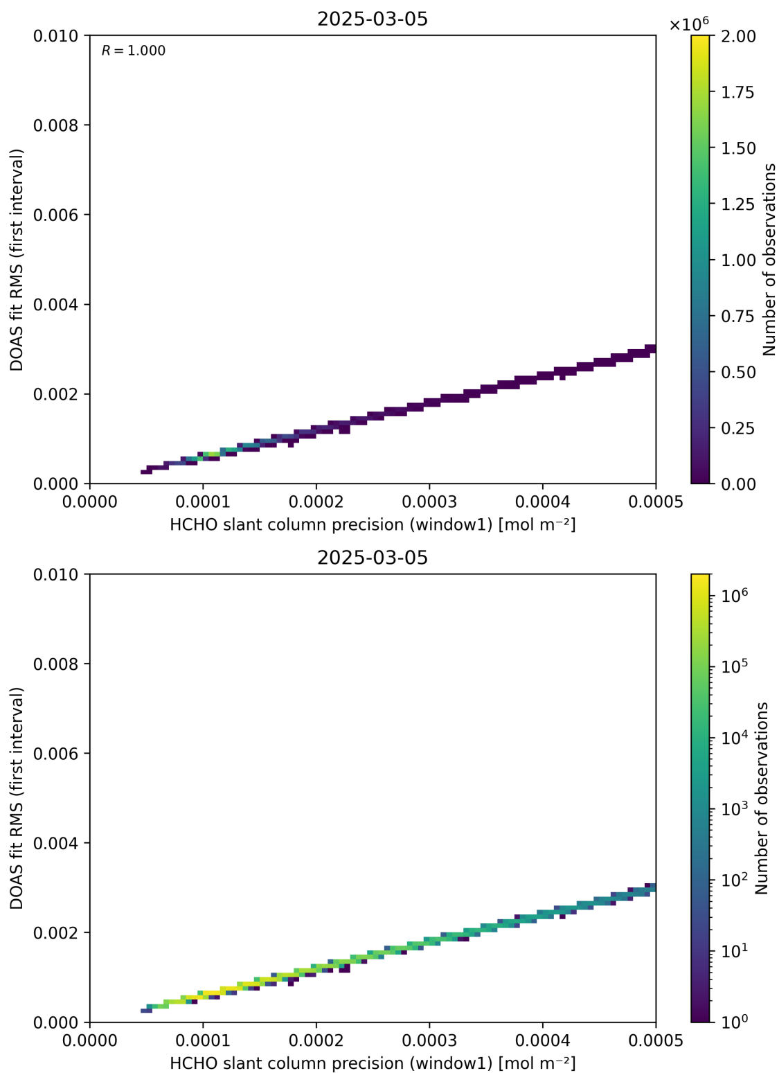
Figure 88: Scatter density plot of “HCHO slant column precision (window1)” against “DOAS fit RMS (first interval)” for 2025-03-04 to 2025-03-06.
