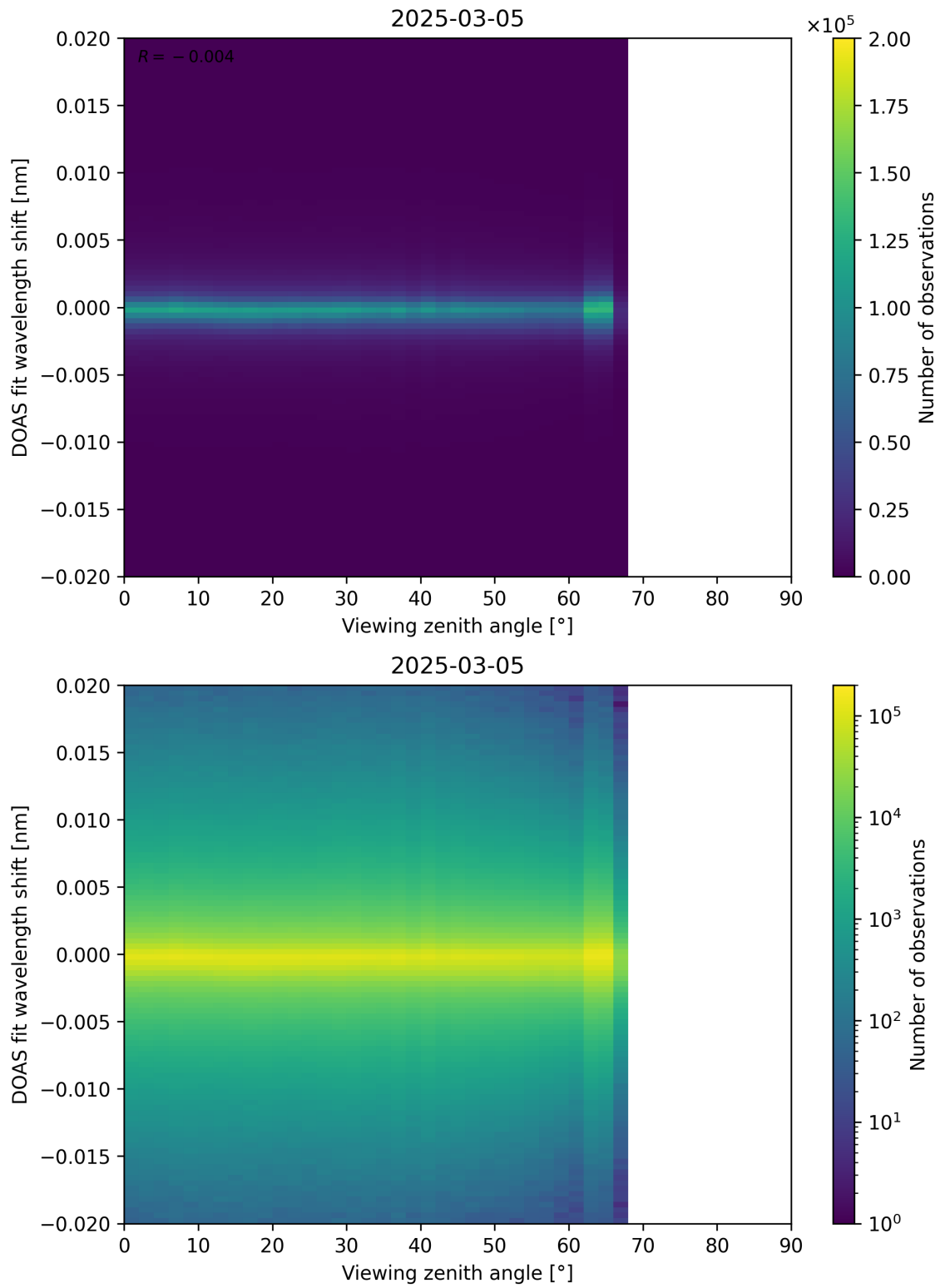
Figure 183: Scatter density plot of “Viewing zenith angle” against “DOAS fit wavelength shift” for 2025-03-04 to 2025-03-06.
