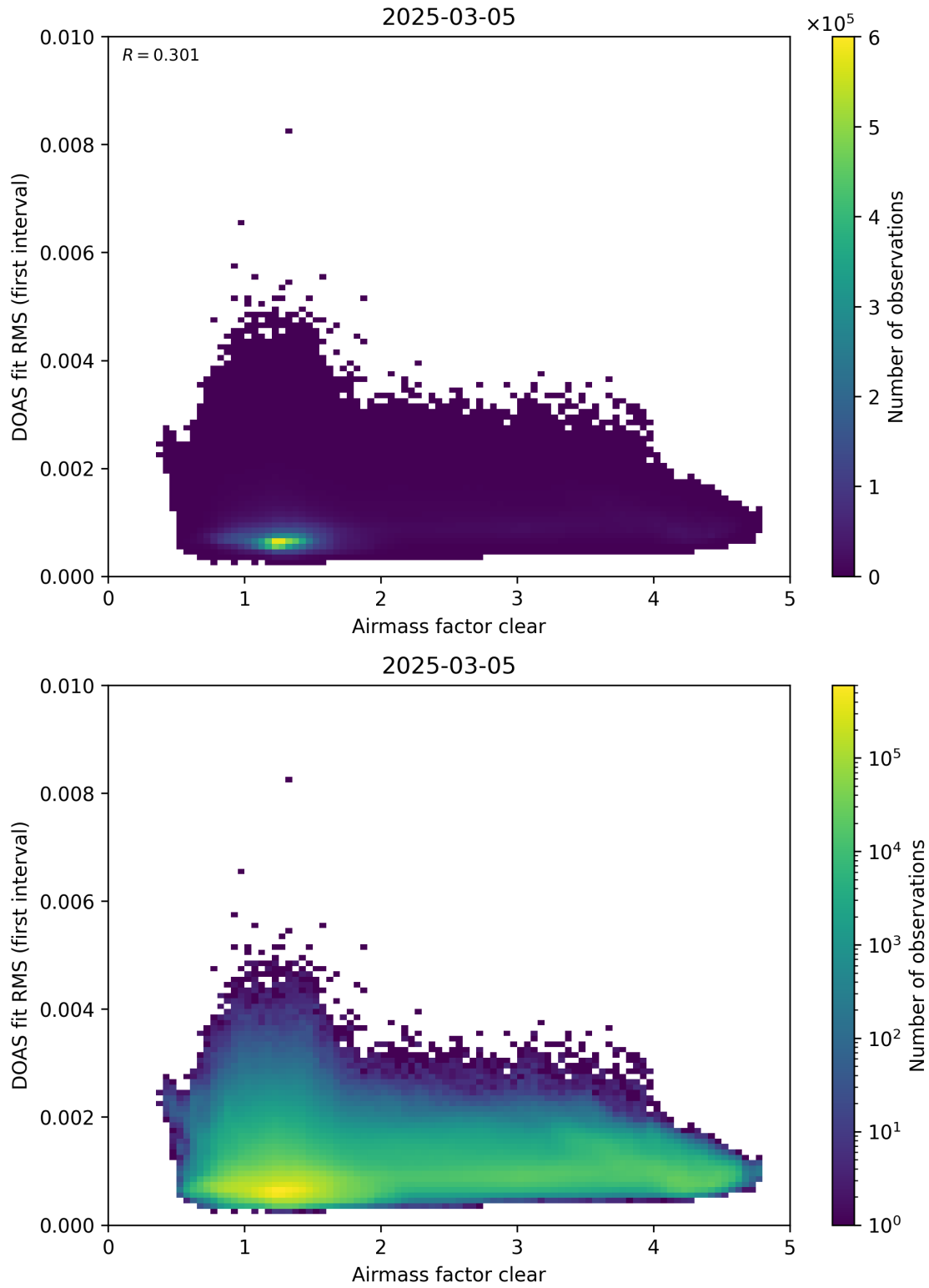
Figure 71: Scatter density plot of “Airmass factor clear” against “DOAS fit RMS (first interval)” for 2025-03-04 to 2025-03-06.
