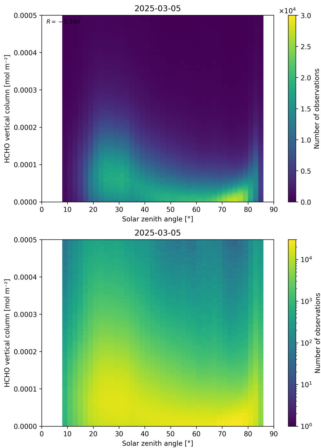
Figure 177: Scatter density plot of “Solar zenith angle” against “HCHO vertical column” for 2025-03-04 to 2025-03-06.
