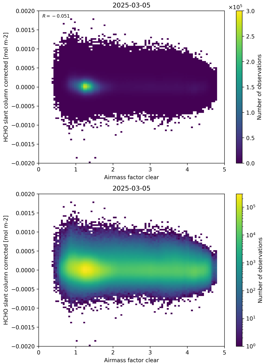
Figure 74: Scatter density plot of “Airmass factor clear” against “HCHO slant column corrected” for 2025-03-04 to 2025-03-06.
