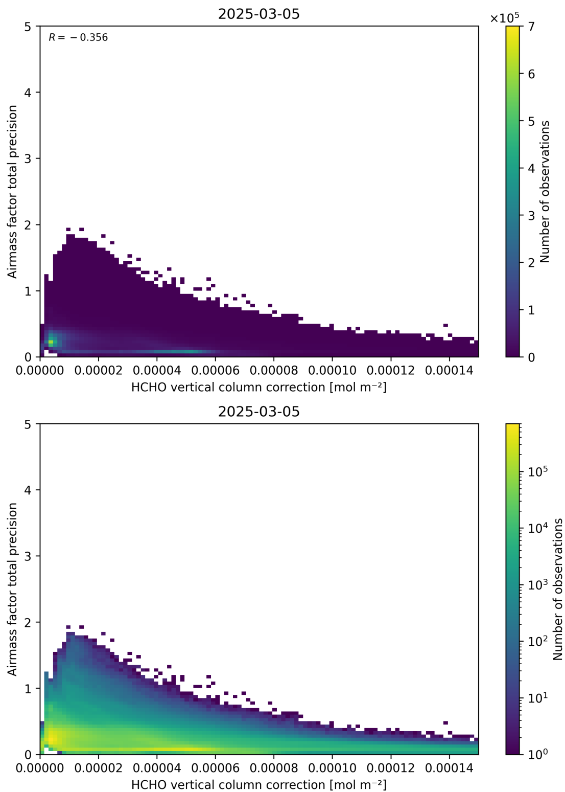
Figure 121: Scatter density plot of “HCHO vertical column correction” against “Airmass factor total precision” for 2025-03-04 to 2025-03-06.
