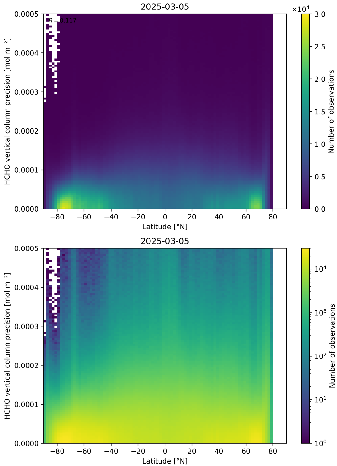
Figure 165: Scatter density plot of “Latitude” against “HCHO vertical column precision” for 2025-03-04 to 2025-03-06.
