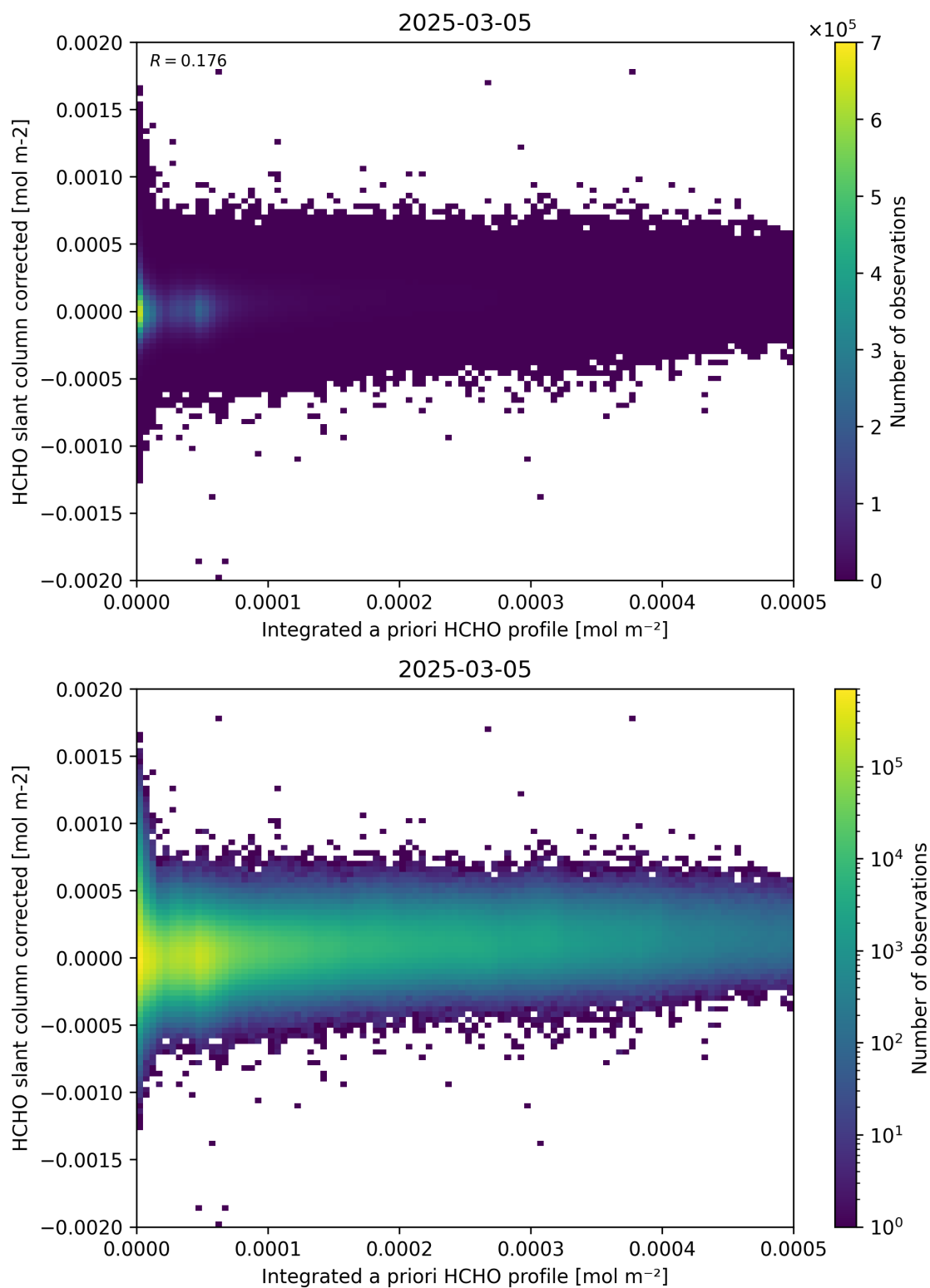
Figure 151: Scatter density plot of “Integrated a priori HCHO profile” against “HCHO slant column corrected” for 2025-03-04 to 2025-03-06.
