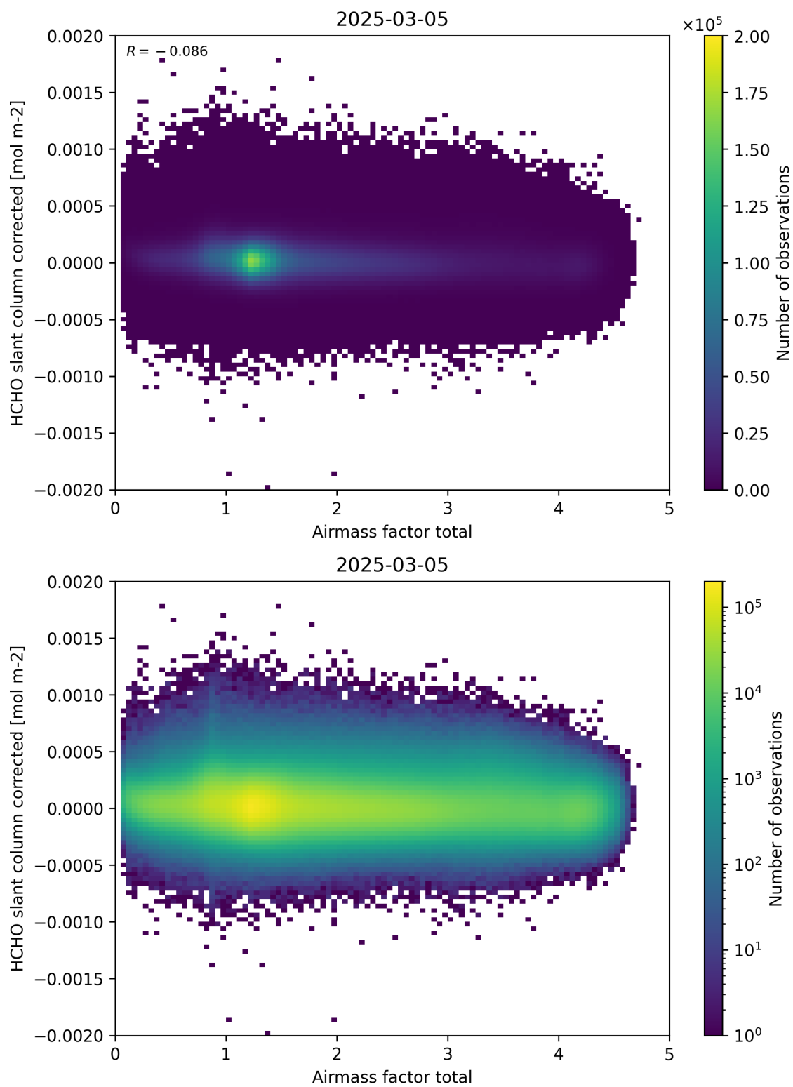
Figure 101: Scatter density plot of “Airmass factor total” against “HCHO slant column corrected” for 2025-03-04 to 2025-03-06.
