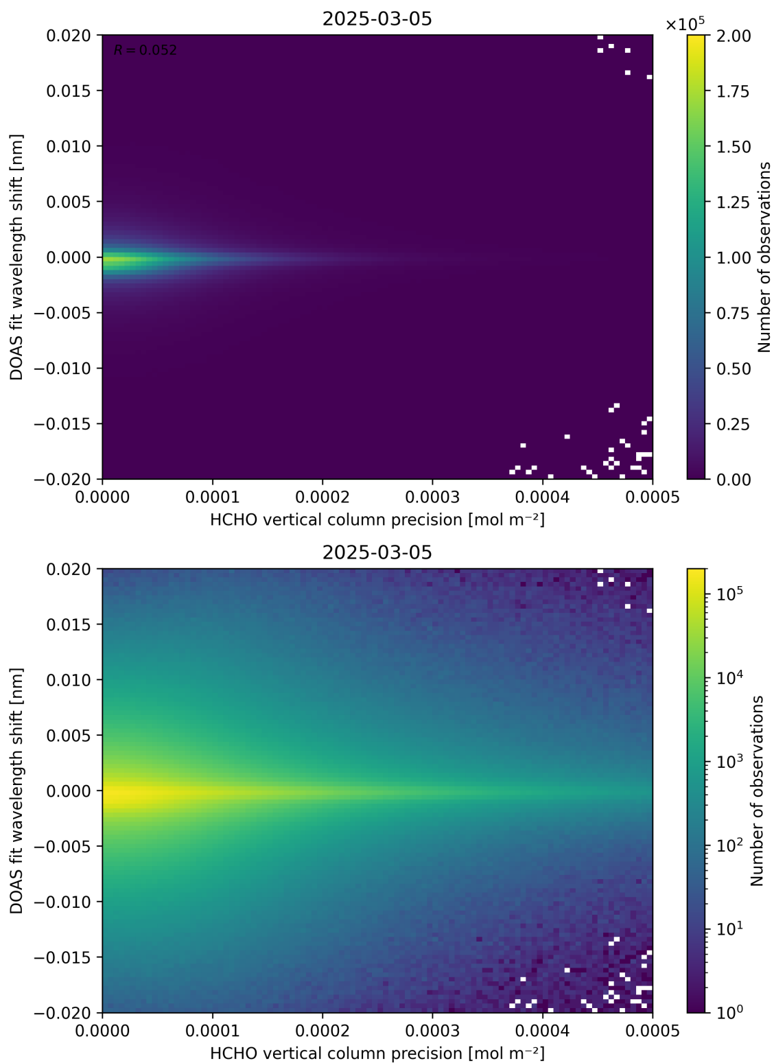
Figure 137: Scatter density plot of “HCHO vertical column precision” against “DOAS fit wavelength shift” for 2025-03-04 to 2025-03-06.
