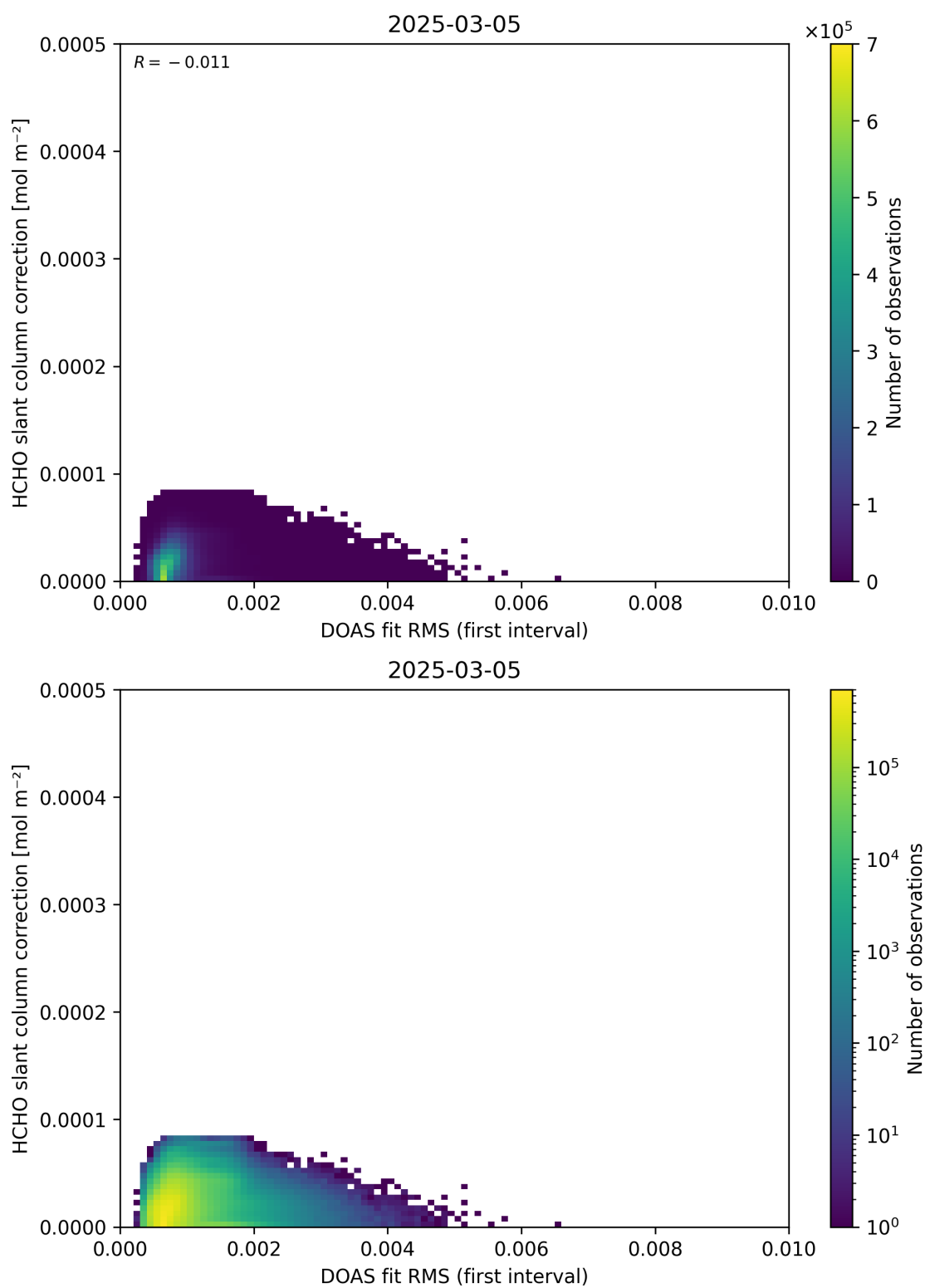
Figure 63: Scatter density plot of “DOAS fit RMS (first interval)” against “HCHO slant column correction” for 2025-03-04 to 2025-03-06.
