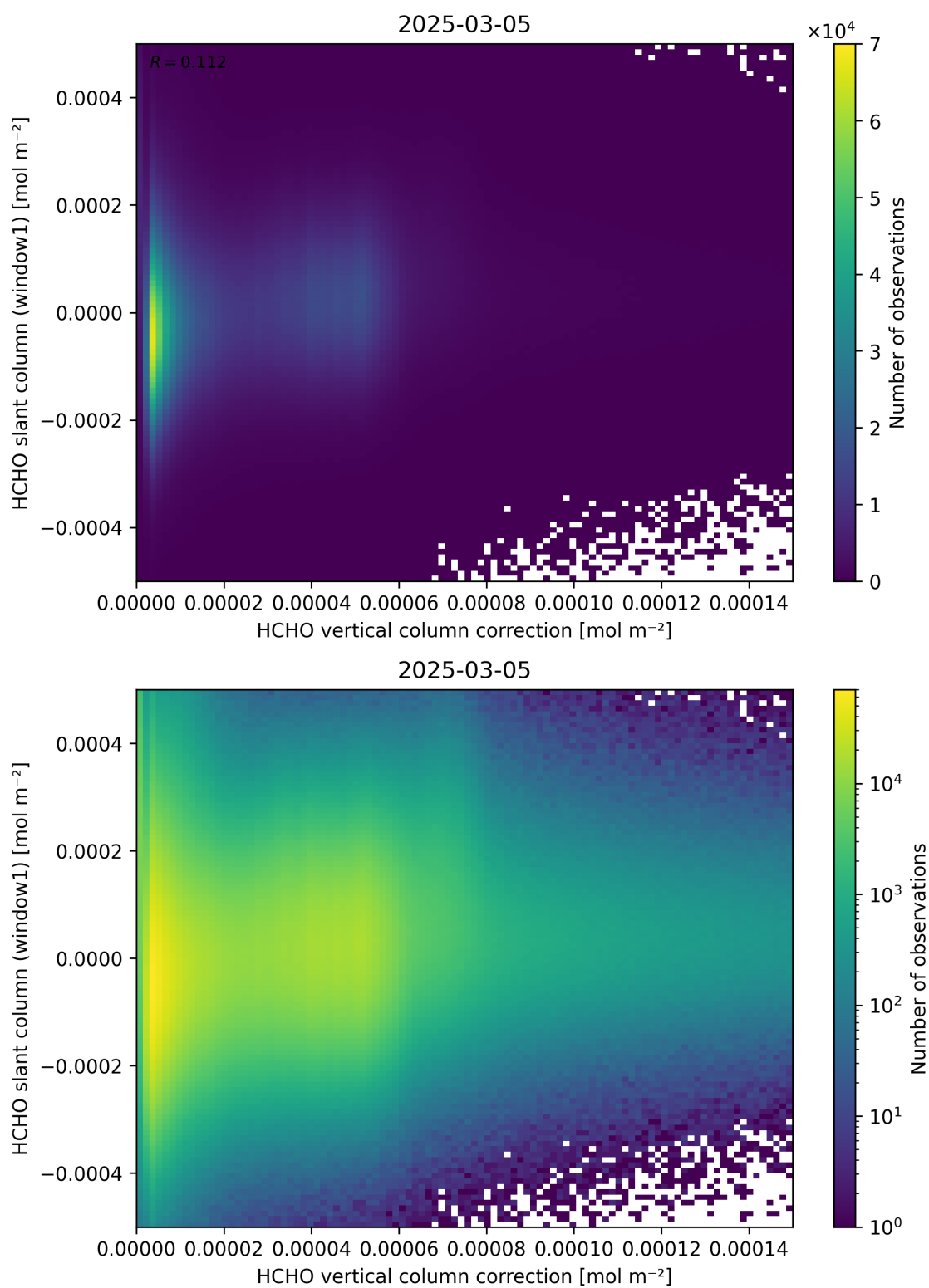
Figure 118: Scatter density plot of “HCHO vertical column correction” against “HCHO slant column (window1)” for 2025-03-04 to 2025-03-06.
