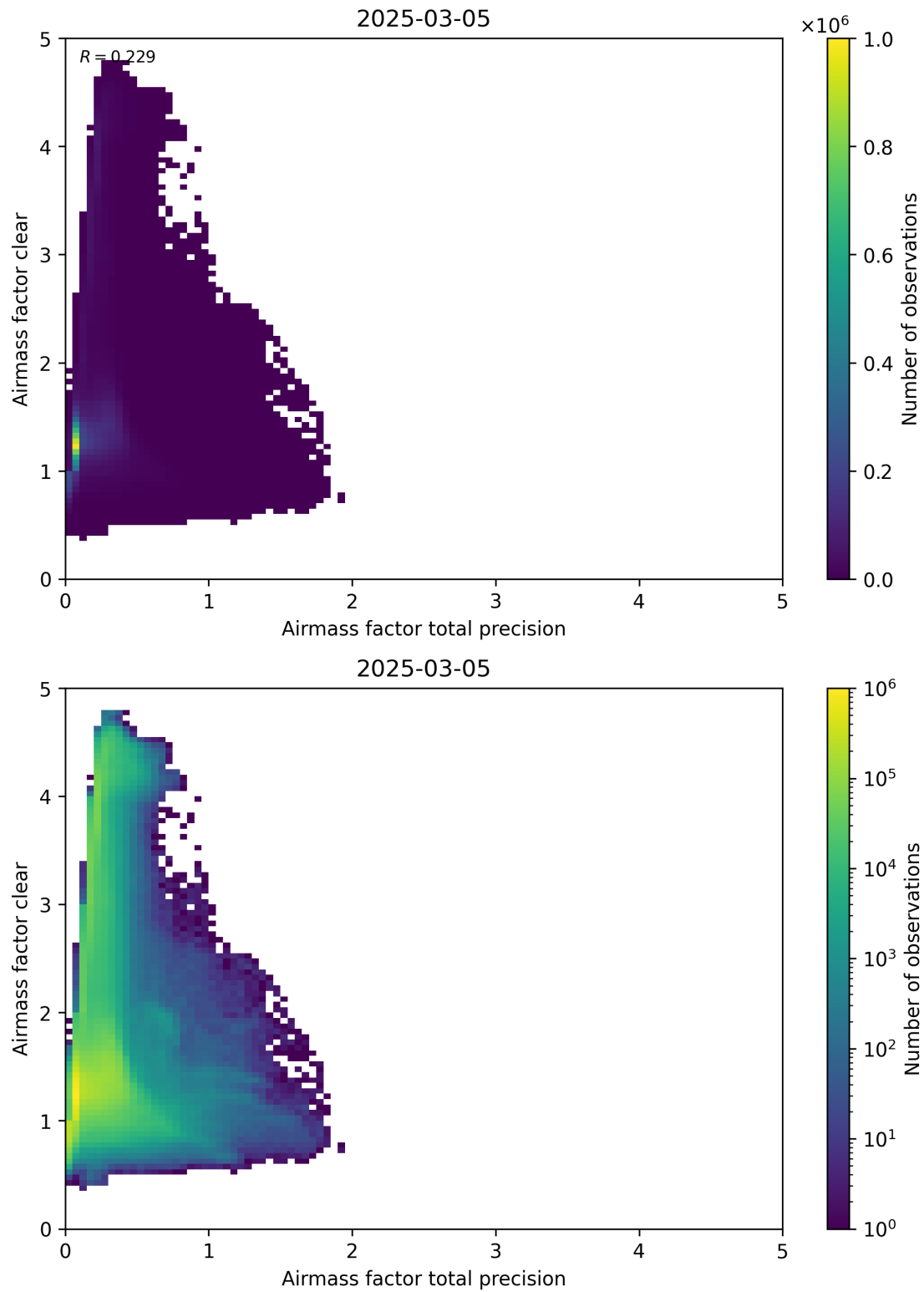
Figure 108: Scatter density plot of “Airmass factor total precision” against “Airmass factor clear” for 2025-03-04 to 2025-03-06.
