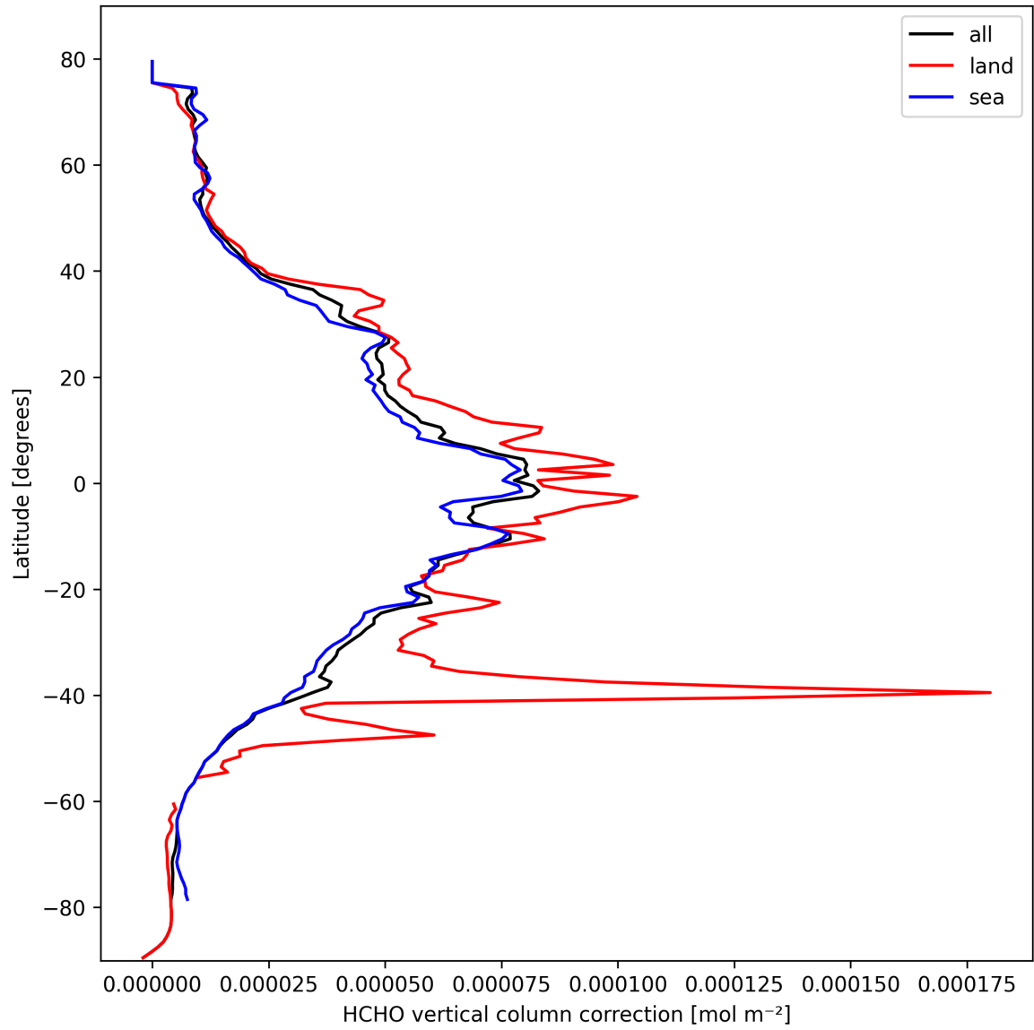
Figure 23: Zonal average of “HCHO vertical column correction” for 2025-03-04 to 2025-03-06.
