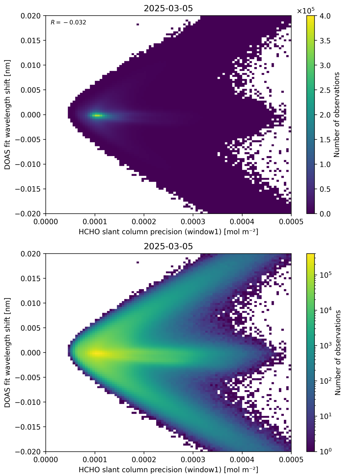
Figure 89: Scatter density plot of “HCHO slant column precision (window1)” against “DOAS fit wavelength shift” for 2025-03-04 to 2025-03-06.
