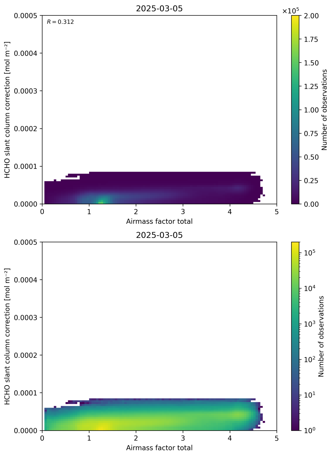
Figure 102: Scatter density plot of “Airmass factor total” against “HCHO slant column correction” for 2025-03-04 to 2025-03-06.
