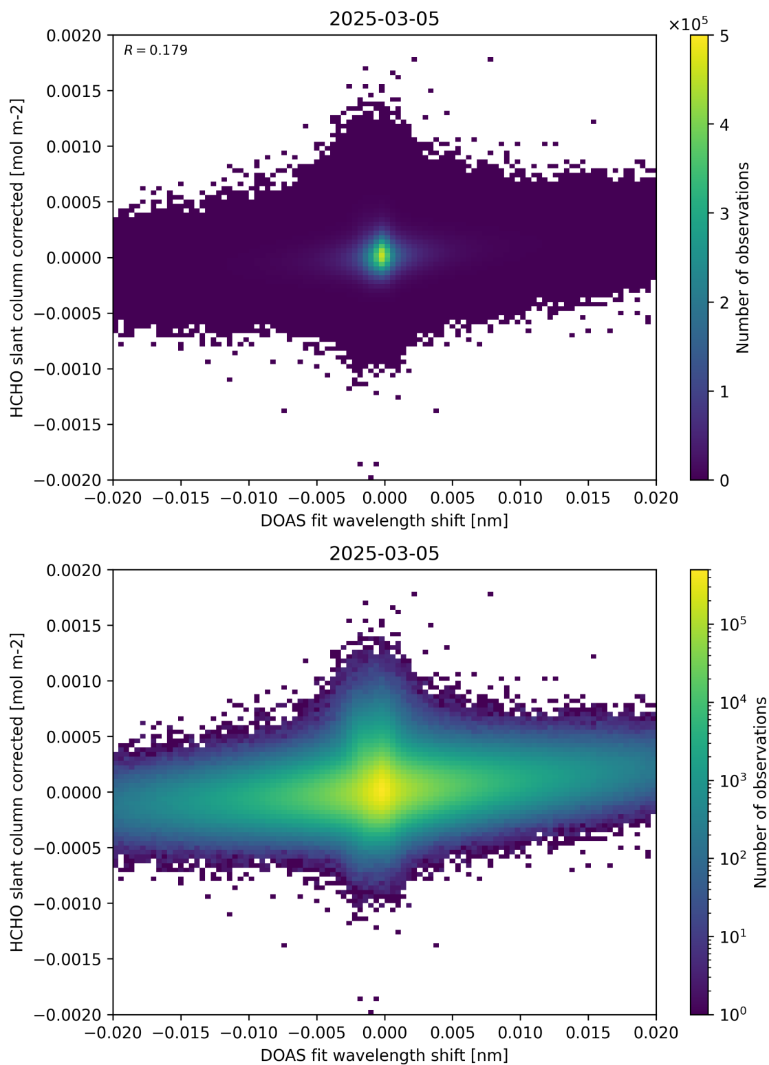
Figure 66: Scatter density plot of “DOAS fit wavelength shift” against “HCHO slant column corrected” for 2025-03-04 to 2025-03-06.
