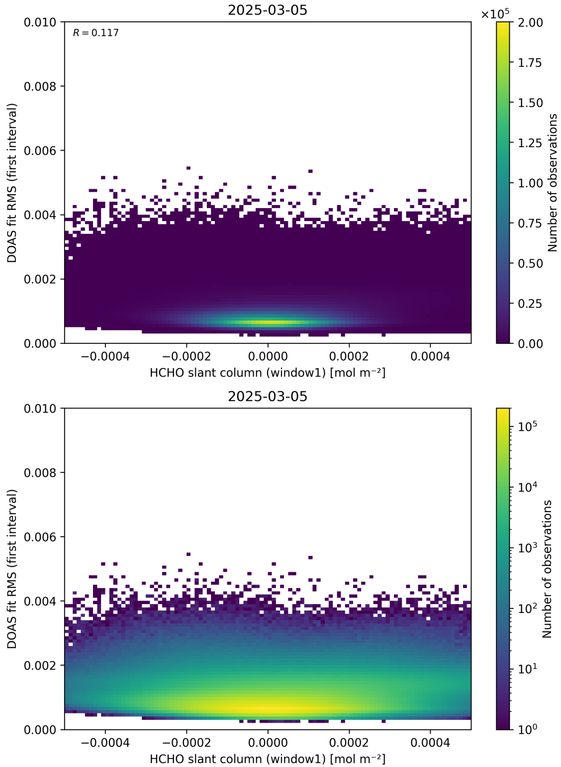
Figure 78: Scatter density plot of “HCHO slant column (window1)” against “DOAS fit RMS (first interval)” for 2025-03-04 to 2025-03-06.
