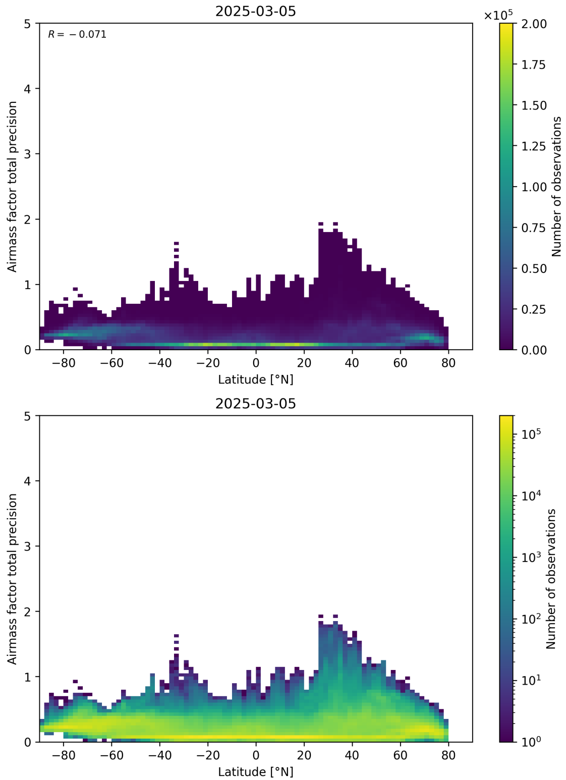
Figure 162: Scatter density plot of “Latitude” against “Airmass factor total precision” for 2025-03-04 to 2025-03-06.
