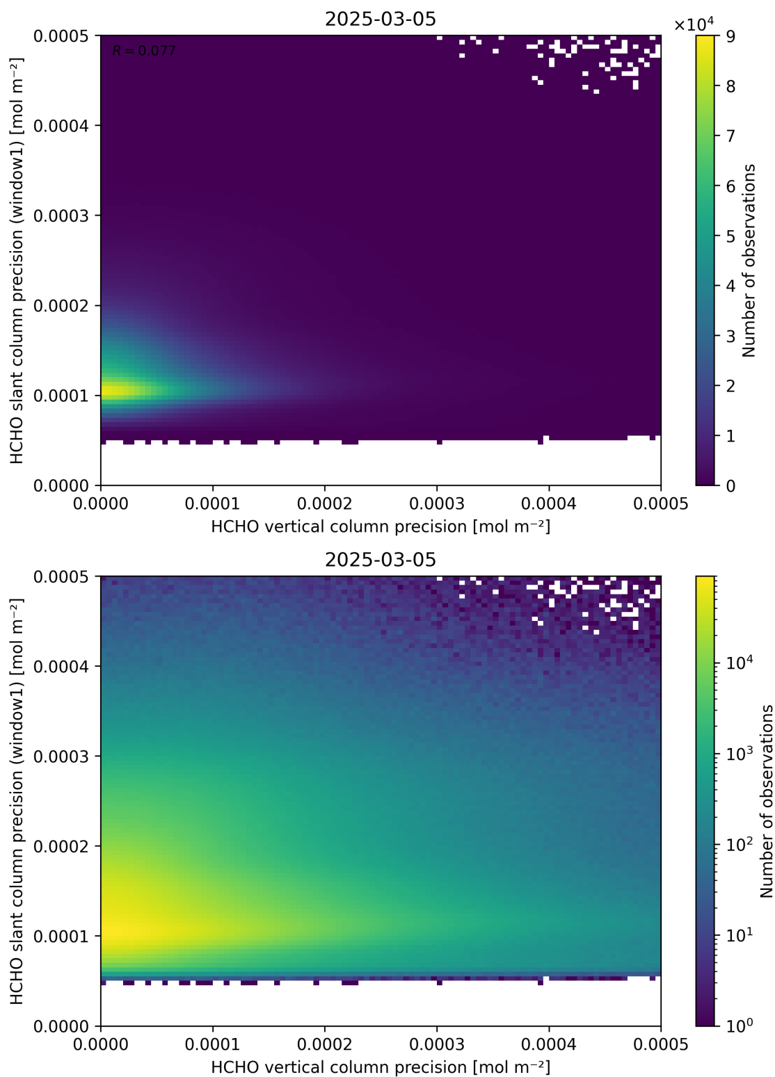
Figure 143: Scatter density plot of “HCHO vertical column precision” against “HCHO slant column precision (window1)” for 2025-03-04 to 2025-03-06.
