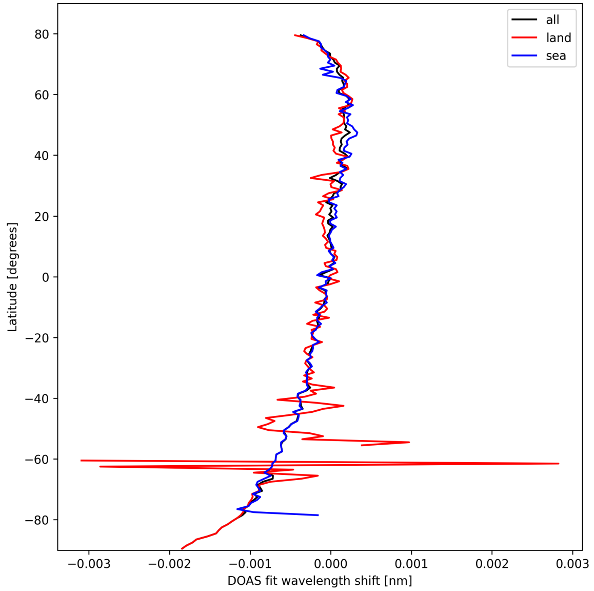
Figure 30: Zonal average of “DOAS fit wavelength shift” for 2025-03-04 to 2025-03-06.
