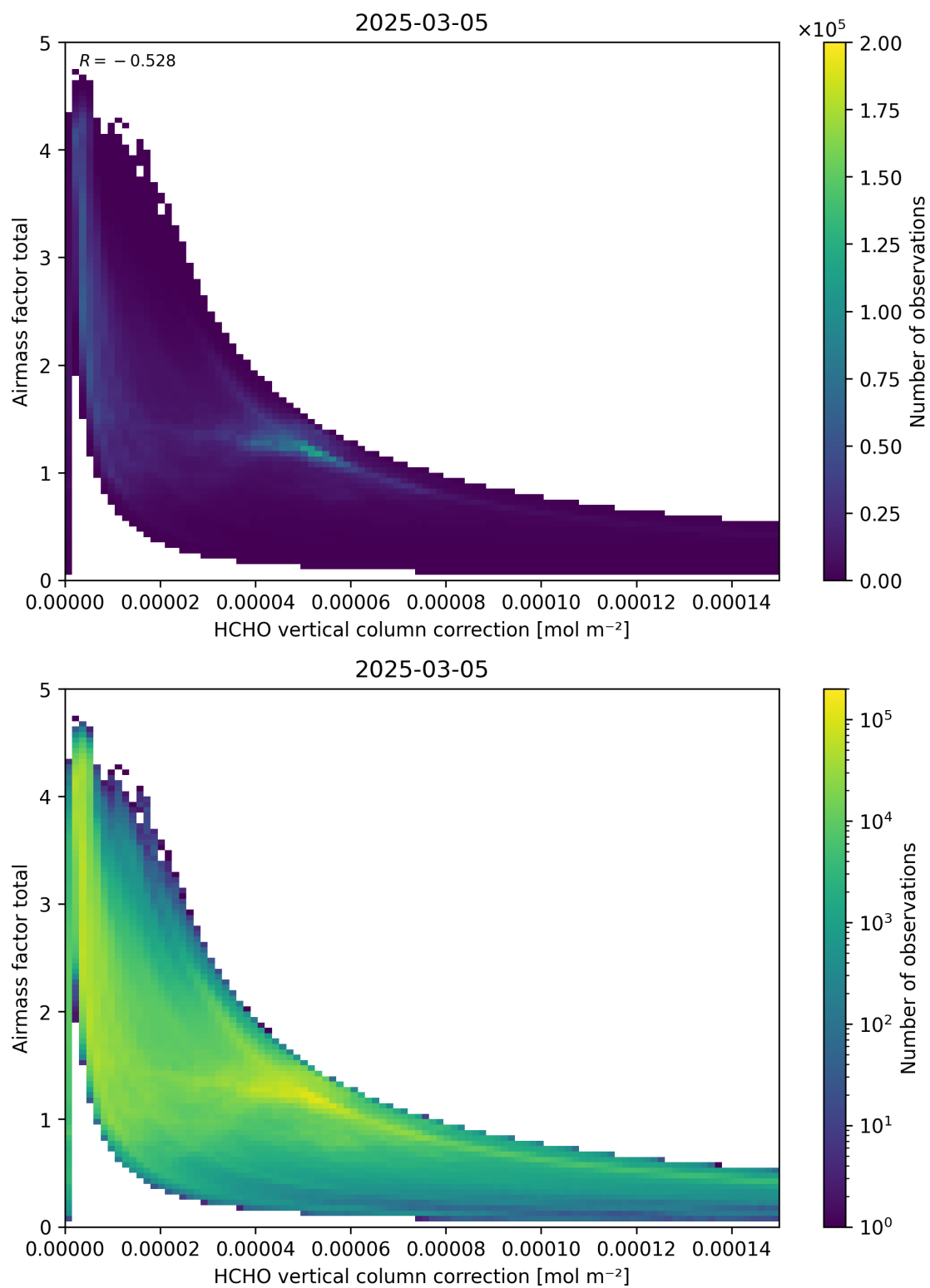
Figure 120: Scatter density plot of “HCHO vertical column correction” against “Airmass factor total” for 2025-03-04 to 2025-03-06.
