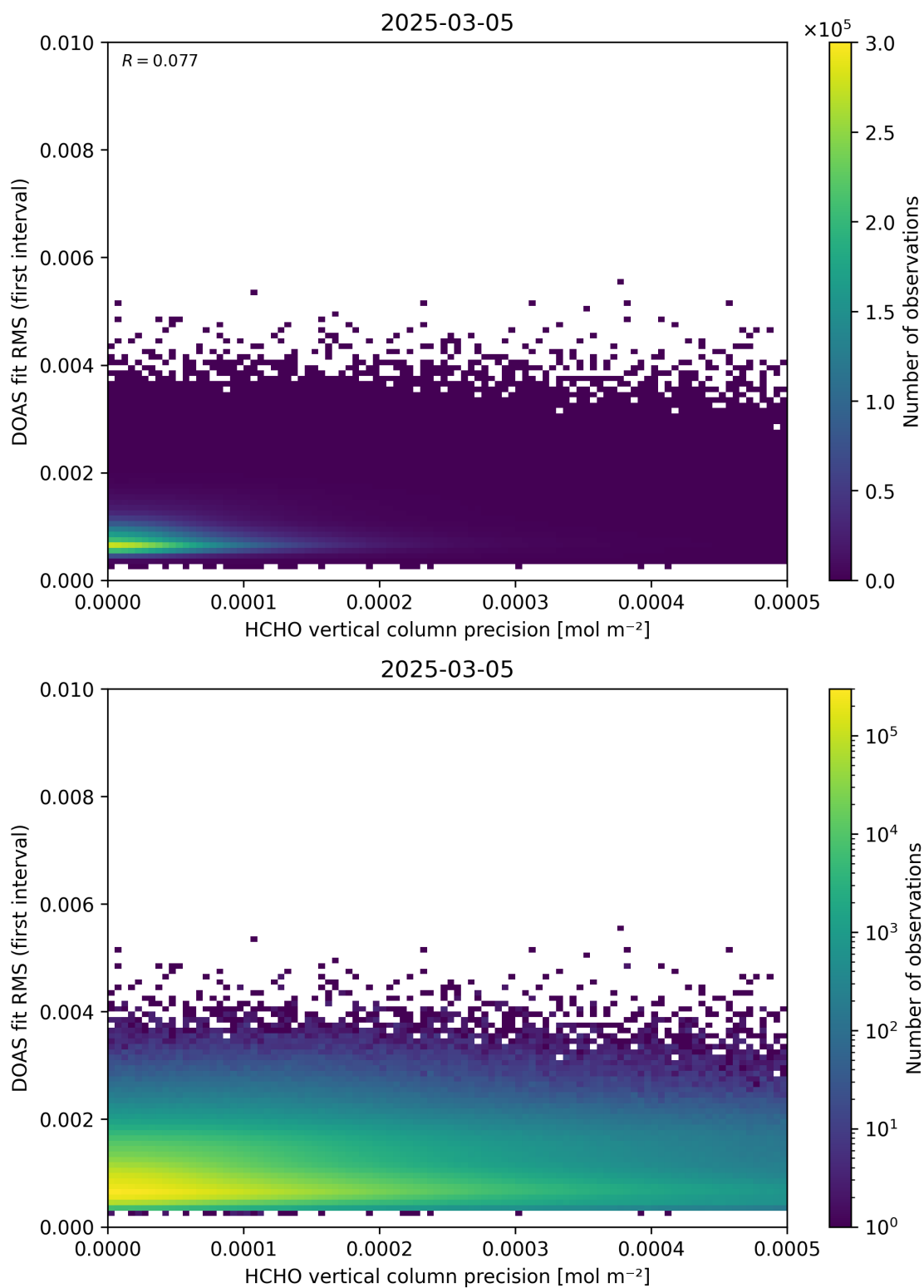
Figure 136: Scatter density plot of “HCHO vertical column precision” against “DOAS fit RMS (first interval)” for 2025-03-04 to 2025-03-06.
