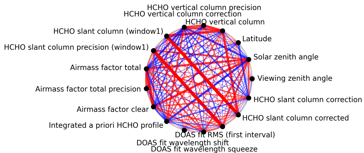
Figure 1: Map of correlation graph for 2025-03-04 to 2025-03-06.
