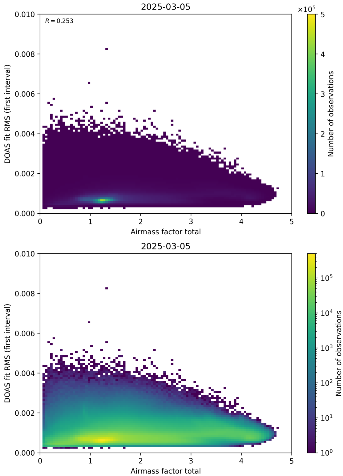
Figure 97: Scatter density plot of “Airmass factor total” against “DOAS fit RMS (first interval)” for 2025-03-04 to 2025-03-06.
