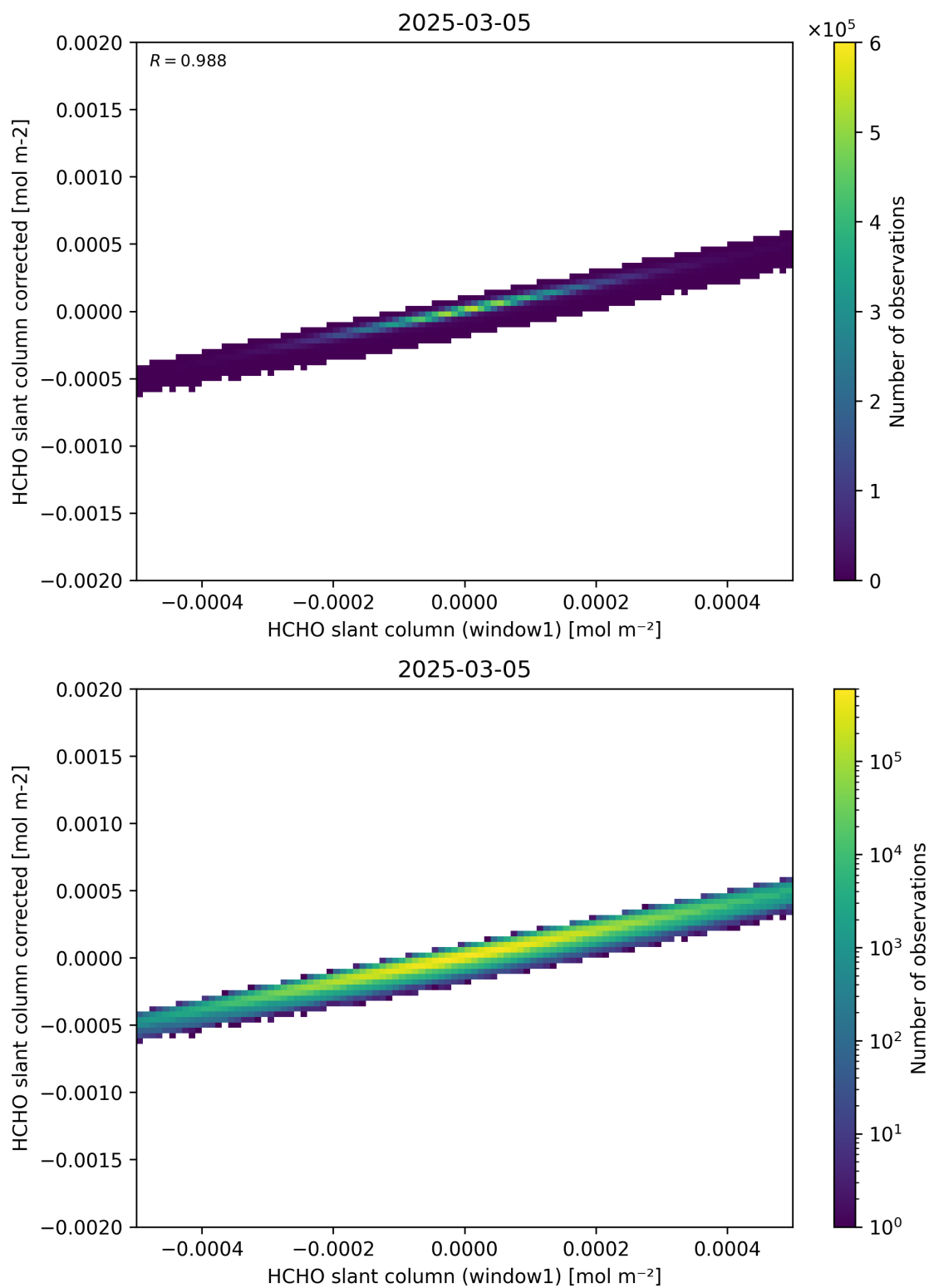
Figure 82: Scatter density plot of “HCHO slant column (window1)” against “HCHO slant column corrected” for 2025-03-04 to 2025-03-06.
