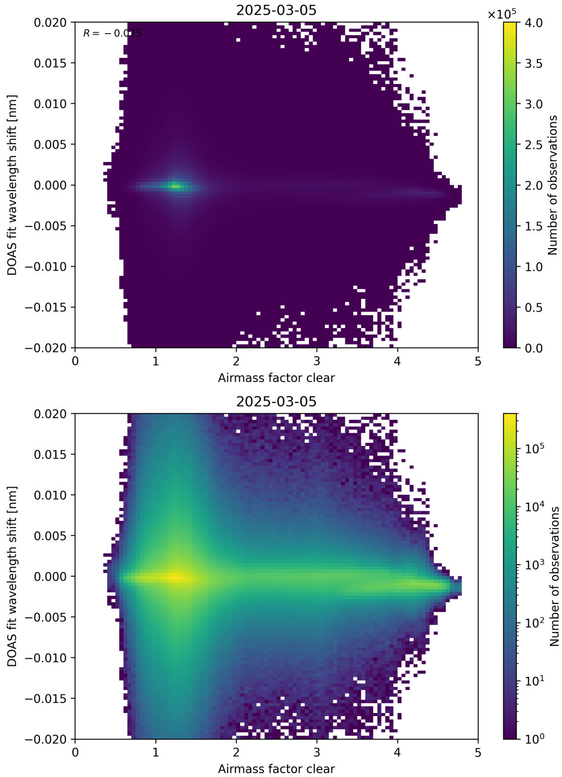
Figure 72: Scatter density plot of “Airmass factor clear” against “DOAS fit wavelength shift” for 2025-03-04 to 2025-03-06.
