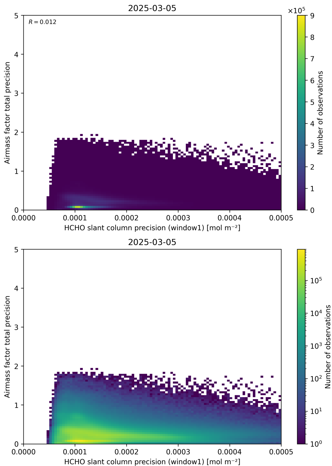
Figure 95: Scatter density plot of “HCHO slant column precision (window1)” against “Airmass factor total precision” for 2025-03-04 to 2025-03-06.
