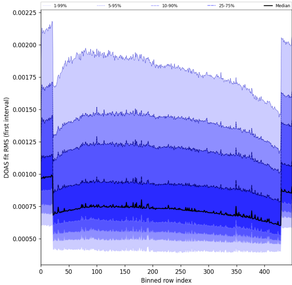
Figure 60: Along track statistics of “DOAS fit RMS (first interval)” for 2025-03-04 to 2025-03-06
