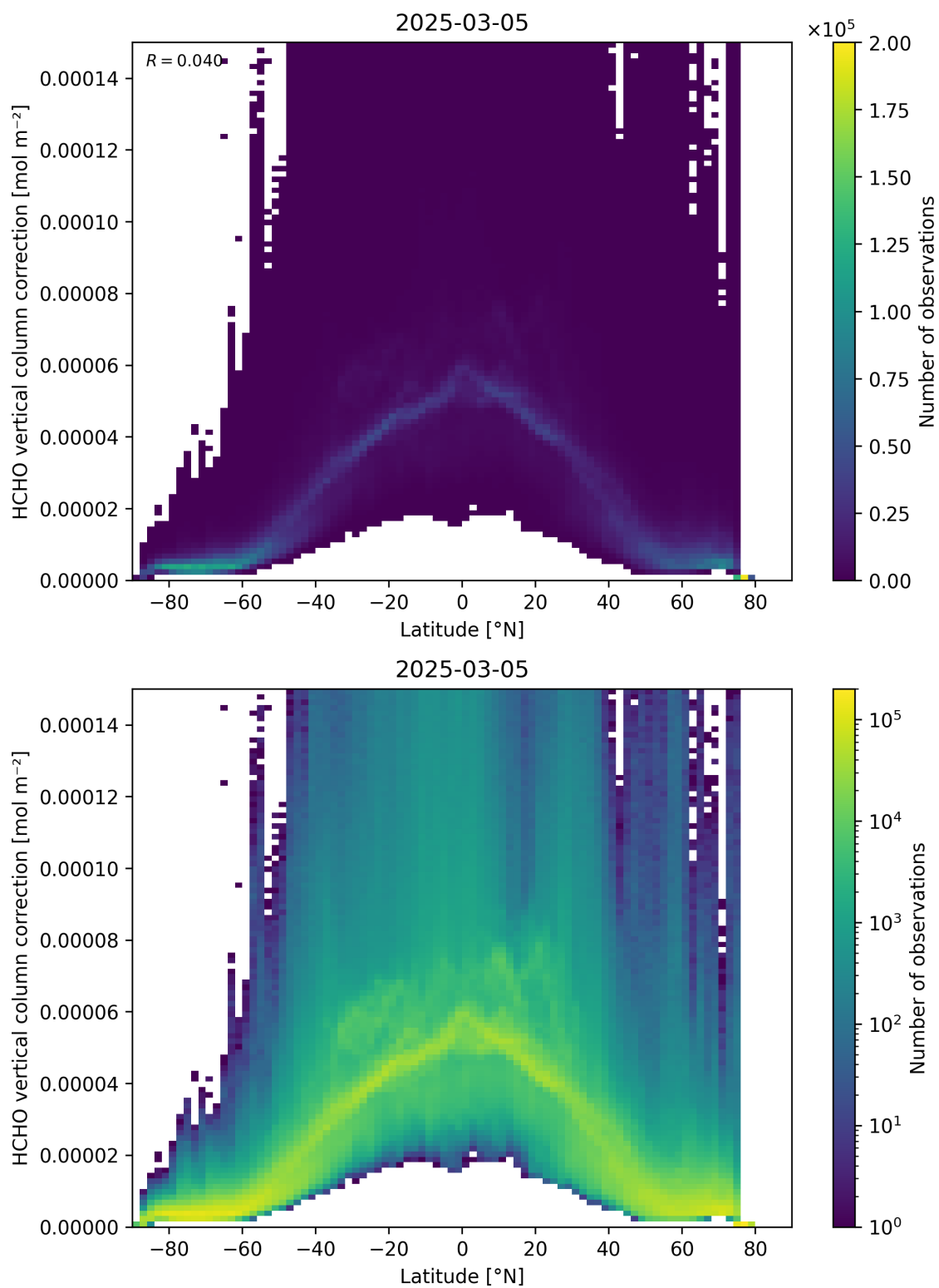
Figure 164: Scatter density plot of “Latitude” against “HCHO vertical column correction” for 2025-03-04 to 2025-03-06.
