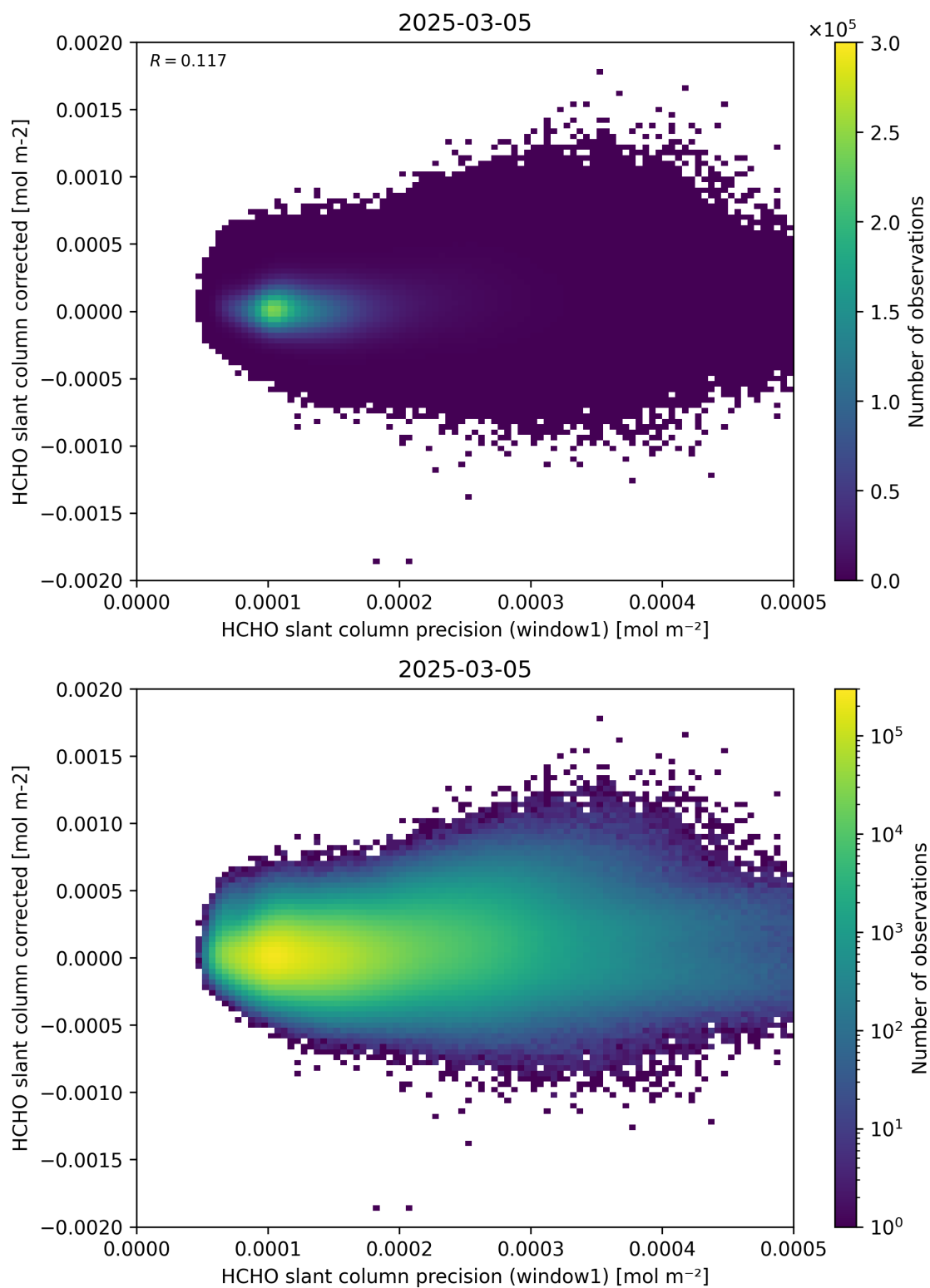
Figure 92: Scatter density plot of “HCHO slant column precision (window1)” against “HCHO slant column corrected” for 2025-03-04 to 2025-03-06.
