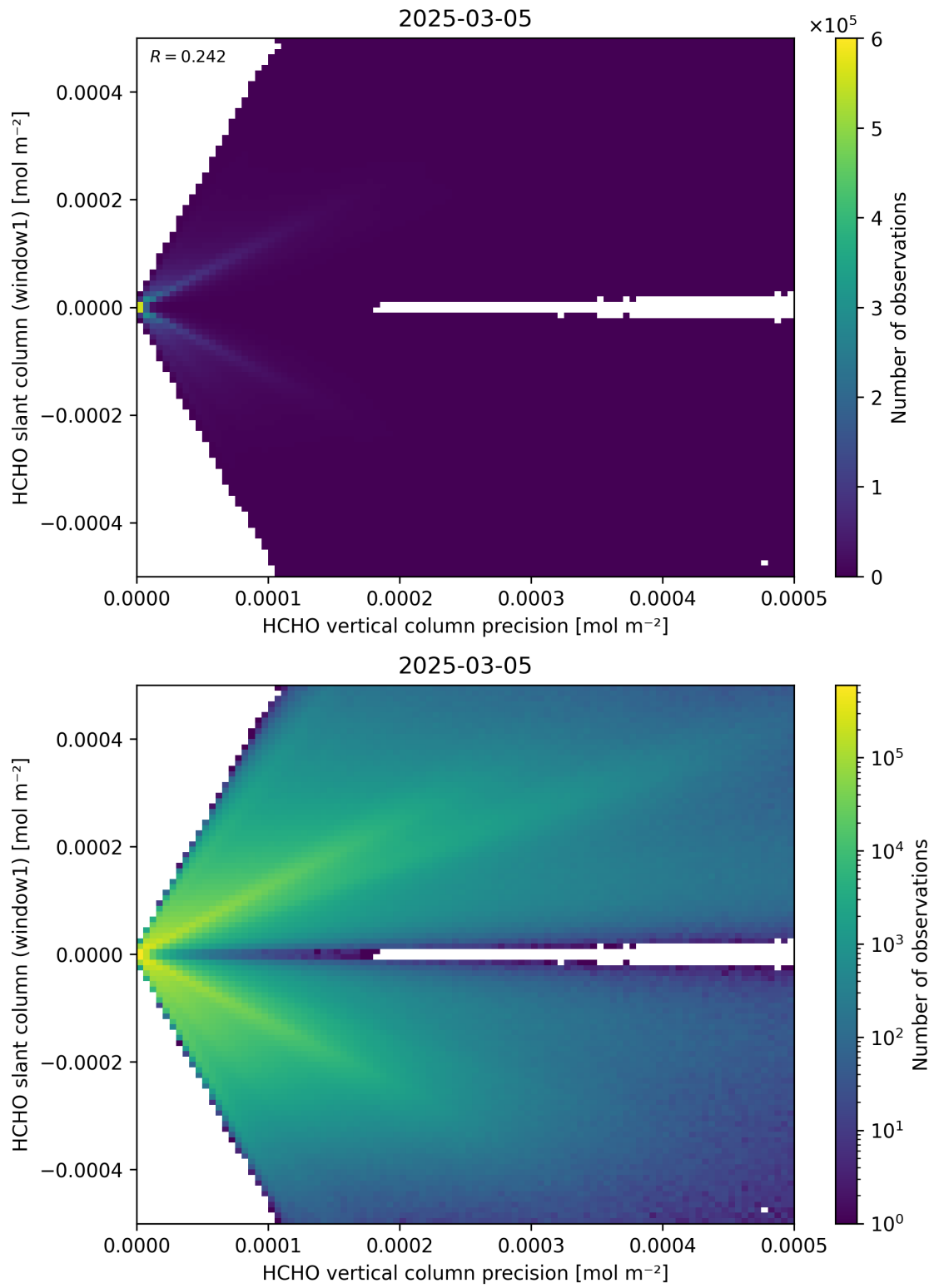
Figure 142: Scatter density plot of “HCHO vertical column precision” against “HCHO slant column (window1)” for 2025-03-04 to 2025-03-06.
