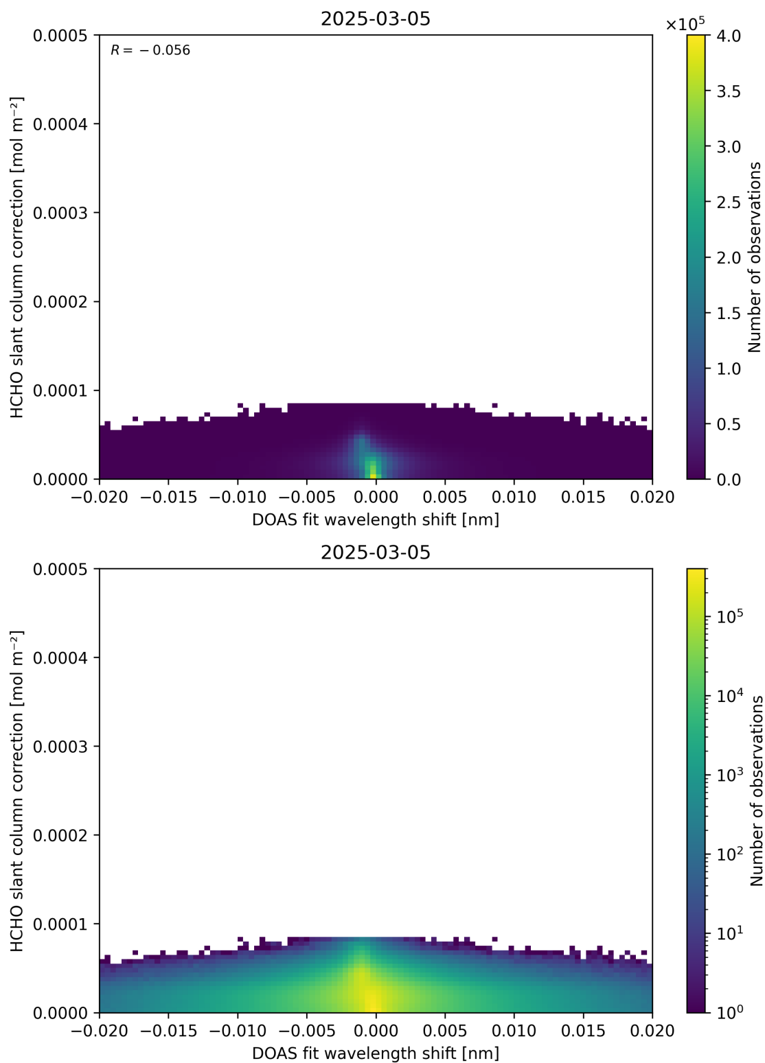
Figure 67: Scatter density plot of “DOAS fit wavelength shift” against “HCHO slant column correction” for 2025-03-04 to 2025-03-06.
