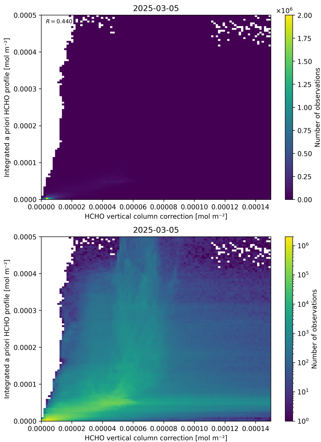
Figure 122: Scatter density plot of “HCHO vertical column correction” against “Integrated a priori HCHO profile” for 2025-03-04 to 2025-03-06.
