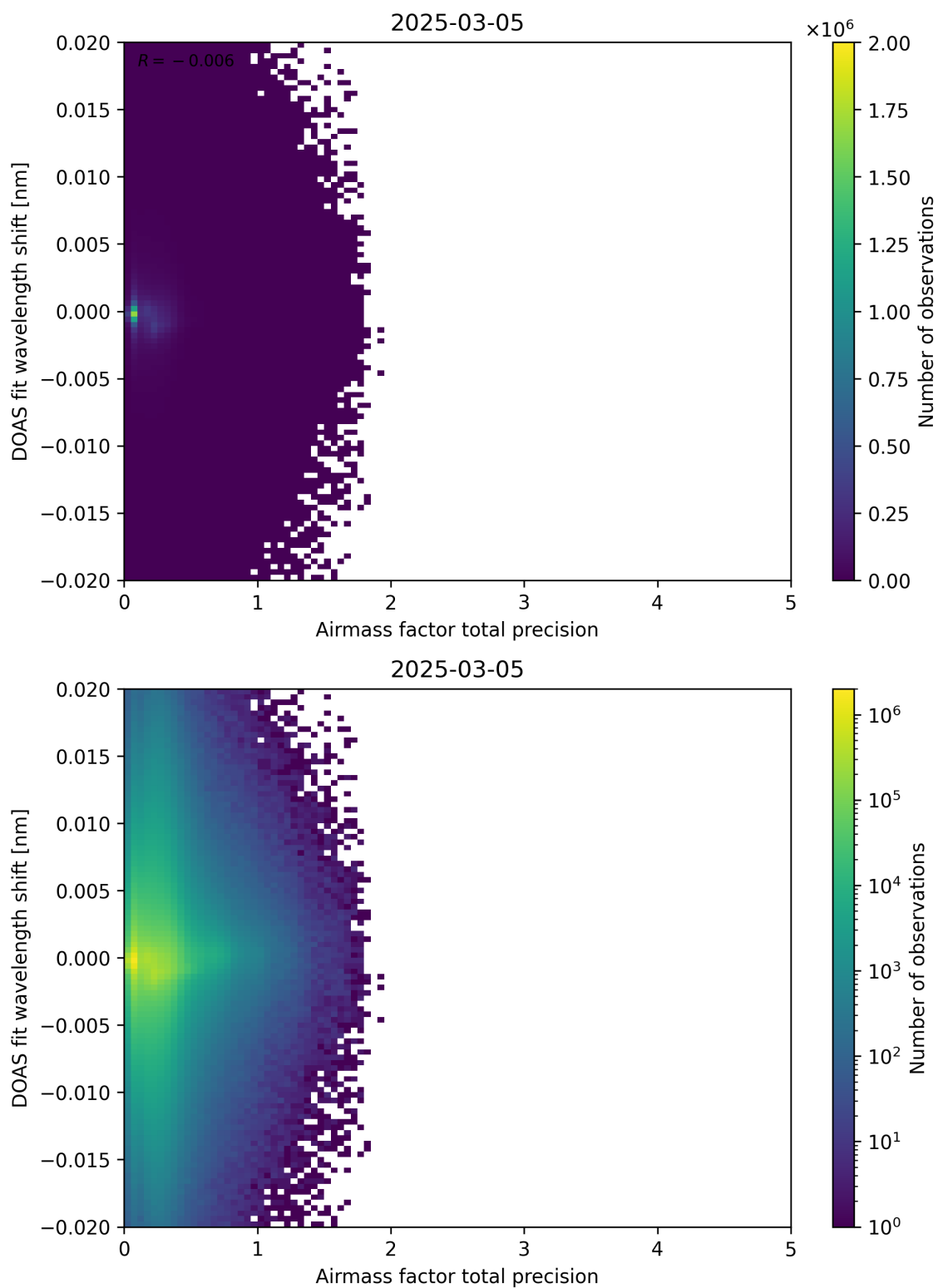
Figure 106: Scatter density plot of “Airmass factor total precision” against “DOAS fit wavelength shift” for 2025-03-04 to 2025-03-06.
