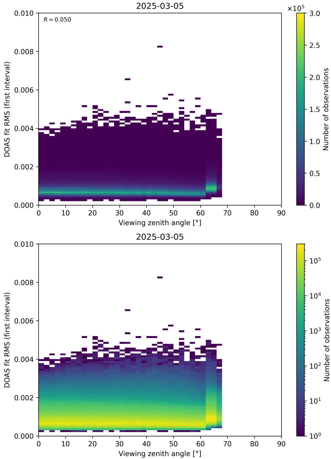
Figure 182: Scatter density plot of “Viewing zenith angle” against “DOAS fit RMS (first interval)” for 2025-03-04 to 2025-03-06.
