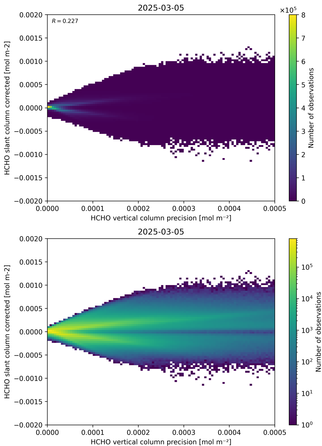
Figure 140: Scatter density plot of “HCHO vertical column precision” against “HCHO slant column corrected” for 2025-03-04 to 2025-03-06.
