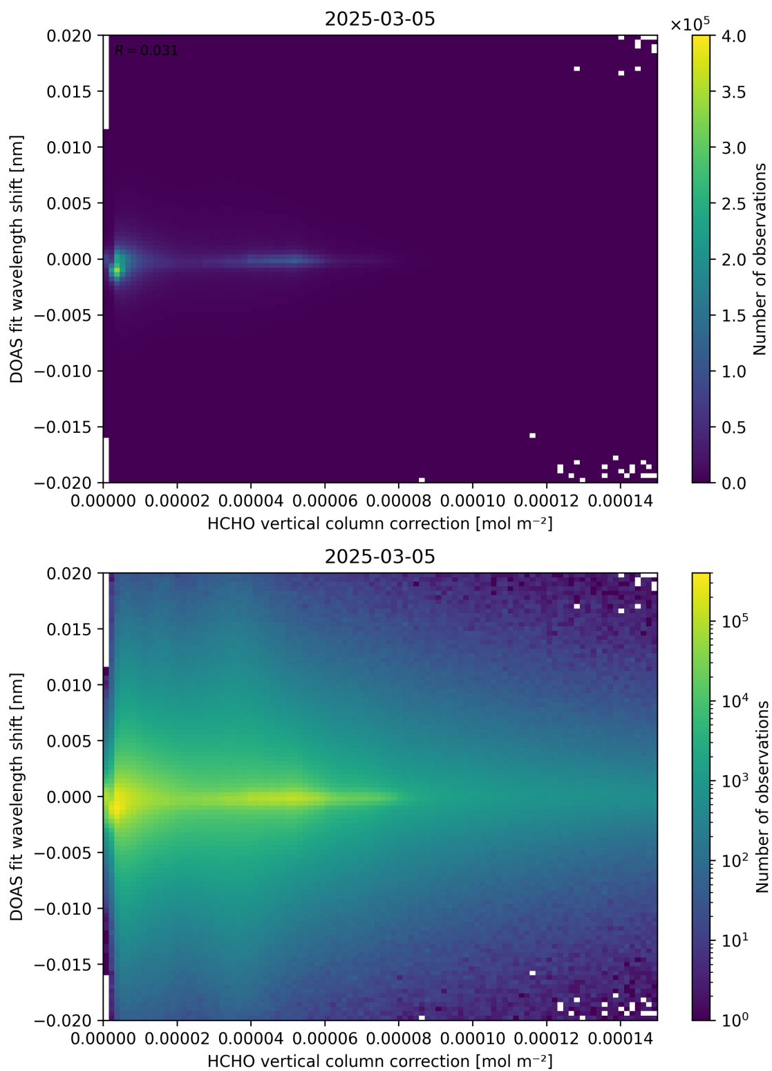
Figure 113: Scatter density plot of “HCHO vertical column correction” against “DOAS fit wavelength shift” for 2025-03-04 to 2025-03-06.
