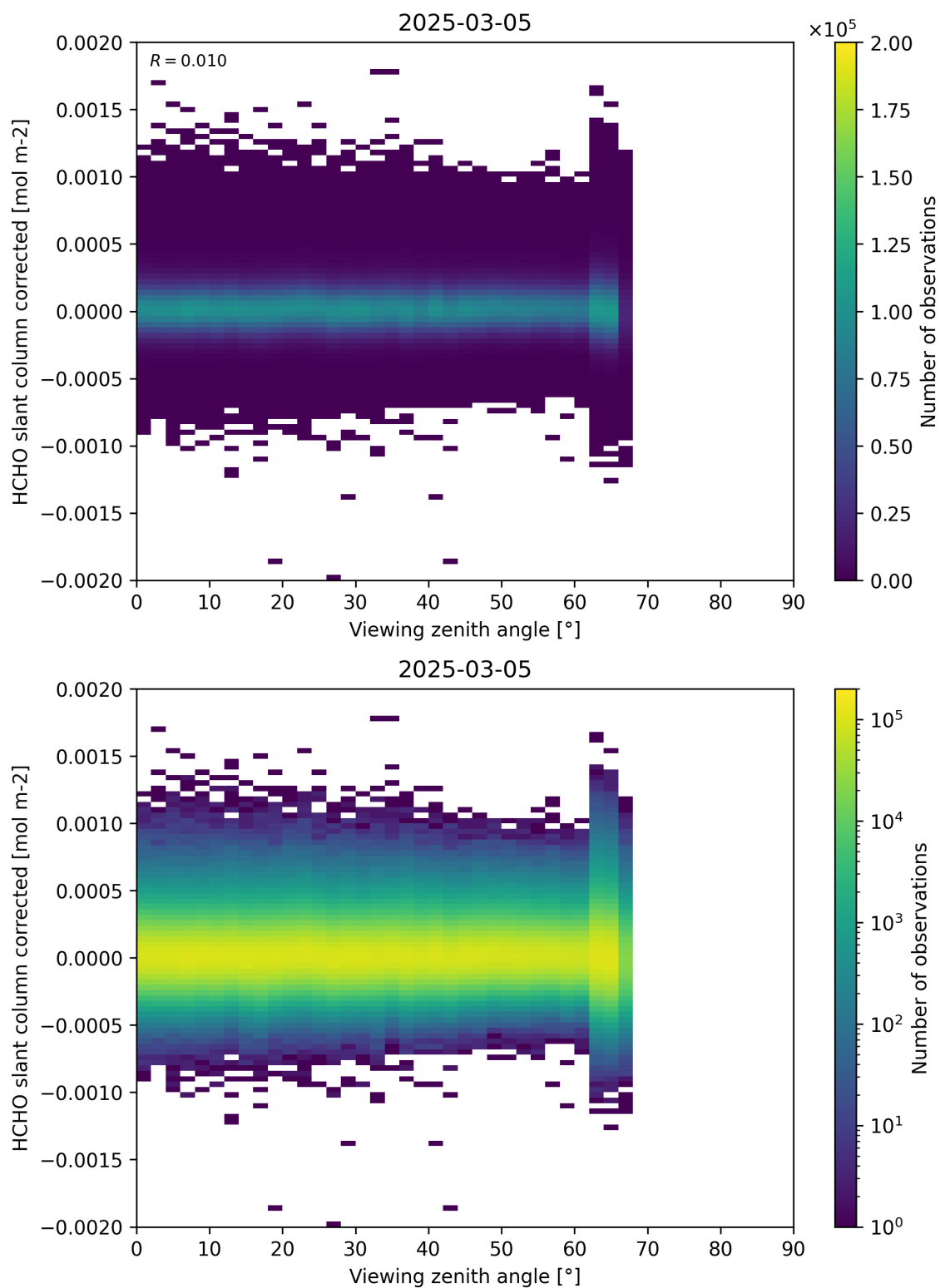
Figure 186: Scatter density plot of “Viewing zenith angle” against “HCHO slant column corrected” for 2025-03-04 to 2025-03-06.
