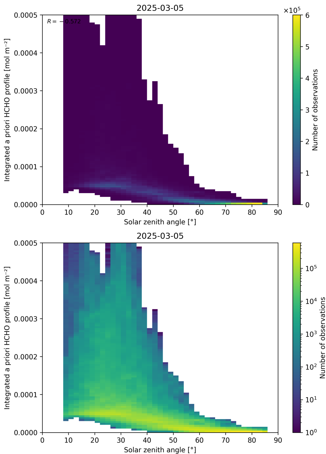
Figure 180: Scatter density plot of “Solar zenith angle” against “Integrated a priori HCHO profile” for 2025-03-04 to 2025-03-06.
