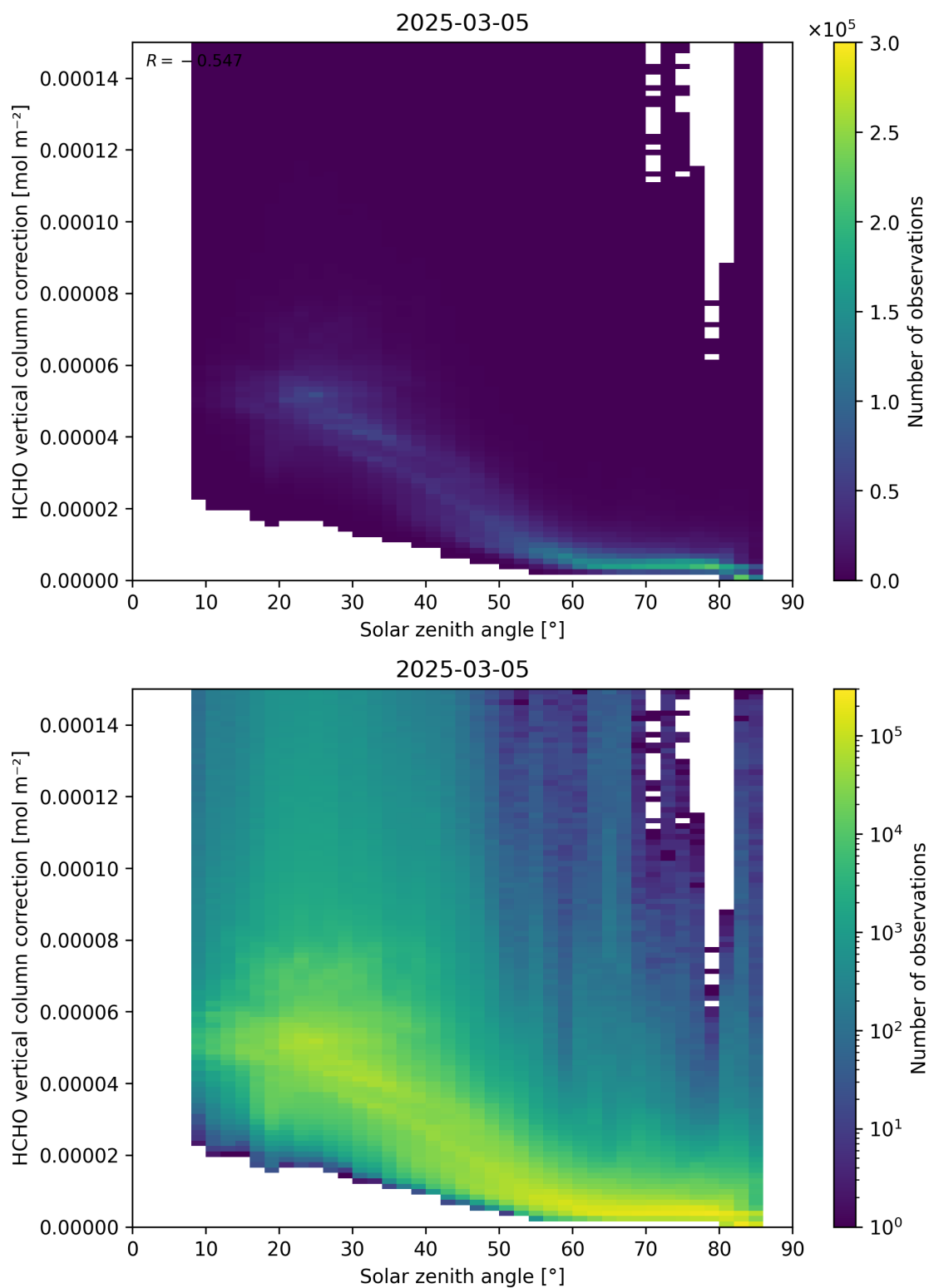
Figure 178: Scatter density plot of “Solar zenith angle” against “HCHO vertical column correction” for 2025-03-04 to 2025-03-06.
