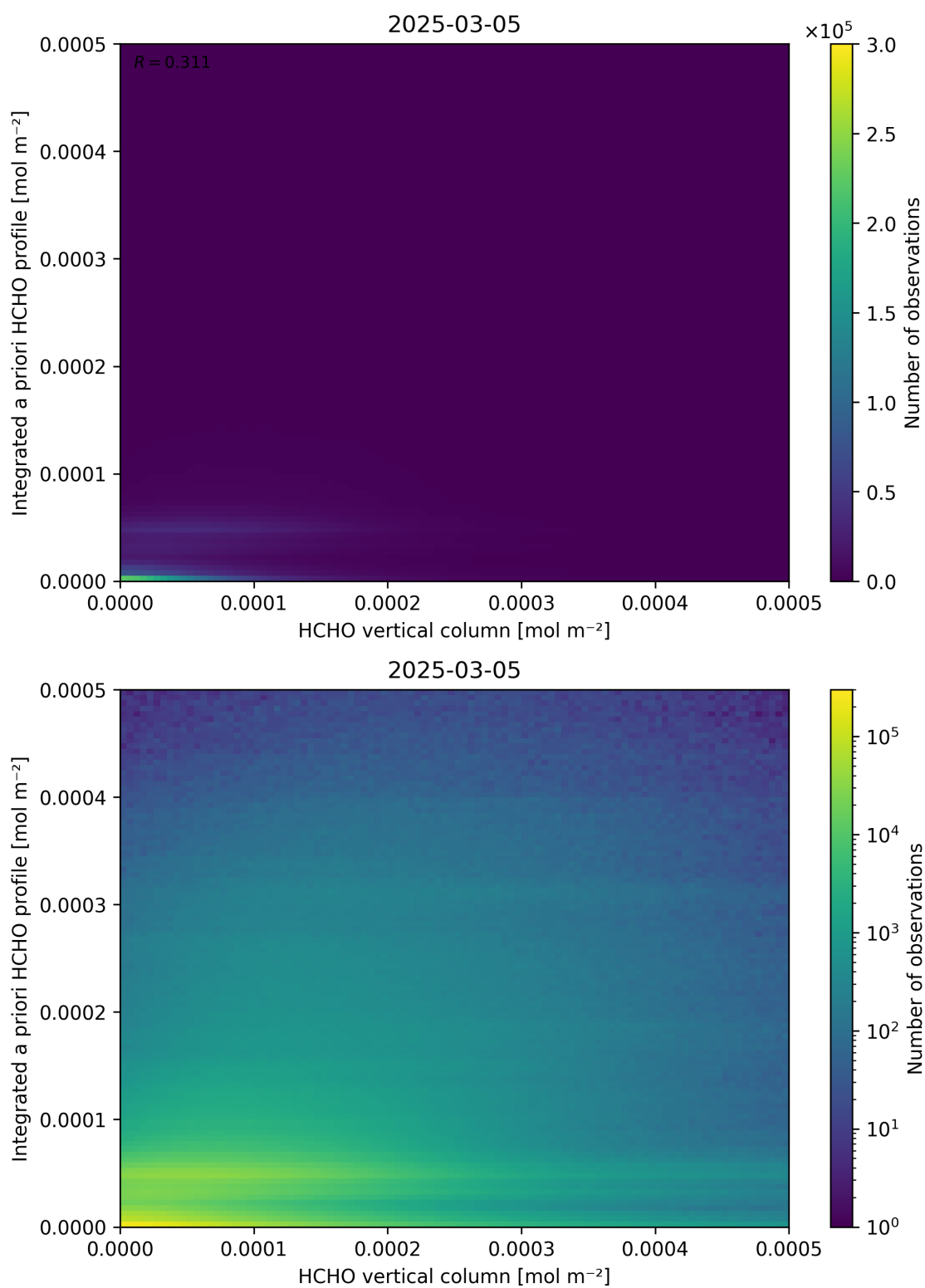
Figure 135: Scatter density plot of “HCHO vertical column” against “Integrated a priori HCHO profile” for 2025-03-04 to 2025-03-06.
