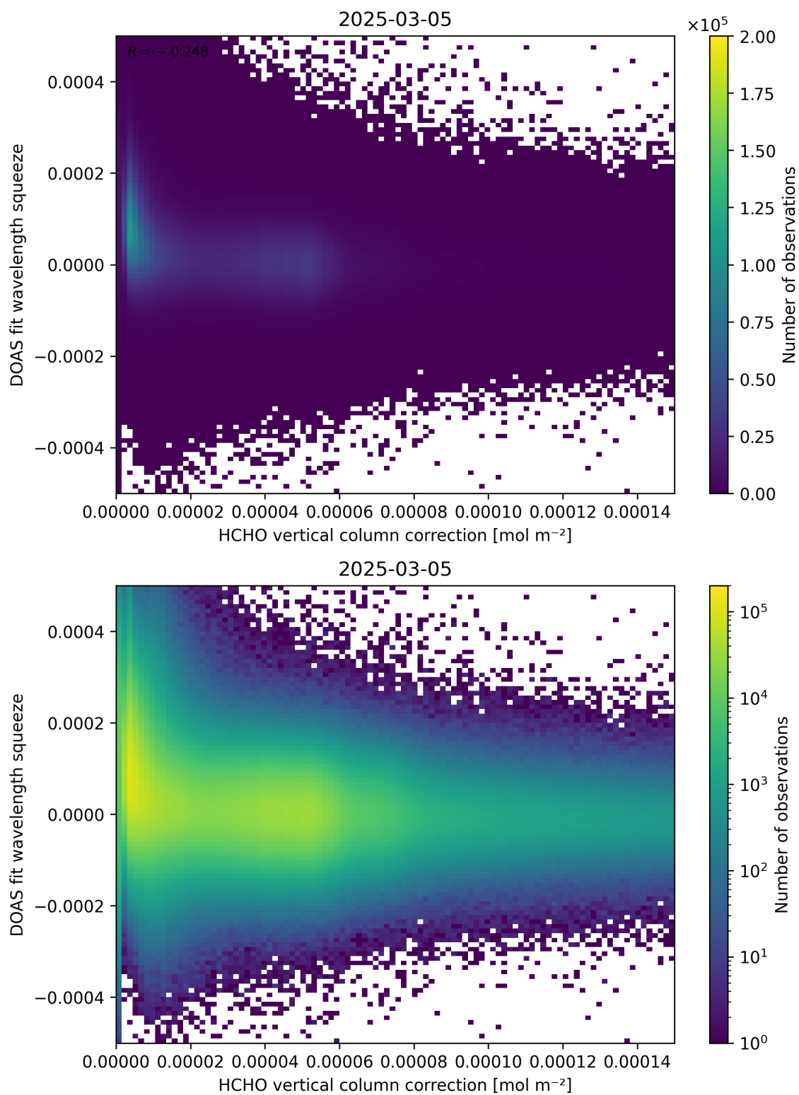
Figure 114: Scatter density plot of “HCHO vertical column correction” against “DOAS fit wavelength squeeze” for 2025-03-04 to 2025-03-06.
