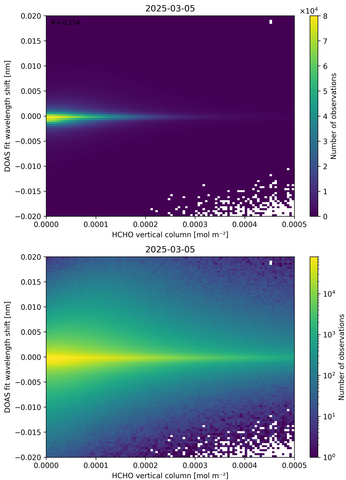
Figure 124: Scatter density plot of “HCHO vertical column” against “DOAS fit wavelength shift” for 2025-03-04 to 2025-03-06.
