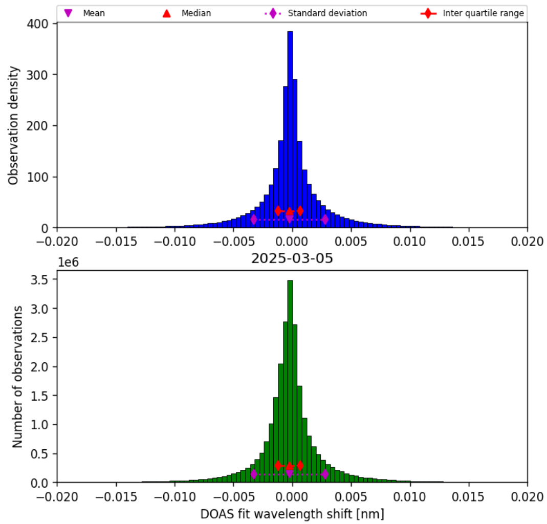
Figure 44: Histogram of “DOAS fit wavelength shift” for 2025-03-04 to 2025-03-06
