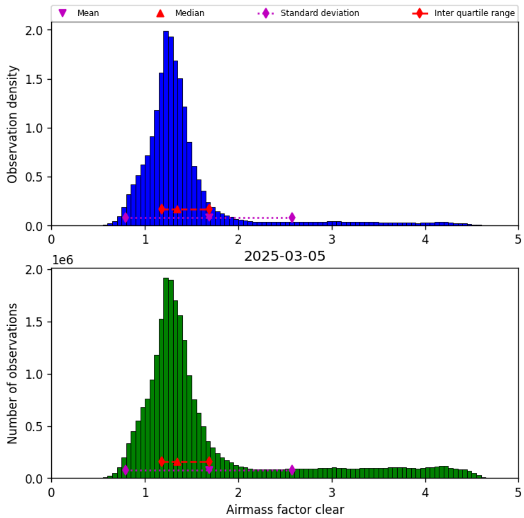
Figure 42: Histogram of “Airmass factor clear” for 2025-03-04 to 2025-03-06
