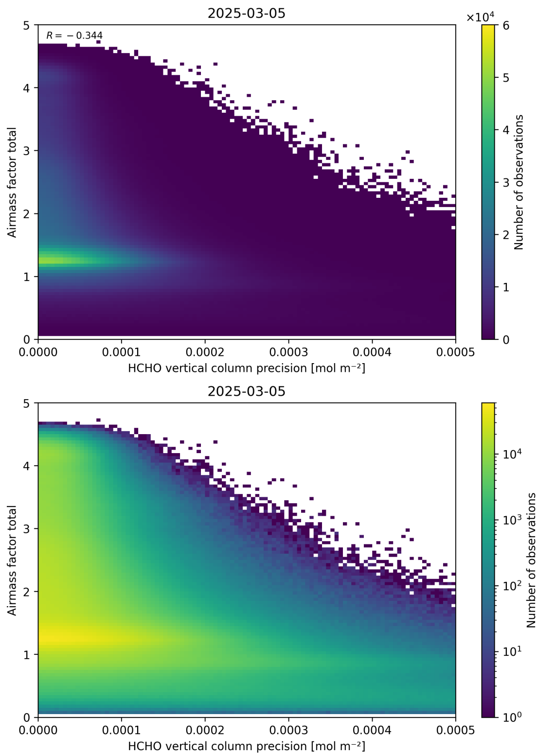
Figure 144: Scatter density plot of “HCHO vertical column precision” against “Airmass factor total” for 2025-03-04 to 2025-03-06.
