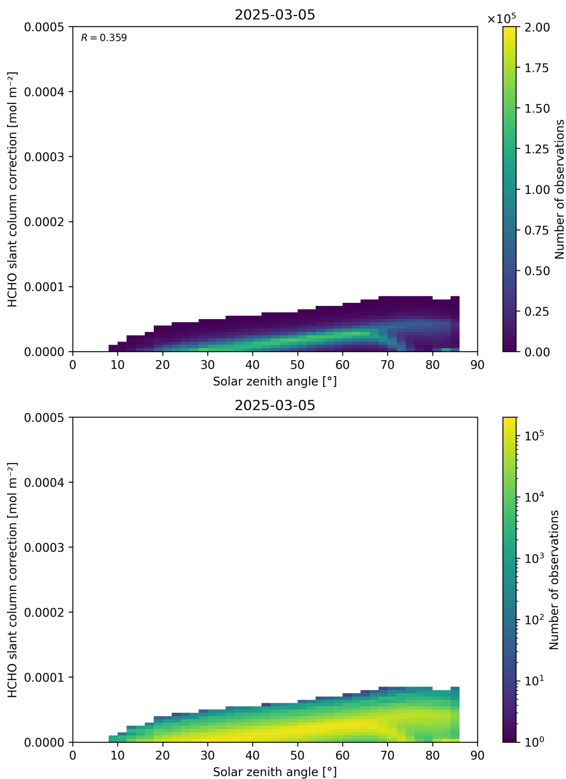
Figure 172: Scatter density plot of “Solar zenith angle” against “HCHO slant column correction” for 2025-03-04 to 2025-03-06.
