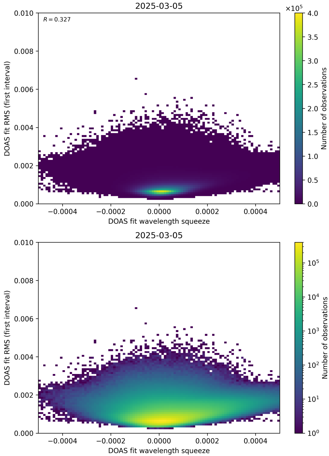
Figure 68: Scatter density plot of “DOAS fit wavelength squeeze” against “DOAS fit RMS (first interval)” for 2025-03-04 to 2025-03-06.
