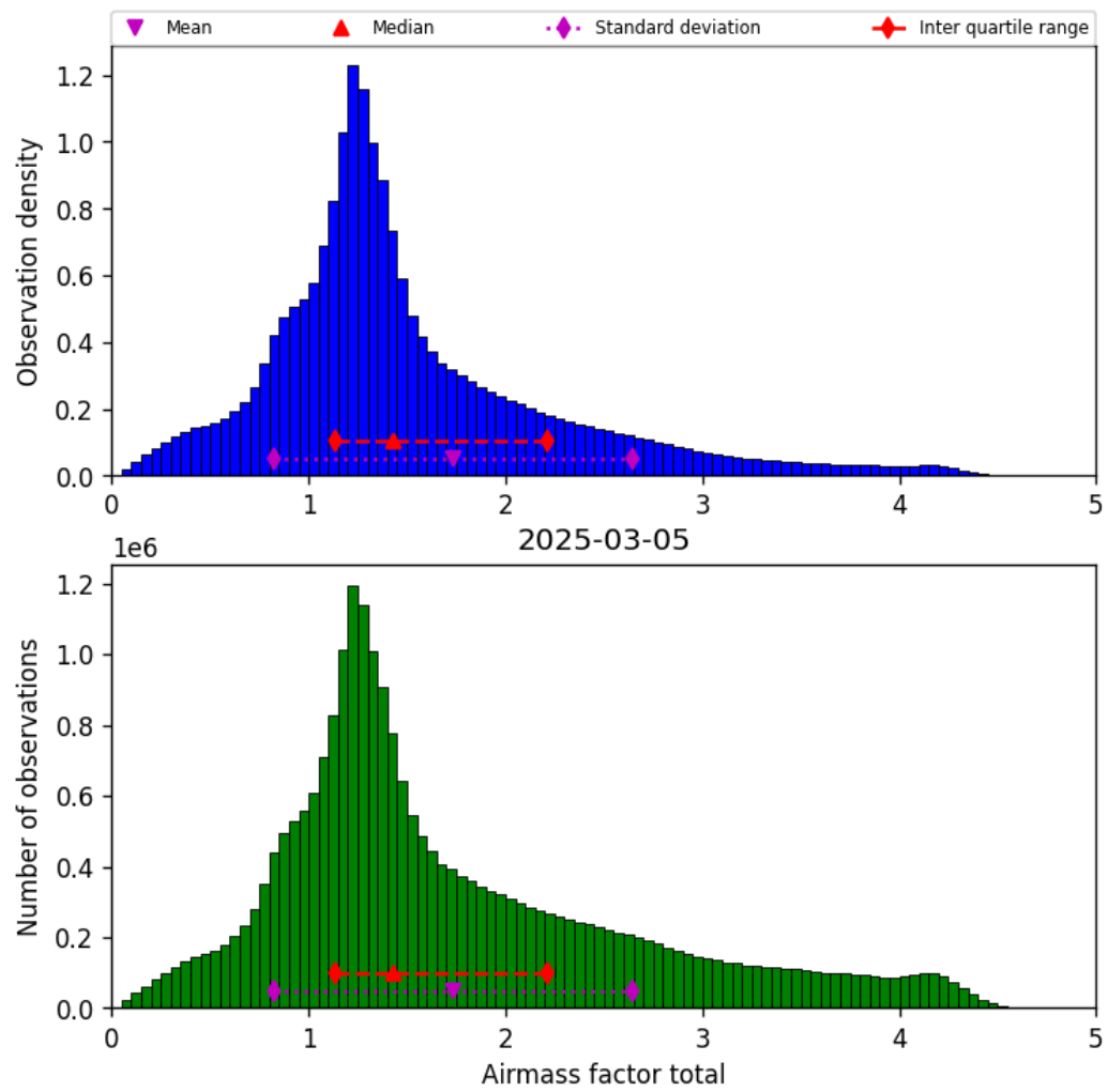
Figure 40: Histogram of “Airmass factor total” for 2025-03-04 to 2025-03-06
