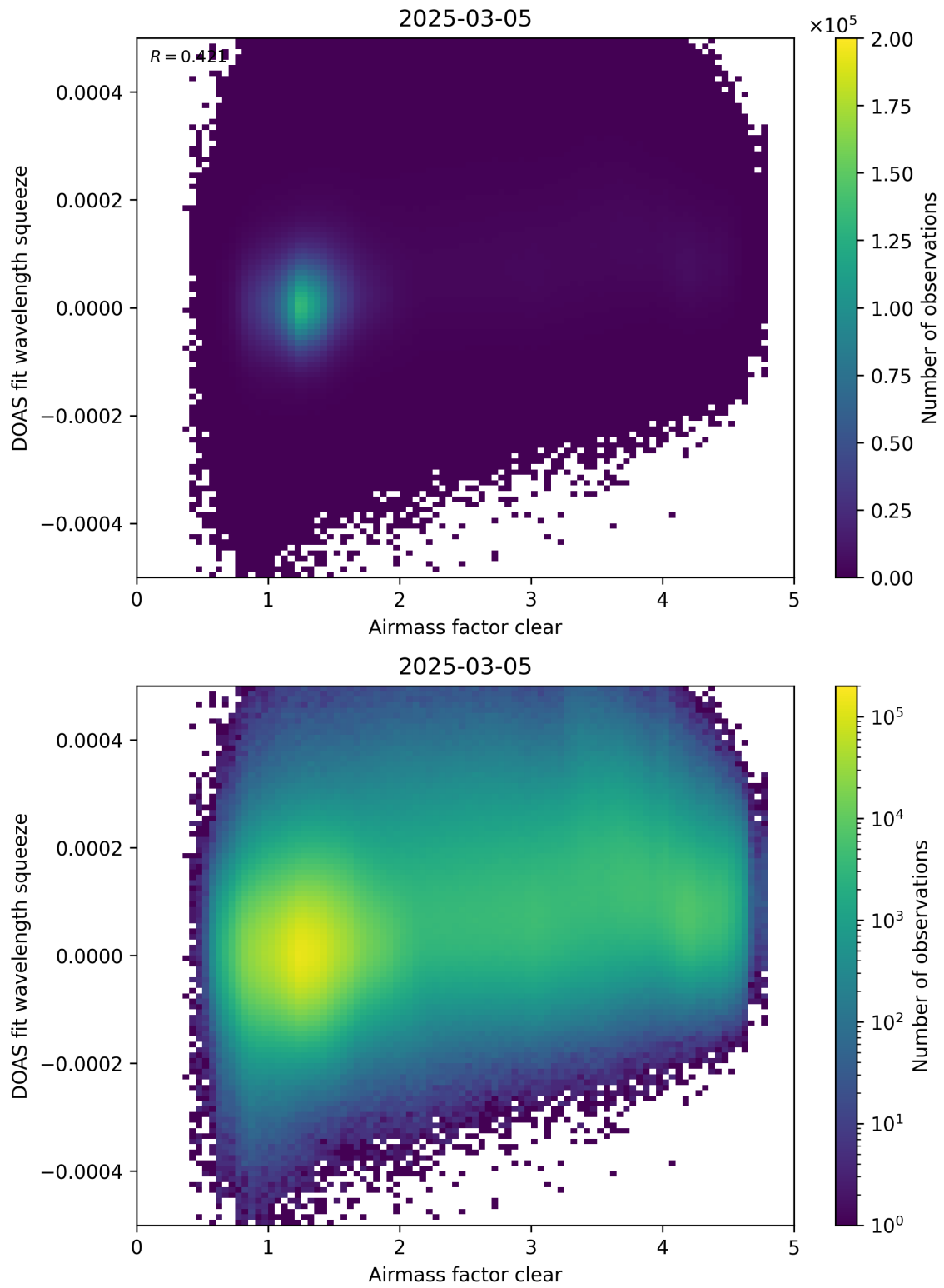
Figure 73: Scatter density plot of “Airmass factor clear” against “DOAS fit wavelength squeeze” for 2025-03-04 to 2025-03-06.
