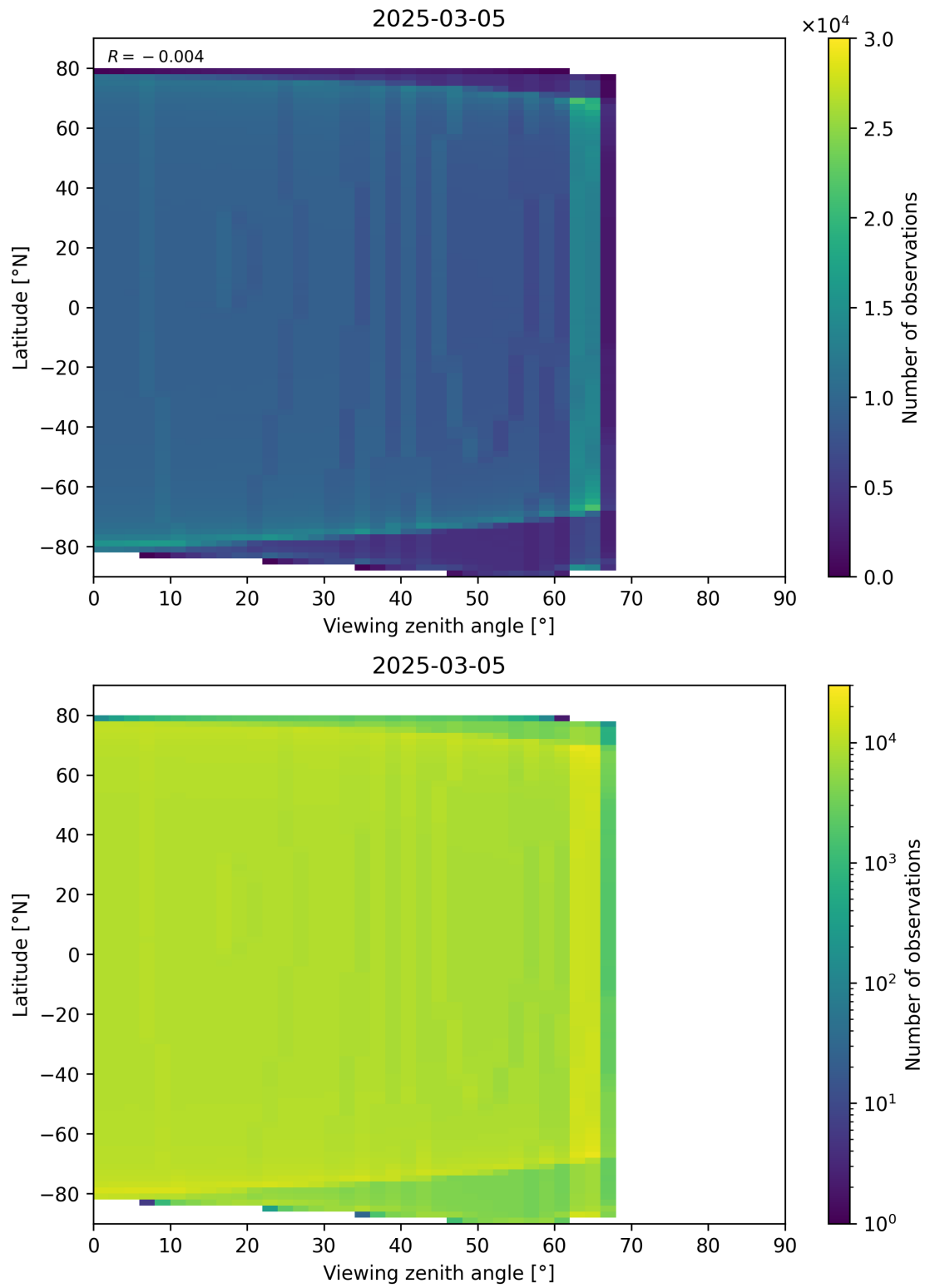
Figure 196: Scatter density plot of “Viewing zenith angle” against “Latitude” for 2025-03-04 to 2025-03-06.
