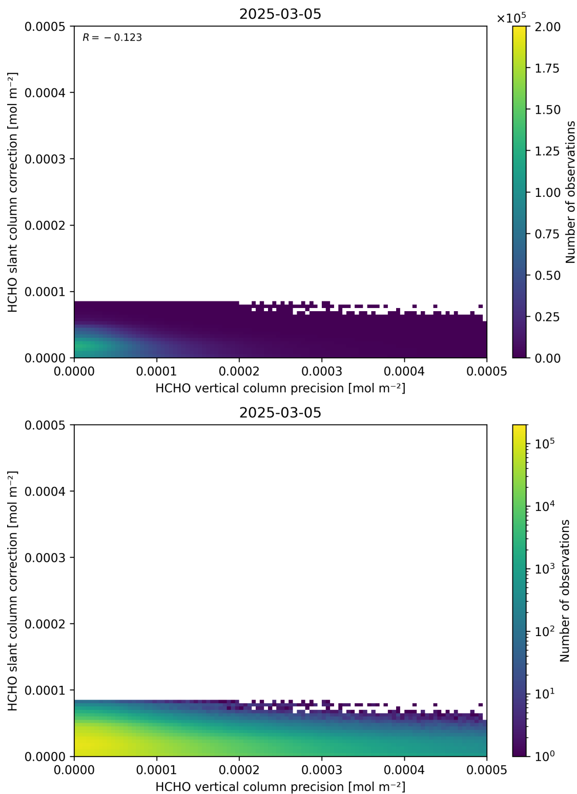
Figure 141: Scatter density plot of “HCHO vertical column precision” against “HCHO slant column correction” for 2025-03-04 to 2025-03-06.
