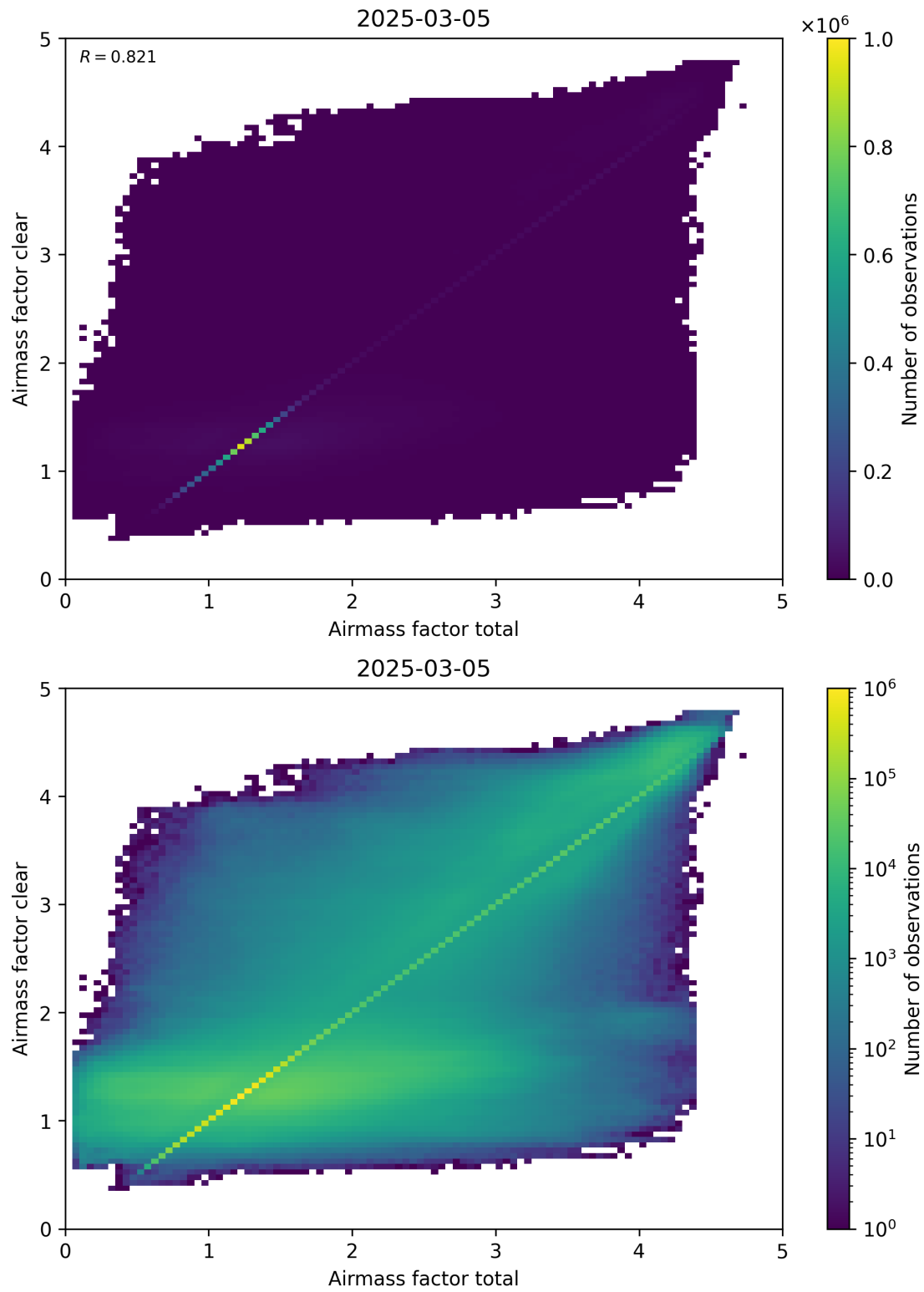
Figure 100: Scatter density plot of “Airmass factor total” against “Airmass factor clear” for 2025-03-04 to 2025-03-06.
