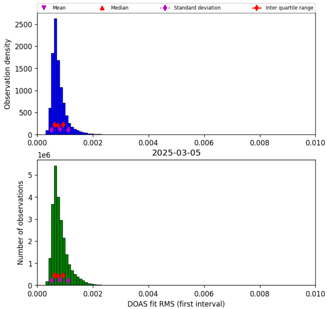
Figure 46: Histogram of “DOAS fit RMS (first interval)” for 2025-03-04 to 2025-03-06
