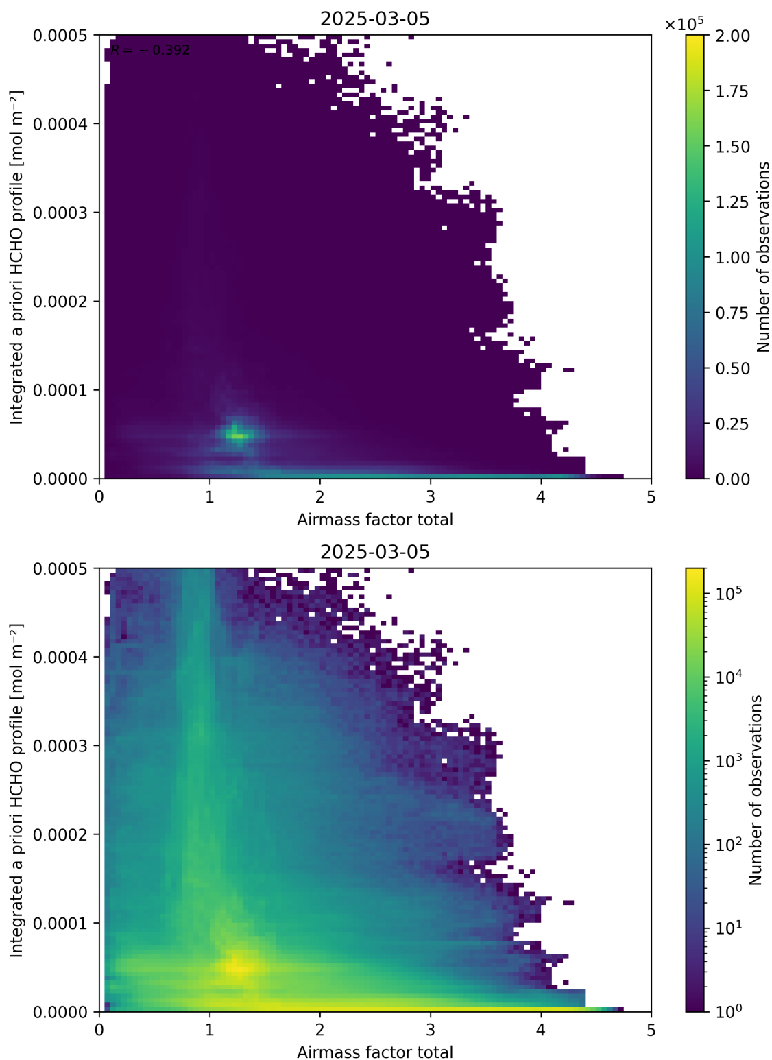
Figure 104: Scatter density plot of “Airmass factor total” against “Integrated a priori HCHO profile” for 2025-03-04 to 2025-03-06.
