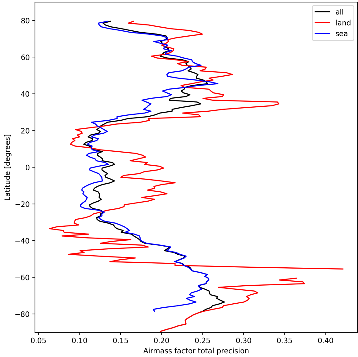
Figure 27: Zonal average of “Airmass factor total precision” for 2025-03-04 to 2025-03-06.
