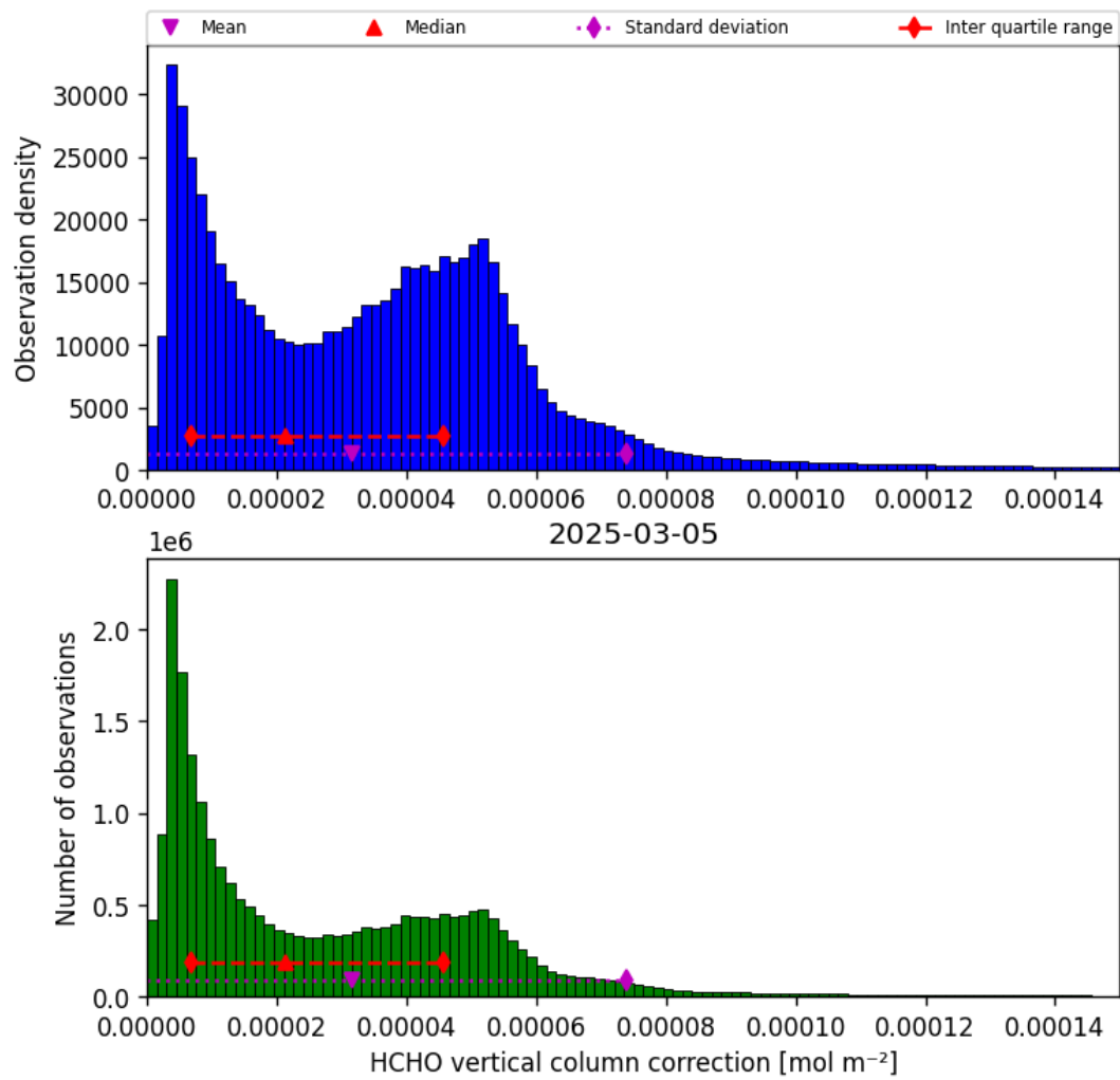
Figure 37: Histogram of “HCHO vertical column correction” for 2025-03-04 to 2025-03-06
