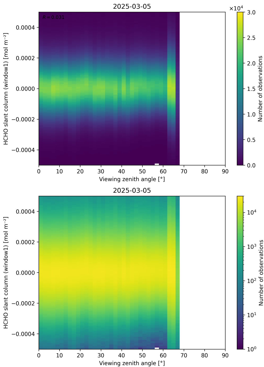
Figure 188: Scatter density plot of “Viewing zenith angle” against “HCHO slant column (window1)” for 2025-03-04 to 2025-03-06.
