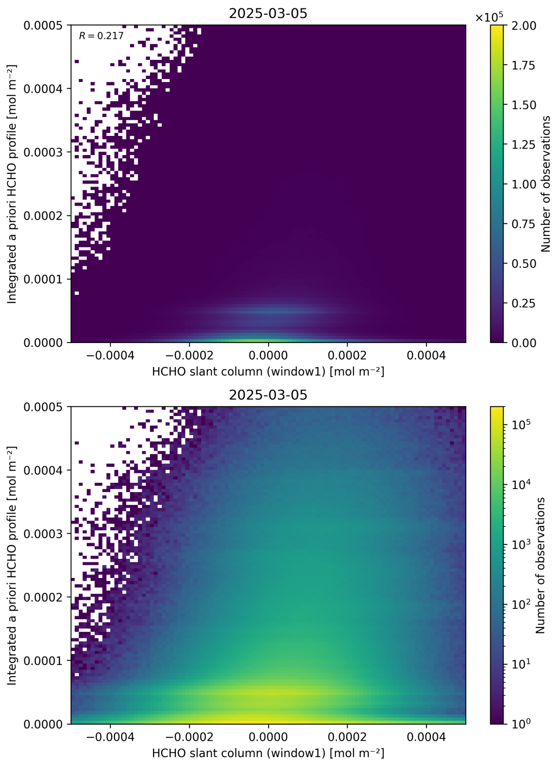
Figure 87: Scatter density plot of “HCHO slant column (window1)” against “Integrated a priori HCHO profile” for 2025-03-04 to 2025-03-06.
