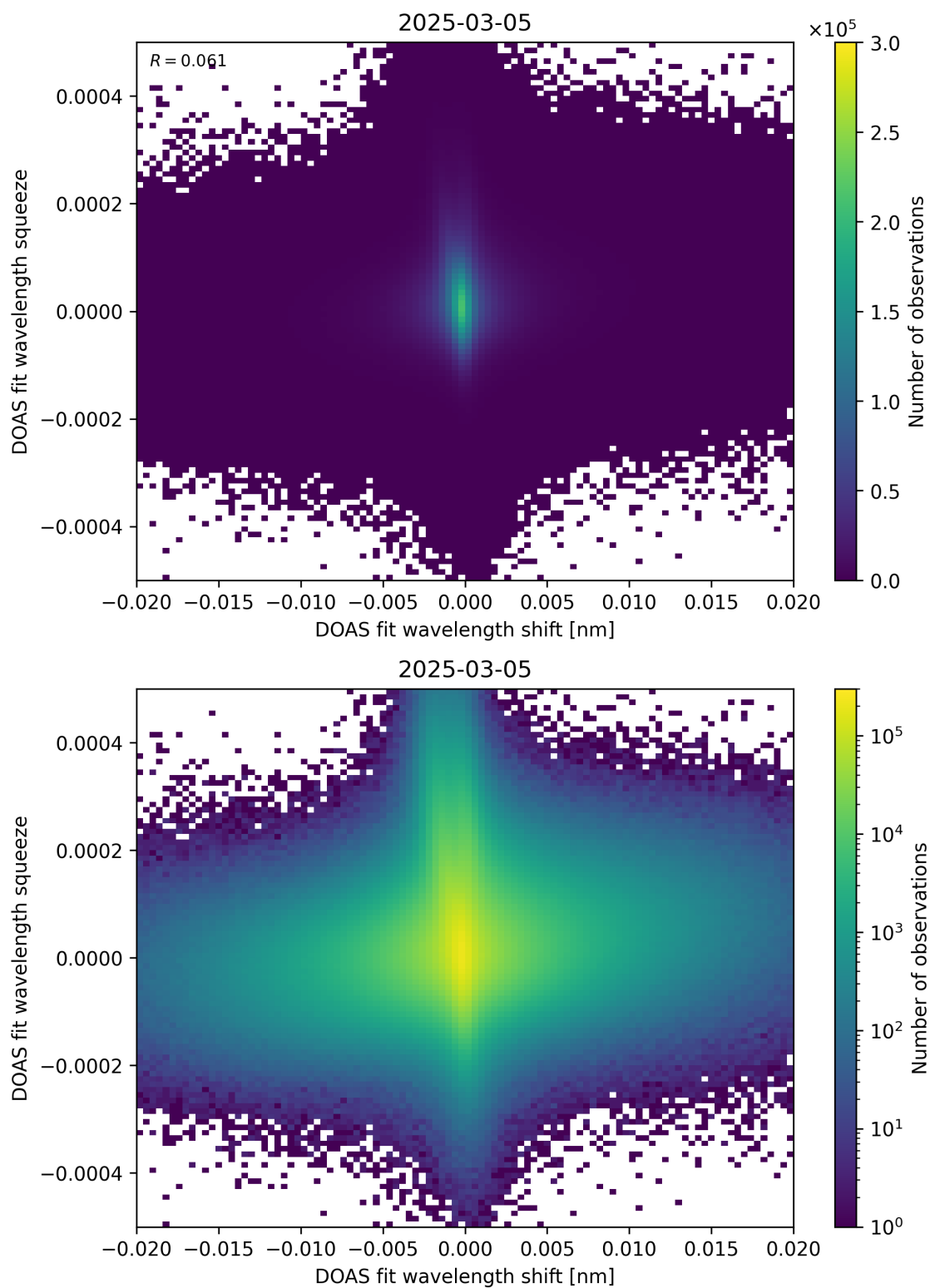
Figure 65: Scatter density plot of “DOAS fit wavelength shift” against “DOAS fit wavelength squeeze” for 2025-03-04 to 2025-03-06.
