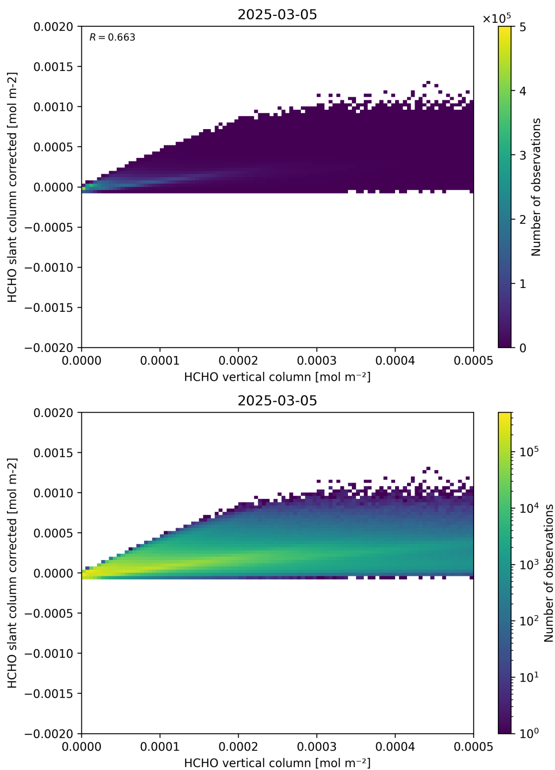
Figure 127: Scatter density plot of “HCHO vertical column” against “HCHO slant column corrected” for 2025-03-04 to 2025-03-06.
