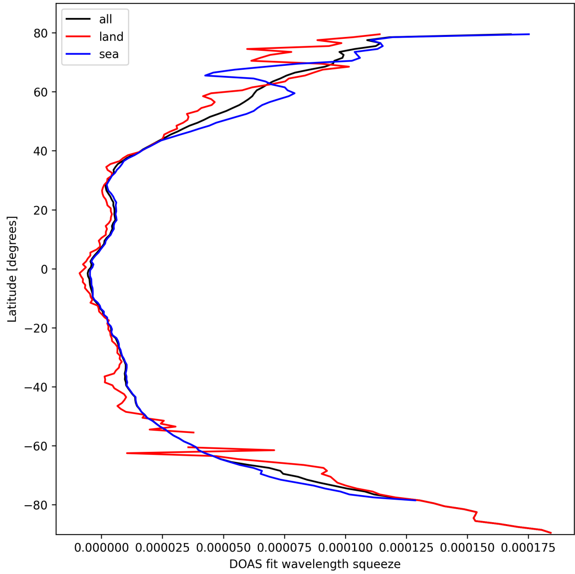
Figure 31: Zonal average of “DOAS fit wavelength squeeze” for 2025-03-04 to 2025-03-06.
