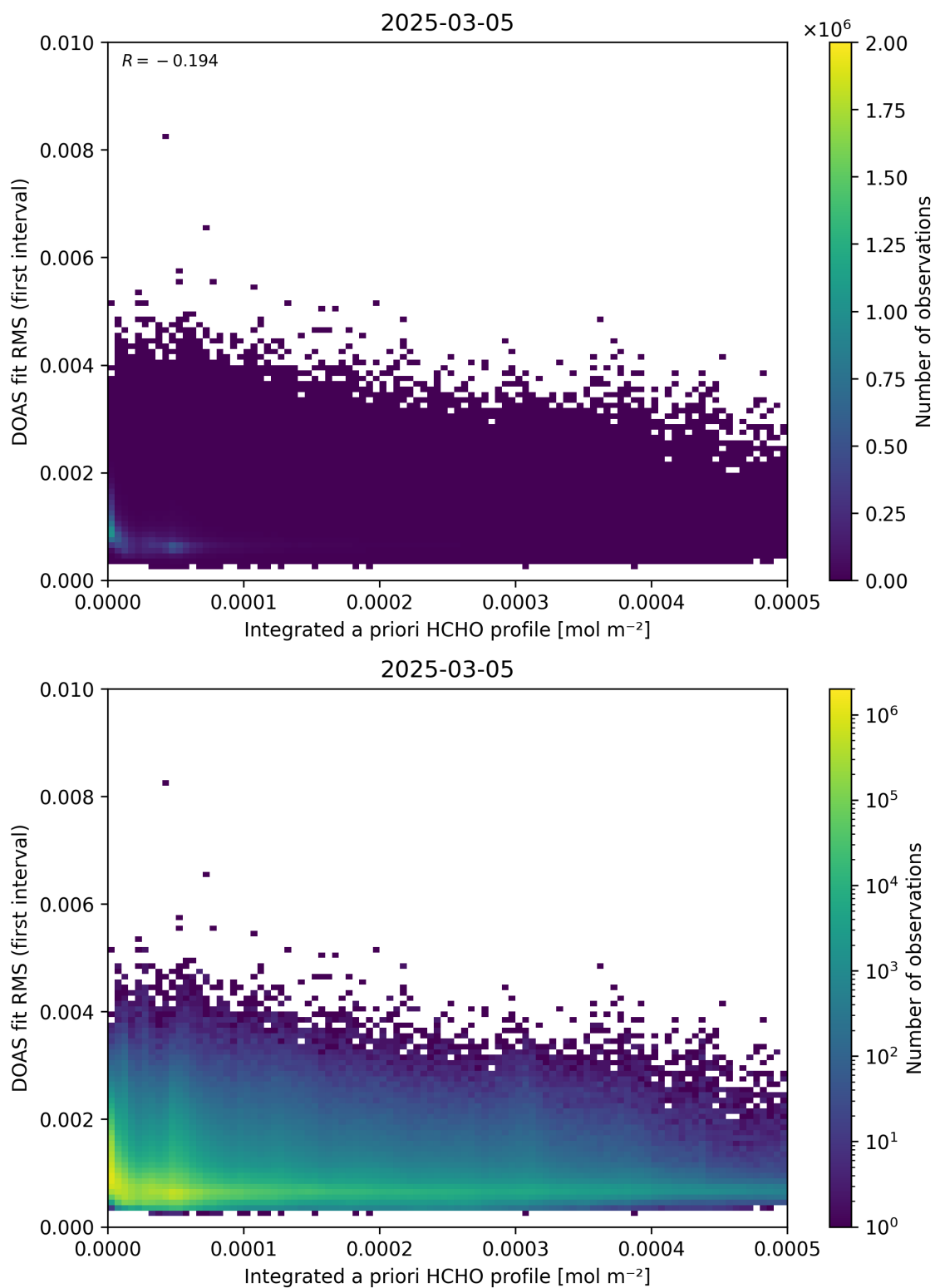
Figure 148: Scatter density plot of “Integrated a priori HCHO profile” against “DOAS fit RMS (first interval)” for 2025-03-04 to 2025-03-06.
