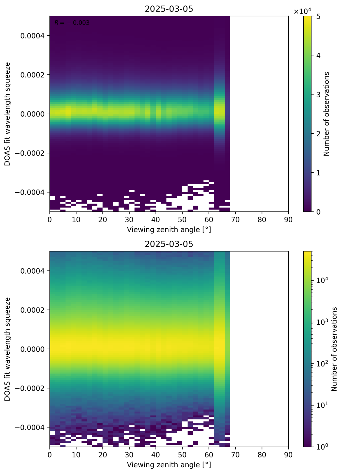
Figure 184: Scatter density plot of “Viewing zenith angle” against “DOAS fit wavelength squeeze” for 2025-03-04 to 2025-03-06.
