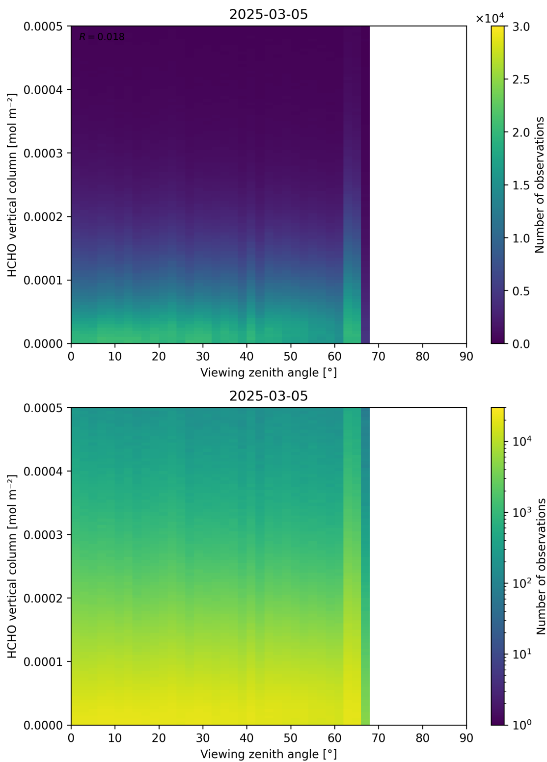
Figure 192: Scatter density plot of “Viewing zenith angle” against “HCHO vertical column” for 2025-03-04 to 2025-03-06.
