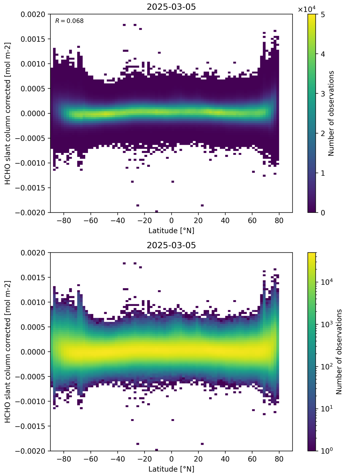
Figure 157: Scatter density plot of “Latitude” against “HCHO slant column corrected” for 2025-03-04 to 2025-03-06.
