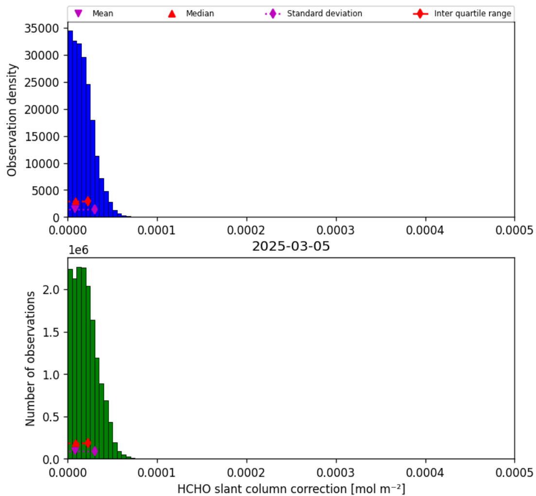
Figure 47: Histogram of “HCHO slant column correction” for 2025-03-04 to 2025-03-06
