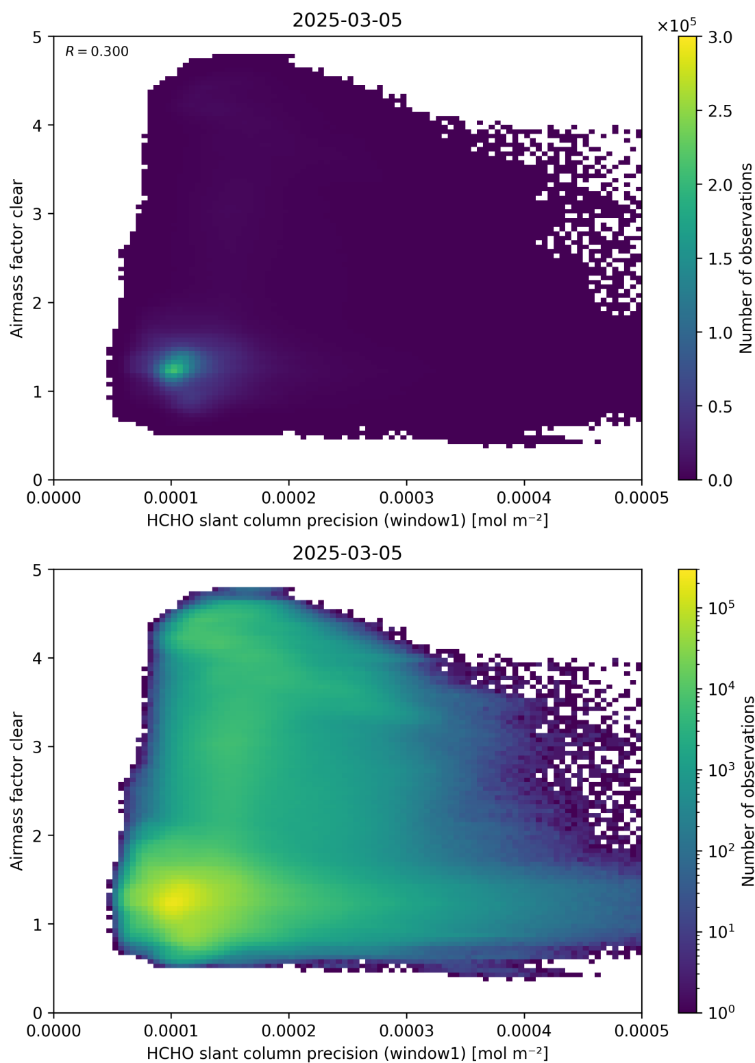
Figure 91: Scatter density plot of “HCHO slant column precision (window1)” against “Airmass factor clear” for 2025-03-04 to 2025-03-06.
