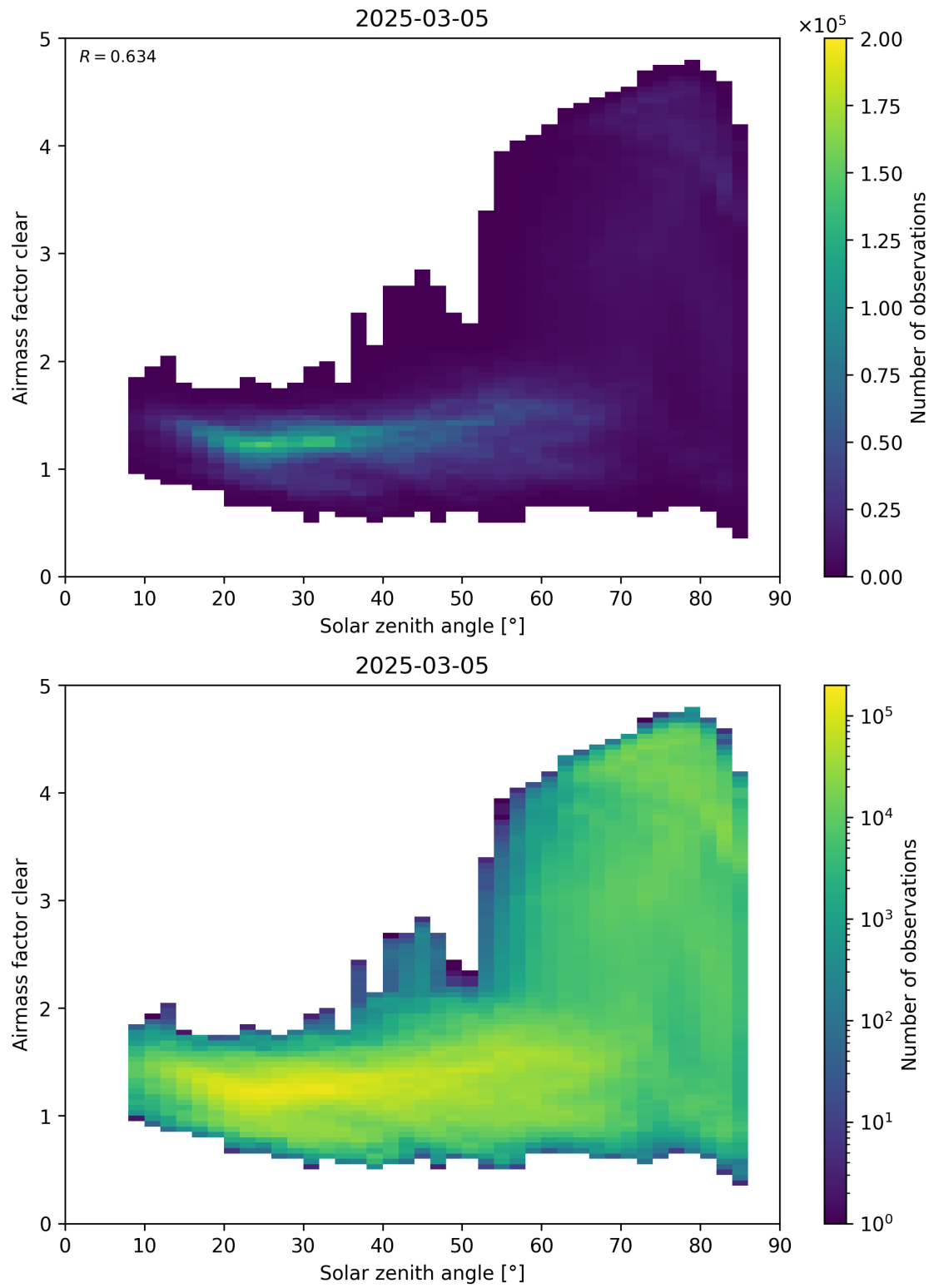
Figure 170: Scatter density plot of “Solar zenith angle” against “Airmass factor clear” for 2025-03-04 to 2025-03-06.
