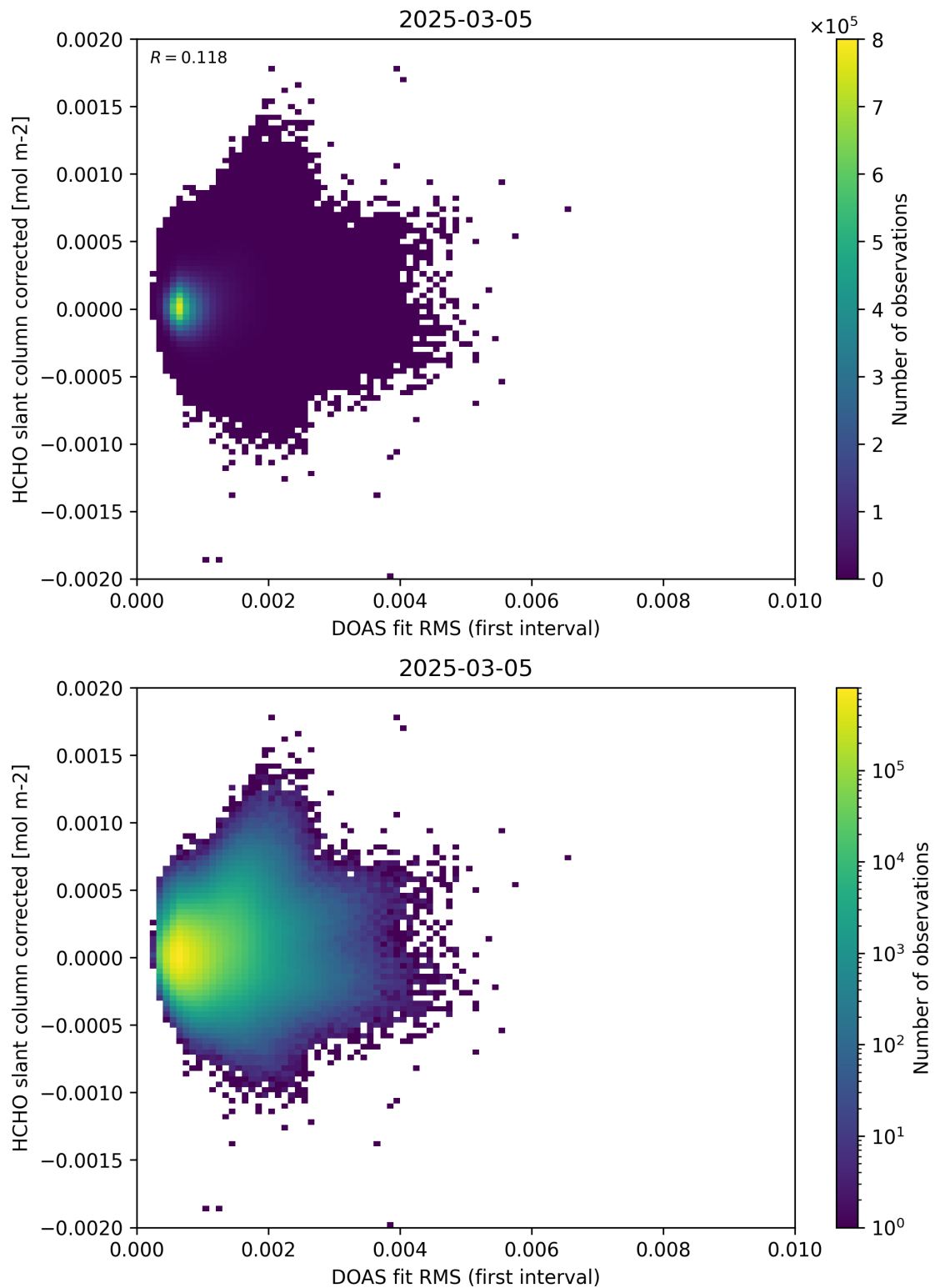
Figure 62: Scatter density plot of “DOAS fit RMS (first interval)” against “HCHO slant column corrected” for 2025-03-04 to 2025-03-06.
