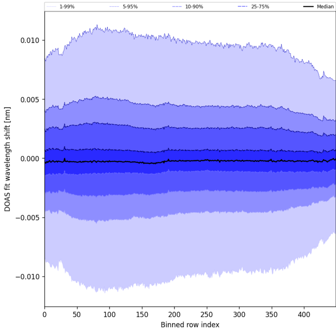
Figure 58: Along track statistics of “DOAS fit wavelength shift” for 2025-03-04 to 2025-03-06
