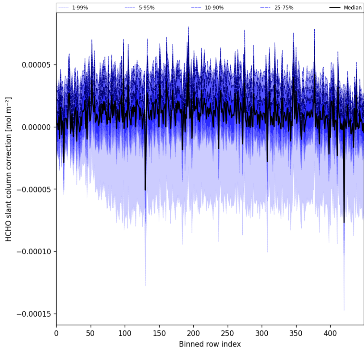
Figure 61: Along track statistics of “HCHO slant column correction” for 2025-03-04 to 2025-03-06
