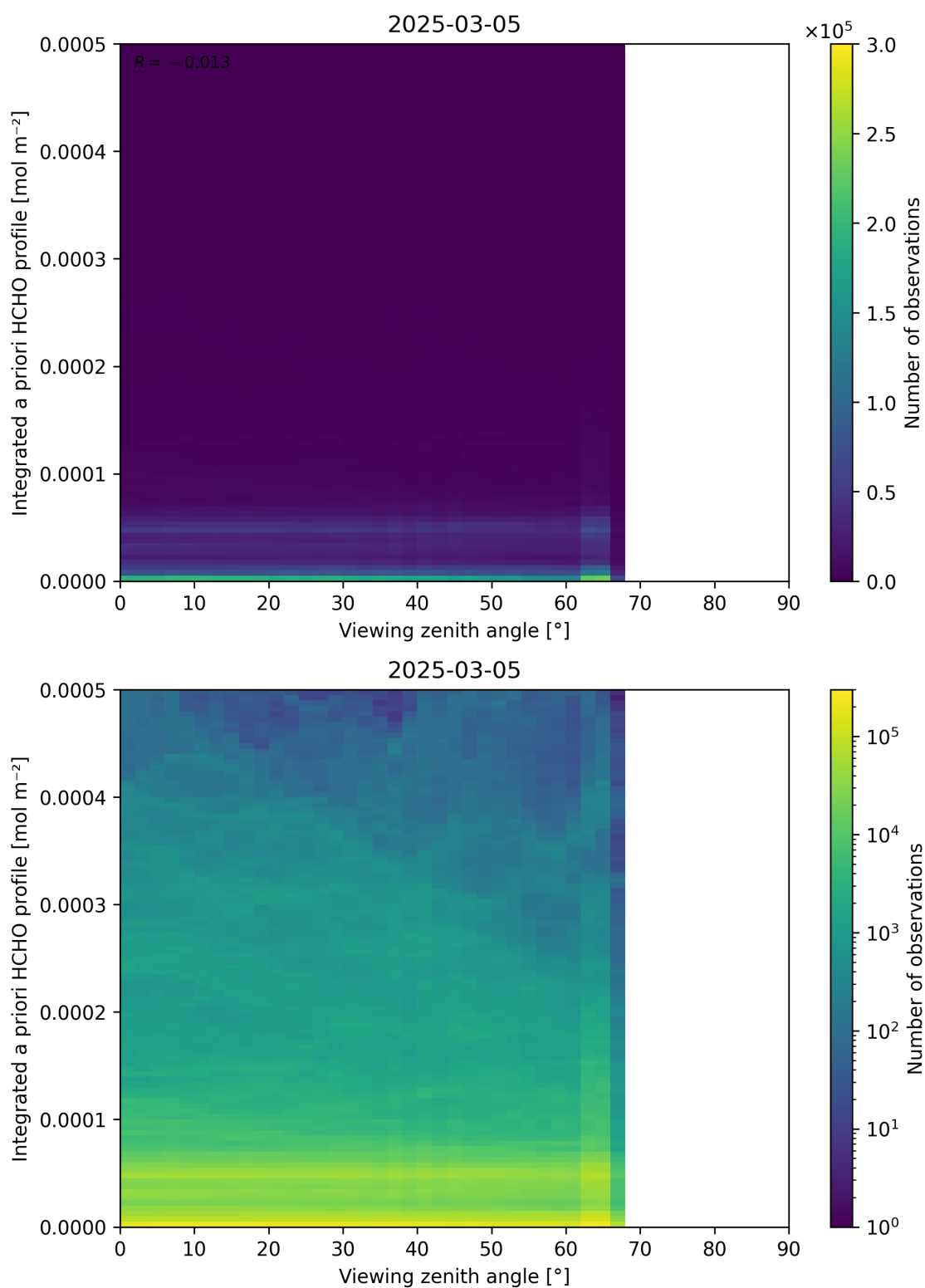
Figure 195: Scatter density plot of “Viewing zenith angle” against “Integrated a priori HCHO profile” for 2025-03-04 to 2025-03-06.
