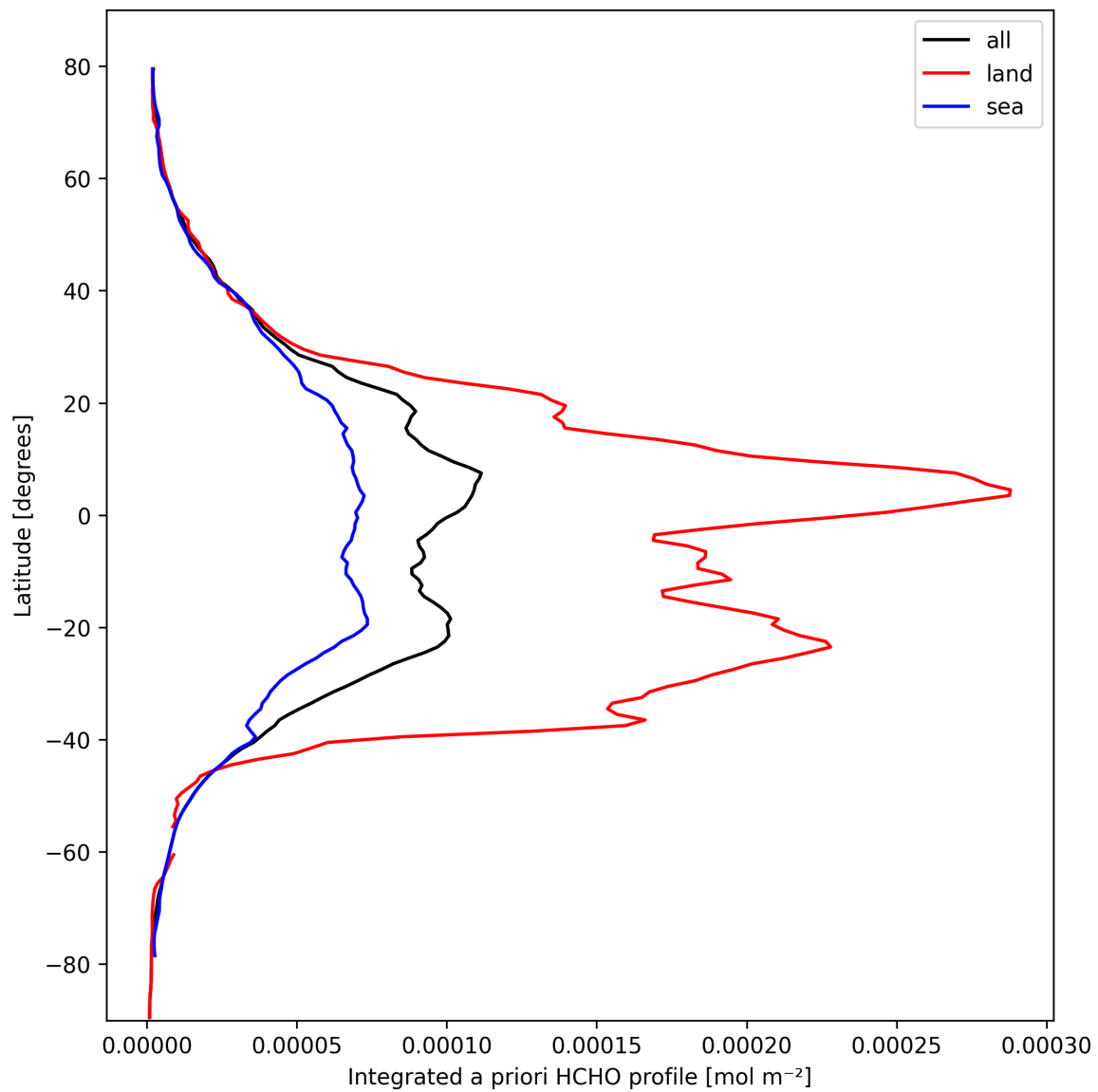
Figure 29: Zonal average of “Integrated a priori HCHO profile” for 2025-03-04 to 2025-03-06.
