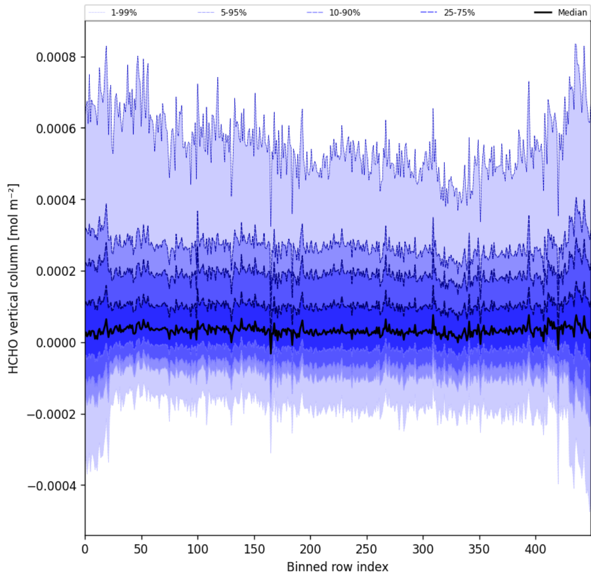
Figure 49: Along track statistics of “HCHO vertical column” for 2025-03-04 to 2025-03-06
