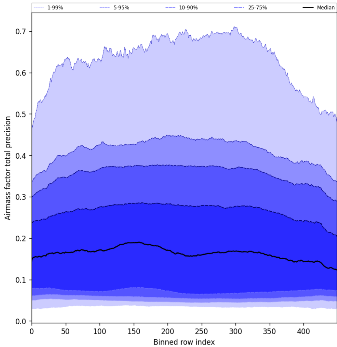
Figure 55: Along track statistics of “Airmass factor total precision” for 2025-03-04 to 2025-03-06
