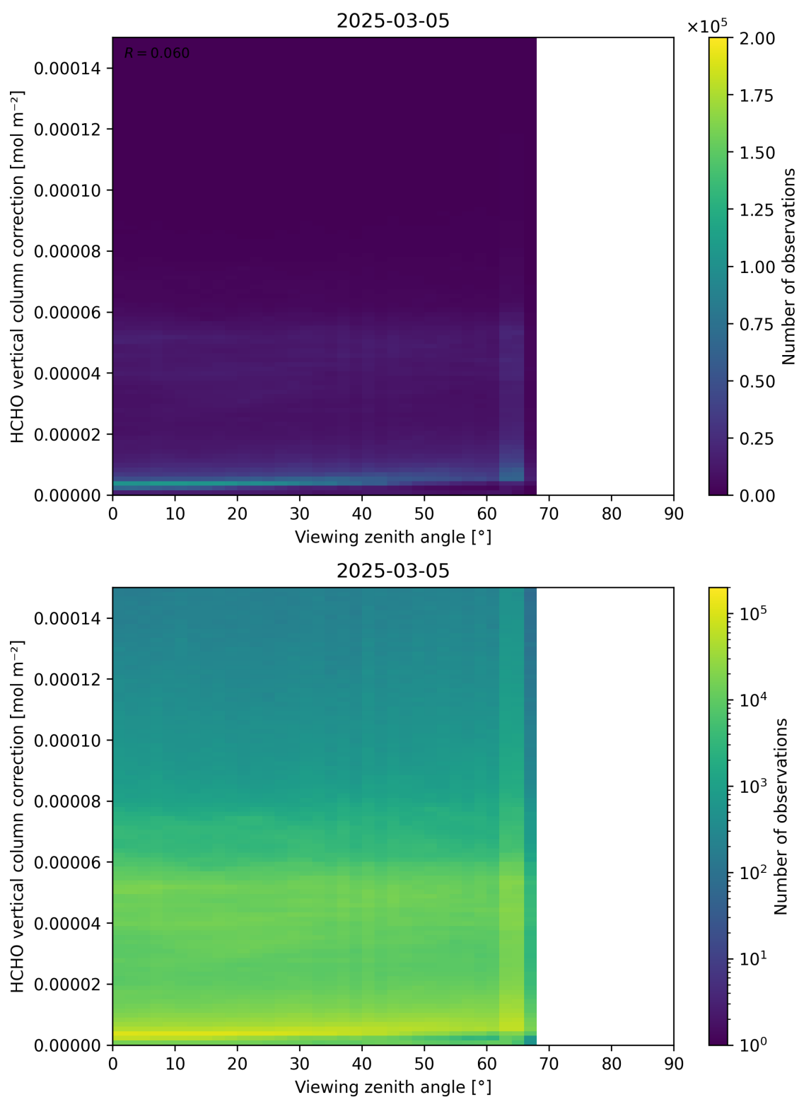
Figure 193: Scatter density plot of “Viewing zenith angle” against “HCHO vertical column correction” for 2025-03-04 to 2025-03-06.
