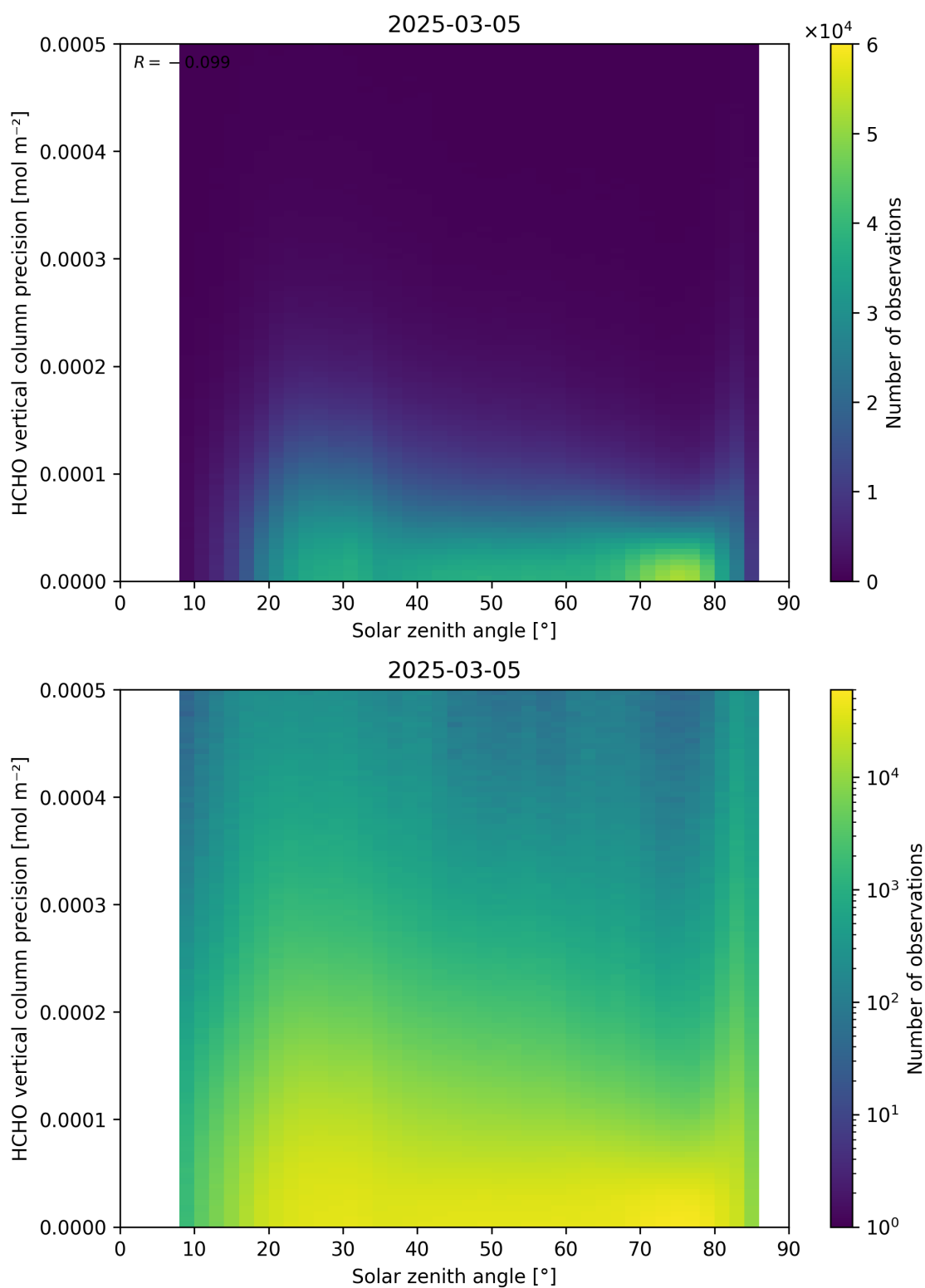
Figure 179: Scatter density plot of “Solar zenith angle” against “HCHO vertical column precision” for 2025-03-04 to 2025-03-06.
