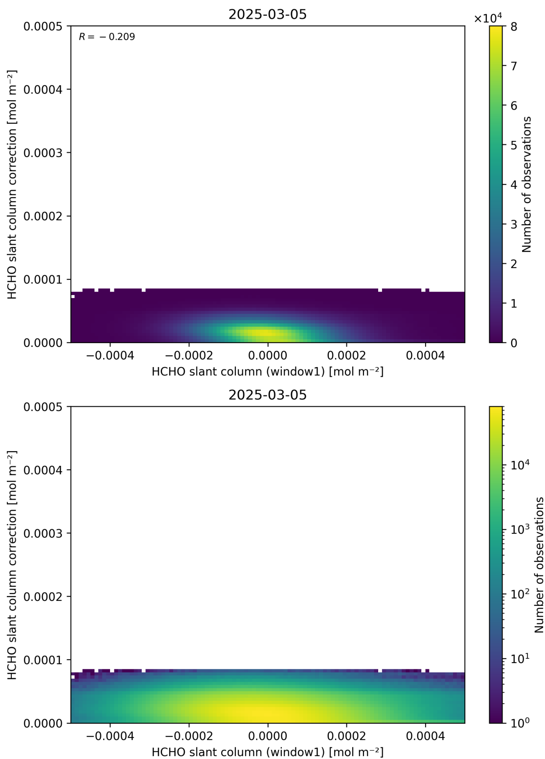
Figure 83: Scatter density plot of “HCHO slant column (window1)” against “HCHO slant column correction” for 2025-03-04 to 2025-03-06.
