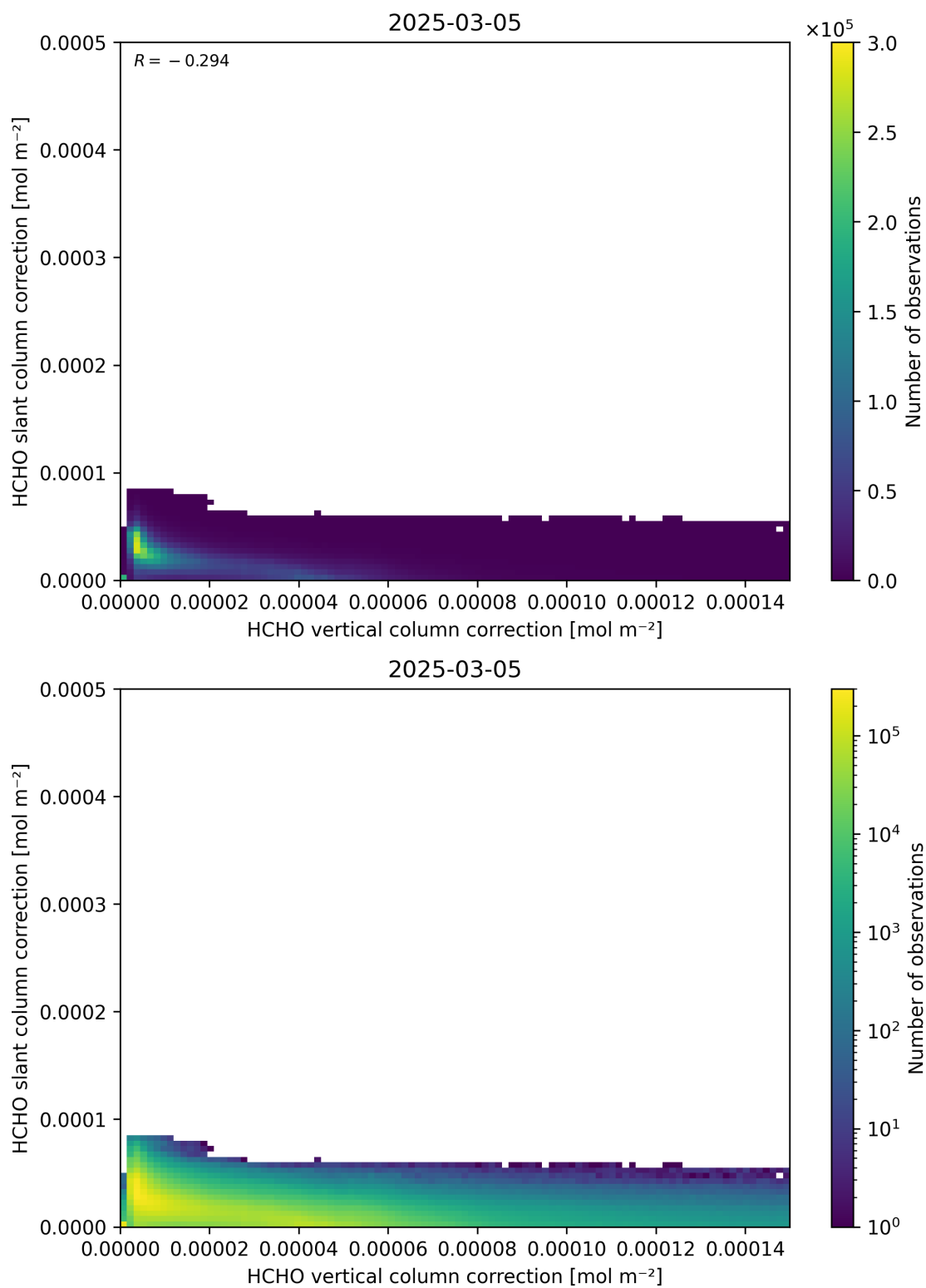
Figure 117: Scatter density plot of “HCHO vertical column correction” against “HCHO slant column correction” for 2025-03-04 to 2025-03-06.
