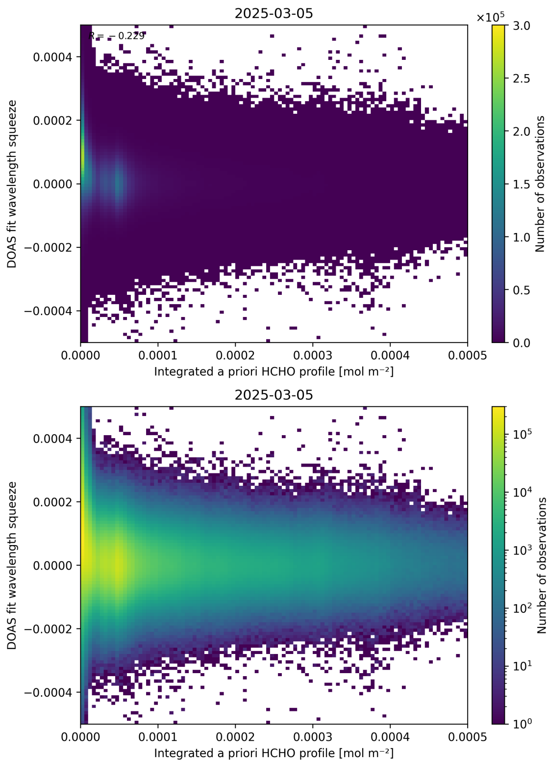
Figure 150: Scatter density plot of “Integrated a priori HCHO profile” against “DOAS fit wavelength squeeze” for 2025-03-04 to 2025-03-06.
