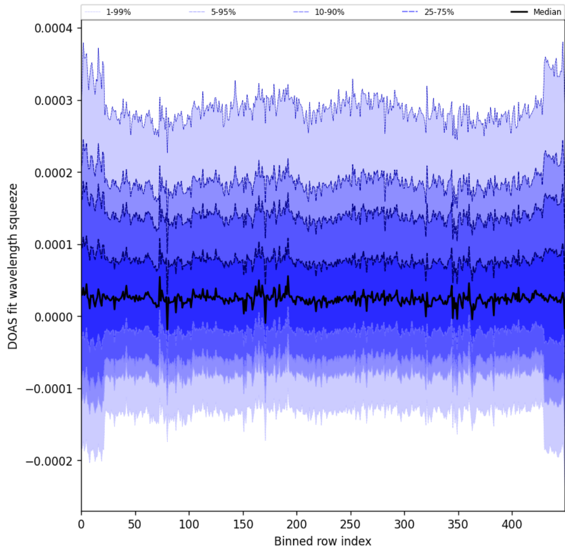
Figure 59: Along track statistics of “DOAS fit wavelength squeeze” for 2025-03-04 to 2025-03-06
