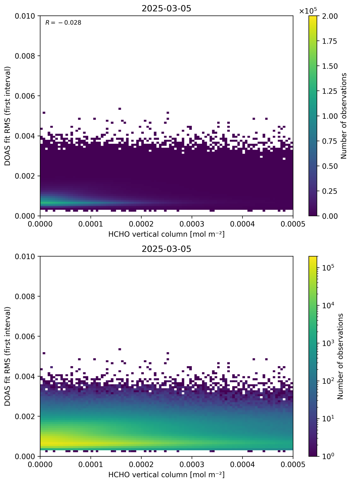
Figure 123: Scatter density plot of “HCHO vertical column” against “DOAS fit RMS (first interval)” for 2025-03-04 to 2025-03-06.
