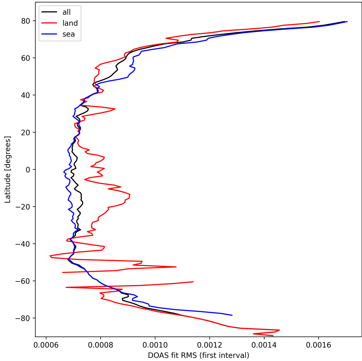
Figure 32: Zonal average of “DOAS fit RMS (first interval)” for 2025-03-04 to 2025-03-06.
