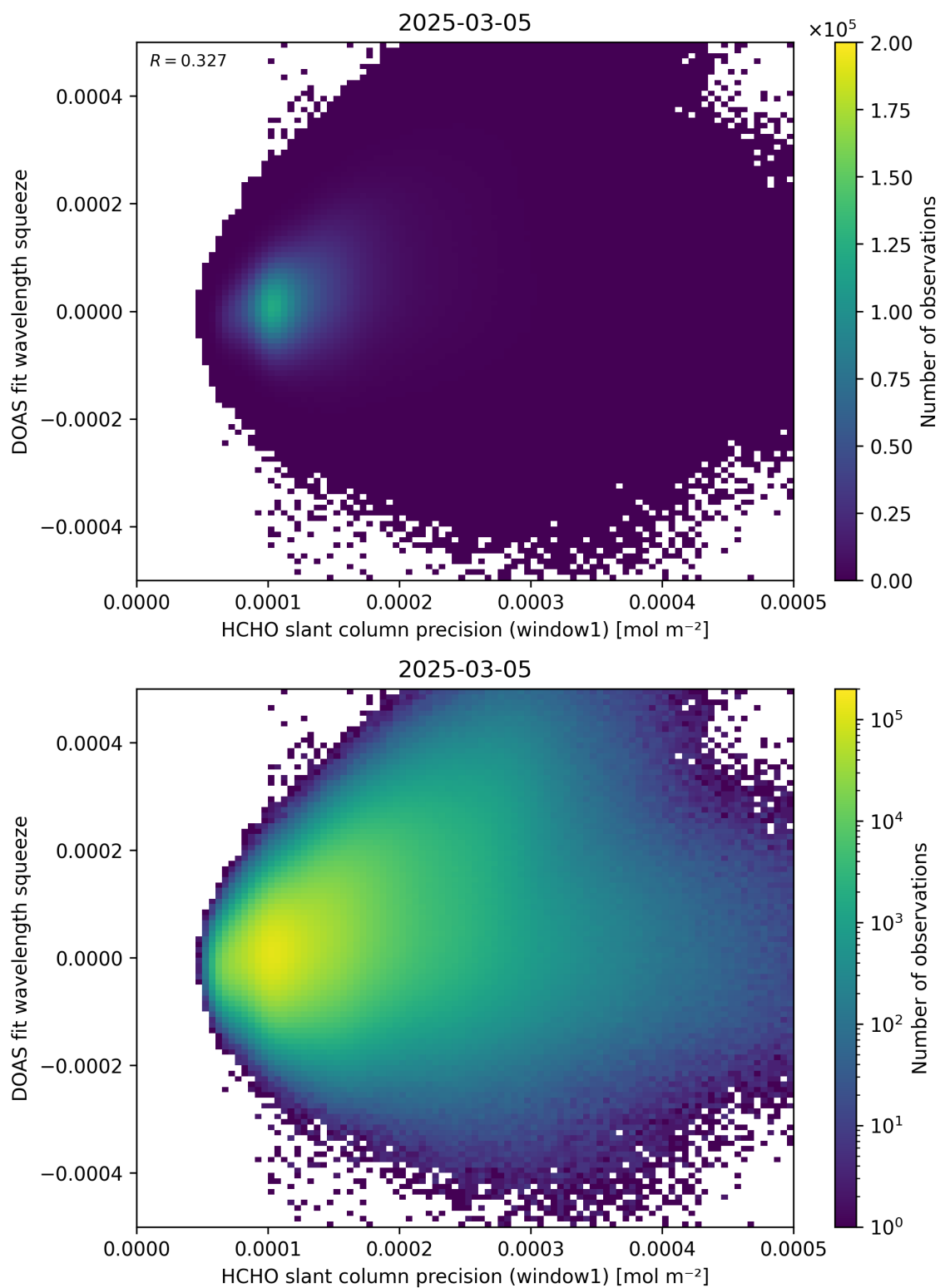
Figure 90: Scatter density plot of “HCHO slant column precision (window1)” against “DOAS fit wavelength squeeze” for 2025-03-04 to 2025-03-06.
