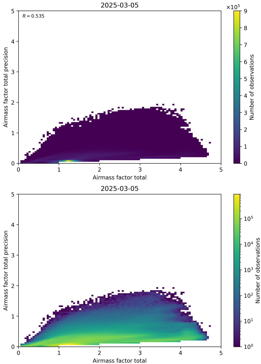
Figure 103: Scatter density plot of “Airmass factor total” against “Airmass factor total precision” for 2025-03-04 to 2025-03-06.
