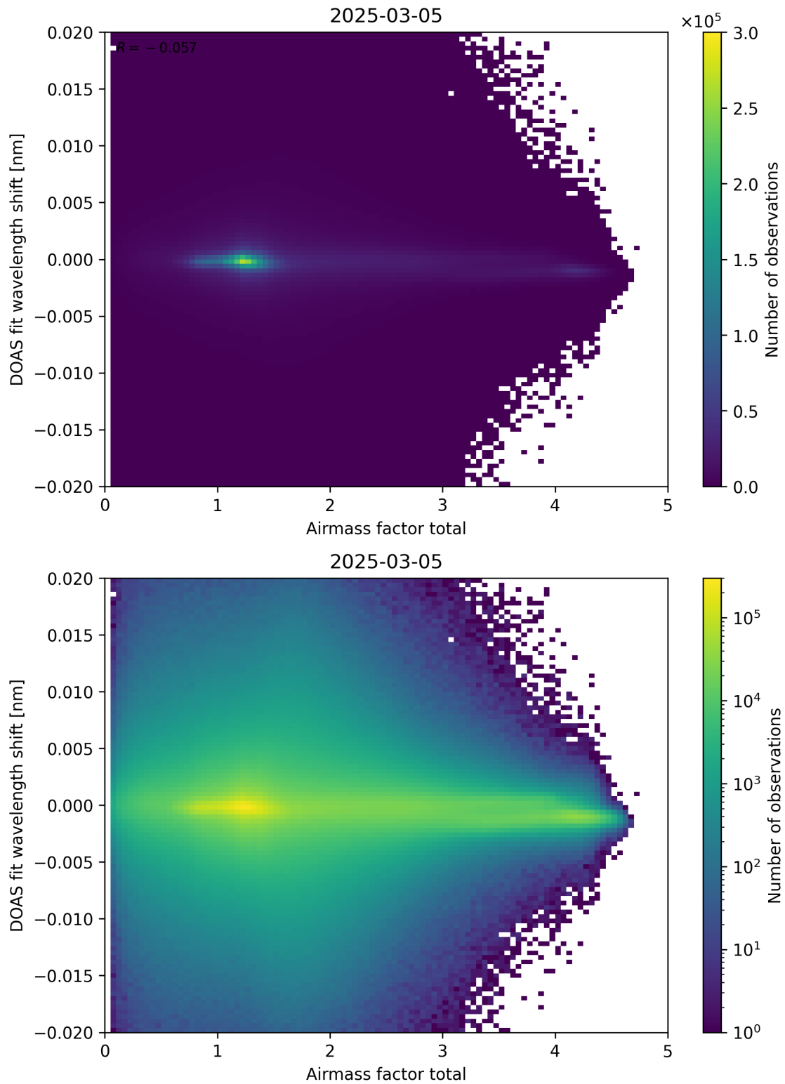
Figure 98: Scatter density plot of “Airmass factor total” against “DOAS fit wavelength shift” for 2025-03-04 to 2025-03-06.
