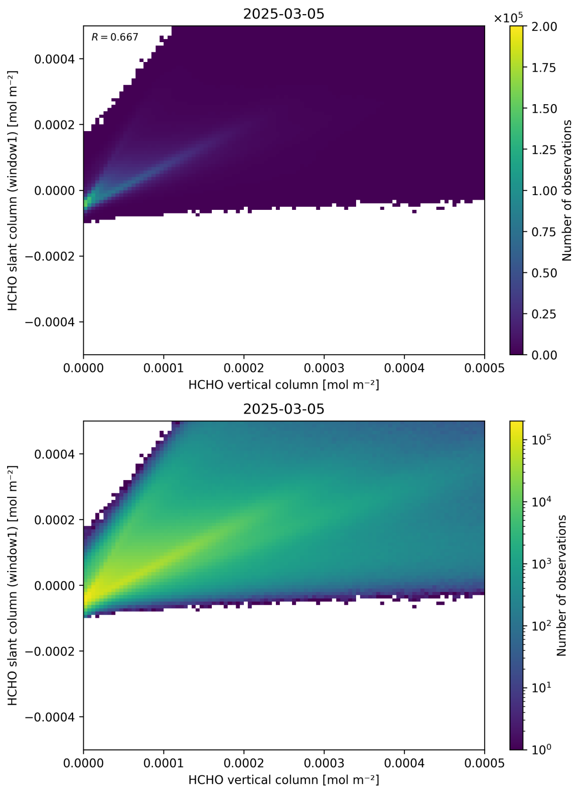
Figure 129: Scatter density plot of “HCHO vertical column” against “HCHO slant column (window1)” for 2025-03-04 to 2025-03-06.
