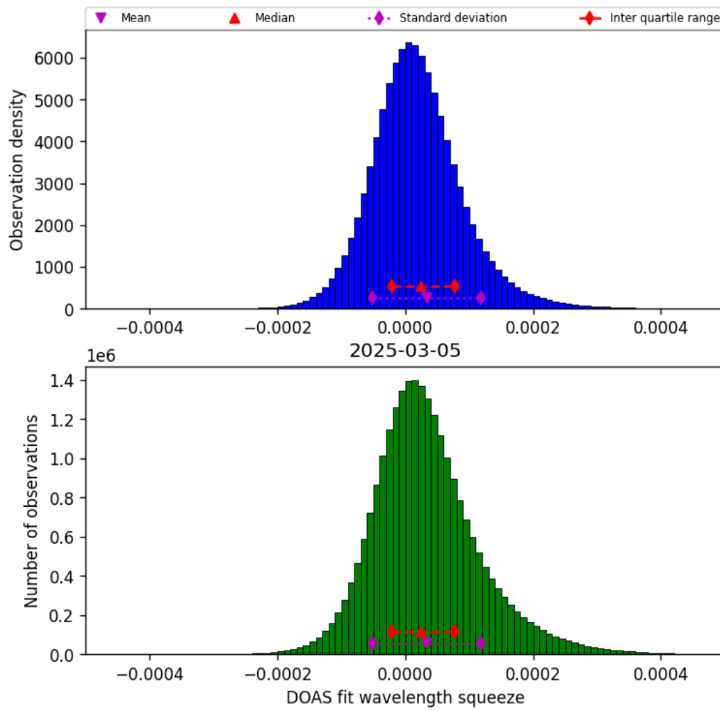
Figure 45: Histogram of “DOAS fit wavelength squeeze” for 2025-03-04 to 2025-03-06
