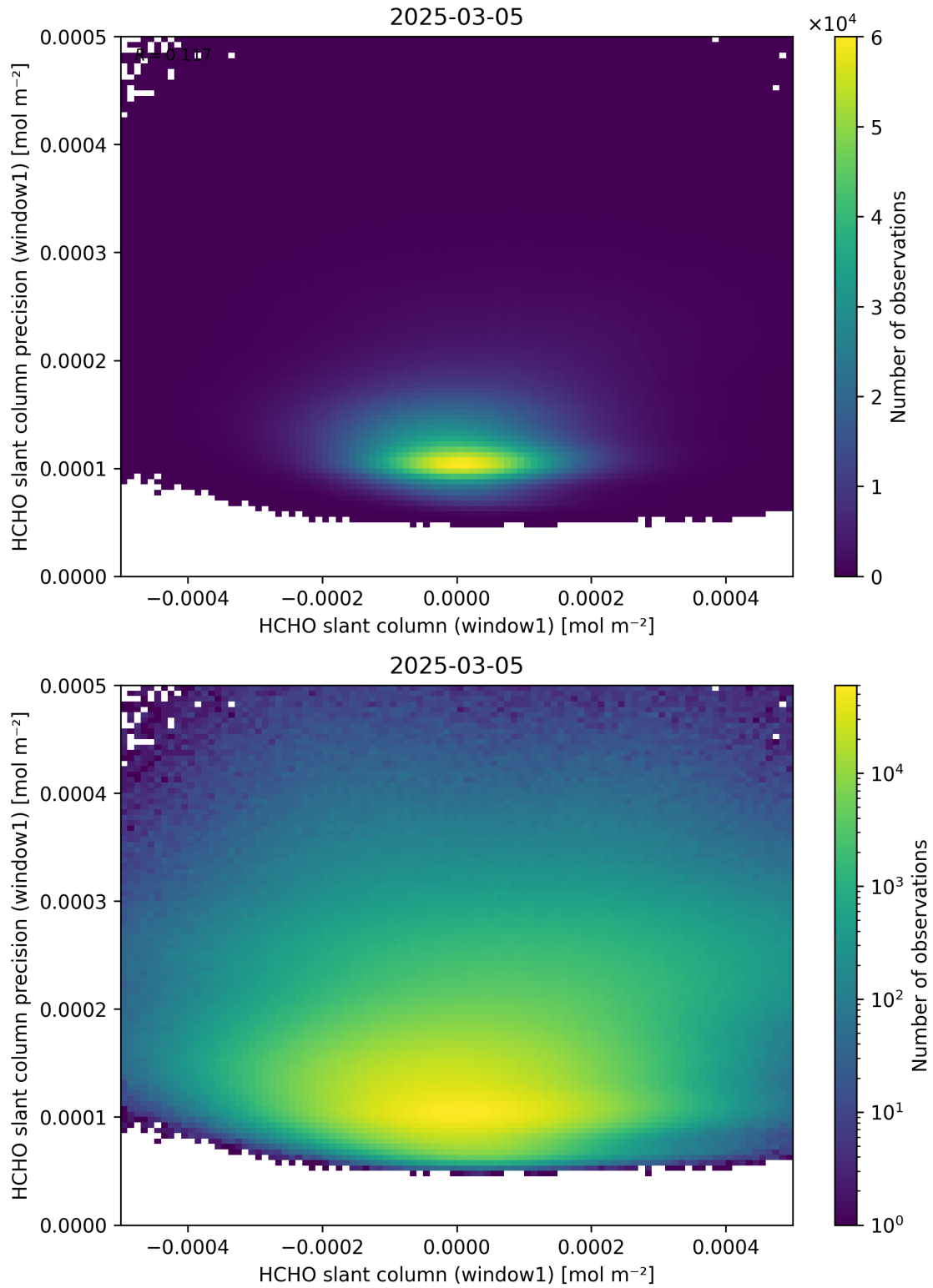
Figure 84: Scatter density plot of “HCHO slant column (window1)” against “HCHO slant column precision (window1)” for 2025-03-04 to 2025-03-06.
