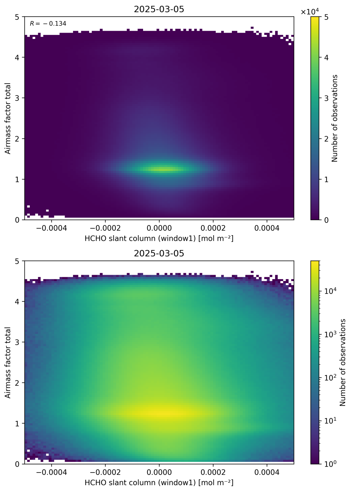
Figure 85: Scatter density plot of “HCHO slant column (window1)” against “Airmass factor total” for 2025-03-04 to 2025-03-06.
