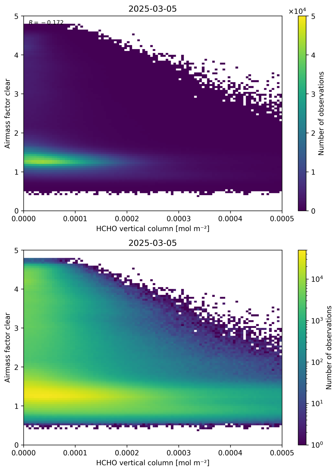
Figure 126: Scatter density plot of “HCHO vertical column” against “Airmass factor clear” for 2025-03-04 to 2025-03-06.
