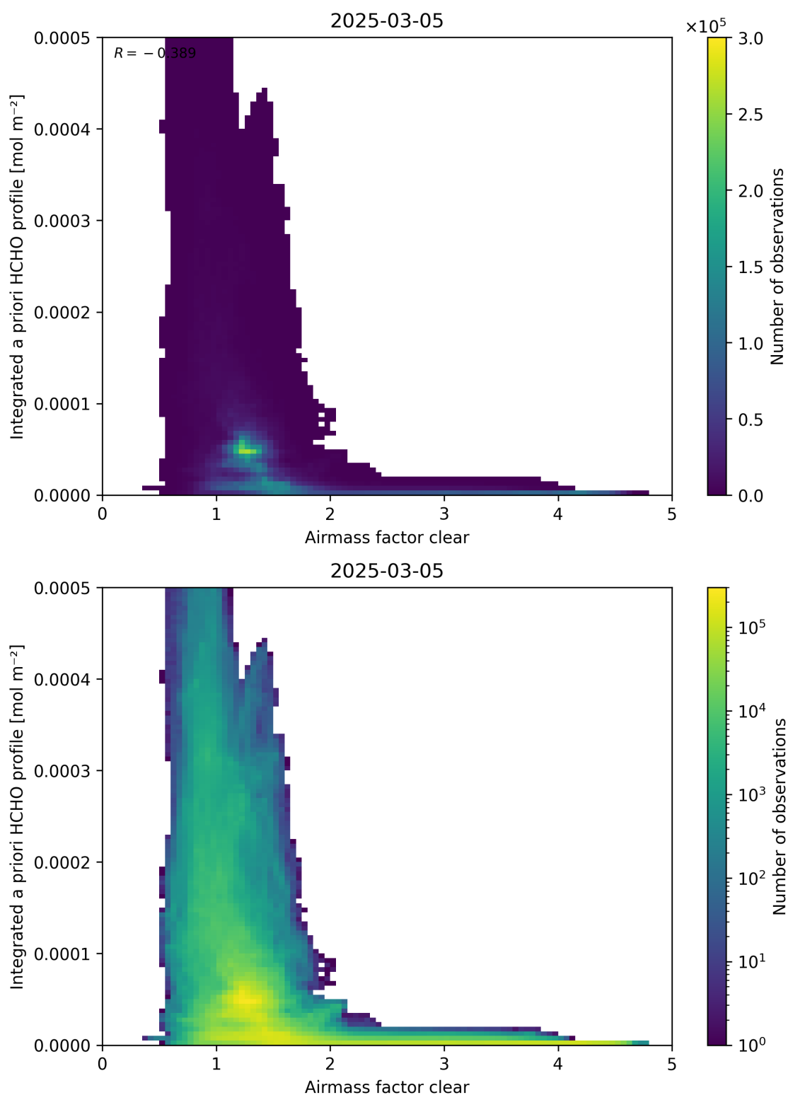
Figure 76: Scatter density plot of “Airmass factor clear” against “Integrated a priori HCHO profile” for 2025-03-04 to 2025-03-06.
