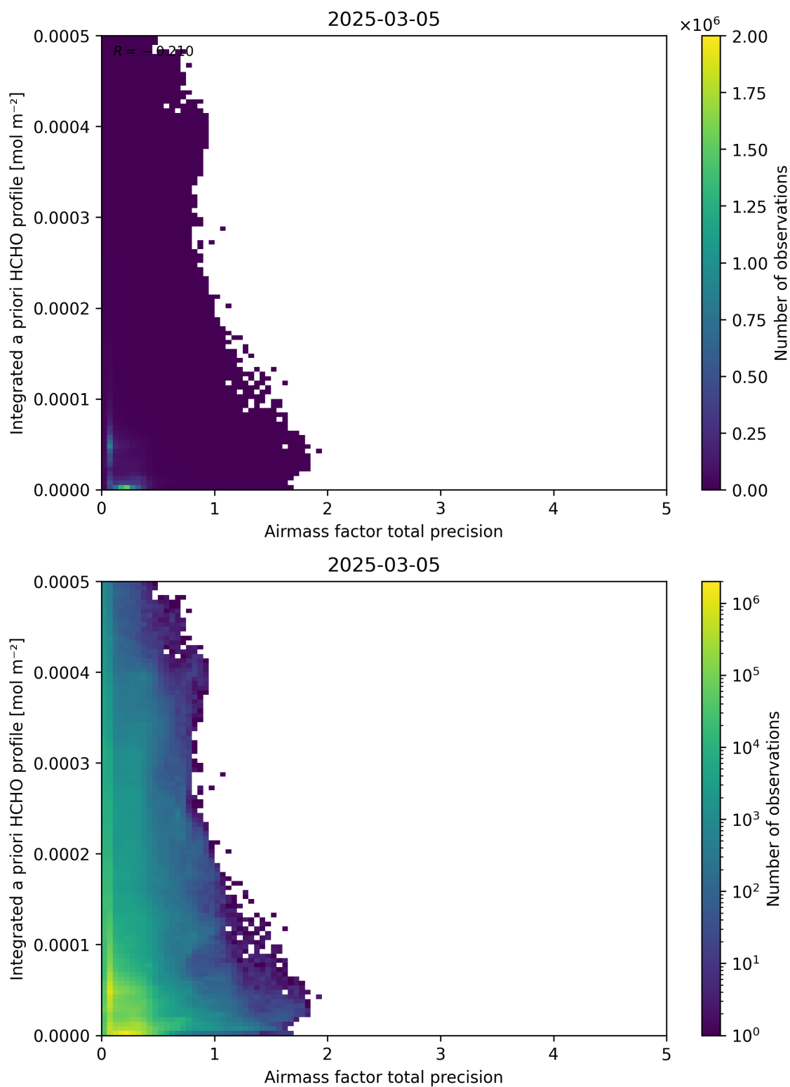
Figure 111: Scatter density plot of “Airmass factor total precision” against “Integrated a priori HCHO profile” for 2025-03-04 to 2025-03-06.
