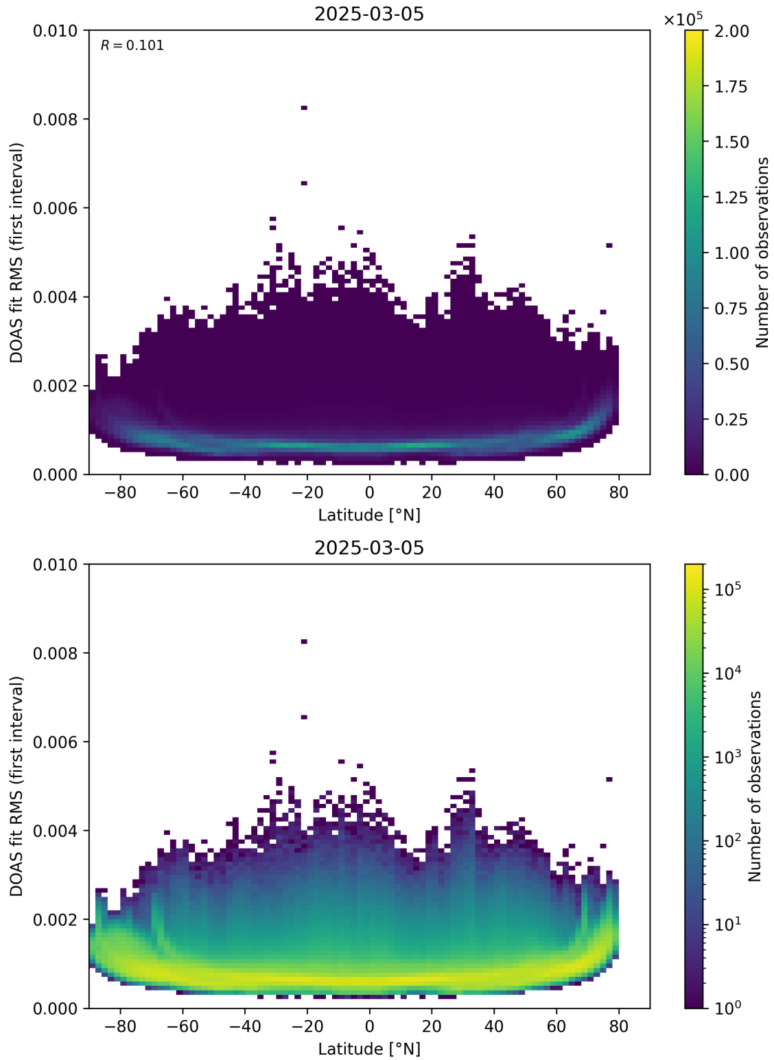
Figure 153: Scatter density plot of “Latitude” against “DOAS fit RMS (first interval)” for 2025-03-04 to 2025-03-06.
