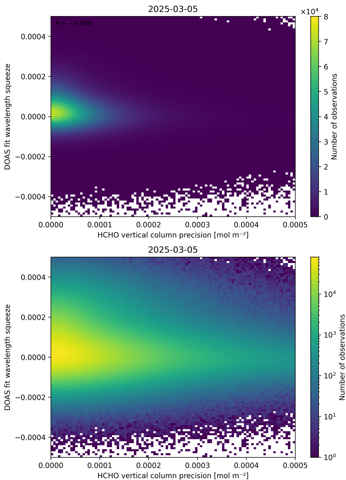
Figure 138: Scatter density plot of “HCHO vertical column precision” against “DOAS fit wavelength squeeze” for 2025-03-04 to 2025-03-06.
