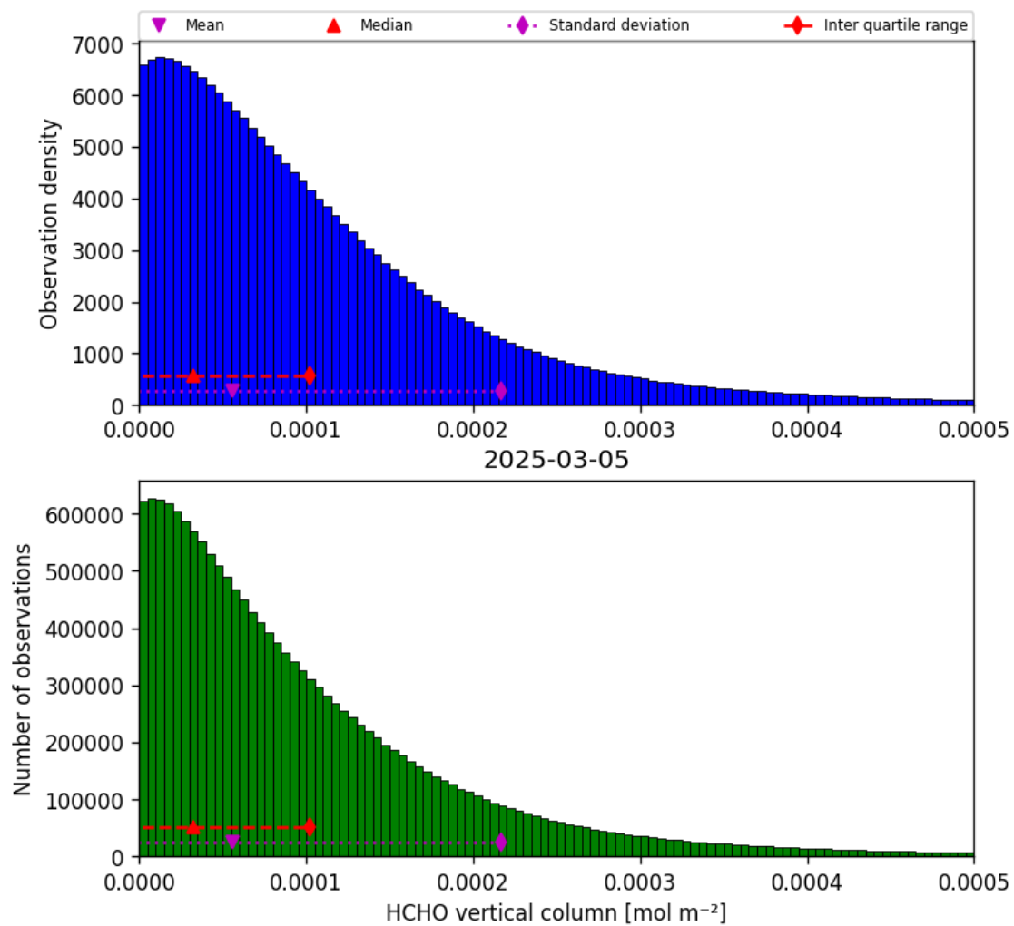
Figure 35: Histogram of “HCHO vertical column” for 2025-03-04 to 2025-03-06
