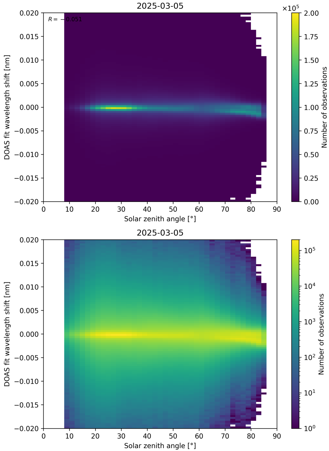
Figure 168: Scatter density plot of “Solar zenith angle” against “DOAS fit wavelength shift” for 2025-03-04 to 2025-03-06.
