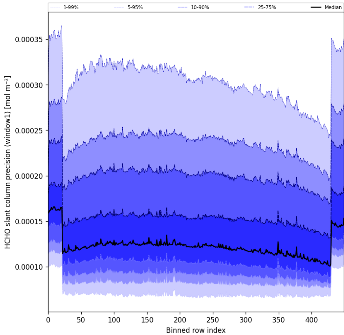
Figure 53: Along track statistics of “HCHO slant column precision (window1)” for 2025-03-04 to 2025-03-06
