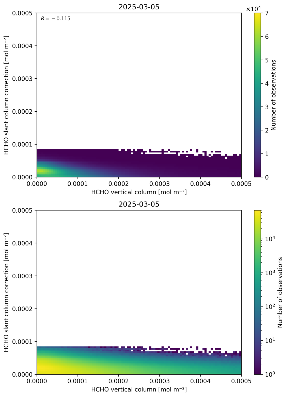
Figure 128: Scatter density plot of “HCHO vertical column” against “HCHO slant column correction” for 2025-03-04 to 2025-03-06.
