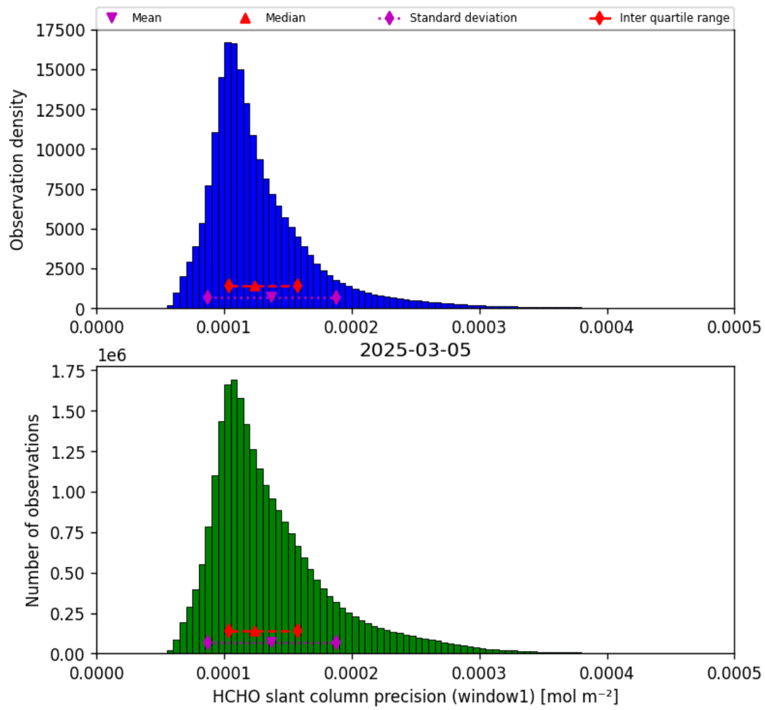
Figure 39: Histogram of “HCHO slant column precision (window1)” for 2025-03-04 to 2025-03-06
