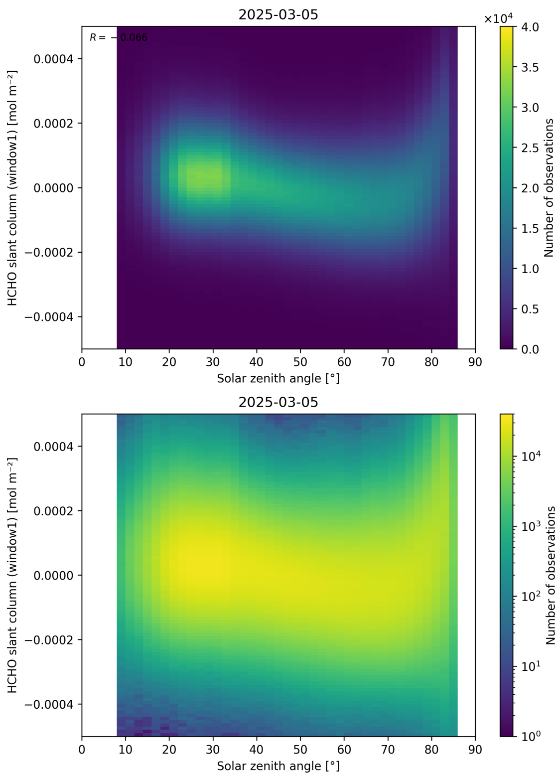
Figure 173: Scatter density plot of “Solar zenith angle” against “HCHO slant column (window1)” for 2025-03-04 to 2025-03-06.
