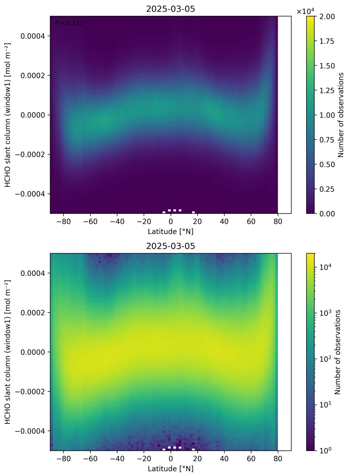
Figure 159: Scatter density plot of “Latitude” against “HCHO slant column (window1)” for 2025-03-04 to 2025-03-06.
