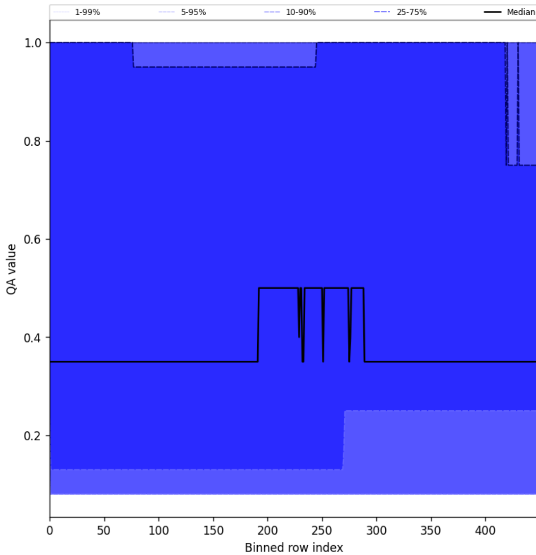
Figure 48: Along track statistics of “QA value” for 2025-03-04 to 2025-03-06
