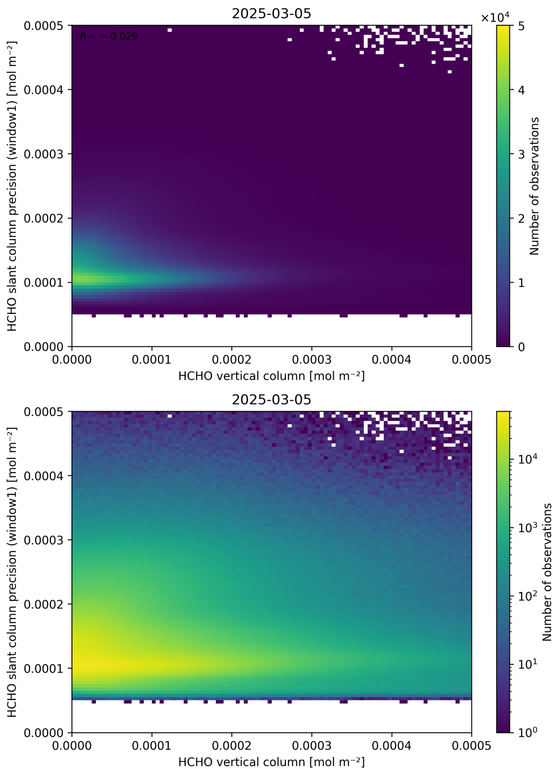
Figure 130: Scatter density plot of “HCHO vertical column” against “HCHO slant column precision (window1)” for 2025-03-04 to 2025-03-06.
