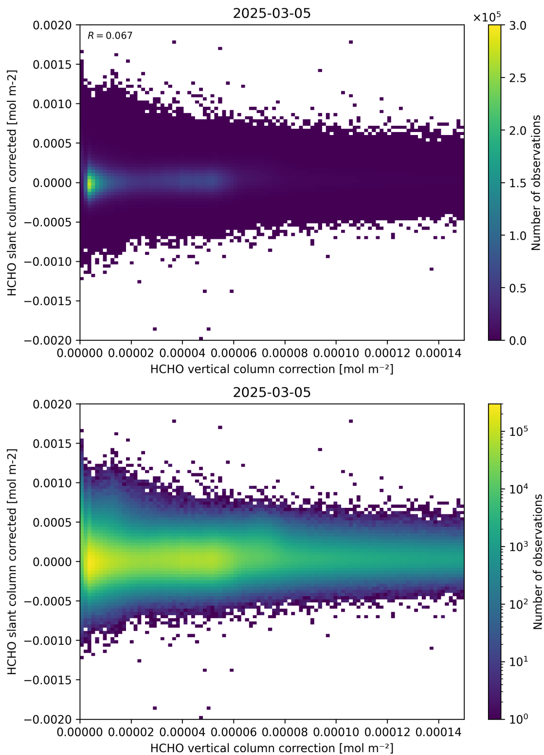
Figure 116: Scatter density plot of “HCHO vertical column correction” against “HCHO slant column corrected” for 2025-03-04 to 2025-03-06.
