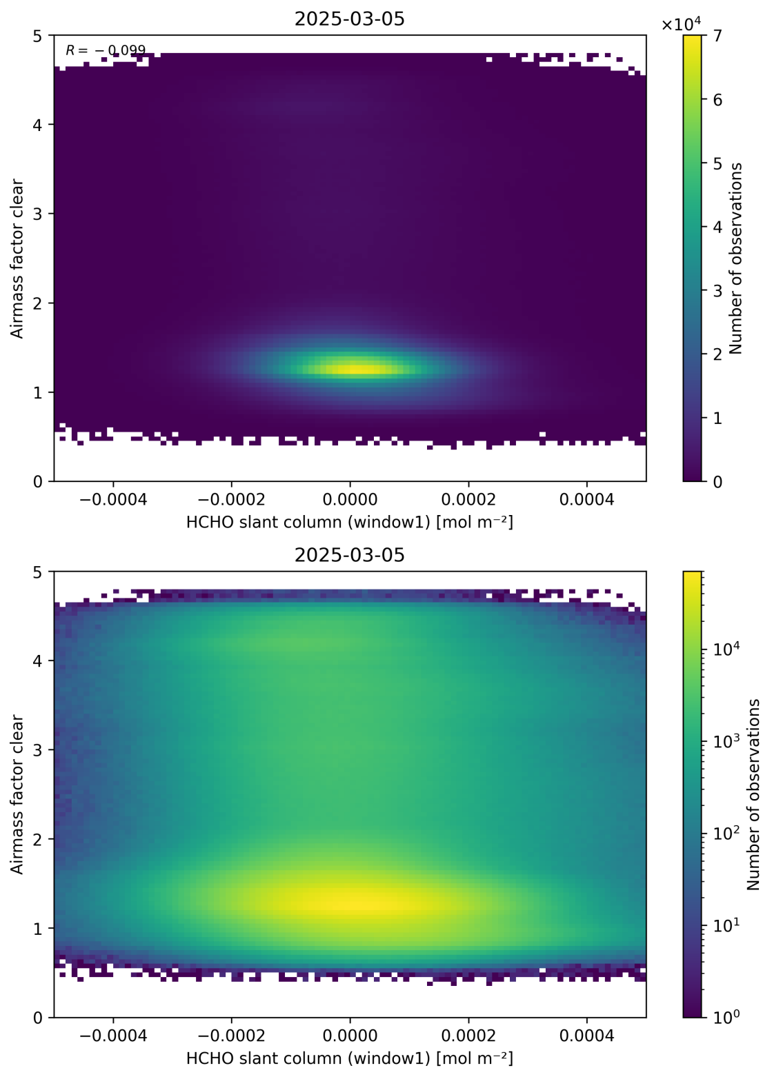
Figure 81: Scatter density plot of “HCHO slant column (window1)” against “Airmass factor clear” for 2025-03-04 to 2025-03-06.
