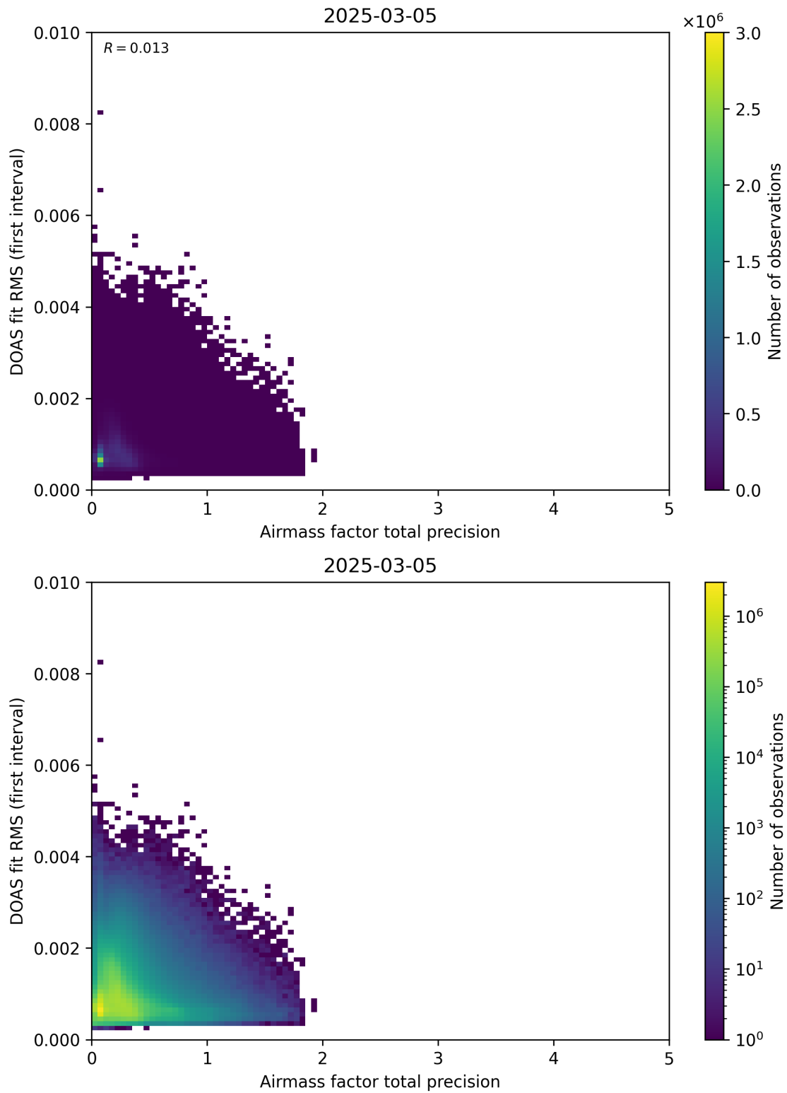
Figure 105: Scatter density plot of “Airmass factor total precision” against “DOAS fit RMS (first interval)” for 2025-03-04 to 2025-03-06.
