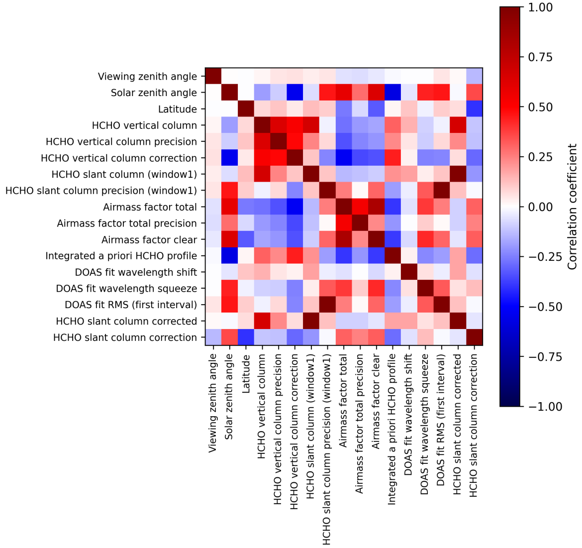
Figure 2: Map of correlation matrix for 2025-03-04 to 2025-03-06.
