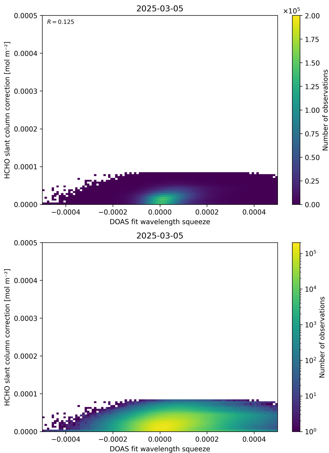
Figure 70: Scatter density plot of “DOAS fit wavelength squeeze” against “HCHO slant column correction” for 2025-03-04 to 2025-03-06.
