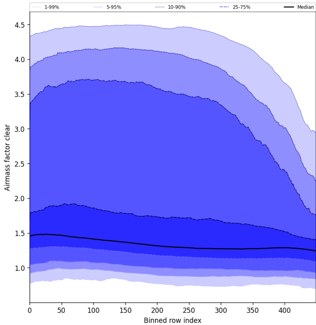
Figure 56: Along track statistics of “Airmass factor clear” for 2025-03-04 to 2025-03-06
