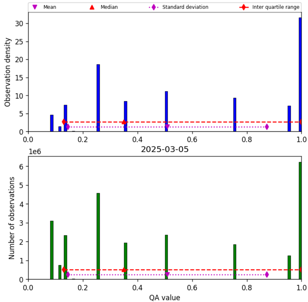
Figure 34: Histogram of “QA value” for 2025-03-04 to 2025-03-06
