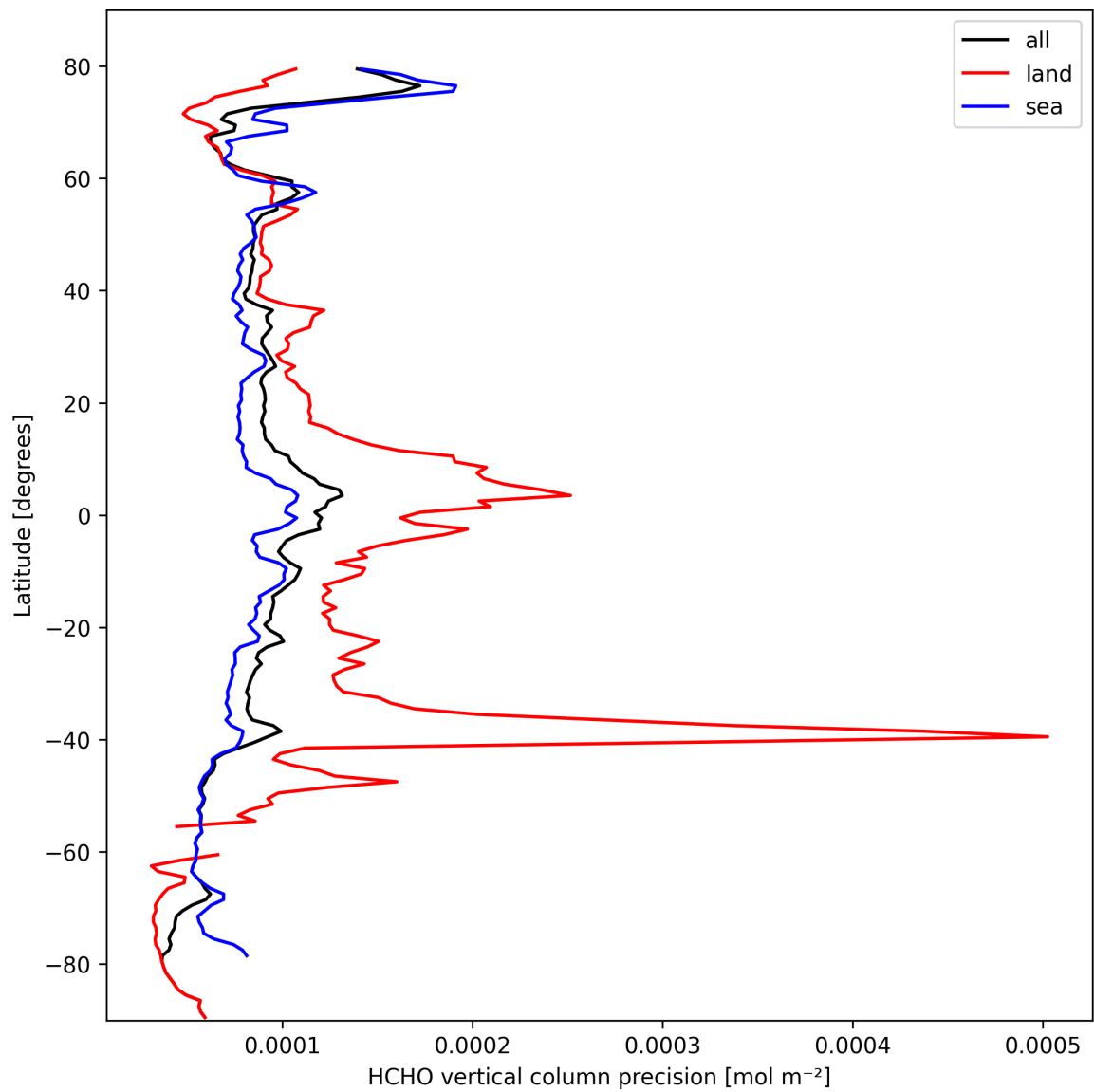
Figure 22: Zonal average of “HCHO vertical column precision” for 2025-03-04 to 2025-03-06.
