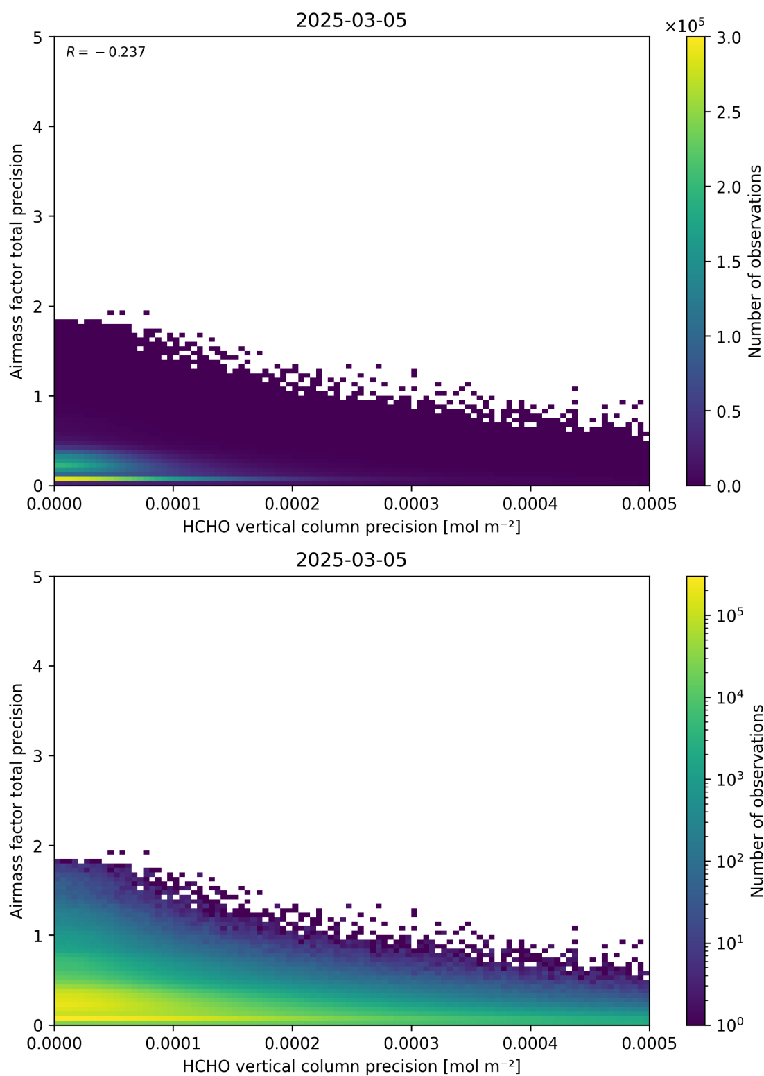
Figure 145: Scatter density plot of “HCHO vertical column precision” against “Airmass factor total precision” for 2025-03-04 to 2025-03-06.
