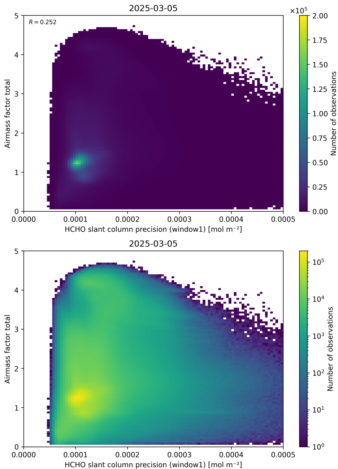
Figure 94: Scatter density plot of “HCHO slant column precision (window1)” against “Airmass factor total” for 2025-03-04 to 2025-03-06.
