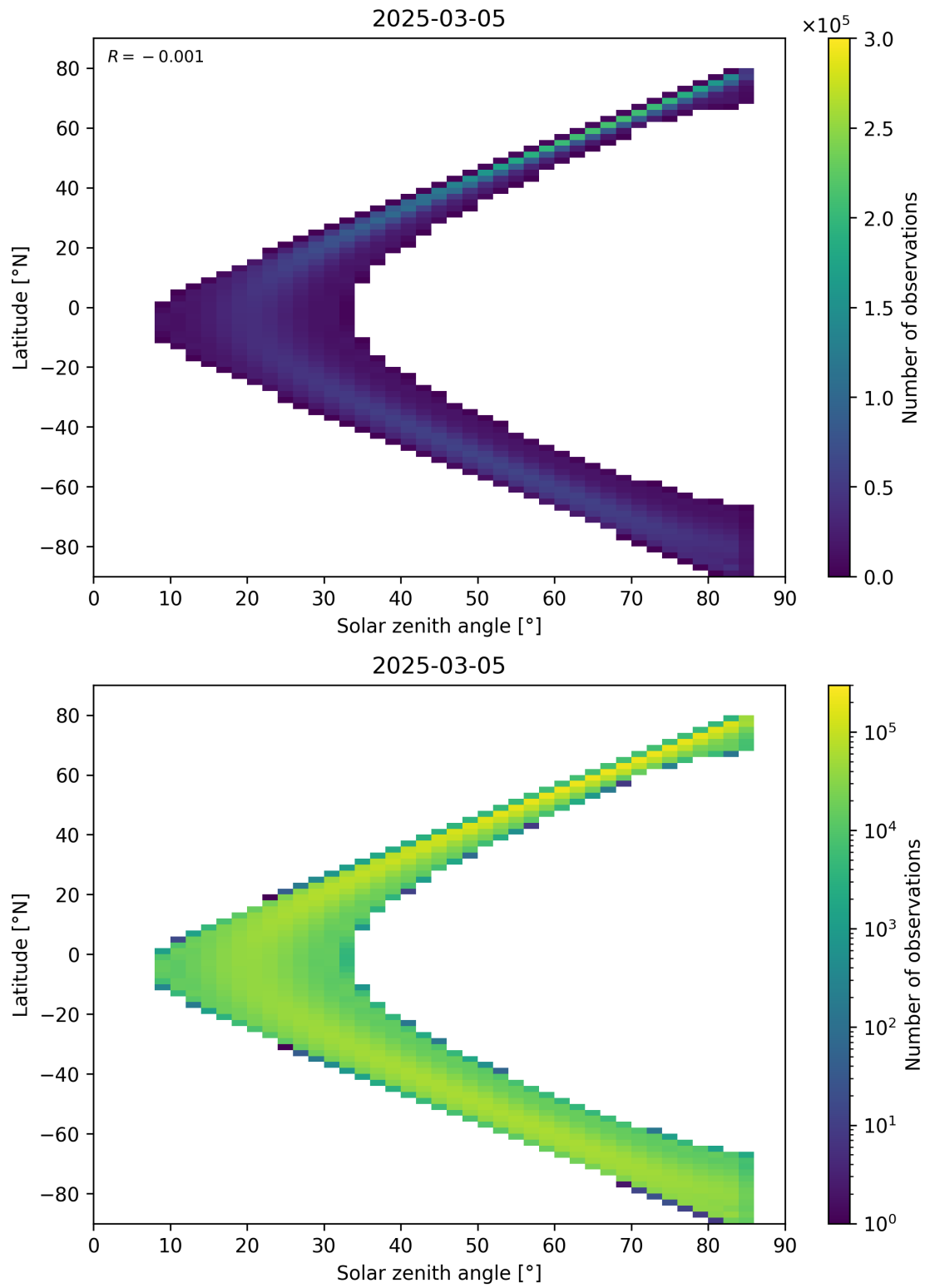
Figure 181: Scatter density plot of “Solar zenith angle” against “Latitude” for 2025-03-04 to 2025-03-06.
