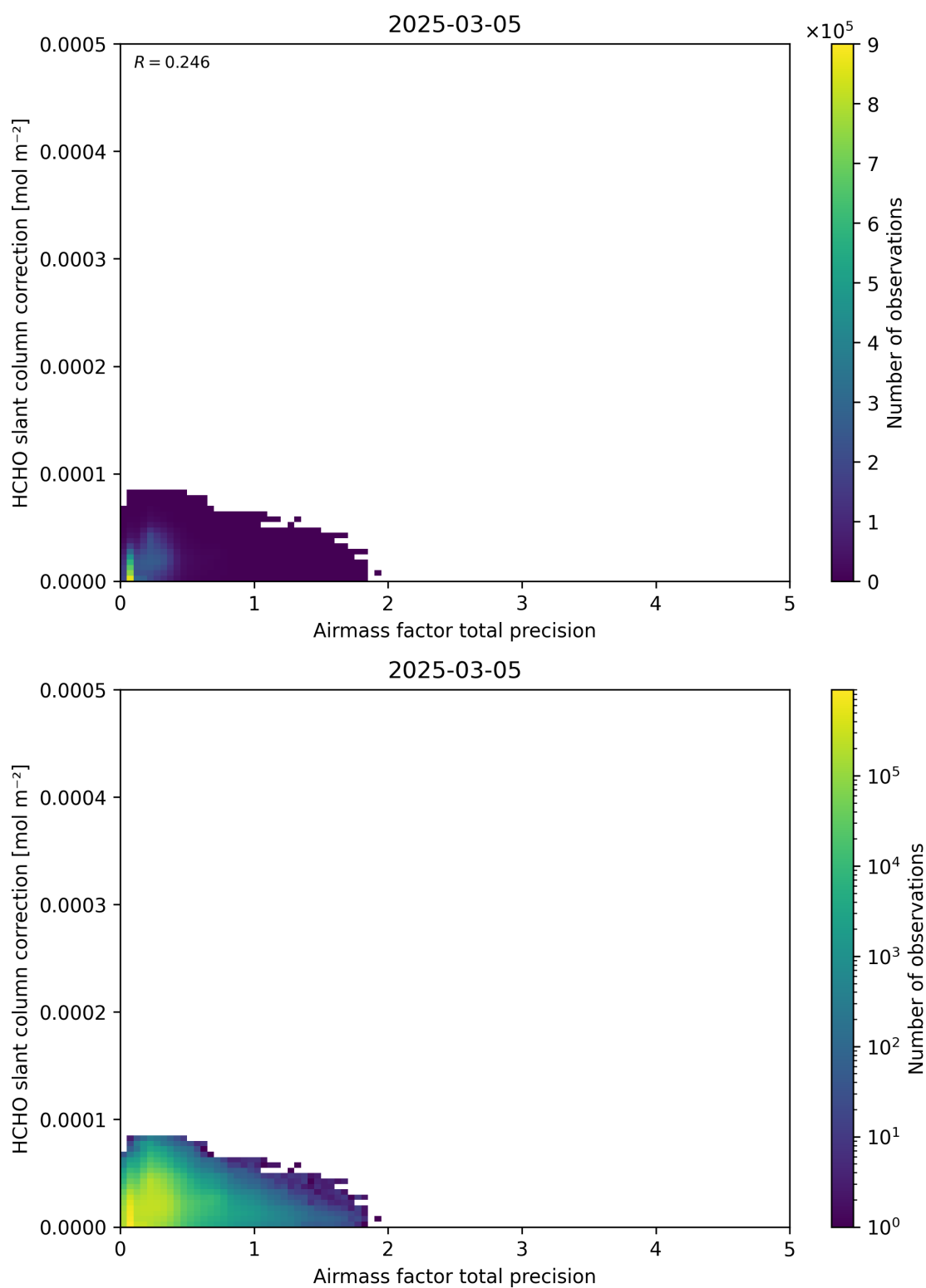
Figure 110: Scatter density plot of “Airmass factor total precision” against “HCHO slant column correction” for 2025-03-04 to 2025-03-06.
