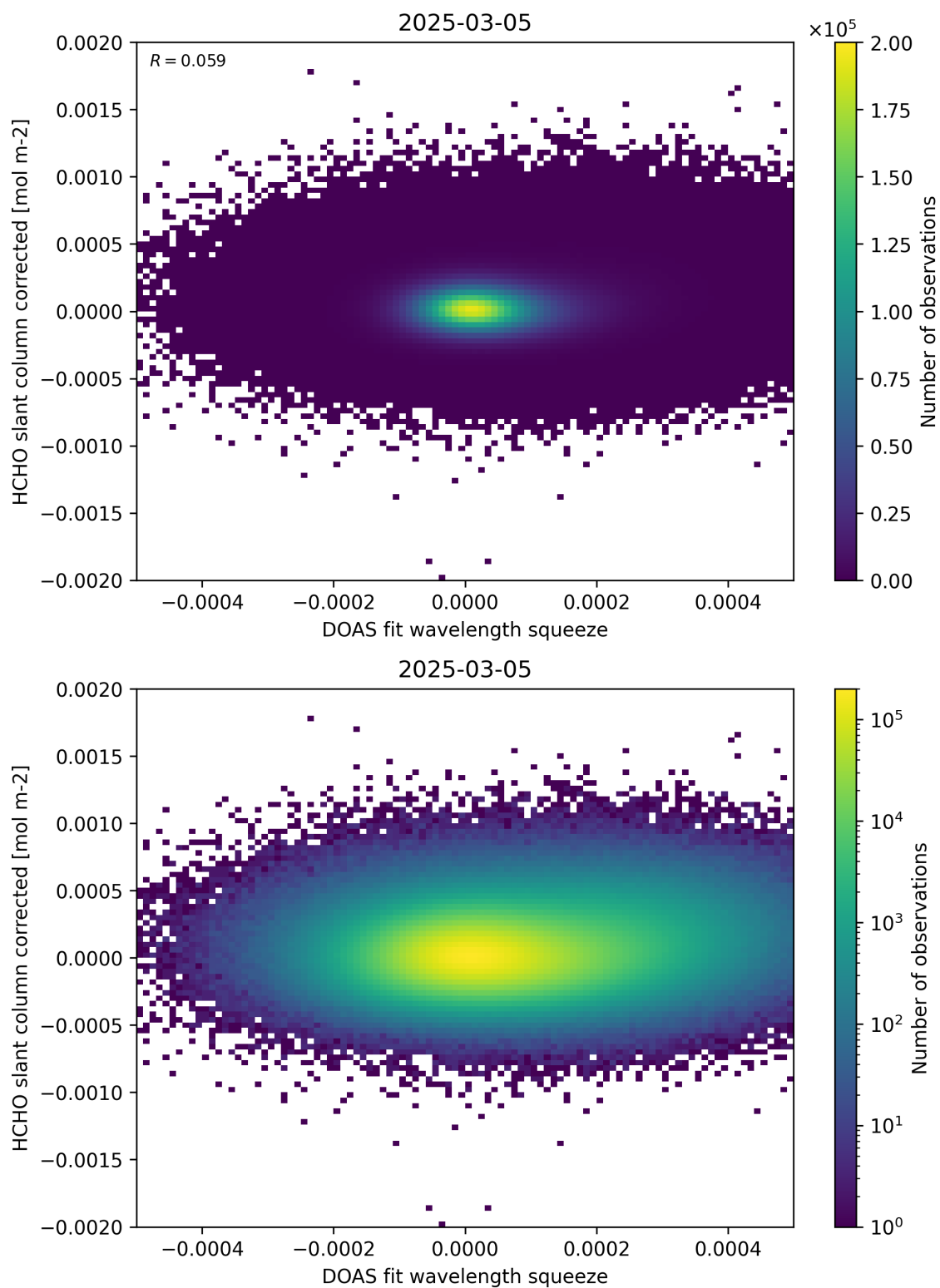
Figure 69: Scatter density plot of “DOAS fit wavelength squeeze” against “HCHO slant column corrected” for 2025-03-04 to 2025-03-06.
