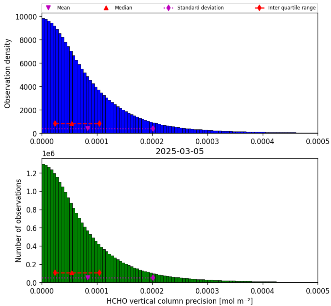
Figure 36: Histogram of “HCHO vertical column precision” for 2025-03-04 to 2025-03-06
