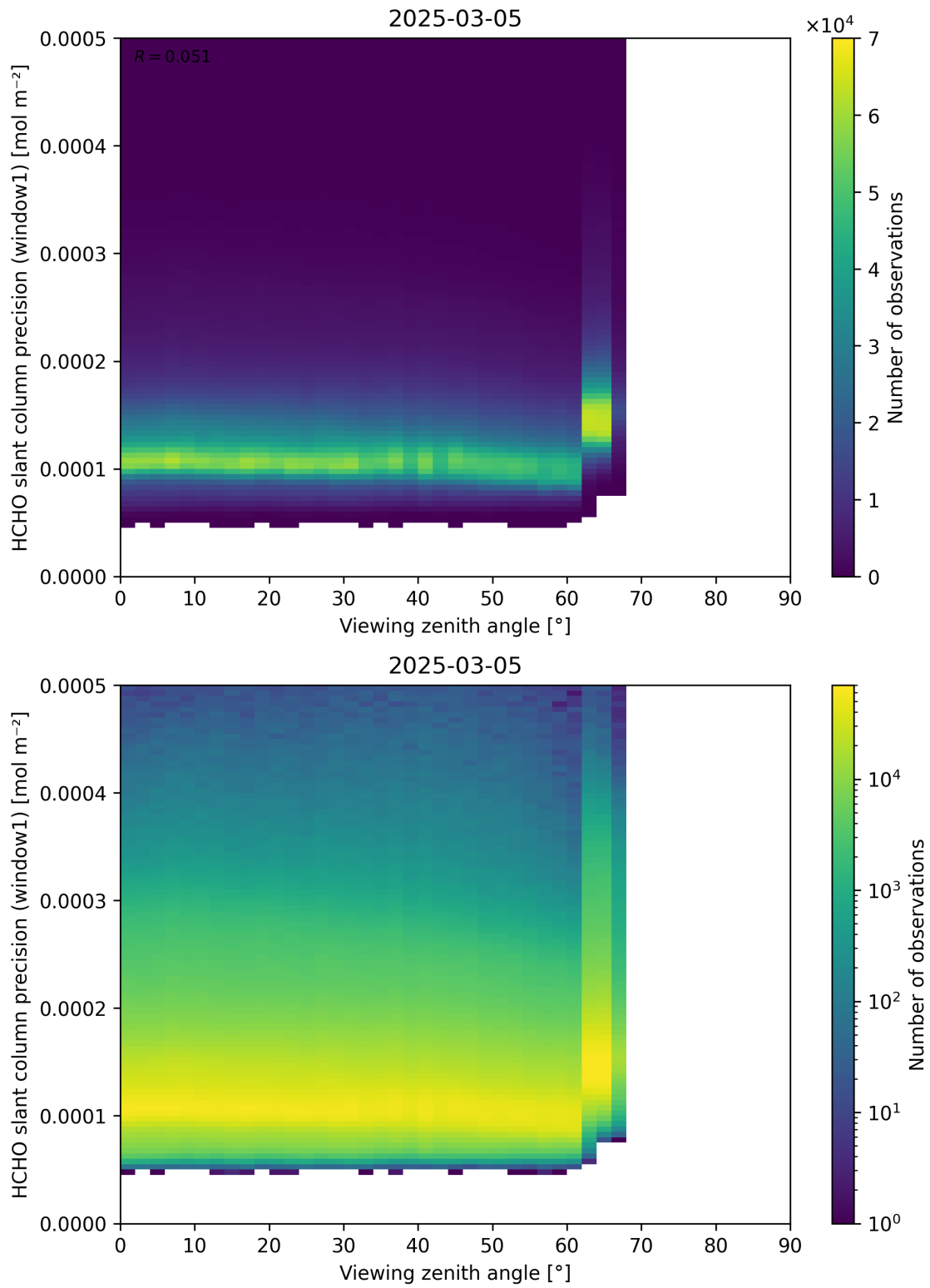
Figure 189: Scatter density plot of “Viewing zenith angle” against “HCHO slant column precision (window1)” for 2025-03-04 to 2025-03-06.
