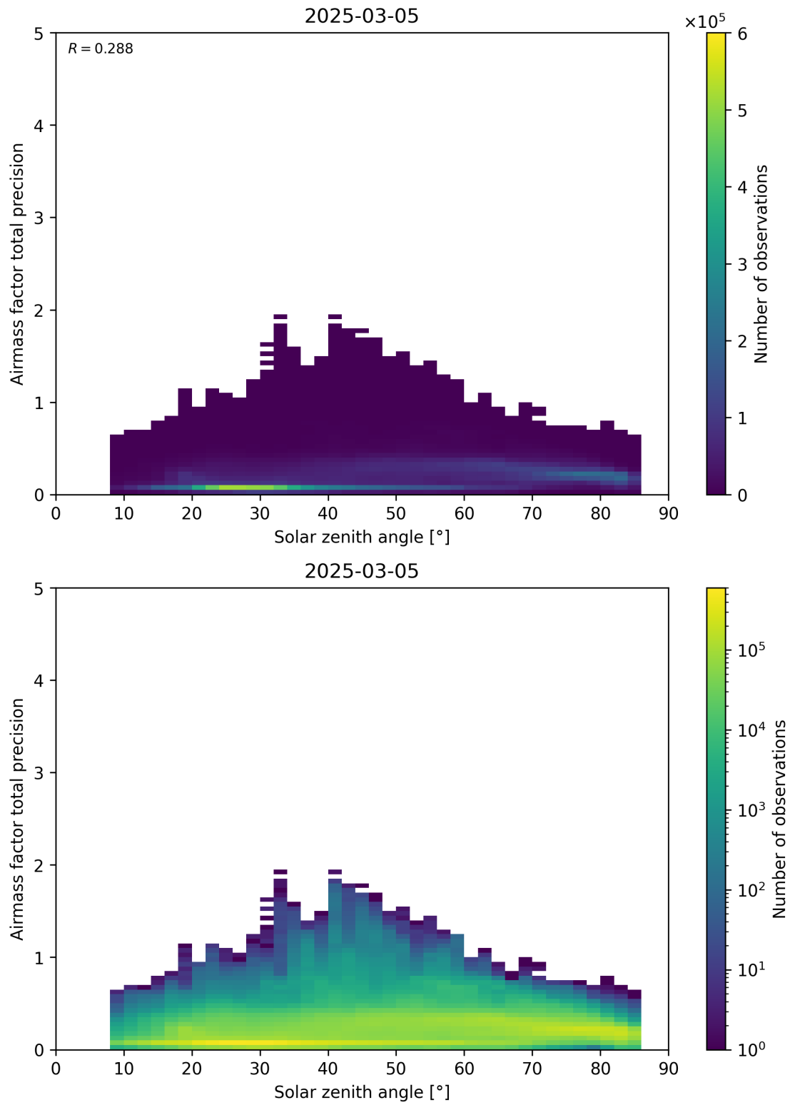
Figure 176: Scatter density plot of “Solar zenith angle” against “Airmass factor total precision” for 2025-03-04 to 2025-03-06.
