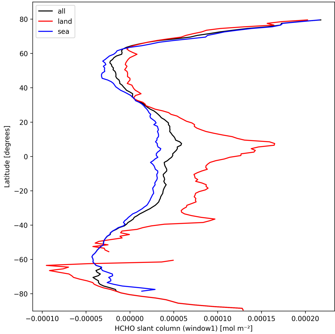
Figure 24: Zonal average of “HCHO slant column (window1)” for 2025-03-04 to 2025-03-06.
