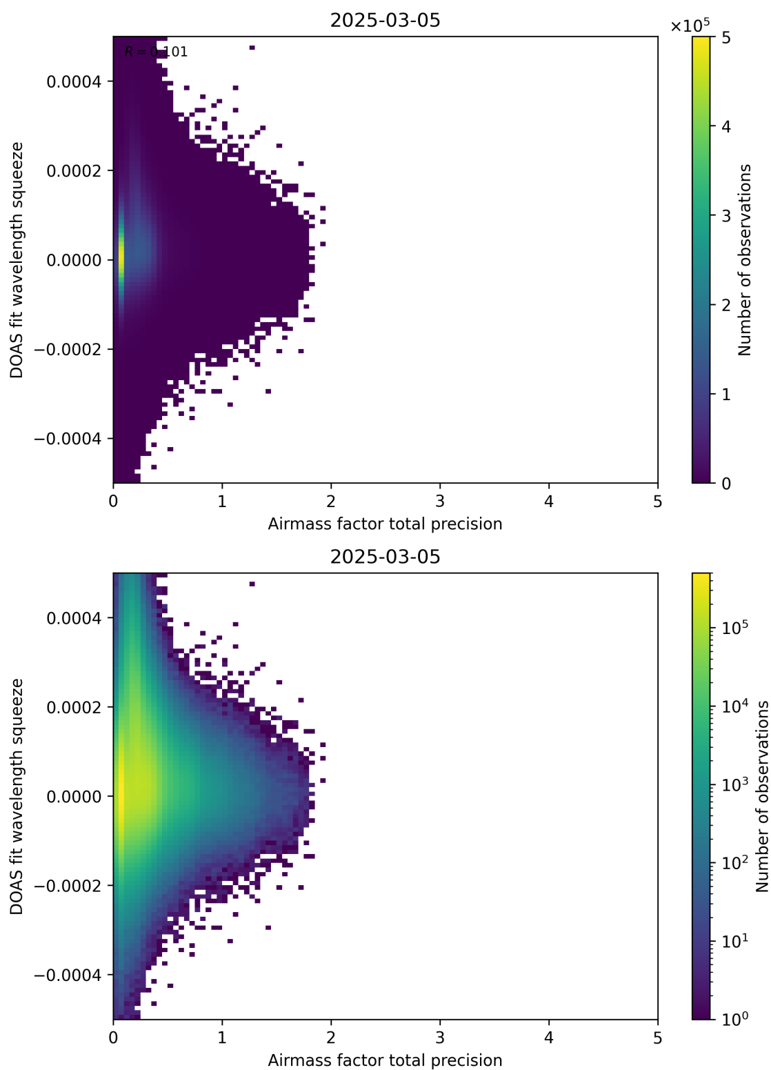
Figure 107: Scatter density plot of “Airmass factor total precision” against “DOAS fit wavelength squeeze” for 2025-03-04 to 2025-03-06.
