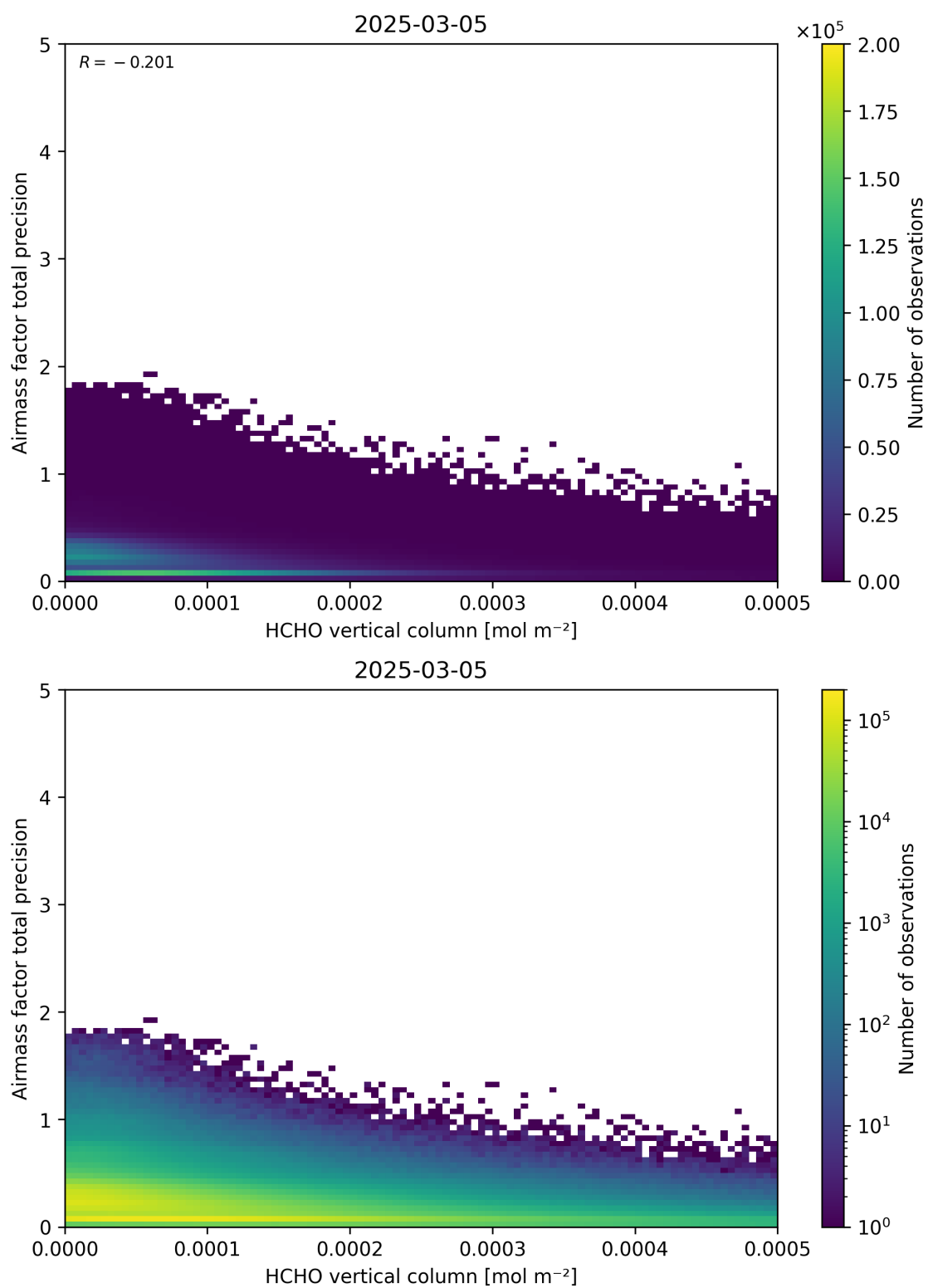
Figure 132: Scatter density plot of “HCHO vertical column” against “Airmass factor total precision” for 2025-03-04 to 2025-03-06.
