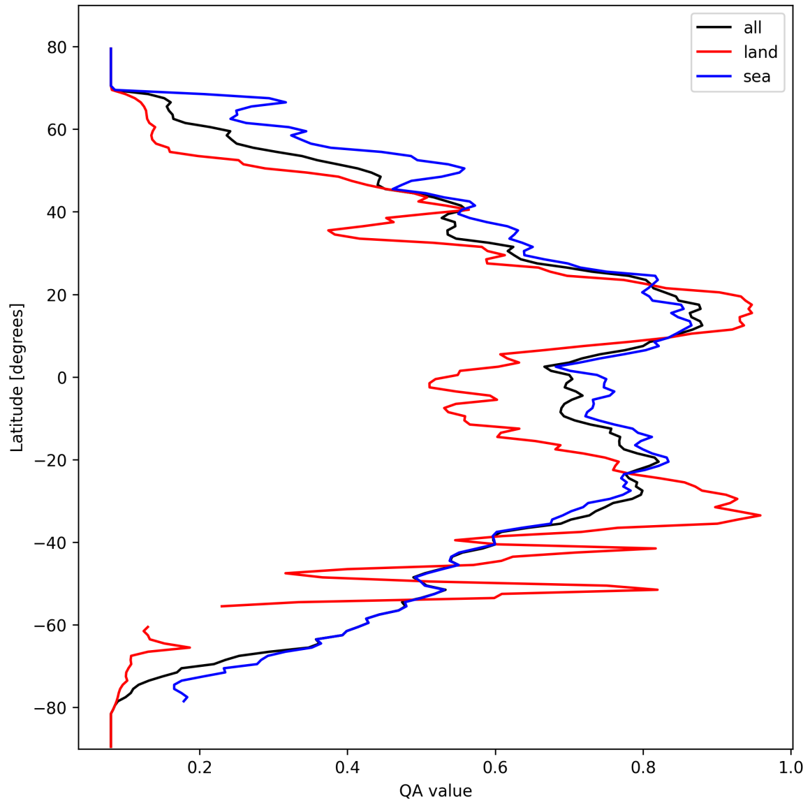
Figure 20: Zonal average of “QA value” for 2025-03-04 to 2025-03-06.
