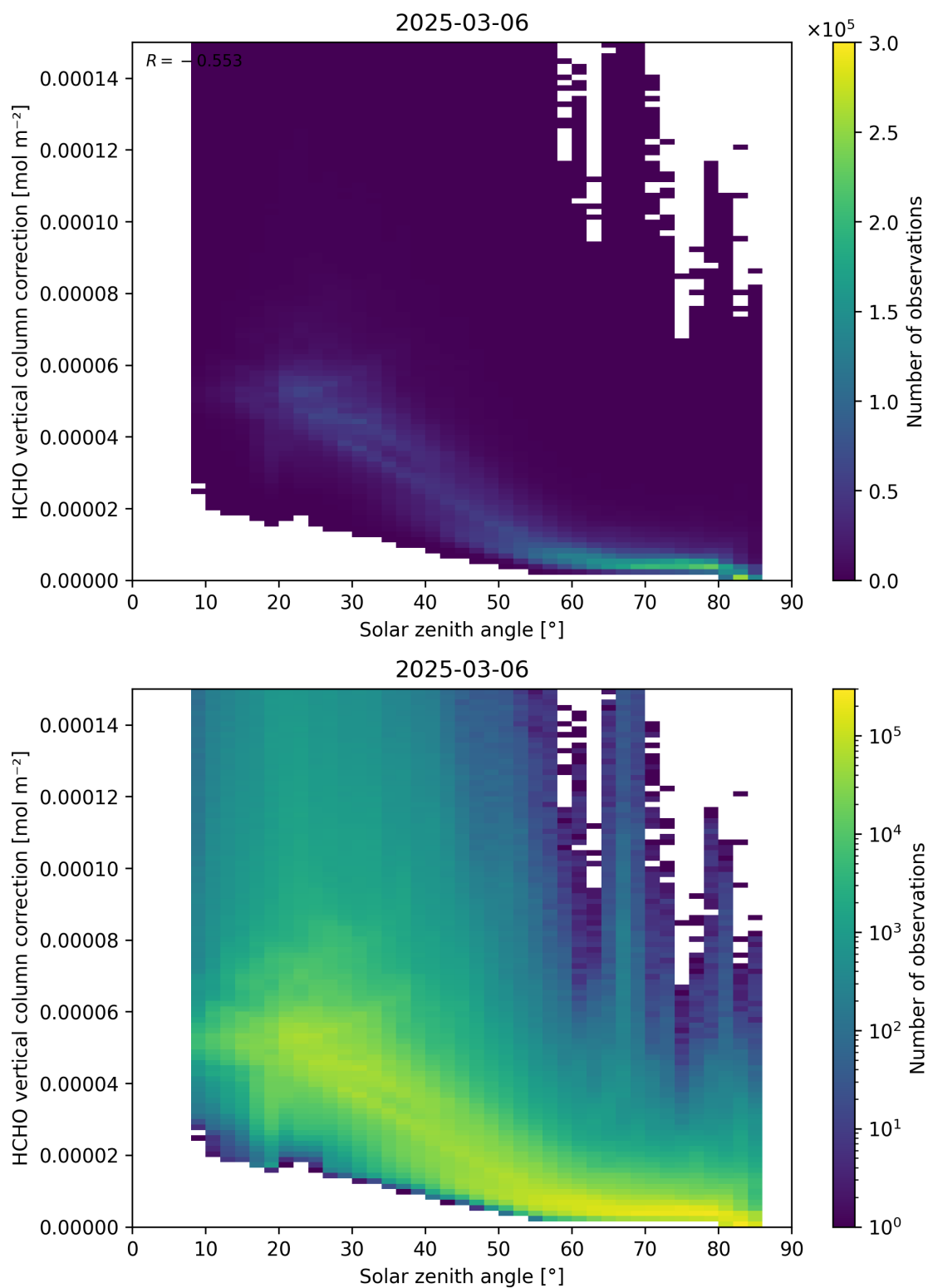
Figure 178: Scatter density plot of “Solar zenith angle” against “HCHO vertical column correction” for 2025-03-05 to 2025-03-07.
