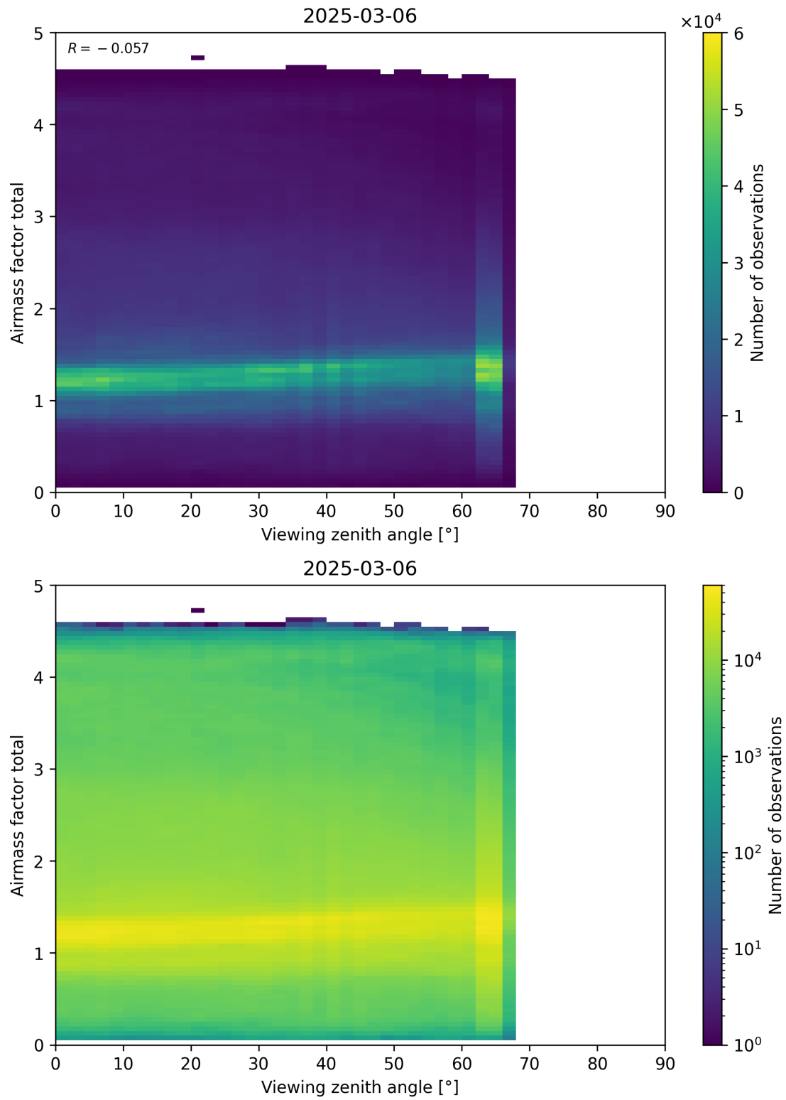
Figure 190: Scatter density plot of “Viewing zenith angle” against “Airmass factor total” for 2025-03-05 to 2025-03-07.
