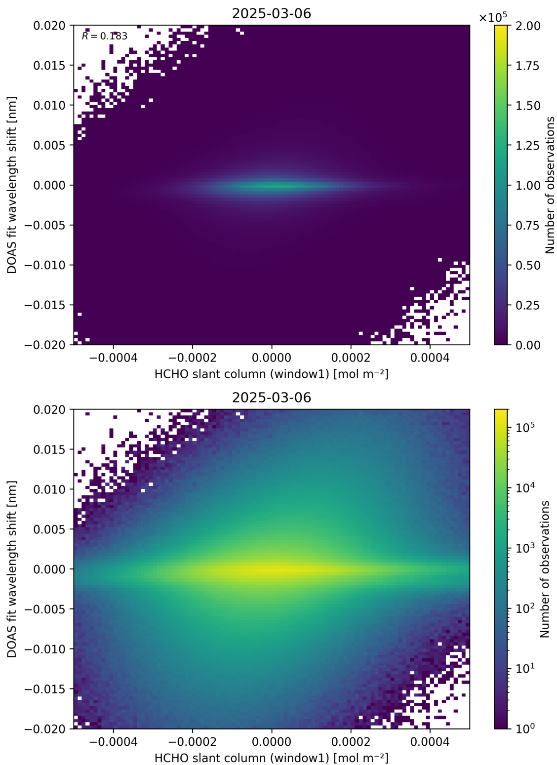
Figure 79: Scatter density plot of “HCHO slant column (window1)” against “DOAS fit wavelength shift” for 2025-03-05 to 2025-03-07.
