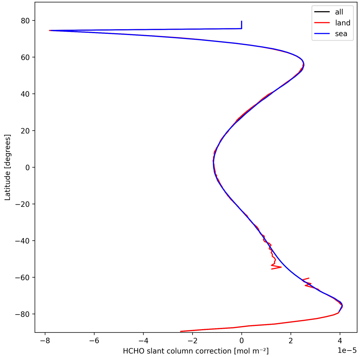
Figure 33: Zonal average of “HCHO slant column correction” for 2025-03-05 to 2025-03-07.
