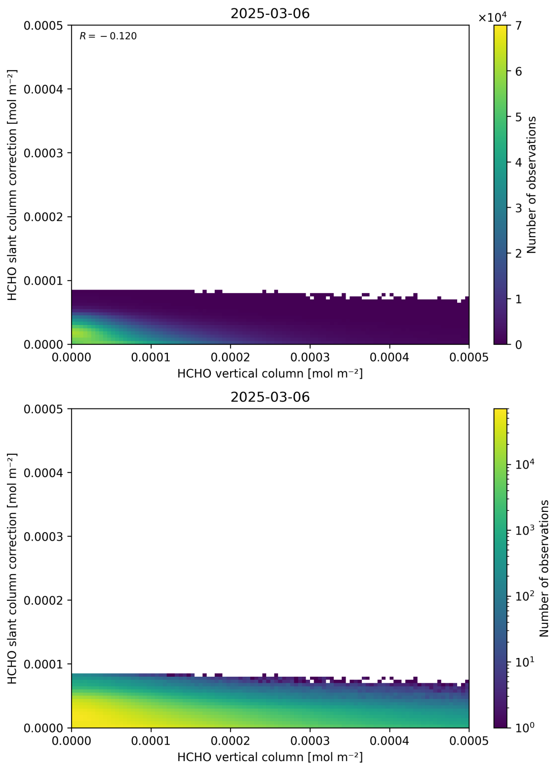
Figure 128: Scatter density plot of “HCHO vertical column” against “HCHO slant column correction” for 2025-03-05 to 2025-03-07.
