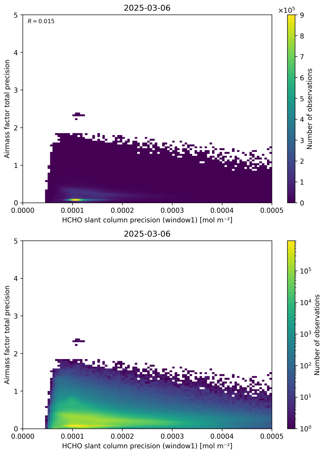
Figure 95: Scatter density plot of “HCHO slant column precision (window1)” against “Airmass factor total precision” for 2025-03-05 to 2025-03-07.
