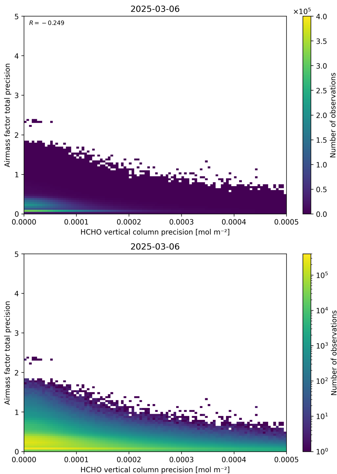
Figure 145: Scatter density plot of “HCHO vertical column precision” against “Airmass factor total precision” for 2025-03-05 to 2025-03-07.
