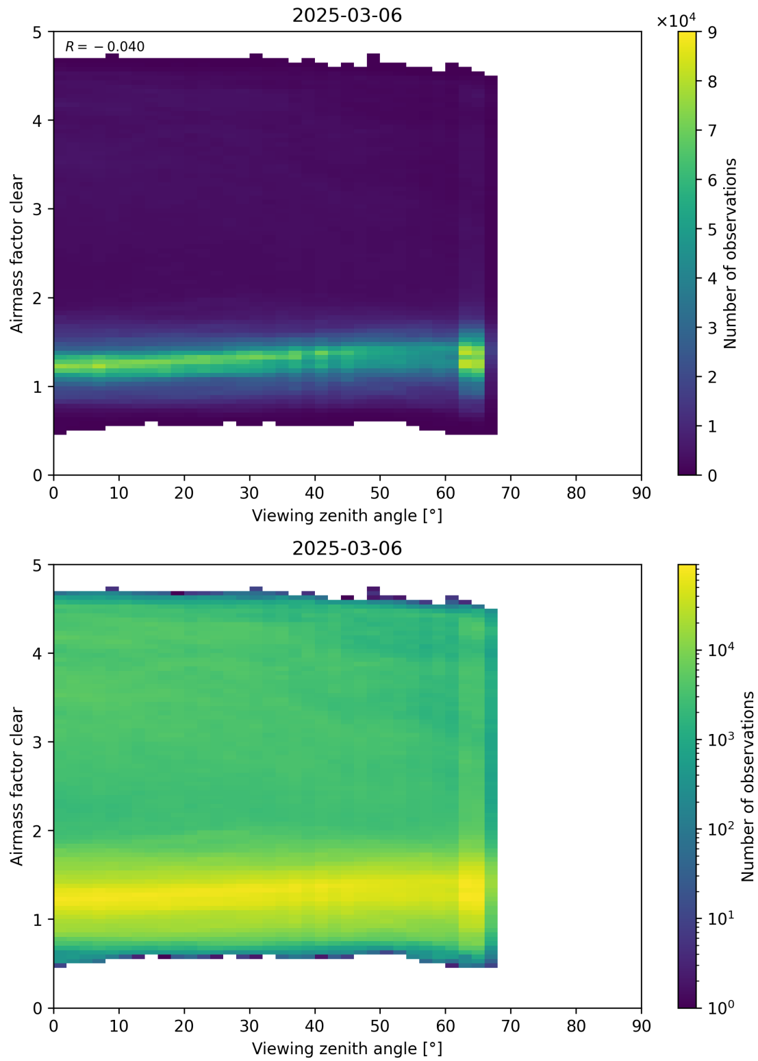
Figure 185: Scatter density plot of “Viewing zenith angle” against “Airmass factor clear” for 2025-03-05 to 2025-03-07.
