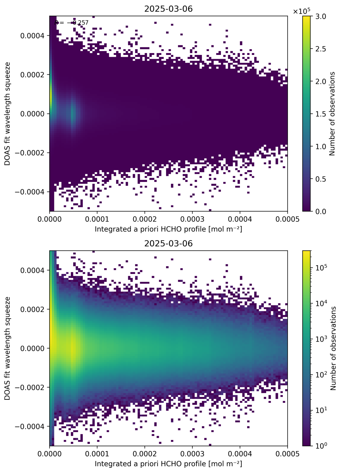
Figure 150: Scatter density plot of “Integrated a priori HCHO profile” against “DOAS fit wavelength squeeze” for 2025-03-05 to 2025-03-07.
