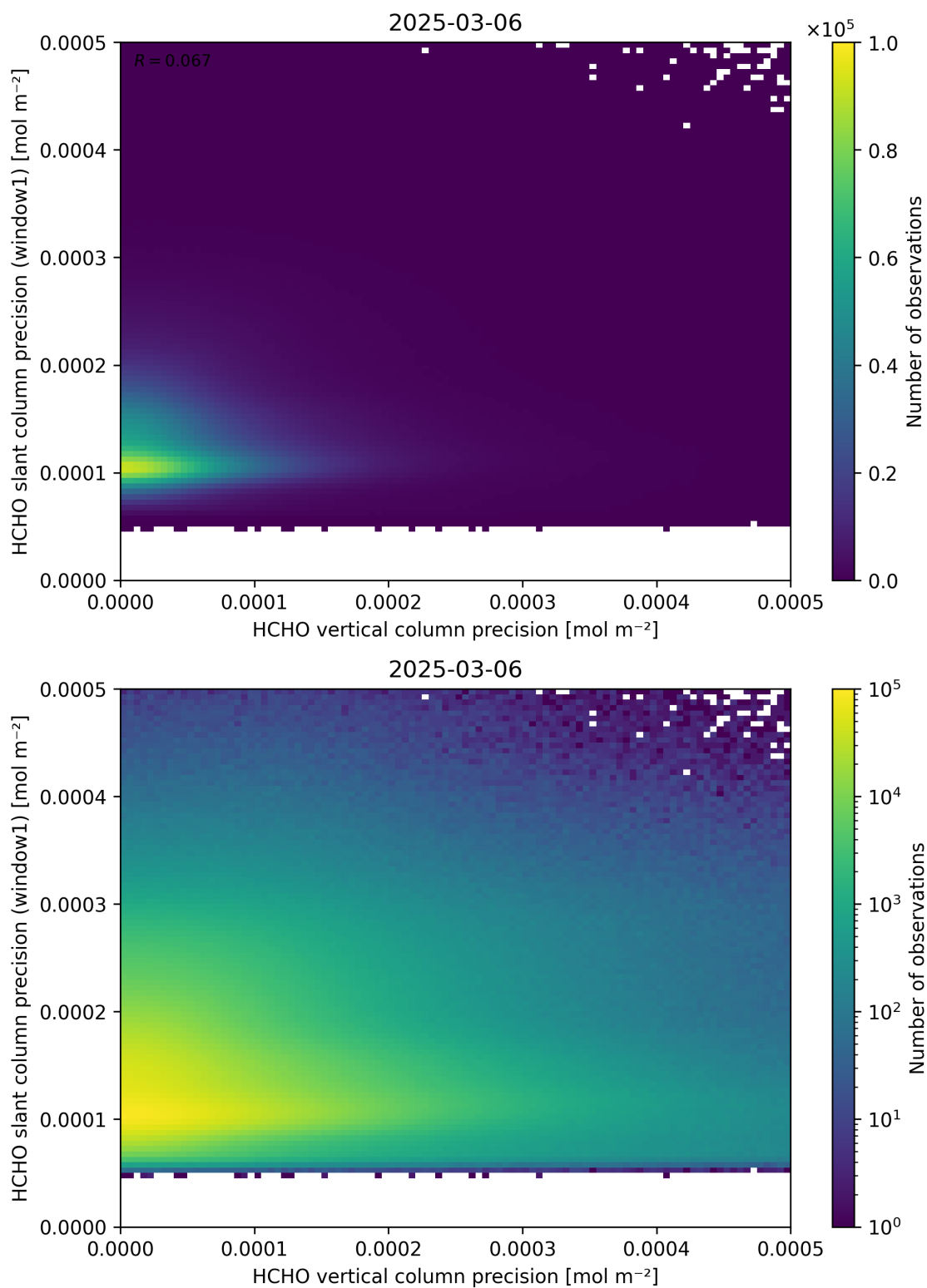
Figure 143: Scatter density plot of “HCHO vertical column precision” against “HCHO slant column precision (window1)” for 2025-03-05 to 2025-03-07.
