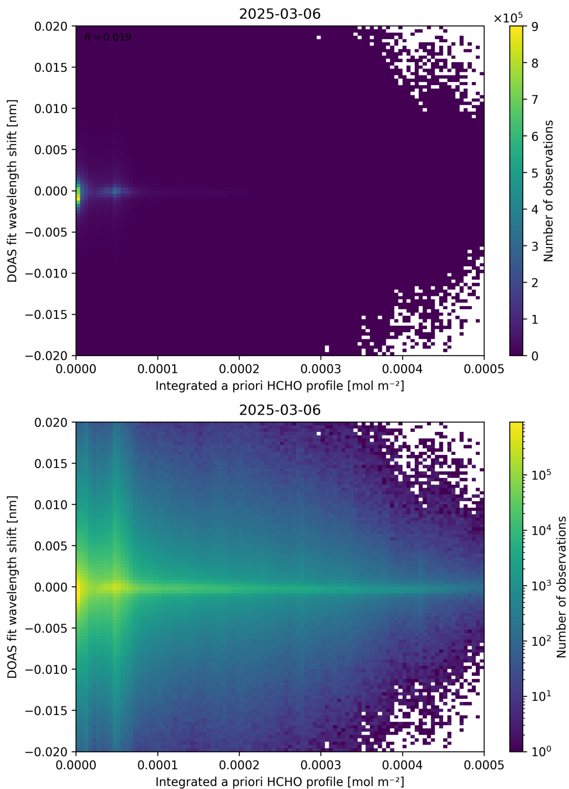
Figure 149: Scatter density plot of “Integrated a priori HCHO profile” against “DOAS fit wavelength shift” for 2025-03-05 to 2025-03-07.
