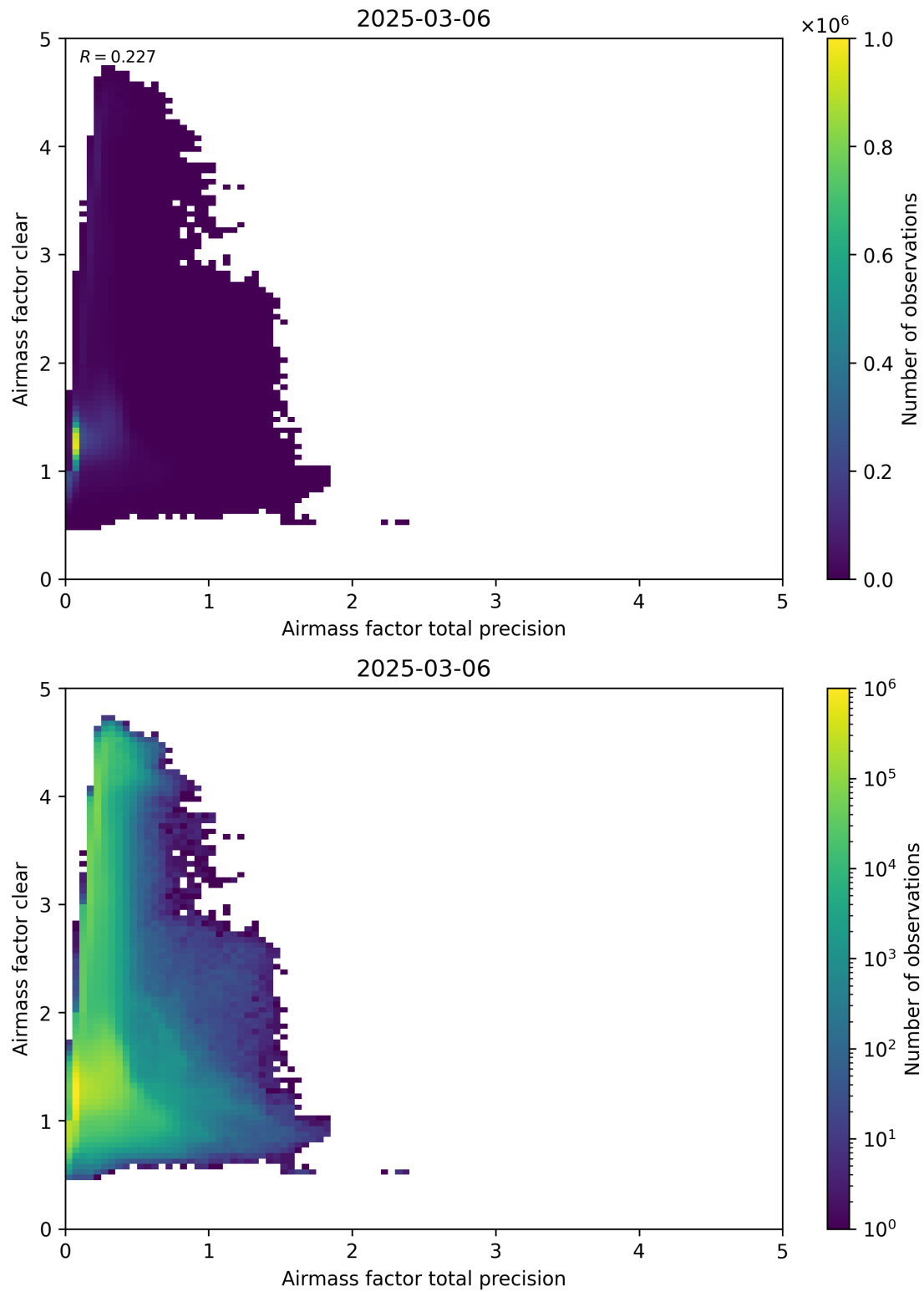
Figure 108: Scatter density plot of “Airmass factor total precision” against “Airmass factor clear” for 2025-03-05 to 2025-03-07.
