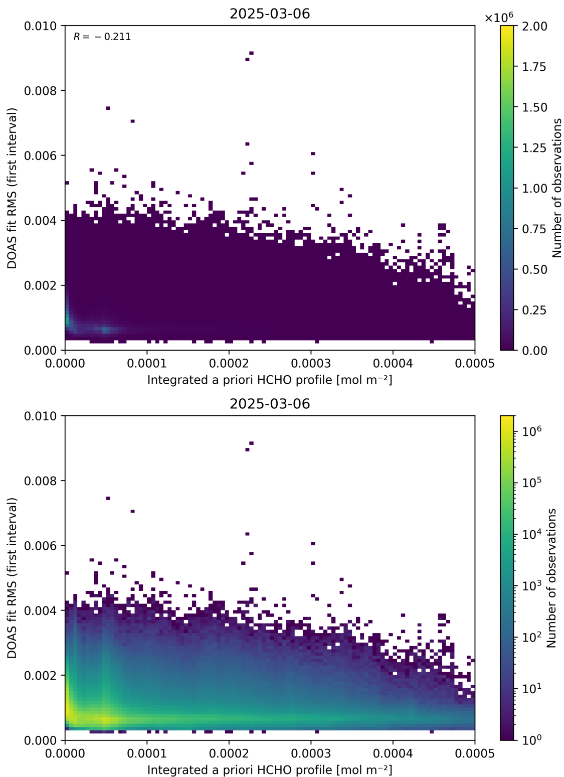
Figure 148: Scatter density plot of “Integrated a priori HCHO profile” against “DOAS fit RMS (first interval)” for 2025-03-05 to 2025-03-07.
