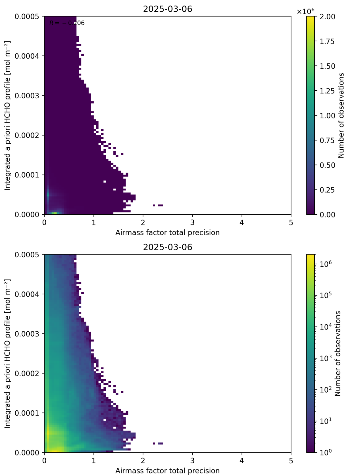
Figure 111: Scatter density plot of “Airmass factor total precision” against “Integrated a priori HCHO profile” for 2025-03-05 to 2025-03-07.
