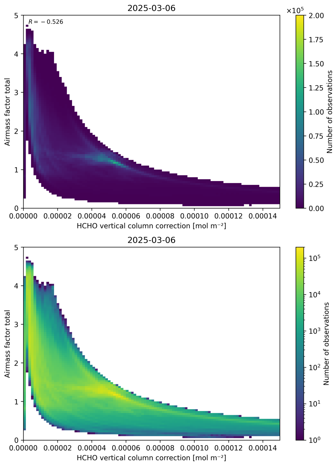
Figure 120: Scatter density plot of “HCHO vertical column correction” against “Airmass factor total” for 2025-03-05 to 2025-03-07.
