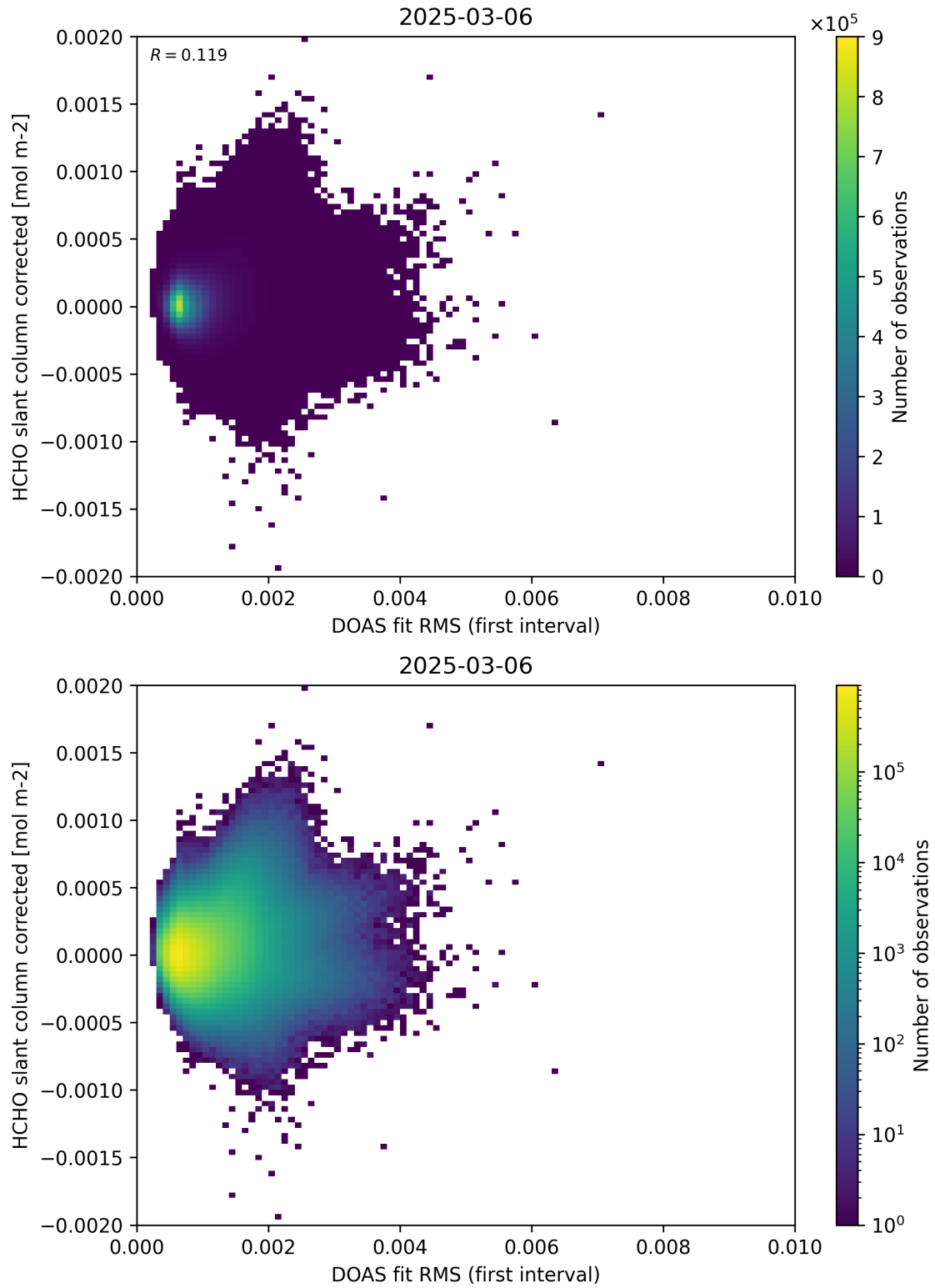
Figure 62: Scatter density plot of “DOAS fit RMS (first interval)” against “HCHO slant column corrected” for 2025-03-05 to 2025-03-07.
