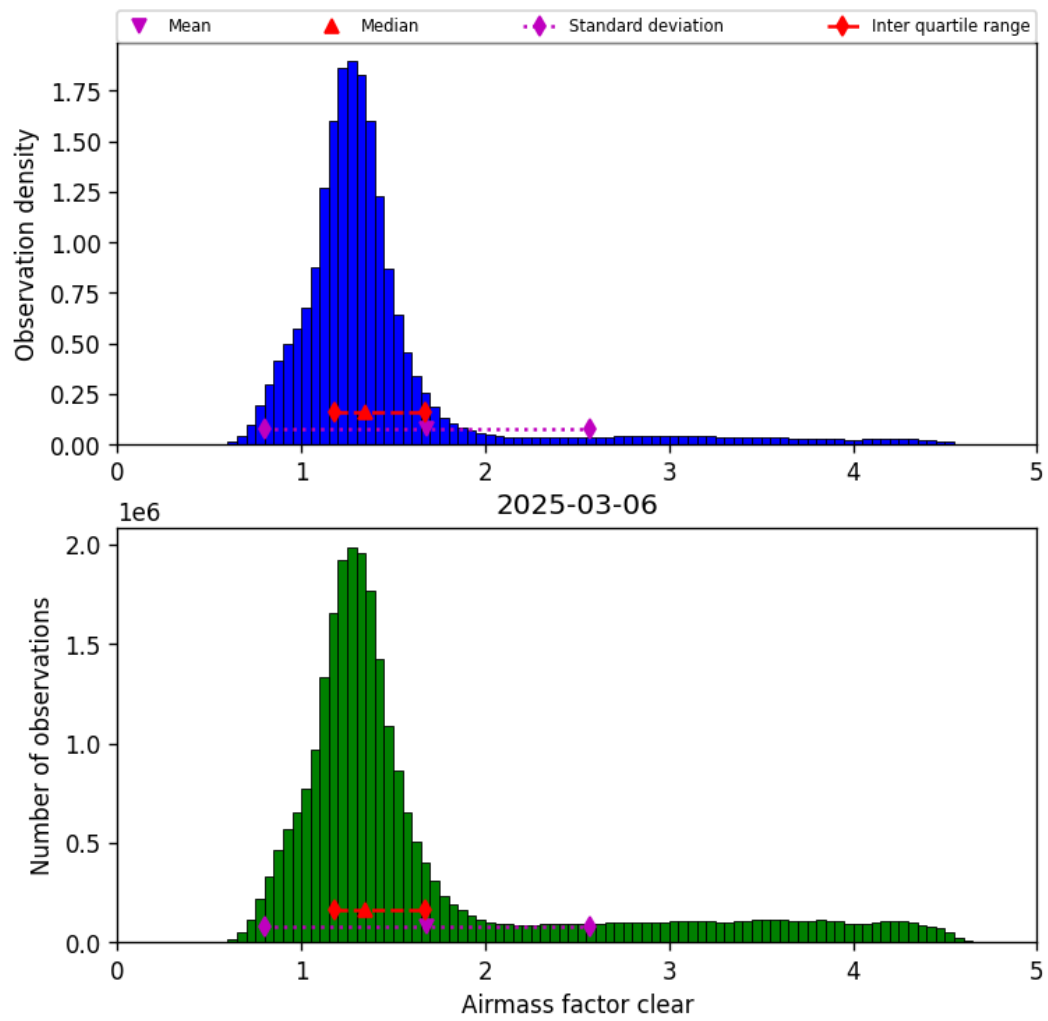
Figure 42: Histogram of “Airmass factor clear” for 2025-03-05 to 2025-03-07
