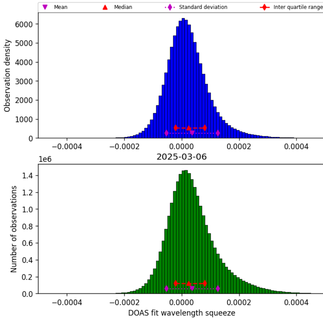
Figure 45: Histogram of “DOAS fit wavelength squeeze” for 2025-03-05 to 2025-03-07
