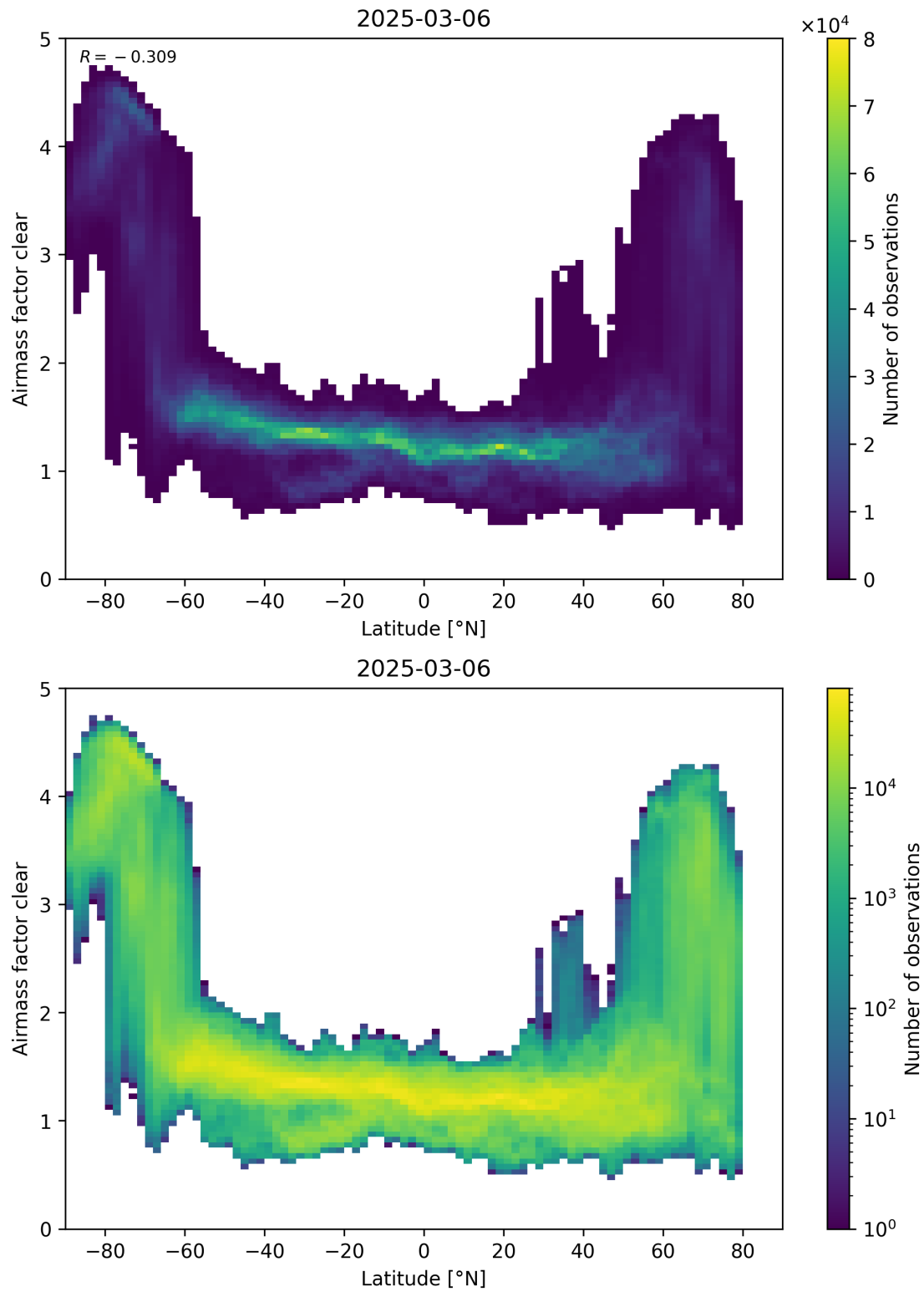
Figure 156: Scatter density plot of “Latitude” against “Airmass factor clear” for 2025-03-05 to 2025-03-07.
