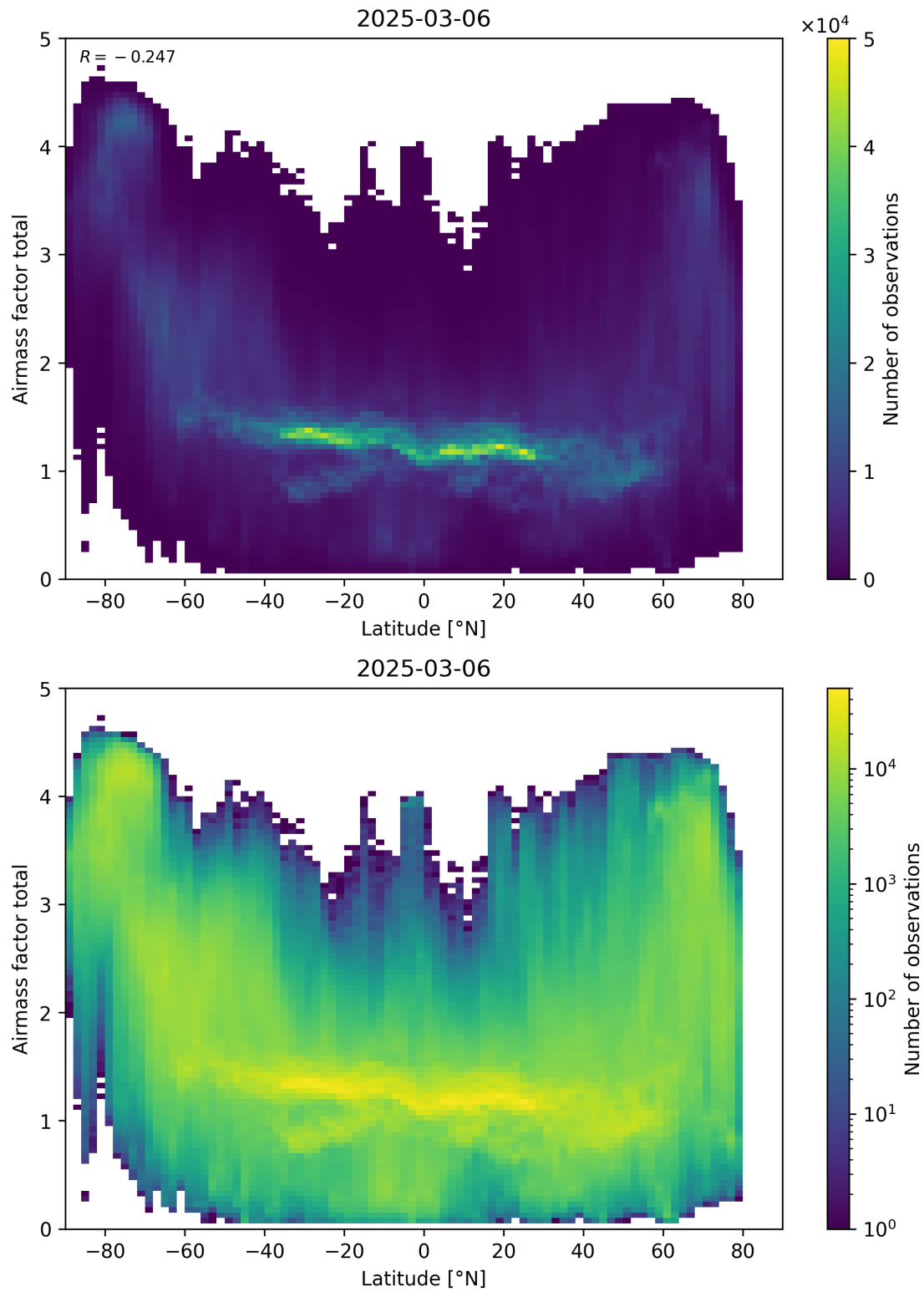
Figure 161: Scatter density plot of “Latitude” against “Airmass factor total” for 2025-03-05 to 2025-03-07.
