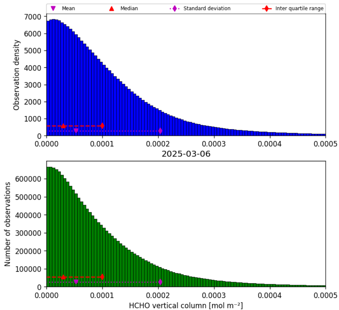
Figure 35: Histogram of “HCHO vertical column” for 2025-03-05 to 2025-03-07
