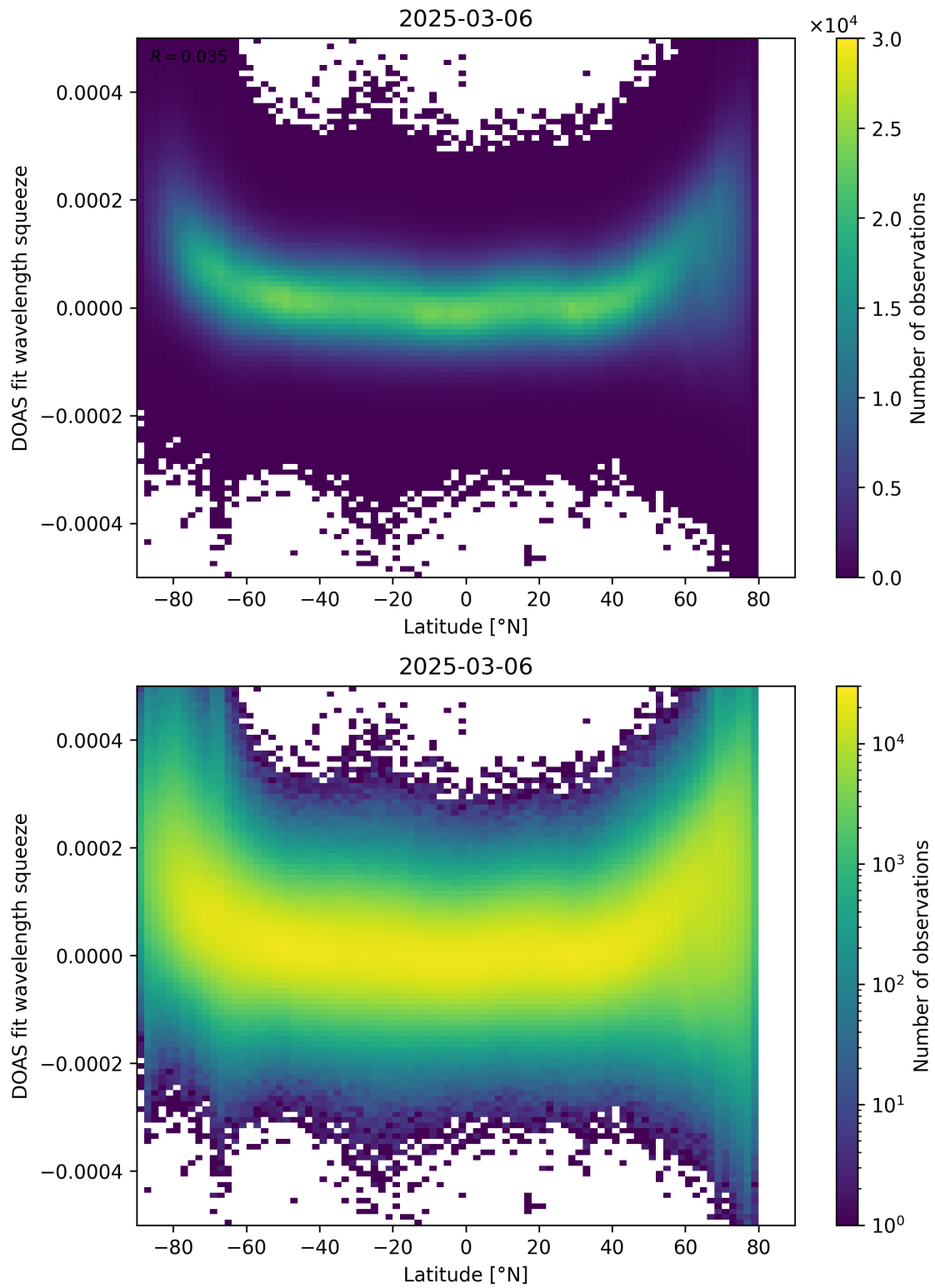
Figure 155: Scatter density plot of “Latitude” against “DOAS fit wavelength squeeze” for 2025-03-05 to 2025-03-07.
