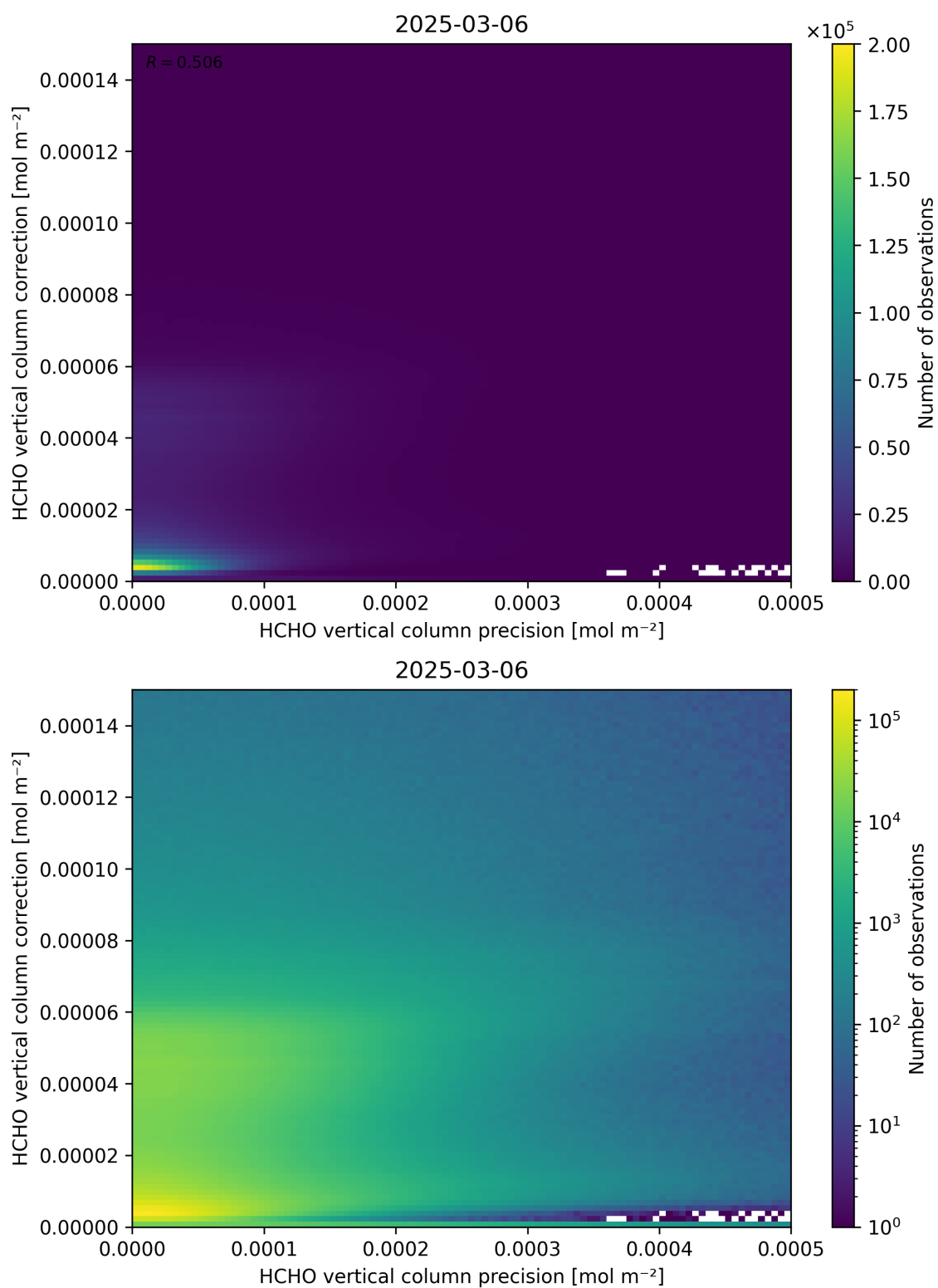
Figure 146: Scatter density plot of “HCHO vertical column precision” against “HCHO vertical column correction” for 2025-03-05 to 2025-03-07.
