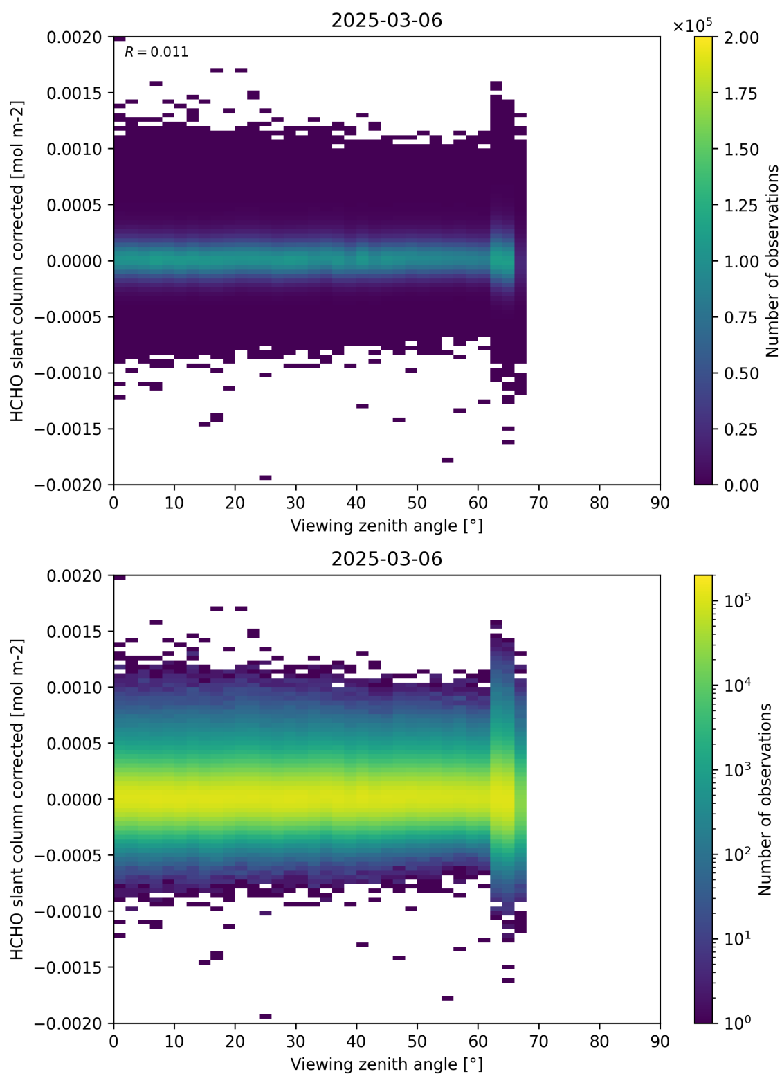
Figure 186: Scatter density plot of “Viewing zenith angle” against “HCHO slant column corrected” for 2025-03-05 to 2025-03-07.
