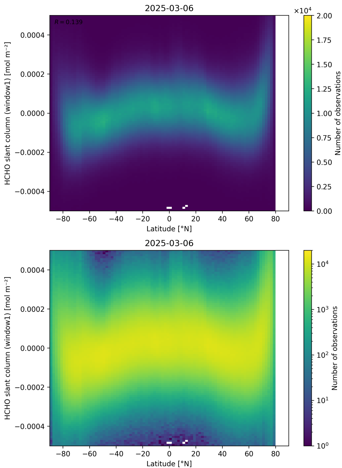
Figure 159: Scatter density plot of “Latitude” against “HCHO slant column (window1)” for 2025-03-05 to 2025-03-07.
