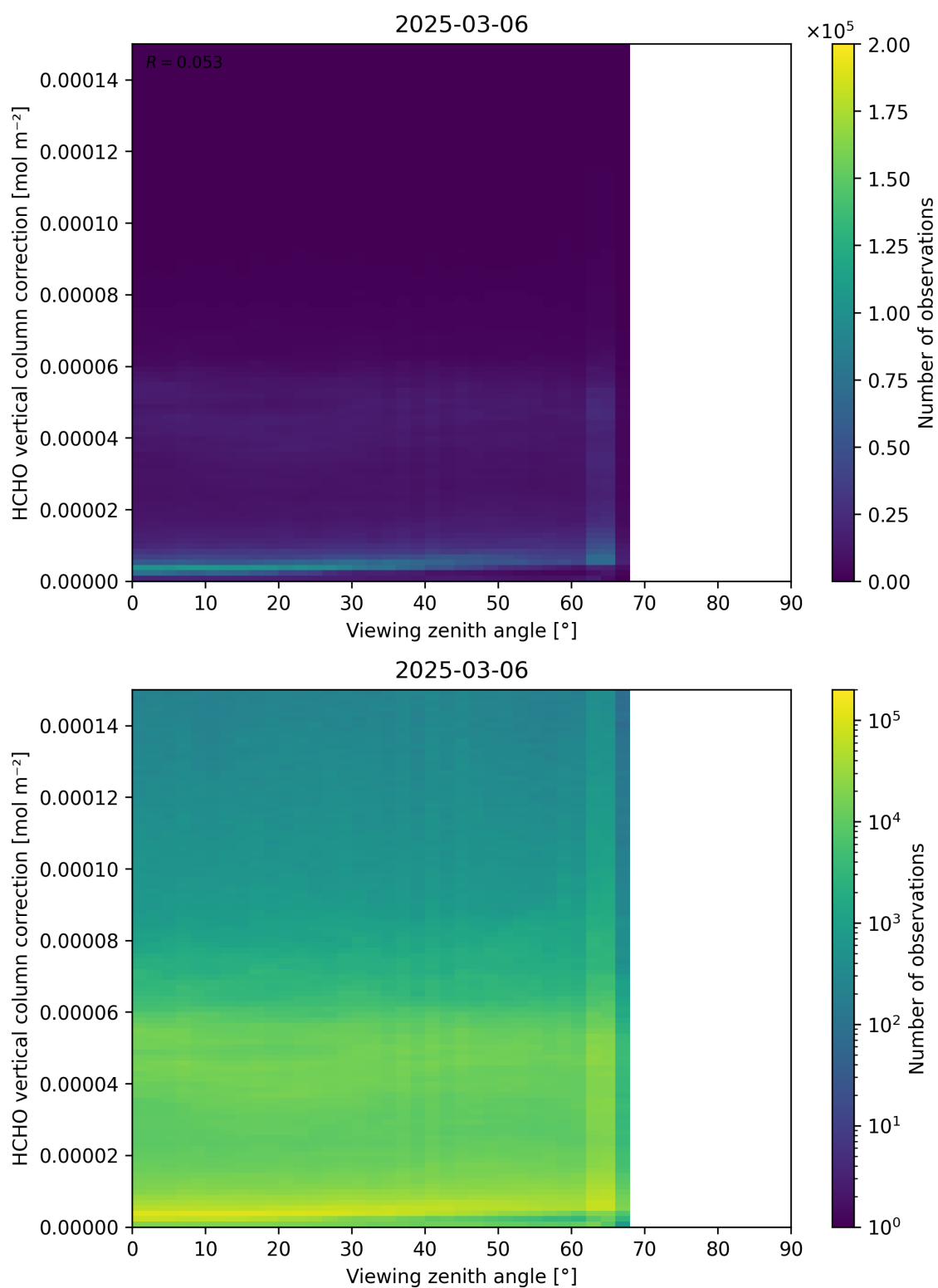
Figure 193: Scatter density plot of “Viewing zenith angle” against “HCHO vertical column correction” for 2025-03-05 to 2025-03-07.
