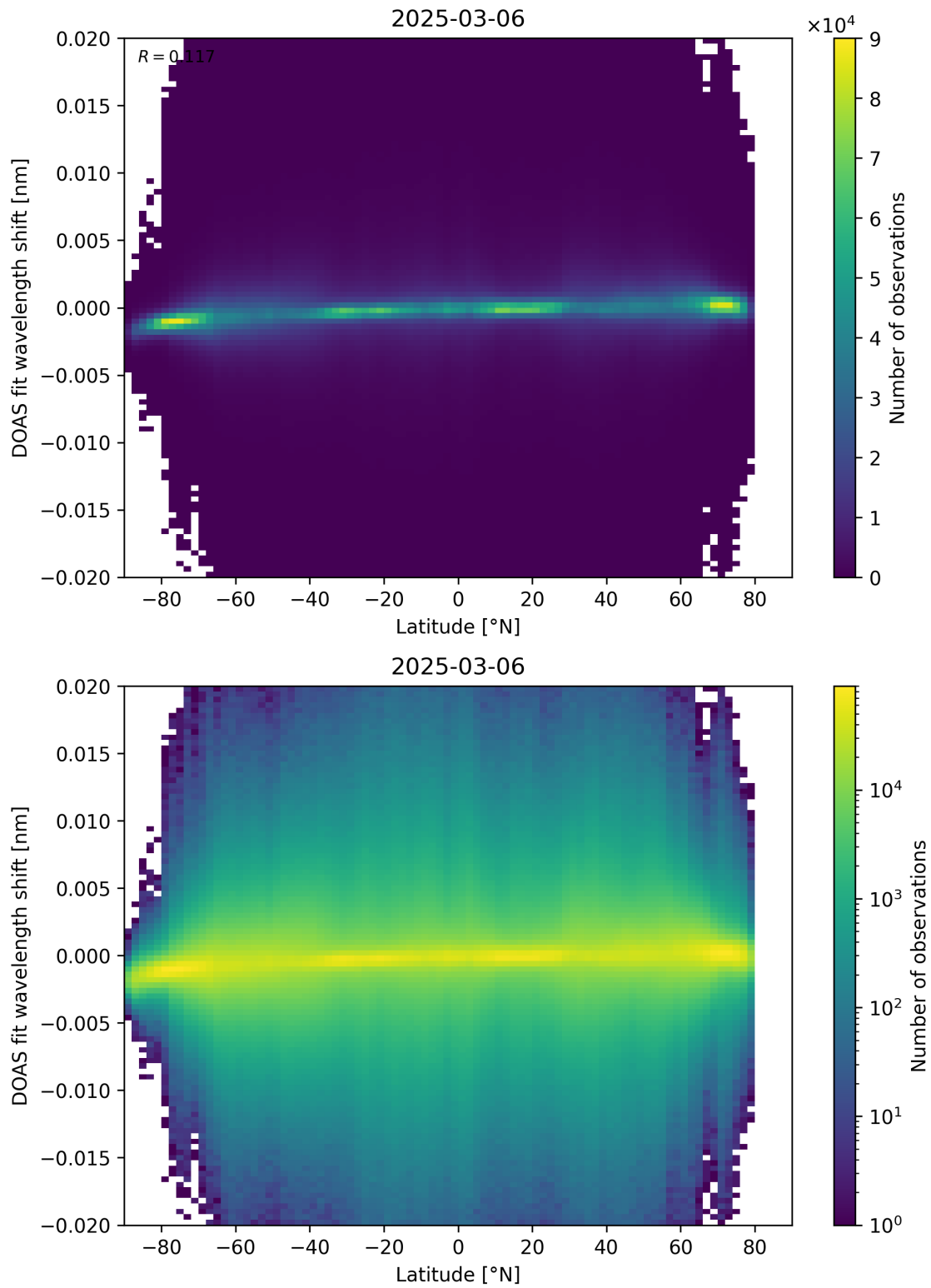
Figure 154: Scatter density plot of “Latitude” against “DOAS fit wavelength shift” for 2025-03-05 to 2025-03-07.
