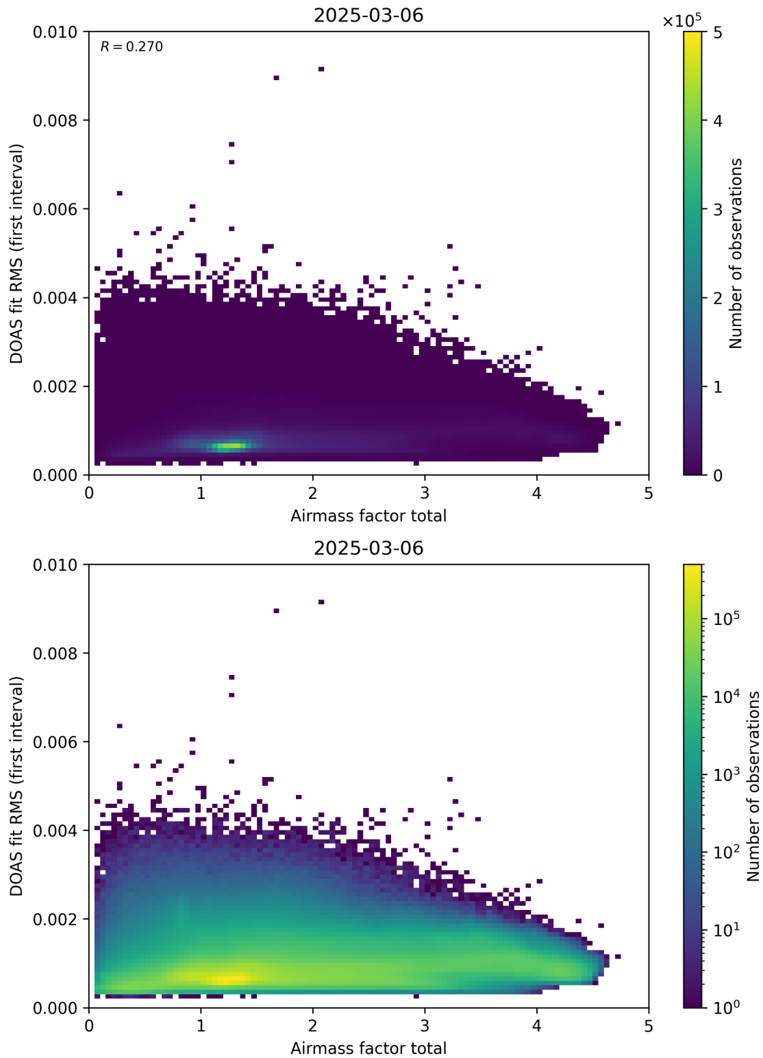
Figure 97: Scatter density plot of “Airmass factor total” against “DOAS fit RMS (first interval)” for 2025-03-05 to 2025-03-07.
