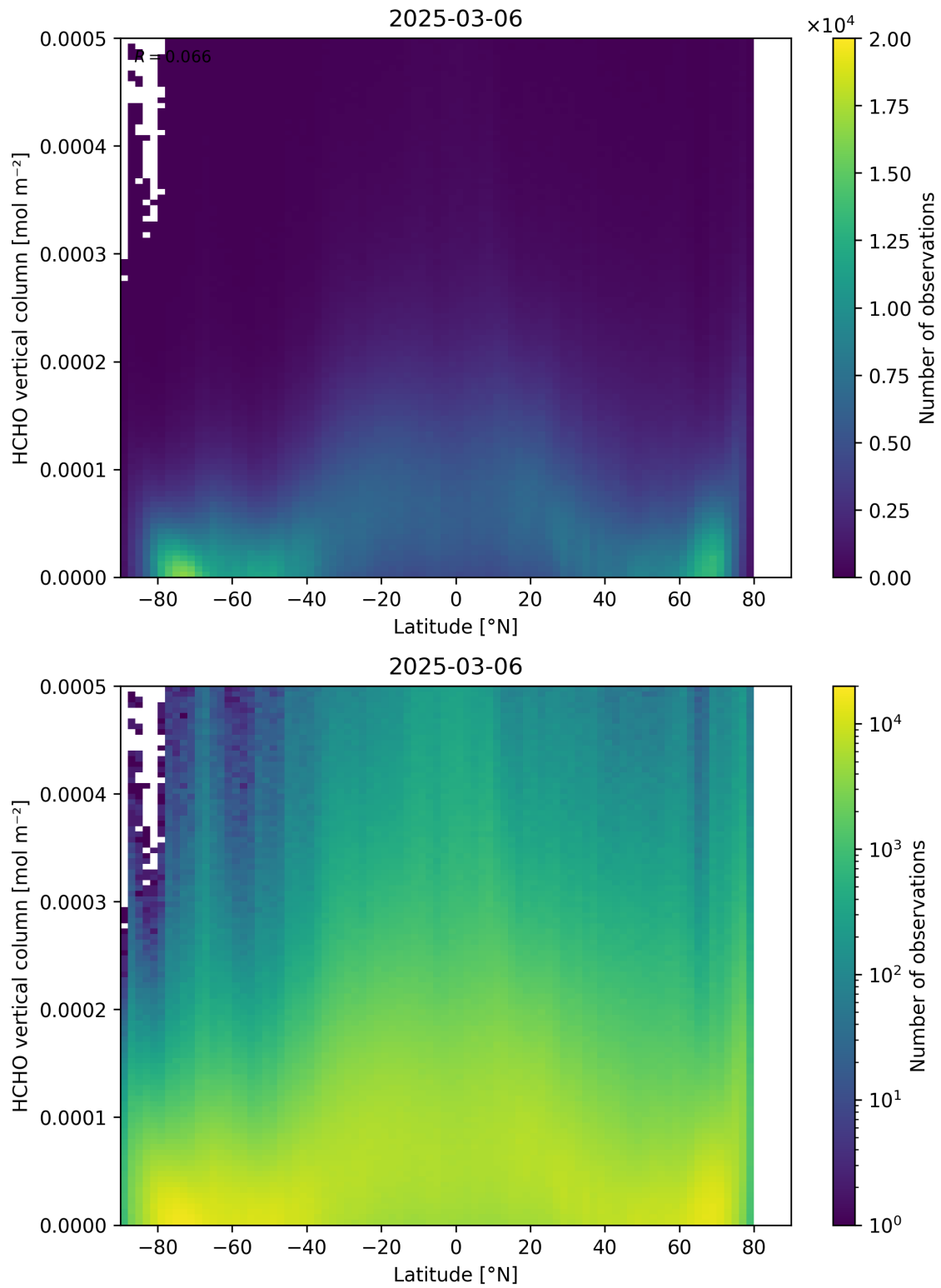
Figure 163: Scatter density plot of “Latitude” against “HCHO vertical column” for 2025-03-05 to 2025-03-07.
