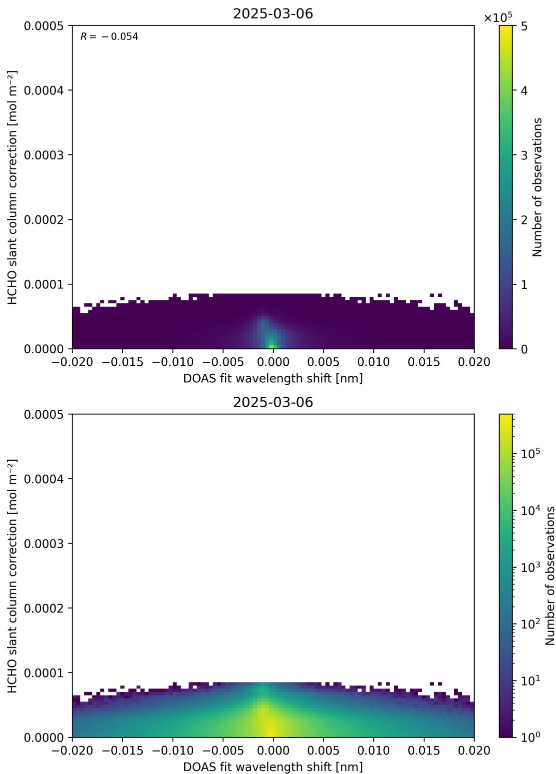
Figure 67: Scatter density plot of “DOAS fit wavelength shift” against “HCHO slant column correction” for 2025-03-05 to 2025-03-07.
