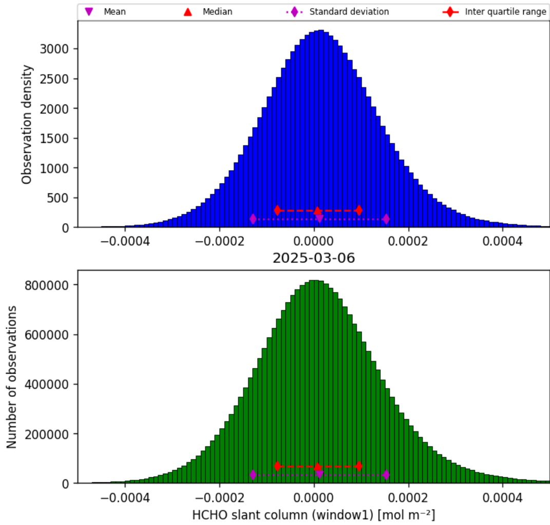
Figure 38: Histogram of “HCHO slant column (window1)” for 2025-03-05 to 2025-03-07
