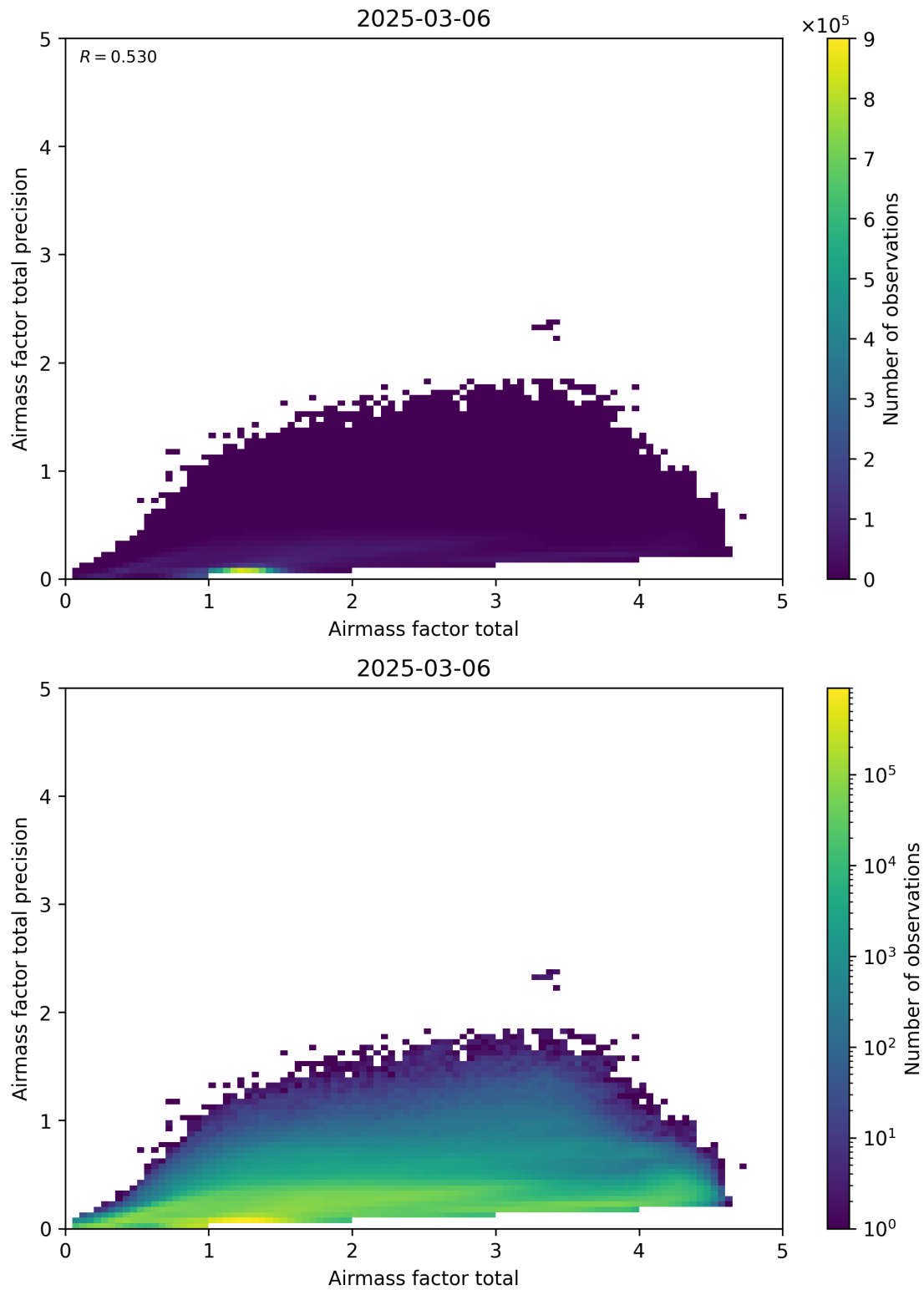
Figure 103: Scatter density plot of “Airmass factor total” against “Airmass factor total precision” for 2025-03-05 to 2025-03-07.
