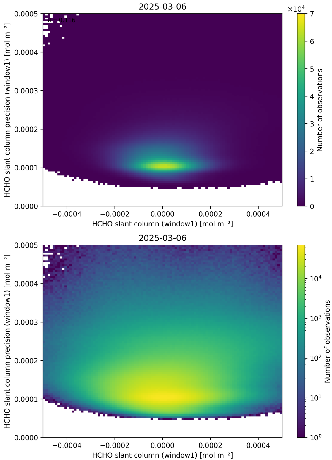
Figure 84: Scatter density plot of “HCHO slant column (window1)” against “HCHO slant column precision (window1)” for 2025-03-05 to 2025-03-07.
