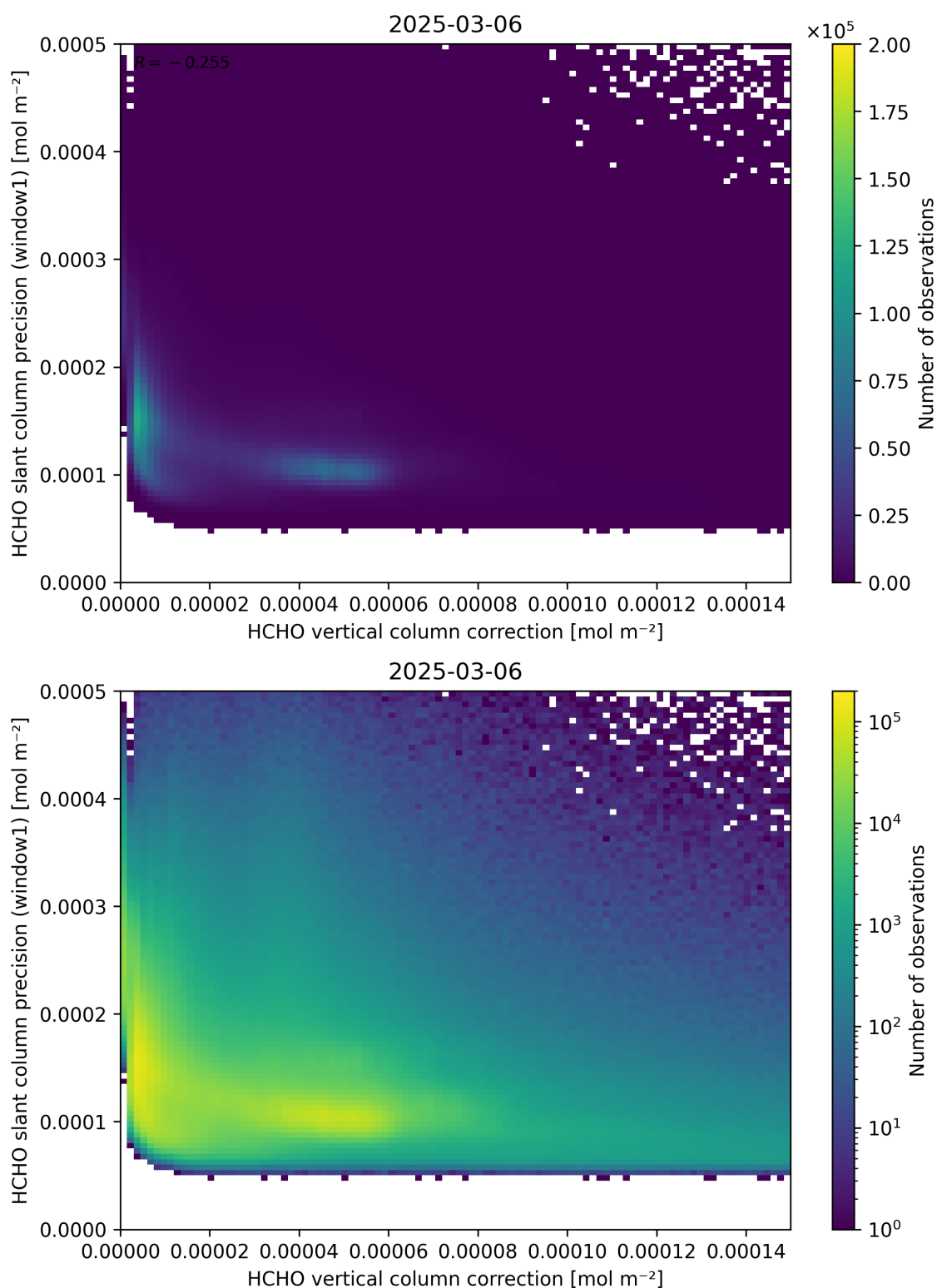
Figure 119: Scatter density plot of “HCHO vertical column correction” against “HCHO slant column precision (window1)” for 2025-03-05 to 2025-03-07.
