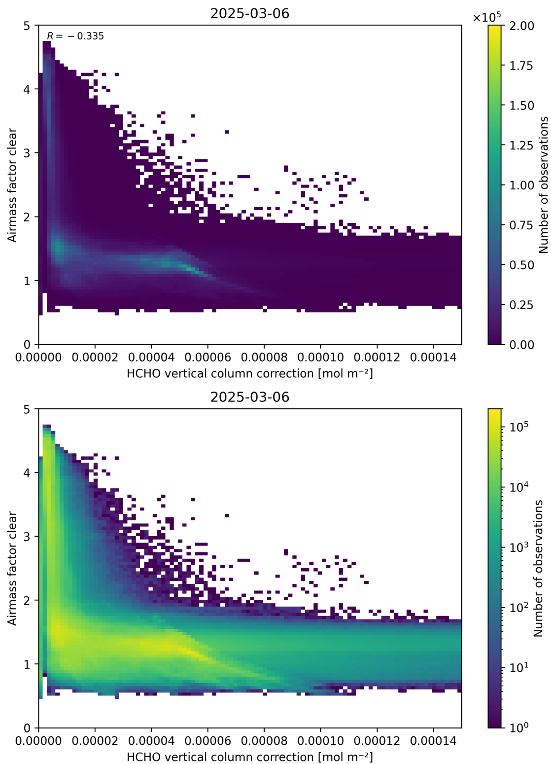
Figure 115: Scatter density plot of “HCHO vertical column correction” against “Airmass factor clear” for 2025-03-05 to 2025-03-07.
