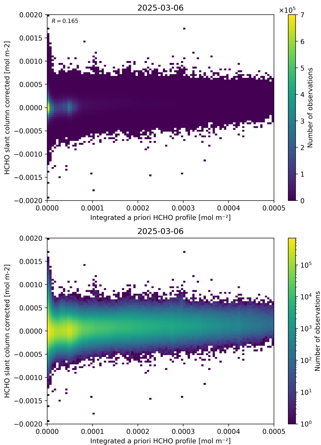
Figure 151: Scatter density plot of “Integrated a priori HCHO profile” against “HCHO slant column corrected” for 2025-03-05 to 2025-03-07.
