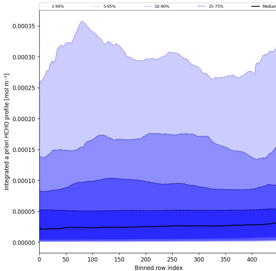
Figure 57: Along track statistics of "Integrated a priori HCHO profile" for 2025-03-05 to 2025-03-07
