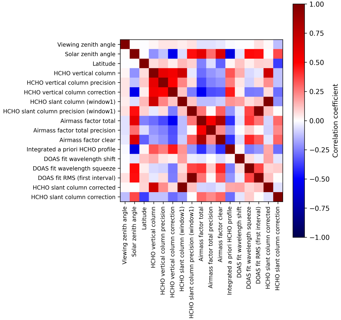
Figure 2: Map of correlation matrix for 2025-03-05 to 2025-03-07.
