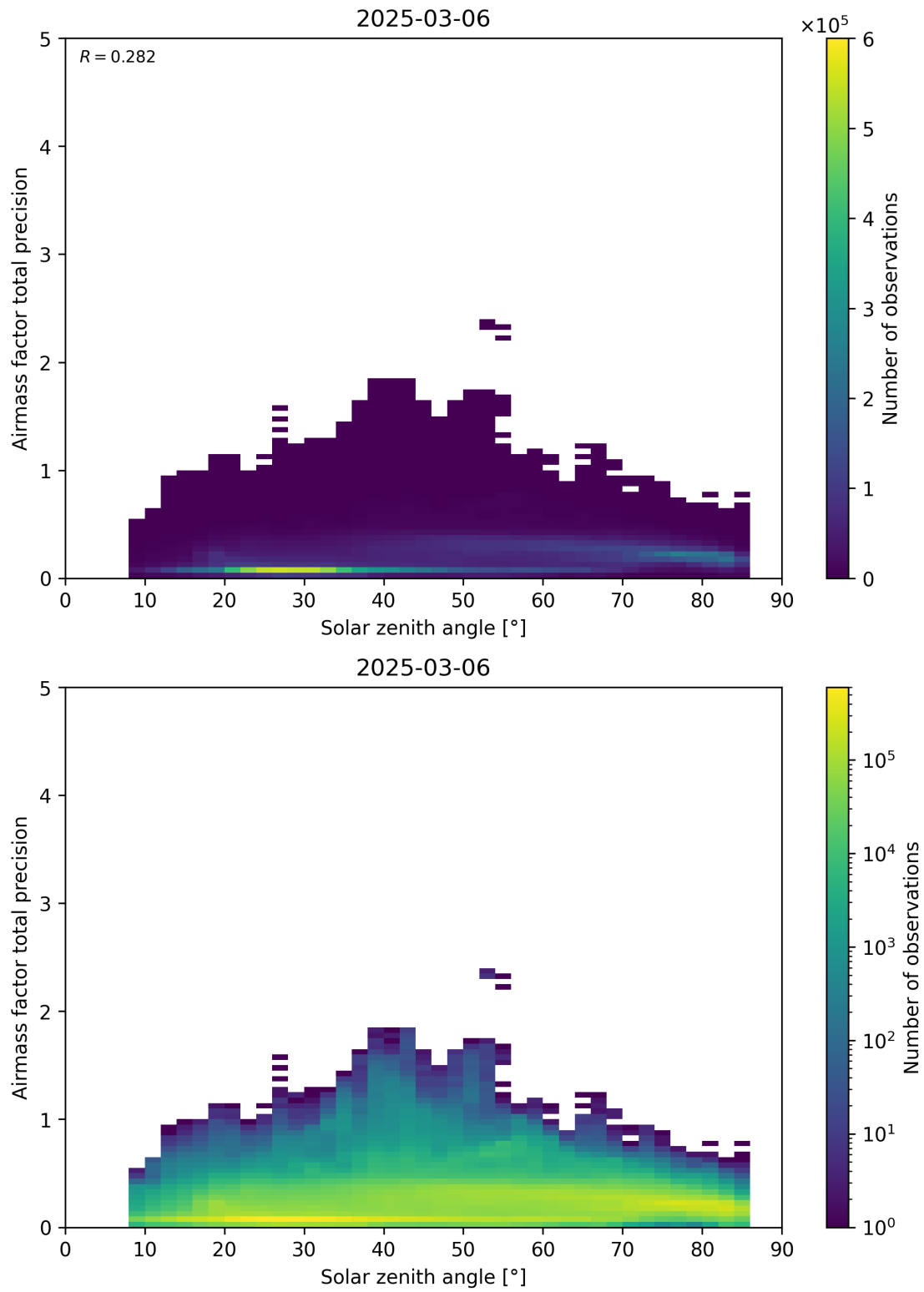
Figure 176: Scatter density plot of “Solar zenith angle” against “Airmass factor total precision” for 2025-03-05 to 2025-03-07.
