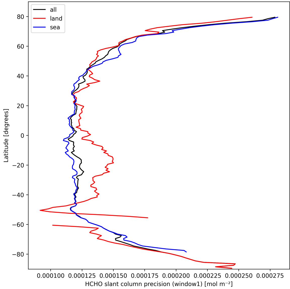
Figure 25: Zonal average of “HCHO slant column precision (window1)” for 2025-03-05 to 2025-03-07.
