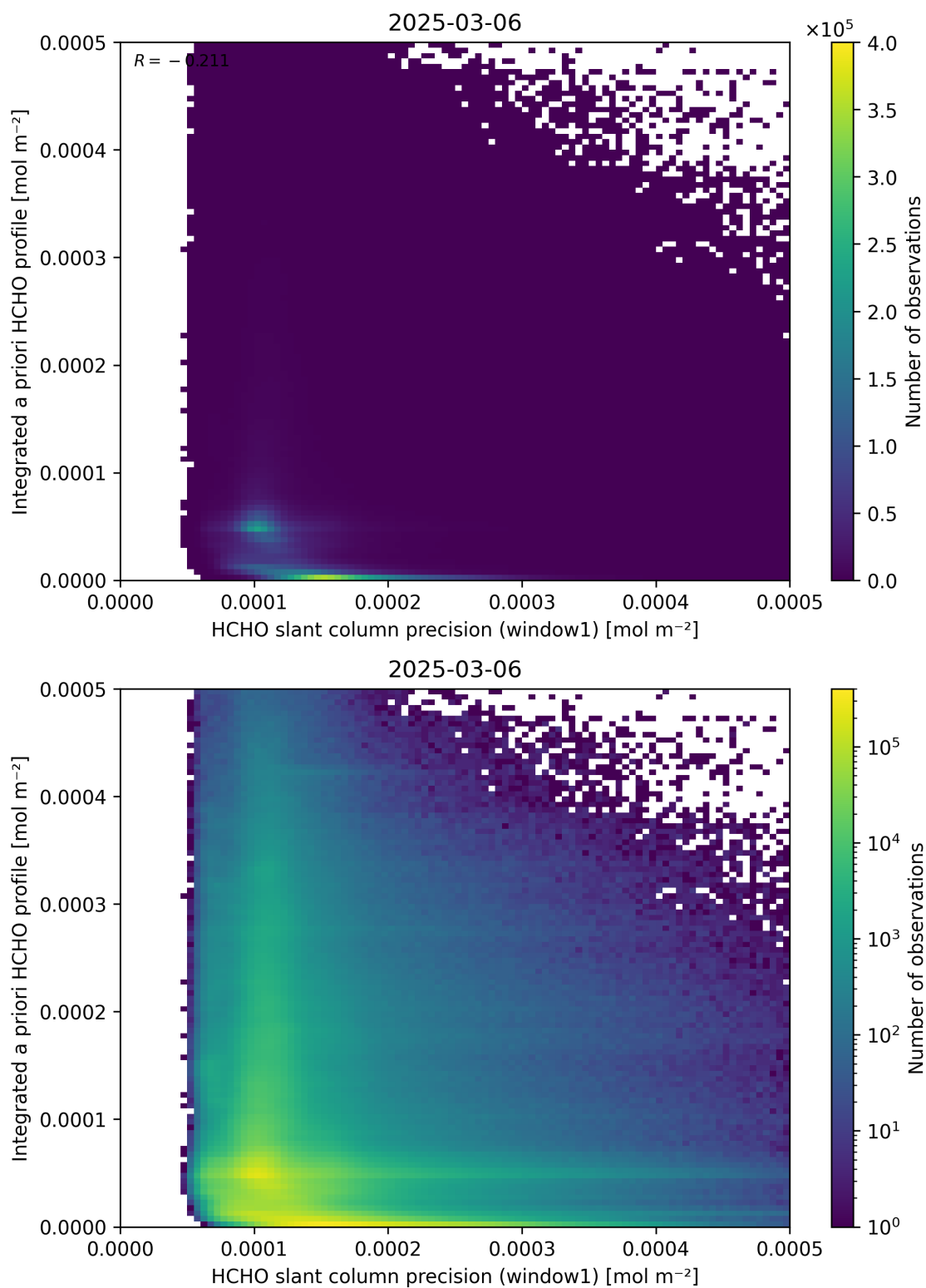
Figure 96: Scatter density plot of “HCHO slant column precision (window1)” against “Integrated a priori HCHO profile” for 2025-03-05 to 2025-03-07.
