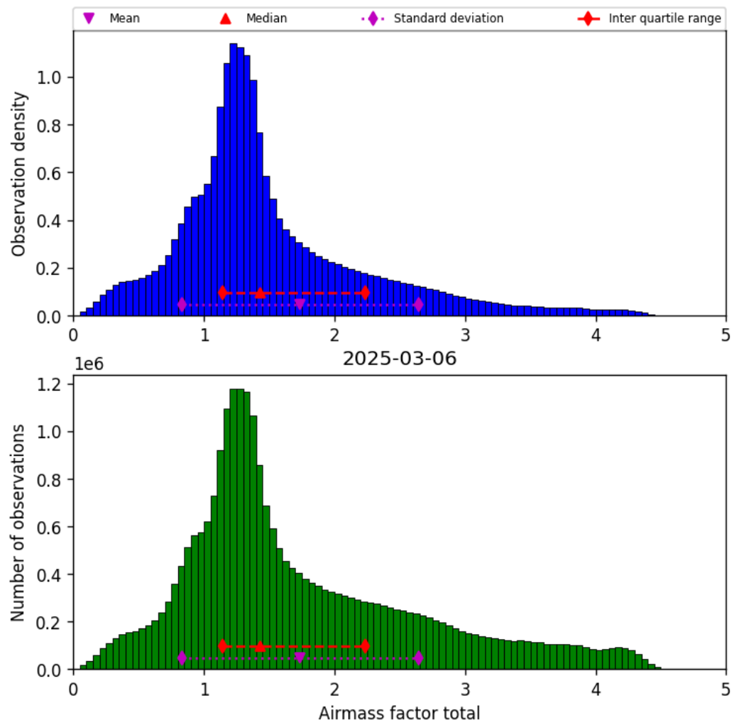
Figure 40: Histogram of “Airmass factor total” for 2025-03-05 to 2025-03-07
