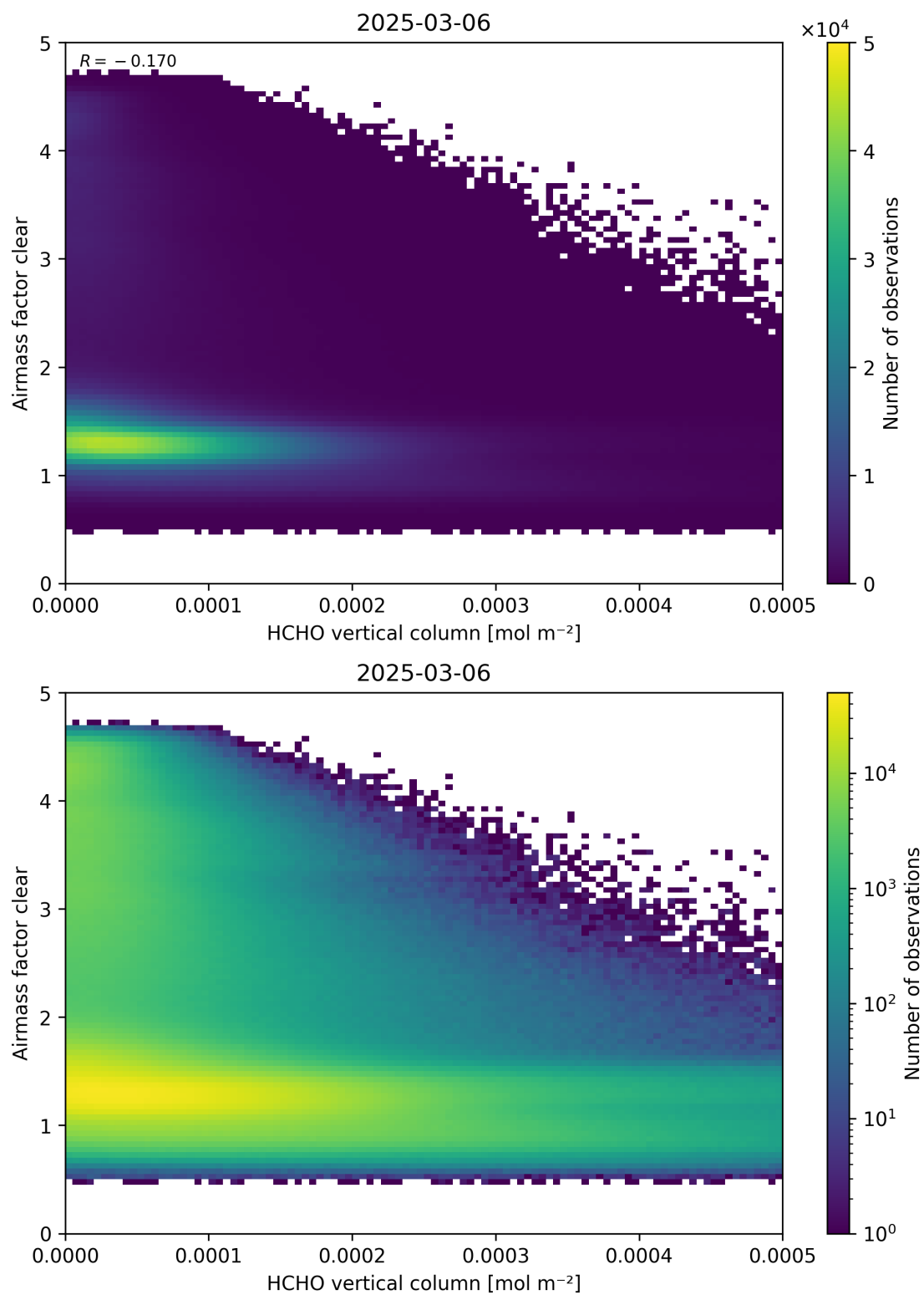
Figure 126: Scatter density plot of “HCHO vertical column” against “Airmass factor clear” for 2025-03-05 to 2025-03-07.
