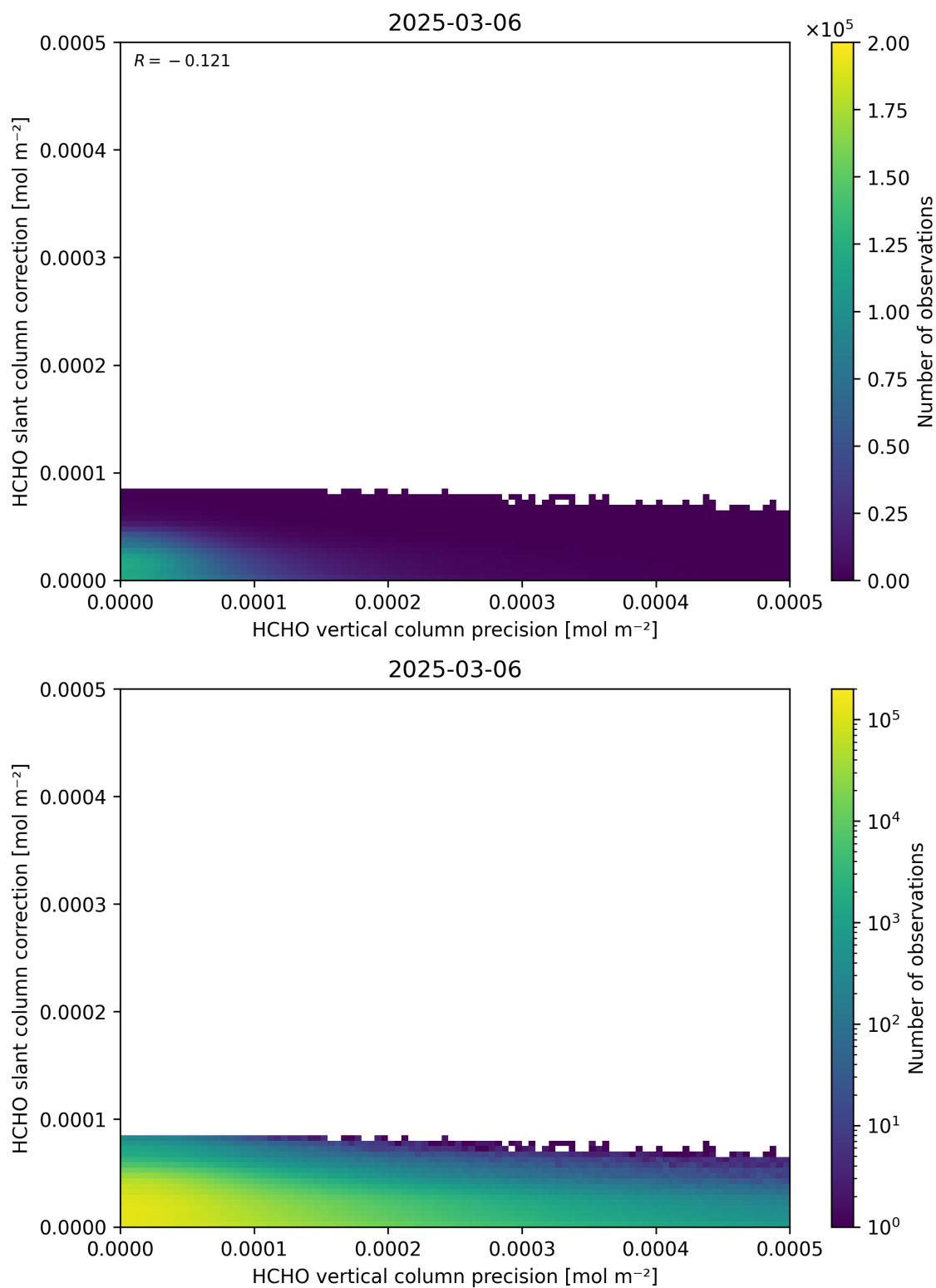
Figure 141: Scatter density plot of “HCHO vertical column precision” against “HCHO slant column correction” for 2025-03-05 to 2025-03-07.
