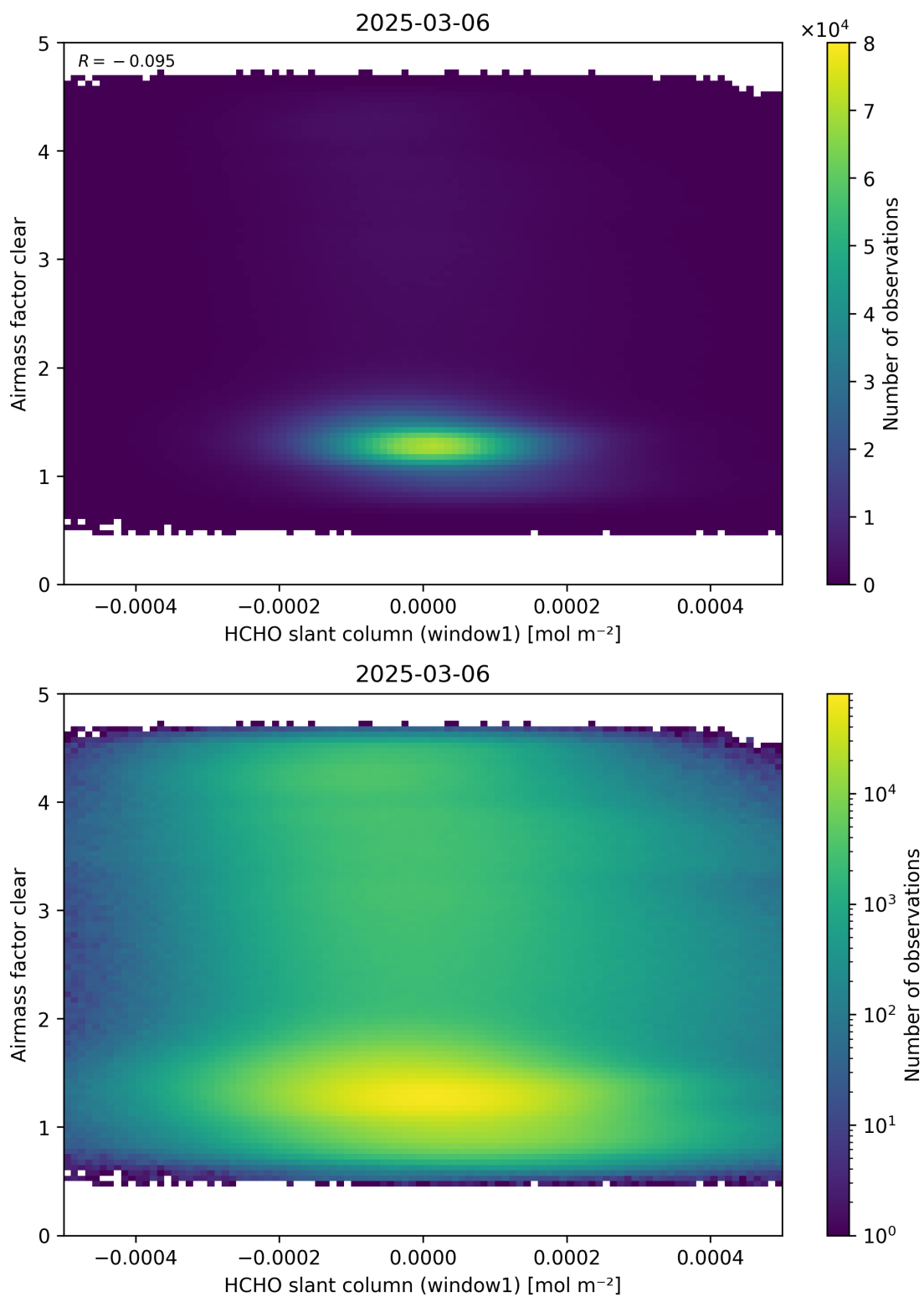
Figure 81: Scatter density plot of “HCHO slant column (window1)” against “Airmass factor clear” for 2025-03-05 to 2025-03-07.
