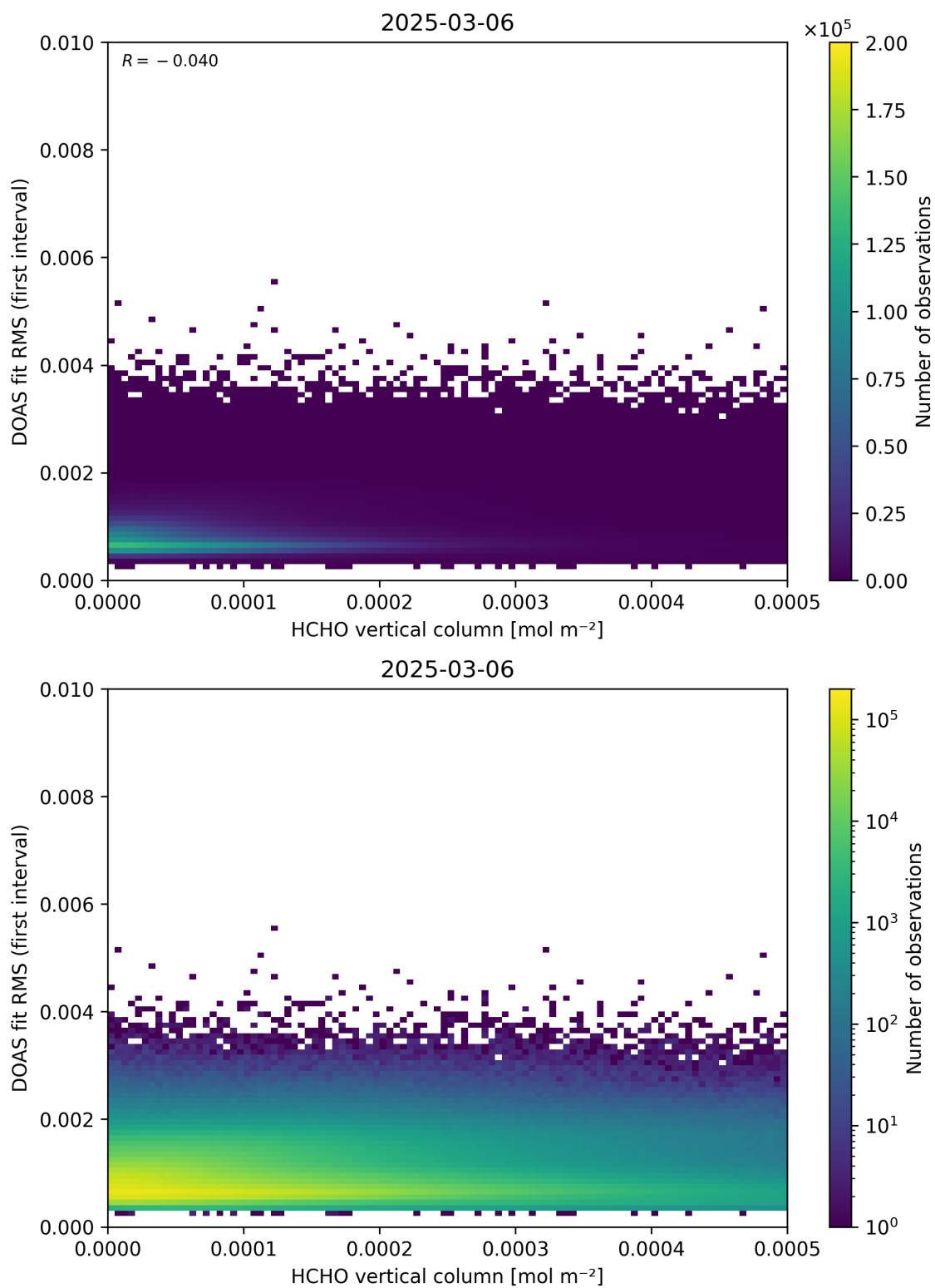
Figure 123: Scatter density plot of “HCHO vertical column” against “DOAS fit RMS (first interval)” for 2025-03-05 to 2025-03-07.
