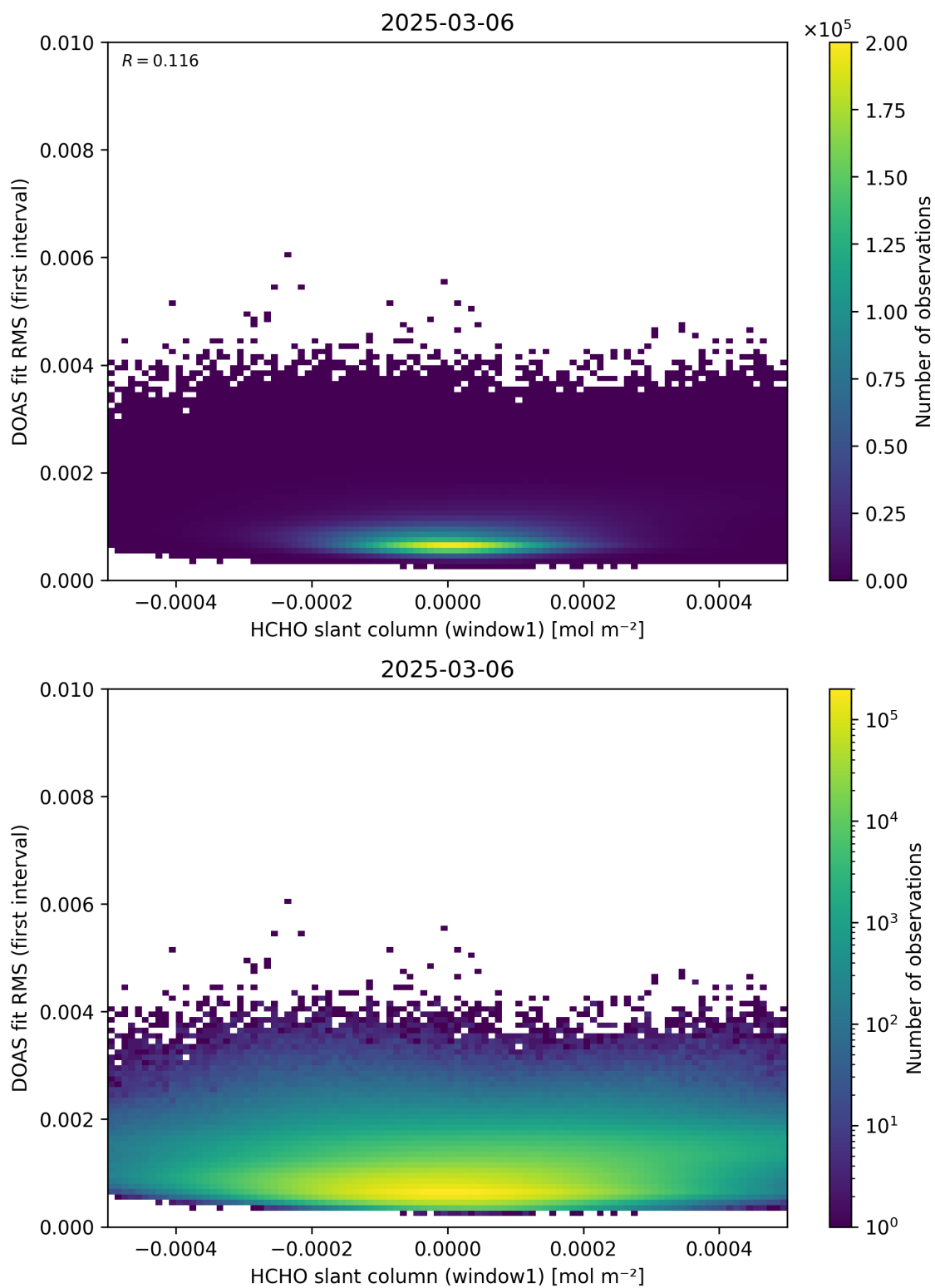
Figure 78: Scatter density plot of “HCHO slant column (window1)” against “DOAS fit RMS (first interval)” for 2025-03-05 to 2025-03-07.
