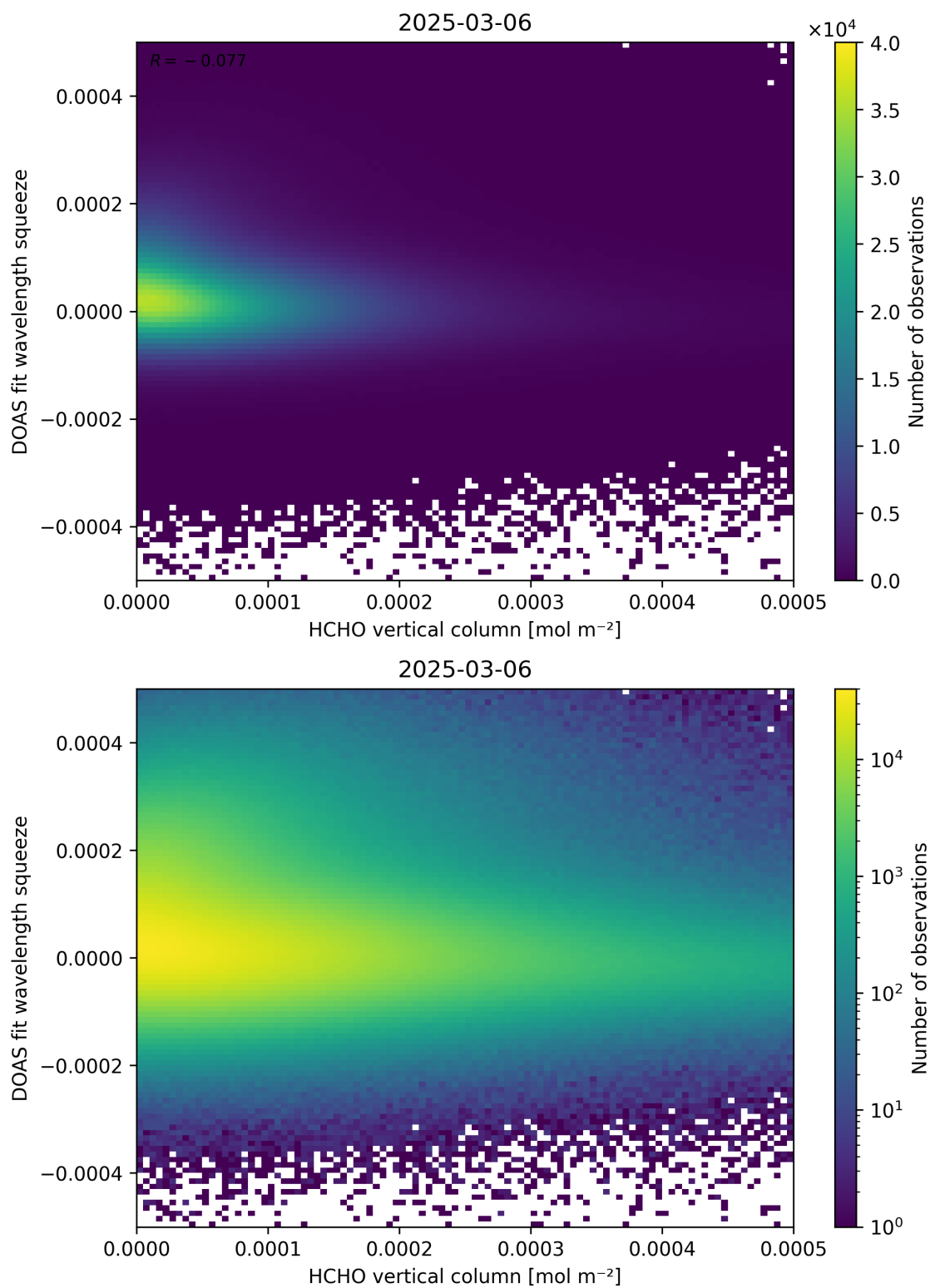
Figure 125: Scatter density plot of “HCHO vertical column” against “DOAS fit wavelength squeeze” for 2025-03-05 to 2025-03-07.
