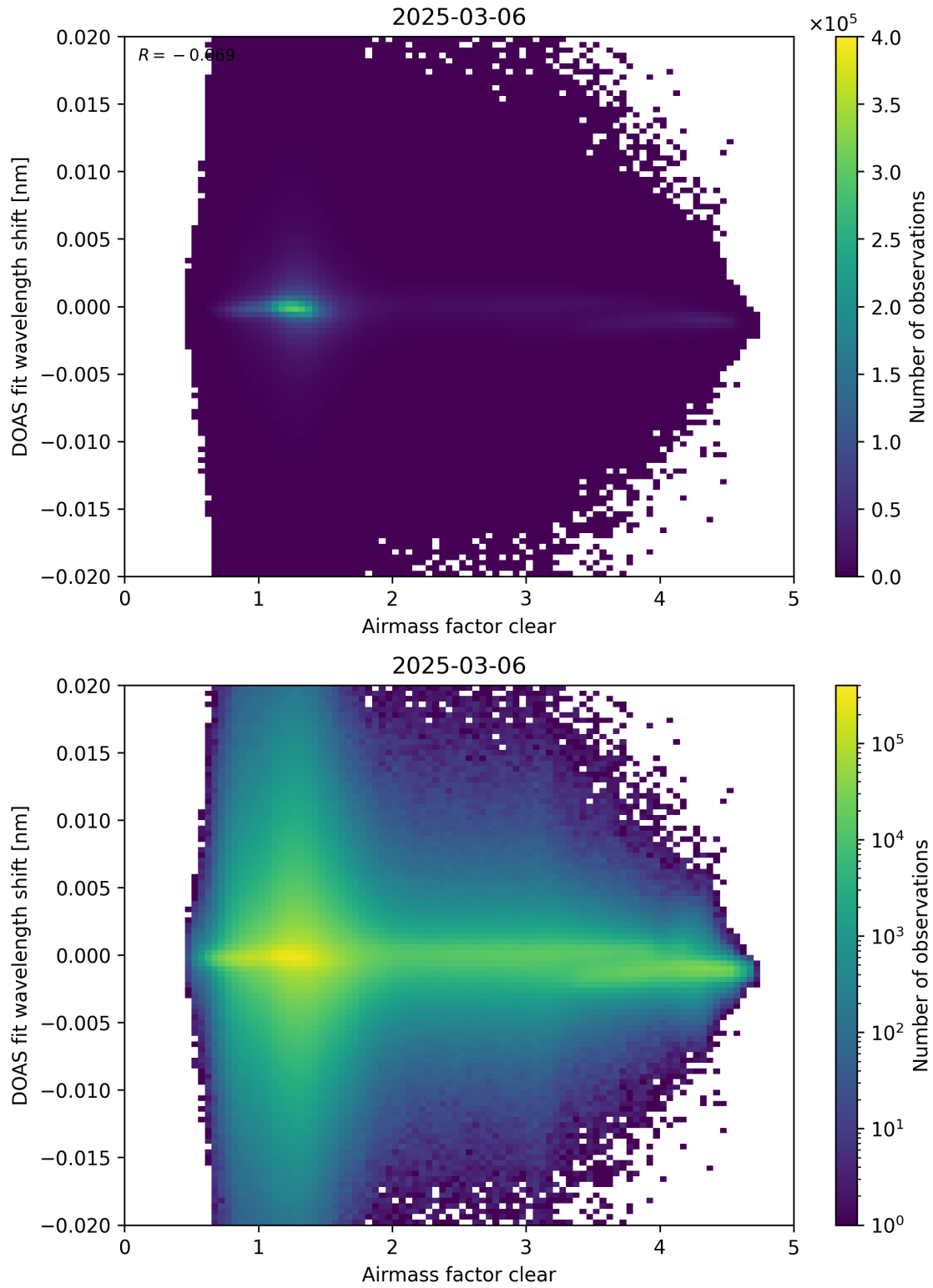
Figure 72: Scatter density plot of “Airmass factor clear” against “DOAS fit wavelength shift” for 2025-03-05 to 2025-03-07.
