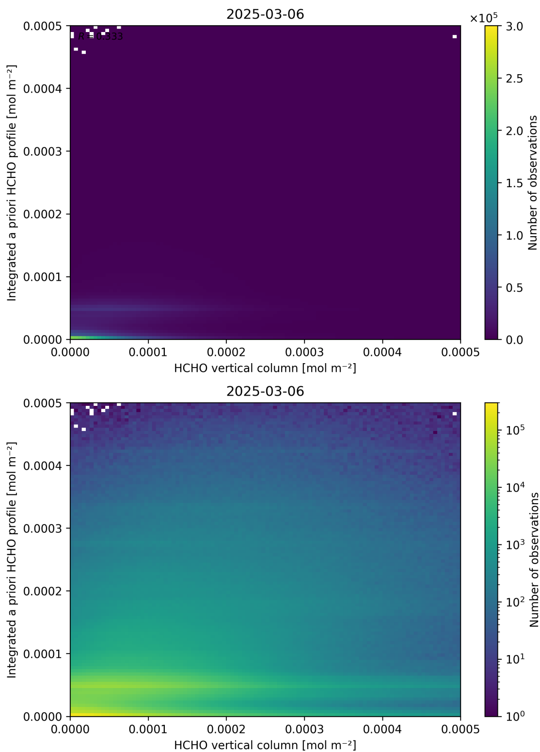
Figure 135: Scatter density plot of “HCHO vertical column” against “Integrated a priori HCHO profile” for 2025-03-05 to 2025-03-07.
