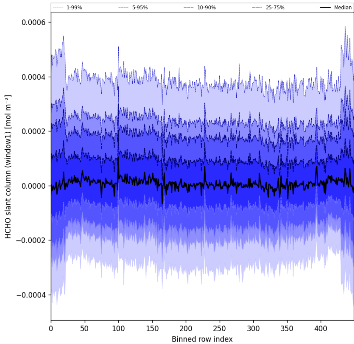
Figure 52: Along track statistics of “HCHO slant column (window1)” for 2025-03-05 to 2025-03-07
