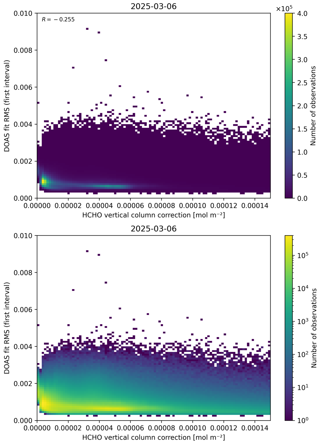
Figure 112: Scatter density plot of “HCHO vertical column correction” against “DOAS fit RMS (first interval)” for 2025-03-05 to 2025-03-07.
