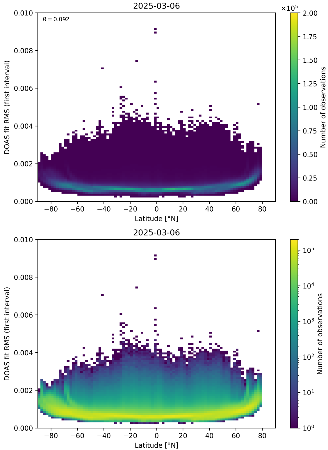
Figure 153: Scatter density plot of “Latitude” against “DOAS fit RMS (first interval)” for 2025-03-05 to 2025-03-07.
