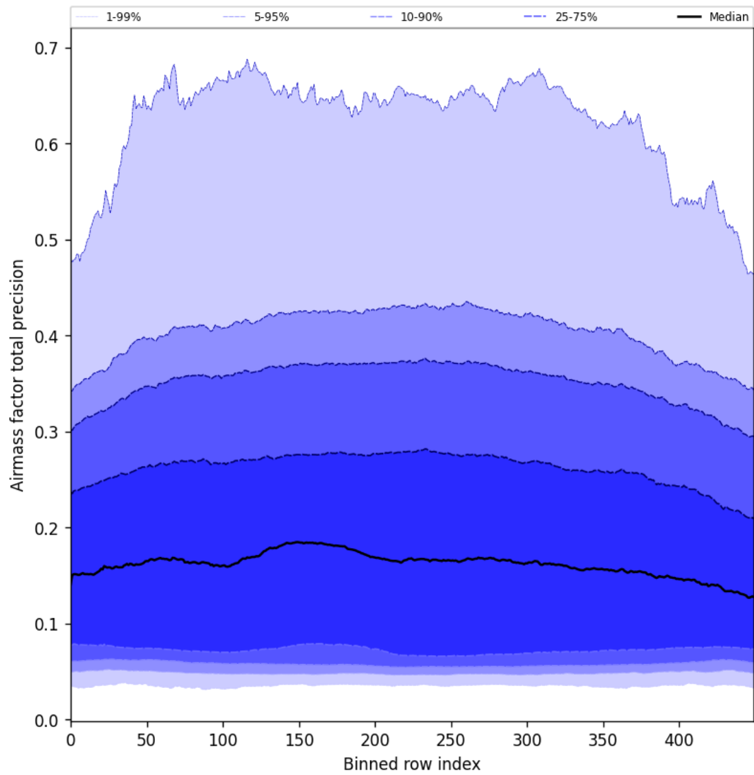
Figure 55: Along track statistics of “Airmass factor total precision” for 2025-03-05 to 2025-03-07
