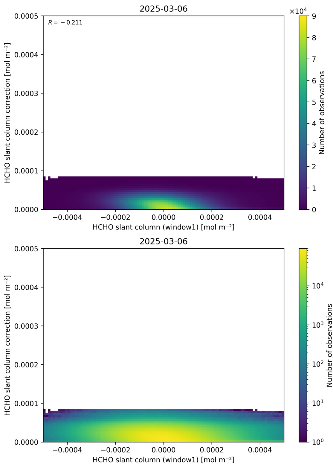
Figure 83: Scatter density plot of “HCHO slant column (window1)” against “HCHO slant column correction” for 2025-03-05 to 2025-03-07.
