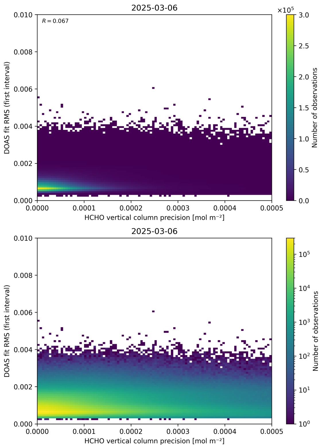
Figure 136: Scatter density plot of “HCHO vertical column precision” against “DOAS fit RMS (first interval)” for 2025-03-05 to 2025-03-07.
