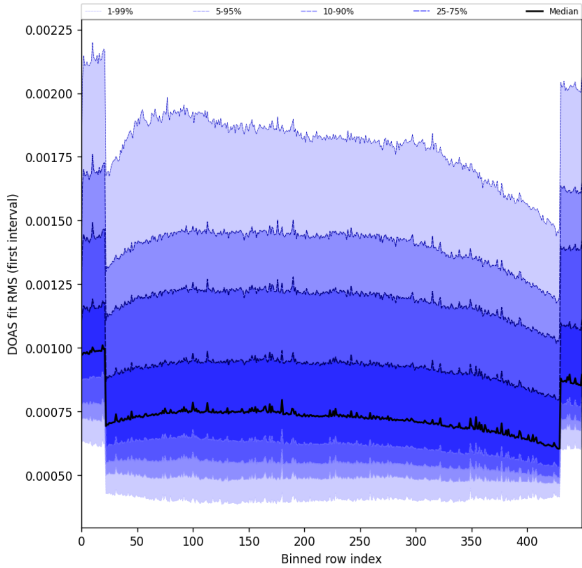
Figure 60: Along track statistics of “DOAS fit RMS (first interval)” for 2025-03-05 to 2025-03-07
