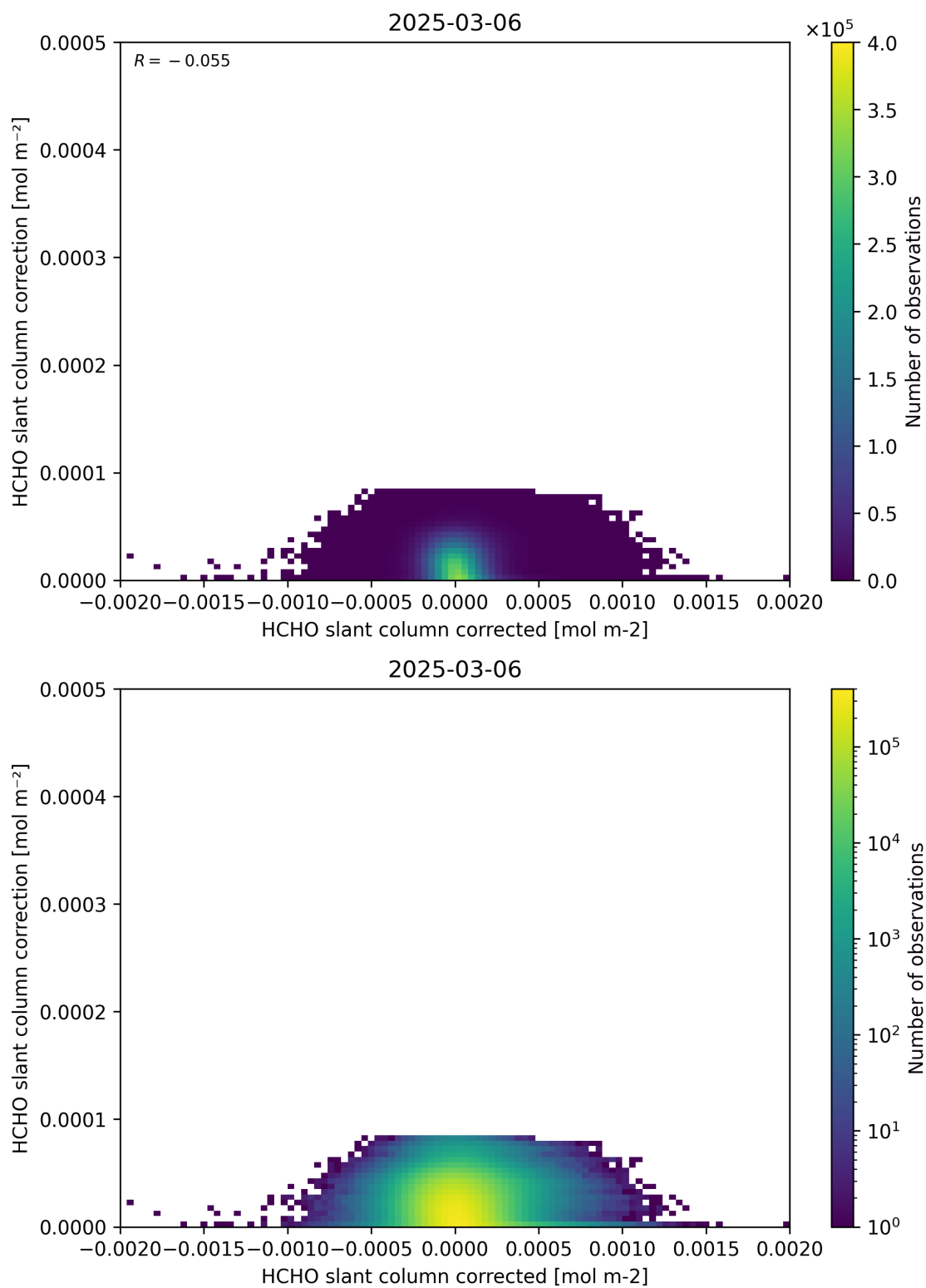
Figure 77: Scatter density plot of “HCHO slant column corrected” against “HCHO slant column correction” for 2025-03-05 to 2025-03-07.
