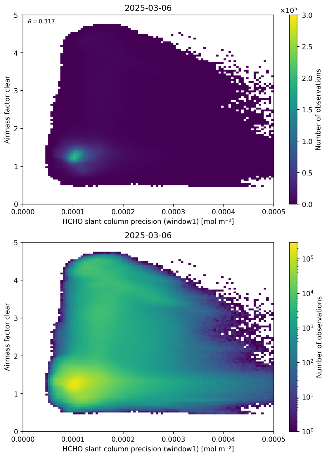
Figure 91: Scatter density plot of “HCHO slant column precision (window1)” against “Airmass factor clear” for 2025-03-05 to 2025-03-07.
