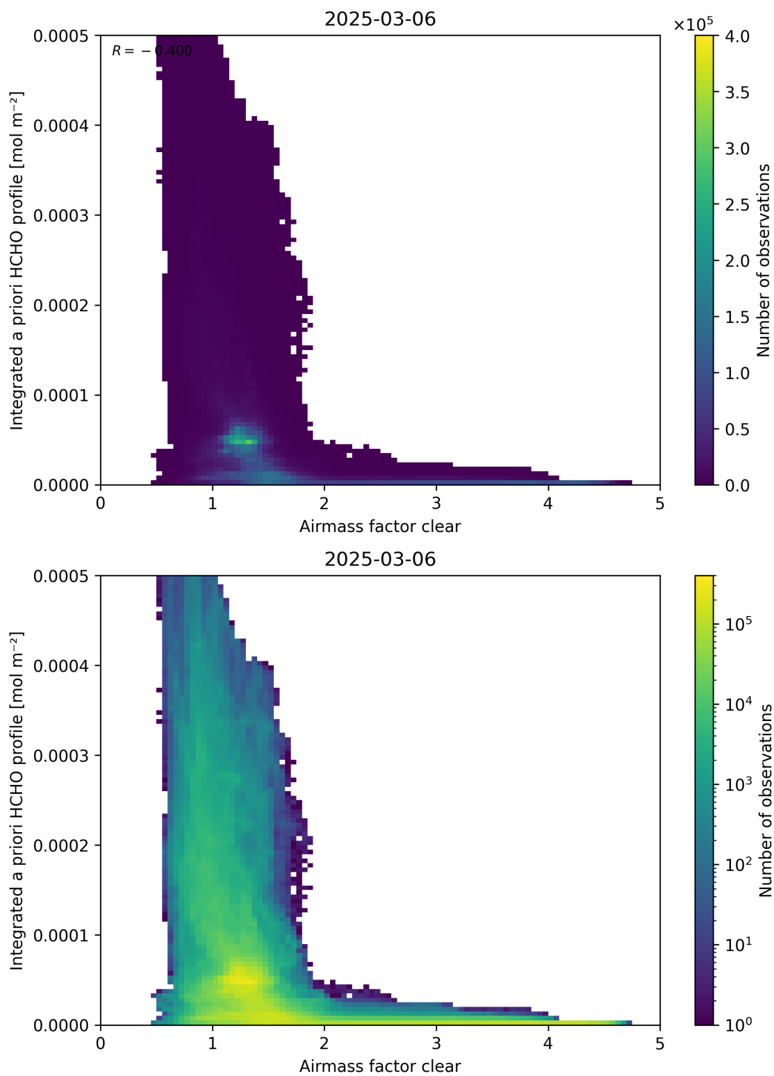
Figure 76: Scatter density plot of “Airmass factor clear” against “Integrated a priori HCHO profile” for 2025-03-05 to 2025-03-07.
