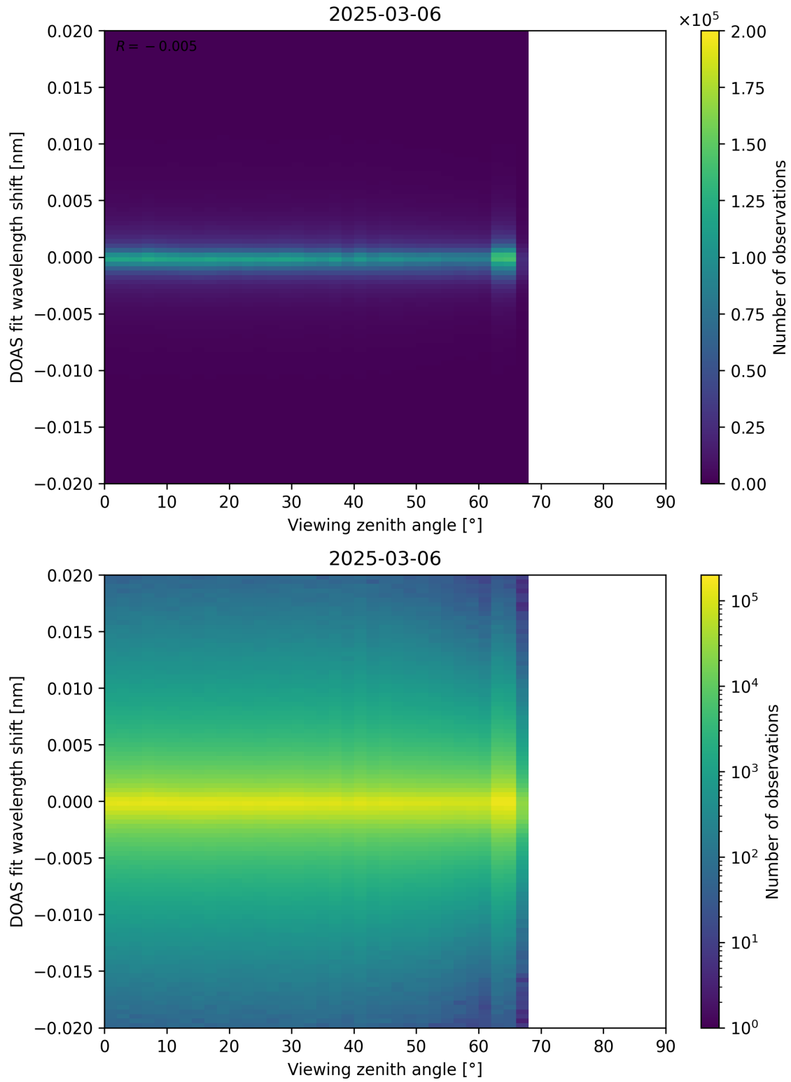
Figure 183: Scatter density plot of “Viewing zenith angle” against “DOAS fit wavelength shift” for 2025-03-05 to 2025-03-07.
