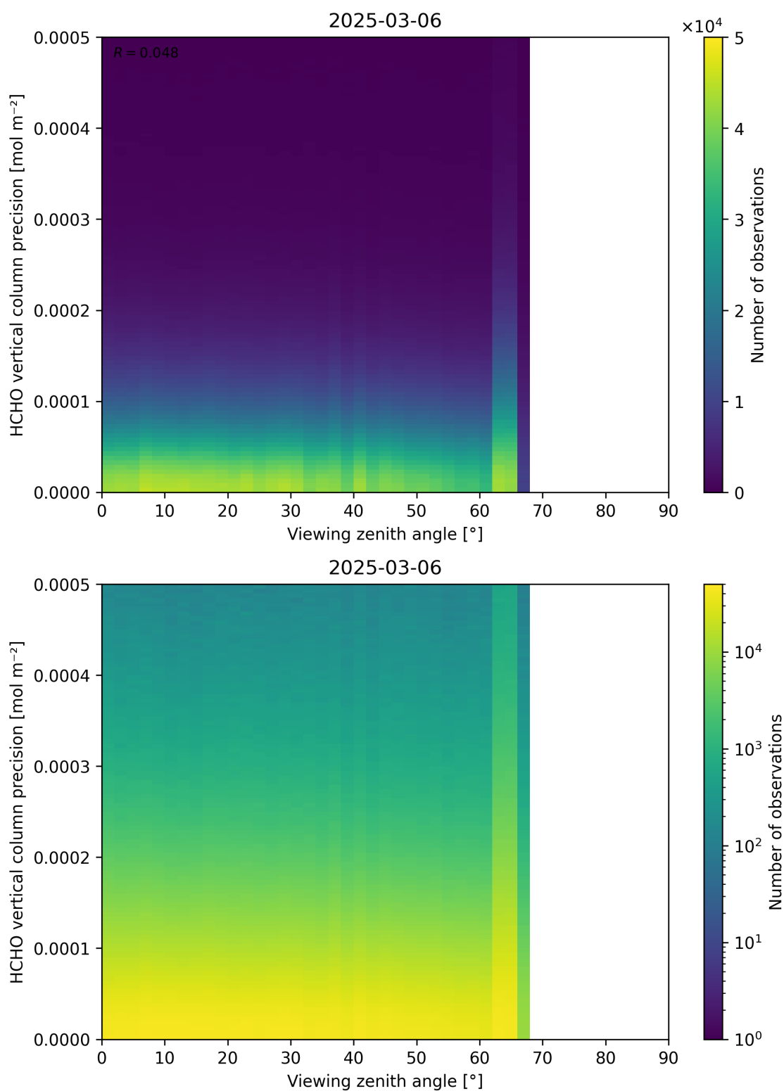
Figure 194: Scatter density plot of “Viewing zenith angle” against “HCHO vertical column precision” for 2025-03-05 to 2025-03-07.
