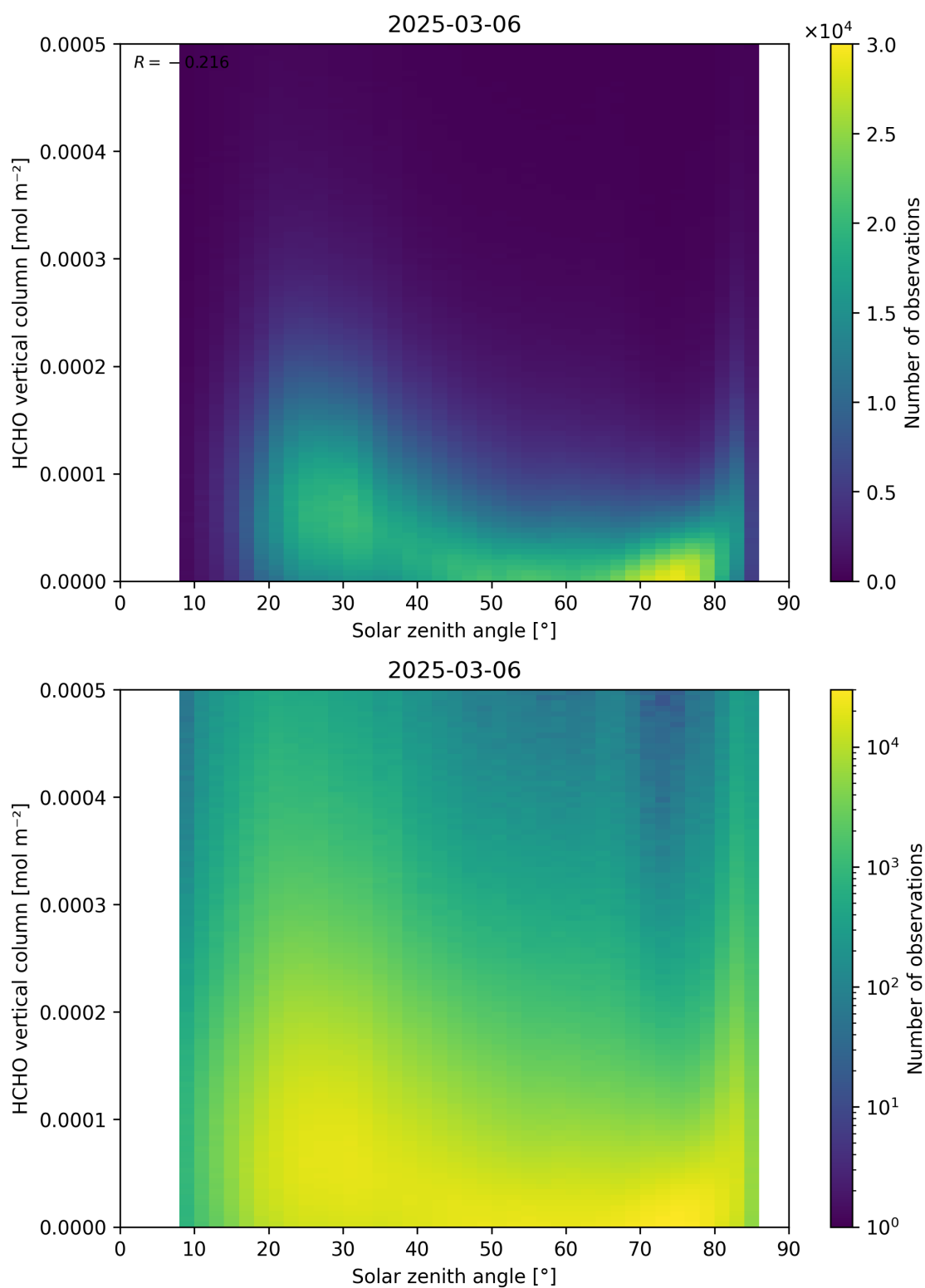
Figure 177: Scatter density plot of “Solar zenith angle” against “HCHO vertical column” for 2025-03-05 to 2025-03-07.
