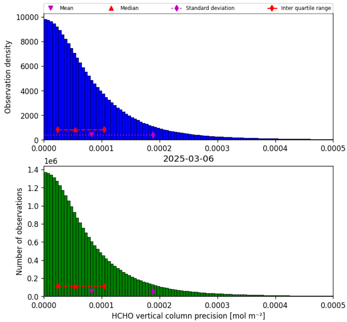
Figure 36: Histogram of “HCHO vertical column precision” for 2025-03-05 to 2025-03-07
