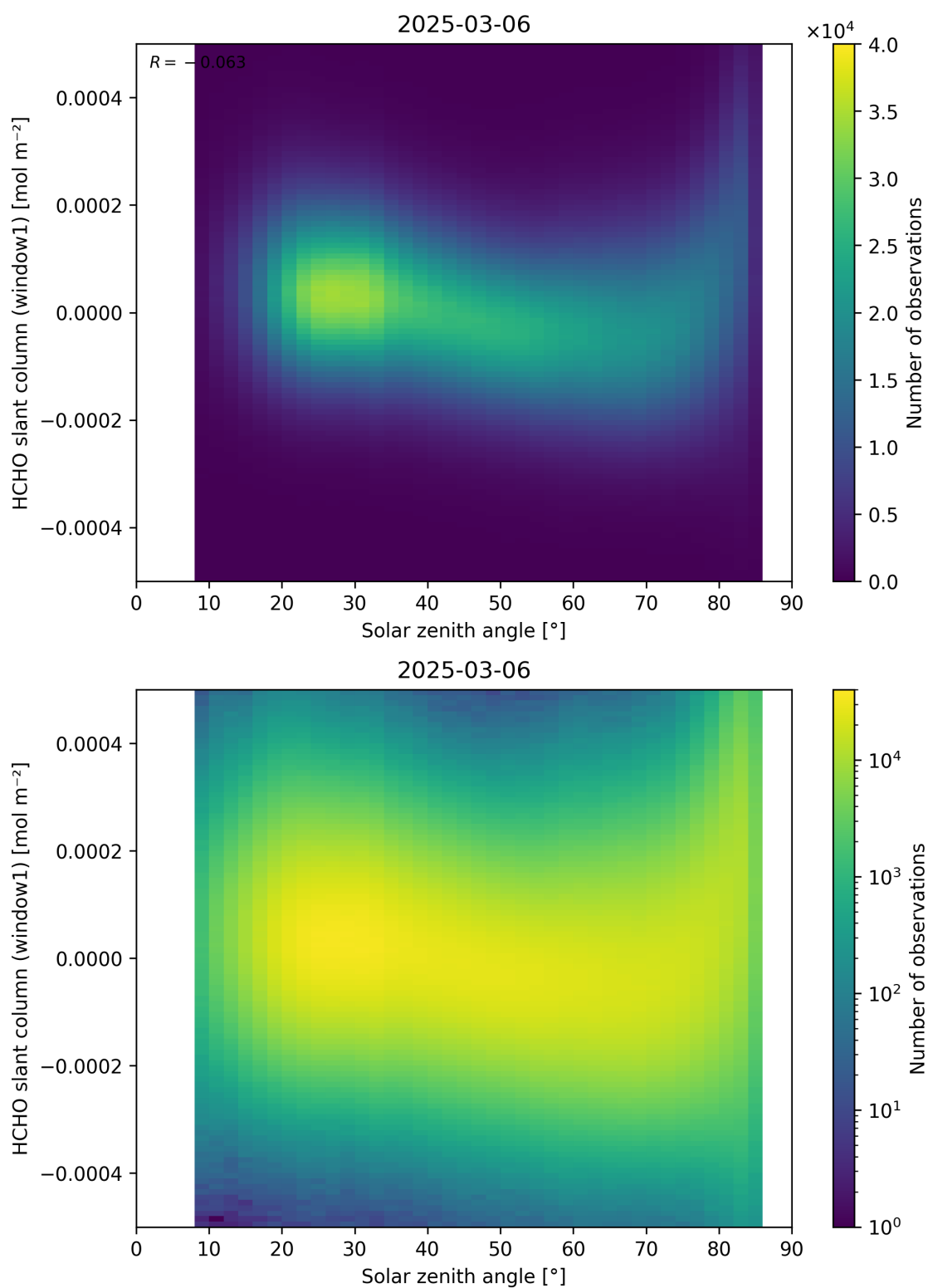
Figure 173: Scatter density plot of “Solar zenith angle” against “HCHO slant column (window1)” for 2025-03-05 to 2025-03-07.
