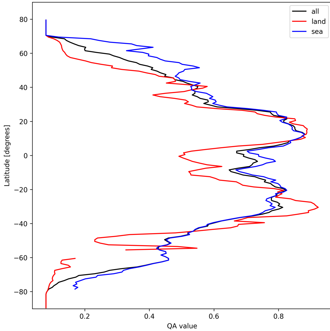
Figure 20: Zonal average of “QA value” for 2025-03-05 to 2025-03-07.
