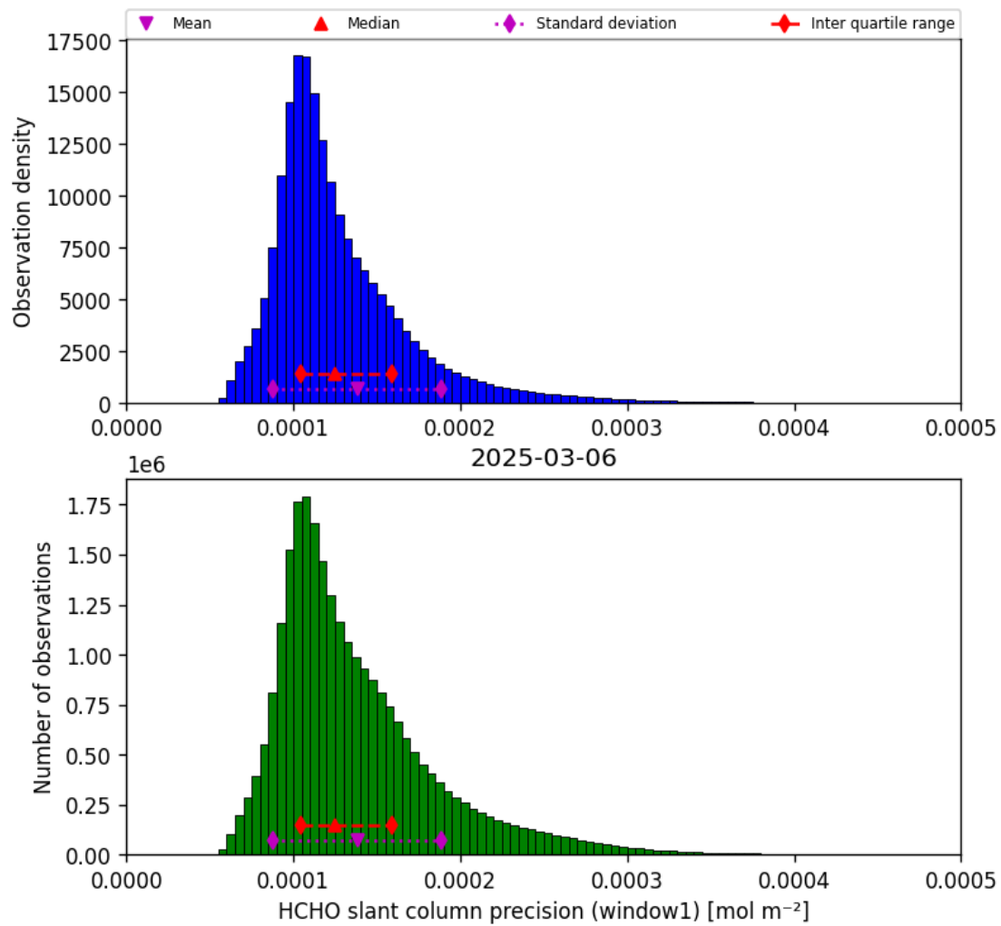
Figure 39: Histogram of “HCHO slant column precision (window1)” for 2025-03-05 to 2025-03-07
