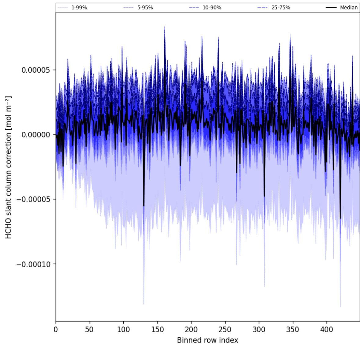
Figure 61: Along track statistics of “HCHO slant column correction” for 2025-03-05 to 2025-03-07
