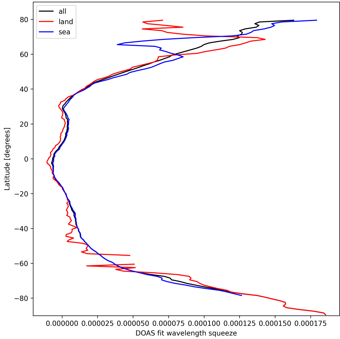
Figure 31: Zonal average of “DOAS fit wavelength squeeze” for 2025-03-05 to 2025-03-07.
