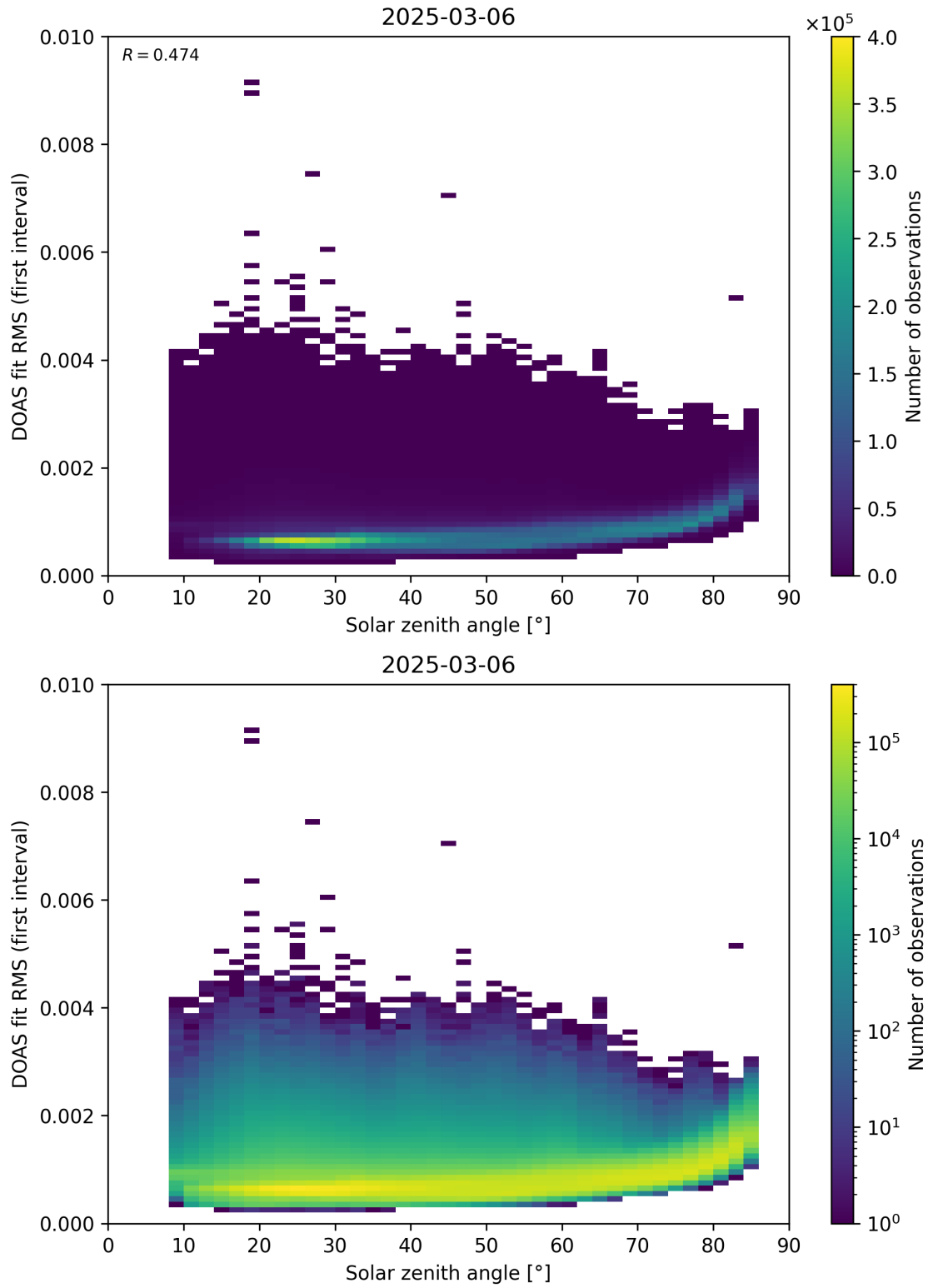
Figure 167: Scatter density plot of “Solar zenith angle” against “DOAS fit RMS (first interval)” for 2025-03-05 to 2025-03-07.
