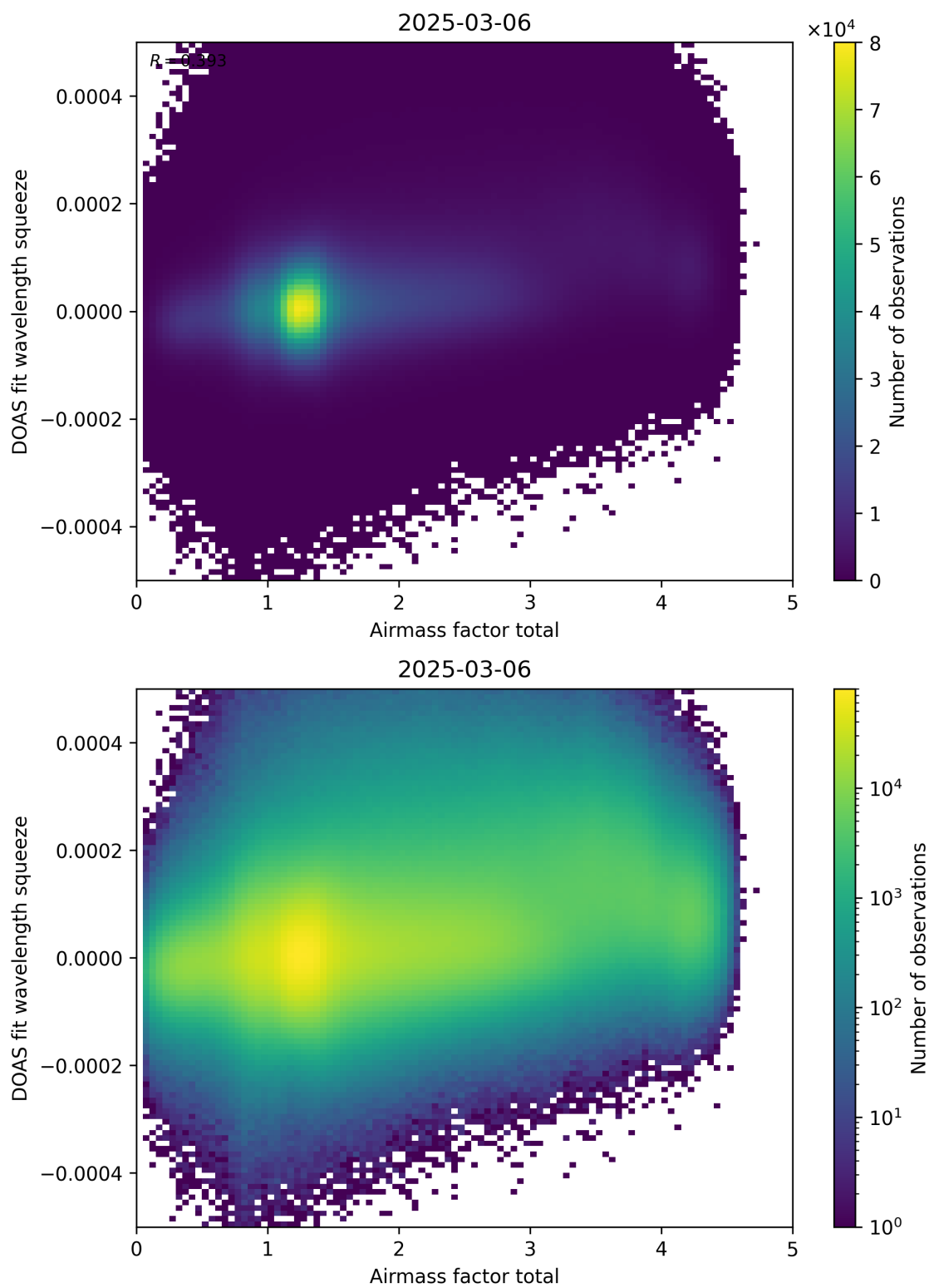
Figure 99: Scatter density plot of “Airmass factor total” against “DOAS fit wavelength squeeze” for 2025-03-05 to 2025-03-07.
