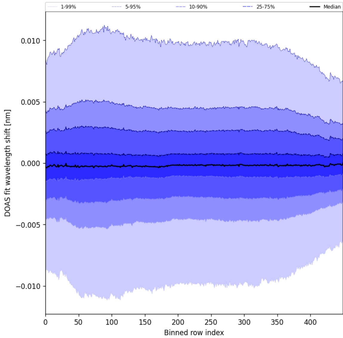
Figure 58: Along track statistics of “DOAS fit wavelength shift” for 2025-03-05 to 2025-03-07
