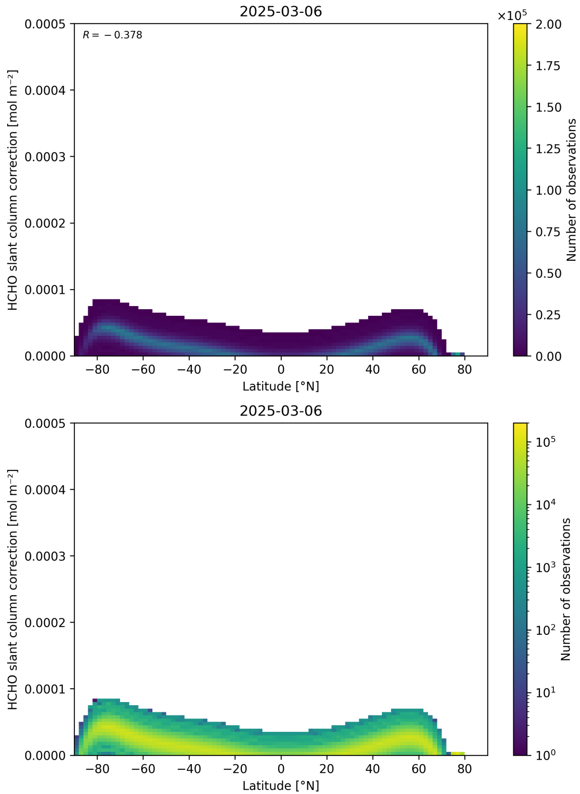
Figure 158: Scatter density plot of “Latitude” against “HCHO slant column correction” for 2025-03-05 to 2025-03-07.
