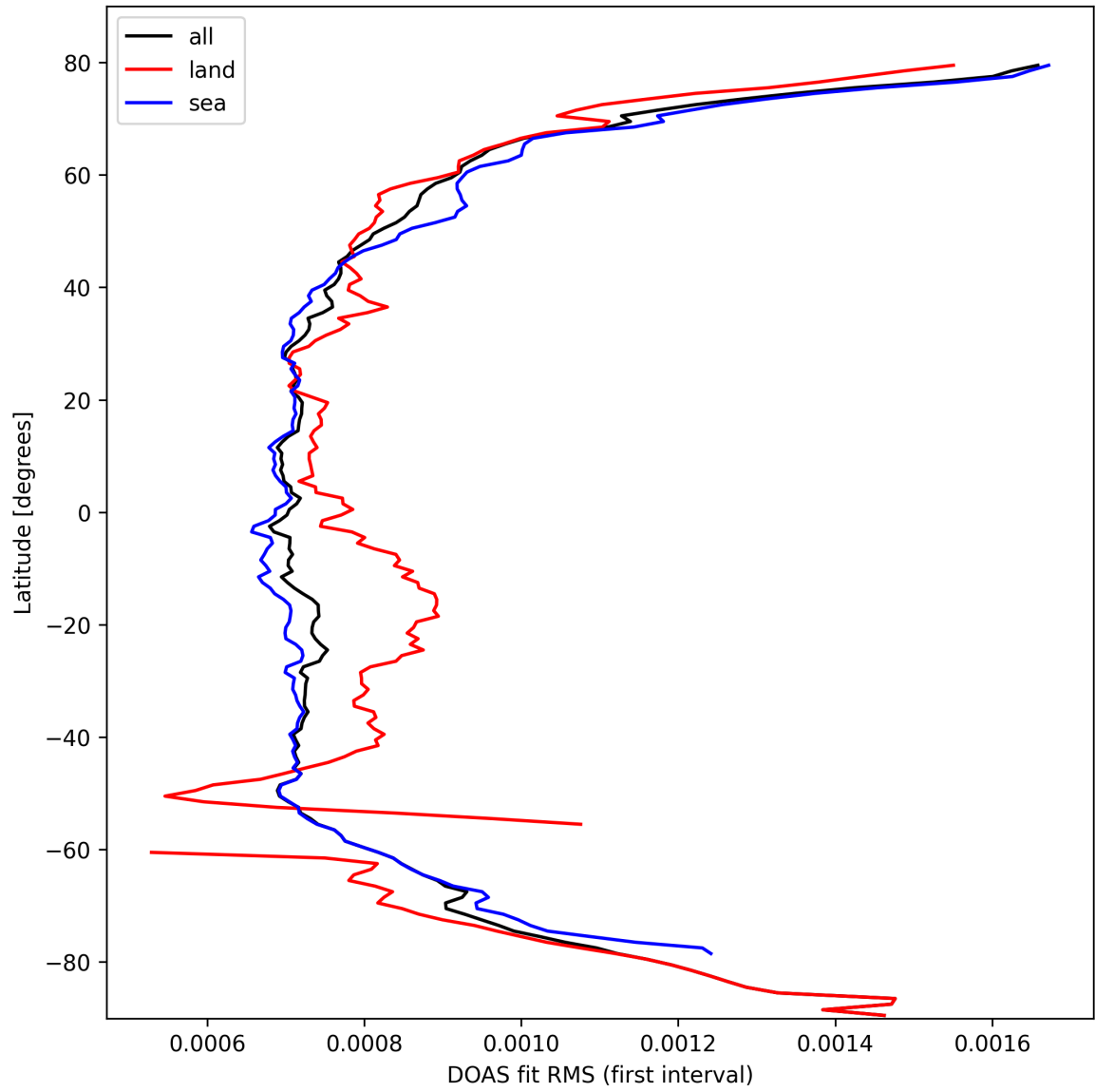
Figure 32: Zonal average of “DOAS fit RMS (first interval)” for 2025-03-05 to 2025-03-07.
