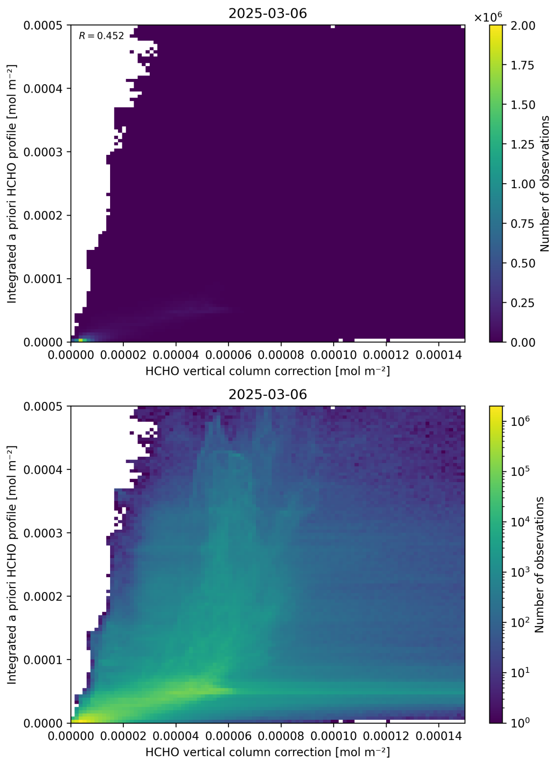
Figure 122: Scatter density plot of “HCHO vertical column correction” against “Integrated a priori HCHO profile” for 2025-03-05 to 2025-03-07.
