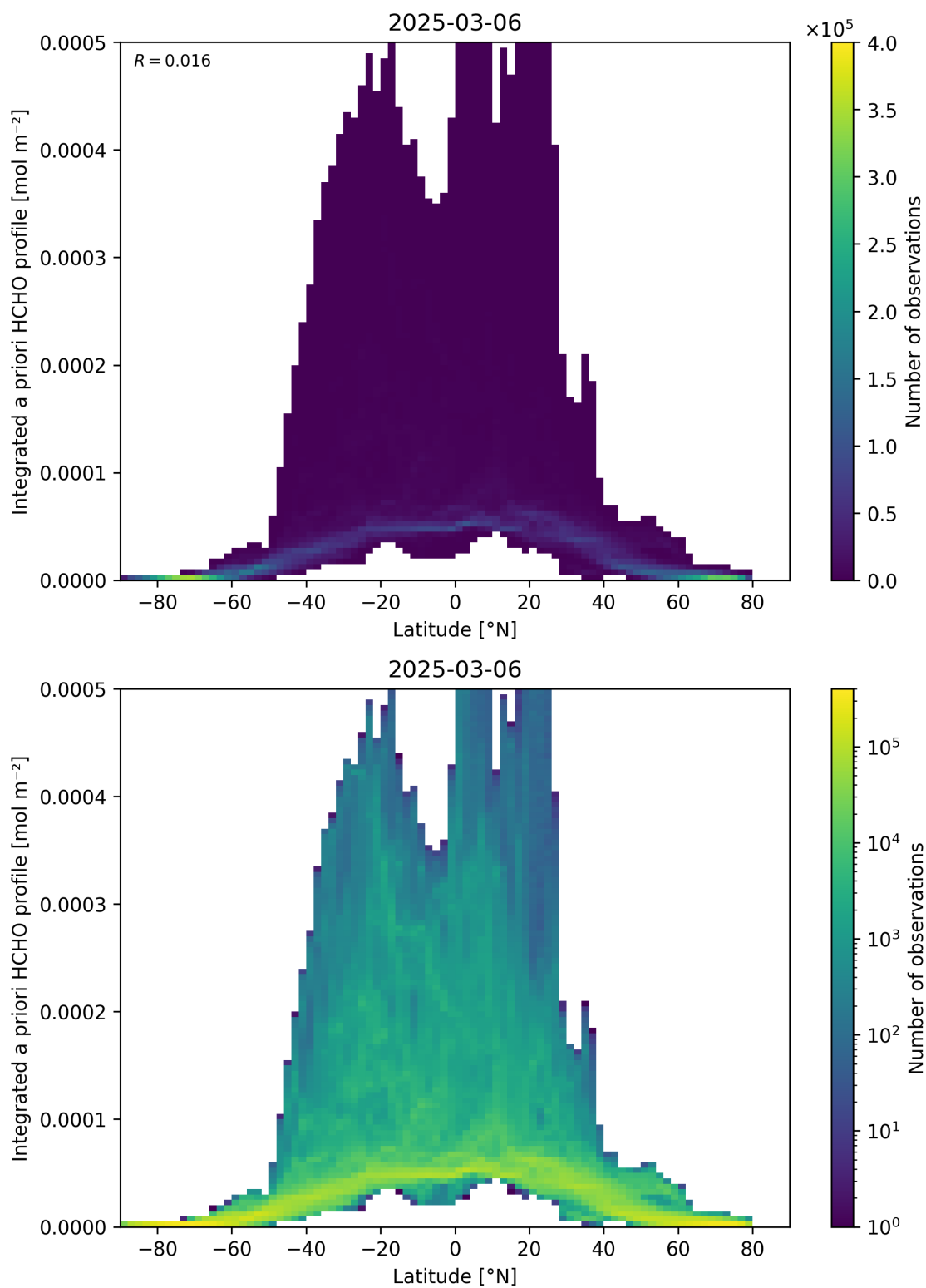
Figure 166: Scatter density plot of “Latitude” against “Integrated a priori HCHO profile” for 2025-03-05 to 2025-03-07.
