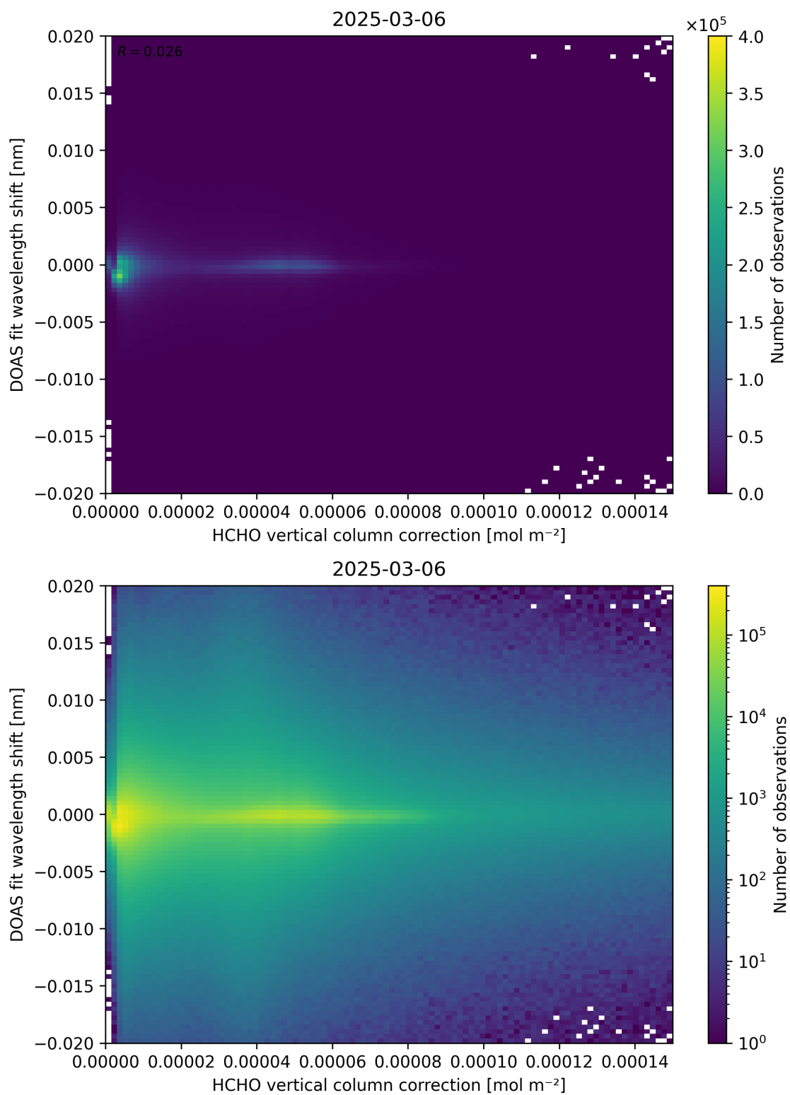
Figure 113: Scatter density plot of “HCHO vertical column correction” against “DOAS fit wavelength shift” for 2025-03-05 to 2025-03-07.
