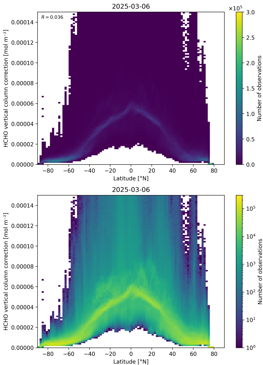
Figure 164: Scatter density plot of “Latitude” against “HCHO vertical column correction” for 2025-03-05 to 2025-03-07.
