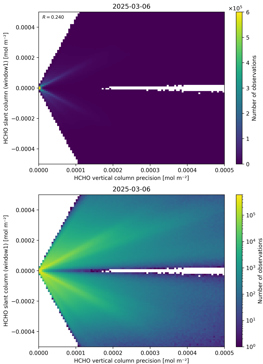
Figure 142: Scatter density plot of “HCHO vertical column precision” against “HCHO slant column (window1)” for 2025-03-05 to 2025-03-07.
