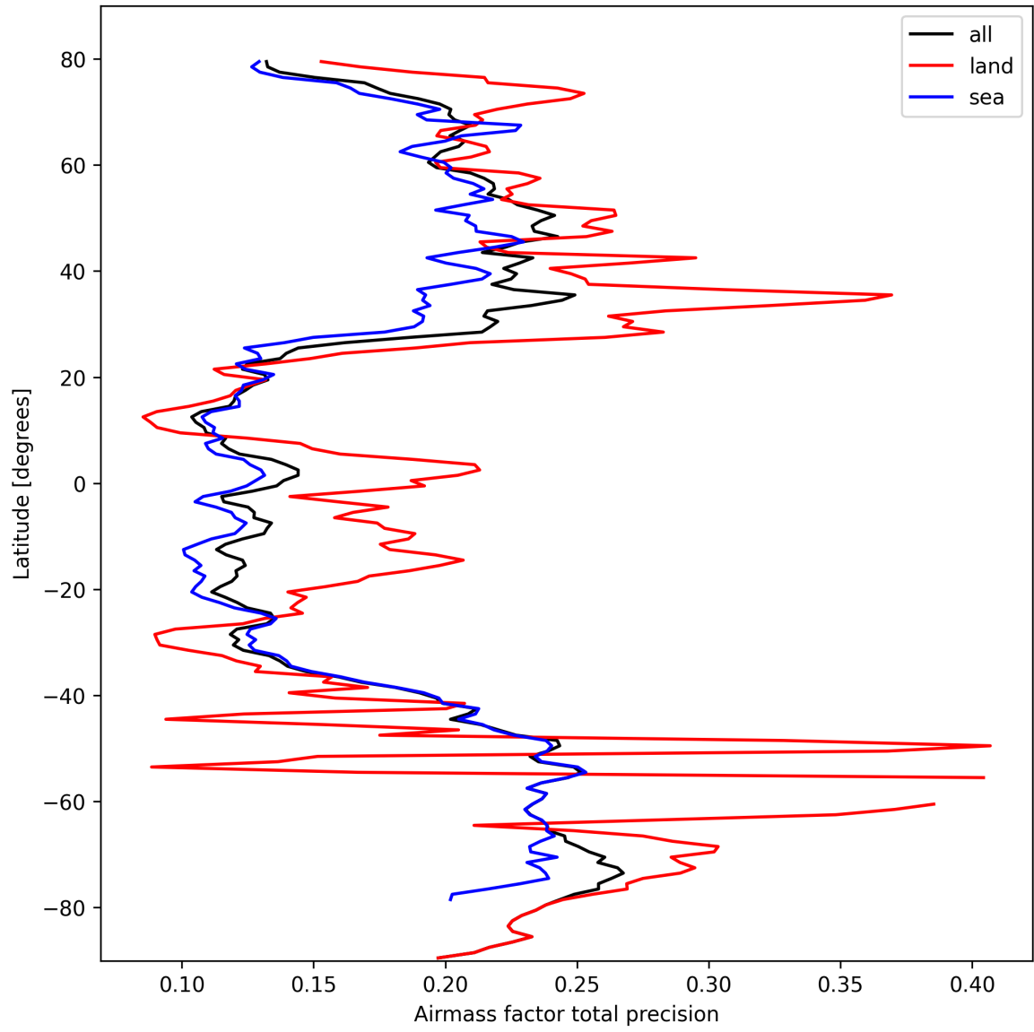
Figure 27: Zonal average of “Airmass factor total precision” for 2025-03-05 to 2025-03-07.
