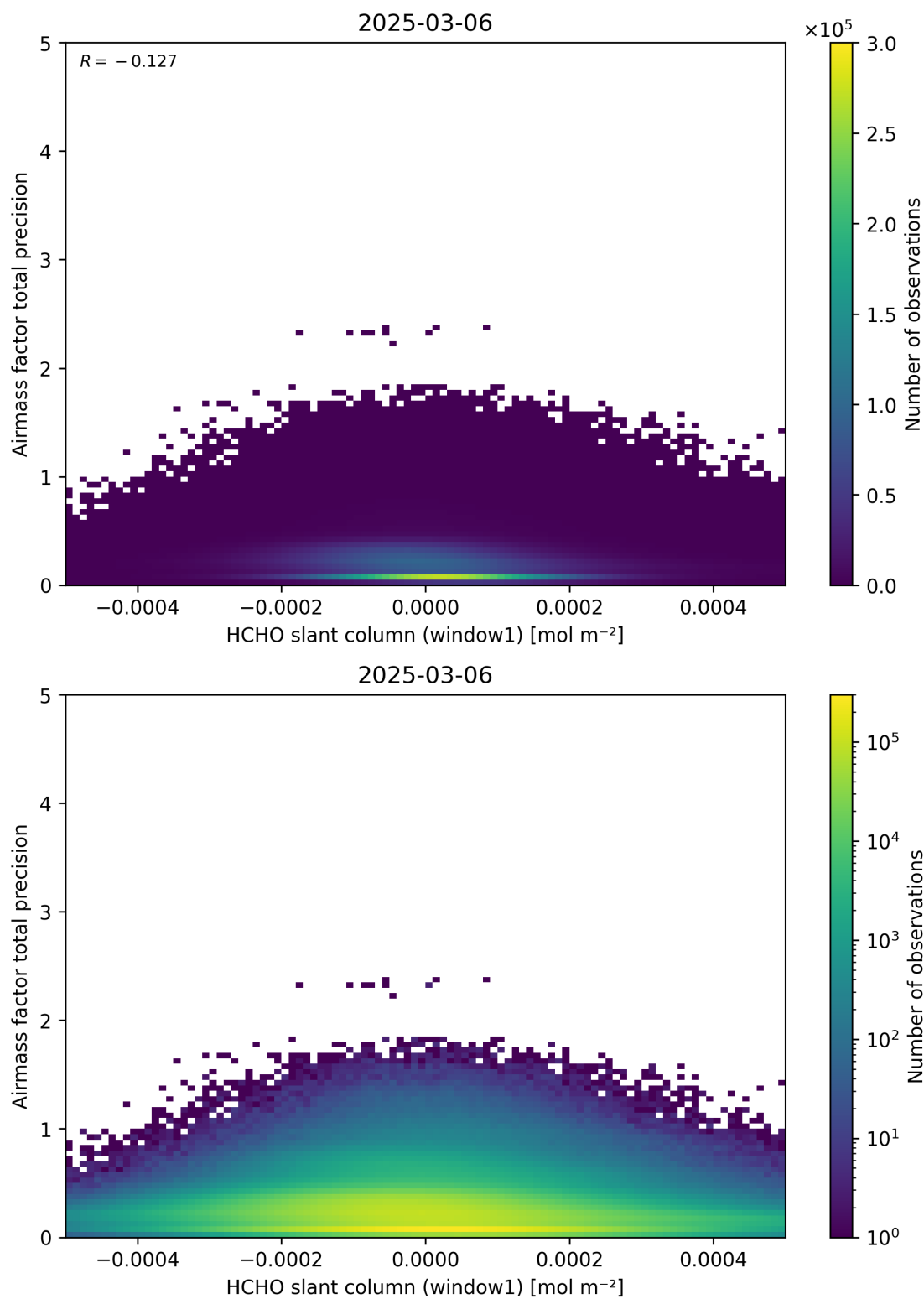
Figure 86: Scatter density plot of “HCHO slant column (window1)” against “Airmass factor total precision” for 2025-03-05 to 2025-03-07.
