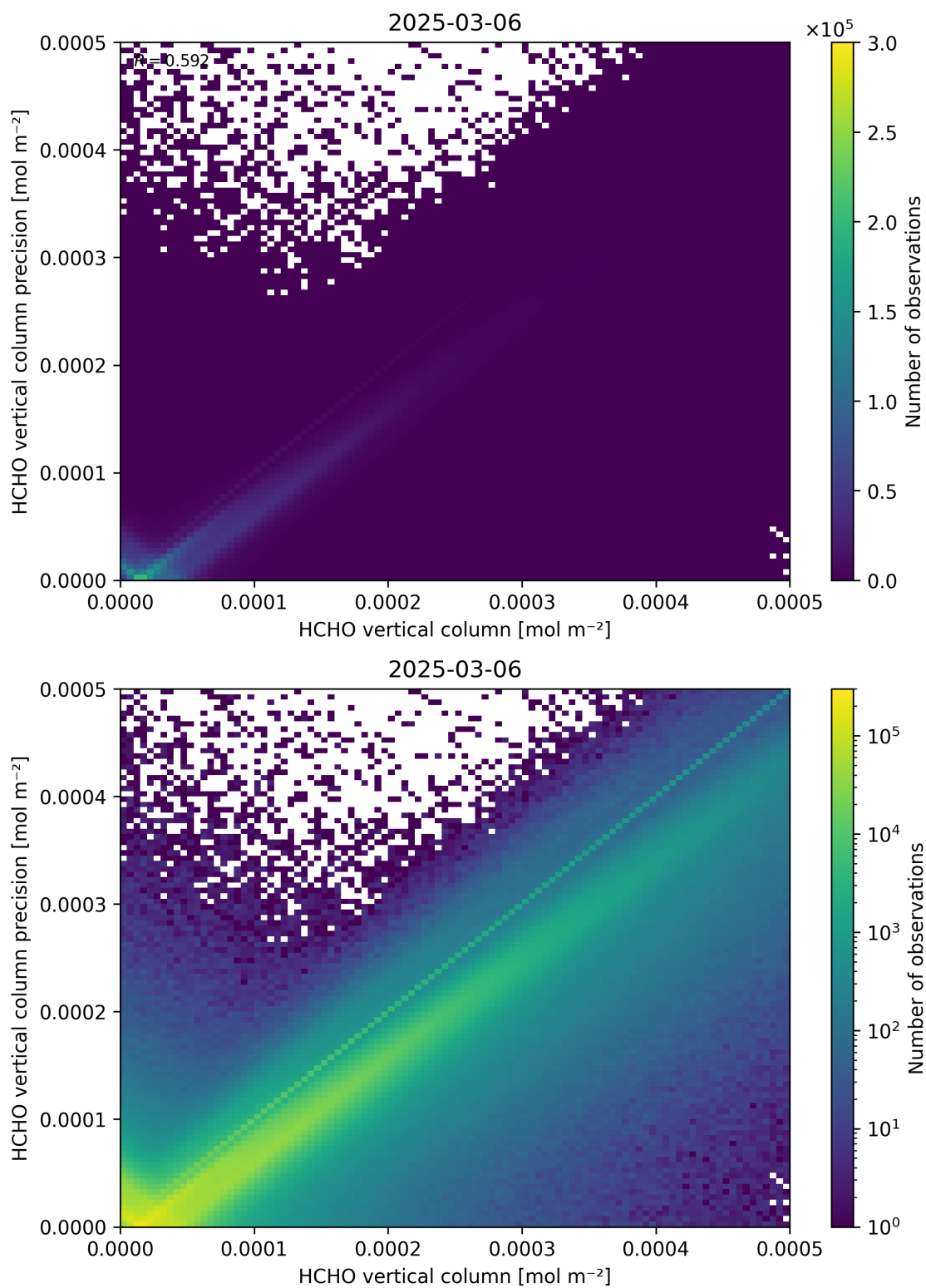
Figure 134: Scatter density plot of “HCHO vertical column” against “HCHO vertical column precision” for 2025-03-05 to 2025-03-07.
