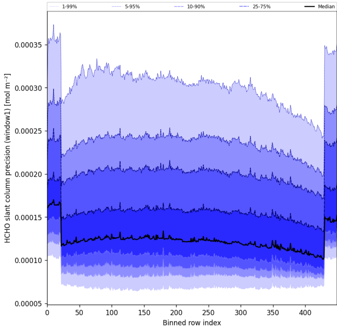
Figure 53: Along track statistics of “HCHO slant column precision (window1)” for 2025-03-05 to 2025-03-07
