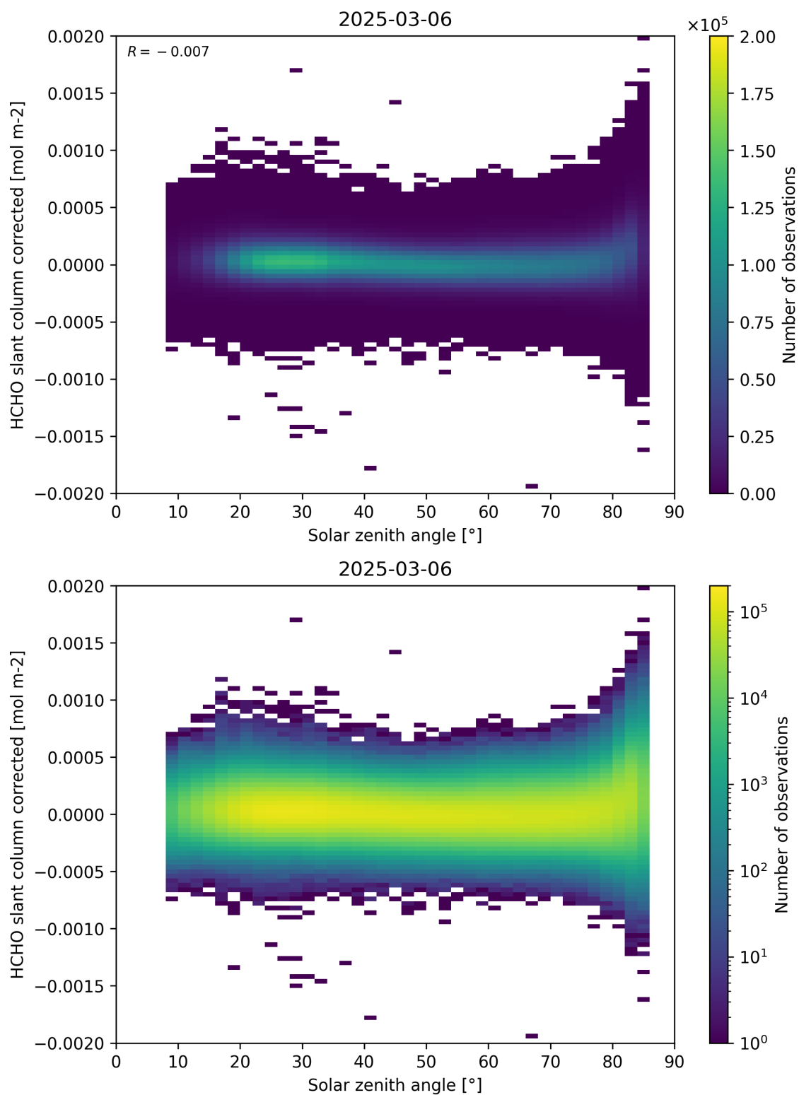
Figure 171: Scatter density plot of “Solar zenith angle” against “HCHO slant column corrected” for 2025-03-05 to 2025-03-07.
