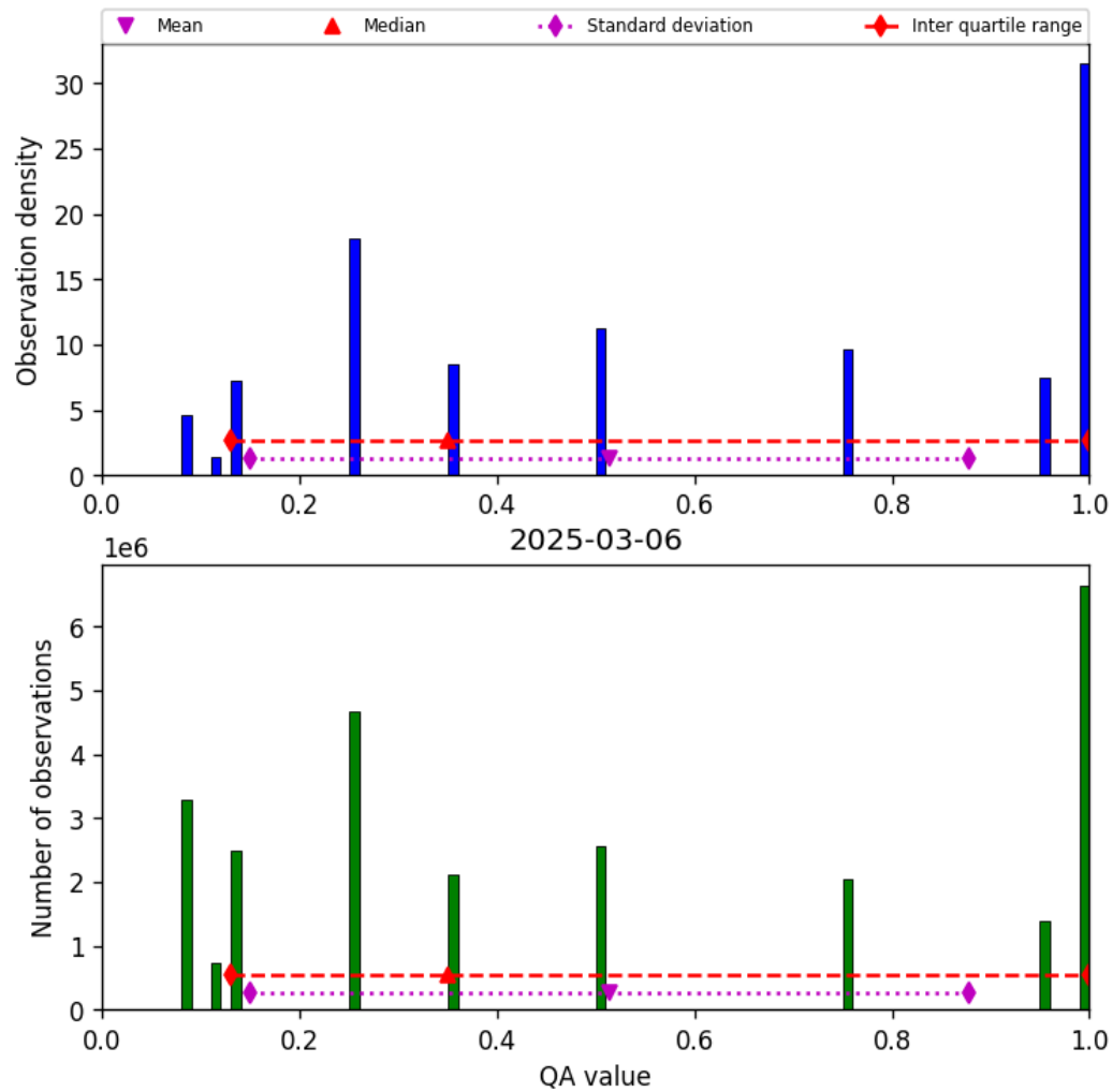
Figure 34: Histogram of “QA value” for 2025-03-05 to 2025-03-07
