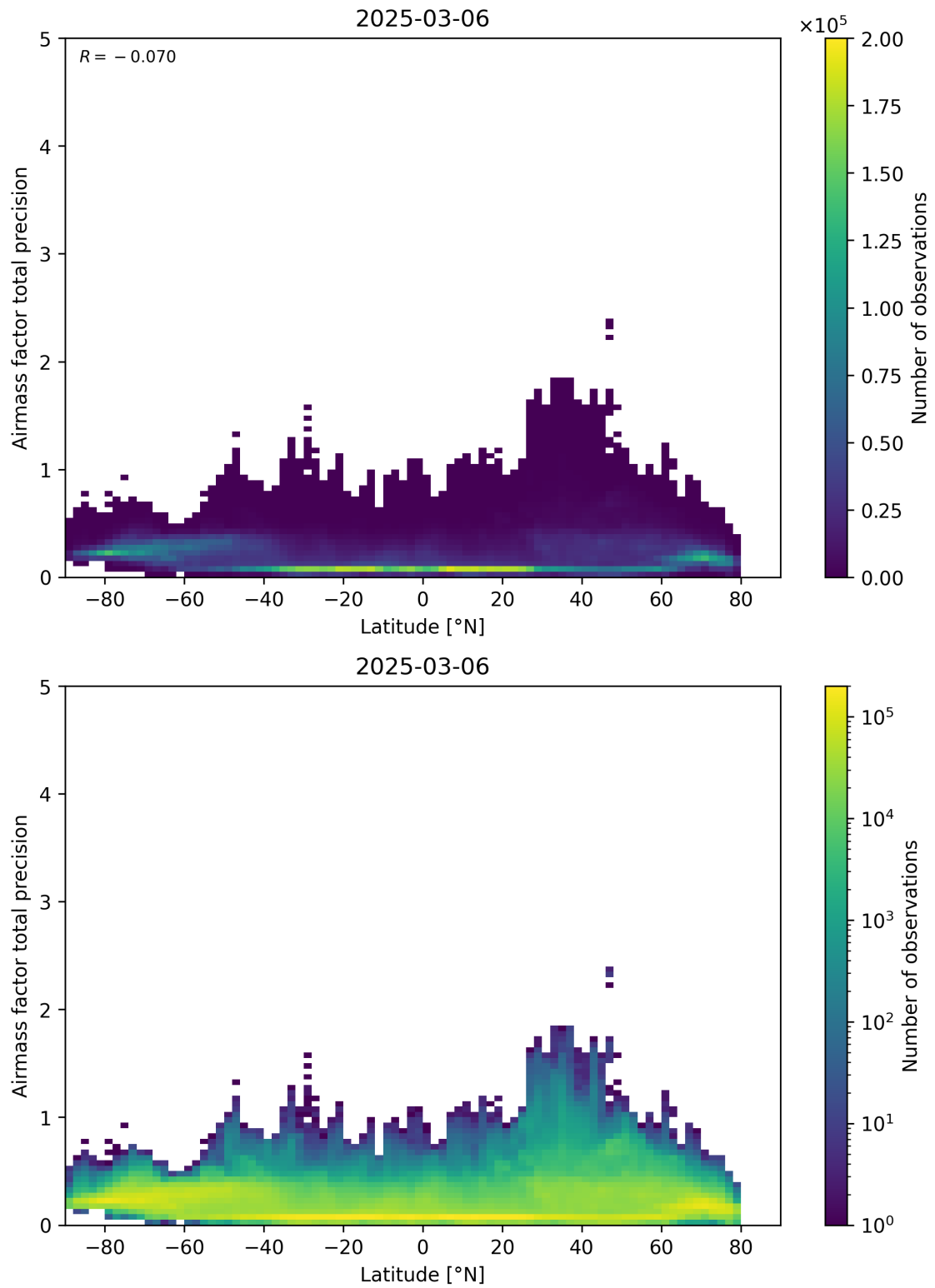
Figure 162: Scatter density plot of “Latitude” against “Airmass factor total precision” for 2025-03-05 to 2025-03-07.
