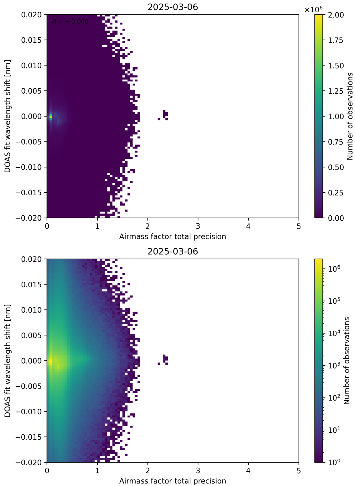
Figure 106: Scatter density plot of “Airmass factor total precision” against “DOAS fit wavelength shift” for 2025-03-05 to 2025-03-07.
