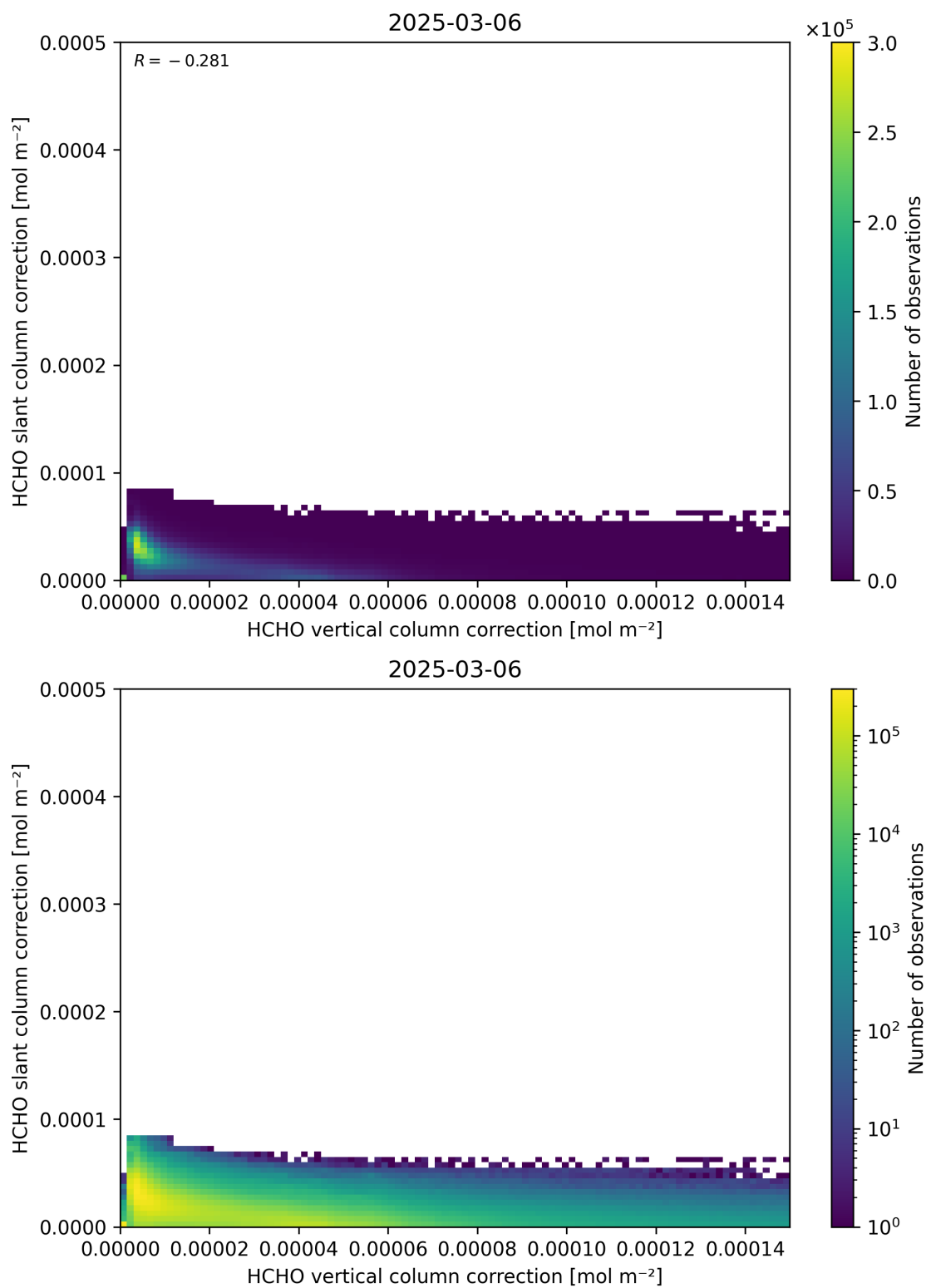
Figure 117: Scatter density plot of “HCHO vertical column correction” against “HCHO slant column correction” for 2025-03-05 to 2025-03-07.
