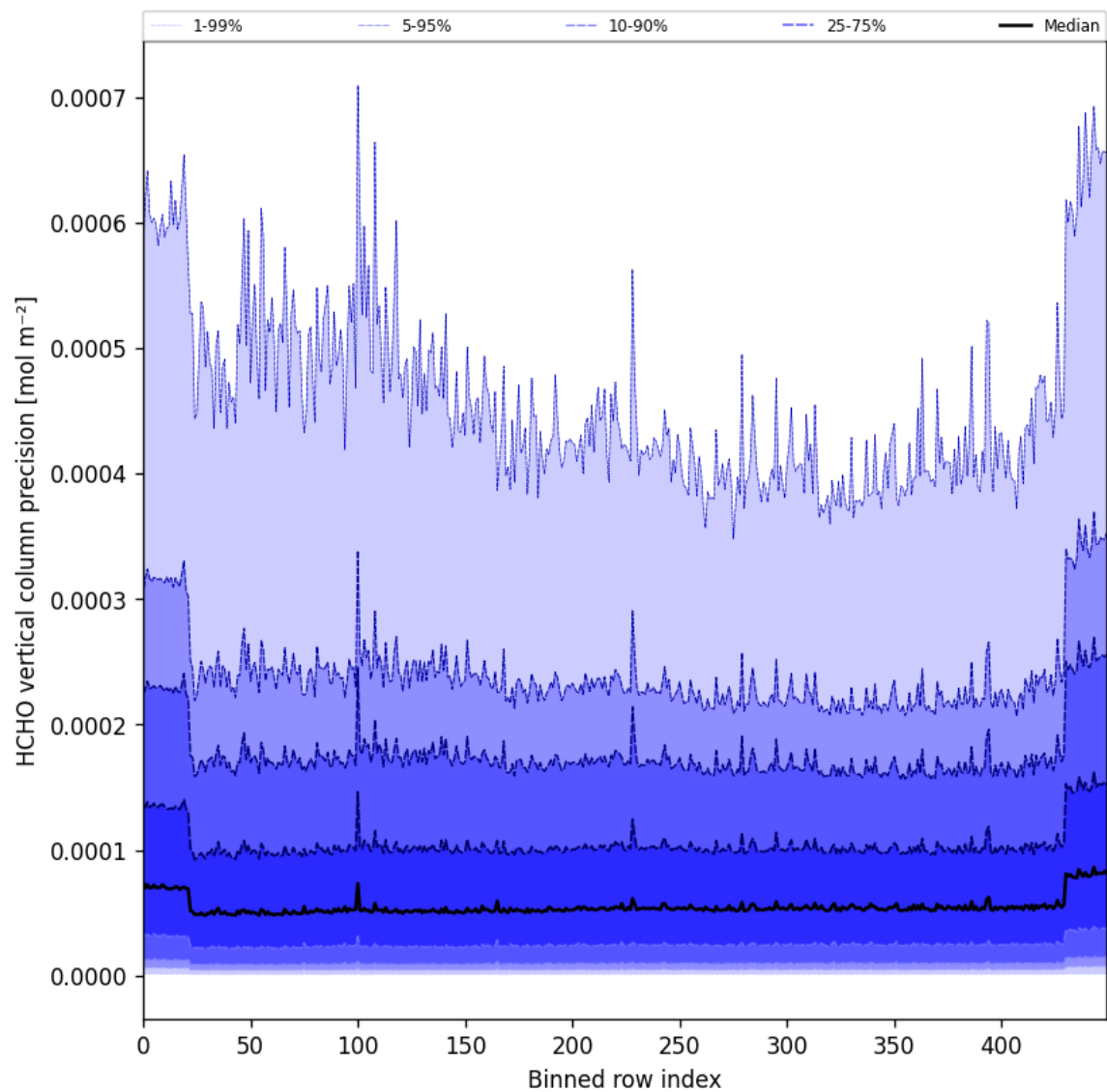
Figure 50: Along track statistics of “HCHO vertical column precision” for 2025-03-05 to 2025-03-07
