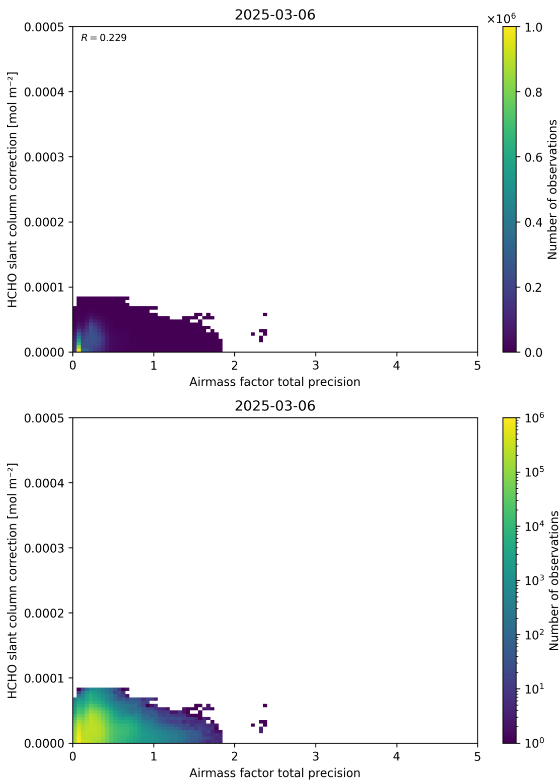
Figure 110: Scatter density plot of “Airmass factor total precision” against “HCHO slant column correction” for 2025-03-05 to 2025-03-07.
