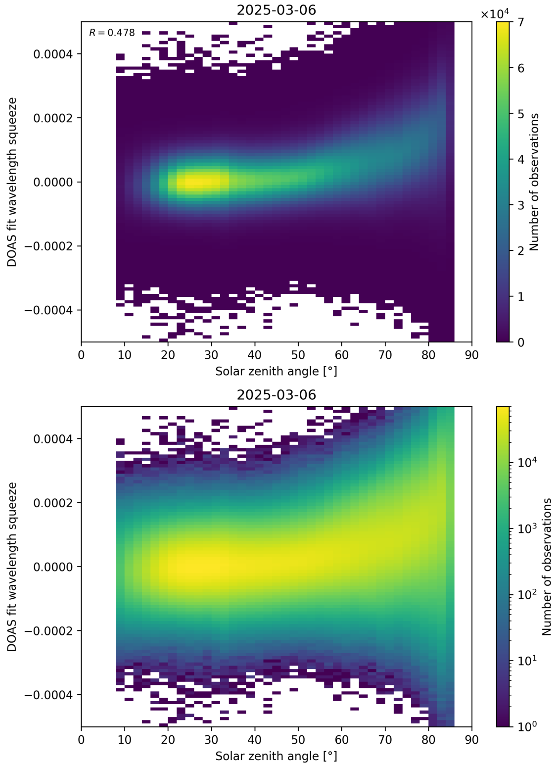
Figure 169: Scatter density plot of “Solar zenith angle” against “DOAS fit wavelength squeeze” for 2025-03-05 to 2025-03-07.
