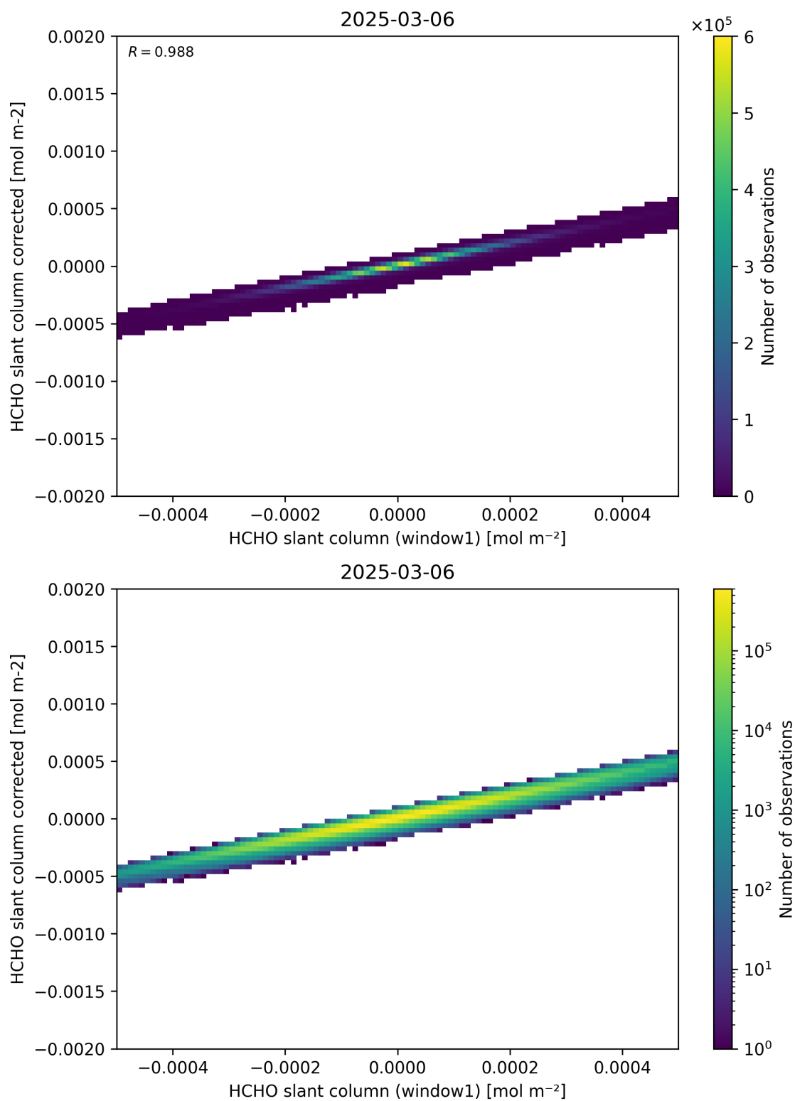
Figure 82: Scatter density plot of “HCHO slant column (window1)” against “HCHO slant column corrected” for 2025-03-05 to 2025-03-07.
