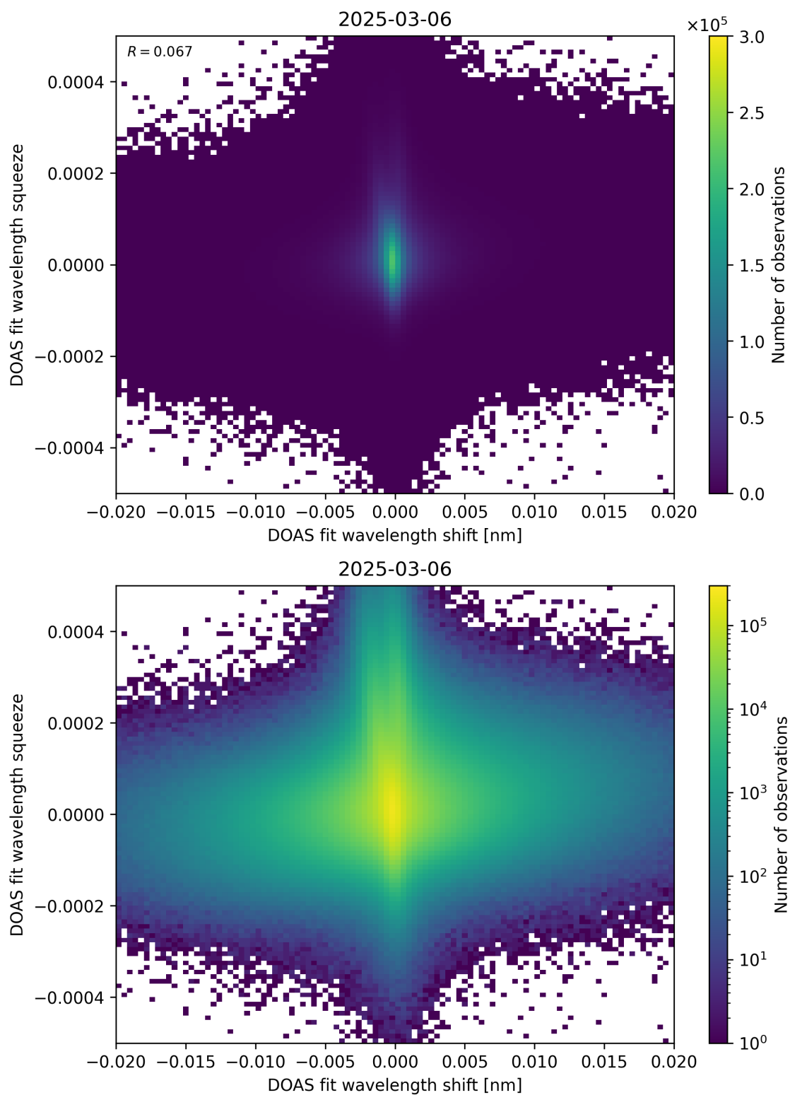
Figure 65: Scatter density plot of “DOAS fit wavelength shift” against “DOAS fit wavelength squeeze” for 2025-03-05 to 2025-03-07.
