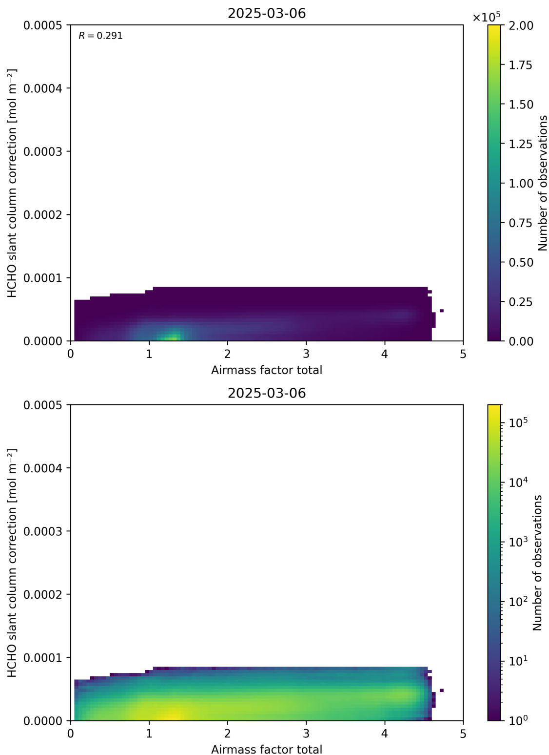
Figure 102: Scatter density plot of “Airmass factor total” against “HCHO slant column correction” for 2025-03-05 to 2025-03-07.
