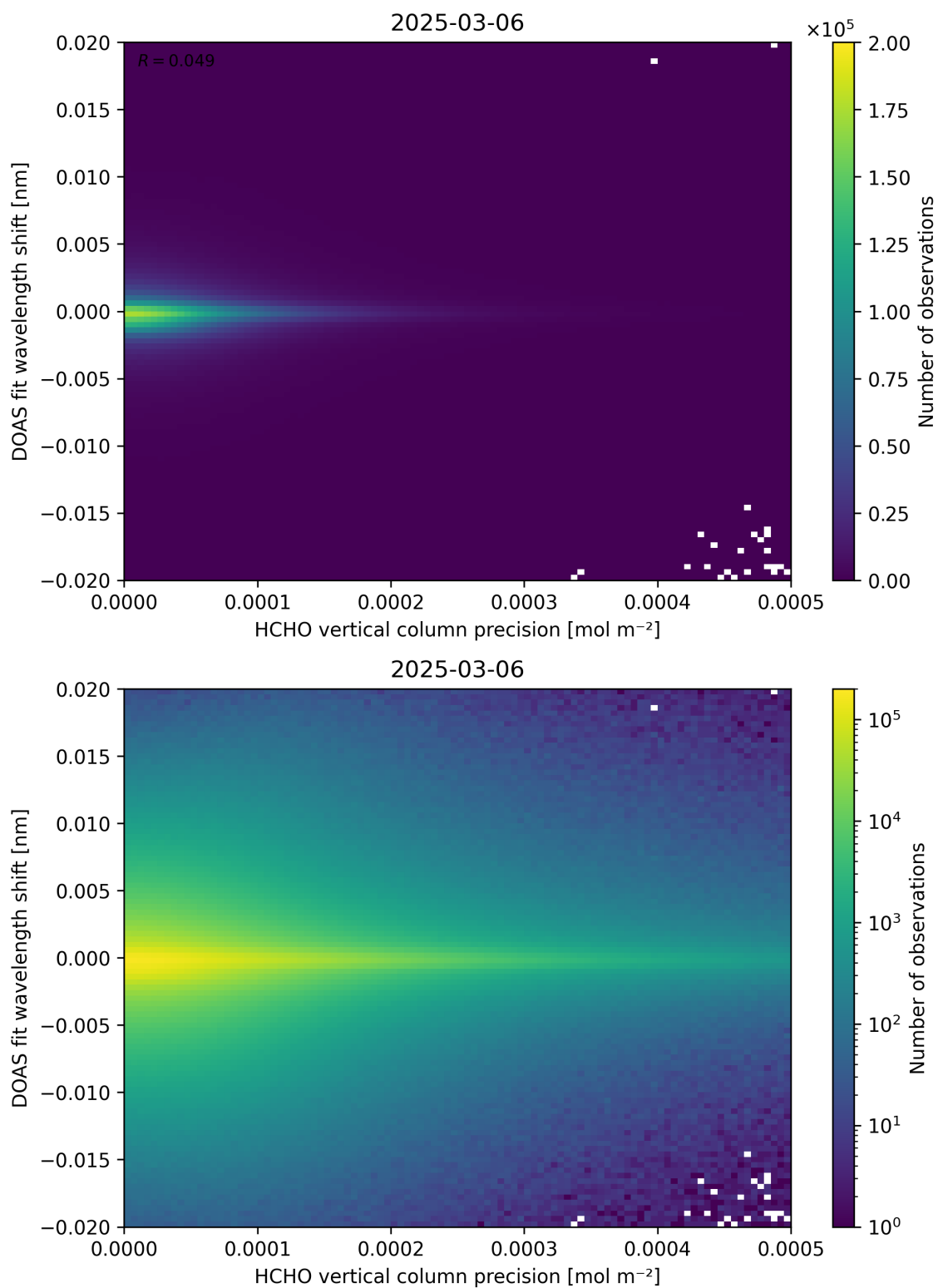
Figure 137: Scatter density plot of “HCHO vertical column precision” against “DOAS fit wavelength shift” for 2025-03-05 to 2025-03-07.
