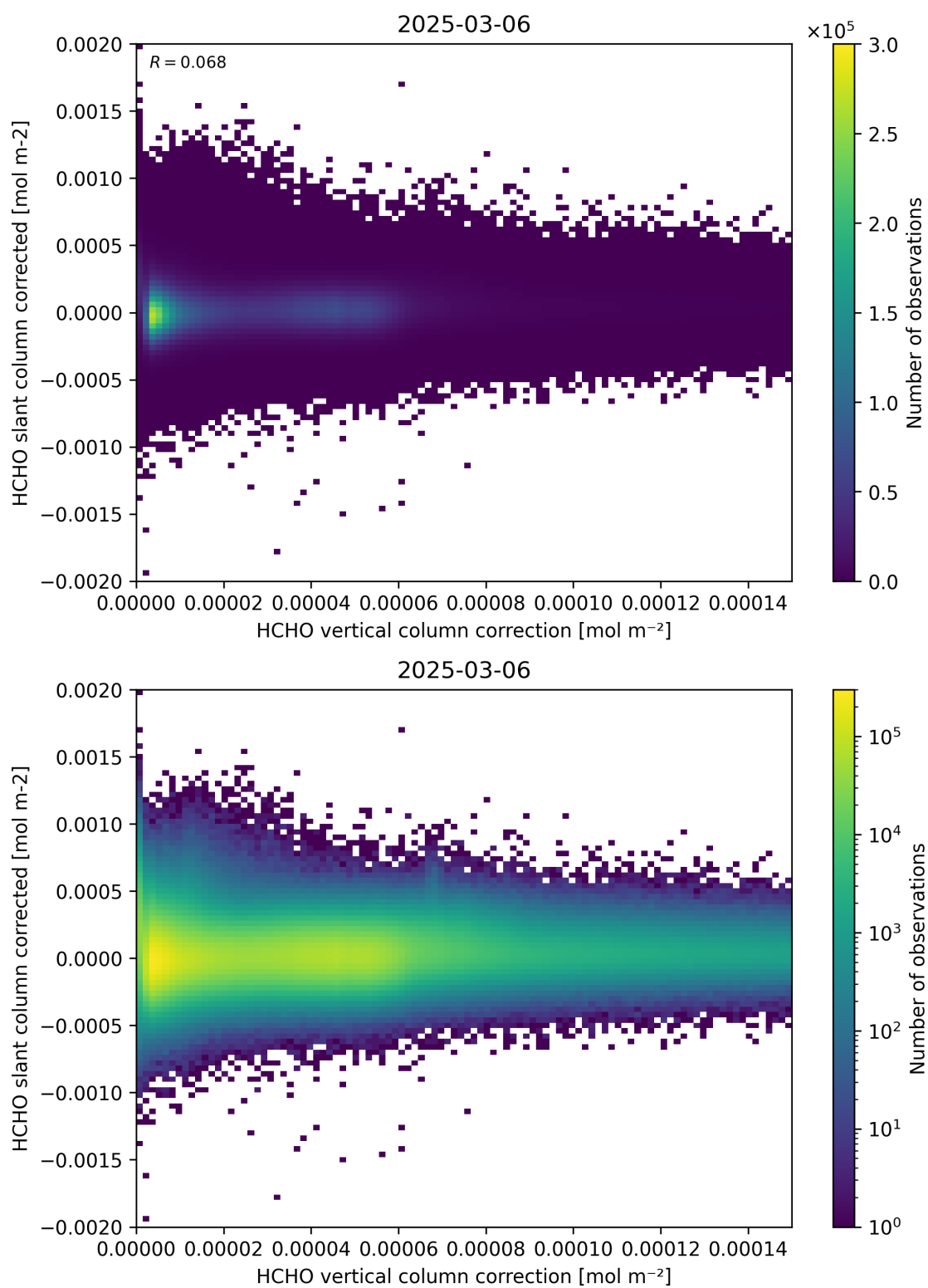
Figure 116: Scatter density plot of “HCHO vertical column correction” against “HCHO slant column corrected” for 2025-03-05 to 2025-03-07.
