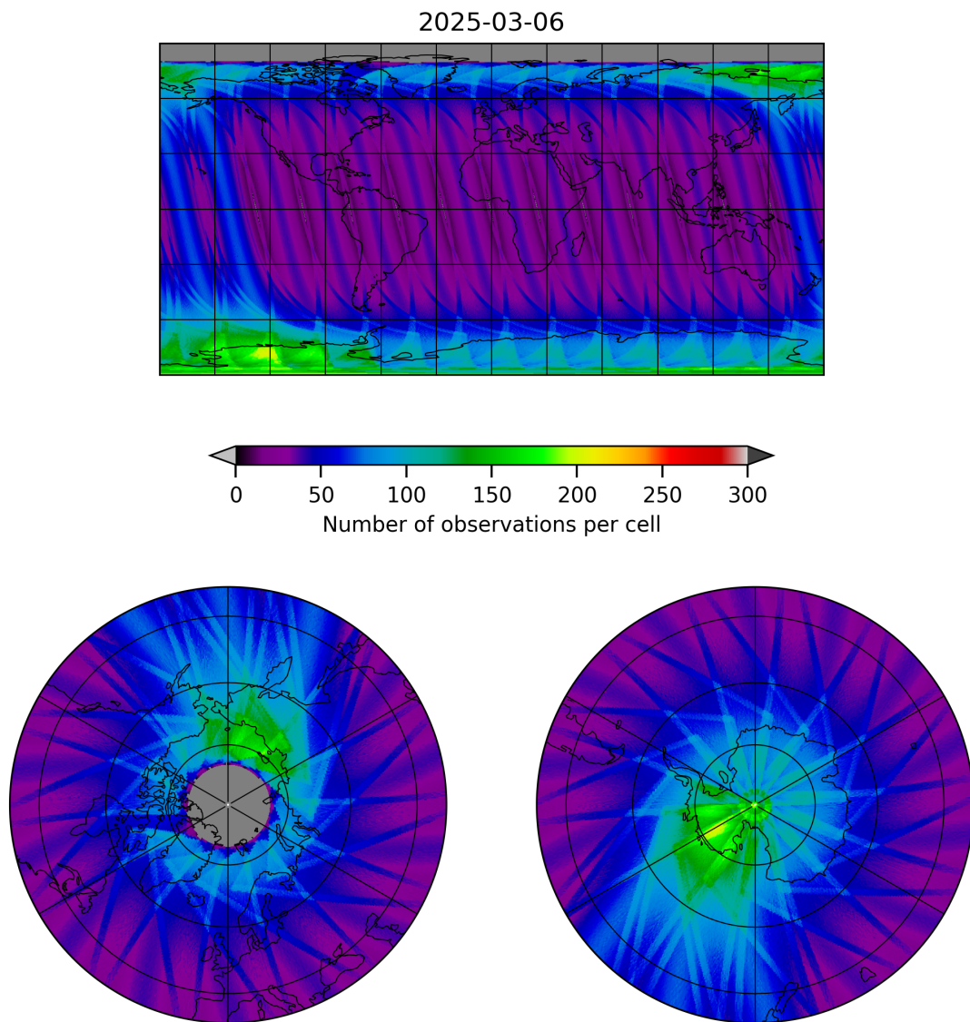
Figure 19: Map of the number of observations for 2025-03-05 to 2025-03-07
