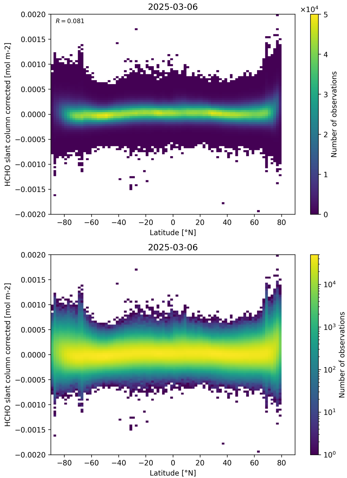
Figure 157: Scatter density plot of “Latitude” against “HCHO slant column corrected” for 2025-03-05 to 2025-03-07.
