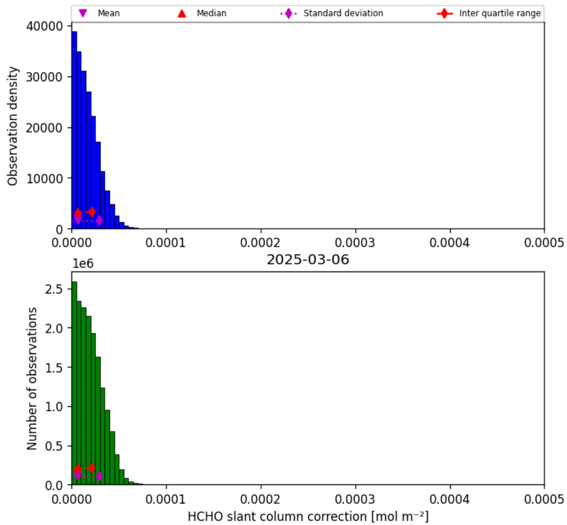
Figure 47: Histogram of “HCHO slant column correction” for 2025-03-05 to 2025-03-07
