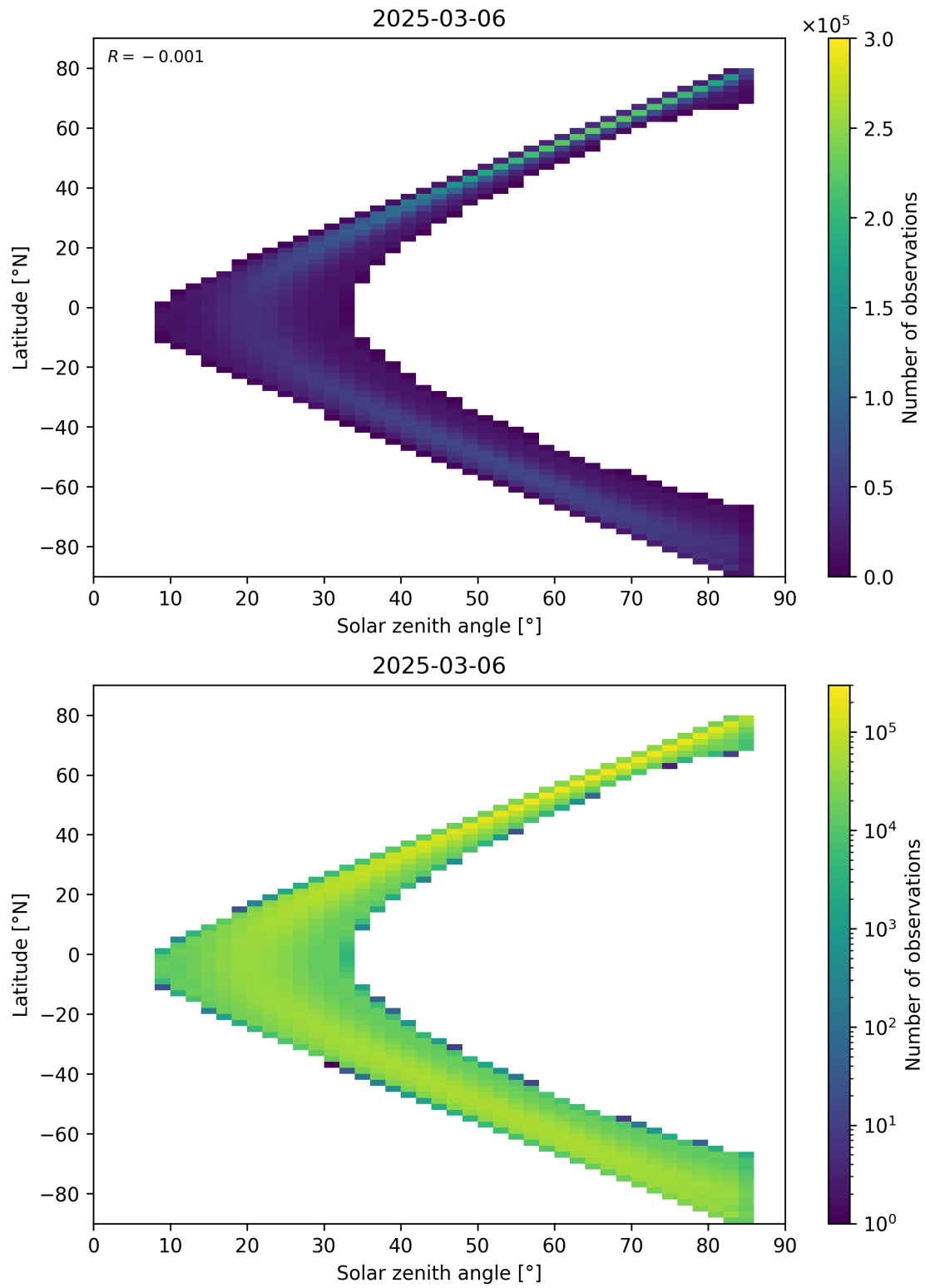
Figure 181: Scatter density plot of “Solar zenith angle” against “Latitude” for 2025-03-05 to 2025-03-07.
