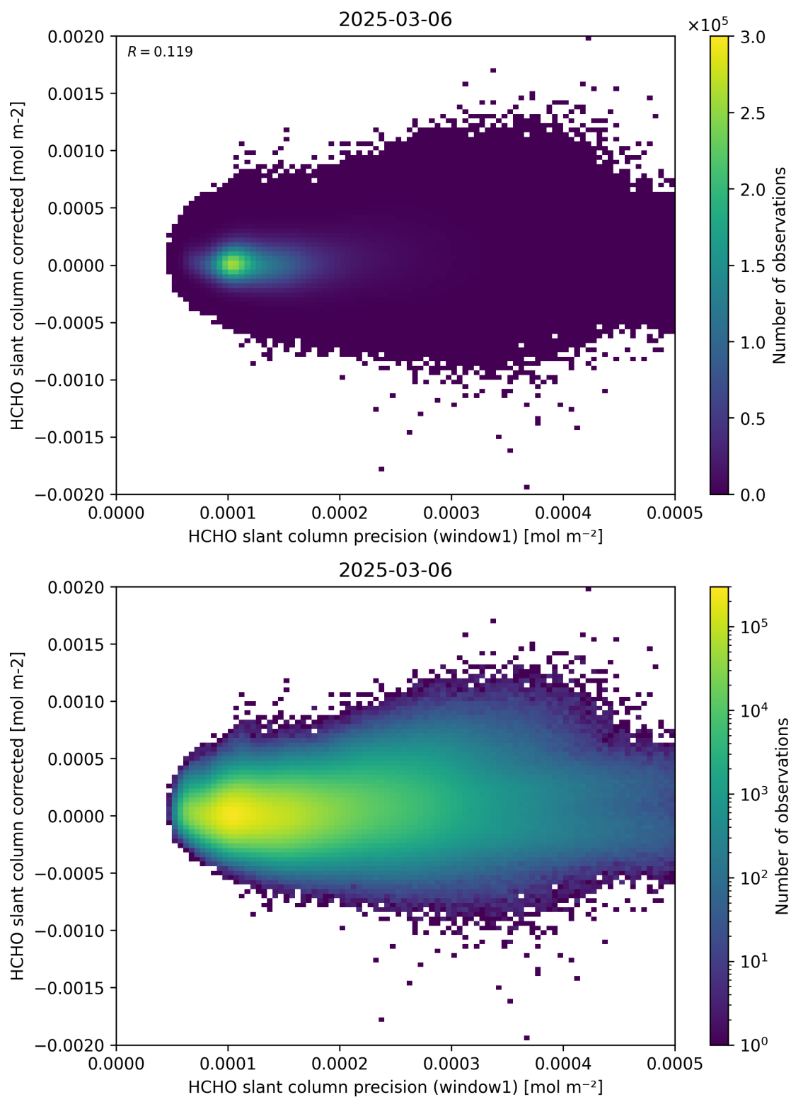
Figure 92: Scatter density plot of “HCHO slant column precision (window1)” against “HCHO slant column corrected” for 2025-03-05 to 2025-03-07.
