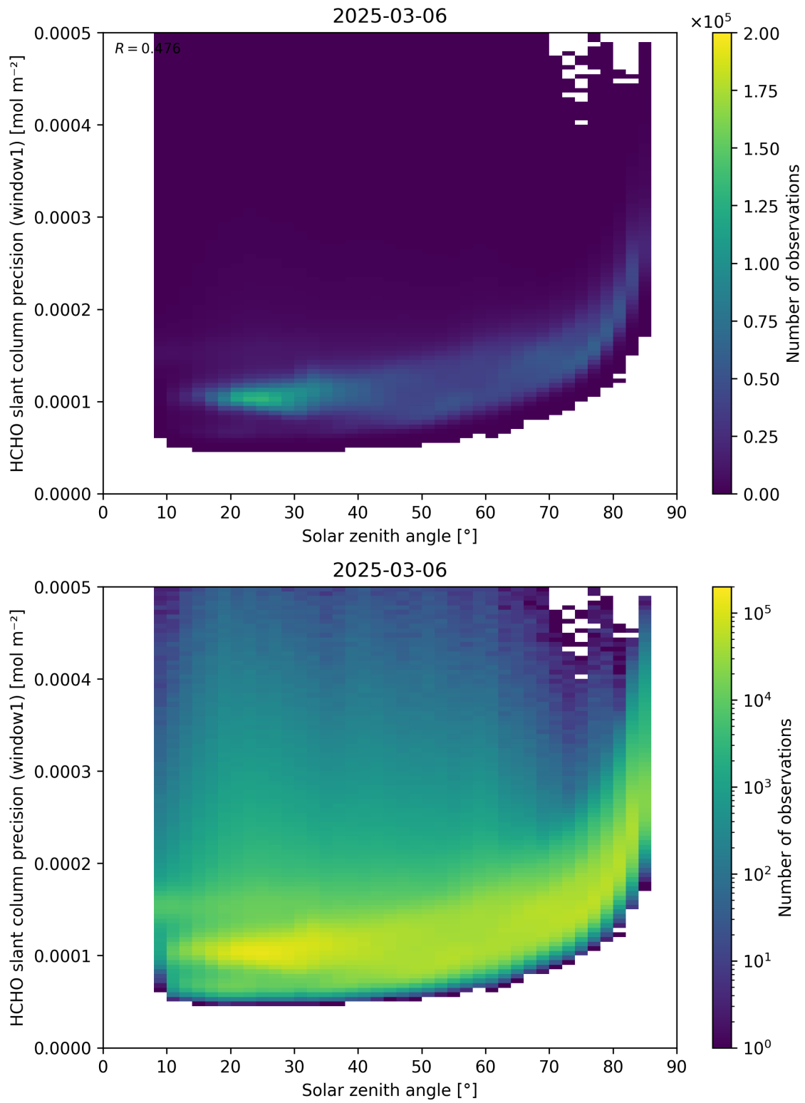
Figure 174: Scatter density plot of “Solar zenith angle” against “HCHO slant column precision (window1)” for 2025-03-05 to 2025-03-07.
