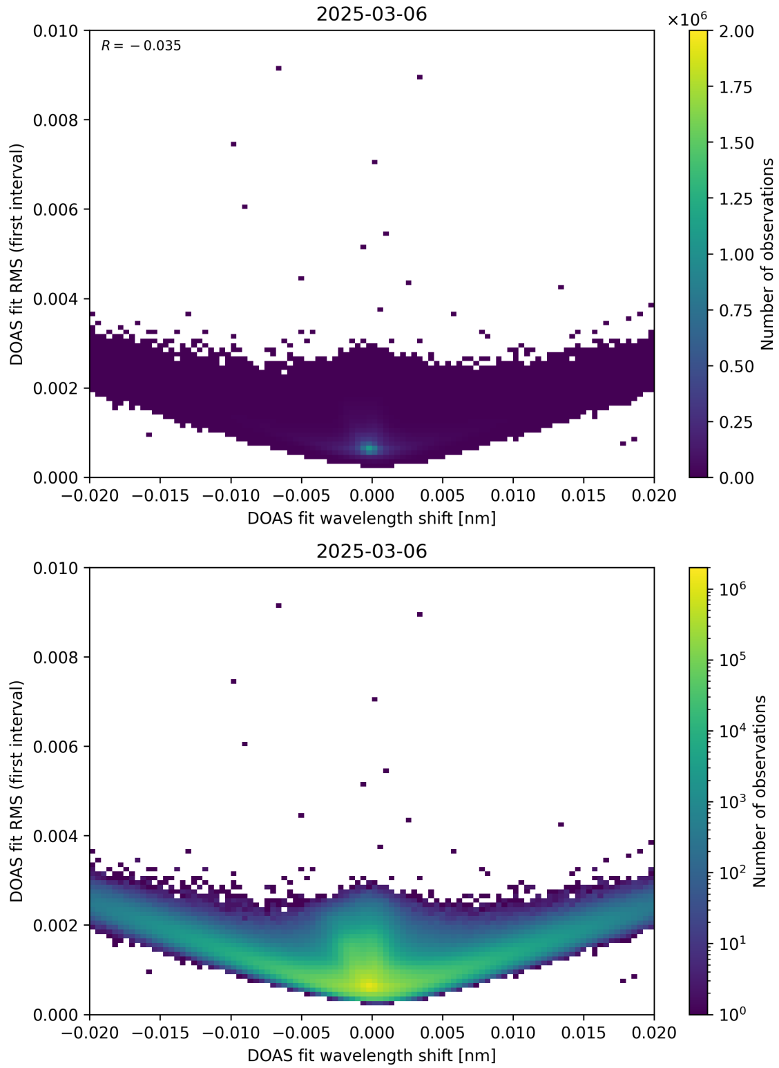
Figure 64: Scatter density plot of “DOAS fit wavelength shift” against “DOAS fit RMS (first interval)” for 2025-03-05 to 2025-03-07.
