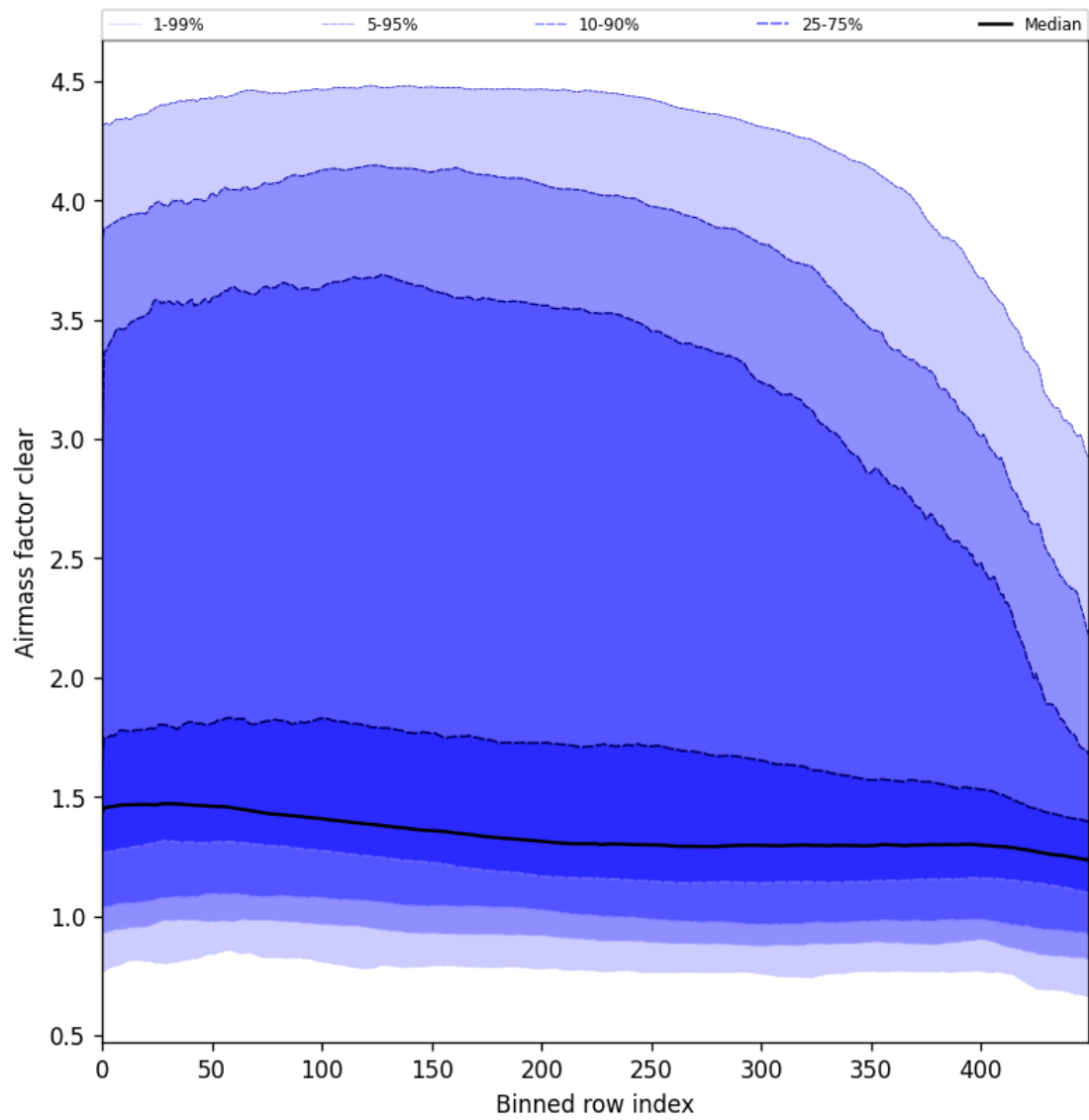
Figure 56: Along track statistics of “Air mass factor clear” for 2025-03-05 to 2025-03-07
