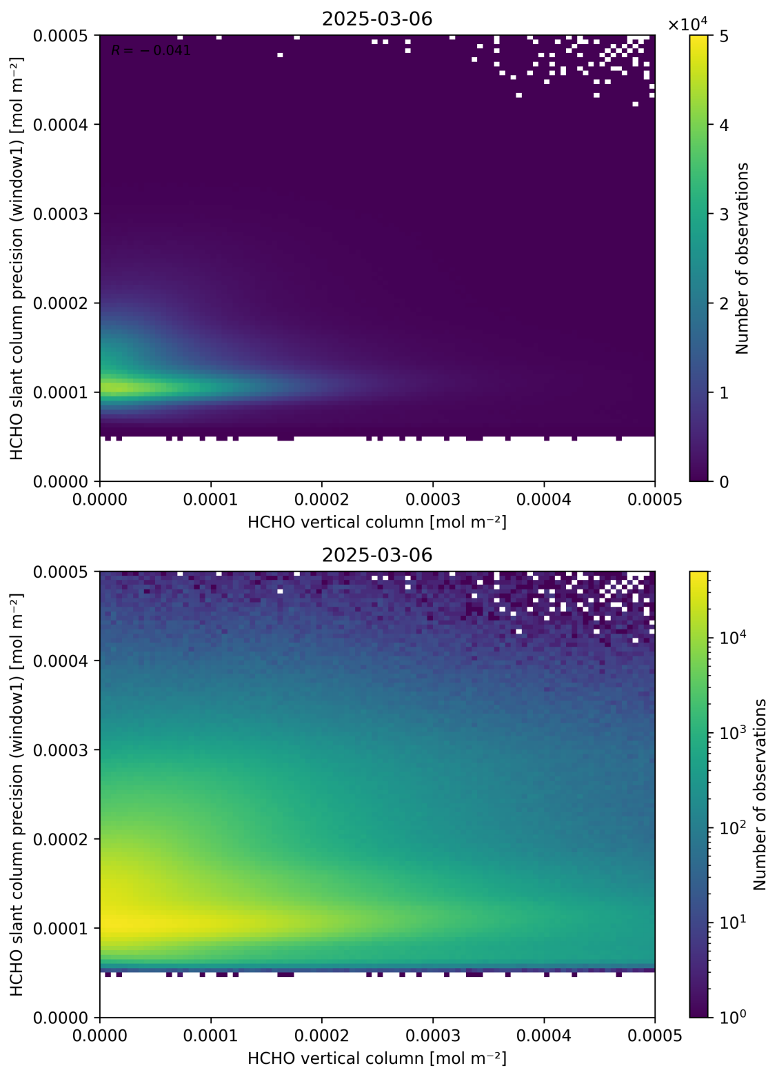
Figure 130: Scatter density plot of “HCHO vertical column” against “HCHO slant column precision (window1)” for 2025-03-05 to 2025-03-07.
