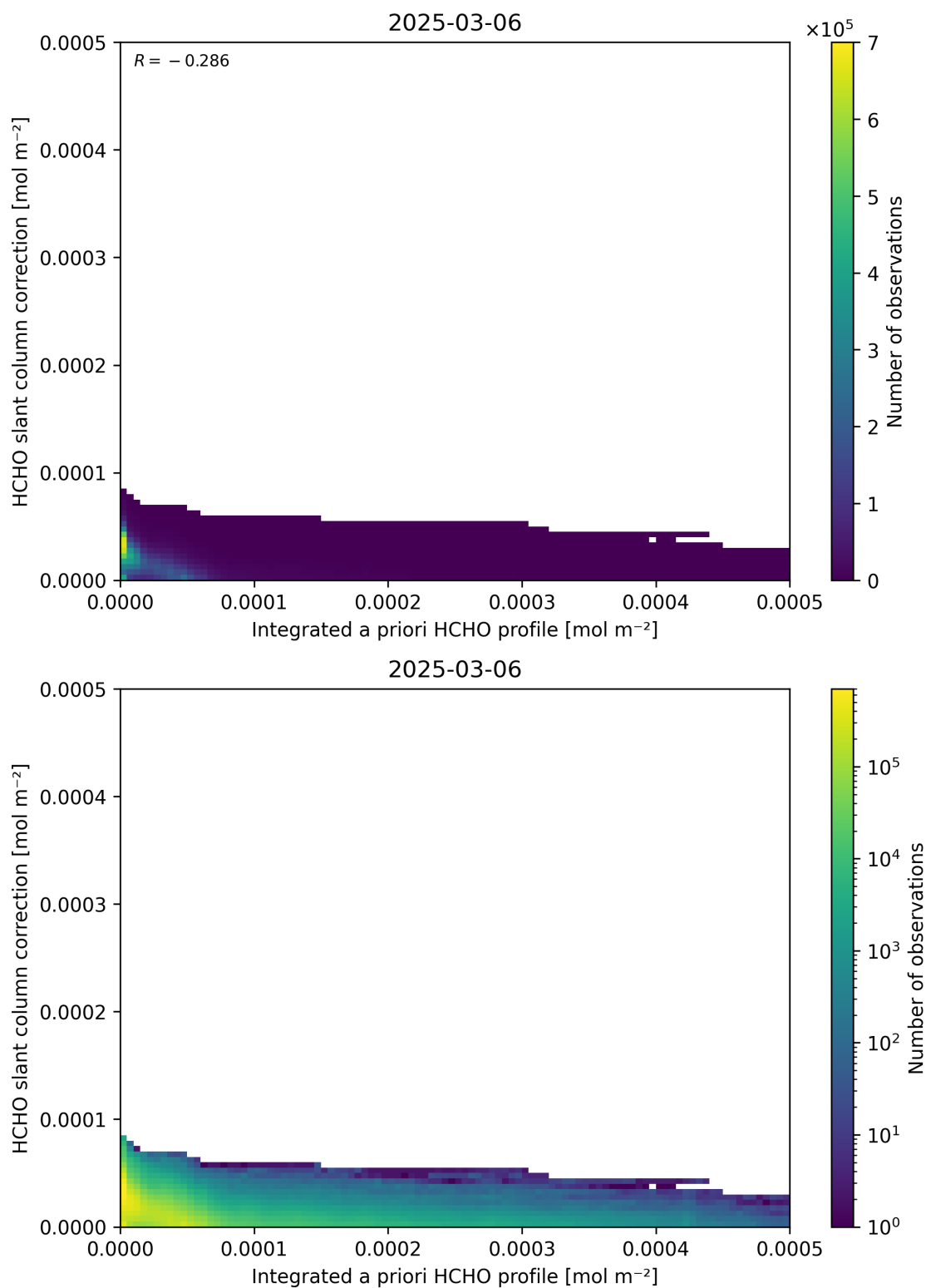
Figure 152: Scatter density plot of “Integrated a priori HCHO profile” against “HCHO slant column correction” for 2025-03-05 to 2025-03-07.
