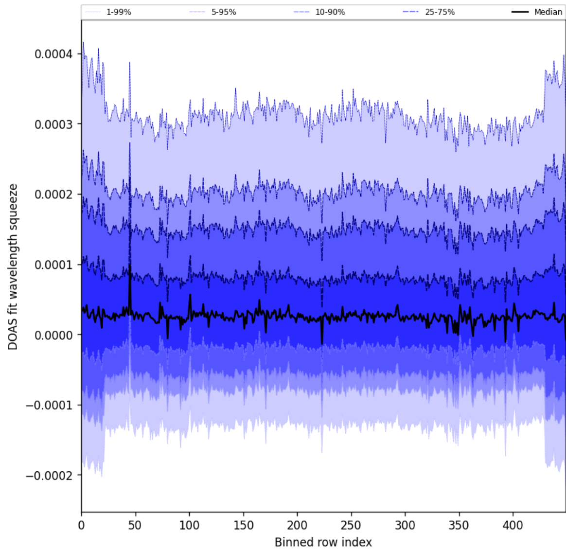
Figure 59: Along track statistics of “DOAS fit wavelength squeeze” for 2025-03-05 to 2025-03-07
