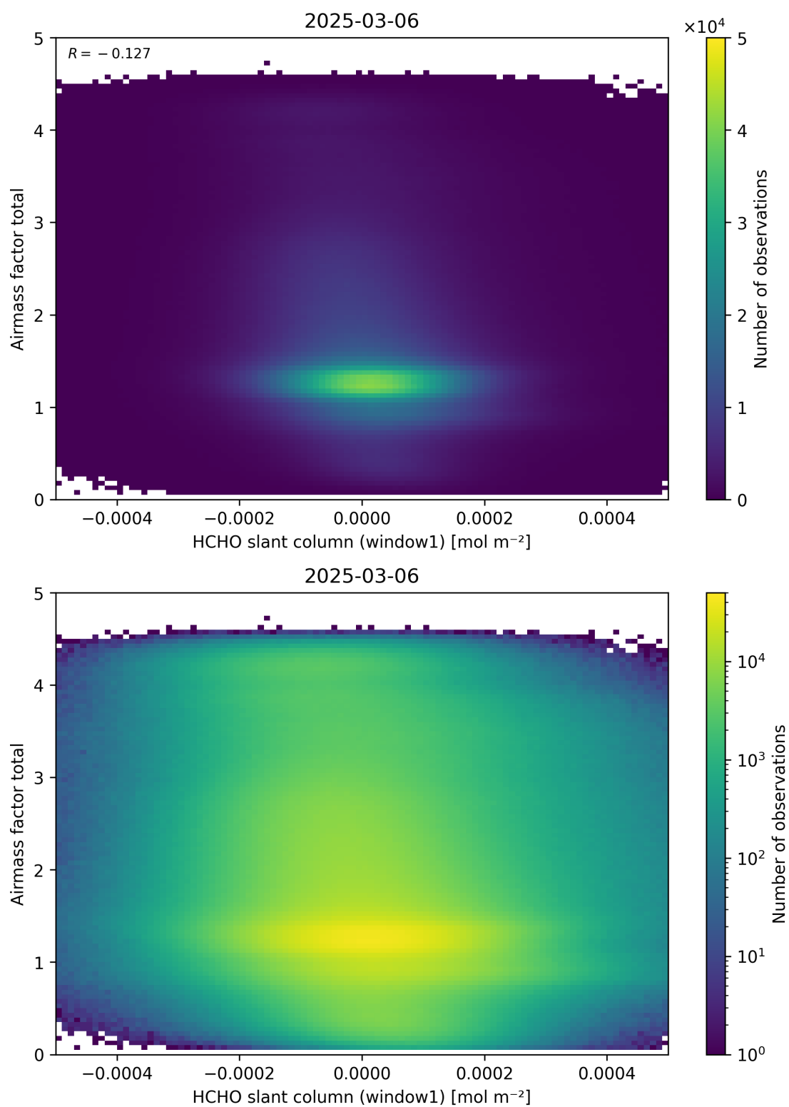
Figure 85: Scatter density plot of “HCHO slant column (window1)” against “Airmass factor total” for 2025-03-05 to 2025-03-07.
