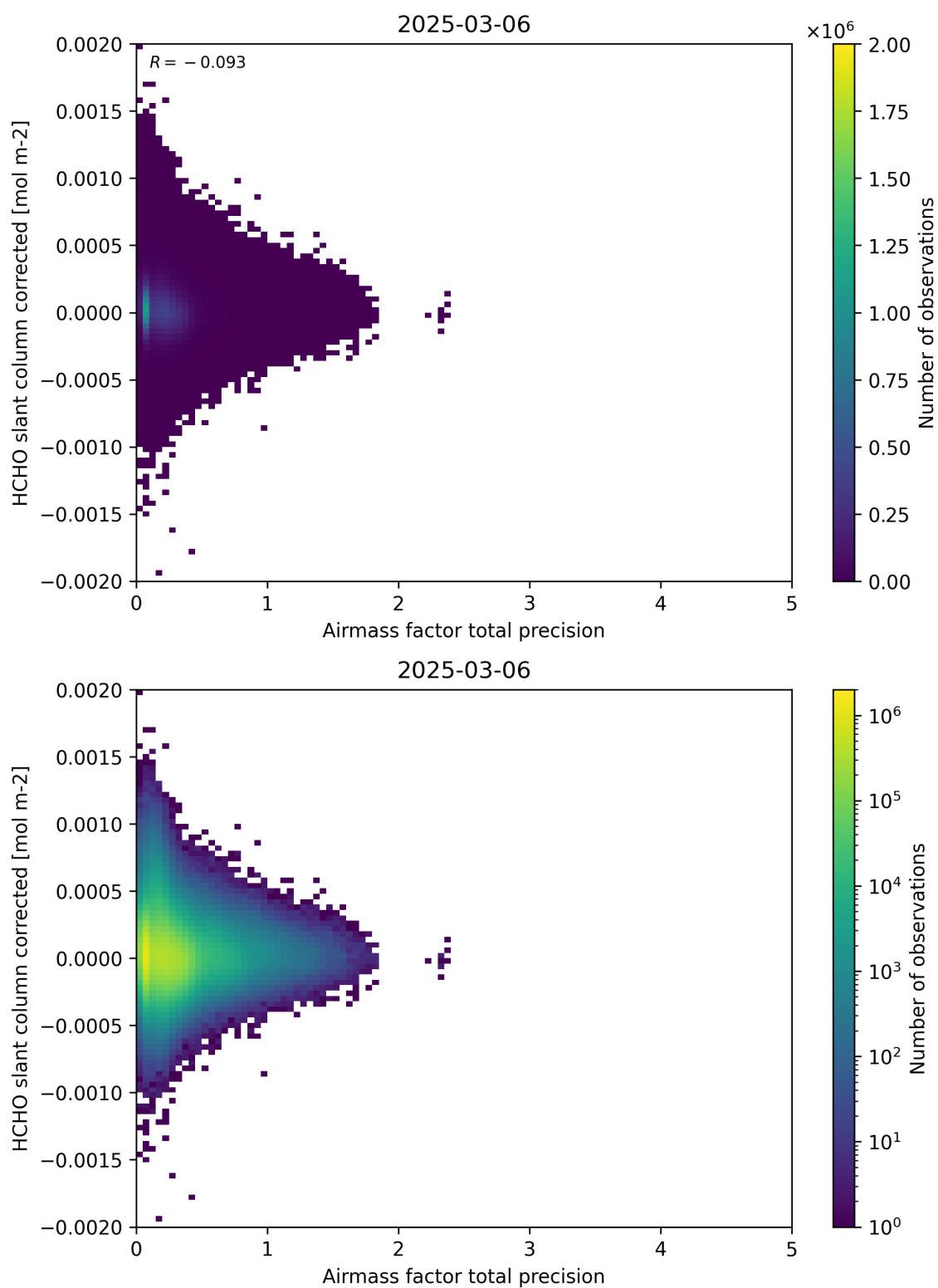
Figure 109: Scatter density plot of “Airmass factor total precision” against “HCHO slant column corrected” for 2025-03-05 to 2025-03-07.
