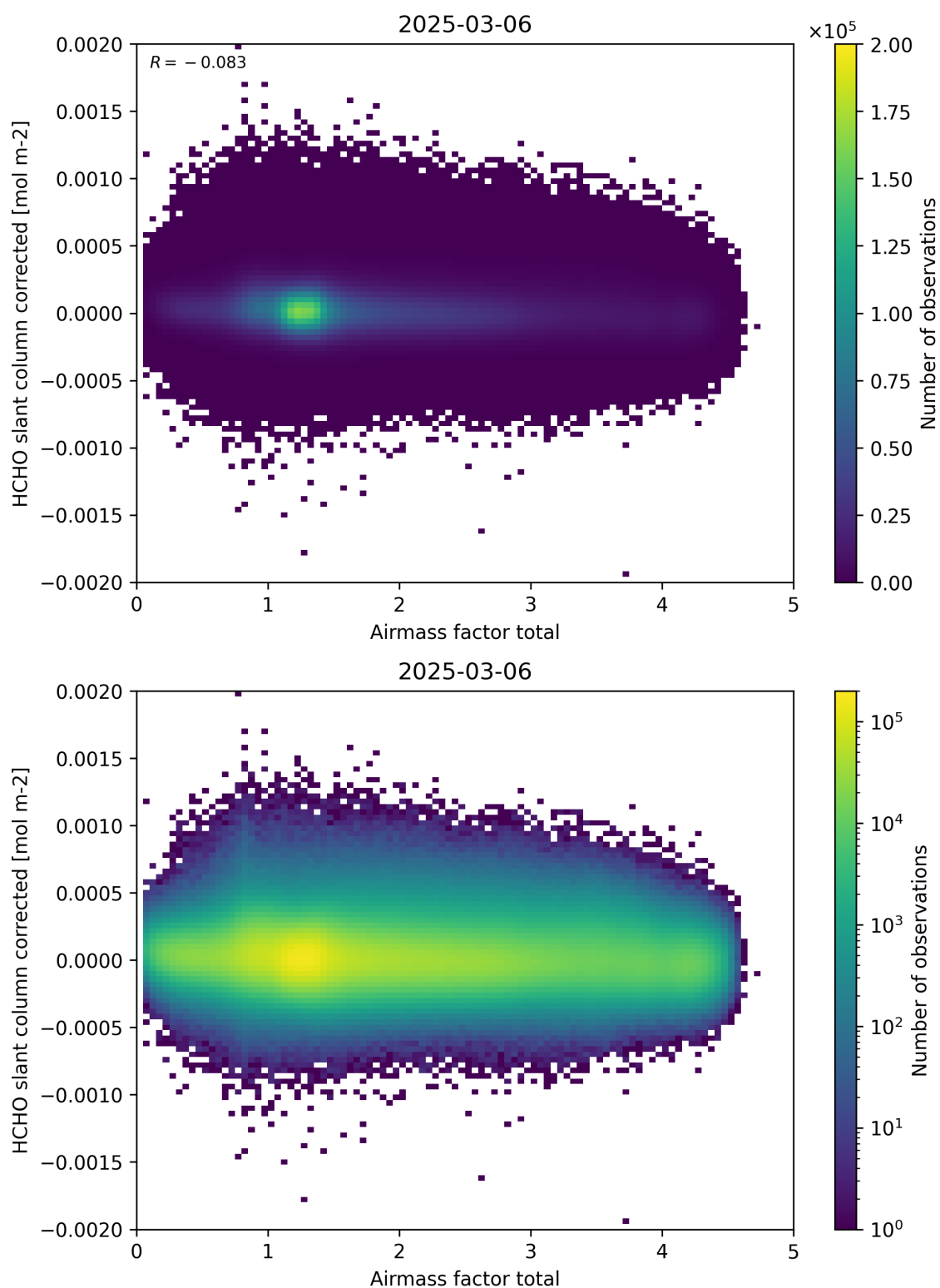
Figure 101: Scatter density plot of “Airmass factor total” against “HCHO slant column corrected” for 2025-03-05 to 2025-03-07.
