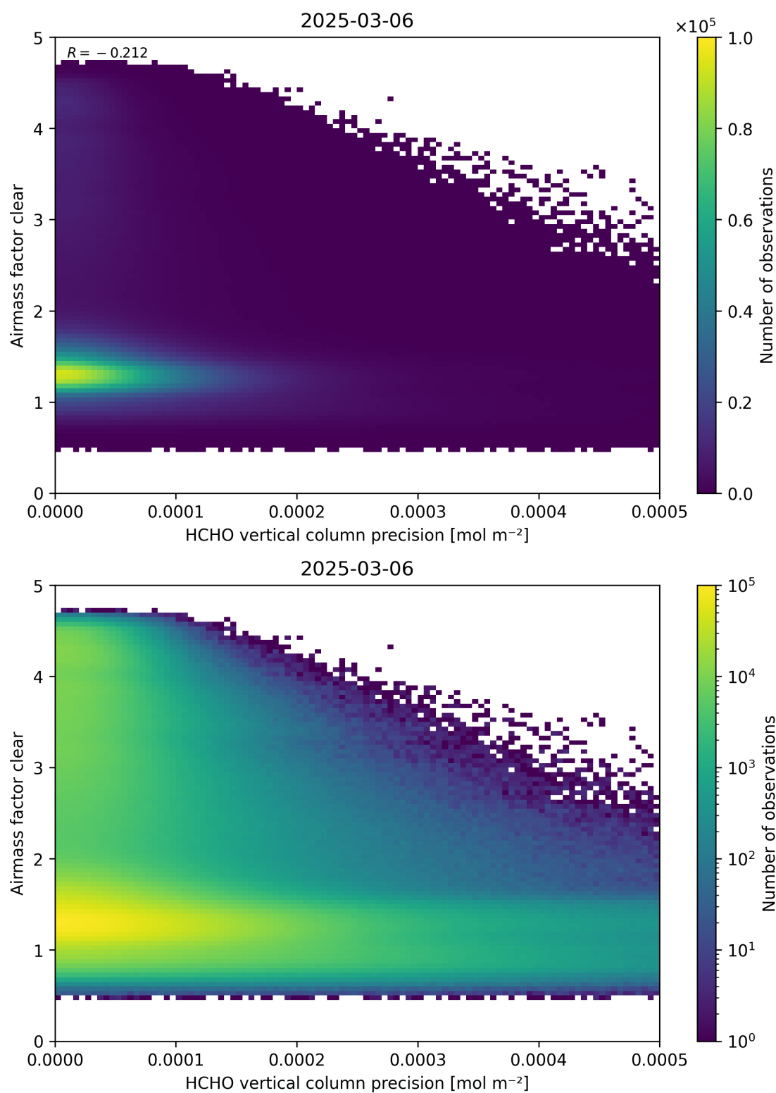
Figure 139: Scatter density plot of “HCHO vertical column precision” against “Airmass factor clear” for 2025-03-05 to 2025-03-07.
