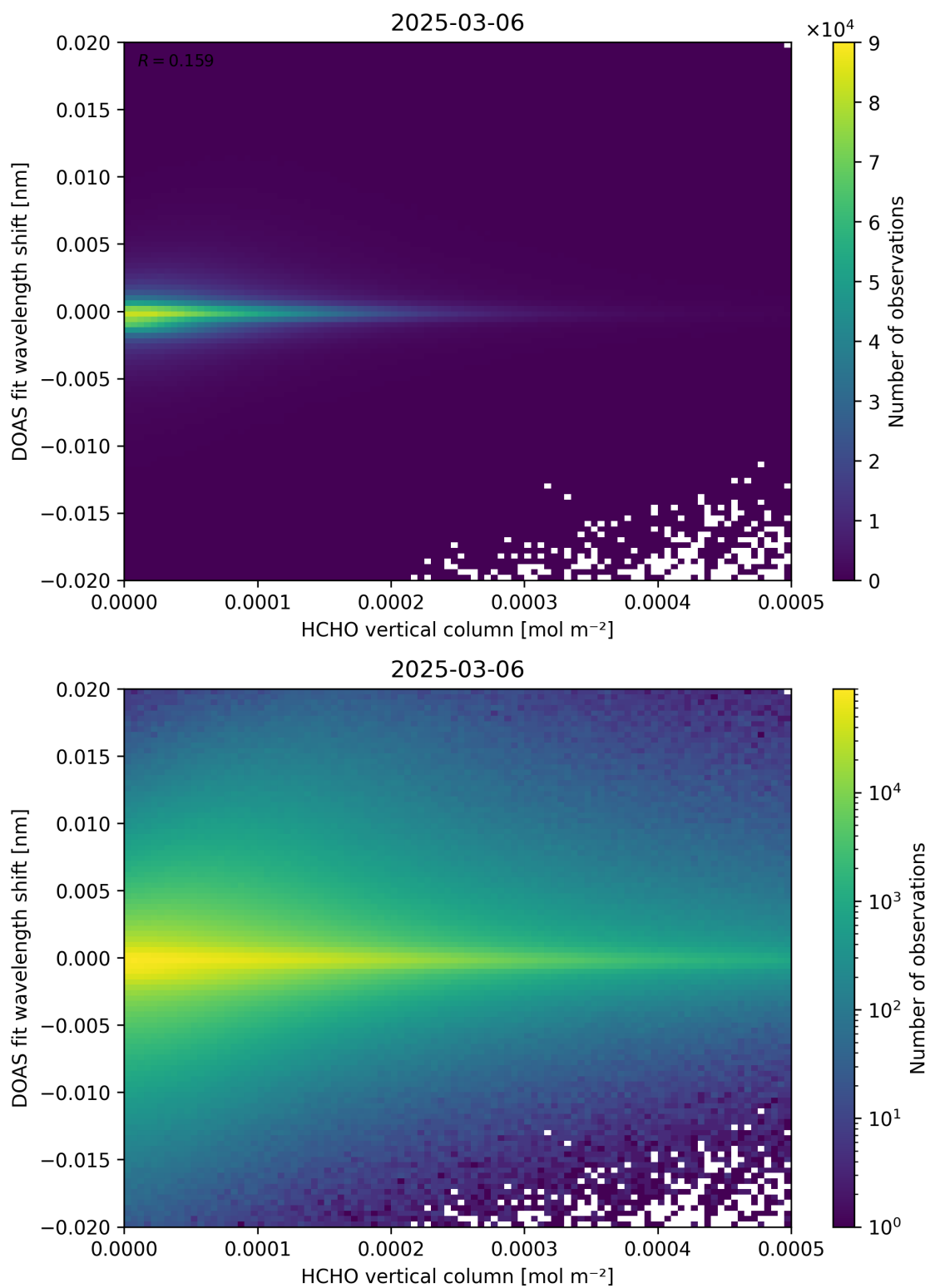
Figure 124: Scatter density plot of “HCHO vertical column” against “DOAS fit wavelength shift” for 2025-03-05 to 2025-03-07.
