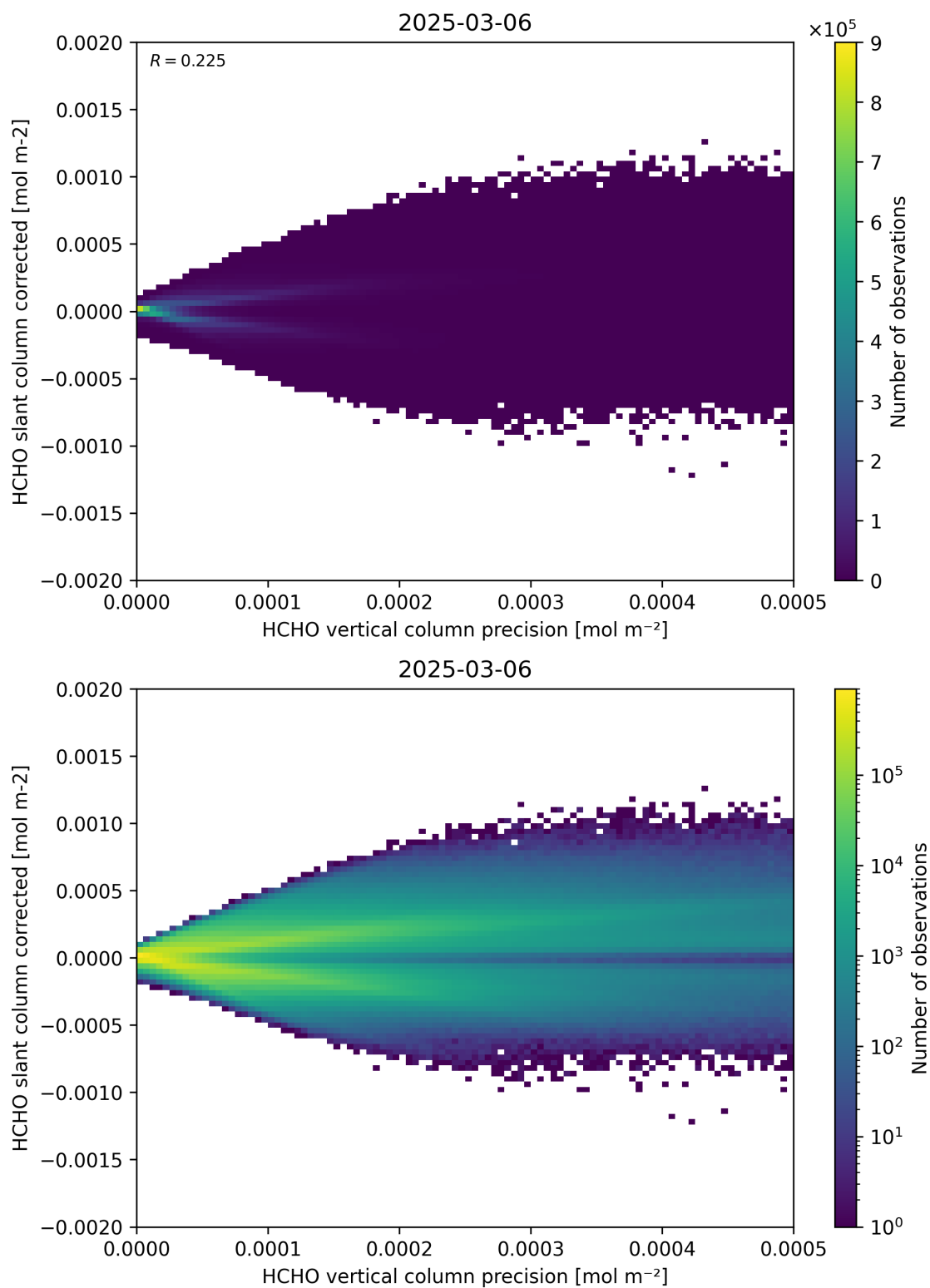
Figure 140: Scatter density plot of “HCHO vertical column precision” against “HCHO slant column corrected” for 2025-03-05 to 2025-03-07.
