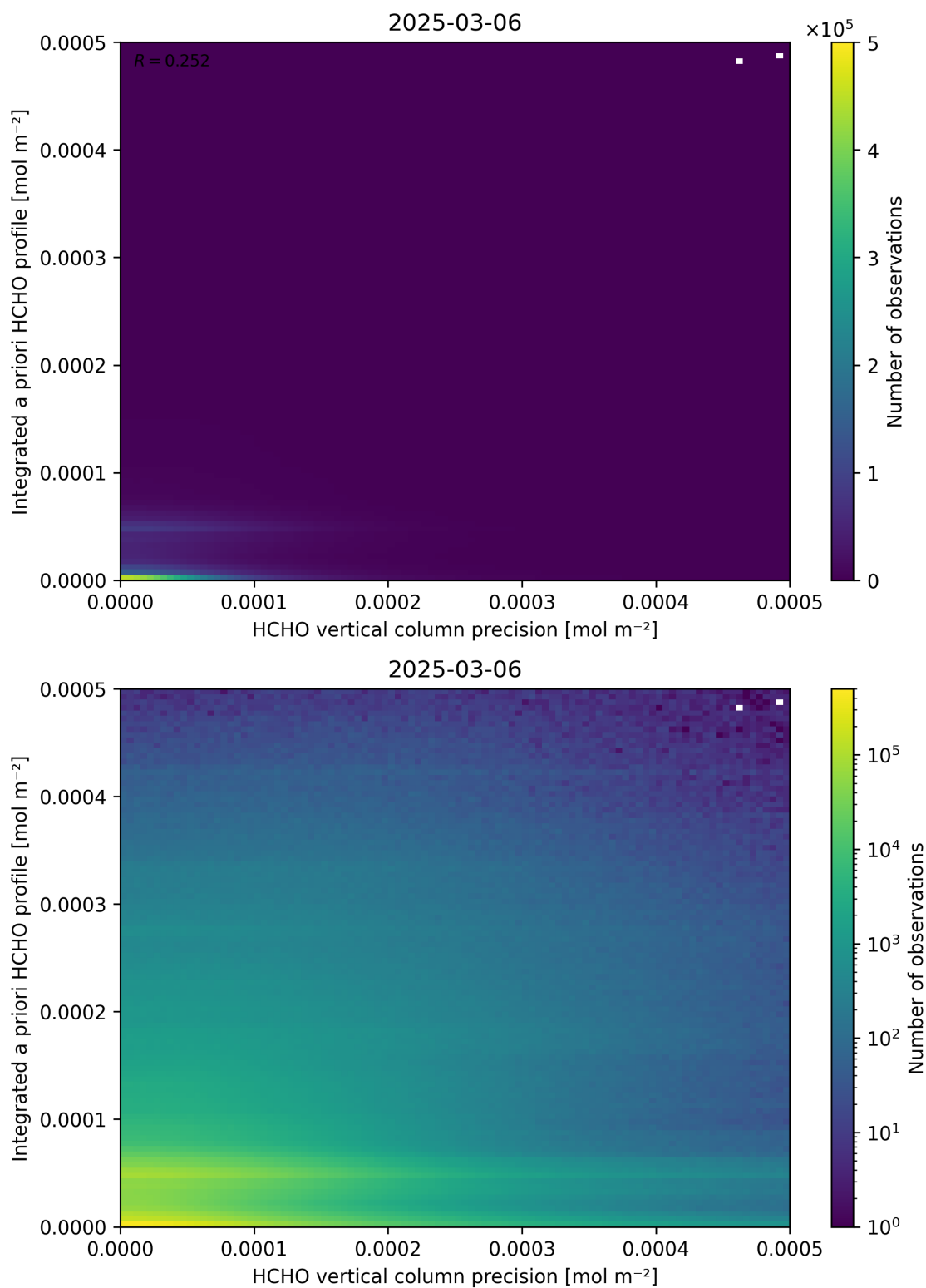
Figure 147: Scatter density plot of “HCHO vertical column precision” against “Integrated a priori HCHO profile” for 2025-03-05 to 2025-03-07.
