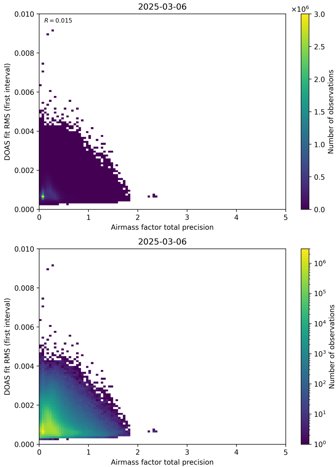
Figure 105: Scatter density plot of “Airmass factor total precision” against “DOAS fit RMS (first interval)” for 2025-03-05 to 2025-03-07.
