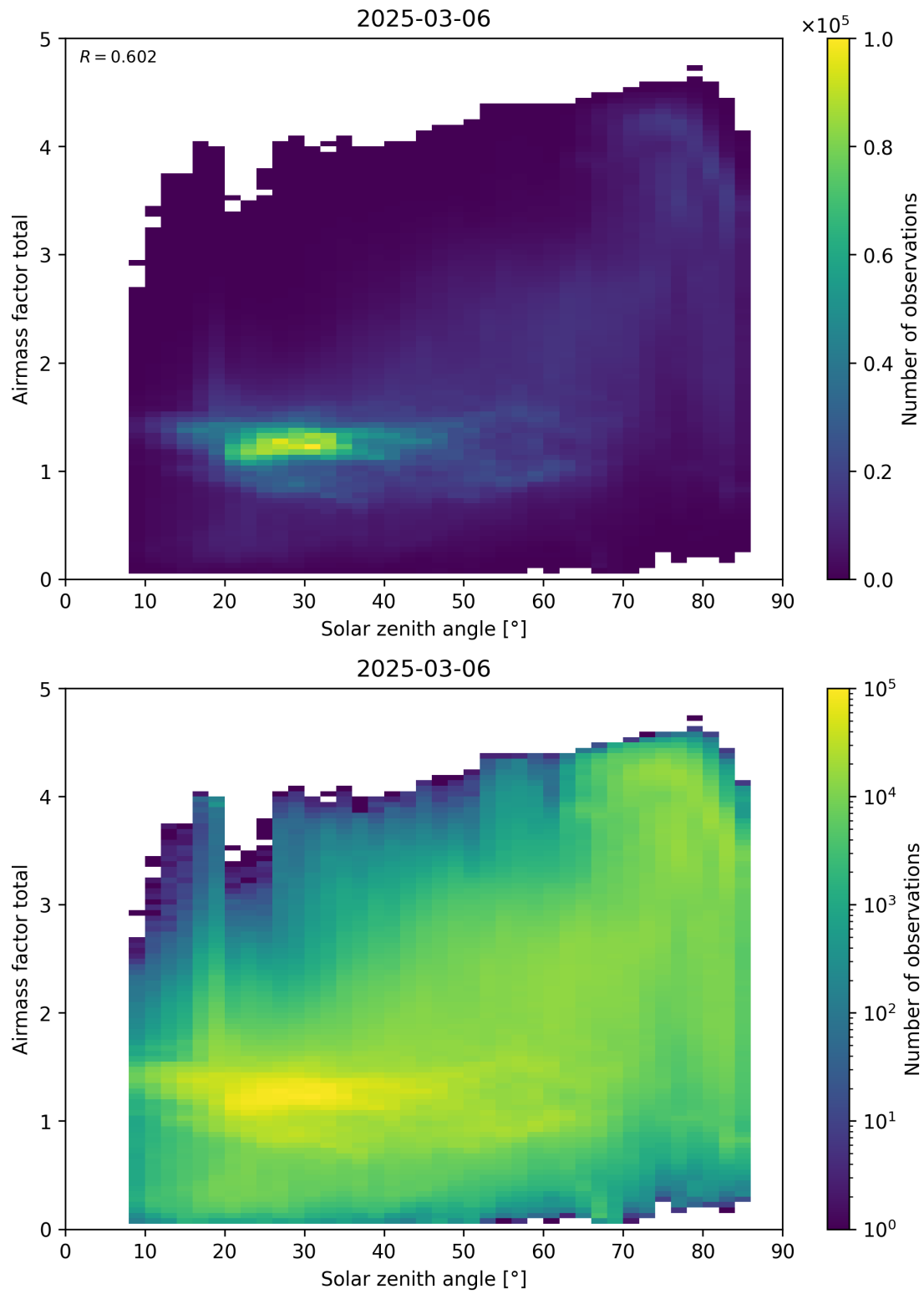
Figure 175: Scatter density plot of “Solar zenith angle” against “Airmass factor total” for 2025-03-05 to 2025-03-07.
