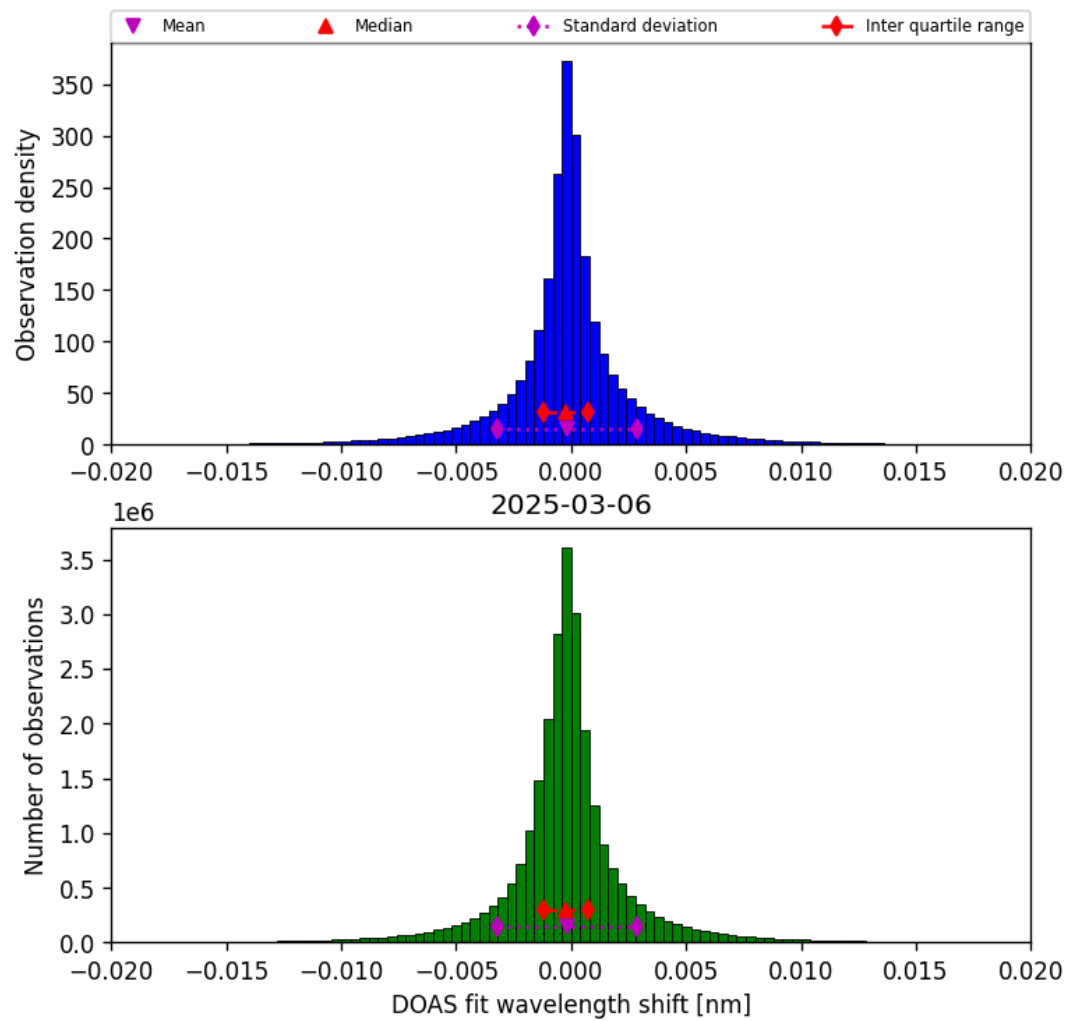
Figure 44: Histogram of “DOAS fit wavelength shift” for 2025-03-05 to 2025-03-07
