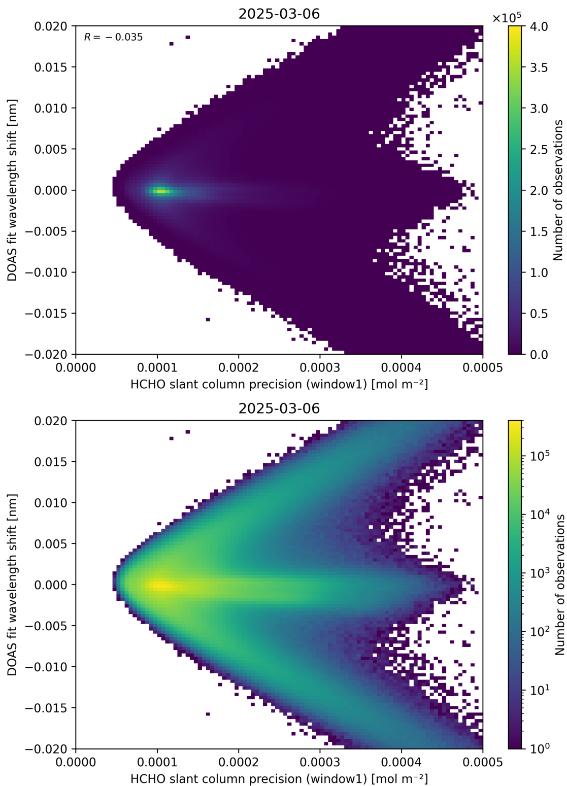
Figure 89: Scatter density plot of “HCHO slant column precision (window1)” against “DOAS fit wavelength shift” for 2025-03-05 to 2025-03-07.
