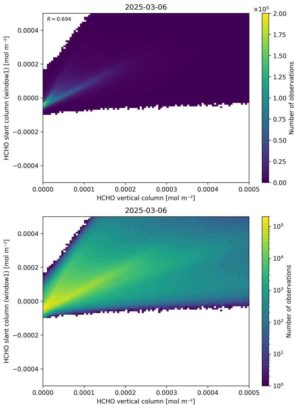
Figure 129: Scatter density plot of “HCHO vertical column” against “HCHO slant column (window1)” for 2025-03-05 to 2025-03-07.
