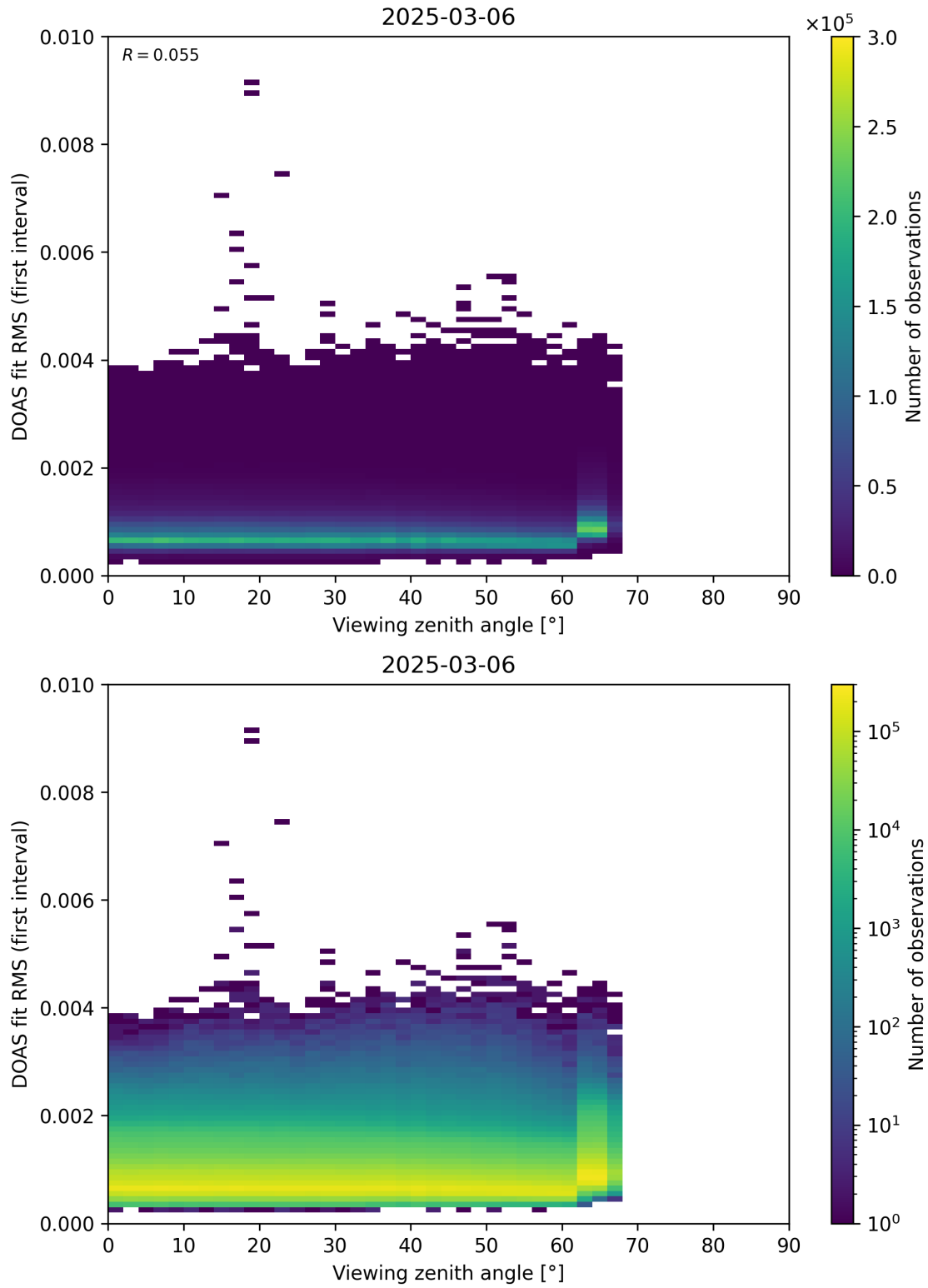
Figure 182: Scatter density plot of “Viewing zenith angle” against “DOAS fit RMS (first interval)” for 2025-03-05 to 2025-03-07.
