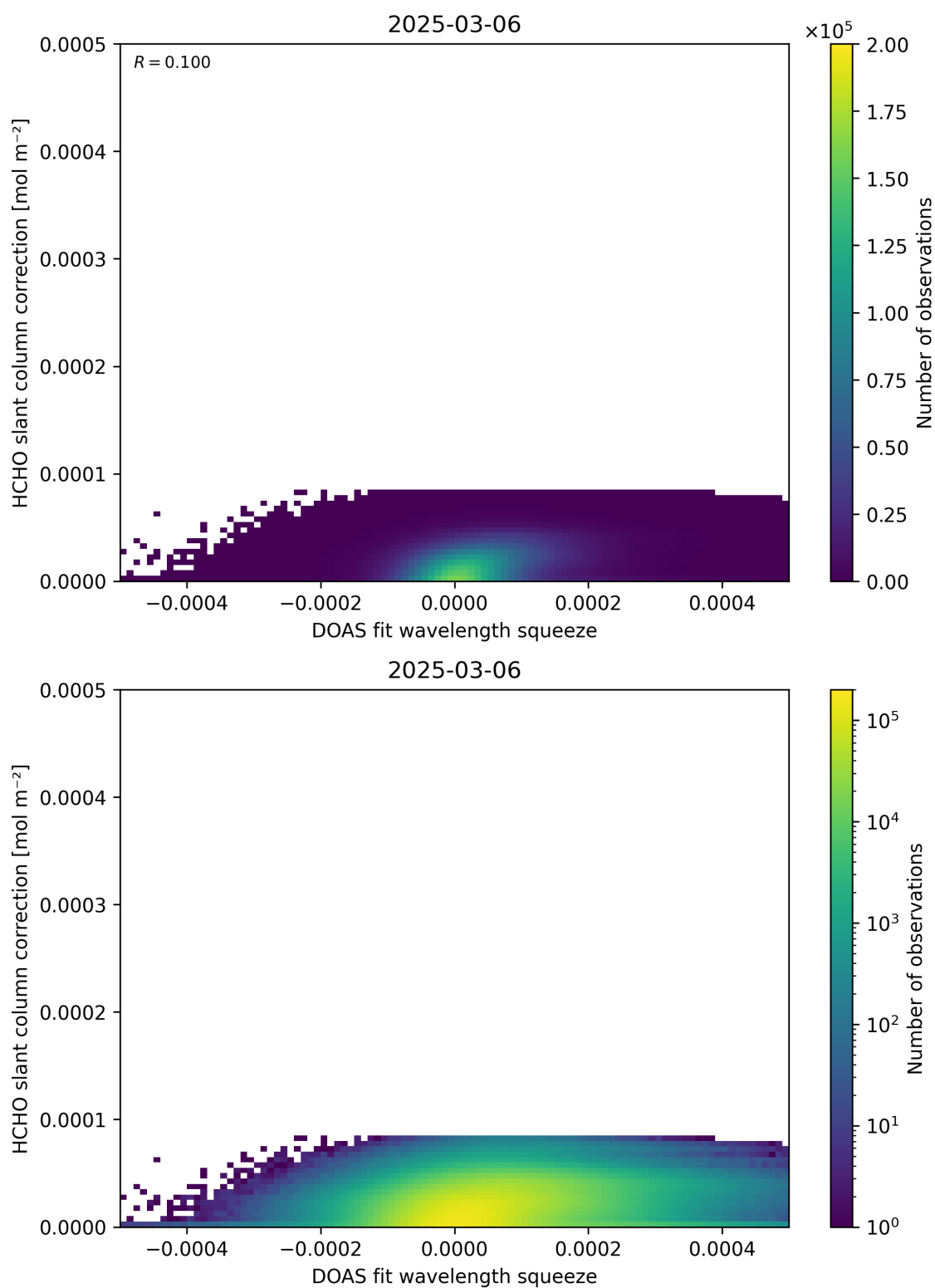
Figure 70: Scatter density plot of “DOAS fit wavelength squeeze” against “HCHO slant column correction” for 2025-03-05 to 2025-03-07.
