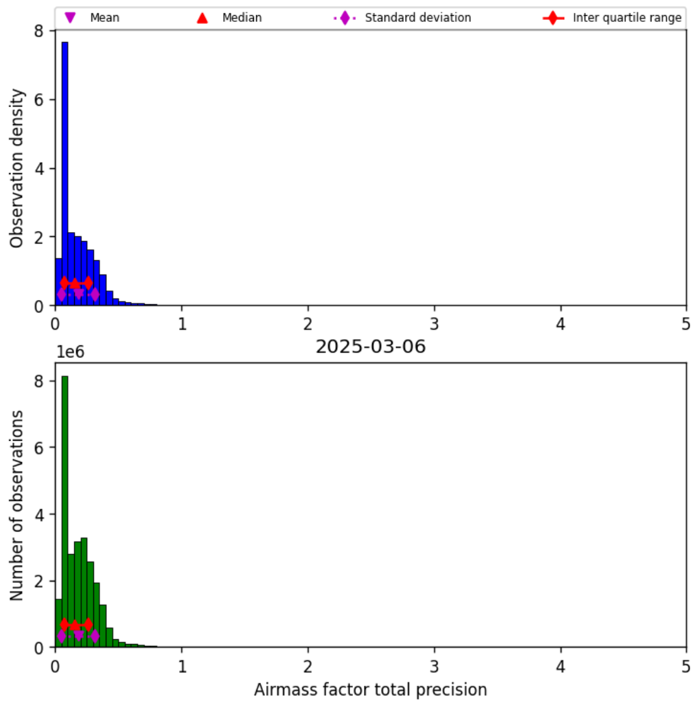
Figure 41: Histogram of “Airmass factor total precision” for 2025-03-05 to 2025-03-07
