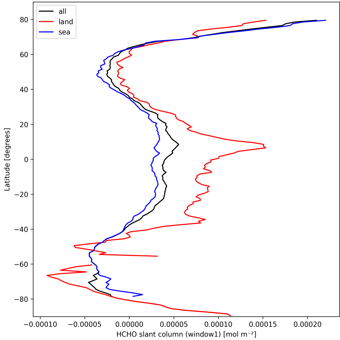
Figure 24: Zonal average of “HCHO slant column (window1)” for 2025-03-05 to 2025-03-07.
