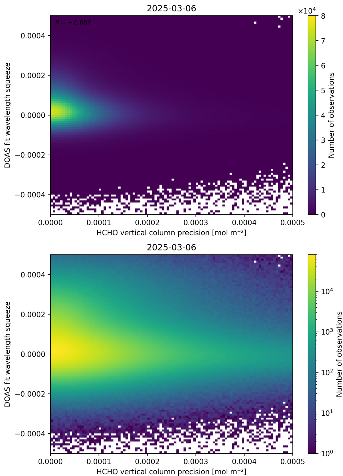
Figure 138: Scatter density plot of “HCHO vertical column precision” against “DOAS fit wavelength squeeze” for 2025-03-05 to 2025-03-07.
