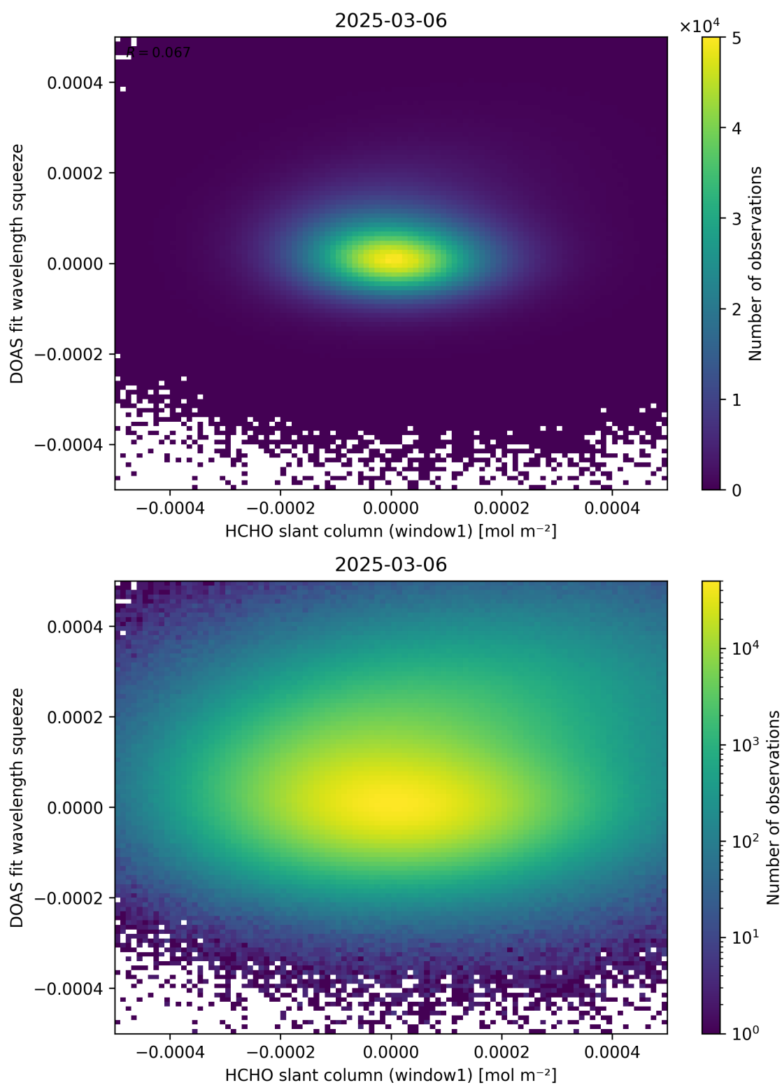
Figure 80: Scatter density plot of “HCHO slant column (window1)” against “DOAS fit wavelength squeeze” for 2025-03-05 to 2025-03-07.
