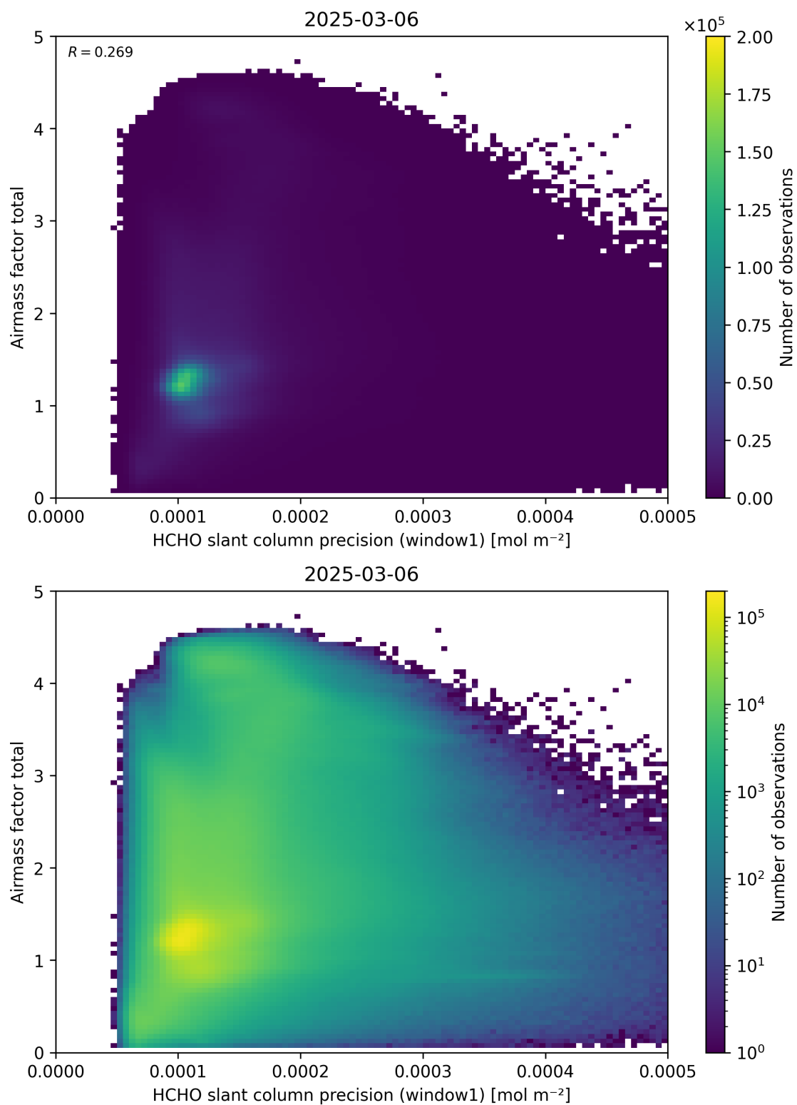
Figure 94: Scatter density plot of “HCHO slant column precision (window1)” against “Airmass factor total” for 2025-03-05 to 2025-03-07.
