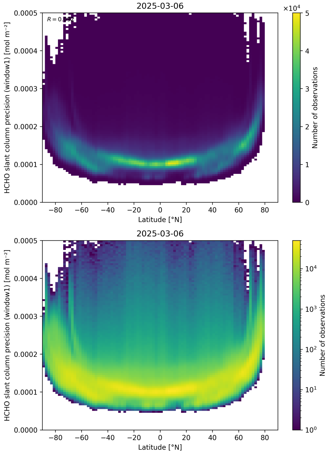
Figure 160: Scatter density plot of “Latitude” against “HCHO slant column precision (window1)” for 2025-03-05 to 2025-03-07.
