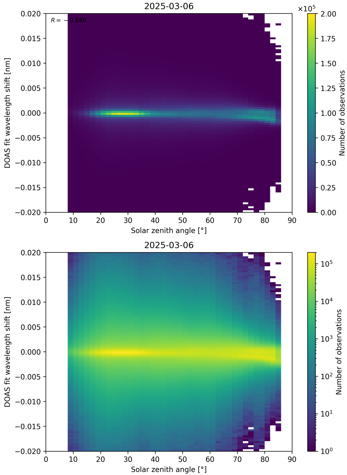
Figure 168: Scatter density plot of “Solar zenith angle” against “DOAS fit wavelength shift” for 2025-03-05 to 2025-03-07.
