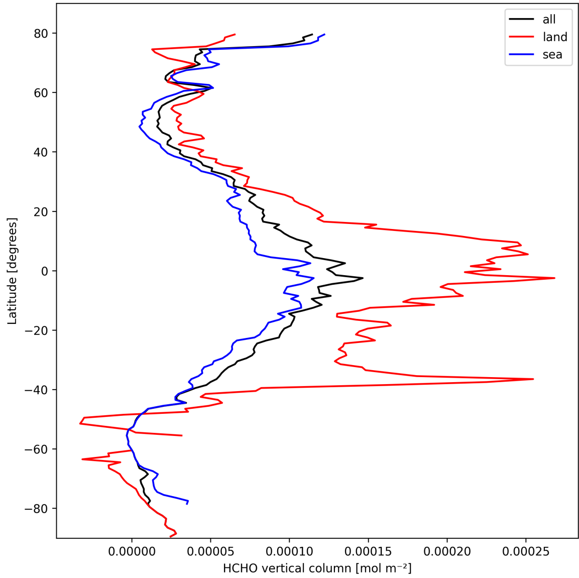
Figure 21: Zonal average of “HCHO vertical column” for 2025-03-05 to 2025-03-07.
