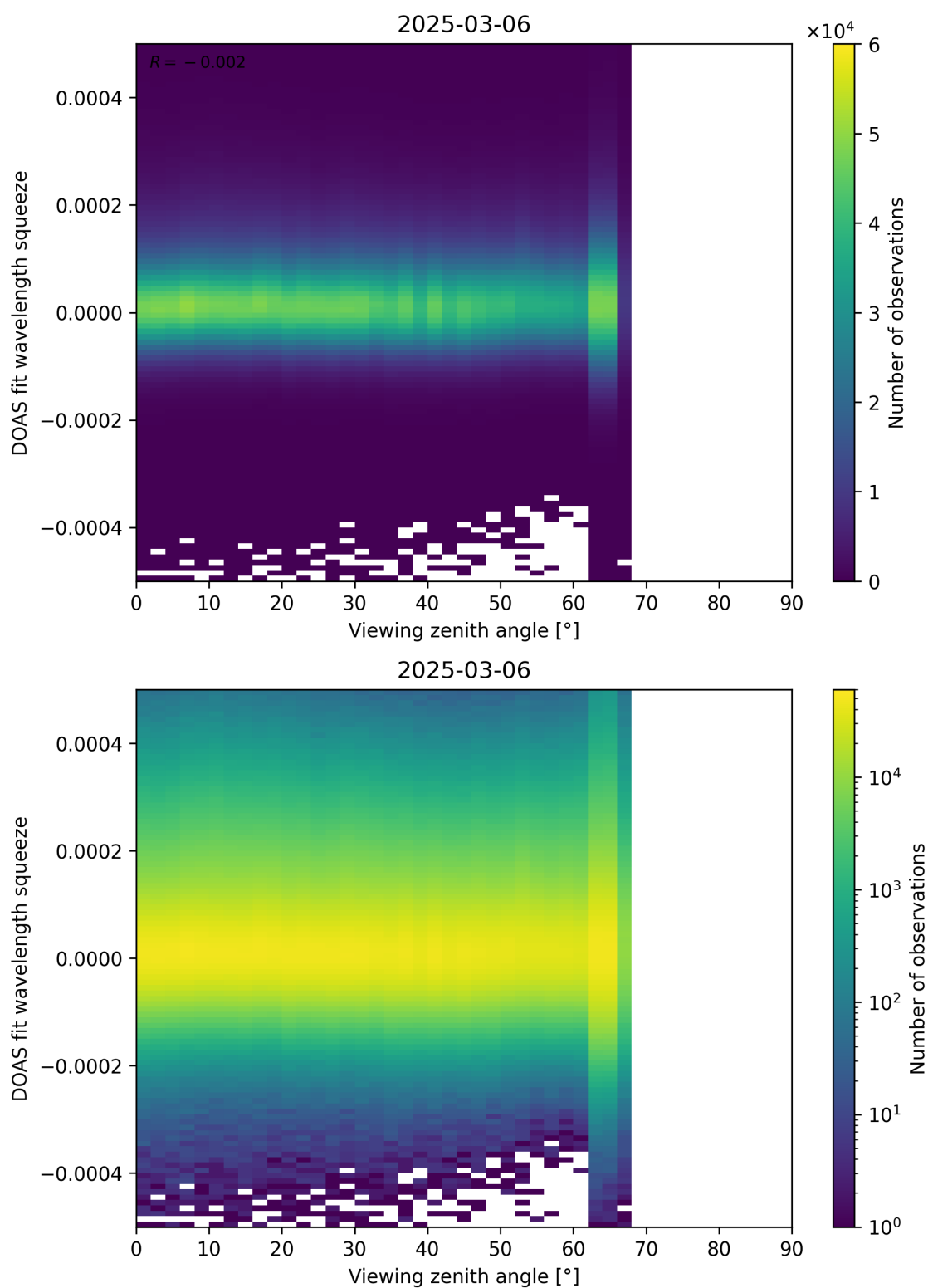
Figure 184: Scatter density plot of “Viewing zenith angle” against “DOAS fit wavelength squeeze” for 2025-03-05 to 2025-03-07.
