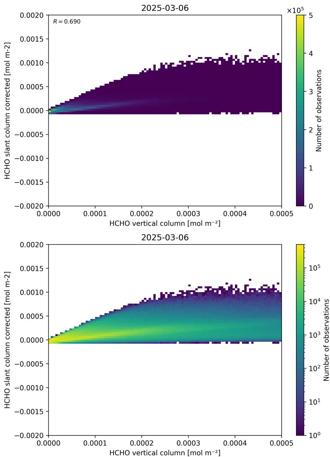
Figure 127: Scatter density plot of “HCHO vertical column” against “HCHO slant column corrected” for 2025-03-05 to 2025-03-07.
