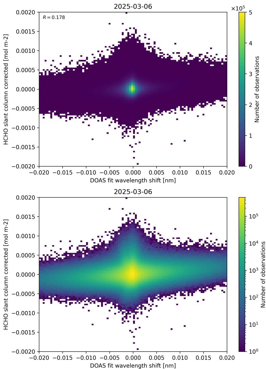
Figure 66: Scatter density plot of “DOAS fit wavelength shift” against “HCHO slant column corrected” for 2025-03-05 to 2025-03-07.
