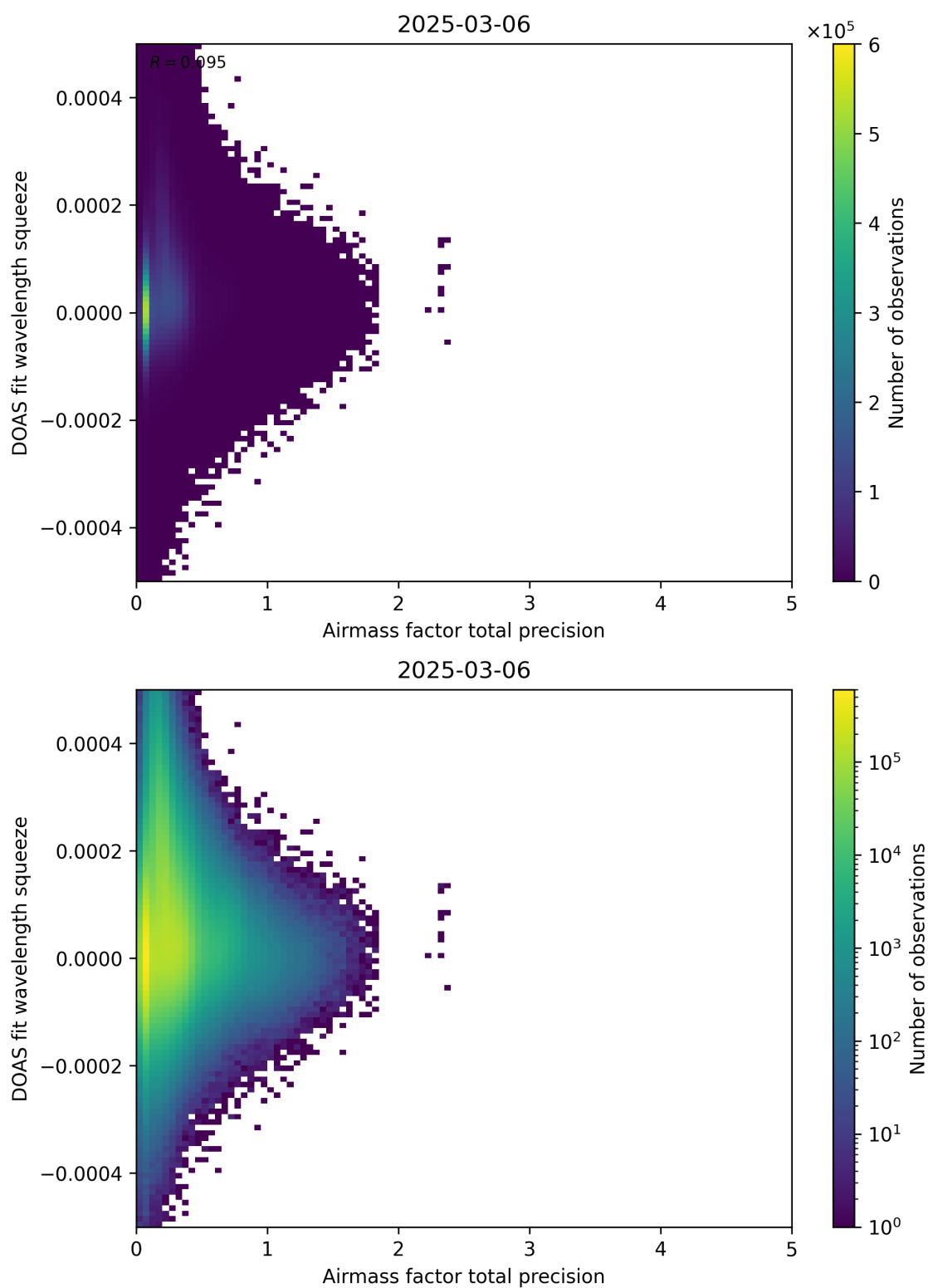
Figure 107: Scatter density plot of “Airmass factor total precision” against “DOAS fit wavelength squeeze” for 2025-03-05 to 2025-03-07.
