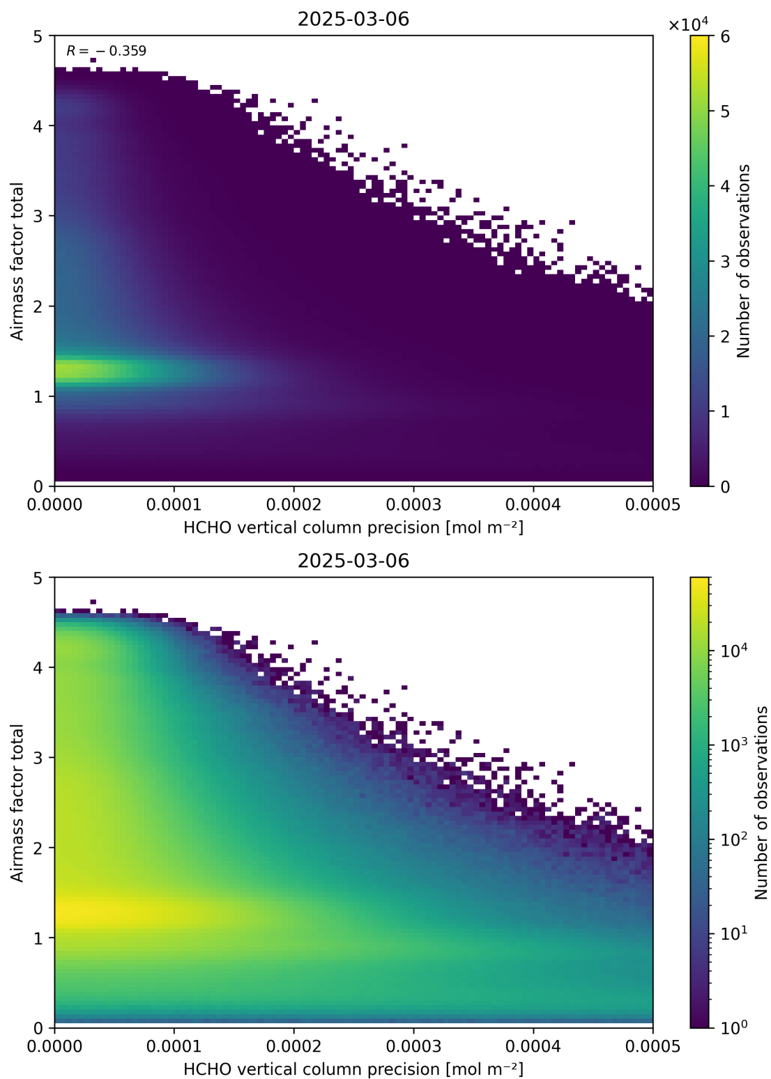
Figure 144: Scatter density plot of “HCHO vertical column precision” against “Airmass factor total” for 2025-03-05 to 2025-03-07.
