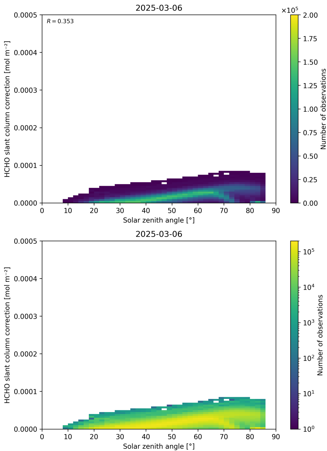
Figure 172: Scatter density plot of “Solar zenith angle” against “HCHO slant column correction” for 2025-03-05 to 2025-03-07.
