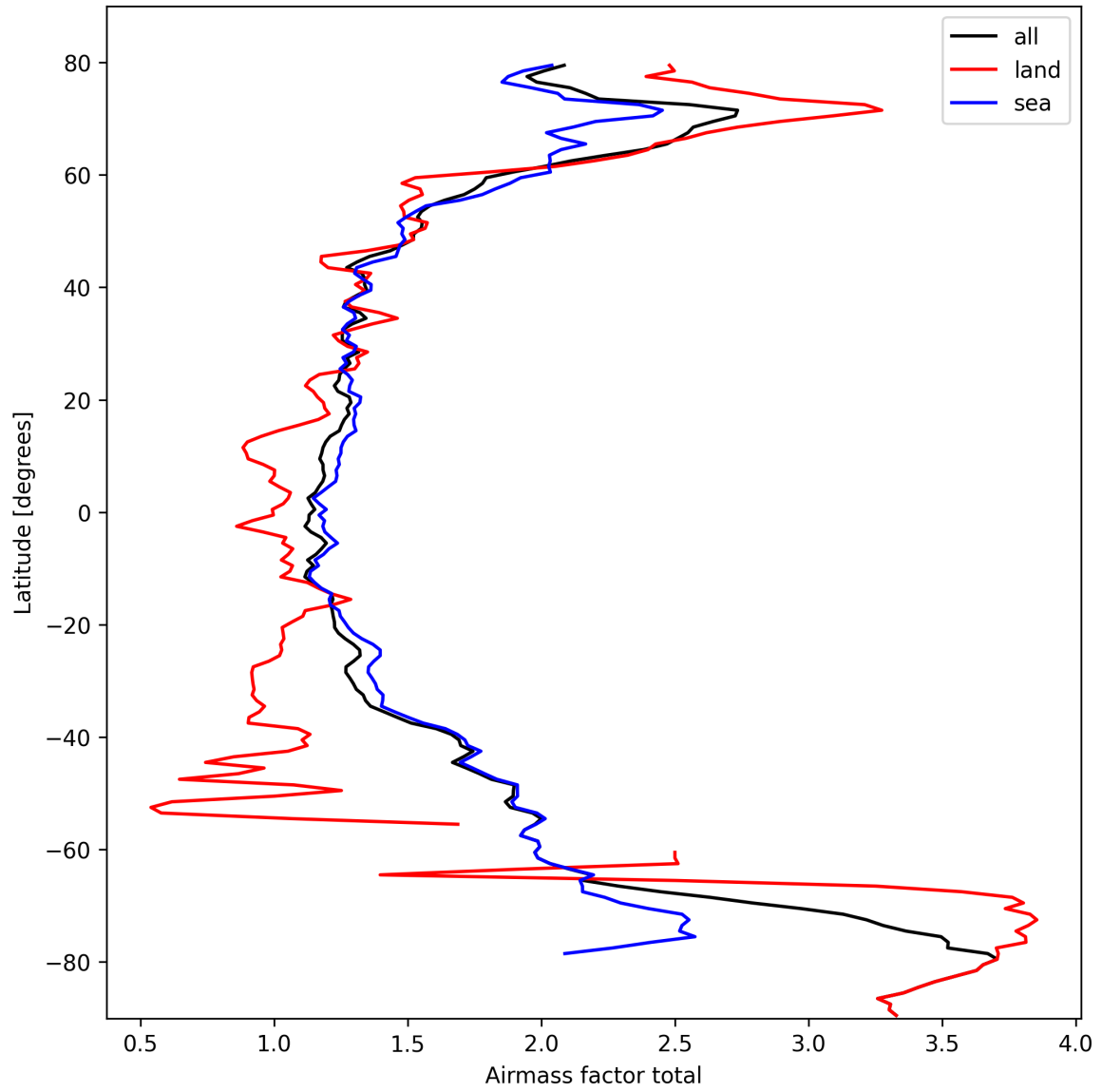
Figure 26: Zonal average of “Airmass factor total” for 2025-03-05 to 2025-03-07.
