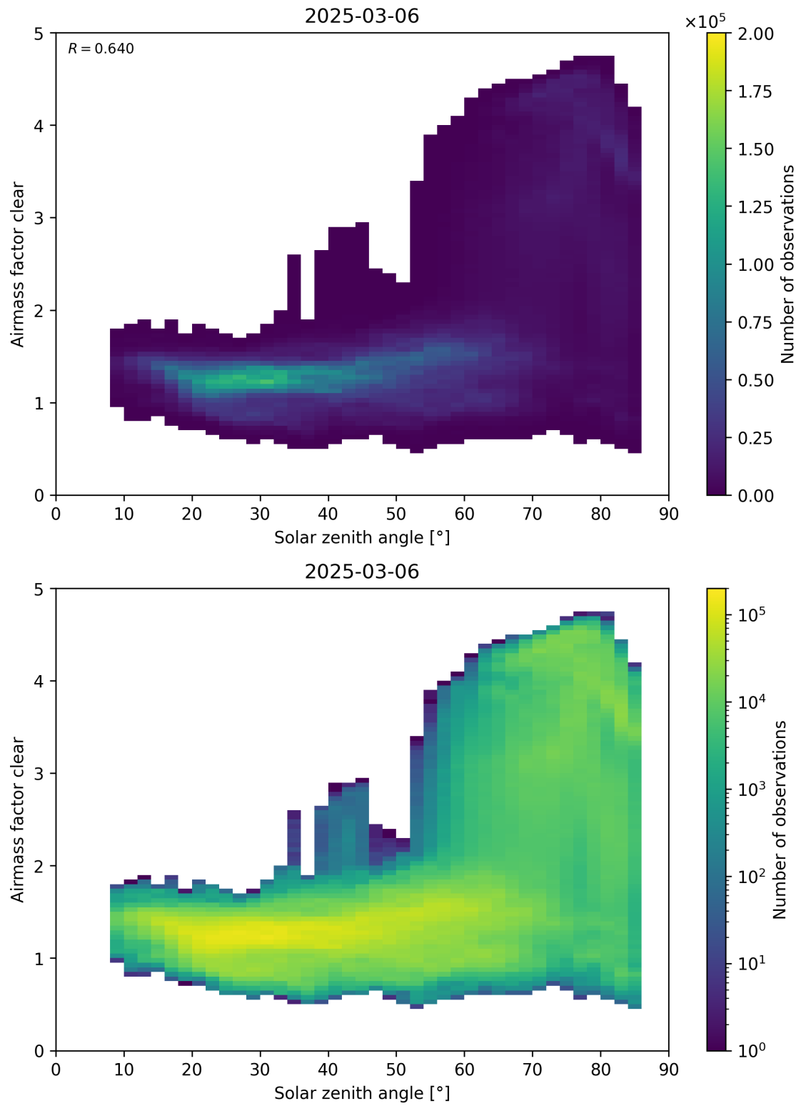
Figure 170: Scatter density plot of “Solar zenith angle” against “Airmass factor clear” for 2025-03-05 to 2025-03-07.
