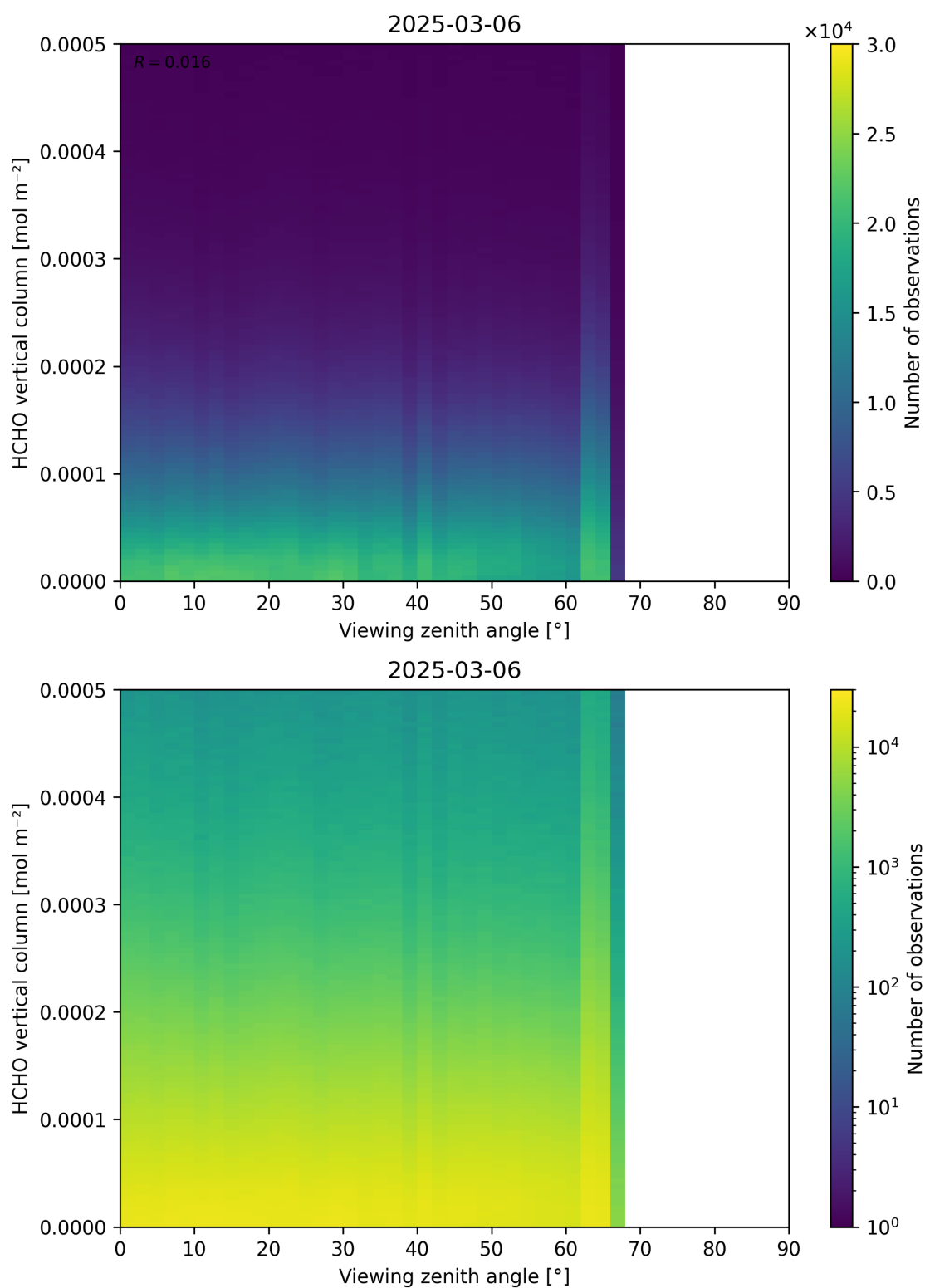
Figure 192: Scatter density plot of “Viewing zenith angle” against “HCHO vertical column” for 2025-03-05 to 2025-03-07.
