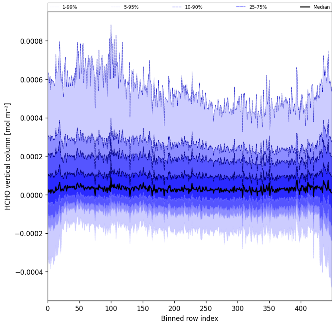
Figure 49: Along track statistics of “HCHO vertical column” for 2025-03-05 to 2025-03-07
