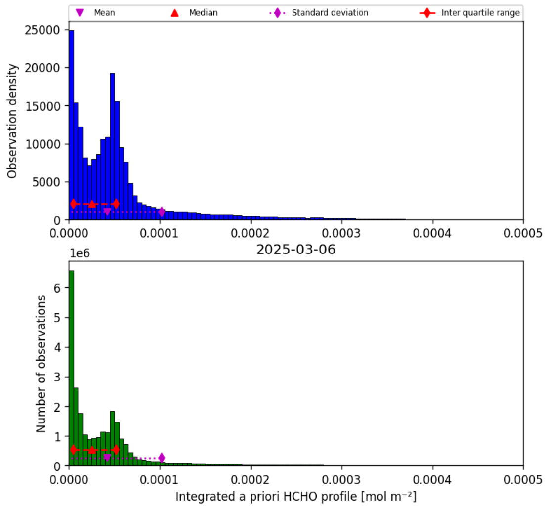
Figure 43: Histogram of “Integrated a priori HCHO profile” for 2025-03-05 to 2025-03-07
