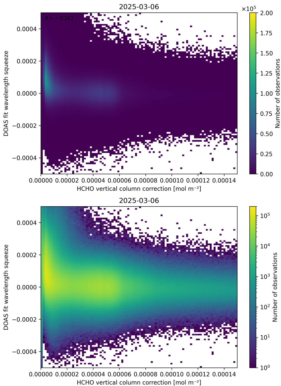
Figure 114: Scatter density plot of “HCHO vertical column correction” against “DOAS fit wavelength squeeze” for 2025-03-05 to 2025-03-07.
