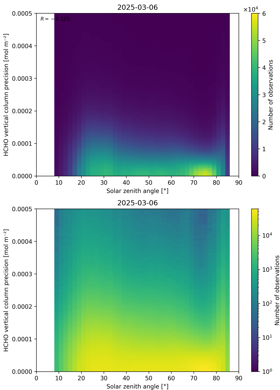
Figure 179: Scatter density plot of “Solar zenith angle” against “HCHO vertical column precision” for 2025-03-05 to 2025-03-07.
