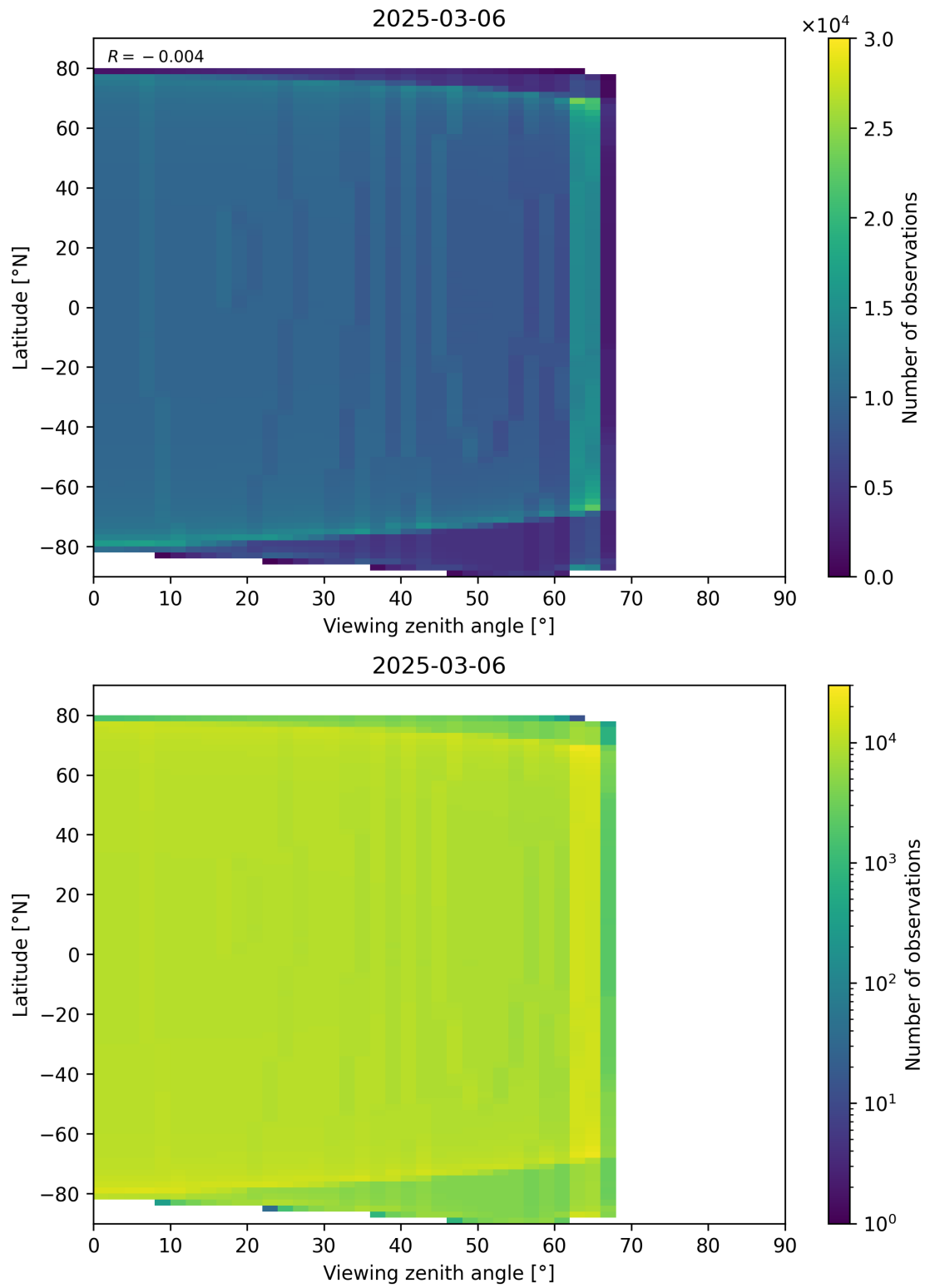
Figure 196: Scatter density plot of “Viewing zenith angle” against “Latitude” for 2025-03-05 to 2025-03-07.
