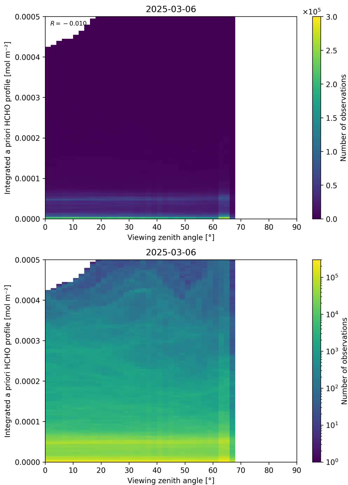
Figure 195: Scatter density plot of “Viewing zenith angle” against “Integrated a priori HCHO profile” for 2025-03-05 to 2025-03-07.
