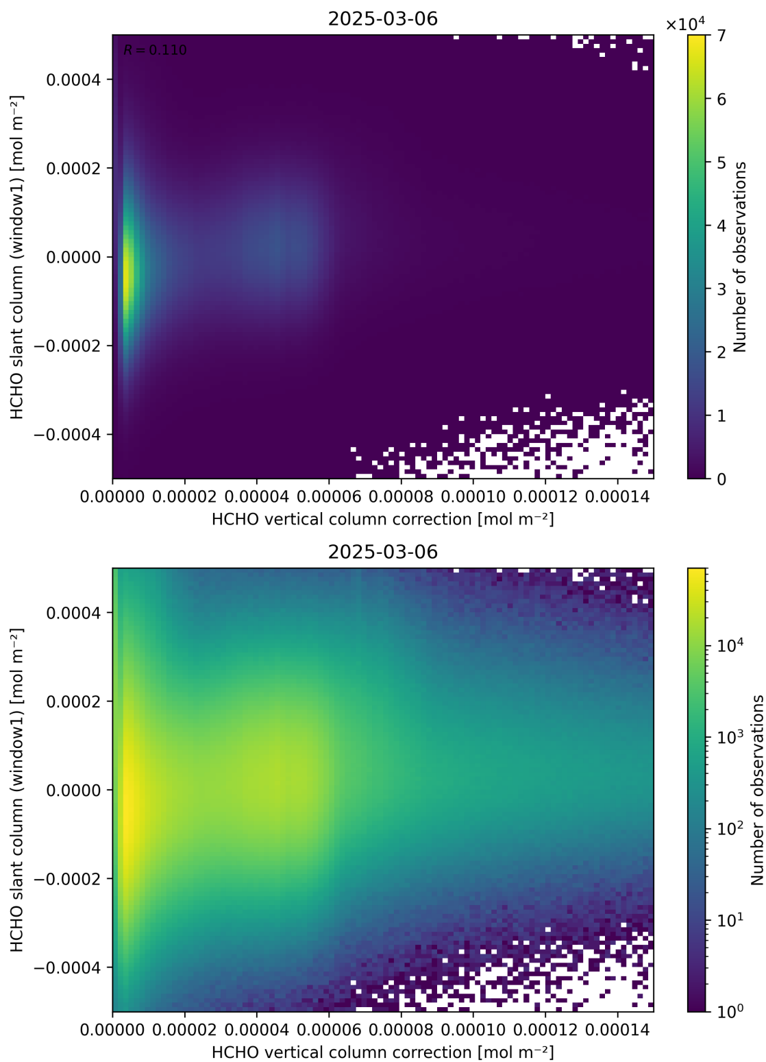
Figure 118: Scatter density plot of “HCHO vertical column correction” against “HCHO slant column (window1)” for 2025-03-05 to 2025-03-07.
