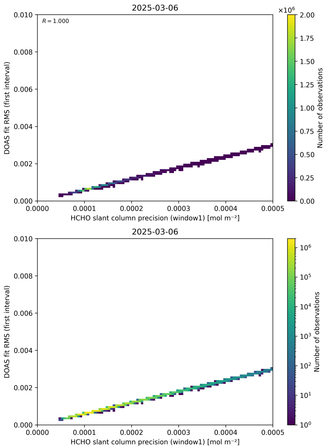
Figure 88: Scatter density plot of “HCHO slant column precision (window1)” against “DOAS fit RMS (first interval)” for 2025-03-05 to 2025-03-07.
