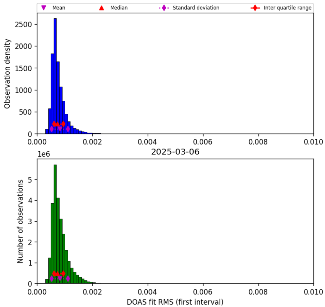
Figure 46: Histogram of “DOAS fit RMS (first interval)” for 2025-03-05 to 2025-03-07
