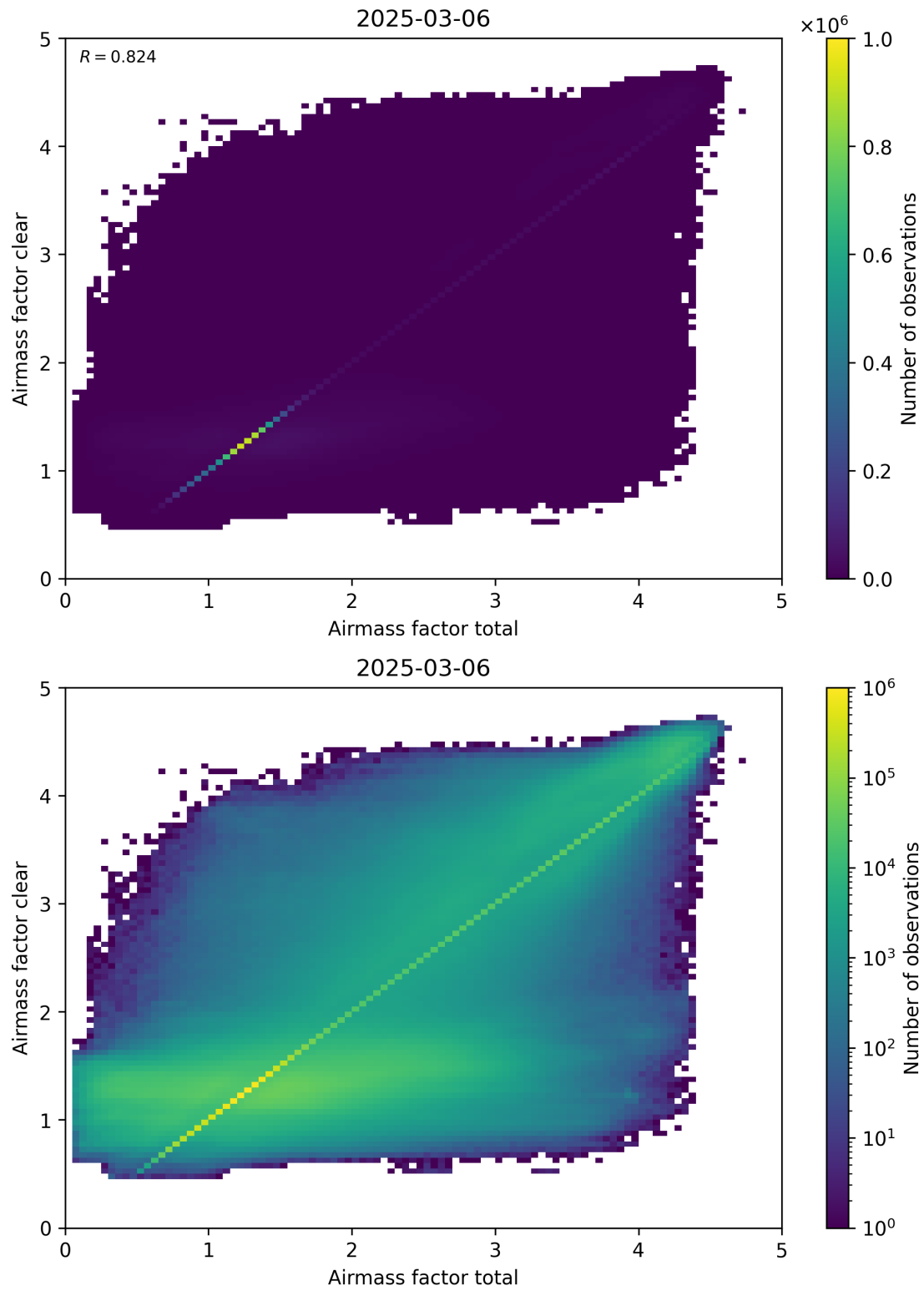
Figure 100: Scatter density plot of “Airmass factor total” against “Airmass factor clear” for 2025-03-05 to 2025-03-07.
