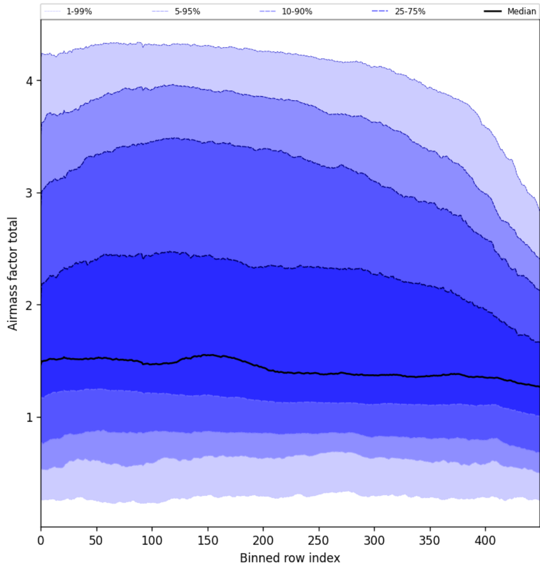
Figure 54: Along track statistics of “Airmass factor total” for 2025-03-05 to 2025-03-07
