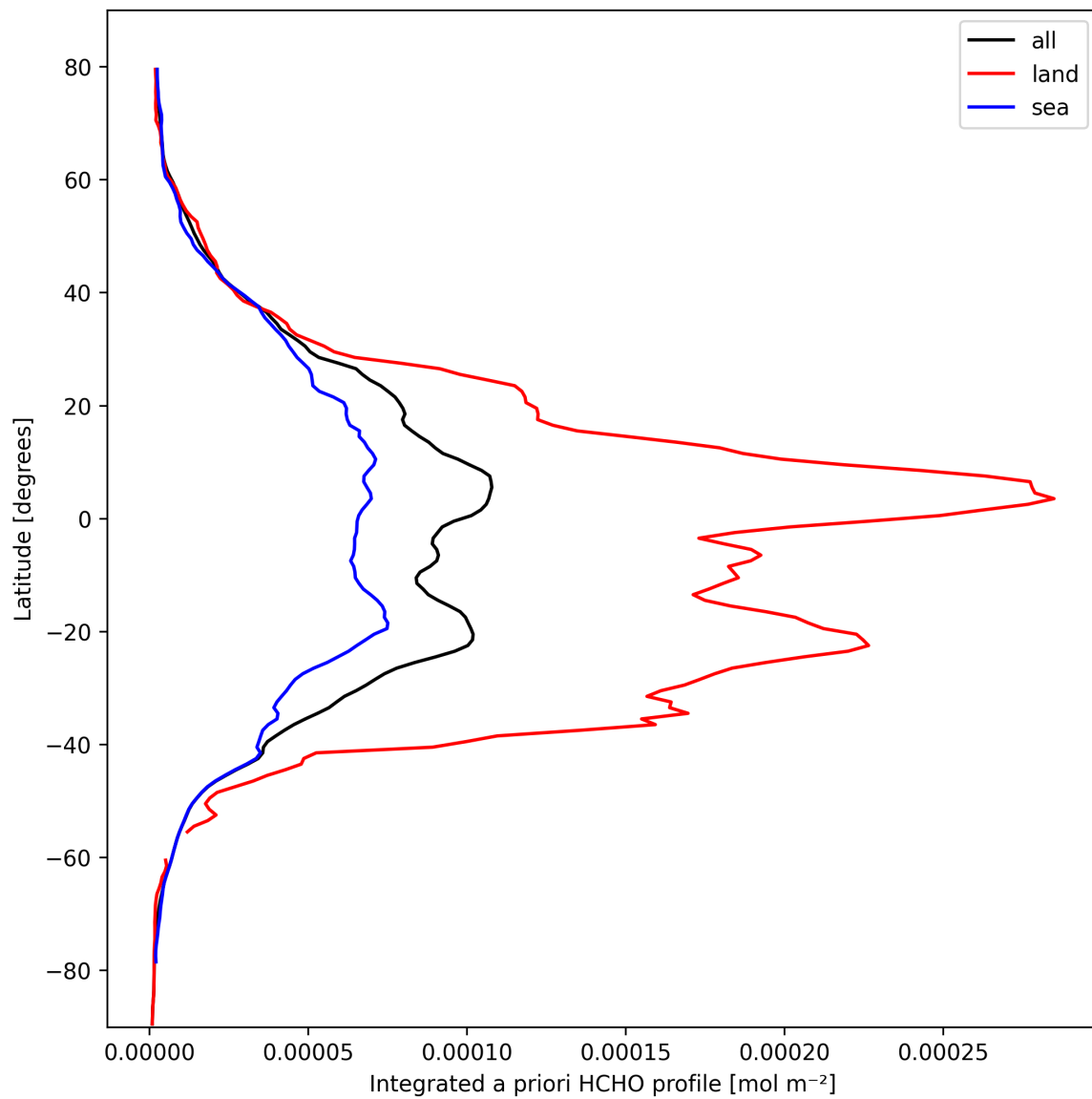
Figure 29: Zonal average of “Integrated a priori HCHO profile” for 2025-03-05 to 2025-03-07.
