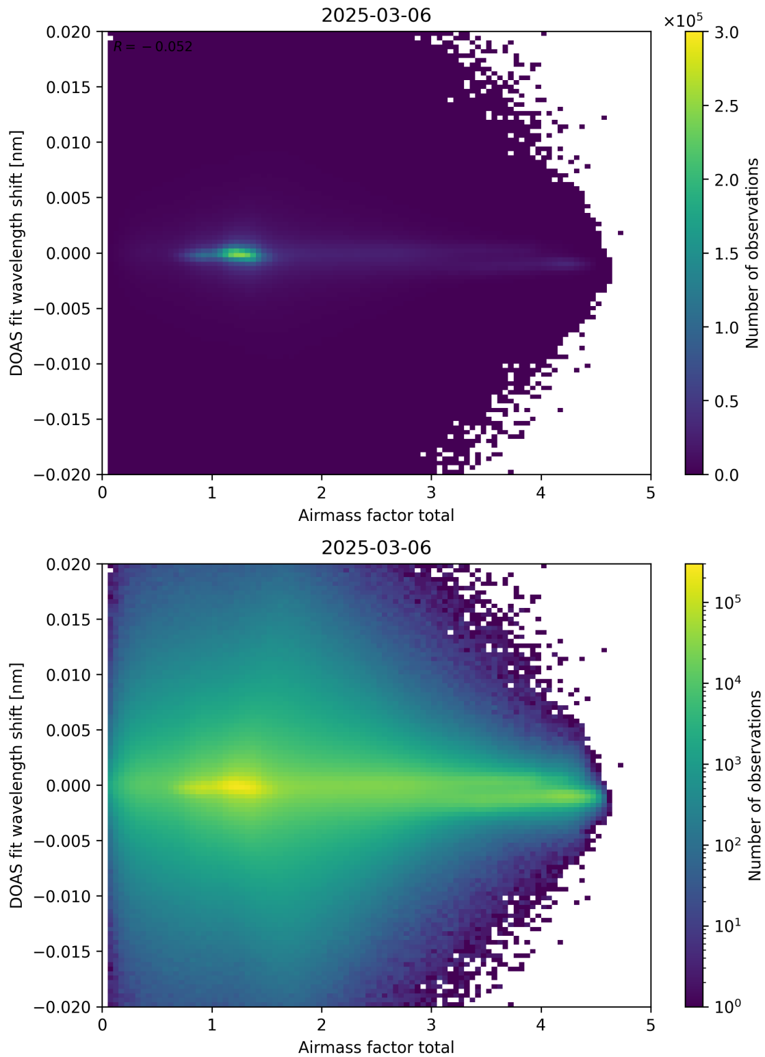
Figure 98: Scatter density plot of “Airmass factor total” against “DOAS fit wavelength shift” for 2025-03-05 to 2025-03-07.
