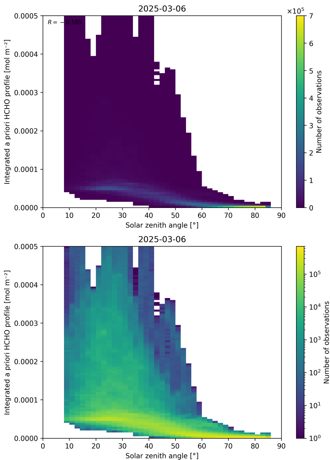
Figure 180: Scatter density plot of “Solar zenith angle” against “Integrated a priori HCHO profile” for 2025-03-05 to 2025-03-07.
