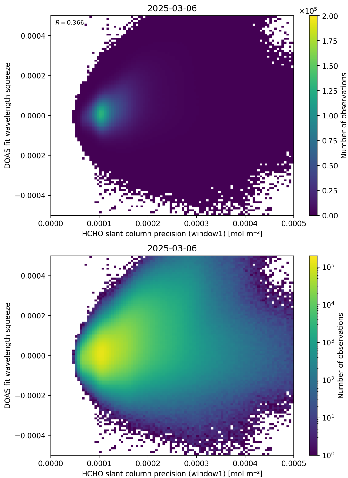
Figure 90: Scatter density plot of “HCHO slant column precision (window1)” against “DOAS fit wavelength squeeze” for 2025-03-05 to 2025-03-07.
