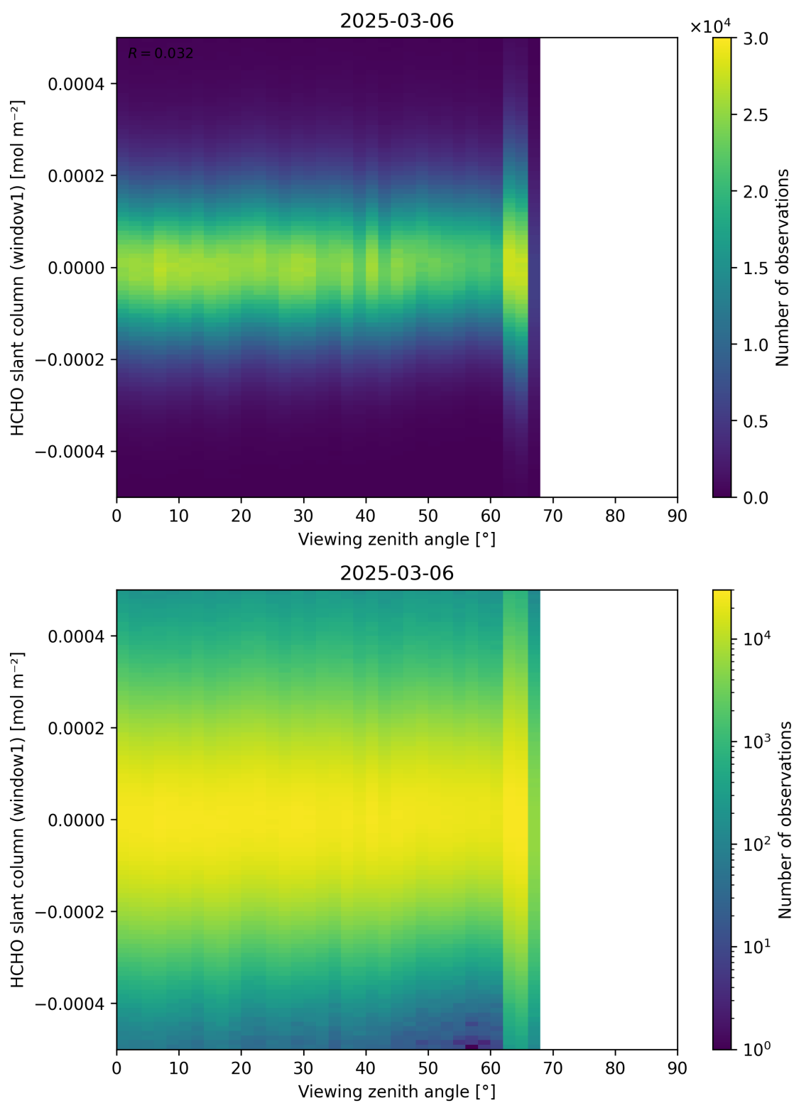
Figure 188: Scatter density plot of “Viewing zenith angle” against “HCHO slant column (window1)” for 2025-03-05 to 2025-03-07.
