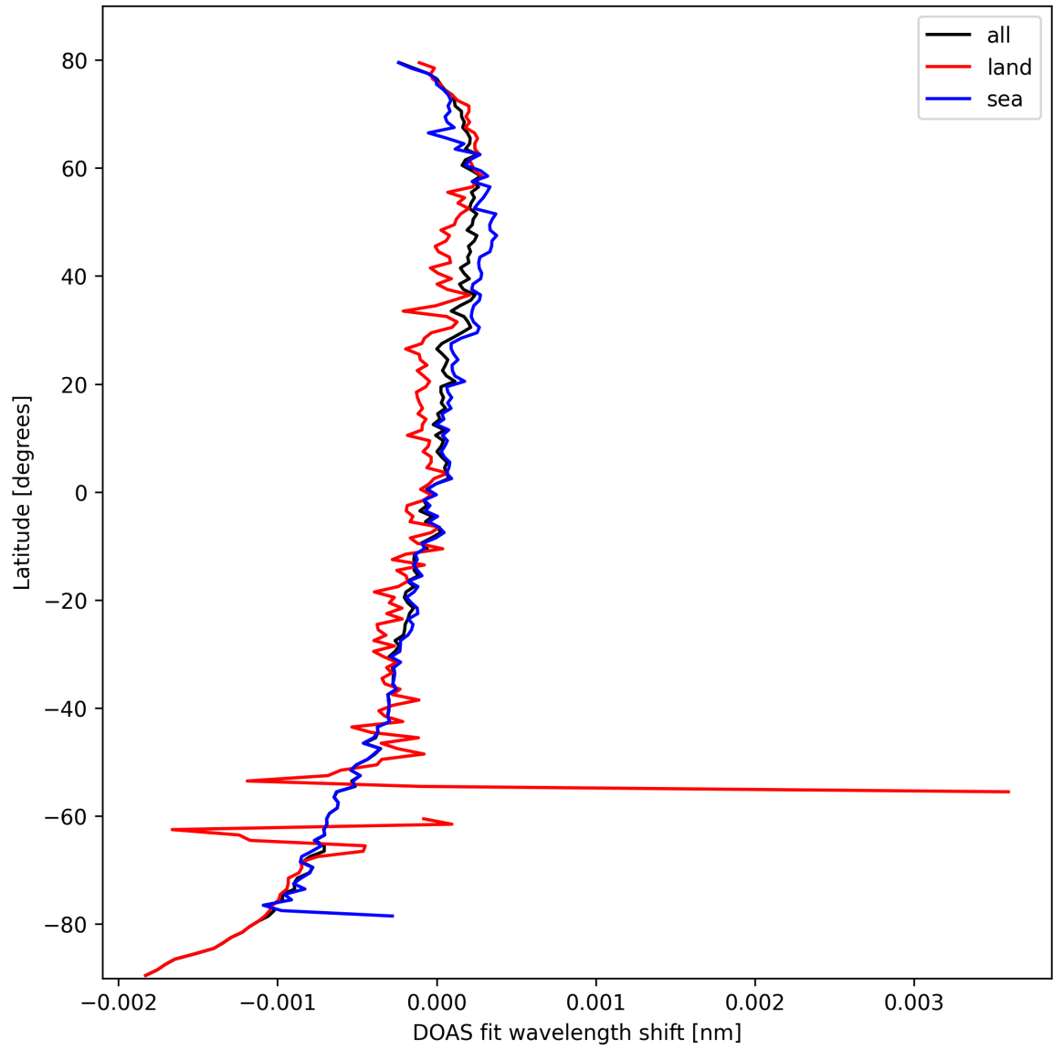
Figure 30: Zonal average of "DOAS fit wavelength shift" for 2025-03-05 to 2025-03-07.
