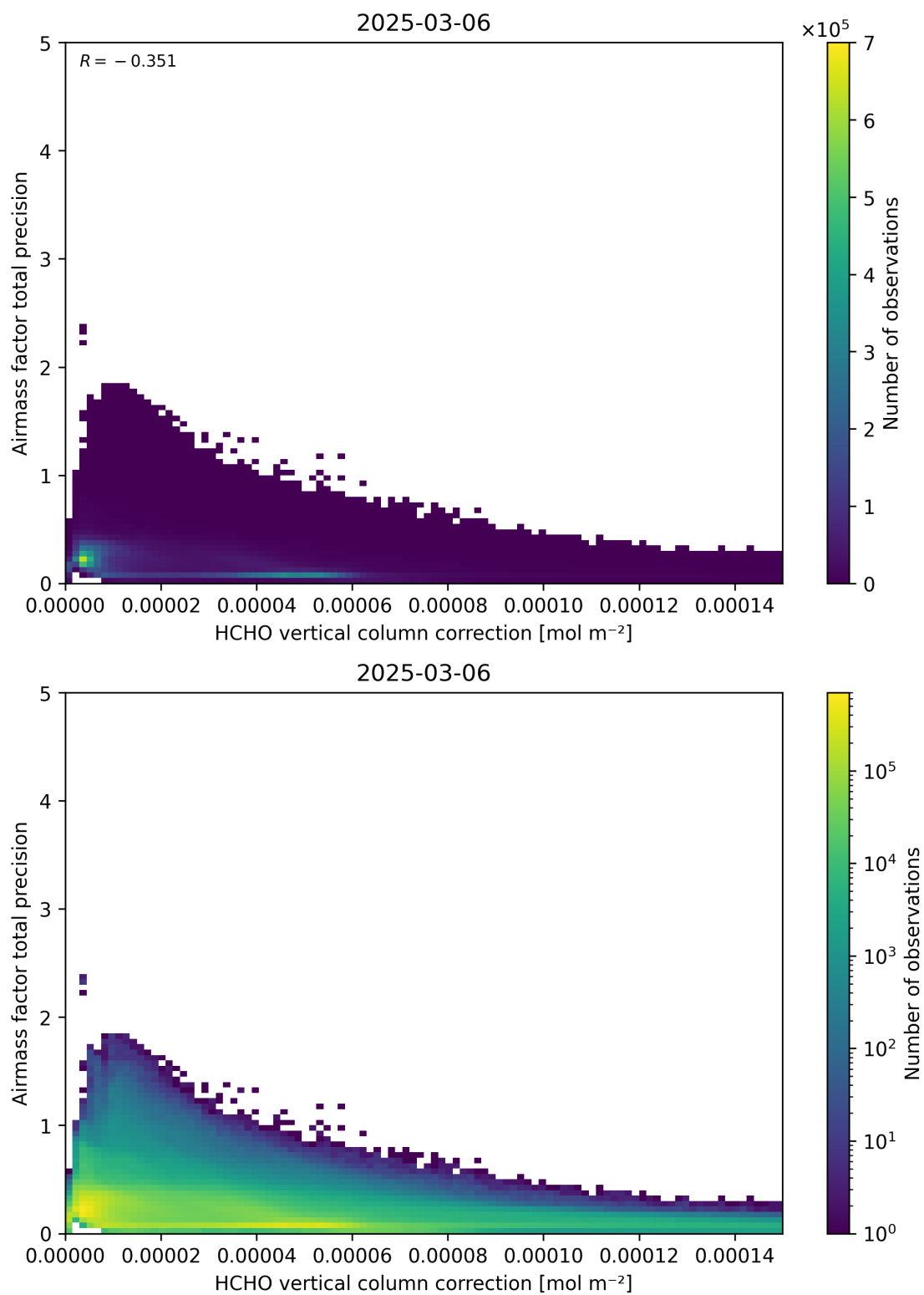
Figure 121: Scatter density plot of “HCHO vertical column correction” against “Airmass factor total precision” for 2025-03-05 to 2025-03-07.
