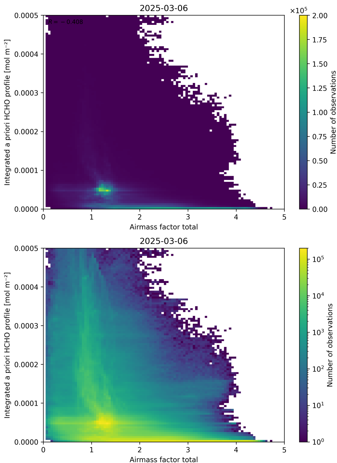
Figure 104: Scatter density plot of “Airmass factor total” against “Integrated a priori HCHO profile” for 2025-03-05 to 2025-03-07.
