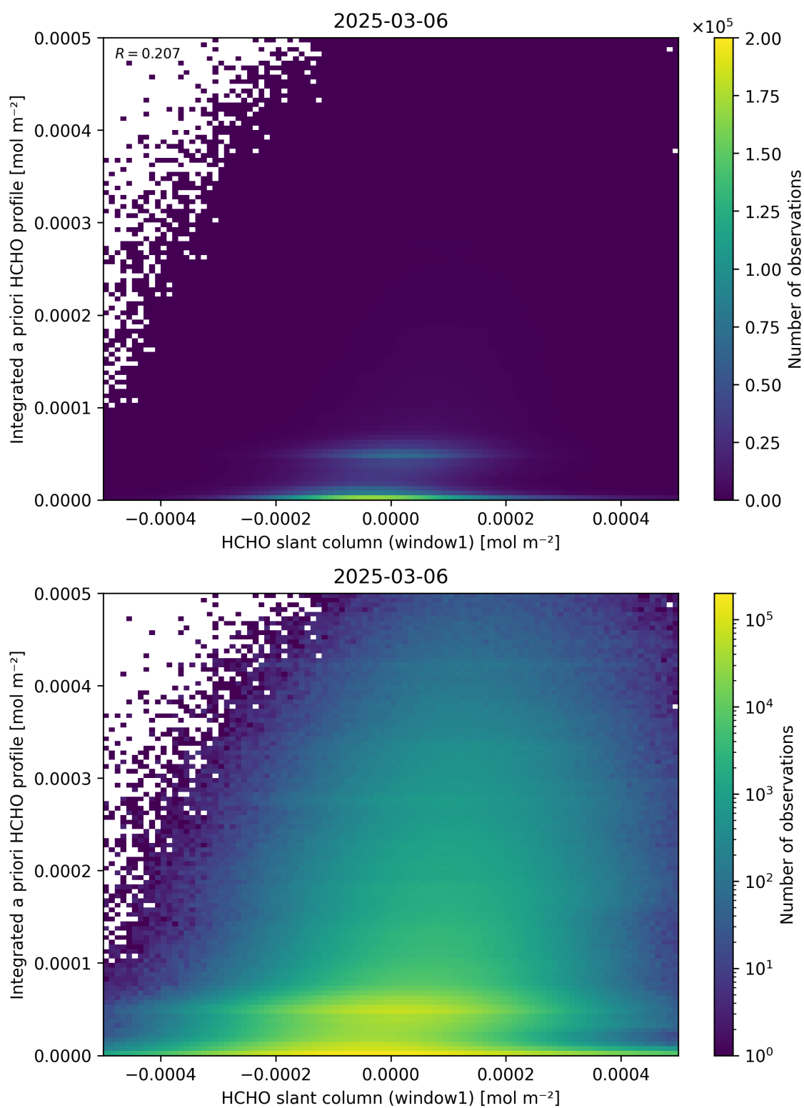
Figure 87: Scatter density plot of “HCHO slant column (window1)” against “Integrated a priori HCHO profile” for 2025-03-05 to 2025-03-07.
