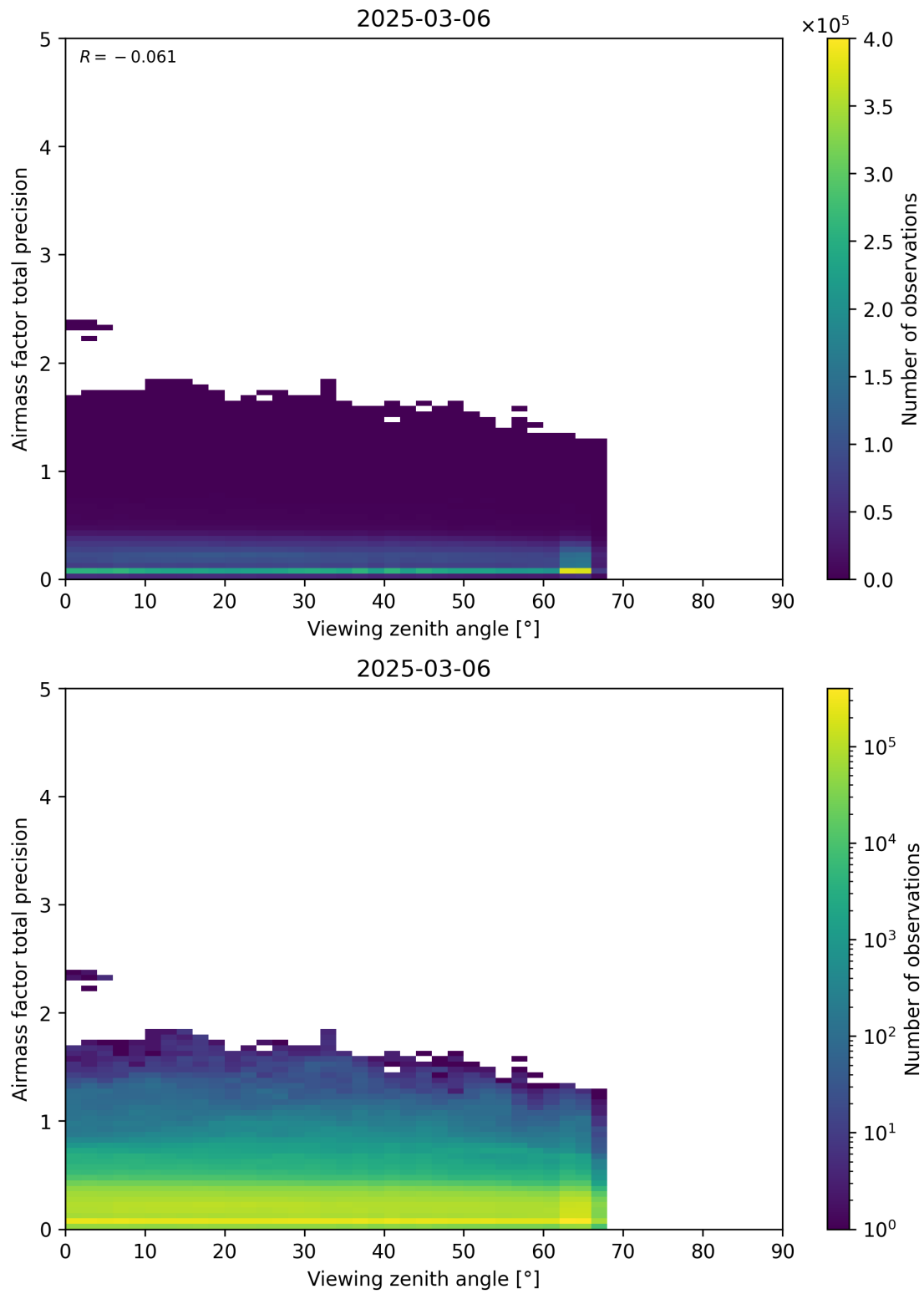
Figure 191: Scatter density plot of “Viewing zenith angle” against “Airmass factor total precision” for 2025-03-05 to 2025-03-07.
