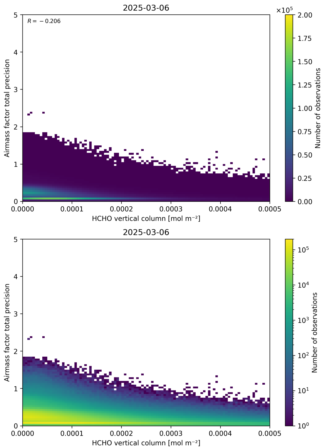
Figure 132: Scatter density plot of “HCHO vertical column” against “Airmass factor total precision” for 2025-03-05 to 2025-03-07.
