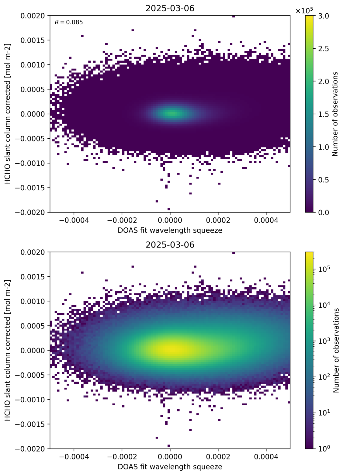
Figure 69: Scatter density plot of “DOAS fit wavelength squeeze” against “HCHO slant column corrected” for 2025-03-05 to 2025-03-07.
