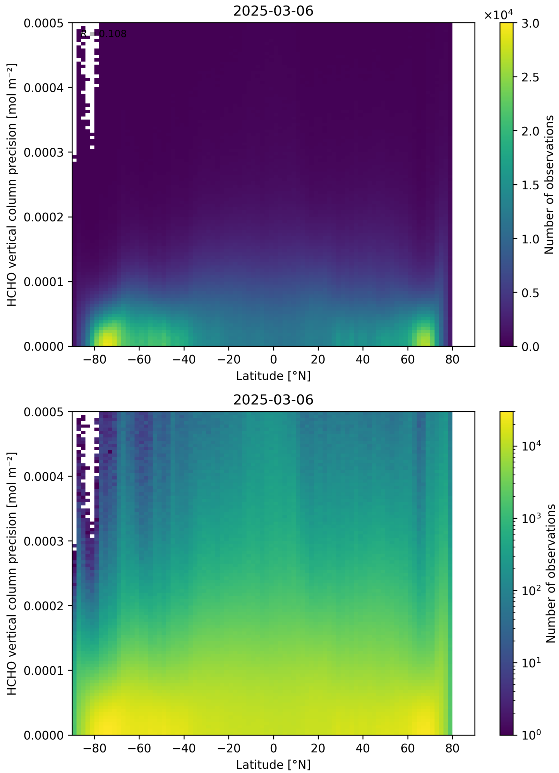
Figure 165: Scatter density plot of “Latitude” against “HCHO vertical column precision” for 2025-03-05 to 2025-03-07.
