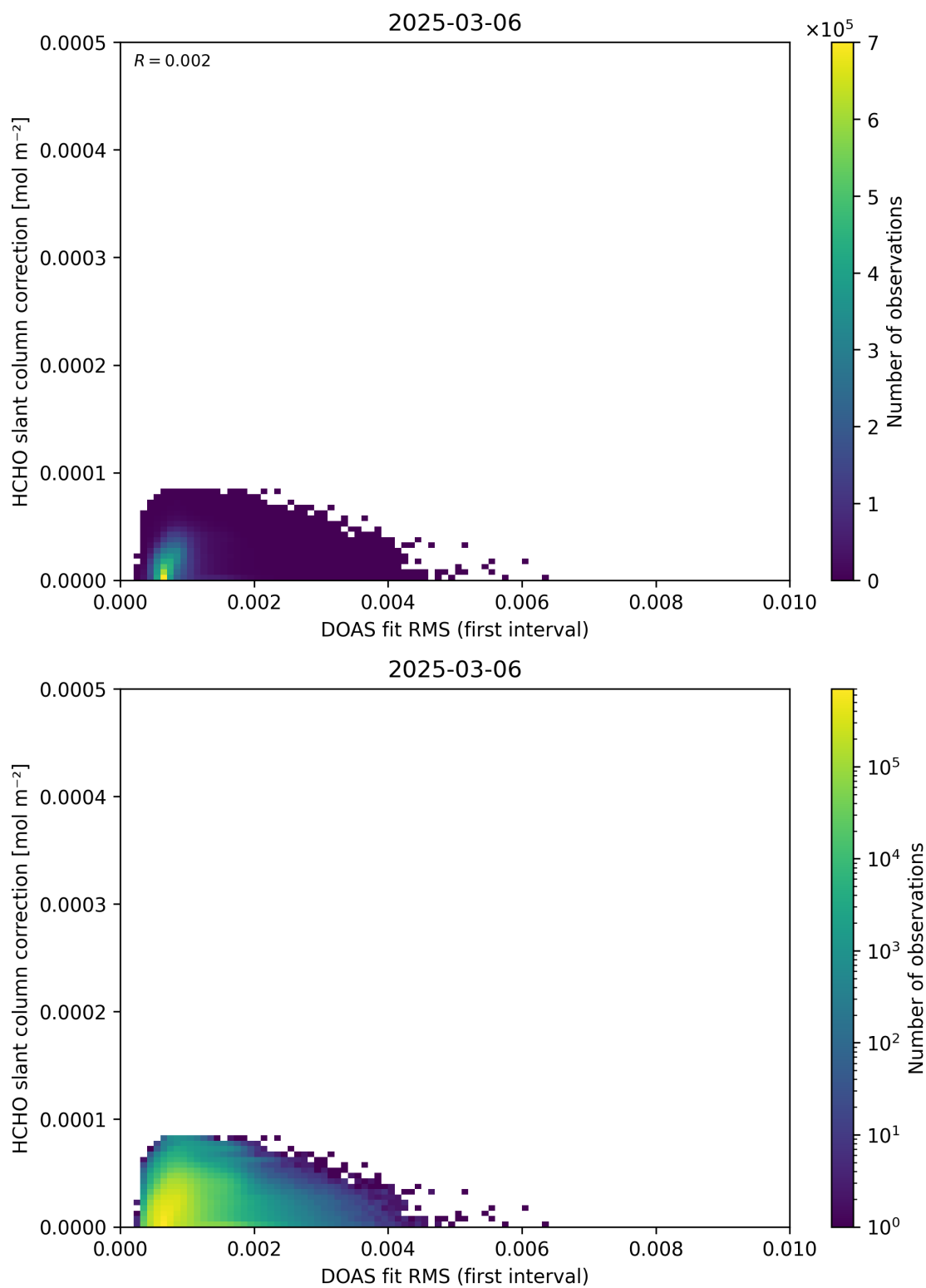
Figure 63: Scatter density plot of “DOAS fit RMS (first interval)” against “HCHO slant column correction” for 2025-03-05 to 2025-03-07.
