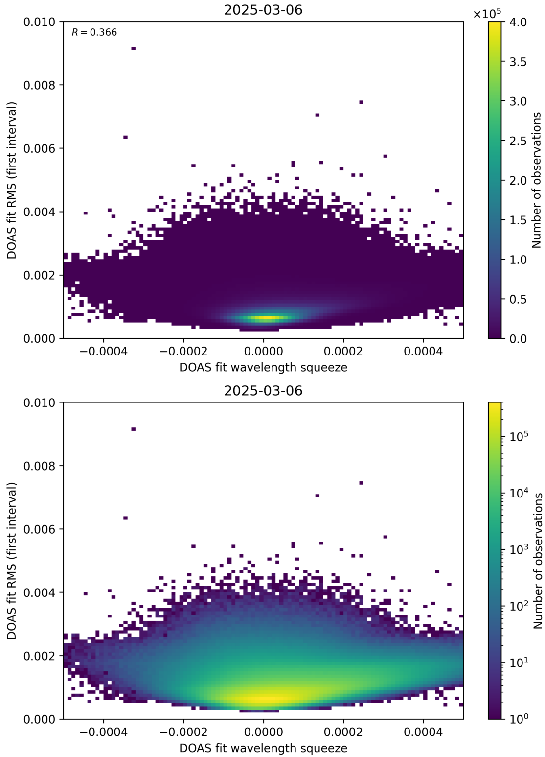
Figure 68: Scatter density plot of “DOAS fit wavelength squeeze” against “DOAS fit RMS (first interval)” for 2025-03-05 to 2025-03-07.
