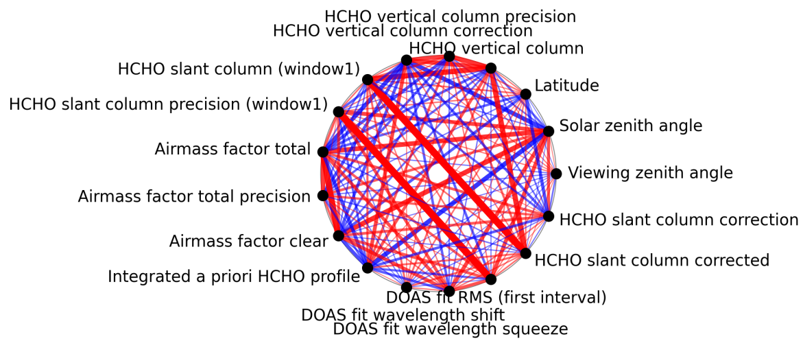
Figure 1: Map of correlation graph for 2025-03-05 to 2025-03-07.
