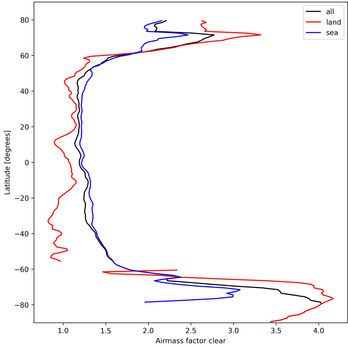
Figure 28: Zonal average of “Airmass factor clear” for 2025-03-05 to 2025-03-07.
