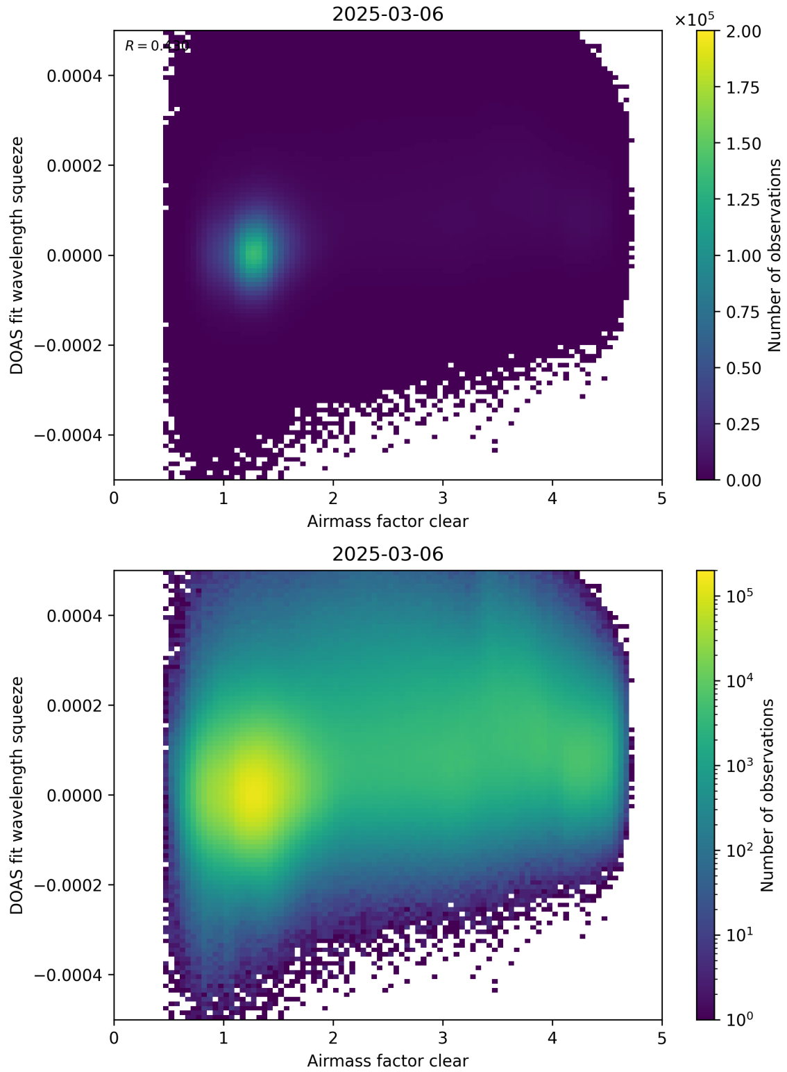
Figure 73: Scatter density plot of “Airmass factor clear” against “DOAS fit wavelength squeeze” for 2025-03-05 to 2025-03-07.
