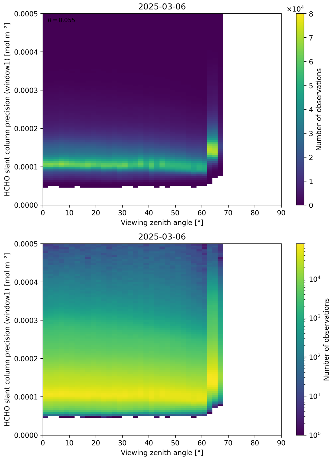
Figure 189: Scatter density plot of “Viewing zenith angle” against “HCHO slant column precision (window1)” for 2025-03-05 to 2025-03-07.
