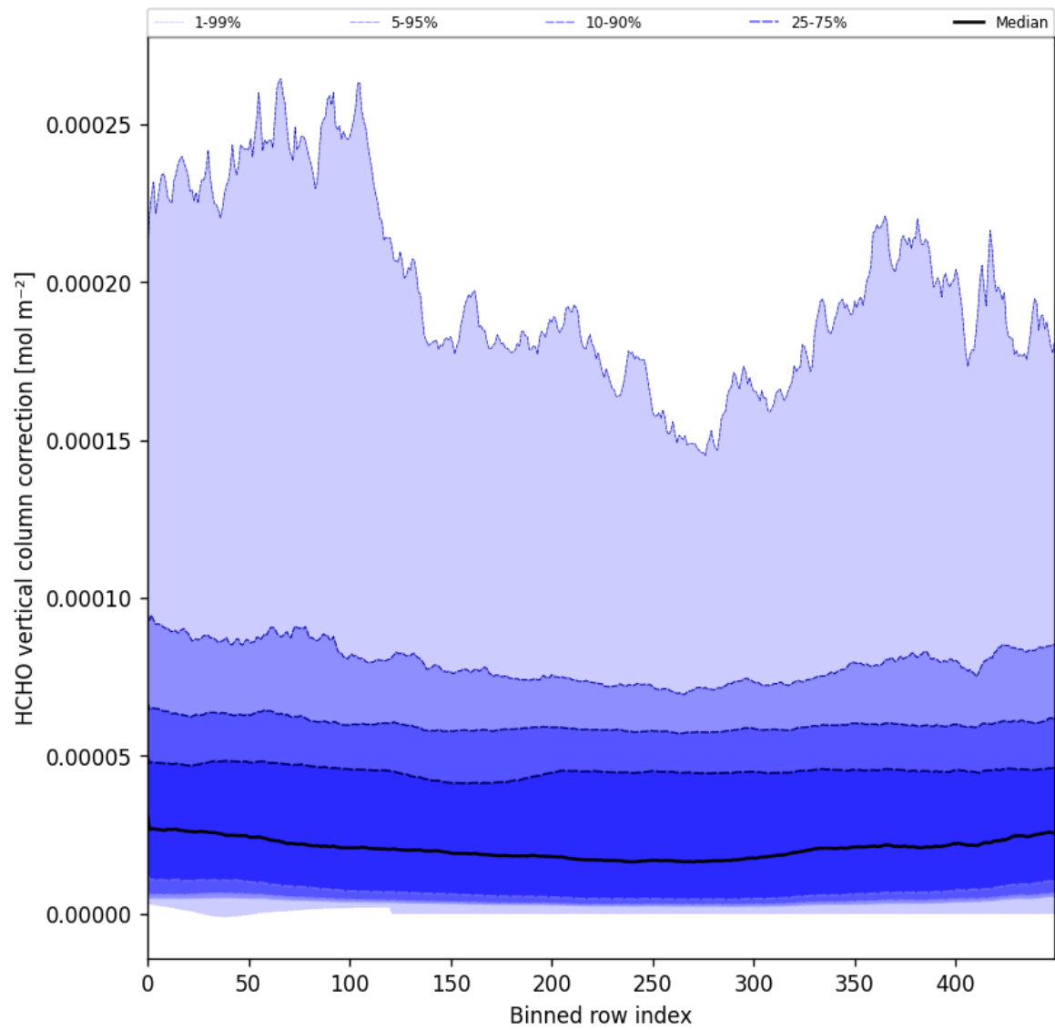
Figure 51: Along track statistics of “HCHO vertical column correction” for 2025-03-05 to 2025-03-07
