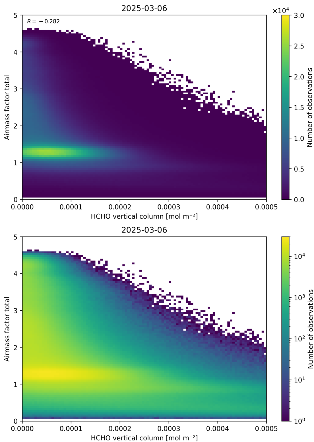
Figure 131: Scatter density plot of “HCHO vertical column” against “Airmass factor total” for 2025-03-05 to 2025-03-07.
