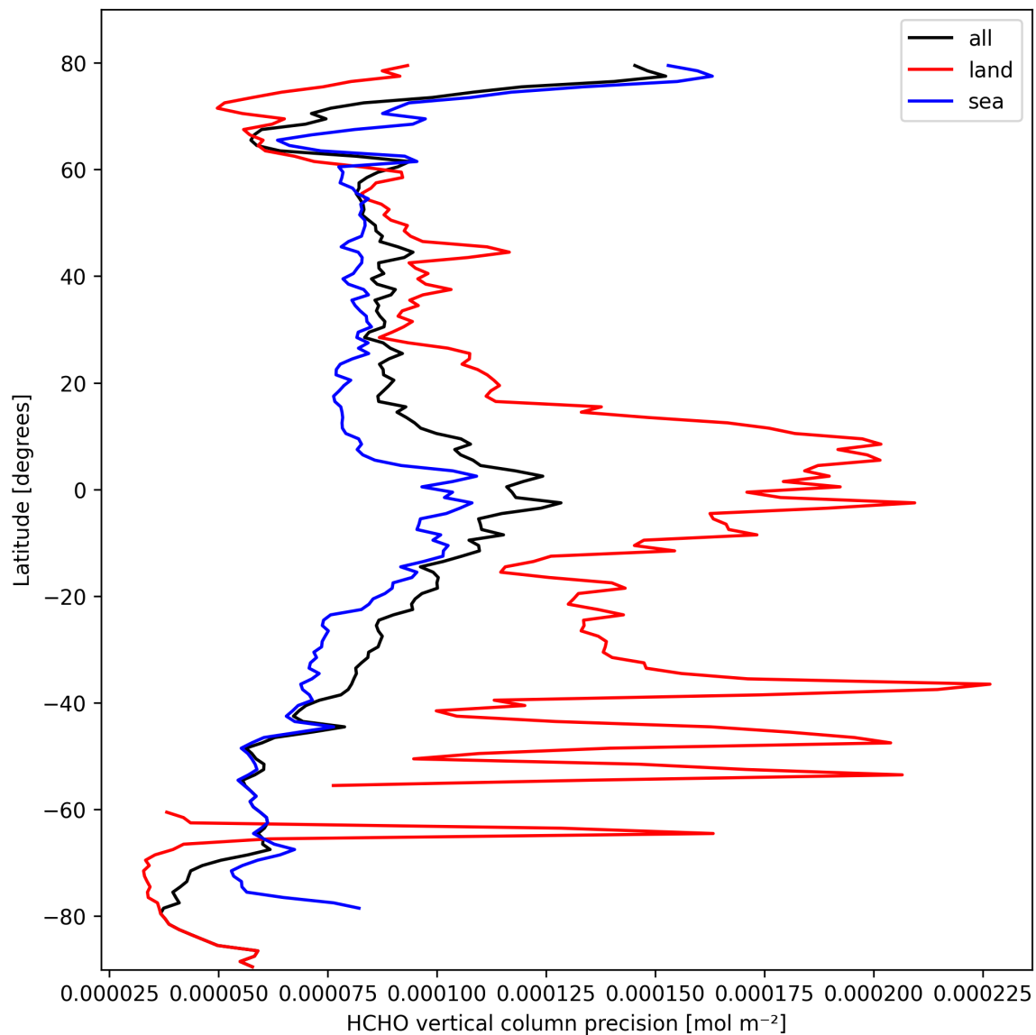
Figure 22: Zonal average of “HCHO vertical column precision” for 2025-03-05 to 2025-03-07.
