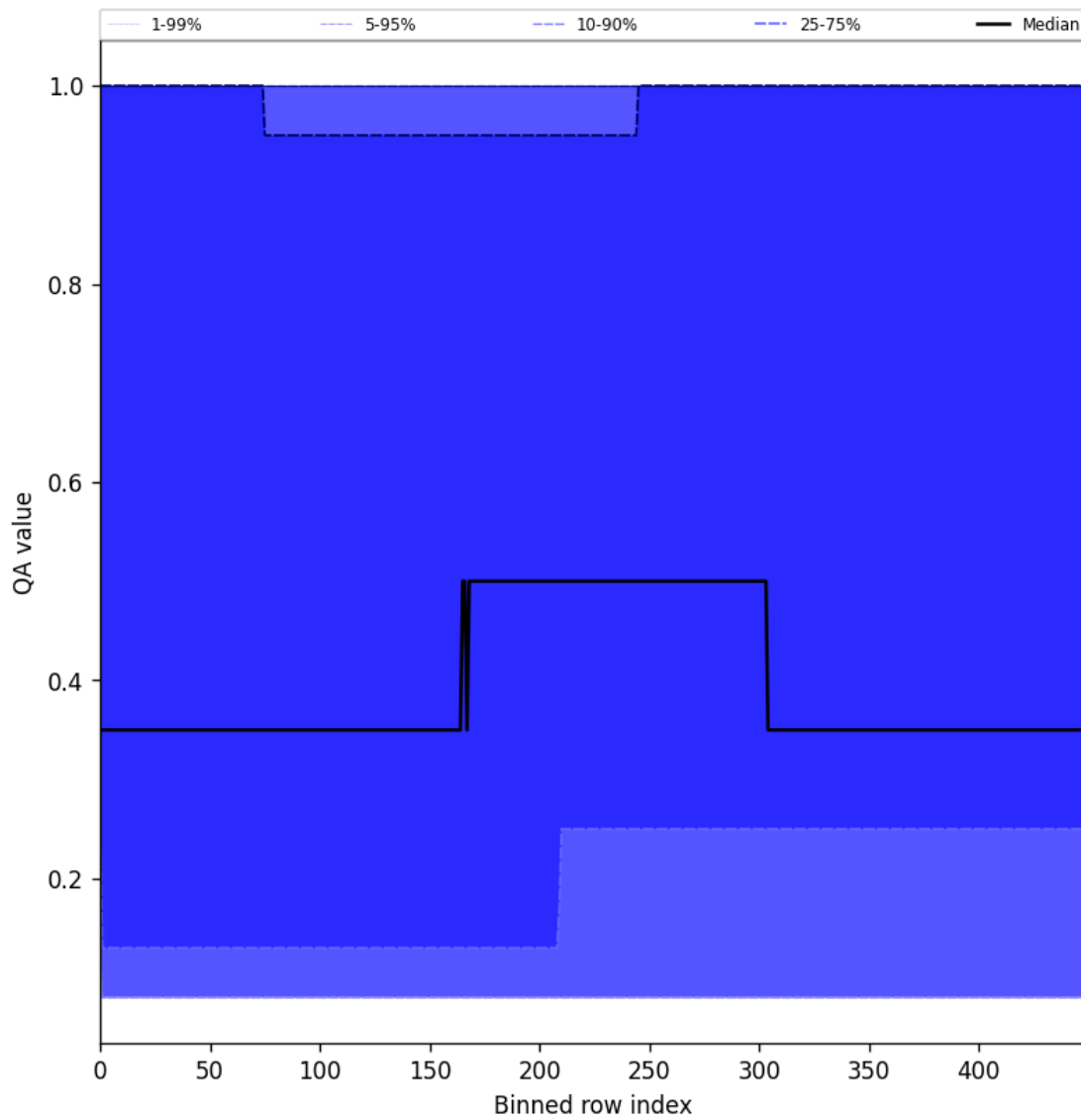
Figure 48: Along track statistics of “QA value” for 2025-03-05 to 2025-03-07
