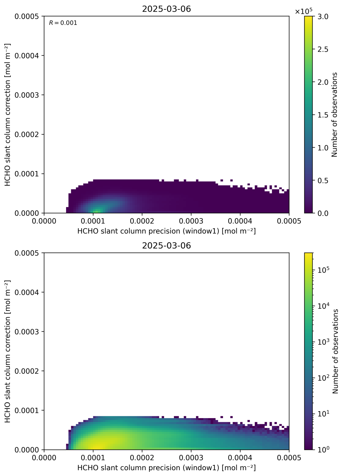
Figure 93: Scatter density plot of “HCHO slant column precision (window1)” against “HCHO slant column correction” for 2025-03-05 to 2025-03-07.
