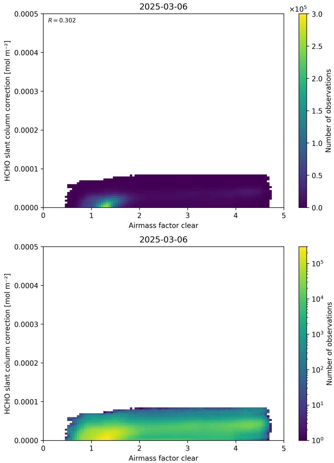
Figure 75: Scatter density plot of “Airmass factor clear” against “HCHO slant column correction” for 2025-03-05 to 2025-03-07.
