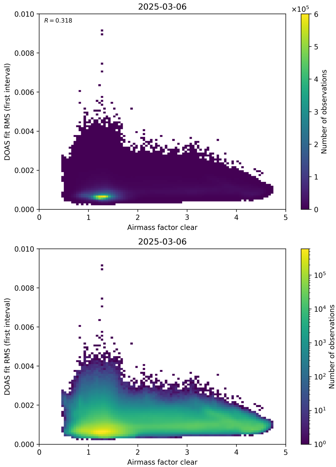
Figure 71: Scatter density plot of “Airmass factor clear” against “DOAS fit RMS (first interval)” for 2025-03-05 to 2025-03-07.
