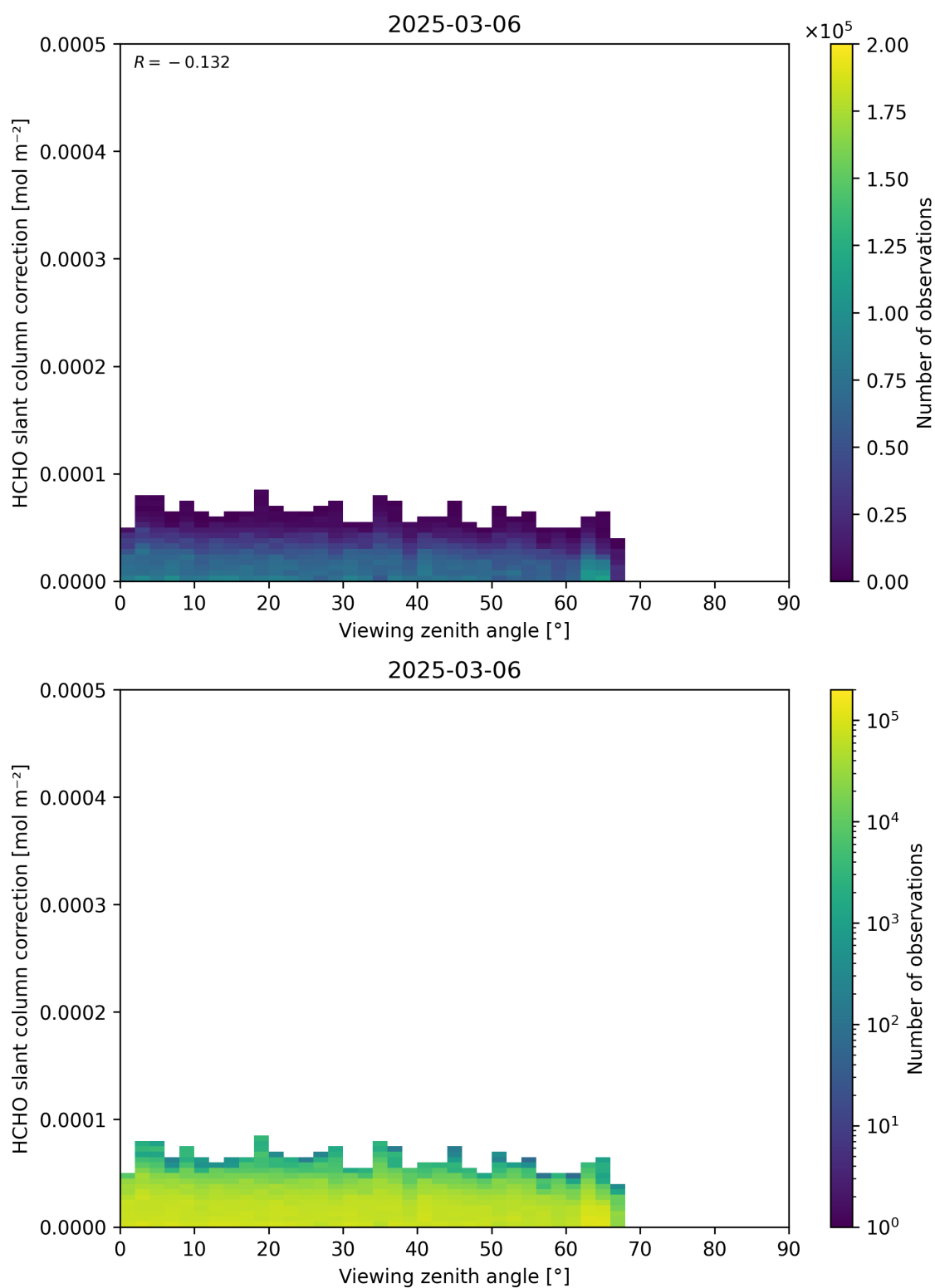
Figure 187: Scatter density plot of “Viewing zenith angle” against “HCHO slant column correction” for 2025-03-05 to 2025-03-07.
