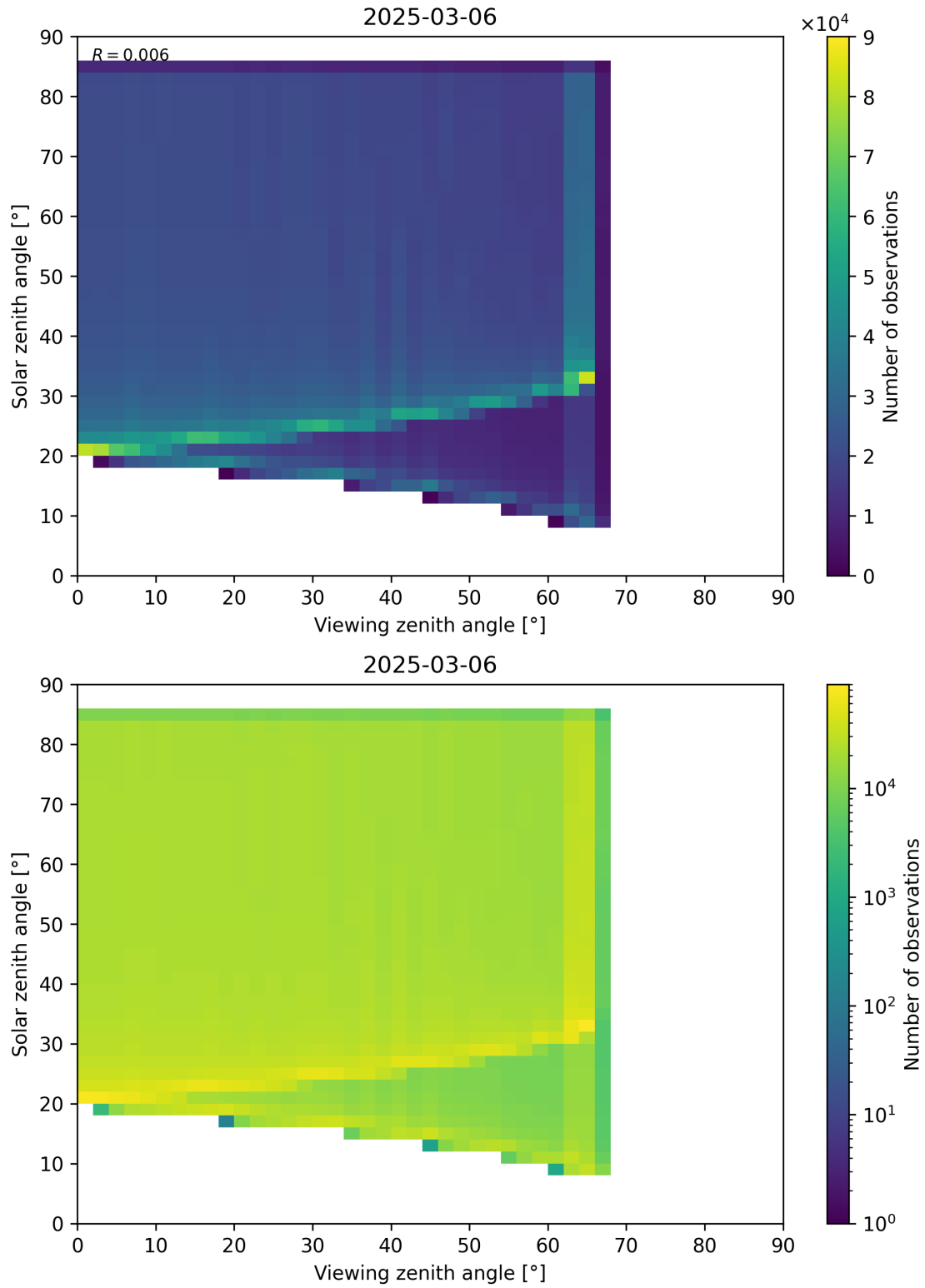
Figure 197: Scatter density plot of “Viewing zenith angle” against “Solar zenith angle” for 2025-03-05 to 2025-03-07.
