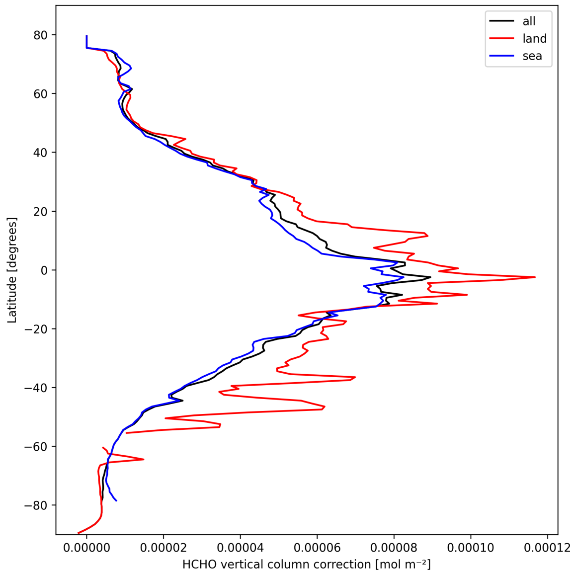
Figure 23: Zonal average of “HCHO vertical column correction” for 2025-03-05 to 2025-03-07.
