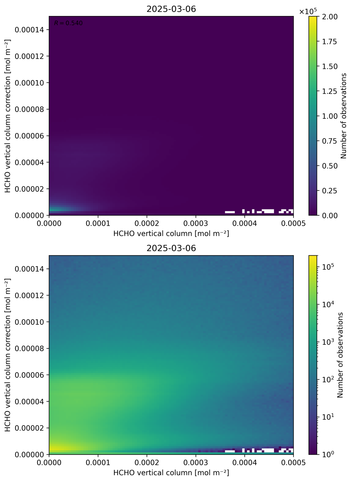
Figure 133: Scatter density plot of “HCHO vertical column” against “HCHO vertical column correction” for 2025-03-05 to 2025-03-07.
