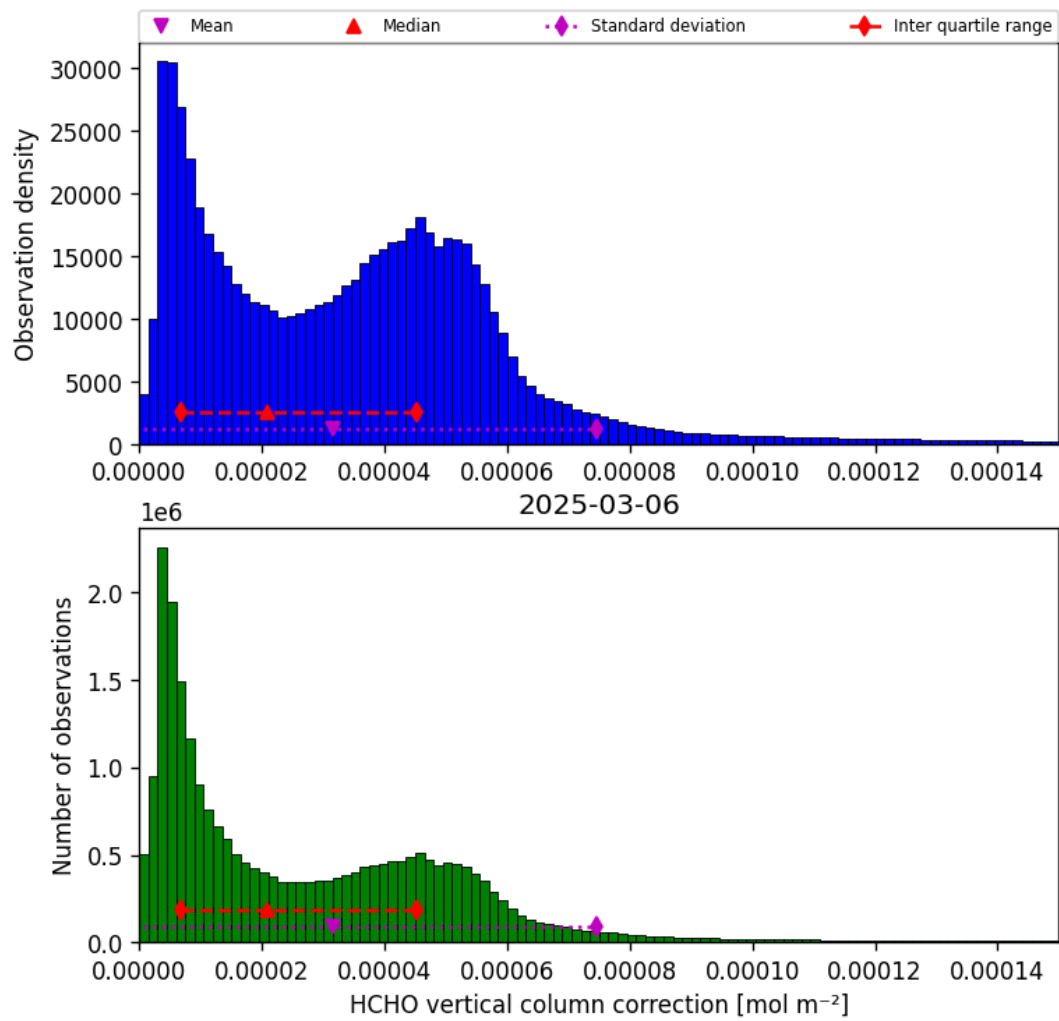
Figure 37: Histogram of “HCHO vertical column correction” for 2025-03-05 to 2025-03-07
