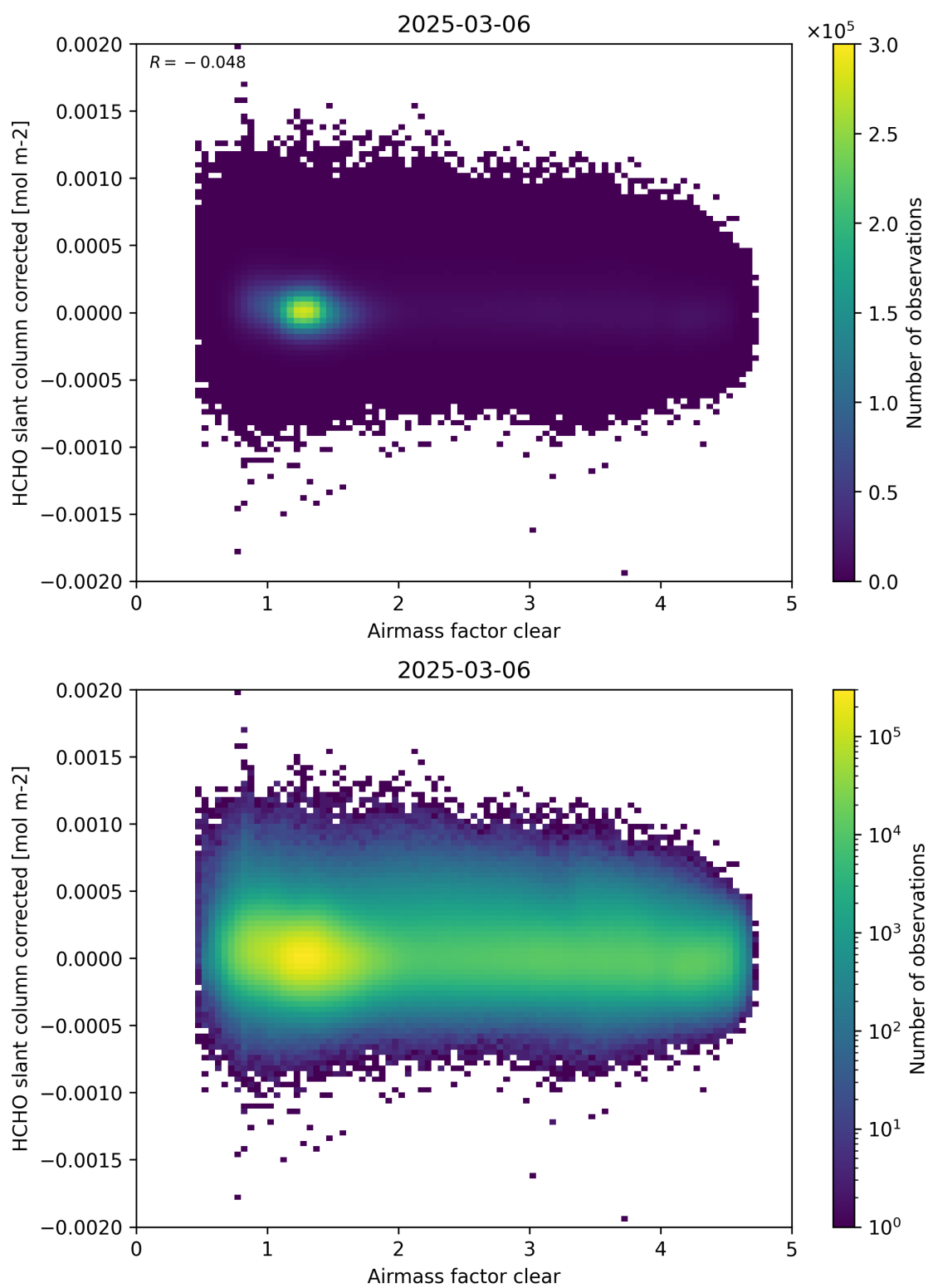
Figure 74: Scatter density plot of “Airmass factor clear” against “HCHO slant column corrected” for 2025-03-05 to 2025-03-07.
