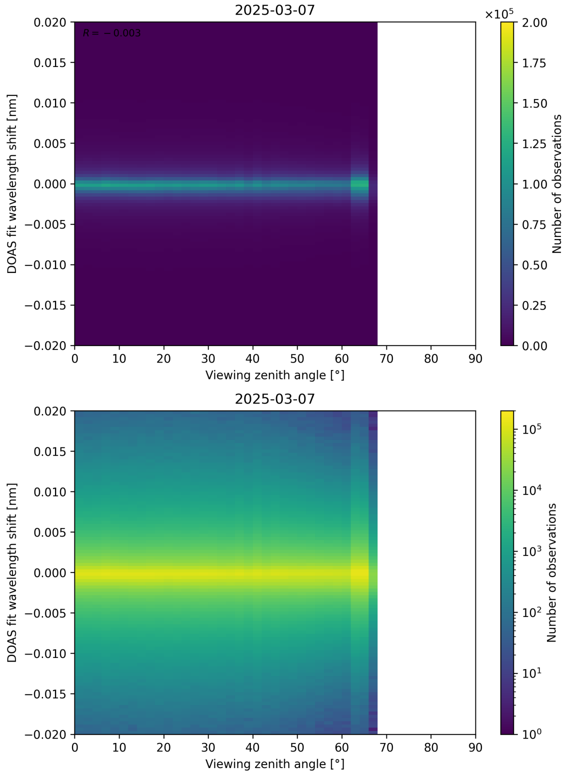
Figure 183: Scatter density plot of “Viewing zenith angle” against “DOAS fit wavelength shift” for 2025-03-07 to 2025-03-08.
