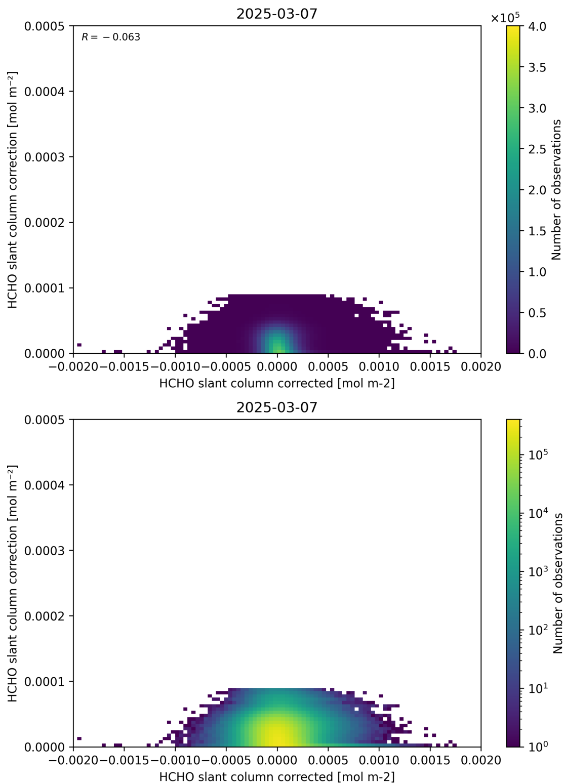
Figure 77: Scatter density plot of “HCHO slant column corrected” against “HCHO slant column correction” for 2025-03-07 to 2025-03-08.
