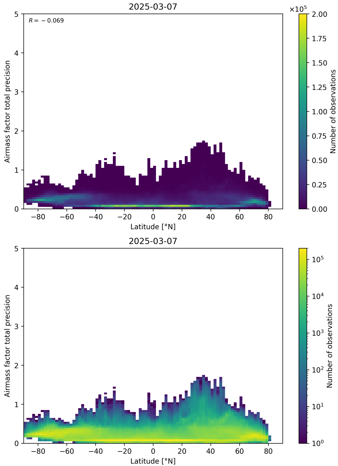
Figure 162: Scatter density plot of “Latitude” against “Airmass factor total precision” for 2025-03-07 to 2025-03-08.
