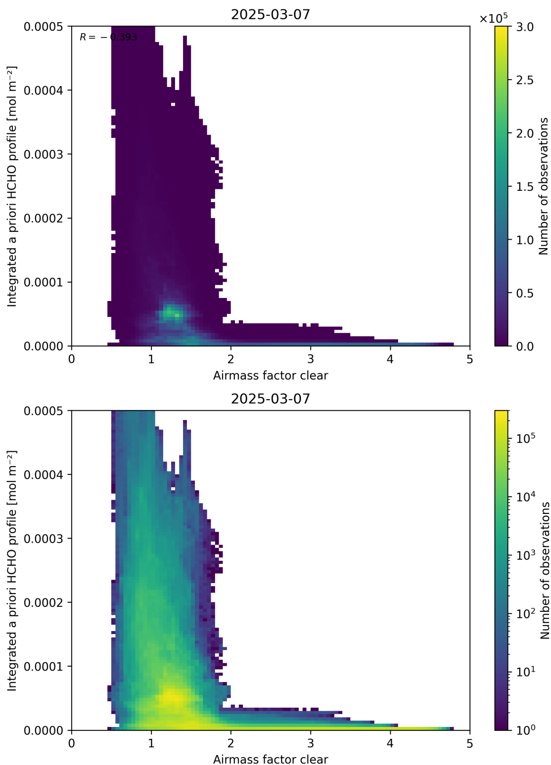
Figure 76: Scatter density plot of “Airmass factor clear” against “Integrated a priori HCHO profile” for 2025-03-07 to 2025-03-08.
