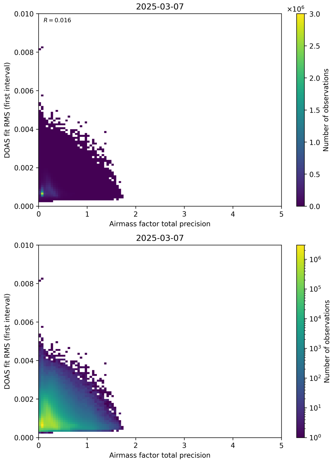
Figure 105: Scatter density plot of “Airmass factor total precision” against “DOAS fit RMS (first interval)” for 2025-03-07 to 2025-03-08.
