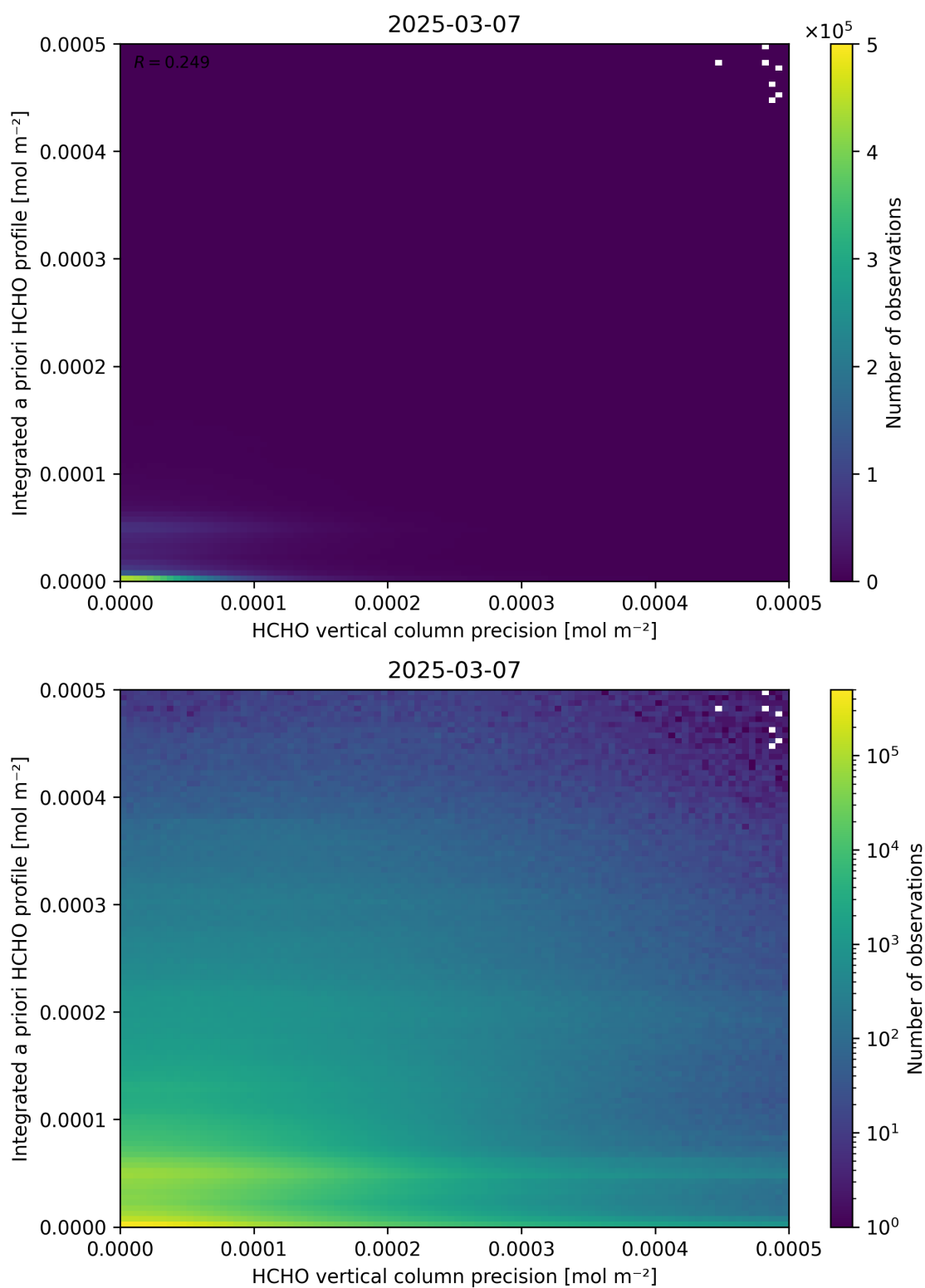
Figure 147: Scatter density plot of “HCHO vertical column precision” against “Integrated a priori HCHO profile” for 2025-03-07 to 2025-03-08.
