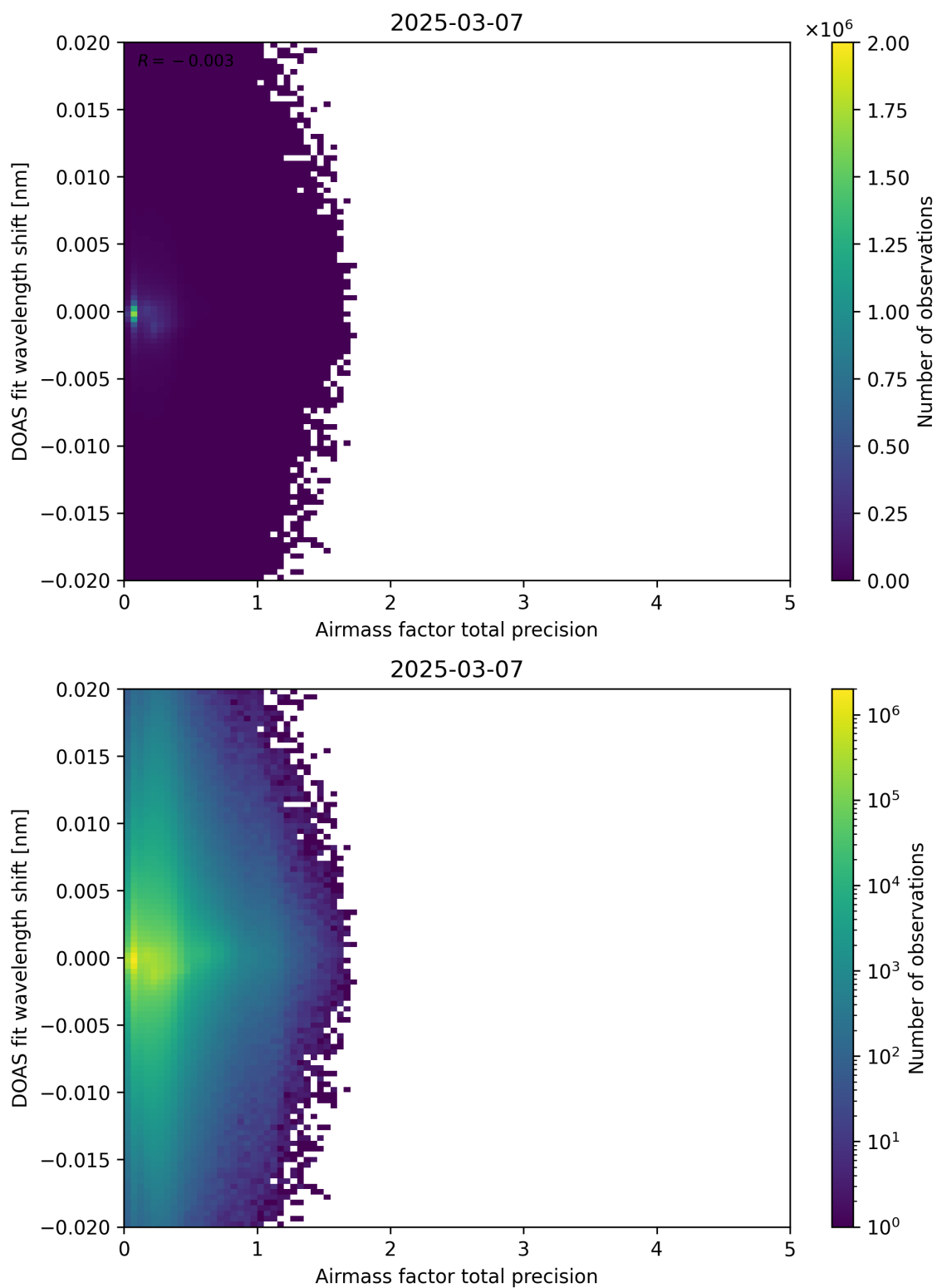
Figure 106: Scatter density plot of “Airmass factor total precision” against “DOAS fit wavelength shift” for 2025-03-07 to 2025-03-08.
