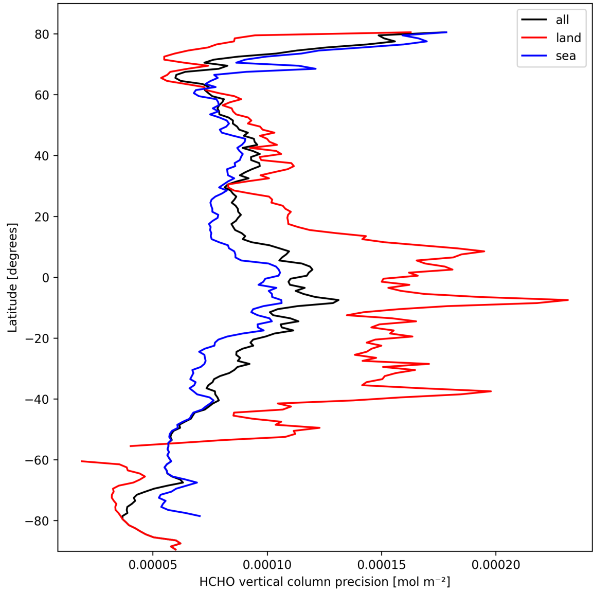
Figure 22: Zonal average of “HCHO vertical column precision” for 2025-03-07 to 2025-03-08.
