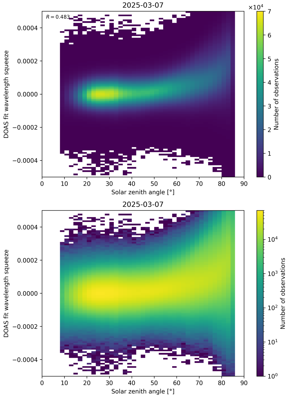
Figure 169: Scatter density plot of “Solar zenith angle” against “DOAS fit wavelength squeeze” for 2025-03-07 to 2025-03-08.
