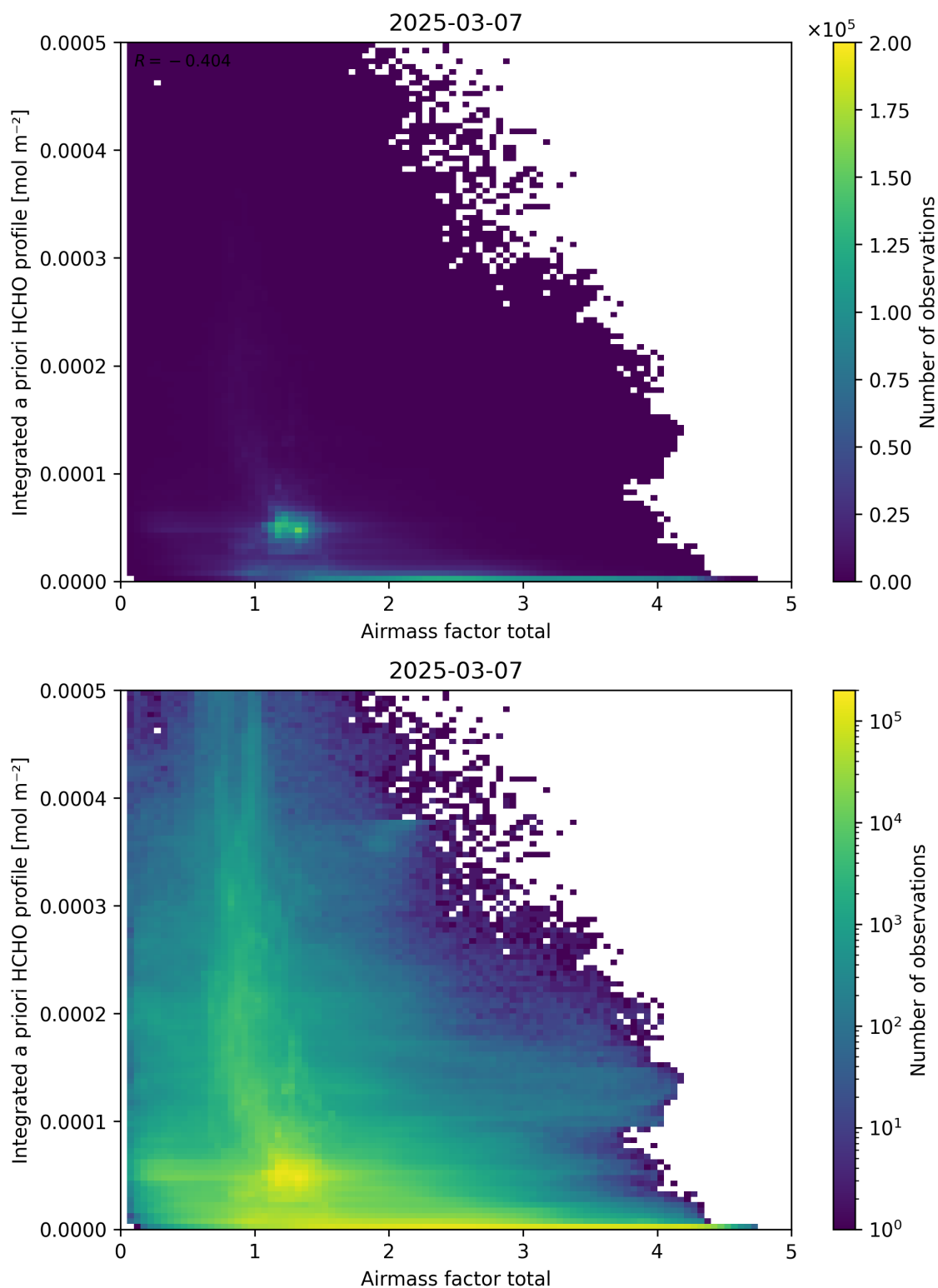
Figure 104: Scatter density plot of “Airmass factor total” against “Integrated a priori HCHO profile” for 2025-03-07 to 2025-03-08.
