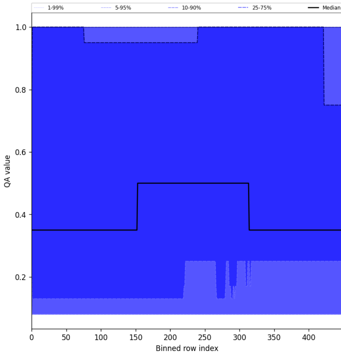
Figure 48: Along track statistics of “QA value” for 2025-03-07 to 2025-03-08
