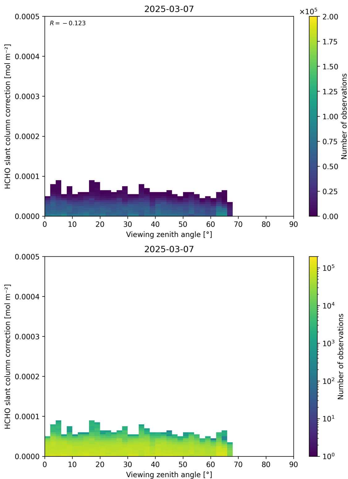
Figure 187: Scatter density plot of “Viewing zenith angle” against “HCHO slant column correction” for 2025-03-07 to 2025-03-08.
