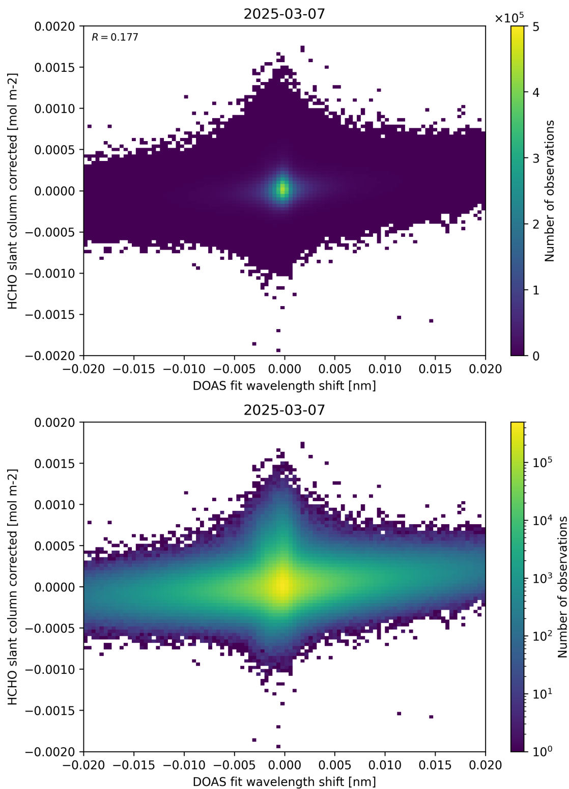
Figure 66: Scatter density plot of “DOAS fit wavelength shift” against “HCHO slant column corrected” for 2025-03-07 to 2025-03-08.
