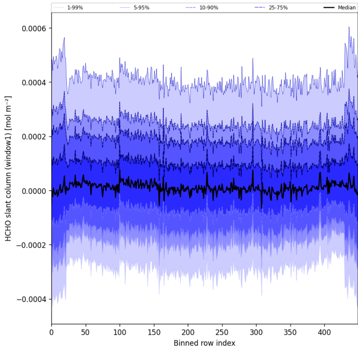
Figure 52: Along track statistics of “HCHO slant column (window1)” for 2025-03-07 to 2025-03-08
