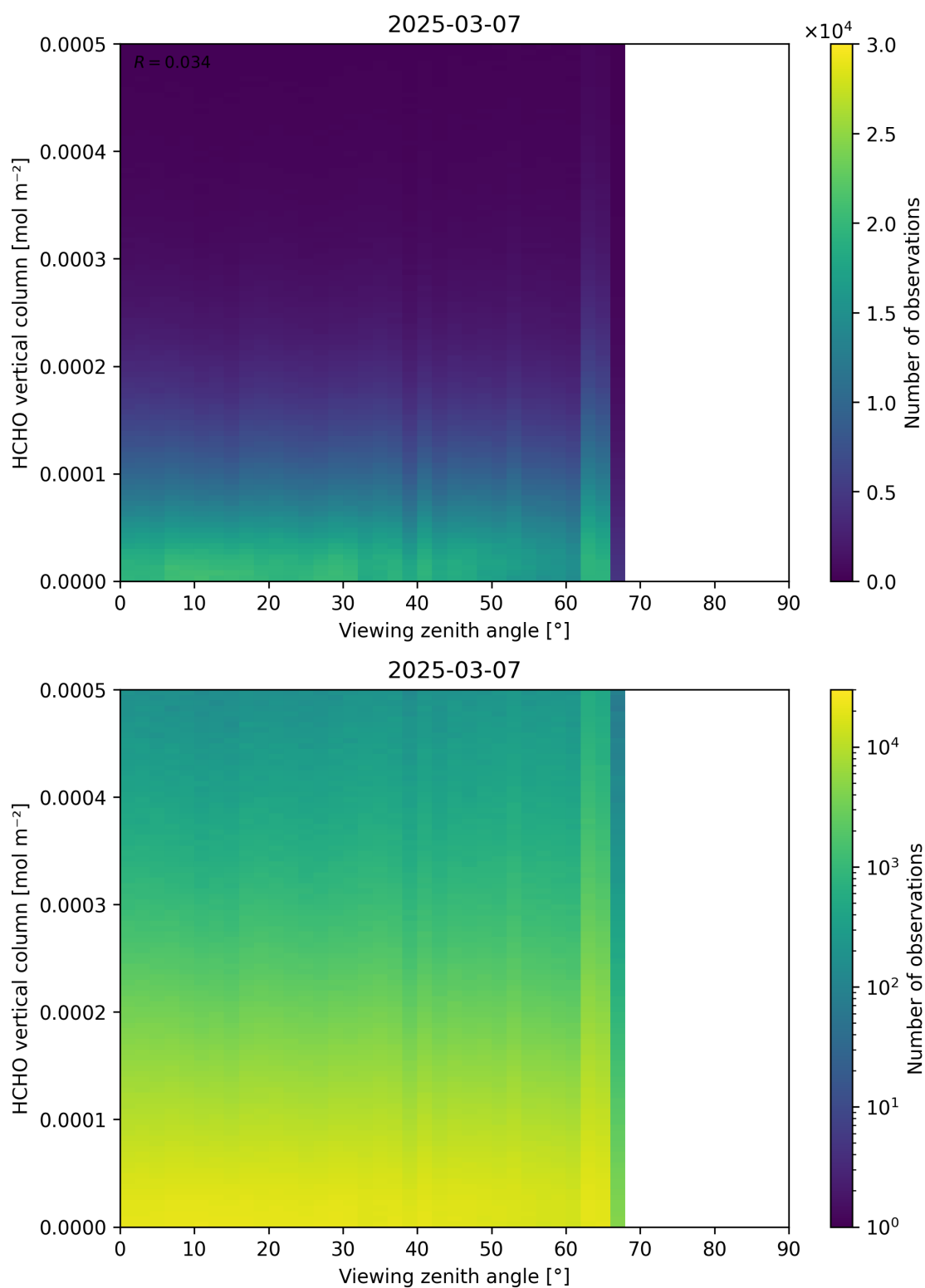
Figure 192: Scatter density plot of “Viewing zenith angle” against “HCHO vertical column” for 2025-03-07 to 2025-03-08.
