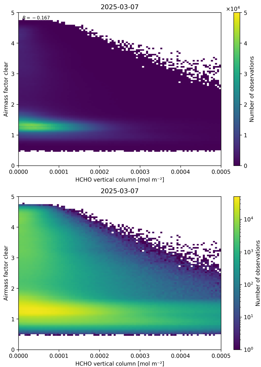
Figure 126: Scatter density plot of “HCHO vertical column” against “Airmass factor clear” for 2025-03-07 to 2025-03-08.
