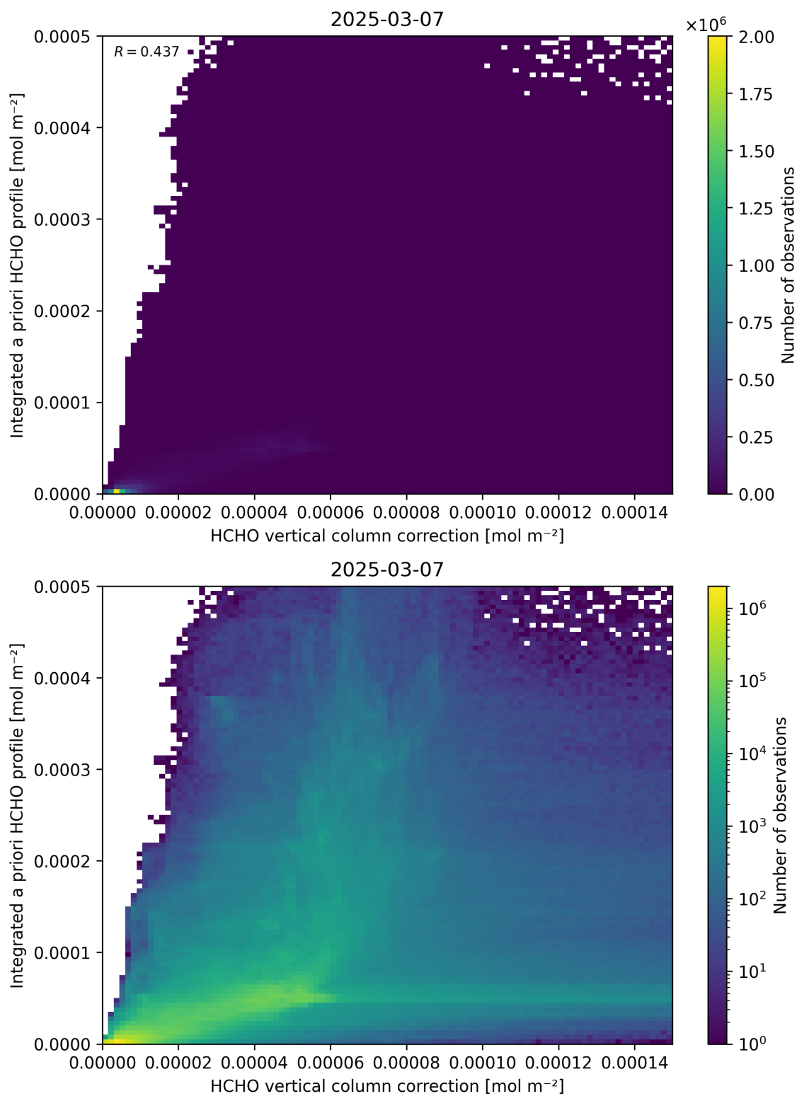
Figure 122: Scatter density plot of “HCHO vertical column correction” against “Integrated a priori HCHO profile” for 2025-03-07 to 2025-03-08.
