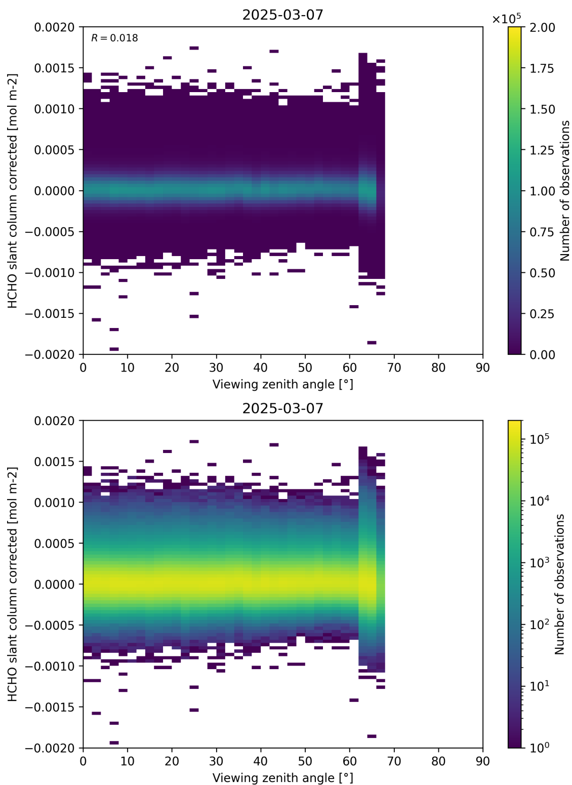
Figure 186: Scatter density plot of “Viewing zenith angle” against “HCHO slant column corrected” for 2025-03-07 to 2025-03-08.
