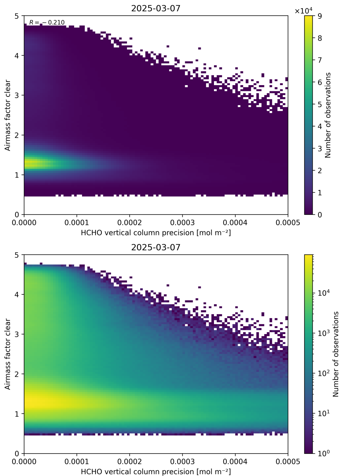
Figure 139: Scatter density plot of “HCHO vertical column precision” against “Airmass factor clear” for 2025-03-07 to 2025-03-08.
