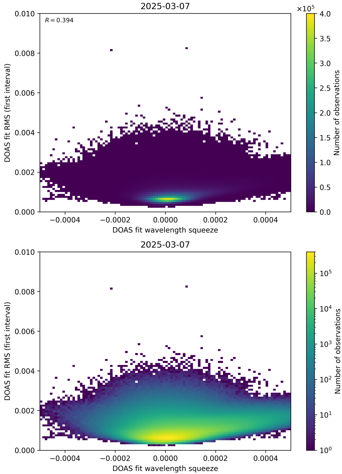
Figure 68: Scatter density plot of “DOAS fit wavelength squeeze” against “DOAS fit RMS (first interval)” for 2025-03-07 to 2025-03-08.
