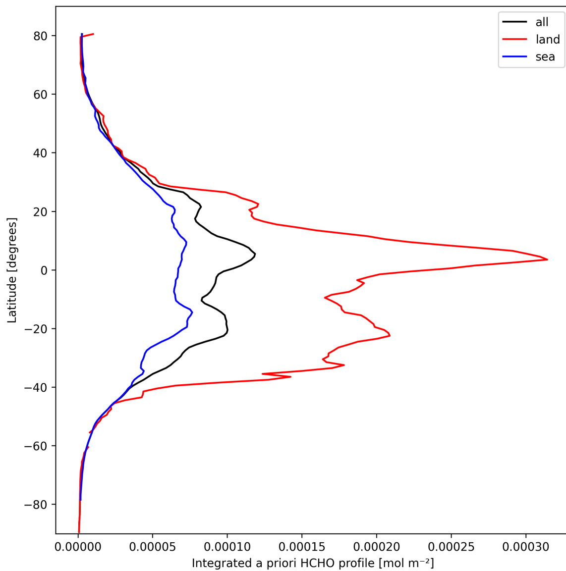
Figure 29: Zonal average of “Integrated a priori HCHO profile” for 2025-03-07 to 2025-03-08.
