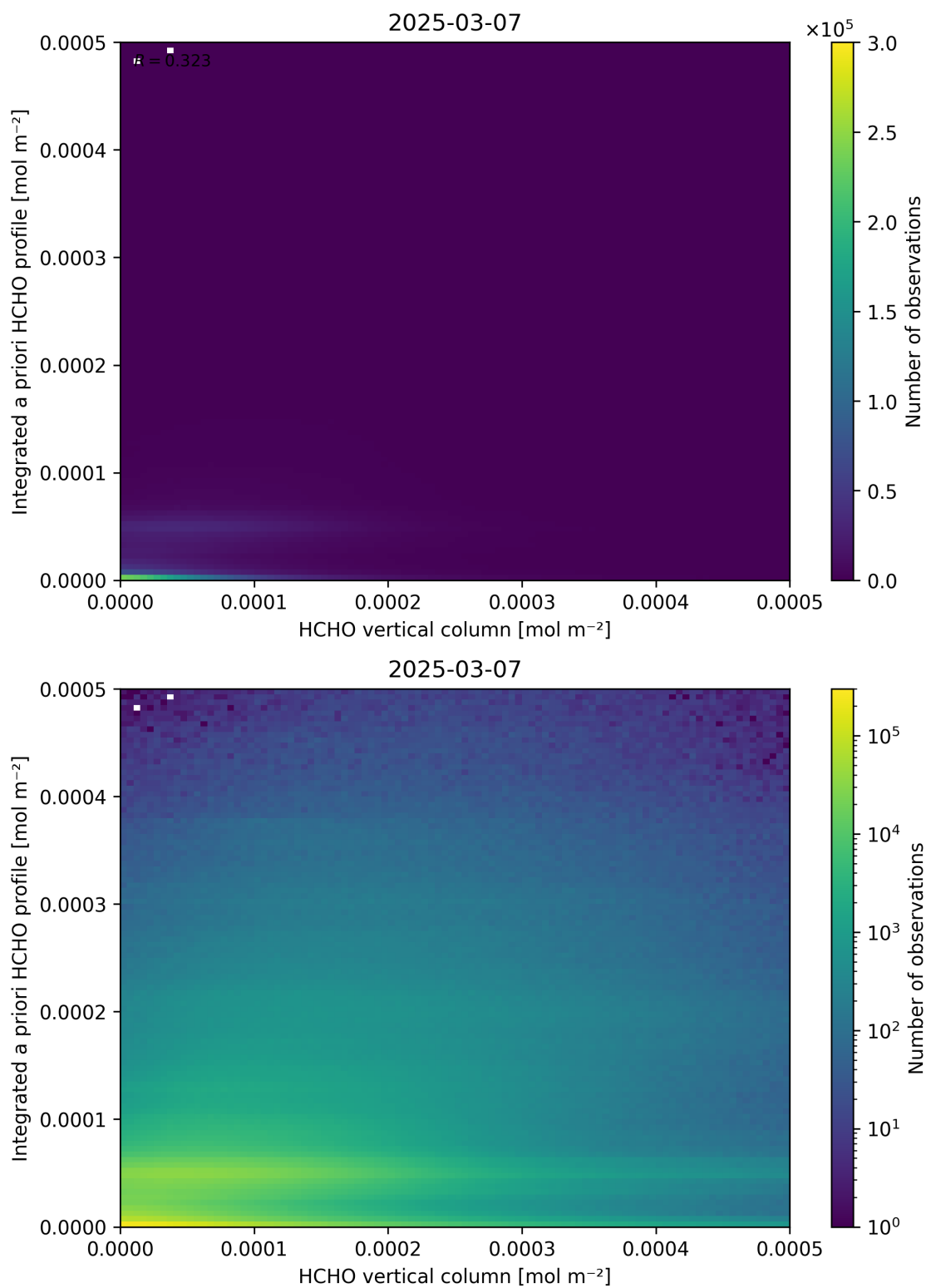
Figure 135: Scatter density plot of “HCHO vertical column” against “Integrated a priori HCHO profile” for 2025-03-07 to 2025-03-08.
