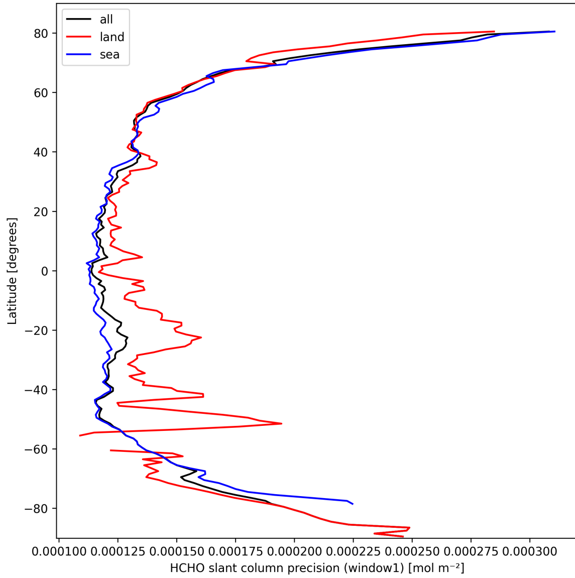
Figure 25: Zonal average of “HCHO slant column precision (window1)” for 2025-03-07 to 2025-03-08.
