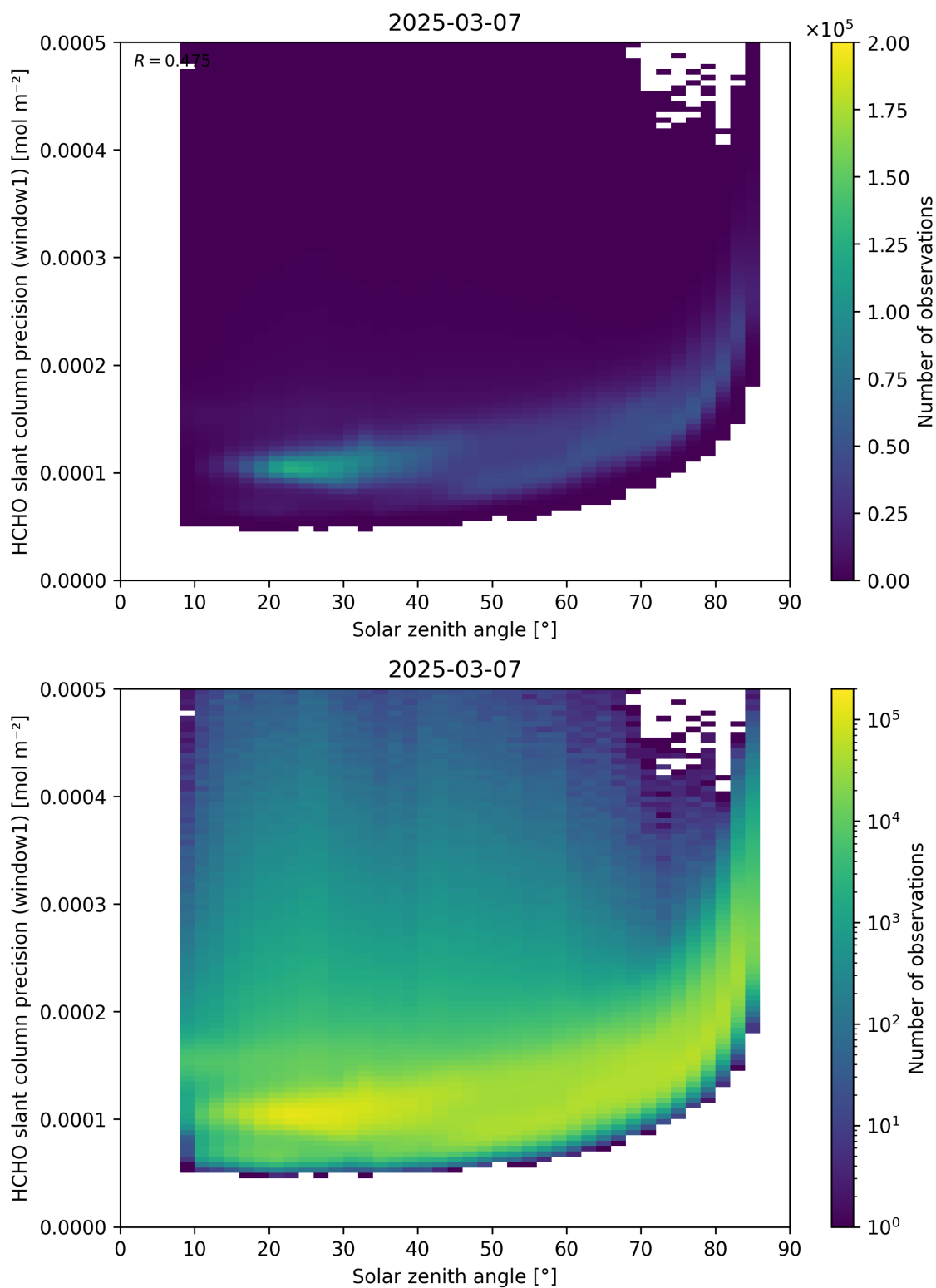
Figure 174: Scatter density plot of “Solar zenith angle” against “HCHO slant column precision (window1)” for 2025-03-07 to 2025-03-08.
