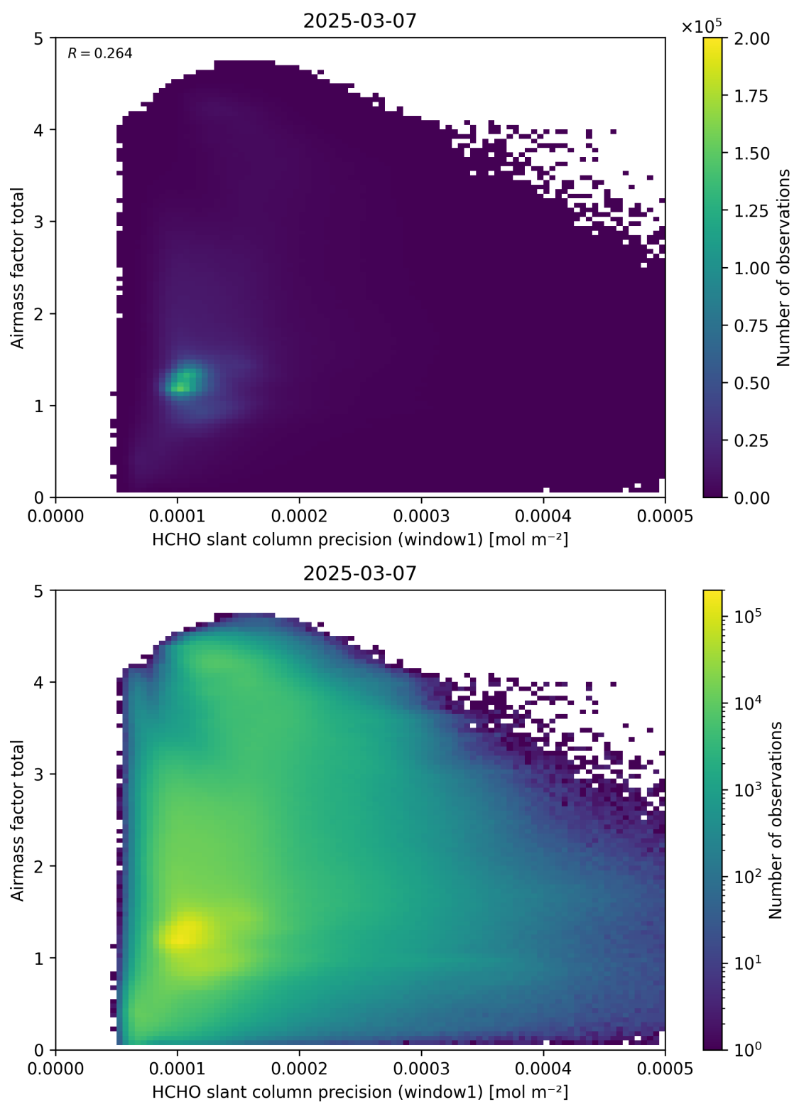
Figure 94: Scatter density plot of “HCHO slant column precision (window1)” against “Airmass factor total” for 2025-03-07 to 2025-03-08.
