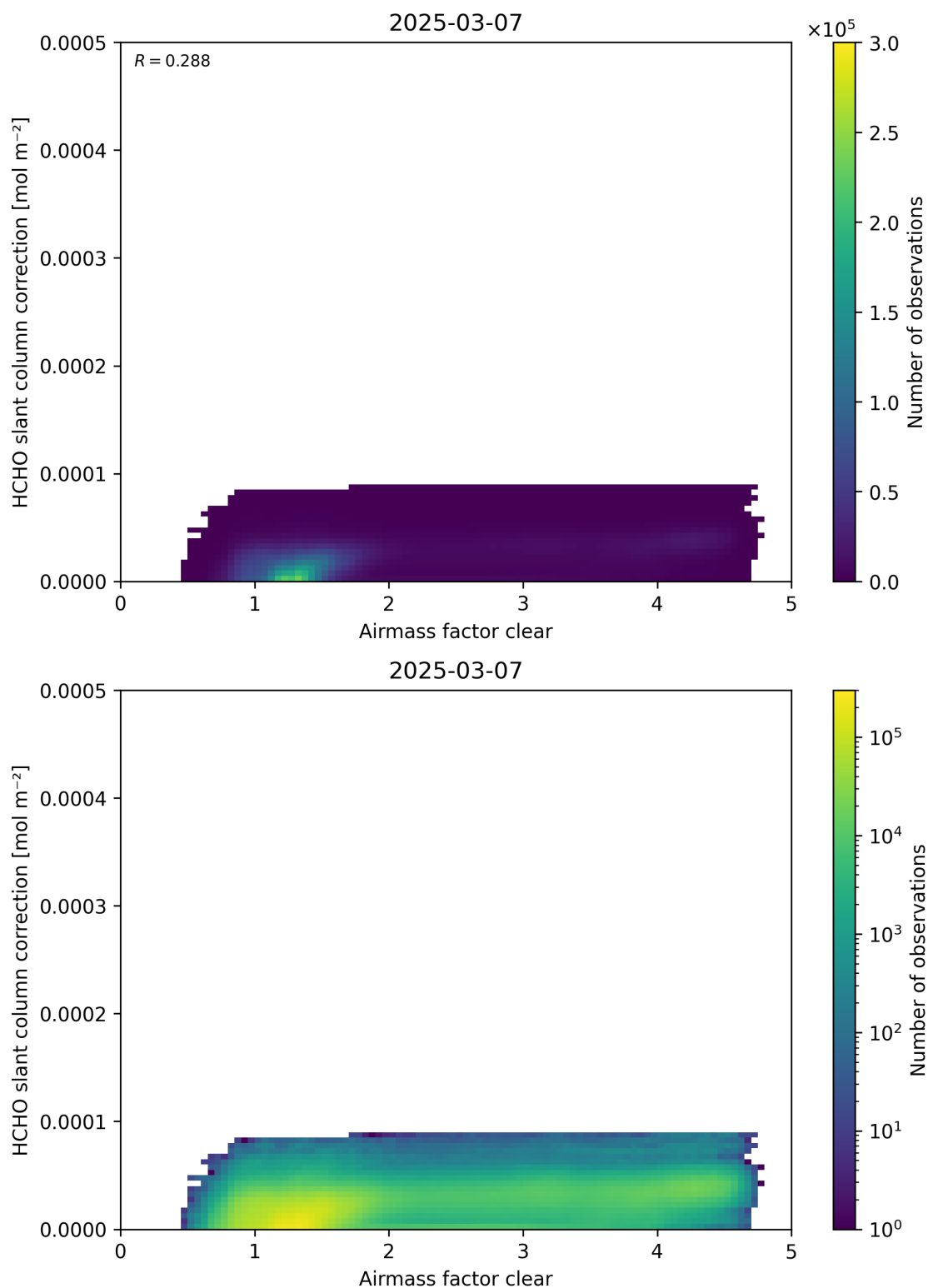
Figure 75: Scatter density plot of “Airmass factor clear” against “HCHO slant column correction” for 2025-03-07 to 2025-03-08.
