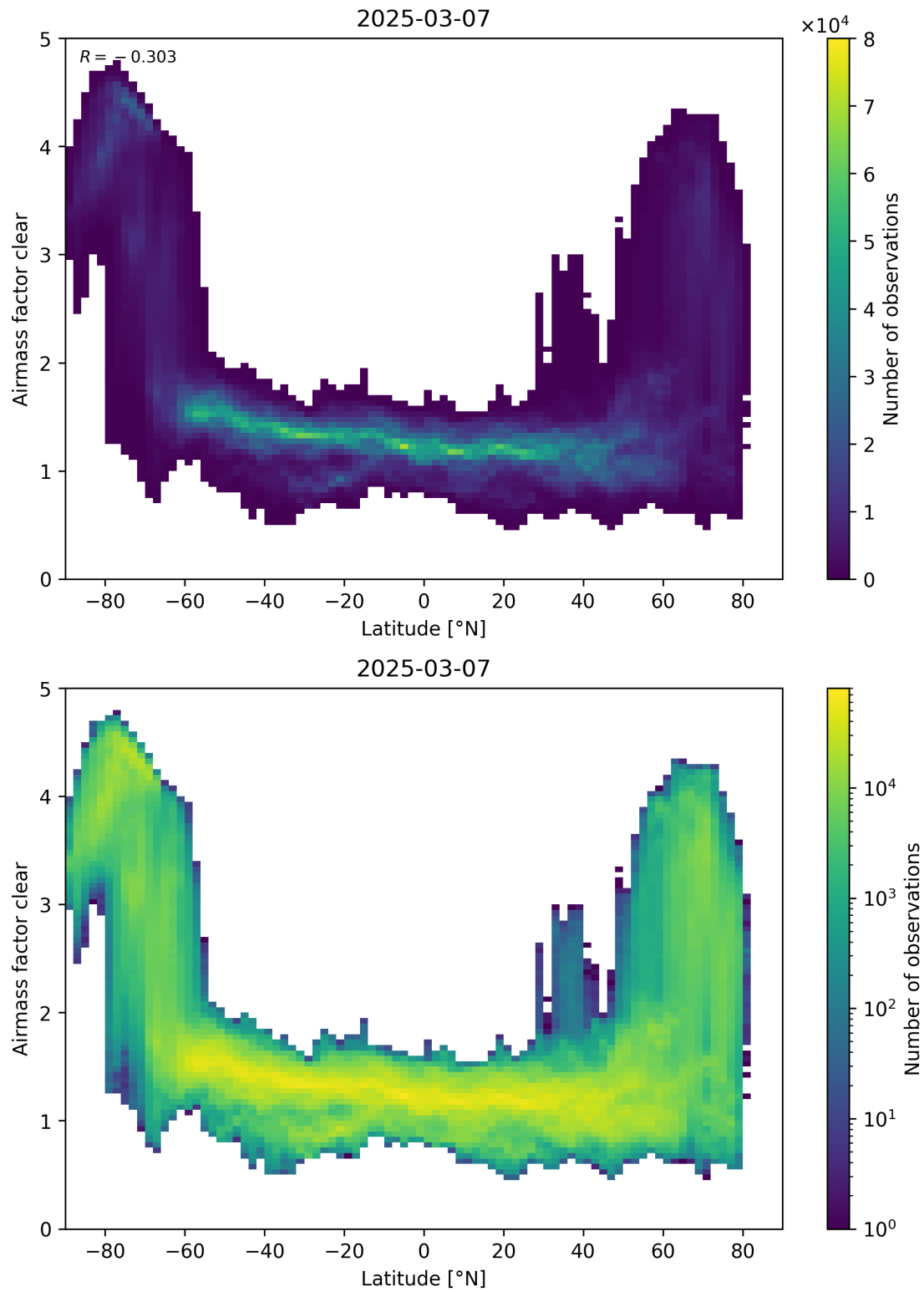
Figure 156: Scatter density plot of “Latitude” against “Airmass factor clear” for 2025-03-07 to 2025-03-08.
