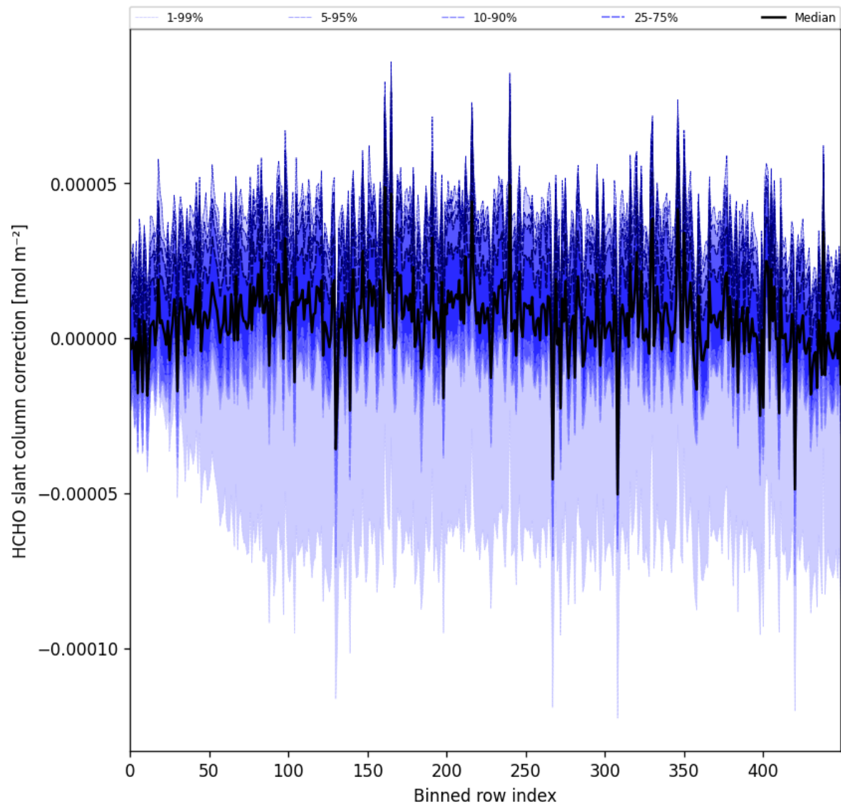
Figure 61: Along track statistics of “HCHO slant column correction” for 2025-03-07 to 2025-03-08
