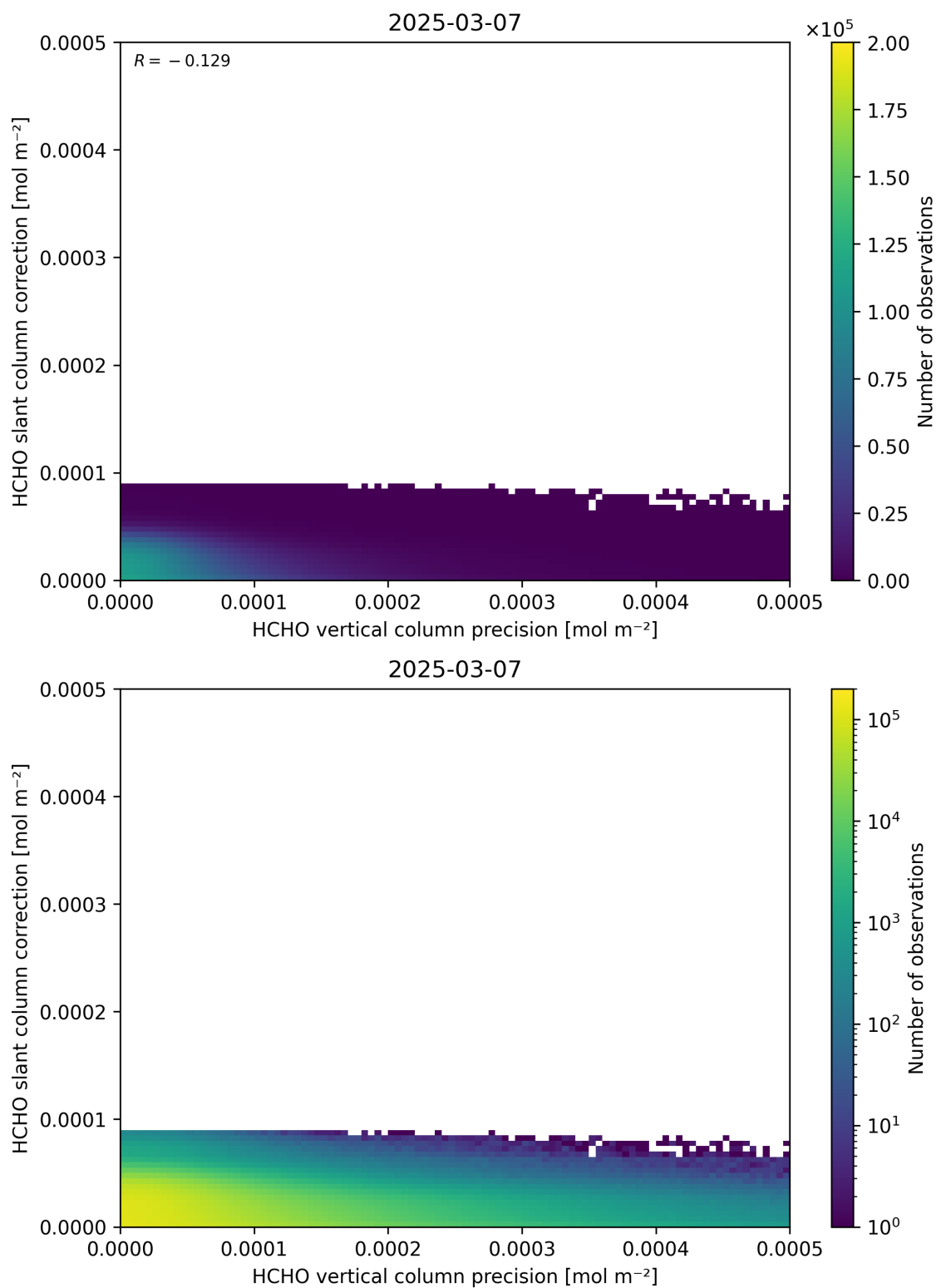
Figure 141: Scatter density plot of “HCHO vertical column precision” against “HCHO slant column correction” for 2025-03-07 to 2025-03-08.
