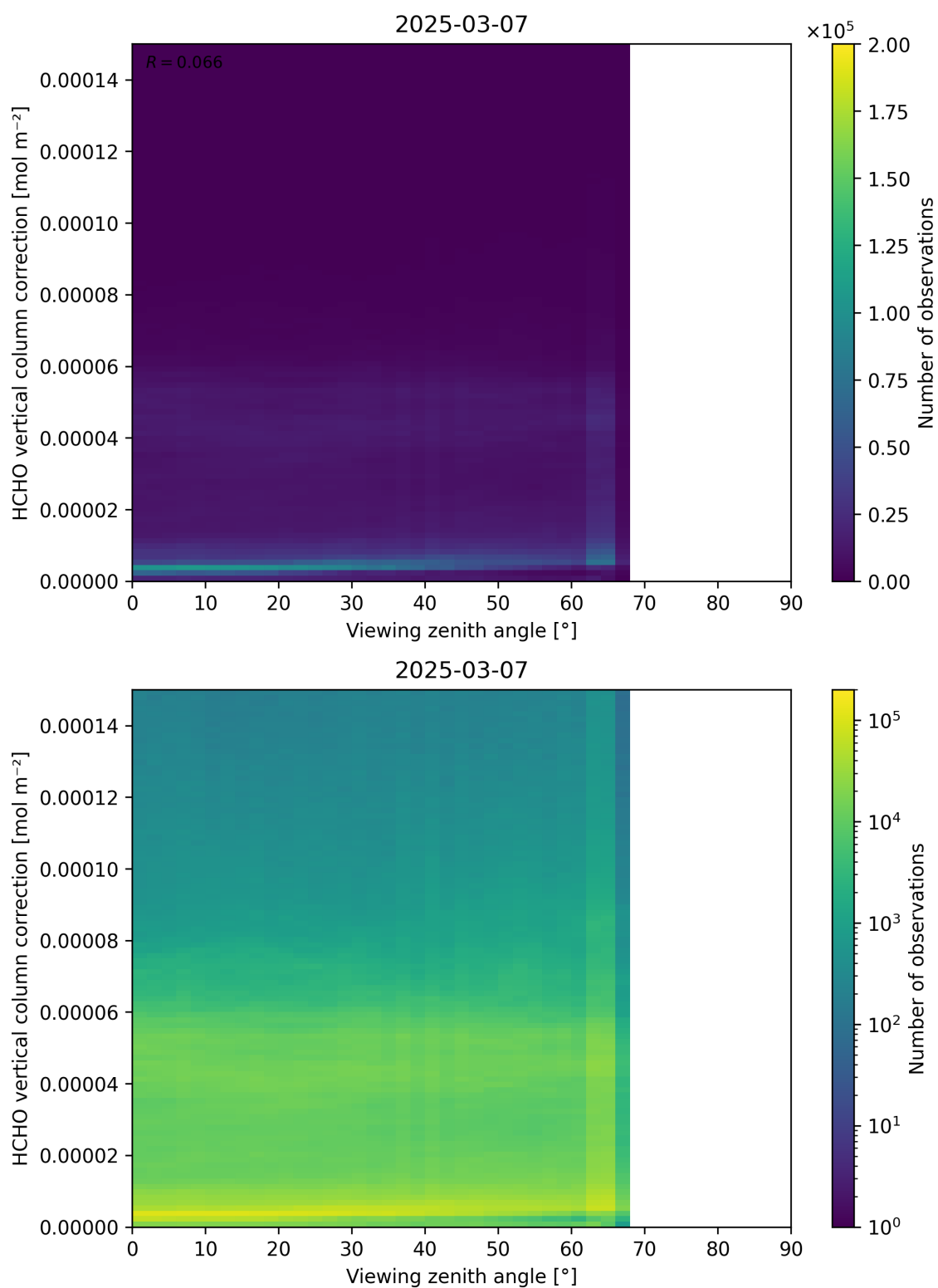
Figure 193: Scatter density plot of “Viewing zenith angle” against “HCHO vertical column correction” for 2025-03-07 to 2025-03-08.
