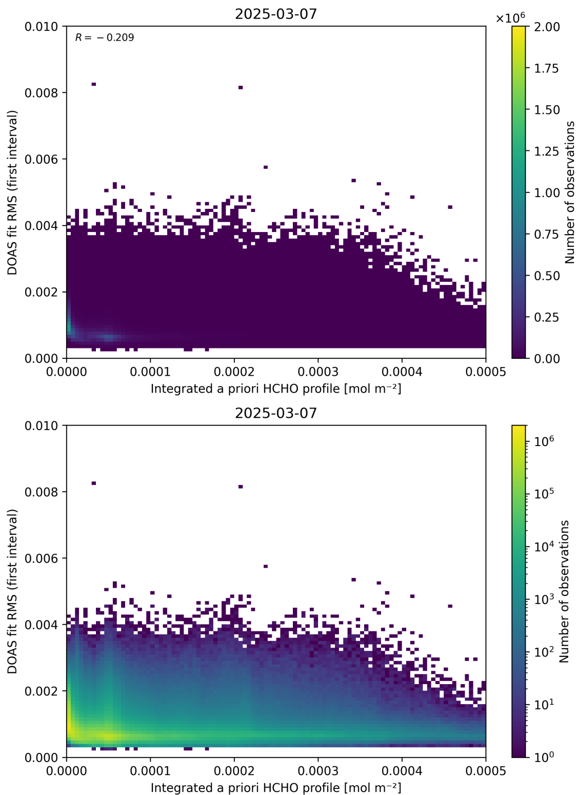
Figure 148: Scatter density plot of “Integrated a priori HCHO profile” against “DOAS fit RMS (first interval)” for 2025-03-07 to 2025-03-08.
