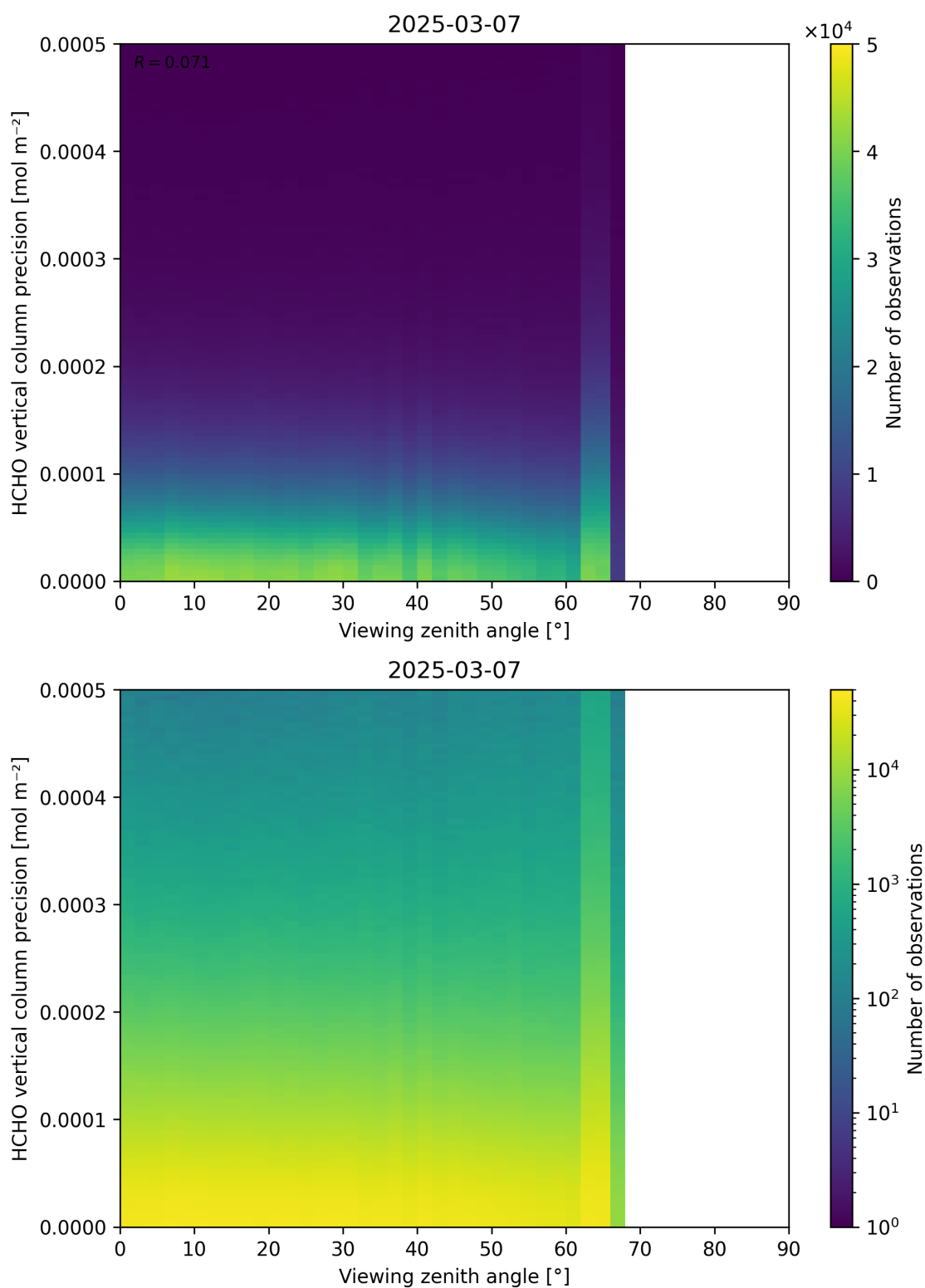
Figure 194: Scatter density plot of “Viewing zenith angle” against “HCHO vertical column precision” for 2025-03-07 to 2025-03-08.
