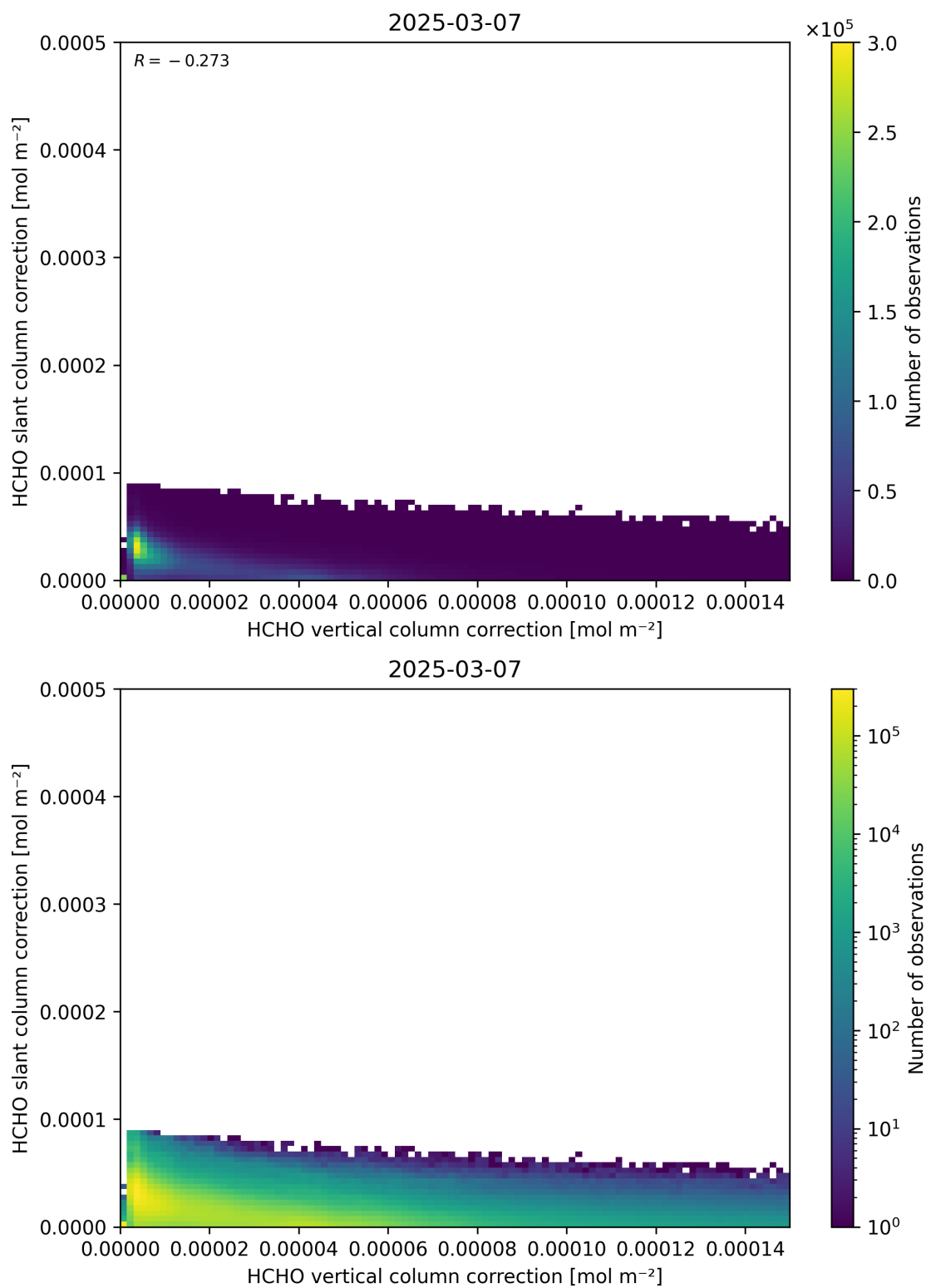
Figure 117: Scatter density plot of “HCHO vertical column correction” against “HCHO slant column correction” for 2025-03-07 to 2025-03-08.
