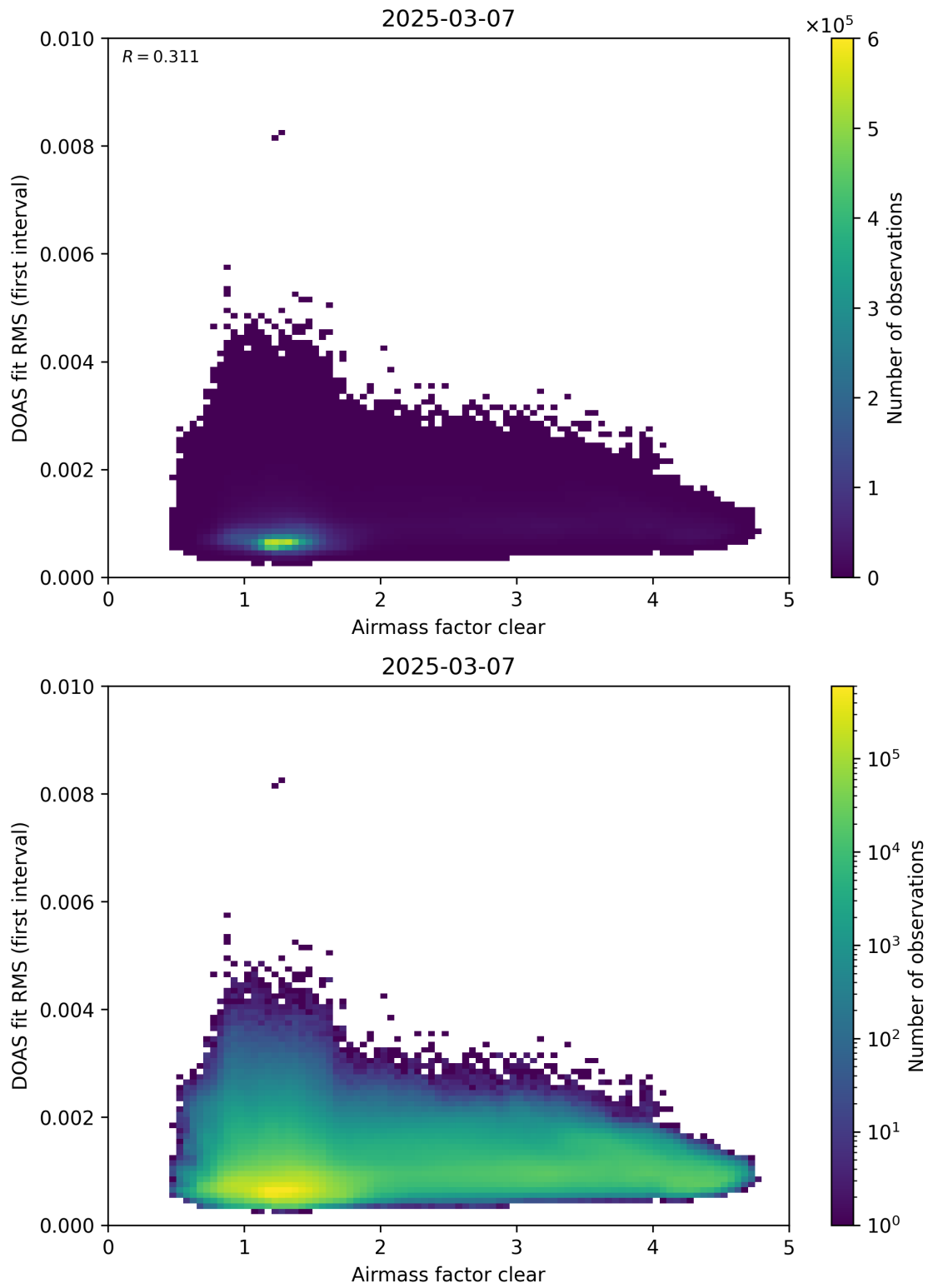
Figure 71: Scatter density plot of “Airmass factor clear” against “DOAS fit RMS (first interval)” for 2025-03-07 to 2025-03-08.
