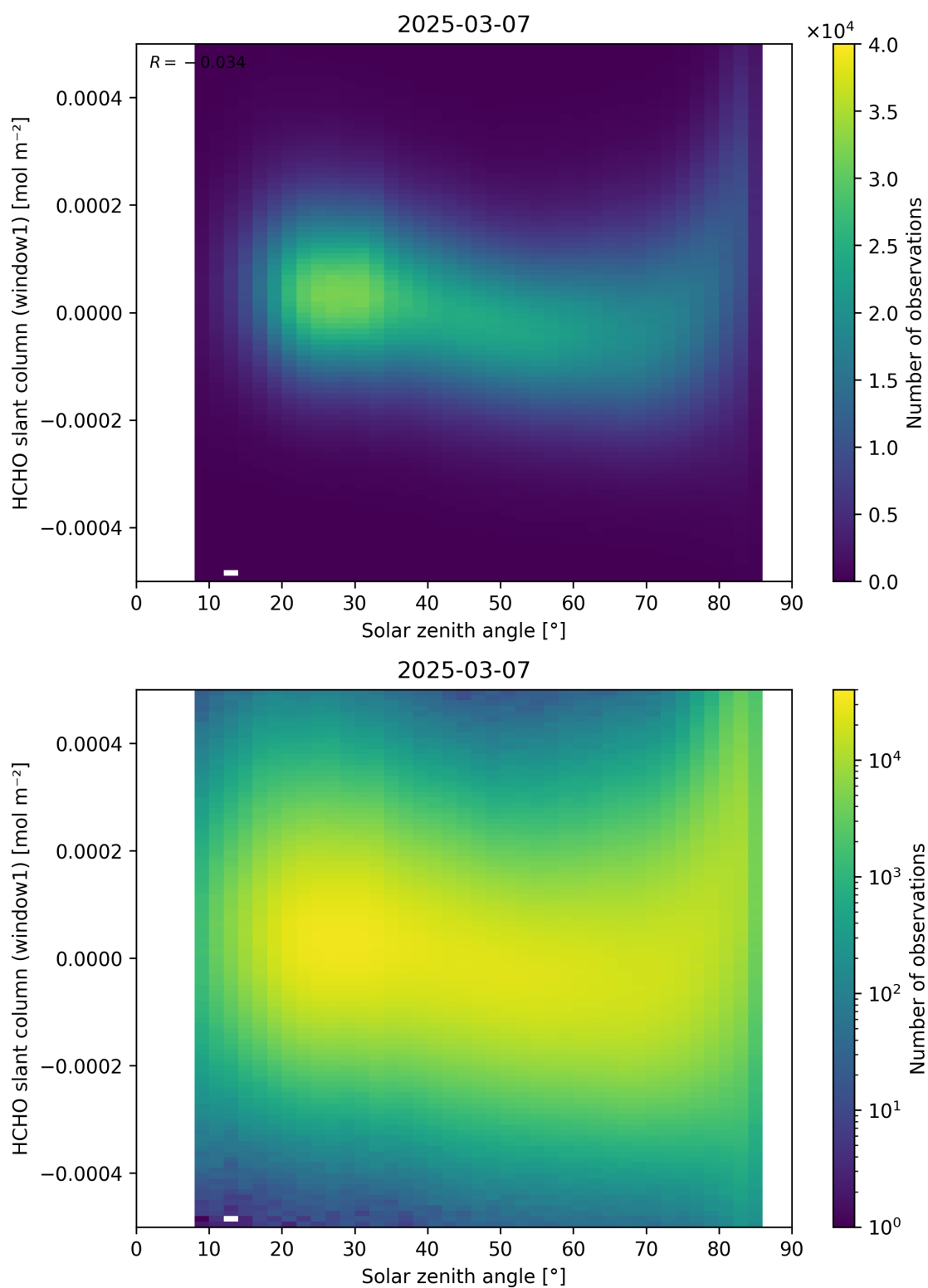
Figure 173: Scatter density plot of “Solar zenith angle” against “HCHO slant column (window1)” for 2025-03-07 to 2025-03-08.
