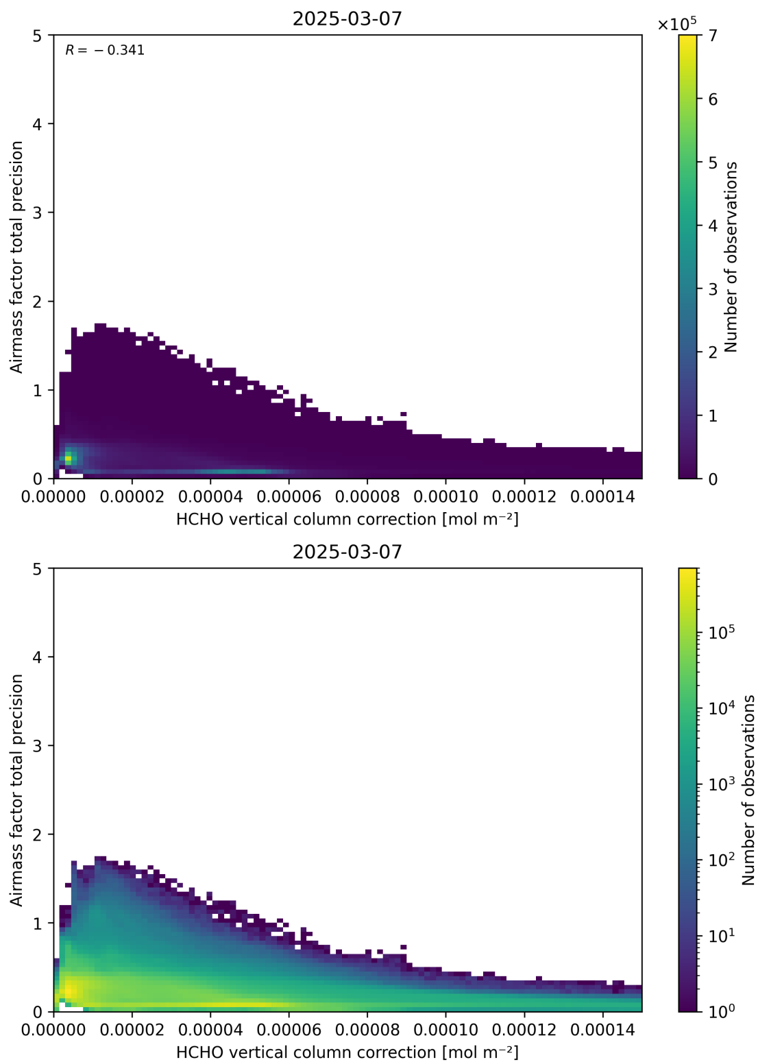
Figure 121: Scatter density plot of “HCHO vertical column correction” against “Airmass factor total precision” for 2025-03-07 to 2025-03-08.
