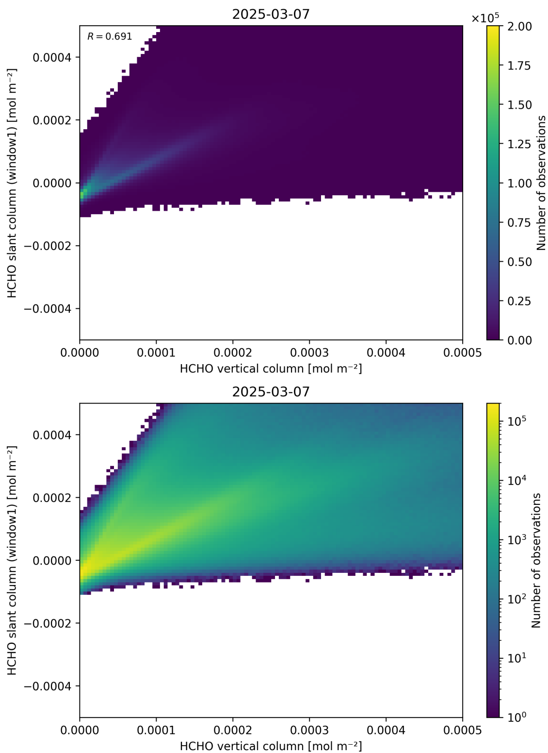
Figure 129: Scatter density plot of “HCHO vertical column” against “HCHO slant column (window1)” for 2025-03-07 to 2025-03-08.
