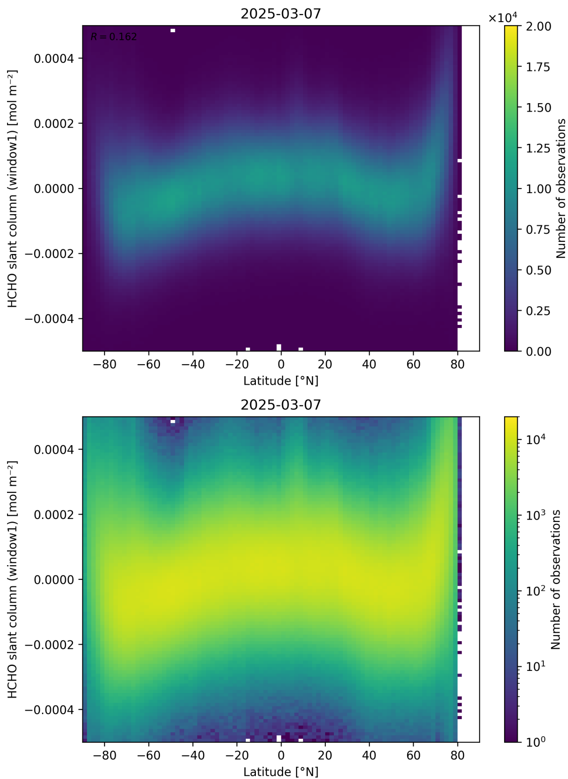
Figure 159: Scatter density plot of “Latitude” against “HCHO slant column (window1)” for 2025-03-07 to 2025-03-08.
