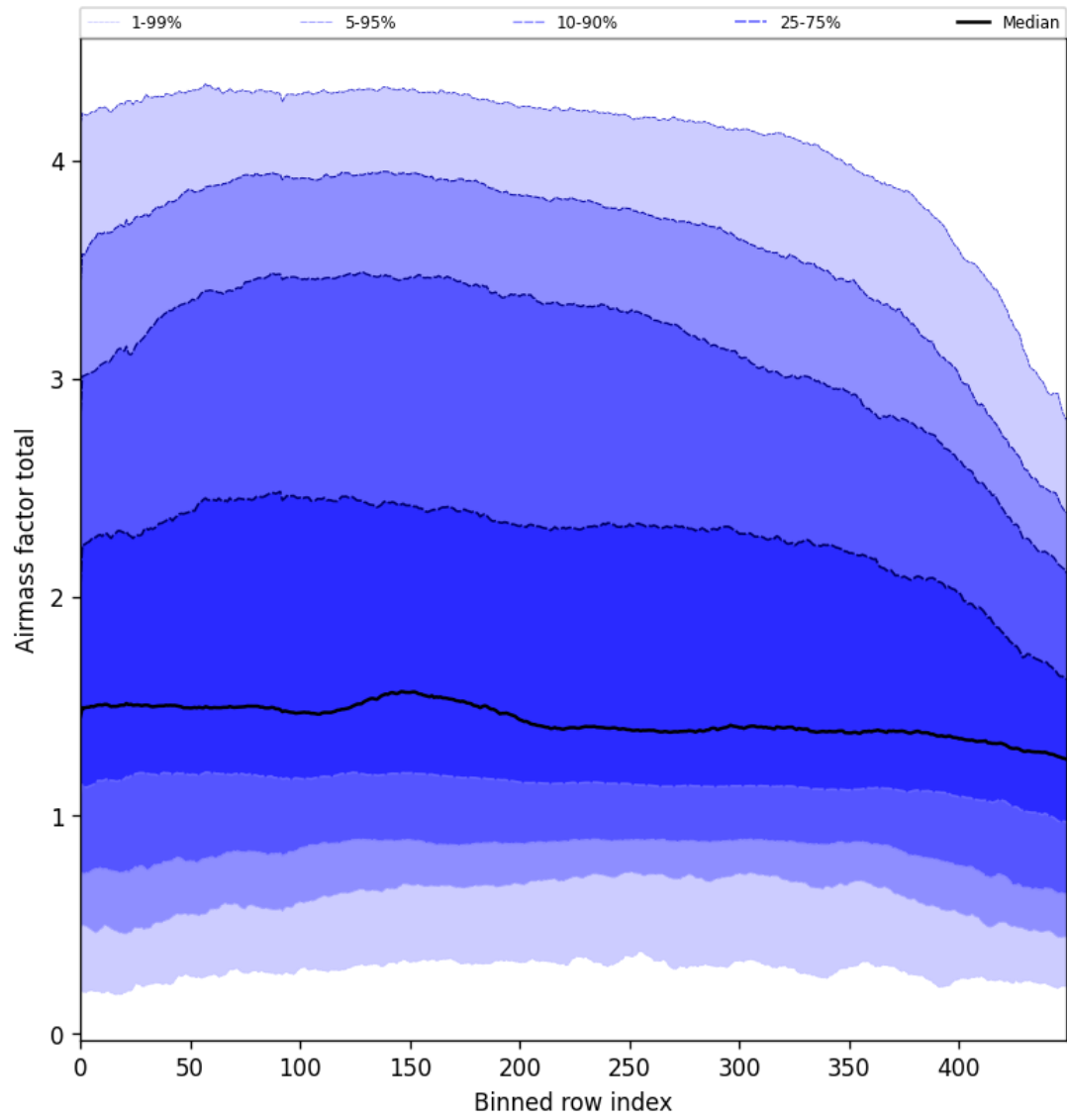
Figure 54: Along track statistics of “Airmass factor total” for 2025-03-07 to 2025-03-08
