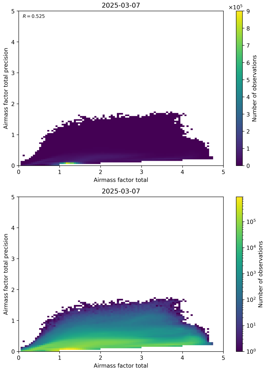
Figure 103: Scatter density plot of “Airmass factor total” against “Airmass factor total precision” for 2025-03-07 to 2025-03-08.
