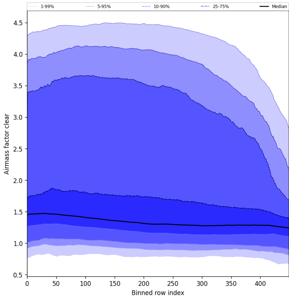
Figure 56: Along track statistics of “Airmass factor clear” for 2025-03-07 to 2025-03-08
