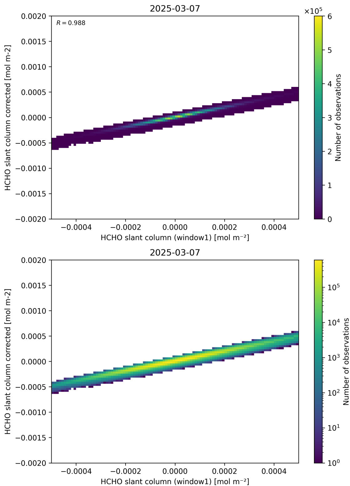
Figure 82: Scatter density plot of “HCHO slant column (window1)” against “HCHO slant column corrected” for 2025-03-07 to 2025-03-08.
