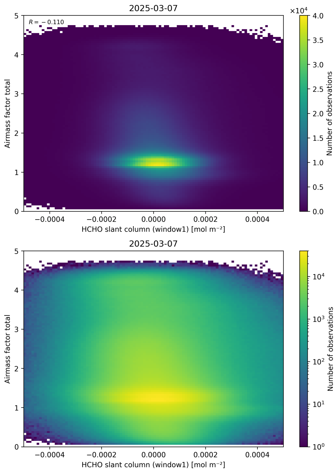
Figure 85: Scatter density plot of “HCHO slant column (window1)” against “Airmass factor total” for 2025-03-07 to 2025-03-08.
