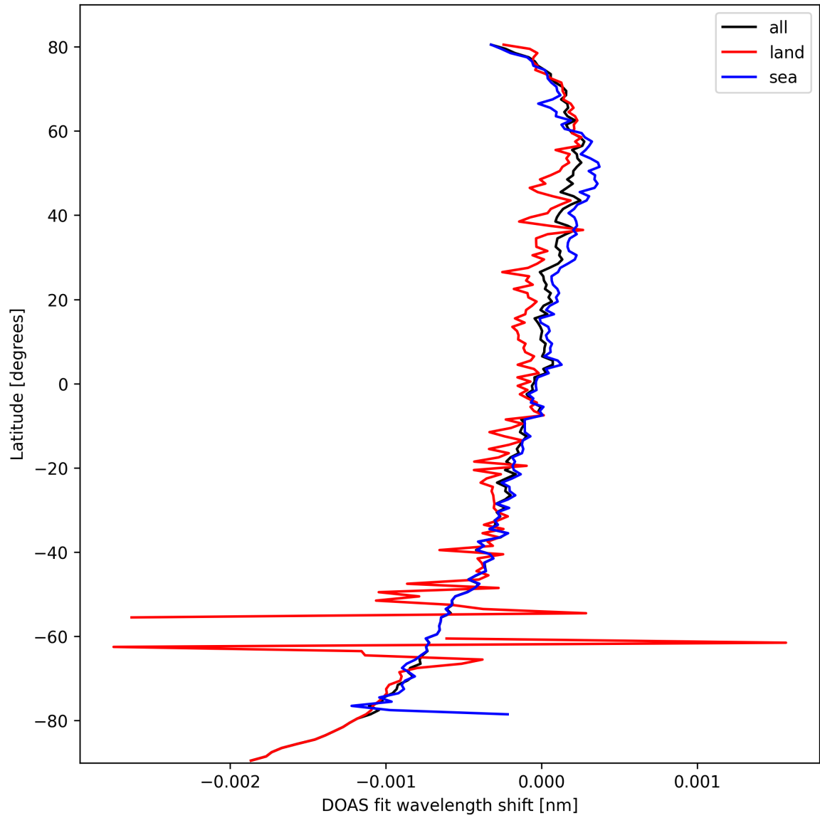
Figure 30: Zonal average of "DOAS fit wavelength shift" for 2025-03-07 to 2025-03-08.
