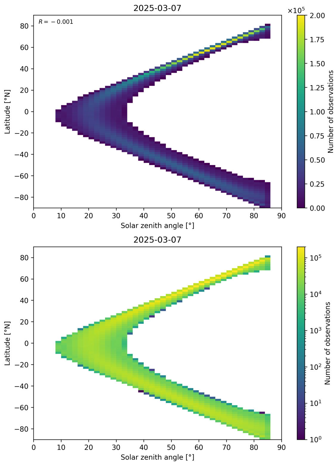
Figure 181: Scatter density plot of “Solar zenith angle” against “Latitude” for 2025-03-07 to 2025-03-08.
