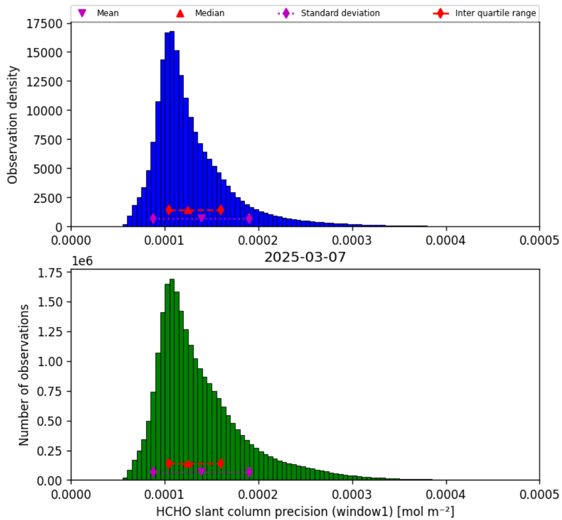
Figure 39: Histogram of “HCHO slant column precision (window1)” for 2025-03-07 to 2025-03-08
