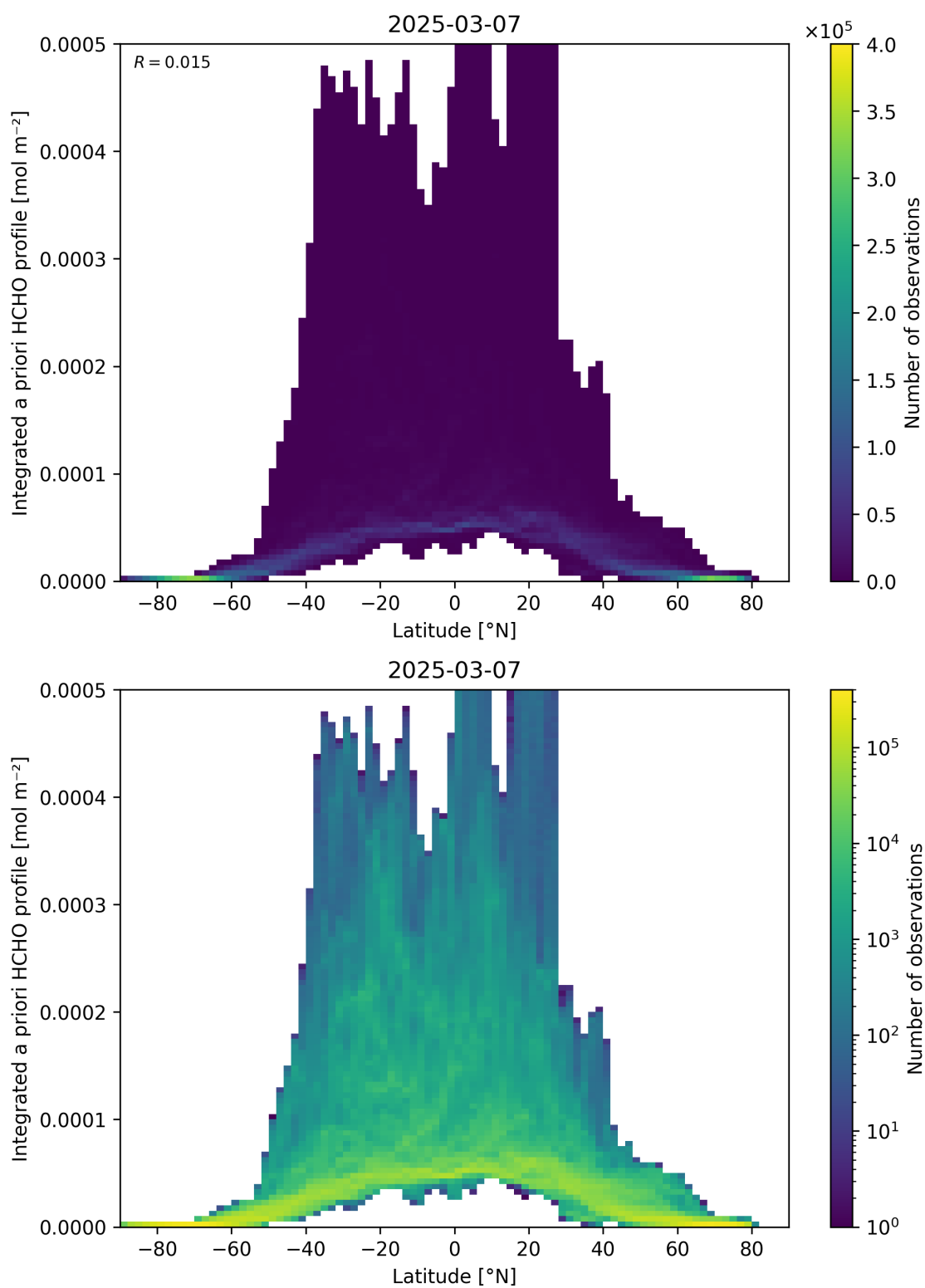
Figure 166: Scatter density plot of “Latitude” against “Integrated a priori HCHO profile” for 2025-03-07 to 2025-03-08.
