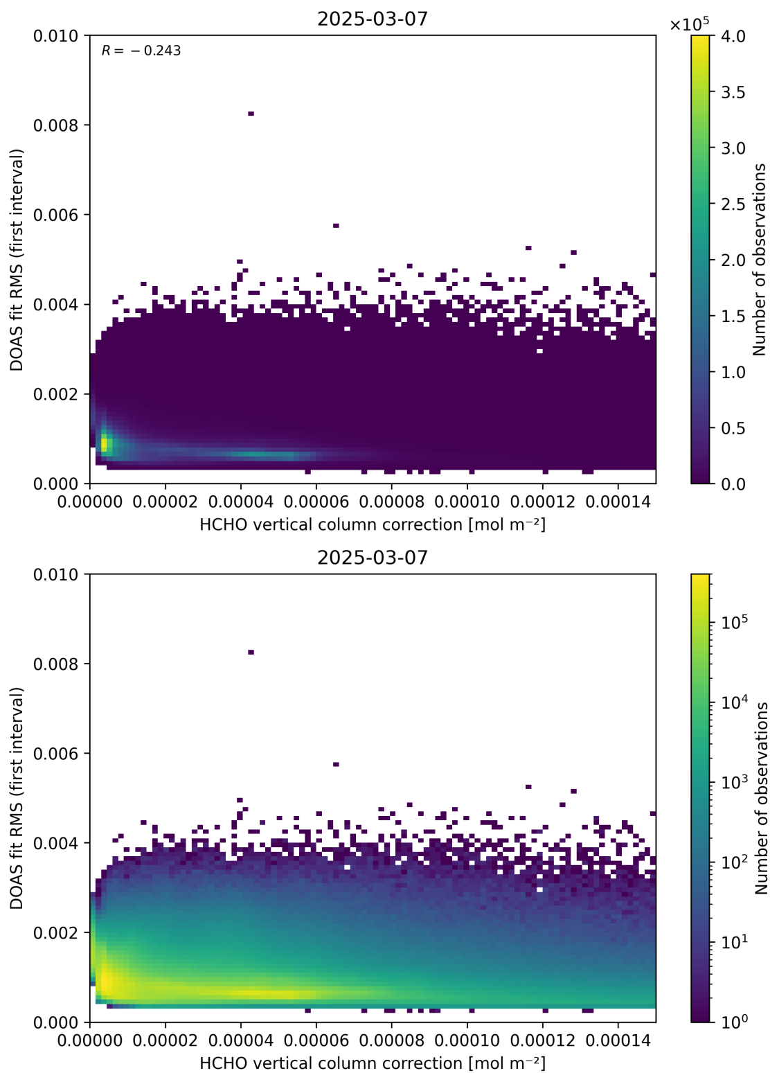
Figure 112: Scatter density plot of “HCHO vertical column correction” against “DOAS fit RMS (first interval)” for 2025-03-07 to 2025-03-08.
