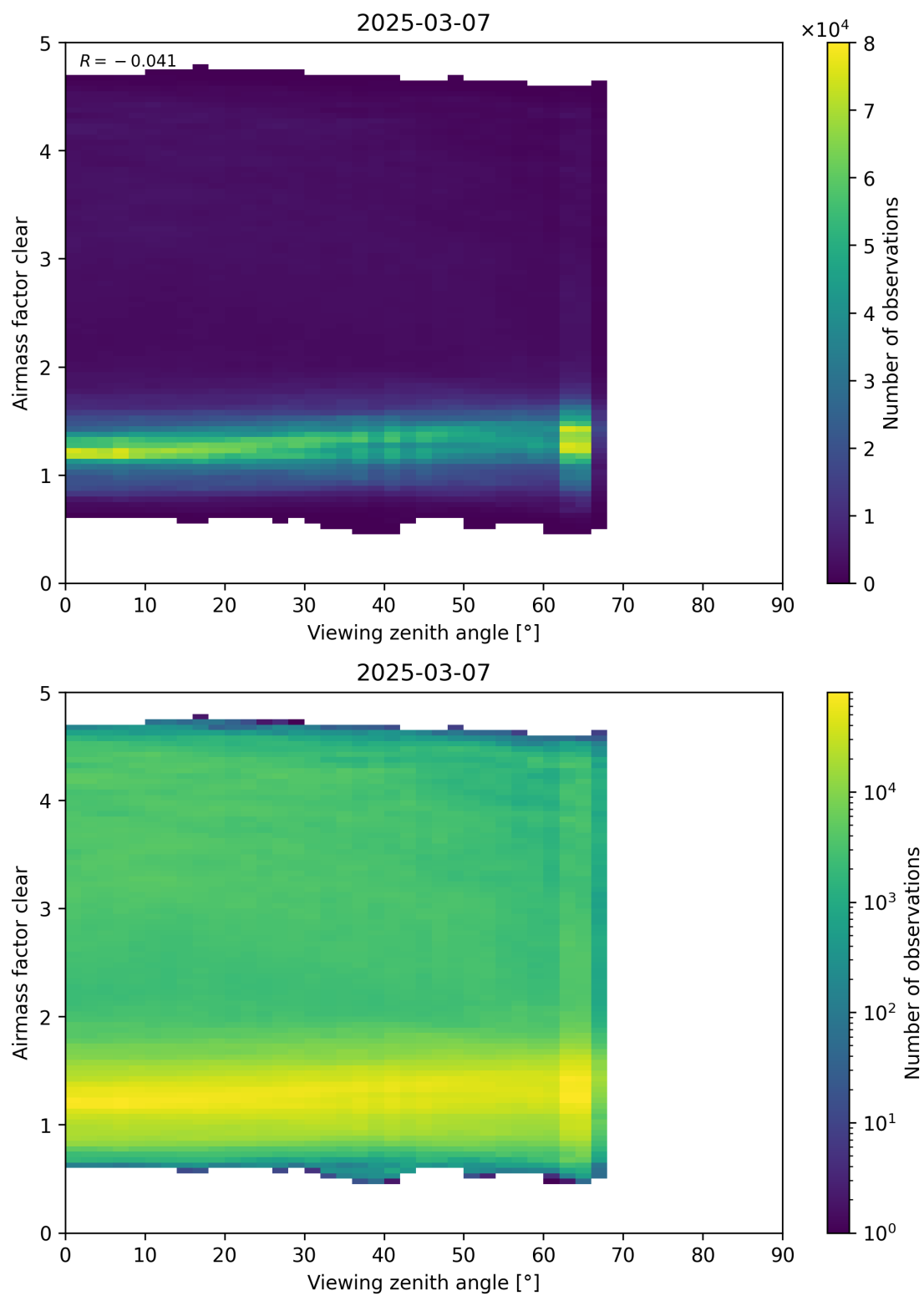
Figure 185: Scatter density plot of “Viewing zenith angle” against “Airmass factor clear” for 2025-03-07 to 2025-03-08.
