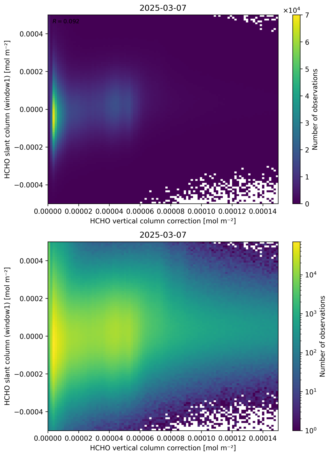
Figure 118: Scatter density plot of “HCHO vertical column correction” against “HCHO slant column (window1)” for 2025-03-07 to 2025-03-08.
