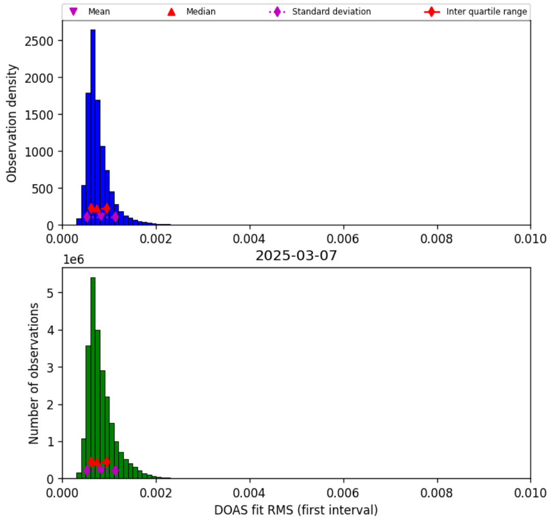
Figure 46: Histogram of “DOAS fit RMS (first interval)” for 2025-03-07 to 2025-03-08
