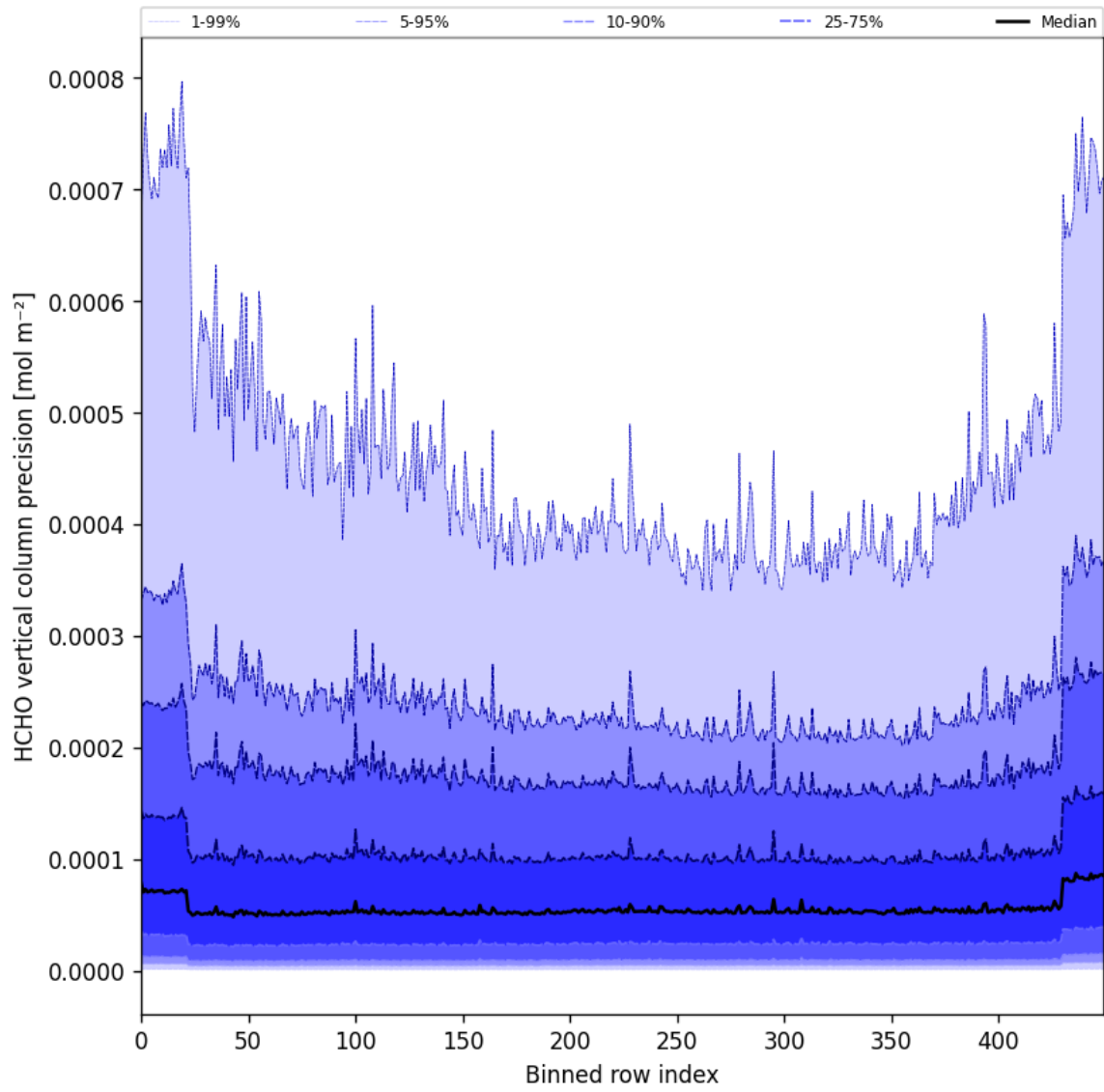
Figure 50: Along track statistics of “HCHO vertical column precision” for 2025-03-07 to 2025-03-08
