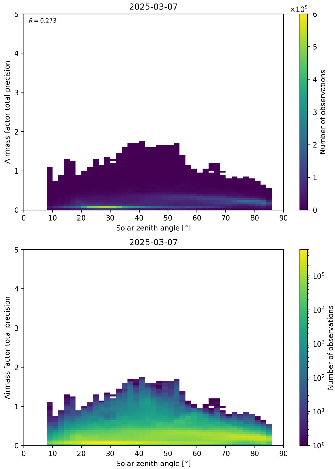
Figure 176: Scatter density plot of “Solar zenith angle” against “Airmass factor total precision” for 2025-03-07 to 2025-03-08.
