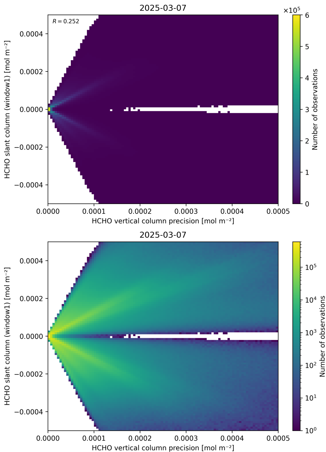
Figure 142: Scatter density plot of “HCHO vertical column precision” against “HCHO slant column (window1)” for 2025-03-07 to 2025-03-08.
