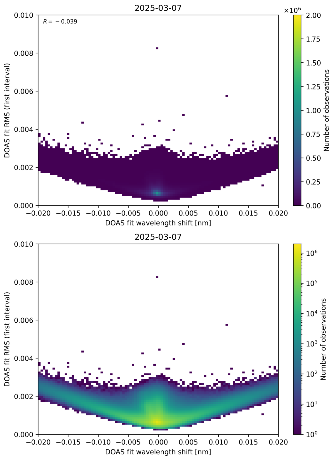
Figure 64: Scatter density plot of “DOAS fit wavelength shift” against “DOAS fit RMS (first interval)” for 2025-03-07 to 2025-03-08.
