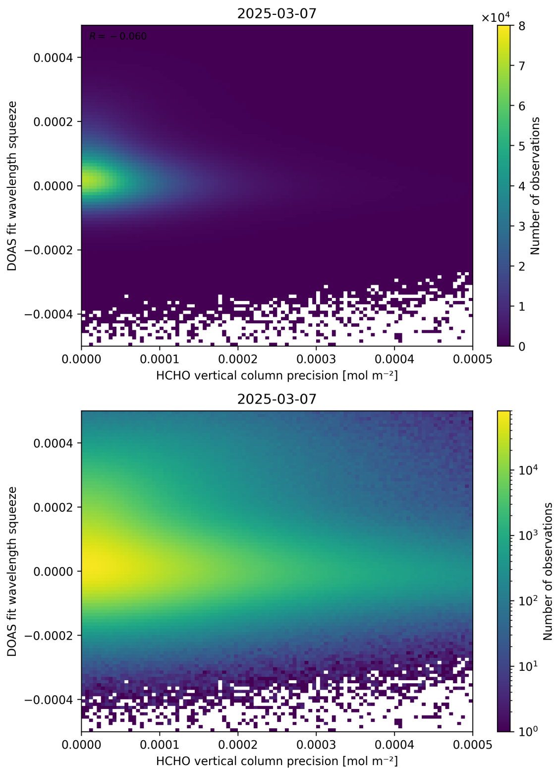
Figure 138: Scatter density plot of “HCHO vertical column precision” against “DOAS fit wavelength squeeze” for 2025-03-07 to 2025-03-08.
