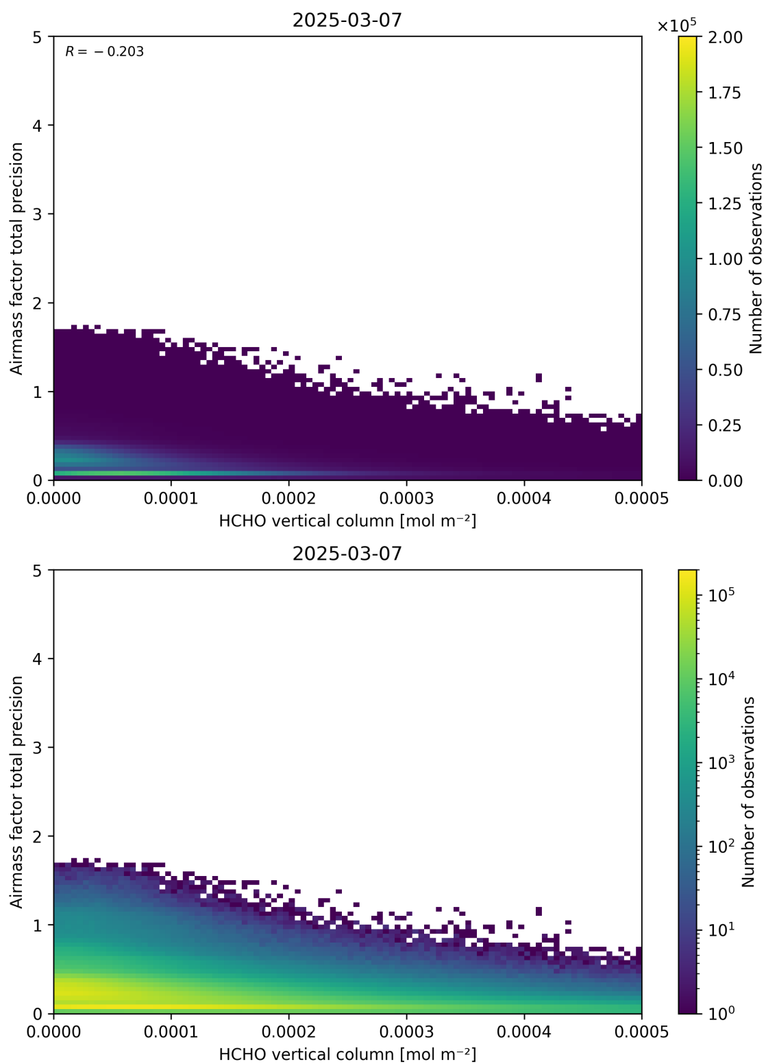
Figure 132: Scatter density plot of “HCHO vertical column” against “Airmass factor total precision” for 2025-03-07 to 2025-03-08.
