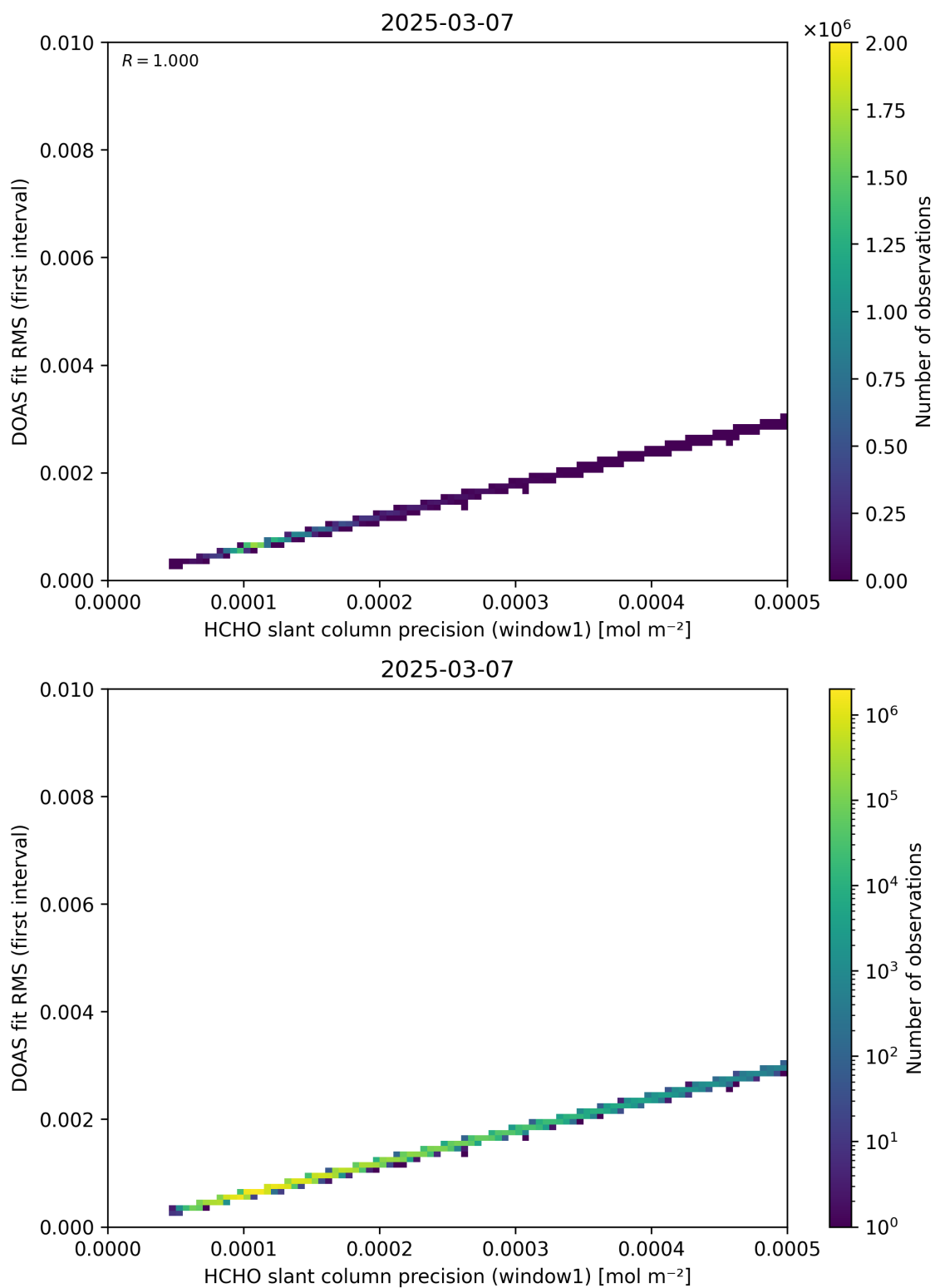
Figure 88: Scatter density plot of “HCHO slant column precision (window1)” against “DOAS fit RMS (first interval)” for 2025-03-07 to 2025-03-08.
