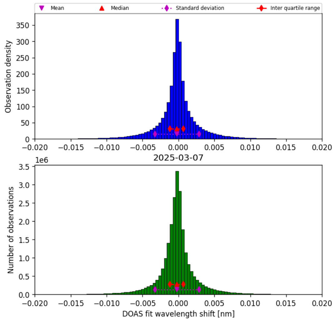
Figure 44: Histogram of “DOAS fit wavelength shift” for 2025-03-07 to 2025-03-08
