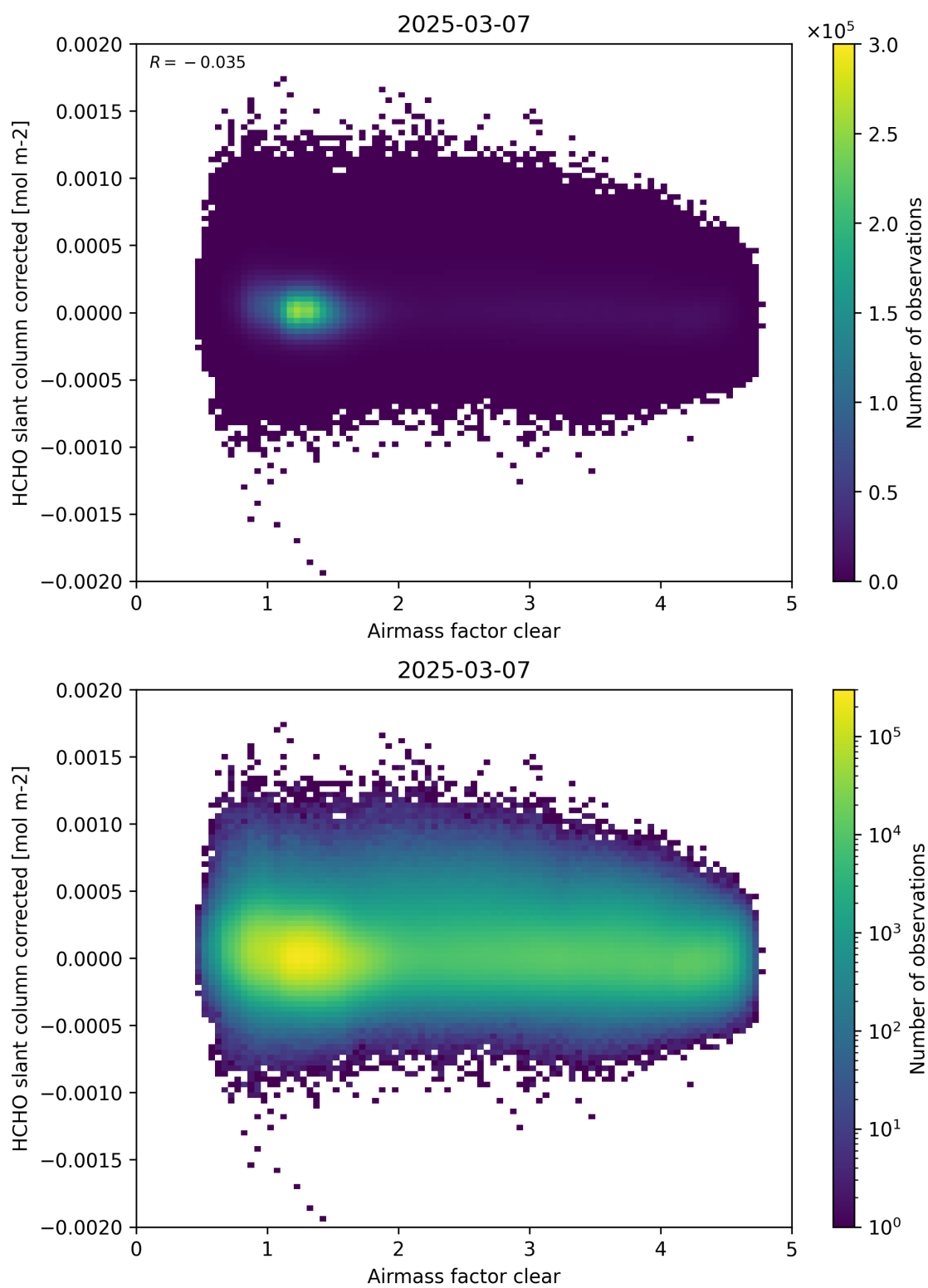
Figure 74: Scatter density plot of “Airmass factor clear” against “HCHO slant column corrected” for 2025-03-07 to 2025-03-08.
