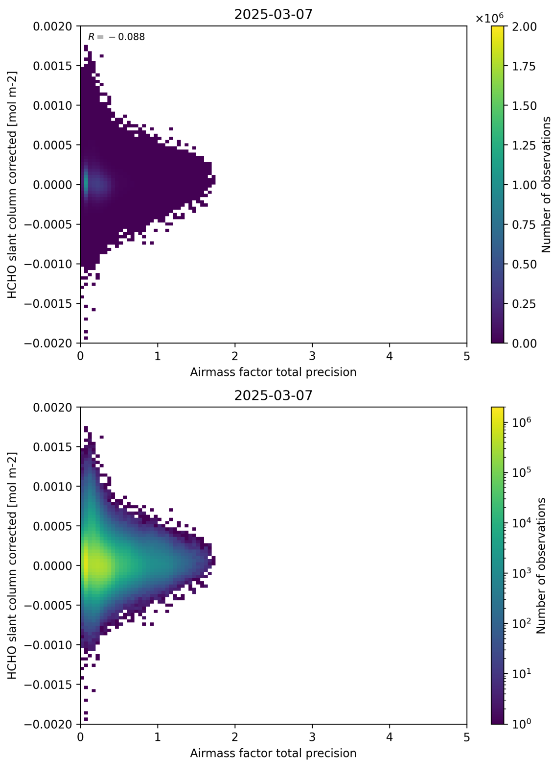
Figure 109: Scatter density plot of “Airmass factor total precision” against “HCHO slant column corrected” for 2025-03-07 to 2025-03-08.
