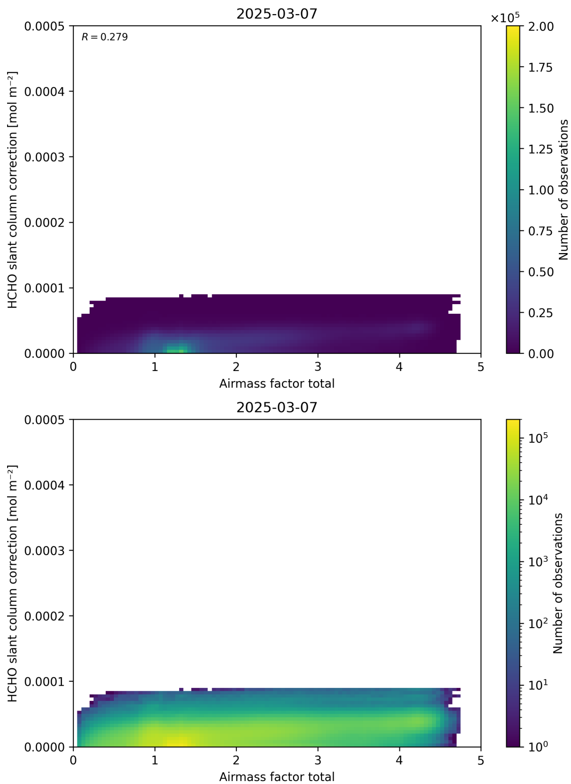
Figure 102: Scatter density plot of “Airmass factor total” against “HCHO slant column correction” for 2025-03-07 to 2025-03-08.
