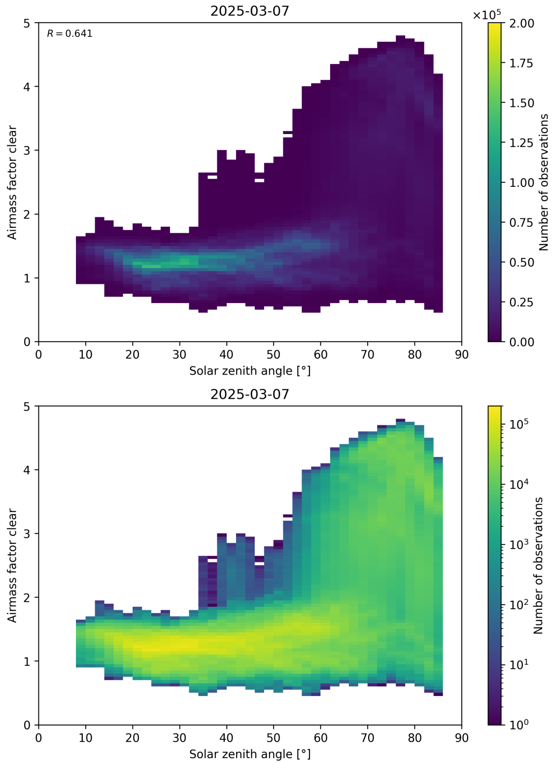
Figure 170: Scatter density plot of “Solar zenith angle” against “Airmass factor clear” for 2025-03-07 to 2025-03-08.
