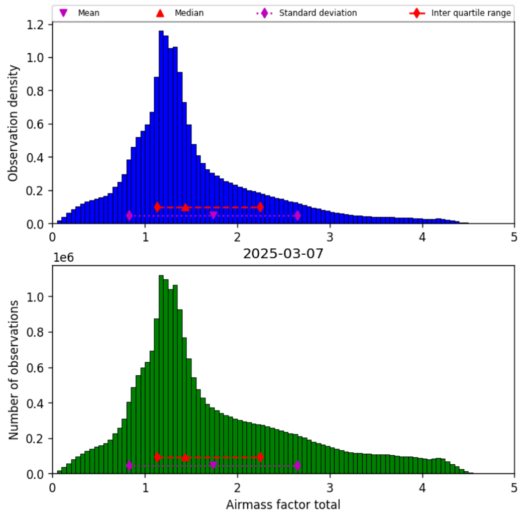
Figure 40: Histogram of “Airmass factor total” for 2025-03-07 to 2025-03-08
