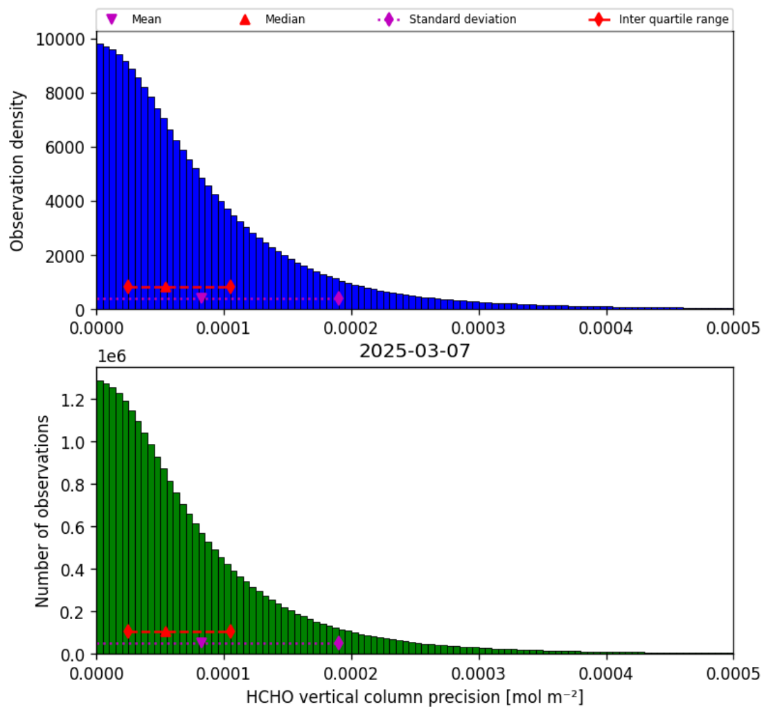
Figure 36: Histogram of “HCHO vertical column precision” for 2025-03-07 to 2025-03-08
