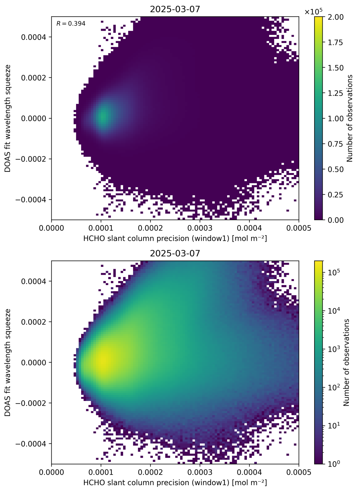
Figure 90: Scatter density plot of “HCHO slant column precision (window1)” against “DOAS fit wavelength squeeze” for 2025-03-07 to 2025-03-08.
