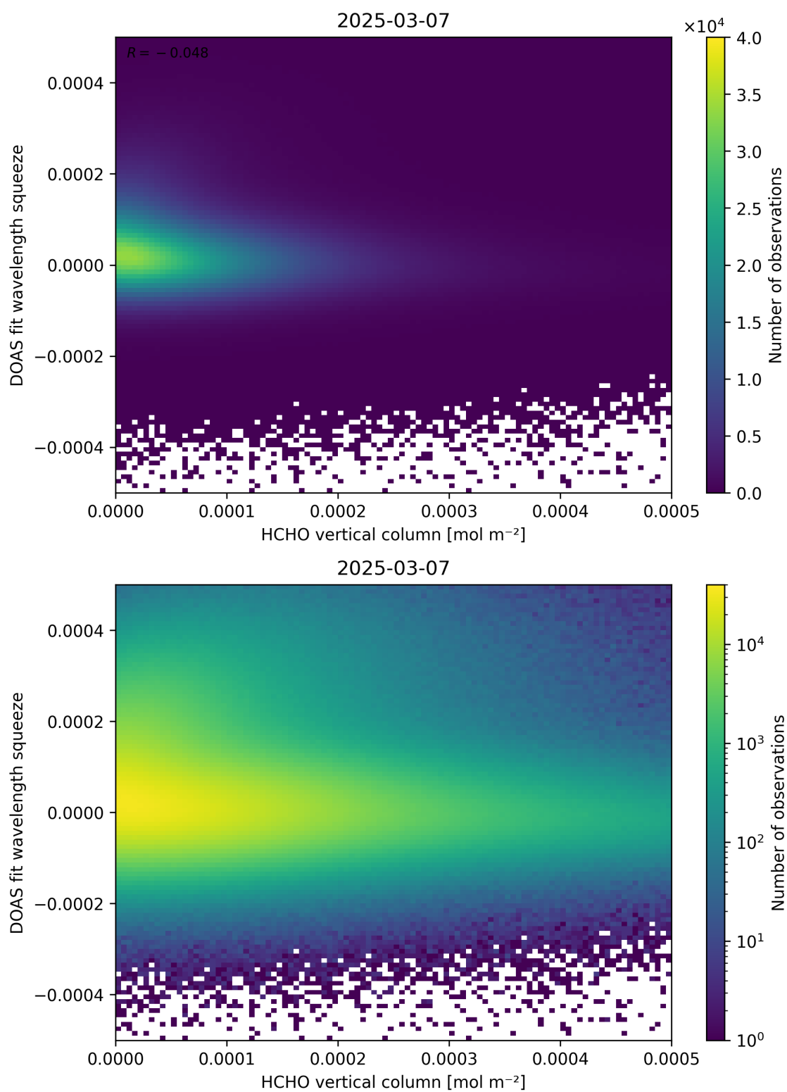
Figure 125: Scatter density plot of “HCHO vertical column” against “DOAS fit wavelength squeeze” for 2025-03-07 to 2025-03-08.
