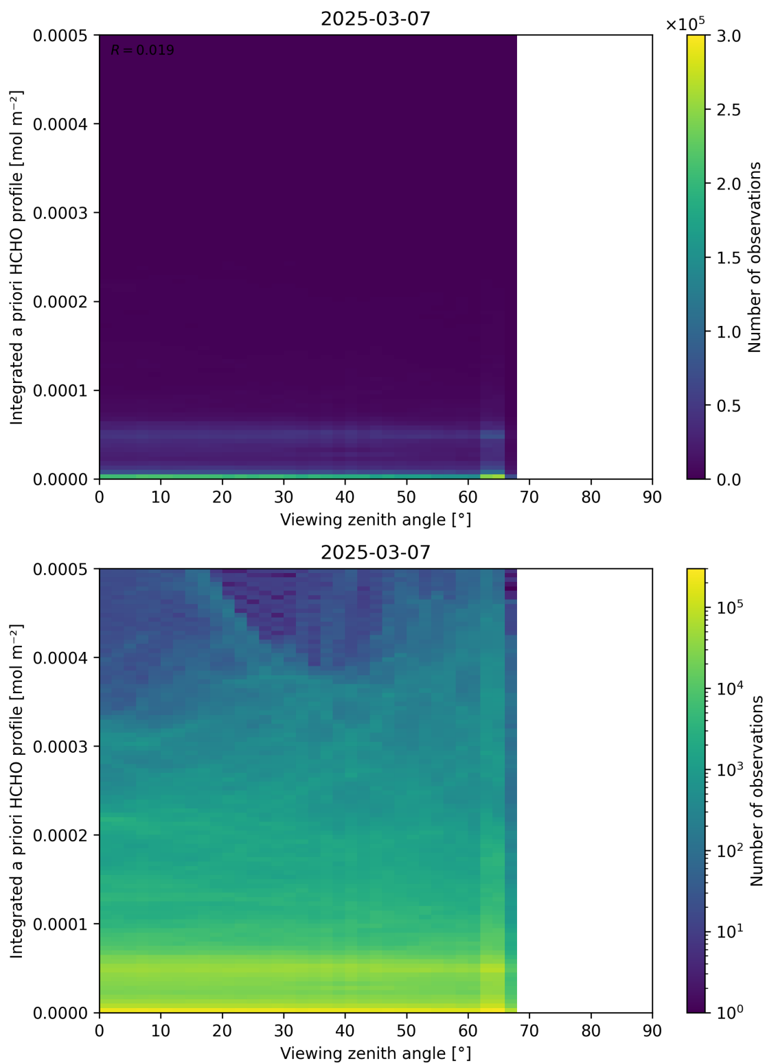
Figure 195: Scatter density plot of “Viewing zenith angle” against “Integrated a priori HCHO profile” for 2025-03-07 to 2025-03-08.
