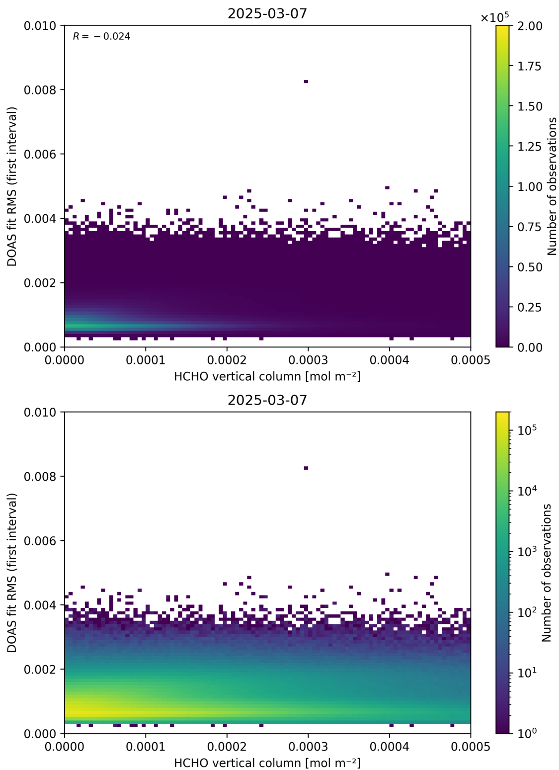
Figure 123: Scatter density plot of “HCHO vertical column” against “DOAS fit RMS (first interval)” for 2025-03-07 to 2025-03-08.
