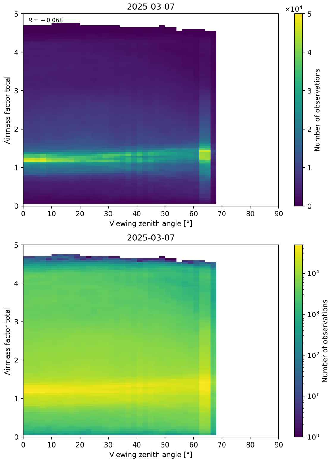
Figure 190: Scatter density plot of “Viewing zenith angle” against “Airmass factor total” for 2025-03-07 to 2025-03-08.
