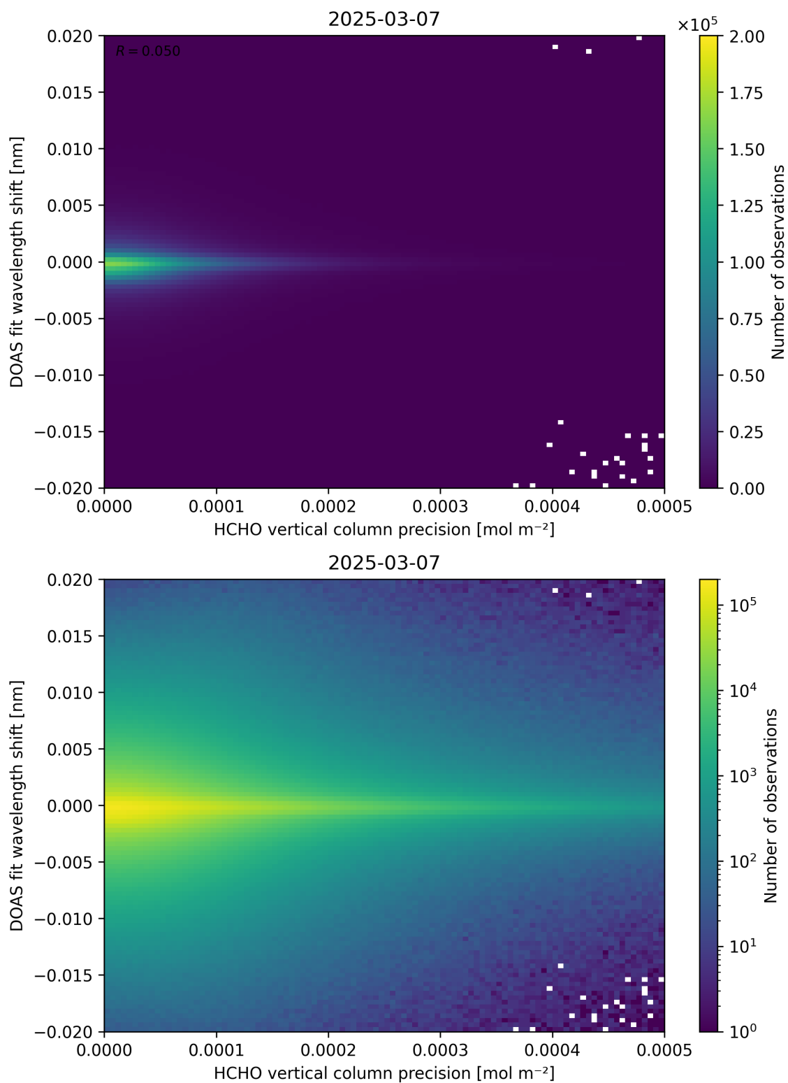
Figure 137: Scatter density plot of “HCHO vertical column precision” against “DOAS fit wavelength shift” for 2025-03-07 to 2025-03-08.
