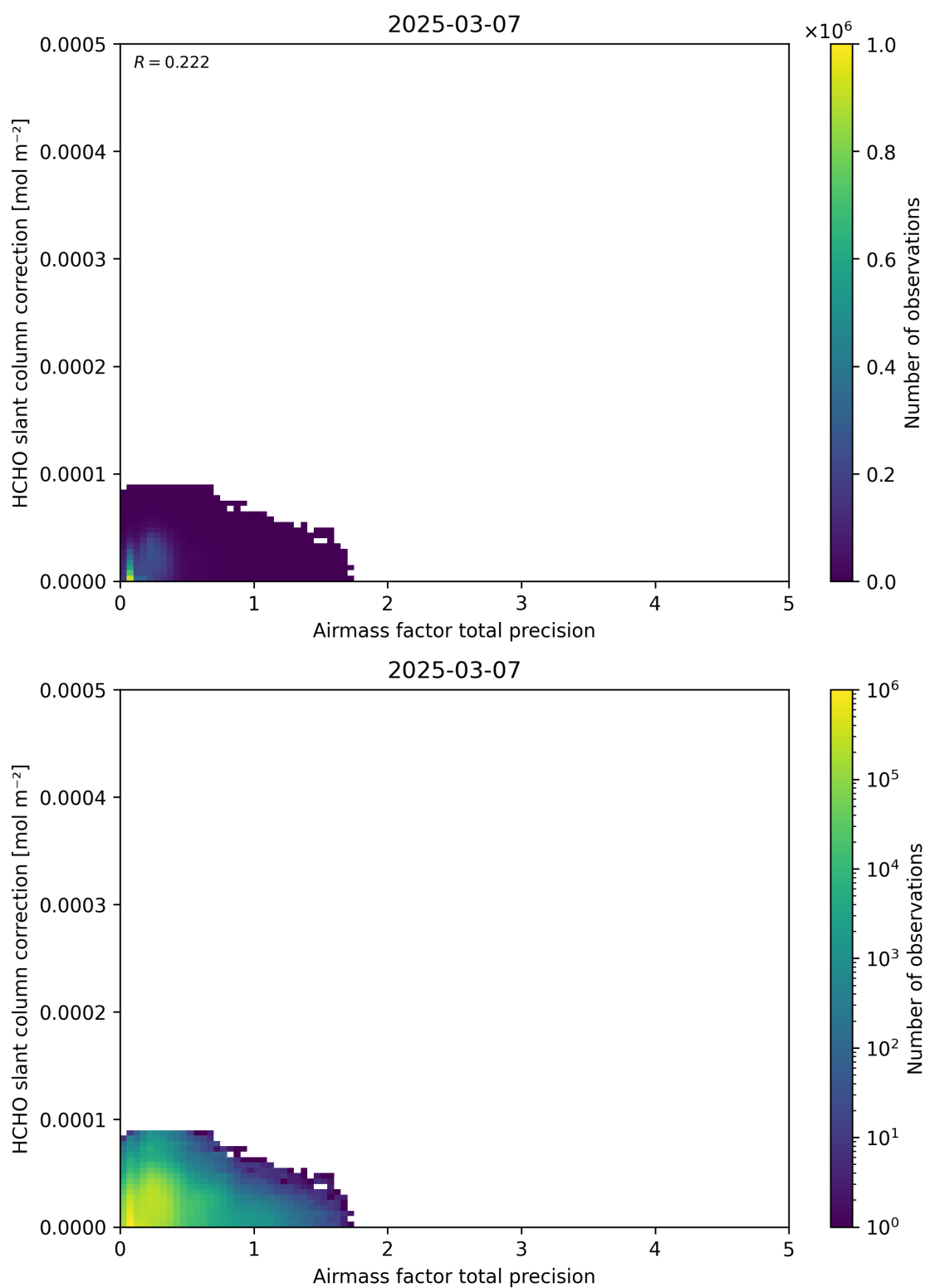
Figure 110: Scatter density plot of “Airmass factor total precision” against “HCHO slant column correction” for 2025-03-07 to 2025-03-08.
