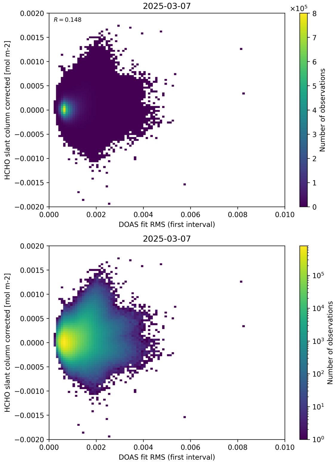
Figure 62: Scatter density plot of “DOAS fit RMS (first interval)” against “HCHO slant column corrected” for 2025-03-07 to 2025-03-08.
