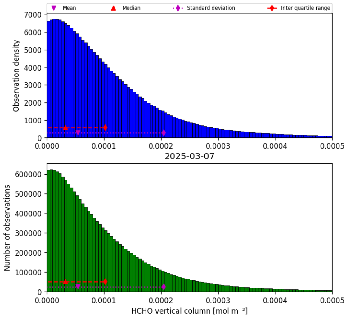
Figure 35: Histogram of “HCHO vertical column” for 2025-03-07 to 2025-03-08
