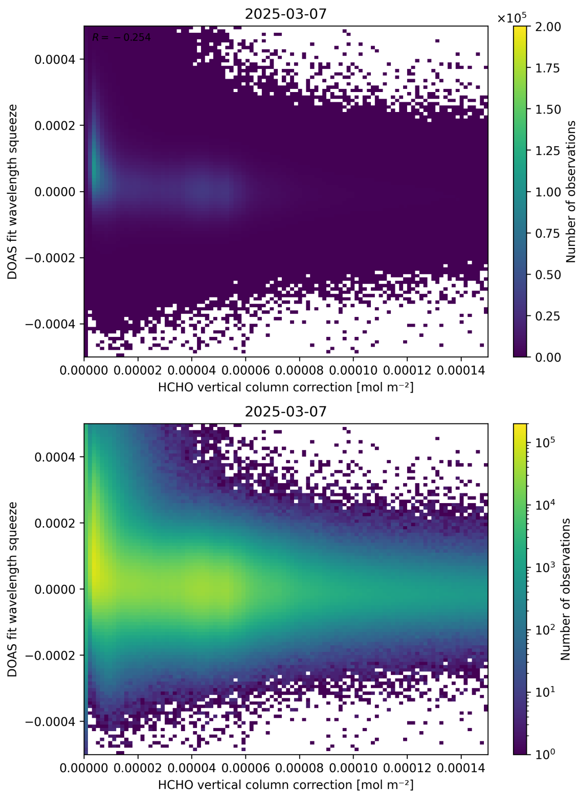
Figure 114: Scatter density plot of “HCHO vertical column correction” against “DOAS fit wavelength squeeze” for 2025-03-07 to 2025-03-08.
