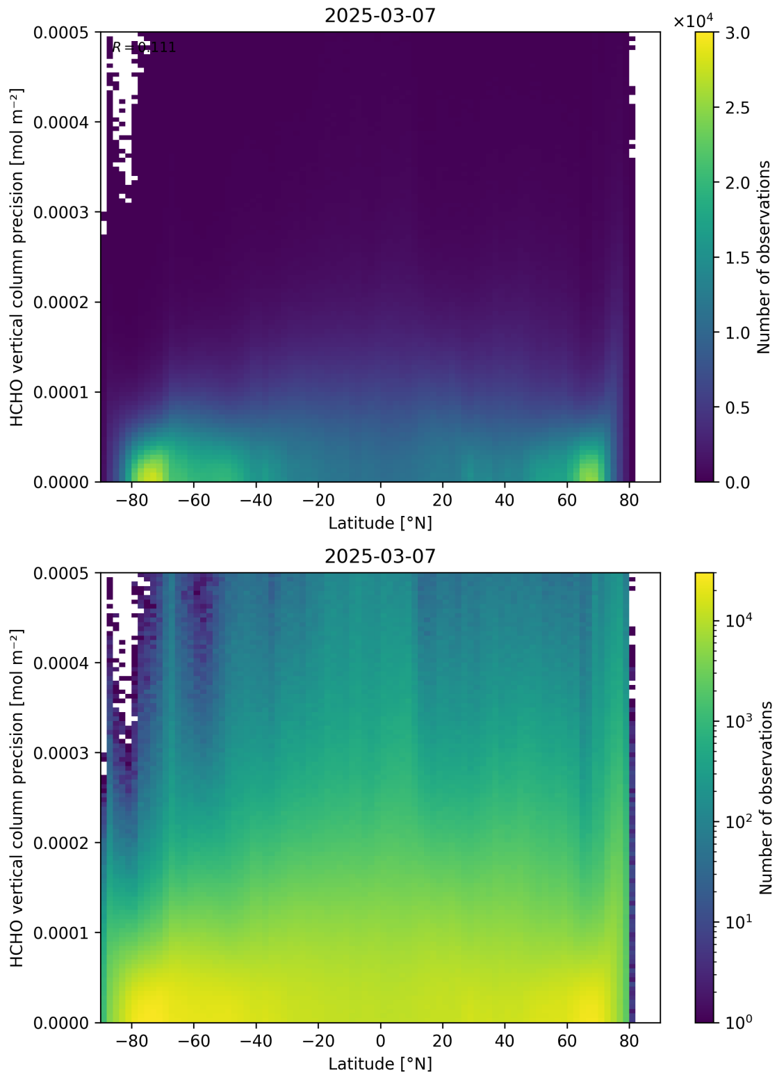
Figure 165: Scatter density plot of “Latitude” against “HCHO vertical column precision” for 2025-03-07 to 2025-03-08.
