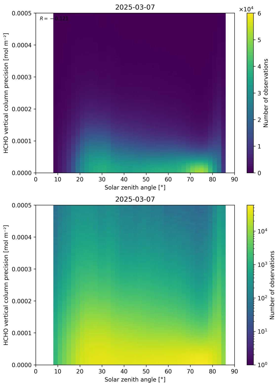
Figure 179: Scatter density plot of “Solar zenith angle” against “HCHO vertical column precision” for 2025-03-07 to 2025-03-08.
