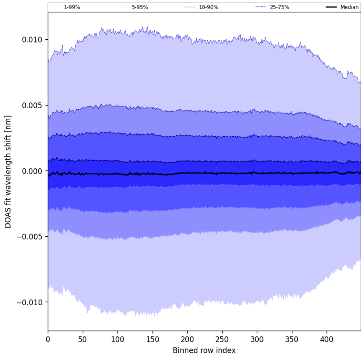
Figure 58: Along track statistics of “DOAS fit wavelength shift” for 2025-03-07 to 2025-03-08
