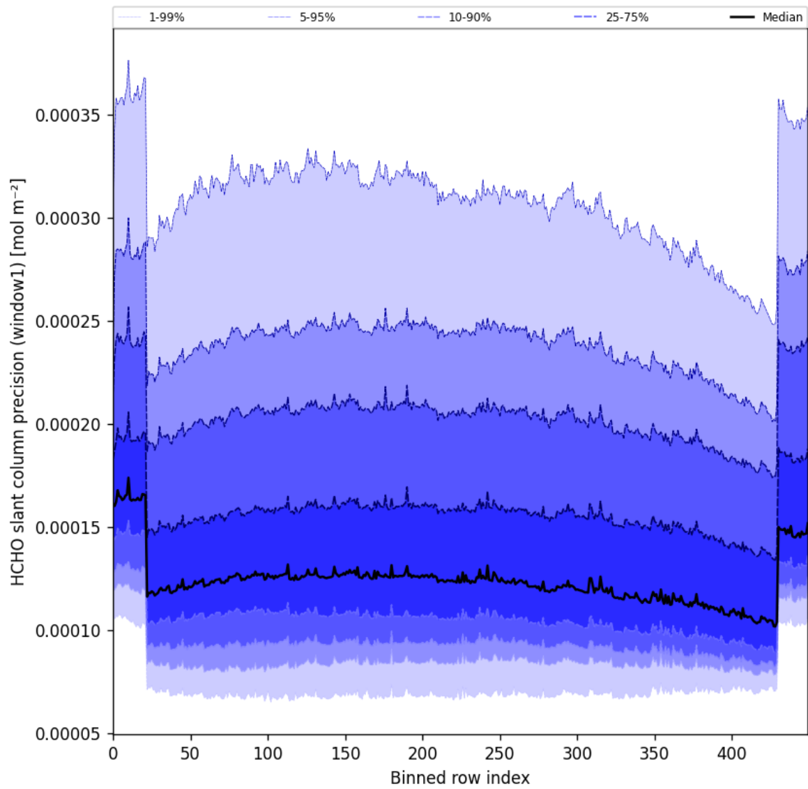
Figure 53: Along track statistics of “HCHO slant column precision (window1)” for 2025-03-07 to 2025-03-08
