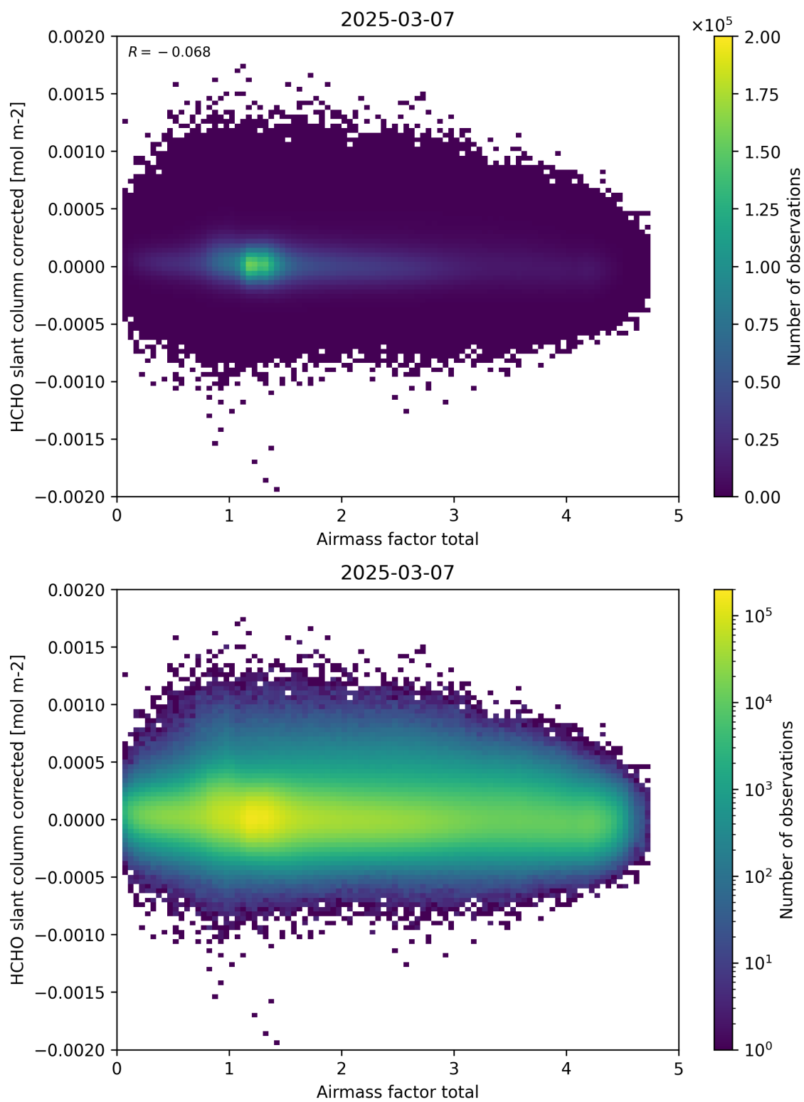
Figure 101: Scatter density plot of “Airmass factor total” against “HCHO slant column corrected” for 2025-03-07 to 2025-03-08.
