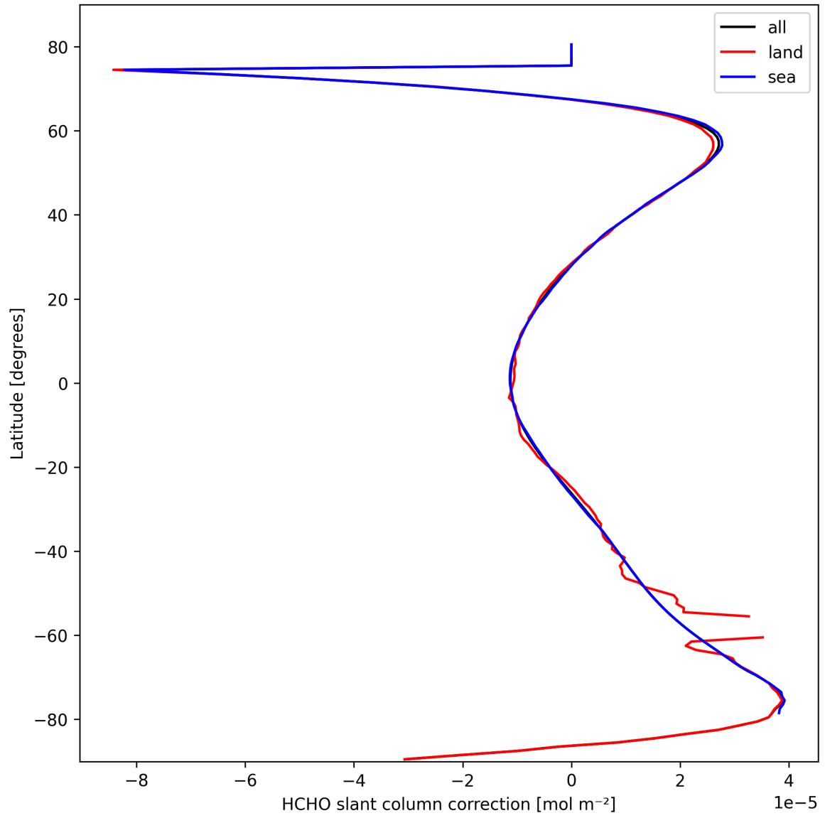
Figure 33: Zonal average of “HCHO slant column correction” for 2025-03-07 to 2025-03-08.
