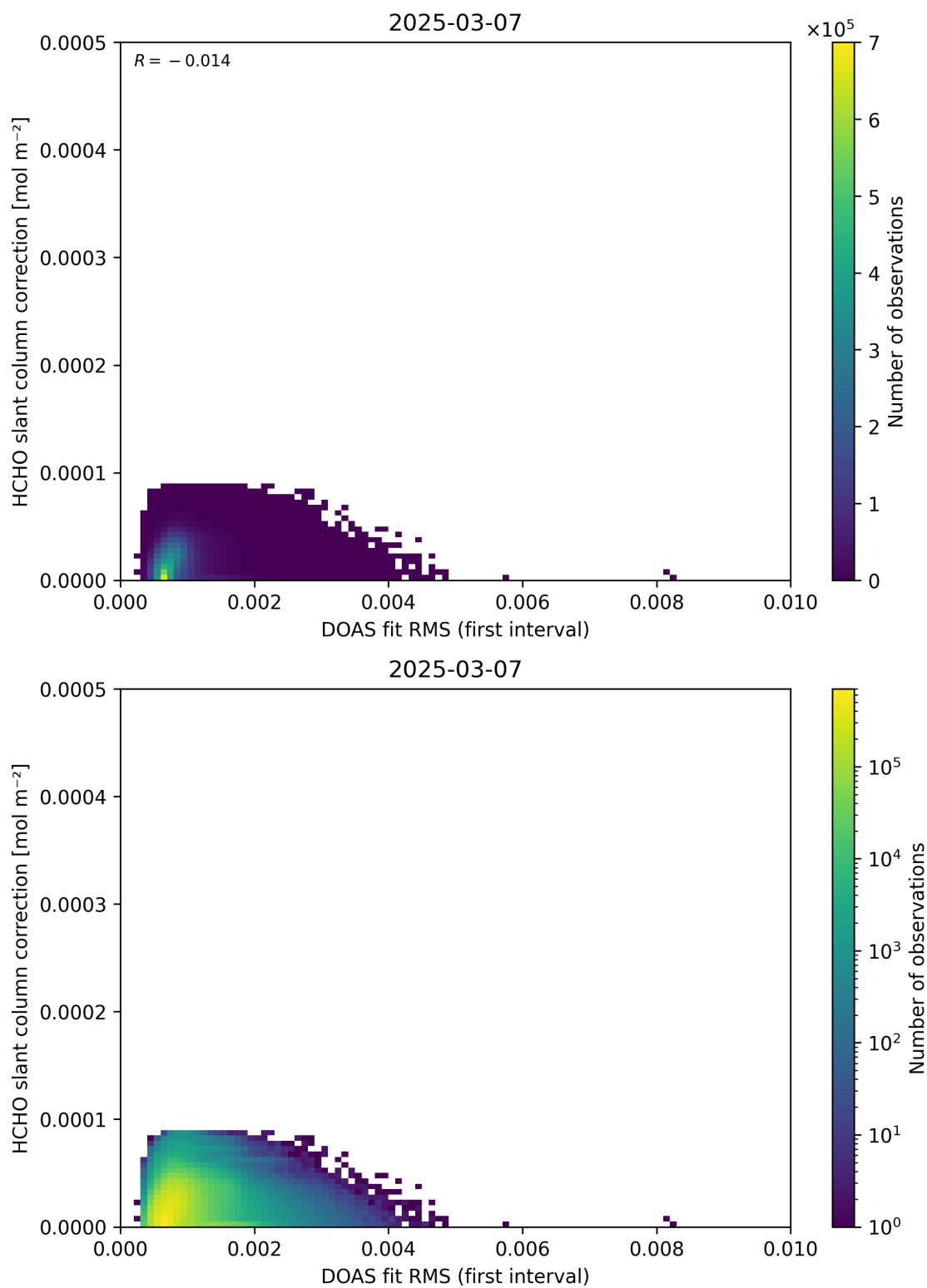
Figure 63: Scatter density plot of “DOAS fit RMS (first interval)” against “HCHO slant column correction” for 2025-03-07 to 2025-03-08.
