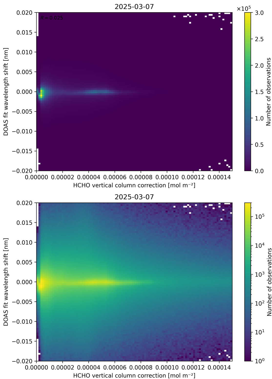
Figure 113: Scatter density plot of “HCHO vertical column correction” against “DOAS fit wavelength shift” for 2025-03-07 to 2025-03-08.
