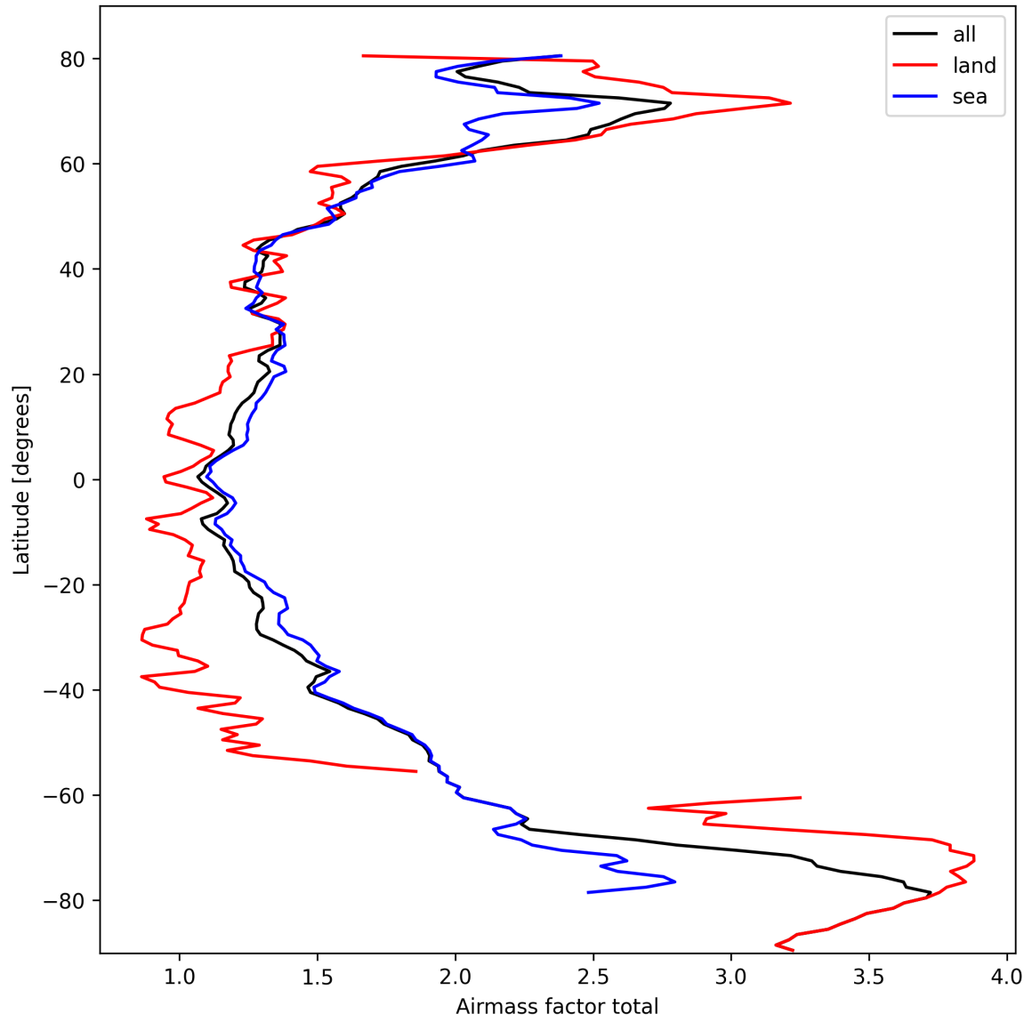
Figure 26: Zonal average of “Airmass factor total” for 2025-03-07 to 2025-03-08.
