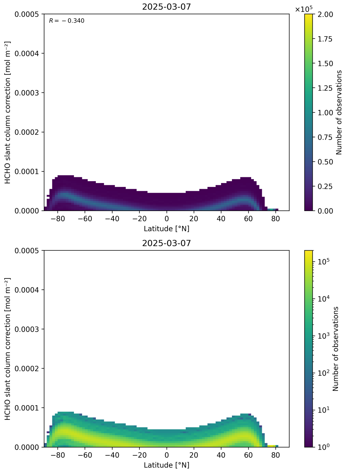
Figure 158: Scatter density plot of “Latitude” against “HCHO slant column correction” for 2025-03-07 to 2025-03-08.
