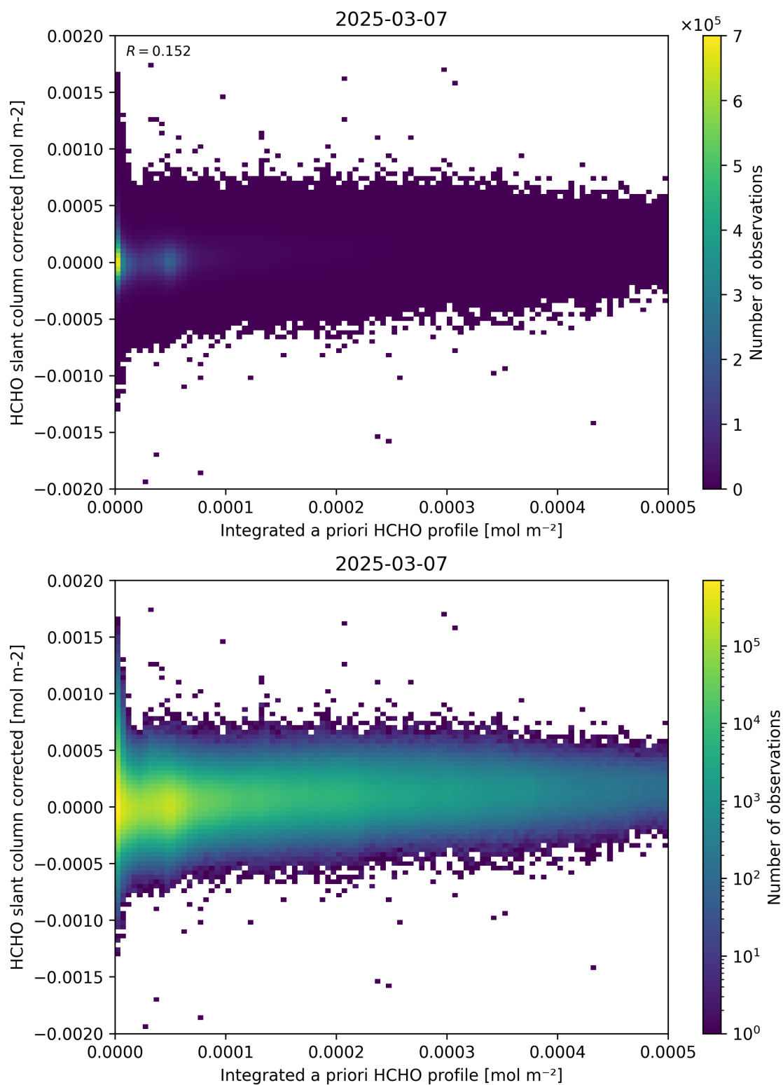
Figure 151: Scatter density plot of “Integrated a priori HCHO profile” against “HCHO slant column corrected” for 2025-03-07 to 2025-03-08.
