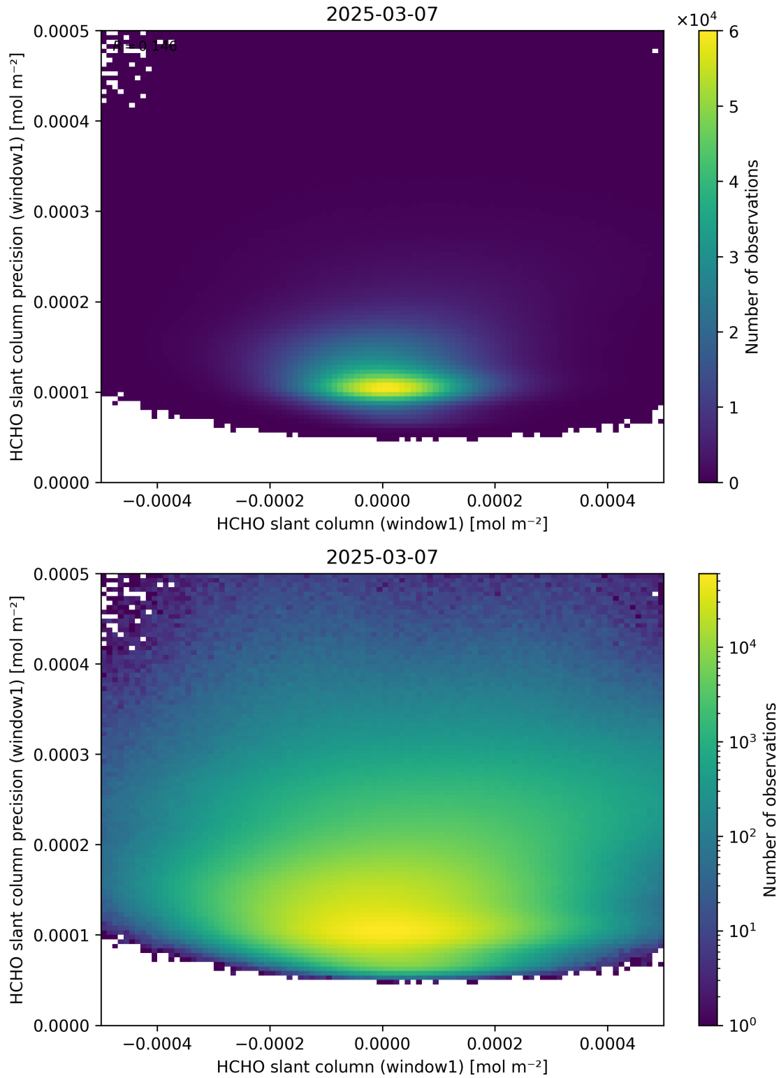
Figure 84: Scatter density plot of “HCHO slant column (window1)” against “HCHO slant column precision (window1)” for 2025-03-07 to 2025-03-08.
