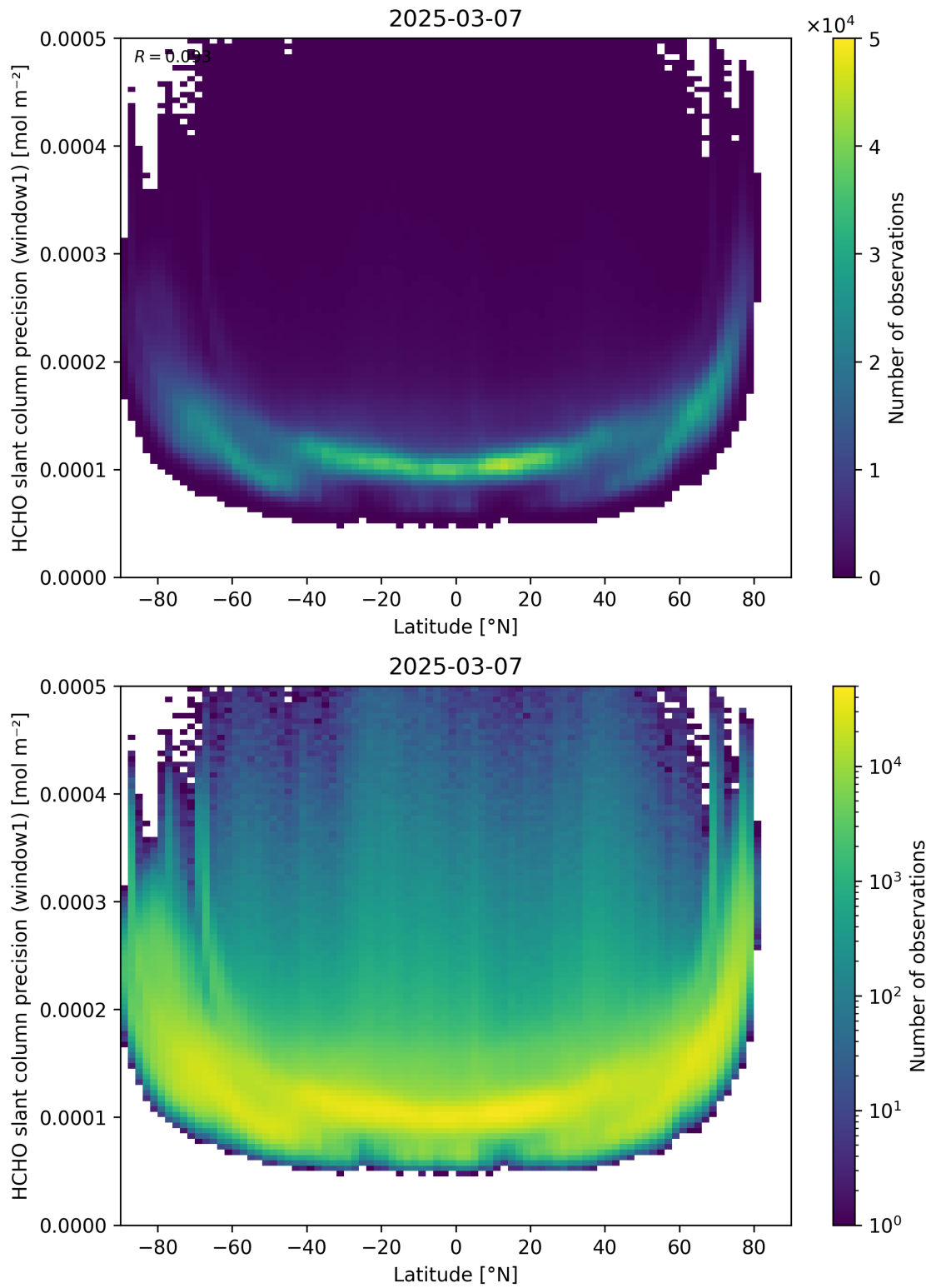
Figure 160: Scatter density plot of “Latitude” against “HCHO slant column precision (window1)” for 2025-03-07 to 2025-03-08.
