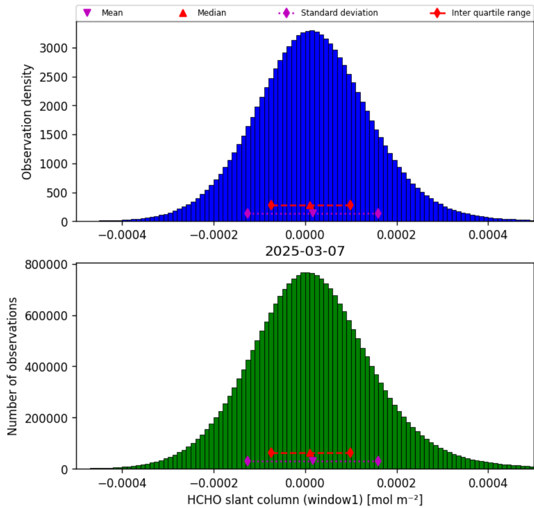
Figure 38: Histogram of “HCHO slant column (window1)” for 2025-03-07 to 2025-03-08
