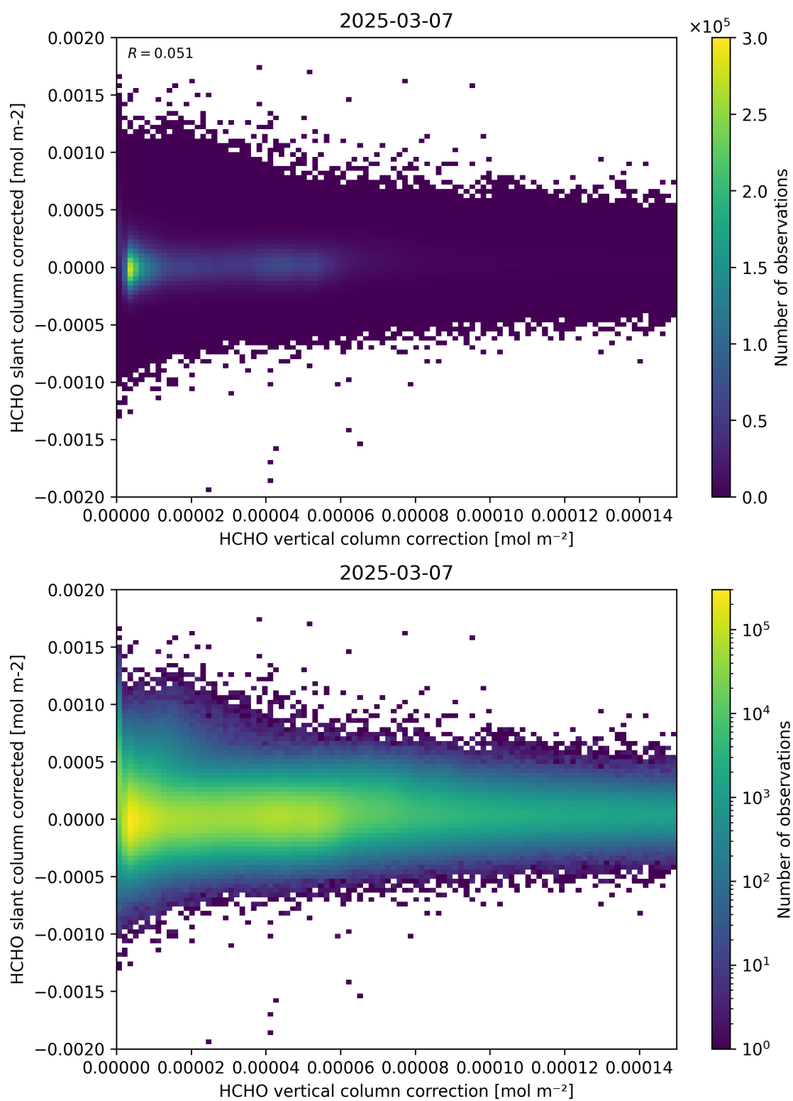
Figure 116: Scatter density plot of “HCHO vertical column correction” against “HCHO slant column corrected” for 2025-03-07 to 2025-03-08.
