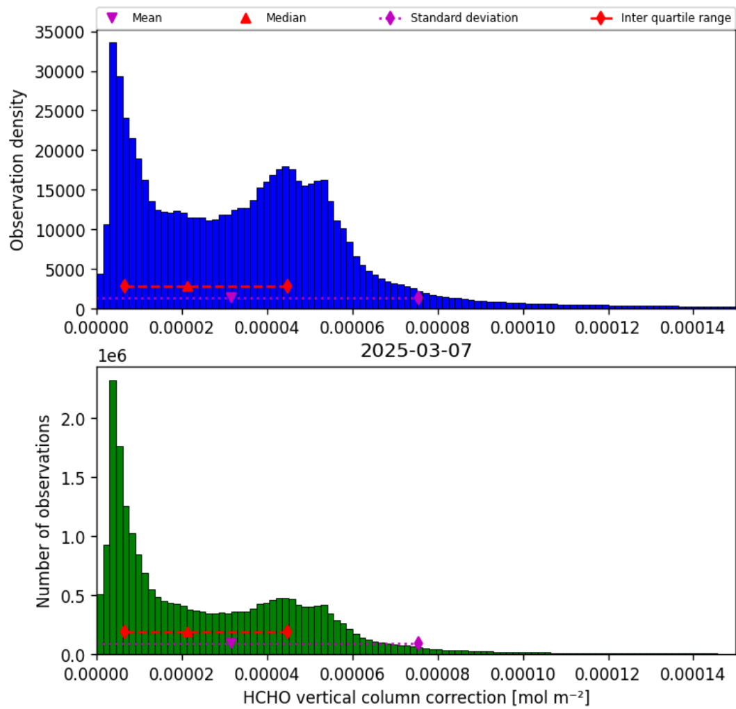
Figure 37: Histogram of “HCHO vertical column correction” for 2025-03-07 to 2025-03-08
