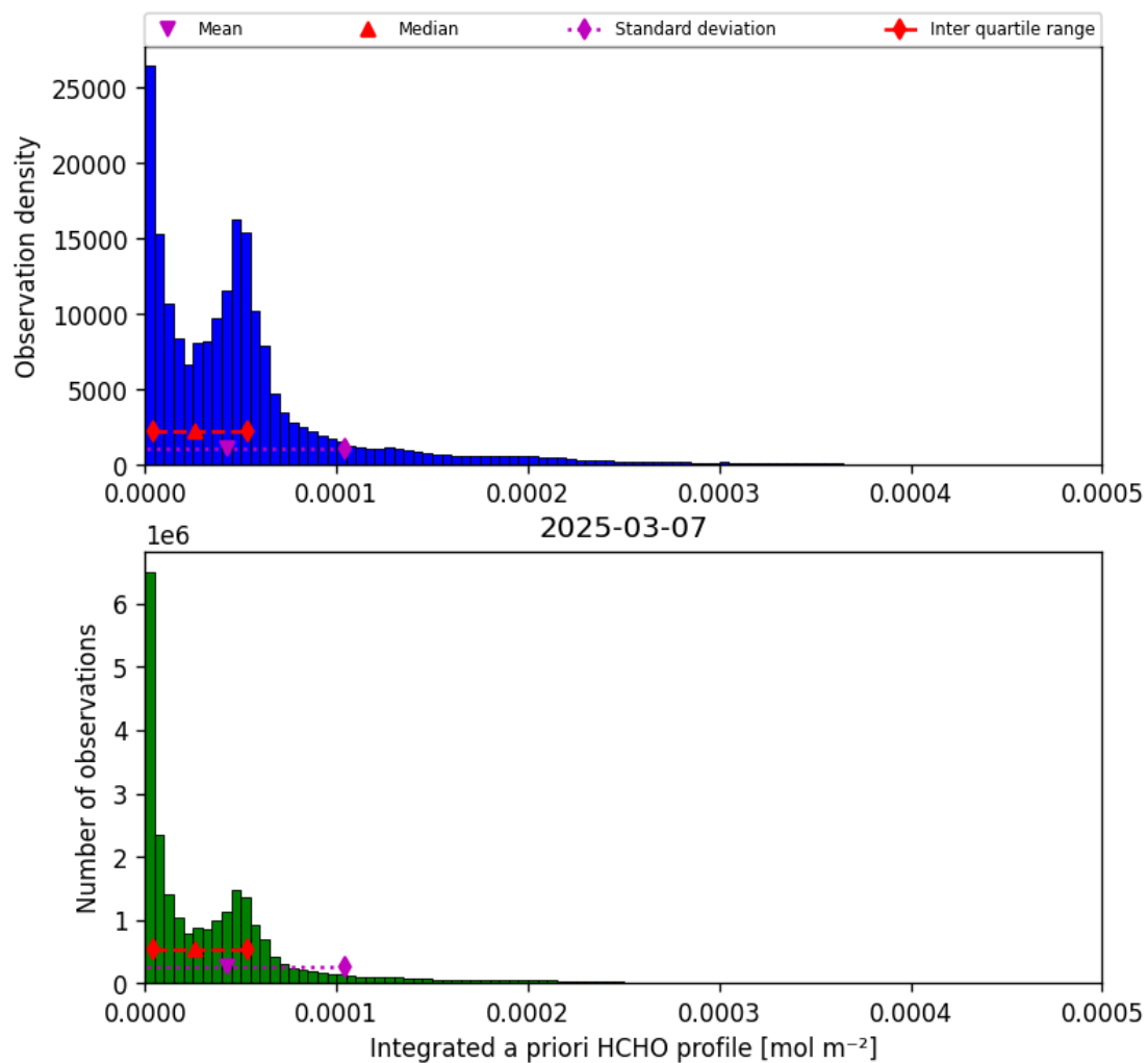
Figure 43: Histogram of “Integrated a priori HCHO profile” for 2025-03-07 to 2025-03-08
