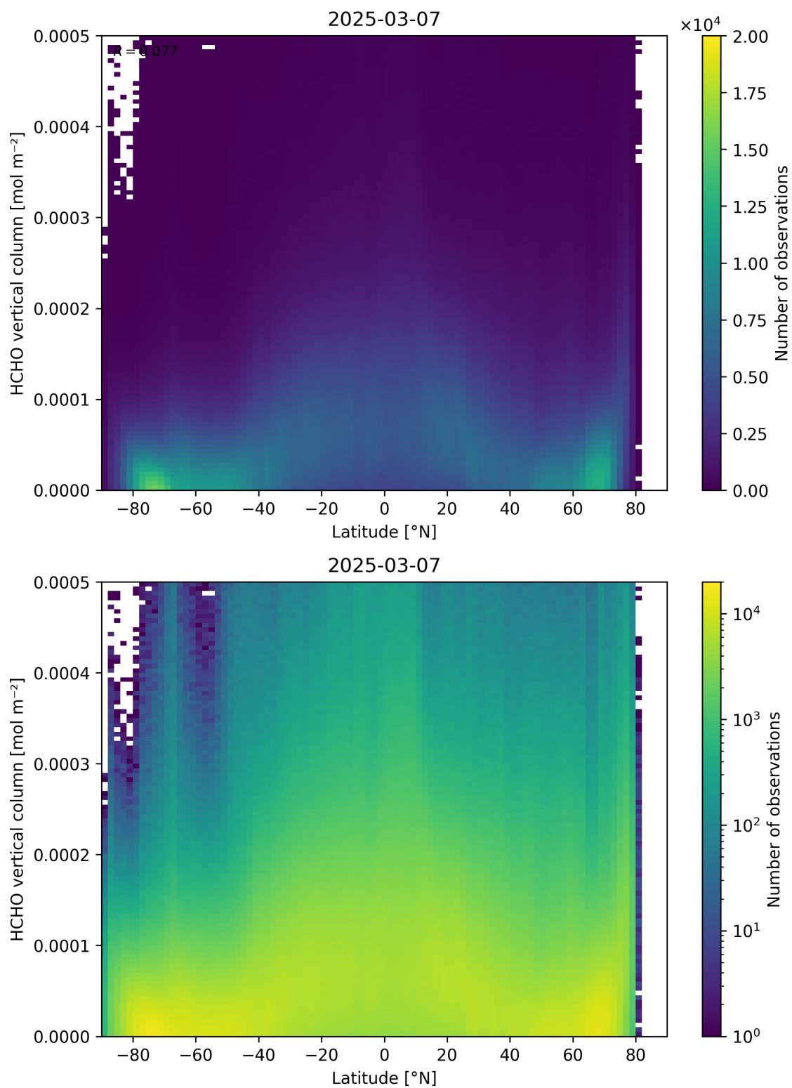
Figure 163: Scatter density plot of “Latitude” against “HCHO vertical column” for 2025-03-07 to 2025-03-08.
