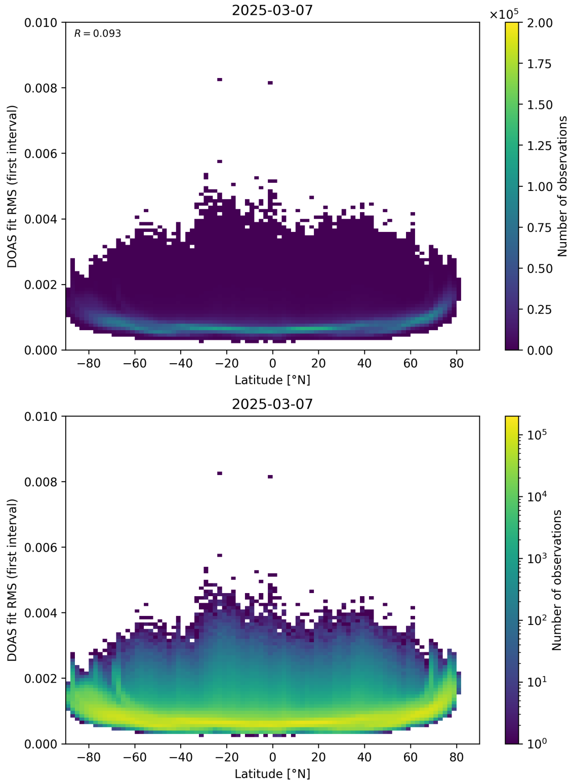
Figure 153: Scatter density plot of “Latitude” against “DOAS fit RMS (first interval)” for 2025-03-07 to 2025-03-08.
