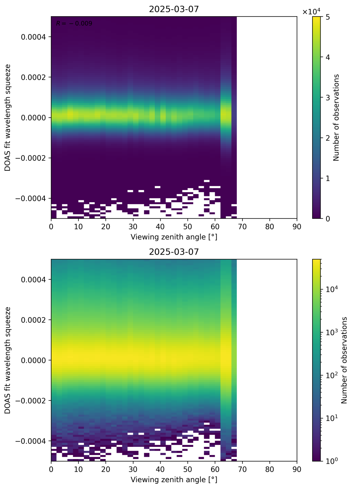
Figure 184: Scatter density plot of “Viewing zenith angle” against “DOAS fit wavelength squeeze” for 2025-03-07 to 2025-03-08.
