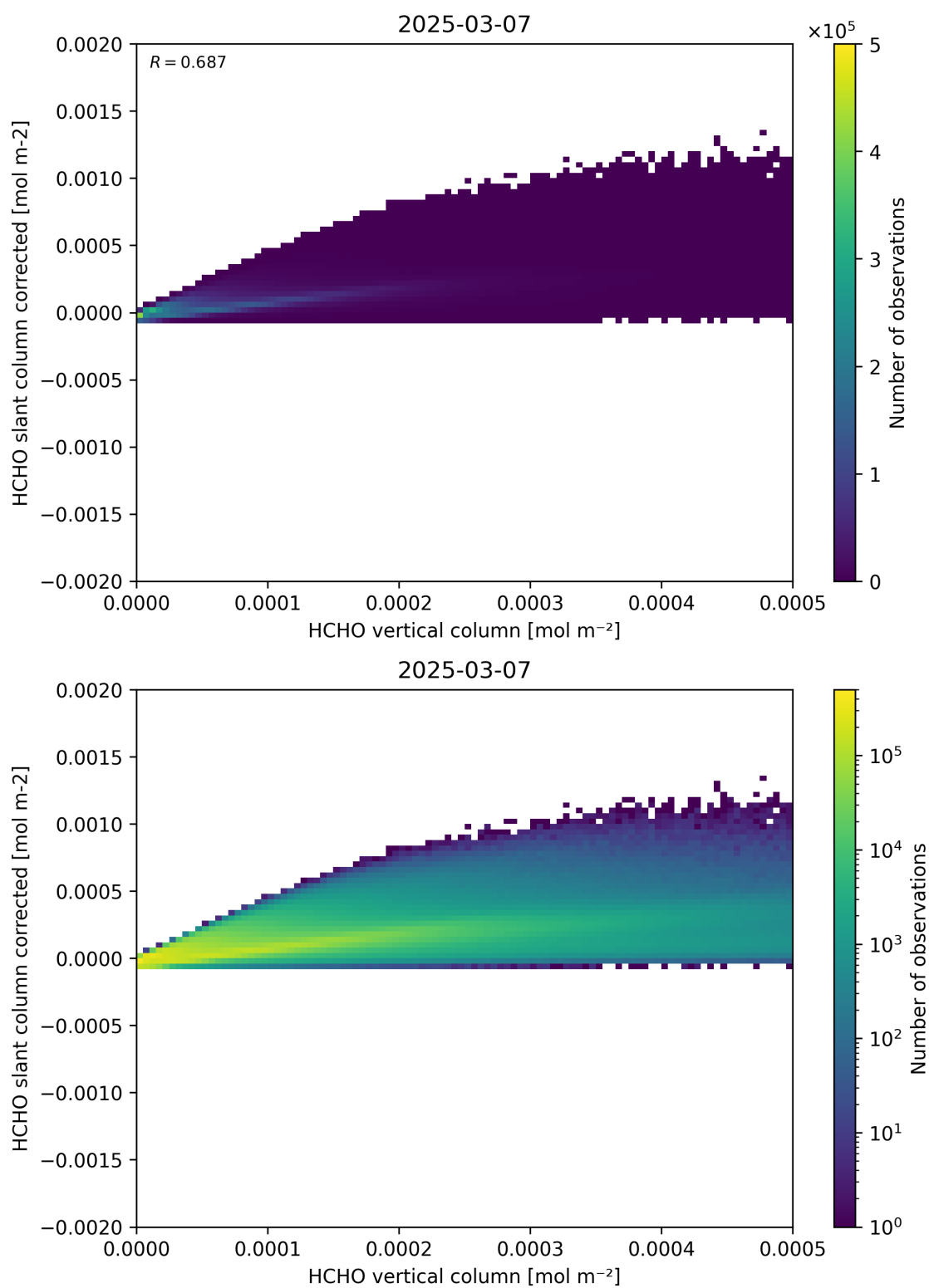
Figure 127: Scatter density plot of “HCHO vertical column” against “HCHO slant column corrected” for 2025-03-07 to 2025-03-08.
