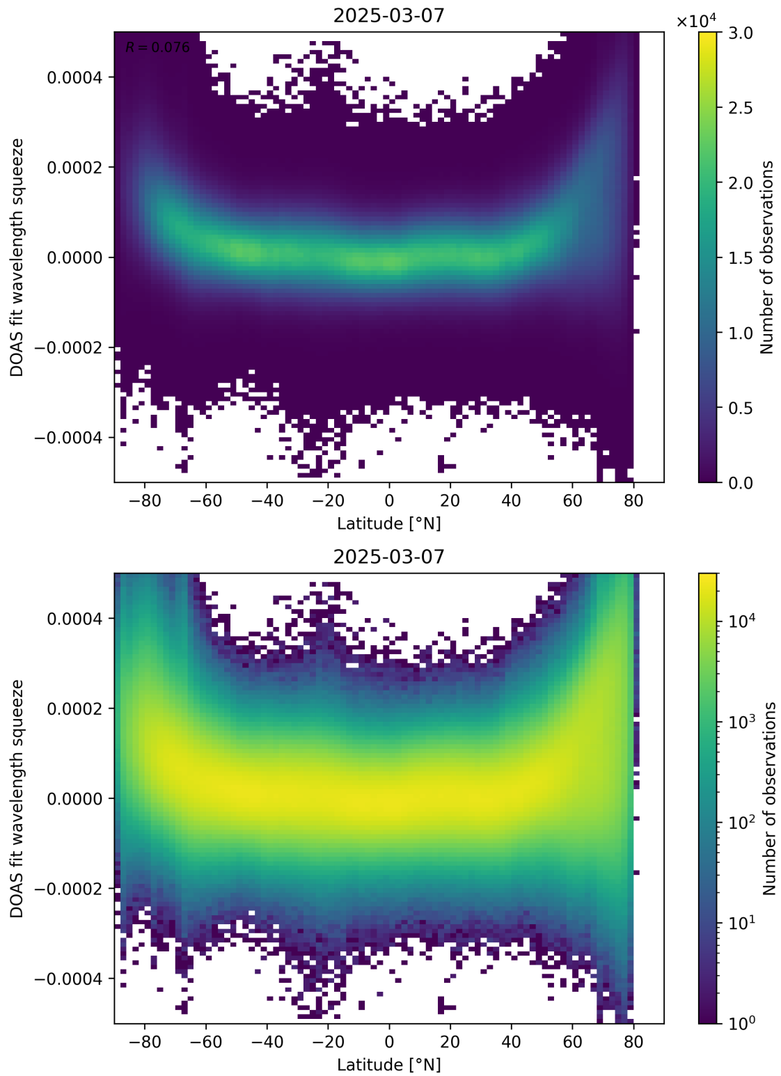
Figure 155: Scatter density plot of “Latitude” against “DOAS fit wavelength squeeze” for 2025-03-07 to 2025-03-08.
