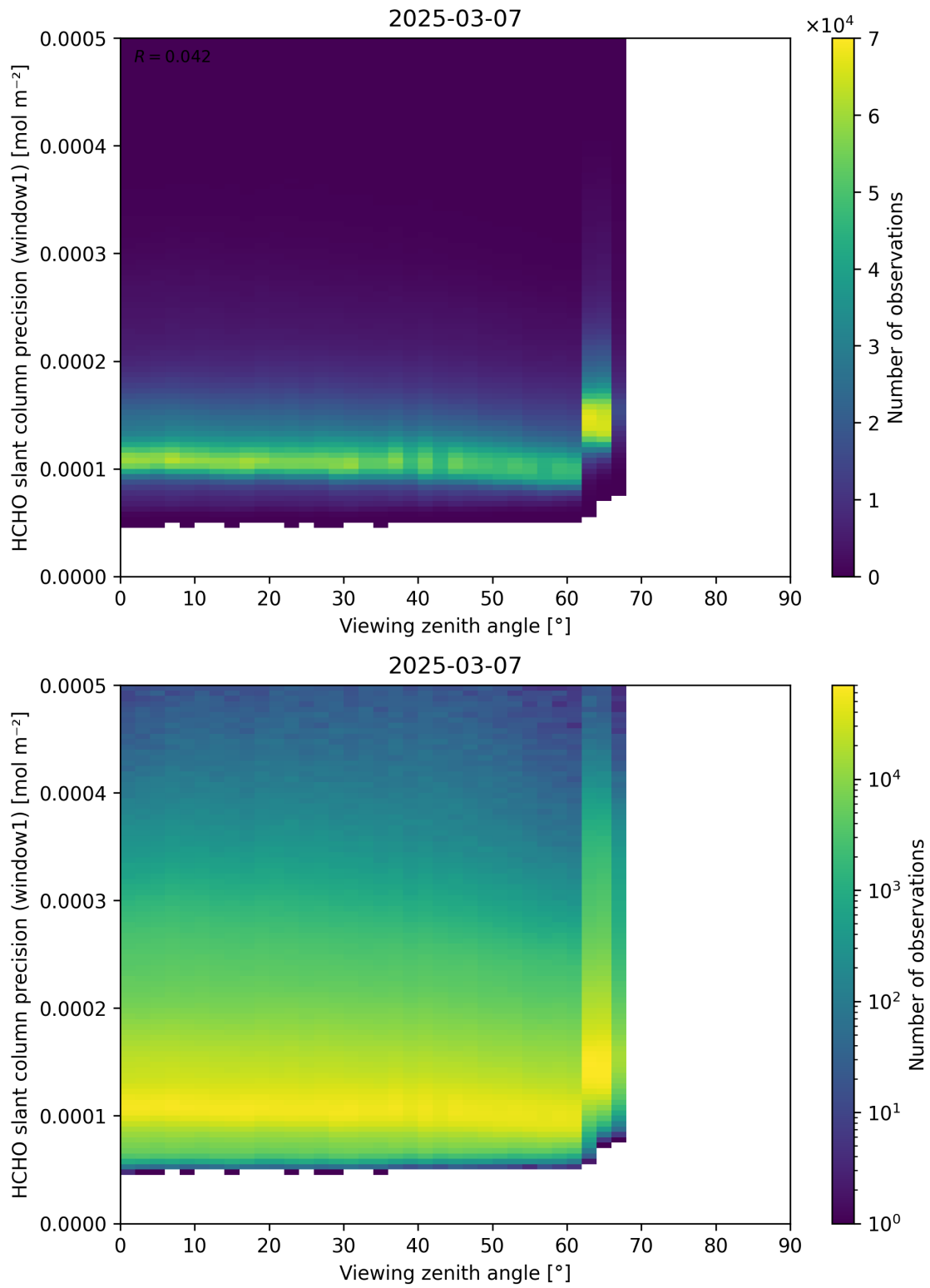
Figure 189: Scatter density plot of “Viewing zenith angle” against “HCHO slant column precision (window1)” for 2025-03-07 to 2025-03-08.
