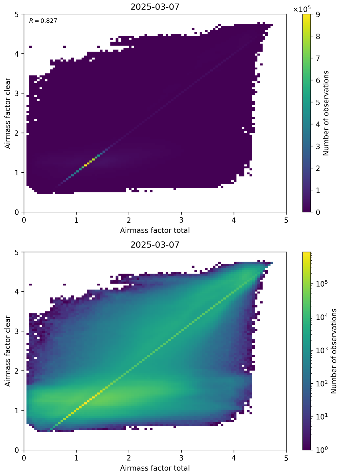
Figure 100: Scatter density plot of “Airmass factor total” against “Airmass factor clear” for 2025-03-07 to 2025-03-08.
