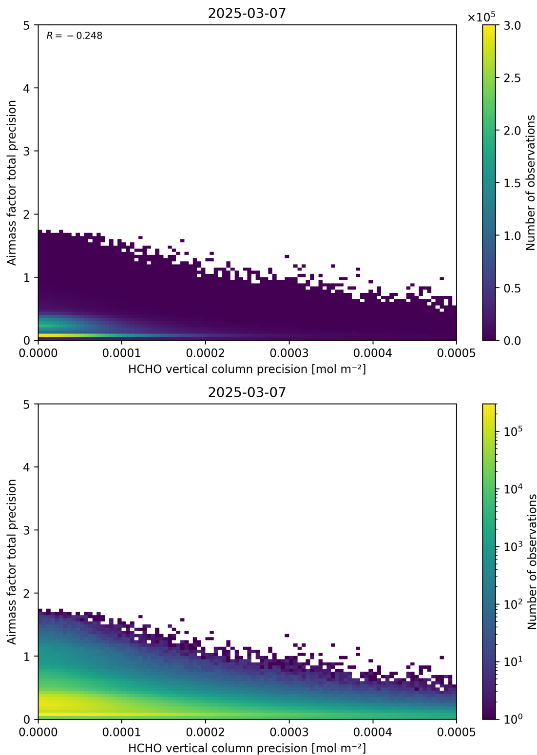
Figure 145: Scatter density plot of “HCHO vertical column precision” against “Airmass factor total precision” for 2025-03-07 to 2025-03-08.
