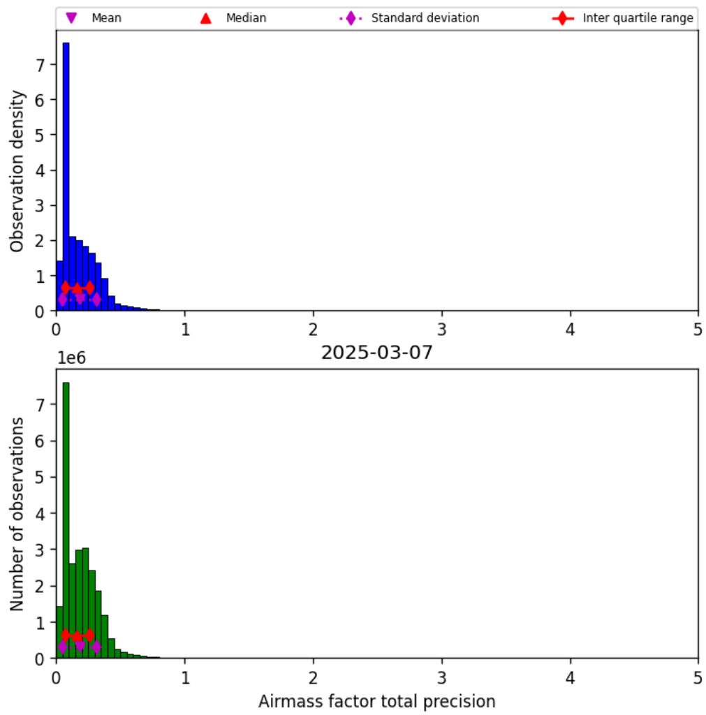
Figure 41: Histogram of “Airmass factor total precision” for 2025-03-07 to 2025-03-08
