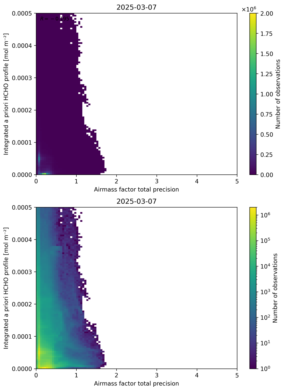
Figure 111: Scatter density plot of “Airmass factor total precision” against “Integrated a priori HCHO profile” for 2025-03-07 to 2025-03-08.
