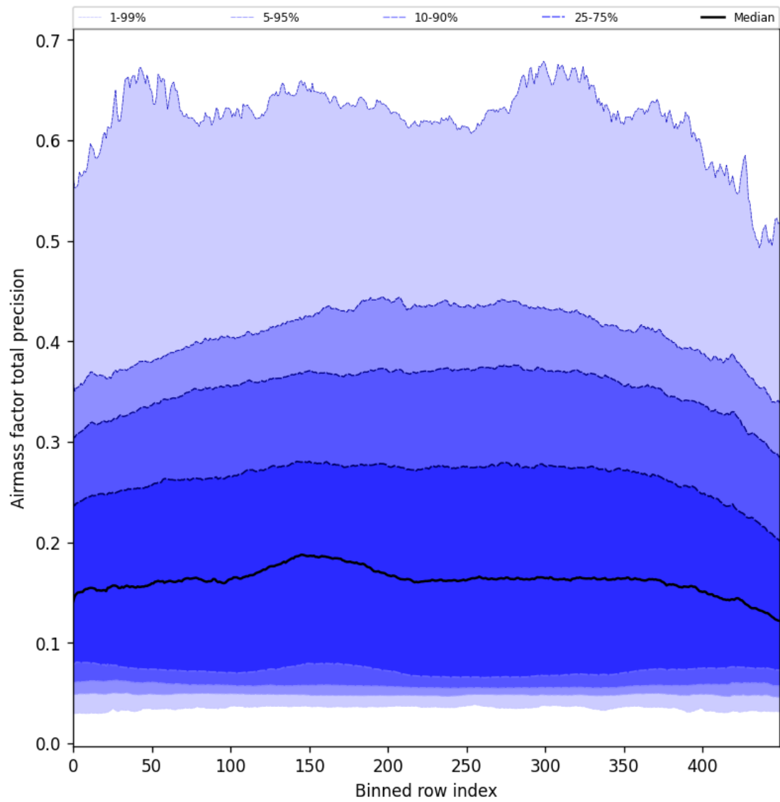
Figure 55: Along track statistics of “Airmass factor total precision” for 2025-03-07 to 2025-03-08
