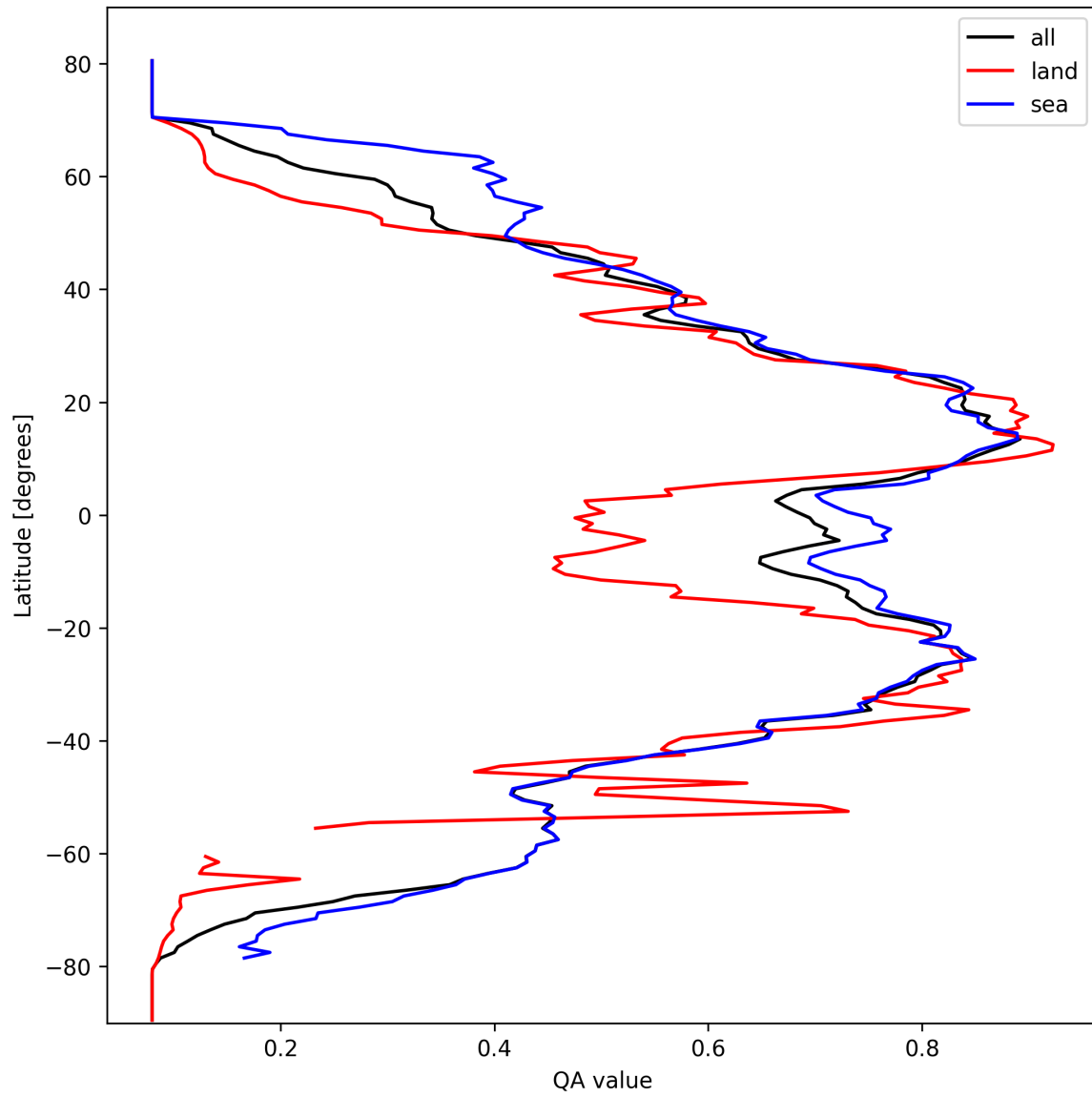
Figure 20: Zonal average of “QA value” for 2025-03-07 to 2025-03-08.
