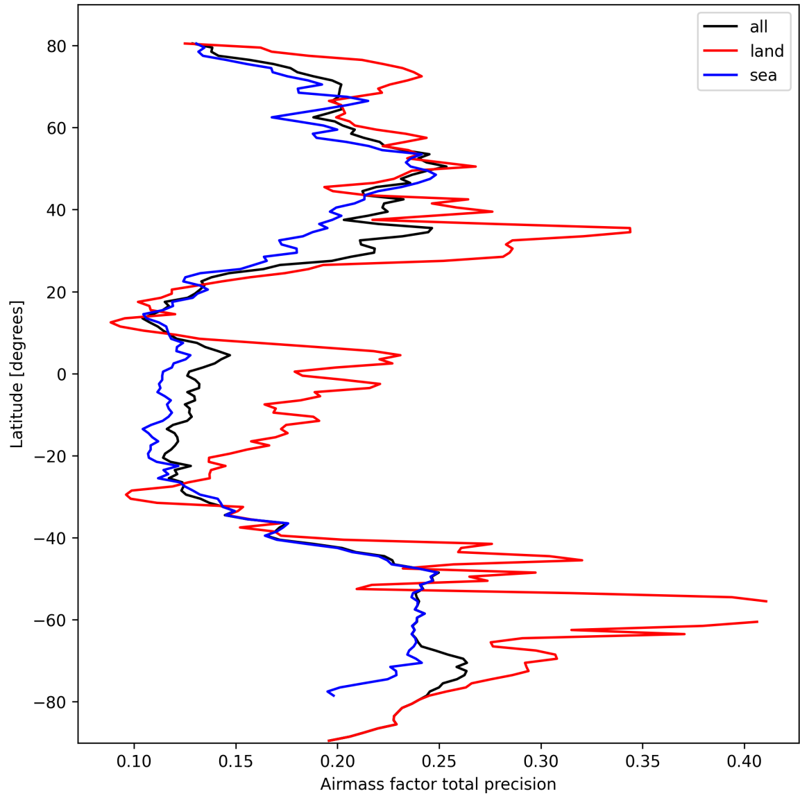
Figure 27: Zonal average of “Airmass factor total precision” for 2025-03-07 to 2025-03-08.
