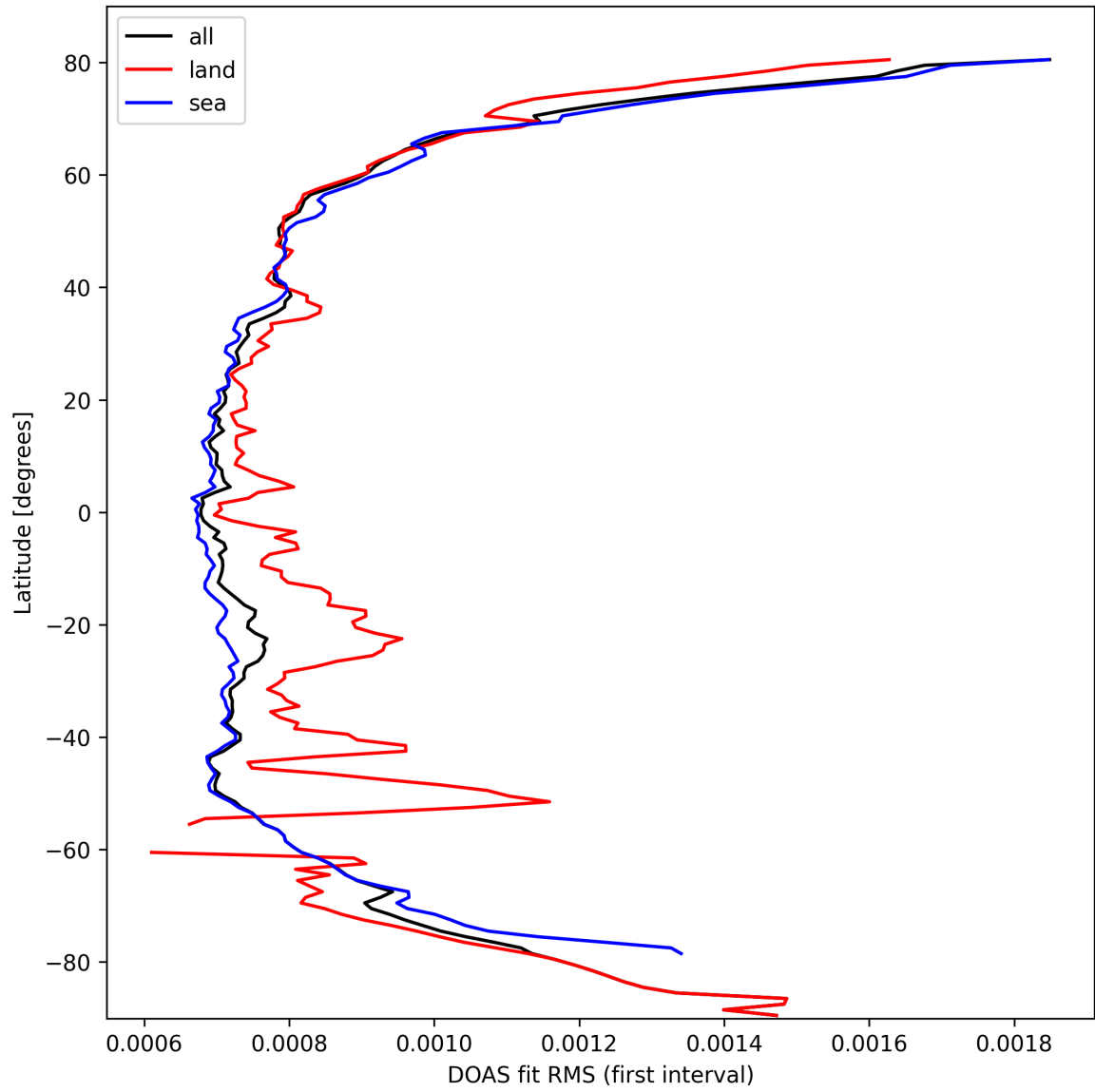
Figure 32: Zonal average of “DOAS fit RMS (first interval)” for 2025-03-07 to 2025-03-08.
