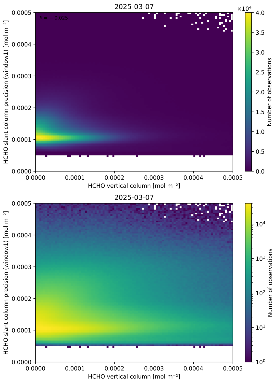
Figure 130: Scatter density plot of “HCHO vertical column” against “HCHO slant column precision (window1)” for 2025-03-07 to 2025-03-08.
