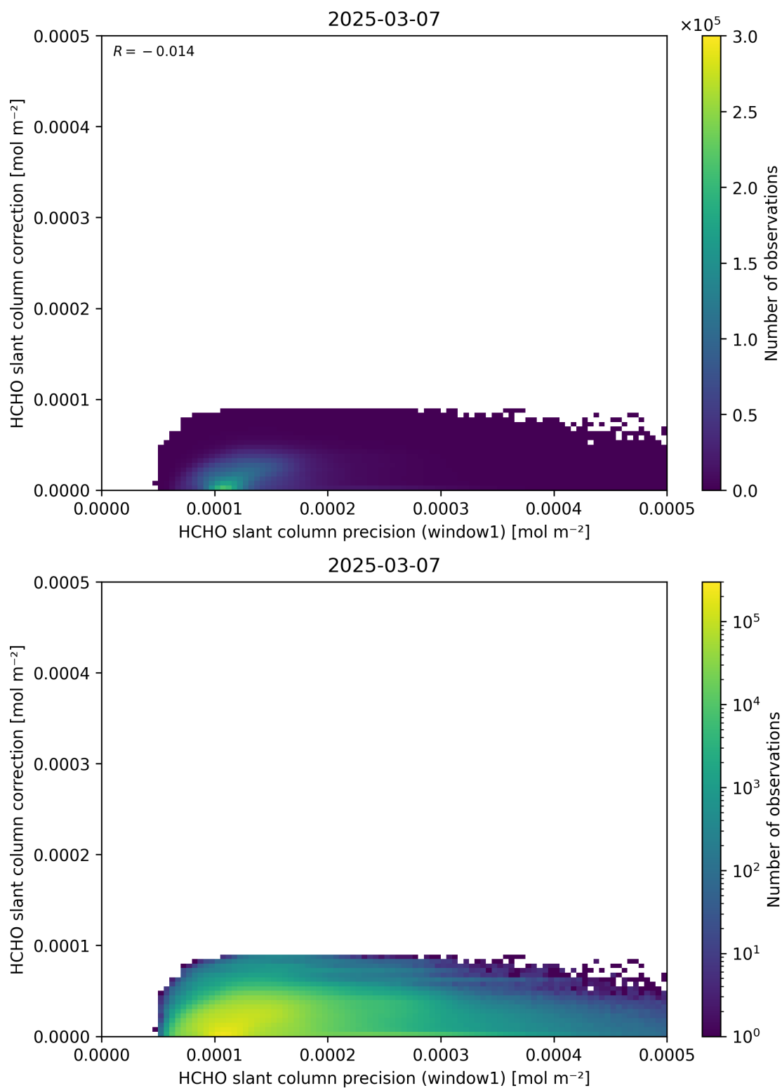
Figure 93: Scatter density plot of “HCHO slant column precision (window1)” against “HCHO slant column correction” for 2025-03-07 to 2025-03-08.
