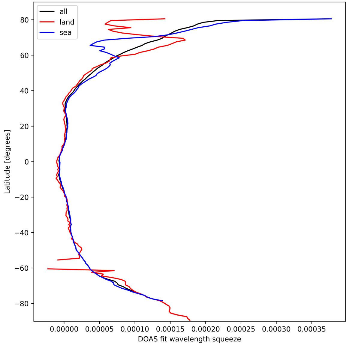
Figure 31: Zonal average of “DOAS fit wavelength squeeze” for 2025-03-07 to 2025-03-08.
