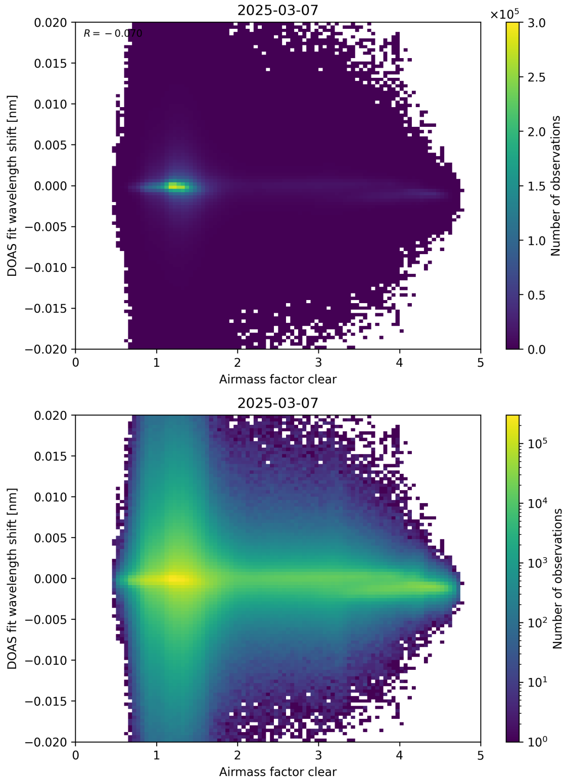
Figure 72: Scatter density plot of “Airmass factor clear” against “DOAS fit wavelength shift” for 2025-03-07 to 2025-03-08.
