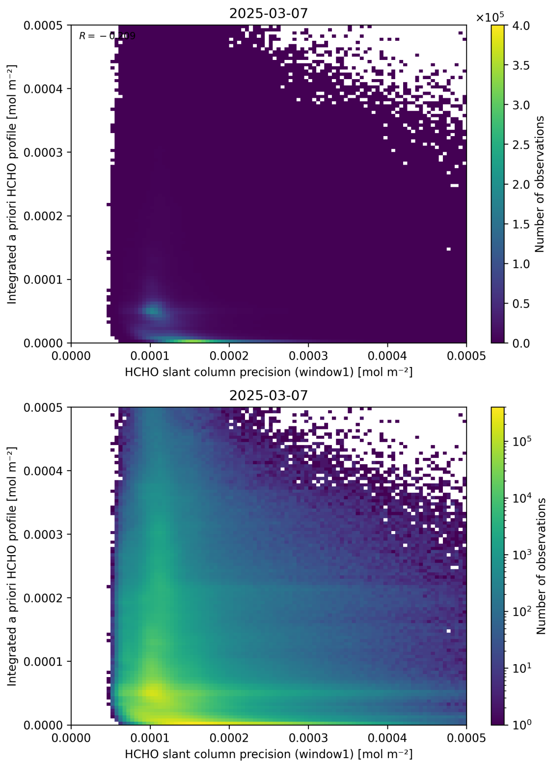
Figure 96: Scatter density plot of “HCHO slant column precision (window1)” against “Integrated a priori HCHO profile” for 2025-03-07 to 2025-03-08.
