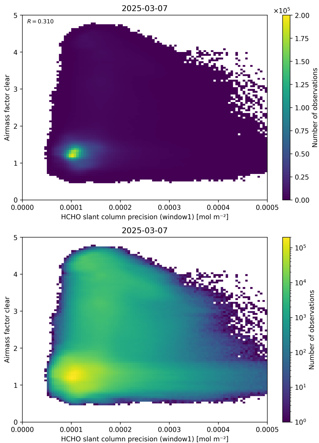
Figure 91: Scatter density plot of “HCHO slant column precision (window1)” against “Airmass factor clear” for 2025-03-07 to 2025-03-08.
