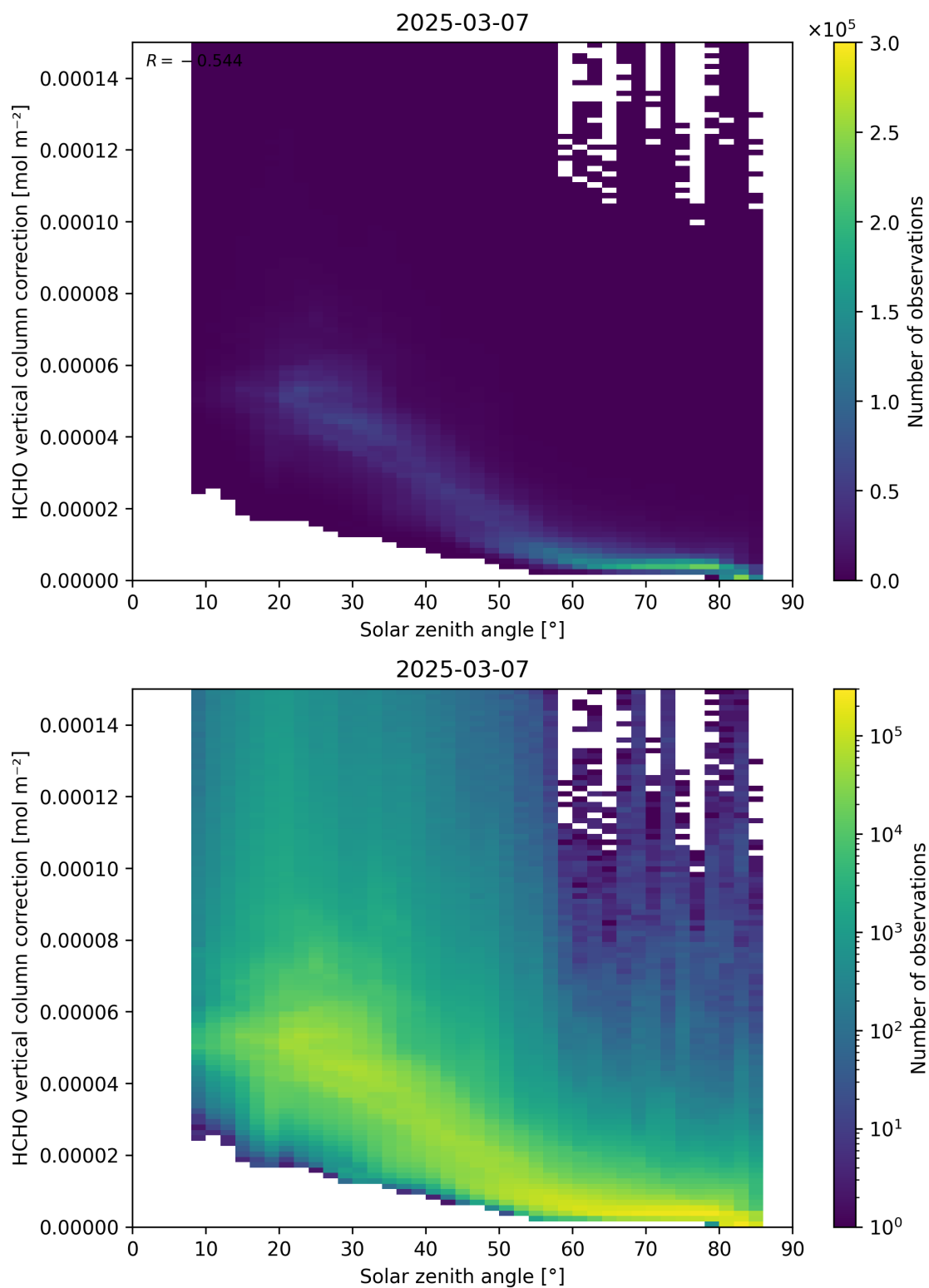
Figure 178: Scatter density plot of “Solar zenith angle” against “HCHO vertical column correction” for 2025-03-07 to 2025-03-08.
