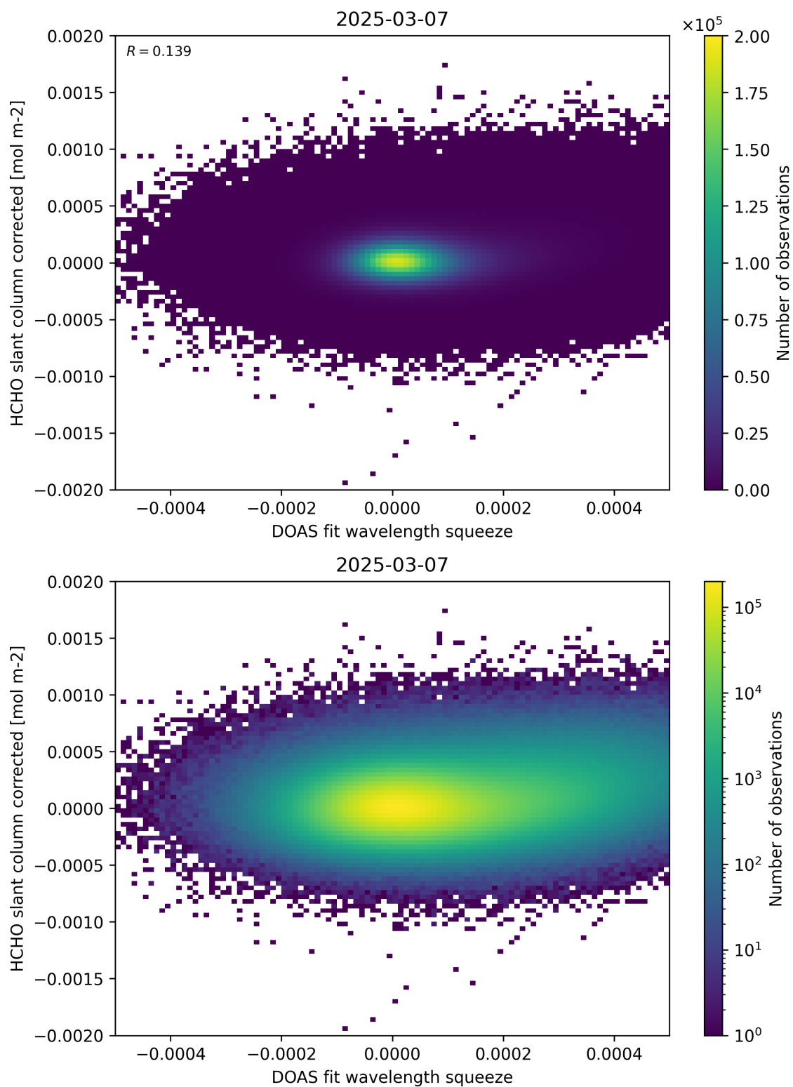
Figure 69: Scatter density plot of “DOAS fit wavelength squeeze” against “HCHO slant column corrected” for 2025-03-07 to 2025-03-08.
