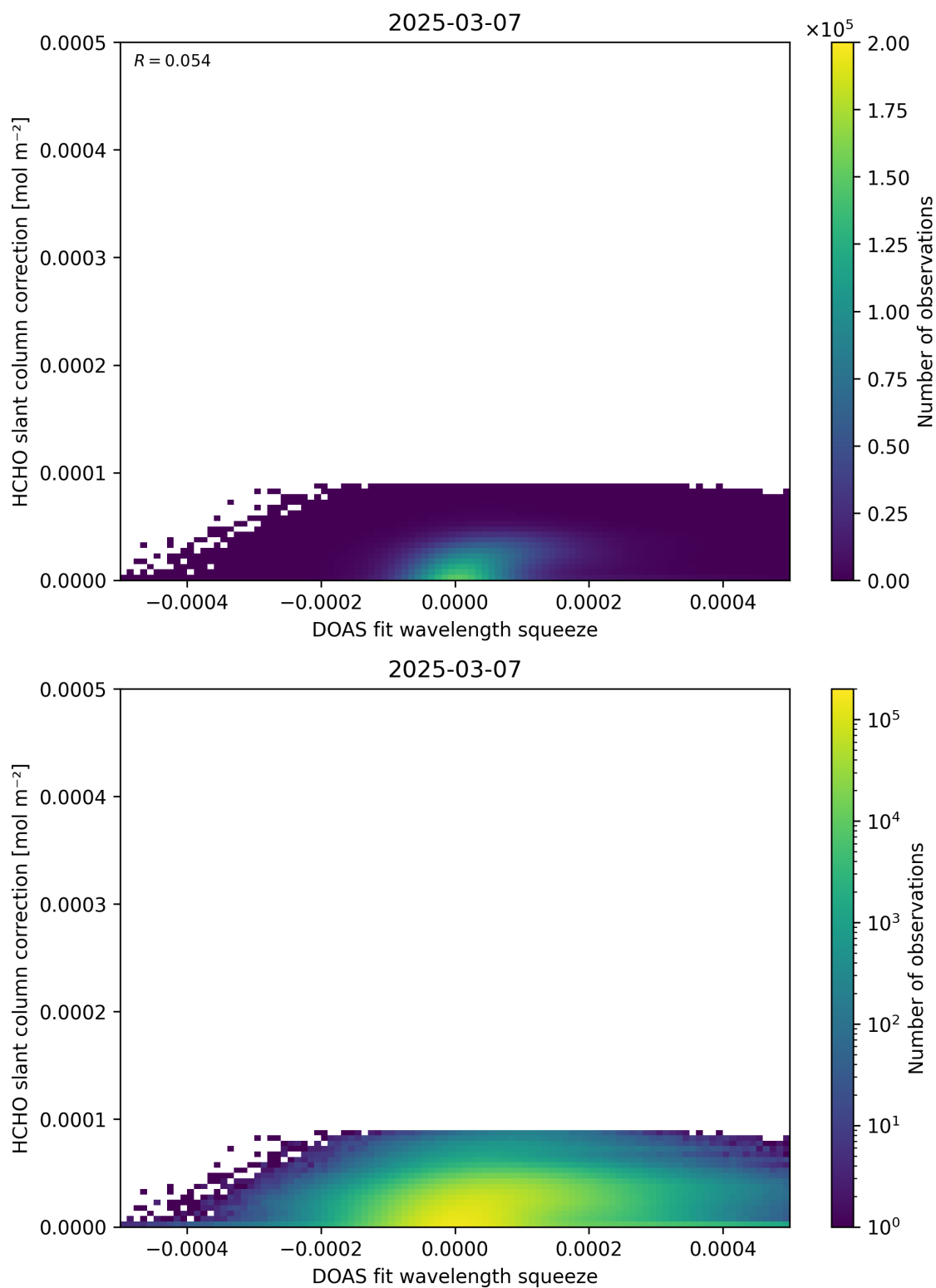
Figure 70: Scatter density plot of “DOAS fit wavelength squeeze” against “HCHO slant column correction” for 2025-03-07 to 2025-03-08.
