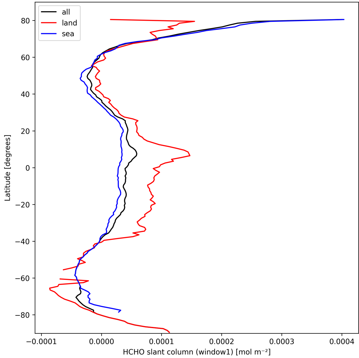
Figure 24: Zonal average of “HCHO slant column (window1)” for 2025-03-07 to 2025-03-08.
