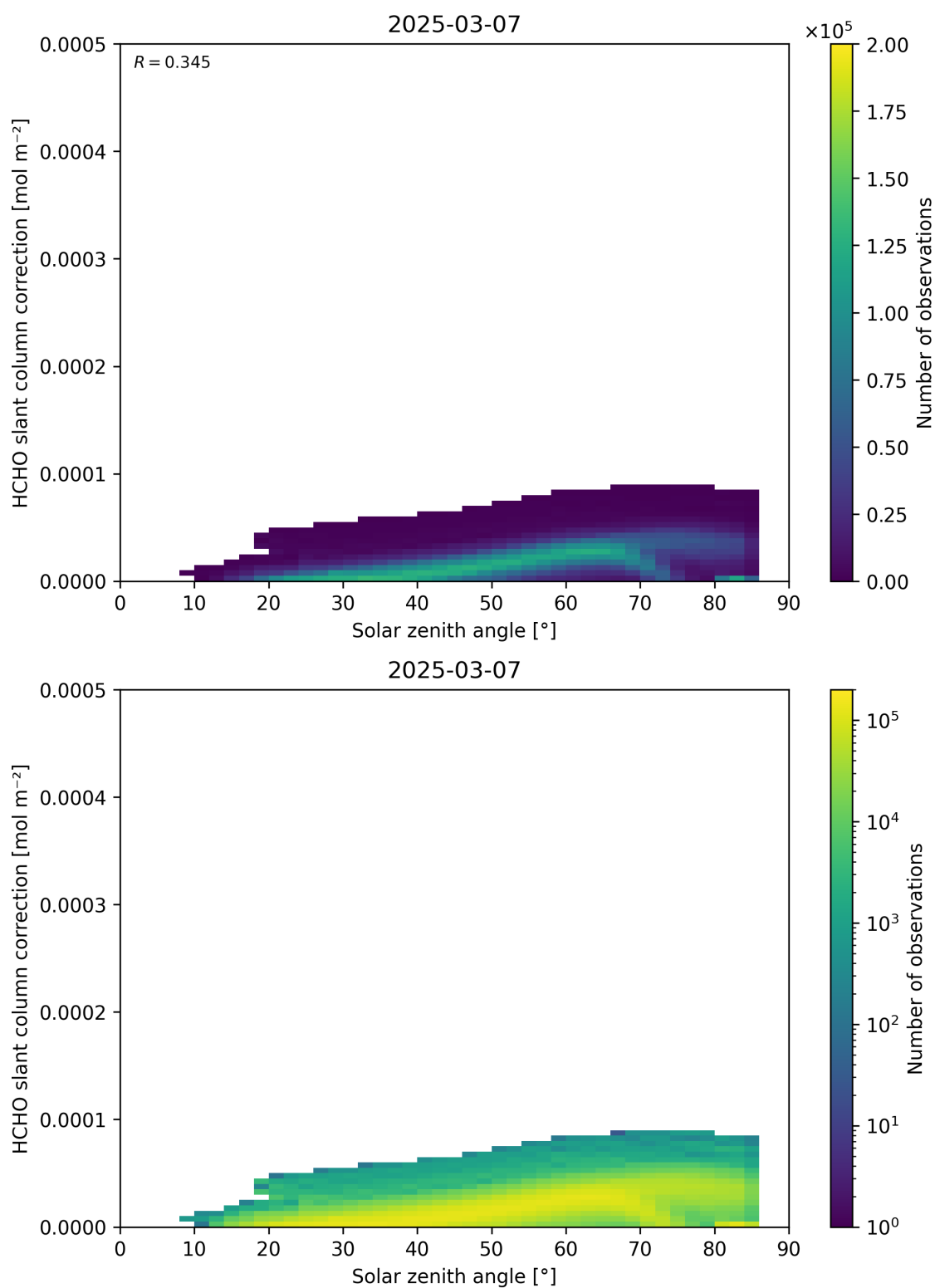
Figure 172: Scatter density plot of “Solar zenith angle” against “HCHO slant column correction” for 2025-03-07 to 2025-03-08.
