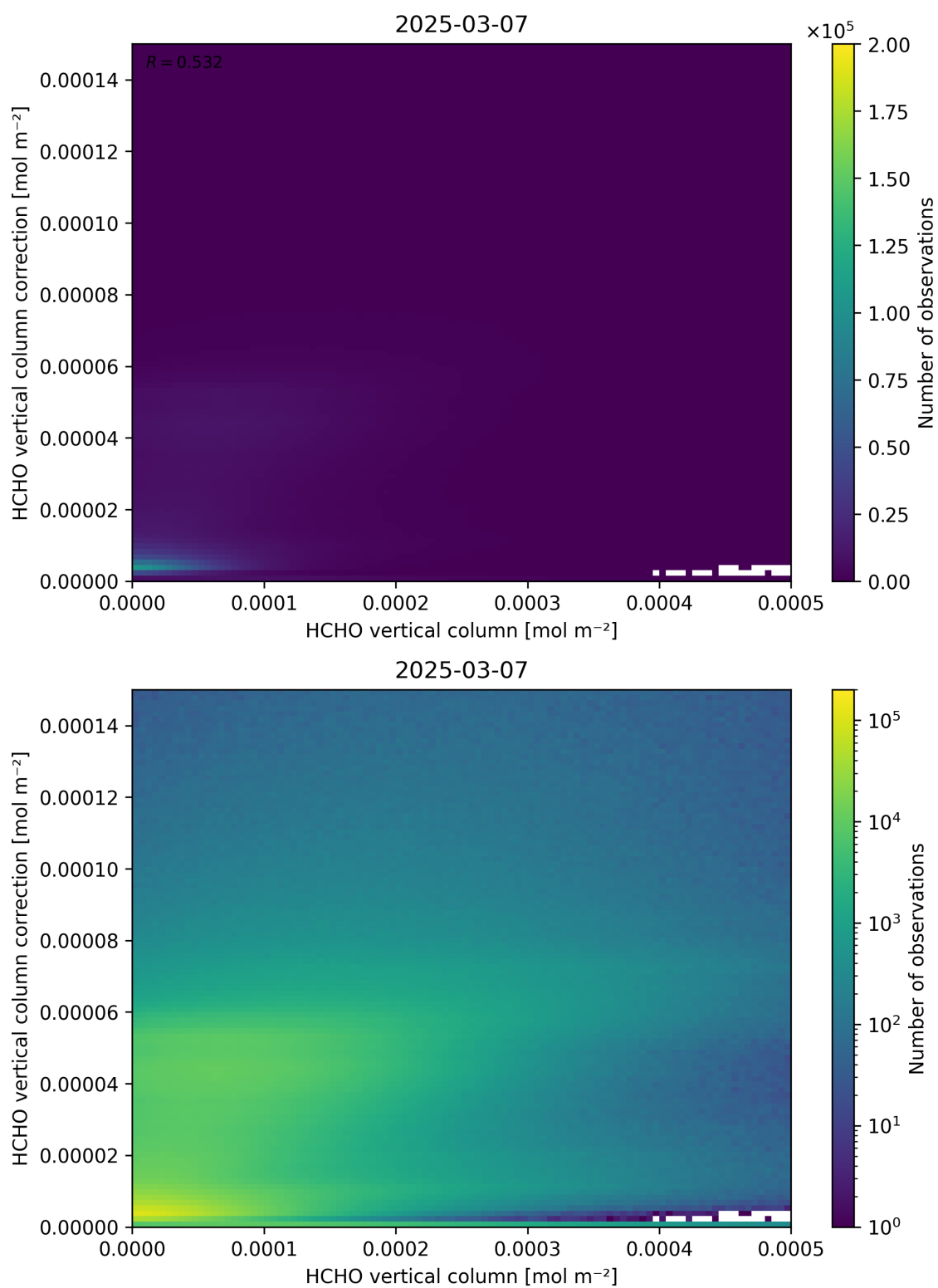
Figure 133: Scatter density plot of “HCHO vertical column” against “HCHO vertical column correction” for 2025-03-07 to 2025-03-08.
