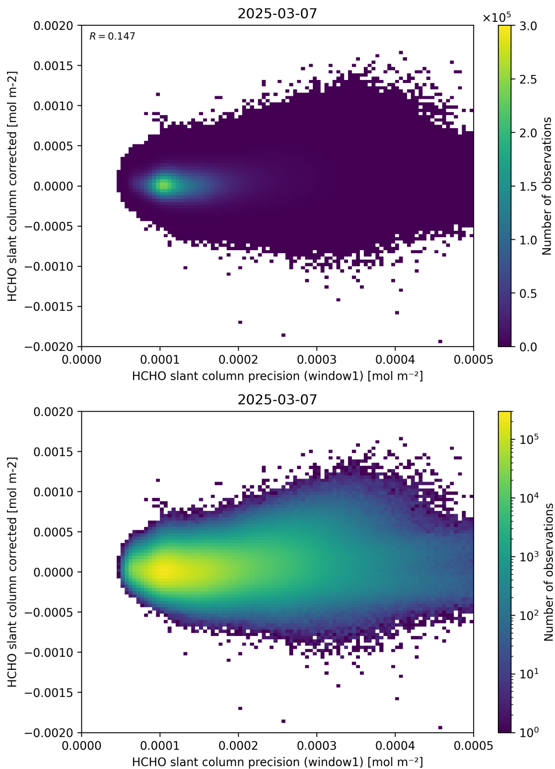
Figure 92: Scatter density plot of “HCHO slant column precision (window1)” against “HCHO slant column corrected” for 2025-03-07 to 2025-03-08.
