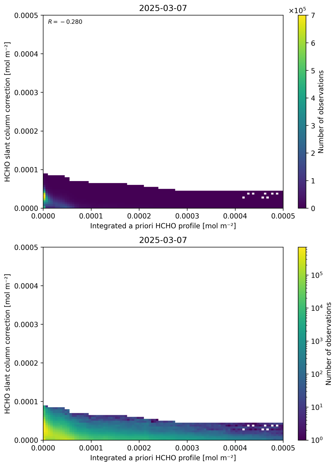
Figure 152: Scatter density plot of “Integrated a priori HCHO profile” against “HCHO slant column correction” for 2025-03-07 to 2025-03-08.
