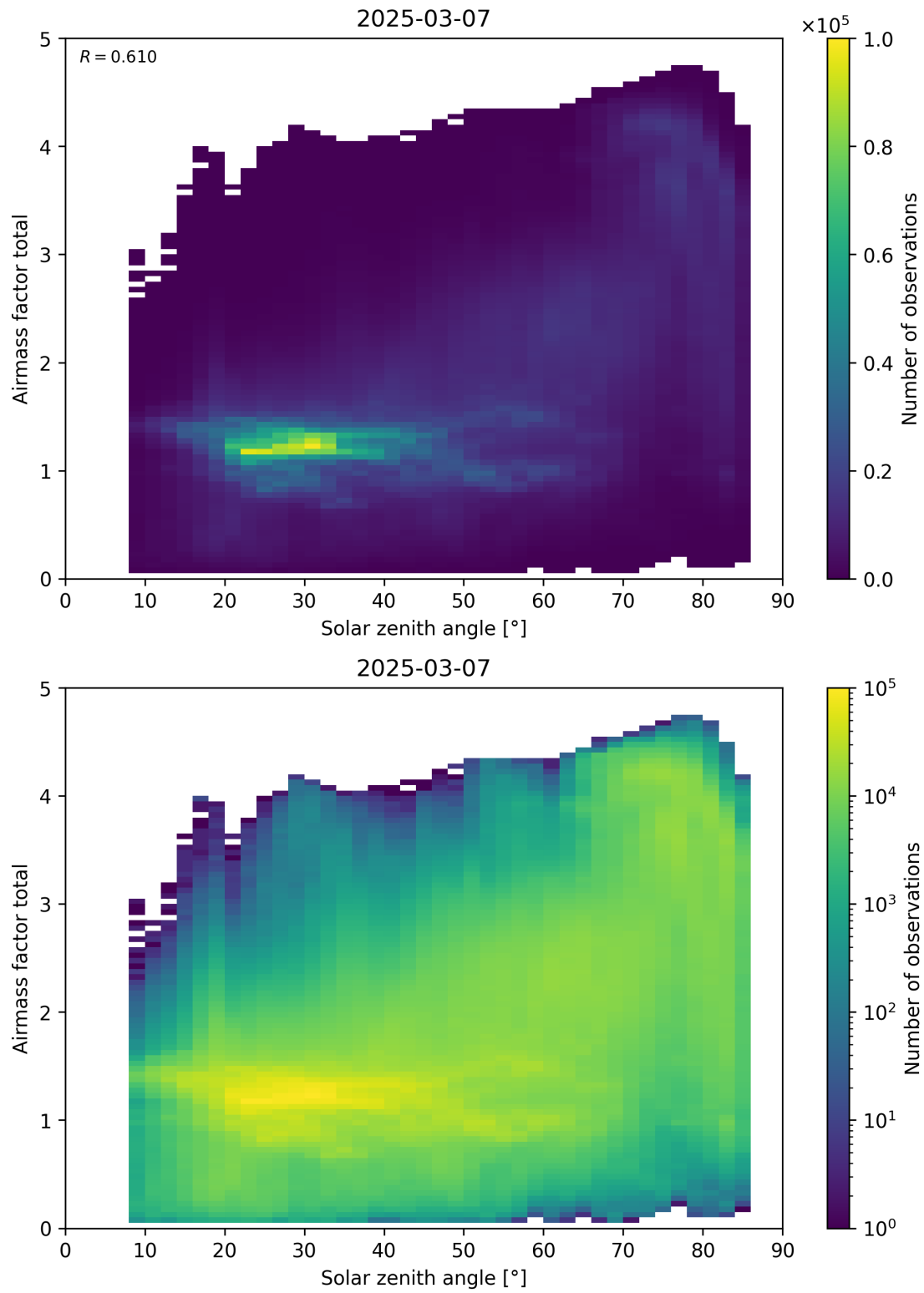
Figure 175: Scatter density plot of “Solar zenith angle” against “Airmass factor total” for 2025-03-07 to 2025-03-08.
