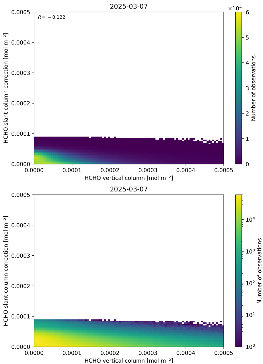
Figure 128: Scatter density plot of “HCHO vertical column” against “HCHO slant column correction” for 2025-03-07 to 2025-03-08.
