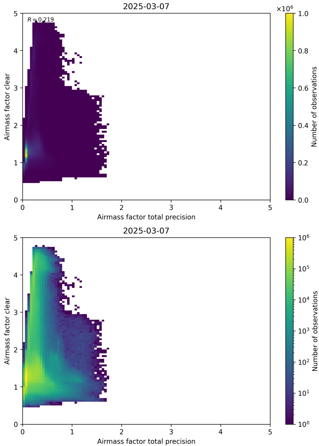
Figure 108: Scatter density plot of “Airmass factor total precision” against “Airmass factor clear” for 2025-03-07 to 2025-03-08.
