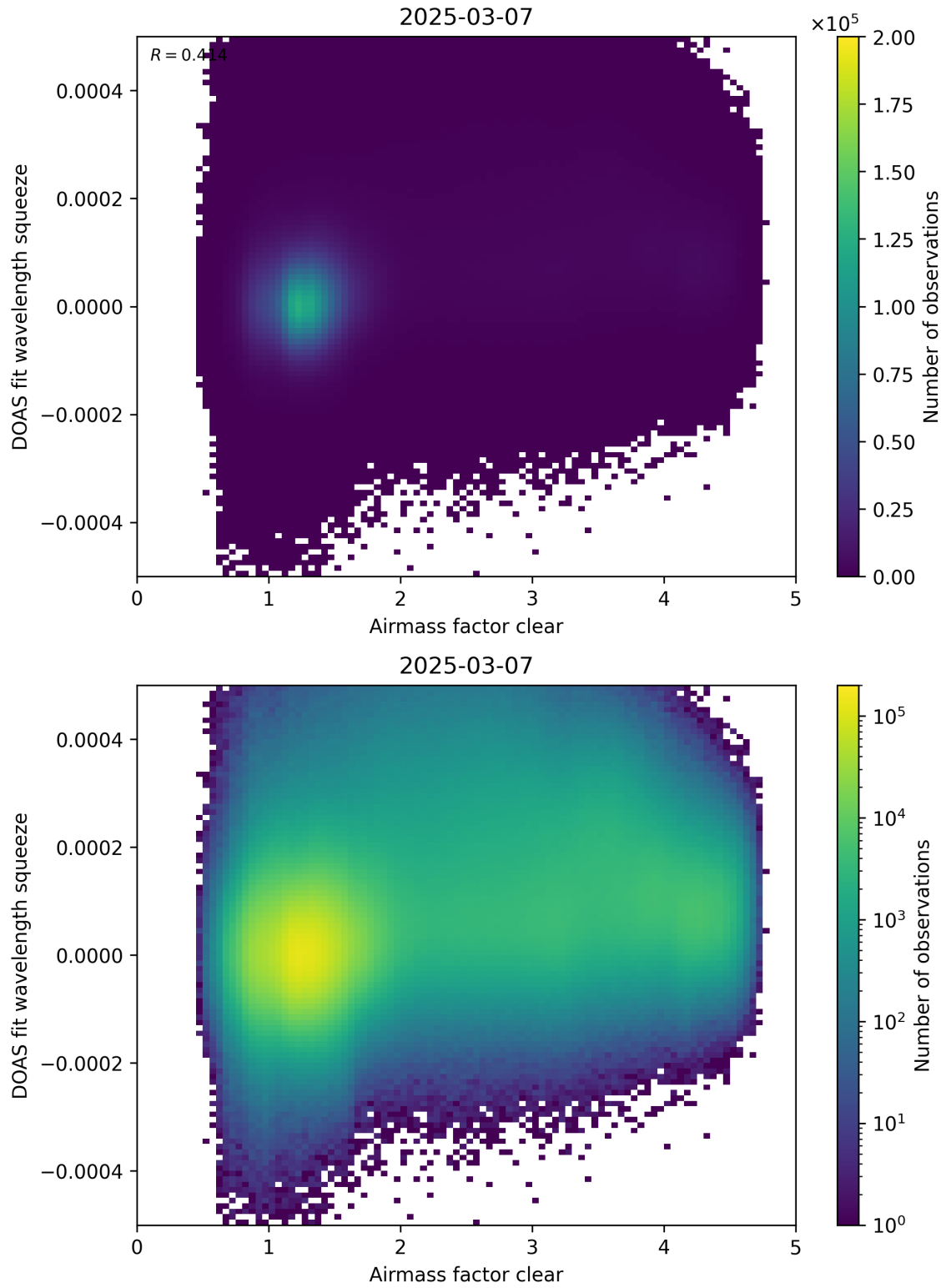
Figure 73: Scatter density plot of “Airmass factor clear” against “DOAS fit wavelength squeeze” for 2025-03-07 to 2025-03-08.
