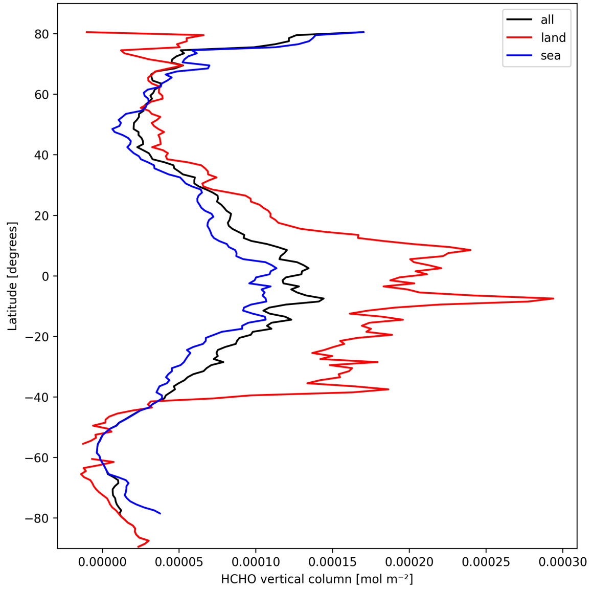
Figure 21: Zonal average of “HCHO vertical column” for 2025-03-07 to 2025-03-08.
