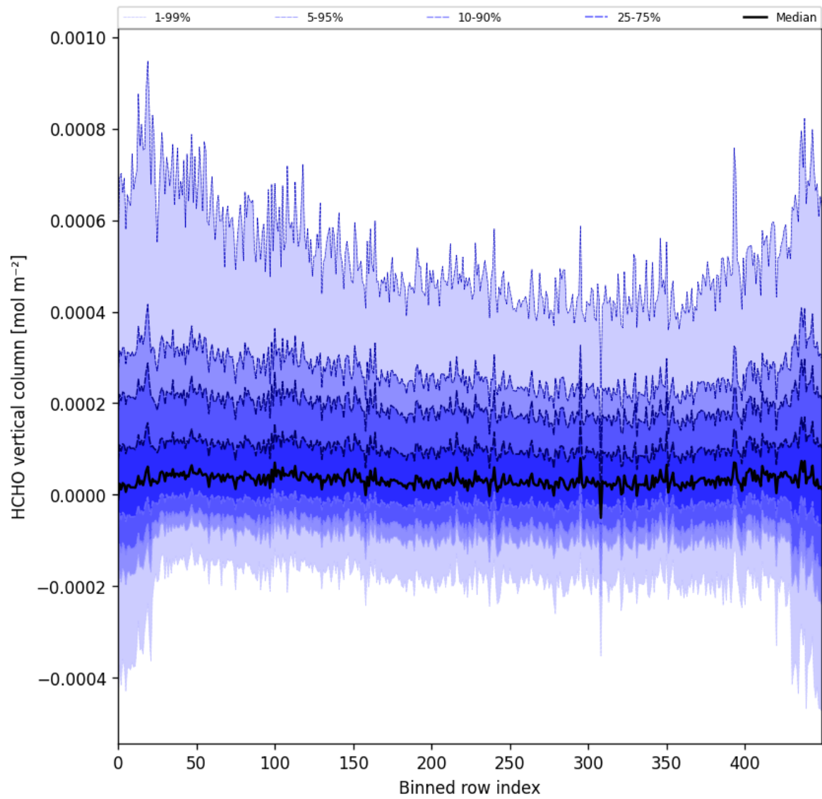
Figure 49: Along track statistics of “HCHO vertical column” for 2025-03-07 to 2025-03-08
