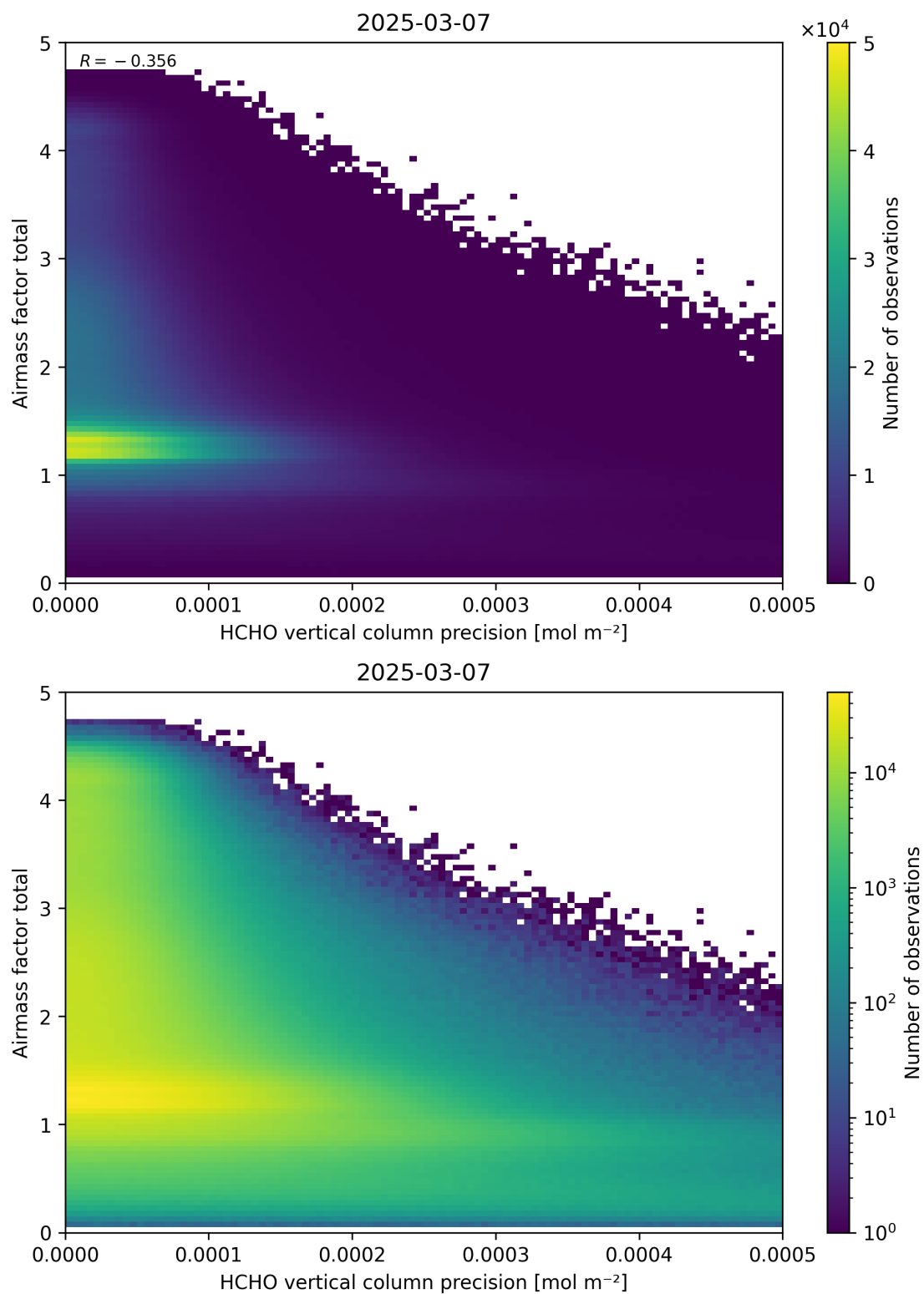
Figure 144: Scatter density plot of “HCHO vertical column precision” against “Airmass factor total” for 2025-03-07 to 2025-03-08.
