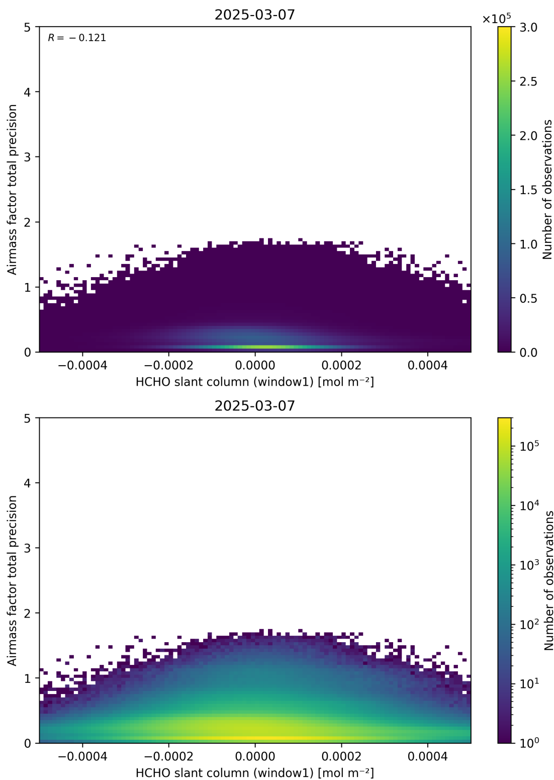
Figure 86: Scatter density plot of “HCHO slant column (window1)” against “Airmass factor total precision” for 2025-03-07 to 2025-03-08.
