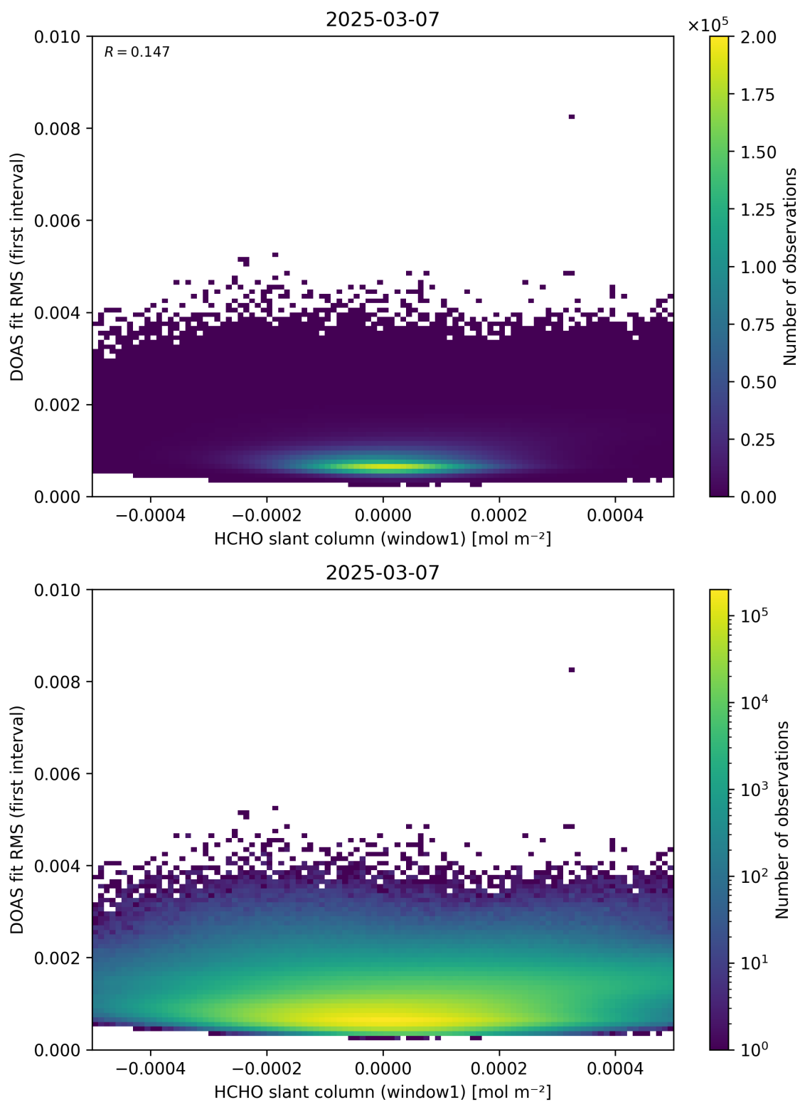
Figure 78: Scatter density plot of “HCHO slant column (window1)” against “DOAS fit RMS (first interval)” for 2025-03-07 to 2025-03-08.
