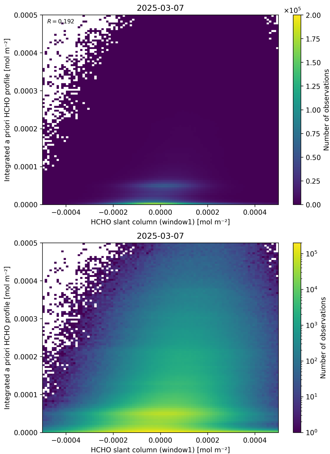
Figure 87: Scatter density plot of “HCHO slant column (window1)” against “Integrated a priori HCHO profile” for 2025-03-07 to 2025-03-08.
