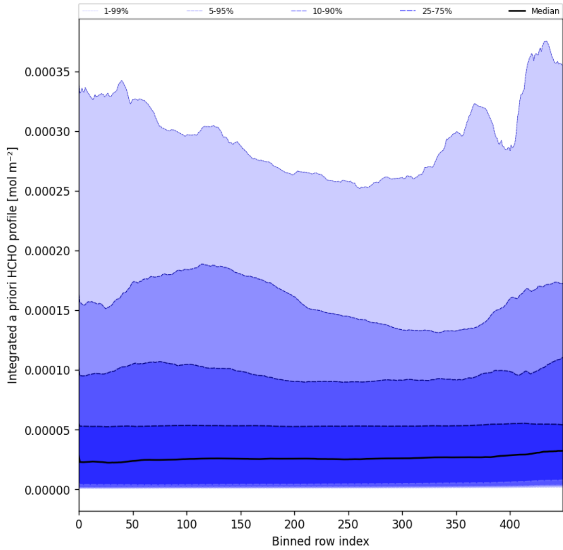
Figure 57: Along track statistics of "Integrated a priori HCHO profile" for 2025-03-07 to 2025-03-08
