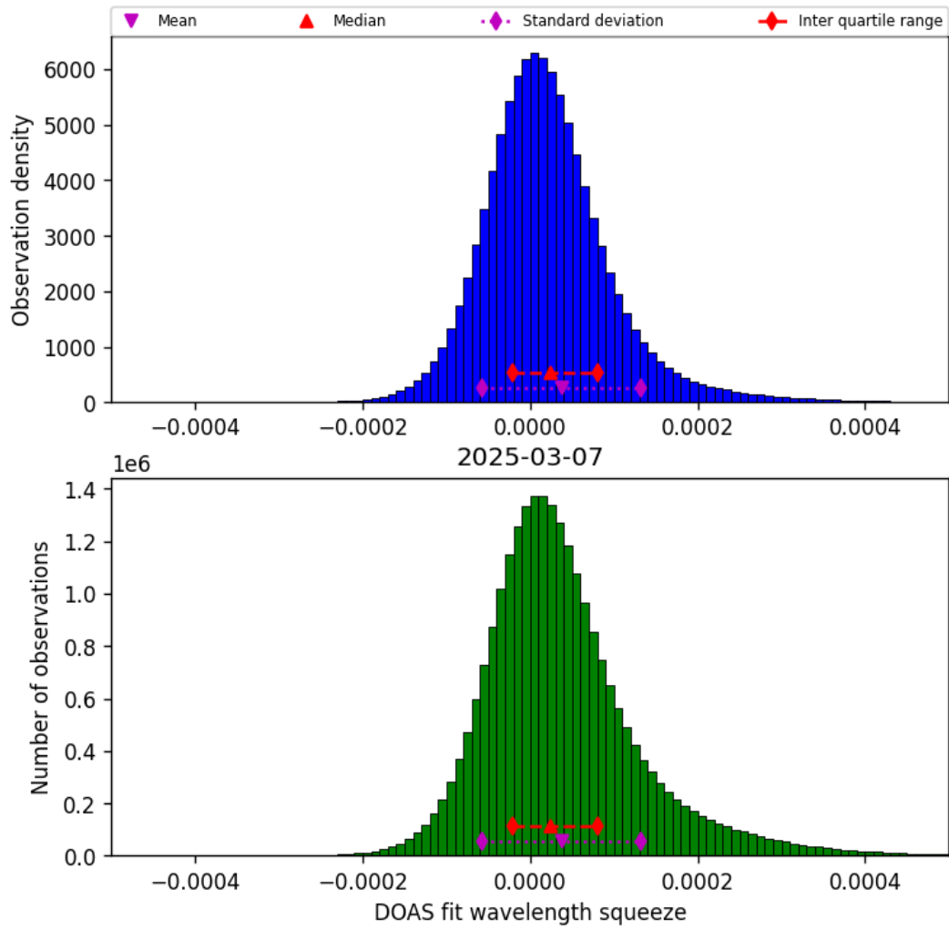
Figure 45: Histogram of “DOAS fit wavelength squeeze” for 2025-03-07 to 2025-03-08
