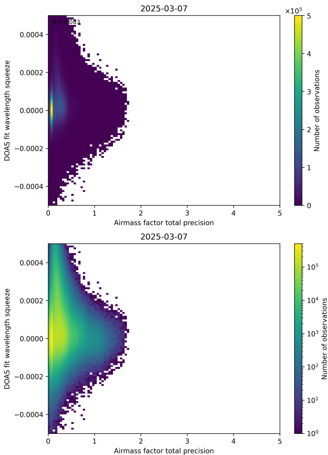
Figure 107: Scatter density plot of “Airmass factor total precision” against “DOAS fit wavelength squeeze” for 2025-03-07 to 2025-03-08.
