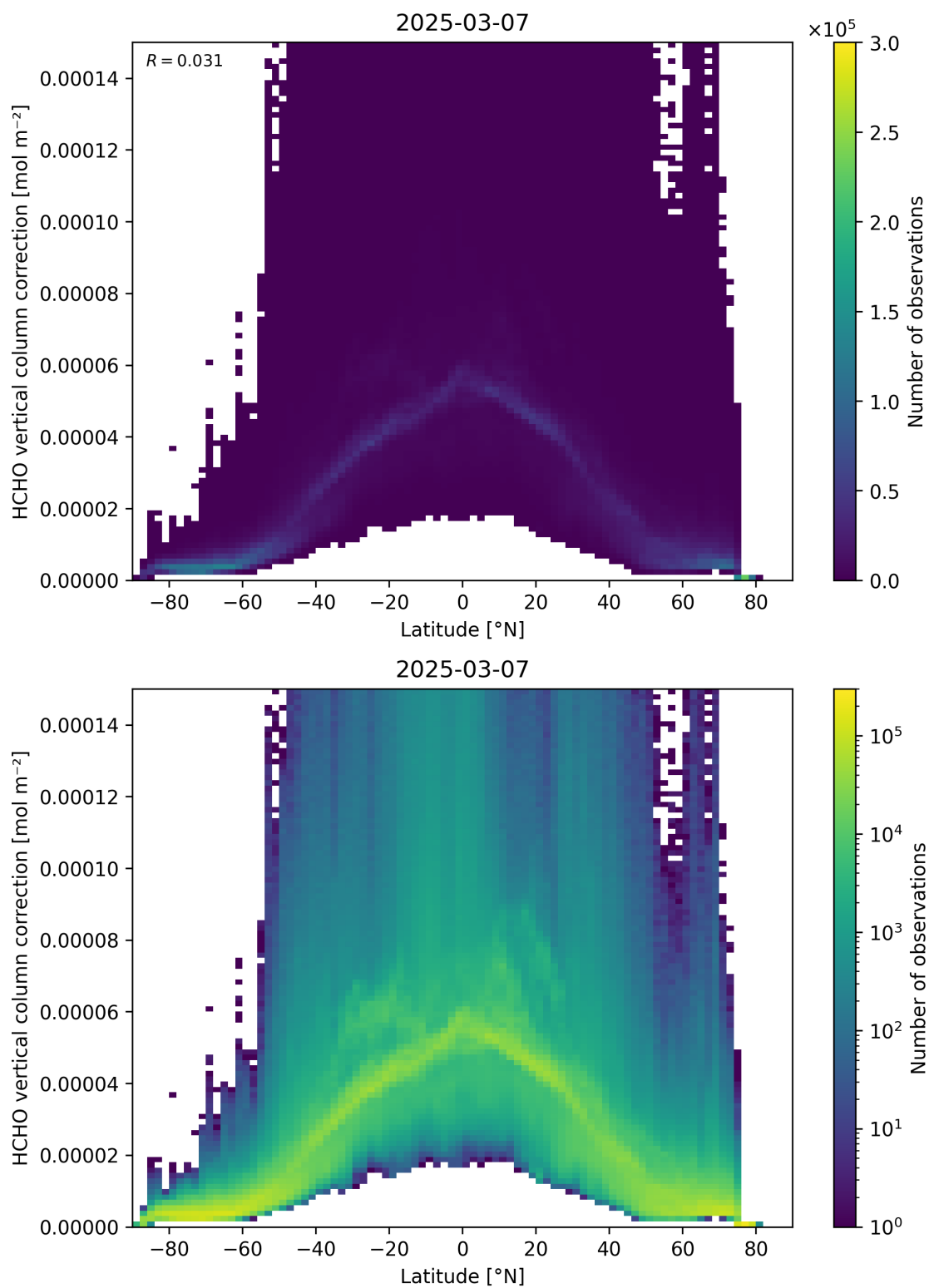
Figure 164: Scatter density plot of “Latitude” against “HCHO vertical column correction” for 2025-03-07 to 2025-03-08.
