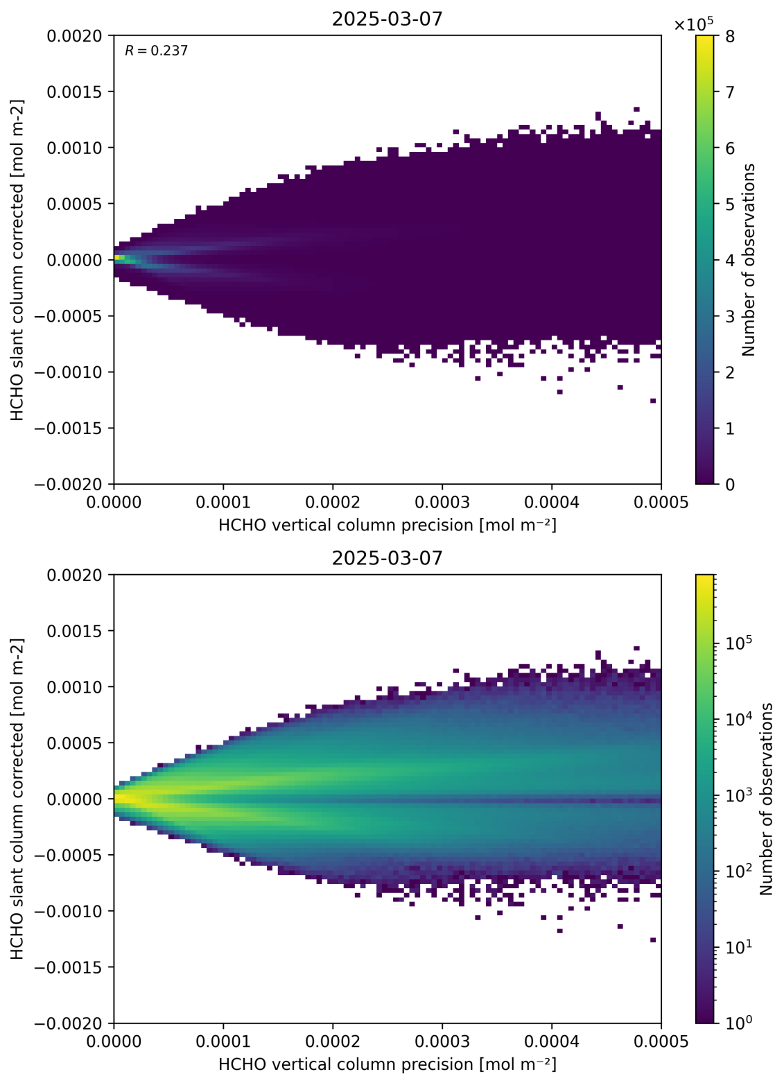
Figure 140: Scatter density plot of “HCHO vertical column precision” against “HCHO slant column corrected” for 2025-03-07 to 2025-03-08.
