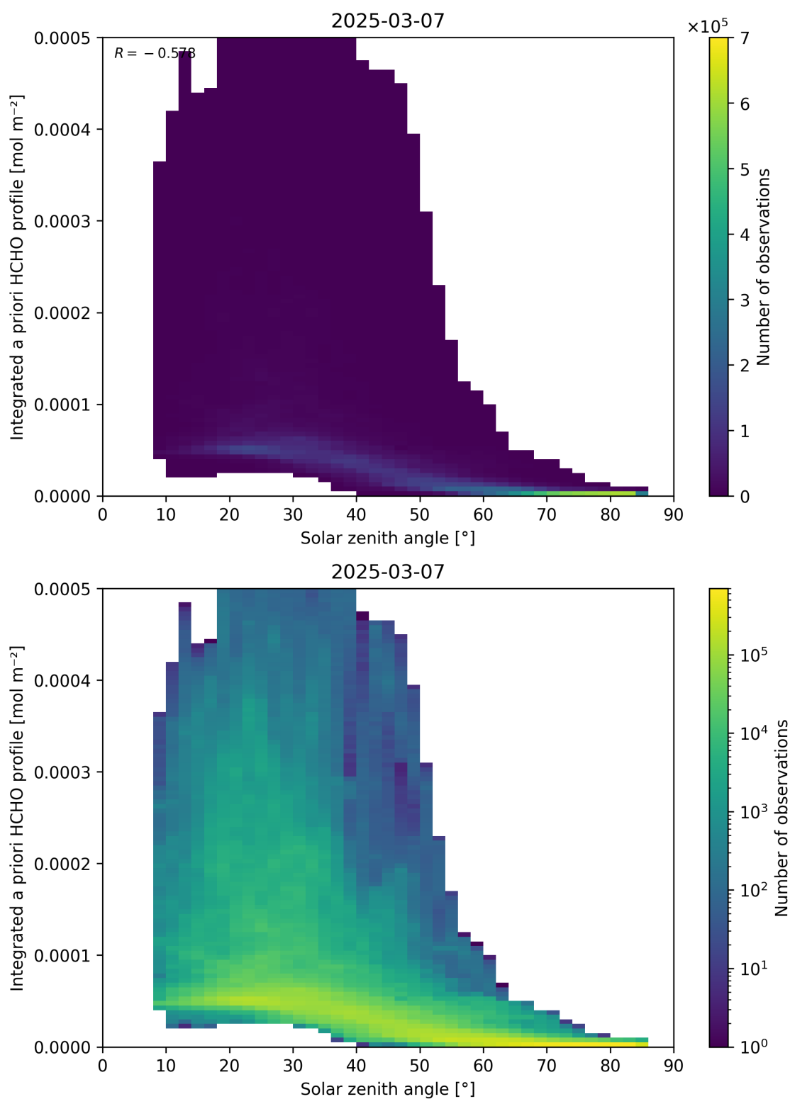
Figure 180: Scatter density plot of “Solar zenith angle” against “Integrated a priori HCHO profile” for 2025-03-07 to 2025-03-08.
