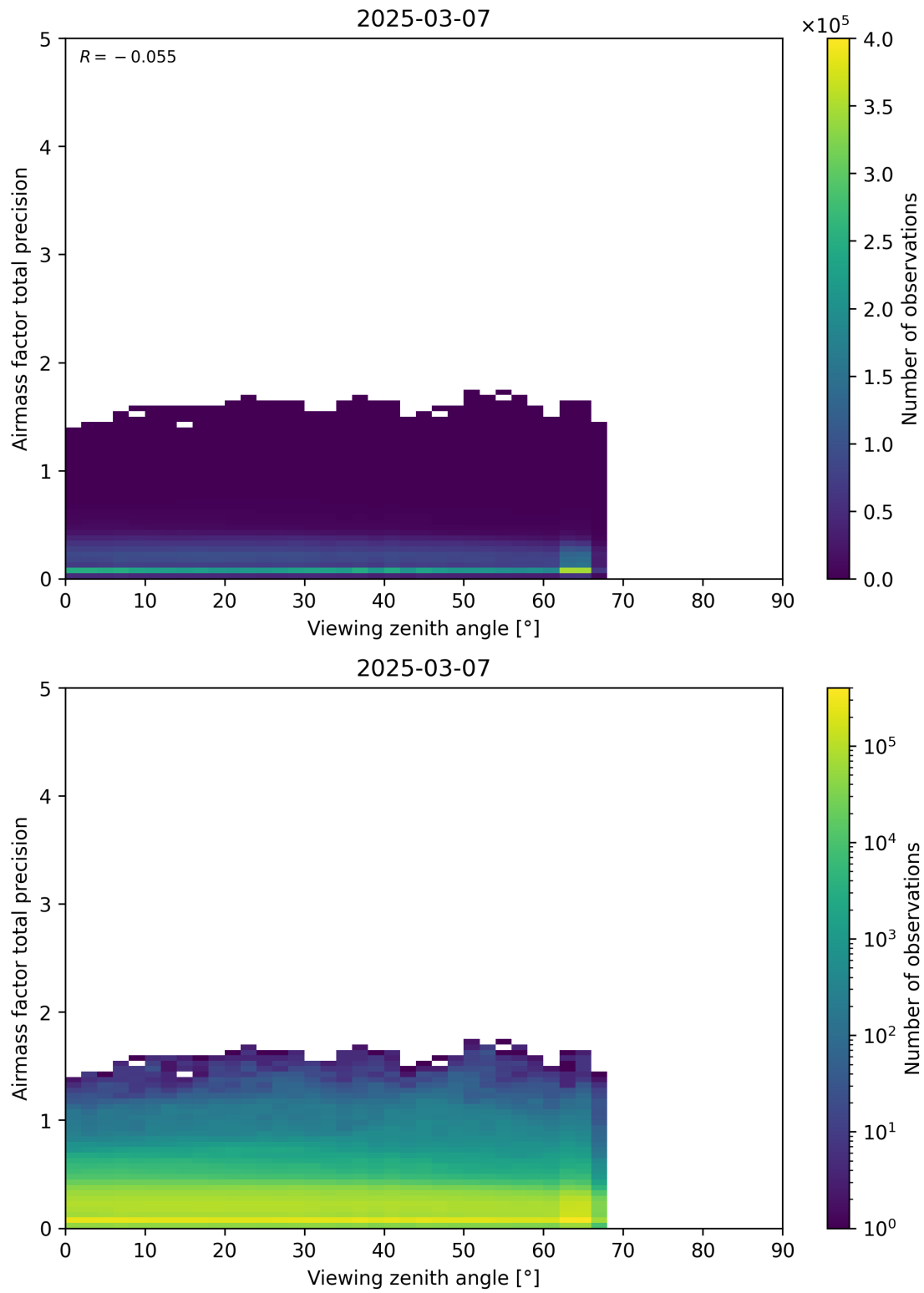
Figure 191: Scatter density plot of “Viewing zenith angle” against “Airmass factor total precision” for 2025-03-07 to 2025-03-08.
