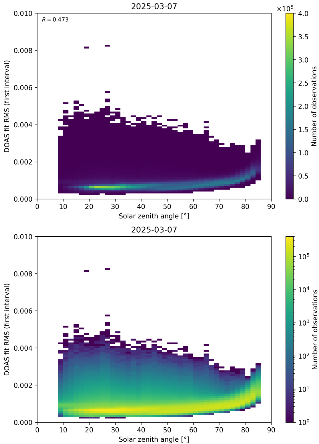
Figure 167: Scatter density plot of “Solar zenith angle” against “DOAS fit RMS (first interval)” for 2025-03-07 to 2025-03-08.
