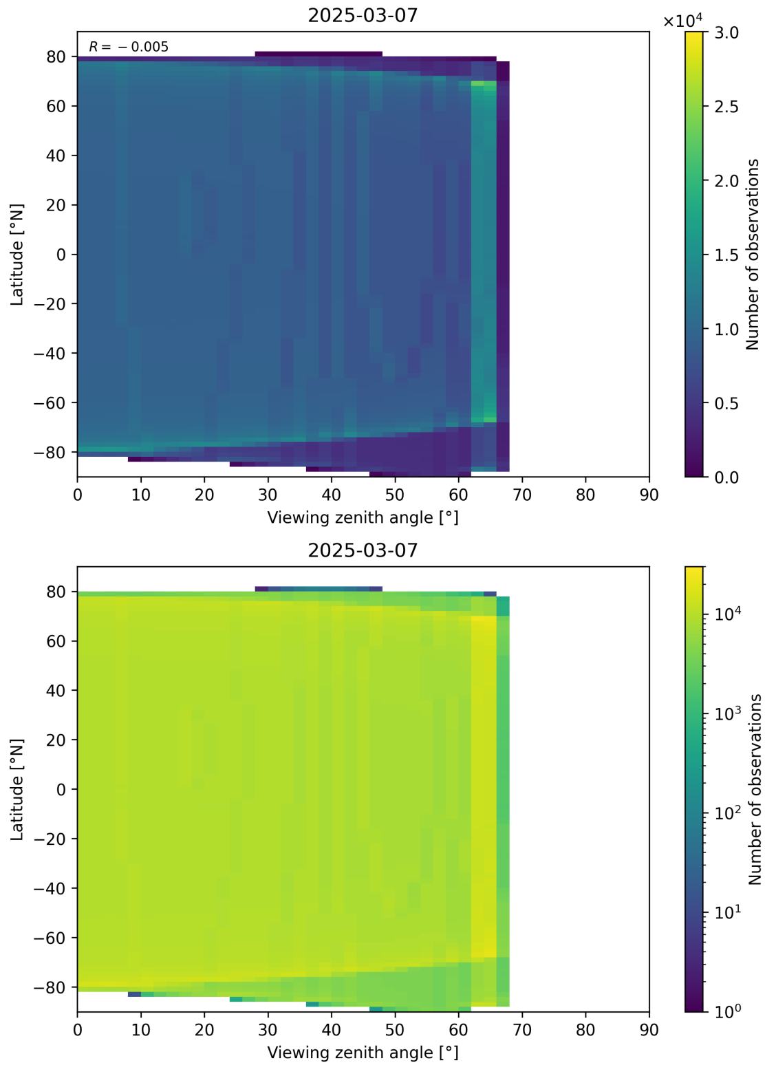
Figure 196: Scatter density plot of “Viewing zenith angle” against “Latitude” for 2025-03-07 to 2025-03-08.
