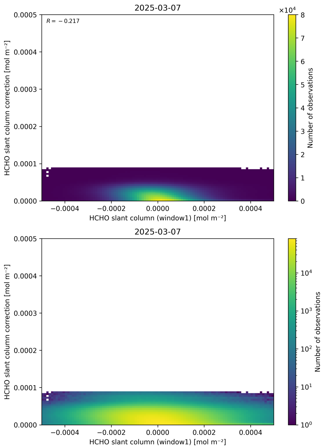
Figure 83: Scatter density plot of “HCHO slant column (window1)” against “HCHO slant column correction” for 2025-03-07 to 2025-03-08.
