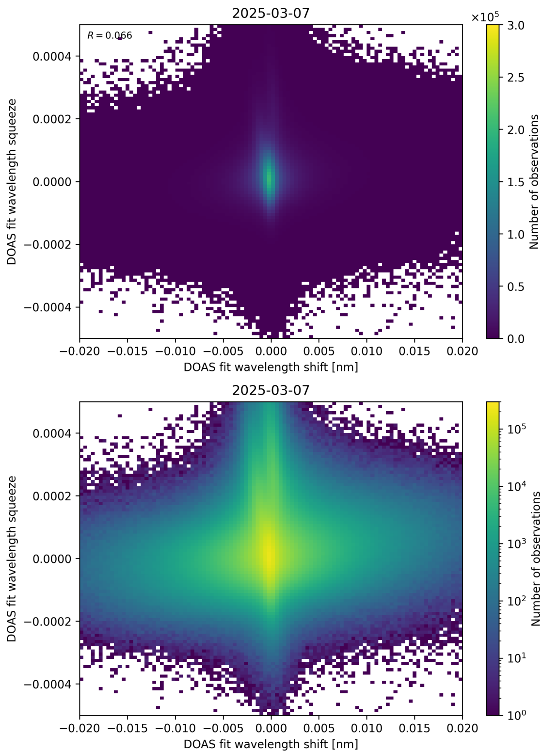
Figure 65: Scatter density plot of “DOAS fit wavelength shift” against “DOAS fit wavelength squeeze” for 2025-03-07 to 2025-03-08.
