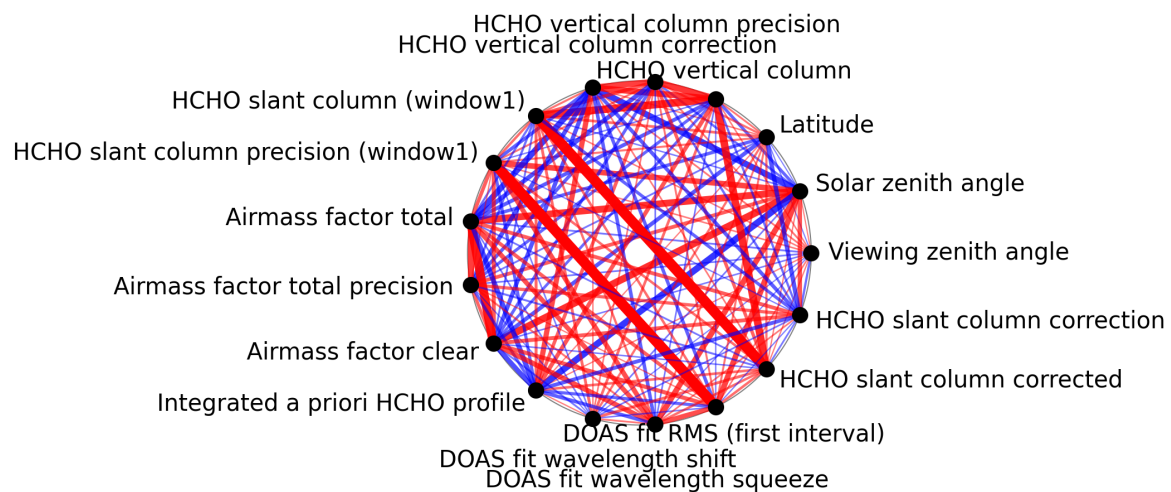
Figure 1: Map of correlation graph for 2025-03-07 to 2025-03-08.
