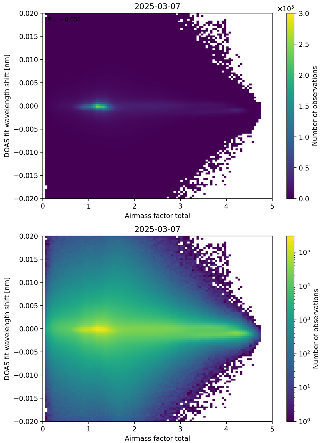
Figure 98: Scatter density plot of “Airmass factor total” against “DOAS fit wavelength shift” for 2025-03-07 to 2025-03-08.
