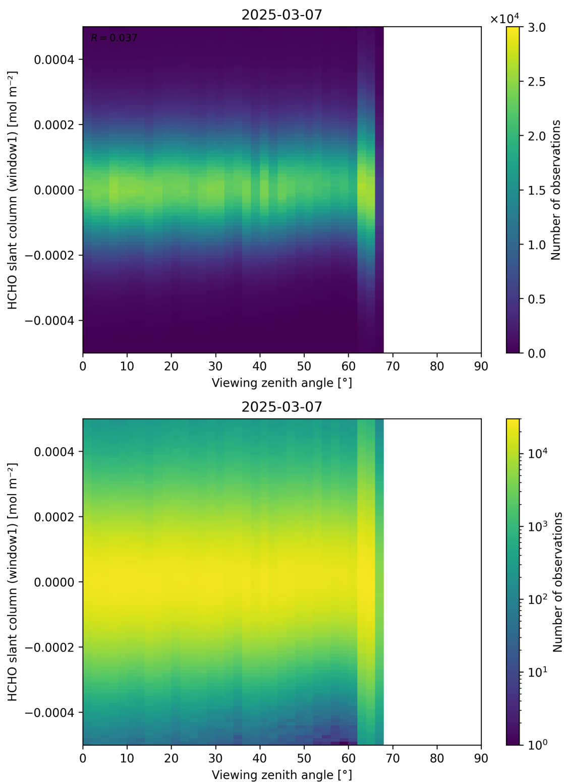
Figure 188: Scatter density plot of “Viewing zenith angle” against “HCHO slant column (window1)” for 2025-03-07 to 2025-03-08.
