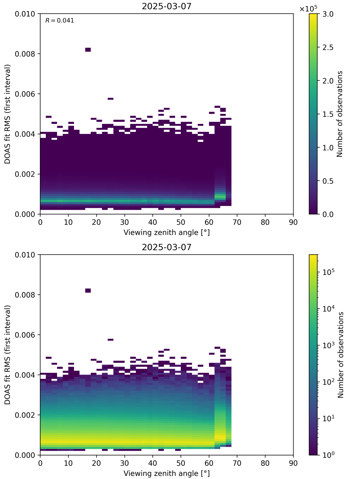
Figure 182: Scatter density plot of “Viewing zenith angle” against “DOAS fit RMS (first interval)” for 2025-03-07 to 2025-03-08.
