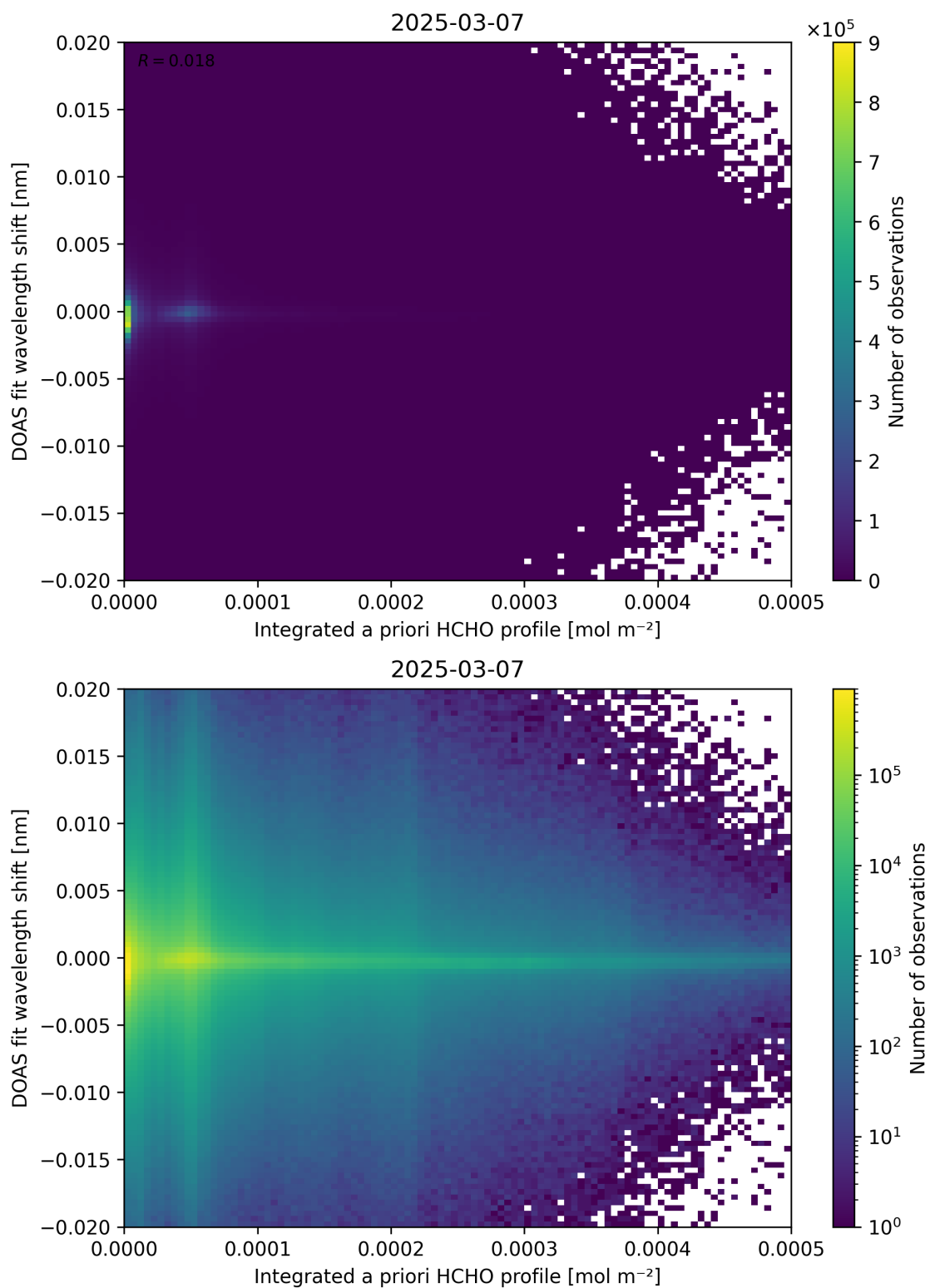
Figure 149: Scatter density plot of “Integrated a priori HCHO profile” against “DOAS fit wavelength shift” for 2025-03-07 to 2025-03-08.
