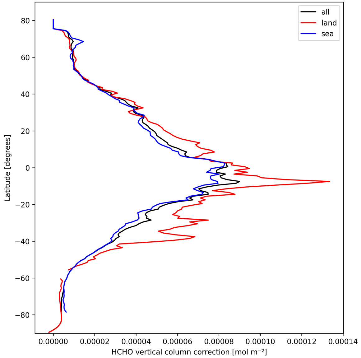
Figure 23: Zonal average of “HCHO vertical column correction” for 2025-03-07 to 2025-03-08.
