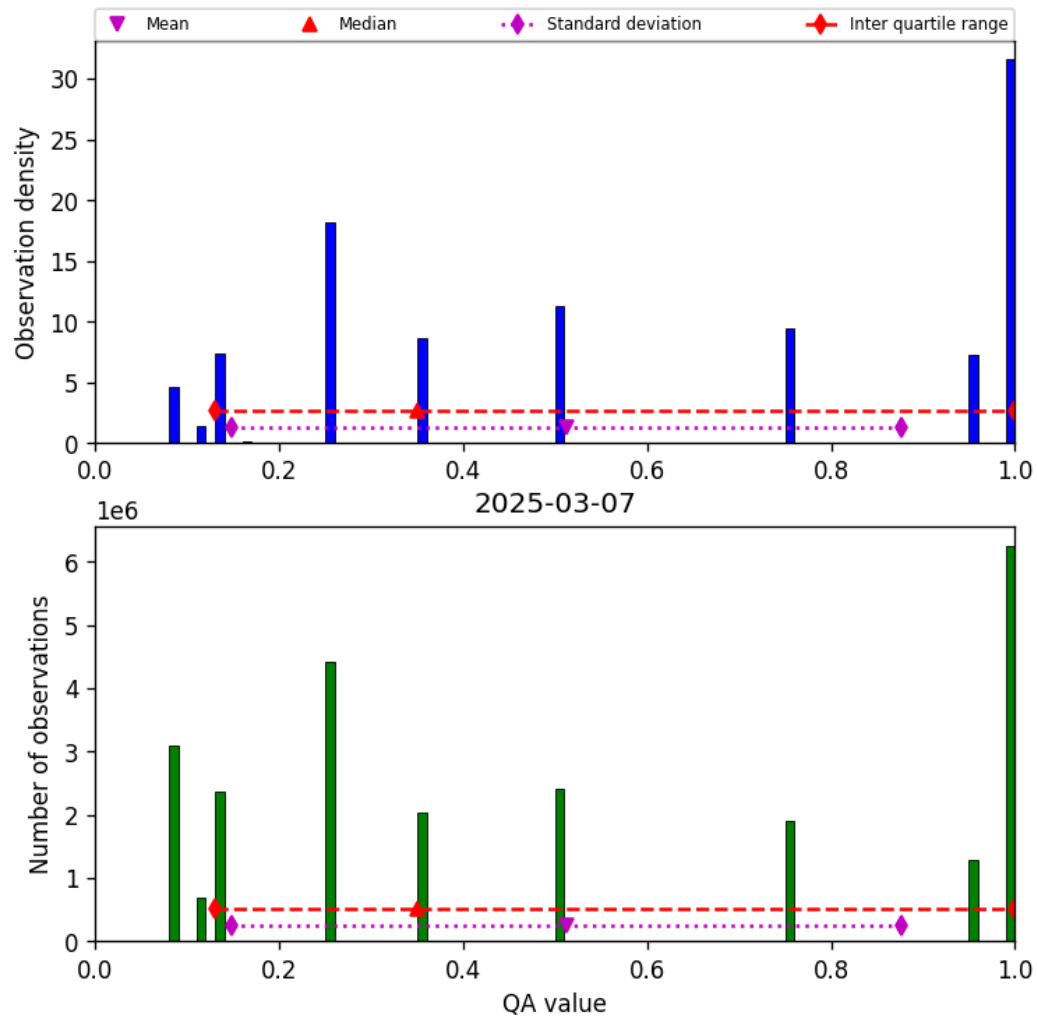
Figure 34: Histogram of “QA value” for 2025-03-07 to 2025-03-08
