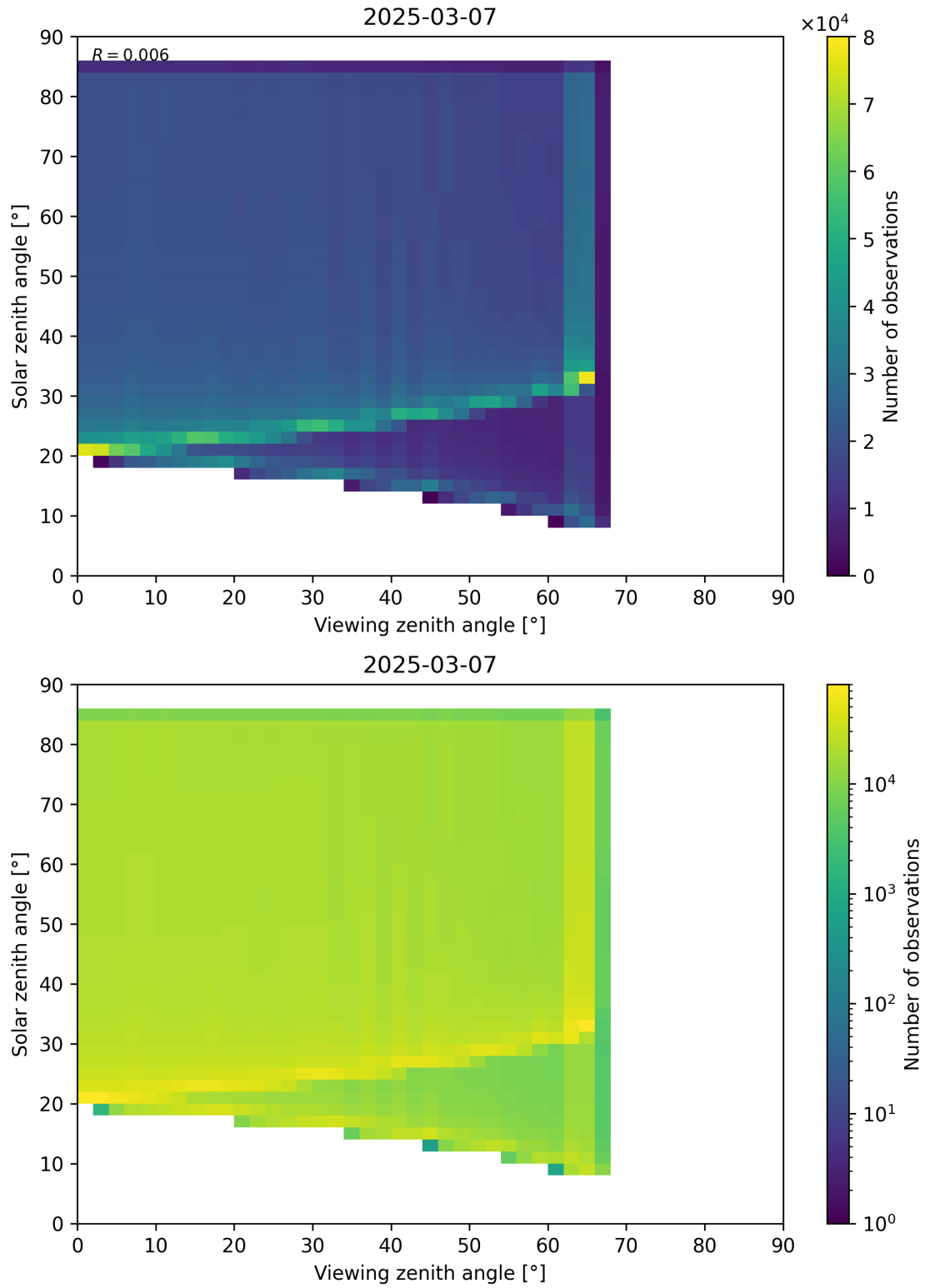
Figure 197: Scatter density plot of “Viewing zenith angle” against “Solar zenith angle” for 2025-03-07 to 2025-03-08.
