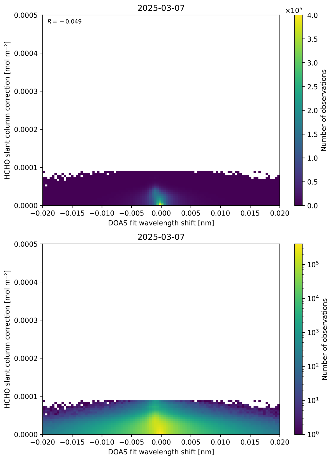
Figure 67: Scatter density plot of “DOAS fit wavelength shift” against “HCHO slant column correction” for 2025-03-07 to 2025-03-08.
