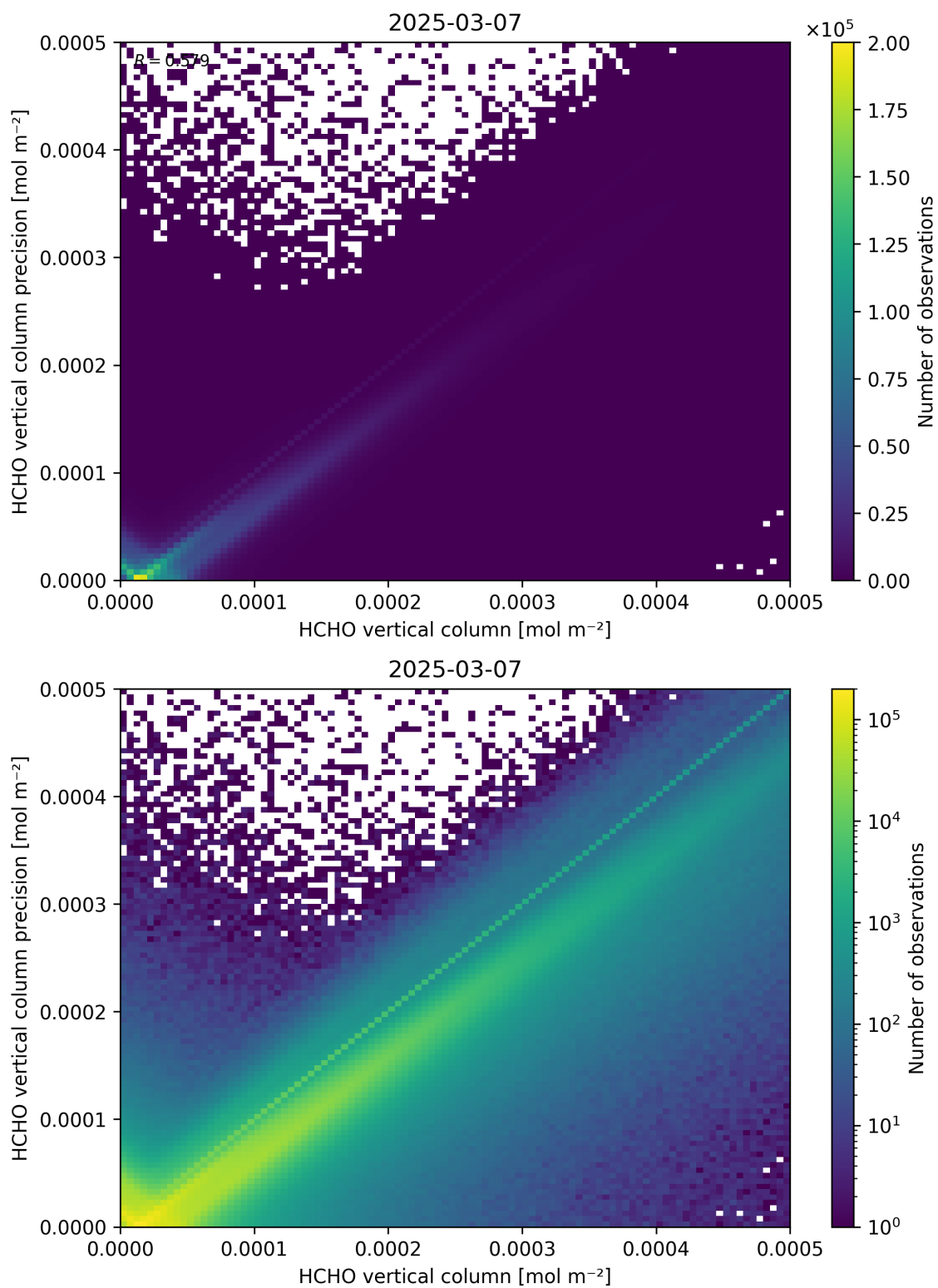
Figure 134: Scatter density plot of “HCHO vertical column” against “HCHO vertical column precision” for 2025-03-07 to 2025-03-08.
