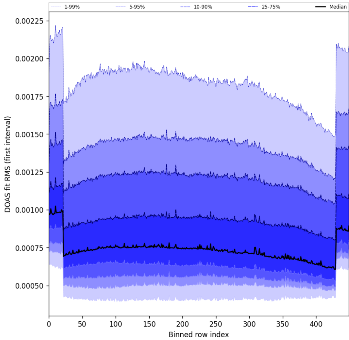
Figure 60: Along track statistics of “DOAS fit RMS (first interval)” for 2025-03-07 to 2025-03-08
