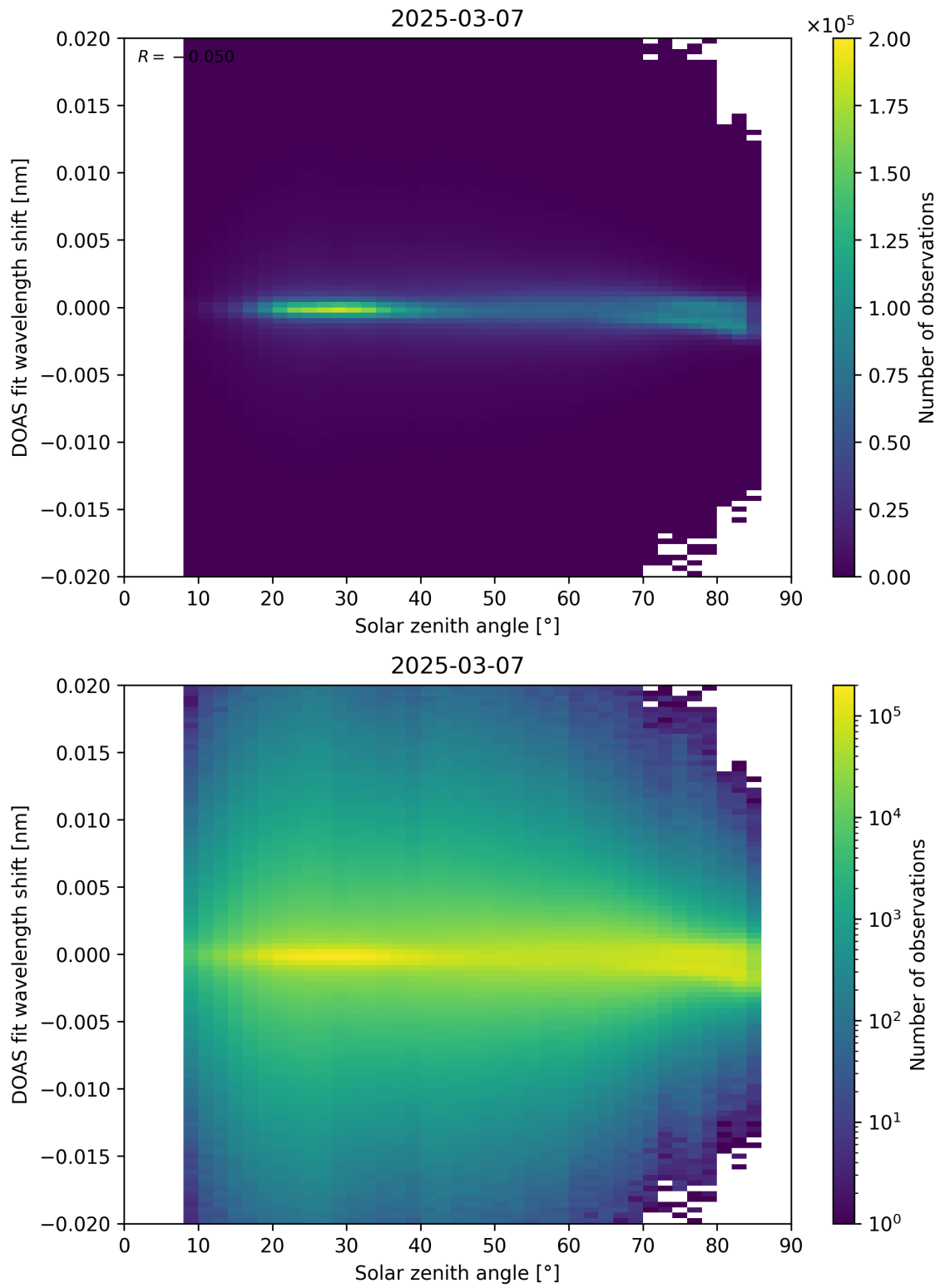
Figure 168: Scatter density plot of “Solar zenith angle” against “DOAS fit wavelength shift” for 2025-03-07 to 2025-03-08.
