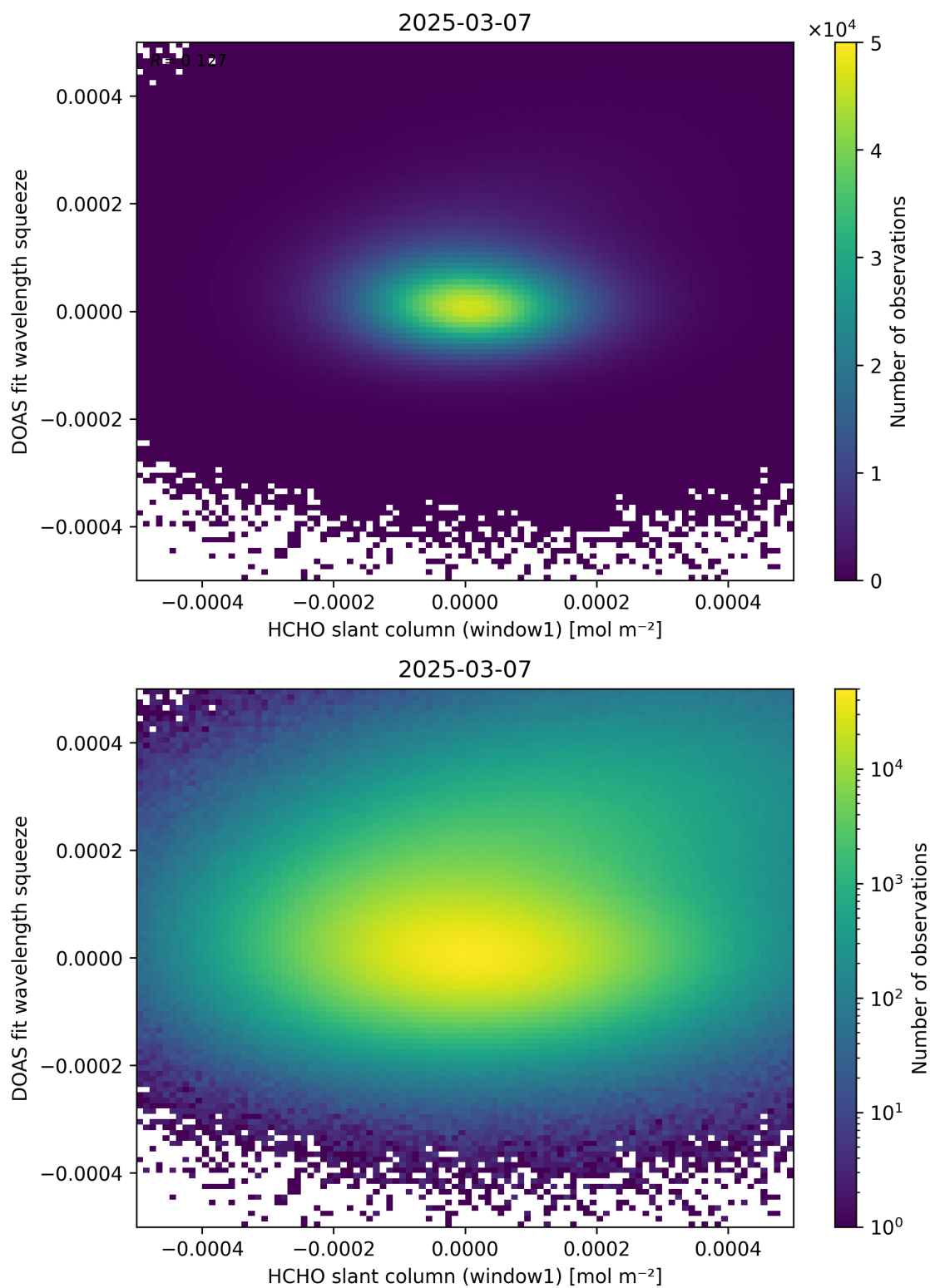
Figure 80: Scatter density plot of “HCHO slant column (window1)” against “DOAS fit wavelength squeeze” for 2025-03-07 to 2025-03-08.
