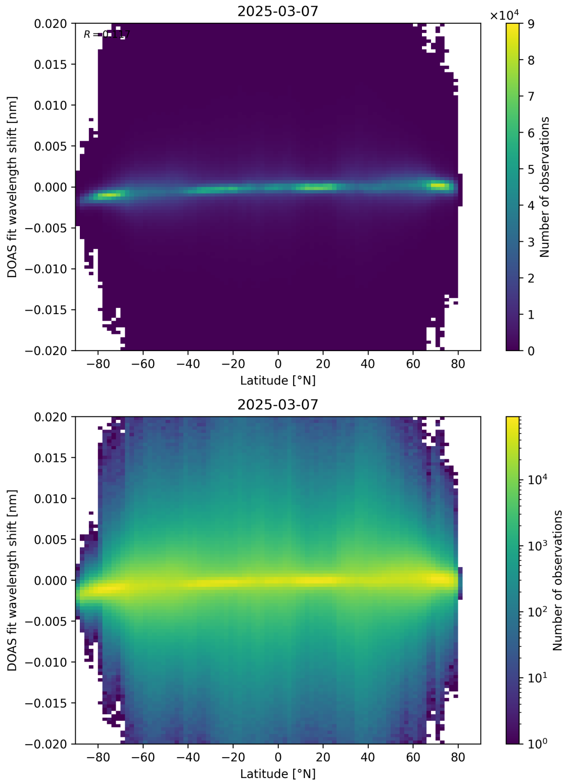
Figure 154: Scatter density plot of “Latitude” against “DOAS fit wavelength shift” for 2025-03-07 to 2025-03-08.
