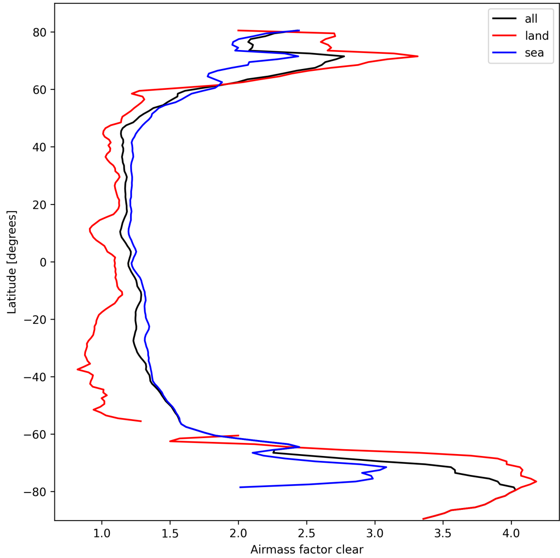
Figure 28: Zonal average of “Airmass factor clear” for 2025-03-07 to 2025-03-08.
