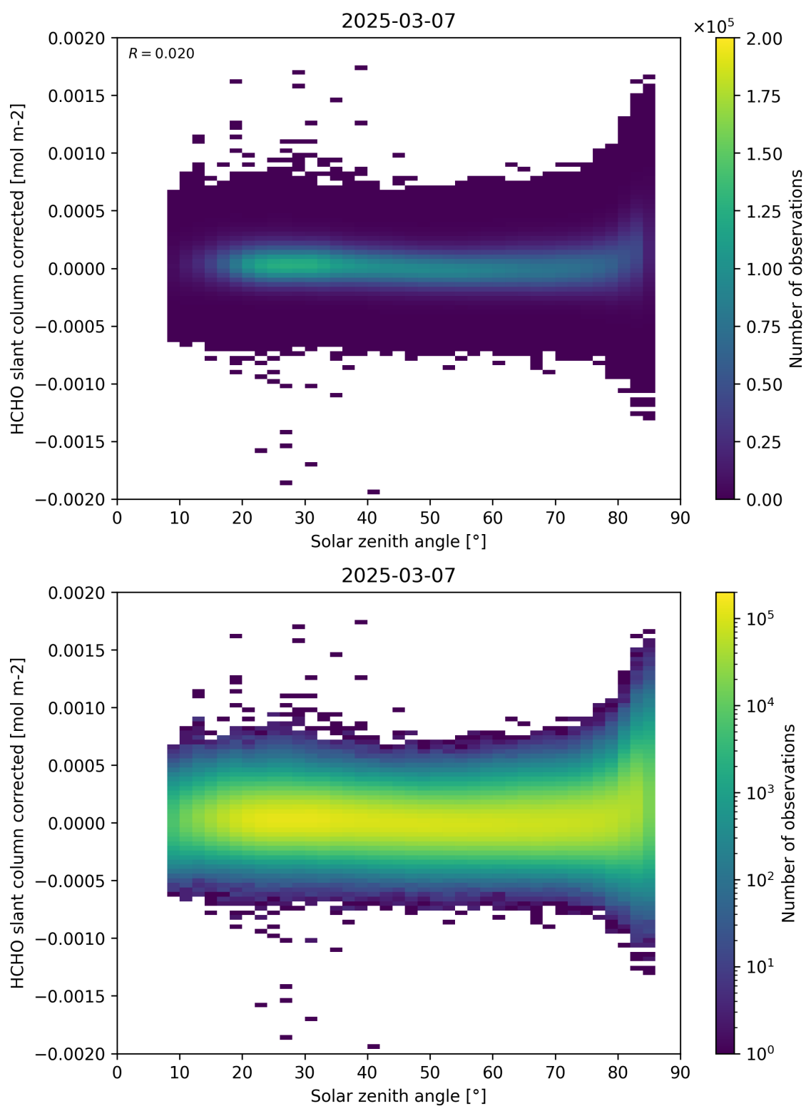
Figure 171: Scatter density plot of “Solar zenith angle” against “HCHO slant column corrected” for 2025-03-07 to 2025-03-08.
