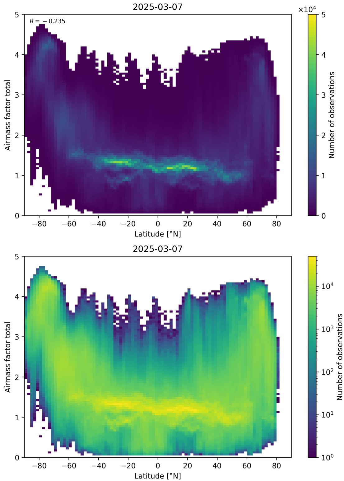
Figure 161: Scatter density plot of “Latitude” against “Airmass factor total” for 2025-03-07 to 2025-03-08.
