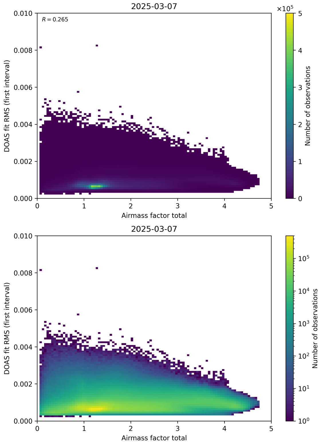
Figure 97: Scatter density plot of “Airmass factor total” against “DOAS fit RMS (first interval)” for 2025-03-07 to 2025-03-08.
