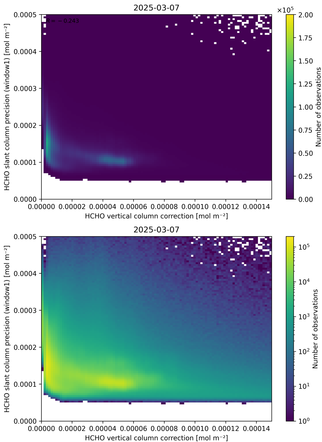
Figure 119: Scatter density plot of “HCHO vertical column correction” against “HCHO slant column precision (window1)” for 2025-03-07 to 2025-03-08.
