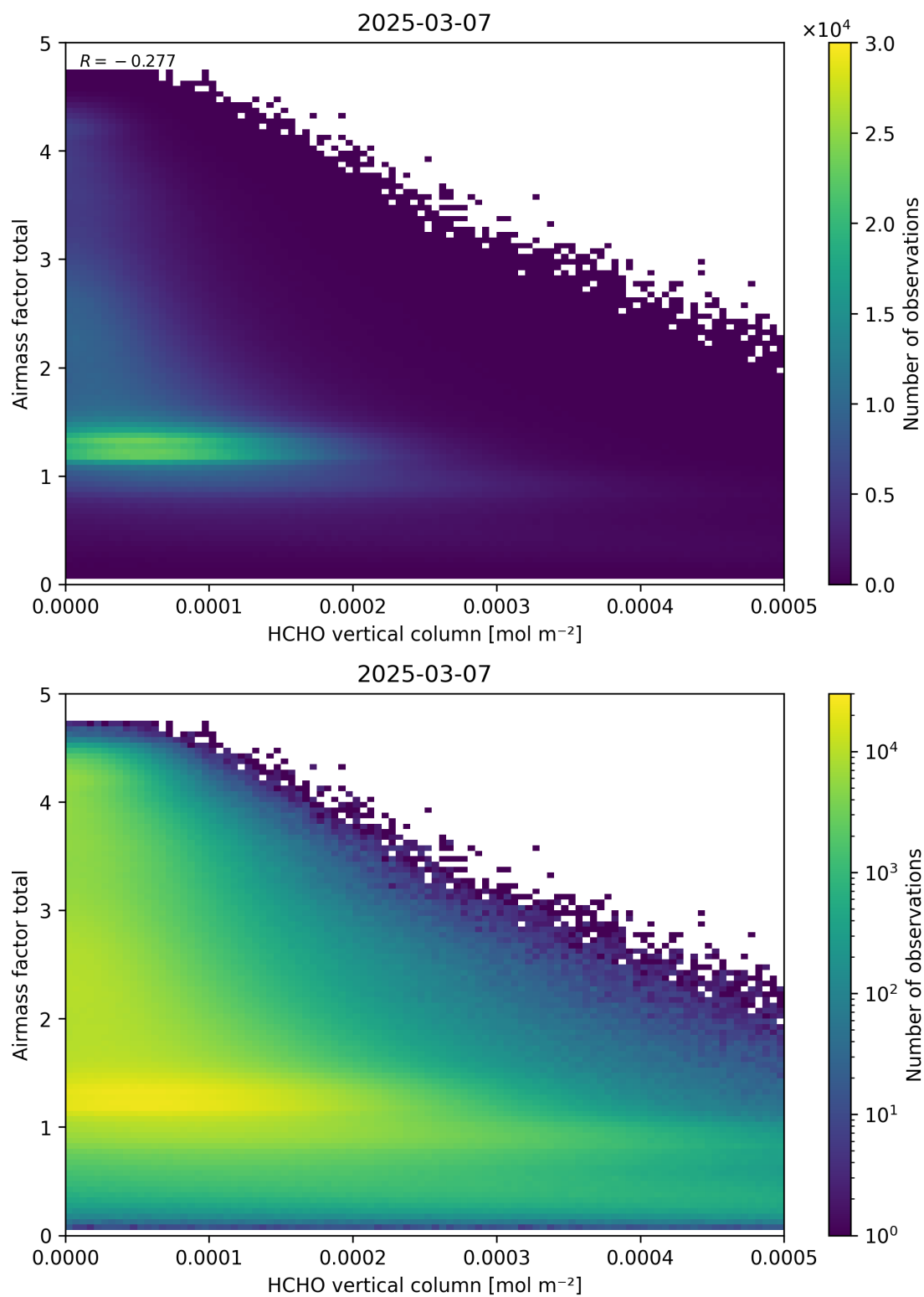
Figure 131: Scatter density plot of “HCHO vertical column” against “Airmass factor total” for 2025-03-07 to 2025-03-08.
