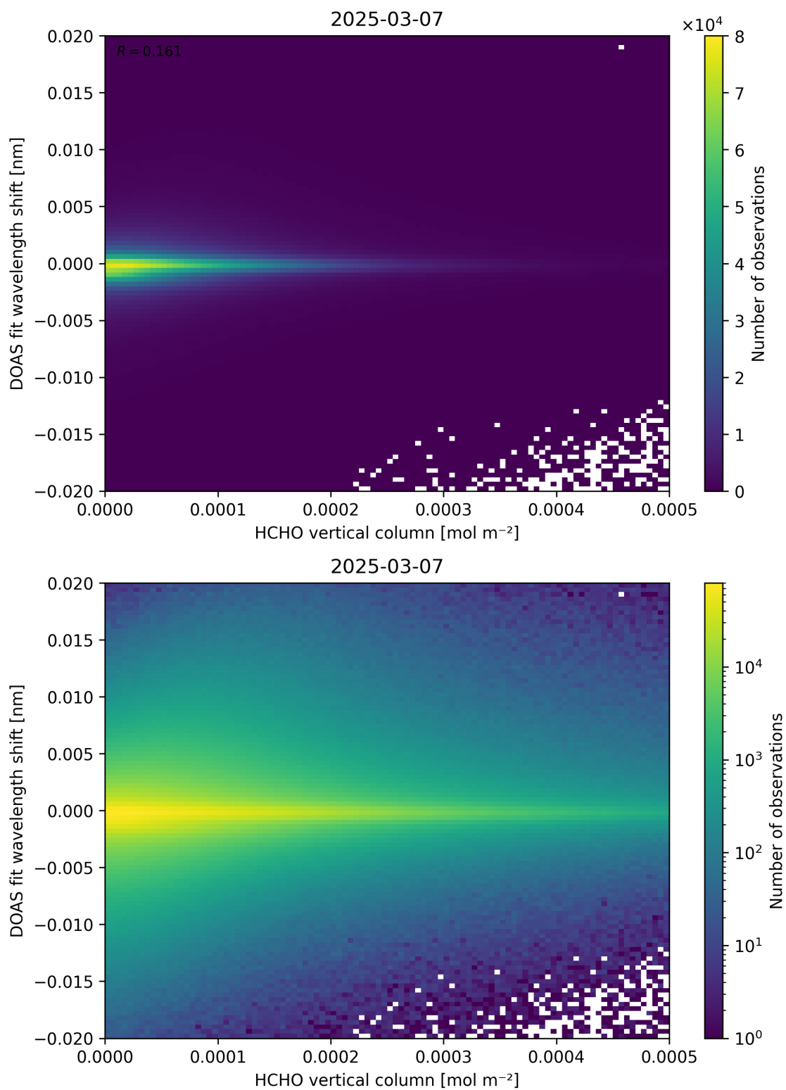
Figure 124: Scatter density plot of “HCHO vertical column” against “DOAS fit wavelength shift” for 2025-03-07 to 2025-03-08.
