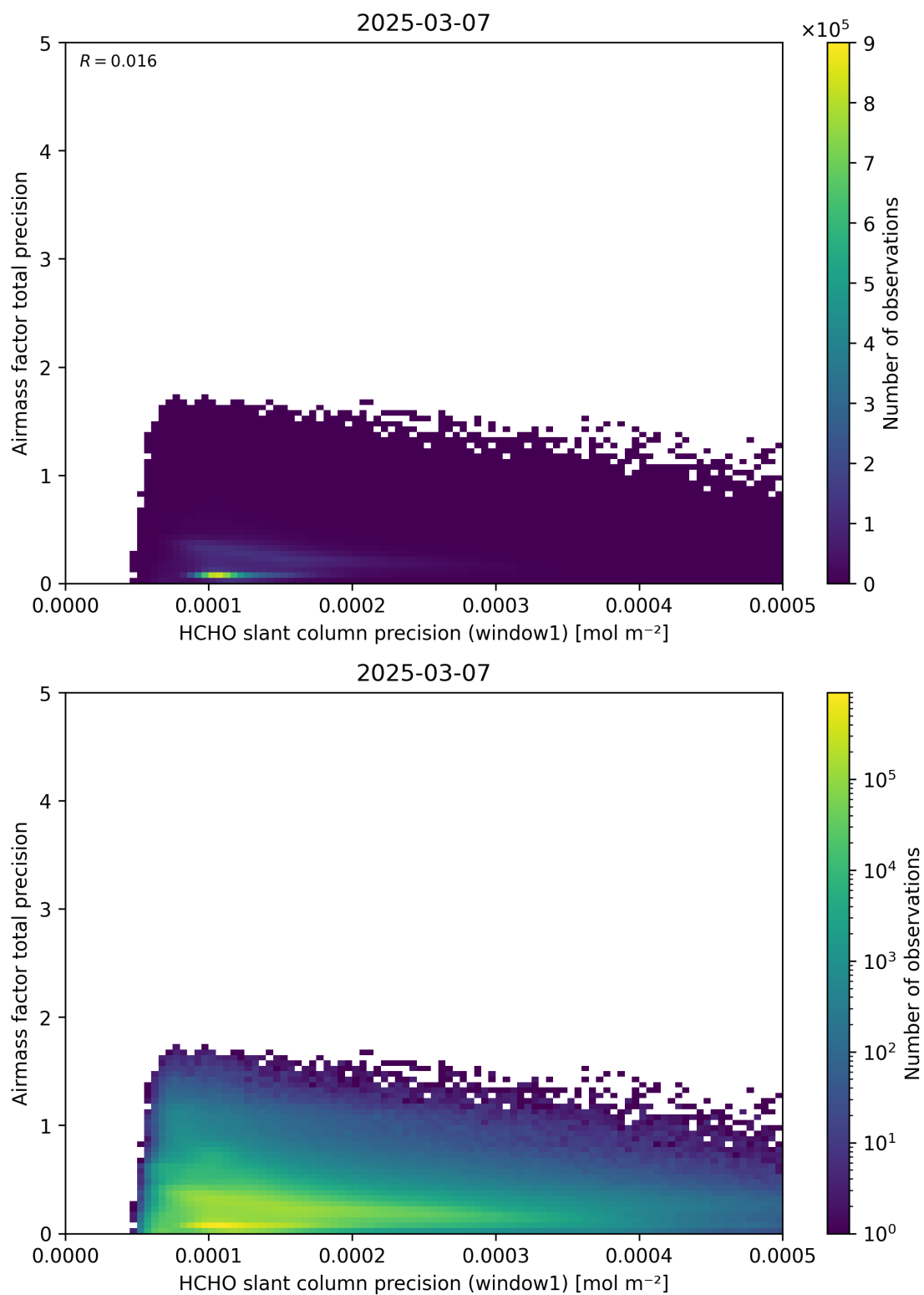
Figure 95: Scatter density plot of “HCHO slant column precision (window1)” against “Airmass factor total precision” for 2025-03-07 to 2025-03-08.
