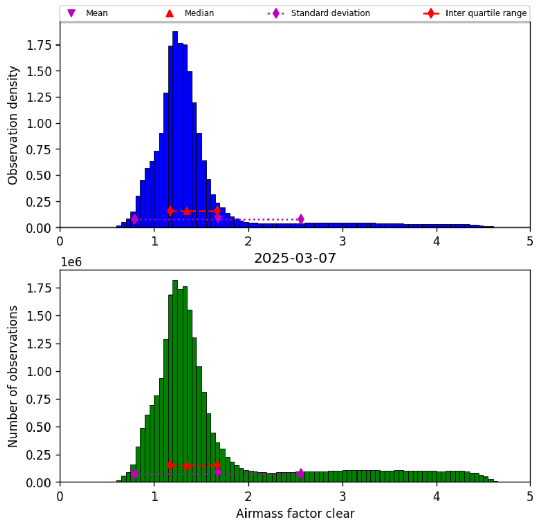
Figure 42: Histogram of “Airmass factor clear” for 2025-03-07 to 2025-03-08
