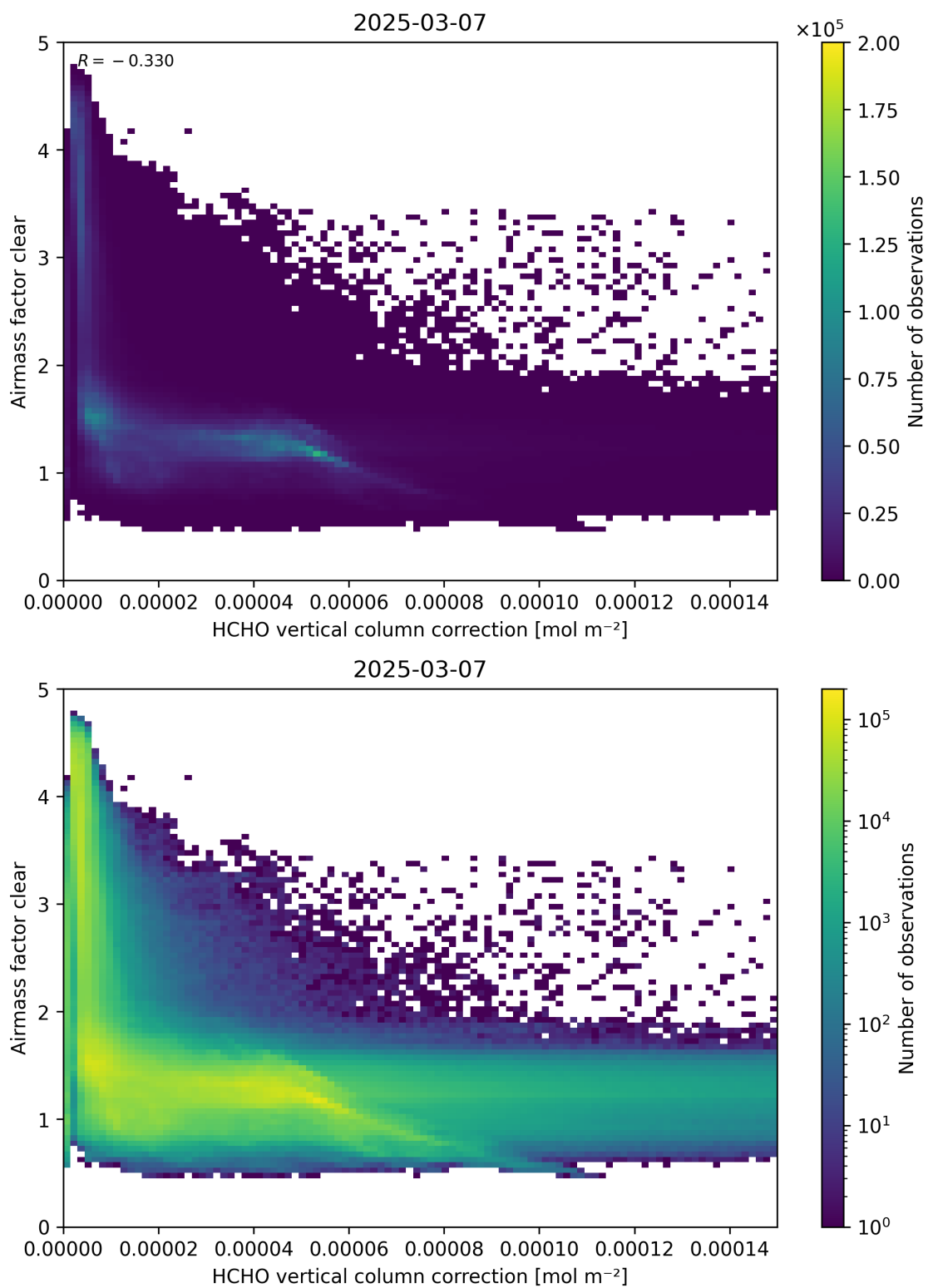
Figure 115: Scatter density plot of “HCHO vertical column correction” against “Airmass factor clear” for 2025-03-07 to 2025-03-08.
