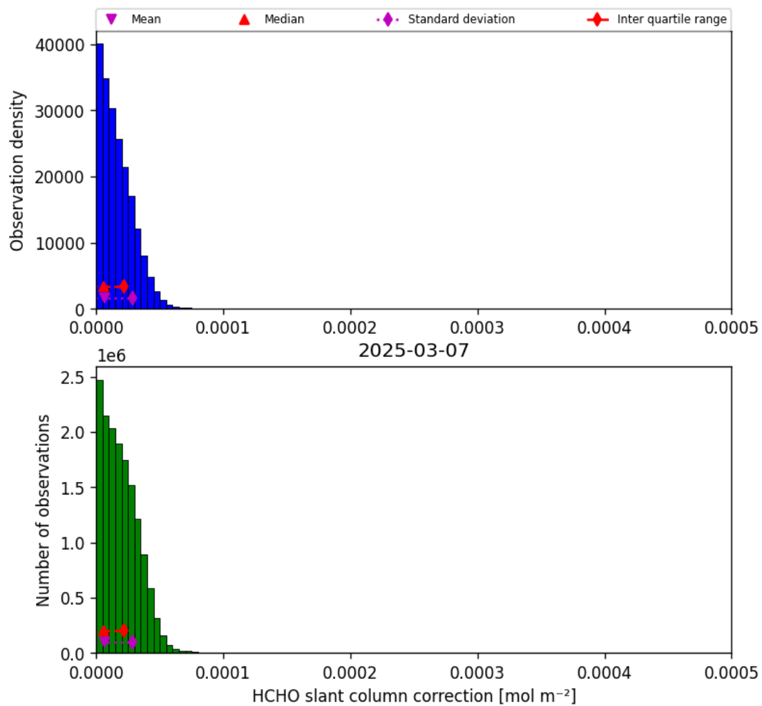
Figure 47: Histogram of “HCHO slant column correction” for 2025-03-07 to 2025-03-08
