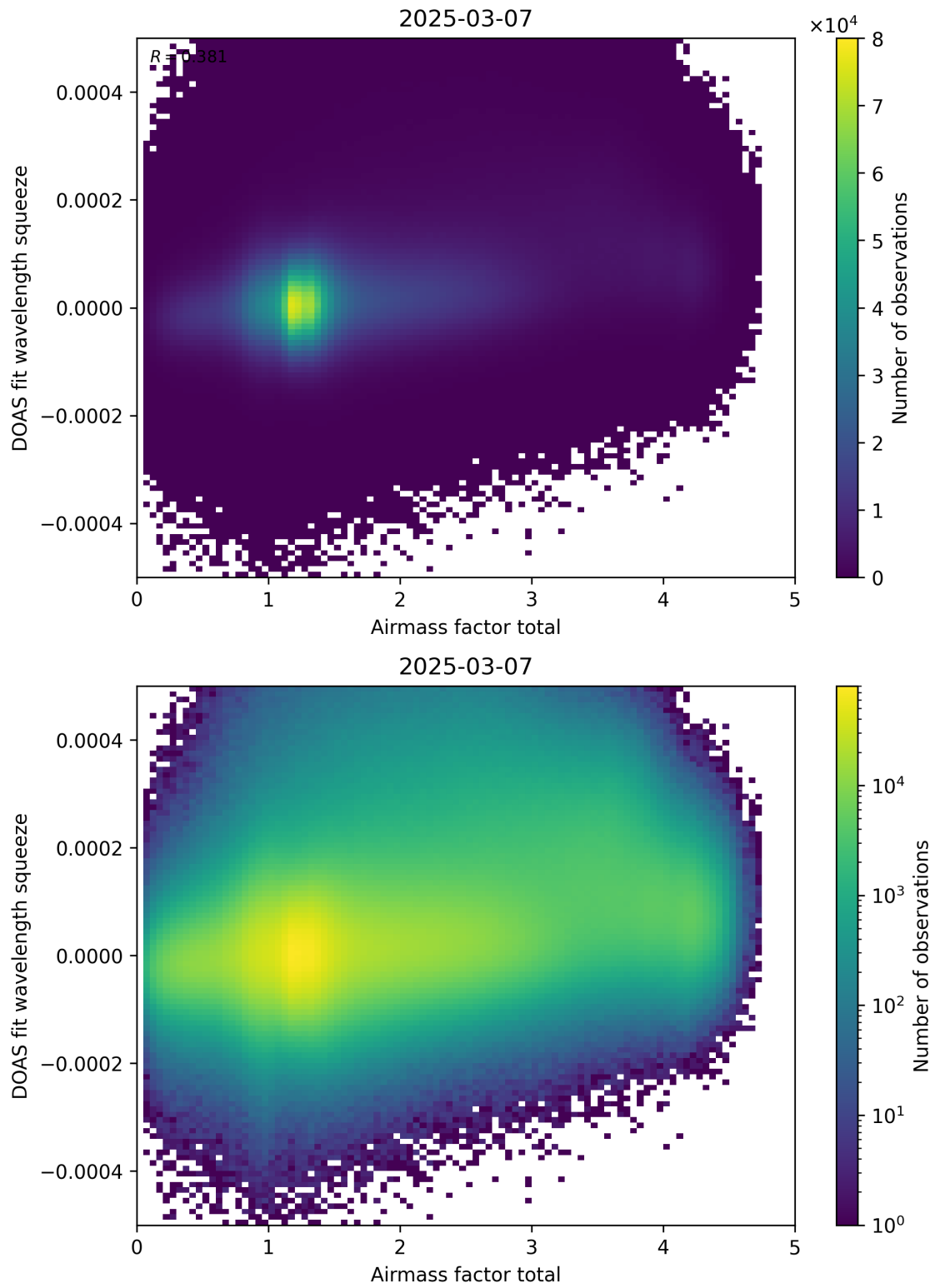
Figure 99: Scatter density plot of “Airmass factor total” against “DOAS fit wavelength squeeze” for 2025-03-07 to 2025-03-08.
