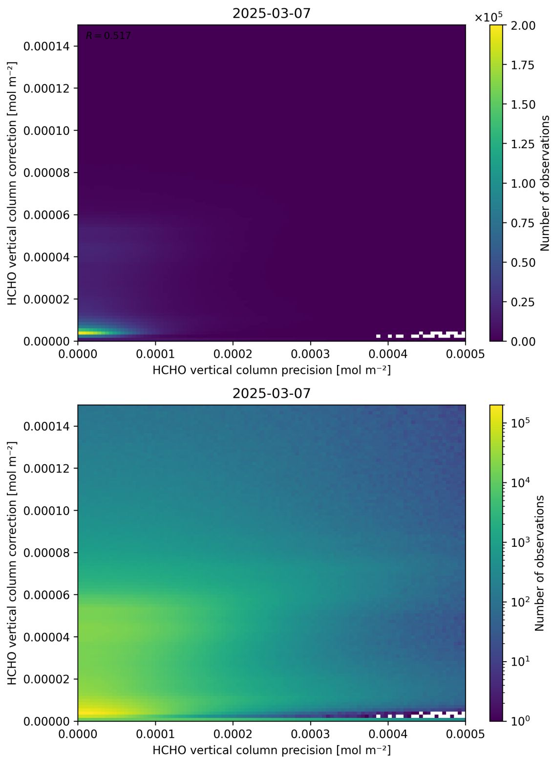
Figure 146: Scatter density plot of “HCHO vertical column precision” against “HCHO vertical column correction” for 2025-03-07 to 2025-03-08.
