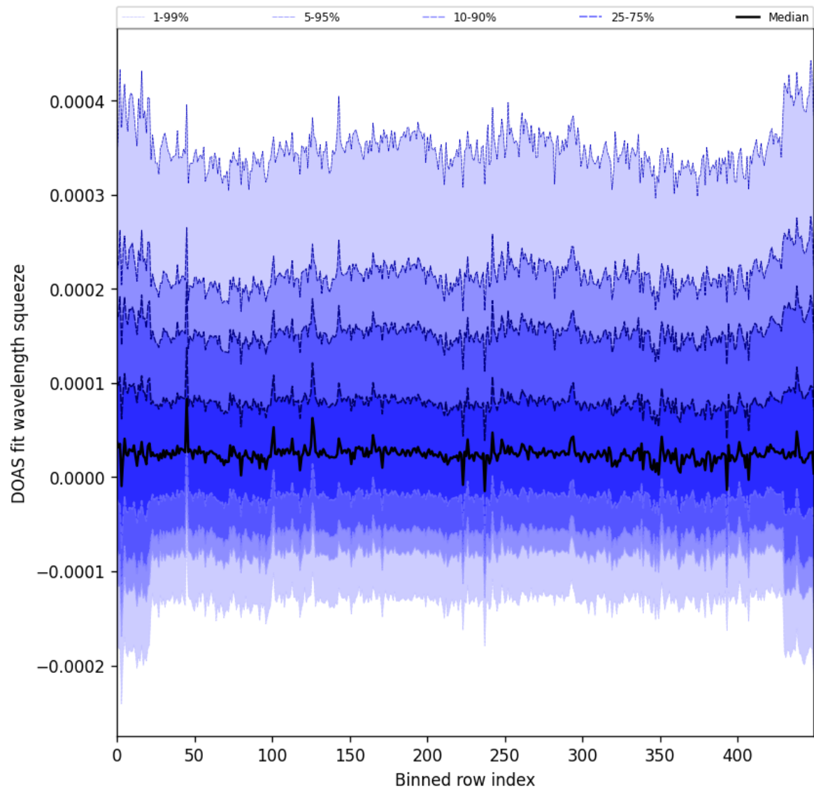
Figure 59: Along track statistics of “DOAS fit wavelength squeeze” for 2025-03-07 to 2025-03-08
