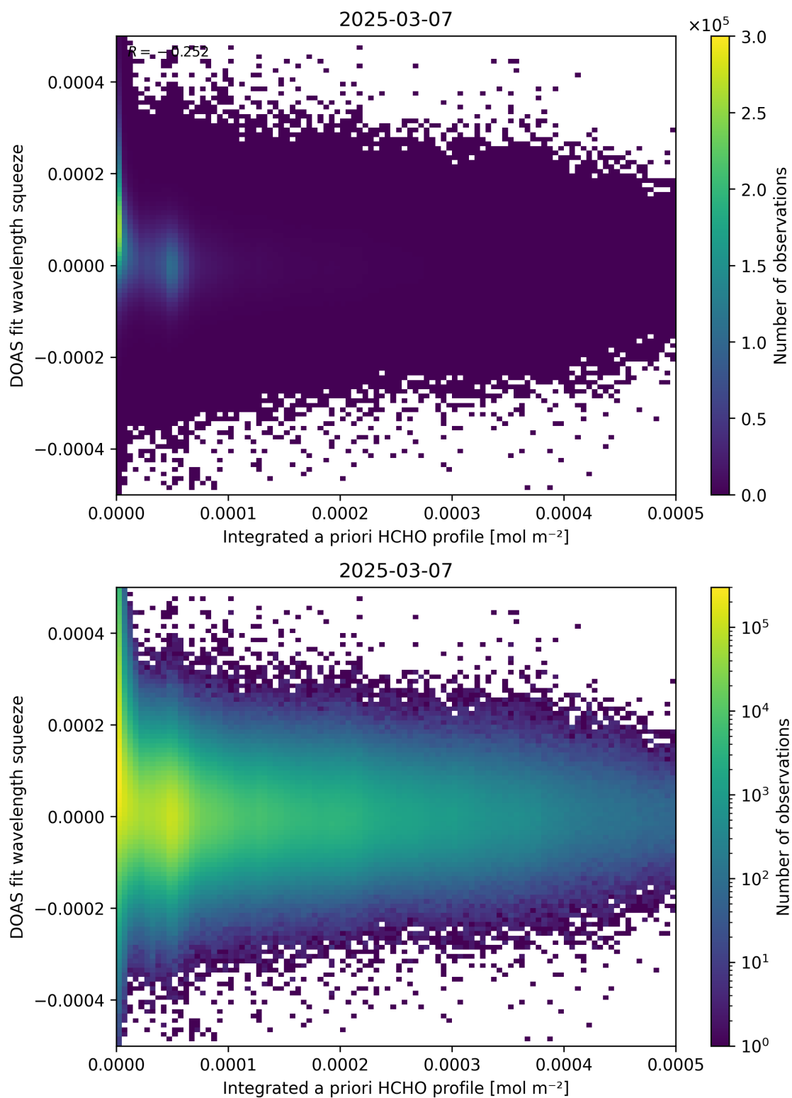
Figure 150: Scatter density plot of “Integrated a priori HCHO profile” against “DOAS fit wavelength squeeze” for 2025-03-07 to 2025-03-08.
