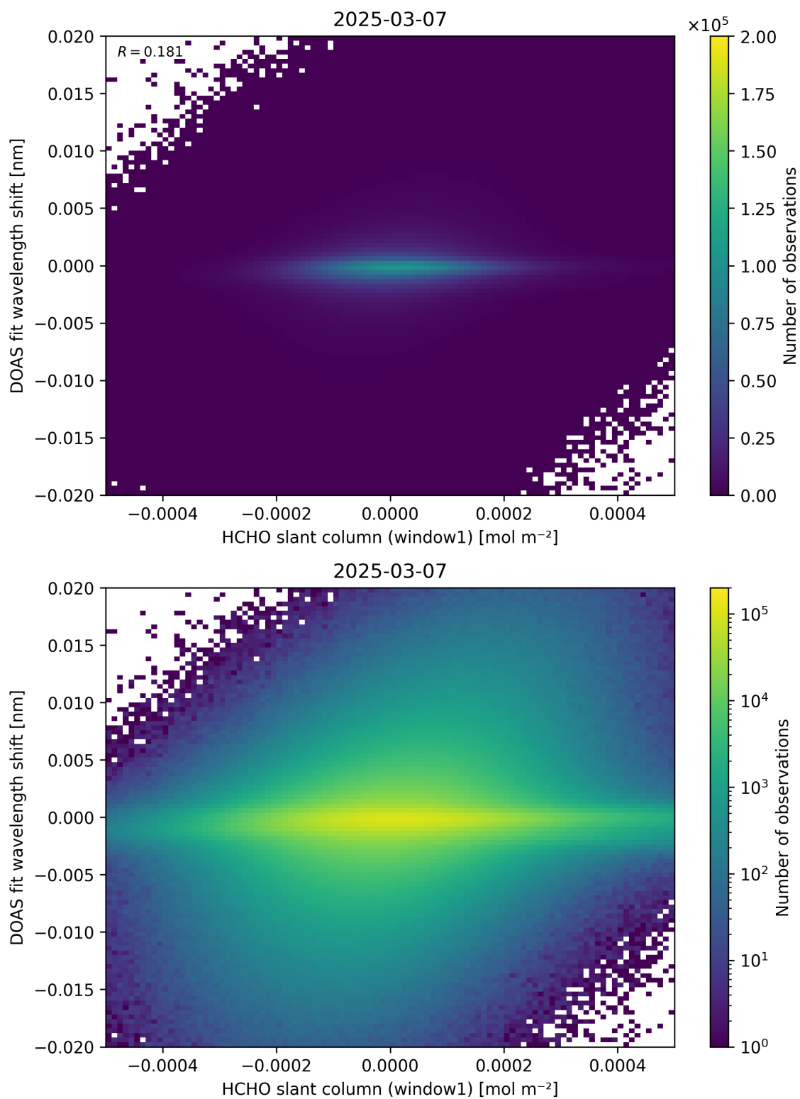
Figure 79: Scatter density plot of “HCHO slant column (window1)” against “DOAS fit wavelength shift” for 2025-03-07 to 2025-03-08.
