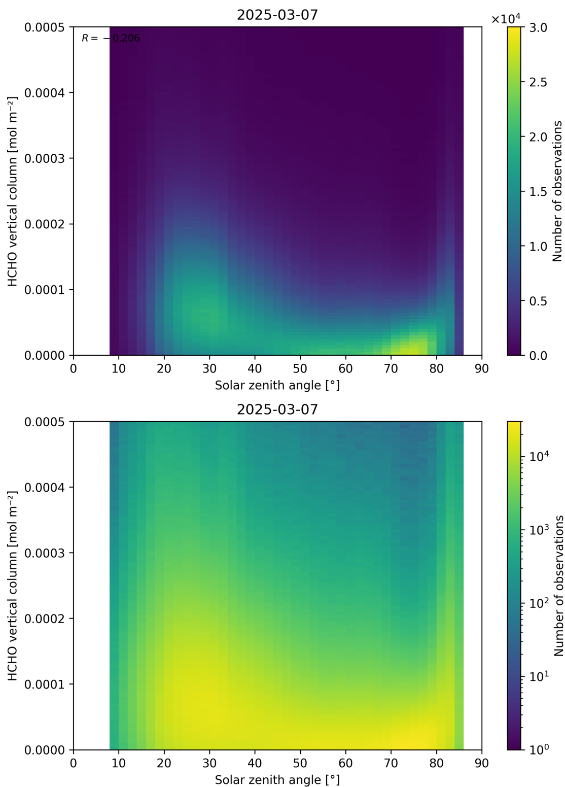
Figure 177: Scatter density plot of “Solar zenith angle” against “HCHO vertical column” for 2025-03-07 to 2025-03-08.
