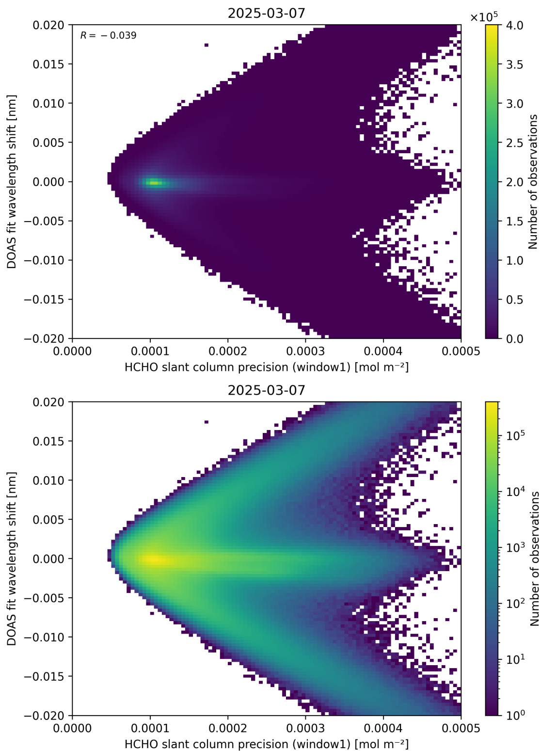
Figure 89: Scatter density plot of “HCHO slant column precision (window1)” against “DOAS fit wavelength shift” for 2025-03-07 to 2025-03-08.
