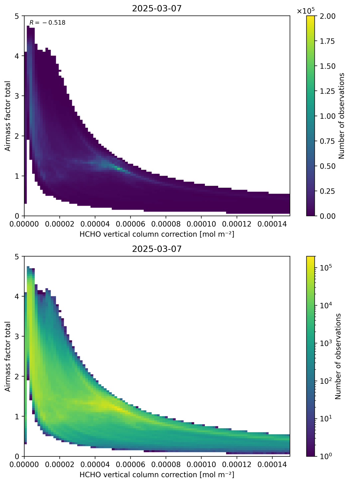
Figure 120: Scatter density plot of “HCHO vertical column correction” against “Airmass factor total” for 2025-03-07 to 2025-03-08.
