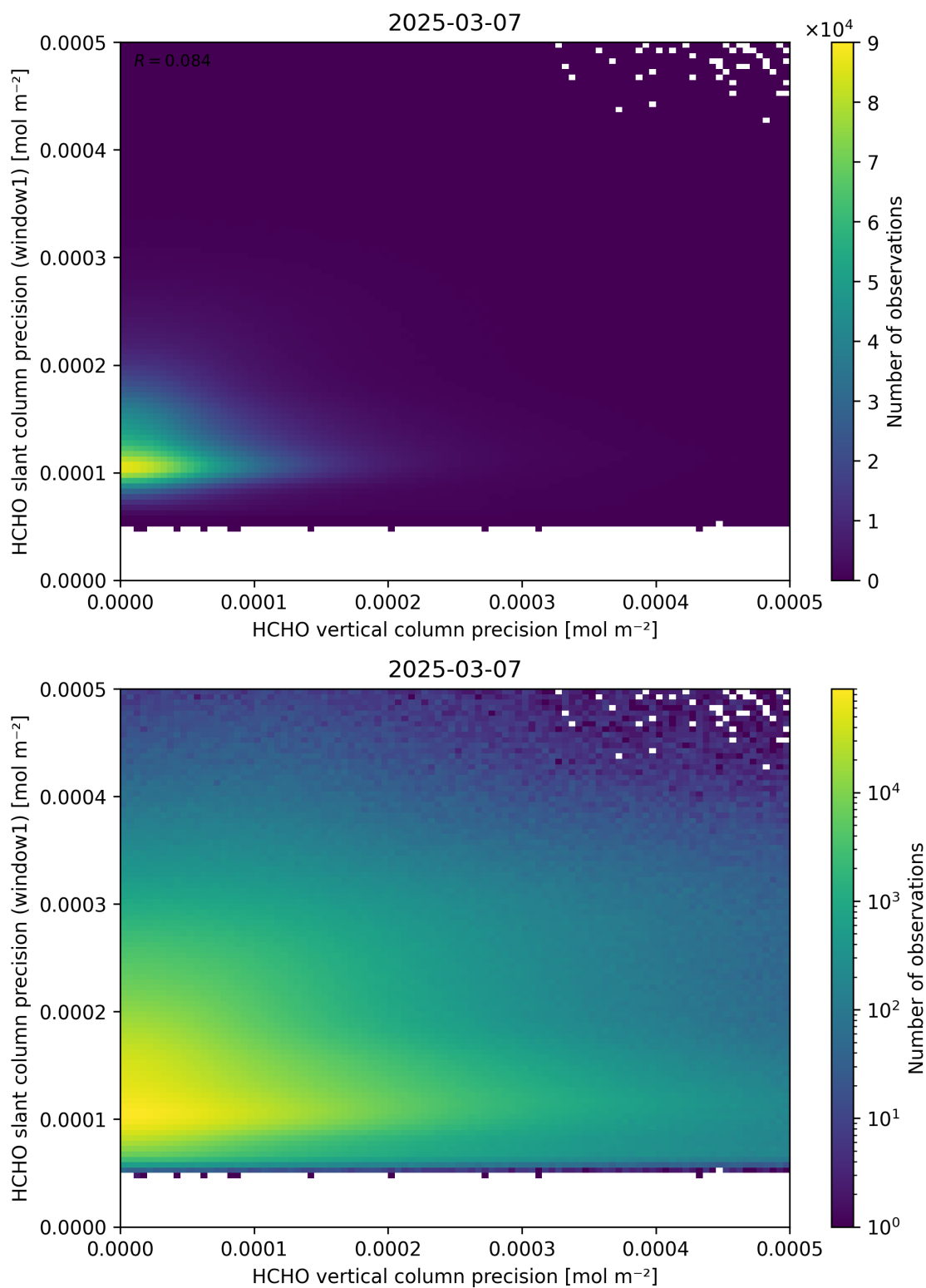
Figure 143: Scatter density plot of “HCHO vertical column precision” against “HCHO slant column precision (window1)” for 2025-03-07 to 2025-03-08.
