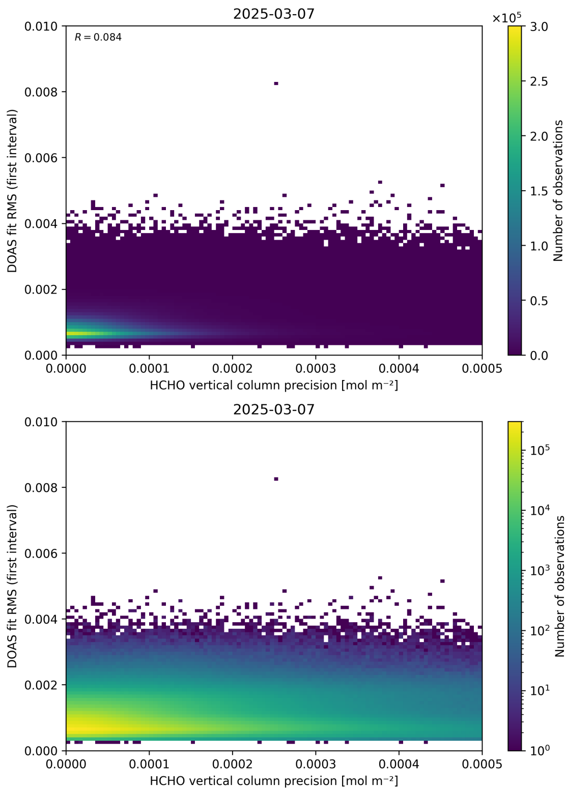
Figure 136: Scatter density plot of “HCHO vertical column precision” against “DOAS fit RMS (first interval)” for 2025-03-07 to 2025-03-08.
