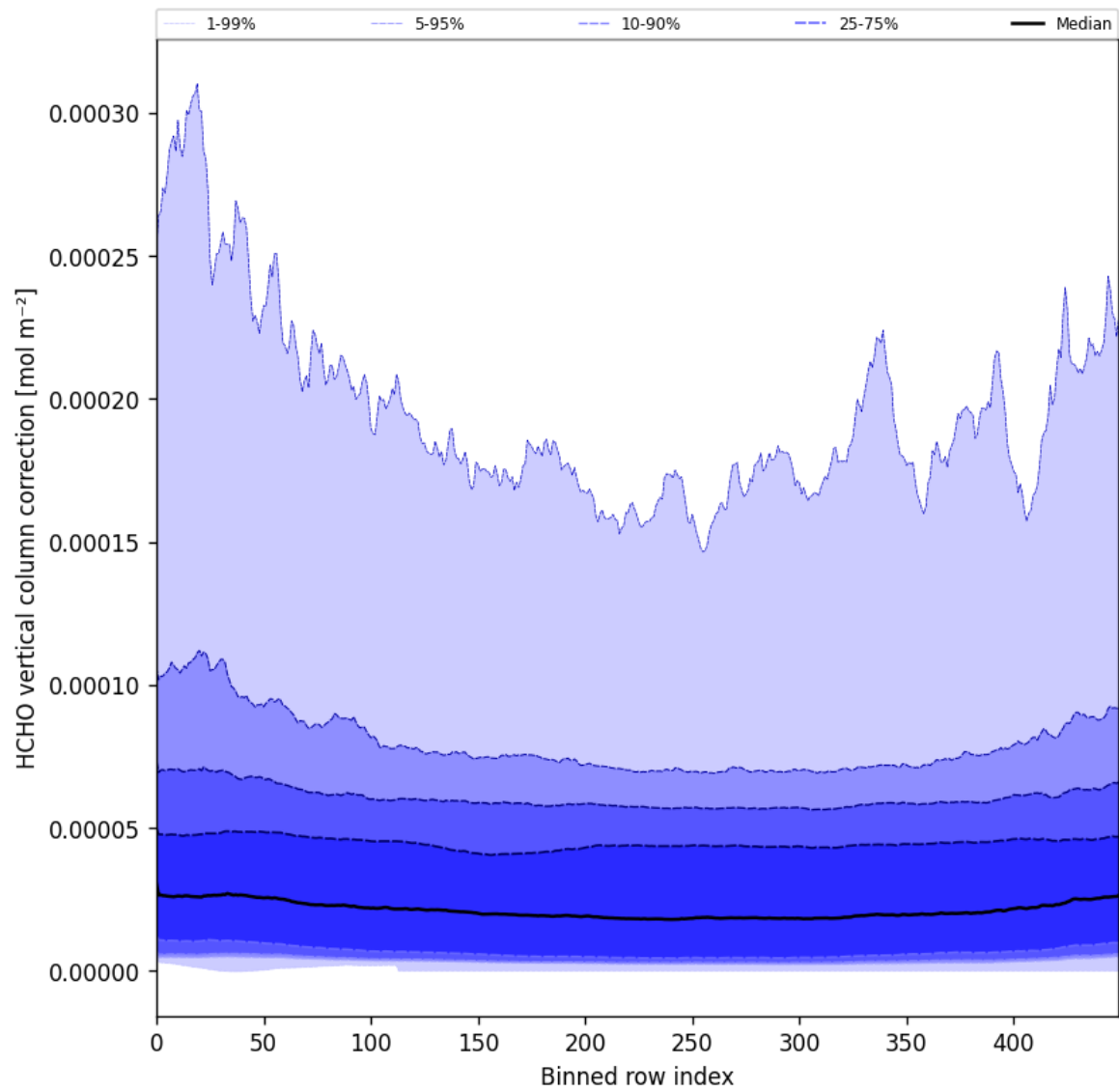
Figure 51: Along track statistics of “HCHO vertical column correction” for 2025-03-07 to 2025-03-08
