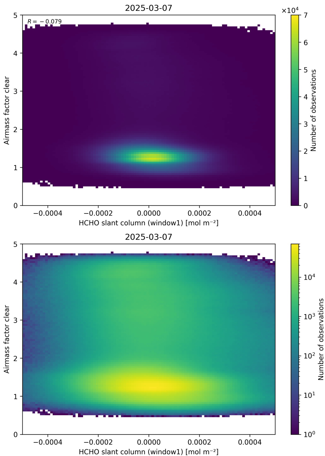
Figure 81: Scatter density plot of “HCHO slant column (window1)” against “Airmass factor clear” for 2025-03-07 to 2025-03-08.
