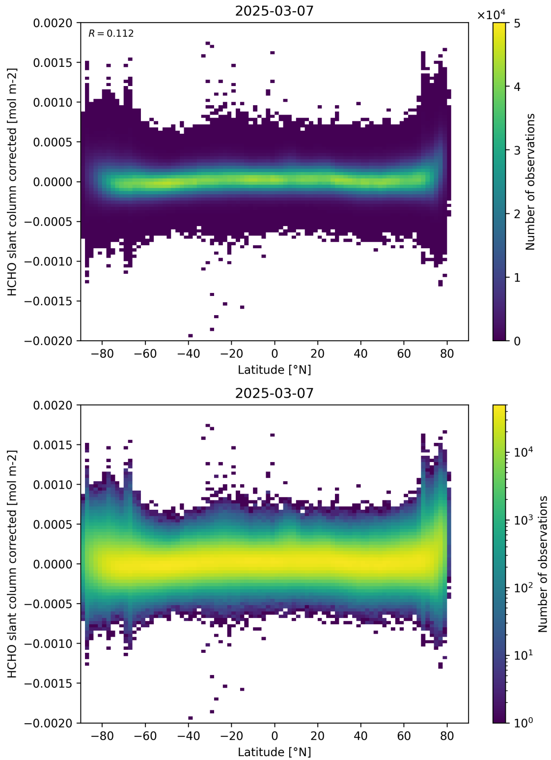
Figure 157: Scatter density plot of “Latitude” against “HCHO slant column corrected” for 2025-03-07 to 2025-03-08.
