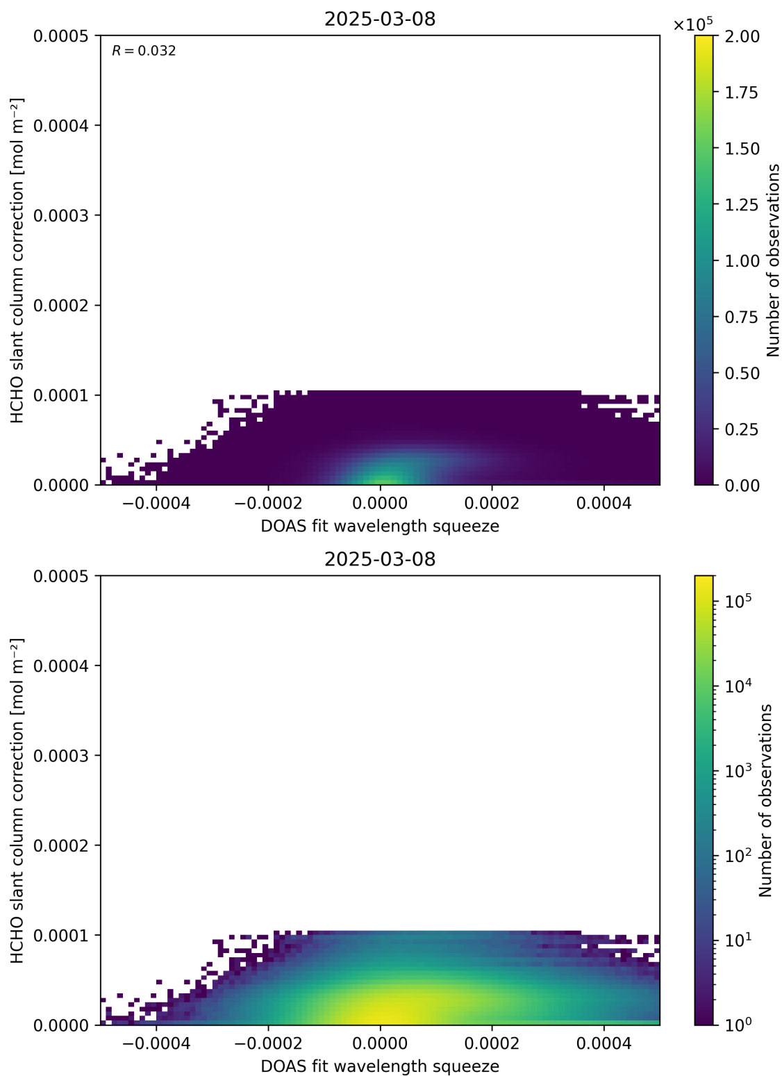
Figure 70: Scatter density plot of “DOAS fit wavelength squeeze” against “HCHO slant column correction” for 2025-03-07 to 2025-03-09.
