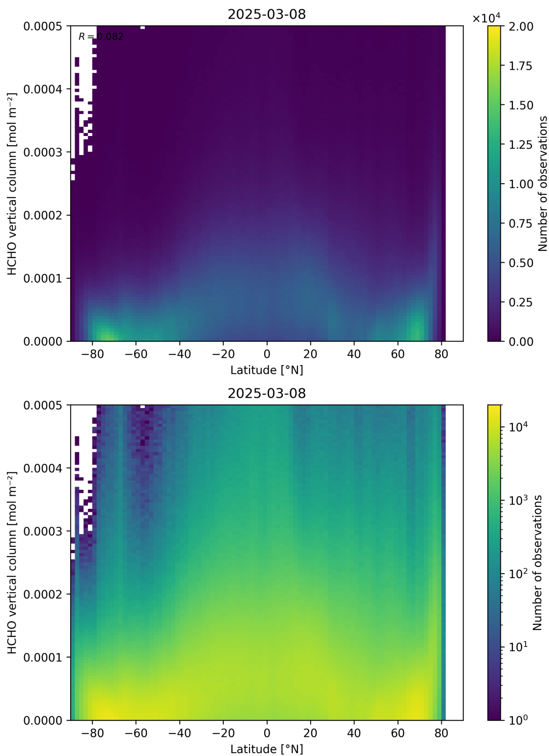
Figure 163: Scatter density plot of “Latitude” against “HCHO vertical column” for 2025-03-07 to 2025-03-09.
