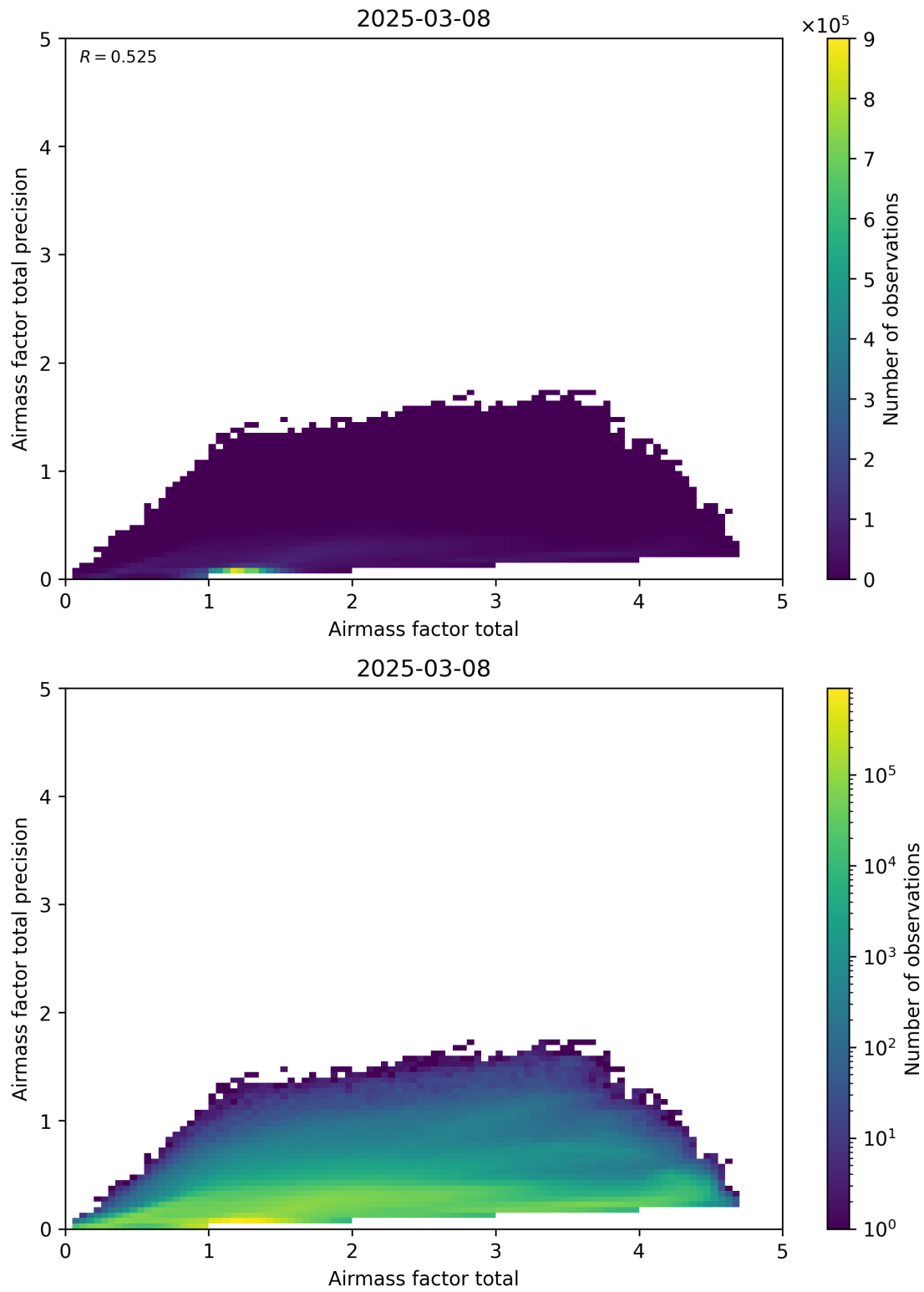
Figure 103: Scatter density plot of “Airmass factor total” against “Airmass factor total precision” for 2025-03-07 to 2025-03-09.
