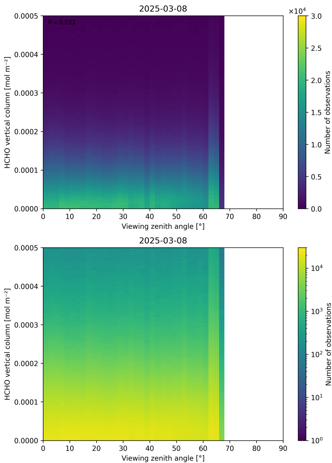
Figure 192: Scatter density plot of “Viewing zenith angle” against “HCHO vertical column” for 2025-03-07 to 2025-03-09.
