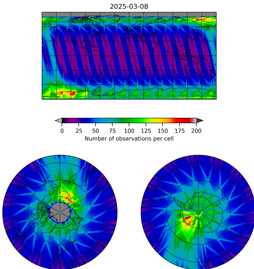
Figure 19: Map of the number of observations for 2025-03-07 to 2025-03-09
