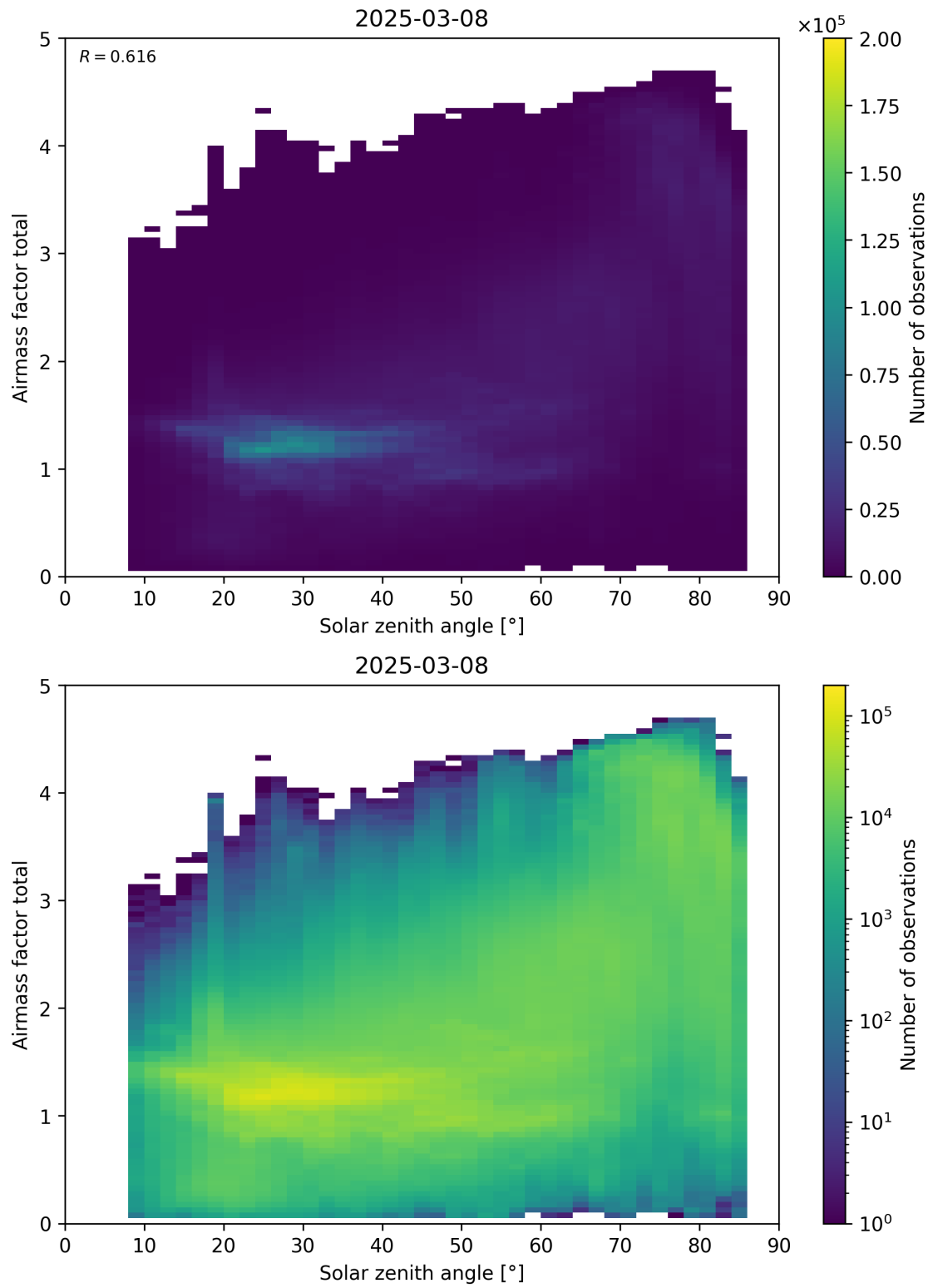
Figure 175: Scatter density plot of “Solar zenith angle” against “Airmass factor total” for 2025-03-07 to 2025-03-09.
