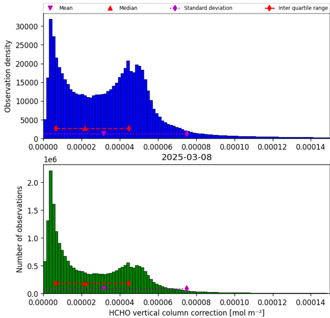
Figure 37: Histogram of “HCHO vertical column correction” for 2025-03-07 to 2025-03-09
