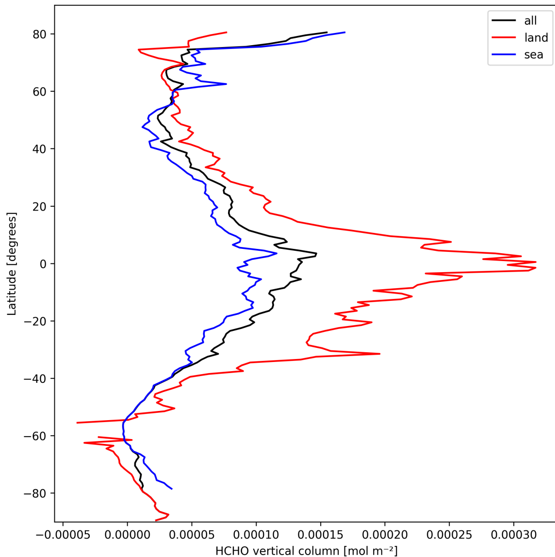
Figure 21: Zonal average of “HCHO vertical column” for 2025-03-07 to 2025-03-09.
