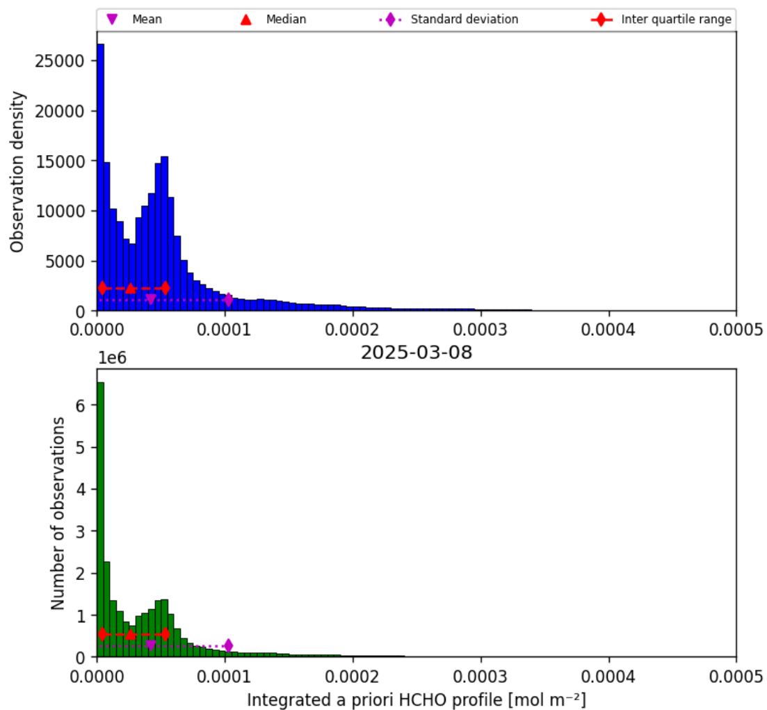
Figure 43: Histogram of “Integrated a priori HCHO profile” for 2025-03-07 to 2025-03-09
