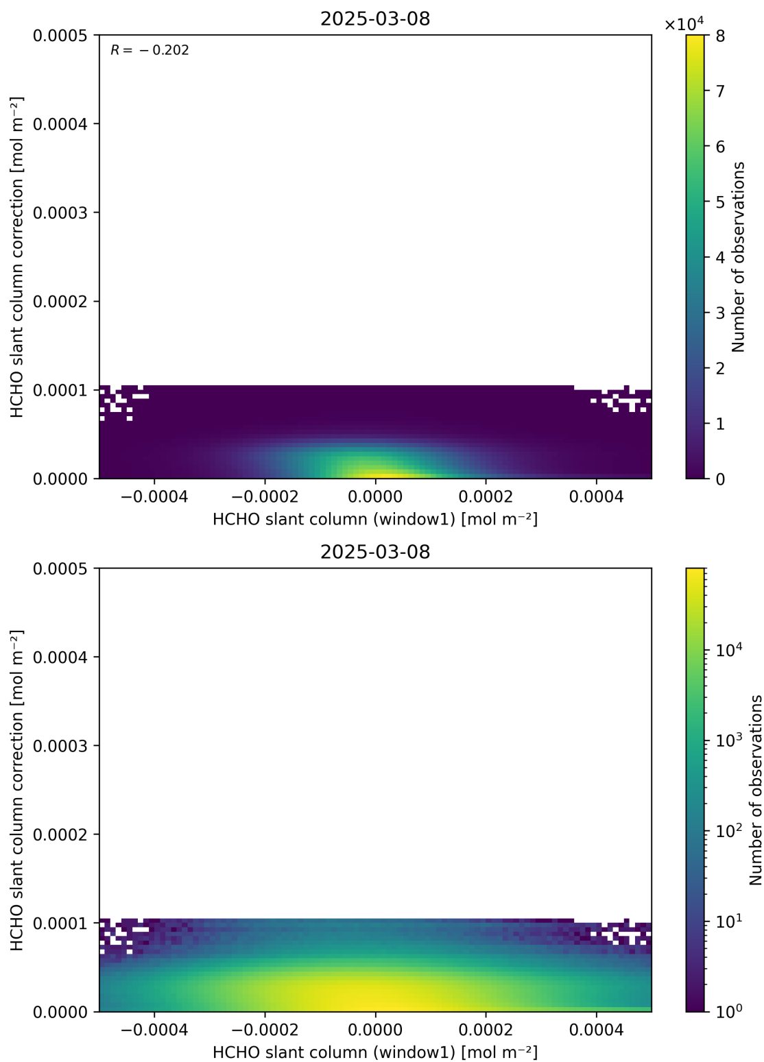
Figure 83: Scatter density plot of “HCHO slant column (window1)” against “HCHO slant column correction” for 2025-03-07 to 2025-03-09.
