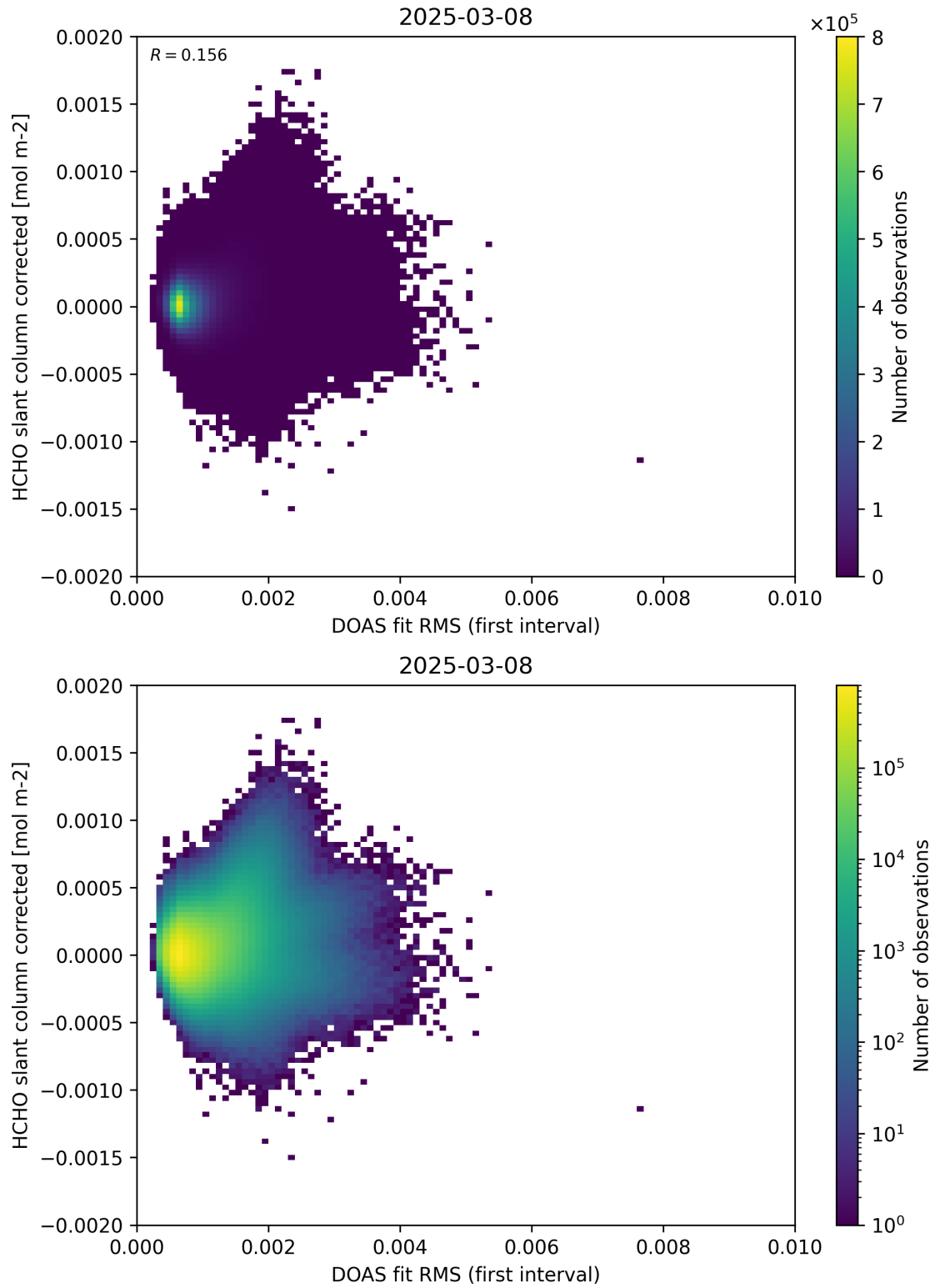
Figure 62: Scatter density plot of “DOAS fit RMS (first interval)” against “HCHO slant column corrected” for 2025-03-07 to 2025-03-09.
