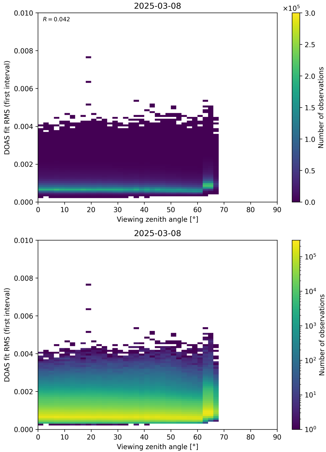
Figure 182: Scatter density plot of “Viewing zenith angle” against “DOAS fit RMS (first interval)” for 2025-03-07 to 2025-03-09.
