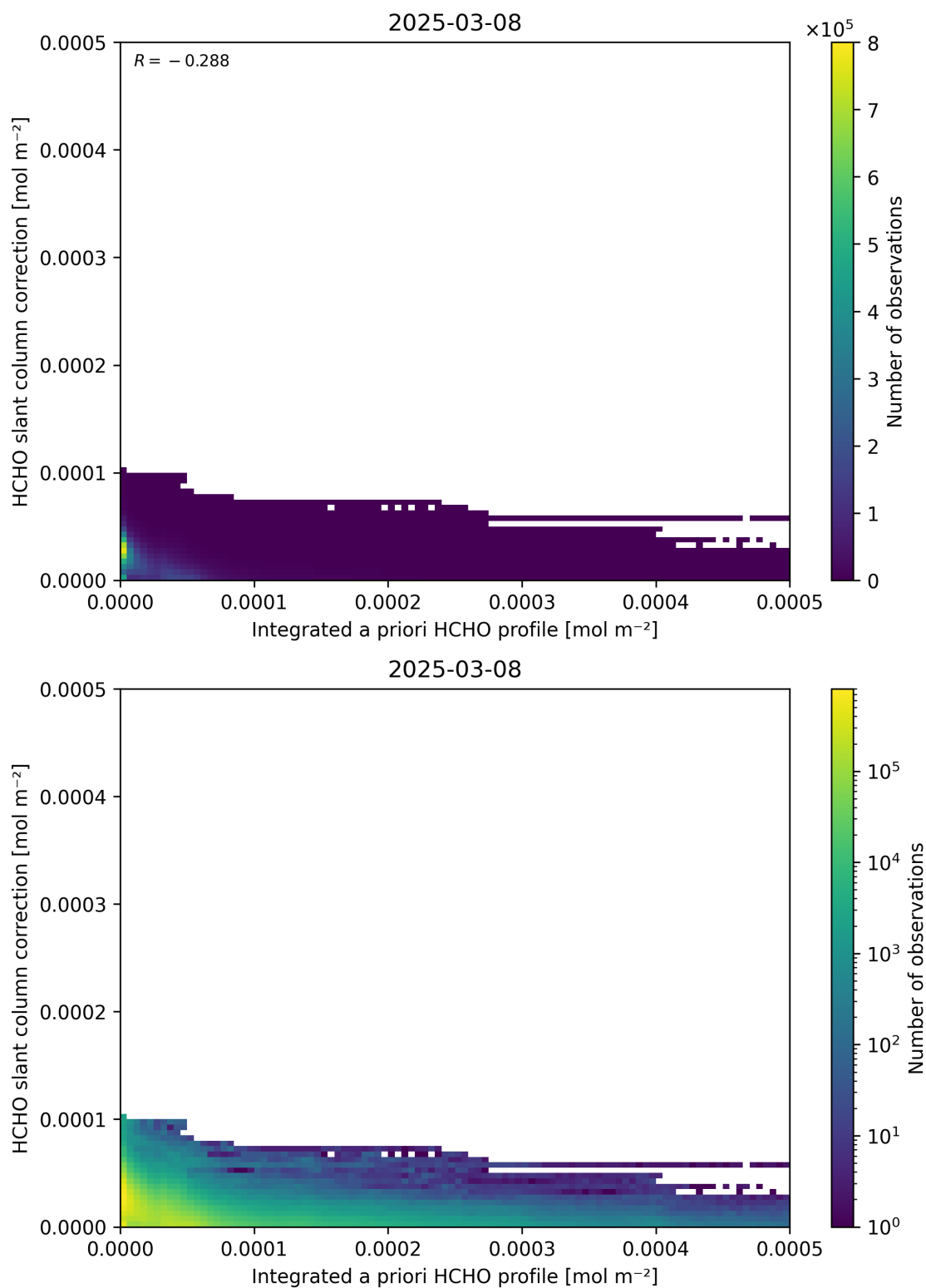
Figure 152: Scatter density plot of “Integrated a priori HCHO profile” against “HCHO slant column correction” for 2025-03-07 to 2025-03-09.
