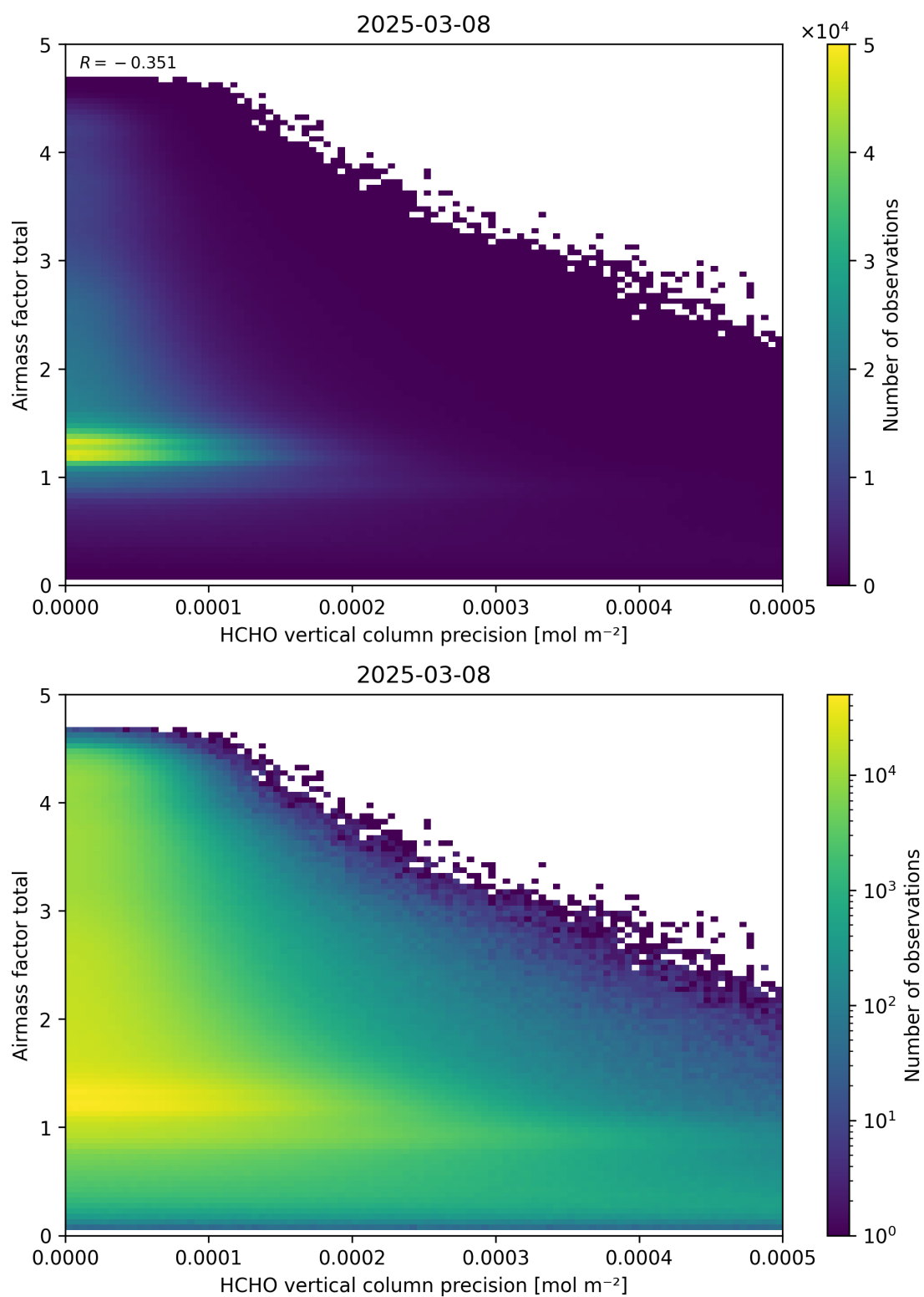
Figure 144: Scatter density plot of “HCHO vertical column precision” against “Airmass factor total” for 2025-03-07 to 2025-03-09.
