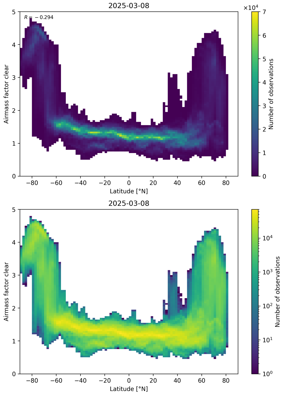
Figure 156: Scatter density plot of “Latitude” against “Airmass factor clear” for 2025-03-07 to 2025-03-09.
