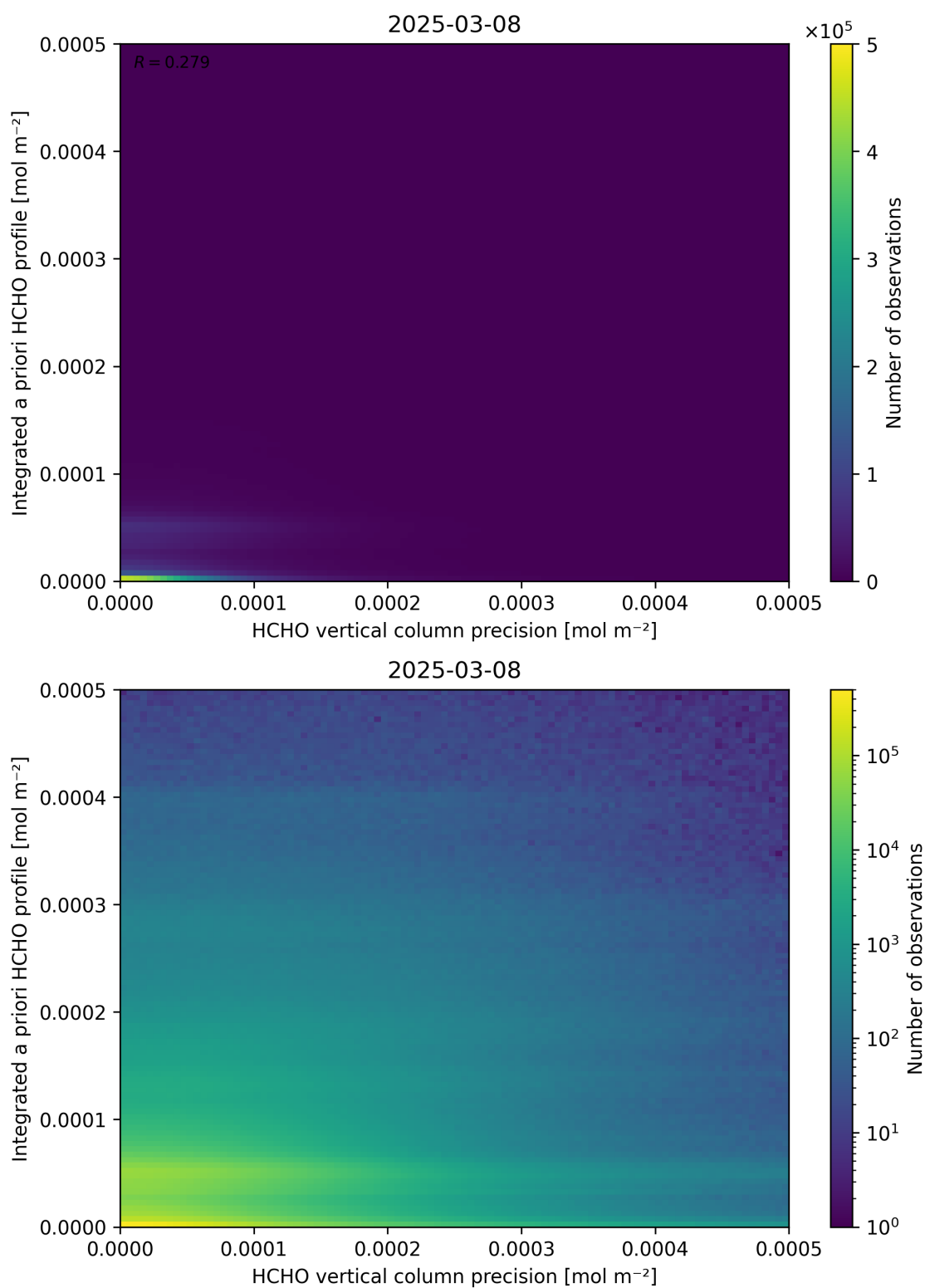
Figure 147: Scatter density plot of “HCHO vertical column precision” against “Integrated a priori HCHO profile” for 2025-03-07 to 2025-03-09.
