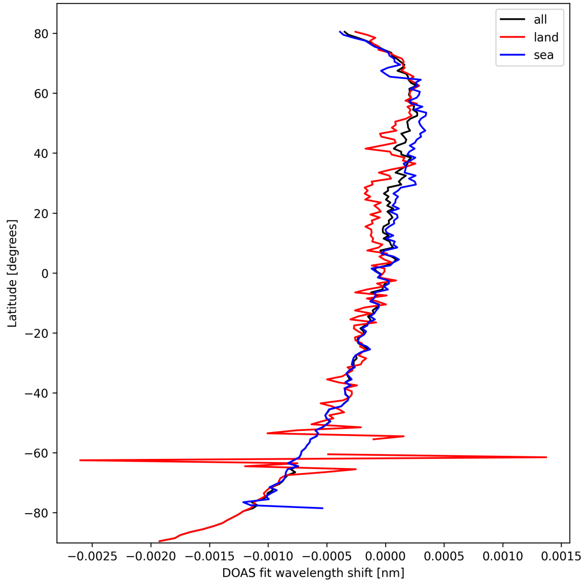
Figure 30: Zonal average of "DOAS fit wavelength shift" for 2025-03-07 to 2025-03-09.
