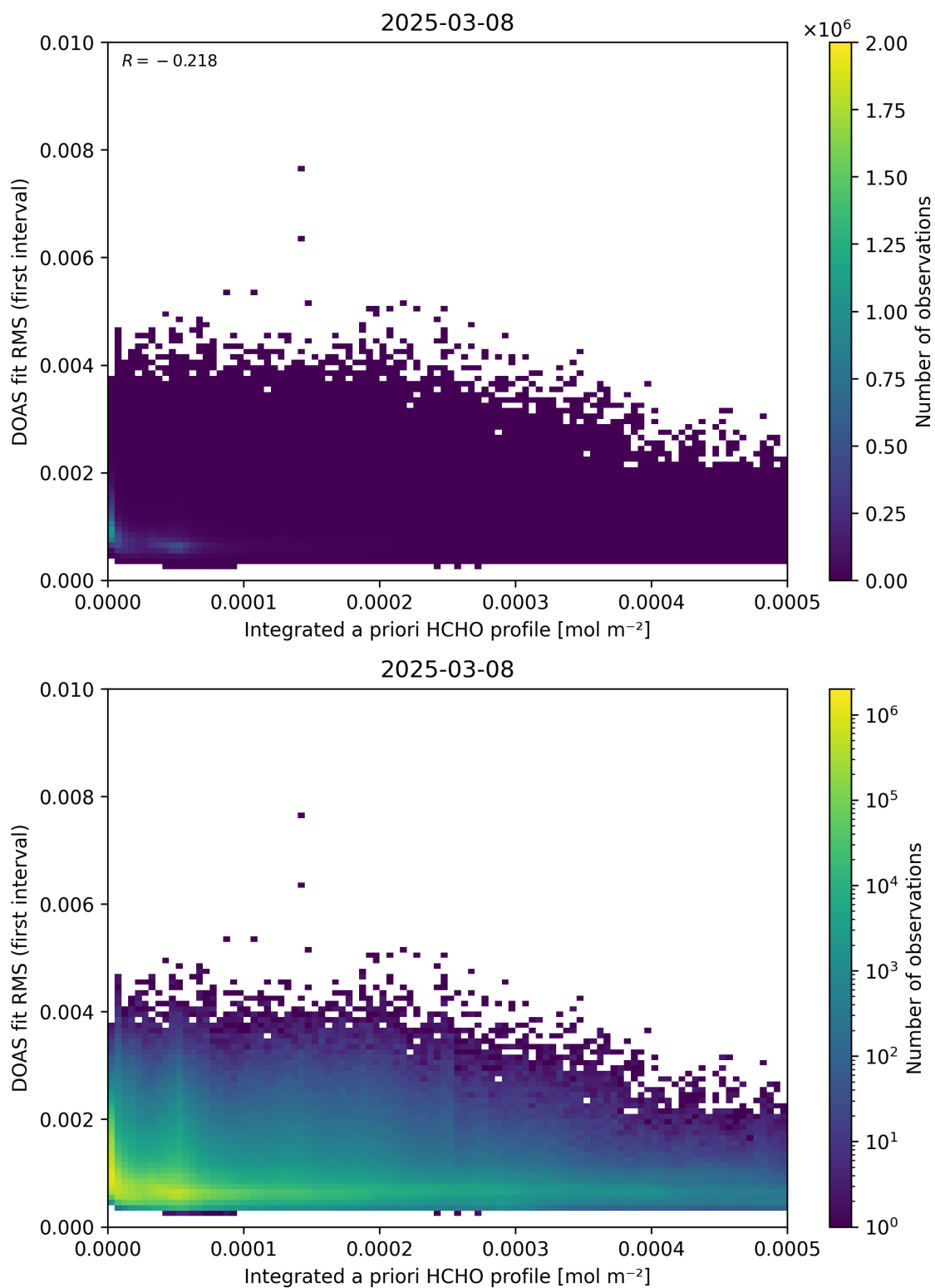
Figure 148: Scatter density plot of “Integrated a priori HCHO profile” against “DOAS fit RMS (first interval)” for 2025-03-07 to 2025-03-09.
