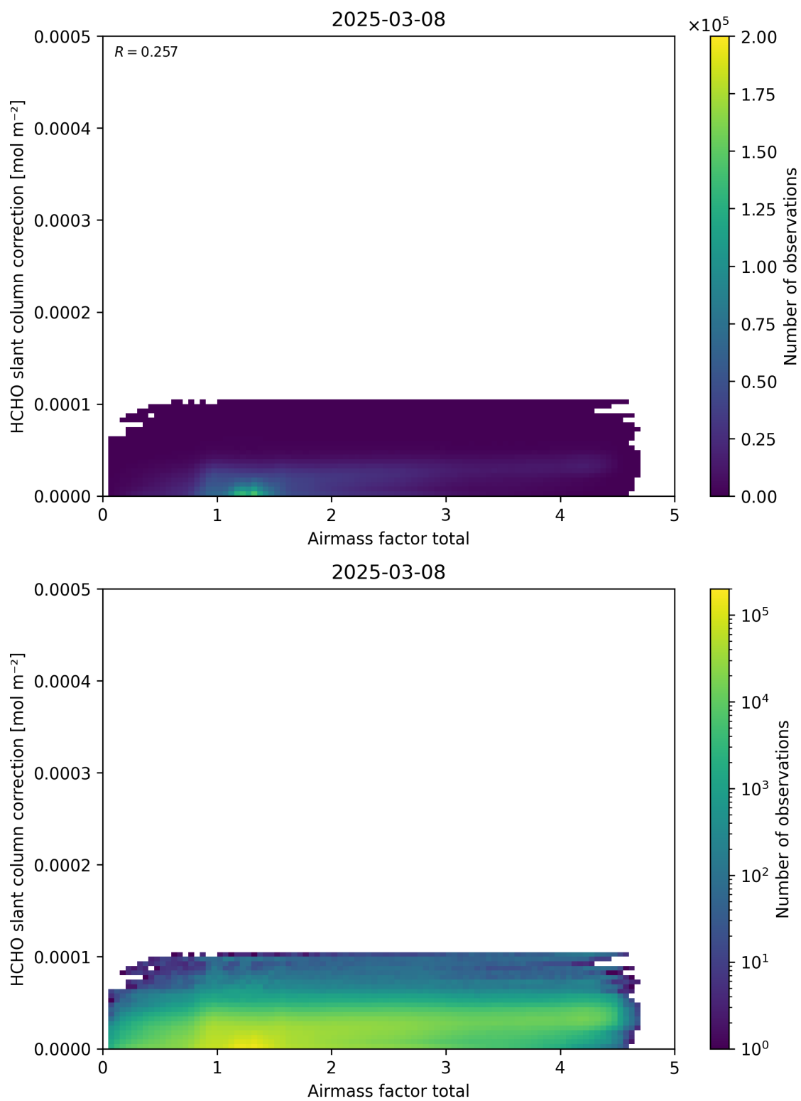
Figure 102: Scatter density plot of “Airmass factor total” against “HCHO slant column correction” for 2025-03-07 to 2025-03-09.
