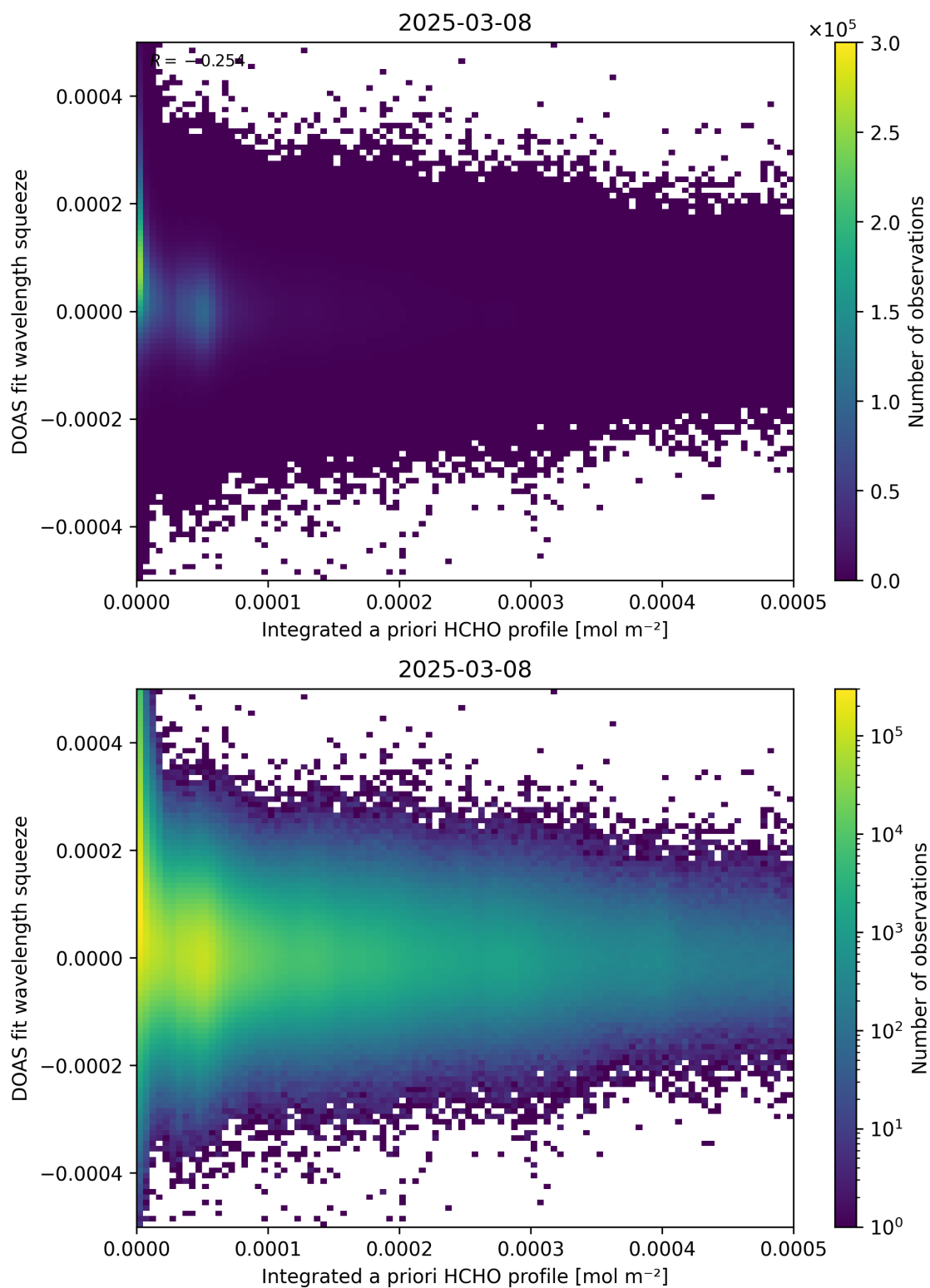
Figure 150: Scatter density plot of “Integrated a priori HCHO profile” against “DOAS fit wavelength squeeze” for 2025-03-07 to 2025-03-09.
