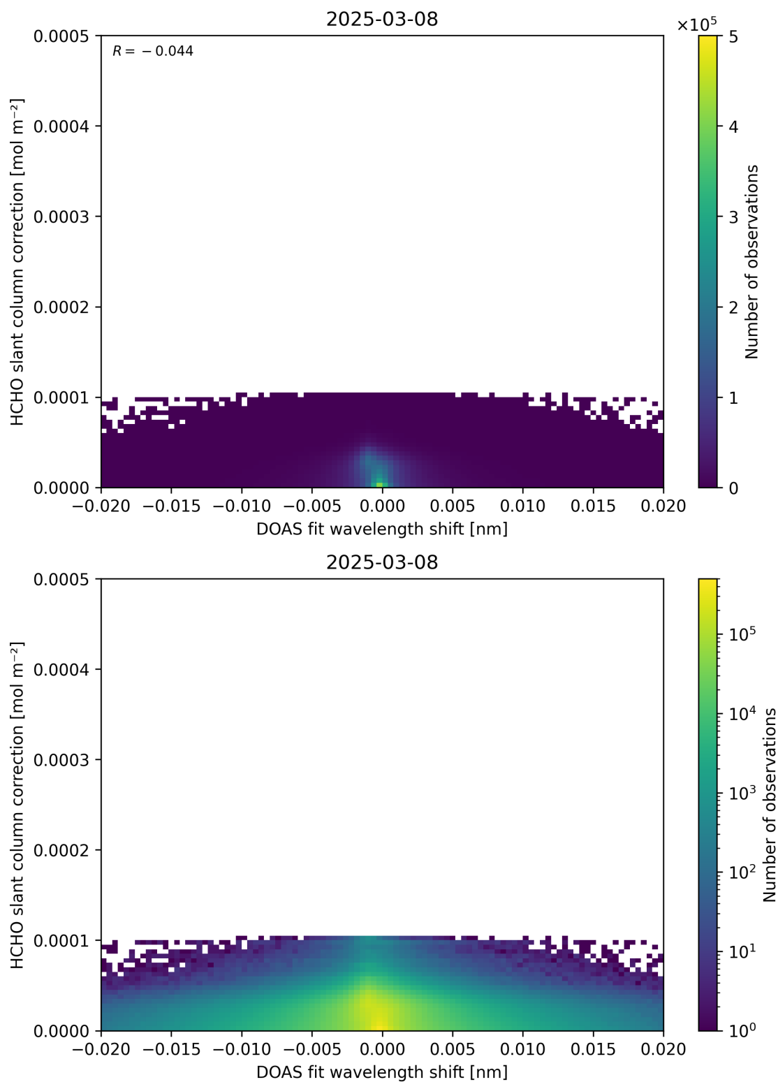
Figure 67: Scatter density plot of “DOAS fit wavelength shift” against “HCHO slant column correction” for 2025-03-07 to 2025-03-09.
