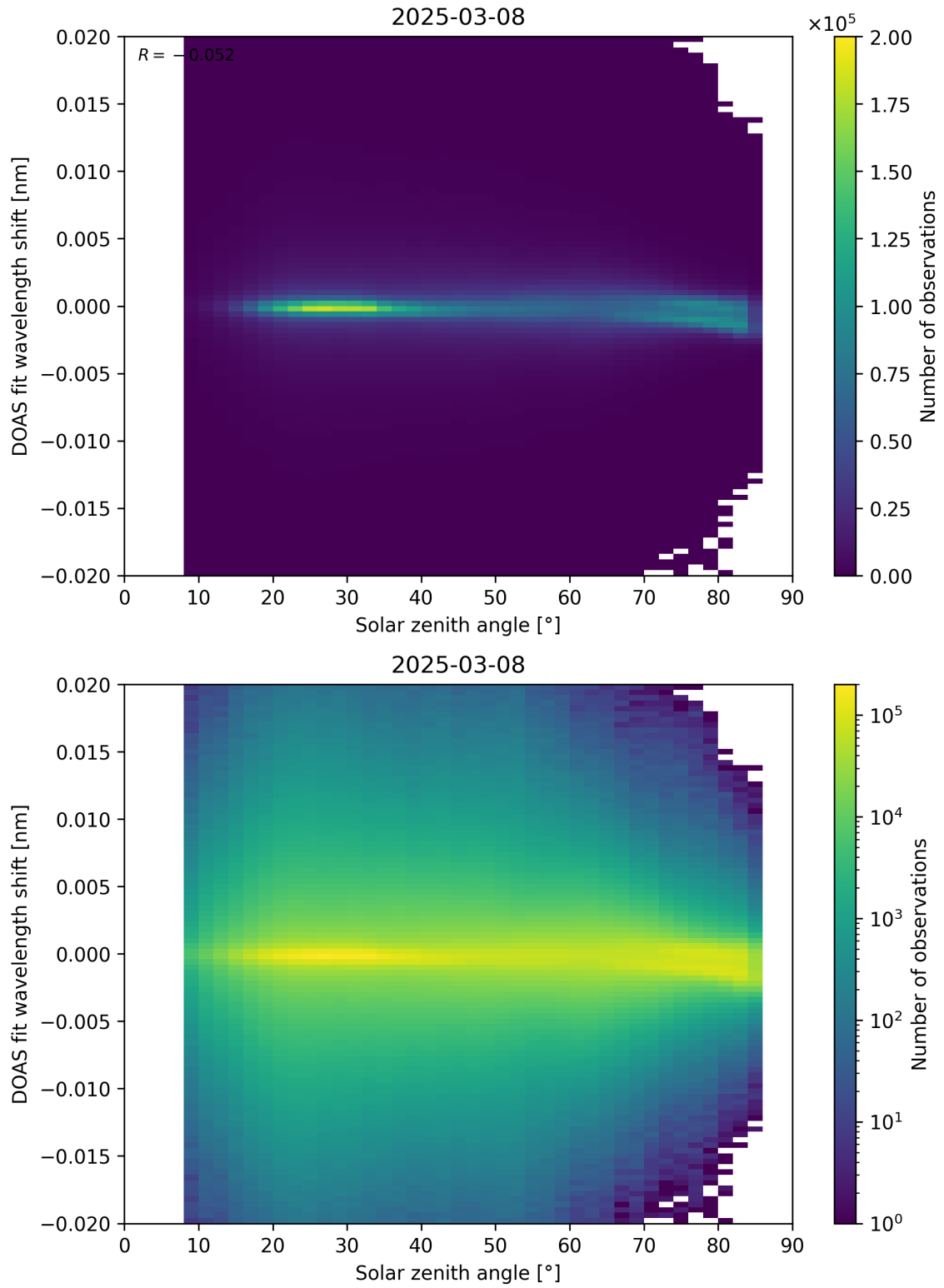
Figure 168: Scatter density plot of “Solar zenith angle” against “DOAS fit wavelength shift” for 2025-03-07 to 2025-03-09.
