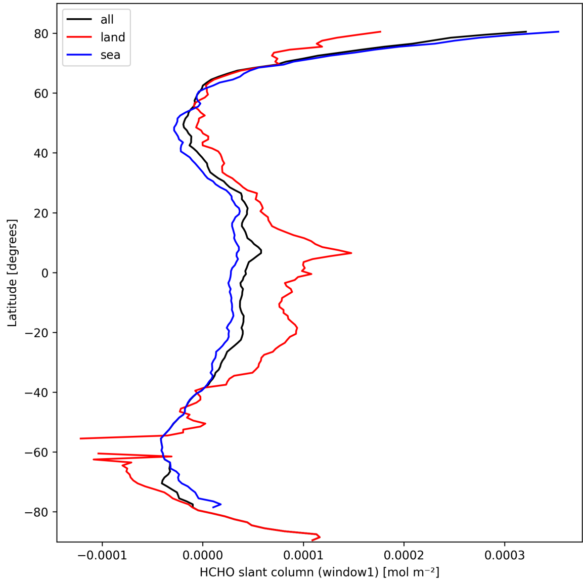
Figure 24: Zonal average of “HCHO slant column (window1)” for 2025-03-07 to 2025-03-09.
