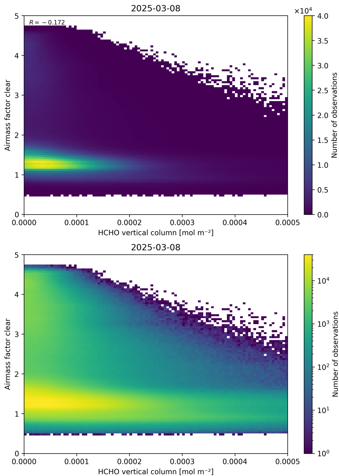
Figure 126: Scatter density plot of “HCHO vertical column” against “Airmass factor clear” for 2025-03-07 to 2025-03-09.
