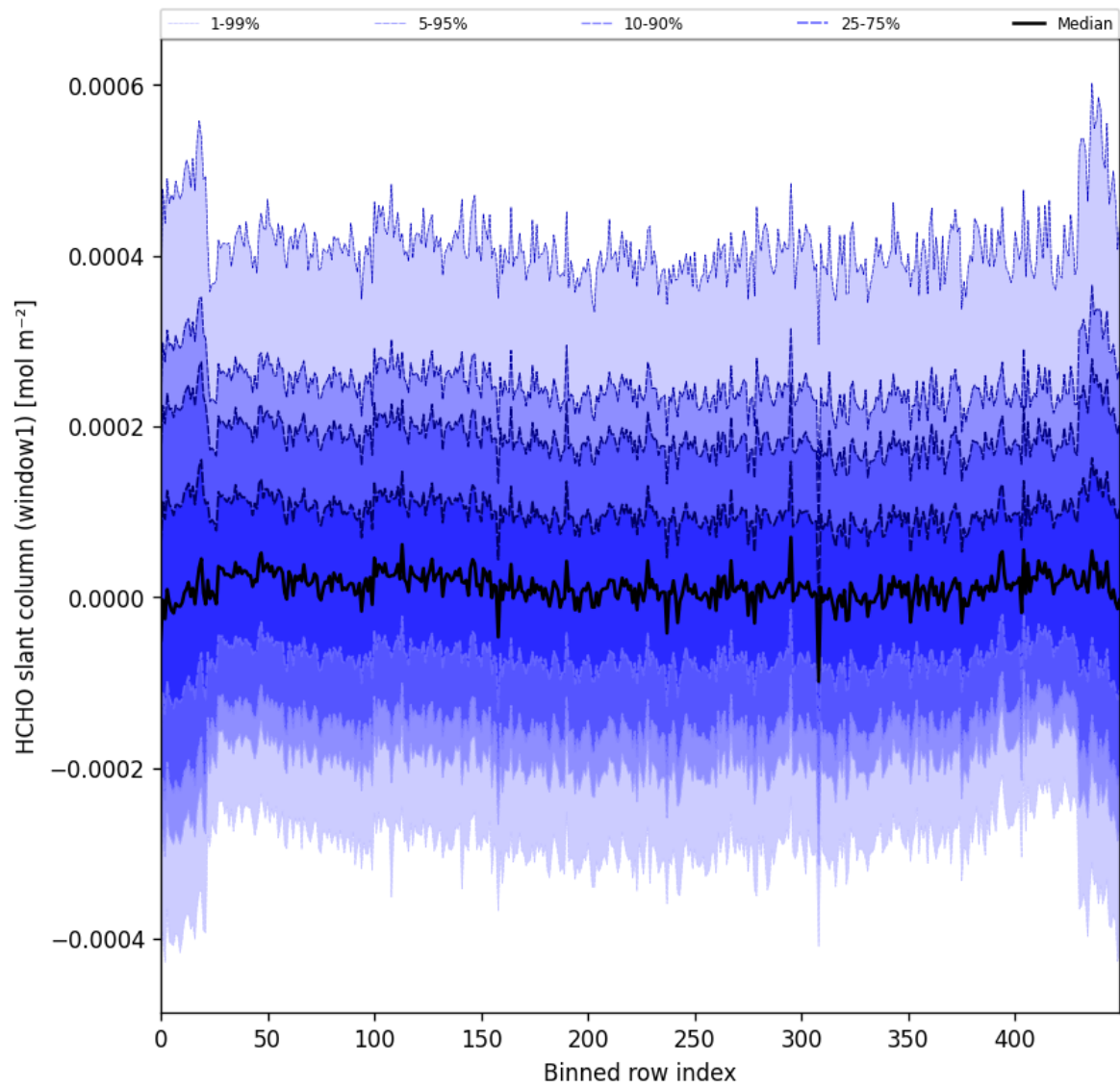
Figure 52: Along track statistics of “HCHO slant column (window1)” for 2025-03-07 to 2025-03-09
