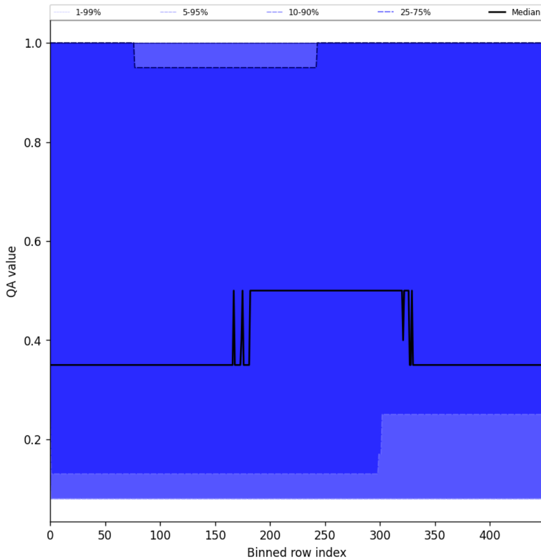
Figure 48: Along track statistics of “QA value” for 2025-03-07 to 2025-03-09
