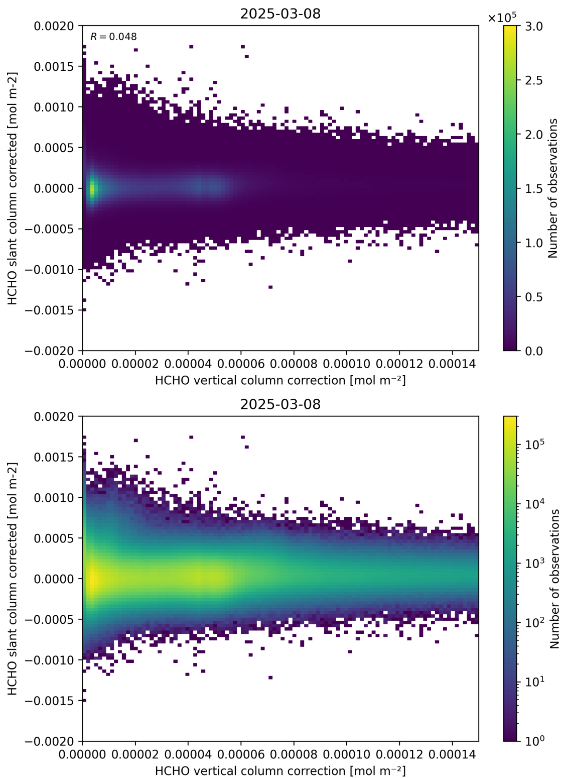
Figure 116: Scatter density plot of “HCHO vertical column correction” against “HCHO slant column corrected” for 2025-03-07 to 2025-03-09.
