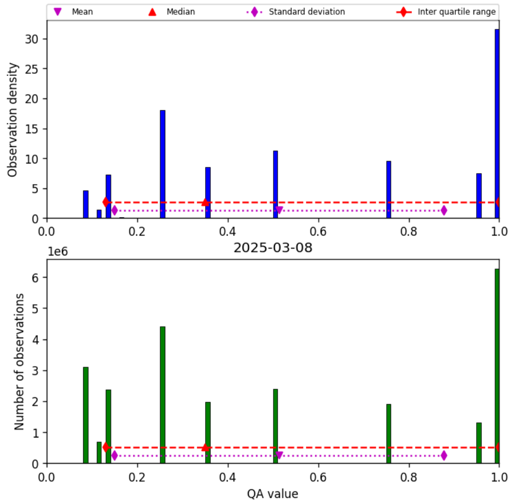
Figure 34: Histogram of “QA value” for 2025-03-07 to 2025-03-09
