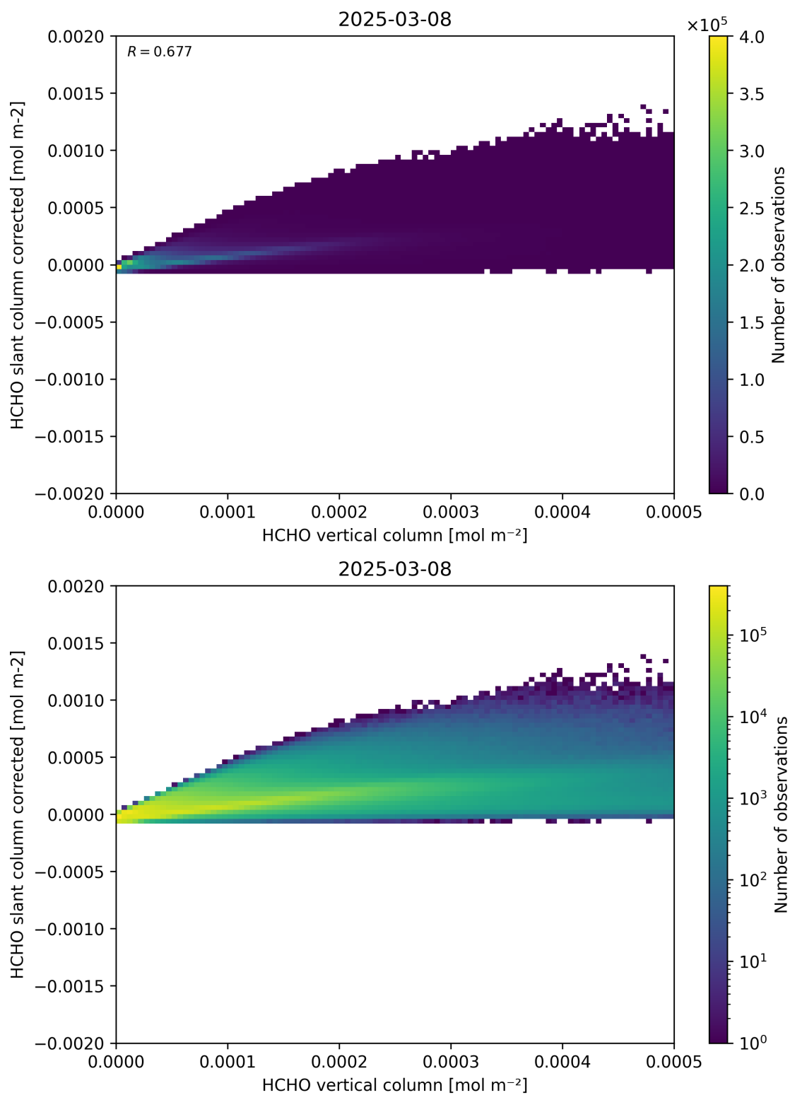
Figure 127: Scatter density plot of “HCHO vertical column” against “HCHO slant column corrected” for 2025-03-07 to 2025-03-09.
