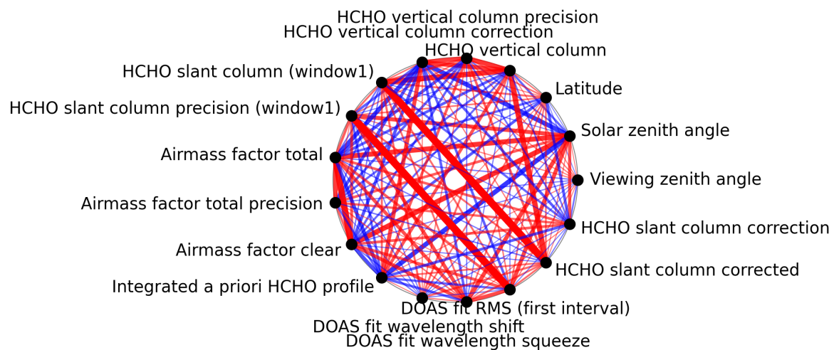
Figure 1: Map of correlation graph for 2025-03-07 to 2025-03-09.
