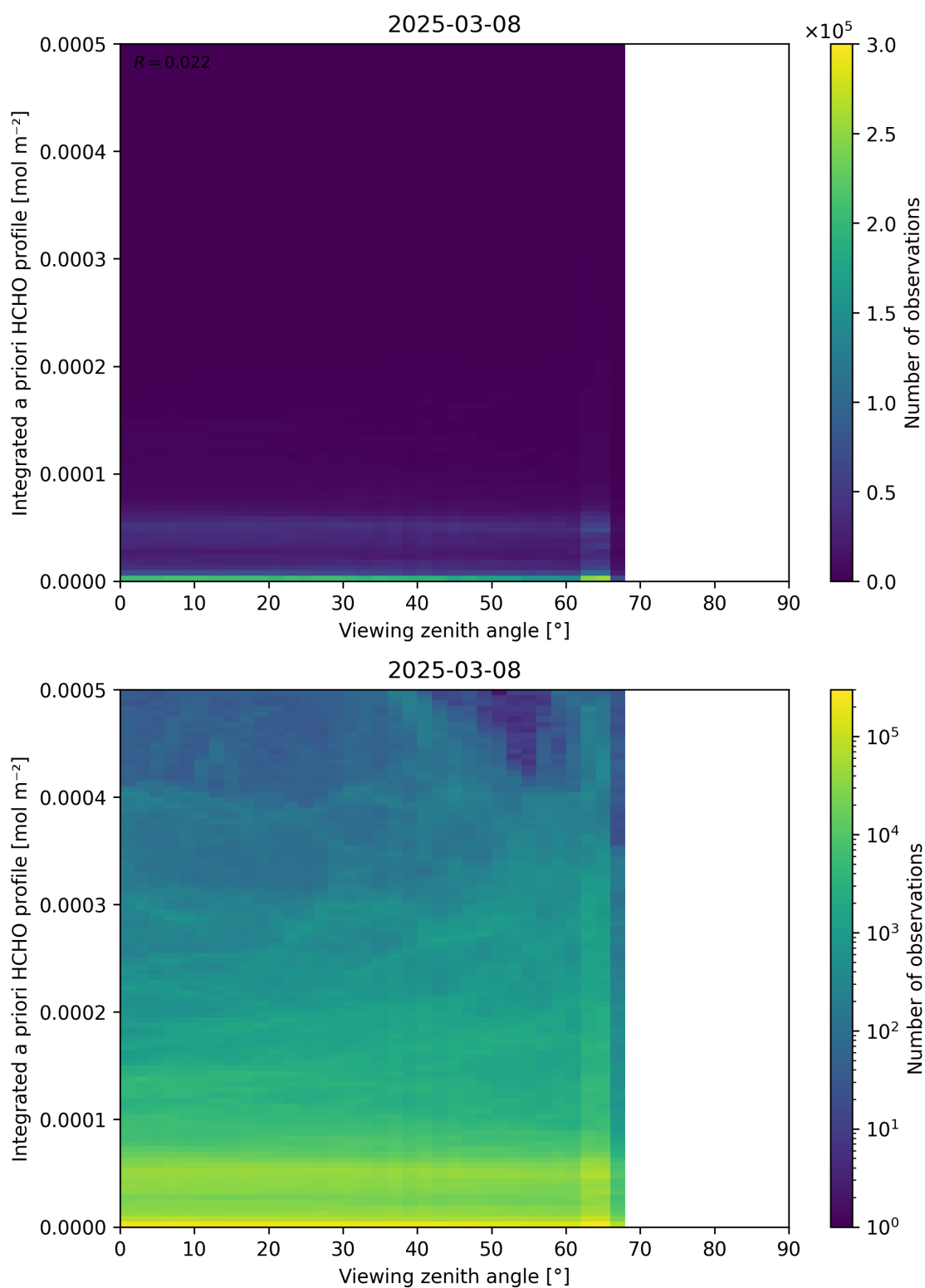
Figure 195: Scatter density plot of “Viewing zenith angle” against “Integrated a priori HCHO profile” for 2025-03-07 to 2025-03-09.
