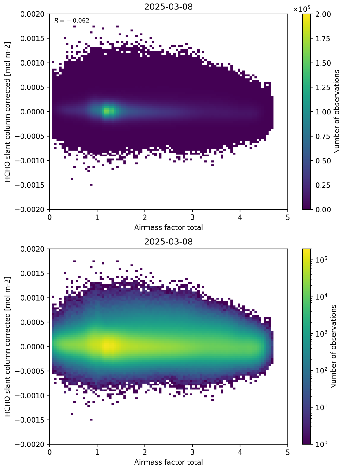
Figure 101: Scatter density plot of “Airmass factor total” against “HCHO slant column corrected” for 2025-03-07 to 2025-03-09.
