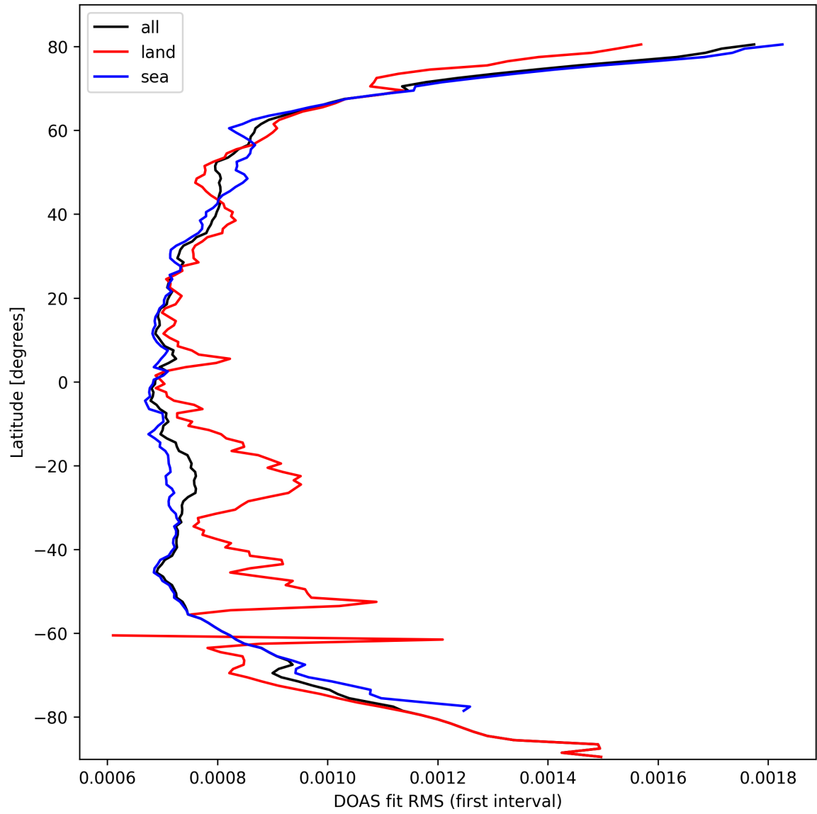
Figure 32: Zonal average of “DOAS fit RMS (first interval)” for 2025-03-07 to 2025-03-09.
