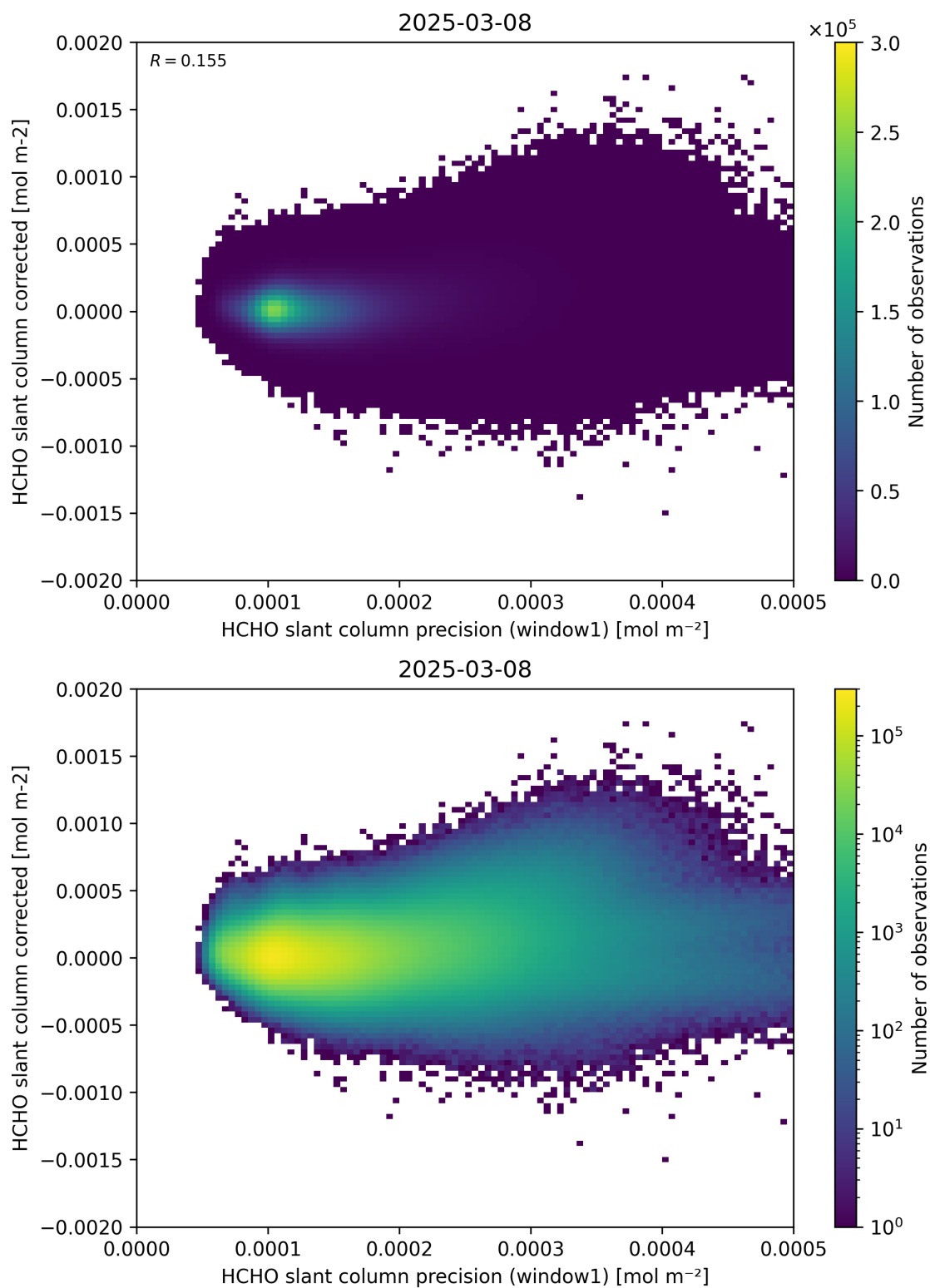
Figure 92: Scatter density plot of “HCHO slant column precision (window1)” against “HCHO slant column corrected” for 2025-03-07 to 2025-03-09.
