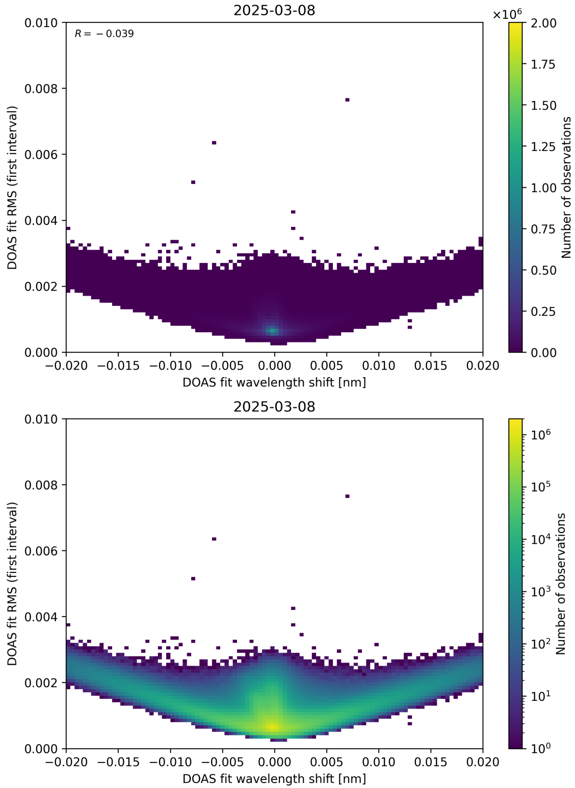
Figure 64: Scatter density plot of “DOAS fit wavelength shift” against “DOAS fit RMS (first interval)” for 2025-03-07 to 2025-03-09.
