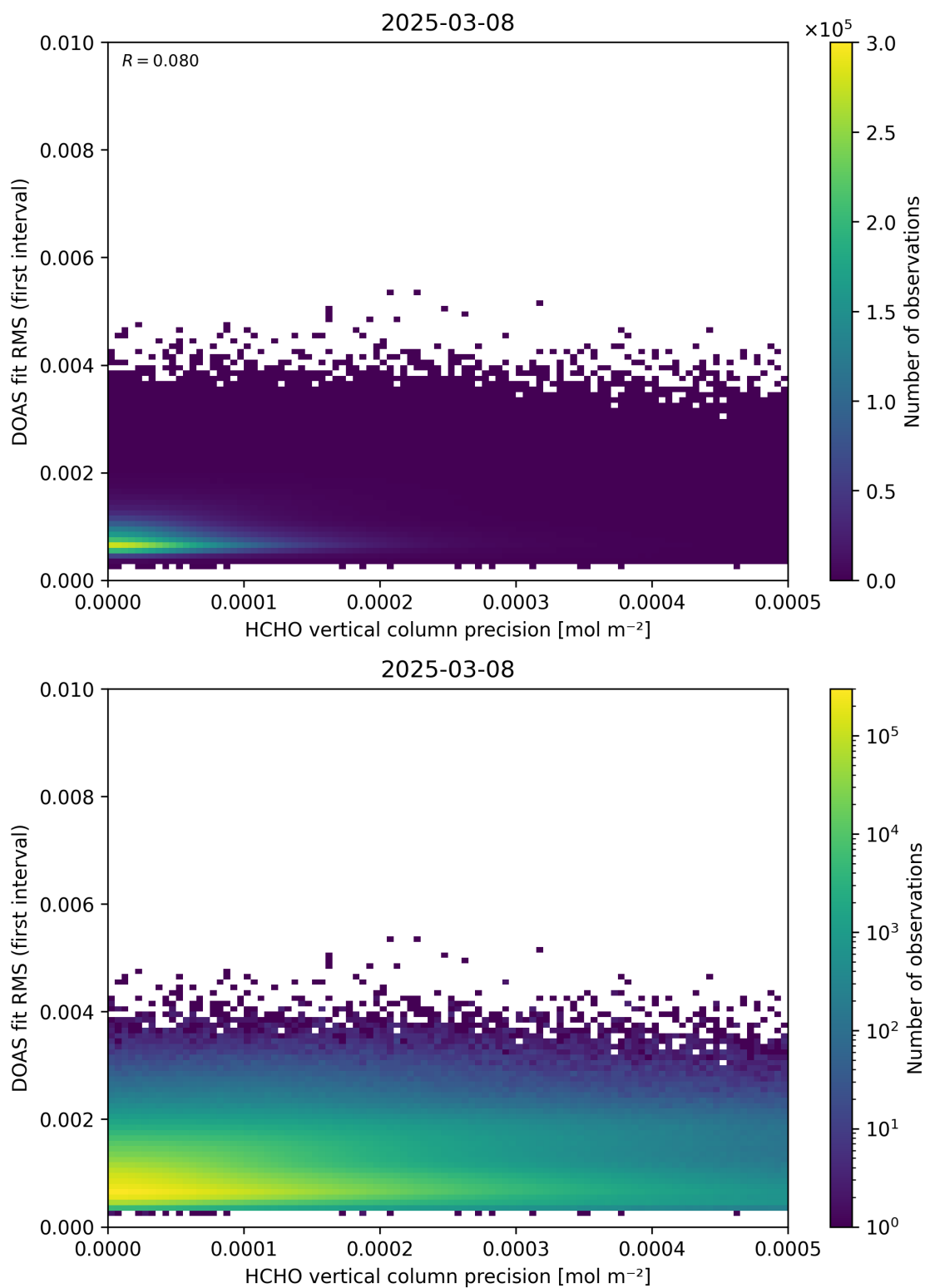
Figure 136: Scatter density plot of “HCHO vertical column precision” against “DOAS fit RMS (first interval)” for 2025-03-07 to 2025-03-09.
