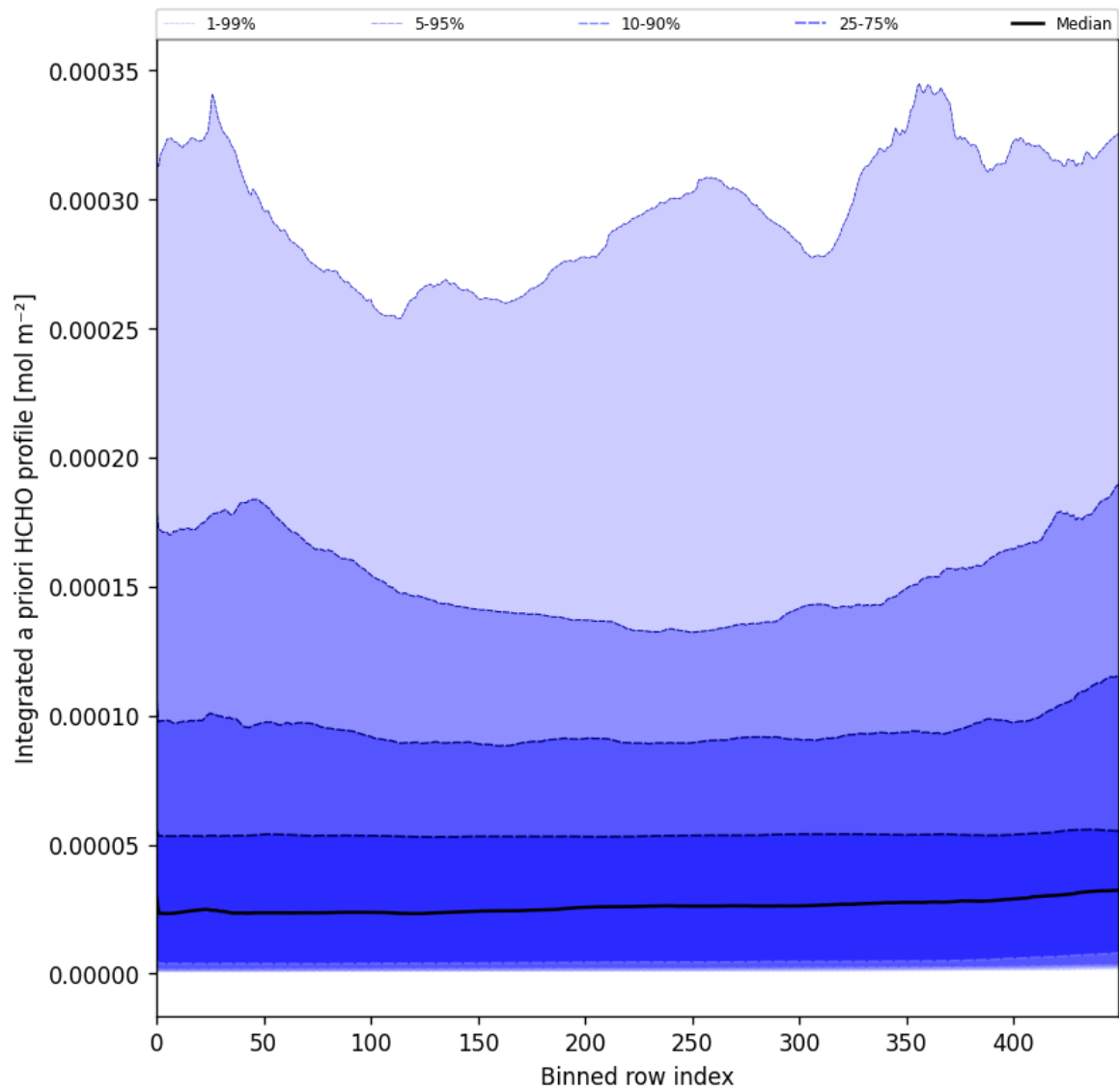
Figure 57: Along track statistics of “Integrated a priori HCHO profile” for 2025-03-07 to 2025-03-09
