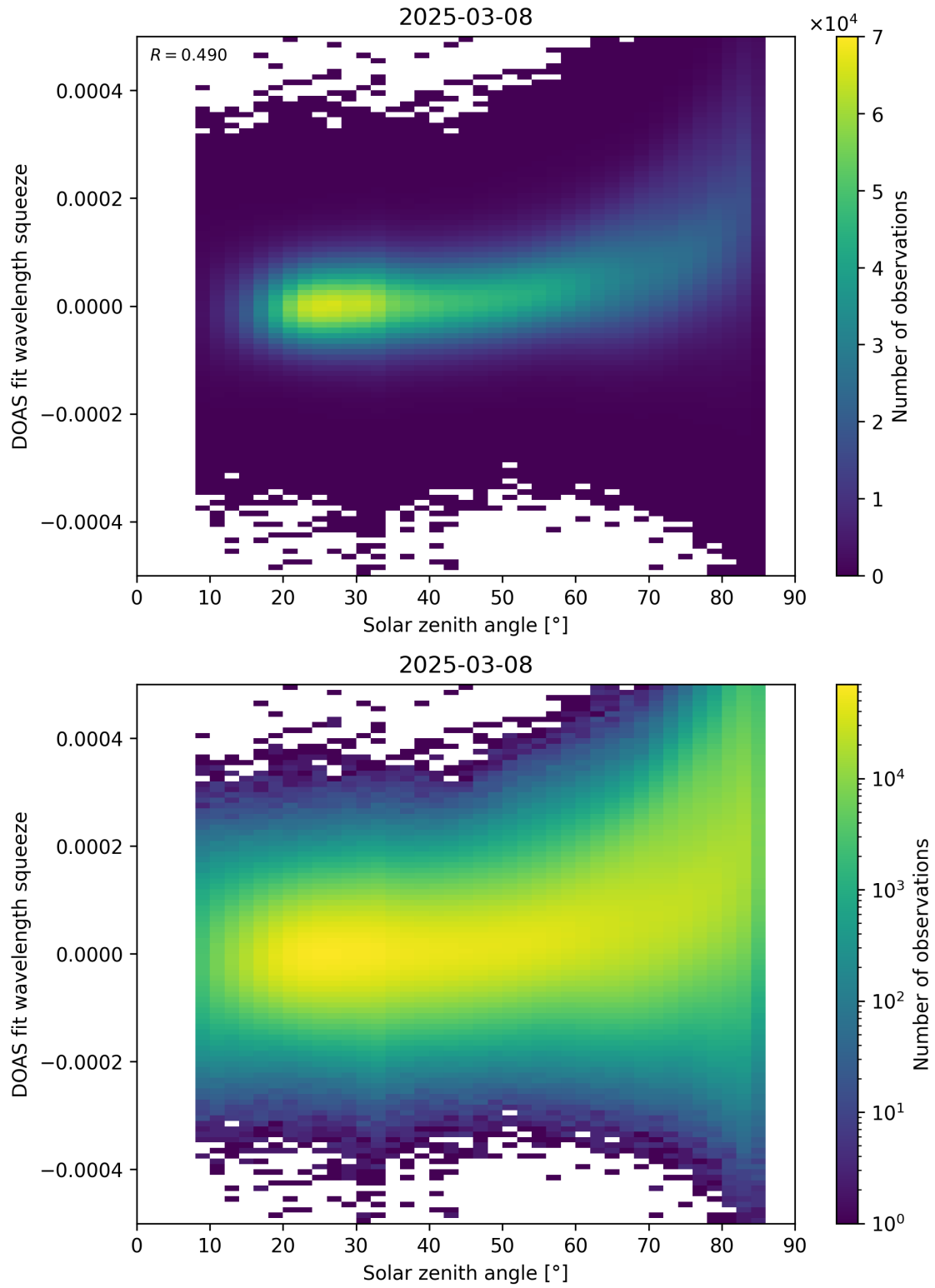
Figure 169: Scatter density plot of “Solar zenith angle” against “DOAS fit wavelength squeeze” for 2025-03-07 to 2025-03-09.
