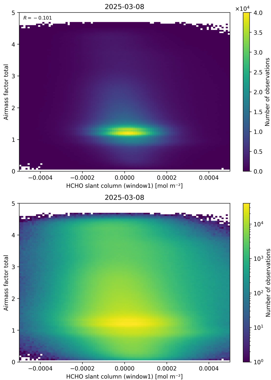
Figure 85: Scatter density plot of “HCHO slant column (window1)” against “Airmass factor total” for 2025-03-07 to 2025-03-09.
