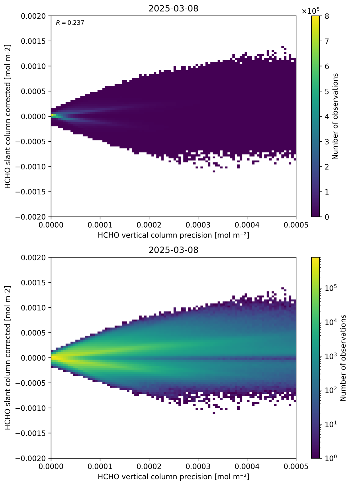
Figure 140: Scatter density plot of “HCHO vertical column precision” against “HCHO slant column corrected” for 2025-03-07 to 2025-03-09.
