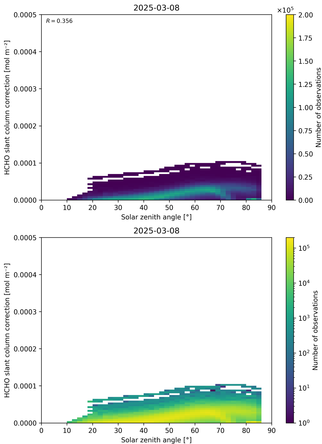
Figure 172: Scatter density plot of “Solar zenith angle” against “HCHO slant column correction” for 2025-03-07 to 2025-03-09.
