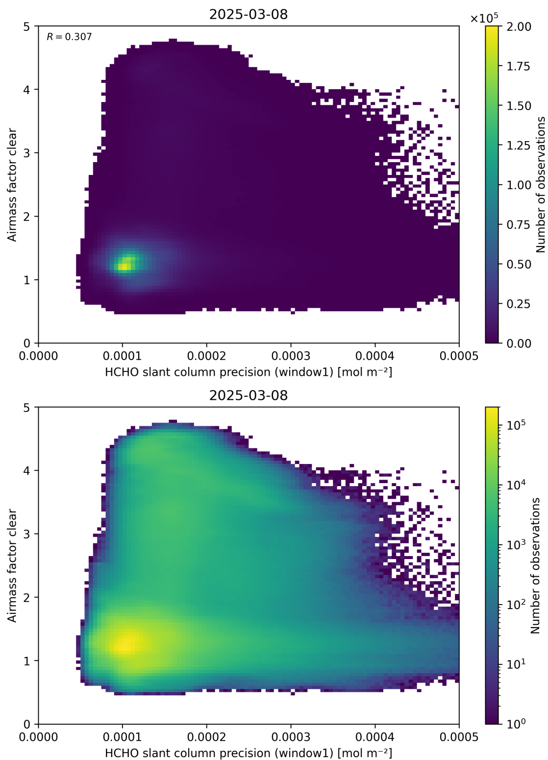
Figure 91: Scatter density plot of “HCHO slant column precision (window1)” against “Airmass factor clear” for 2025-03-07 to 2025-03-09.
