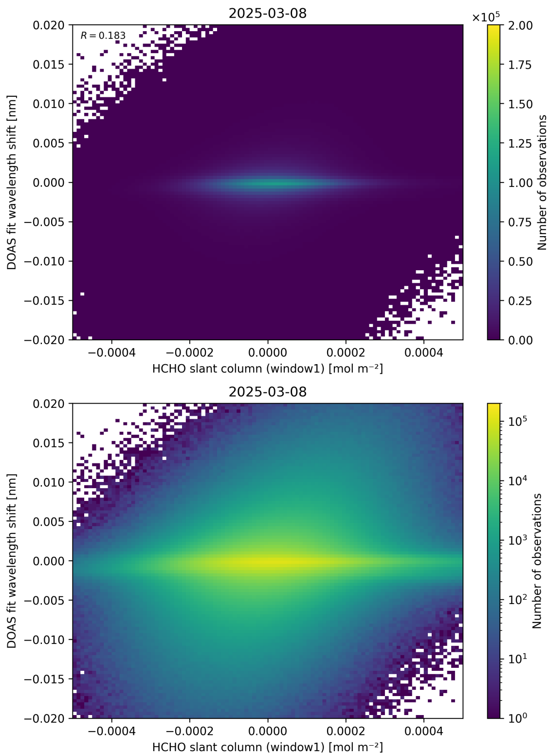
Figure 79: Scatter density plot of “HCHO slant column (window1)” against “DOAS fit wavelength shift” for 2025-03-07 to 2025-03-09.
