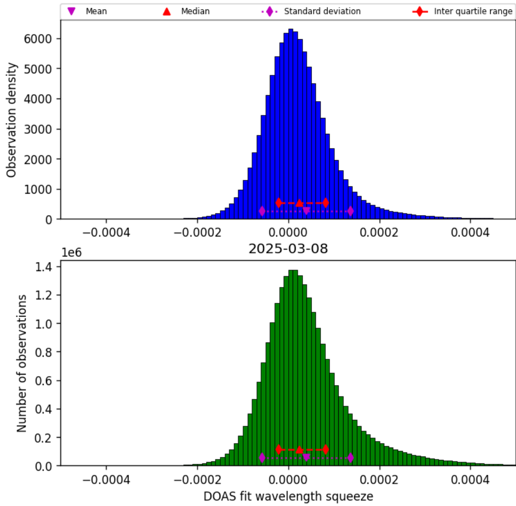
Figure 45: Histogram of “DOAS fit wavelength squeeze” for 2025-03-07 to 2025-03-09
