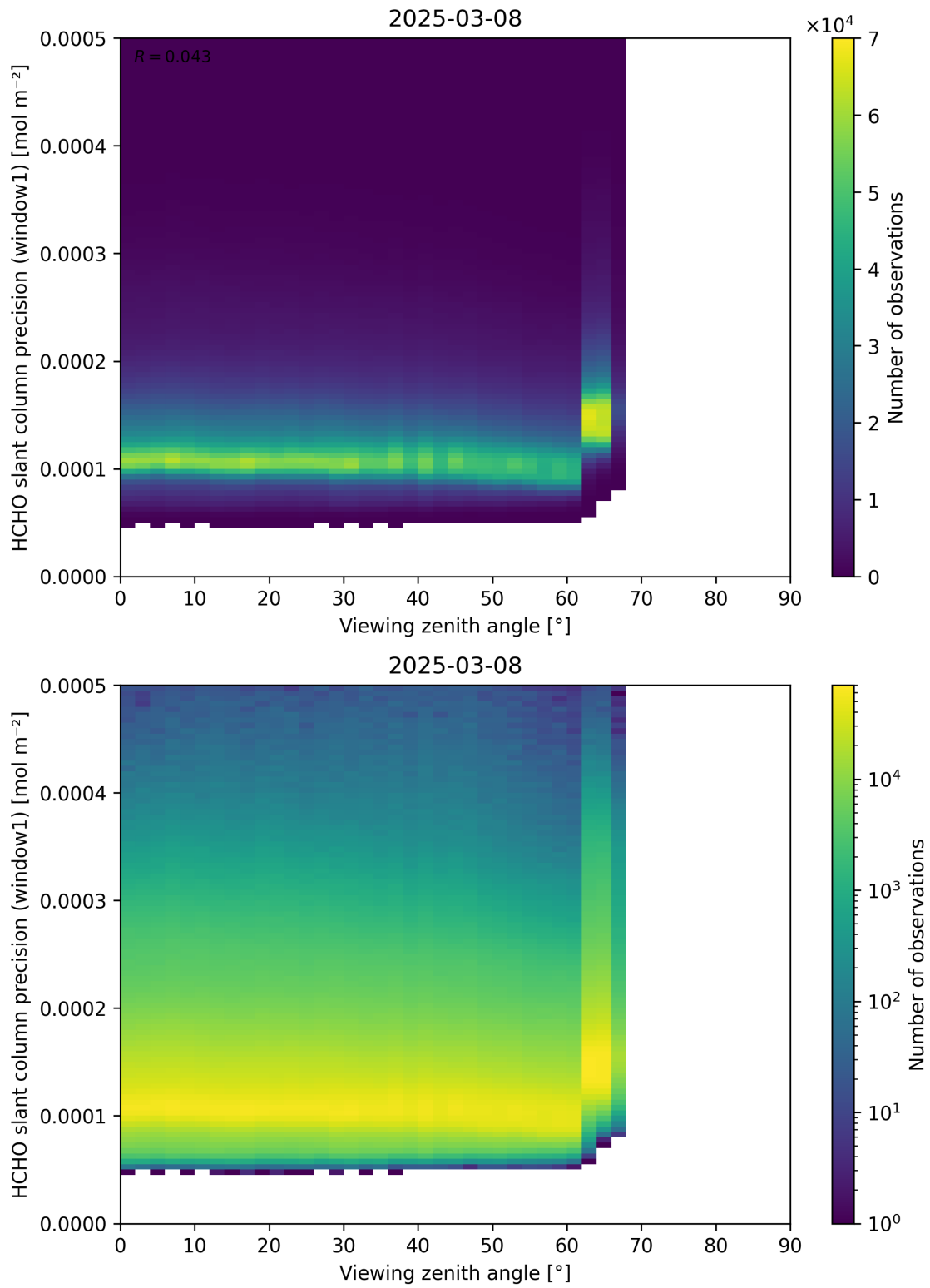
Figure 189: Scatter density plot of “Viewing zenith angle” against “HCHO slant column precision (window1)” for 2025-03-07 to 2025-03-09.
