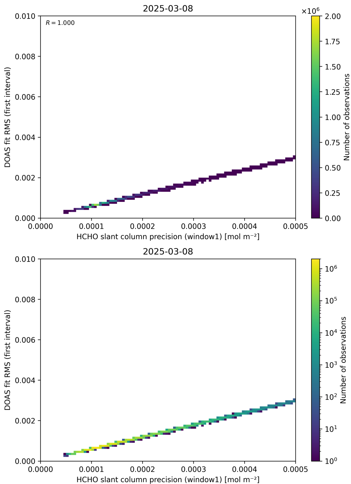
Figure 88: Scatter density plot of “HCHO slant column precision (window1)” against “DOAS fit RMS (first interval)” for 2025-03-07 to 2025-03-09.
