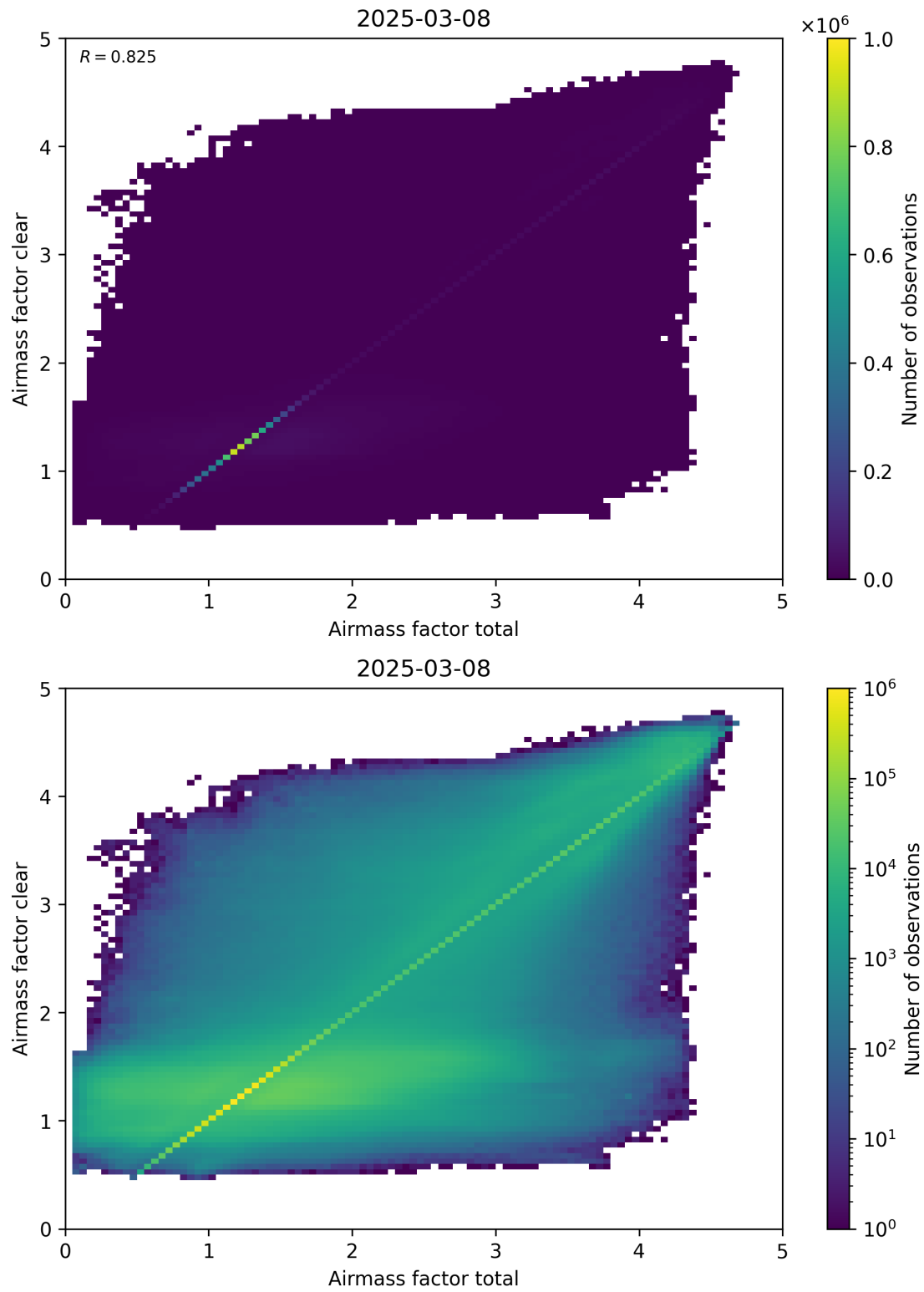
Figure 100: Scatter density plot of “Airmass factor total” against “Airmass factor clear” for 2025-03-07 to 2025-03-09.
