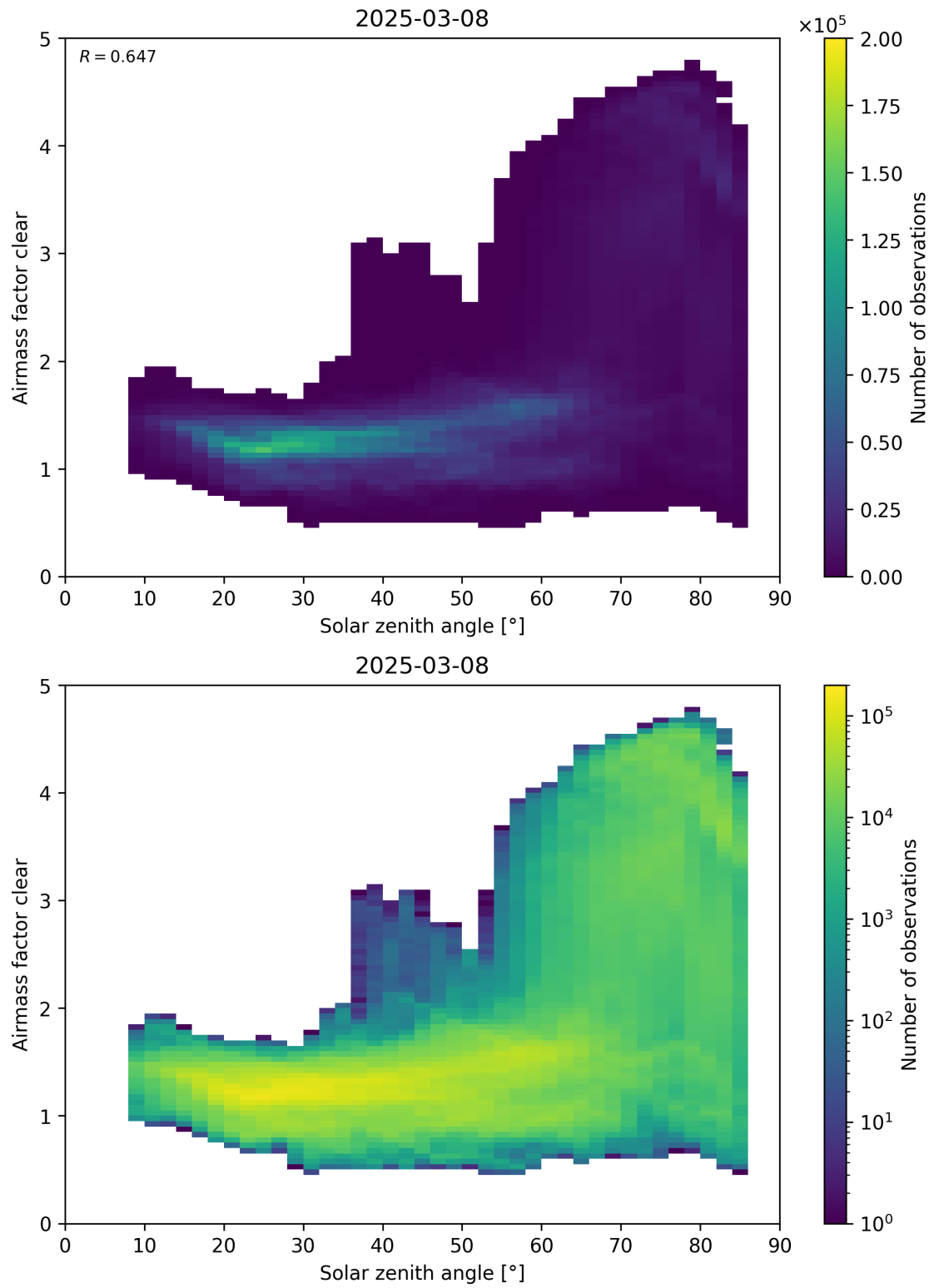
Figure 170: Scatter density plot of “Solar zenith angle” against “Airmass factor clear” for 2025-03-07 to 2025-03-09.
