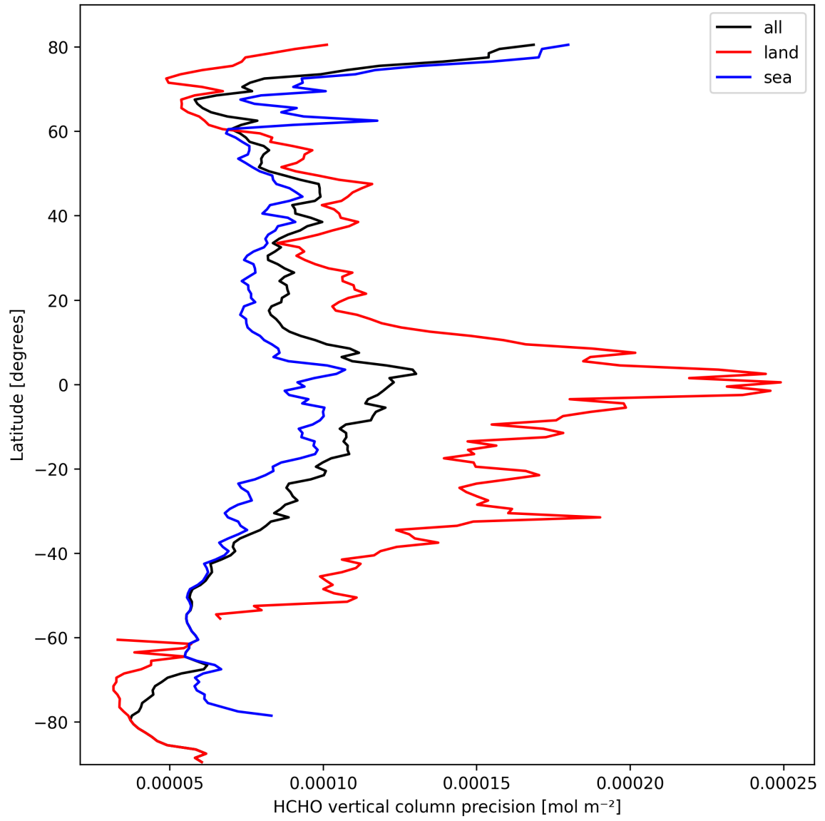
Figure 22: Zonal average of “HCHO vertical column precision” for 2025-03-07 to 2025-03-09.
