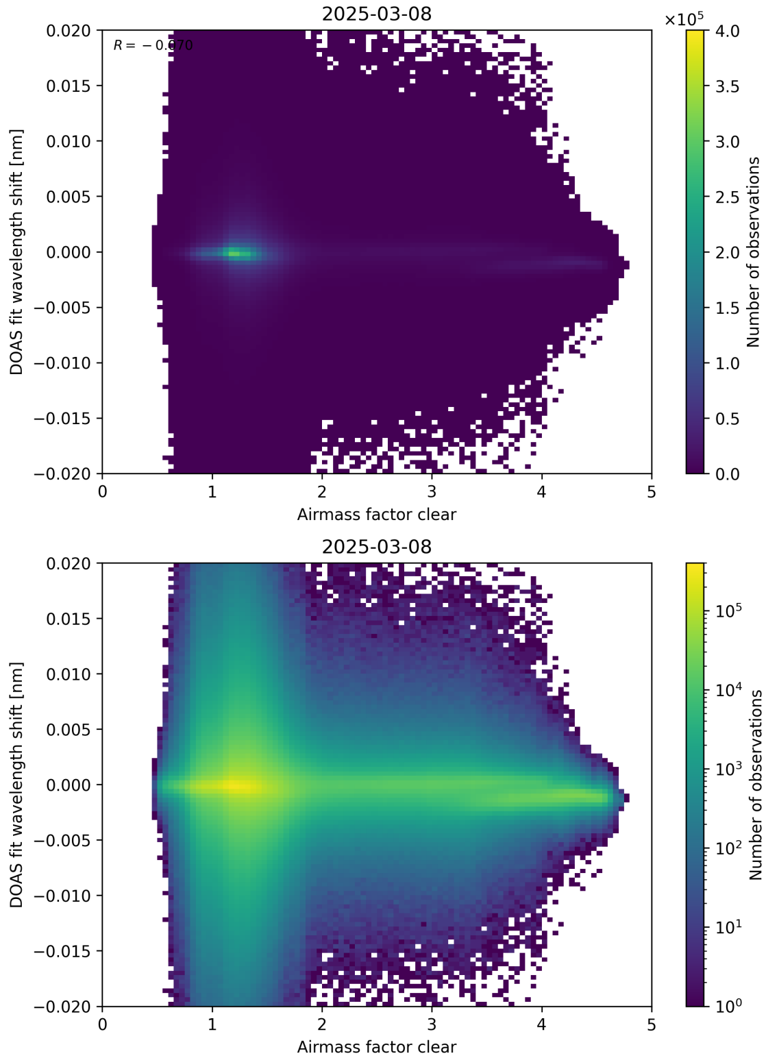
Figure 72: Scatter density plot of “Airmass factor clear” against “DOAS fit wavelength shift” for 2025-03-07 to 2025-03-09.
