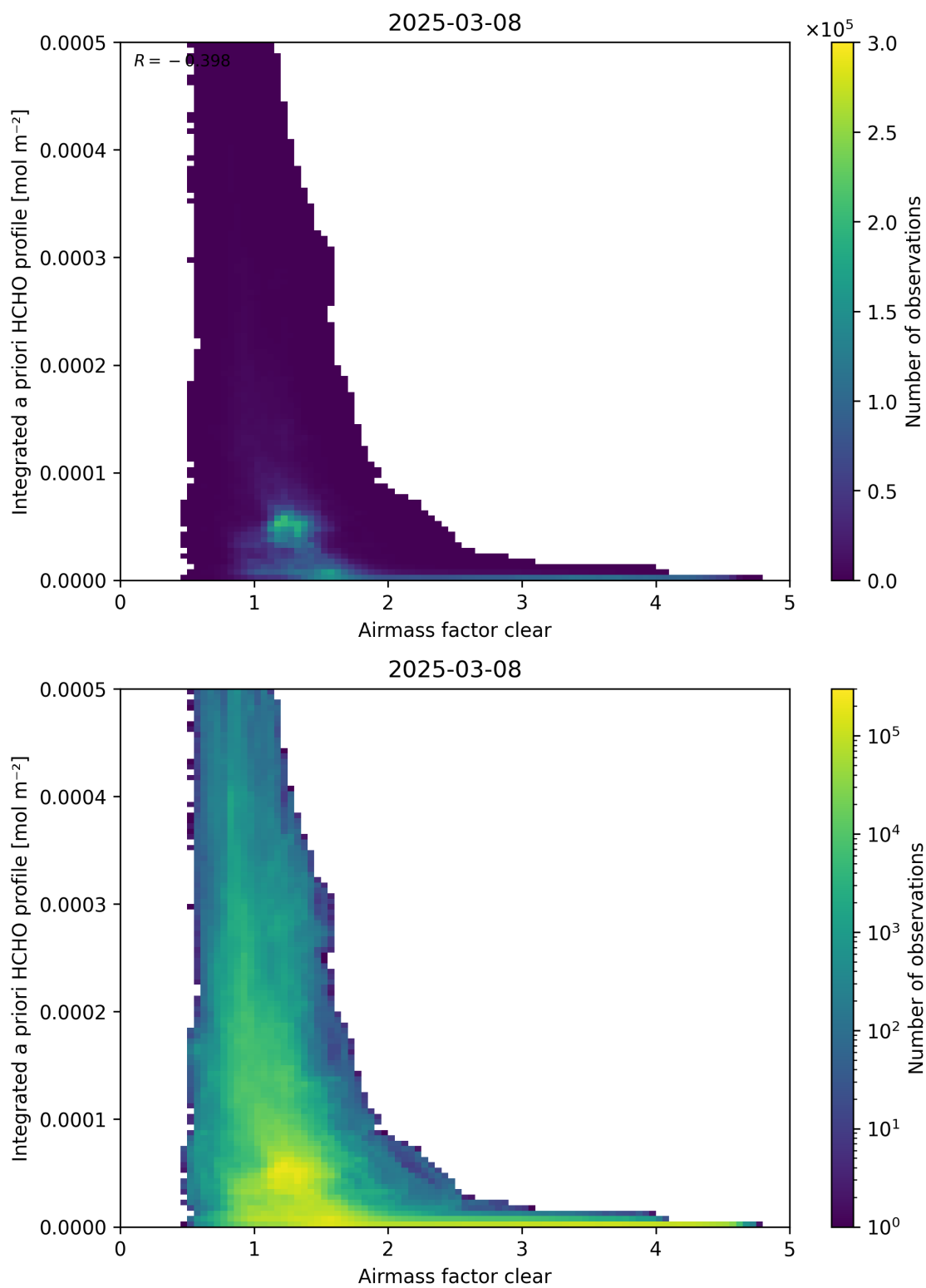
Figure 76: Scatter density plot of “Airmass factor clear” against “Integrated a priori HCHO profile” for 2025-03-07 to 2025-03-09.
