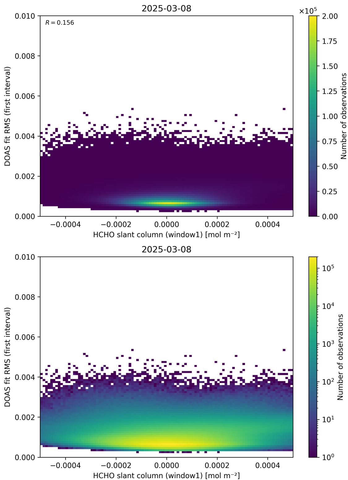
Figure 78: Scatter density plot of “HCHO slant column (window1)” against “DOAS fit RMS (first interval)” for 2025-03-07 to 2025-03-09.
