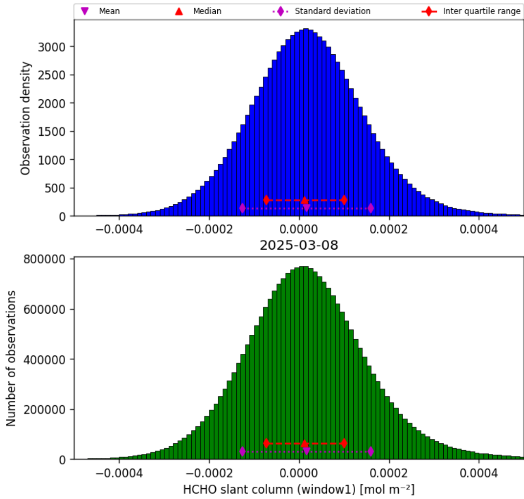
Figure 38: Histogram of “HCHO slant column (window1)” for 2025-03-07 to 2025-03-09
