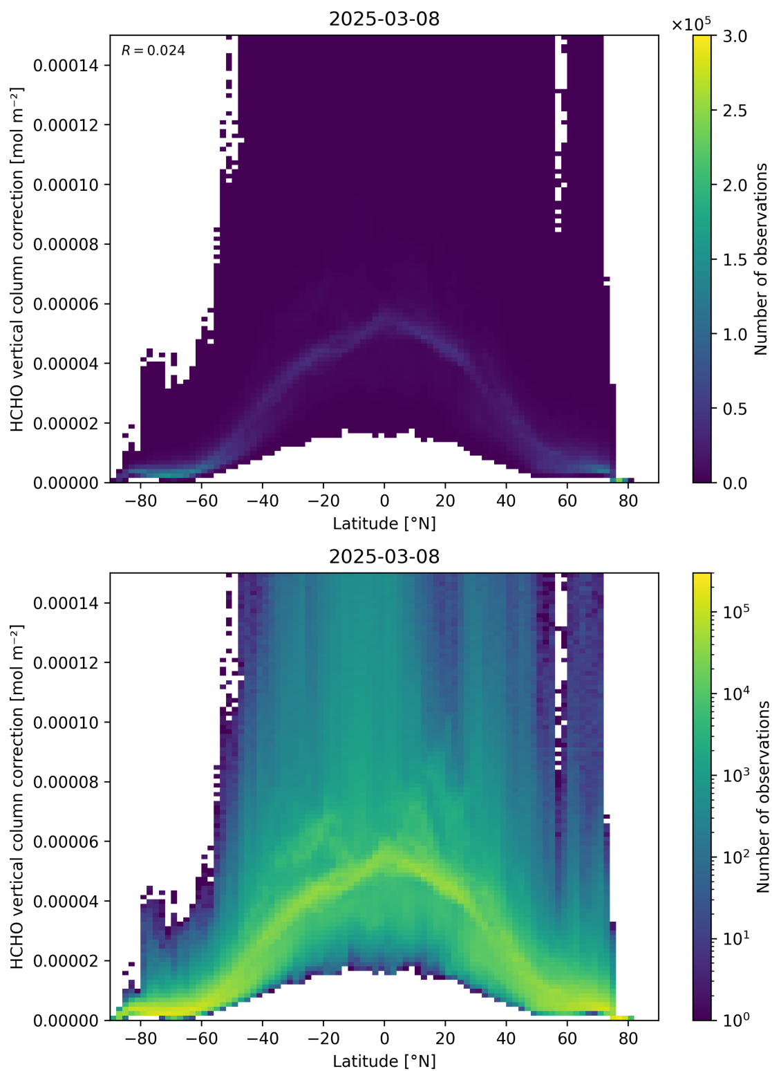
Figure 164: Scatter density plot of “Latitude” against “HCHO vertical column correction” for 2025-03-07 to 2025-03-09.
