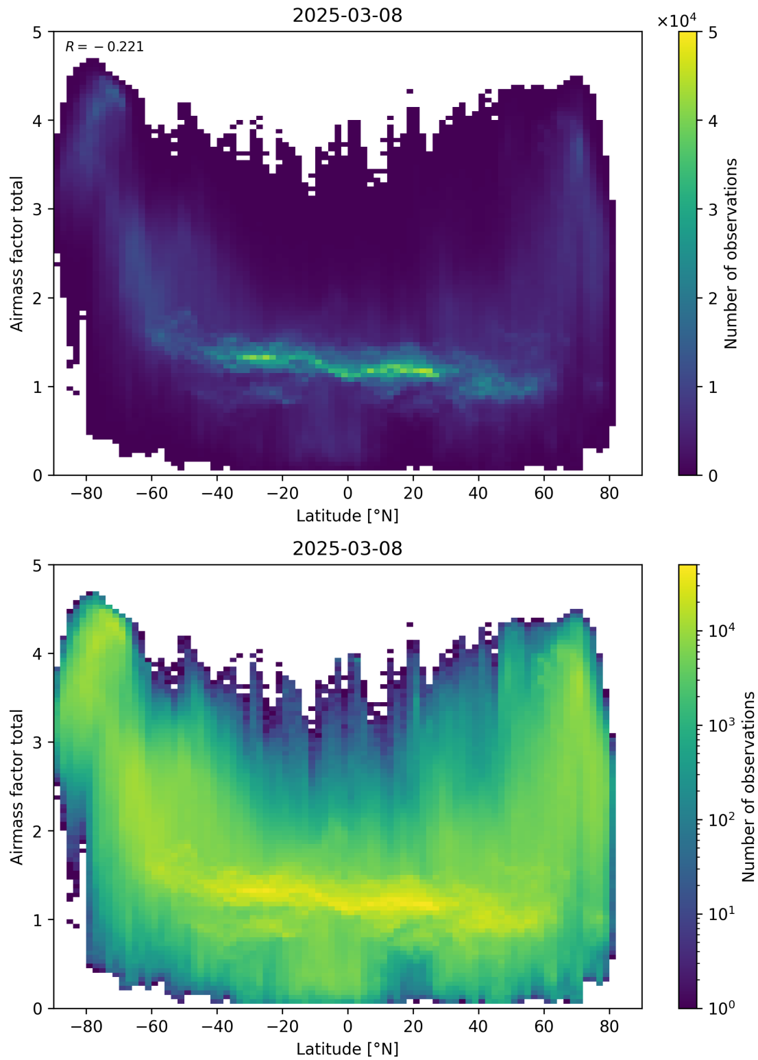
Figure 161: Scatter density plot of “Latitude” against “Airmass factor total” for 2025-03-07 to 2025-03-09.
