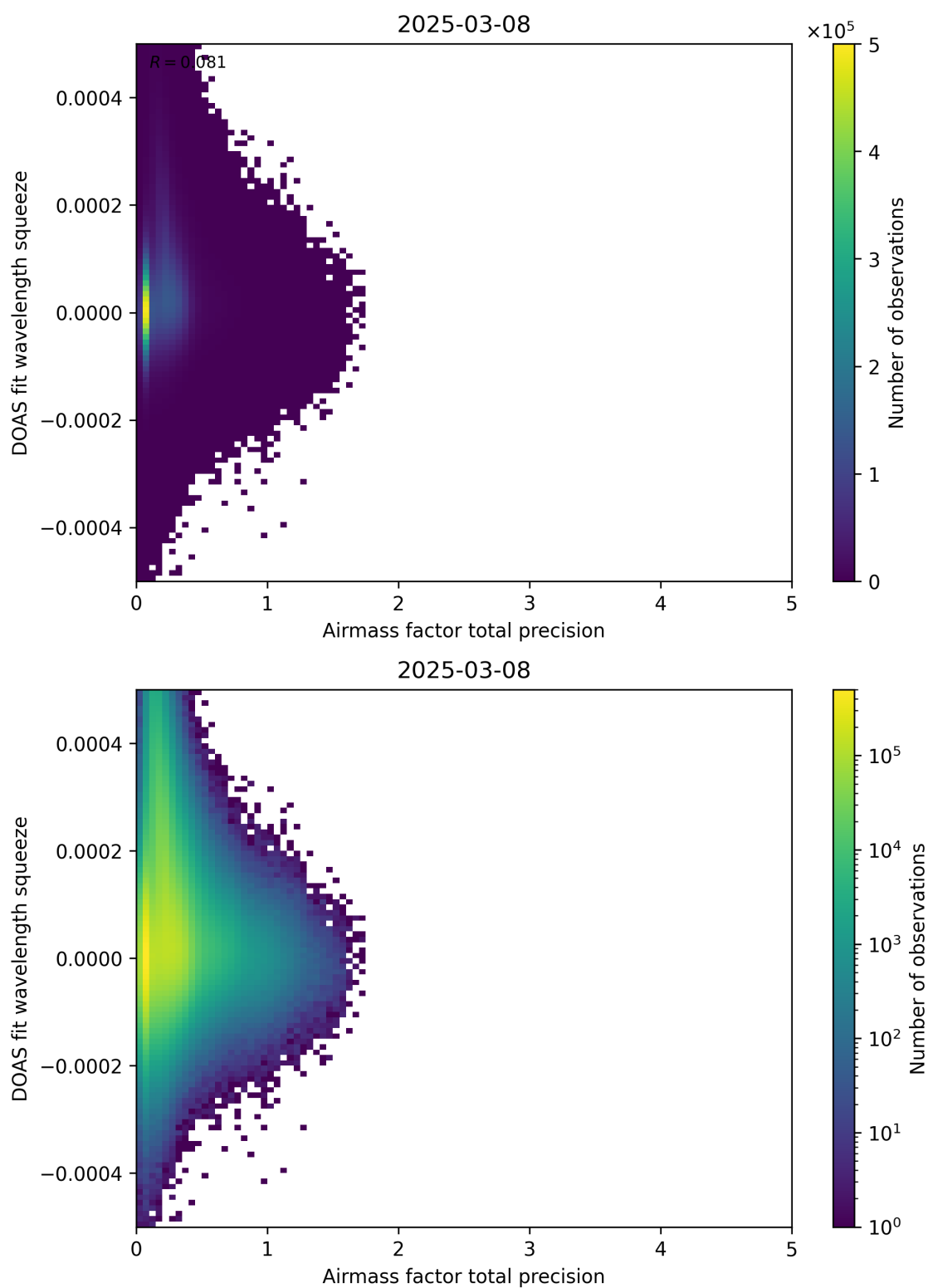
Figure 107: Scatter density plot of “Airmass factor total precision” against “DOAS fit wavelength squeeze” for 2025-03-07 to 2025-03-09.
