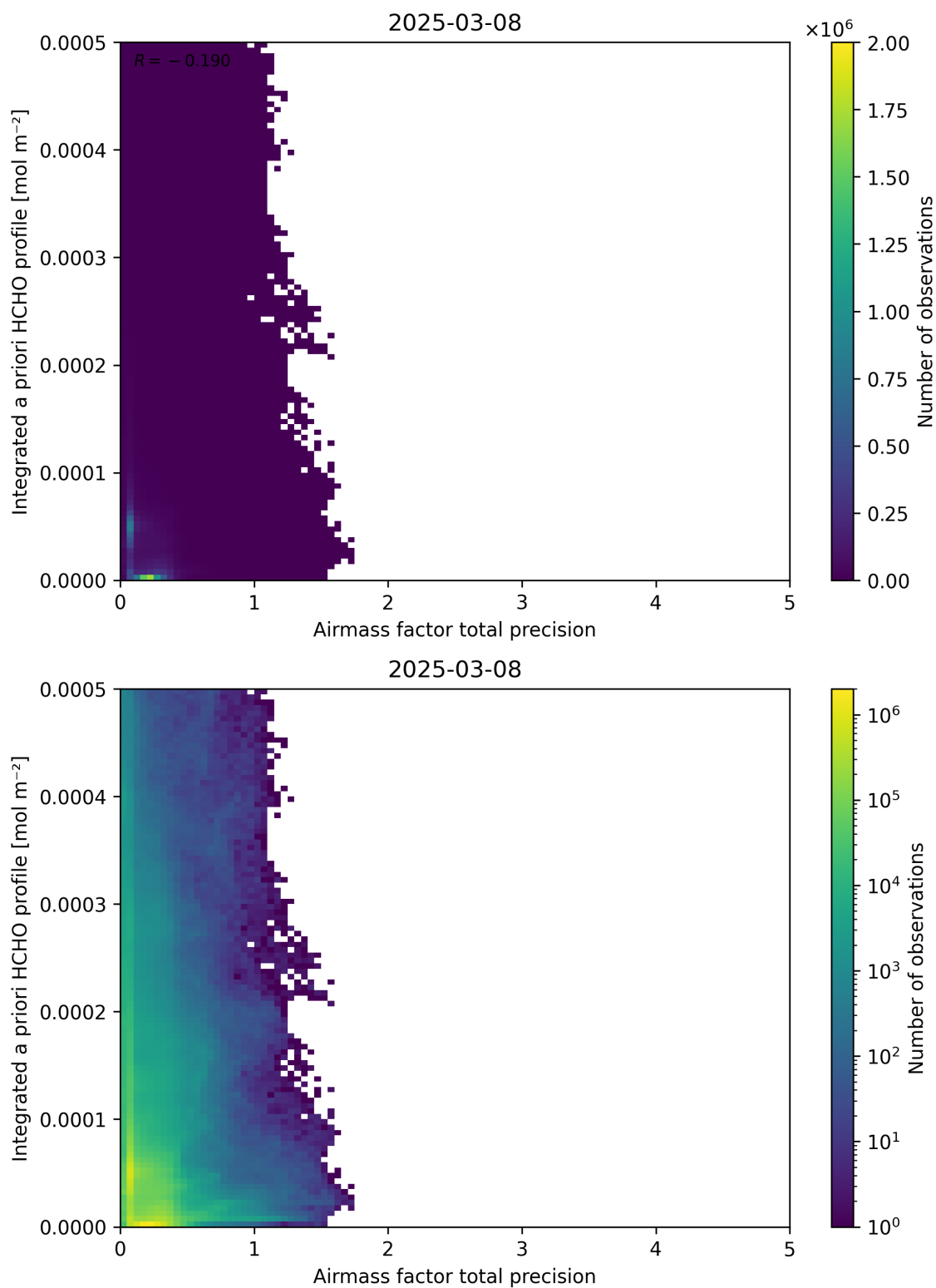
Figure 111: Scatter density plot of “Airmass factor total precision” against “Integrated a priori HCHO profile” for 2025-03-07 to 2025-03-09.
