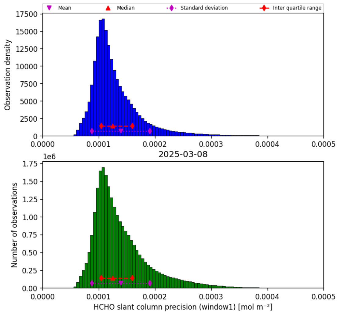
Figure 39: Histogram of “HCHO slant column precision (window1)” for 2025-03-07 to 2025-03-09
