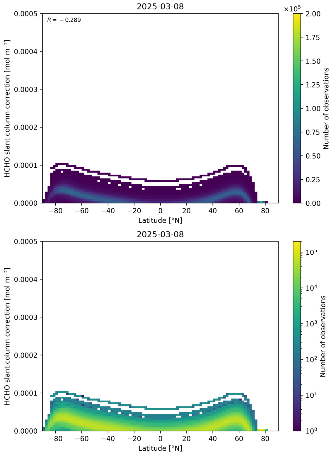
Figure 158: Scatter density plot of “Latitude” against “HCHO slant column correction” for 2025-03-07 to 2025-03-09.
