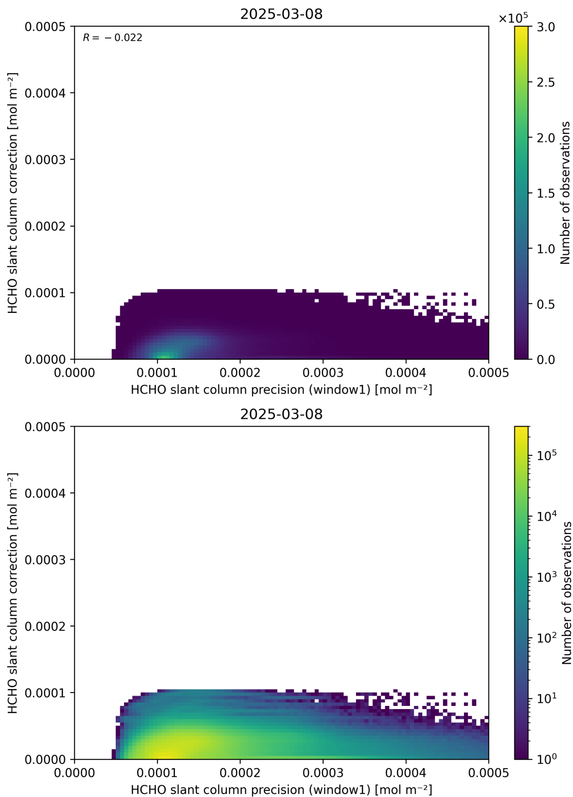
Figure 93: Scatter density plot of “HCHO slant column precision (window1)” against “HCHO slant column correction” for 2025-03-07 to 2025-03-09.
