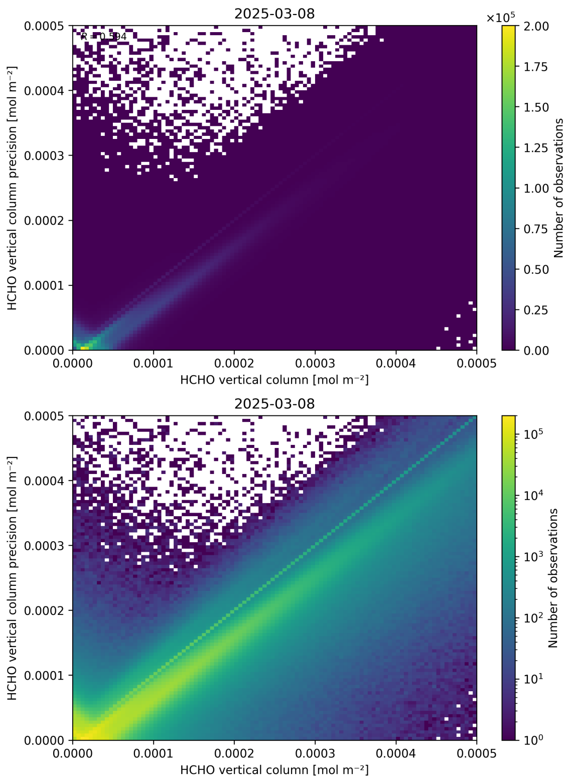
Figure 134: Scatter density plot of “HCHO vertical column” against “HCHO vertical column precision” for 2025-03-07 to 2025-03-09.
