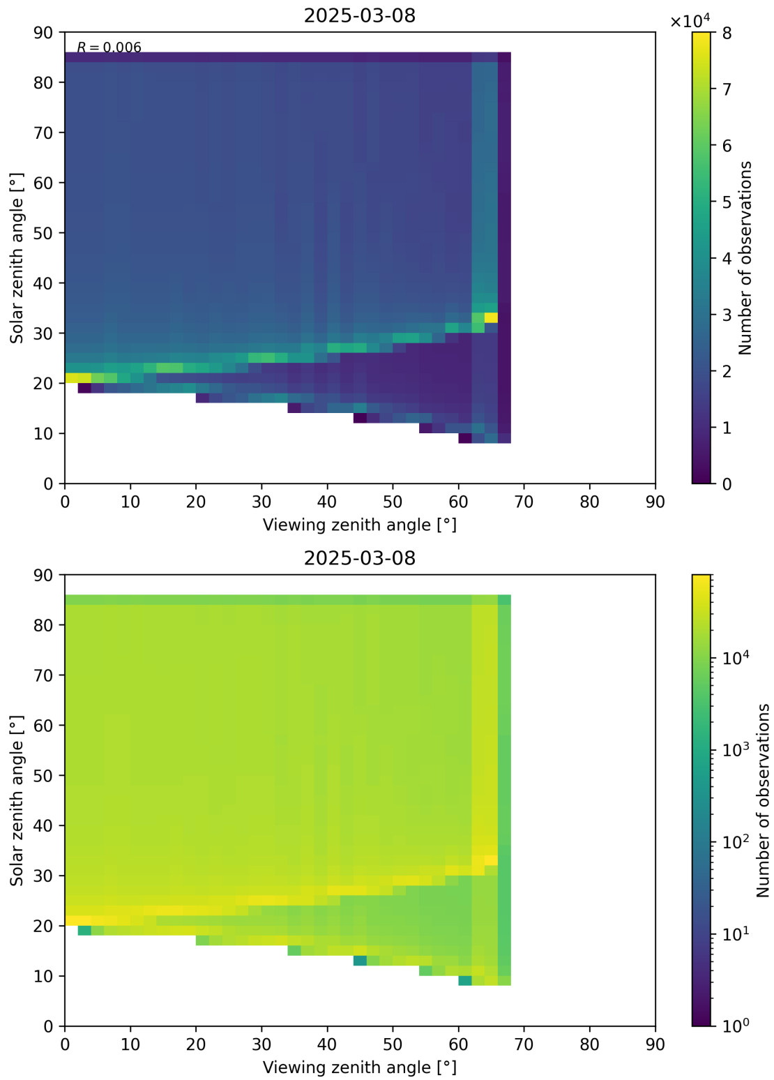
Figure 197: Scatter density plot of “Viewing zenith angle” against “Solar zenith angle” for 2025-03-07 to 2025-03-09.
