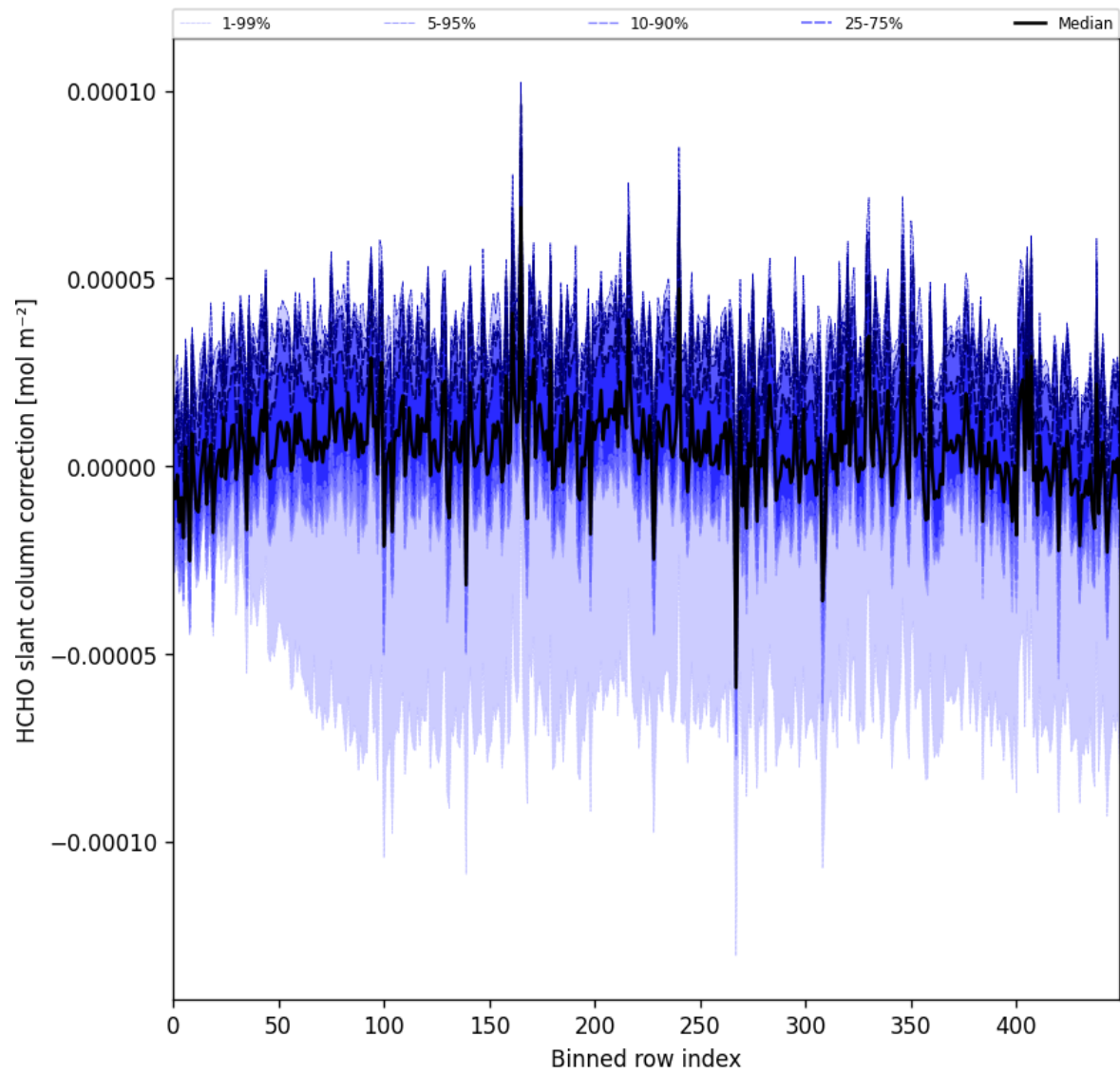
Figure 61: Along track statistics of “HCHO slant column correction” for 2025-03-07 to 2025-03-09
