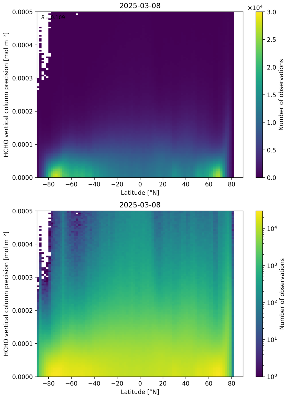
Figure 165: Scatter density plot of “Latitude” against “HCHO vertical column precision” for 2025-03-07 to 2025-03-09.
