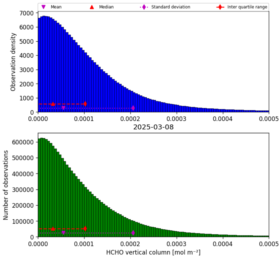
Figure 35: Histogram of “HCHO vertical column” for 2025-03-07 to 2025-03-09
