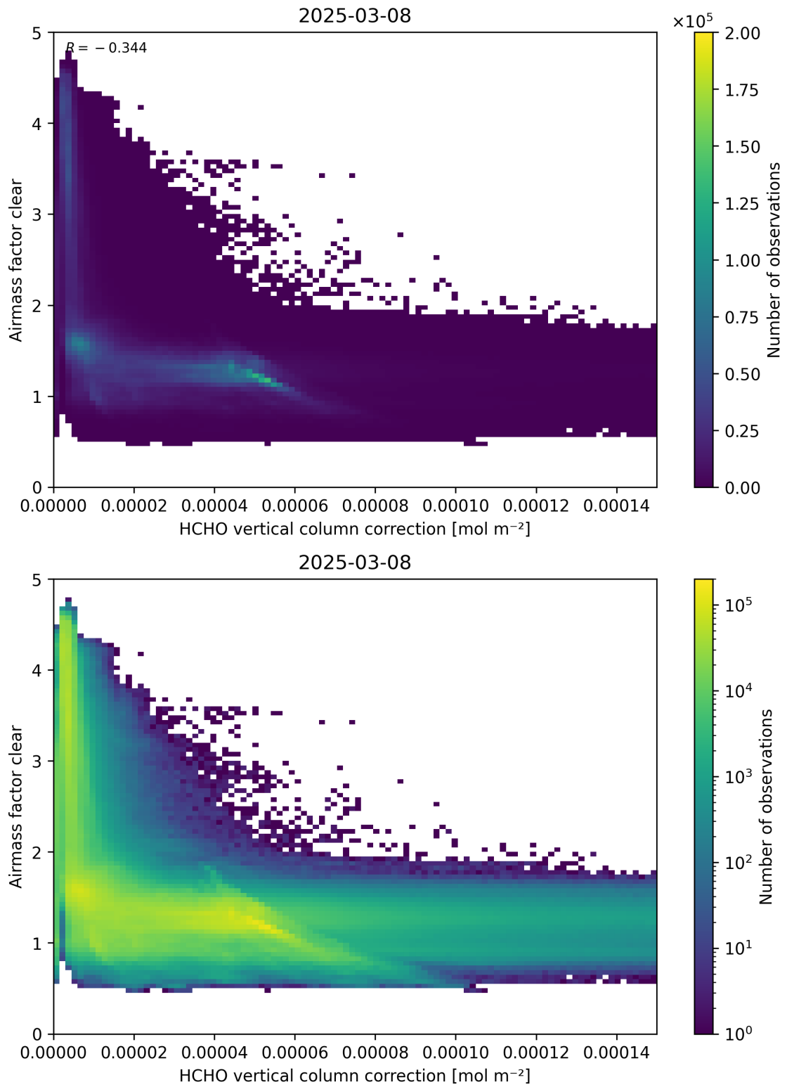
Figure 115: Scatter density plot of “HCHO vertical column correction” against “Airmass factor clear” for 2025-03-07 to 2025-03-09.
