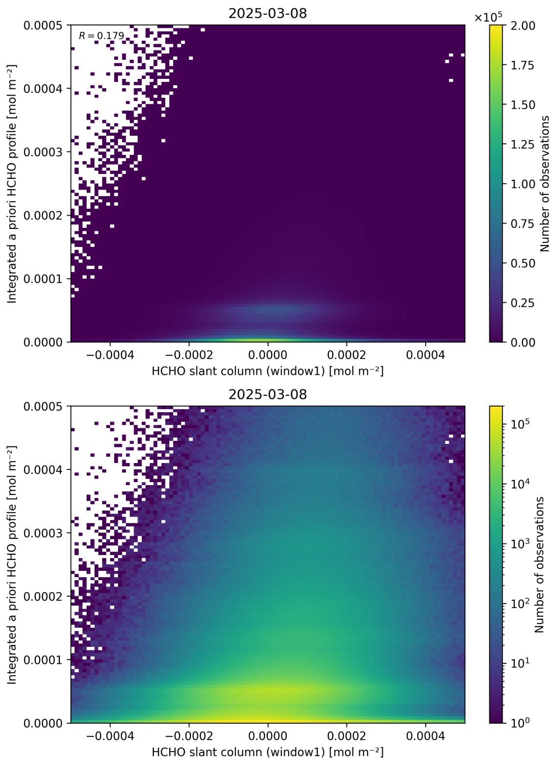
Figure 87: Scatter density plot of “HCHO slant column (window1)” against “Integrated a priori HCHO profile” for 2025-03-07 to 2025-03-09.
