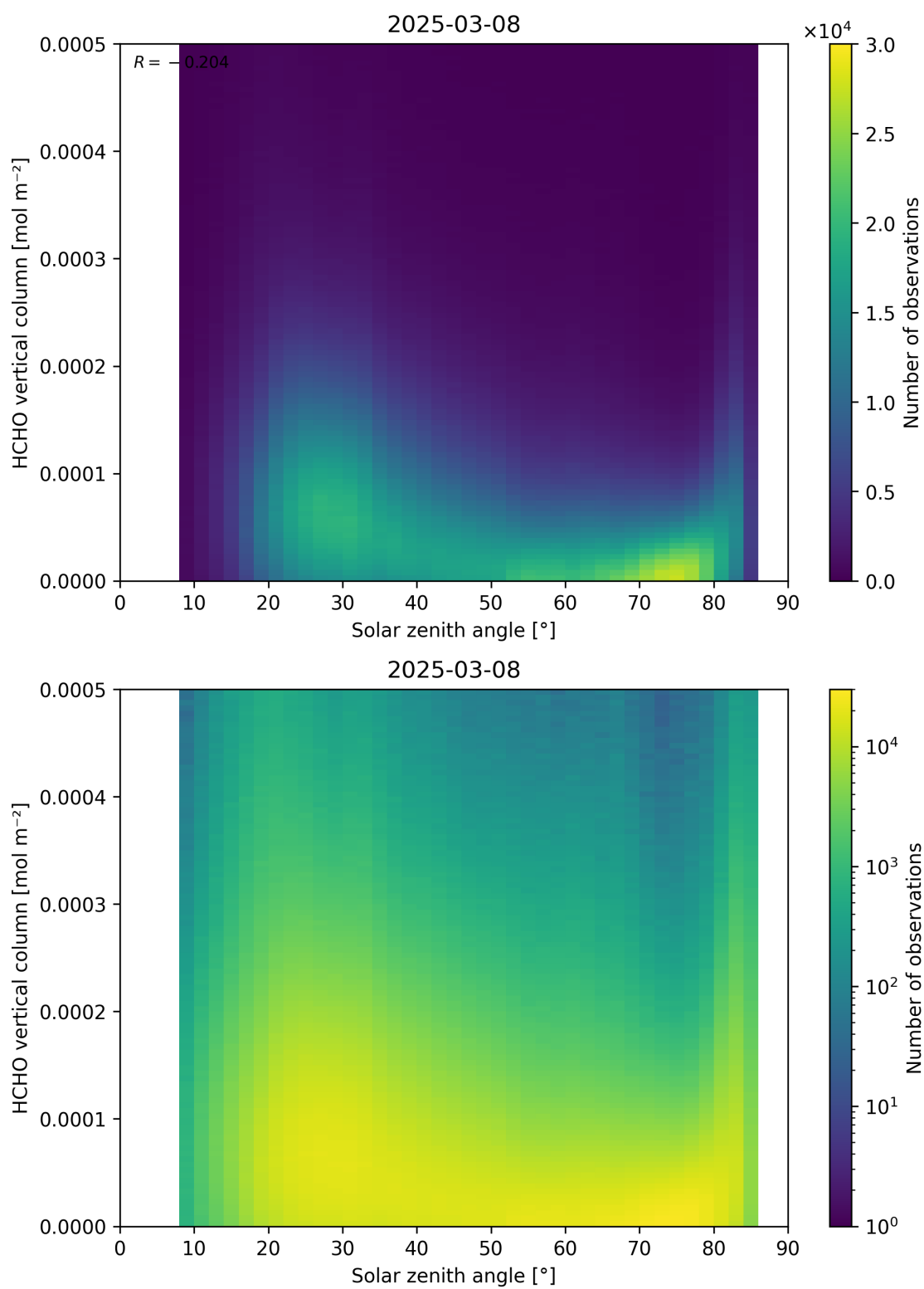
Figure 177: Scatter density plot of “Solar zenith angle” against “HCHO vertical column” for 2025-03-07 to 2025-03-09.
