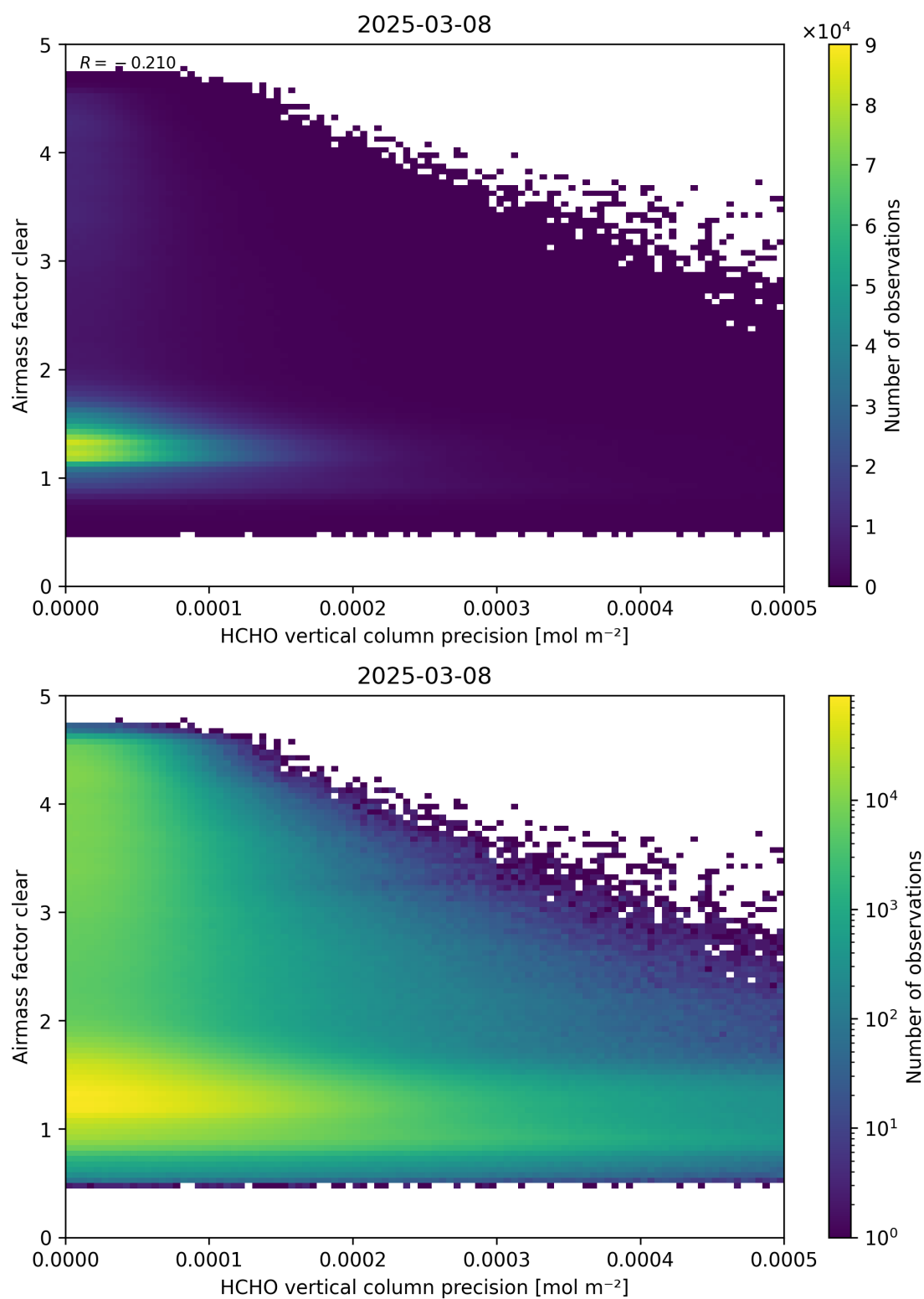
Figure 139: Scatter density plot of “HCHO vertical column precision” against “Airmass factor clear” for 2025-03-07 to 2025-03-09.
