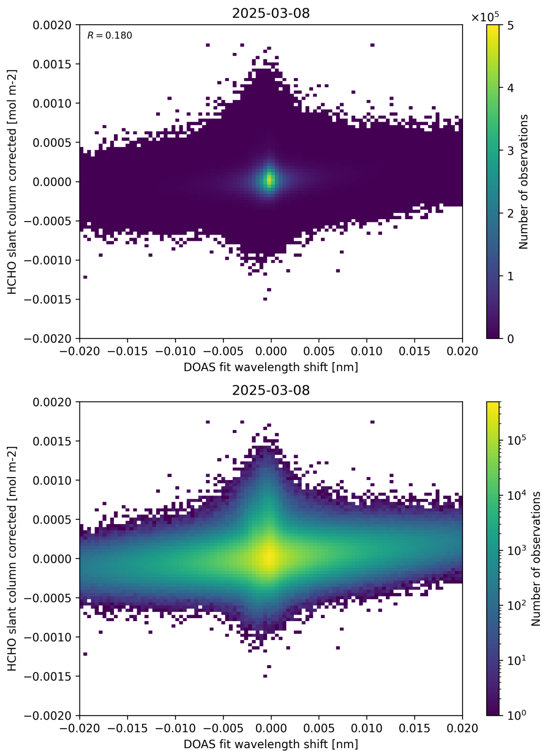
Figure 66: Scatter density plot of “DOAS fit wavelength shift” against “HCHO slant column corrected” for 2025-03-07 to 2025-03-09.
