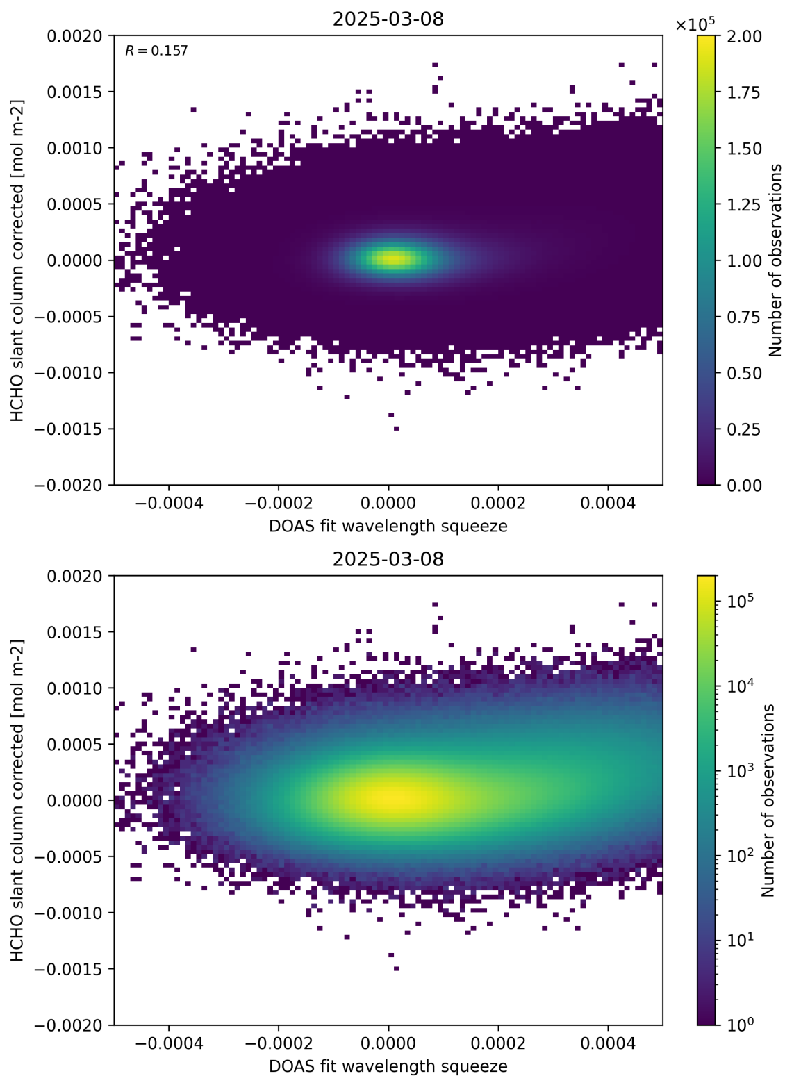
Figure 69: Scatter density plot of “DOAS fit wavelength squeeze” against “HCHO slant column corrected” for 2025-03-07 to 2025-03-09.
