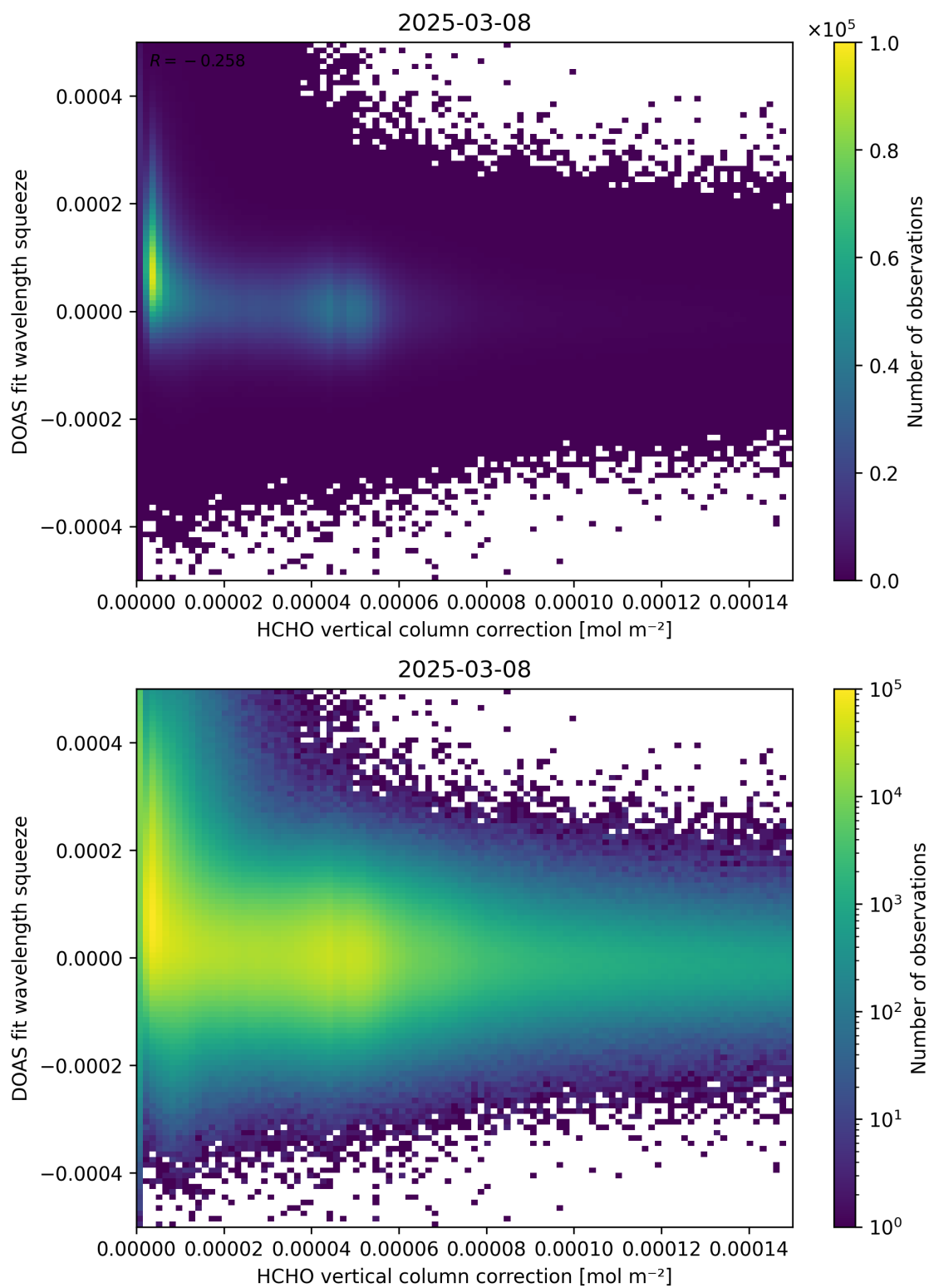
Figure 114: Scatter density plot of “HCHO vertical column correction” against “DOAS fit wavelength squeeze” for 2025-03-07 to 2025-03-09.
