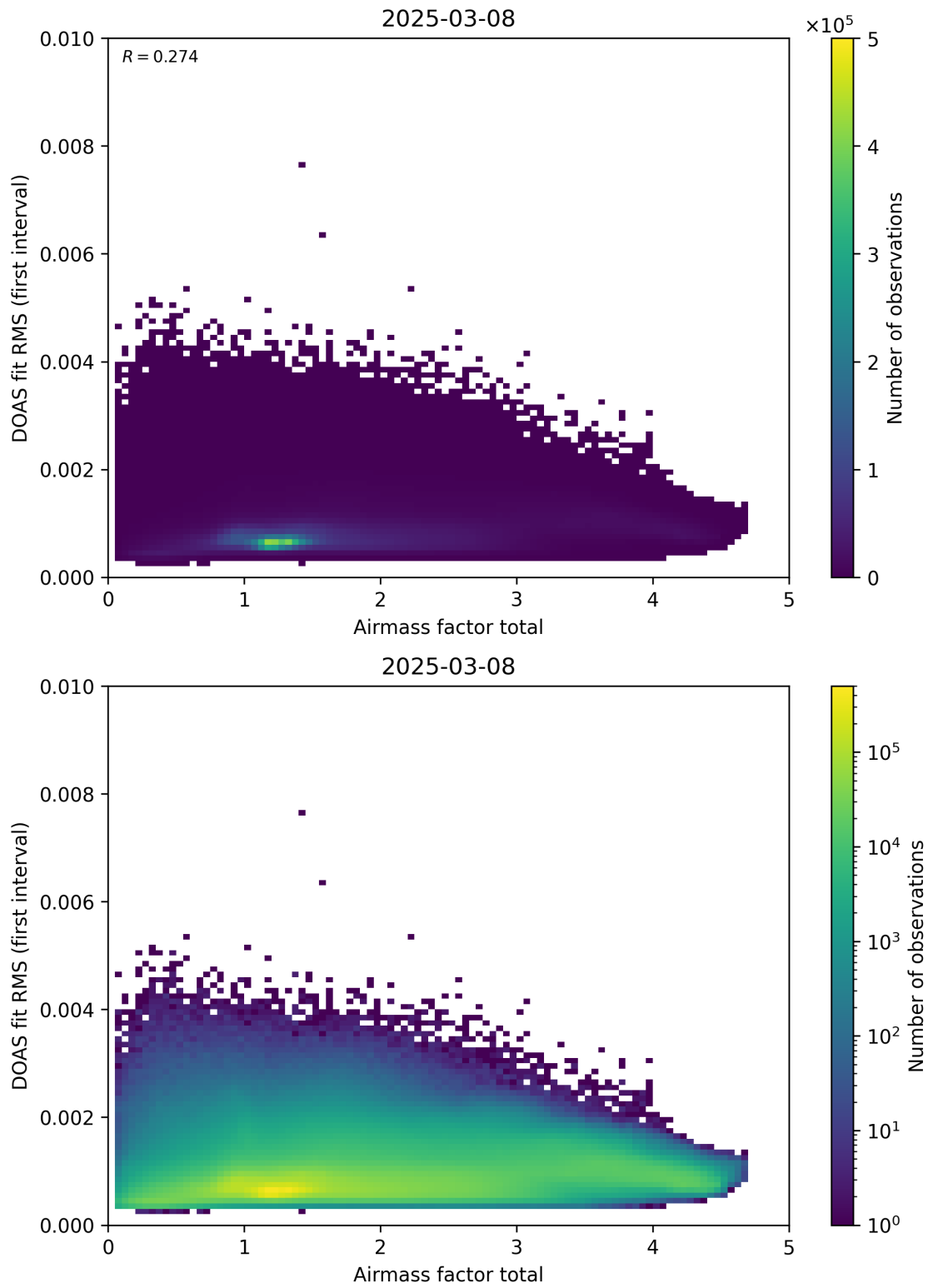
Figure 97: Scatter density plot of “Airmass factor total” against “DOAS fit RMS (first interval)” for 2025-03-07 to 2025-03-09.
