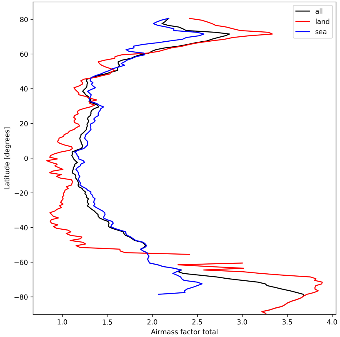
Figure 26: Zonal average of “Airmass factor total” for 2025-03-07 to 2025-03-09.
