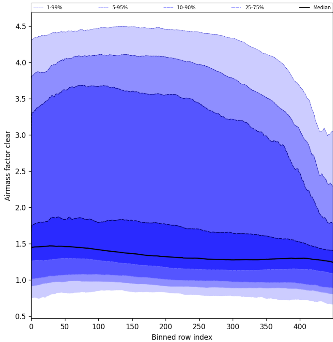
Figure 56: Along track statistics of “Air mass factor clear” for 2025-03-07 to 2025-03-09
