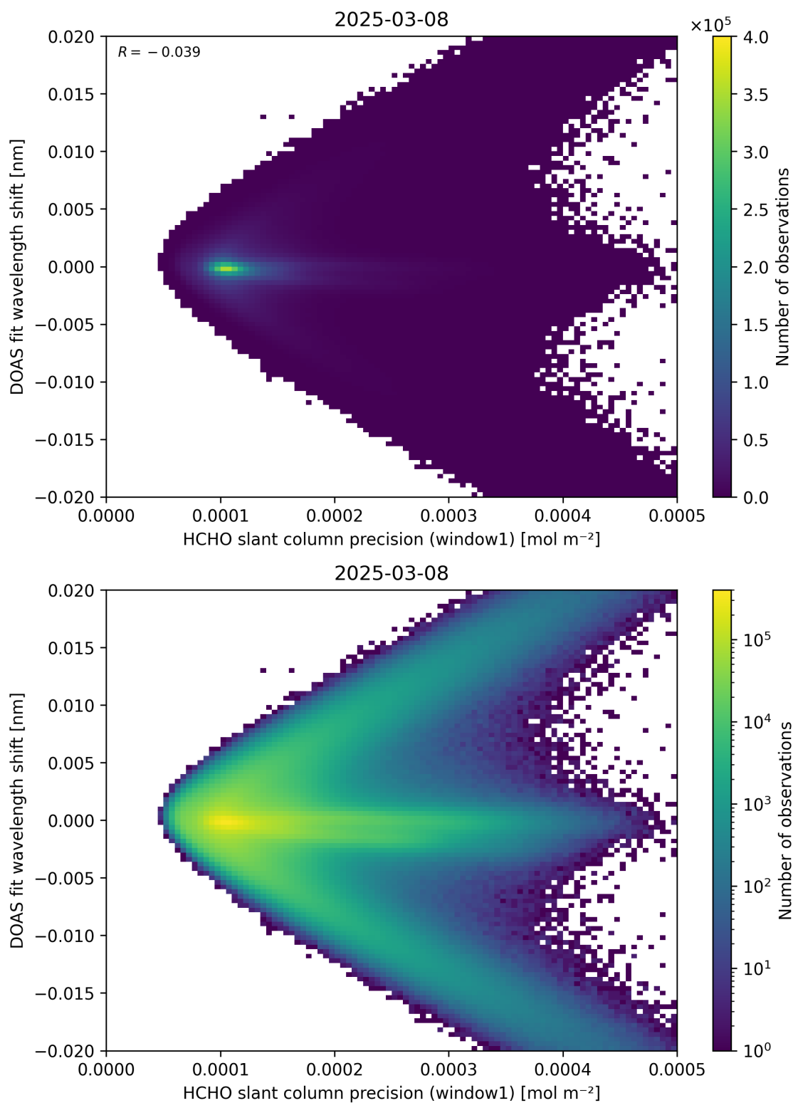
Figure 89: Scatter density plot of “HCHO slant column precision (window1)” against “DOAS fit wavelength shift” for 2025-03-07 to 2025-03-09.
