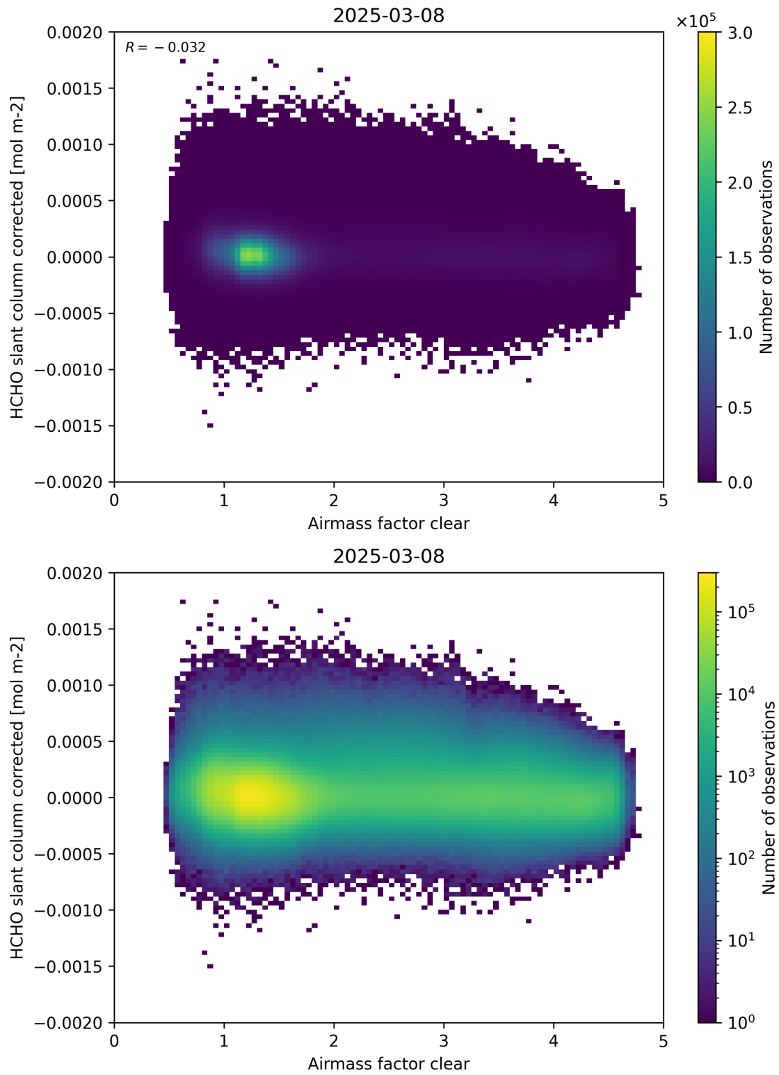
Figure 74: Scatter density plot of “Airmass factor clear” against “HCHO slant column corrected” for 2025-03-07 to 2025-03-09.
