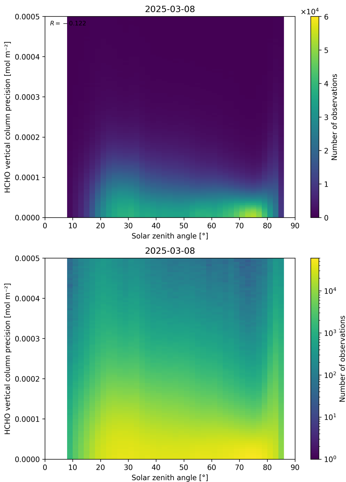
Figure 179: Scatter density plot of “Solar zenith angle” against “HCHO vertical column precision” for 2025-03-07 to 2025-03-09.
