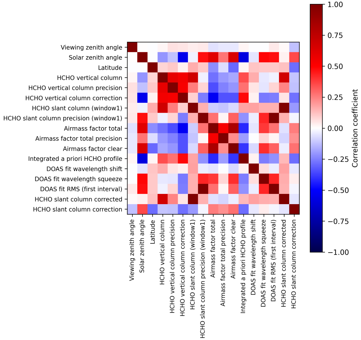
Figure 2: Map of correlation matrix for 2025-03-07 to 2025-03-09.
