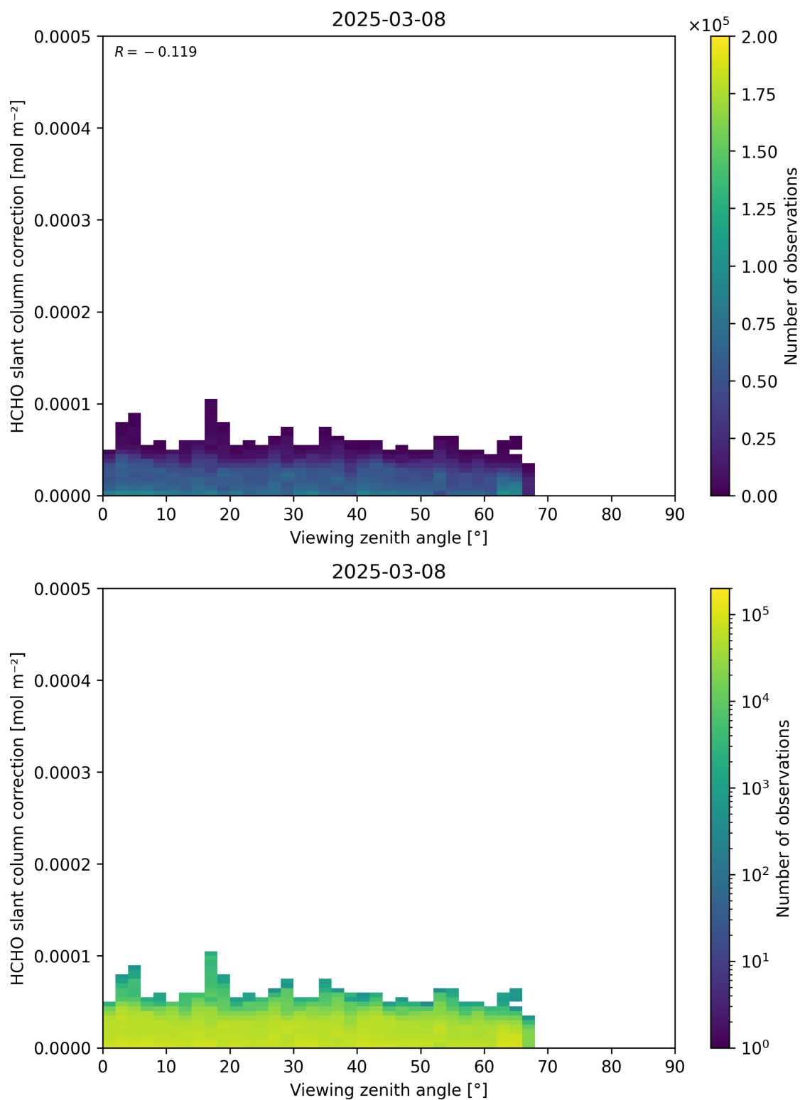
Figure 187: Scatter density plot of “Viewing zenith angle” against “HCHO slant column correction” for 2025-03-07 to 2025-03-09.
