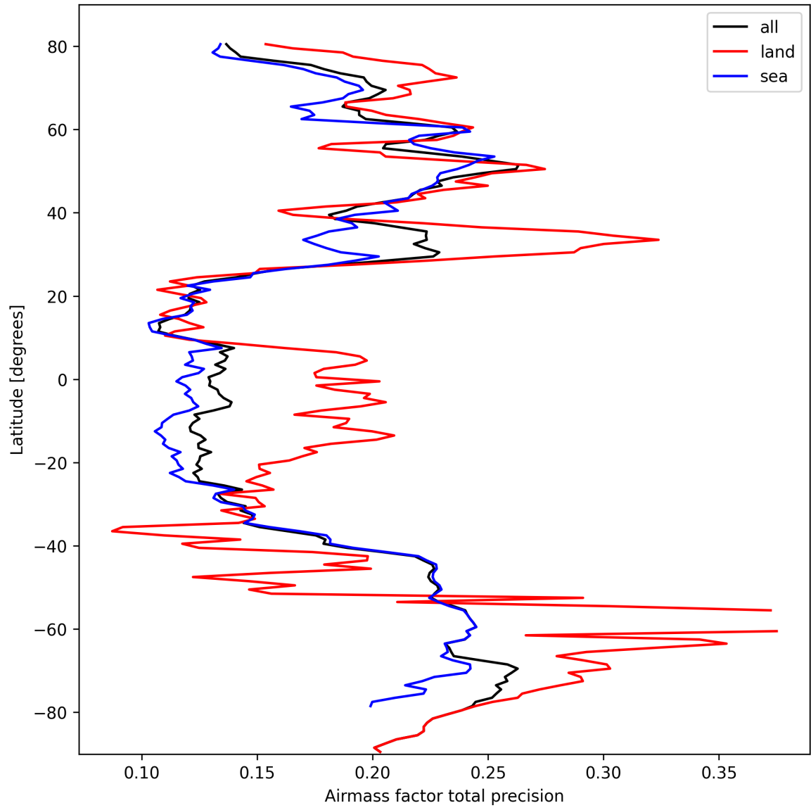
Figure 27: Zonal average of “Airmass factor total precision” for 2025-03-07 to 2025-03-09.
