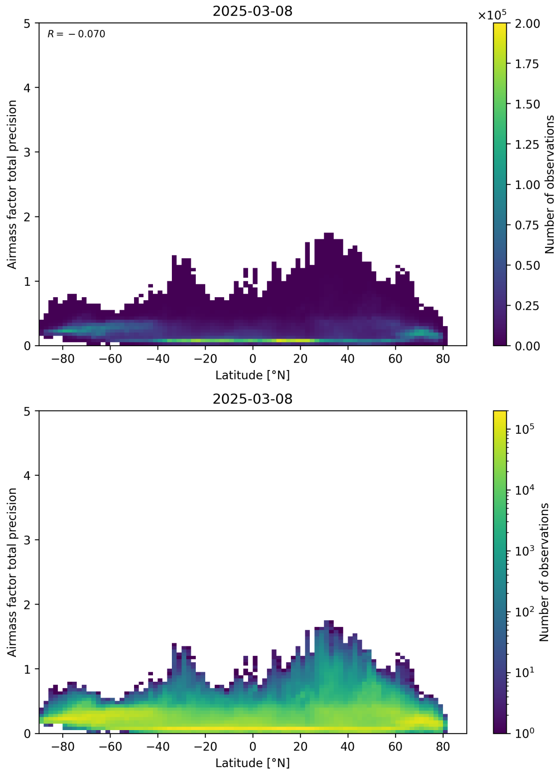
Figure 162: Scatter density plot of “Latitude” against “Airmass factor total precision” for 2025-03-07 to 2025-03-09.
