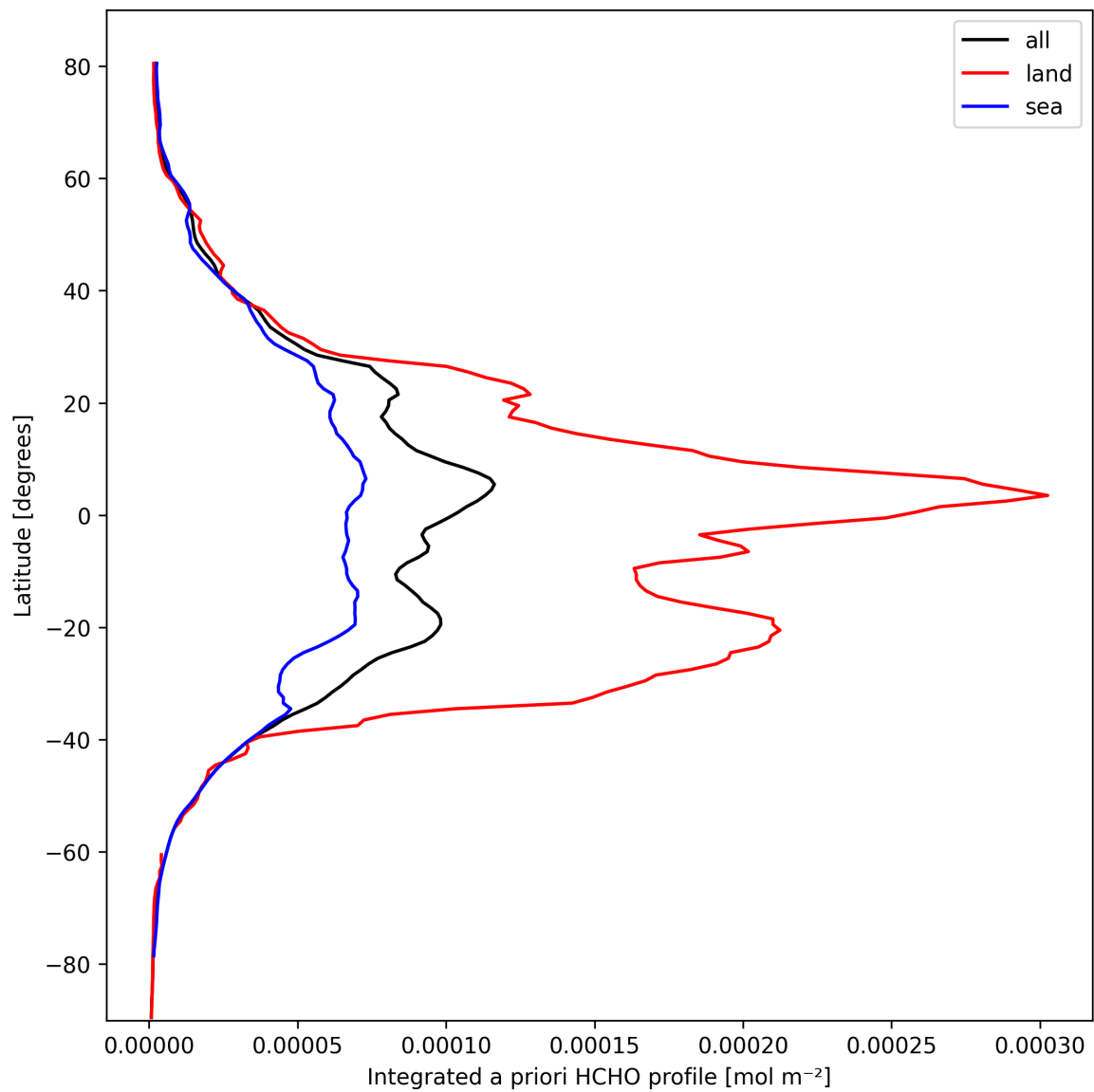
Figure 29: Zonal average of “Integrated a priori HCHO profile” for 2025-03-07 to 2025-03-09.
