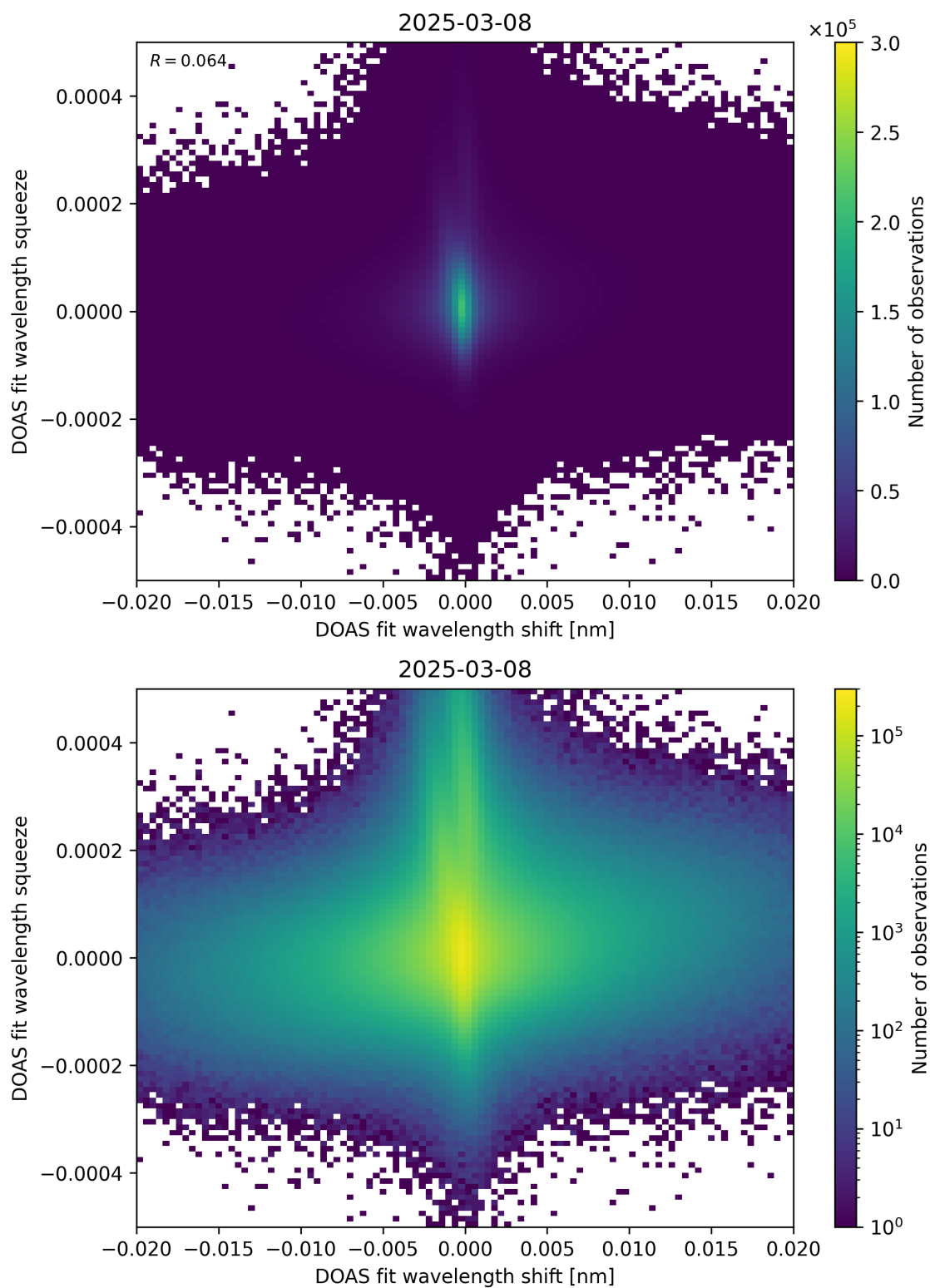
Figure 65: Scatter density plot of “DOAS fit wavelength shift” against “DOAS fit wavelength squeeze” for 2025-03-07 to 2025-03-09.
