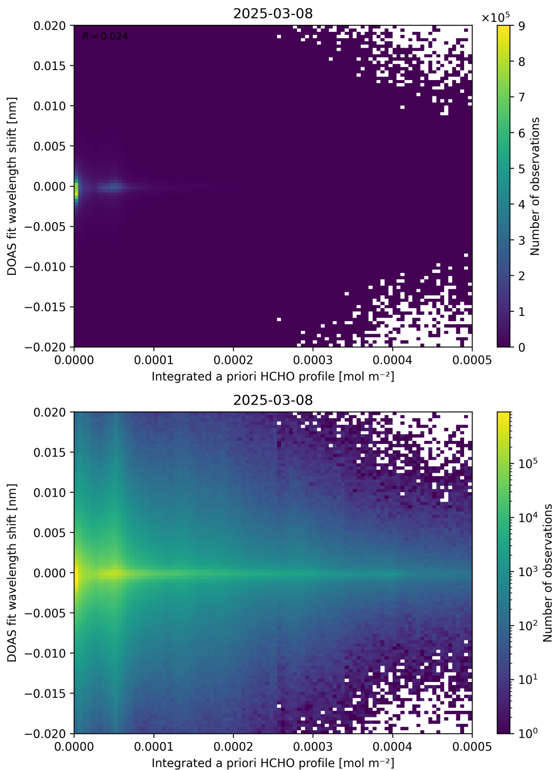
Figure 149: Scatter density plot of “Integrated a priori HCHO profile” against “DOAS fit wavelength shift” for 2025-03-07 to 2025-03-09.
