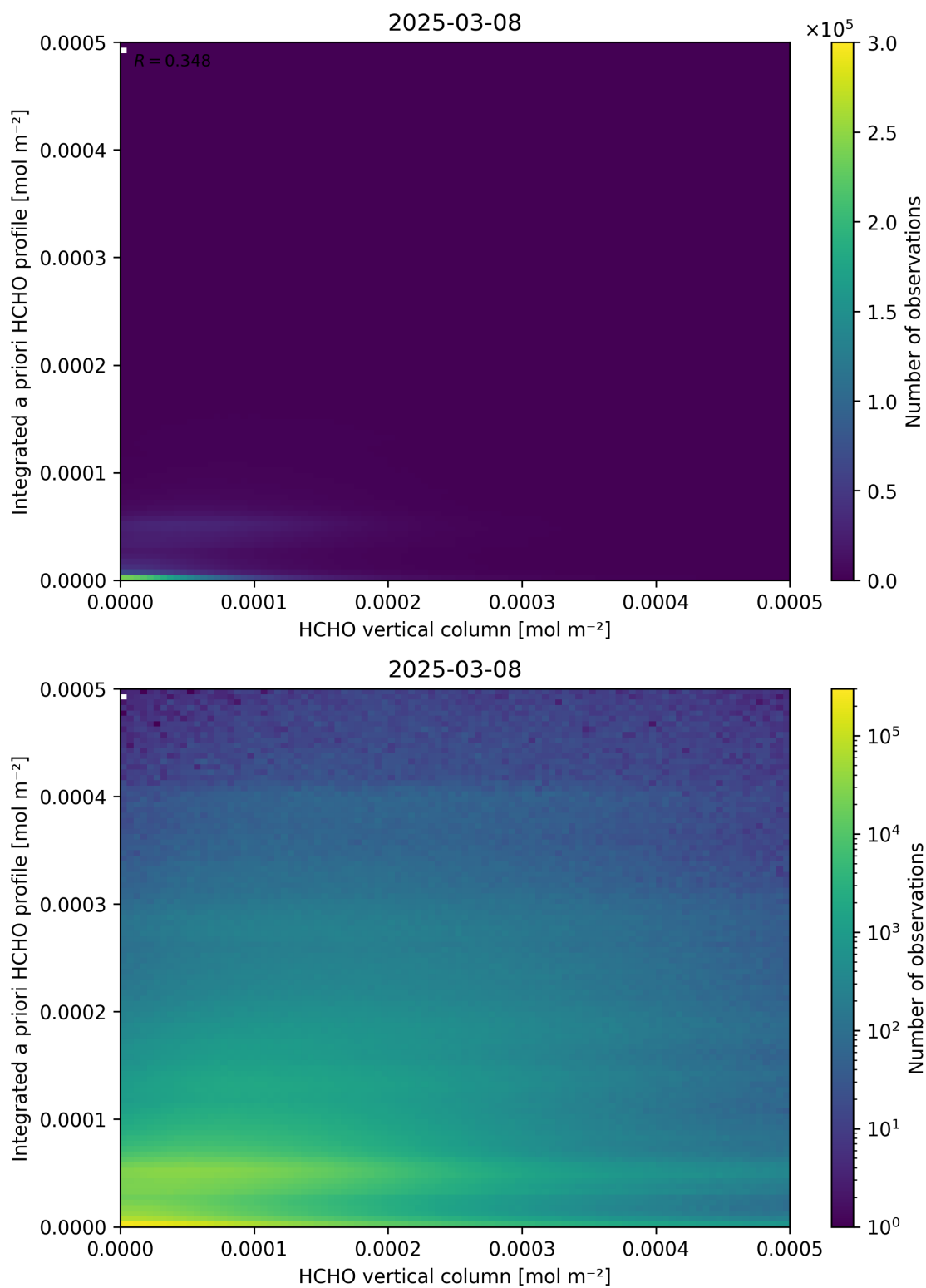
Figure 135: Scatter density plot of “HCHO vertical column” against “Integrated a priori HCHO profile” for 2025-03-07 to 2025-03-09.
