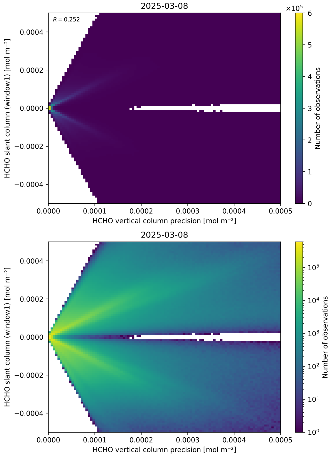
Figure 142: Scatter density plot of “HCHO vertical column precision” against “HCHO slant column (window1)” for 2025-03-07 to 2025-03-09.
