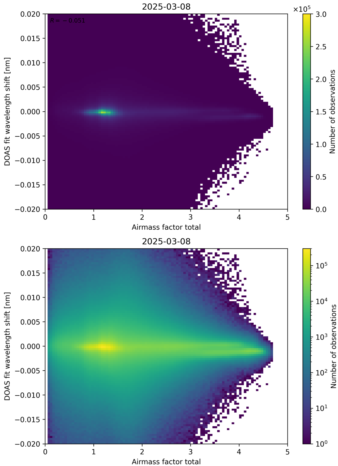
Figure 98: Scatter density plot of “Airmass factor total” against “DOAS fit wavelength shift” for 2025-03-07 to 2025-03-09.
