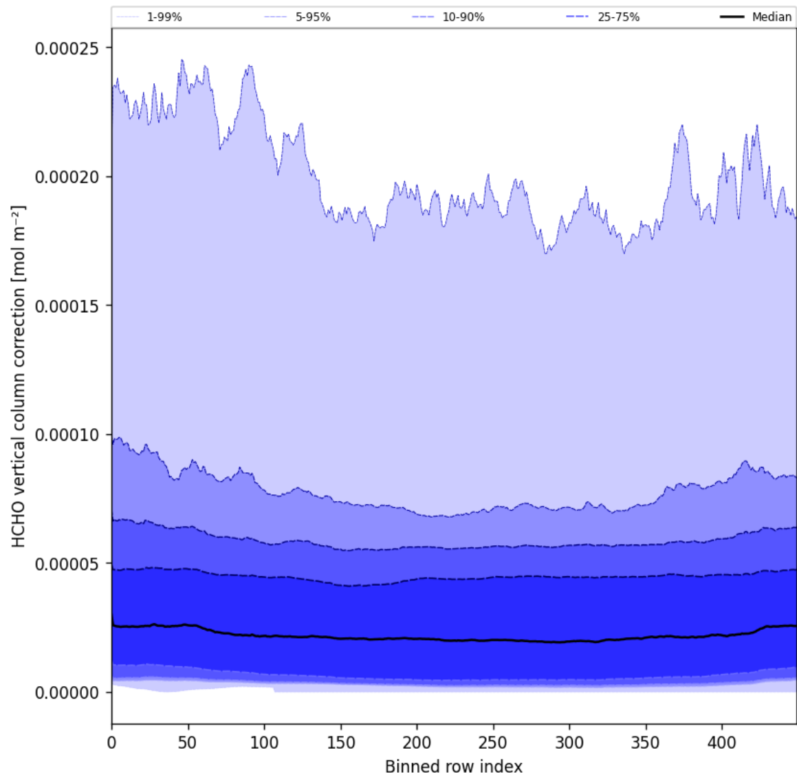
Figure 51: Along track statistics of “HCHO vertical column correction” for 2025-03-07 to 2025-03-09
