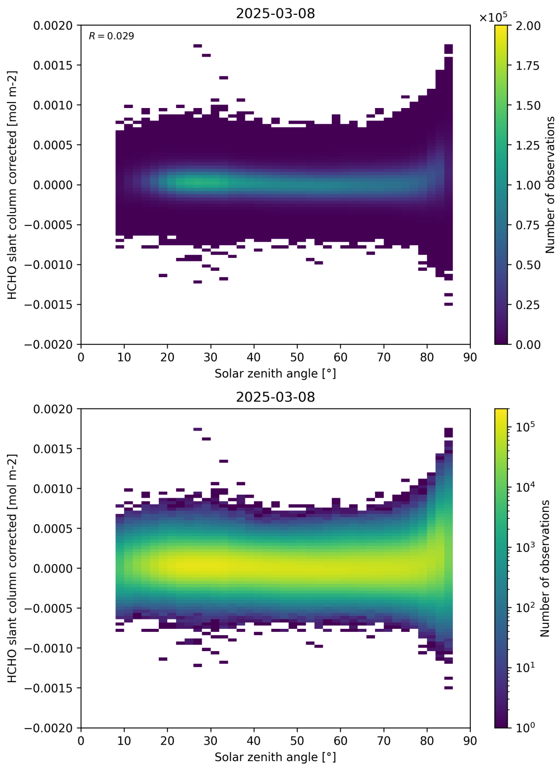
Figure 171: Scatter density plot of “Solar zenith angle” against “HCHO slant column corrected” for 2025-03-07 to 2025-03-09.
