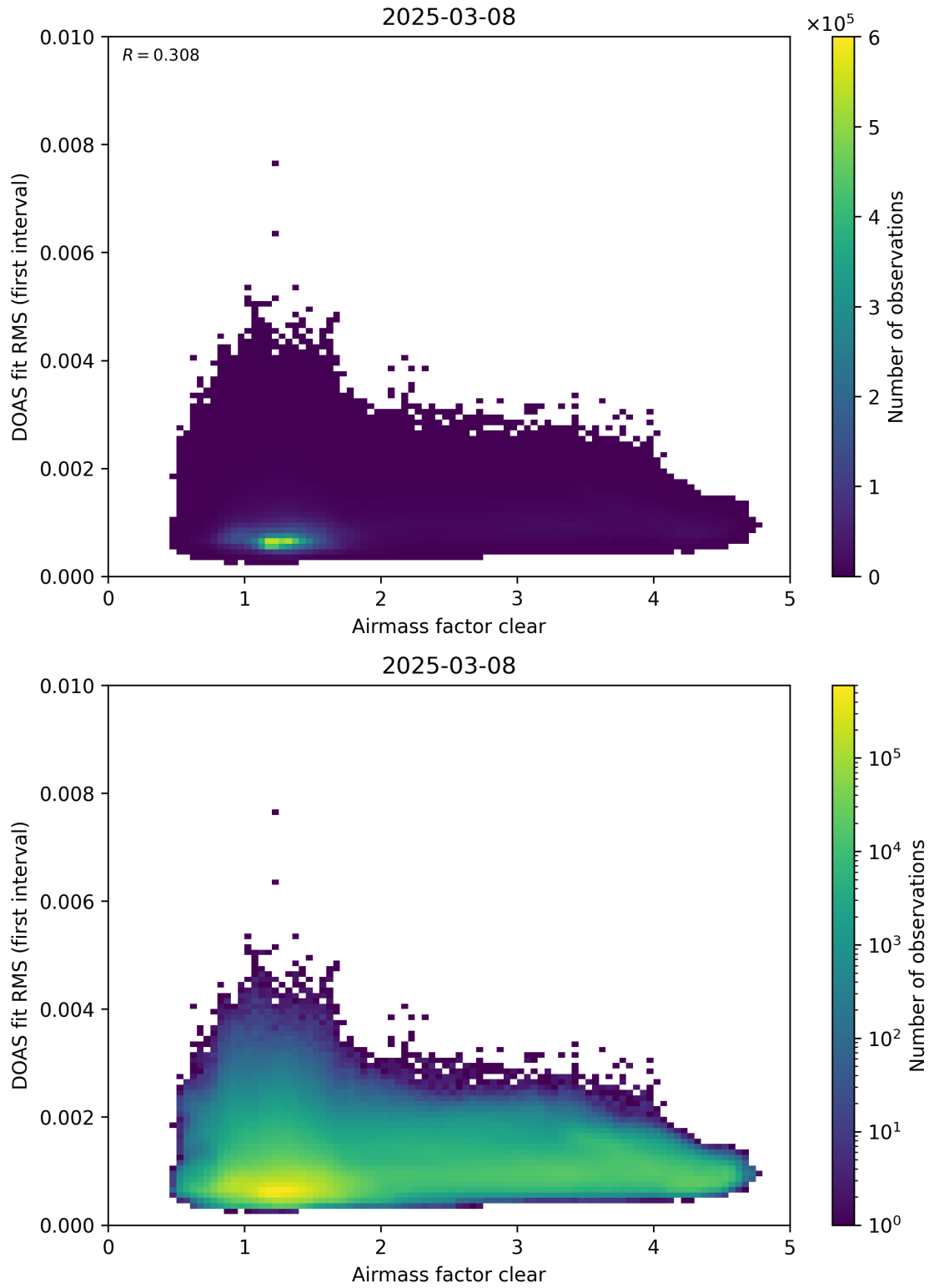
Figure 71: Scatter density plot of “Airmass factor clear” against “DOAS fit RMS (first interval)” for 2025-03-07 to 2025-03-09.
