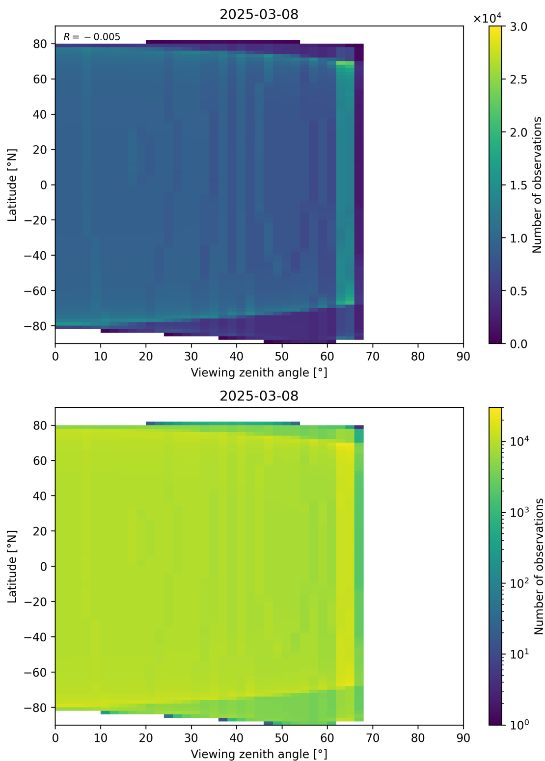
Figure 196: Scatter density plot of “Viewing zenith angle” against “Latitude” for 2025-03-07 to 2025-03-09.
