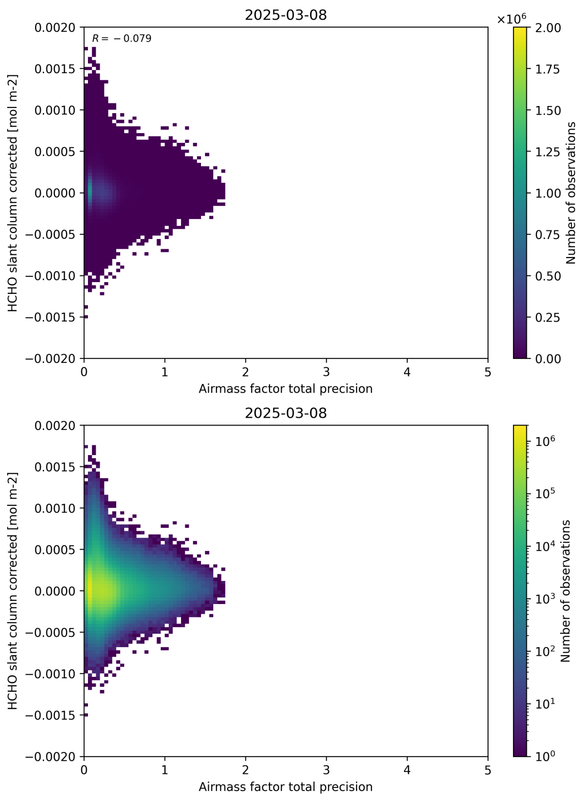
Figure 109: Scatter density plot of “Airmass factor total precision” against “HCHO slant column corrected” for 2025-03-07 to 2025-03-09.
