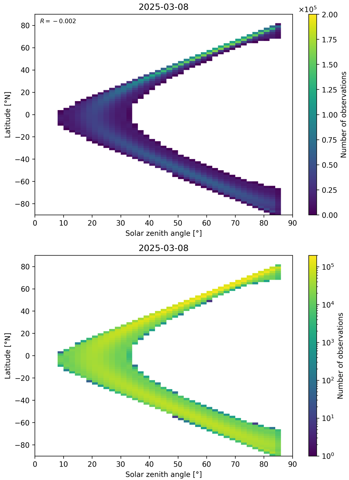
Figure 181: Scatter density plot of “Solar zenith angle” against “Latitude” for 2025-03-07 to 2025-03-09.
