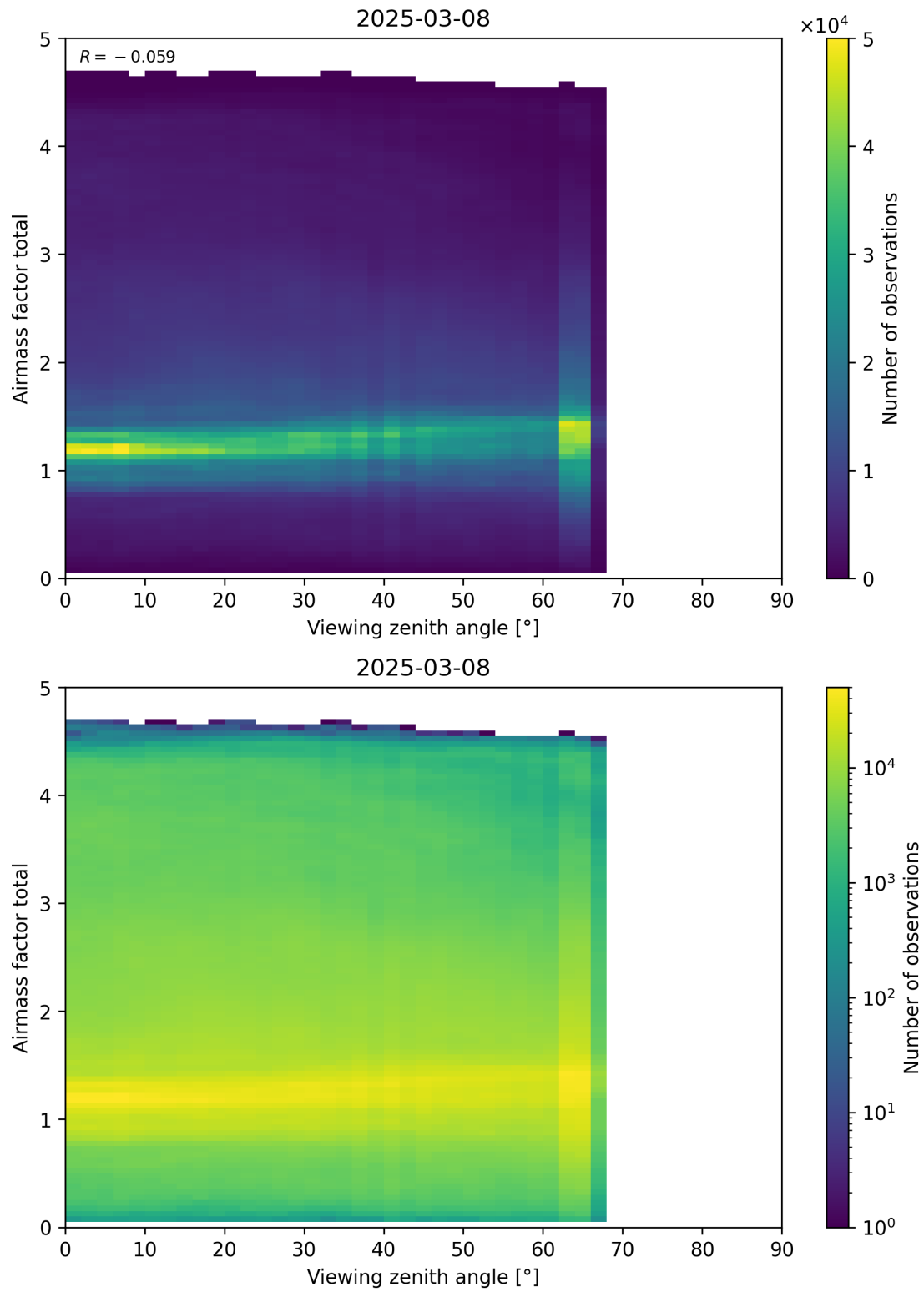
Figure 190: Scatter density plot of “Viewing zenith angle” against “Airmass factor total” for 2025-03-07 to 2025-03-09.
