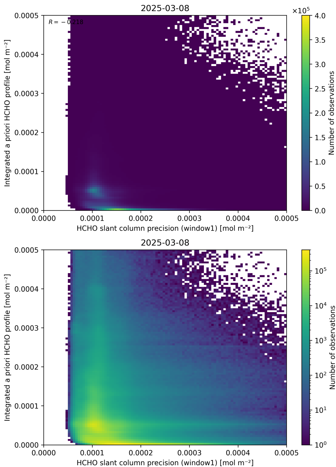
Figure 96: Scatter density plot of “HCHO slant column precision (window1)” against “Integrated a priori HCHO profile” for 2025-03-07 to 2025-03-09.
