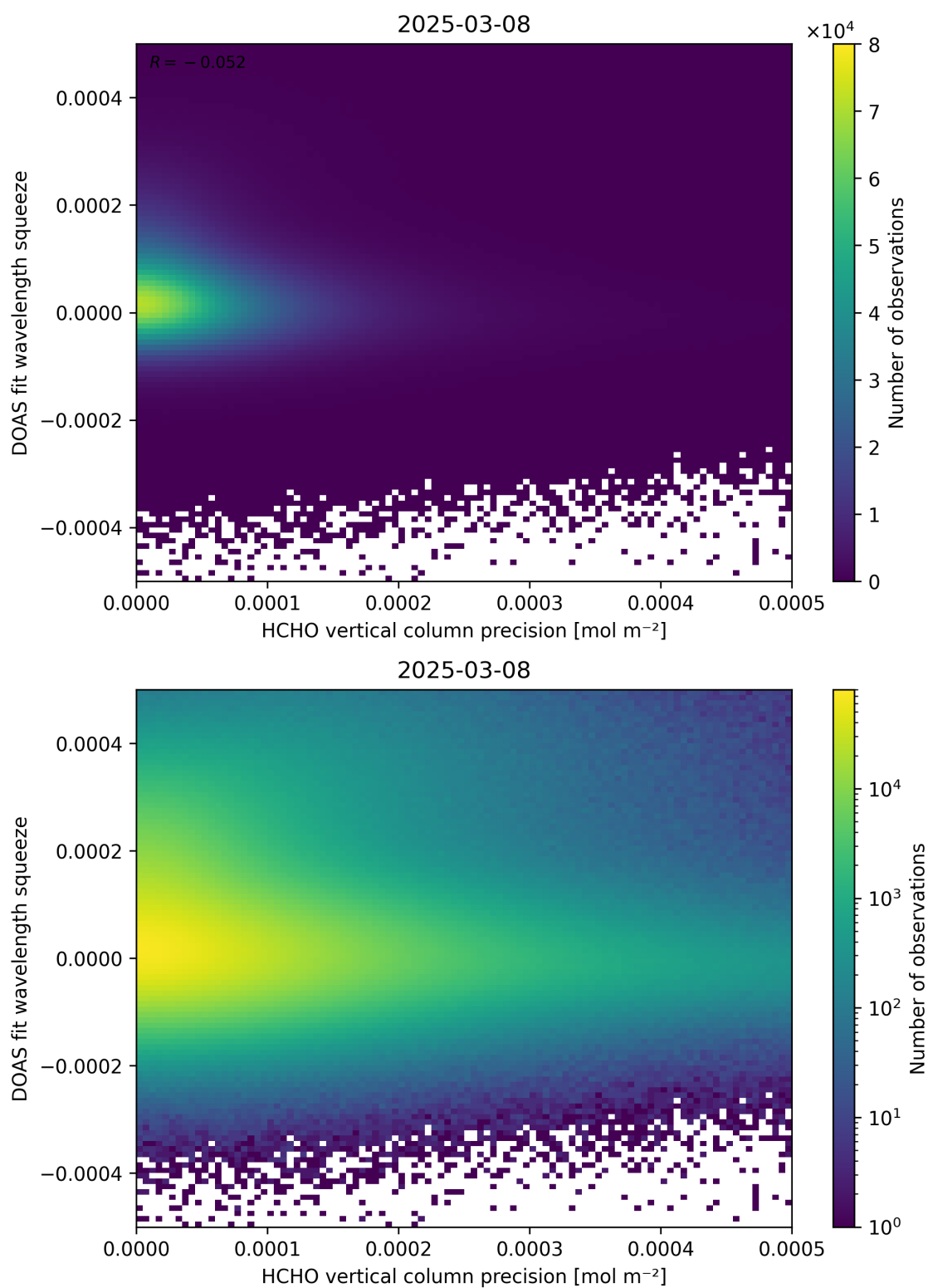
Figure 138: Scatter density plot of “HCHO vertical column precision” against “DOAS fit wavelength squeeze” for 2025-03-07 to 2025-03-09.
