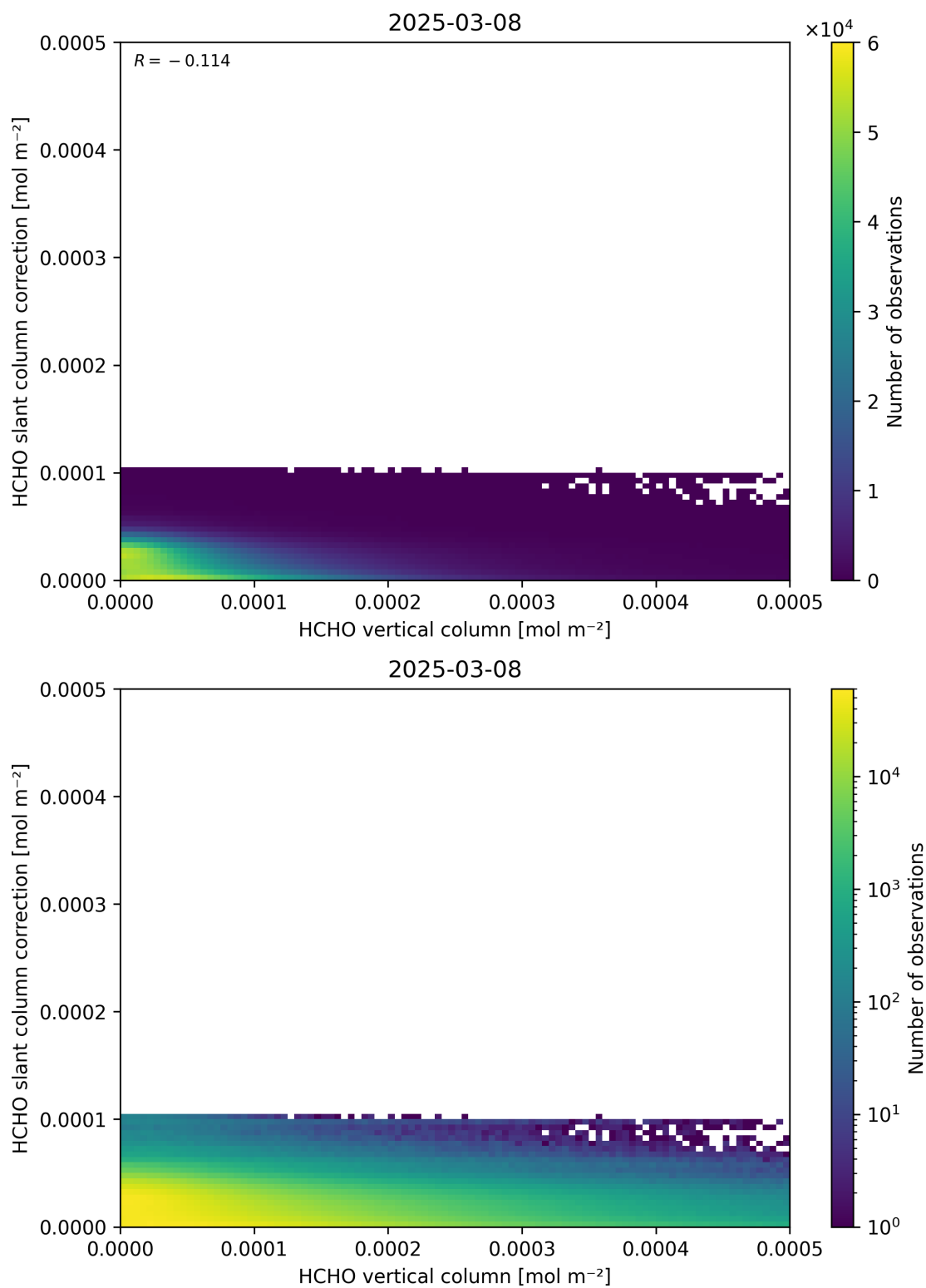
Figure 128: Scatter density plot of “HCHO vertical column” against “HCHO slant column correction” for 2025-03-07 to 2025-03-09.
