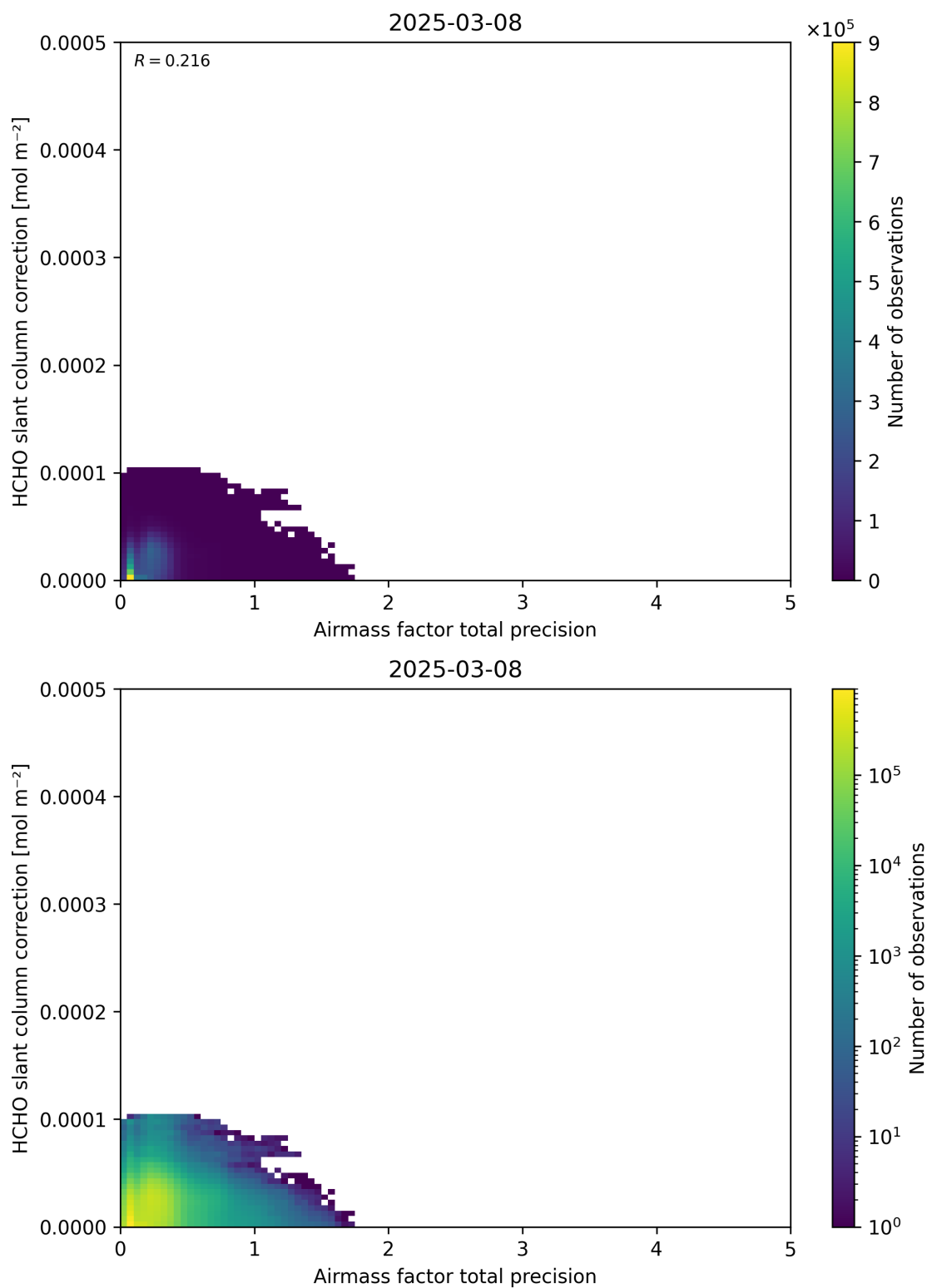
Figure 110: Scatter density plot of “Airmass factor total precision” against “HCHO slant column correction” for 2025-03-07 to 2025-03-09.
