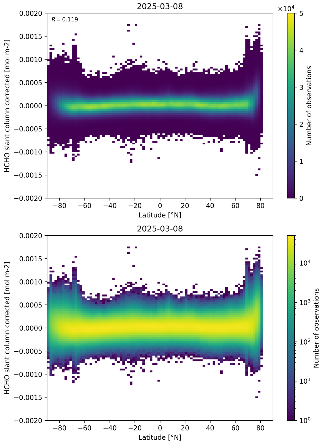
Figure 157: Scatter density plot of “Latitude” against “HCHO slant column corrected” for 2025-03-07 to 2025-03-09.
