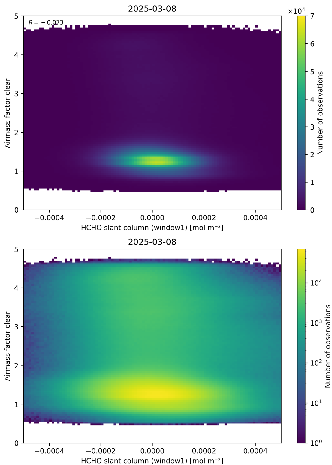
Figure 81: Scatter density plot of “HCHO slant column (window1)” against “Airmass factor clear” for 2025-03-07 to 2025-03-09.
