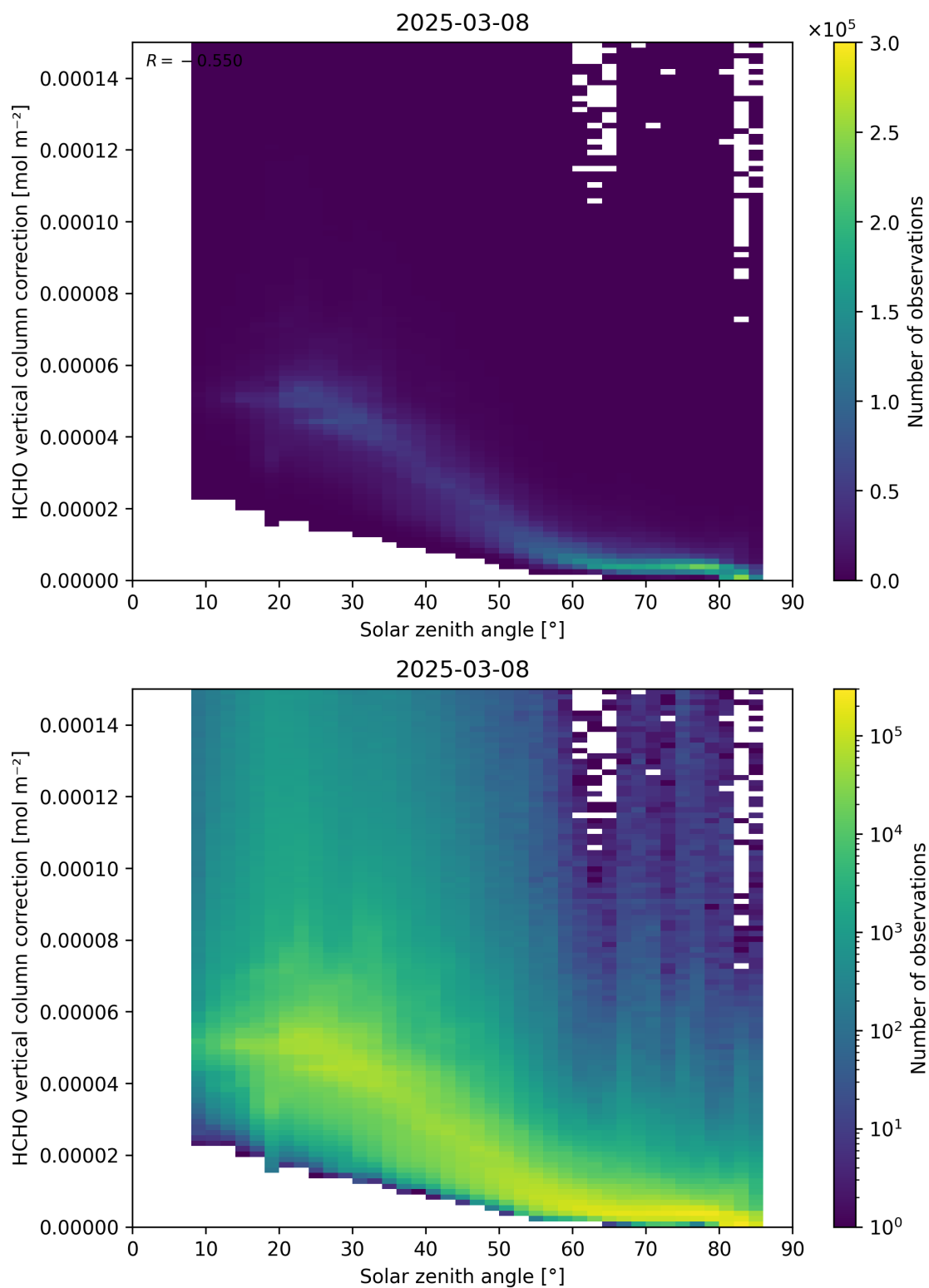
Figure 178: Scatter density plot of “Solar zenith angle” against “HCHO vertical column correction” for 2025-03-07 to 2025-03-09.
