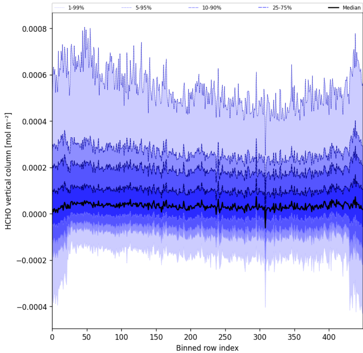
Figure 49: Along track statistics of “HCHO vertical column” for 2025-03-07 to 2025-03-09
