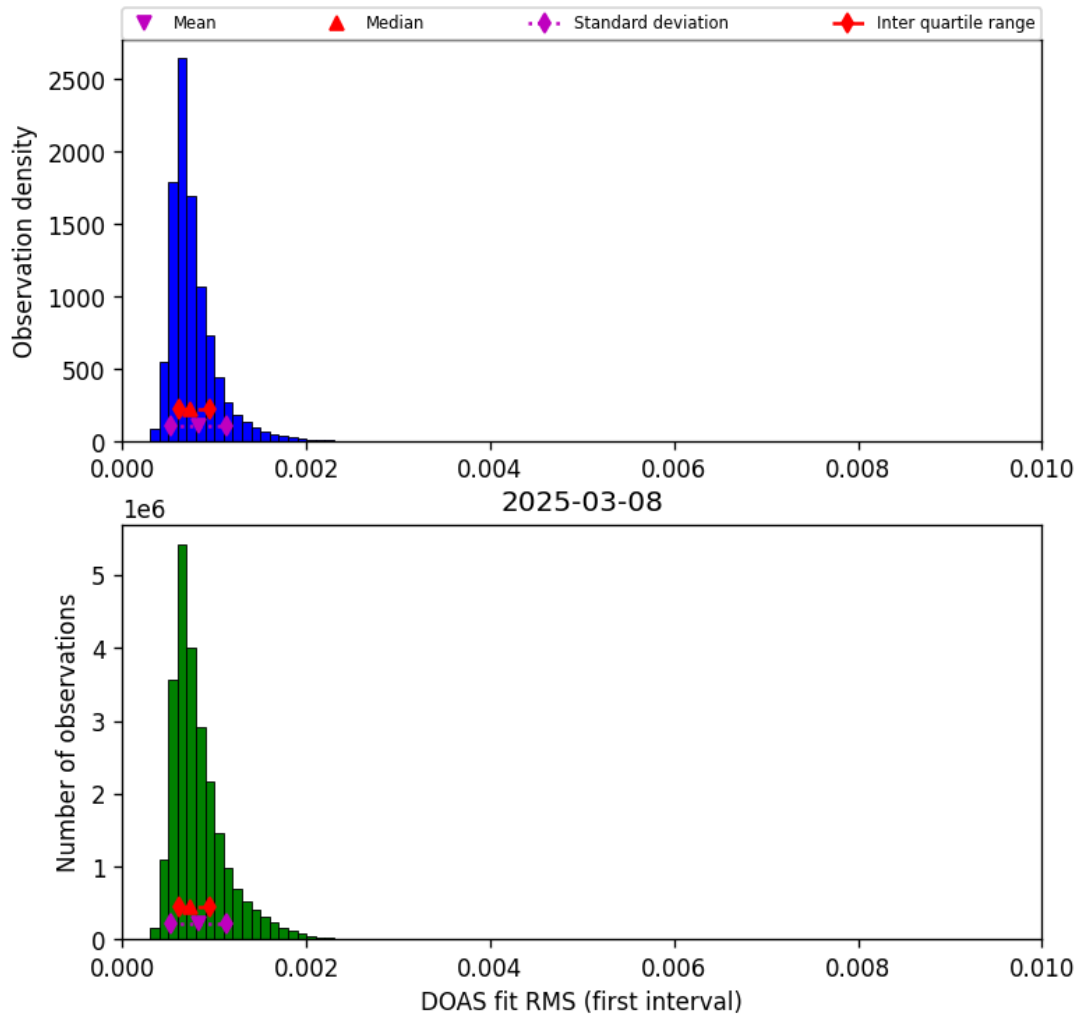
Figure 46: Histogram of “DOAS fit RMS (first interval)” for 2025-03-07 to 2025-03-09
