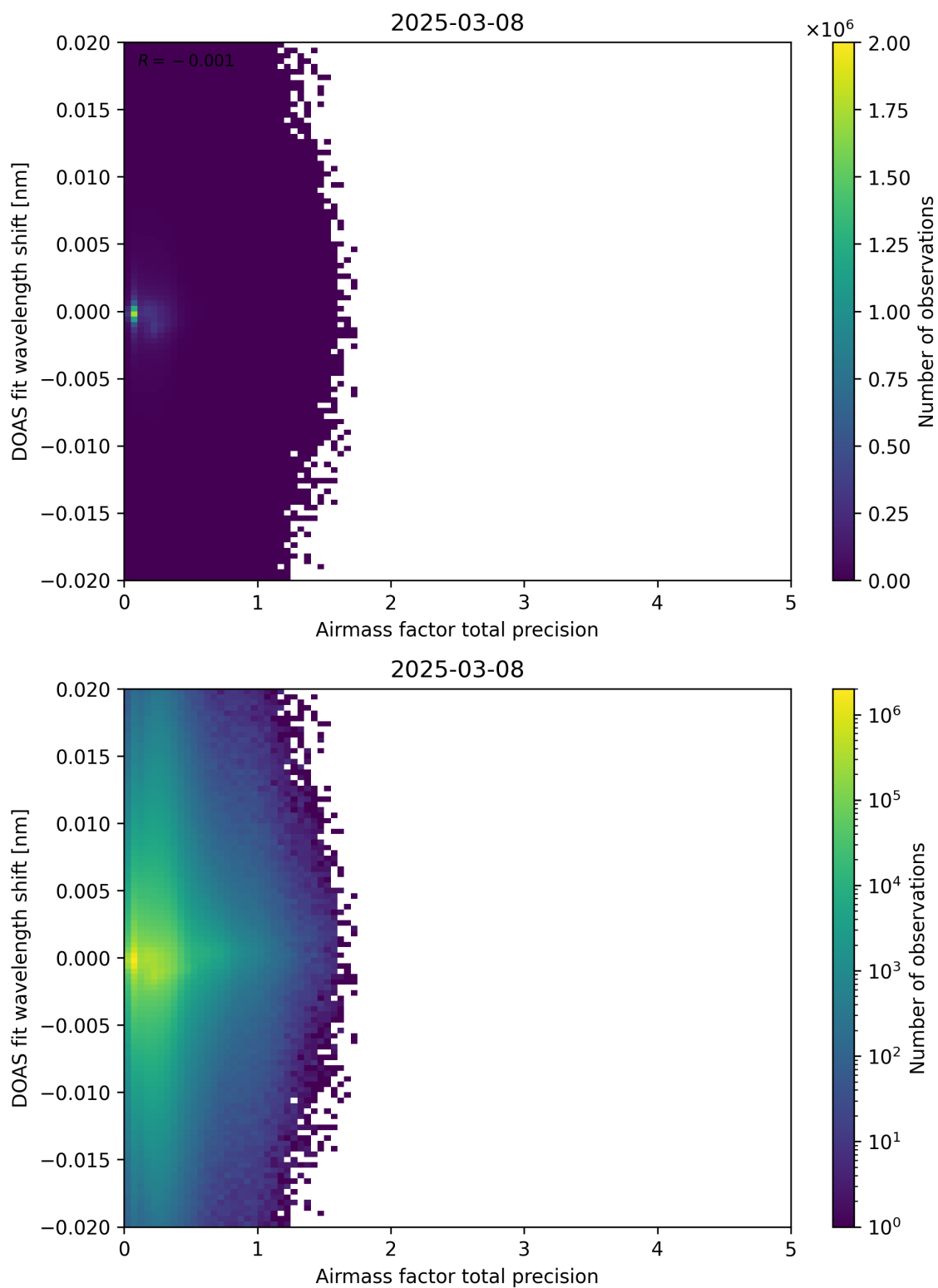
Figure 106: Scatter density plot of “Airmass factor total precision” against “DOAS fit wavelength shift” for 2025-03-07 to 2025-03-09.
