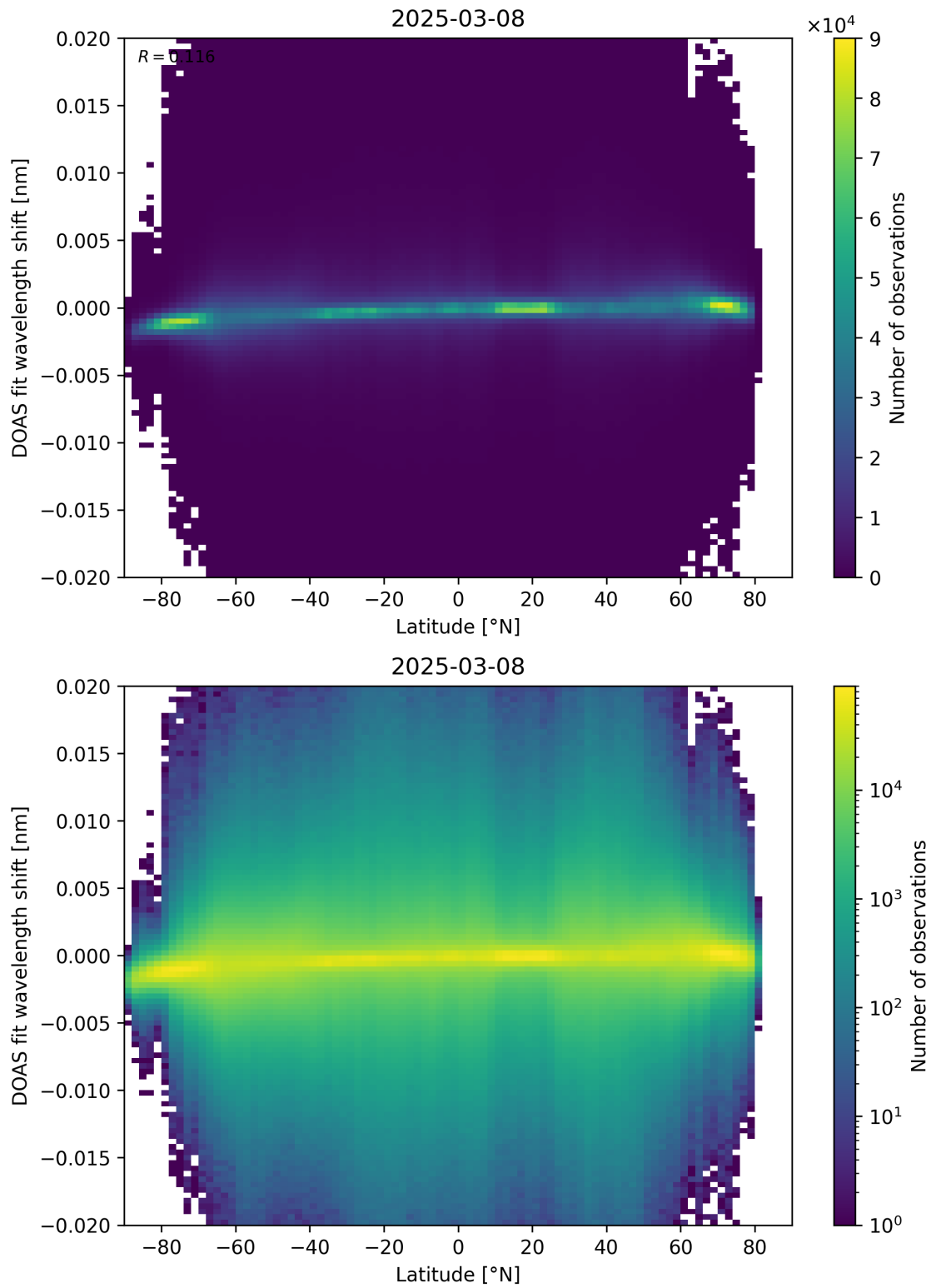
Figure 154: Scatter density plot of “Latitude” against “DOAS fit wavelength shift” for 2025-03-07 to 2025-03-09.
