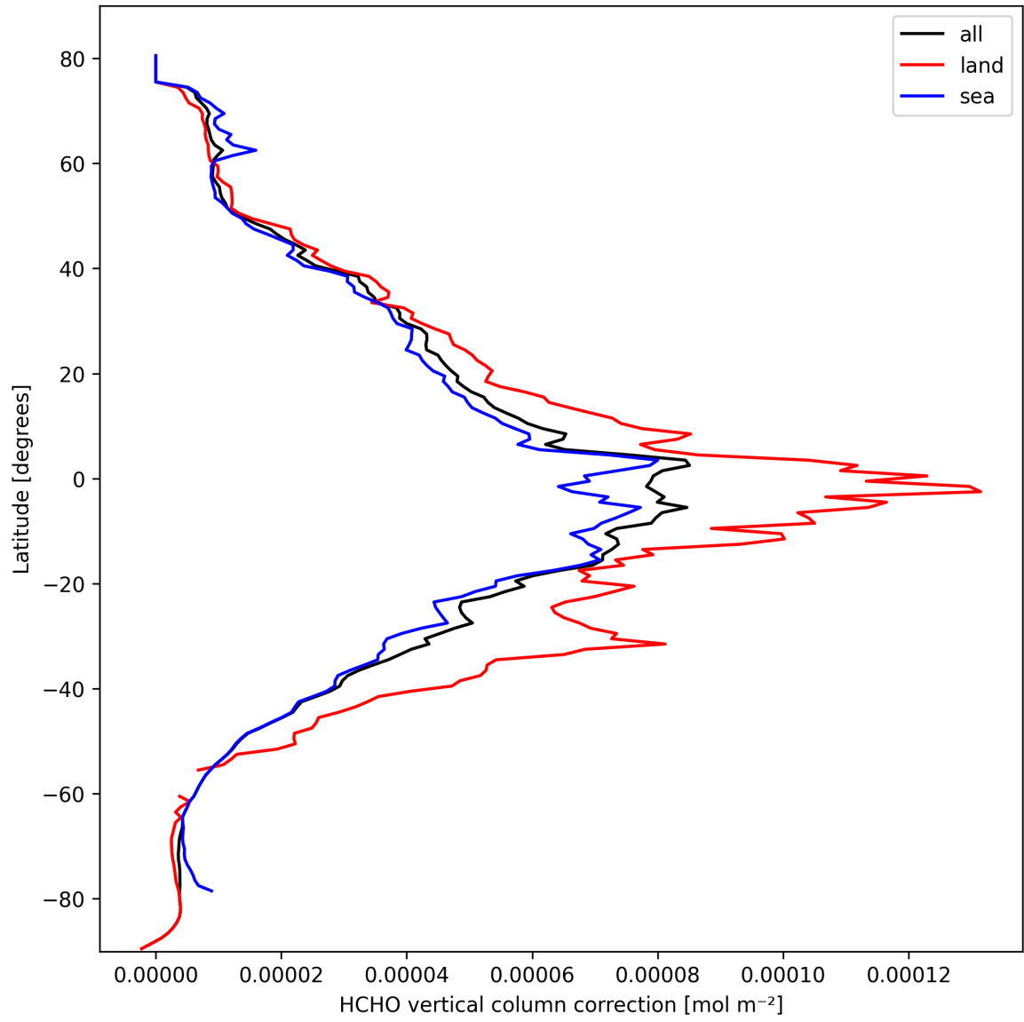
Figure 23: Zonal average of “HCHO vertical column correction” for 2025-03-07 to 2025-03-09.
