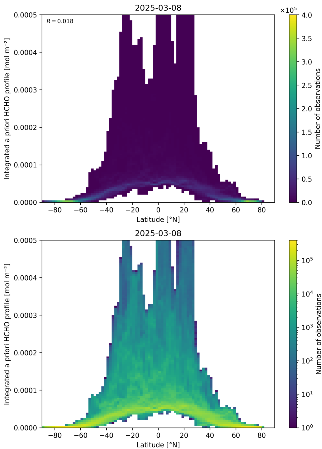
Figure 166: Scatter density plot of “Latitude” against “Integrated a priori HCHO profile” for 2025-03-07 to 2025-03-09.
