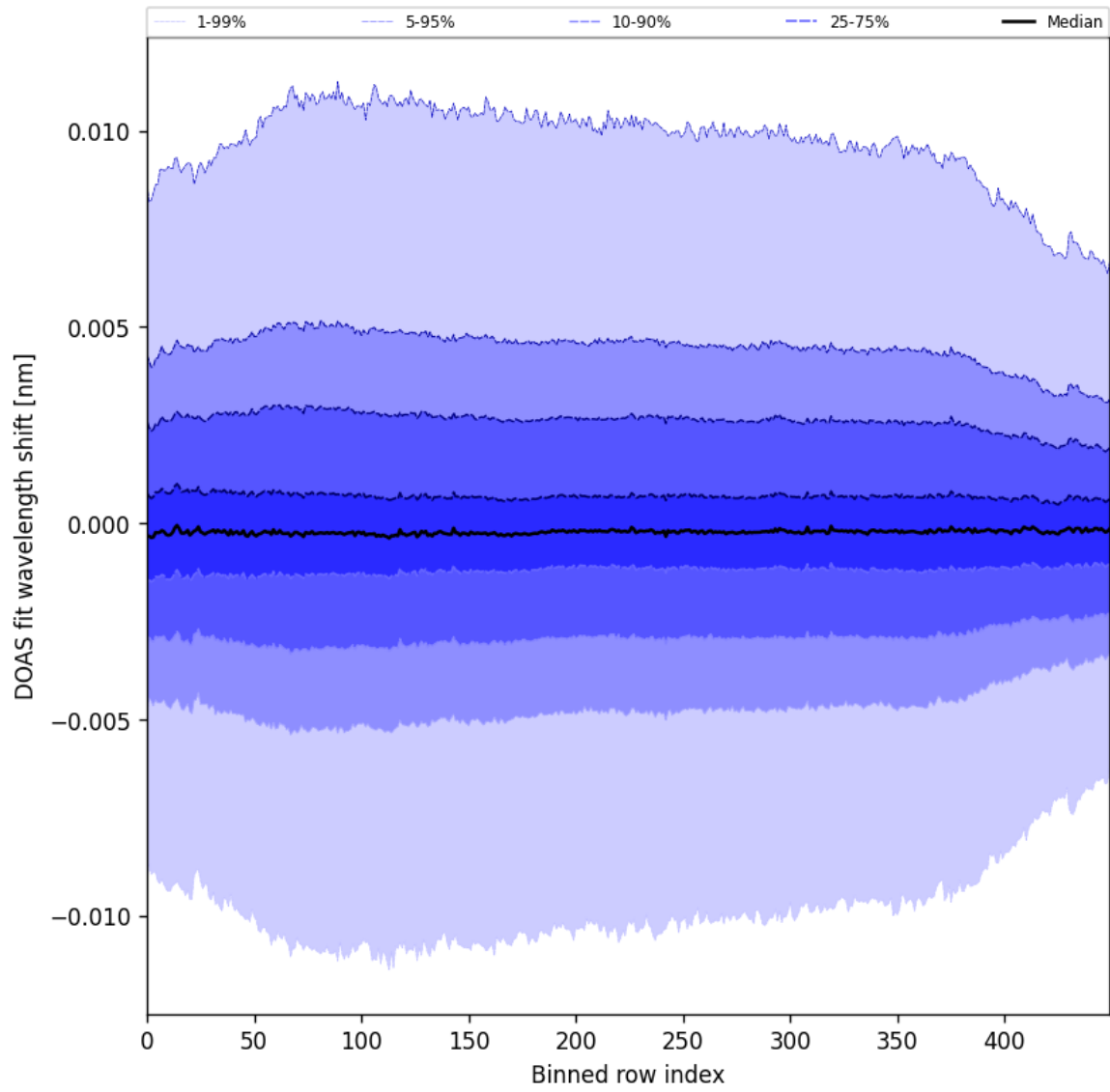
Figure 58: Along track statistics of “DOAS fit wavelength shift” for 2025-03-07 to 2025-03-09
