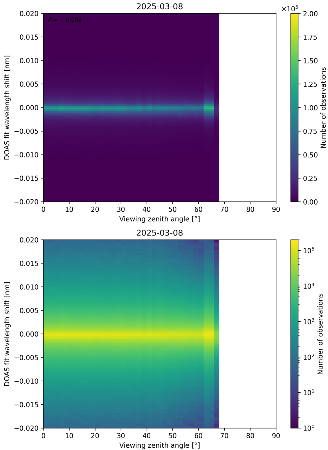
Figure 183: Scatter density plot of “Viewing zenith angle” against “DOAS fit wavelength shift” for 2025-03-07 to 2025-03-09.
