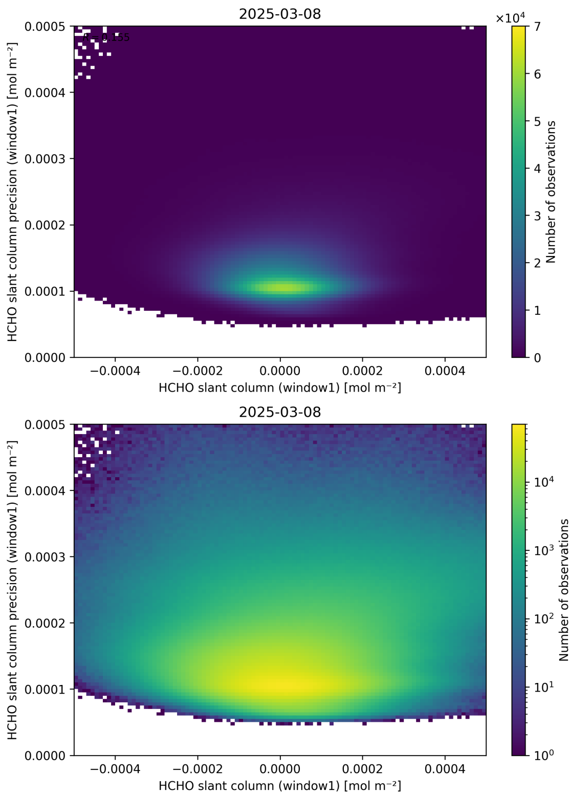
Figure 84: Scatter density plot of “HCHO slant column (window1)” against “HCHO slant column precision (window1)” for 2025-03-07 to 2025-03-09.
