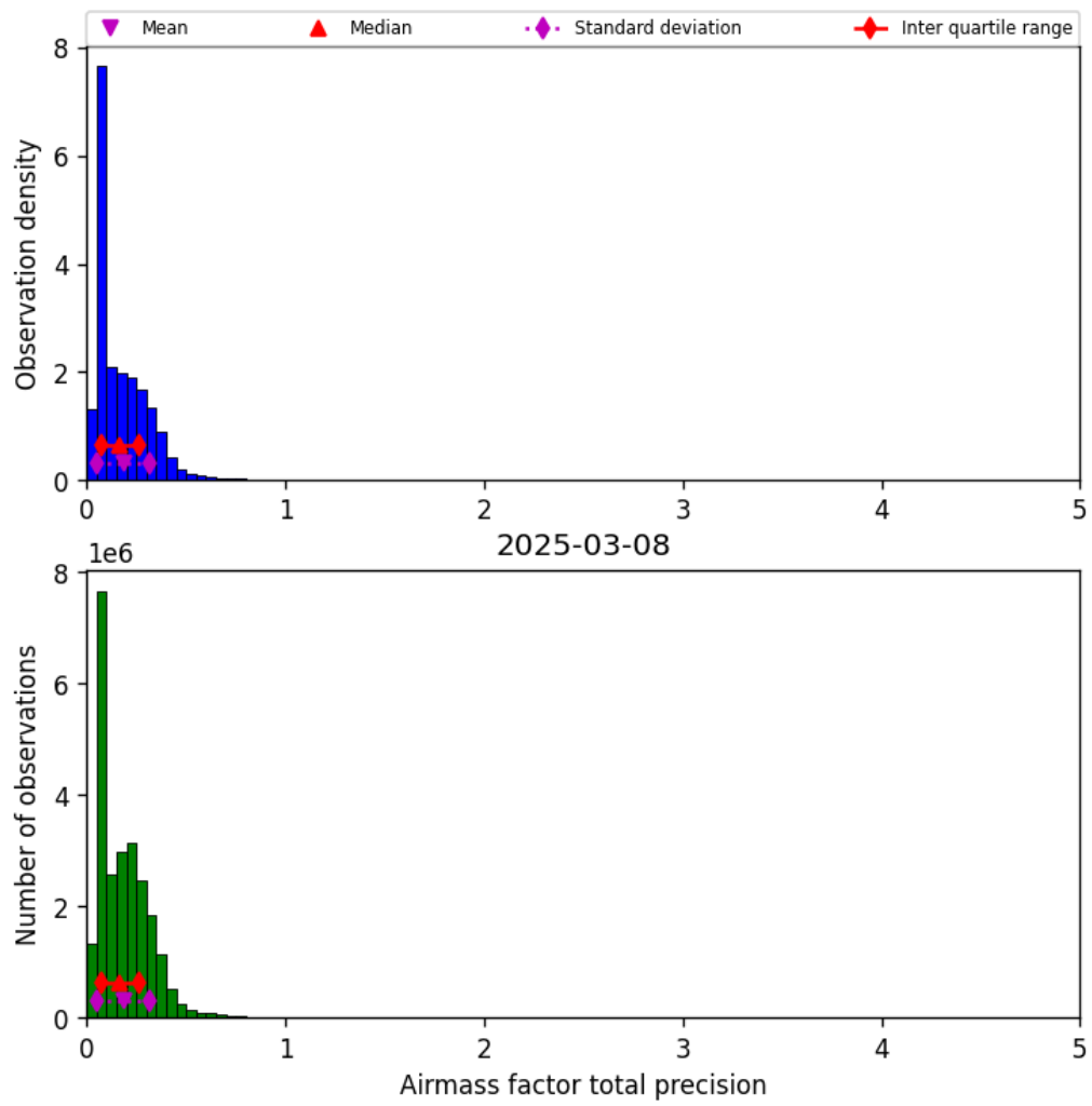
Figure 41: Histogram of “Airmass factor total precision” for 2025-03-07 to 2025-03-09
