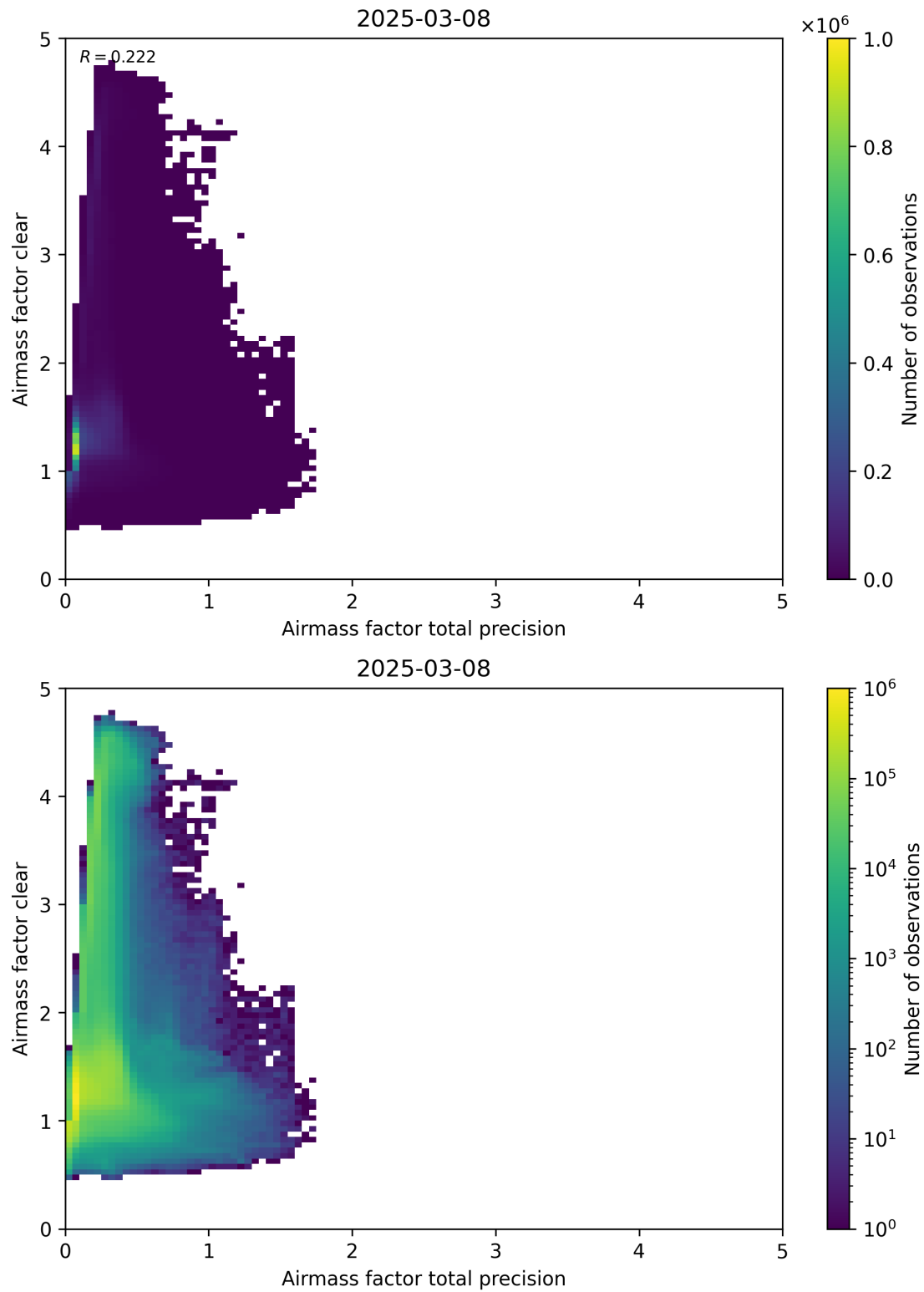
Figure 108: Scatter density plot of “Airmass factor total precision” against “Airmass factor clear” for 2025-03-07 to 2025-03-09.
