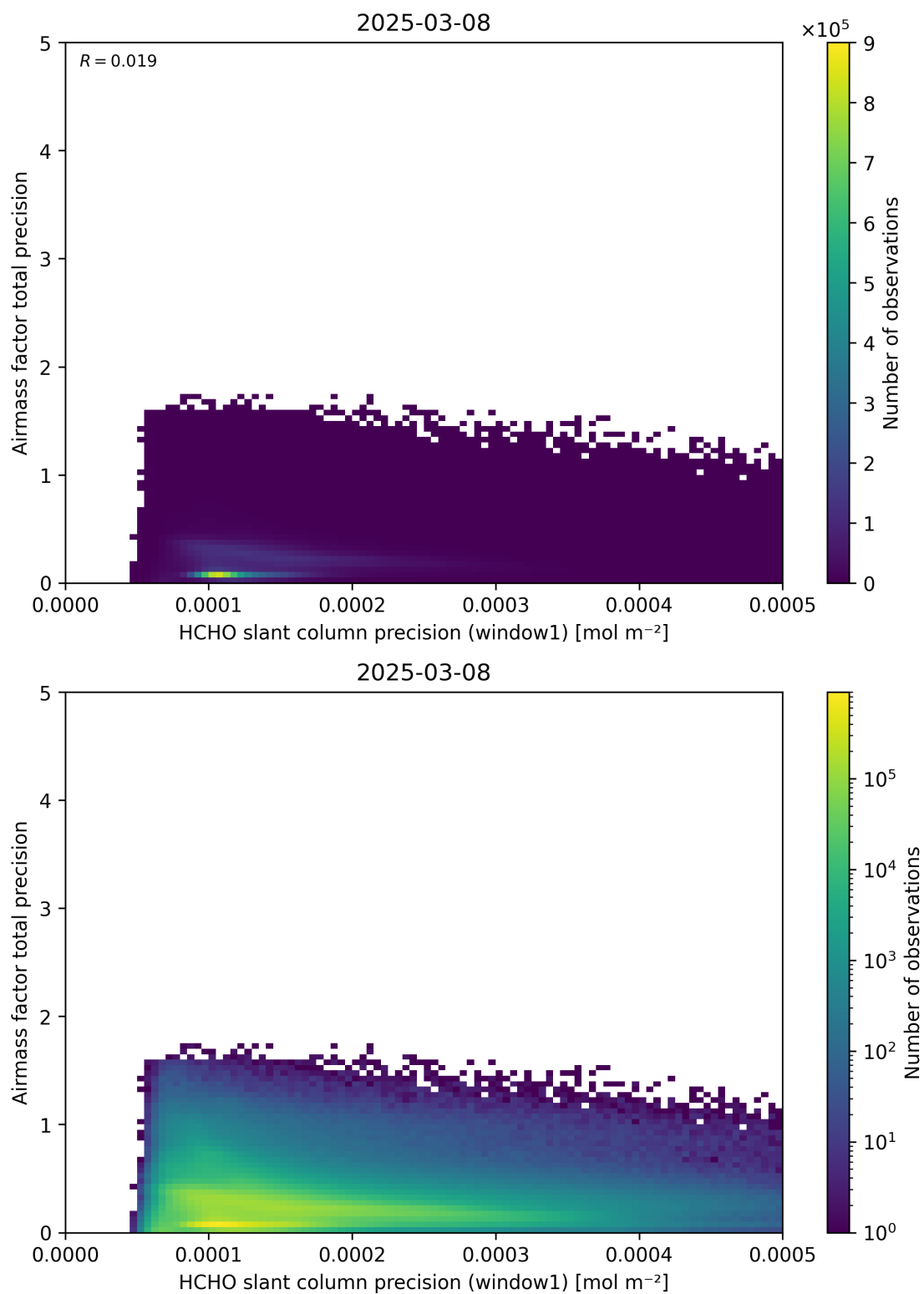
Figure 95: Scatter density plot of “HCHO slant column precision (window1)” against “Airmass factor total precision” for 2025-03-07 to 2025-03-09.
