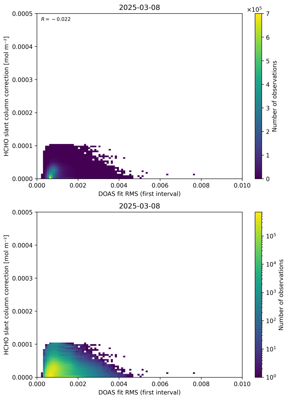
Figure 63: Scatter density plot of “DOAS fit RMS (first interval)” against “HCHO slant column correction” for 2025-03-07 to 2025-03-09.
