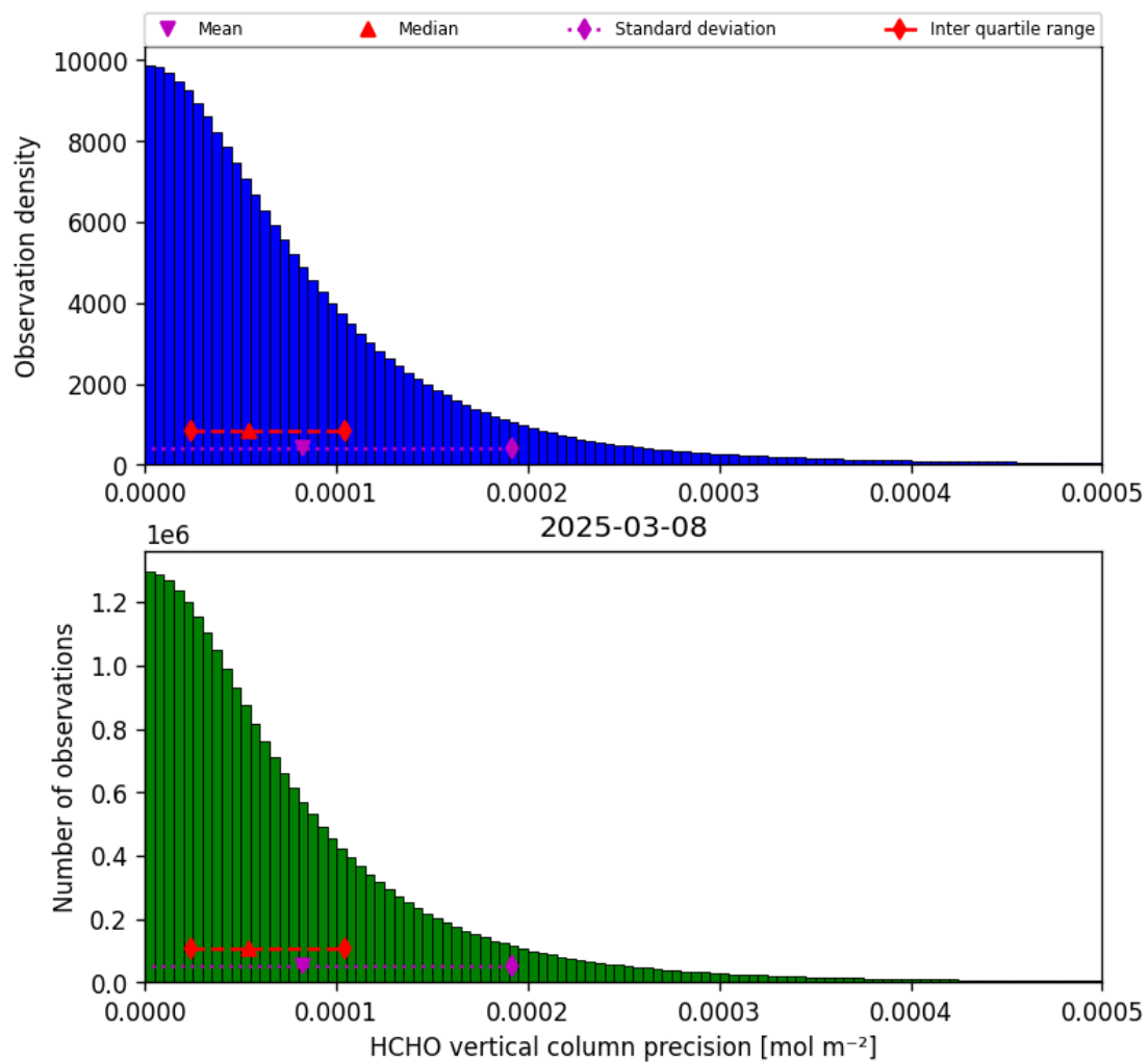
Figure 36: Histogram of “HCHO vertical column precision” for 2025-03-07 to 2025-03-09
