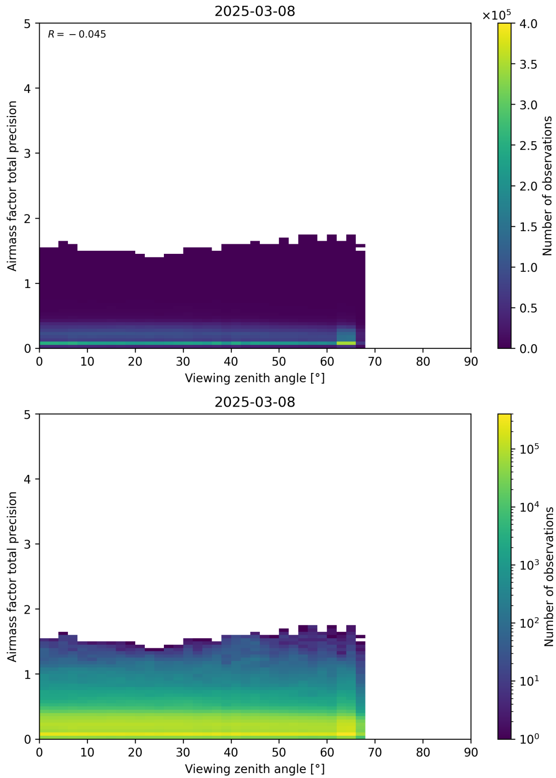
Figure 191: Scatter density plot of “Viewing zenith angle” against “Airmass factor total precision” for 2025-03-07 to 2025-03-09.
