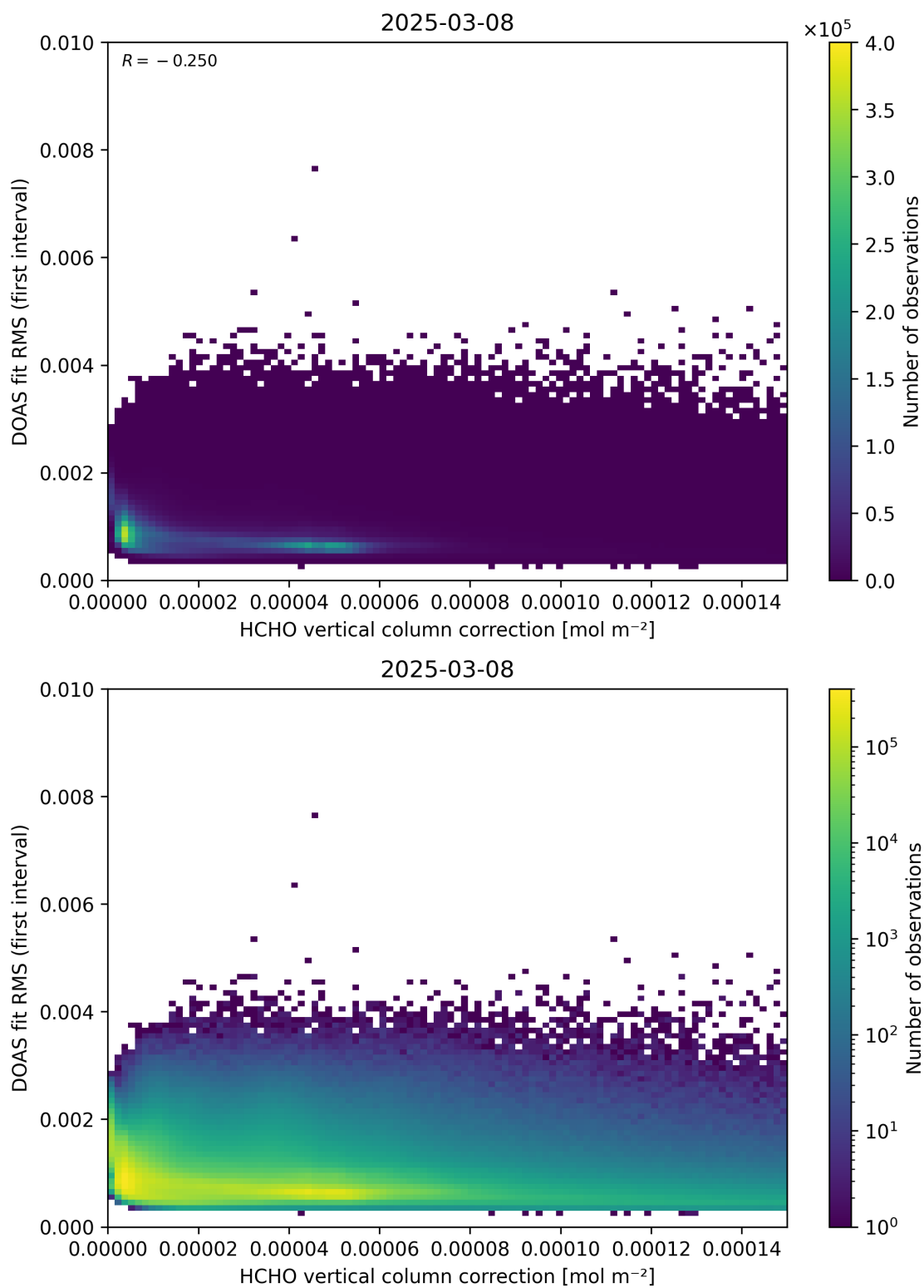
Figure 112: Scatter density plot of “HCHO vertical column correction” against “DOAS fit RMS (first interval)” for 2025-03-07 to 2025-03-09.
