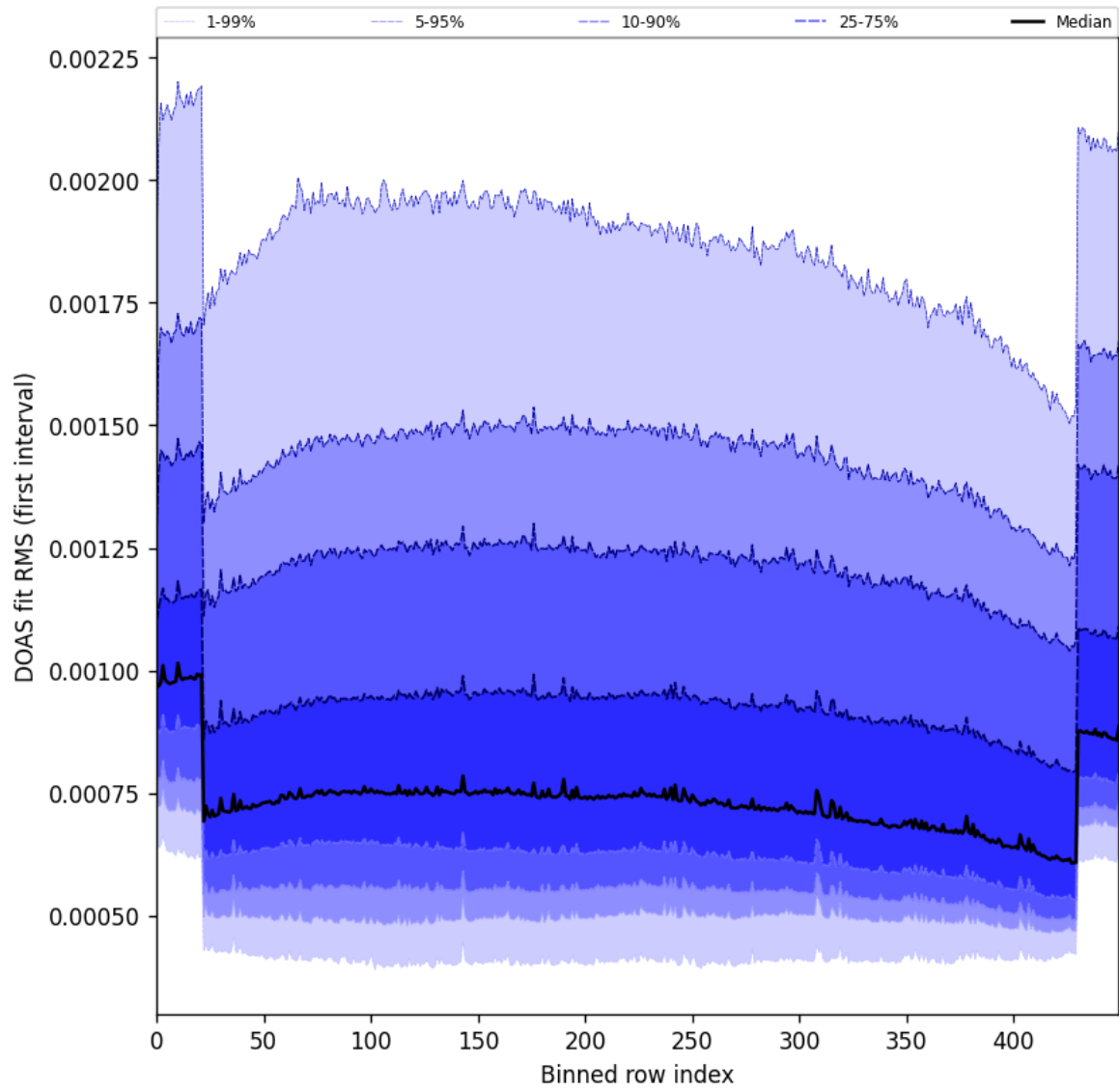
Figure 60: Along track statistics of “DOAS fit RMS (first interval)” for 2025-03-07 to 2025-03-09
