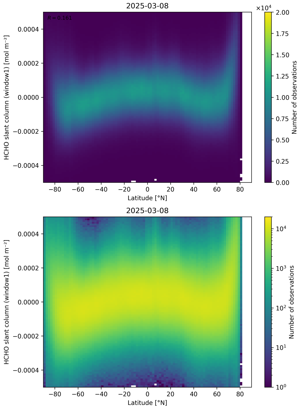
Figure 159: Scatter density plot of “Latitude” against “HCHO slant column (window1)” for 2025-03-07 to 2025-03-09.
