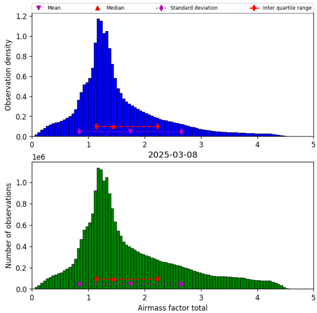
Figure 40: Histogram of “Airmass factor total” for 2025-03-07 to 2025-03-09
