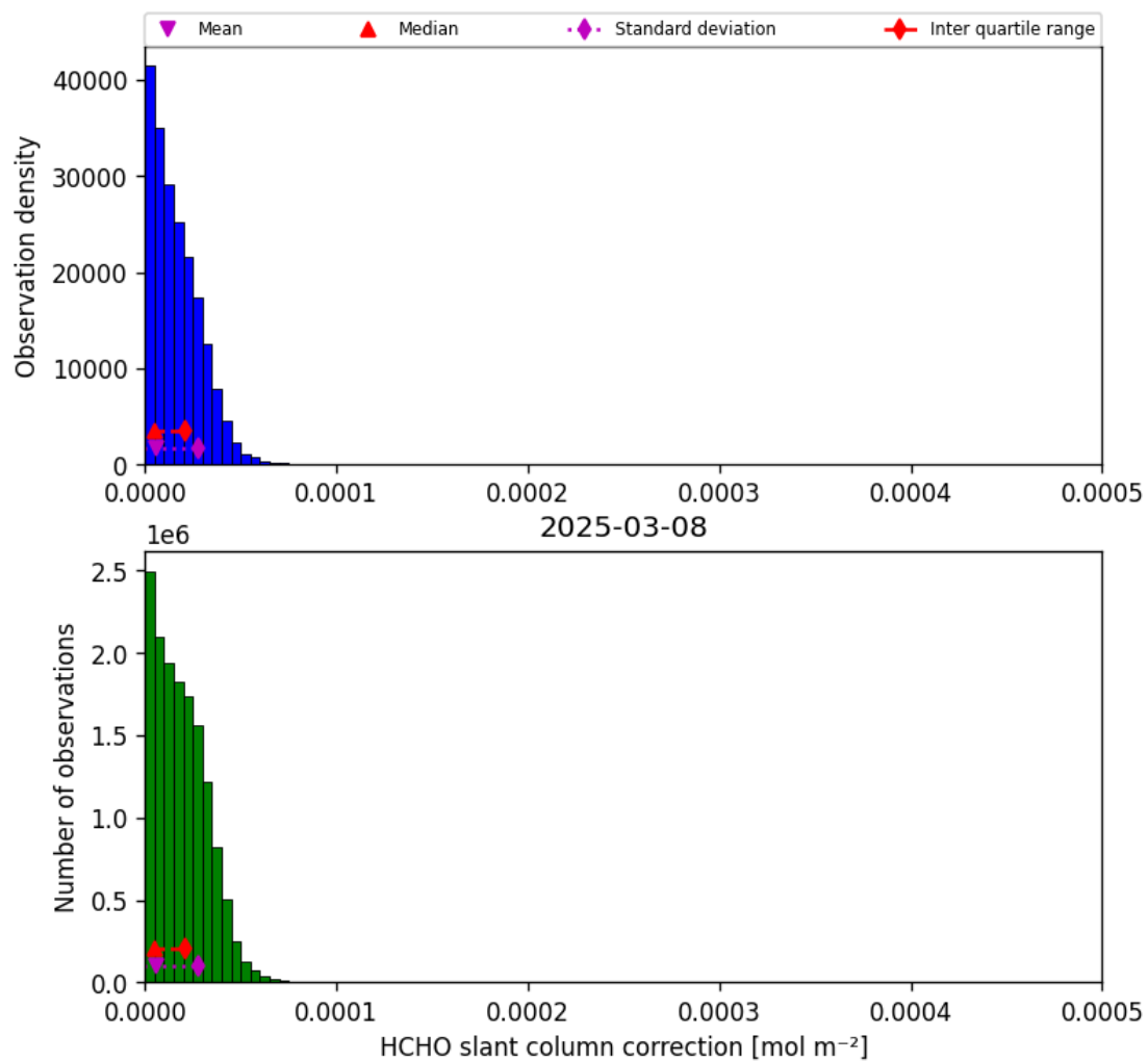
Figure 47: Histogram of “HCHO slant column correction” for 2025-03-07 to 2025-03-09
