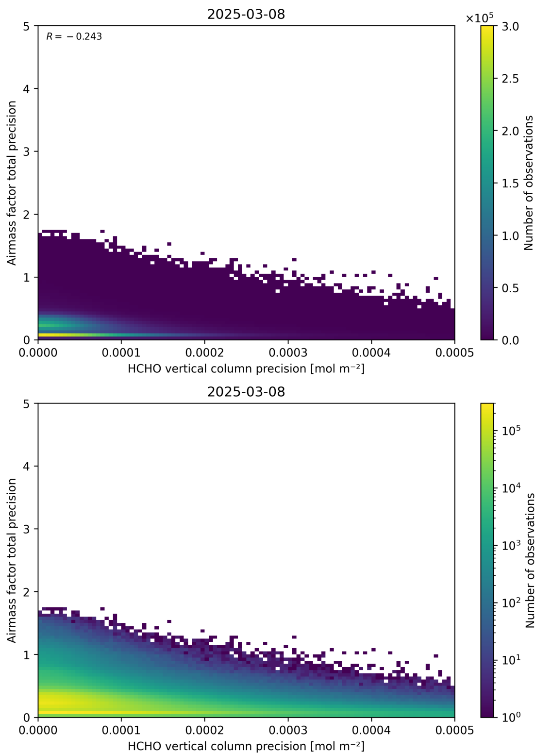
Figure 145: Scatter density plot of “HCHO vertical column precision” against “Airmass factor total precision” for 2025-03-07 to 2025-03-09.
