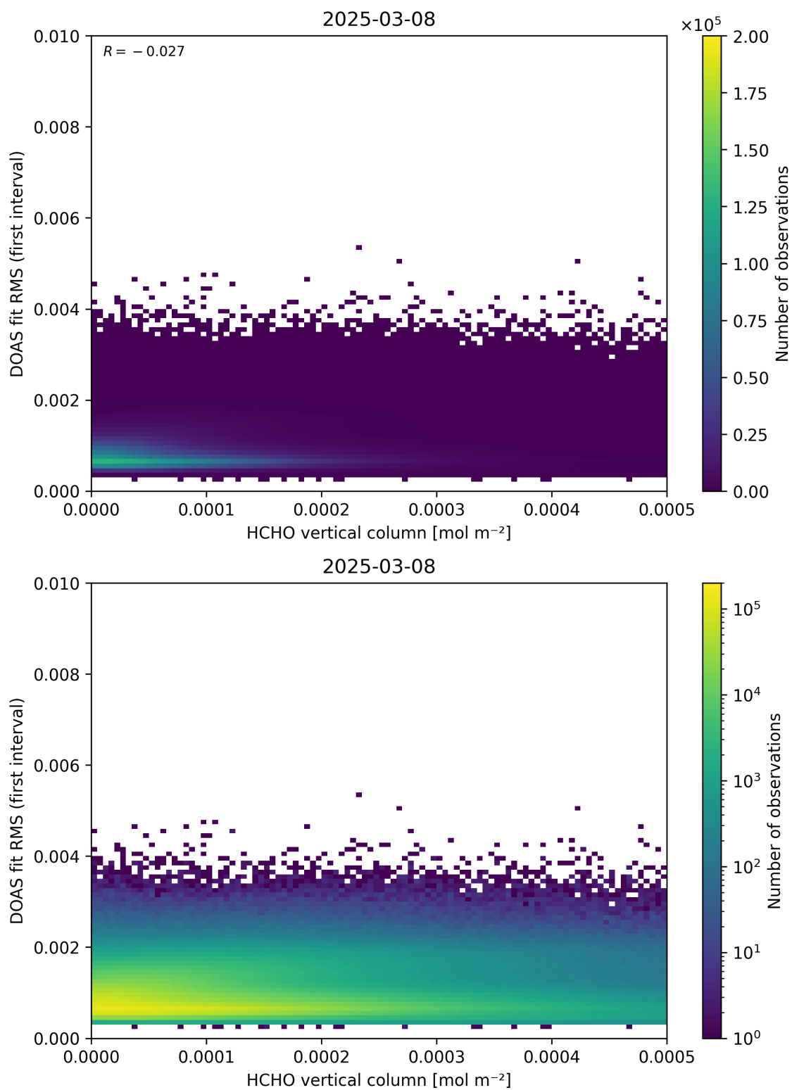
Figure 123: Scatter density plot of “HCHO vertical column” against “DOAS fit RMS (first interval)” for 2025-03-07 to 2025-03-09.
