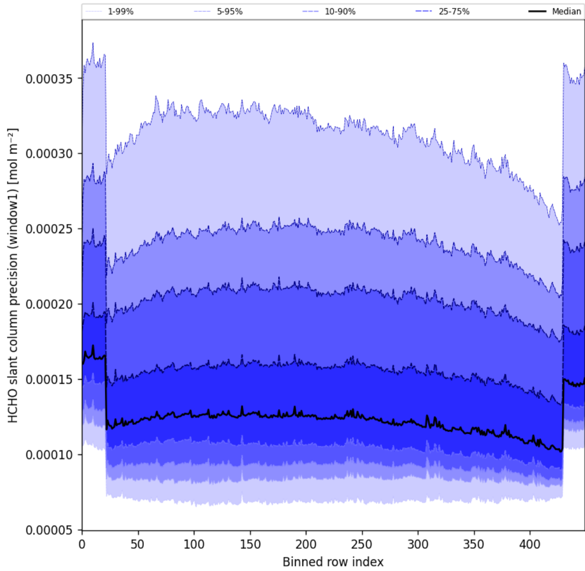
Figure 53: Along track statistics of “HCHO slant column precision (window1)” for 2025-03-07 to 2025-03-09
