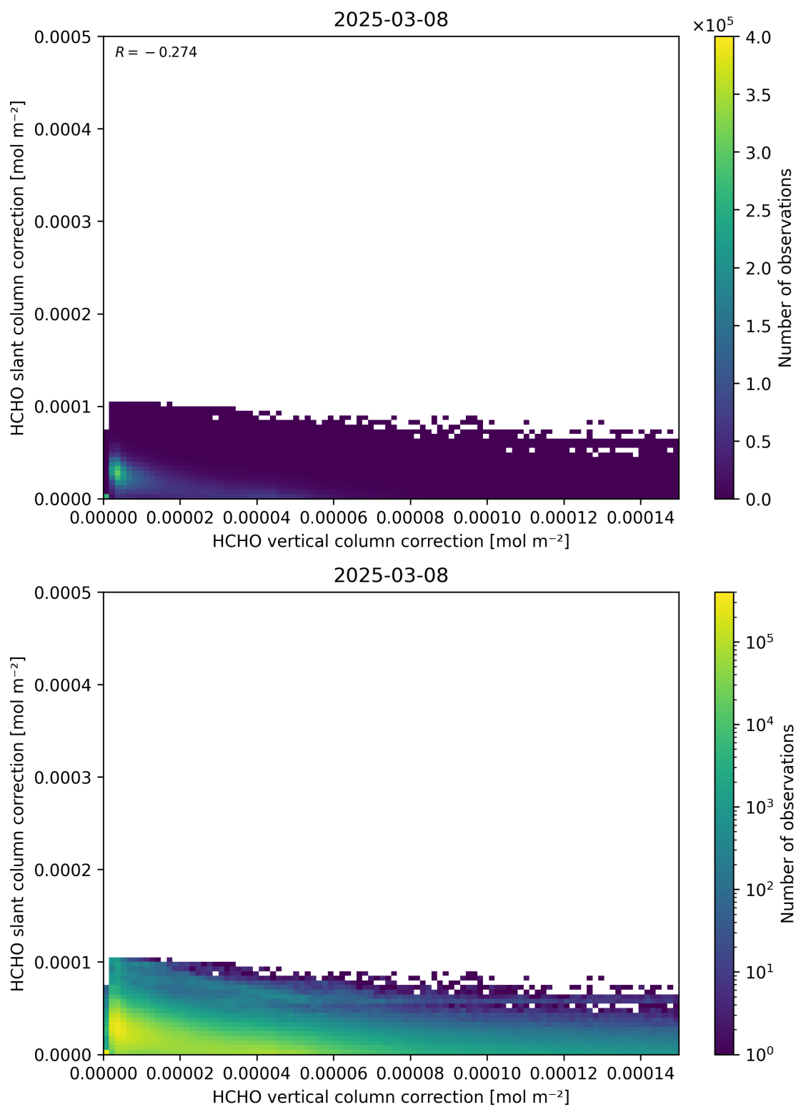
Figure 117: Scatter density plot of “HCHO vertical column correction” against “HCHO slant column correction” for 2025-03-07 to 2025-03-09.
