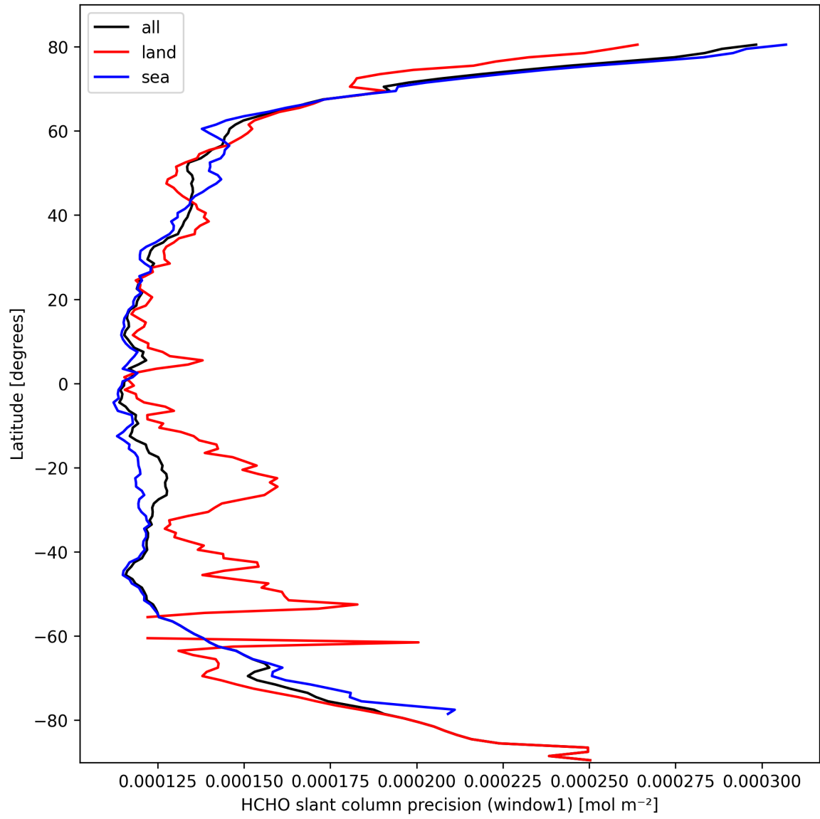
Figure 25: Zonal average of “HCHO slant column precision (window1)” for 2025-03-07 to 2025-03-09.
