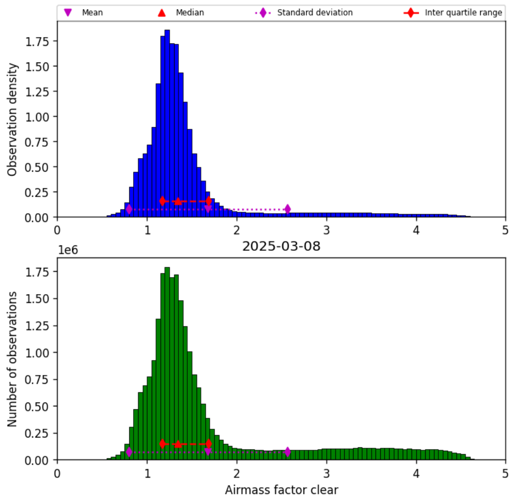
Figure 42: Histogram of “Airmass factor clear” for 2025-03-07 to 2025-03-09
