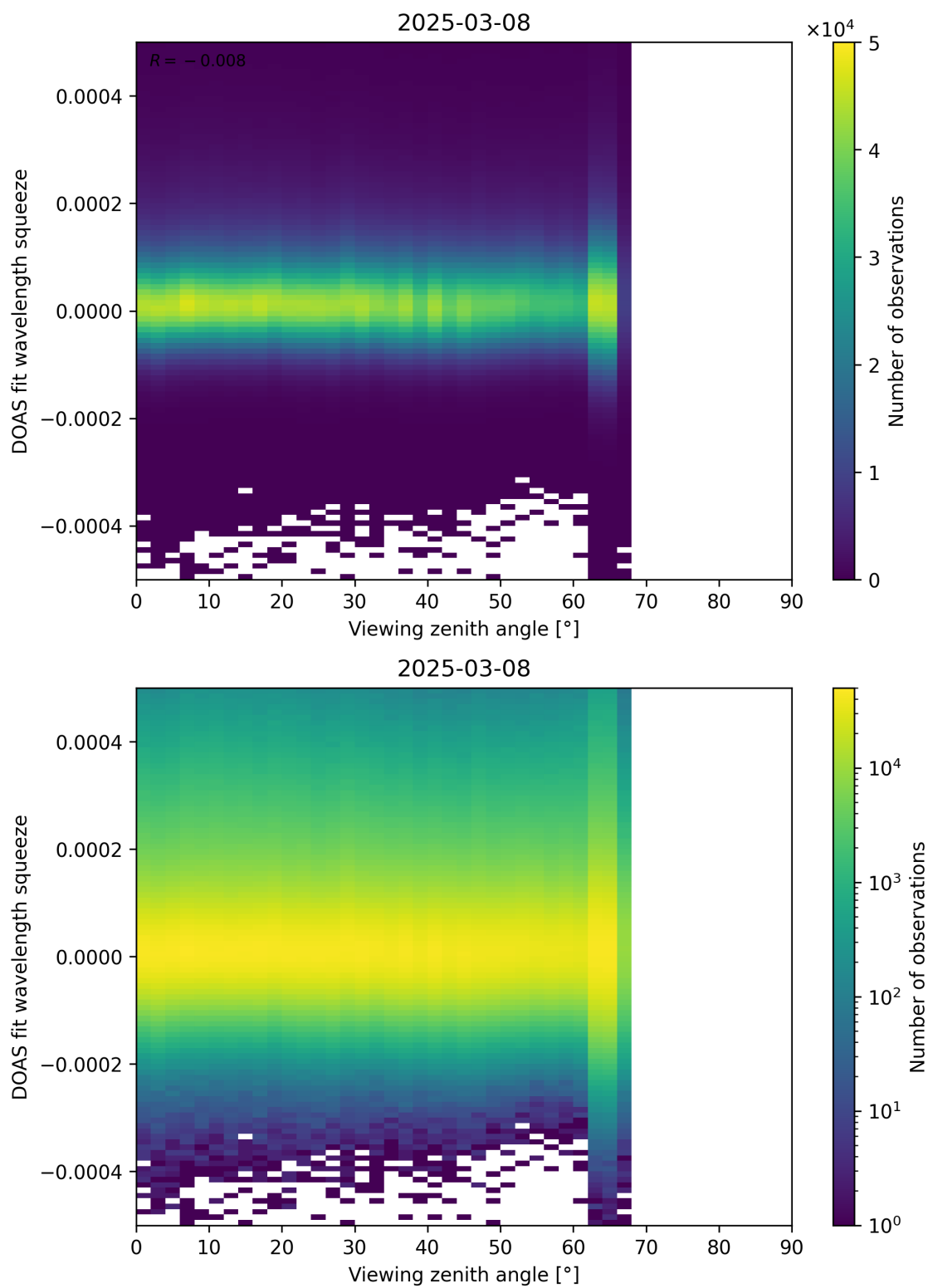
Figure 184: Scatter density plot of “Viewing zenith angle” against “DOAS fit wavelength squeeze” for 2025-03-07 to 2025-03-09.
