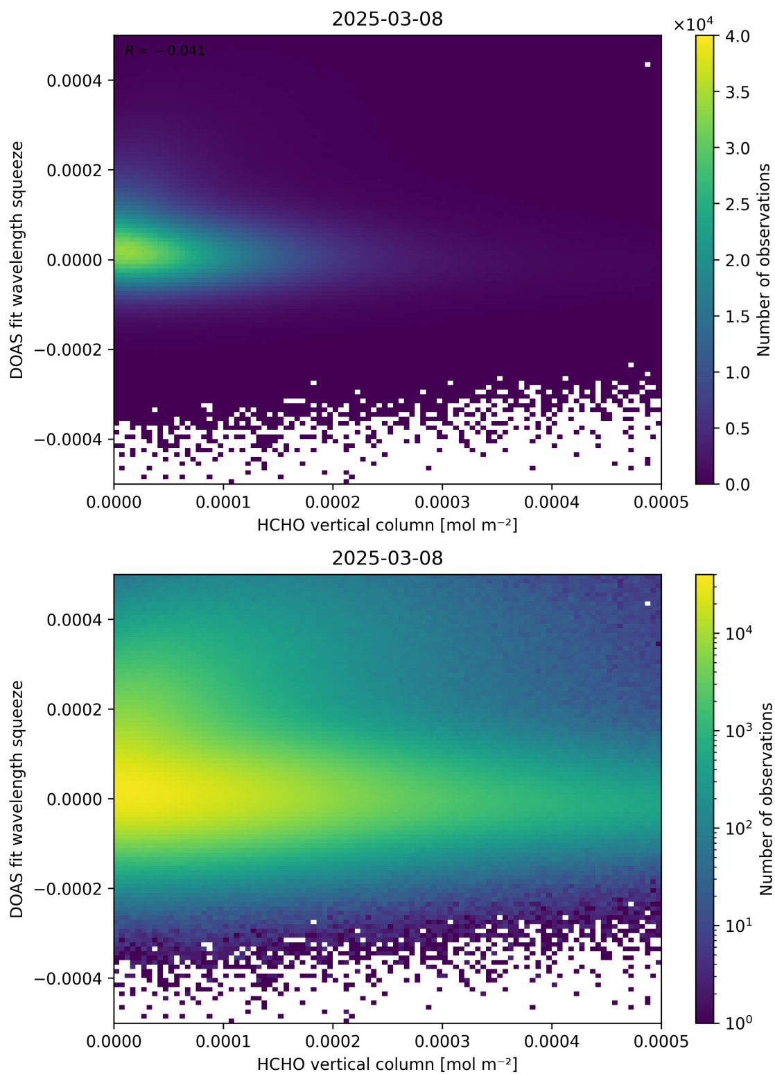
Figure 125: Scatter density plot of “HCHO vertical column” against “DOAS fit wavelength squeeze” for 2025-03-07 to 2025-03-09.
