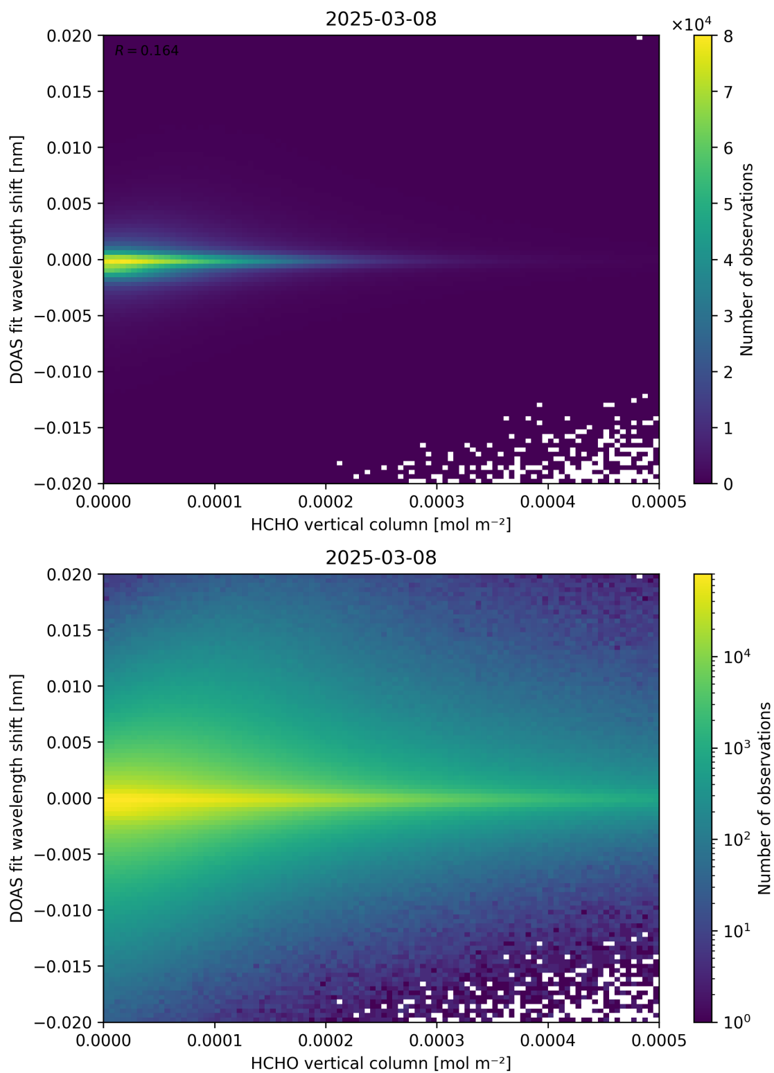
Figure 124: Scatter density plot of “HCHO vertical column” against “DOAS fit wavelength shift” for 2025-03-07 to 2025-03-09.
