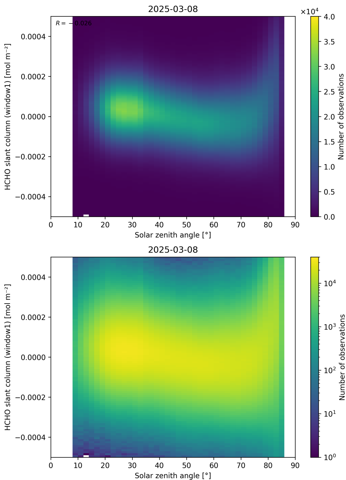
Figure 173: Scatter density plot of “Solar zenith angle” against “HCHO slant column (window1)” for 2025-03-07 to 2025-03-09.
