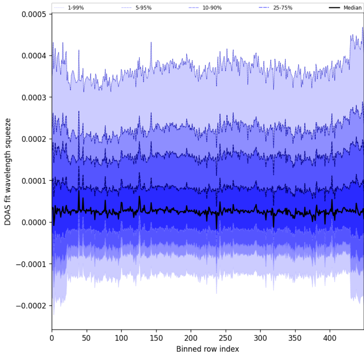
Figure 59: Along track statistics of “DOAS fit wavelength squeeze” for 2025-03-07 to 2025-03-09
