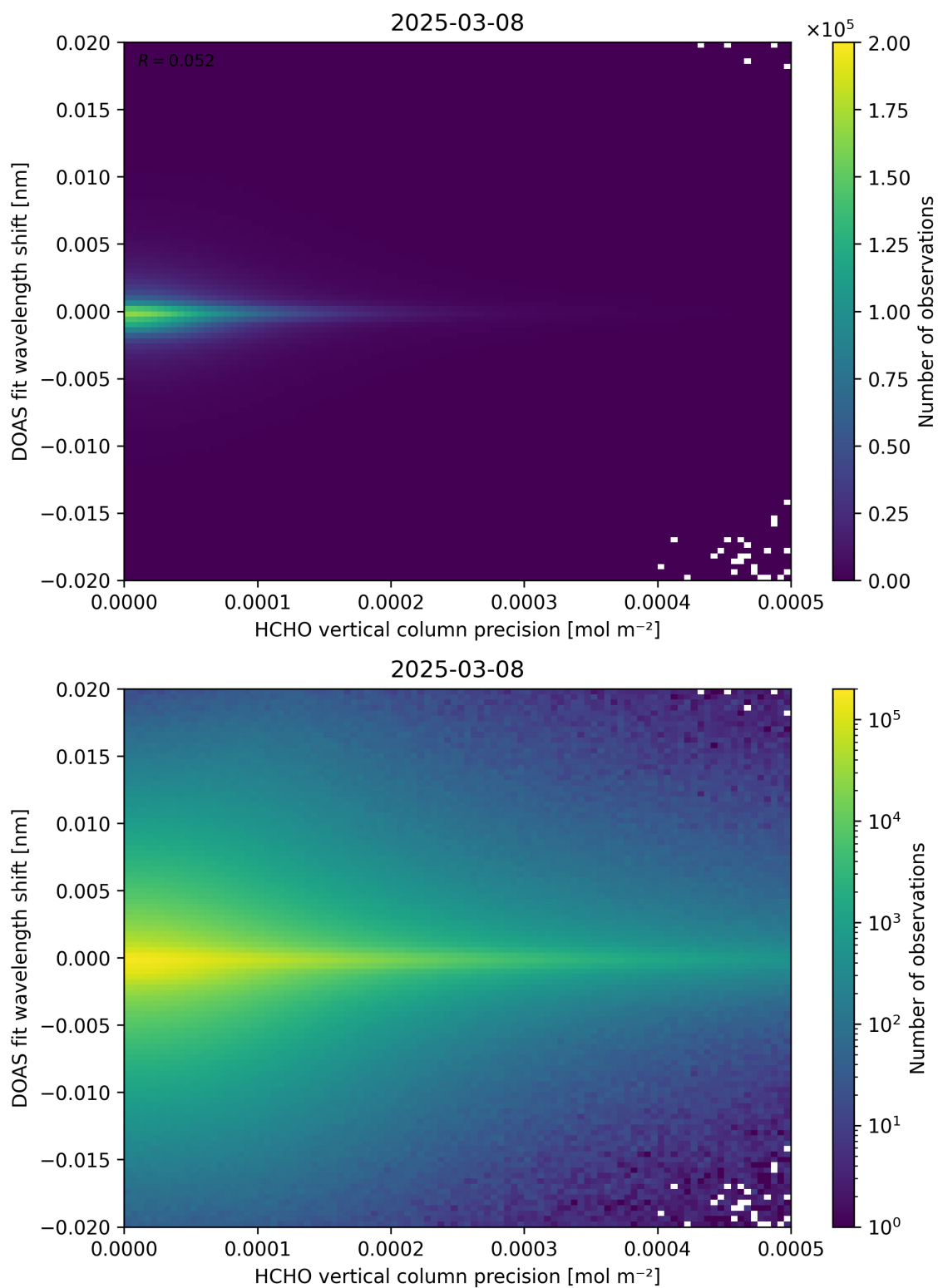
Figure 137: Scatter density plot of “HCHO vertical column precision” against “DOAS fit wavelength shift” for 2025-03-07 to 2025-03-09.
