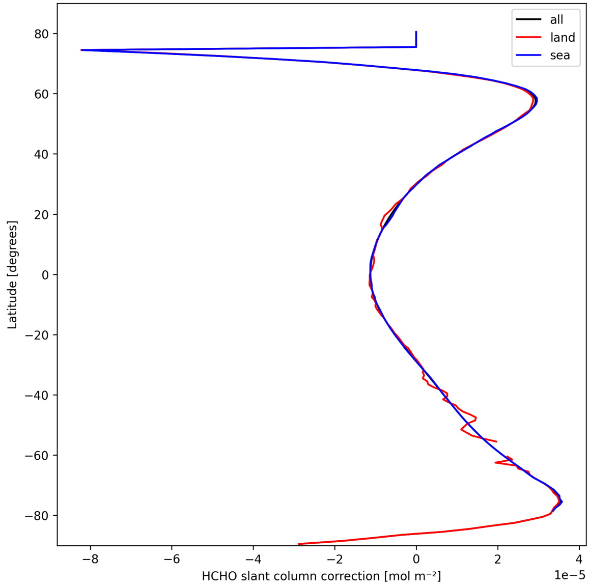
Figure 33: Zonal average of “HCHO slant column correction” for 2025-03-07 to 2025-03-09.
