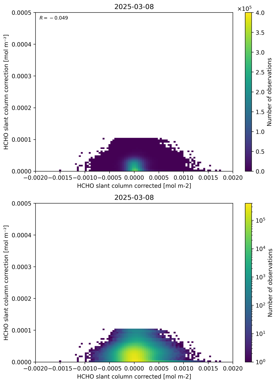
Figure 77: Scatter density plot of “HCHO slant column corrected” against “HCHO slant column correction” for 2025-03-07 to 2025-03-09.
