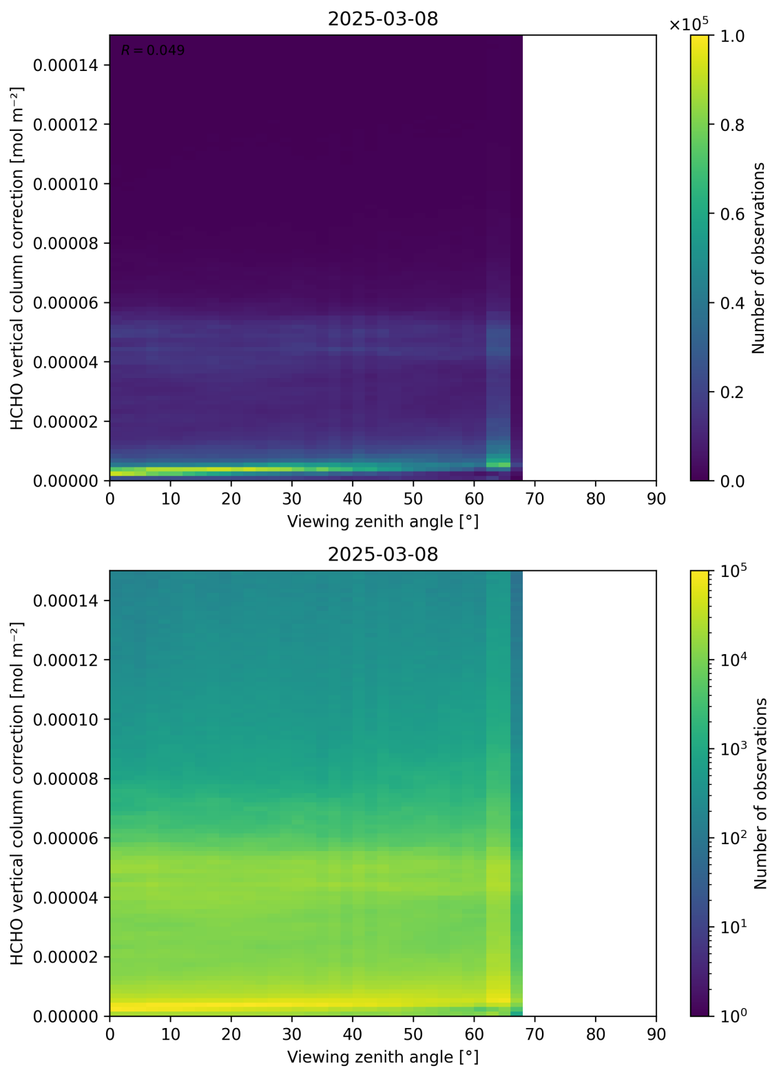
Figure 193: Scatter density plot of “Viewing zenith angle” against “HCHO vertical column correction” for 2025-03-07 to 2025-03-09.
