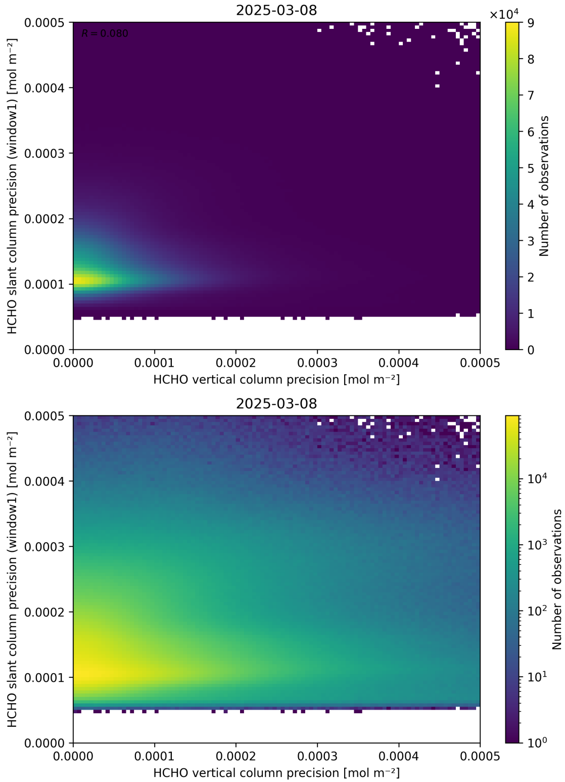
Figure 143: Scatter density plot of “HCHO vertical column precision” against “HCHO slant column precision (window1)” for 2025-03-07 to 2025-03-09.
