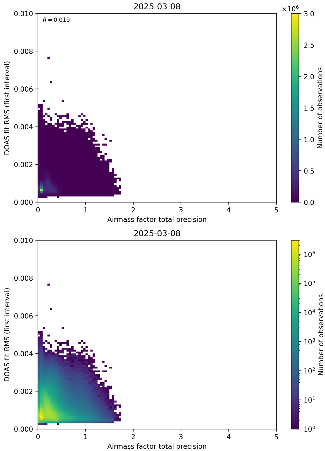
Figure 105: Scatter density plot of “Airmass factor total precision” against “DOAS fit RMS (first interval)” for 2025-03-07 to 2025-03-09.
