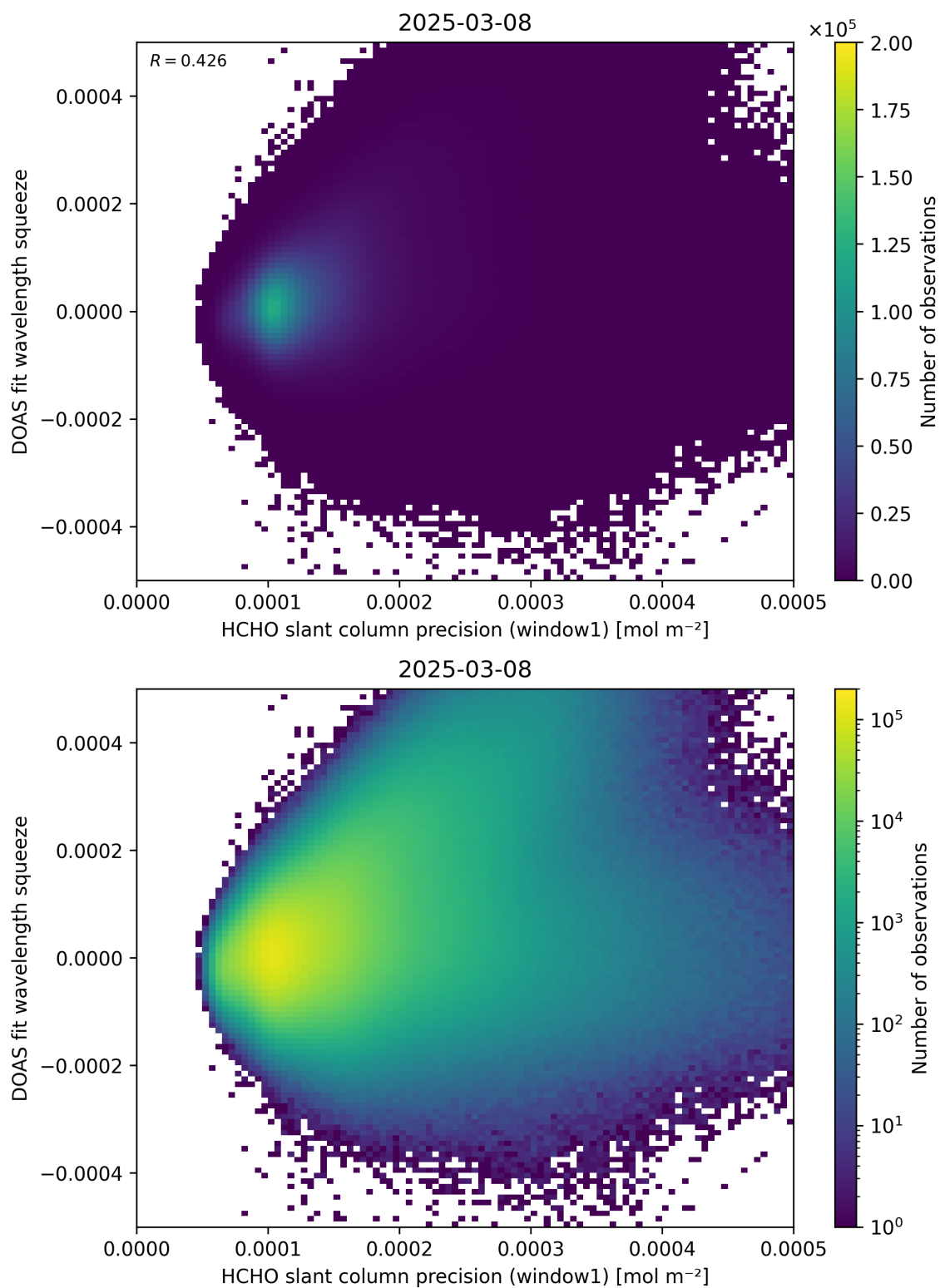
Figure 90: Scatter density plot of “HCHO slant column precision (window1)” against “DOAS fit wavelength squeeze” for 2025-03-07 to 2025-03-09.
