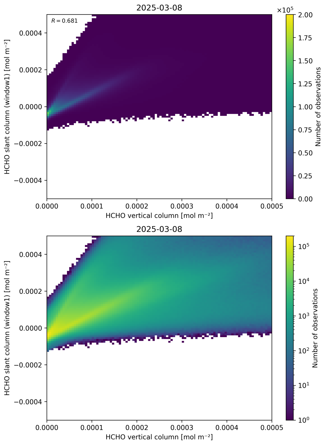
Figure 129: Scatter density plot of “HCHO vertical column” against “HCHO slant column (window1)” for 2025-03-07 to 2025-03-09.
