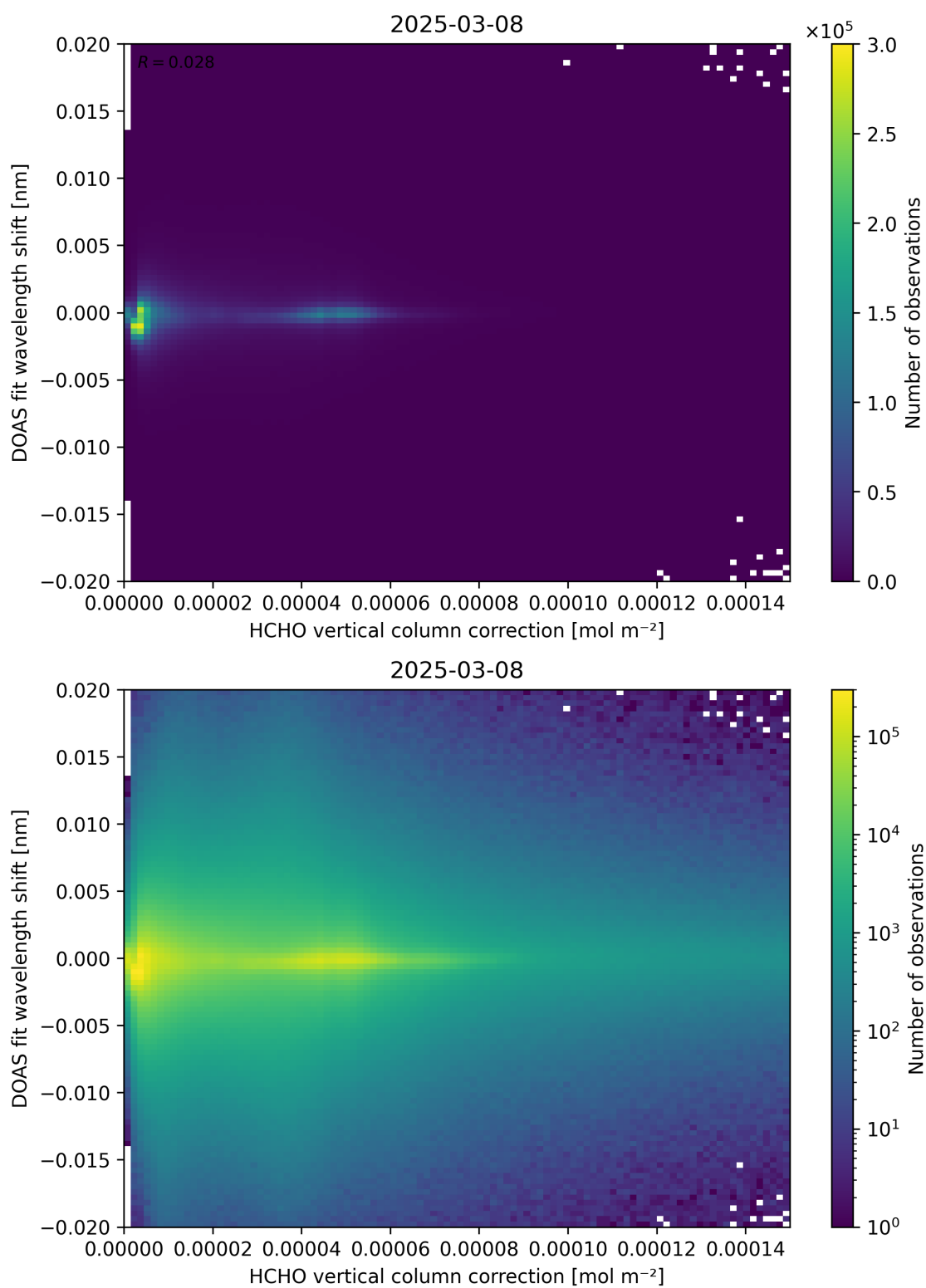
Figure 113: Scatter density plot of “HCHO vertical column correction” against “DOAS fit wavelength shift” for 2025-03-07 to 2025-03-09.
