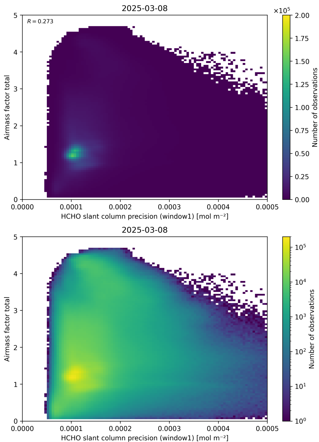
Figure 94: Scatter density plot of “HCHO slant column precision (window1)” against “Airmass factor total” for 2025-03-07 to 2025-03-09.
