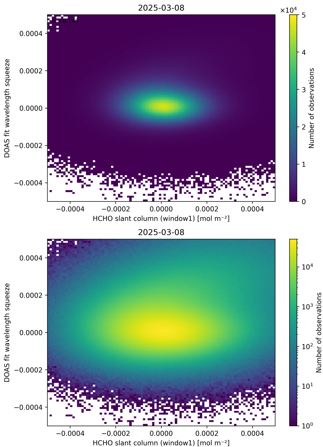
Figure 80: Scatter density plot of “HCHO slant column (window1)” against “DOAS fit wavelength squeeze” for 2025-03-07 to 2025-03-09.
