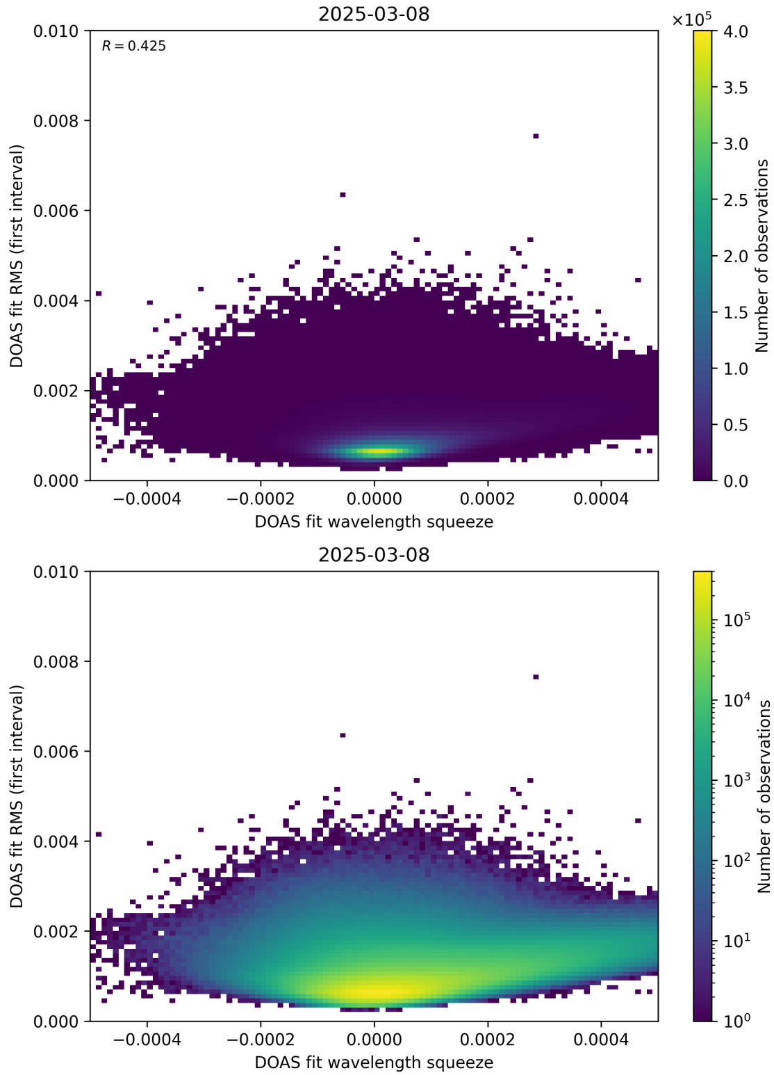
Figure 68: Scatter density plot of “DOAS fit wavelength squeeze” against “DOAS fit RMS (first interval)” for 2025-03-07 to 2025-03-09.
