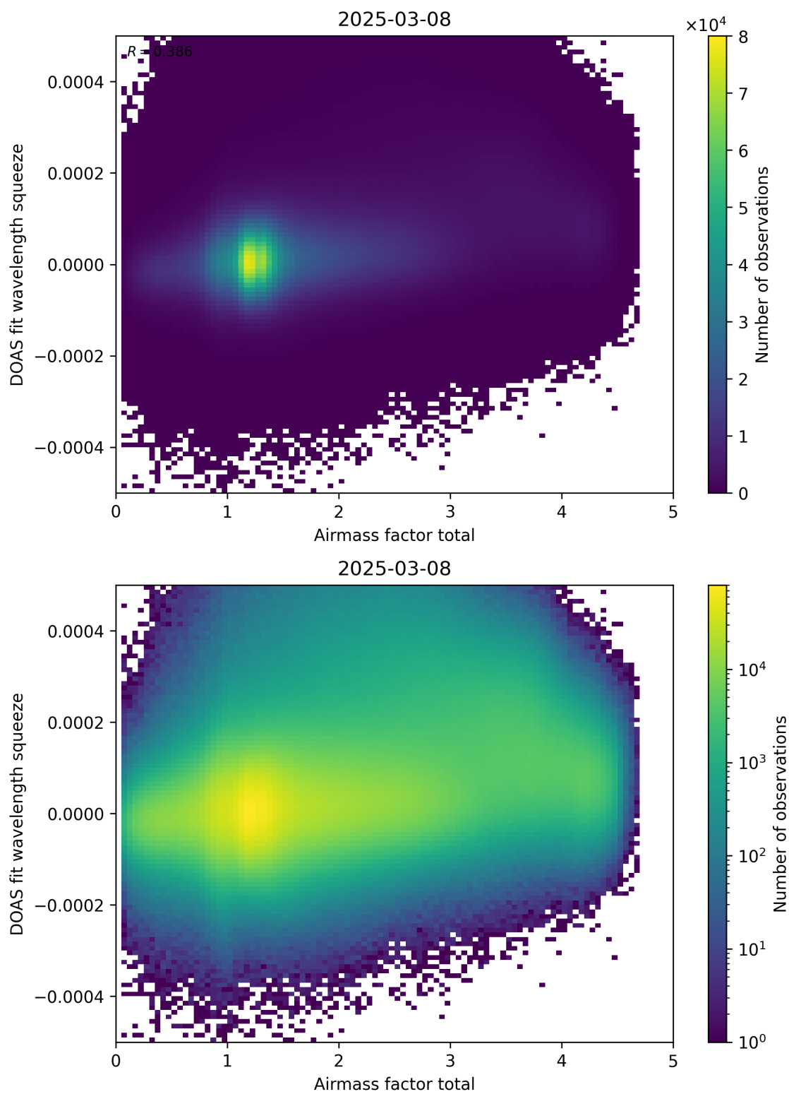
Figure 99: Scatter density plot of “Airmass factor total” against “DOAS fit wavelength squeeze” for 2025-03-07 to 2025-03-09.
