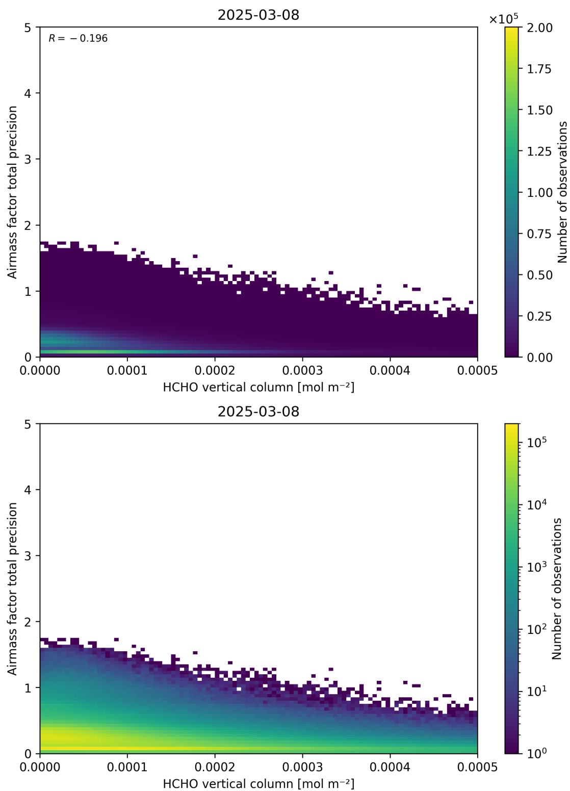
Figure 132: Scatter density plot of “HCHO vertical column” against “Airmass factor total precision” for 2025-03-07 to 2025-03-09.
