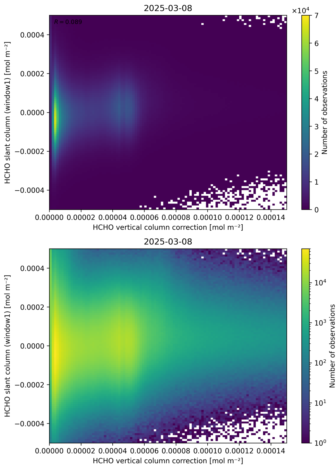
Figure 118: Scatter density plot of “HCHO vertical column correction” against “HCHO slant column (window1)” for 2025-03-07 to 2025-03-09.
