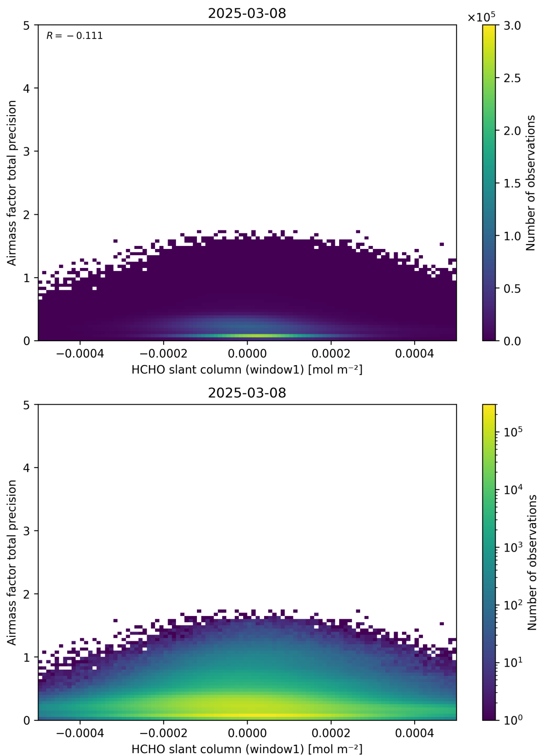
Figure 86: Scatter density plot of “HCHO slant column (window1)” against “Airmass factor total precision” for 2025-03-07 to 2025-03-09.
