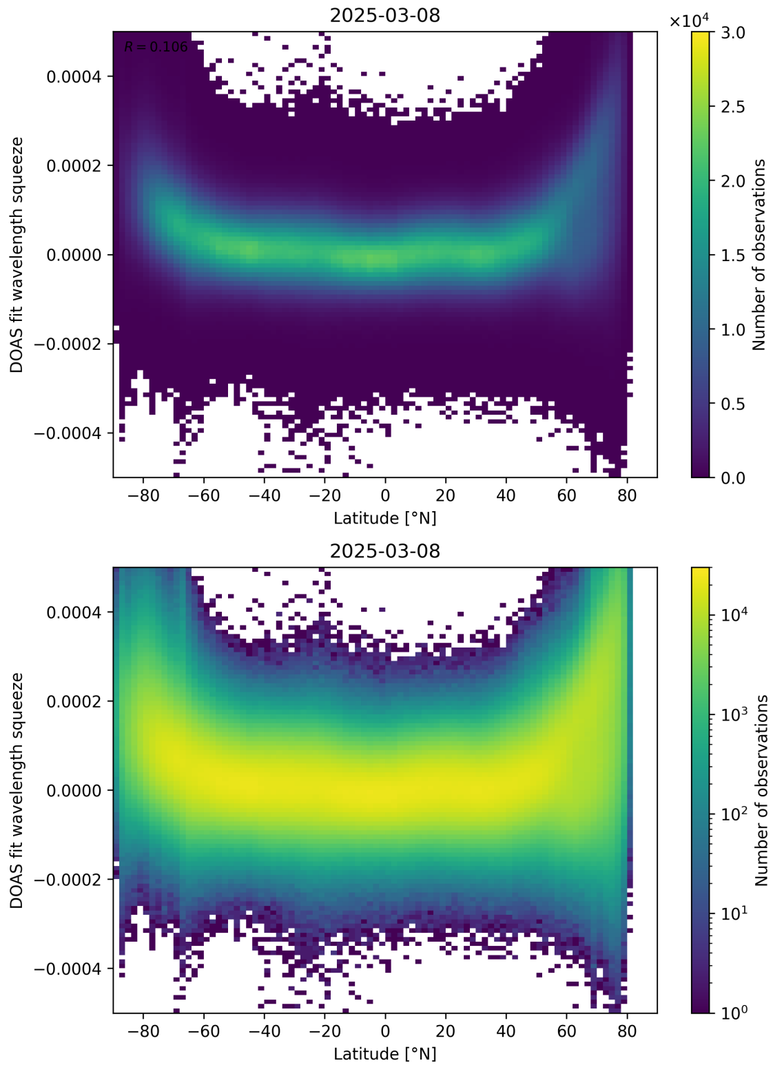
Figure 155: Scatter density plot of “Latitude” against “DOAS fit wavelength squeeze” for 2025-03-07 to 2025-03-09.
