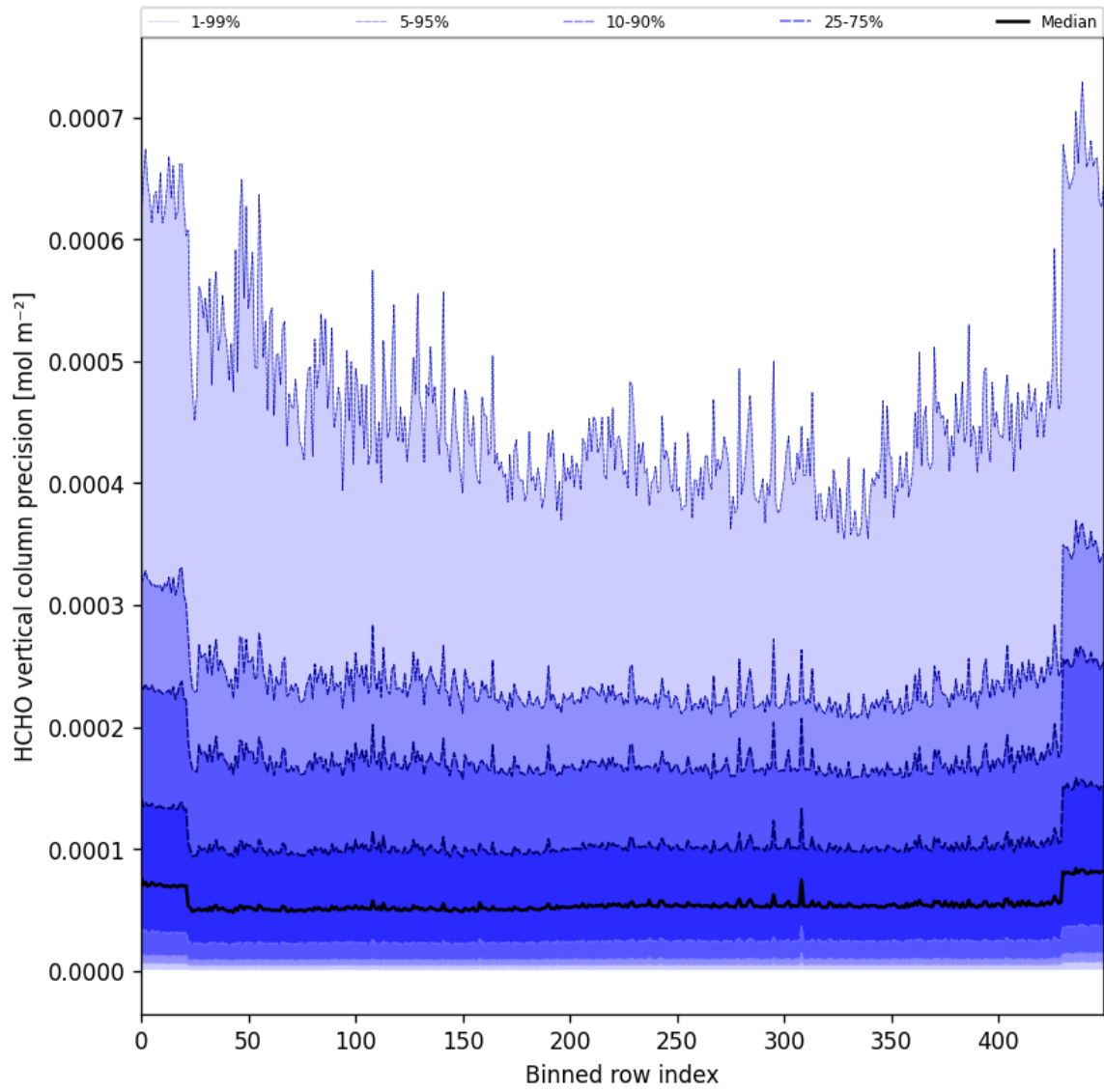
Figure 50: Along track statistics of “HCHO vertical column precision” for 2025-03-07 to 2025-03-09
