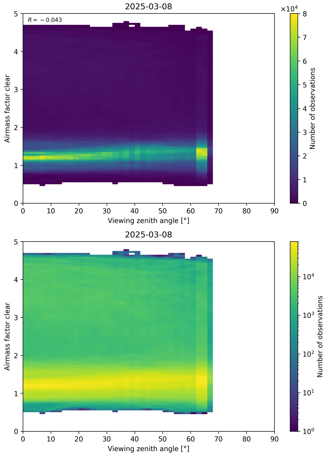
Figure 185: Scatter density plot of “Viewing zenith angle” against “Airmass factor clear” for 2025-03-07 to 2025-03-09.
