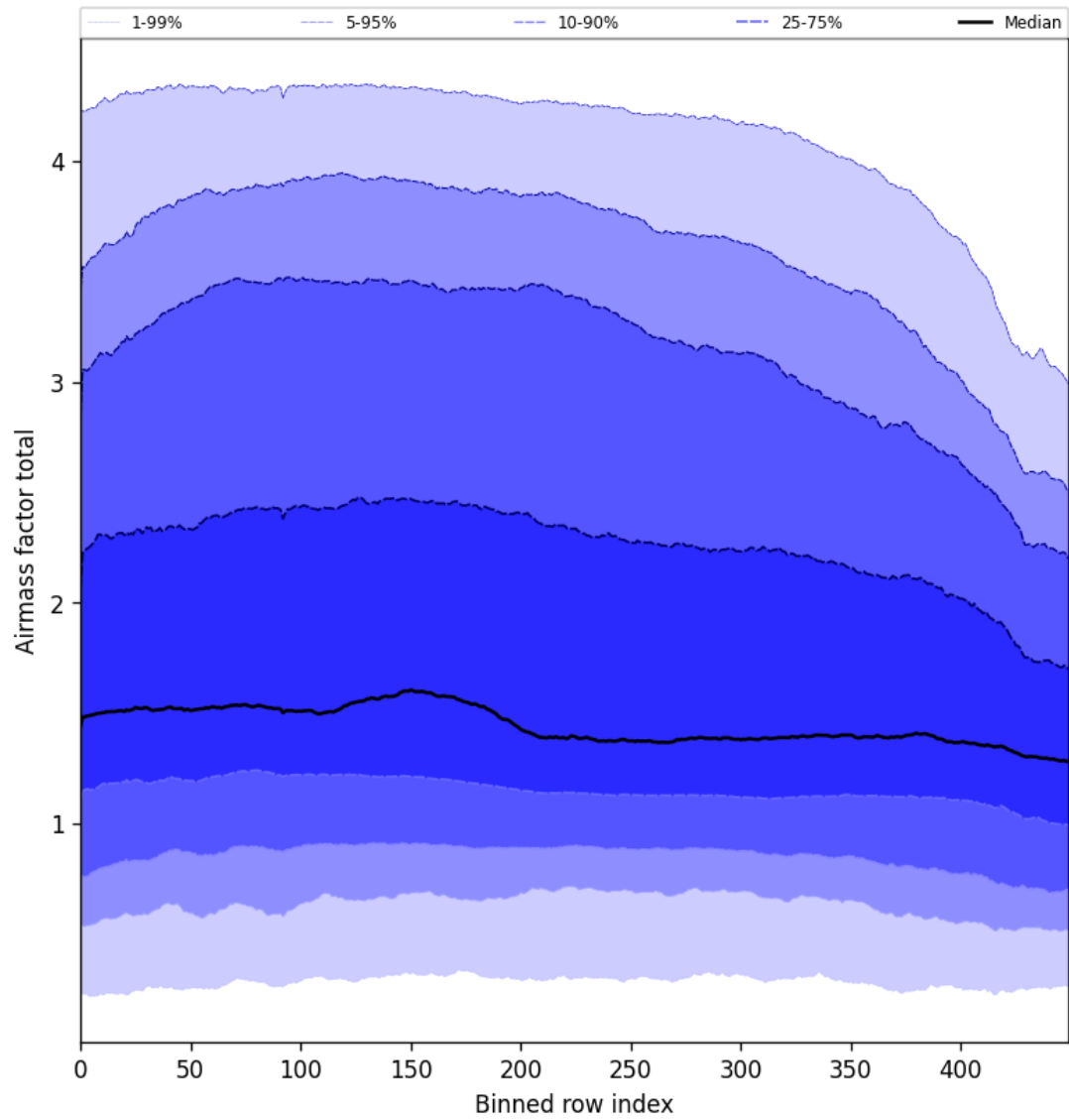
Figure 54: Along track statistics of “Airmass factor total” for 2025-03-07 to 2025-03-09
