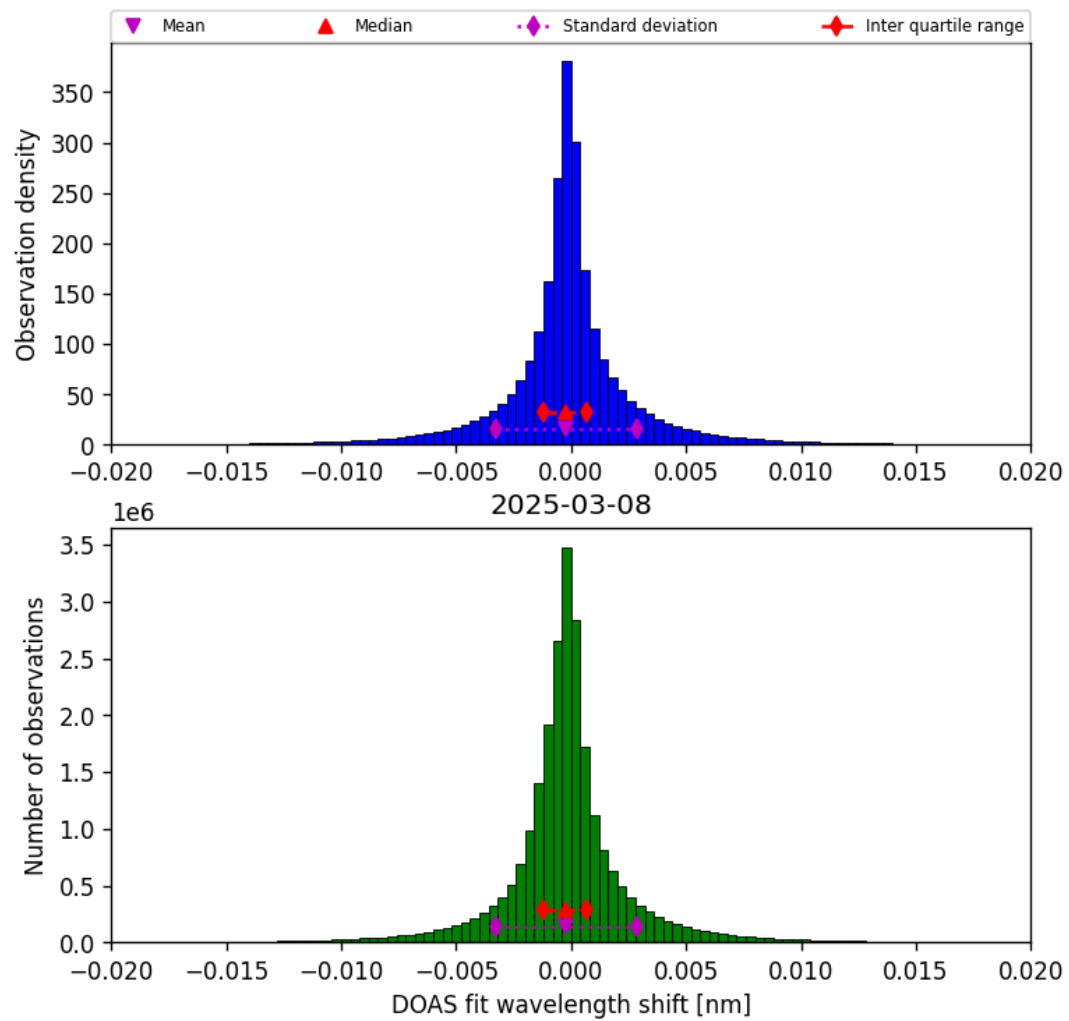
Figure 44: Histogram of “DOAS fit wavelength shift” for 2025-03-07 to 2025-03-09
