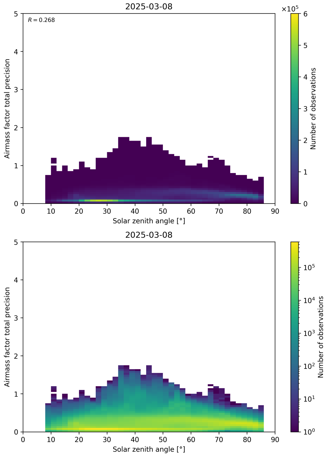
Figure 176: Scatter density plot of “Solar zenith angle” against “Airmass factor total precision” for 2025-03-07 to 2025-03-09.
