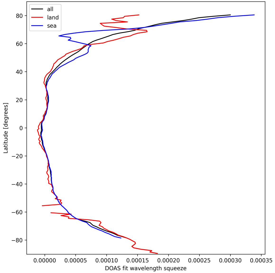
Figure 31: Zonal average of “DOAS fit wavelength squeeze” for 2025-03-07 to 2025-03-09.
