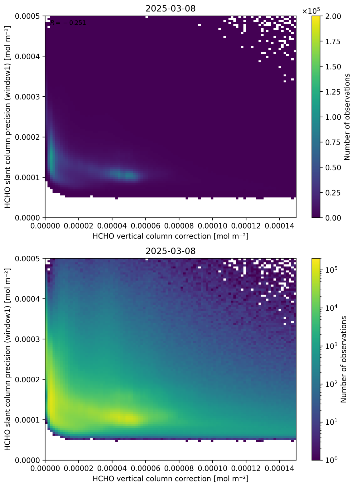
Figure 119: Scatter density plot of “HCHO vertical column correction” against “HCHO slant column precision (window1)” for 2025-03-07 to 2025-03-09.
