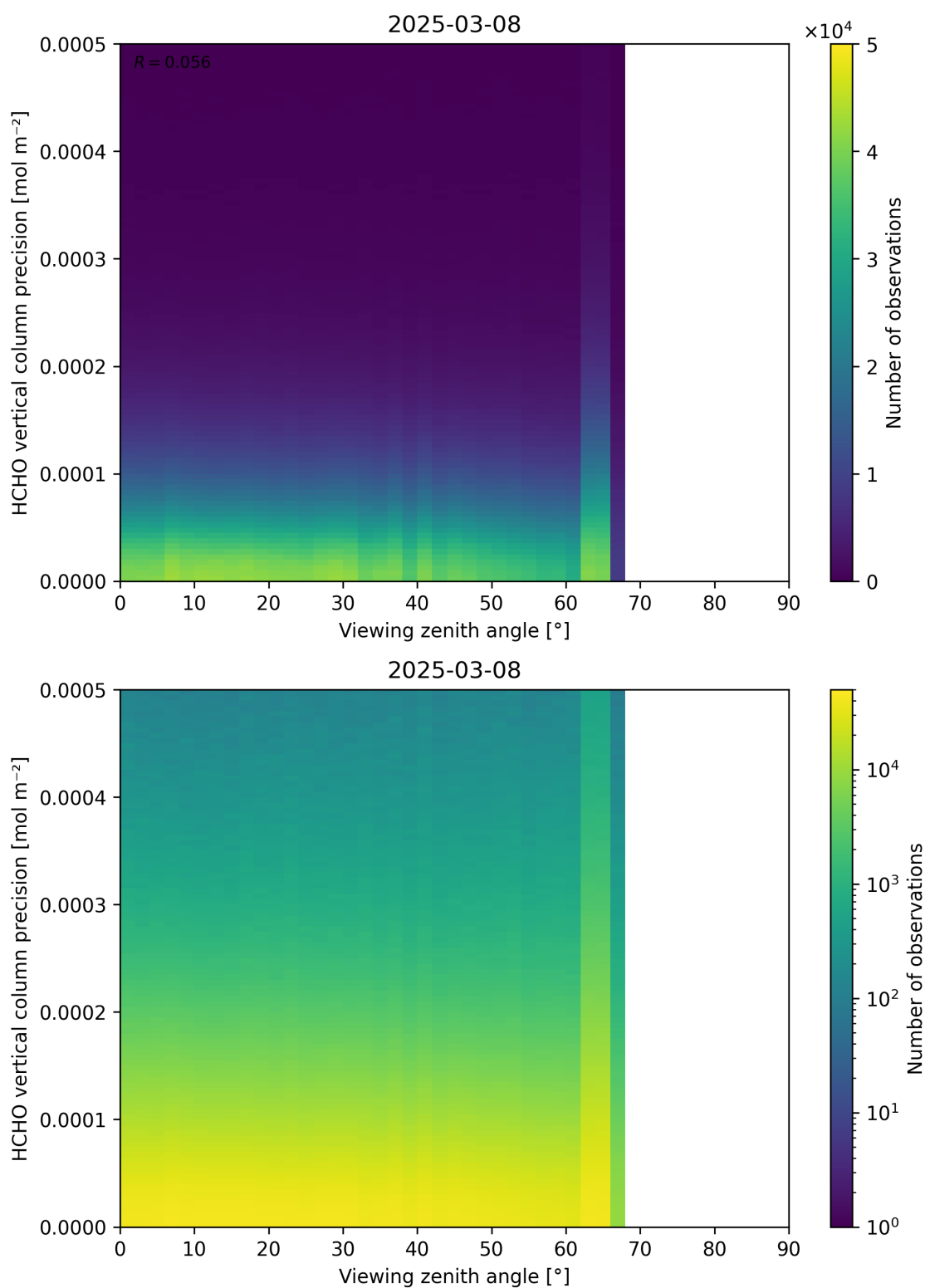
Figure 194: Scatter density plot of “Viewing zenith angle” against “HCHO vertical column precision” for 2025-03-07 to 2025-03-09.
