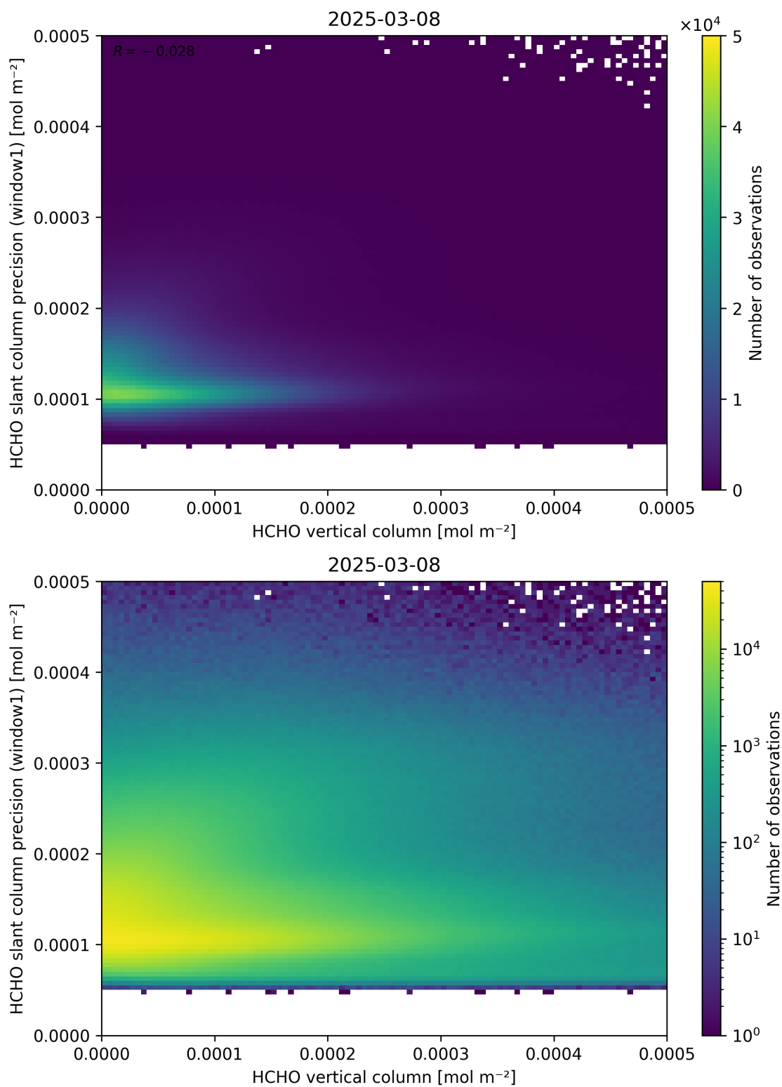
Figure 130: Scatter density plot of “HCHO vertical column” against “HCHO slant column precision (window1)” for 2025-03-07 to 2025-03-09.
