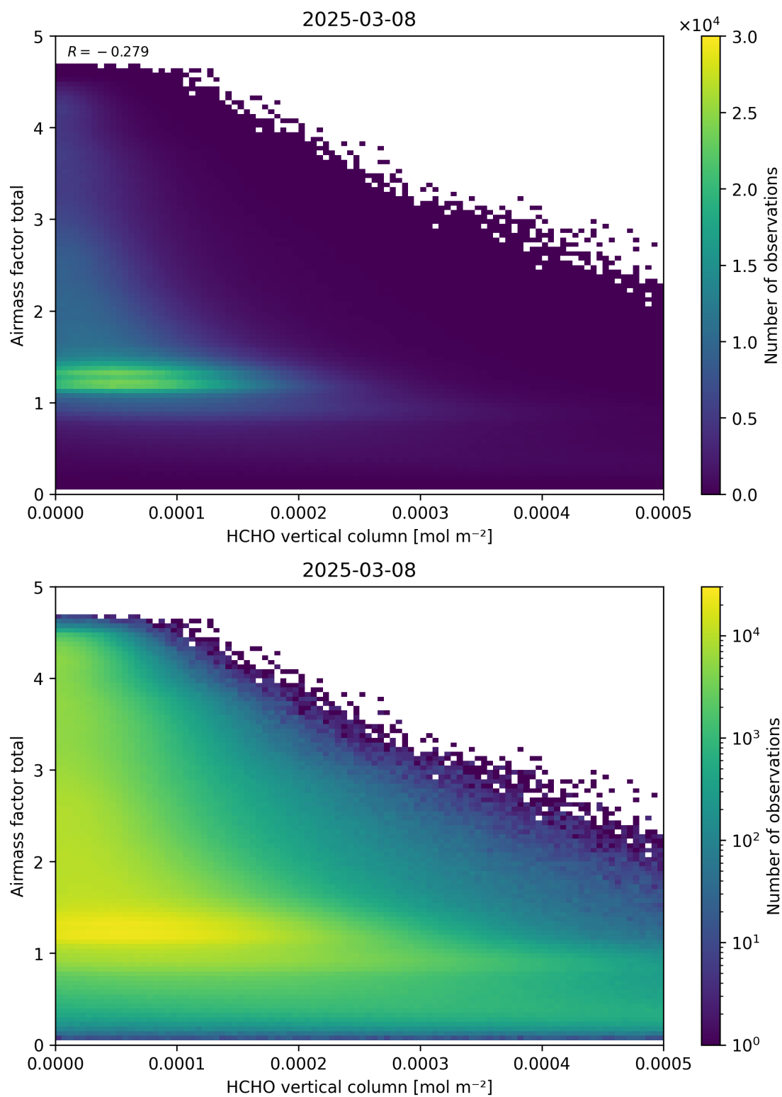
Figure 131: Scatter density plot of “HCHO vertical column” against “Airmass factor total” for 2025-03-07 to 2025-03-09.
