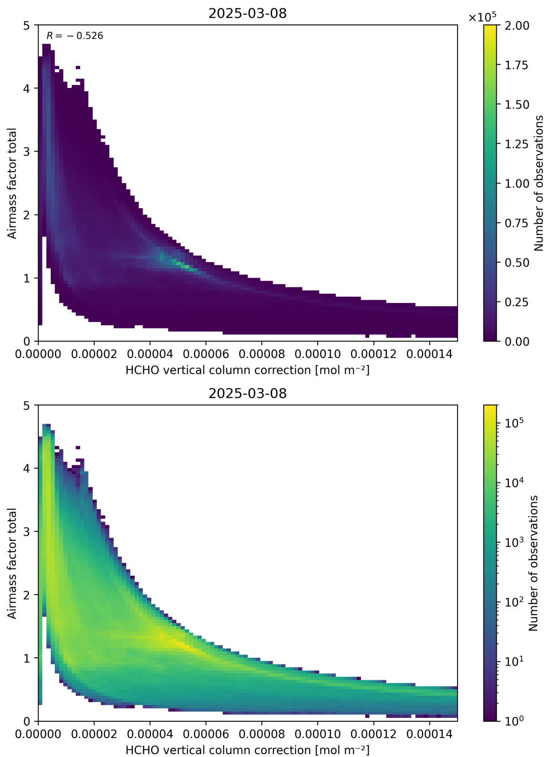
Figure 120: Scatter density plot of “HCHO vertical column correction” against “Airmass factor total” for 2025-03-07 to 2025-03-09.
