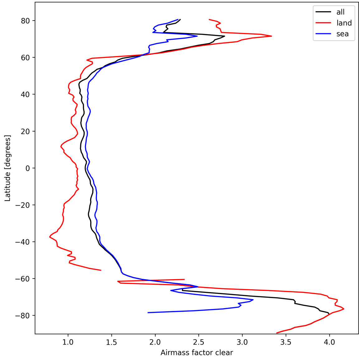
Figure 28: Zonal average of “Airmass factor clear” for 2025-03-07 to 2025-03-09.
