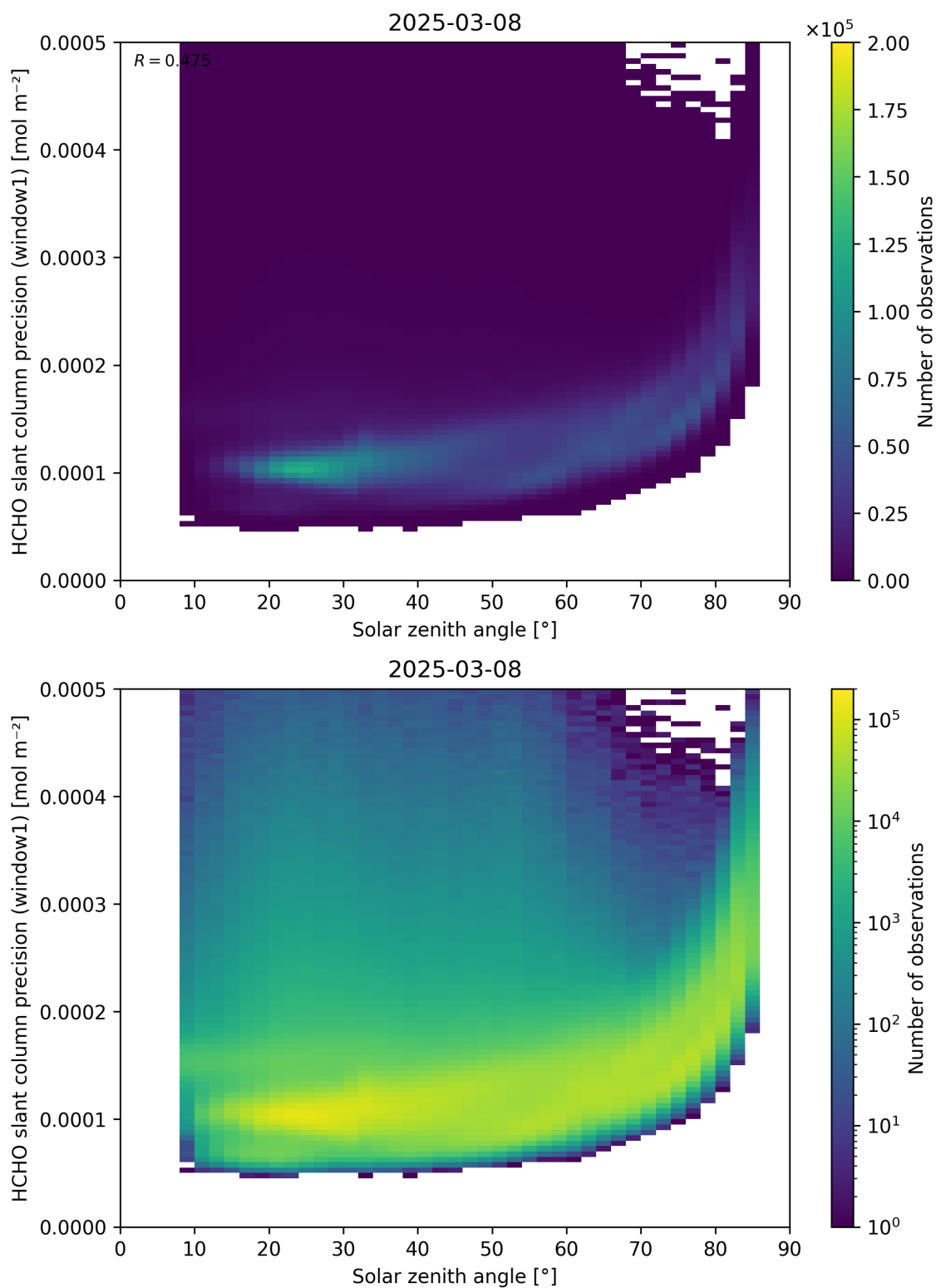
Figure 174: Scatter density plot of “Solar zenith angle” against “HCHO slant column precision (window1)” for 2025-03-07 to 2025-03-09.
