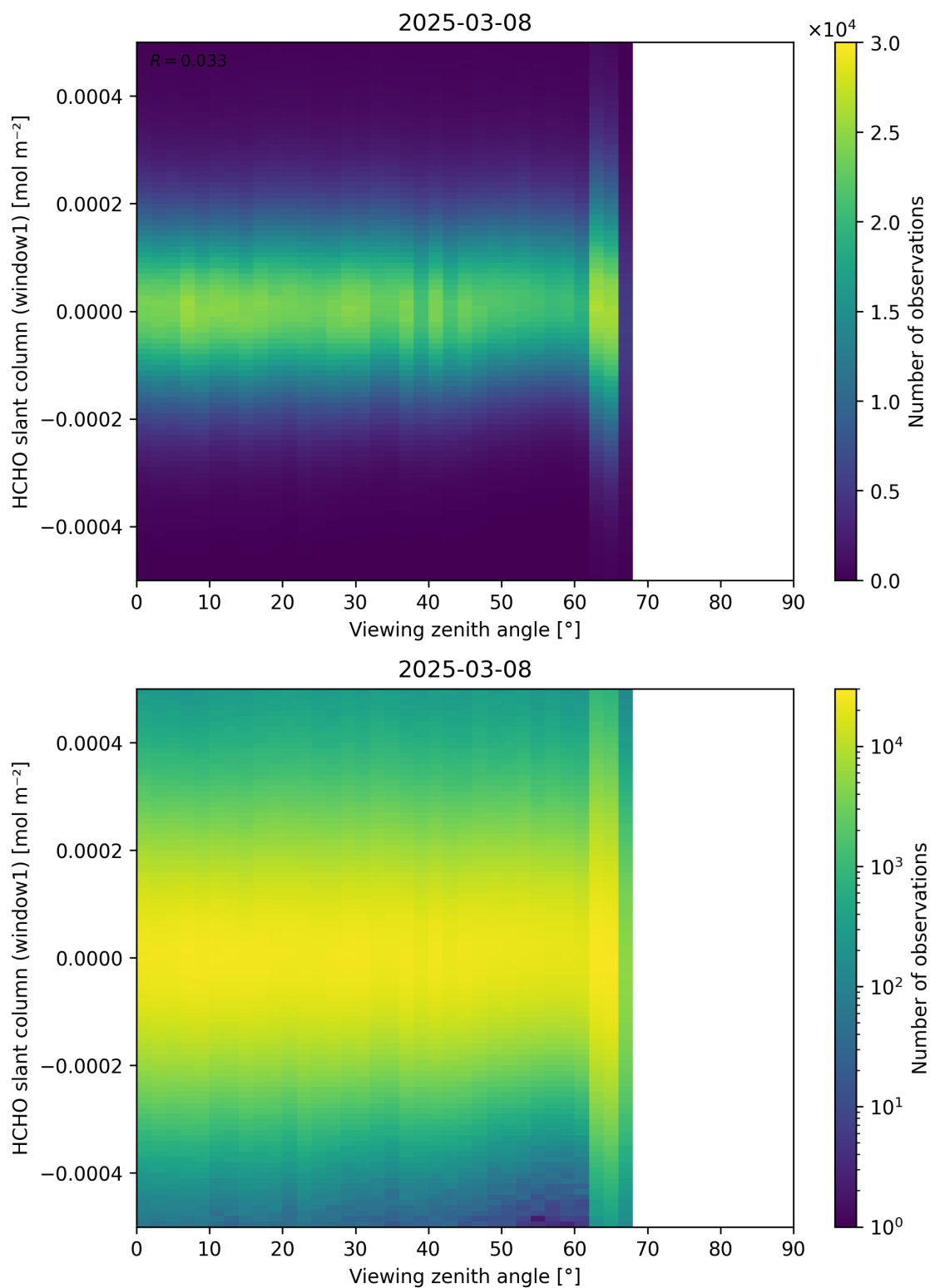
Figure 188: Scatter density plot of “Viewing zenith angle” against “HCHO slant column (window1)” for 2025-03-07 to 2025-03-09.
