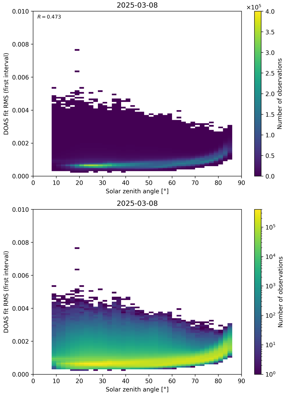
Figure 167: Scatter density plot of “Solar zenith angle” against “DOAS fit RMS (first interval)” for 2025-03-07 to 2025-03-09.
