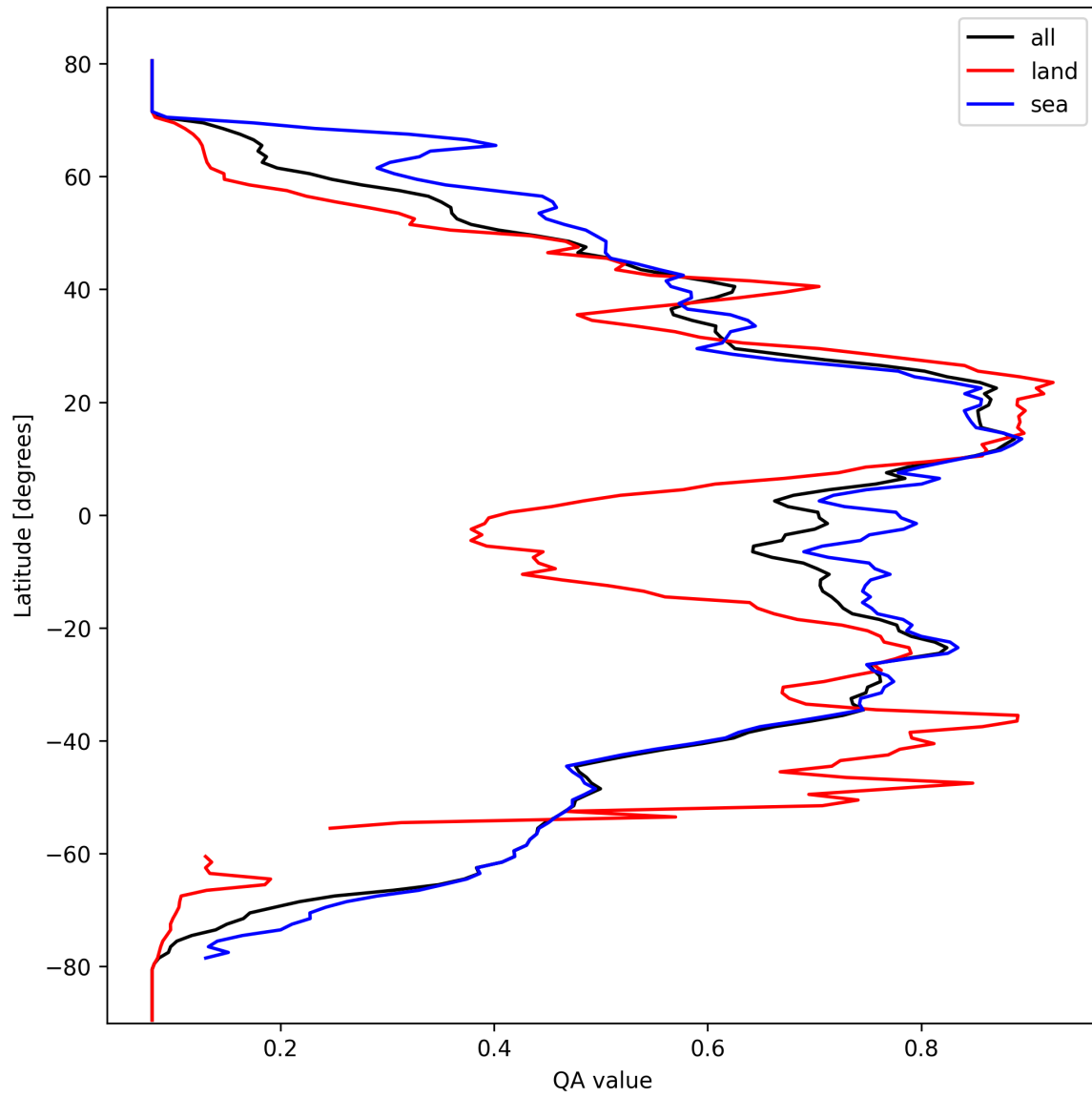
Figure 20: Zonal average of “QA value” for 2025-03-07 to 2025-03-09.
