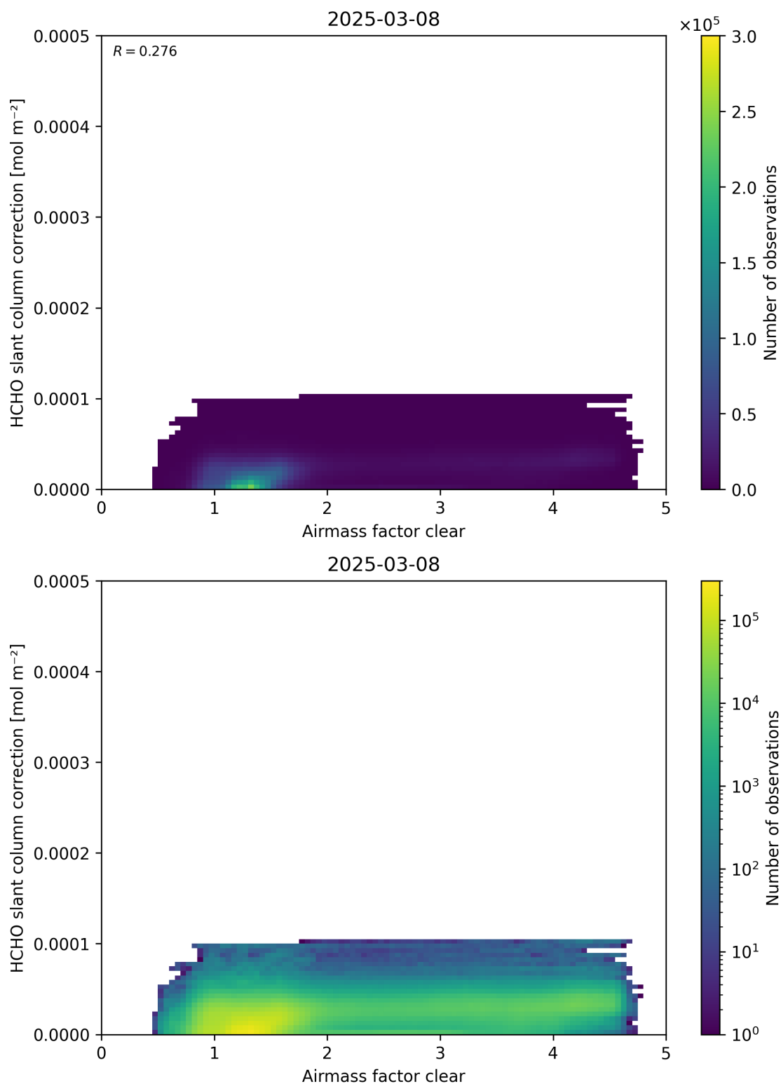
Figure 75: Scatter density plot of “Airmass factor clear” against “HCHO slant column correction” for 2025-03-07 to 2025-03-09.
