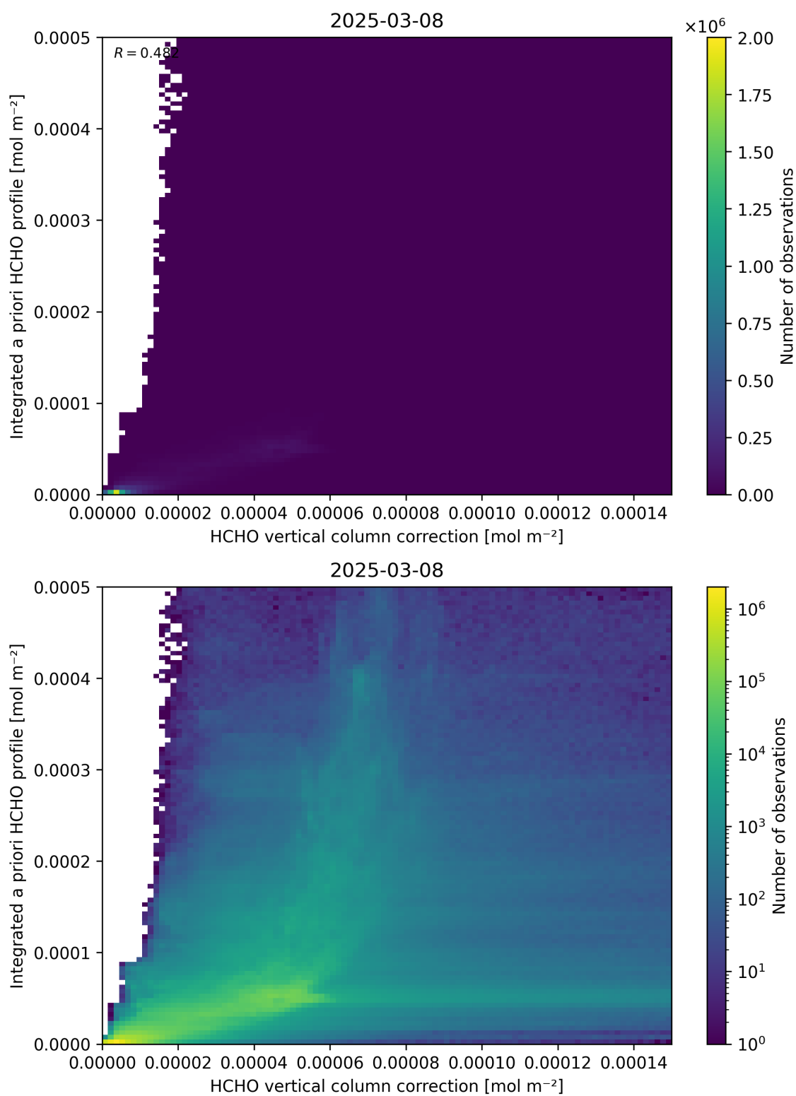
Figure 122: Scatter density plot of “HCHO vertical column correction” against “Integrated a priori HCHO profile” for 2025-03-07 to 2025-03-09.
