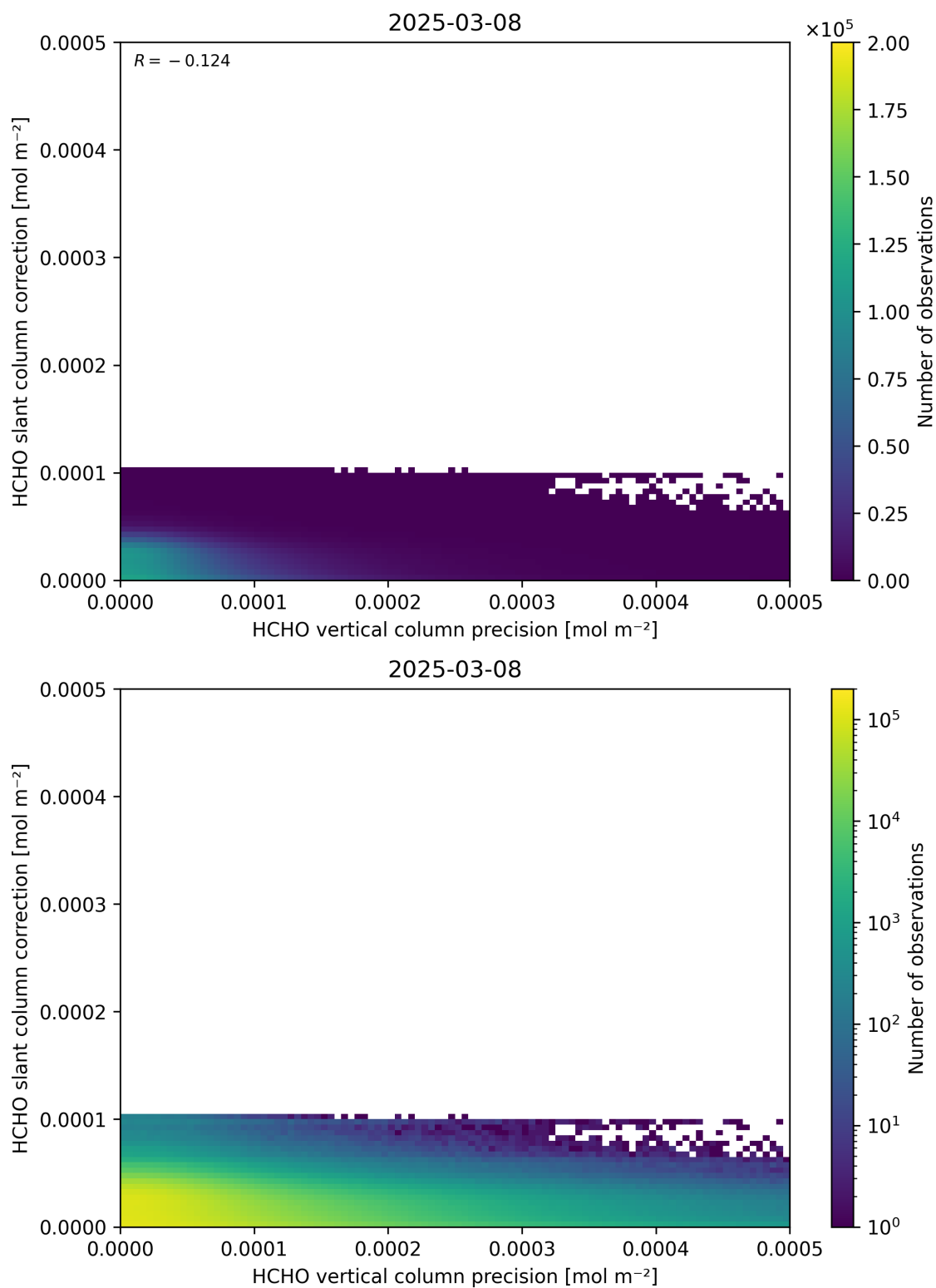
Figure 141: Scatter density plot of “HCHO vertical column precision” against “HCHO slant column correction” for 2025-03-07 to 2025-03-09.
