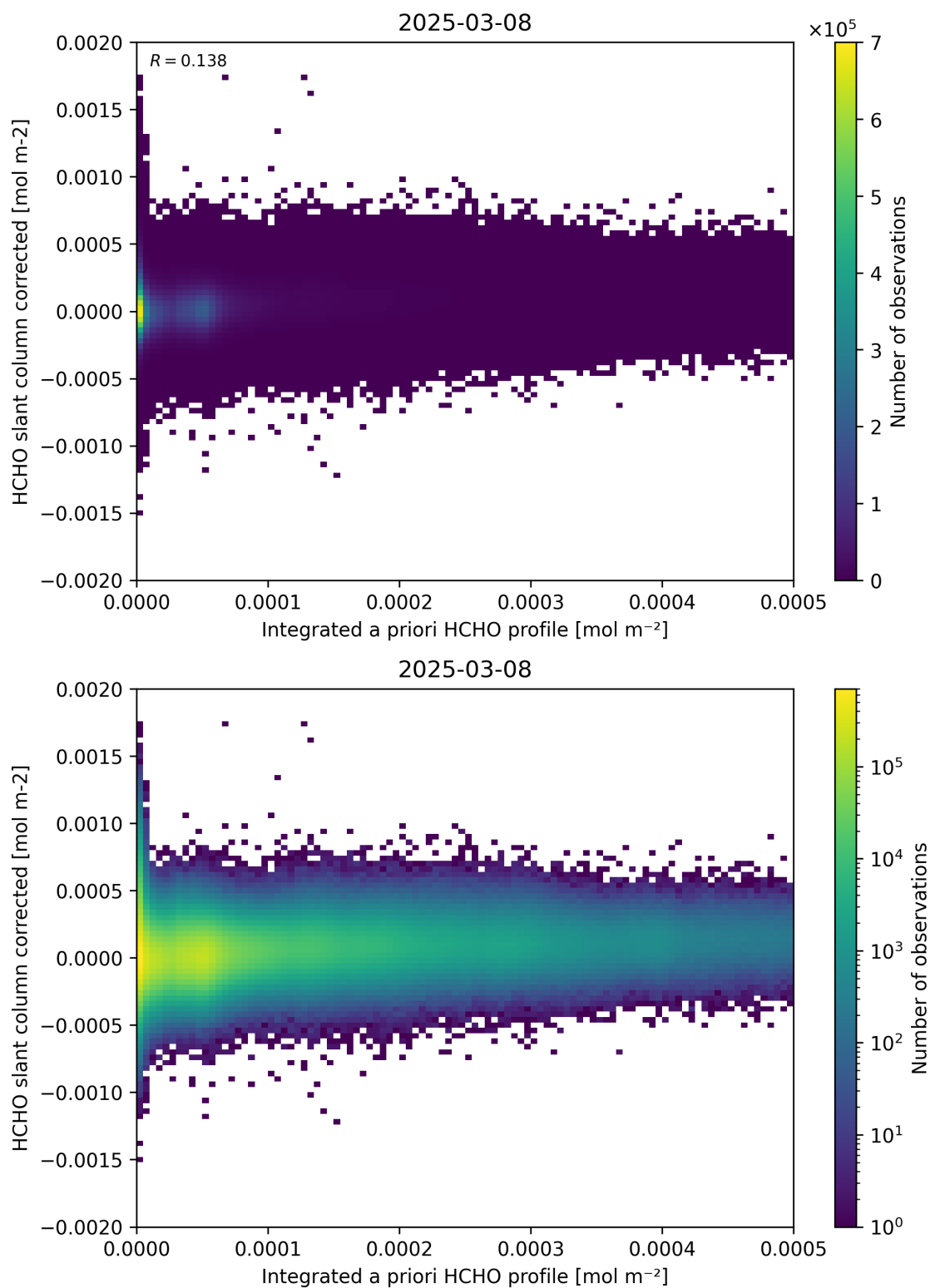
Figure 151: Scatter density plot of “Integrated a priori HCHO profile” against “HCHO slant column corrected” for 2025-03-07 to 2025-03-09.
