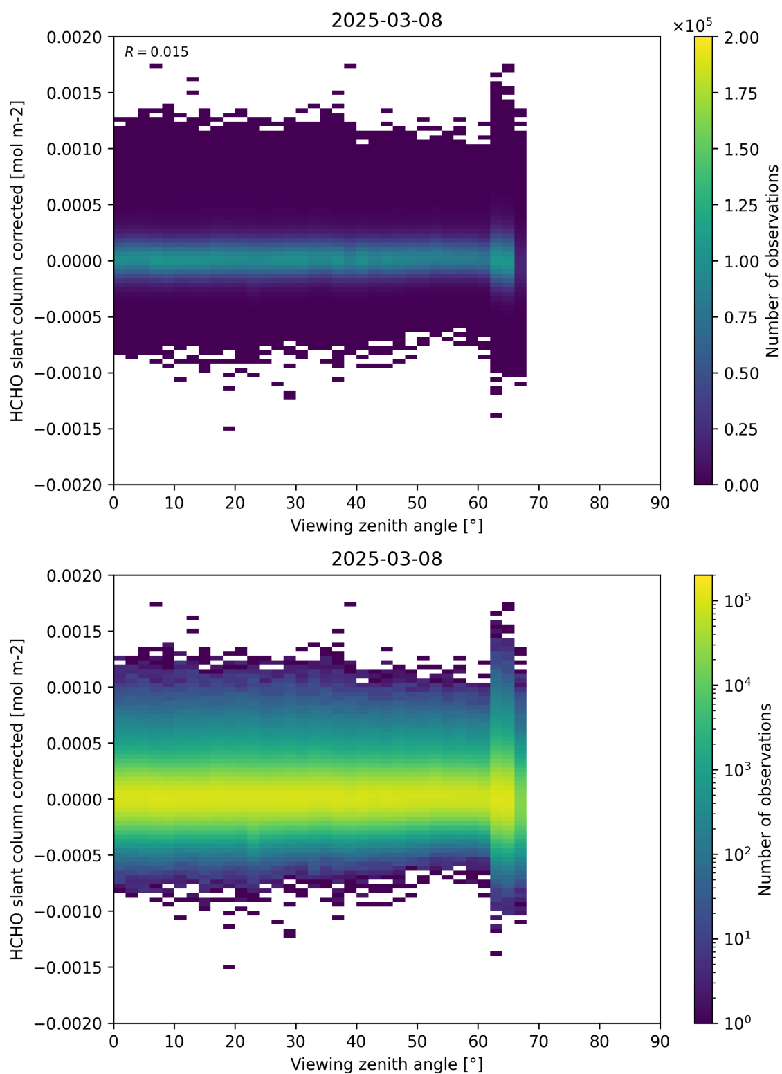
Figure 186: Scatter density plot of “Viewing zenith angle” against “HCHO slant column corrected” for 2025-03-07 to 2025-03-09.
