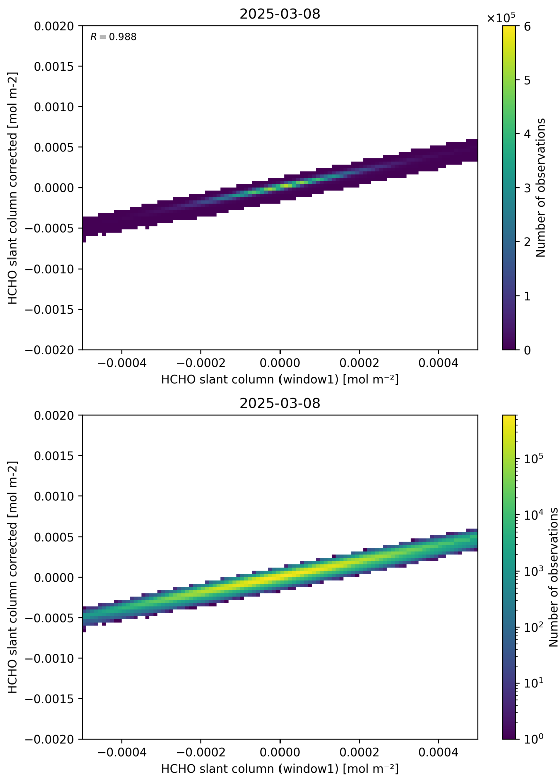
Figure 82: Scatter density plot of “HCHO slant column (window1)” against “HCHO slant column corrected” for 2025-03-07 to 2025-03-09.
