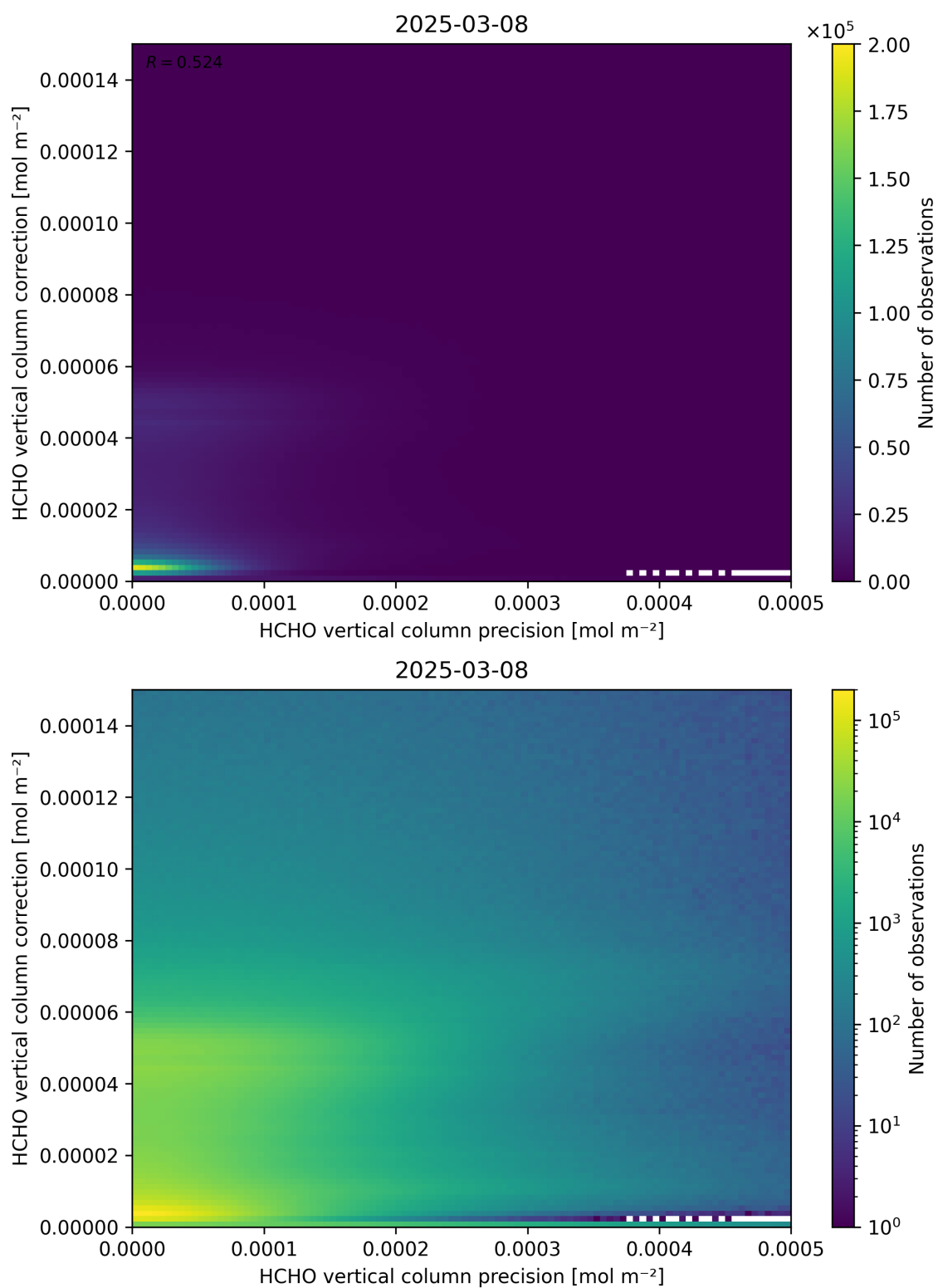
Figure 146: Scatter density plot of “HCHO vertical column precision” against “HCHO vertical column correction” for 2025-03-07 to 2025-03-09.
