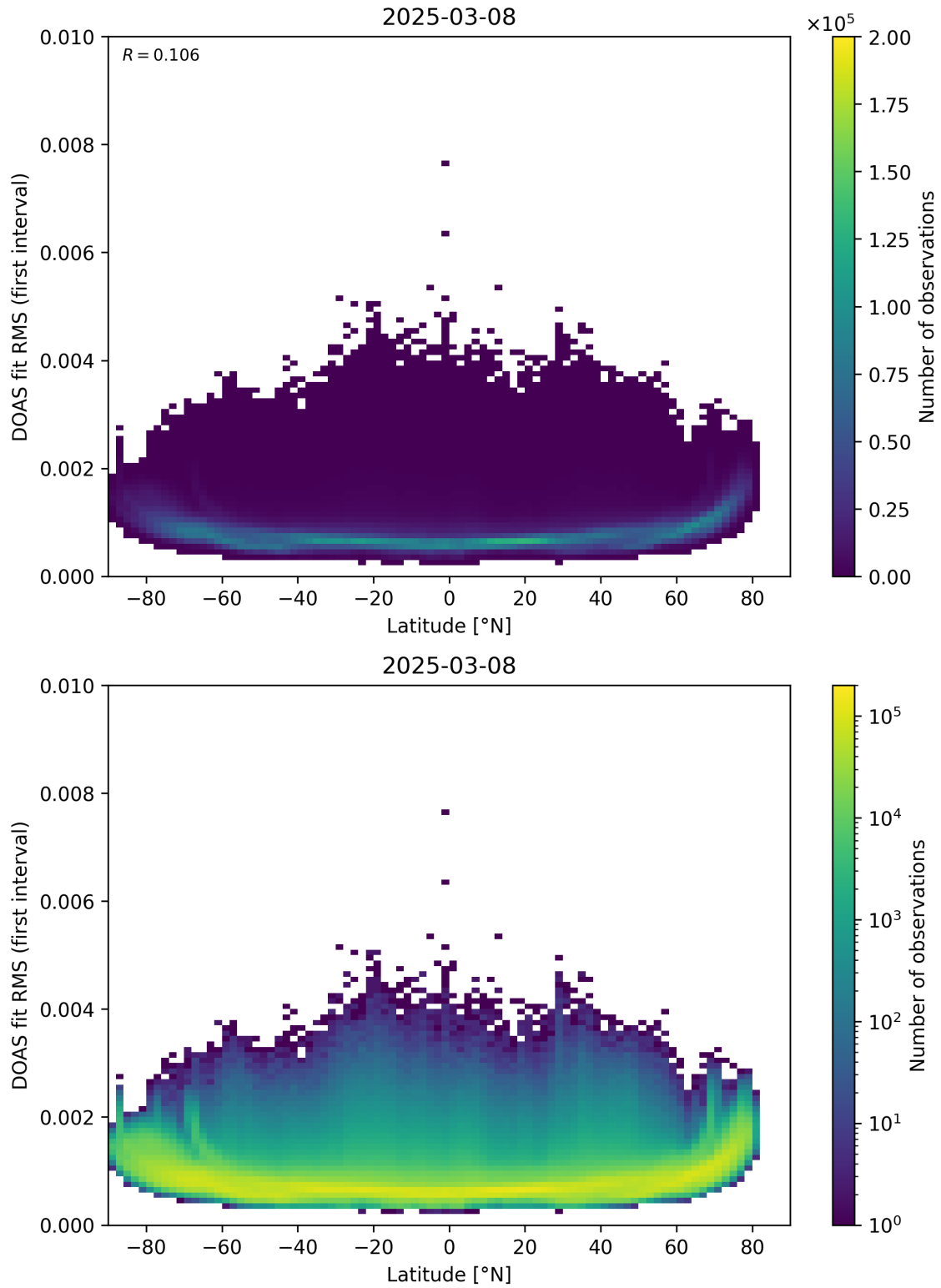
Figure 153: Scatter density plot of “Latitude” against “DOAS fit RMS (first interval)” for 2025-03-07 to 2025-03-09.
