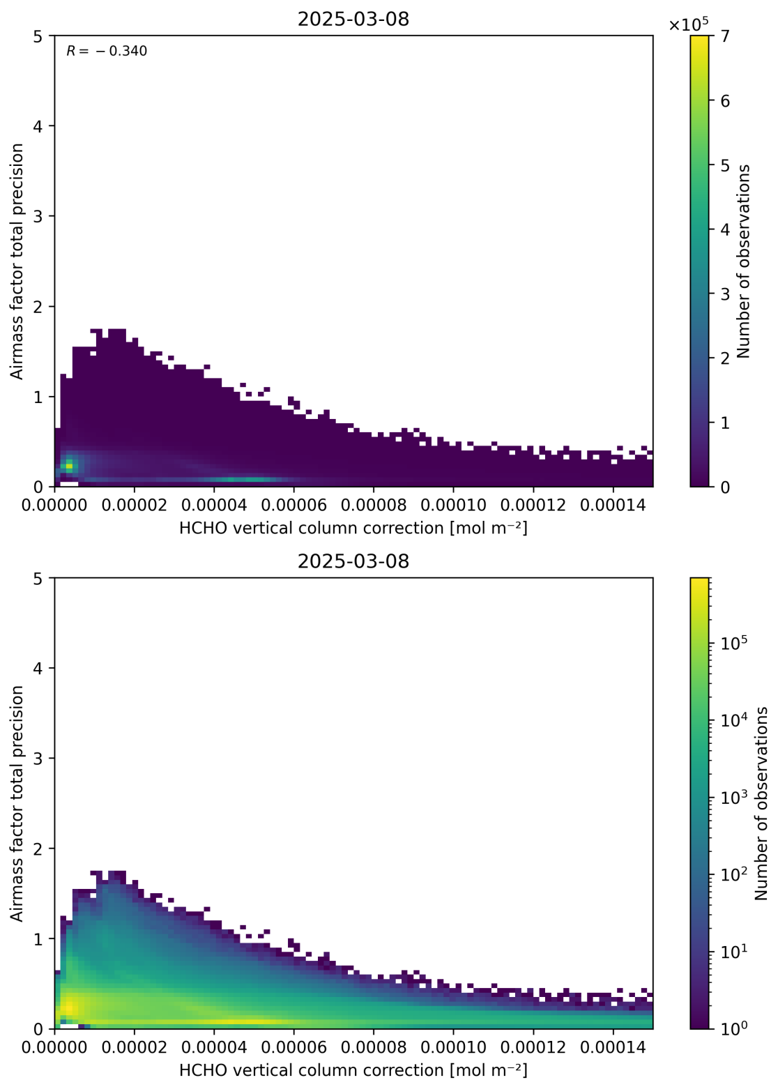
Figure 121: Scatter density plot of “HCHO vertical column correction” against “Airmass factor total precision” for 2025-03-07 to 2025-03-09.
