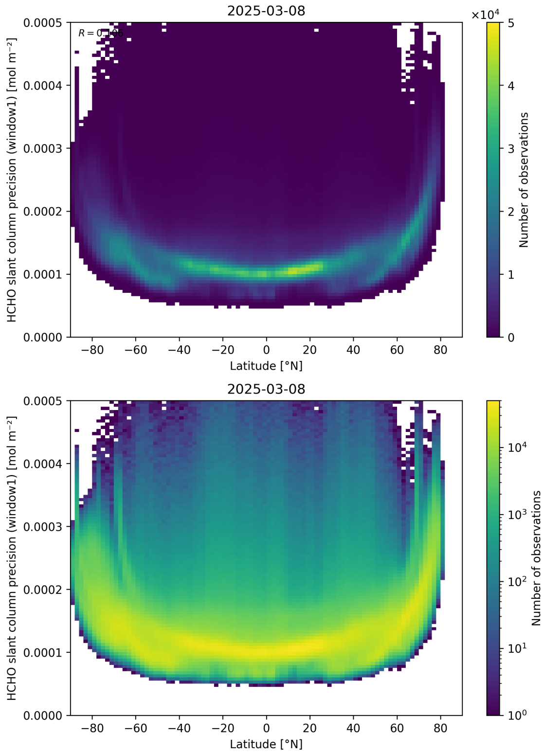
Figure 160: Scatter density plot of “Latitude” against “HCHO slant column precision (window1)” for 2025-03-07 to 2025-03-09.
