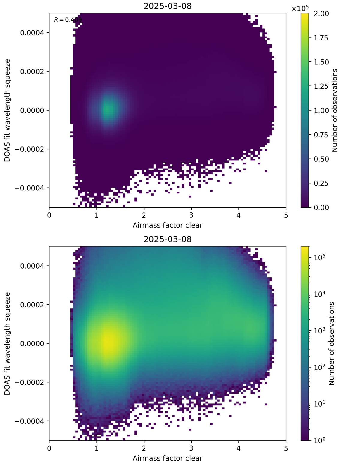
Figure 73: Scatter density plot of “Airmass factor clear” against “DOAS fit wavelength squeeze” for 2025-03-07 to 2025-03-09.
