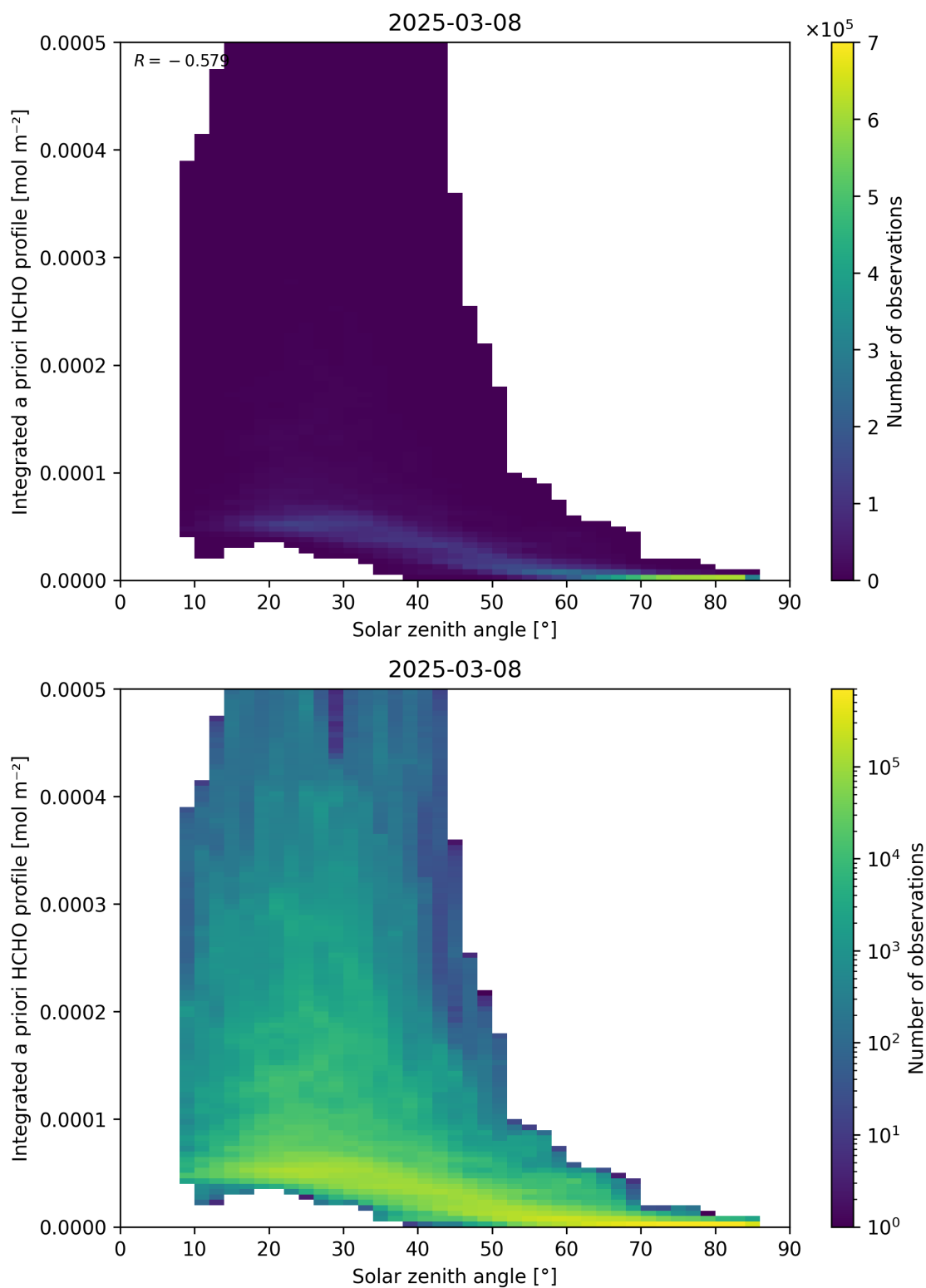
Figure 180: Scatter density plot of “Solar zenith angle” against “Integrated a priori HCHO profile” for 2025-03-07 to 2025-03-09.
