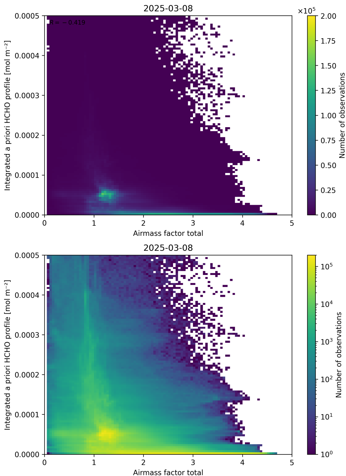
Figure 104: Scatter density plot of “Airmass factor total” against “Integrated a priori HCHO profile” for 2025-03-07 to 2025-03-09.
