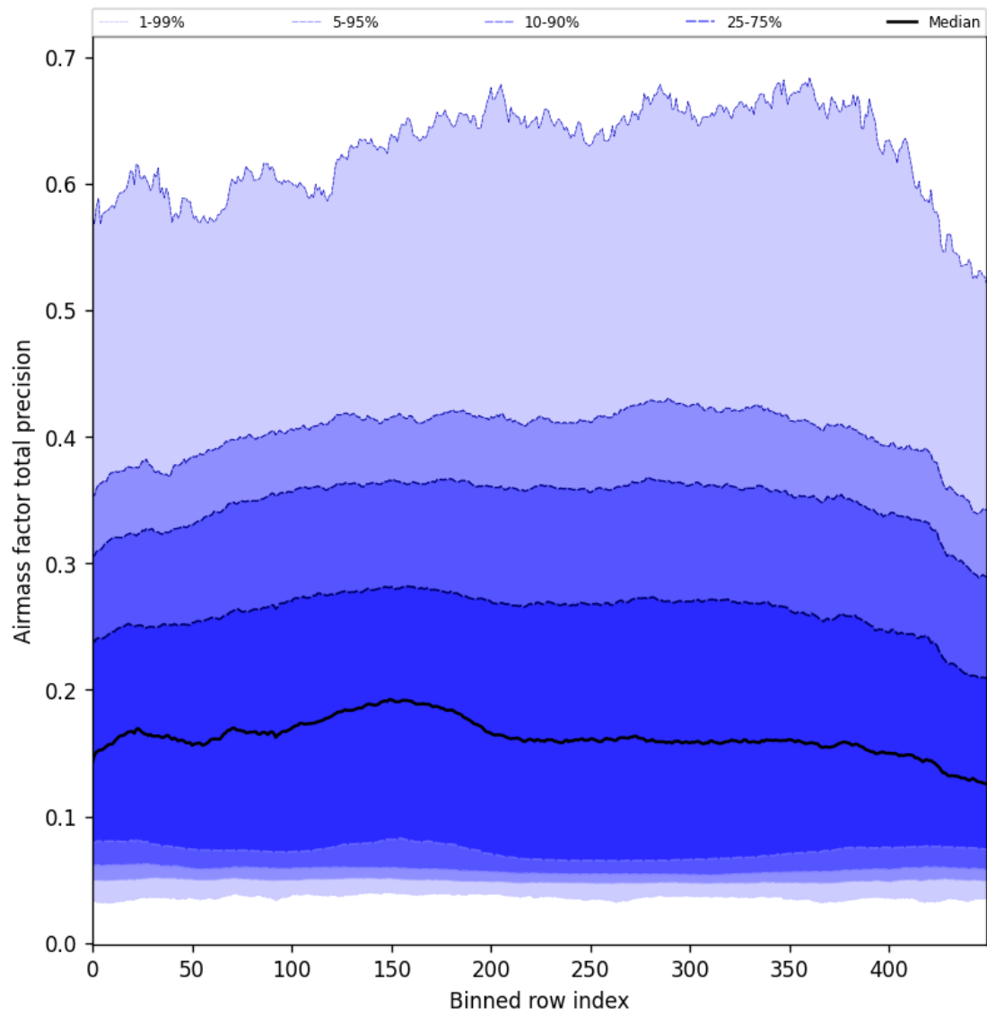
Figure 55: Along track statistics of “Airmass factor total precision” for 2025-03-07 to 2025-03-09
