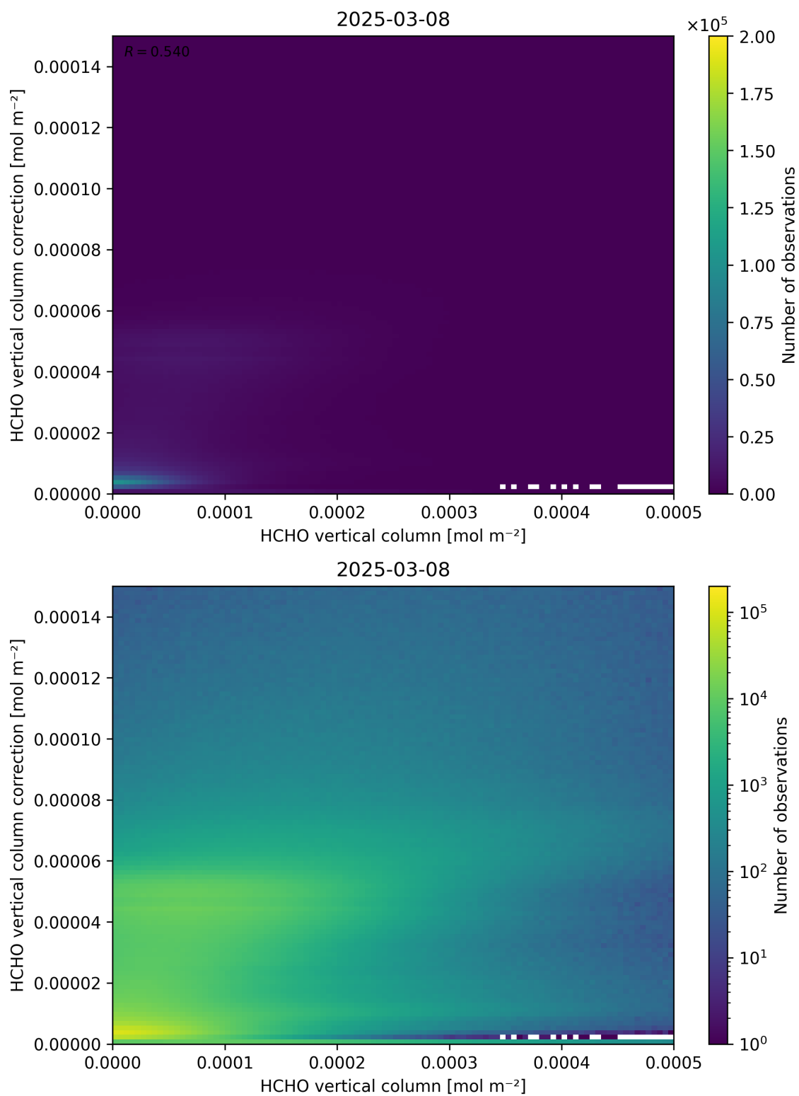
Figure 133: Scatter density plot of “HCHO vertical column” against “HCHO vertical column correction” for 2025-03-07 to 2025-03-09.
