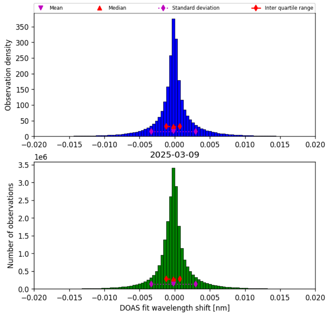
Figure 44: Histogram of “DOAS fit wavelength shift” for 2025-03-08 to 2025-03-10
