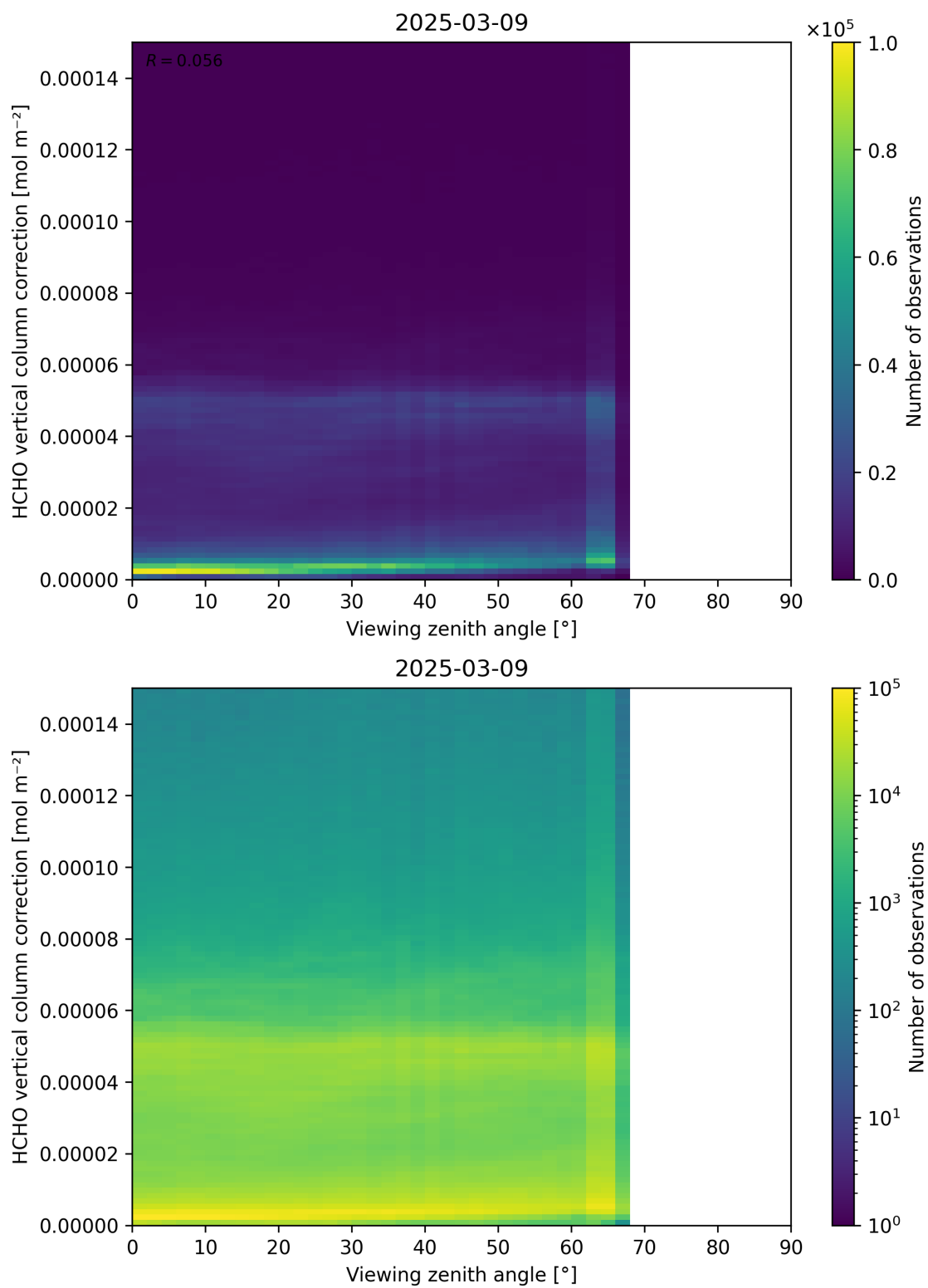
Figure 193: Scatter density plot of “Viewing zenith angle” against “HCHO vertical column correction” for 2025-03-08 to 2025-03-10.
