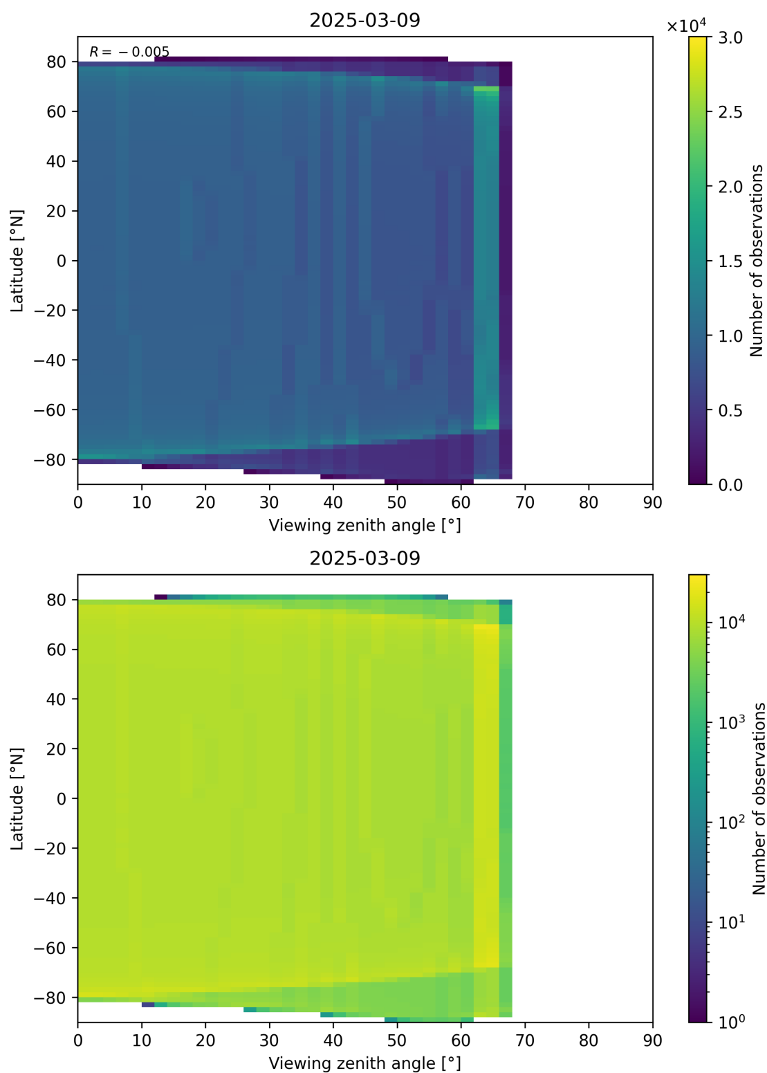
Figure 196: Scatter density plot of “Viewing zenith angle” against “Latitude” for 2025-03-08 to 2025-03-10.
