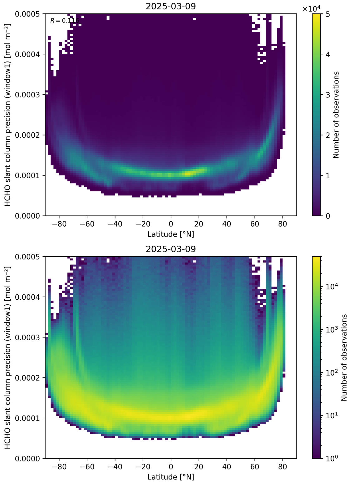
Figure 160: Scatter density plot of “Latitude” against “HCHO slant column precision (window1)” for 2025-03-08 to 2025-03-10.
