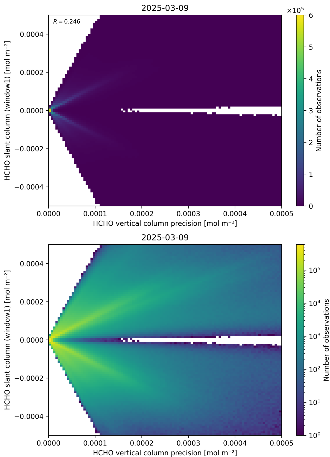
Figure 142: Scatter density plot of “HCHO vertical column precision” against “HCHO slant column (window1)” for 2025-03-08 to 2025-03-10.
