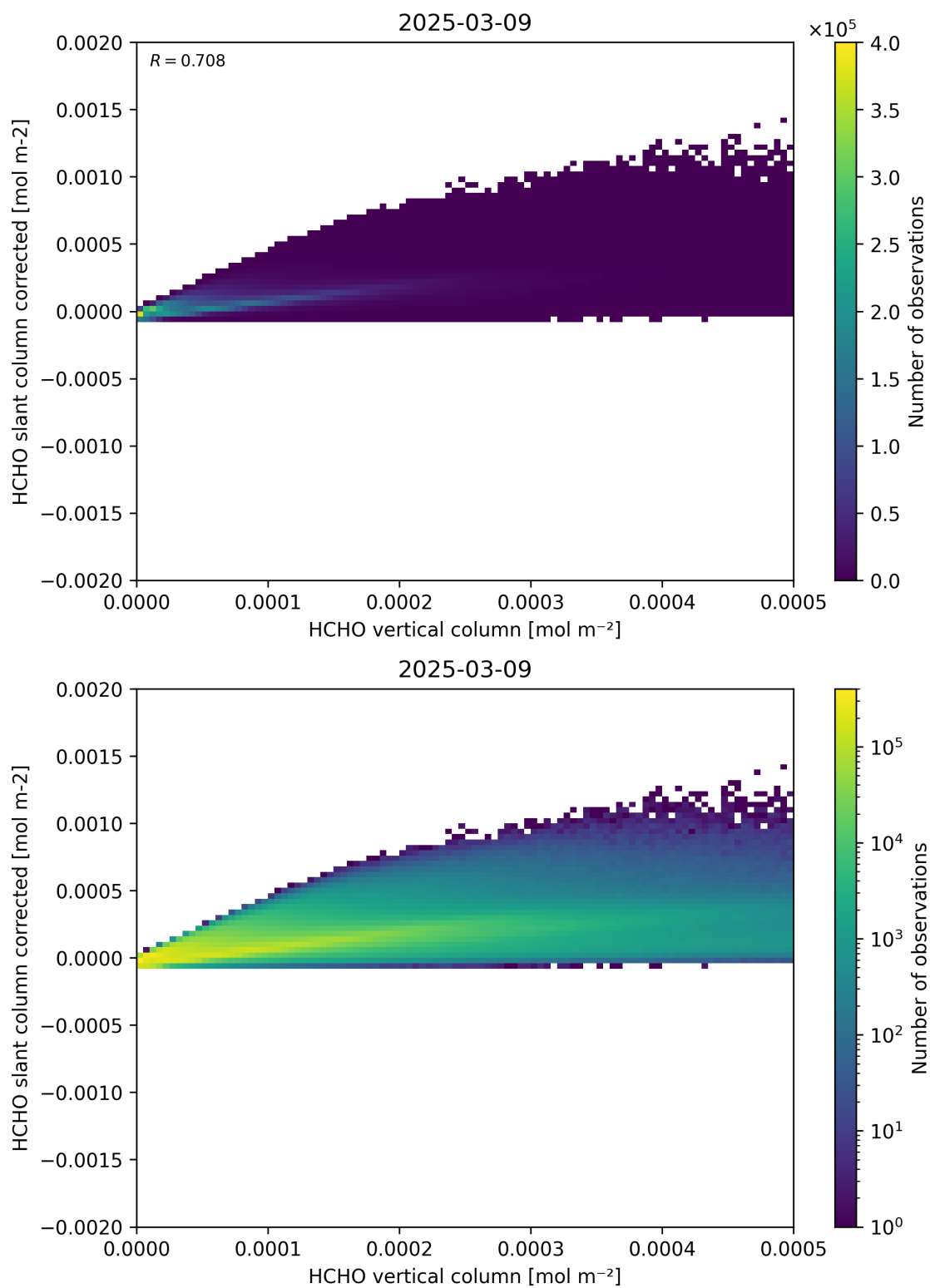
Figure 127: Scatter density plot of “HCHO vertical column” against “HCHO slant column corrected” for 2025-03-08 to 2025-03-10.
