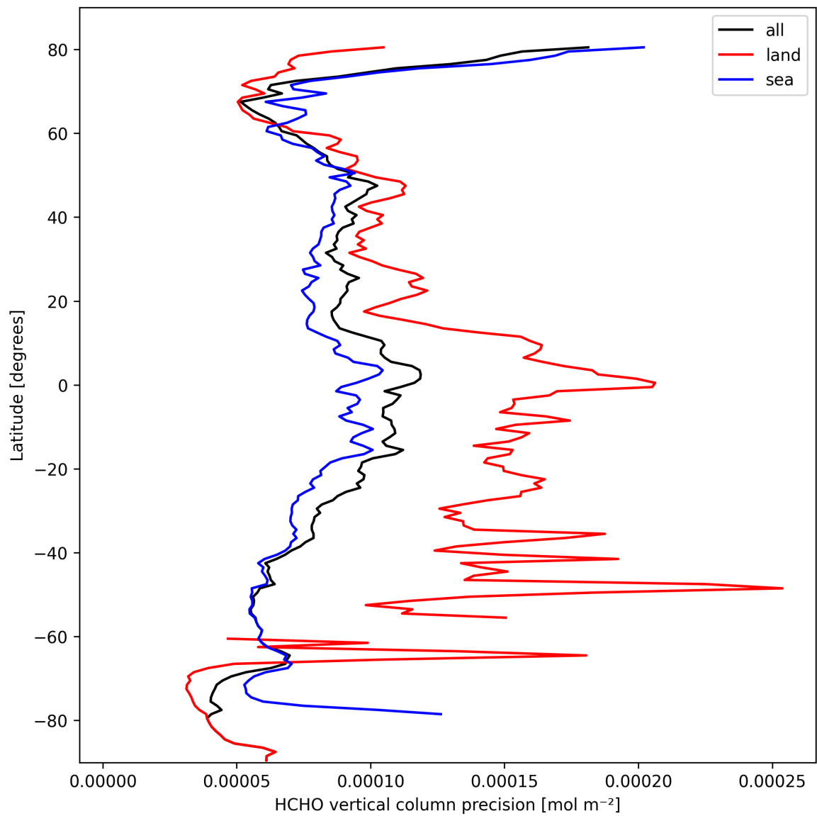
Figure 22: Zonal average of “HCHO vertical column precision” for 2025-03-08 to 2025-03-10.
