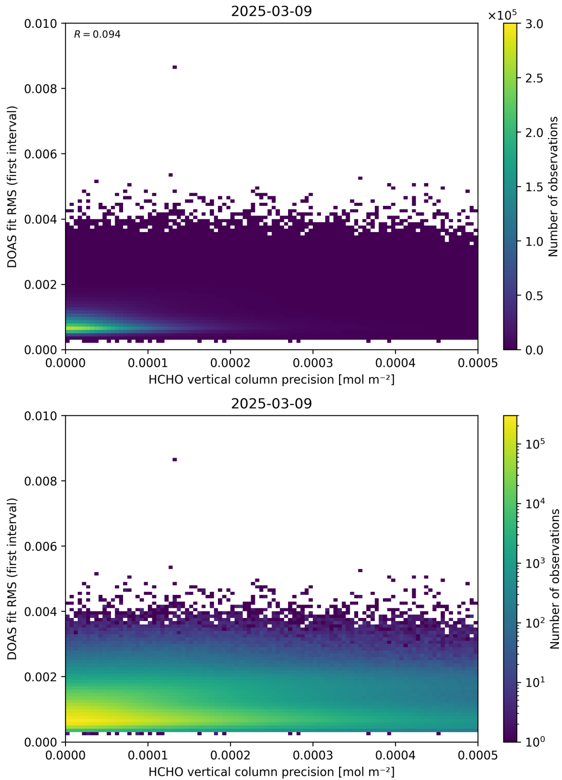
Figure 136: Scatter density plot of “HCHO vertical column precision” against “DOAS fit RMS (first interval)” for 2025-03-08 to 2025-03-10.
