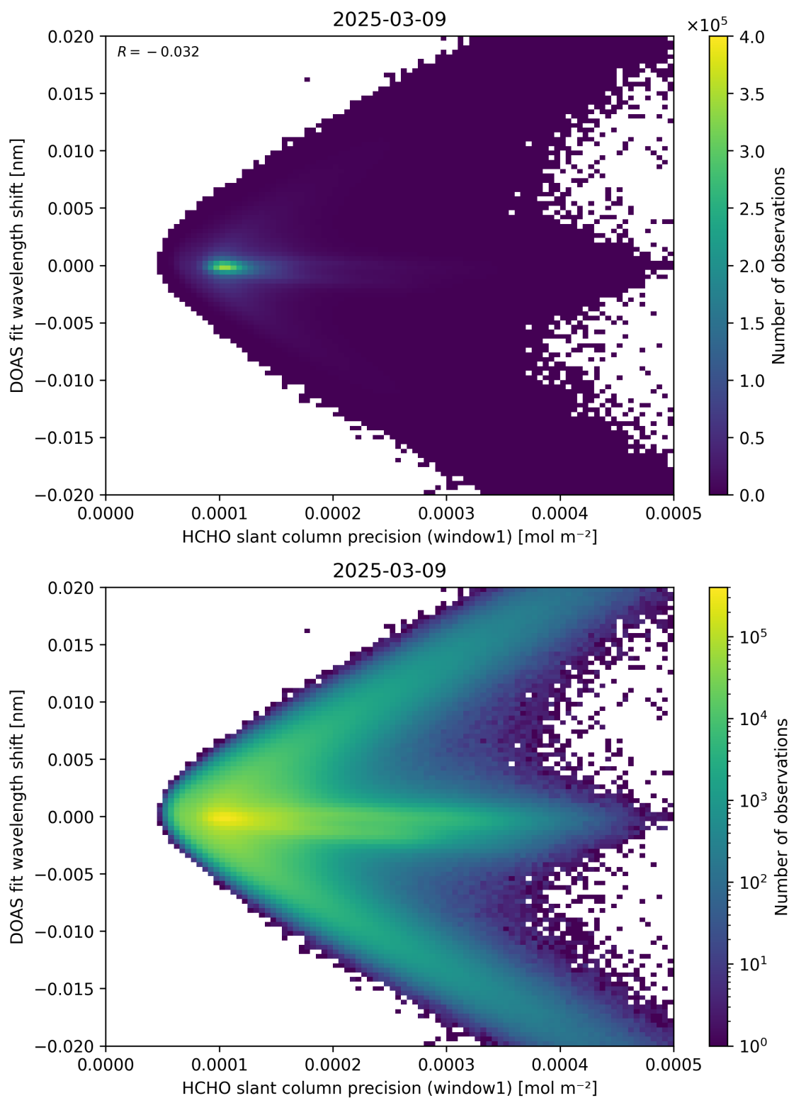
Figure 89: Scatter density plot of “HCHO slant column precision (window1)” against “DOAS fit wavelength shift” for 2025-03-08 to 2025-03-10.
