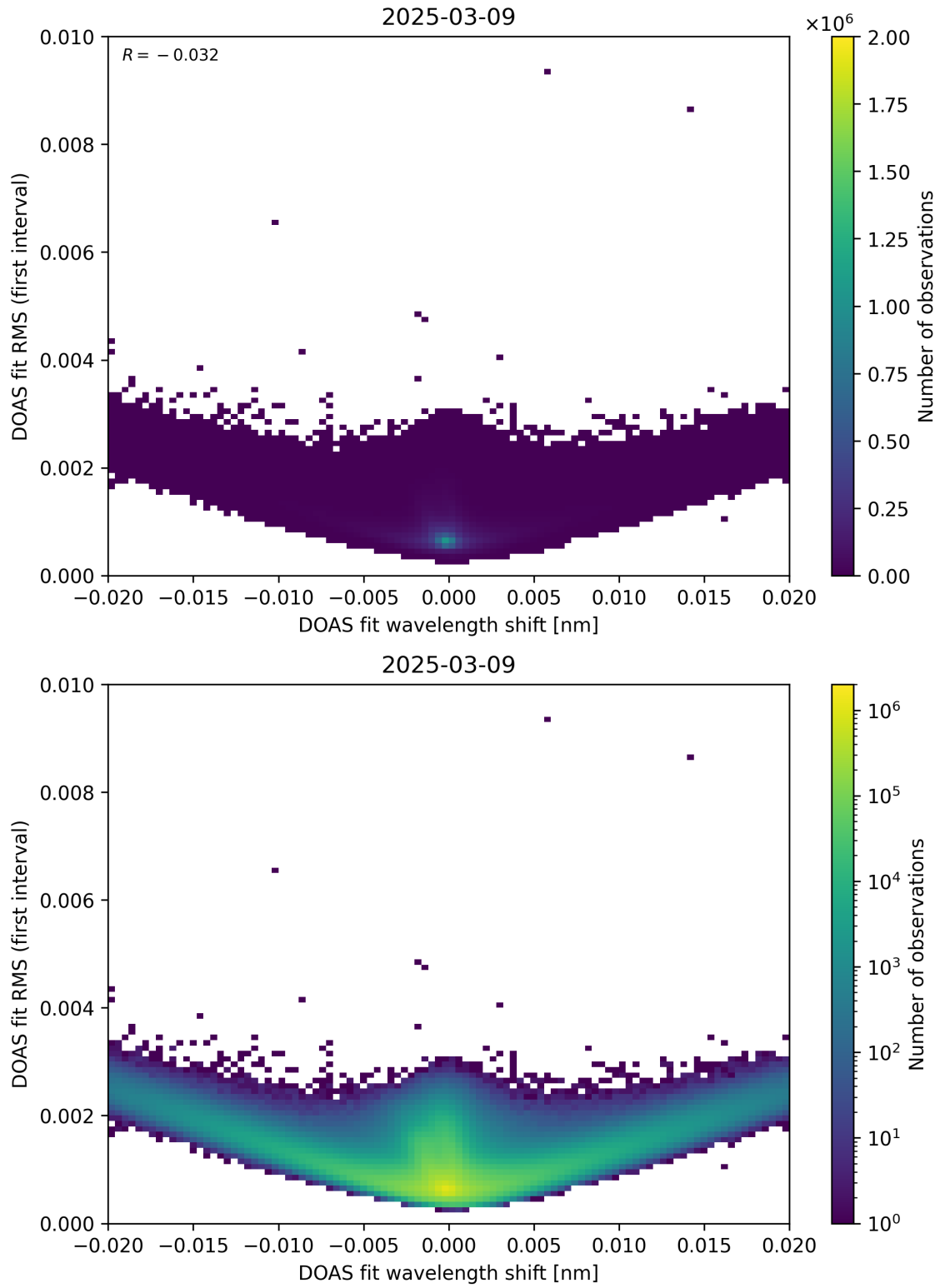
Figure 64: Scatter density plot of “DOAS fit wavelength shift” against “DOAS fit RMS (first interval)” for 2025-03-08 to 2025-03-10.
