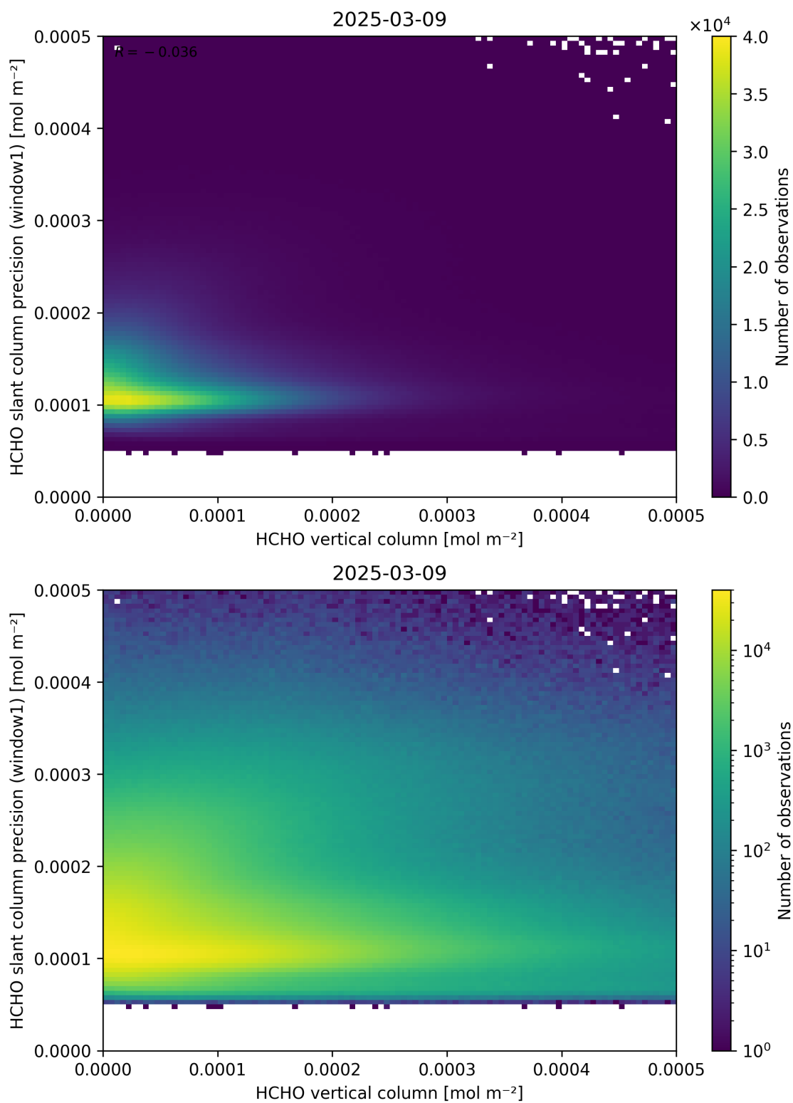
Figure 130: Scatter density plot of “HCHO vertical column” against “HCHO slant column precision (window1)” for 2025-03-08 to 2025-03-10.
