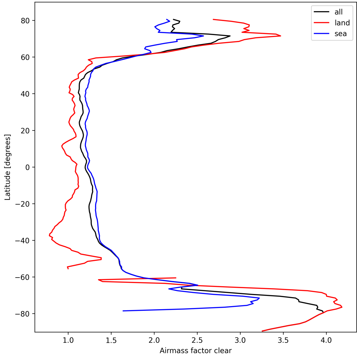
Figure 28: Zonal average of “Airmass factor clear” for 2025-03-08 to 2025-03-10.
