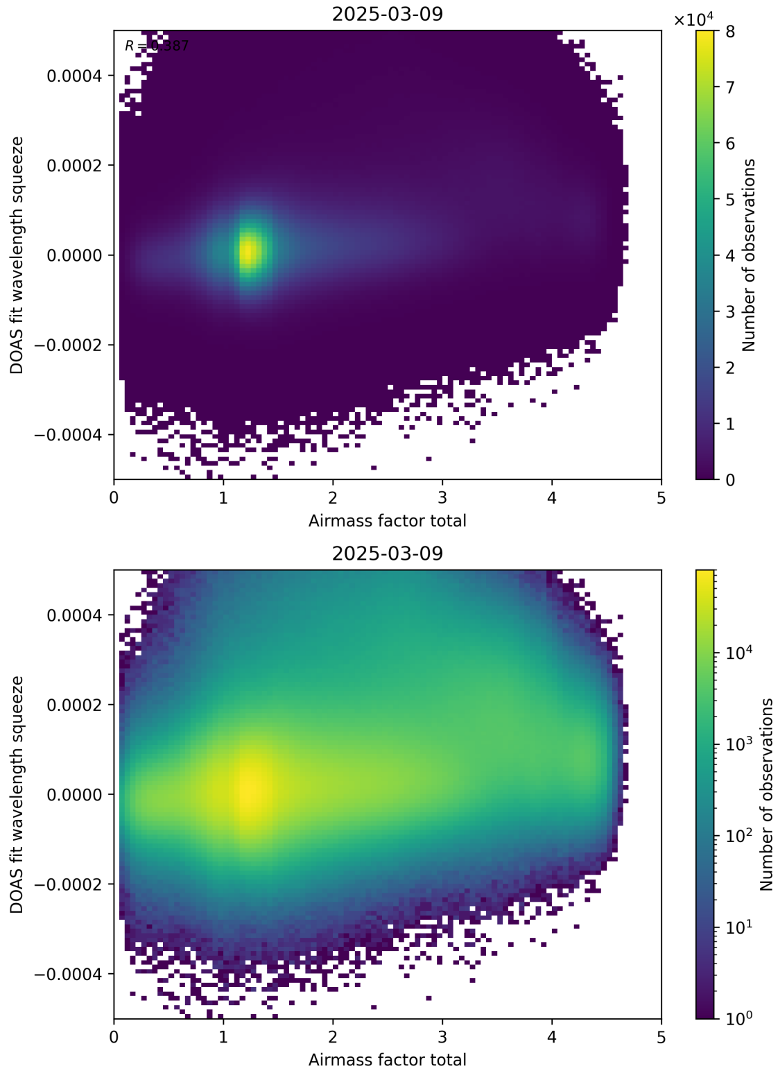
Figure 99: Scatter density plot of “Airmass factor total” against “DOAS fit wavelength squeeze” for 2025-03-08 to 2025-03-10.
