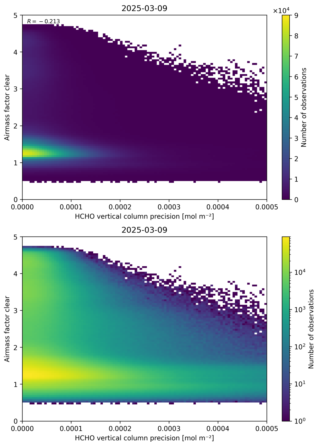
Figure 139: Scatter density plot of “HCHO vertical column precision” against “Airmass factor clear” for 2025-03-08 to 2025-03-10.
