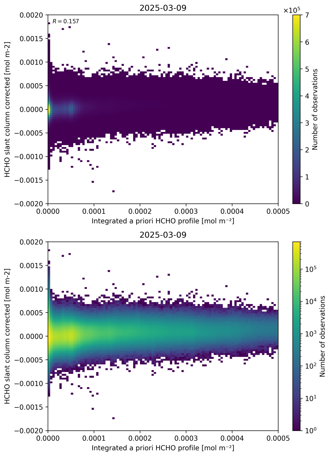
Figure 151: Scatter density plot of “Integrated a priori HCHO profile” against “HCHO slant column corrected” for 2025-03-08 to 2025-03-10.
