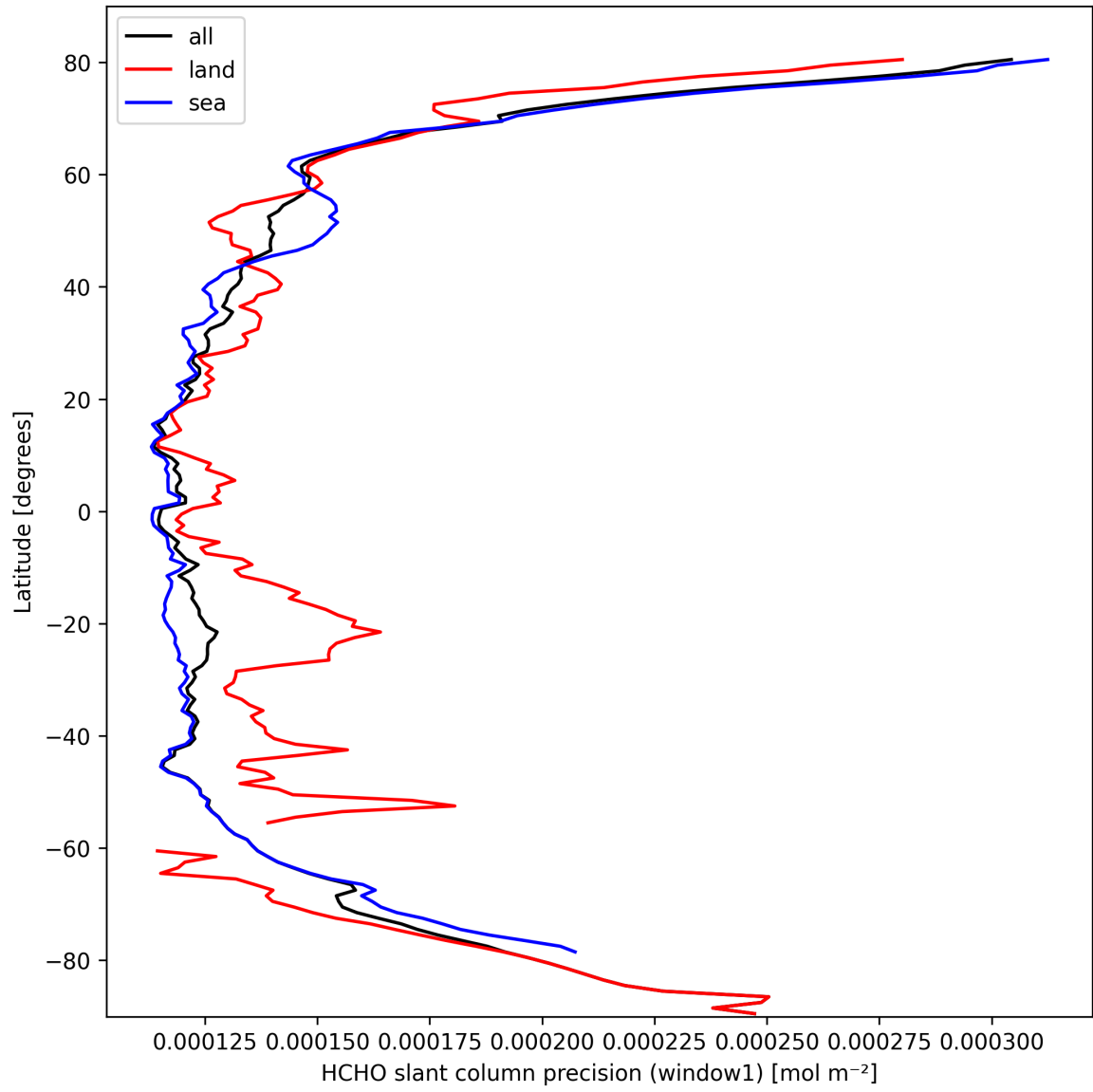
Figure 25: Zonal average of “HCHO slant column precision (window1)” for 2025-03-08 to 2025-03-10.
