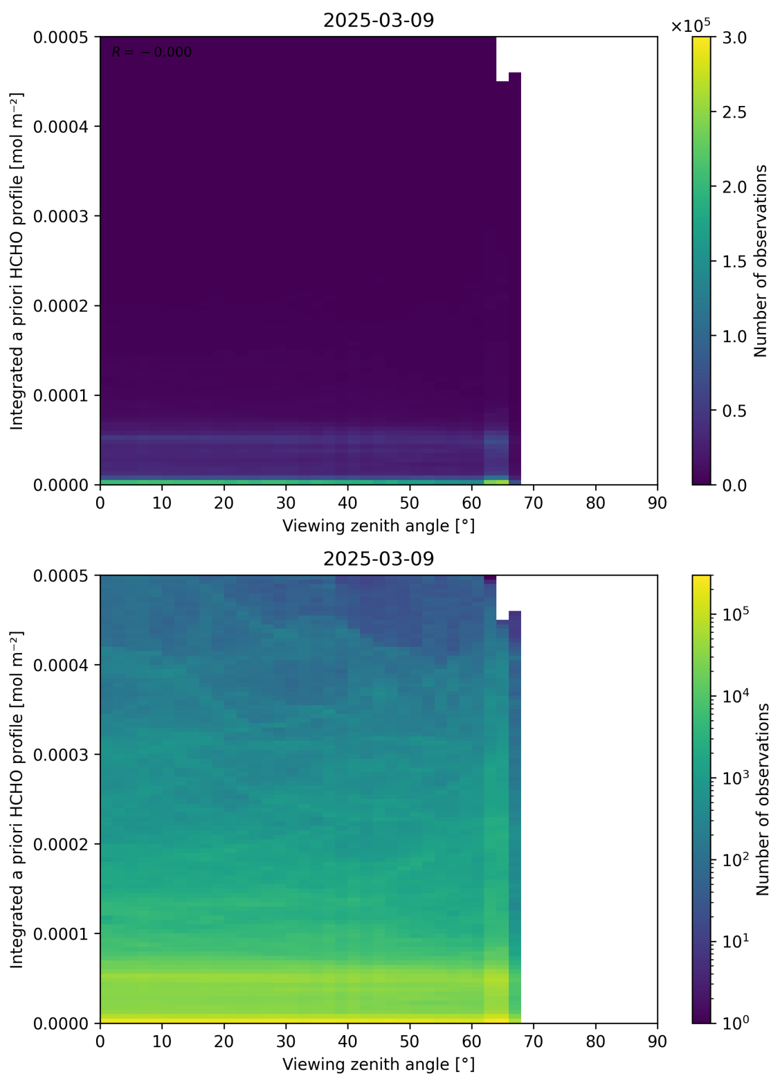
Figure 195: Scatter density plot of “Viewing zenith angle” against “Integrated a priori HCHO profile” for 2025-03-08 to 2025-03-10.
