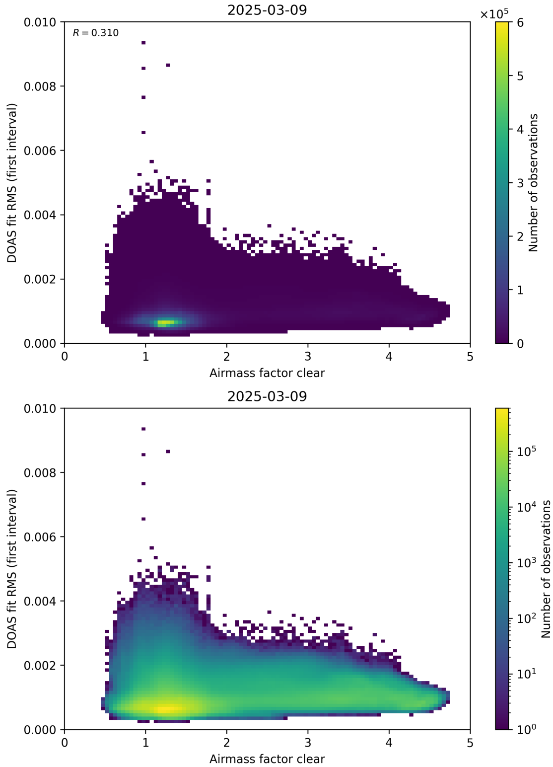
Figure 71: Scatter density plot of “Airmass factor clear” against “DOAS fit RMS (first interval)” for 2025-03-08 to 2025-03-10.
