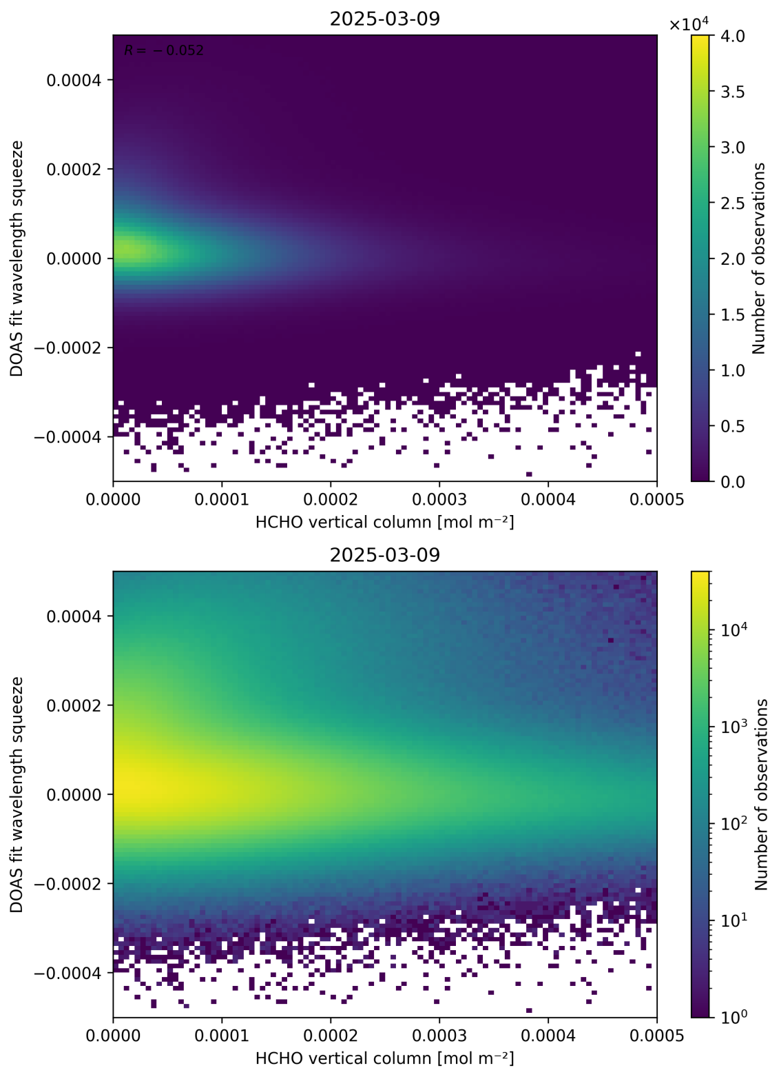
Figure 125: Scatter density plot of “HCHO vertical column” against “DOAS fit wavelength squeeze” for 2025-03-08 to 2025-03-10.
