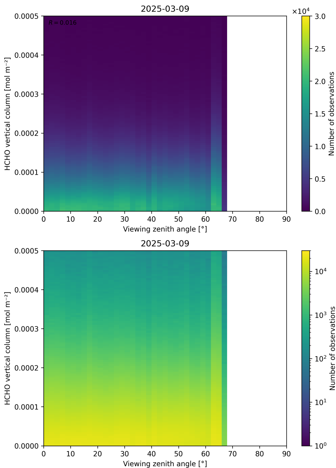
Figure 192: Scatter density plot of “Viewing zenith angle” against “HCHO vertical column” for 2025-03-08 to 2025-03-10.
