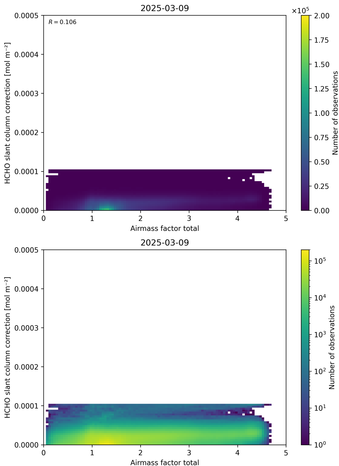
Figure 102: Scatter density plot of “Airmass factor total” against “HCHO slant column correction” for 2025-03-08 to 2025-03-10.
