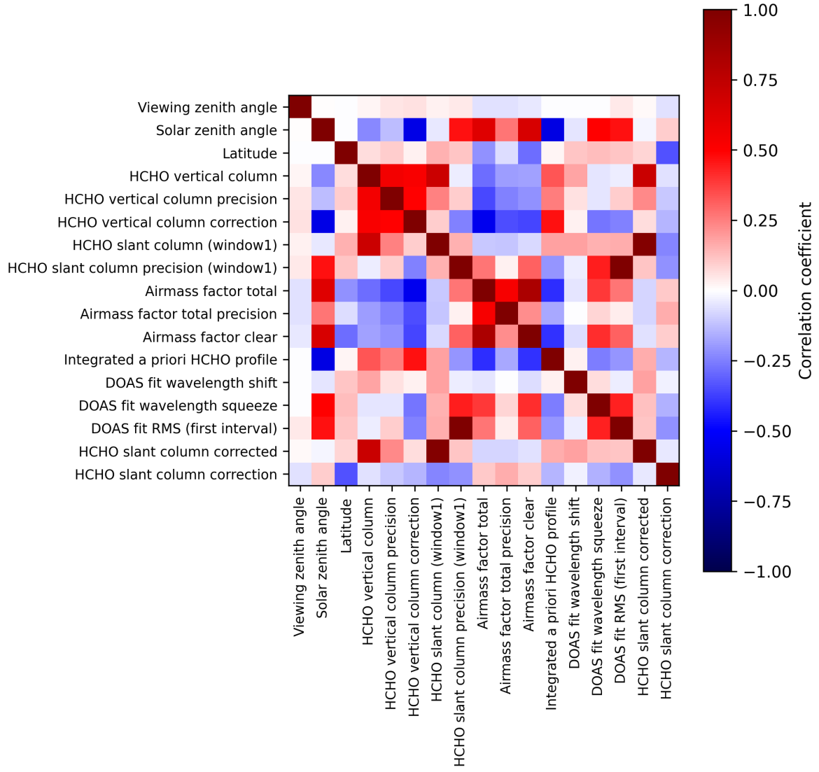
Figure 2: Map of correlation matrix for 2025-03-08 to 2025-03-10.
