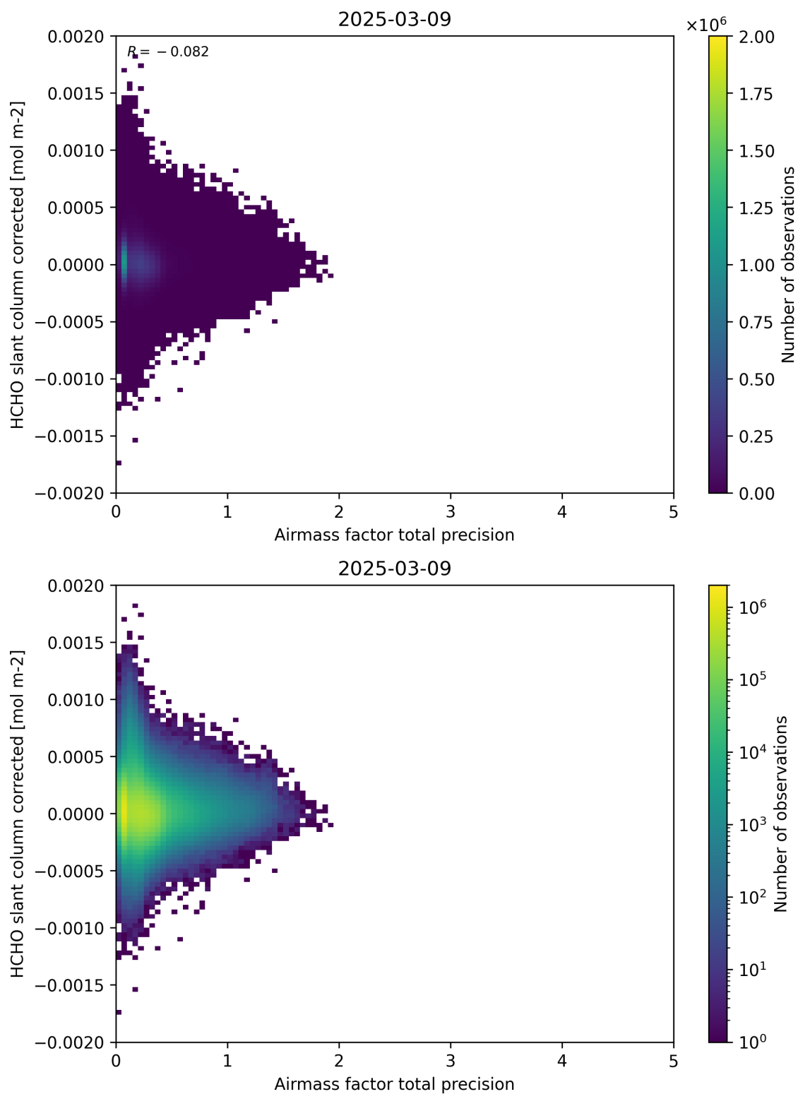
Figure 109: Scatter density plot of “Airmass factor total precision” against “HCHO slant column corrected” for 2025-03-08 to 2025-03-10.
