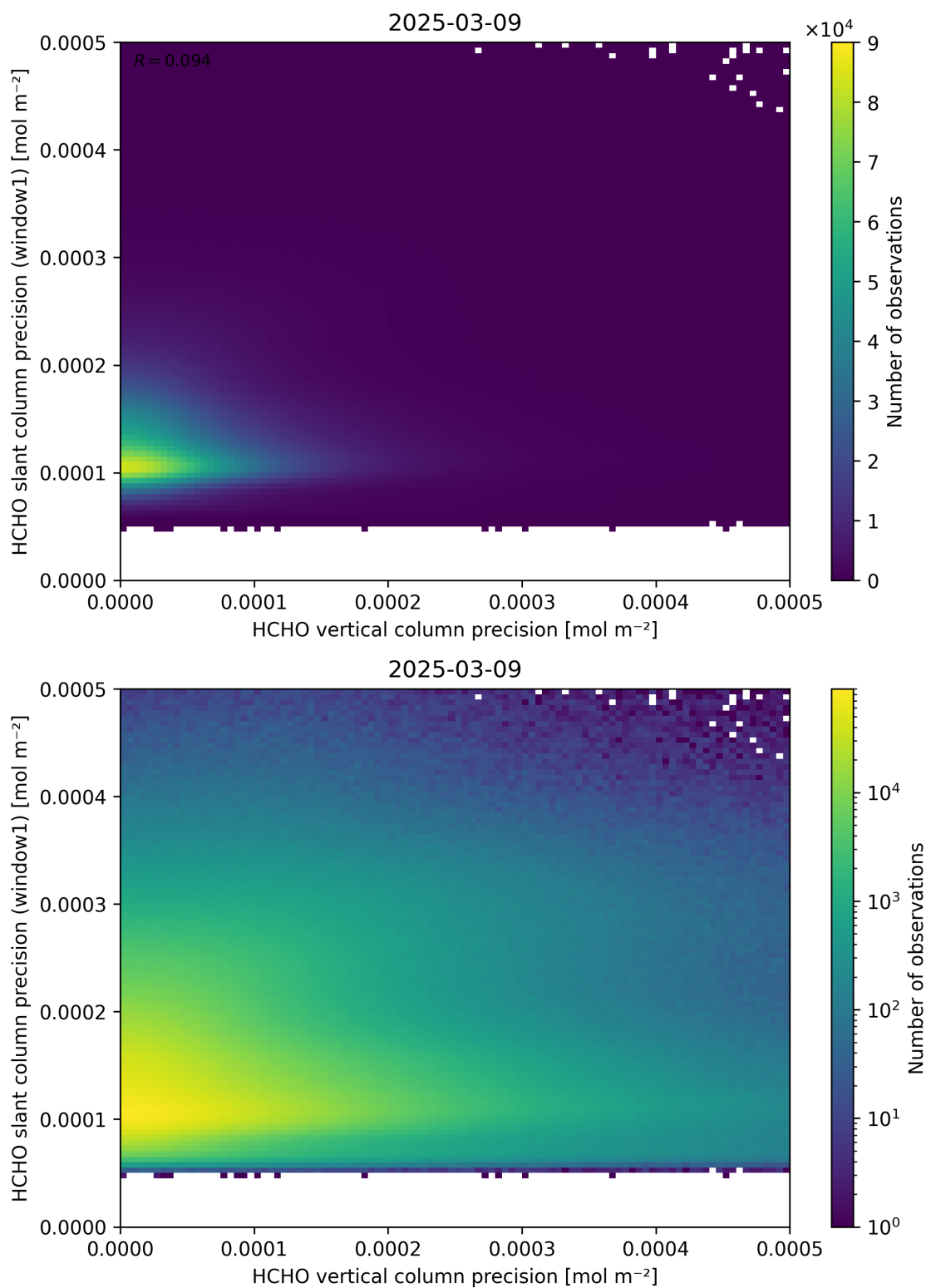
Figure 143: Scatter density plot of “HCHO vertical column precision” against “HCHO slant column precision (window1)” for 2025-03-08 to 2025-03-10.
