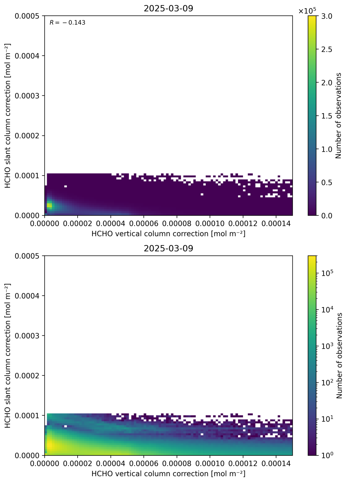
Figure 117: Scatter density plot of “HCHO vertical column correction” against “HCHO slant column correction” for 2025-03-08 to 2025-03-10.
