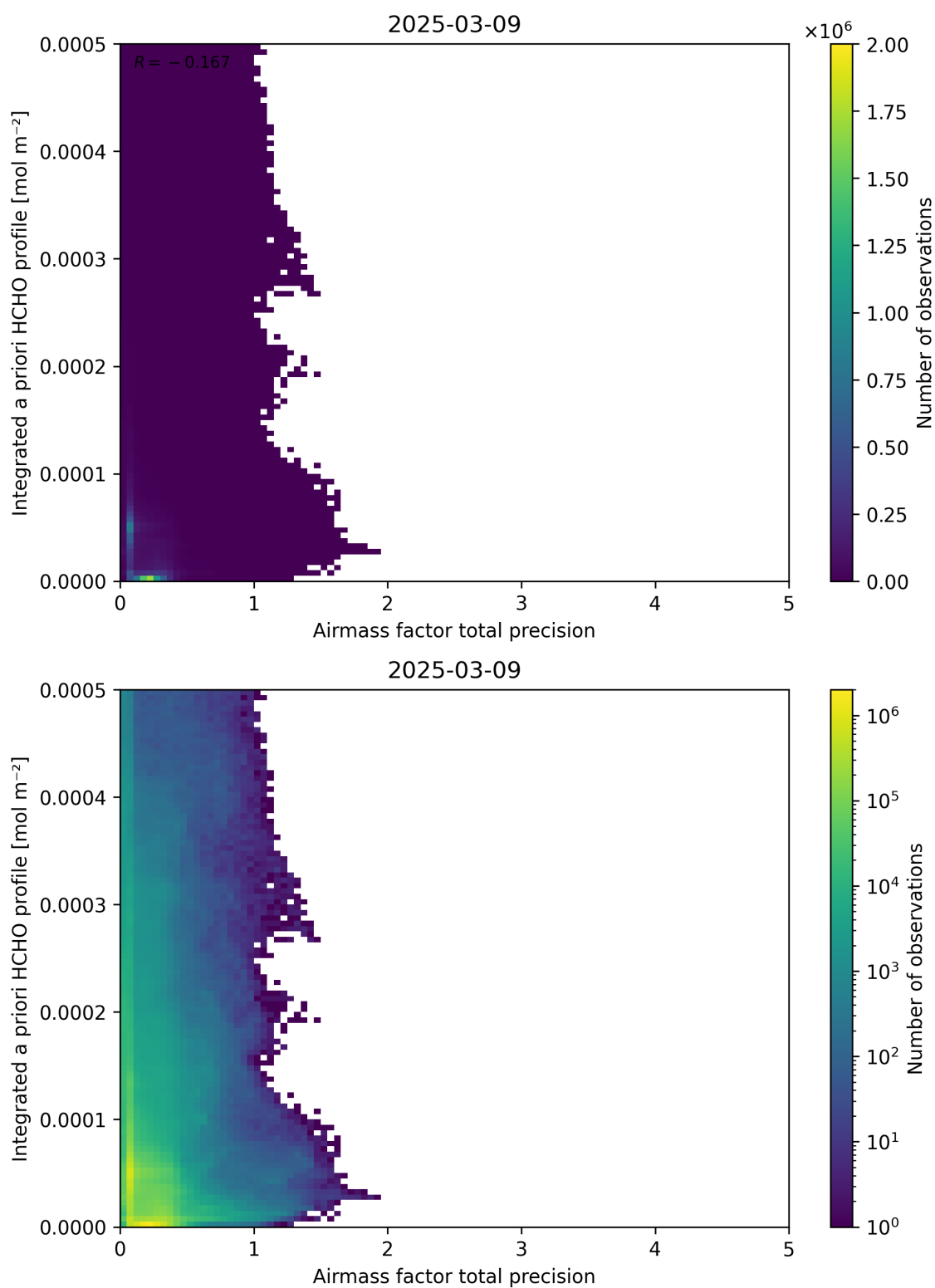
Figure 111: Scatter density plot of “Airmass factor total precision” against “Integrated a priori HCHO profile” for 2025-03-08 to 2025-03-10.
