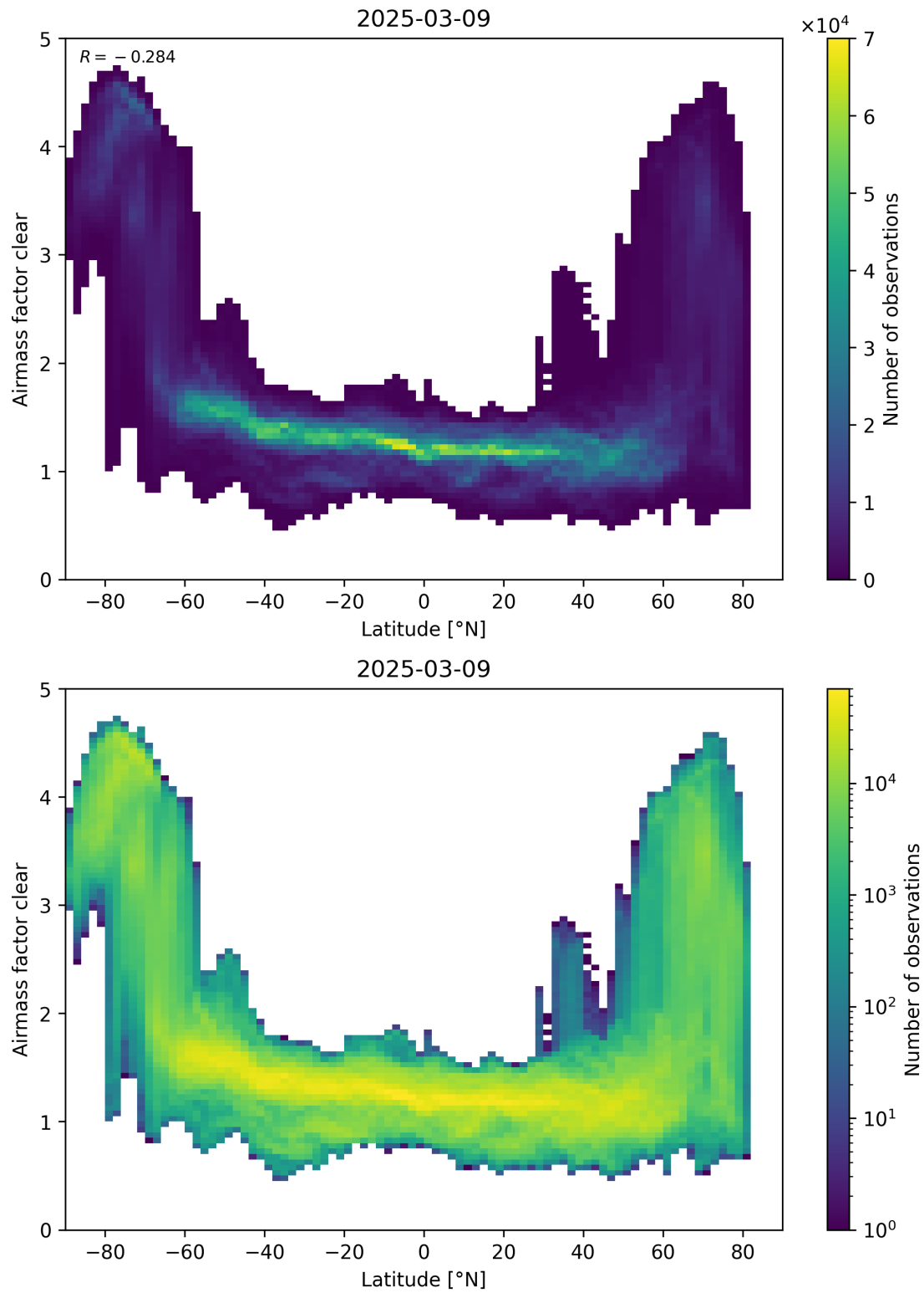
Figure 156: Scatter density plot of “Latitude” against “Airmass factor clear” for 2025-03-08 to 2025-03-10.
