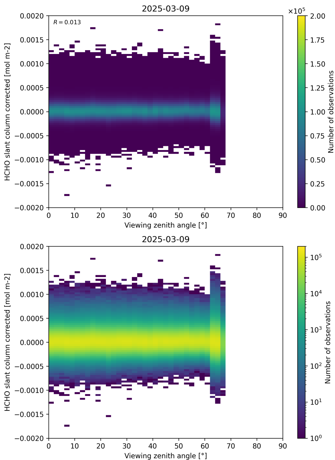
Figure 186: Scatter density plot of “Viewing zenith angle” against “HCHO slant column corrected” for 2025-03-08 to 2025-03-10.
