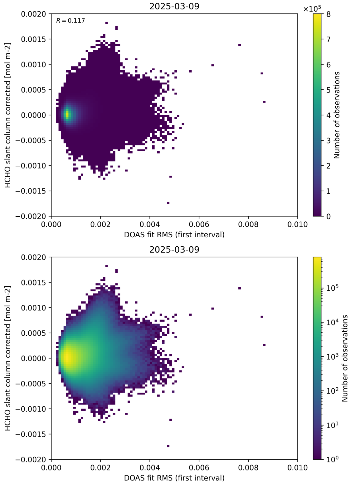
Figure 62: Scatter density plot of “DOAS fit RMS (first interval)” against “HCHO slant column corrected” for 2025-03-08 to 2025-03-10.
