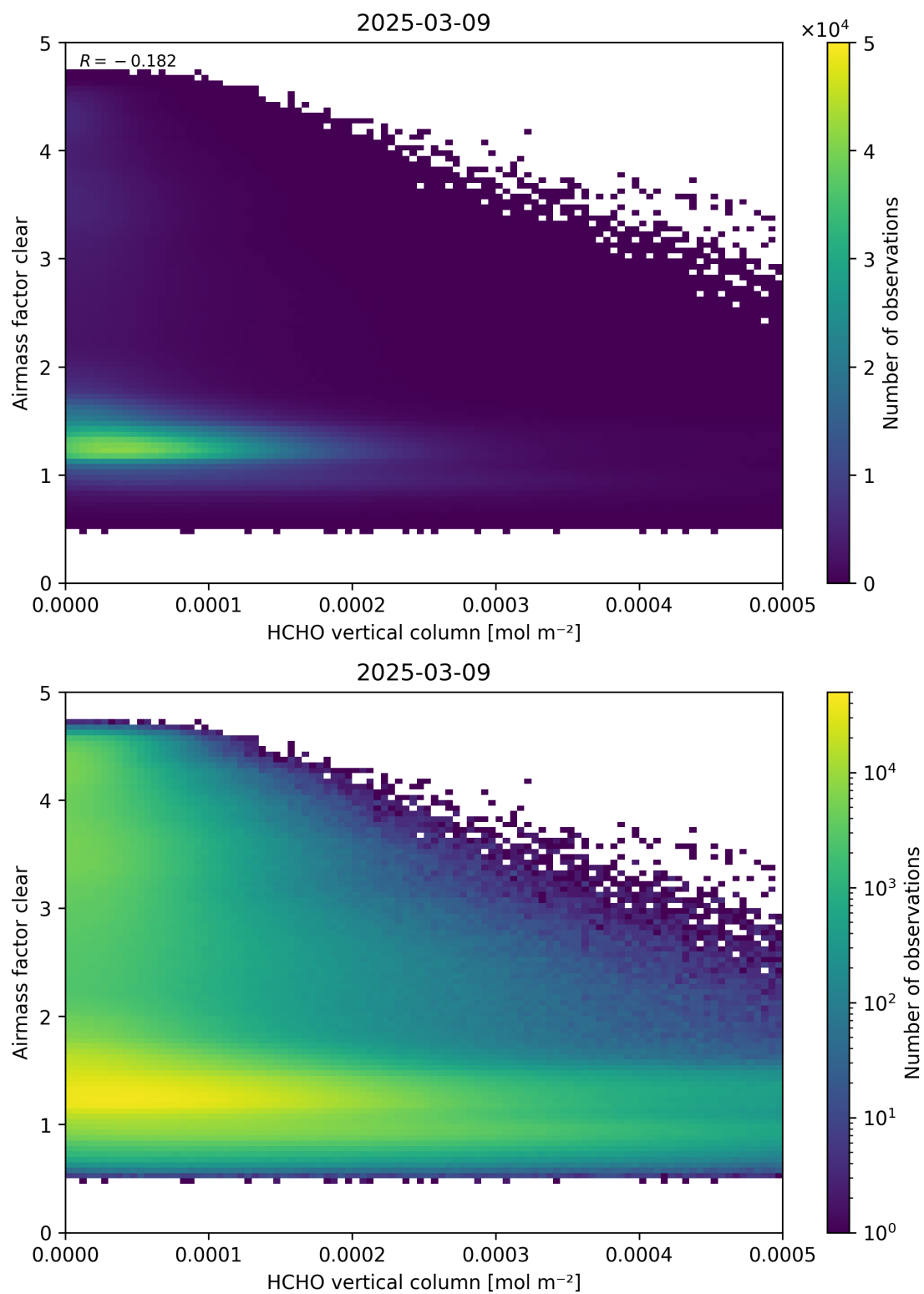
Figure 126: Scatter density plot of “HCHO vertical column” against “Airmass factor clear” for 2025-03-08 to 2025-03-10.
