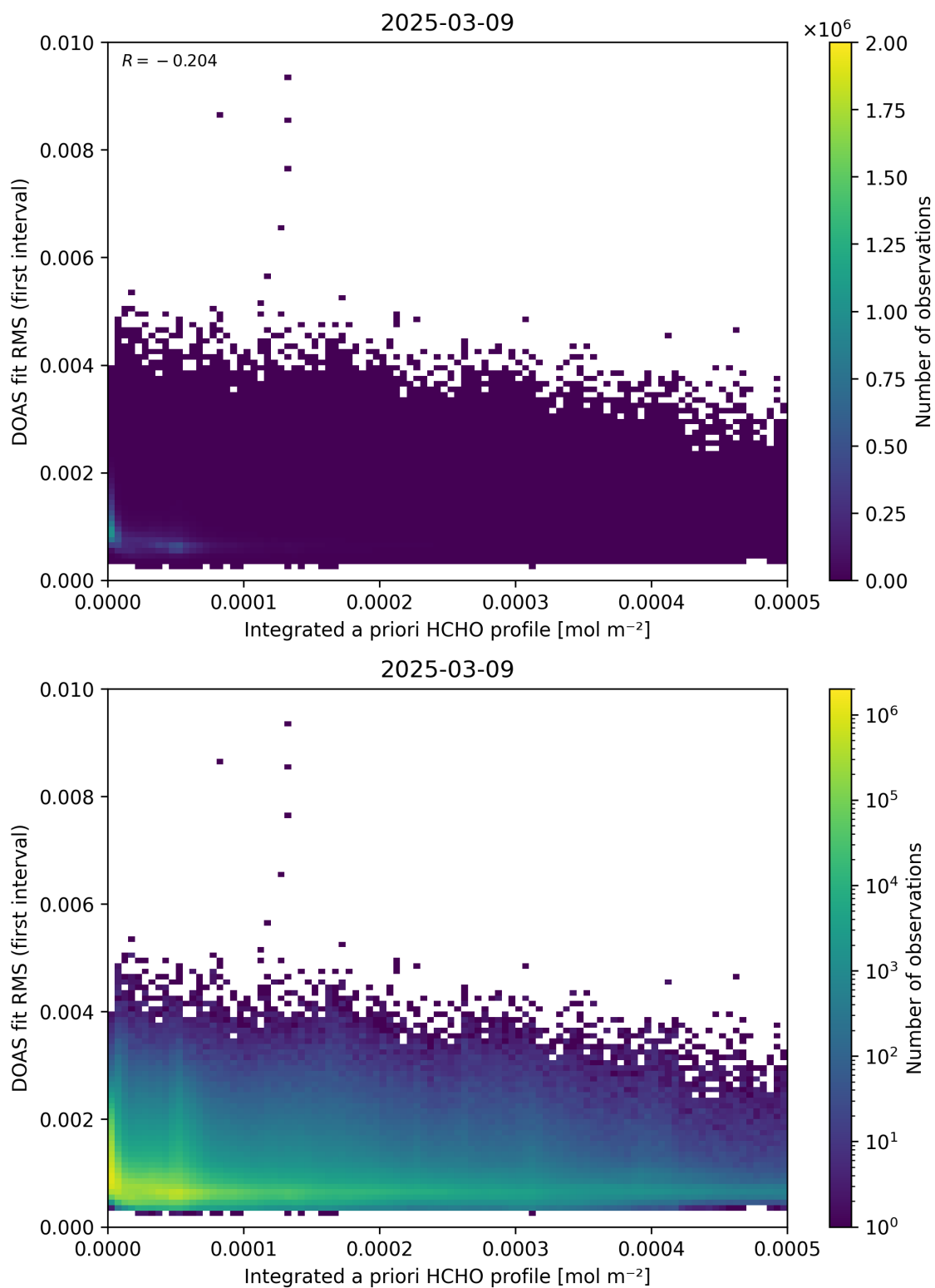
Figure 148: Scatter density plot of “Integrated a priori HCHO profile” against “DOAS fit RMS (first interval)” for 2025-03-08 to 2025-03-10.
