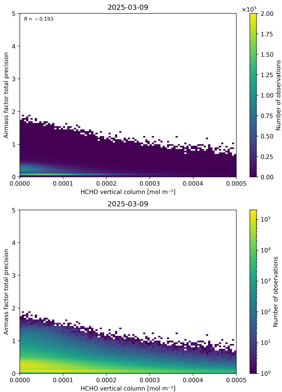
Figure 132: Scatter density plot of “HCHO vertical column” against “Airmass factor total precision” for 2025-03-08 to 2025-03-10.
