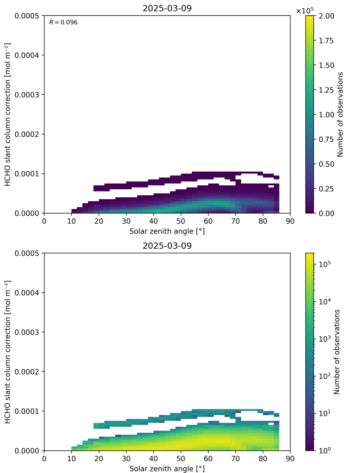
Figure 172: Scatter density plot of “Solar zenith angle” against “HCHO slant column correction” for 2025-03-08 to 2025-03-10.
