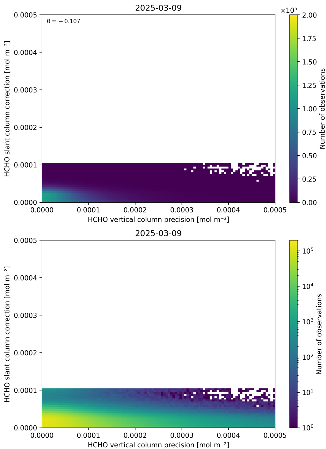
Figure 141: Scatter density plot of “HCHO vertical column precision” against “HCHO slant column correction” for 2025-03-08 to 2025-03-10.
