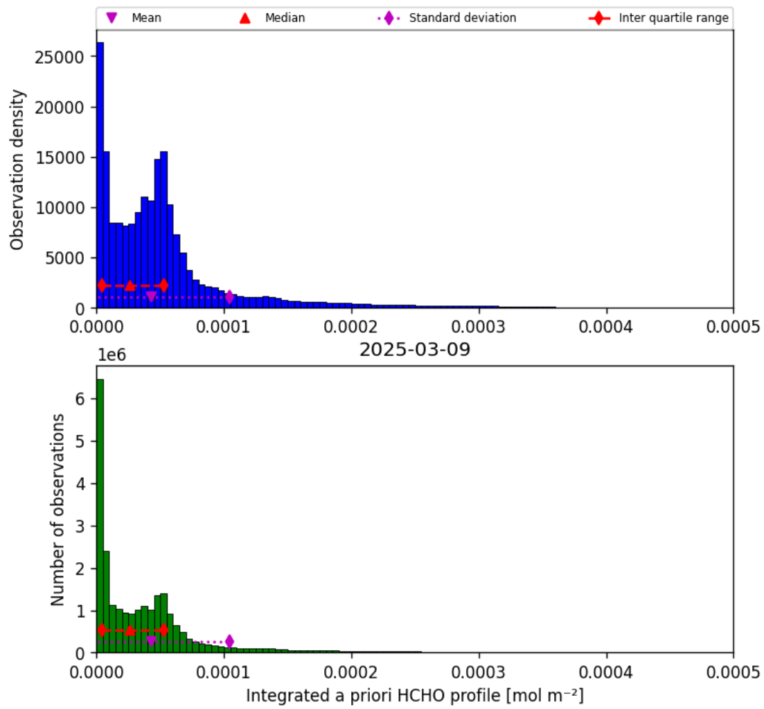
Figure 43: Histogram of “Integrated a priori HCHO profile” for 2025-03-08 to 2025-03-10
