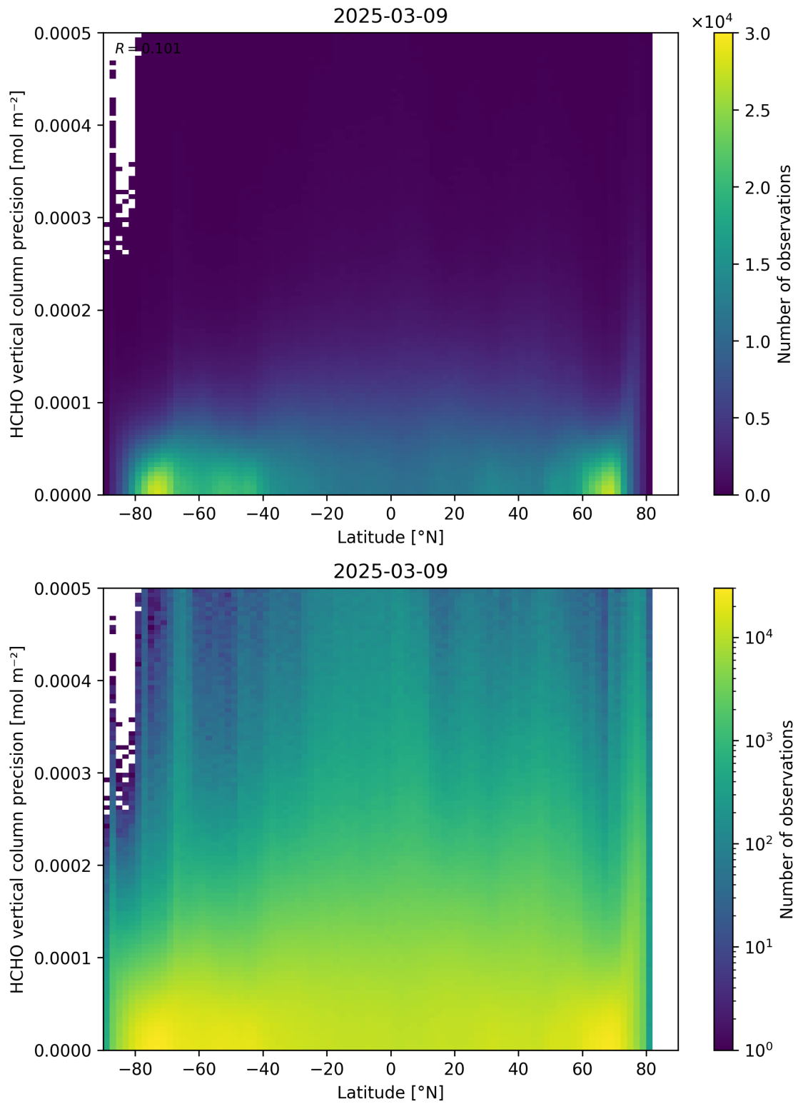
Figure 165: Scatter density plot of “Latitude” against “HCHO vertical column precision” for 2025-03-08 to 2025-03-10.
