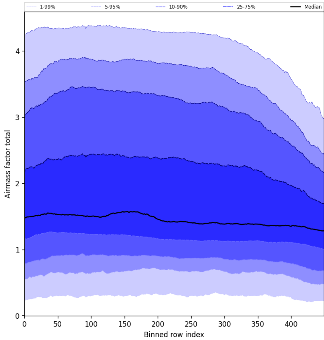
Figure 54: Along track statistics of “Airmass factor total” for 2025-03-08 to 2025-03-10
