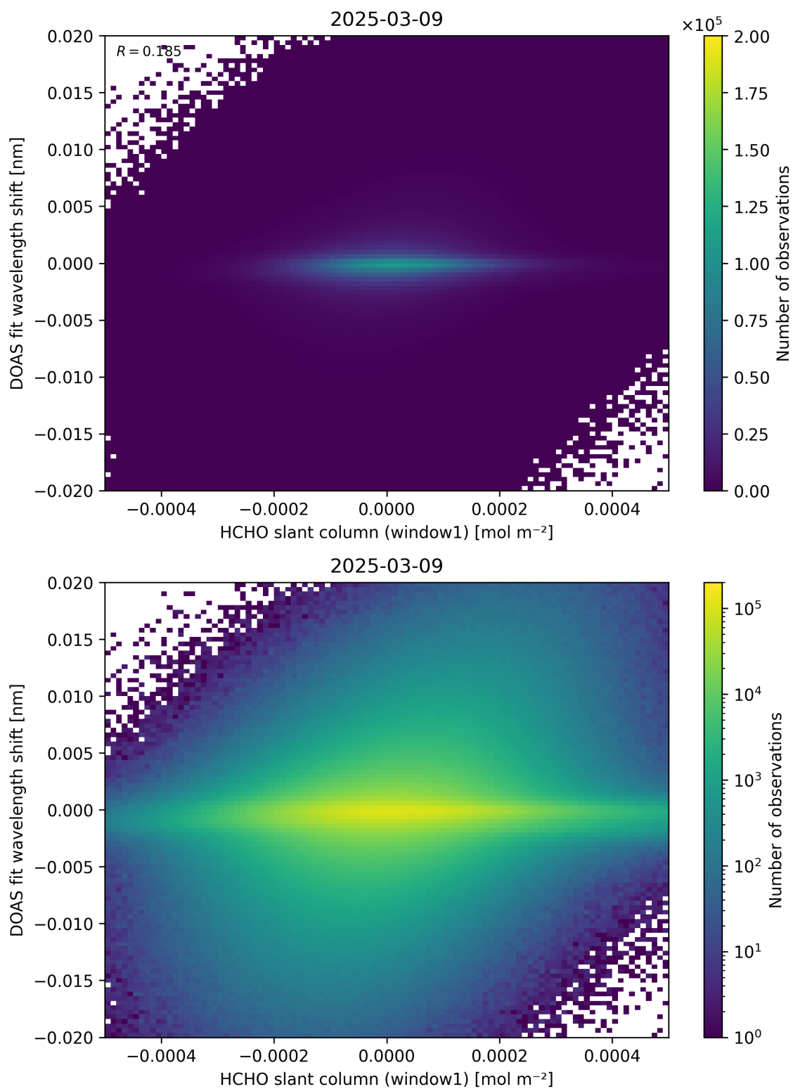
Figure 79: Scatter density plot of “HCHO slant column (window1)” against “DOAS fit wavelength shift” for 2025-03-08 to 2025-03-10.
