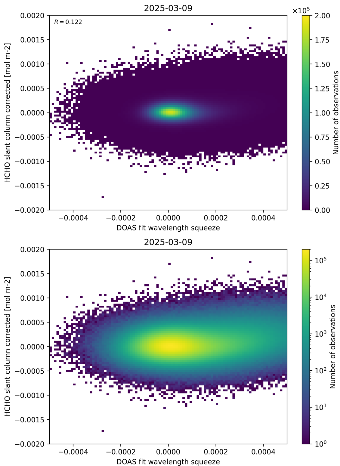
Figure 69: Scatter density plot of “DOAS fit wavelength squeeze” against “HCHO slant column corrected” for 2025-03-08 to 2025-03-10.
