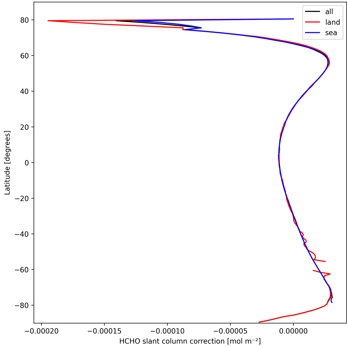
Figure 33: Zonal average of “HCHO slant column correction” for 2025-03-08 to 2025-03-10.
