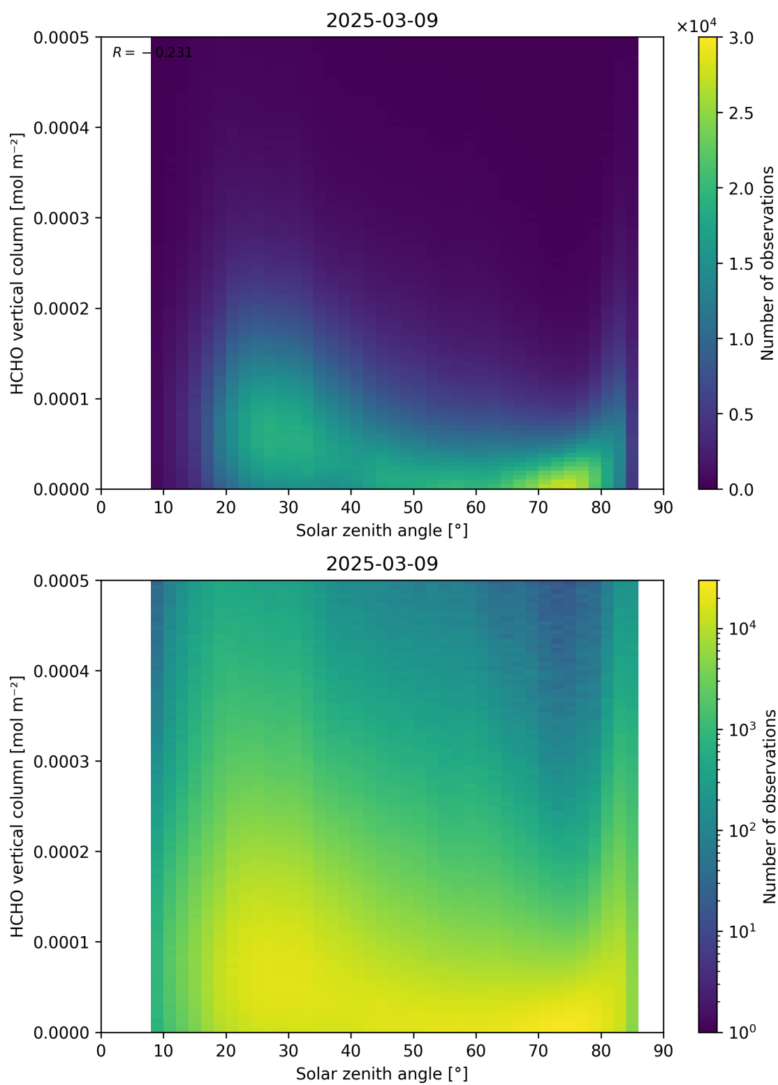
Figure 177: Scatter density plot of “Solar zenith angle” against “HCHO vertical column” for 2025-03-08 to 2025-03-10.
