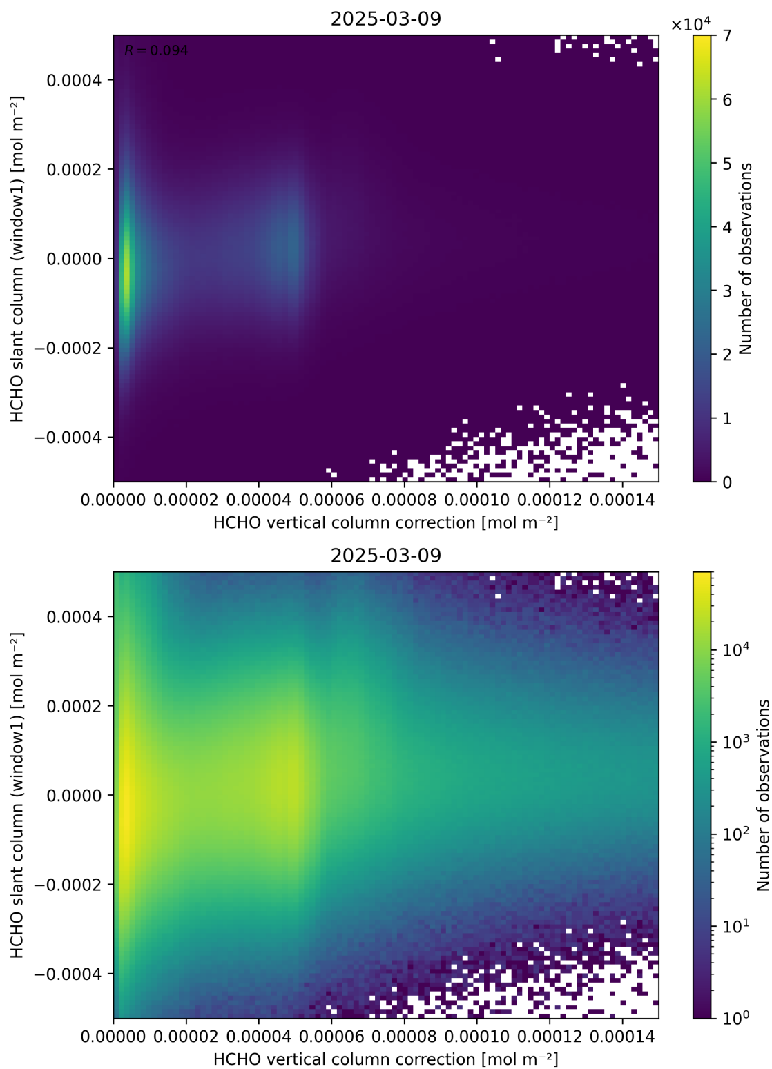
Figure 118: Scatter density plot of “HCHO vertical column correction” against “HCHO slant column (window1)” for 2025-03-08 to 2025-03-10.
