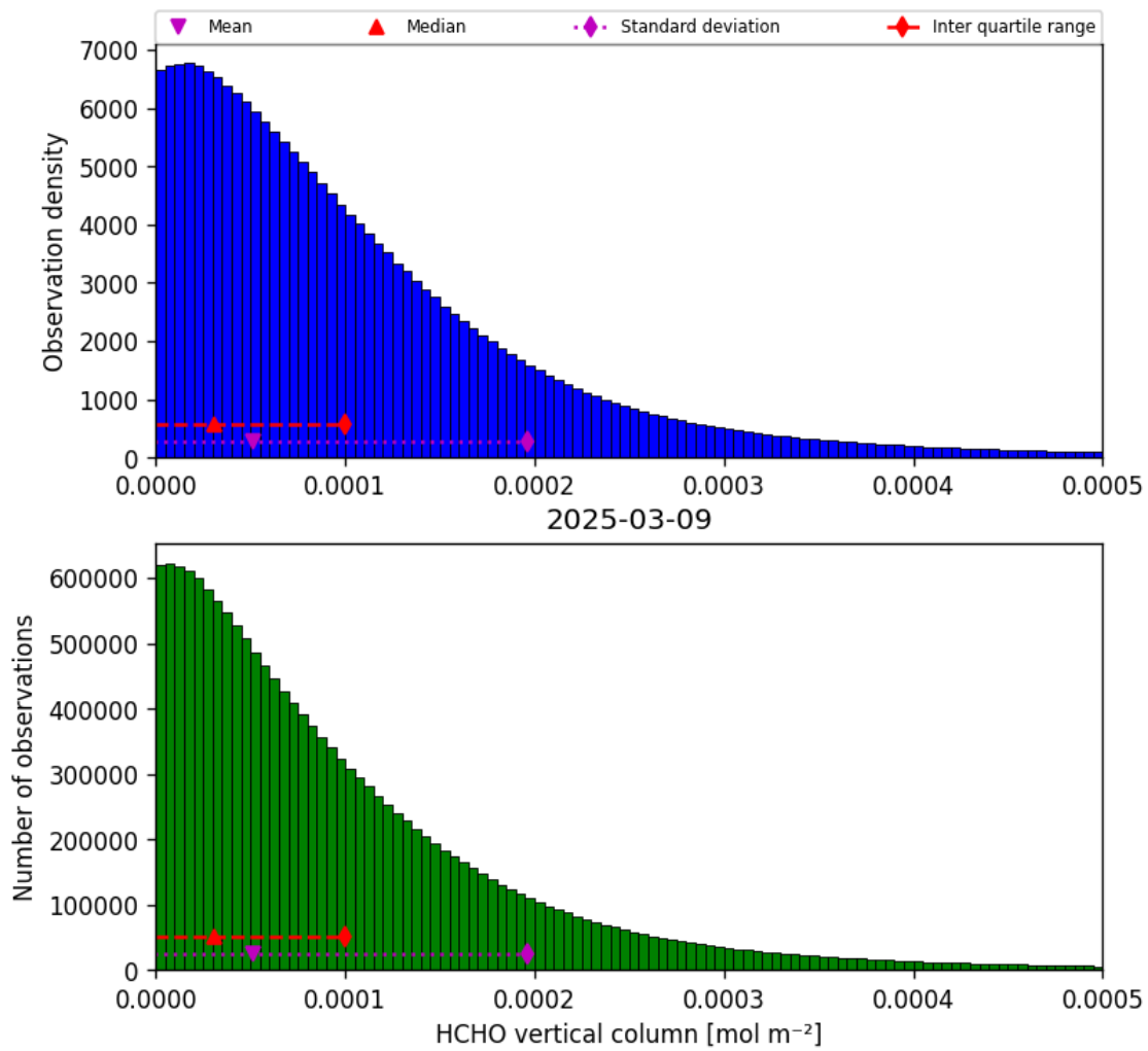
Figure 35: Histogram of “HCHO vertical column” for 2025-03-08 to 2025-03-10
