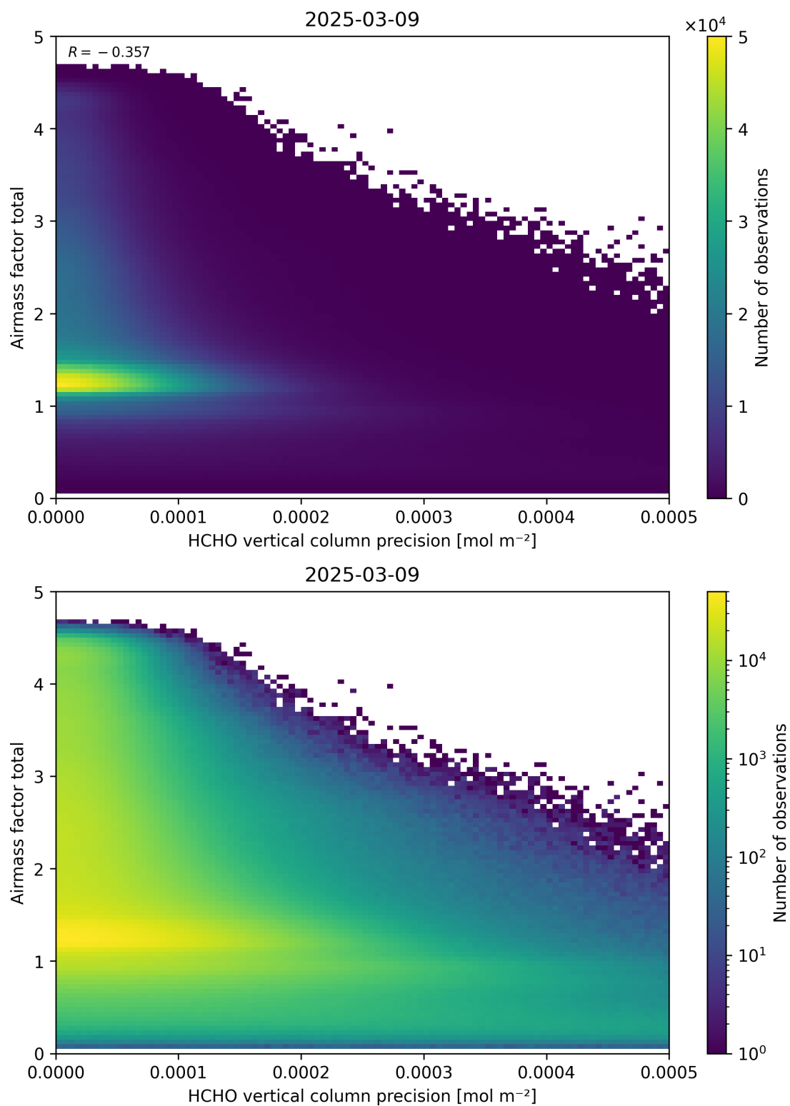
Figure 144: Scatter density plot of “HCHO vertical column precision” against “Airmass factor total” for 2025-03-08 to 2025-03-10.
