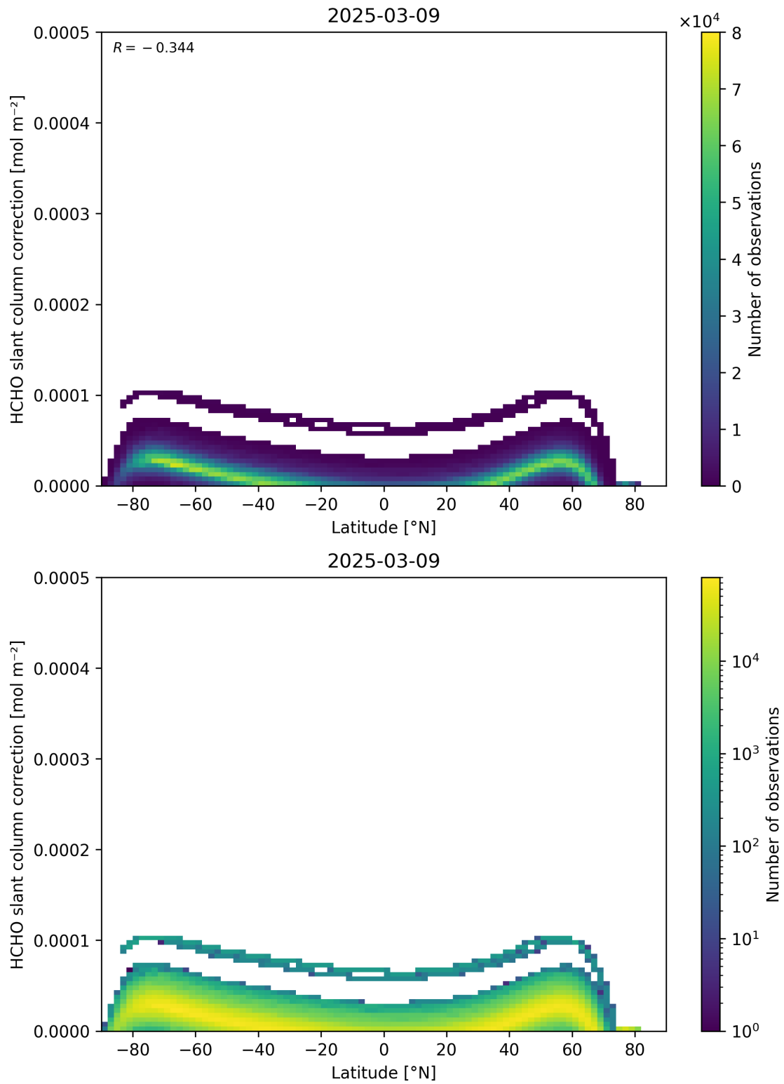
Figure 158: Scatter density plot of “Latitude” against “HCHO slant column correction” for 2025-03-08 to 2025-03-10.
