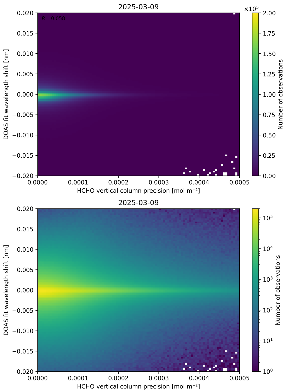
Figure 137: Scatter density plot of “HCHO vertical column precision” against “DOAS fit wavelength shift” for 2025-03-08 to 2025-03-10.
