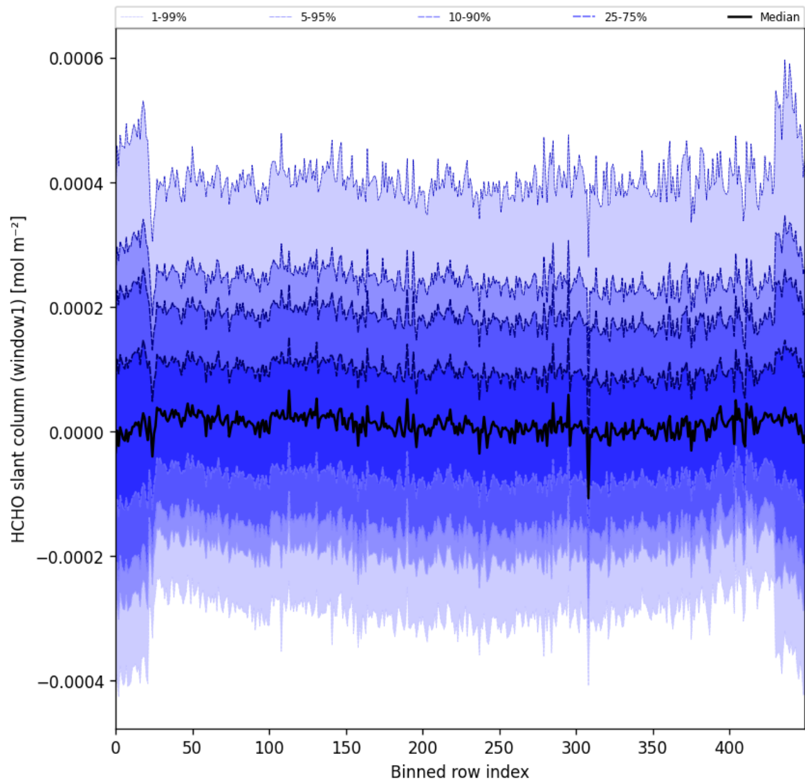
Figure 52: Along track statistics of “HCHO slant column (window1)” for 2025-03-08 to 2025-03-10
