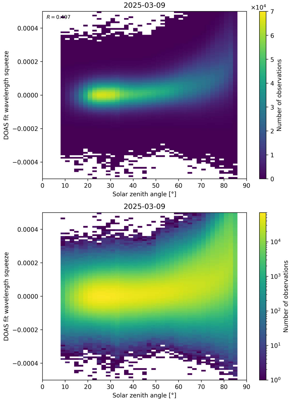
Figure 169: Scatter density plot of “Solar zenith angle” against “DOAS fit wavelength squeeze” for 2025-03-08 to 2025-03-10.
