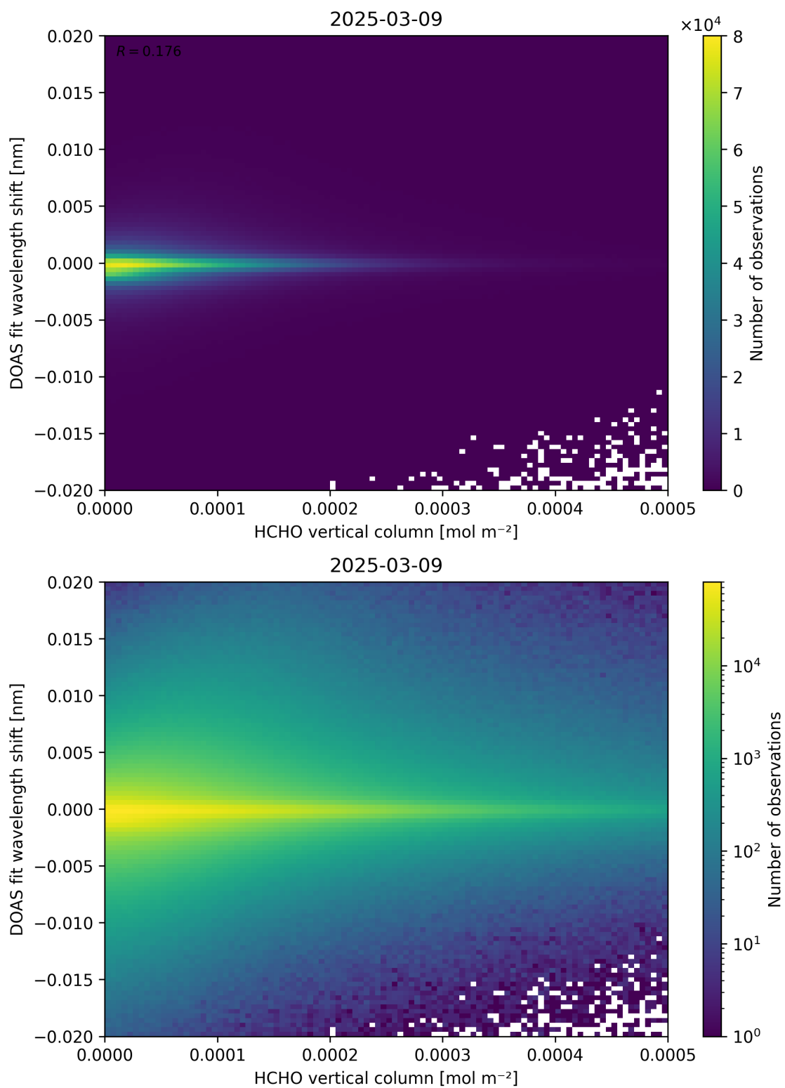
Figure 124: Scatter density plot of “HCHO vertical column” against “DOAS fit wavelength shift” for 2025-03-08 to 2025-03-10.
