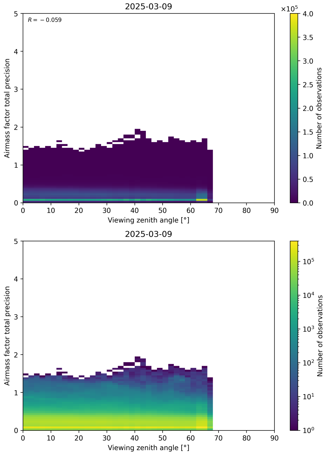
Figure 191: Scatter density plot of “Viewing zenith angle” against “Airmass factor total precision” for 2025-03-08 to 2025-03-10.
