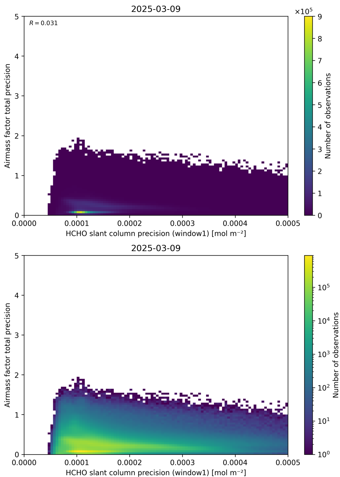
Figure 95: Scatter density plot of “HCHO slant column precision (window1)” against “Airmass factor total precision” for 2025-03-08 to 2025-03-10.
