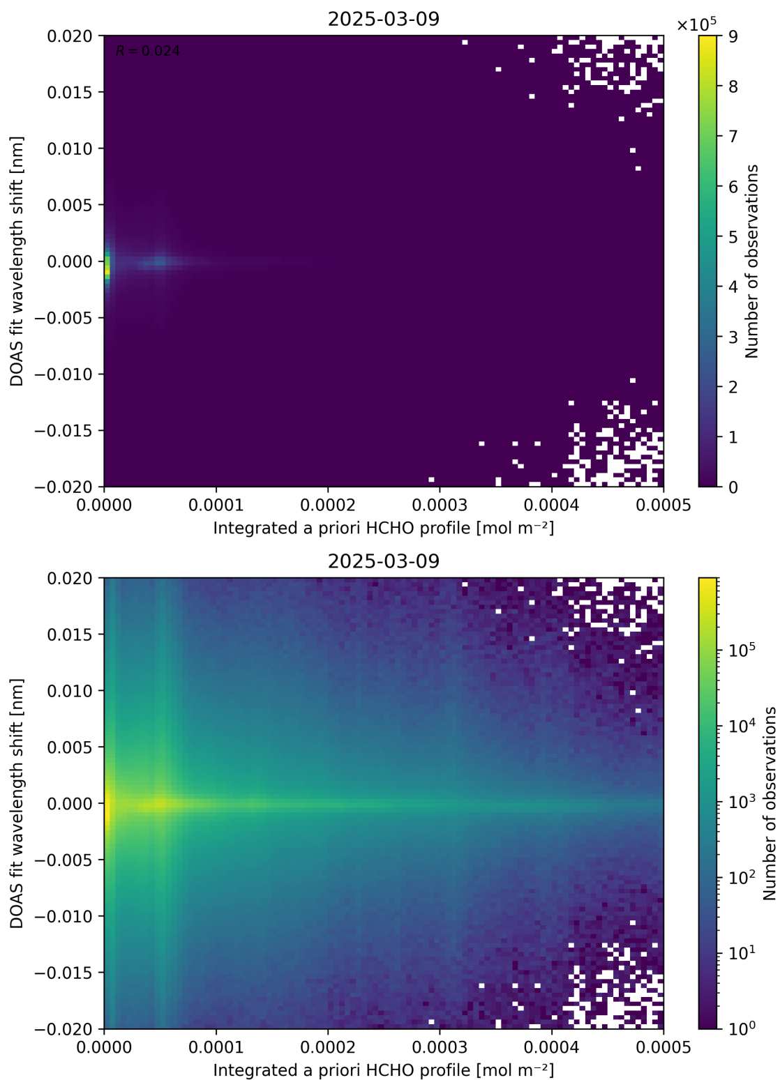
Figure 149: Scatter density plot of “Integrated a priori HCHO profile” against “DOAS fit wavelength shift” for 2025-03-08 to 2025-03-10.
