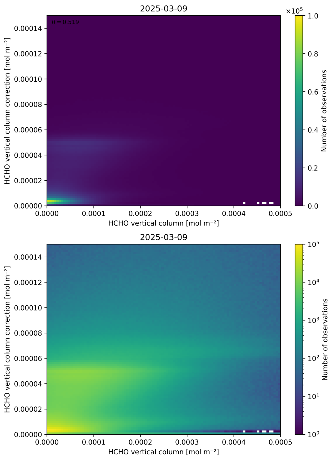
Figure 133: Scatter density plot of “HCHO vertical column” against “HCHO vertical column correction” for 2025-03-08 to 2025-03-10.
