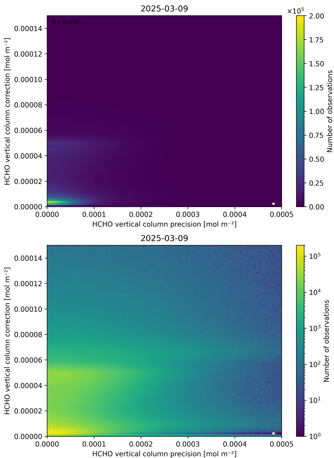
Figure 146: Scatter density plot of “HCHO vertical column precision” against “HCHO vertical column correction” for 2025-03-08 to 2025-03-10.
