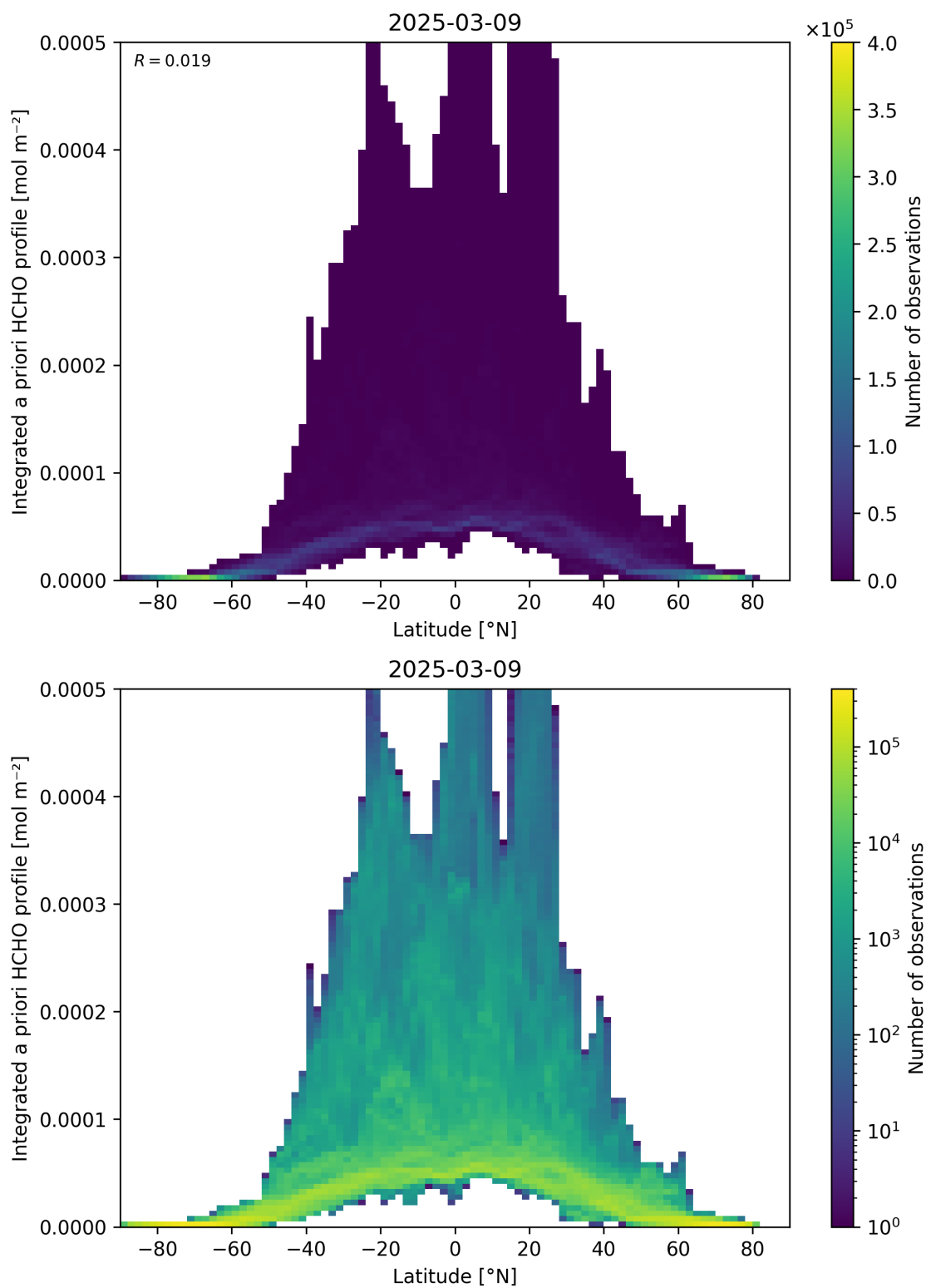
Figure 166: Scatter density plot of “Latitude” against “Integrated a priori HCHO profile” for 2025-03-08 to 2025-03-10.
