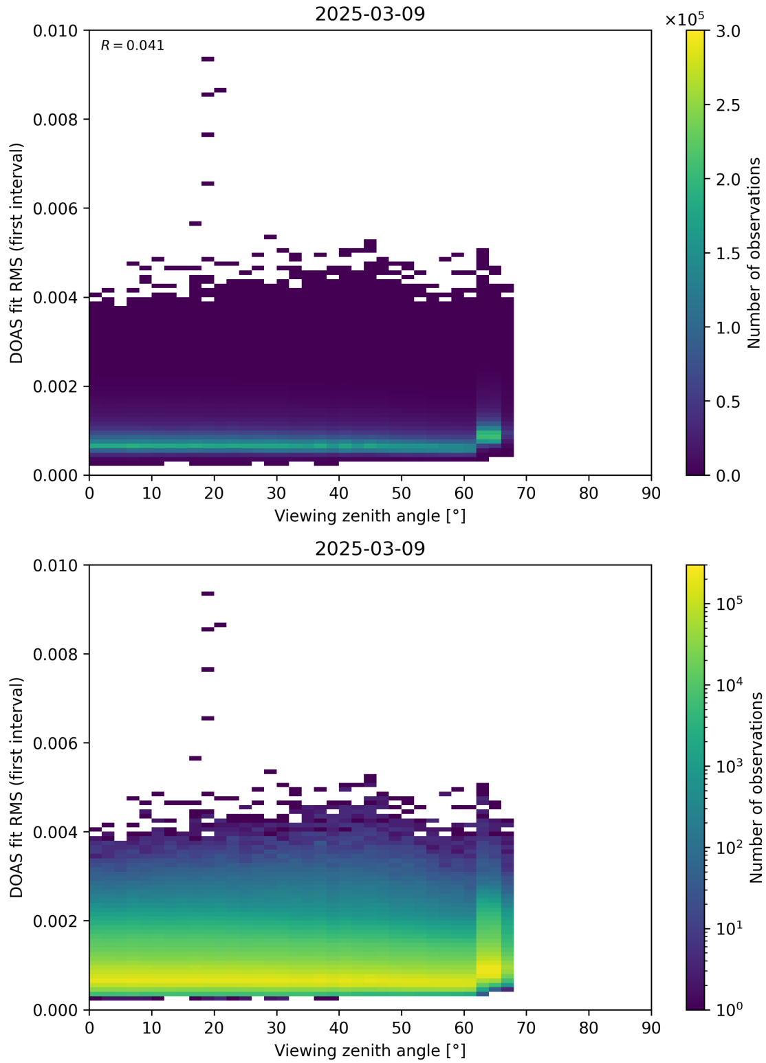
Figure 182: Scatter density plot of “Viewing zenith angle” against “DOAS fit RMS (first interval)” for 2025-03-08 to 2025-03-10.
