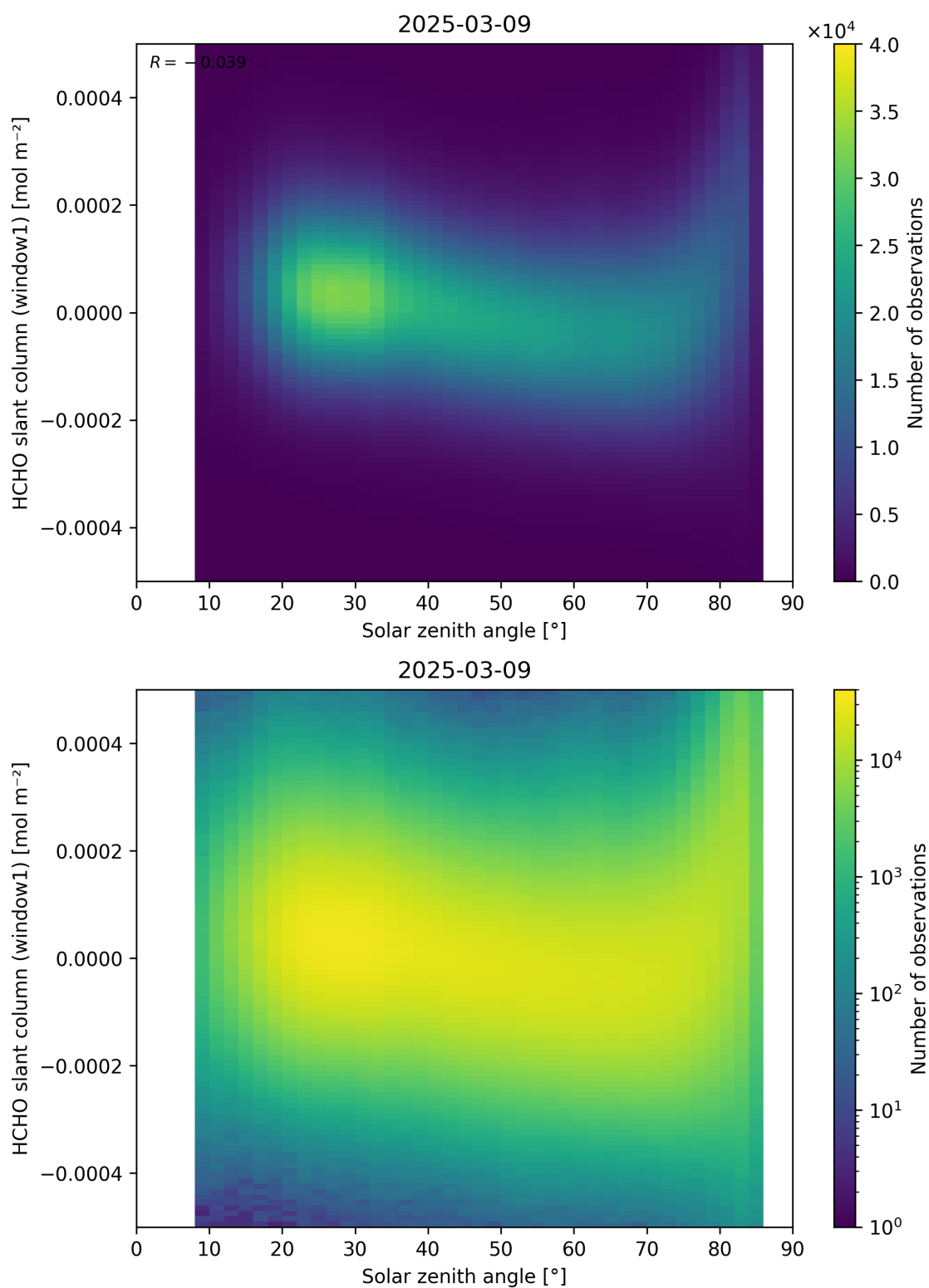
Figure 173: Scatter density plot of “Solar zenith angle” against “HCHO slant column (window1)” for 2025-03-08 to 2025-03-10.
