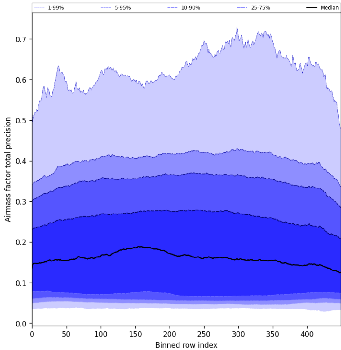
Figure 55: Along track statistics of “Airmass factor total precision” for 2025-03-08 to 2025-03-10
