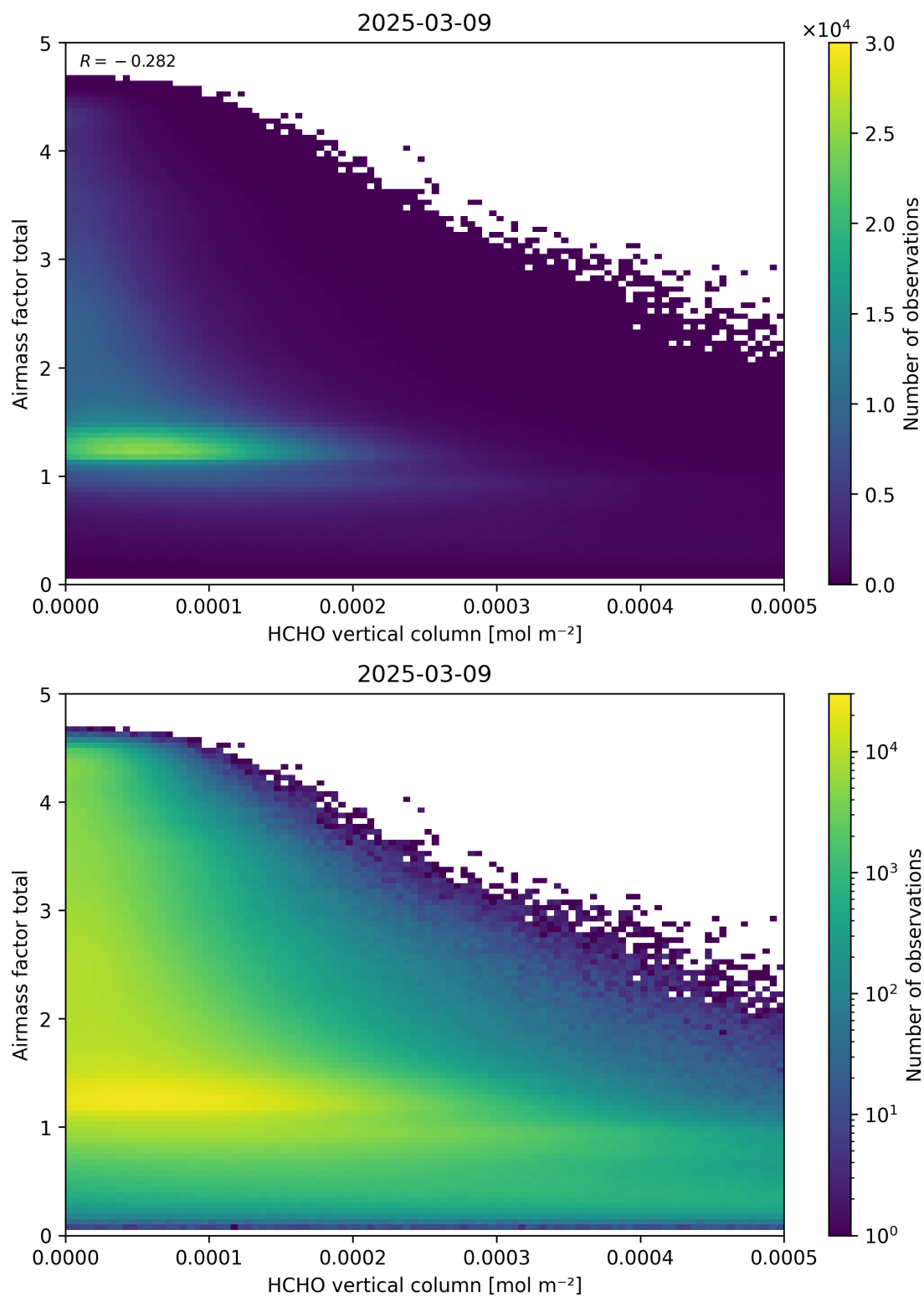
Figure 131: Scatter density plot of “HCHO vertical column” against “Airmass factor total” for 2025-03-08 to 2025-03-10.
