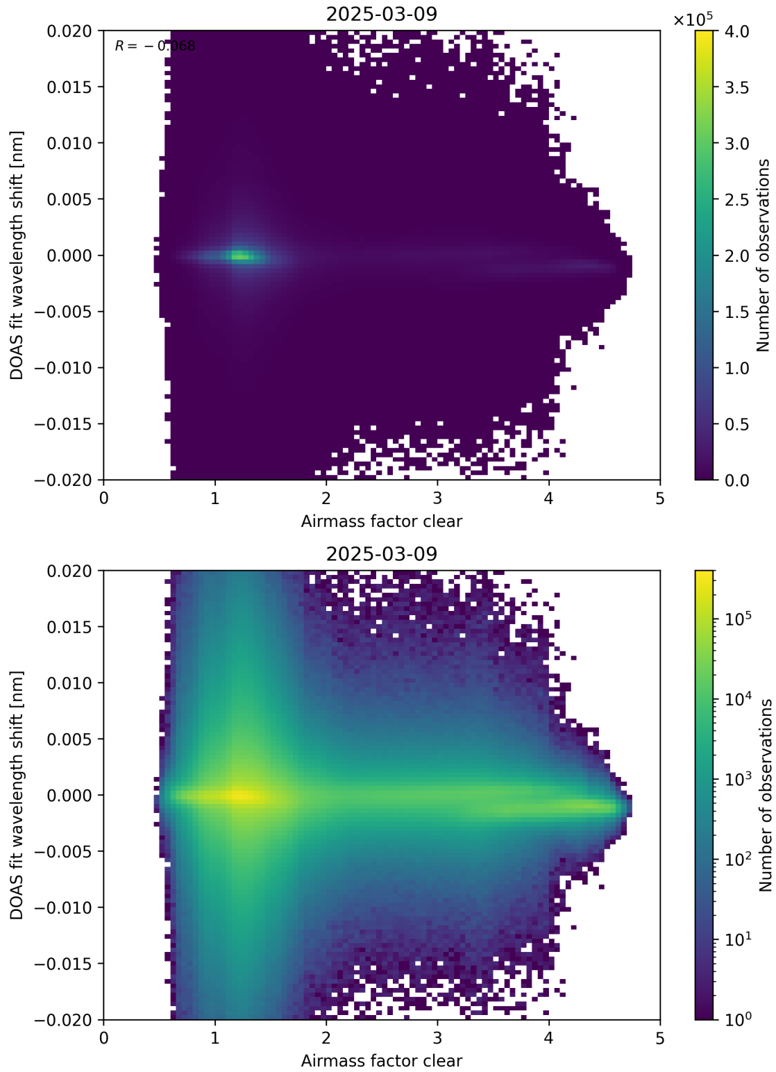
Figure 72: Scatter density plot of “Airmass factor clear” against “DOAS fit wavelength shift” for 2025-03-08 to 2025-03-10.
