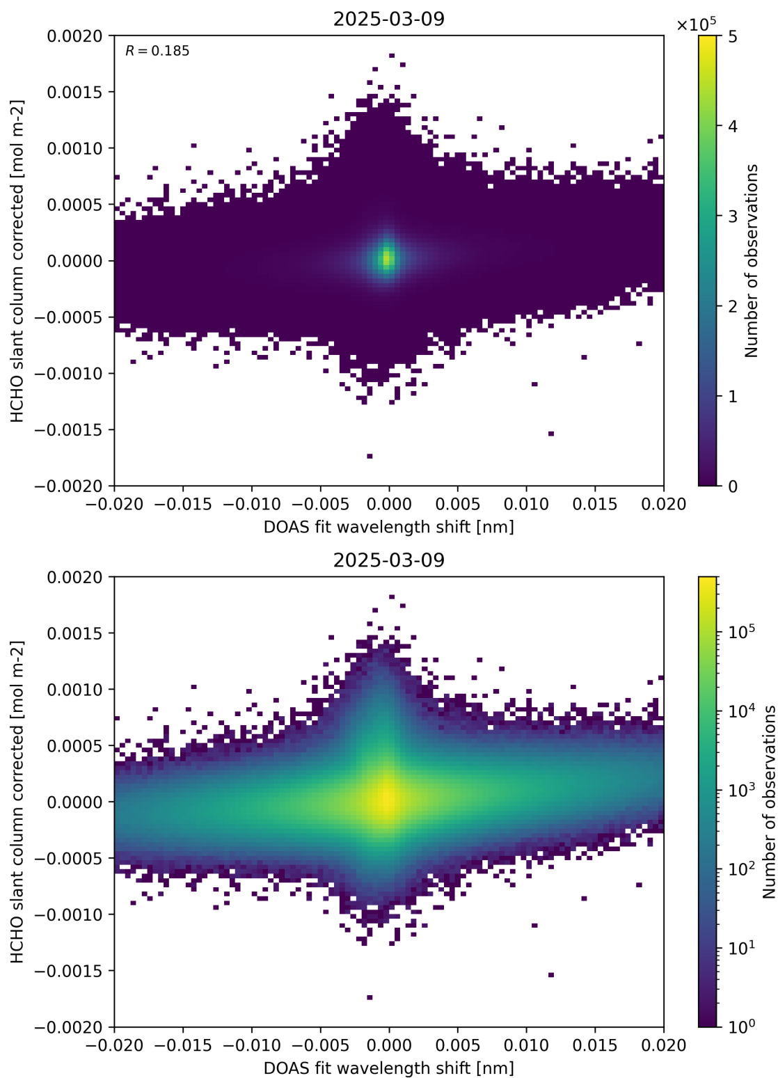
Figure 66: Scatter density plot of “DOAS fit wavelength shift” against “HCHO slant column corrected” for 2025-03-08 to 2025-03-10.
