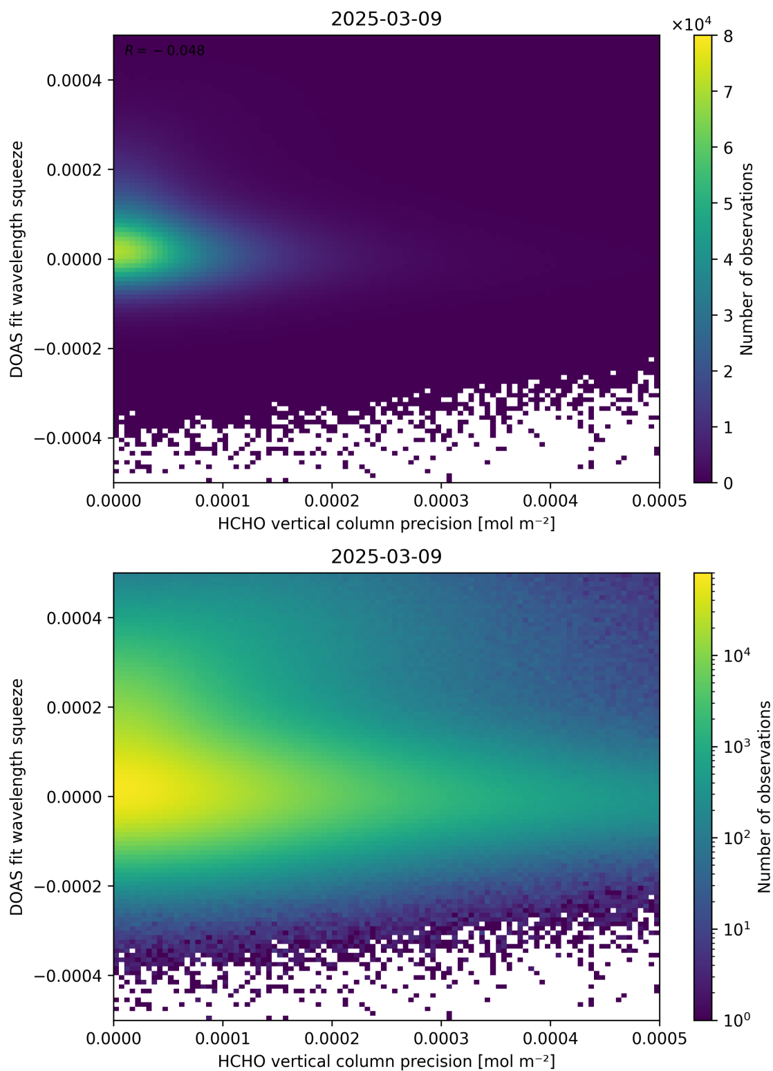
Figure 138: Scatter density plot of “HCHO vertical column precision” against “DOAS fit wavelength squeeze” for 2025-03-08 to 2025-03-10.
