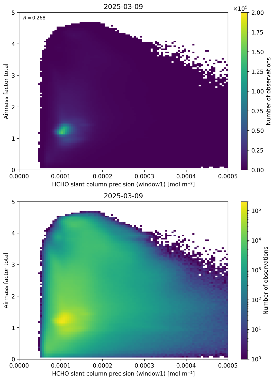
Figure 94: Scatter density plot of “HCHO slant column precision (window1)” against “Airmass factor total” for 2025-03-08 to 2025-03-10.
