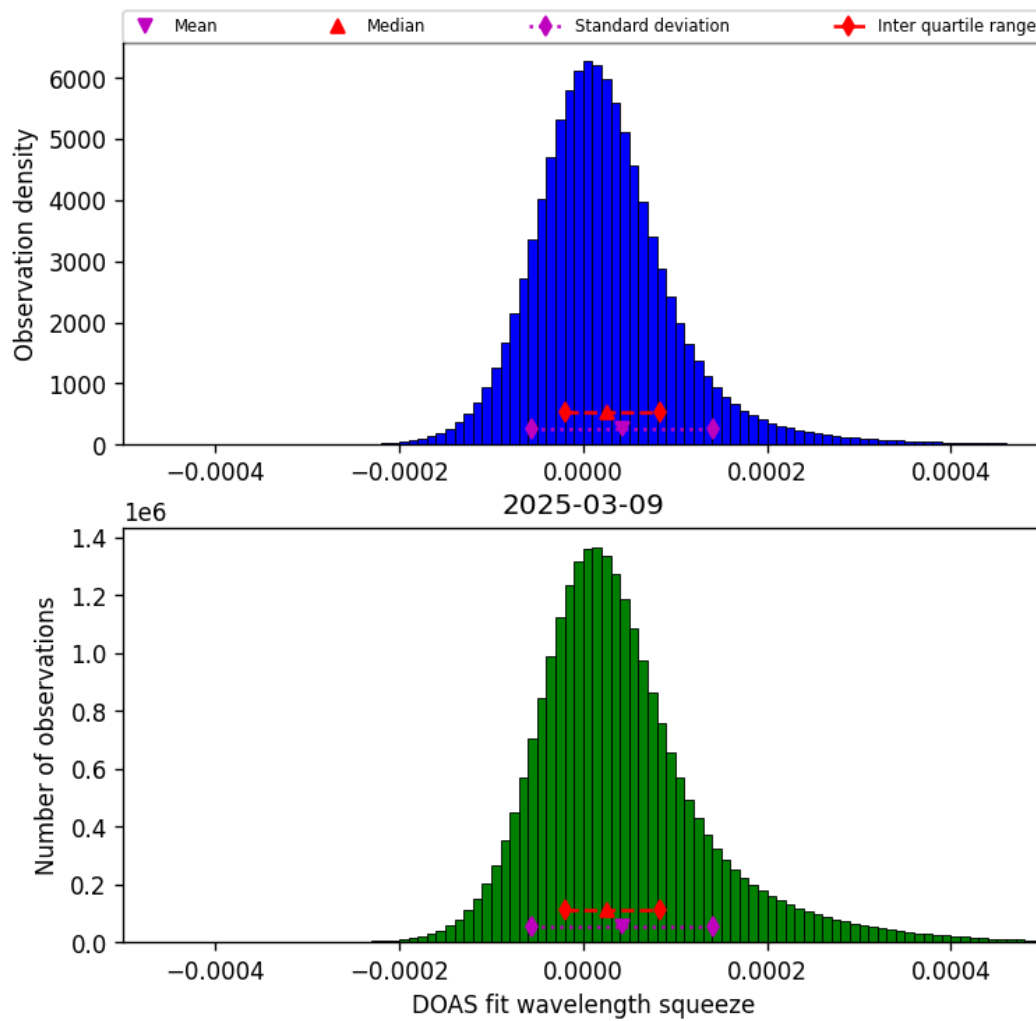
Figure 45: Histogram of “DOAS fit wavelength squeeze” for 2025-03-08 to 2025-03-10
