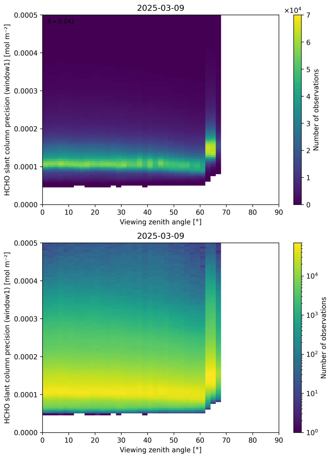
Figure 189: Scatter density plot of “Viewing zenith angle” against “HCHO slant column precision (window1)” for 2025-03-08 to 2025-03-10.
