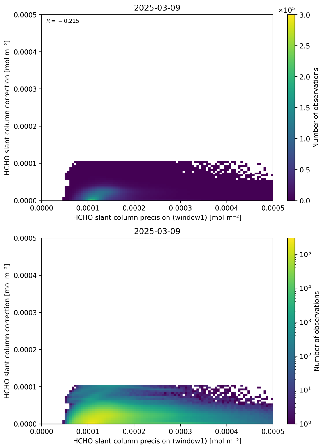
Figure 93: Scatter density plot of “HCHO slant column precision (window1)” against “HCHO slant column correction” for 2025-03-08 to 2025-03-10.
