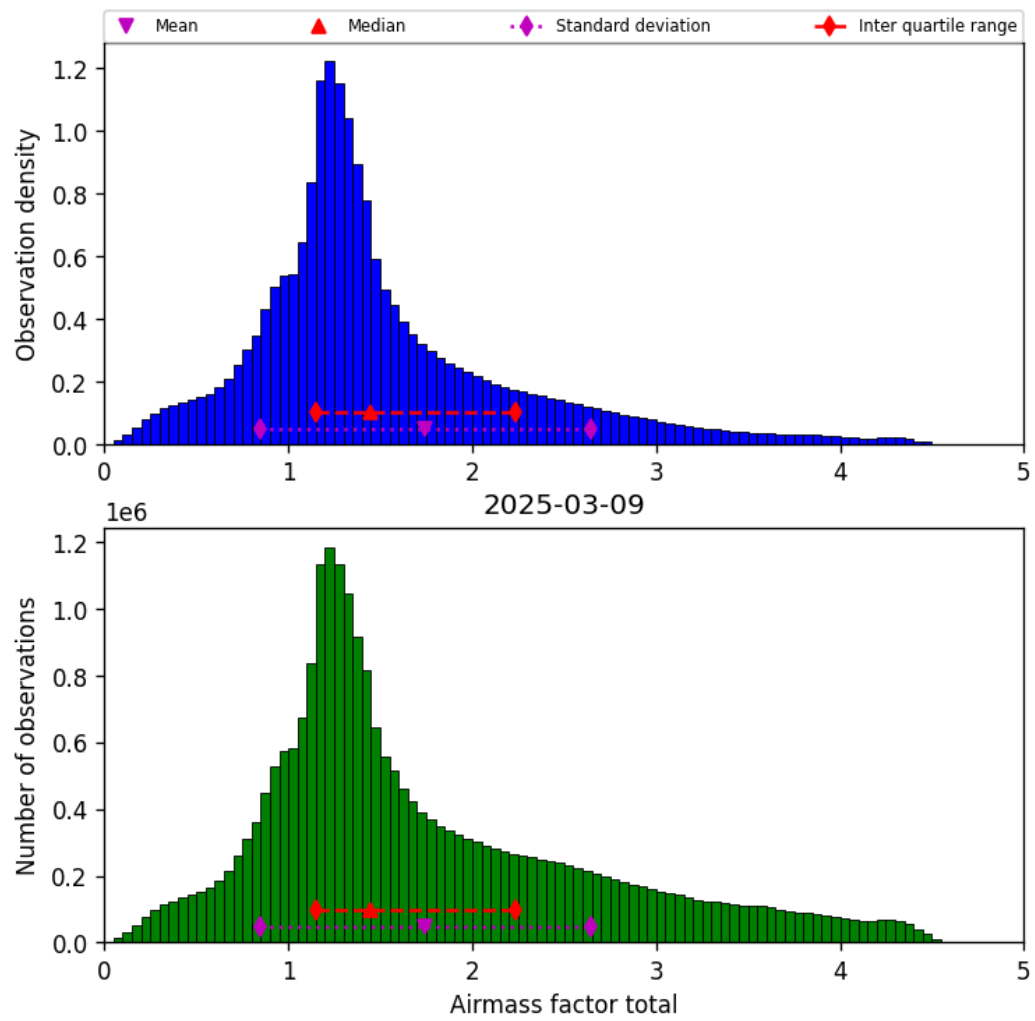
Figure 40: Histogram of “Airmass factor total” for 2025-03-08 to 2025-03-10
