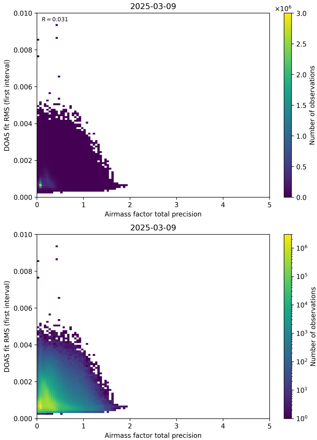
Figure 105: Scatter density plot of “Airmass factor total precision” against “DOAS fit RMS (first interval)” for 2025-03-08 to 2025-03-10.
