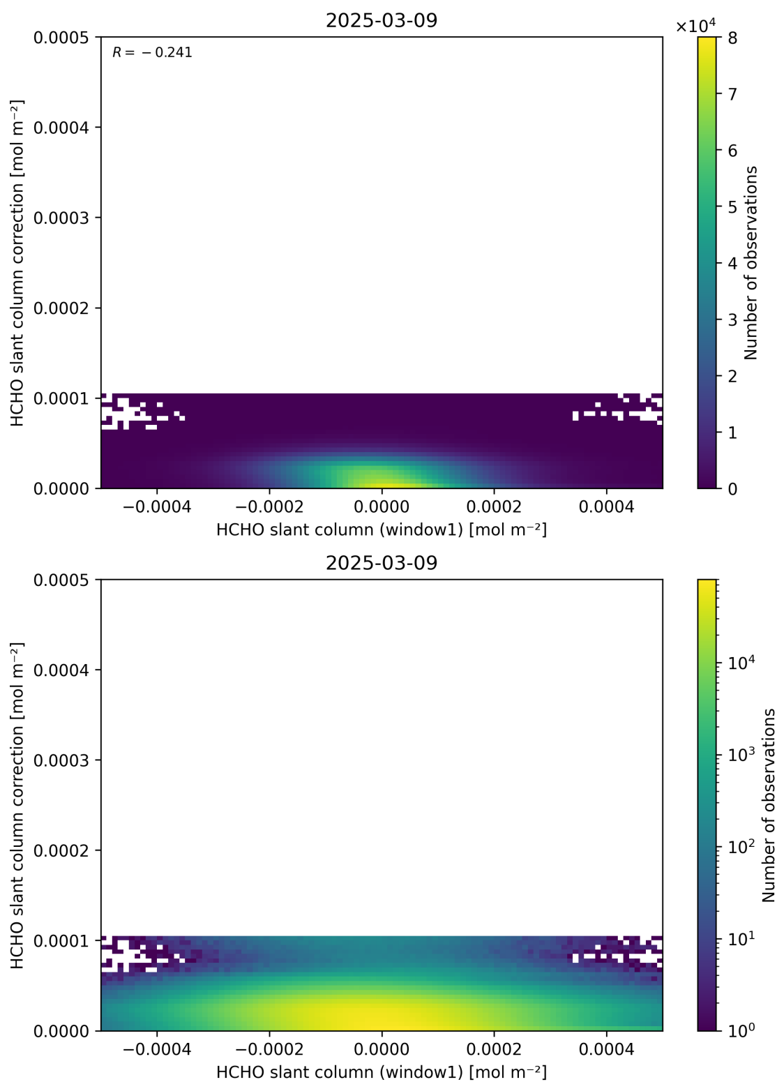
Figure 83: Scatter density plot of “HCHO slant column (window1)” against “HCHO slant column correction” for 2025-03-08 to 2025-03-10.
