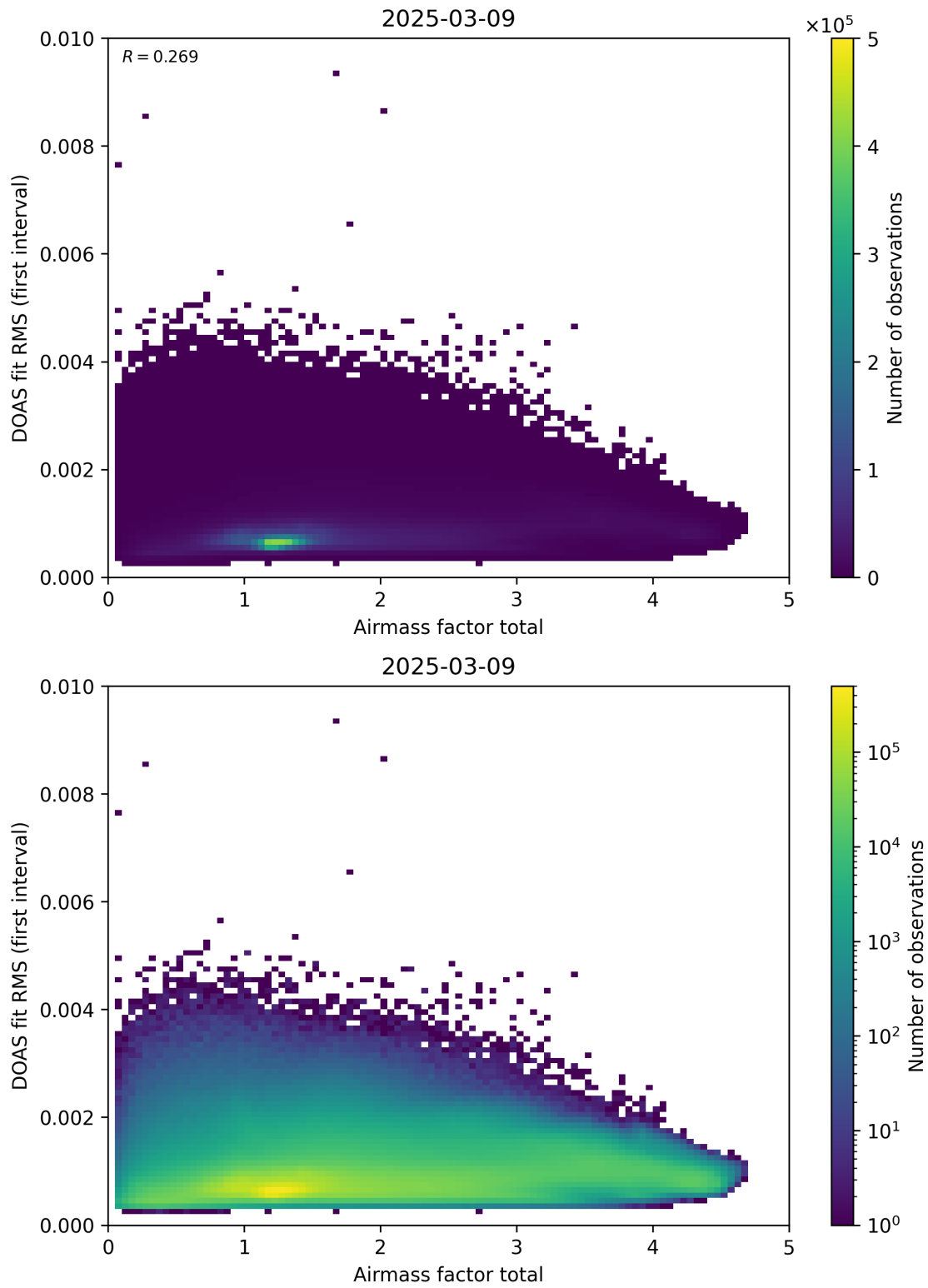
Figure 97: Scatter density plot of “Airmass factor total” against “DOAS fit RMS (first interval)” for 2025-03-08 to 2025-03-10.
