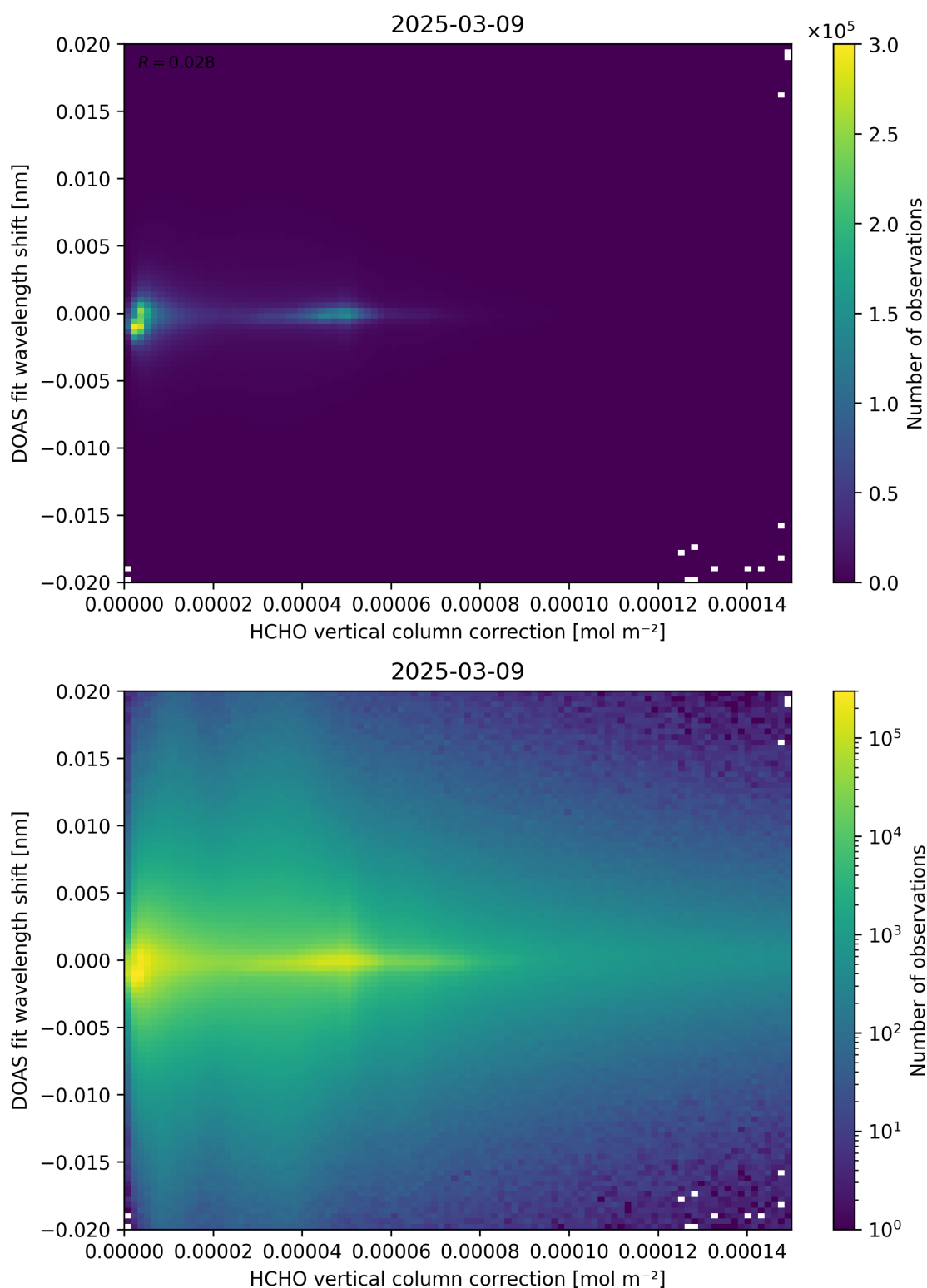
Figure 113: Scatter density plot of “HCHO vertical column correction” against “DOAS fit wavelength shift” for 2025-03-08 to 2025-03-10.
