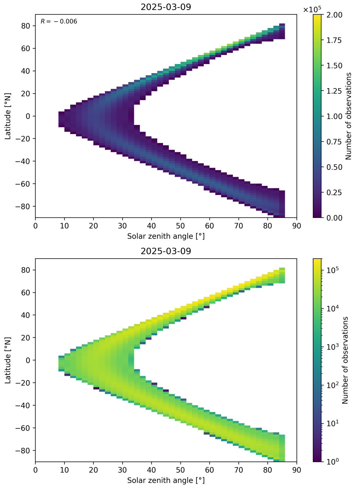
Figure 181: Scatter density plot of “Solar zenith angle” against “Latitude” for 2025-03-08 to 2025-03-10.
