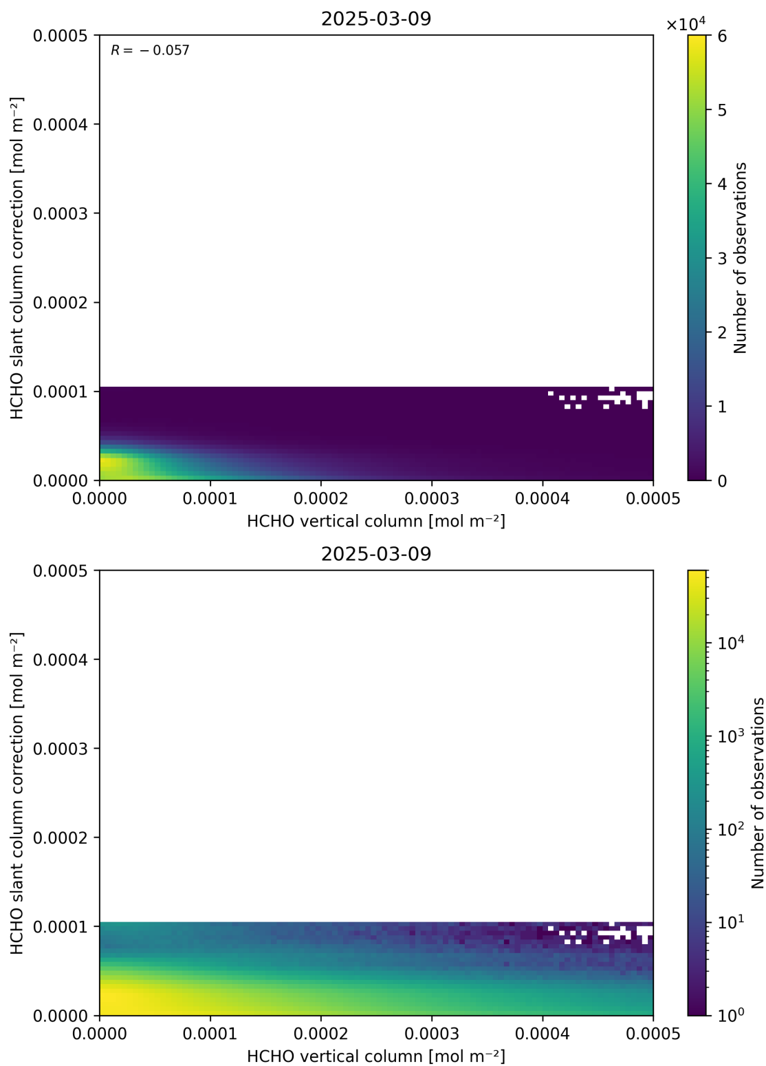
Figure 128: Scatter density plot of “HCHO vertical column” against “HCHO slant column correction” for 2025-03-08 to 2025-03-10.
