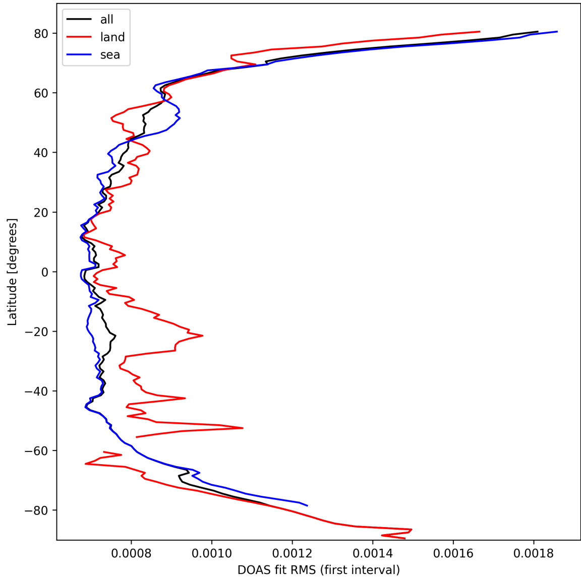
Figure 32: Zonal average of “DOAS fit RMS (first interval)” for 2025-03-08 to 2025-03-10.
