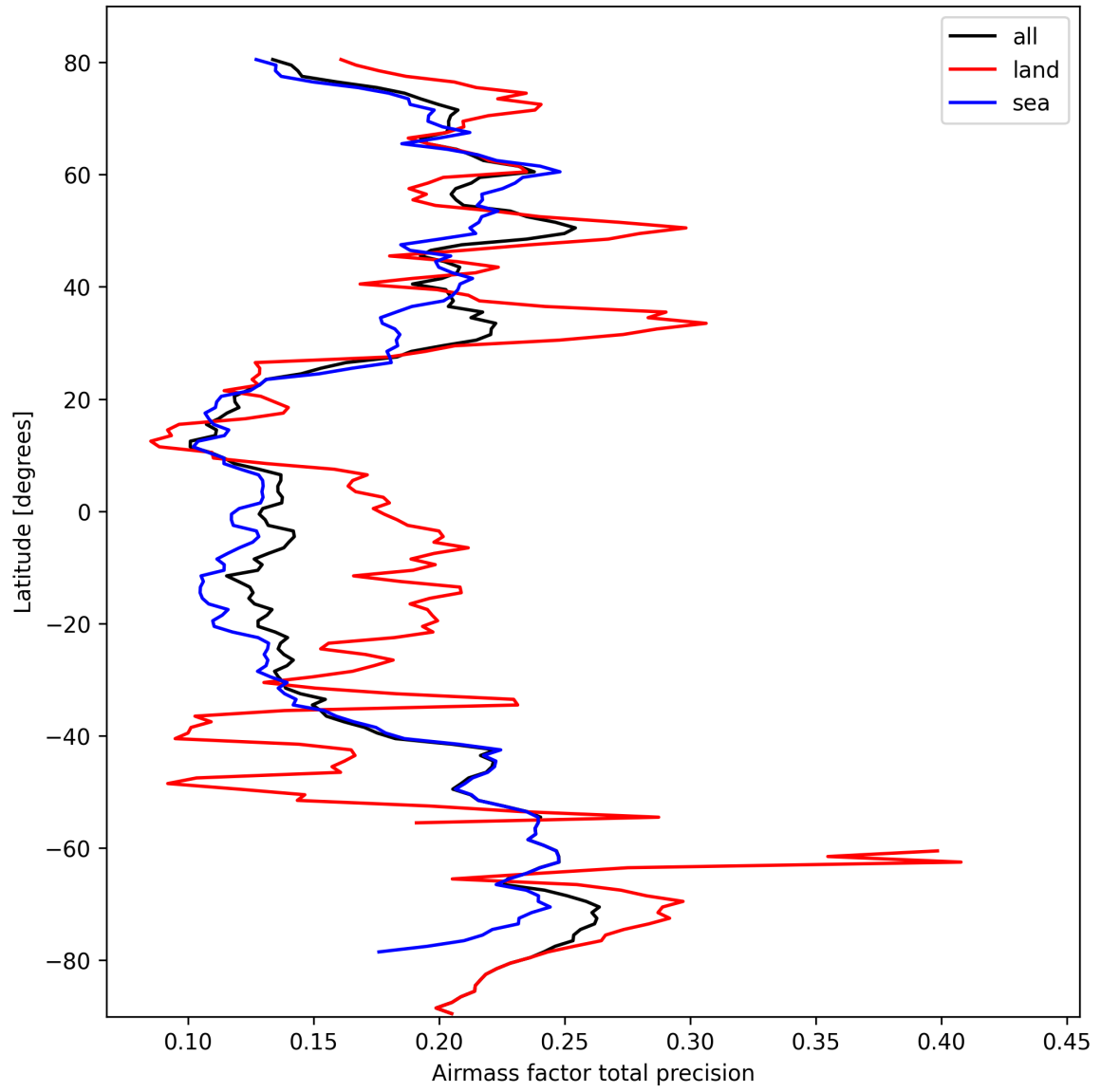
Figure 27: Zonal average of “Airmass factor total precision” for 2025-03-08 to 2025-03-10.
