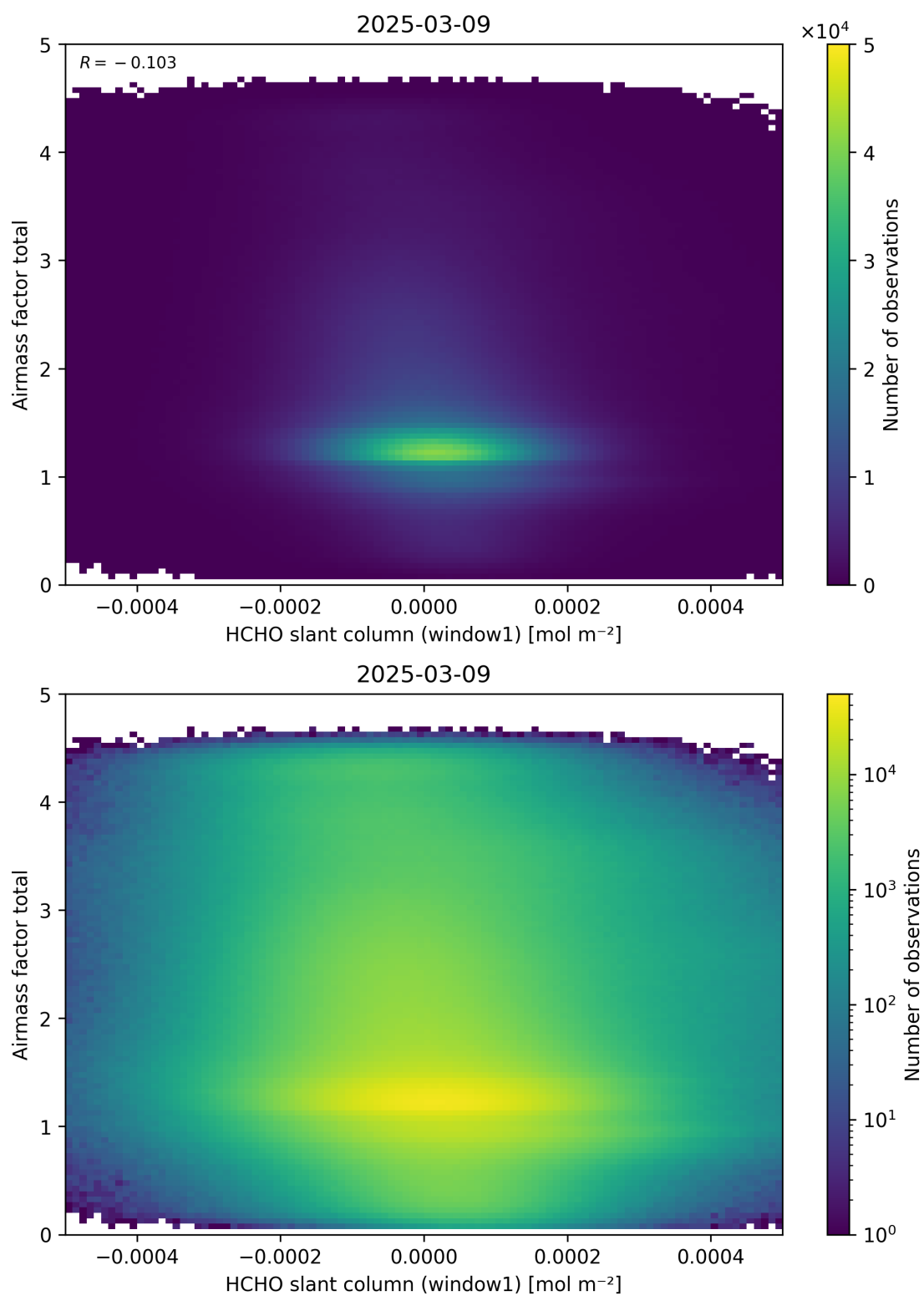
Figure 85: Scatter density plot of “HCHO slant column (window1)” against “Airmass factor total” for 2025-03-08 to 2025-03-10.
