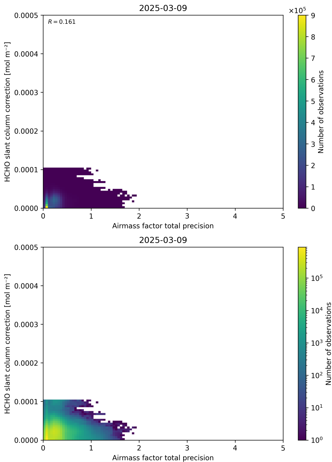
Figure 110: Scatter density plot of “Airmass factor total precision” against “HCHO slant column correction” for 2025-03-08 to 2025-03-10.
