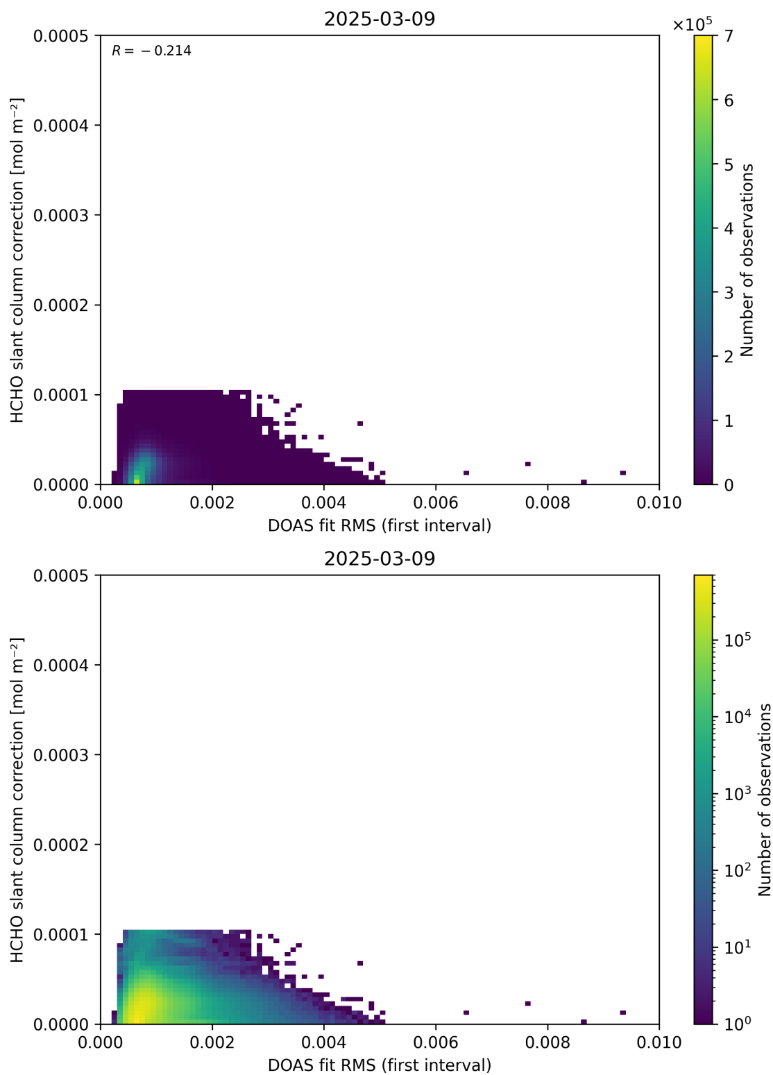
Figure 63: Scatter density plot of “DOAS fit RMS (first interval)” against “HCHO slant column correction” for 2025-03-08 to 2025-03-10.
