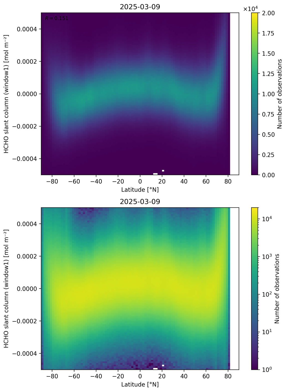
Figure 159: Scatter density plot of “Latitude” against “HCHO slant column (window1)” for 2025-03-08 to 2025-03-10.
