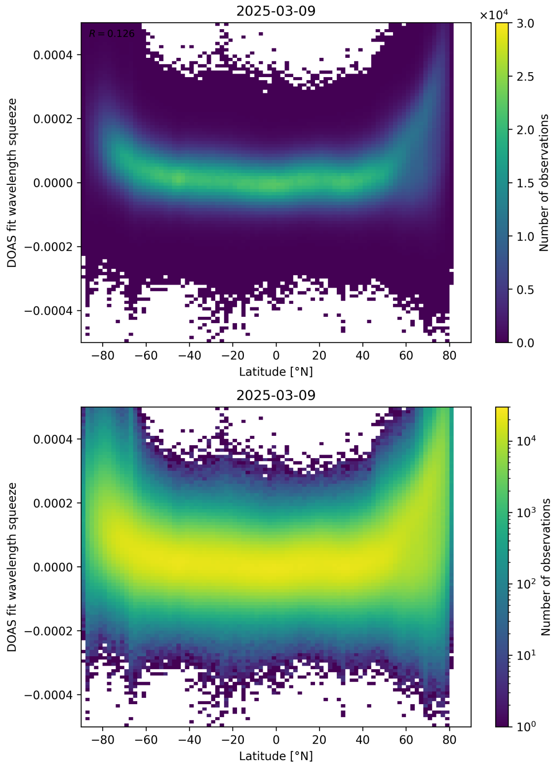
Figure 155: Scatter density plot of “Latitude” against “DOAS fit wavelength squeeze” for 2025-03-08 to 2025-03-10.
