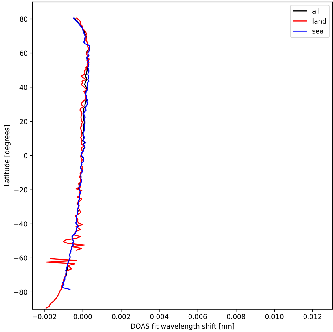
Figure 30: Zonal average of “DOAS fit wavelength shift” for 2025-03-08 to 2025-03-10.
