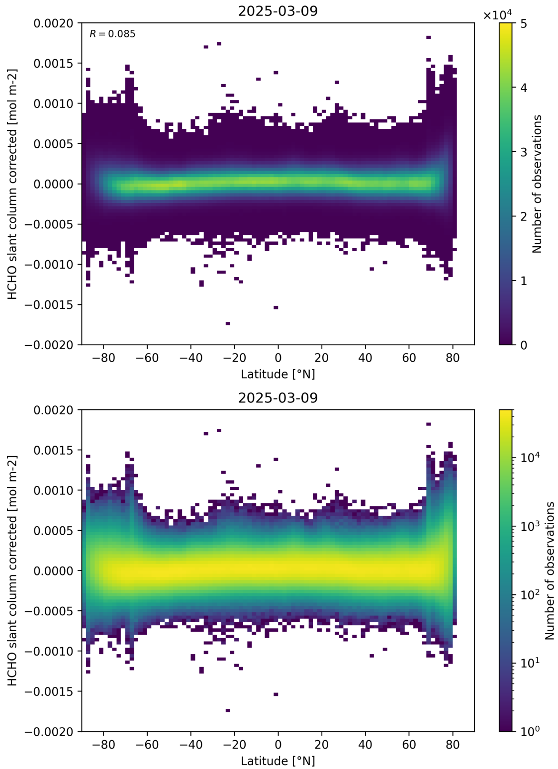
Figure 157: Scatter density plot of “Latitude” against “HCHO slant column corrected” for 2025-03-08 to 2025-03-10.
