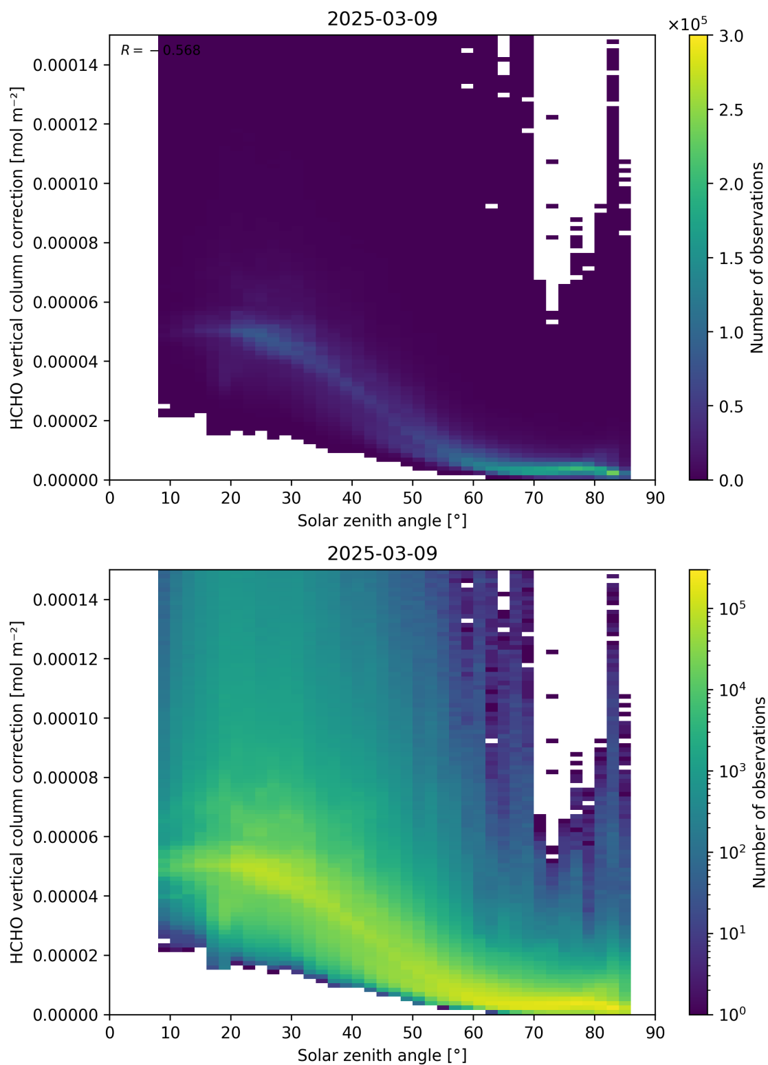
Figure 178: Scatter density plot of “Solar zenith angle” against “HCHO vertical column correction” for 2025-03-08 to 2025-03-10.
