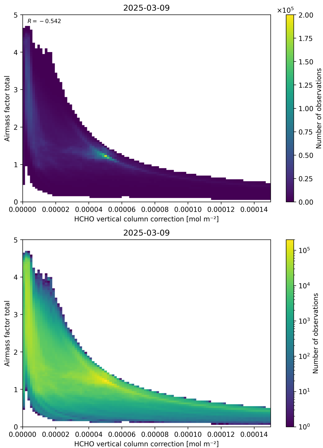
Figure 120: Scatter density plot of “HCHO vertical column correction” against “Airmass factor total” for 2025-03-08 to 2025-03-10.
