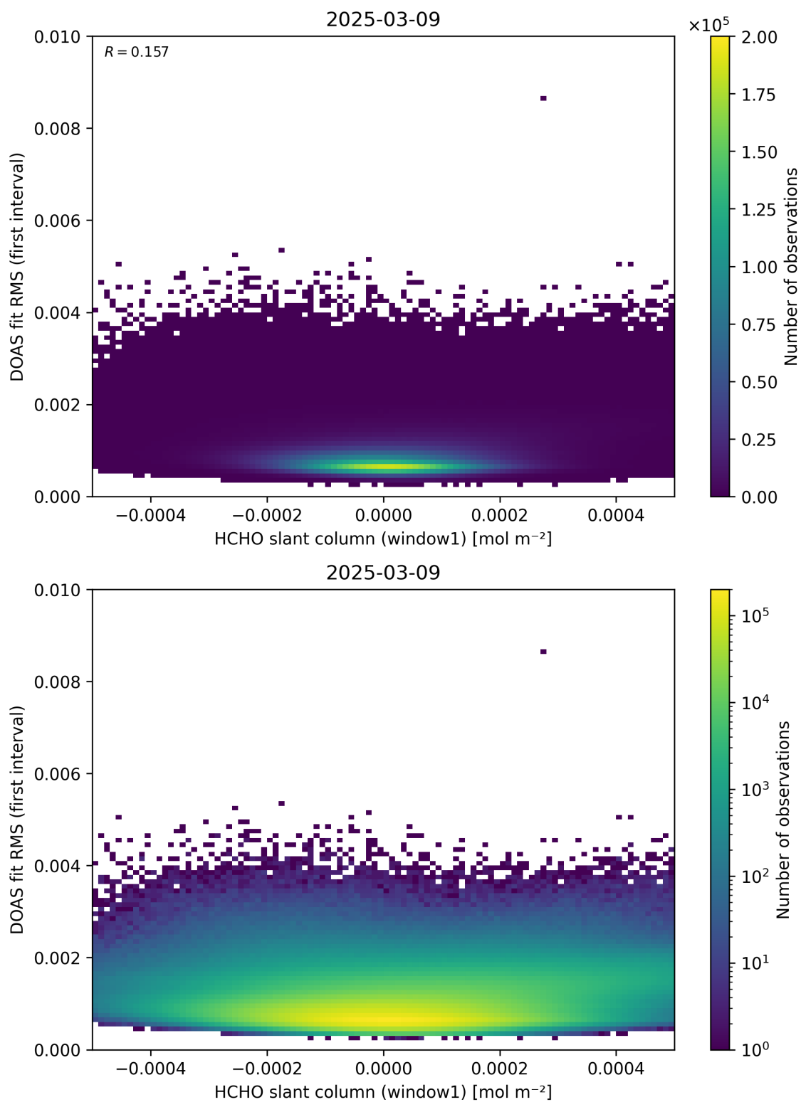
Figure 78: Scatter density plot of “HCHO slant column (window1)” against “DOAS fit RMS (first interval)” for 2025-03-08 to 2025-03-10.
