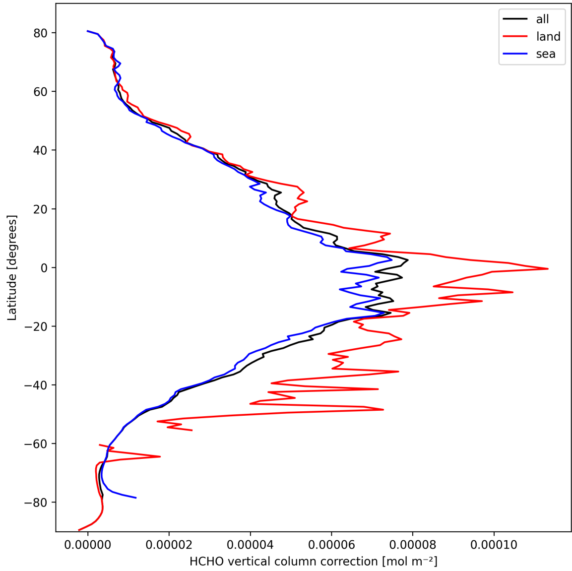
Figure 23: Zonal average of “HCHO vertical column correction” for 2025-03-08 to 2025-03-10.
