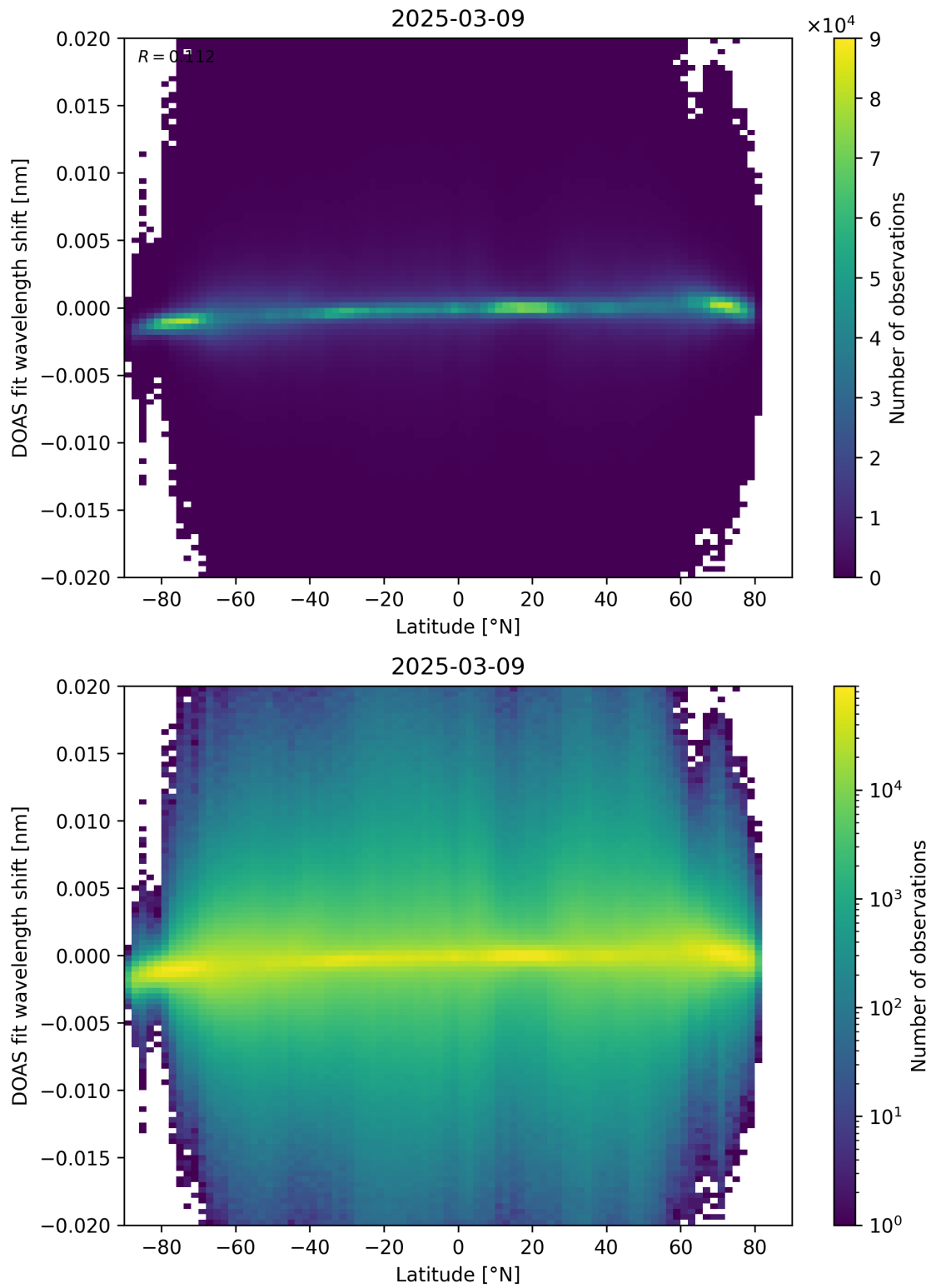
Figure 154: Scatter density plot of “Latitude” against “DOAS fit wavelength shift” for 2025-03-08 to 2025-03-10.
