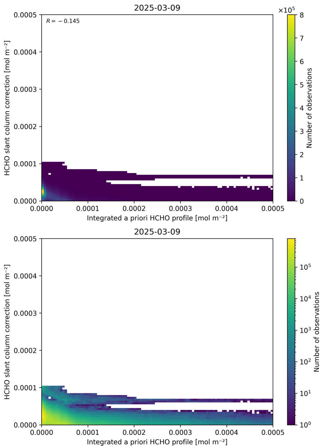
Figure 152: Scatter density plot of “Integrated a priori HCHO profile” against “HCHO slant column correction” for 2025-03-08 to 2025-03-10.
