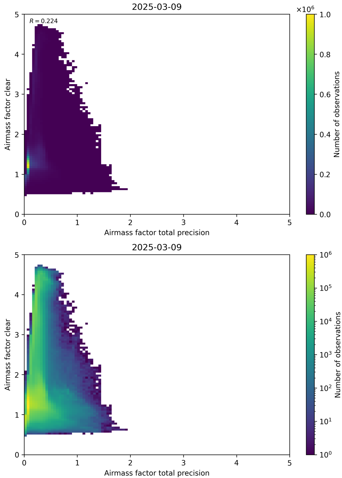
Figure 108: Scatter density plot of “Airmass factor total precision” against “Airmass factor clear” for 2025-03-08 to 2025-03-10.
