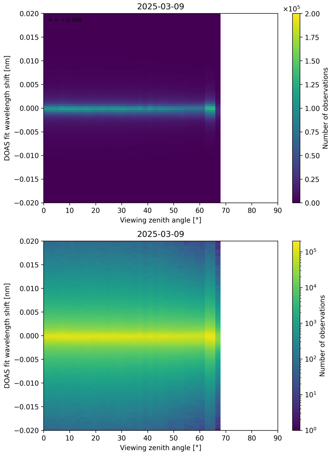
Figure 183: Scatter density plot of “Viewing zenith angle” against “DOAS fit wavelength shift” for 2025-03-08 to 2025-03-10.
