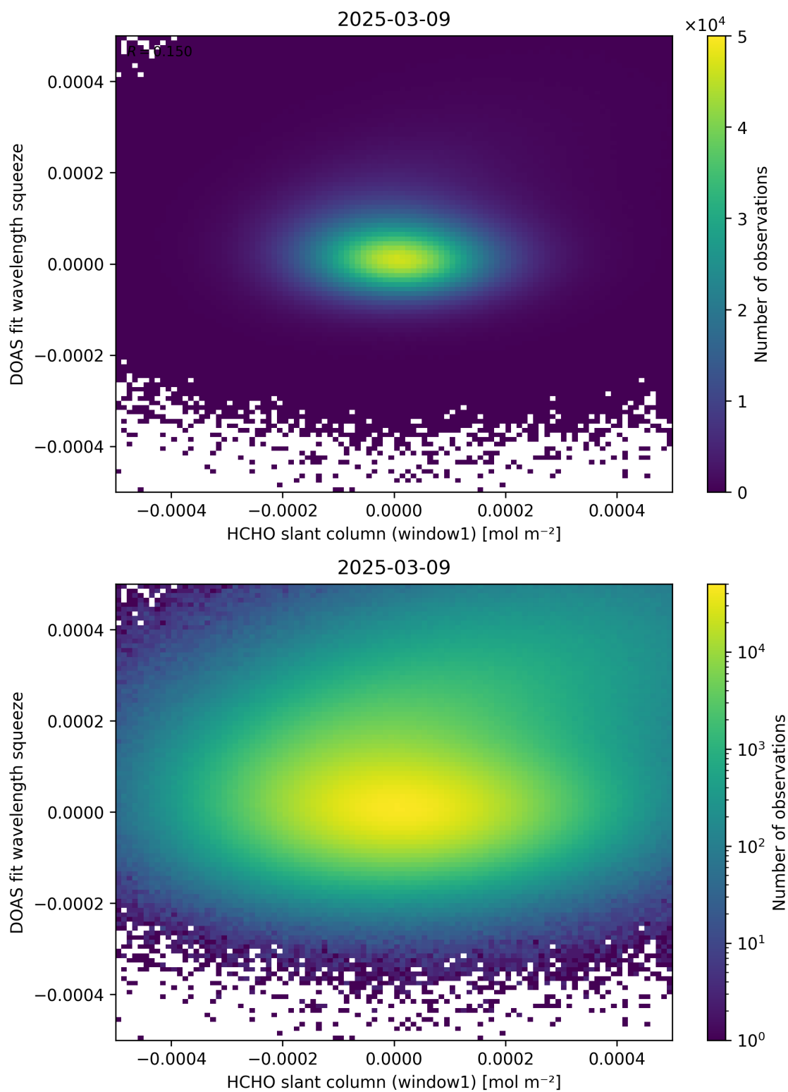
Figure 80: Scatter density plot of “HCHO slant column (window1)” against “DOAS fit wavelength squeeze” for 2025-03-08 to 2025-03-10.
