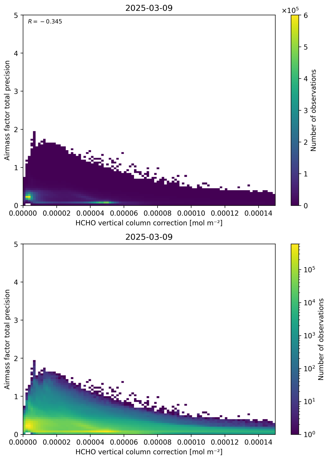
Figure 121: Scatter density plot of “HCHO vertical column correction” against “Airmass factor total precision” for 2025-03-08 to 2025-03-10.
