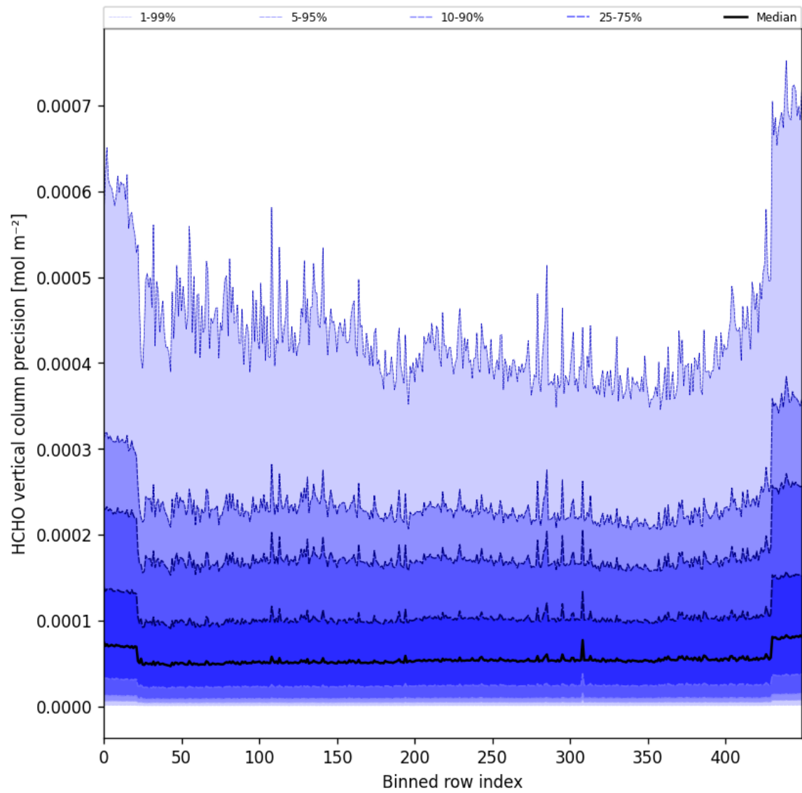
Figure 50: Along track statistics of “HCHO vertical column precision” for 2025-03-08 to 2025-03-10
