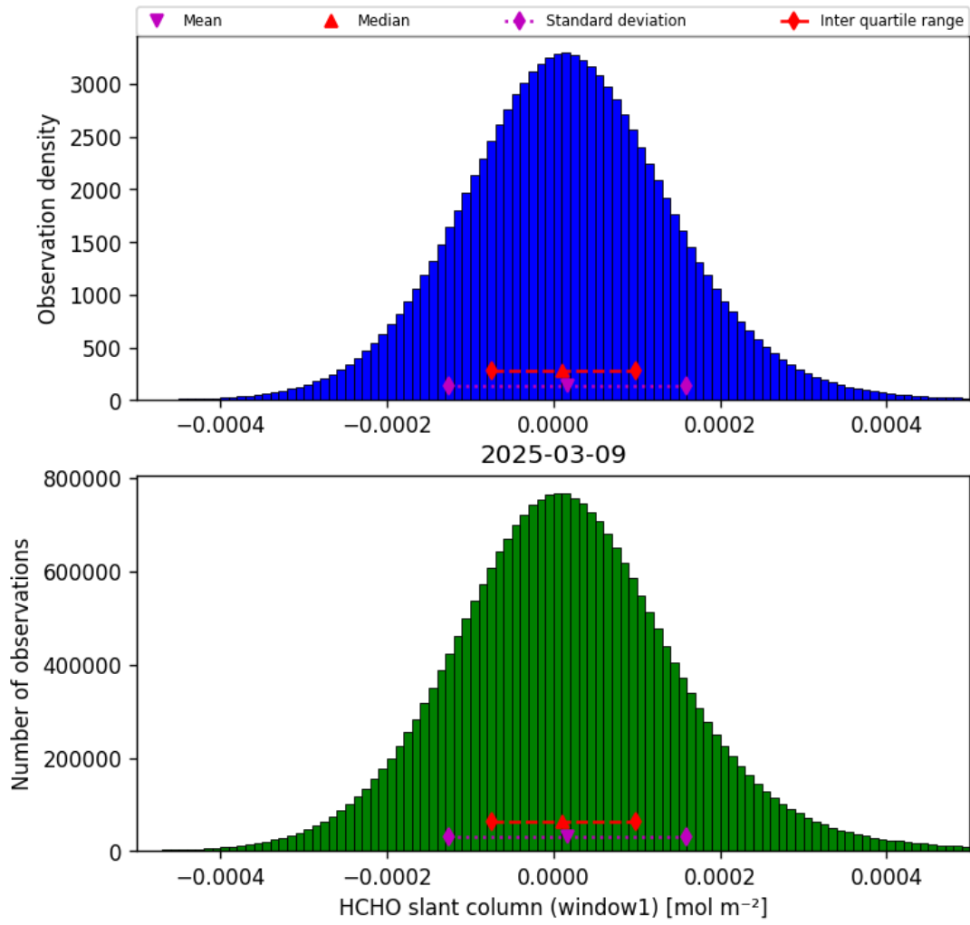
Figure 38: Histogram of “HCHO slant column (window1)” for 2025-03-08 to 2025-03-10
