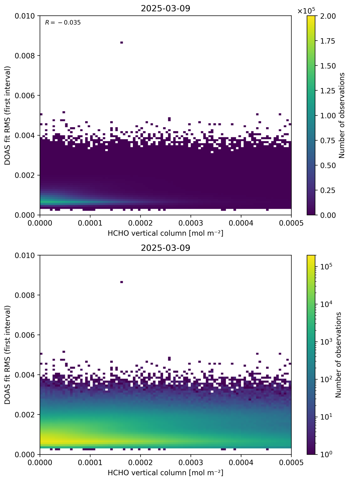
Figure 123: Scatter density plot of “HCHO vertical column” against “DOAS fit RMS (first interval)” for 2025-03-08 to 2025-03-10.
