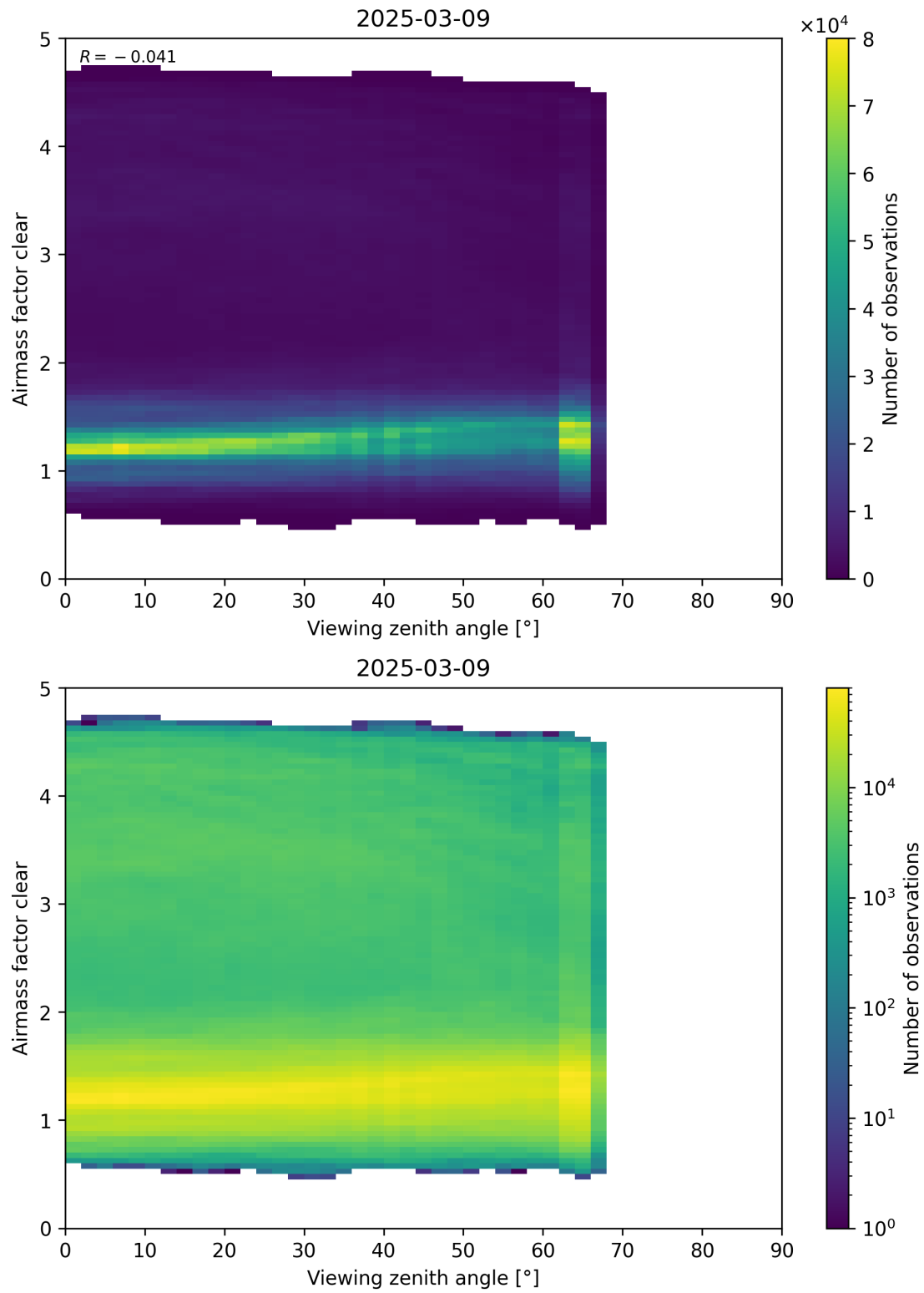
Figure 185: Scatter density plot of “Viewing zenith angle” against “Airmass factor clear” for 2025-03-08 to 2025-03-10.
