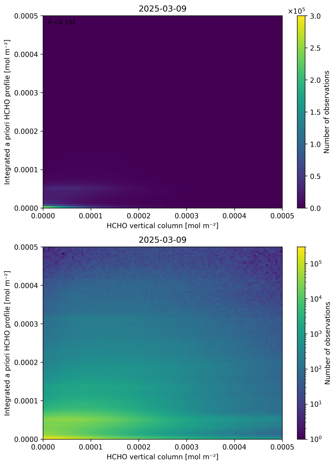
Figure 135: Scatter density plot of “HCHO vertical column” against “Integrated a priori HCHO profile” for 2025-03-08 to 2025-03-10.
