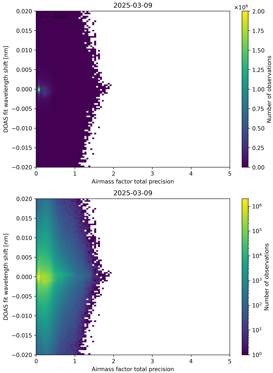
Figure 106: Scatter density plot of “Airmass factor total precision” against “DOAS fit wavelength shift” for 2025-03-08 to 2025-03-10.
