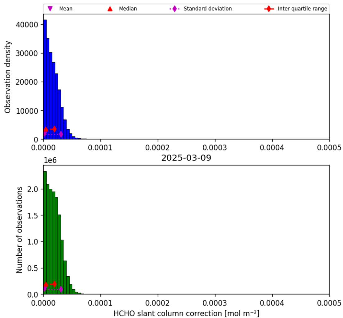
Figure 47: Histogram of “HCHO slant column correction” for 2025-03-08 to 2025-03-10
