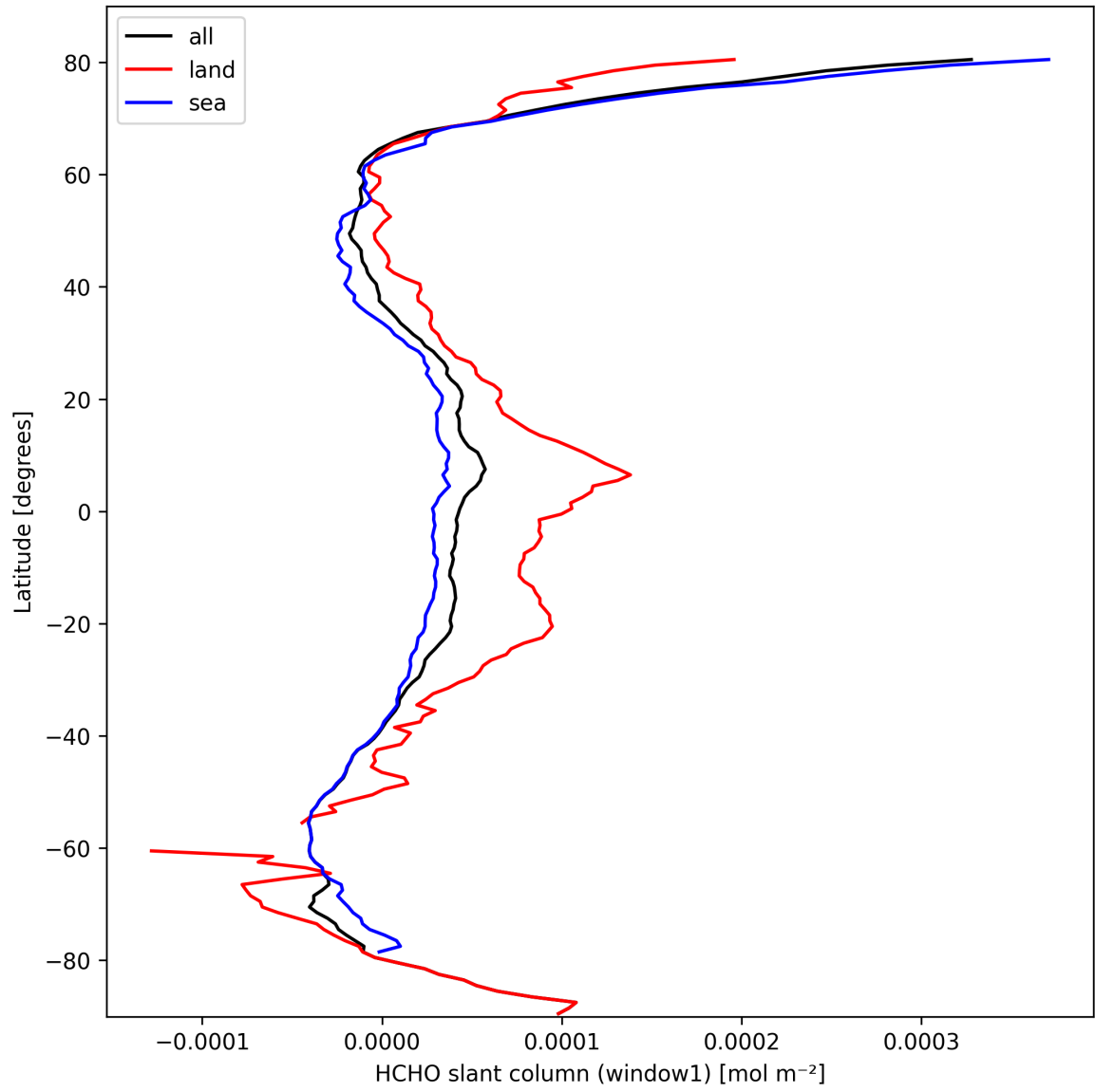
Figure 24: Zonal average of “HCHO slant column (window1)” for 2025-03-08 to 2025-03-10.
