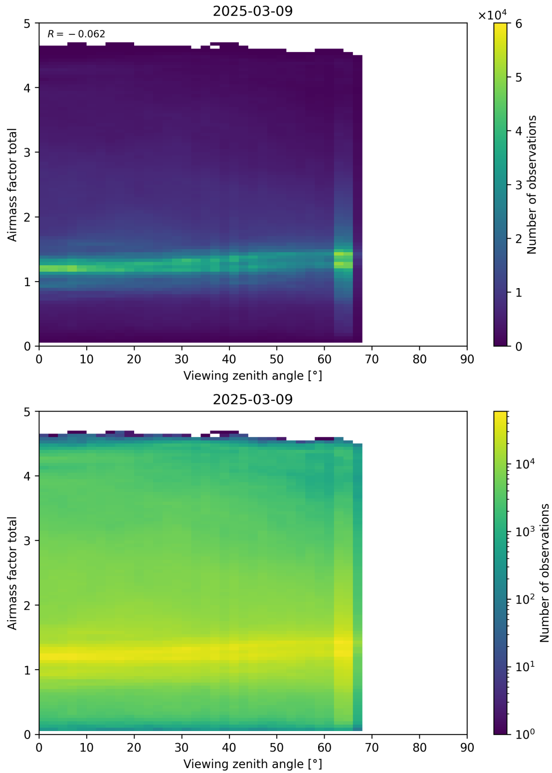
Figure 190: Scatter density plot of “Viewing zenith angle” against “Airmass factor total” for 2025-03-08 to 2025-03-10.
