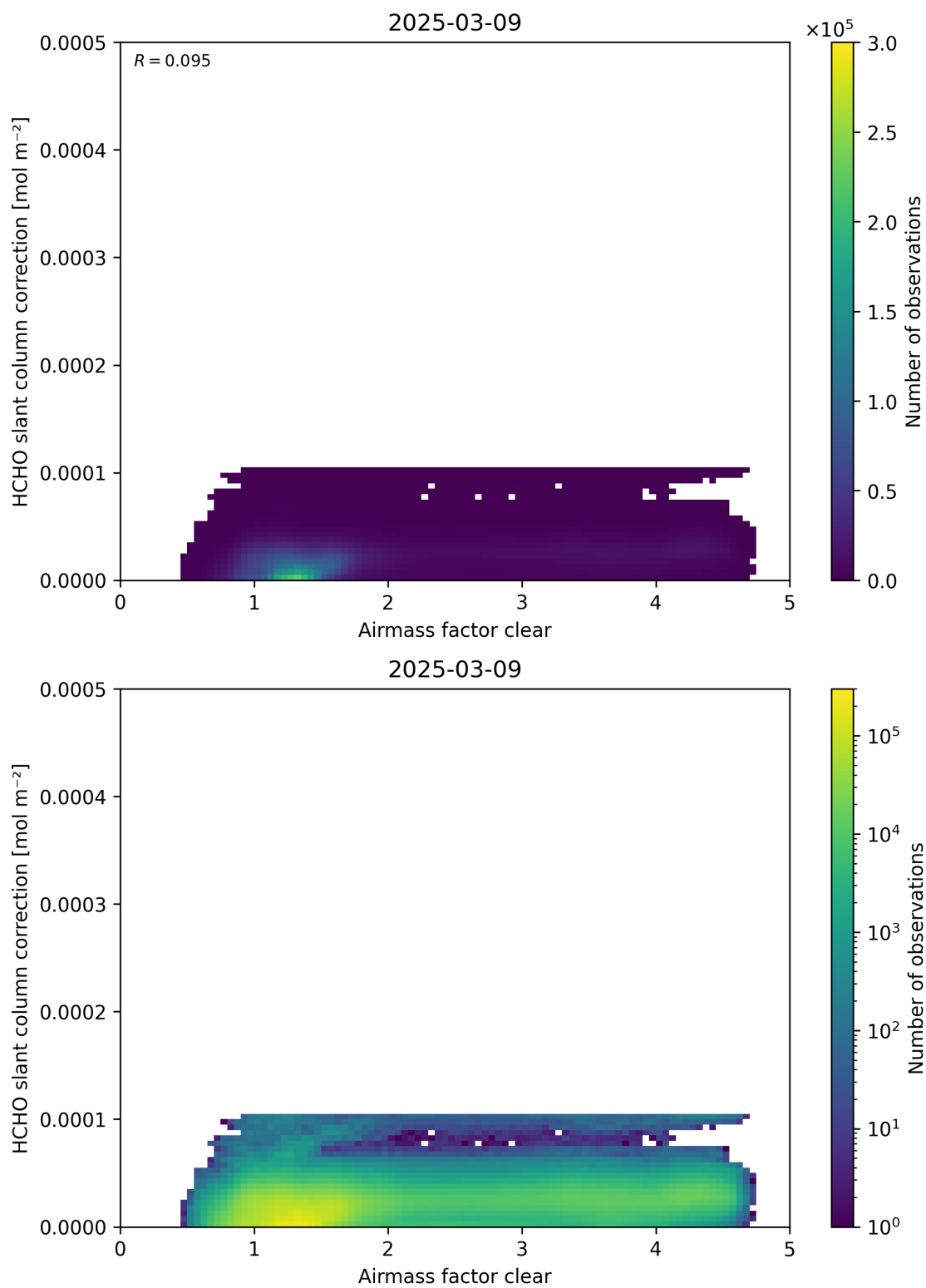
Figure 75: Scatter density plot of “Airmass factor clear” against “HCHO slant column correction” for 2025-03-08 to 2025-03-10.
