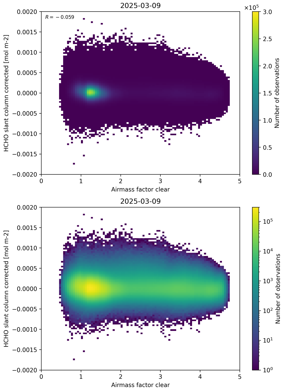
Figure 74: Scatter density plot of “Airmass factor clear” against “HCHO slant column corrected” for 2025-03-08 to 2025-03-10.
