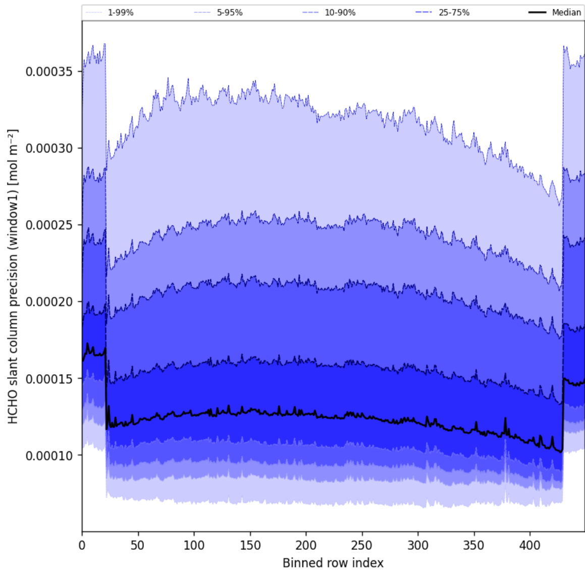
Figure 53: Along track statistics of “HCHO slant column precision (window1)” for 2025-03-08 to 2025-03-10
