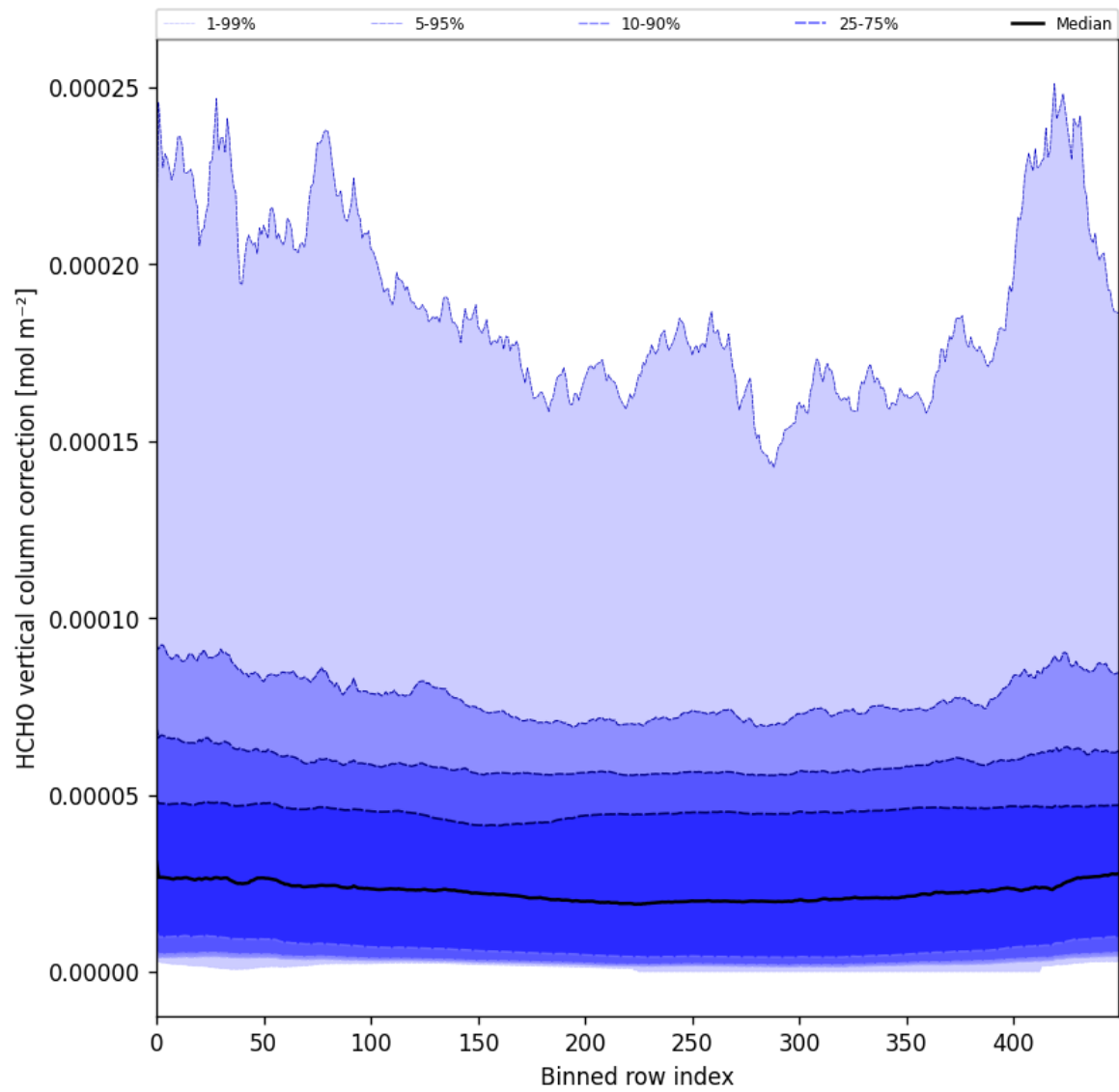
Figure 51: Along track statistics of “HCHO vertical column correction” for 2025-03-08 to 2025-03-10
