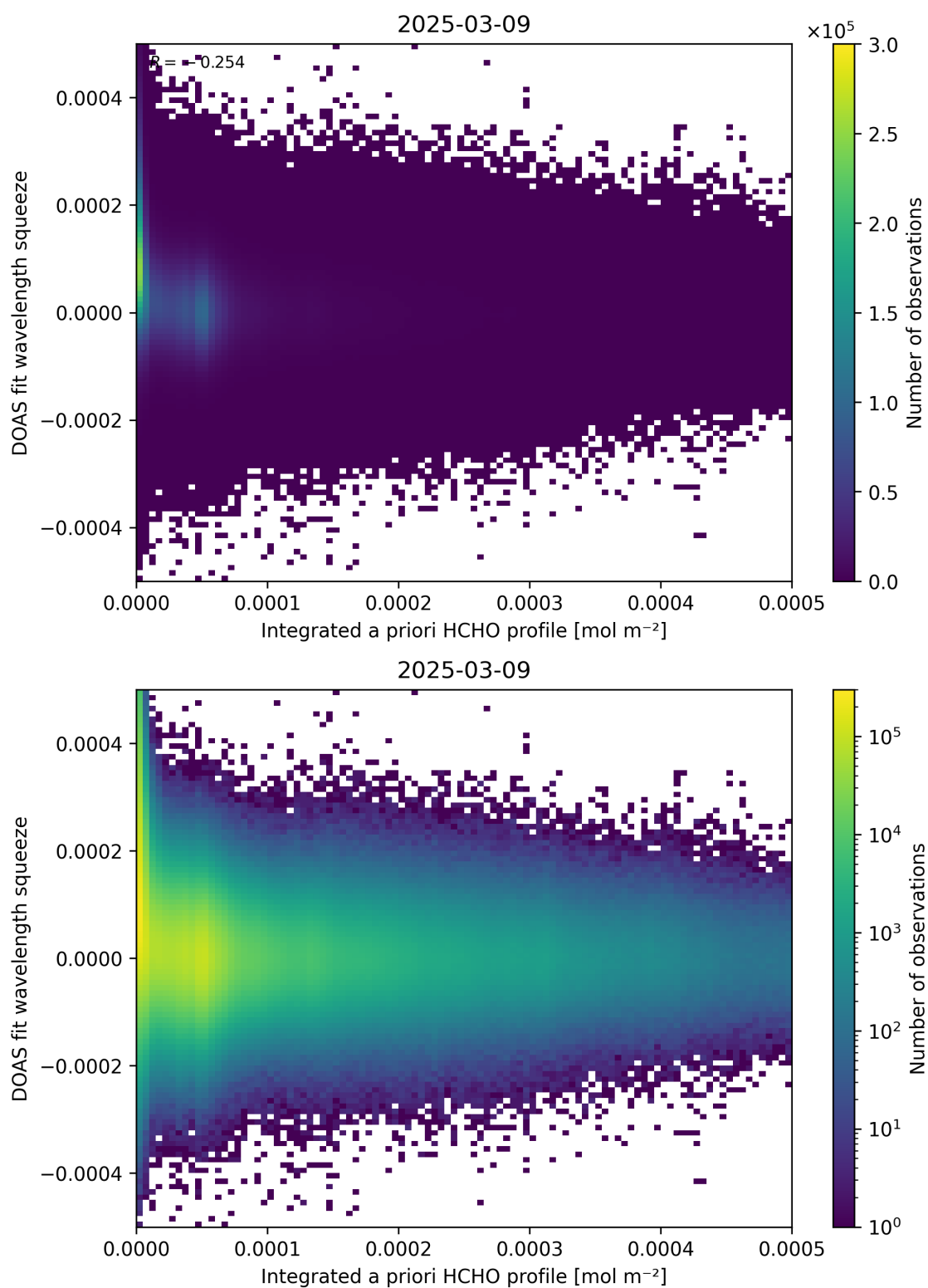
Figure 150: Scatter density plot of “Integrated a priori HCHO profile” against “DOAS fit wavelength squeeze” for 2025-03-08 to 2025-03-10.
