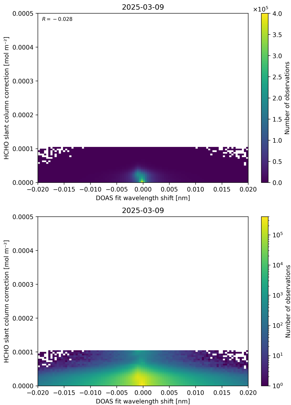
Figure 67: Scatter density plot of “DOAS fit wavelength shift” against “HCHO slant column correction” for 2025-03-08 to 2025-03-10.
