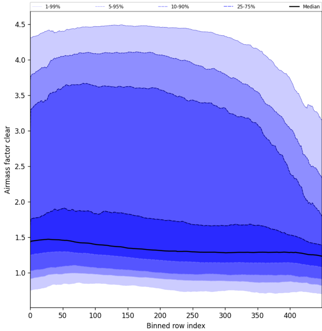
Figure 56: Along track statistics of “Airmass factor clear” for 2025-03-08 to 2025-03-10
