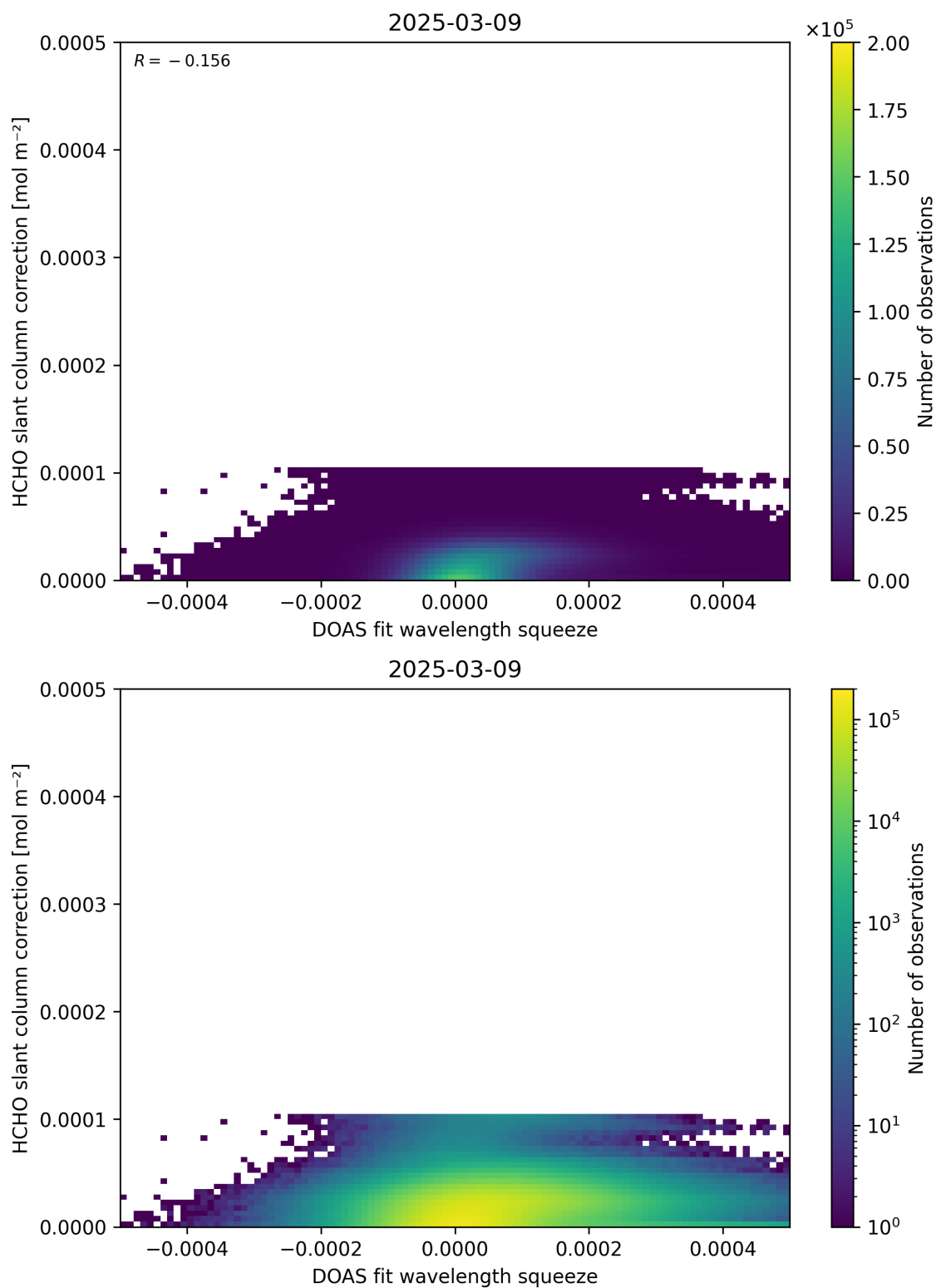
Figure 70: Scatter density plot of “DOAS fit wavelength squeeze” against “HCHO slant column correction” for 2025-03-08 to 2025-03-10.
