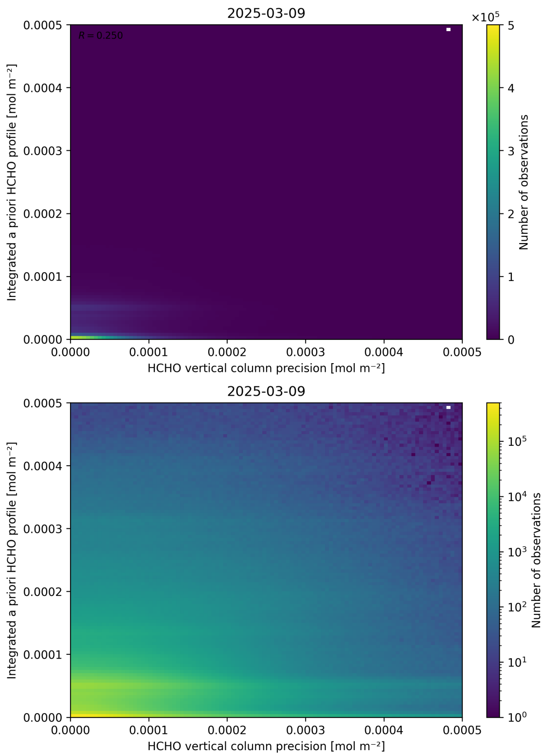
Figure 147: Scatter density plot of “HCHO vertical column precision” against “Integrated a priori HCHO profile” for 2025-03-08 to 2025-03-10.
