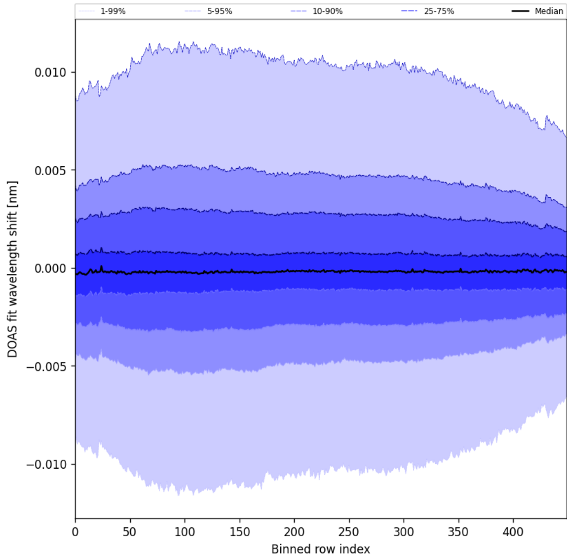
Figure 58: Along track statistics of “DOAS fit wavelength shift” for 2025-03-08 to 2025-03-10
