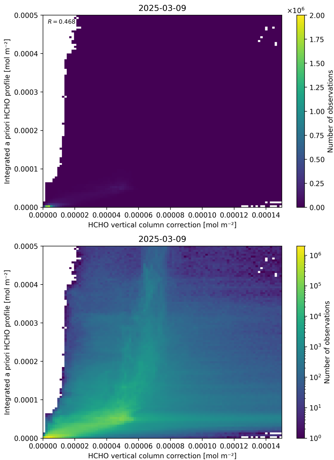
Figure 122: Scatter density plot of “HCHO vertical column correction” against “Integrated a priori HCHO profile” for 2025-03-08 to 2025-03-10.
