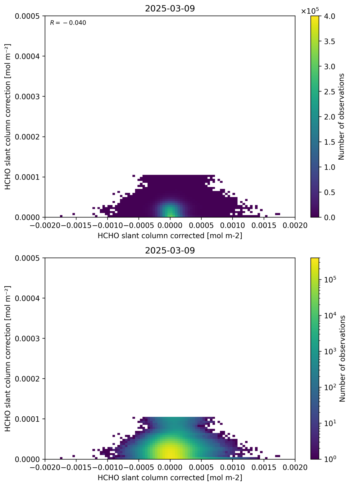
Figure 77: Scatter density plot of “HCHO slant column corrected” against “HCHO slant column correction” for 2025-03-08 to 2025-03-10.
