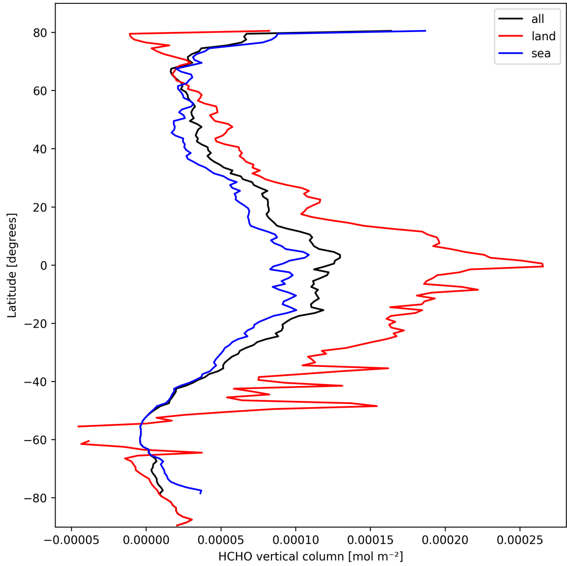
Figure 21: Zonal average of “HCHO vertical column” for 2025-03-08 to 2025-03-10.
