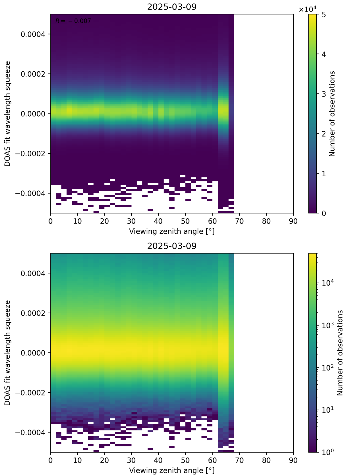
Figure 184: Scatter density plot of “Viewing zenith angle” against “DOAS fit wavelength squeeze” for 2025-03-08 to 2025-03-10.
