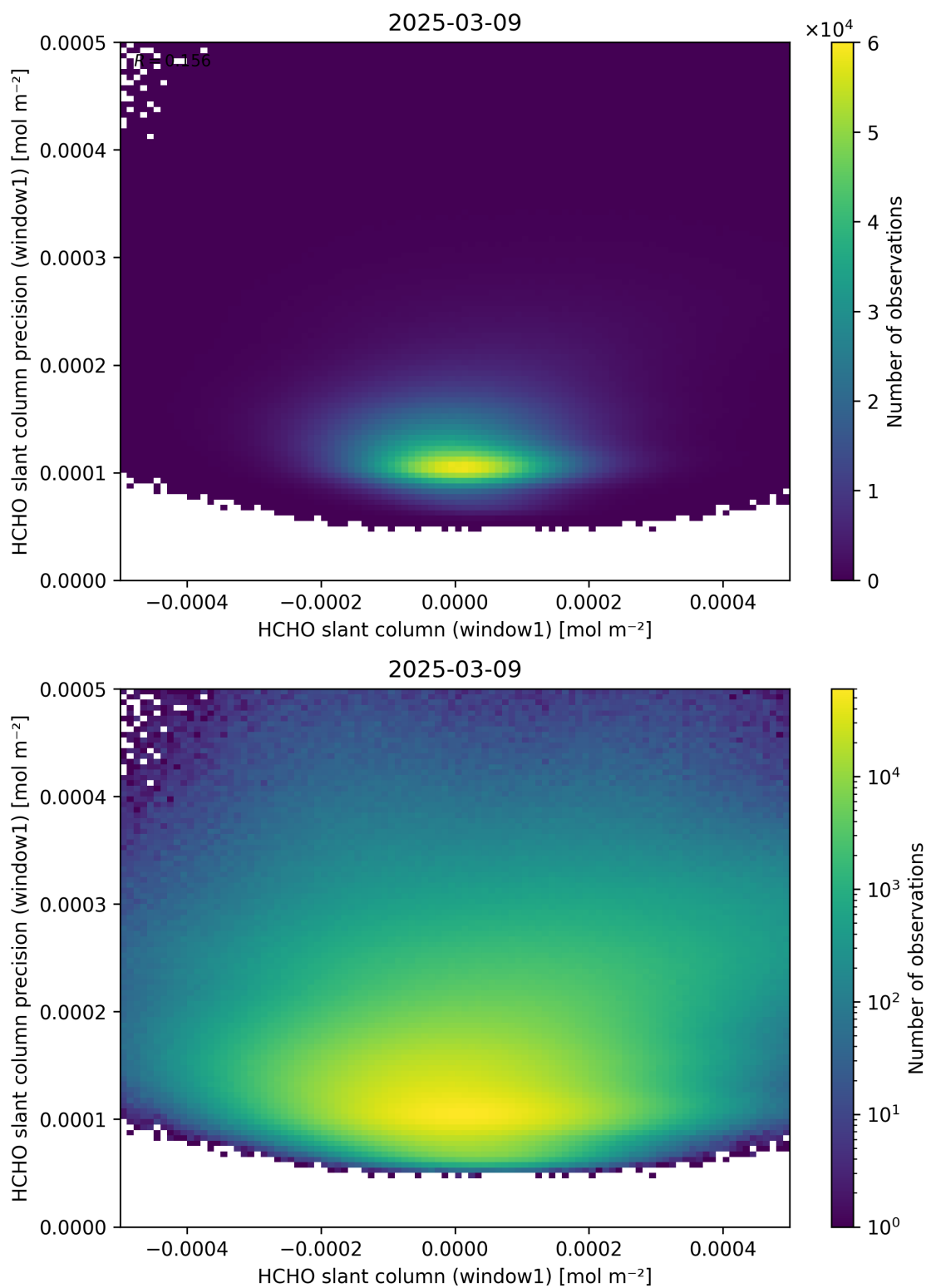
Figure 84: Scatter density plot of “HCHO slant column (window1)” against “HCHO slant column precision (window1)” for 2025-03-08 to 2025-03-10.
