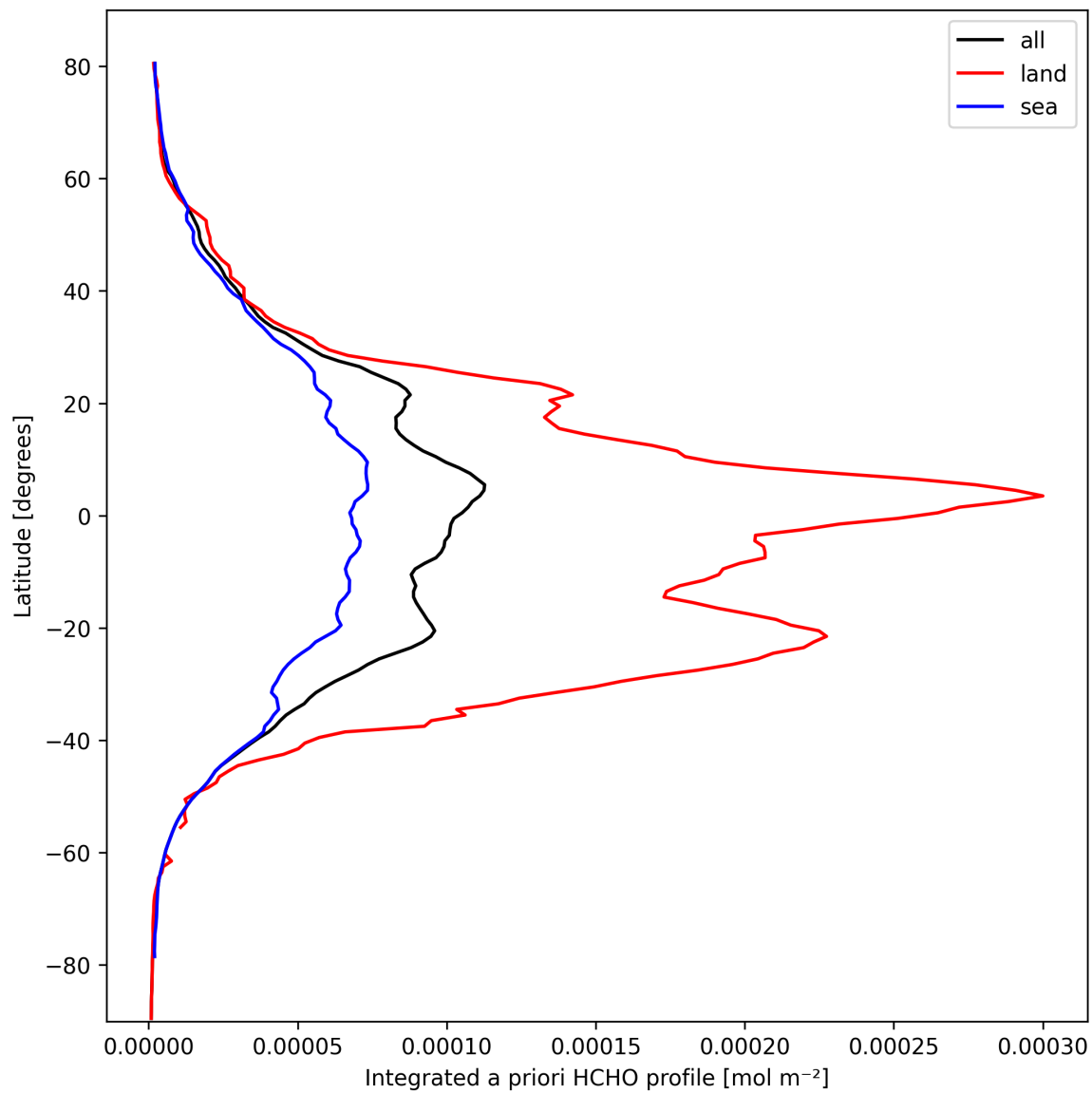
Figure 29: Zonal average of “Integrated a priori HCHO profile” for 2025-03-08 to 2025-03-10.
