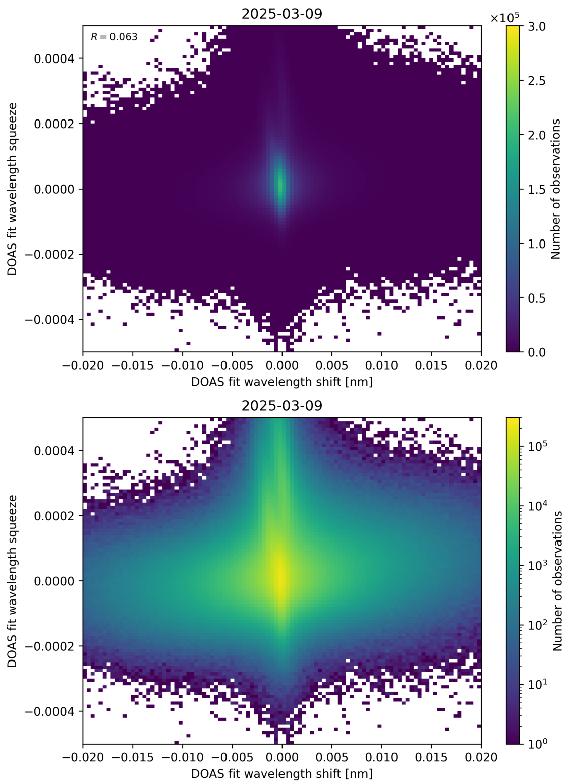
Figure 65: Scatter density plot of “DOAS fit wavelength shift” against “DOAS fit wavelength squeeze” for 2025-03-08 to 2025-03-10.
