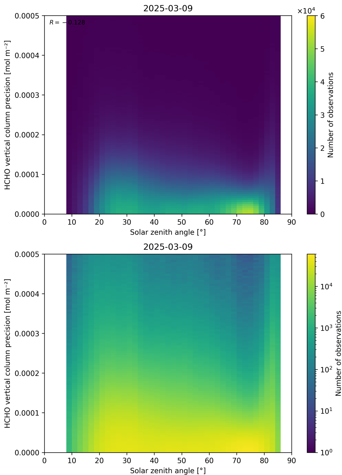
Figure 179: Scatter density plot of “Solar zenith angle” against “HCHO vertical column precision” for 2025-03-08 to 2025-03-10.
