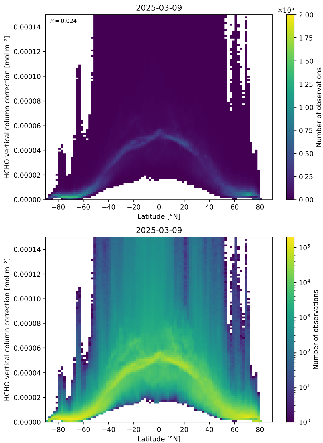
Figure 164: Scatter density plot of “Latitude” against “HCHO vertical column correction” for 2025-03-08 to 2025-03-10.
