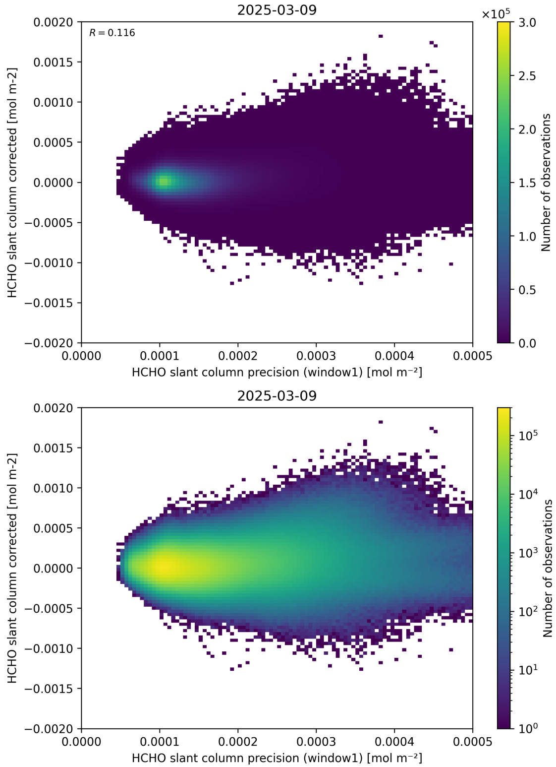
Figure 92: Scatter density plot of “HCHO slant column precision (window1)” against “HCHO slant column corrected” for 2025-03-08 to 2025-03-10.
