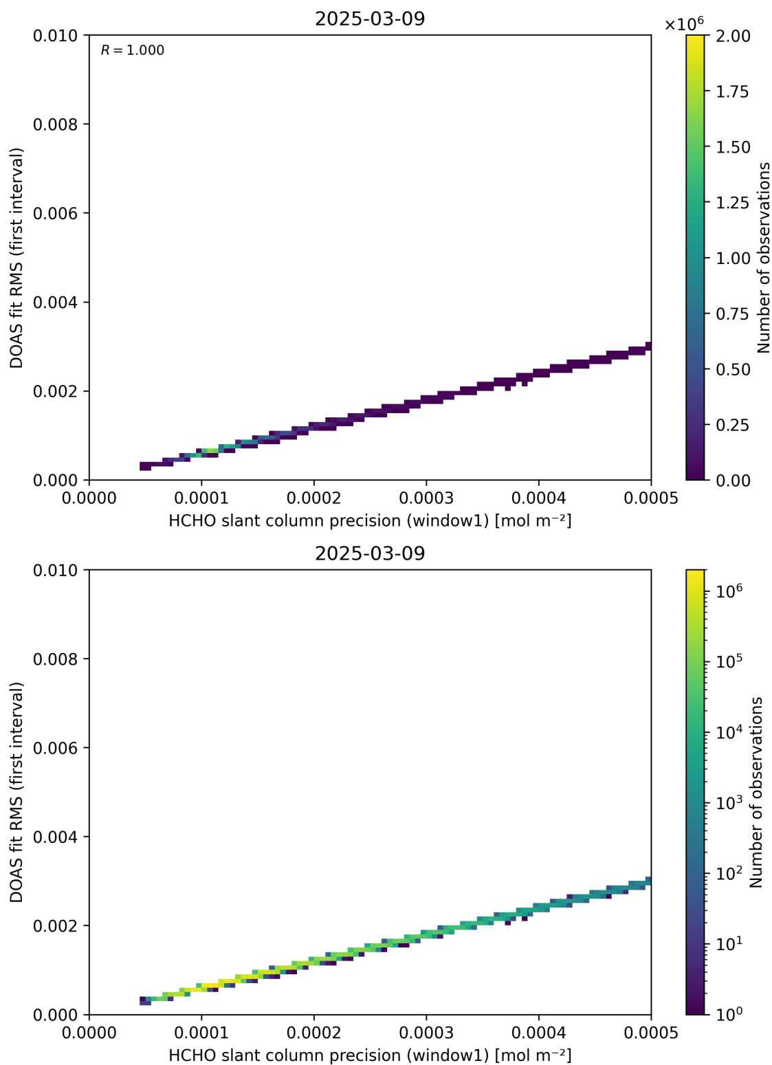
Figure 88: Scatter density plot of “HCHO slant column precision (window1)” against “DOAS fit RMS (first interval)” for 2025-03-08 to 2025-03-10.
