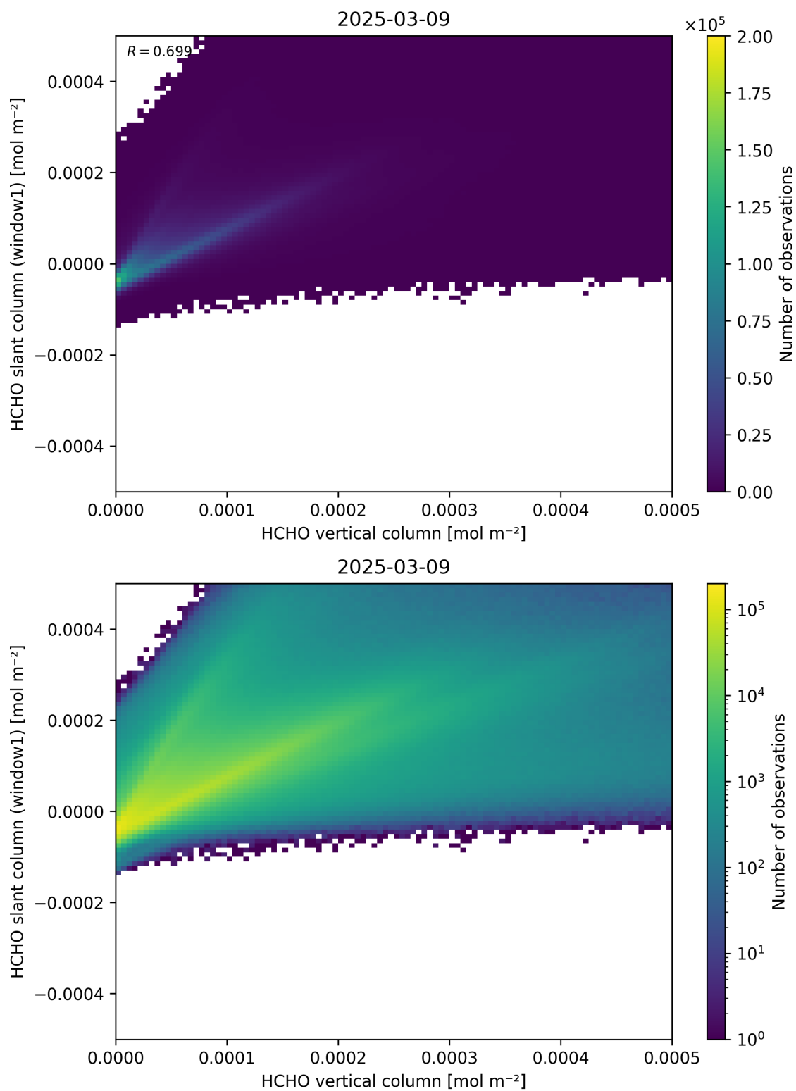
Figure 129: Scatter density plot of “HCHO vertical column” against “HCHO slant column (window1)” for 2025-03-08 to 2025-03-10.
