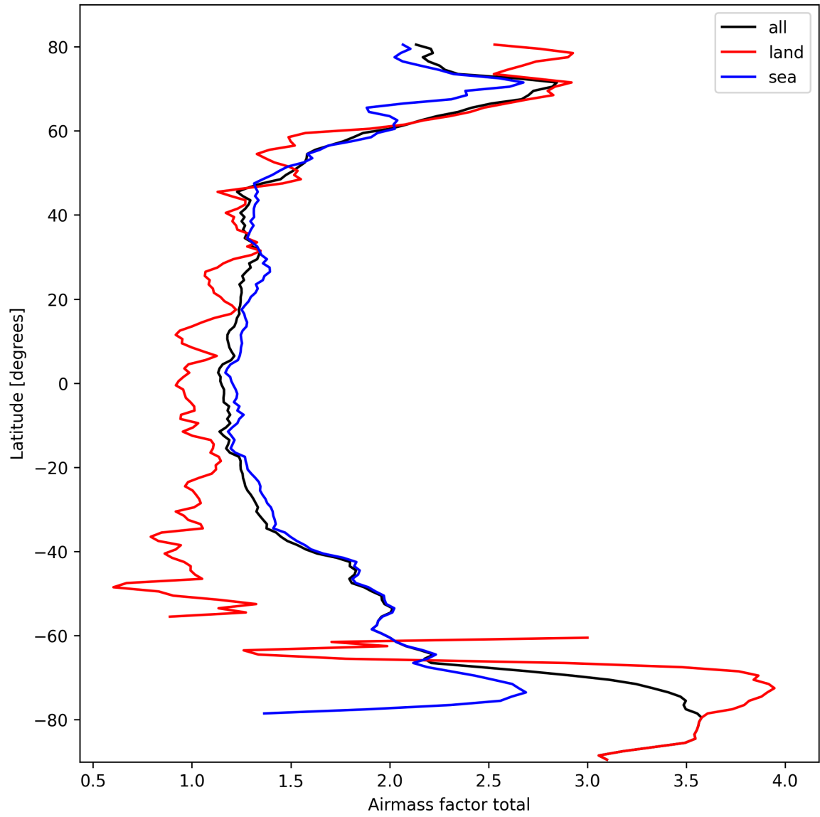
Figure 26: Zonal average of “Airmass factor total” for 2025-03-08 to 2025-03-10.
