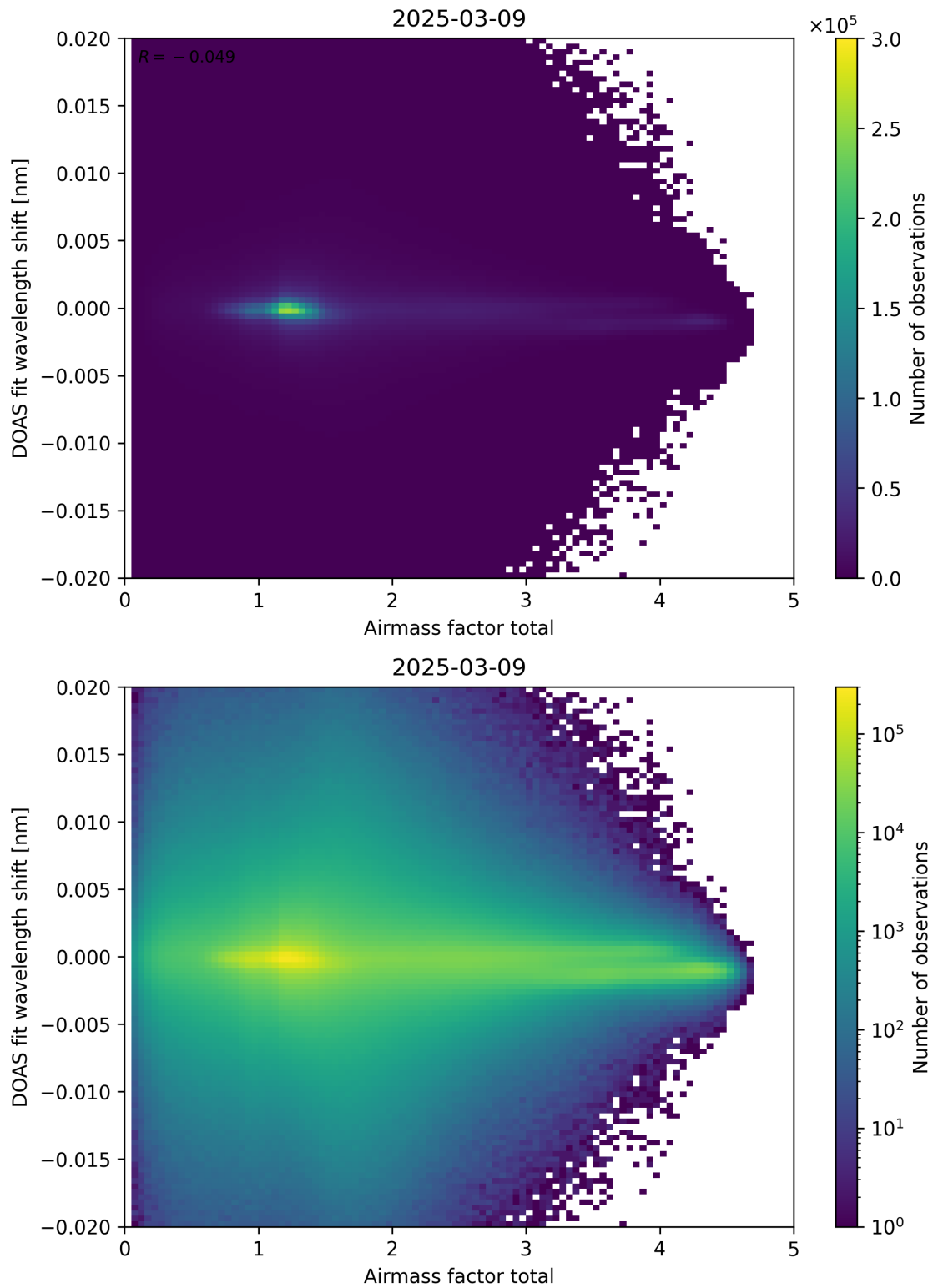
Figure 98: Scatter density plot of “Airmass factor total” against “DOAS fit wavelength shift” for 2025-03-08 to 2025-03-10.
