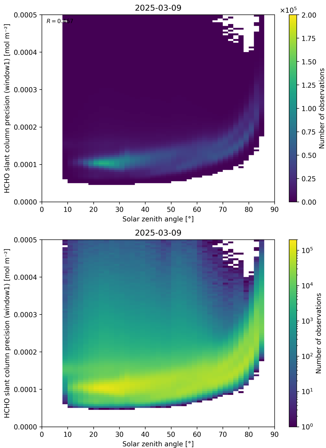
Figure 174: Scatter density plot of “Solar zenith angle” against “HCHO slant column precision (window1)” for 2025-03-08 to 2025-03-10.
