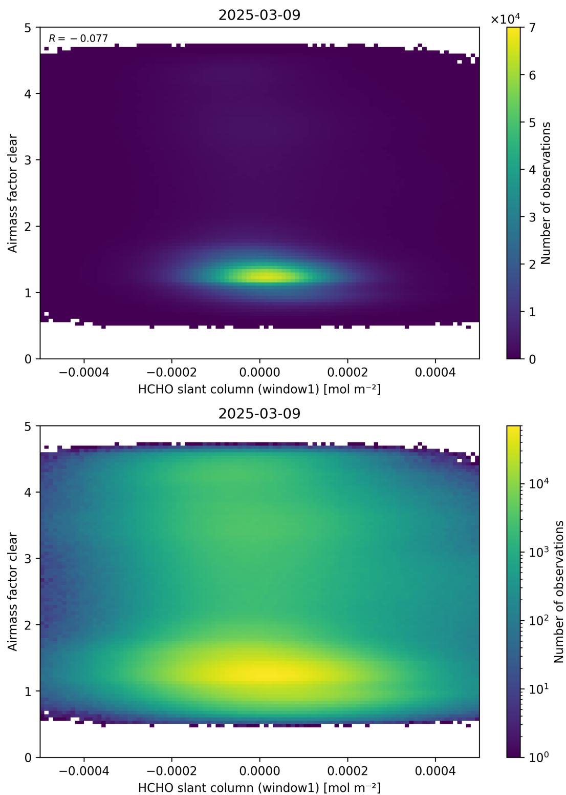
Figure 81: Scatter density plot of “HCHO slant column (window1)” against “Airmass factor clear” for 2025-03-08 to 2025-03-10.
