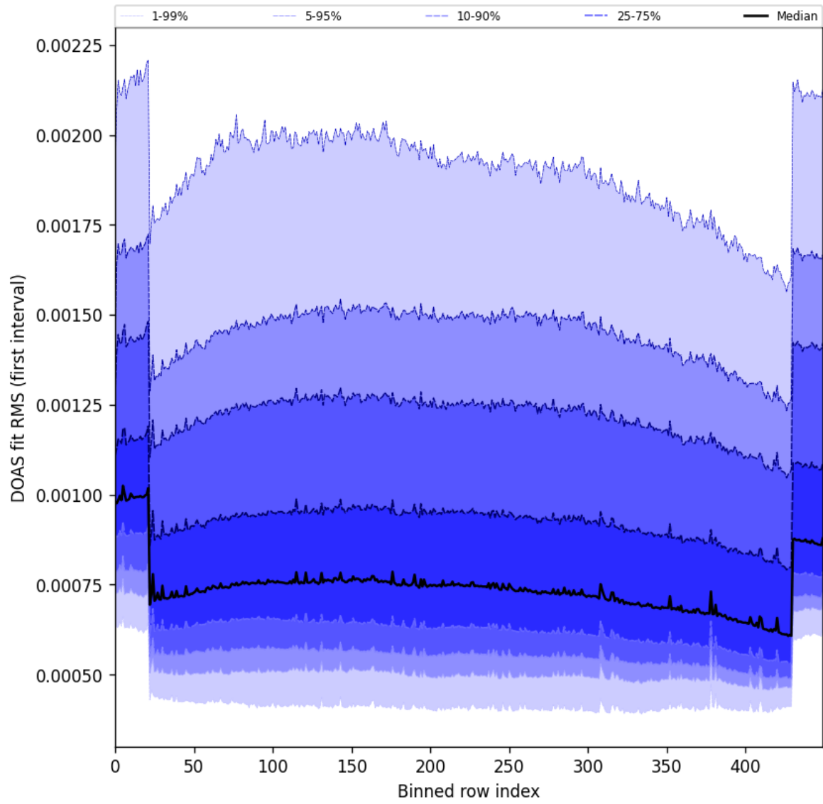
Figure 60: Along track statistics of “DOAS fit RMS (first interval)” for 2025-03-08 to 2025-03-10
