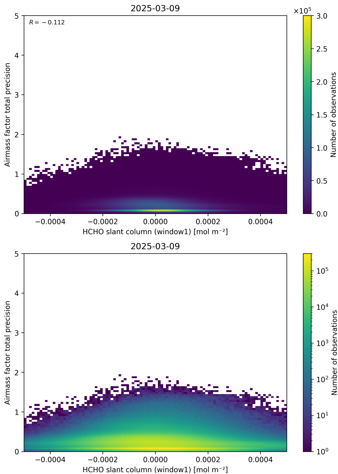
Figure 86: Scatter density plot of “HCHO slant column (window1)” against “Airmass factor total precision” for 2025-03-08 to 2025-03-10.
