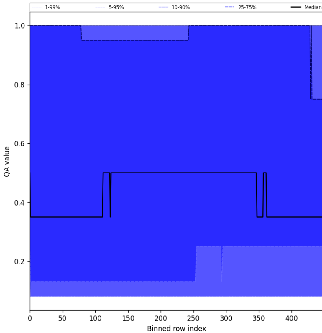
Figure 48: Along track statistics of “QA value” for 2025-03-08 to 2025-03-10
