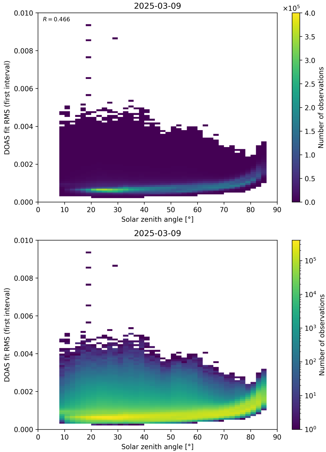
Figure 167: Scatter density plot of “Solar zenith angle” against “DOAS fit RMS (first interval)” for 2025-03-08 to 2025-03-10.
