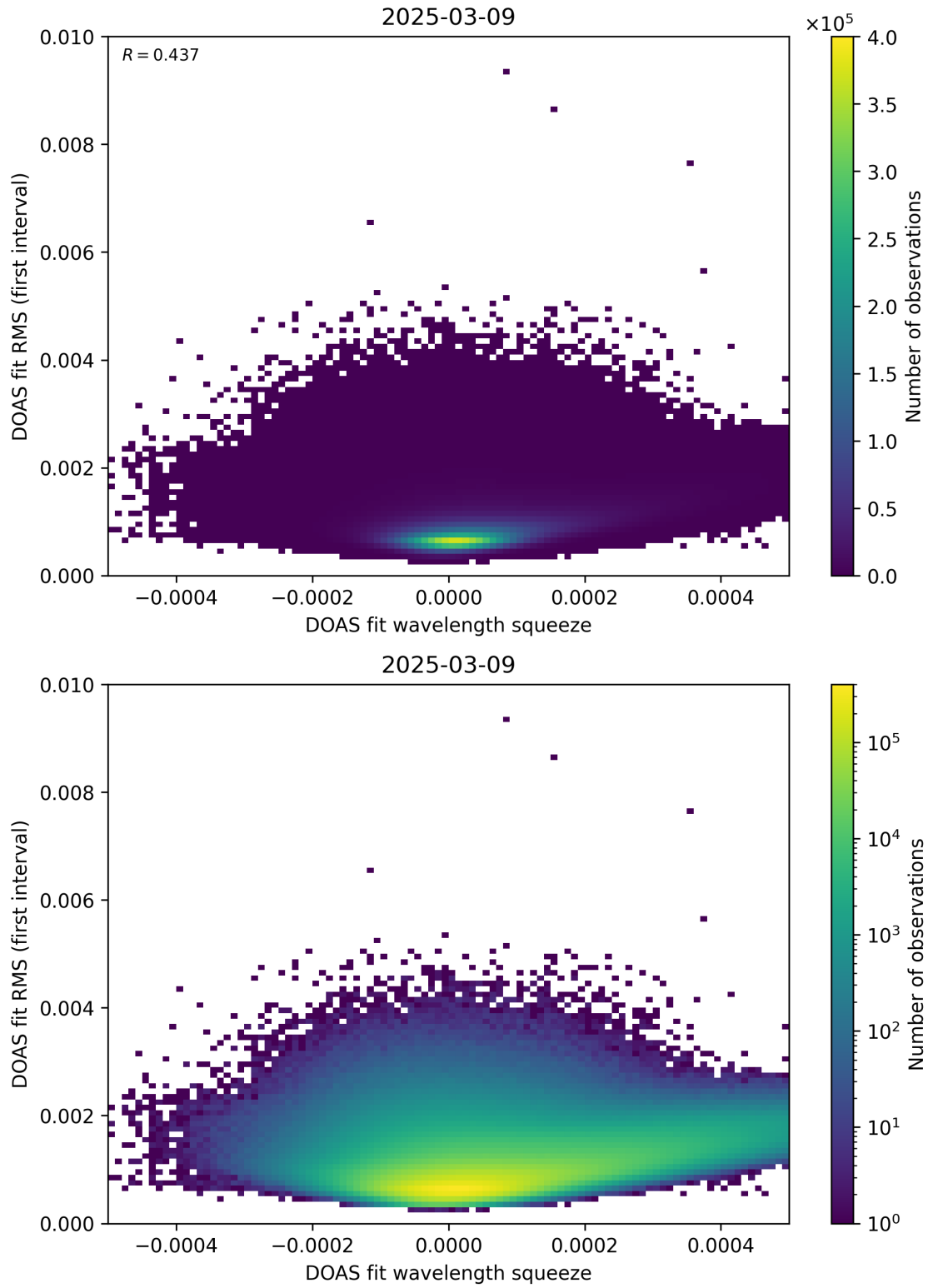
Figure 68: Scatter density plot of “DOAS fit wavelength squeeze” against “DOAS fit RMS (first interval)” for 2025-03-08 to 2025-03-10.
