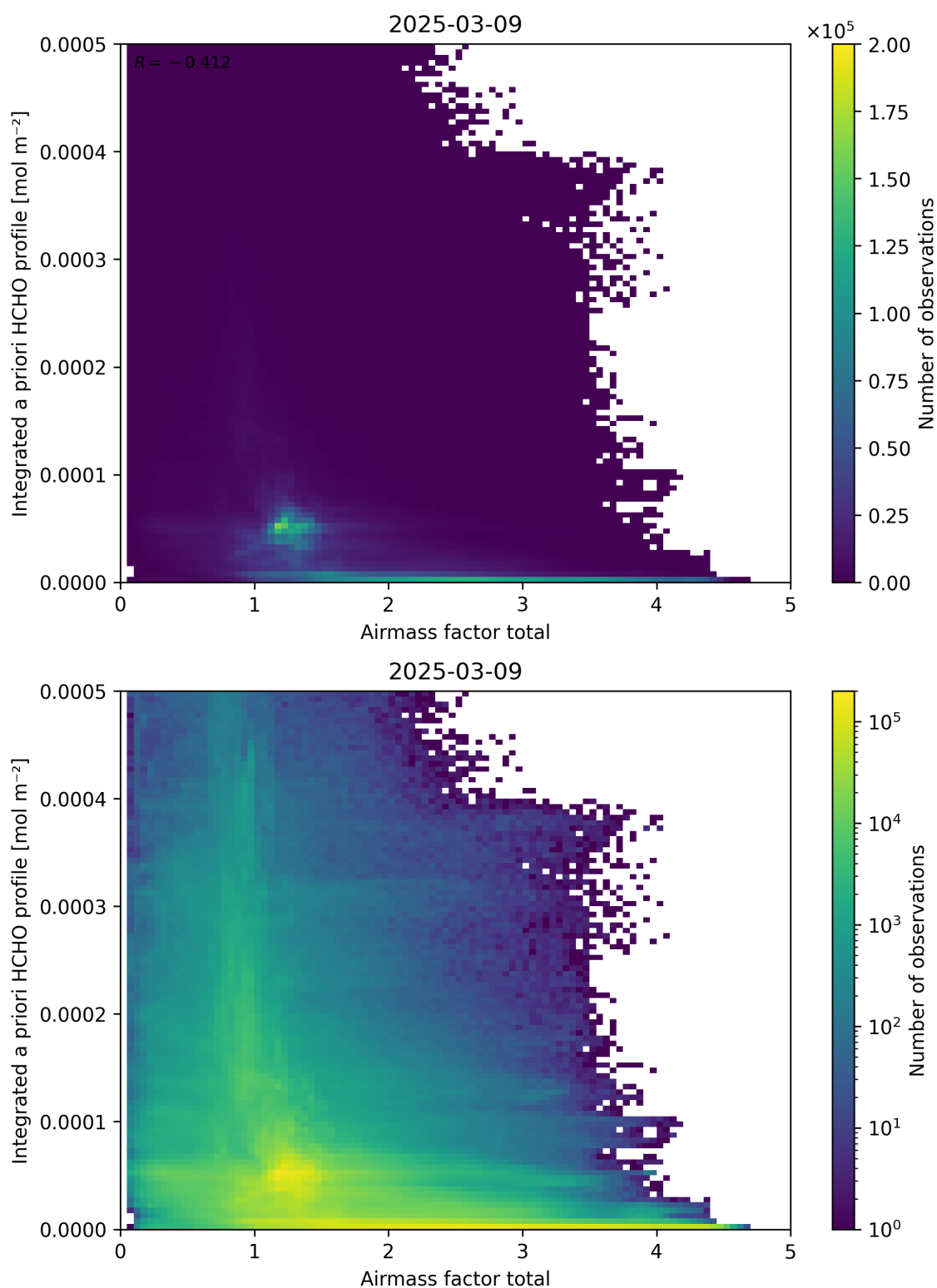
Figure 104: Scatter density plot of “Airmass factor total” against “Integrated a priori HCHO profile” for 2025-03-08 to 2025-03-10.
