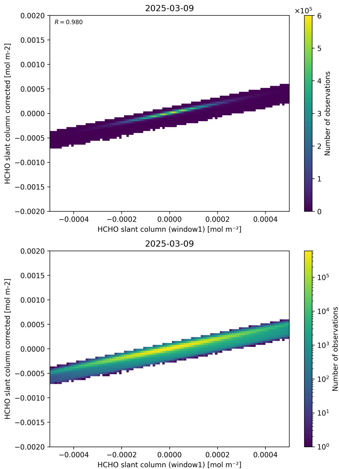
Figure 82: Scatter density plot of “HCHO slant column (window1)” against “HCHO slant column corrected” for 2025-03-08 to 2025-03-10.
