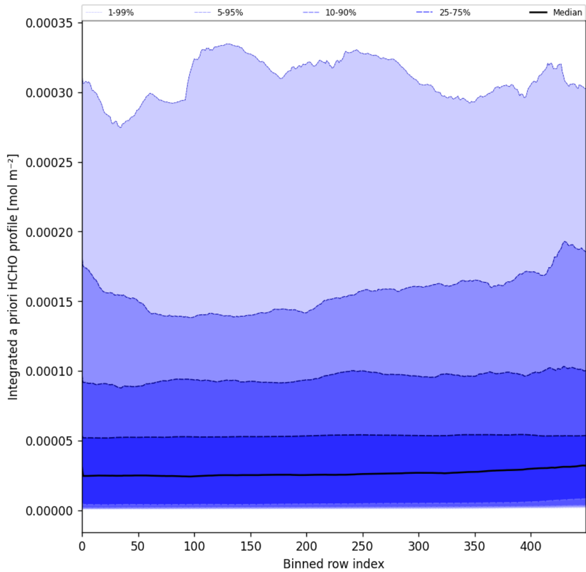
Figure 57: Along track statistics of "Integrated a priori HCHO profile" for 2025-03-08 to 2025-03-10
