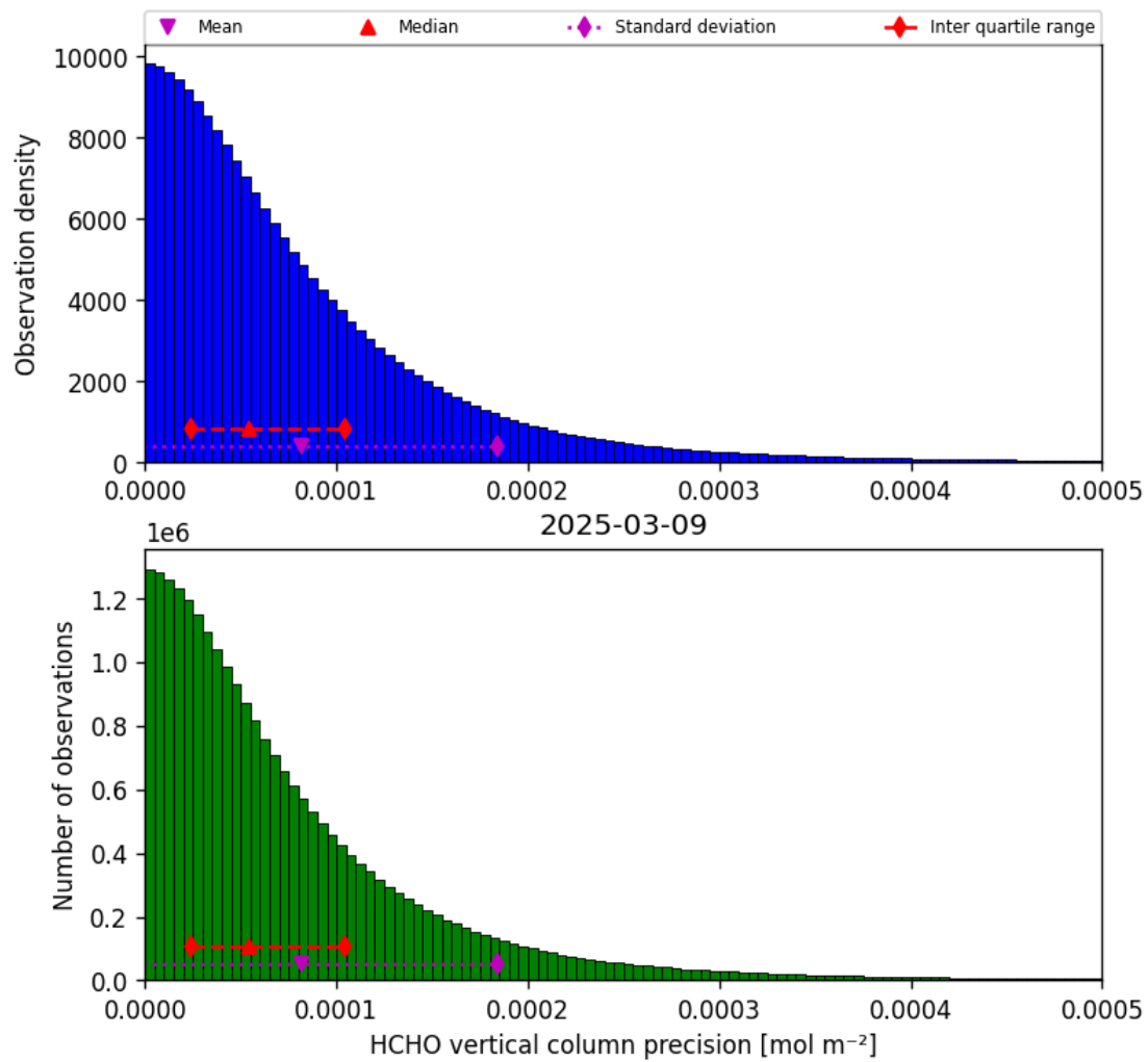
Figure 36: Histogram of “HCHO vertical column precision” for 2025-03-08 to 2025-03-10
