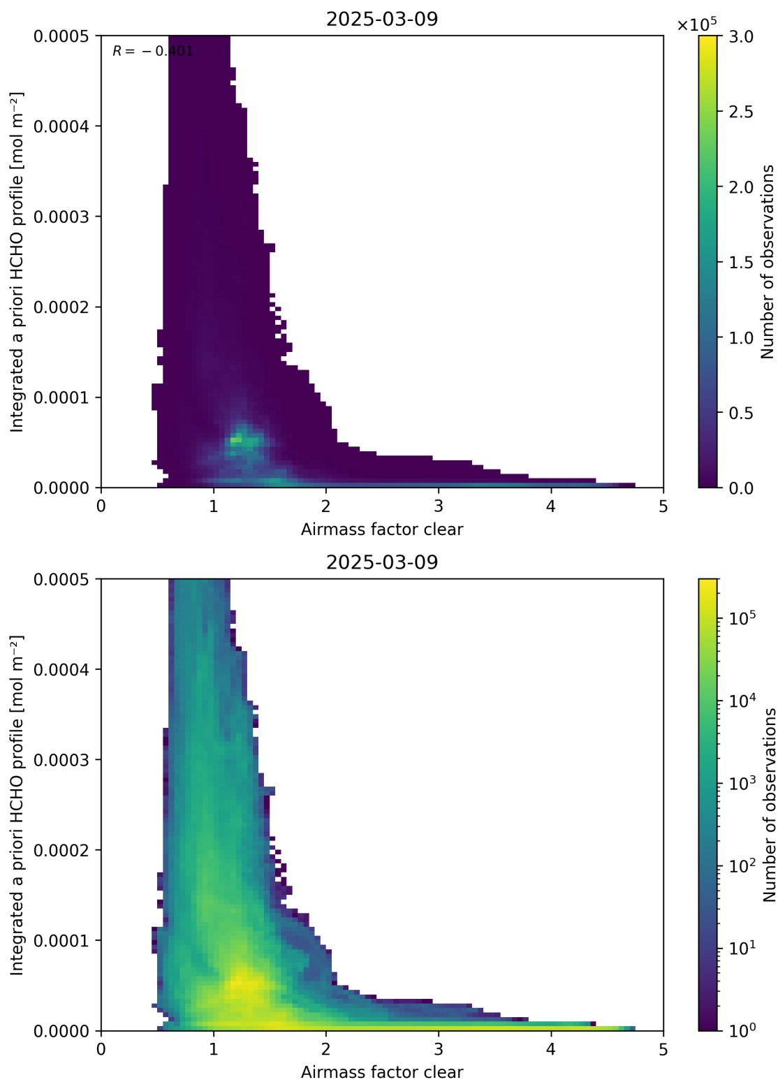
Figure 76: Scatter density plot of “Airmass factor clear” against “Integrated a priori HCHO profile” for 2025-03-08 to 2025-03-10.
