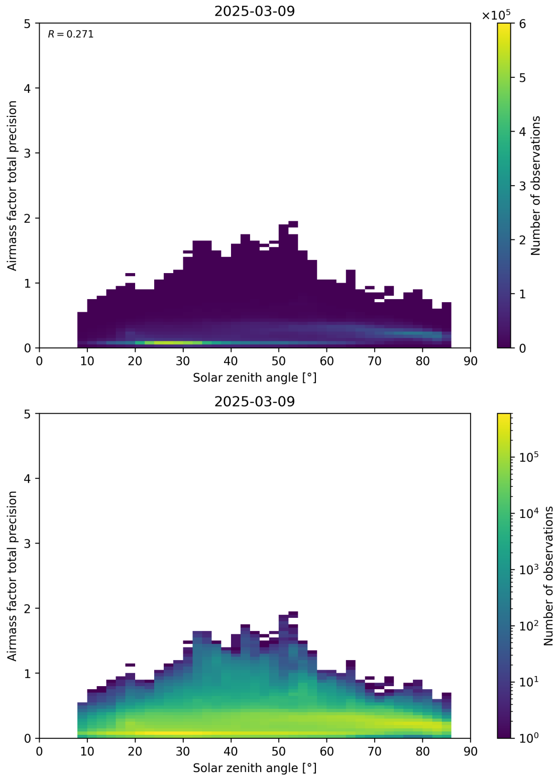
Figure 176: Scatter density plot of “Solar zenith angle” against “Airmass factor total precision” for 2025-03-08 to 2025-03-10.
