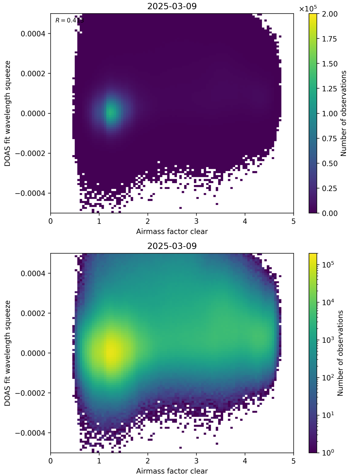
Figure 73: Scatter density plot of “Airmass factor clear” against “DOAS fit wavelength squeeze” for 2025-03-08 to 2025-03-10.
