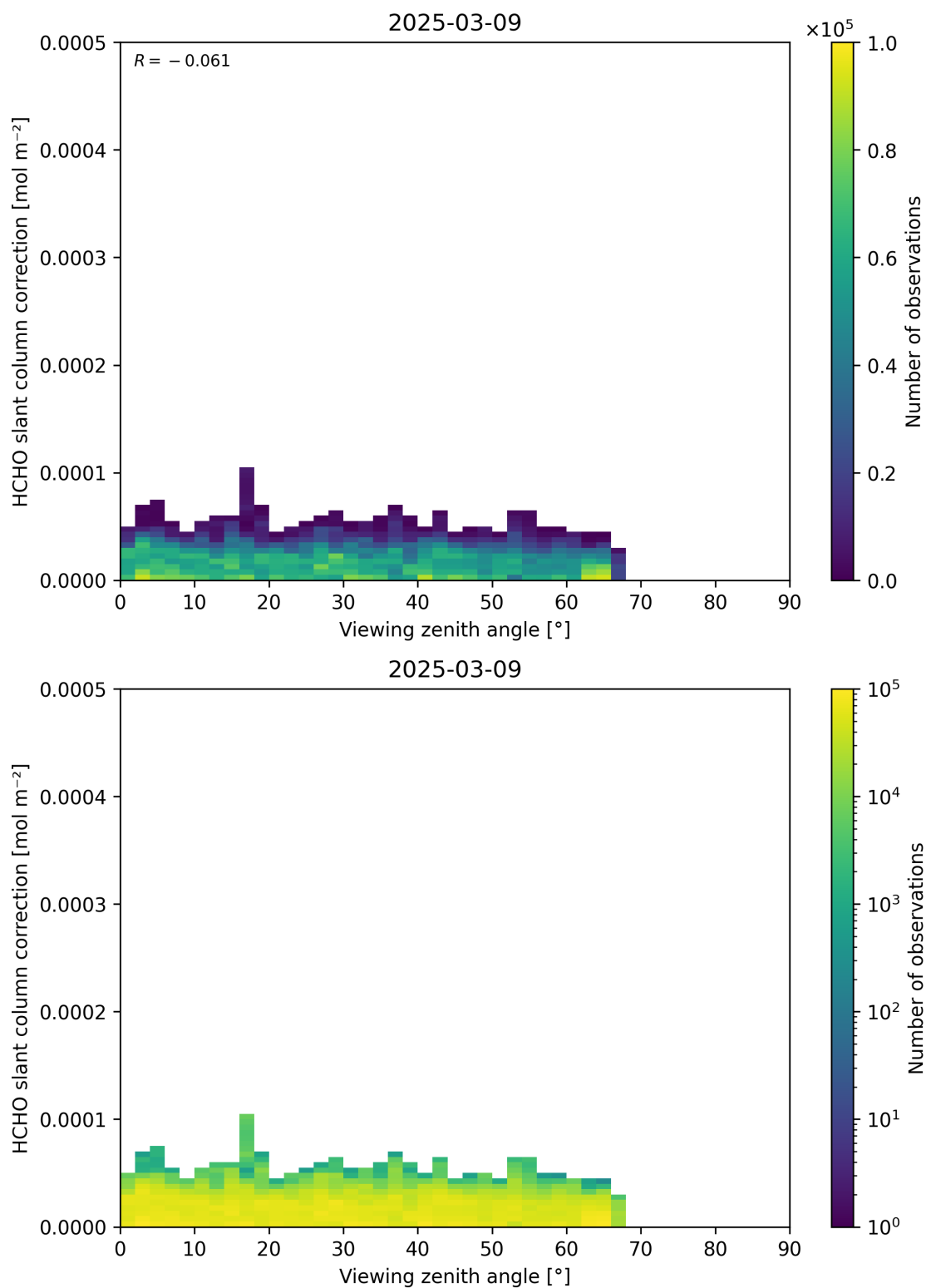
Figure 187: Scatter density plot of “Viewing zenith angle” against “HCHO slant column correction” for 2025-03-08 to 2025-03-10.
