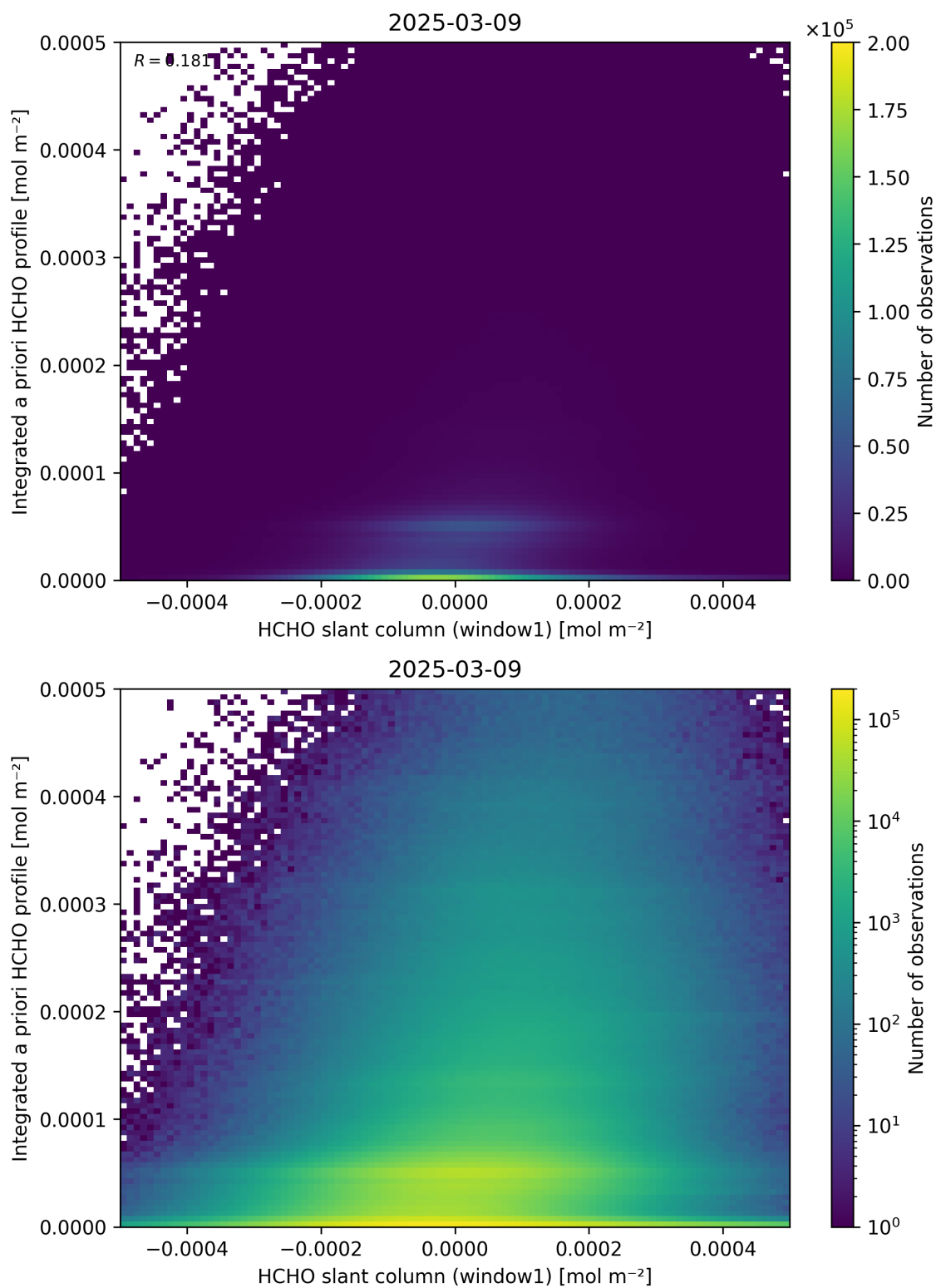
Figure 87: Scatter density plot of “HCHO slant column (window1)” against “Integrated a priori HCHO profile” for 2025-03-08 to 2025-03-10.
