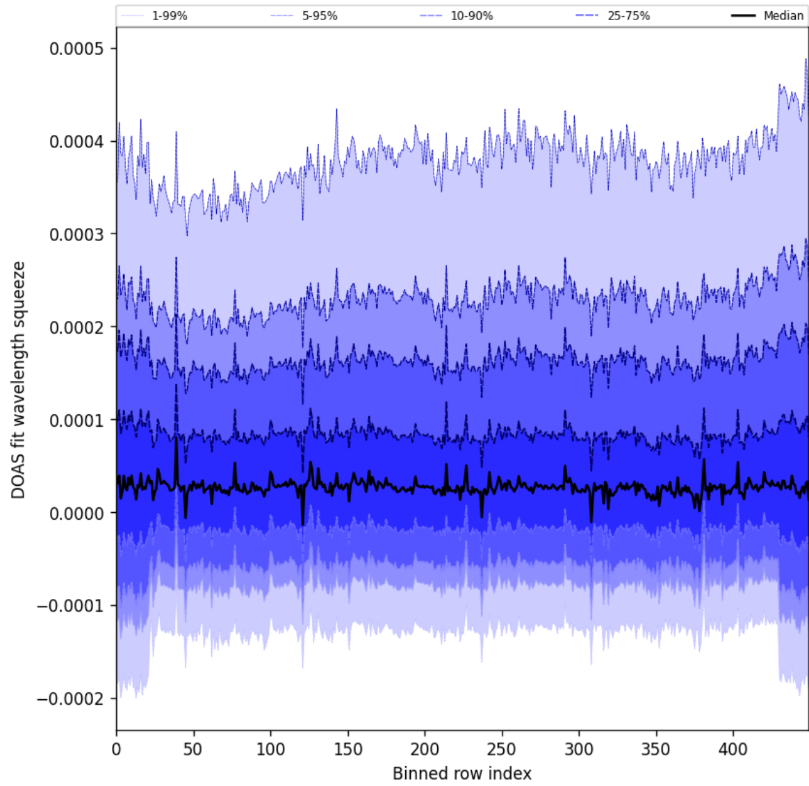
Figure 59: Along track statistics of “DOAS fit wavelength squeeze” for 2025-03-08 to 2025-03-10
