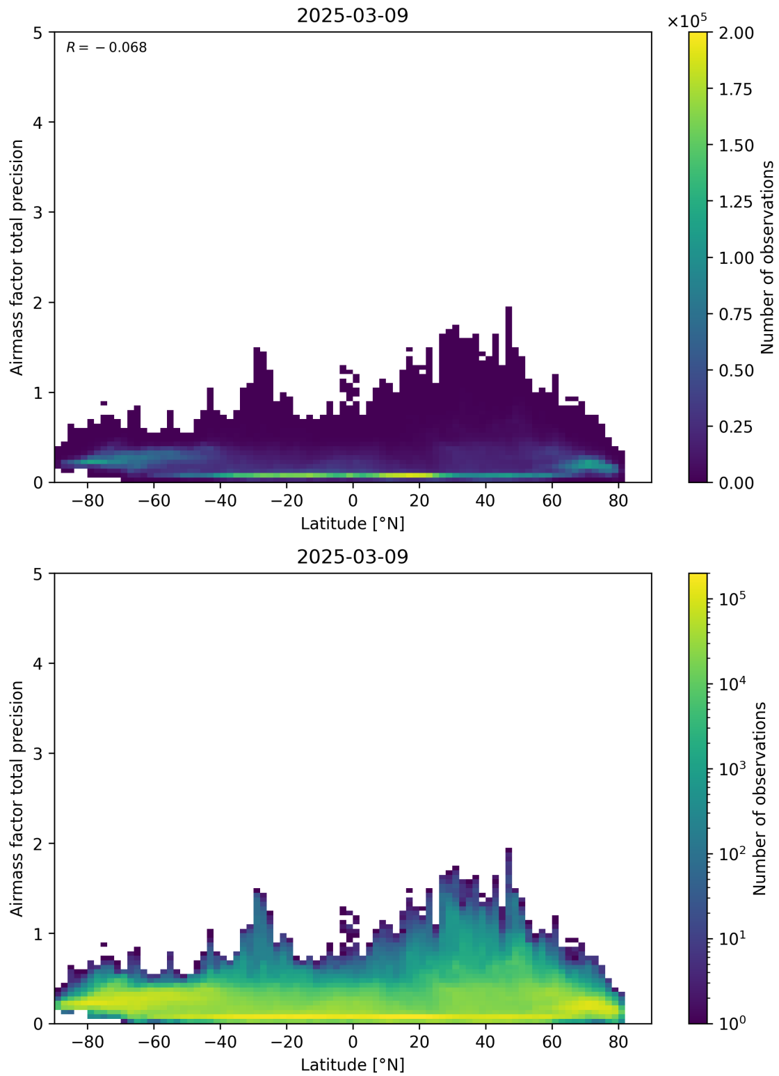
Figure 162: Scatter density plot of “Latitude” against “Airmass factor total precision” for 2025-03-08 to 2025-03-10.
