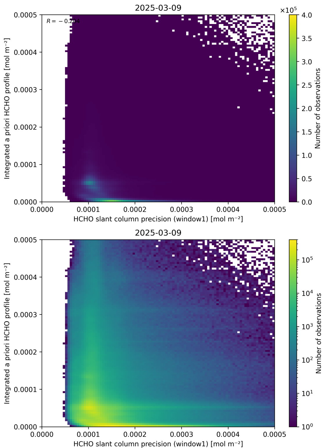
Figure 96: Scatter density plot of “HCHO slant column precision (window1)” against “Integrated a priori HCHO profile” for 2025-03-08 to 2025-03-10.
