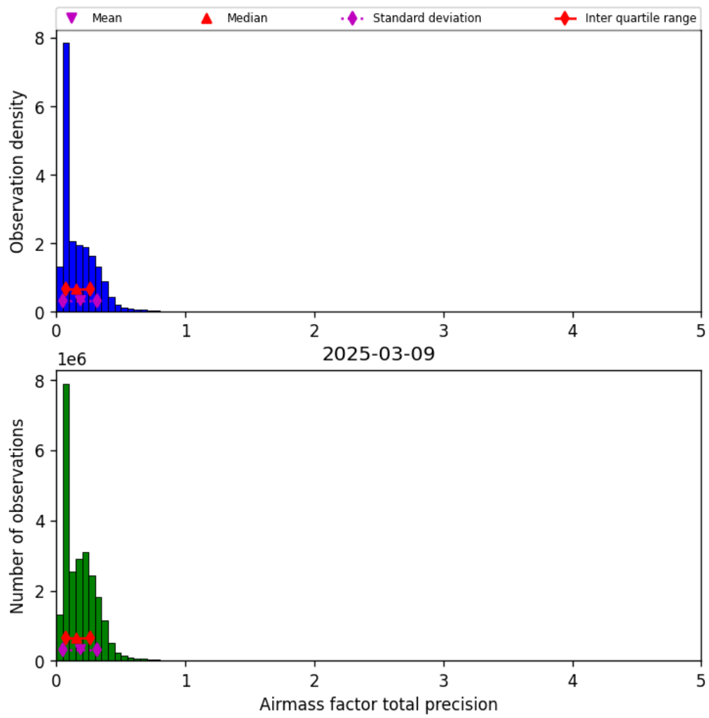
Figure 41: Histogram of “Airmass factor total precision” for 2025-03-08 to 2025-03-10
