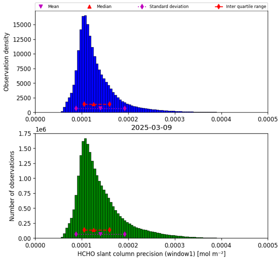
Figure 39: Histogram of “HCHO slant column precision (window1)” for 2025-03-08 to 2025-03-10
