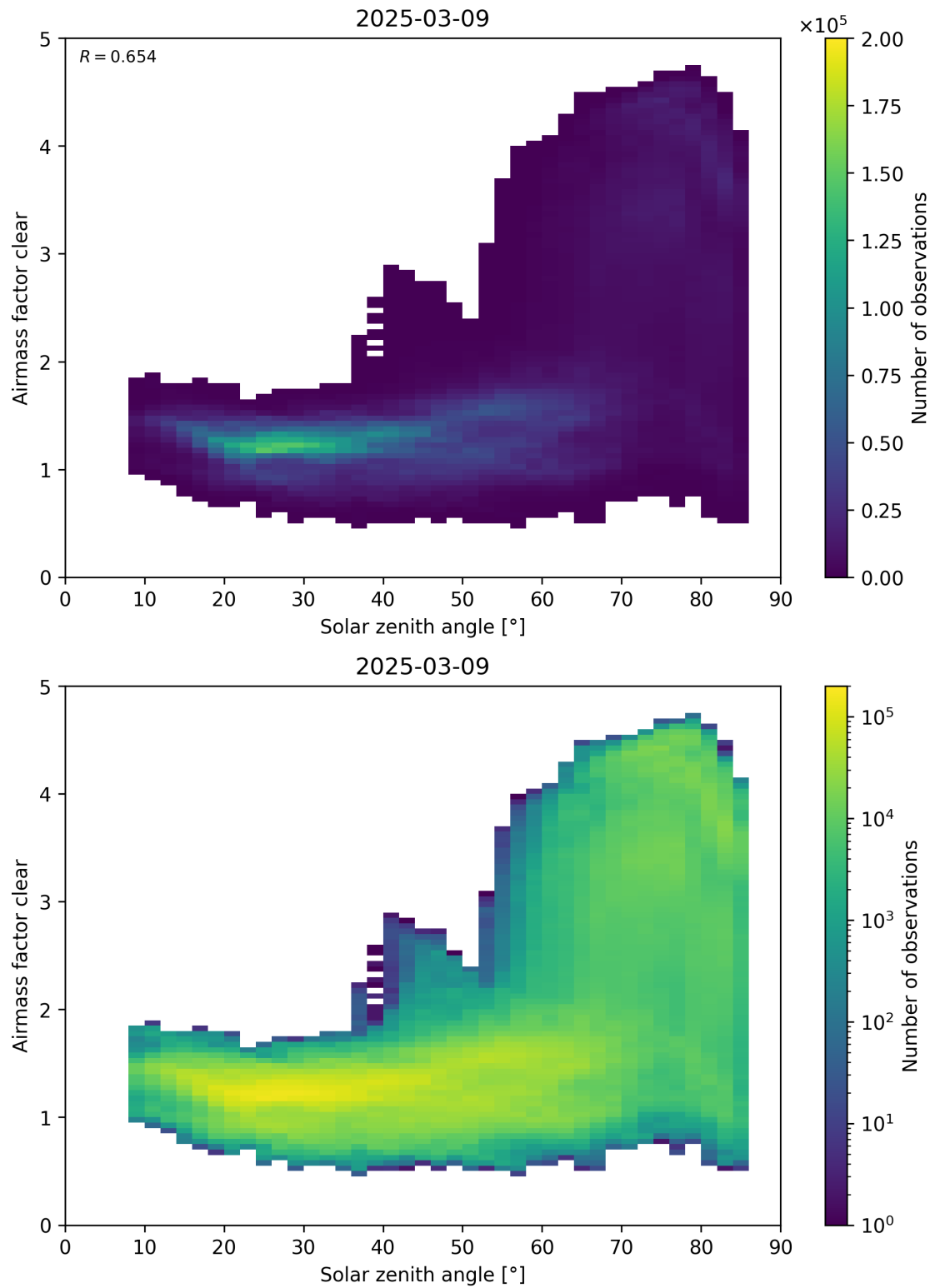
Figure 170: Scatter density plot of “Solar zenith angle” against “Airmass factor clear” for 2025-03-08 to 2025-03-10.
