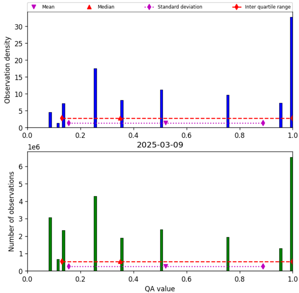
Figure 34: Histogram of “QA value” for 2025-03-08 to 2025-03-10
