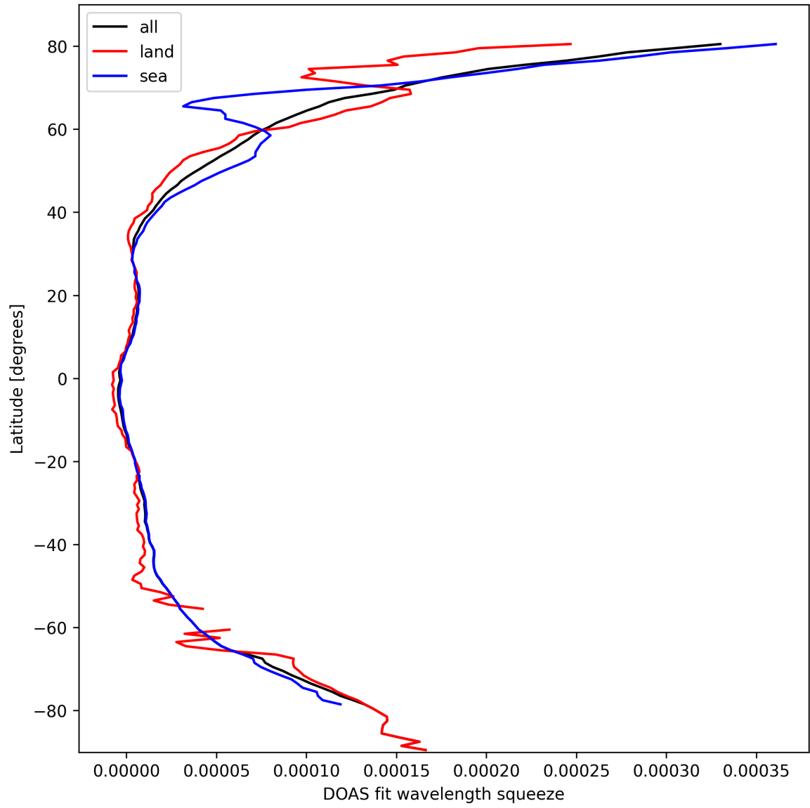
Figure 31: Zonal average of “DOAS fit wavelength squeeze” for 2025-03-08 to 2025-03-10.
