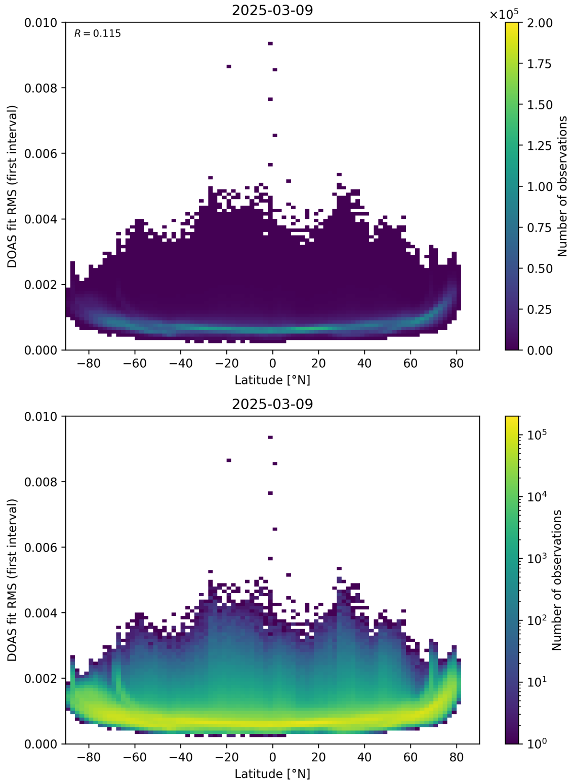
Figure 153: Scatter density plot of “Latitude” against “DOAS fit RMS (first interval)” for 2025-03-08 to 2025-03-10.
