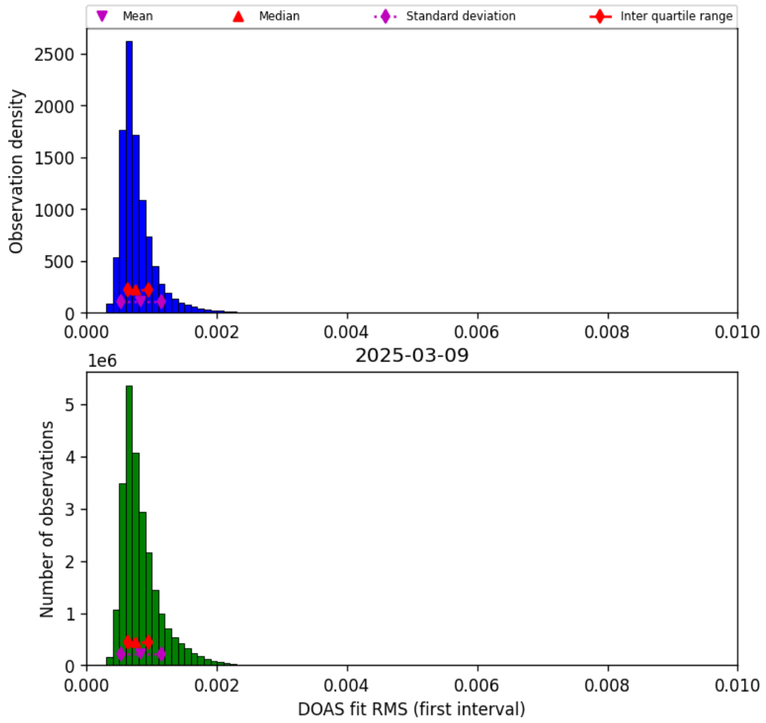
Figure 46: Histogram of “DOAS fit RMS (first interval)” for 2025-03-08 to 2025-03-10
