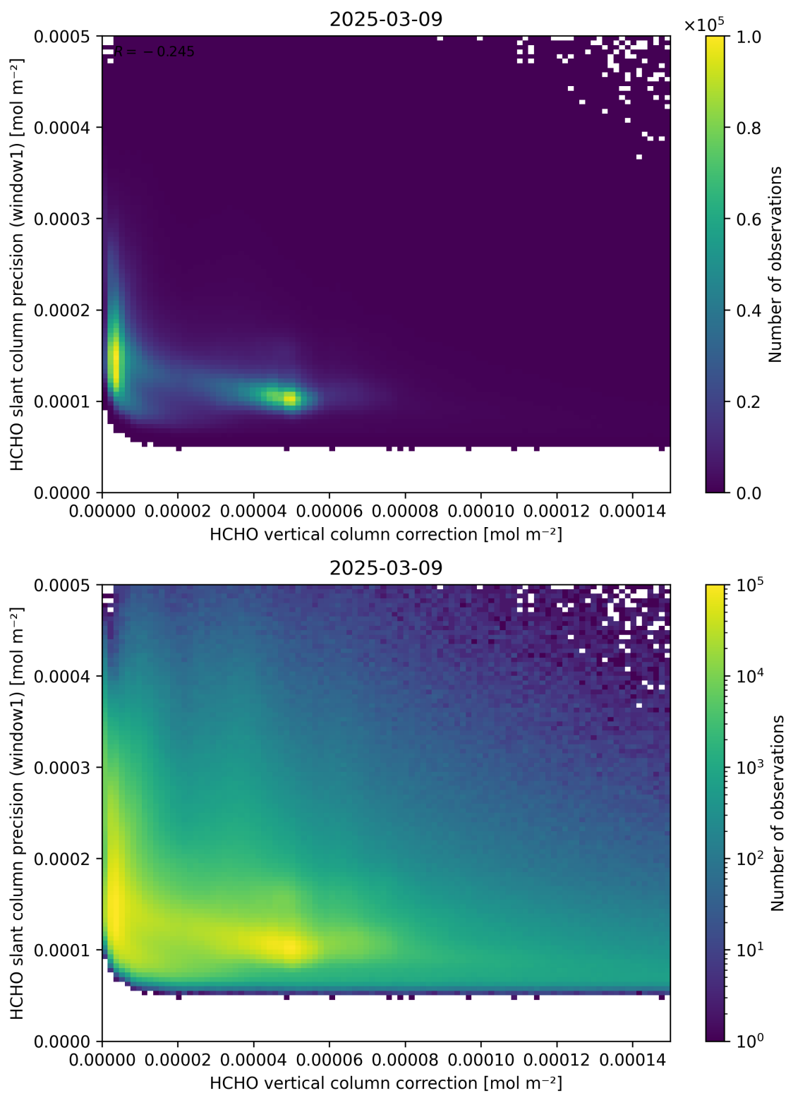
Figure 119: Scatter density plot of “HCHO vertical column correction” against “HCHO slant column precision (window1)” for 2025-03-08 to 2025-03-10.
