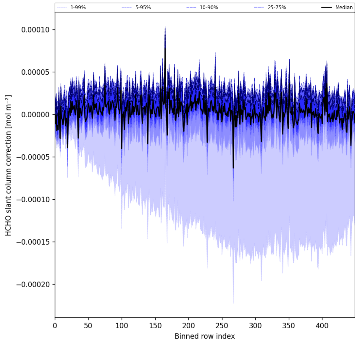
Figure 61: Along track statistics of “HCHO slant column correction” for 2025-03-08 to 2025-03-10
