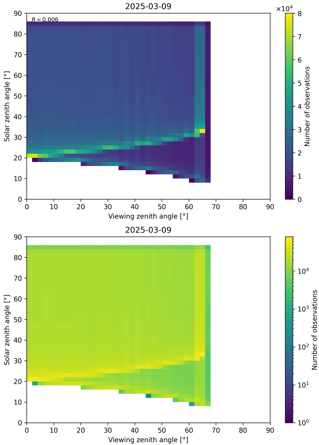
Figure 197: Scatter density plot of “Viewing zenith angle” against “Solar zenith angle” for 2025-03-08 to 2025-03-10.
