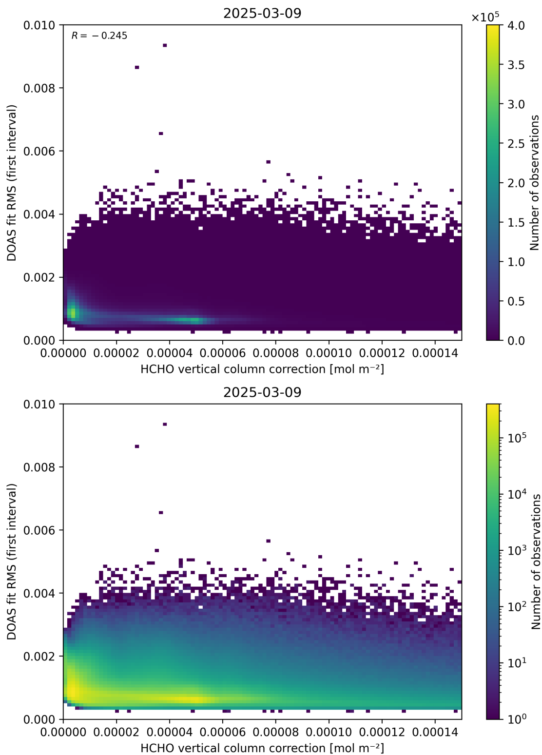
Figure 112: Scatter density plot of “HCHO vertical column correction” against “DOAS fit RMS (first interval)” for 2025-03-08 to 2025-03-10.
