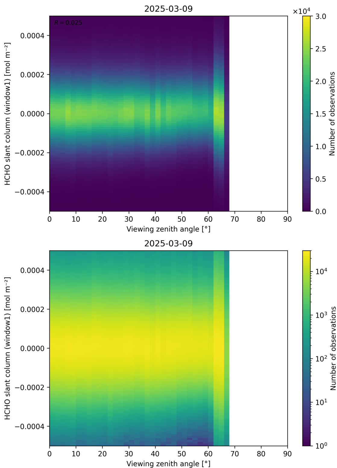
Figure 188: Scatter density plot of “Viewing zenith angle” against “HCHO slant column (window1)” for 2025-03-08 to 2025-03-10.
