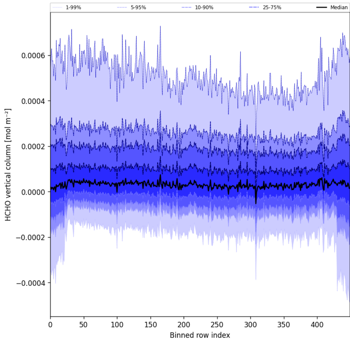
Figure 49: Along track statistics of “HCHO vertical column” for 2025-03-08 to 2025-03-10
