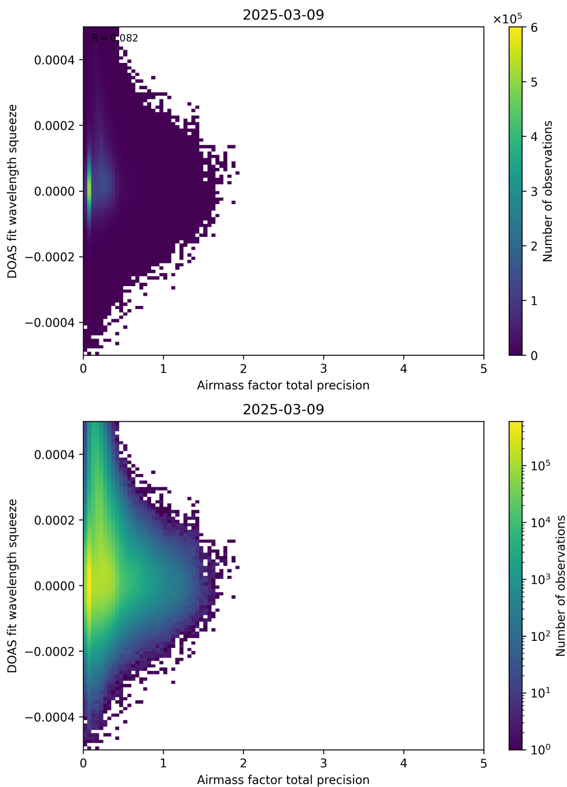
Figure 107: Scatter density plot of “Airmass factor total precision” against “DOAS fit wavelength squeeze” for 2025-03-08 to 2025-03-10.
