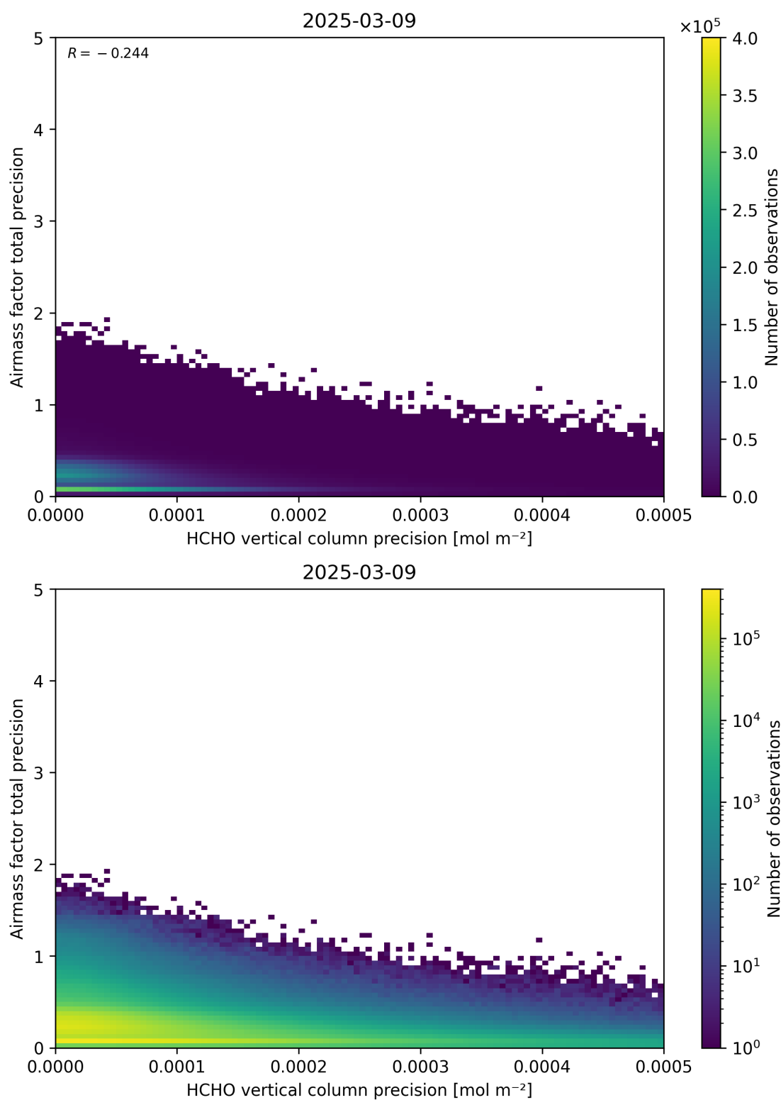
Figure 145: Scatter density plot of “HCHO vertical column precision” against “Airmass factor total precision” for 2025-03-08 to 2025-03-10.
