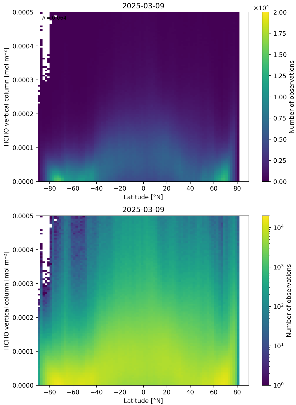
Figure 163: Scatter density plot of “Latitude” against “HCHO vertical column” for 2025-03-08 to 2025-03-10.
