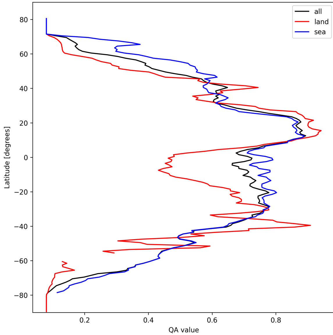
Figure 20: Zonal average of “QA value” for 2025-03-08 to 2025-03-10.
