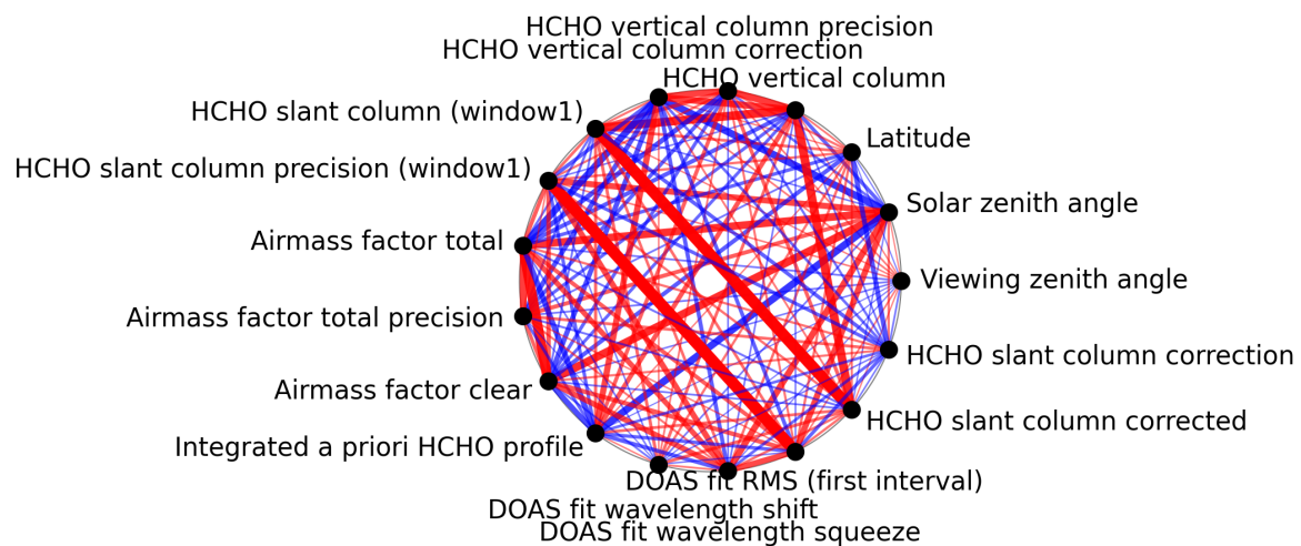
Figure 1: Map of correlation graph for 2025-03-08 to 2025-03-10.
