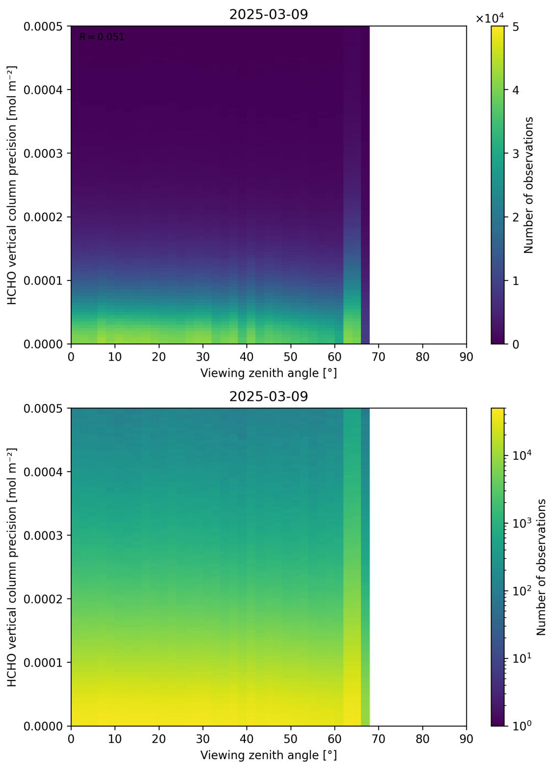
Figure 194: Scatter density plot of “Viewing zenith angle” against “HCHO vertical column precision” for 2025-03-08 to 2025-03-10.
