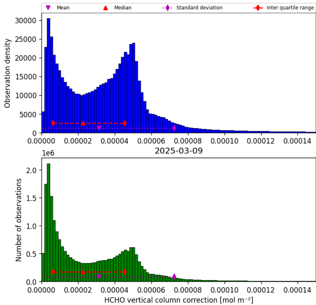
Figure 37: Histogram of “HCHO vertical column correction” for 2025-03-08 to 2025-03-10
