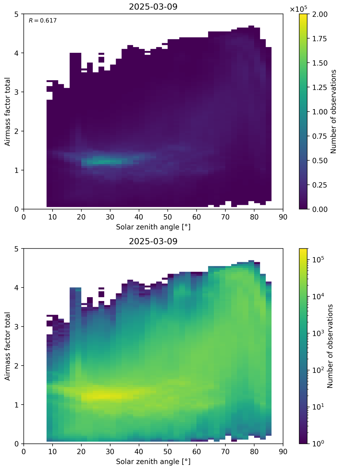
Figure 175: Scatter density plot of “Solar zenith angle” against “Airmass factor total” for 2025-03-08 to 2025-03-10.
