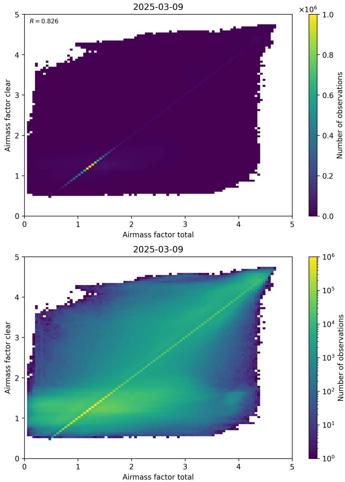
Figure 100: Scatter density plot of “Airmass factor total” against “Airmass factor clear” for 2025-03-08 to 2025-03-10.
