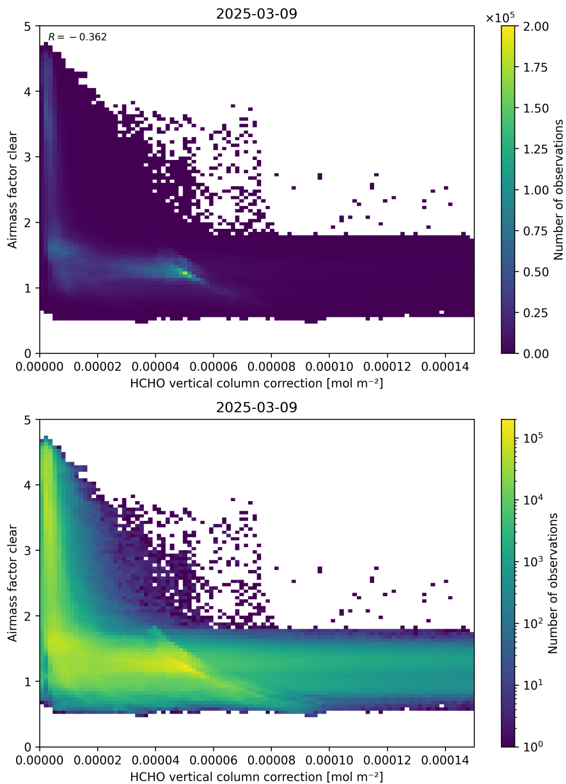
Figure 115: Scatter density plot of “HCHO vertical column correction” against “Airmass factor clear” for 2025-03-08 to 2025-03-10.
