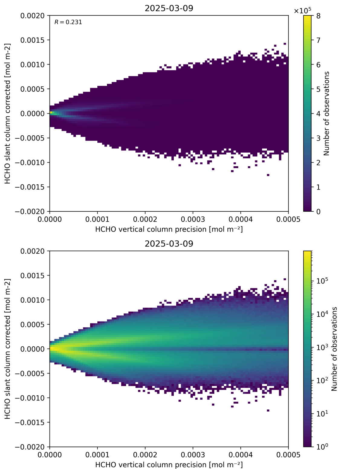
Figure 140: Scatter density plot of “HCHO vertical column precision” against “HCHO slant column corrected” for 2025-03-08 to 2025-03-10.
