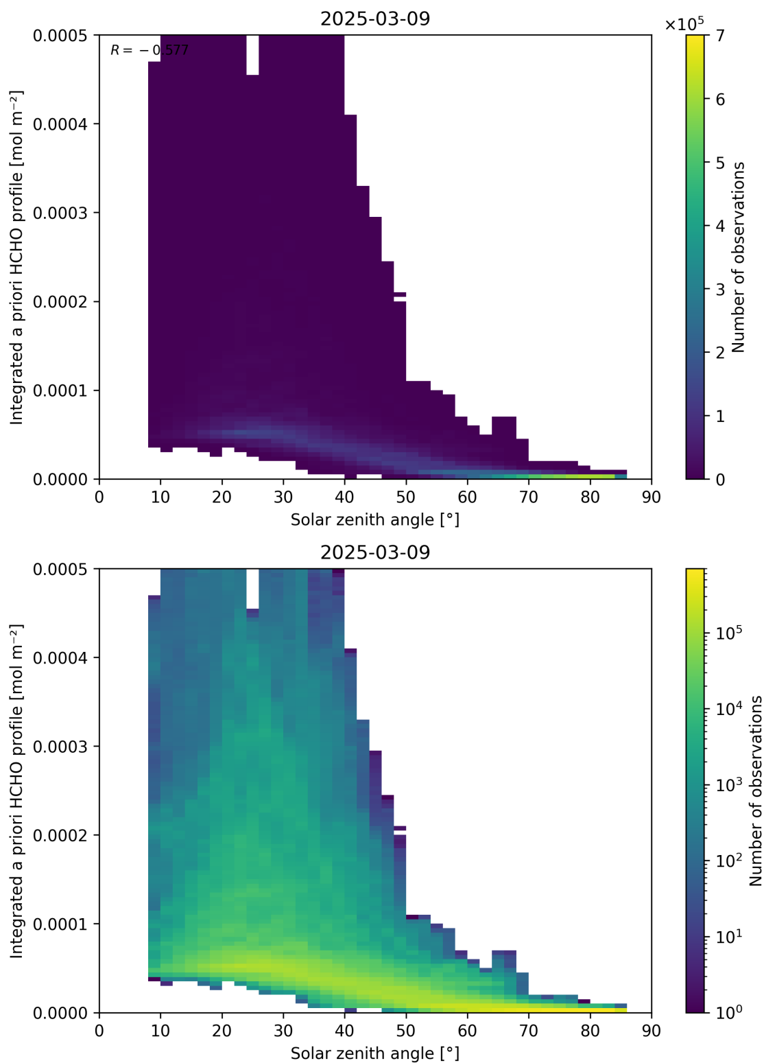
Figure 180: Scatter density plot of “Solar zenith angle” against “Integrated a priori HCHO profile” for 2025-03-08 to 2025-03-10.
