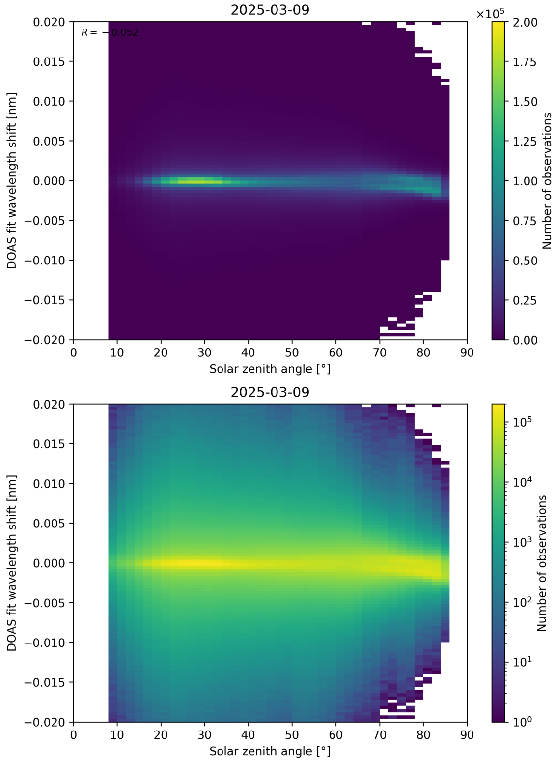
Figure 168: Scatter density plot of “Solar zenith angle” against “DOAS fit wavelength shift” for 2025-03-08 to 2025-03-10.
