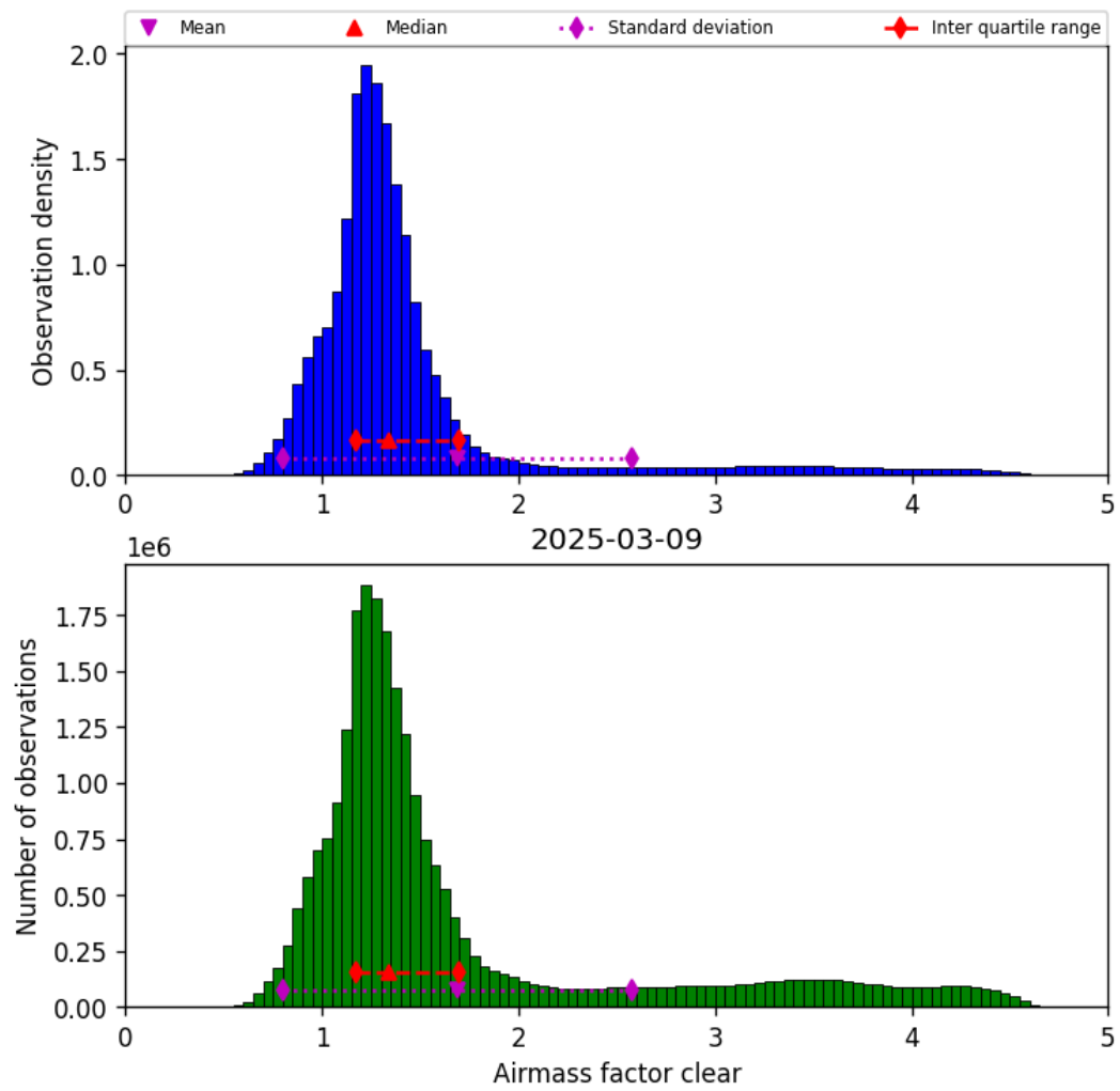
Figure 42: Histogram of “Airmass factor clear” for 2025-03-08 to 2025-03-10
