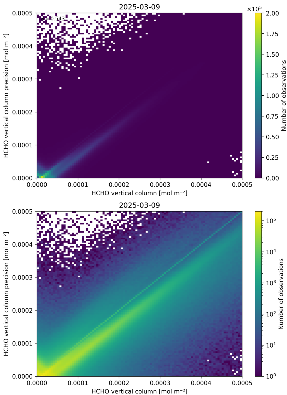
Figure 134: Scatter density plot of “HCHO vertical column” against “HCHO vertical column precision” for 2025-03-08 to 2025-03-10.
