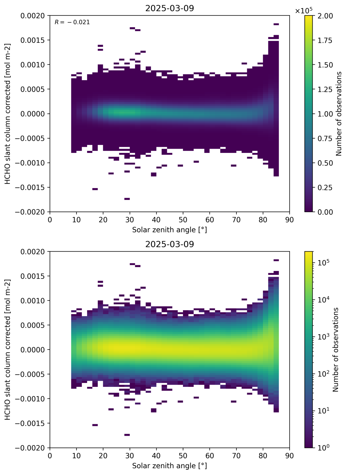
Figure 171: Scatter density plot of “Solar zenith angle” against “HCHO slant column corrected” for 2025-03-08 to 2025-03-10.
