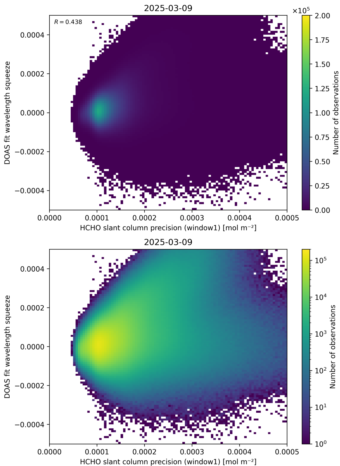
Figure 90: Scatter density plot of “HCHO slant column precision (window1)” against “DOAS fit wavelength squeeze” for 2025-03-08 to 2025-03-10.
