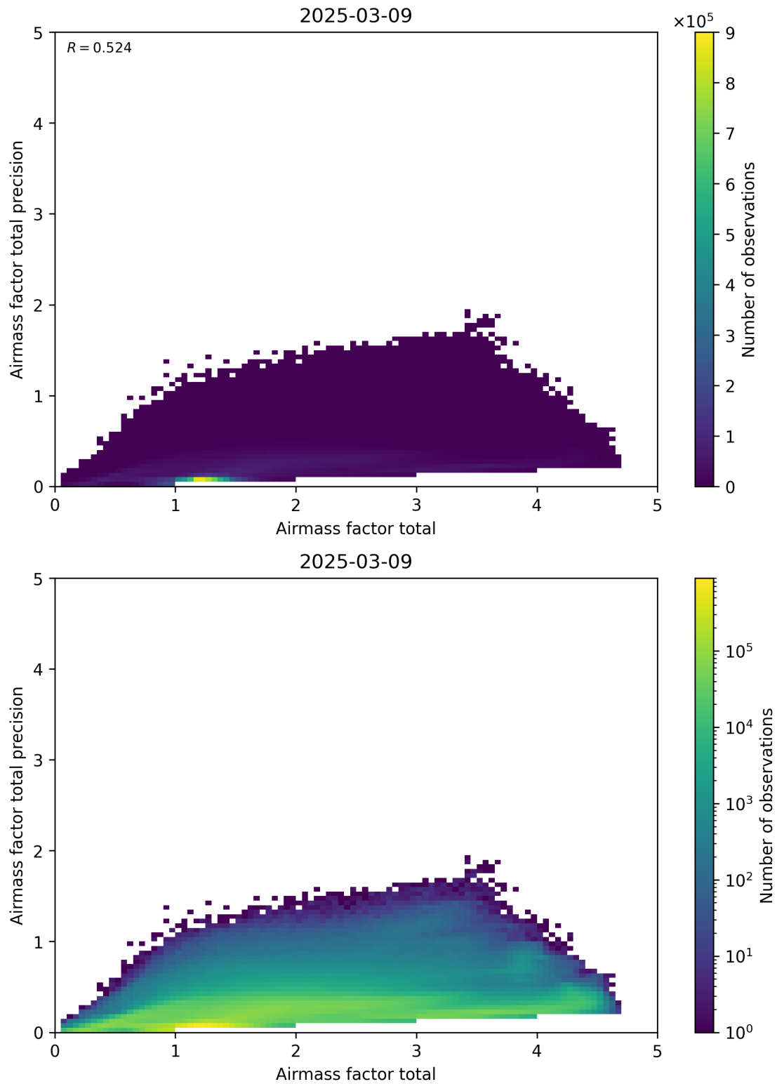
Figure 103: Scatter density plot of “Airmass factor total” against “Airmass factor total precision” for 2025-03-08 to 2025-03-10.
