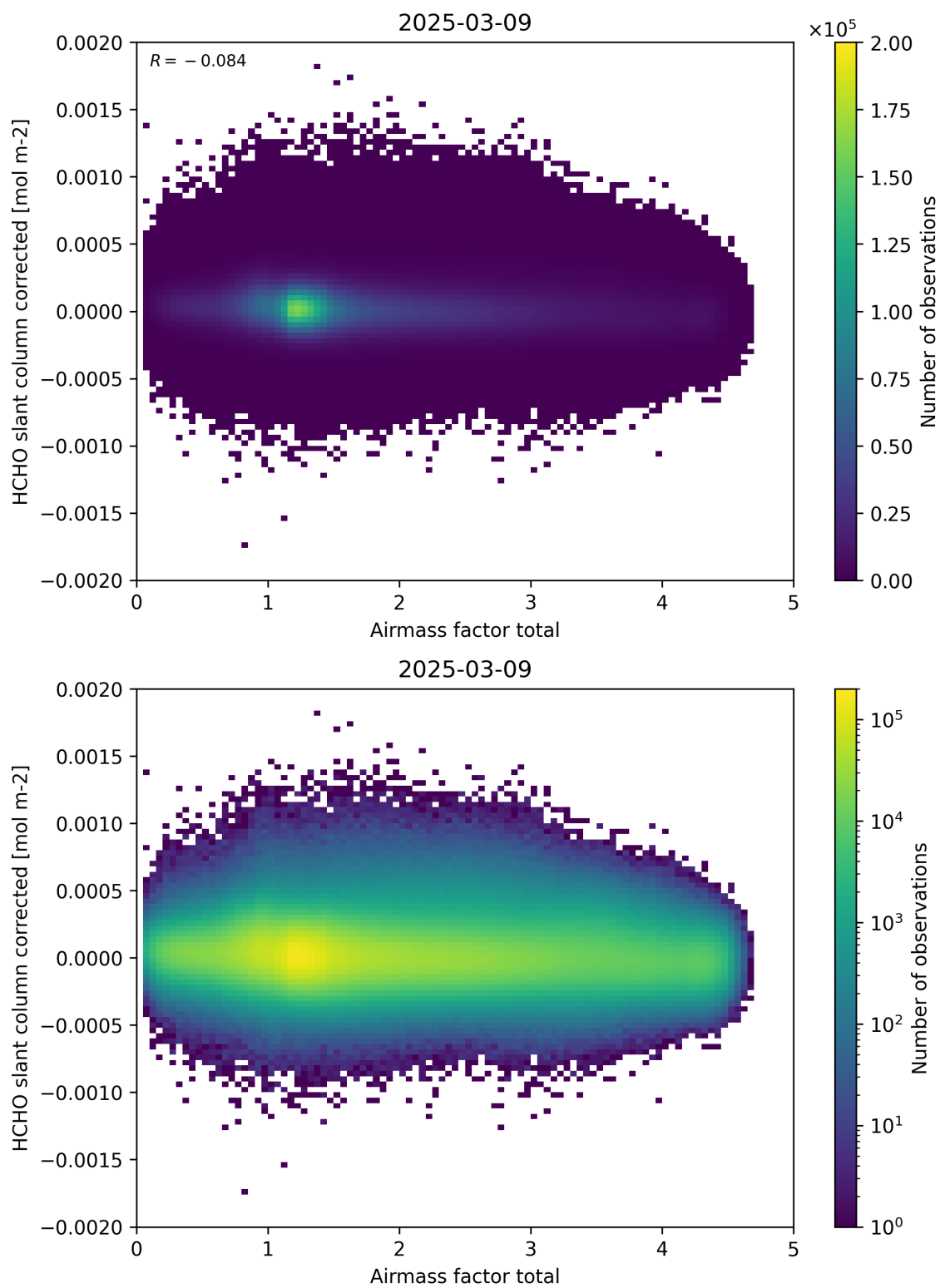
Figure 101: Scatter density plot of “Airmass factor total” against “HCHO slant column corrected” for 2025-03-08 to 2025-03-10.
