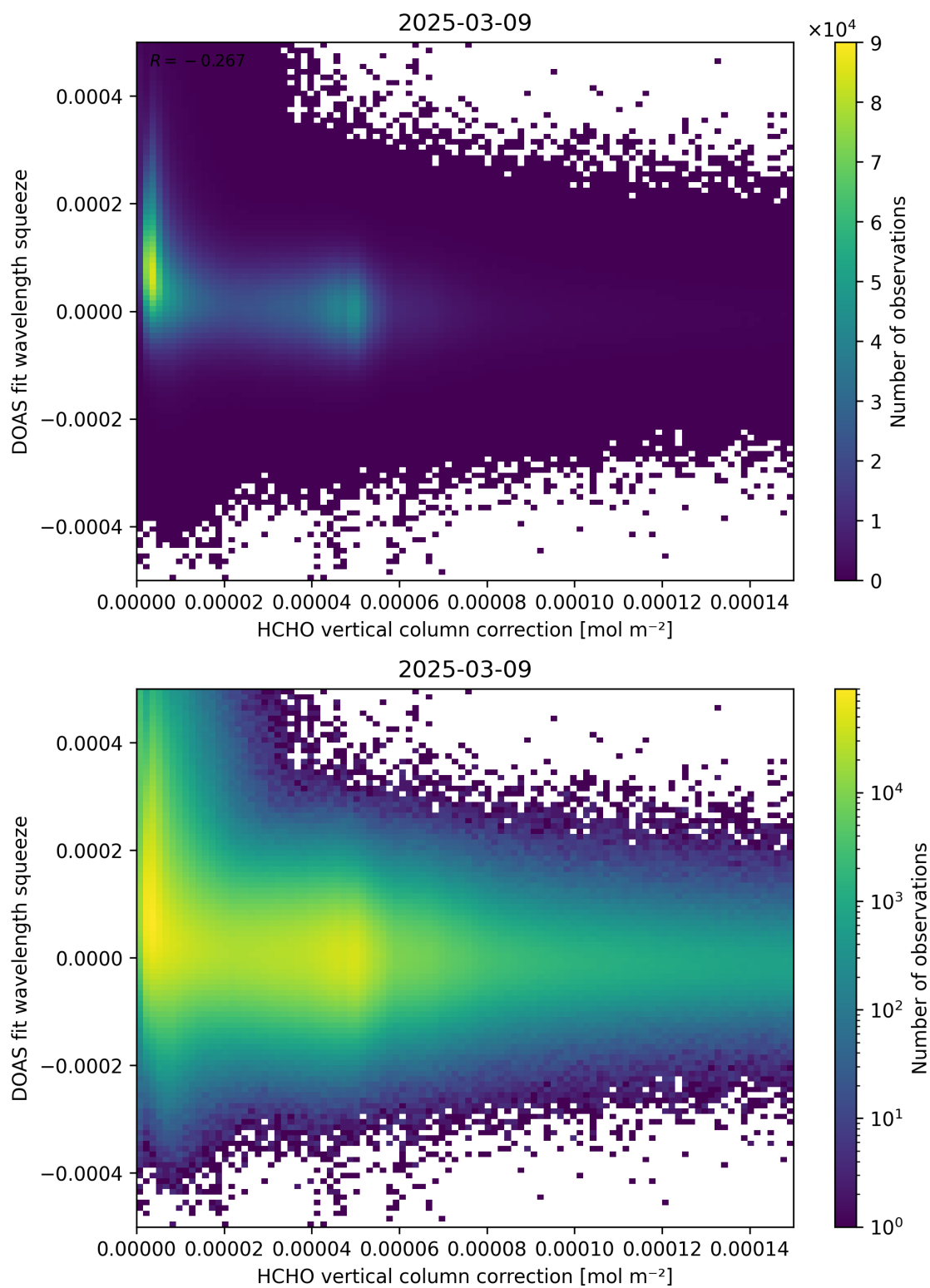
Figure 114: Scatter density plot of “HCHO vertical column correction” against “DOAS fit wavelength squeeze” for 2025-03-08 to 2025-03-10.
