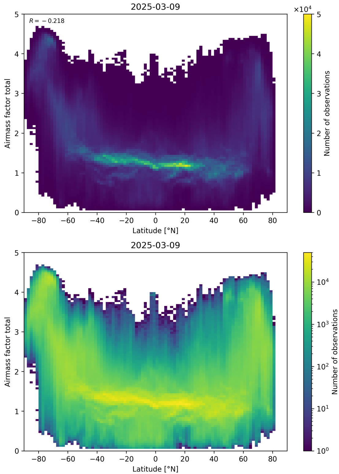
Figure 161: Scatter density plot of “Latitude” against “Airmass factor total” for 2025-03-08 to 2025-03-10.
