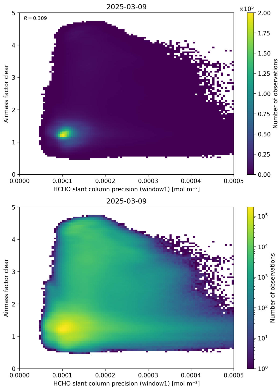
Figure 91: Scatter density plot of “HCHO slant column precision (window1)” against “Airmass factor clear” for 2025-03-08 to 2025-03-10.
