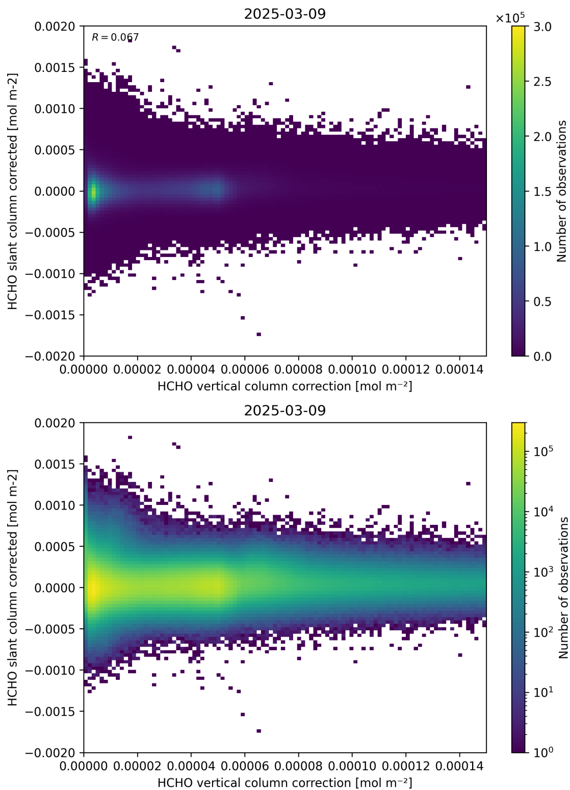
Figure 116: Scatter density plot of “HCHO vertical column correction” against “HCHO slant column corrected” for 2025-03-08 to 2025-03-10.
