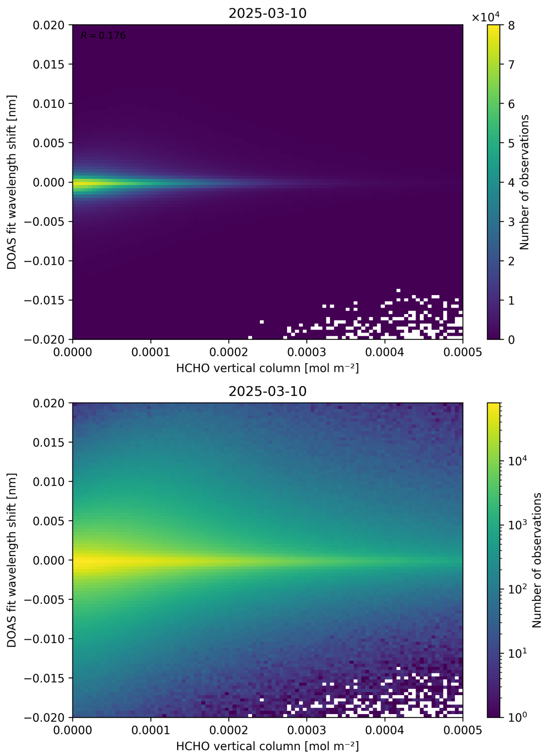
Figure 124: Scatter density plot of “HCHO vertical column” against “DOAS fit wavelength shift” for 2025-03-09 to 2025-03-11.
