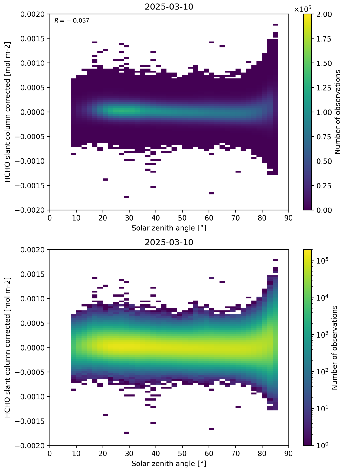
Figure 171: Scatter density plot of “Solar zenith angle” against “HCHO slant column corrected” for 2025-03-09 to 2025-03-11.
