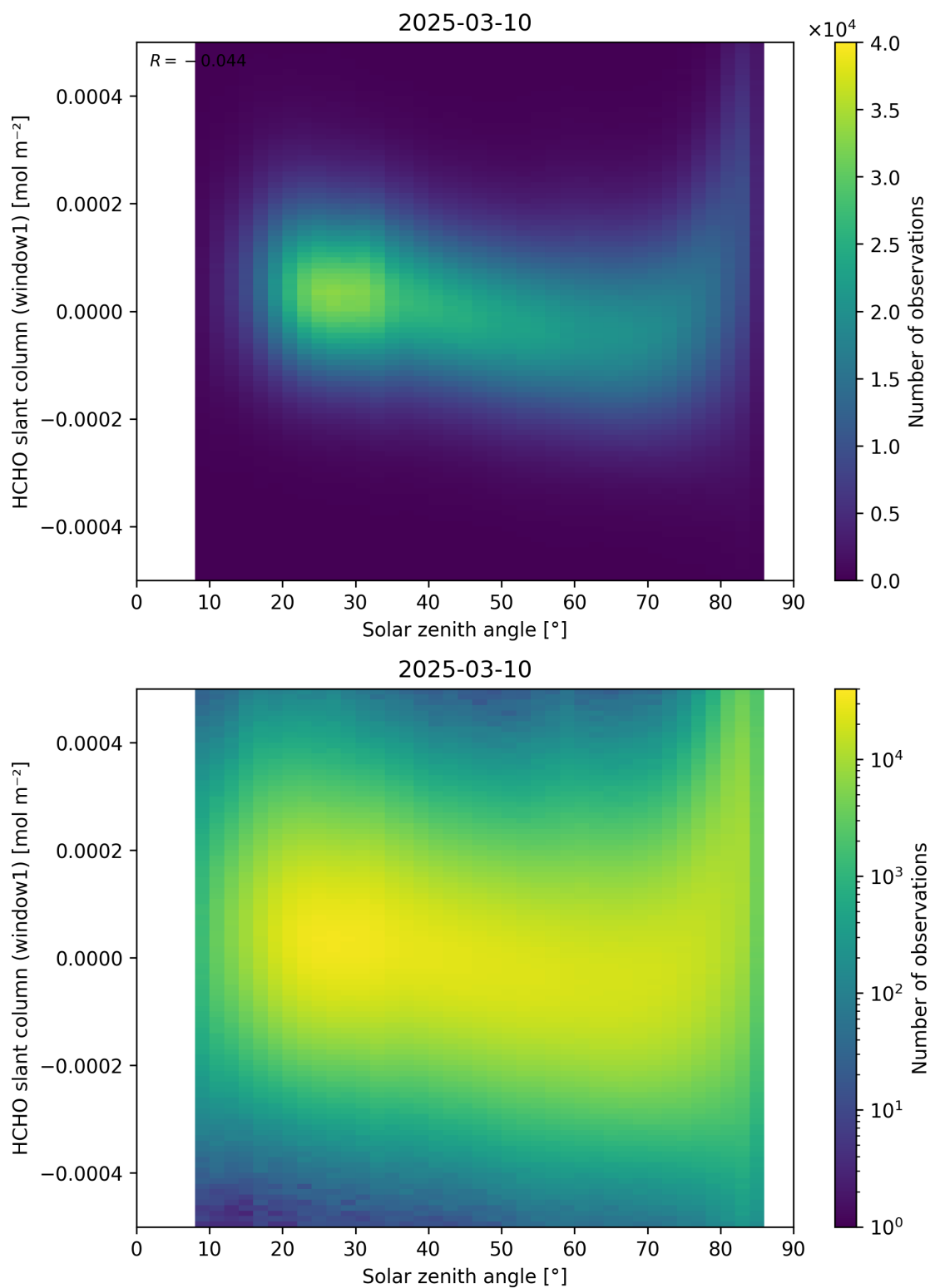
Figure 173: Scatter density plot of “Solar zenith angle” against “HCHO slant column (window1)” for 2025-03-09 to 2025-03-11.
