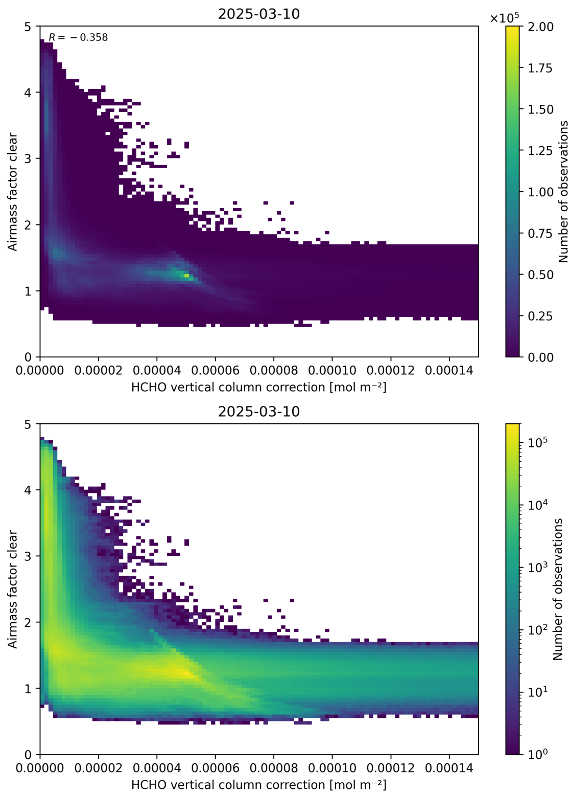
Figure 115: Scatter density plot of “HCHO vertical column correction” against “Airmass factor clear” for 2025-03-09 to 2025-03-11.
