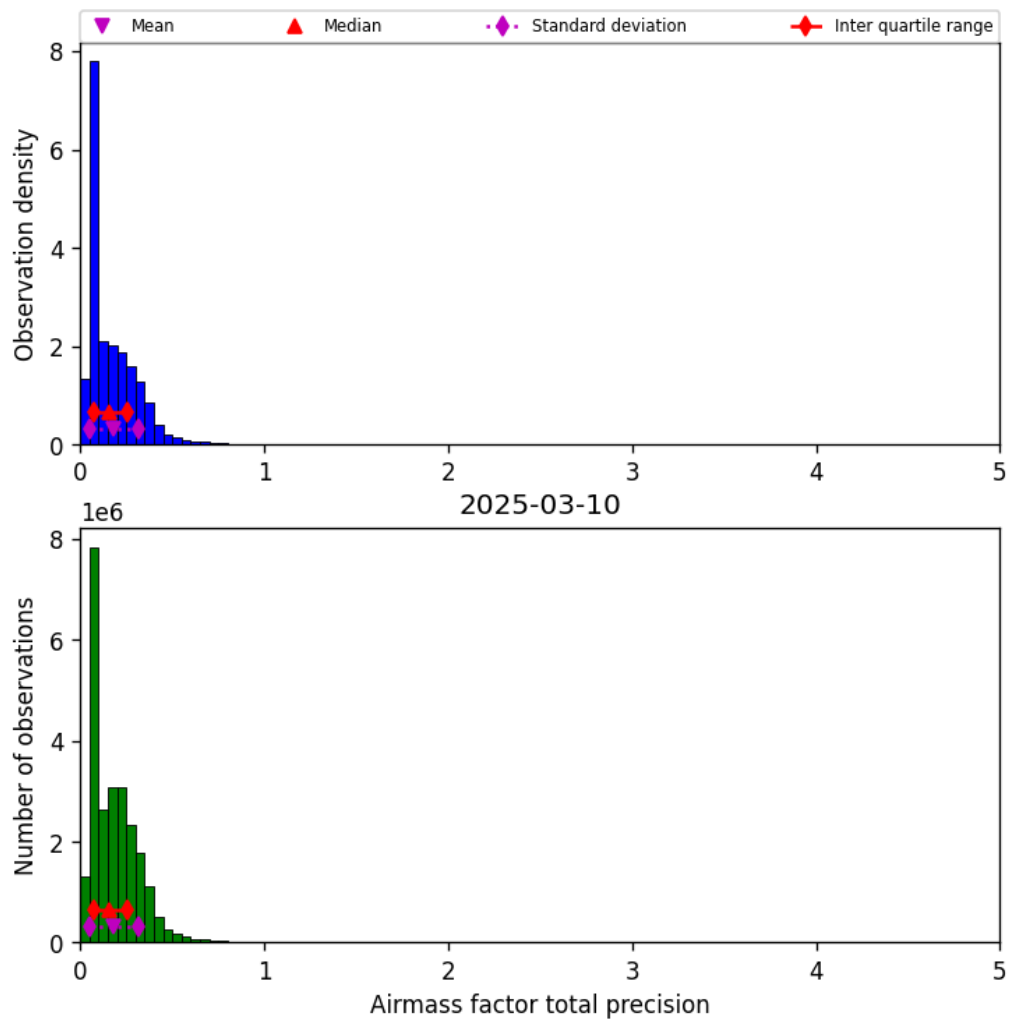
Figure 41: Histogram of “Airmass factor total precision” for 2025-03-09 to 2025-03-11
