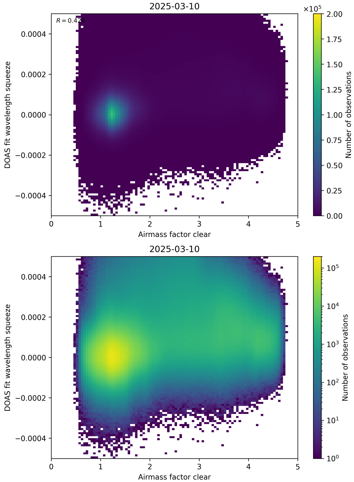
Figure 73: Scatter density plot of “Airmass factor clear” against “DOAS fit wavelength squeeze” for 2025-03-09 to 2025-03-11.
