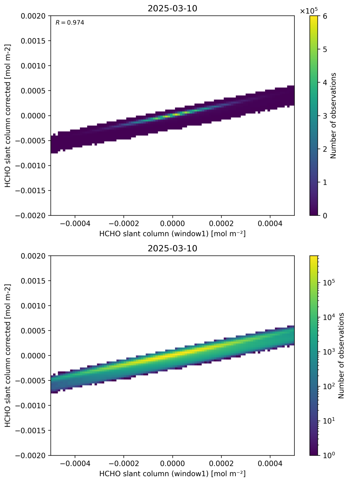
Figure 82: Scatter density plot of “HCHO slant column (window1)” against “HCHO slant column corrected” for 2025-03-09 to 2025-03-11.
