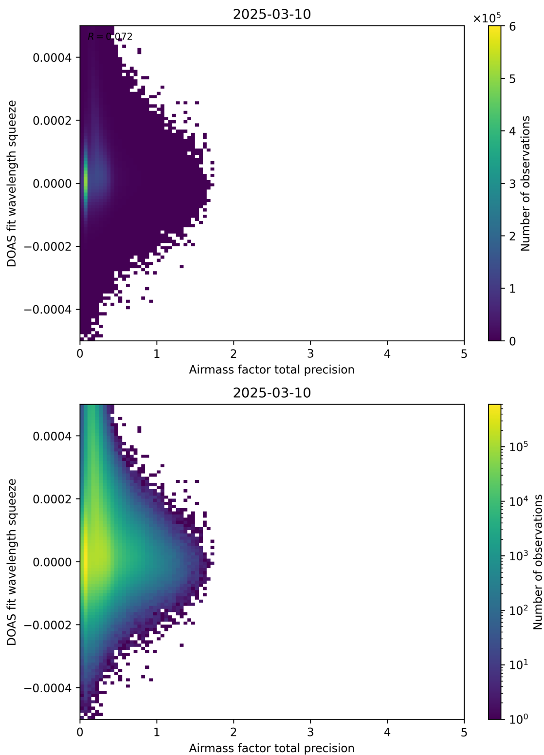
Figure 107: Scatter density plot of “Airmass factor total precision” against “DOAS fit wavelength squeeze” for 2025-03-09 to 2025-03-11.
