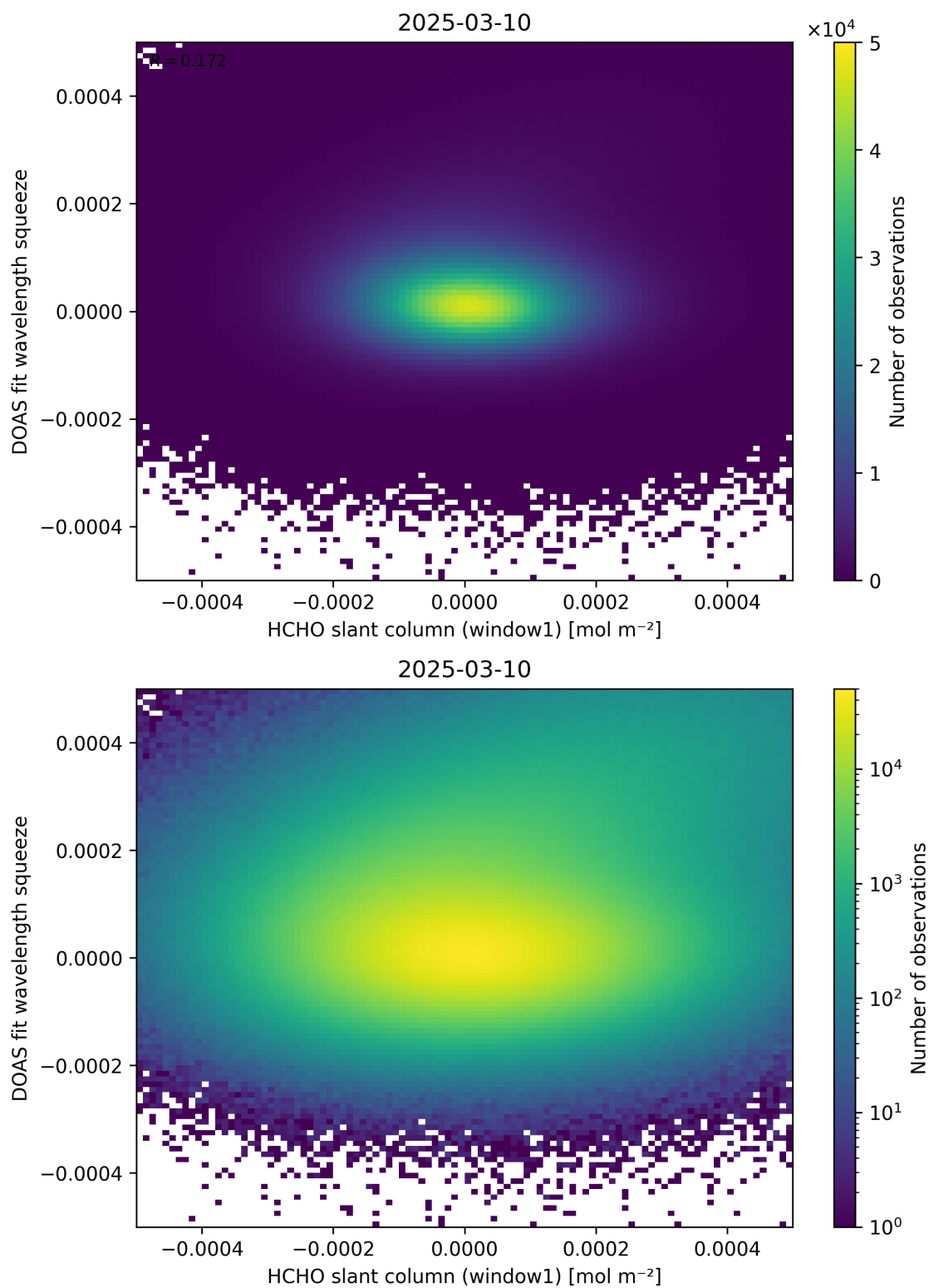
Figure 80: Scatter density plot of “HCHO slant column (window1)” against “DOAS fit wavelength squeeze” for 2025-03-09 to 2025-03-11.
