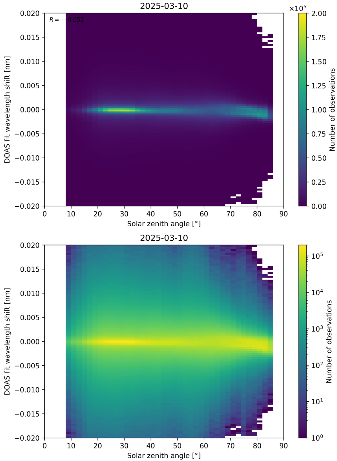
Figure 168: Scatter density plot of “Solar zenith angle” against “DOAS fit wavelength shift” for 2025-03-09 to 2025-03-11.
