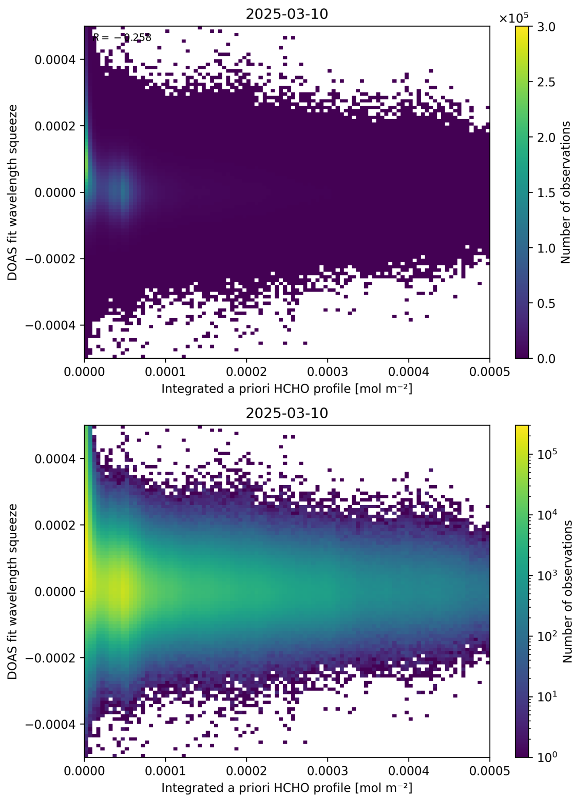
Figure 150: Scatter density plot of “Integrated a priori HCHO profile” against “DOAS fit wavelength squeeze” for 2025-03-09 to 2025-03-11.
