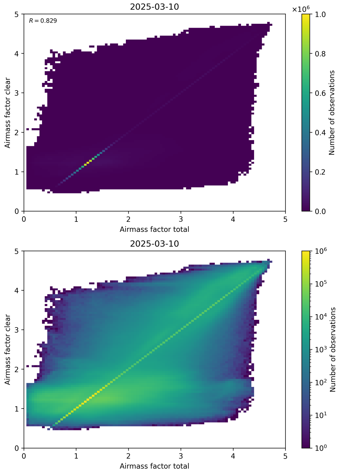
Figure 100: Scatter density plot of “Airmass factor total” against “Airmass factor clear” for 2025-03-09 to 2025-03-11.
