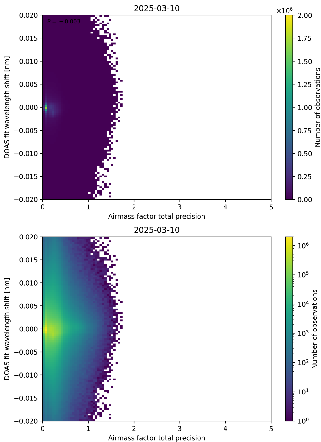
Figure 106: Scatter density plot of “Airmass factor total precision” against “DOAS fit wavelength shift” for 2025-03-09 to 2025-03-11.
