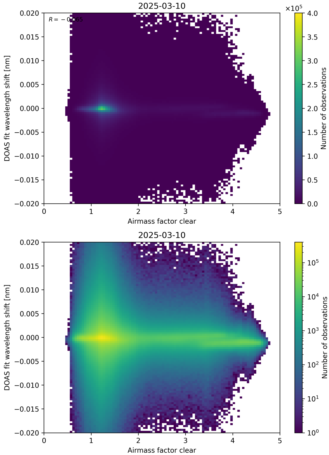
Figure 72: Scatter density plot of “Airmass factor clear” against “DOAS fit wavelength shift” for 2025-03-09 to 2025-03-11.
