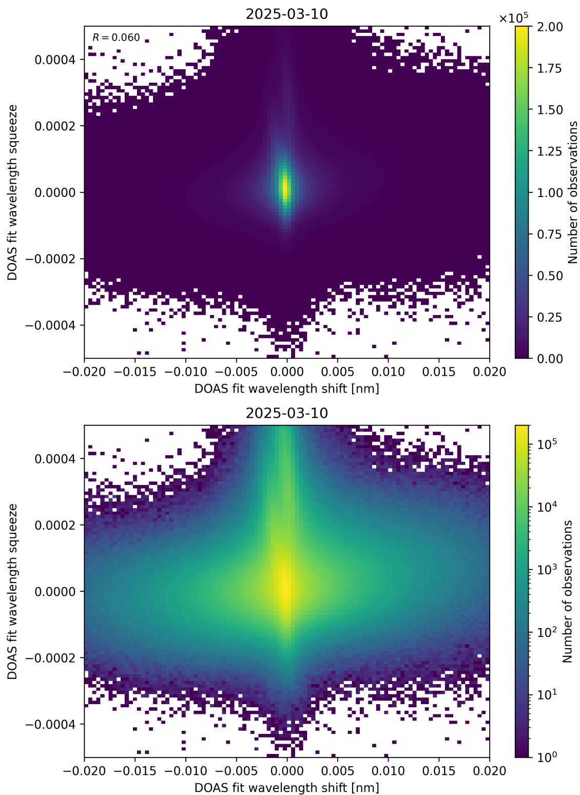
Figure 65: Scatter density plot of “DOAS fit wavelength shift” against “DOAS fit wavelength squeeze” for 2025-03-09 to 2025-03-11.
