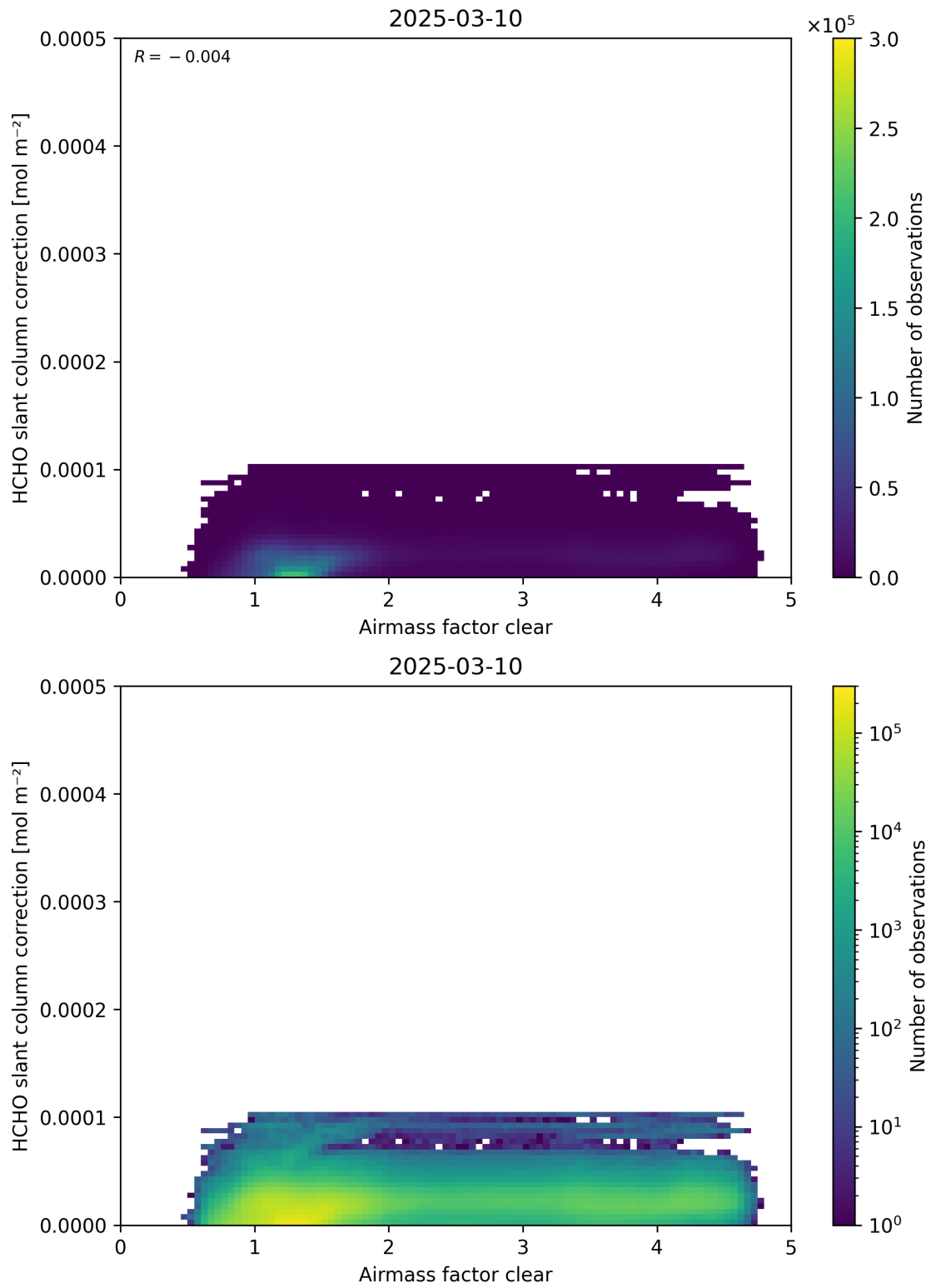
Figure 75: Scatter density plot of “Airmass factor clear” against “HCHO slant column correction” for 2025-03-09 to 2025-03-11.
