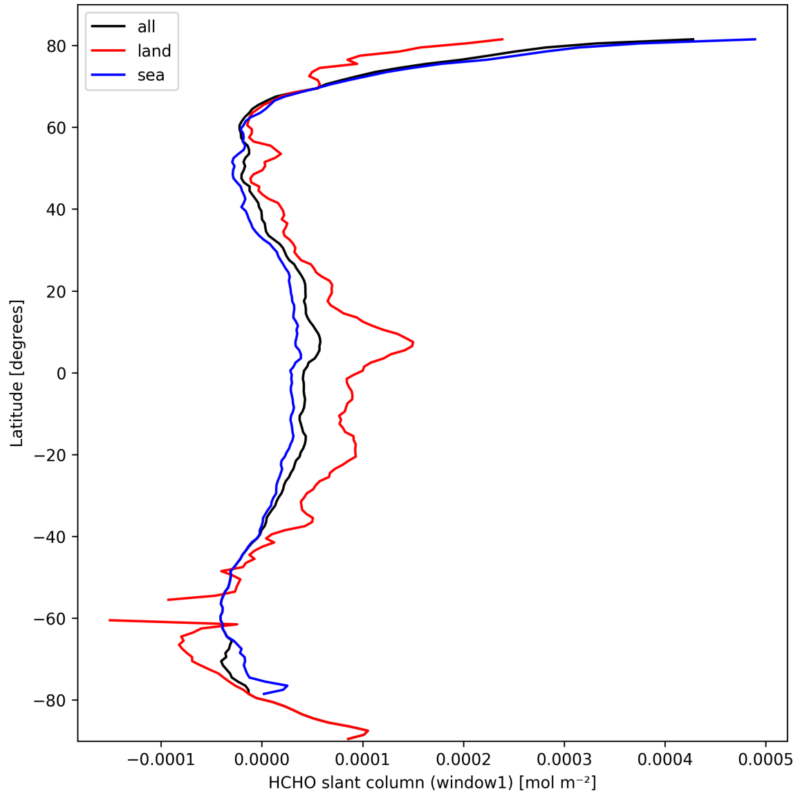
Figure 24: Zonal average of “HCHO slant column (window1)” for 2025-03-09 to 2025-03-11.
