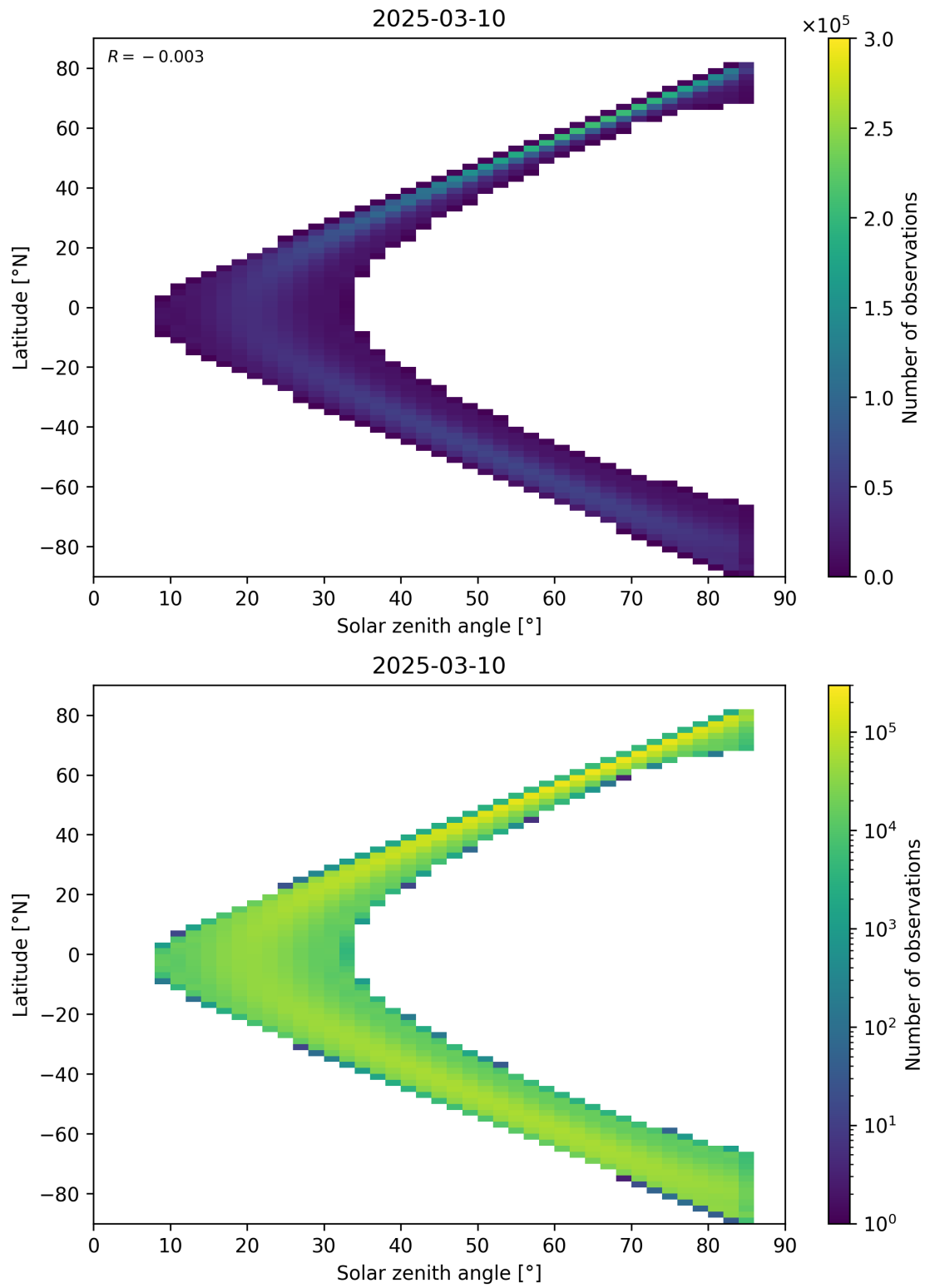
Figure 181: Scatter density plot of “Solar zenith angle” against “Latitude” for 2025-03-09 to 2025-03-11.
