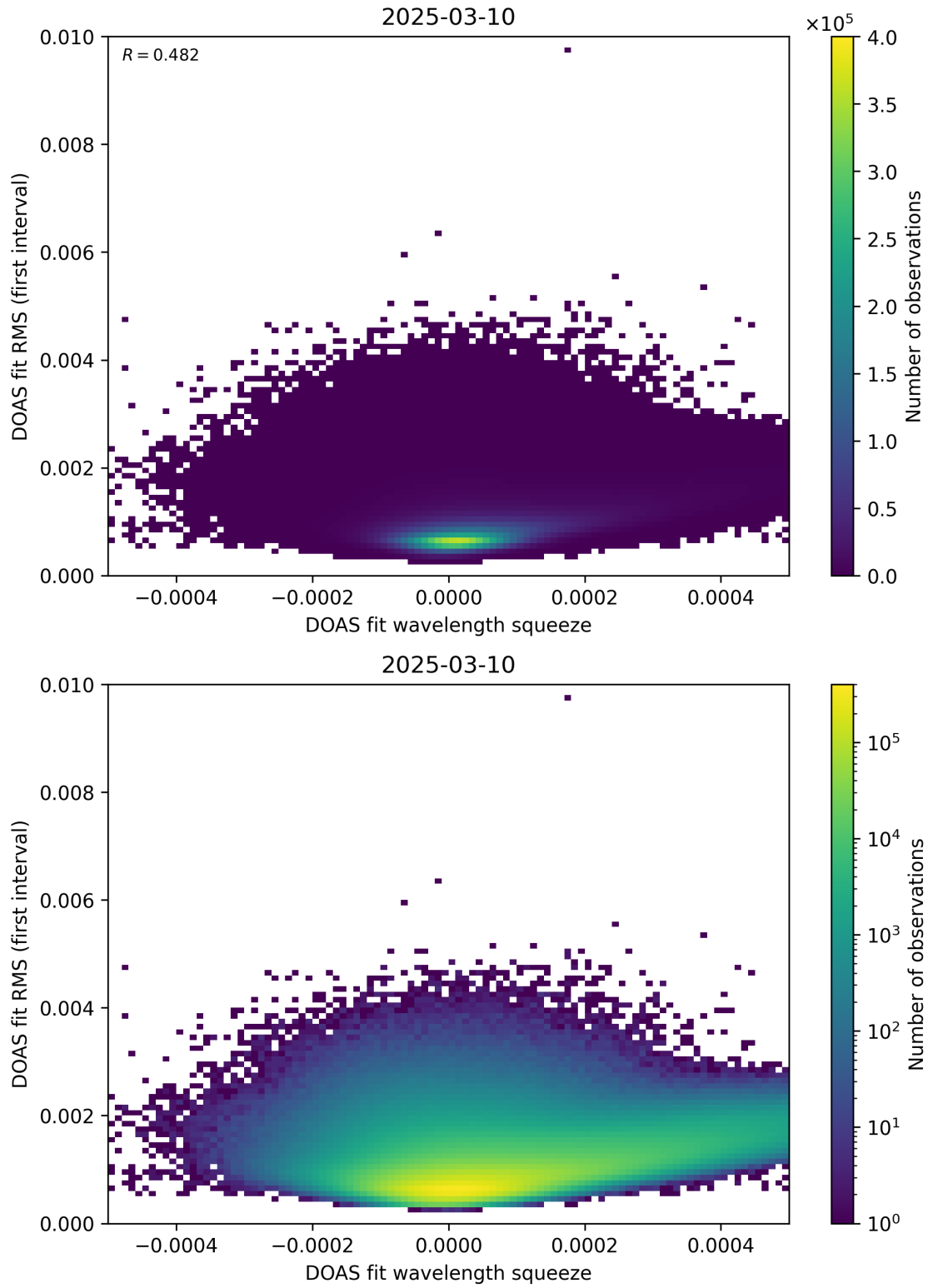
Figure 68: Scatter density plot of “DOAS fit wavelength squeeze” against “DOAS fit RMS (first interval)” for 2025-03-09 to 2025-03-11.
