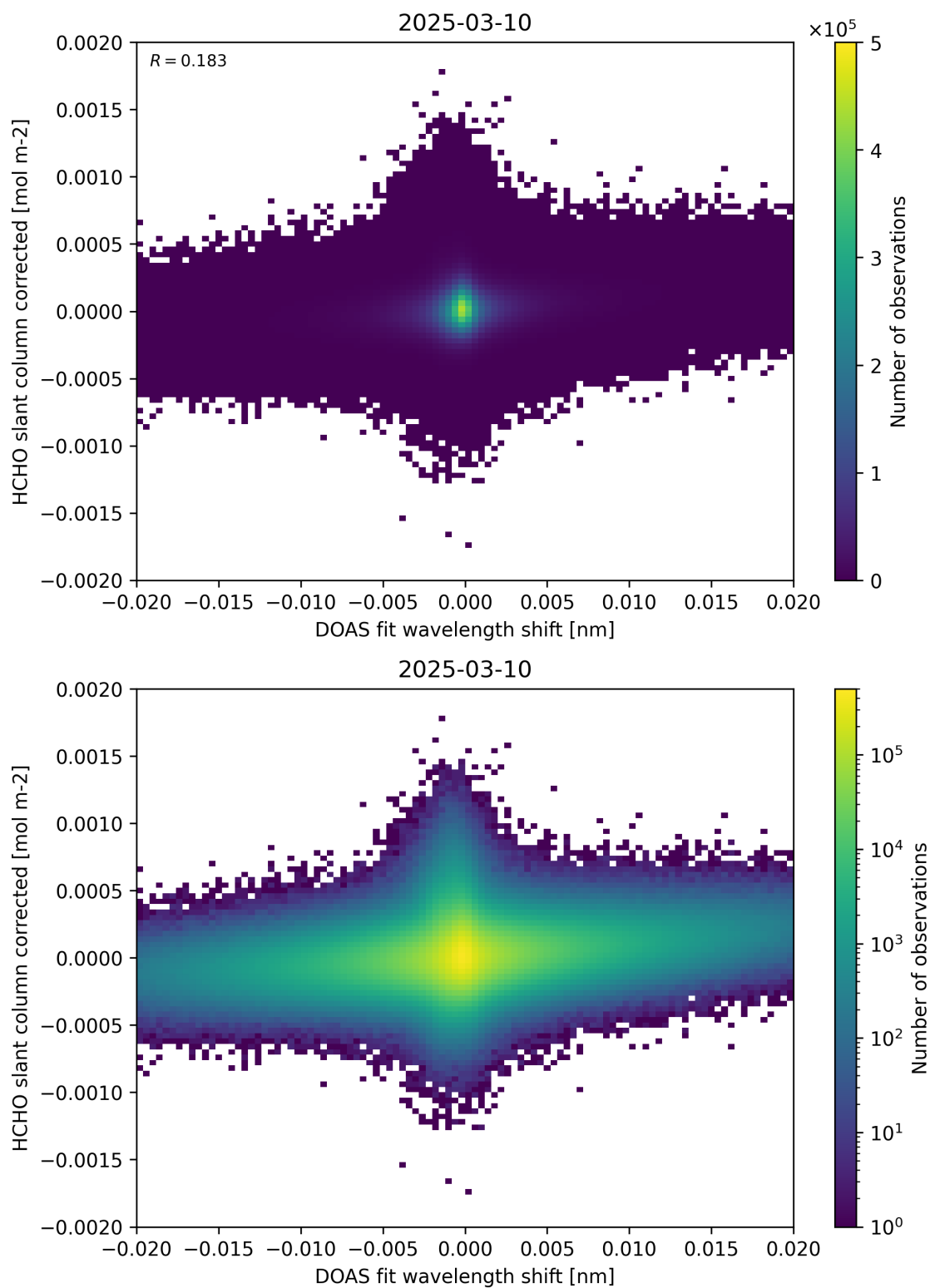
Figure 66: Scatter density plot of “DOAS fit wavelength shift” against “HCHO slant column corrected” for 2025-03-09 to 2025-03-11.
