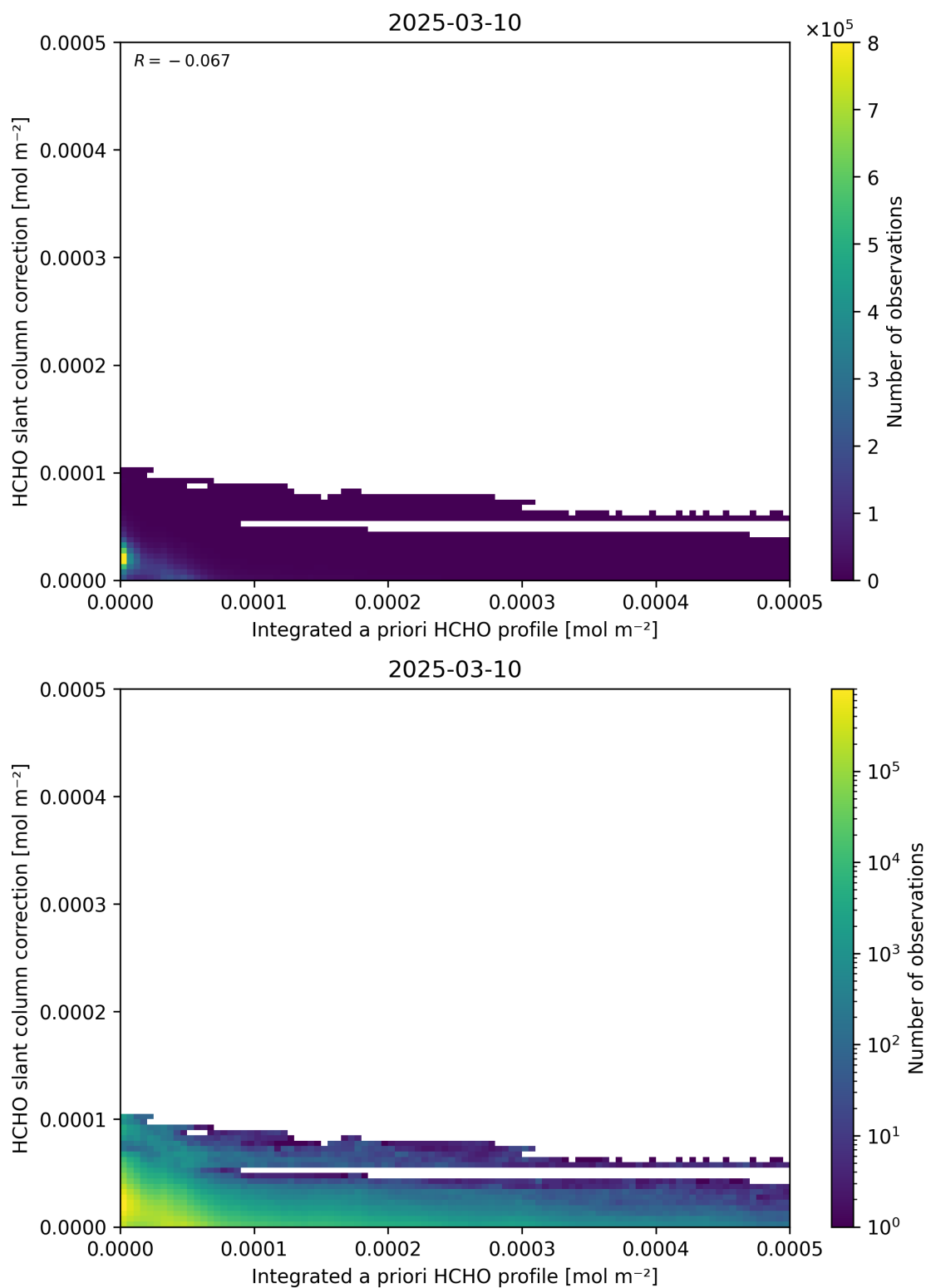
Figure 152: Scatter density plot of “Integrated a priori HCHO profile” against “HCHO slant column correction” for 2025-03-09 to 2025-03-11.
