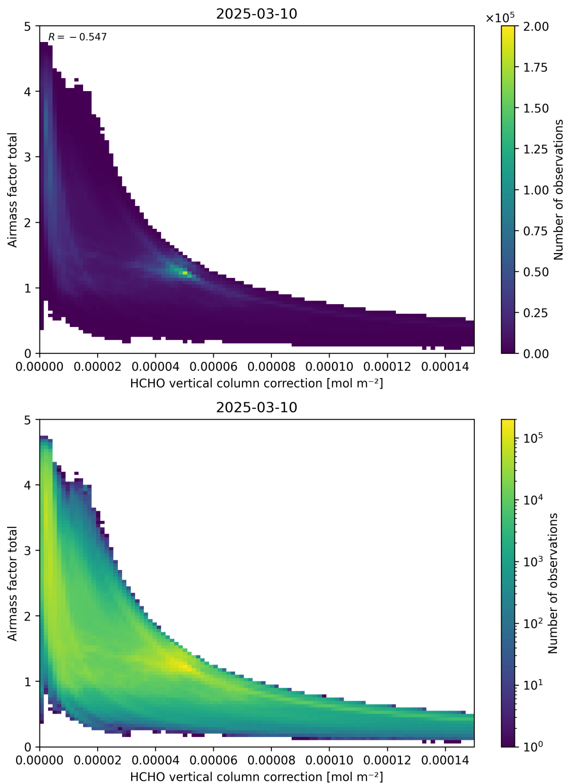
Figure 120: Scatter density plot of “HCHO vertical column correction” against “Airmass factor total” for 2025-03-09 to 2025-03-11.
