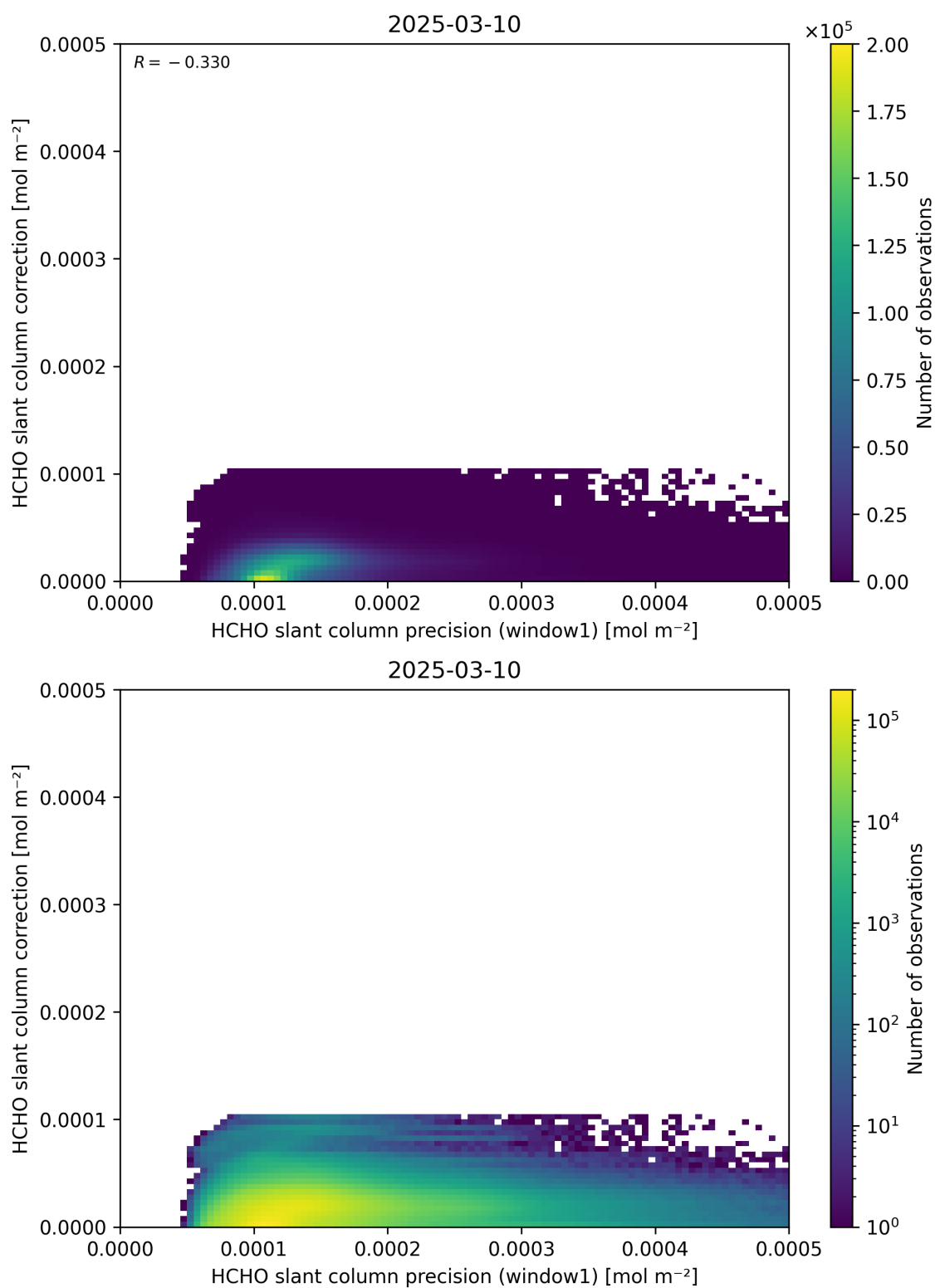
Figure 93: Scatter density plot of “HCHO slant column precision (window1)” against “HCHO slant column correction” for 2025-03-09 to 2025-03-11.
