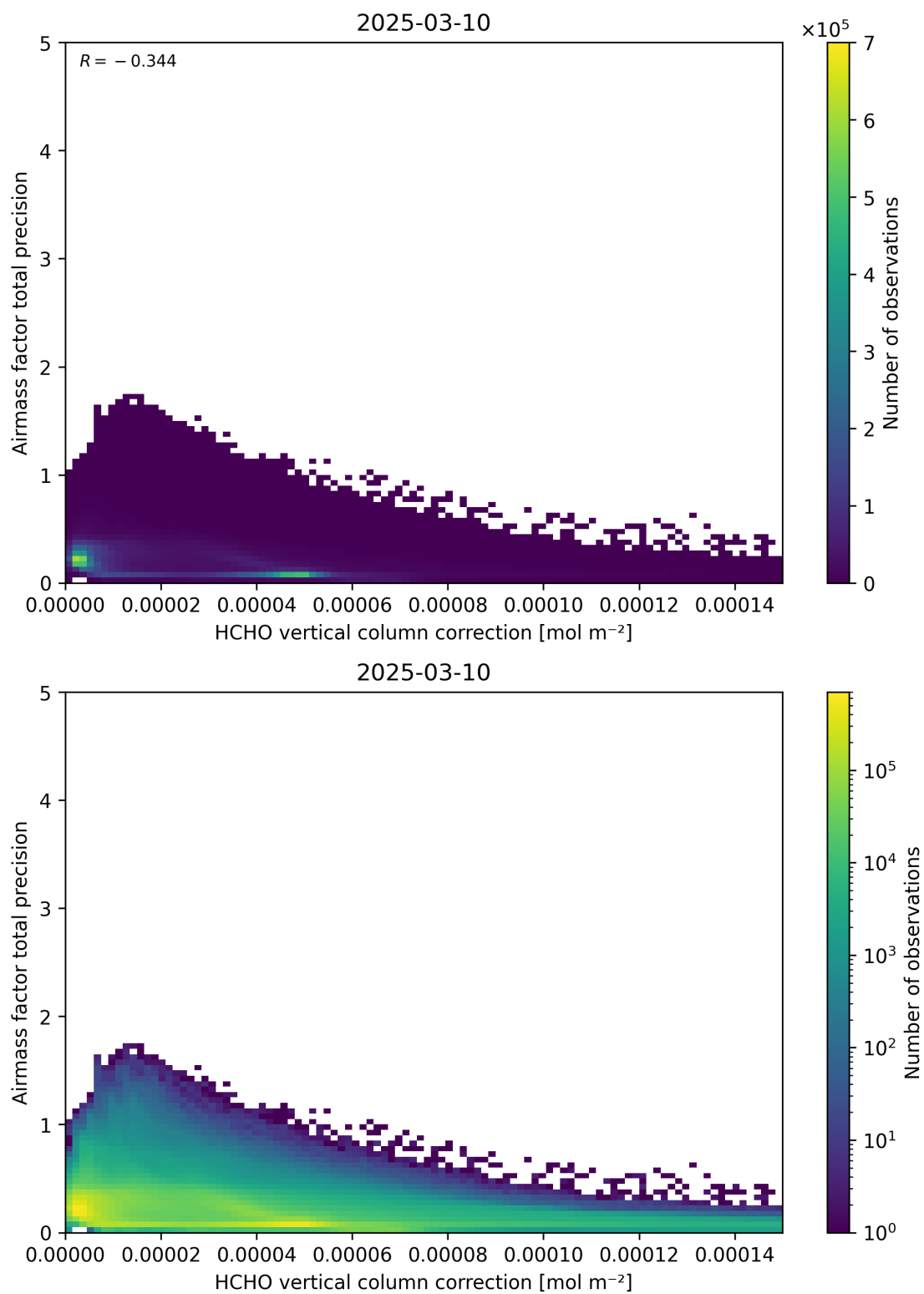
Figure 121: Scatter density plot of “HCHO vertical column correction” against “Airmass factor total precision” for 2025-03-09 to 2025-03-11.
