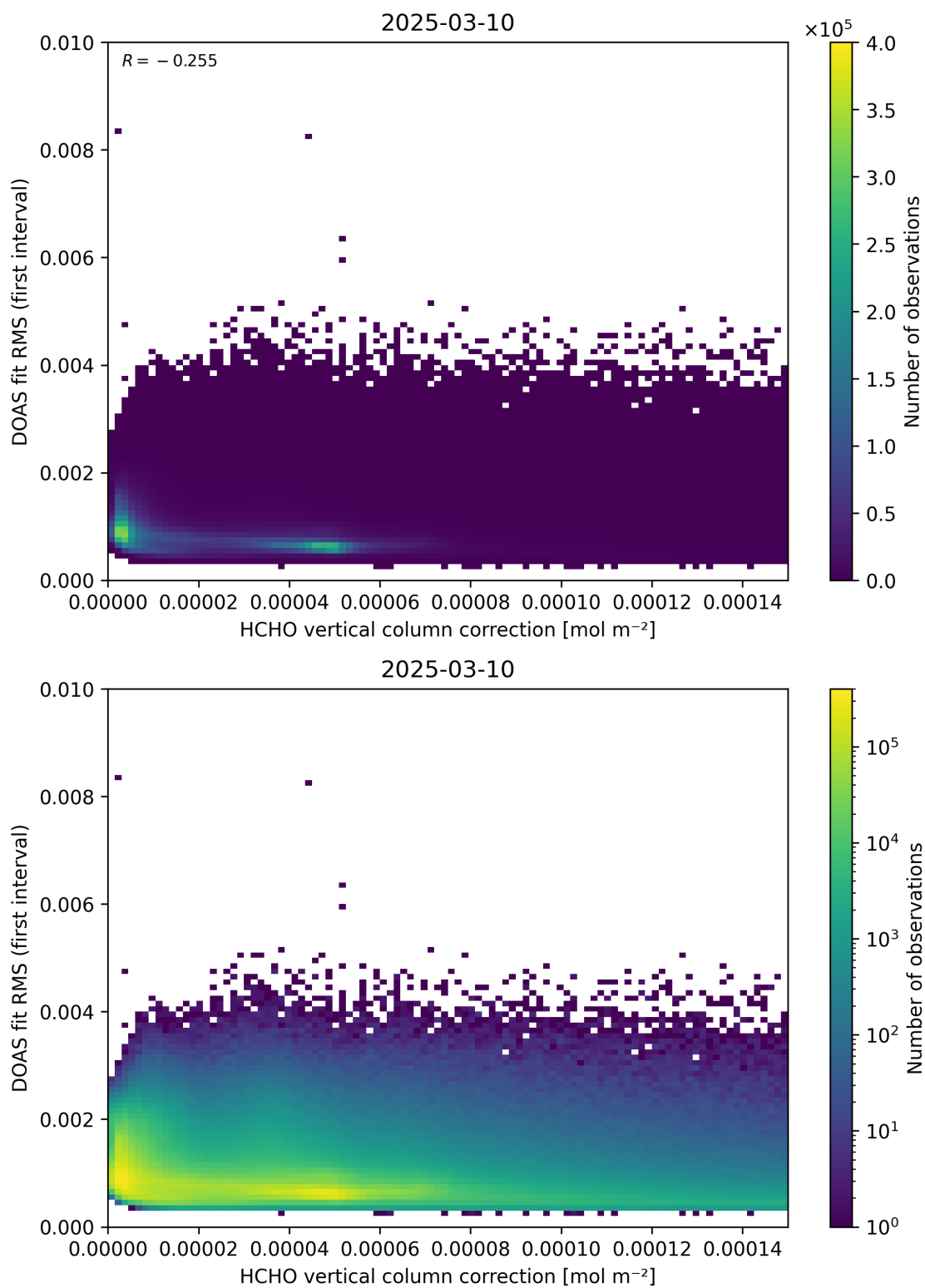
Figure 112: Scatter density plot of “HCHO vertical column correction” against “DOAS fit RMS (first interval)” for 2025-03-09 to 2025-03-11.
