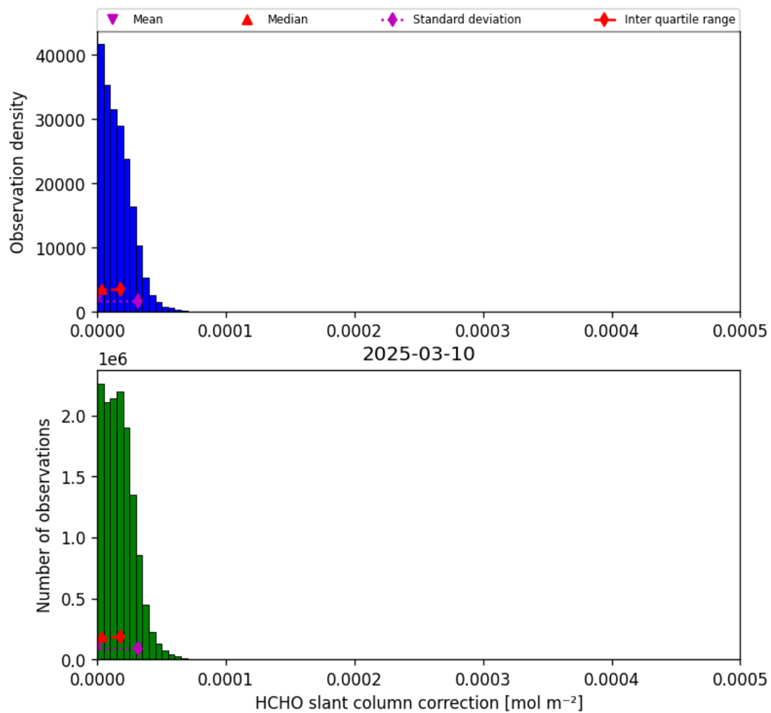
Figure 47: Histogram of “HCHO slant column correction” for 2025-03-09 to 2025-03-11
