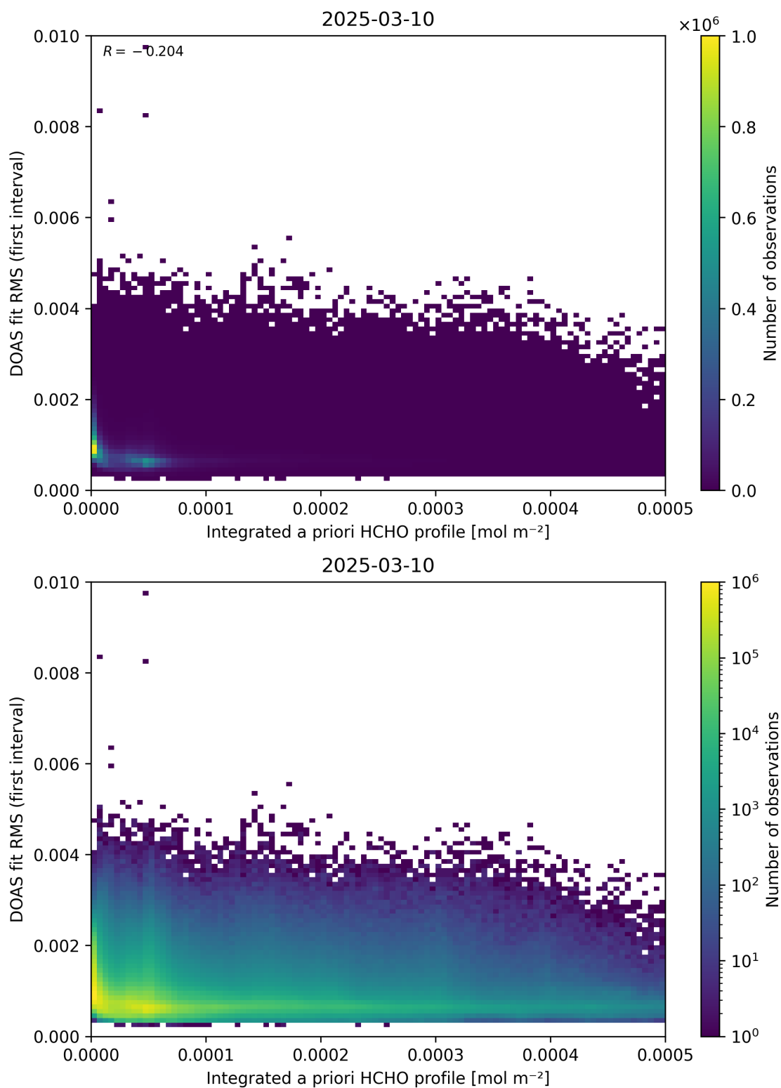
Figure 148: Scatter density plot of “Integrated a priori HCHO profile” against “DOAS fit RMS (first interval)” for 2025-03-09 to 2025-03-11.
