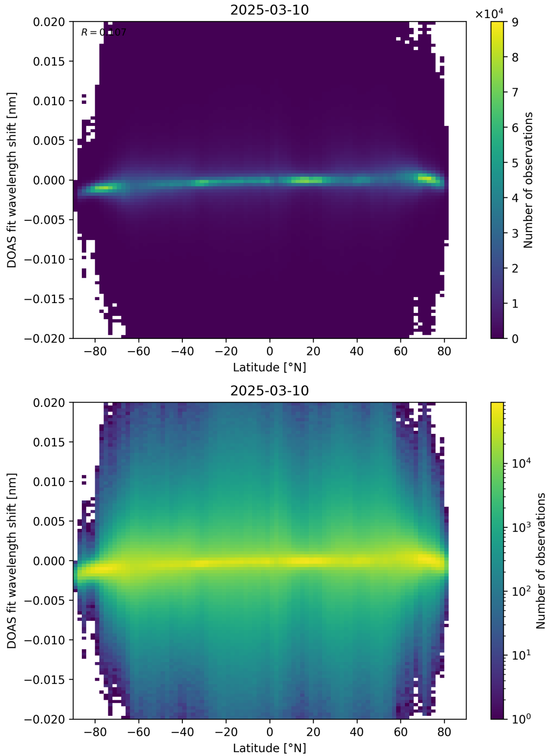
Figure 154: Scatter density plot of “Latitude” against “DOAS fit wavelength shift” for 2025-03-09 to 2025-03-11.
