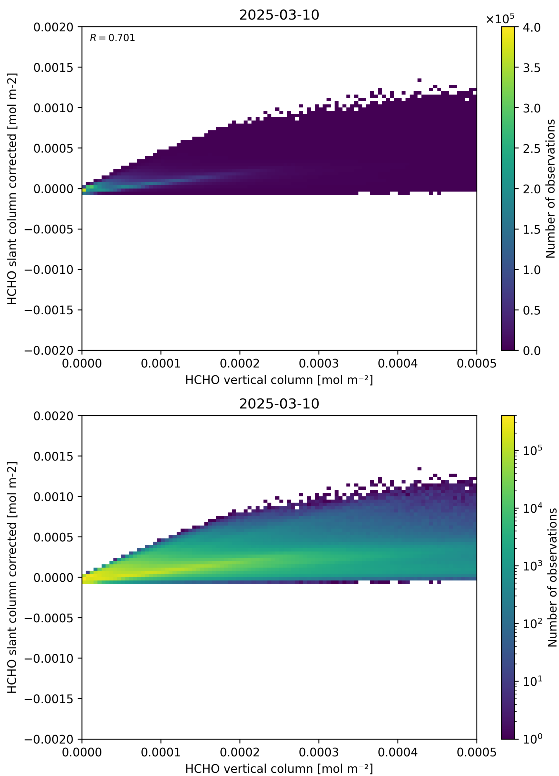
Figure 127: Scatter density plot of “HCHO vertical column” against “HCHO slant column corrected” for 2025-03-09 to 2025-03-11.
