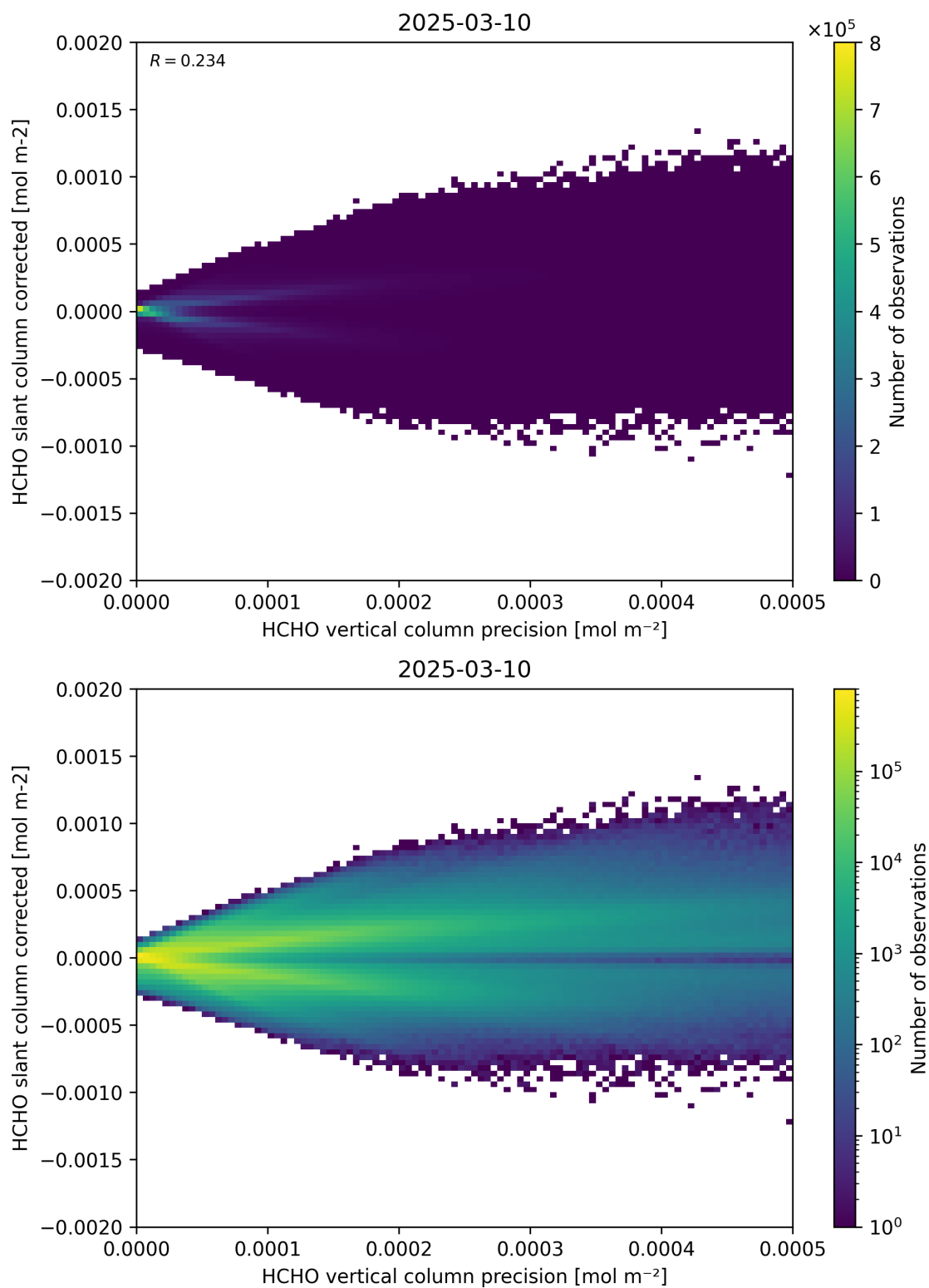
Figure 140: Scatter density plot of “HCHO vertical column precision” against “HCHO slant column corrected” for 2025-03-09 to 2025-03-11.
