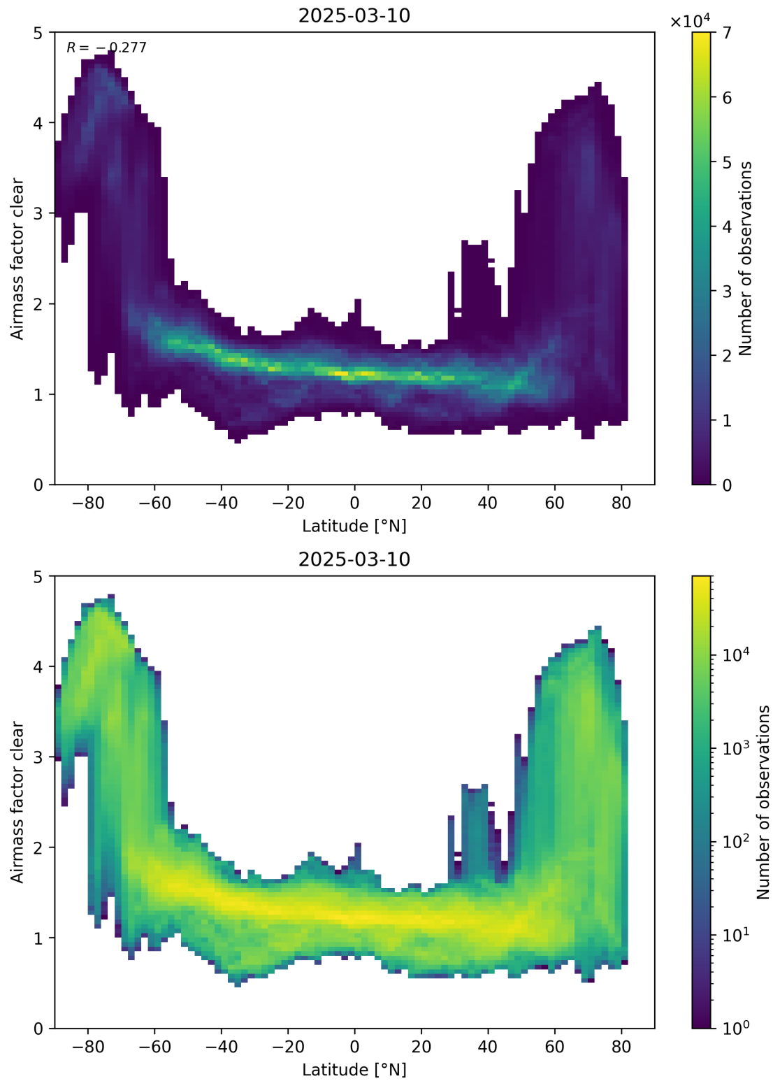
Figure 156: Scatter density plot of “Latitude” against “Airmass factor clear” for 2025-03-09 to 2025-03-11.
