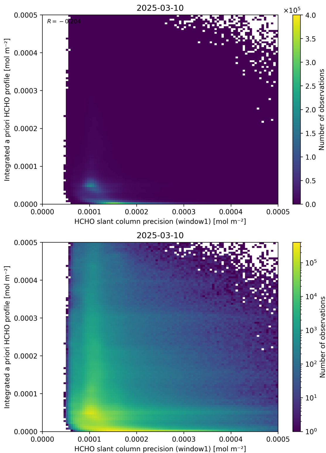
Figure 96: Scatter density plot of “HCHO slant column precision (window1)” against “Integrated a priori HCHO profile” for 2025-03-09 to 2025-03-11.
