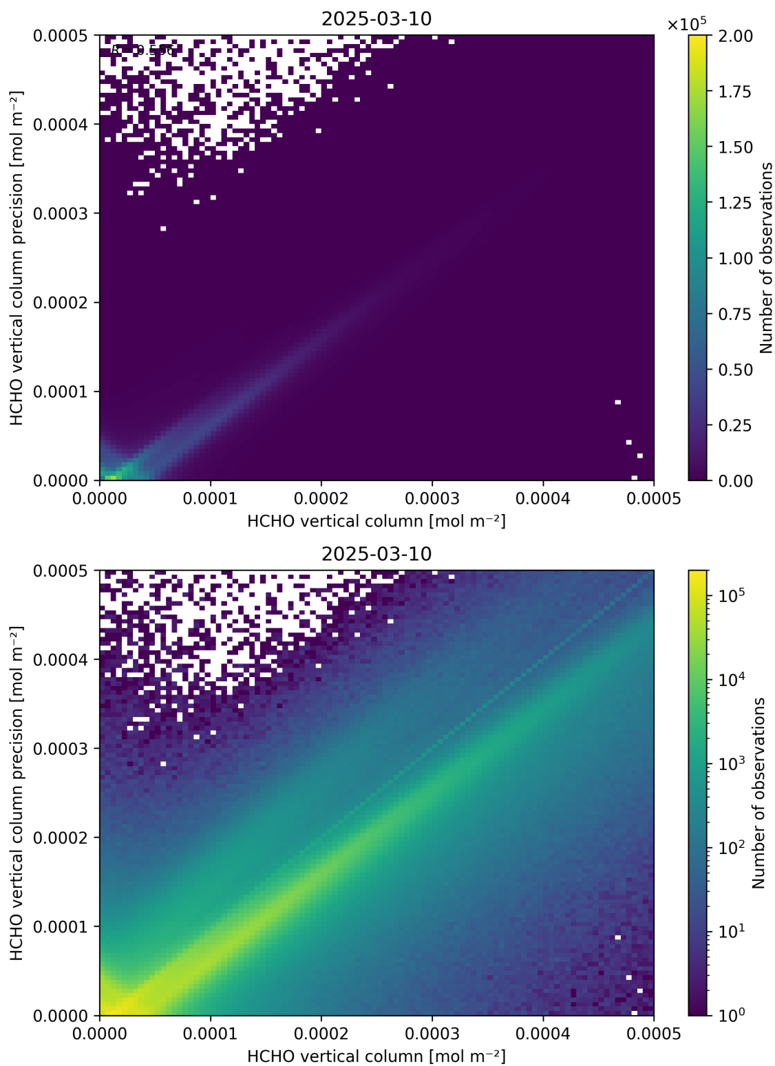
Figure 134: Scatter density plot of “HCHO vertical column” against “HCHO vertical column precision” for 2025-03-09 to 2025-03-11.
