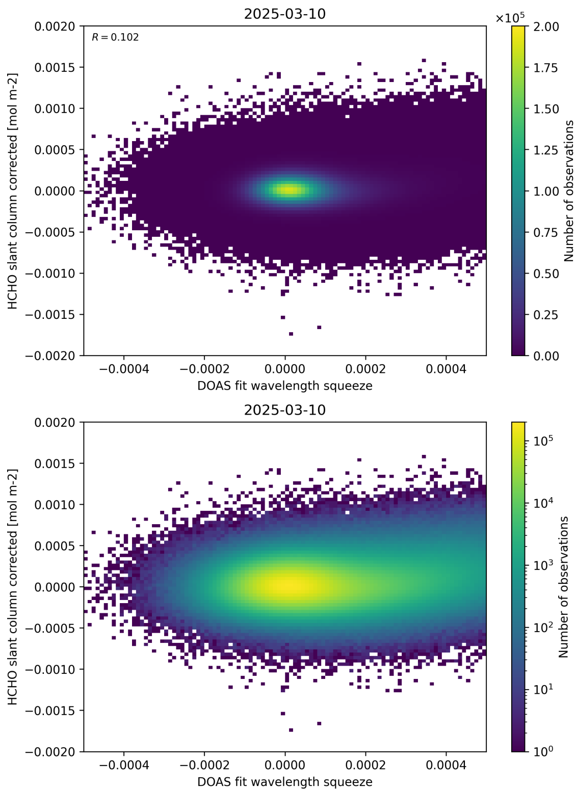
Figure 69: Scatter density plot of “DOAS fit wavelength squeeze” against “HCHO slant column corrected” for 2025-03-09 to 2025-03-11.
