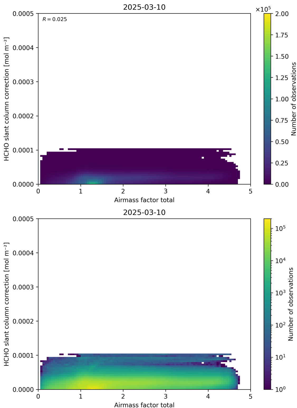
Figure 102: Scatter density plot of “Airmass factor total” against “HCHO slant column correction” for 2025-03-09 to 2025-03-11.
