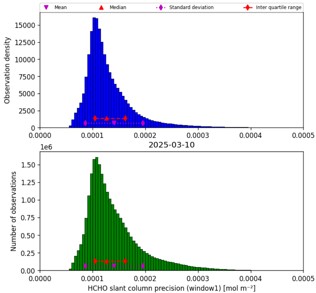
Figure 39: Histogram of “HCHO slant column precision (window1)” for 2025-03-09 to 2025-03-11
