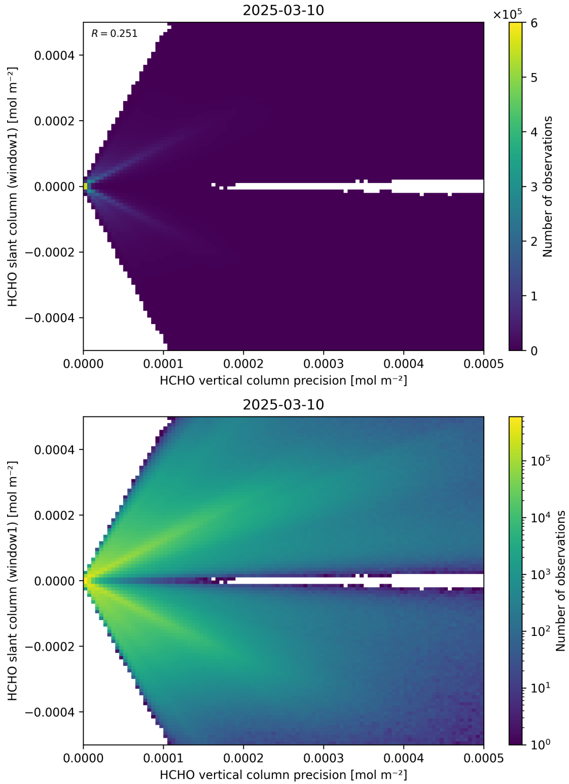
Figure 142: Scatter density plot of “HCHO vertical column precision” against “HCHO slant column (window1)” for 2025-03-09 to 2025-03-11.
