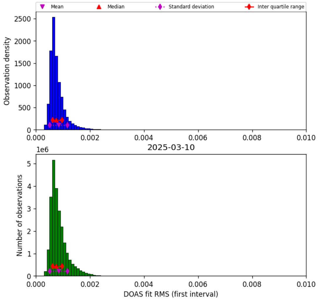
Figure 46: Histogram of “DOAS fit RMS (first interval)” for 2025-03-09 to 2025-03-11
