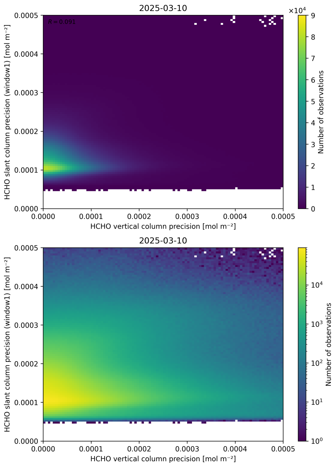
Figure 143: Scatter density plot of “HCHO vertical column precision” against “HCHO slant column precision (window1)” for 2025-03-09 to 2025-03-11.
