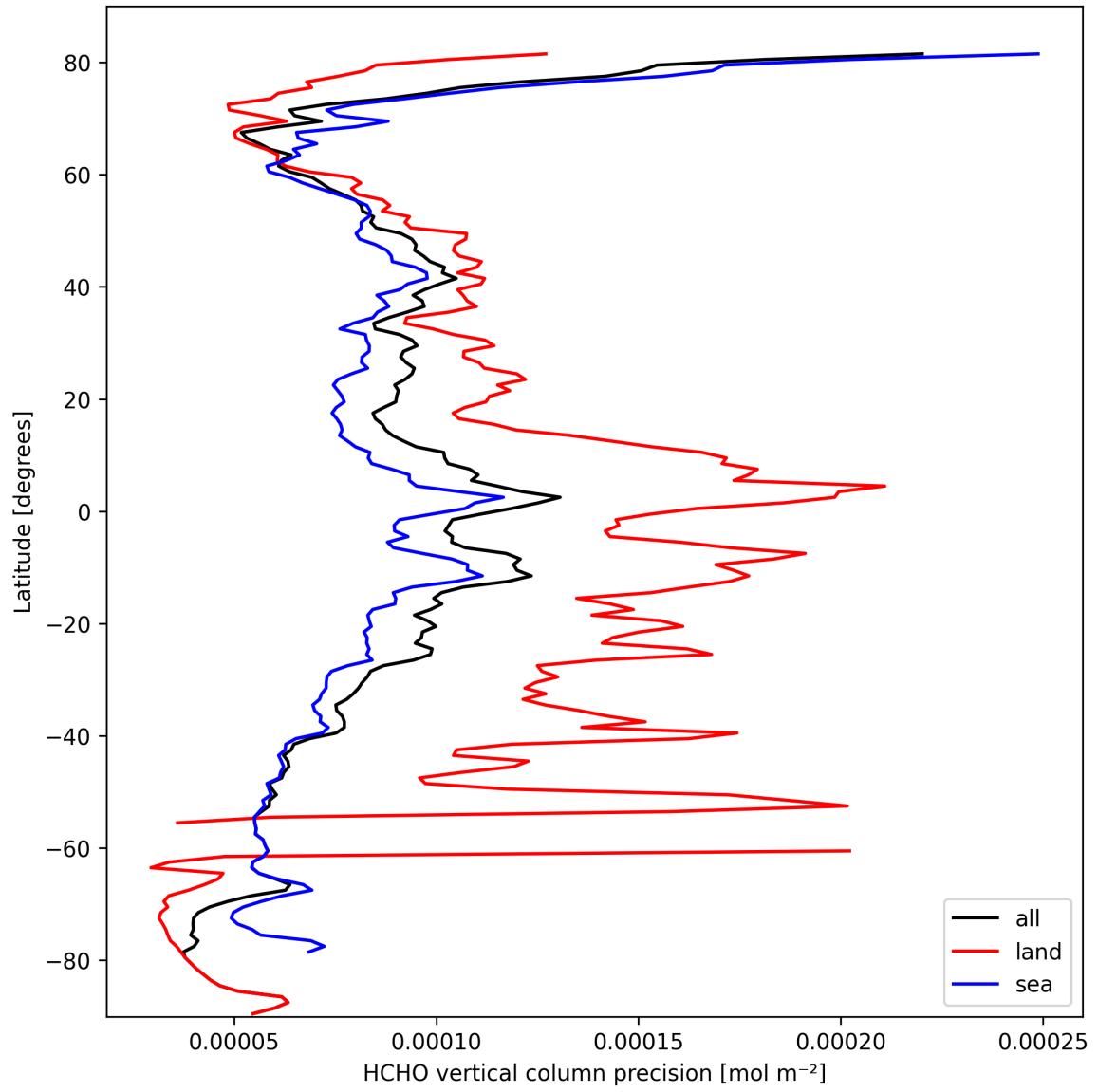
Figure 22: Zonal average of "HCHO vertical column precision" for 2025-03-09 to 2025-03-11.
