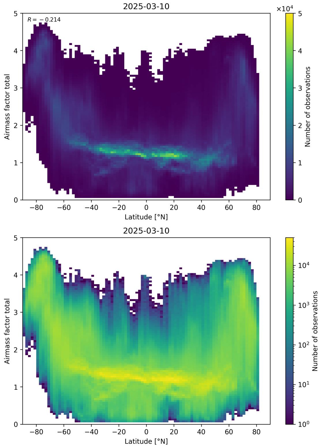
Figure 161: Scatter density plot of “Latitude” against “Airmass factor total” for 2025-03-09 to 2025-03-11.
