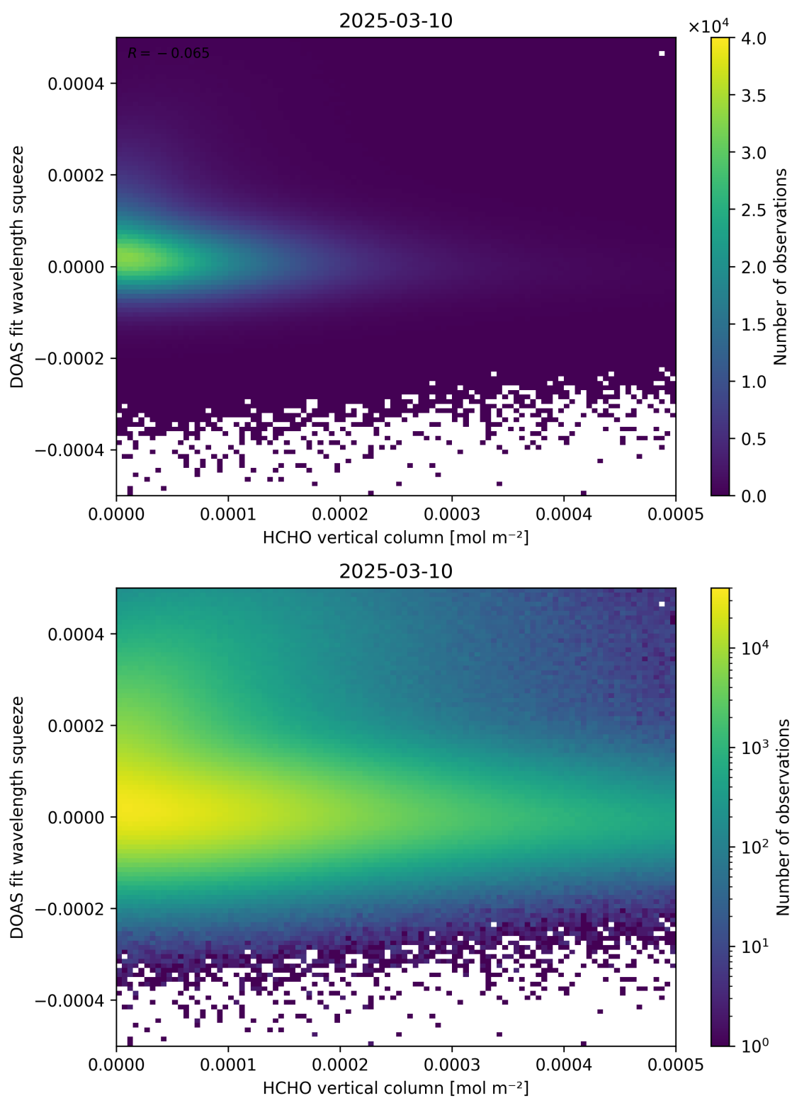
Figure 125: Scatter density plot of “HCHO vertical column” against “DOAS fit wavelength squeeze” for 2025-03-09 to 2025-03-11.
