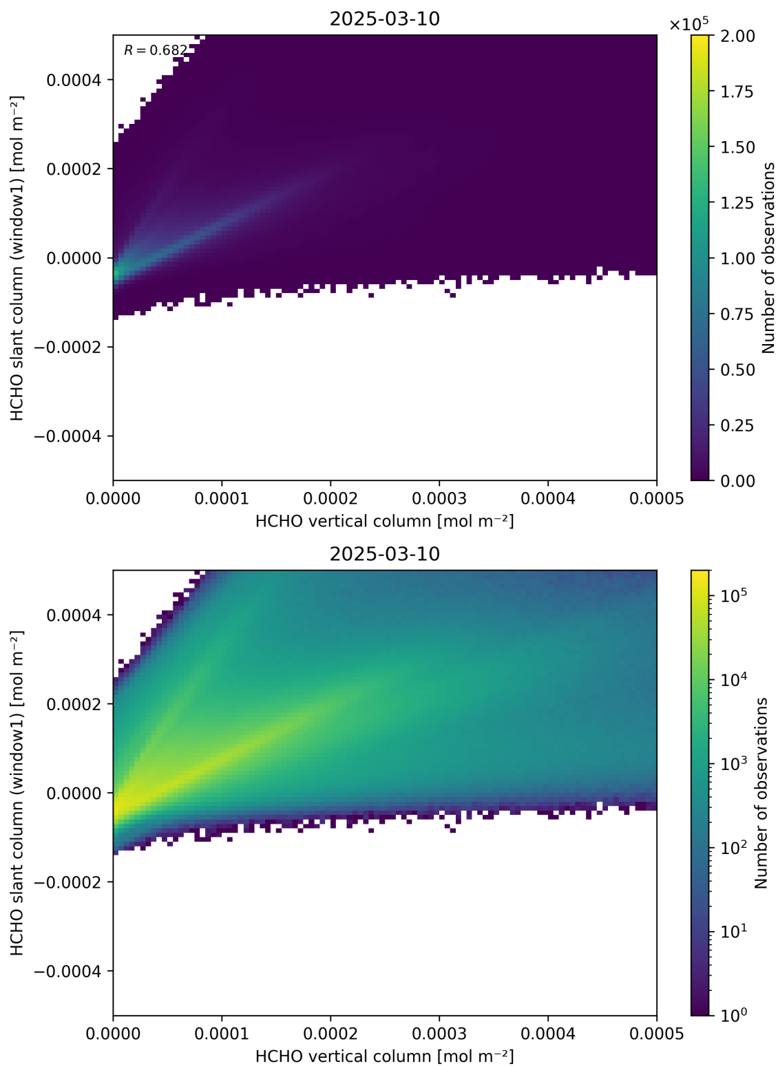
Figure 129: Scatter density plot of “HCHO vertical column” against “HCHO slant column (window1)” for 2025-03-09 to 2025-03-11.
