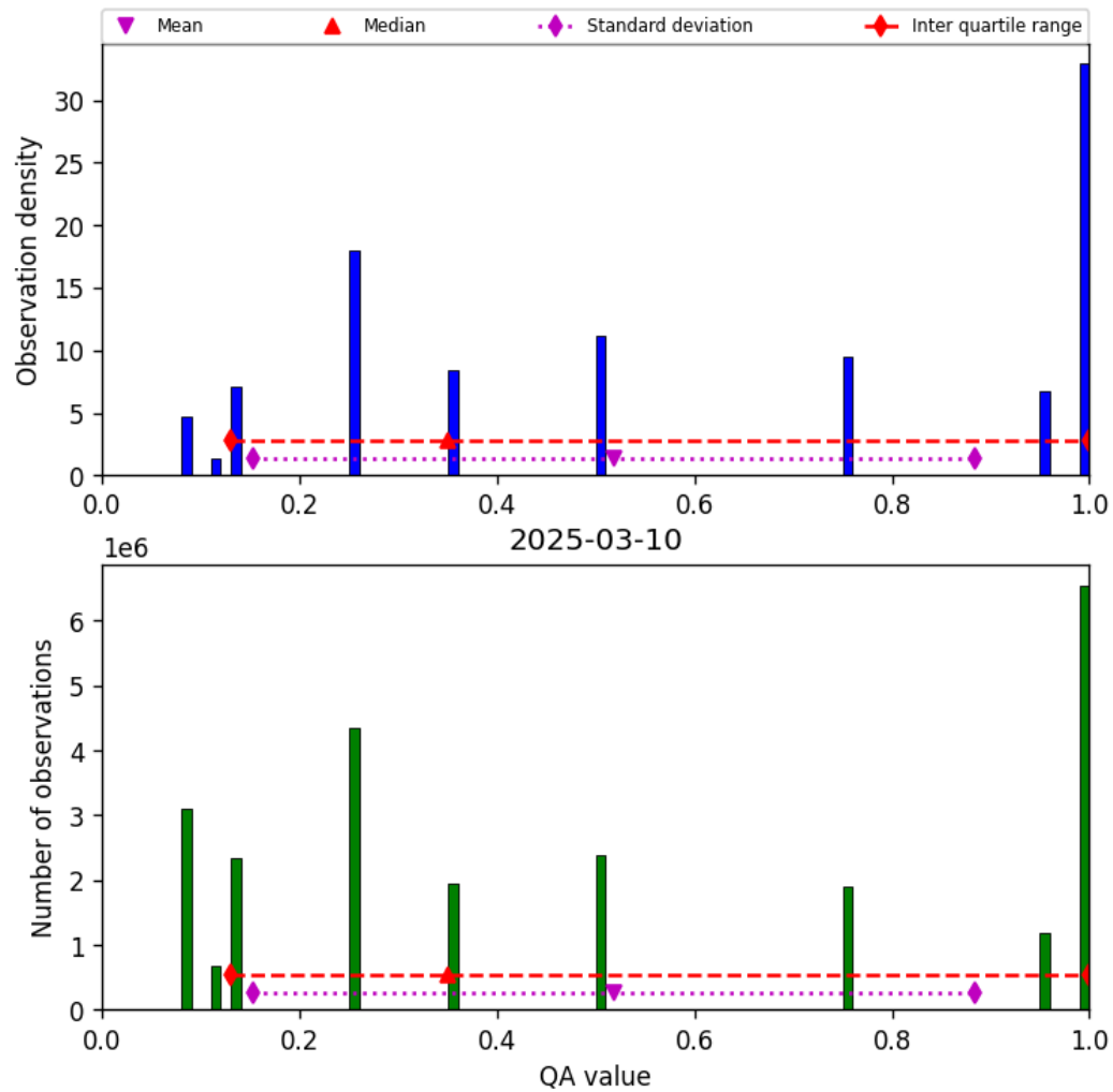
Figure 34: Histogram of “QA value” for 2025-03-09 to 2025-03-11
