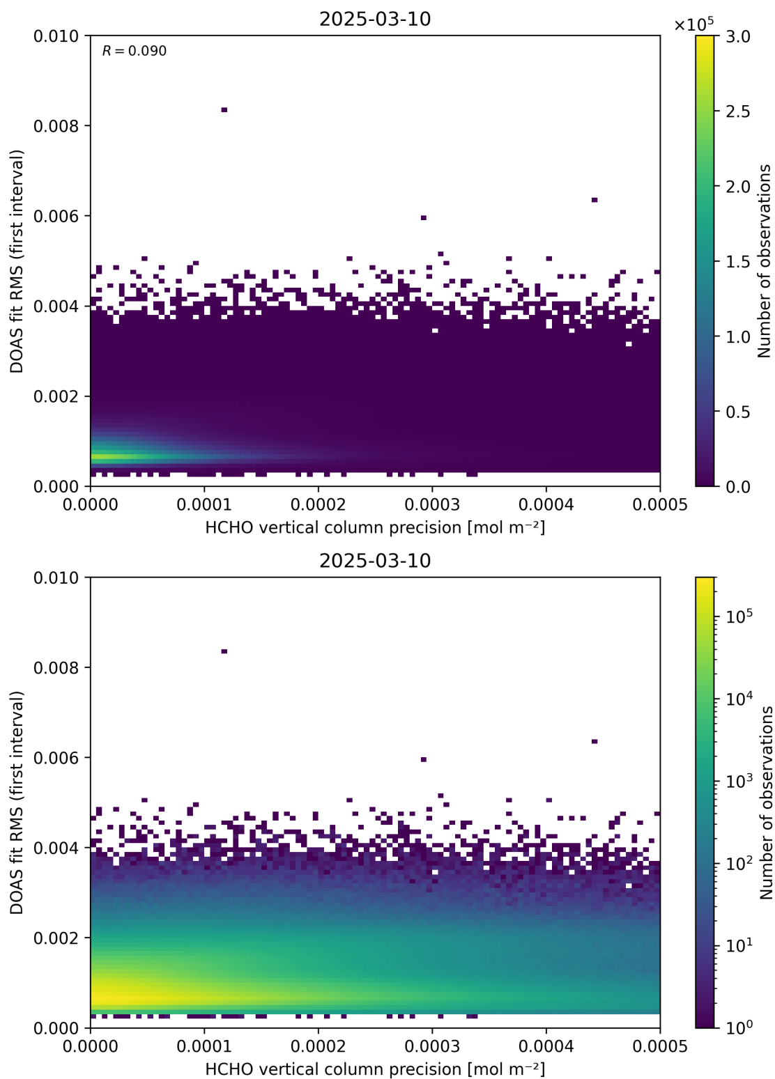
Figure 136: Scatter density plot of “HCHO vertical column precision” against “DOAS fit RMS (first interval)” for 2025-03-09 to 2025-03-11.
