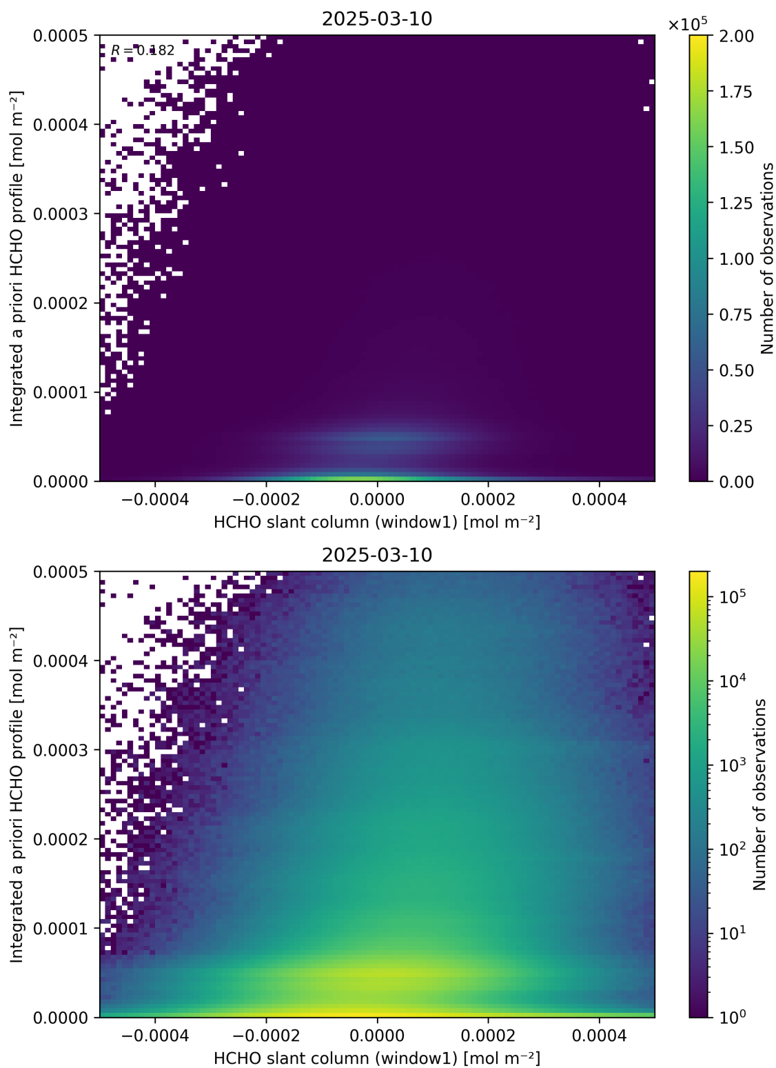
Figure 87: Scatter density plot of “HCHO slant column (window1)” against “Integrated a priori HCHO profile” for 2025-03-09 to 2025-03-11.
