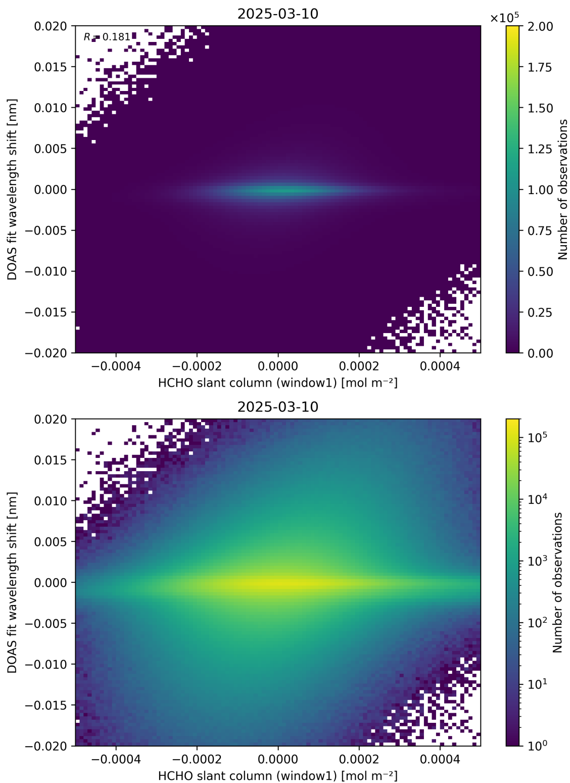
Figure 79: Scatter density plot of “HCHO slant column (window1)” against “DOAS fit wavelength shift” for 2025-03-09 to 2025-03-11.
