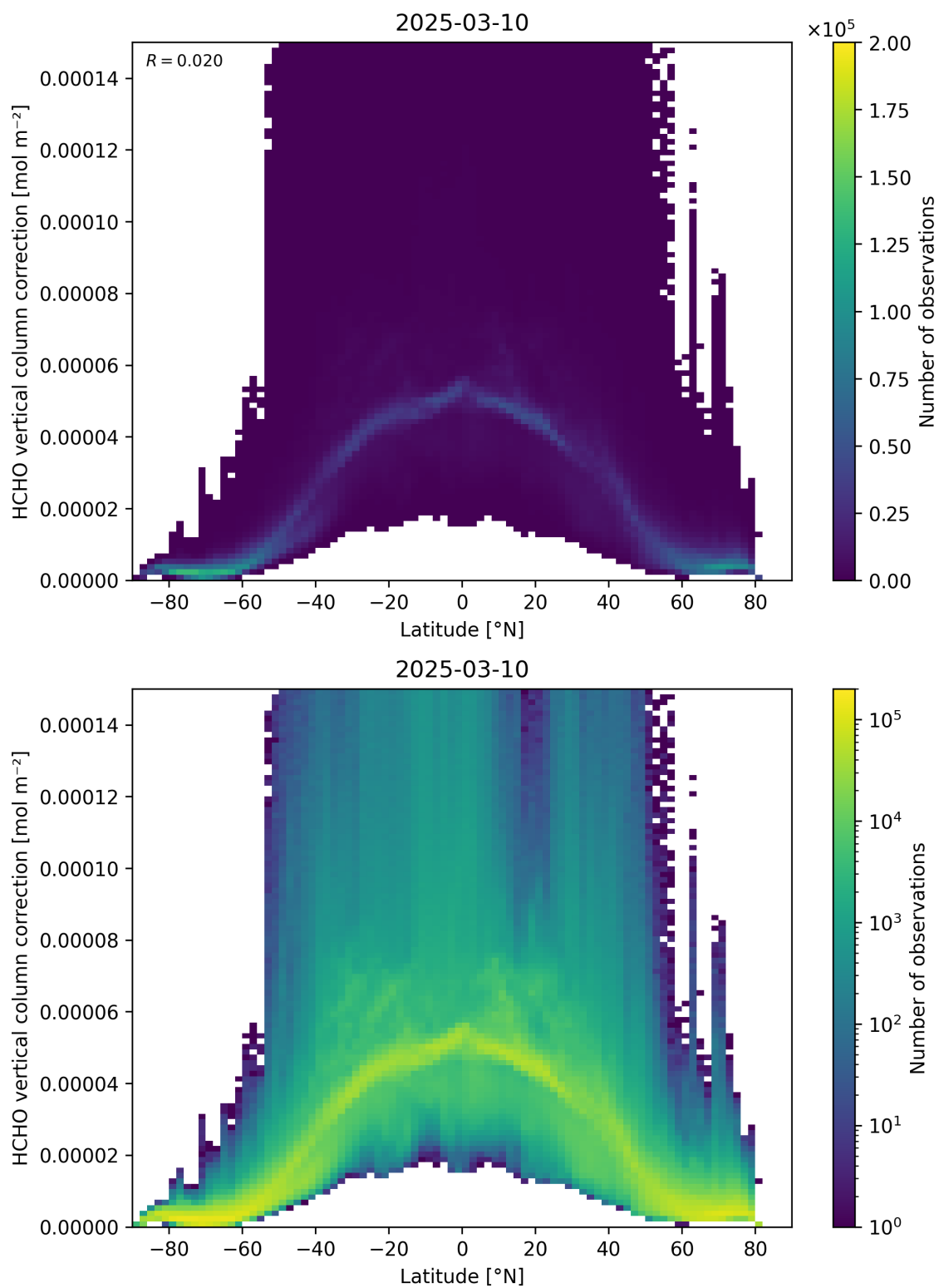
Figure 164: Scatter density plot of “Latitude” against “HCHO vertical column correction” for 2025-03-09 to 2025-03-11.
