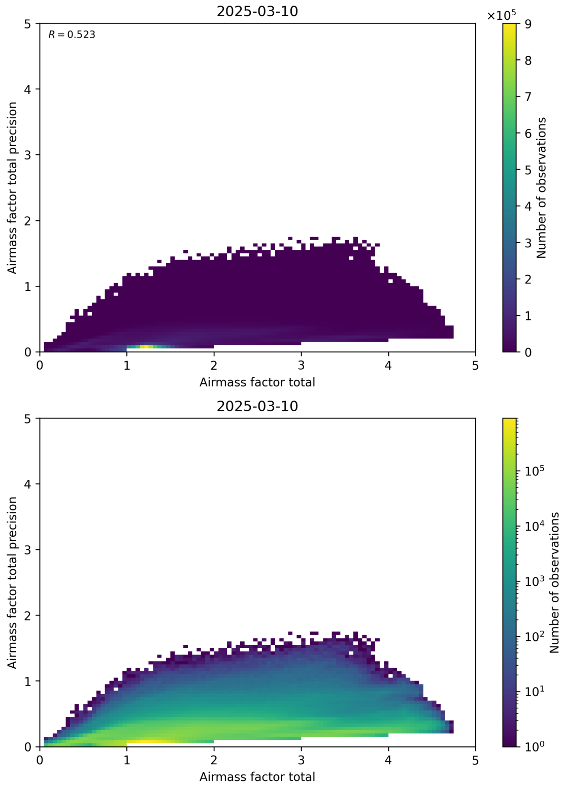
Figure 103: Scatter density plot of “Airmass factor total” against “Airmass factor total precision” for 2025-03-09 to 2025-03-11.
