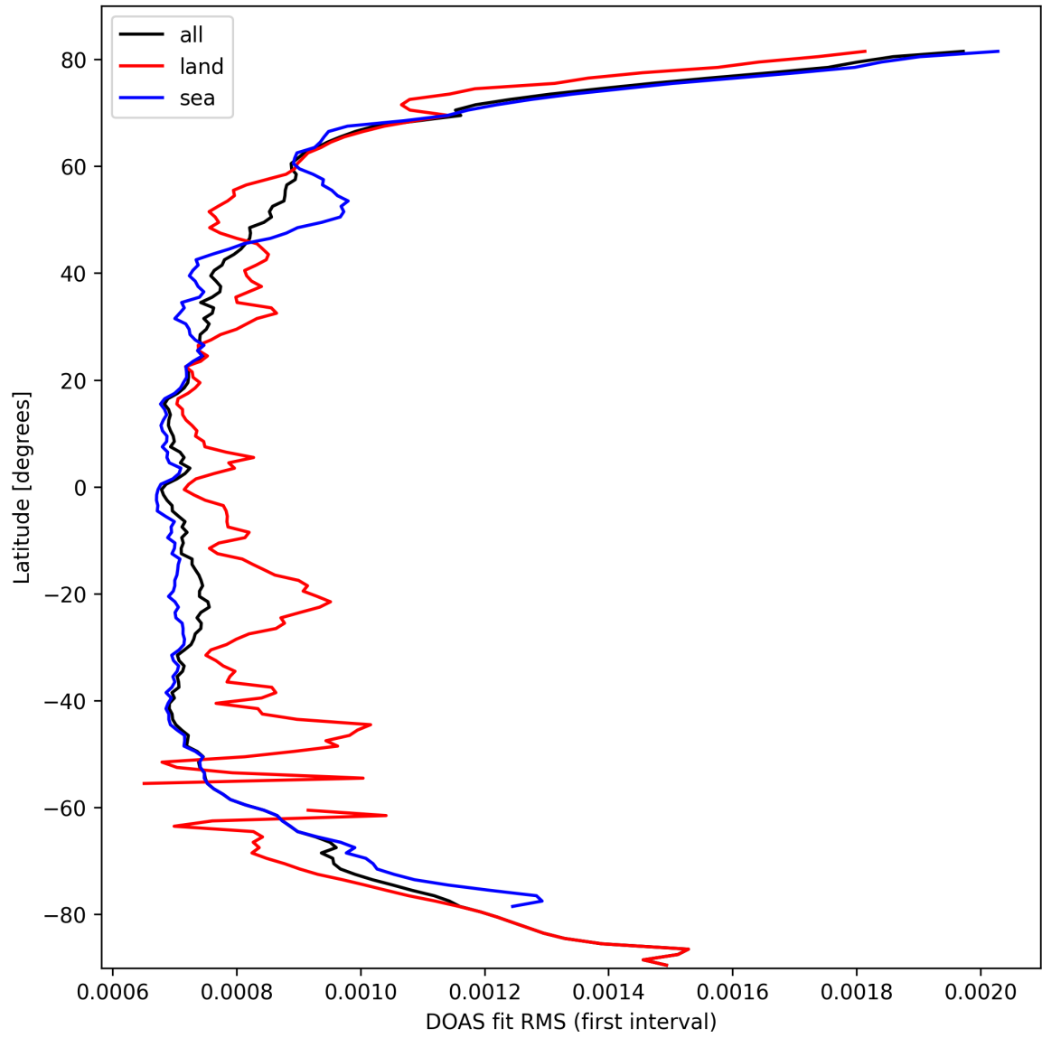
Figure 32: Zonal average of “DOAS fit RMS (first interval)” for 2025-03-09 to 2025-03-11.
