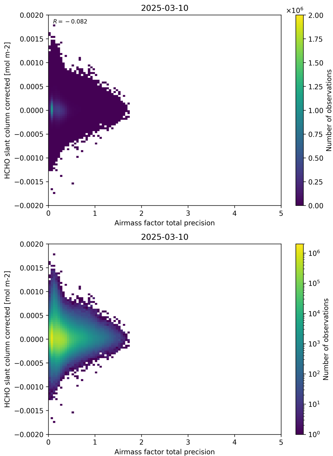
Figure 109: Scatter density plot of “Airmass factor total precision” against “HCHO slant column corrected” for 2025-03-09 to 2025-03-11.
