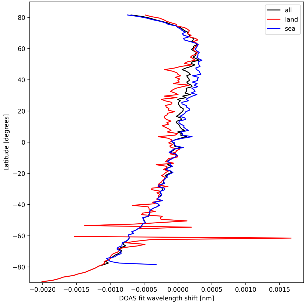
Figure 30: Zonal average of "DOAS fit wavelength shift" for 2025-03-09 to 2025-03-11.
