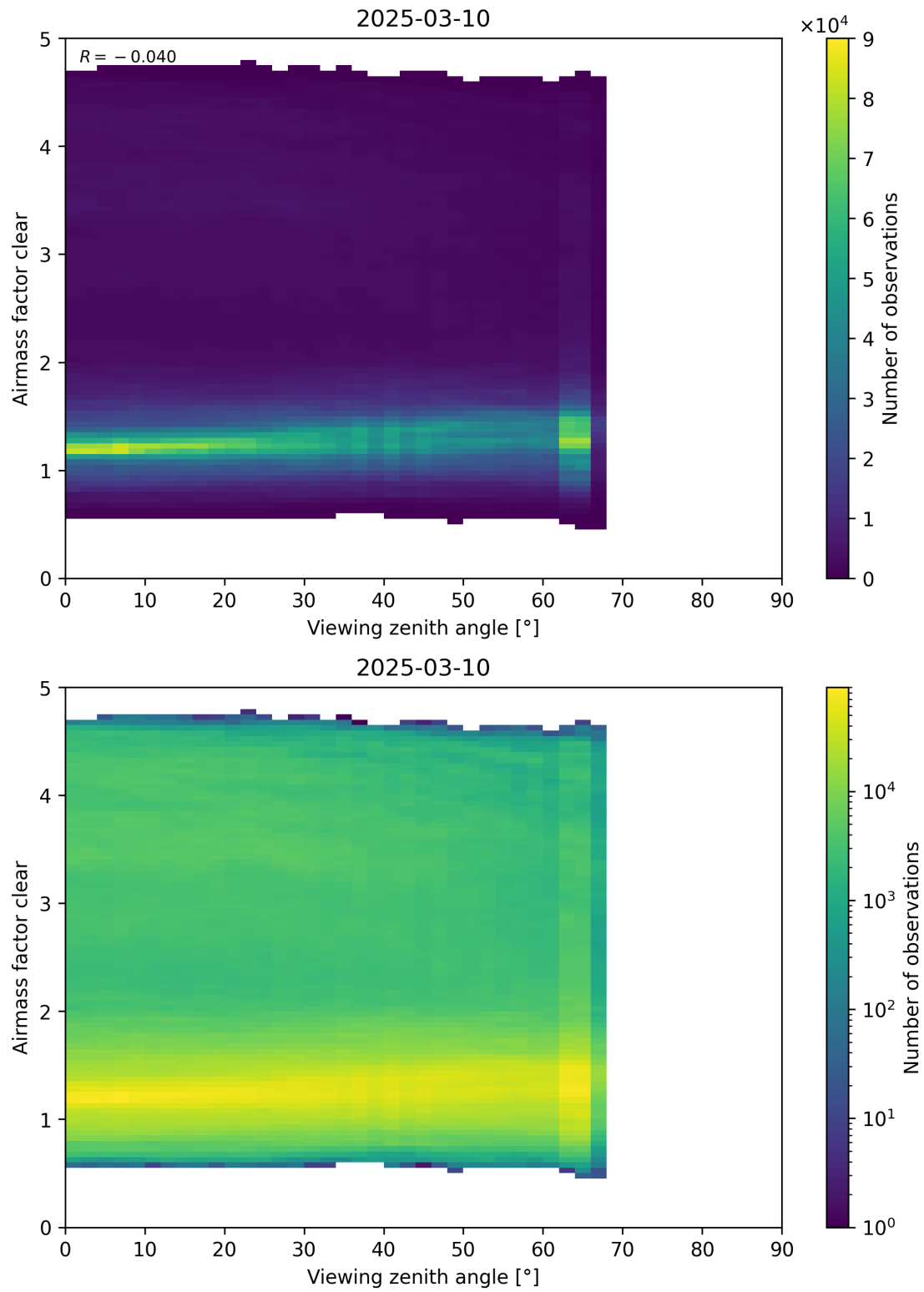
Figure 185: Scatter density plot of “Viewing zenith angle” against “Airmass factor clear” for 2025-03-09 to 2025-03-11.
