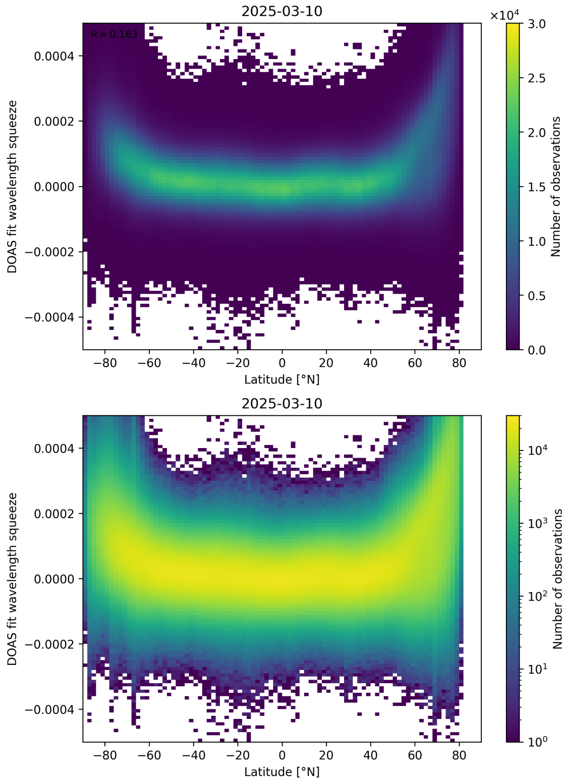
Figure 155: Scatter density plot of “Latitude” against “DOAS fit wavelength squeeze” for 2025-03-09 to 2025-03-11.
