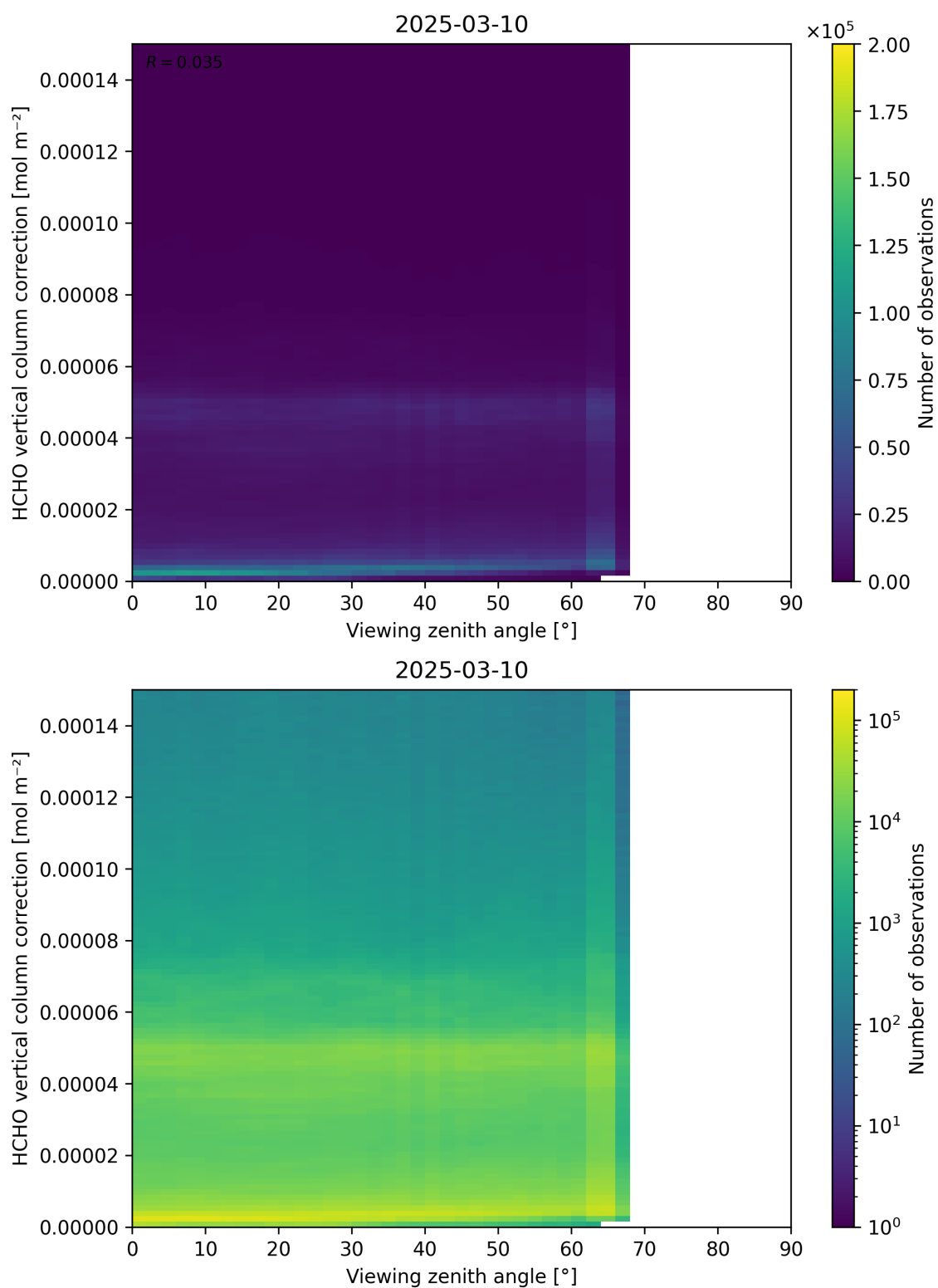
Figure 193: Scatter density plot of “Viewing zenith angle” against “HCHO vertical column correction” for 2025-03-09 to 2025-03-11.
