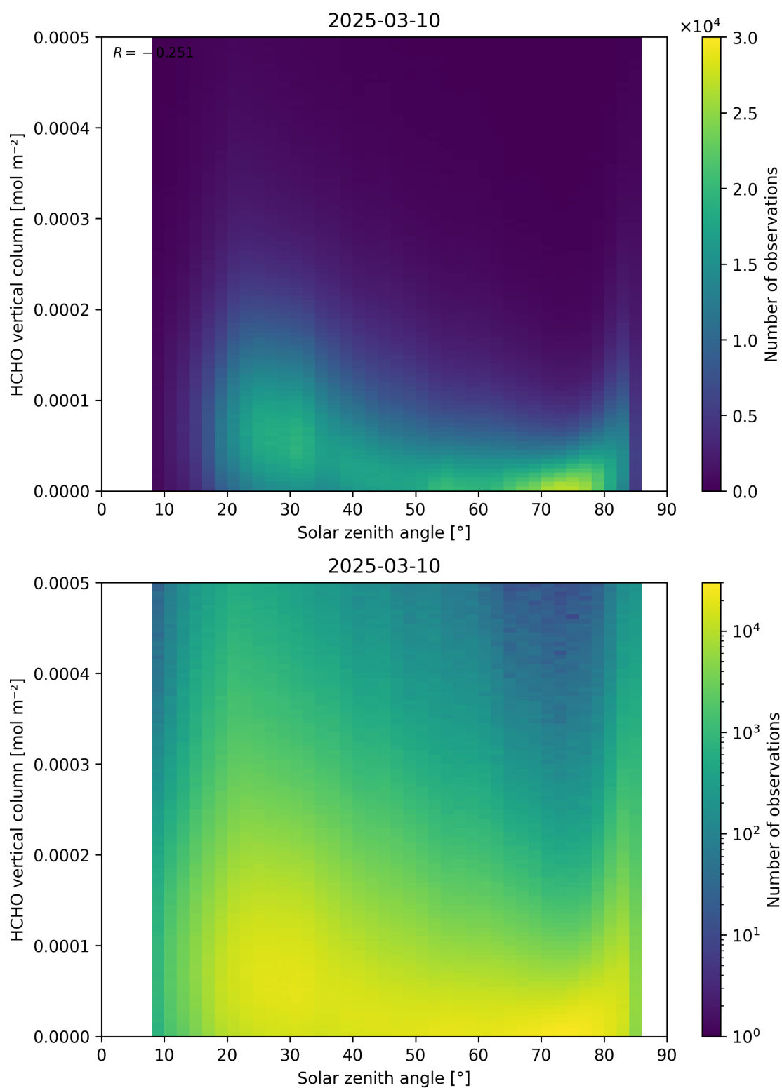
Figure 177: Scatter density plot of “Solar zenith angle” against “HCHO vertical column” for 2025-03-09 to 2025-03-11.
