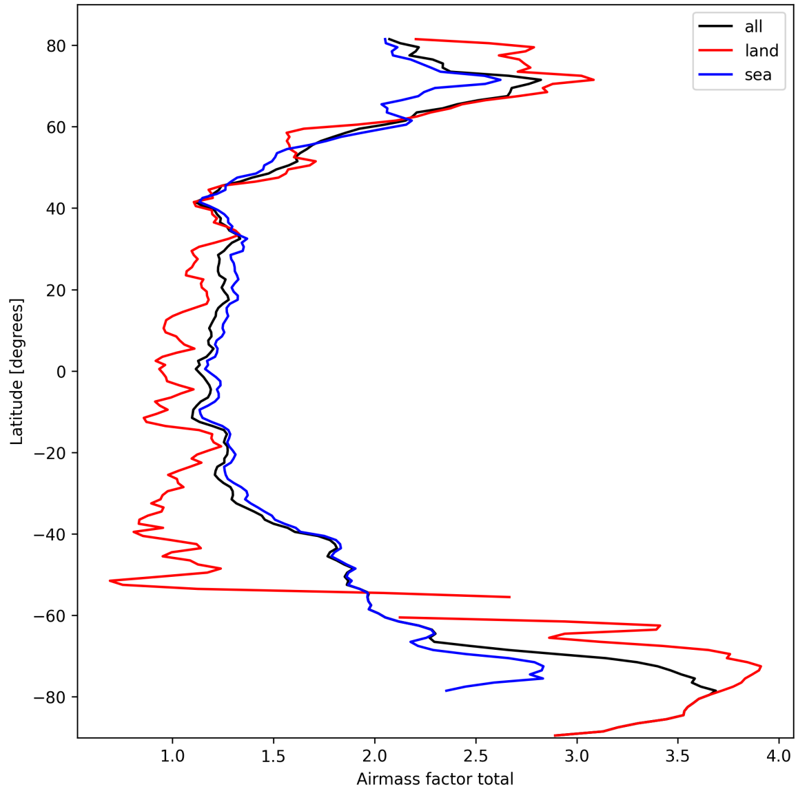
Figure 26: Zonal average of “Airmass factor total” for 2025-03-09 to 2025-03-11.
