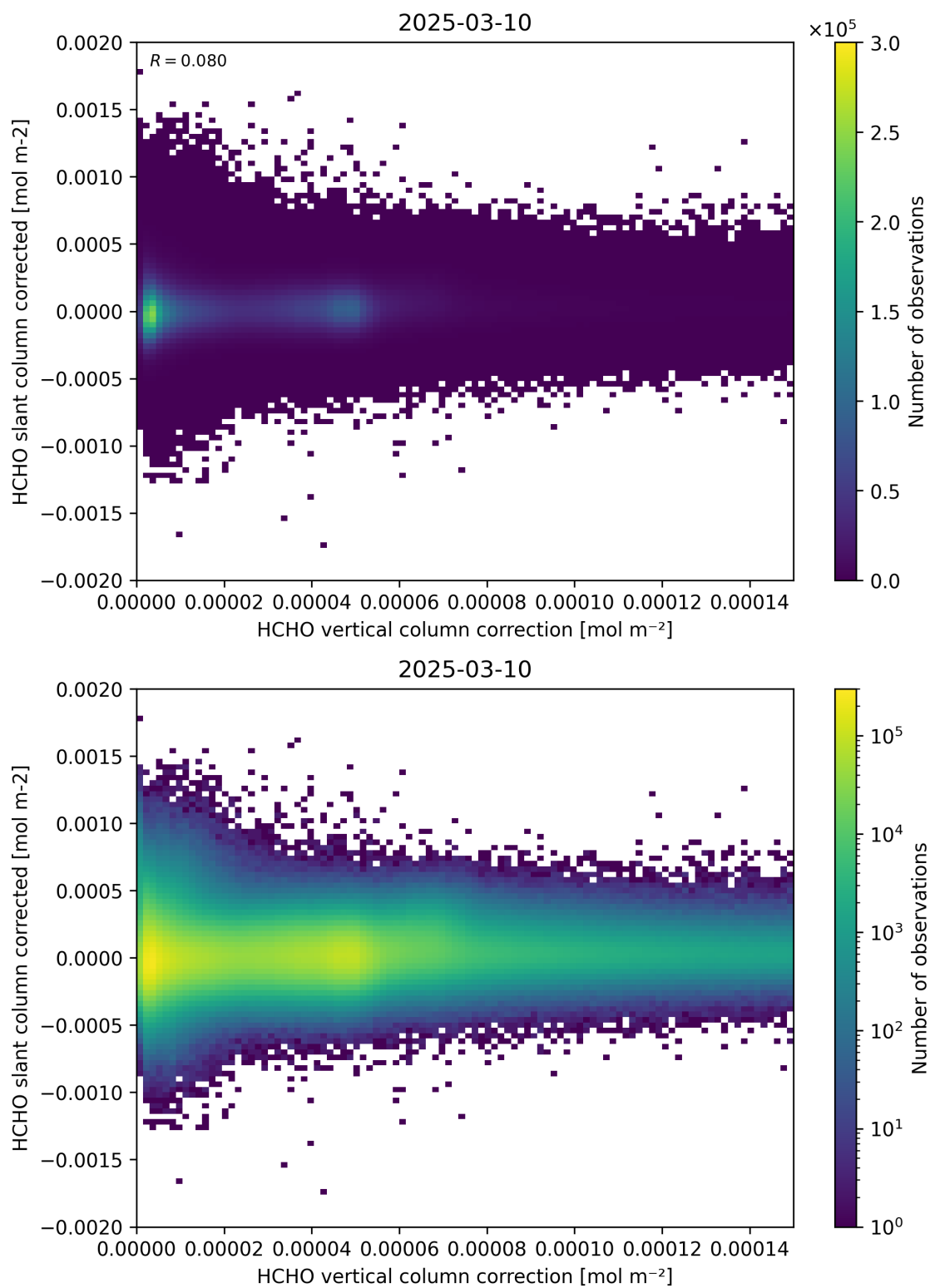
Figure 116: Scatter density plot of “HCHO vertical column correction” against “HCHO slant column corrected” for 2025-03-09 to 2025-03-11.
