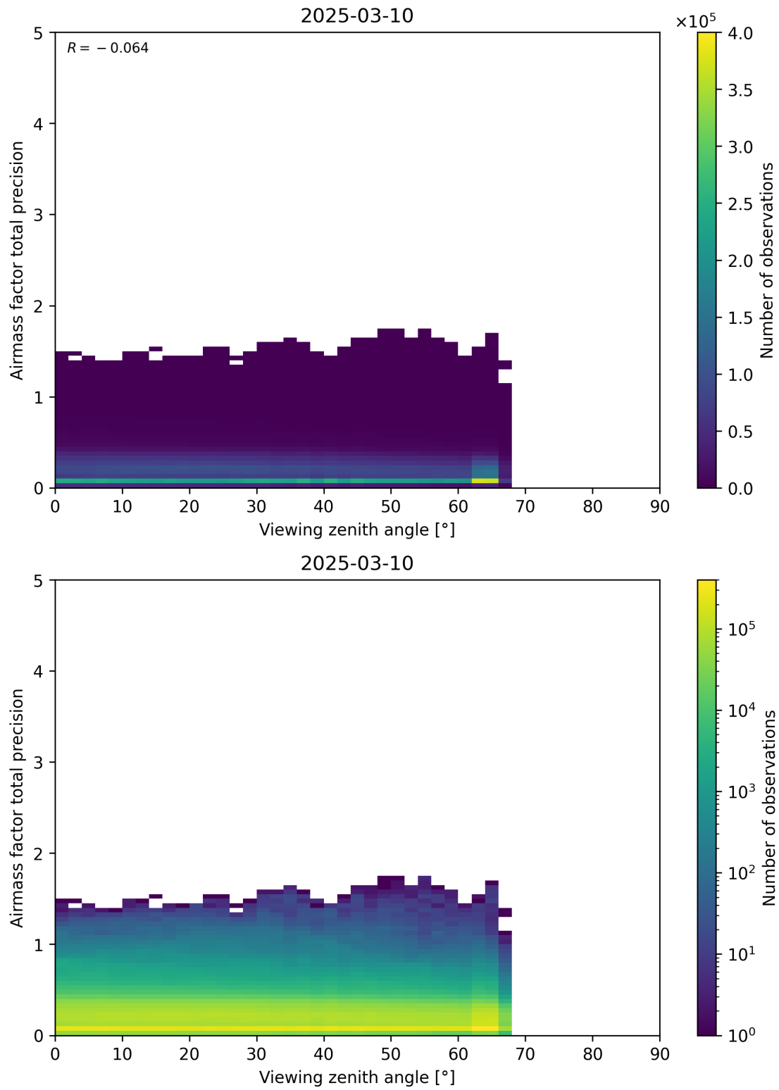
Figure 191: Scatter density plot of “Viewing zenith angle” against “Airmass factor total precision” for 2025-03-09 to 2025-03-11.
