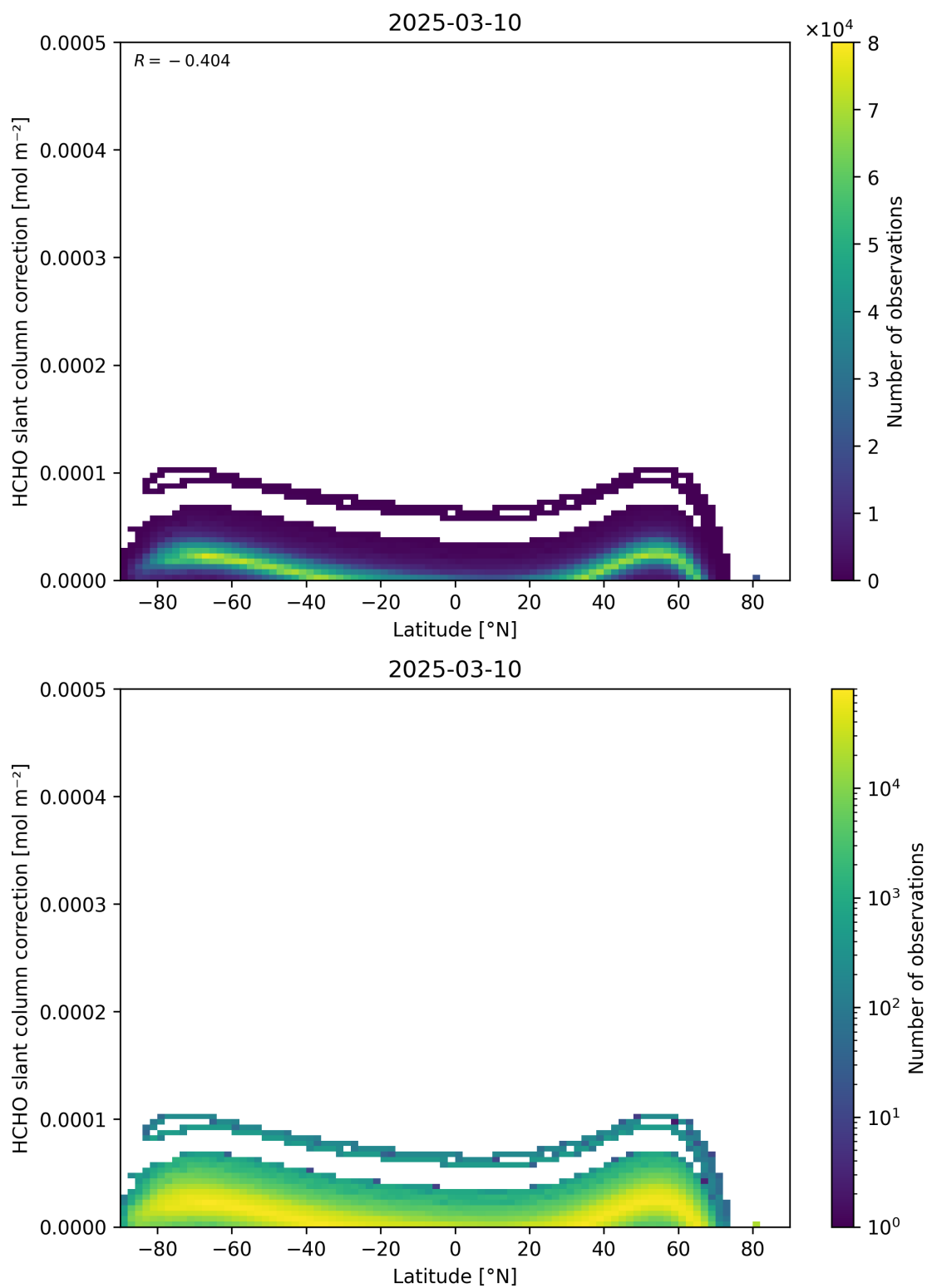
Figure 158: Scatter density plot of “Latitude” against “HCHO slant column correction” for 2025-03-09 to 2025-03-11.
