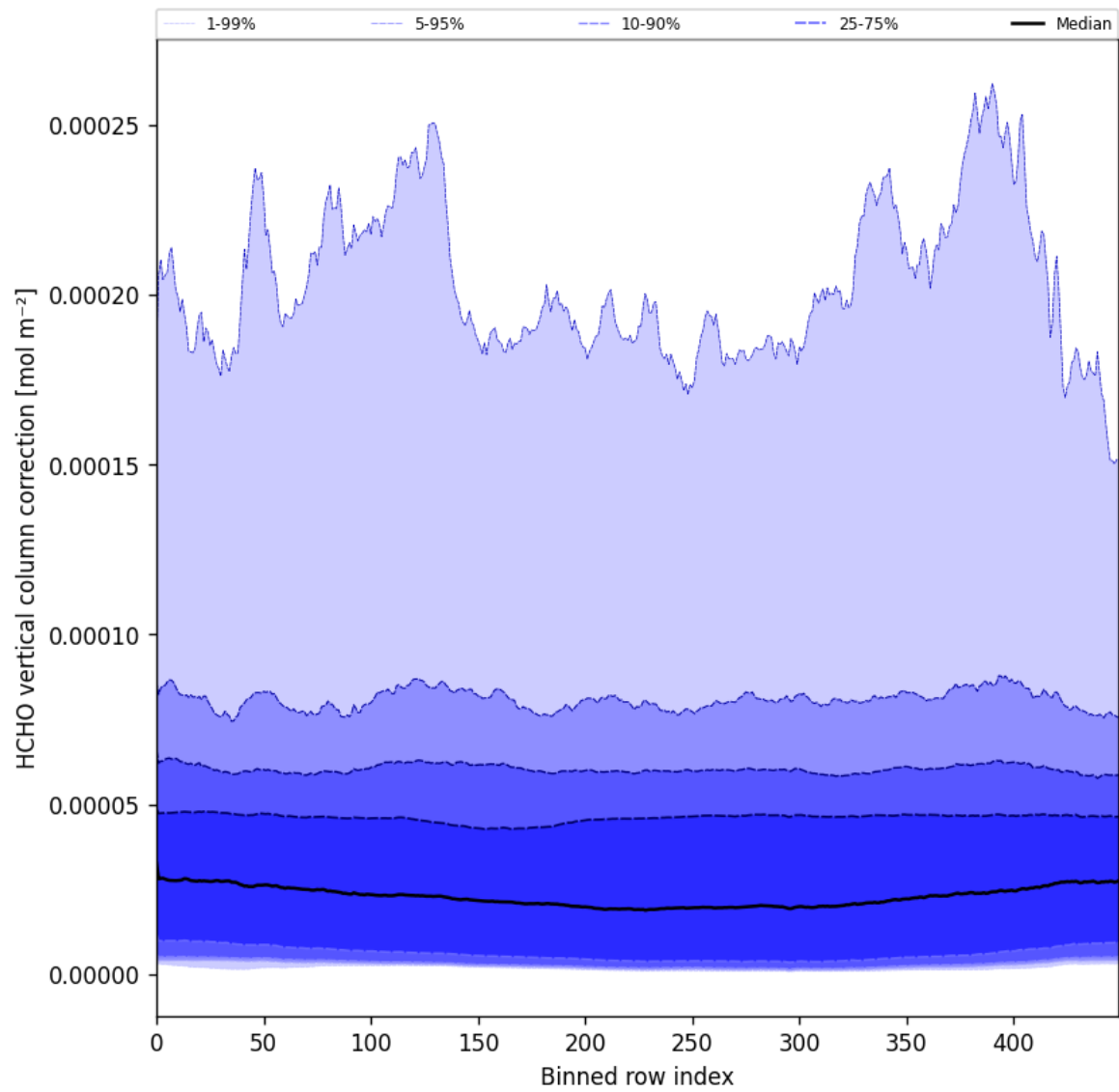
Figure 51: Along track statistics of “HCHO vertical column correction” for 2025-03-09 to 2025-03-11
