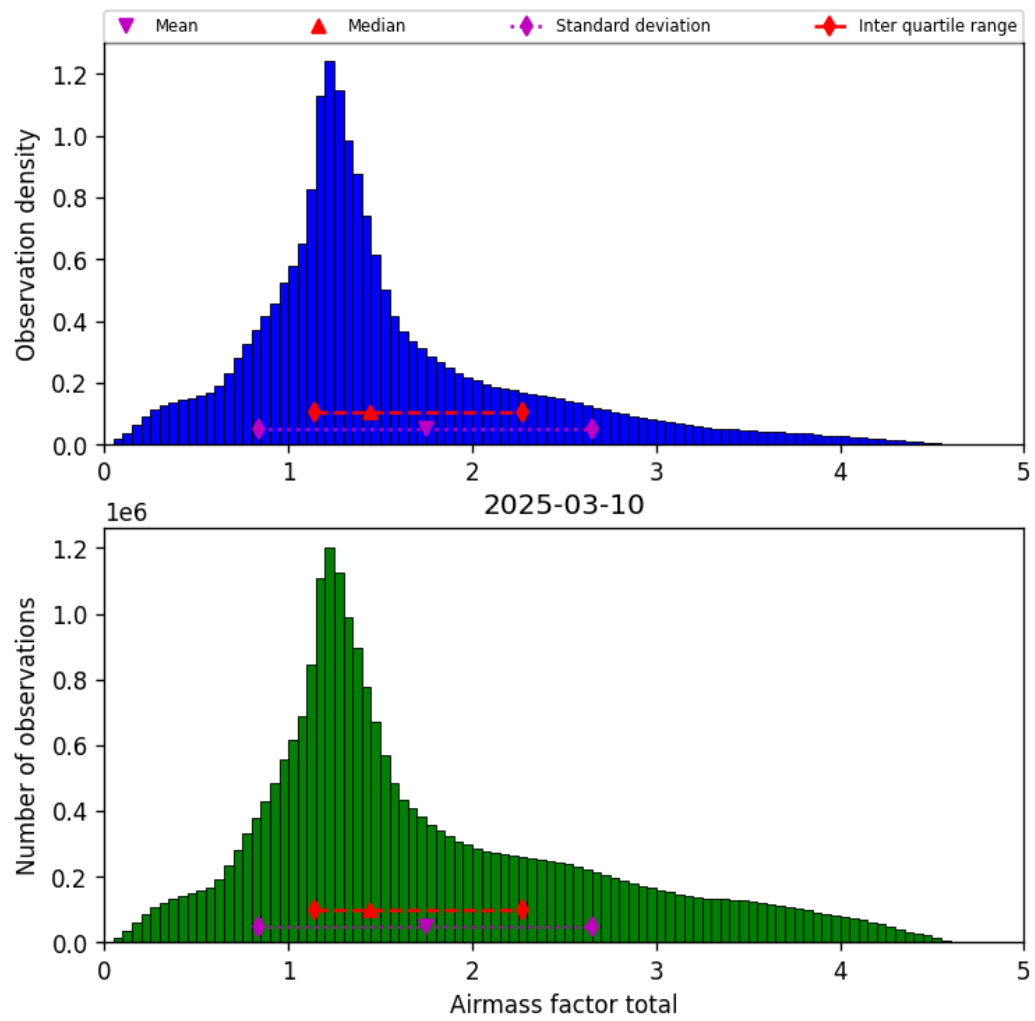
Figure 40: Histogram of “Airmass factor total” for 2025-03-09 to 2025-03-11
