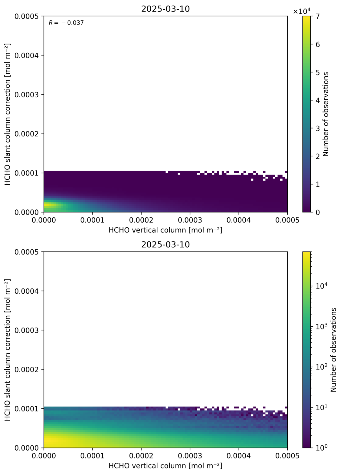
Figure 128: Scatter density plot of “HCHO vertical column” against “HCHO slant column correction” for 2025-03-09 to 2025-03-11.
