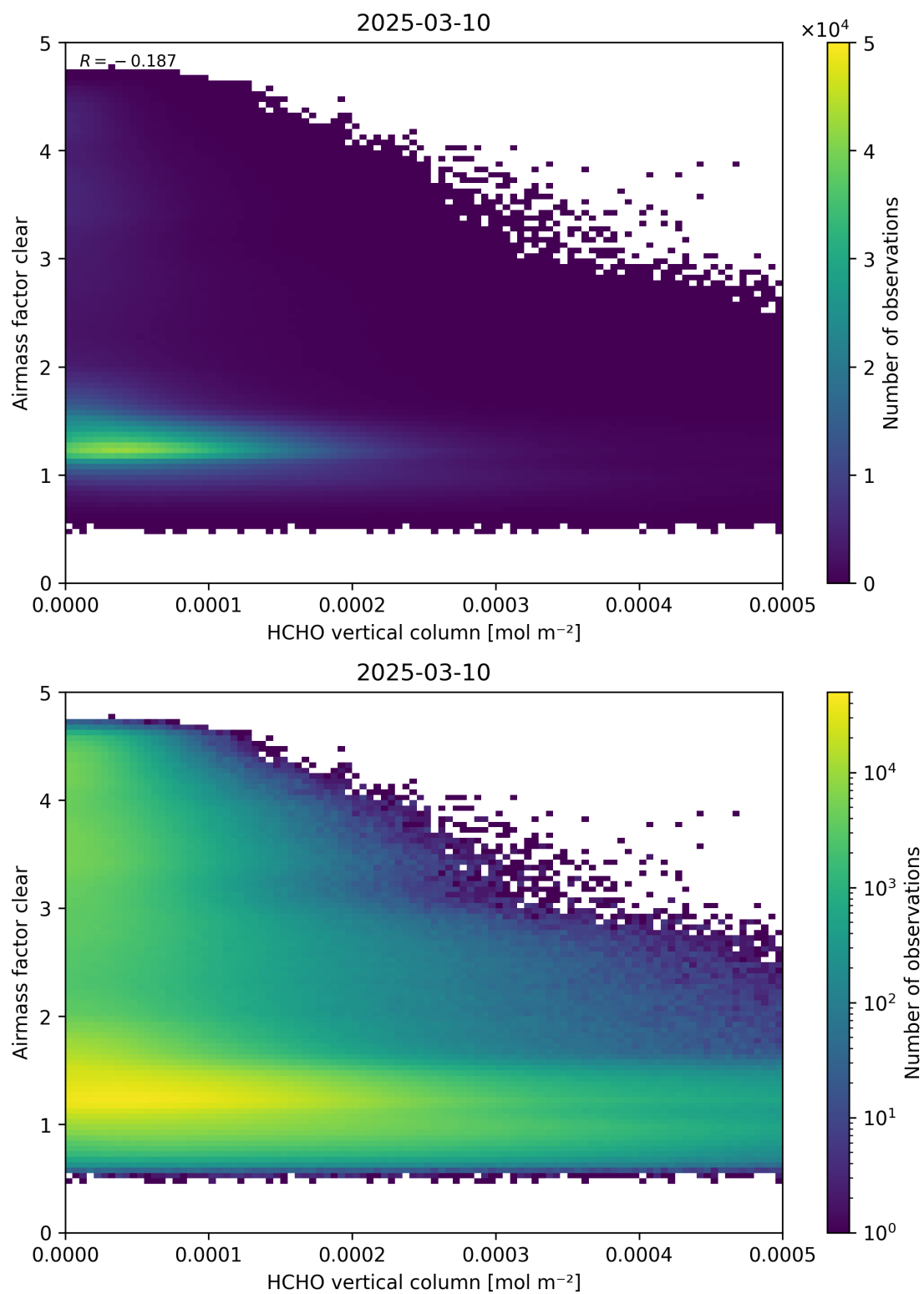
Figure 126: Scatter density plot of “HCHO vertical column” against “Airmass factor clear” for 2025-03-09 to 2025-03-11.
