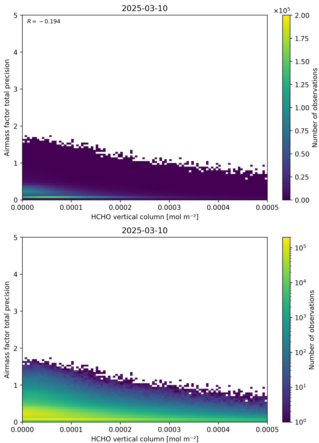
Figure 132: Scatter density plot of “HCHO vertical column” against “Airmass factor total precision” for 2025-03-09 to 2025-03-11.
