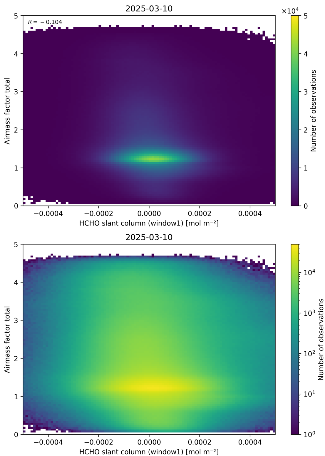
Figure 85: Scatter density plot of “HCHO slant column (window1)” against “Airmass factor total” for 2025-03-09 to 2025-03-11.
