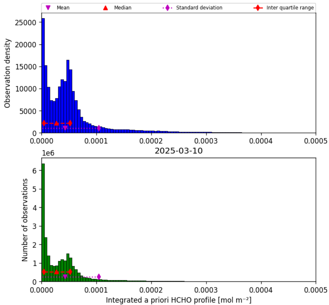
Figure 43: Histogram of “Integrated a priori HCHO profile” for 2025-03-09 to 2025-03-11
