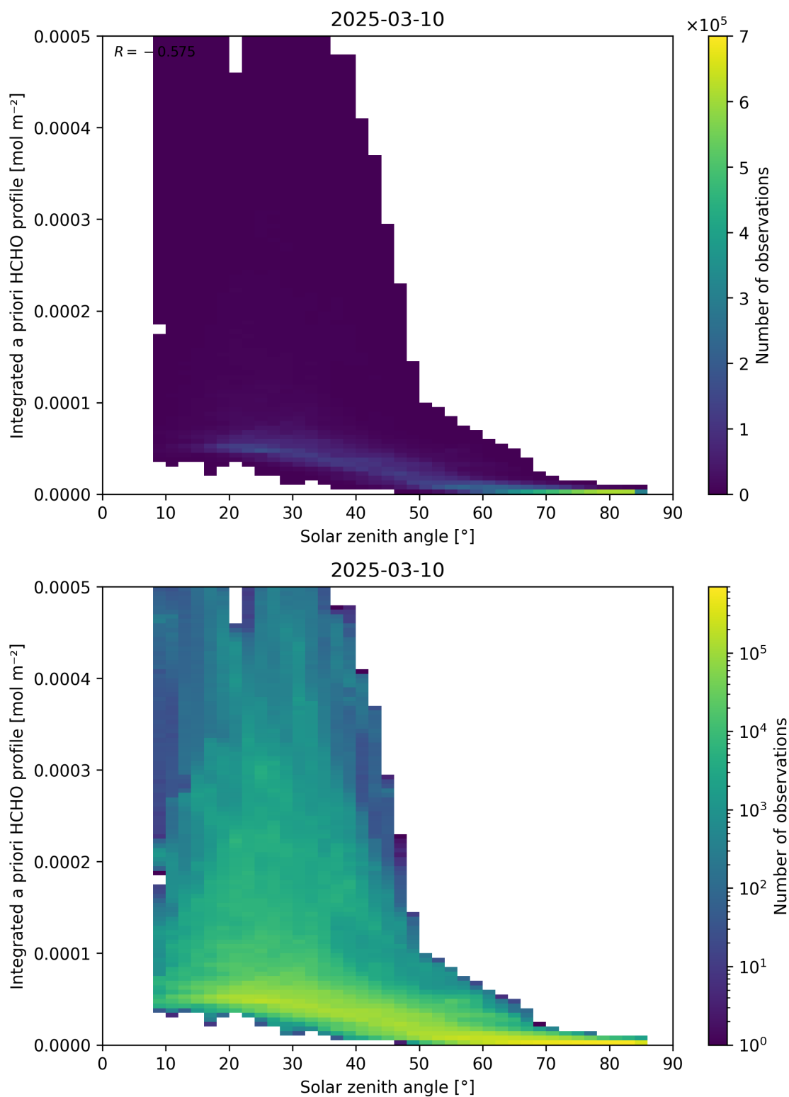
Figure 180: Scatter density plot of “Solar zenith angle” against “Integrated a priori HCHO profile” for 2025-03-09 to 2025-03-11.
