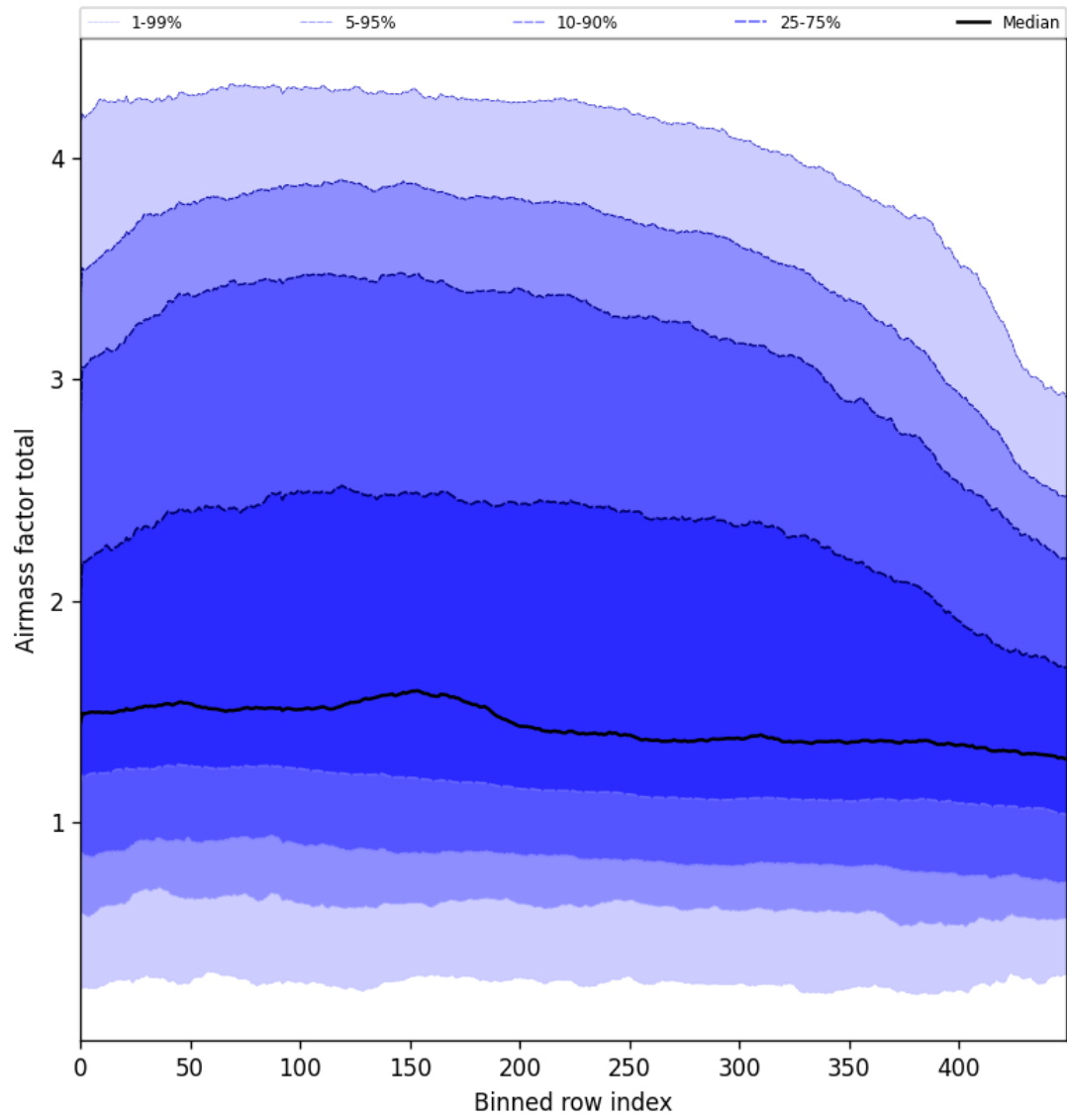
Figure 54: Along track statistics of “Airmass factor total” for 2025-03-09 to 2025-03-11
