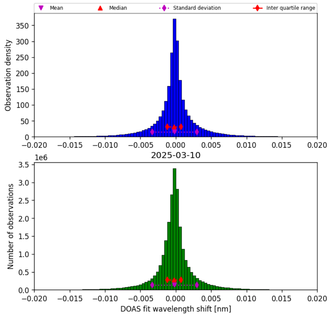
Figure 44: Histogram of “DOAS fit wavelength shift” for 2025-03-09 to 2025-03-11
