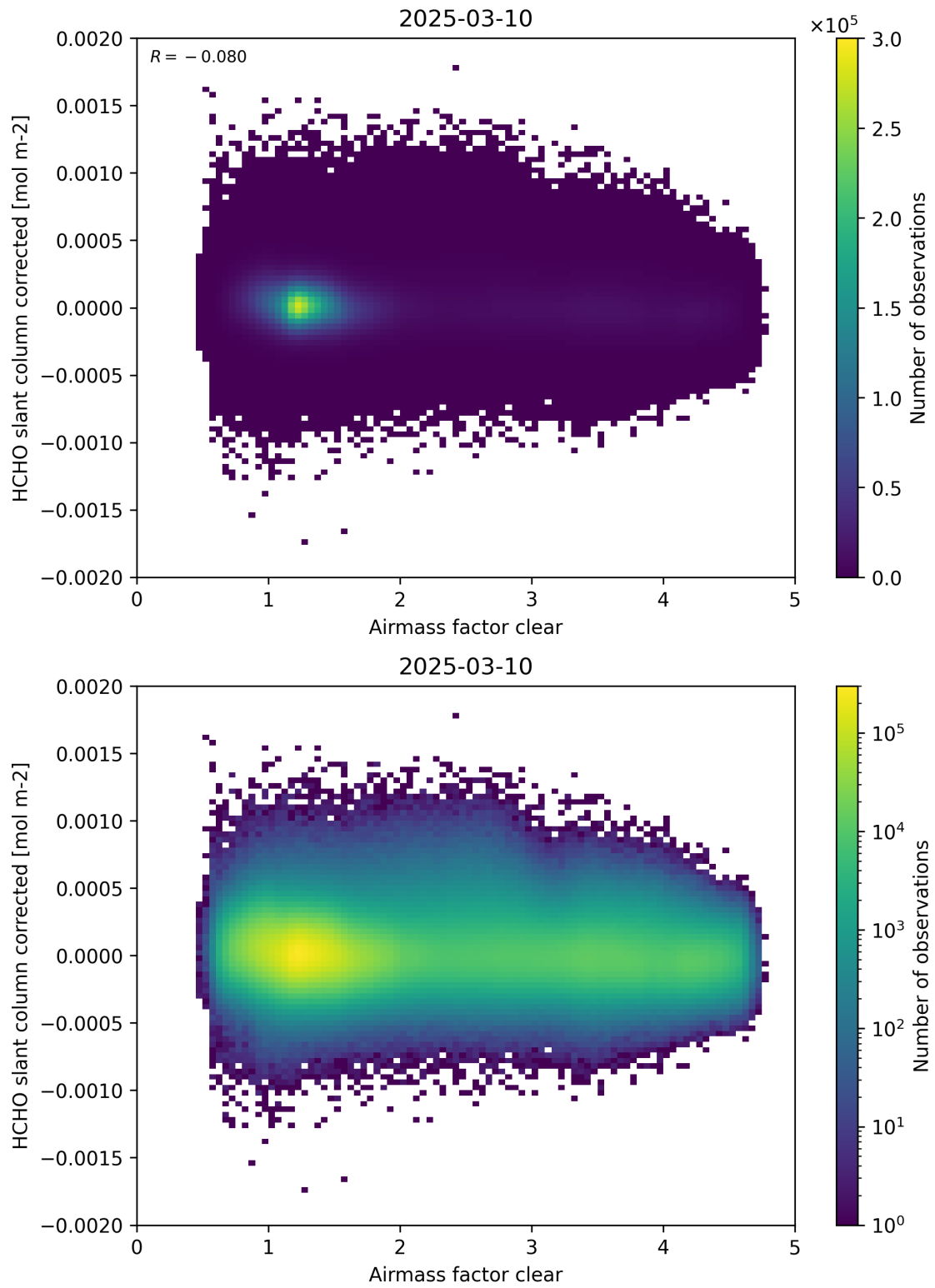
Figure 74: Scatter density plot of “Airmass factor clear” against “HCHO slant column corrected” for 2025-03-09 to 2025-03-11.
