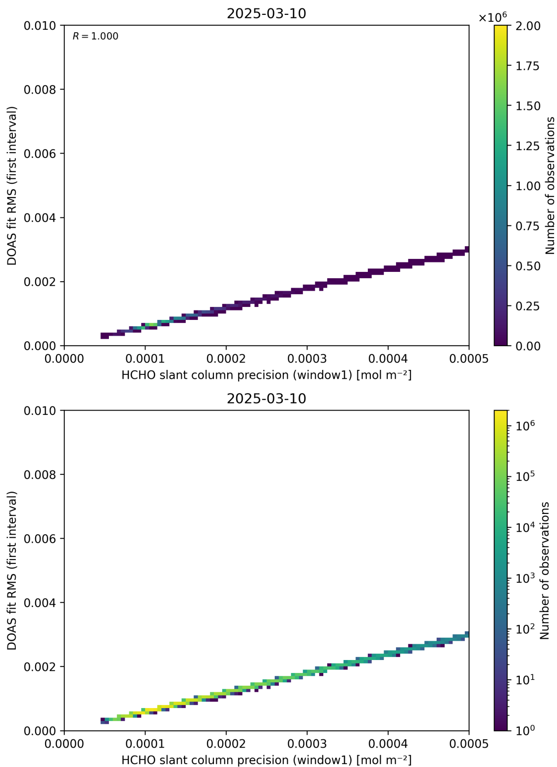
Figure 88: Scatter density plot of “HCHO slant column precision (window1)” against “DOAS fit RMS (first interval)” for 2025-03-09 to 2025-03-11.
