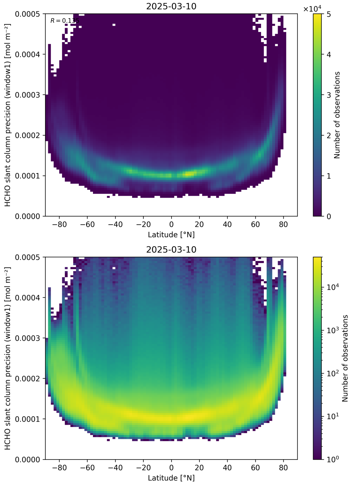
Figure 160: Scatter density plot of “Latitude” against “HCHO slant column precision (window1)” for 2025-03-09 to 2025-03-11.
