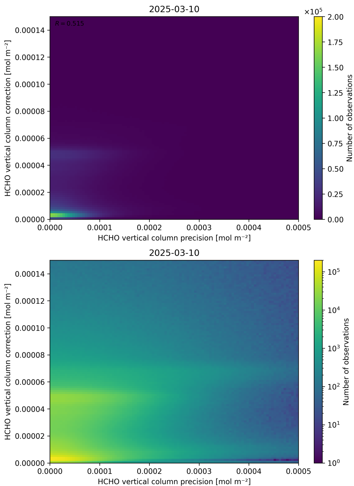
Figure 146: Scatter density plot of “HCHO vertical column precision” against “HCHO vertical column correction” for 2025-03-09 to 2025-03-11.
