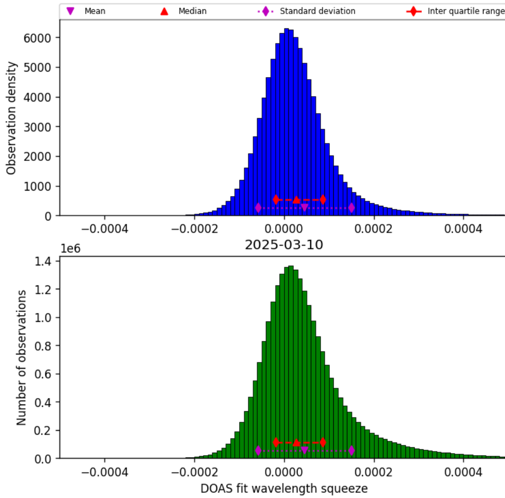
Figure 45: Histogram of “DOAS fit wavelength squeeze” for 2025-03-09 to 2025-03-11
