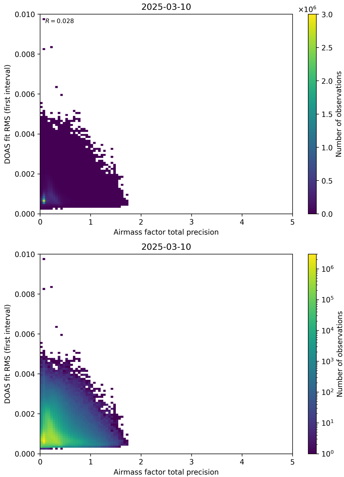
Figure 105: Scatter density plot of “Airmass factor total precision” against “DOAS fit RMS (first interval)” for 2025-03-09 to 2025-03-11.
