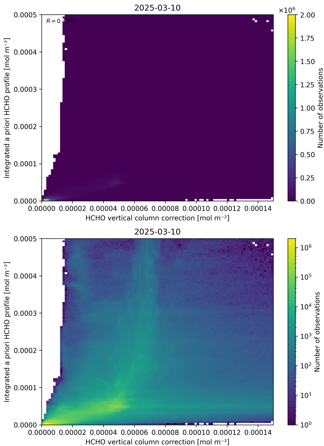
Figure 122: Scatter density plot of “HCHO vertical column correction” against “Integrated a priori HCHO profile” for 2025-03-09 to 2025-03-11.
