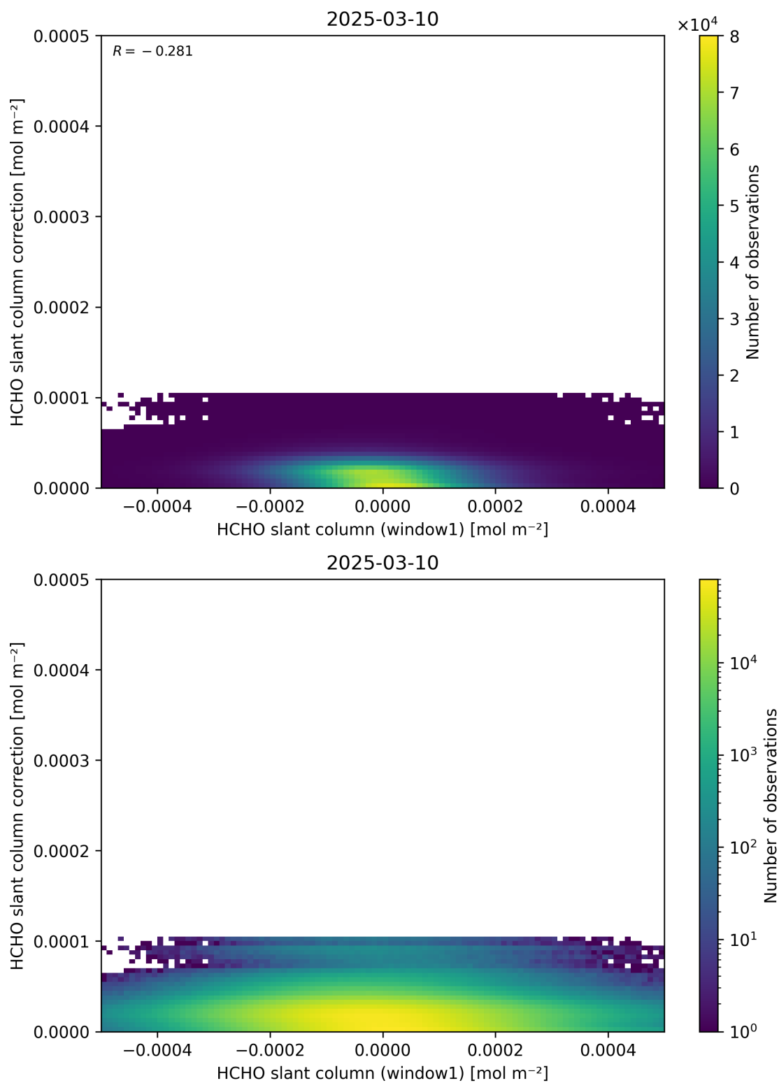
Figure 83: Scatter density plot of “HCHO slant column (window1)” against “HCHO slant column correction” for 2025-03-09 to 2025-03-11.
