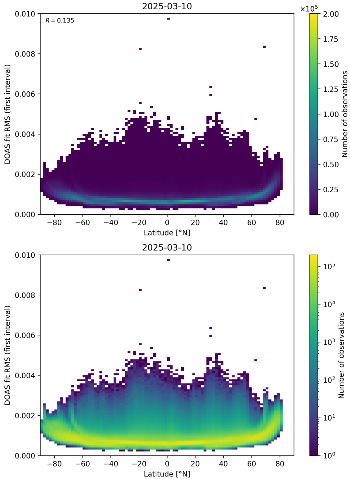
Figure 153: Scatter density plot of “Latitude” against “DOAS fit RMS (first interval)” for 2025-03-09 to 2025-03-11.
