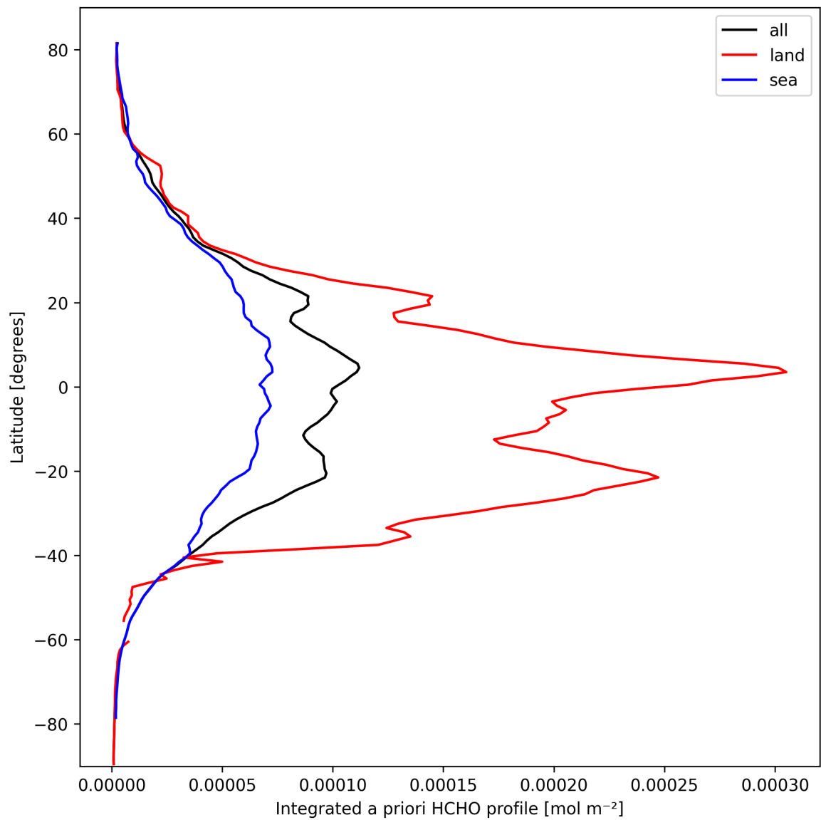
Figure 29: Zonal average of “Integrated a priori HCHO profile” for 2025-03-09 to 2025-03-11.
