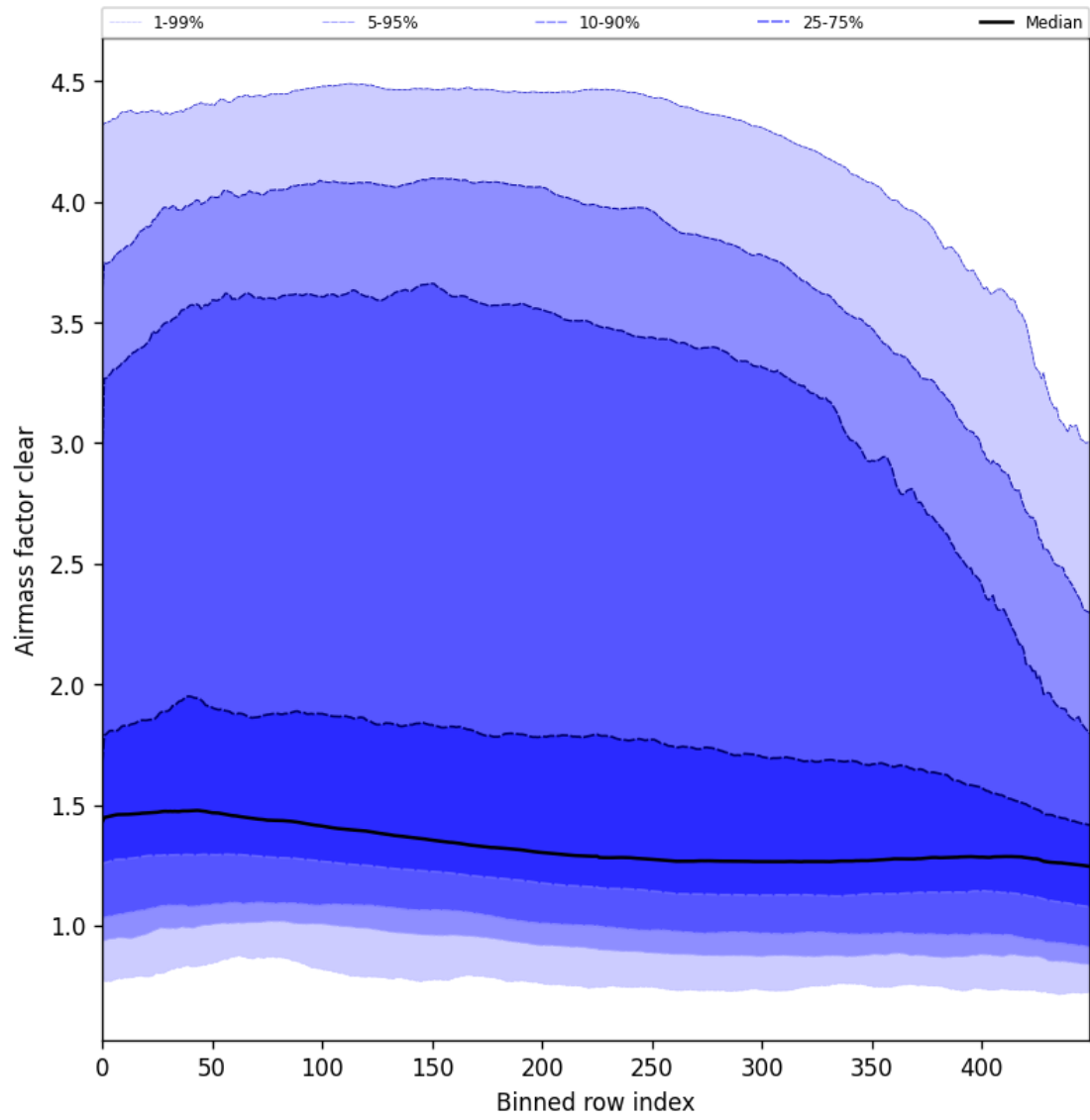
Figure 56: Along track statistics of “Airmass factor clear” for 2025-03-09 to 2025-03-11
