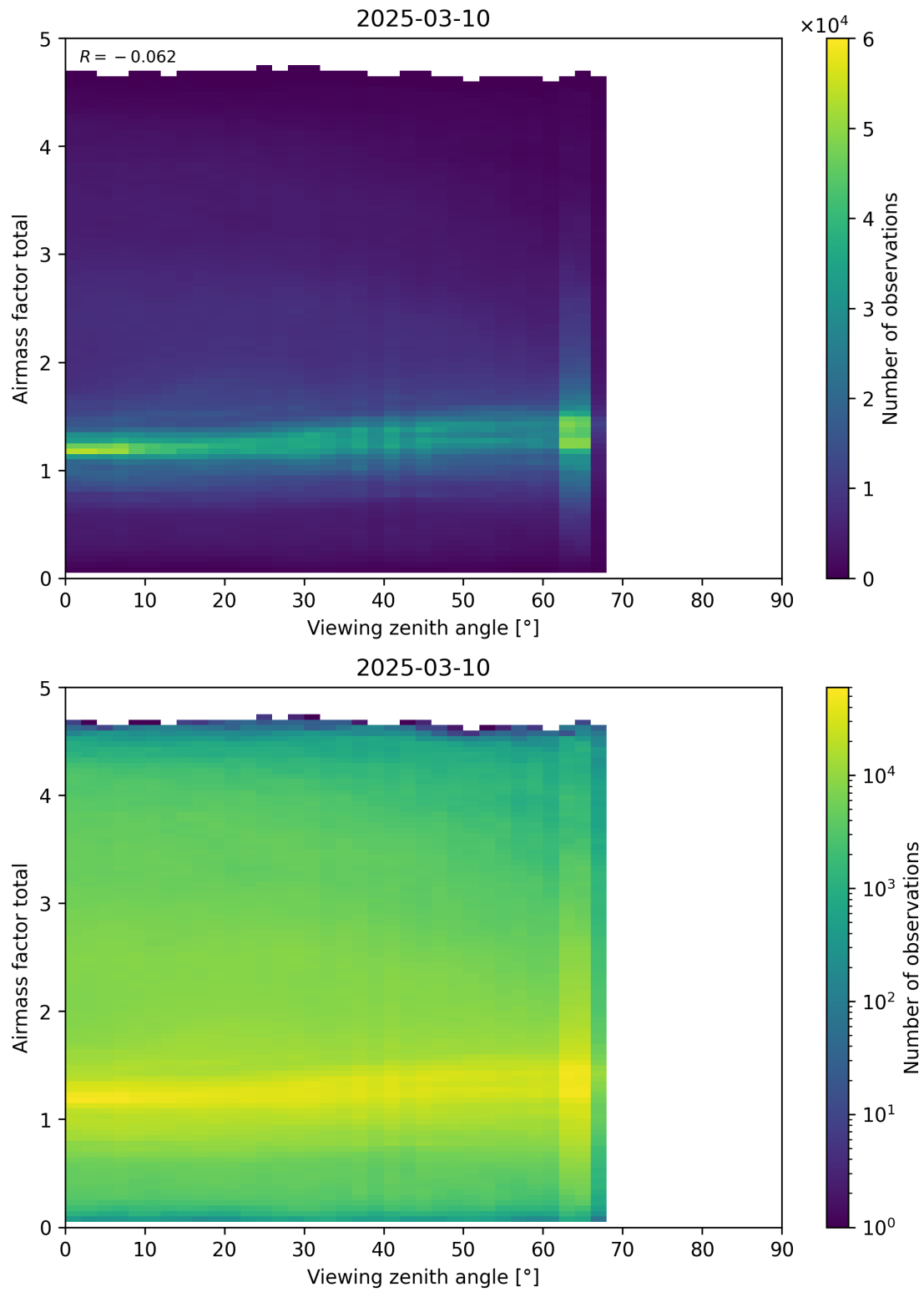
Figure 190: Scatter density plot of “Viewing zenith angle” against “Airmass factor total” for 2025-03-09 to 2025-03-11.
