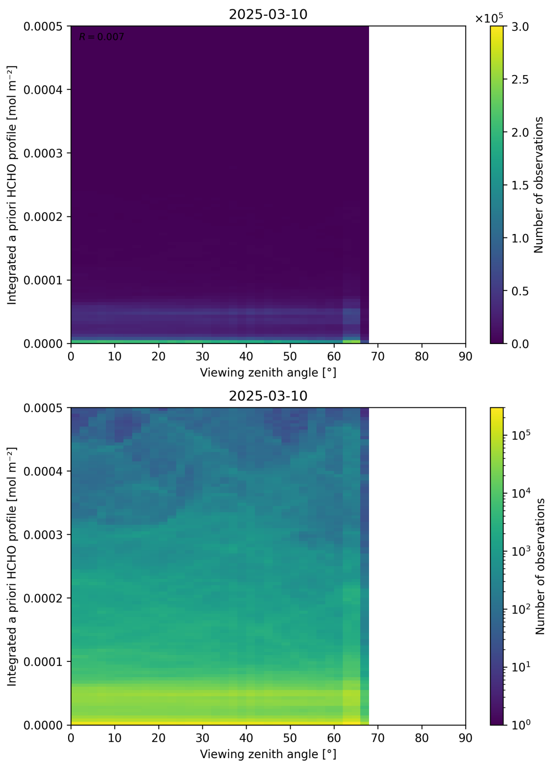
Figure 195: Scatter density plot of “Viewing zenith angle” against “Integrated a priori HCHO profile” for 2025-03-09 to 2025-03-11.
