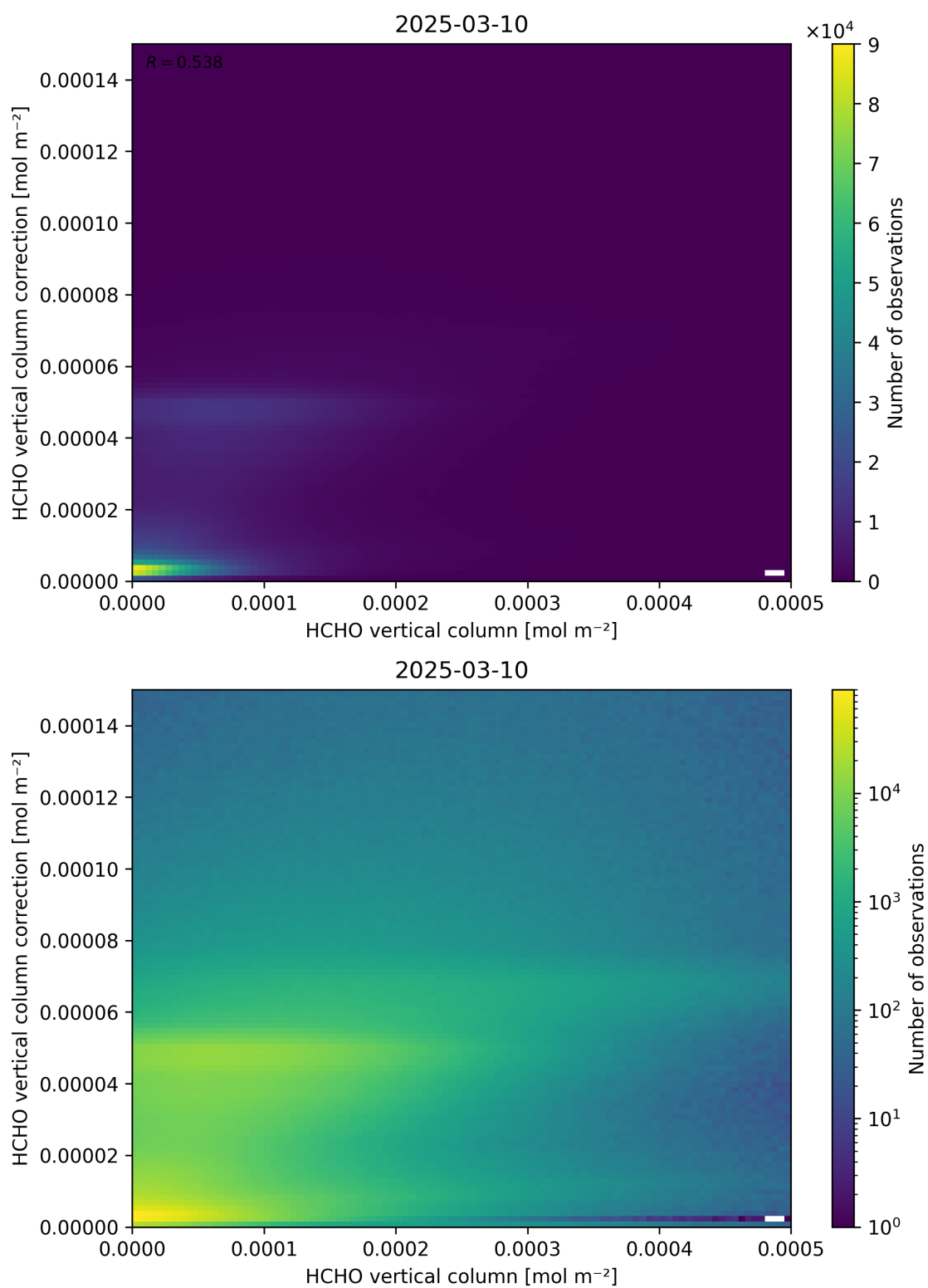
Figure 133: Scatter density plot of “HCHO vertical column” against “HCHO vertical column correction” for 2025-03-09 to 2025-03-11.
