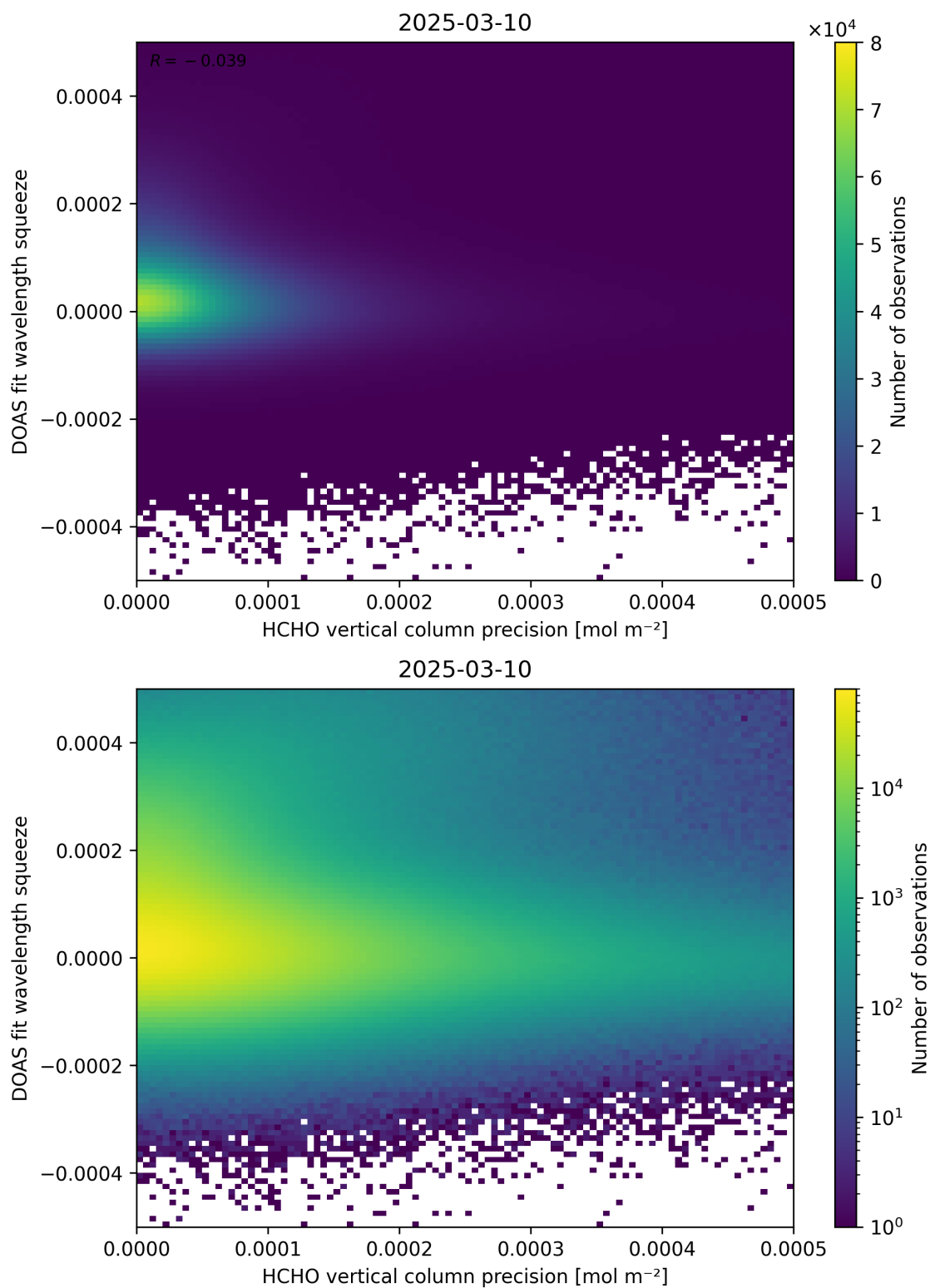
Figure 138: Scatter density plot of “HCHO vertical column precision” against “DOAS fit wavelength squeeze” for 2025-03-09 to 2025-03-11.
