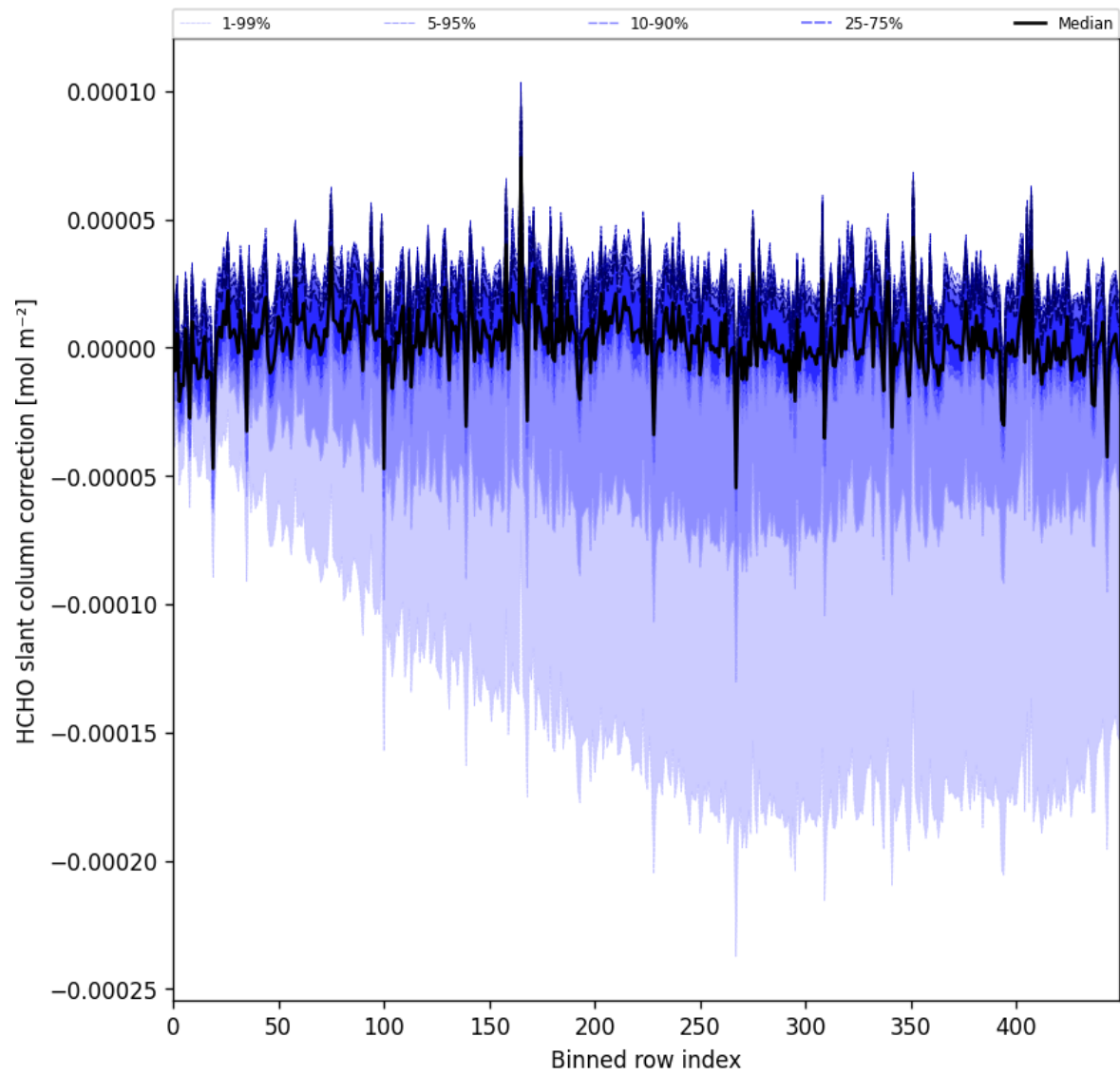
Figure 61: Along track statistics of “HCHO slant column correction” for 2025-03-09 to 2025-03-11
