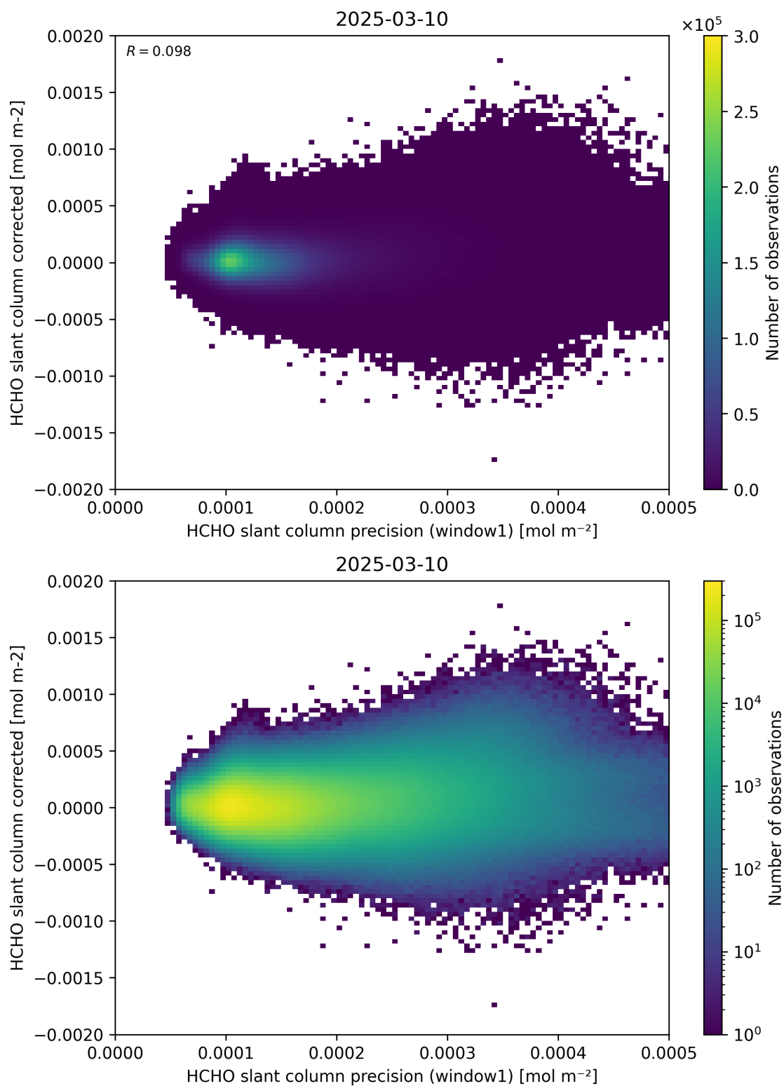
Figure 92: Scatter density plot of “HCHO slant column precision (window1)” against “HCHO slant column corrected” for 2025-03-09 to 2025-03-11.
