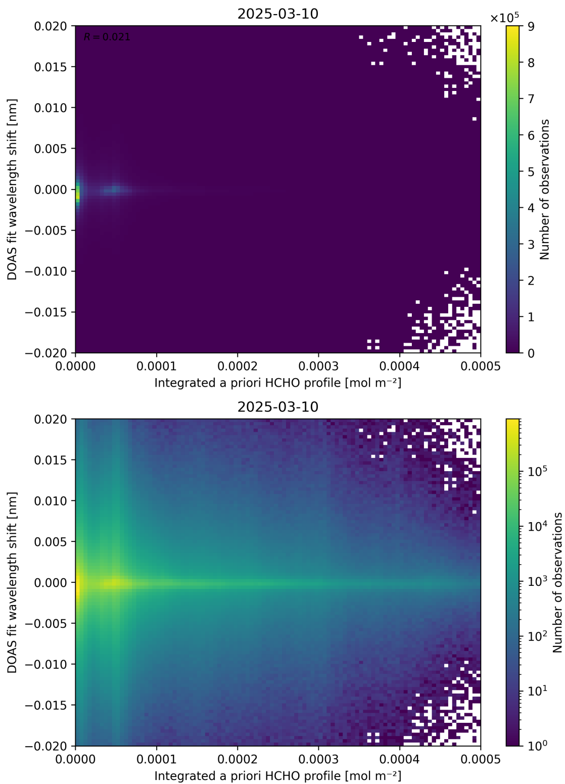
Figure 149: Scatter density plot of “Integrated a priori HCHO profile” against “DOAS fit wavelength shift” for 2025-03-09 to 2025-03-11.
