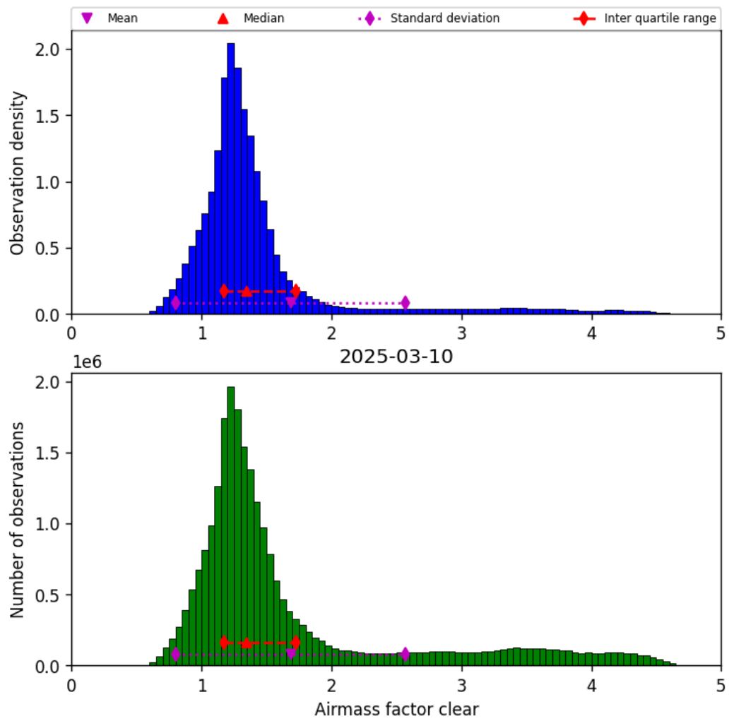
Figure 42: Histogram of “Airmass factor clear” for 2025-03-09 to 2025-03-11
