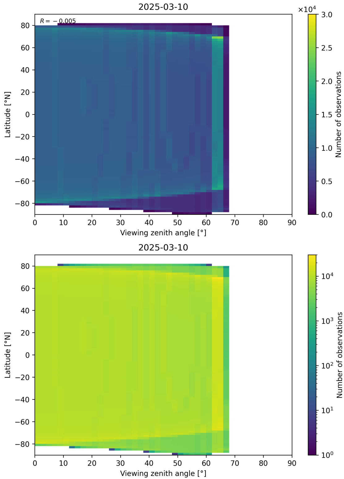
Figure 196: Scatter density plot of “Viewing zenith angle” against “Latitude” for 2025-03-09 to 2025-03-11.
