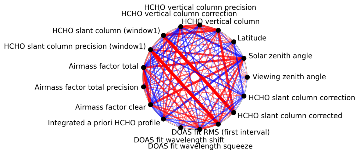
Figure 1: Map of correlation graph for 2025-03-09 to 2025-03-11.
