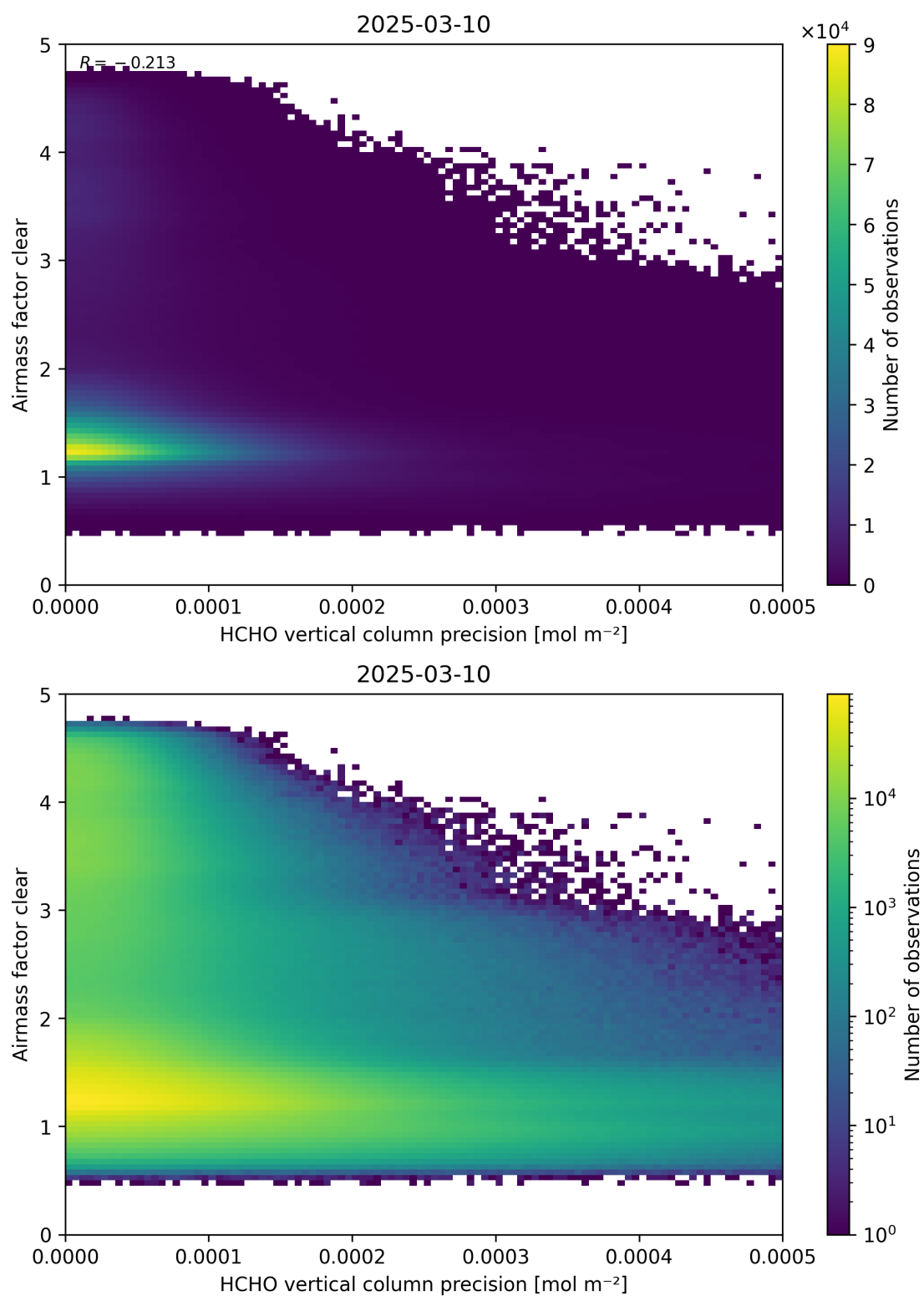
Figure 139: Scatter density plot of “HCHO vertical column precision” against “Airmass factor clear” for 2025-03-09 to 2025-03-11.
