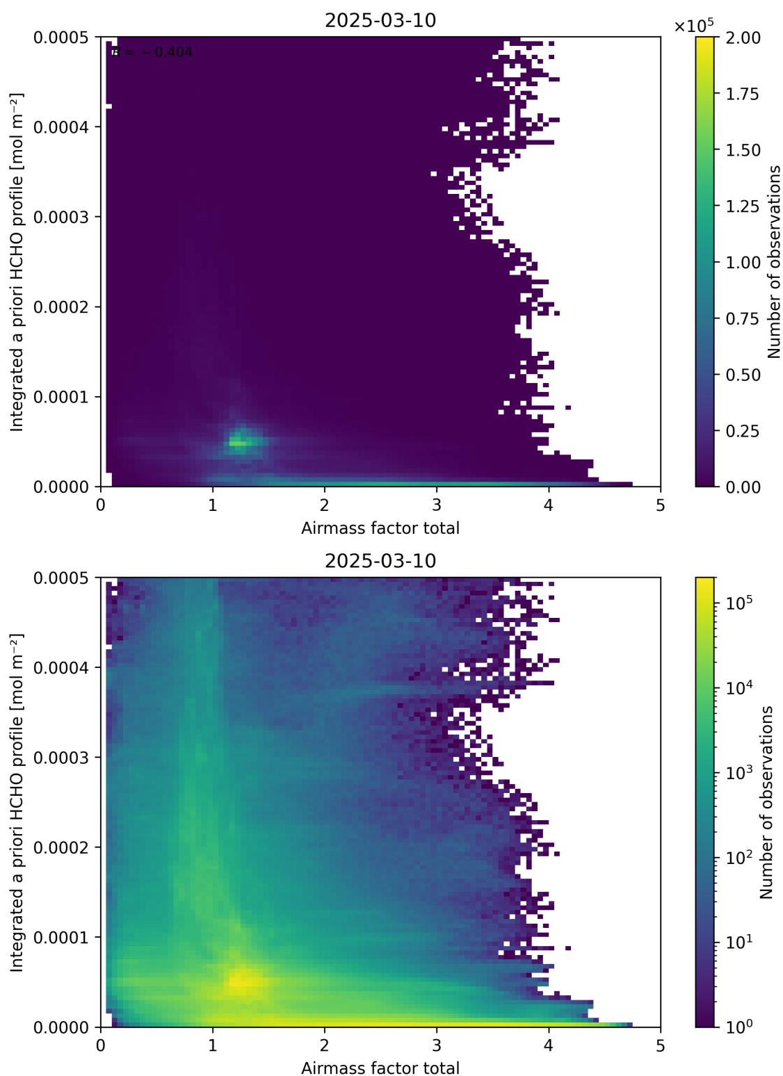
Figure 104: Scatter density plot of “Airmass factor total” against “Integrated a priori HCHO profile” for 2025-03-09 to 2025-03-11.
