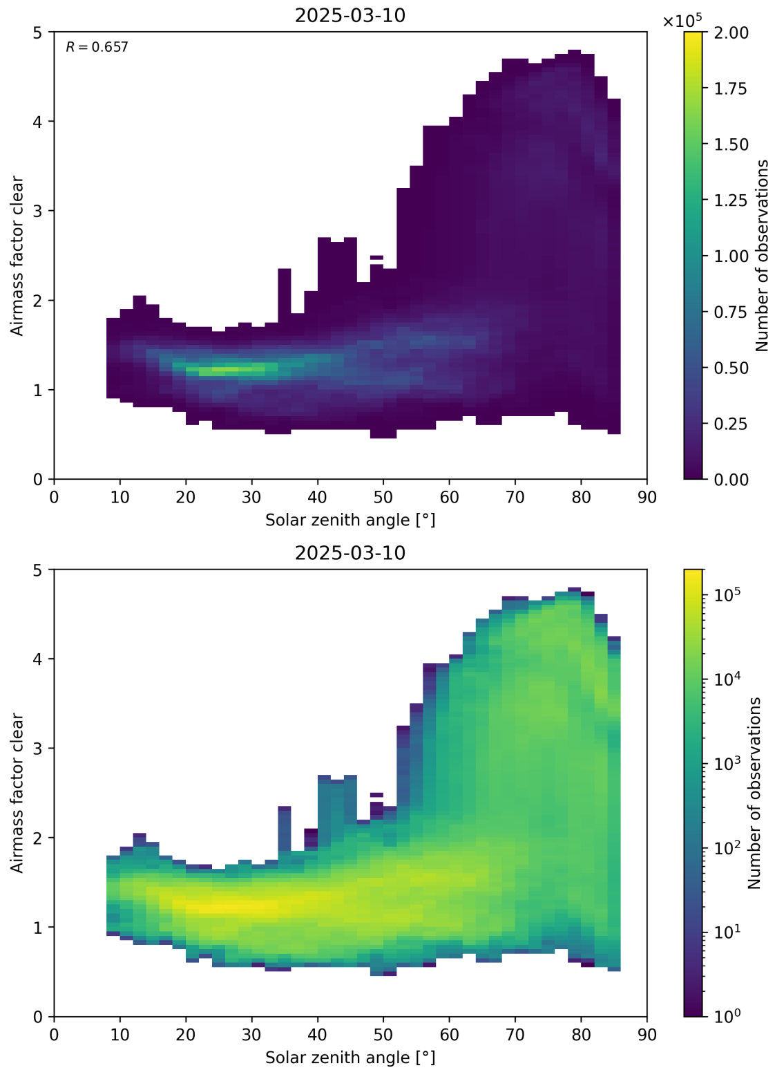
Figure 170: Scatter density plot of “Solar zenith angle” against “Airmass factor clear” for 2025-03-09 to 2025-03-11.
