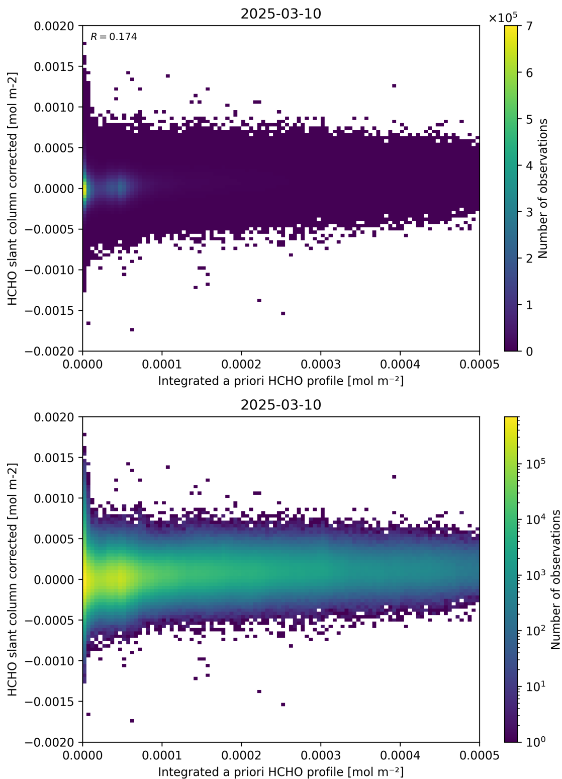
Figure 151: Scatter density plot of “Integrated a priori HCHO profile” against “HCHO slant column corrected” for 2025-03-09 to 2025-03-11.
