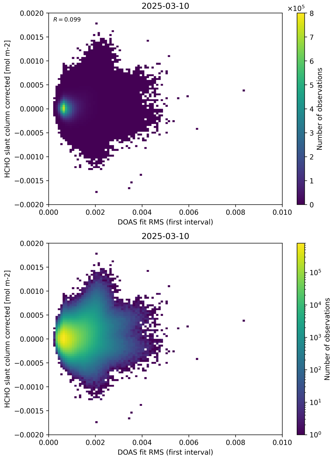
Figure 62: Scatter density plot of “DOAS fit RMS (first interval)” against “HCHO slant column corrected” for 2025-03-09 to 2025-03-11.
