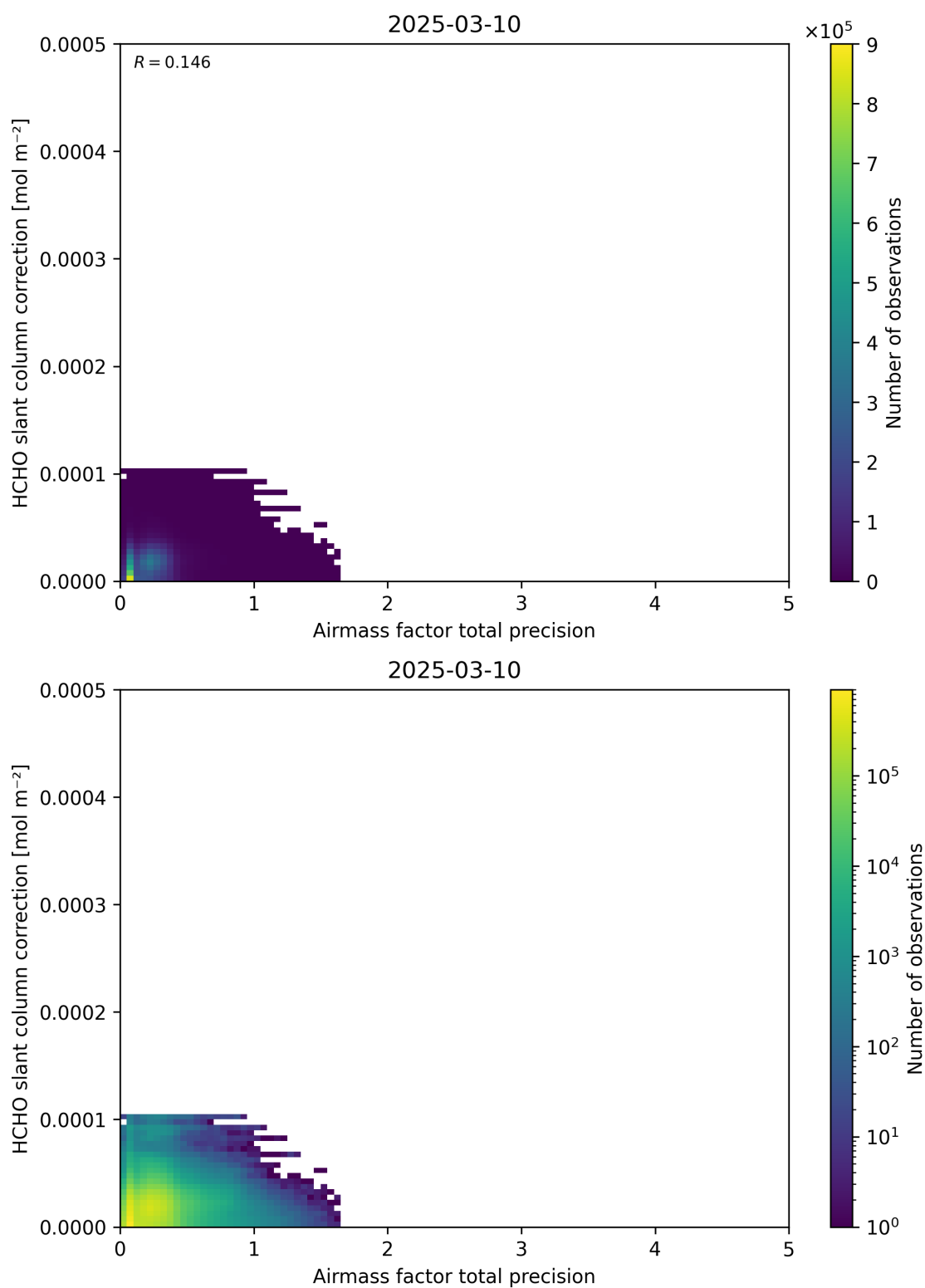
Figure 110: Scatter density plot of “Airmass factor total precision” against “HCHO slant column correction” for 2025-03-09 to 2025-03-11.
