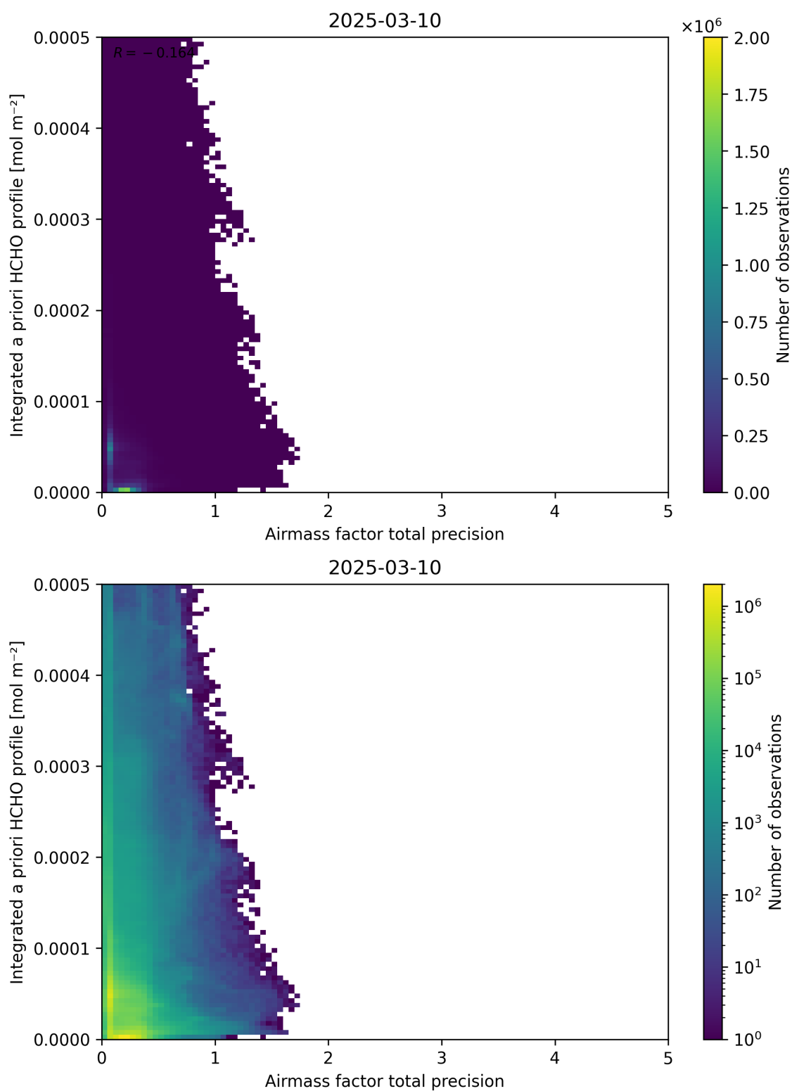
Figure 111: Scatter density plot of “Airmass factor total precision” against “Integrated a priori HCHO profile” for 2025-03-09 to 2025-03-11.
