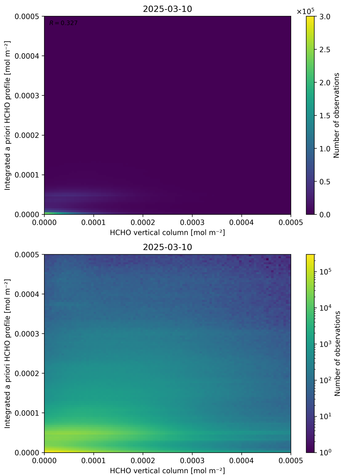
Figure 135: Scatter density plot of “HCHO vertical column” against “Integrated a priori HCHO profile” for 2025-03-09 to 2025-03-11.
