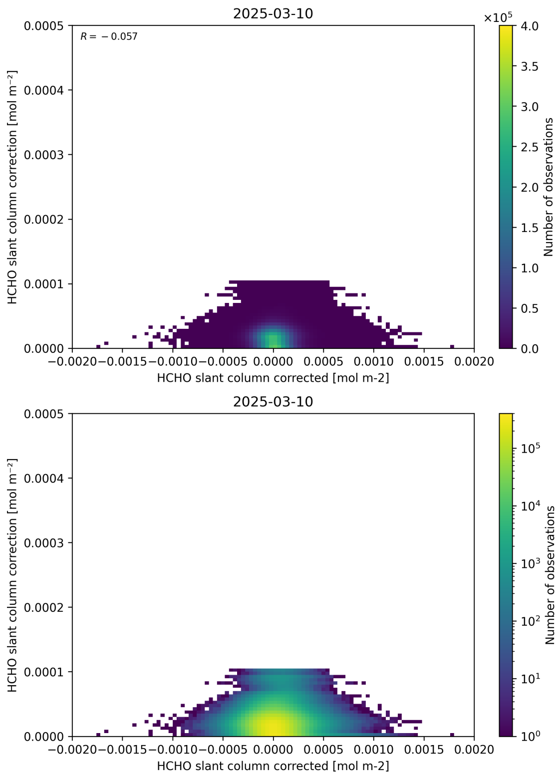
Figure 77: Scatter density plot of “HCHO slant column corrected” against “HCHO slant column correction” for 2025-03-09 to 2025-03-11.
