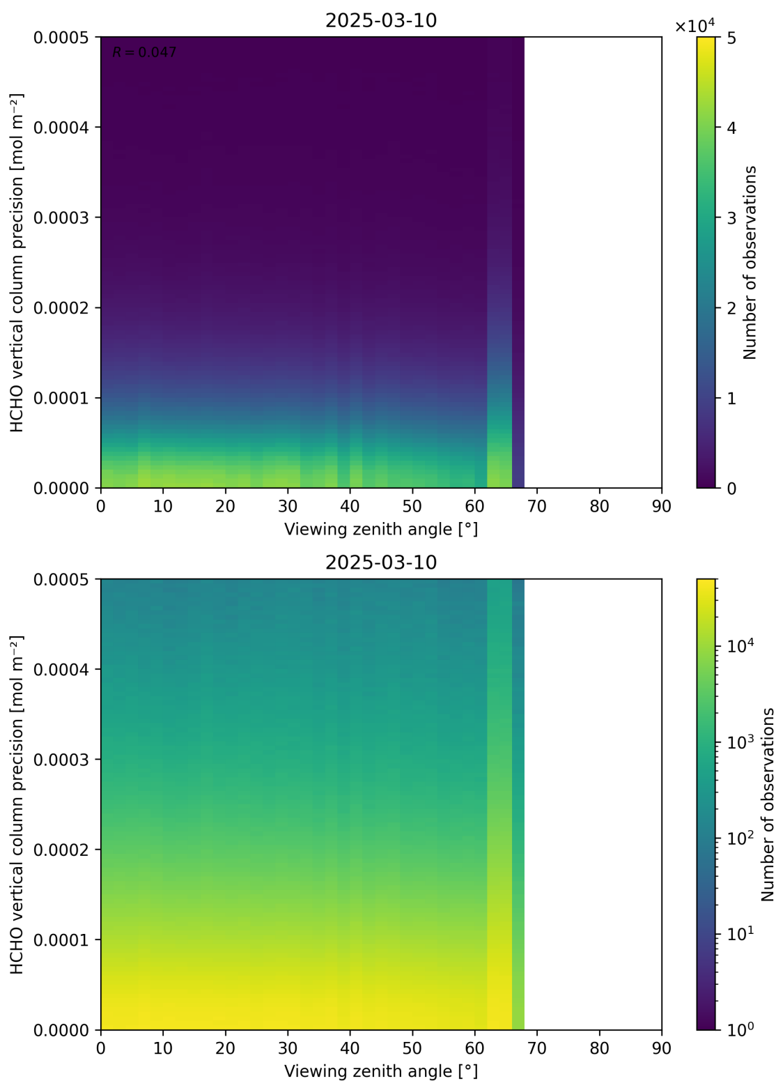
Figure 194: Scatter density plot of “Viewing zenith angle” against “HCHO vertical column precision” for 2025-03-09 to 2025-03-11.
