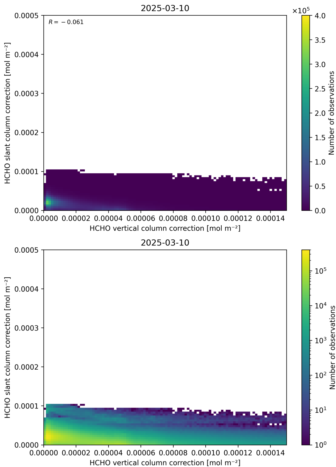
Figure 117: Scatter density plot of “HCHO vertical column correction” against “HCHO slant column correction” for 2025-03-09 to 2025-03-11.
