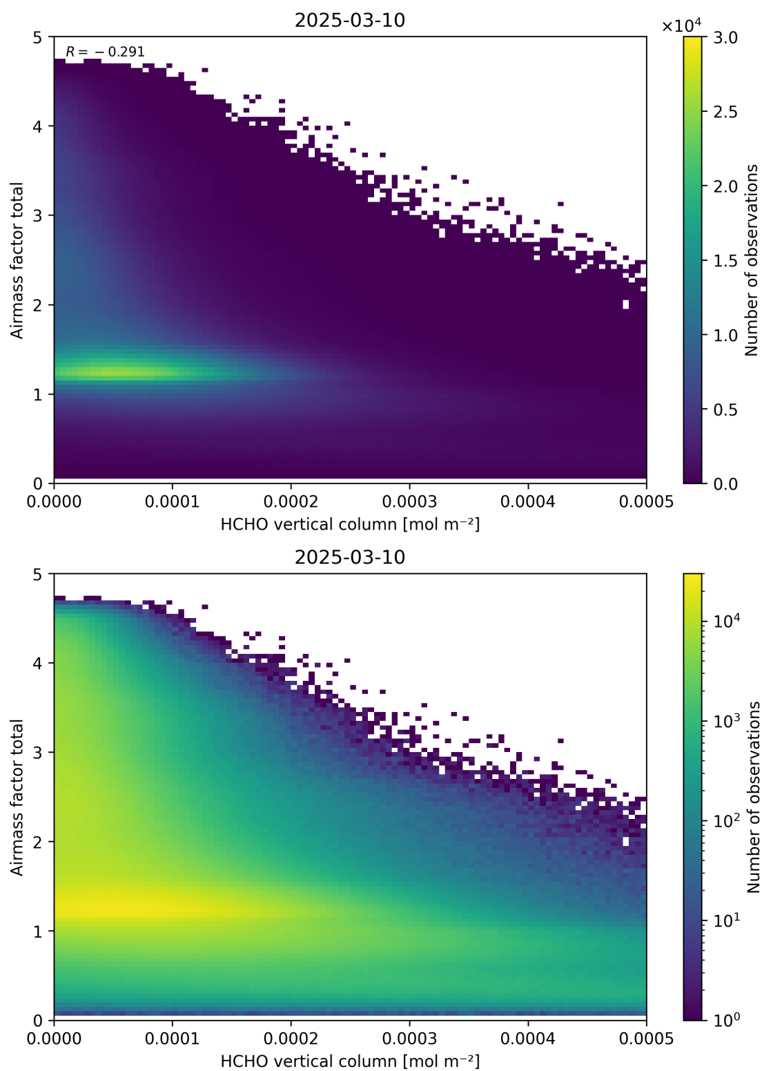
Figure 131: Scatter density plot of “HCHO vertical column” against “Airmass factor total” for 2025-03-09 to 2025-03-11.
