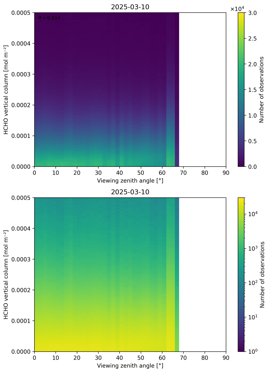
Figure 192: Scatter density plot of “Viewing zenith angle” against “HCHO vertical column” for 2025-03-09 to 2025-03-11.
