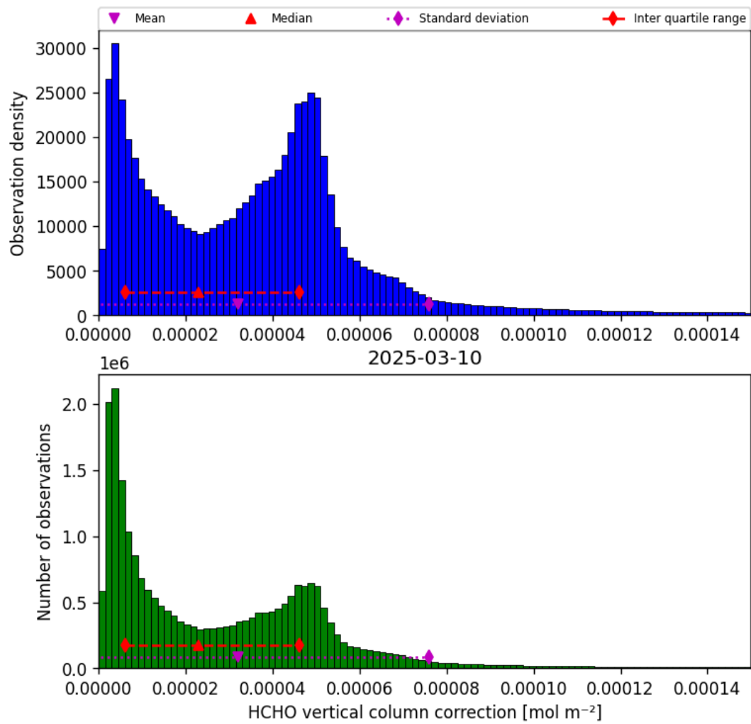
Figure 37: Histogram of “HCHO vertical column correction” for 2025-03-09 to 2025-03-11
