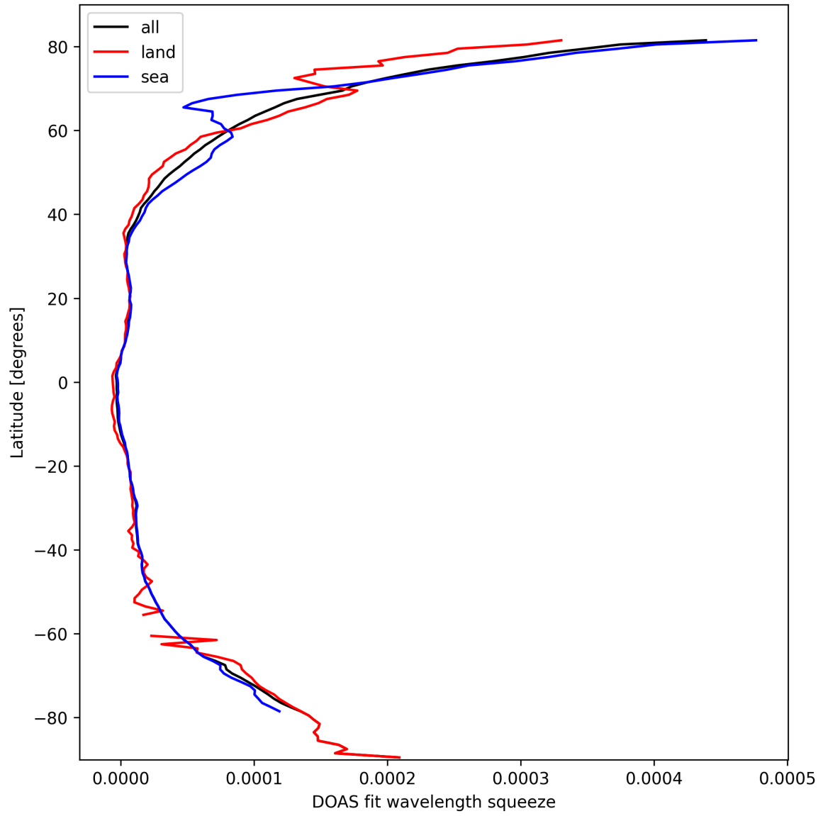
Figure 31: Zonal average of “DOAS fit wavelength squeeze” for 2025-03-09 to 2025-03-11.
