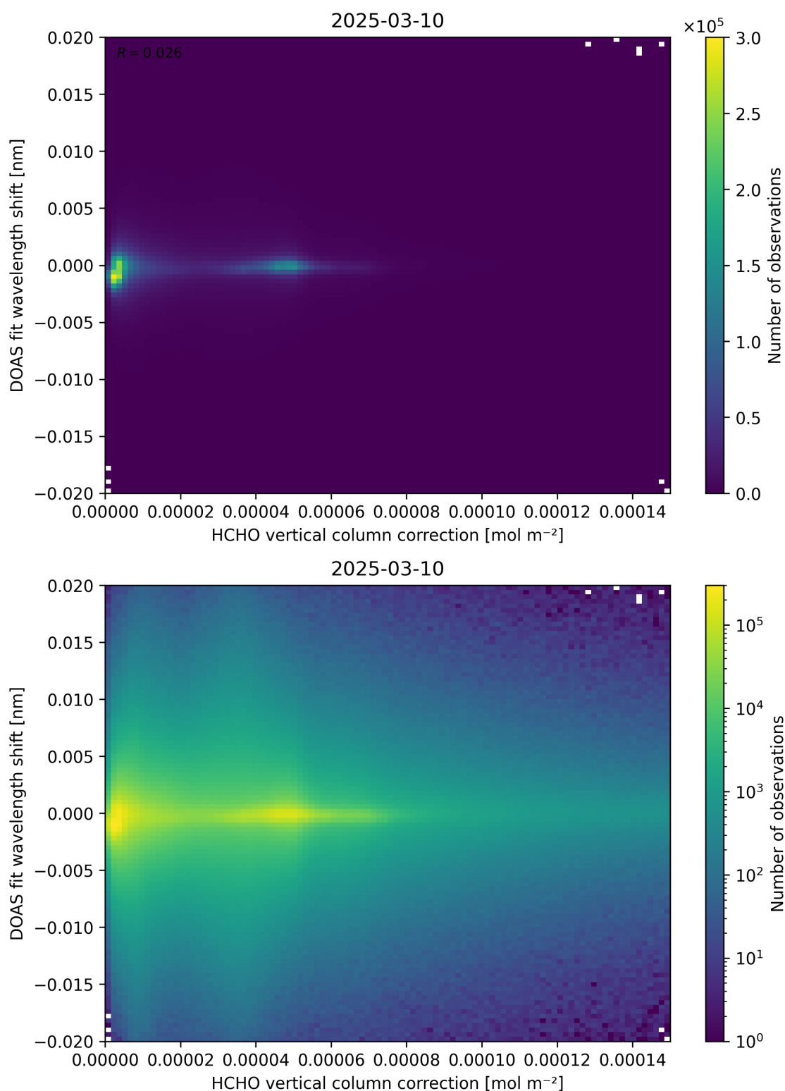
Figure 113: Scatter density plot of “HCHO vertical column correction” against “DOAS fit wavelength shift” for 2025-03-09 to 2025-03-11.
