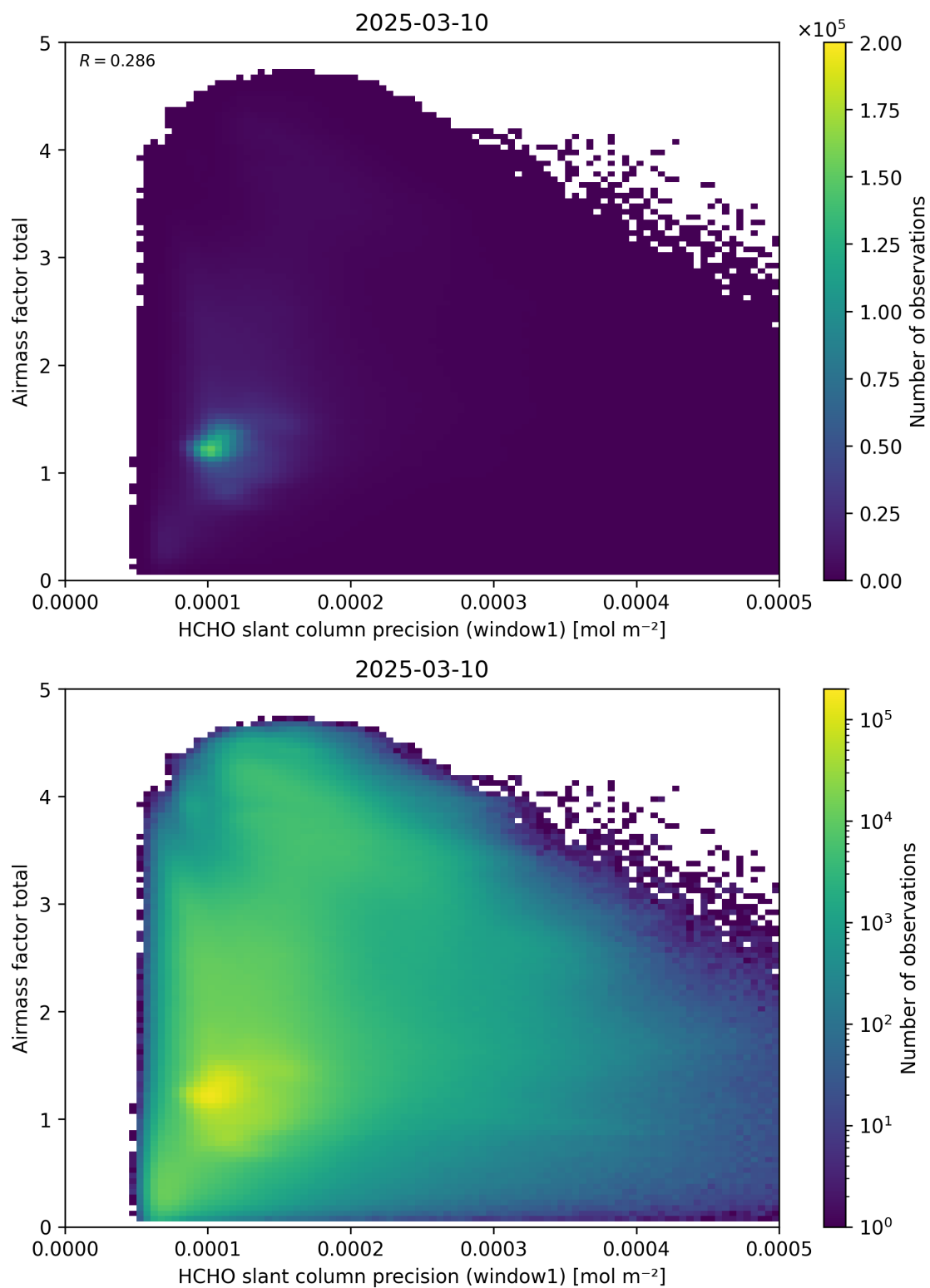
Figure 94: Scatter density plot of “HCHO slant column precision (window1)” against “Airmass factor total” for 2025-03-09 to 2025-03-11.
