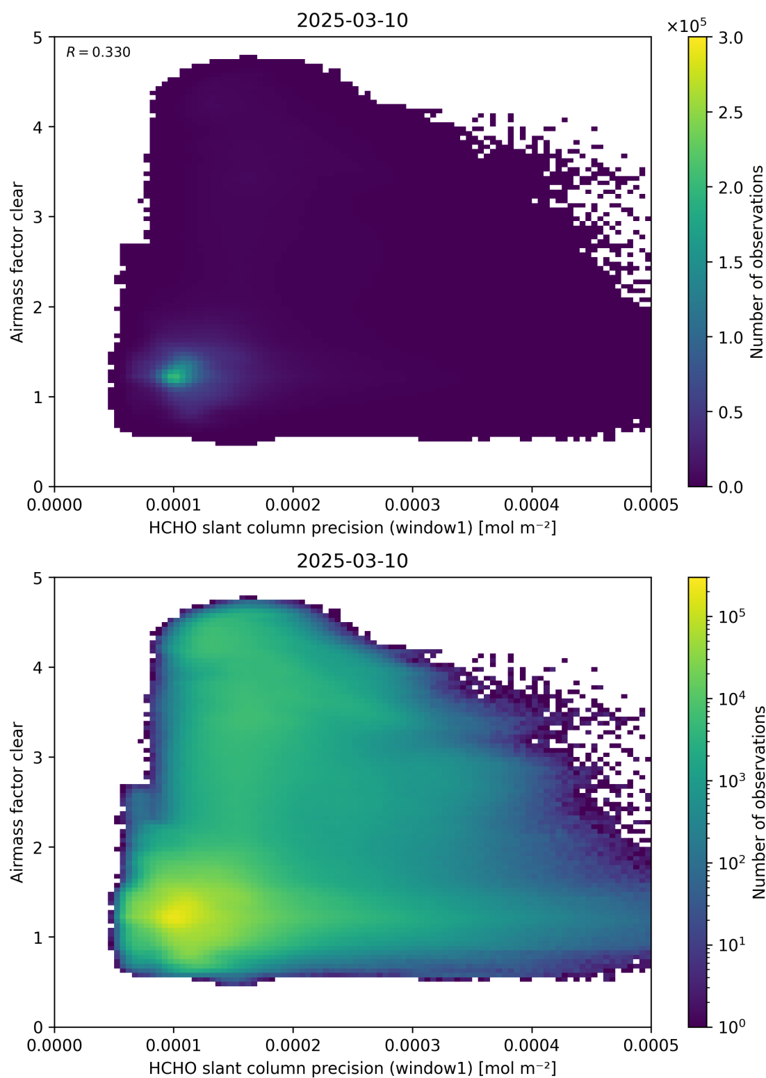
Figure 91: Scatter density plot of “HCHO slant column precision (window1)” against “Airmass factor clear” for 2025-03-09 to 2025-03-11.
