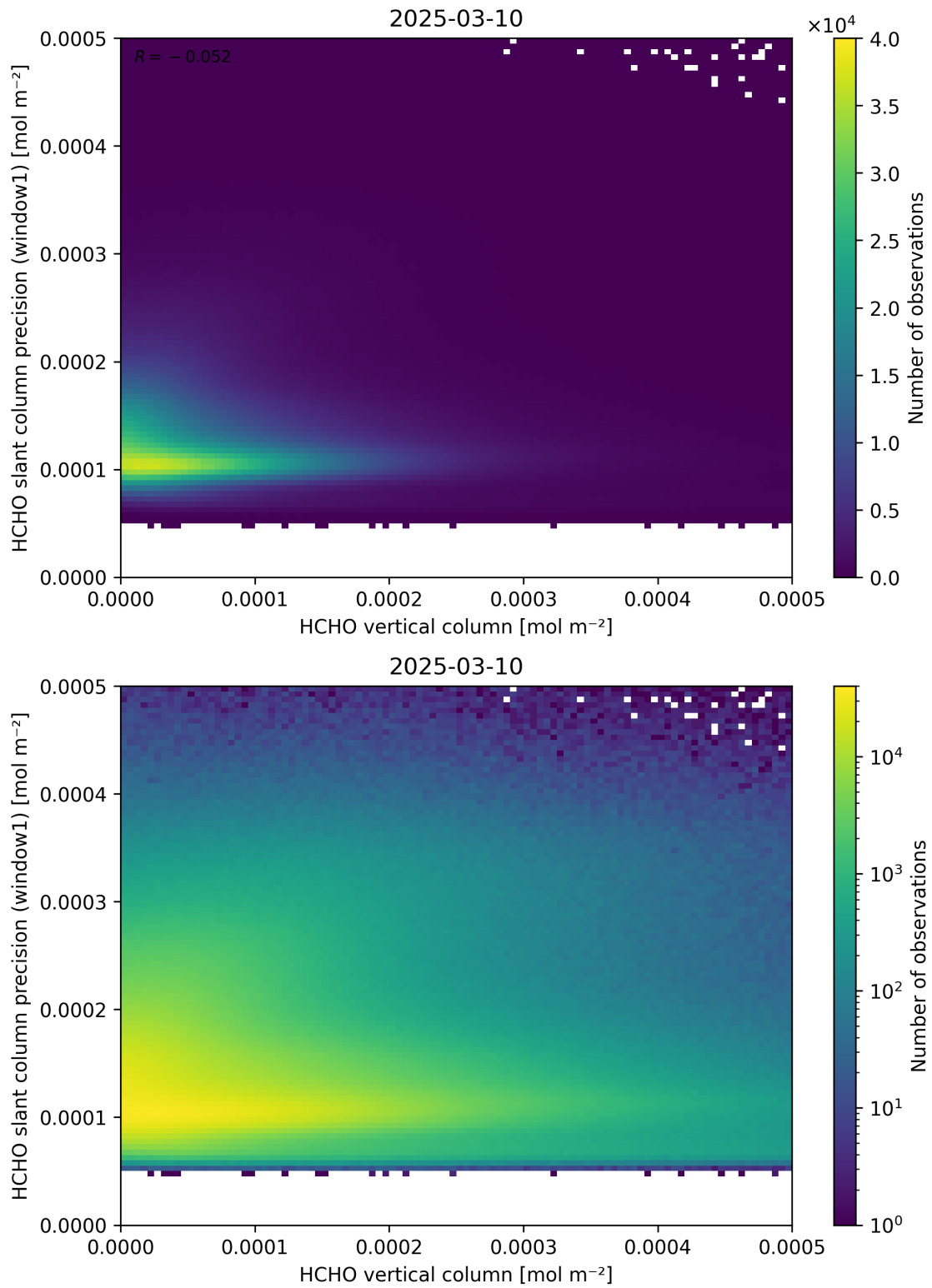
Figure 130: Scatter density plot of “HCHO vertical column” against “HCHO slant column precision (window1)” for 2025-03-09 to 2025-03-11.
