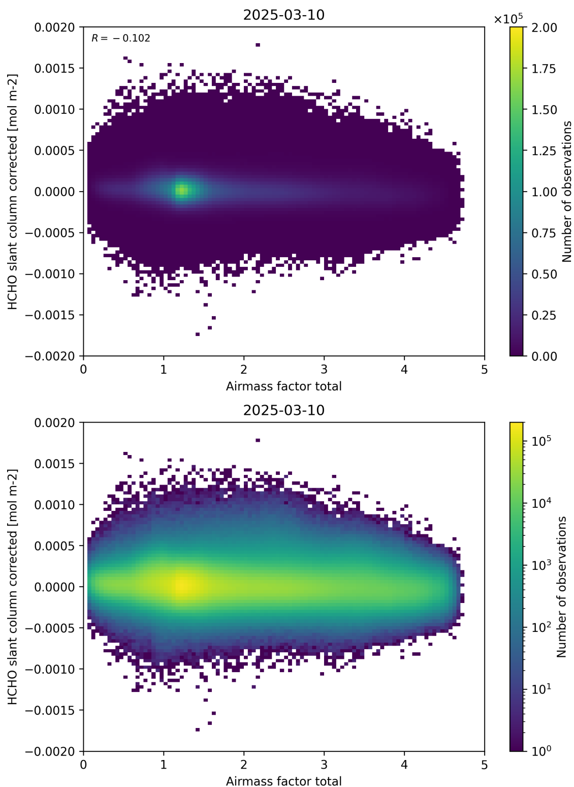
Figure 101: Scatter density plot of “Airmass factor total” against “HCHO slant column corrected” for 2025-03-09 to 2025-03-11.
