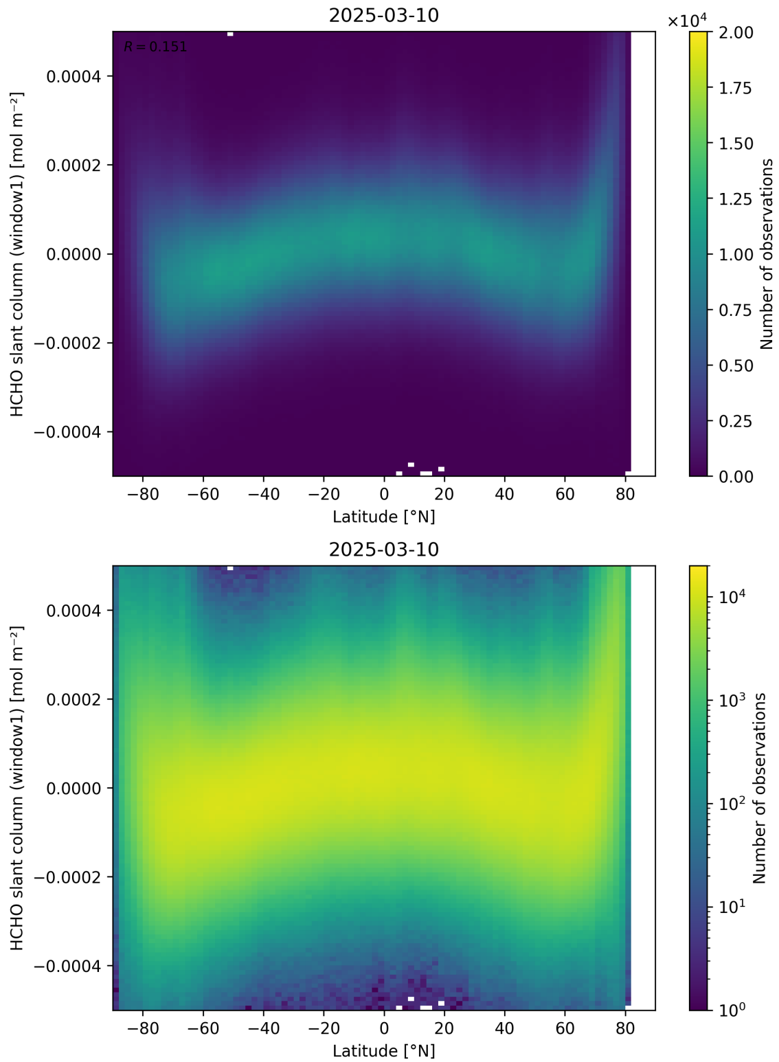
Figure 159: Scatter density plot of “Latitude” against “HCHO slant column (window1)” for 2025-03-09 to 2025-03-11.
