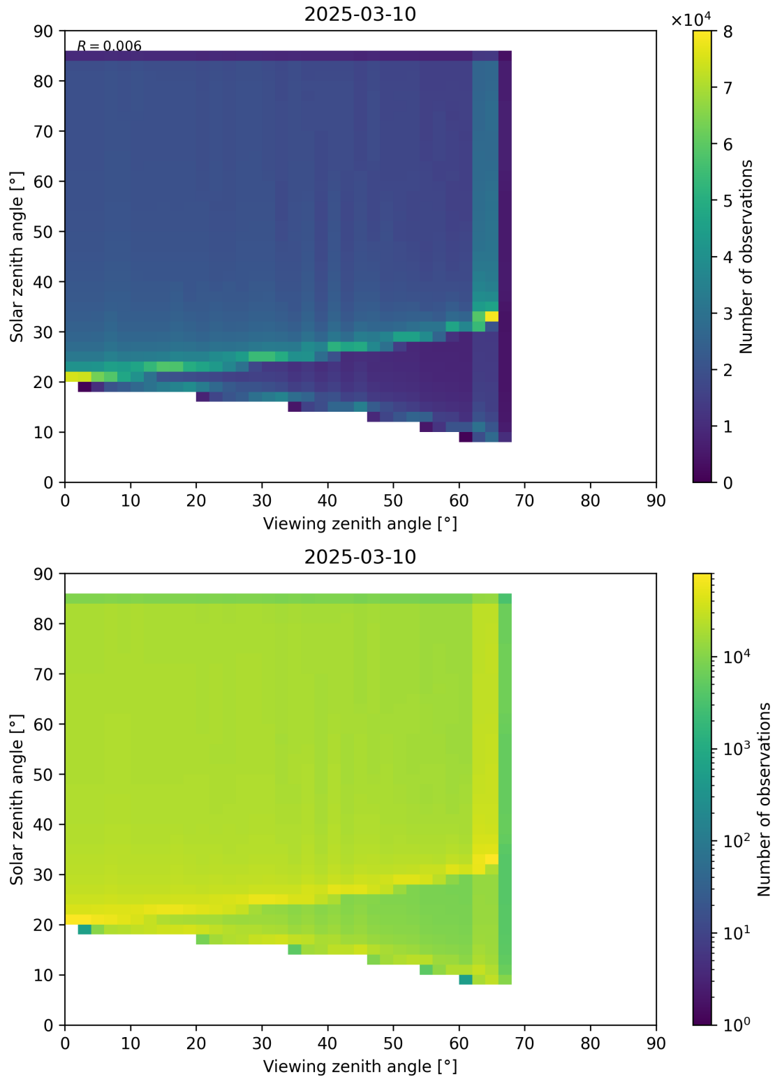
Figure 197: Scatter density plot of “Viewing zenith angle” against “Solar zenith angle” for 2025-03-09 to 2025-03-11.
