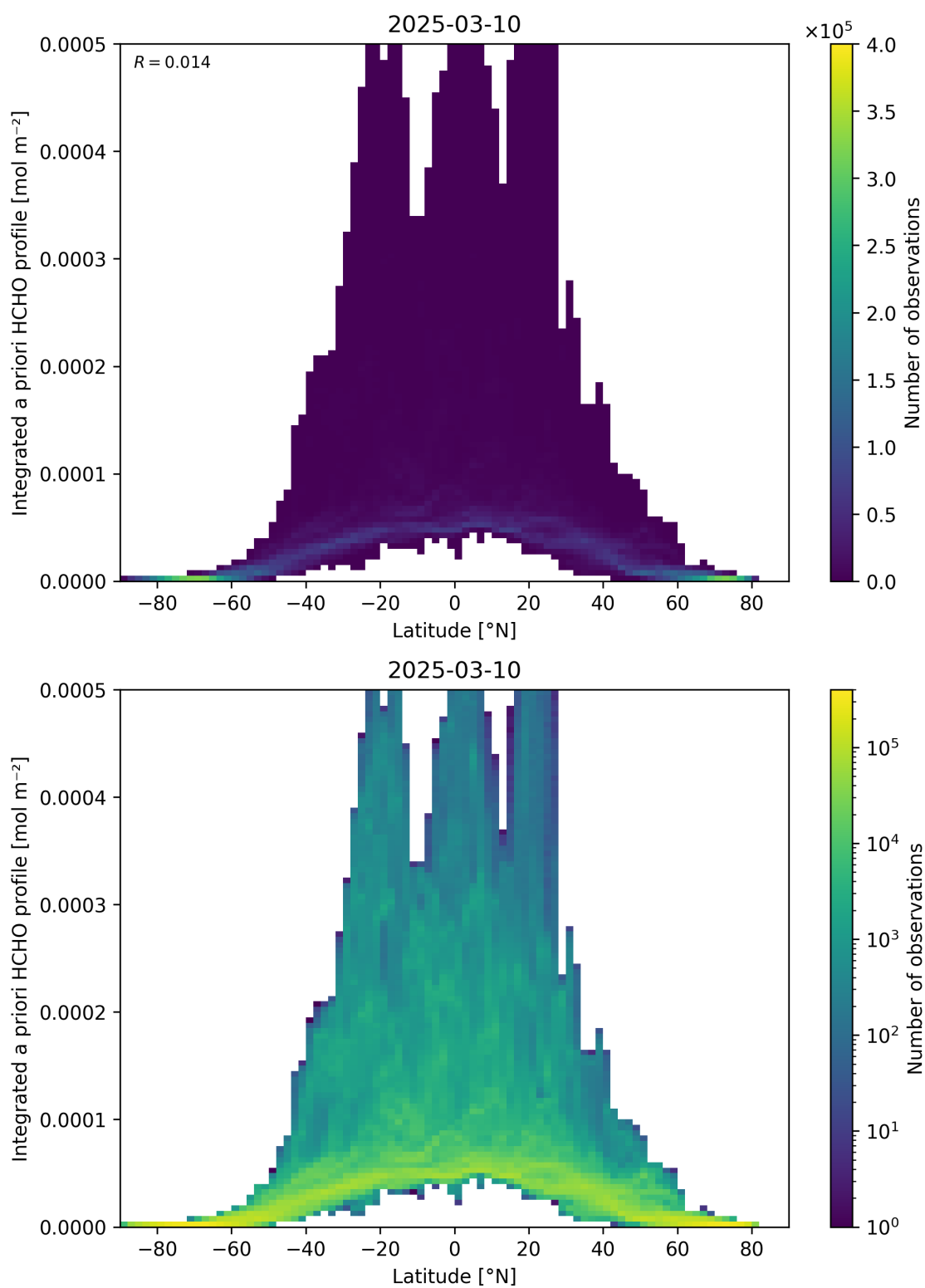
Figure 166: Scatter density plot of “Latitude” against “Integrated a priori HCHO profile” for 2025-03-09 to 2025-03-11.
