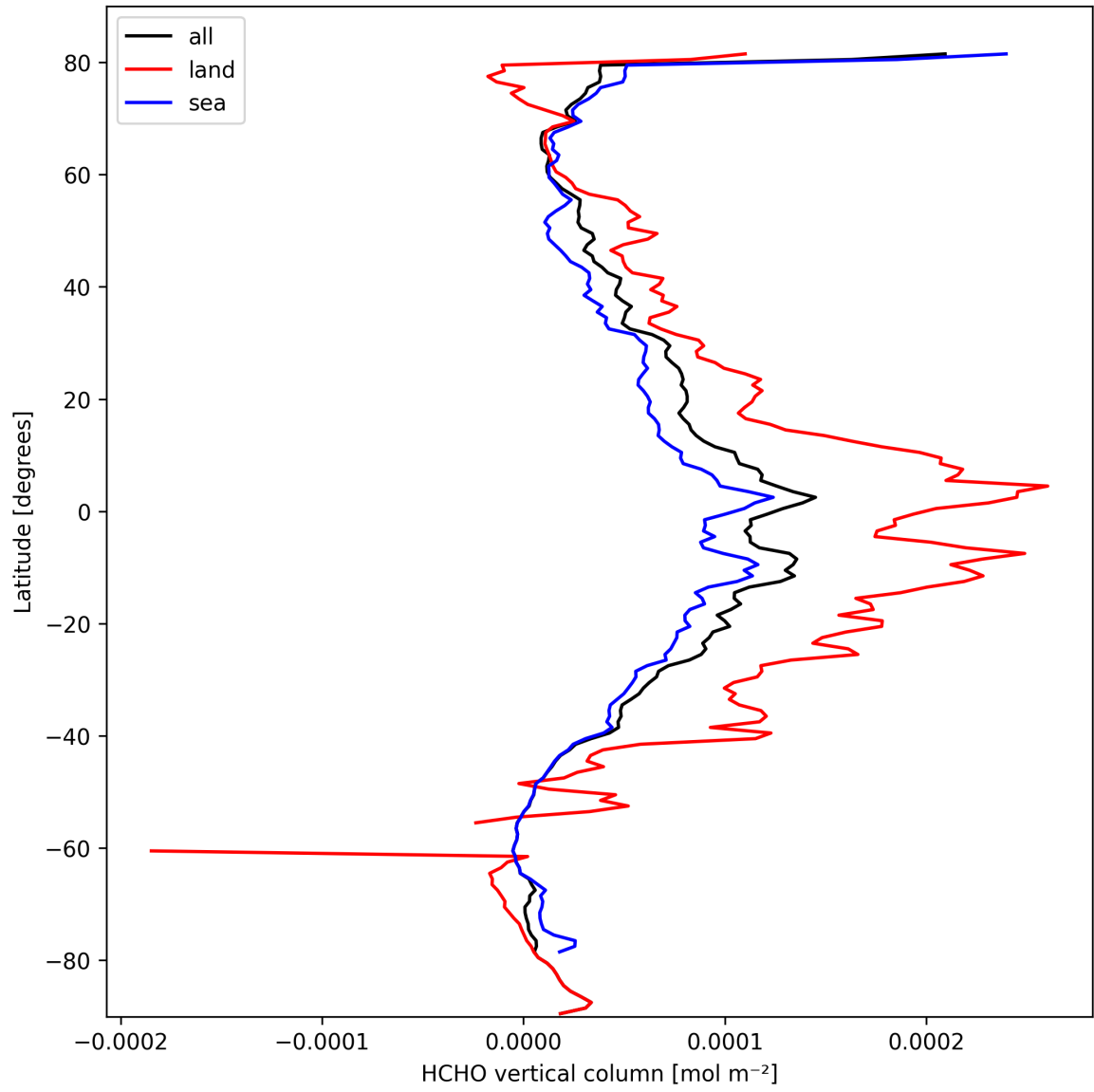
Figure 21: Zonal average of “HCHO vertical column” for 2025-03-09 to 2025-03-11.
