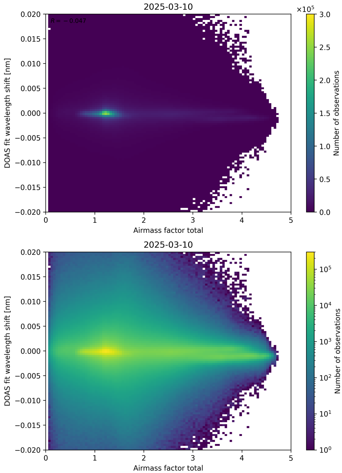
Figure 98: Scatter density plot of “Airmass factor total” against “DOAS fit wavelength shift” for 2025-03-09 to 2025-03-11.
