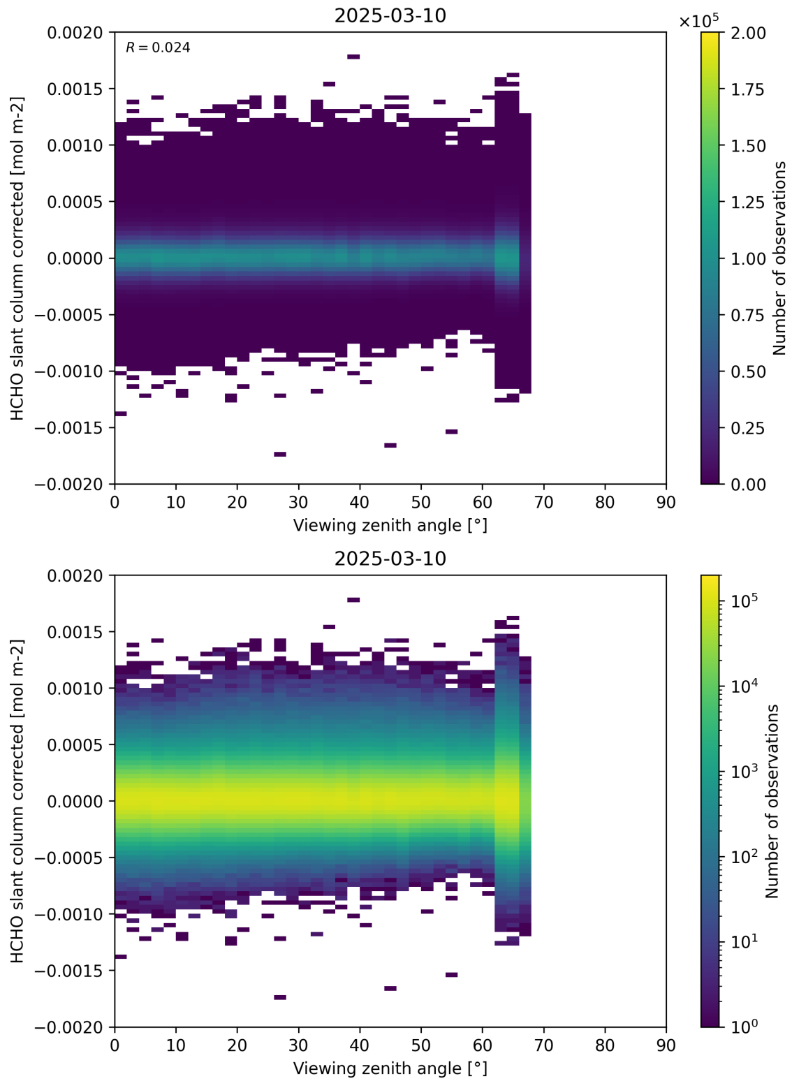
Figure 186: Scatter density plot of “Viewing zenith angle” against “HCHO slant column corrected” for 2025-03-09 to 2025-03-11.
