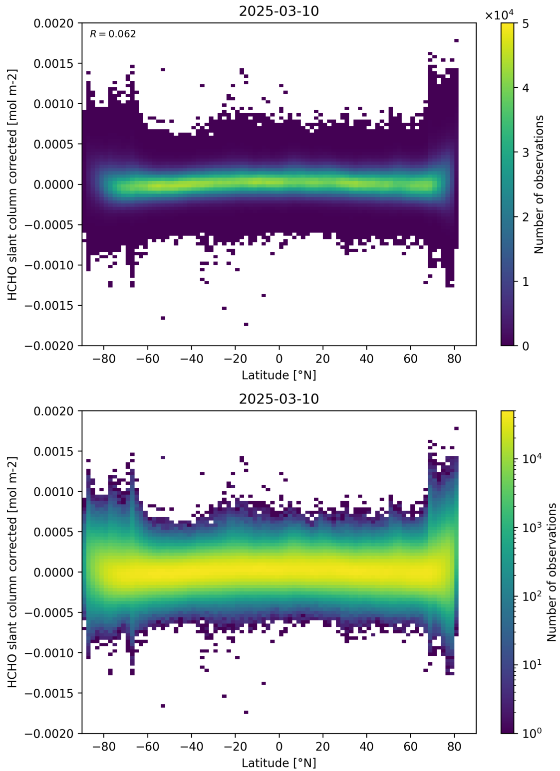
Figure 157: Scatter density plot of “Latitude” against “HCHO slant column corrected” for 2025-03-09 to 2025-03-11.
