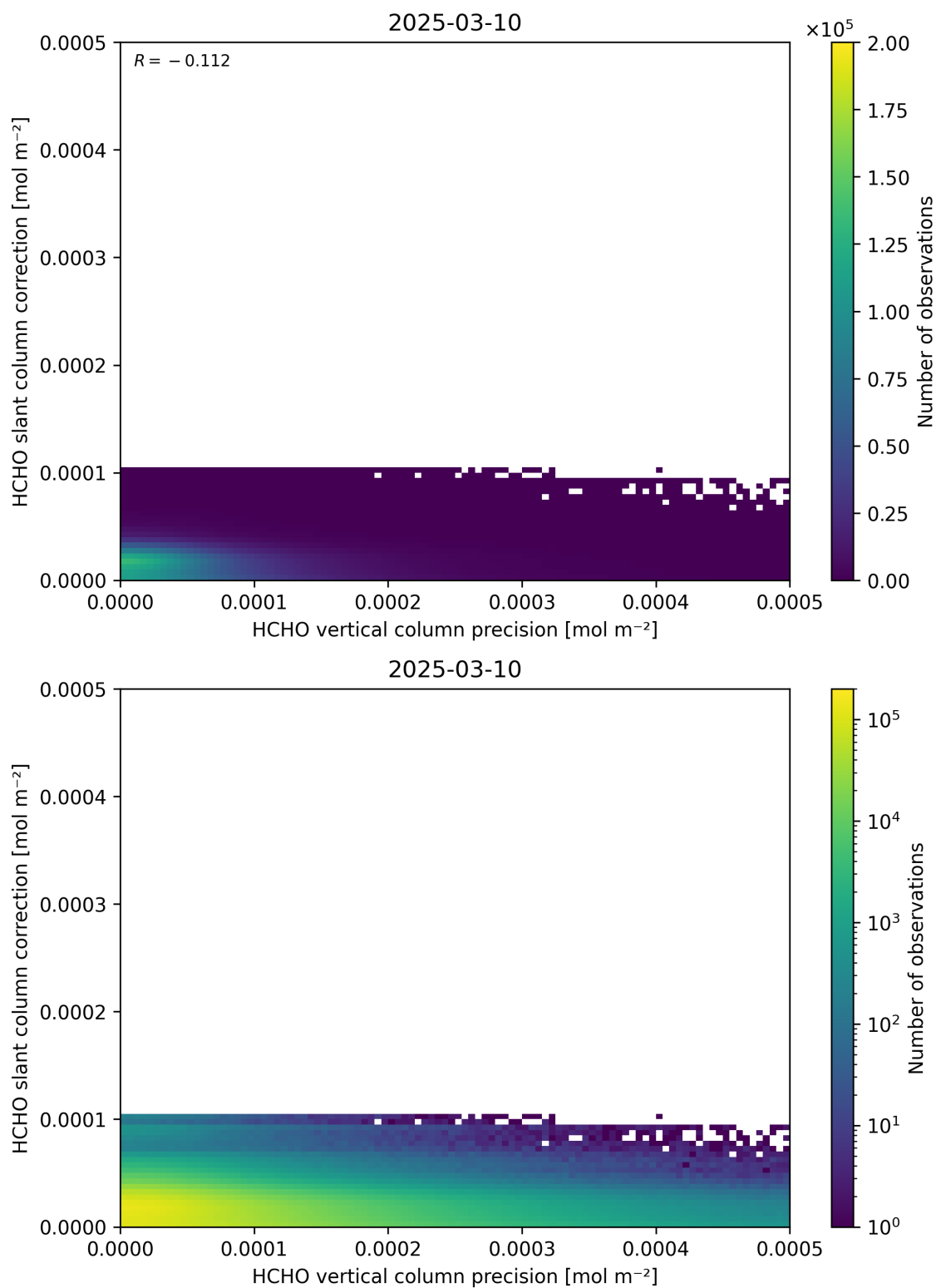
Figure 141: Scatter density plot of “HCHO vertical column precision” against “HCHO slant column correction” for 2025-03-09 to 2025-03-11.
