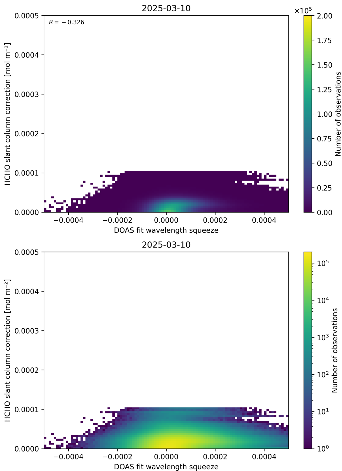
Figure 70: Scatter density plot of “DOAS fit wavelength squeeze” against “HCHO slant column correction” for 2025-03-09 to 2025-03-11.
