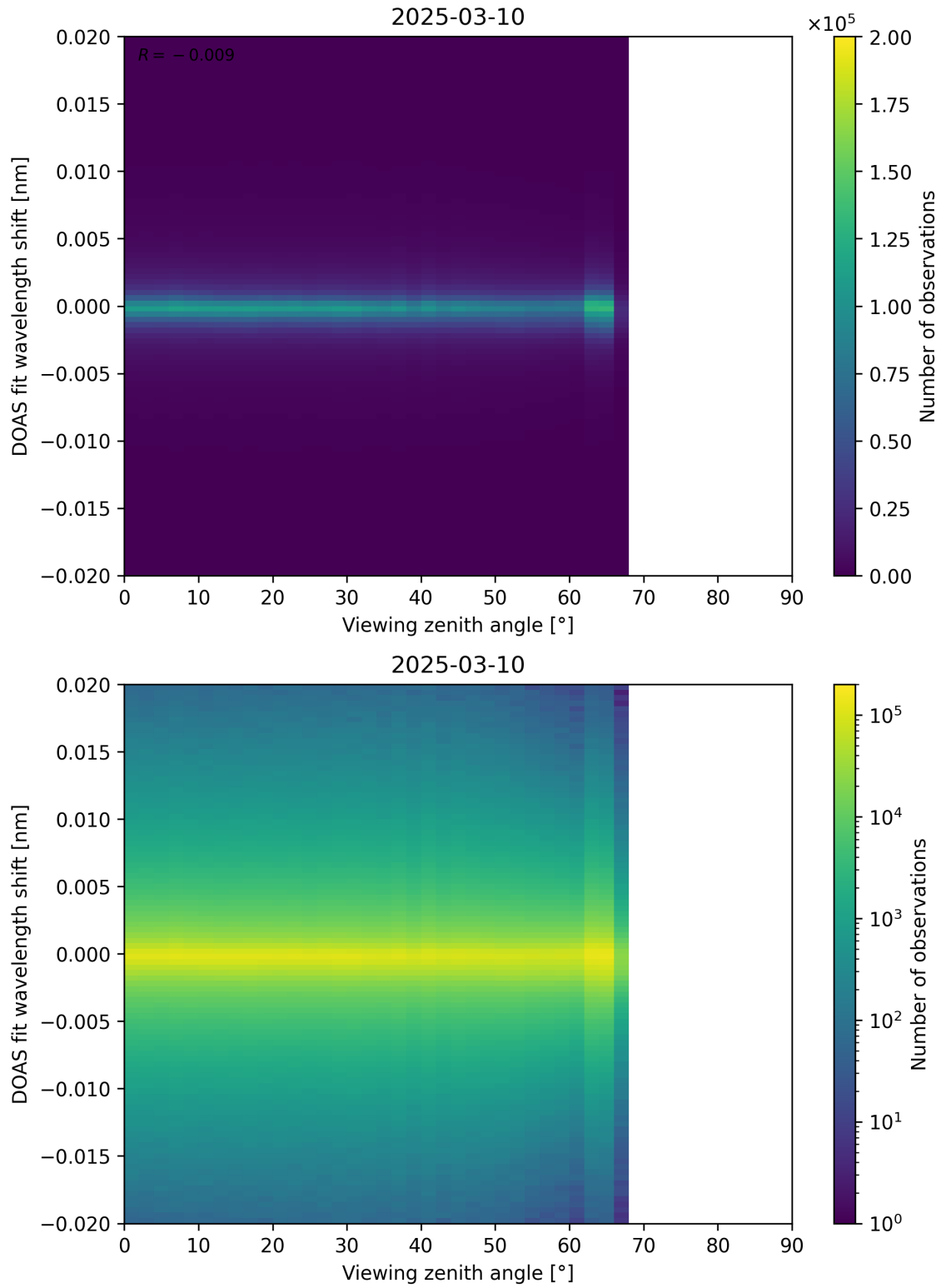
Figure 183: Scatter density plot of “Viewing zenith angle” against “DOAS fit wavelength shift” for 2025-03-09 to 2025-03-11.
