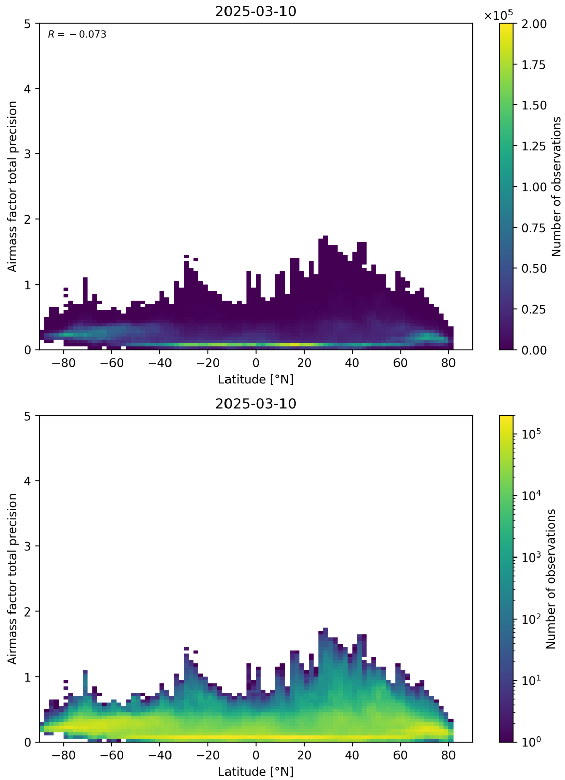
Figure 162: Scatter density plot of “Latitude” against “Airmass factor total precision” for 2025-03-09 to 2025-03-11.
