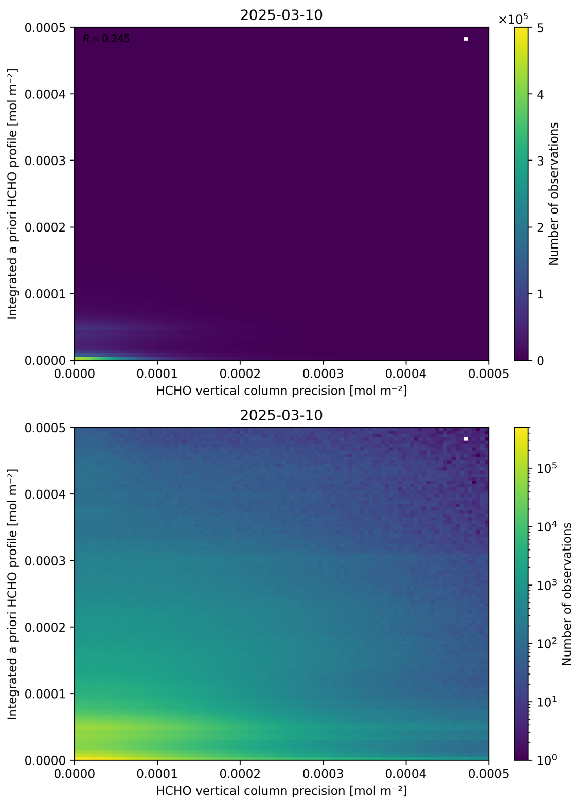
Figure 147: Scatter density plot of “HCHO vertical column precision” against “Integrated a priori HCHO profile” for 2025-03-09 to 2025-03-11.
