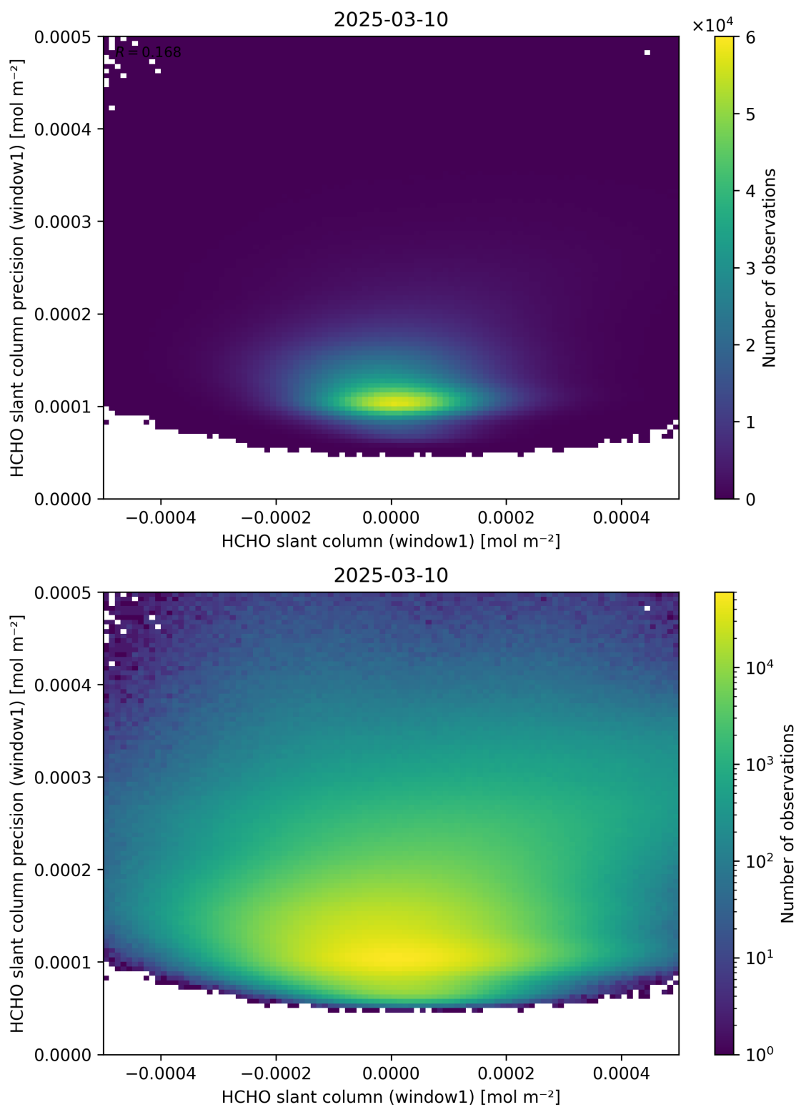
Figure 84: Scatter density plot of “HCHO slant column (window1)” against “HCHO slant column precision (window1)” for 2025-03-09 to 2025-03-11.
