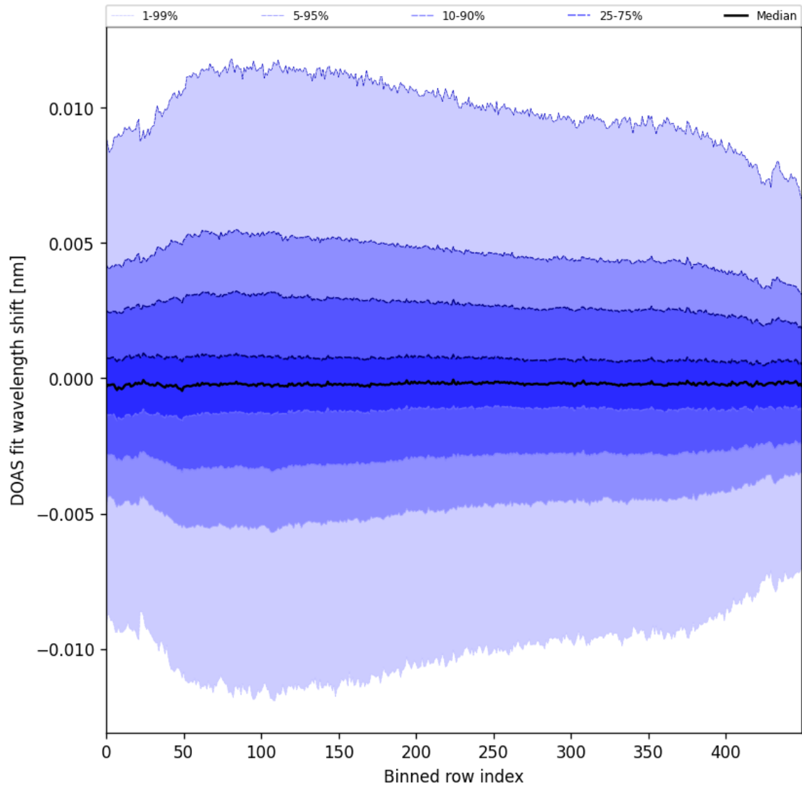
Figure 58: Along track statistics of “DOAS fit wavelength shift” for 2025-03-09 to 2025-03-11
