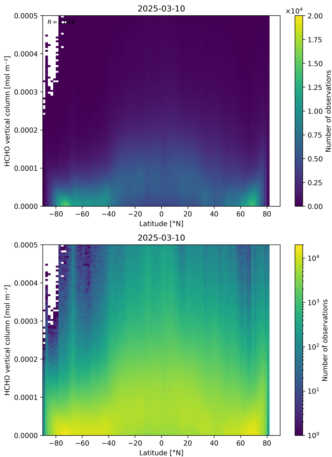
Figure 163: Scatter density plot of “Latitude” against “HCHO vertical column” for 2025-03-09 to 2025-03-11.
