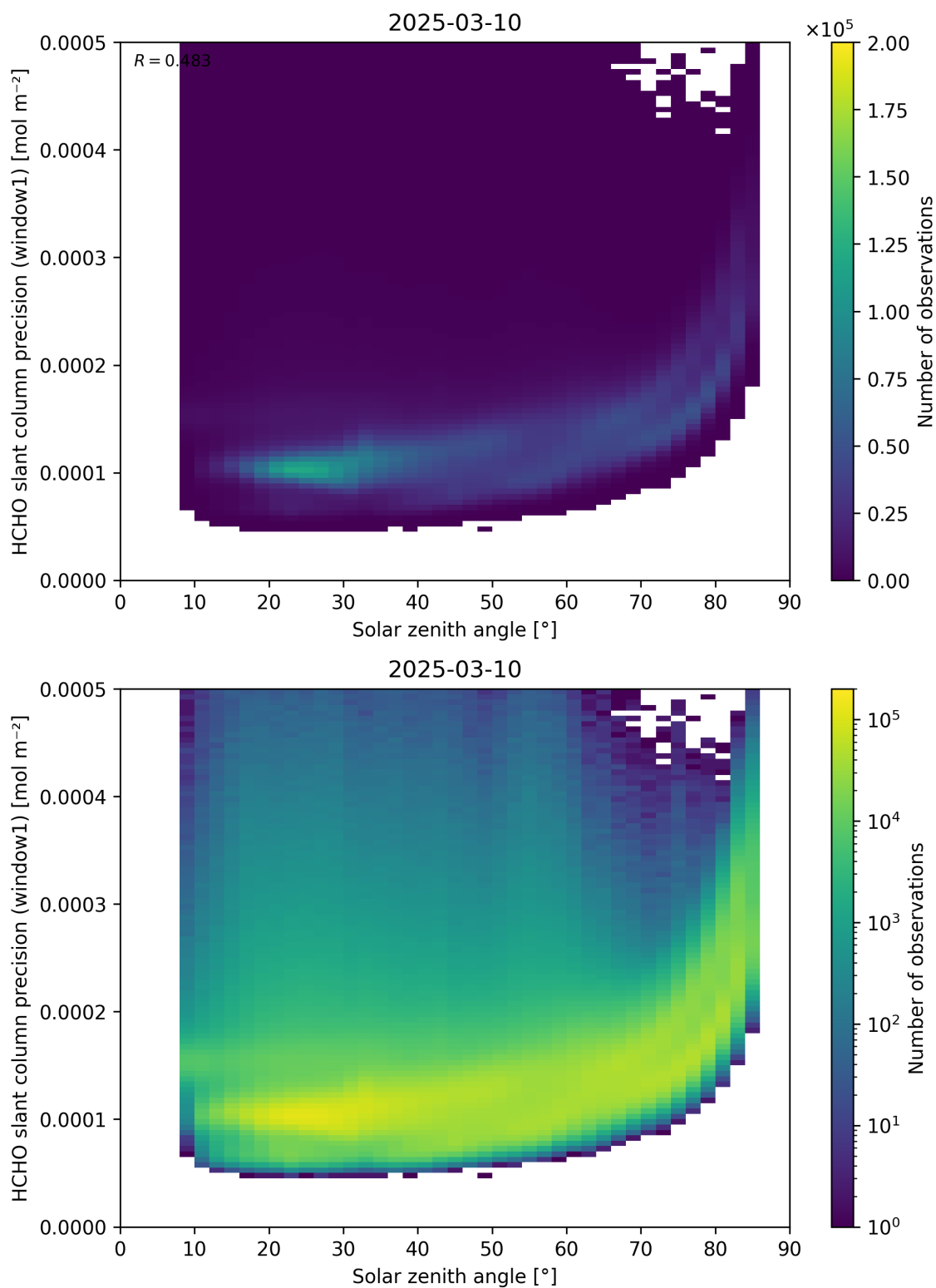
Figure 174: Scatter density plot of “Solar zenith angle” against “HCHO slant column precision (window1)” for 2025-03-09 to 2025-03-11.
