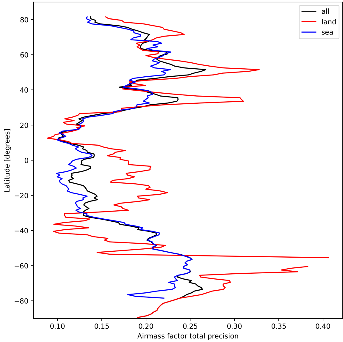
Figure 27: Zonal average of “Airmass factor total precision” for 2025-03-09 to 2025-03-11.
