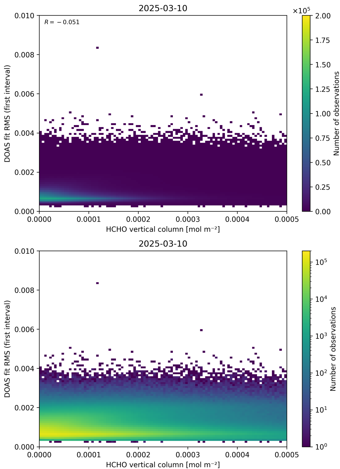
Figure 123: Scatter density plot of “HCHO vertical column” against “DOAS fit RMS (first interval)” for 2025-03-09 to 2025-03-11.
