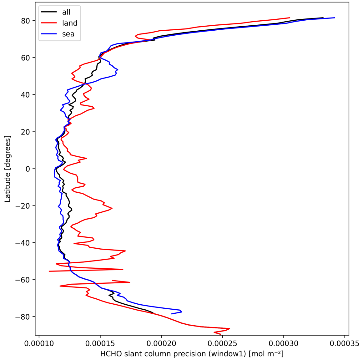
Figure 25: Zonal average of “HCHO slant column precision (window1)” for 2025-03-09 to 2025-03-11.
