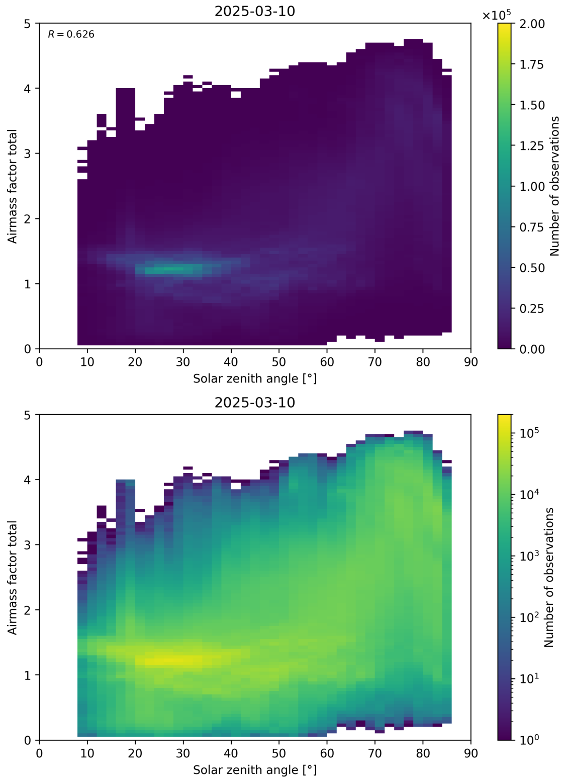
Figure 175: Scatter density plot of “Solar zenith angle” against “Airmass factor total” for 2025-03-09 to 2025-03-11.
