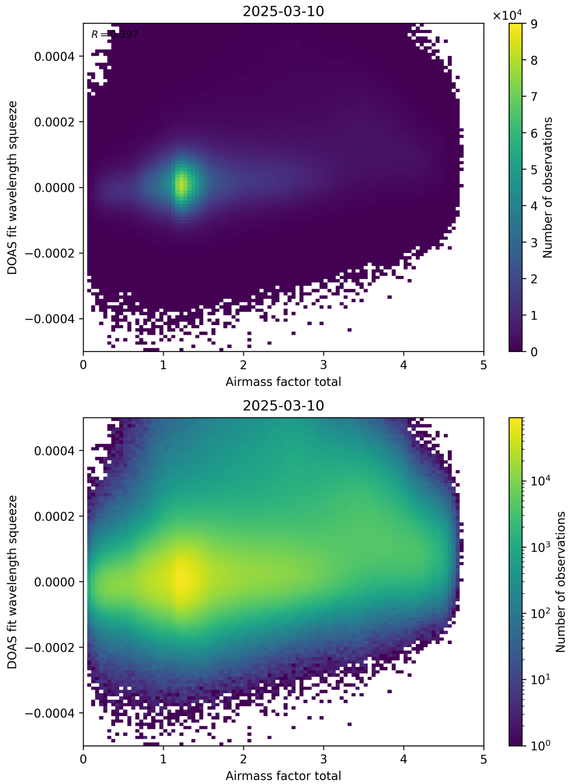
Figure 99: Scatter density plot of “Airmass factor total” against “DOAS fit wavelength squeeze” for 2025-03-09 to 2025-03-11.
