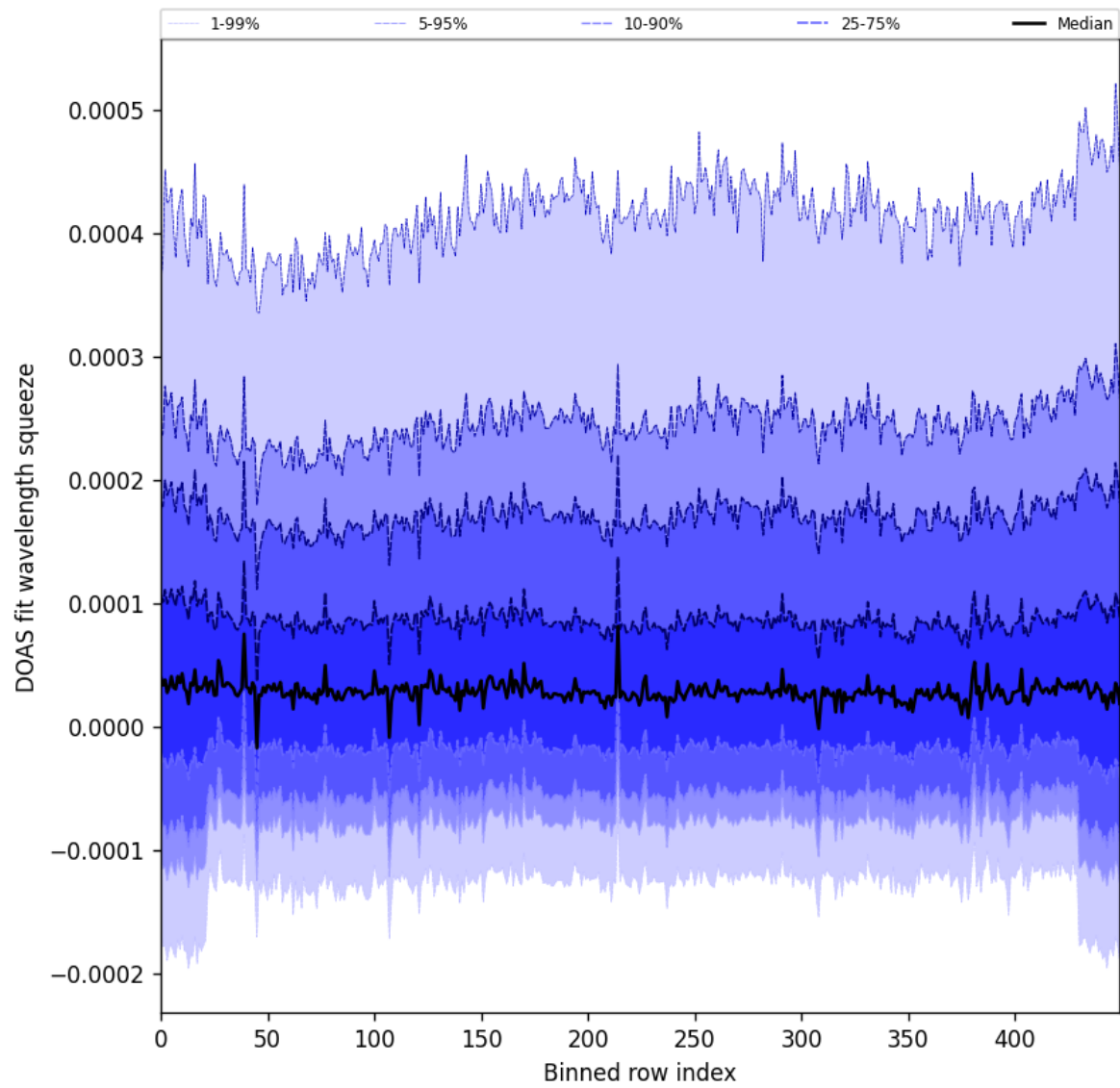
Figure 59: Along track statistics of “DOAS fit wavelength squeeze” for 2025-03-09 to 2025-03-11
