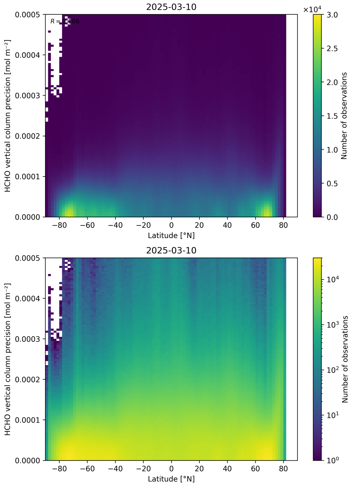
Figure 165: Scatter density plot of “Latitude” against “HCHO vertical column precision” for 2025-03-09 to 2025-03-11.
