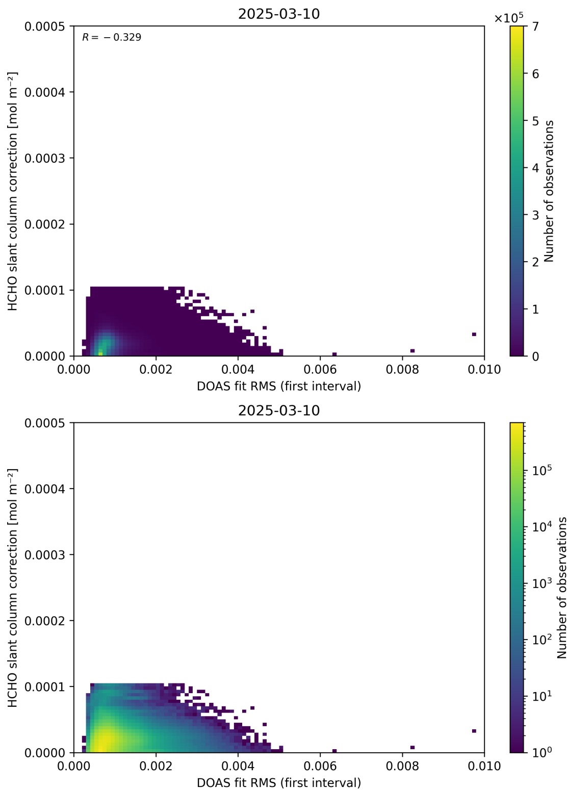
Figure 63: Scatter density plot of “DOAS fit RMS (first interval)” against “HCHO slant column correction” for 2025-03-09 to 2025-03-11.
