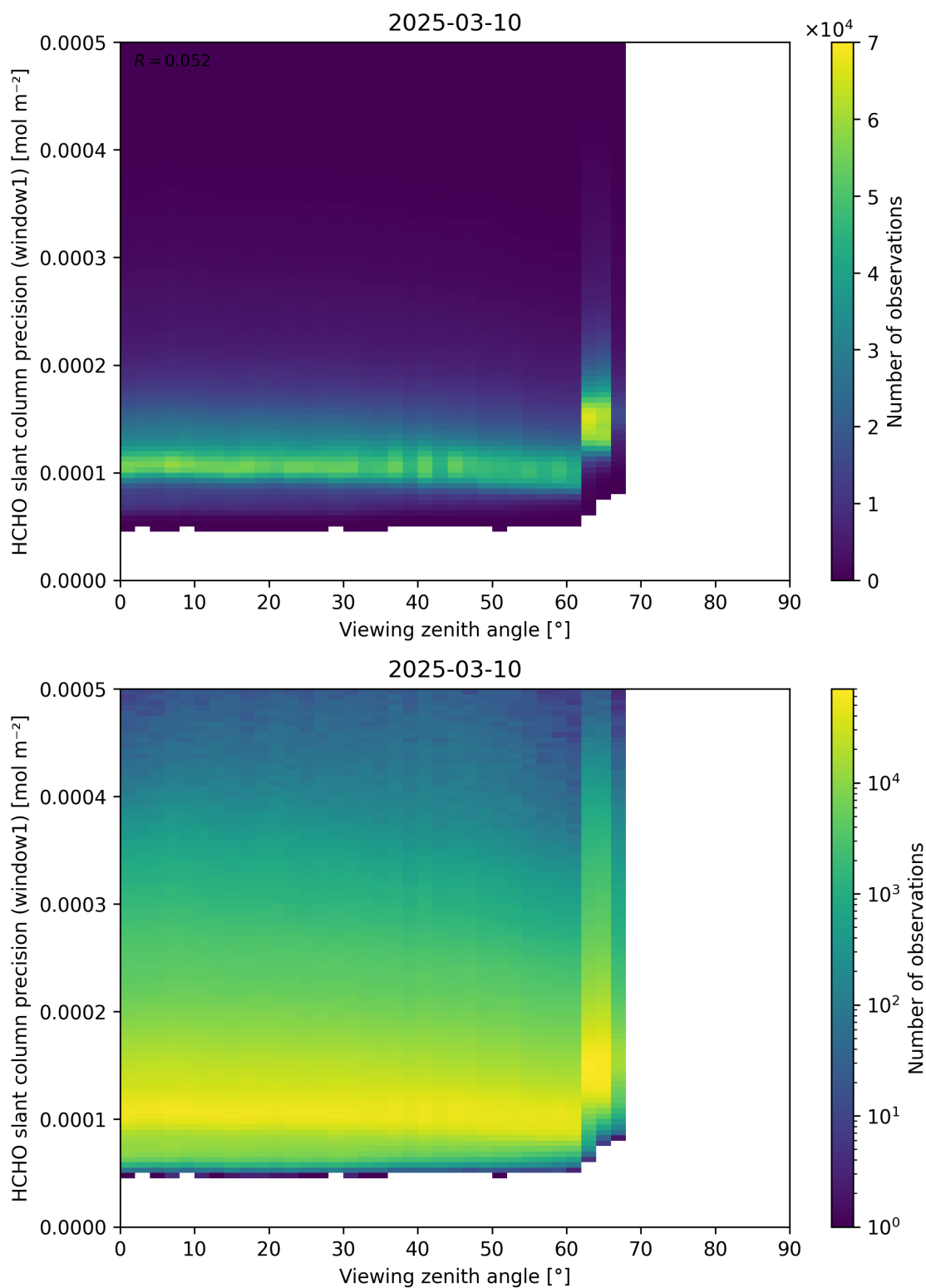
Figure 189: Scatter density plot of “Viewing zenith angle” against “HCHO slant column precision (window1)” for 2025-03-09 to 2025-03-11.
