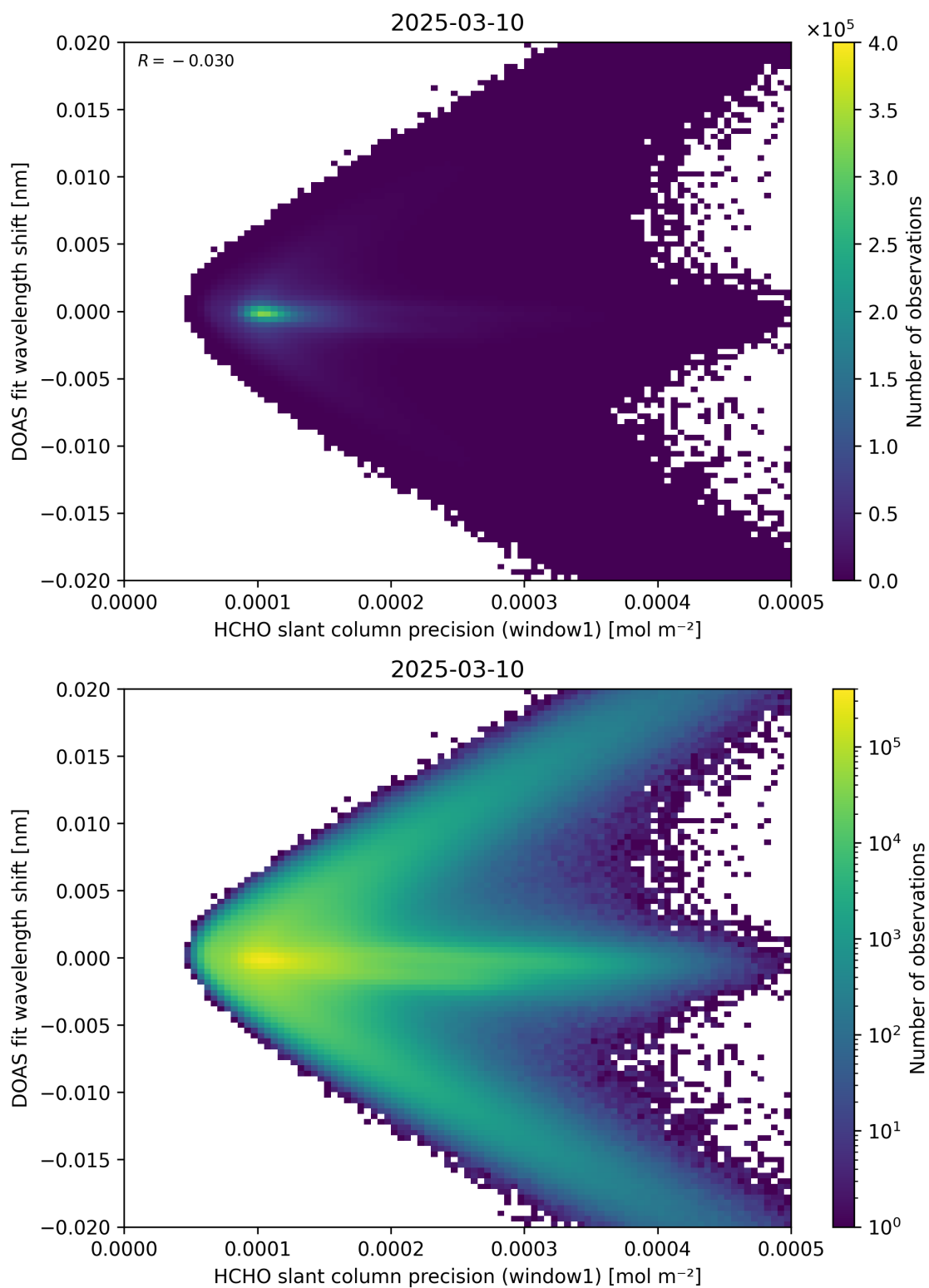
Figure 89: Scatter density plot of “HCHO slant column precision (window1)” against “DOAS fit wavelength shift” for 2025-03-09 to 2025-03-11.
