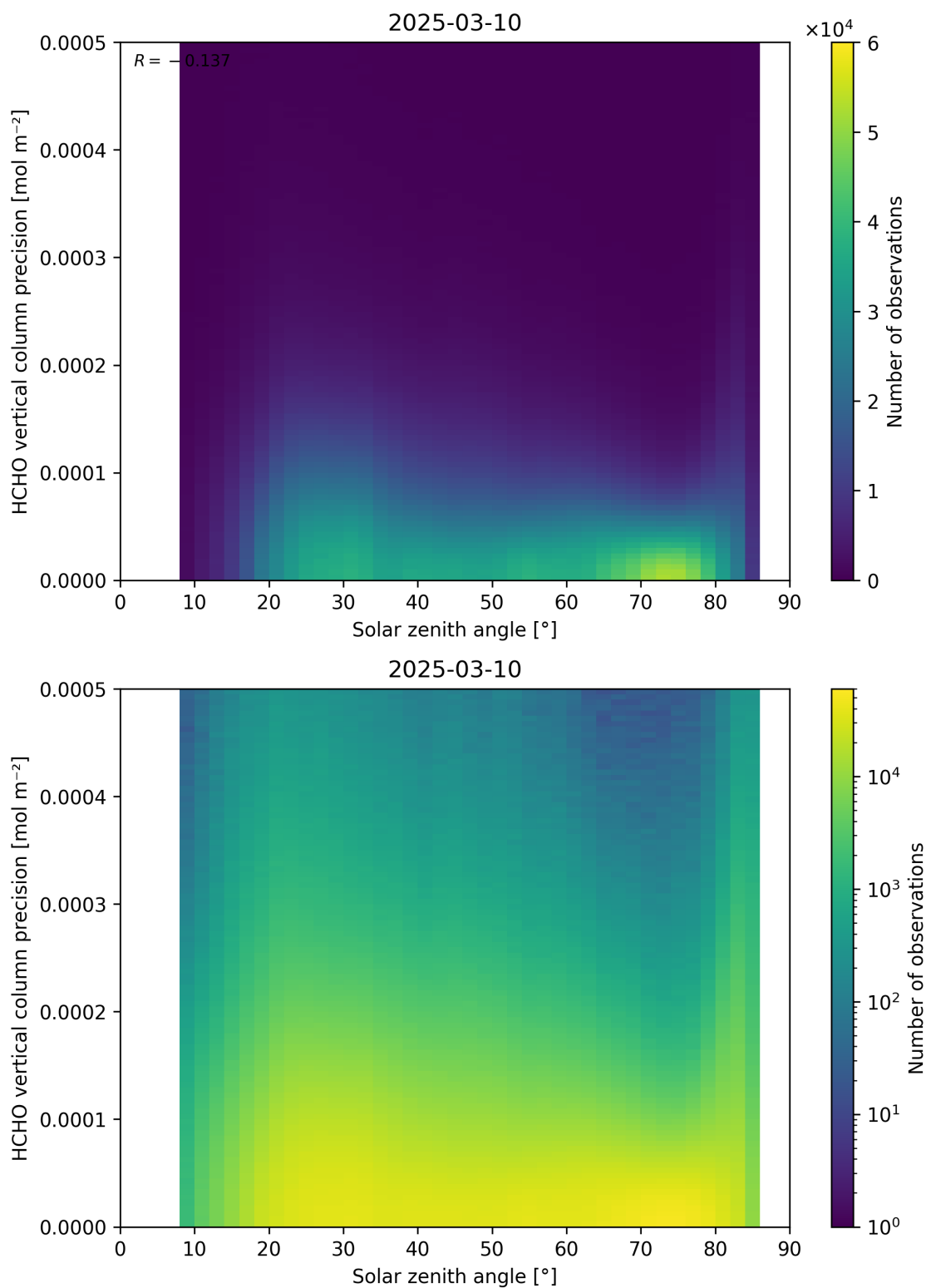
Figure 179: Scatter density plot of “Solar zenith angle” against “HCHO vertical column precision” for 2025-03-09 to 2025-03-11.
