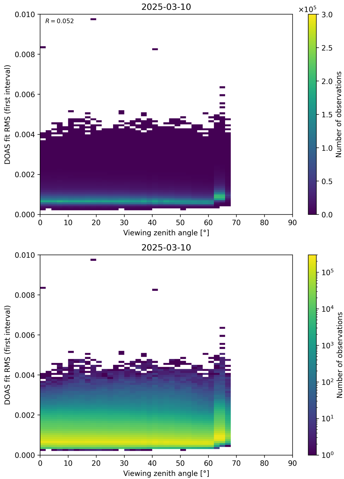
Figure 182: Scatter density plot of “Viewing zenith angle” against “DOAS fit RMS (first interval)” for 2025-03-09 to 2025-03-11.
