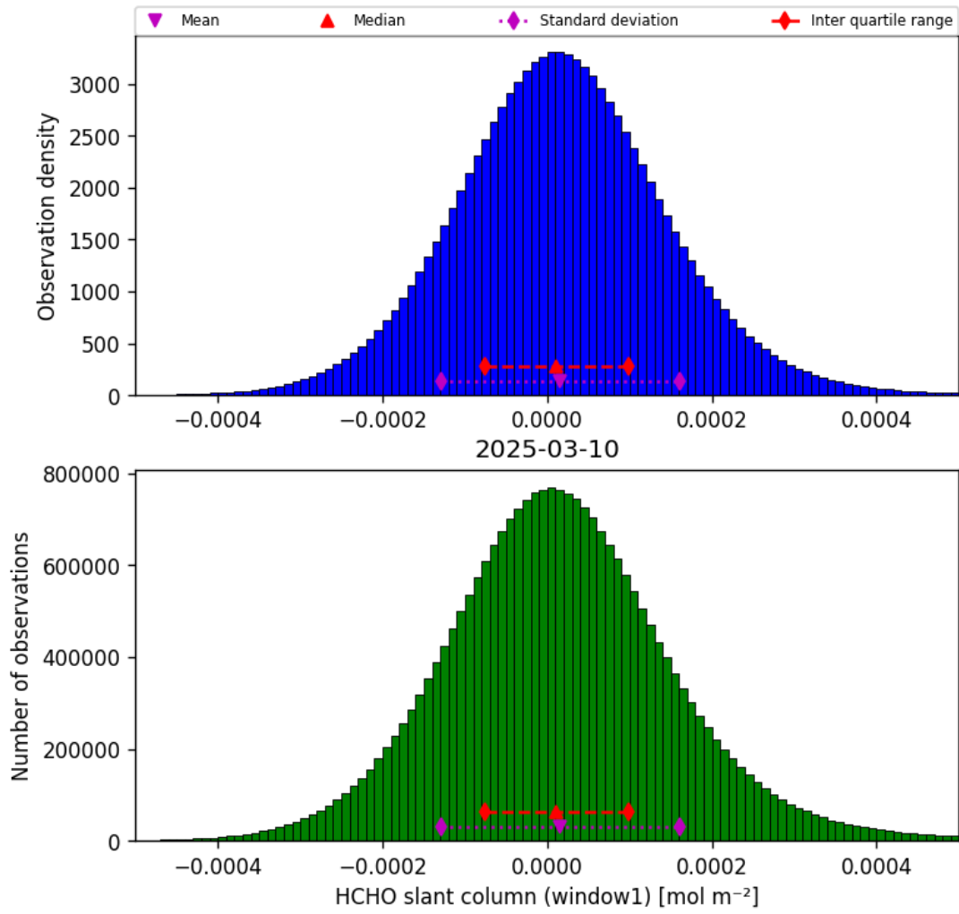
Figure 38: Histogram of “HCHO slant column (window1)” for 2025-03-09 to 2025-03-11
