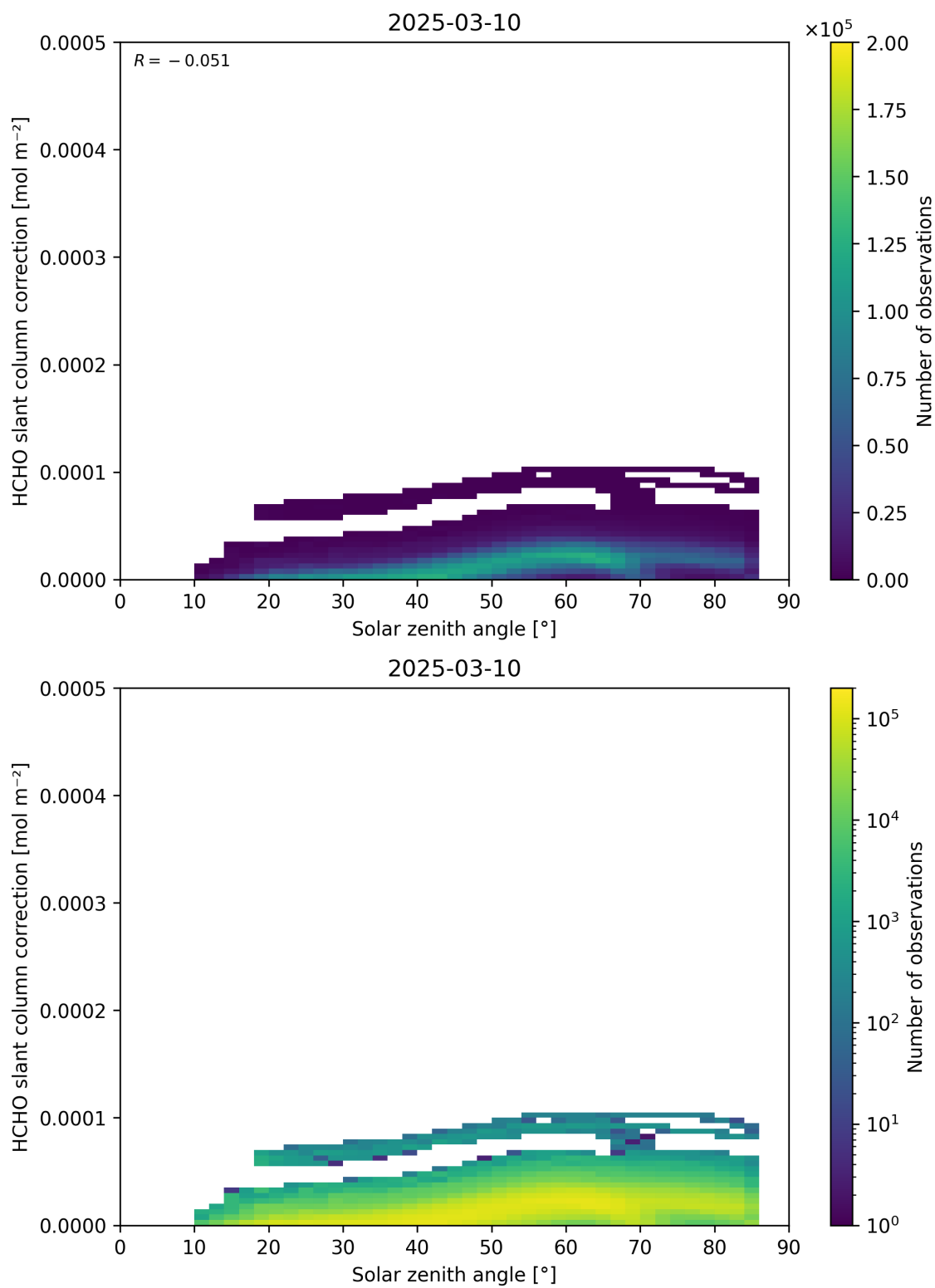
Figure 172: Scatter density plot of “Solar zenith angle” against “HCHO slant column correction” for 2025-03-09 to 2025-03-11.
