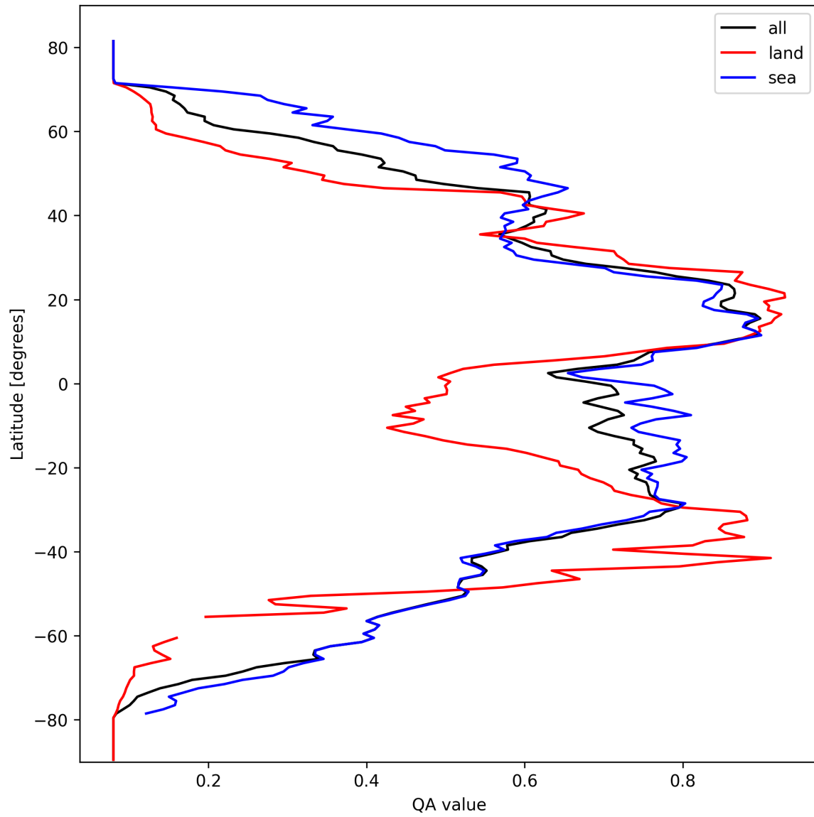
Figure 20: Zonal average of “QA value” for 2025-03-09 to 2025-03-11.
