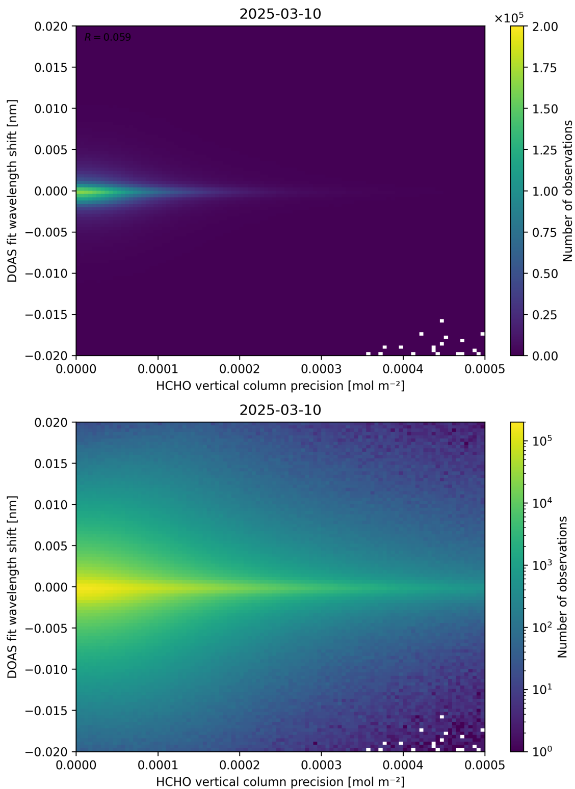
Figure 137: Scatter density plot of “HCHO vertical column precision” against “DOAS fit wavelength shift” for 2025-03-09 to 2025-03-11.
