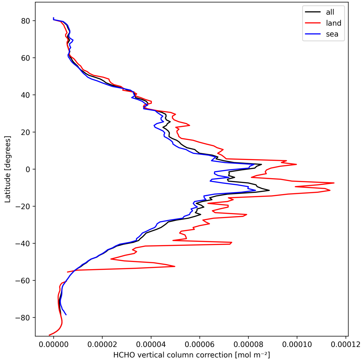
Figure 23: Zonal average of “HCHO vertical column correction” for 2025-03-09 to 2025-03-11.
