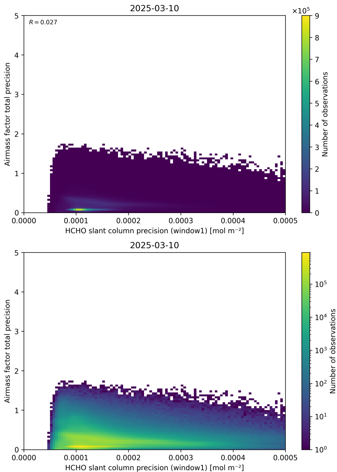
Figure 95: Scatter density plot of “HCHO slant column precision (window1)” against “Airmass factor total precision” for 2025-03-09 to 2025-03-11.
