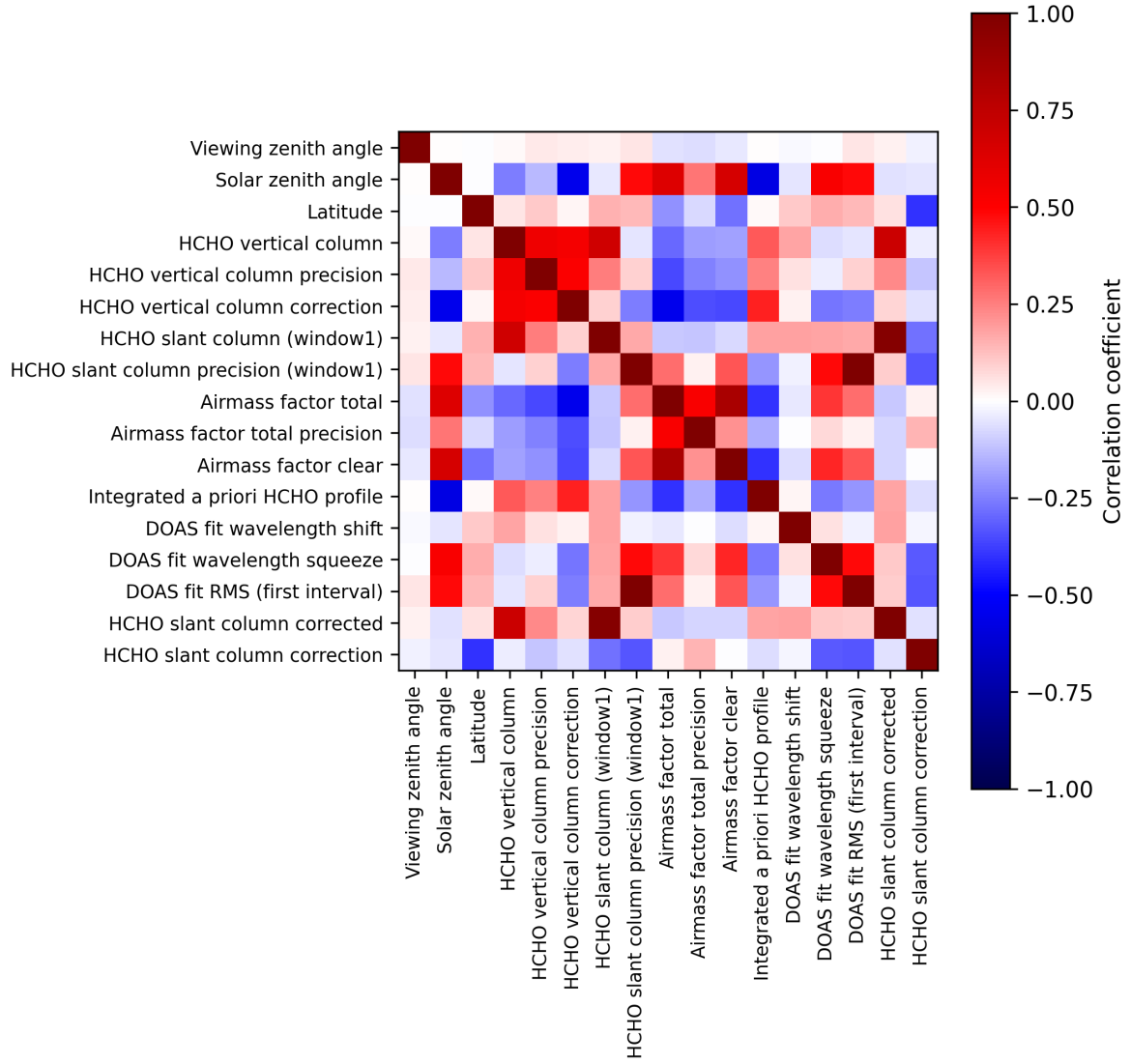
Figure 2: Map of correlation matrix for 2025-03-09 to 2025-03-11.
