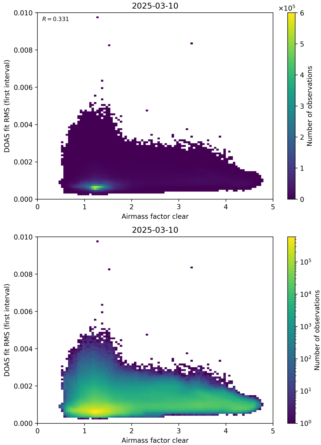
Figure 71: Scatter density plot of “Airmass factor clear” against “DOAS fit RMS (first interval)” for 2025-03-09 to 2025-03-11.
