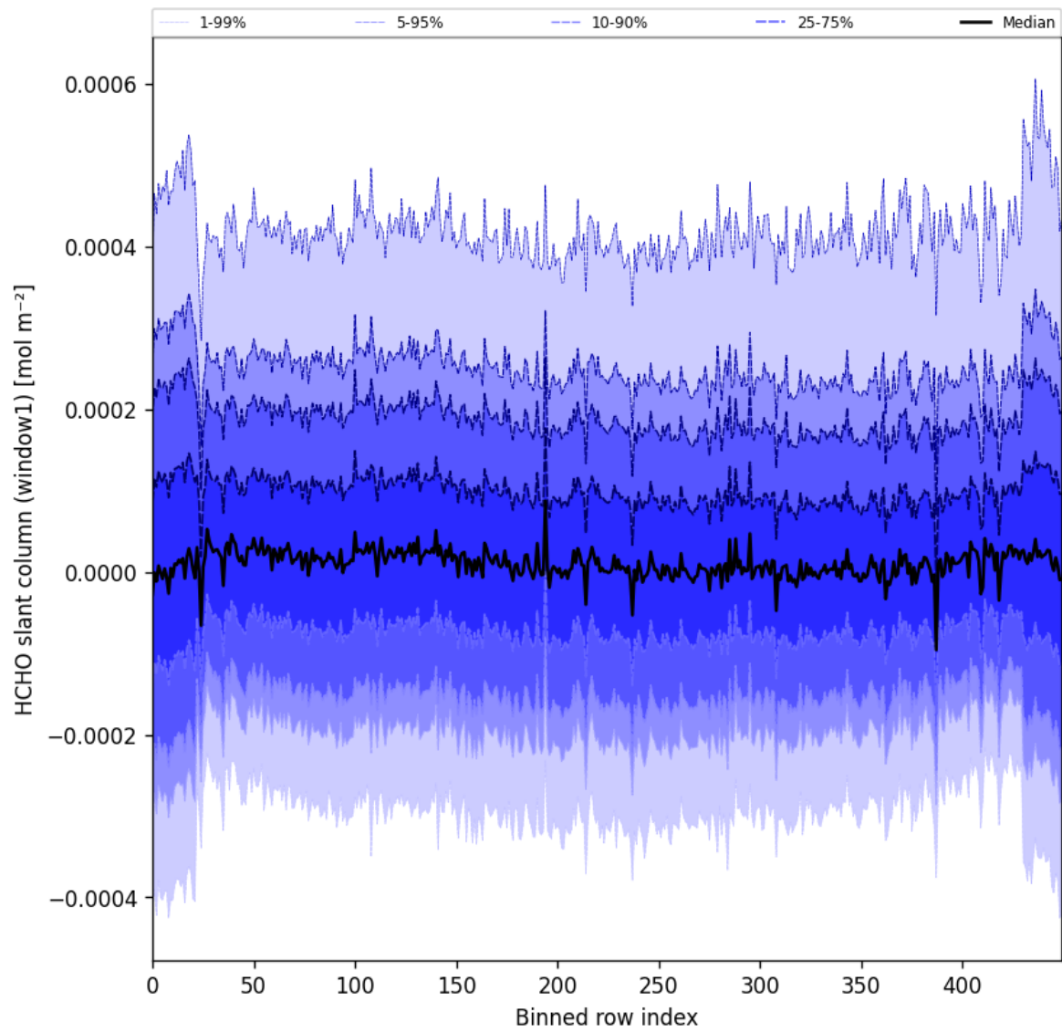
Figure 52: Along track statistics of “HCHO slant column (window1)” for 2025-03-09 to 2025-03-11
