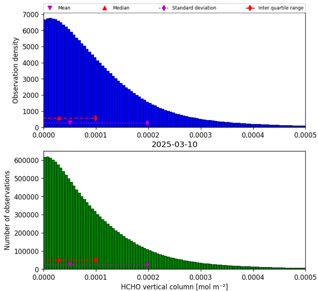
Figure 35: Histogram of “HCHO vertical column” for 2025-03-09 to 2025-03-11
