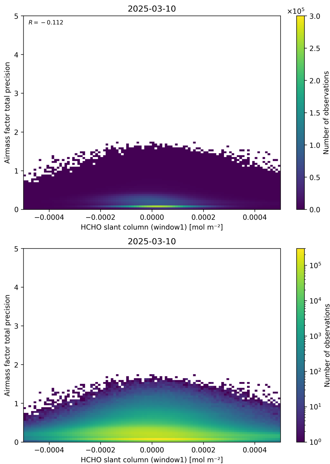
Figure 86: Scatter density plot of “HCHO slant column (window1)” against “Airmass factor total precision” for 2025-03-09 to 2025-03-11.
