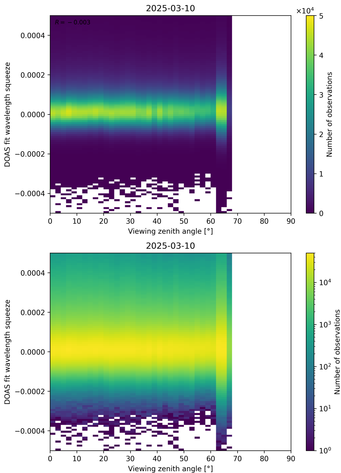
Figure 184: Scatter density plot of “Viewing zenith angle” against “DOAS fit wavelength squeeze” for 2025-03-09 to 2025-03-11.
