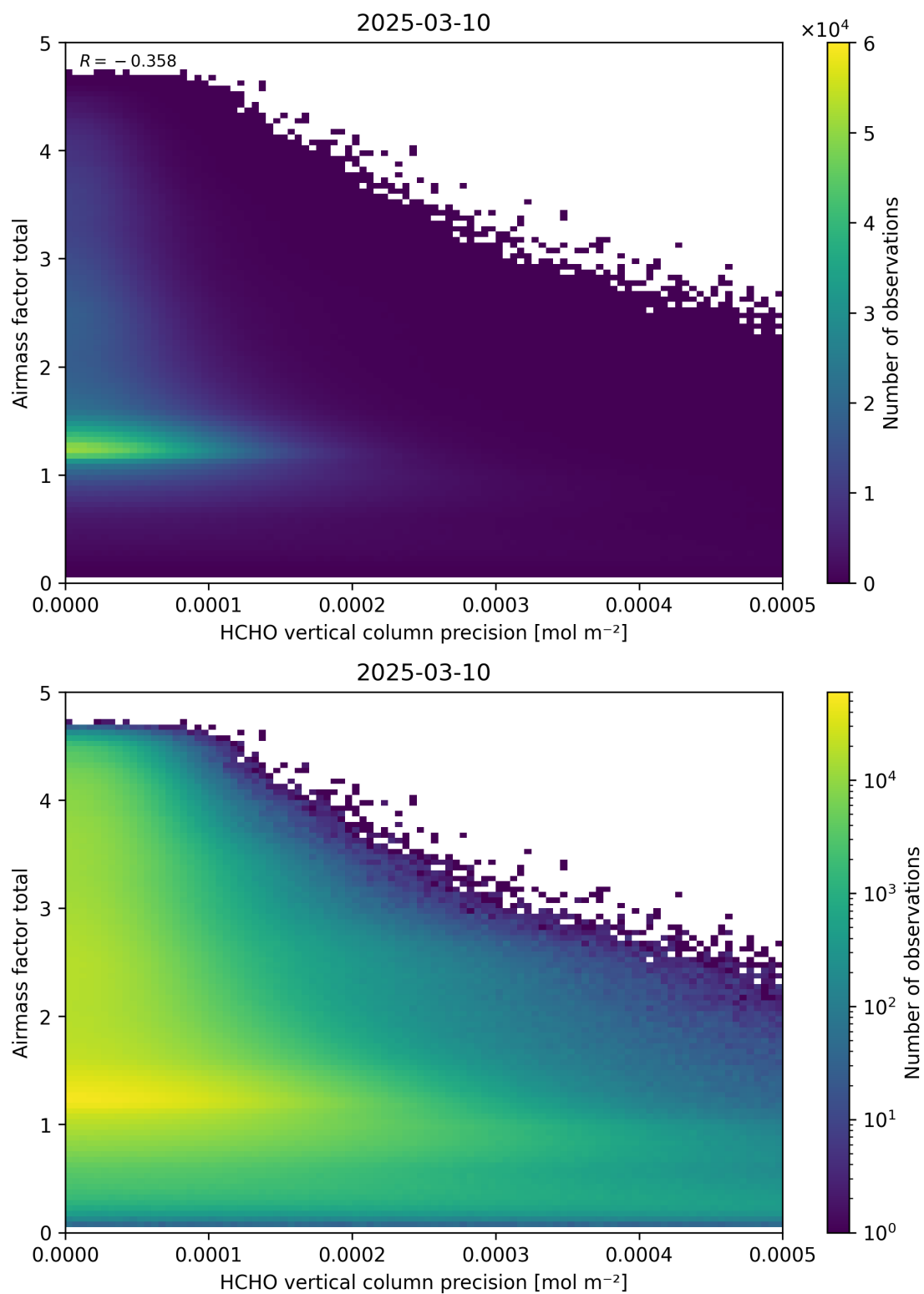
Figure 144: Scatter density plot of “HCHO vertical column precision” against “Airmass factor total” for 2025-03-09 to 2025-03-11.
