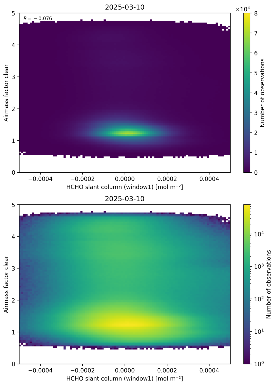
Figure 81: Scatter density plot of “HCHO slant column (window1)” against “Airmass factor clear” for 2025-03-09 to 2025-03-11.
