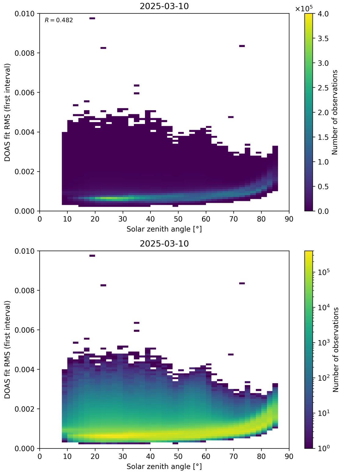
Figure 167: Scatter density plot of “Solar zenith angle” against “DOAS fit RMS (first interval)” for 2025-03-09 to 2025-03-11.
