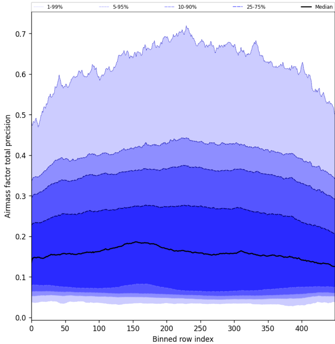
Figure 55: Along track statistics of “Airmass factor total precision” for 2025-03-09 to 2025-03-11
