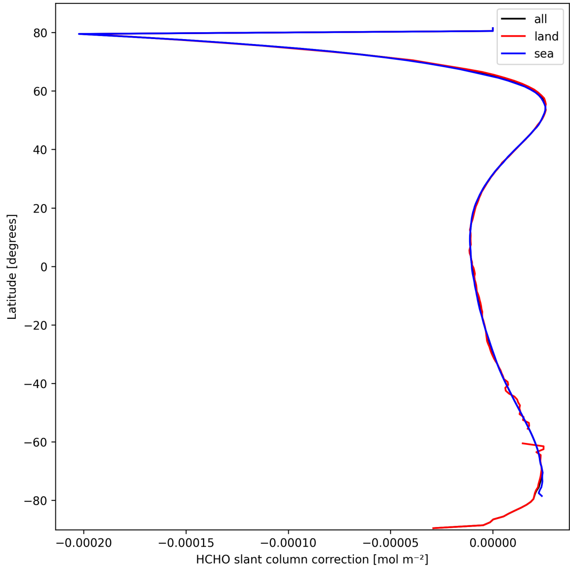
Figure 33: Zonal average of “HCHO slant column correction” for 2025-03-09 to 2025-03-11.
