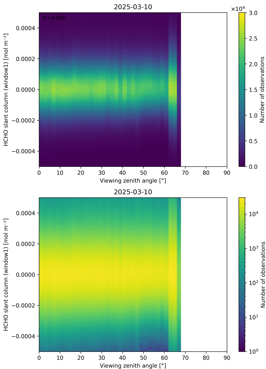
Figure 188: Scatter density plot of “Viewing zenith angle” against “HCHO slant column (window1)” for 2025-03-09 to 2025-03-11.
