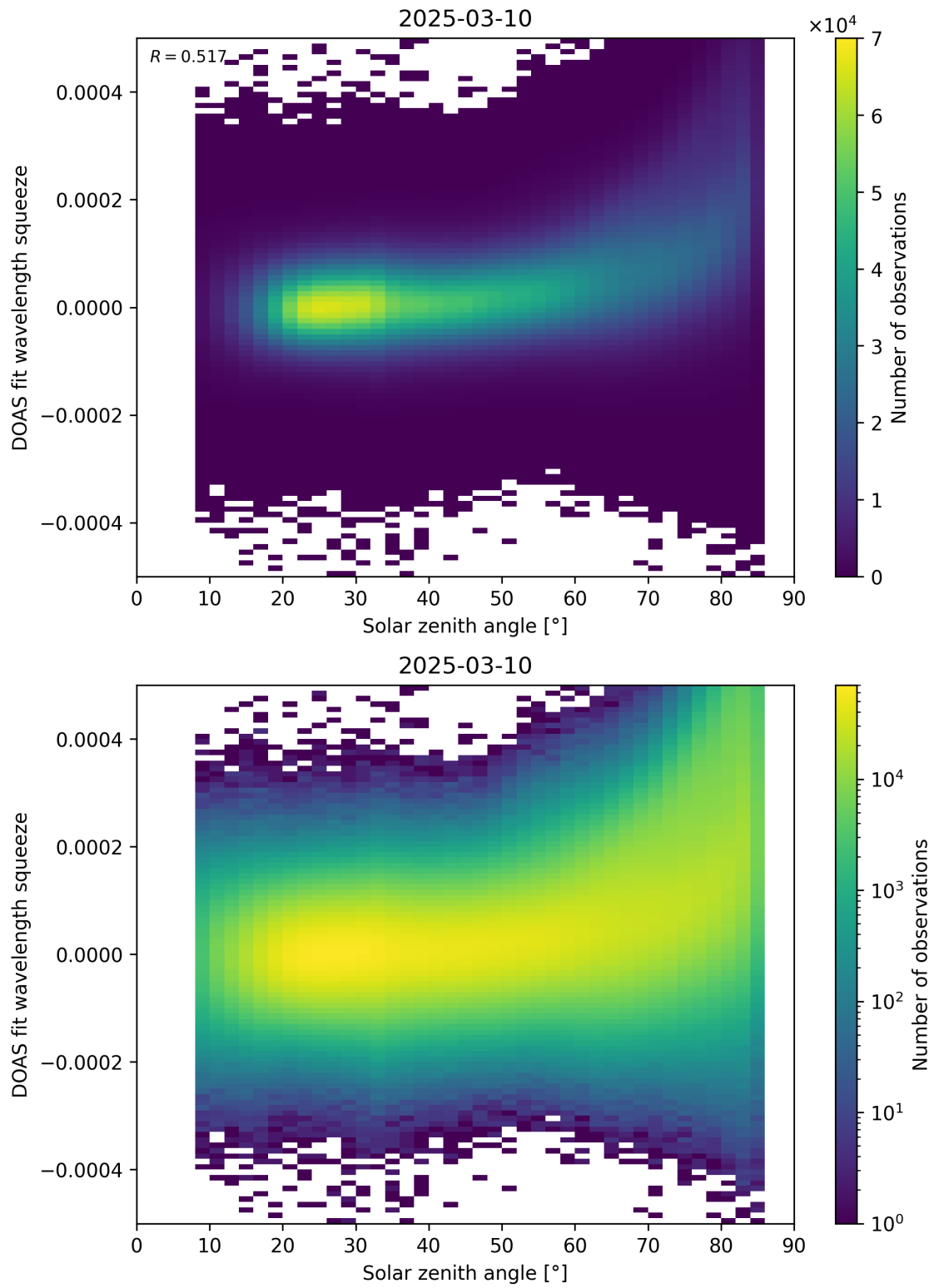
Figure 169: Scatter density plot of “Solar zenith angle” against “DOAS fit wavelength squeeze” for 2025-03-09 to 2025-03-11.
