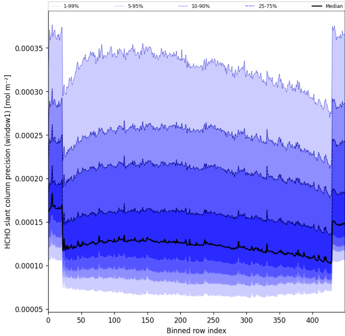
Figure 53: Along track statistics of “HCHO slant column precision (window1)” for 2025-03-09 to 2025-03-11
