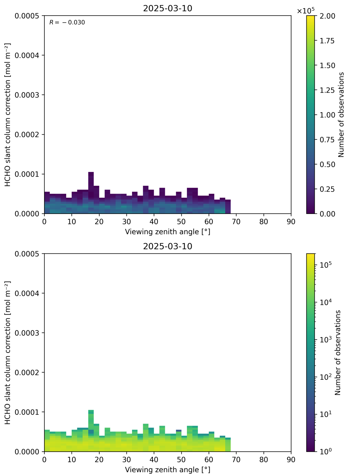
Figure 187: Scatter density plot of “Viewing zenith angle” against “HCHO slant column correction” for 2025-03-09 to 2025-03-11.
