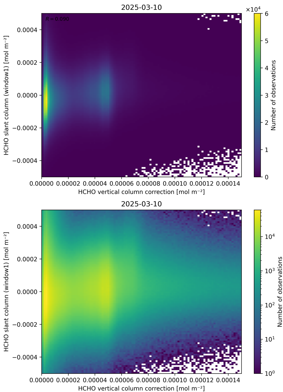
Figure 118: Scatter density plot of “HCHO vertical column correction” against “HCHO slant column (window1)” for 2025-03-09 to 2025-03-11.
