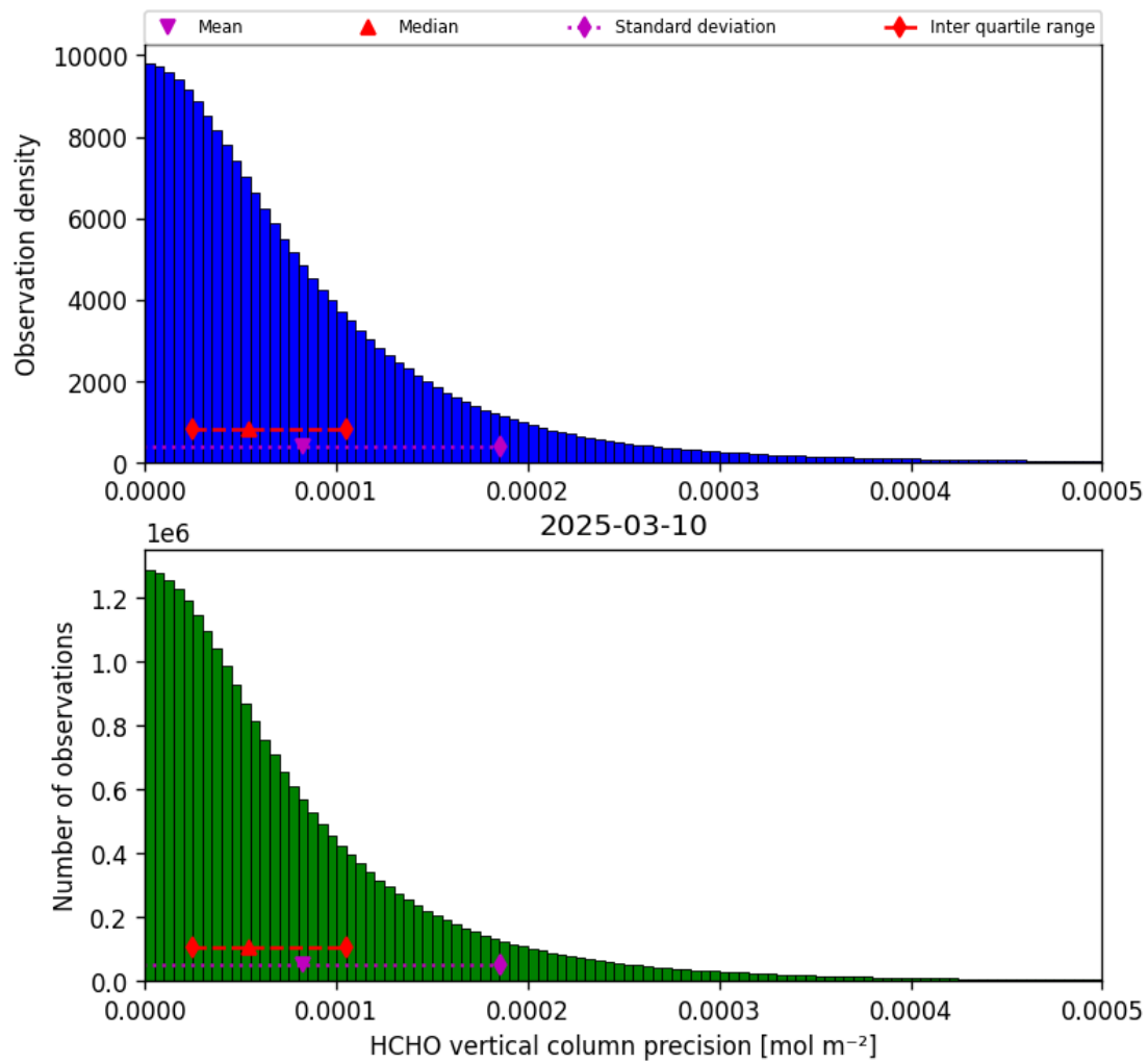
Figure 36: Histogram of “HCHO vertical column precision” for 2025-03-09 to 2025-03-11
