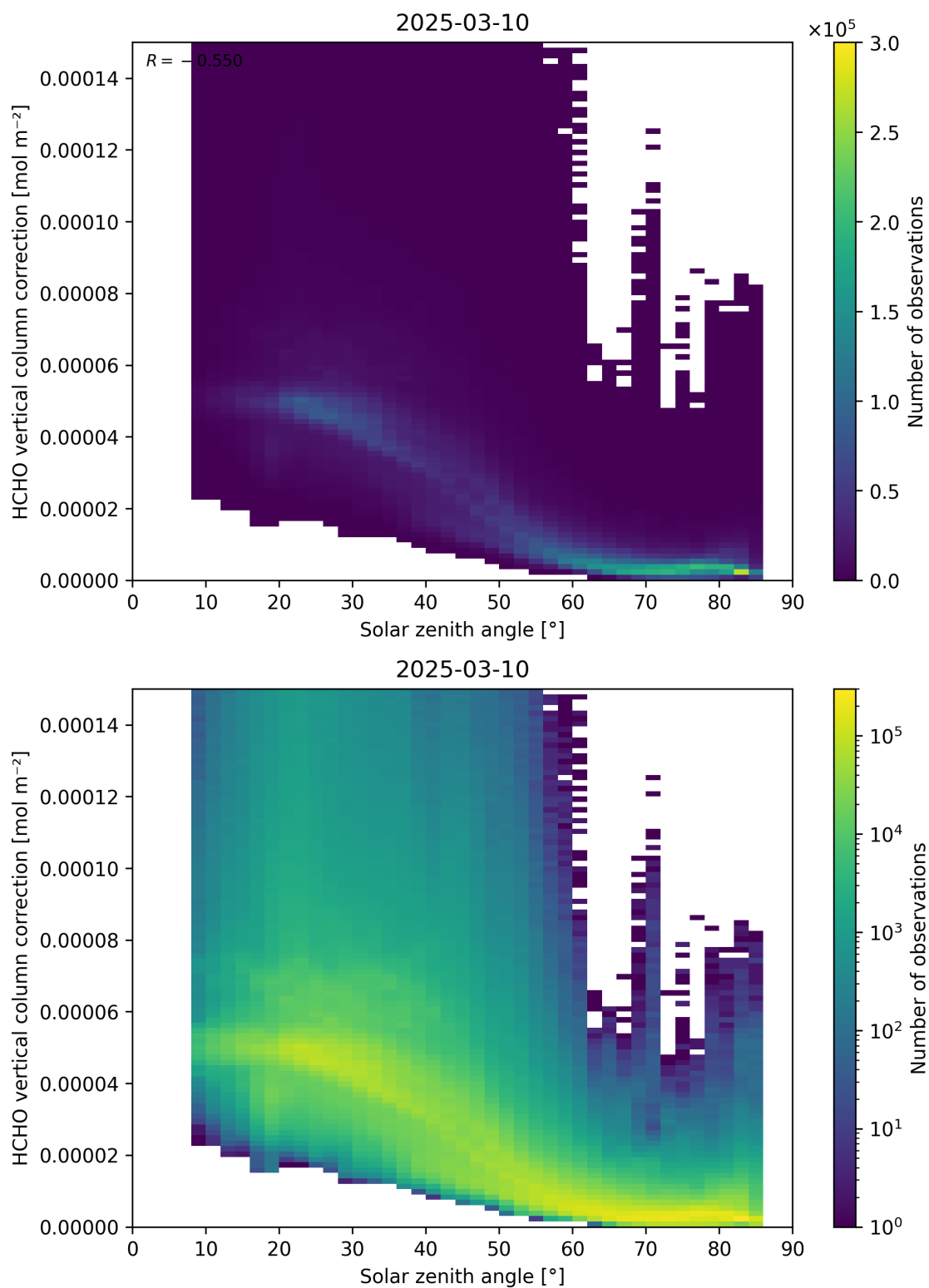
Figure 178: Scatter density plot of “Solar zenith angle” against “HCHO vertical column correction” for 2025-03-09 to 2025-03-11.
