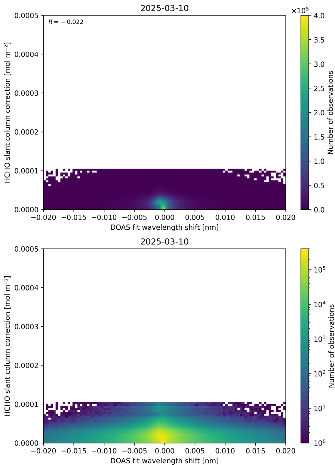
Figure 67: Scatter density plot of “DOAS fit wavelength shift” against “HCHO slant column correction” for 2025-03-09 to 2025-03-11.
