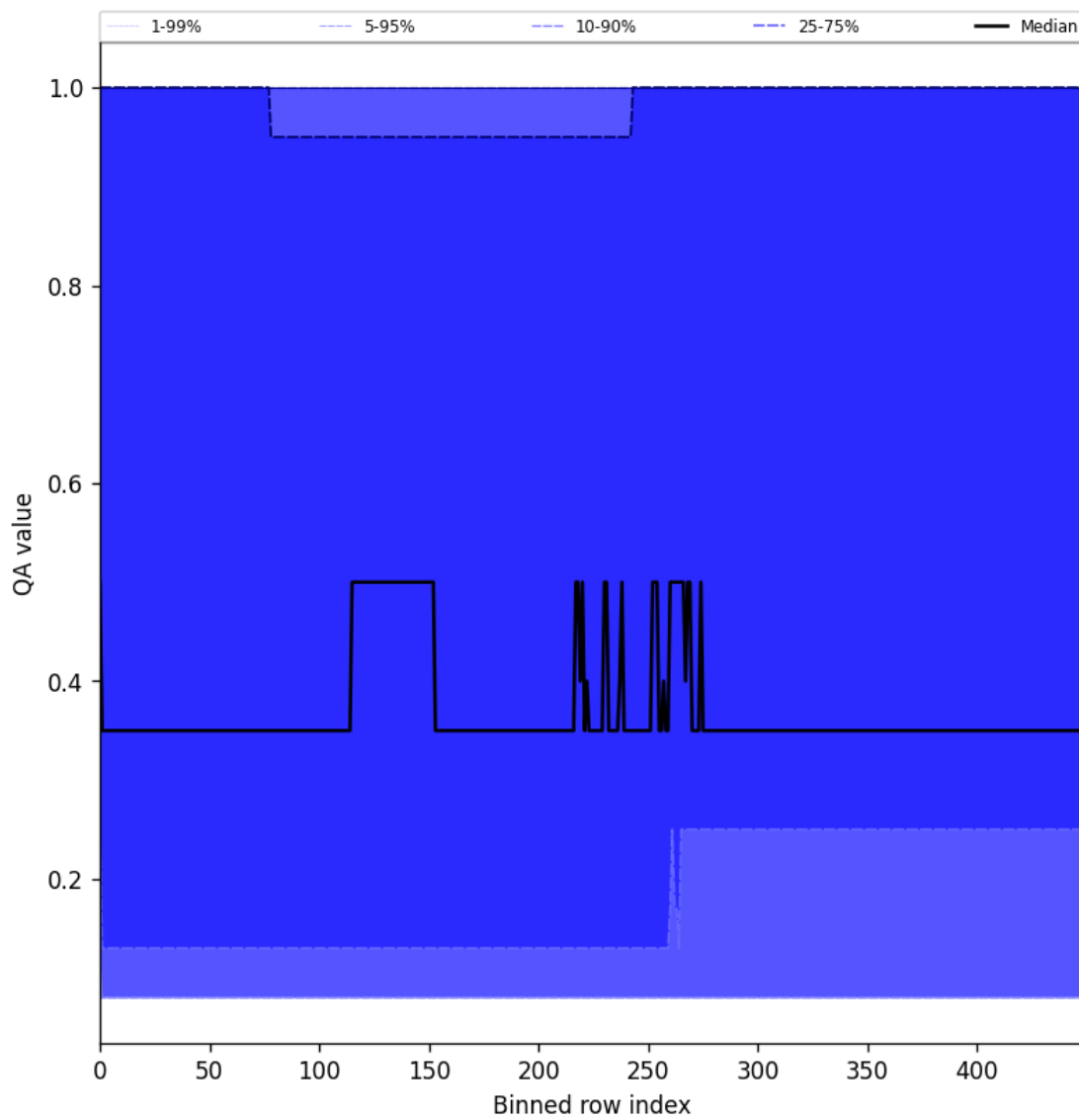
Figure 48: Along track statistics of “QA value” for 2025-03-09 to 2025-03-11
