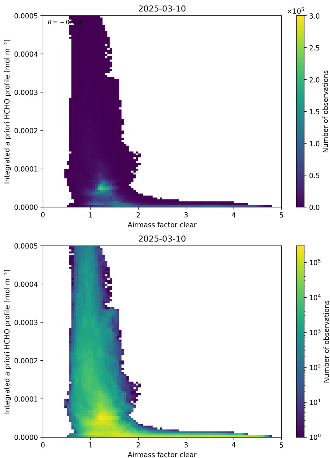
Figure 76: Scatter density plot of “Airmass factor clear” against “Integrated a priori HCHO profile” for 2025-03-09 to 2025-03-11.
