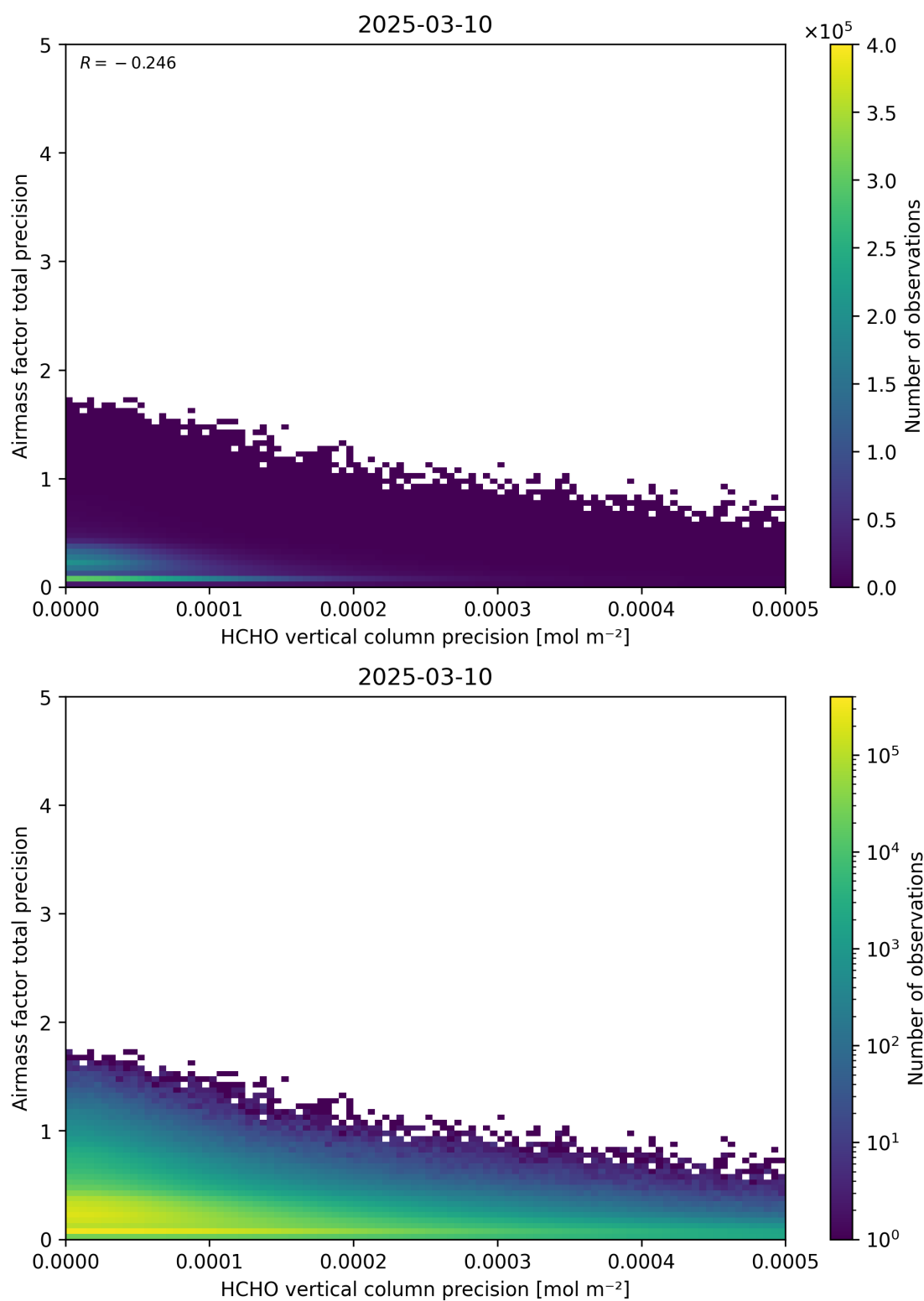
Figure 145: Scatter density plot of “HCHO vertical column precision” against “Airmass factor total precision” for 2025-03-09 to 2025-03-11.
