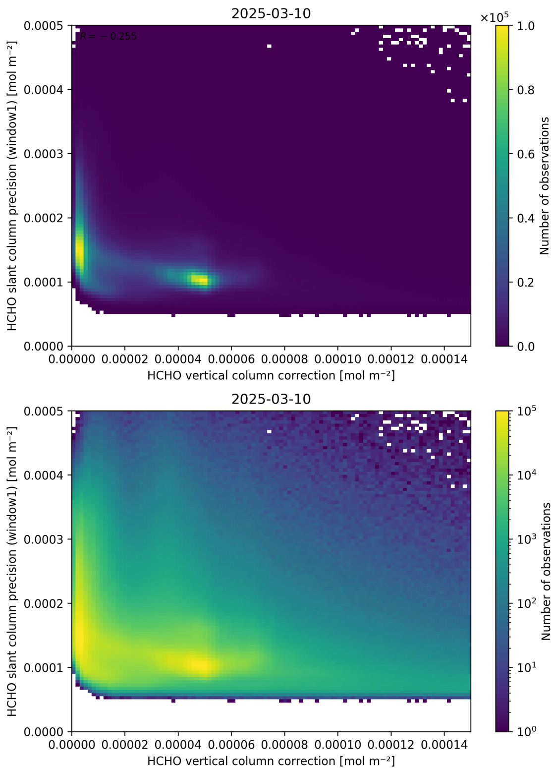
Figure 119: Scatter density plot of “HCHO vertical column correction” against “HCHO slant column precision (window1)” for 2025-03-09 to 2025-03-11.
