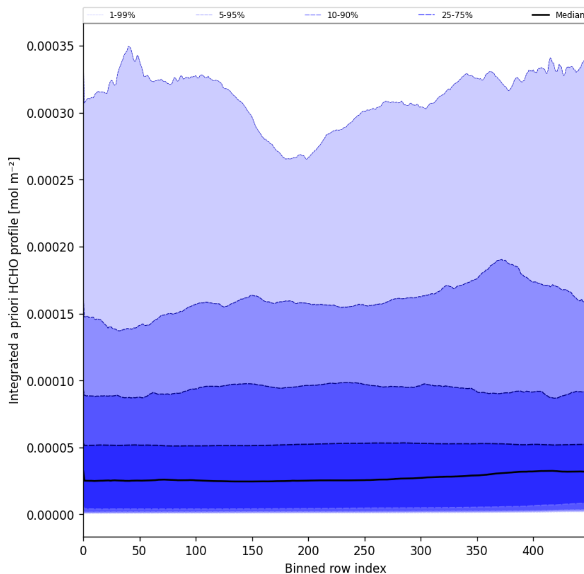
Figure 57: Along track statistics of "Integrated a priori HCHO profile" for 2025-03-09 to 2025-03-11
