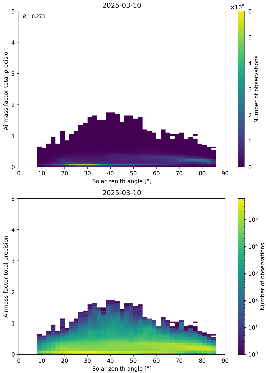
Figure 176: Scatter density plot of “Solar zenith angle” against “Airmass factor total precision” for 2025-03-09 to 2025-03-11.
