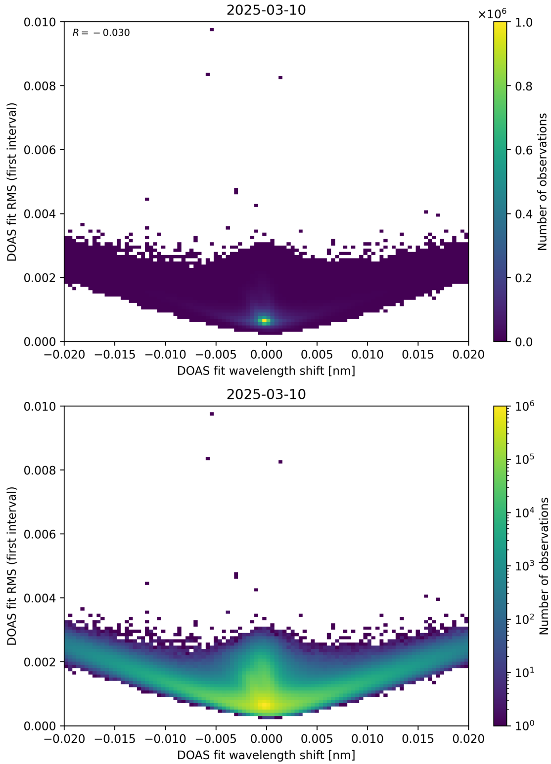
Figure 64: Scatter density plot of “DOAS fit wavelength shift” against “DOAS fit RMS (first interval)” for 2025-03-09 to 2025-03-11.
