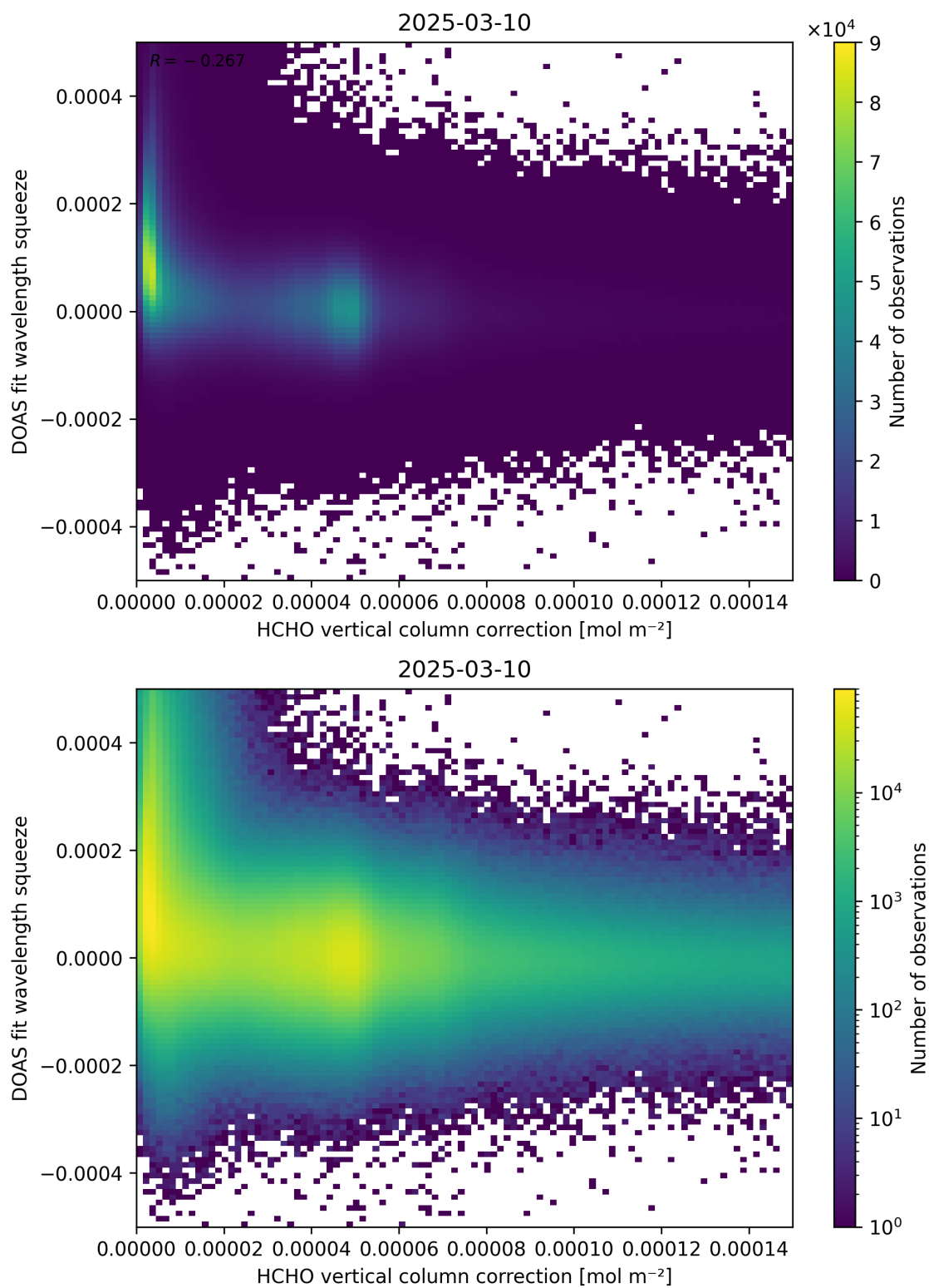
Figure 114: Scatter density plot of “HCHO vertical column correction” against “DOAS fit wavelength squeeze” for 2025-03-09 to 2025-03-11.
