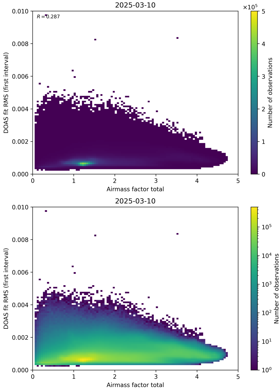
Figure 97: Scatter density plot of “Airmass factor total” against “DOAS fit RMS (first interval)” for 2025-03-09 to 2025-03-11.
