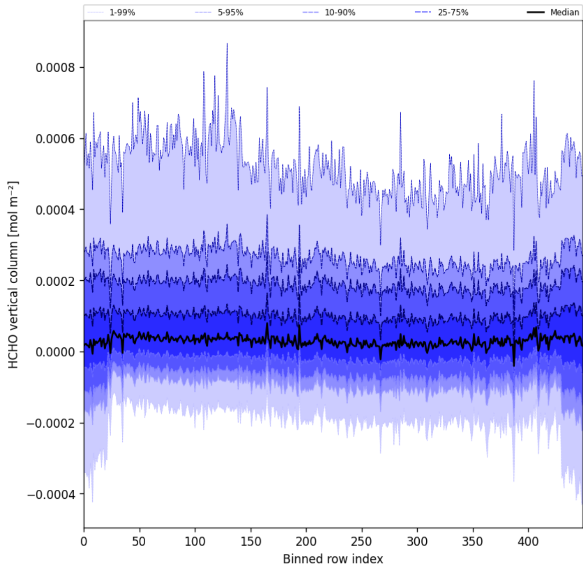
Figure 49: Along track statistics of “HCHO vertical column” for 2025-03-09 to 2025-03-11
