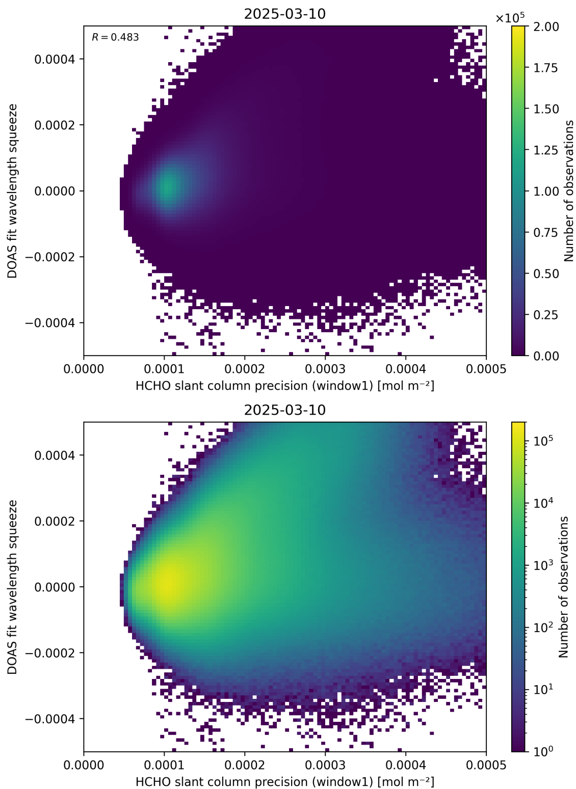
Figure 90: Scatter density plot of “HCHO slant column precision (window1)” against “DOAS fit wavelength squeeze” for 2025-03-09 to 2025-03-11.
