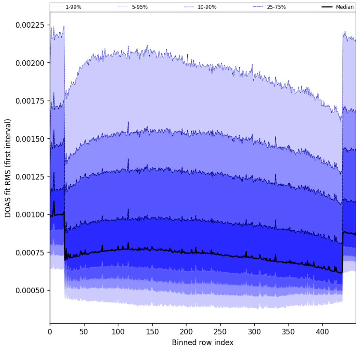
Figure 60: Along track statistics of “DOAS fit RMS (first interval)” for 2025-03-09 to 2025-03-11
