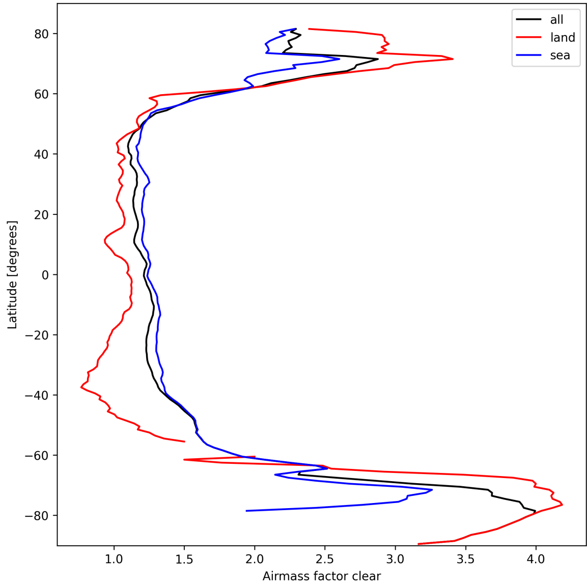
Figure 28: Zonal average of “Airmass factor clear” for 2025-03-09 to 2025-03-11.
