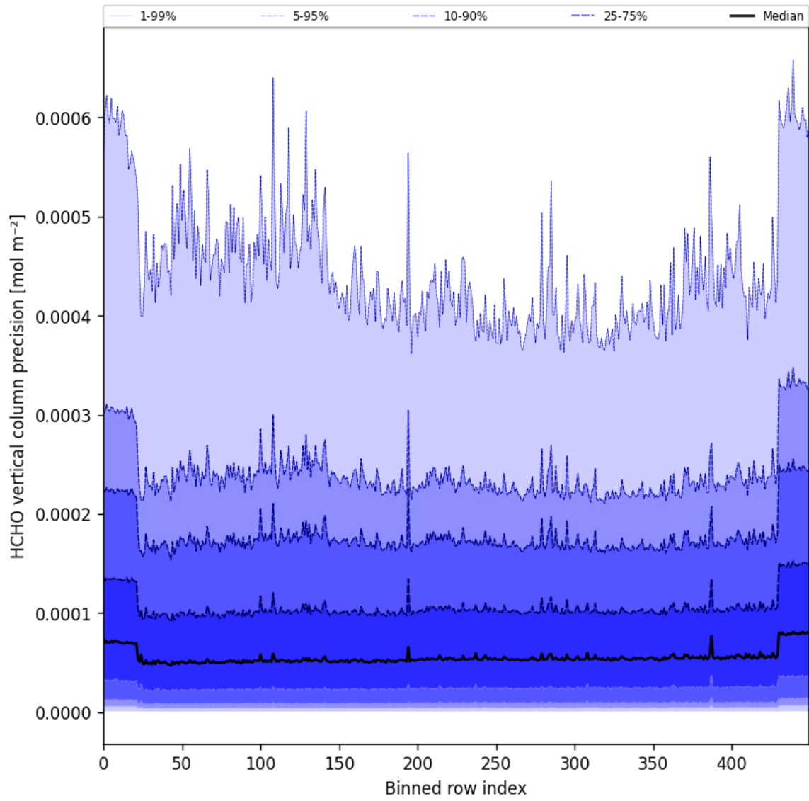
Figure 50: Along track statistics of “HCHO vertical column precision” for 2025-03-09 to 2025-03-11
