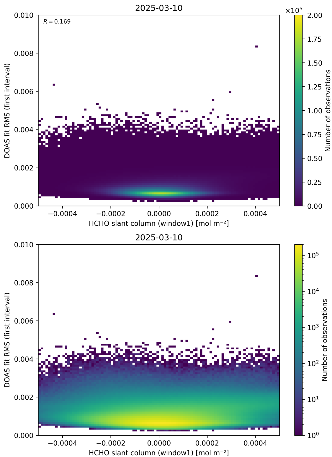
Figure 78: Scatter density plot of “HCHO slant column (window1)” against “DOAS fit RMS (first interval)” for 2025-03-09 to 2025-03-11.
