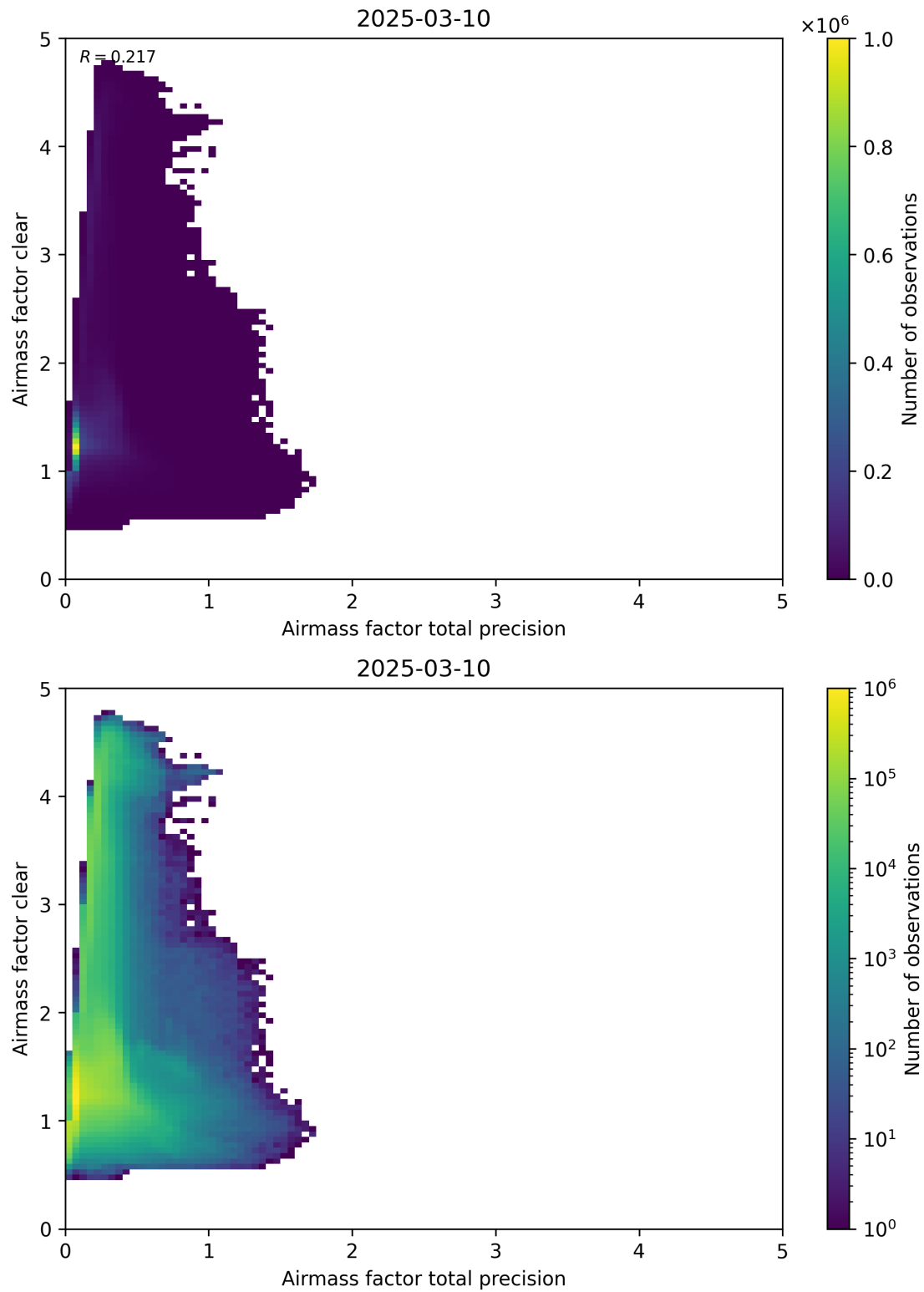
Figure 108: Scatter density plot of “Airmass factor total precision” against “Airmass factor clear” for 2025-03-09 to 2025-03-11.
