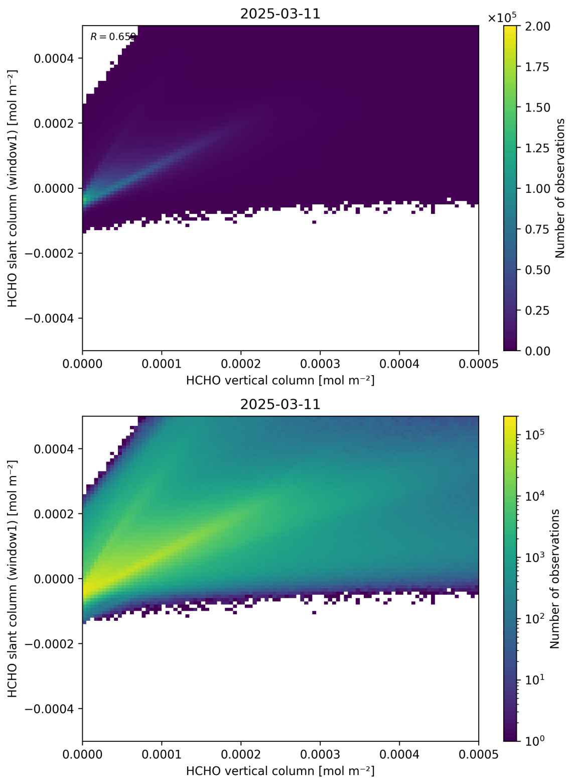
Figure 129: Scatter density plot of “HCHO vertical column” against “HCHO slant column (window1)” for 2025-03-10 to 2025-03-12.
