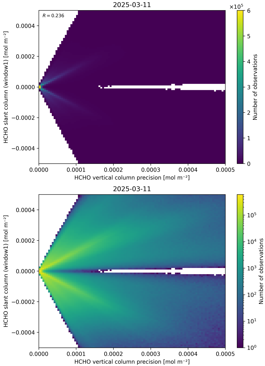
Figure 142: Scatter density plot of “HCHO vertical column precision” against “HCHO slant column (window1)” for 2025-03-10 to 2025-03-12.
