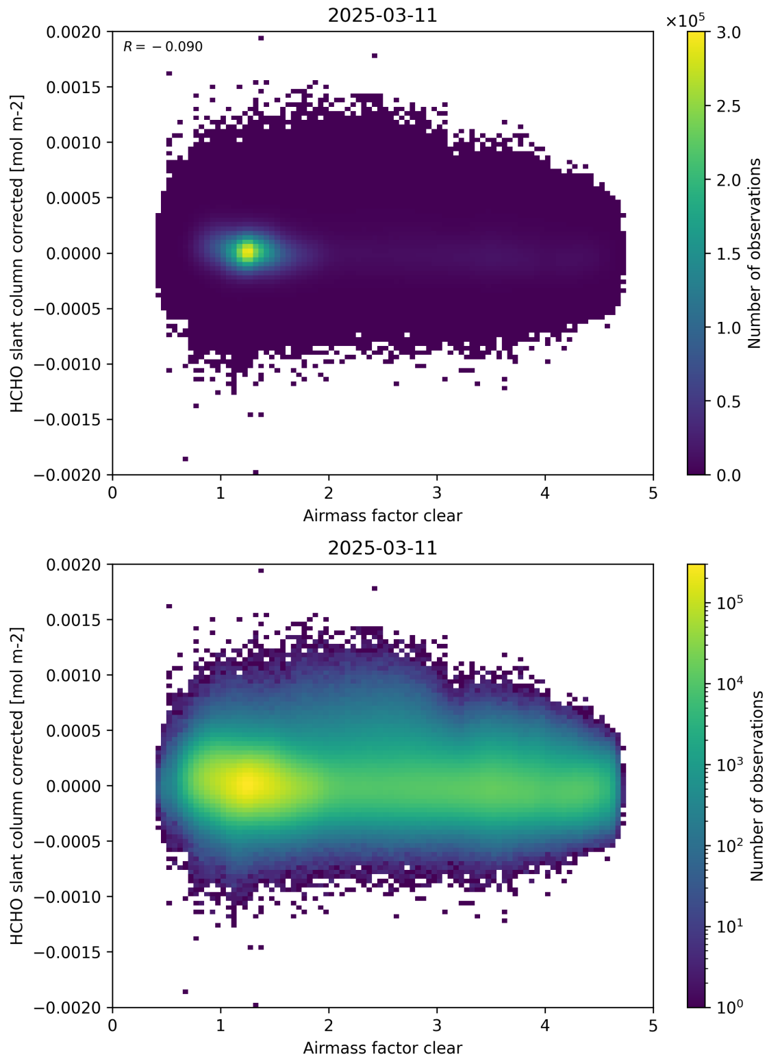
Figure 74: Scatter density plot of “Airmass factor clear” against “HCHO slant column corrected” for 2025-03-10 to 2025-03-12.
