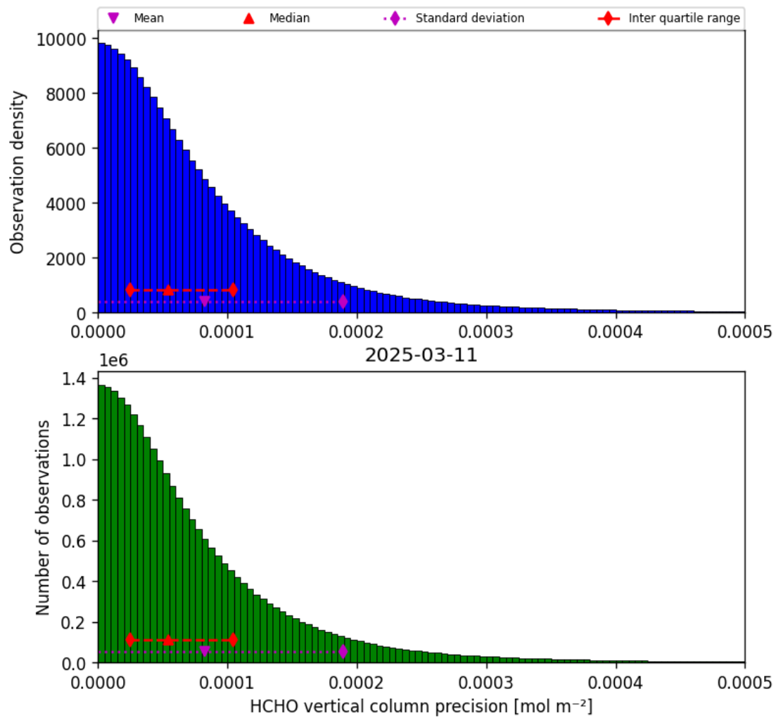
Figure 36: Histogram of “HCHO vertical column precision” for 2025-03-10 to 2025-03-12
