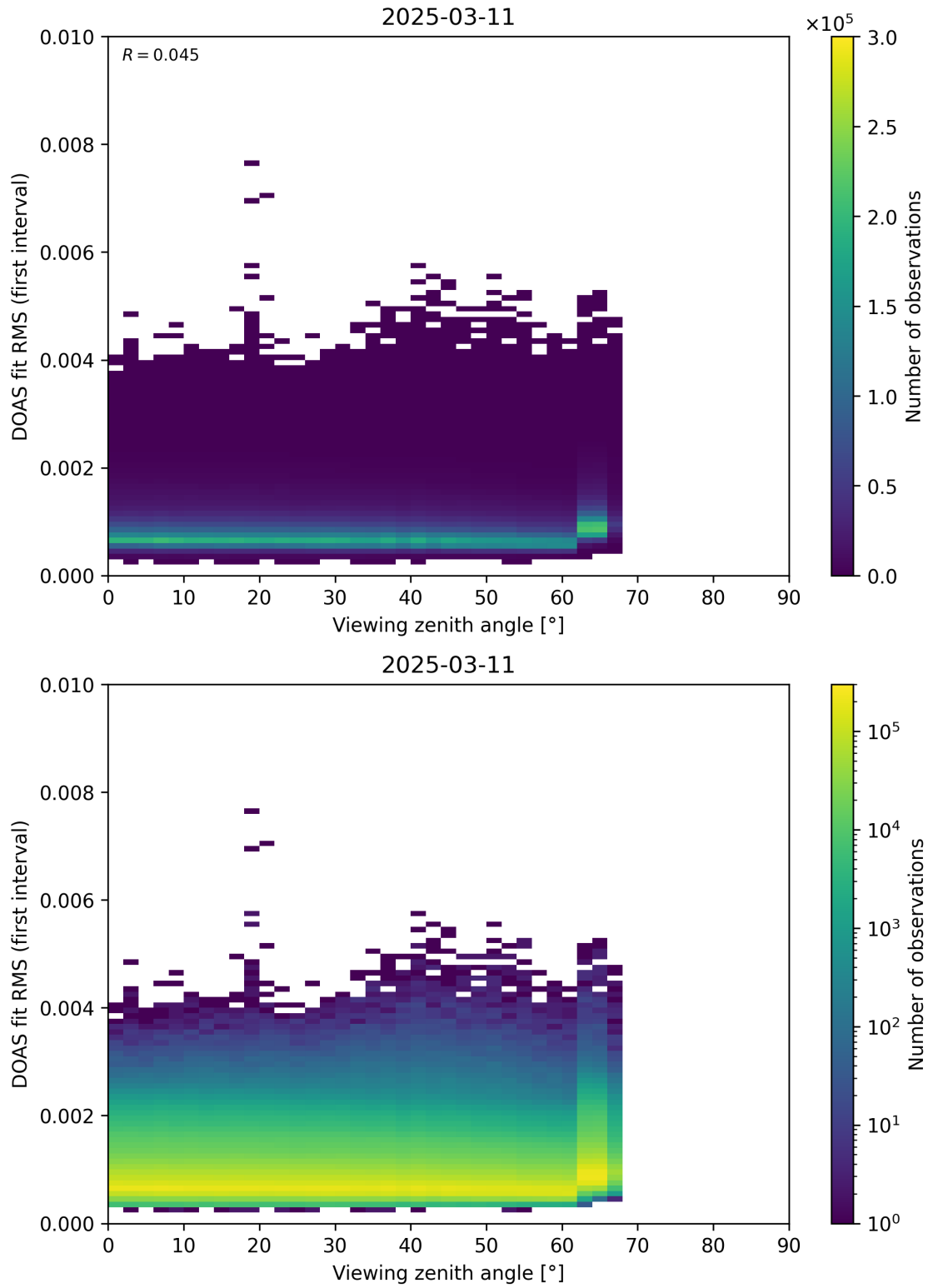
Figure 182: Scatter density plot of “Viewing zenith angle” against “DOAS fit RMS (first interval)” for 2025-03-10 to 2025-03-12.
