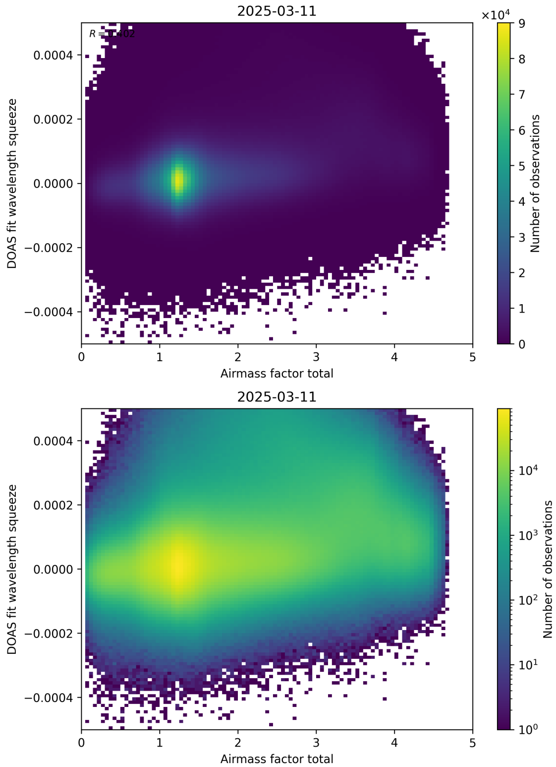
Figure 99: Scatter density plot of “Airmass factor total” against “DOAS fit wavelength squeeze” for 2025-03-10 to 2025-03-12.
