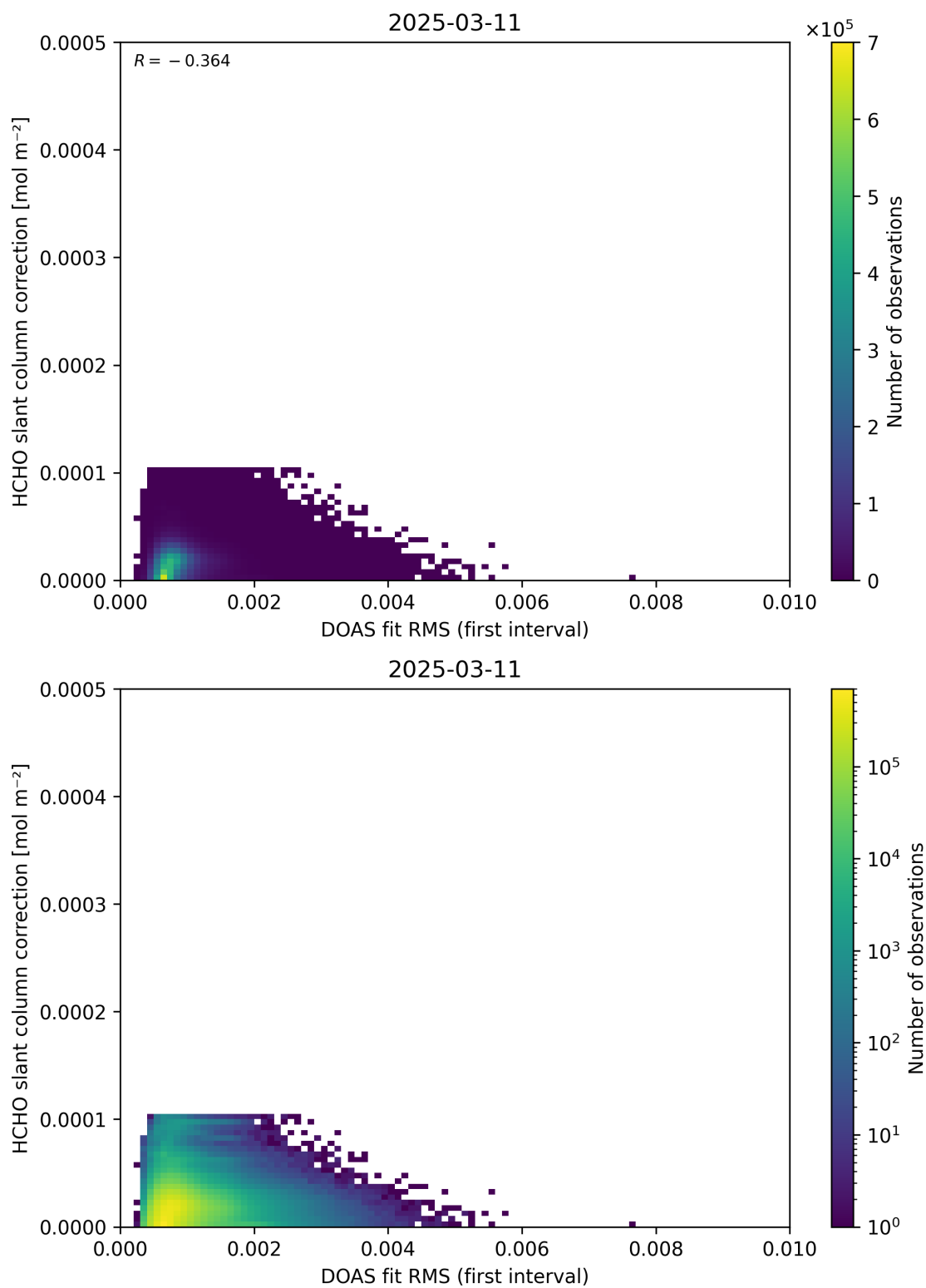
Figure 63: Scatter density plot of “DOAS fit RMS (first interval)” against “HCHO slant column correction” for 2025-03-10 to 2025-03-12.
