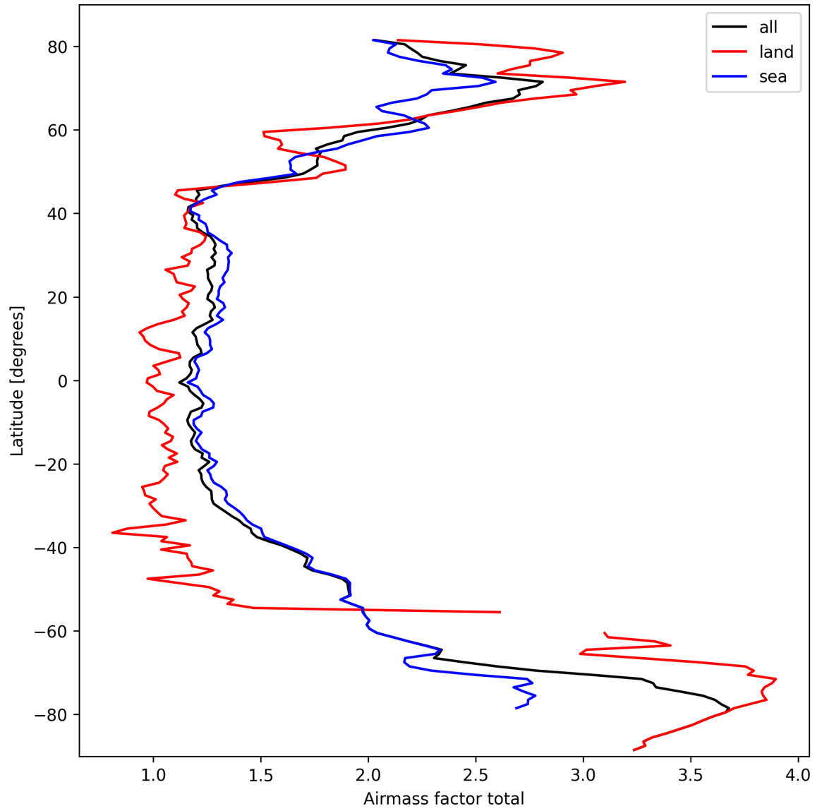
Figure 26: Zonal average of “Airmass factor total” for 2025-03-10 to 2025-03-12.
