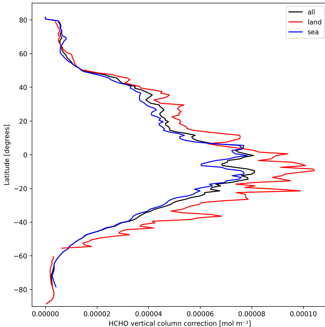
Figure 23: Zonal average of “HCHO vertical column correction” for 2025-03-10 to 2025-03-12.
