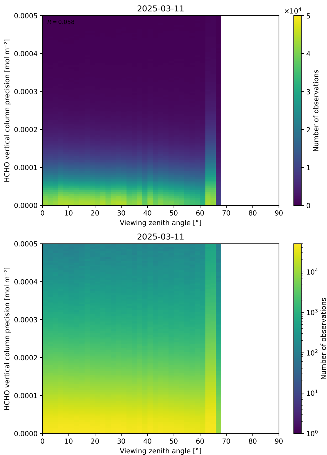
Figure 194: Scatter density plot of “Viewing zenith angle” against “HCHO vertical column precision” for 2025-03-10 to 2025-03-12.
