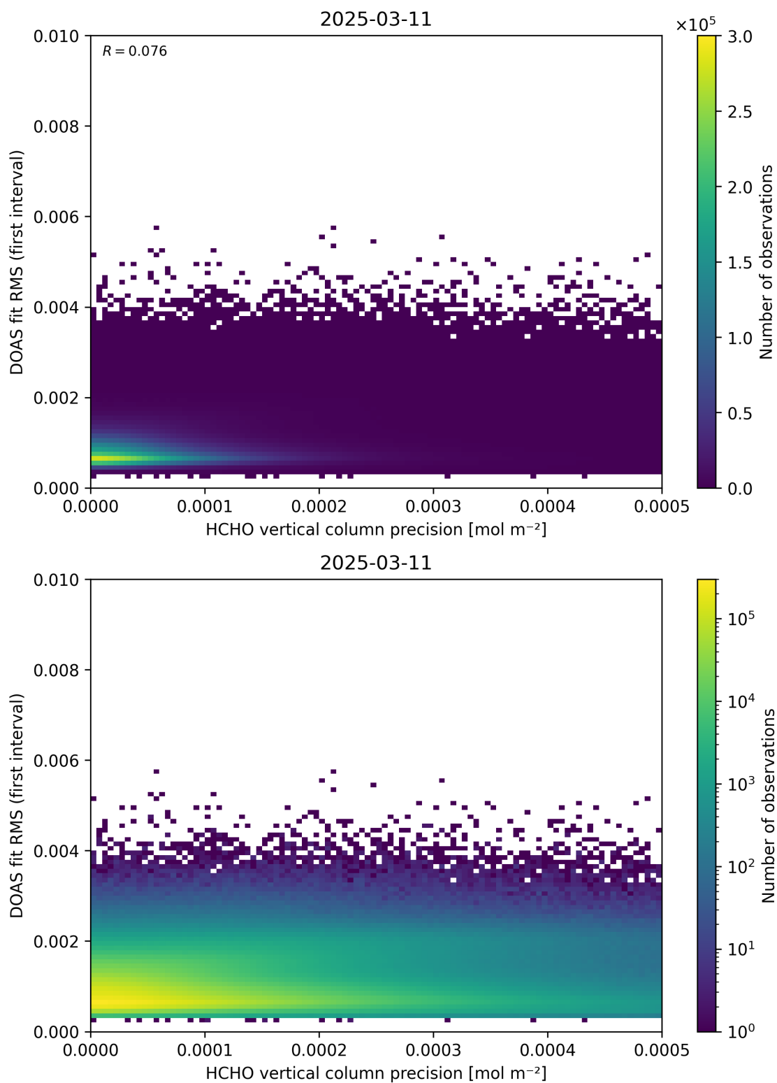
Figure 136: Scatter density plot of “HCHO vertical column precision” against “DOAS fit RMS (first interval)” for 2025-03-10 to 2025-03-12.
