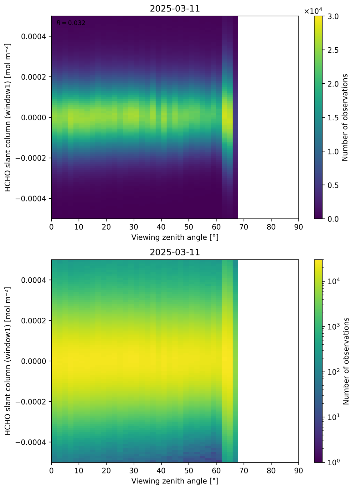
Figure 188: Scatter density plot of “Viewing zenith angle” against “HCHO slant column (window1)” for 2025-03-10 to 2025-03-12.
