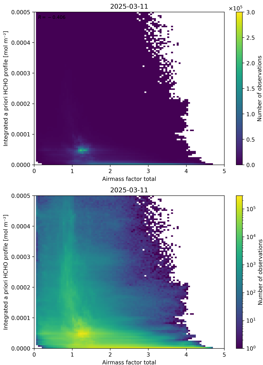
Figure 104: Scatter density plot of “Airmass factor total” against “Integrated a priori HCHO profile” for 2025-03-10 to 2025-03-12.
