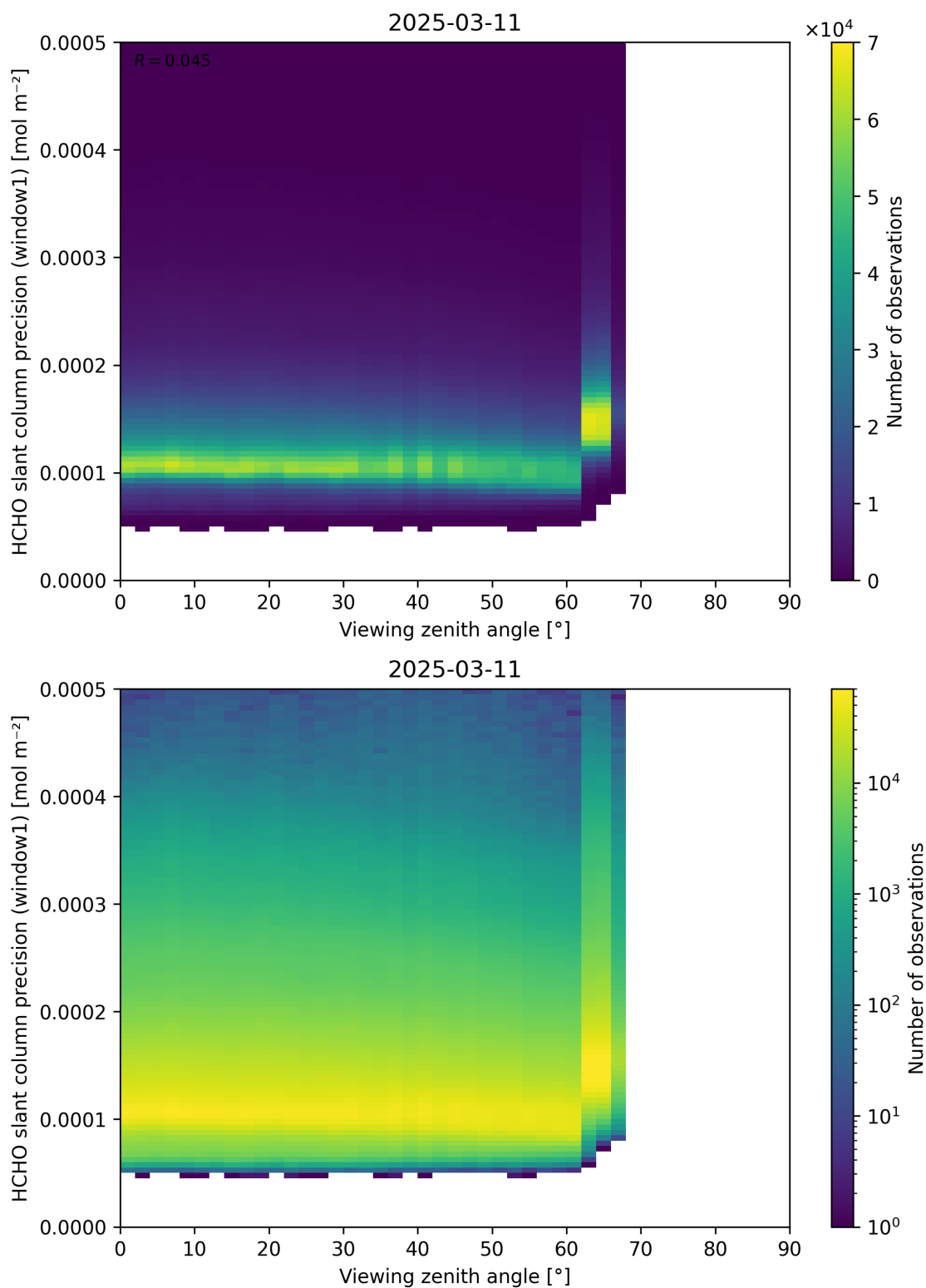
Figure 189: Scatter density plot of “Viewing zenith angle” against “HCHO slant column precision (window1)” for 2025-03-10 to 2025-03-12.
