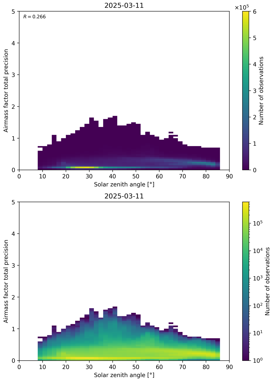
Figure 176: Scatter density plot of “Solar zenith angle” against “Airmass factor total precision” for 2025-03-10 to 2025-03-12.
