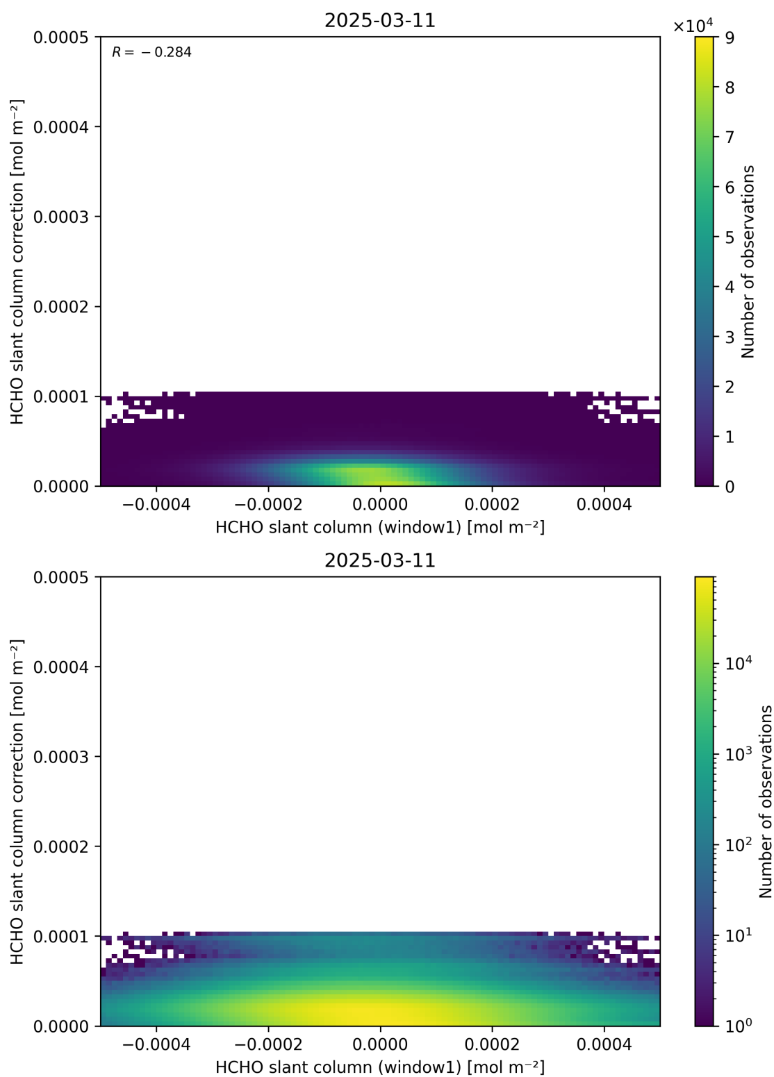
Figure 83: Scatter density plot of “HCHO slant column (window1)” against “HCHO slant column correction” for 2025-03-10 to 2025-03-12.
