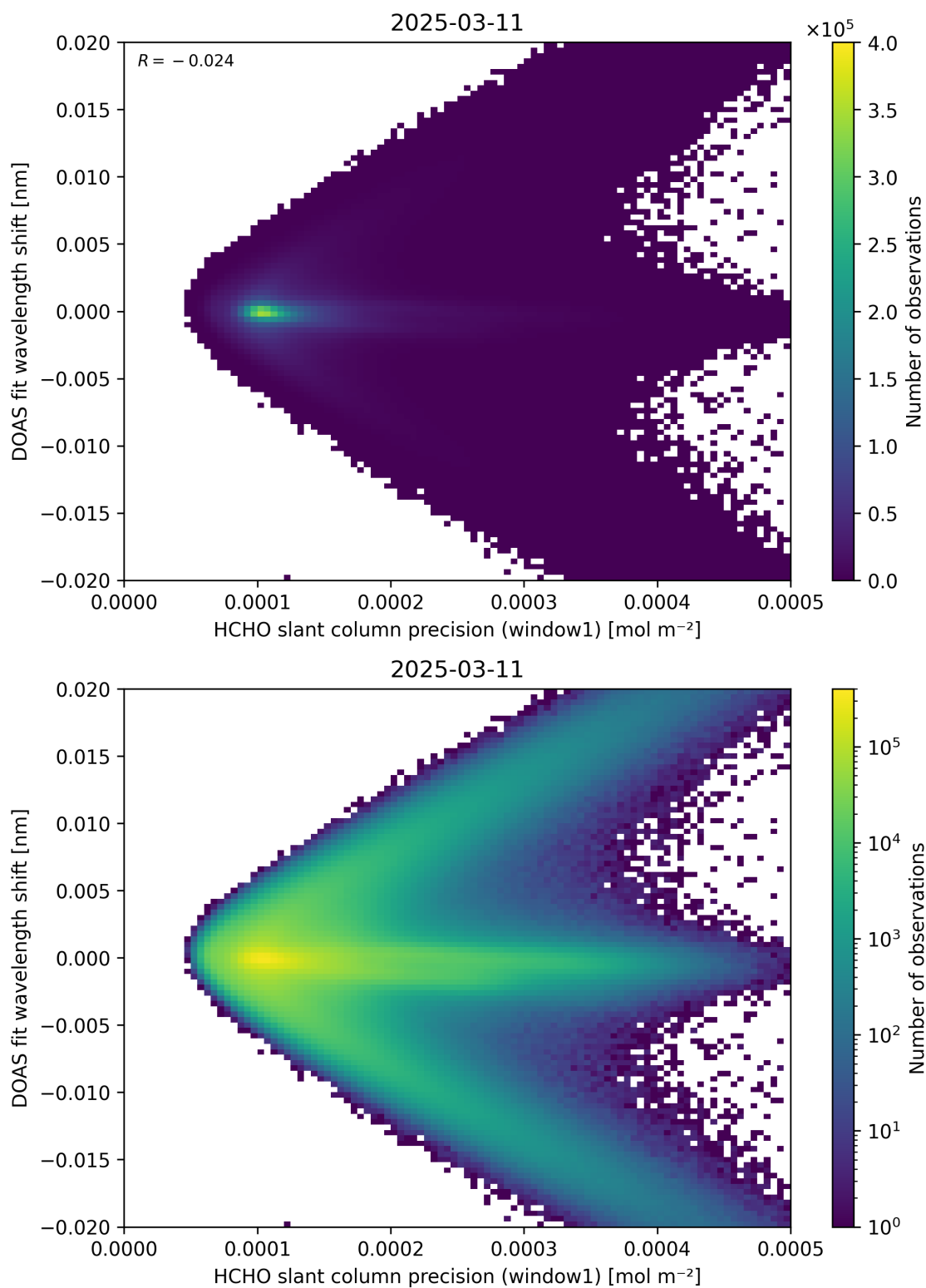
Figure 89: Scatter density plot of “HCHO slant column precision (window1)” against “DOAS fit wavelength shift” for 2025-03-10 to 2025-03-12.
