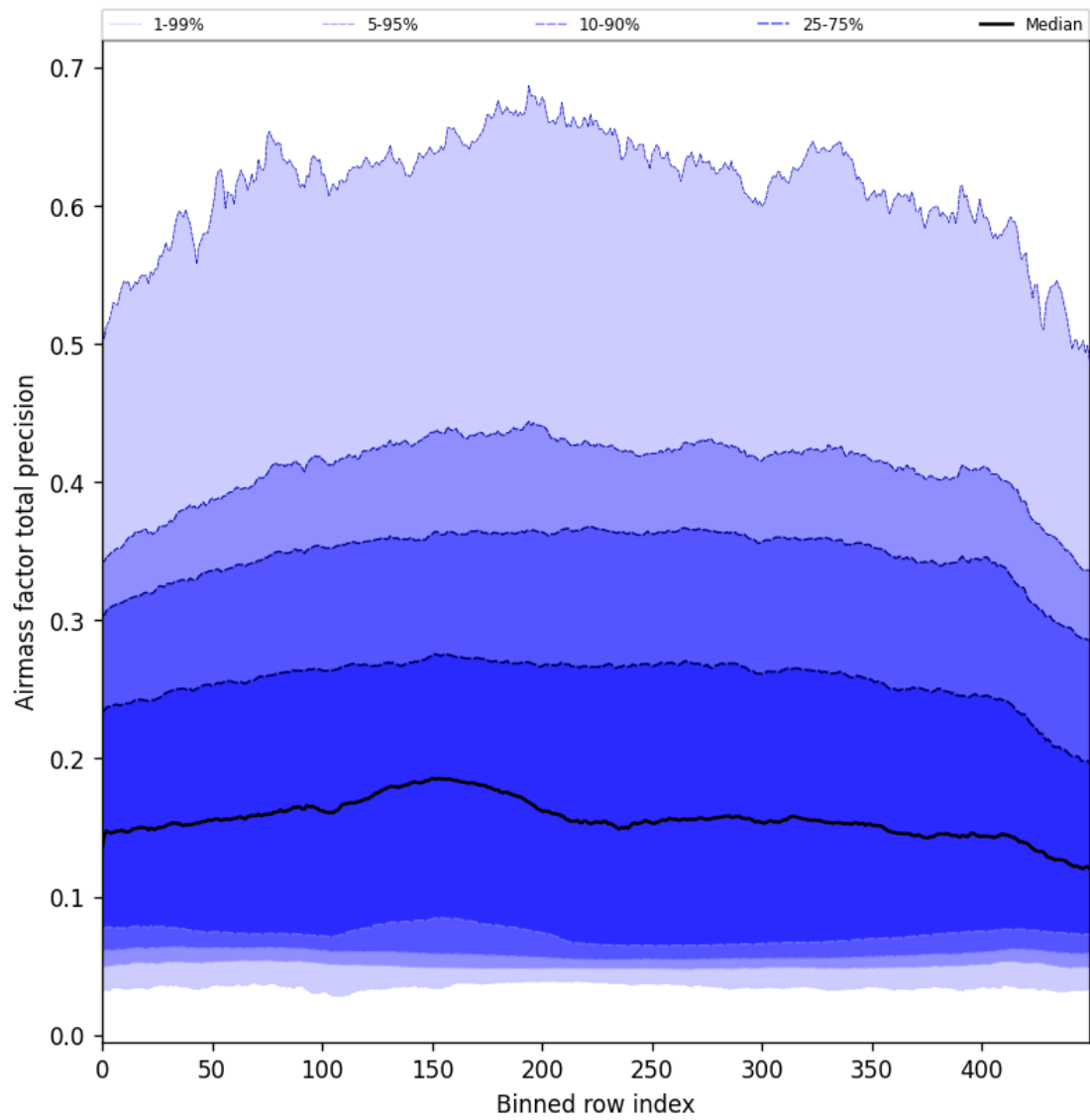
Figure 55: Along track statistics of “Airmass factor total precision” for 2025-03-10 to 2025-03-12
