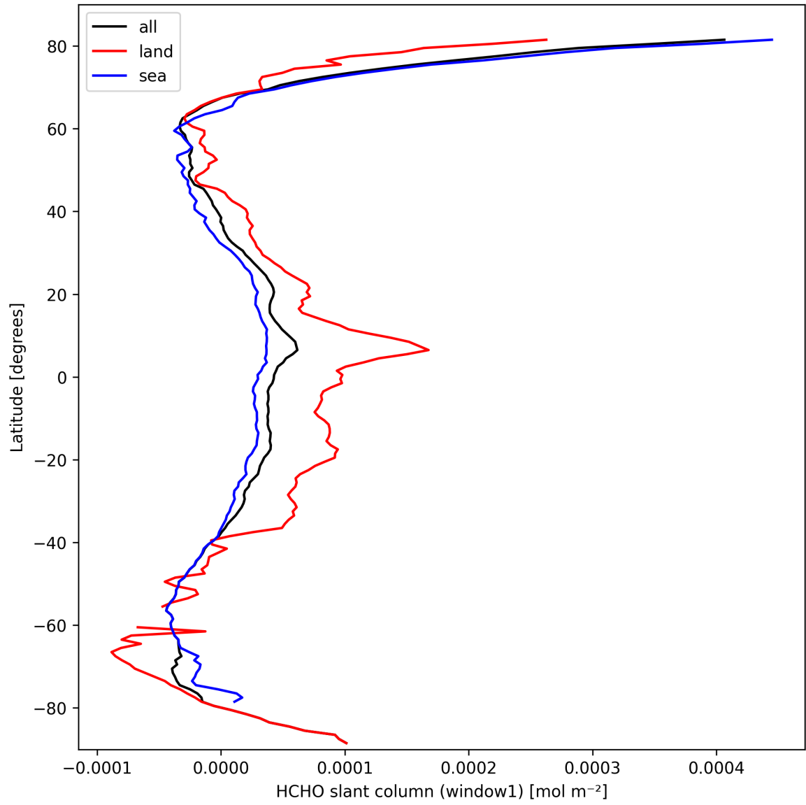
Figure 24: Zonal average of “HCHO slant column (window1)” for 2025-03-10 to 2025-03-12.
