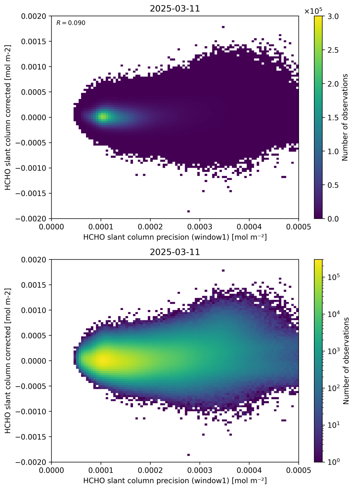
Figure 92: Scatter density plot of “HCHO slant column precision (window1)” against “HCHO slant column corrected” for 2025-03-10 to 2025-03-12.
