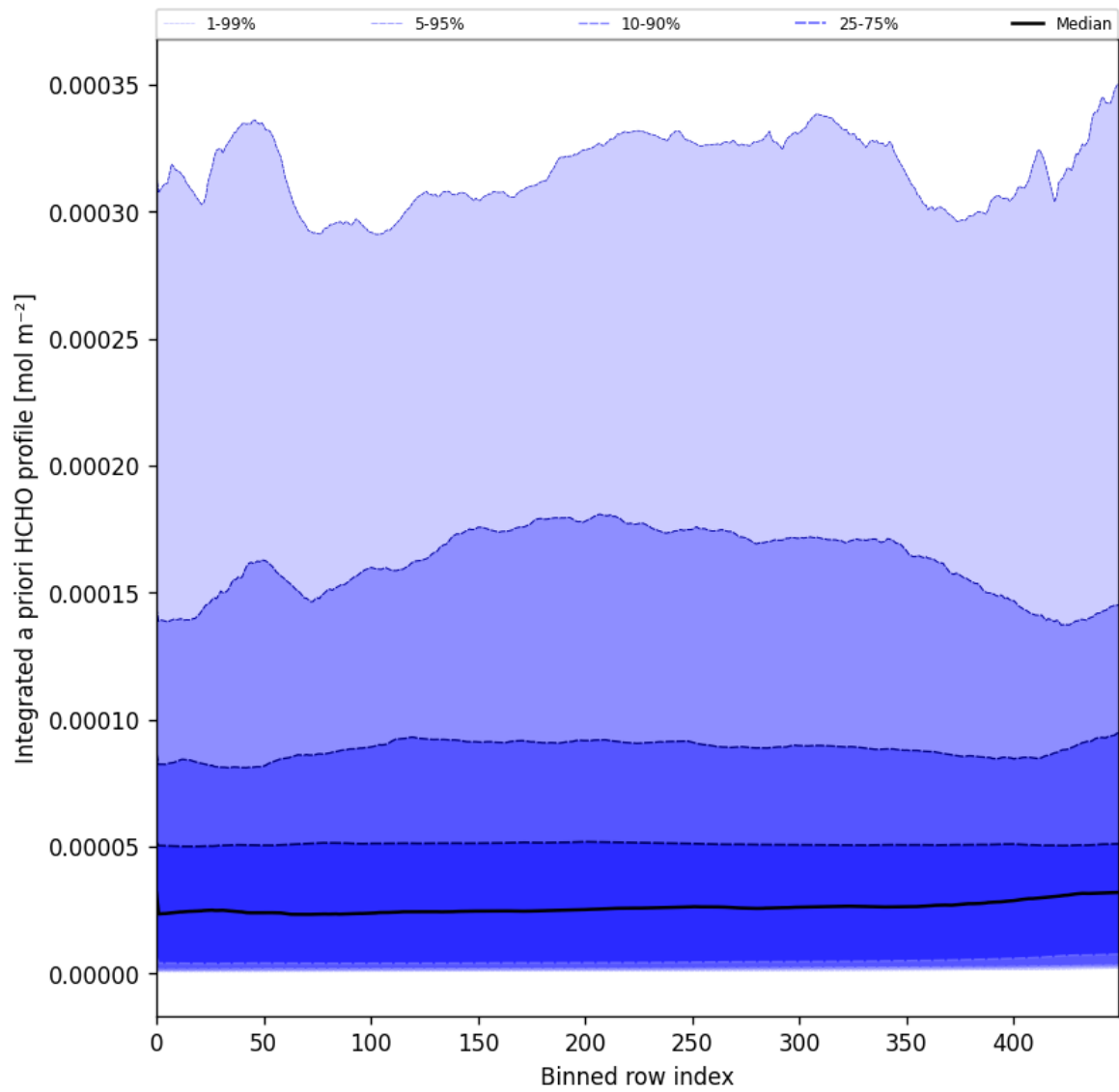
Figure 57: Along track statistics of “Integrated a priori HCHO profile” for 2025-03-10 to 2025-03-12
