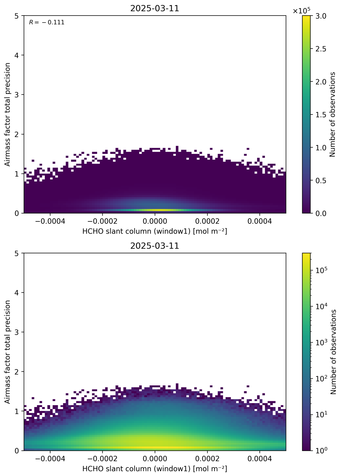
Figure 86: Scatter density plot of “HCHO slant column (window1)” against “Airmass factor total precision” for 2025-03-10 to 2025-03-12.
