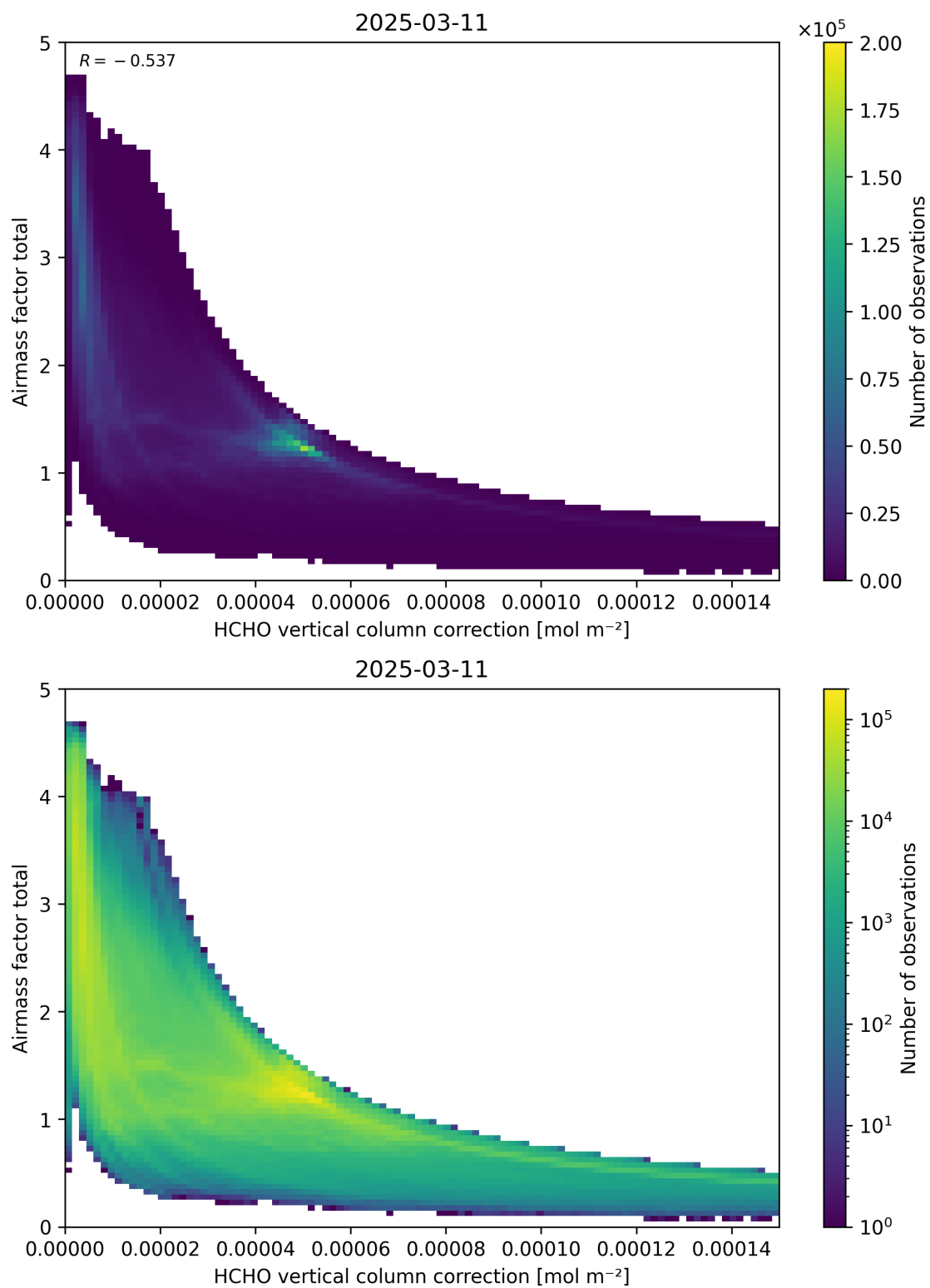
Figure 120: Scatter density plot of “HCHO vertical column correction” against “Airmass factor total” for 2025-03-10 to 2025-03-12.
