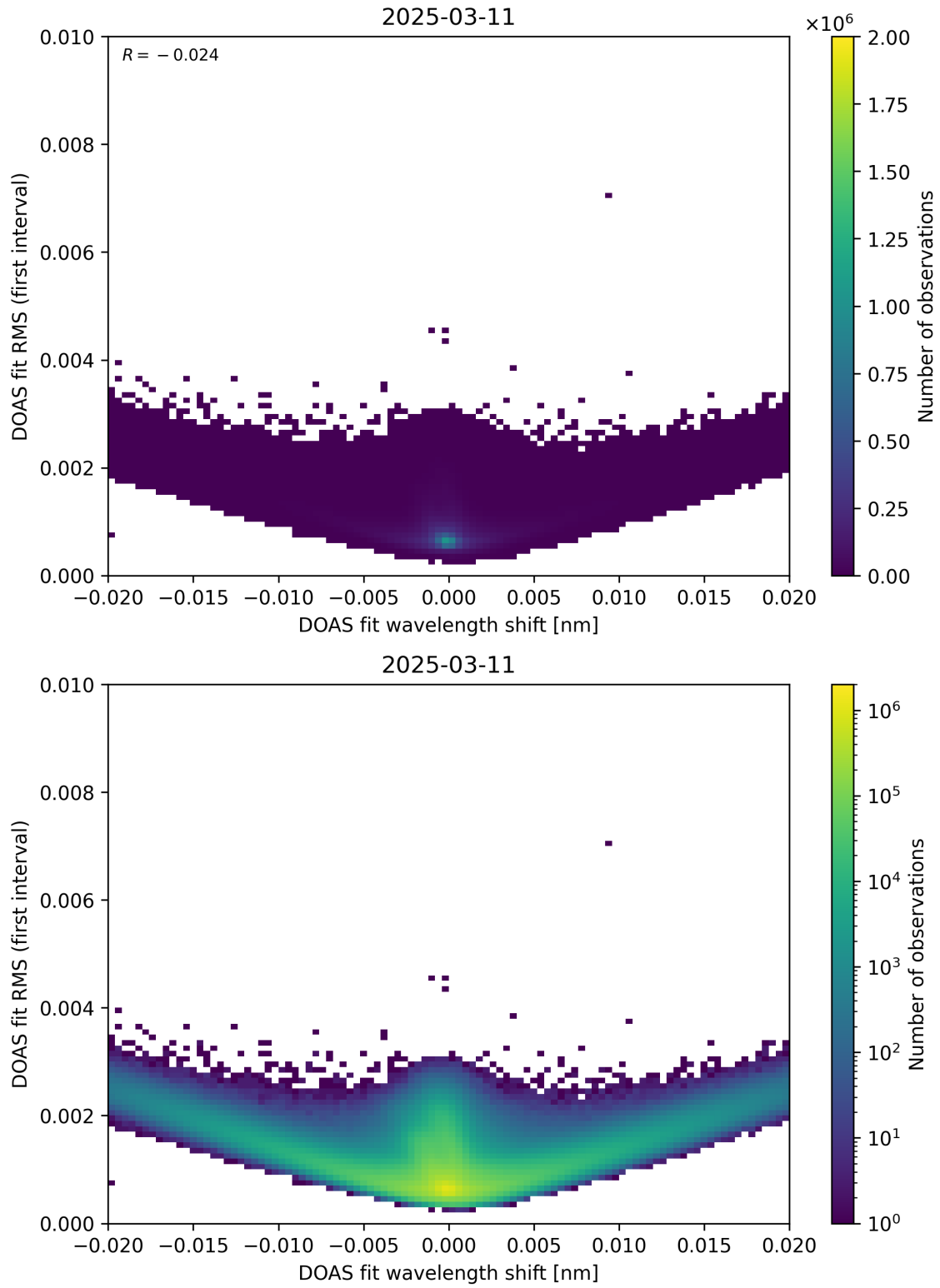
Figure 64: Scatter density plot of “DOAS fit wavelength shift” against “DOAS fit RMS (first interval)” for 2025-03-10 to 2025-03-12.
