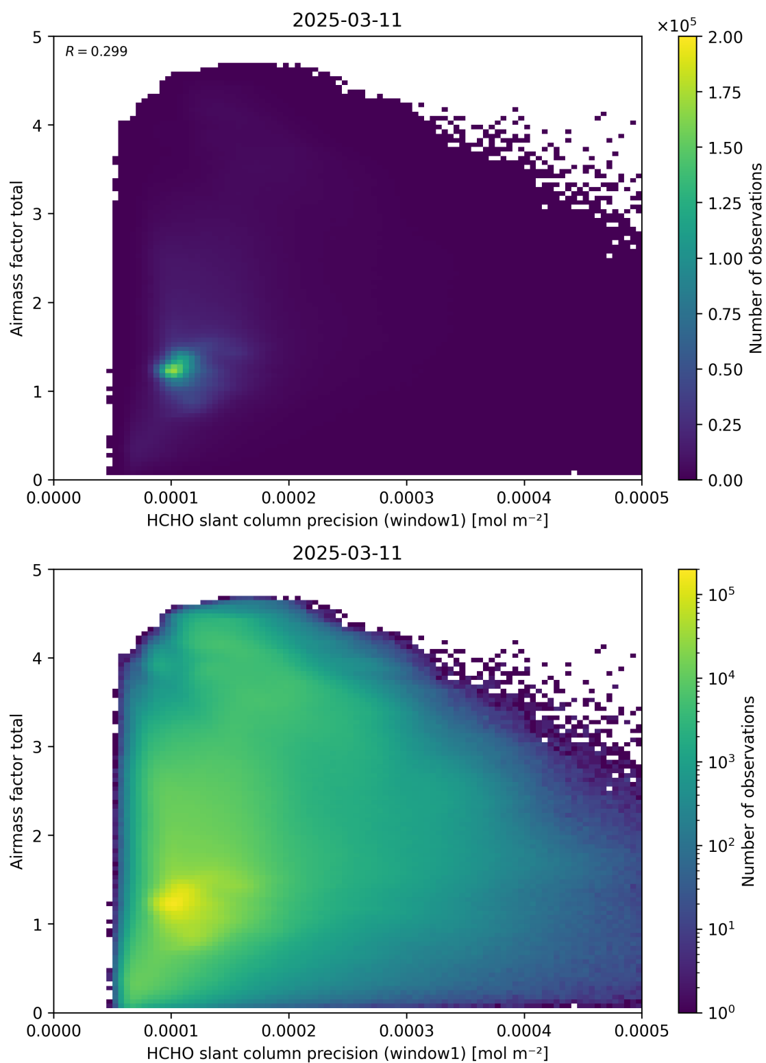
Figure 94: Scatter density plot of “HCHO slant column precision (window1)” against “Airmass factor total” for 2025-03-10 to 2025-03-12.
