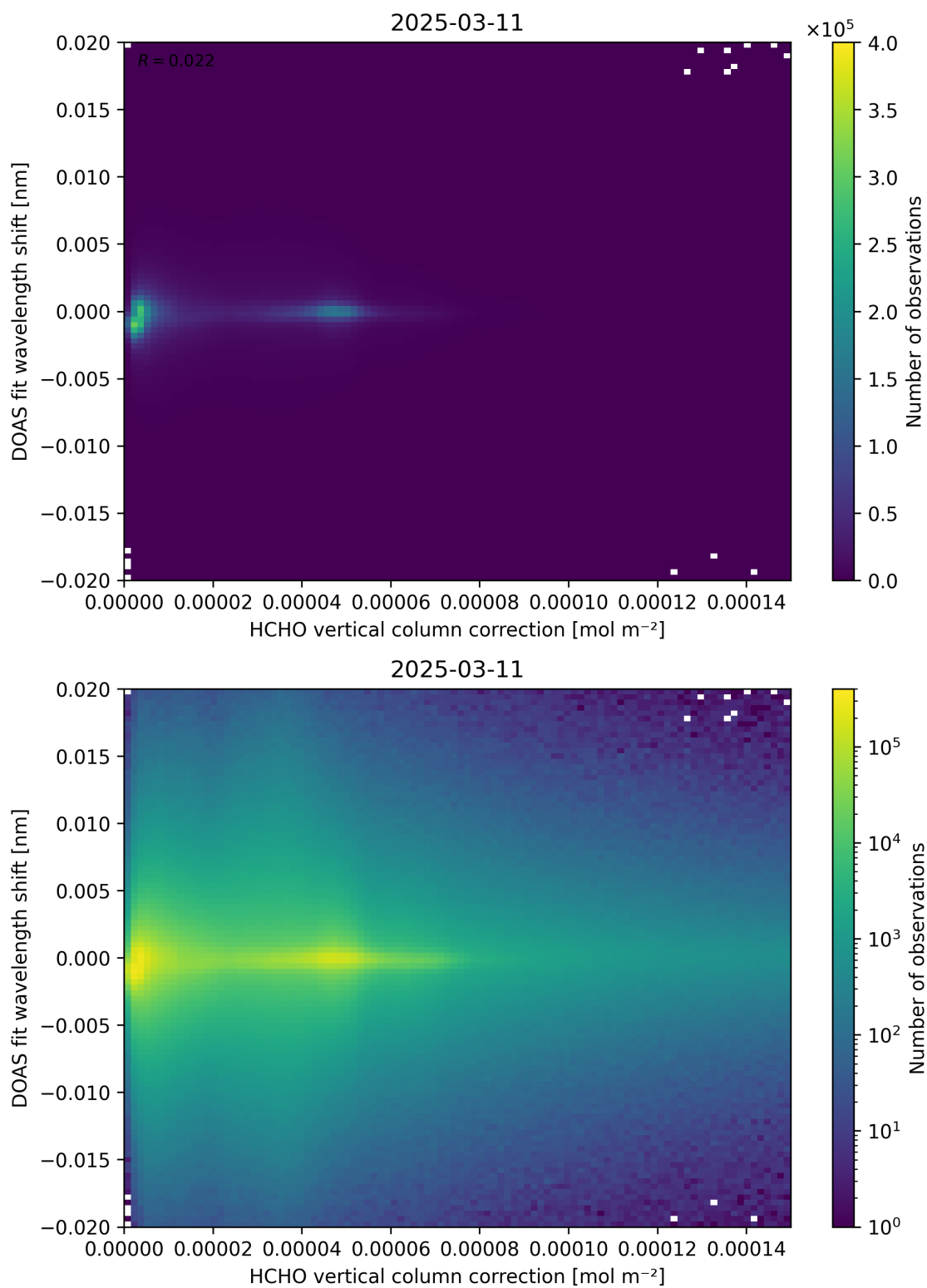
Figure 113: Scatter density plot of “HCHO vertical column correction” against “DOAS fit wavelength shift” for 2025-03-10 to 2025-03-12.
