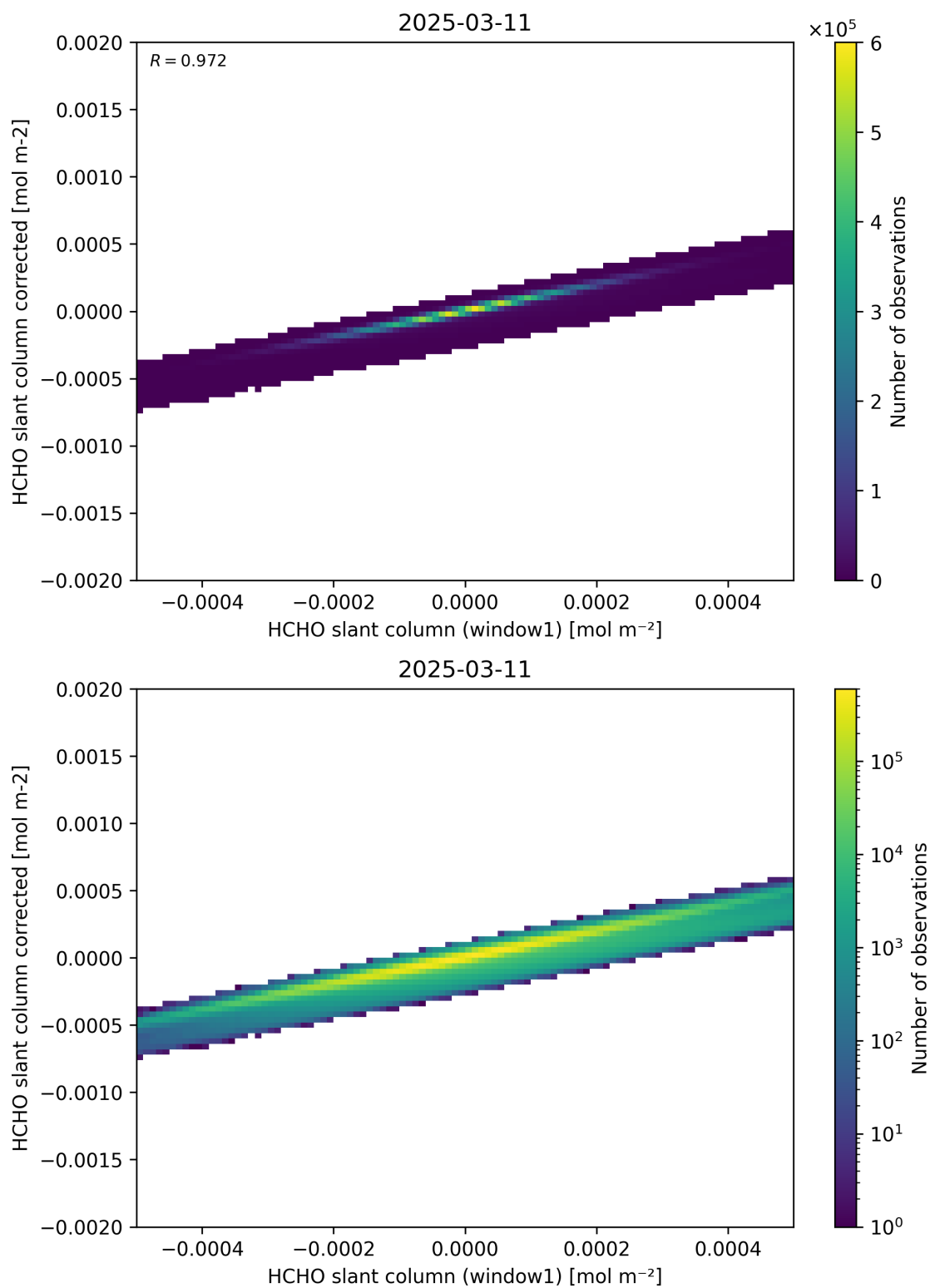
Figure 82: Scatter density plot of “HCHO slant column (window1)” against “HCHO slant column corrected” for 2025-03-10 to 2025-03-12.
