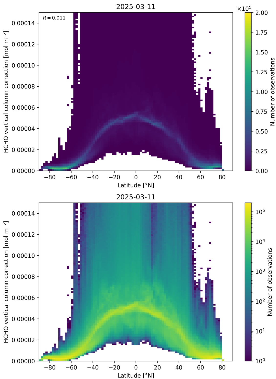
Figure 164: Scatter density plot of “Latitude” against “HCHO vertical column correction” for 2025-03-10 to 2025-03-12.
