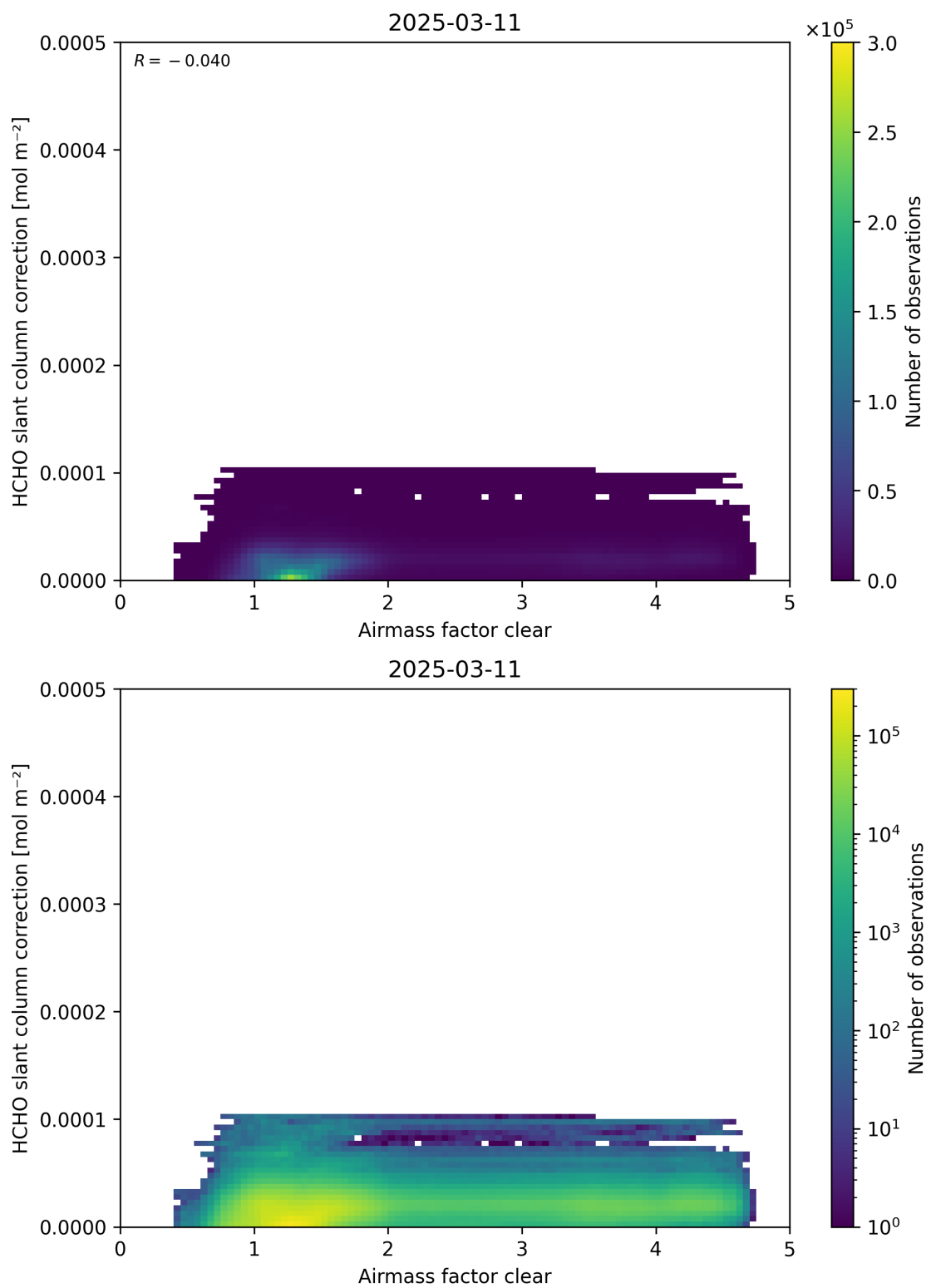
Figure 75: Scatter density plot of “Airmass factor clear” against “HCHO slant column correction” for 2025-03-10 to 2025-03-12.
