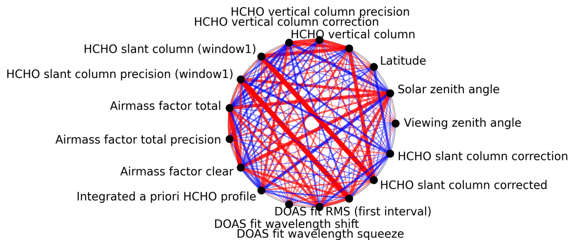
Figure 1: Map of correlation graph for 2025-03-10 to 2025-03-12.
