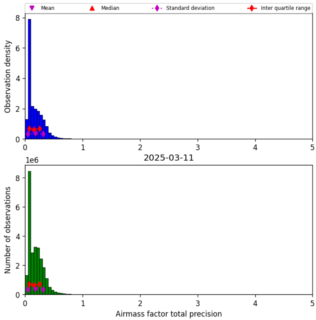
Figure 41: Histogram of “Airmass factor total precision” for 2025-03-10 to 2025-03-12
