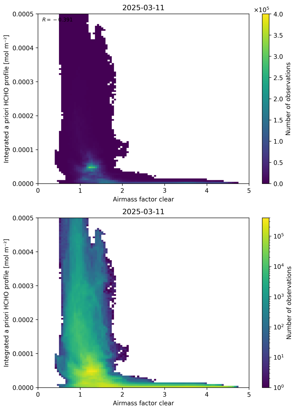
Figure 76: Scatter density plot of “Airmass factor clear” against “Integrated a priori HCHO profile” for 2025-03-10 to 2025-03-12.
