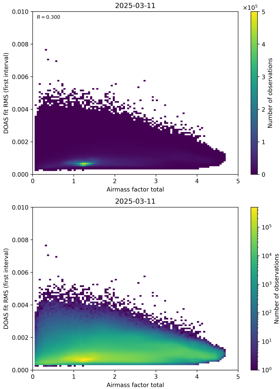
Figure 97: Scatter density plot of “Airmass factor total” against “DOAS fit RMS (first interval)” for 2025-03-10 to 2025-03-12.
