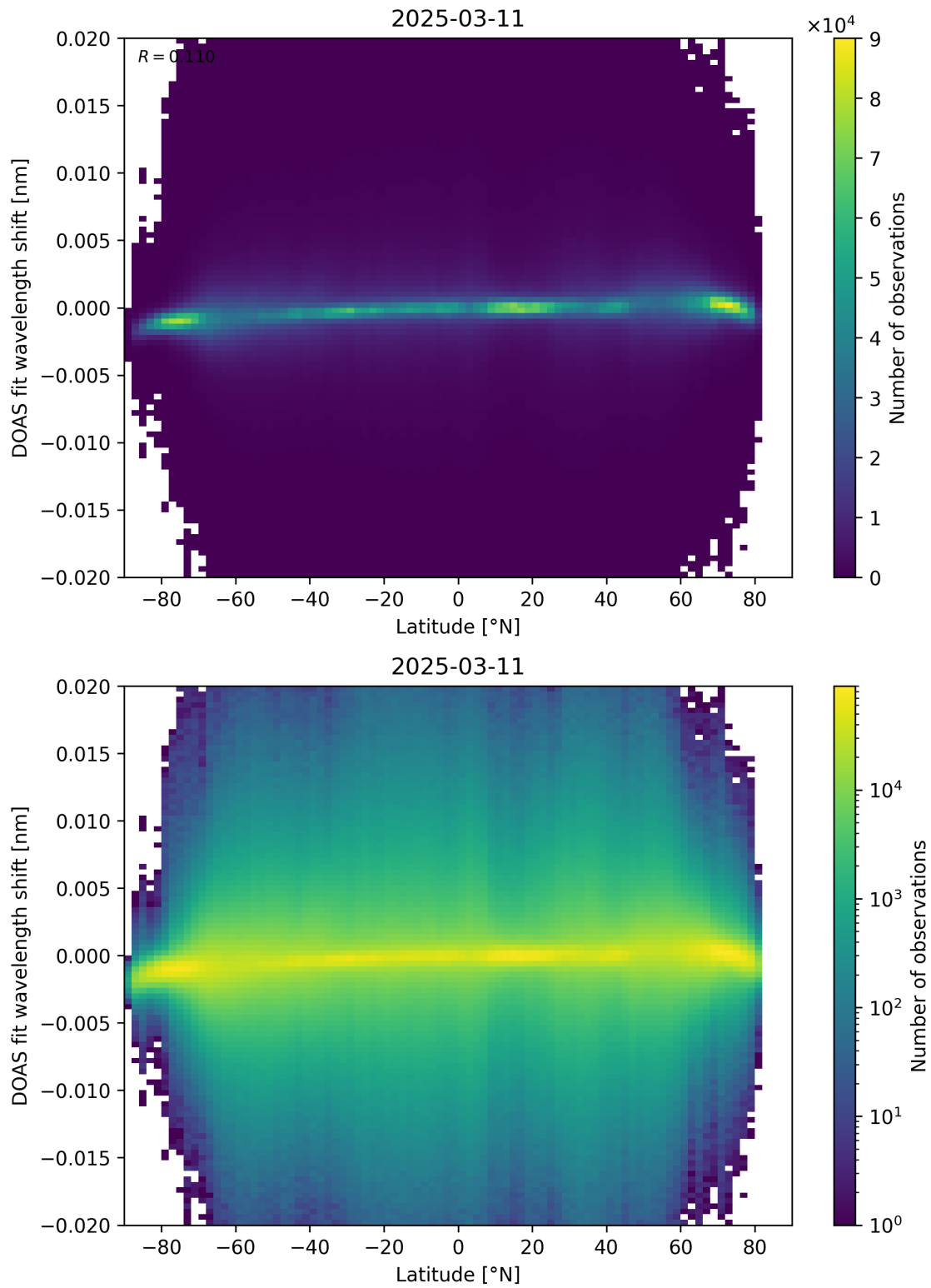
Figure 154: Scatter density plot of “Latitude” against “DOAS fit wavelength shift” for 2025-03-10 to 2025-03-12.
