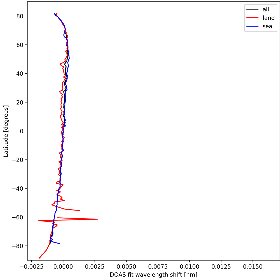
Figure 30: Zonal average of "DOAS fit wavelength shift" for 2025-03-10 to 2025-03-12.
