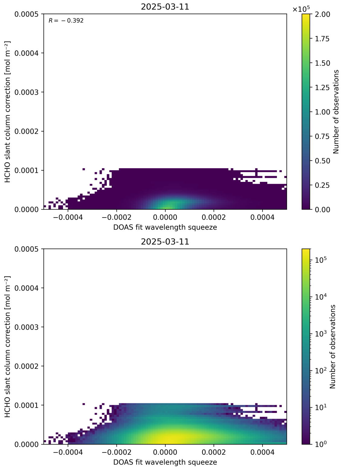
Figure 70: Scatter density plot of “DOAS fit wavelength squeeze” against “HCHO slant column correction” for 2025-03-10 to 2025-03-12.
