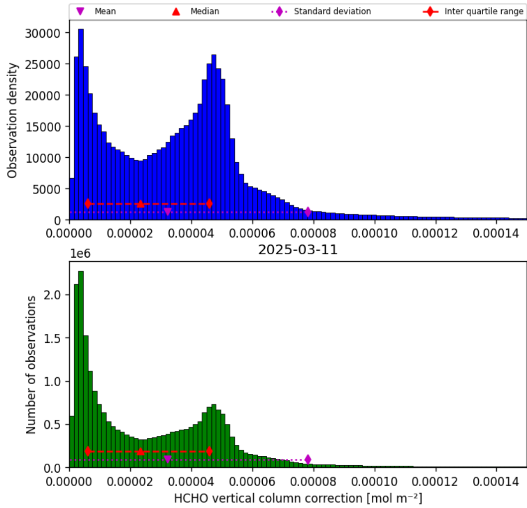
Figure 37: Histogram of “HCHO vertical column correction” for 2025-03-10 to 2025-03-12
