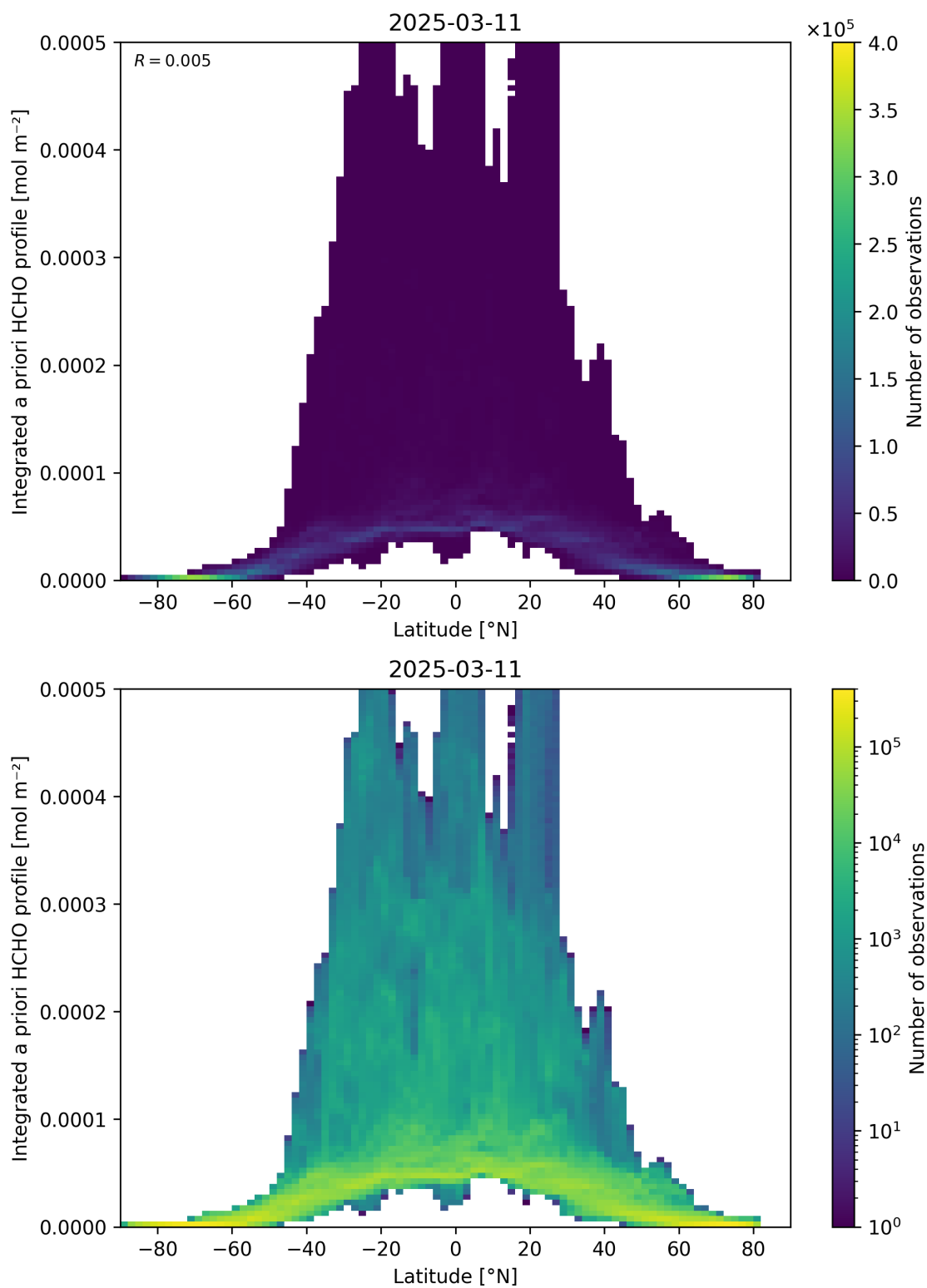
Figure 166: Scatter density plot of “Latitude” against “Integrated a priori HCHO profile” for 2025-03-10 to 2025-03-12.
