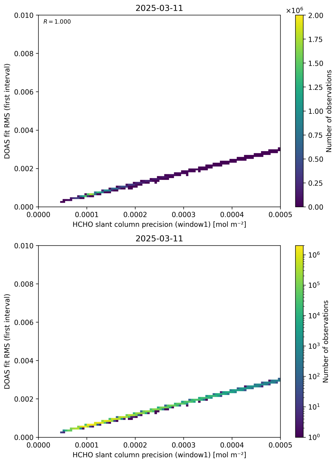
Figure 88: Scatter density plot of “HCHO slant column precision (window1)” against “DOAS fit RMS (first interval)” for 2025-03-10 to 2025-03-12.
