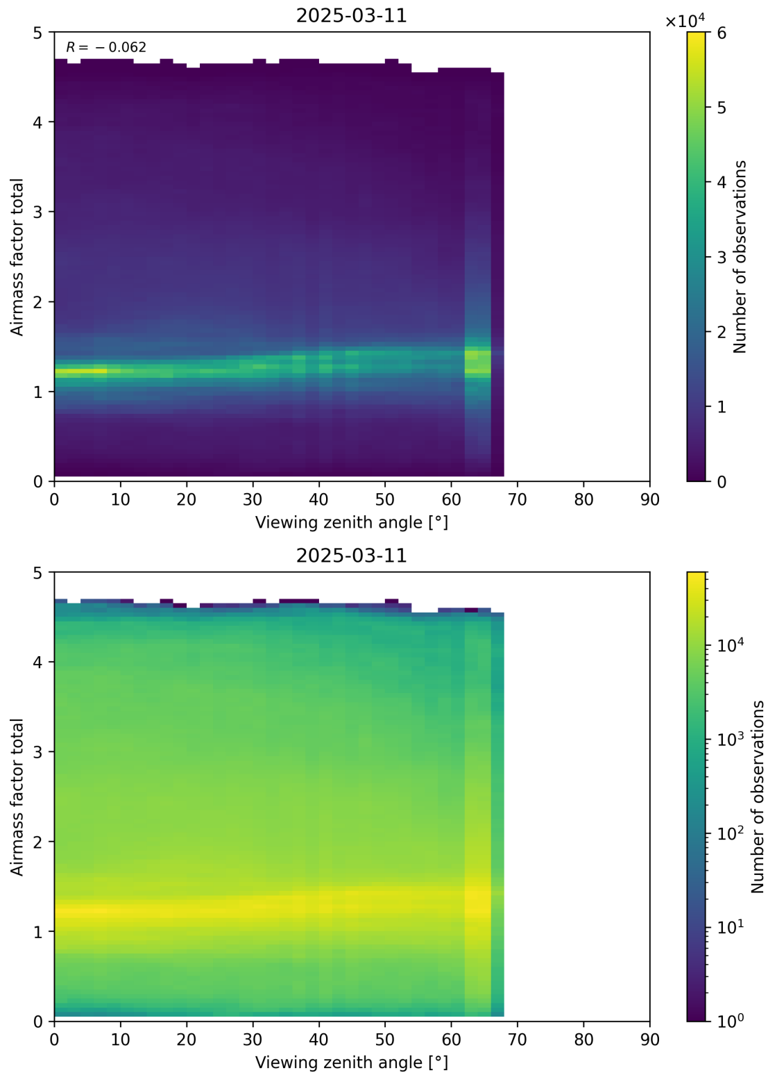
Figure 190: Scatter density plot of “Viewing zenith angle” against “Airmass factor total” for 2025-03-10 to 2025-03-12.
