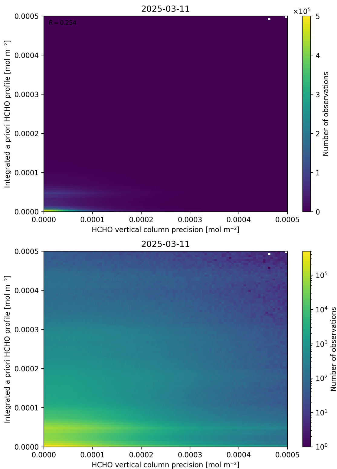
Figure 147: Scatter density plot of “HCHO vertical column precision” against “Integrated a priori HCHO profile” for 2025-03-10 to 2025-03-12.
