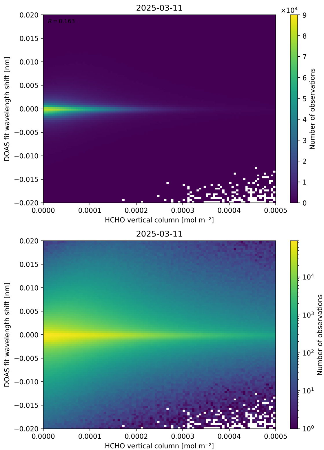
Figure 124: Scatter density plot of “HCHO vertical column” against “DOAS fit wavelength shift” for 2025-03-10 to 2025-03-12.
