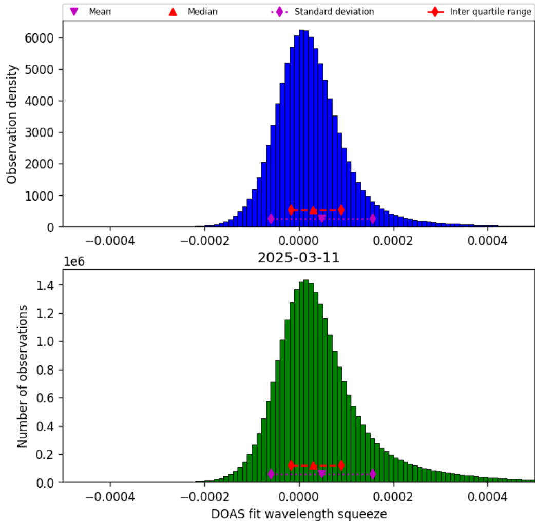
Figure 45: Histogram of “DOAS fit wavelength squeeze” for 2025-03-10 to 2025-03-12
