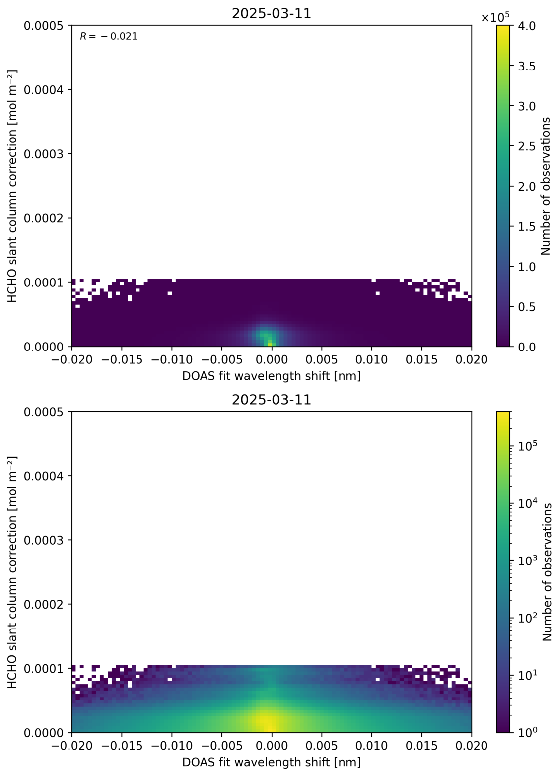
Figure 67: Scatter density plot of “DOAS fit wavelength shift” against “HCHO slant column correction” for 2025-03-10 to 2025-03-12.
