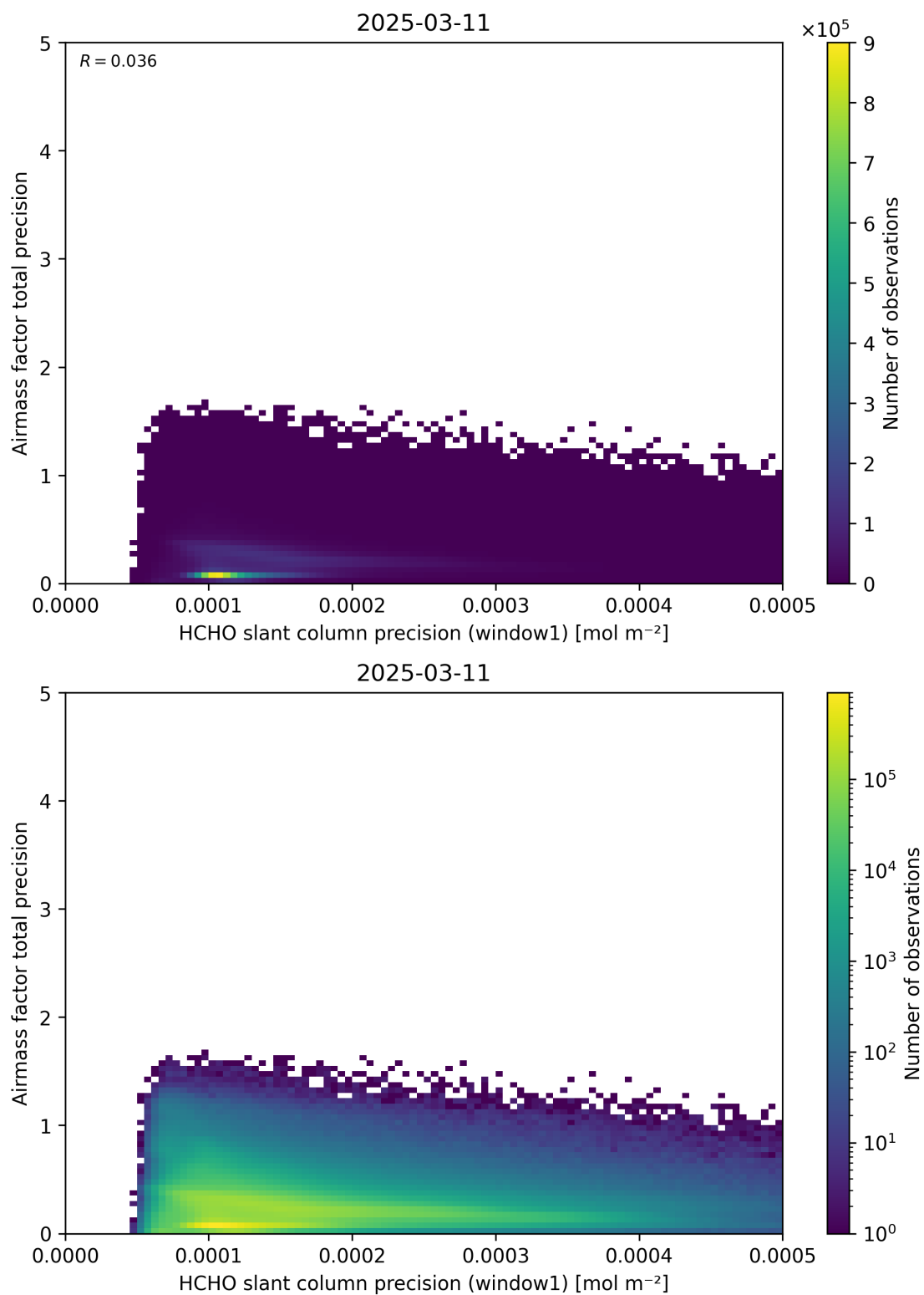
Figure 95: Scatter density plot of “HCHO slant column precision (window1)” against “Airmass factor total precision” for 2025-03-10 to 2025-03-12.
