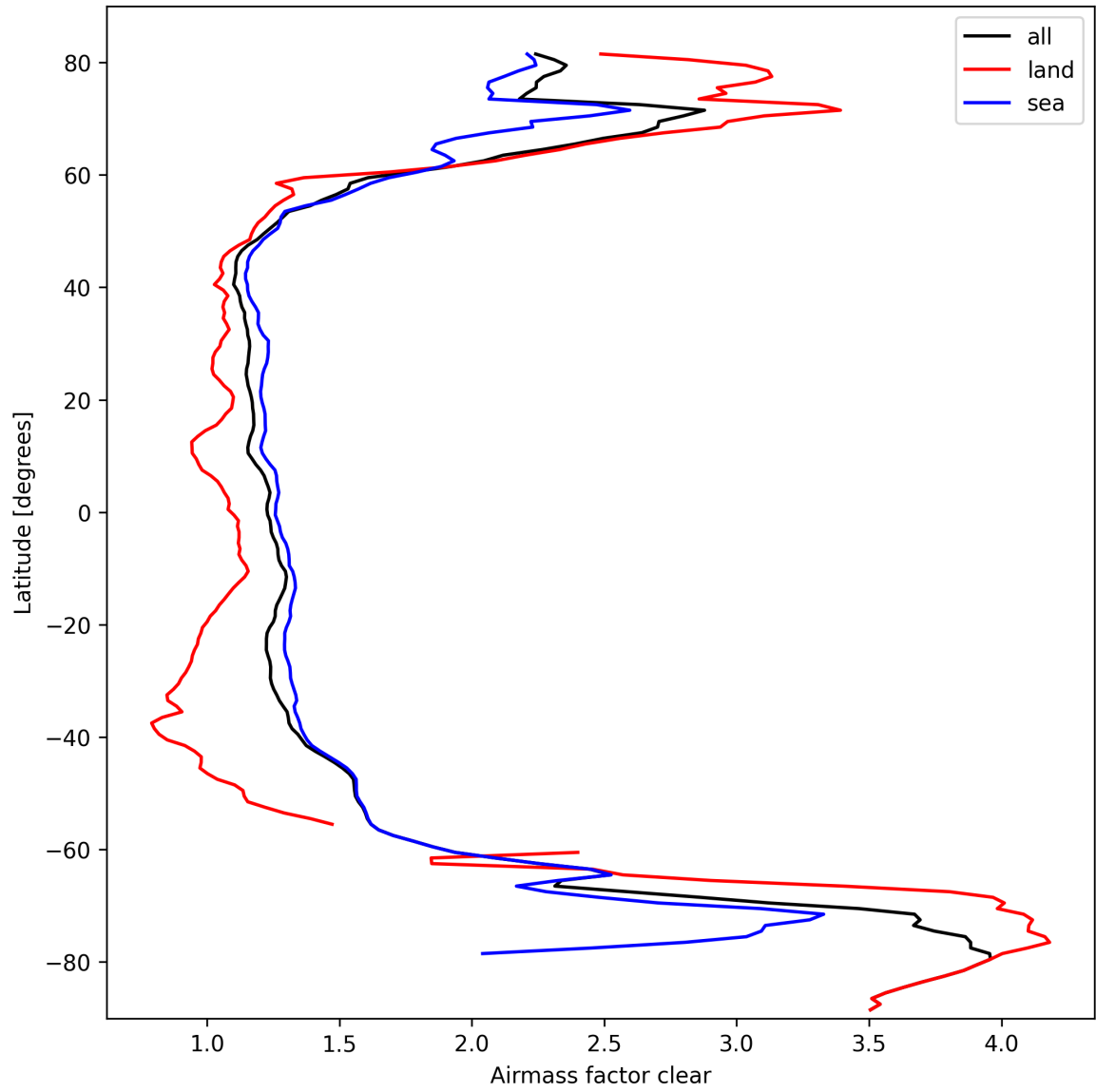
Figure 28: Zonal average of “Airmass factor clear” for 2025-03-10 to 2025-03-12.
