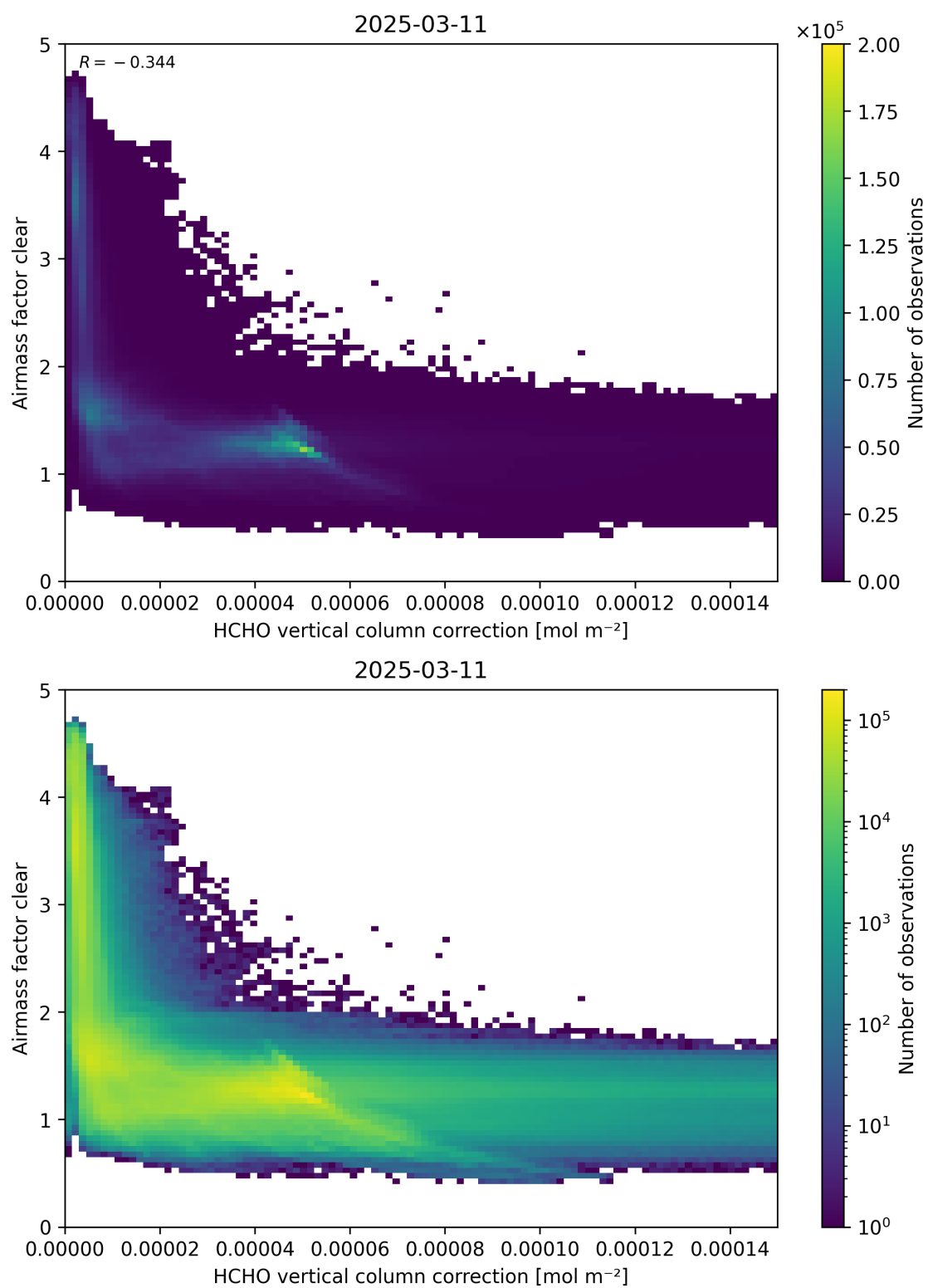
Figure 115: Scatter density plot of “HCHO vertical column correction” against “Airmass factor clear” for 2025-03-10 to 2025-03-12.
