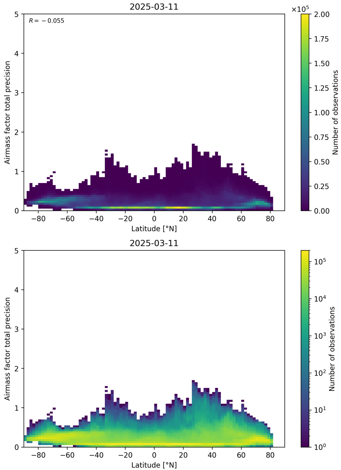
Figure 162: Scatter density plot of “Latitude” against “Airmass factor total precision” for 2025-03-10 to 2025-03-12.
