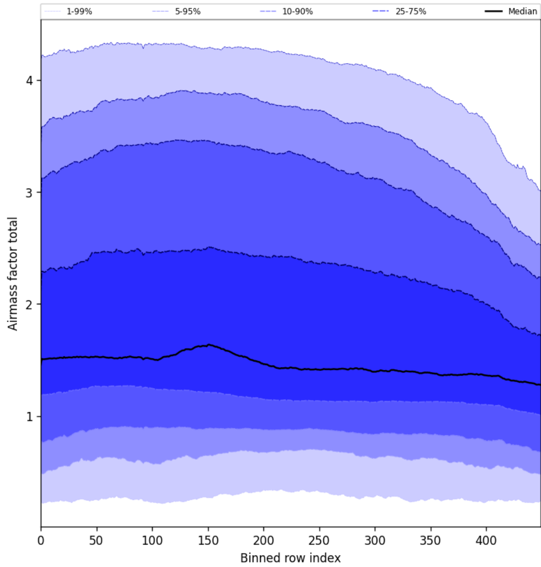
Figure 54: Along track statistics of “Airmass factor total” for 2025-03-10 to 2025-03-12
