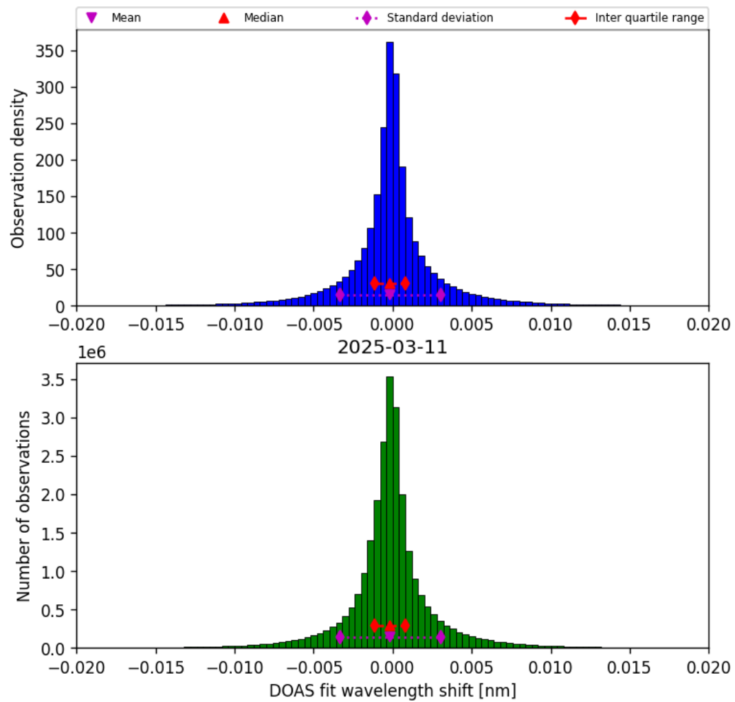
Figure 44: Histogram of “DOAS fit wavelength shift” for 2025-03-10 to 2025-03-12
