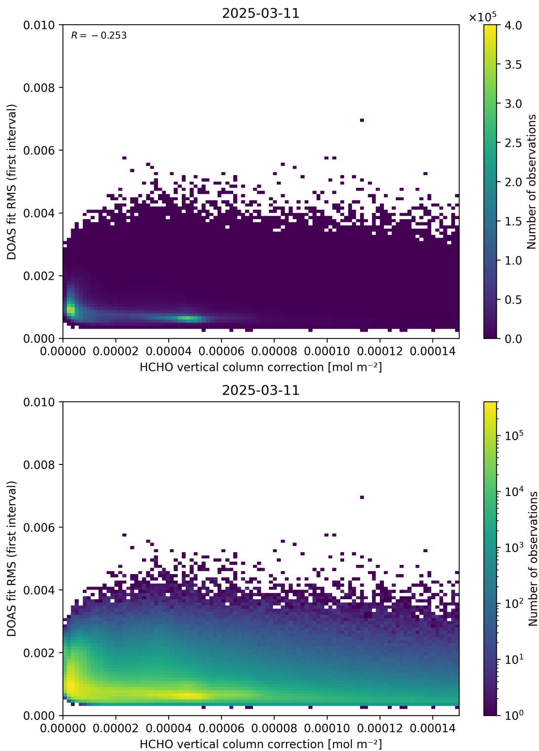
Figure 112: Scatter density plot of “HCHO vertical column correction” against “DOAS fit RMS (first interval)” for 2025-03-10 to 2025-03-12.
