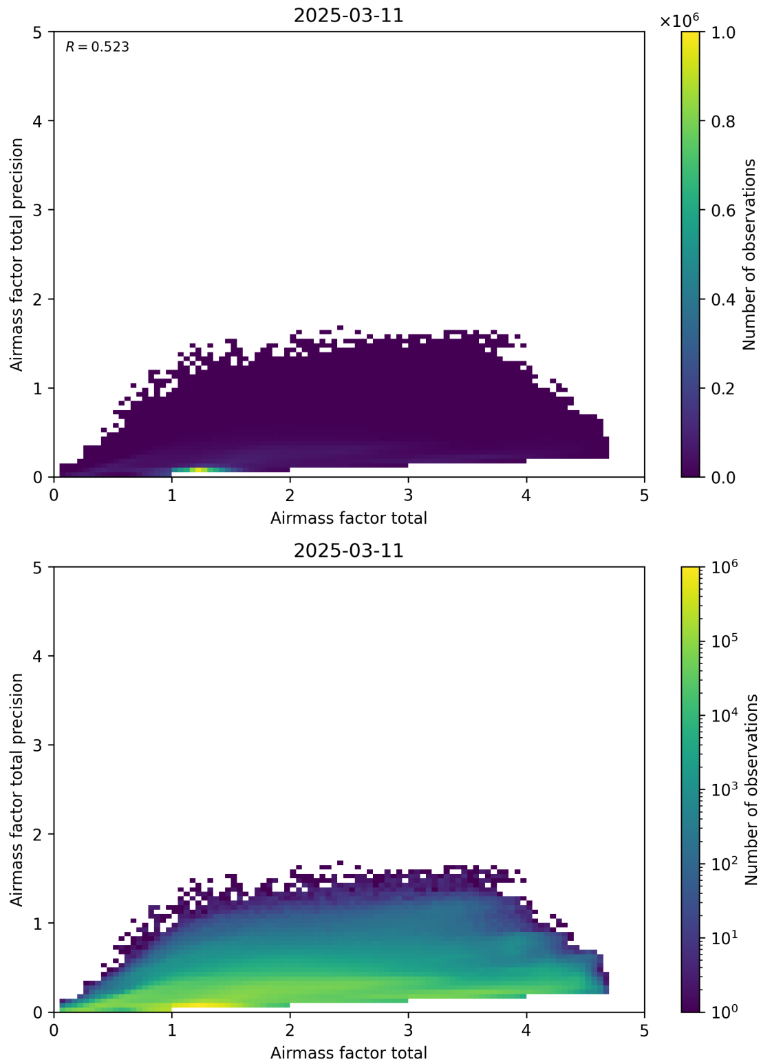
Figure 103: Scatter density plot of “Airmass factor total” against “Airmass factor total precision” for 2025-03-10 to 2025-03-12.
