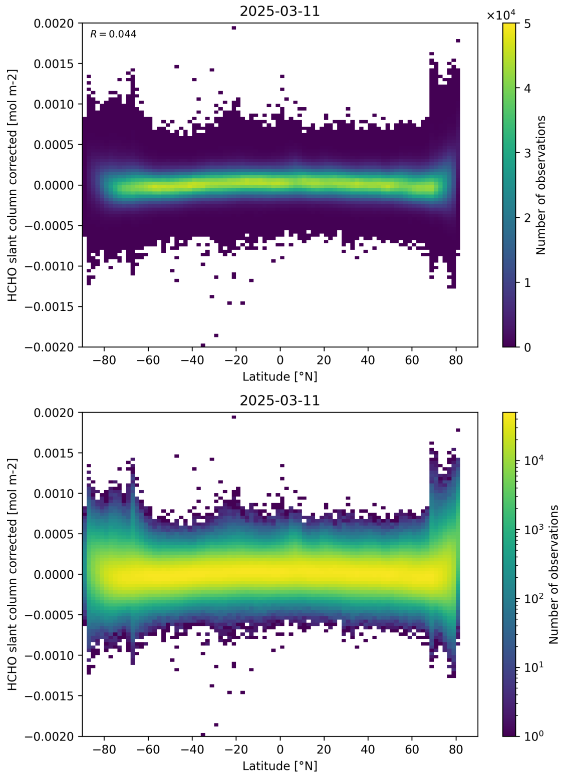
Figure 157: Scatter density plot of “Latitude” against “HCHO slant column corrected” for 2025-03-10 to 2025-03-12.
