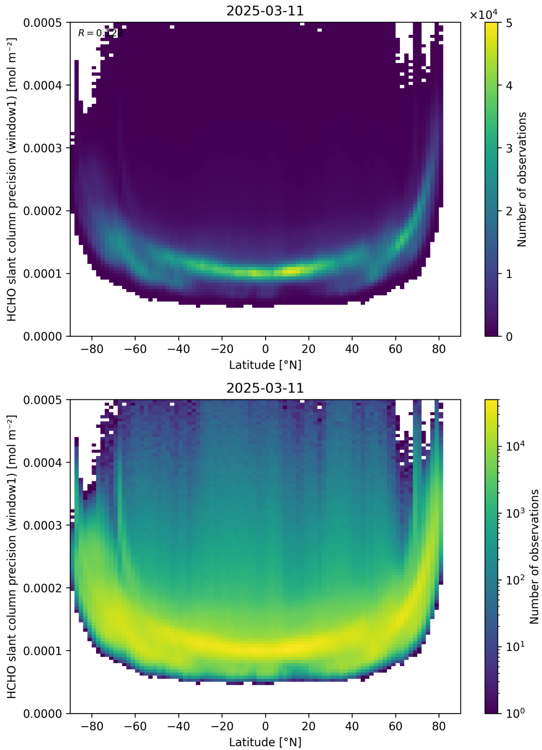
Figure 160: Scatter density plot of “Latitude” against “HCHO slant column precision (window1)” for 2025-03-10 to 2025-03-12.
