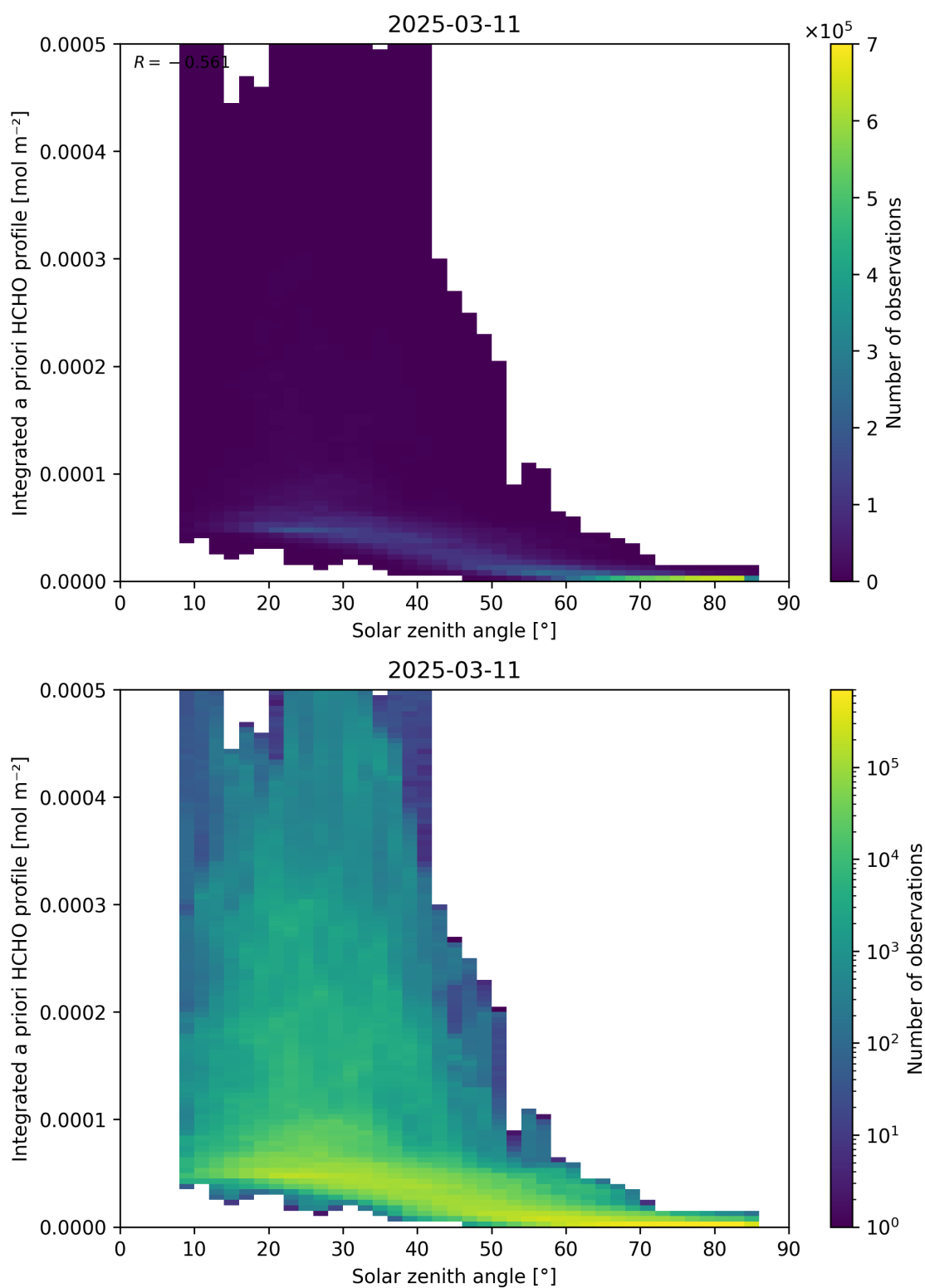
Figure 180: Scatter density plot of “Solar zenith angle” against “Integrated a priori HCHO profile” for 2025-03-10 to 2025-03-12.
