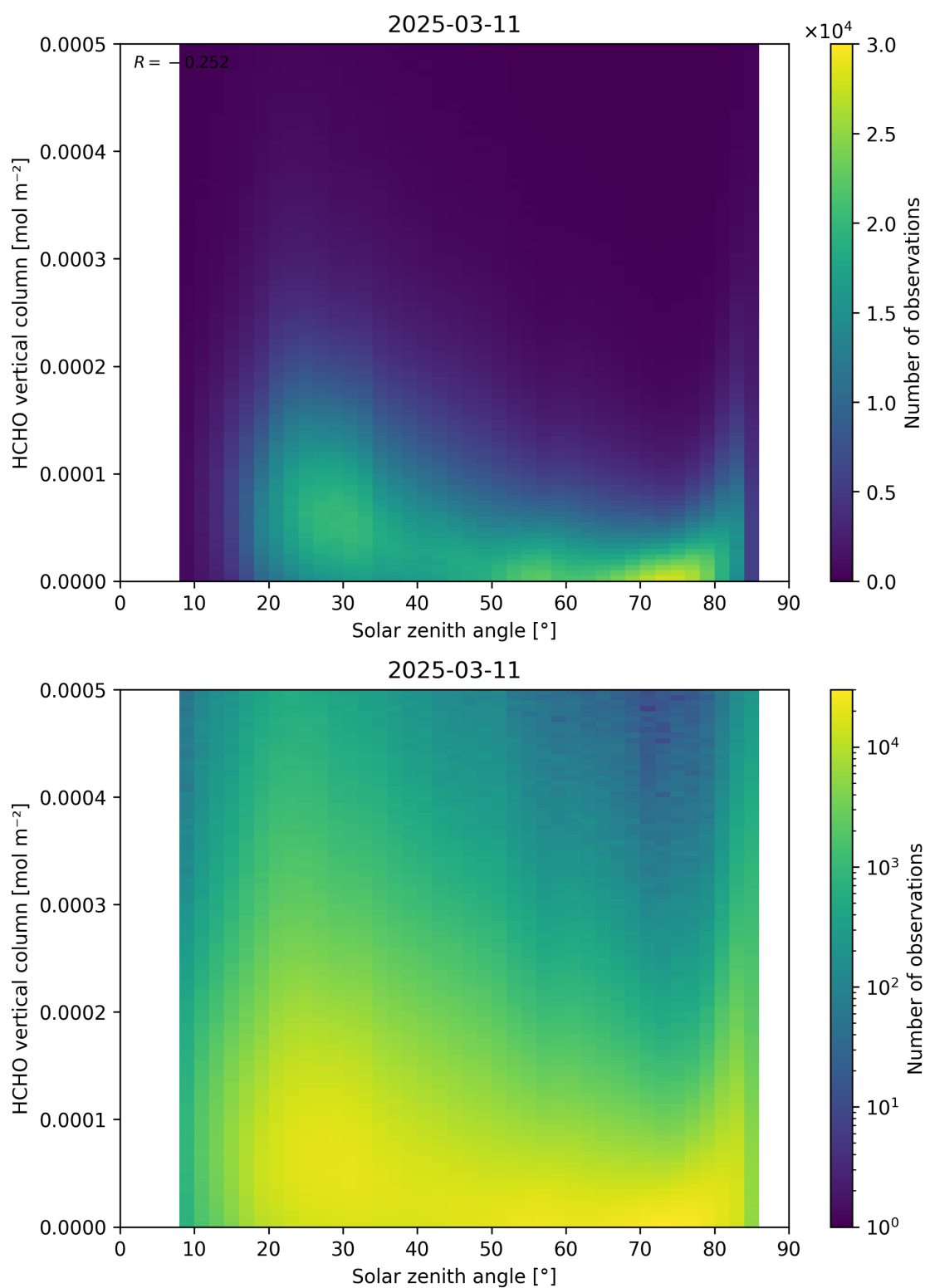
Figure 177: Scatter density plot of “Solar zenith angle” against “HCHO vertical column” for 2025-03-10 to 2025-03-12.
