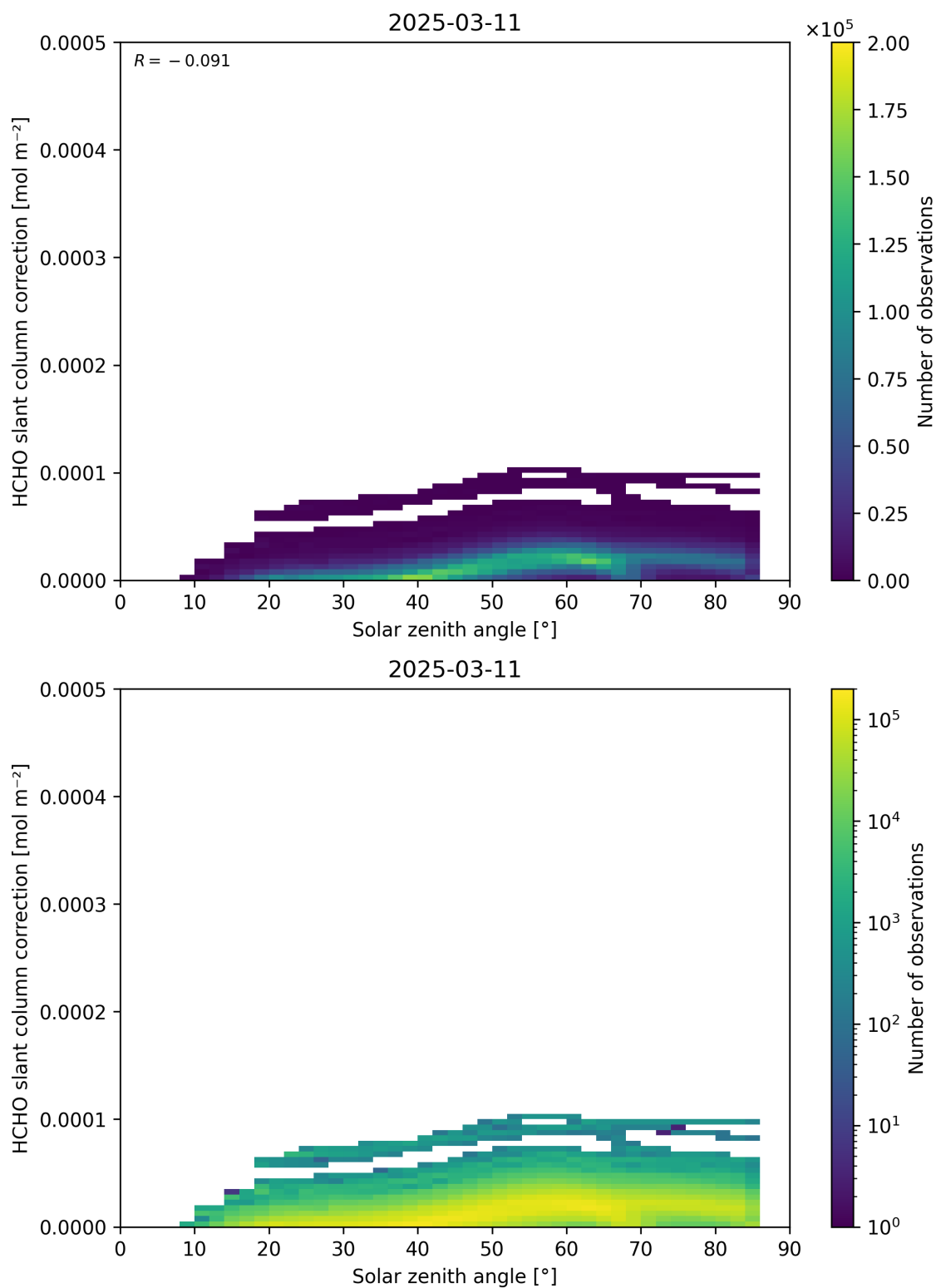
Figure 172: Scatter density plot of “Solar zenith angle” against “HCHO slant column correction” for 2025-03-10 to 2025-03-12.
