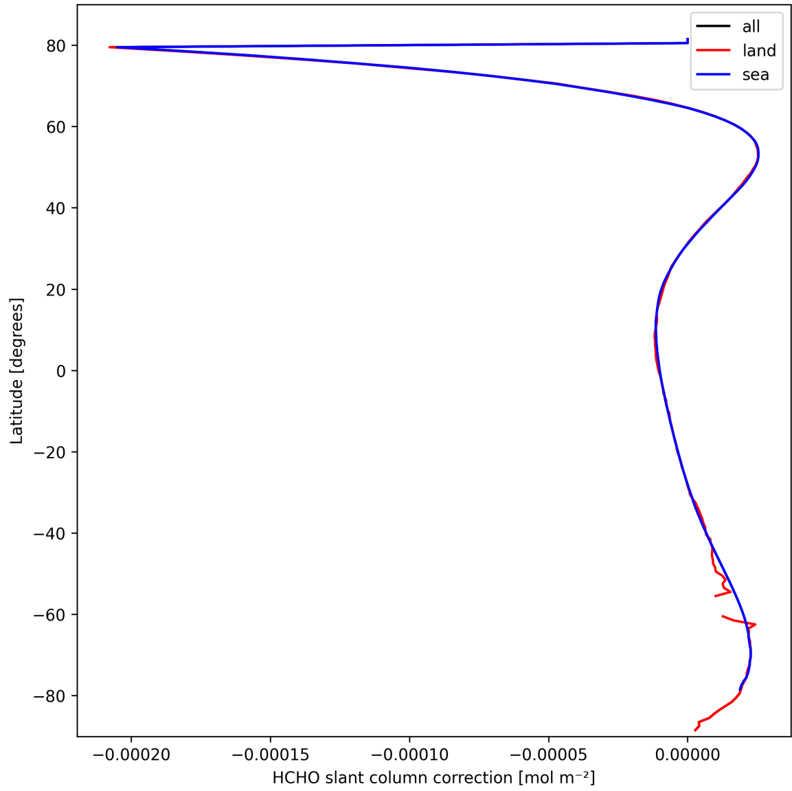
Figure 33: Zonal average of “HCHO slant column correction” for 2025-03-10 to 2025-03-12.
