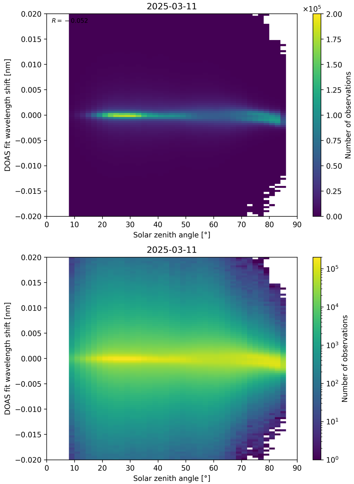
Figure 168: Scatter density plot of “Solar zenith angle” against “DOAS fit wavelength shift” for 2025-03-10 to 2025-03-12.
