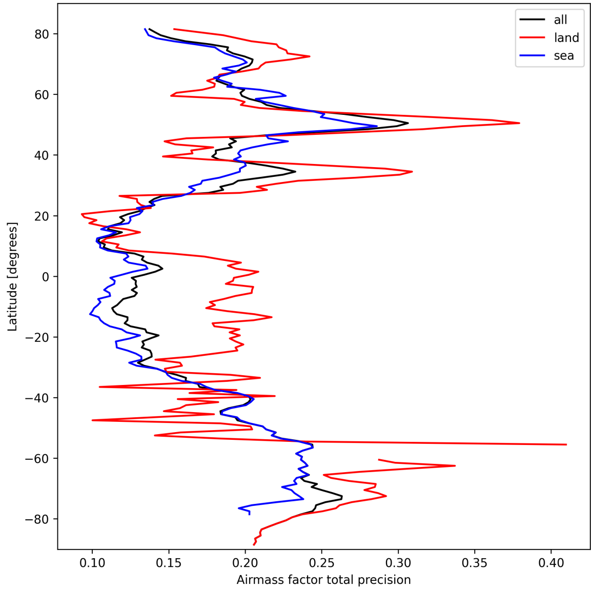
Figure 27: Zonal average of “Airmass factor total precision” for 2025-03-10 to 2025-03-12.
