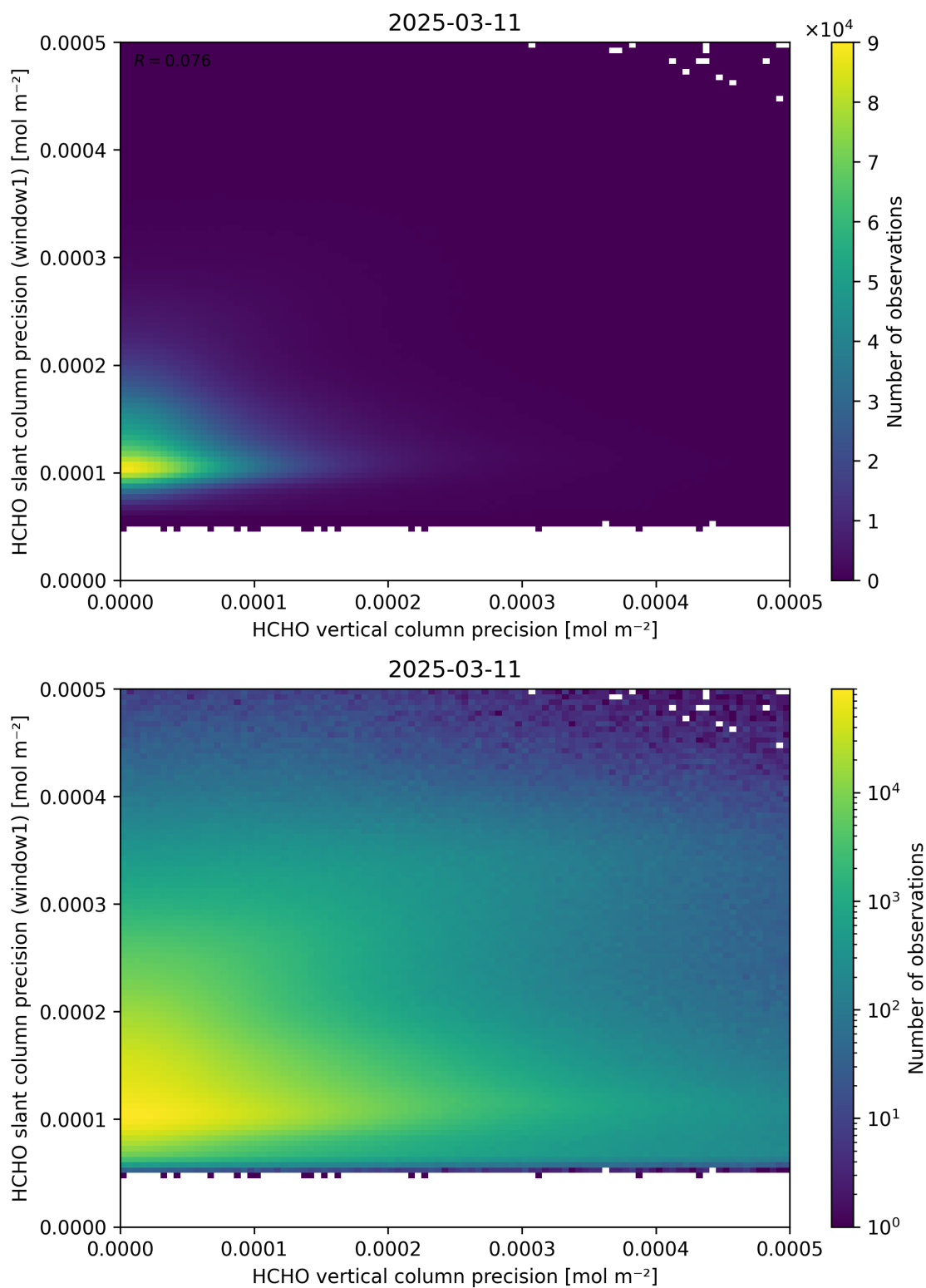
Figure 143: Scatter density plot of “HCHO vertical column precision” against “HCHO slant column precision (window1)” for 2025-03-10 to 2025-03-12.
