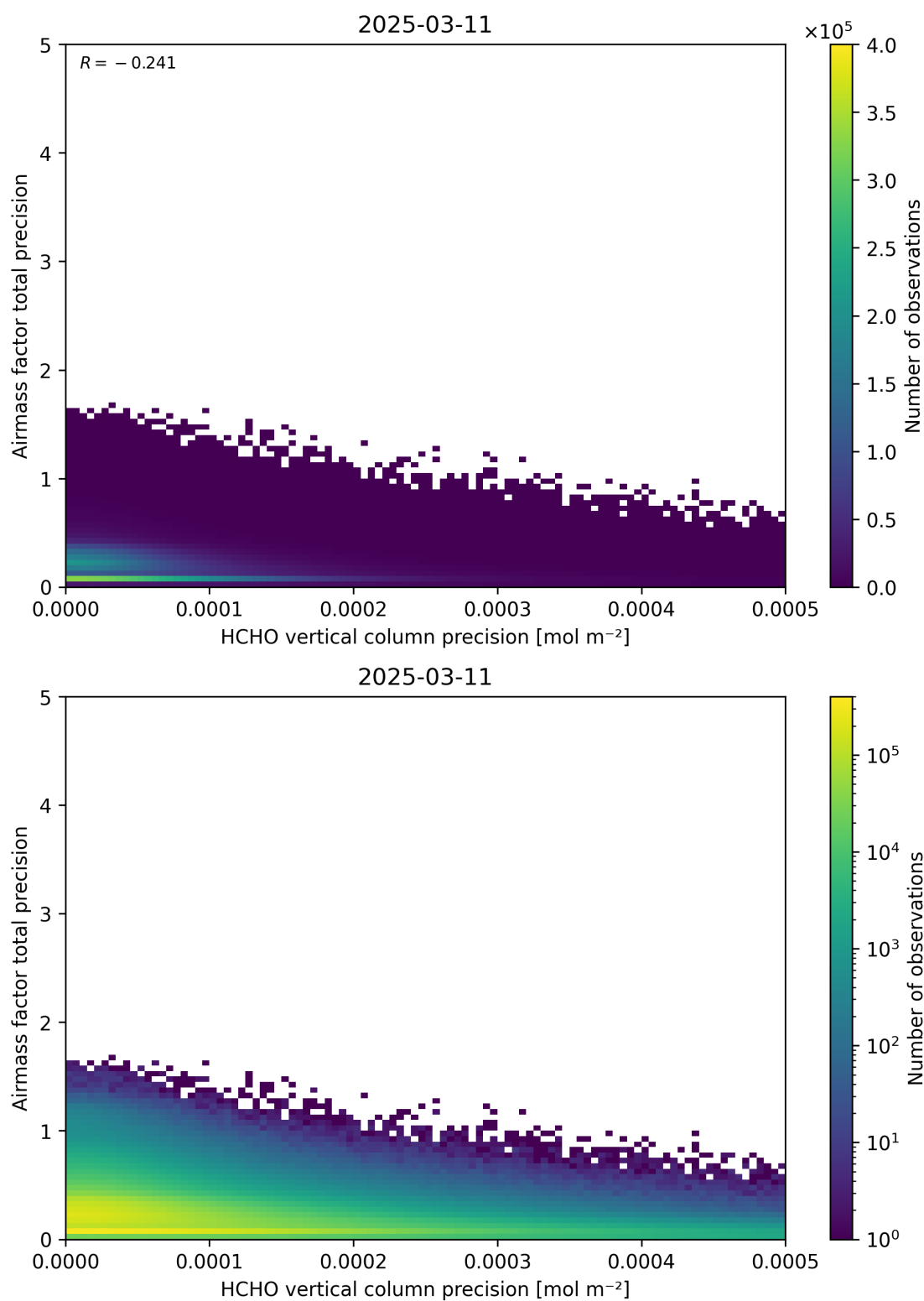
Figure 145: Scatter density plot of “HCHO vertical column precision” against “Airmass factor total precision” for 2025-03-10 to 2025-03-12.
