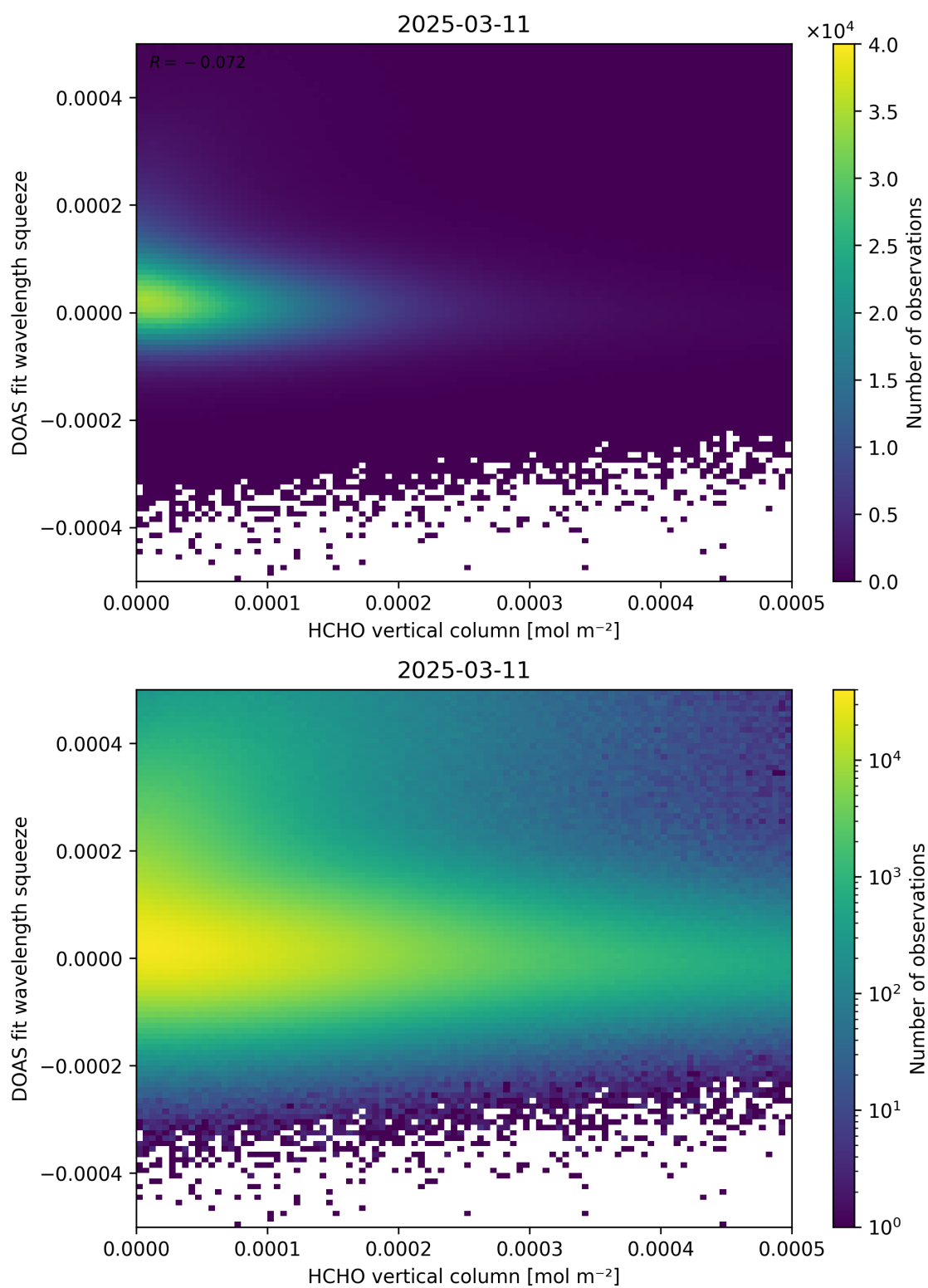
Figure 125: Scatter density plot of “HCHO vertical column” against “DOAS fit wavelength squeeze” for 2025-03-10 to 2025-03-12.
