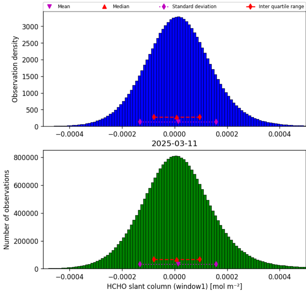
Figure 38: Histogram of “HCHO slant column (window1)” for 2025-03-10 to 2025-03-12
