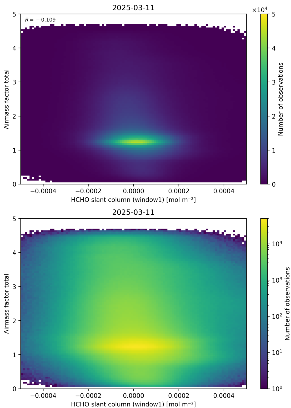
Figure 85: Scatter density plot of “HCHO slant column (window1)” against “Airmass factor total” for 2025-03-10 to 2025-03-12.
