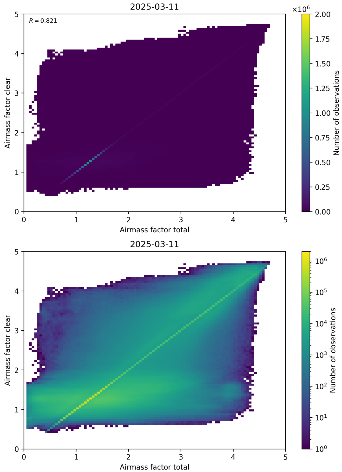
Figure 100: Scatter density plot of “Airmass factor total” against “Airmass factor clear” for 2025-03-10 to 2025-03-12.
