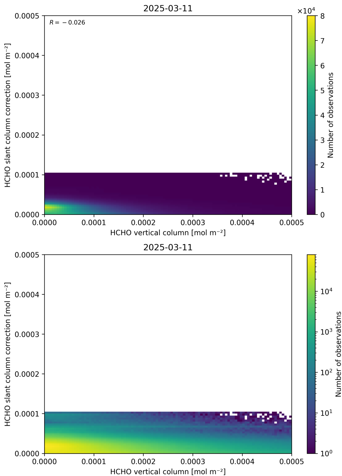
Figure 128: Scatter density plot of “HCHO vertical column” against “HCHO slant column correction” for 2025-03-10 to 2025-03-12.
