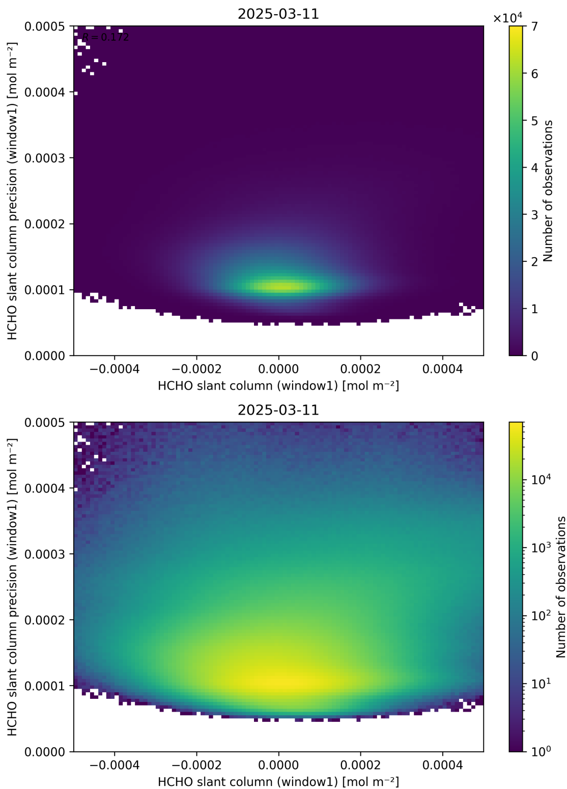
Figure 84: Scatter density plot of “HCHO slant column (window1)” against “HCHO slant column precision (window1)” for 2025-03-10 to 2025-03-12.
