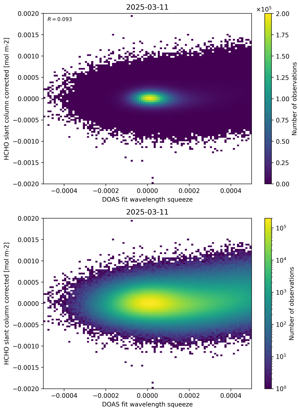
Figure 69: Scatter density plot of “DOAS fit wavelength squeeze” against “HCHO slant column corrected” for 2025-03-10 to 2025-03-12.
