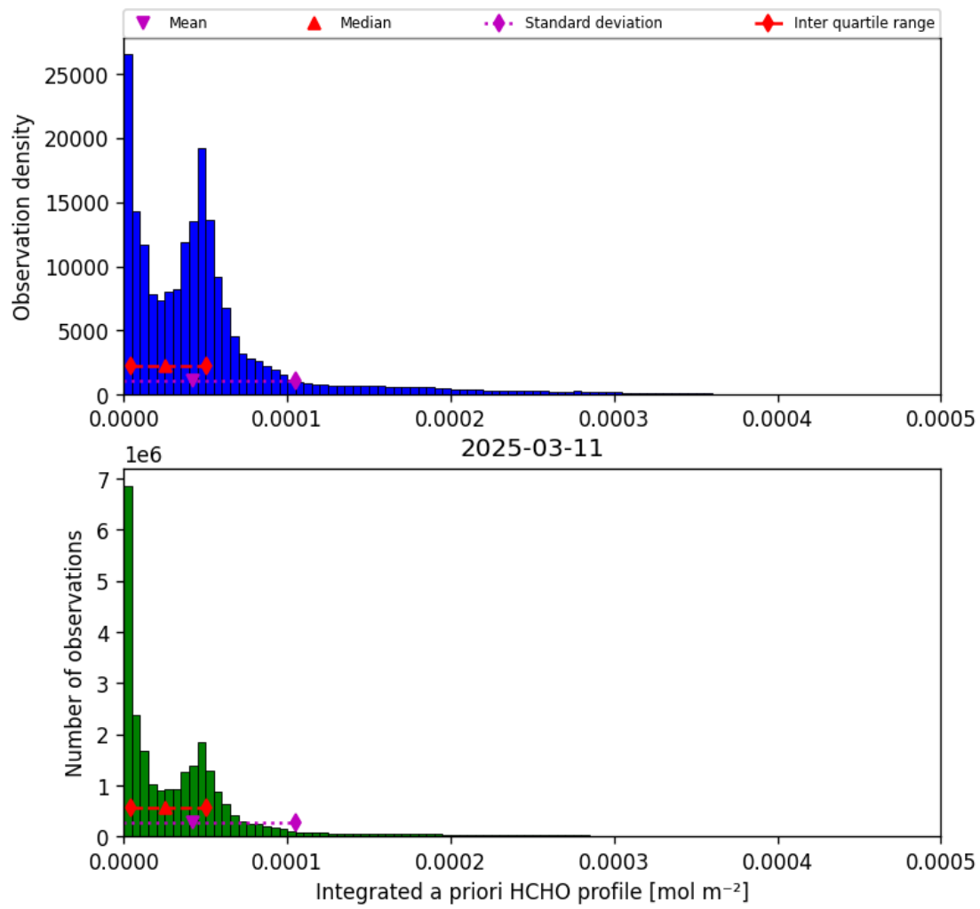
Figure 43: Histogram of “Integrated a priori HCHO profile” for 2025-03-10 to 2025-03-12
