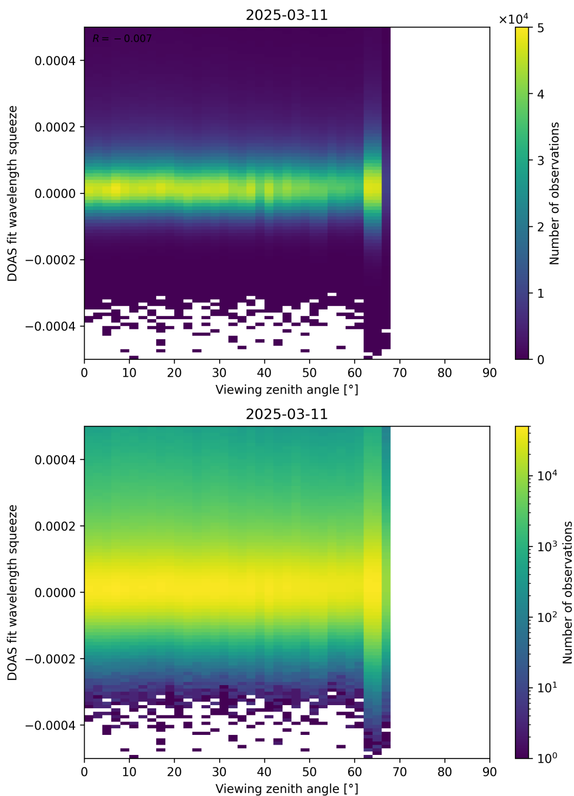
Figure 184: Scatter density plot of “Viewing zenith angle” against “DOAS fit wavelength squeeze” for 2025-03-10 to 2025-03-12.
