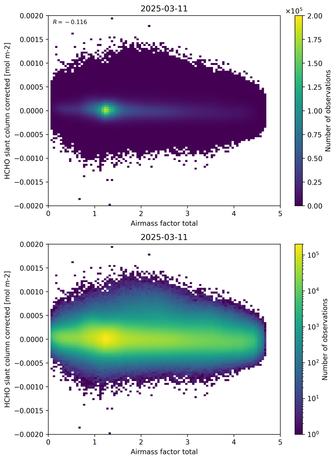
Figure 101: Scatter density plot of “Airmass factor total” against “HCHO slant column corrected” for 2025-03-10 to 2025-03-12.
