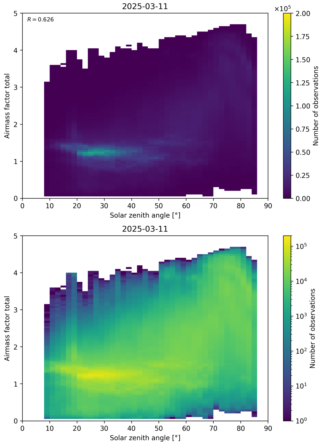
Figure 175: Scatter density plot of “Solar zenith angle” against “Airmass factor total” for 2025-03-10 to 2025-03-12.
