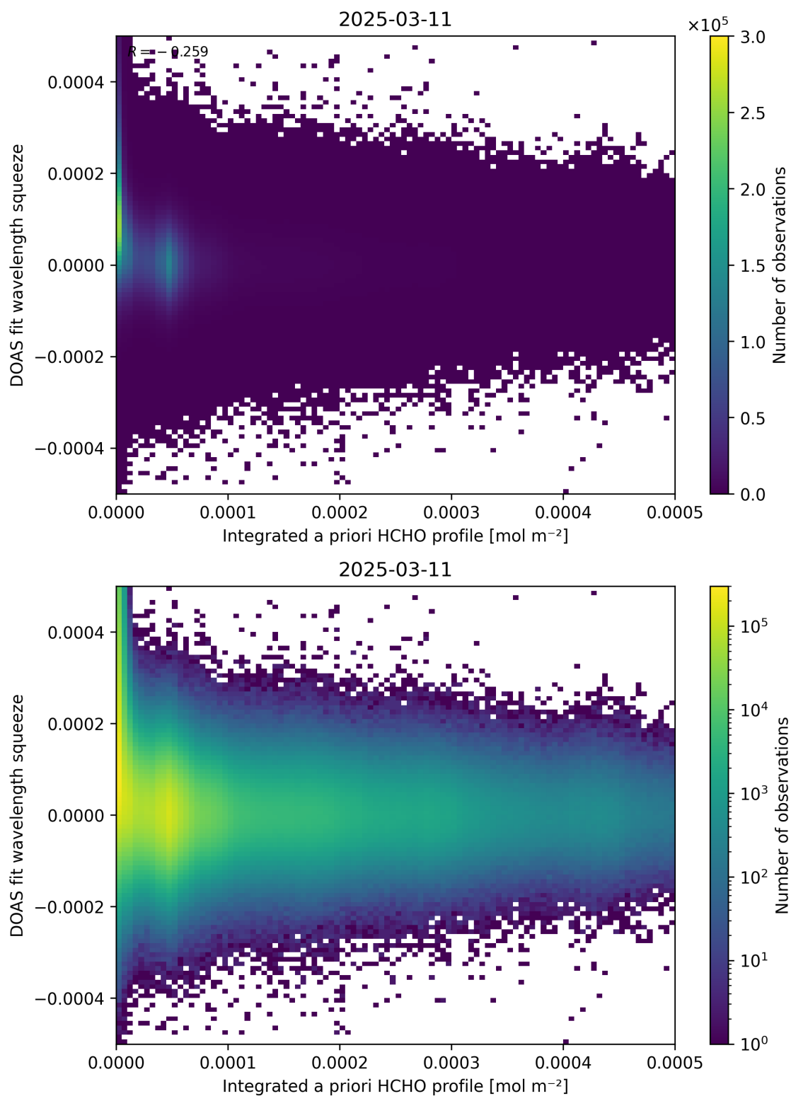
Figure 150: Scatter density plot of “Integrated a priori HCHO profile” against “DOAS fit wavelength squeeze” for 2025-03-10 to 2025-03-12.
