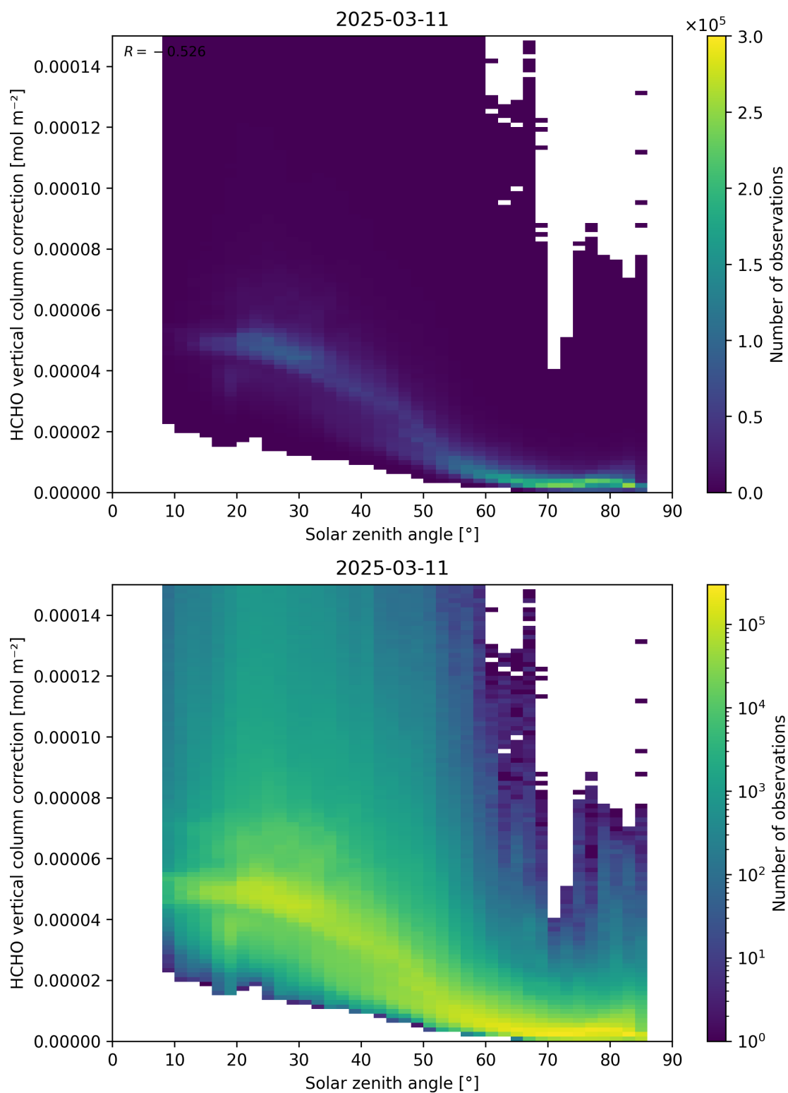
Figure 178: Scatter density plot of “Solar zenith angle” against “HCHO vertical column correction” for 2025-03-10 to 2025-03-12.
