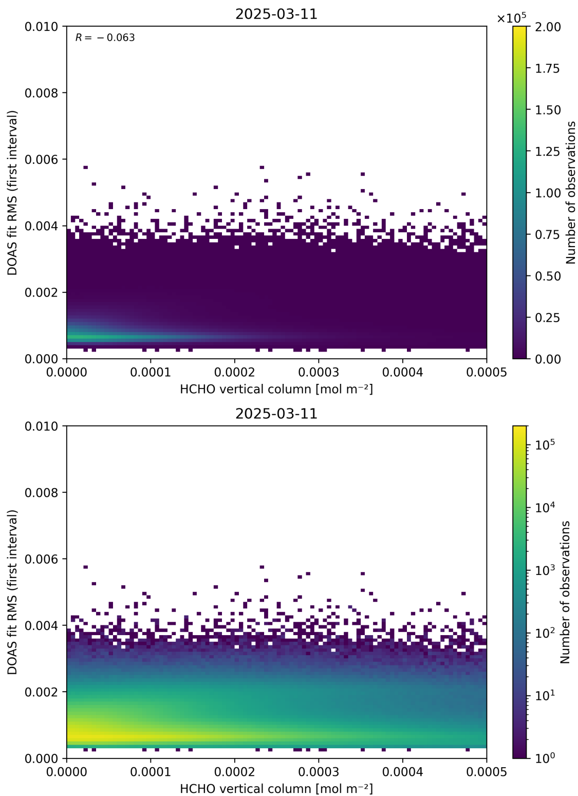
Figure 123: Scatter density plot of “HCHO vertical column” against “DOAS fit RMS (first interval)” for 2025-03-10 to 2025-03-12.
