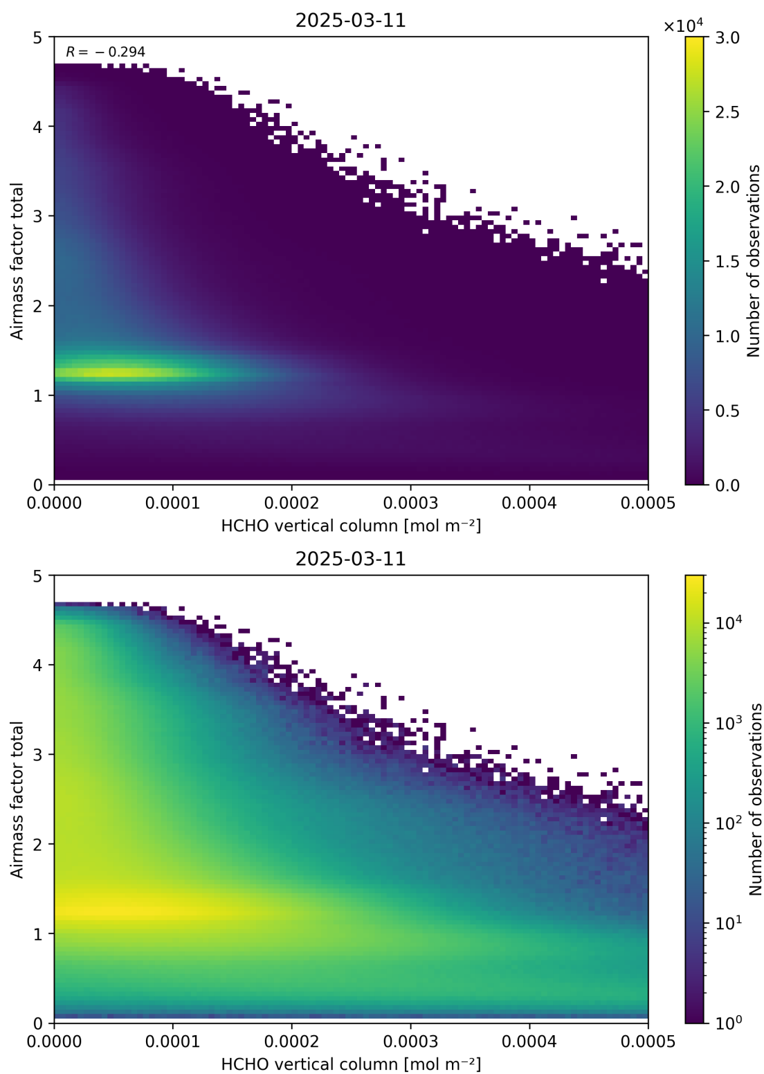
Figure 131: Scatter density plot of “HCHO vertical column” against “Airmass factor total” for 2025-03-10 to 2025-03-12.
