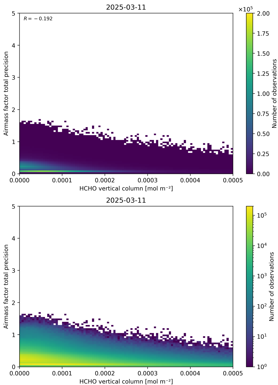
Figure 132: Scatter density plot of “HCHO vertical column” against “Airmass factor total precision” for 2025-03-10 to 2025-03-12.
