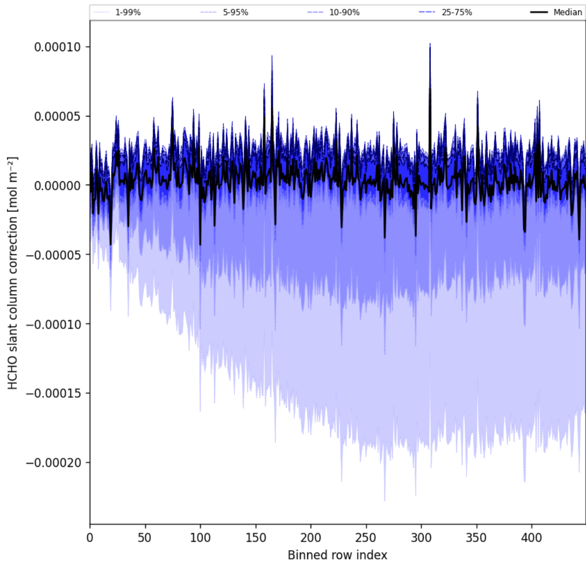
Figure 61: Along track statistics of “HCHO slant column correction” for 2025-03-10 to 2025-03-12
