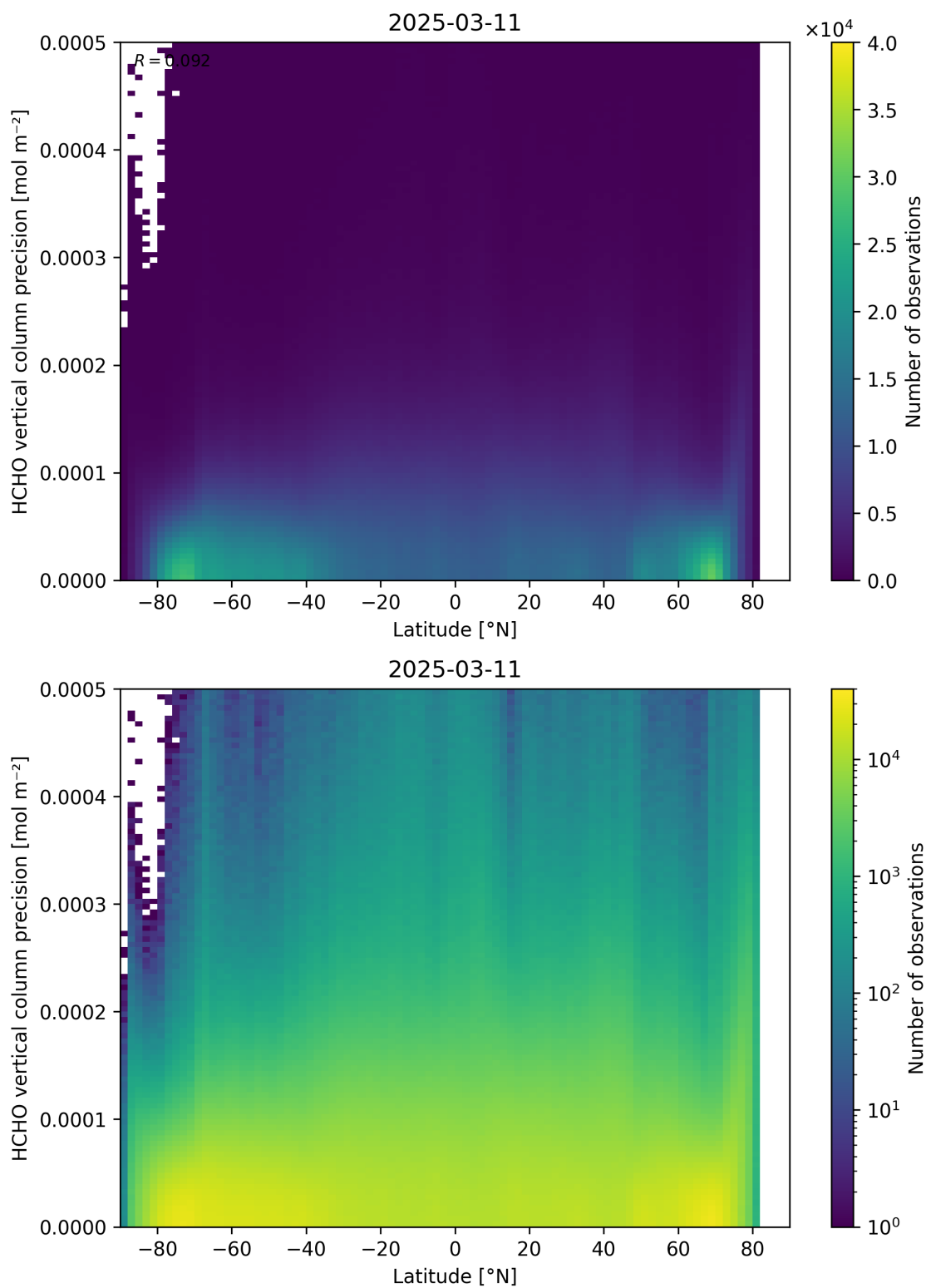
Figure 165: Scatter density plot of “Latitude” against “HCHO vertical column precision” for 2025-03-10 to 2025-03-12.
