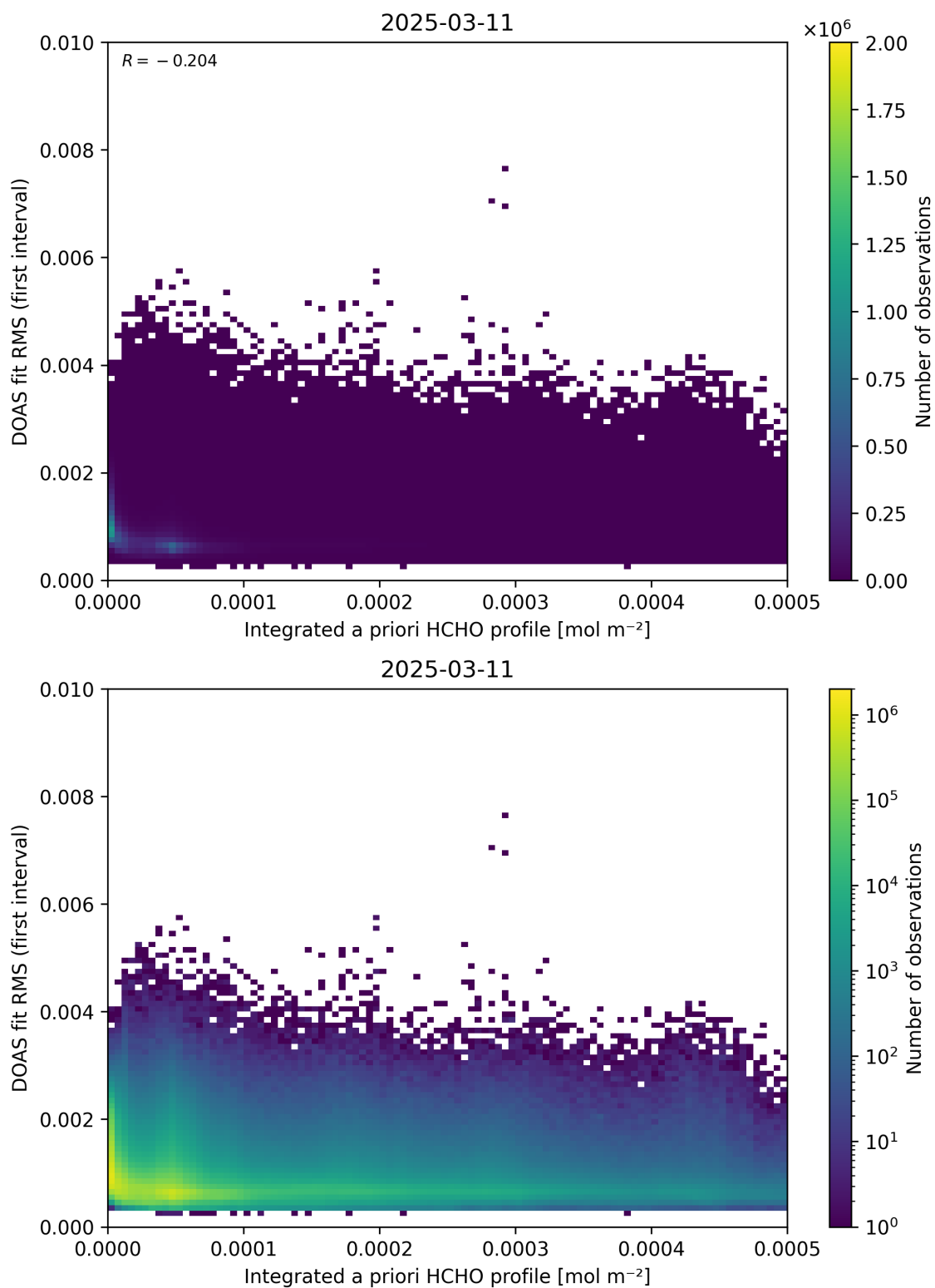
Figure 148: Scatter density plot of “Integrated a priori HCHO profile” against “DOAS fit RMS (first interval)” for 2025-03-10 to 2025-03-12.
