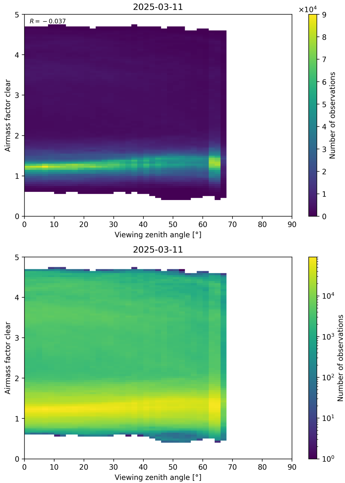
Figure 185: Scatter density plot of “Viewing zenith angle” against “Airmass factor clear” for 2025-03-10 to 2025-03-12.
