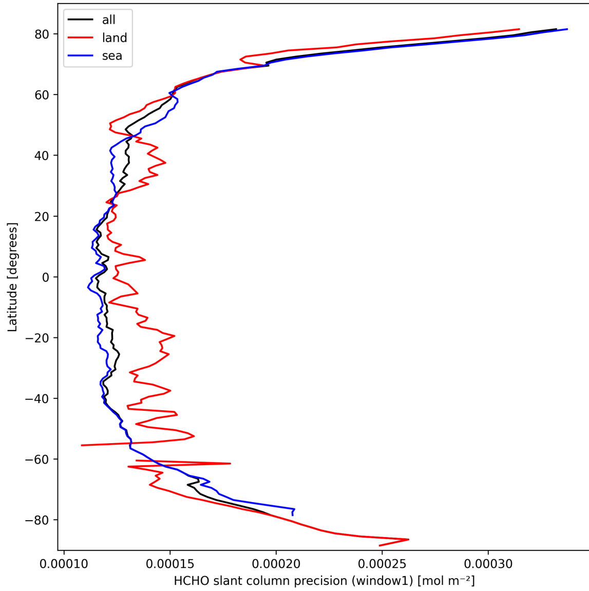
Figure 25: Zonal average of “HCHO slant column precision (window1)” for 2025-03-10 to 2025-03-12.
