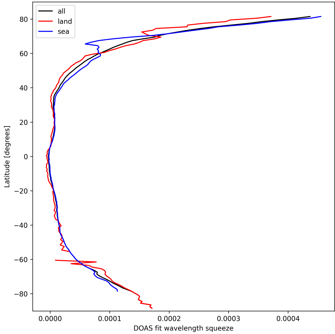
Figure 31: Zonal average of “DOAS fit wavelength squeeze” for 2025-03-10 to 2025-03-12.
