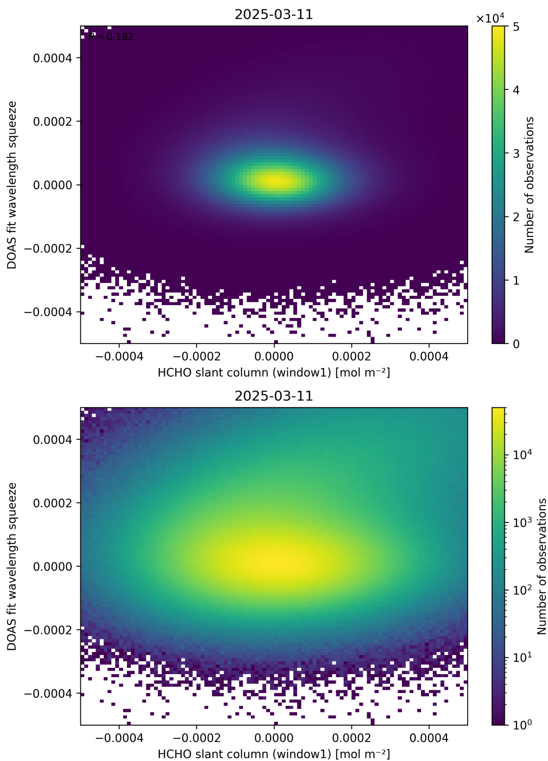
Figure 80: Scatter density plot of “HCHO slant column (window1)” against “DOAS fit wavelength squeeze” for 2025-03-10 to 2025-03-12.
