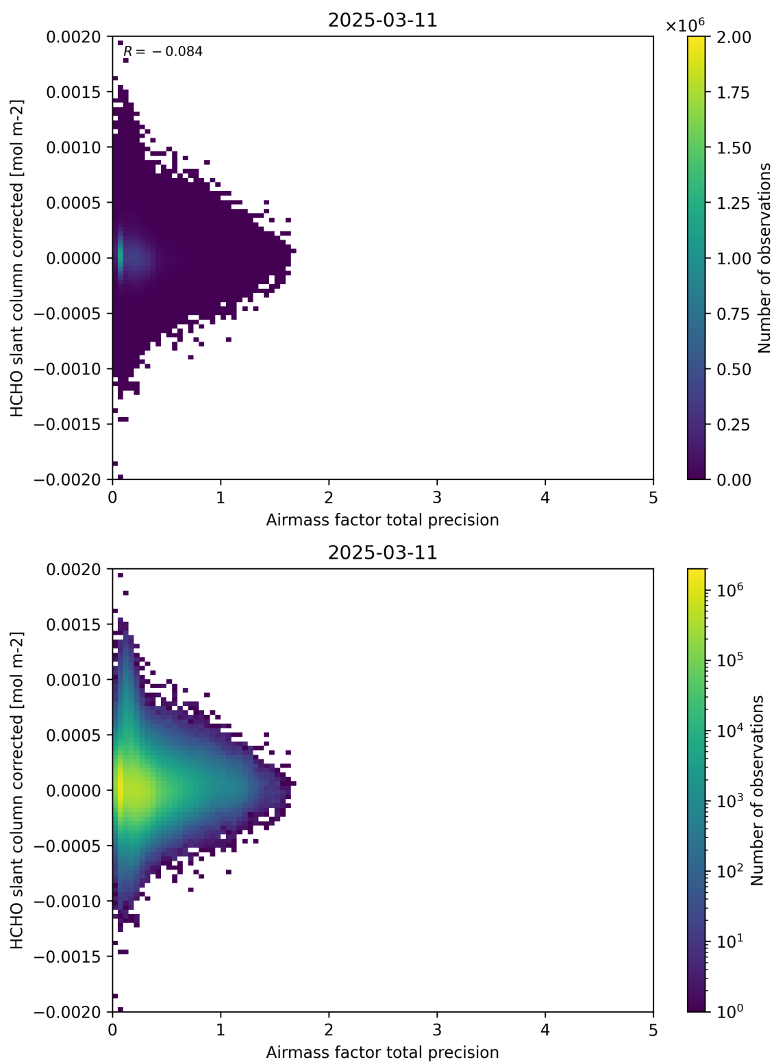
Figure 109: Scatter density plot of “Airmass factor total precision” against “HCHO slant column corrected” for 2025-03-10 to 2025-03-12.
