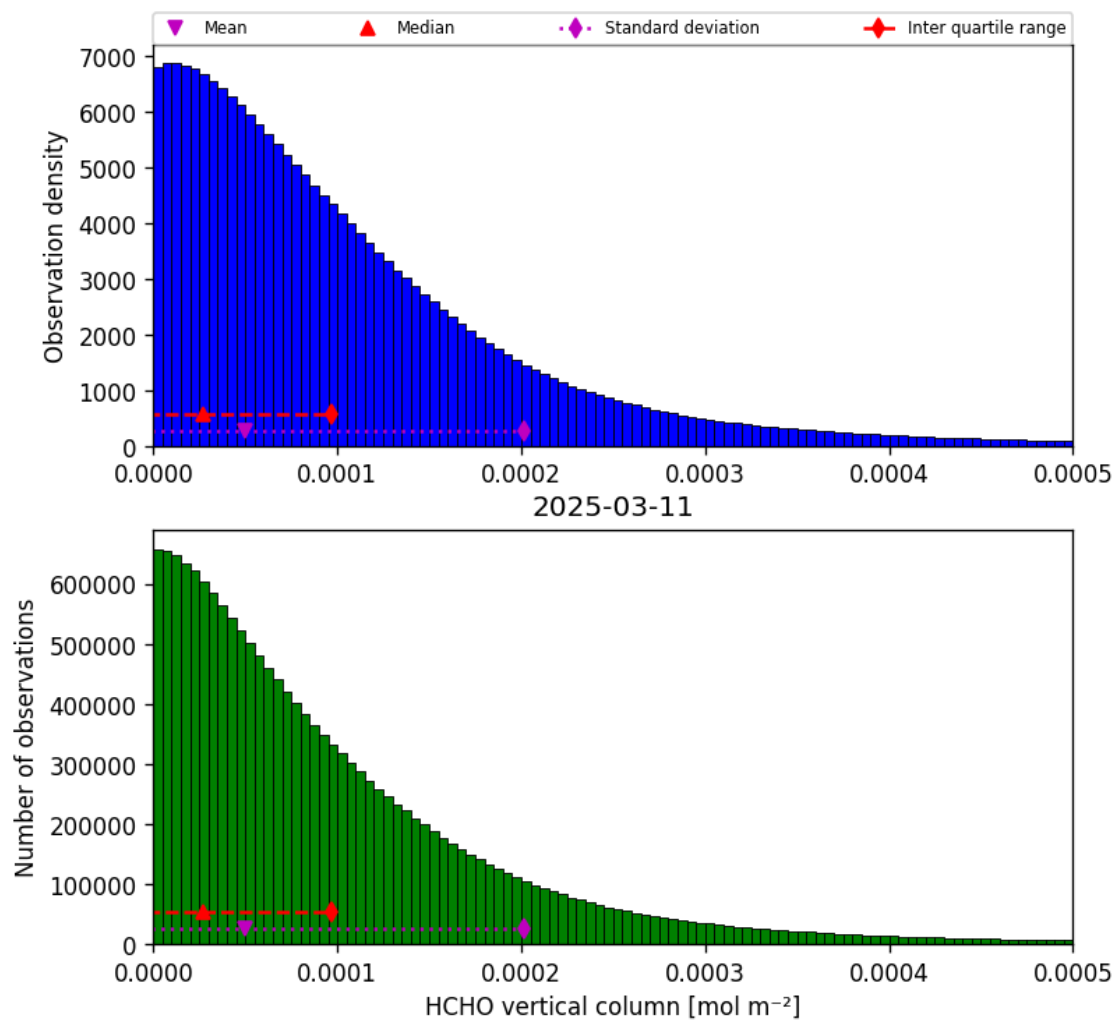
Figure 35: Histogram of “HCHO vertical column” for 2025-03-10 to 2025-03-12
