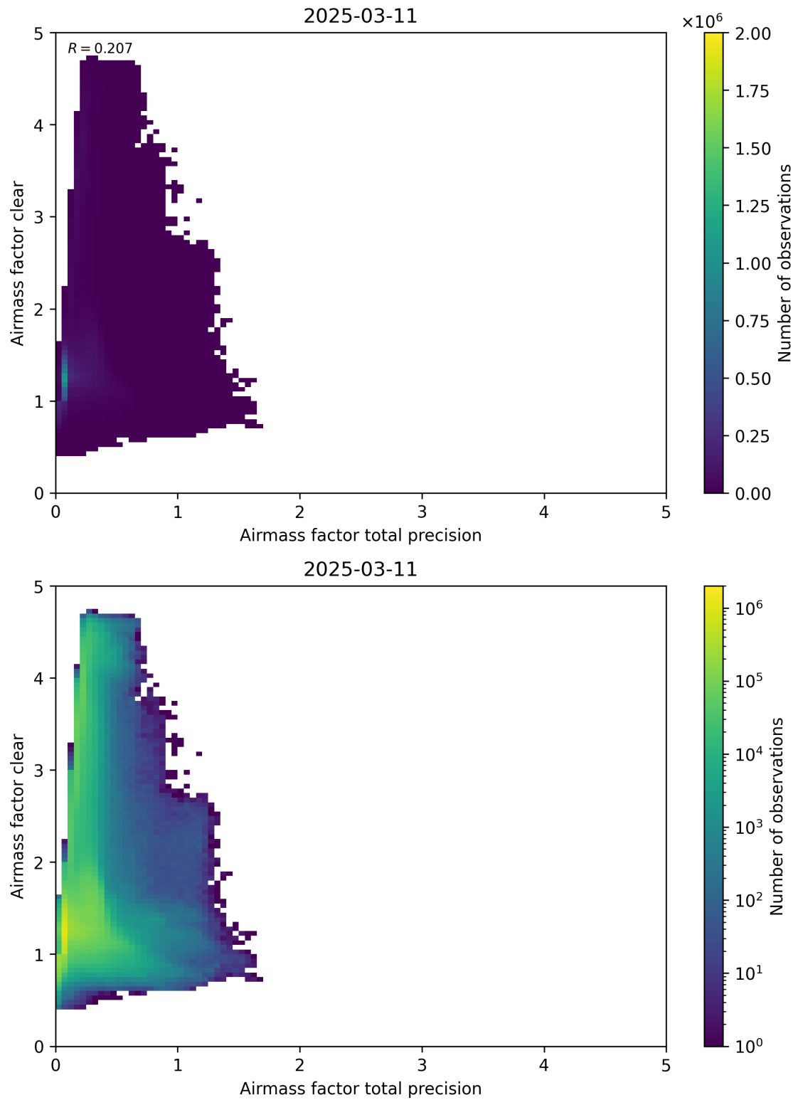
Figure 108: Scatter density plot of “Airmass factor total precision” against “Airmass factor clear” for 2025-03-10 to 2025-03-12.
