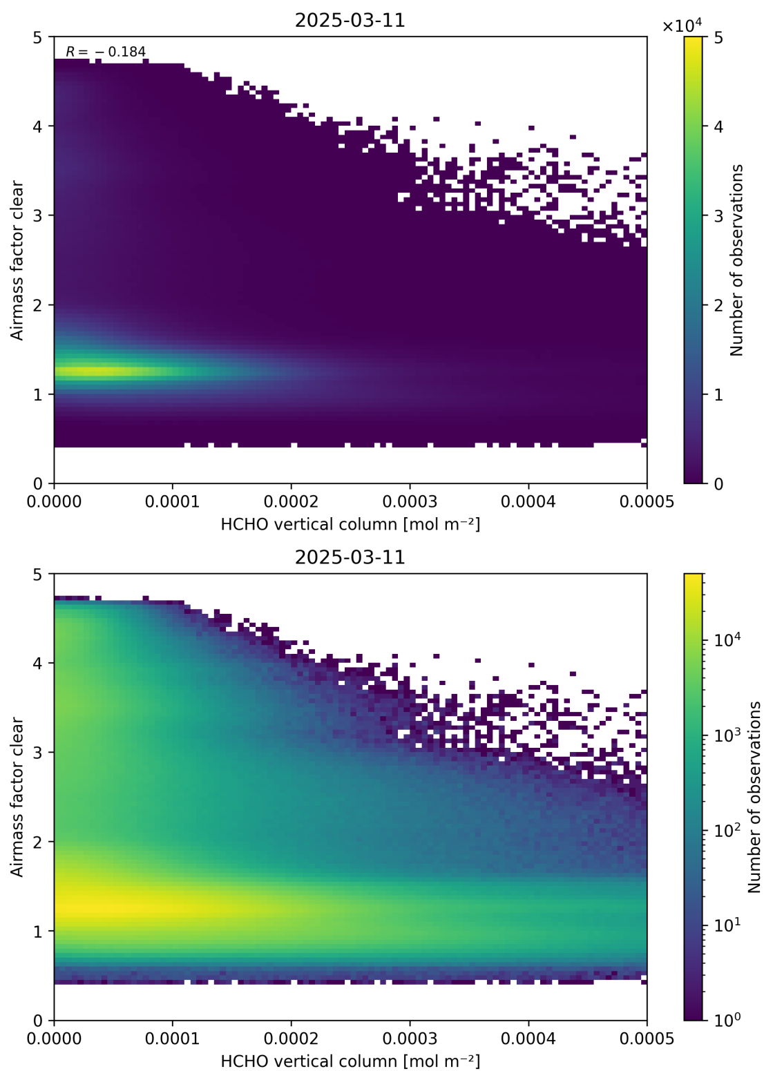
Figure 126: Scatter density plot of “HCHO vertical column” against “Airmass factor clear” for 2025-03-10 to 2025-03-12.
