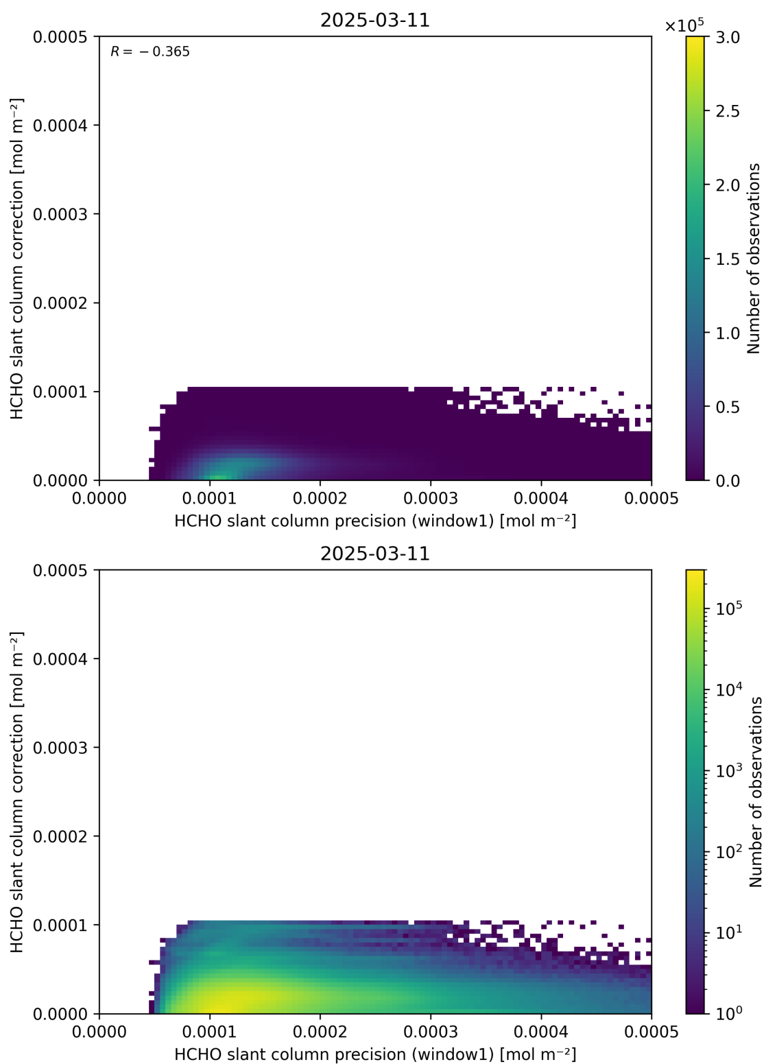
Figure 93: Scatter density plot of “HCHO slant column precision (window1)” against “HCHO slant column correction” for 2025-03-10 to 2025-03-12.
