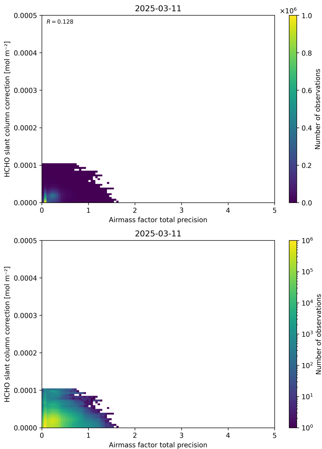
Figure 110: Scatter density plot of “Airmass factor total precision” against “HCHO slant column correction” for 2025-03-10 to 2025-03-12.
