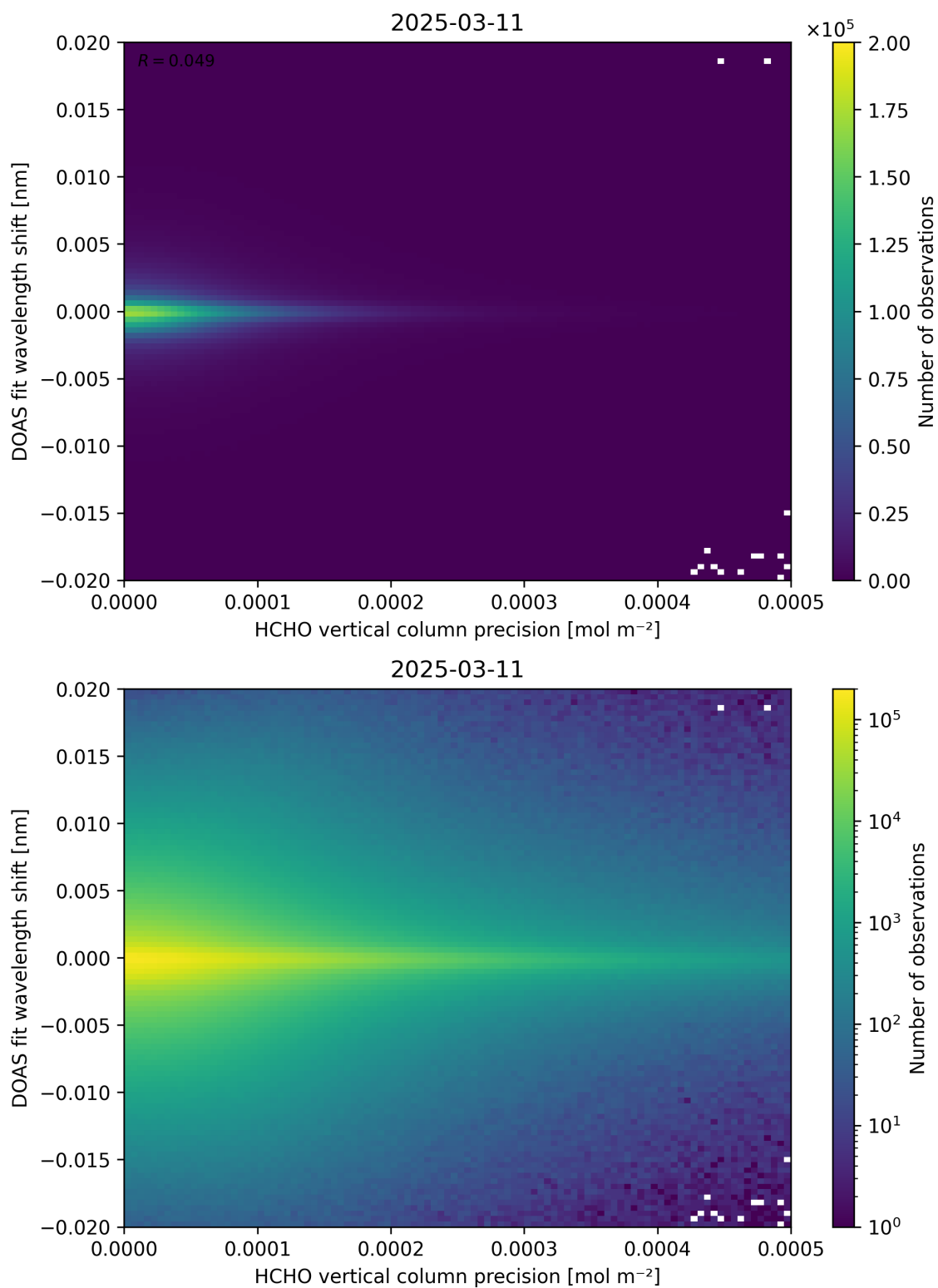
Figure 137: Scatter density plot of “HCHO vertical column precision” against “DOAS fit wavelength shift” for 2025-03-10 to 2025-03-12.
