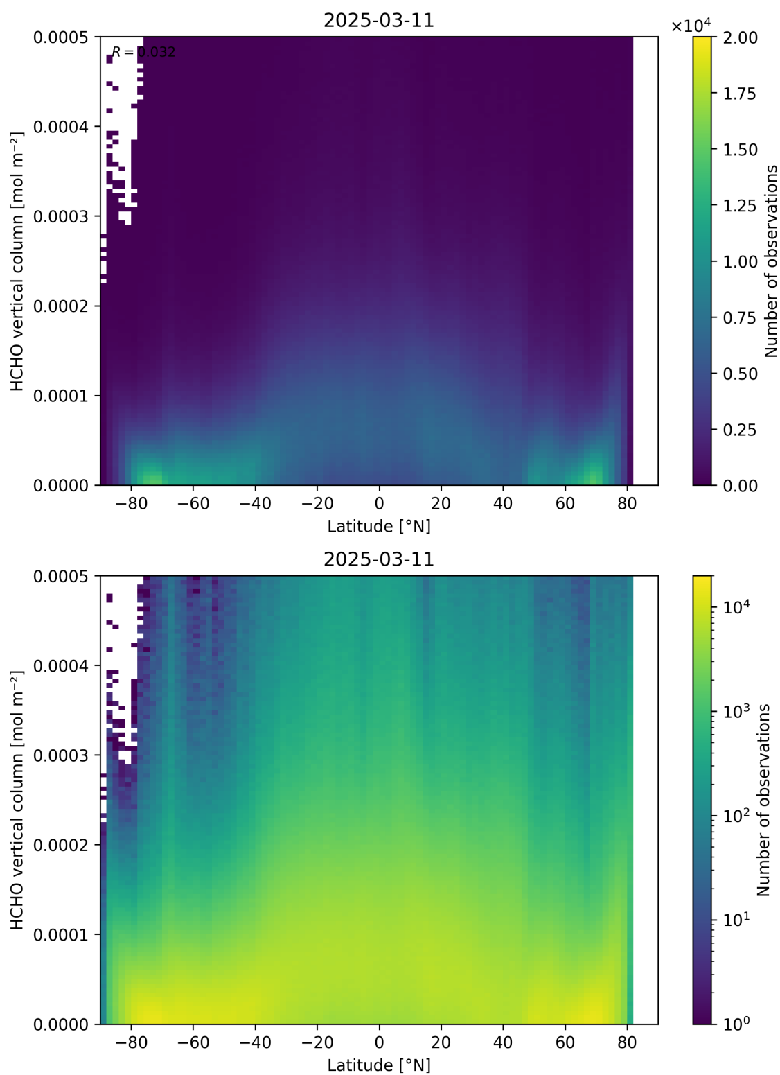
Figure 163: Scatter density plot of “Latitude” against “HCHO vertical column” for 2025-03-10 to 2025-03-12.
