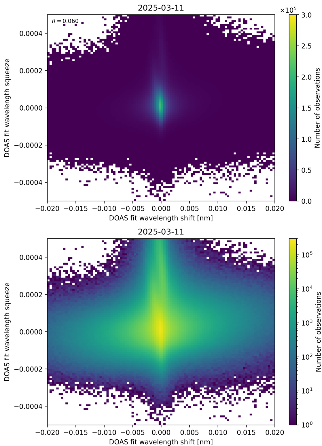
Figure 65: Scatter density plot of “DOAS fit wavelength shift” against “DOAS fit wavelength squeeze” for 2025-03-10 to 2025-03-12.
