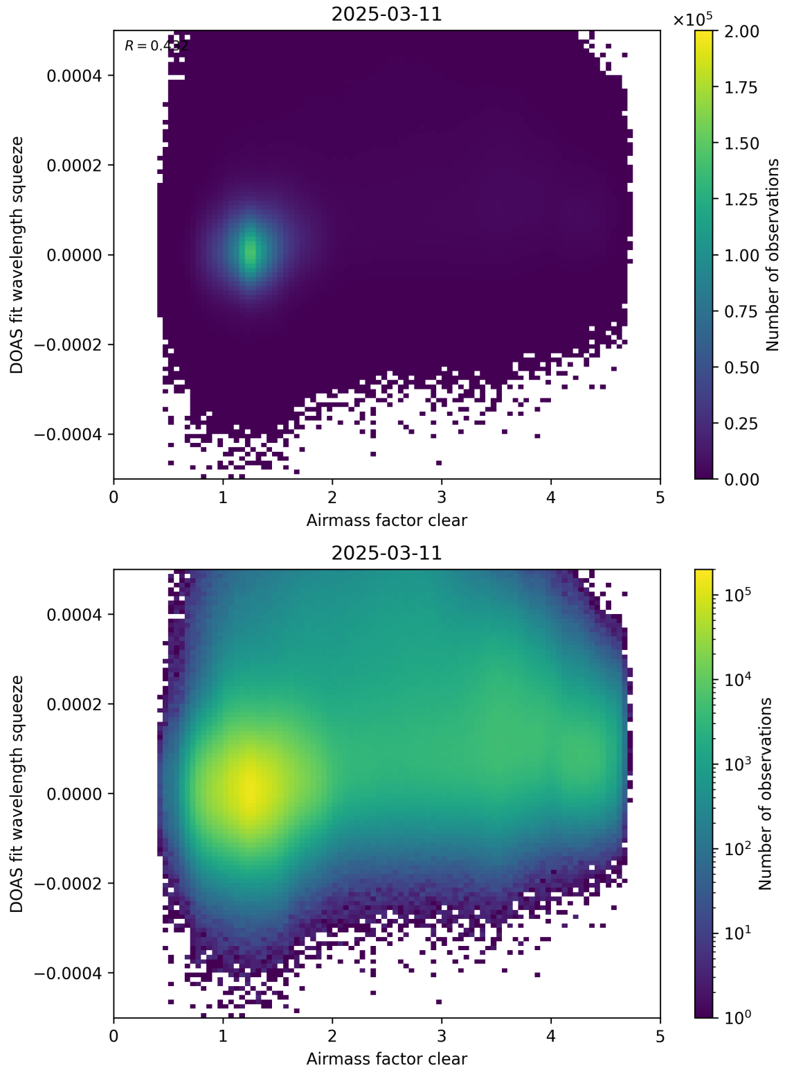
Figure 73: Scatter density plot of “Airmass factor clear” against “DOAS fit wavelength squeeze” for 2025-03-10 to 2025-03-12.
