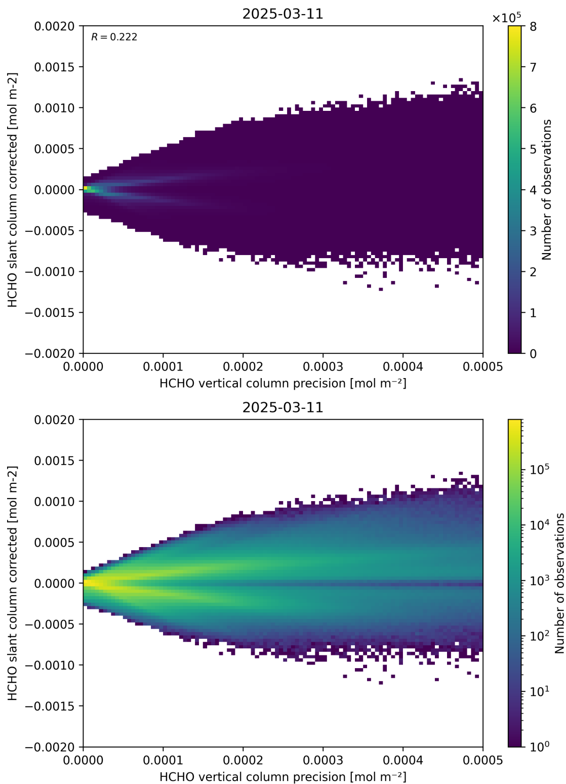
Figure 140: Scatter density plot of “HCHO vertical column precision” against “HCHO slant column corrected” for 2025-03-10 to 2025-03-12.
