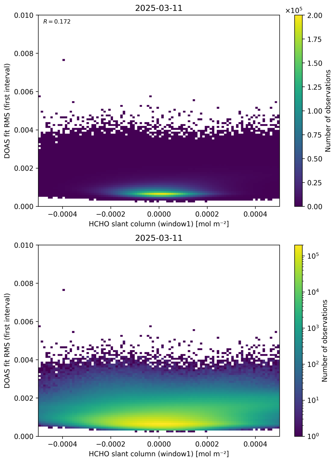
Figure 78: Scatter density plot of “HCHO slant column (window1)” against “DOAS fit RMS (first interval)” for 2025-03-10 to 2025-03-12.
