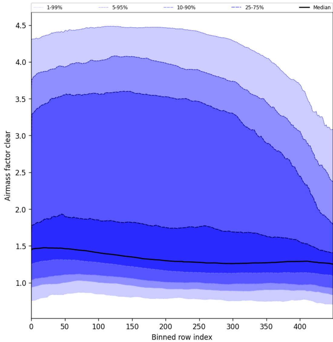
Figure 56: Along track statistics of “Airmass factor clear” for 2025-03-10 to 2025-03-12
