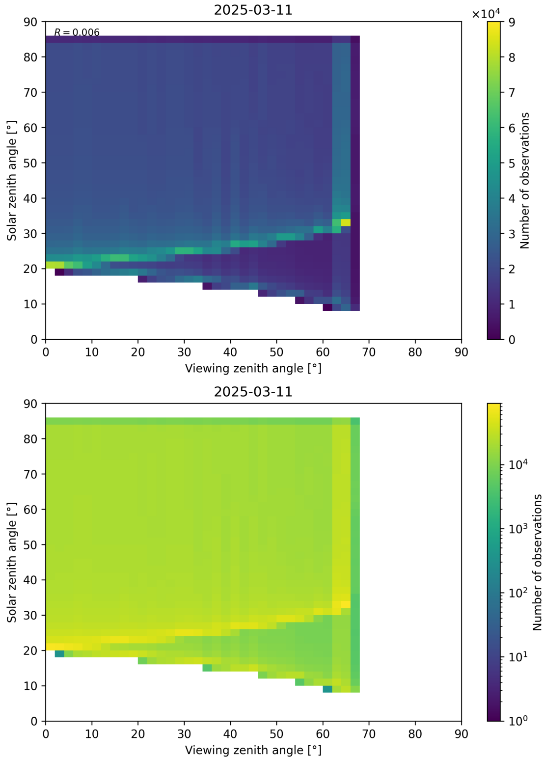
Figure 197: Scatter density plot of “Viewing zenith angle” against “Solar zenith angle” for 2025-03-10 to 2025-03-12.
