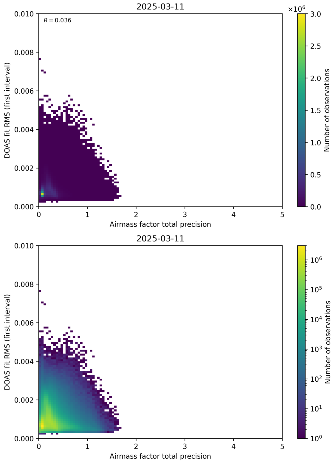
Figure 105: Scatter density plot of “Airmass factor total precision” against “DOAS fit RMS (first interval)” for 2025-03-10 to 2025-03-12.
