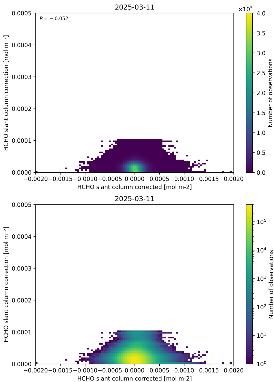
Figure 77: Scatter density plot of “HCHO slant column corrected” against “HCHO slant column correction” for 2025-03-10 to 2025-03-12.
