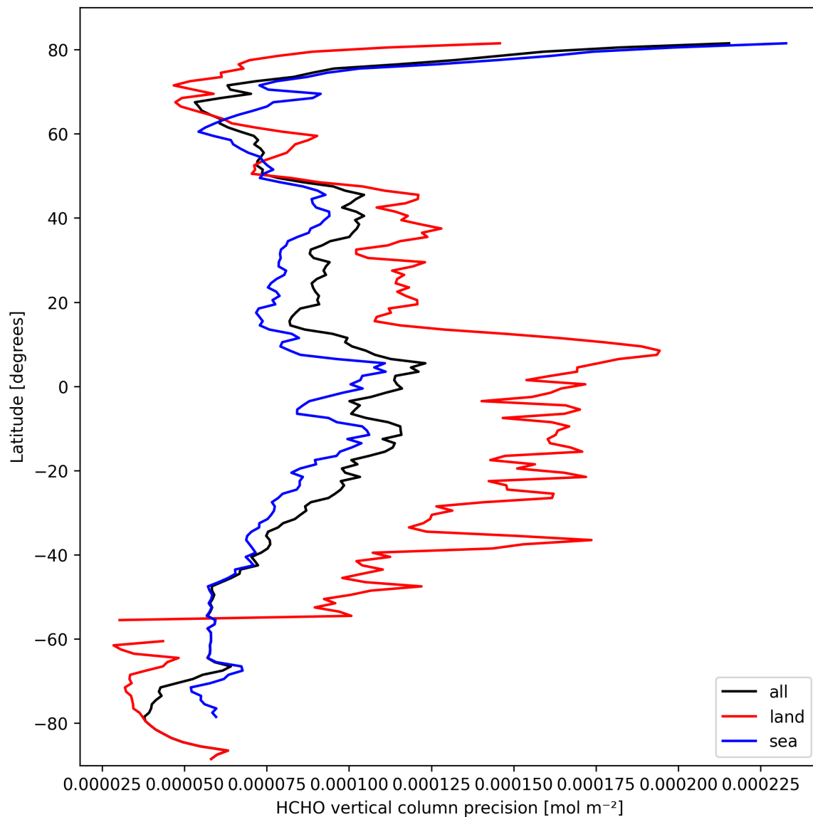
Figure 22: Zonal average of “HCHO vertical column precision” for 2025-03-10 to 2025-03-12.
