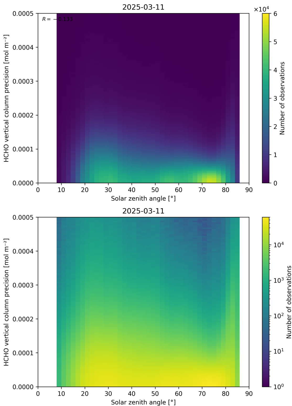
Figure 179: Scatter density plot of “Solar zenith angle” against “HCHO vertical column precision” for 2025-03-10 to 2025-03-12.
