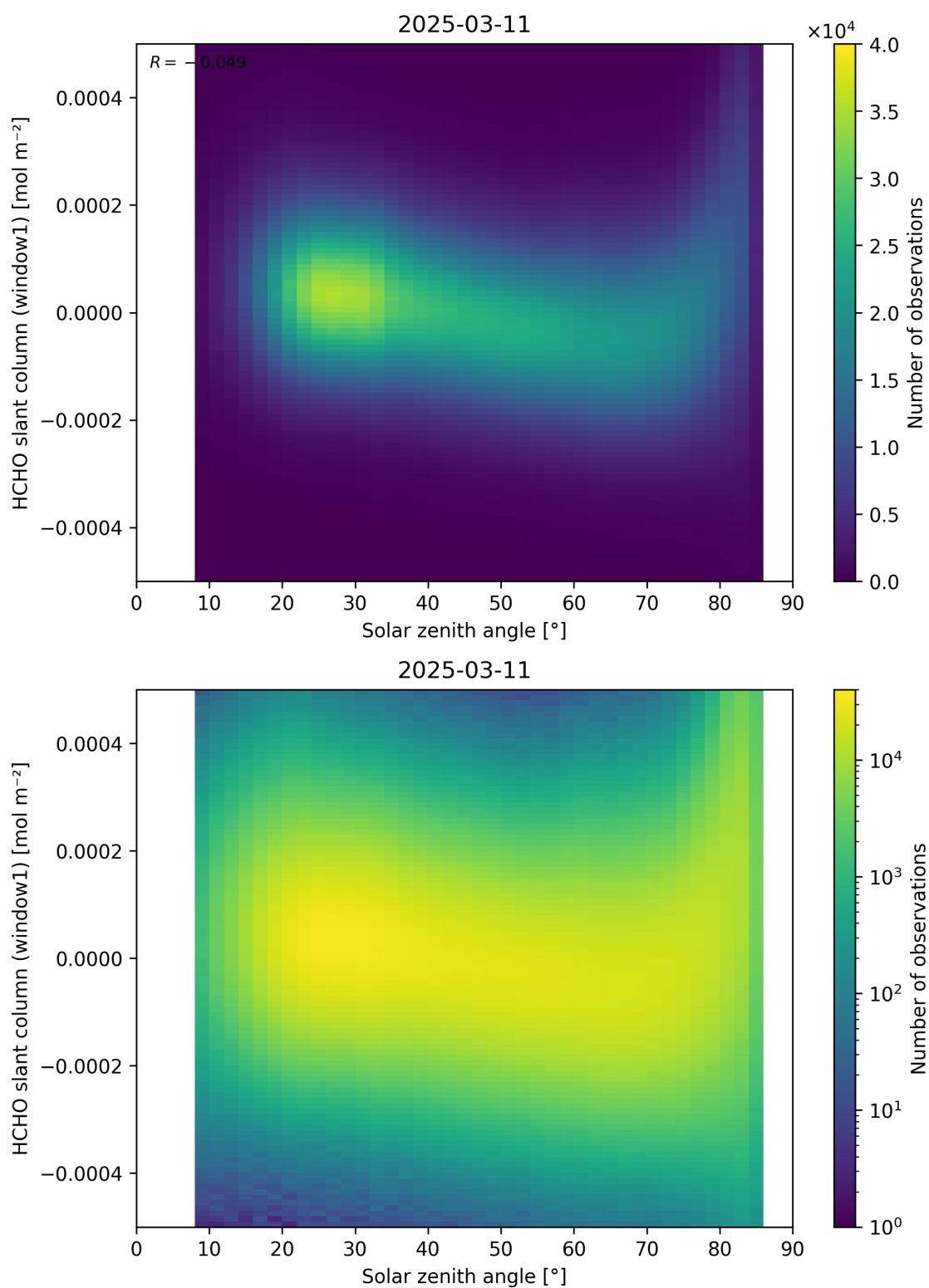
Figure 173: Scatter density plot of “Solar zenith angle” against “HCHO slant column (window1)” for 2025-03-10 to 2025-03-12.
