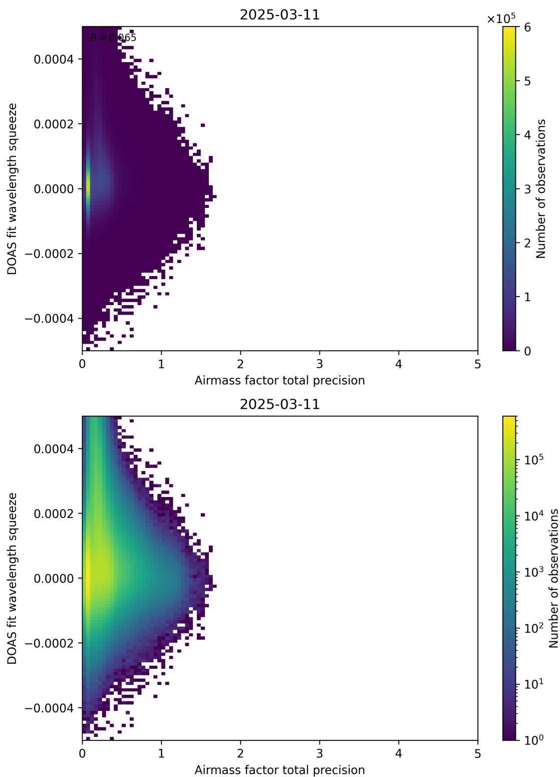
Figure 107: Scatter density plot of “Airmass factor total precision” against “DOAS fit wavelength squeeze” for 2025-03-10 to 2025-03-12.
