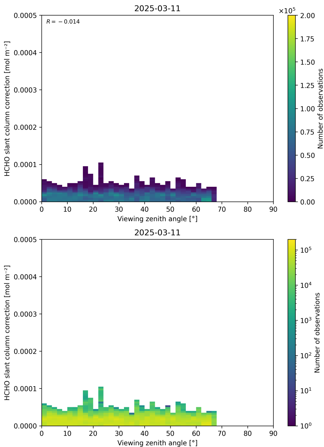
Figure 187: Scatter density plot of “Viewing zenith angle” against “HCHO slant column correction” for 2025-03-10 to 2025-03-12.
