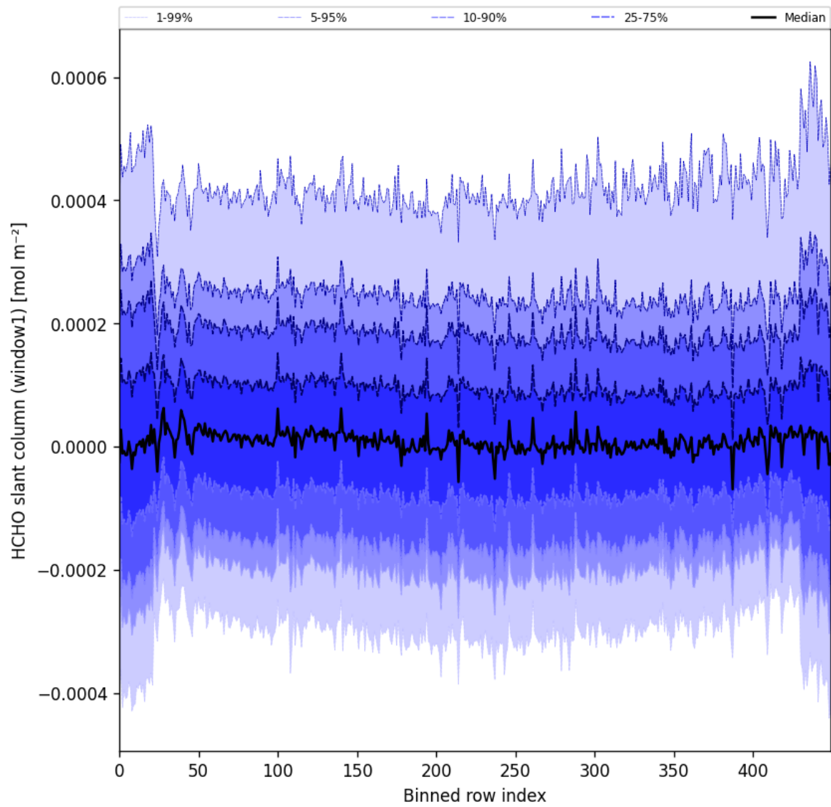
Figure 52: Along track statistics of “HCHO slant column (window1)” for 2025-03-10 to 2025-03-12
