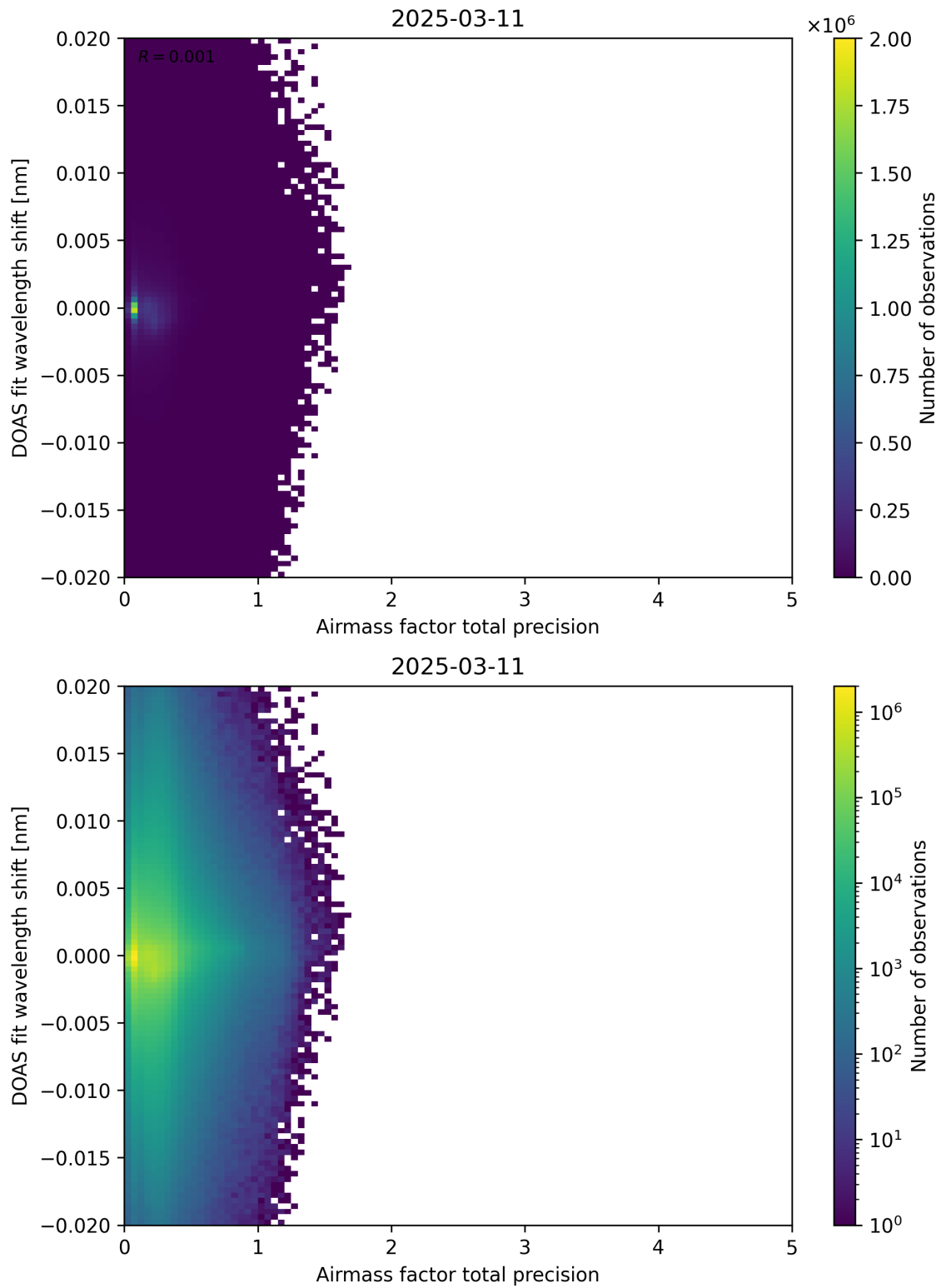
Figure 106: Scatter density plot of “Airmass factor total precision” against “DOAS fit wavelength shift” for 2025-03-10 to 2025-03-12.
