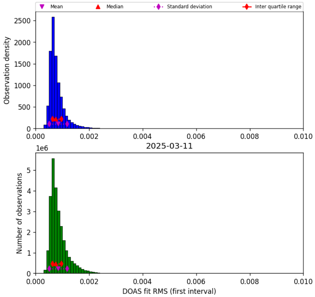
Figure 46: Histogram of “DOAS fit RMS (first interval)” for 2025-03-10 to 2025-03-12
