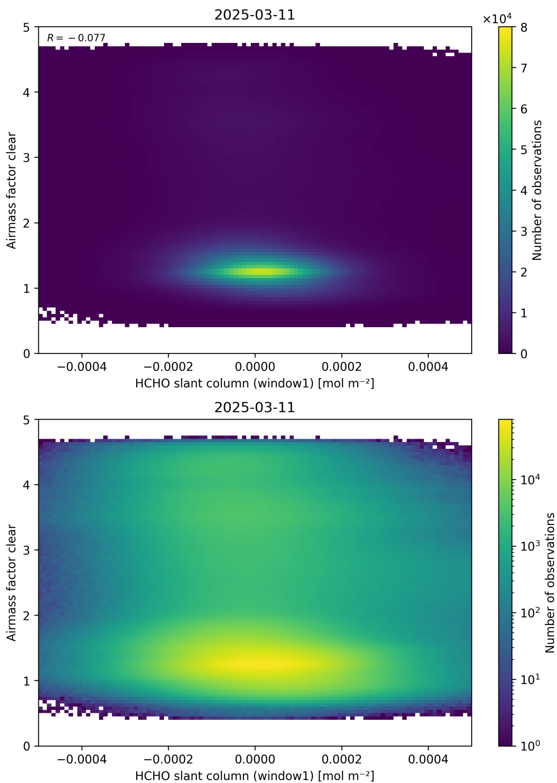
Figure 81: Scatter density plot of “HCHO slant column (window1)” against “Airmass factor clear” for 2025-03-10 to 2025-03-12.
