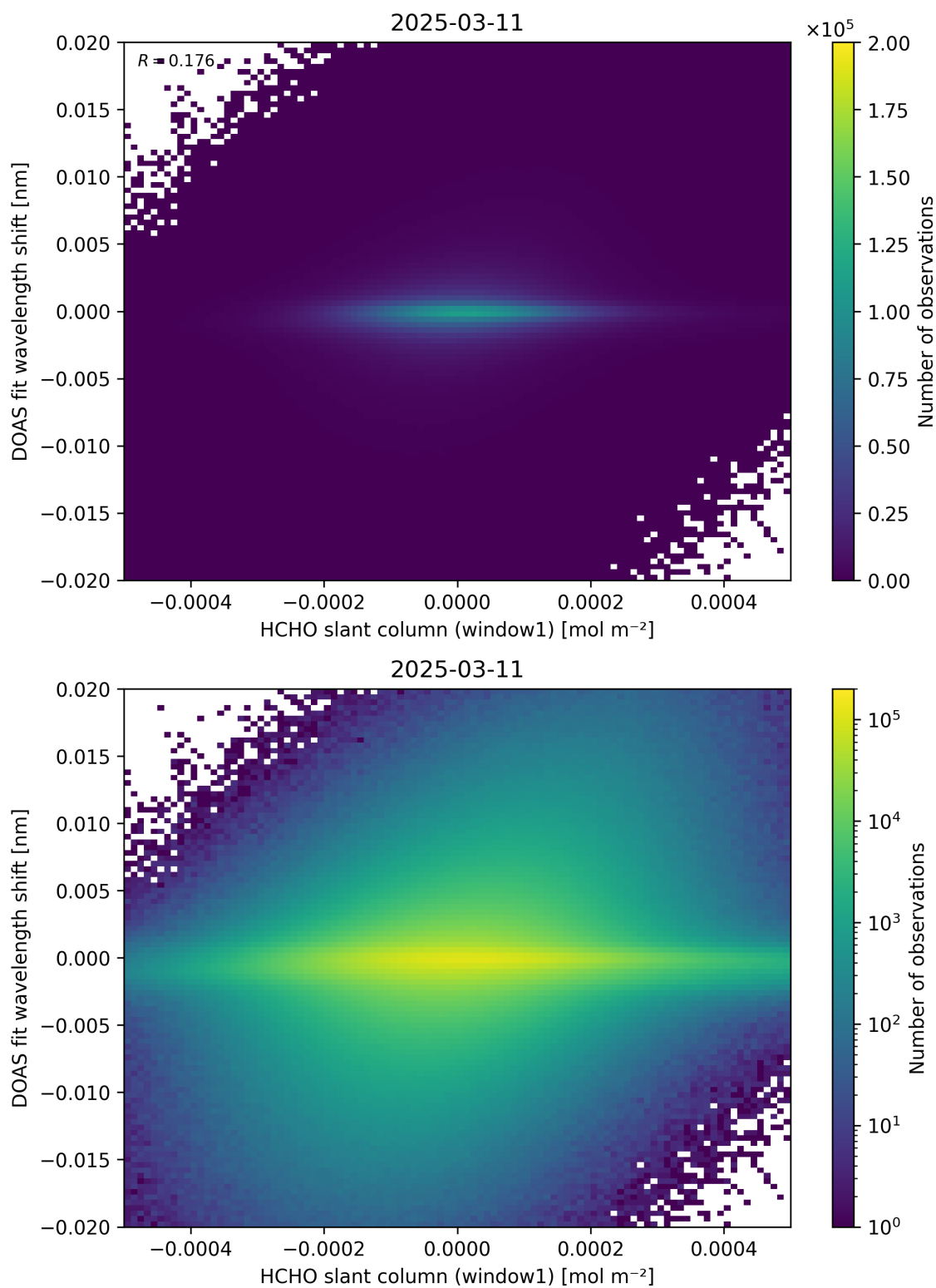
Figure 79: Scatter density plot of “HCHO slant column (window1)” against “DOAS fit wavelength shift” for 2025-03-10 to 2025-03-12.
