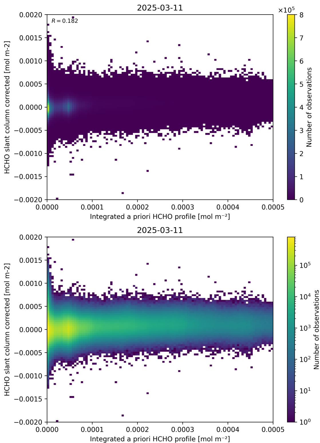
Figure 151: Scatter density plot of “Integrated a priori HCHO profile” against “HCHO slant column corrected” for 2025-03-10 to 2025-03-12.
