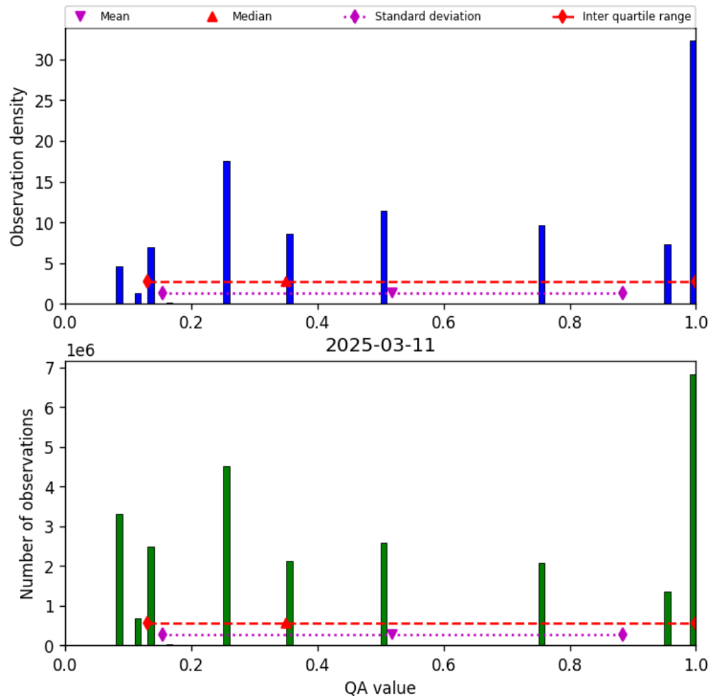
Figure 34: Histogram of “QA value” for 2025-03-10 to 2025-03-12
