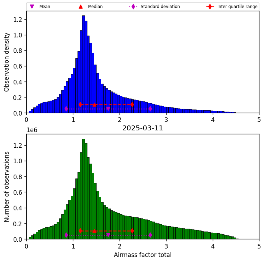
Figure 40: Histogram of “Airmass factor total” for 2025-03-10 to 2025-03-12
