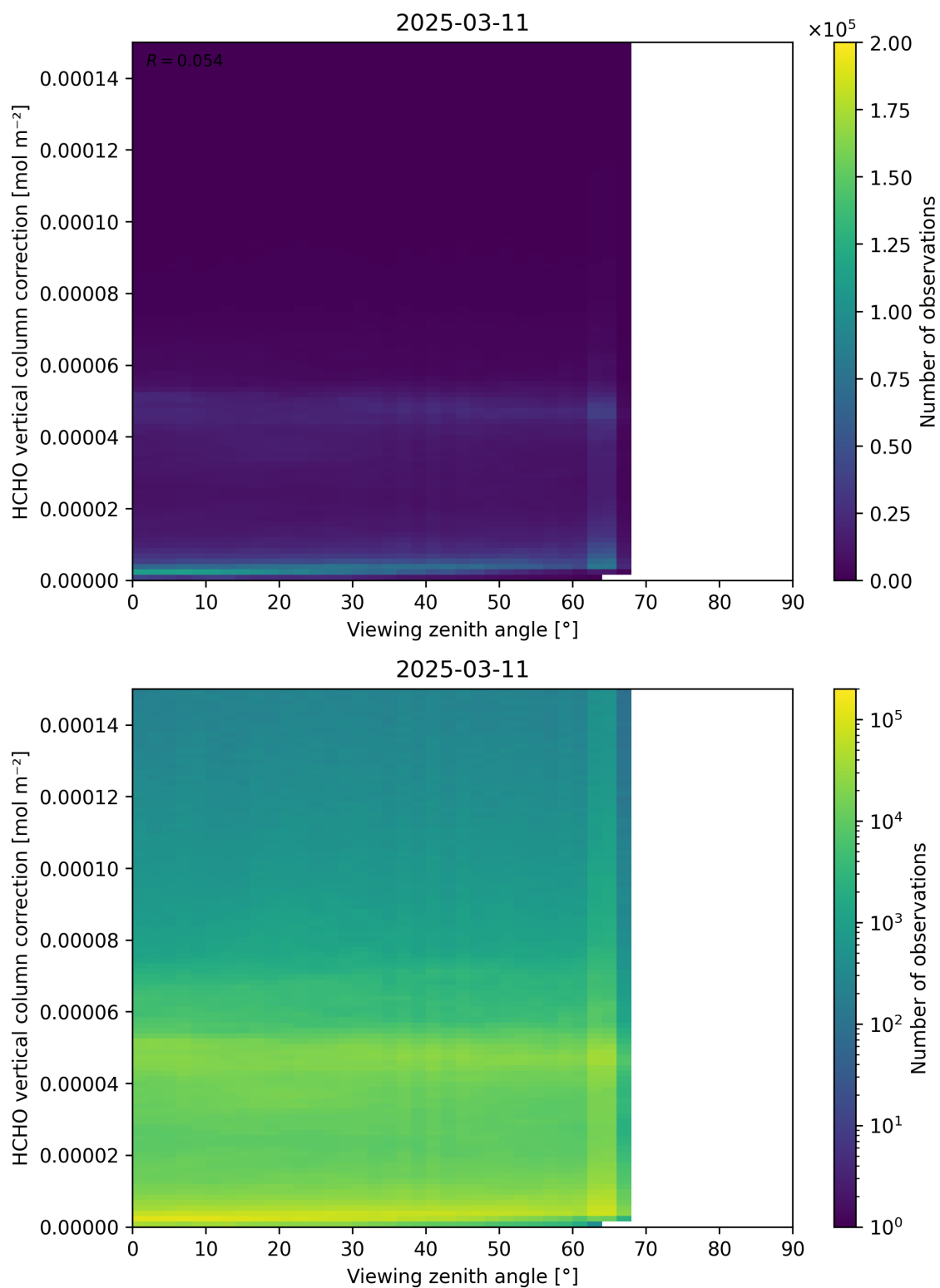
Figure 193: Scatter density plot of “Viewing zenith angle” against “HCHO vertical column correction” for 2025-03-10 to 2025-03-12.
