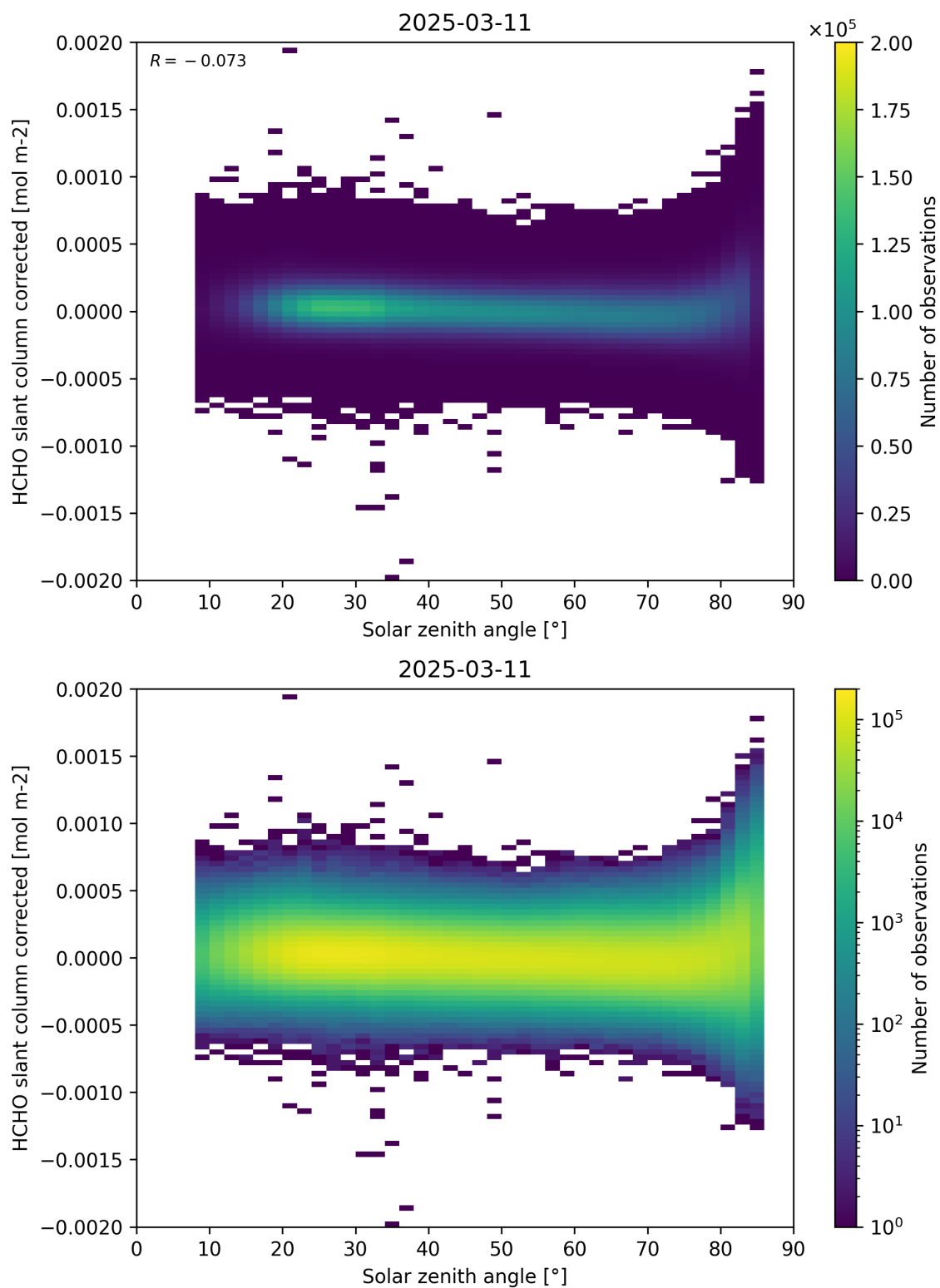
Figure 171: Scatter density plot of “Solar zenith angle” against “HCHO slant column corrected” for 2025-03-10 to 2025-03-12.
