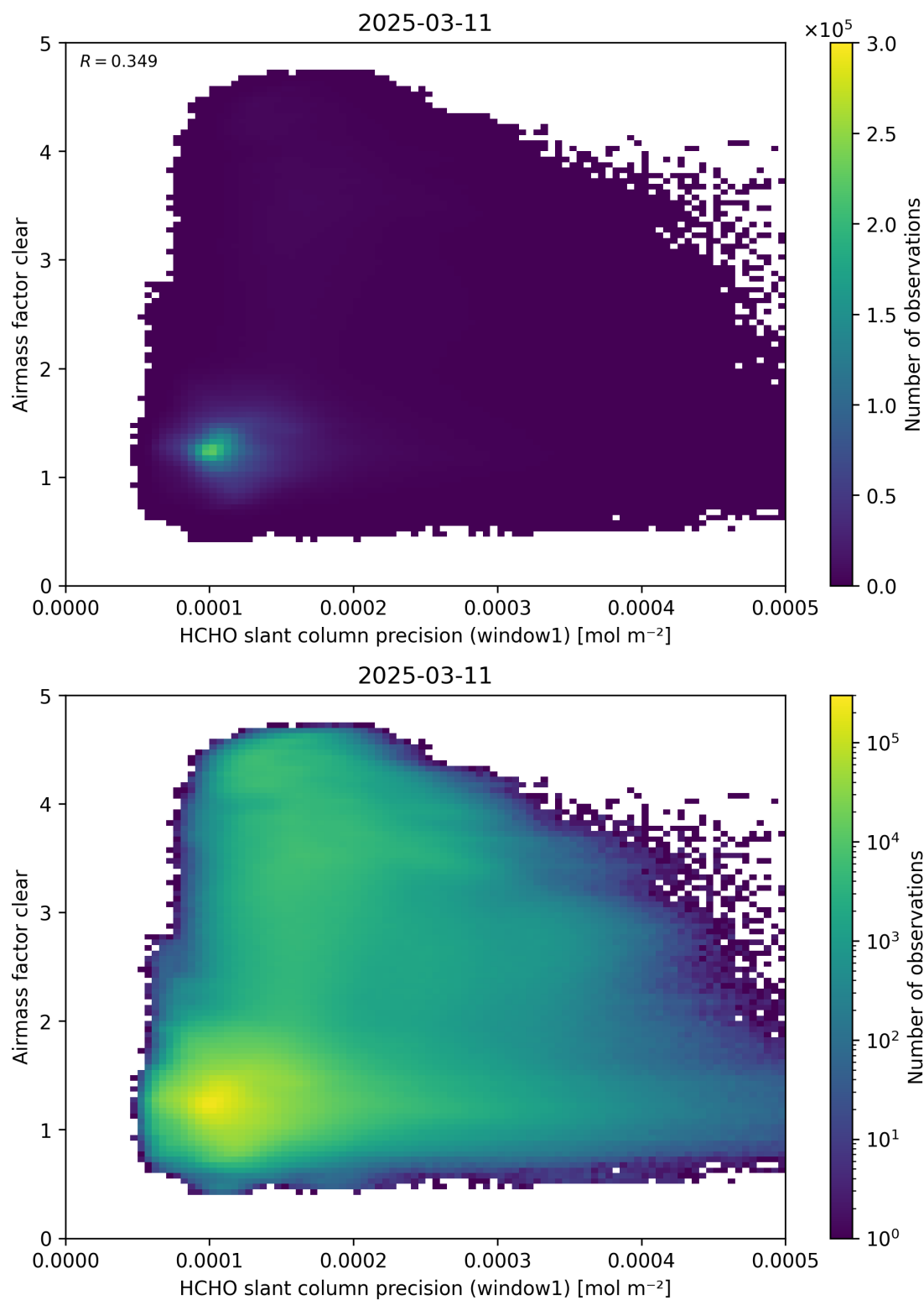
Figure 91: Scatter density plot of “HCHO slant column precision (window1)” against “Airmass factor clear” for 2025-03-10 to 2025-03-12.
