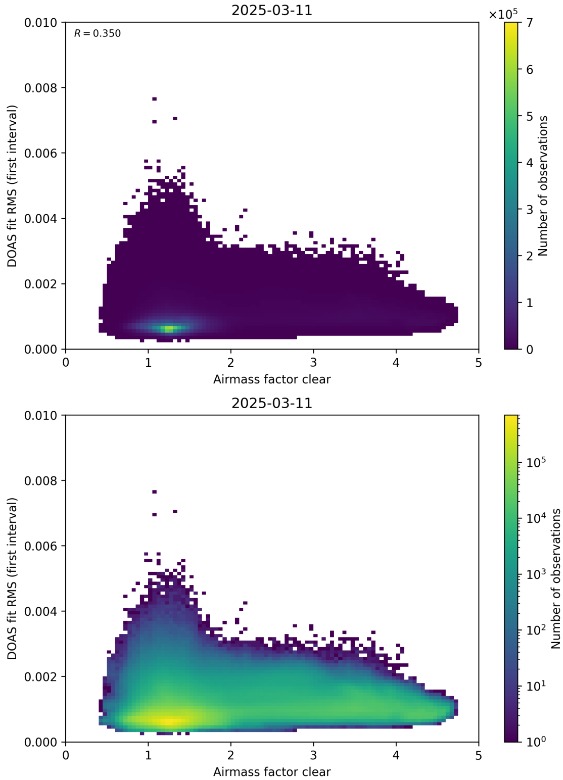
Figure 71: Scatter density plot of “Airmass factor clear” against “DOAS fit RMS (first interval)” for 2025-03-10 to 2025-03-12.
