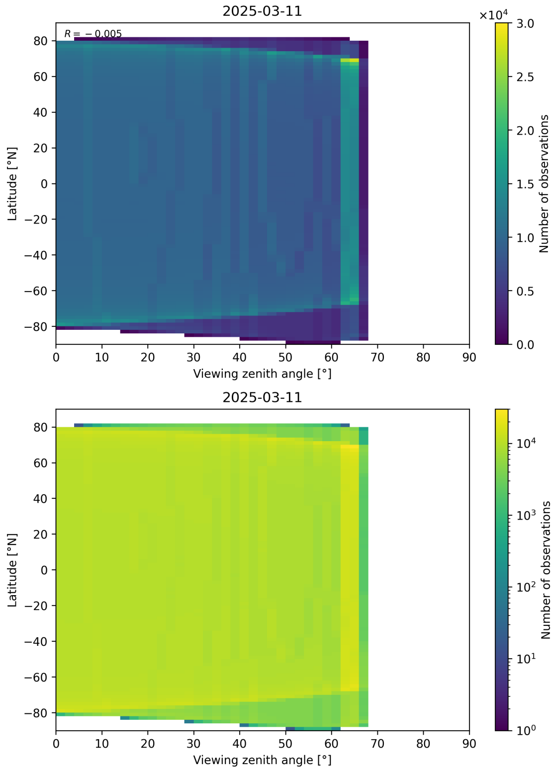
Figure 196: Scatter density plot of “Viewing zenith angle” against “Latitude” for 2025-03-10 to 2025-03-12.
