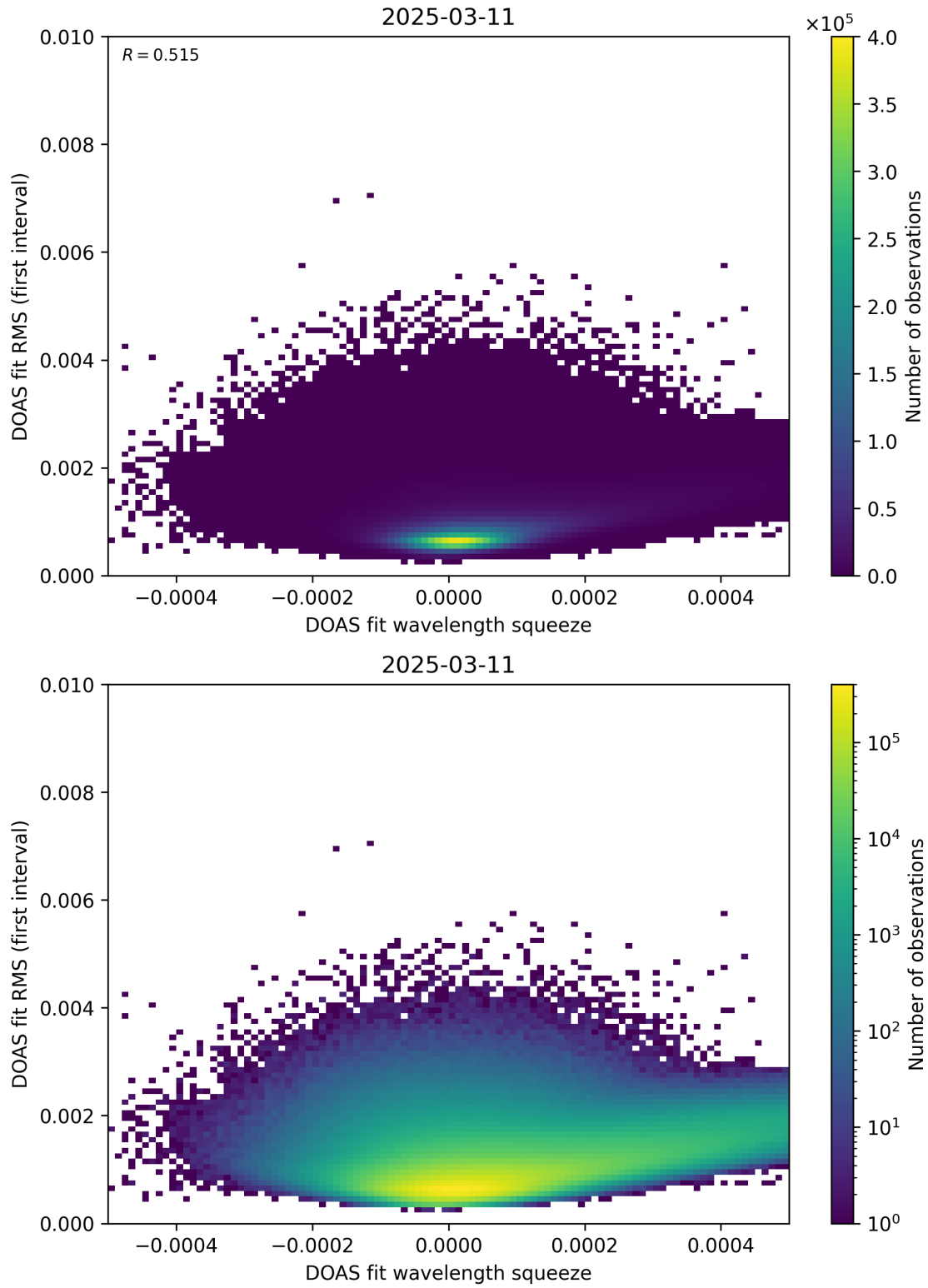
Figure 68: Scatter density plot of “DOAS fit wavelength squeeze” against “DOAS fit RMS (first interval)” for 2025-03-10 to 2025-03-12.
