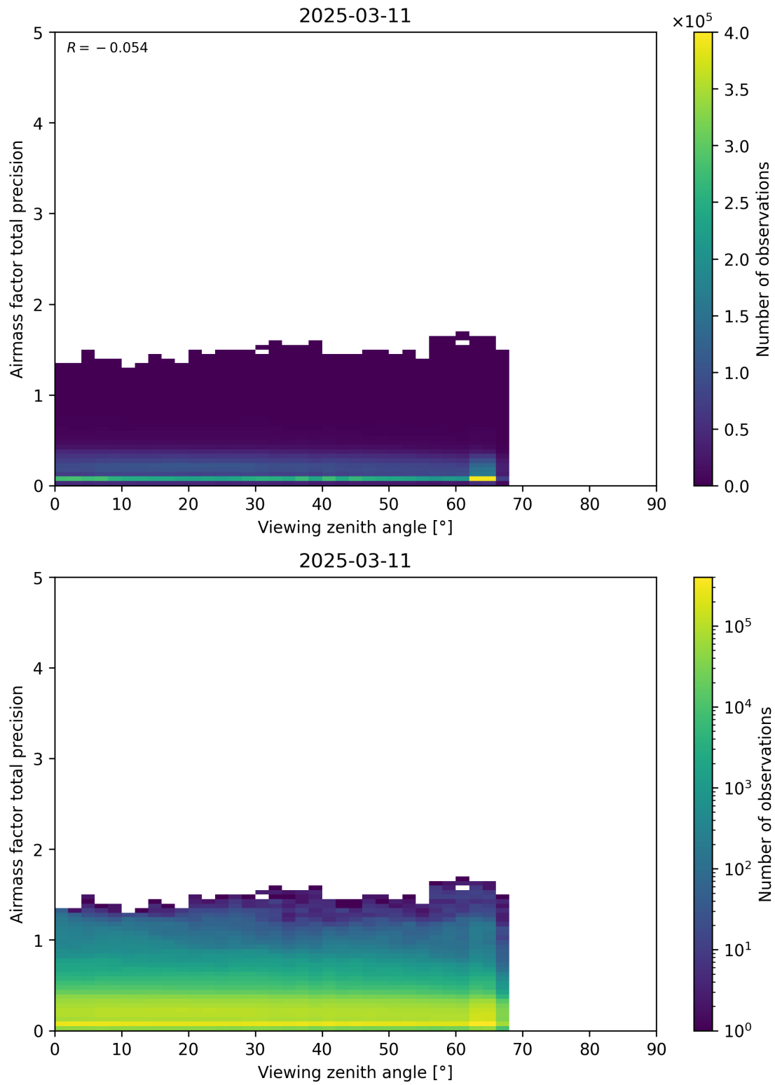
Figure 191: Scatter density plot of “Viewing zenith angle” against “Airmass factor total precision” for 2025-03-10 to 2025-03-12.
