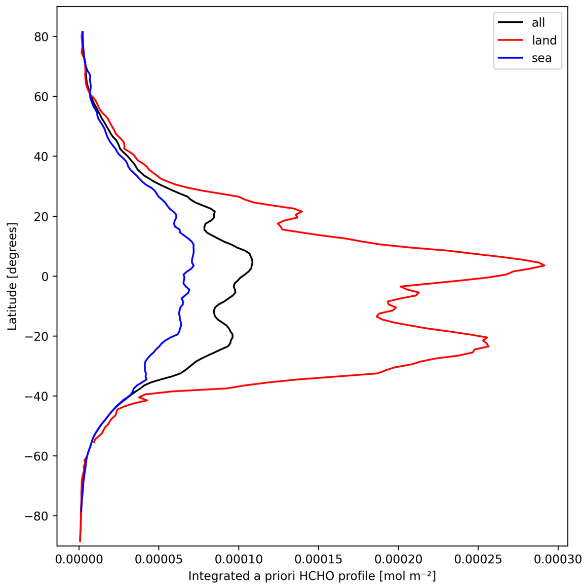
Figure 29: Zonal average of “Integrated a priori HCHO profile” for 2025-03-10 to 2025-03-12.
