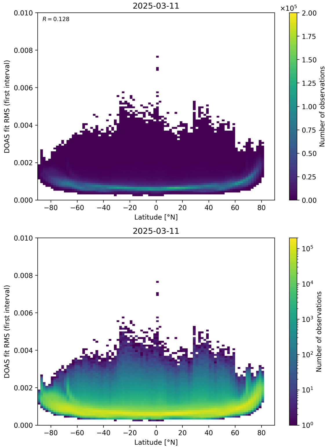
Figure 153: Scatter density plot of “Latitude” against “DOAS fit RMS (first interval)” for 2025-03-10 to 2025-03-12.
