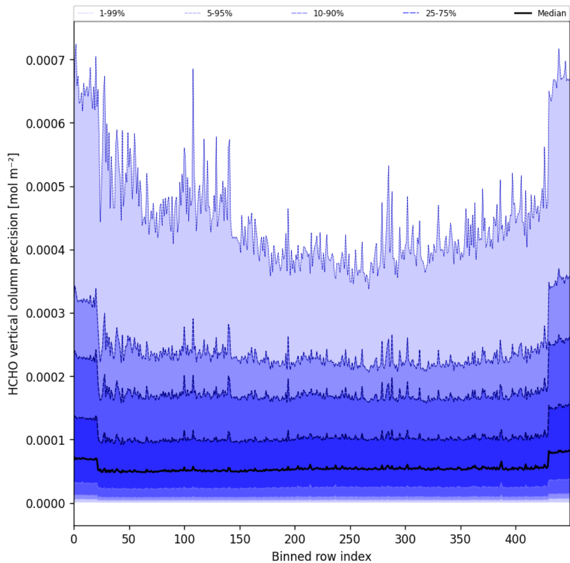
Figure 50: Along track statistics of “HCHO vertical column precision” for 2025-03-10 to 2025-03-12
