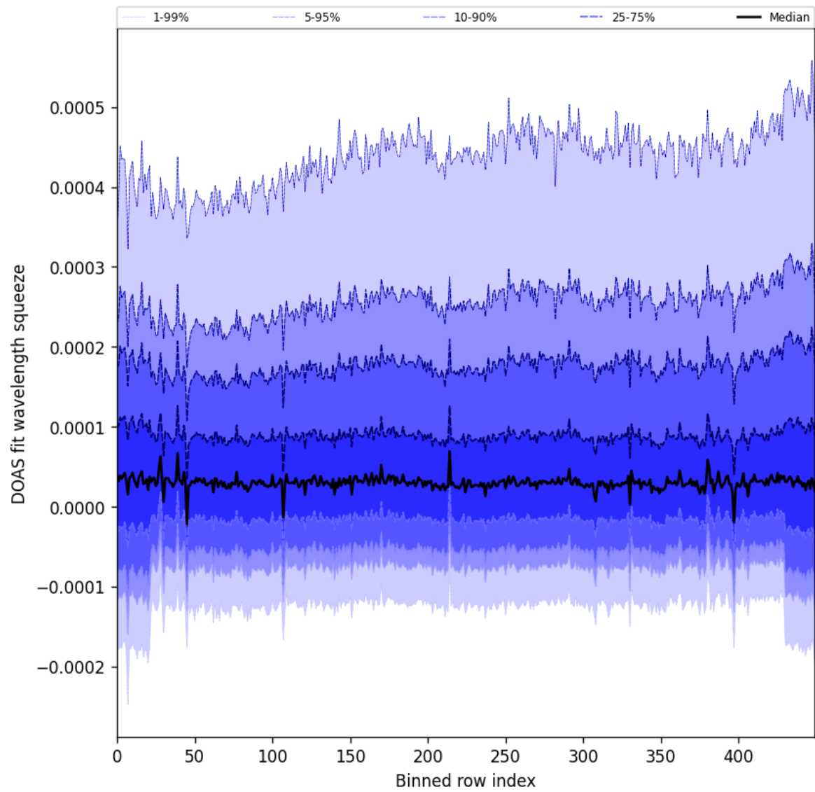
Figure 59: Along track statistics of “DOAS fit wavelength squeeze” for 2025-03-10 to 2025-03-12
