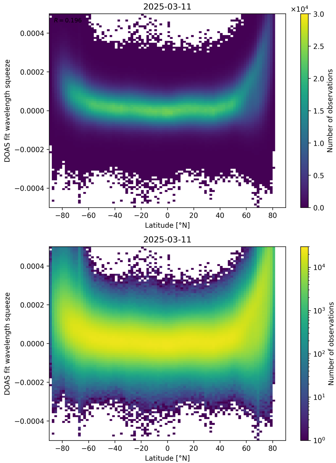
Figure 155: Scatter density plot of “Latitude” against “DOAS fit wavelength squeeze” for 2025-03-10 to 2025-03-12.
