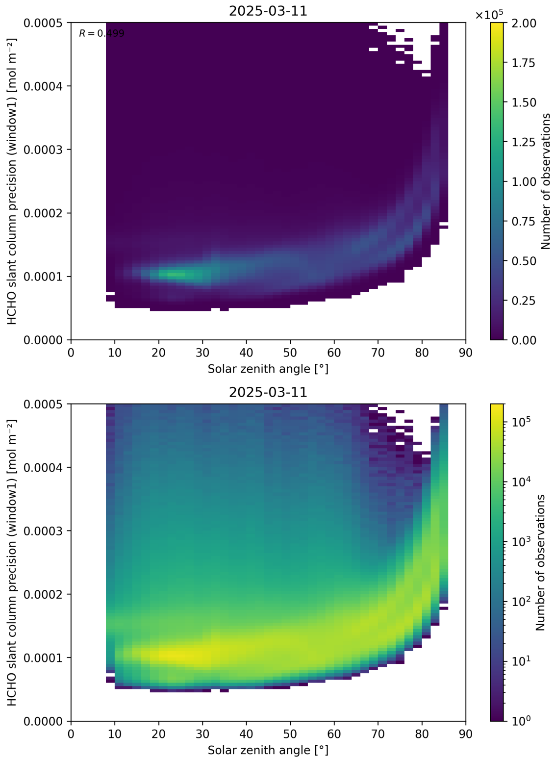
Figure 174: Scatter density plot of “Solar zenith angle” against “HCHO slant column precision (window1)” for 2025-03-10 to 2025-03-12.
