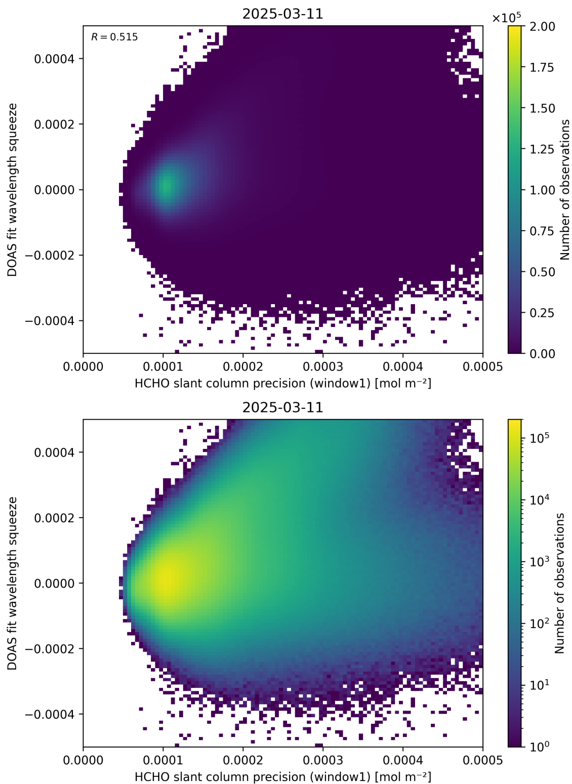
Figure 90: Scatter density plot of “HCHO slant column precision (window1)” against “DOAS fit wavelength squeeze” for 2025-03-10 to 2025-03-12.
