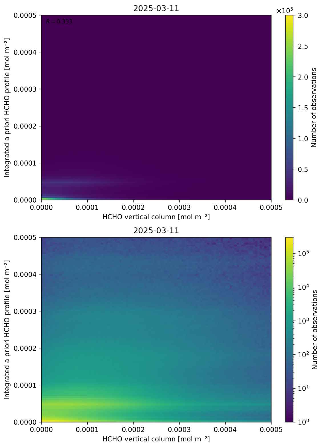
Figure 135: Scatter density plot of “HCHO vertical column” against “Integrated a priori HCHO profile” for 2025-03-10 to 2025-03-12.
