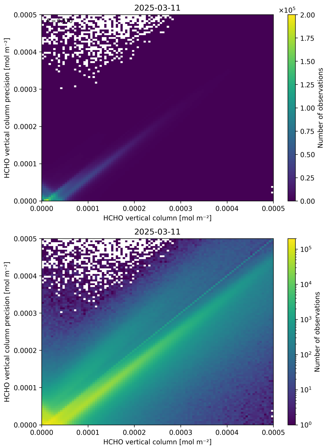
Figure 134: Scatter density plot of “HCHO vertical column” against “HCHO vertical column precision” for 2025-03-10 to 2025-03-12.
