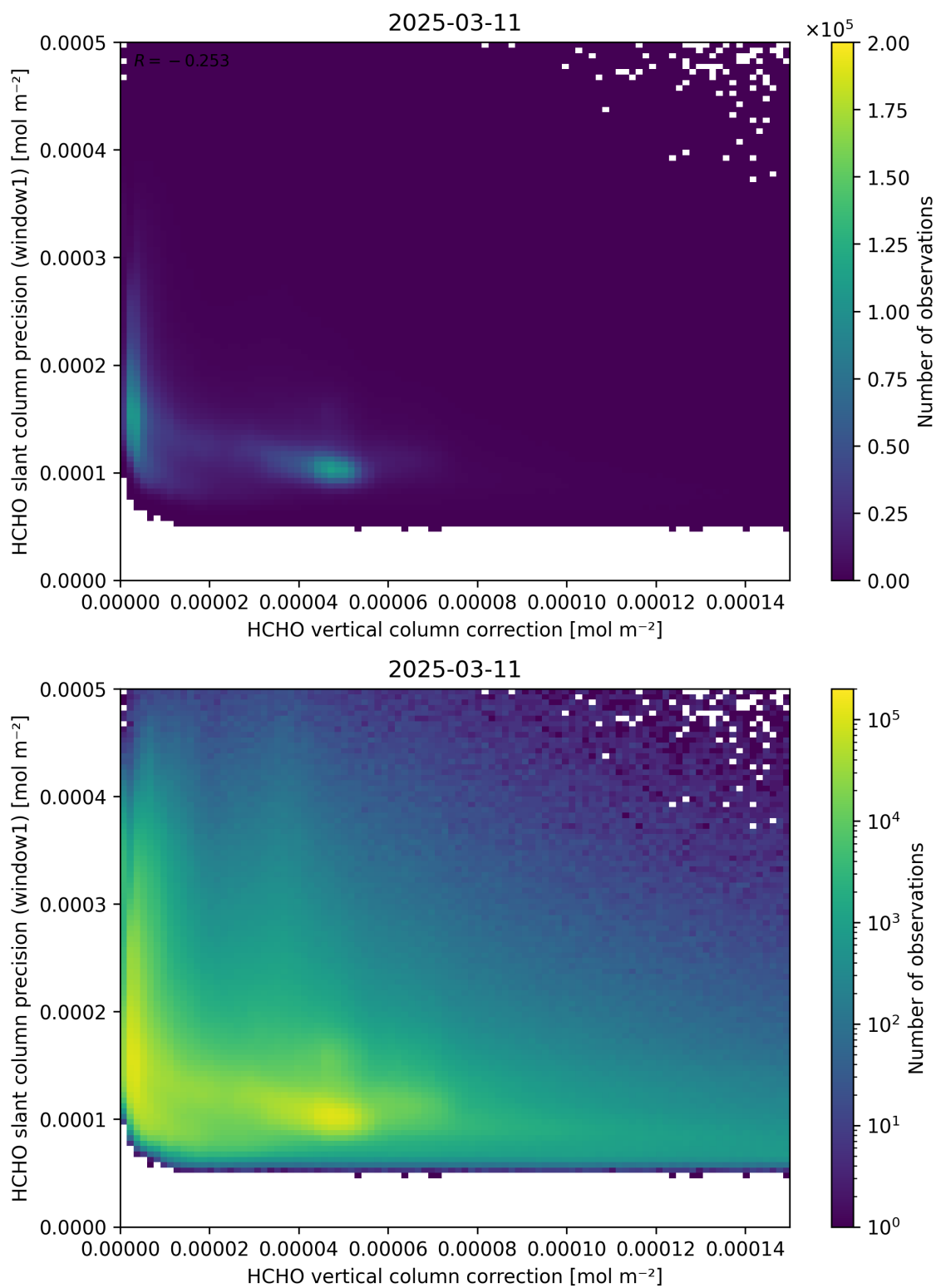
Figure 119: Scatter density plot of “HCHO vertical column correction” against “HCHO slant column precision (window1)” for 2025-03-10 to 2025-03-12.
