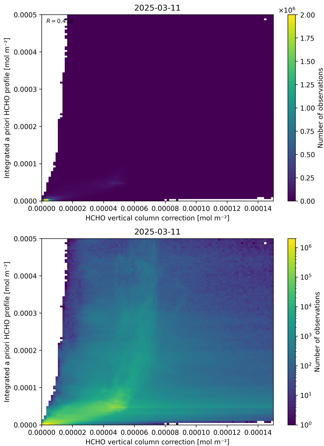
Figure 122: Scatter density plot of “HCHO vertical column correction” against “Integrated a priori HCHO profile” for 2025-03-10 to 2025-03-12.
