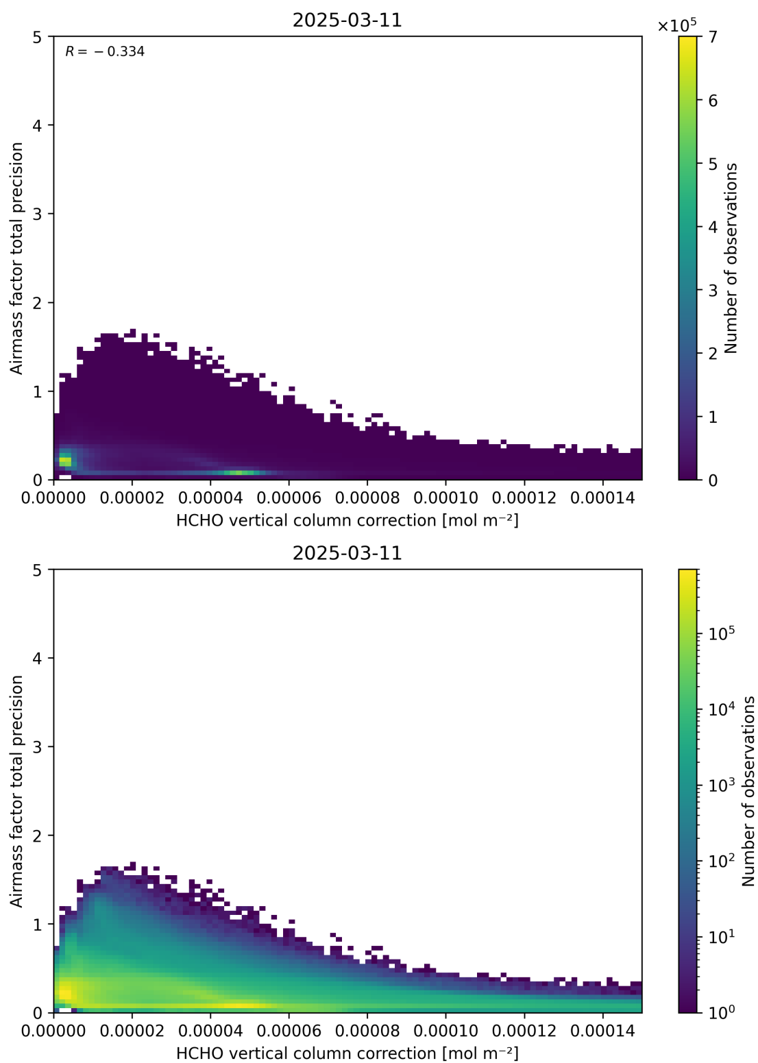
Figure 121: Scatter density plot of “HCHO vertical column correction” against “Airmass factor total precision” for 2025-03-10 to 2025-03-12.
