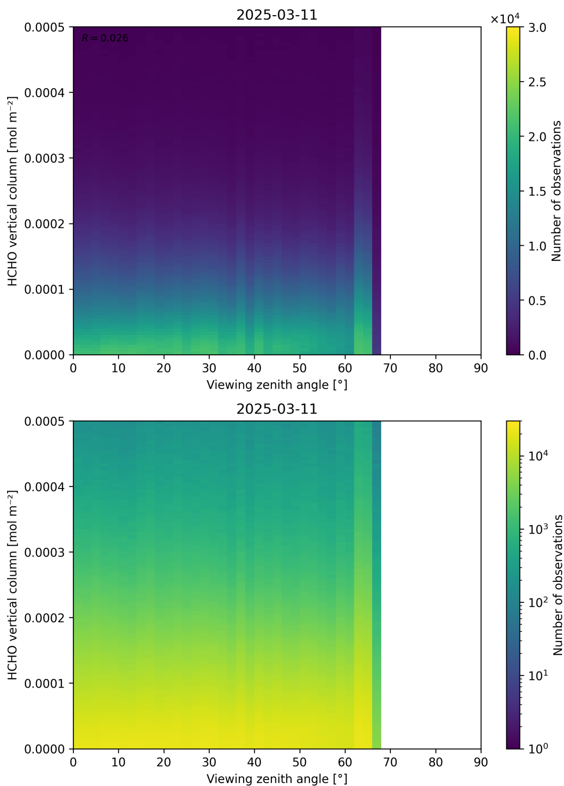
Figure 192: Scatter density plot of “Viewing zenith angle” against “HCHO vertical column” for 2025-03-10 to 2025-03-12.
