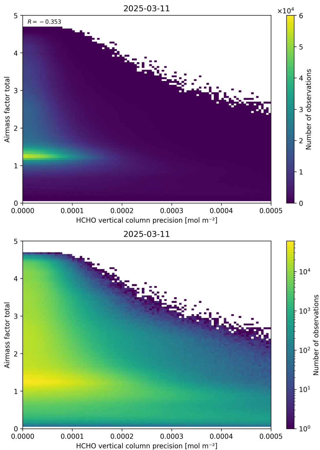
Figure 144: Scatter density plot of “HCHO vertical column precision” against “Airmass factor total” for 2025-03-10 to 2025-03-12.
