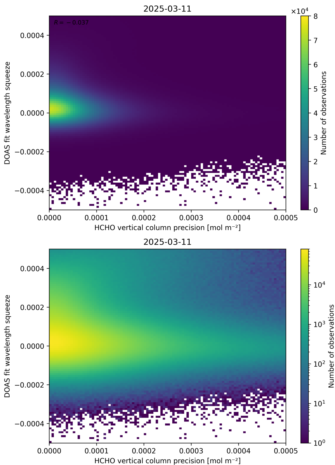
Figure 138: Scatter density plot of “HCHO vertical column precision” against “DOAS fit wavelength squeeze” for 2025-03-10 to 2025-03-12.
