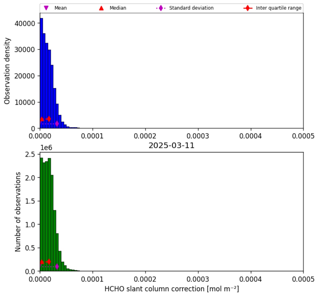
Figure 47: Histogram of “HCHO slant column correction” for 2025-03-10 to 2025-03-12
