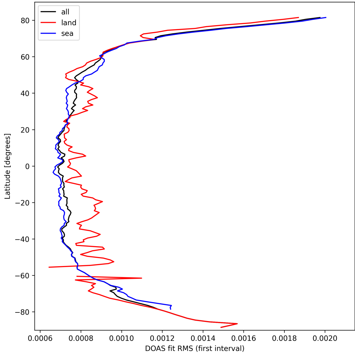
Figure 32: Zonal average of “DOAS fit RMS (first interval)” for 2025-03-10 to 2025-03-12.
