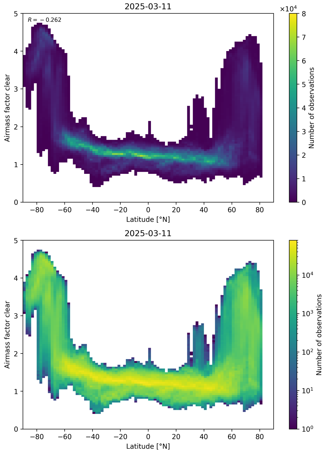
Figure 156: Scatter density plot of “Latitude” against “Airmass factor clear” for 2025-03-10 to 2025-03-12.
