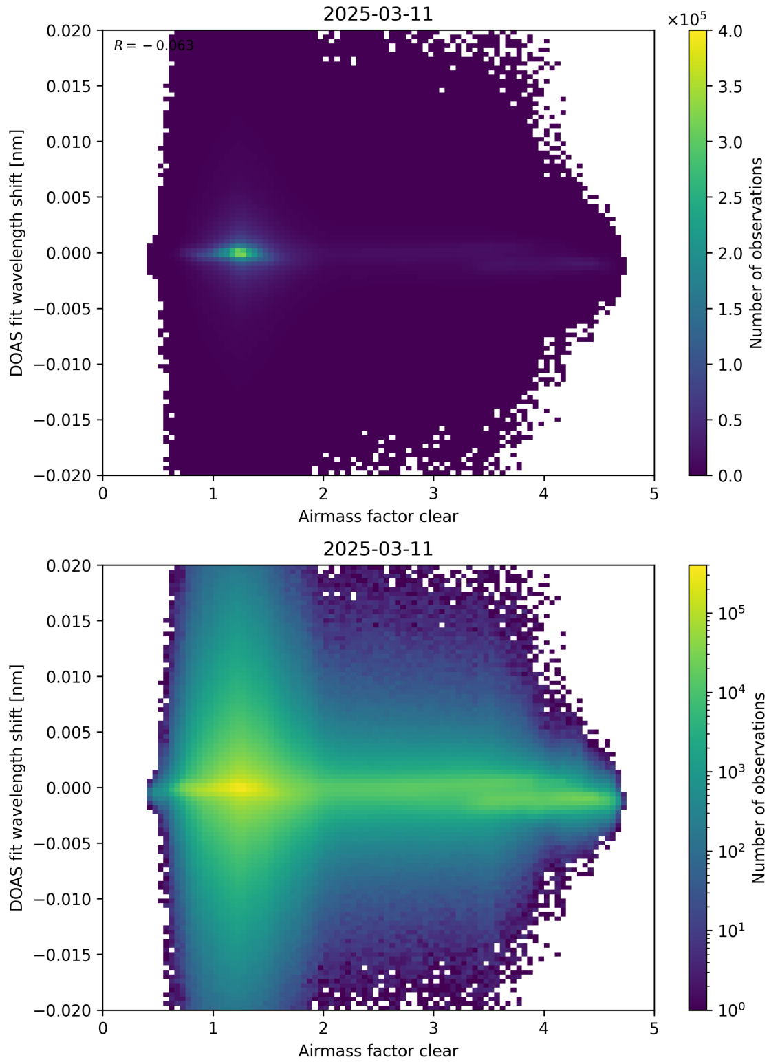
Figure 72: Scatter density plot of “Airmass factor clear” against “DOAS fit wavelength shift” for 2025-03-10 to 2025-03-12.
