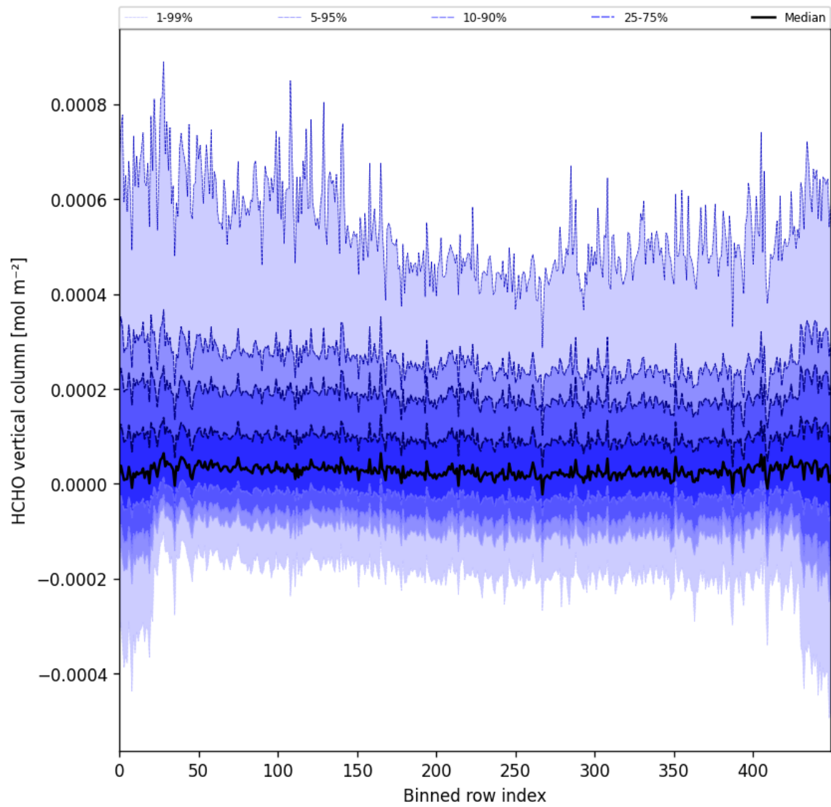
Figure 49: Along track statistics of “HCHO vertical column” for 2025-03-10 to 2025-03-12
