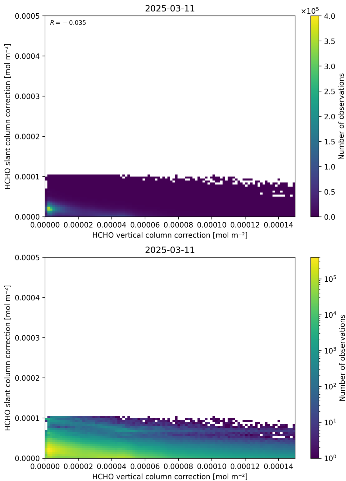
Figure 117: Scatter density plot of “HCHO vertical column correction” against “HCHO slant column correction” for 2025-03-10 to 2025-03-12.
