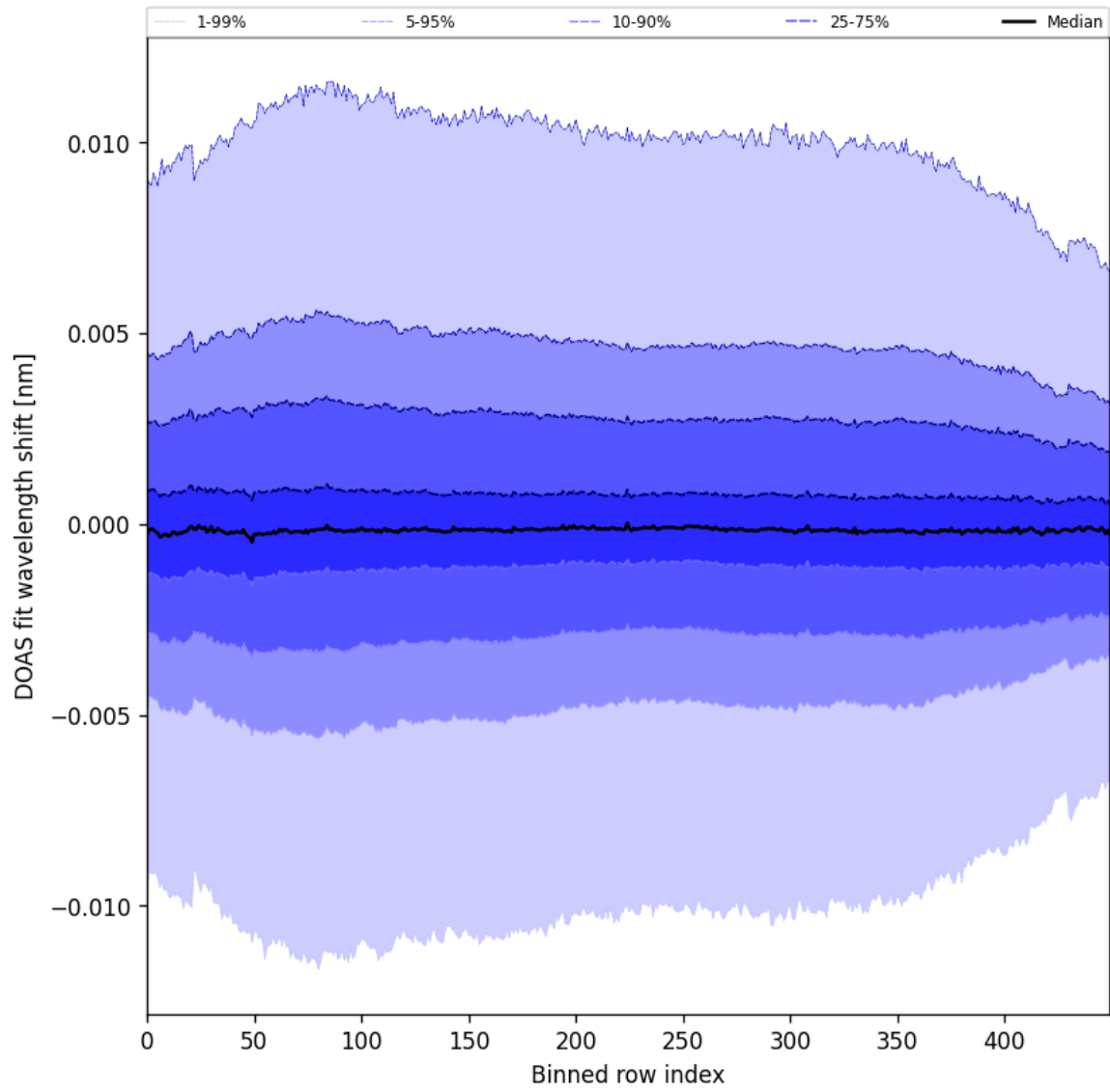
Figure 58: Along track statistics of “DOAS fit wavelength shift” for 2025-03-10 to 2025-03-12
