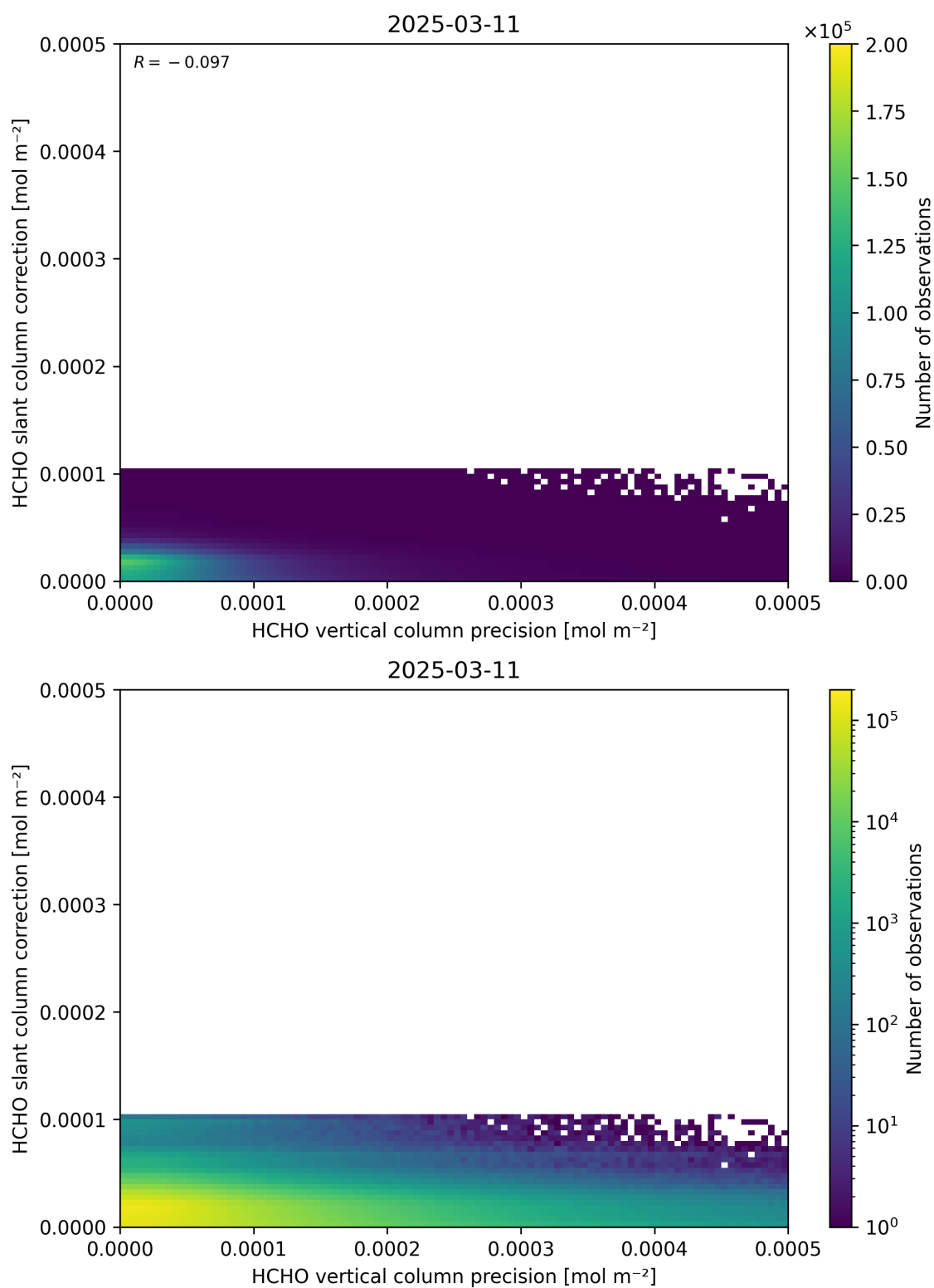
Figure 141: Scatter density plot of “HCHO vertical column precision” against “HCHO slant column correction” for 2025-03-10 to 2025-03-12.
