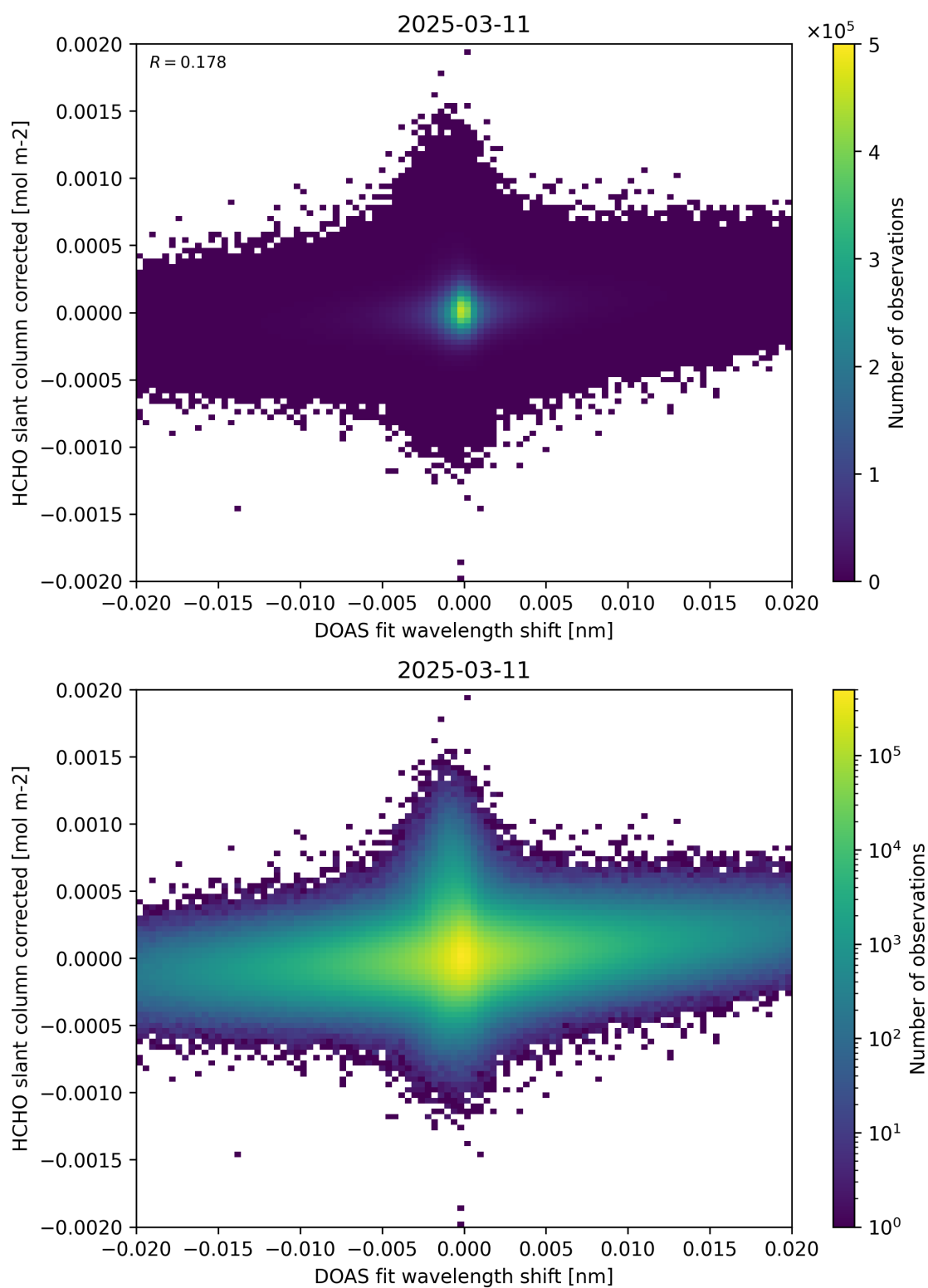
Figure 66: Scatter density plot of “DOAS fit wavelength shift” against “HCHO slant column corrected” for 2025-03-10 to 2025-03-12.
