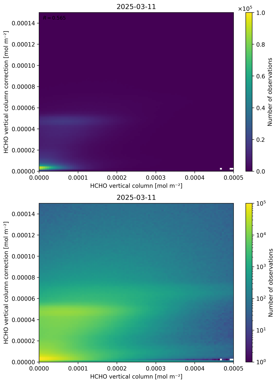
Figure 133: Scatter density plot of “HCHO vertical column” against “HCHO vertical column correction” for 2025-03-10 to 2025-03-12.
