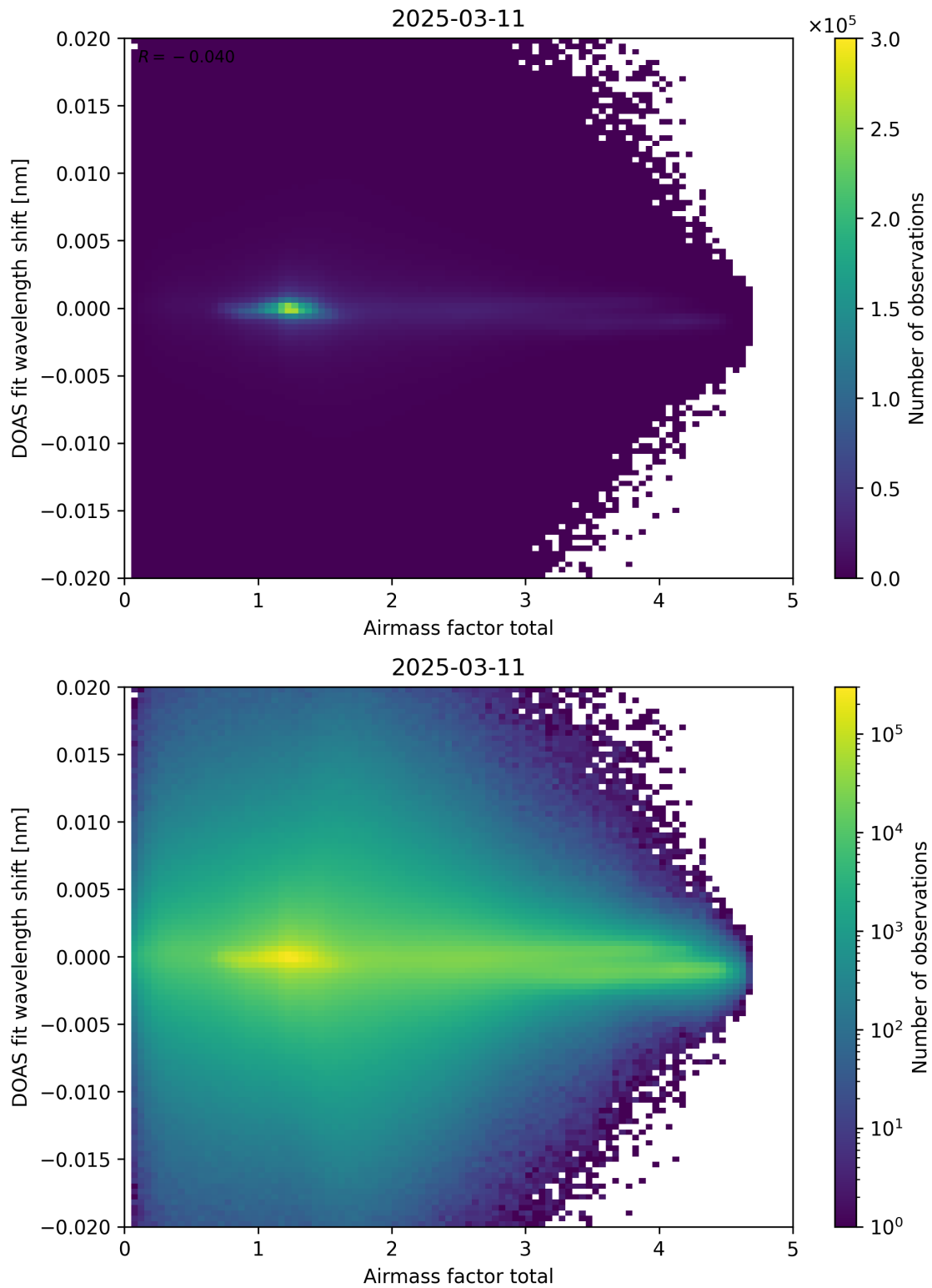
Figure 98: Scatter density plot of “Airmass factor total” against “DOAS fit wavelength shift” for 2025-03-10 to 2025-03-12.
