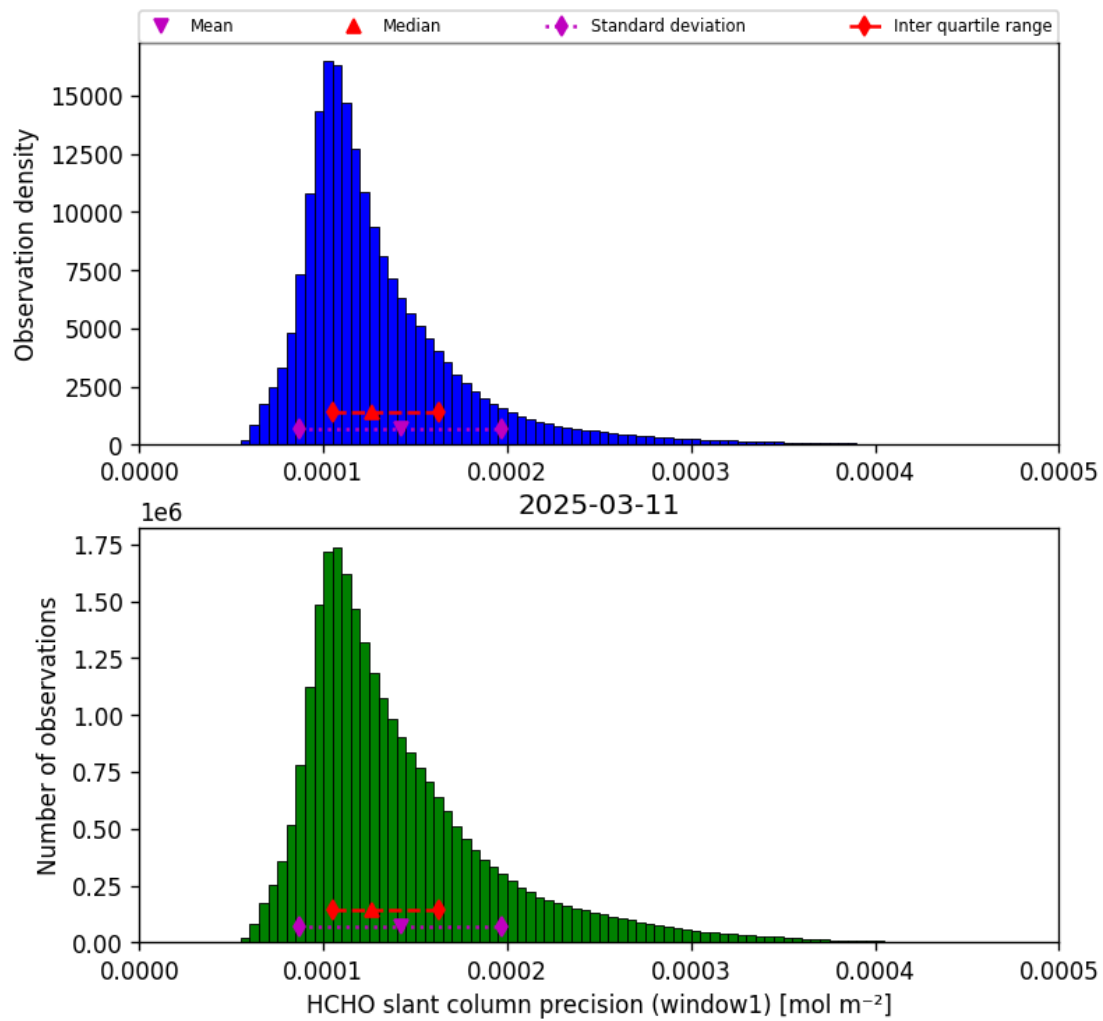
Figure 39: Histogram of “HCHO slant column precision (window1)” for 2025-03-10 to 2025-03-12
