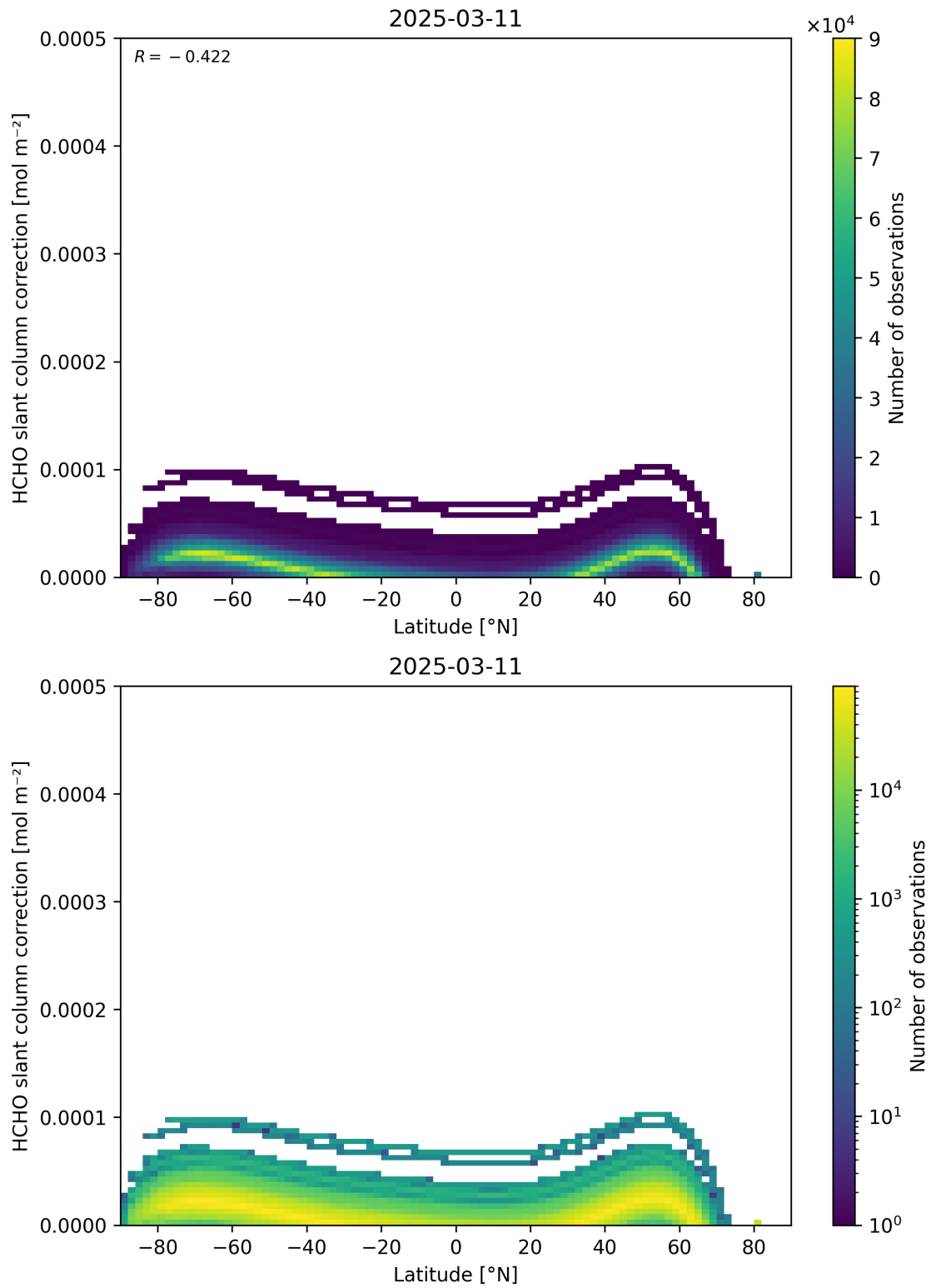
Figure 158: Scatter density plot of “Latitude” against “HCHO slant column correction” for 2025-03-10 to 2025-03-12.
