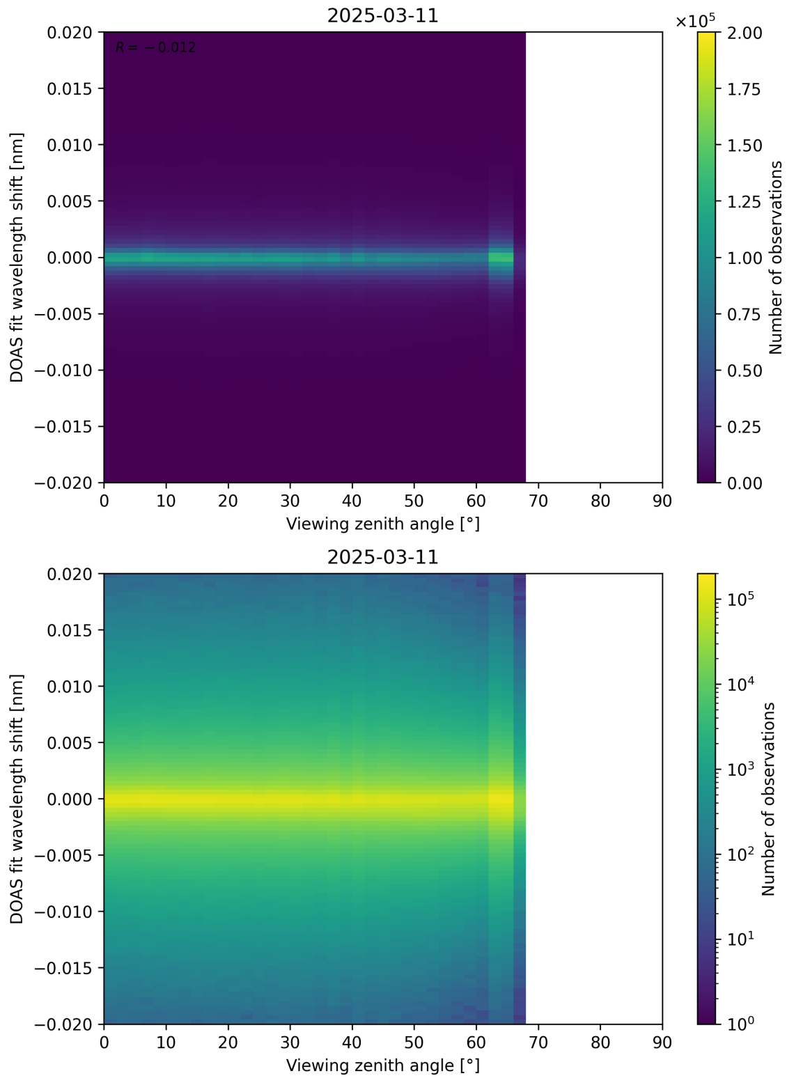
Figure 183: Scatter density plot of “Viewing zenith angle” against “DOAS fit wavelength shift” for 2025-03-10 to 2025-03-12.
