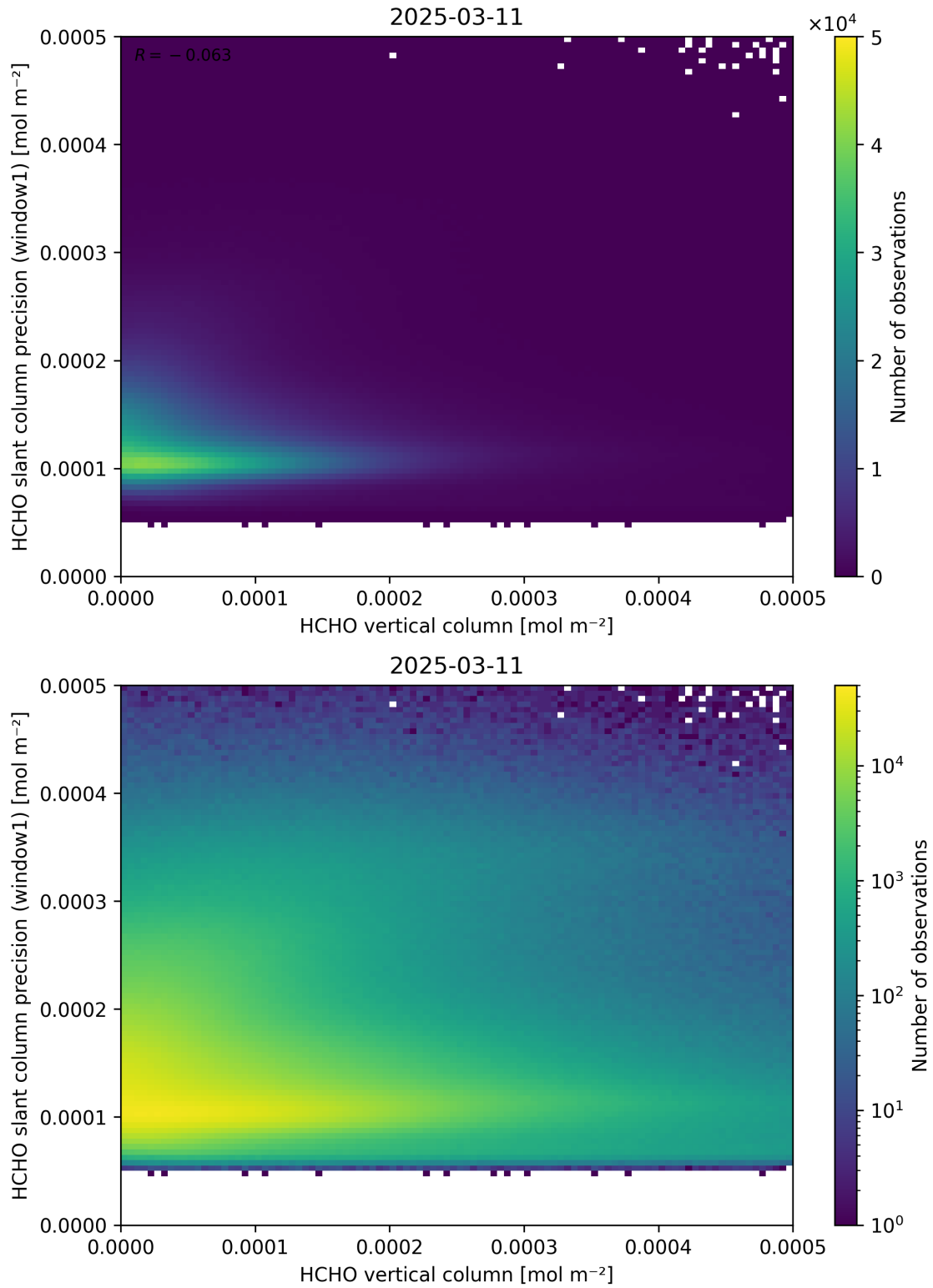
Figure 130: Scatter density plot of “HCHO vertical column” against “HCHO slant column precision (window1)” for 2025-03-10 to 2025-03-12.
