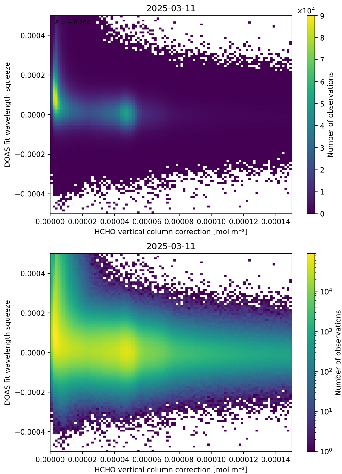
Figure 114: Scatter density plot of “HCHO vertical column correction” against “DOAS fit wavelength squeeze” for 2025-03-10 to 2025-03-12.
