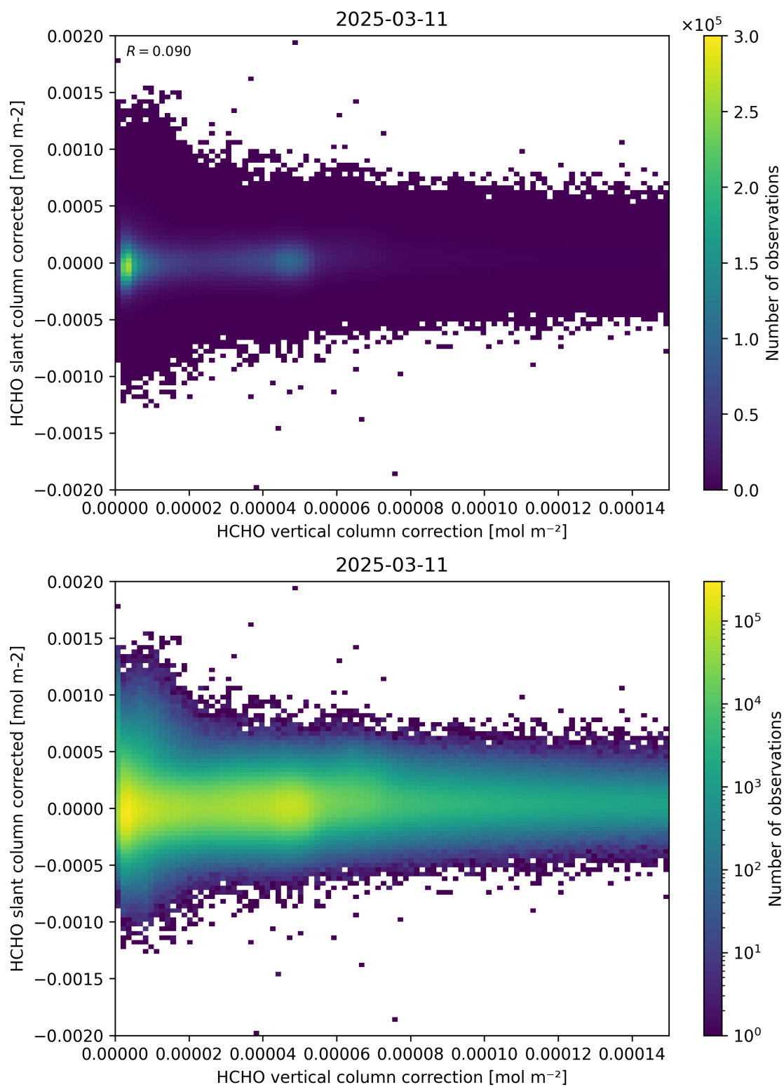
Figure 116: Scatter density plot of “HCHO vertical column correction” against “HCHO slant column corrected” for 2025-03-10 to 2025-03-12.
