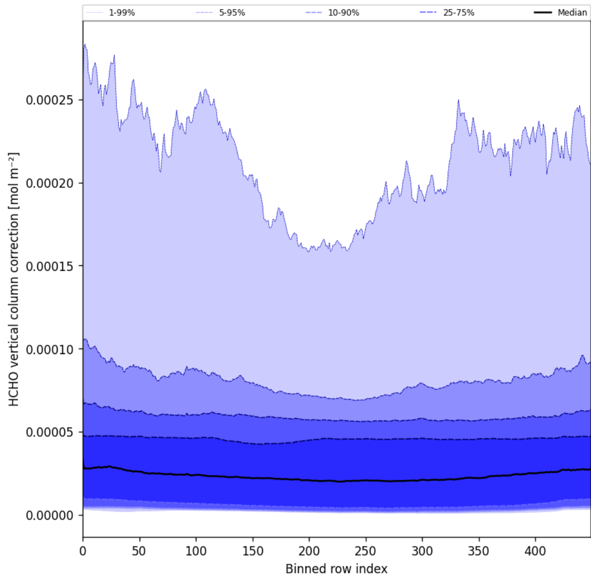
Figure 51: Along track statistics of "HCHO vertical column correction" for 2025-03-10 to 2025-03-12
