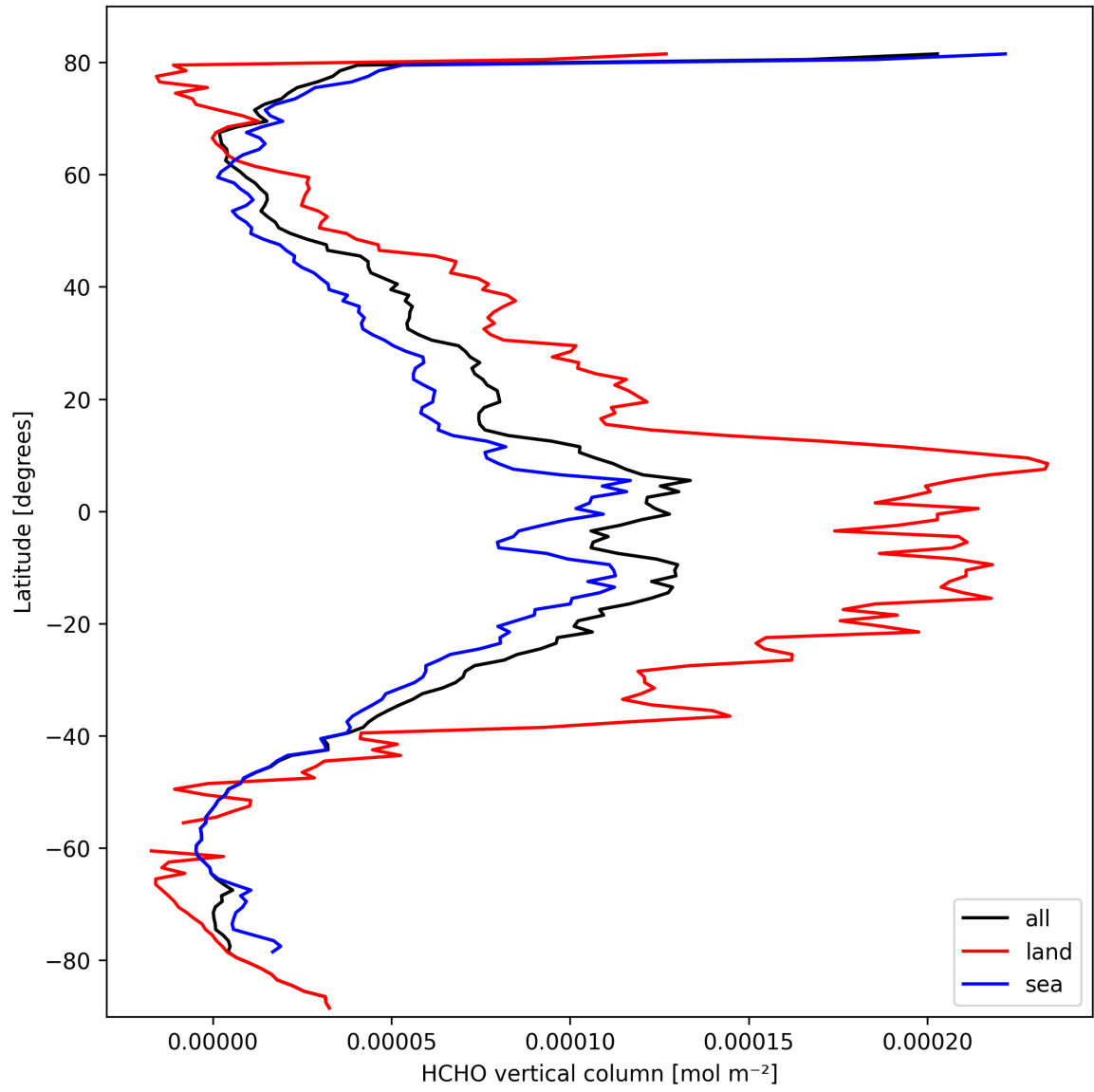
Figure 21: Zonal average of “HCHO vertical column” for 2025-03-10 to 2025-03-12.
