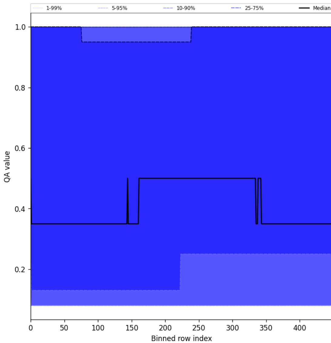
Figure 48: Along track statistics of “QA value” for 2025-03-10 to 2025-03-12
