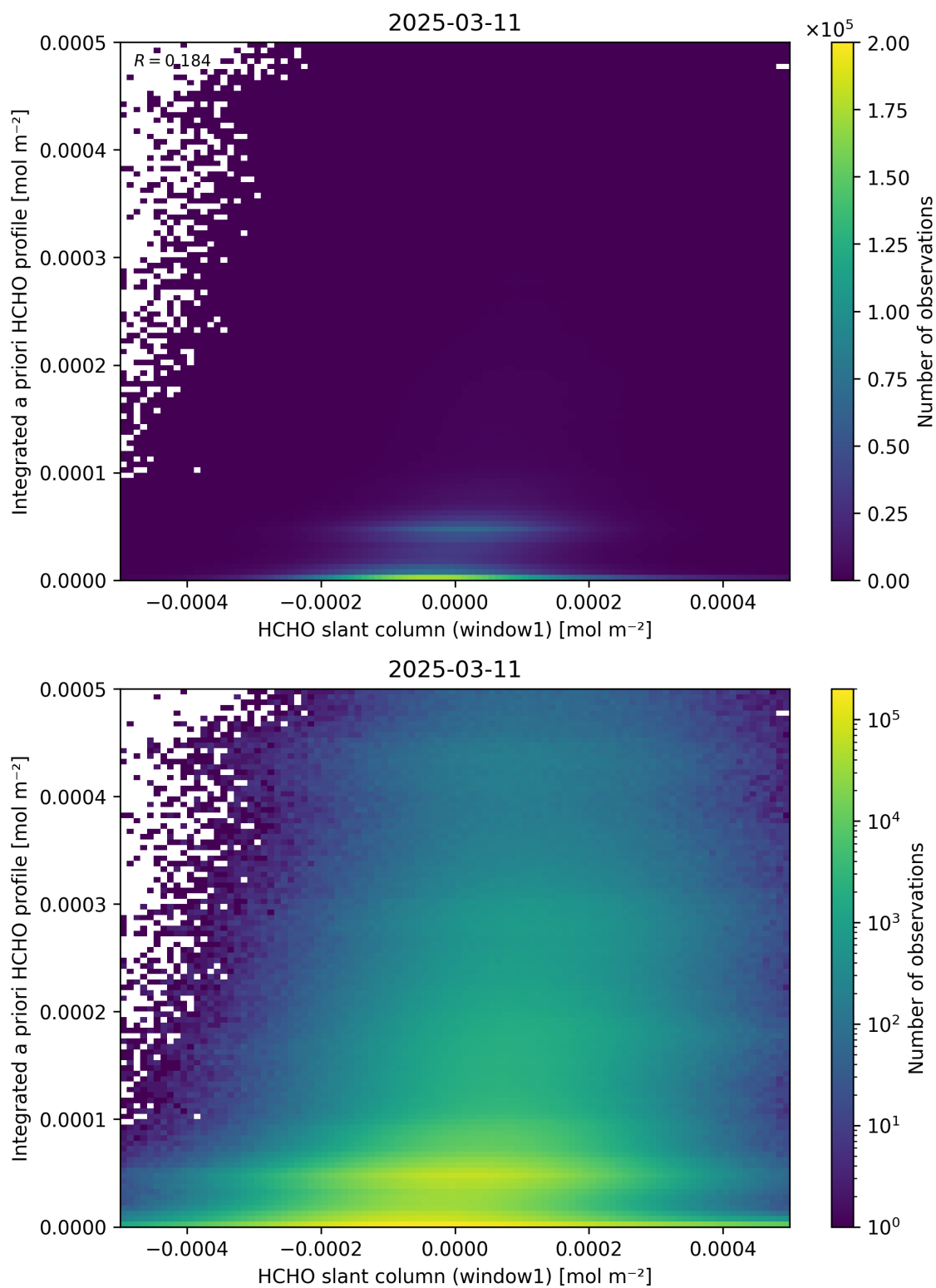
Figure 87: Scatter density plot of “HCHO slant column (window1)” against “Integrated a priori HCHO profile” for 2025-03-10 to 2025-03-12.
