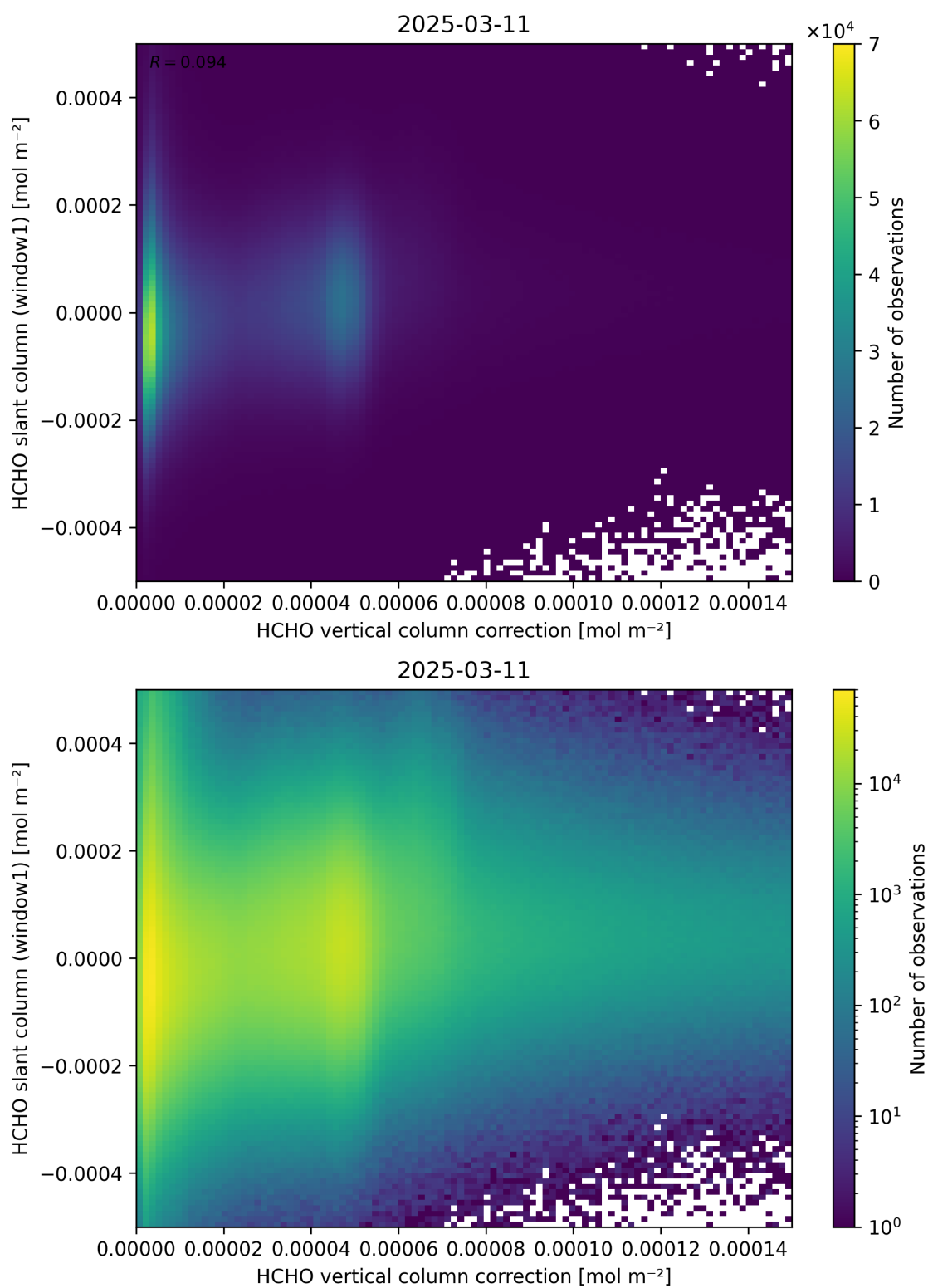
Figure 118: Scatter density plot of “HCHO vertical column correction” against “HCHO slant column (window1)” for 2025-03-10 to 2025-03-12.
