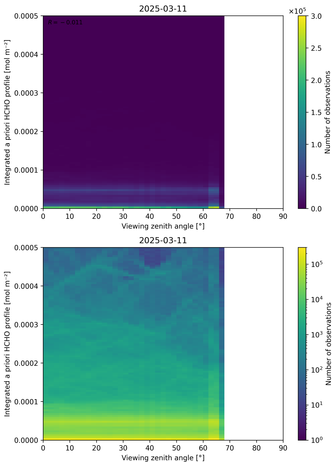
Figure 195: Scatter density plot of “Viewing zenith angle” against “Integrated a priori HCHO profile” for 2025-03-10 to 2025-03-12.
