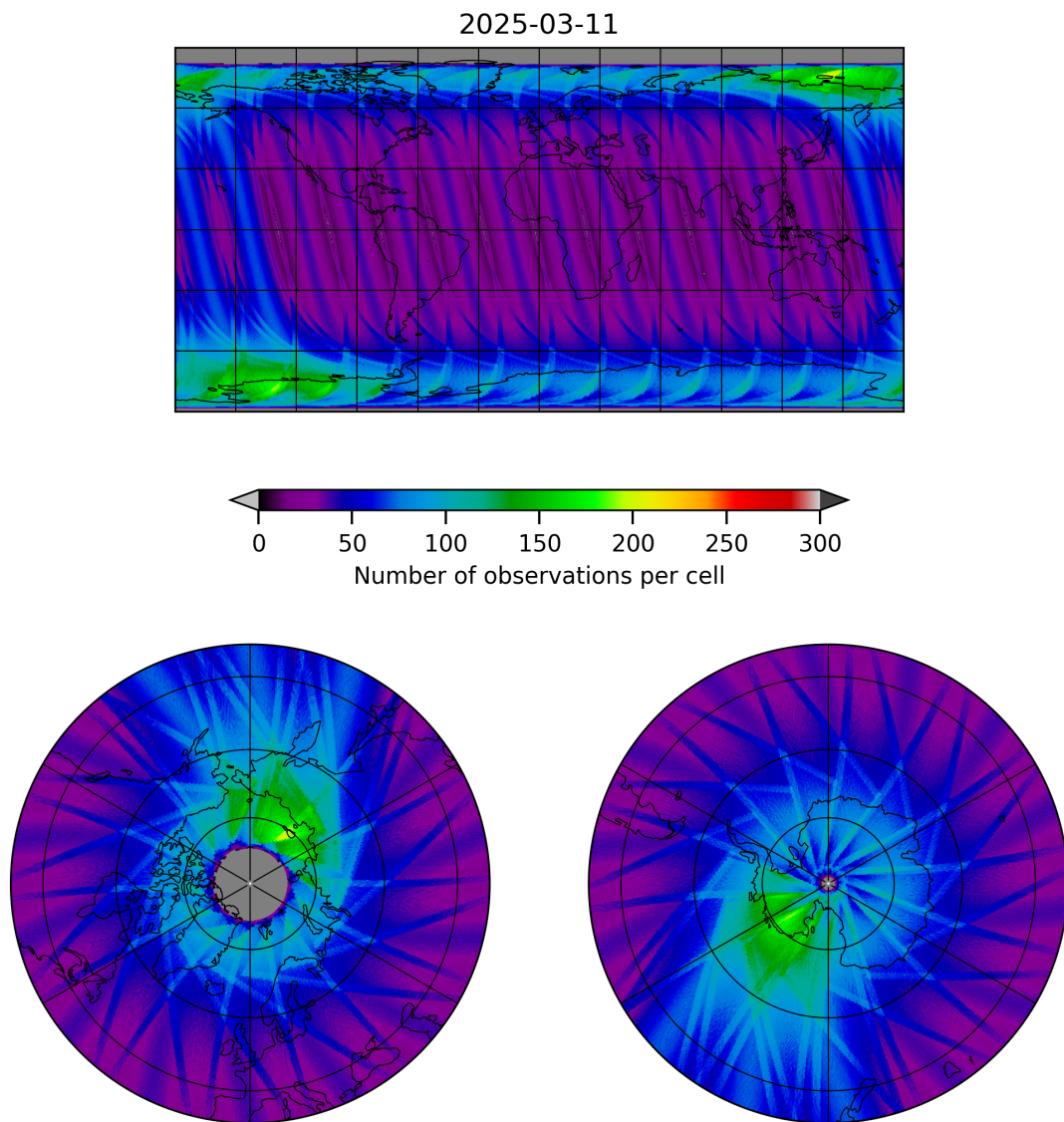
Figure 19: Map of the number of observations for 2025-03-10 to 2025-03-12
