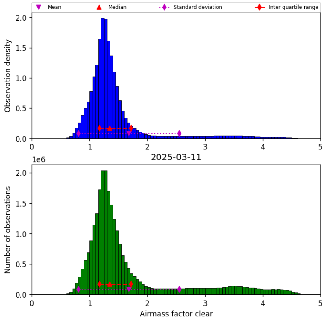
Figure 42: Histogram of “Airmass factor clear” for 2025-03-10 to 2025-03-12
