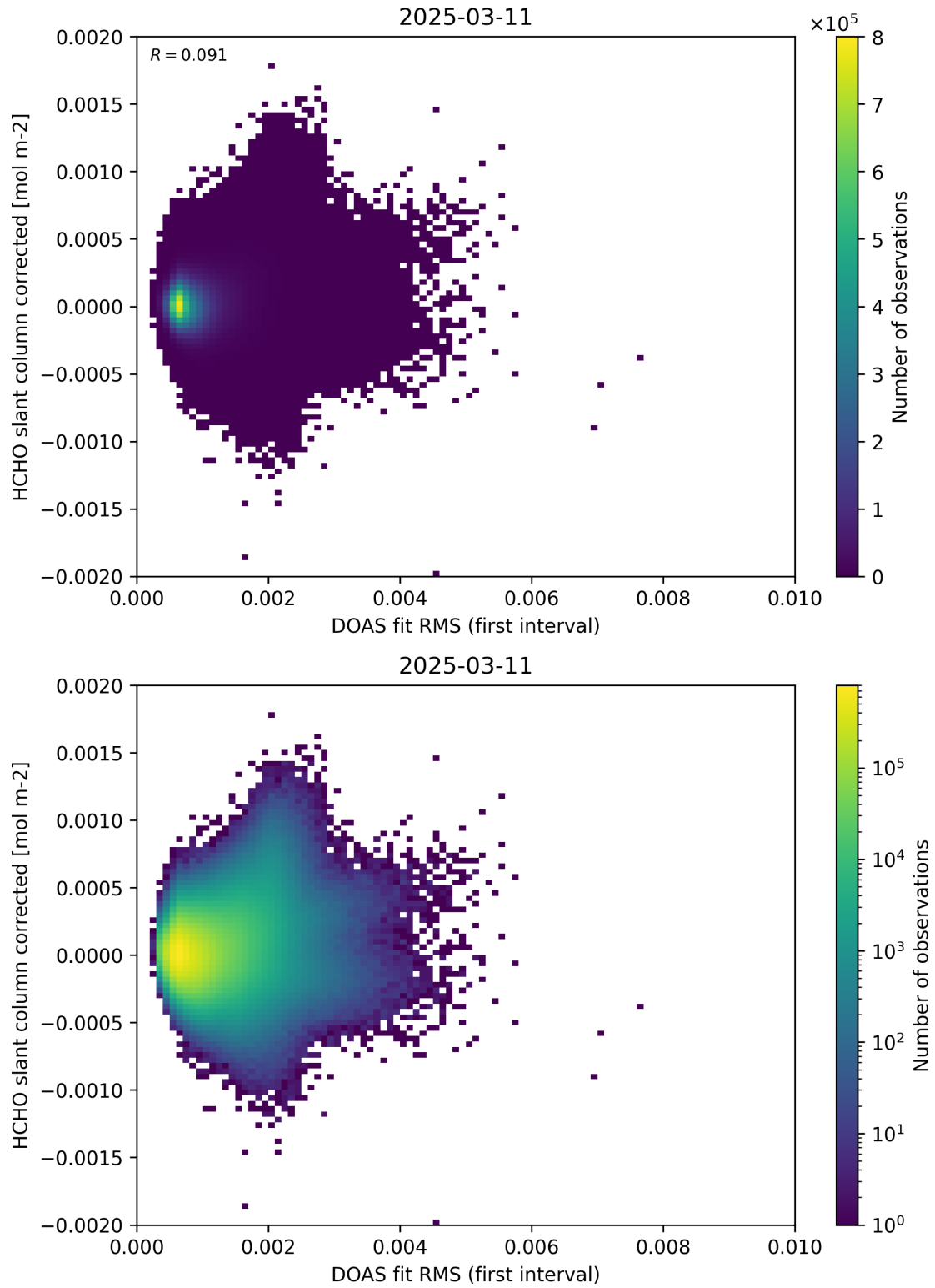
Figure 62: Scatter density plot of “DOAS fit RMS (first interval)” against “HCHO slant column corrected” for 2025-03-10 to 2025-03-12.
