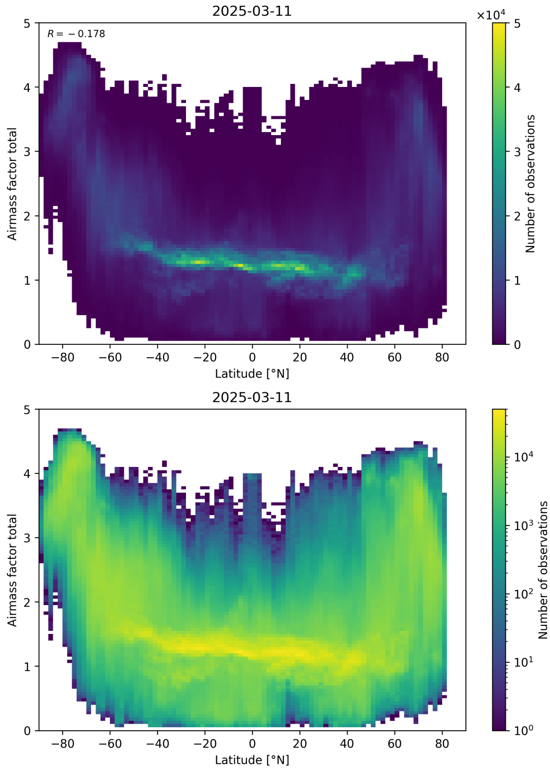
Figure 161: Scatter density plot of “Latitude” against “Airmass factor total” for 2025-03-10 to 2025-03-12.
