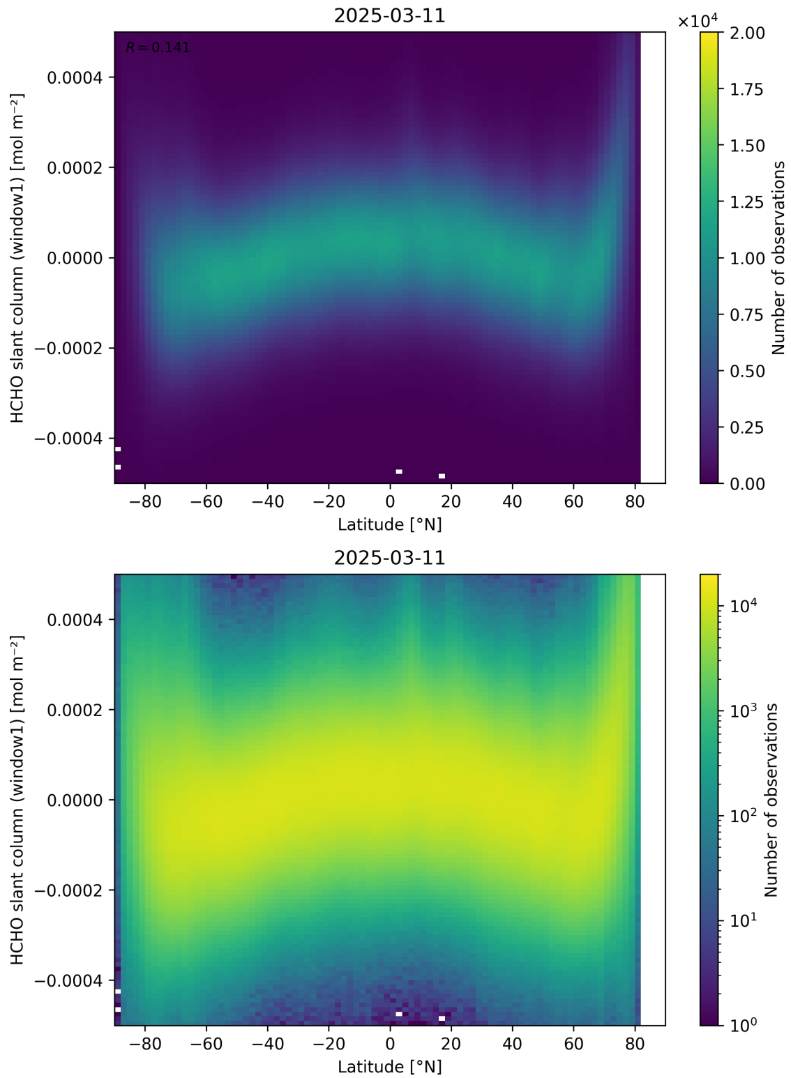
Figure 159: Scatter density plot of “Latitude” against “HCHO slant column (window1)” for 2025-03-10 to 2025-03-12.
