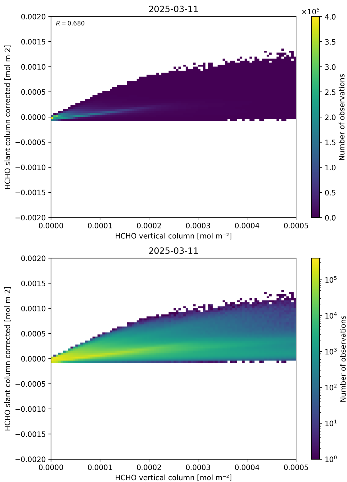
Figure 127: Scatter density plot of “HCHO vertical column” against “HCHO slant column corrected” for 2025-03-10 to 2025-03-12.
