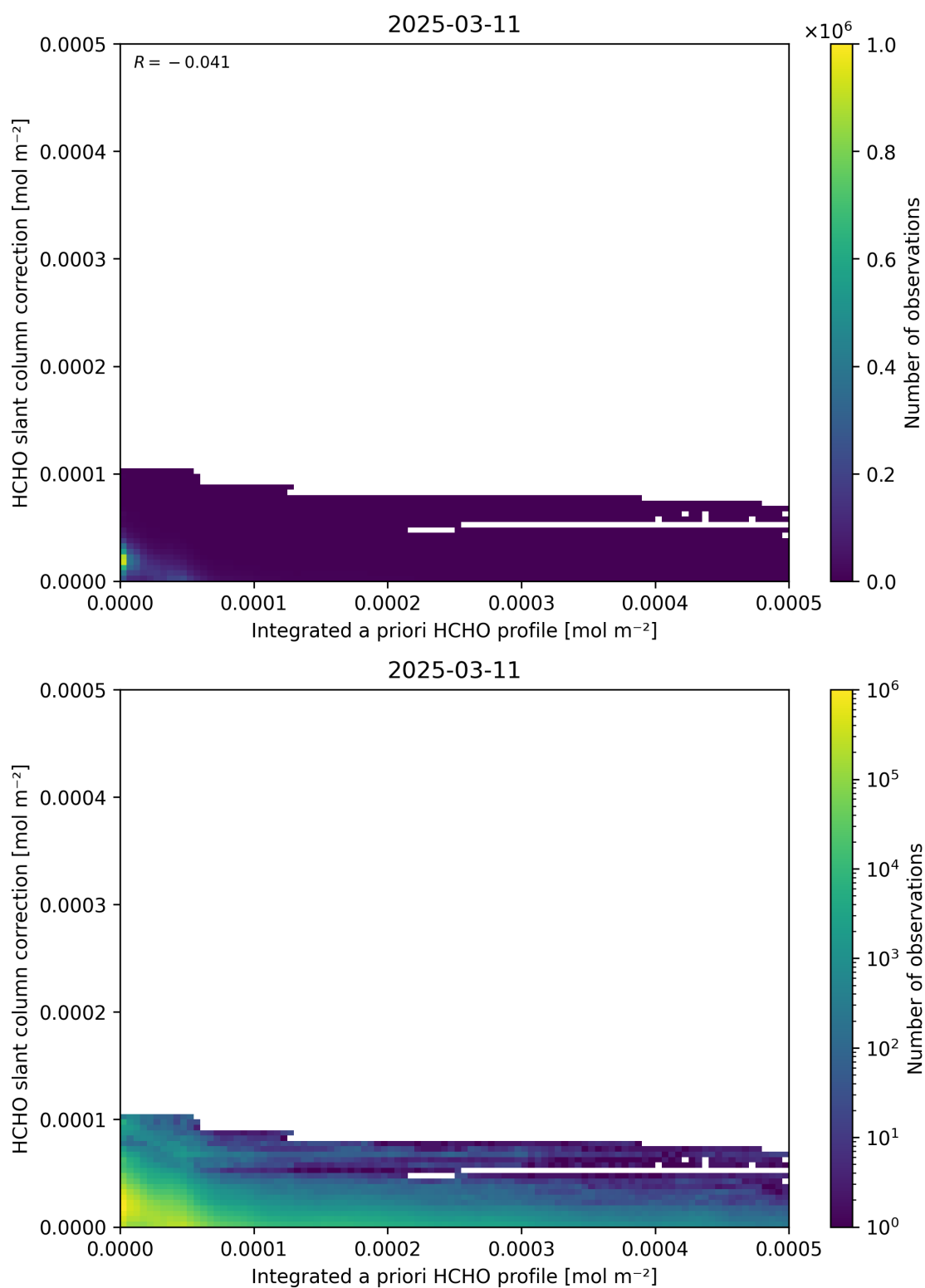
Figure 152: Scatter density plot of “Integrated a priori HCHO profile” against “HCHO slant column correction” for 2025-03-10 to 2025-03-12.
