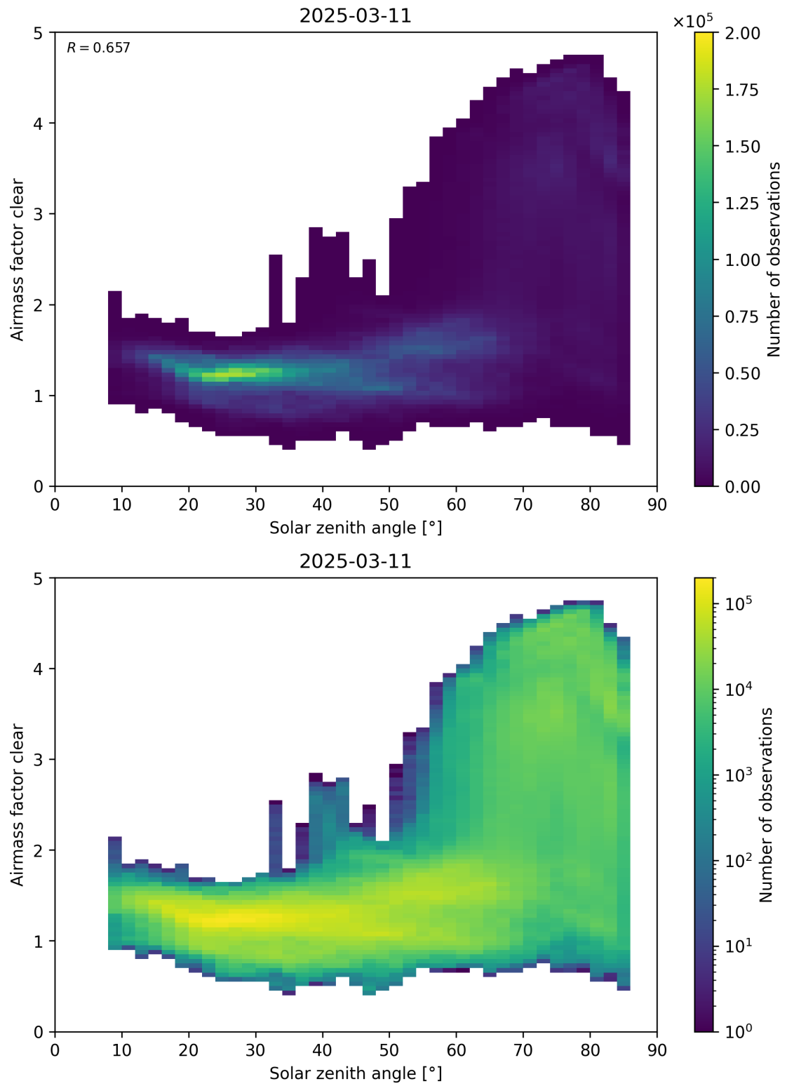
Figure 170: Scatter density plot of “Solar zenith angle” against “Airmass factor clear” for 2025-03-10 to 2025-03-12.
