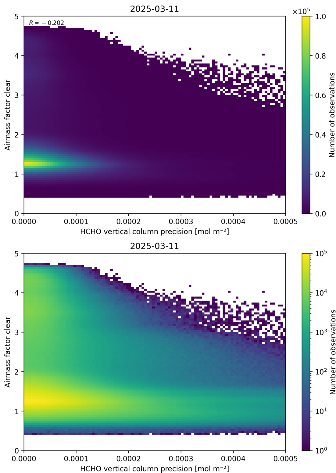
Figure 139: Scatter density plot of “HCHO vertical column precision” against “Airmass factor clear” for 2025-03-10 to 2025-03-12.
