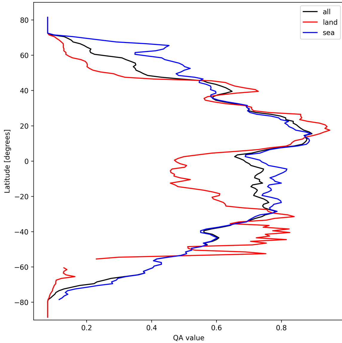
Figure 20: Zonal average of “QA value” for 2025-03-10 to 2025-03-12.
