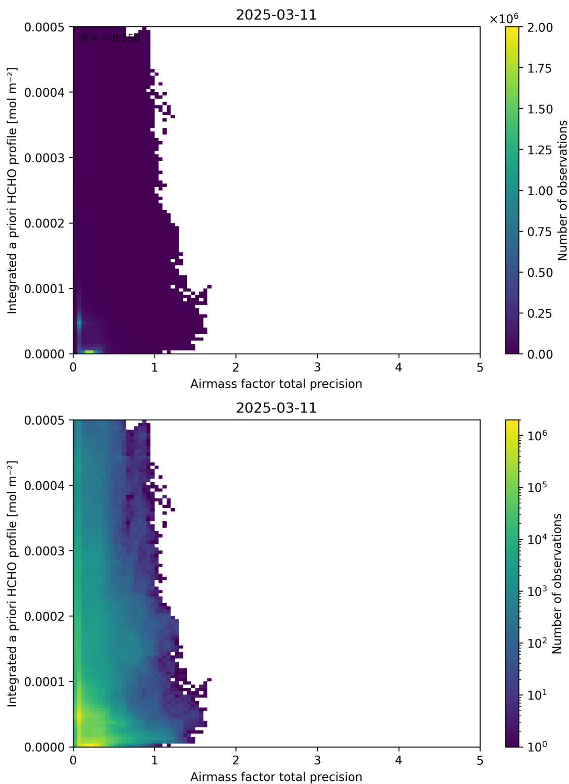
Figure 111: Scatter density plot of “Airmass factor total precision” against “Integrated a priori HCHO profile” for 2025-03-10 to 2025-03-12.
