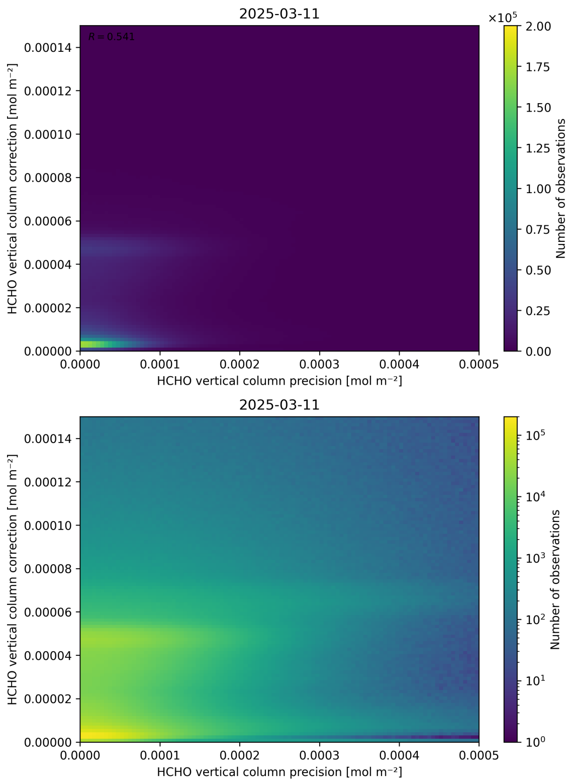
Figure 146: Scatter density plot of “HCHO vertical column precision” against “HCHO vertical column correction” for 2025-03-10 to 2025-03-12.
