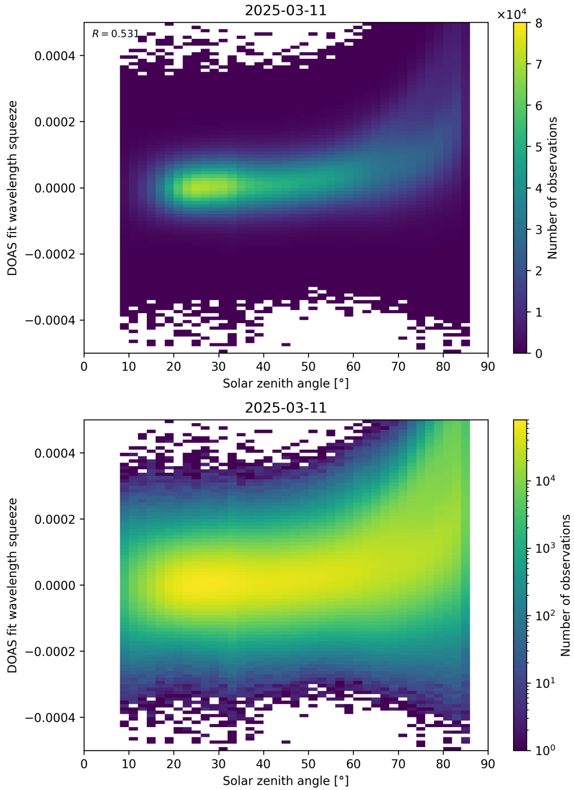
Figure 169: Scatter density plot of “Solar zenith angle” against “DOAS fit wavelength squeeze” for 2025-03-10 to 2025-03-12.
