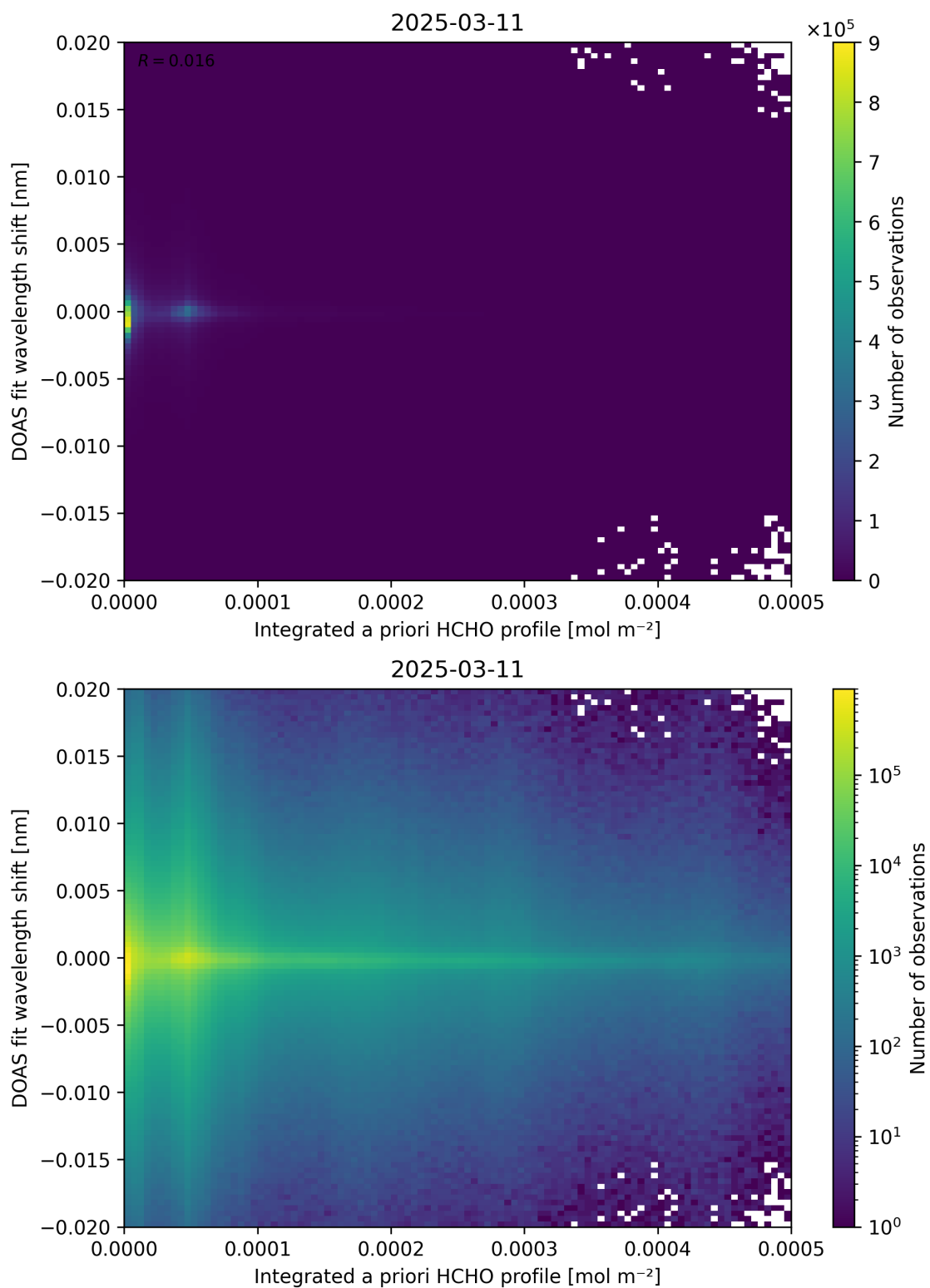
Figure 149: Scatter density plot of “Integrated a priori HCHO profile” against “DOAS fit wavelength shift” for 2025-03-10 to 2025-03-12.
