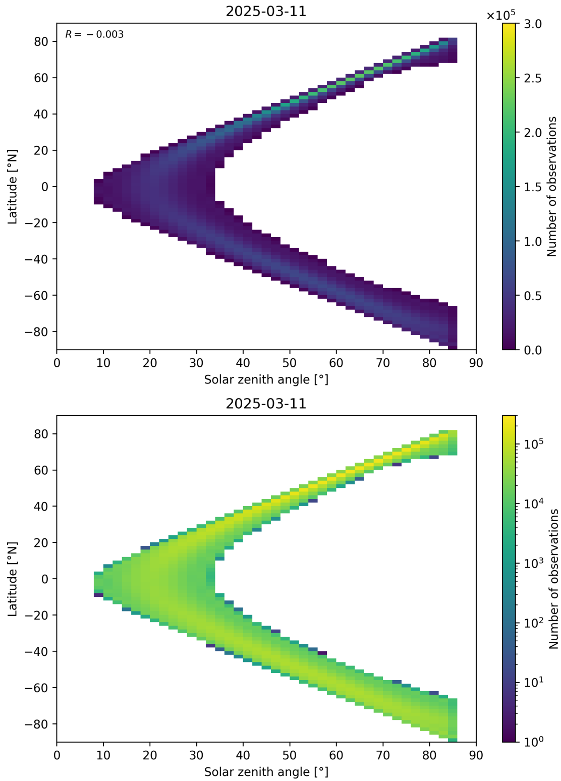
Figure 181: Scatter density plot of “Solar zenith angle” against “Latitude” for 2025-03-10 to 2025-03-12.
