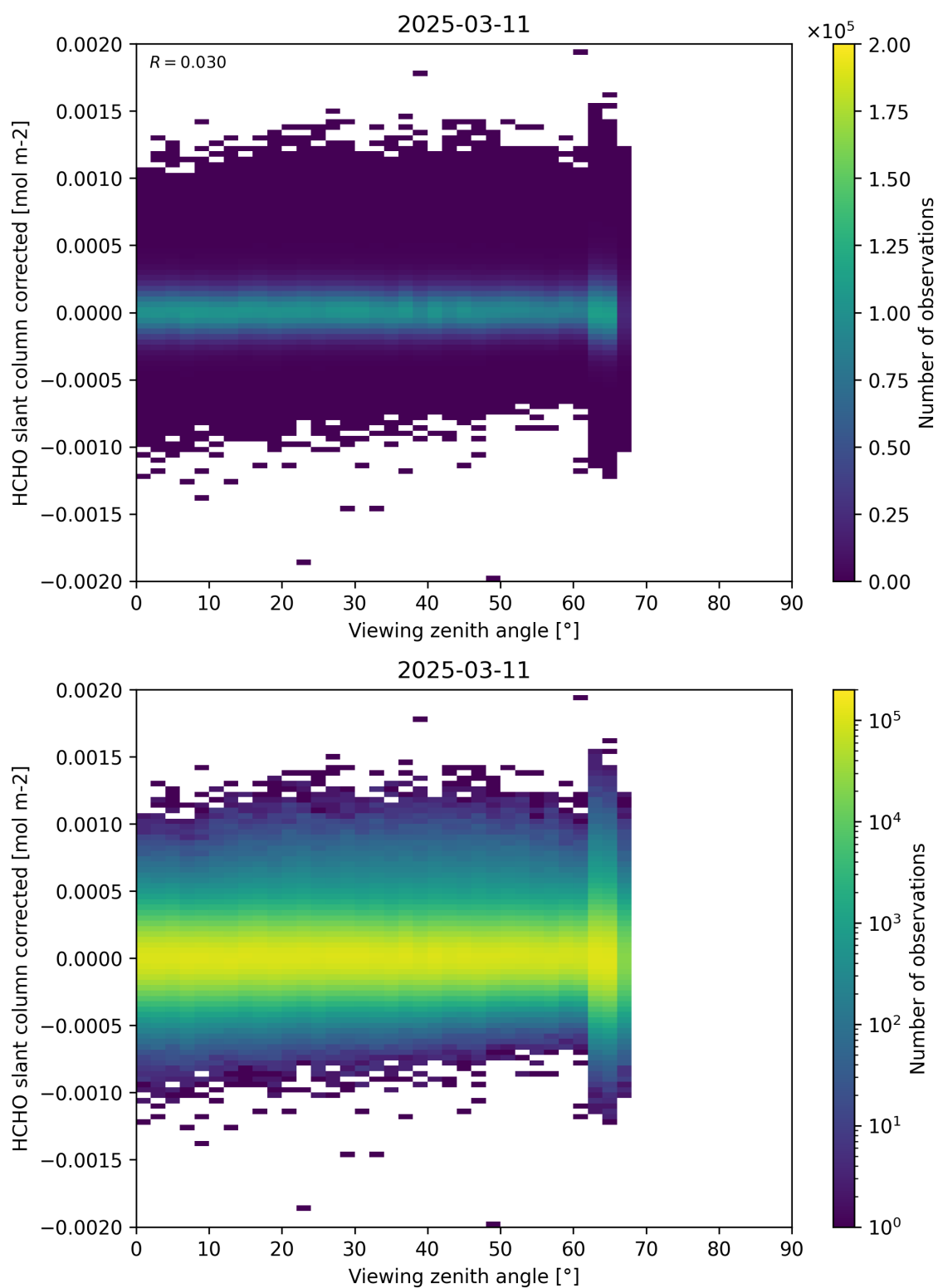
Figure 186: Scatter density plot of “Viewing zenith angle” against “HCHO slant column corrected” for 2025-03-10 to 2025-03-12.
