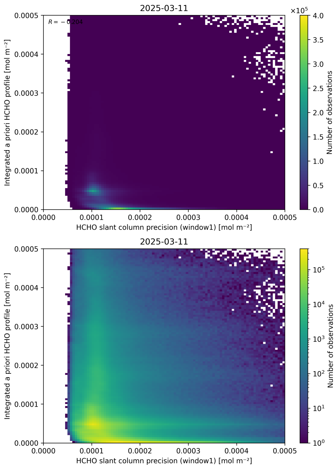
Figure 96: Scatter density plot of “HCHO slant column precision (window1)” against “Integrated a priori HCHO profile” for 2025-03-10 to 2025-03-12.
