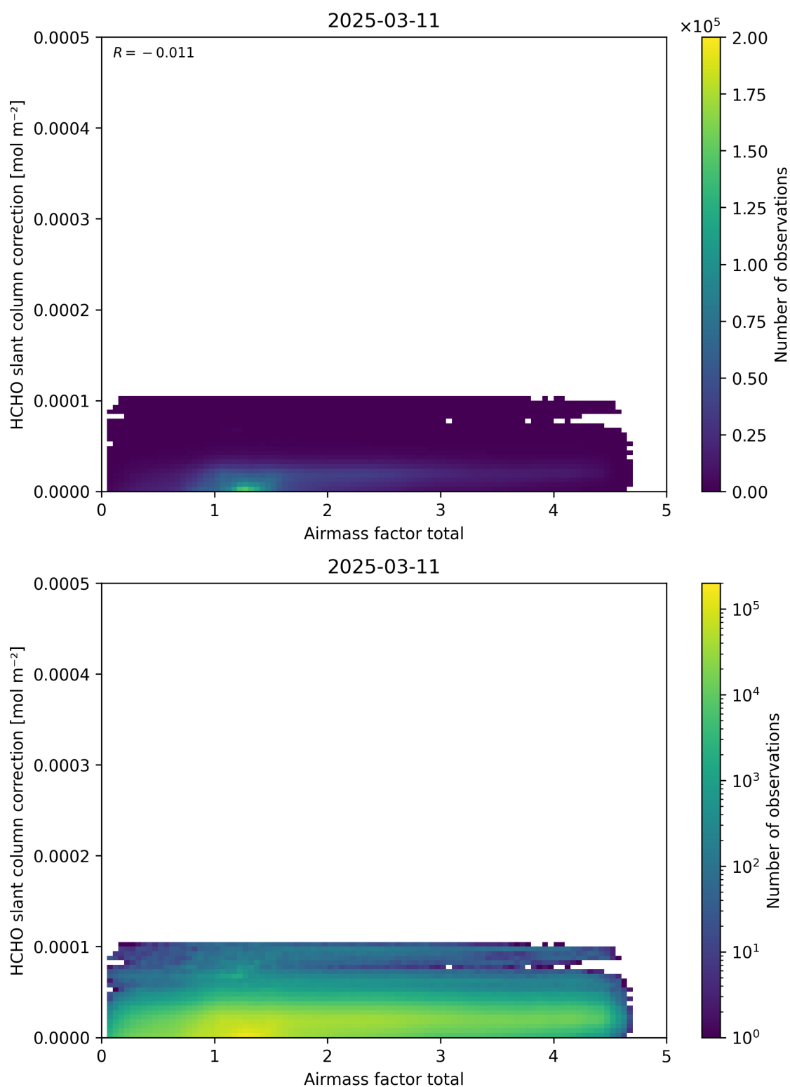
Figure 102: Scatter density plot of “Airmass factor total” against “HCHO slant column correction” for 2025-03-10 to 2025-03-12.
