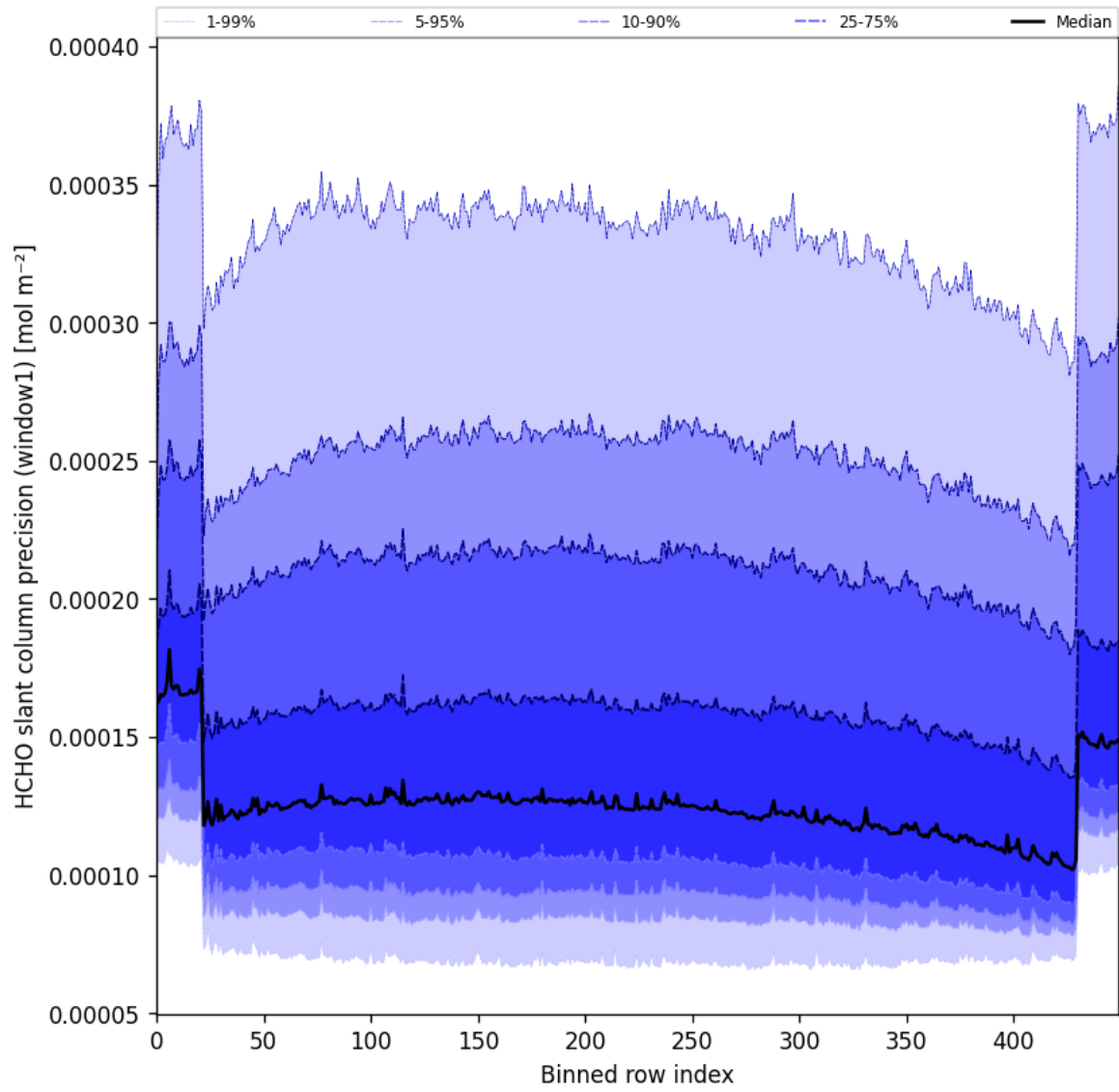
Figure 53: Along track statistics of “HCHO slant column precision (window1)” for 2025-03-10 to 2025-03-12
