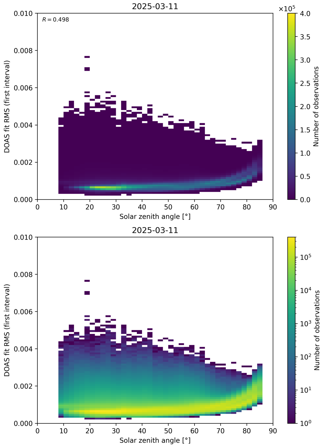
Figure 167: Scatter density plot of “Solar zenith angle” against “DOAS fit RMS (first interval)” for 2025-03-10 to 2025-03-12.
