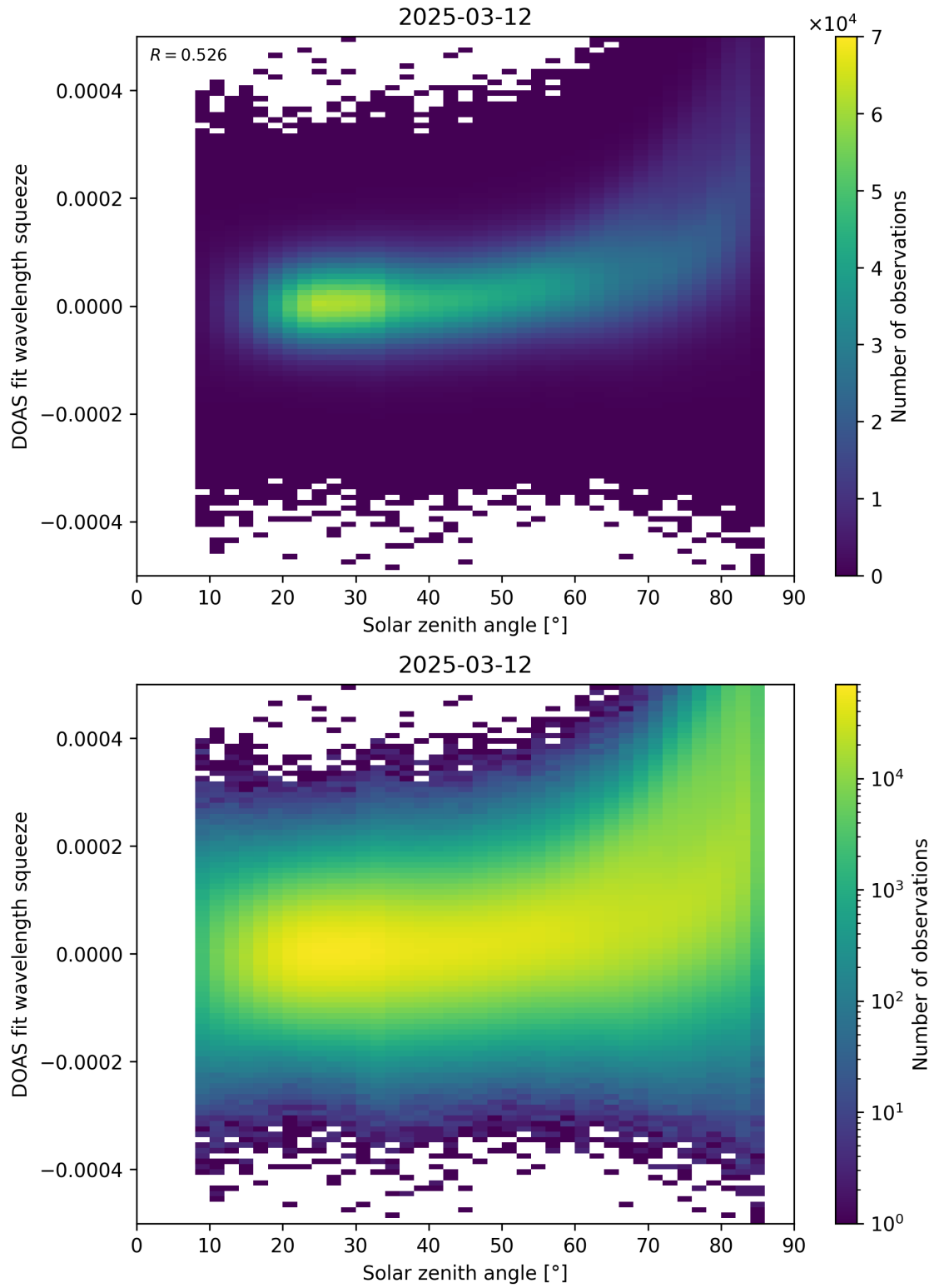
Figure 169: Scatter density plot of “Solar zenith angle” against “DOAS fit wavelength squeeze” for 2025-03-12 to 2025-03-13.
