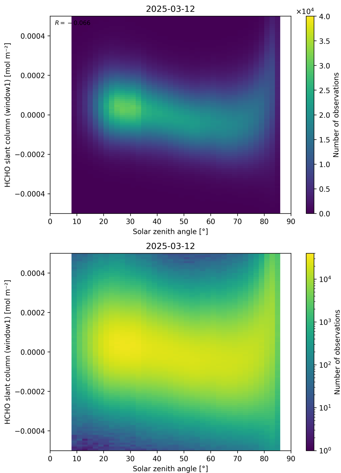
Figure 173: Scatter density plot of “Solar zenith angle” against “HCHO slant column (window1)” for 2025-03-12 to 2025-03-13.
