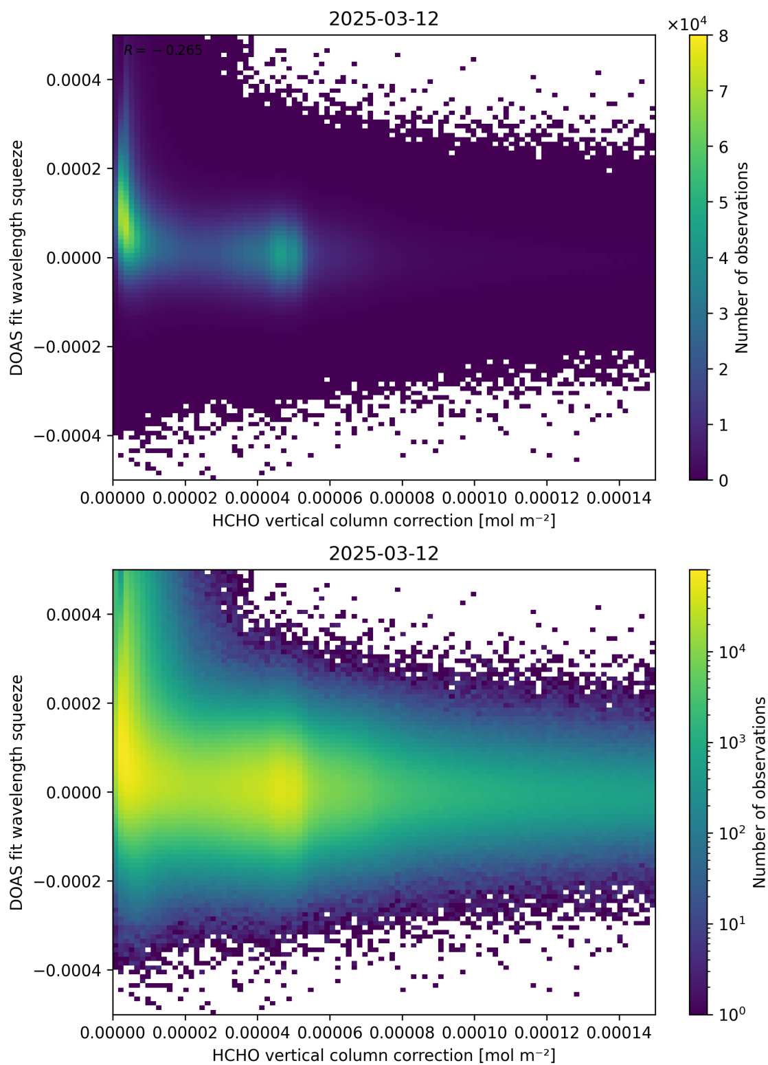
Figure 114: Scatter density plot of “HCHO vertical column correction” against “DOAS fit wavelength squeeze” for 2025-03-12 to 2025-03-13.
