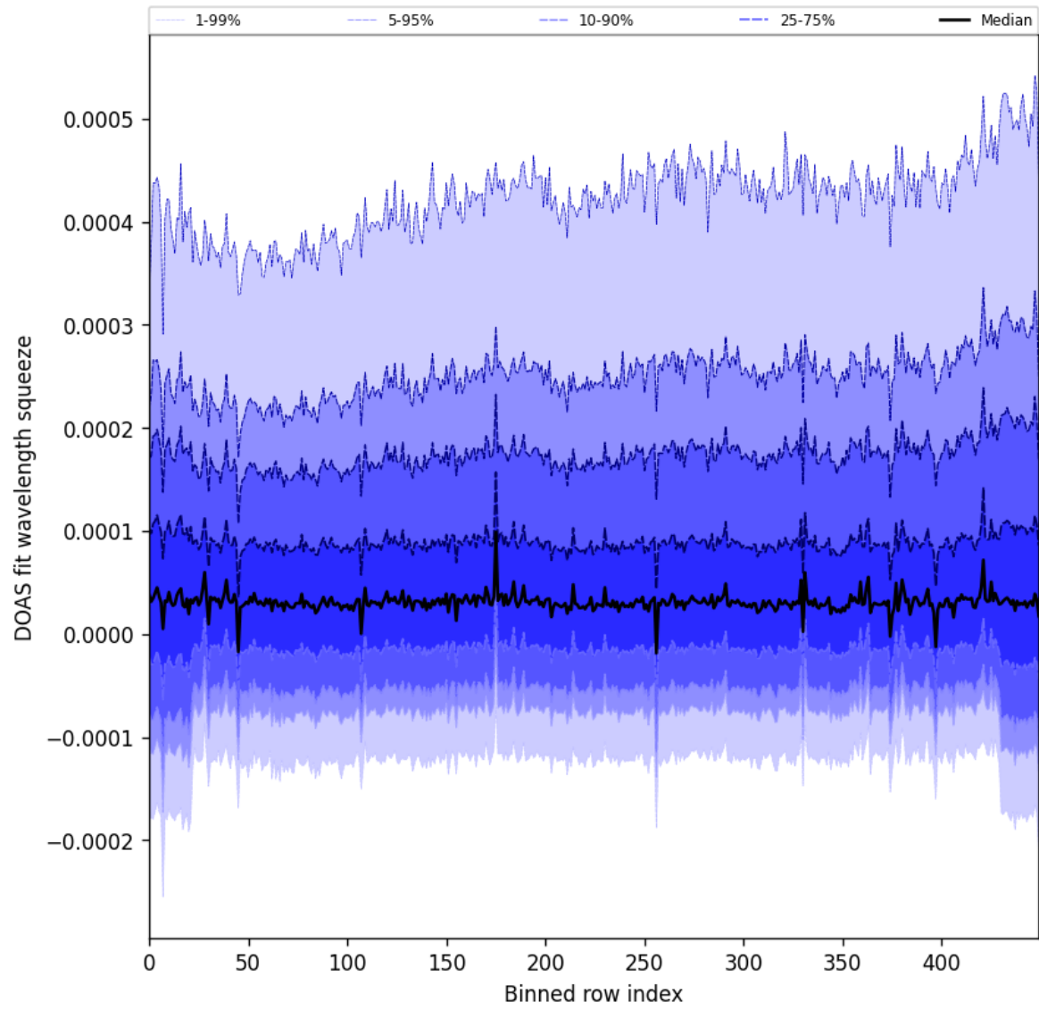
Figure 59: Along track statistics of “DOAS fit wavelength squeeze” for 2025-03-12 to 2025-03-13
