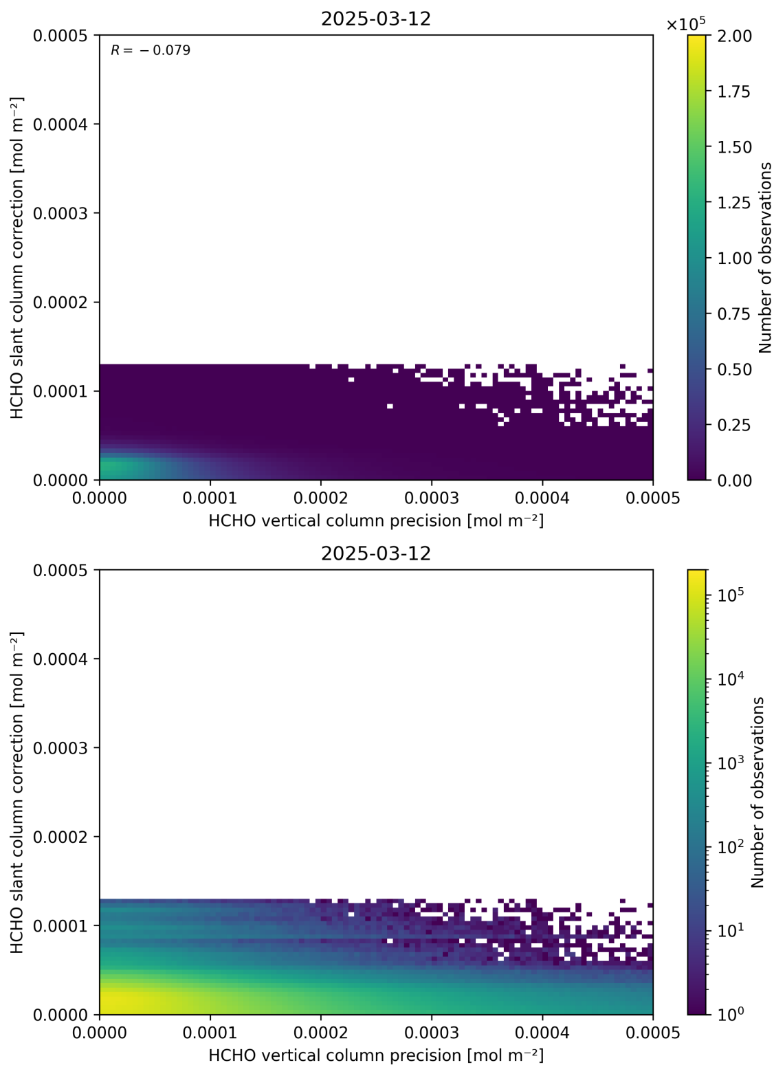
Figure 141: Scatter density plot of “HCHO vertical column precision” against “HCHO slant column correction” for 2025-03-12 to 2025-03-13.
