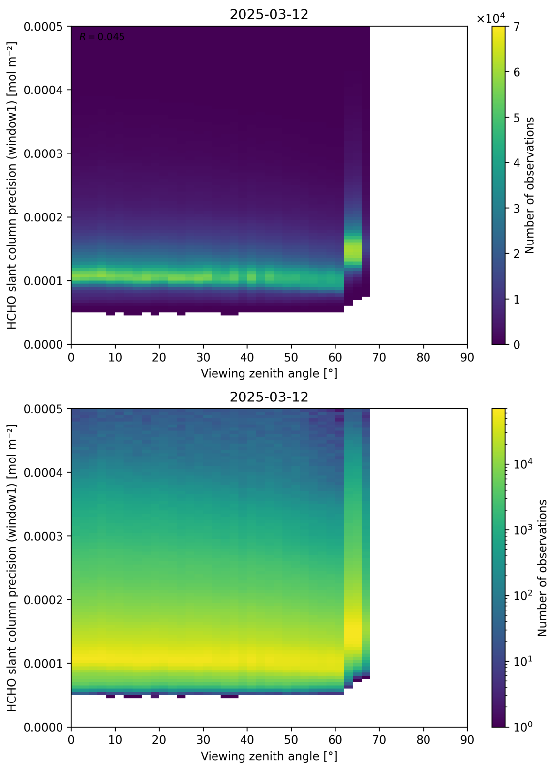
Figure 189: Scatter density plot of “Viewing zenith angle” against “HCHO slant column precision (window1)” for 2025-03-12 to 2025-03-13.
