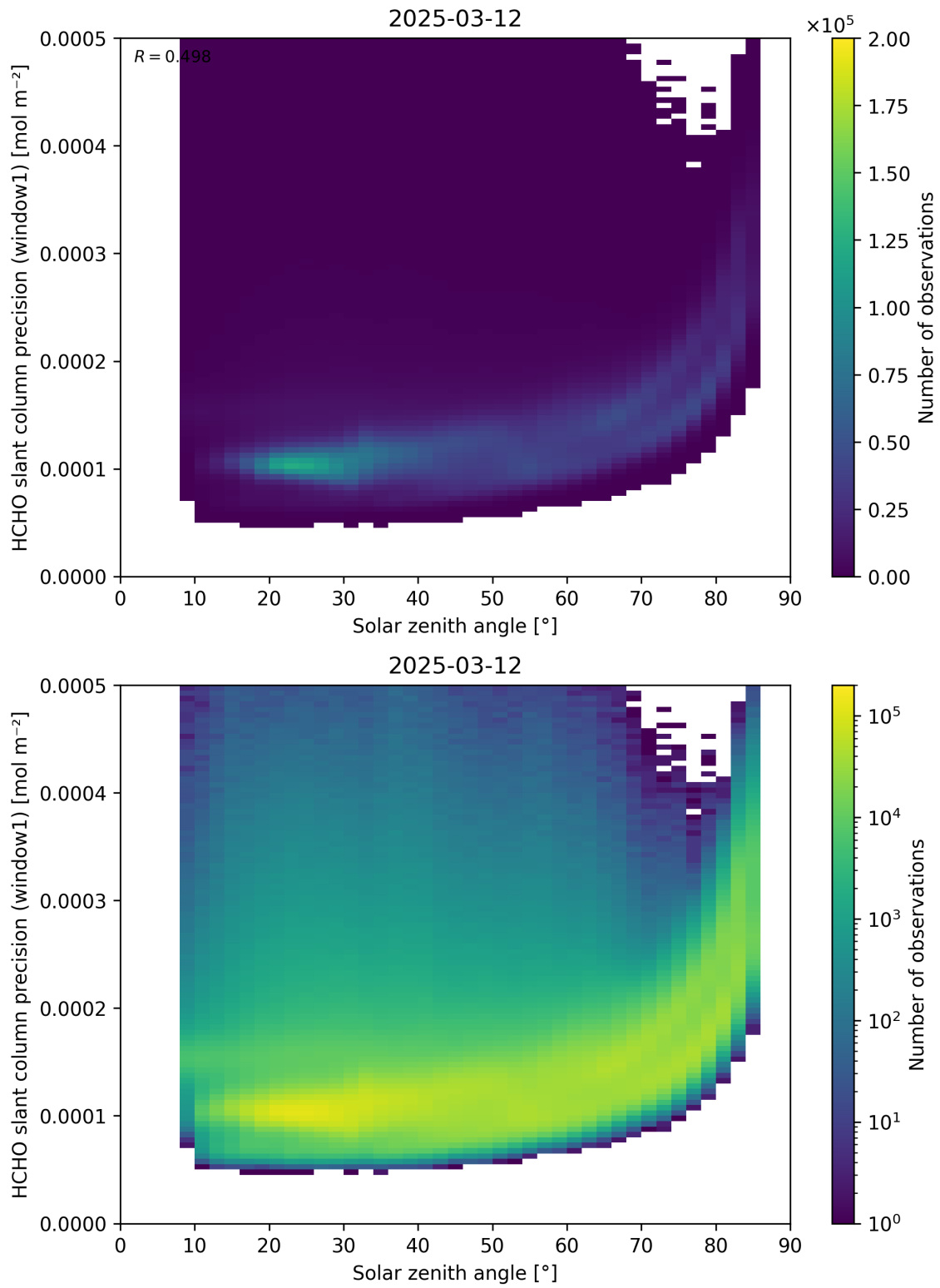
Figure 174: Scatter density plot of “Solar zenith angle” against “HCHO slant column precision (window1)” for 2025-03-12 to 2025-03-13.
