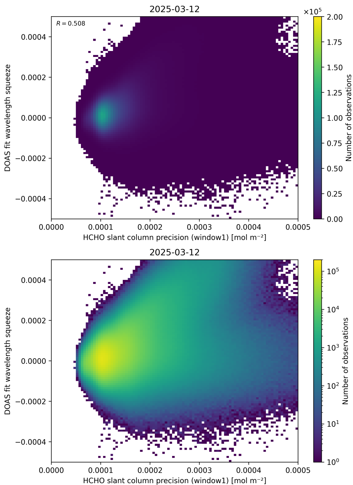
Figure 90: Scatter density plot of “HCHO slant column precision (window1)” against “DOAS fit wavelength squeeze” for 2025-03-12 to 2025-03-13.
