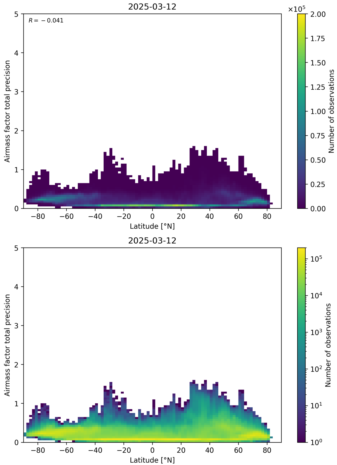
Figure 162: Scatter density plot of “Latitude” against “Airmass factor total precision” for 2025-03-12 to 2025-03-13.
