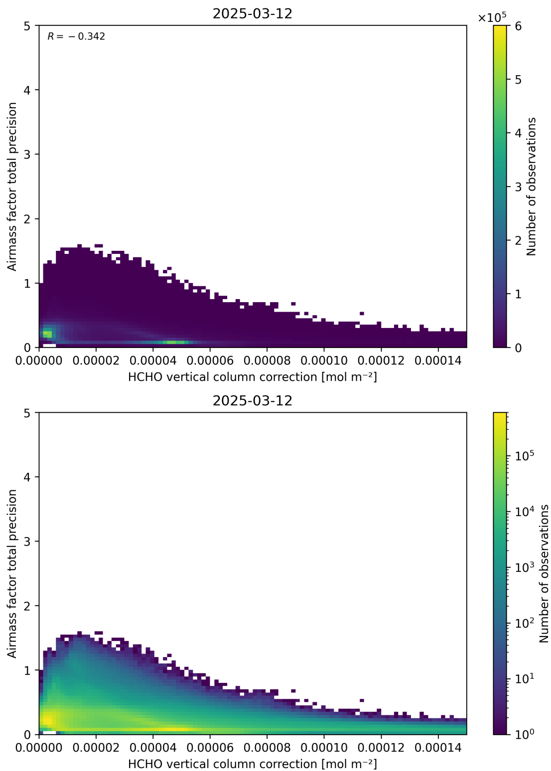
Figure 121: Scatter density plot of “HCHO vertical column correction” against “Airmass factor total precision” for 2025-03-12 to 2025-03-13.
