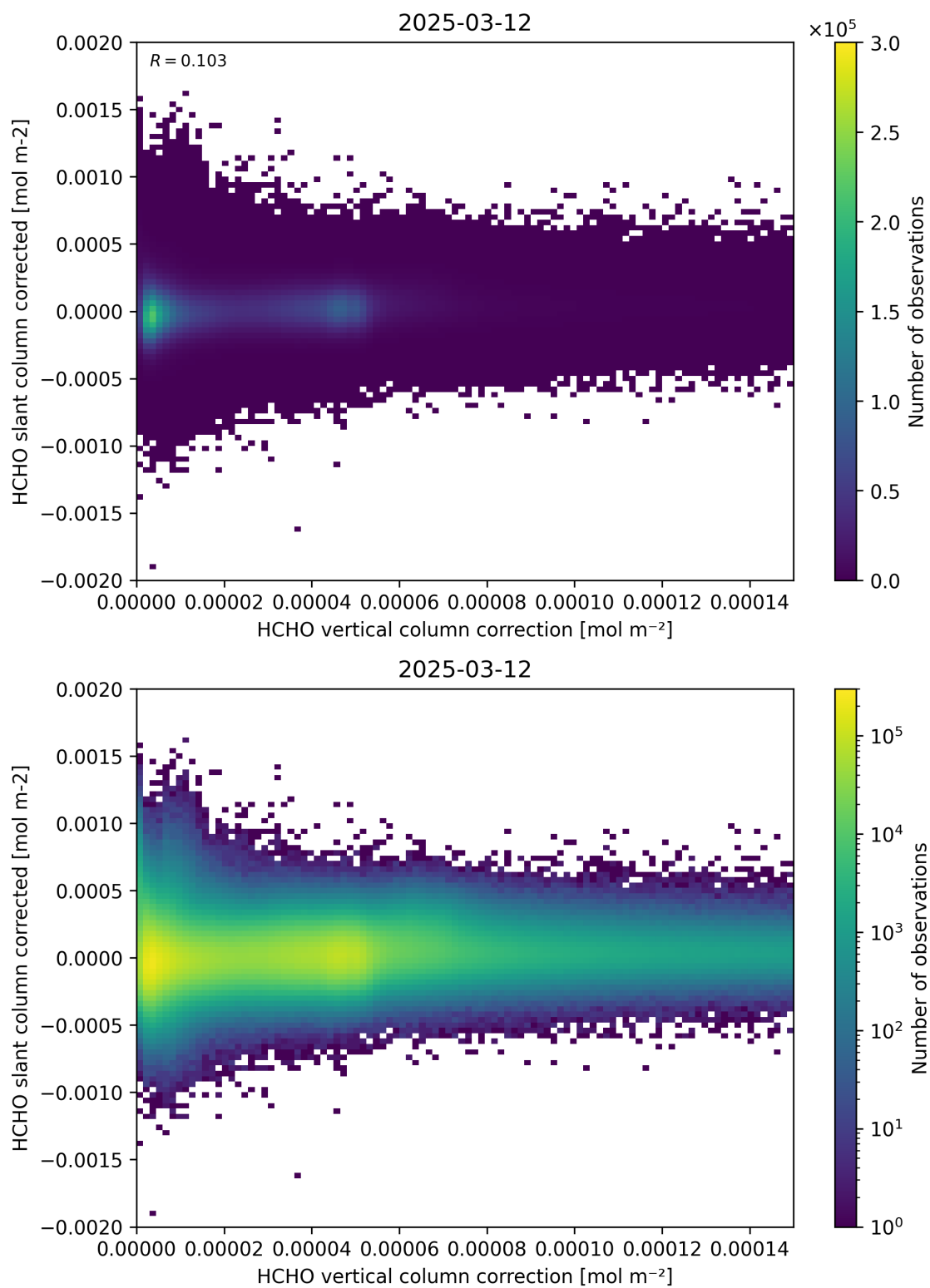
Figure 116: Scatter density plot of “HCHO vertical column correction” against “HCHO slant column corrected” for 2025-03-12 to 2025-03-13.
