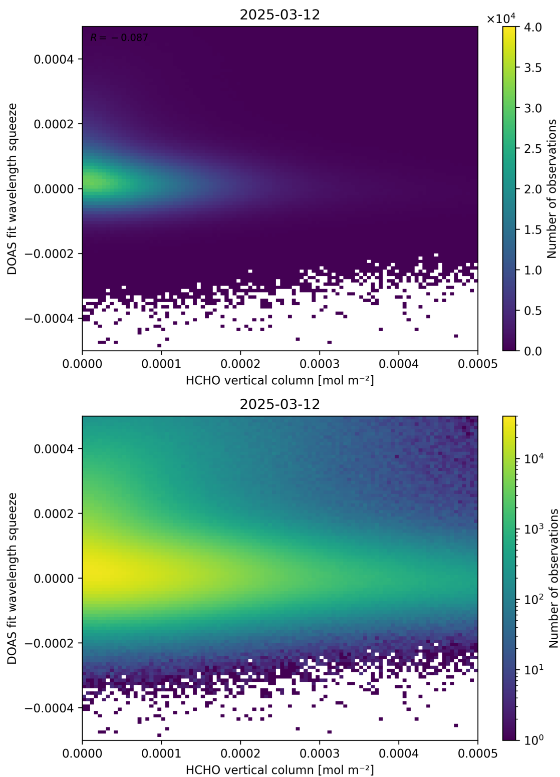
Figure 125: Scatter density plot of “HCHO vertical column” against “DOAS fit wavelength squeeze” for 2025-03-12 to 2025-03-13.
