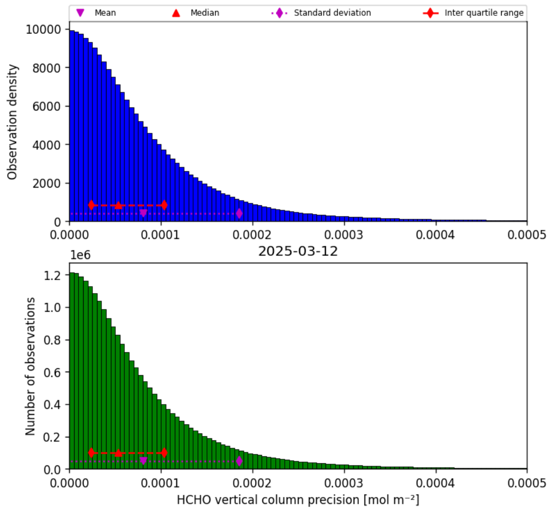
Figure 36: Histogram of “HCHO vertical column precision” for 2025-03-12 to 2025-03-13
