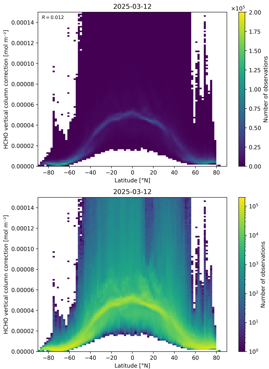
Figure 164: Scatter density plot of “Latitude” against “HCHO vertical column correction” for 2025-03-12 to 2025-03-13.
