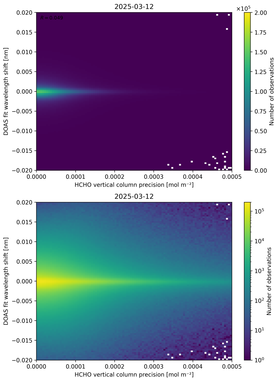
Figure 137: Scatter density plot of “HCHO vertical column precision” against “DOAS fit wavelength shift” for 2025-03-12 to 2025-03-13.
