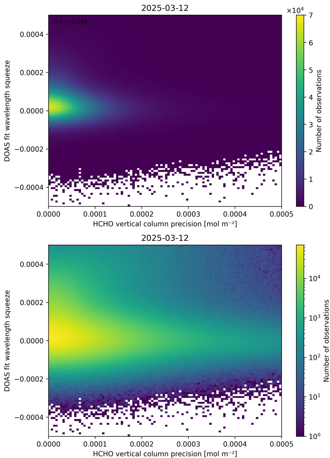
Figure 138: Scatter density plot of “HCHO vertical column precision” against “DOAS fit wavelength squeeze” for 2025-03-12 to 2025-03-13.
