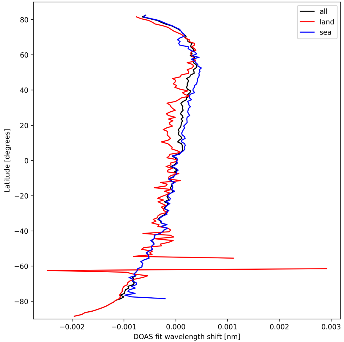
Figure 30: Zonal average of "DOAS fit wavelength shift" for 2025-03-12 to 2025-03-13.
