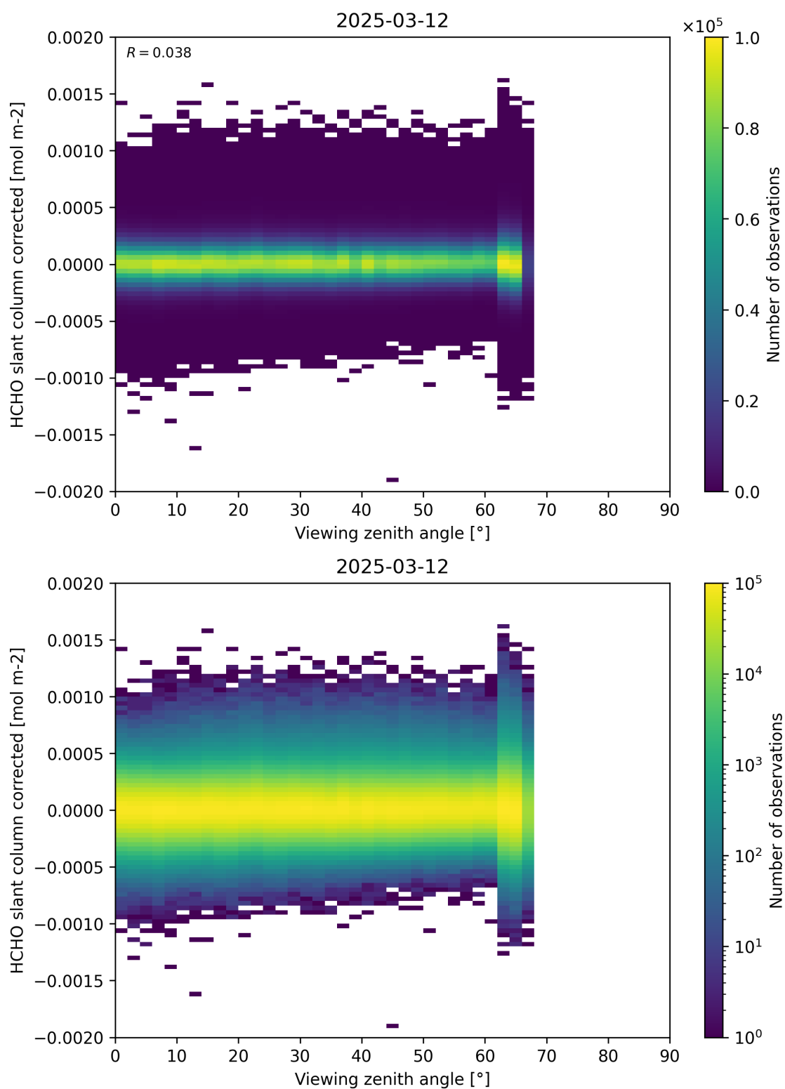
Figure 186: Scatter density plot of “Viewing zenith angle” against “HCHO slant column corrected” for 2025-03-12 to 2025-03-13.
