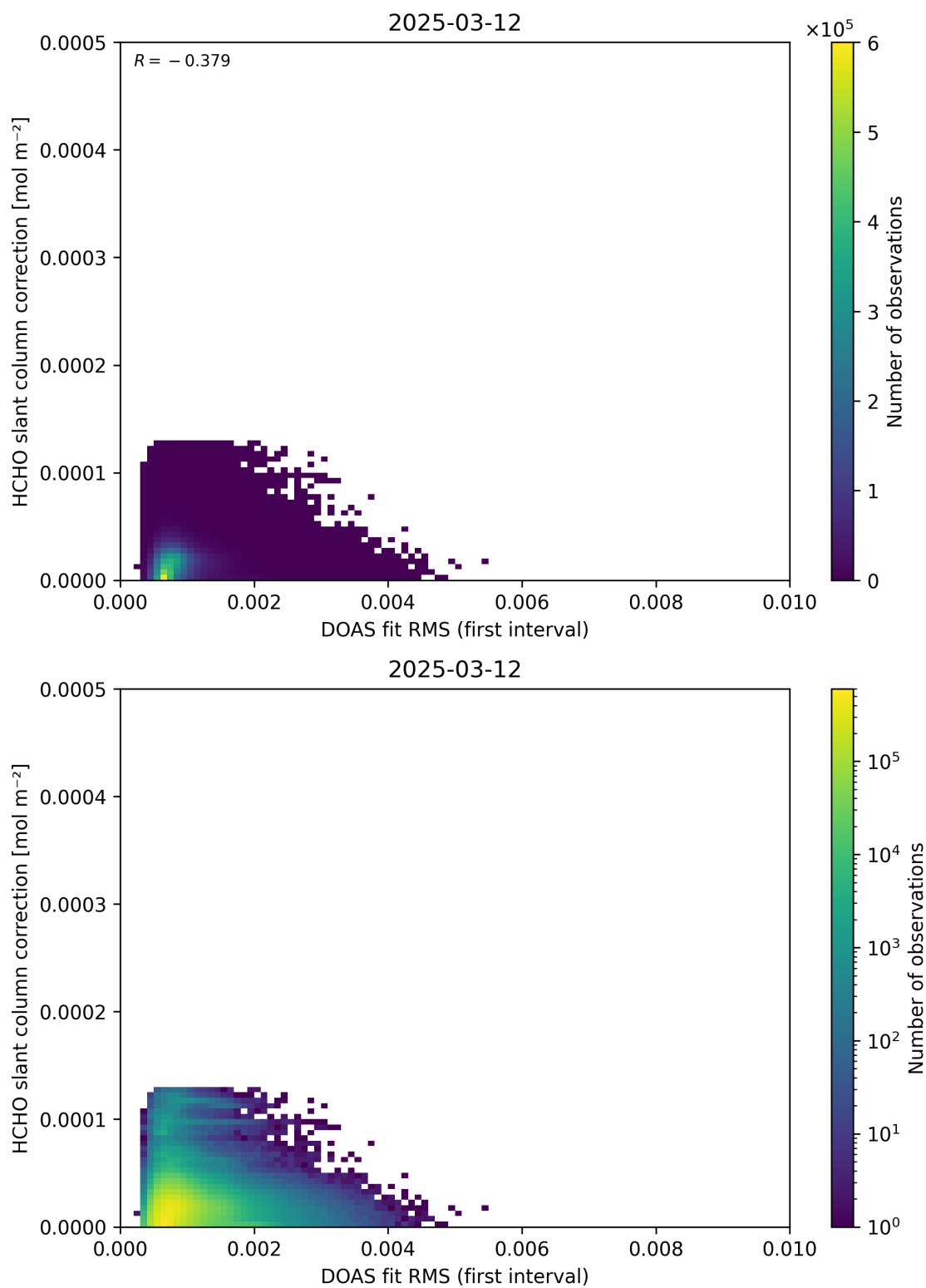
Figure 63: Scatter density plot of “DOAS fit RMS (first interval)” against “HCHO slant column correction” for 2025-03-12 to 2025-03-13.
