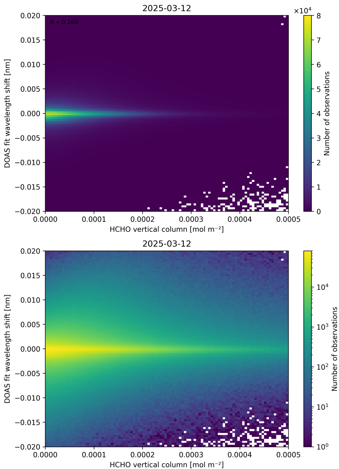
Figure 124: Scatter density plot of “HCHO vertical column” against “DOAS fit wavelength shift” for 2025-03-12 to 2025-03-13.
