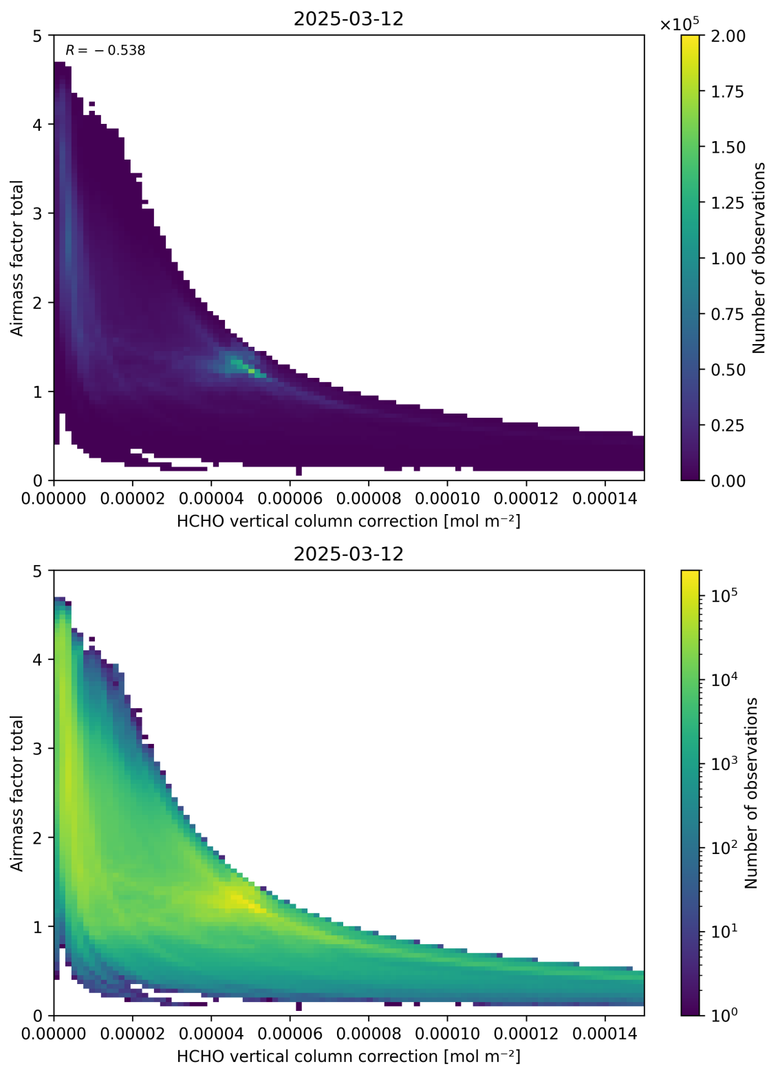
Figure 120: Scatter density plot of “HCHO vertical column correction” against “Airmass factor total” for 2025-03-12 to 2025-03-13.
