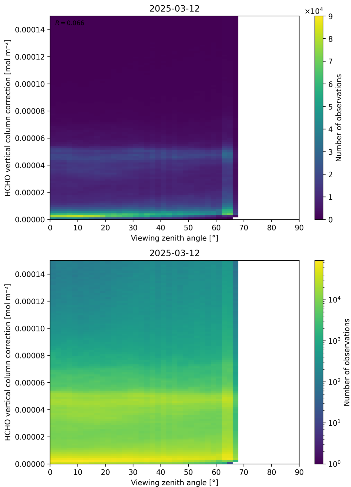
Figure 193: Scatter density plot of “Viewing zenith angle” against “HCHO vertical column correction” for 2025-03-12 to 2025-03-13.
