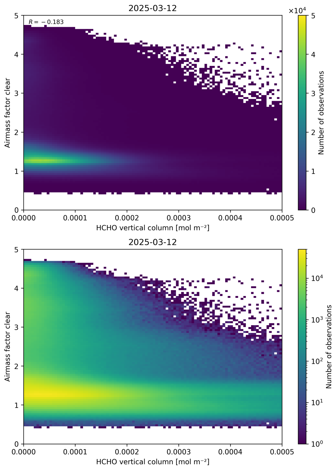
Figure 126: Scatter density plot of “HCHO vertical column” against “Airmass factor clear” for 2025-03-12 to 2025-03-13.
