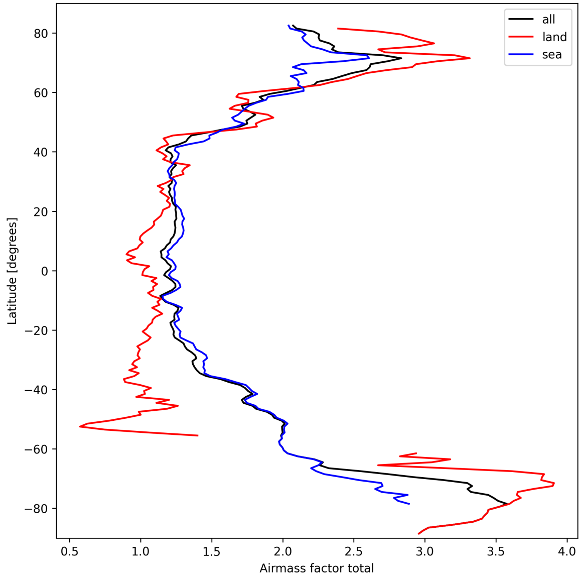
Figure 26: Zonal average of “Airmass factor total” for 2025-03-12 to 2025-03-13.
