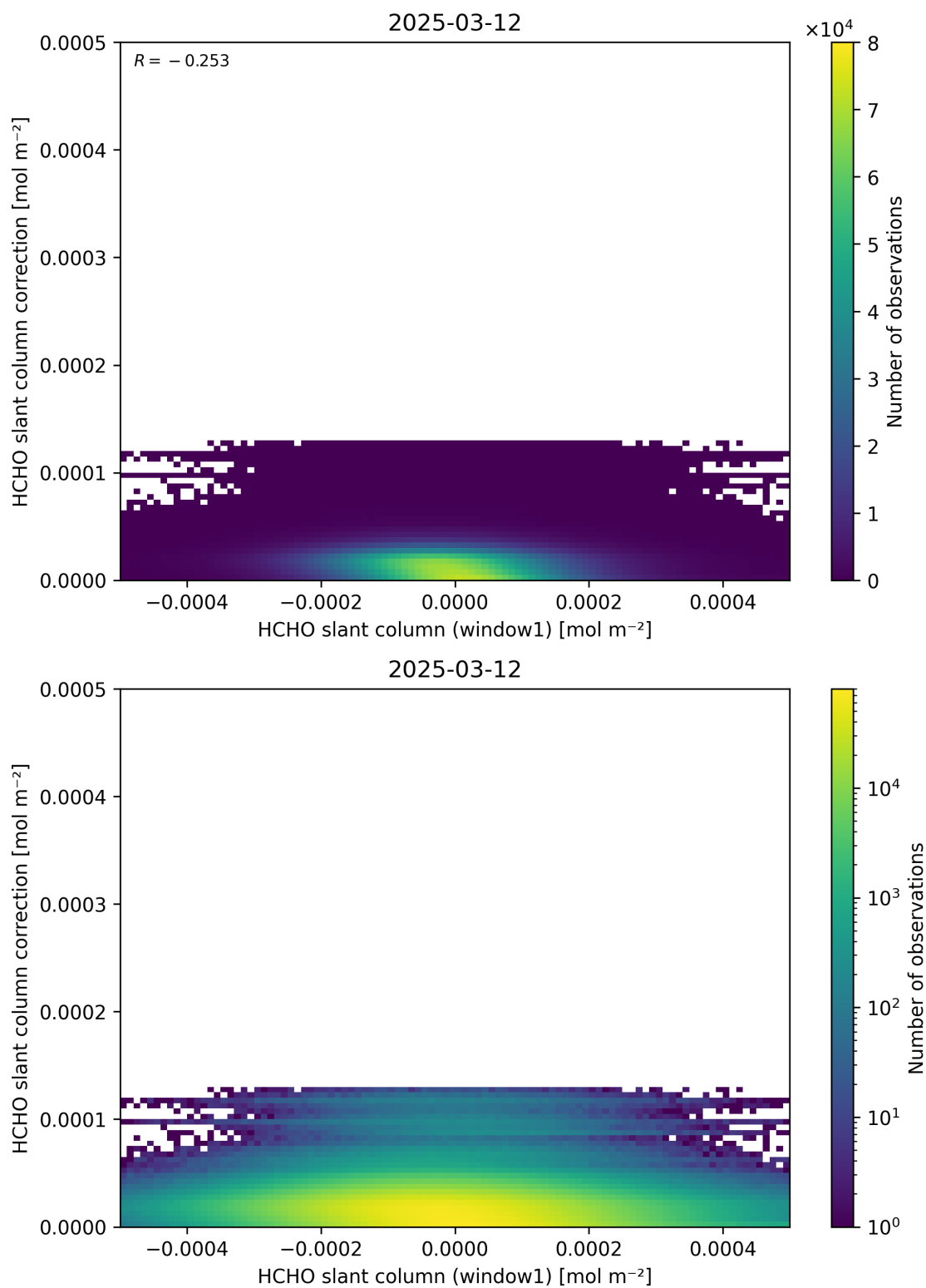
Figure 83: Scatter density plot of “HCHO slant column (window1)” against “HCHO slant column correction” for 2025-03-12 to 2025-03-13.
