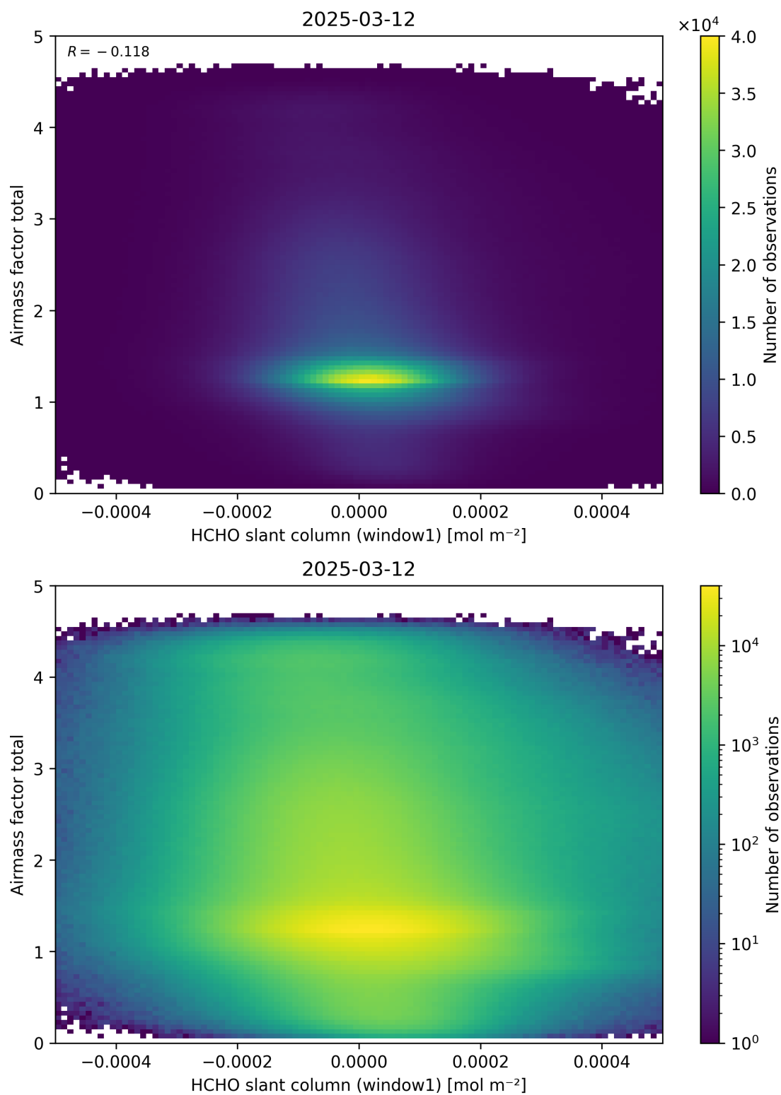
Figure 85: Scatter density plot of “HCHO slant column (window1)” against “Airmass factor total” for 2025-03-12 to 2025-03-13.
