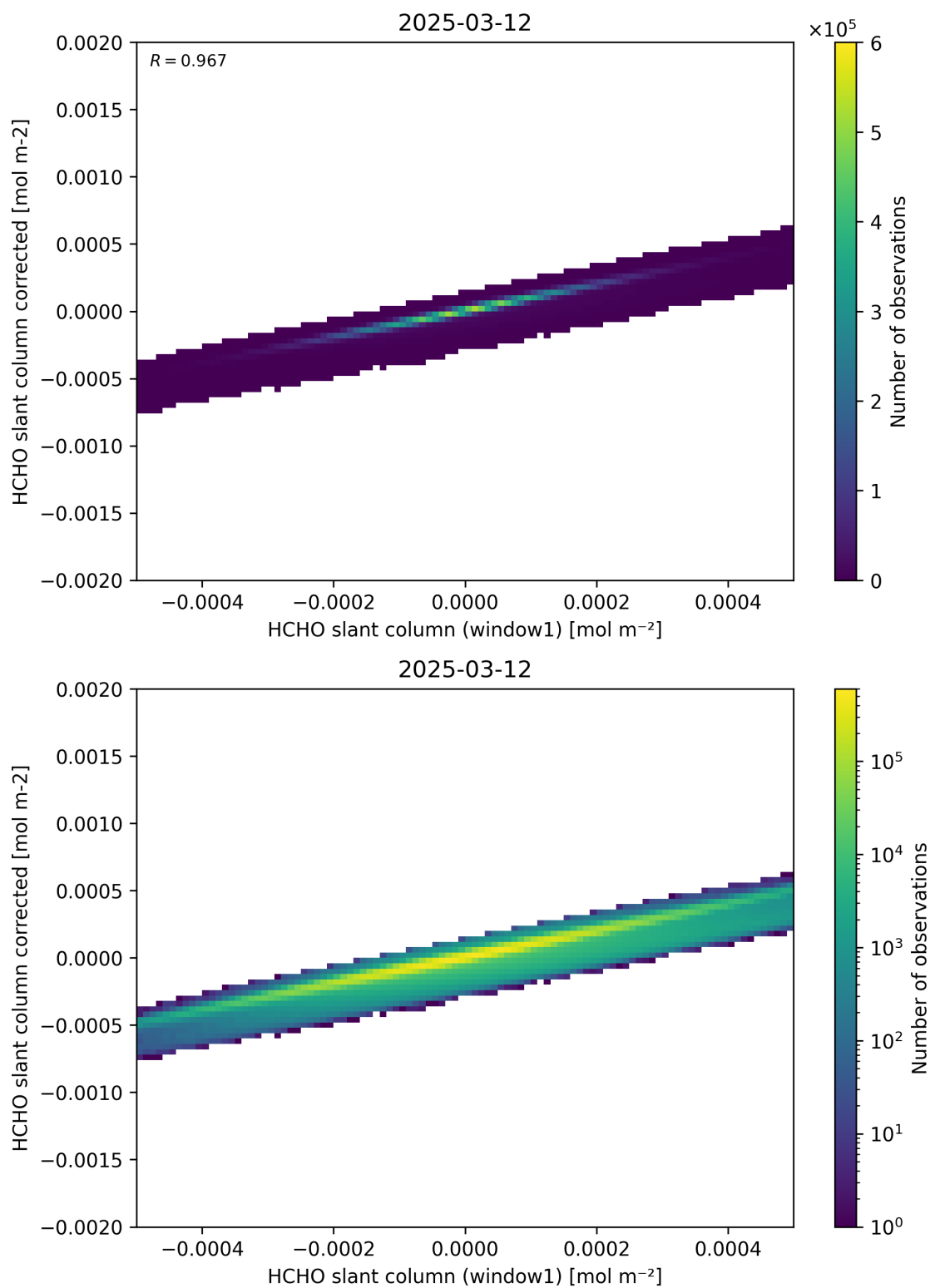
Figure 82: Scatter density plot of “HCHO slant column (window1)” against “HCHO slant column corrected” for 2025-03-12 to 2025-03-13.
