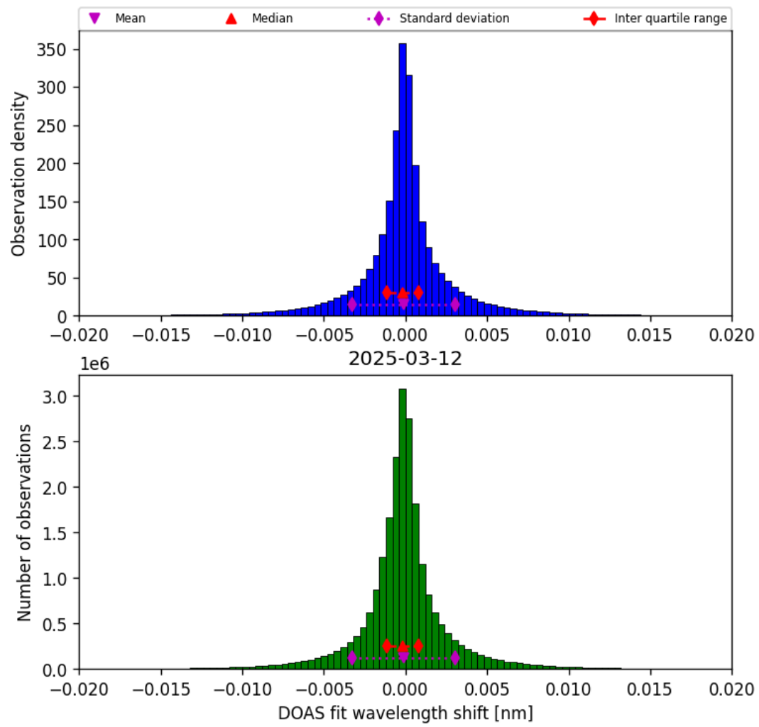
Figure 44: Histogram of “DOAS fit wavelength shift” for 2025-03-12 to 2025-03-13
