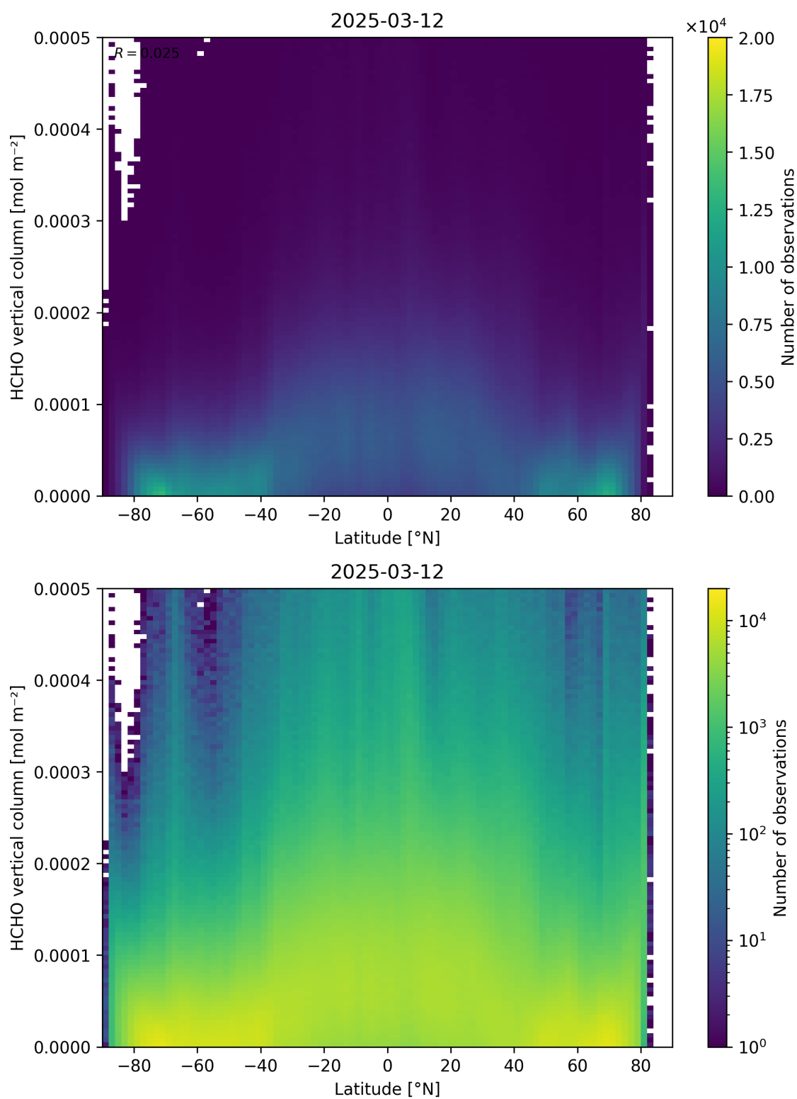
Figure 163: Scatter density plot of “Latitude” against “HCHO vertical column” for 2025-03-12 to 2025-03-13.
