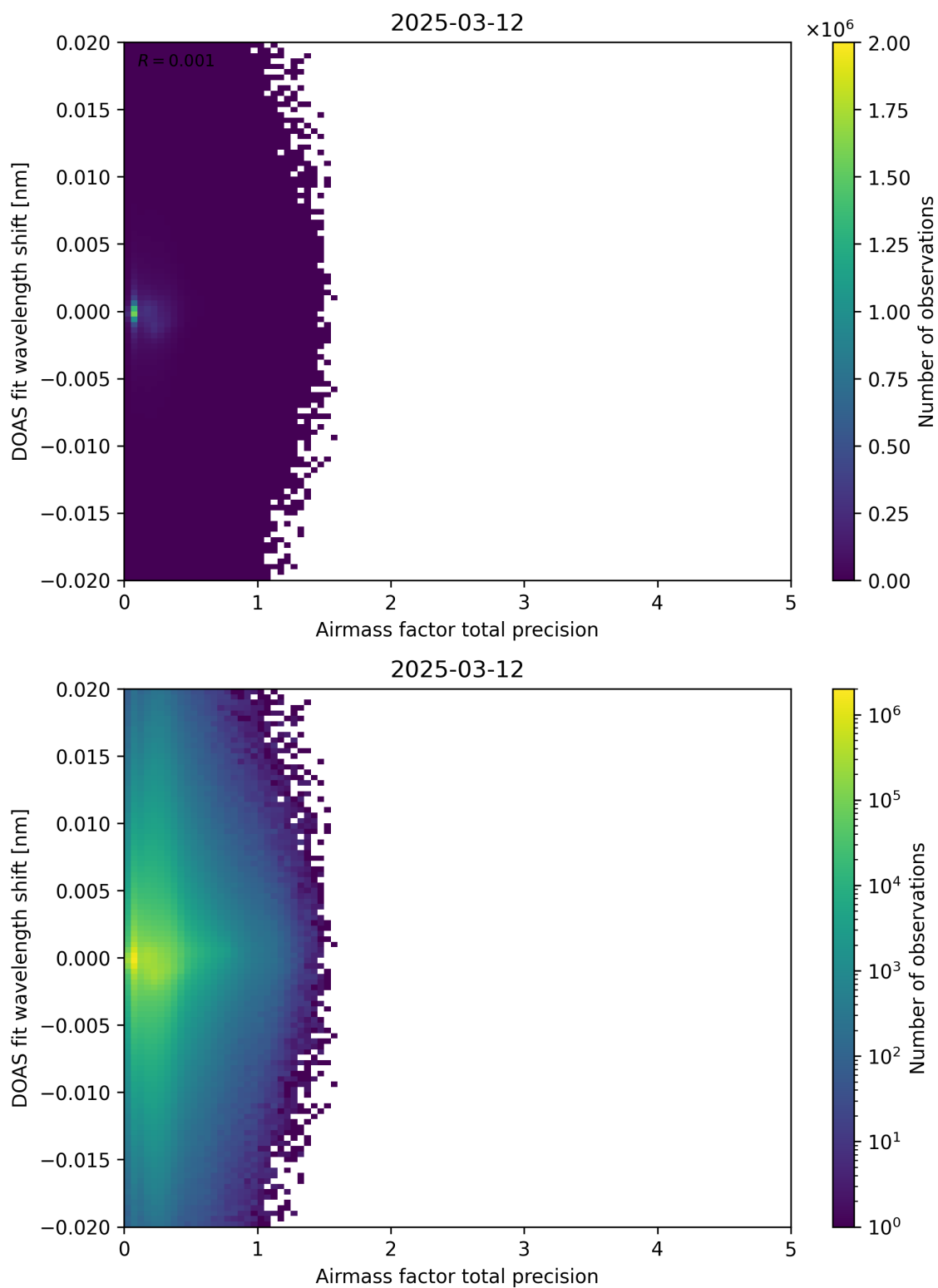
Figure 106: Scatter density plot of “Airmass factor total precision” against “DOAS fit wavelength shift” for 2025-03-12 to 2025-03-13.
