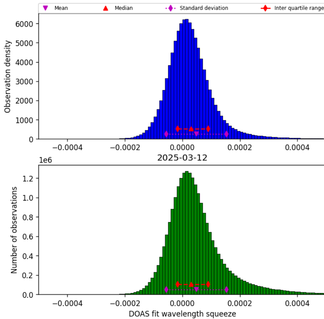
Figure 45: Histogram of “DOAS fit wavelength squeeze” for 2025-03-12 to 2025-03-13
