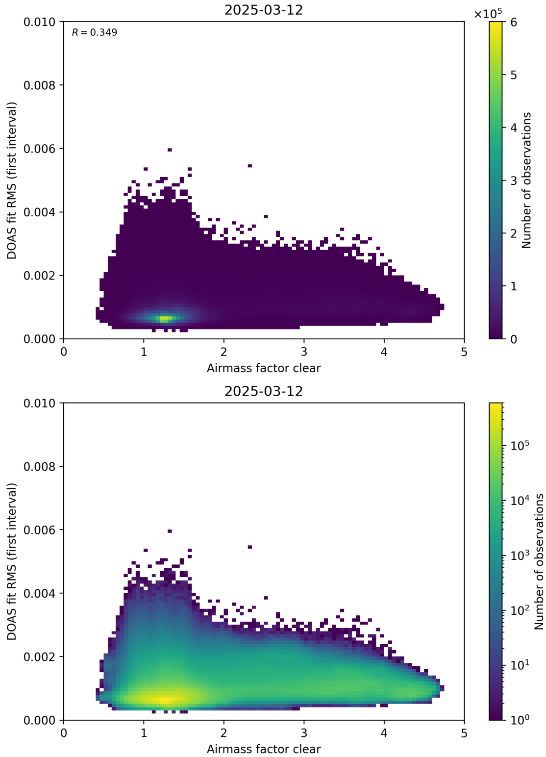
Figure 71: Scatter density plot of “Airmass factor clear” against “DOAS fit RMS (first interval)” for 2025-03-12 to 2025-03-13.
