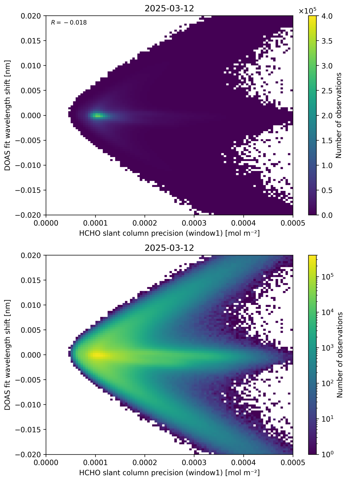
Figure 89: Scatter density plot of “HCHO slant column precision (window1)” against “DOAS fit wavelength shift” for 2025-03-12 to 2025-03-13.
