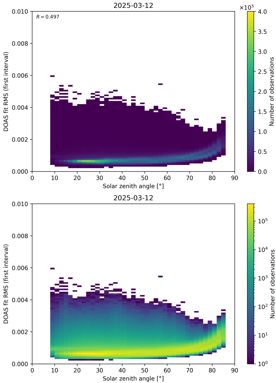
Figure 167: Scatter density plot of “Solar zenith angle” against “DOAS fit RMS (first interval)” for 2025-03-12 to 2025-03-13.
