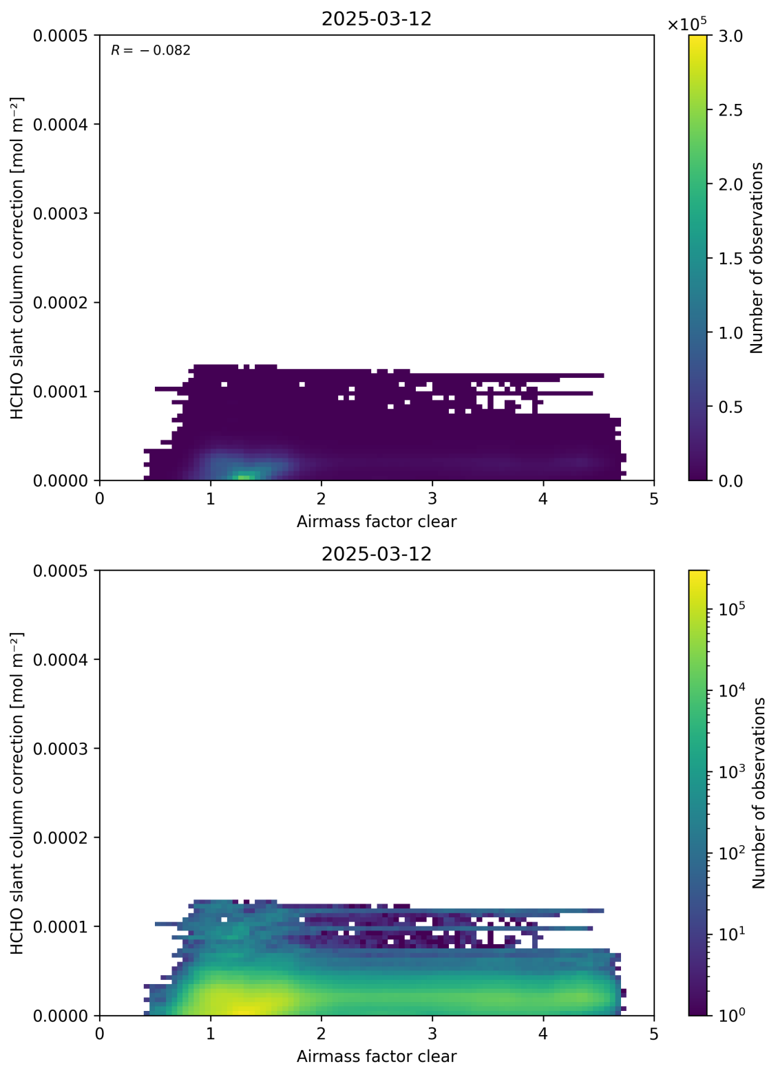
Figure 75: Scatter density plot of “Airmass factor clear” against “HCHO slant column correction” for 2025-03-12 to 2025-03-13.
