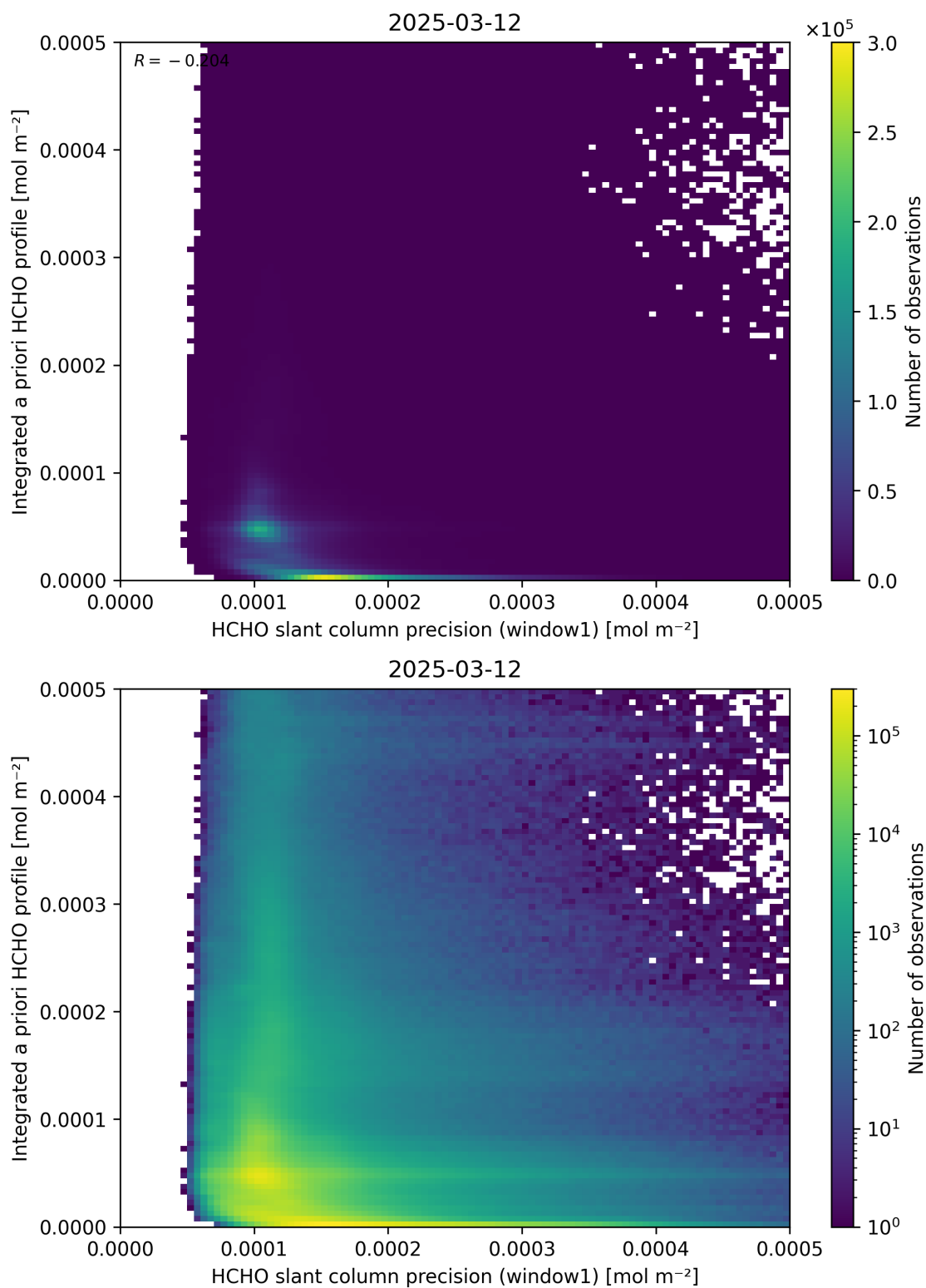
Figure 96: Scatter density plot of “HCHO slant column precision (window1)” against “Integrated a priori HCHO profile” for 2025-03-12 to 2025-03-13.
