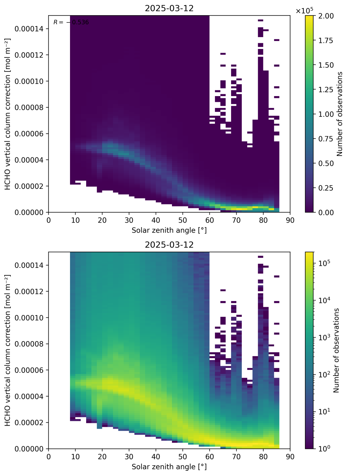
Figure 178: Scatter density plot of “Solar zenith angle” against “HCHO vertical column correction” for 2025-03-12 to 2025-03-13.
