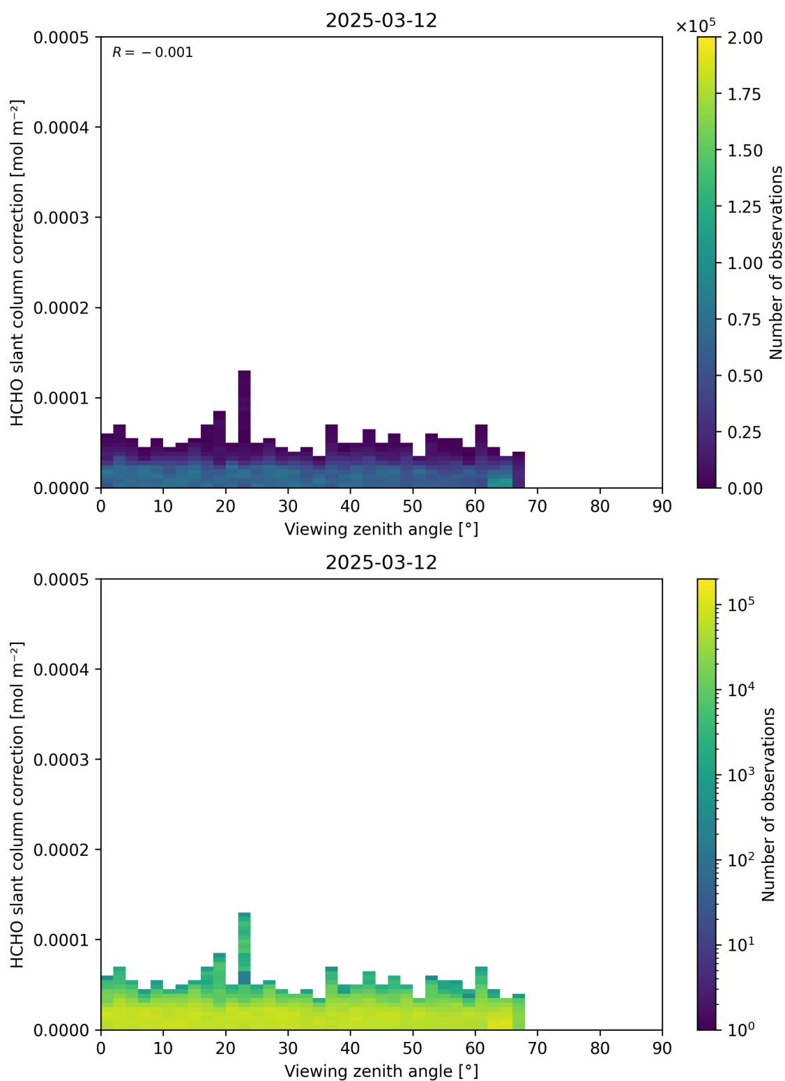
Figure 187: Scatter density plot of “Viewing zenith angle” against “HCHO slant column correction” for 2025-03-12 to 2025-03-13.
