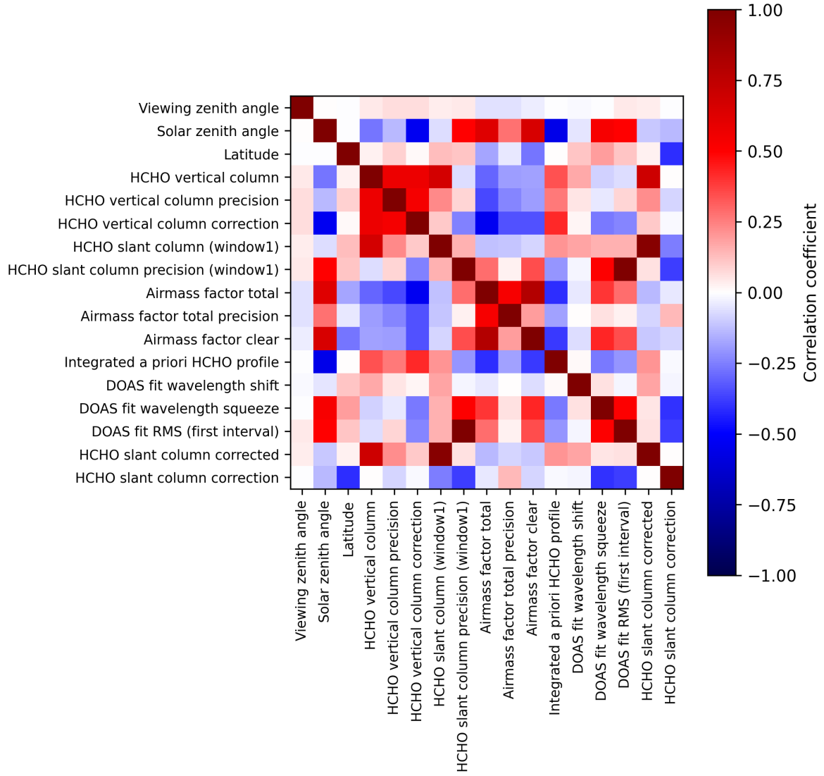
Figure 2: Map of correlation matrix for 2025-03-12 to 2025-03-13.
