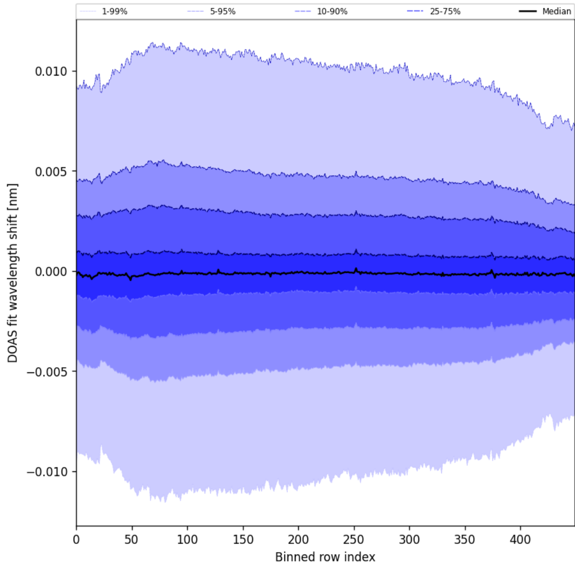
Figure 58: Along track statistics of “DOAS fit wavelength shift” for 2025-03-12 to 2025-03-13
