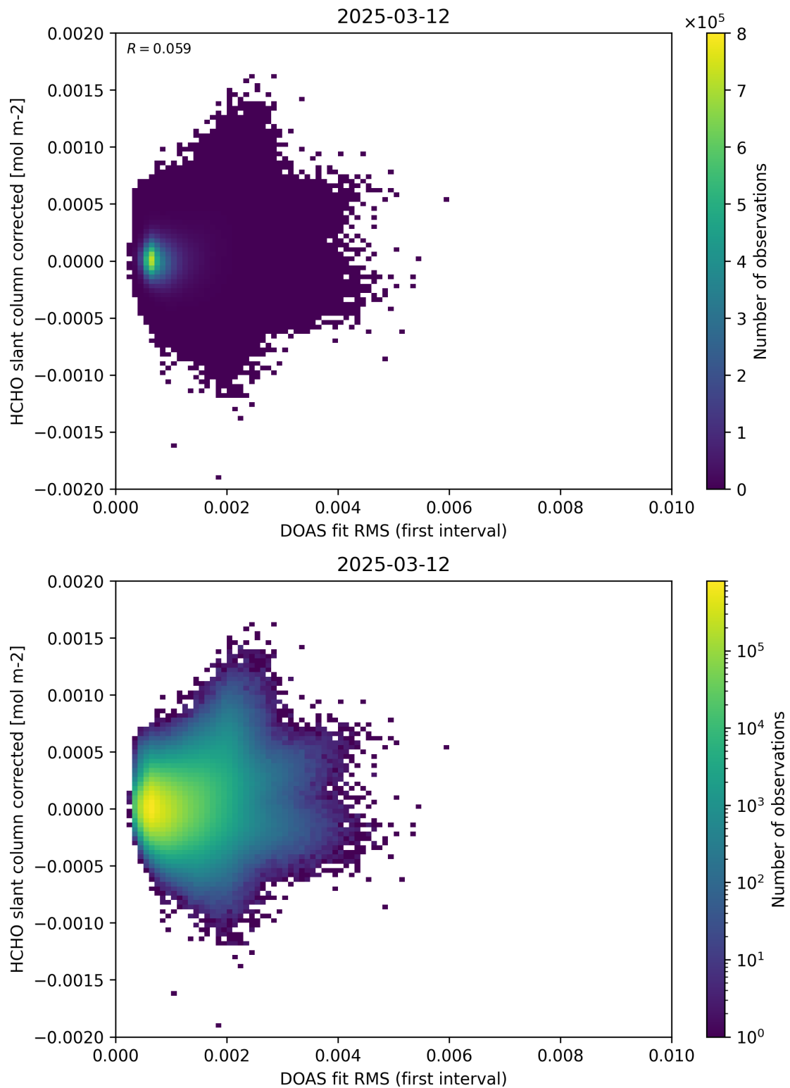
Figure 62: Scatter density plot of “DOAS fit RMS (first interval)” against “HCHO slant column corrected” for 2025-03-12 to 2025-03-13.
