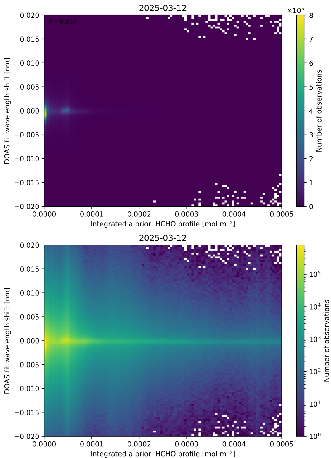
Figure 149: Scatter density plot of “Integrated a priori HCHO profile” against “DOAS fit wavelength shift” for 2025-03-12 to 2025-03-13.
