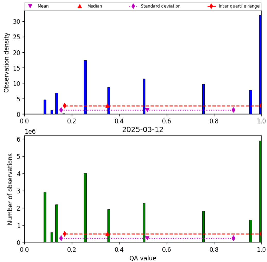
Figure 34: Histogram of “QA value” for 2025-03-12 to 2025-03-13
