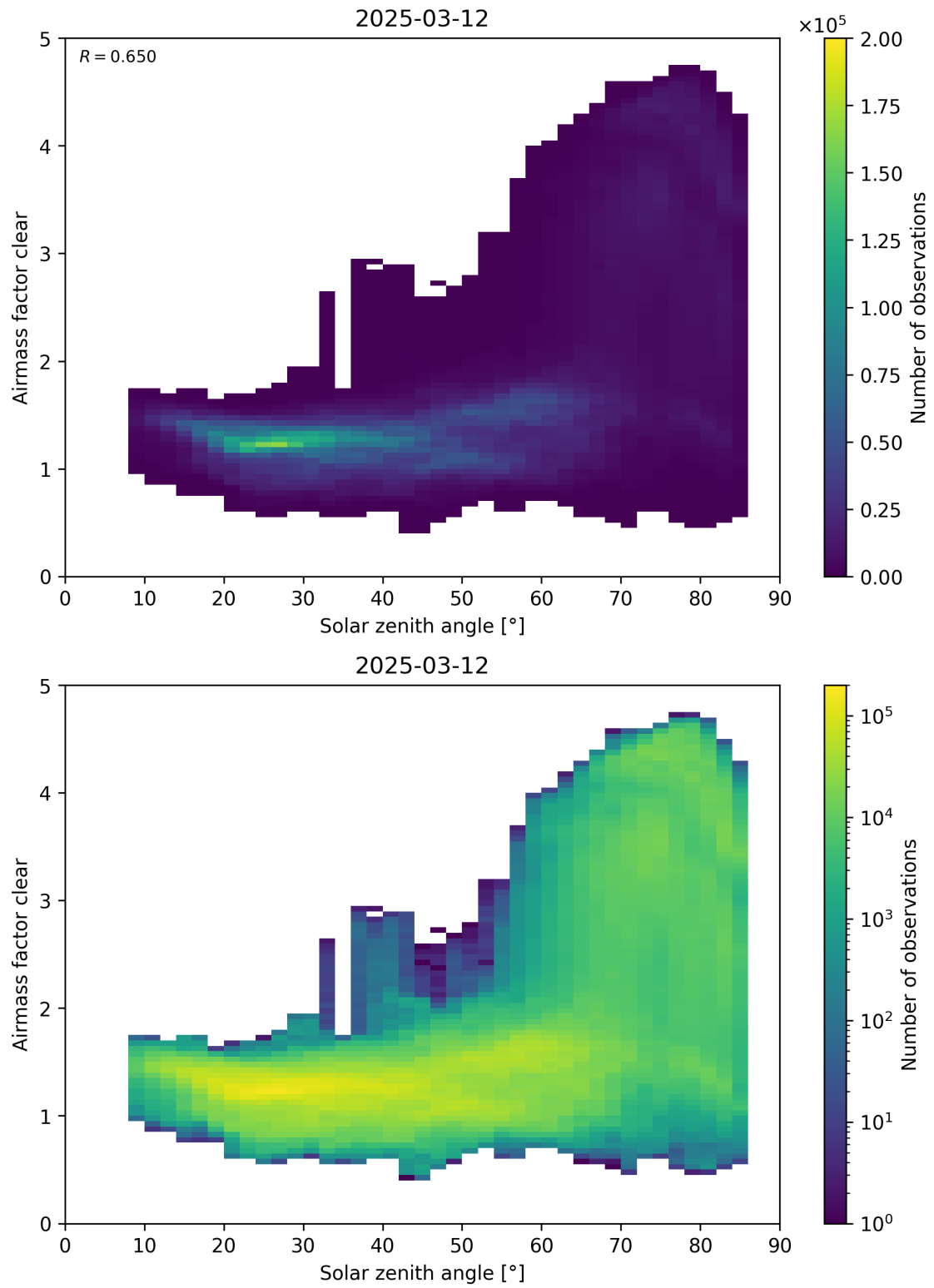
Figure 170: Scatter density plot of “Solar zenith angle” against “Airmass factor clear” for 2025-03-12 to 2025-03-13.
