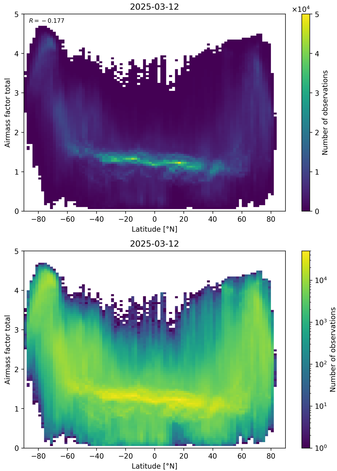
Figure 161: Scatter density plot of “Latitude” against “Airmass factor total” for 2025-03-12 to 2025-03-13.
