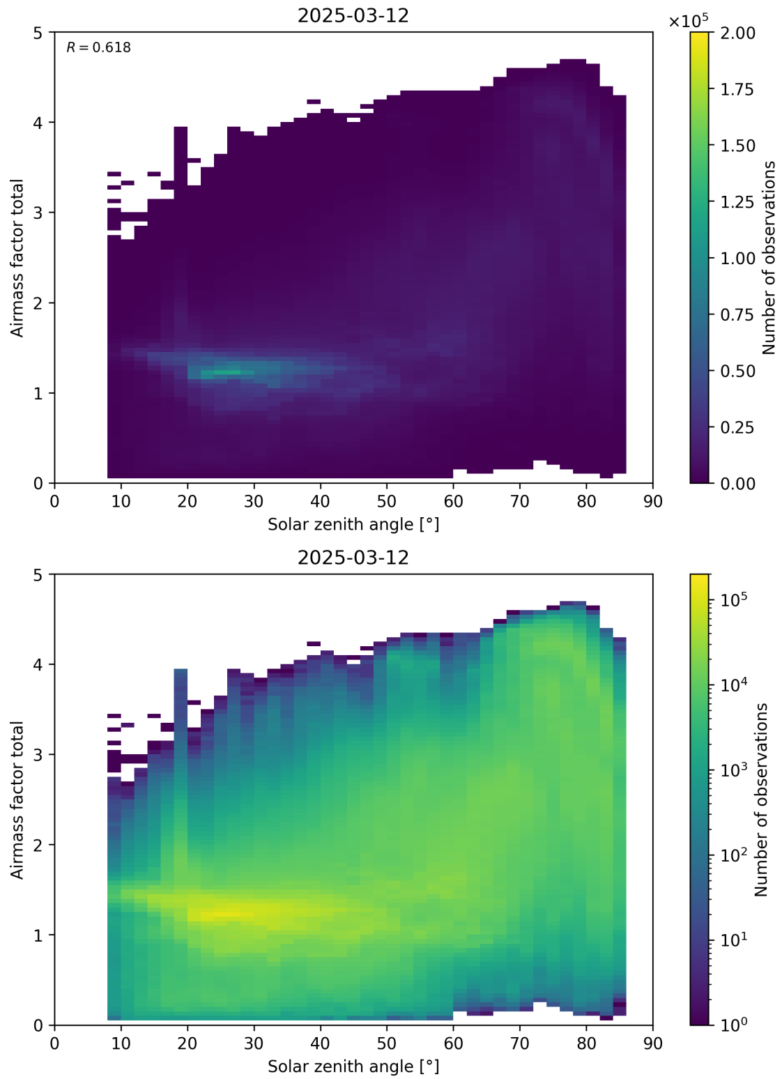
Figure 175: Scatter density plot of “Solar zenith angle” against “Airmass factor total” for 2025-03-12 to 2025-03-13.
