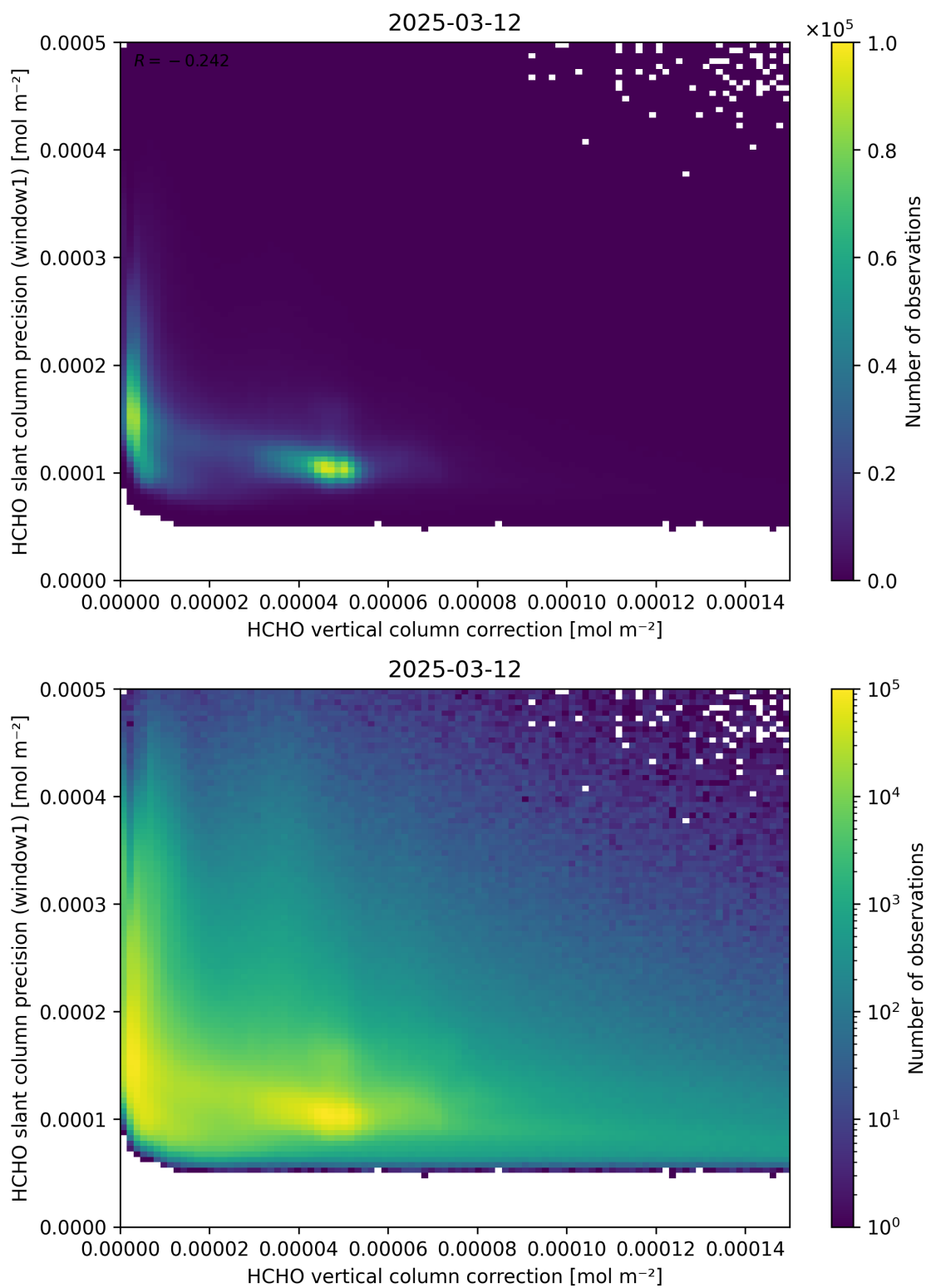
Figure 119: Scatter density plot of “HCHO vertical column correction” against “HCHO slant column precision (window1)” for 2025-03-12 to 2025-03-13.
