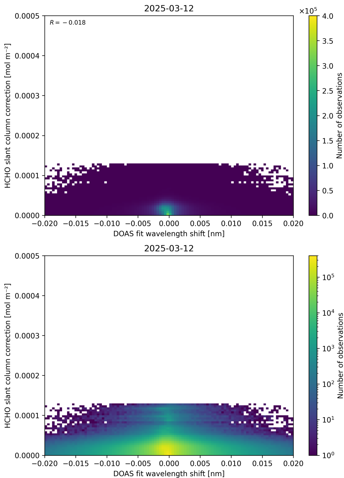
Figure 67: Scatter density plot of “DOAS fit wavelength shift” against “HCHO slant column correction” for 2025-03-12 to 2025-03-13.
