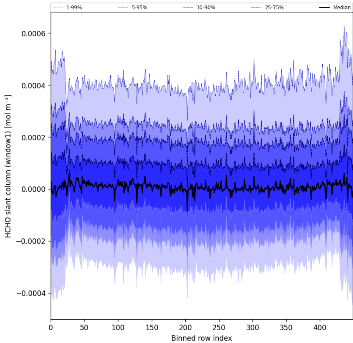
Figure 52: Along track statistics of “HCHO slant column (window1)” for 2025-03-12 to 2025-03-13
