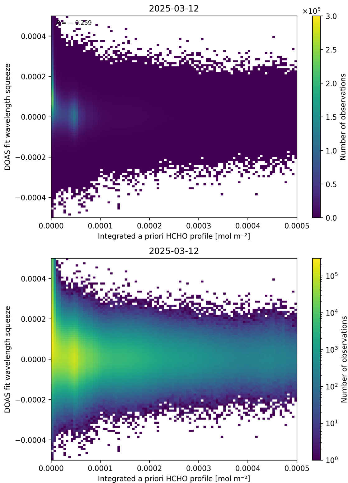
Figure 150: Scatter density plot of “Integrated a priori HCHO profile” against “DOAS fit wavelength squeeze” for 2025-03-12 to 2025-03-13.
