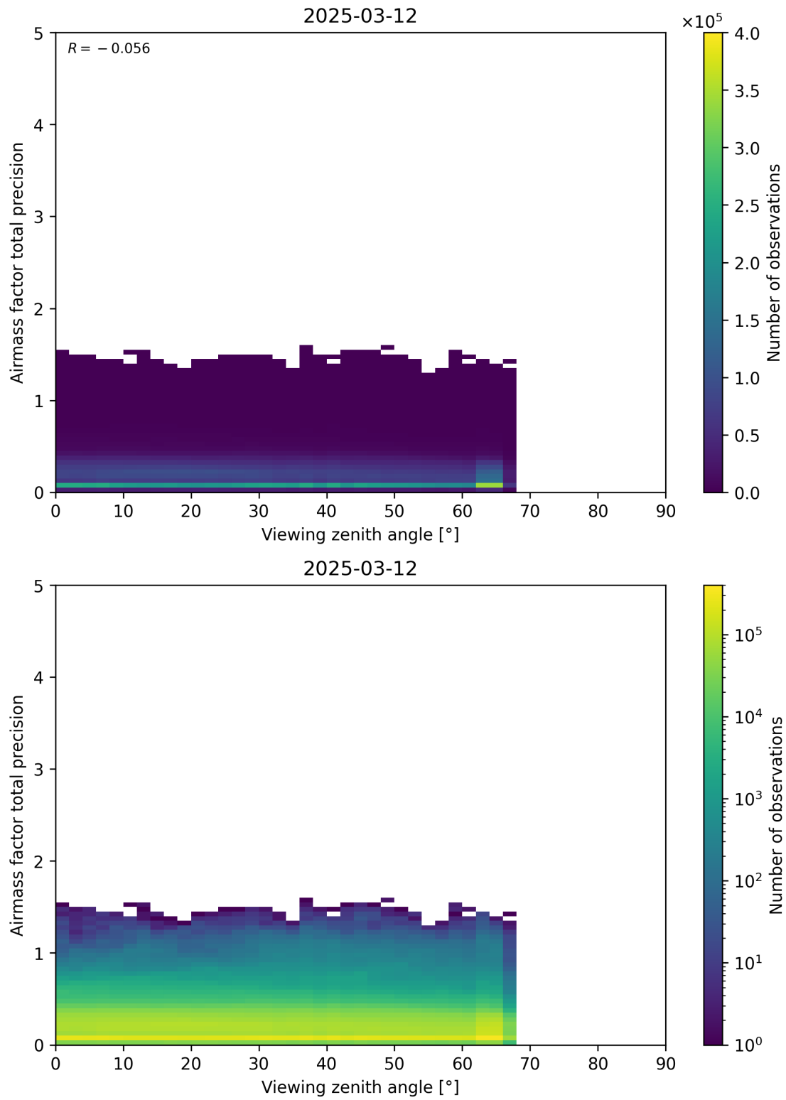
Figure 191: Scatter density plot of “Viewing zenith angle” against “Airmass factor total precision” for 2025-03-12 to 2025-03-13.
