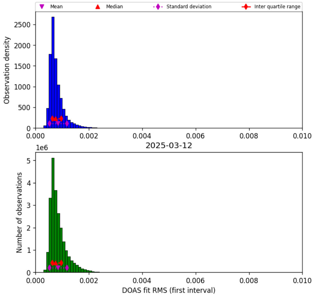
Figure 46: Histogram of “DOAS fit RMS (first interval)” for 2025-03-12 to 2025-03-13
