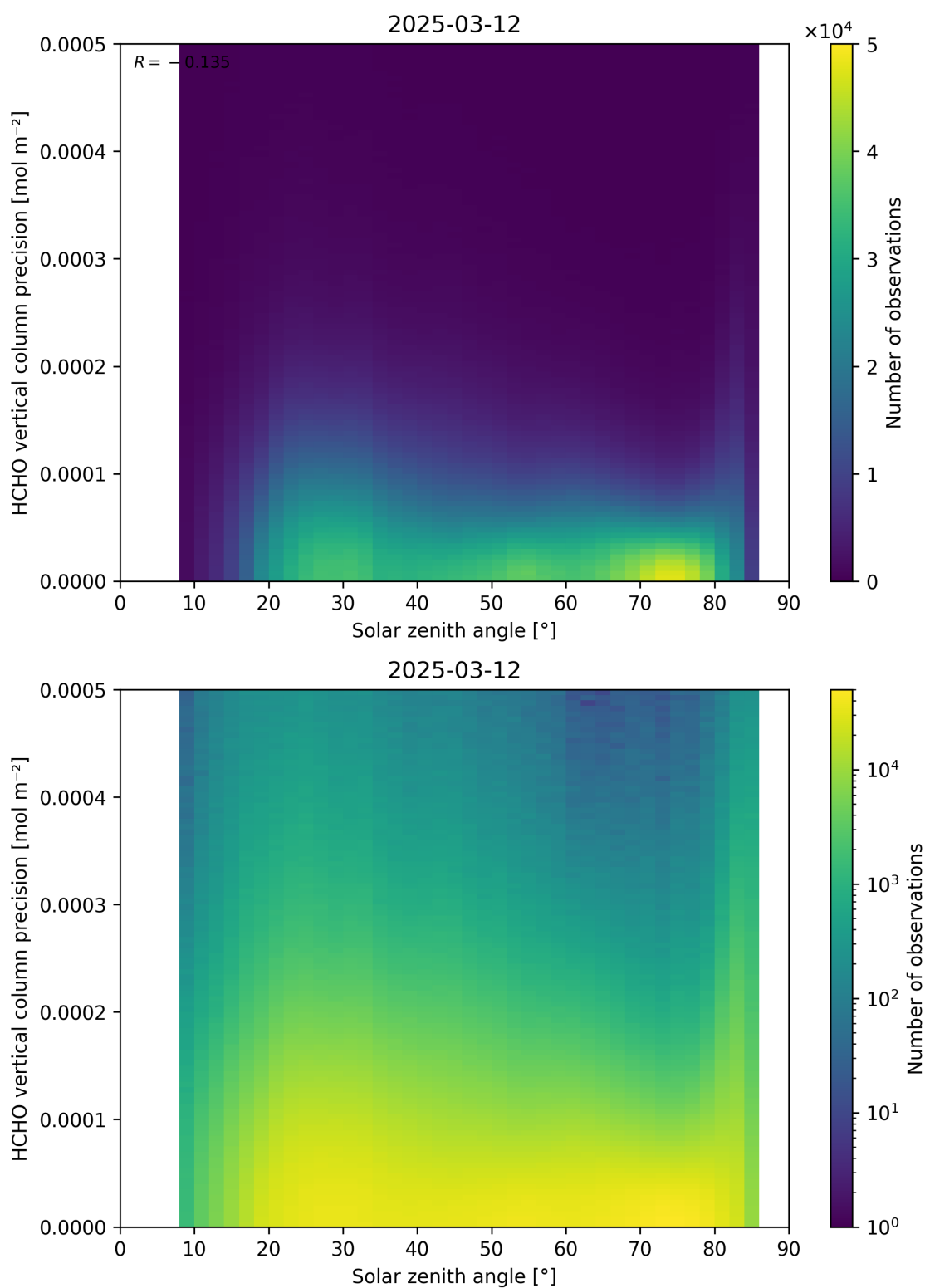
Figure 179: Scatter density plot of “Solar zenith angle” against “HCHO vertical column precision” for 2025-03-12 to 2025-03-13.
