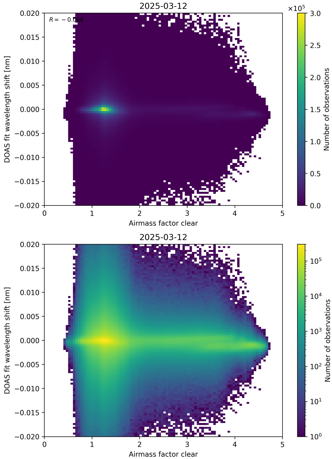
Figure 72: Scatter density plot of “Airmass factor clear” against “DOAS fit wavelength shift” for 2025-03-12 to 2025-03-13.
