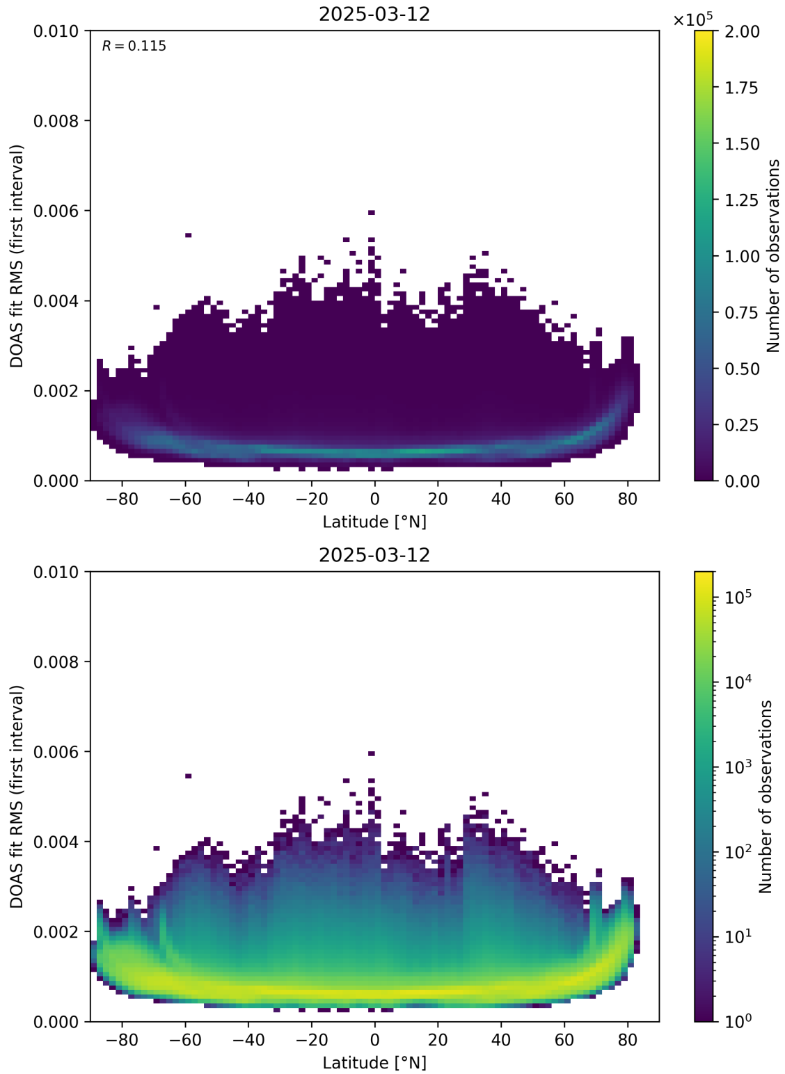
Figure 153: Scatter density plot of “Latitude” against “DOAS fit RMS (first interval)” for 2025-03-12 to 2025-03-13.
