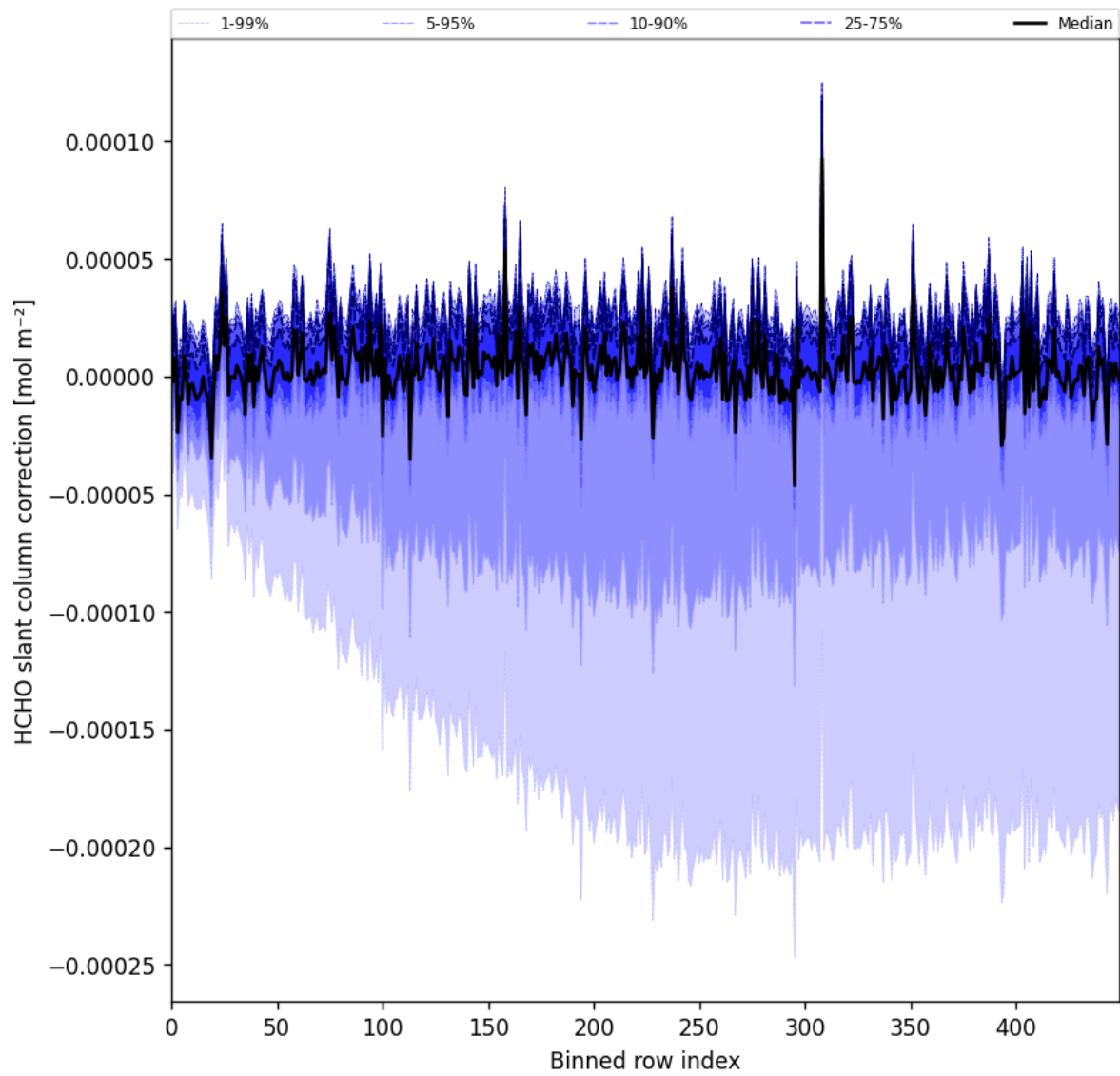
Figure 61: Along track statistics of “HCHO slant column correction” for 2025-03-12 to 2025-03-13
