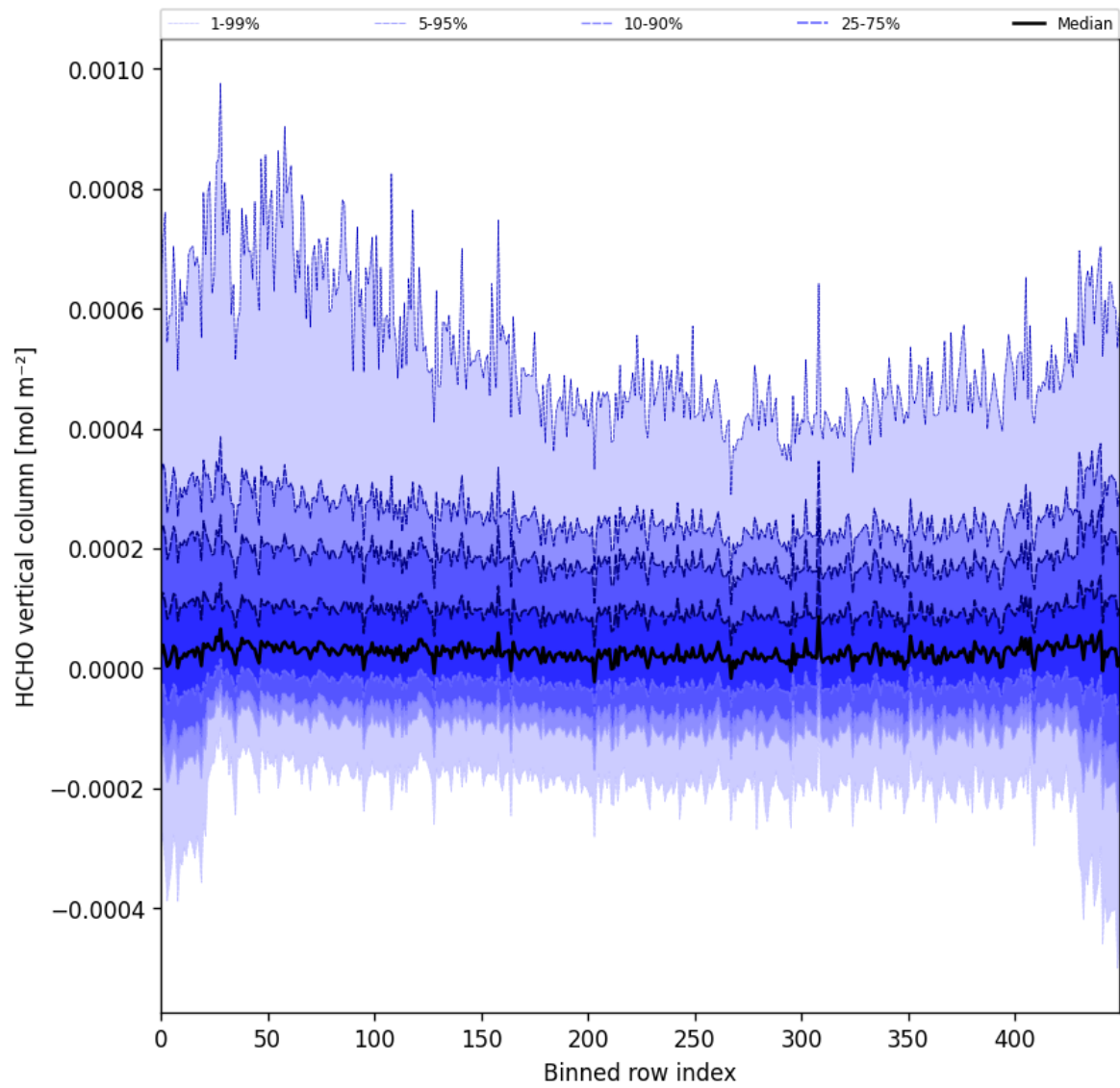
Figure 49: Along track statistics of “HCHO vertical column” for 2025-03-12 to 2025-03-13
