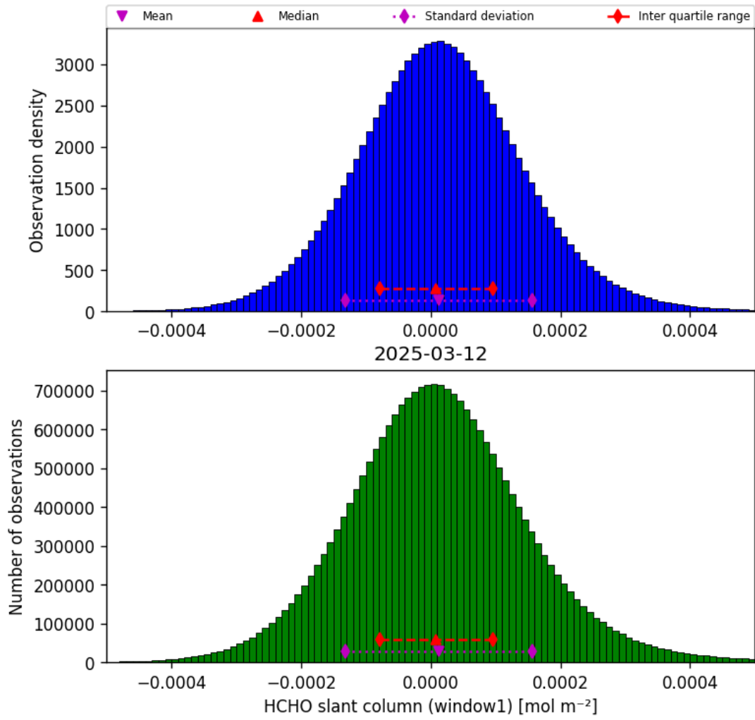
Figure 38: Histogram of “HCHO slant column (window1)” for 2025-03-12 to 2025-03-13
