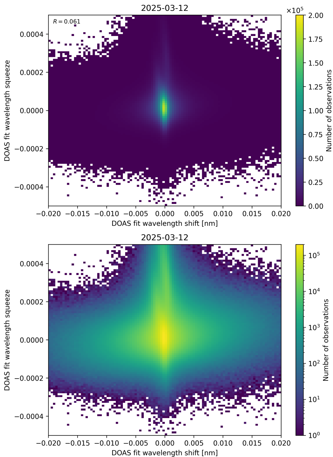
Figure 65: Scatter density plot of “DOAS fit wavelength shift” against “DOAS fit wavelength squeeze” for 2025-03-12 to 2025-03-13.
