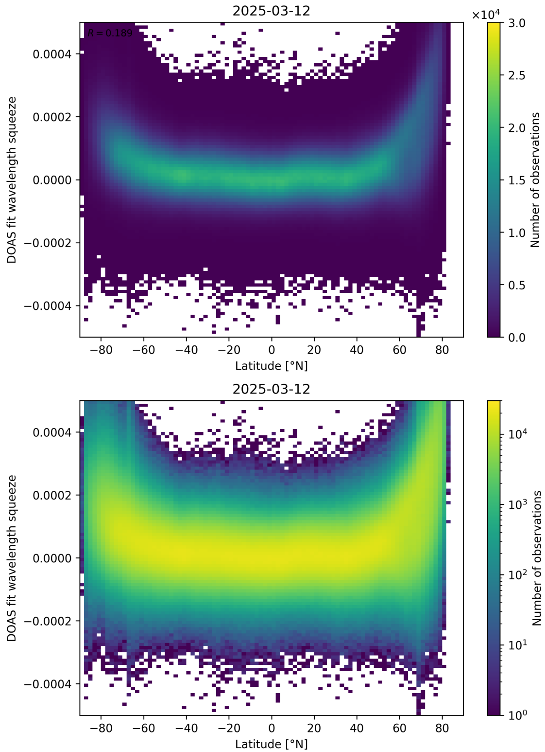
Figure 155: Scatter density plot of “Latitude” against “DOAS fit wavelength squeeze” for 2025-03-12 to 2025-03-13.
