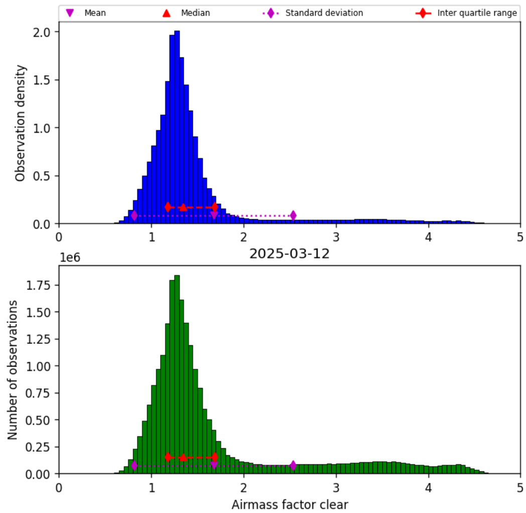
Figure 42: Histogram of “Airmass factor clear” for 2025-03-12 to 2025-03-13
