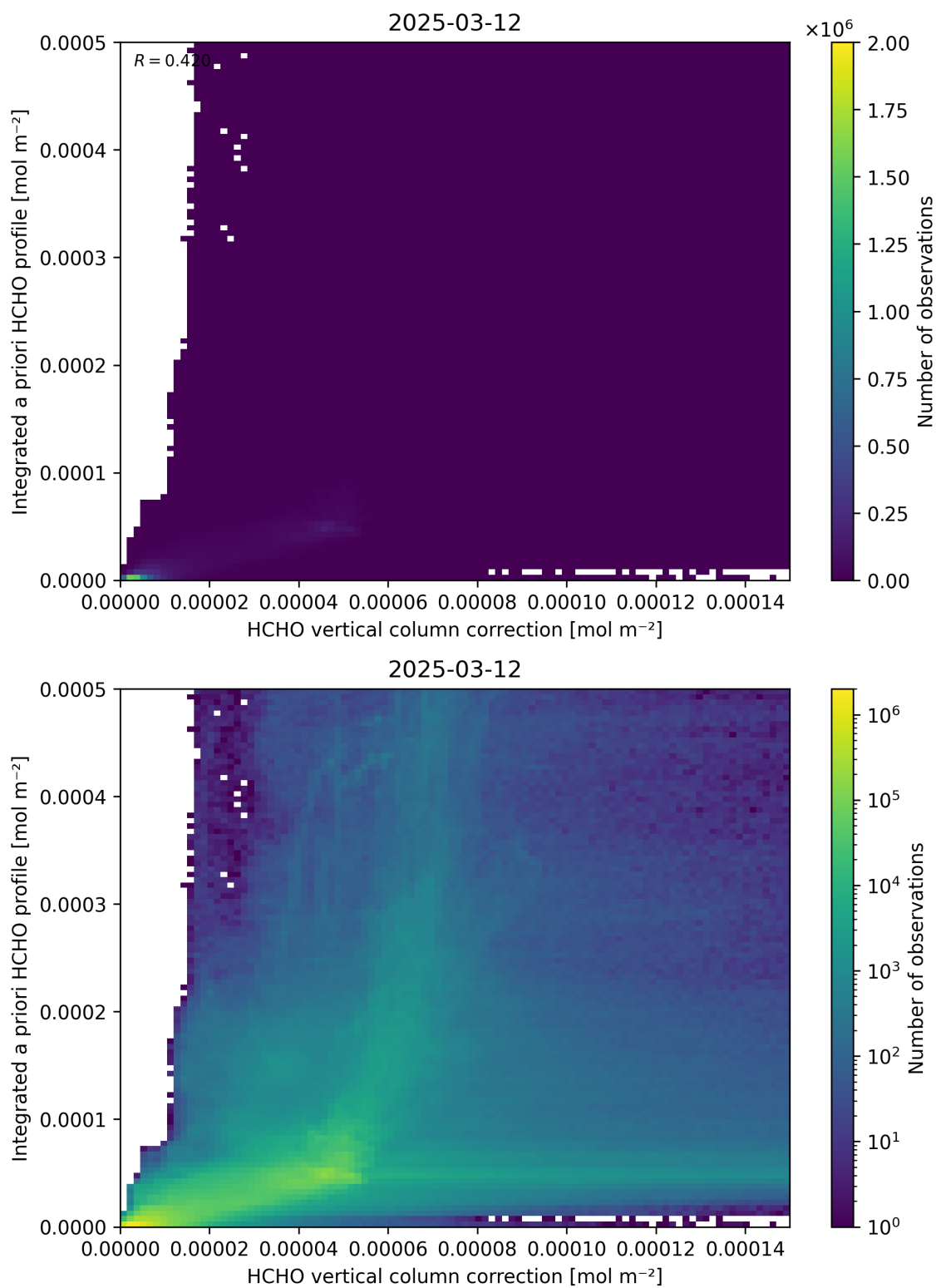
Figure 122: Scatter density plot of “HCHO vertical column correction” against “Integrated a priori HCHO profile” for 2025-03-12 to 2025-03-13.
