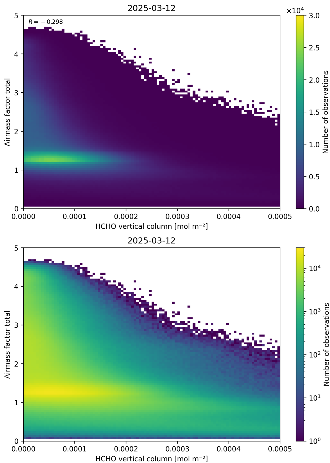
Figure 131: Scatter density plot of “HCHO vertical column” against “Airmass factor total” for 2025-03-12 to 2025-03-13.
