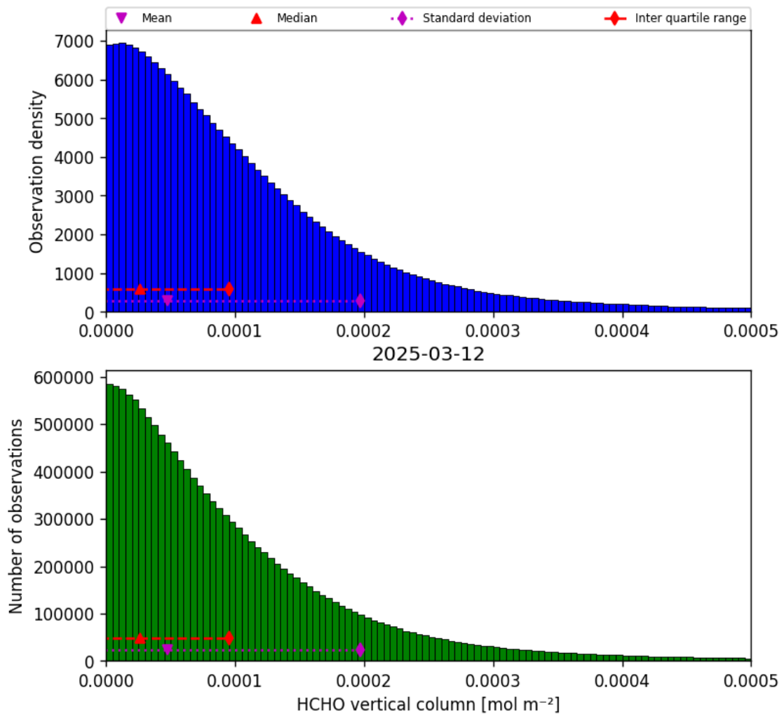
Figure 35: Histogram of “HCHO vertical column” for 2025-03-12 to 2025-03-13
