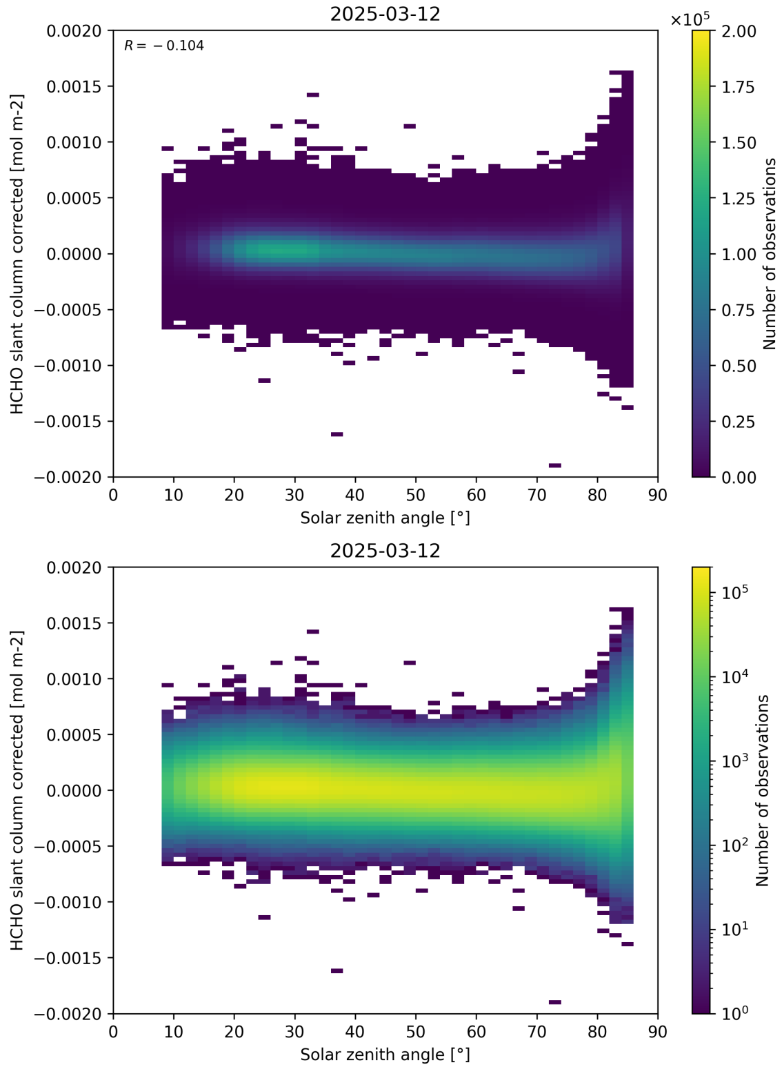
Figure 171: Scatter density plot of “Solar zenith angle” against “HCHO slant column corrected” for 2025-03-12 to 2025-03-13.
