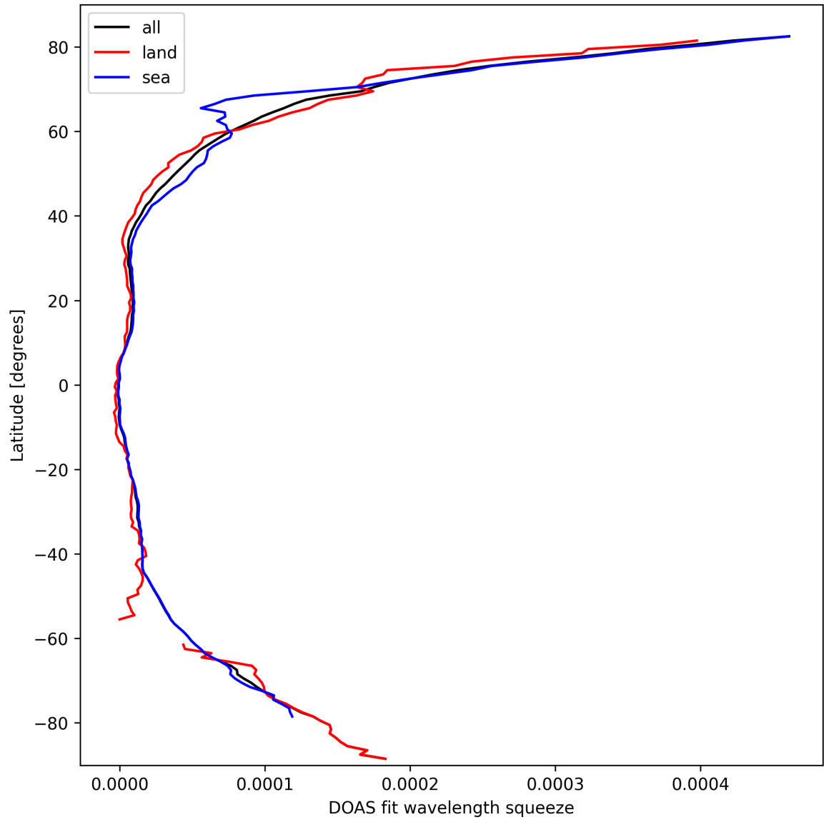
Figure 31: Zonal average of “DOAS fit wavelength squeeze” for 2025-03-12 to 2025-03-13.
