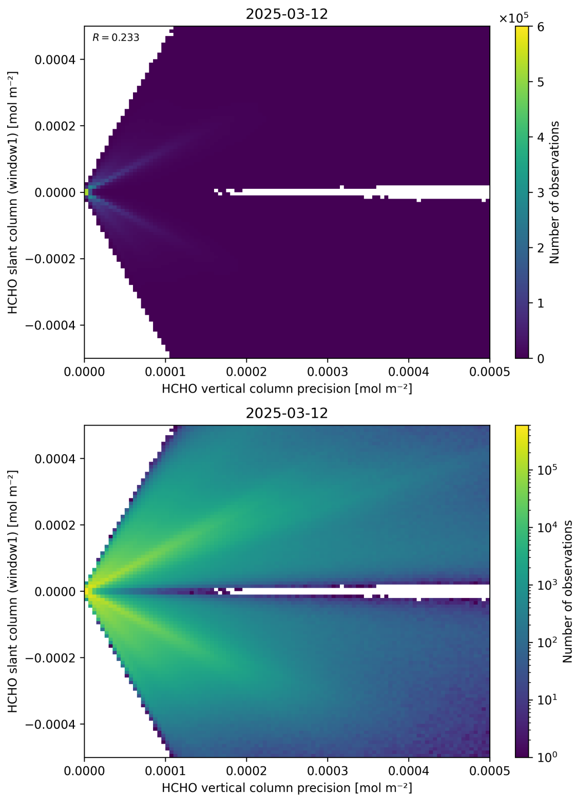
Figure 142: Scatter density plot of “HCHO vertical column precision” against “HCHO slant column (window1)” for 2025-03-12 to 2025-03-13.
