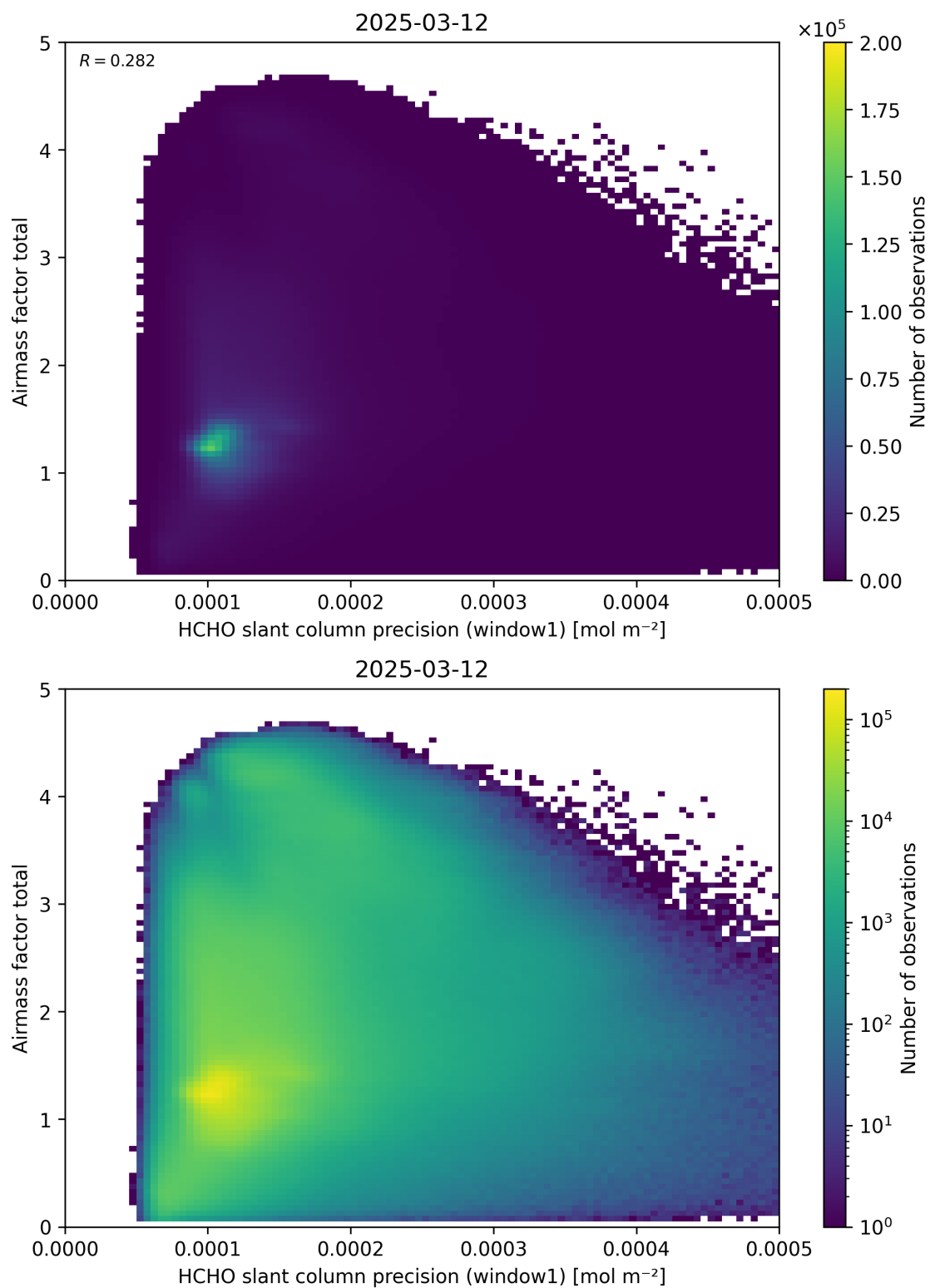
Figure 94: Scatter density plot of “HCHO slant column precision (window1)” against “Airmass factor total” for 2025-03-12 to 2025-03-13.
