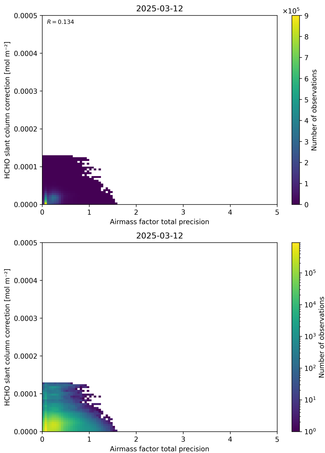
Figure 110: Scatter density plot of “Airmass factor total precision” against “HCHO slant column correction” for 2025-03-12 to 2025-03-13.
