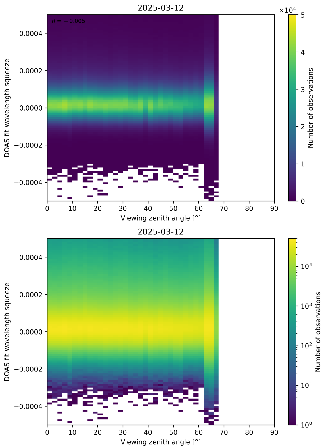
Figure 184: Scatter density plot of “Viewing zenith angle” against “DOAS fit wavelength squeeze” for 2025-03-12 to 2025-03-13.
