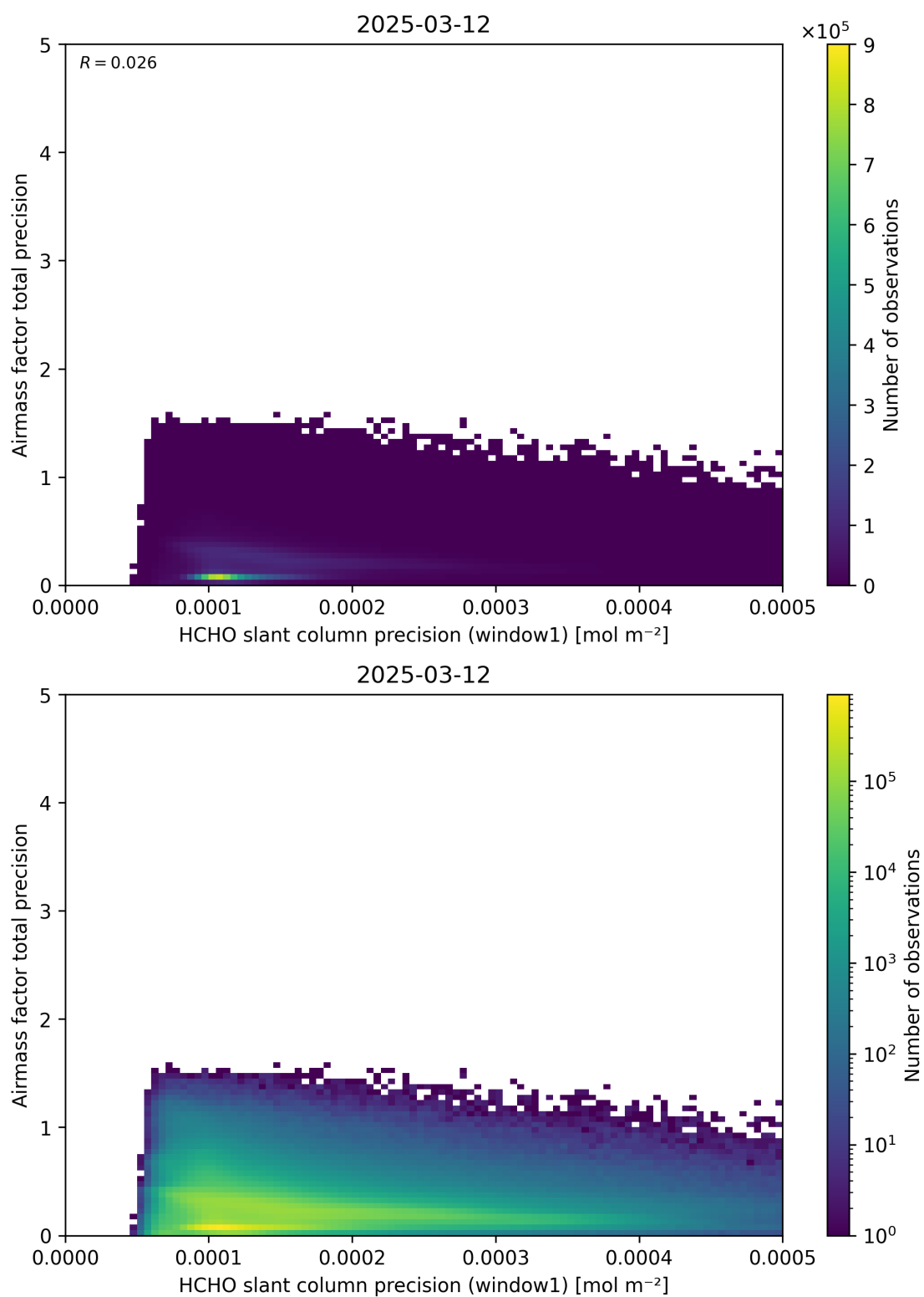
Figure 95: Scatter density plot of “HCHO slant column precision (window1)” against “Airmass factor total precision” for 2025-03-12 to 2025-03-13.
