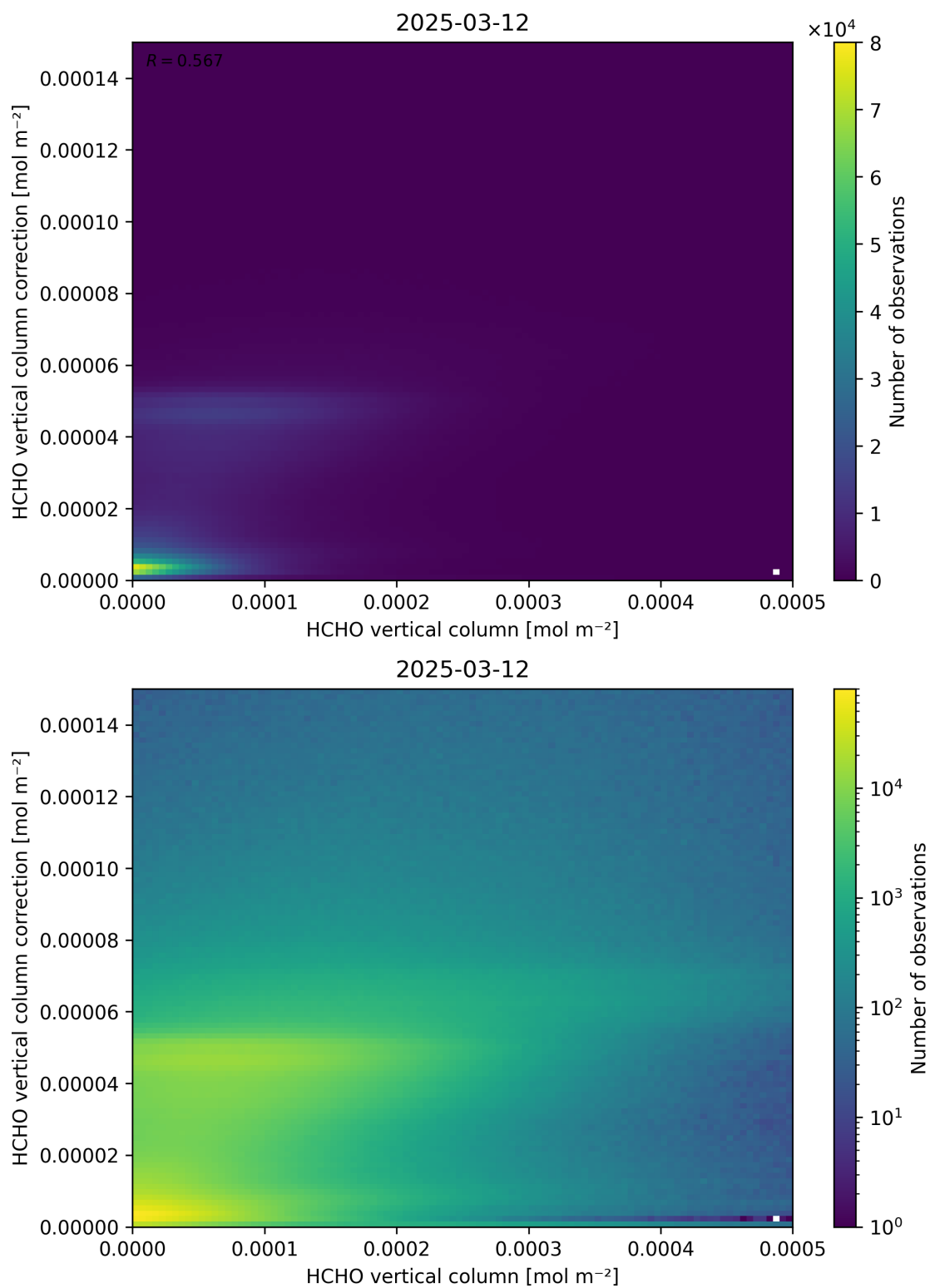
Figure 133: Scatter density plot of “HCHO vertical column” against “HCHO vertical column correction” for 2025-03-12 to 2025-03-13.
