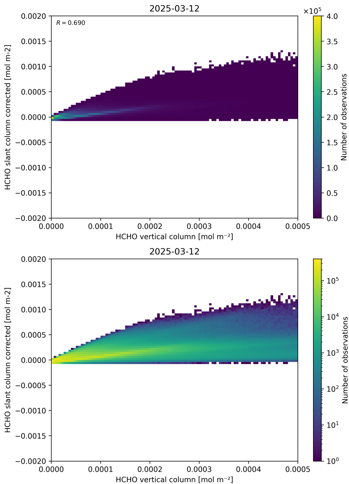
Figure 127: Scatter density plot of “HCHO vertical column” against “HCHO slant column corrected” for 2025-03-12 to 2025-03-13.
