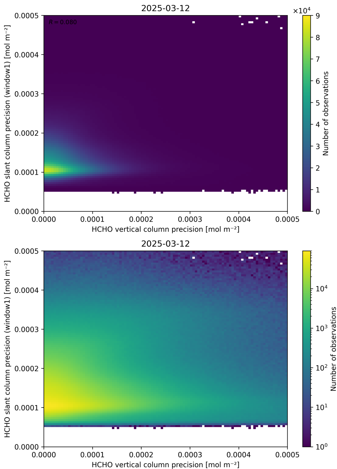
Figure 143: Scatter density plot of “HCHO vertical column precision” against “HCHO slant column precision (window1)” for 2025-03-12 to 2025-03-13.
