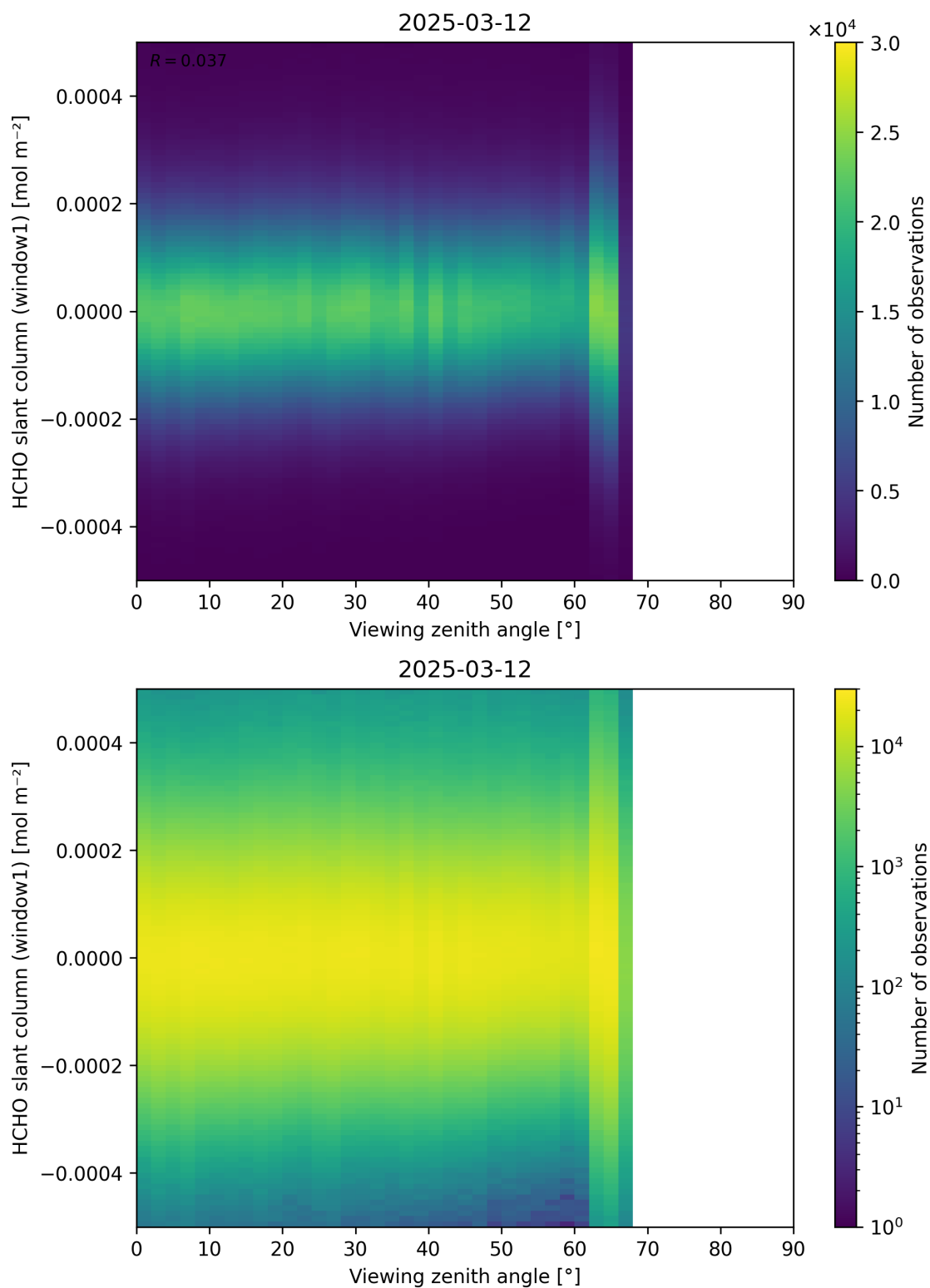
Figure 188: Scatter density plot of “Viewing zenith angle” against “HCHO slant column (window1)” for 2025-03-12 to 2025-03-13.
