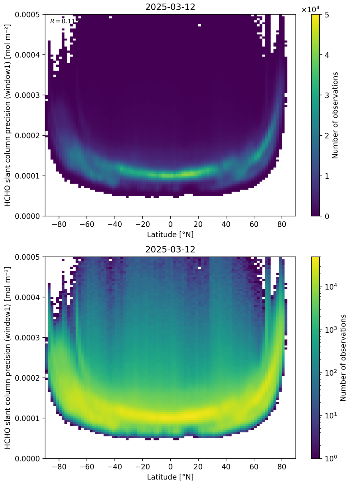
Figure 160: Scatter density plot of “Latitude” against “HCHO slant column precision (window1)” for 2025-03-12 to 2025-03-13.
