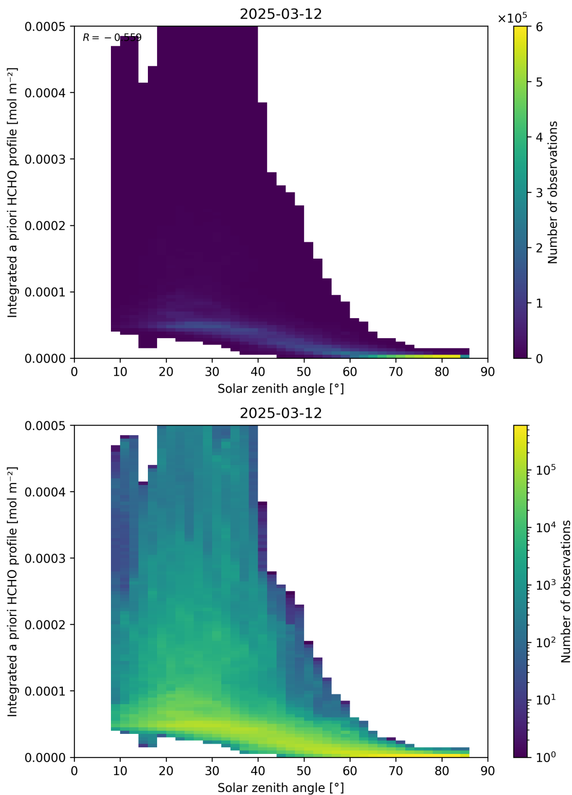
Figure 180: Scatter density plot of “Solar zenith angle” against “Integrated a priori HCHO profile” for 2025-03-12 to 2025-03-13.
