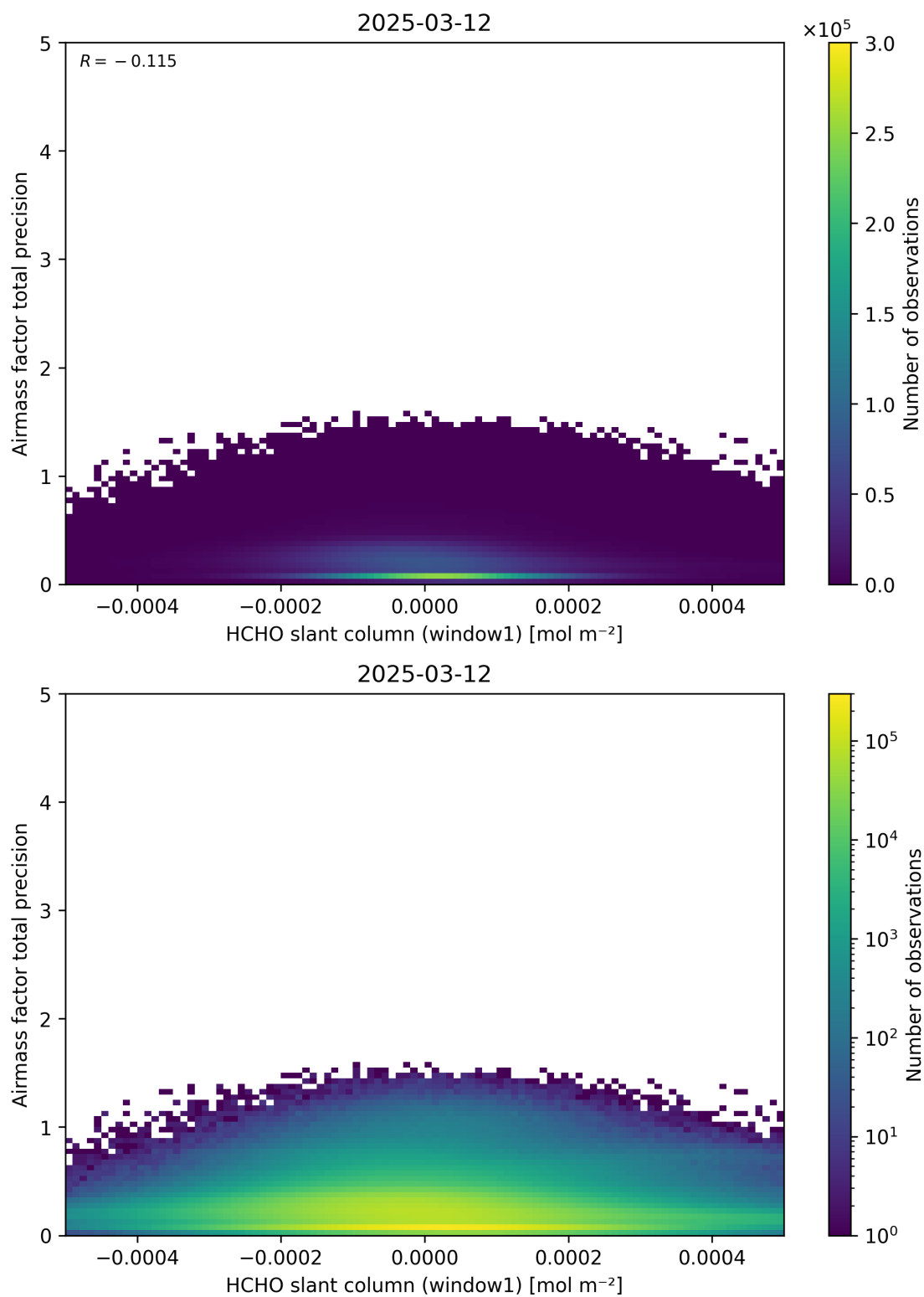
Figure 86: Scatter density plot of “HCHO slant column (window1)” against “Airmass factor total precision” for 2025-03-12 to 2025-03-13.
