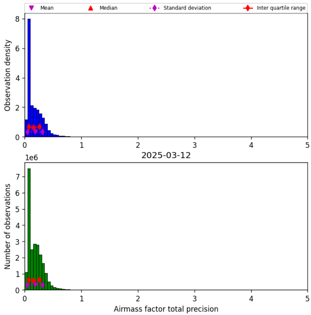
Figure 41: Histogram of “Airmass factor total precision” for 2025-03-12 to 2025-03-13
