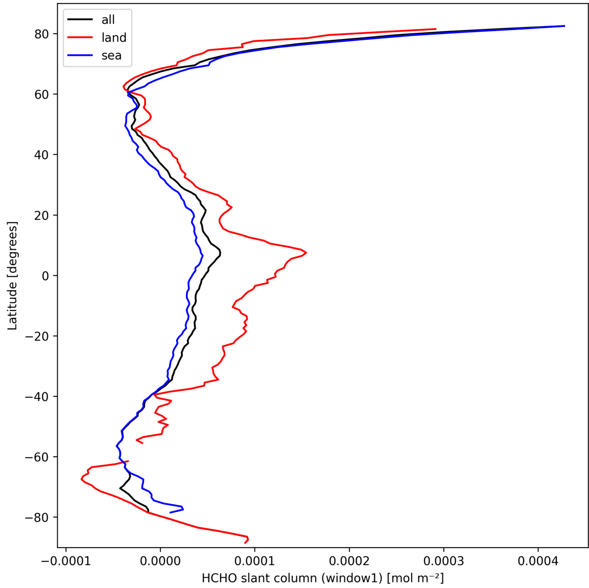
Figure 24: Zonal average of “HCHO slant column (window1)” for 2025-03-12 to 2025-03-13.
