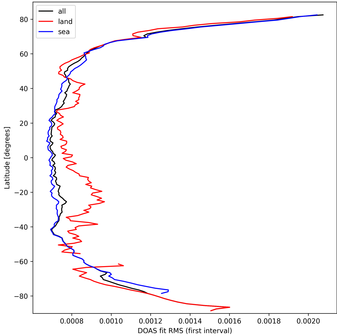
Figure 32: Zonal average of “DOAS fit RMS (first interval)” for 2025-03-12 to 2025-03-13.
