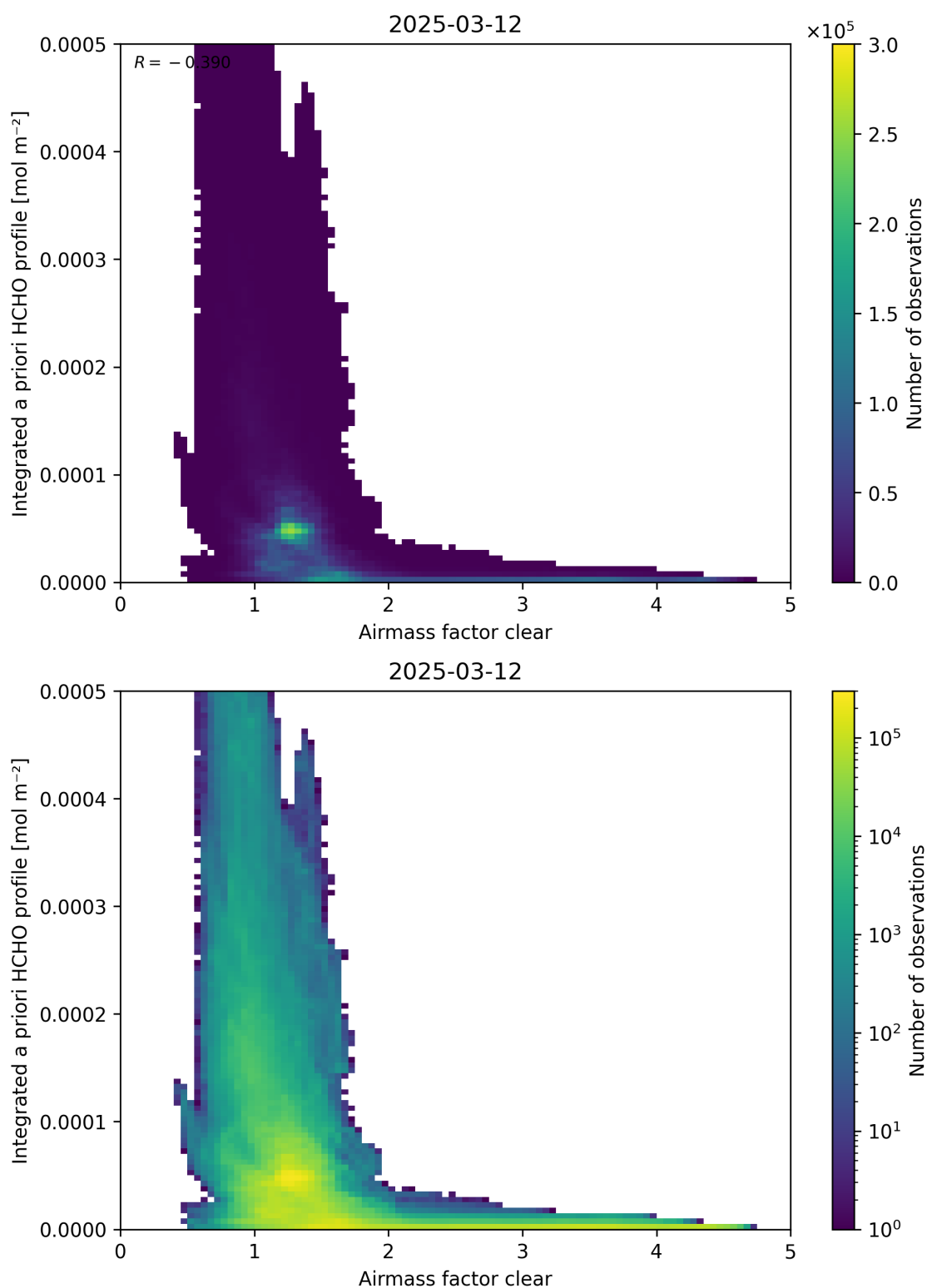
Figure 76: Scatter density plot of “Airmass factor clear” against “Integrated a priori HCHO profile” for 2025-03-12 to 2025-03-13.
