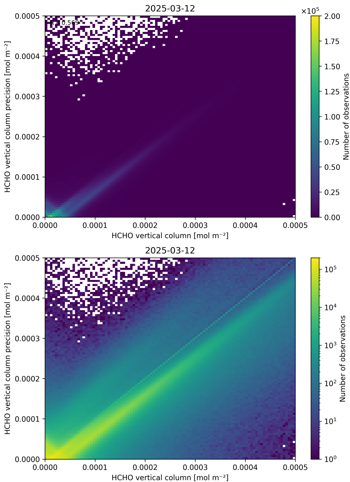
Figure 134: Scatter density plot of “HCHO vertical column” against “HCHO vertical column precision” for 2025-03-12 to 2025-03-13.
