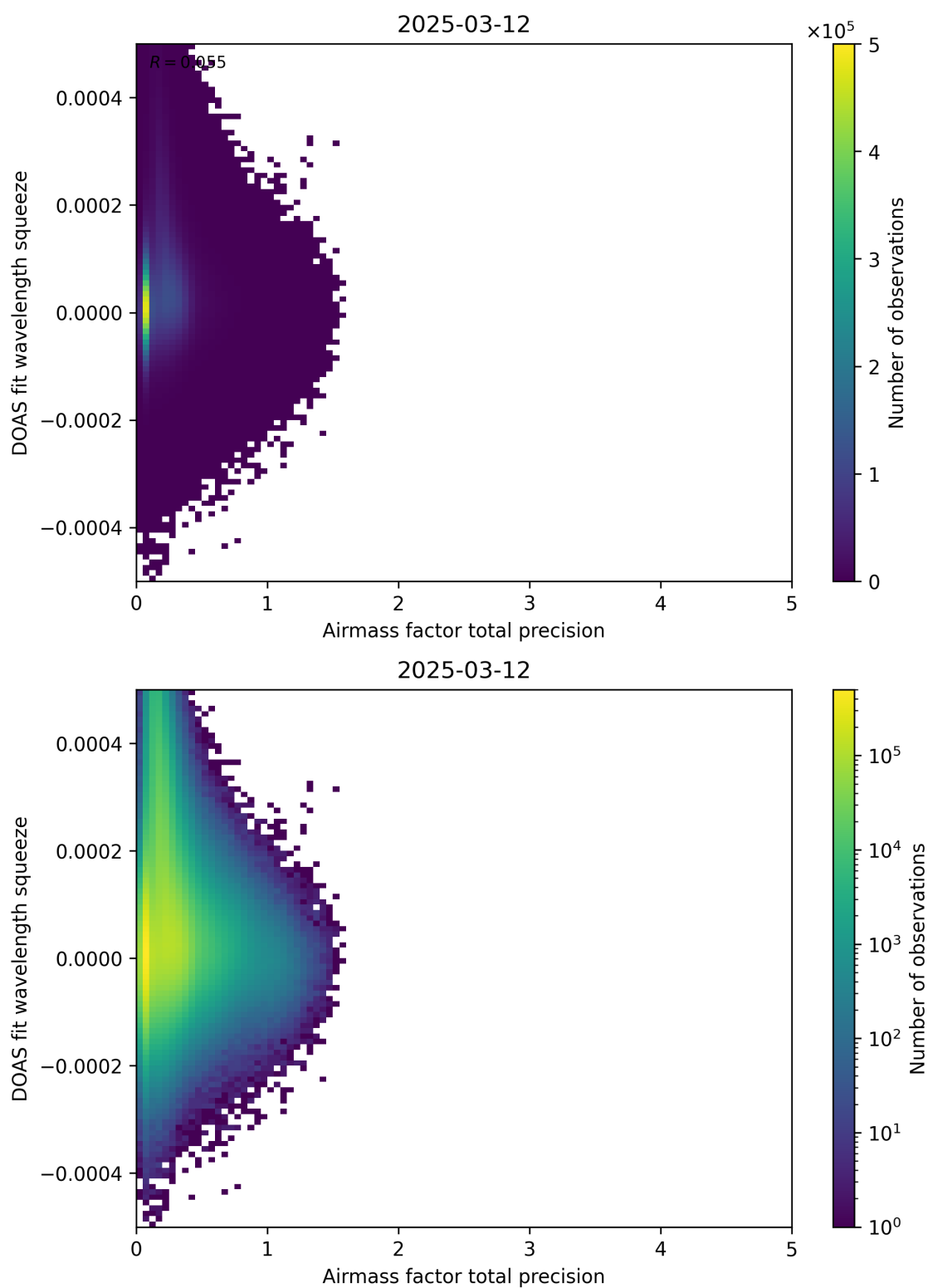
Figure 107: Scatter density plot of “Airmass factor total precision” against “DOAS fit wavelength squeeze” for 2025-03-12 to 2025-03-13.
