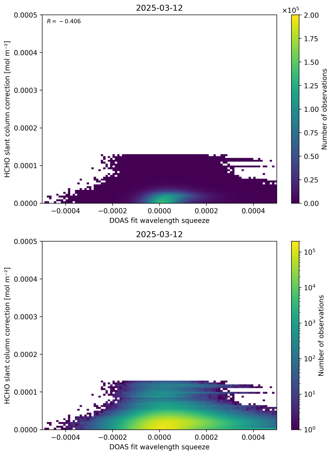
Figure 70: Scatter density plot of “DOAS fit wavelength squeeze” against “HCHO slant column correction” for 2025-03-12 to 2025-03-13.
