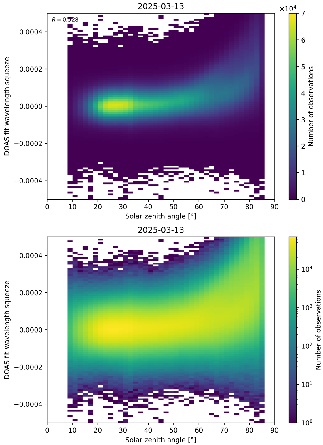
Figure 169: Scatter density plot of “Solar zenith angle” against “DOAS fit wavelength squeeze” for 2025-03-12 to 2025-03-14.
