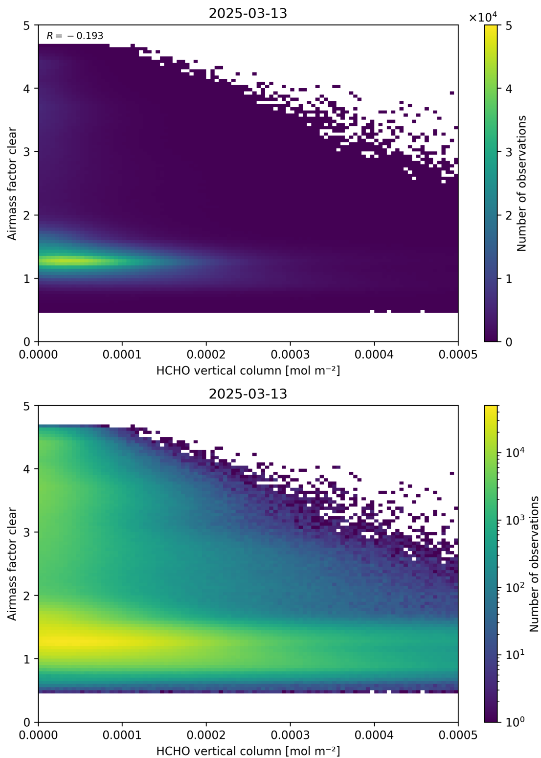
Figure 126: Scatter density plot of “HCHO vertical column” against “Airmass factor clear” for 2025-03-12 to 2025-03-14.
