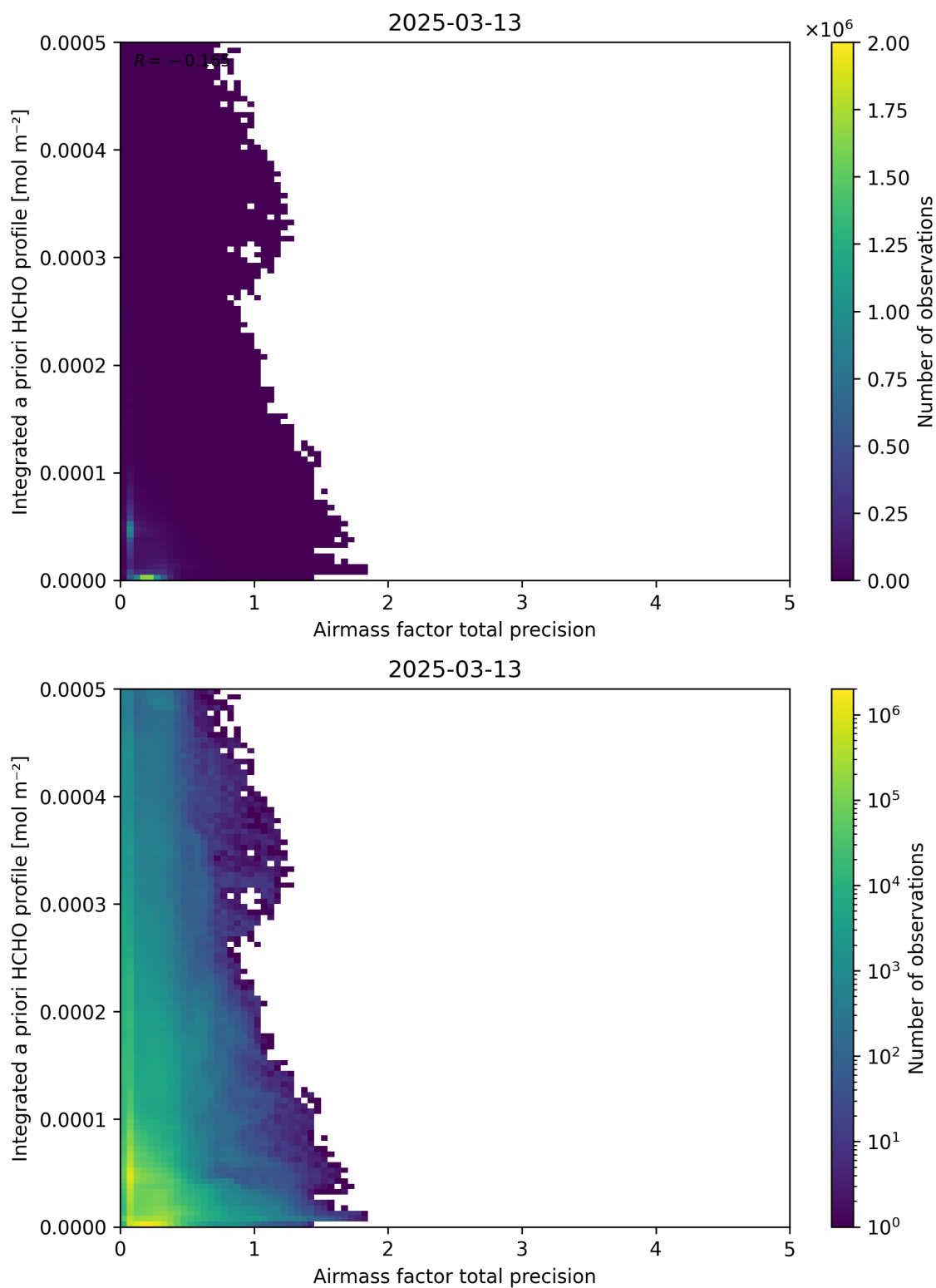
Figure 111: Scatter density plot of “Airmass factor total precision” against “Integrated a priori HCHO profile” for 2025-03-12 to 2025-03-14.
