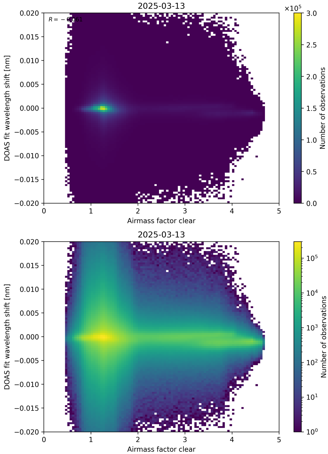
Figure 72: Scatter density plot of “Airmass factor clear” against “DOAS fit wavelength shift” for 2025-03-12 to 2025-03-14.
