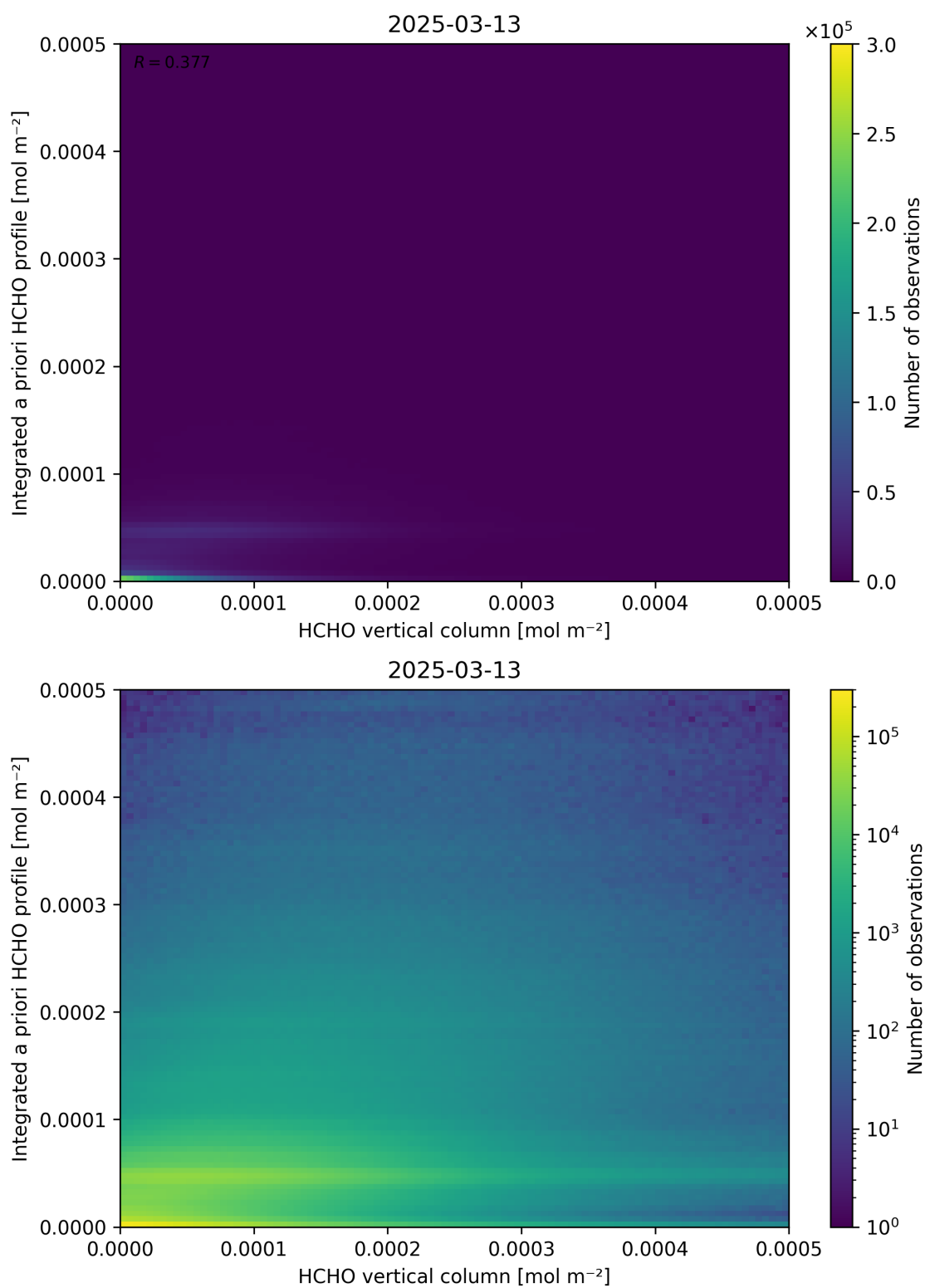
Figure 135: Scatter density plot of “HCHO vertical column” against “Integrated a priori HCHO profile” for 2025-03-12 to 2025-03-14.
