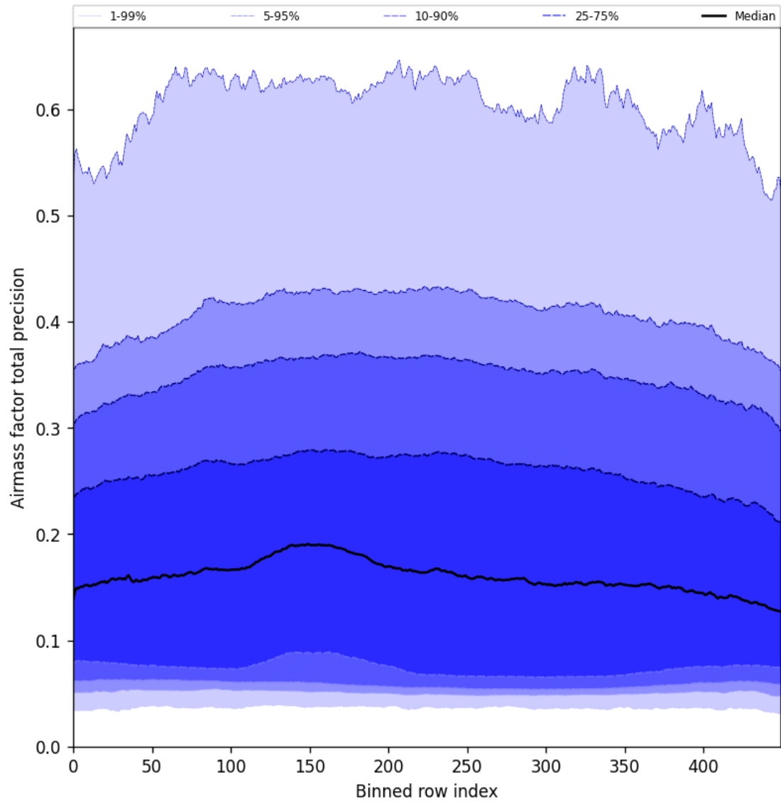
Figure 55: Along track statistics of “Airmass factor total precision” for 2025-03-12 to 2025-03-14
