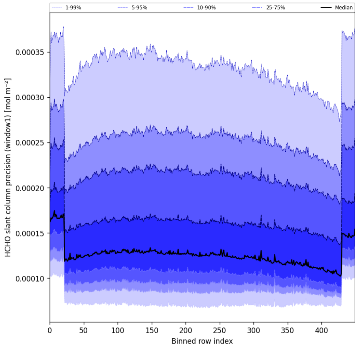
Figure 53: Along track statistics of “HCHO slant column precision (window1)” for 2025-03-12 to 2025-03-14
