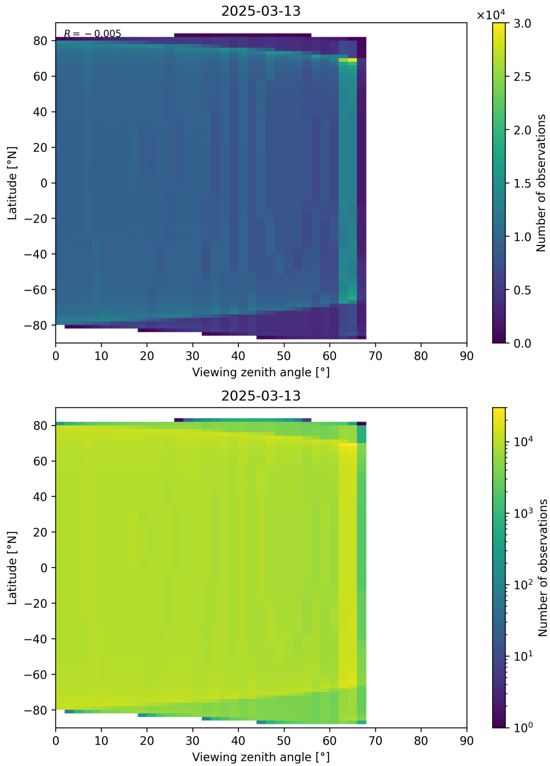
Figure 196: Scatter density plot of “Viewing zenith angle” against “Latitude” for 2025-03-12 to 2025-03-14.
