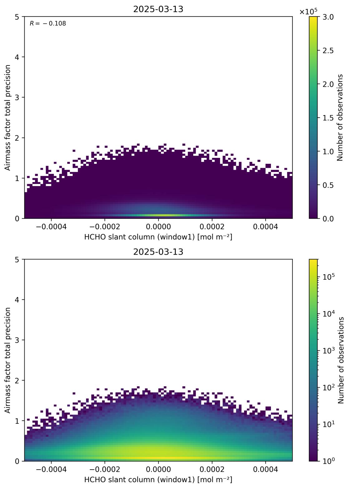
Figure 86: Scatter density plot of “HCHO slant column (window1)” against “Airmass factor total precision” for 2025-03-12 to 2025-03-14.
