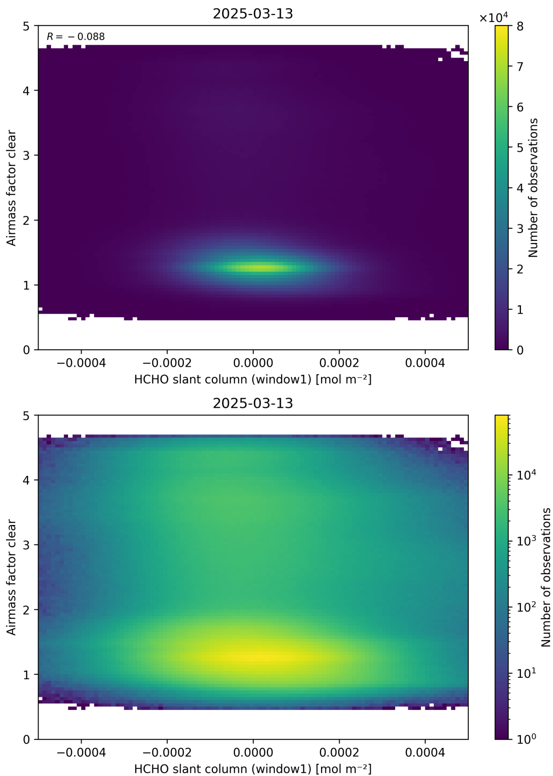
Figure 81: Scatter density plot of “HCHO slant column (window1)” against “Airmass factor clear” for 2025-03-12 to 2025-03-14.
