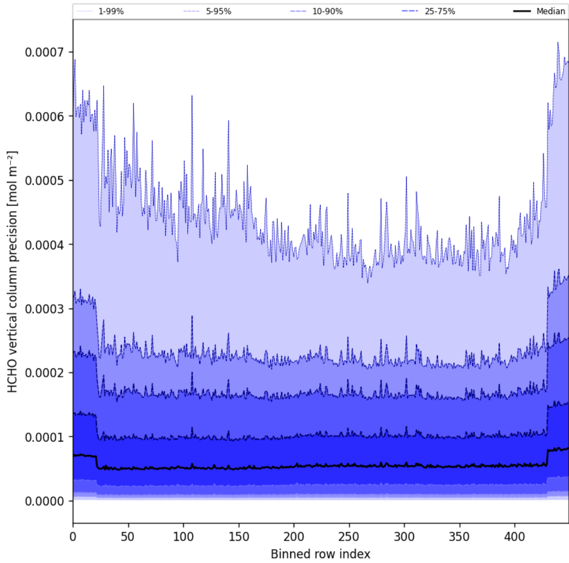
Figure 50: Along track statistics of “HCHO vertical column precision” for 2025-03-12 to 2025-03-14
