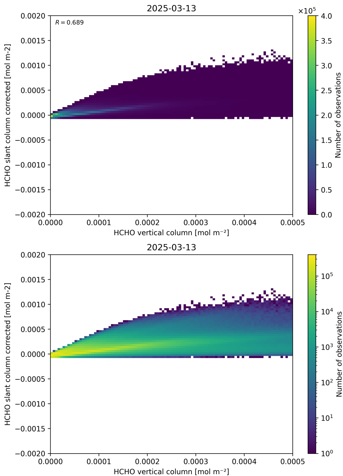
Figure 127: Scatter density plot of “HCHO vertical column” against “HCHO slant column corrected” for 2025-03-12 to 2025-03-14.
