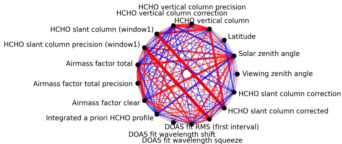
Figure 1: Map of correlation graph for 2025-03-12 to 2025-03-14.
