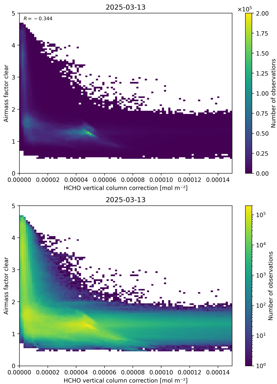
Figure 115: Scatter density plot of “HCHO vertical column correction” against “Airmass factor clear” for 2025-03-12 to 2025-03-14.
