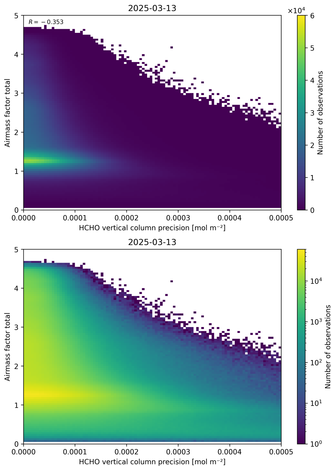
Figure 144: Scatter density plot of “HCHO vertical column precision” against “Airmass factor total” for 2025-03-12 to 2025-03-14.
