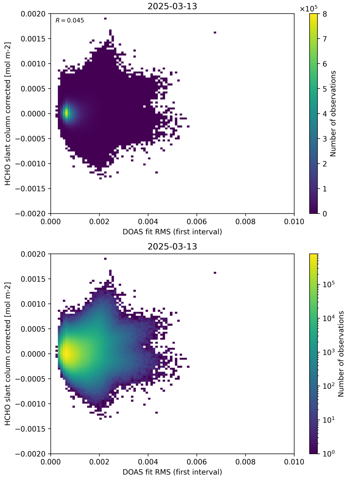
Figure 62: Scatter density plot of “DOAS fit RMS (first interval)” against “HCHO slant column corrected” for 2025-03-12 to 2025-03-14.
