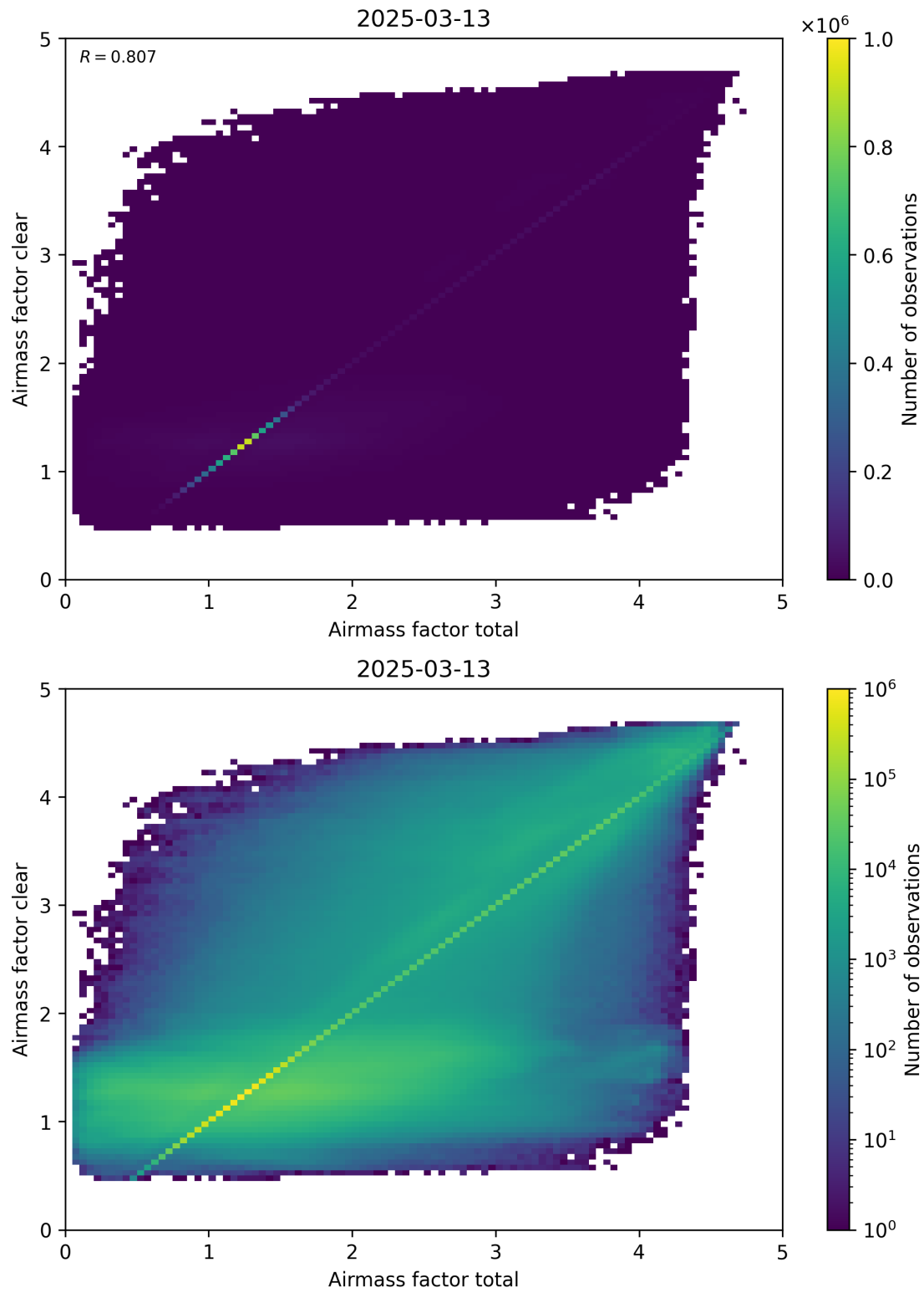
Figure 100: Scatter density plot of “Airmass factor total” against “Airmass factor clear” for 2025-03-12 to 2025-03-14.
