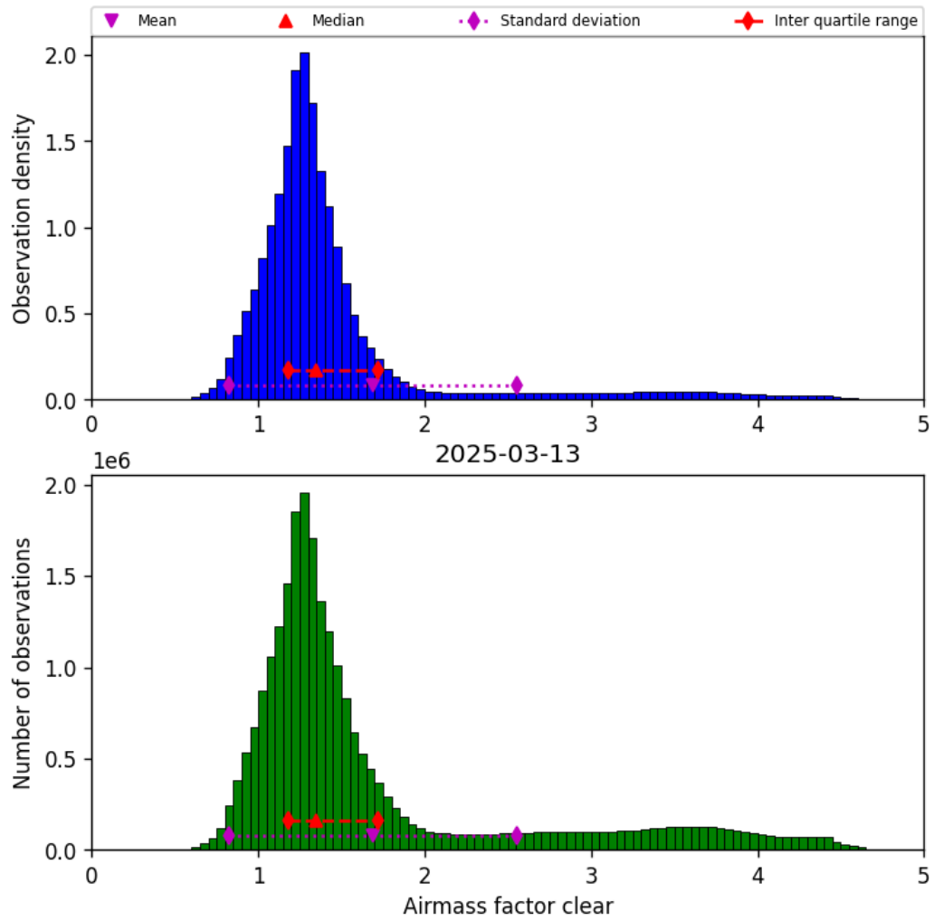
Figure 42: Histogram of “Airmass factor clear” for 2025-03-12 to 2025-03-14
