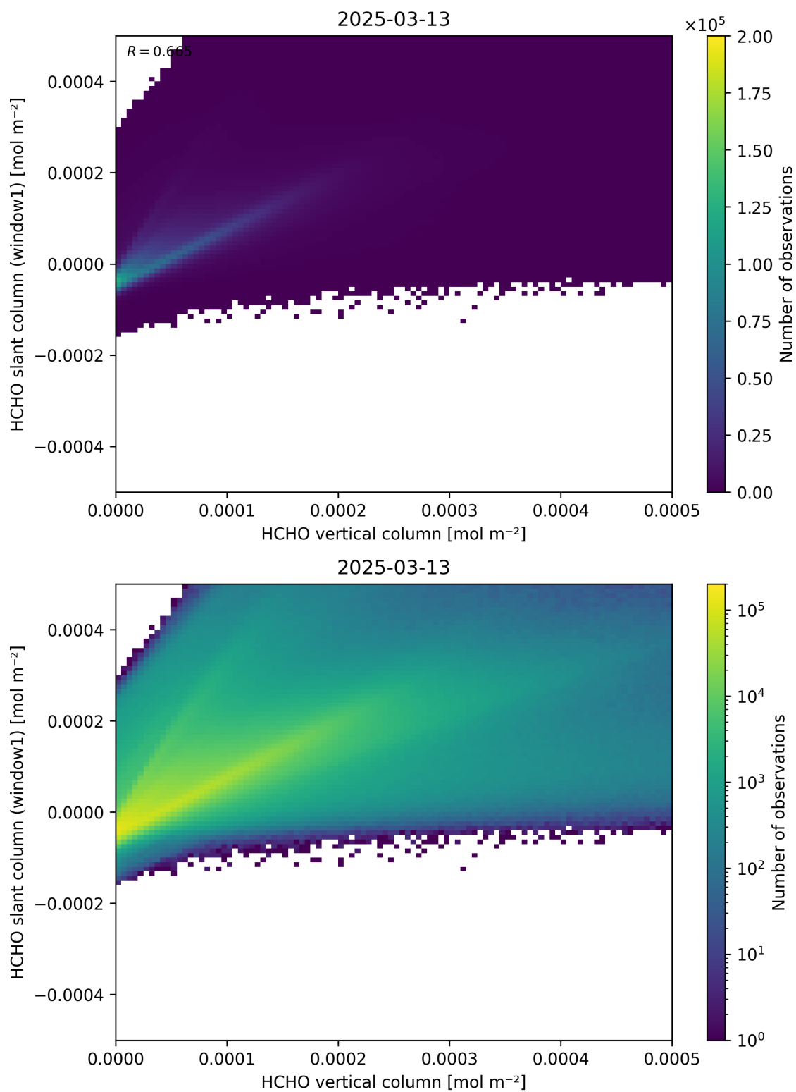
Figure 129: Scatter density plot of “HCHO vertical column” against “HCHO slant column (window1)” for 2025-03-12 to 2025-03-14.
