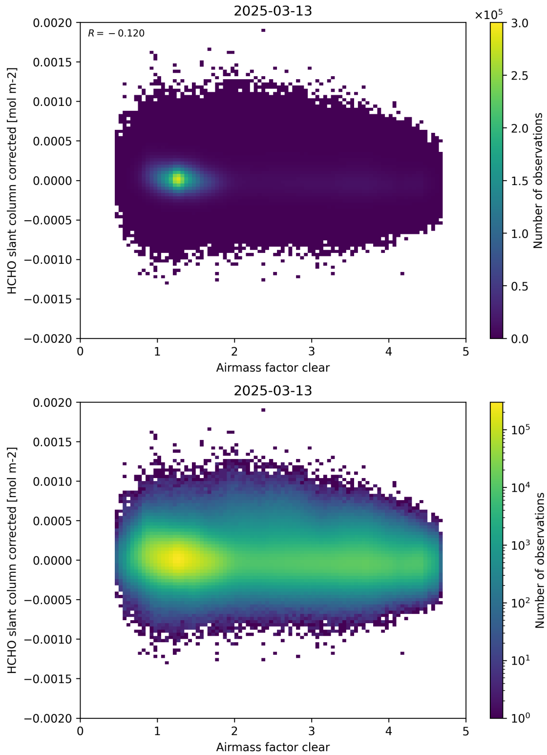
Figure 74: Scatter density plot of “Airmass factor clear” against “HCHO slant column corrected” for 2025-03-12 to 2025-03-14.
