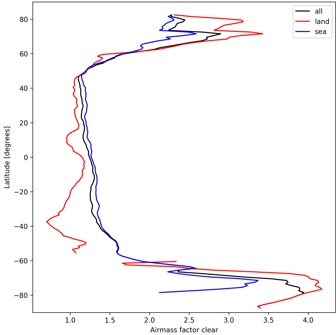
Figure 28: Zonal average of “Airmass factor clear” for 2025-03-12 to 2025-03-14.
