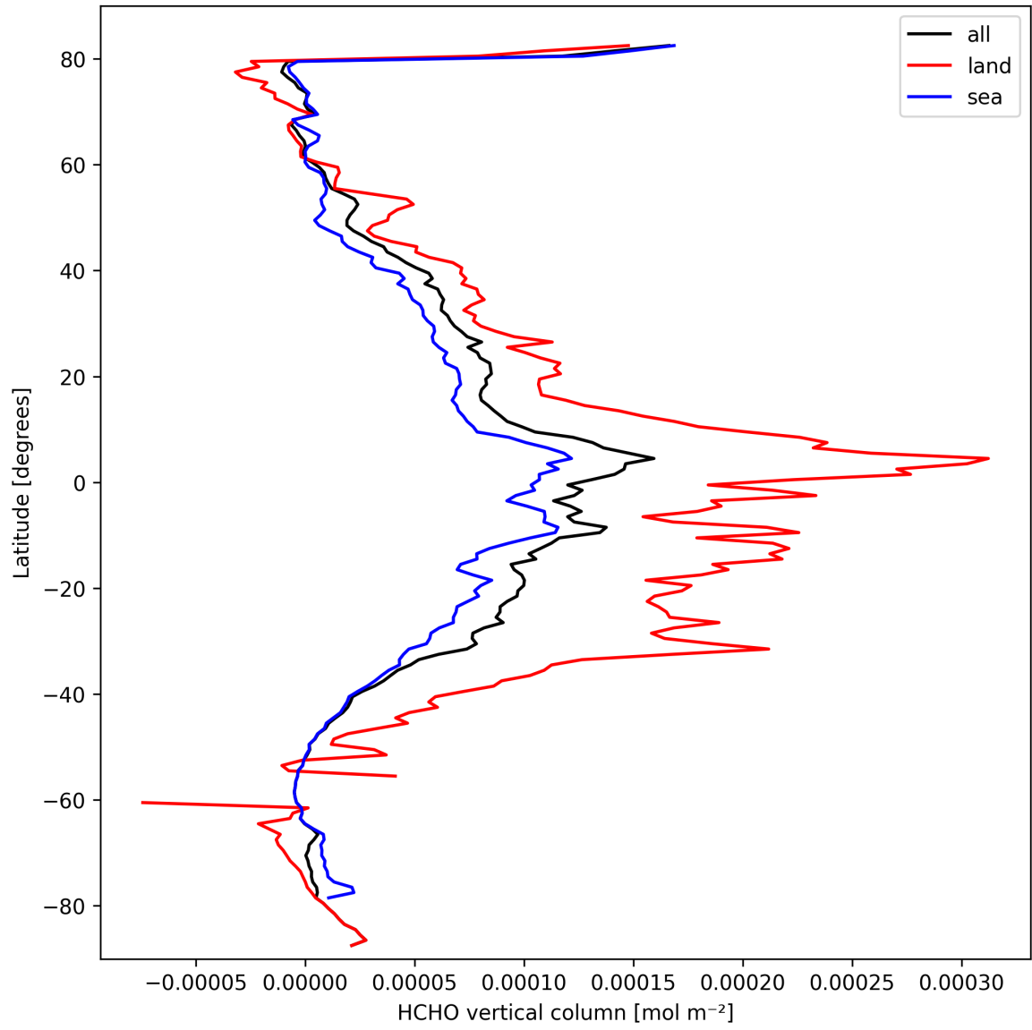
Figure 21: Zonal average of “HCHO vertical column” for 2025-03-12 to 2025-03-14.
