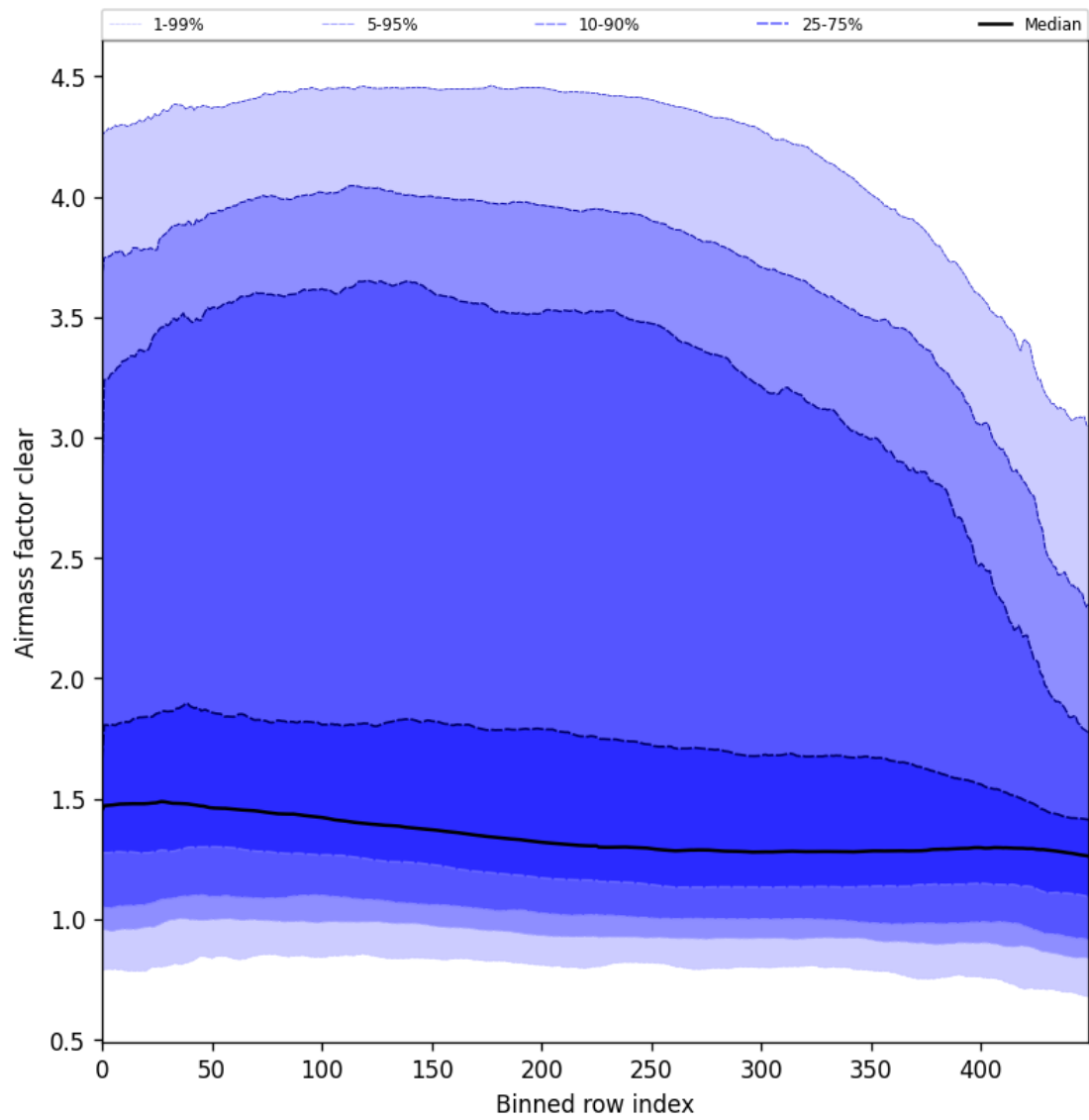
Figure 56: Along track statistics of “Air mass factor clear” for 2025-03-12 to 2025-03-14
