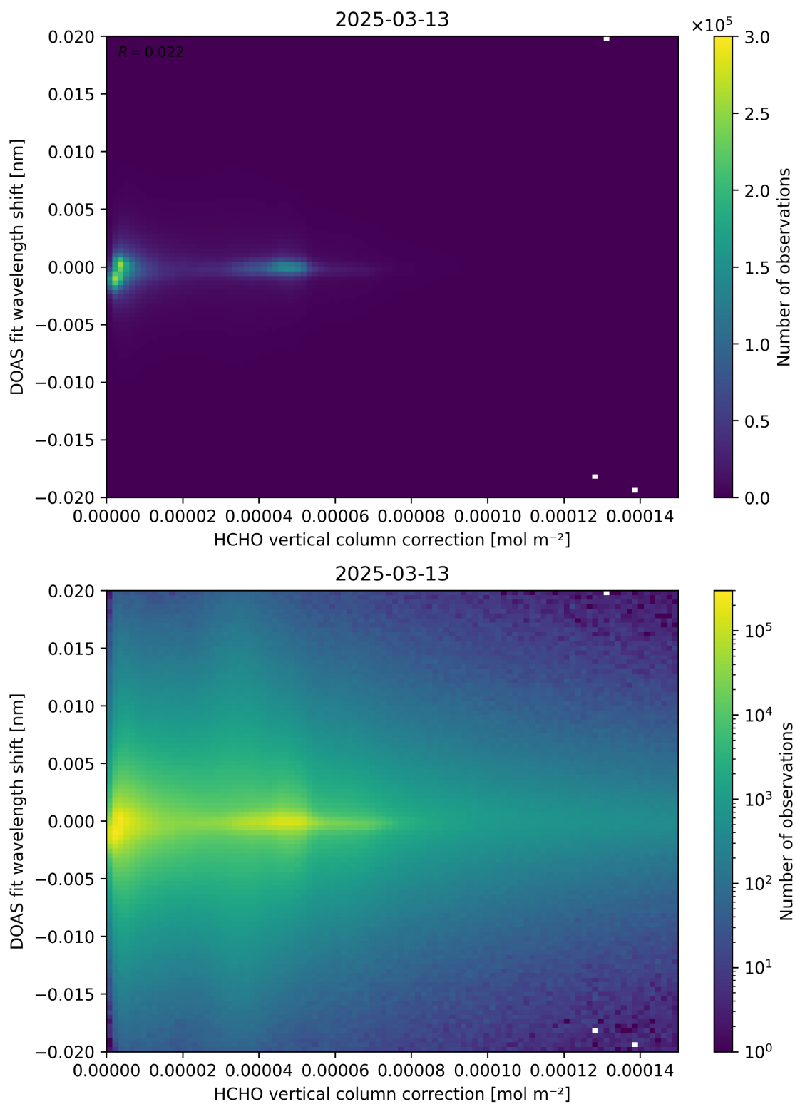
Figure 113: Scatter density plot of “HCHO vertical column correction” against “DOAS fit wavelength shift” for 2025-03-12 to 2025-03-14.
