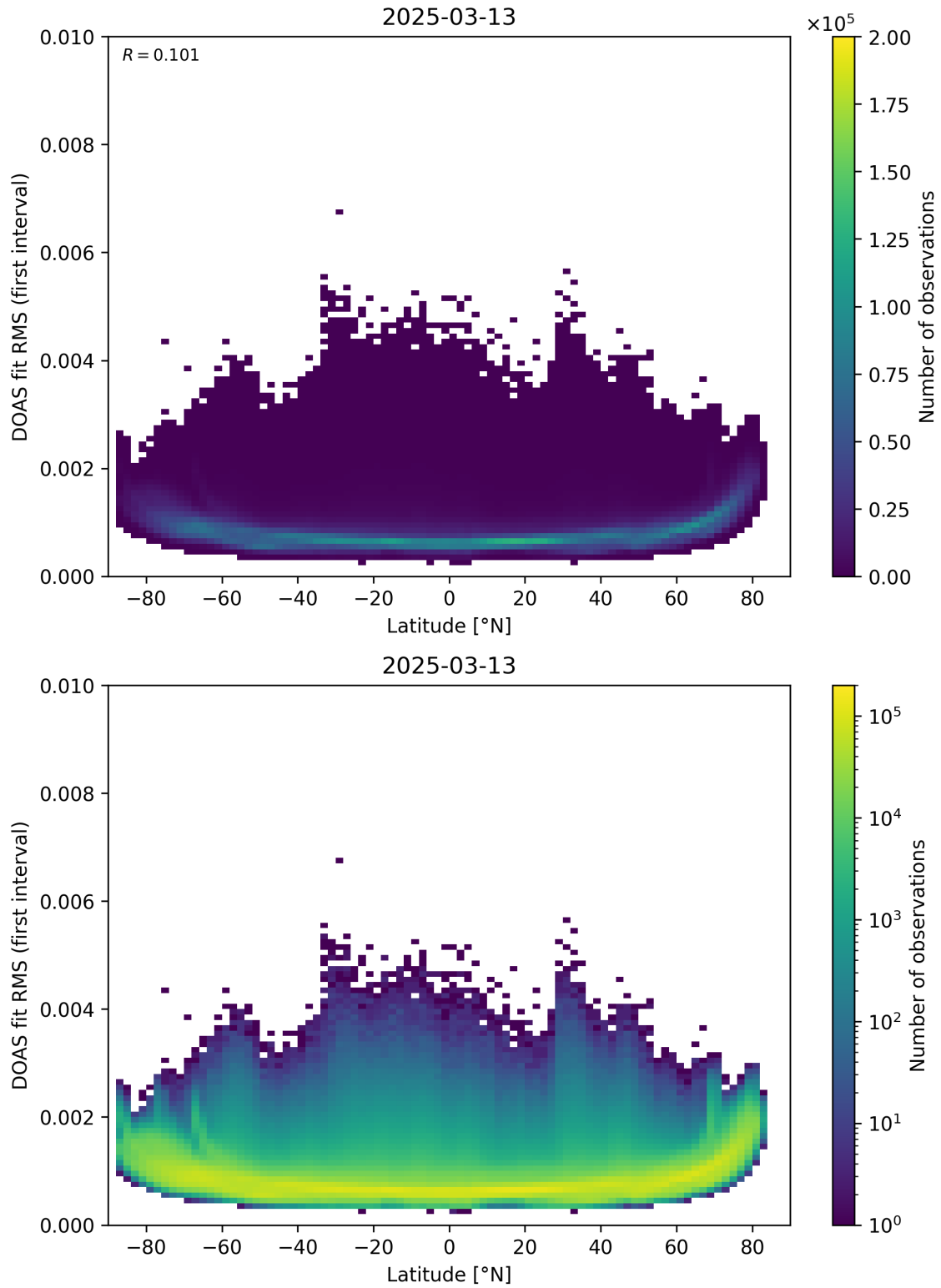
Figure 153: Scatter density plot of “Latitude” against “DOAS fit RMS (first interval)” for 2025-03-12 to 2025-03-14.
