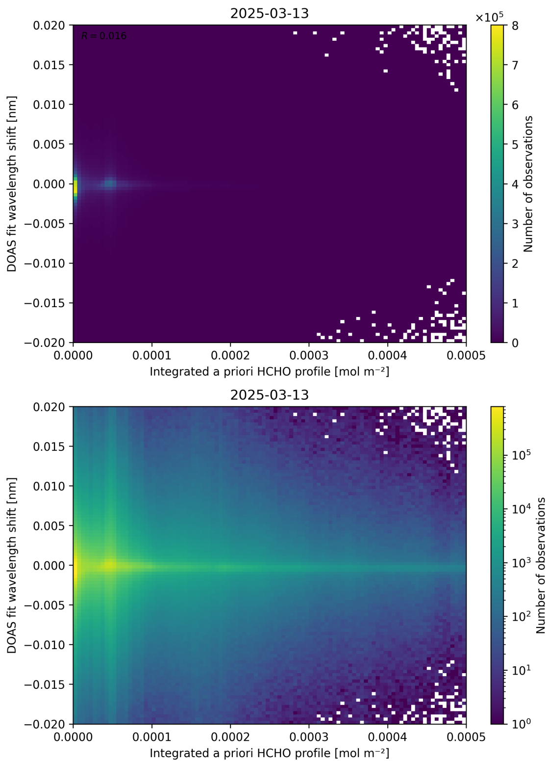
Figure 149: Scatter density plot of “Integrated a priori HCHO profile” against “DOAS fit wavelength shift” for 2025-03-12 to 2025-03-14.
