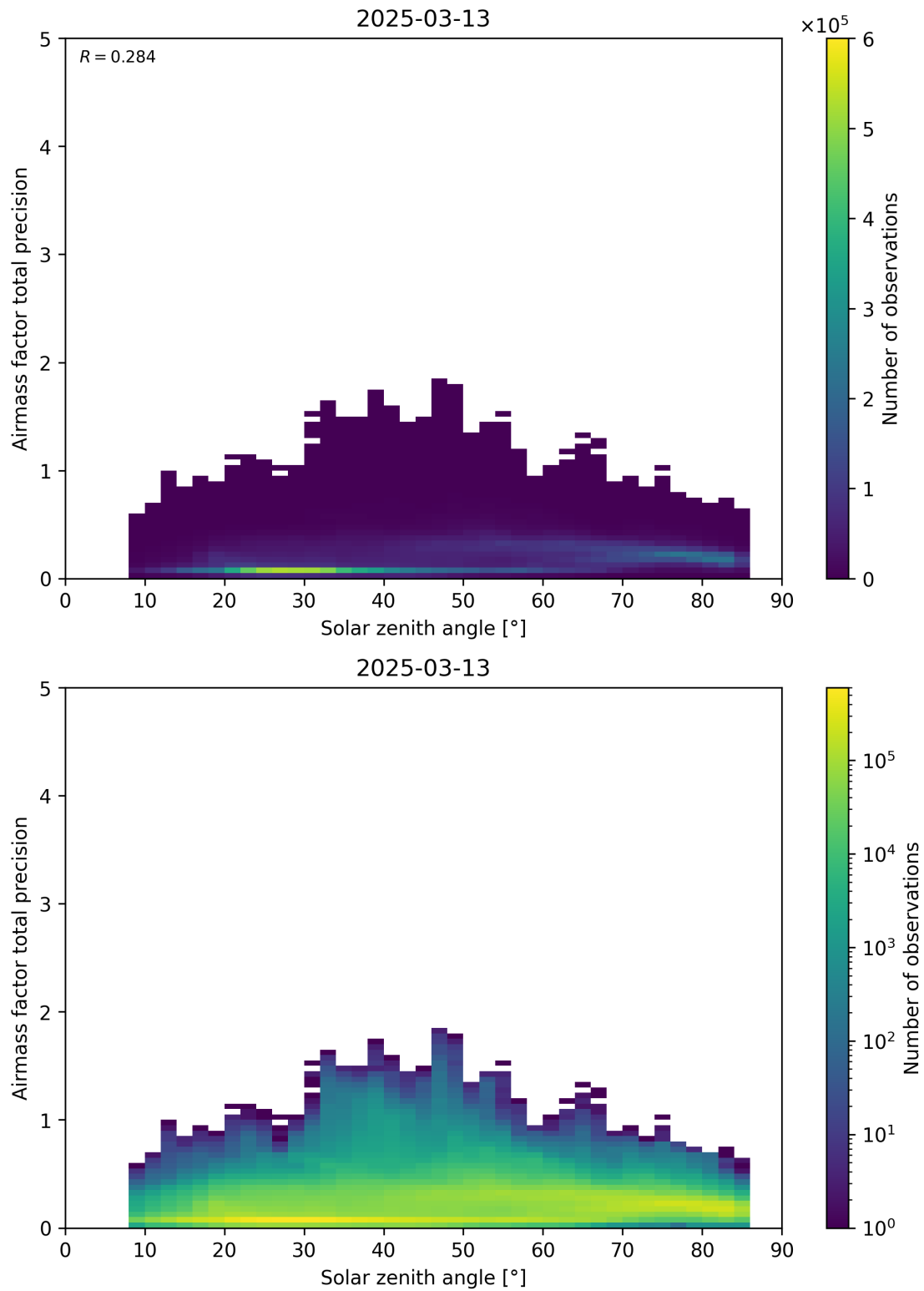
Figure 176: Scatter density plot of “Solar zenith angle” against “Airmass factor total precision” for 2025-03-12 to 2025-03-14.
