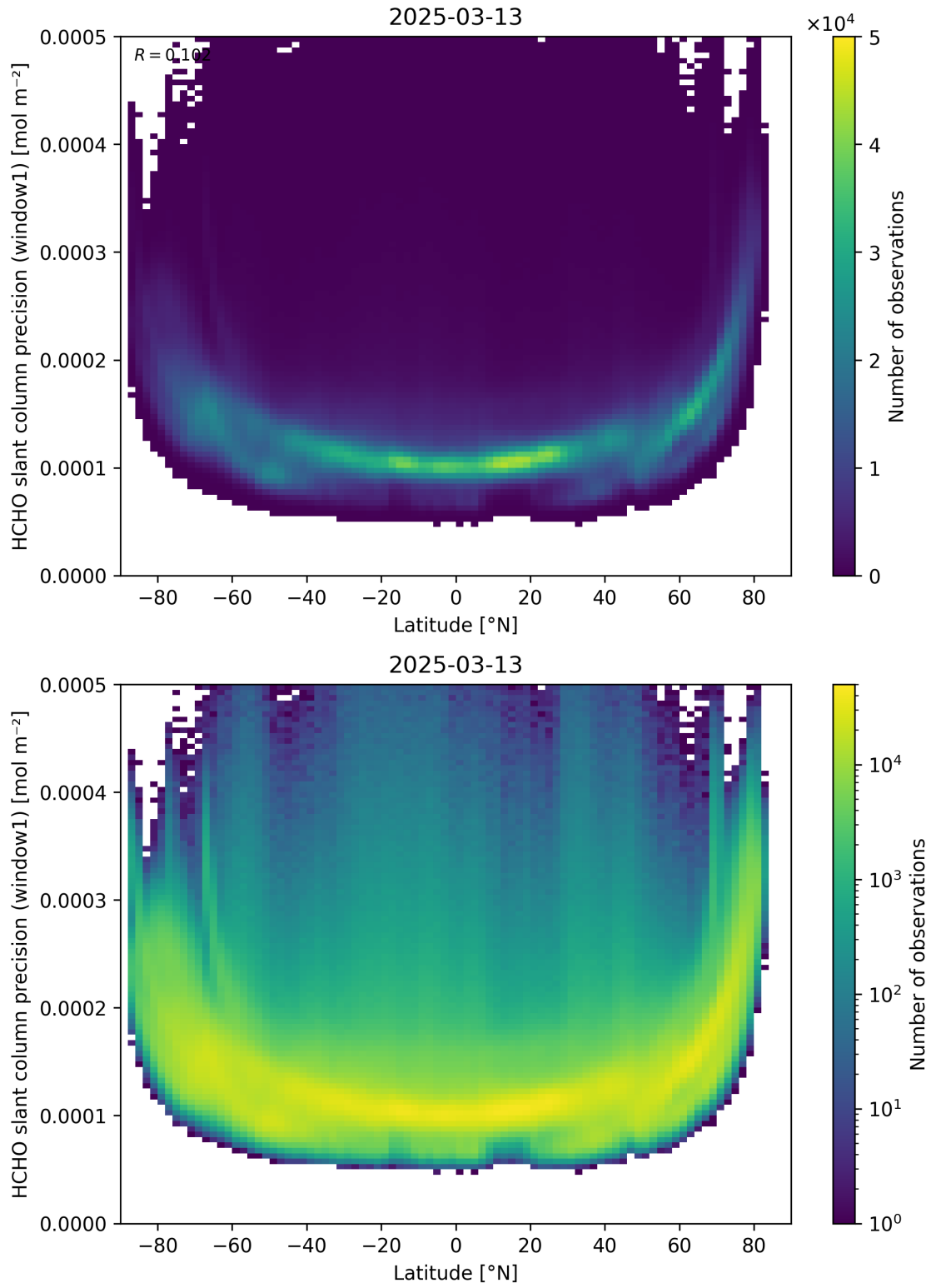
Figure 160: Scatter density plot of “Latitude” against “HCHO slant column precision (window1)” for 2025-03-12 to 2025-03-14.
