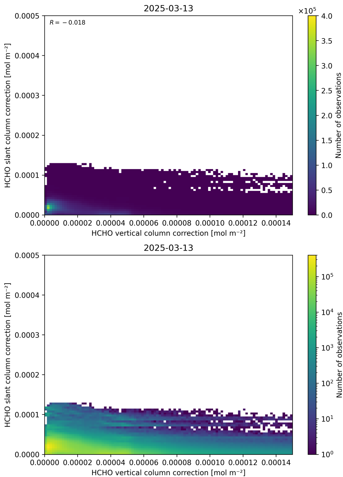
Figure 117: Scatter density plot of “HCHO vertical column correction” against “HCHO slant column correction” for 2025-03-12 to 2025-03-14.
