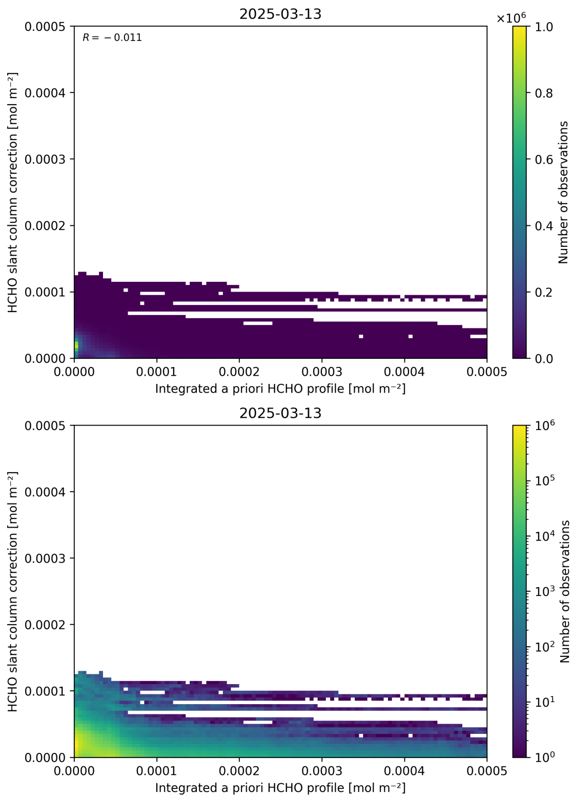
Figure 152: Scatter density plot of “Integrated a priori HCHO profile” against “HCHO slant column correction” for 2025-03-12 to 2025-03-14.
