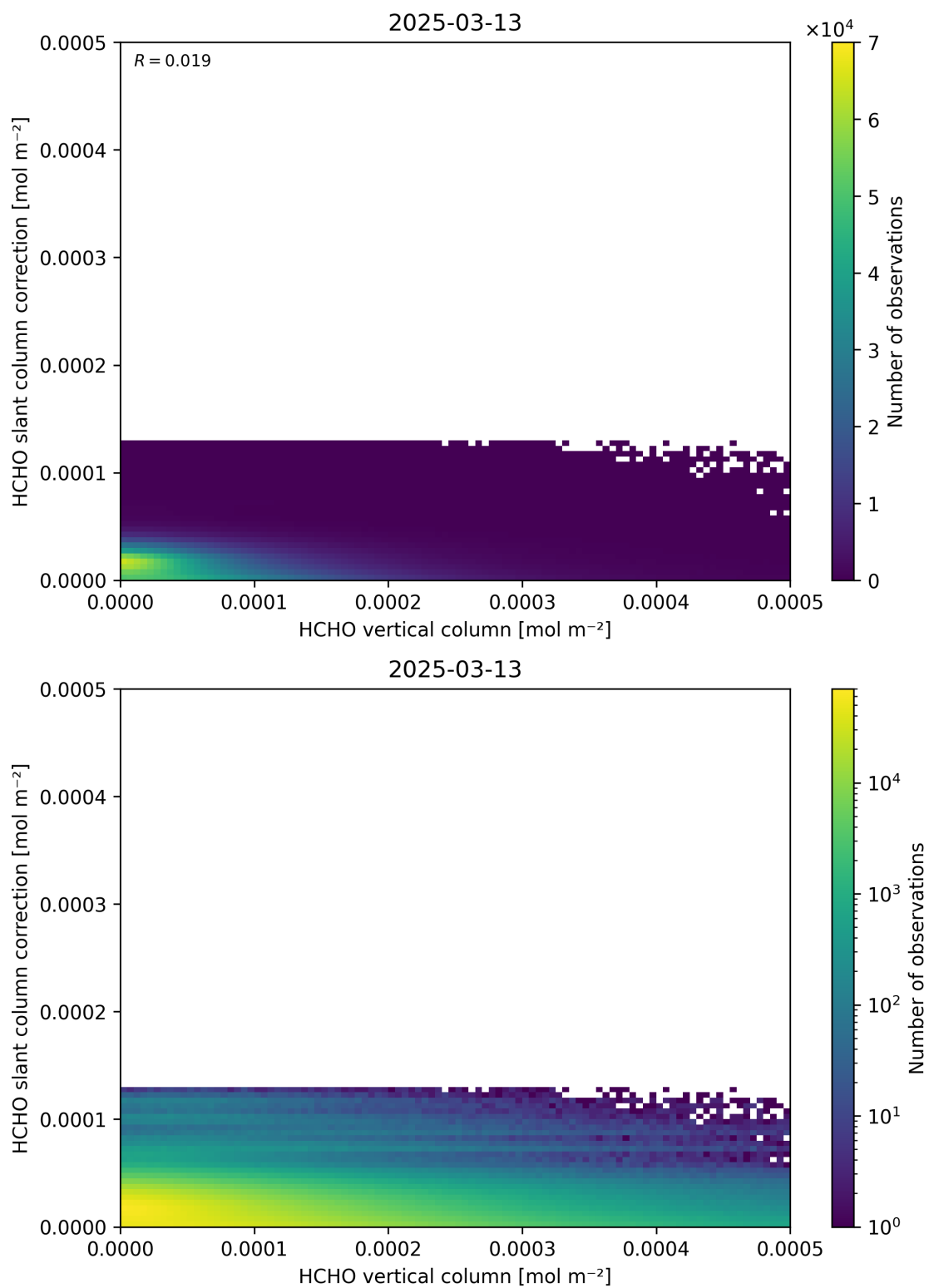
Figure 128: Scatter density plot of “HCHO vertical column” against “HCHO slant column correction” for 2025-03-12 to 2025-03-14.
