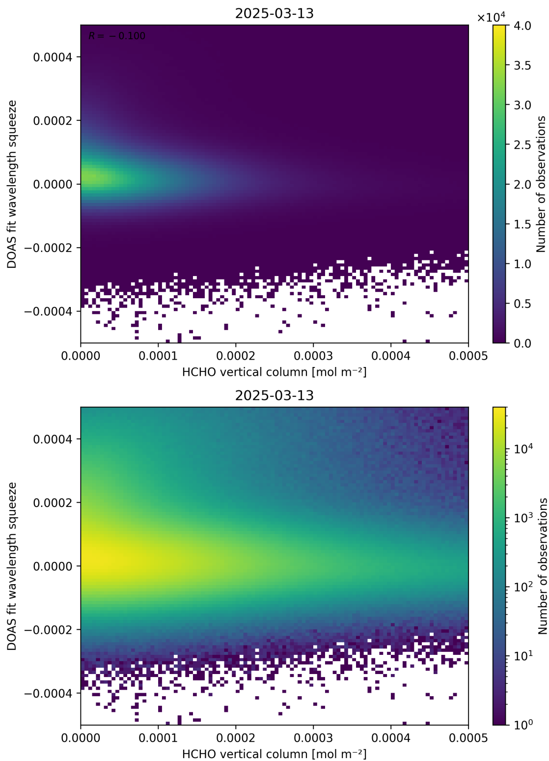
Figure 125: Scatter density plot of “HCHO vertical column” against “DOAS fit wavelength squeeze” for 2025-03-12 to 2025-03-14.
