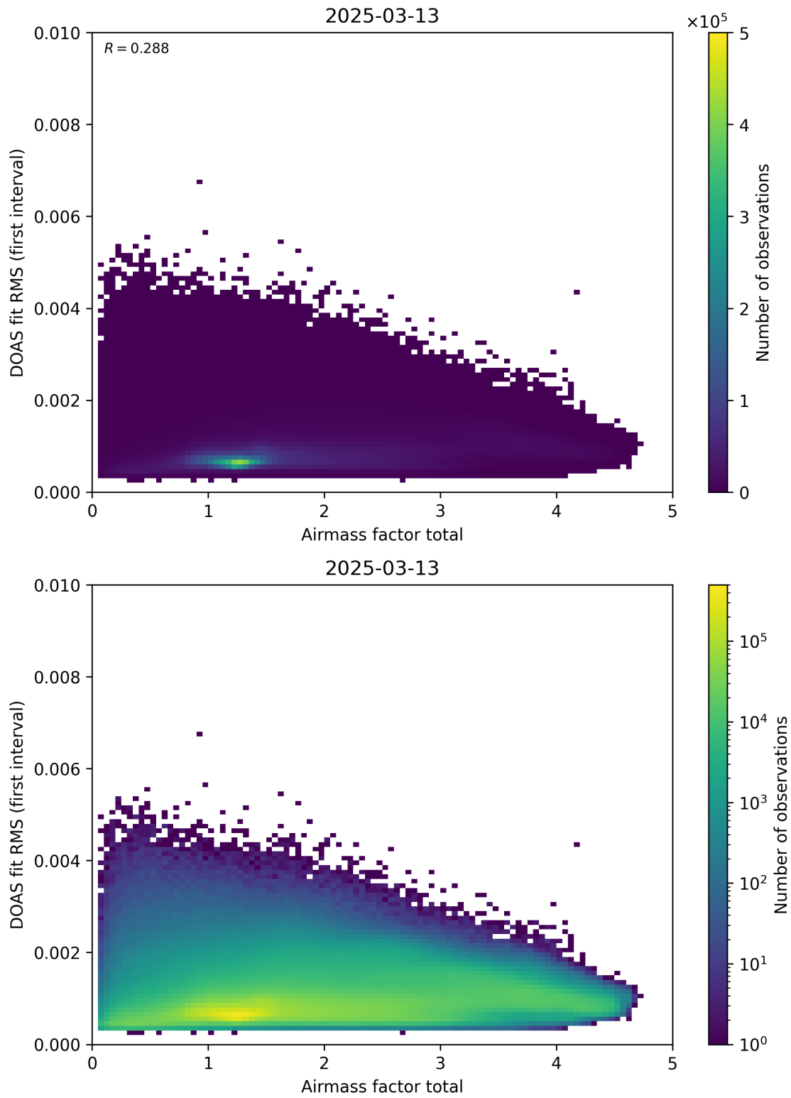
Figure 97: Scatter density plot of “Airmass factor total” against “DOAS fit RMS (first interval)” for 2025-03-12 to 2025-03-14.
