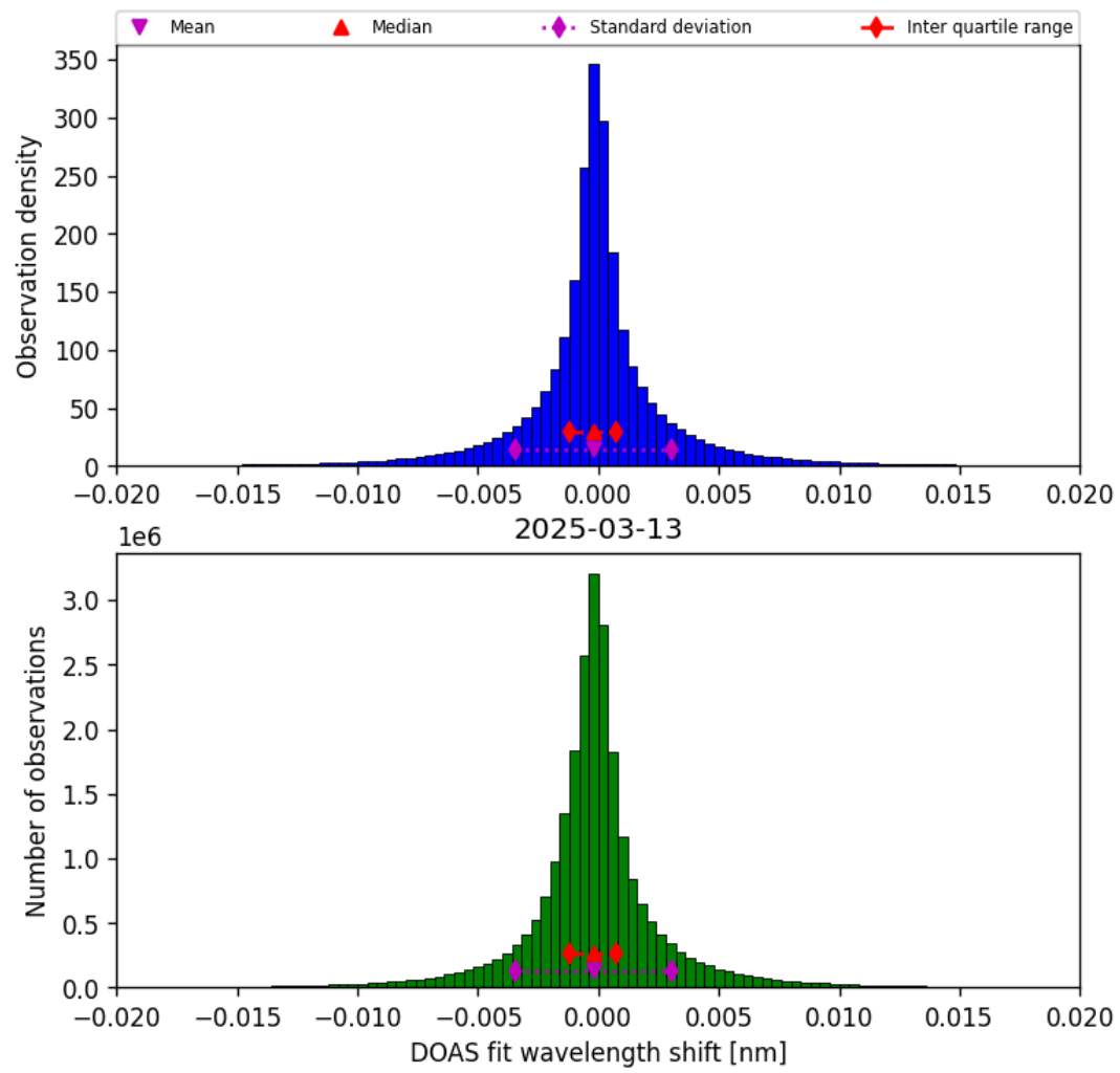
Figure 44: Histogram of “DOAS fit wavelength shift” for 2025-03-12 to 2025-03-14
