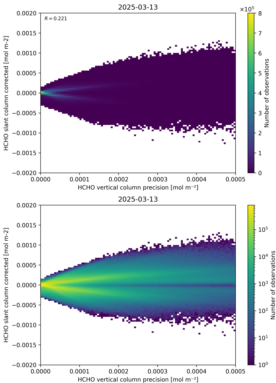
Figure 140: Scatter density plot of “HCHO vertical column precision” against “HCHO slant column corrected” for 2025-03-12 to 2025-03-14.
