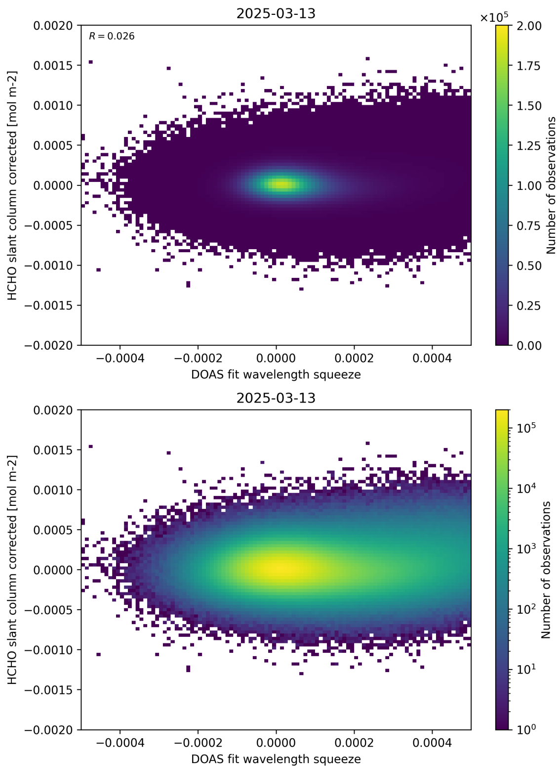
Figure 69: Scatter density plot of “DOAS fit wavelength squeeze” against “HCHO slant column corrected” for 2025-03-12 to 2025-03-14.
