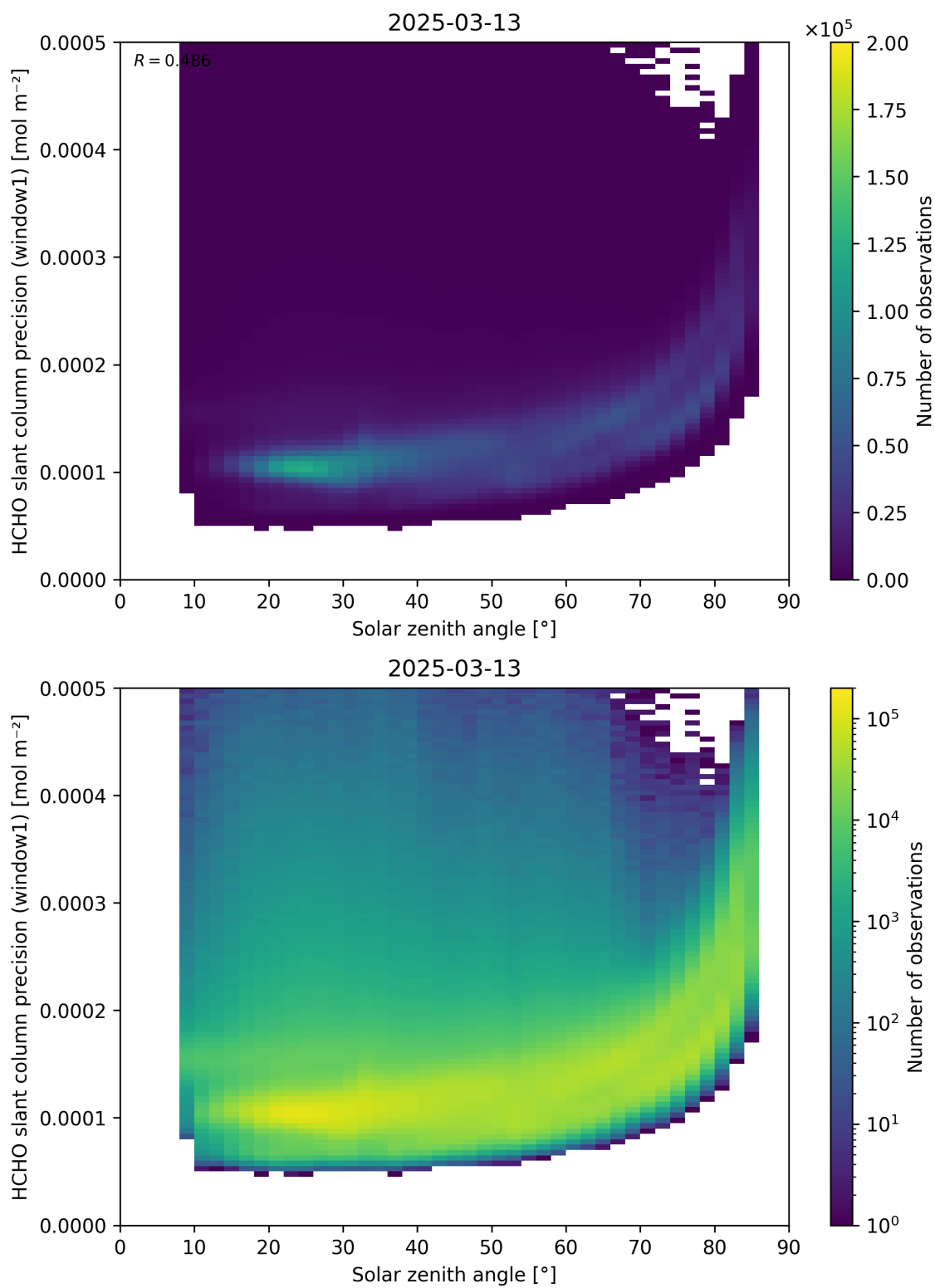
Figure 174: Scatter density plot of “Solar zenith angle” against “HCHO slant column precision (window1)” for 2025-03-12 to 2025-03-14.
