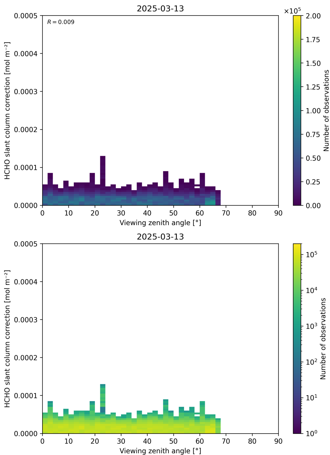
Figure 187: Scatter density plot of “Viewing zenith angle” against “HCHO slant column correction” for 2025-03-12 to 2025-03-14.
