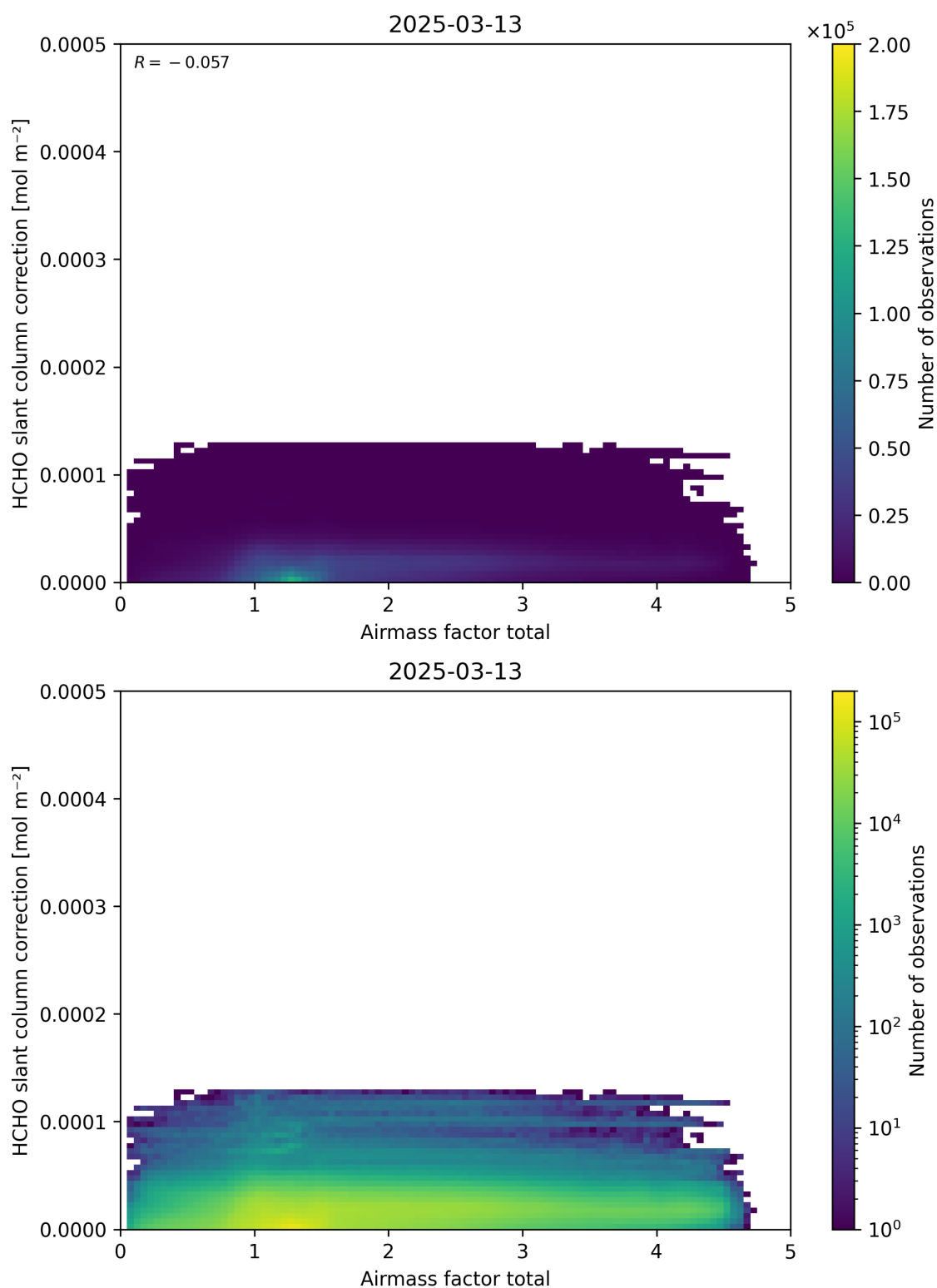
Figure 102: Scatter density plot of “Airmass factor total” against “HCHO slant column correction” for 2025-03-12 to 2025-03-14.
