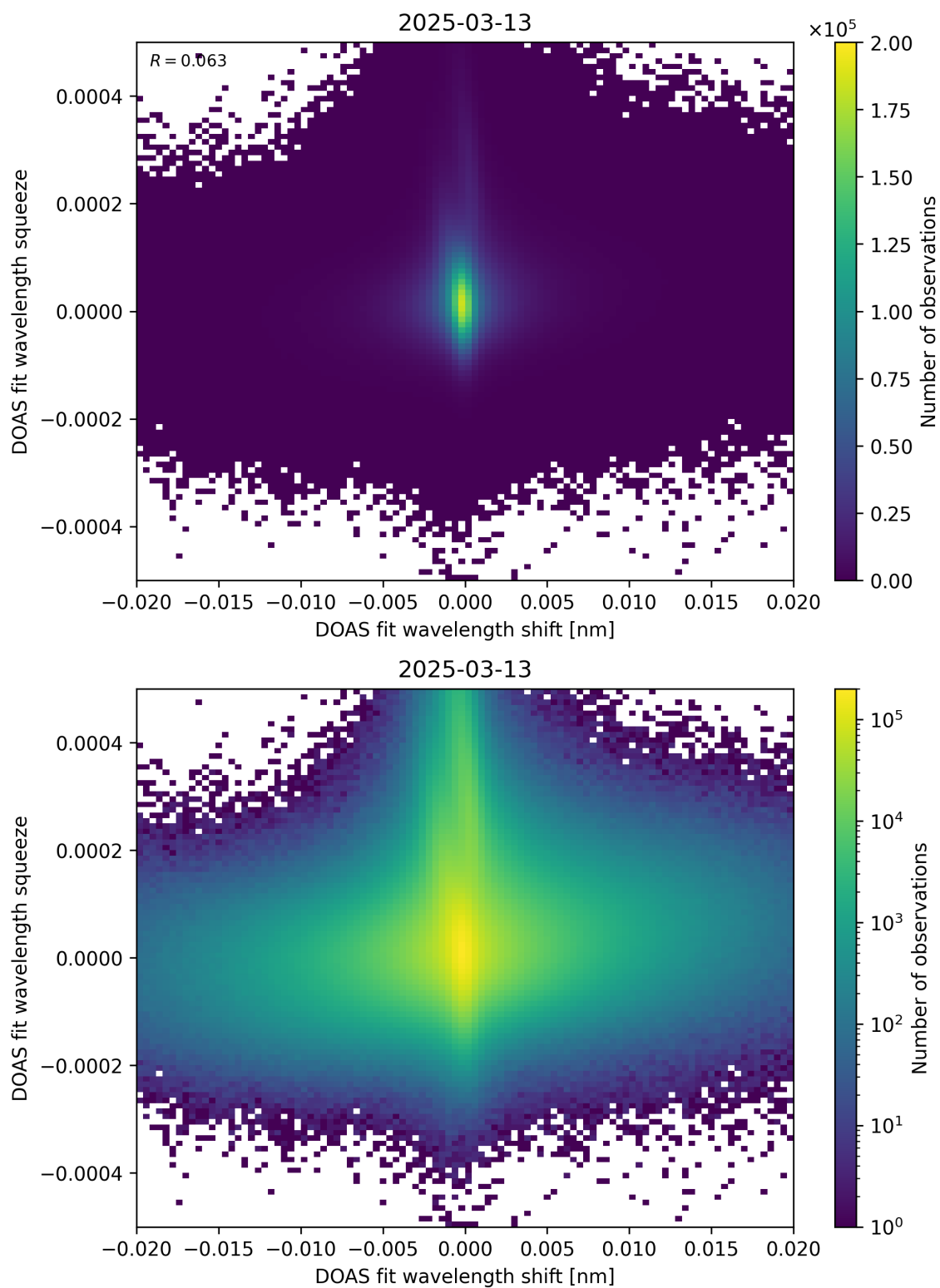
Figure 65: Scatter density plot of “DOAS fit wavelength shift” against “DOAS fit wavelength squeeze” for 2025-03-12 to 2025-03-14.
