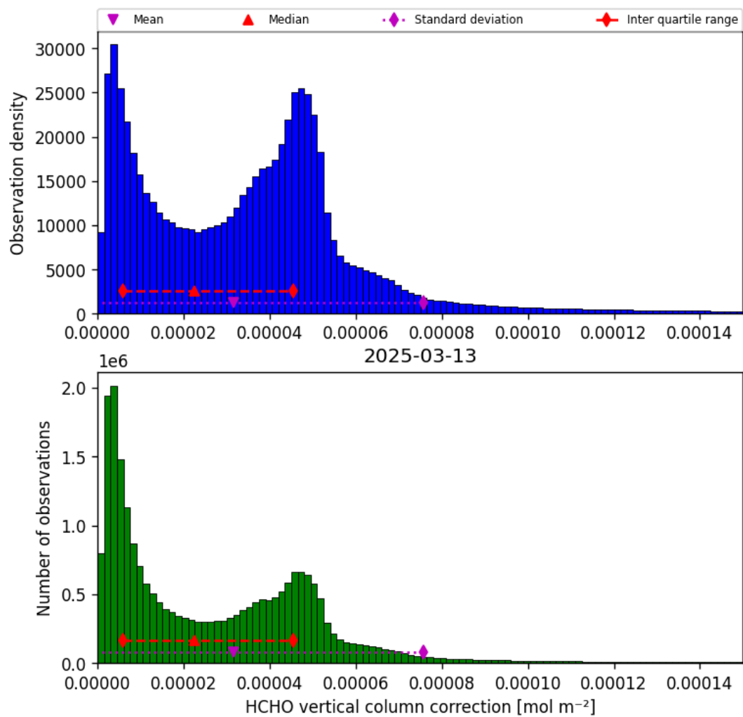
Figure 37: Histogram of “HCHO vertical column correction” for 2025-03-12 to 2025-03-14
