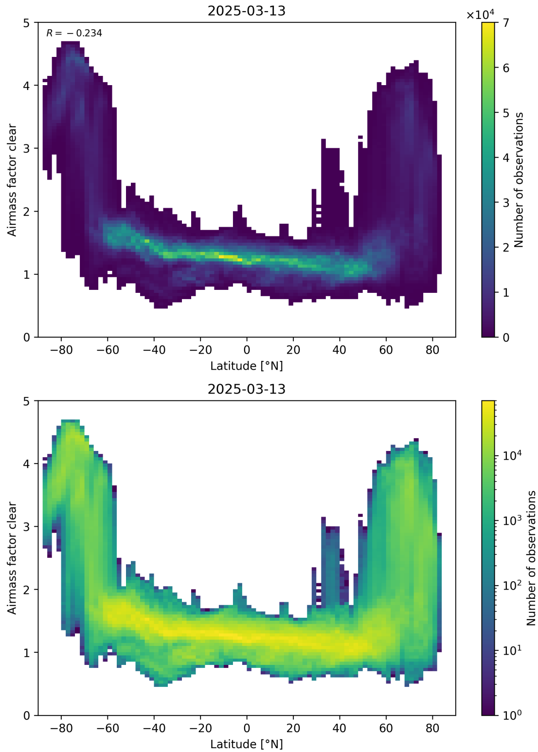
Figure 156: Scatter density plot of “Latitude” against “Airmass factor clear” for 2025-03-12 to 2025-03-14.
