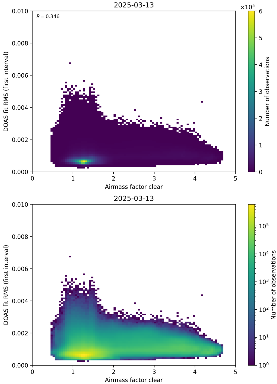
Figure 71: Scatter density plot of “Airmass factor clear” against “DOAS fit RMS (first interval)” for 2025-03-12 to 2025-03-14.
