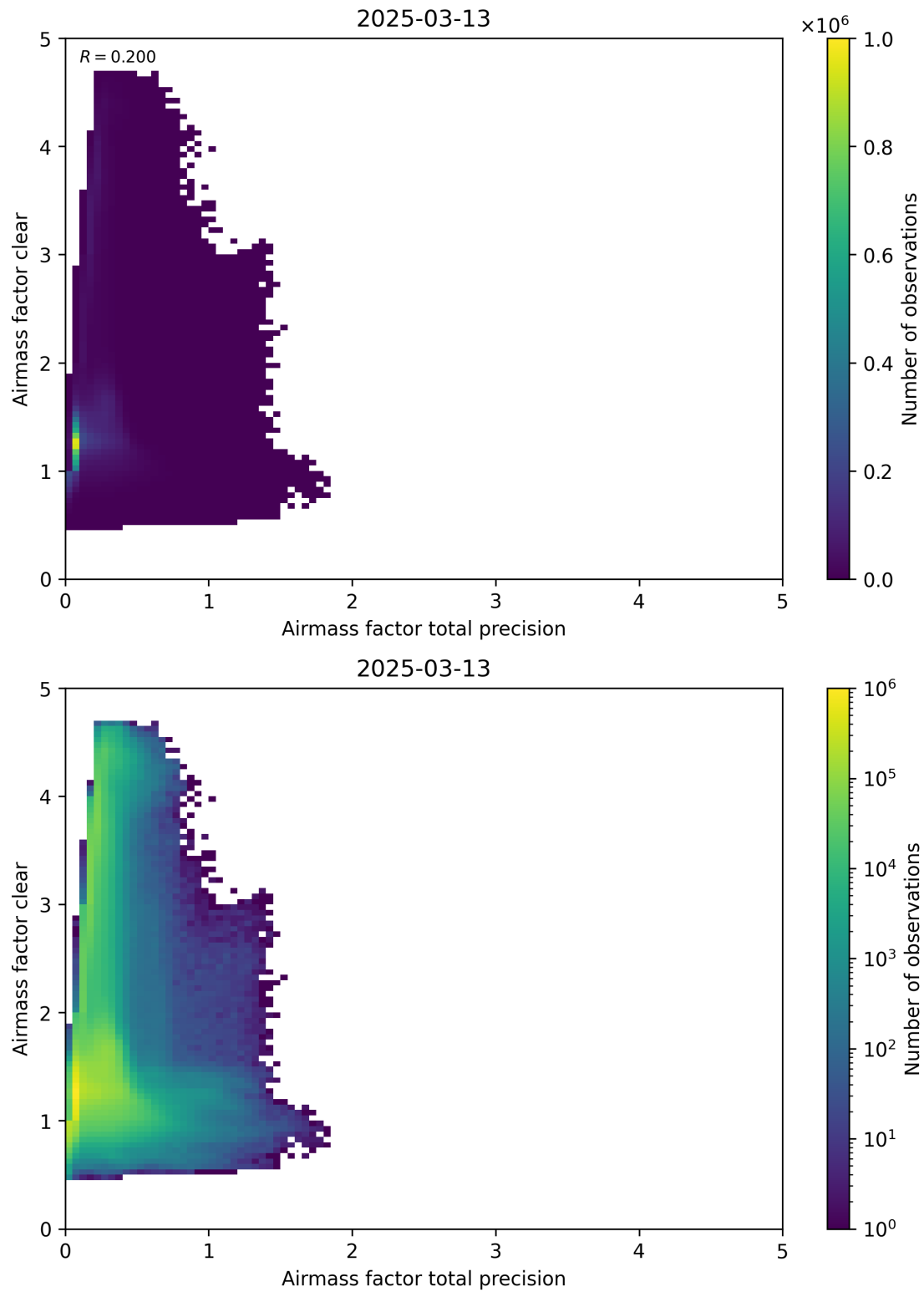
Figure 108: Scatter density plot of “Airmass factor total precision” against “Airmass factor clear” for 2025-03-12 to 2025-03-14.
