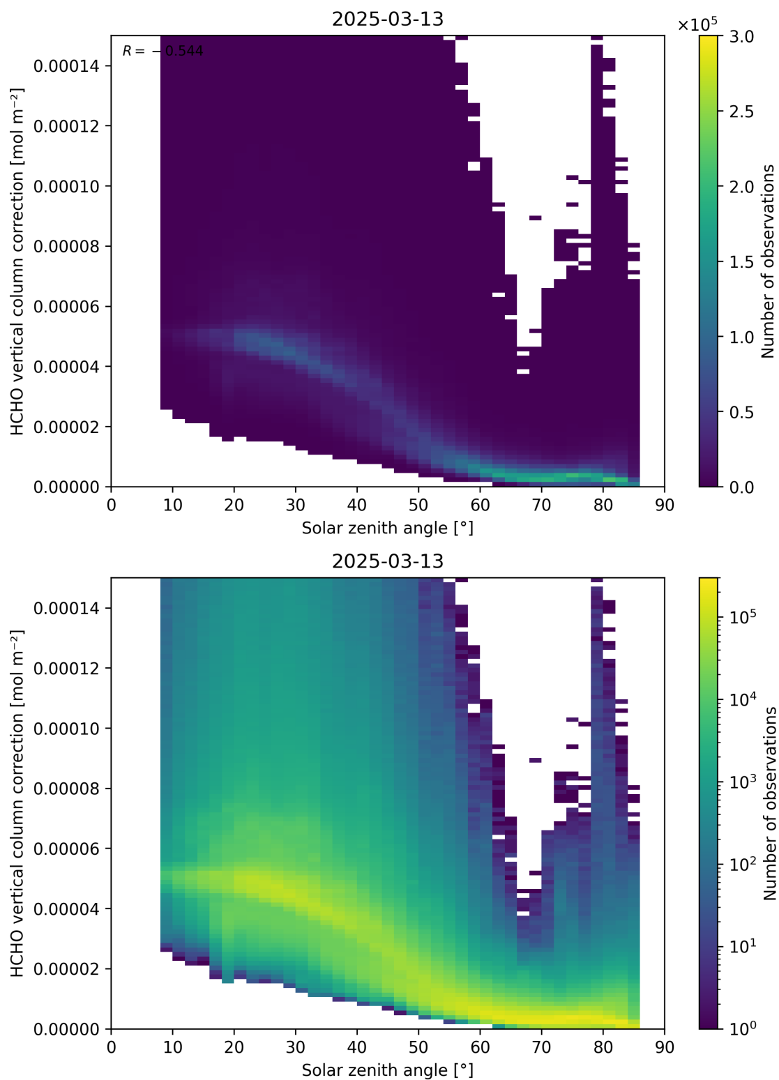
Figure 178: Scatter density plot of “Solar zenith angle” against “HCHO vertical column correction” for 2025-03-12 to 2025-03-14.
