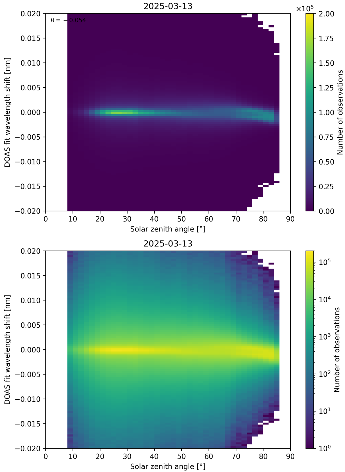
Figure 168: Scatter density plot of “Solar zenith angle” against “DOAS fit wavelength shift” for 2025-03-12 to 2025-03-14.
