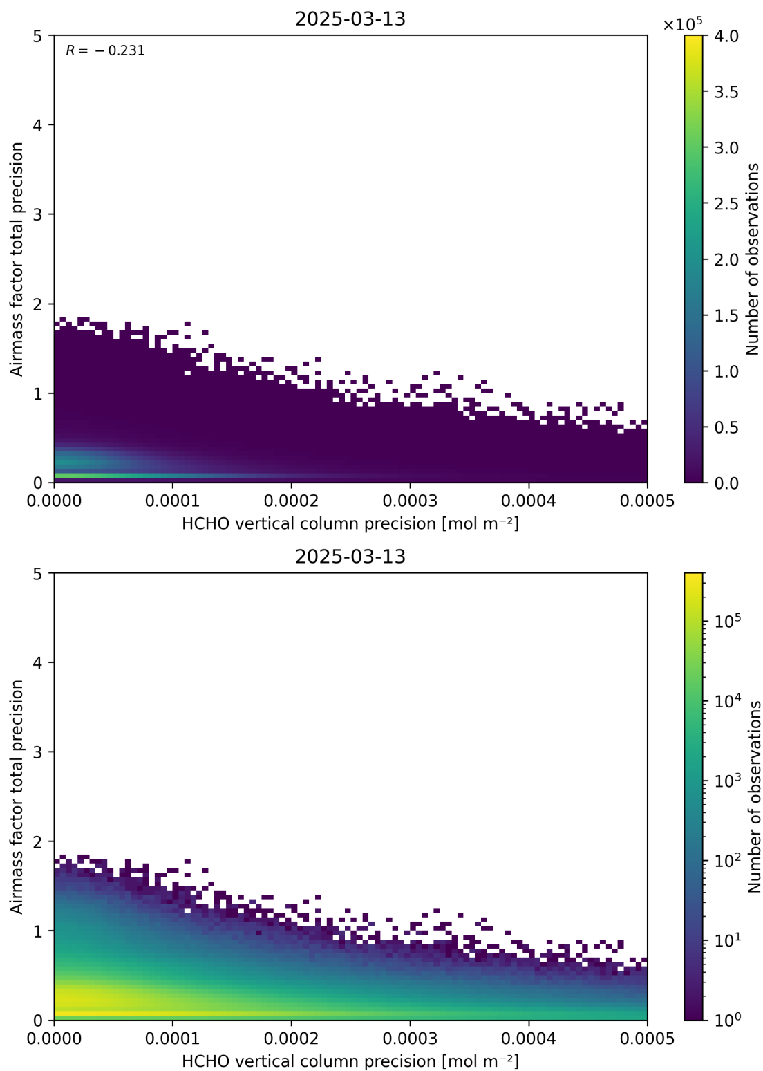
Figure 145: Scatter density plot of “HCHO vertical column precision” against “Airmass factor total precision” for 2025-03-12 to 2025-03-14.
