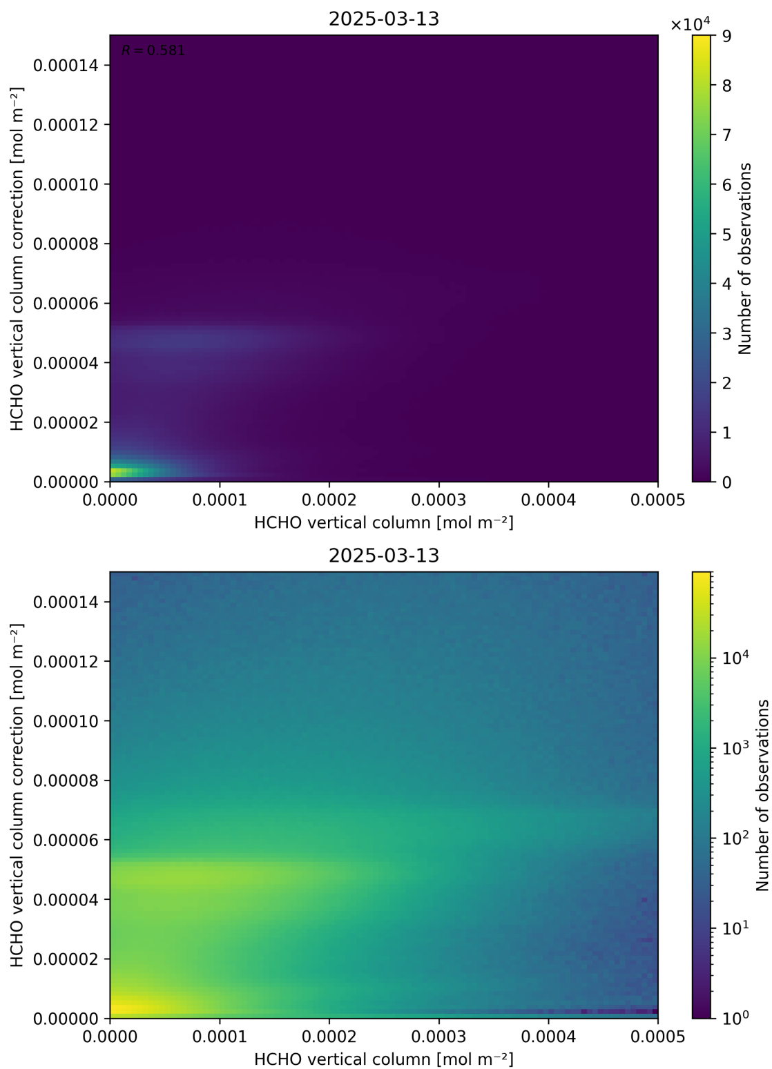
Figure 133: Scatter density plot of “HCHO vertical column” against “HCHO vertical column correction” for 2025-03-12 to 2025-03-14.
