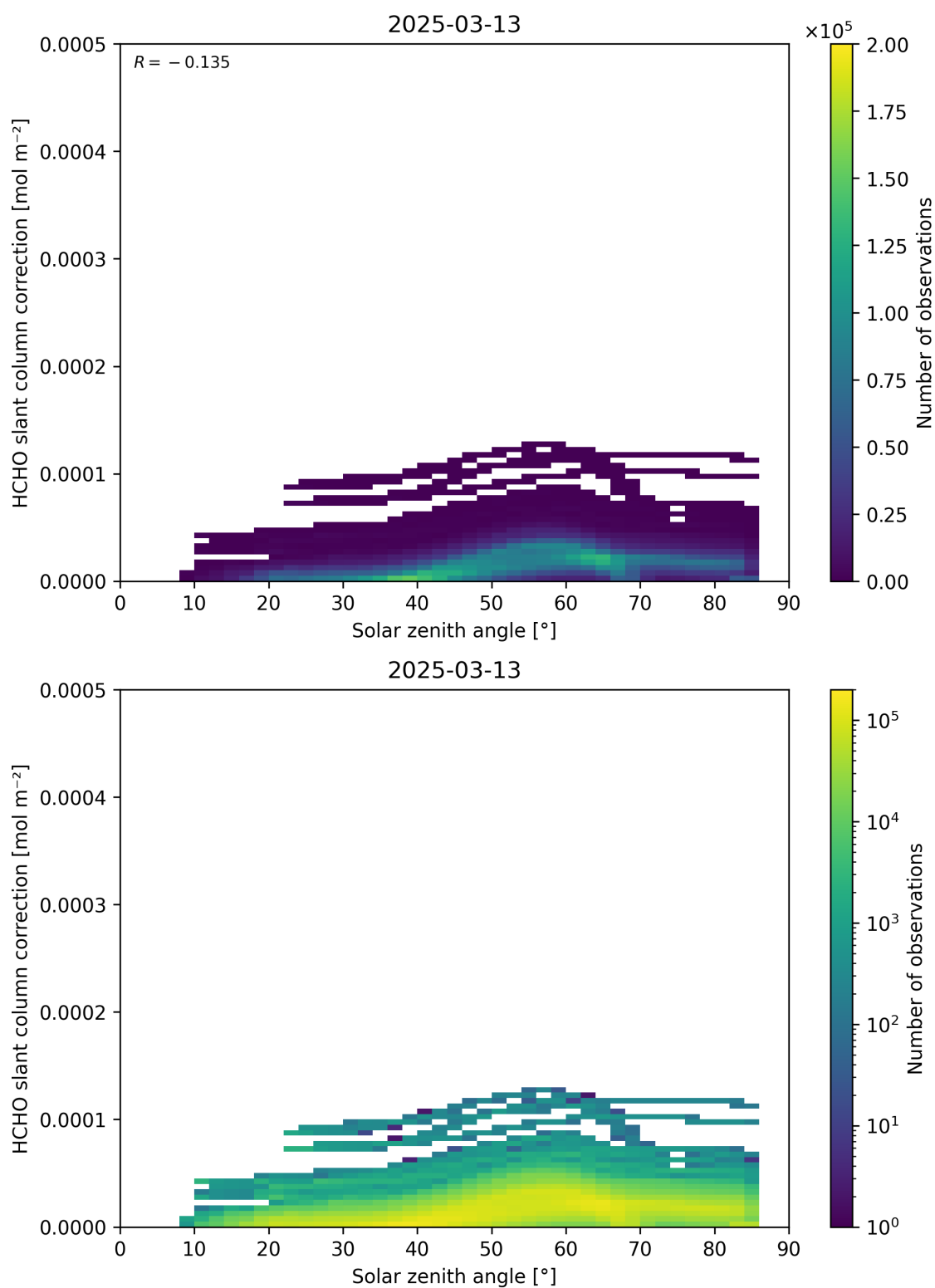
Figure 172: Scatter density plot of “Solar zenith angle” against “HCHO slant column correction” for 2025-03-12 to 2025-03-14.
