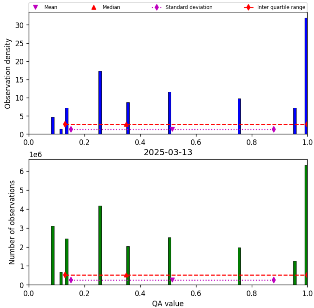
Figure 34: Histogram of “QA value” for 2025-03-12 to 2025-03-14
