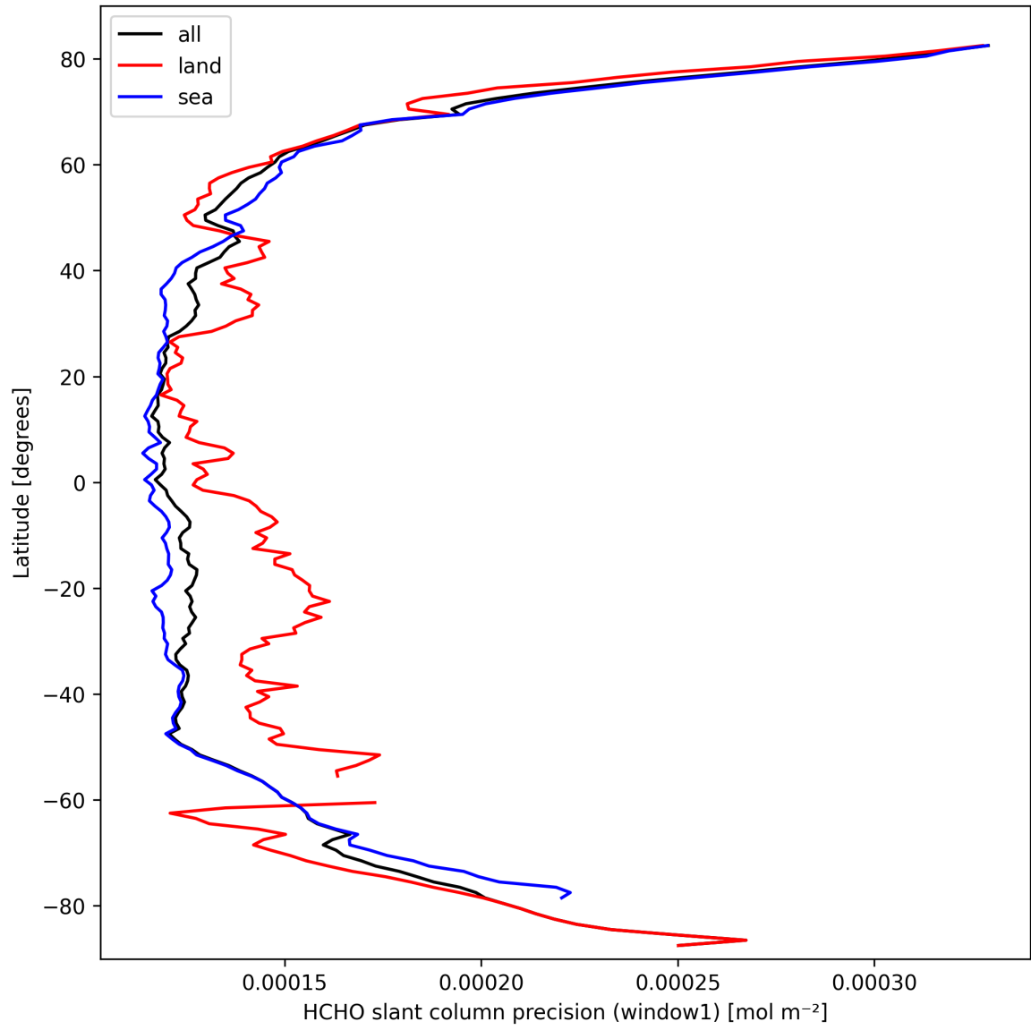
Figure 25: Zonal average of “HCHO slant column precision (window1)” for 2025-03-12 to 2025-03-14.
