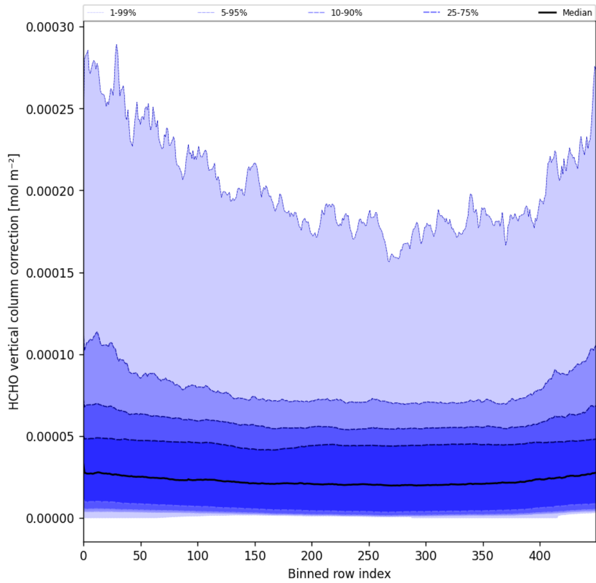
Figure 51: Along track statistics of “HCHO vertical column correction” for 2025-03-12 to 2025-03-14
