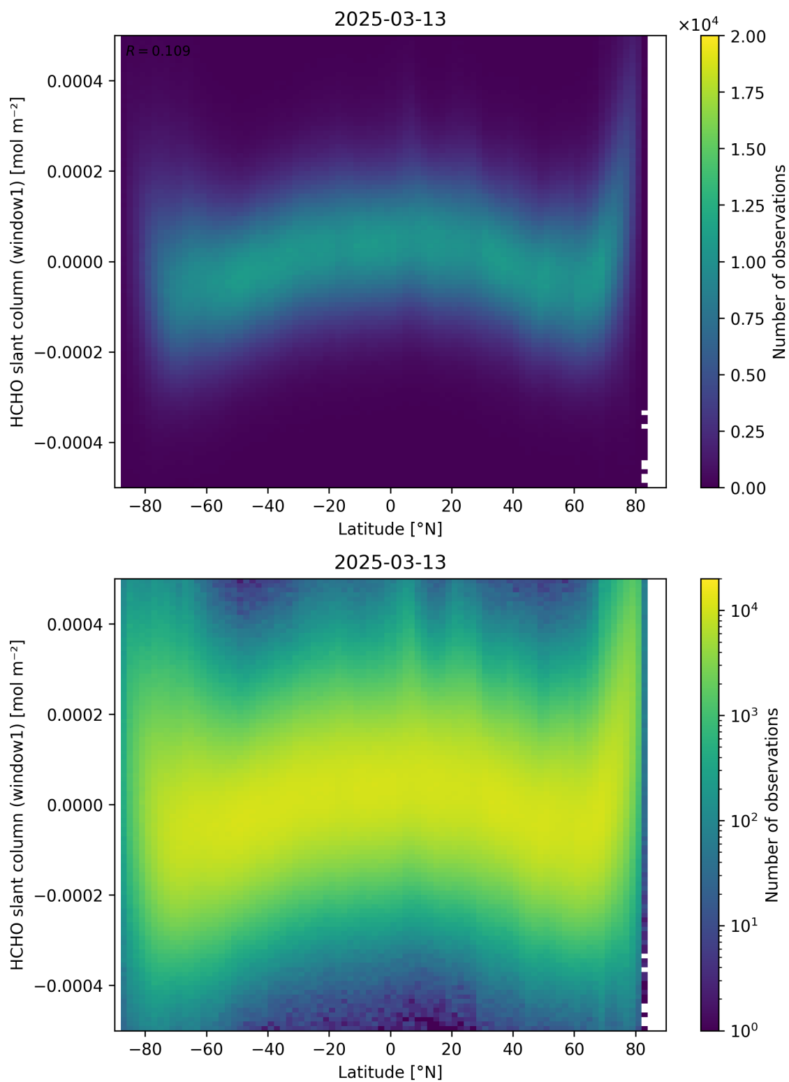
Figure 159: Scatter density plot of “Latitude” against “HCHO slant column (window1)” for 2025-03-12 to 2025-03-14.
