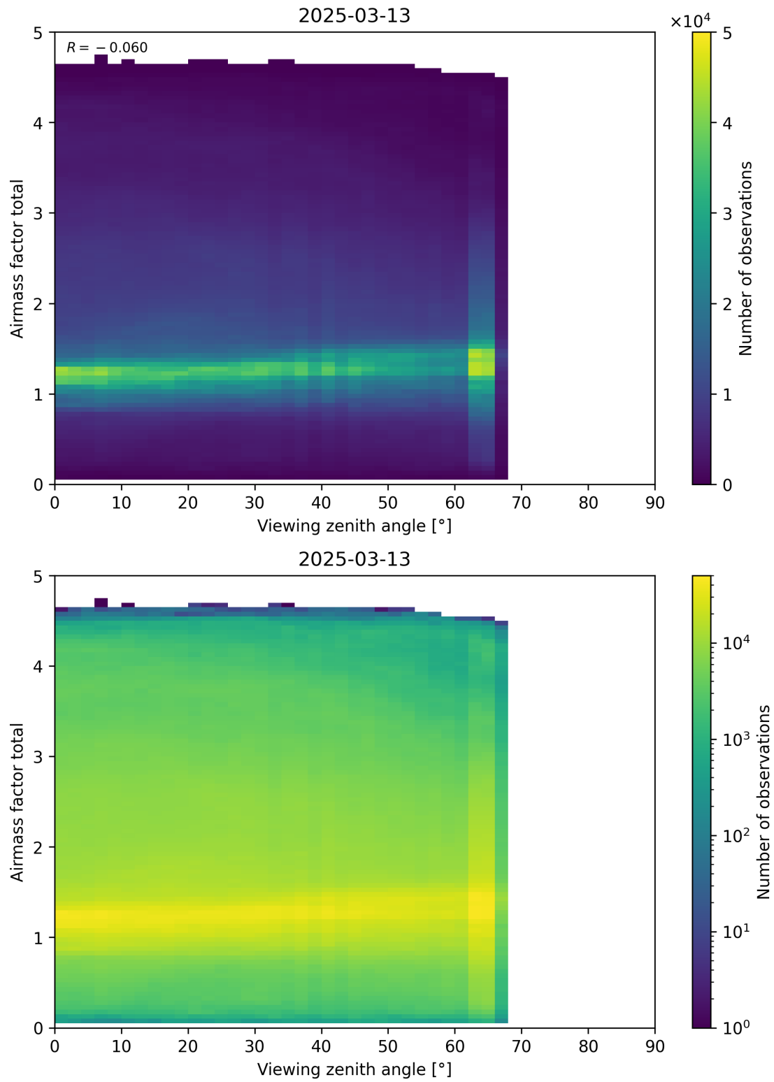
Figure 190: Scatter density plot of “Viewing zenith angle” against “Airmass factor total” for 2025-03-12 to 2025-03-14.
