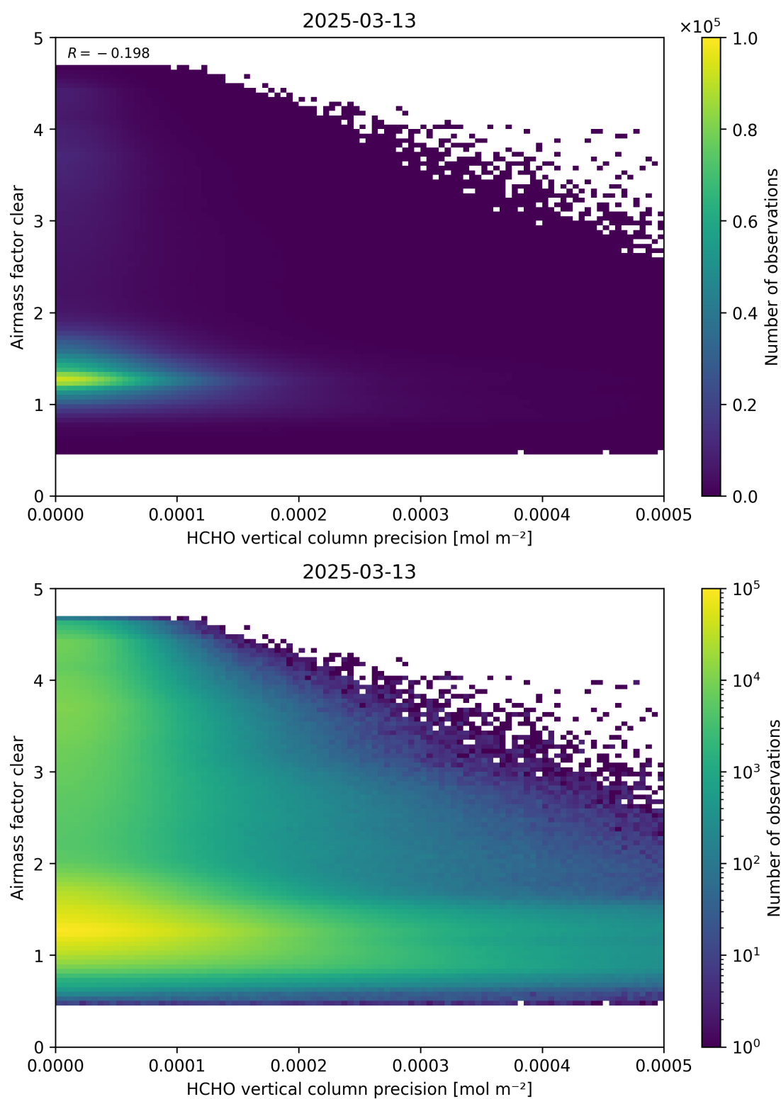
Figure 139: Scatter density plot of “HCHO vertical column precision” against “Airmass factor clear” for 2025-03-12 to 2025-03-14.
