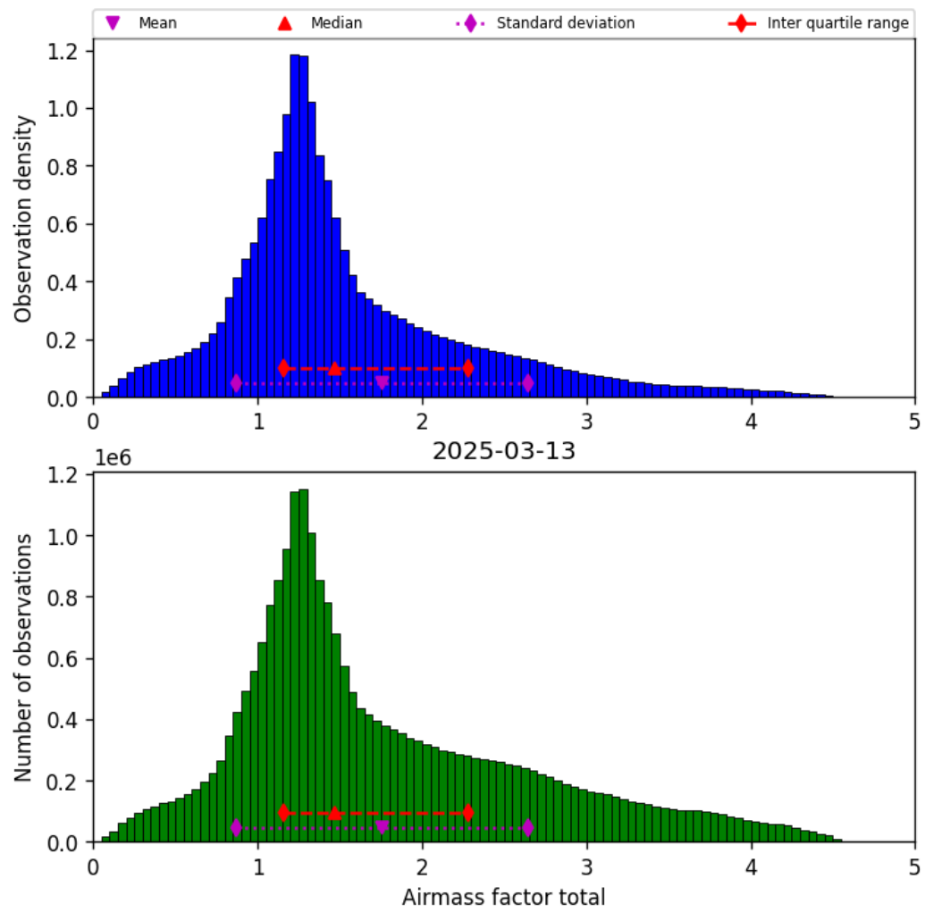
Figure 40: Histogram of “Airmass factor total” for 2025-03-12 to 2025-03-14
