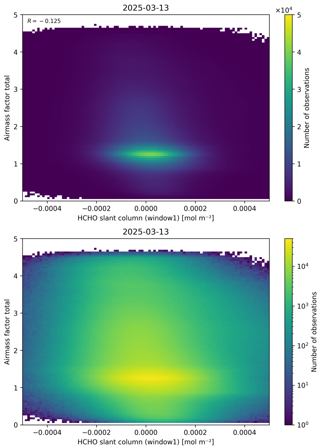
Figure 85: Scatter density plot of “HCHO slant column (window1)” against “Airmass factor total” for 2025-03-12 to 2025-03-14.
