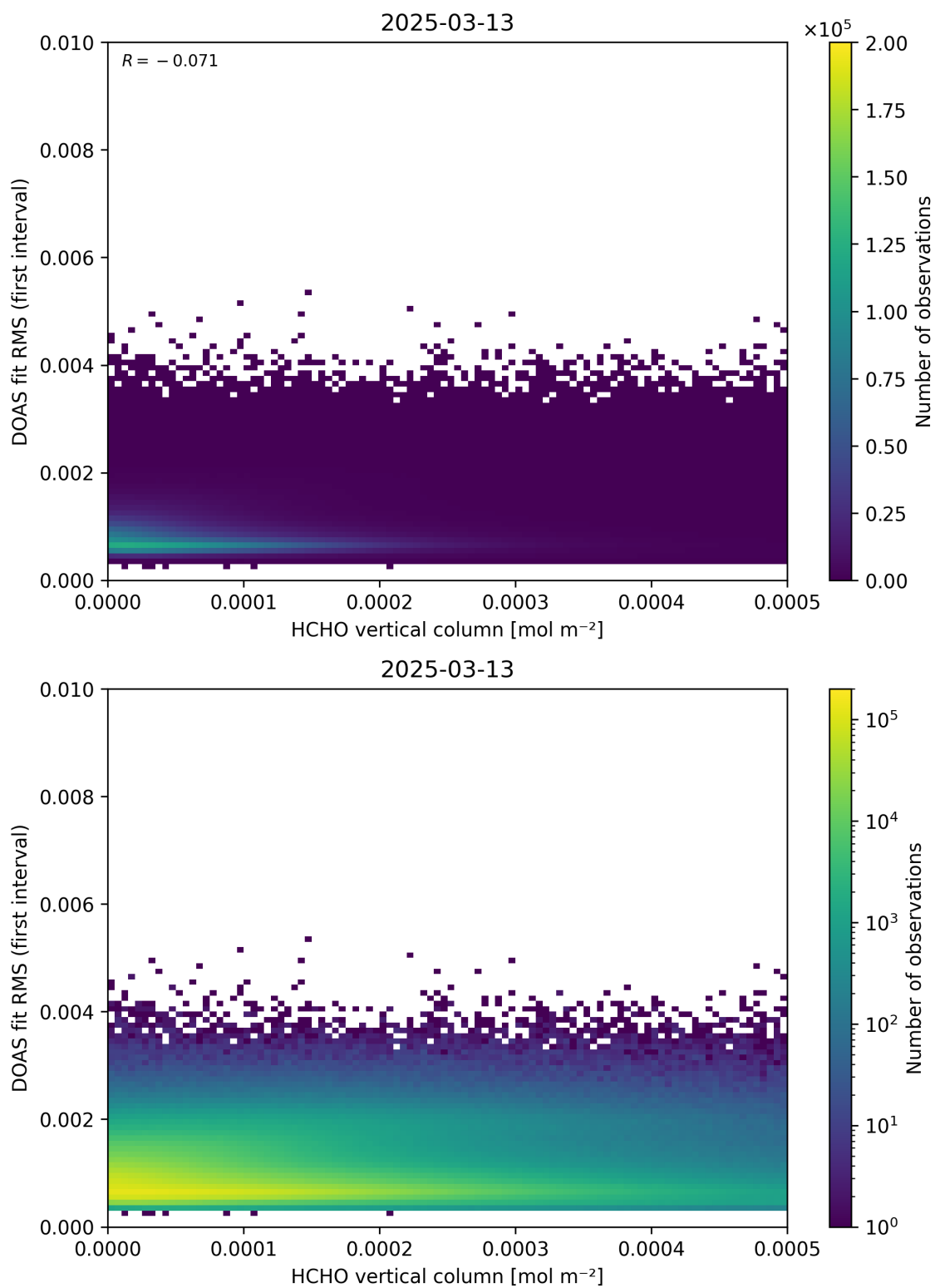
Figure 123: Scatter density plot of “HCHO vertical column” against “DOAS fit RMS (first interval)” for 2025-03-12 to 2025-03-14.
