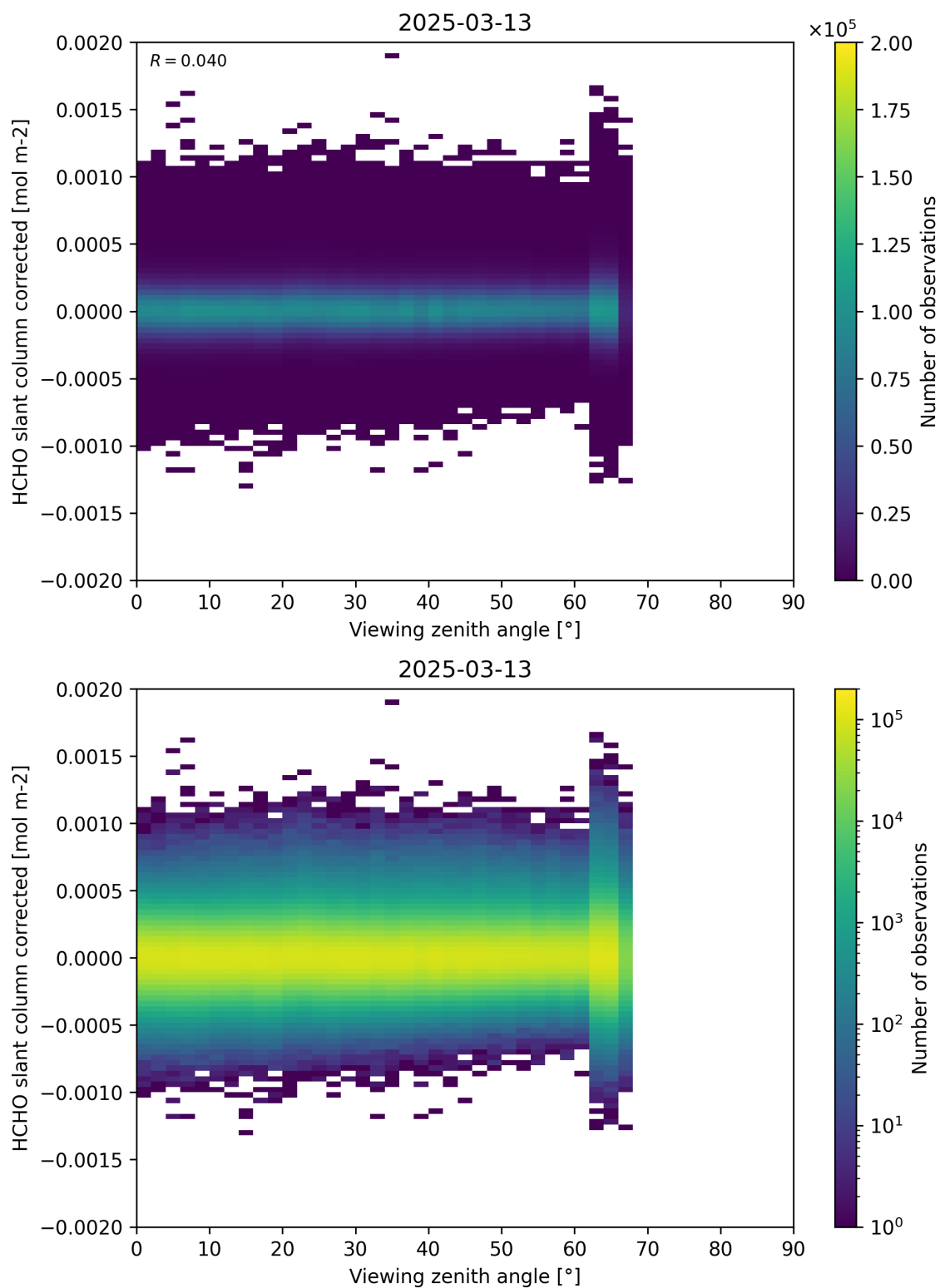
Figure 186: Scatter density plot of “Viewing zenith angle” against “HCHO slant column corrected” for 2025-03-12 to 2025-03-14.
