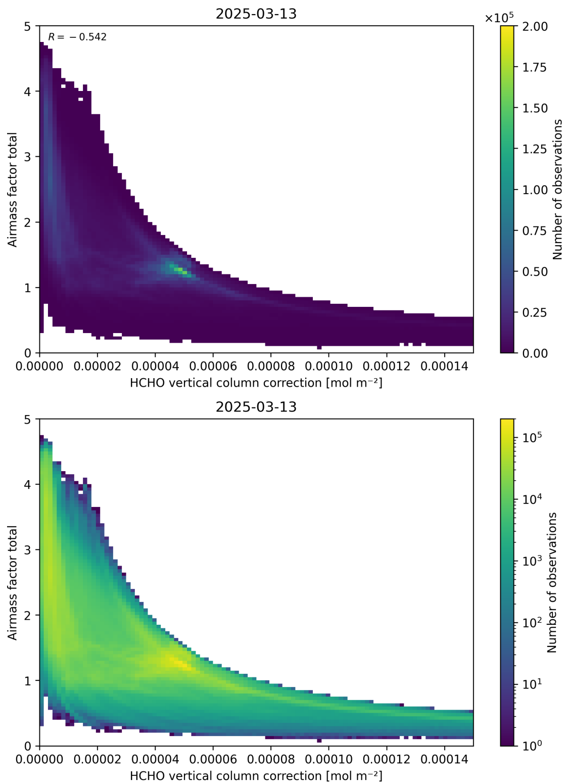
Figure 120: Scatter density plot of “HCHO vertical column correction” against “Airmass factor total” for 2025-03-12 to 2025-03-14.
