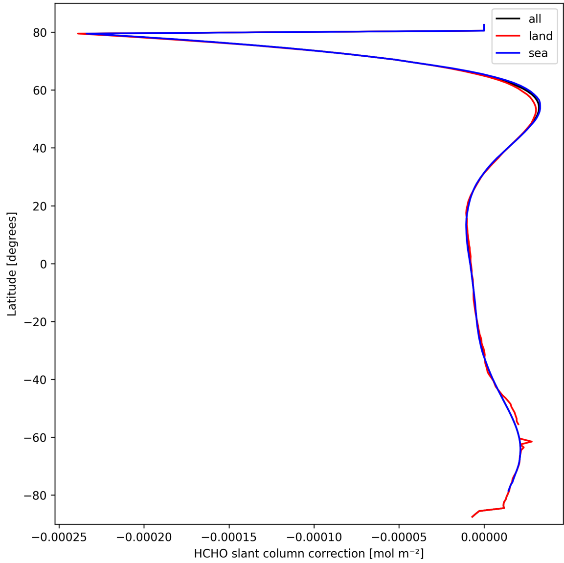
Figure 33: Zonal average of "HCHO slant column correction" for 2025-03-12 to 2025-03-14.
