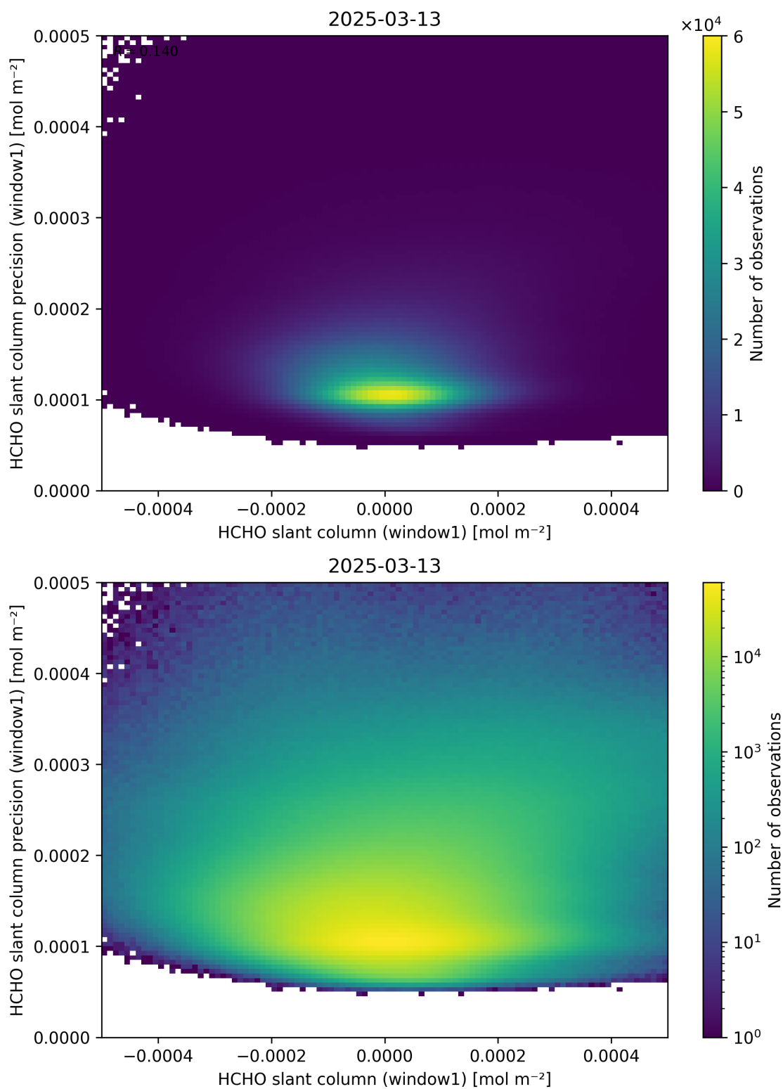
Figure 84: Scatter density plot of “HCHO slant column (window1)” against “HCHO slant column precision (window1)” for 2025-03-12 to 2025-03-14.
