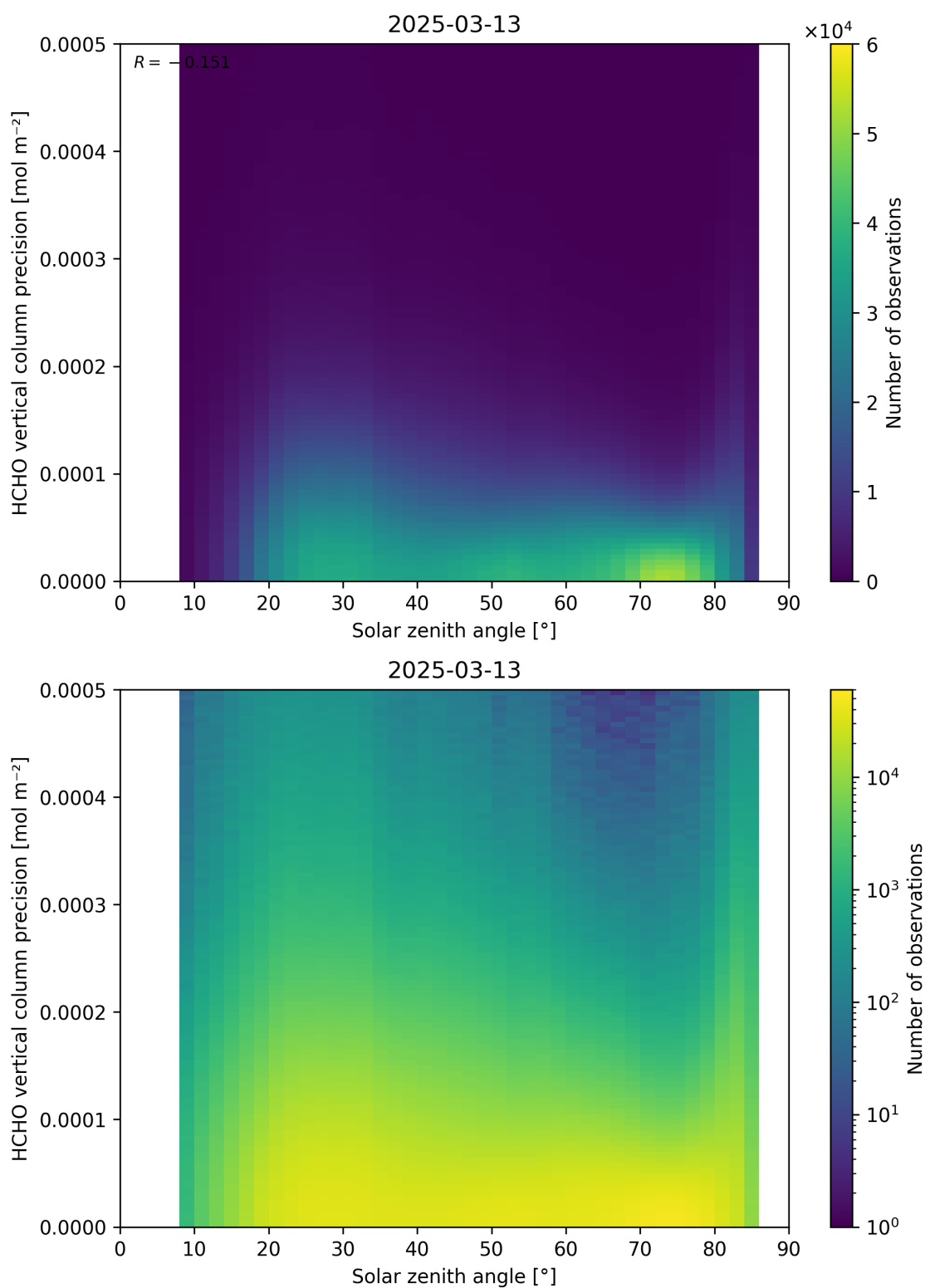
Figure 179: Scatter density plot of “Solar zenith angle” against “HCHO vertical column precision” for 2025-03-12 to 2025-03-14.
