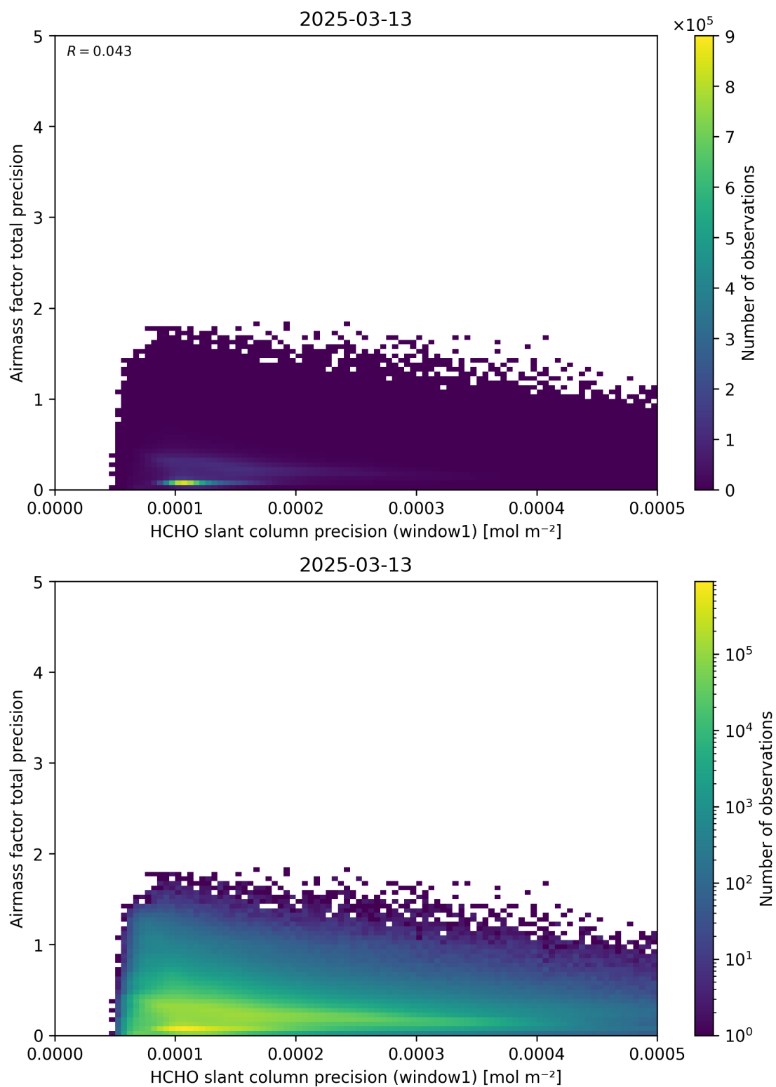
Figure 95: Scatter density plot of “HCHO slant column precision (window1)” against “Airmass factor total precision” for 2025-03-12 to 2025-03-14.
