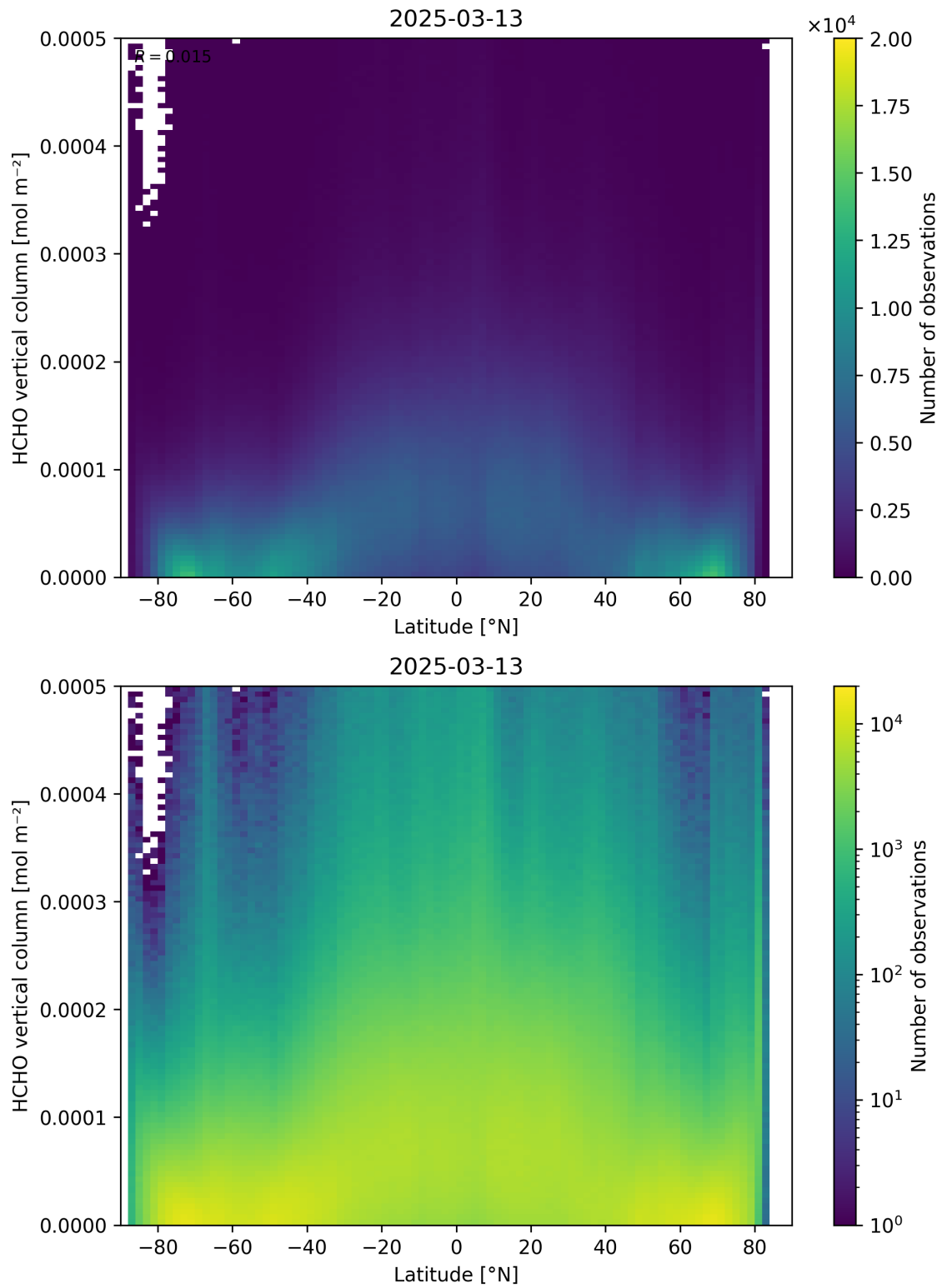
Figure 163: Scatter density plot of “Latitude” against “HCHO vertical column” for 2025-03-12 to 2025-03-14.
