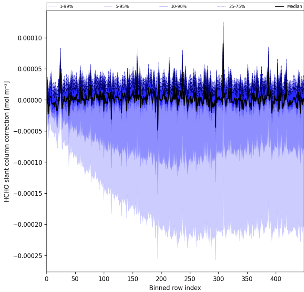
Figure 61: Along track statistics of “HCHO slant column correction” for 2025-03-12 to 2025-03-14
