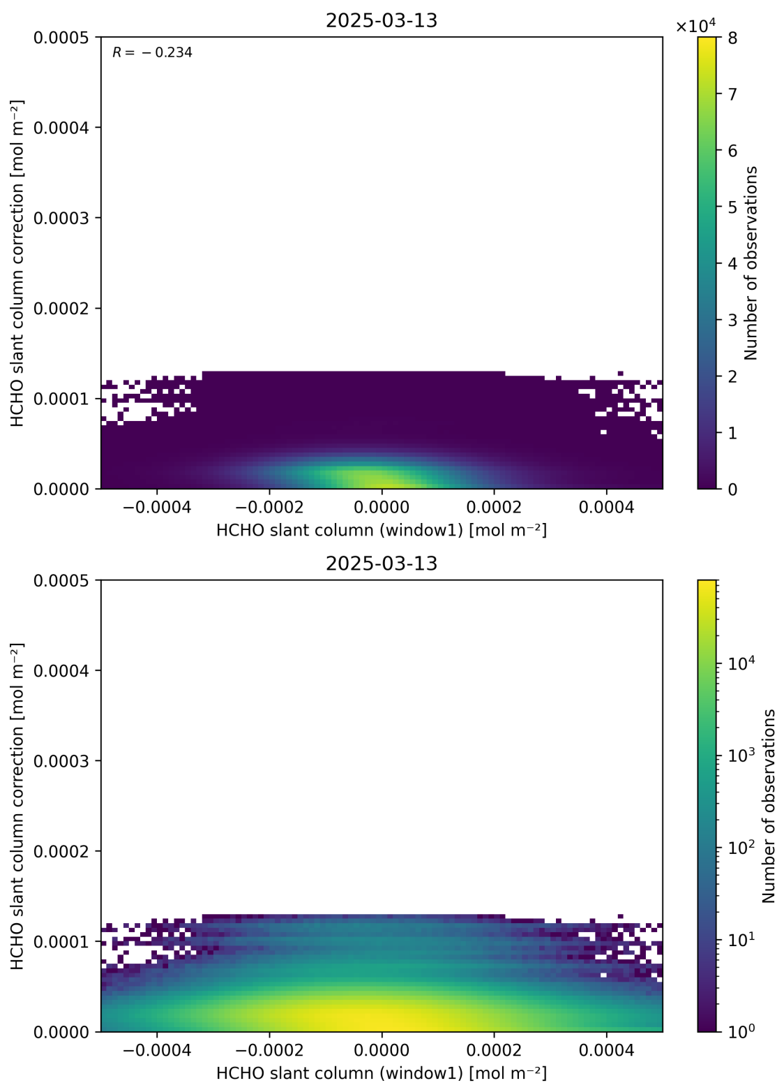
Figure 83: Scatter density plot of “HCHO slant column (window1)” against “HCHO slant column correction” for 2025-03-12 to 2025-03-14.
