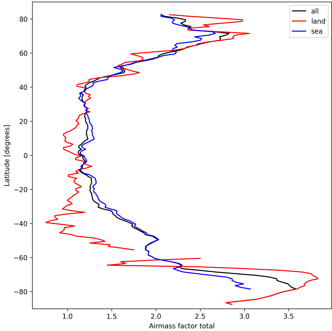
Figure 26: Zonal average of “Airmass factor total” for 2025-03-12 to 2025-03-14.
