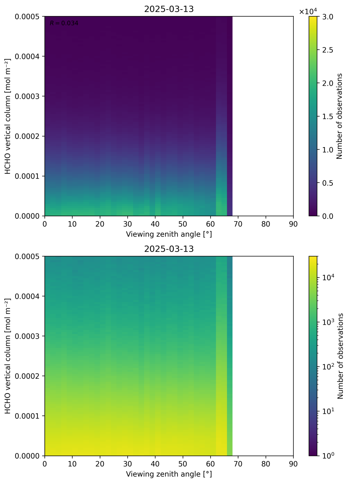
Figure 192: Scatter density plot of “Viewing zenith angle” against “HCHO vertical column” for 2025-03-12 to 2025-03-14.
