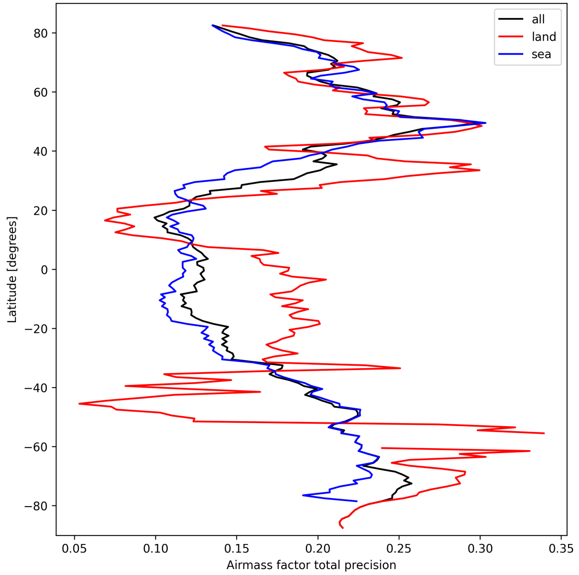
Figure 27: Zonal average of “Airmass factor total precision” for 2025-03-12 to 2025-03-14.
