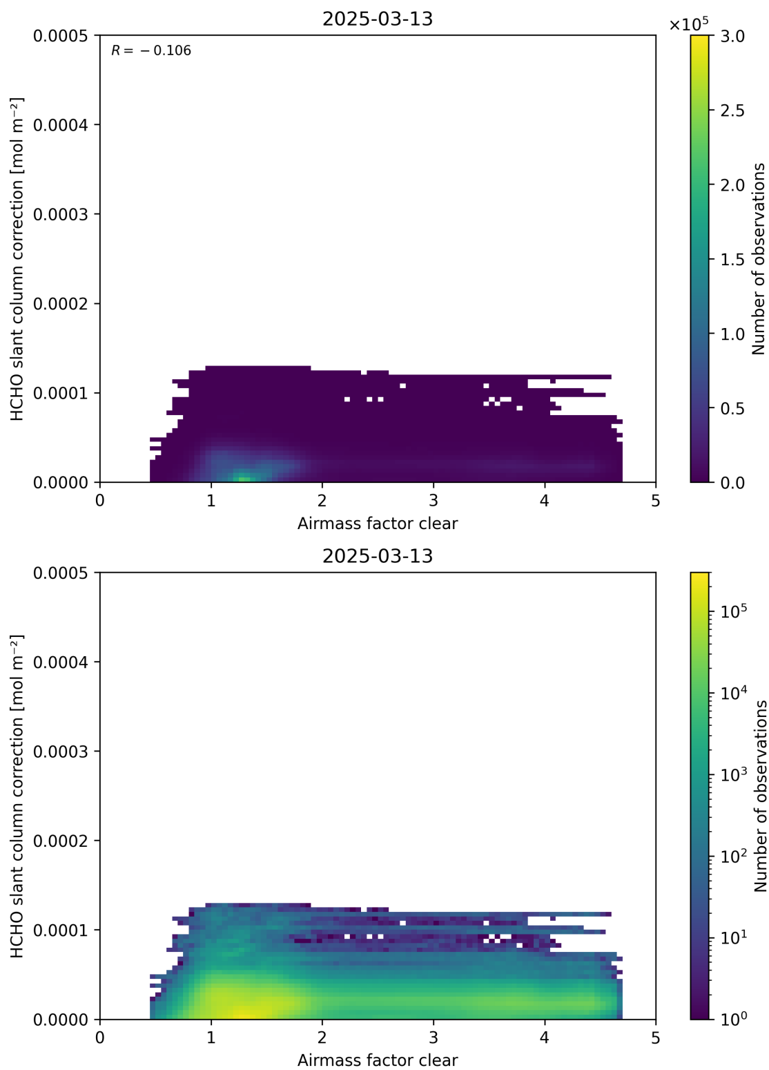
Figure 75: Scatter density plot of “Airmass factor clear” against “HCHO slant column correction” for 2025-03-12 to 2025-03-14.
