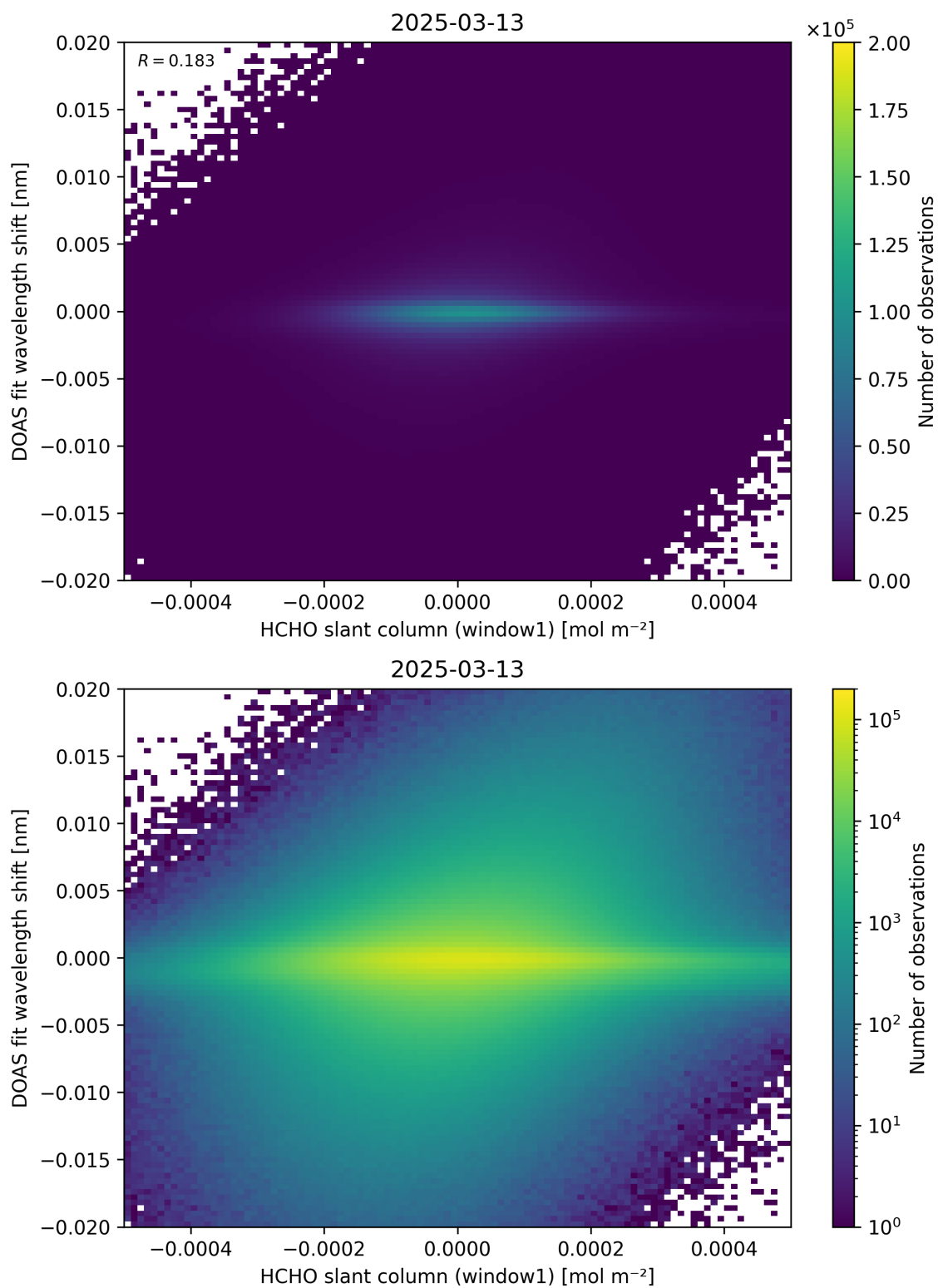
Figure 79: Scatter density plot of “HCHO slant column (window1)” against “DOAS fit wavelength shift” for 2025-03-12 to 2025-03-14.
