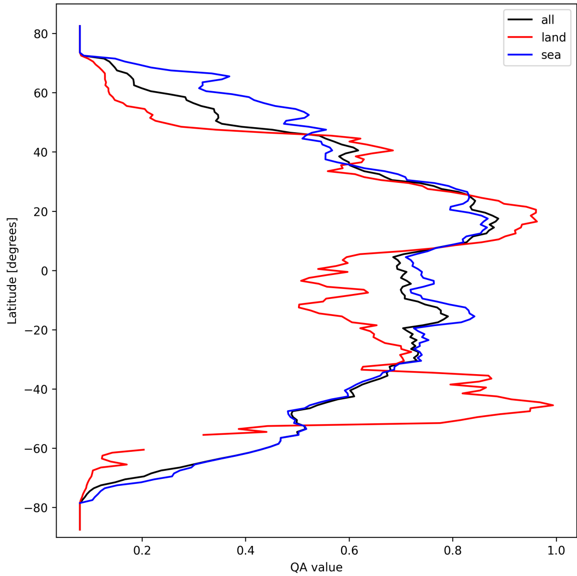
Figure 20: Zonal average of “QA value” for 2025-03-12 to 2025-03-14.
