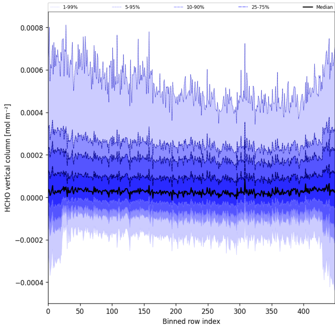
Figure 49: Along track statistics of “HCHO vertical column” for 2025-03-12 to 2025-03-14
