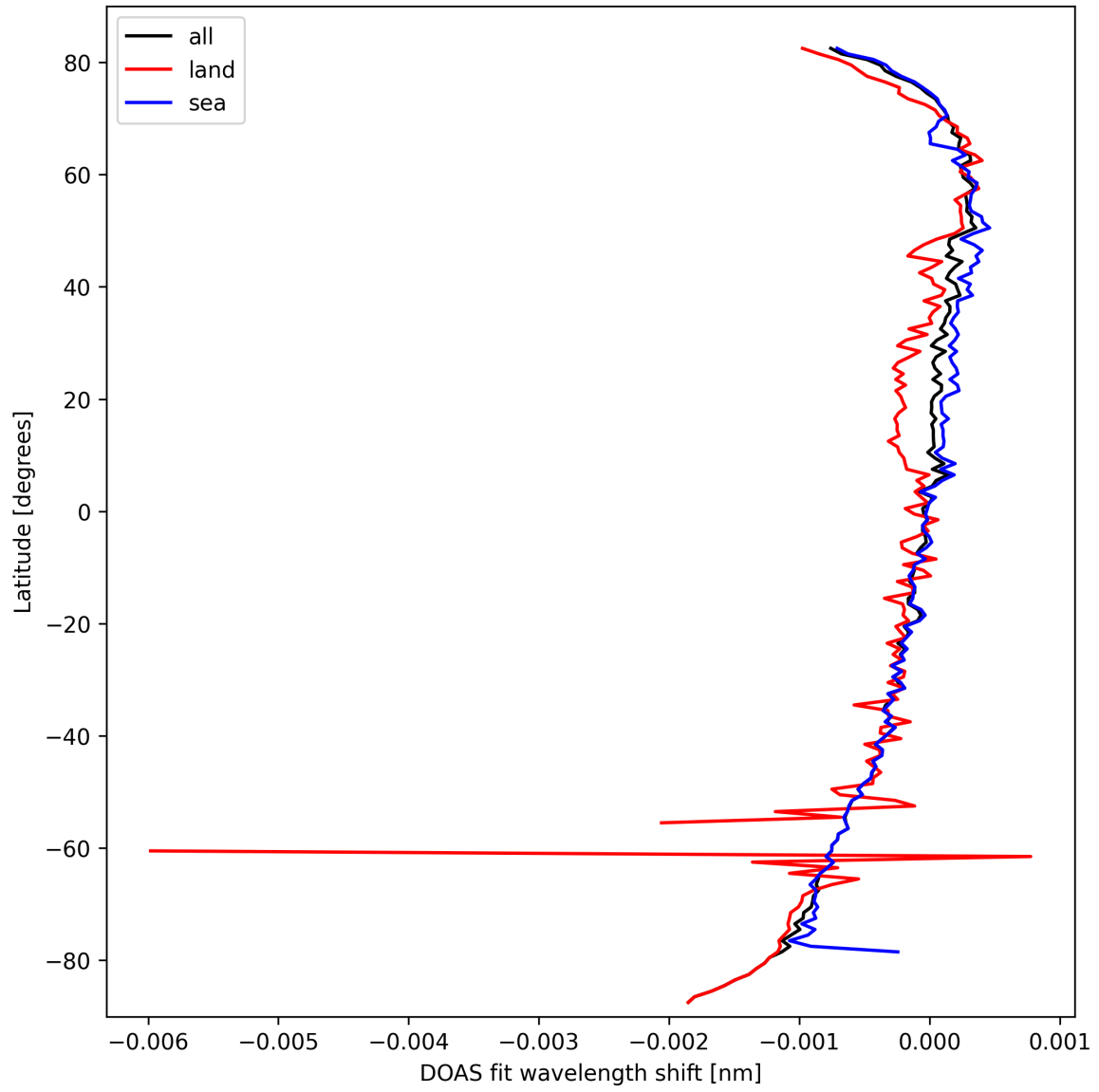
Figure 30: Zonal average of “DOAS fit wavelength shift” for 2025-03-12 to 2025-03-14.
