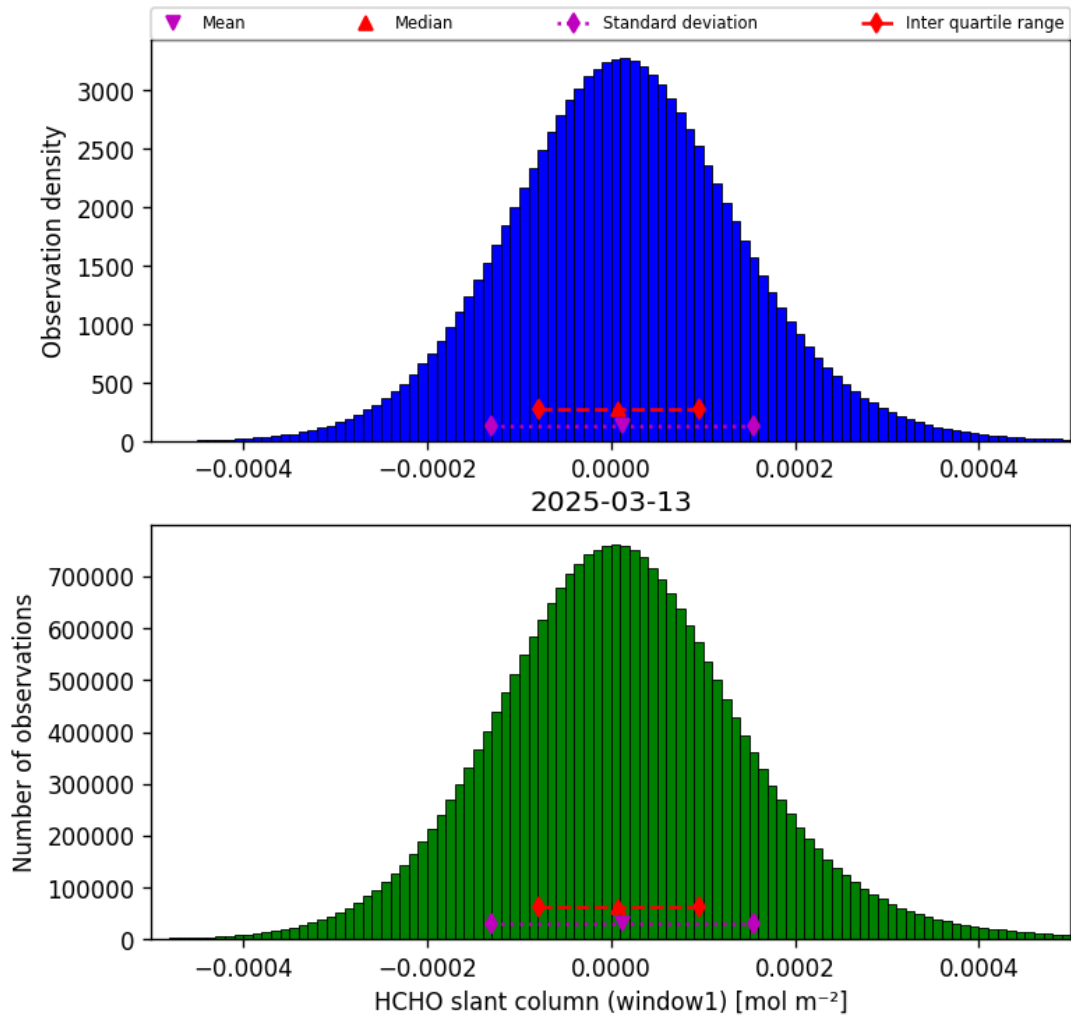
Figure 38: Histogram of “HCHO slant column (window1)” for 2025-03-12 to 2025-03-14
