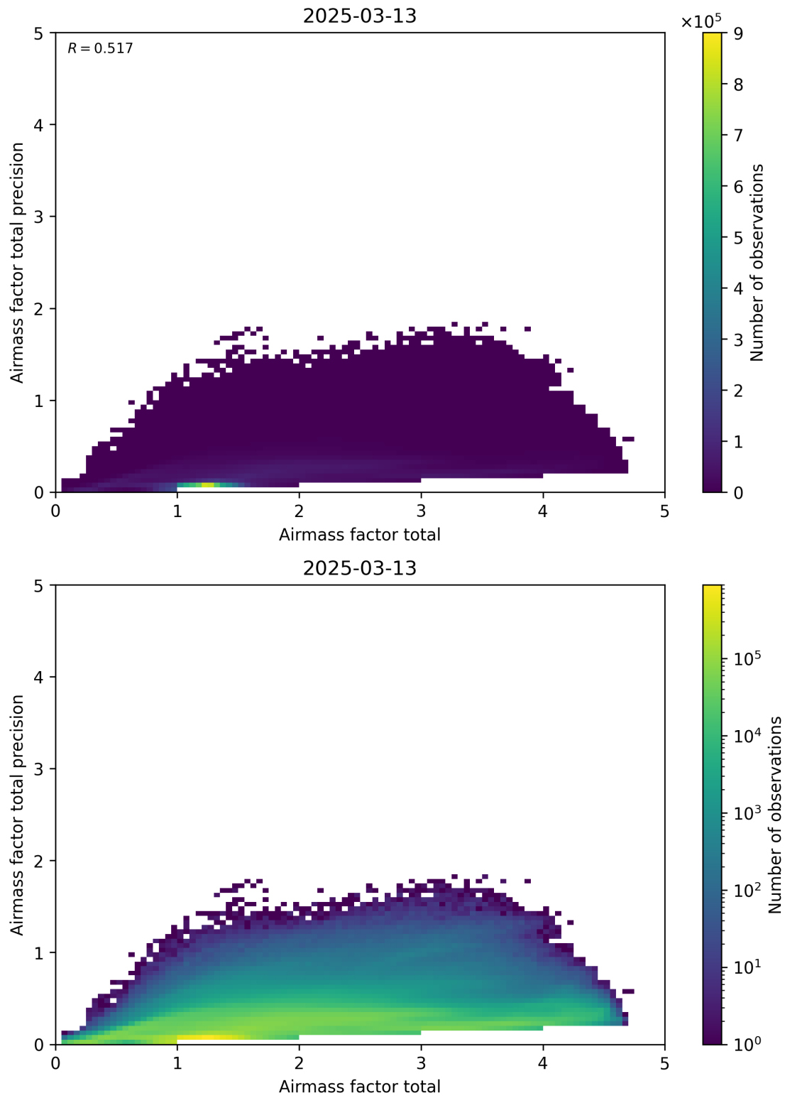
Figure 103: Scatter density plot of “Airmass factor total” against “Airmass factor total precision” for 2025-03-12 to 2025-03-14.
