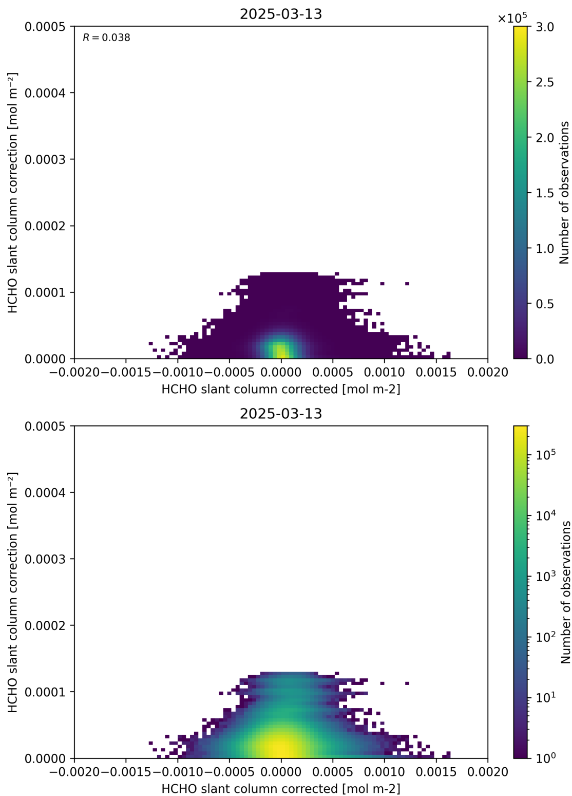
Figure 77: Scatter density plot of “HCHO slant column corrected” against “HCHO slant column correction” for 2025-03-12 to 2025-03-14.
