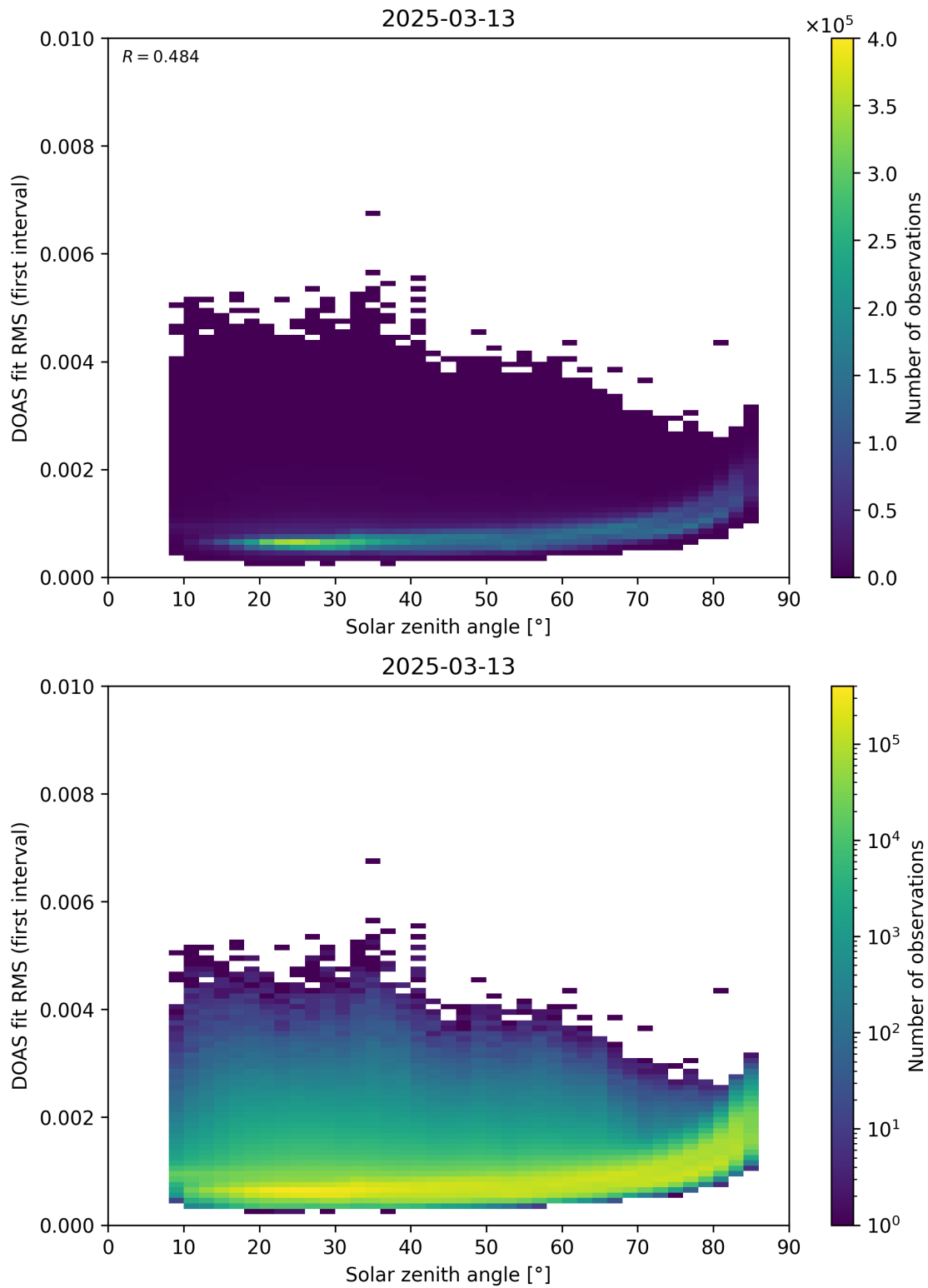
Figure 167: Scatter density plot of “Solar zenith angle” against “DOAS fit RMS (first interval)” for 2025-03-12 to 2025-03-14.
