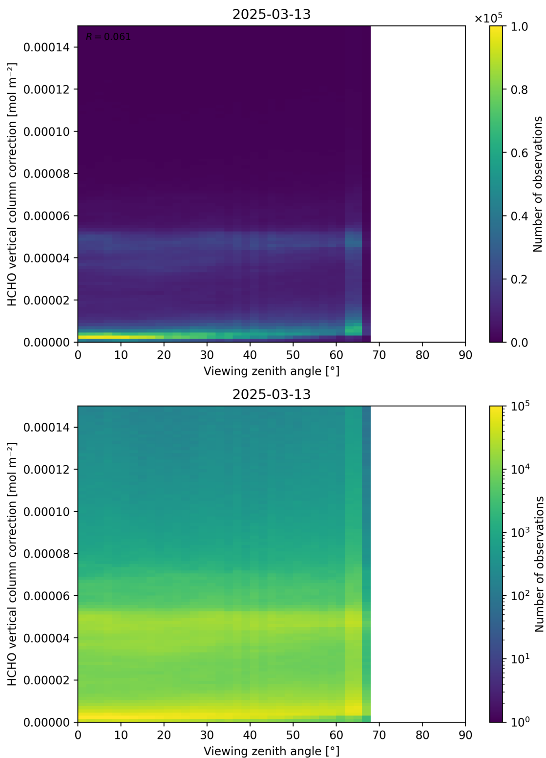
Figure 193: Scatter density plot of “Viewing zenith angle” against “HCHO vertical column correction” for 2025-03-12 to 2025-03-14.
