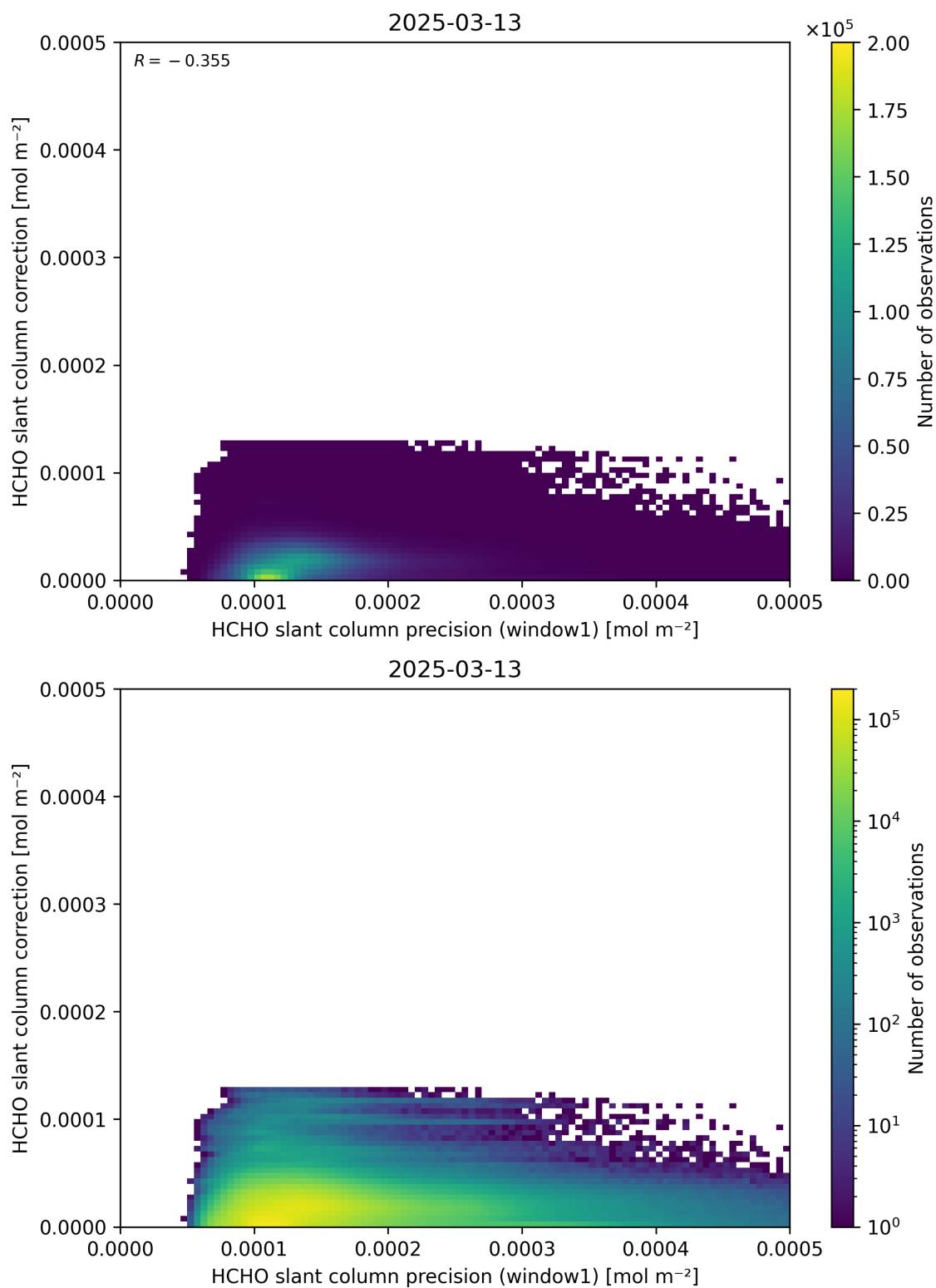
Figure 93: Scatter density plot of “HCHO slant column precision (window1)” against “HCHO slant column correction” for 2025-03-12 to 2025-03-14.
