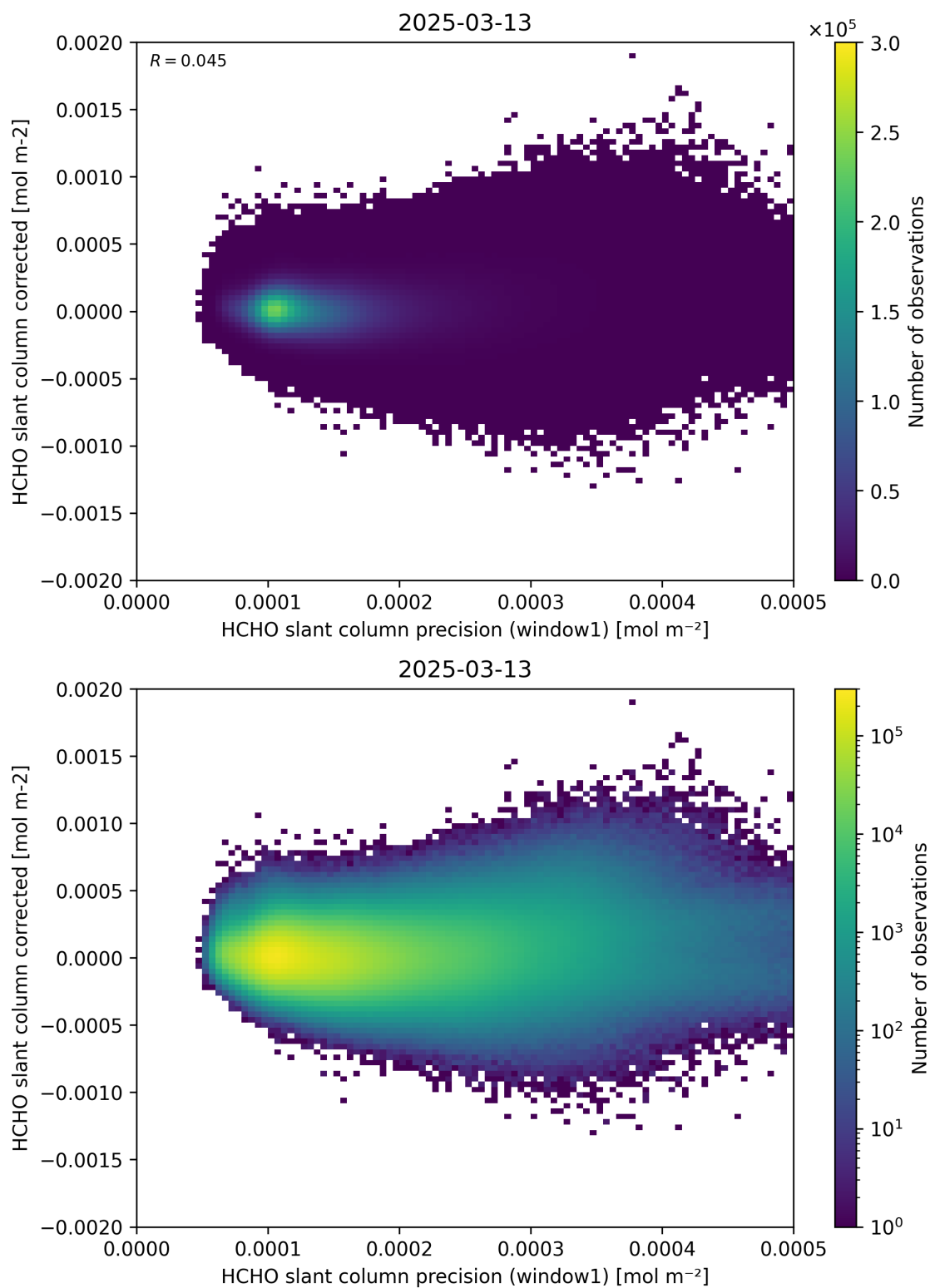
Figure 92: Scatter density plot of “HCHO slant column precision (window1)” against “HCHO slant column corrected” for 2025-03-12 to 2025-03-14.
