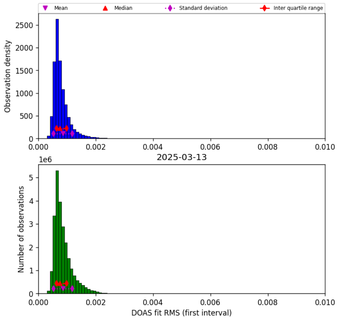
Figure 46: Histogram of “DOAS fit RMS (first interval)” for 2025-03-12 to 2025-03-14
