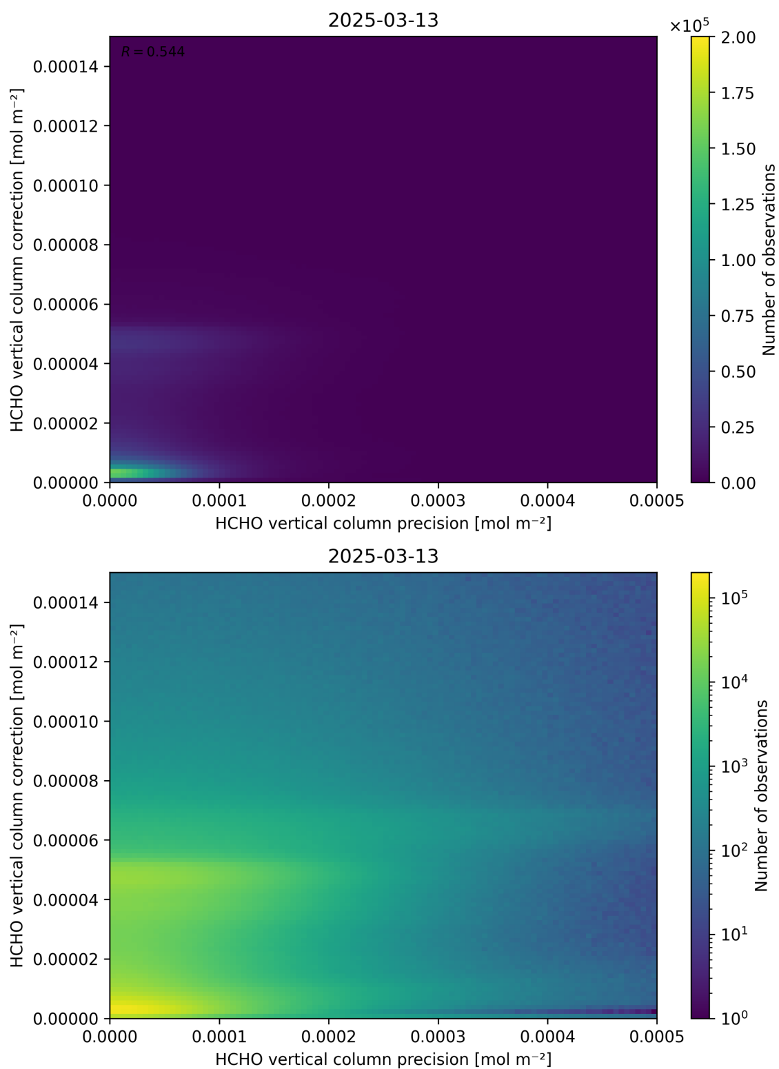
Figure 146: Scatter density plot of “HCHO vertical column precision” against “HCHO vertical column correction” for 2025-03-12 to 2025-03-14.
