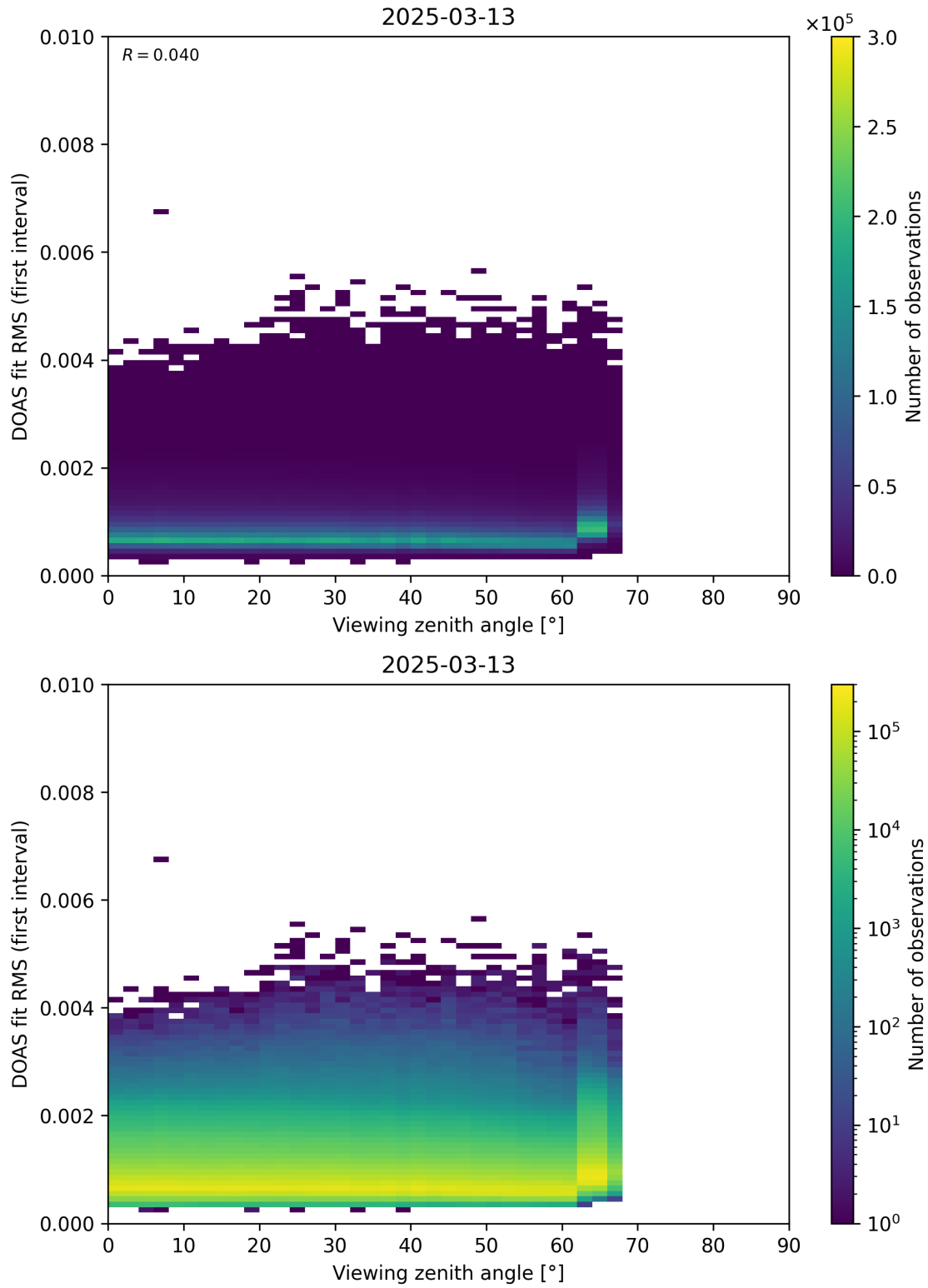
Figure 182: Scatter density plot of “Viewing zenith angle” against “DOAS fit RMS (first interval)” for 2025-03-12 to 2025-03-14.
