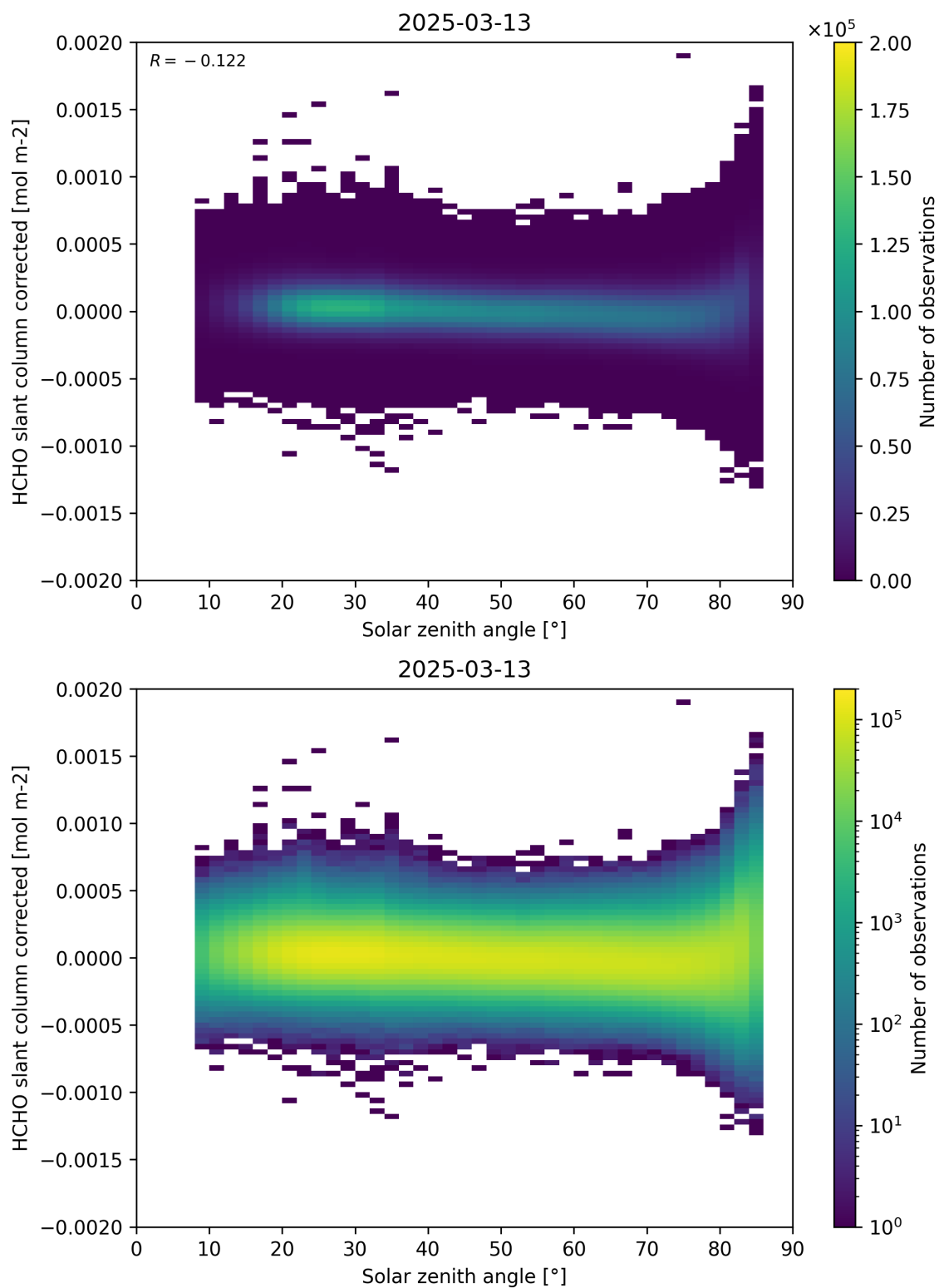
Figure 171: Scatter density plot of “Solar zenith angle” against “HCHO slant column corrected” for 2025-03-12 to 2025-03-14.
