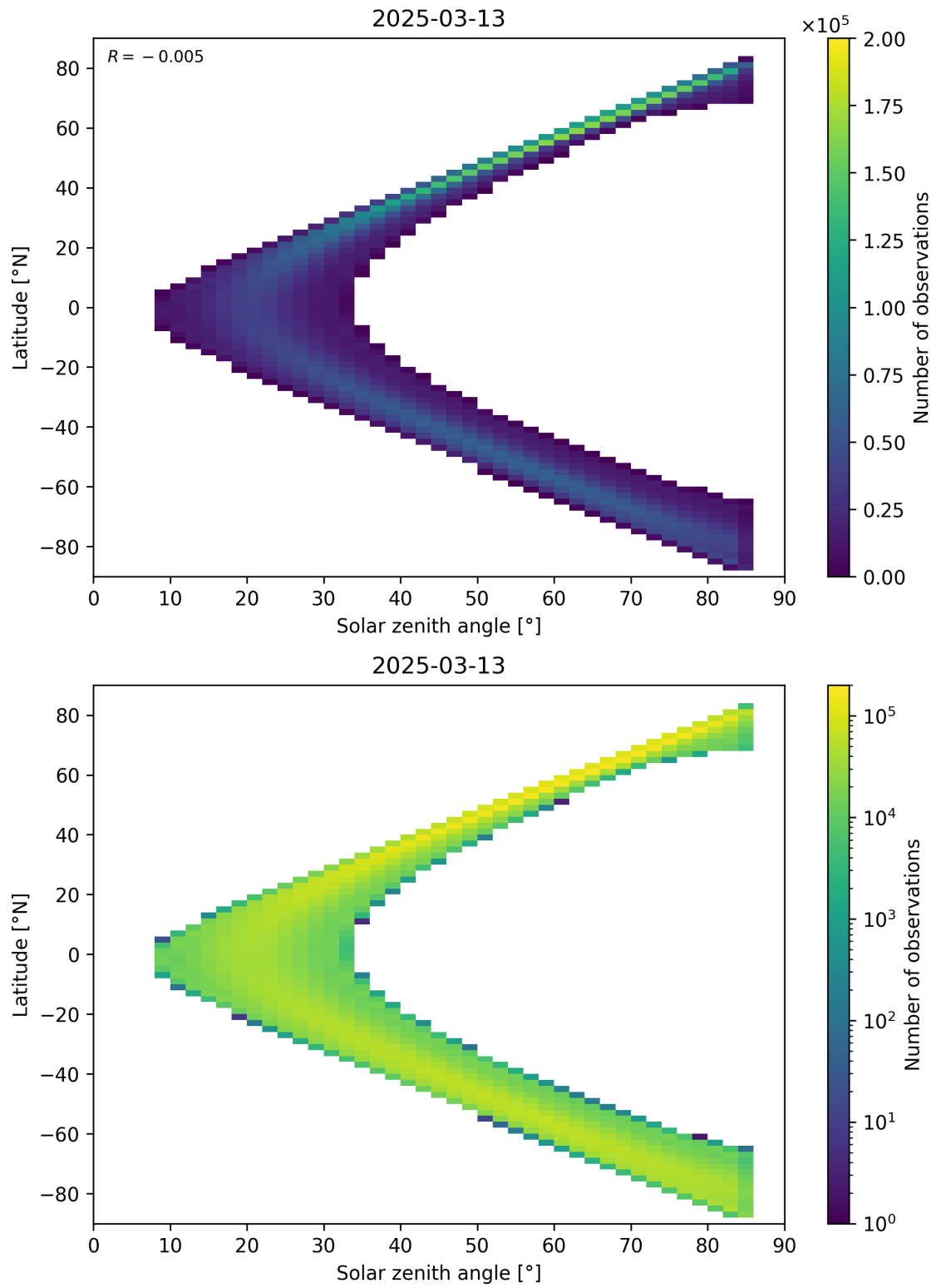
Figure 181: Scatter density plot of “Solar zenith angle” against “Latitude” for 2025-03-12 to 2025-03-14.
