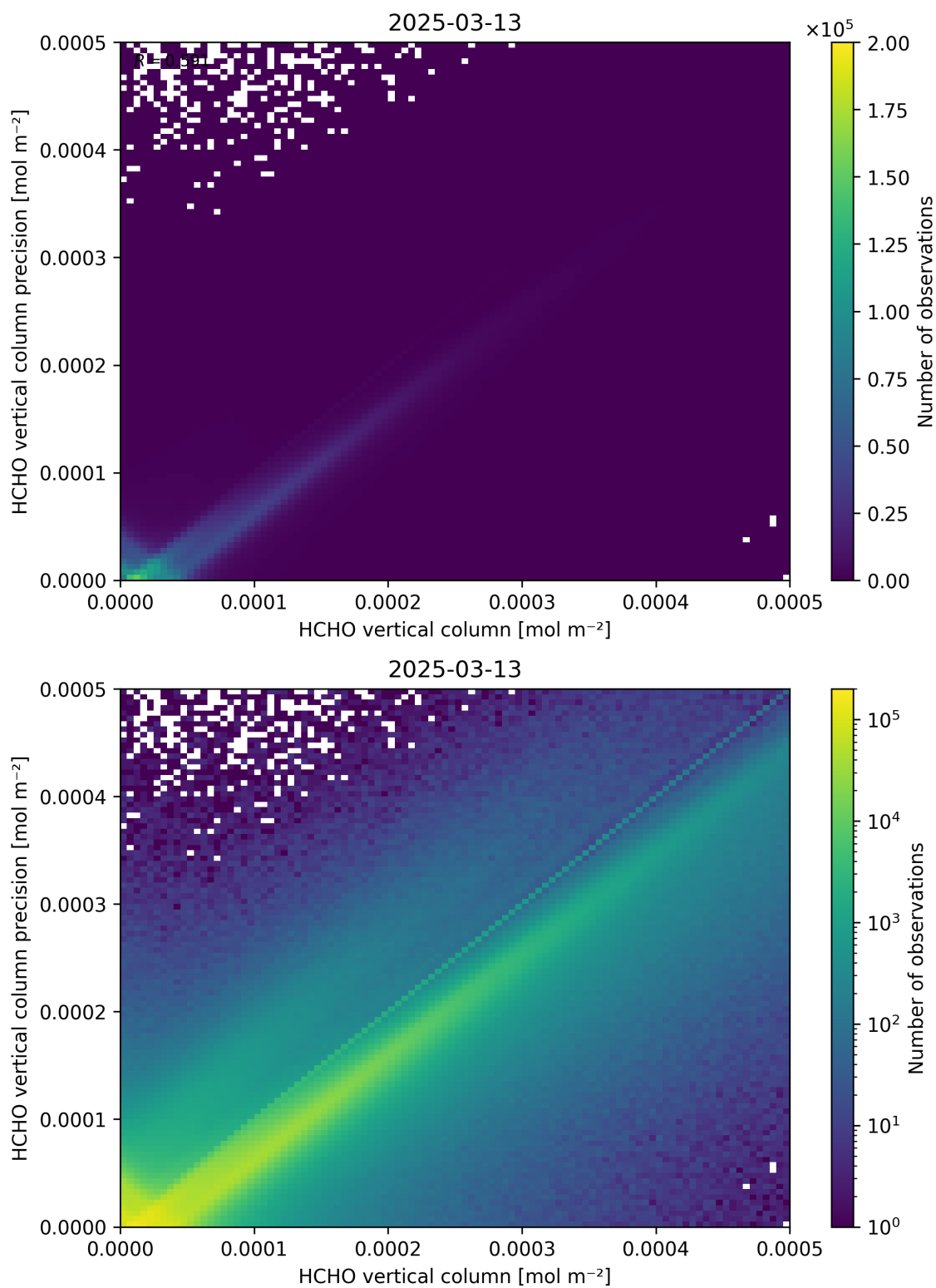
Figure 134: Scatter density plot of “HCHO vertical column” against “HCHO vertical column precision” for 2025-03-12 to 2025-03-14.
