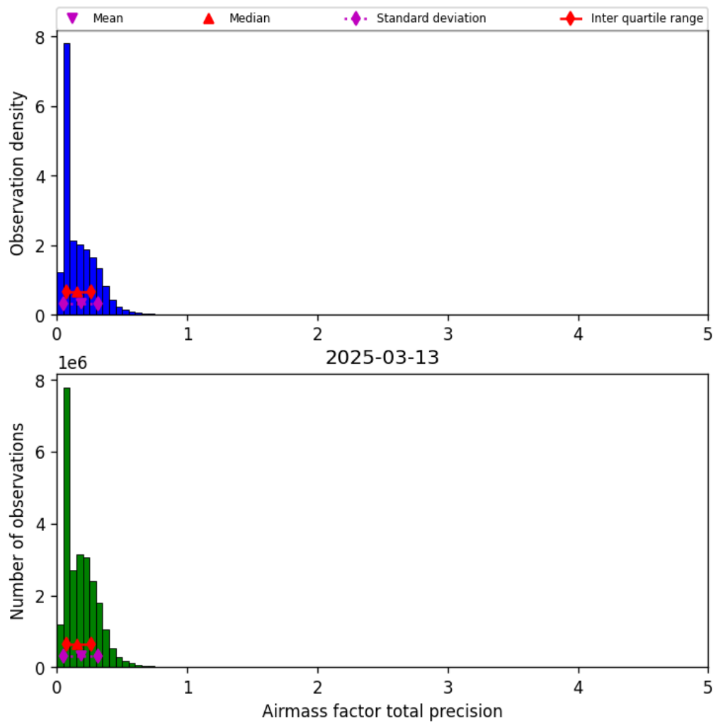
Figure 41: Histogram of “Airmass factor total precision” for 2025-03-12 to 2025-03-14
