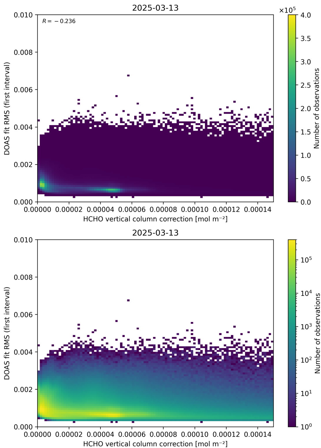
Figure 112: Scatter density plot of “HCHO vertical column correction” against “DOAS fit RMS (first interval)” for 2025-03-12 to 2025-03-14.
