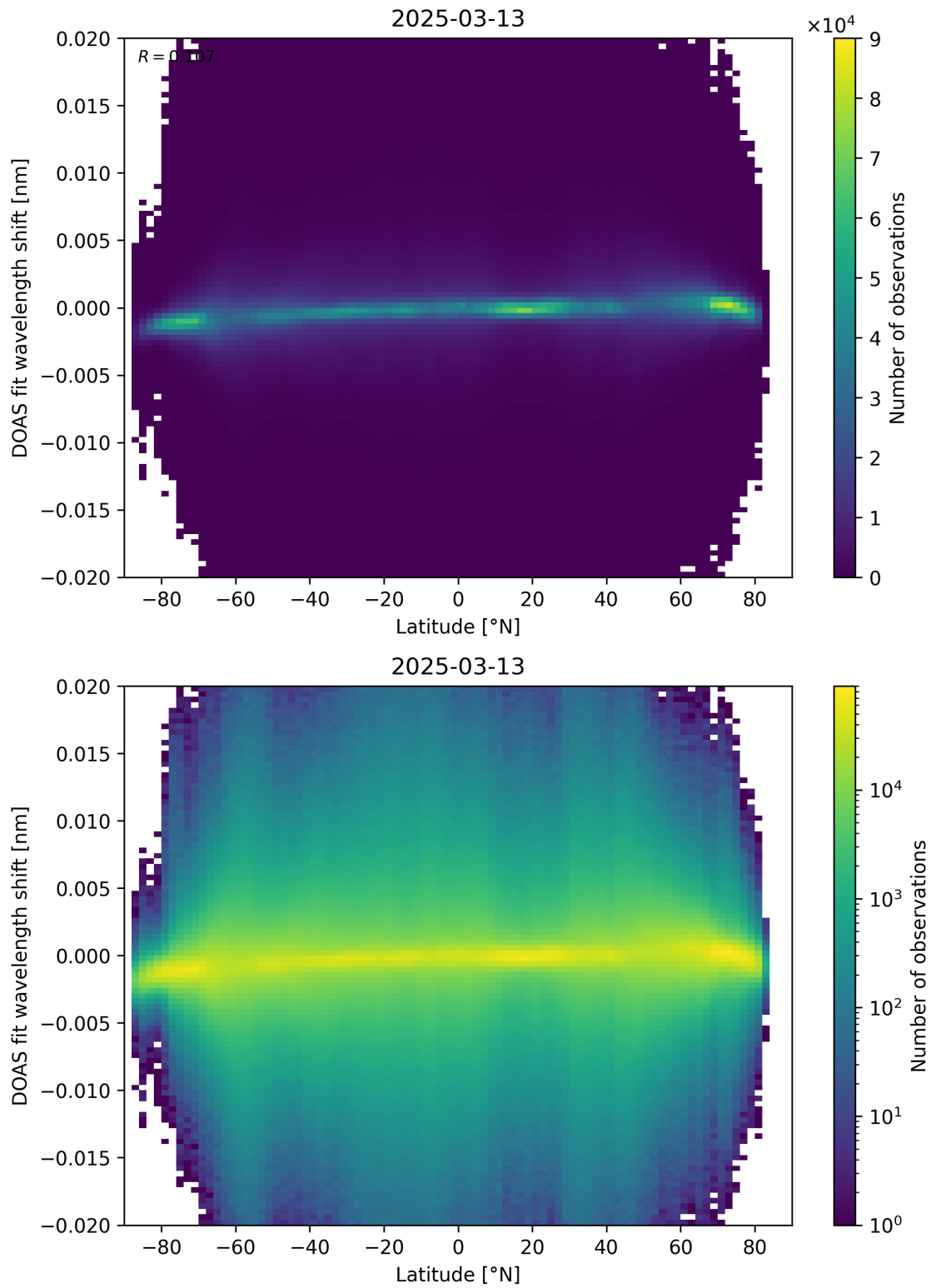
Figure 154: Scatter density plot of “Latitude” against “DOAS fit wavelength shift” for 2025-03-12 to 2025-03-14.
