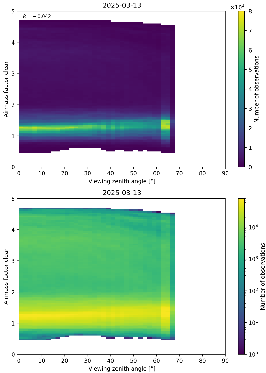
Figure 185: Scatter density plot of “Viewing zenith angle” against “Airmass factor clear” for 2025-03-12 to 2025-03-14.
