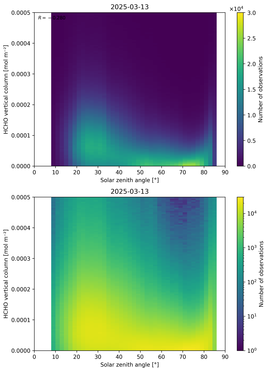
Figure 177: Scatter density plot of “Solar zenith angle” against “HCHO vertical column” for 2025-03-12 to 2025-03-14.
