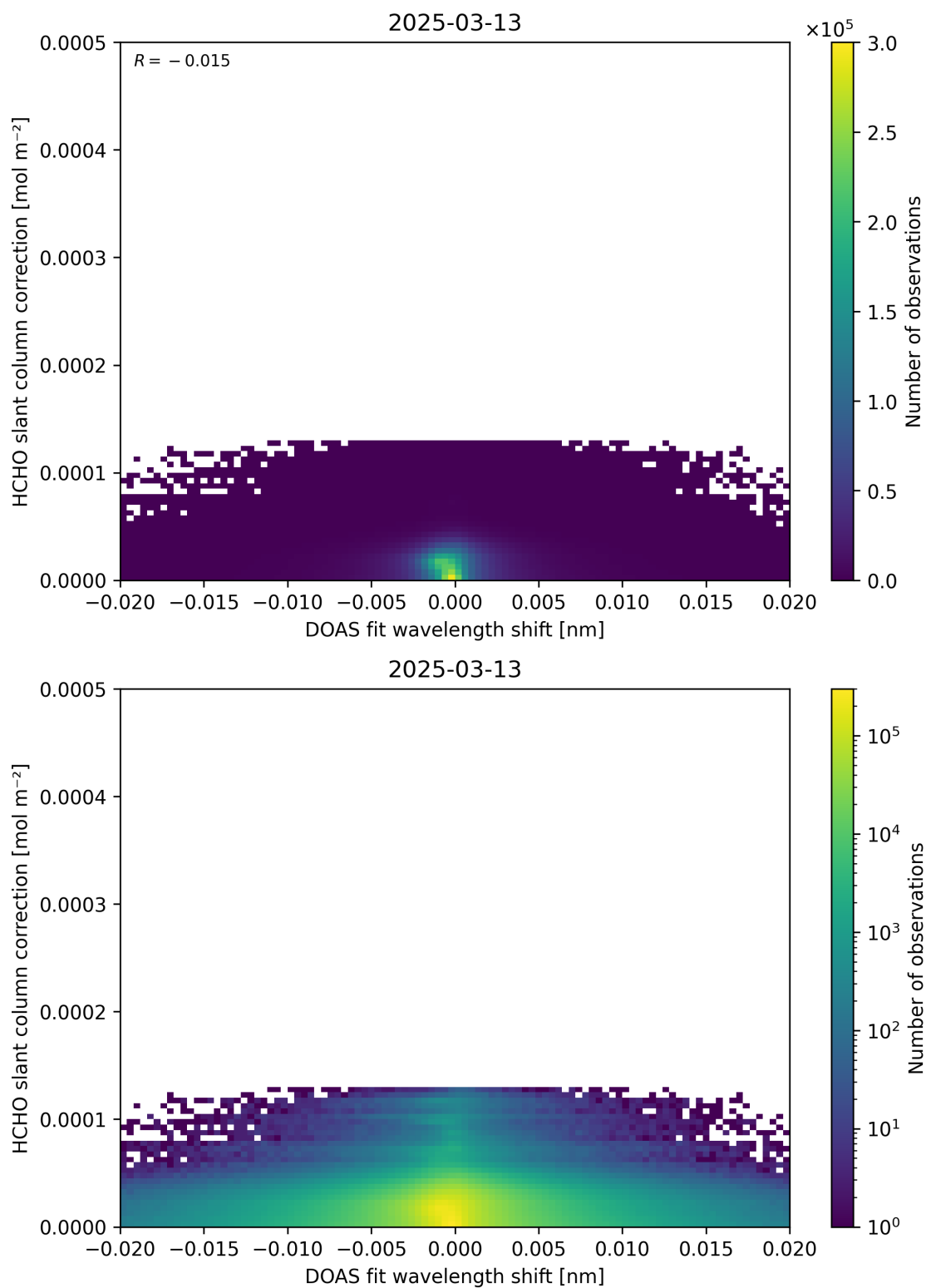
Figure 67: Scatter density plot of “DOAS fit wavelength shift” against “HCHO slant column correction” for 2025-03-12 to 2025-03-14.
