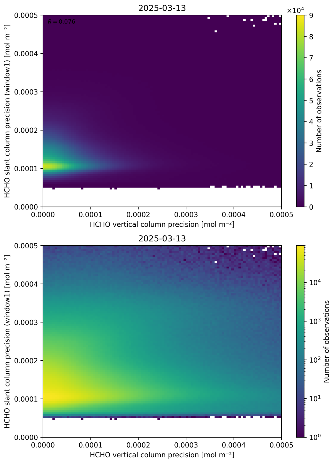
Figure 143: Scatter density plot of “HCHO vertical column precision” against “HCHO slant column precision (window1)” for 2025-03-12 to 2025-03-14.
