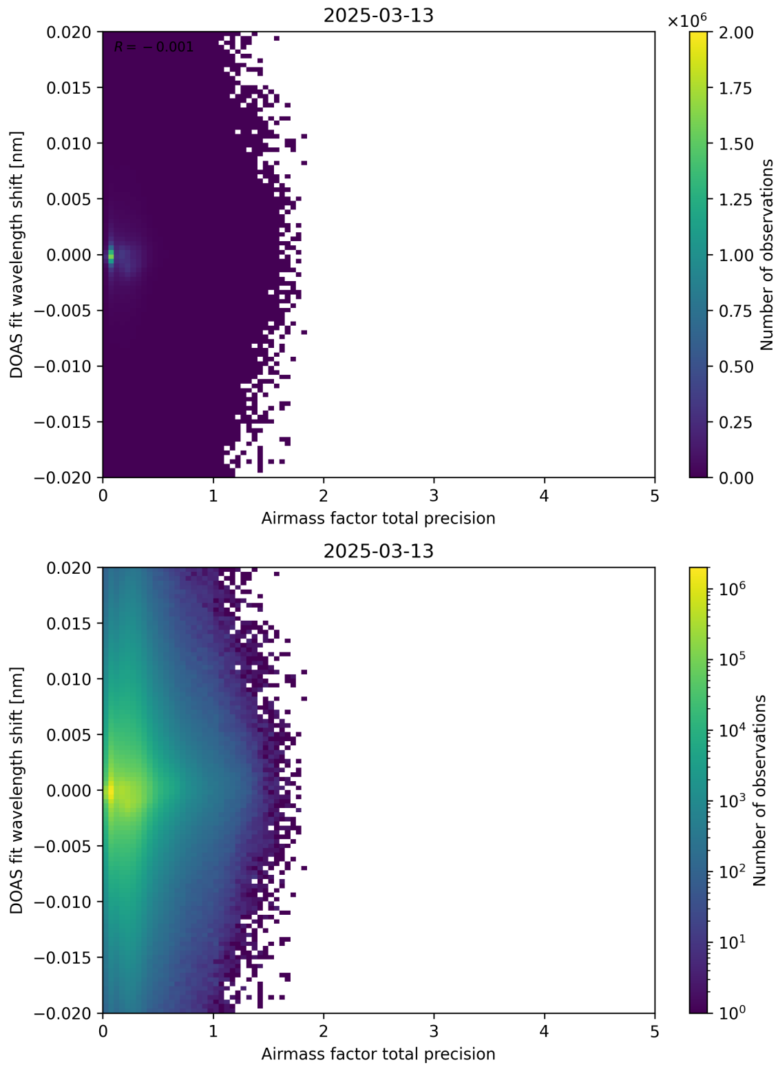
Figure 106: Scatter density plot of “Airmass factor total precision” against “DOAS fit wavelength shift” for 2025-03-12 to 2025-03-14.
