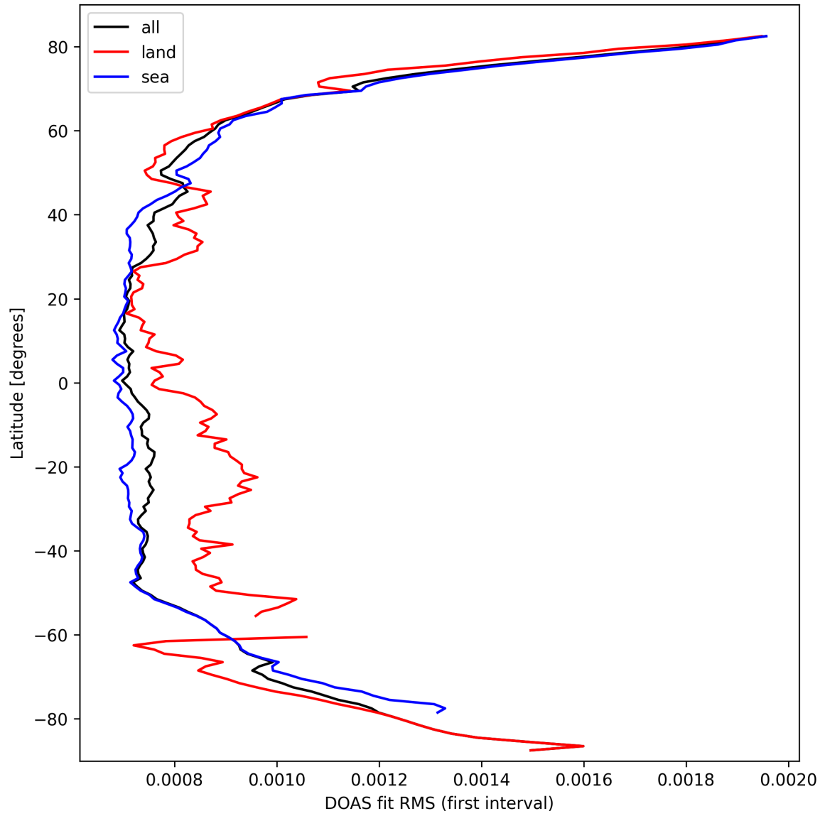
Figure 32: Zonal average of “DOAS fit RMS (first interval)” for 2025-03-12 to 2025-03-14.
