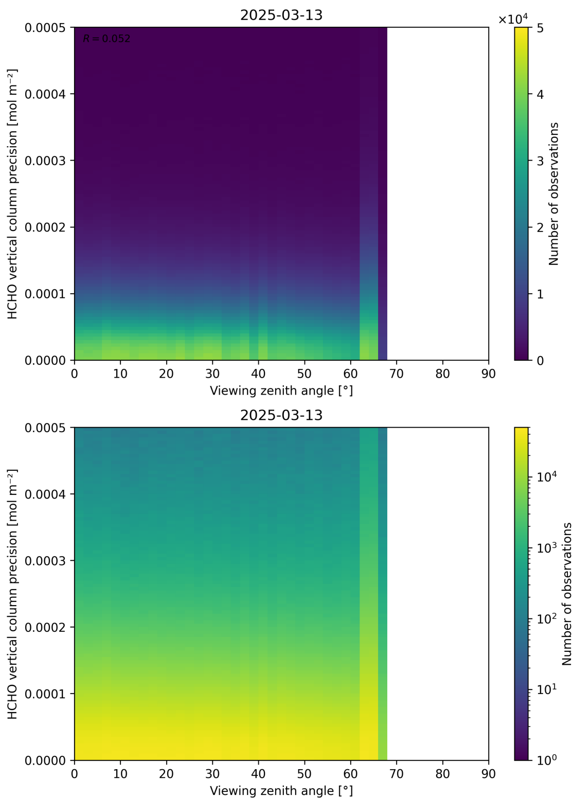
Figure 194: Scatter density plot of “Viewing zenith angle” against “HCHO vertical column precision” for 2025-03-12 to 2025-03-14.
