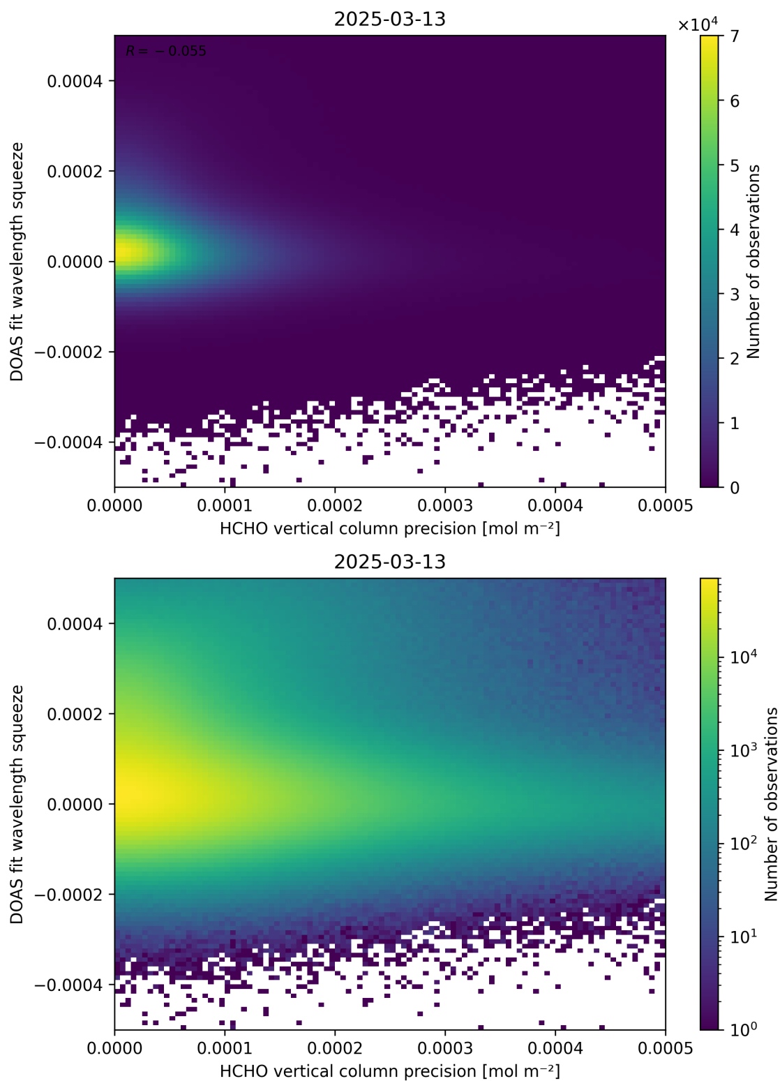
Figure 138: Scatter density plot of “HCHO vertical column precision” against “DOAS fit wavelength squeeze” for 2025-03-12 to 2025-03-14.
