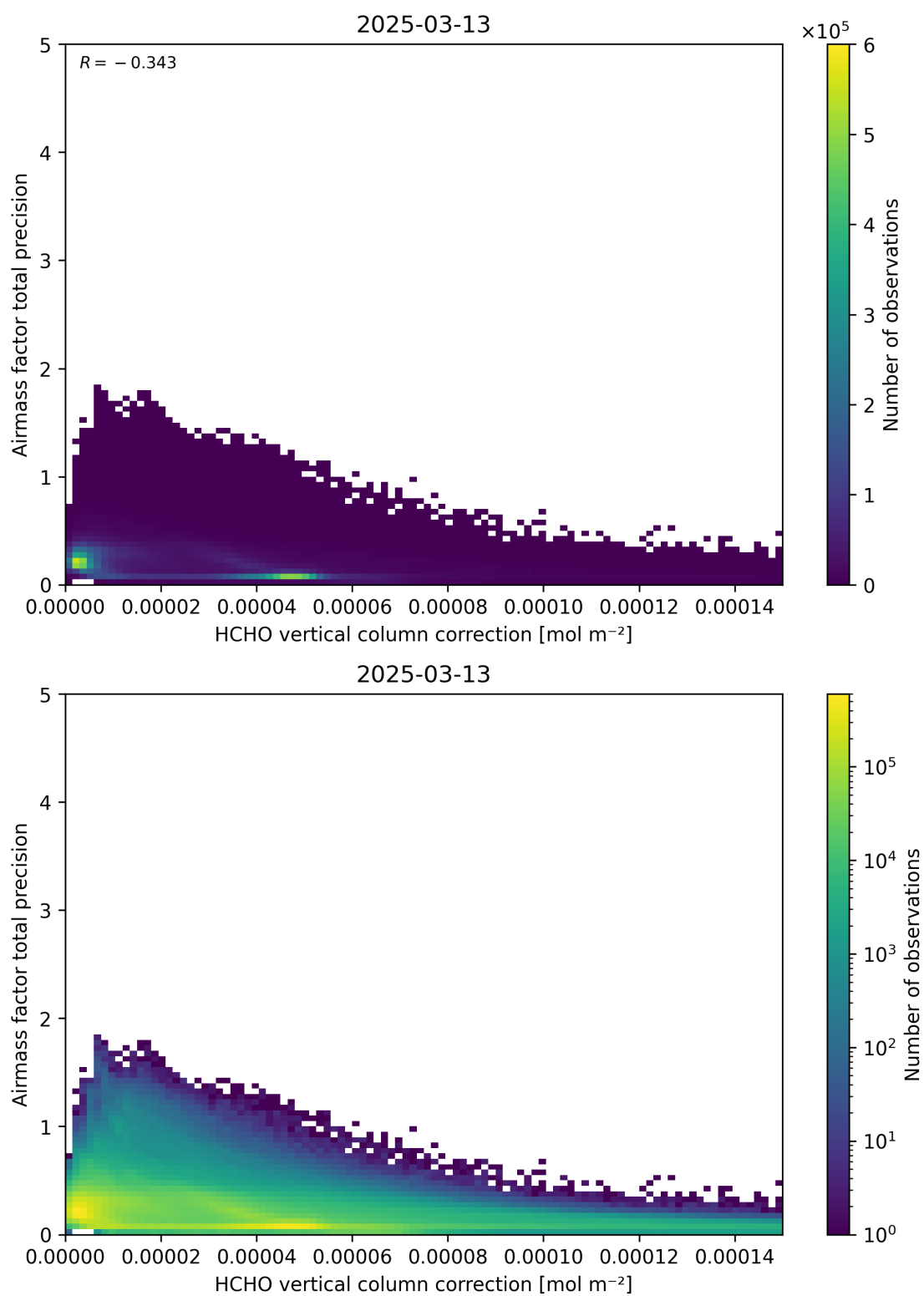
Figure 121: Scatter density plot of “HCHO vertical column correction” against “Airmass factor total precision” for 2025-03-12 to 2025-03-14.
