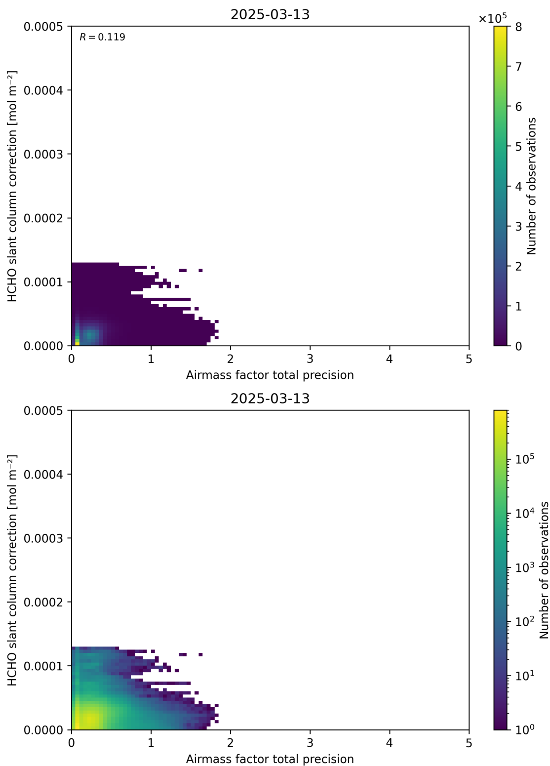
Figure 110: Scatter density plot of “Airmass factor total precision” against “HCHO slant column correction” for 2025-03-12 to 2025-03-14.
