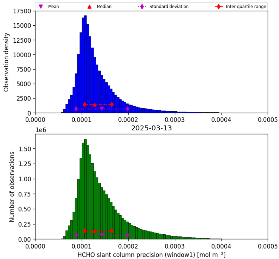
Figure 39: Histogram of “HCHO slant column precision (window1)” for 2025-03-12 to 2025-03-14
