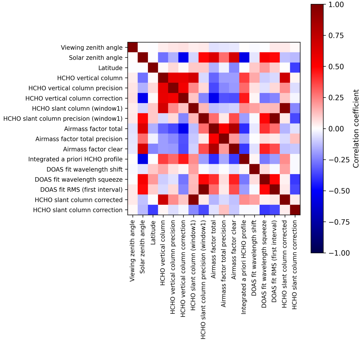
Figure 2: Map of correlation matrix for 2025-03-12 to 2025-03-14.
