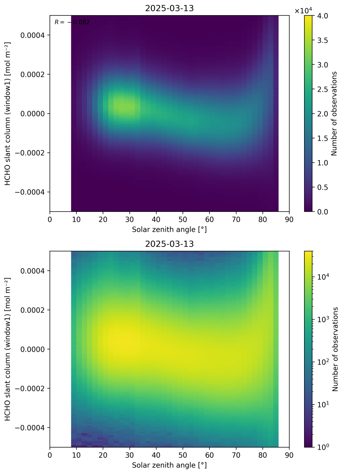
Figure 173: Scatter density plot of “Solar zenith angle” against “HCHO slant column (window1)” for 2025-03-12 to 2025-03-14.
