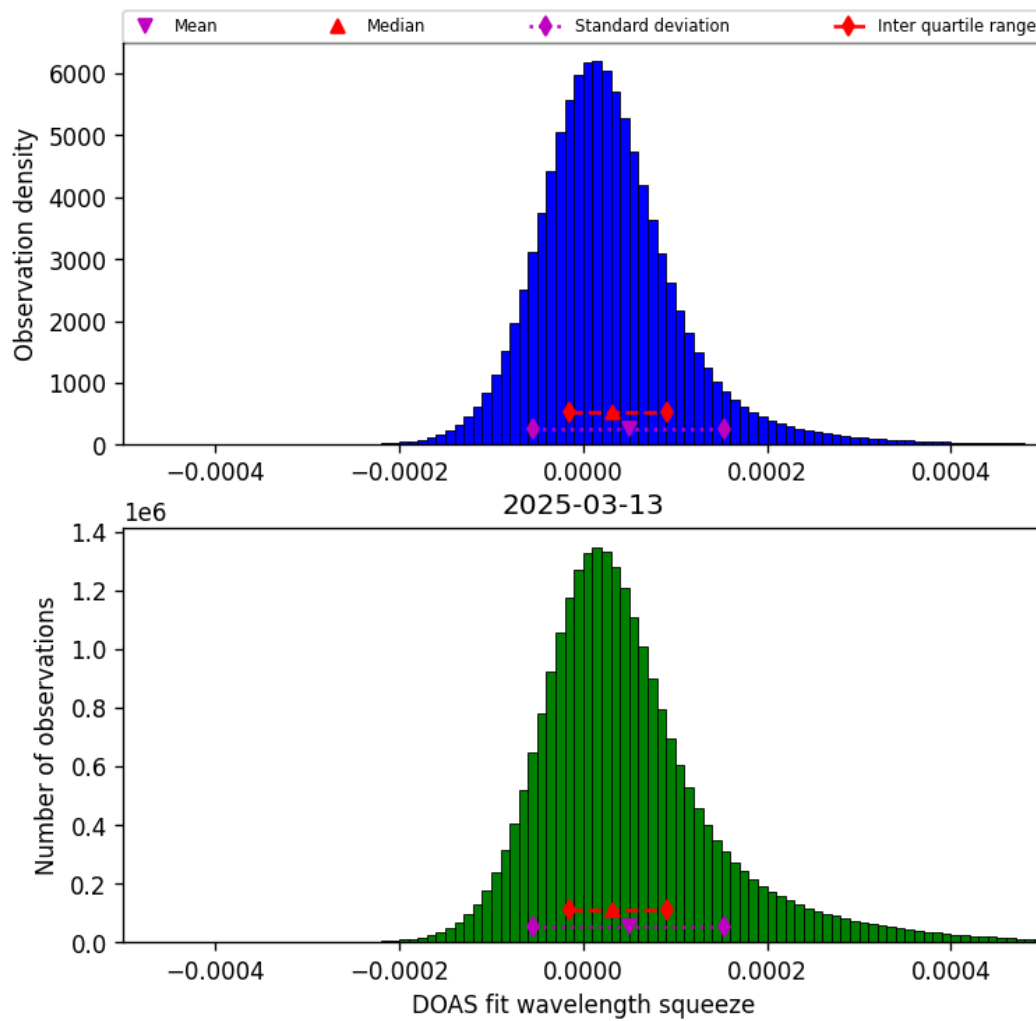
Figure 45: Histogram of “DOAS fit wavelength squeeze” for 2025-03-12 to 2025-03-14
