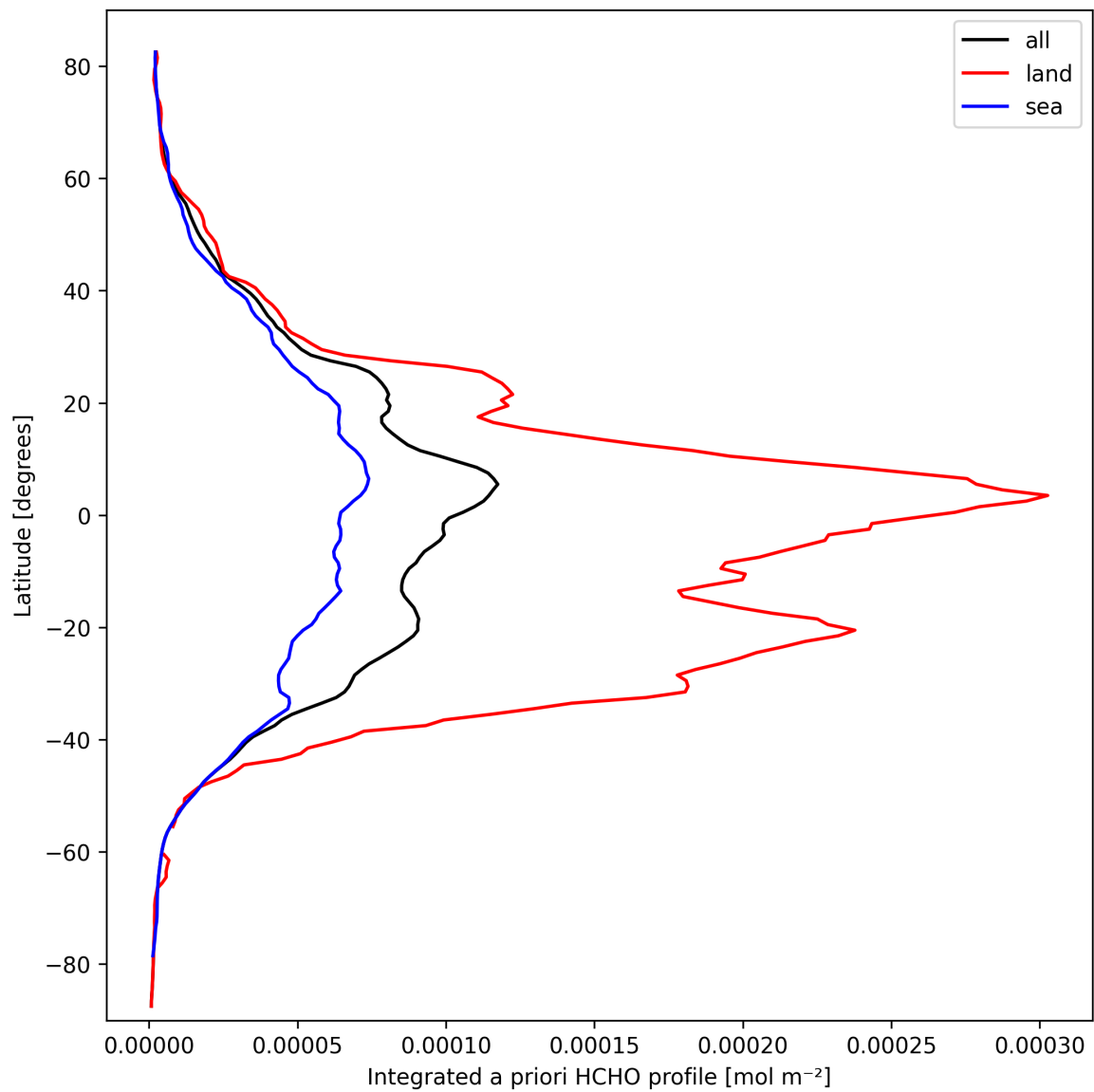
Figure 29: Zonal average of “Integrated a priori HCHO profile” for 2025-03-12 to 2025-03-14.
