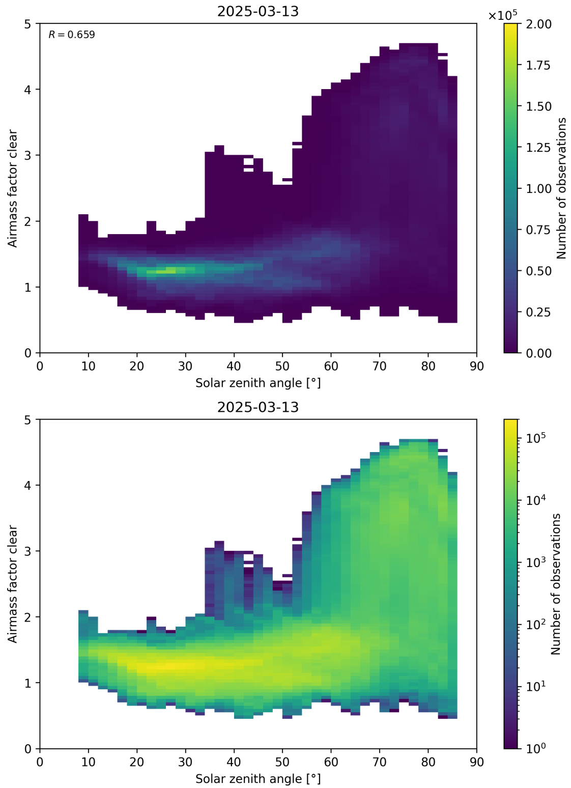
Figure 170: Scatter density plot of “Solar zenith angle” against “Airmass factor clear” for 2025-03-12 to 2025-03-14.
