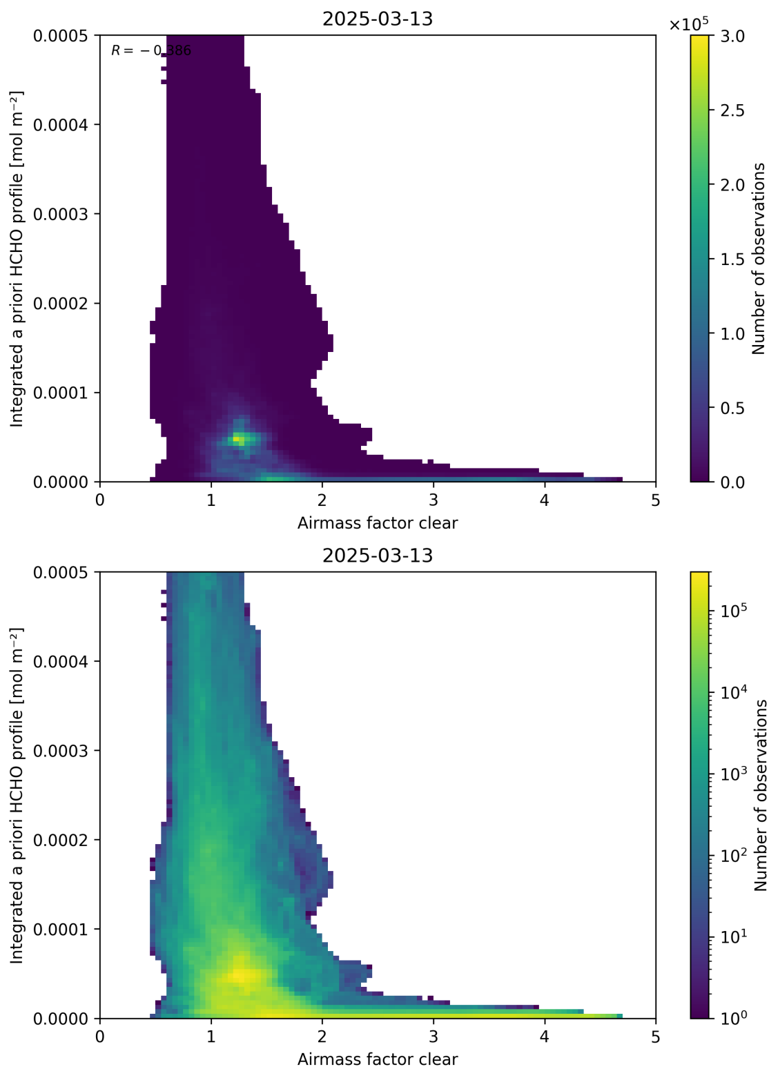
Figure 76: Scatter density plot of “Airmass factor clear” against “Integrated a priori HCHO profile” for 2025-03-12 to 2025-03-14.
