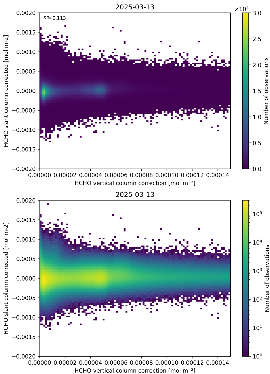
Figure 116: Scatter density plot of “HCHO vertical column correction” against “HCHO slant column corrected” for 2025-03-12 to 2025-03-14.
