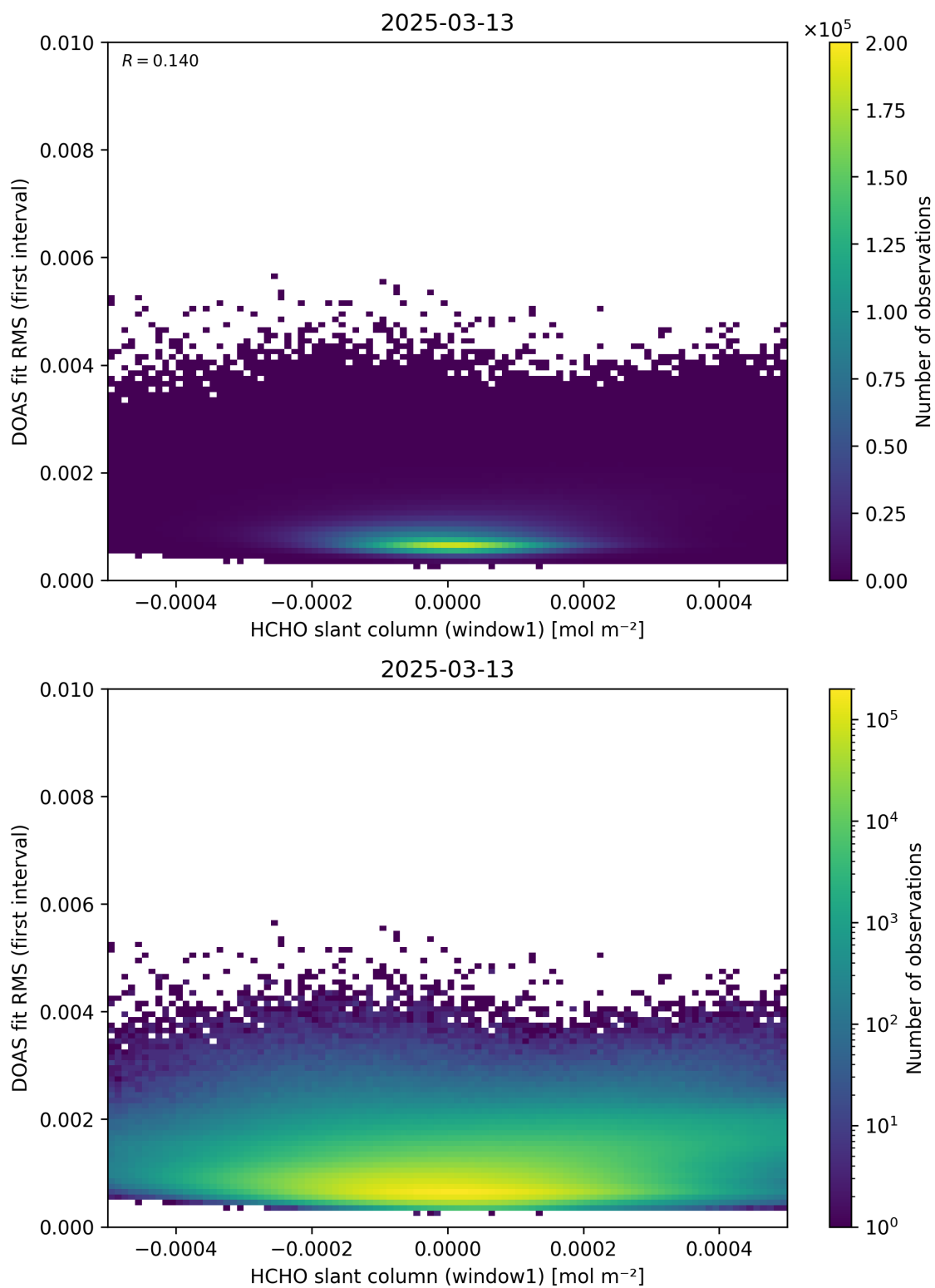
Figure 78: Scatter density plot of “HCHO slant column (window1)” against “DOAS fit RMS (first interval)” for 2025-03-12 to 2025-03-14.
