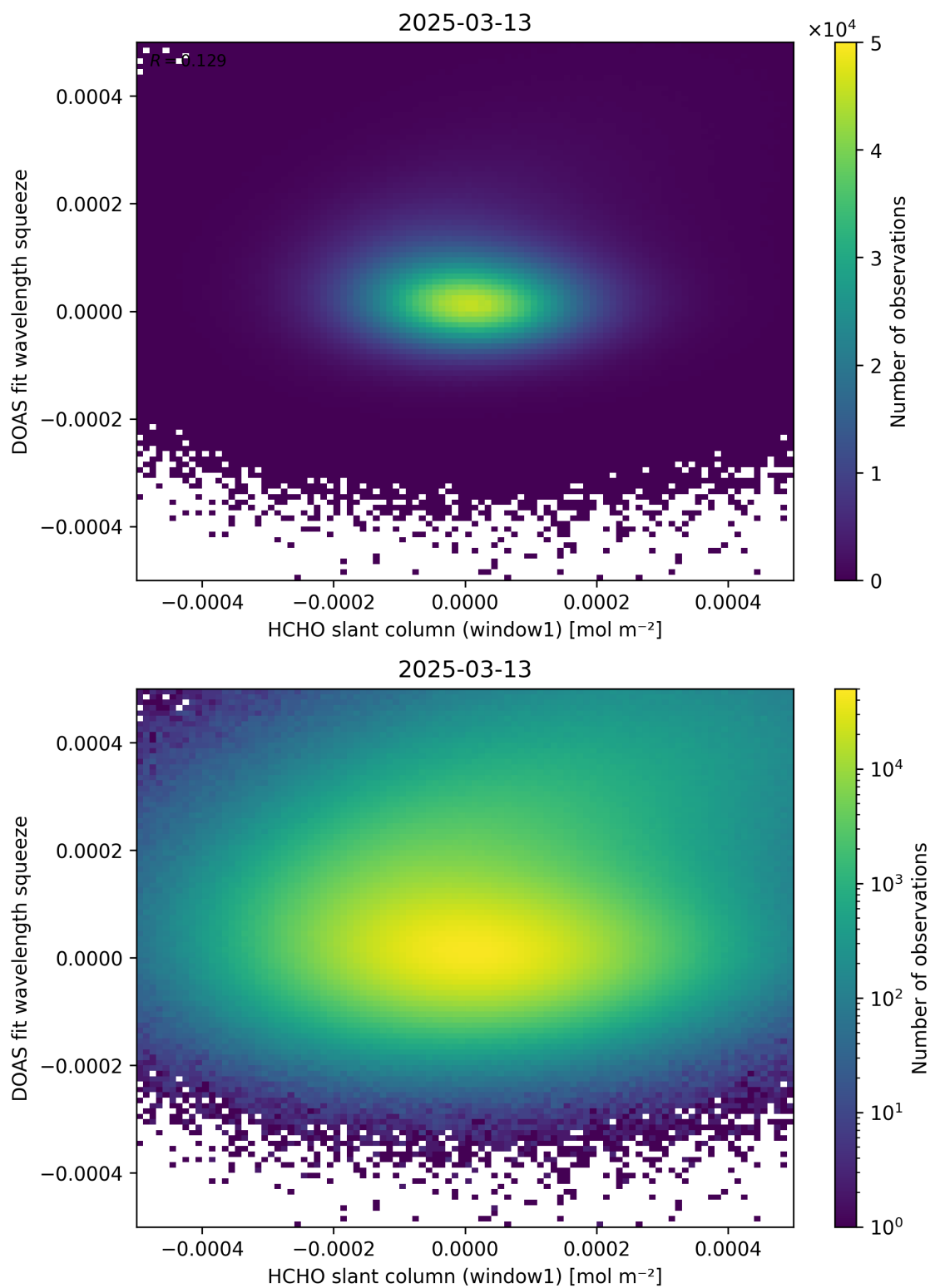
Figure 80: Scatter density plot of “HCHO slant column (window1)” against “DOAS fit wavelength squeeze” for 2025-03-12 to 2025-03-14.
