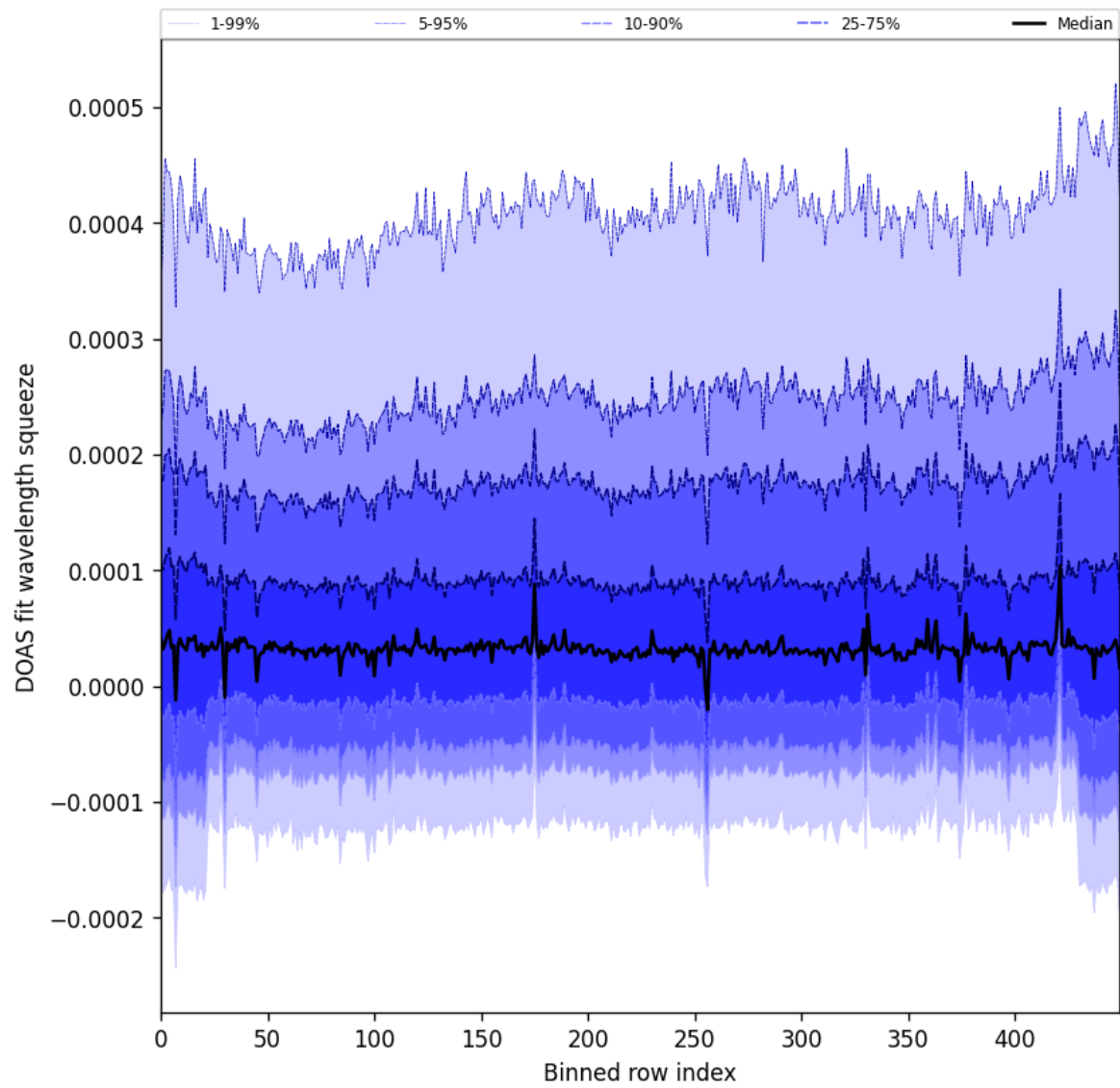
Figure 59: Along track statistics of “DOAS fit wavelength squeeze” for 2025-03-12 to 2025-03-14
