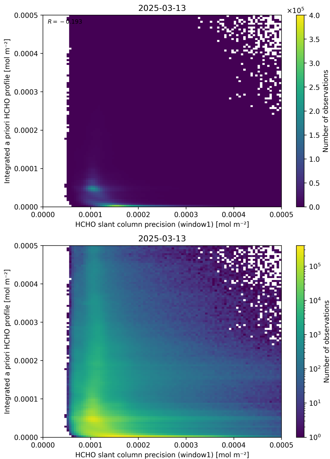
Figure 96: Scatter density plot of “HCHO slant column precision (window1)” against “Integrated a priori HCHO profile” for 2025-03-12 to 2025-03-14.
