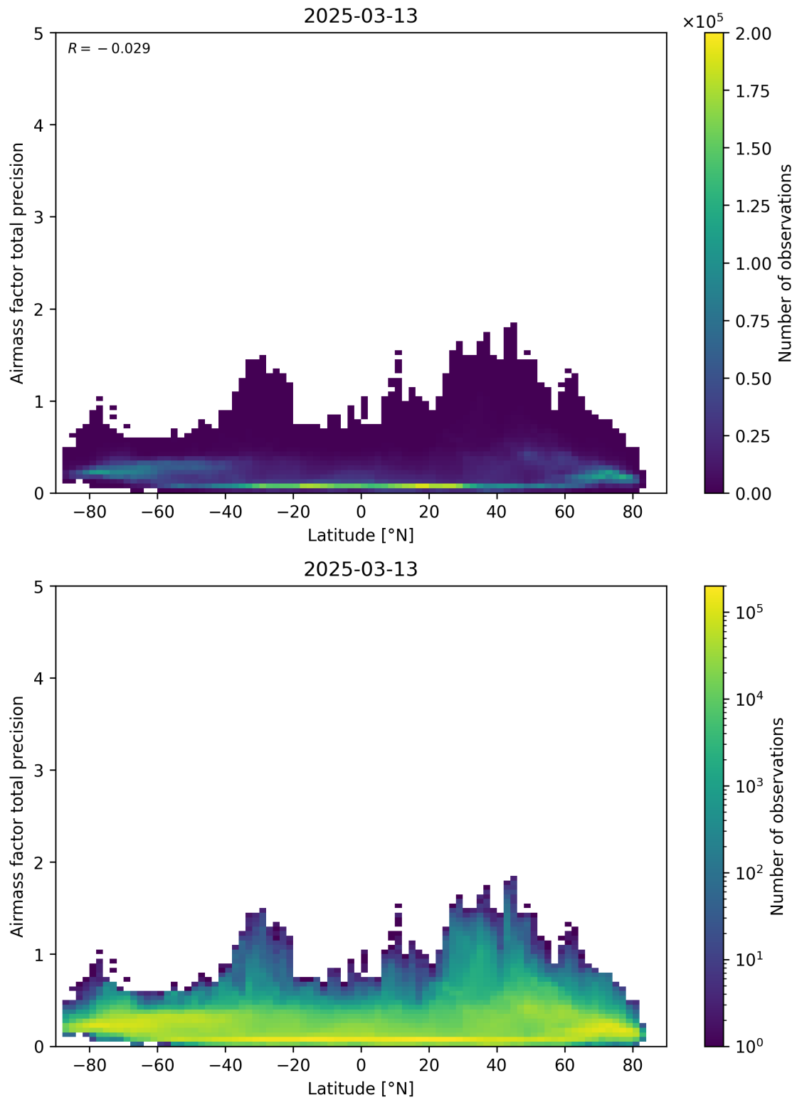
Figure 162: Scatter density plot of “Latitude” against “Airmass factor total precision” for 2025-03-12 to 2025-03-14.
