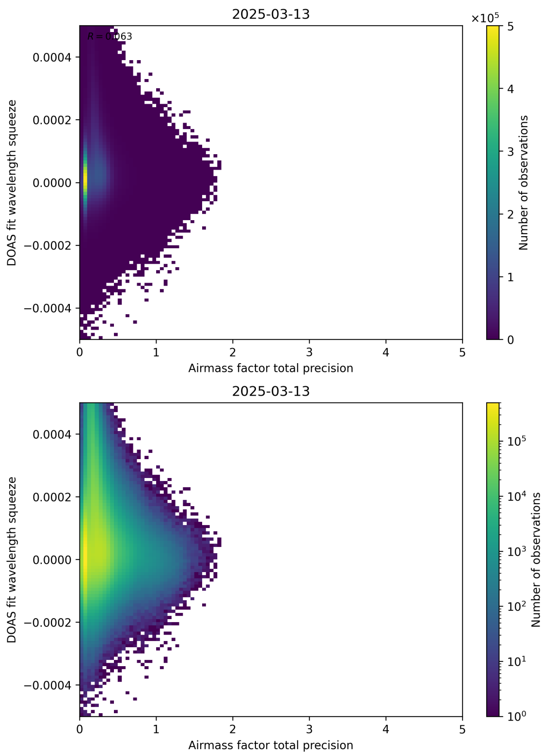
Figure 107: Scatter density plot of “Airmass factor total precision” against “DOAS fit wavelength squeeze” for 2025-03-12 to 2025-03-14.
