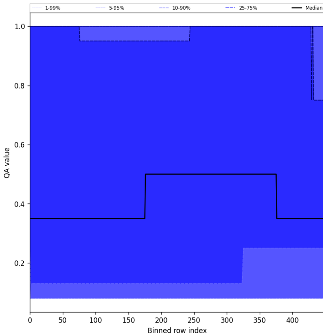
Figure 48: Along track statistics of “QA value” for 2025-03-12 to 2025-03-14
