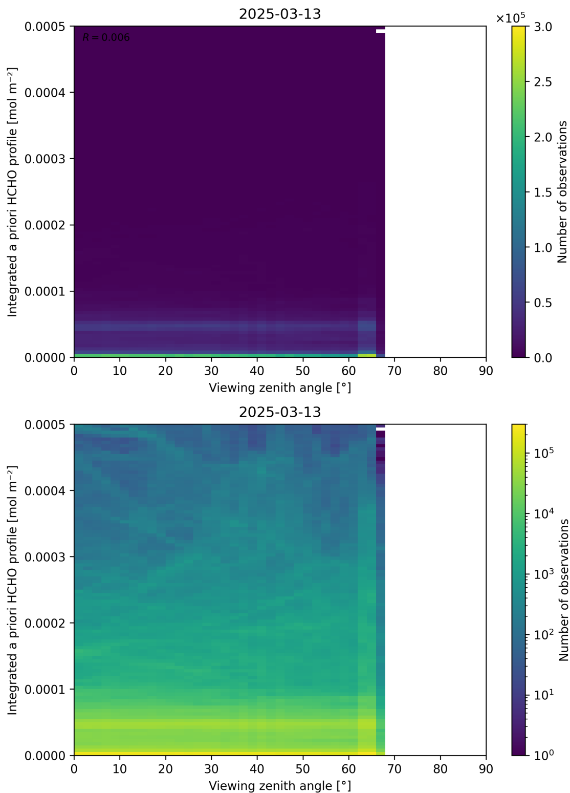
Figure 195: Scatter density plot of “Viewing zenith angle” against “Integrated a priori HCHO profile” for 2025-03-12 to 2025-03-14.
