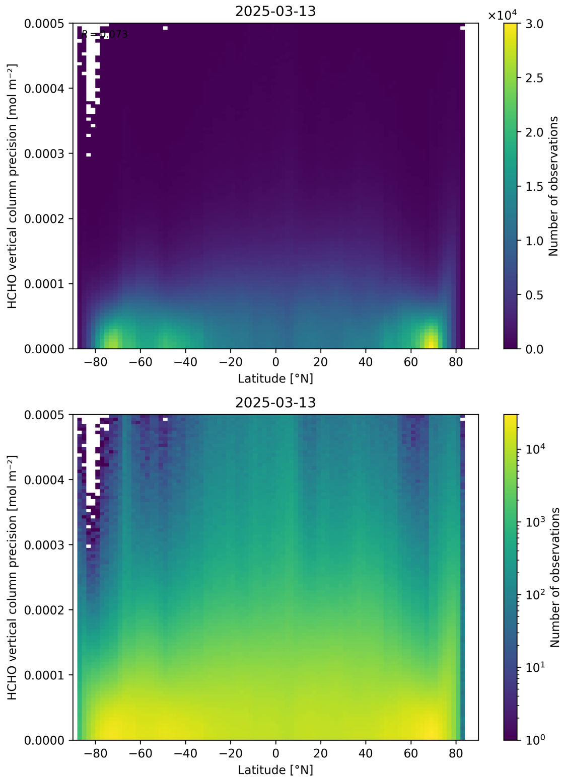
Figure 165: Scatter density plot of “Latitude” against “HCHO vertical column precision” for 2025-03-12 to 2025-03-14.
