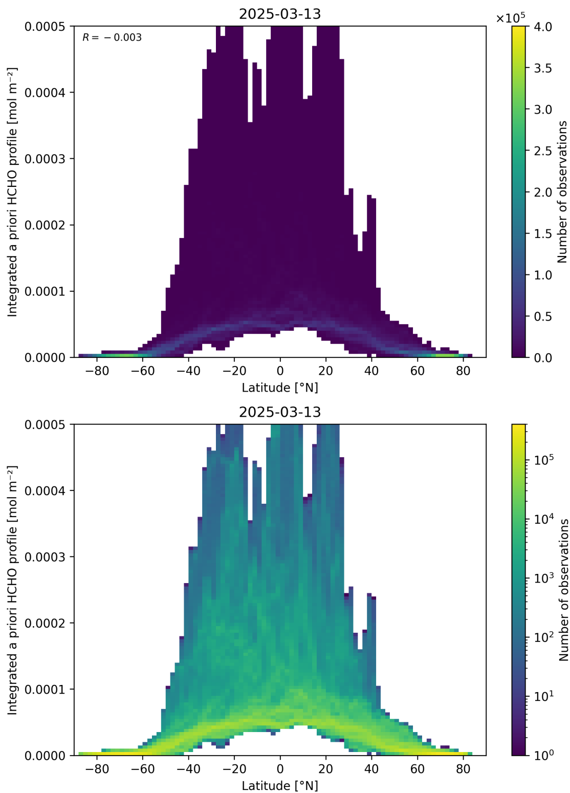
Figure 166: Scatter density plot of “Latitude” against “Integrated a priori HCHO profile” for 2025-03-12 to 2025-03-14.
