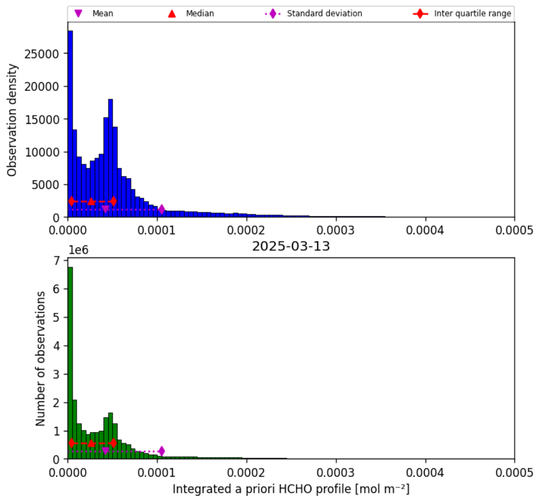
Figure 43: Histogram of “Integrated a priori HCHO profile” for 2025-03-12 to 2025-03-14
