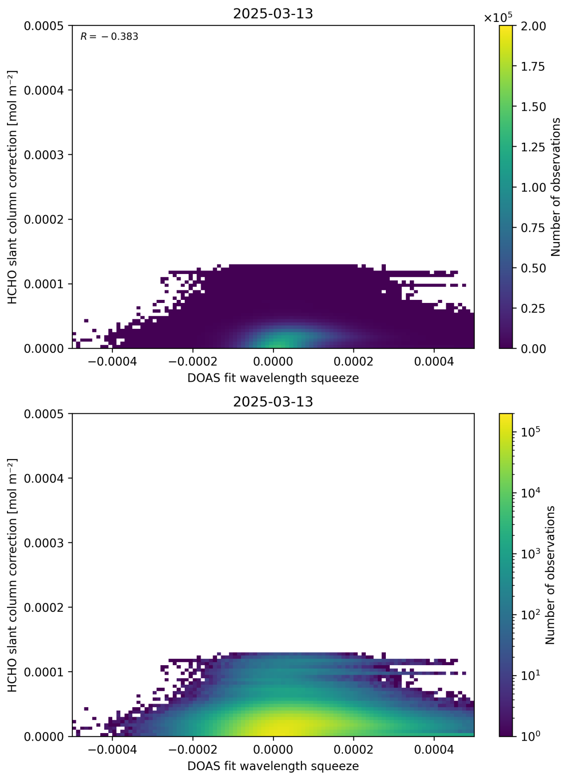
Figure 70: Scatter density plot of “DOAS fit wavelength squeeze” against “HCHO slant column correction” for 2025-03-12 to 2025-03-14.
