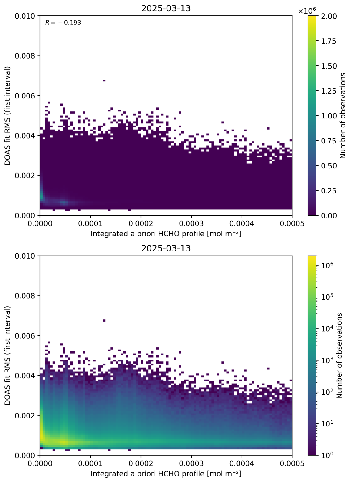
Figure 148: Scatter density plot of “Integrated a priori HCHO profile” against “DOAS fit RMS (first interval)” for 2025-03-12 to 2025-03-14.
