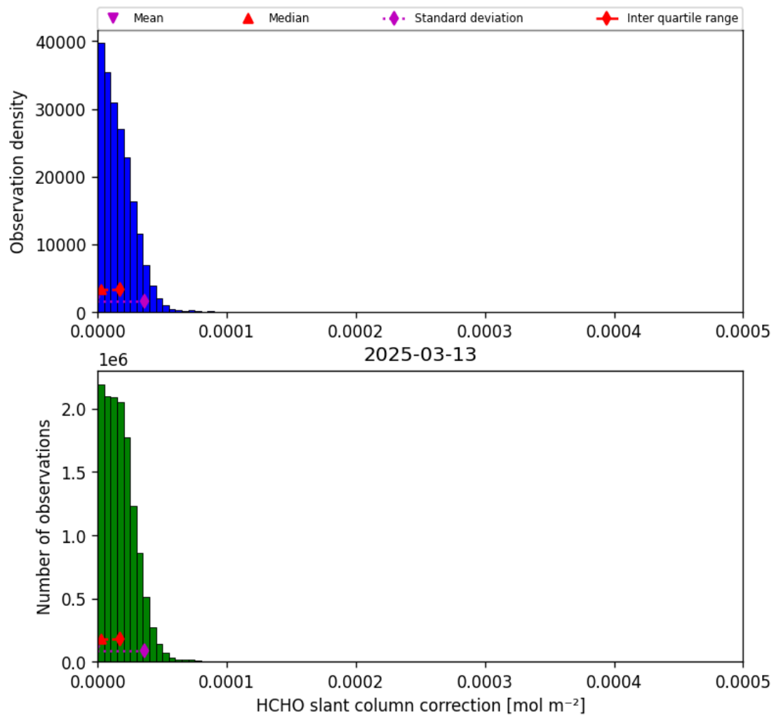
Figure 47: Histogram of “HCHO slant column correction” for 2025-03-12 to 2025-03-14
