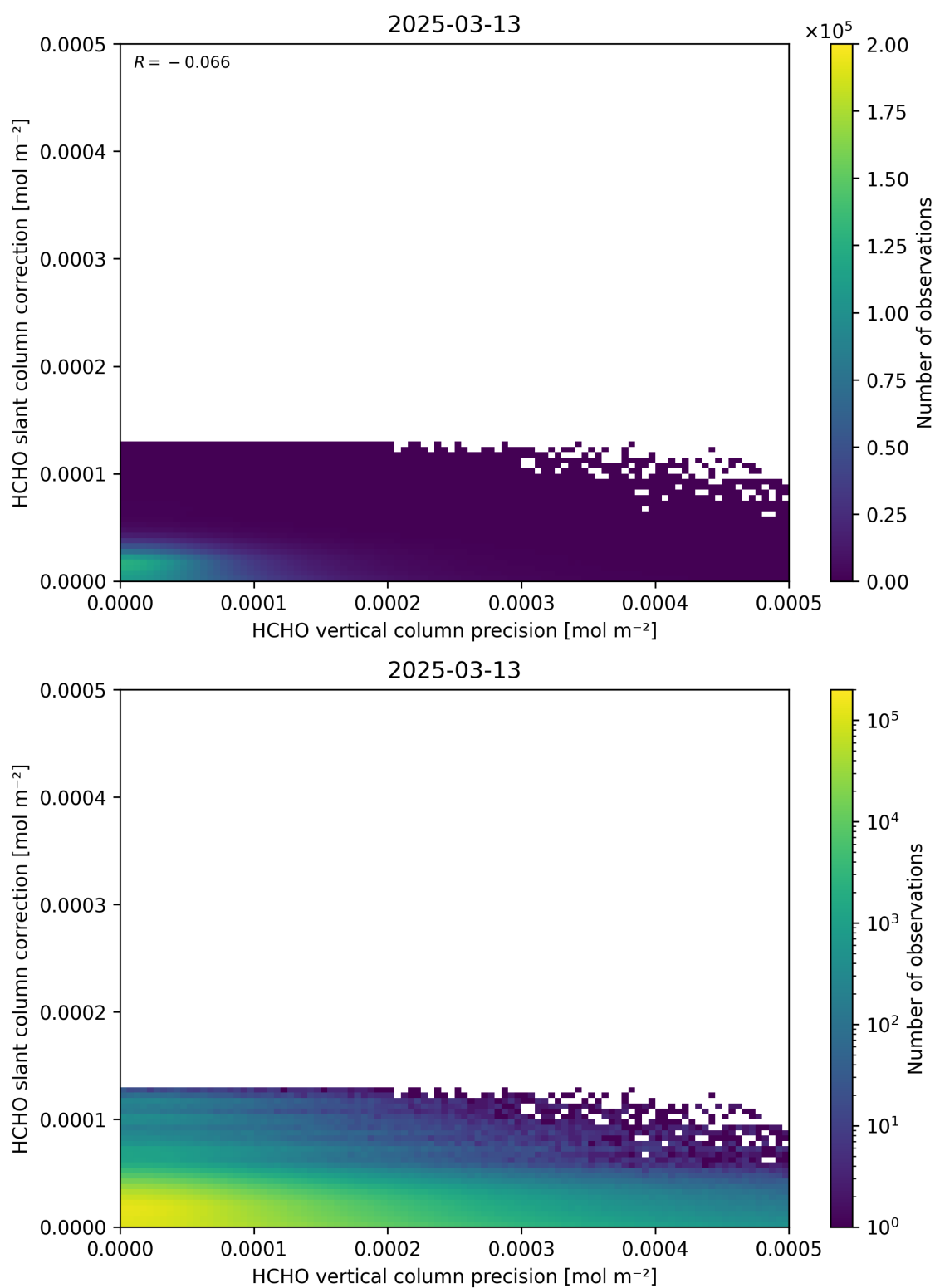
Figure 141: Scatter density plot of “HCHO vertical column precision” against “HCHO slant column correction” for 2025-03-12 to 2025-03-14.
