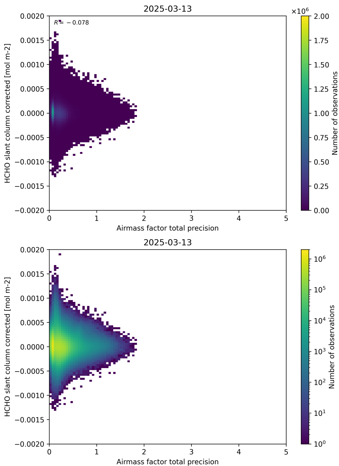
Figure 109: Scatter density plot of “Airmass factor total precision” against “HCHO slant column corrected” for 2025-03-12 to 2025-03-14.
