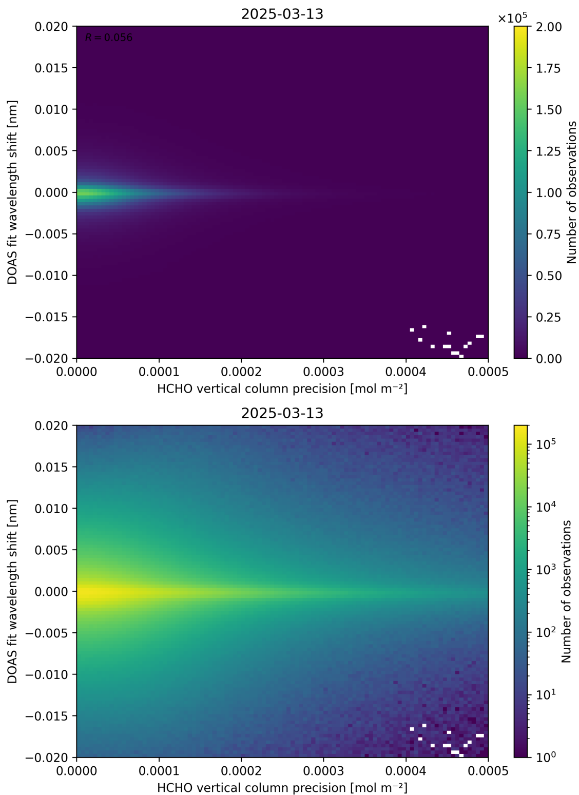
Figure 137: Scatter density plot of “HCHO vertical column precision” against “DOAS fit wavelength shift” for 2025-03-12 to 2025-03-14.
