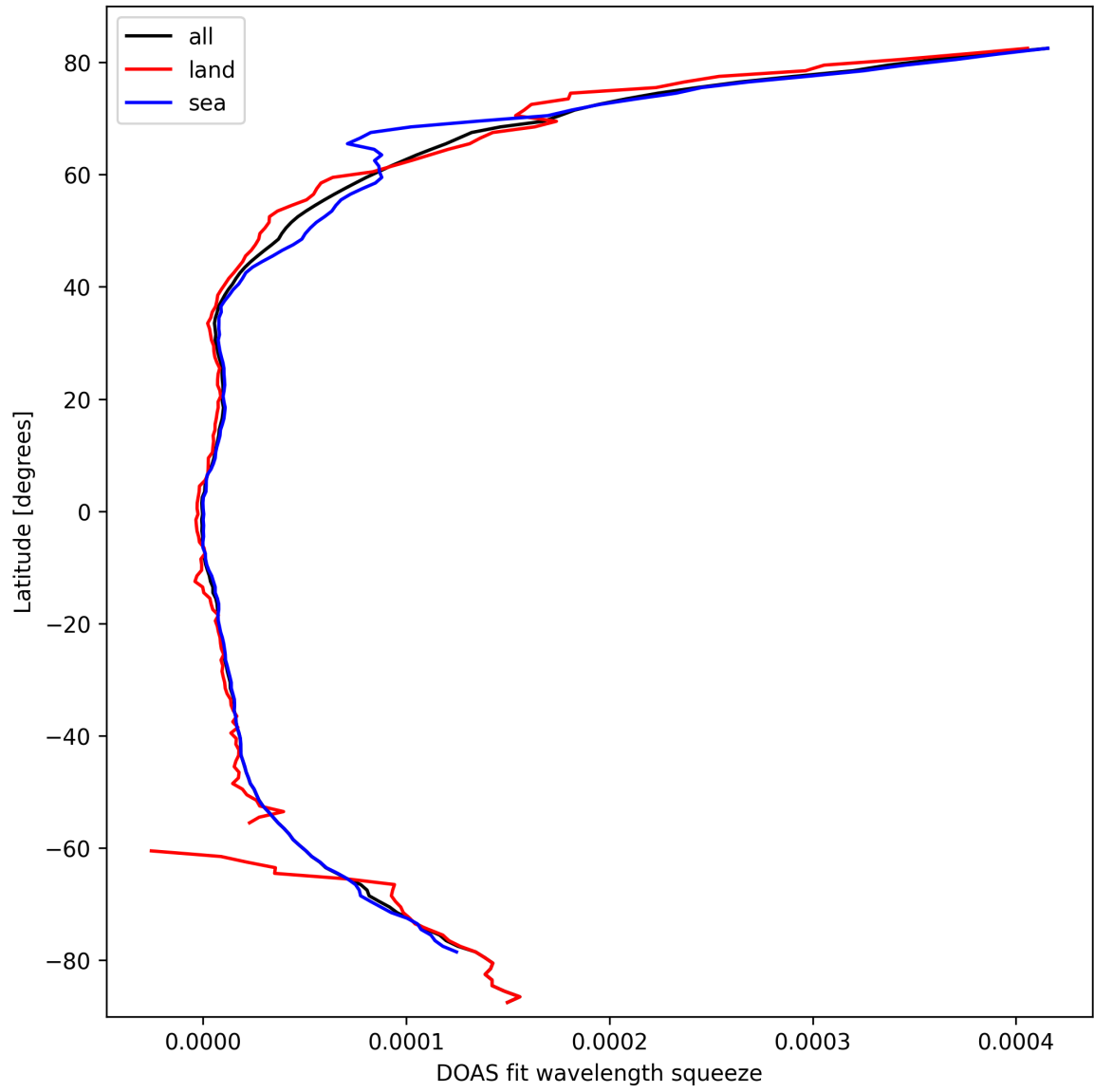
Figure 31: Zonal average of “DOAS fit wavelength squeeze” for 2025-03-12 to 2025-03-14.
