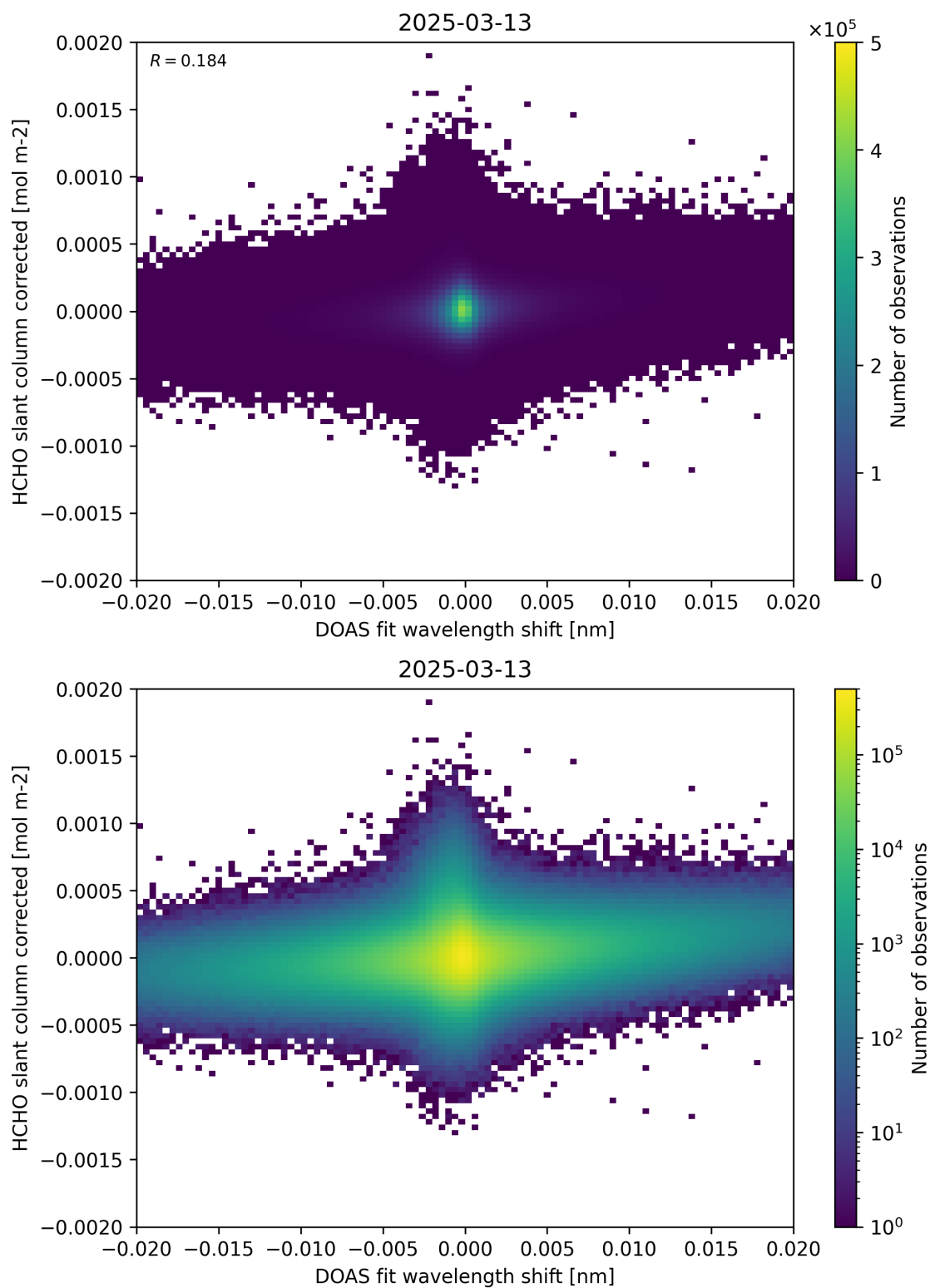
Figure 66: Scatter density plot of “DOAS fit wavelength shift” against “HCHO slant column corrected” for 2025-03-12 to 2025-03-14.
