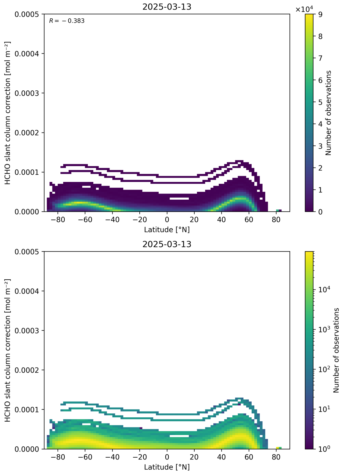
Figure 158: Scatter density plot of “Latitude” against “HCHO slant column correction” for 2025-03-12 to 2025-03-14.
