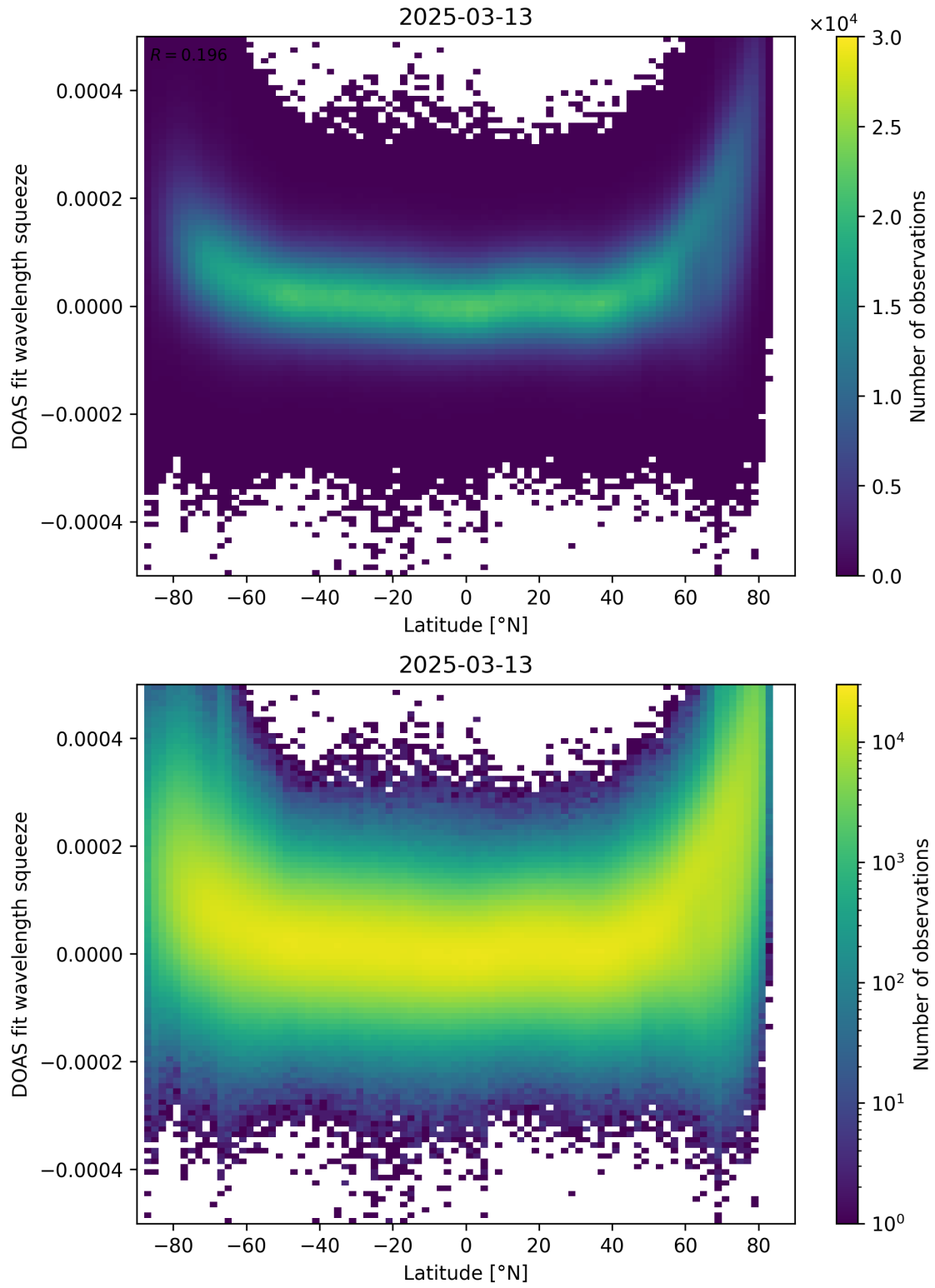
Figure 155: Scatter density plot of “Latitude” against “DOAS fit wavelength squeeze” for 2025-03-12 to 2025-03-14.
