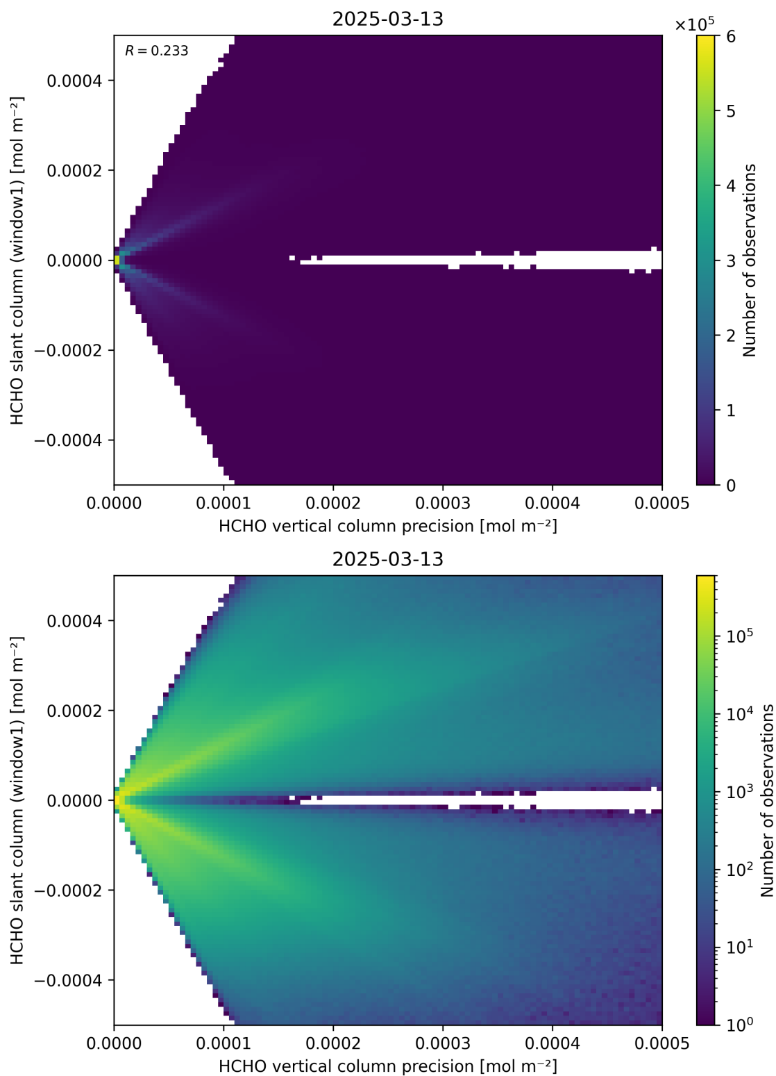
Figure 142: Scatter density plot of “HCHO vertical column precision” against “HCHO slant column (window1)” for 2025-03-12 to 2025-03-14.
