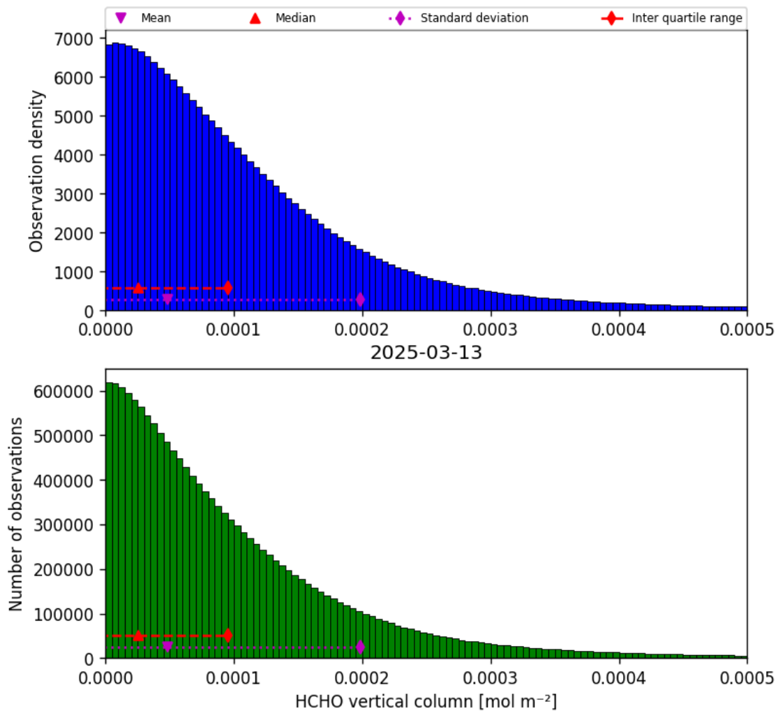
Figure 35: Histogram of “HCHO vertical column” for 2025-03-12 to 2025-03-14
