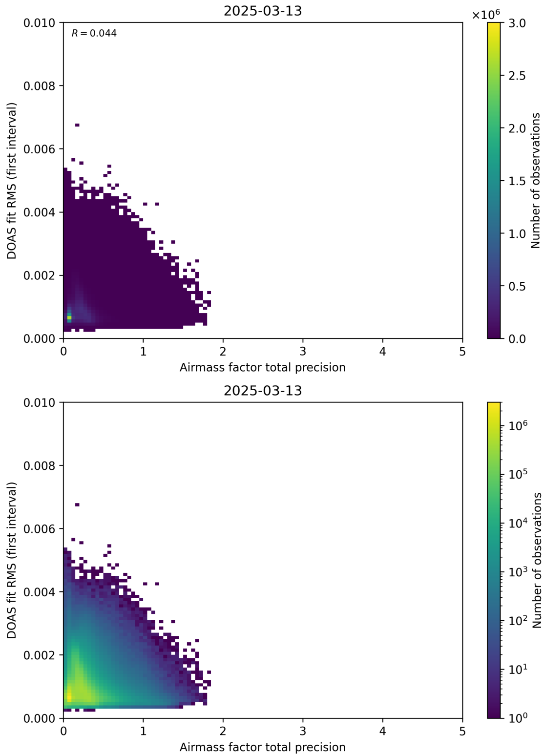
Figure 105: Scatter density plot of “Airmass factor total precision” against “DOAS fit RMS (first interval)” for 2025-03-12 to 2025-03-14.
