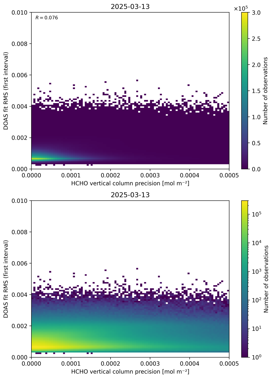
Figure 136: Scatter density plot of “HCHO vertical column precision” against “DOAS fit RMS (first interval)” for 2025-03-12 to 2025-03-14.
