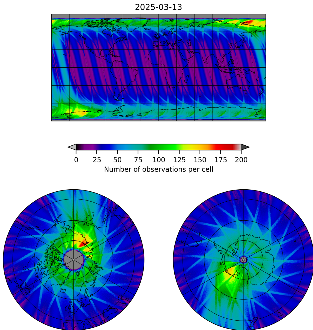
Figure 19: Map of the number of observations for 2025-03-12 to 2025-03-14
