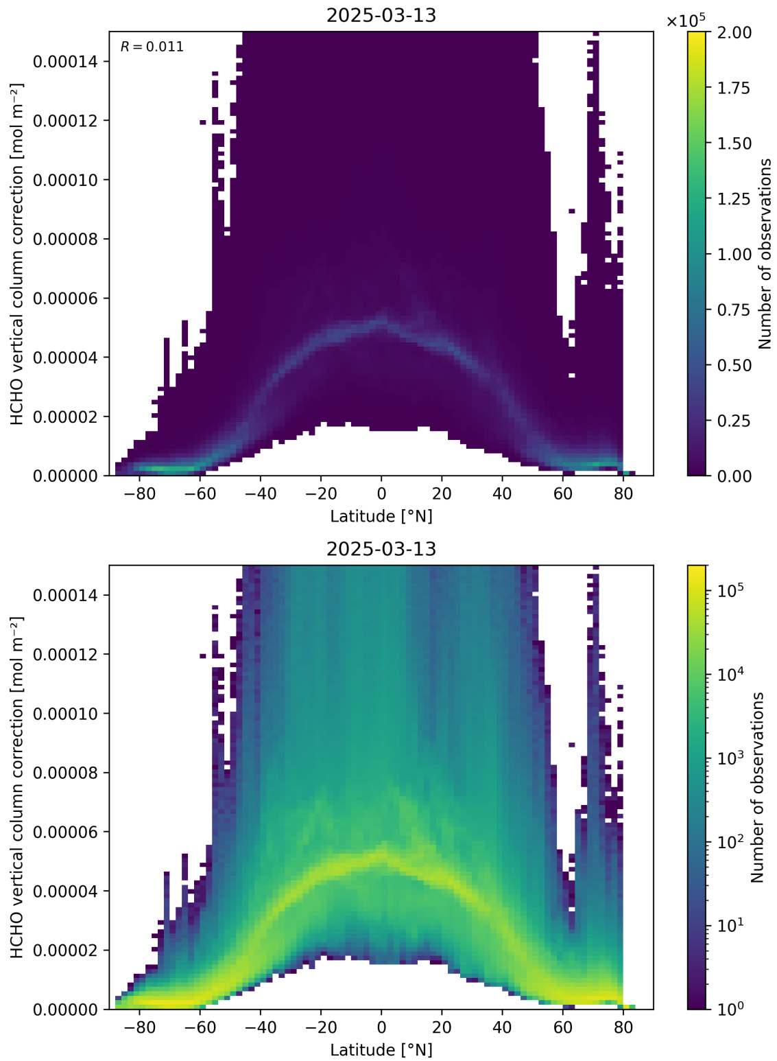
Figure 164: Scatter density plot of “Latitude” against “HCHO vertical column correction” for 2025-03-12 to 2025-03-14.
