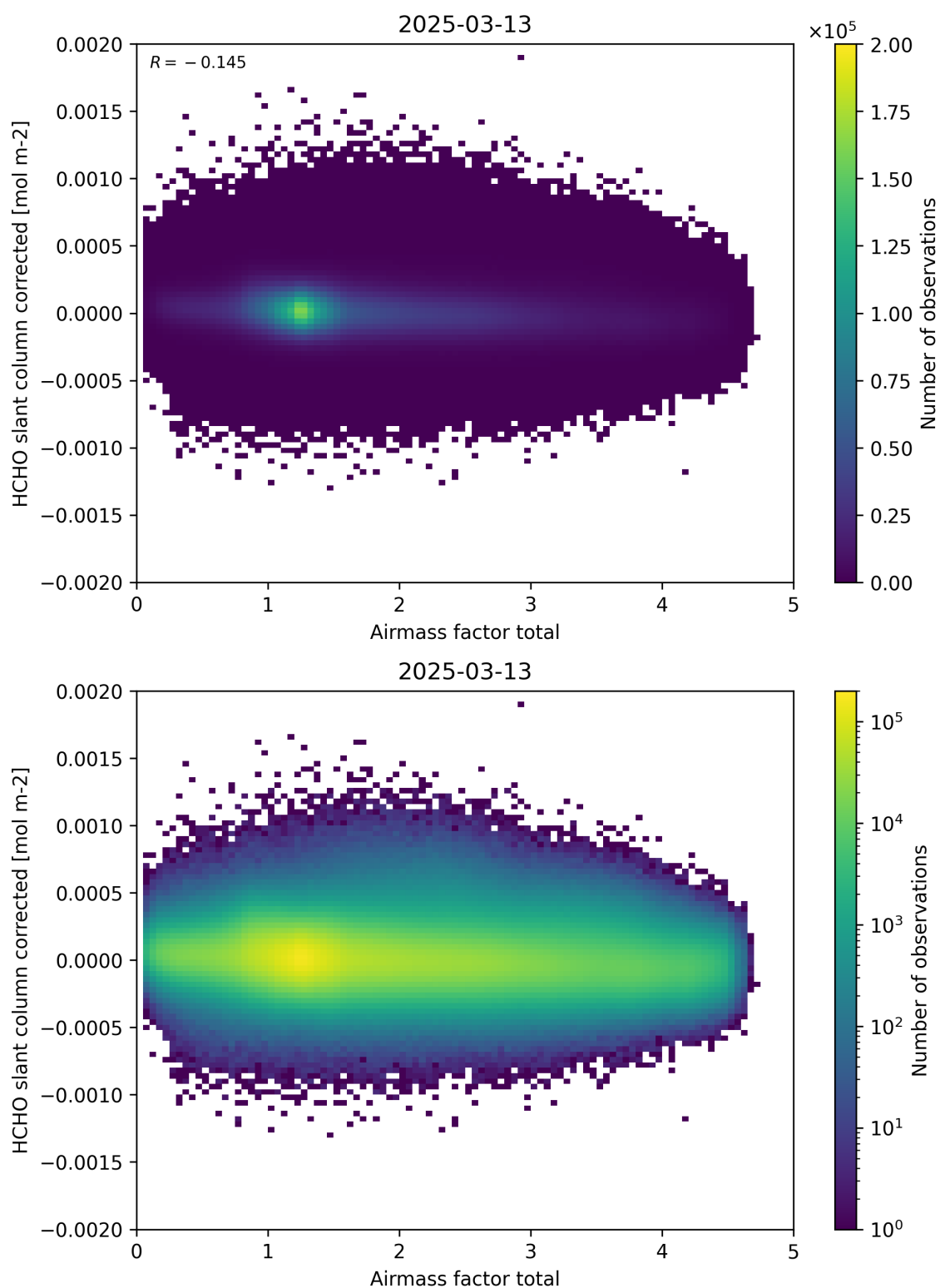
Figure 101: Scatter density plot of “Airmass factor total” against “HCHO slant column corrected” for 2025-03-12 to 2025-03-14.
