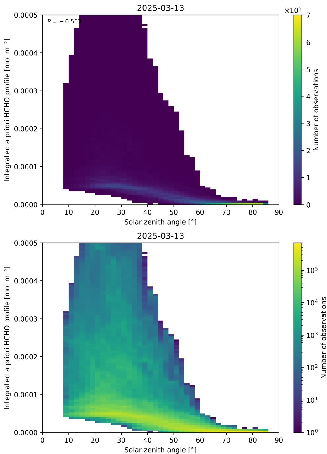
Figure 180: Scatter density plot of “Solar zenith angle” against “Integrated a priori HCHO profile” for 2025-03-12 to 2025-03-14.
