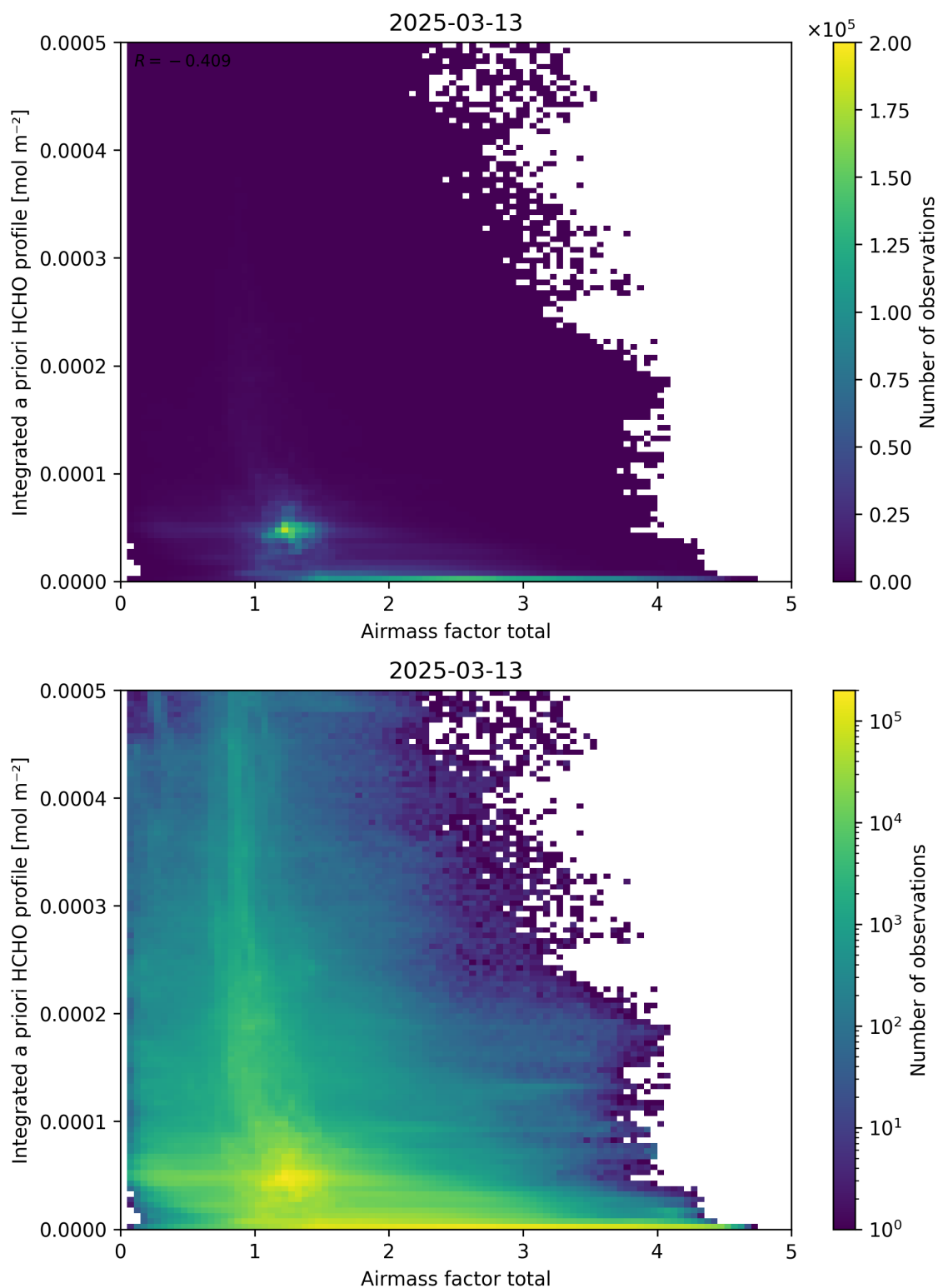
Figure 104: Scatter density plot of “Airmass factor total” against “Integrated a priori HCHO profile” for 2025-03-12 to 2025-03-14.
