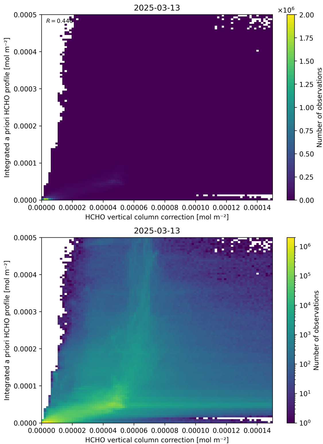
Figure 122: Scatter density plot of “HCHO vertical column correction” against “Integrated a priori HCHO profile” for 2025-03-12 to 2025-03-14.
