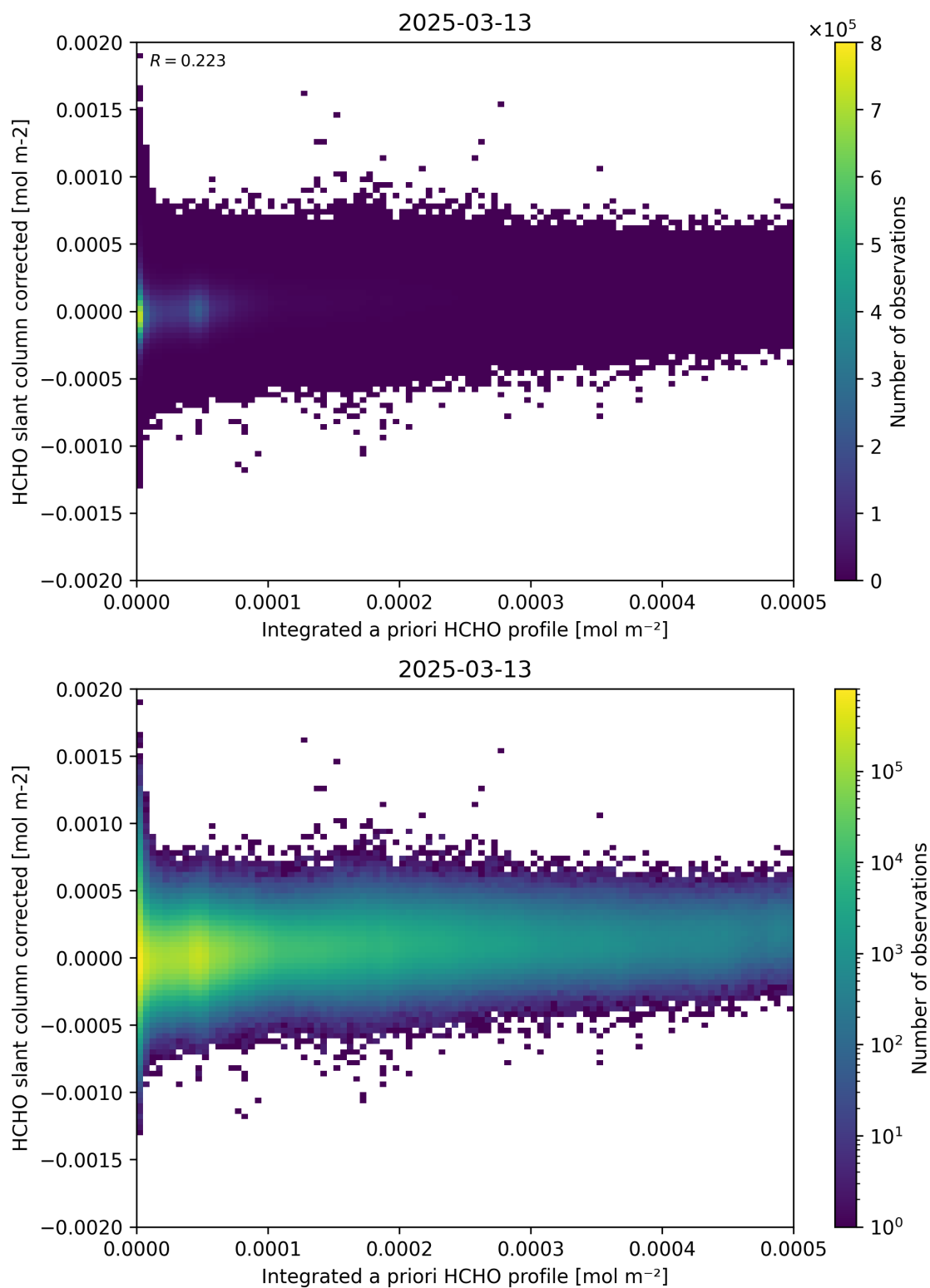
Figure 151: Scatter density plot of “Integrated a priori HCHO profile” against “HCHO slant column corrected” for 2025-03-12 to 2025-03-14.
