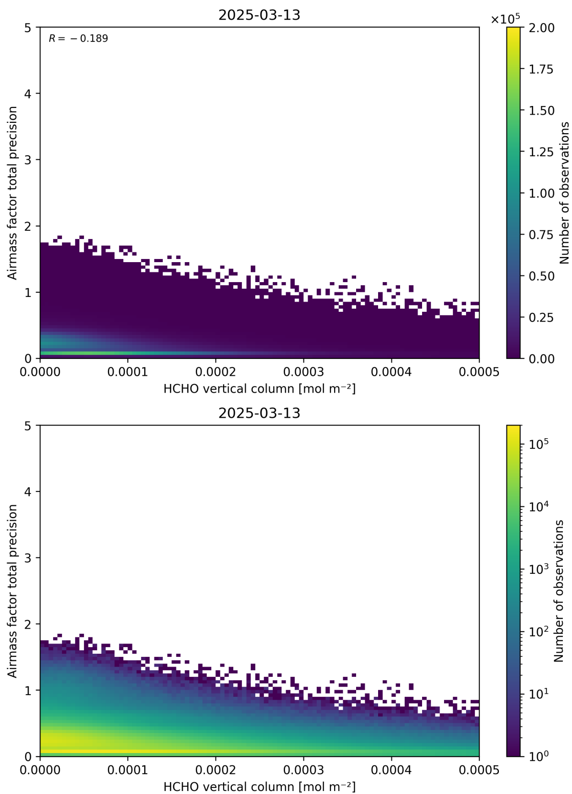
Figure 132: Scatter density plot of “HCHO vertical column” against “Airmass factor total precision” for 2025-03-12 to 2025-03-14.
