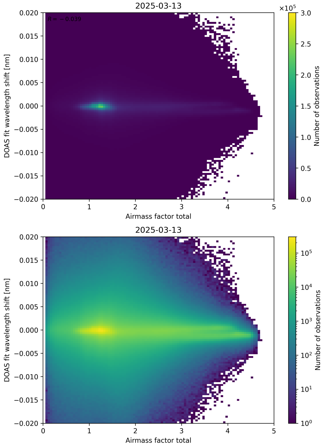
Figure 98: Scatter density plot of “Airmass factor total” against “DOAS fit wavelength shift” for 2025-03-12 to 2025-03-14.
