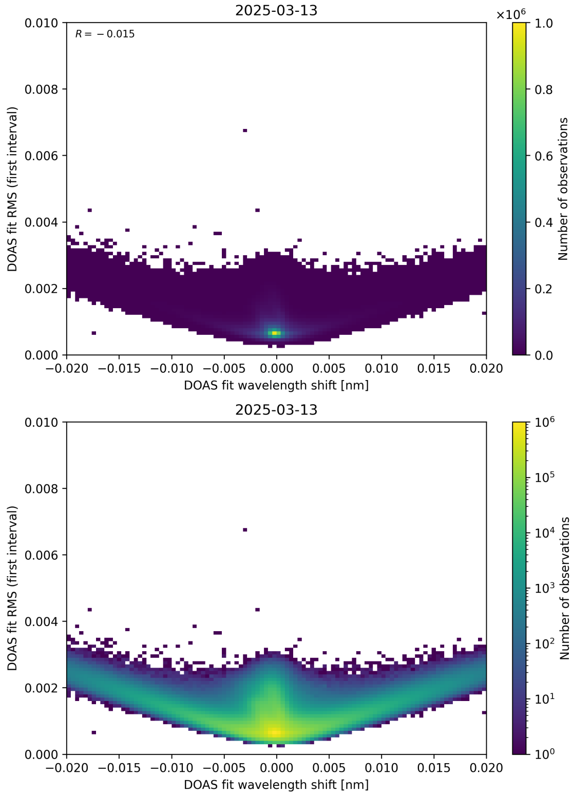
Figure 64: Scatter density plot of “DOAS fit wavelength shift” against “DOAS fit RMS (first interval)” for 2025-03-12 to 2025-03-14.
