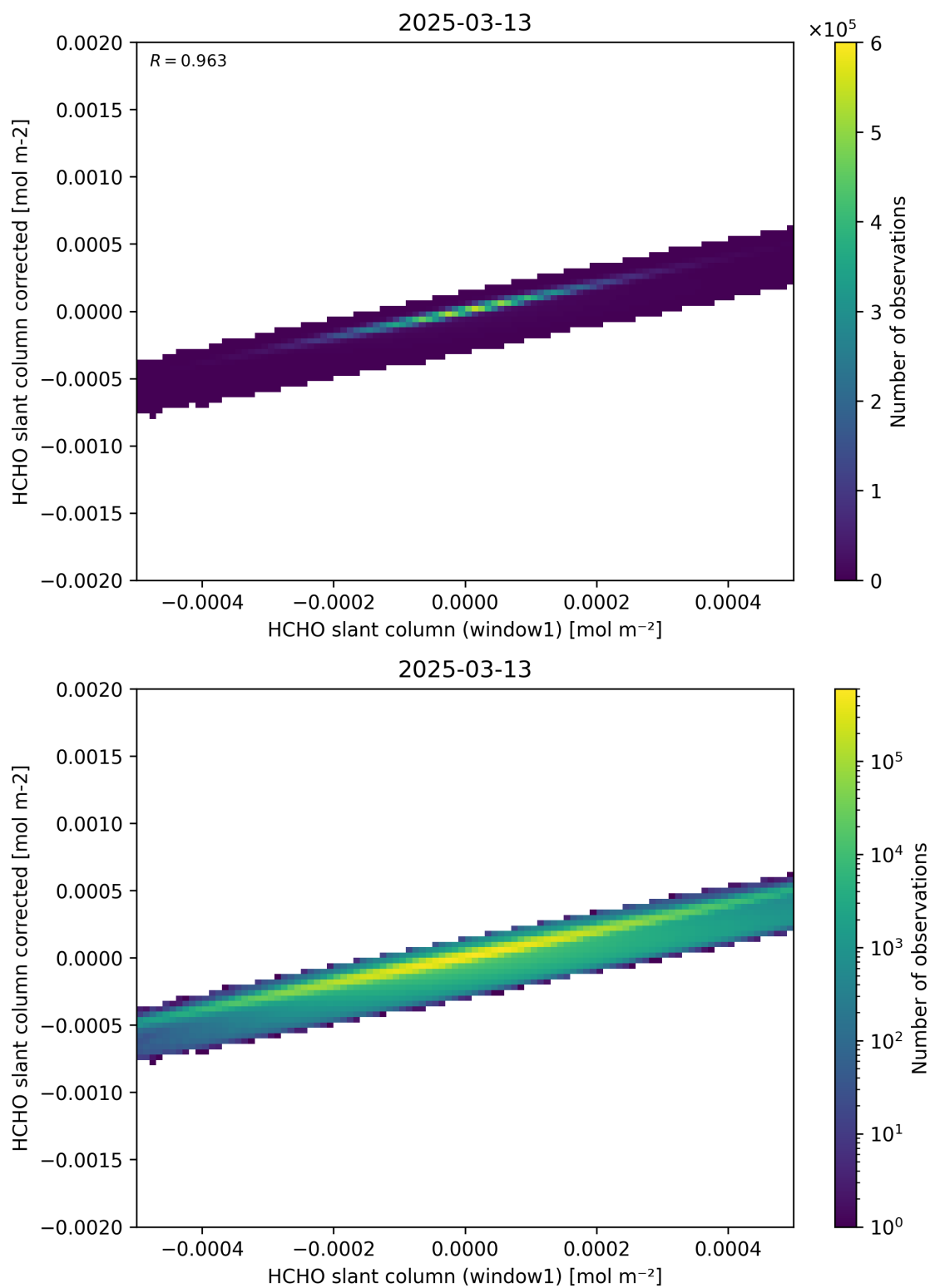
Figure 82: Scatter density plot of “HCHO slant column (window1)” against “HCHO slant column corrected” for 2025-03-12 to 2025-03-14.
