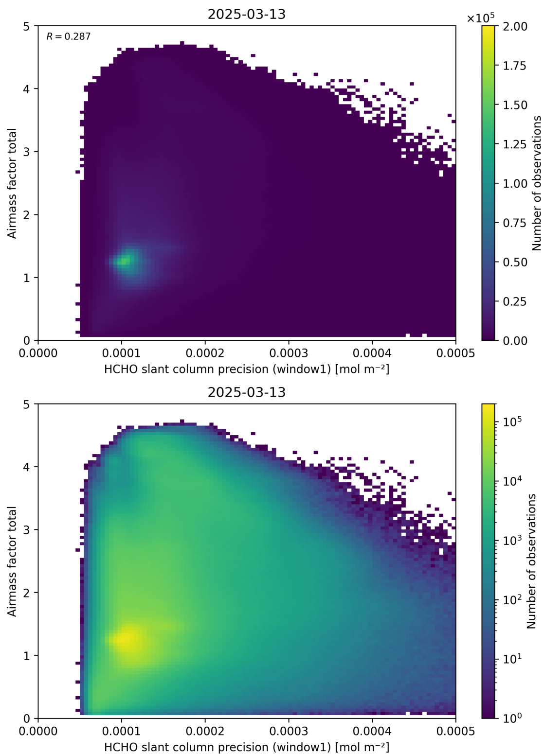
Figure 94: Scatter density plot of “HCHO slant column precision (window1)” against “Airmass factor total” for 2025-03-12 to 2025-03-14.
