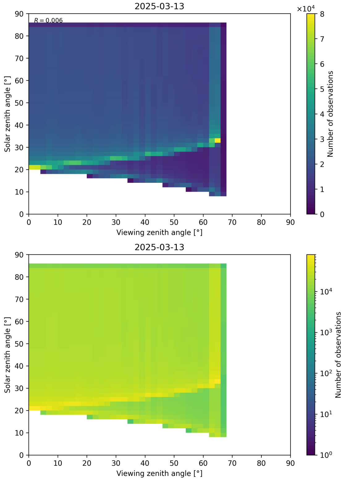
Figure 197: Scatter density plot of “Viewing zenith angle” against “Solar zenith angle” for 2025-03-12 to 2025-03-14.
