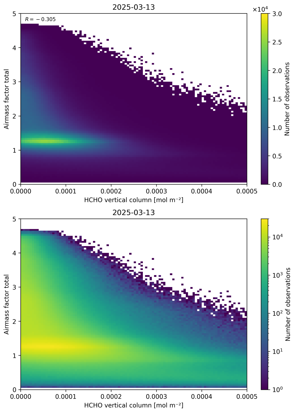
Figure 131: Scatter density plot of “HCHO vertical column” against “Airmass factor total” for 2025-03-12 to 2025-03-14.
