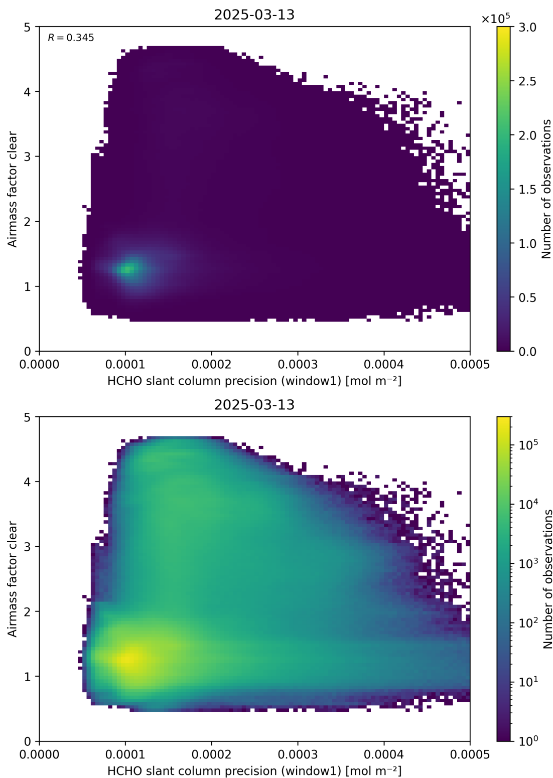
Figure 91: Scatter density plot of “HCHO slant column precision (window1)” against “Airmass factor clear” for 2025-03-12 to 2025-03-14.
