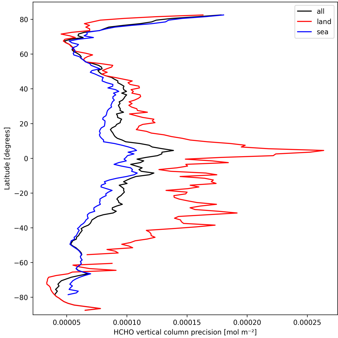
Figure 22: Zonal average of “HCHO vertical column precision” for 2025-03-12 to 2025-03-14.
