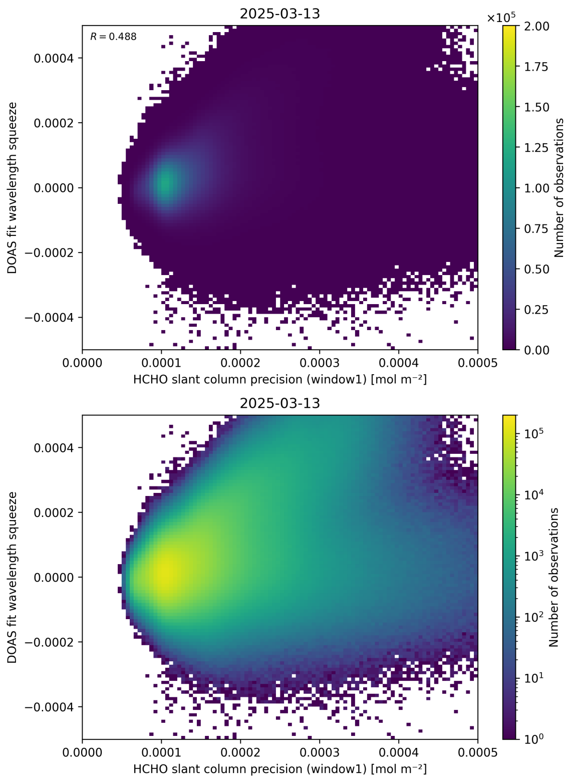
Figure 90: Scatter density plot of “HCHO slant column precision (window1)” against “DOAS fit wavelength squeeze” for 2025-03-12 to 2025-03-14.
