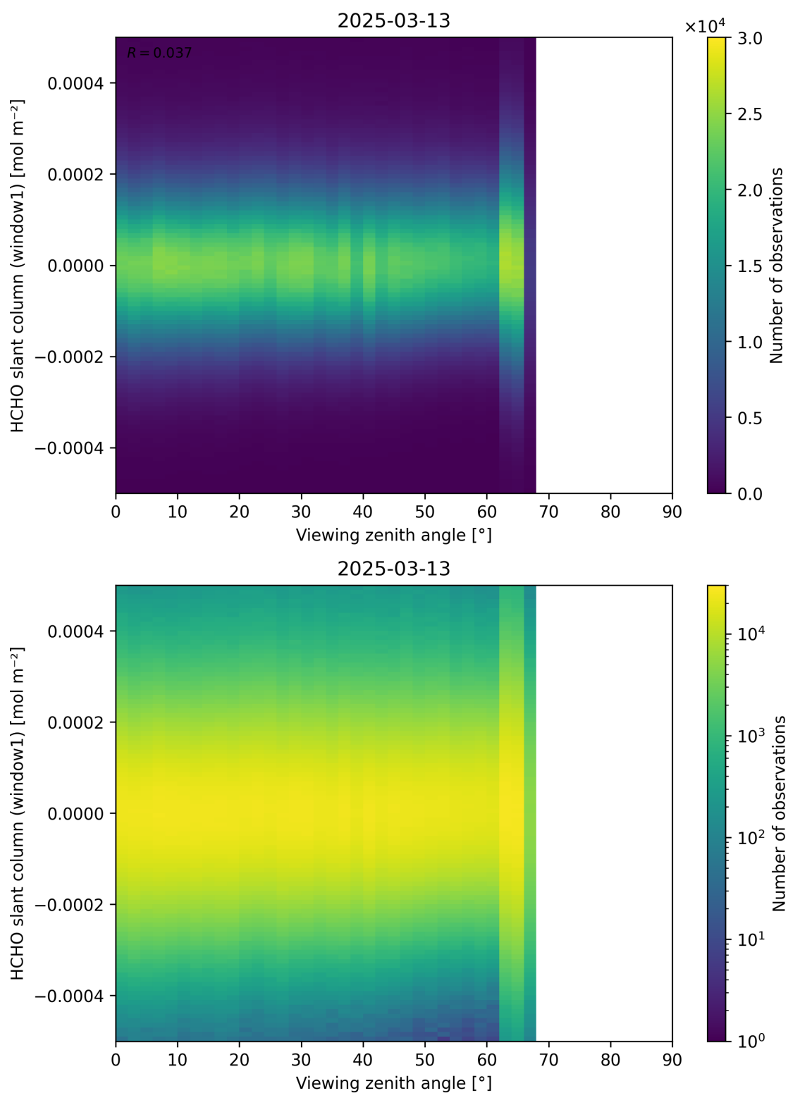
Figure 188: Scatter density plot of “Viewing zenith angle” against “HCHO slant column (window1)” for 2025-03-12 to 2025-03-14.
