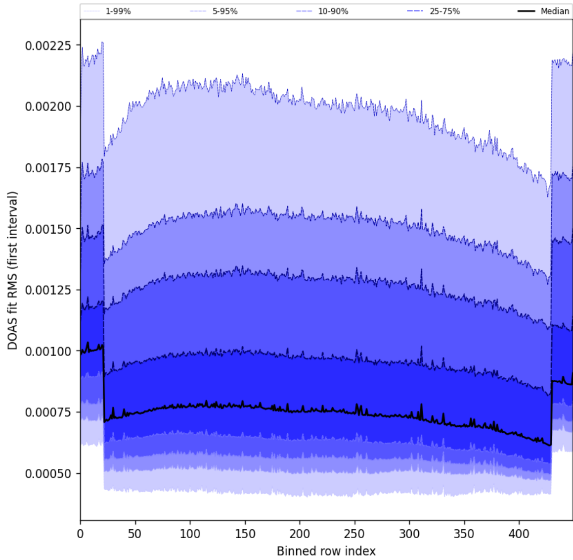
Figure 60: Along track statistics of “DOAS fit RMS (first interval)” for 2025-03-12 to 2025-03-14
