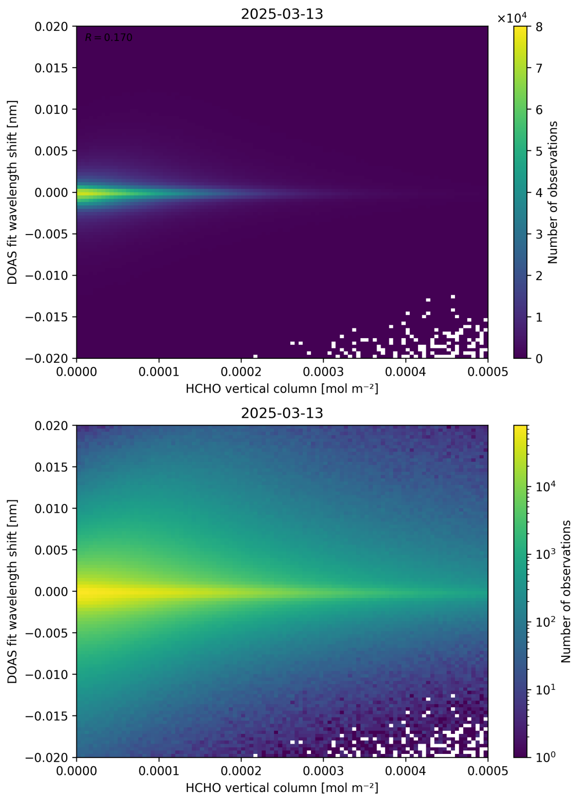
Figure 124: Scatter density plot of “HCHO vertical column” against “DOAS fit wavelength shift” for 2025-03-12 to 2025-03-14.
