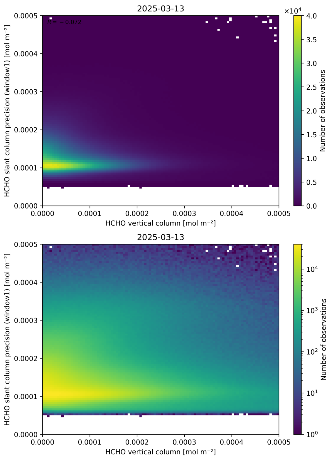
Figure 130: Scatter density plot of “HCHO vertical column” against “HCHO slant column precision (window1)” for 2025-03-12 to 2025-03-14.
