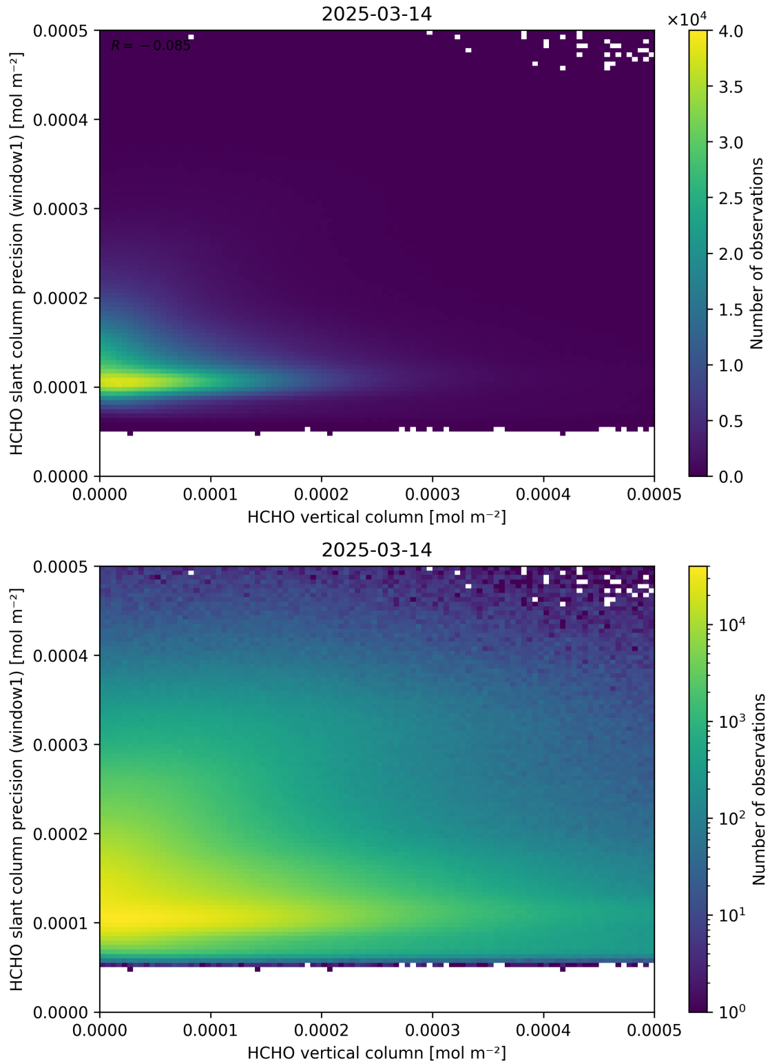
Figure 130: Scatter density plot of “HCHO vertical column” against “HCHO slant column precision (window1)” for 2025-03-13 to 2025-03-15.
