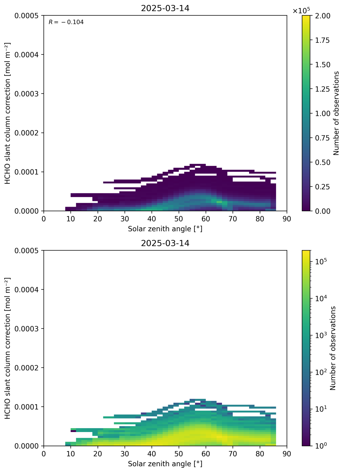
Figure 172: Scatter density plot of “Solar zenith angle” against “HCHO slant column correction” for 2025-03-13 to 2025-03-15.
