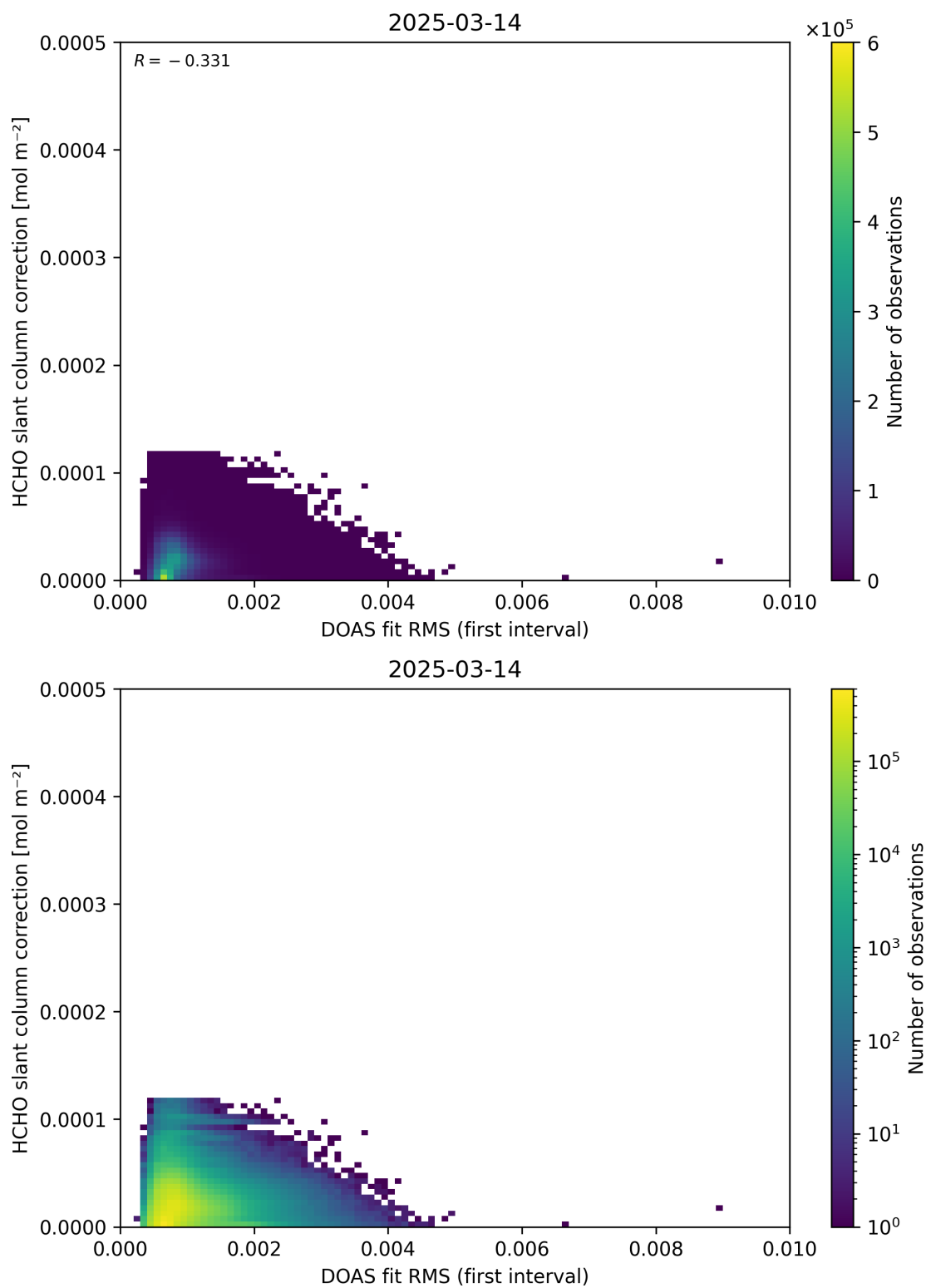
Figure 63: Scatter density plot of “DOAS fit RMS (first interval)” against “HCHO slant column correction” for 2025-03-13 to 2025-03-15.
