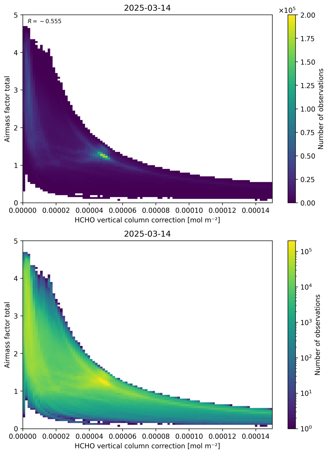
Figure 120: Scatter density plot of “HCHO vertical column correction” against “Airmass factor total” for 2025-03-13 to 2025-03-15.
