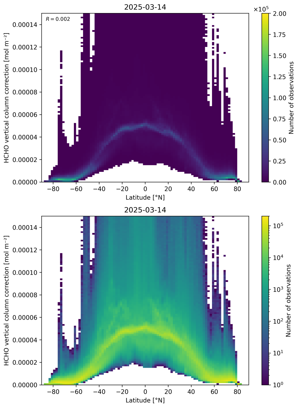
Figure 164: Scatter density plot of “Latitude” against “HCHO vertical column correction” for 2025-03-13 to 2025-03-15.
