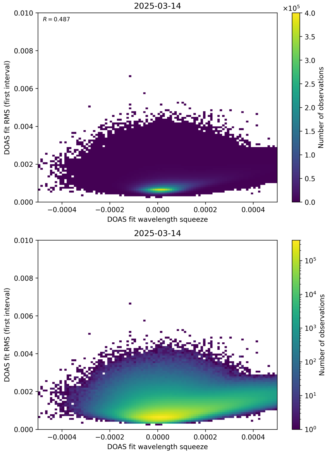
Figure 68: Scatter density plot of “DOAS fit wavelength squeeze” against “DOAS fit RMS (first interval)” for 2025-03-13 to 2025-03-15.
