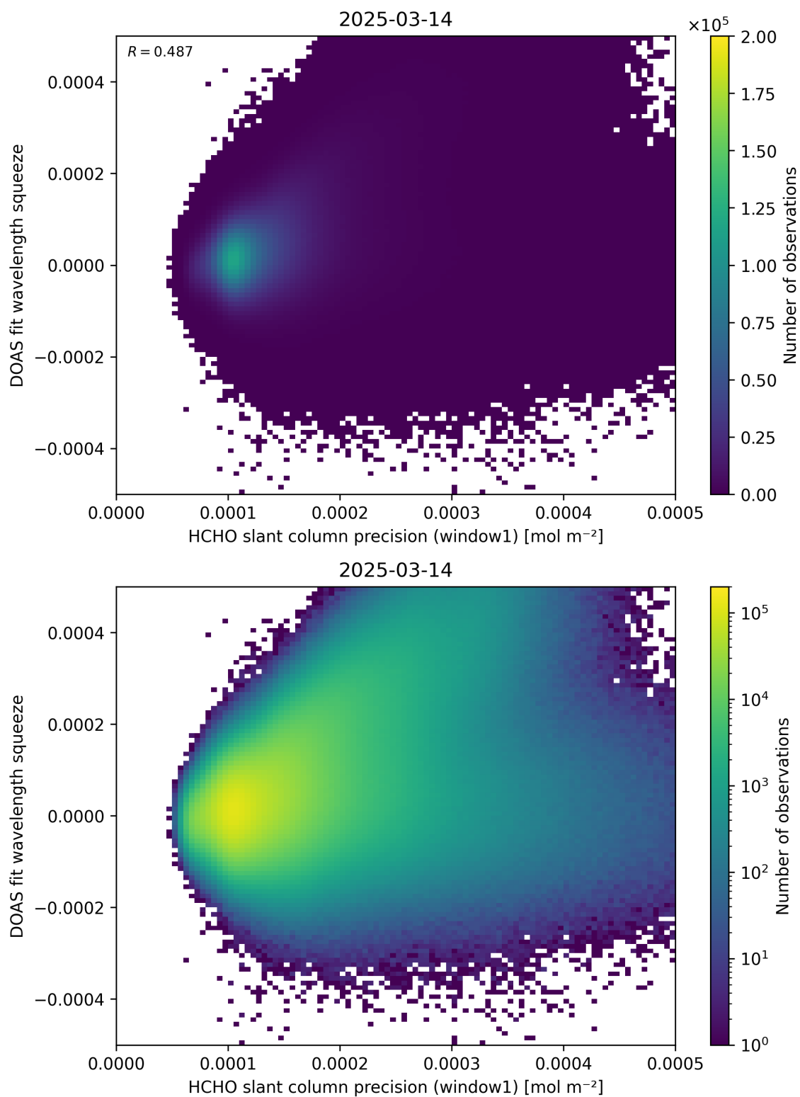
Figure 90: Scatter density plot of “HCHO slant column precision (window1)” against “DOAS fit wavelength squeeze” for 2025-03-13 to 2025-03-15.
