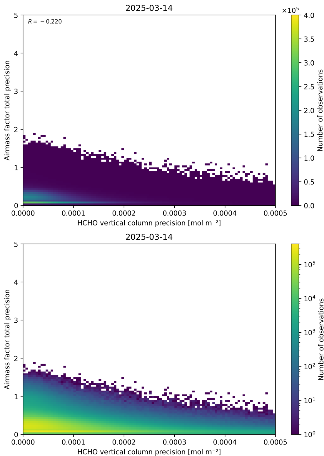
Figure 145: Scatter density plot of “HCHO vertical column precision” against “Airmass factor total precision” for 2025-03-13 to 2025-03-15.
