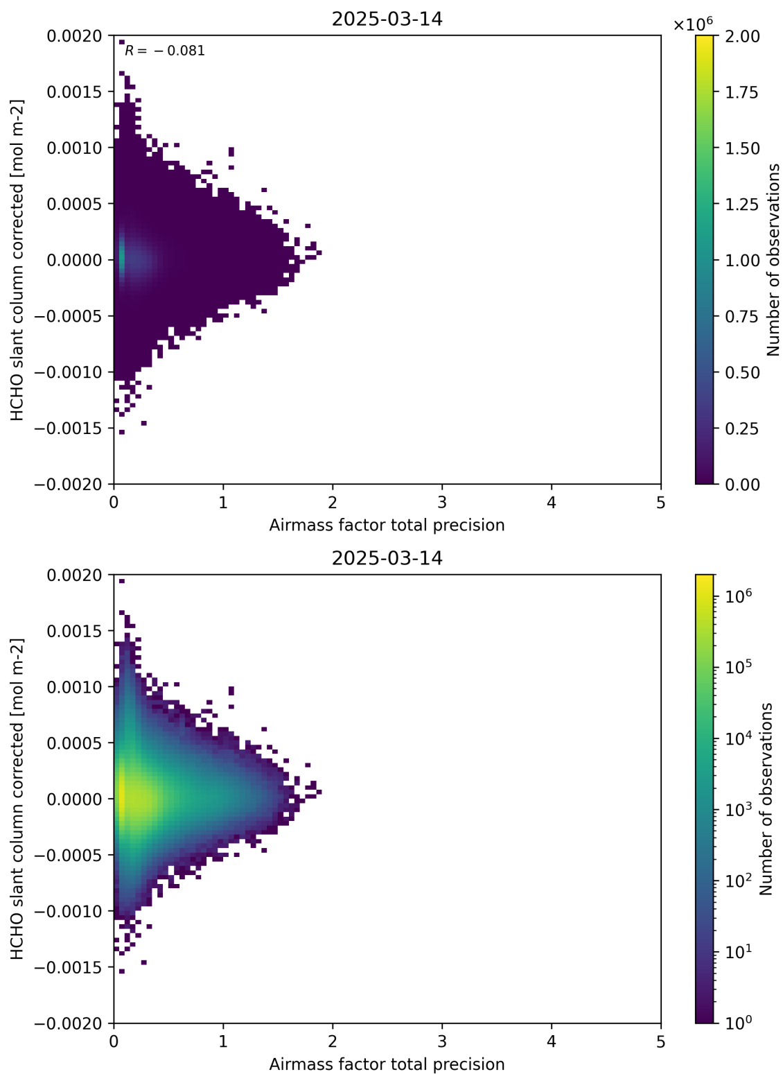
Figure 109: Scatter density plot of “Airmass factor total precision” against “HCHO slant column corrected” for 2025-03-13 to 2025-03-15.
