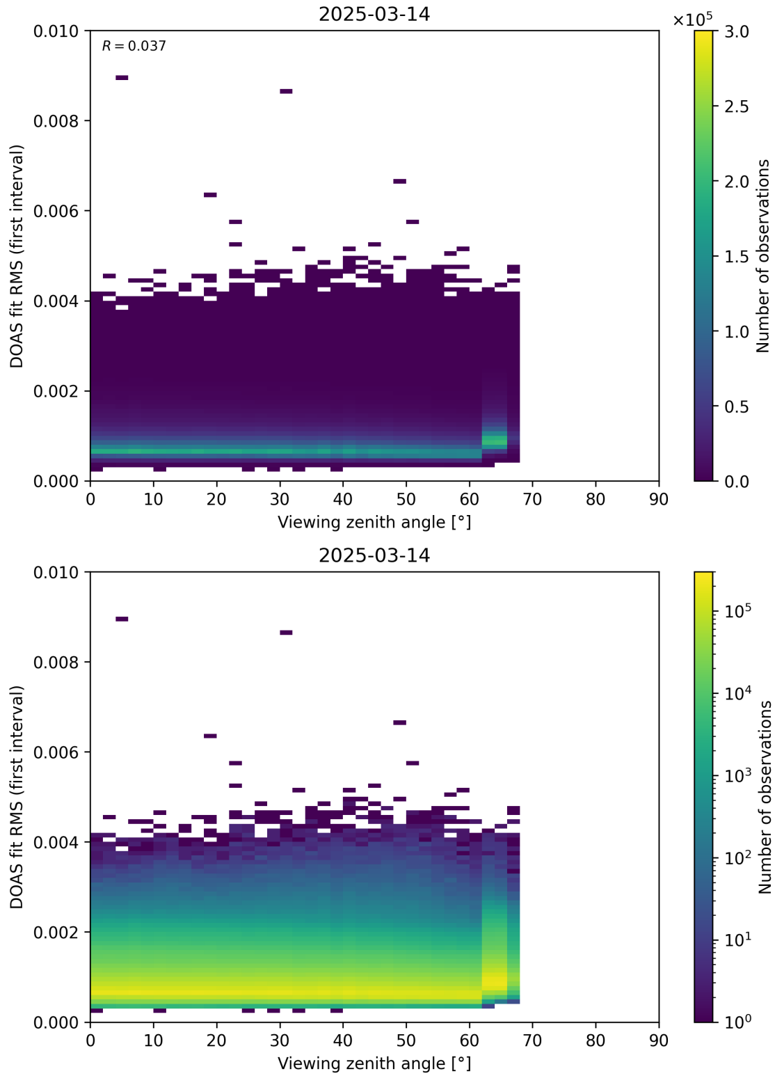
Figure 182: Scatter density plot of “Viewing zenith angle” against “DOAS fit RMS (first interval)” for 2025-03-13 to 2025-03-15.
