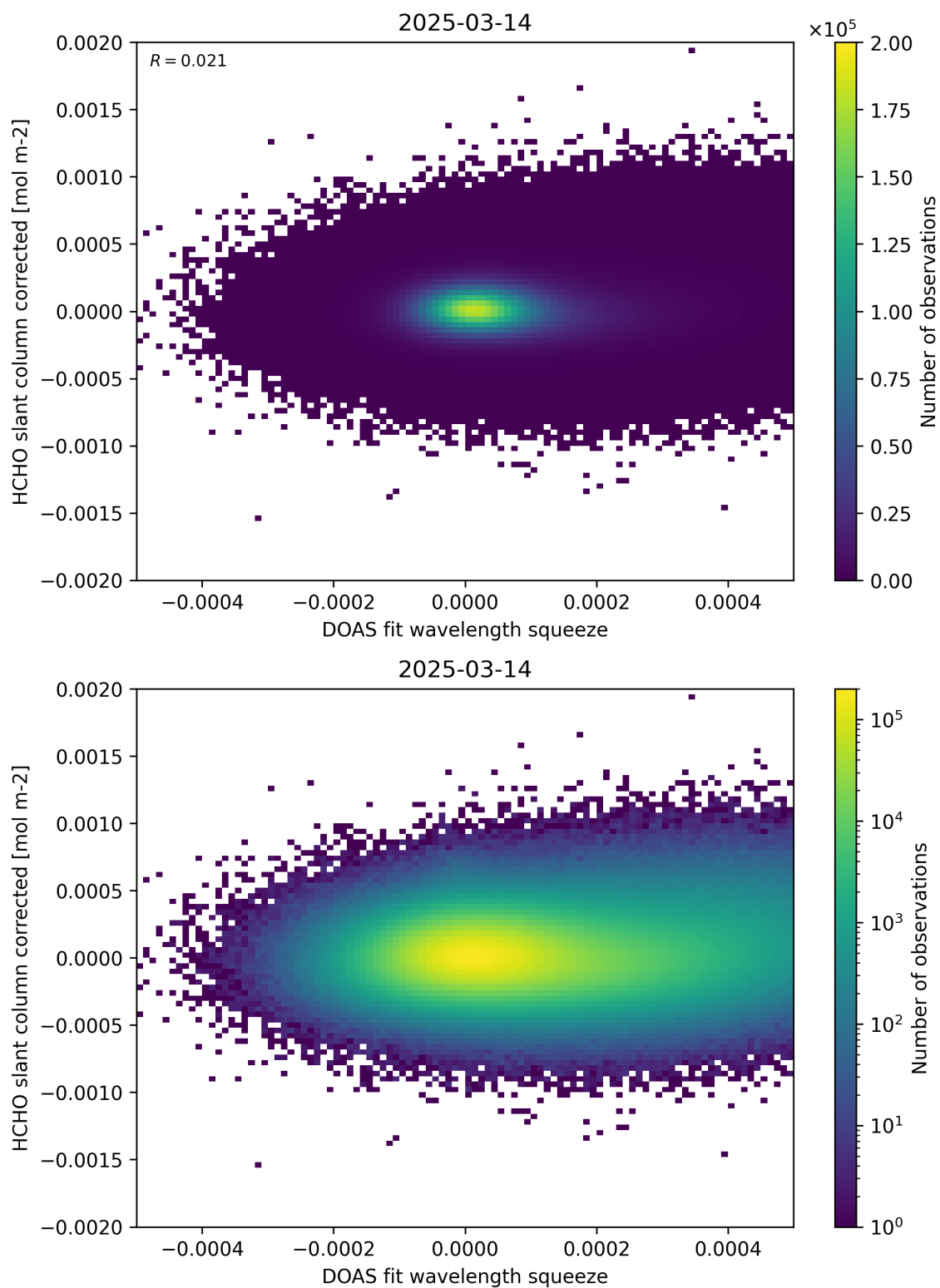
Figure 69: Scatter density plot of “DOAS fit wavelength squeeze” against “HCHO slant column corrected” for 2025-03-13 to 2025-03-15.
