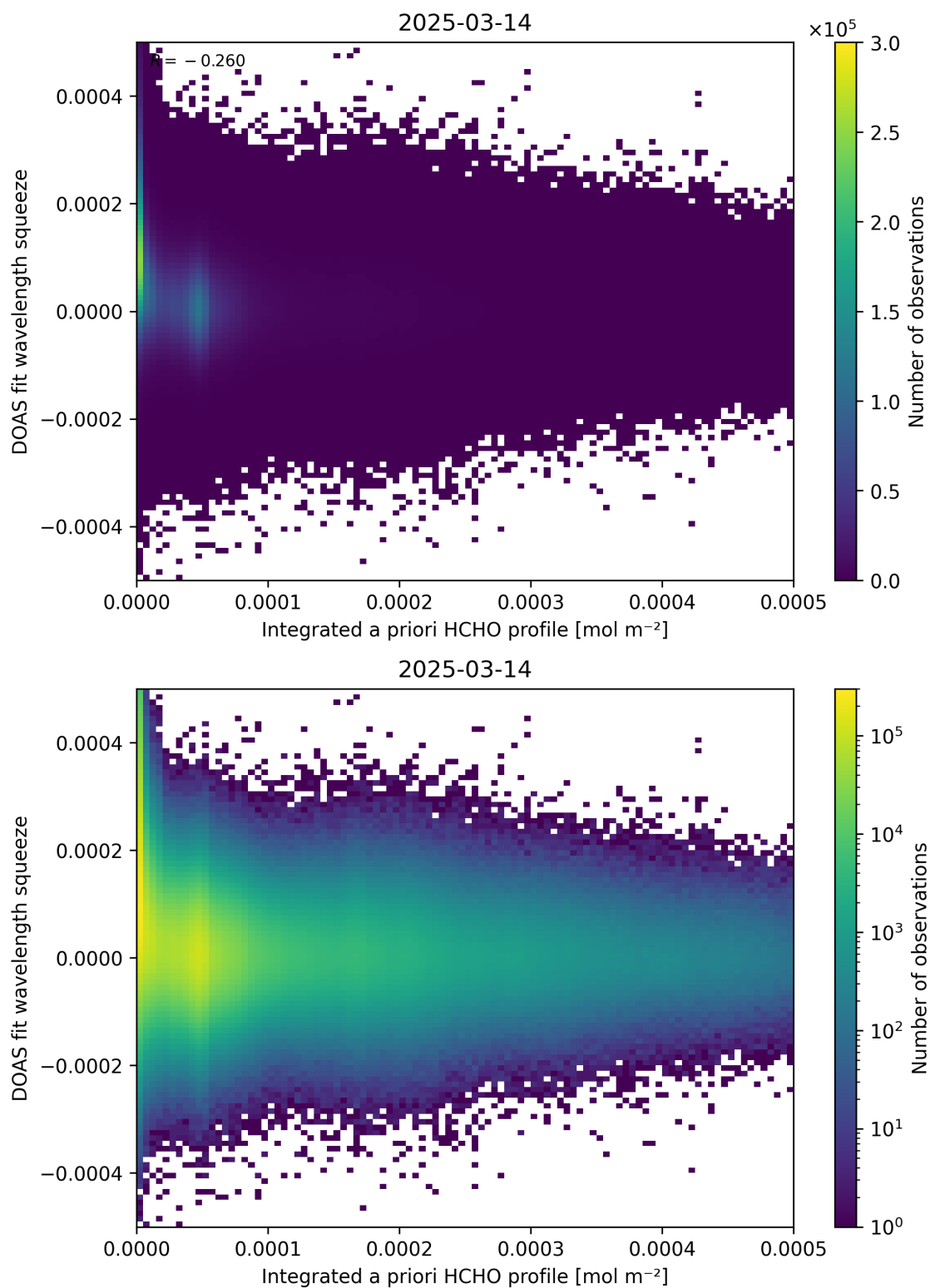
Figure 150: Scatter density plot of “Integrated a priori HCHO profile” against “DOAS fit wavelength squeeze” for 2025-03-13 to 2025-03-15.
