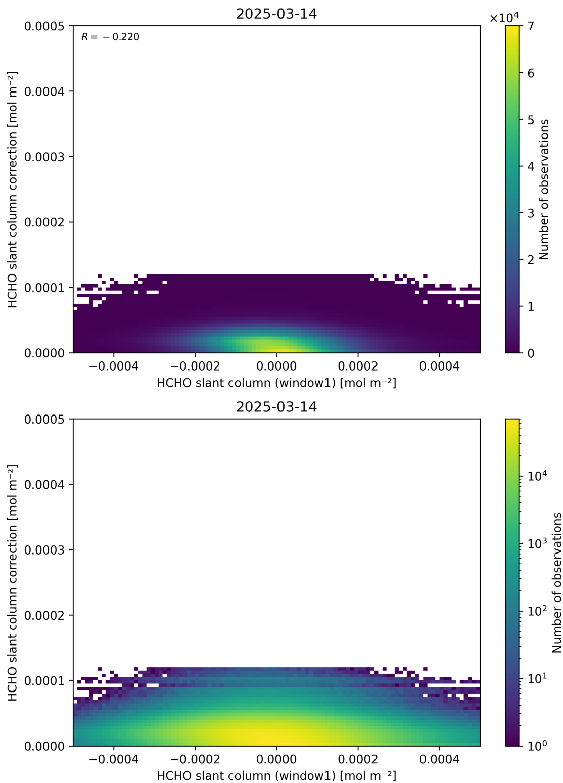
Figure 83: Scatter density plot of “HCHO slant column (window1)” against “HCHO slant column correction” for 2025-03-13 to 2025-03-15.
