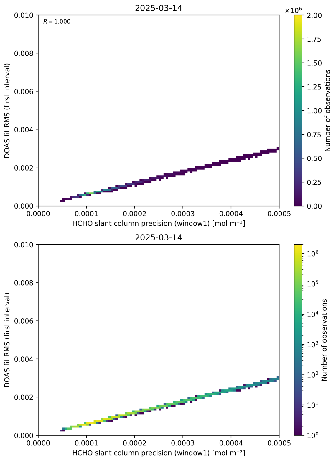
Figure 88: Scatter density plot of “HCHO slant column precision (window1)” against “DOAS fit RMS (first interval)” for 2025-03-13 to 2025-03-15.
