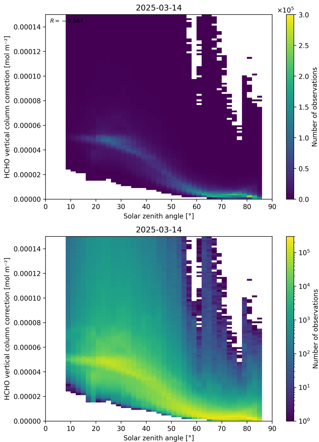
Figure 178: Scatter density plot of “Solar zenith angle” against “HCHO vertical column correction” for 2025-03-13 to 2025-03-15.
