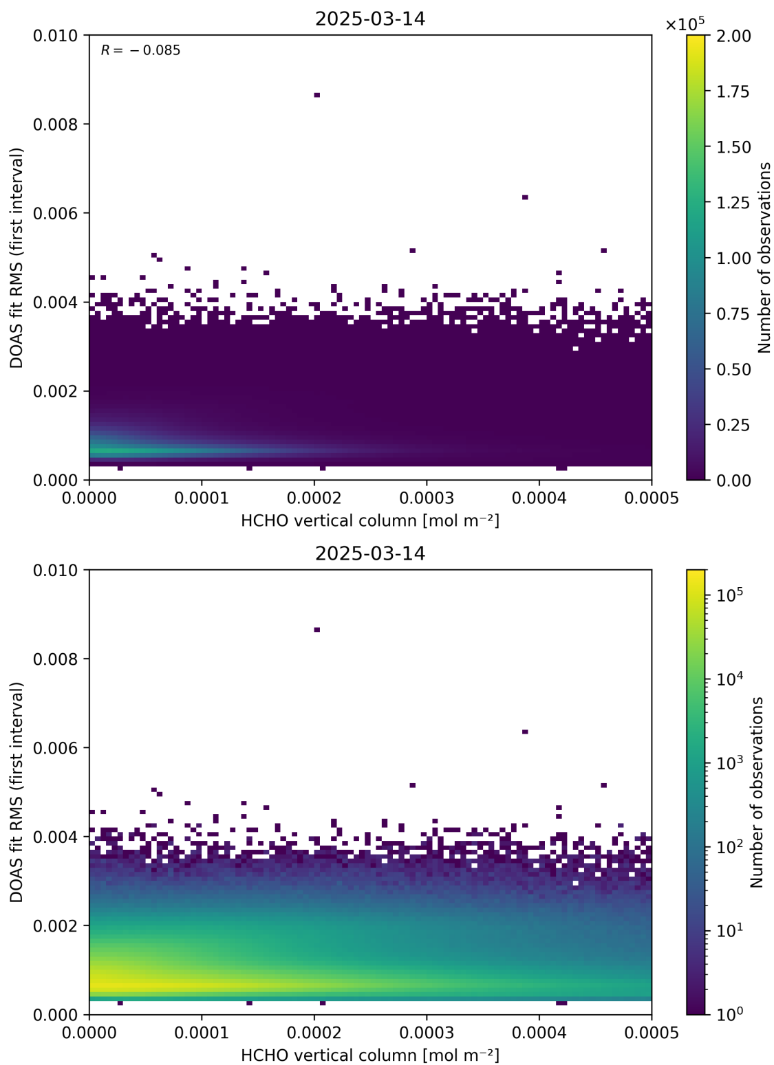
Figure 123: Scatter density plot of “HCHO vertical column” against “DOAS fit RMS (first interval)” for 2025-03-13 to 2025-03-15.
