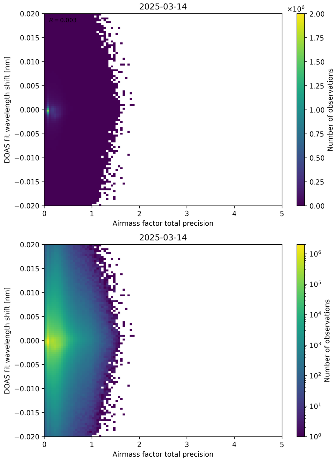
Figure 106: Scatter density plot of “Airmass factor total precision” against “DOAS fit wavelength shift” for 2025-03-13 to 2025-03-15.
