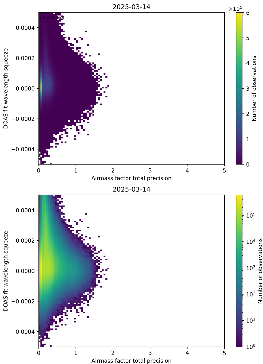
Figure 107: Scatter density plot of “Airmass factor total precision” against “DOAS fit wavelength squeeze” for 2025-03-13 to 2025-03-15.
