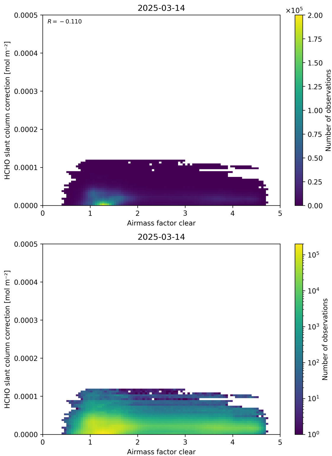
Figure 75: Scatter density plot of “Airmass factor clear” against “HCHO slant column correction” for 2025-03-13 to 2025-03-15.
