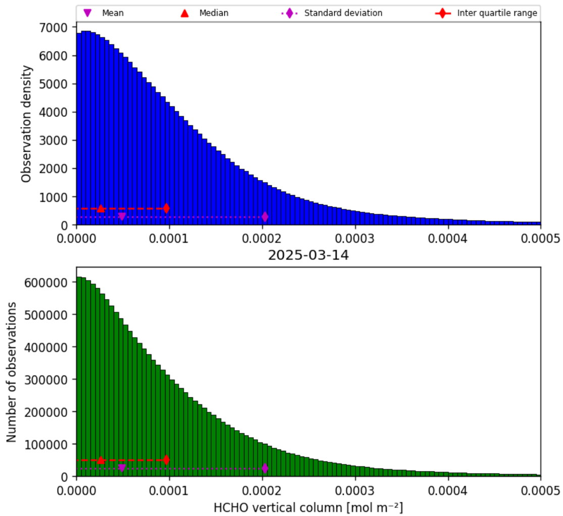
Figure 35: Histogram of “HCHO vertical column” for 2025-03-13 to 2025-03-15
