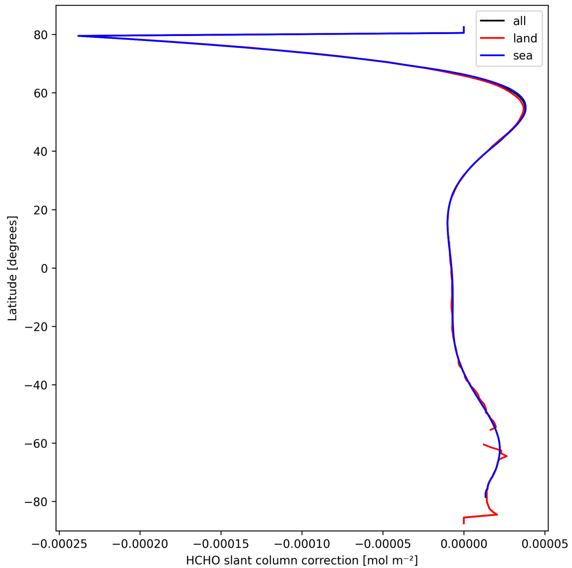
Figure 33: Zonal average of “HCHO slant column correction” for 2025-03-13 to 2025-03-15.
