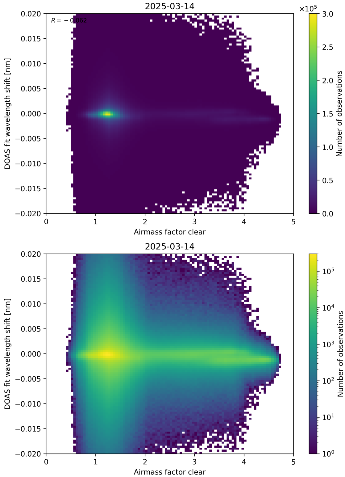
Figure 72: Scatter density plot of “Airmass factor clear” against “DOAS fit wavelength shift” for 2025-03-13 to 2025-03-15.
