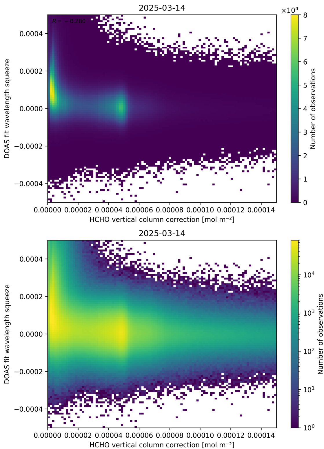
Figure 114: Scatter density plot of “HCHO vertical column correction” against “DOAS fit wavelength squeeze” for 2025-03-13 to 2025-03-15.
