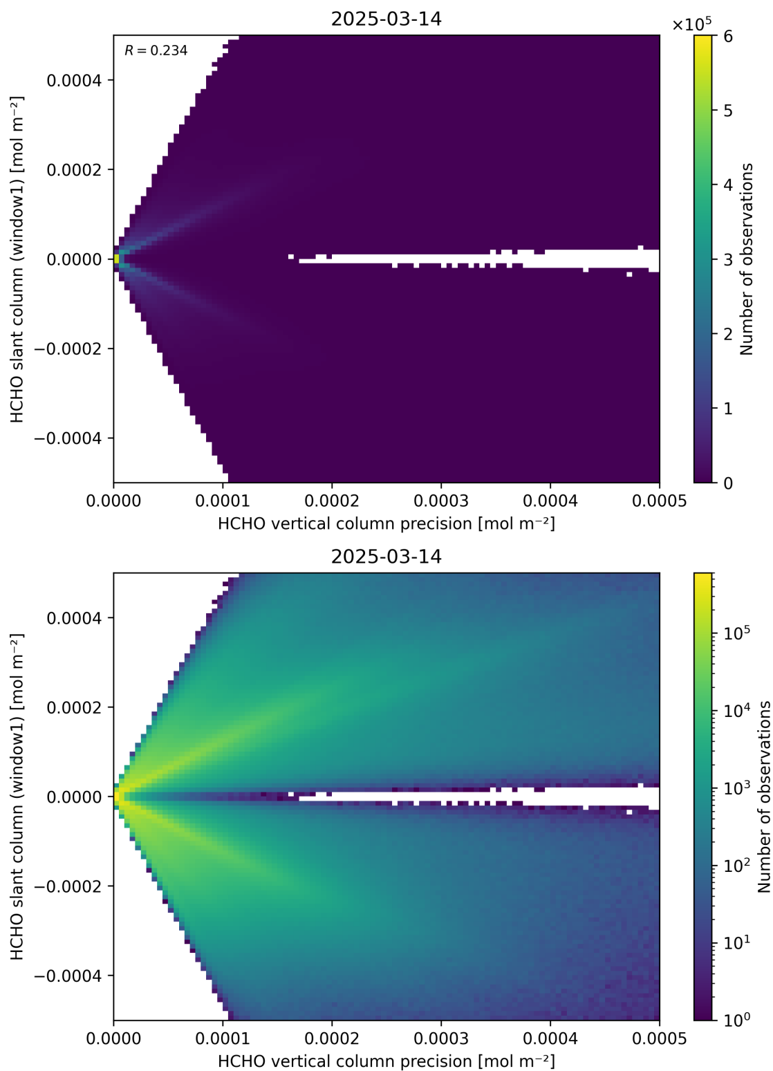
Figure 142: Scatter density plot of “HCHO vertical column precision” against “HCHO slant column (window1)” for 2025-03-13 to 2025-03-15.
