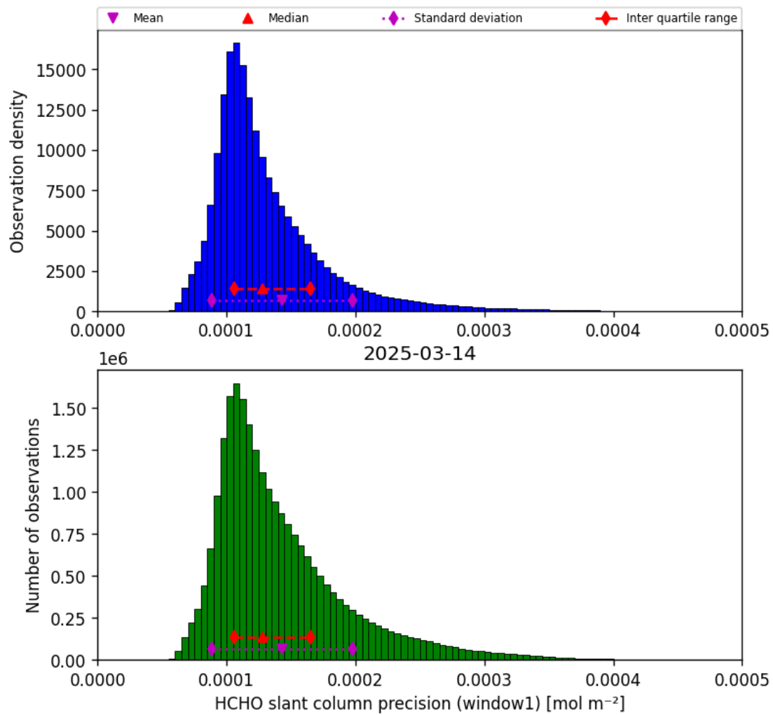
Figure 39: Histogram of “HCHO slant column precision (window1)” for 2025-03-13 to 2025-03-15
