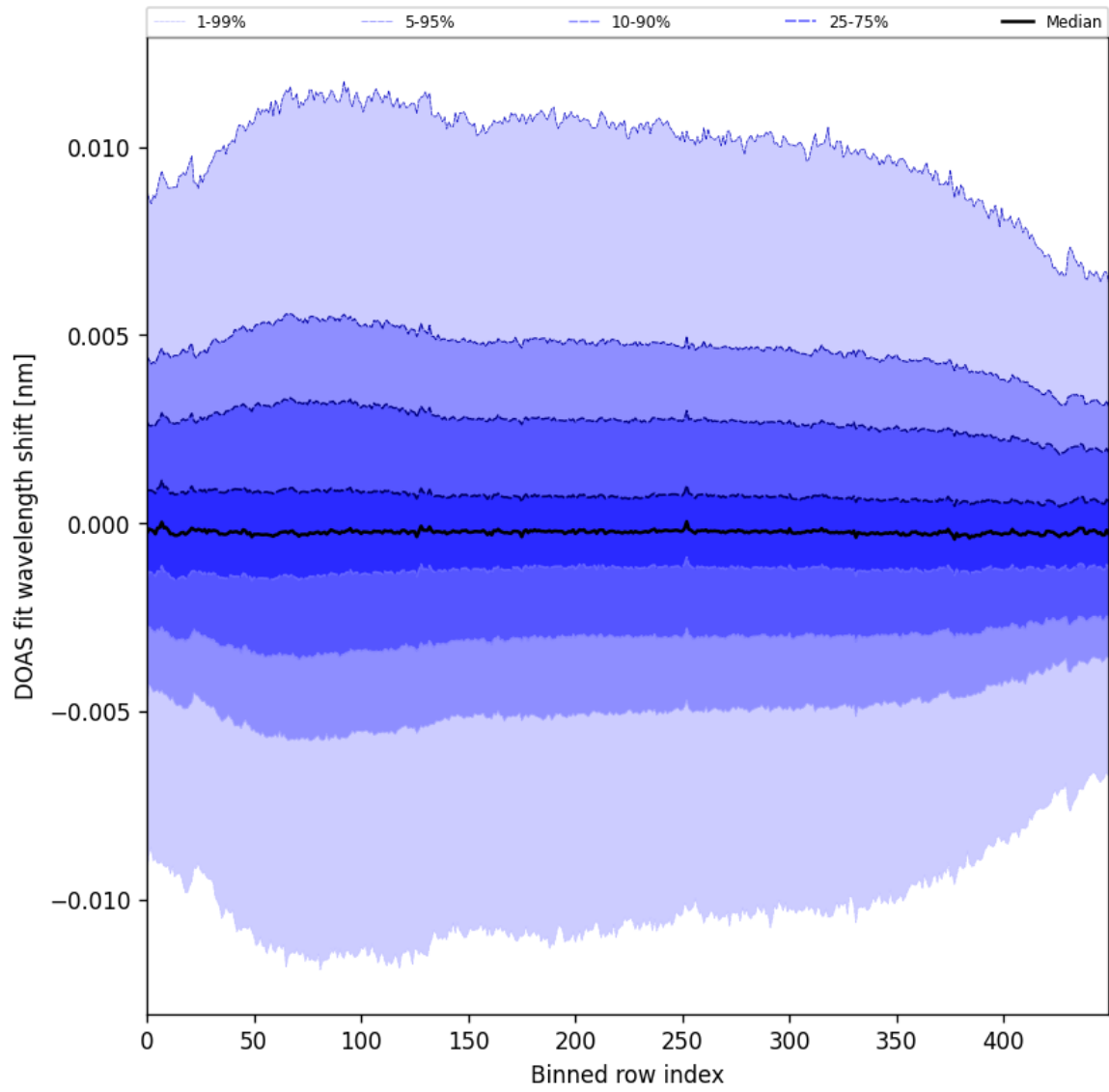
Figure 58: Along track statistics of “DOAS fit wavelength shift” for 2025-03-13 to 2025-03-15
