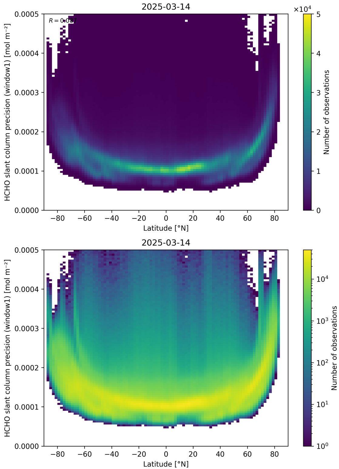
Figure 160: Scatter density plot of “Latitude” against “HCHO slant column precision (window1)” for 2025-03-13 to 2025-03-15.
