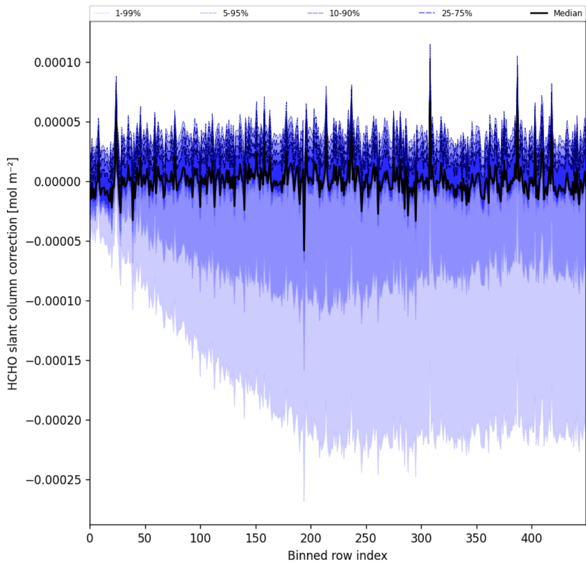
Figure 61: Along track statistics of “HCHO slant column correction” for 2025-03-13 to 2025-03-15
