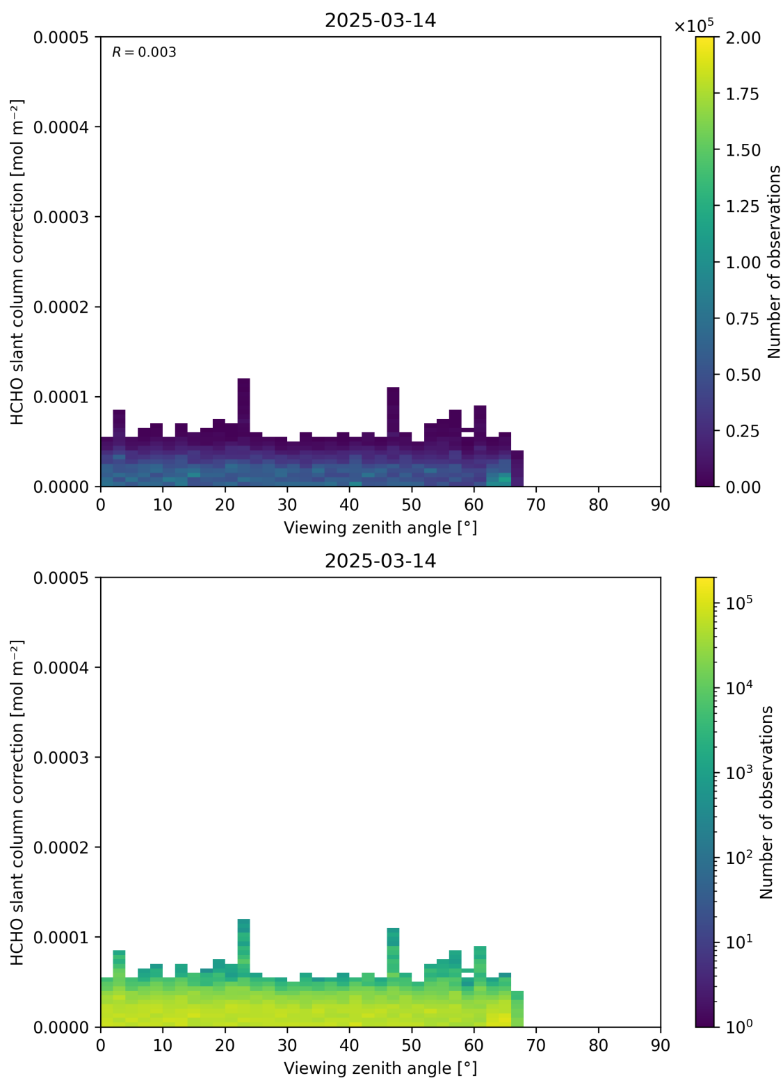
Figure 187: Scatter density plot of “Viewing zenith angle” against “HCHO slant column correction” for 2025-03-13 to 2025-03-15.
