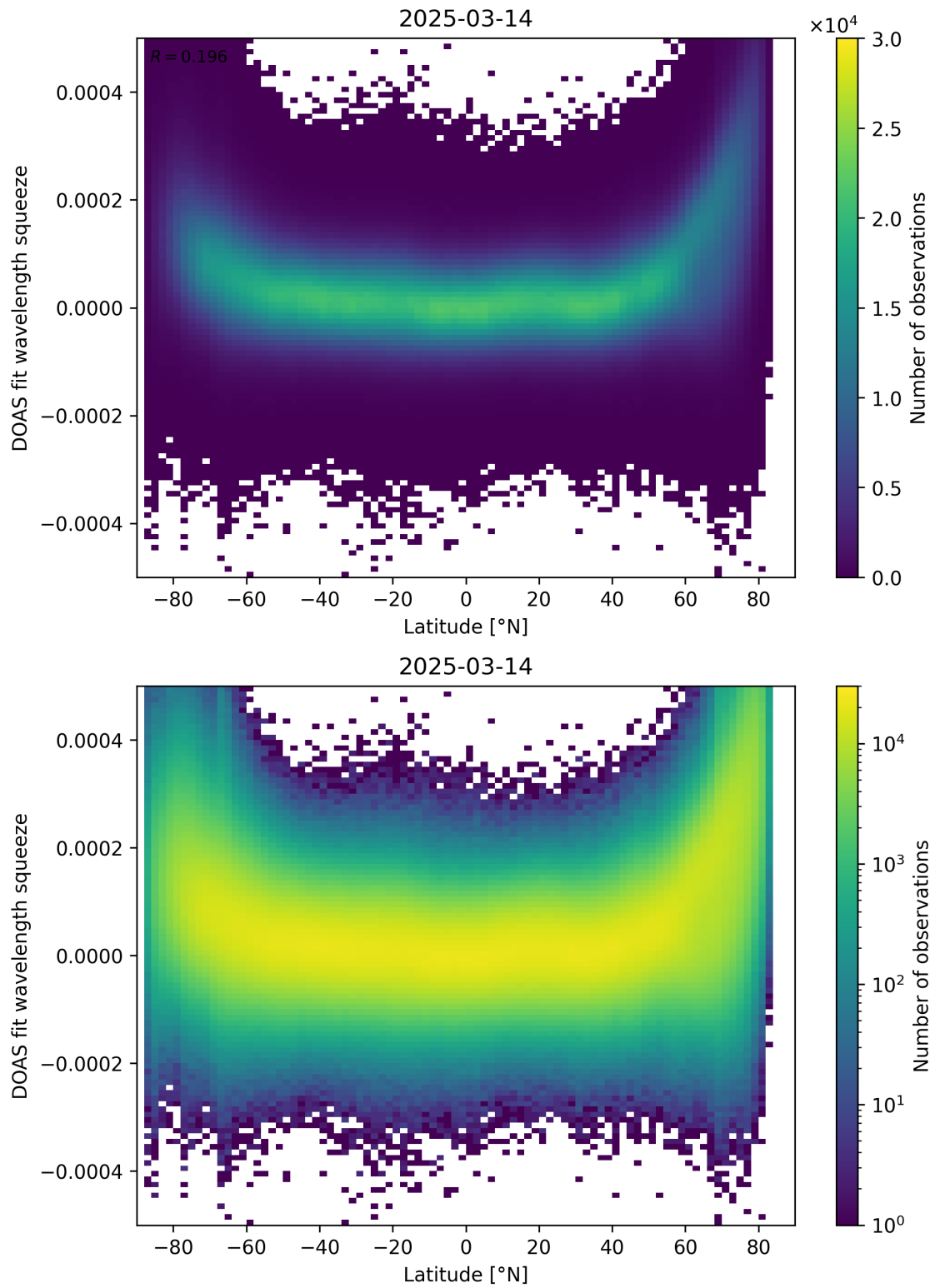
Figure 155: Scatter density plot of “Latitude” against “DOAS fit wavelength squeeze” for 2025-03-13 to 2025-03-15.
