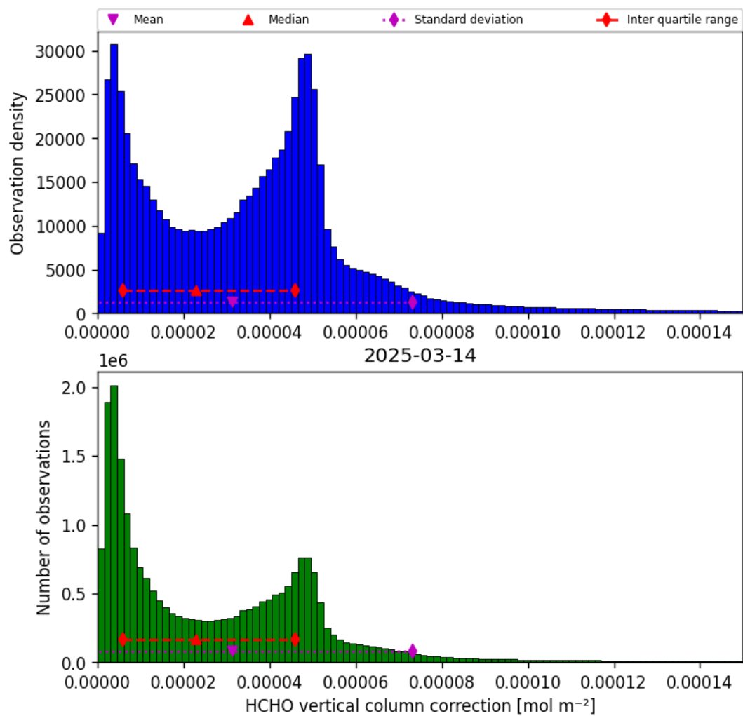
Figure 37: Histogram of “HCHO vertical column correction” for 2025-03-13 to 2025-03-15
