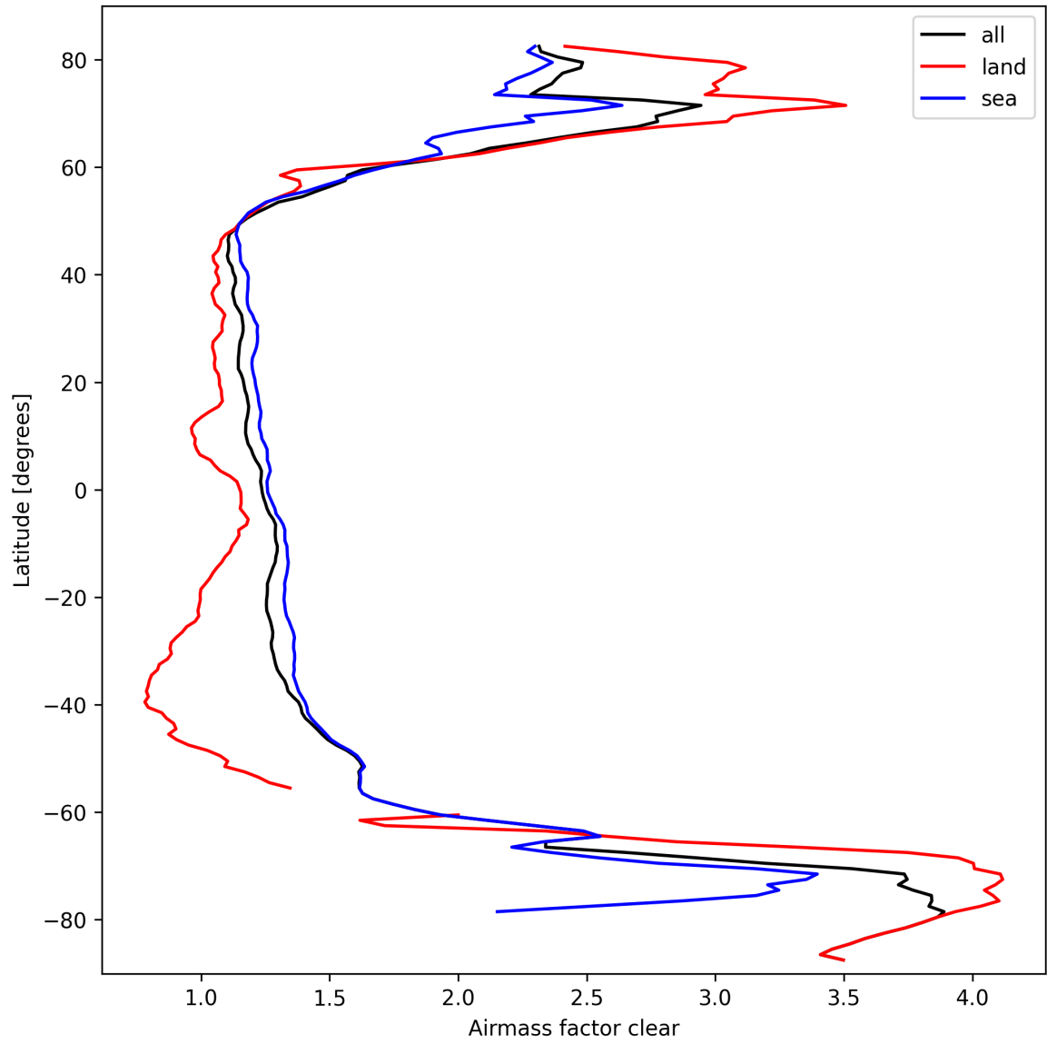
Figure 28: Zonal average of “Airmass factor clear” for 2025-03-13 to 2025-03-15.
