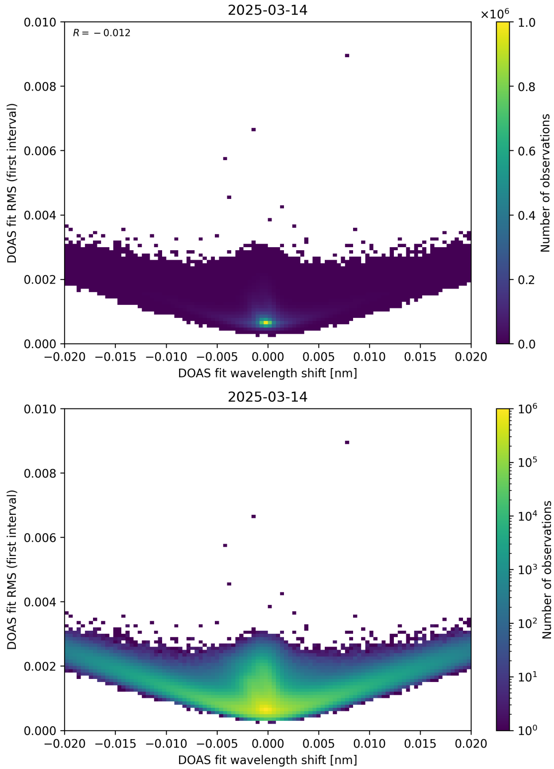
Figure 64: Scatter density plot of “DOAS fit wavelength shift” against “DOAS fit RMS (first interval)” for 2025-03-13 to 2025-03-15.
