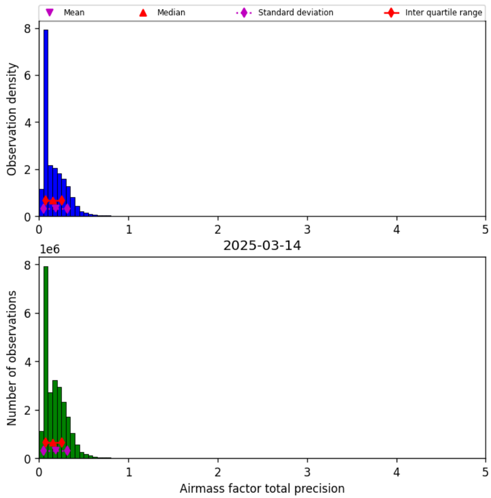
Figure 41: Histogram of “Airmass factor total precision” for 2025-03-13 to 2025-03-15
