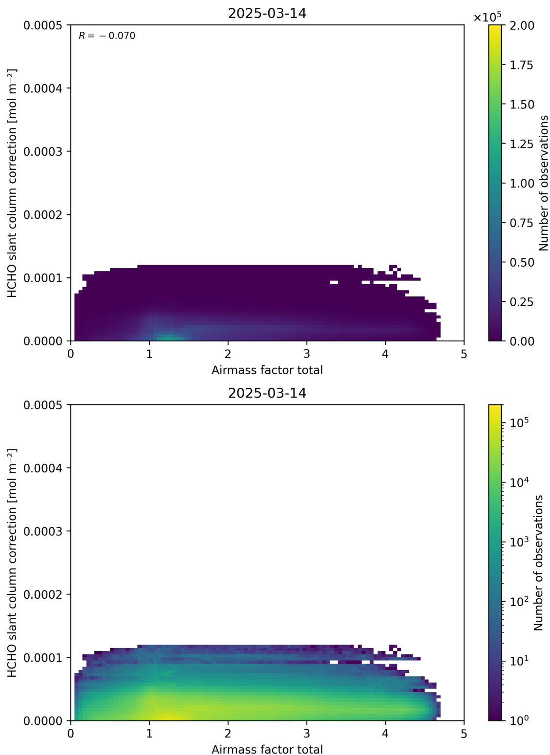
Figure 102: Scatter density plot of “Airmass factor total” against “HCHO slant column correction” for 2025-03-13 to 2025-03-15.
