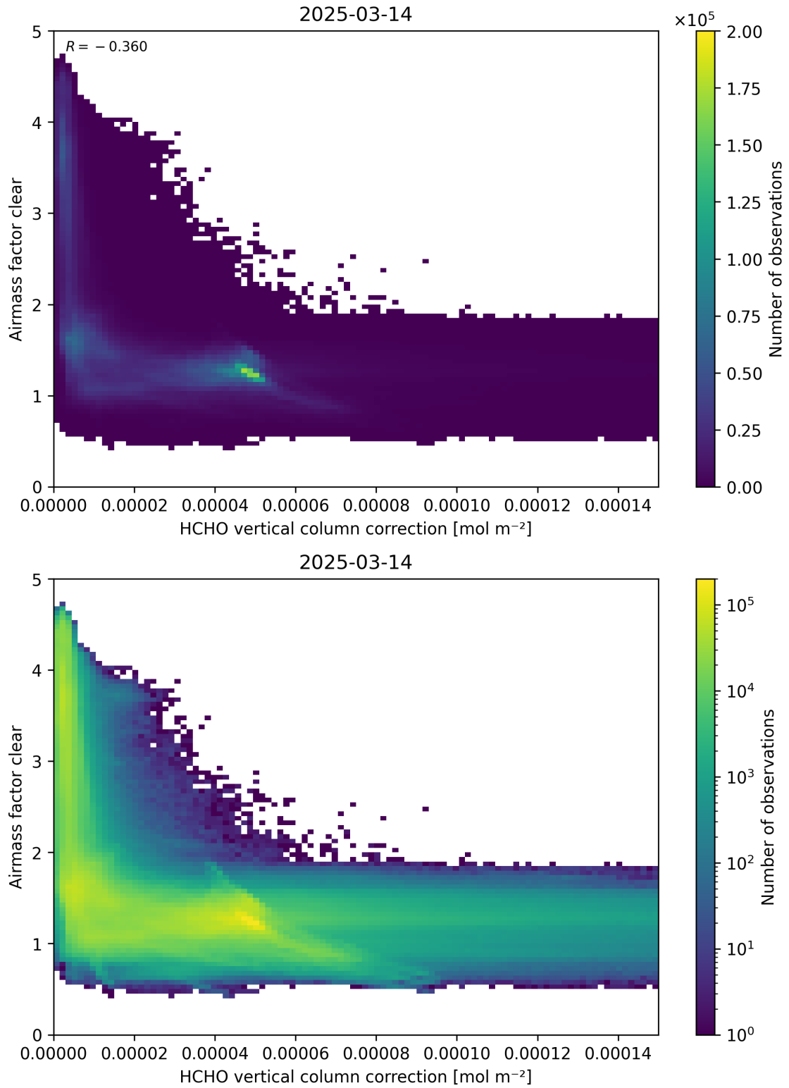
Figure 115: Scatter density plot of “HCHO vertical column correction” against “Airmass factor clear” for 2025-03-13 to 2025-03-15.
