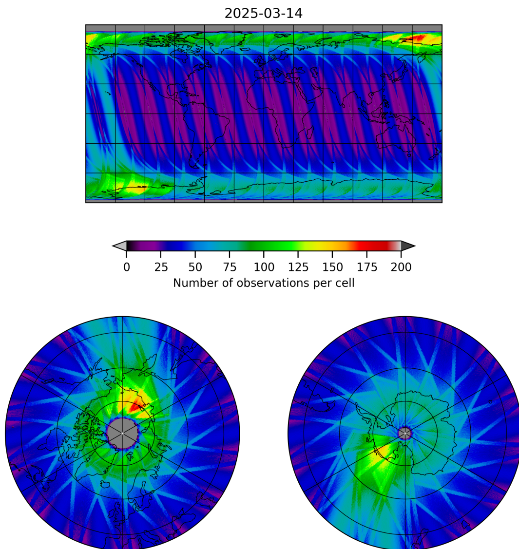
Figure 19: Map of the number of observations for 2025-03-13 to 2025-03-15
