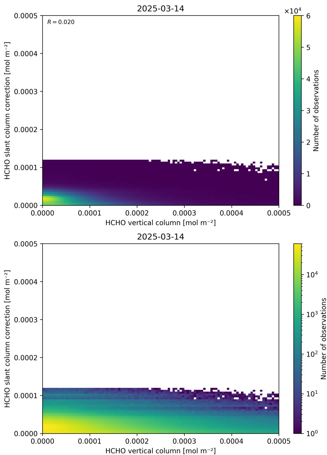
Figure 128: Scatter density plot of “HCHO vertical column” against “HCHO slant column correction” for 2025-03-13 to 2025-03-15.
