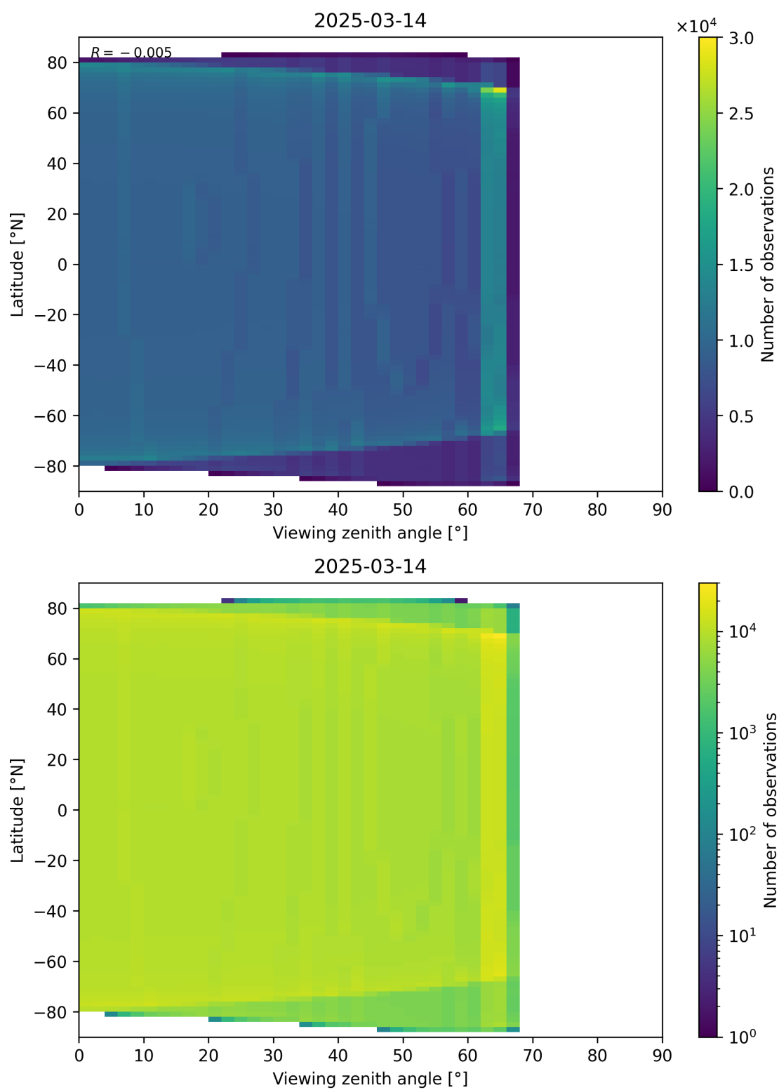
Figure 196: Scatter density plot of “Viewing zenith angle” against “Latitude” for 2025-03-13 to 2025-03-15.
