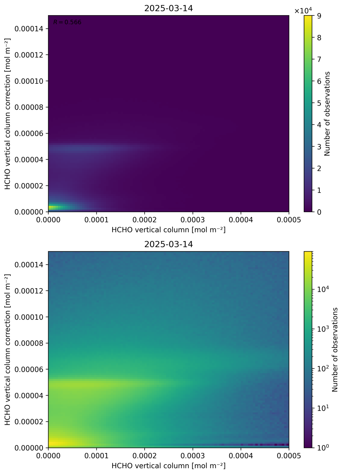
Figure 133: Scatter density plot of “HCHO vertical column” against “HCHO vertical column correction” for 2025-03-13 to 2025-03-15.
