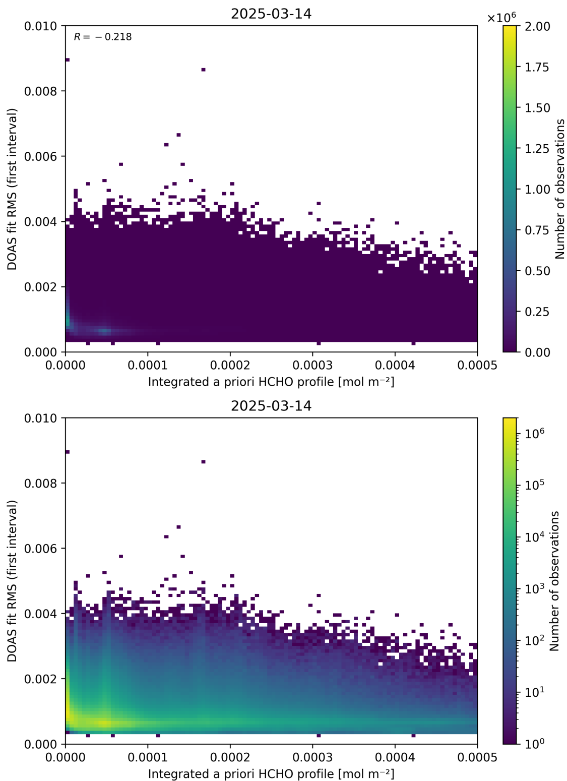
Figure 148: Scatter density plot of “Integrated a priori HCHO profile” against “DOAS fit RMS (first interval)” for 2025-03-13 to 2025-03-15.
