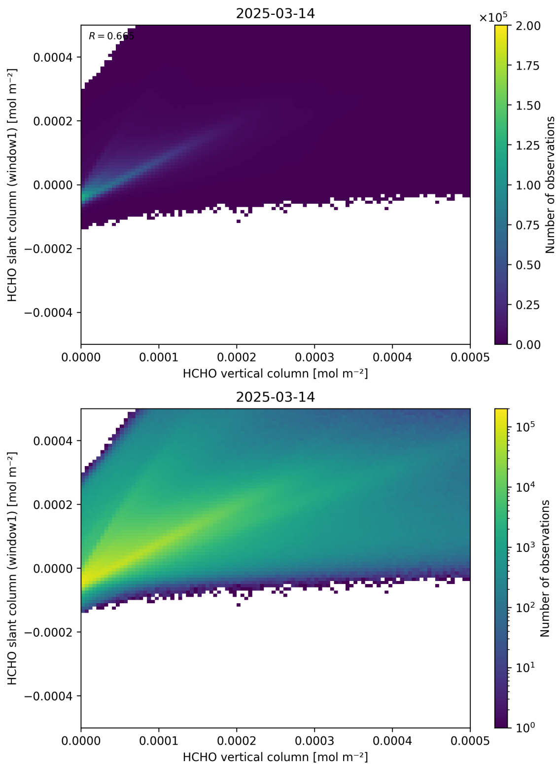
Figure 129: Scatter density plot of “HCHO vertical column” against “HCHO slant column (window1)” for 2025-03-13 to 2025-03-15.
