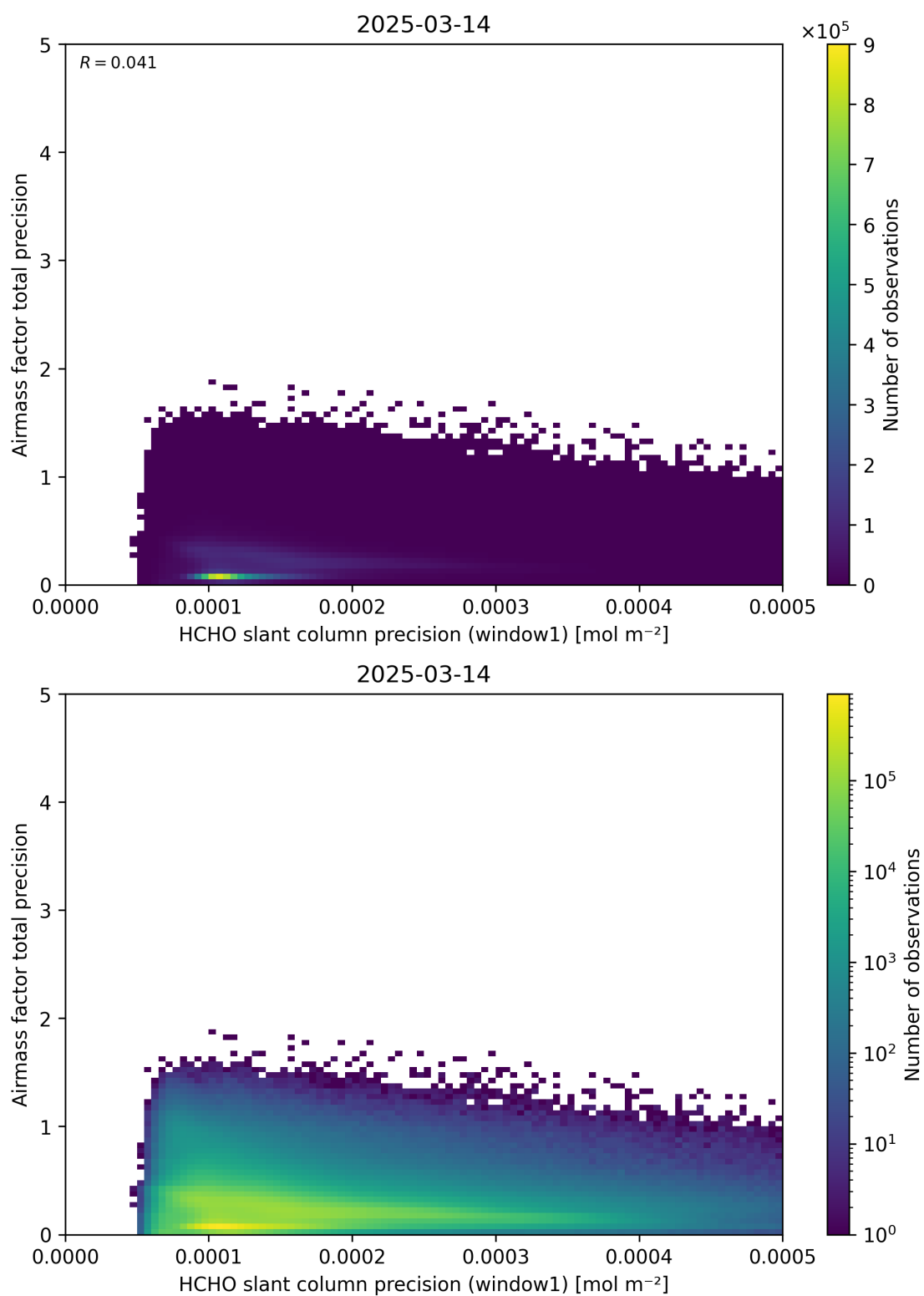
Figure 95: Scatter density plot of “HCHO slant column precision (window1)” against “Airmass factor total precision” for 2025-03-13 to 2025-03-15.
