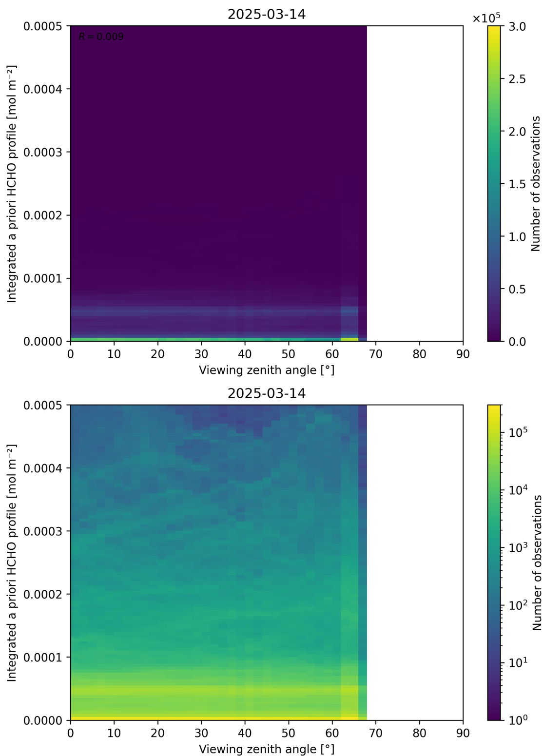
Figure 195: Scatter density plot of “Viewing zenith angle” against “Integrated a priori HCHO profile” for 2025-03-13 to 2025-03-15.
