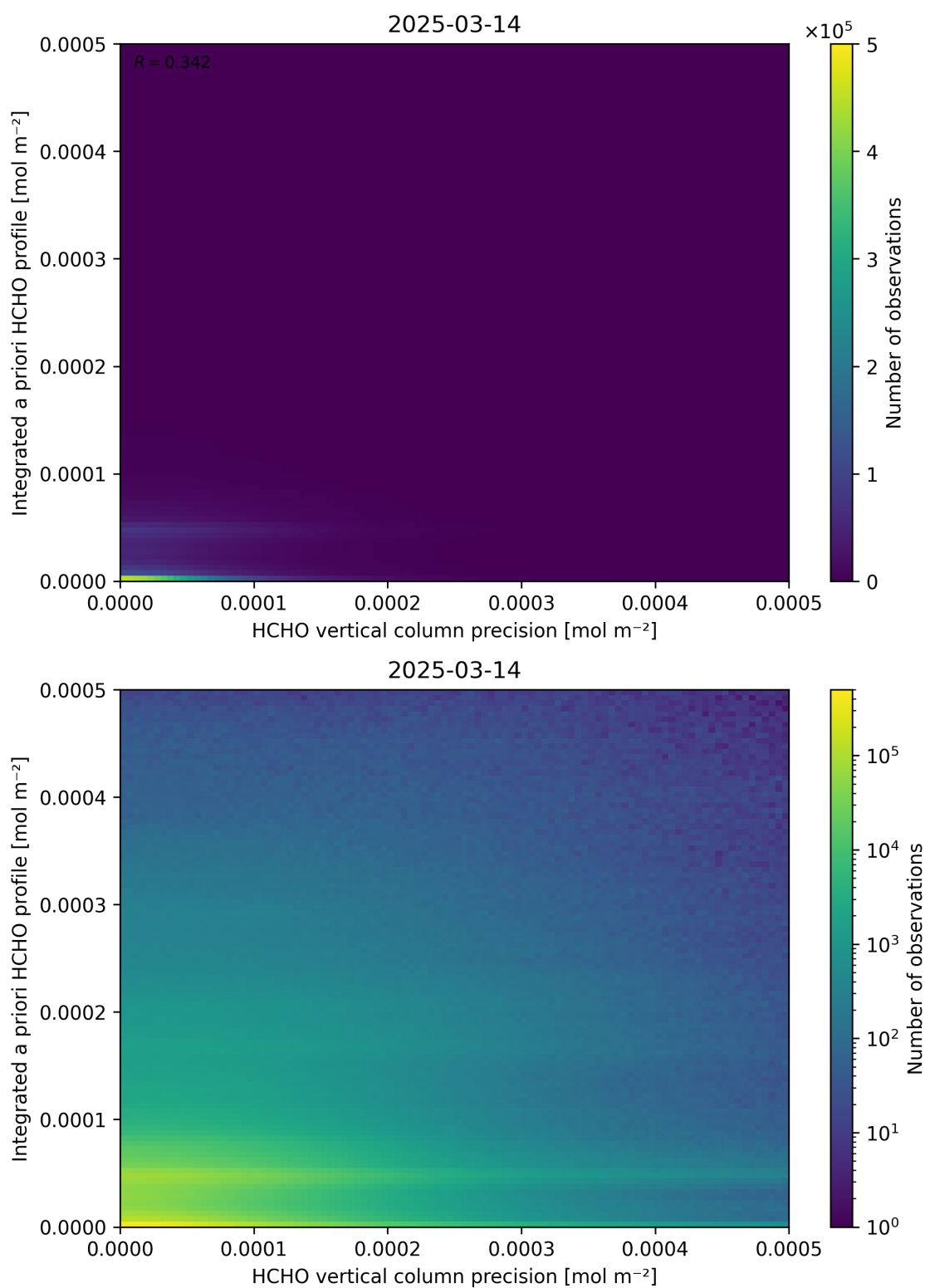
Figure 147: Scatter density plot of “HCHO vertical column precision” against “Integrated a priori HCHO profile” for 2025-03-13 to 2025-03-15.
