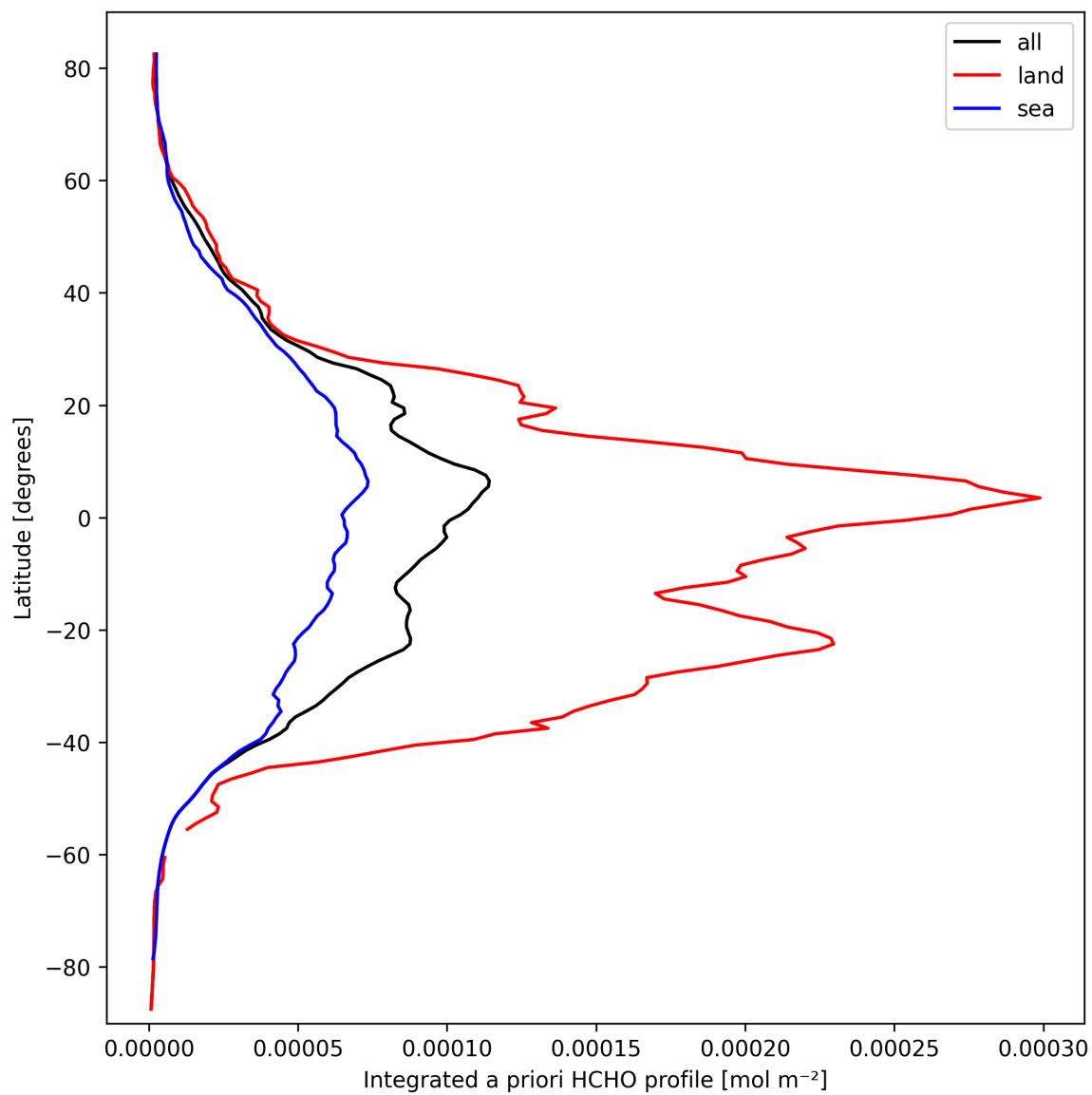
Figure 29: Zonal average of “Integrated a priori HCHO profile” for 2025-03-13 to 2025-03-15.
