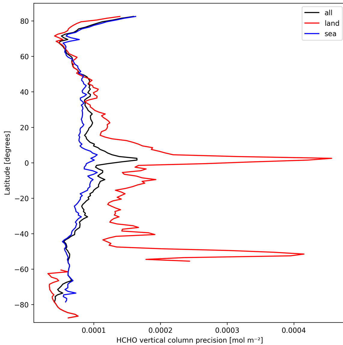
Figure 22: Zonal average of “HCHO vertical column precision” for 2025-03-13 to 2025-03-15.
