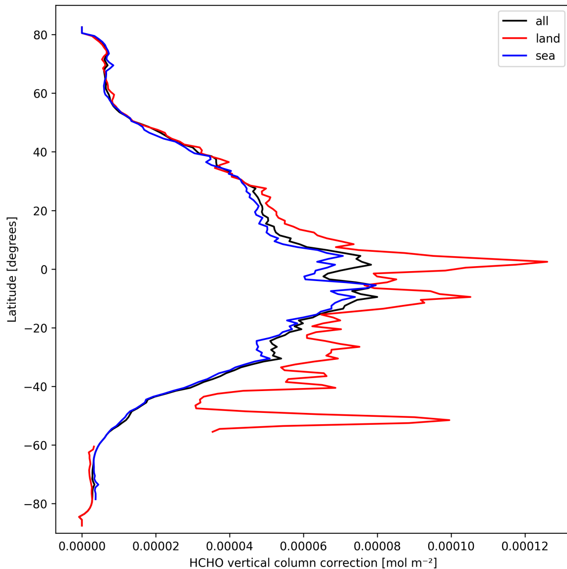
Figure 23: Zonal average of “HCHO vertical column correction” for 2025-03-13 to 2025-03-15.
