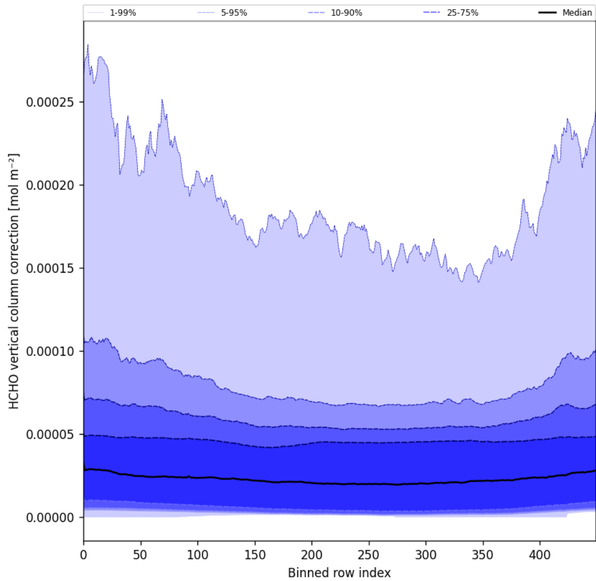
Figure 51: Along track statistics of “HCHO vertical column correction” for 2025-03-13 to 2025-03-15
