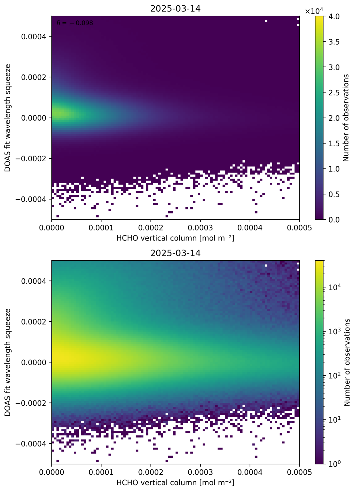
Figure 125: Scatter density plot of “HCHO vertical column” against “DOAS fit wavelength squeeze” for 2025-03-13 to 2025-03-15.
