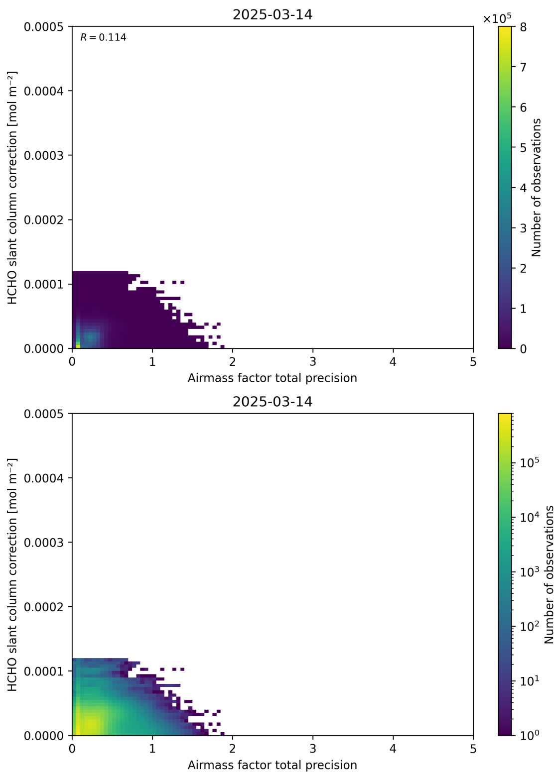
Figure 110: Scatter density plot of “Airmass factor total precision” against “HCHO slant column correction” for 2025-03-13 to 2025-03-15.
