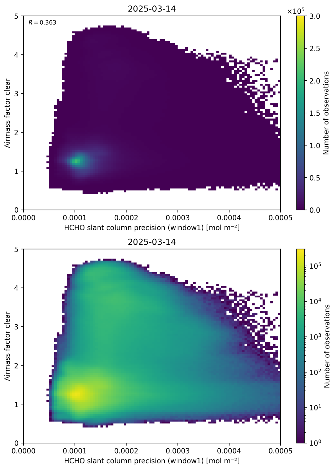
Figure 91: Scatter density plot of “HCHO slant column precision (window1)” against “Airmass factor clear” for 2025-03-13 to 2025-03-15.
