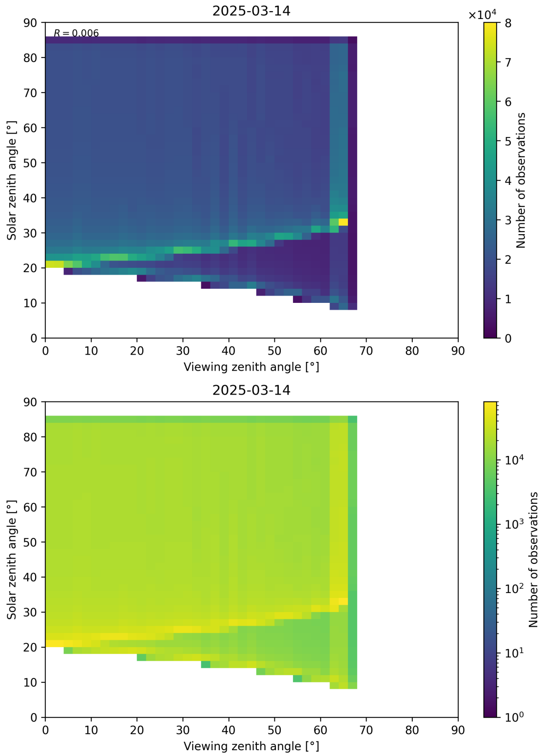
Figure 197: Scatter density plot of “Viewing zenith angle” against “Solar zenith angle” for 2025-03-13 to 2025-03-15.
