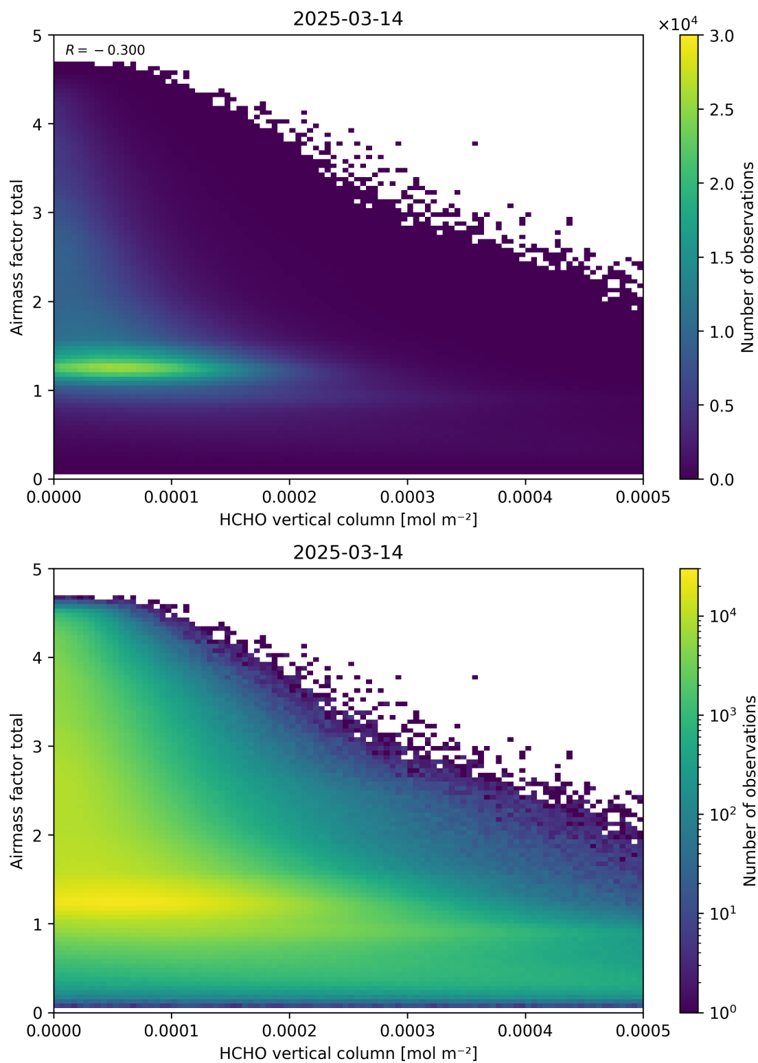
Figure 131: Scatter density plot of “HCHO vertical column” against “Airmass factor total” for 2025-03-13 to 2025-03-15.
