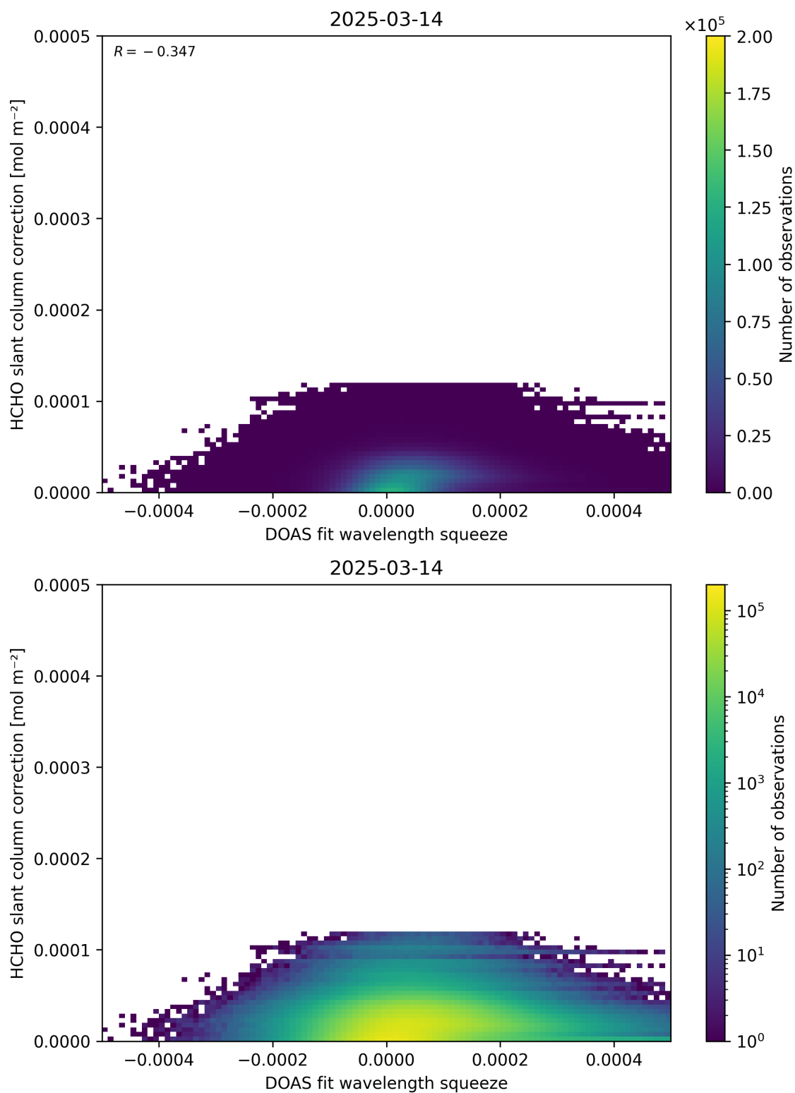
Figure 70: Scatter density plot of “DOAS fit wavelength squeeze” against “HCHO slant column correction” for 2025-03-13 to 2025-03-15.
