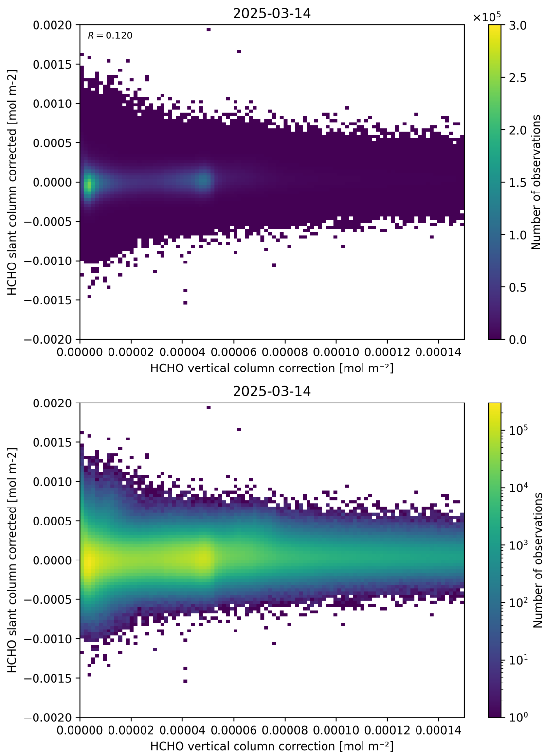
Figure 116: Scatter density plot of “HCHO vertical column correction” against “HCHO slant column corrected” for 2025-03-13 to 2025-03-15.
