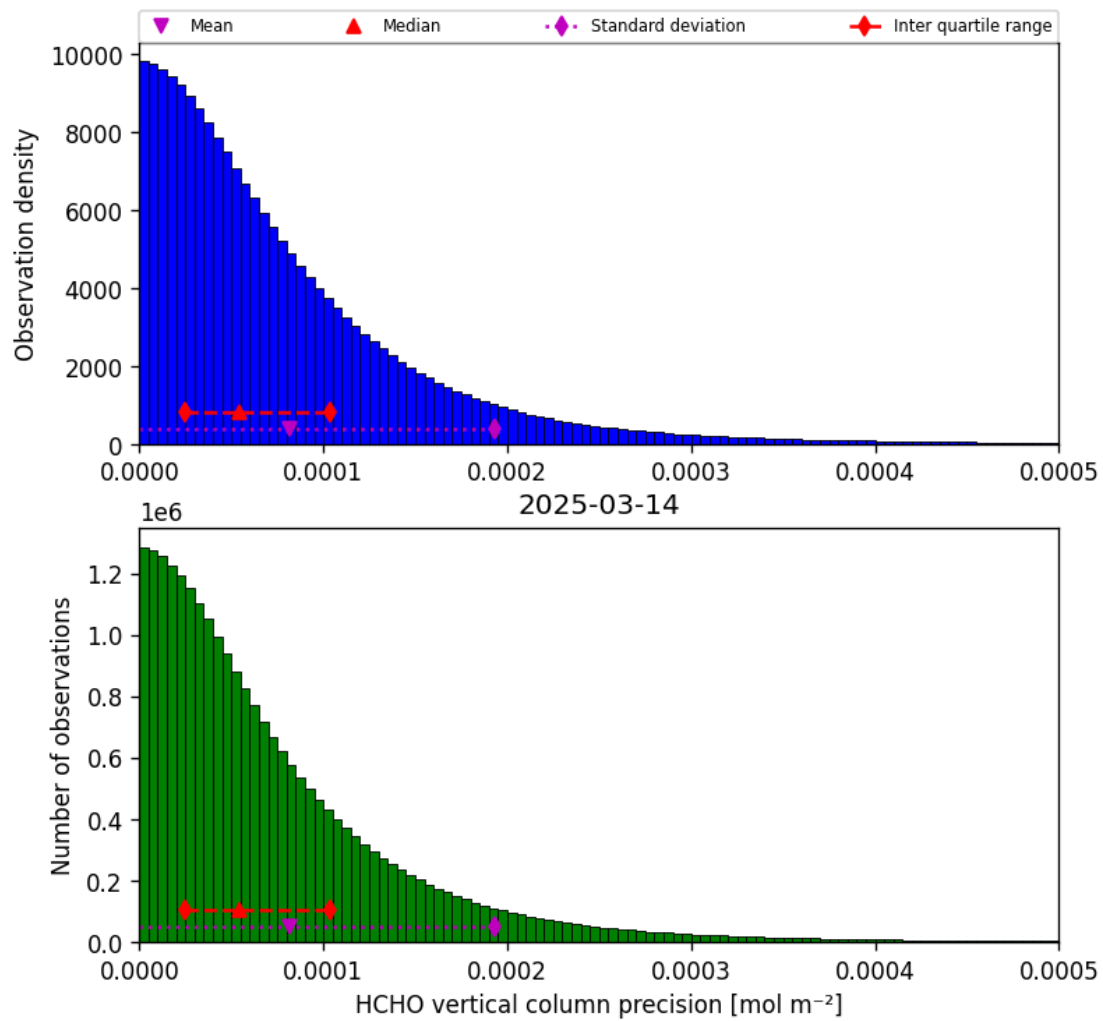
Figure 36: Histogram of “HCHO vertical column precision” for 2025-03-13 to 2025-03-15
