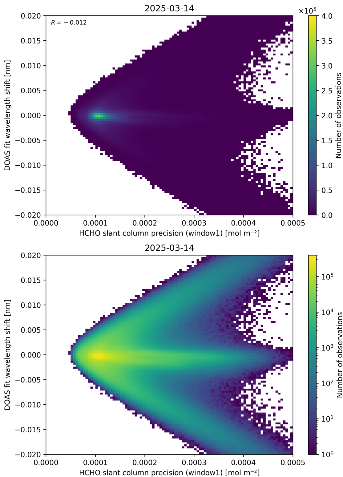
Figure 89: Scatter density plot of “HCHO slant column precision (window1)” against “DOAS fit wavelength shift” for 2025-03-13 to 2025-03-15.
