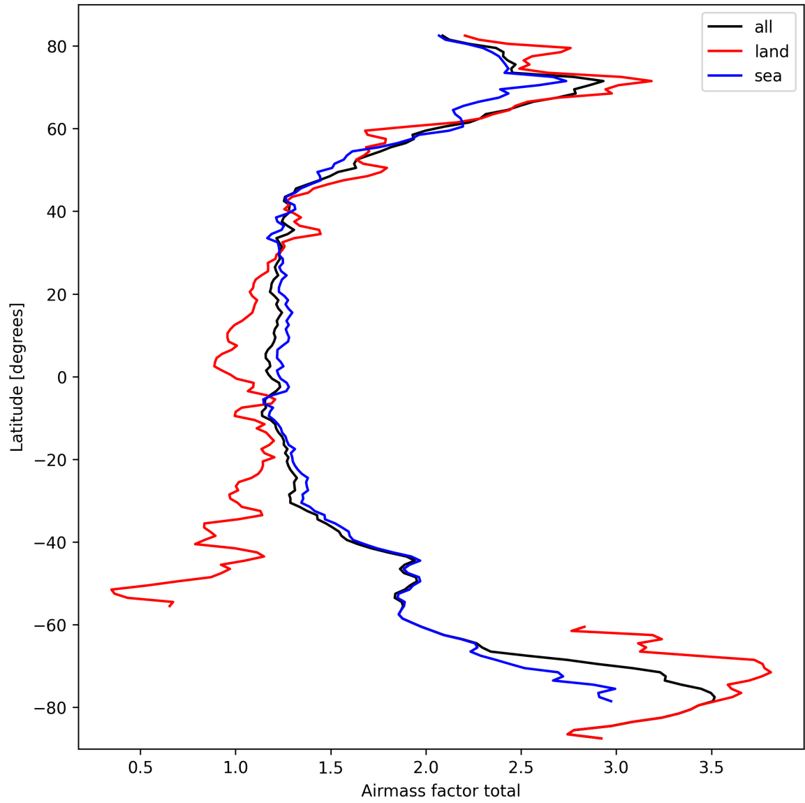
Figure 26: Zonal average of “Airmass factor total” for 2025-03-13 to 2025-03-15.
