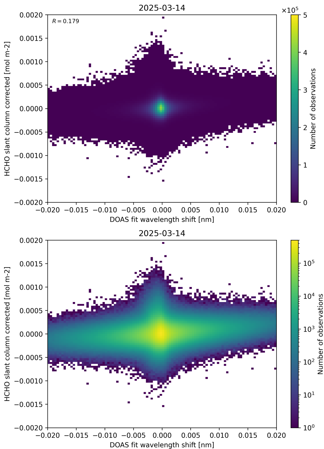
Figure 66: Scatter density plot of “DOAS fit wavelength shift” against “HCHO slant column corrected” for 2025-03-13 to 2025-03-15.
