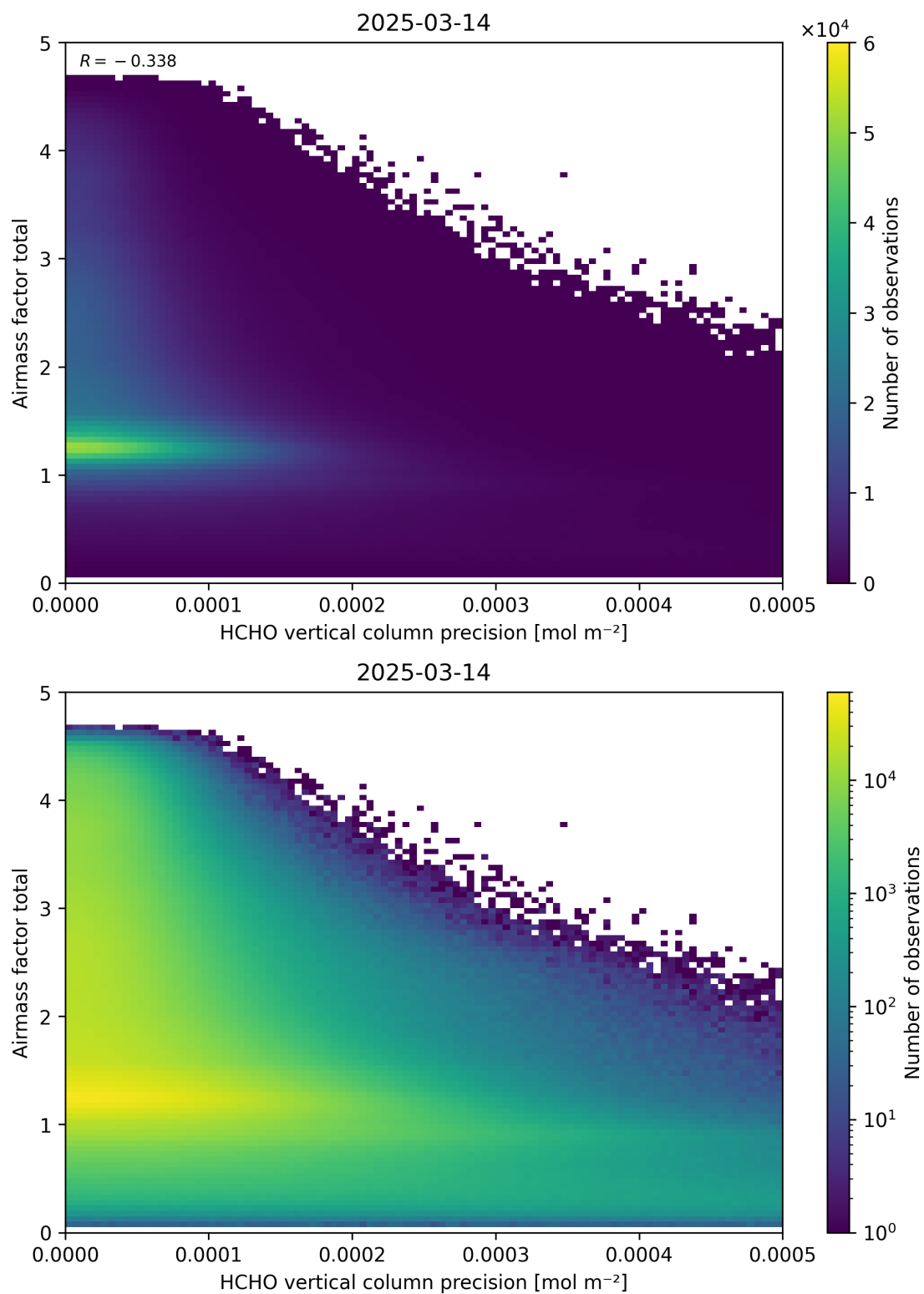
Figure 144: Scatter density plot of “HCHO vertical column precision” against “Airmass factor total” for 2025-03-13 to 2025-03-15.
