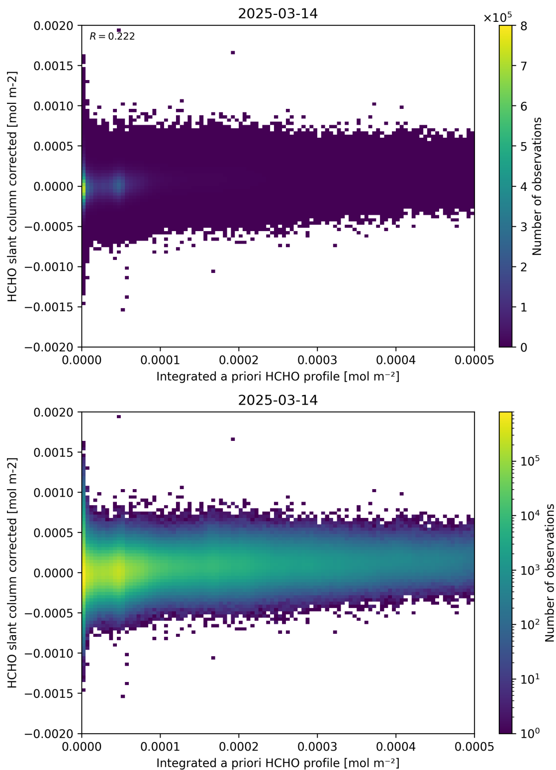
Figure 151: Scatter density plot of “Integrated a priori HCHO profile” against “HCHO slant column corrected” for 2025-03-13 to 2025-03-15.
