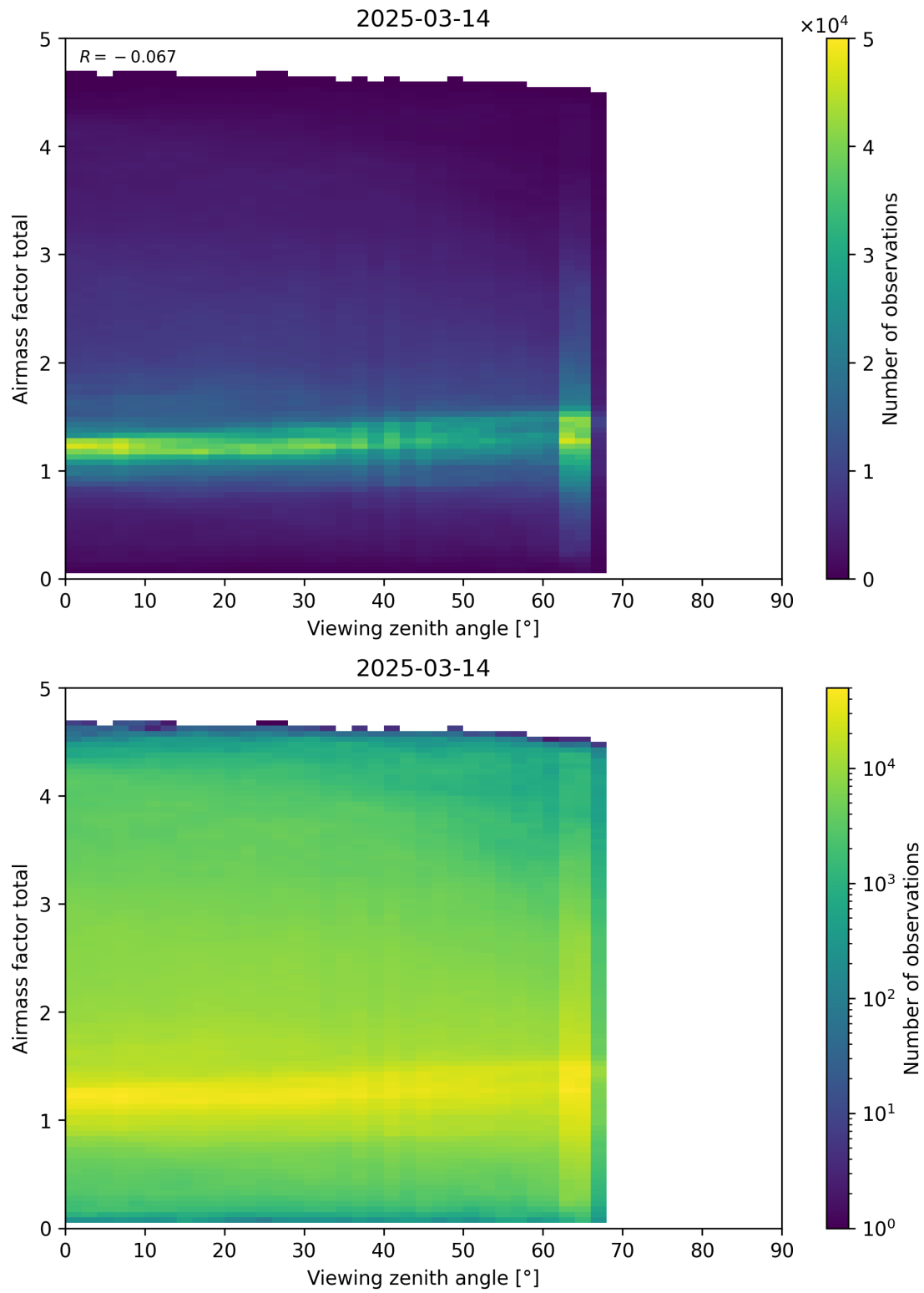
Figure 190: Scatter density plot of “Viewing zenith angle” against “Airmass factor total” for 2025-03-13 to 2025-03-15.
