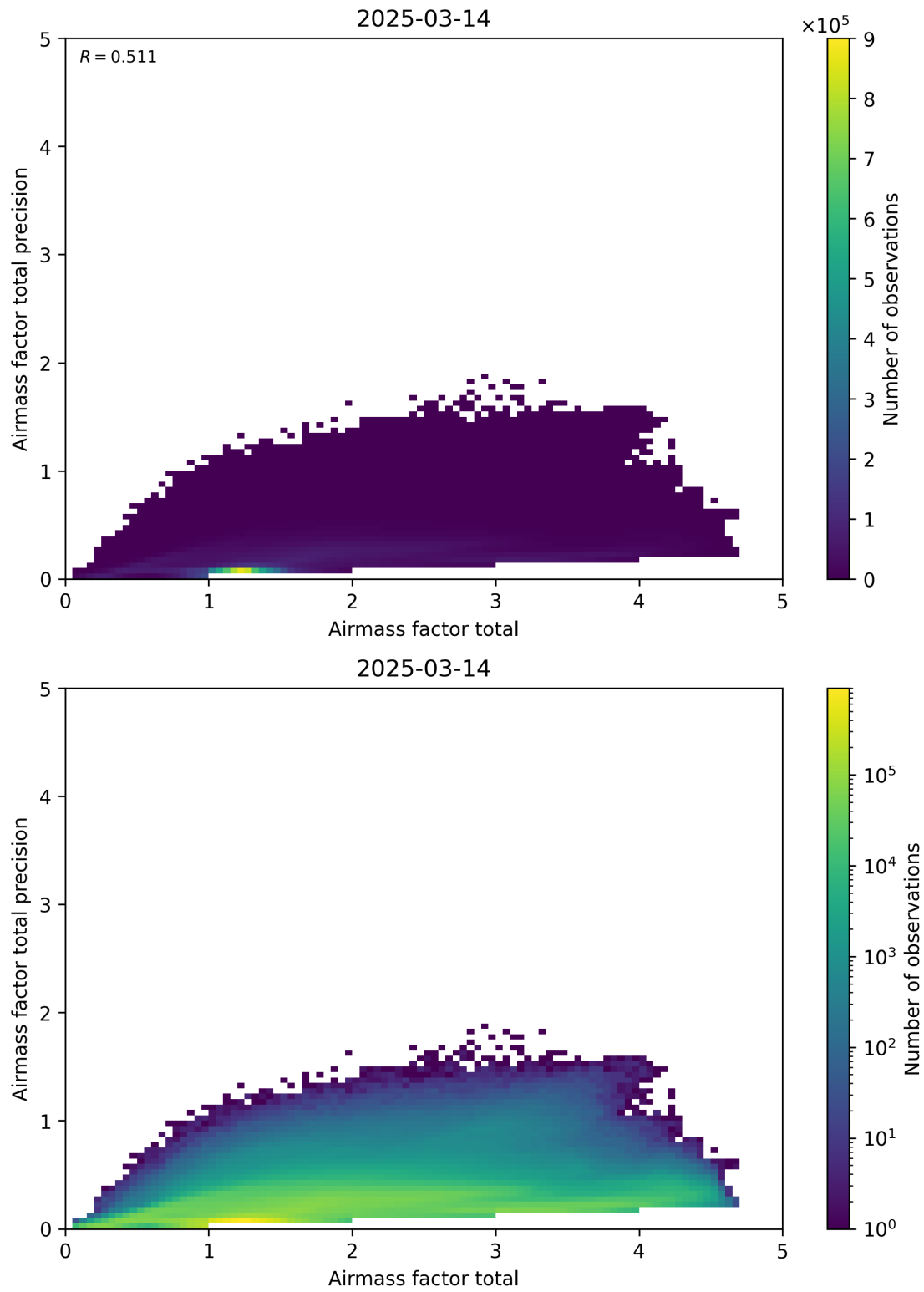
Figure 103: Scatter density plot of “Airmass factor total” against “Airmass factor total precision” for 2025-03-13 to 2025-03-15.
