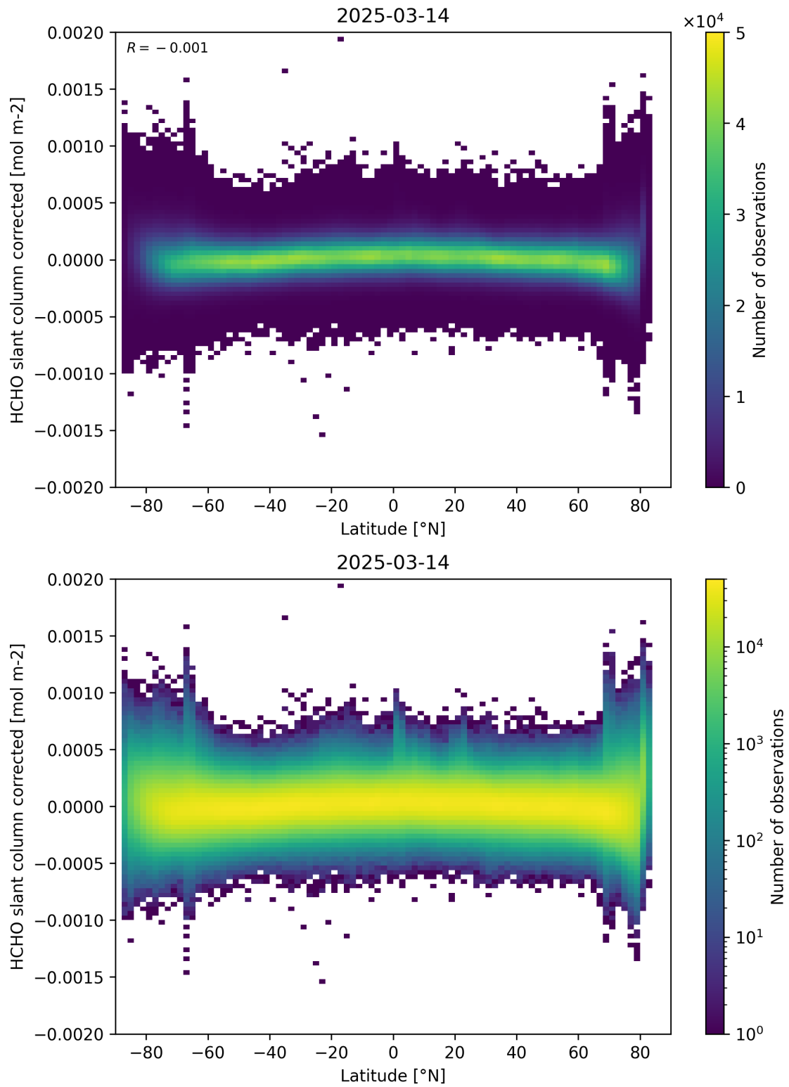
Figure 157: Scatter density plot of “Latitude” against “HCHO slant column corrected” for 2025-03-13 to 2025-03-15.
