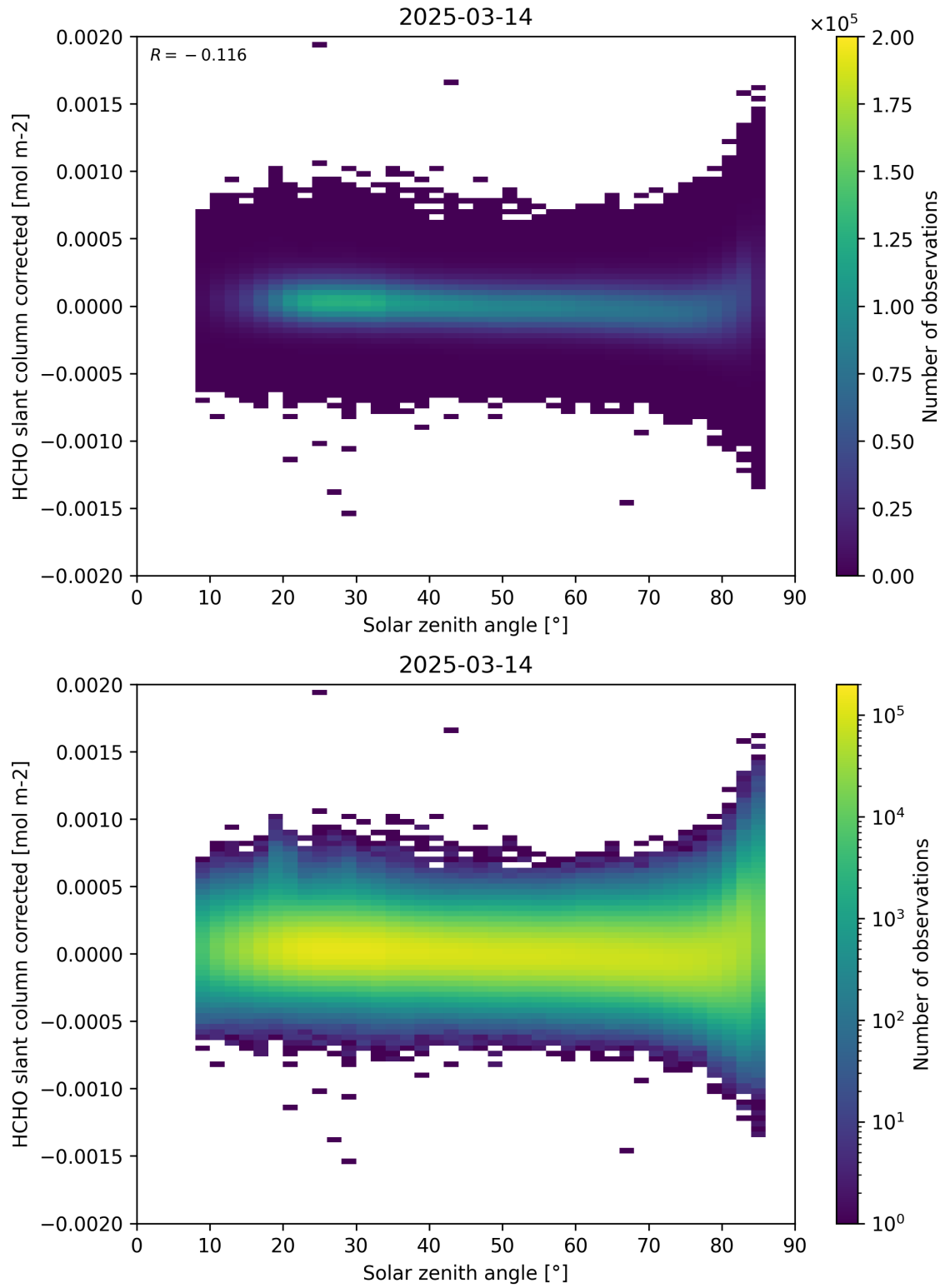
Figure 171: Scatter density plot of “Solar zenith angle” against “HCHO slant column corrected” for 2025-03-13 to 2025-03-15.
