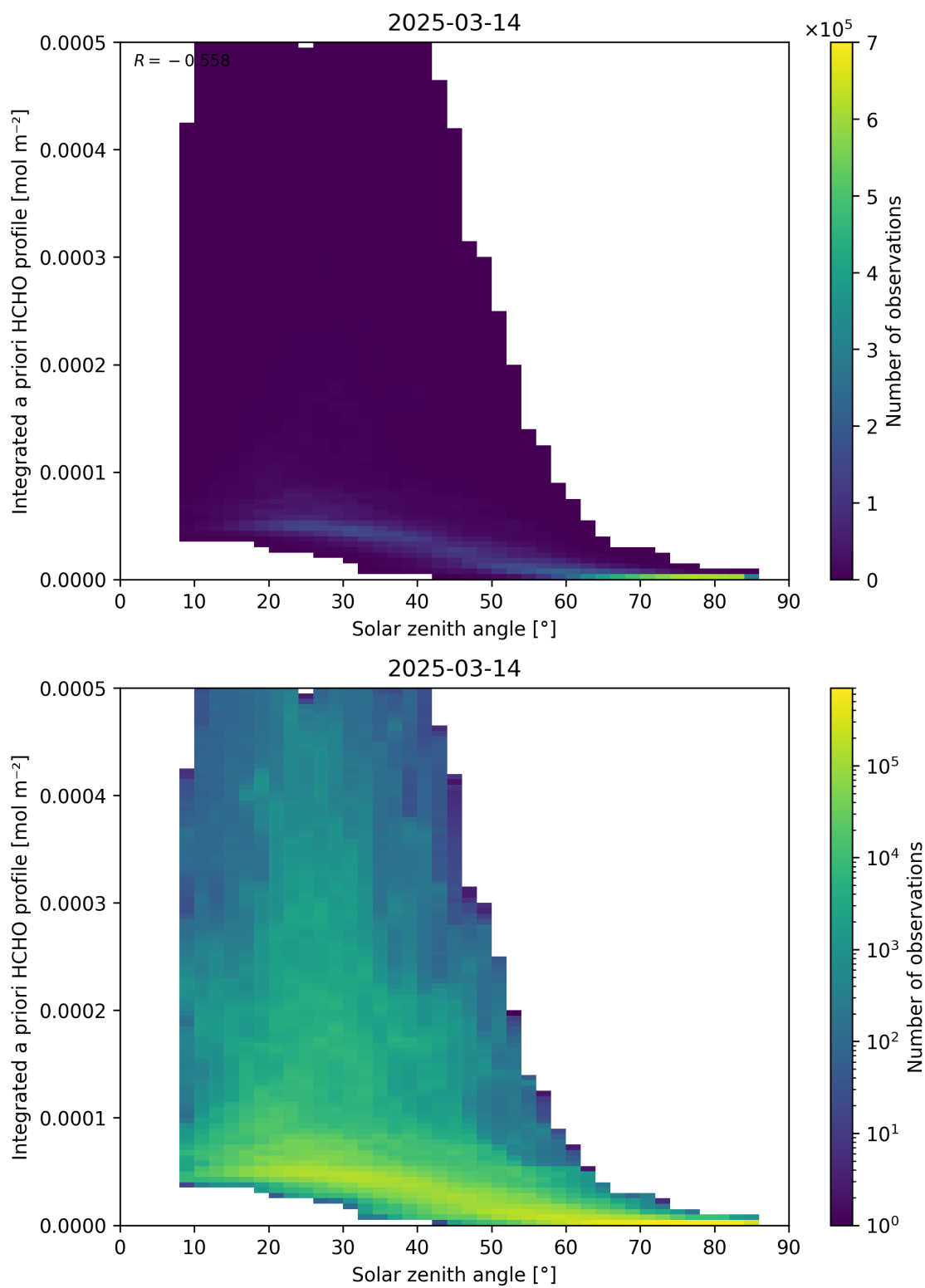
Figure 180: Scatter density plot of “Solar zenith angle” against “Integrated a priori HCHO profile” for 2025-03-13 to 2025-03-15.
