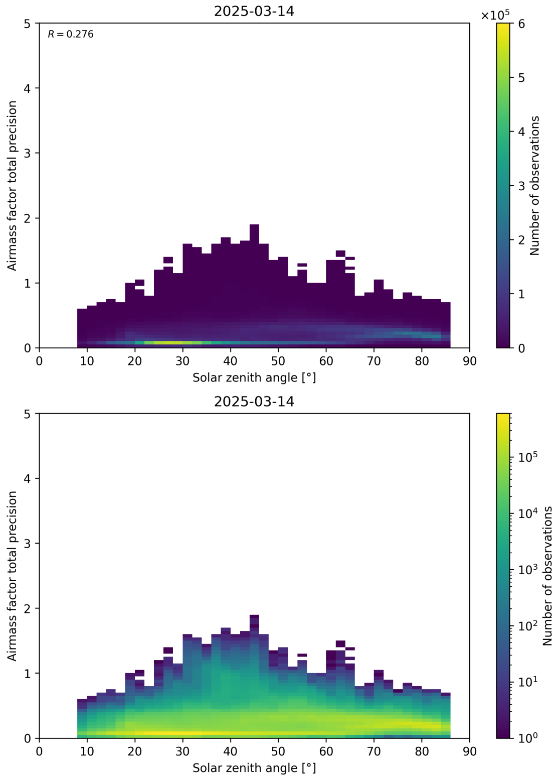
Figure 176: Scatter density plot of “Solar zenith angle” against “Airmass factor total precision” for 2025-03-13 to 2025-03-15.
