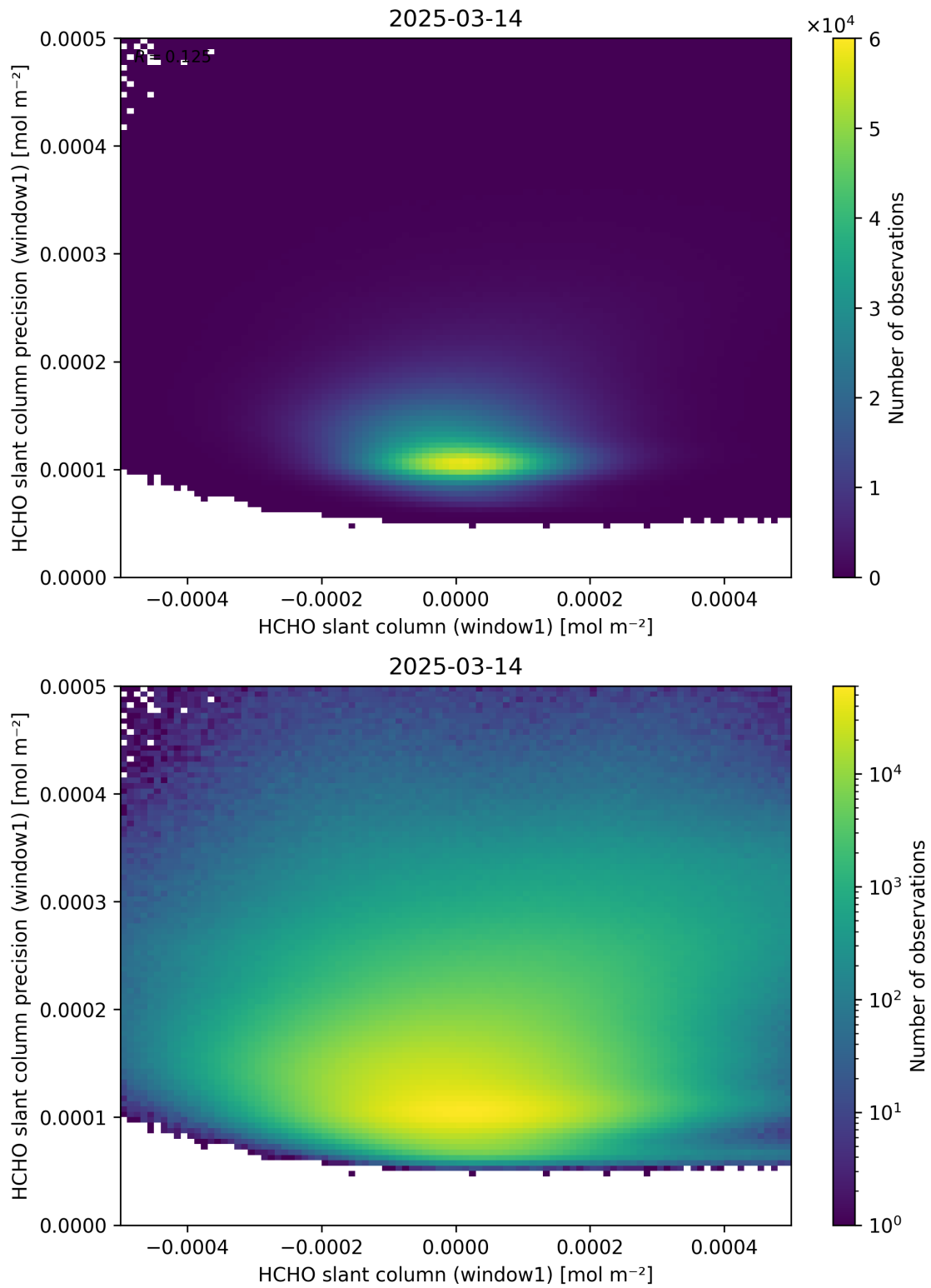
Figure 84: Scatter density plot of “HCHO slant column (window1)” against “HCHO slant column precision (window1)” for 2025-03-13 to 2025-03-15.
