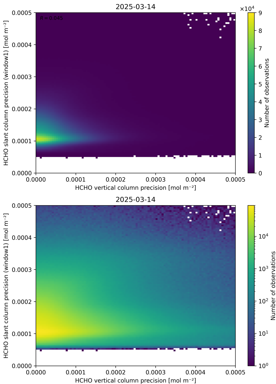
Figure 143: Scatter density plot of “HCHO vertical column precision” against “HCHO slant column precision (window1)” for 2025-03-13 to 2025-03-15.
