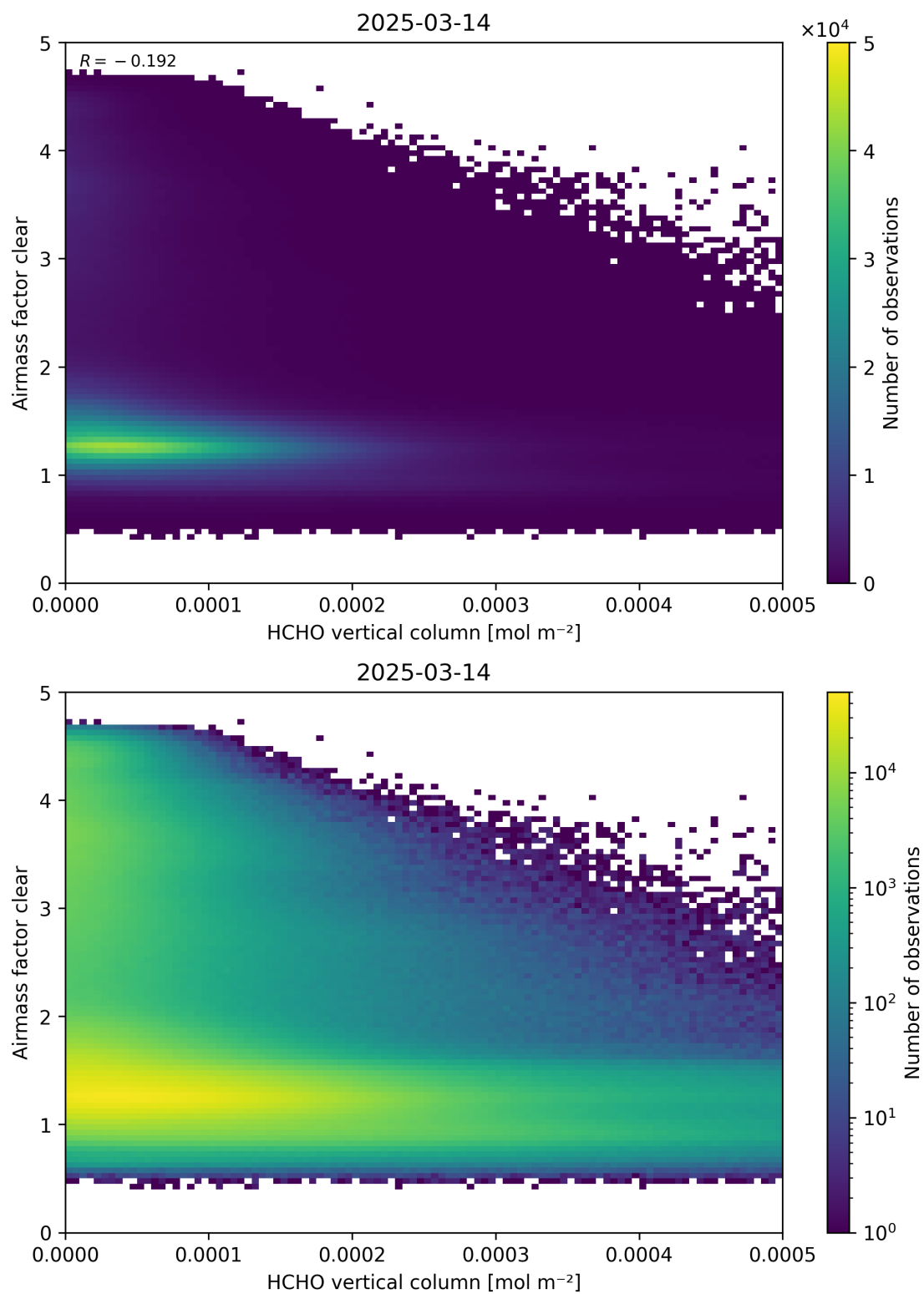
Figure 126: Scatter density plot of “HCHO vertical column” against “Airmass factor clear” for 2025-03-13 to 2025-03-15.
