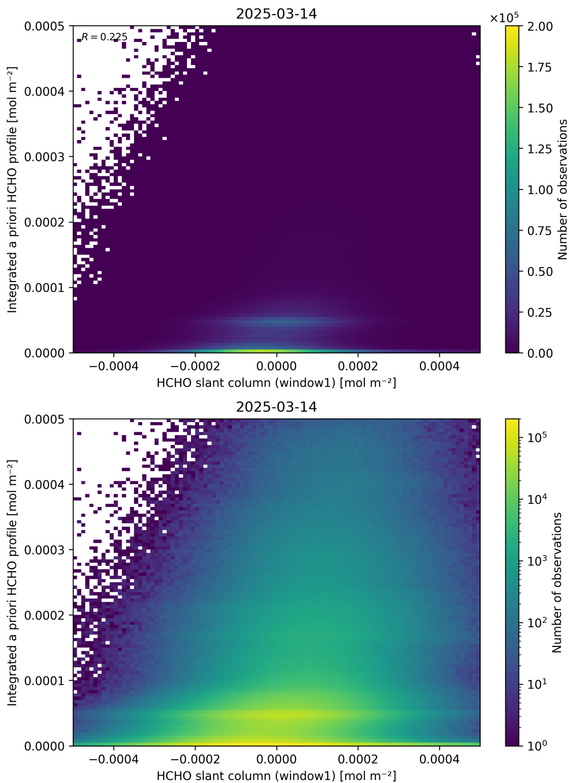
Figure 87: Scatter density plot of “HCHO slant column (window1)” against “Integrated a priori HCHO profile” for 2025-03-13 to 2025-03-15.
