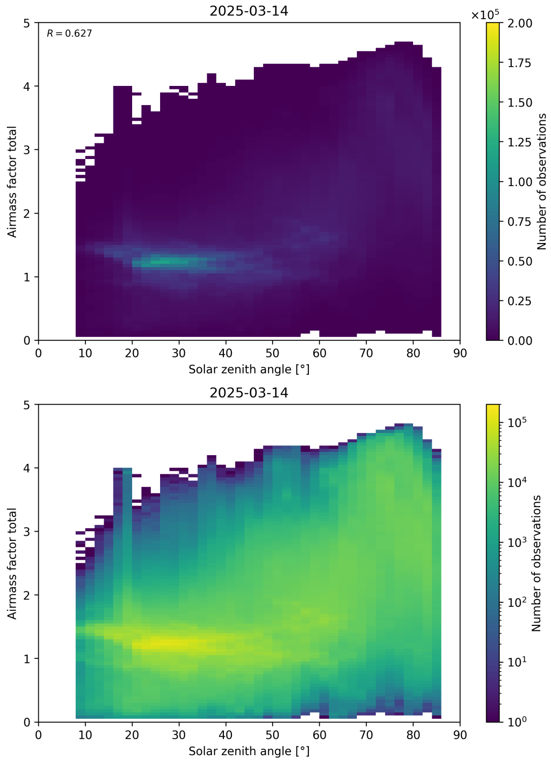
Figure 175: Scatter density plot of “Solar zenith angle” against “Airmass factor total” for 2025-03-13 to 2025-03-15.
