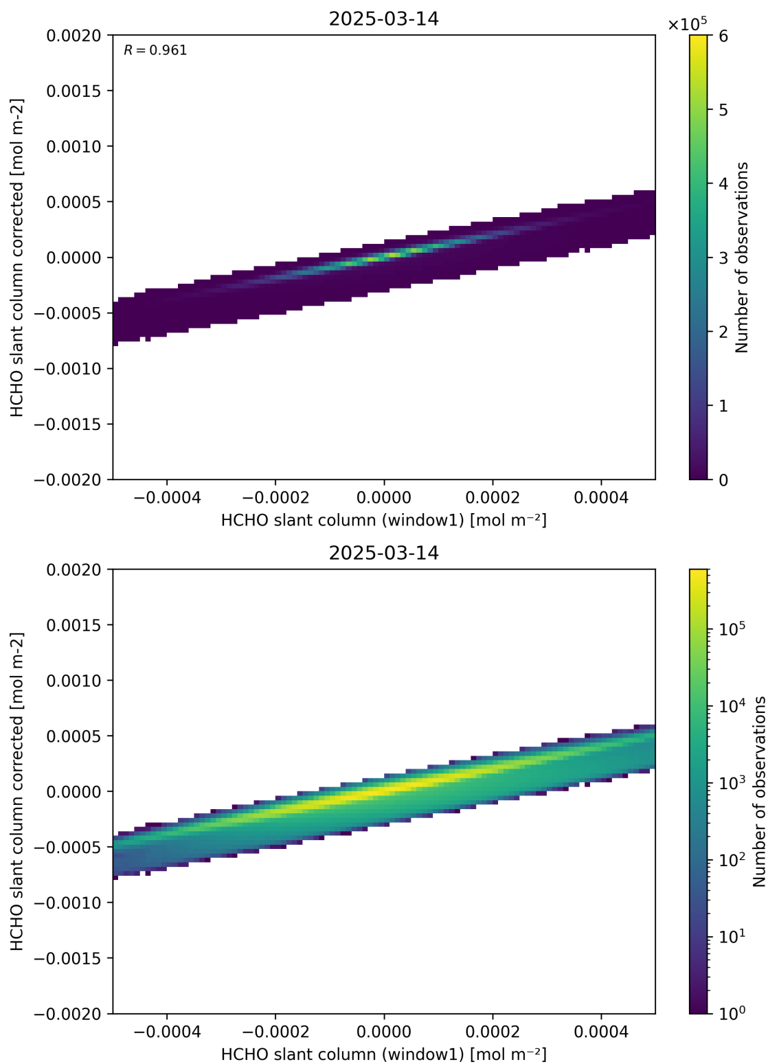
Figure 82: Scatter density plot of “HCHO slant column (window1)” against “HCHO slant column corrected” for 2025-03-13 to 2025-03-15.
