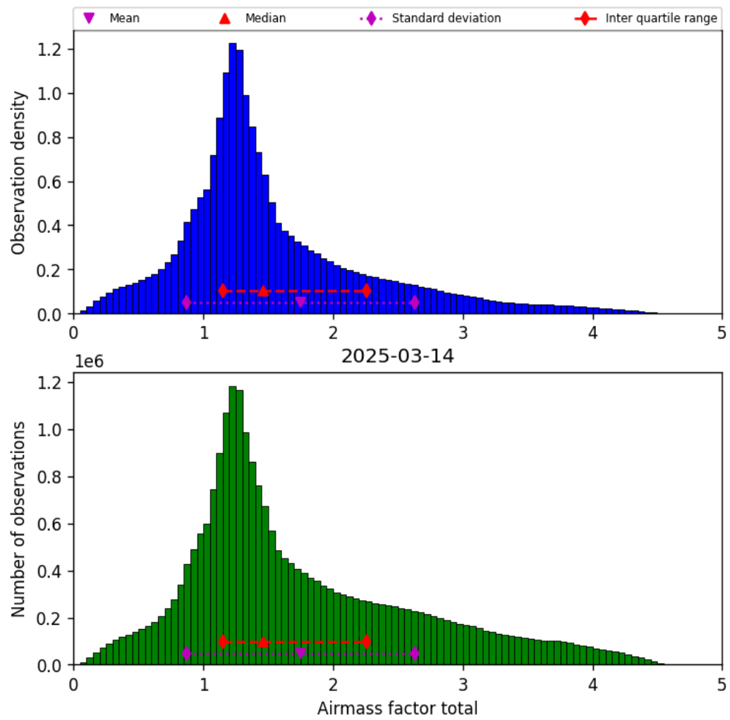
Figure 40: Histogram of “Airmass factor total” for 2025-03-13 to 2025-03-15
