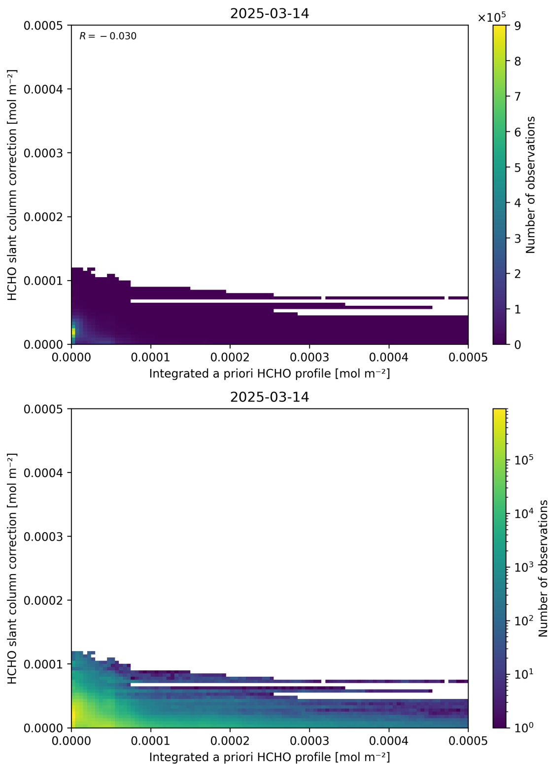
Figure 152: Scatter density plot of “Integrated a priori HCHO profile” against “HCHO slant column correction” for 2025-03-13 to 2025-03-15.
