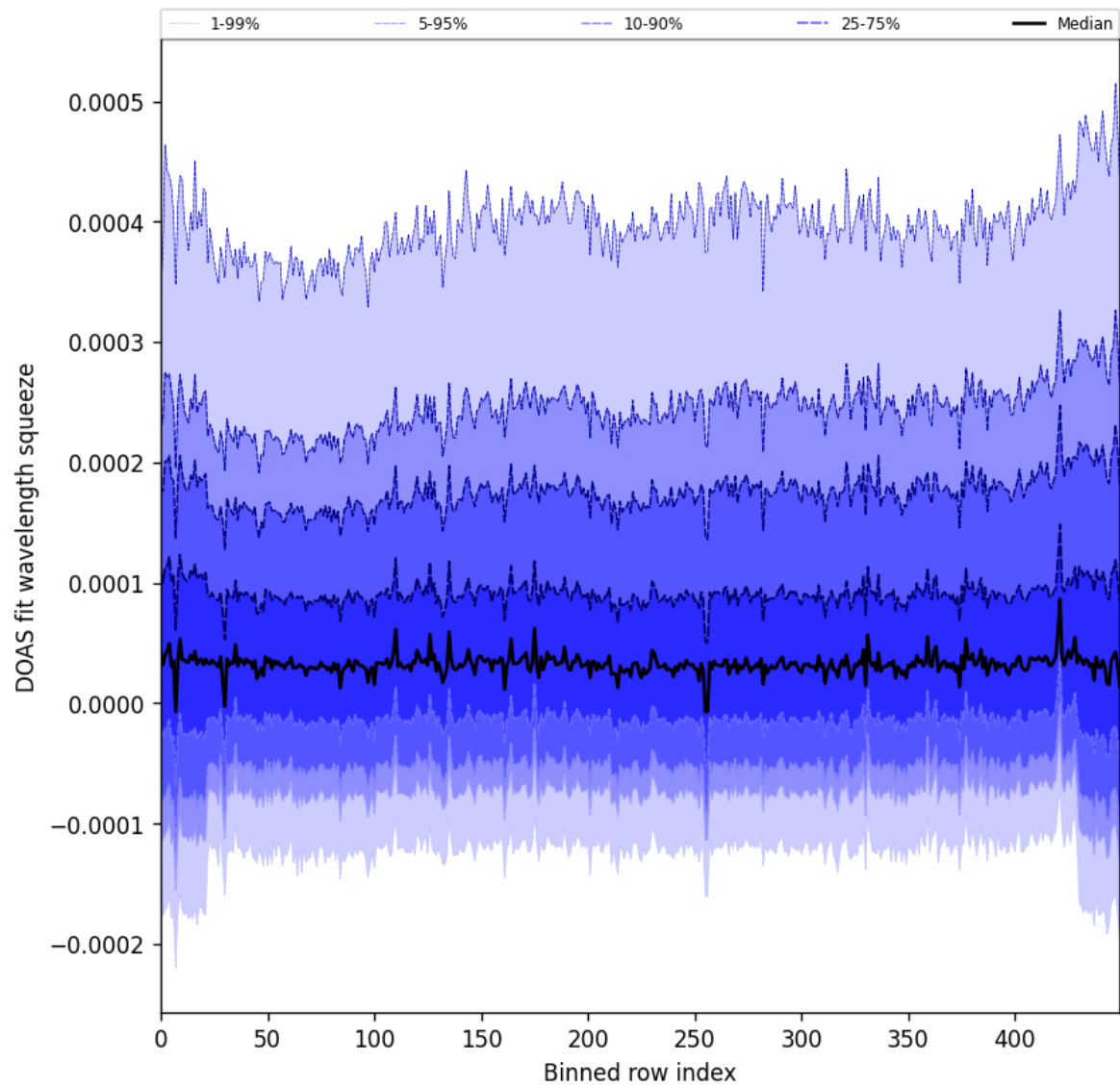
Figure 59: Along track statistics of “DOAS fit wavelength squeeze” for 2025-03-13 to 2025-03-15
