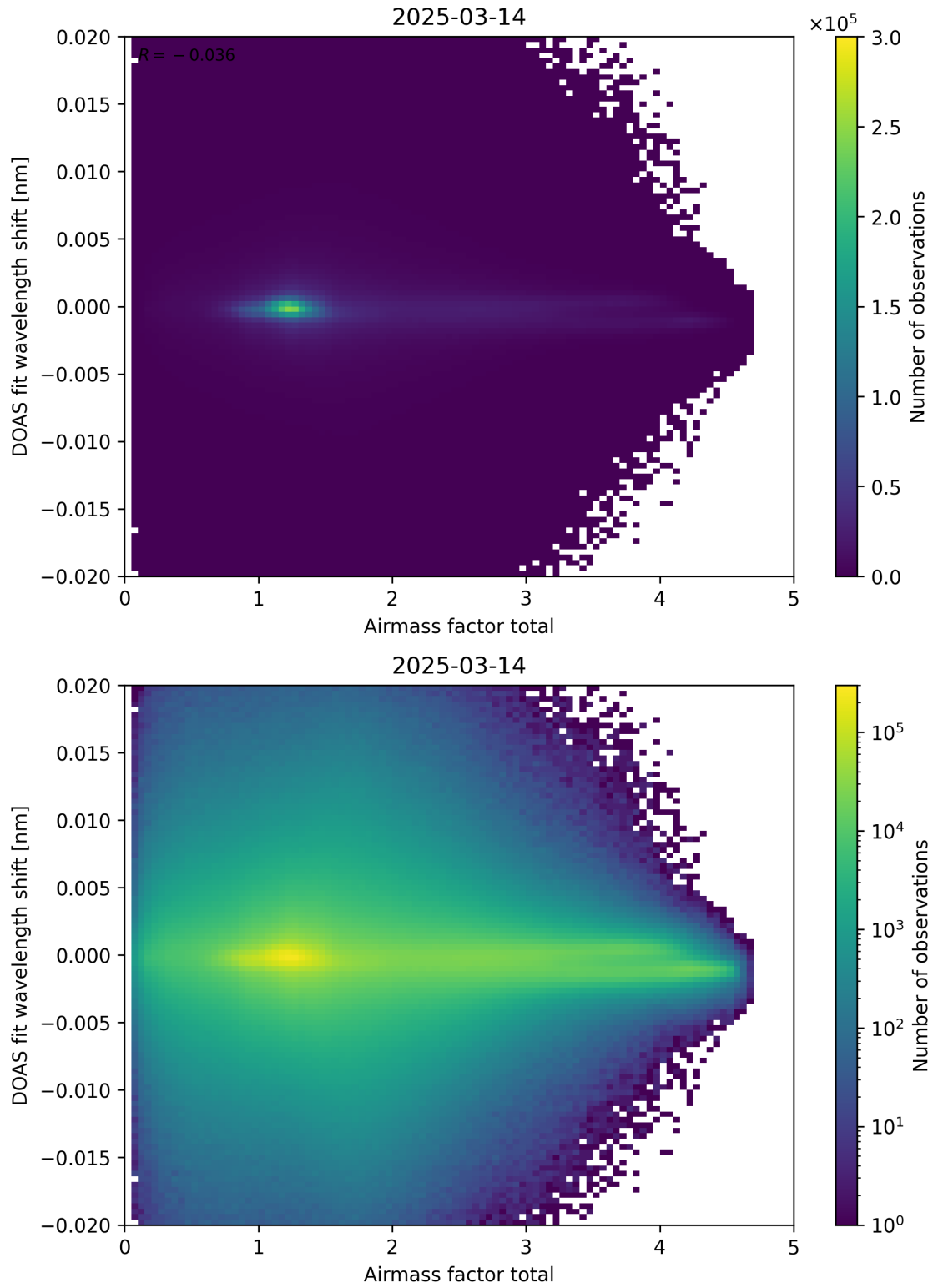
Figure 98: Scatter density plot of “Airmass factor total” against “DOAS fit wavelength shift” for 2025-03-13 to 2025-03-15.
