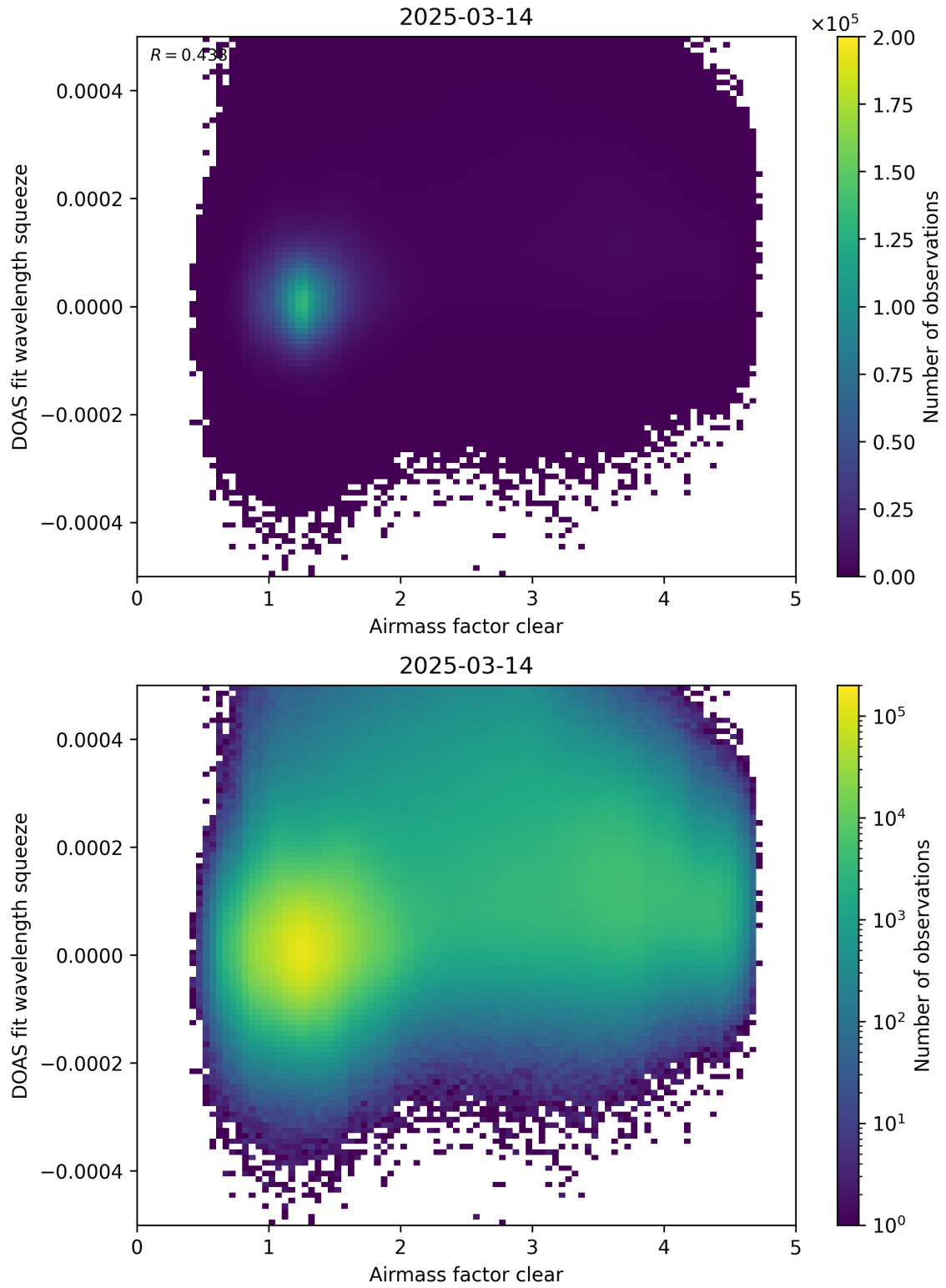
Figure 73: Scatter density plot of “Airmass factor clear” against “DOAS fit wavelength squeeze” for 2025-03-13 to 2025-03-15.
