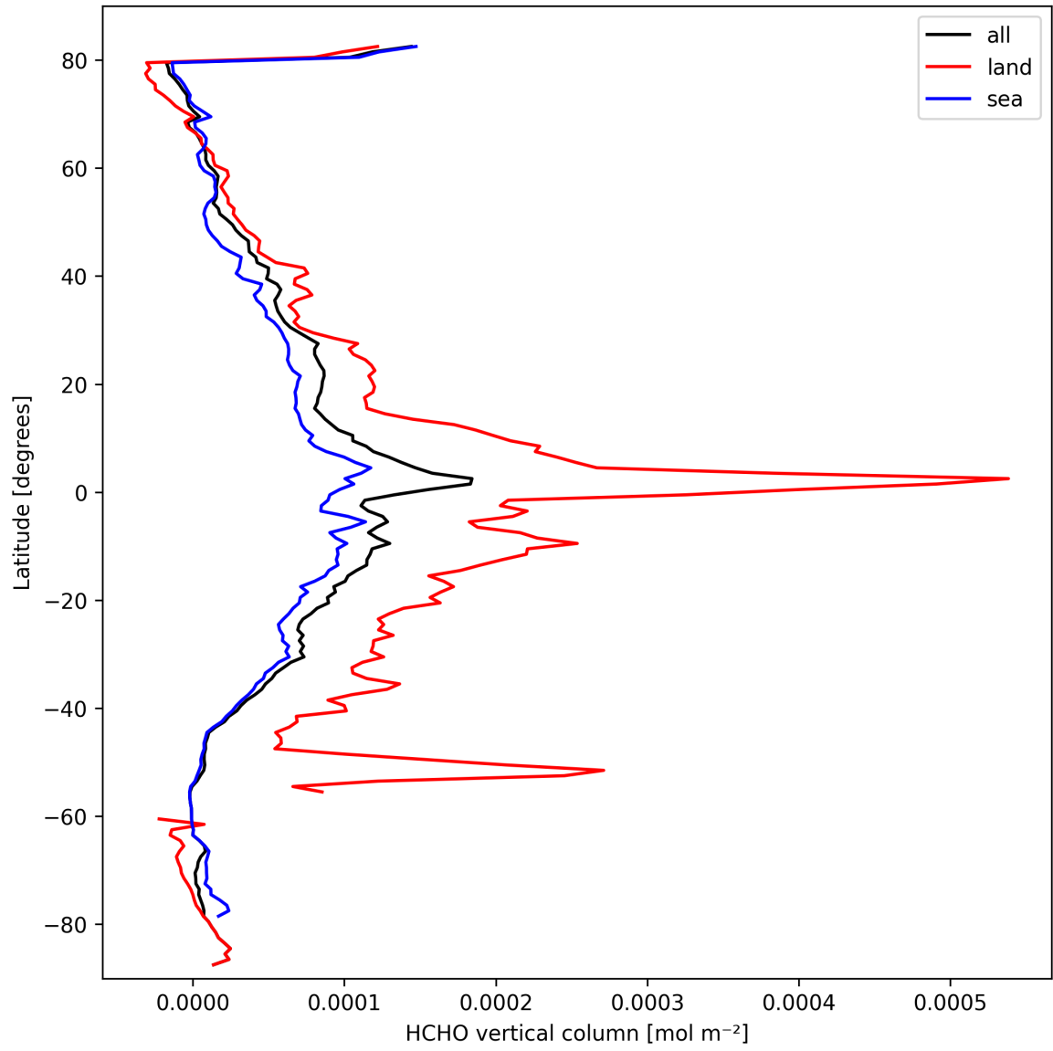
Figure 21: Zonal average of “HCHO vertical column” for 2025-03-13 to 2025-03-15.
