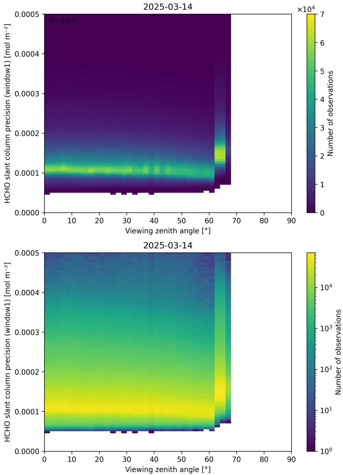
Figure 189: Scatter density plot of “Viewing zenith angle” against “HCHO slant column precision (window1)” for 2025-03-13 to 2025-03-15.
