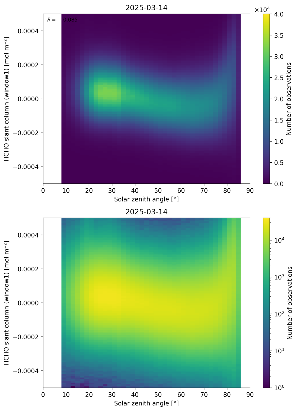
Figure 173: Scatter density plot of “Solar zenith angle” against “HCHO slant column (window1)” for 2025-03-13 to 2025-03-15.
