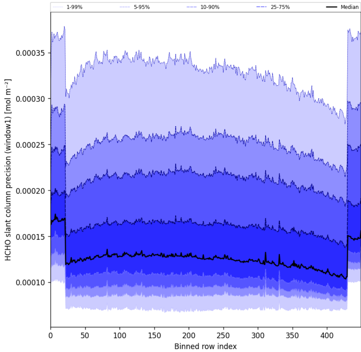
Figure 53: Along track statistics of “HCHO slant column precision (window1)” for 2025-03-13 to 2025-03-15
