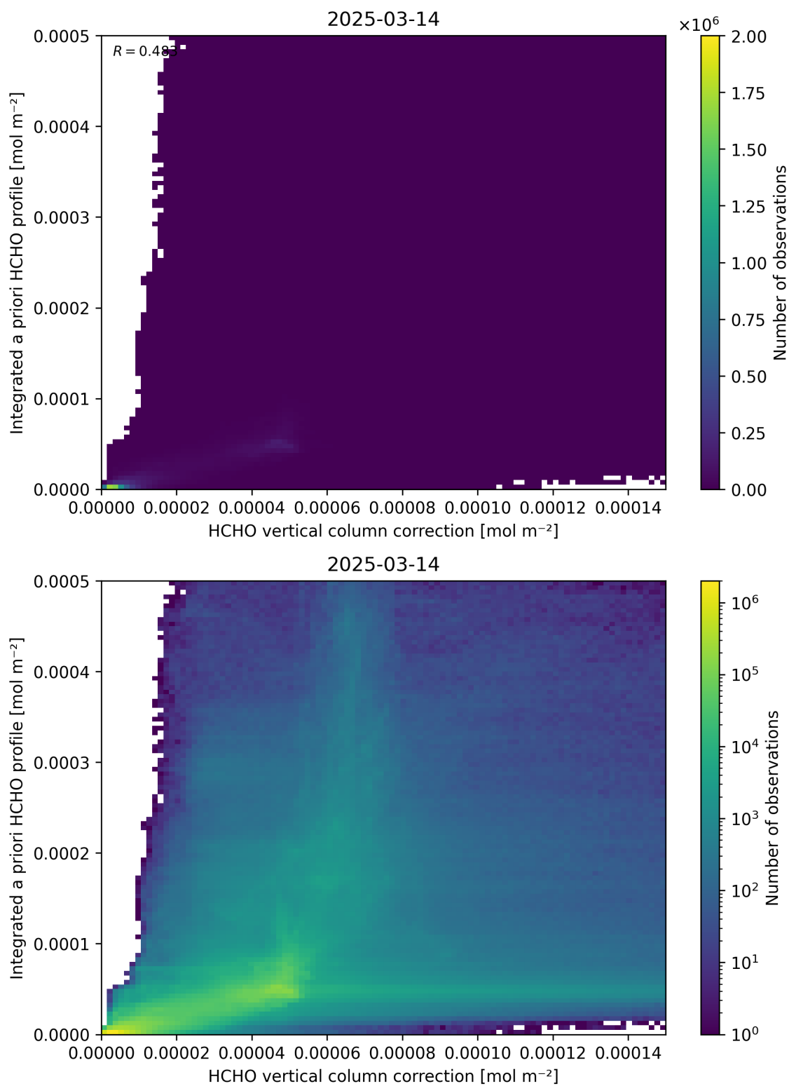
Figure 122: Scatter density plot of “HCHO vertical column correction” against “Integrated a priori HCHO profile” for 2025-03-13 to 2025-03-15.
