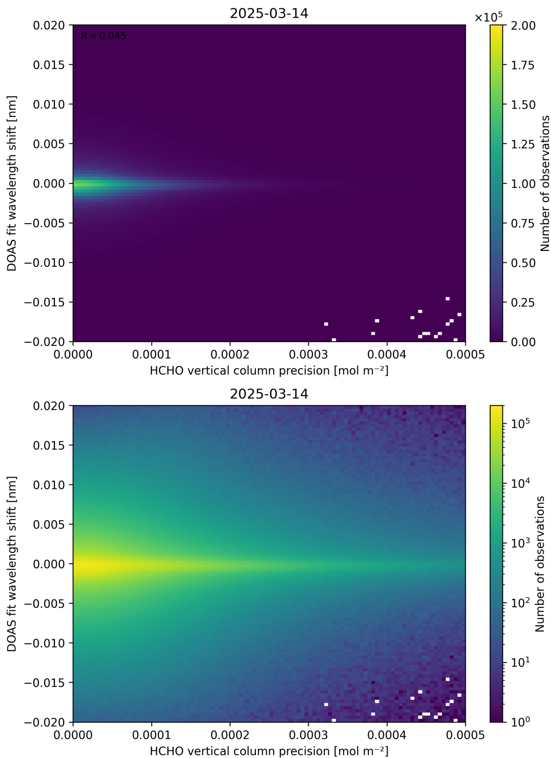
Figure 137: Scatter density plot of “HCHO vertical column precision” against “DOAS fit wavelength shift” for 2025-03-13 to 2025-03-15.
