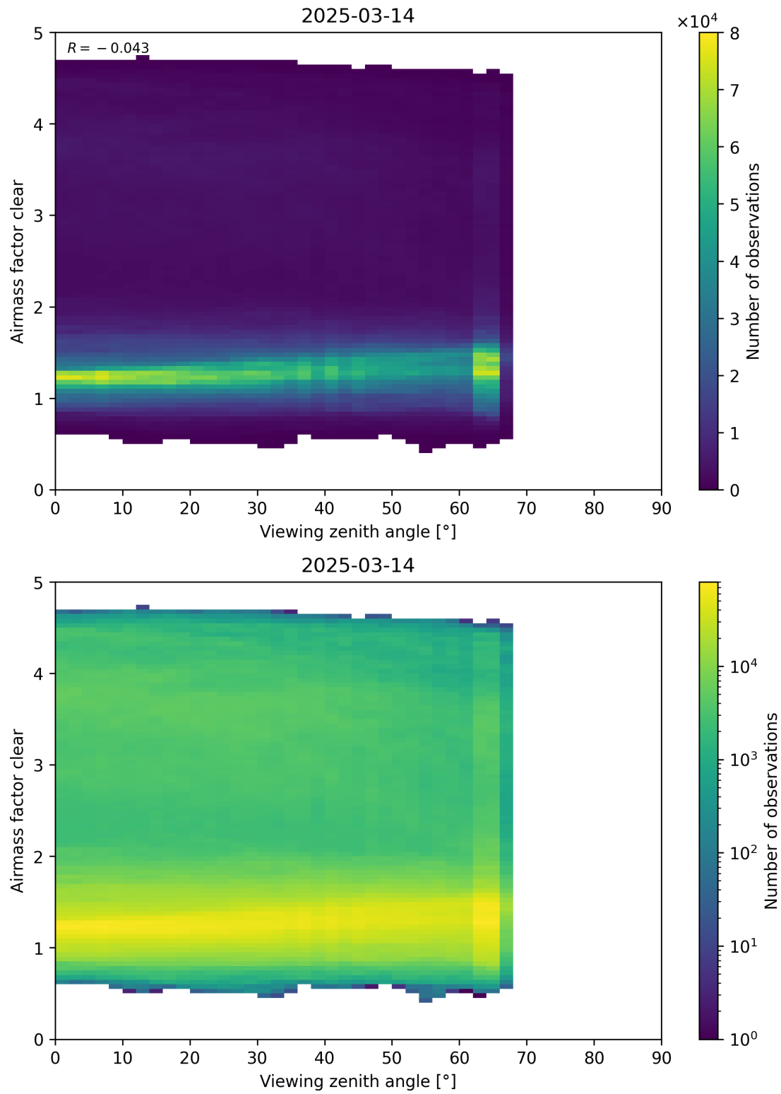
Figure 185: Scatter density plot of “Viewing zenith angle” against “Airmass factor clear” for 2025-03-13 to 2025-03-15.
