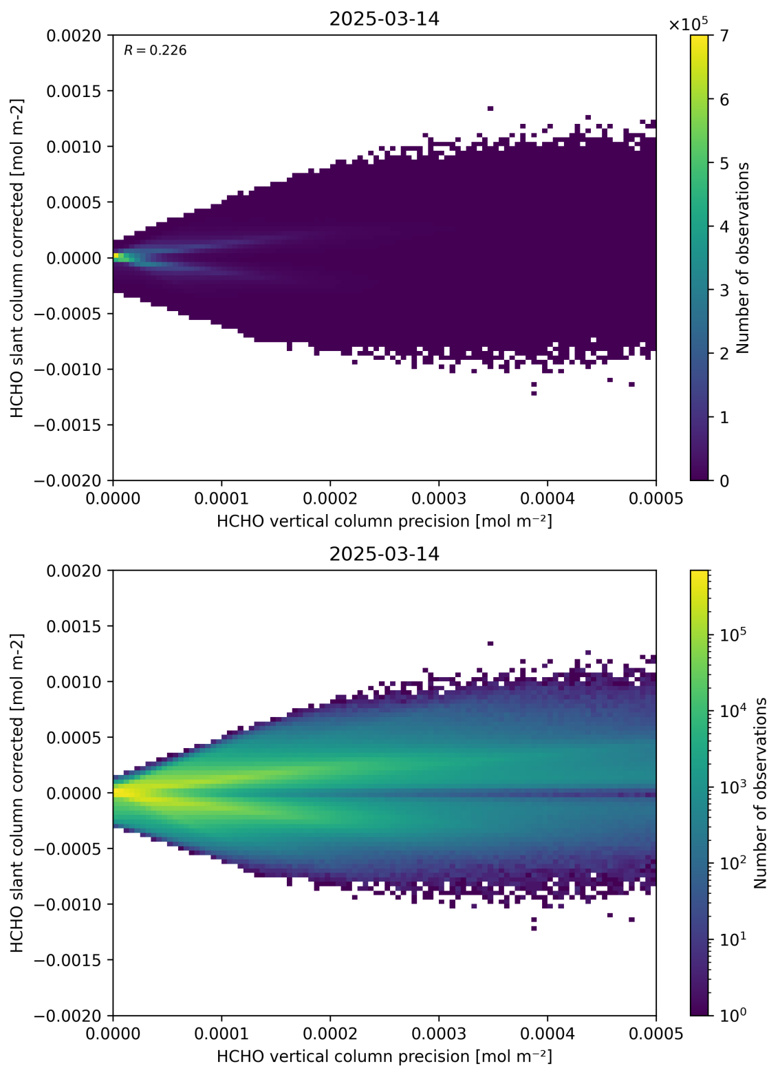
Figure 140: Scatter density plot of “HCHO vertical column precision” against “HCHO slant column corrected” for 2025-03-13 to 2025-03-15.
