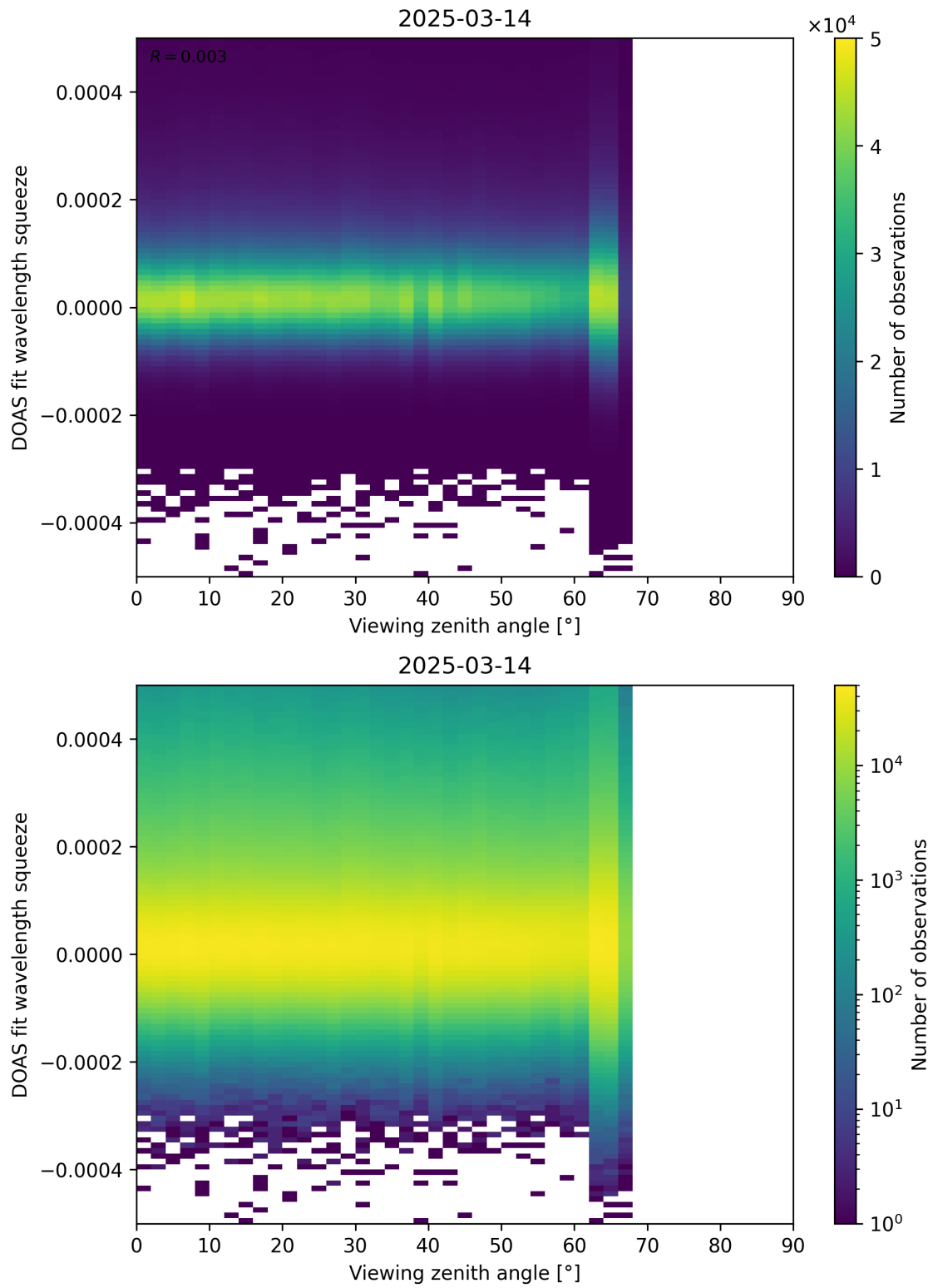
Figure 184: Scatter density plot of “Viewing zenith angle” against “DOAS fit wavelength squeeze” for 2025-03-13 to 2025-03-15.
