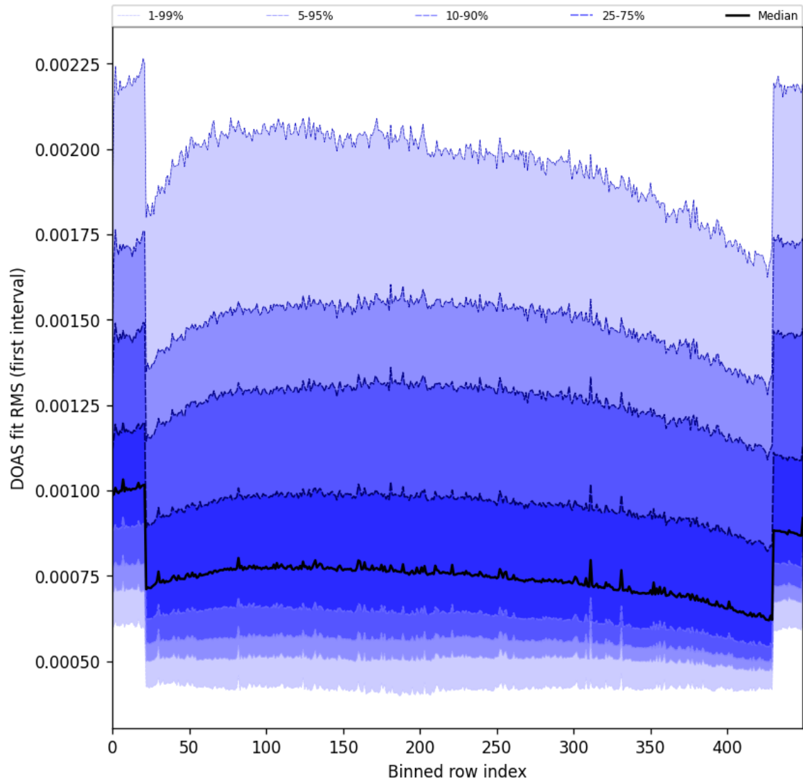
Figure 60: Along track statistics of “DOAS fit RMS (first interval)” for 2025-03-13 to 2025-03-15
