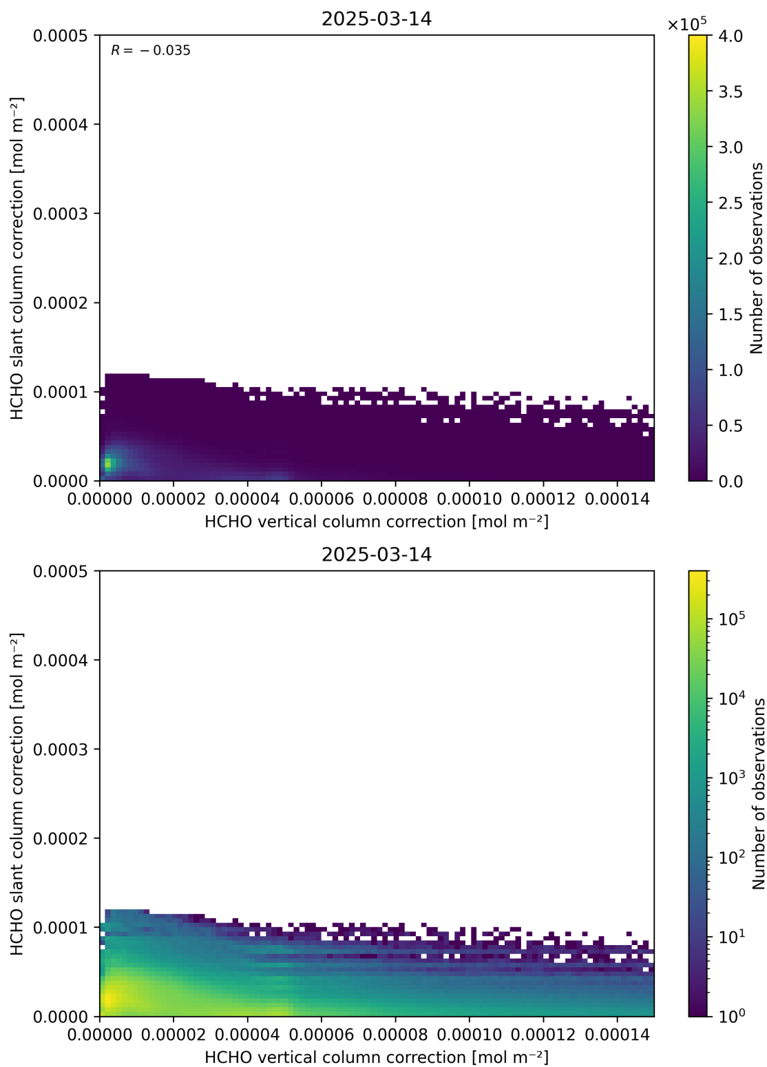
Figure 117: Scatter density plot of “HCHO vertical column correction” against “HCHO slant column correction” for 2025-03-13 to 2025-03-15.
