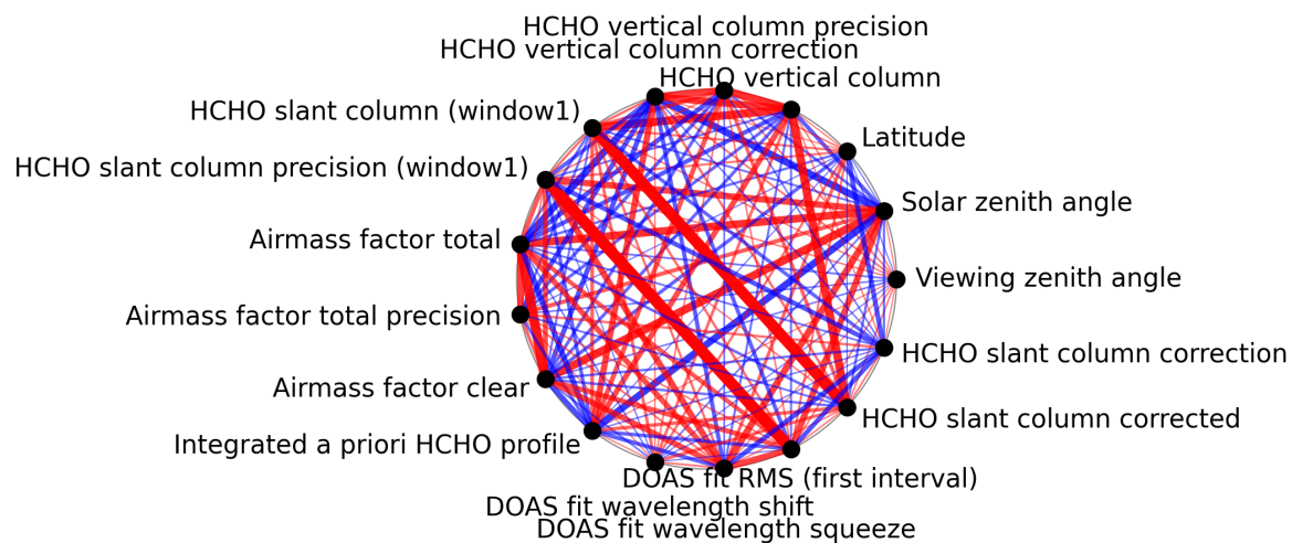
Figure 1: Map of correlation graph for 2025-03-13 to 2025-03-15.
