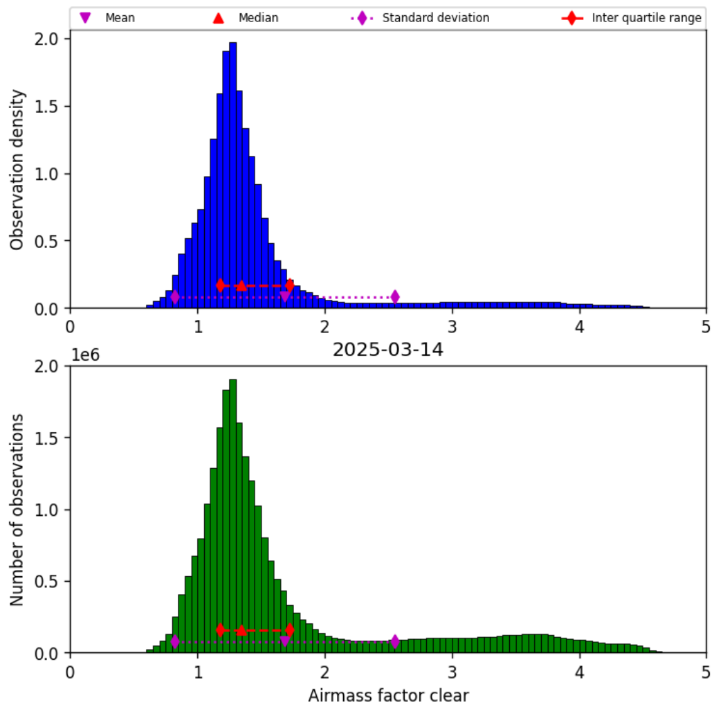
Figure 42: Histogram of “Airmass factor clear” for 2025-03-13 to 2025-03-15
