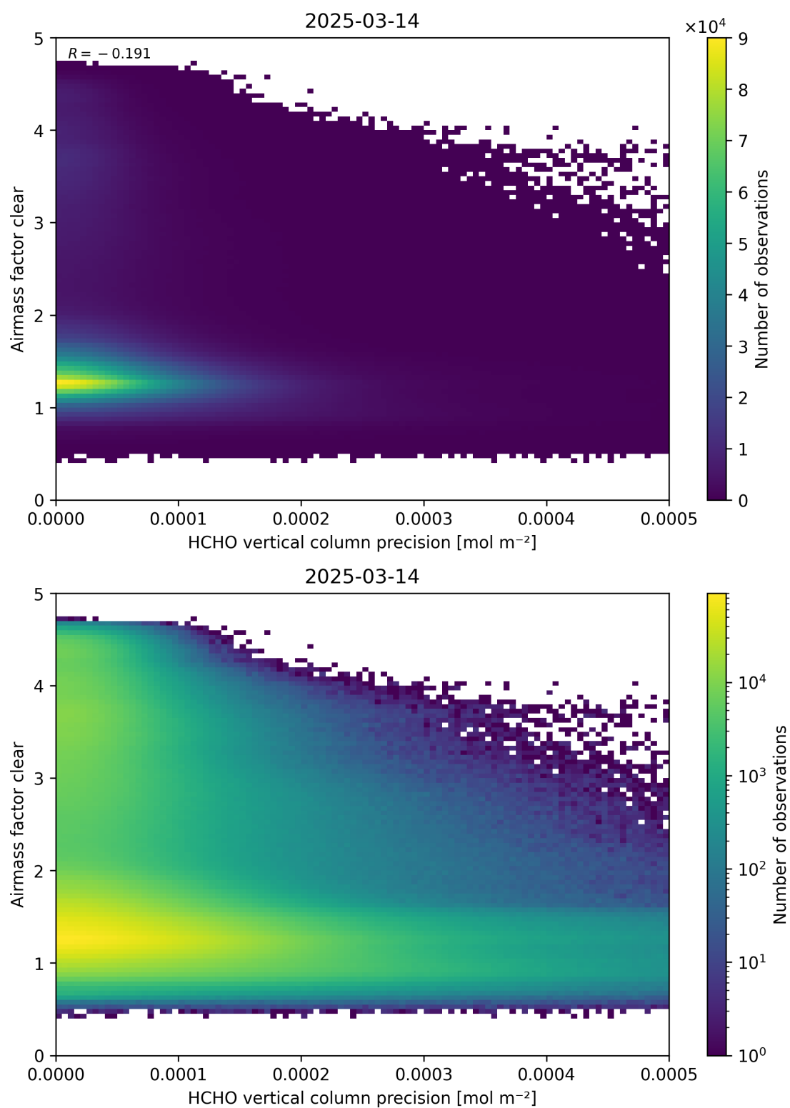
Figure 139: Scatter density plot of “HCHO vertical column precision” against “Airmass factor clear” for 2025-03-13 to 2025-03-15.
