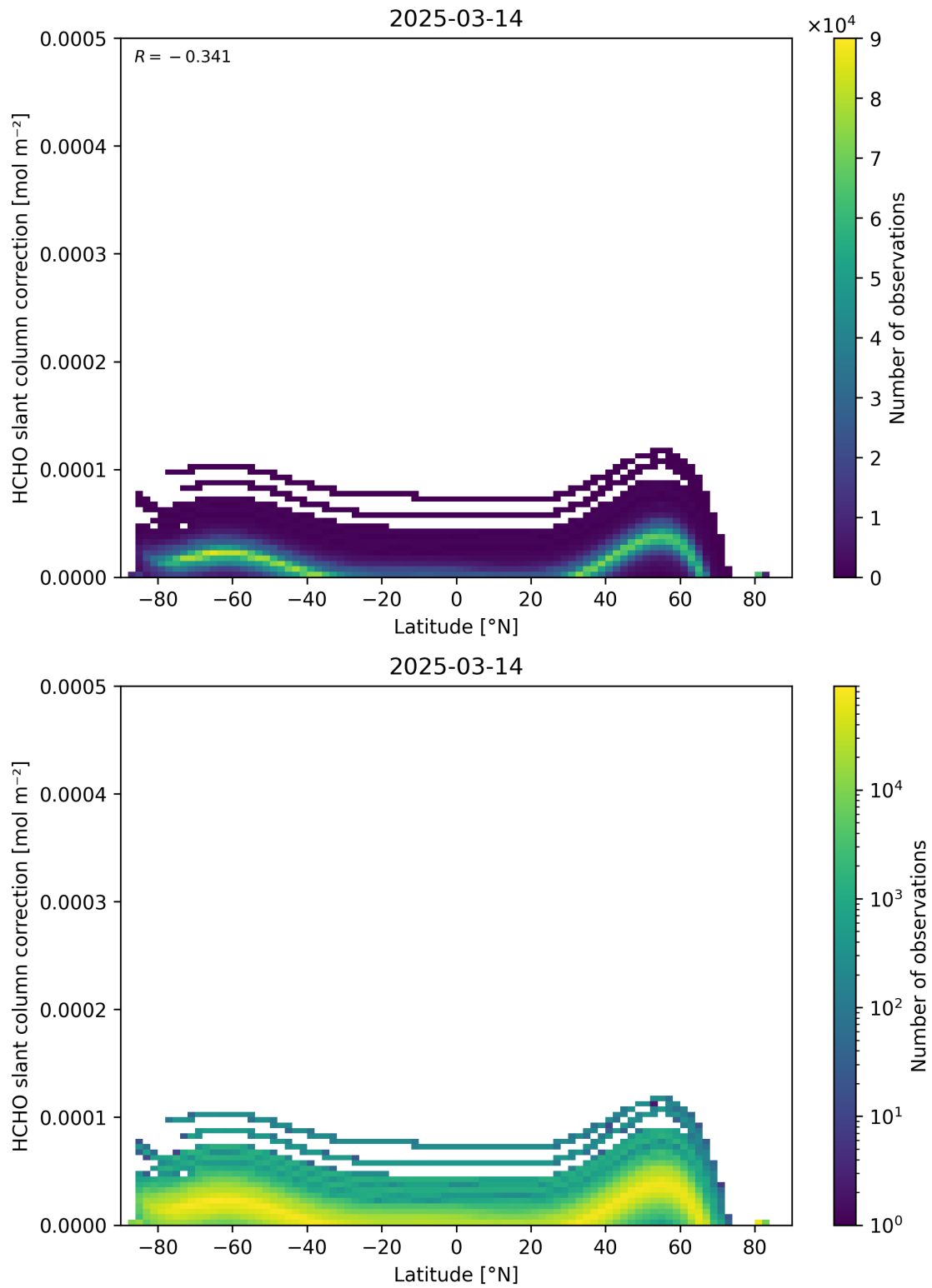
Figure 158: Scatter density plot of “Latitude” against “HCHO slant column correction” for 2025-03-13 to 2025-03-15.
