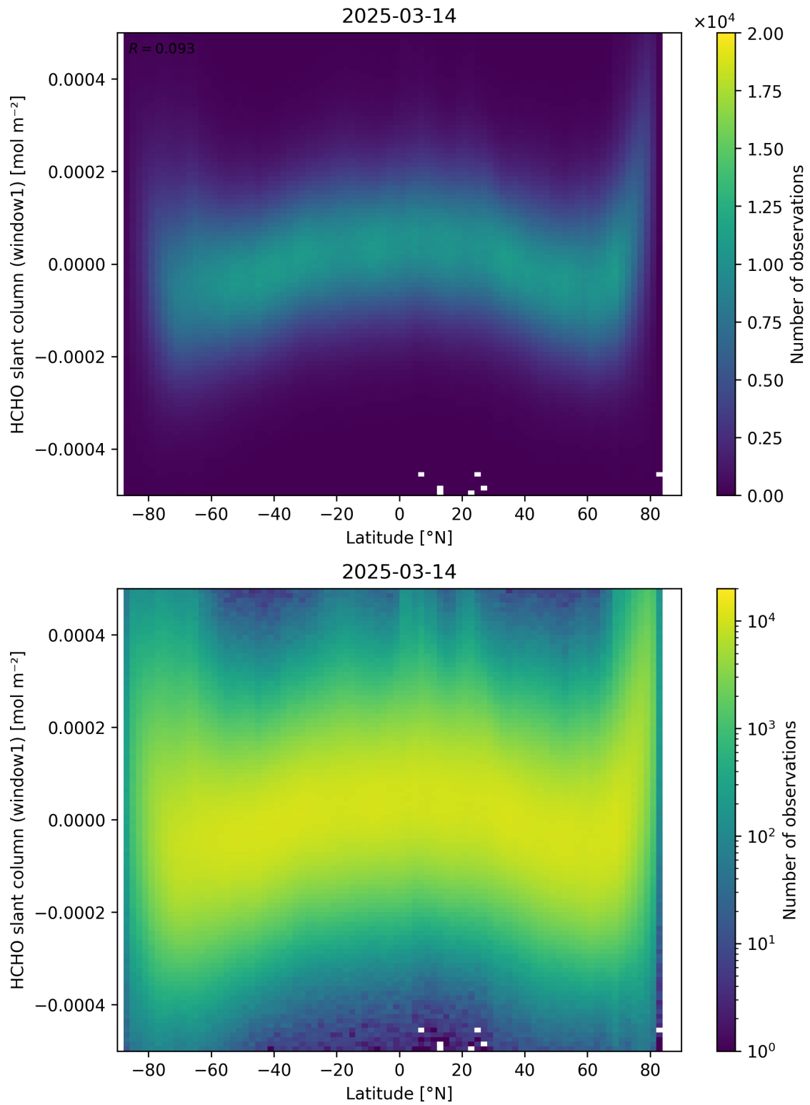
Figure 159: Scatter density plot of “Latitude” against “HCHO slant column (window1)” for 2025-03-13 to 2025-03-15.
