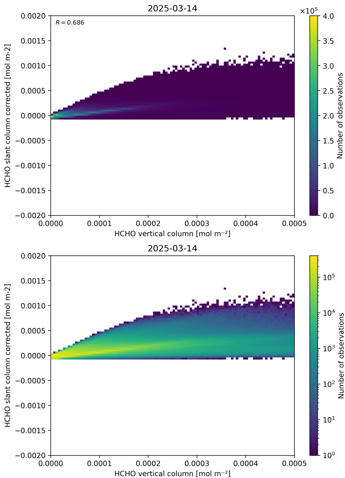
Figure 127: Scatter density plot of “HCHO vertical column” against “HCHO slant column corrected” for 2025-03-13 to 2025-03-15.
