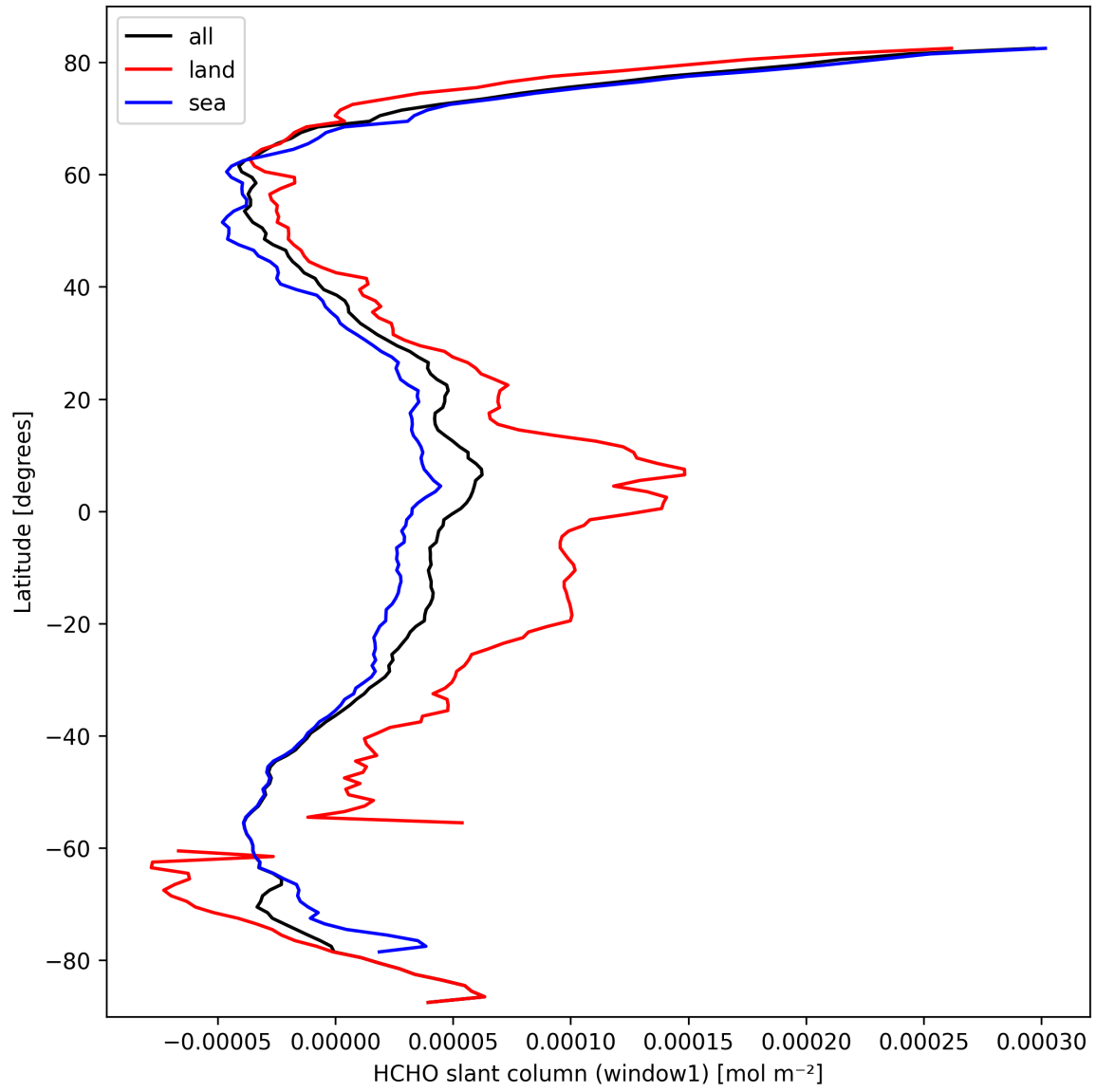
Figure 24: Zonal average of “HCHO slant column (window1)” for 2025-03-13 to 2025-03-15.
