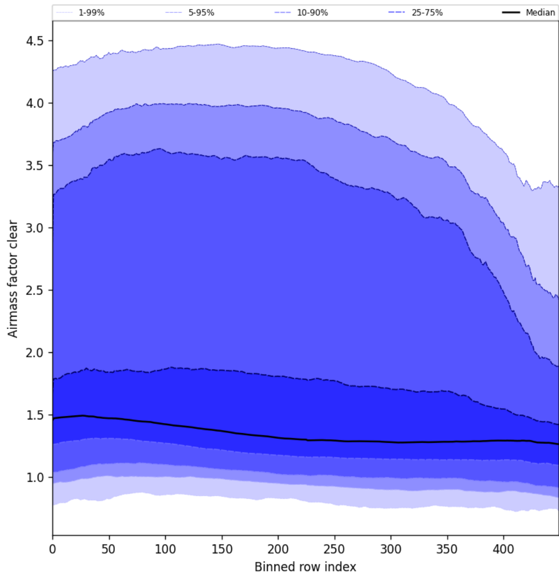
Figure 56: Along track statistics of “Airmass factor clear” for 2025-03-13 to 2025-03-15
