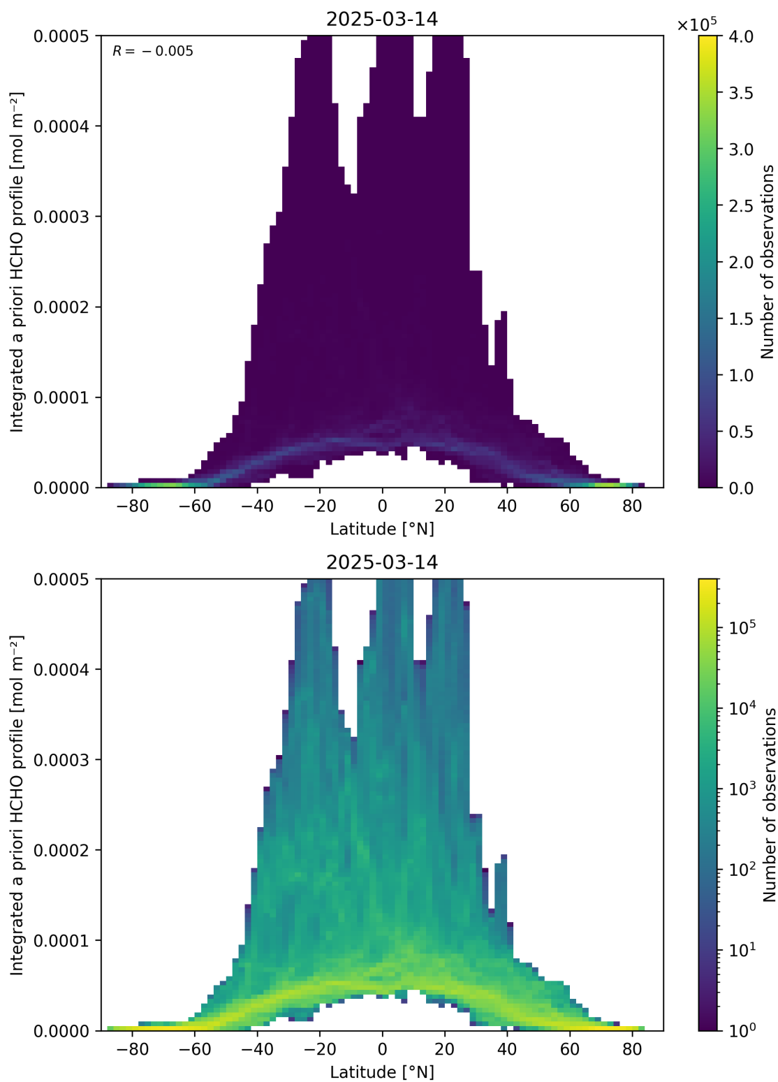
Figure 166: Scatter density plot of “Latitude” against “Integrated a priori HCHO profile” for 2025-03-13 to 2025-03-15.
