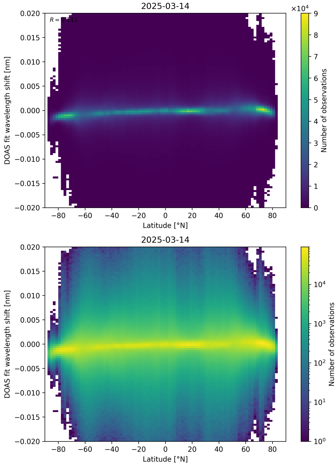
Figure 154: Scatter density plot of “Latitude” against “DOAS fit wavelength shift” for 2025-03-13 to 2025-03-15.
