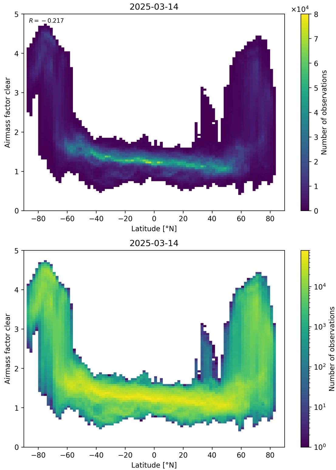
Figure 156: Scatter density plot of “Latitude” against “Airmass factor clear” for 2025-03-13 to 2025-03-15.
