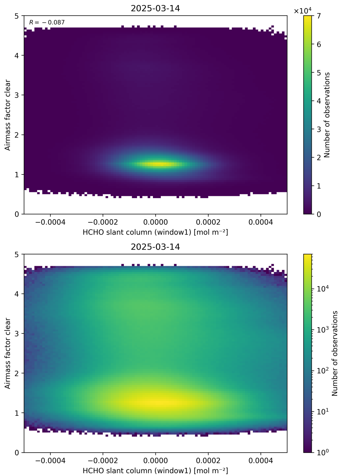
Figure 81: Scatter density plot of “HCHO slant column (window1)” against “Airmass factor clear” for 2025-03-13 to 2025-03-15.
