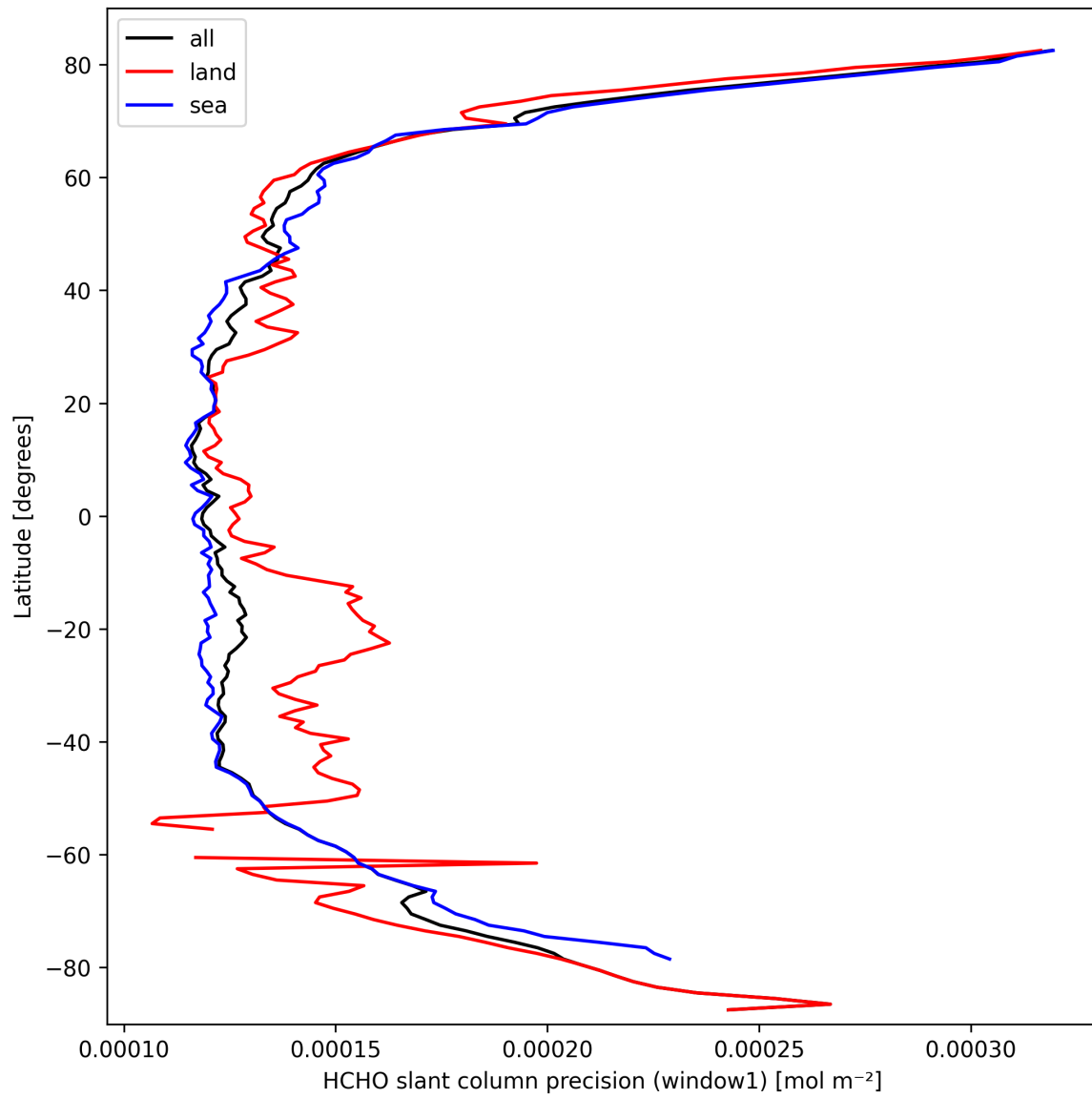
Figure 25: Zonal average of "HCHO slant column precision (window1)" for 2025-03-13 to 2025-03-15.
