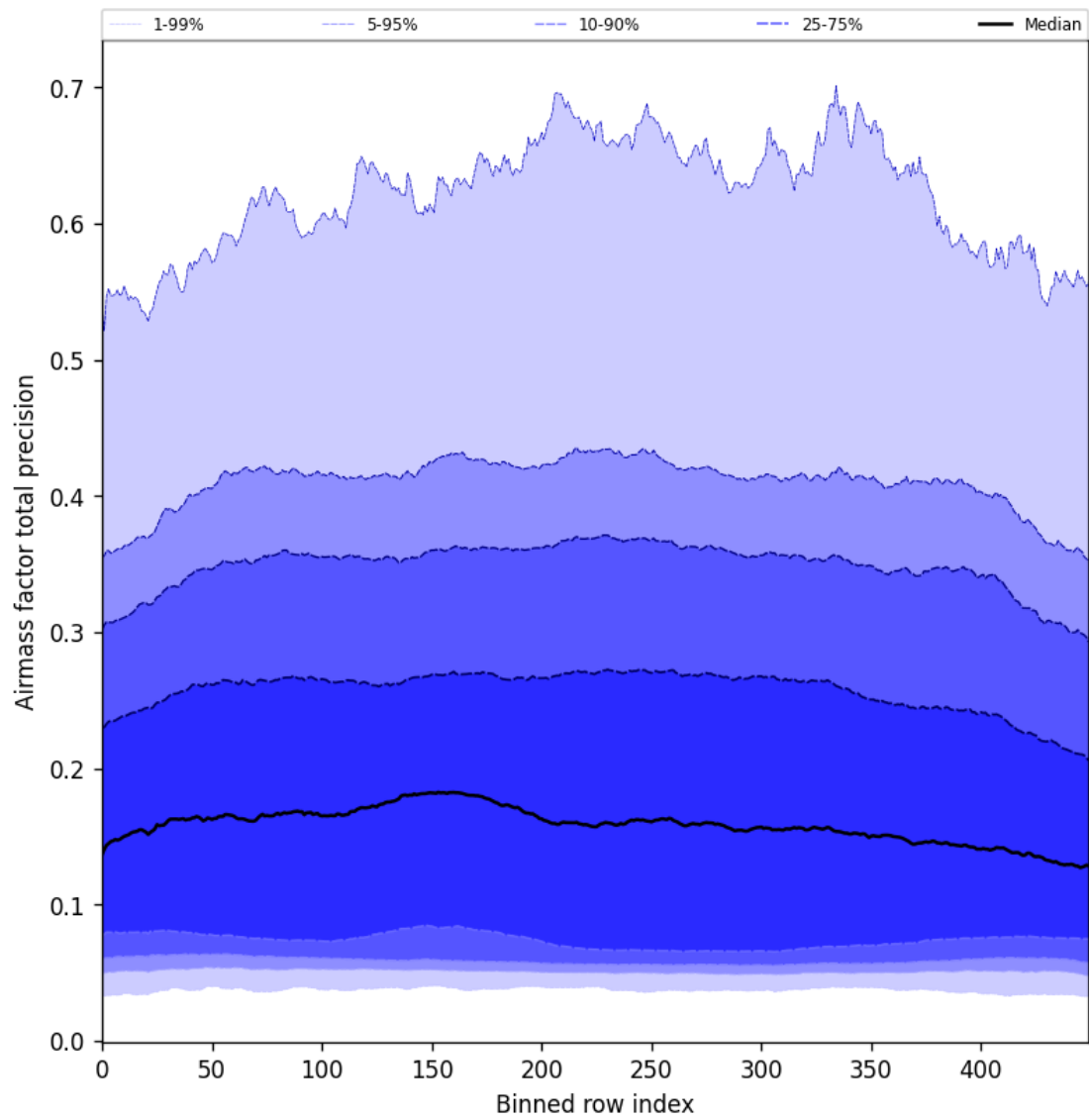
Figure 55: Along track statistics of “Airmass factor total precision” for 2025-03-13 to 2025-03-15
