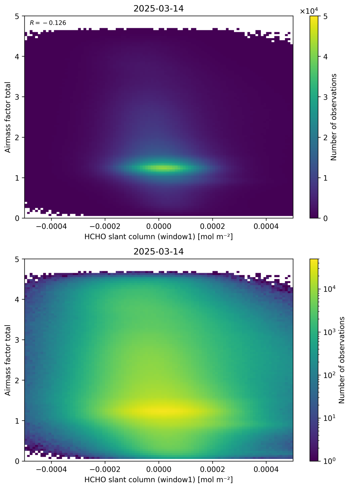
Figure 85: Scatter density plot of “HCHO slant column (window1)” against “Airmass factor total” for 2025-03-13 to 2025-03-15.
