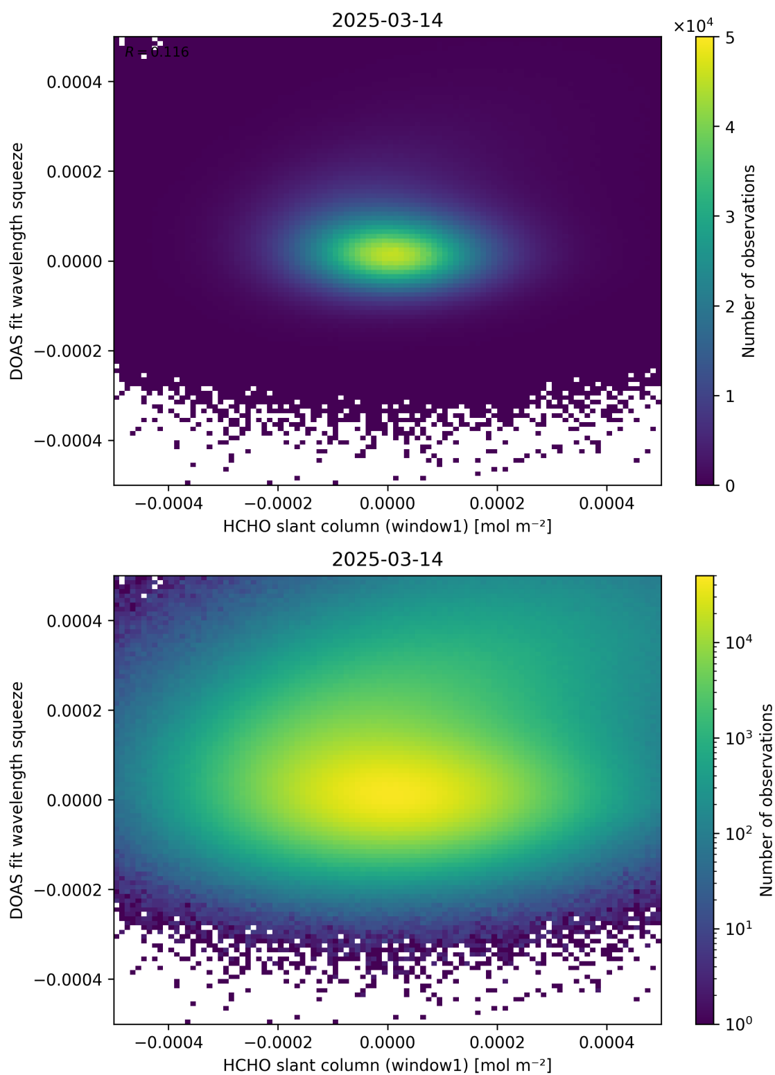
Figure 80: Scatter density plot of “HCHO slant column (window1)” against “DOAS fit wavelength squeeze” for 2025-03-13 to 2025-03-15.
