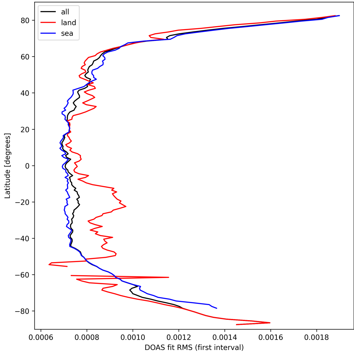
Figure 32: Zonal average of "DOAS fit RMS (first interval)" for 2025-03-13 to 2025-03-15.
