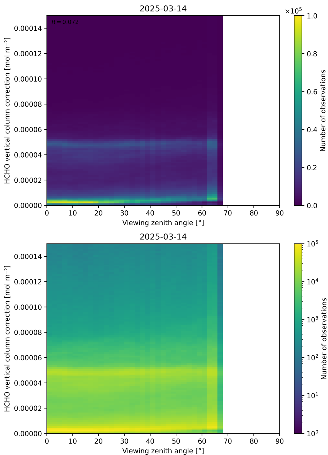
Figure 193: Scatter density plot of “Viewing zenith angle” against “HCHO vertical column correction” for 2025-03-13 to 2025-03-15.
