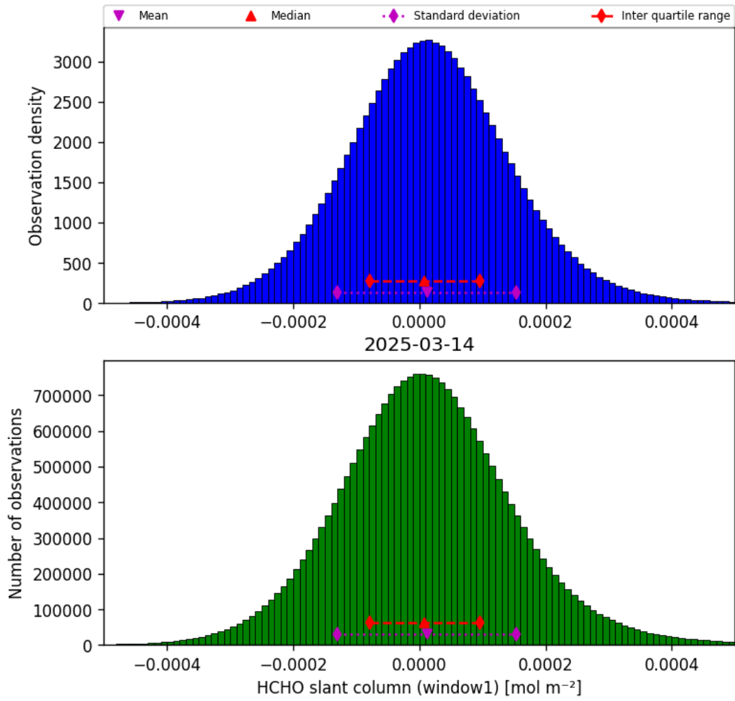
Figure 38: Histogram of “HCHO slant column (window1)” for 2025-03-13 to 2025-03-15
