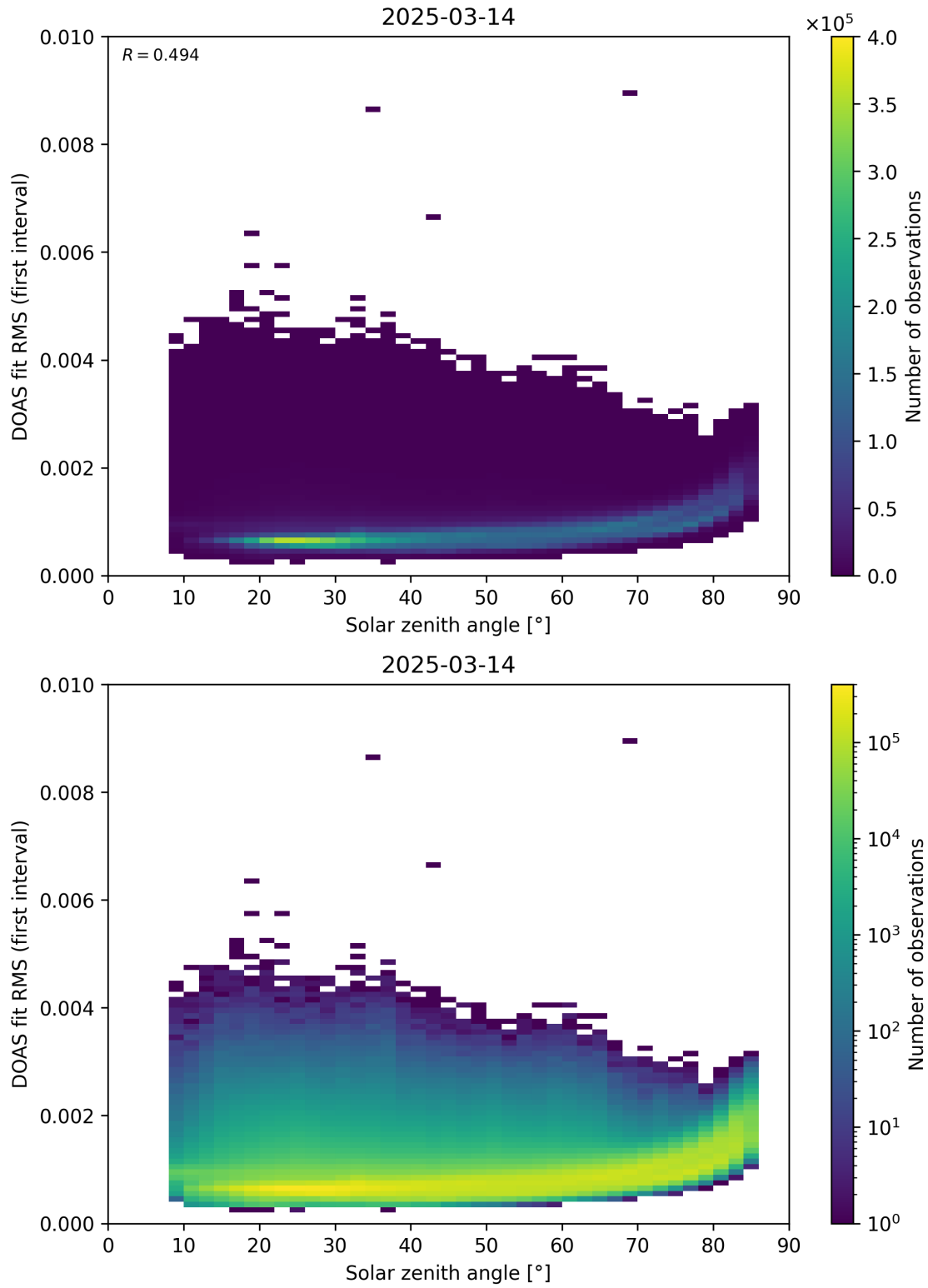
Figure 167: Scatter density plot of “Solar zenith angle” against “DOAS fit RMS (first interval)” for 2025-03-13 to 2025-03-15.
