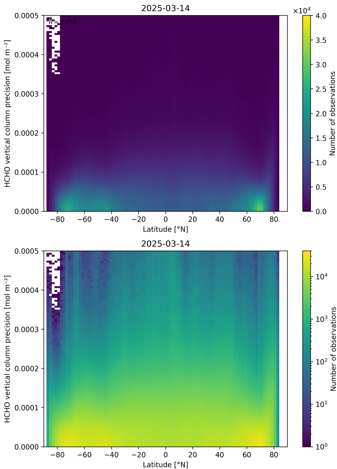
Figure 165: Scatter density plot of “Latitude” against “HCHO vertical column precision” for 2025-03-13 to 2025-03-15.
