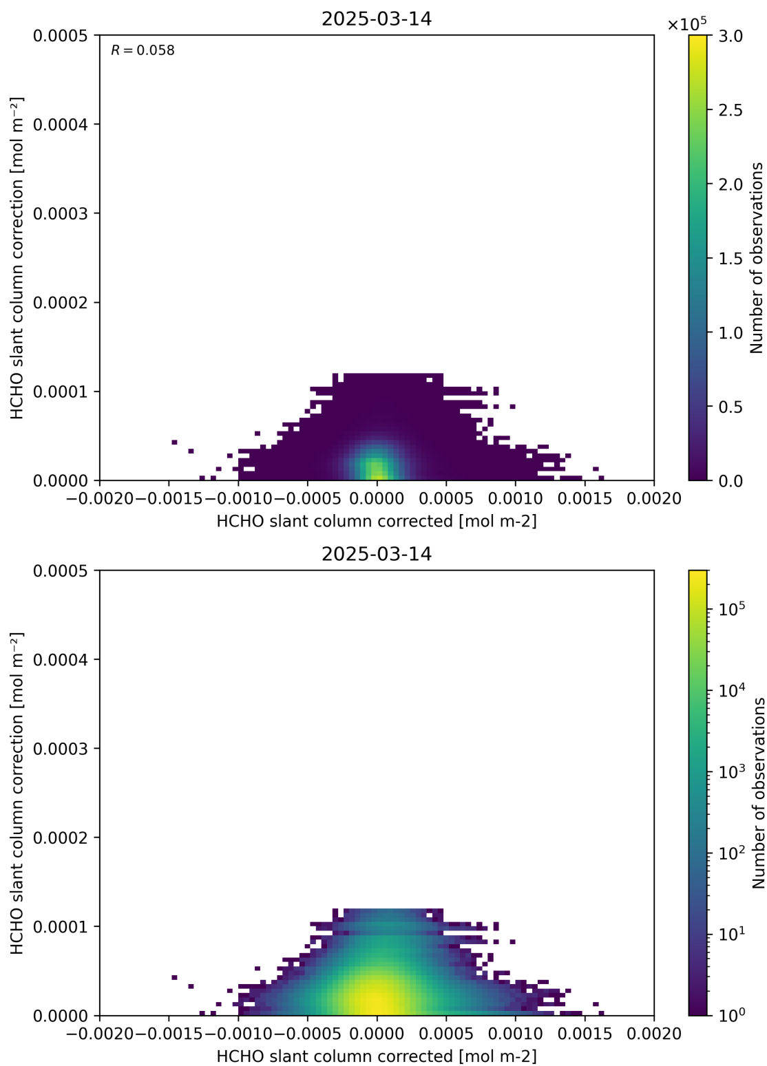
Figure 77: Scatter density plot of “HCHO slant column corrected” against “HCHO slant column correction” for 2025-03-13 to 2025-03-15.
