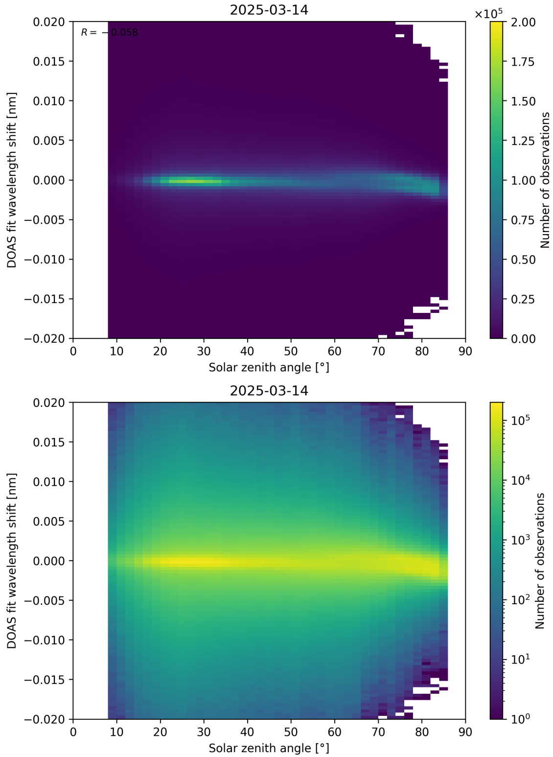
Figure 168: Scatter density plot of “Solar zenith angle” against “DOAS fit wavelength shift” for 2025-03-13 to 2025-03-15.
