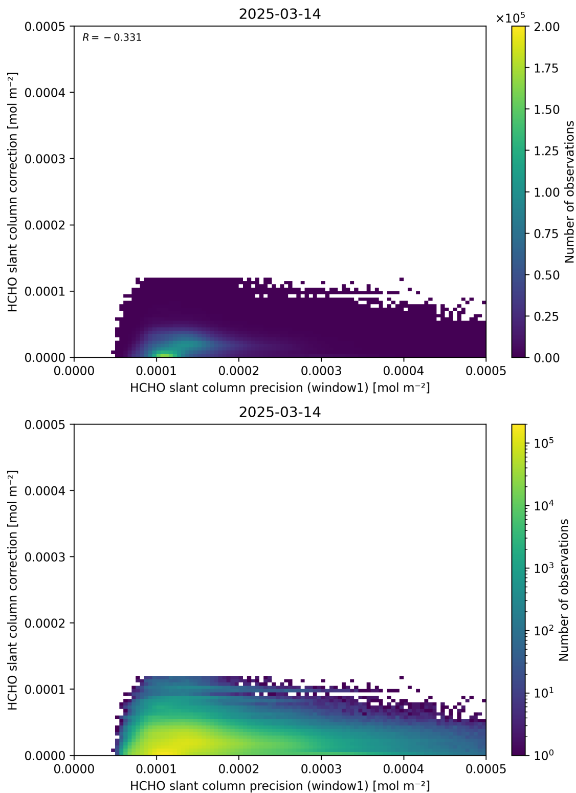
Figure 93: Scatter density plot of “HCHO slant column precision (window1)” against “HCHO slant column correction” for 2025-03-13 to 2025-03-15.
