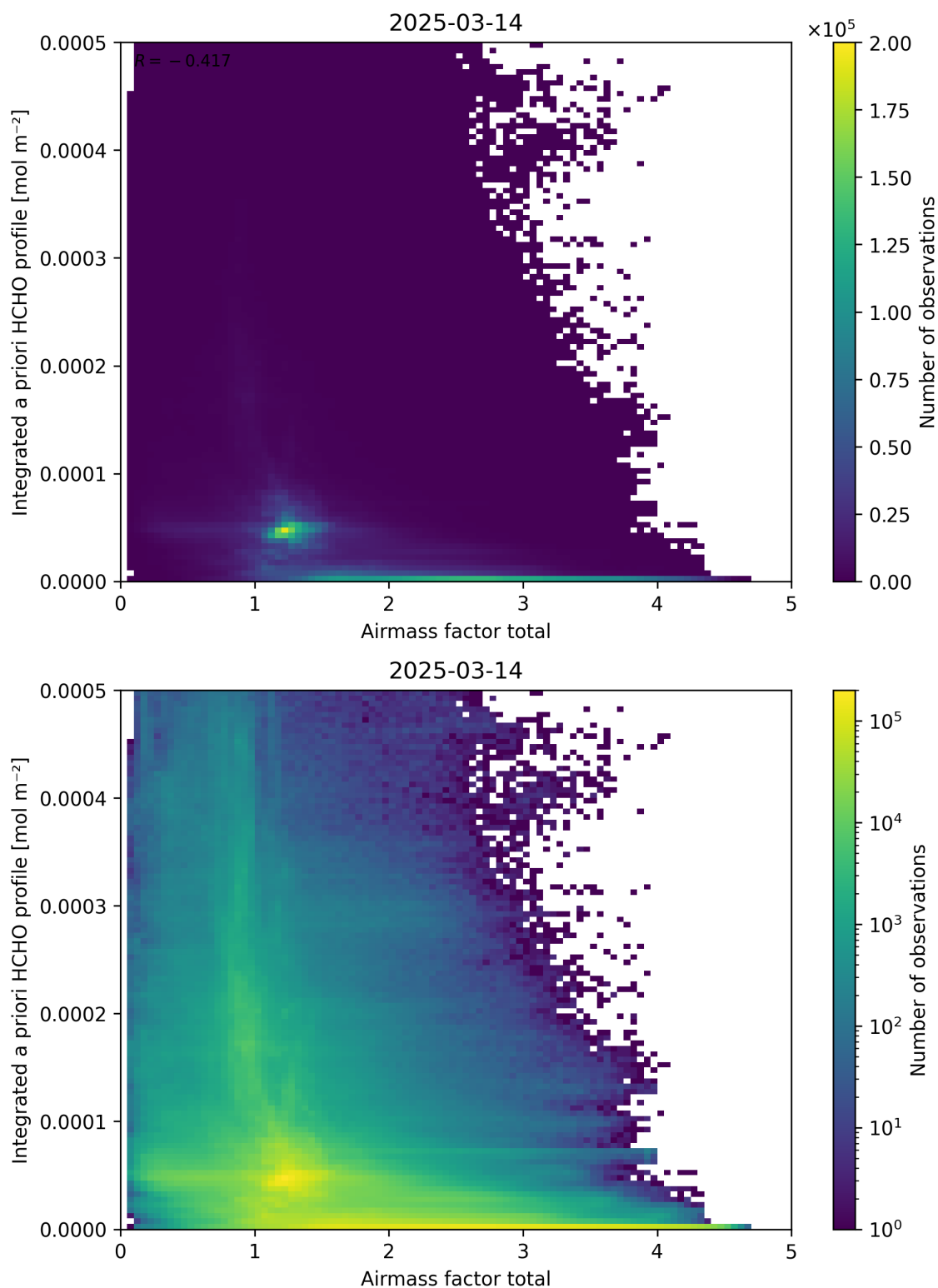
Figure 104: Scatter density plot of “Airmass factor total” against “Integrated a priori HCHO profile” for 2025-03-13 to 2025-03-15.
