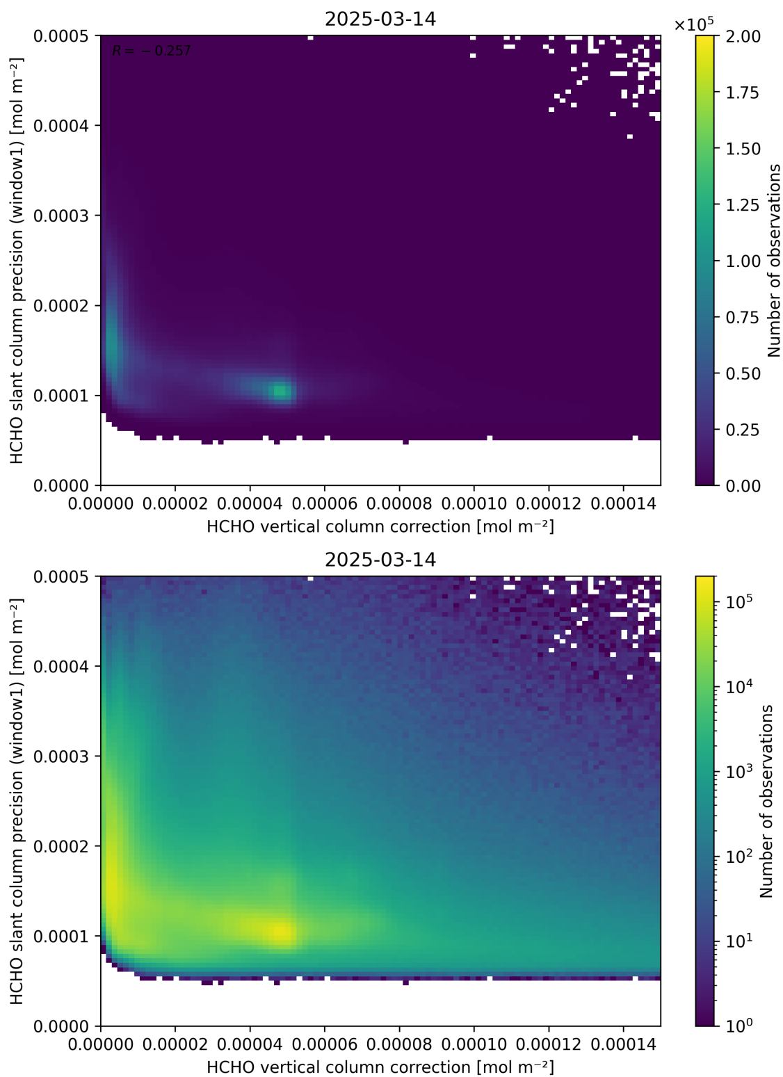
Figure 119: Scatter density plot of “HCHO vertical column correction” against “HCHO slant column precision (window1)” for 2025-03-13 to 2025-03-15.
