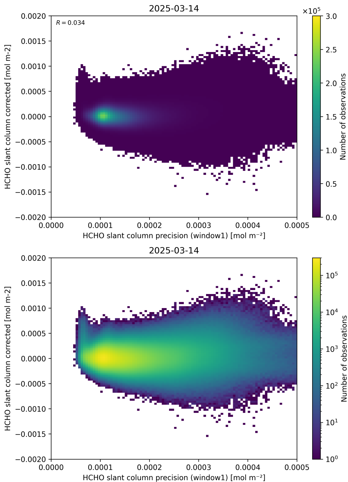
Figure 92: Scatter density plot of “HCHO slant column precision (window1)” against “HCHO slant column corrected” for 2025-03-13 to 2025-03-15.
