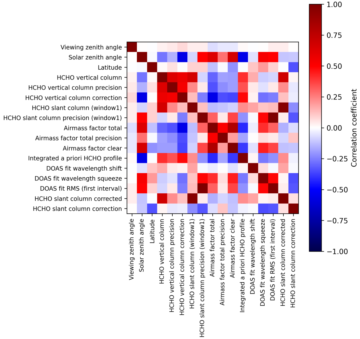
Figure 2: Map of correlation matrix for 2025-03-13 to 2025-03-15.
