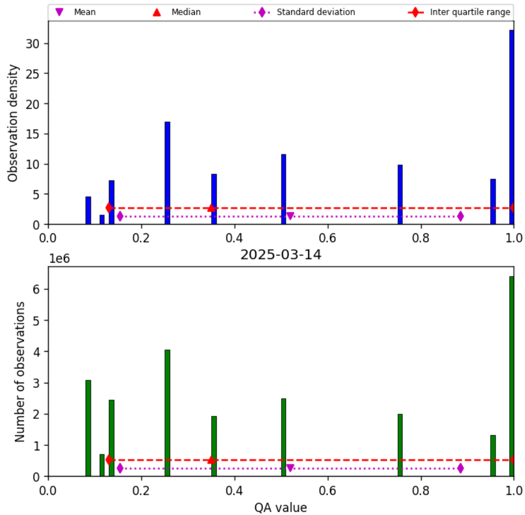
Figure 34: Histogram of “QA value” for 2025-03-13 to 2025-03-15
