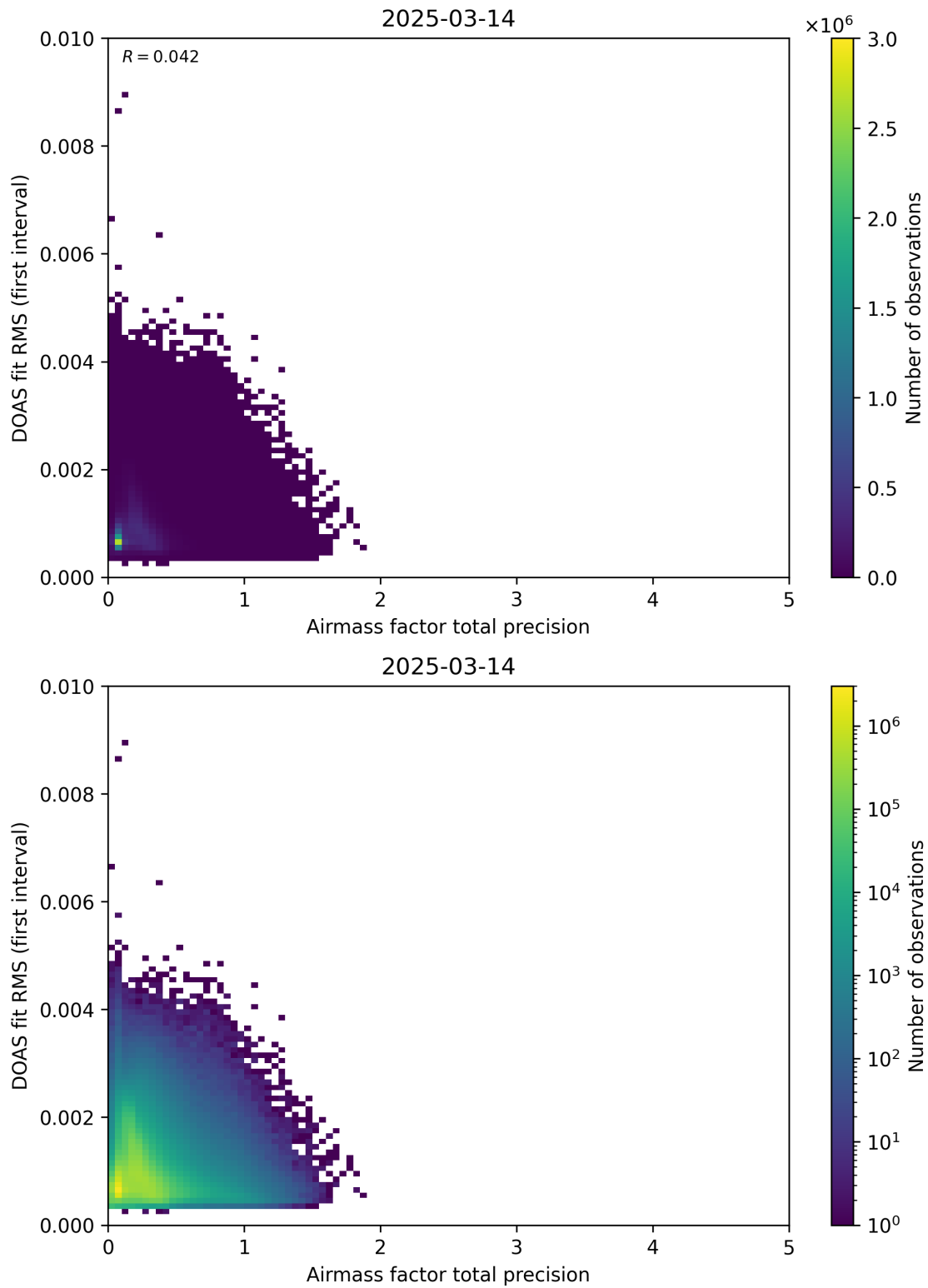
Figure 105: Scatter density plot of “Airmass factor total precision” against “DOAS fit RMS (first interval)” for 2025-03-13 to 2025-03-15.
