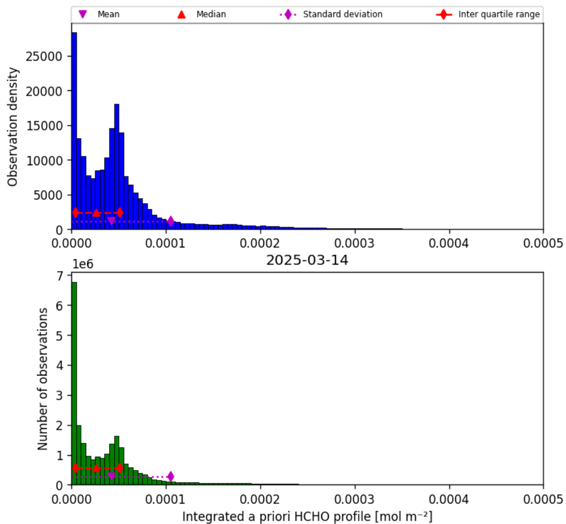
Figure 43: Histogram of “Integrated a priori HCHO profile” for 2025-03-13 to 2025-03-15
