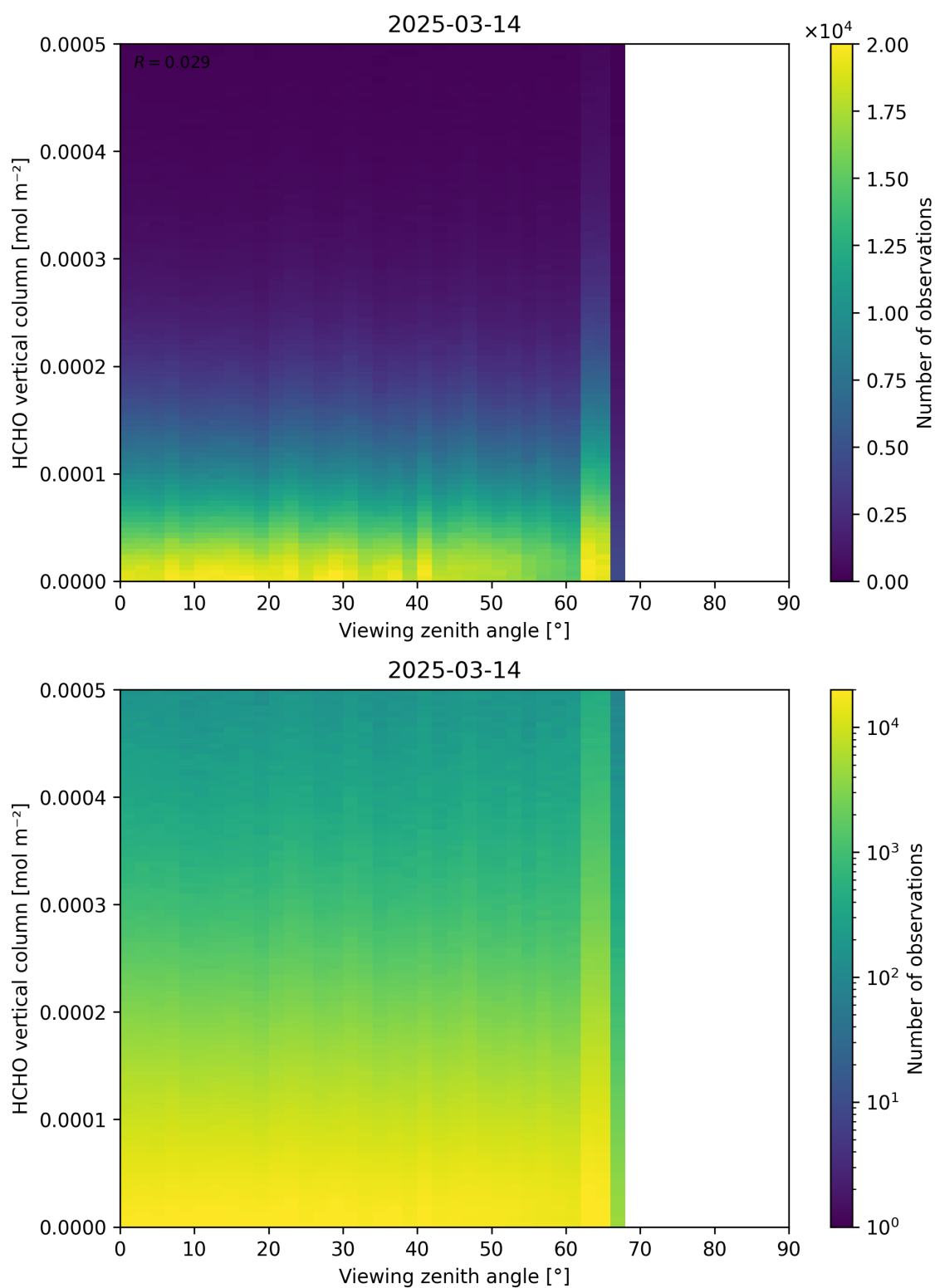
Figure 192: Scatter density plot of “Viewing zenith angle” against “HCHO vertical column” for 2025-03-13 to 2025-03-15.
