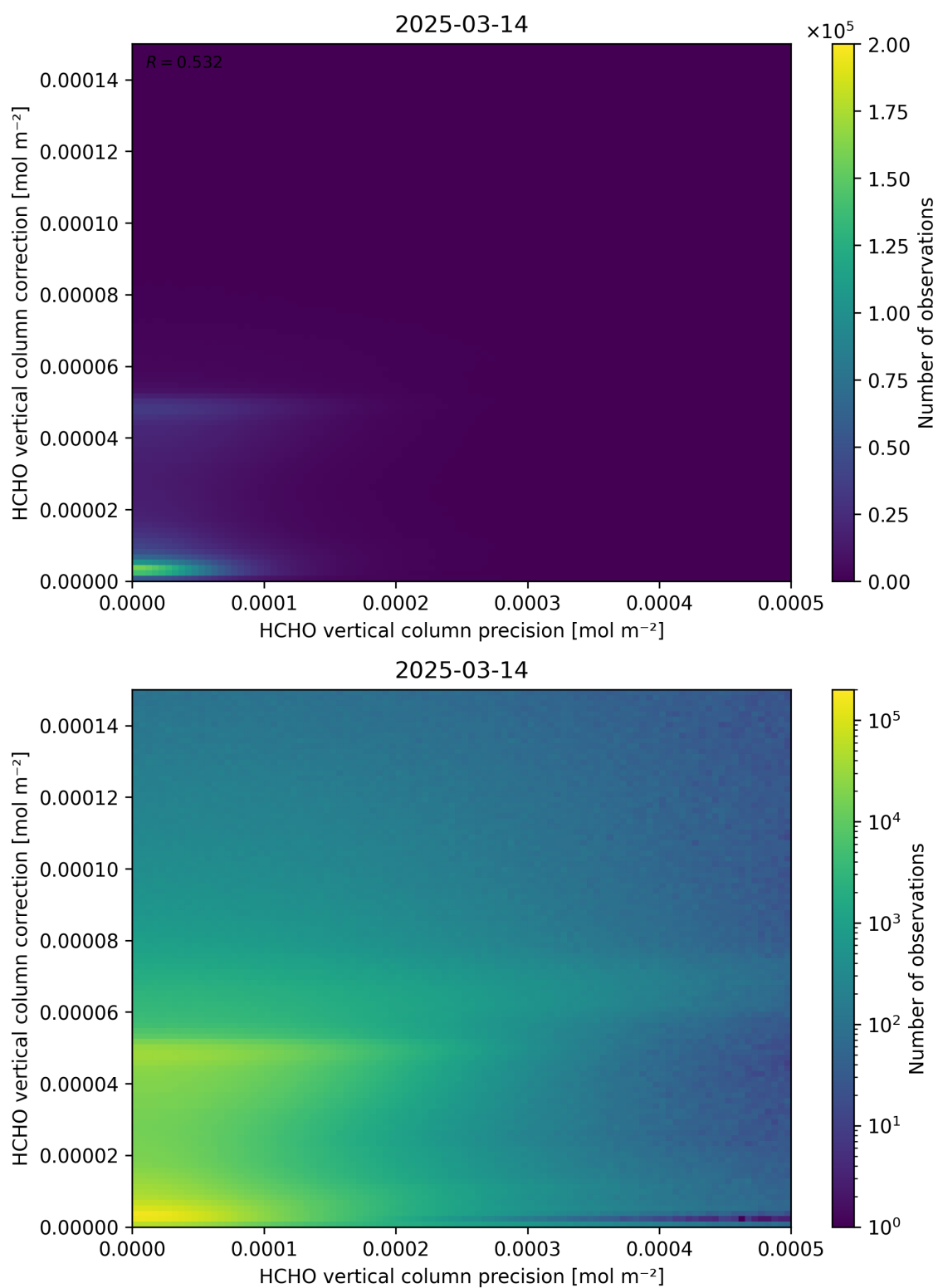
Figure 146: Scatter density plot of “HCHO vertical column precision” against “HCHO vertical column correction” for 2025-03-13 to 2025-03-15.
