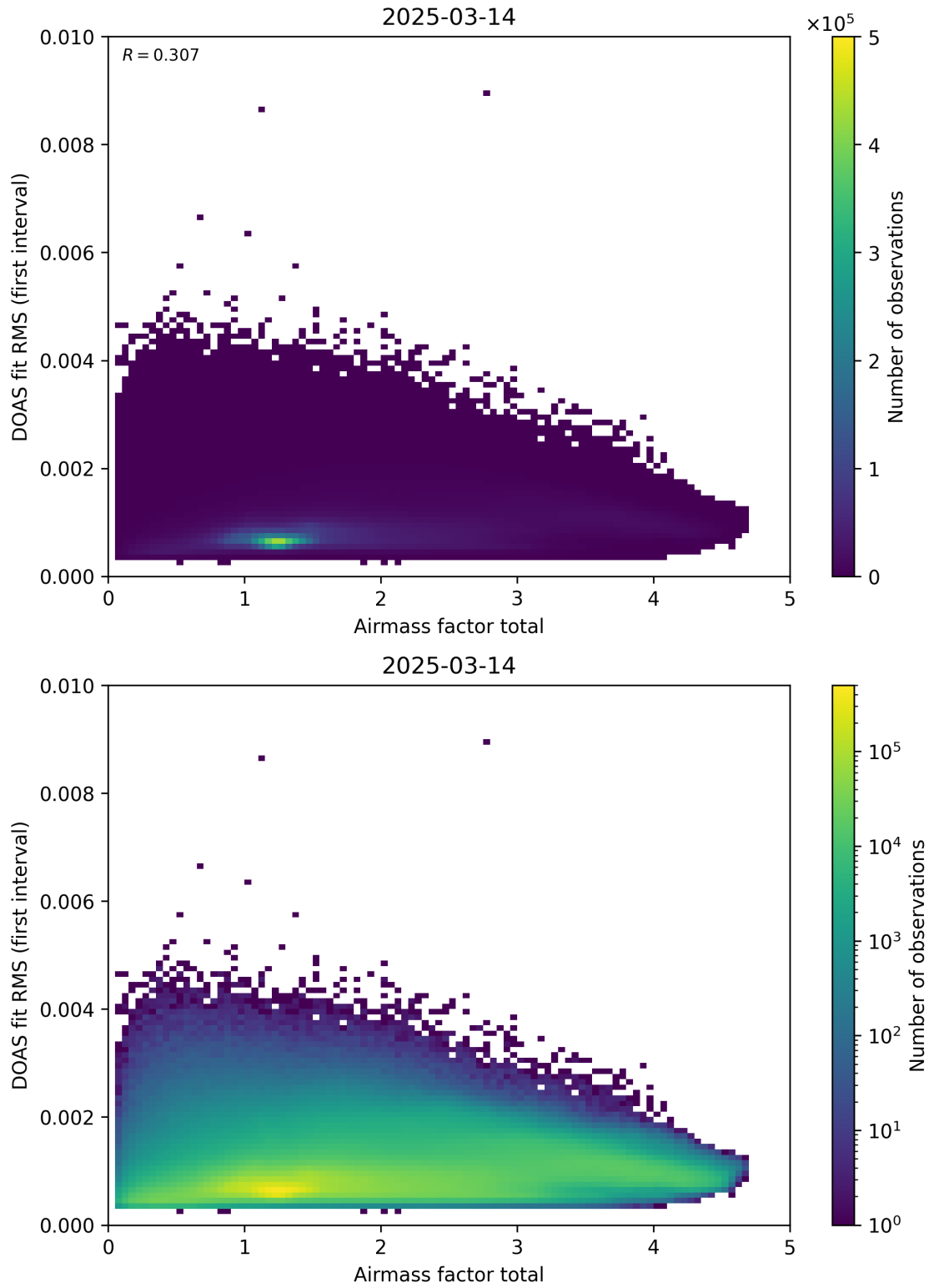
Figure 97: Scatter density plot of “Airmass factor total” against “DOAS fit RMS (first interval)” for 2025-03-13 to 2025-03-15.
