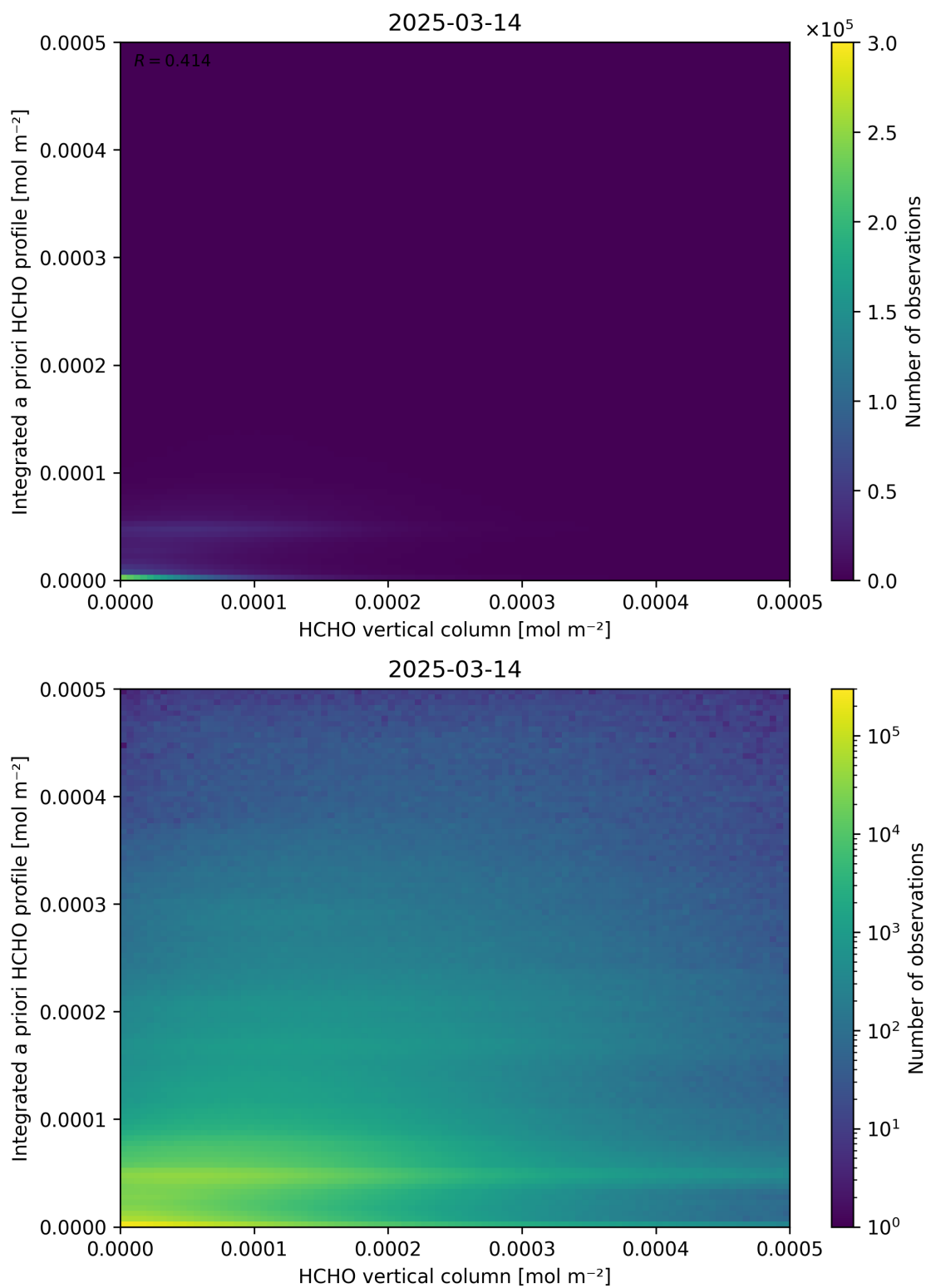
Figure 135: Scatter density plot of “HCHO vertical column” against “Integrated a priori HCHO profile” for 2025-03-13 to 2025-03-15.
