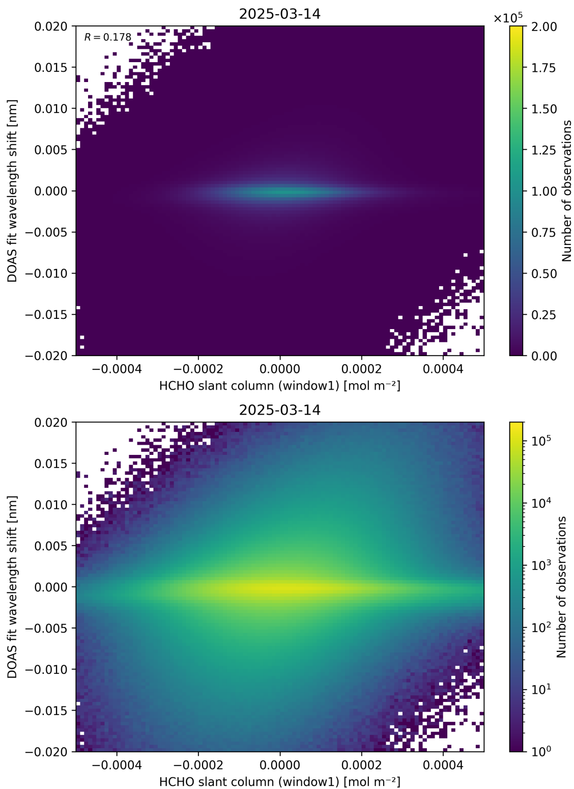
Figure 79: Scatter density plot of “HCHO slant column (window1)” against “DOAS fit wavelength shift” for 2025-03-13 to 2025-03-15.
