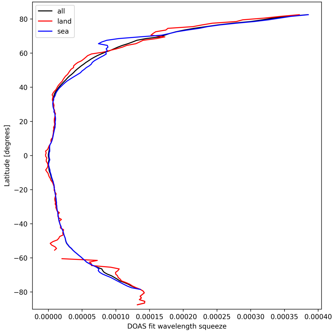
Figure 31: Zonal average of “DOAS fit wavelength squeeze” for 2025-03-13 to 2025-03-15.
