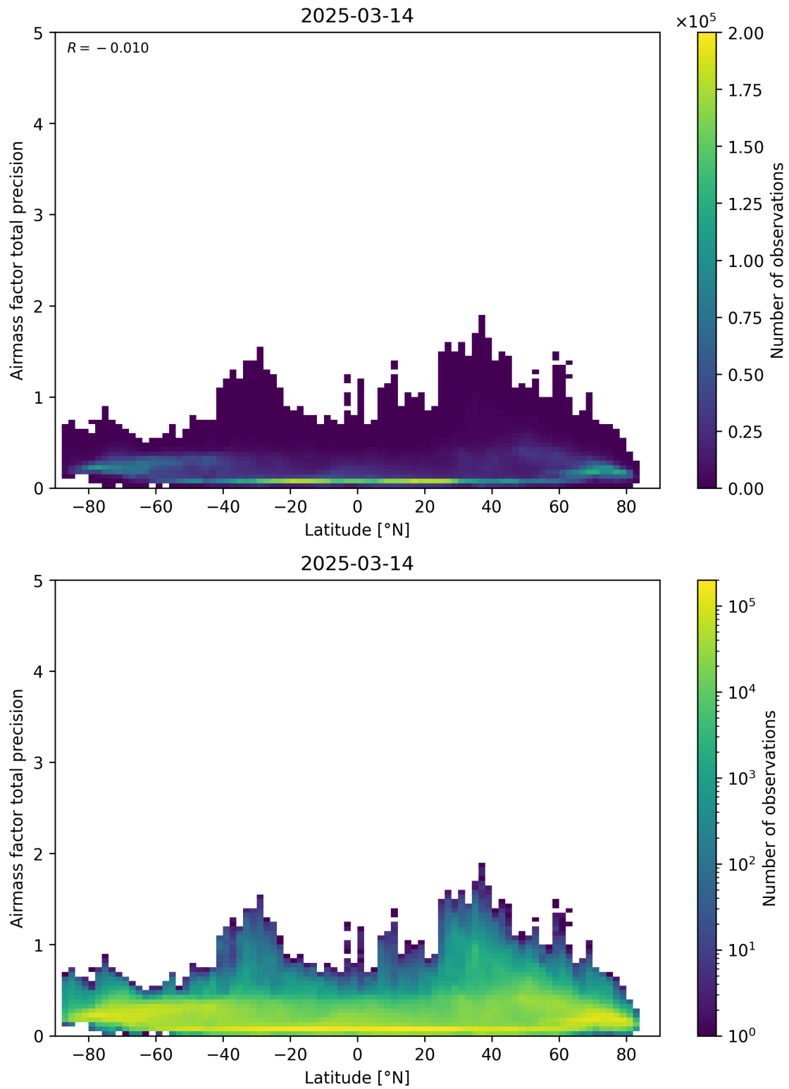
Figure 162: Scatter density plot of “Latitude” against “Airmass factor total precision” for 2025-03-13 to 2025-03-15.
