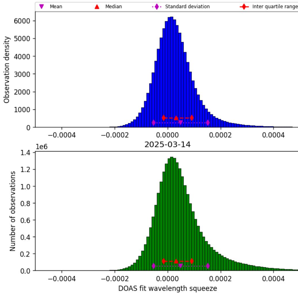
Figure 45: Histogram of “DOAS fit wavelength squeeze” for 2025-03-13 to 2025-03-15
