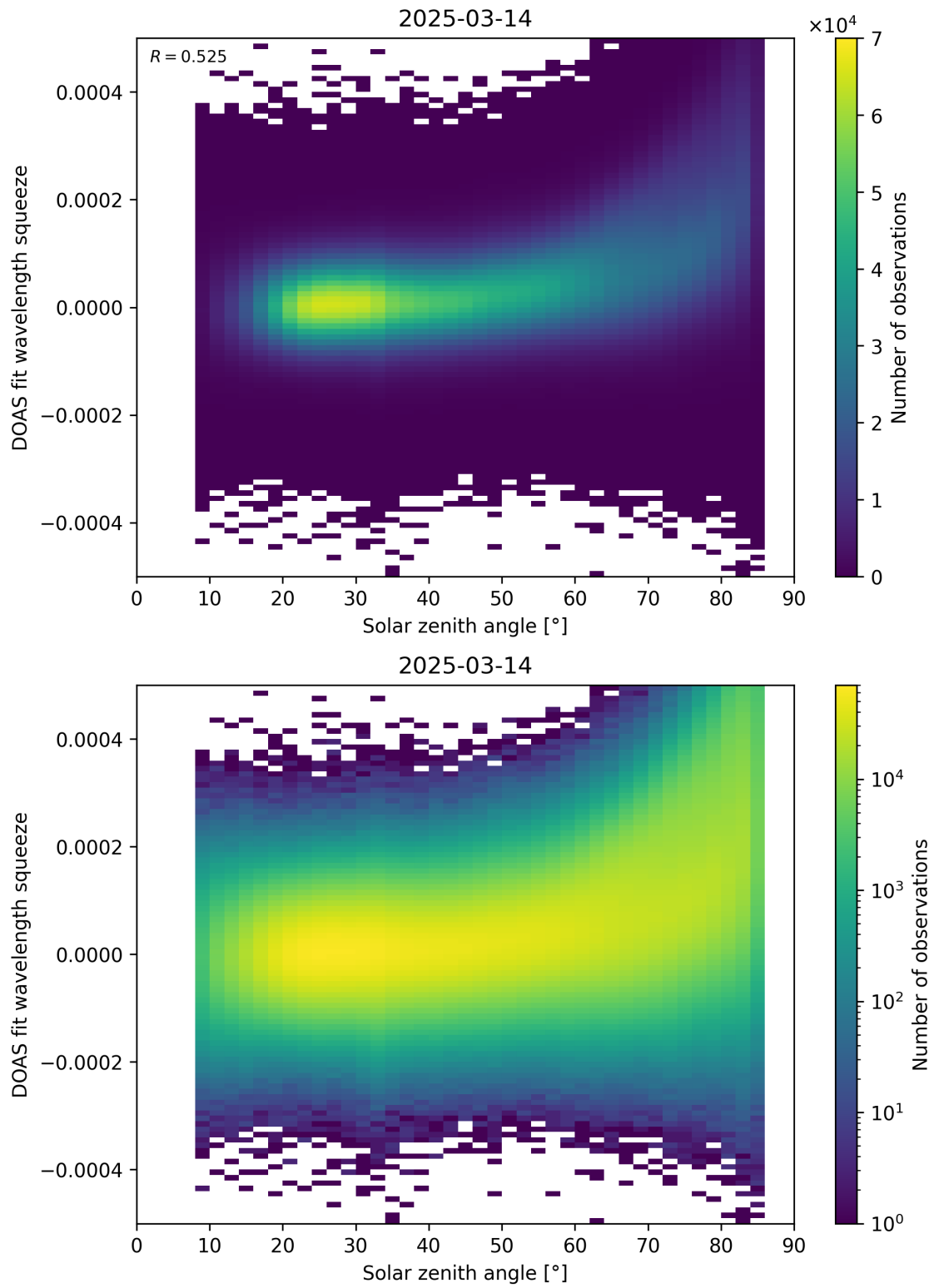
Figure 169: Scatter density plot of “Solar zenith angle” against “DOAS fit wavelength squeeze” for 2025-03-13 to 2025-03-15.
