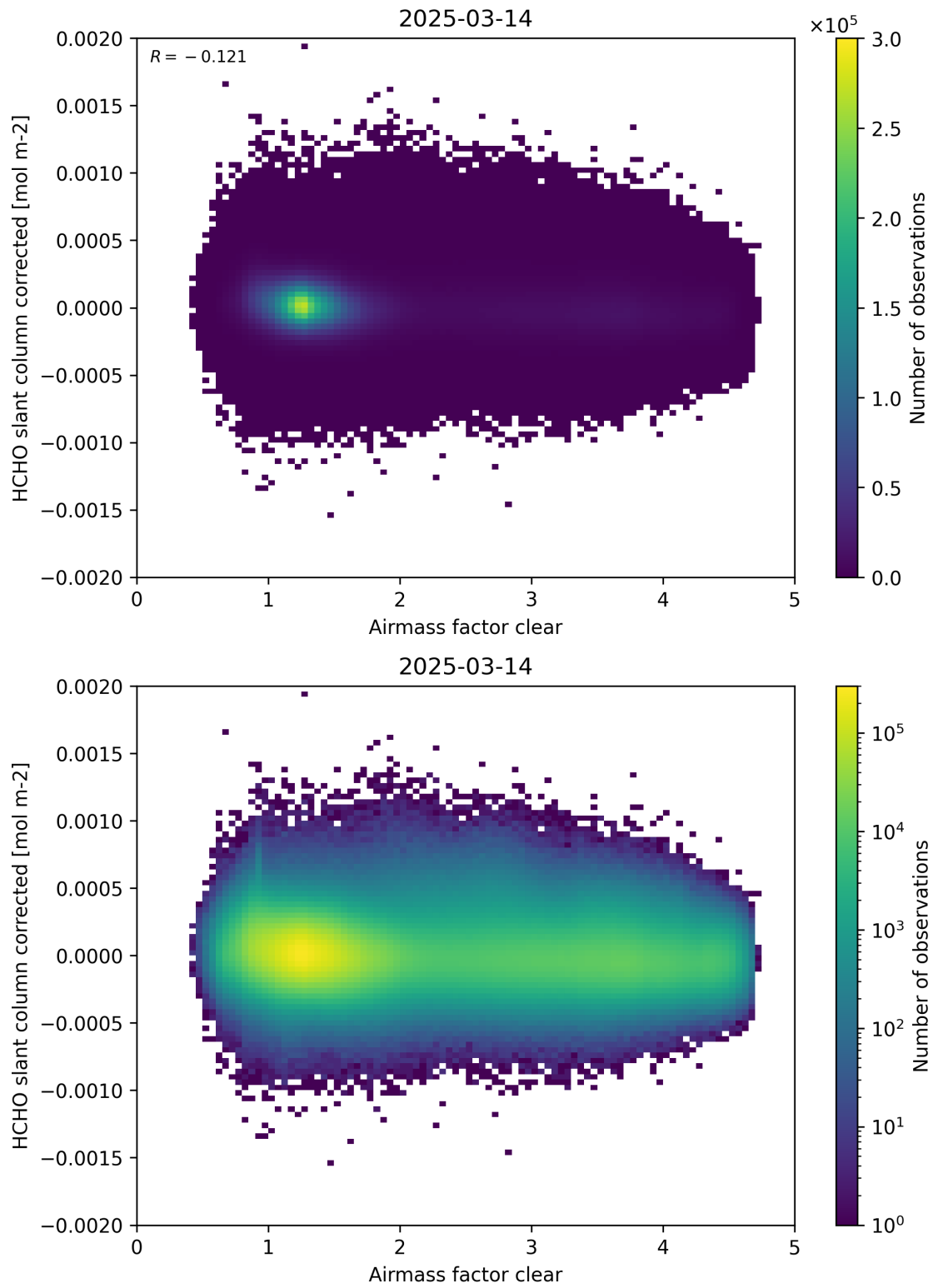
Figure 74: Scatter density plot of “Airmass factor clear” against “HCHO slant column corrected” for 2025-03-13 to 2025-03-15.
