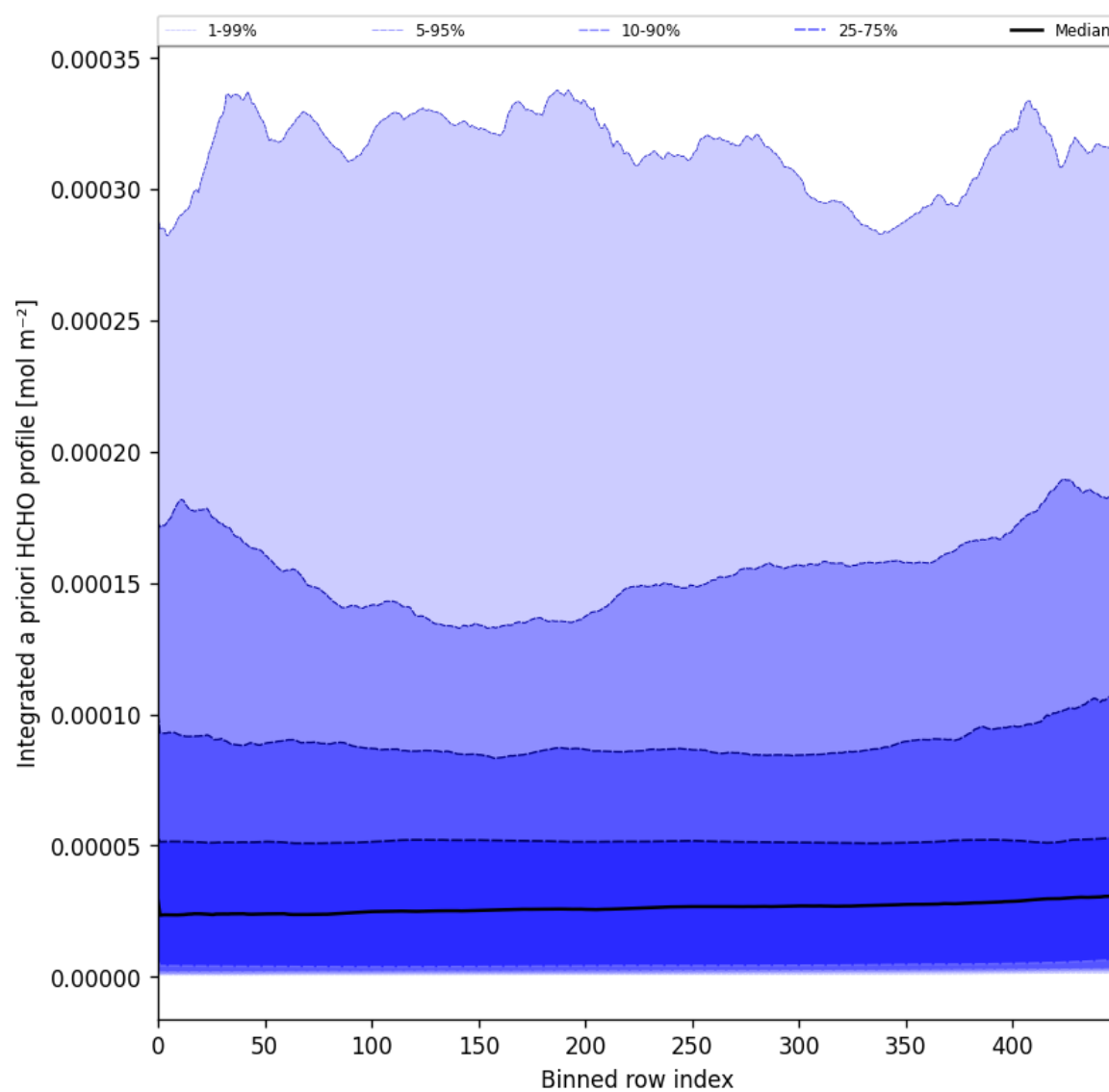
Figure 57: Along track statistics of “Integrated a priori HCHO profile” for 2025-03-13 to 2025-03-15
