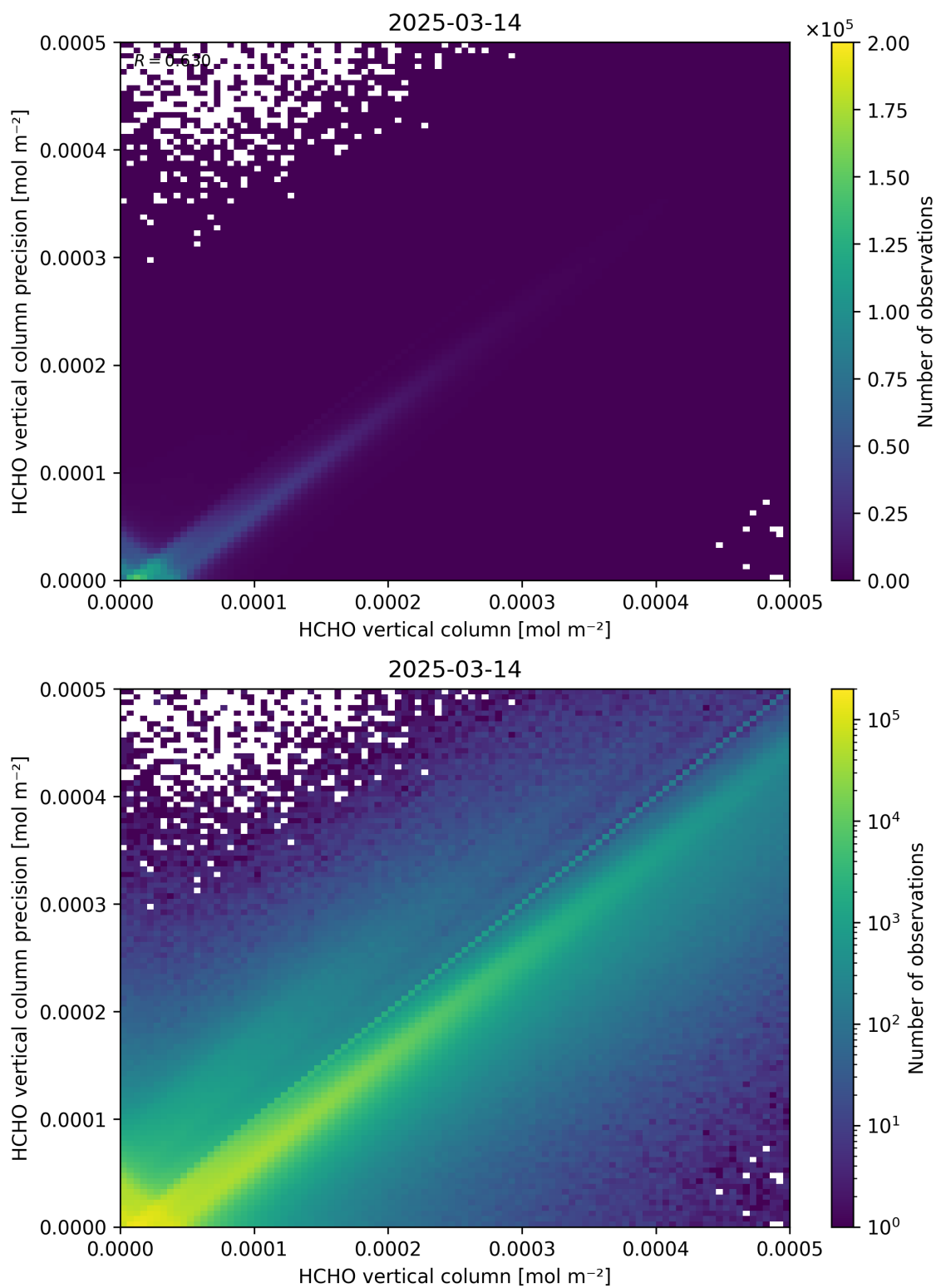
Figure 134: Scatter density plot of “HCHO vertical column” against “HCHO vertical column precision” for 2025-03-13 to 2025-03-15.
