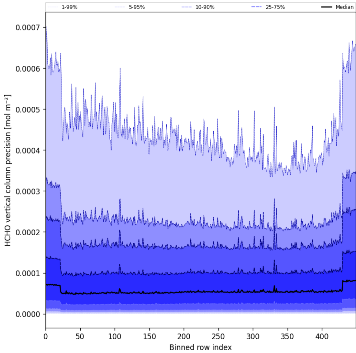
Figure 50: Along track statistics of “HCHO vertical column precision” for 2025-03-13 to 2025-03-15
