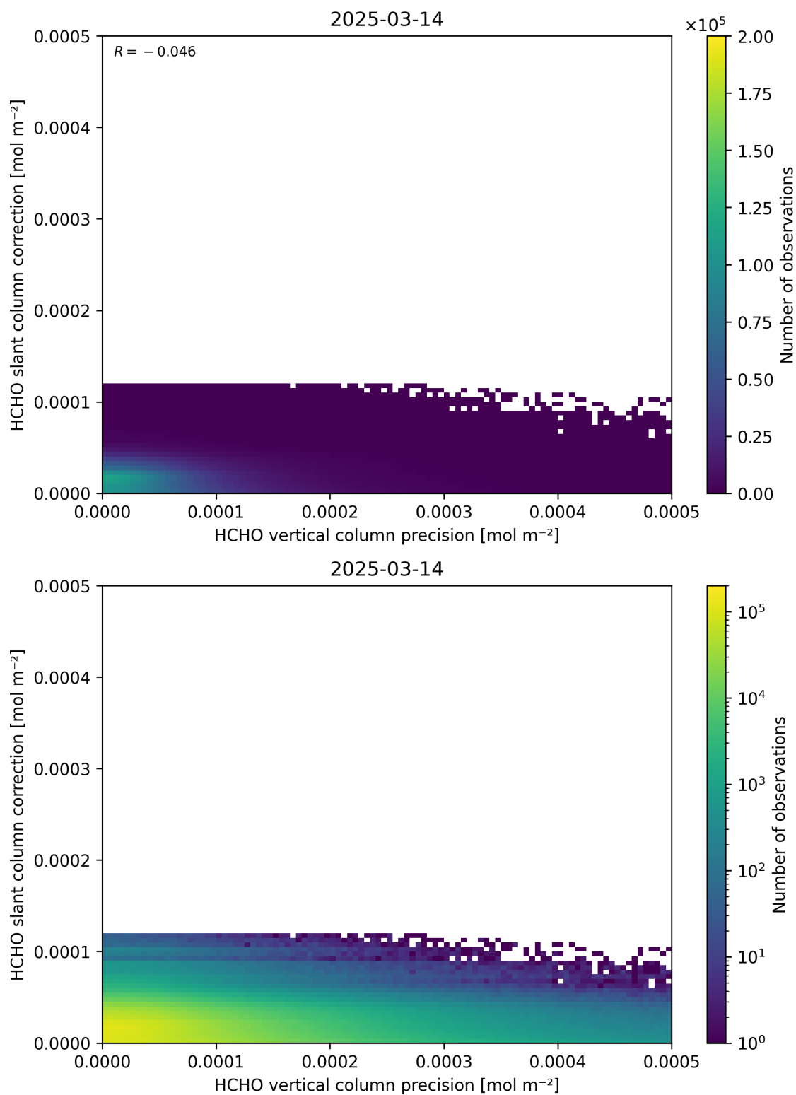
Figure 141: Scatter density plot of “HCHO vertical column precision” against “HCHO slant column correction” for 2025-03-13 to 2025-03-15.
