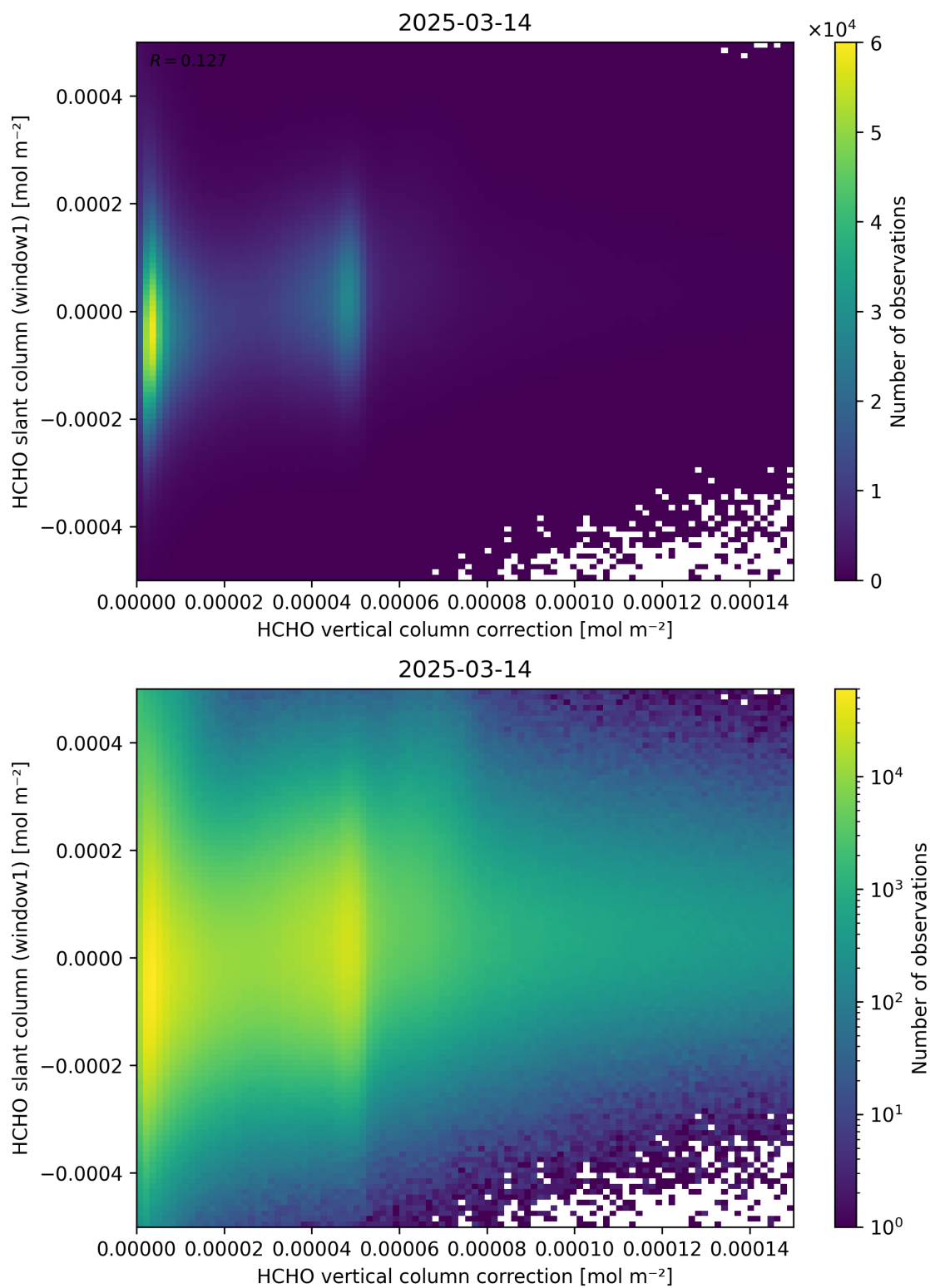
Figure 118: Scatter density plot of “HCHO vertical column correction” against “HCHO slant column (window1)” for 2025-03-13 to 2025-03-15.
