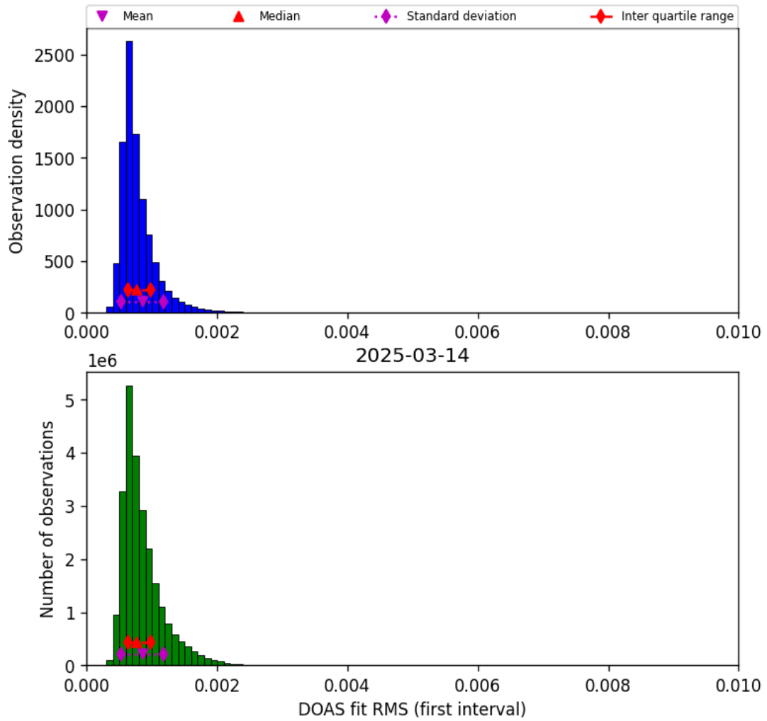
Figure 46: Histogram of “DOAS fit RMS (first interval)” for 2025-03-13 to 2025-03-15
