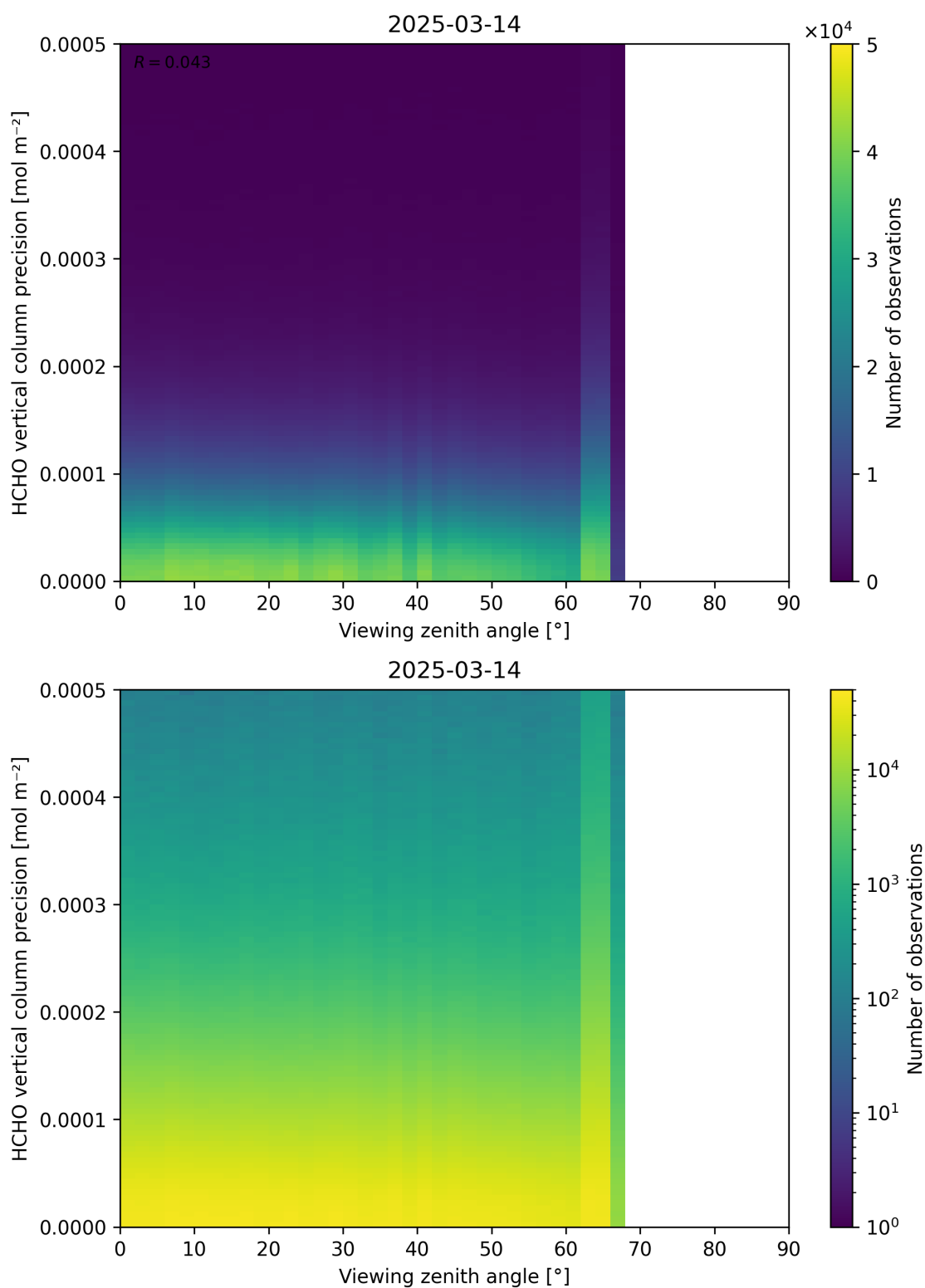
Figure 194: Scatter density plot of “Viewing zenith angle” against “HCHO vertical column precision” for 2025-03-13 to 2025-03-15.
