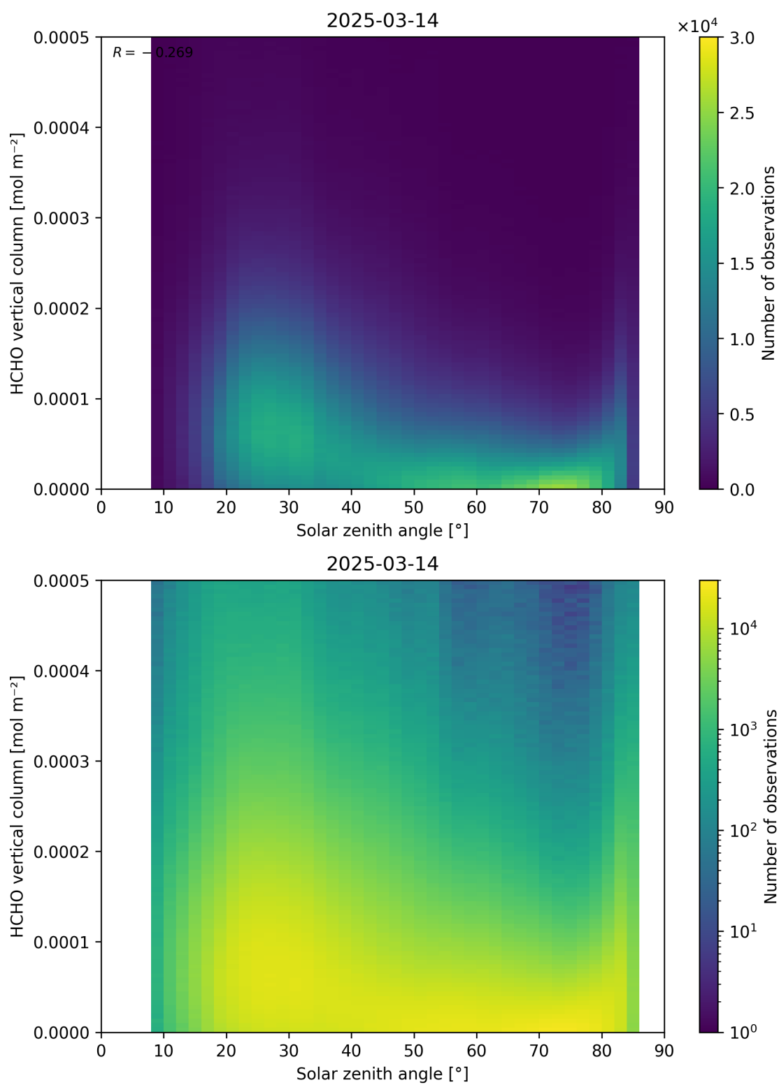
Figure 177: Scatter density plot of “Solar zenith angle” against “HCHO vertical column” for 2025-03-13 to 2025-03-15.
