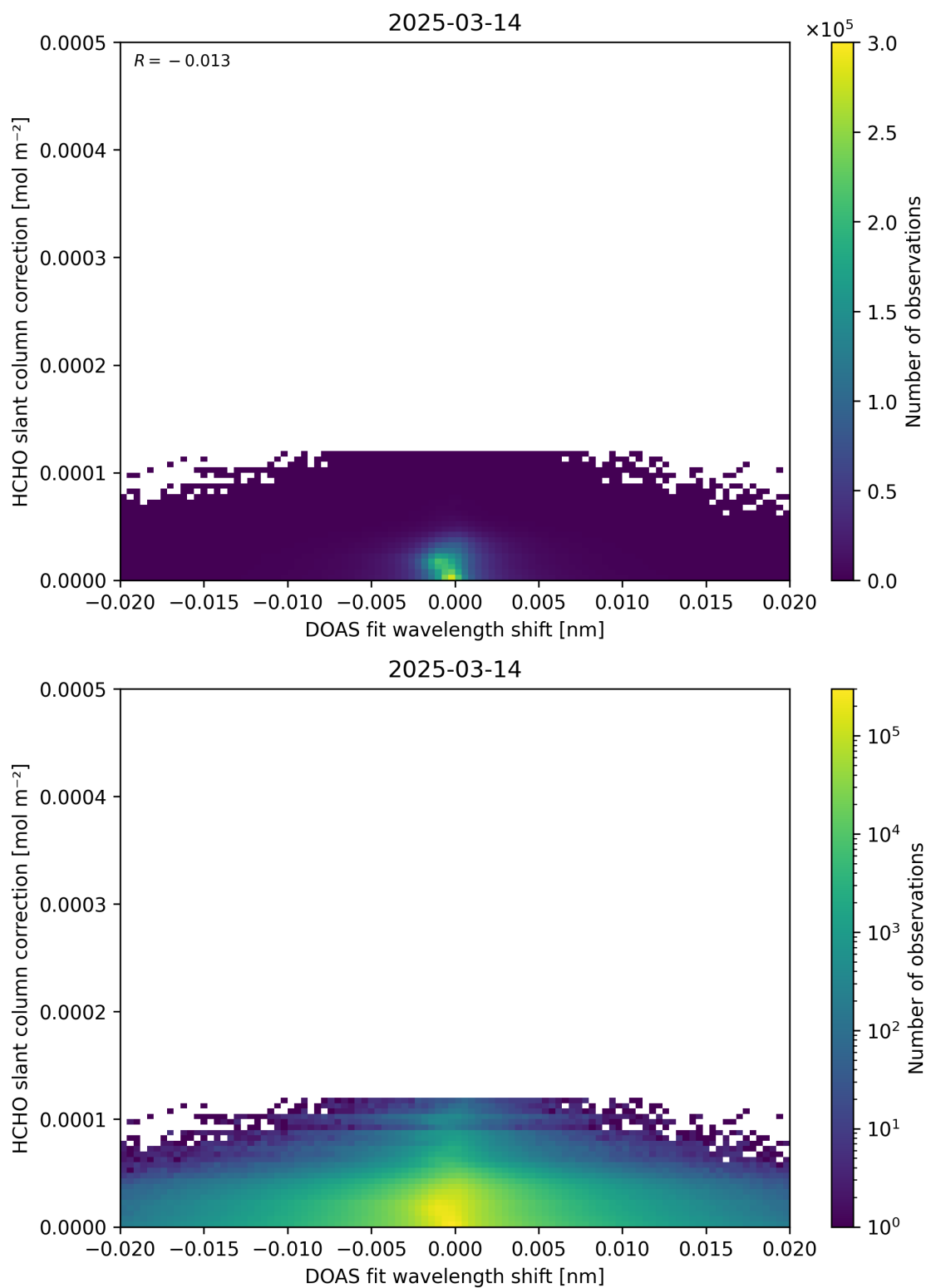
Figure 67: Scatter density plot of “DOAS fit wavelength shift” against “HCHO slant column correction” for 2025-03-13 to 2025-03-15.
