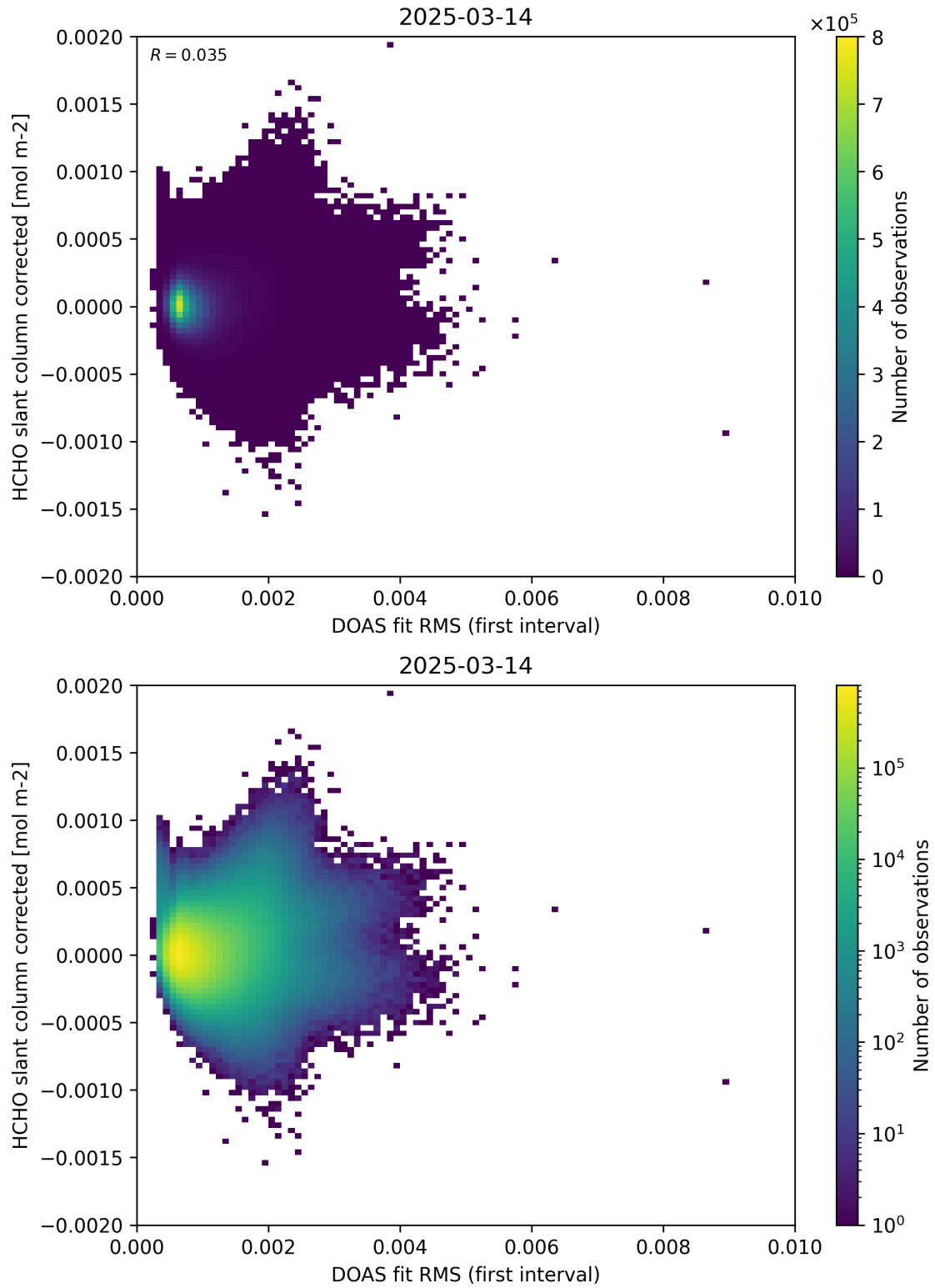
Figure 62: Scatter density plot of “DOAS fit RMS (first interval)” against “HCHO slant column corrected” for 2025-03-13 to 2025-03-15.
