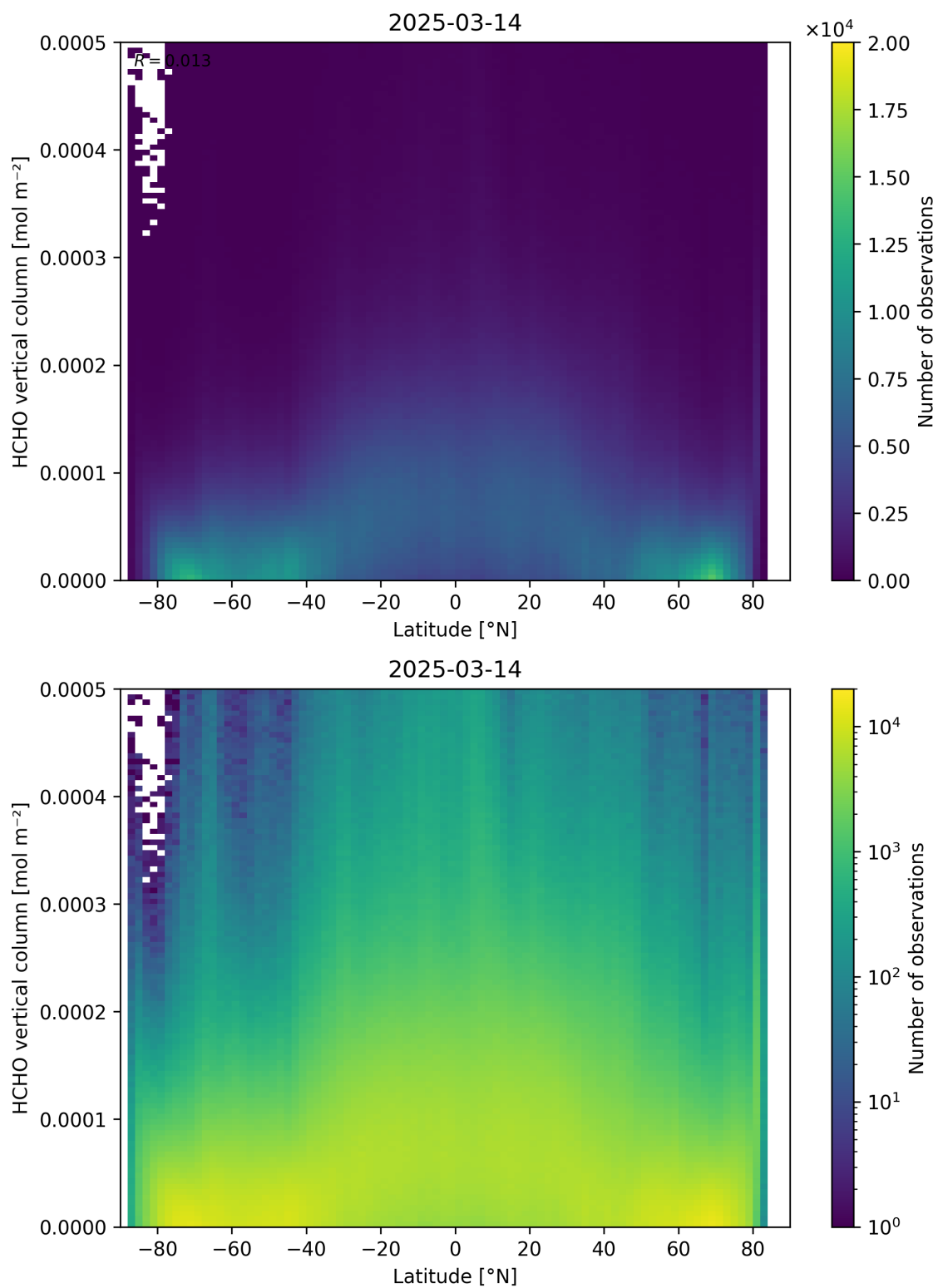
Figure 163: Scatter density plot of “Latitude” against “HCHO vertical column” for 2025-03-13 to 2025-03-15.
