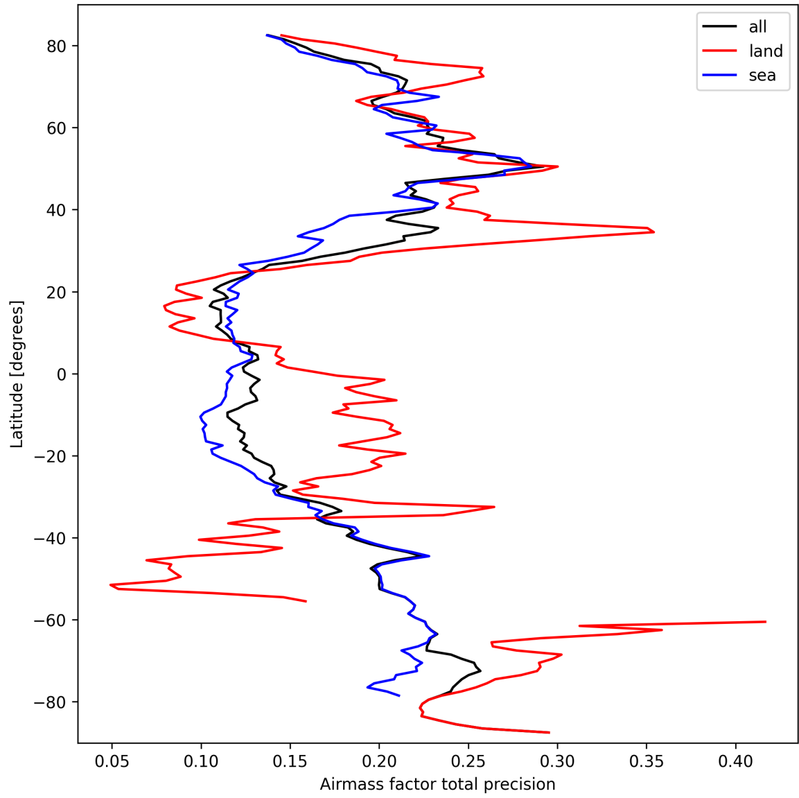
Figure 27: Zonal average of “Airmass factor total precision” for 2025-03-13 to 2025-03-15.
