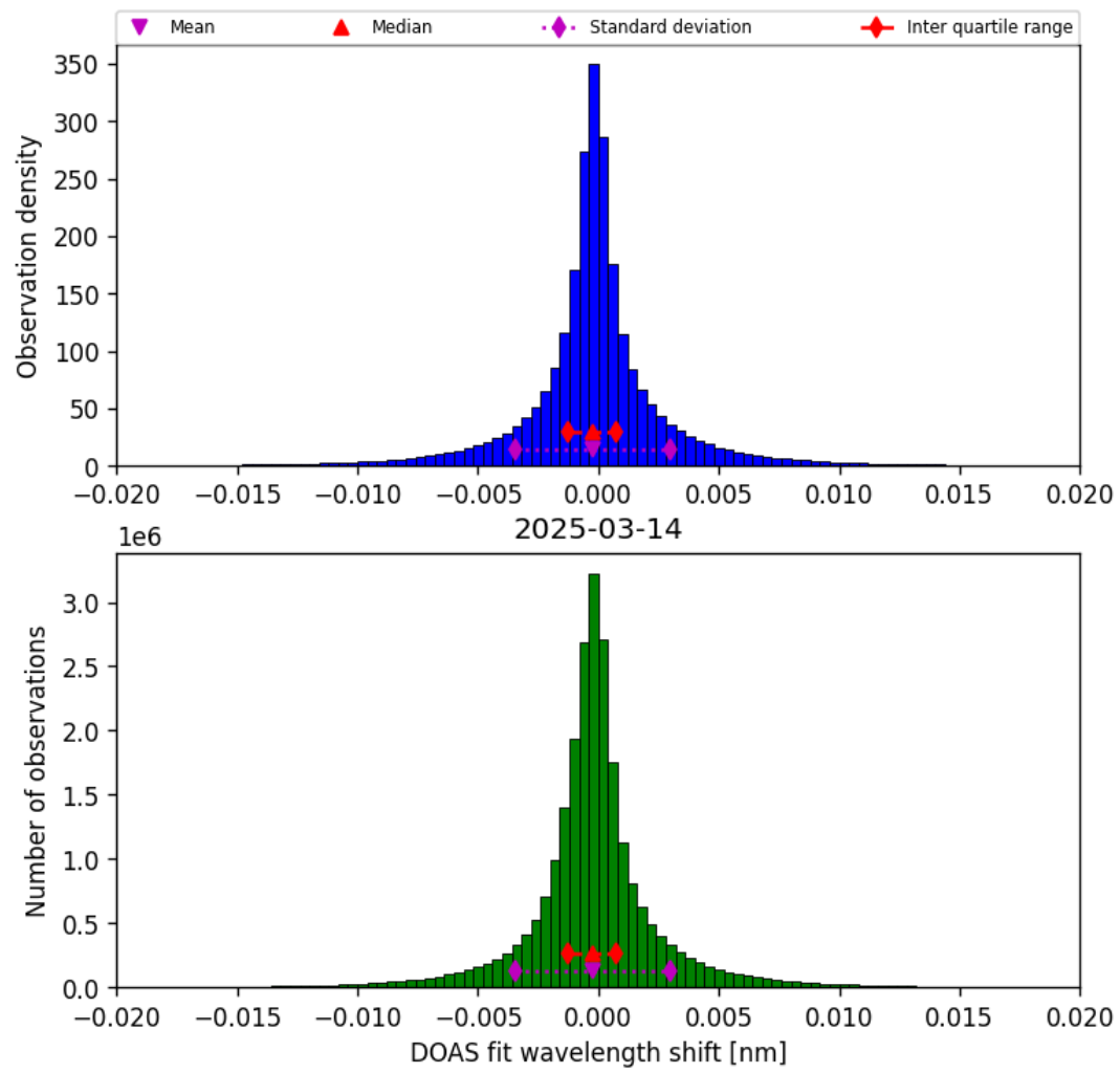
Figure 44: Histogram of “DOAS fit wavelength shift” for 2025-03-13 to 2025-03-15
