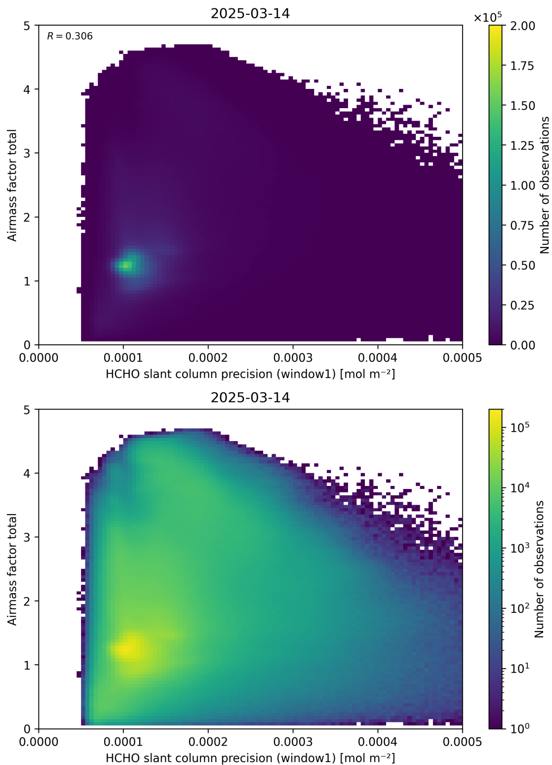
Figure 94: Scatter density plot of “HCHO slant column precision (window1)” against “Airmass factor total” for 2025-03-13 to 2025-03-15.
