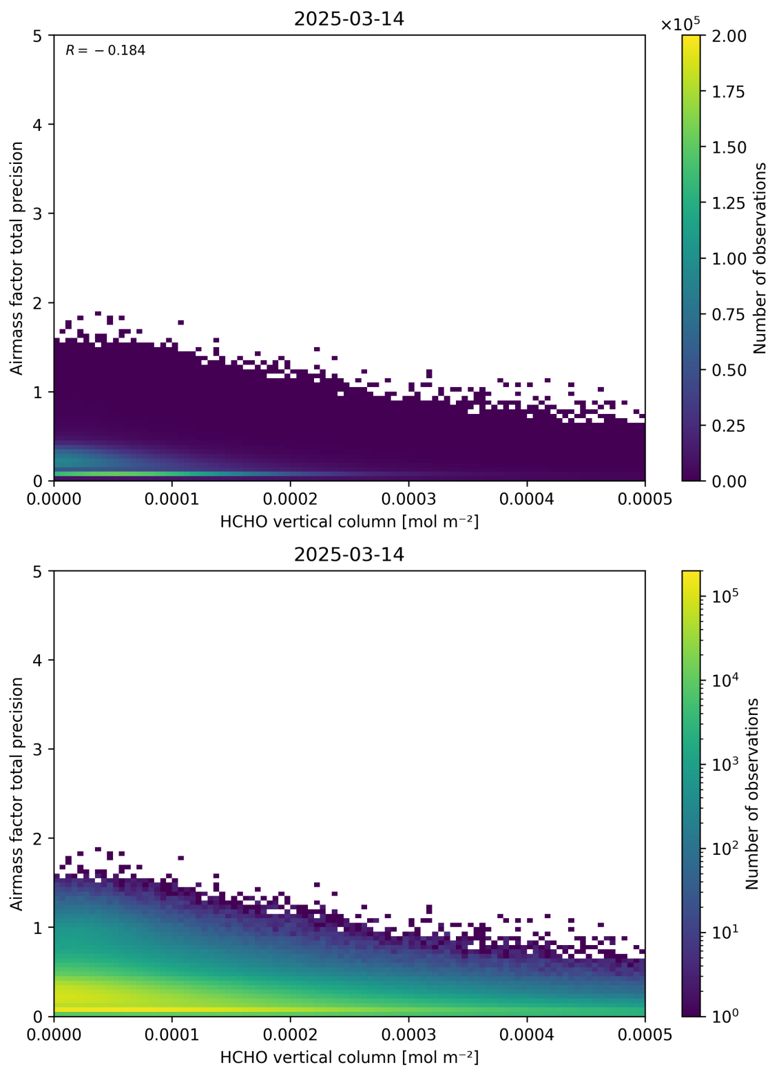
Figure 132: Scatter density plot of “HCHO vertical column” against “Airmass factor total precision” for 2025-03-13 to 2025-03-15.
