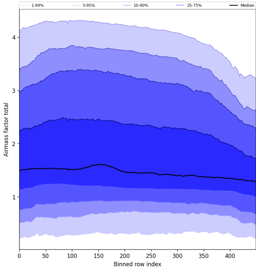
Figure 54: Along track statistics of “Airmass factor total” for 2025-03-13 to 2025-03-15
