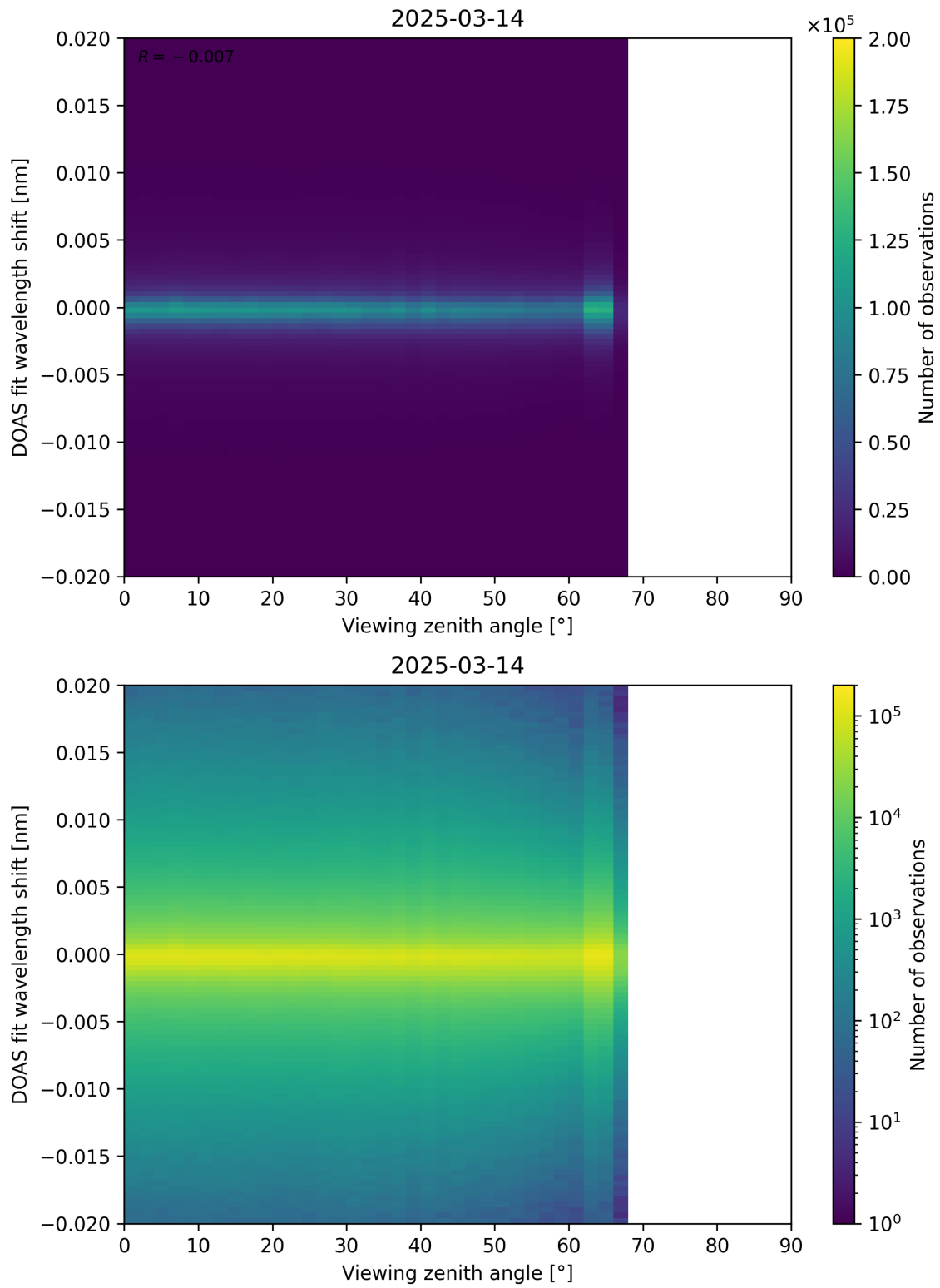
Figure 183: Scatter density plot of “Viewing zenith angle” against “DOAS fit wavelength shift” for 2025-03-13 to 2025-03-15.
