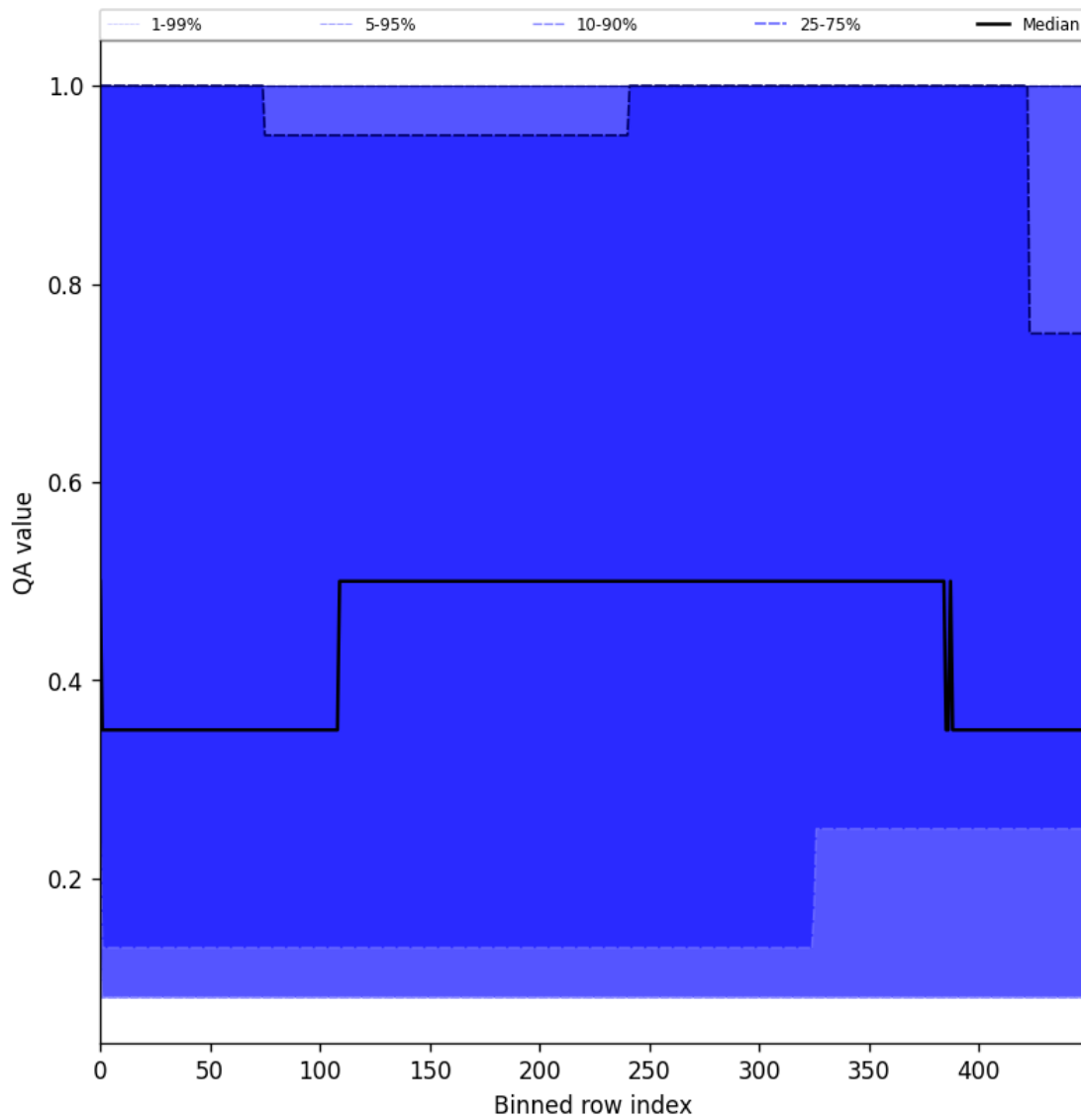
Figure 48: Along track statistics of “QA value” for 2025-03-13 to 2025-03-15
