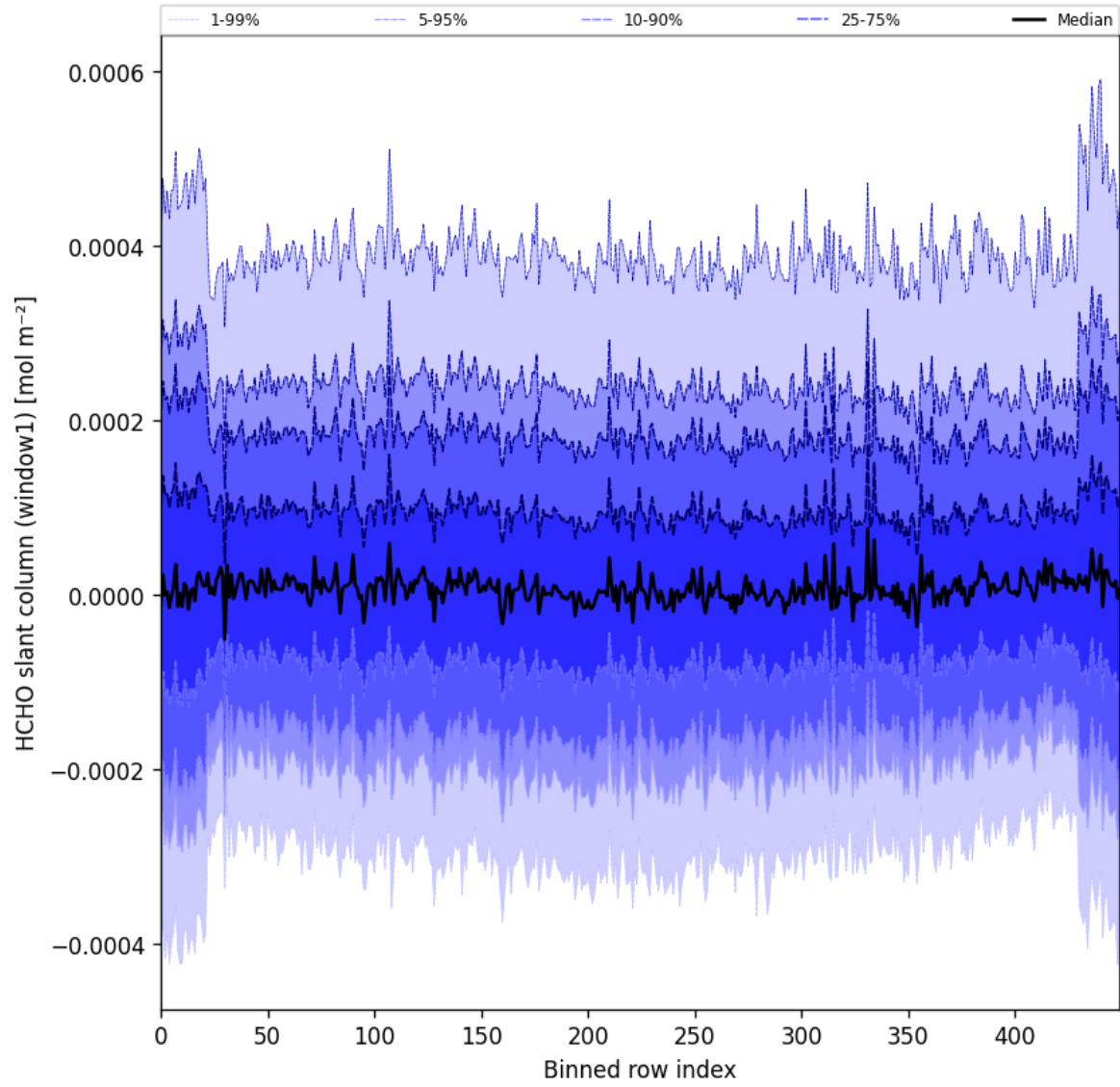
Figure 52: Along track statistics of “HCHO slant column (window1)” for 2025-03-13 to 2025-03-15
