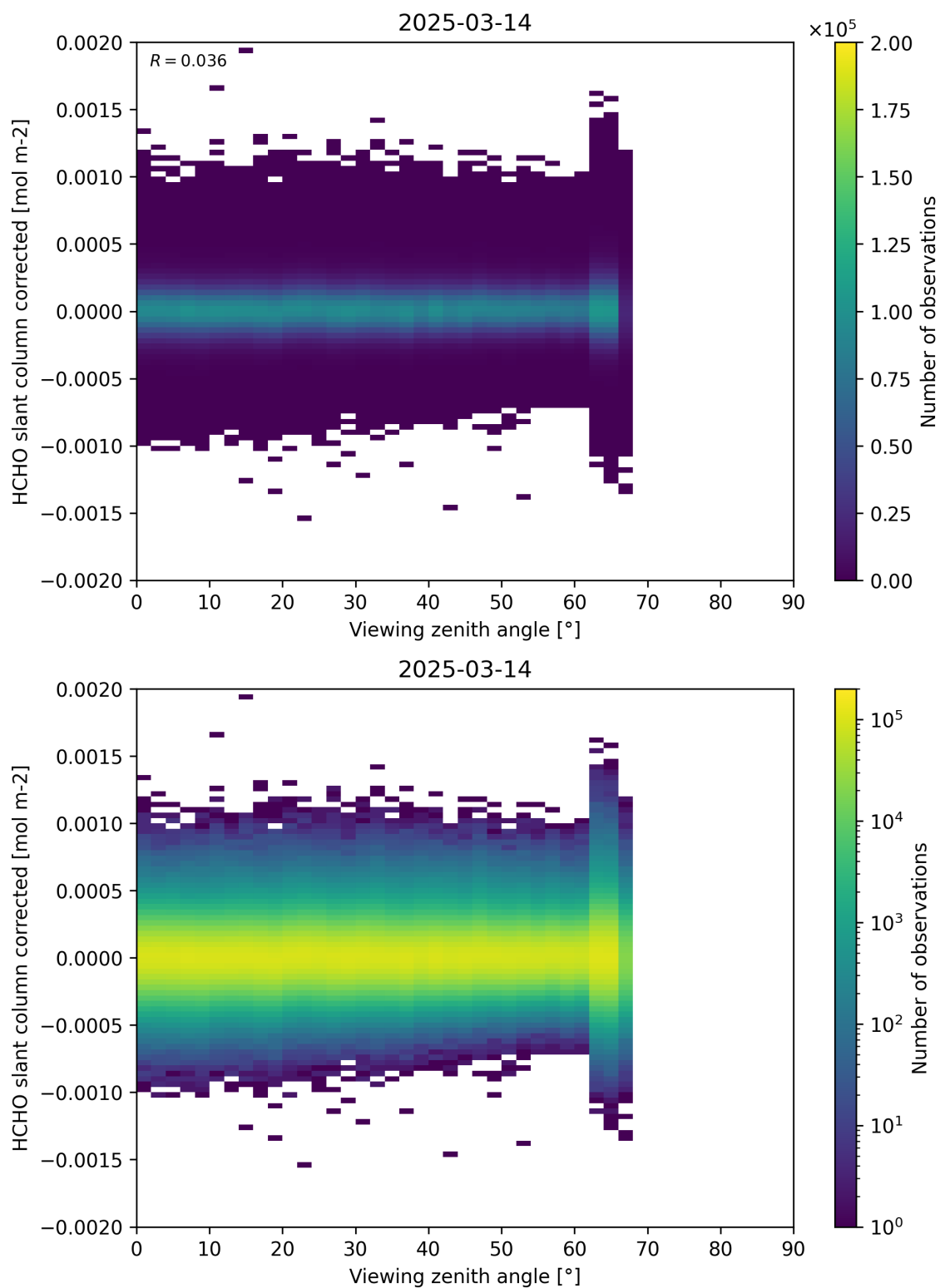
Figure 186: Scatter density plot of “Viewing zenith angle” against “HCHO slant column corrected” for 2025-03-13 to 2025-03-15.
