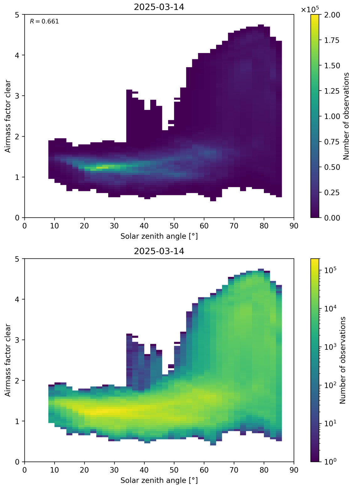
Figure 170: Scatter density plot of “Solar zenith angle” against “Airmass factor clear” for 2025-03-13 to 2025-03-15.
