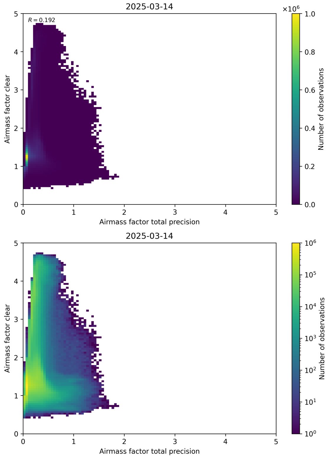
Figure 108: Scatter density plot of “Airmass factor total precision” against “Airmass factor clear” for 2025-03-13 to 2025-03-15.
