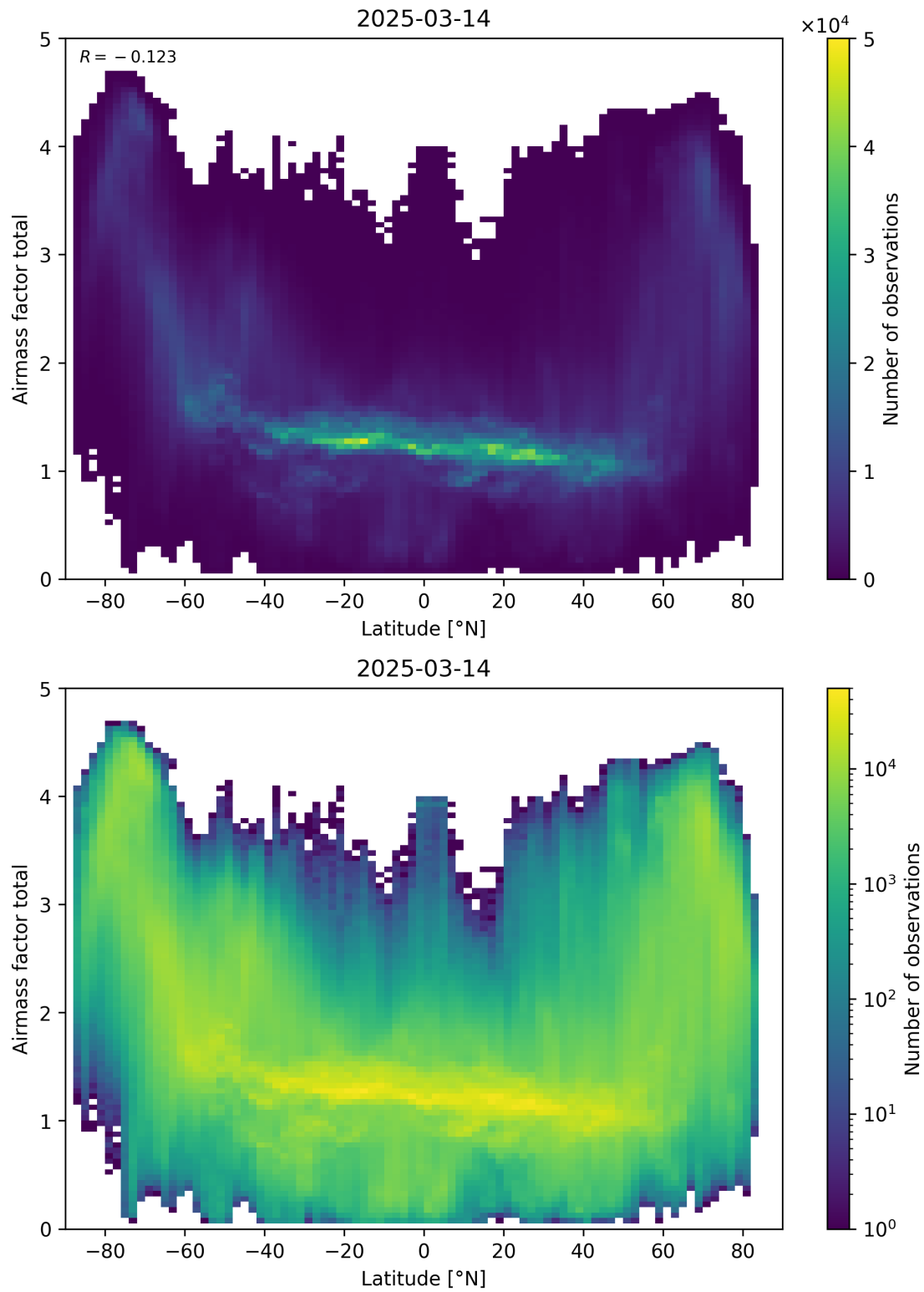
Figure 161: Scatter density plot of “Latitude” against “Airmass factor total” for 2025-03-13 to 2025-03-15.
