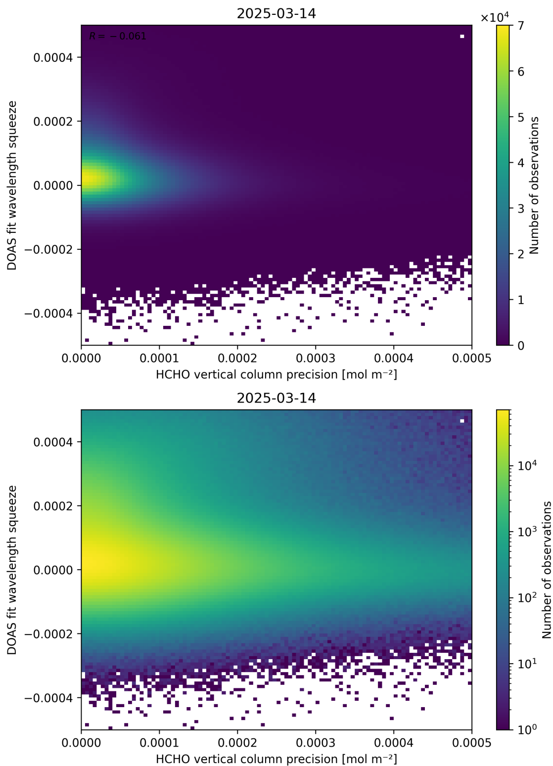
Figure 138: Scatter density plot of “HCHO vertical column precision” against “DOAS fit wavelength squeeze” for 2025-03-13 to 2025-03-15.
