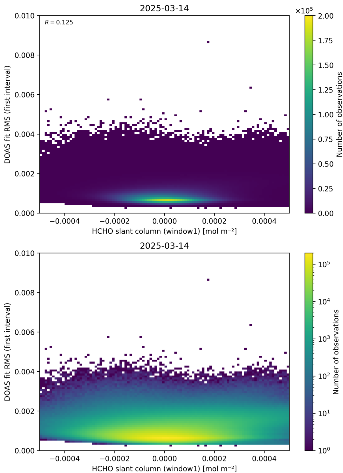
Figure 78: Scatter density plot of “HCHO slant column (window1)” against “DOAS fit RMS (first interval)” for 2025-03-13 to 2025-03-15.
