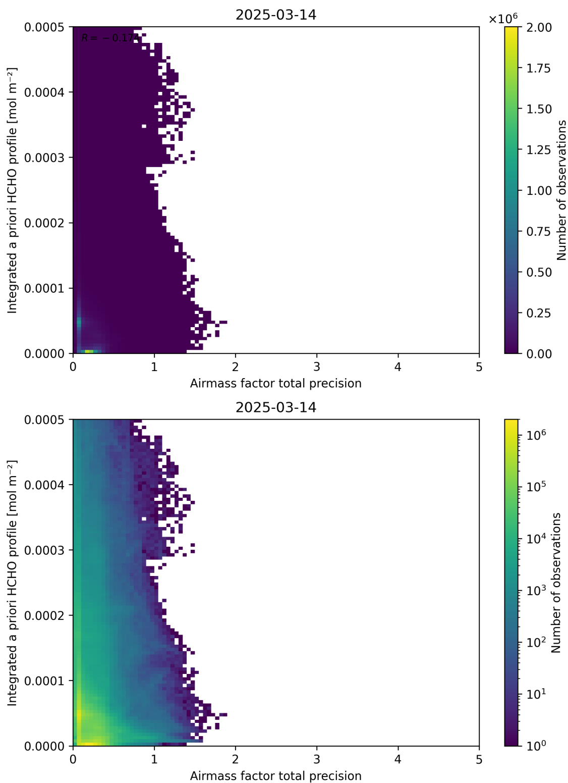
Figure 111: Scatter density plot of “Airmass factor total precision” against “Integrated a priori HCHO profile” for 2025-03-13 to 2025-03-15.
