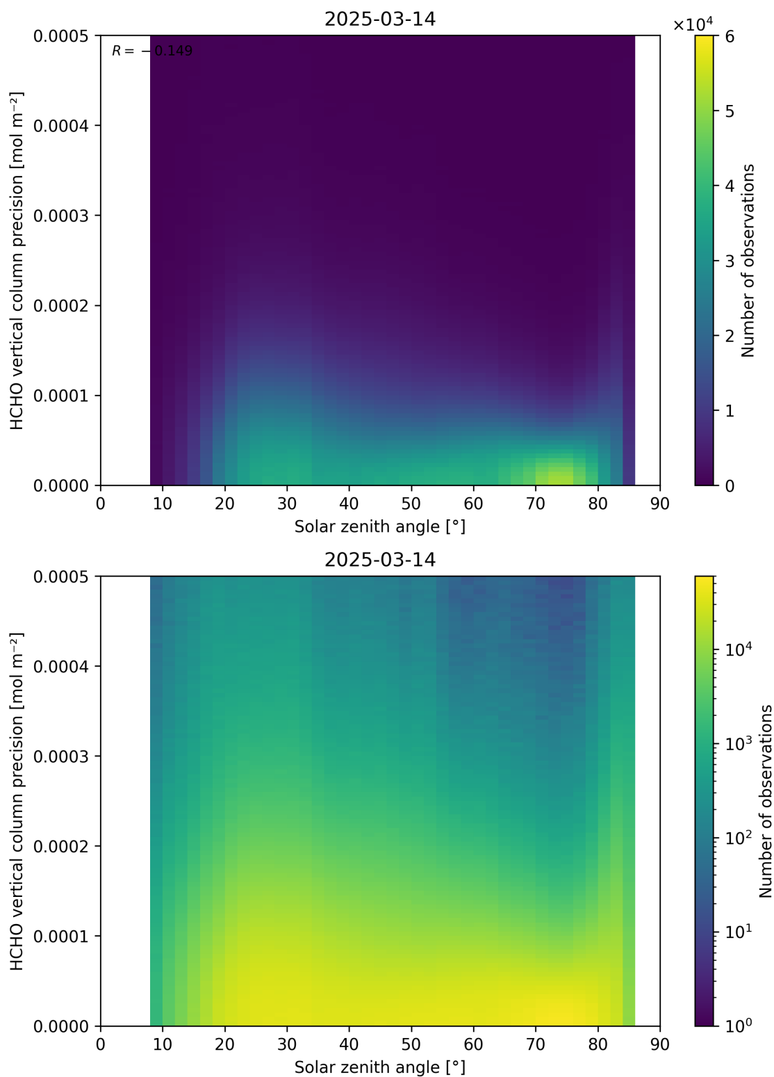
Figure 179: Scatter density plot of “Solar zenith angle” against “HCHO vertical column precision” for 2025-03-13 to 2025-03-15.
