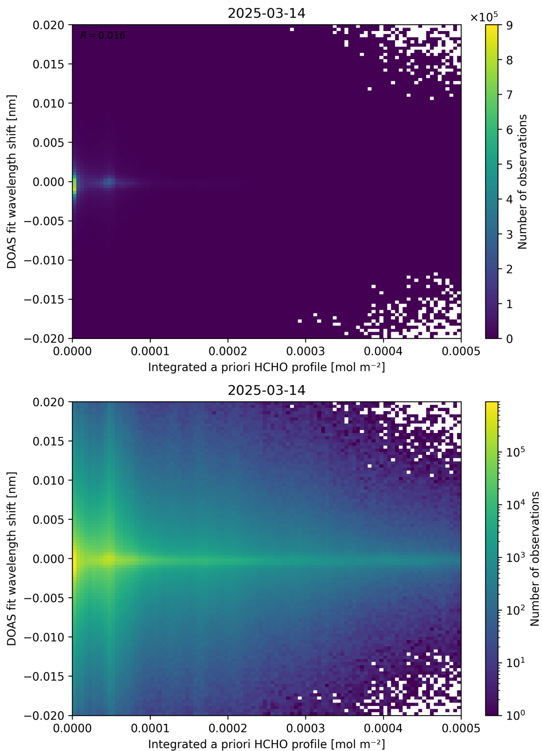
Figure 149: Scatter density plot of “Integrated a priori HCHO profile” against “DOAS fit wavelength shift” for 2025-03-13 to 2025-03-15.
