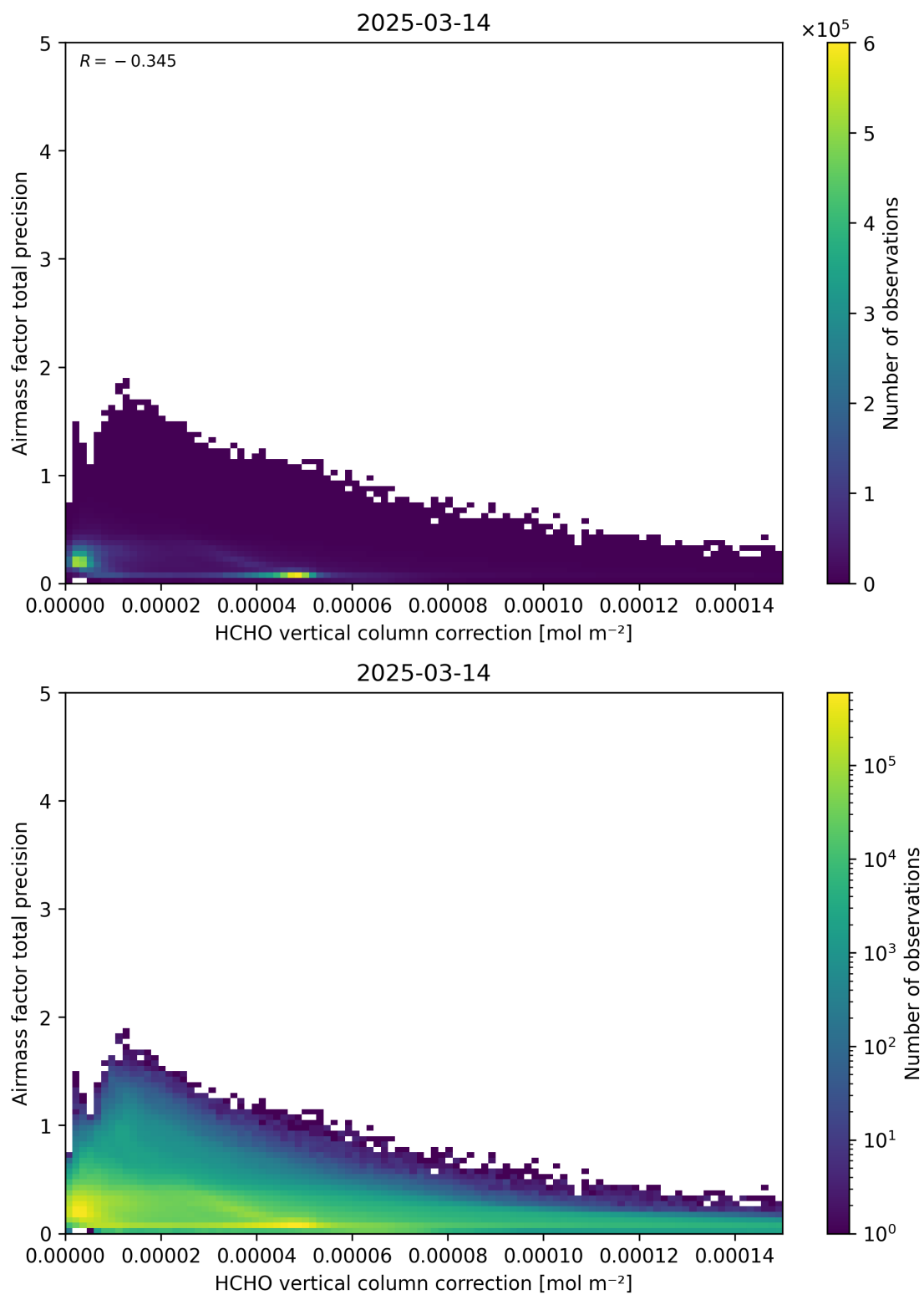
Figure 121: Scatter density plot of “HCHO vertical column correction” against “Airmass factor total precision” for 2025-03-13 to 2025-03-15.
