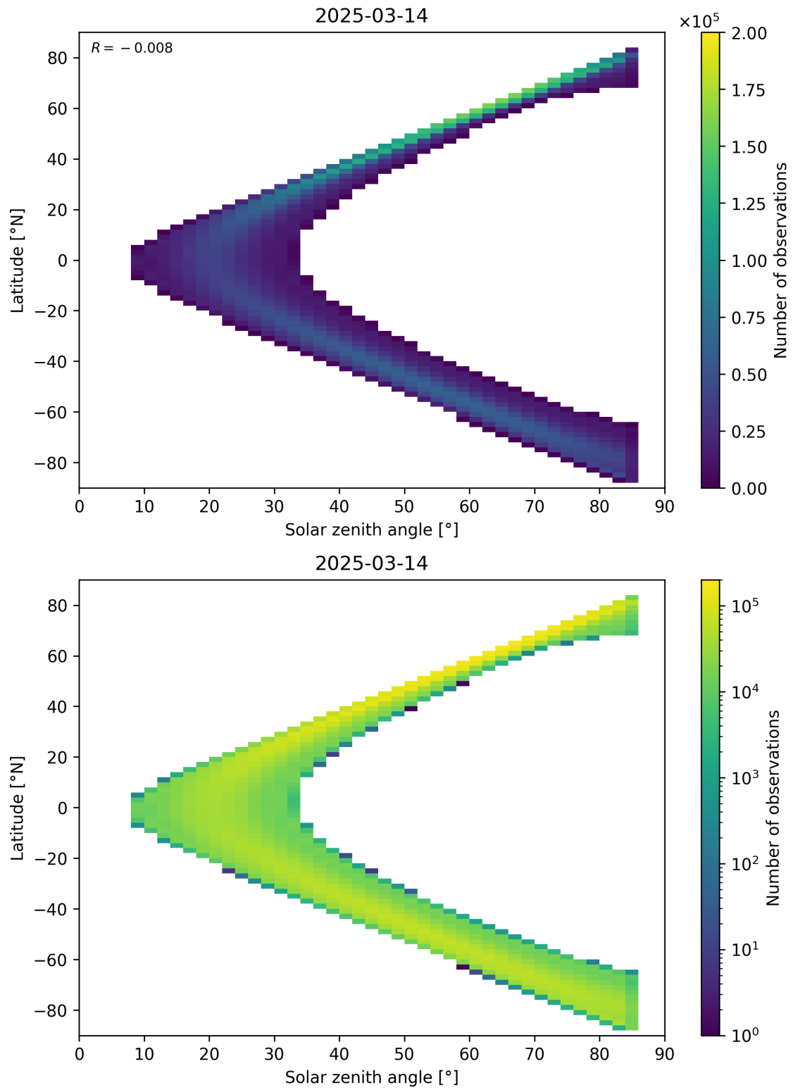
Figure 181: Scatter density plot of “Solar zenith angle” against “Latitude” for 2025-03-13 to 2025-03-15.
