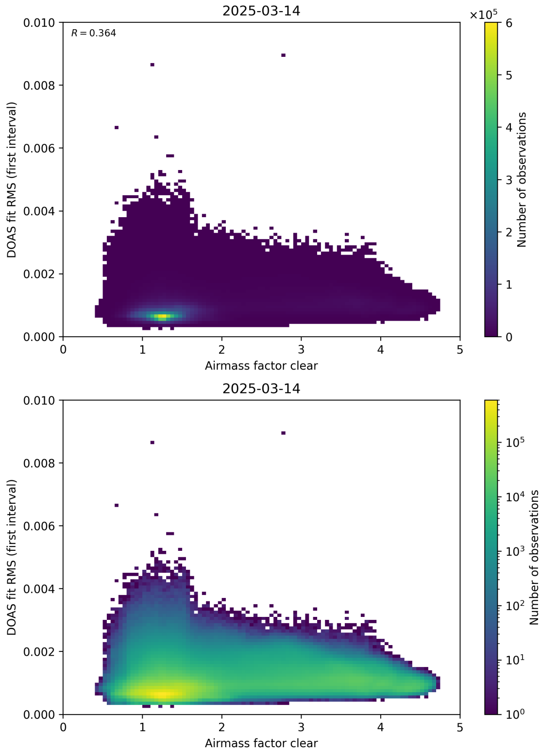
Figure 71: Scatter density plot of “Airmass factor clear” against “DOAS fit RMS (first interval)” for 2025-03-13 to 2025-03-15.
