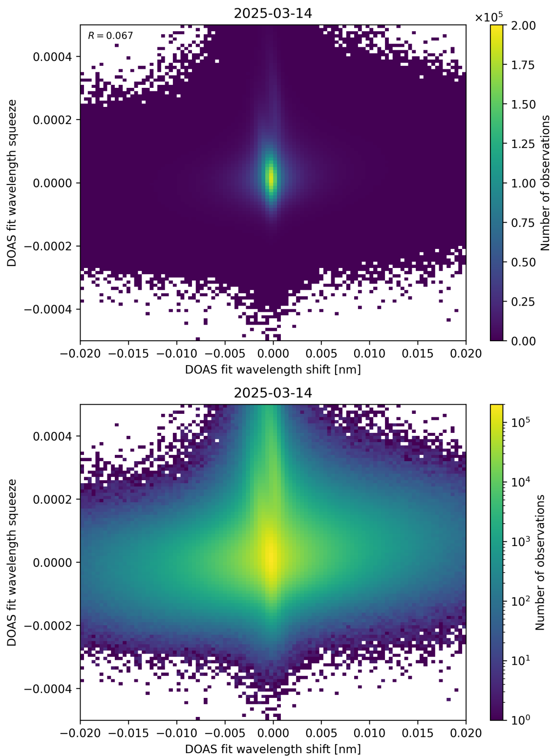
Figure 65: Scatter density plot of “DOAS fit wavelength shift” against “DOAS fit wavelength squeeze” for 2025-03-13 to 2025-03-15.
