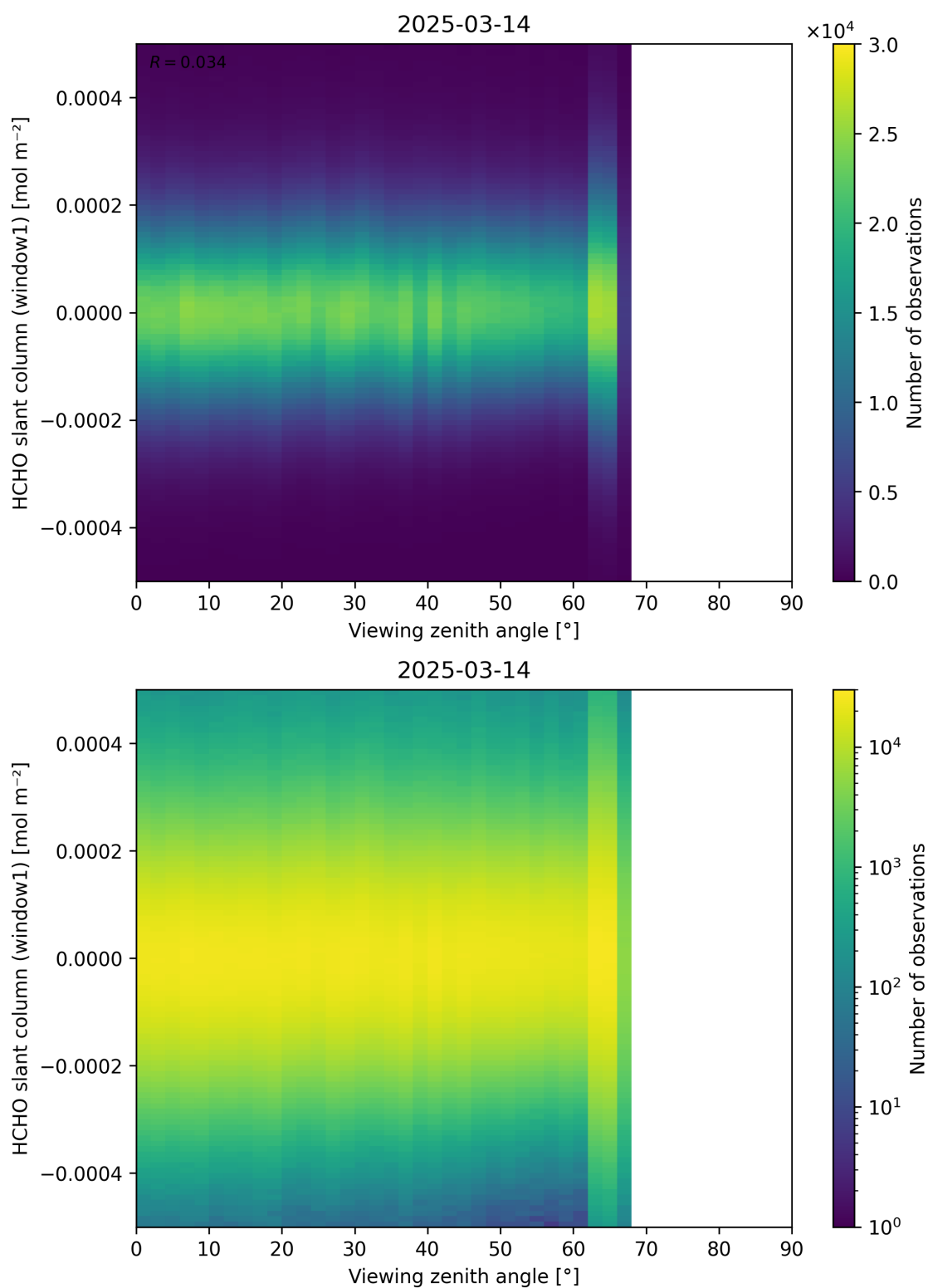
Figure 188: Scatter density plot of “Viewing zenith angle” against “HCHO slant column (window1)” for 2025-03-13 to 2025-03-15.
