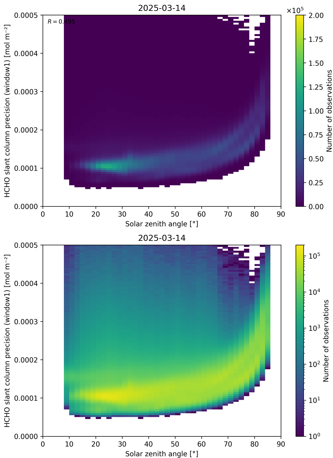
Figure 174: Scatter density plot of “Solar zenith angle” against “HCHO slant column precision (window1)” for 2025-03-13 to 2025-03-15.
