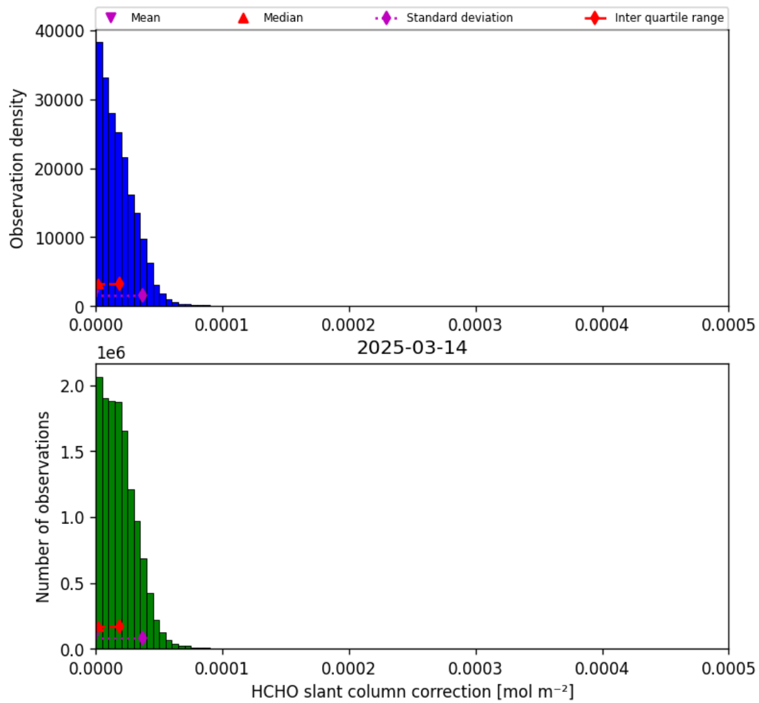
Figure 47: Histogram of “HCHO slant column correction” for 2025-03-13 to 2025-03-15
