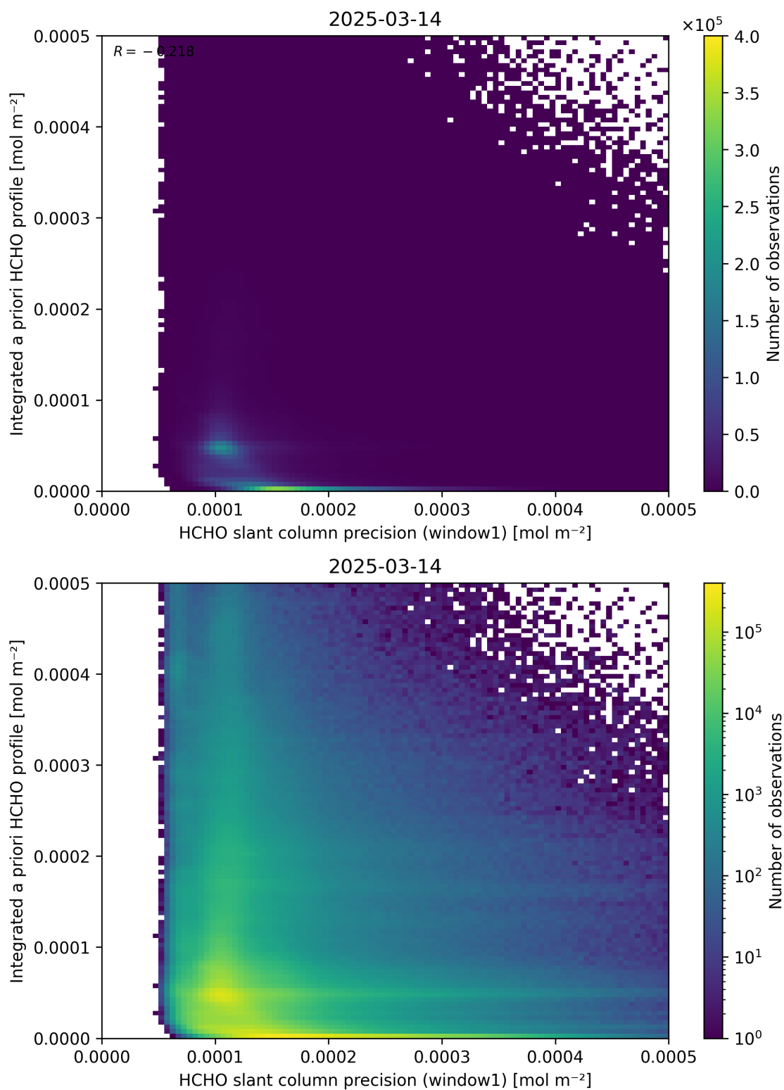
Figure 96: Scatter density plot of “HCHO slant column precision (window1)” against “Integrated a priori HCHO profile” for 2025-03-13 to 2025-03-15.
