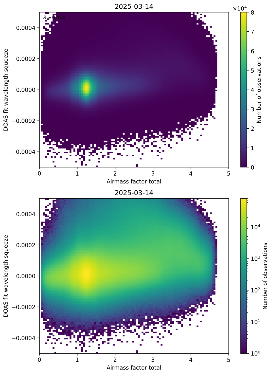
Figure 99: Scatter density plot of “Airmass factor total” against “DOAS fit wavelength squeeze” for 2025-03-13 to 2025-03-15.
