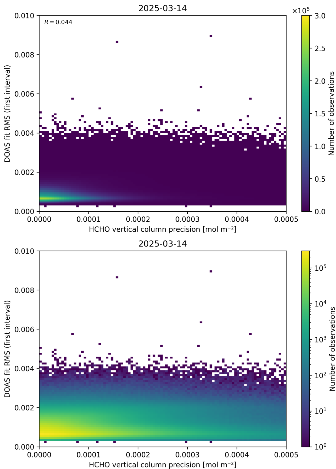
Figure 136: Scatter density plot of “HCHO vertical column precision” against “DOAS fit RMS (first interval)” for 2025-03-13 to 2025-03-15.
