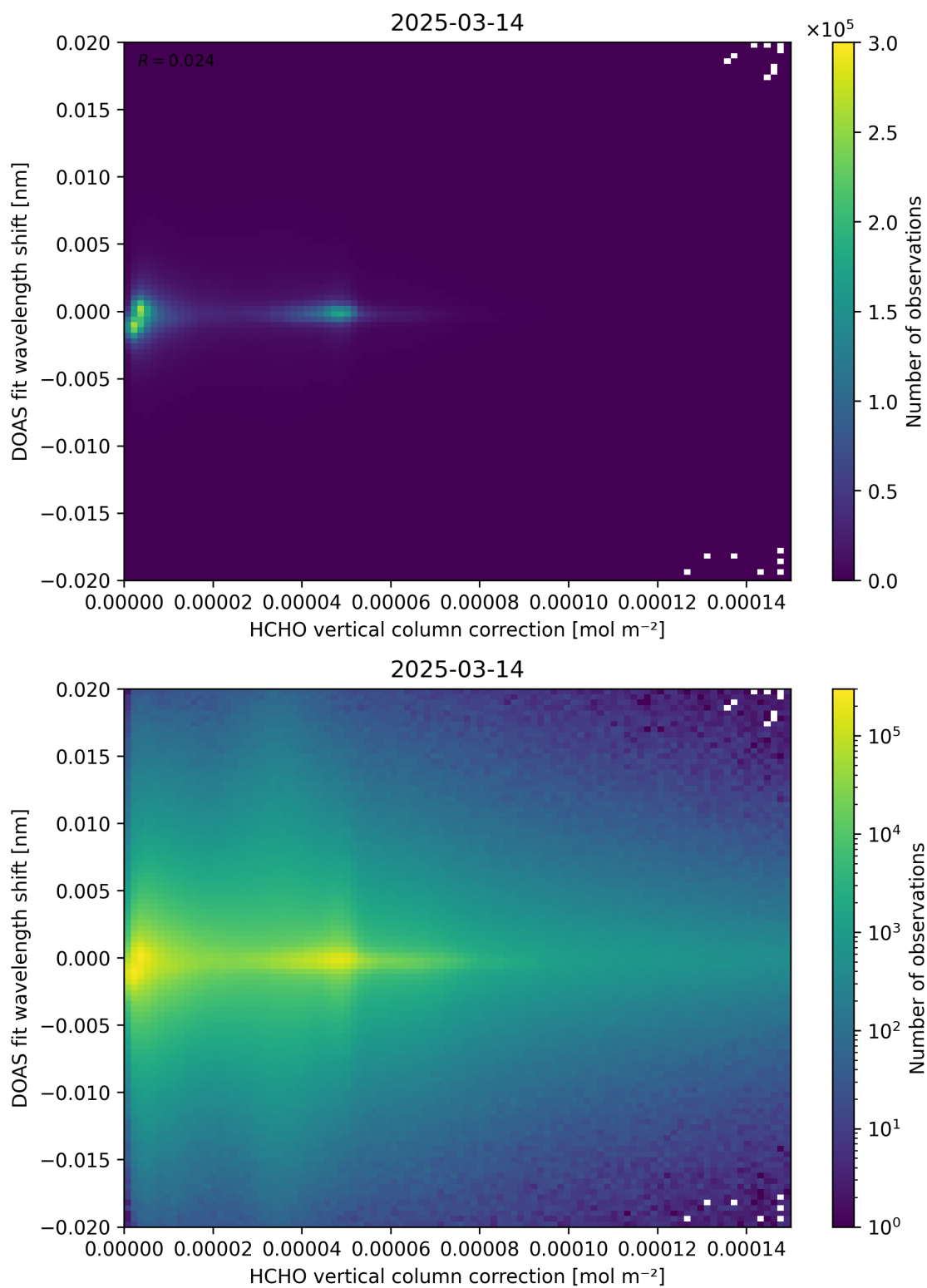
Figure 113: Scatter density plot of “HCHO vertical column correction” against “DOAS fit wavelength shift” for 2025-03-13 to 2025-03-15.
