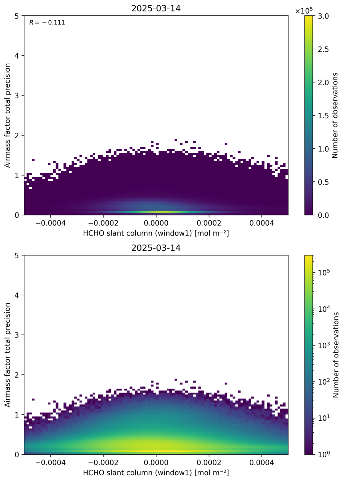
Figure 86: Scatter density plot of “HCHO slant column (window1)” against “Airmass factor total precision” for 2025-03-13 to 2025-03-15.
