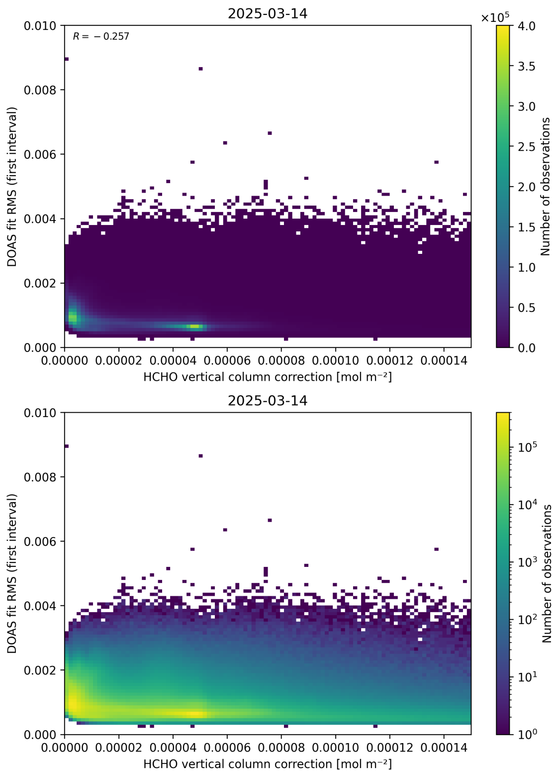
Figure 112: Scatter density plot of “HCHO vertical column correction” against “DOAS fit RMS (first interval)” for 2025-03-13 to 2025-03-15.
