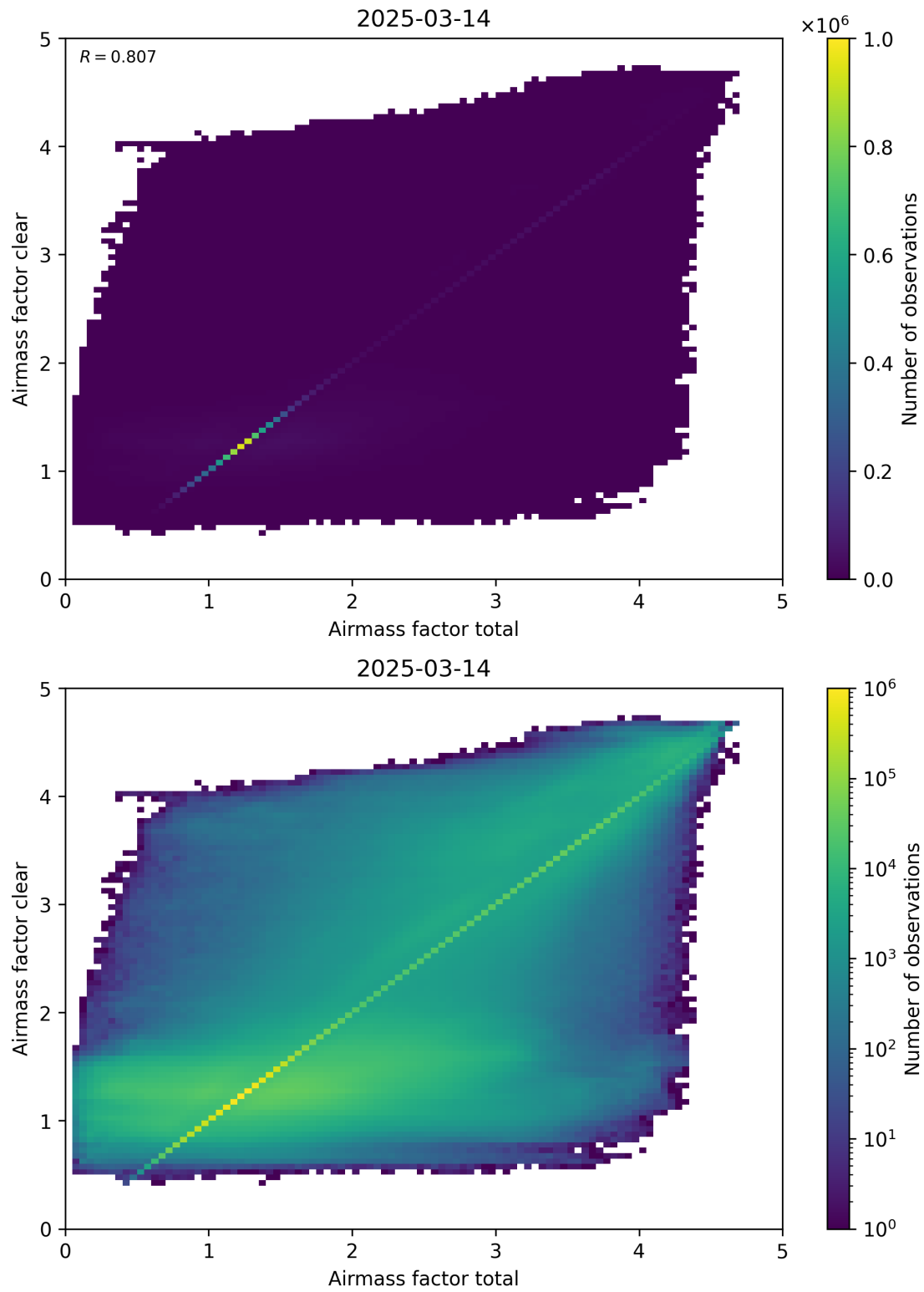
Figure 100: Scatter density plot of “Airmass factor total” against “Airmass factor clear” for 2025-03-13 to 2025-03-15.
