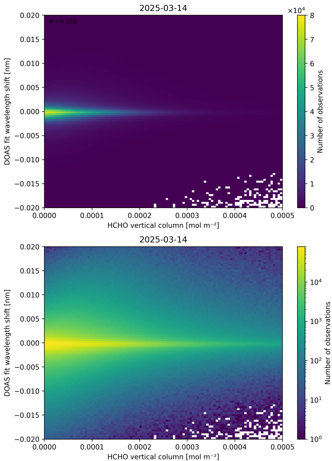
Figure 124: Scatter density plot of “HCHO vertical column” against “DOAS fit wavelength shift” for 2025-03-13 to 2025-03-15.
