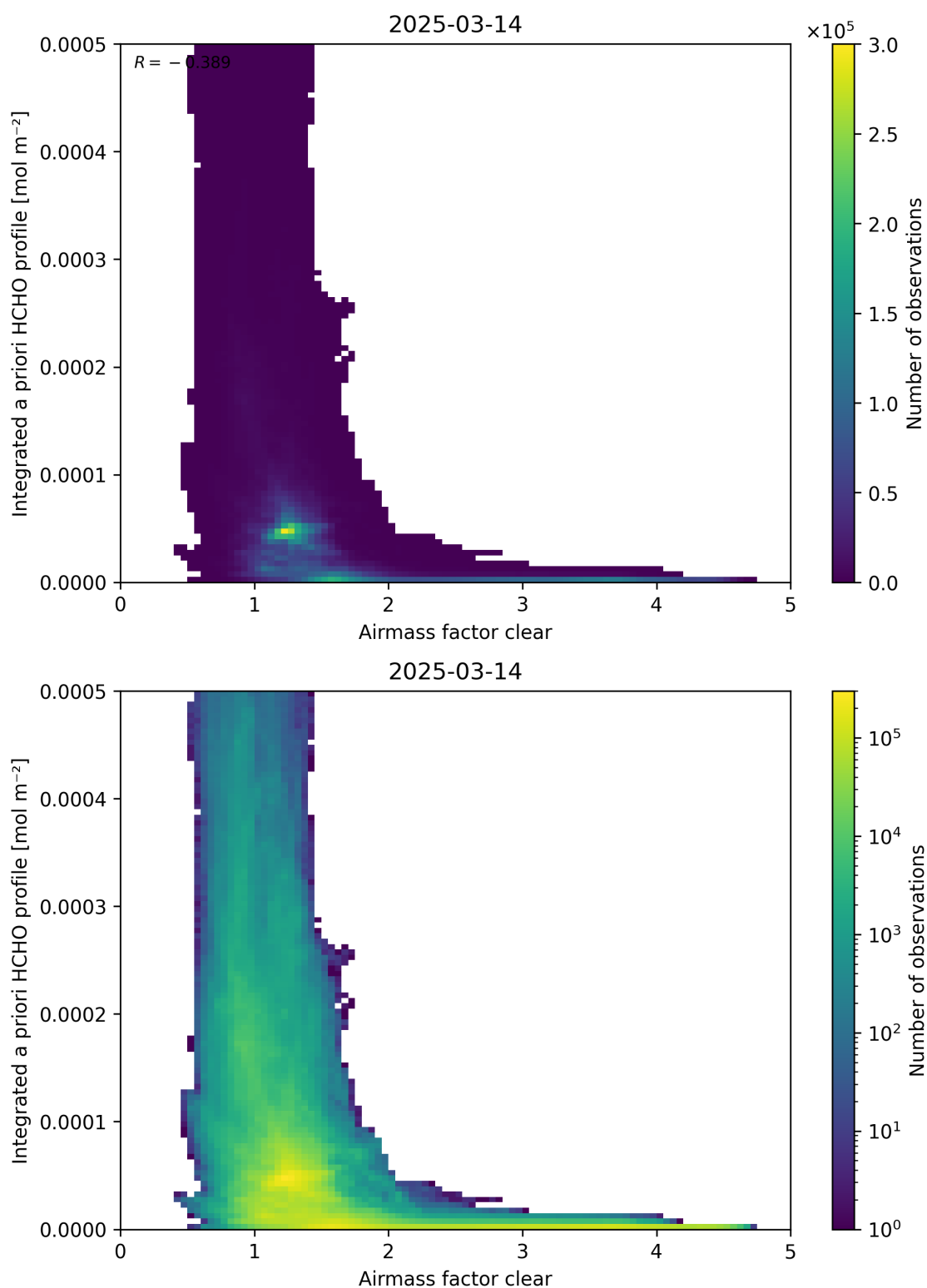
Figure 76: Scatter density plot of “Airmass factor clear” against “Integrated a priori HCHO profile” for 2025-03-13 to 2025-03-15.
