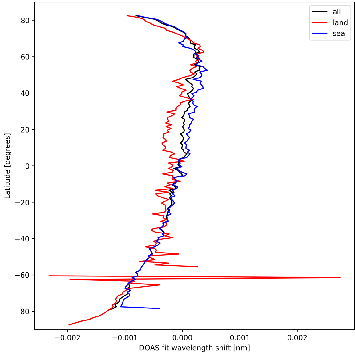
Figure 30: Zonal average of “DOAS fit wavelength shift” for 2025-03-13 to 2025-03-15.
