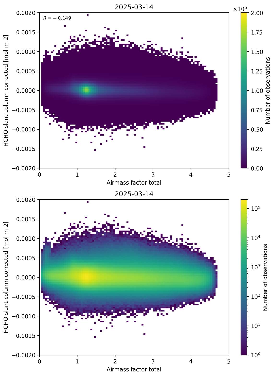
Figure 101: Scatter density plot of “Airmass factor total” against “HCHO slant column corrected” for 2025-03-13 to 2025-03-15.
