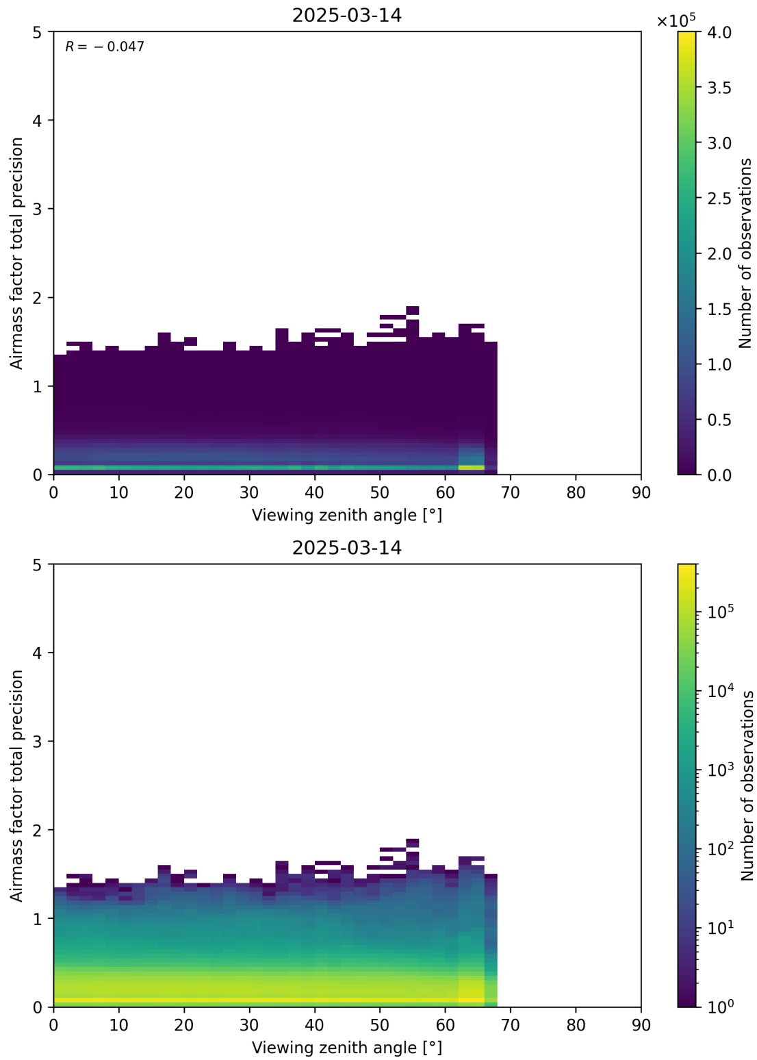
Figure 191: Scatter density plot of “Viewing zenith angle” against “Airmass factor total precision” for 2025-03-13 to 2025-03-15.
