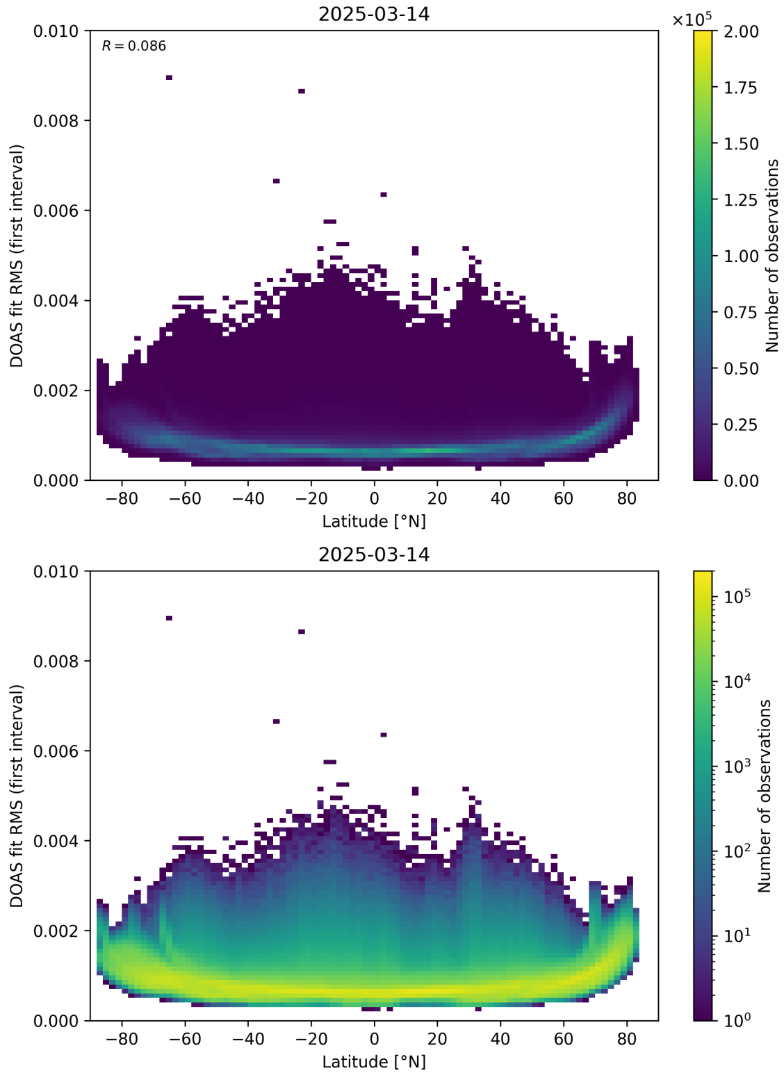
Figure 153: Scatter density plot of “Latitude” against “DOAS fit RMS (first interval)” for 2025-03-13 to 2025-03-15.
