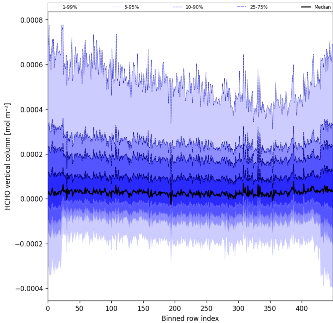
Figure 49: Along track statistics of “HCHO vertical column” for 2025-03-13 to 2025-03-15
