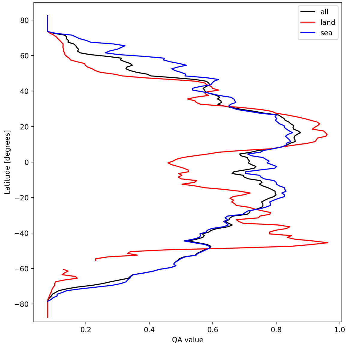
Figure 20: Zonal average of “QA value” for 2025-03-13 to 2025-03-15.
