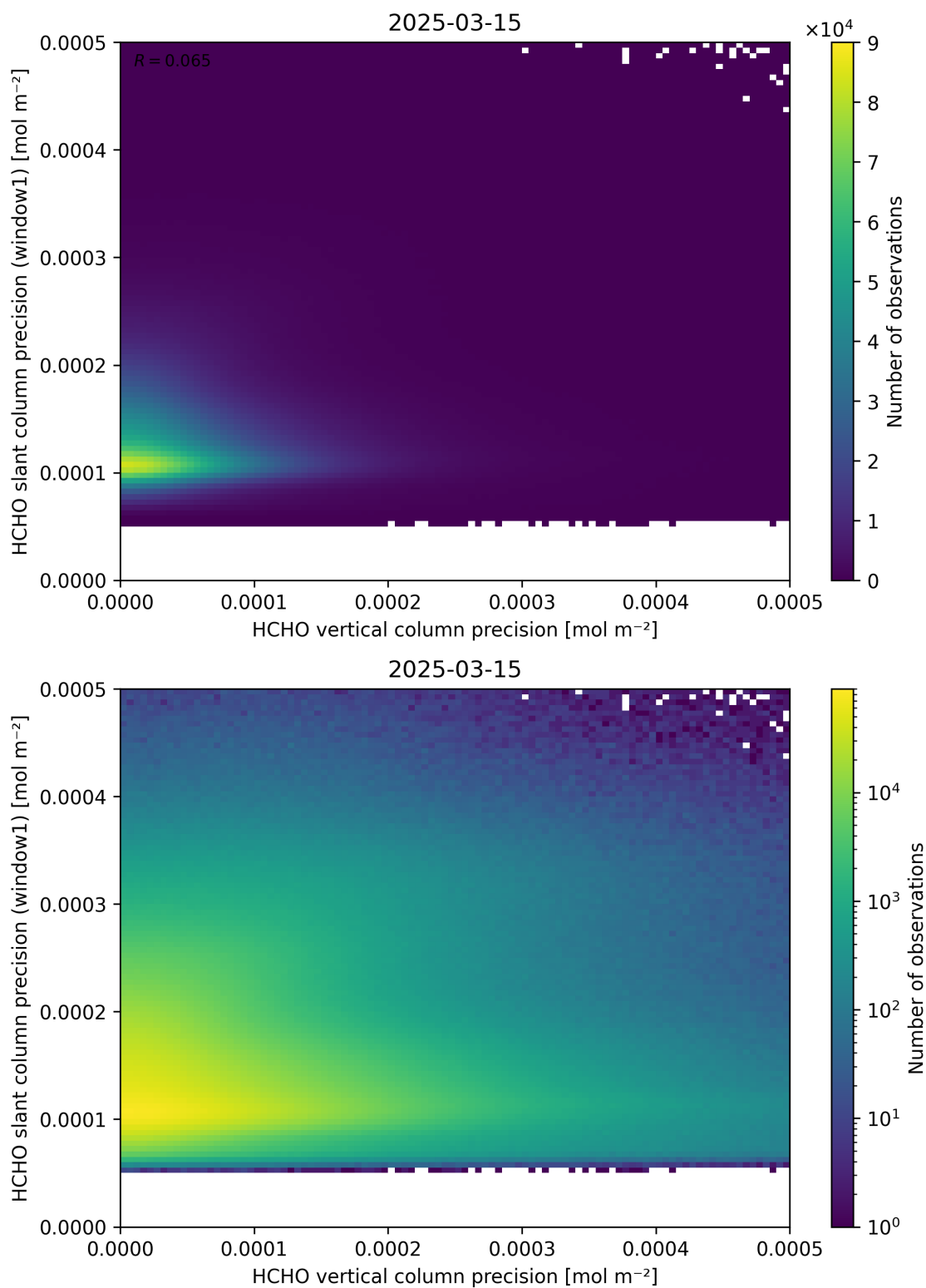
Figure 143: Scatter density plot of “HCHO vertical column precision” against “HCHO slant column precision (window1)” for 2025-03-14 to 2025-03-16.
