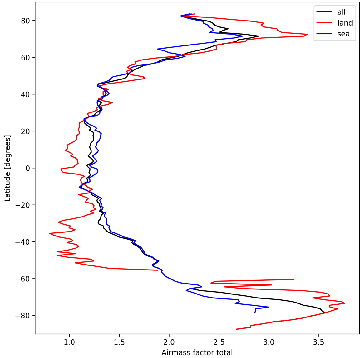
Figure 26: Zonal average of “Airmass factor total” for 2025-03-14 to 2025-03-16.
