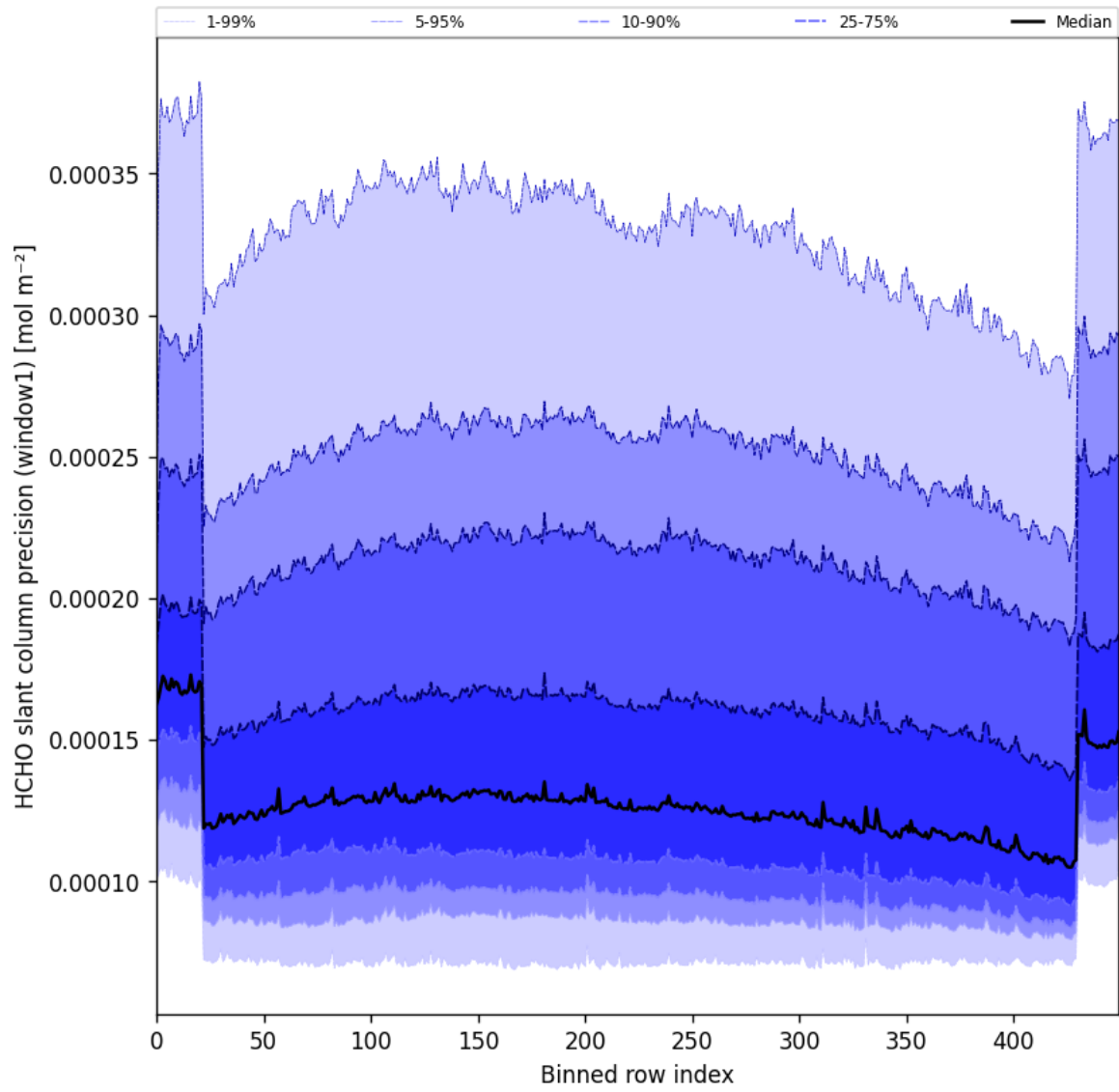
Figure 53: Along track statistics of “HCHO slant column precision (window1)” for 2025-03-14 to 2025-03-16
