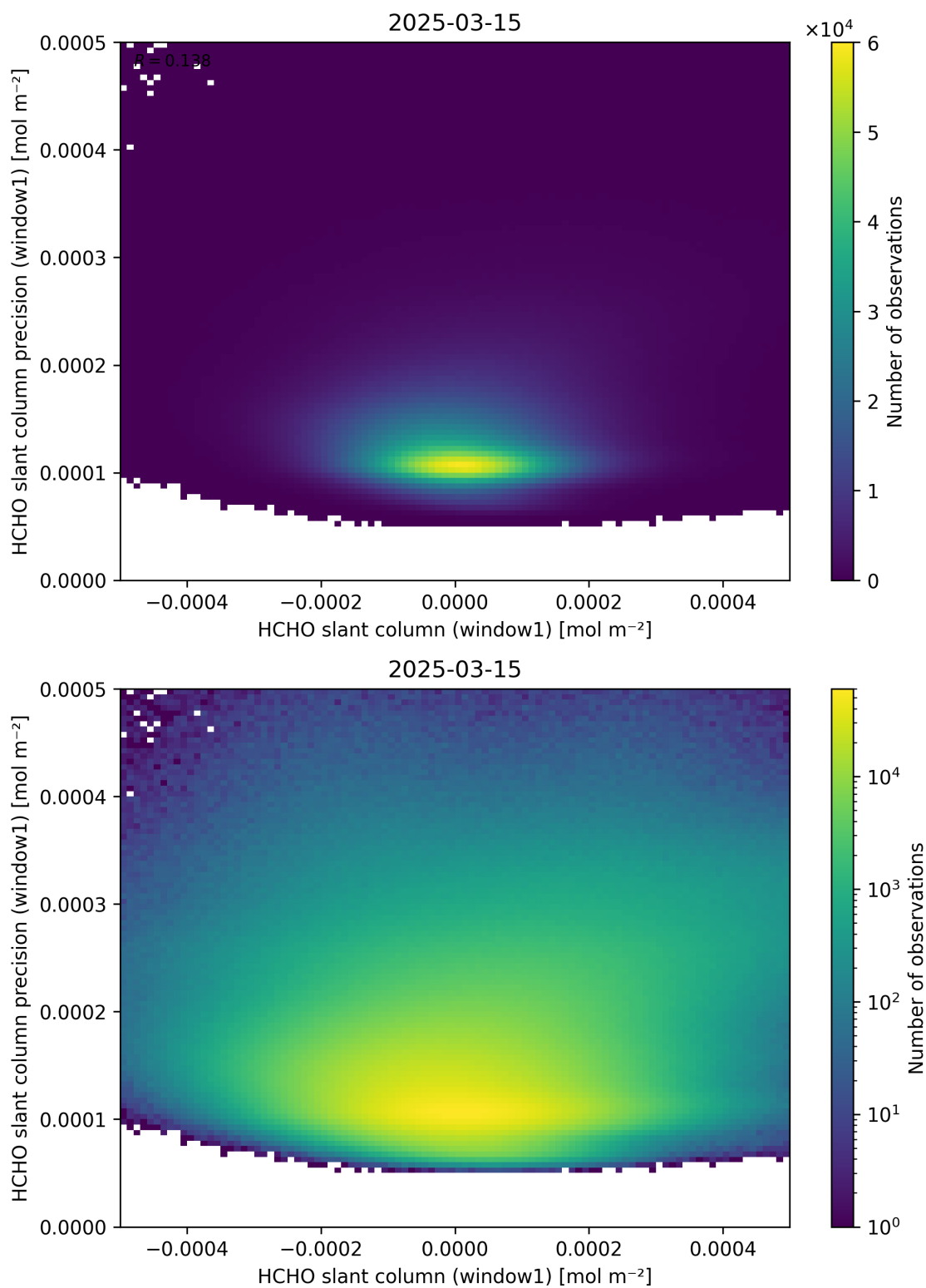
Figure 84: Scatter density plot of “HCHO slant column (window1)” against “HCHO slant column precision (window1)” for 2025-03-14 to 2025-03-16.
