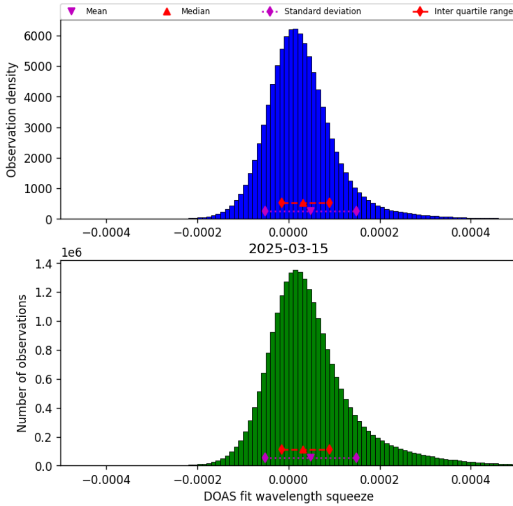
Figure 45: Histogram of “DOAS fit wavelength squeeze” for 2025-03-14 to 2025-03-16
