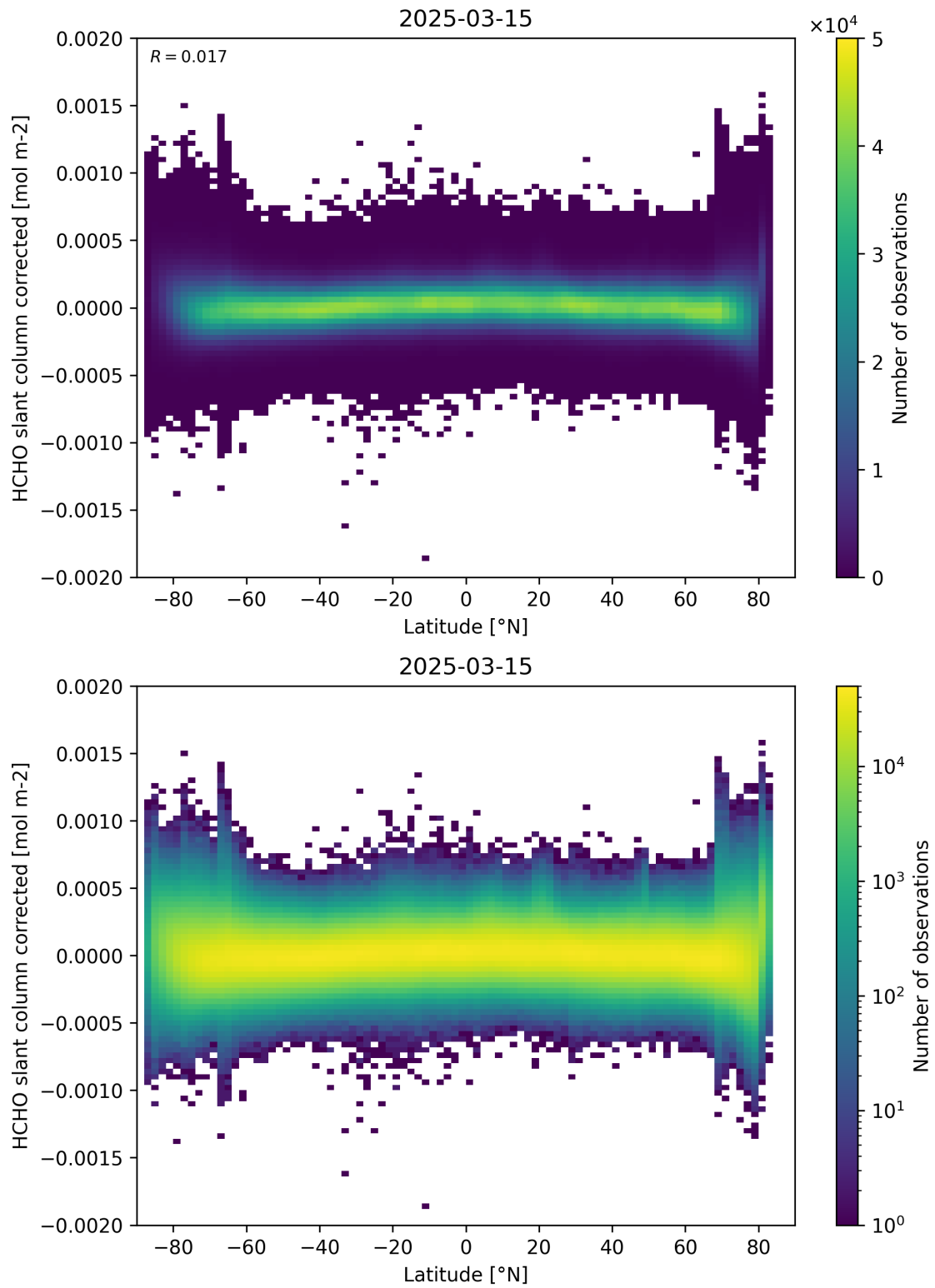
Figure 157: Scatter density plot of “Latitude” against “HCHO slant column corrected” for 2025-03-14 to 2025-03-16.
