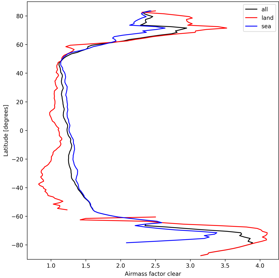
Figure 28: Zonal average of “Airmass factor clear” for 2025-03-14 to 2025-03-16.
