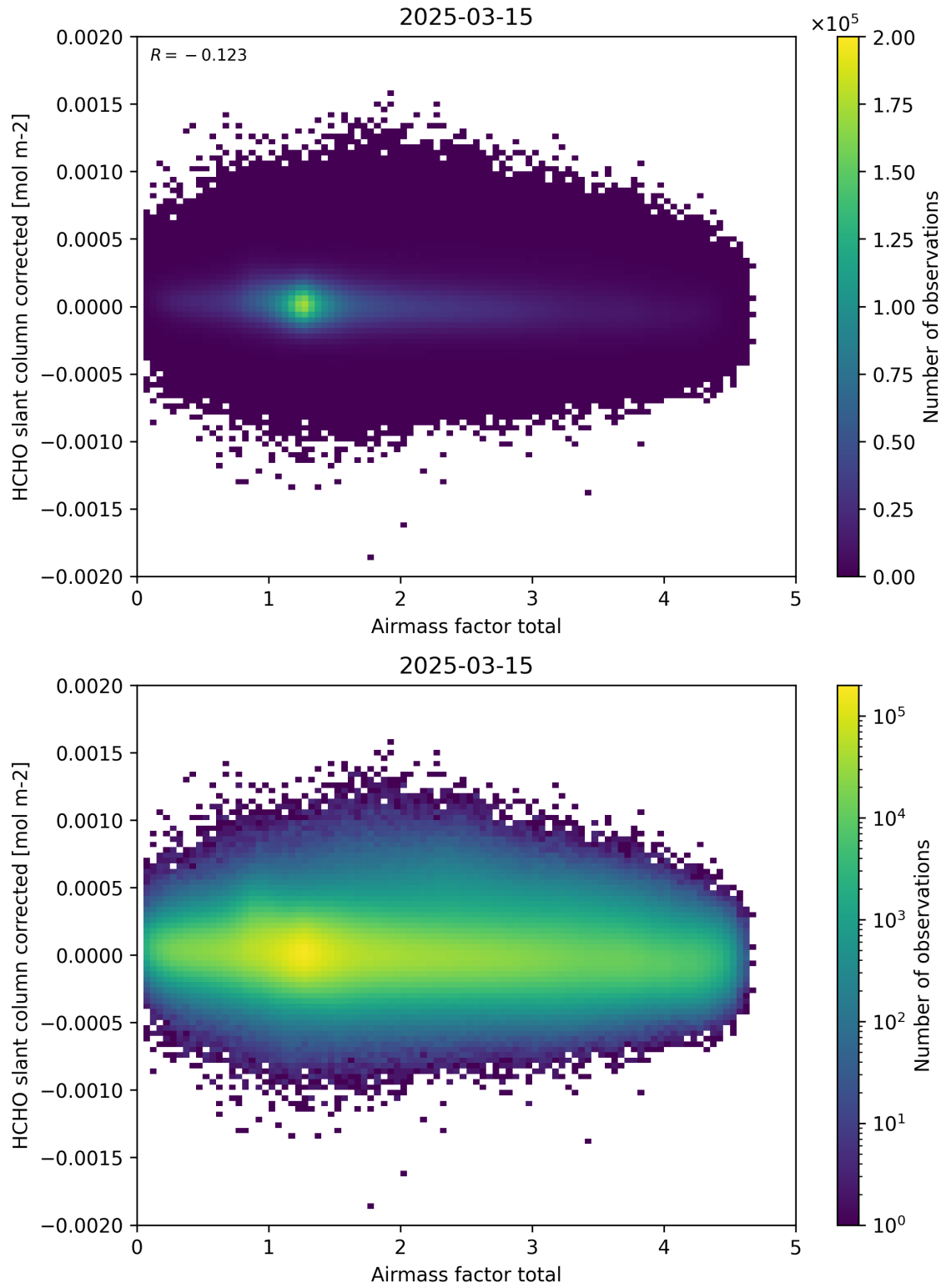
Figure 101: Scatter density plot of “Airmass factor total” against “HCHO slant column corrected” for 2025-03-14 to 2025-03-16.
