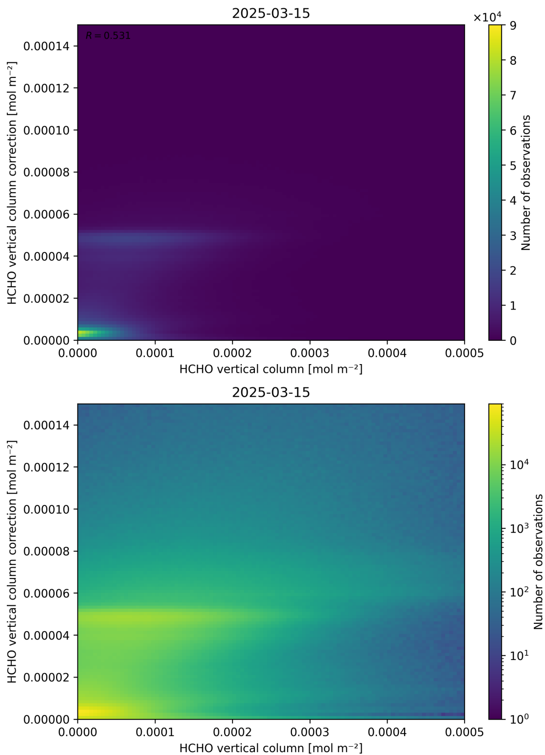
Figure 133: Scatter density plot of “HCHO vertical column” against “HCHO vertical column correction” for 2025-03-14 to 2025-03-16.
