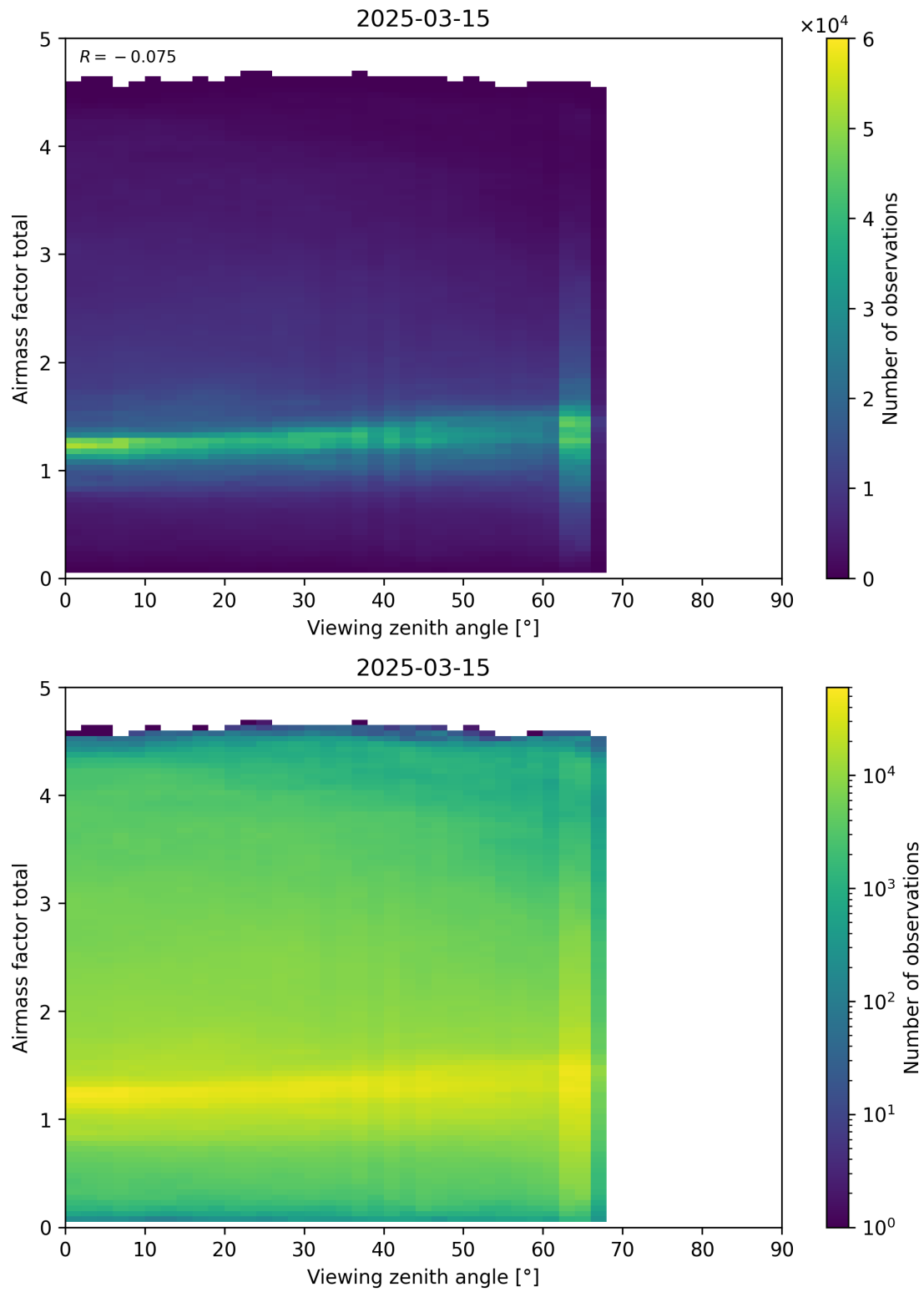
Figure 190: Scatter density plot of “Viewing zenith angle” against “Airmass factor total” for 2025-03-14 to 2025-03-16.
