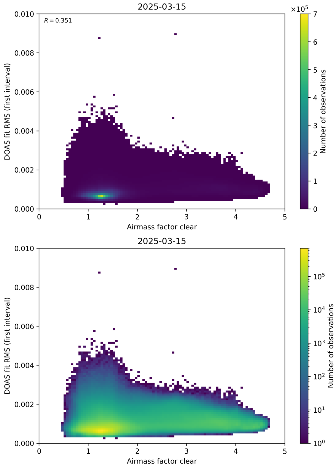
Figure 71: Scatter density plot of “Airmass factor clear” against “DOAS fit RMS (first interval)” for 2025-03-14 to 2025-03-16.
