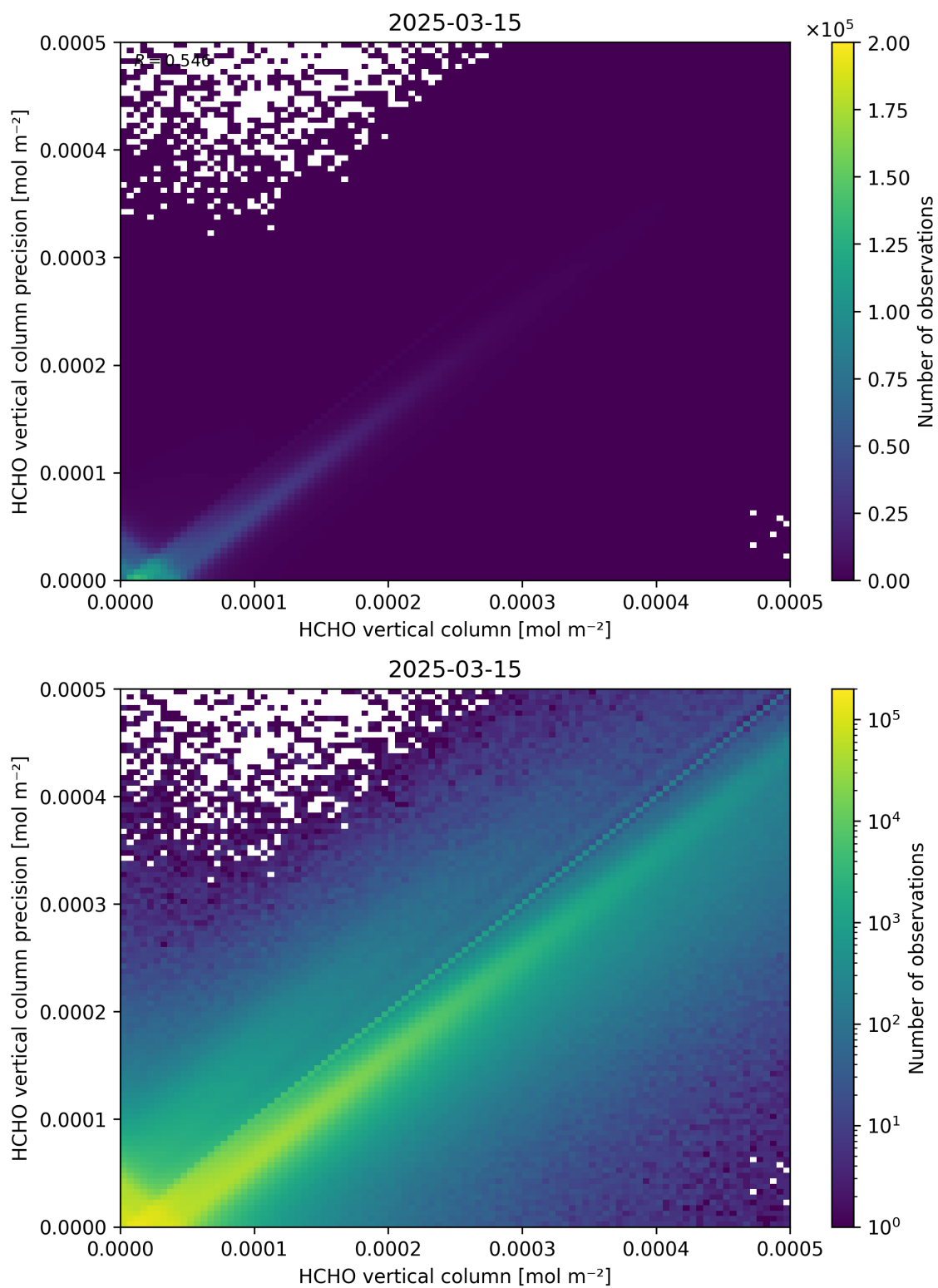
Figure 134: Scatter density plot of “HCHO vertical column” against “HCHO vertical column precision” for 2025-03-14 to 2025-03-16.
