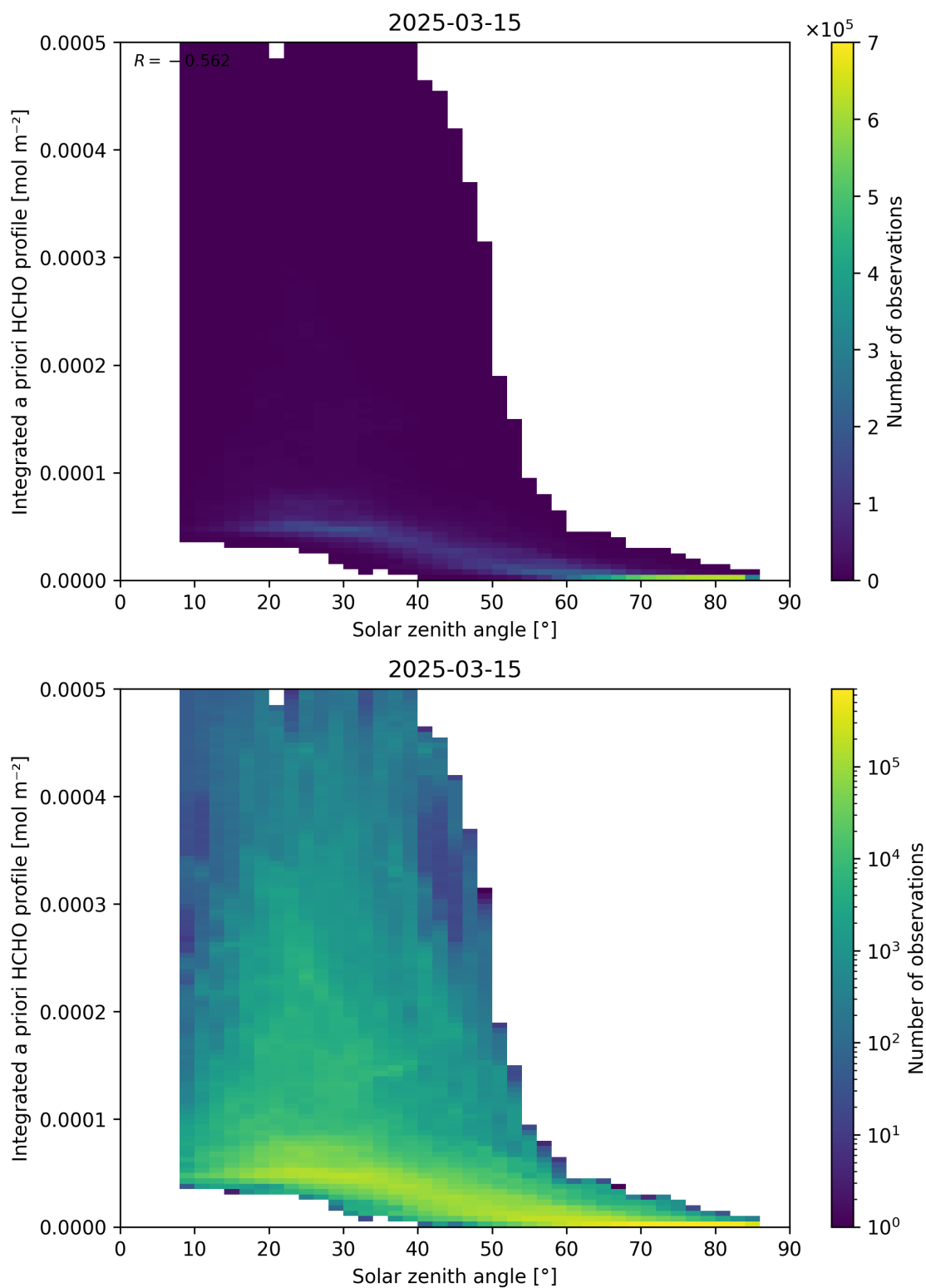
Figure 180: Scatter density plot of “Solar zenith angle” against “Integrated a priori HCHO profile” for 2025-03-14 to 2025-03-16.
