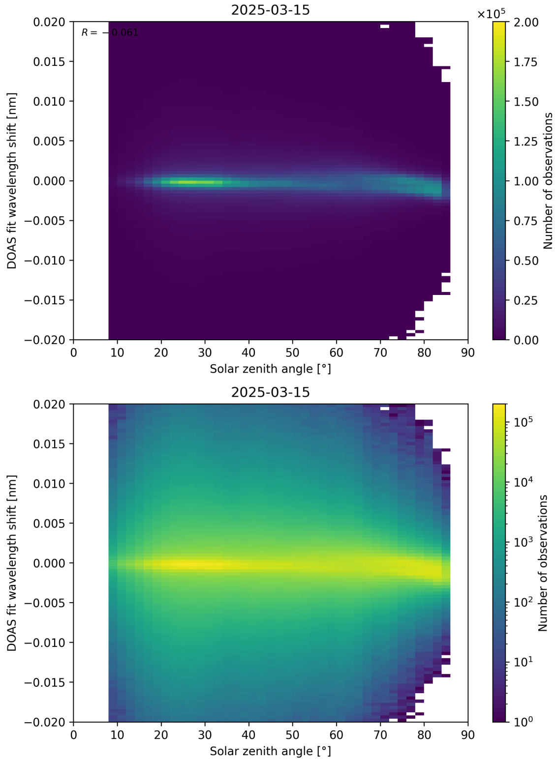
Figure 168: Scatter density plot of “Solar zenith angle” against “DOAS fit wavelength shift” for 2025-03-14 to 2025-03-16.
