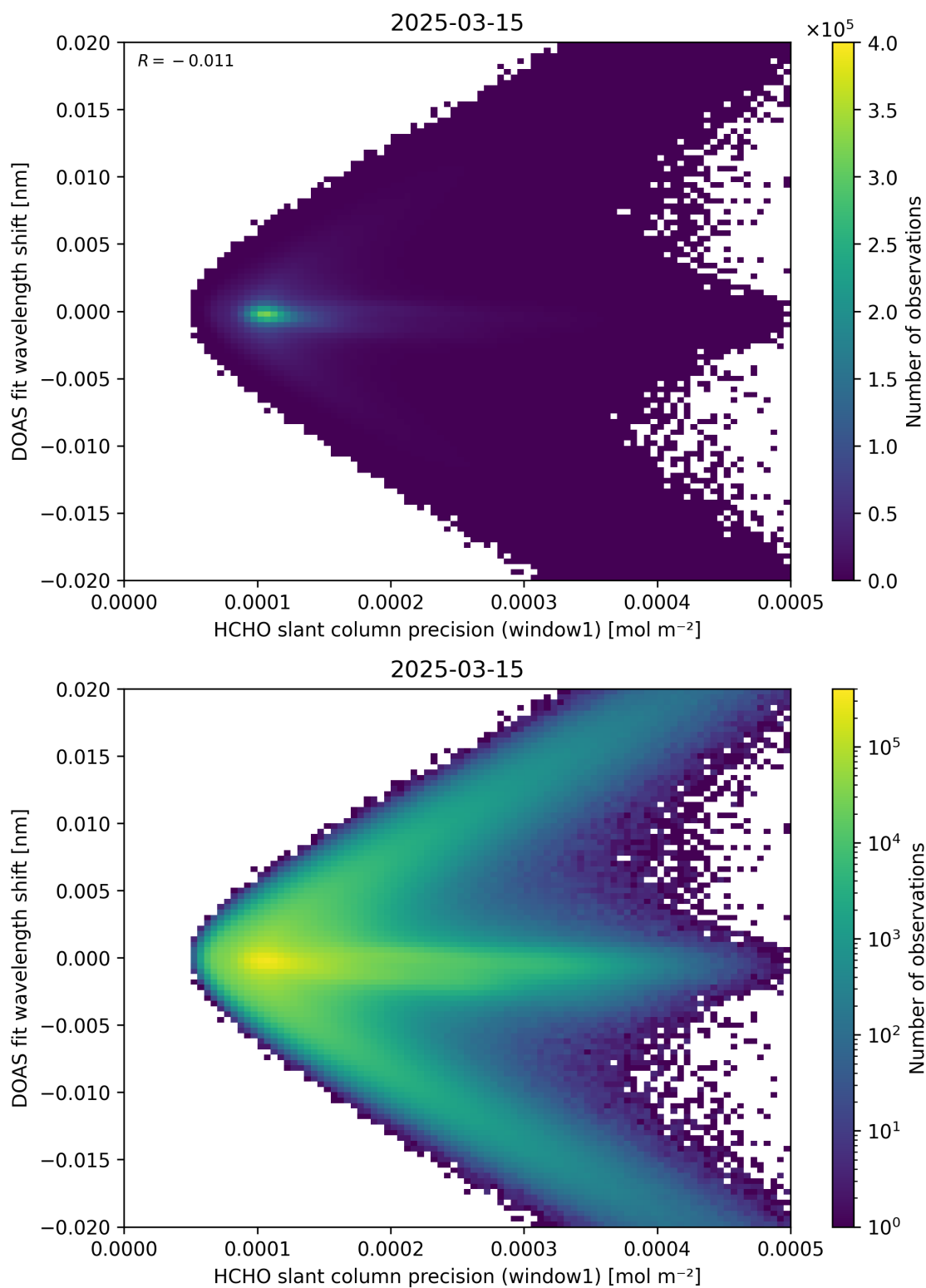
Figure 89: Scatter density plot of “HCHO slant column precision (window1)” against “DOAS fit wavelength shift” for 2025-03-14 to 2025-03-16.
