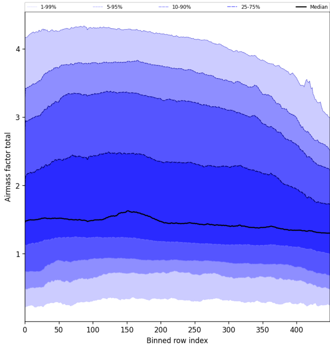
Figure 54: Along track statistics of “Airmass factor total” for 2025-03-14 to 2025-03-16
