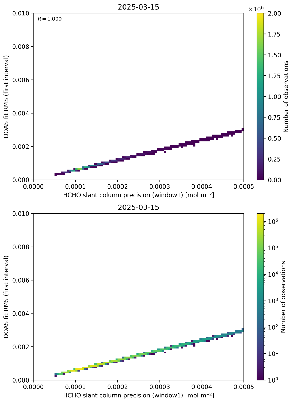
Figure 88: Scatter density plot of “HCHO slant column precision (window1)” against “DOAS fit RMS (first interval)” for 2025-03-14 to 2025-03-16.
