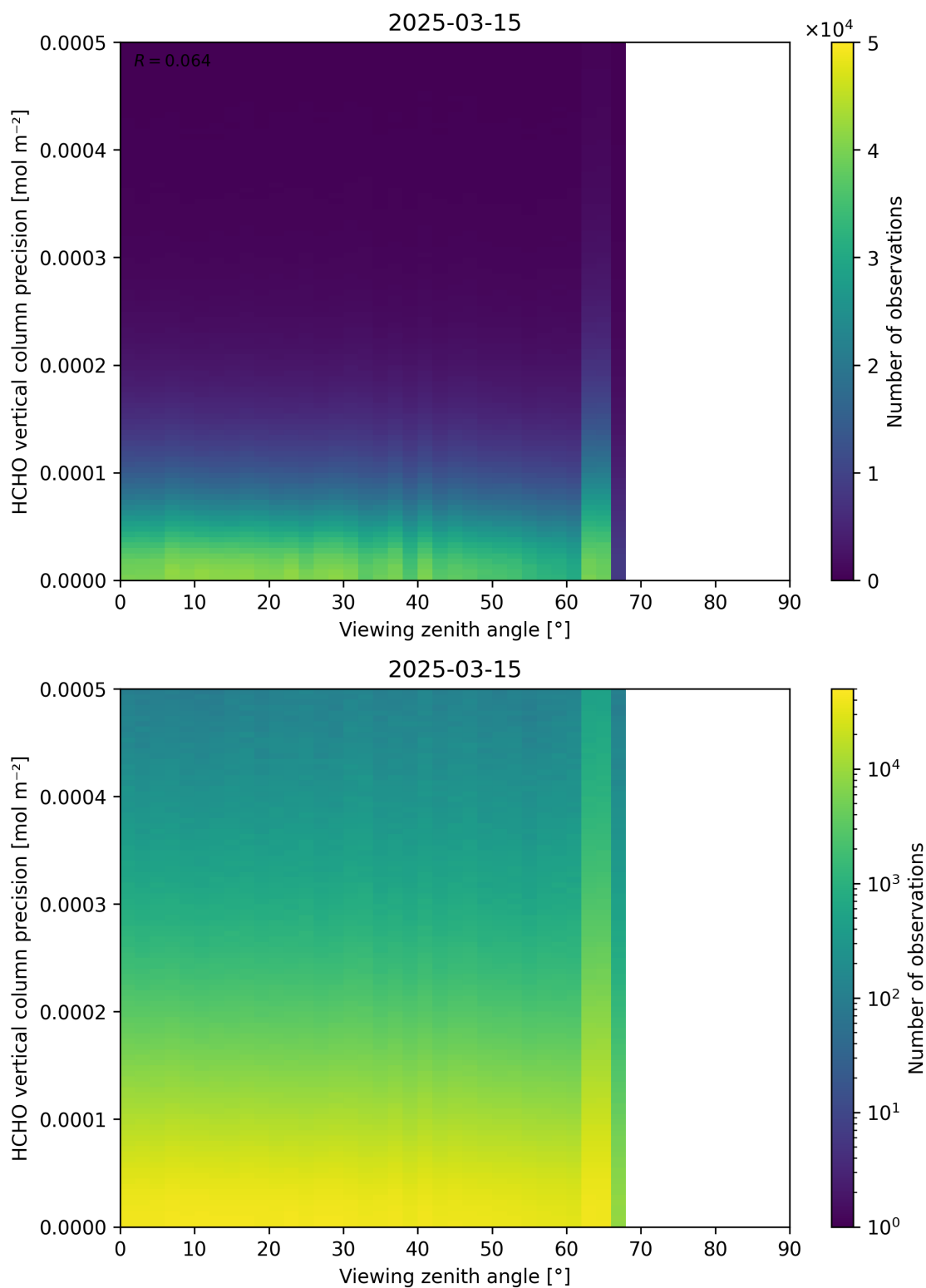
Figure 194: Scatter density plot of “Viewing zenith angle” against “HCHO vertical column precision” for 2025-03-14 to 2025-03-16.
