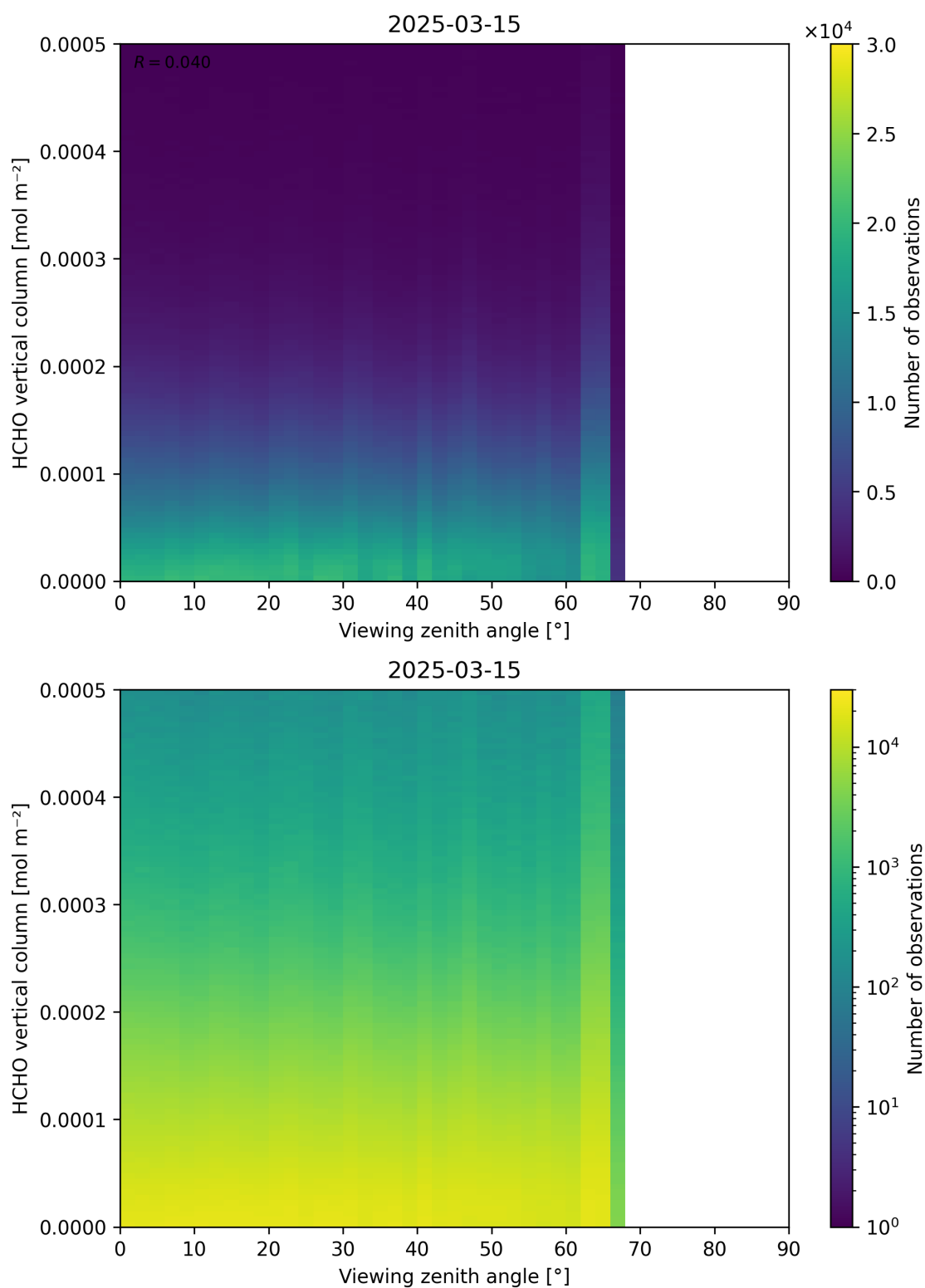
Figure 192: Scatter density plot of “Viewing zenith angle” against “HCHO vertical column” for 2025-03-14 to 2025-03-16.
