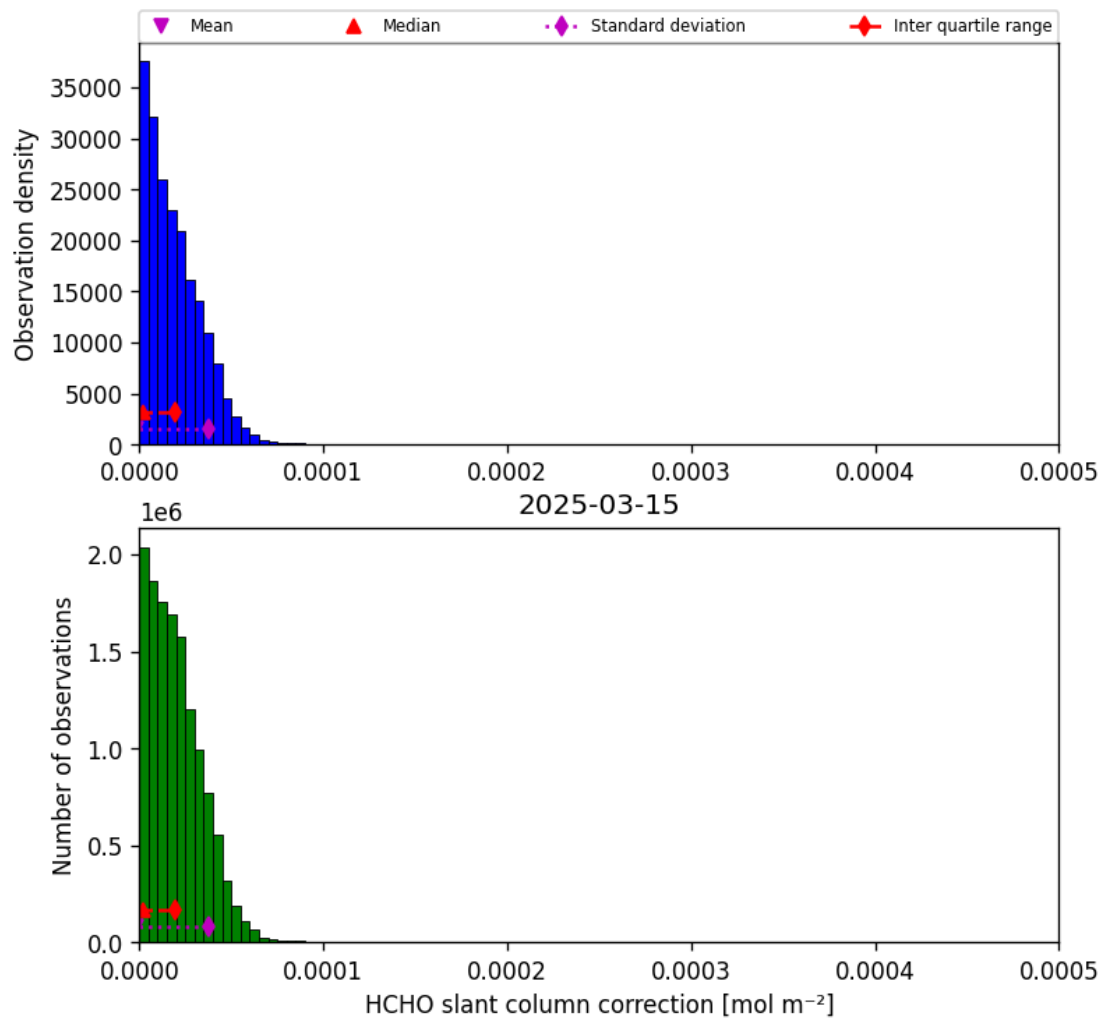
Figure 47: Histogram of “HCHO slant column correction” for 2025-03-14 to 2025-03-16
