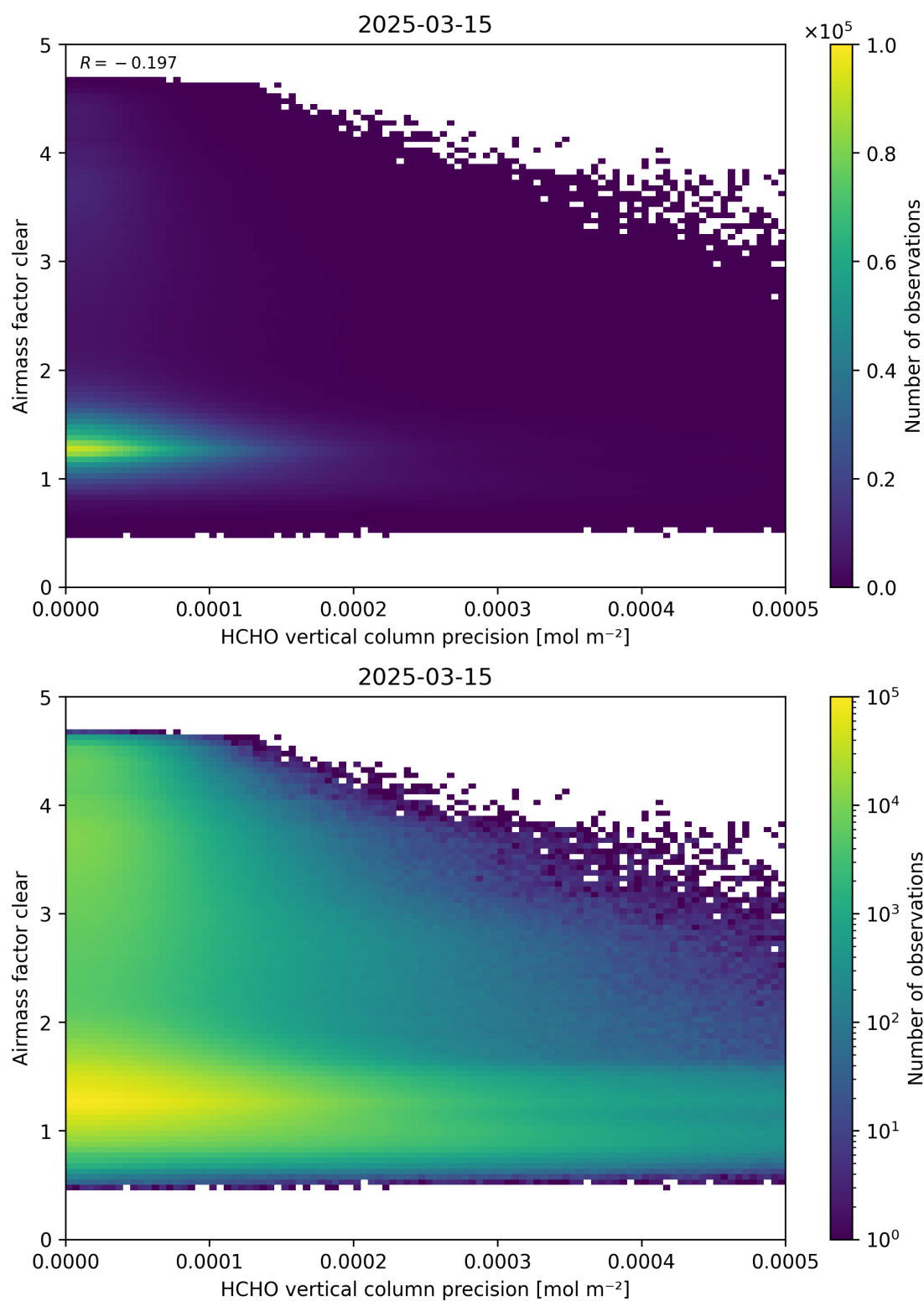
Figure 139: Scatter density plot of “HCHO vertical column precision” against “Airmass factor clear” for 2025-03-14 to 2025-03-16.
