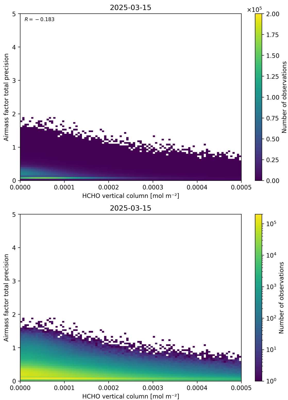
Figure 132: Scatter density plot of “HCHO vertical column” against “Airmass factor total precision” for 2025-03-14 to 2025-03-16.
