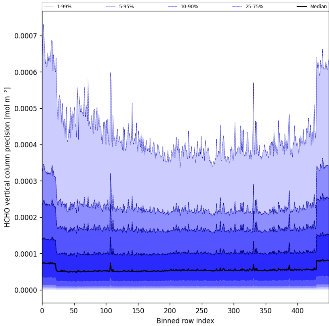
Figure 50: Along track statistics of “HCHO vertical column precision” for 2025-03-14 to 2025-03-16
