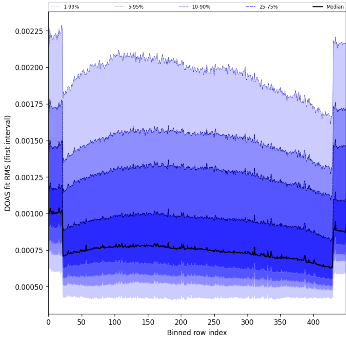
Figure 60: Along track statistics of “DOAS fit RMS (first interval)” for 2025-03-14 to 2025-03-16
