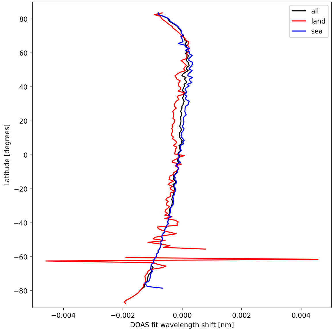
Figure 30: Zonal average of “DOAS fit wavelength shift” for 2025-03-14 to 2025-03-16.
