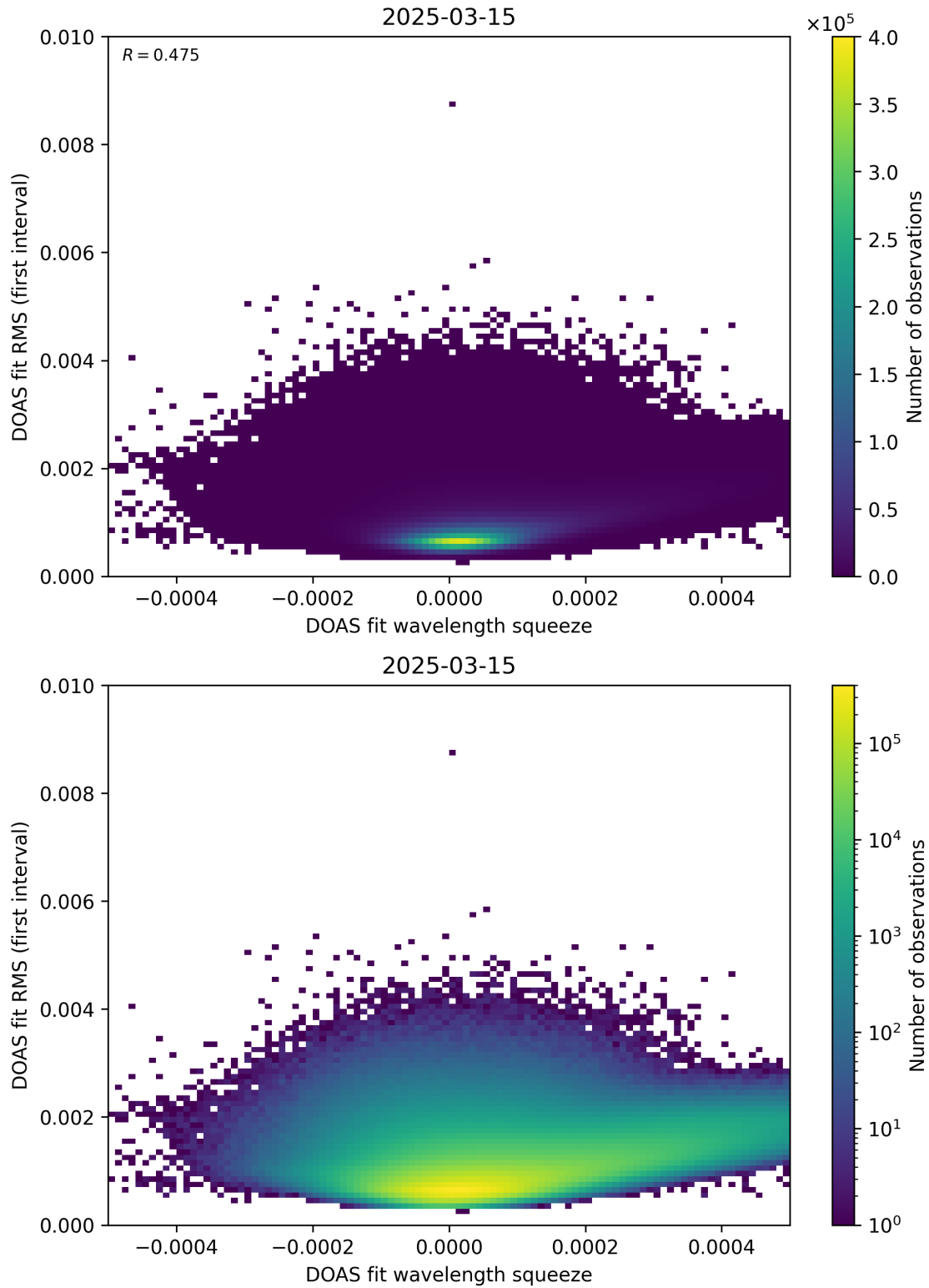
Figure 68: Scatter density plot of “DOAS fit wavelength squeeze” against “DOAS fit RMS (first interval)” for 2025-03-14 to 2025-03-16.
