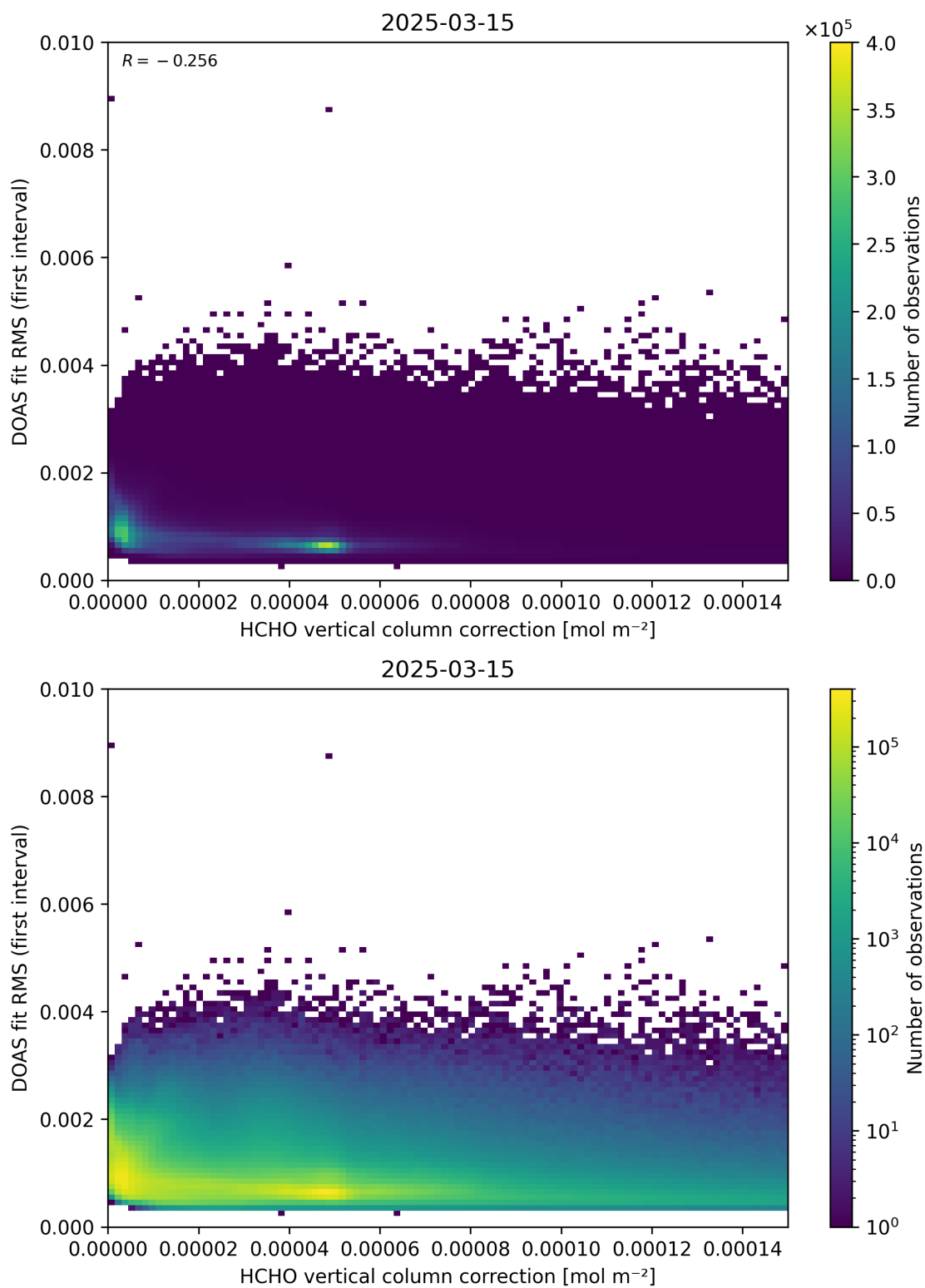
Figure 112: Scatter density plot of “HCHO vertical column correction” against “DOAS fit RMS (first interval)” for 2025-03-14 to 2025-03-16.
