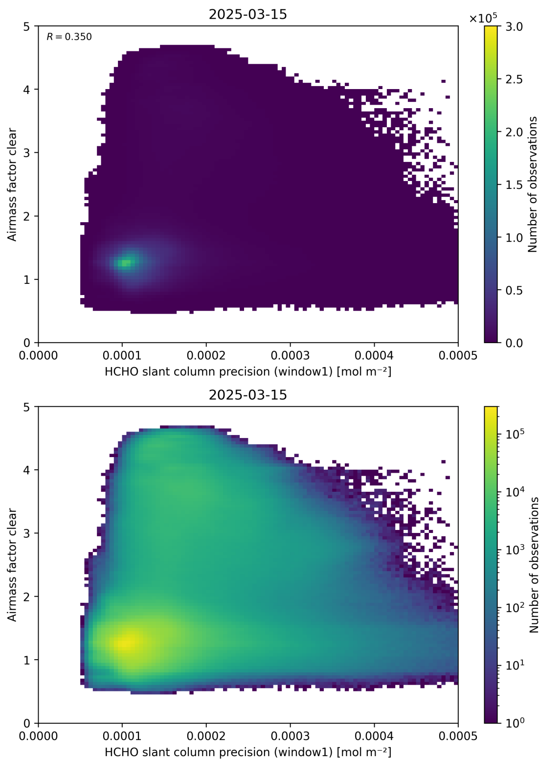
Figure 91: Scatter density plot of “HCHO slant column precision (window1)” against “Airmass factor clear” for 2025-03-14 to 2025-03-16.
