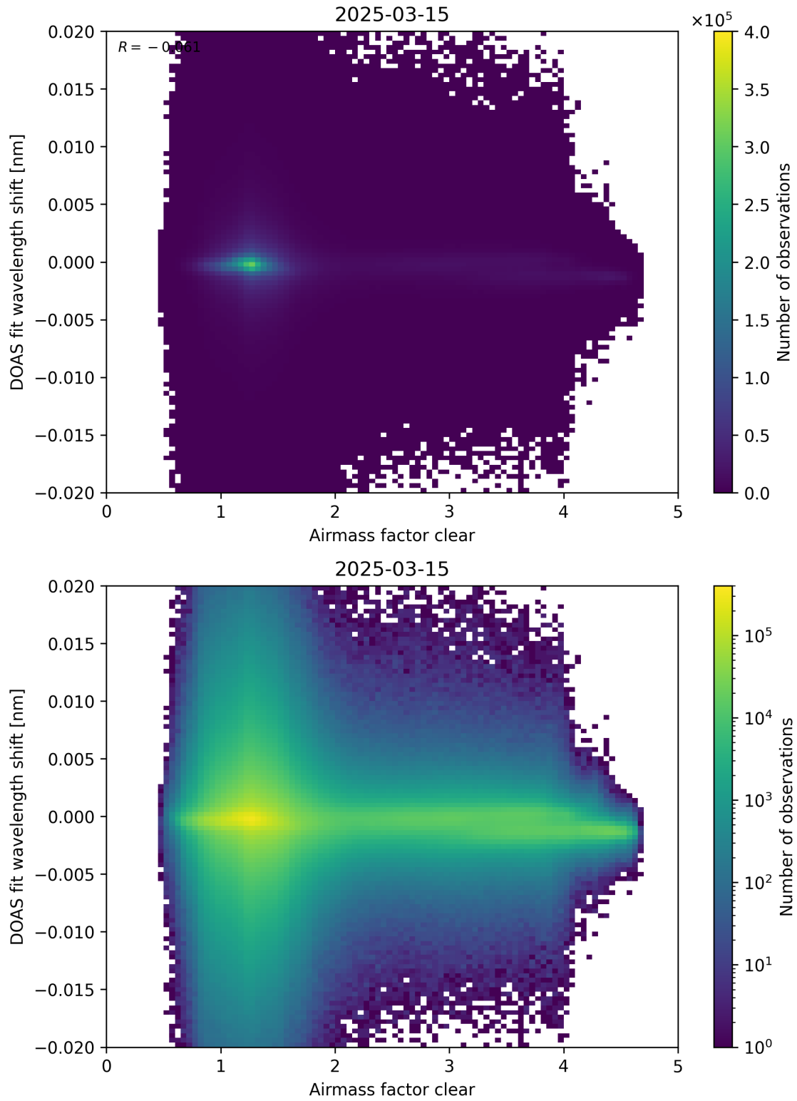
Figure 72: Scatter density plot of “Airmass factor clear” against “DOAS fit wavelength shift” for 2025-03-14 to 2025-03-16.
