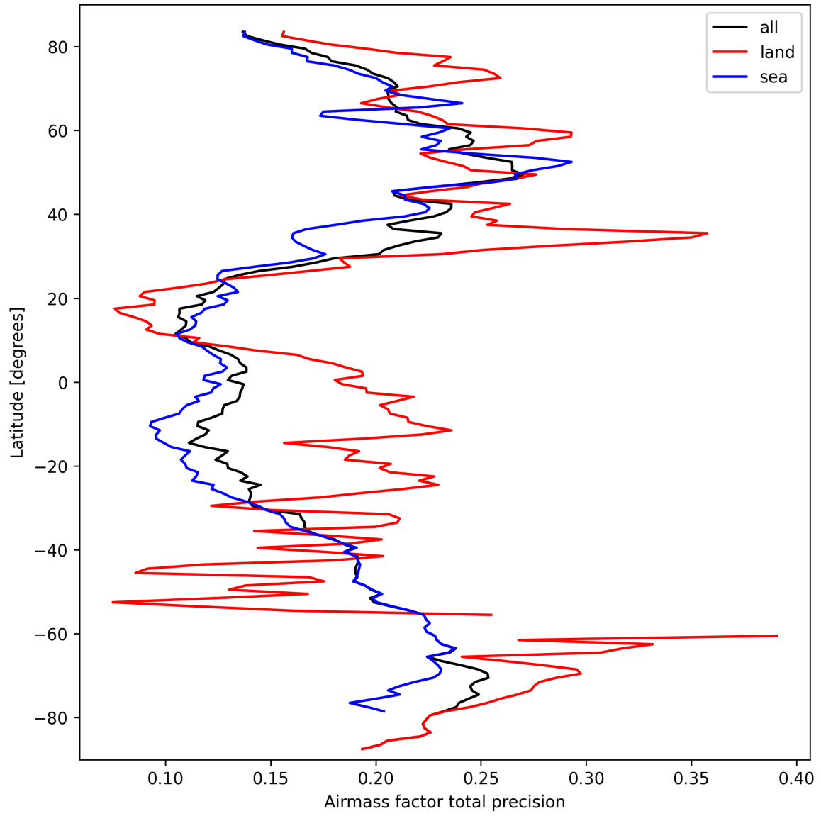
Figure 27: Zonal average of “Airmass factor total precision” for 2025-03-14 to 2025-03-16.
