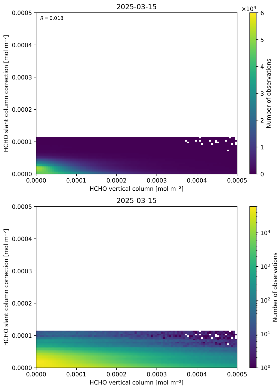
Figure 128: Scatter density plot of “HCHO vertical column” against “HCHO slant column correction” for 2025-03-14 to 2025-03-16.
