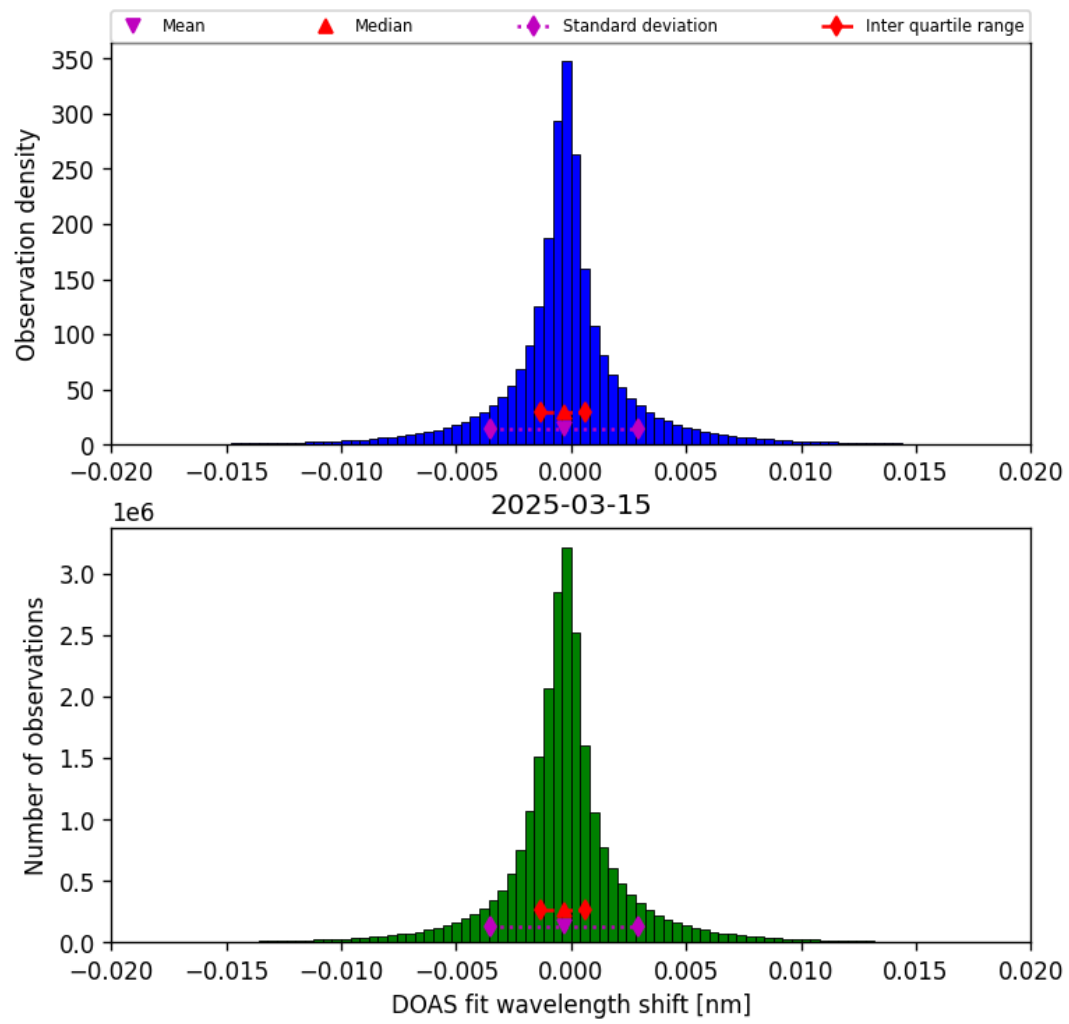
Figure 44: Histogram of “DOAS fit wavelength shift” for 2025-03-14 to 2025-03-16
