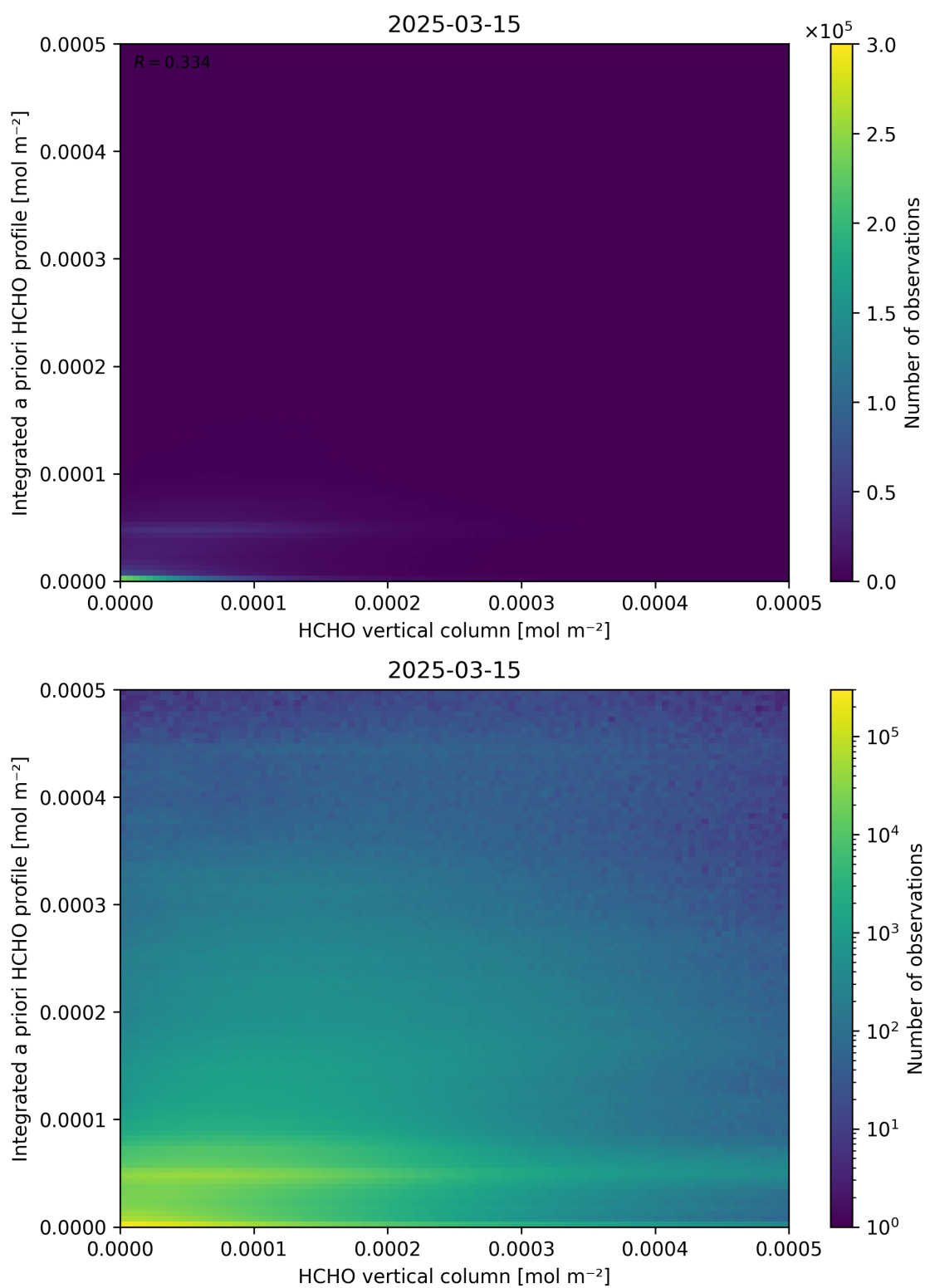
Figure 135: Scatter density plot of “HCHO vertical column” against “Integrated a priori HCHO profile” for 2025-03-14 to 2025-03-16.
