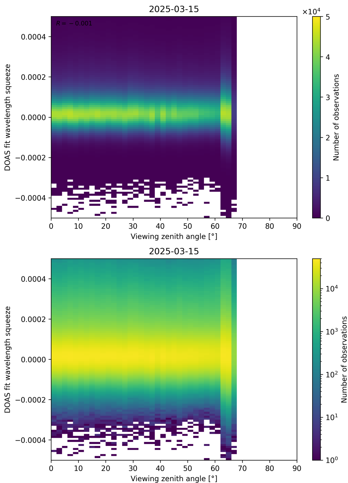
Figure 184: Scatter density plot of “Viewing zenith angle” against “DOAS fit wavelength squeeze” for 2025-03-14 to 2025-03-16.
