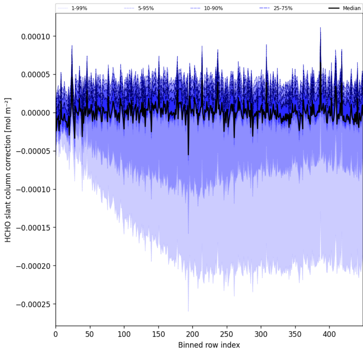
Figure 61: Along track statistics of “HCHO slant column correction” for 2025-03-14 to 2025-03-16
