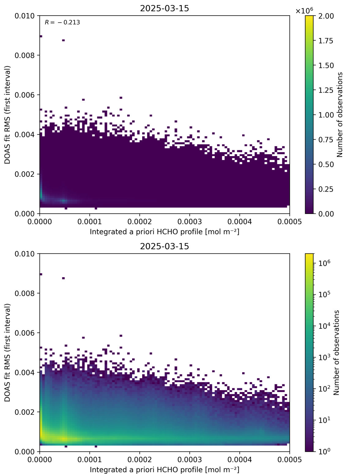
Figure 148: Scatter density plot of “Integrated a priori HCHO profile” against “DOAS fit RMS (first interval)” for 2025-03-14 to 2025-03-16.
