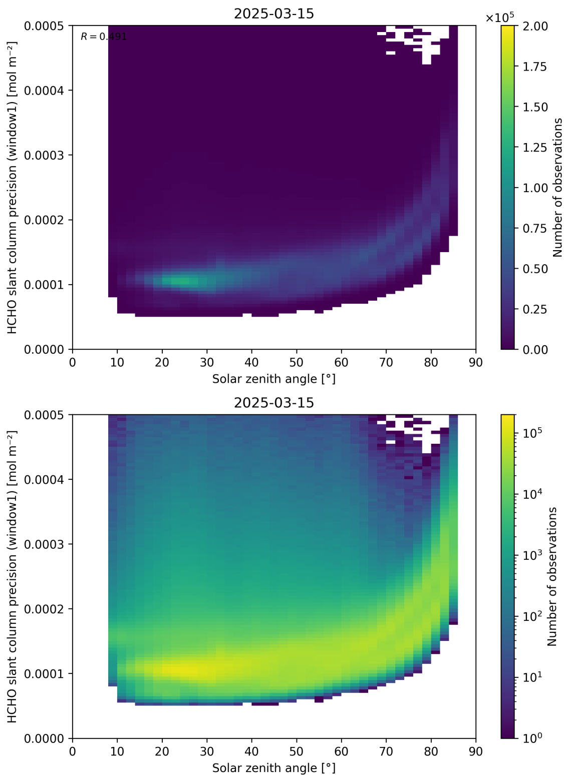
Figure 174: Scatter density plot of “Solar zenith angle” against “HCHO slant column precision (window1)” for 2025-03-14 to 2025-03-16.
