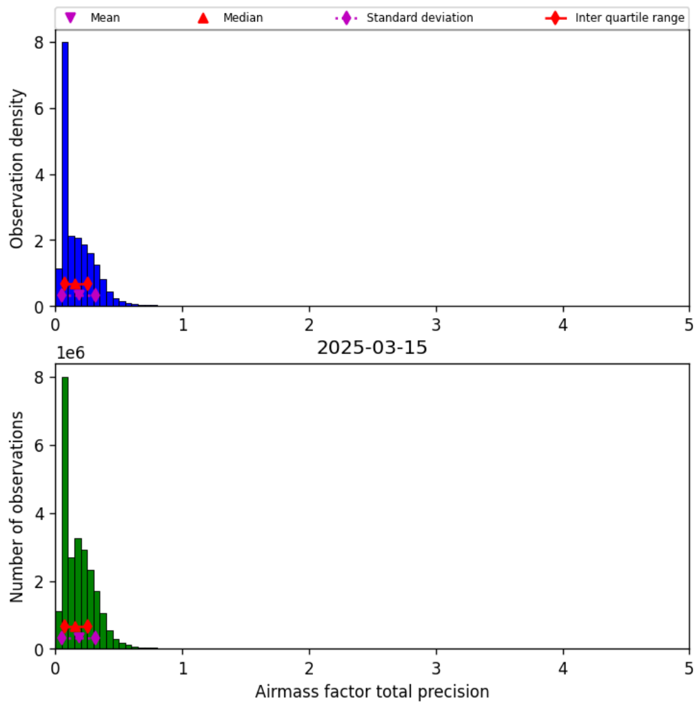
Figure 41: Histogram of “Airmass factor total precision” for 2025-03-14 to 2025-03-16
