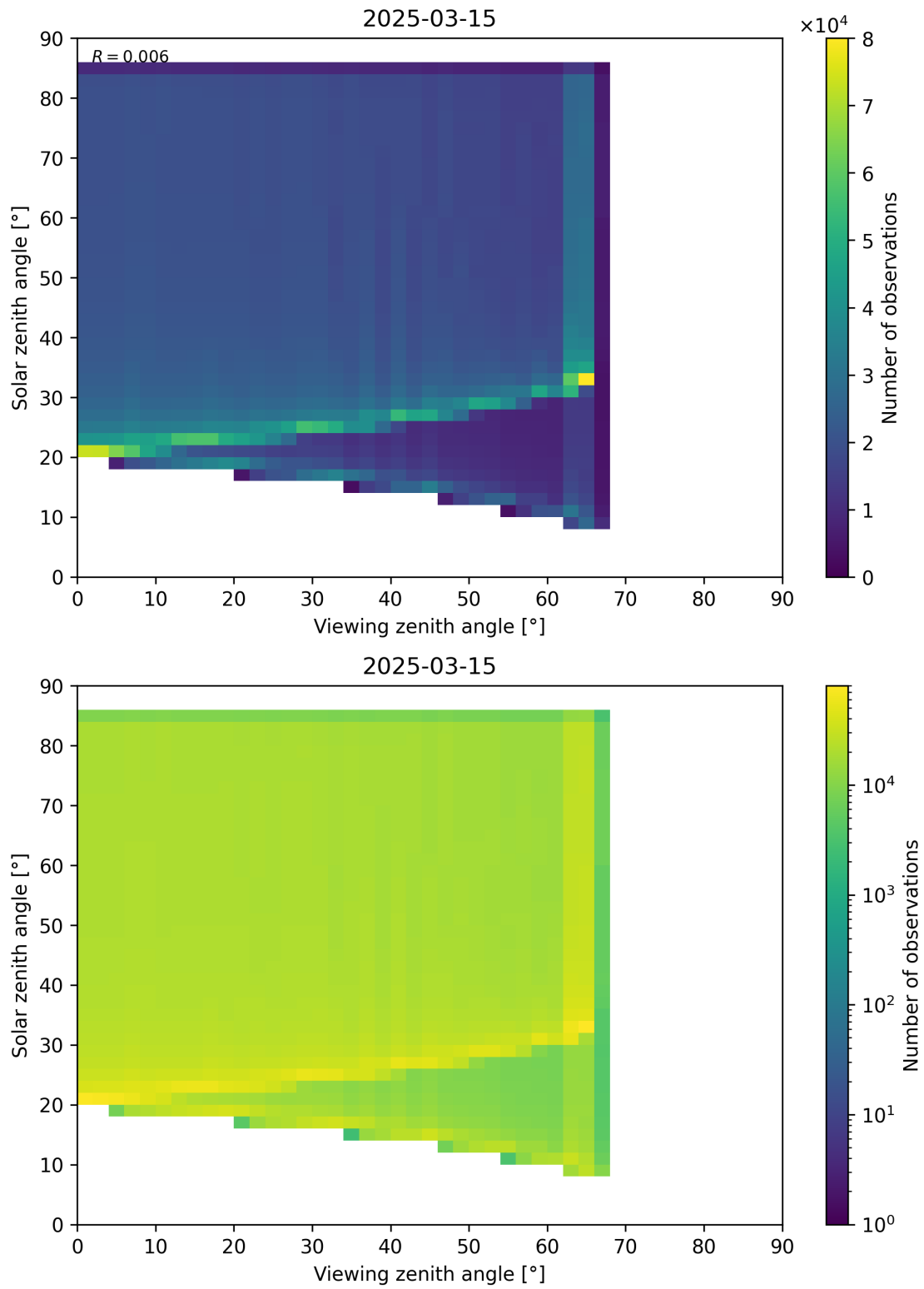
Figure 197: Scatter density plot of “Viewing zenith angle” against “Solar zenith angle” for 2025-03-14 to 2025-03-16.
