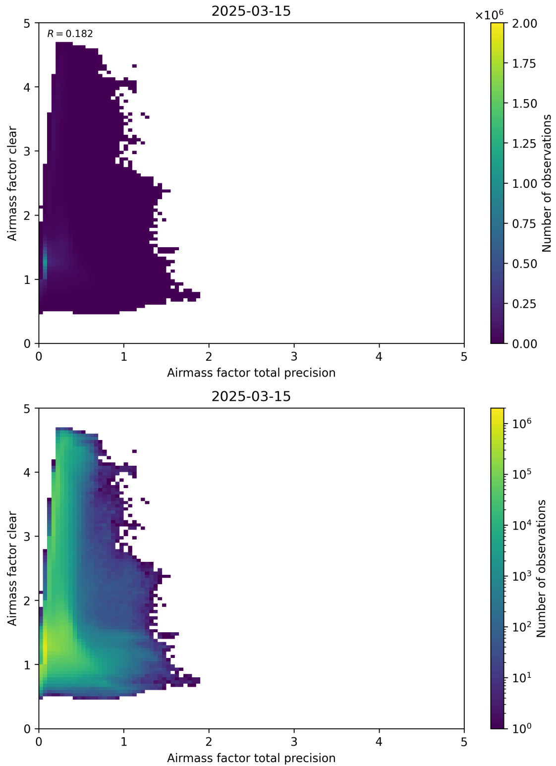
Figure 108: Scatter density plot of “Airmass factor total precision” against “Airmass factor clear” for 2025-03-14 to 2025-03-16.
