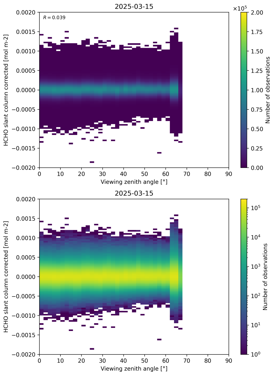
Figure 186: Scatter density plot of “Viewing zenith angle” against “HCHO slant column corrected” for 2025-03-14 to 2025-03-16.
