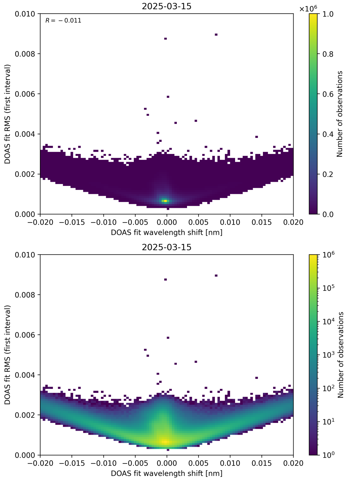
Figure 64: Scatter density plot of “DOAS fit wavelength shift” against “DOAS fit RMS (first interval)” for 2025-03-14 to 2025-03-16.
