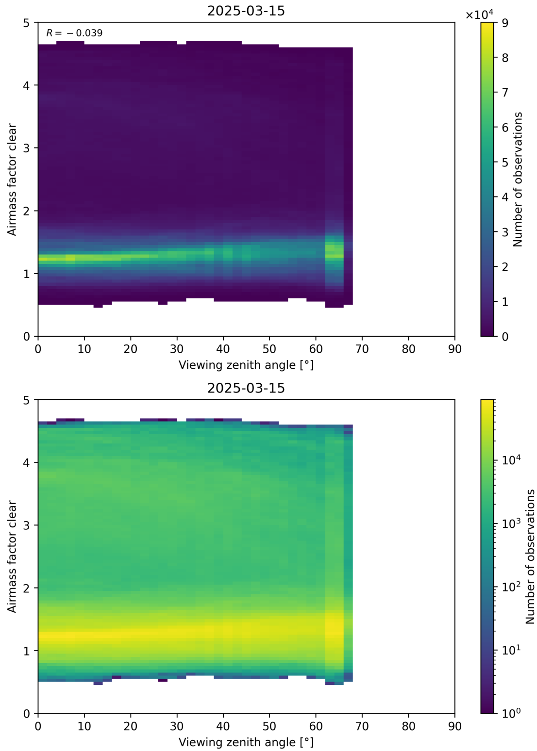
Figure 185: Scatter density plot of “Viewing zenith angle” against “Airmass factor clear” for 2025-03-14 to 2025-03-16.
