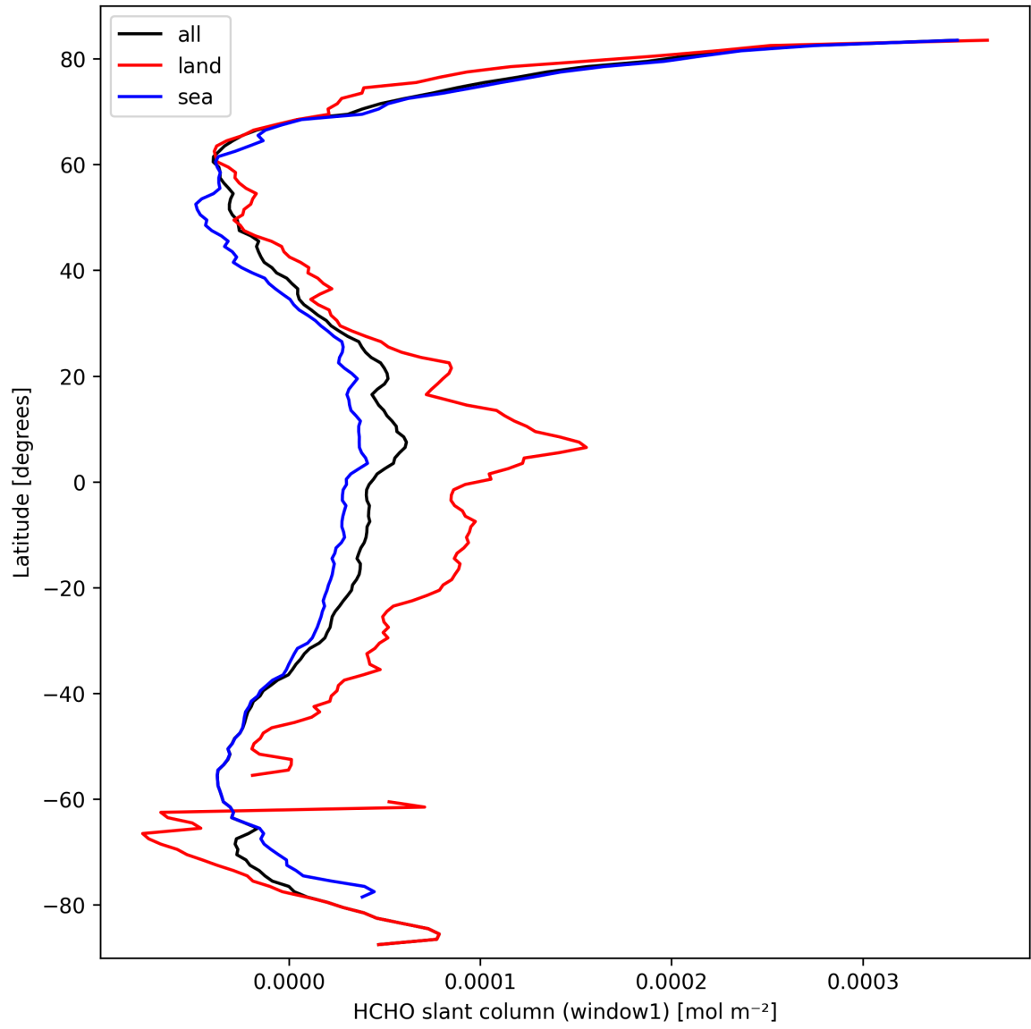
Figure 24: Zonal average of “HCHO slant column (window1)” for 2025-03-14 to 2025-03-16.
