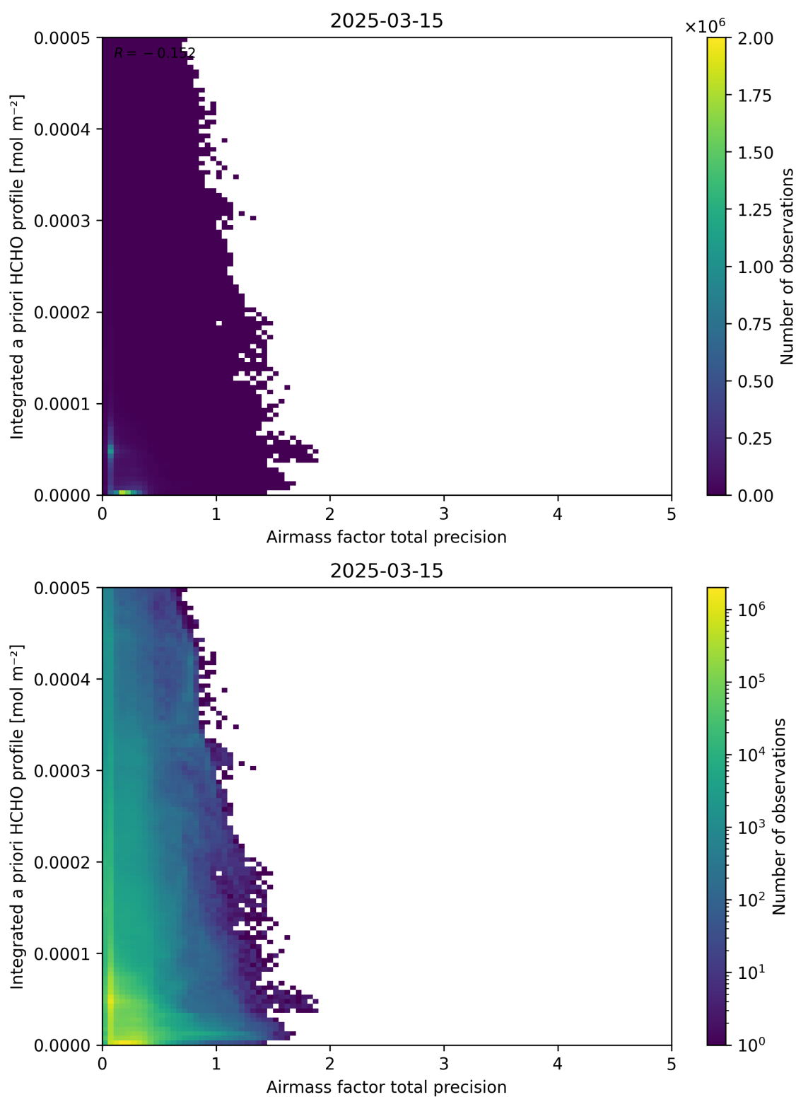
Figure 111: Scatter density plot of “Airmass factor total precision” against “Integrated a priori HCHO profile” for 2025-03-14 to 2025-03-16.
