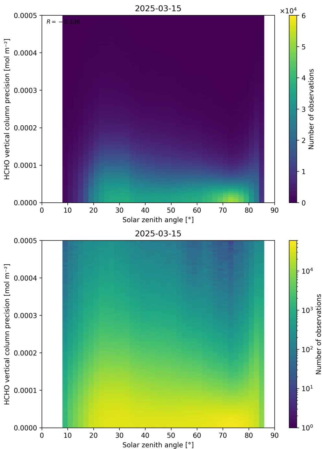
Figure 179: Scatter density plot of “Solar zenith angle” against “HCHO vertical column precision” for 2025-03-14 to 2025-03-16.
