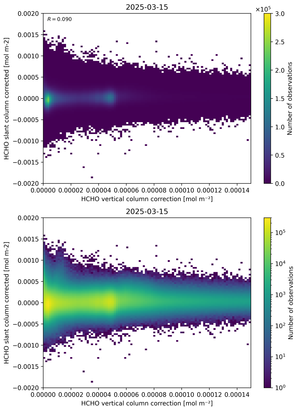
Figure 116: Scatter density plot of “HCHO vertical column correction” against “HCHO slant column corrected” for 2025-03-14 to 2025-03-16.
