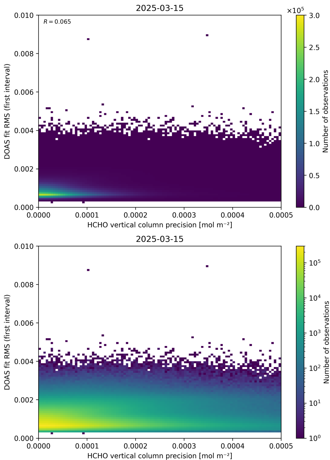
Figure 136: Scatter density plot of “HCHO vertical column precision” against “DOAS fit RMS (first interval)” for 2025-03-14 to 2025-03-16.
