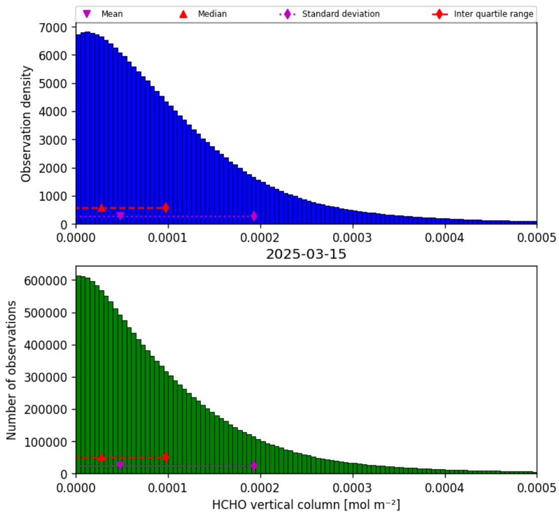
Figure 35: Histogram of “HCHO vertical column” for 2025-03-14 to 2025-03-16
