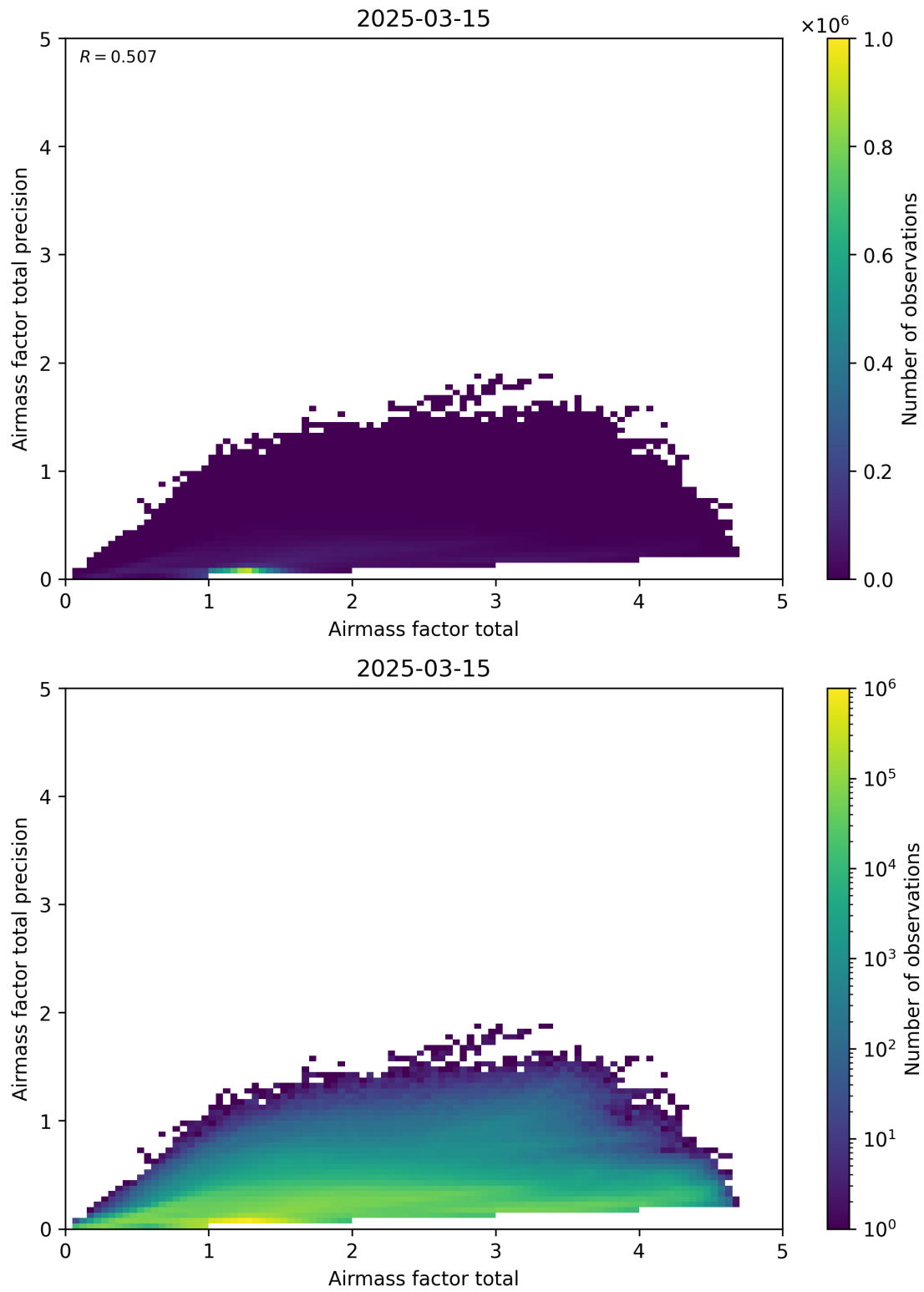
Figure 103: Scatter density plot of “Airmass factor total” against “Airmass factor total precision” for 2025-03-14 to 2025-03-16.
