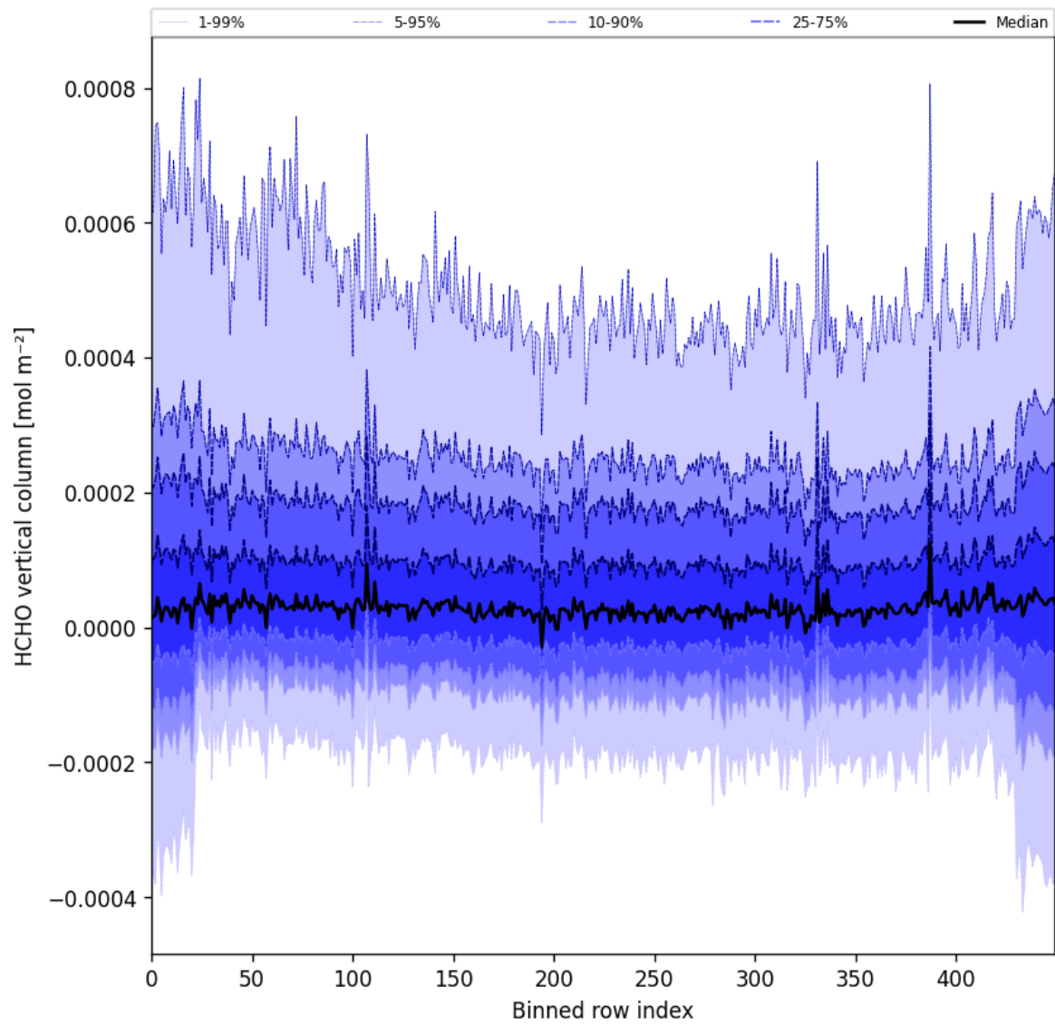
Figure 49: Along track statistics of “HCHO vertical column” for 2025-03-14 to 2025-03-16
