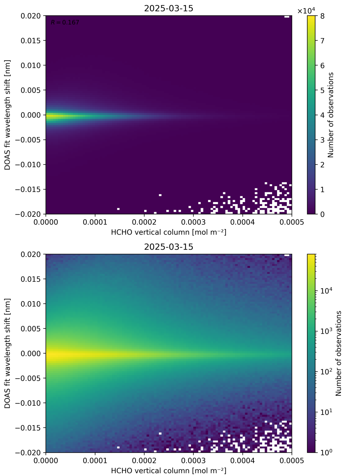
Figure 124: Scatter density plot of “HCHO vertical column” against “DOAS fit wavelength shift” for 2025-03-14 to 2025-03-16.
