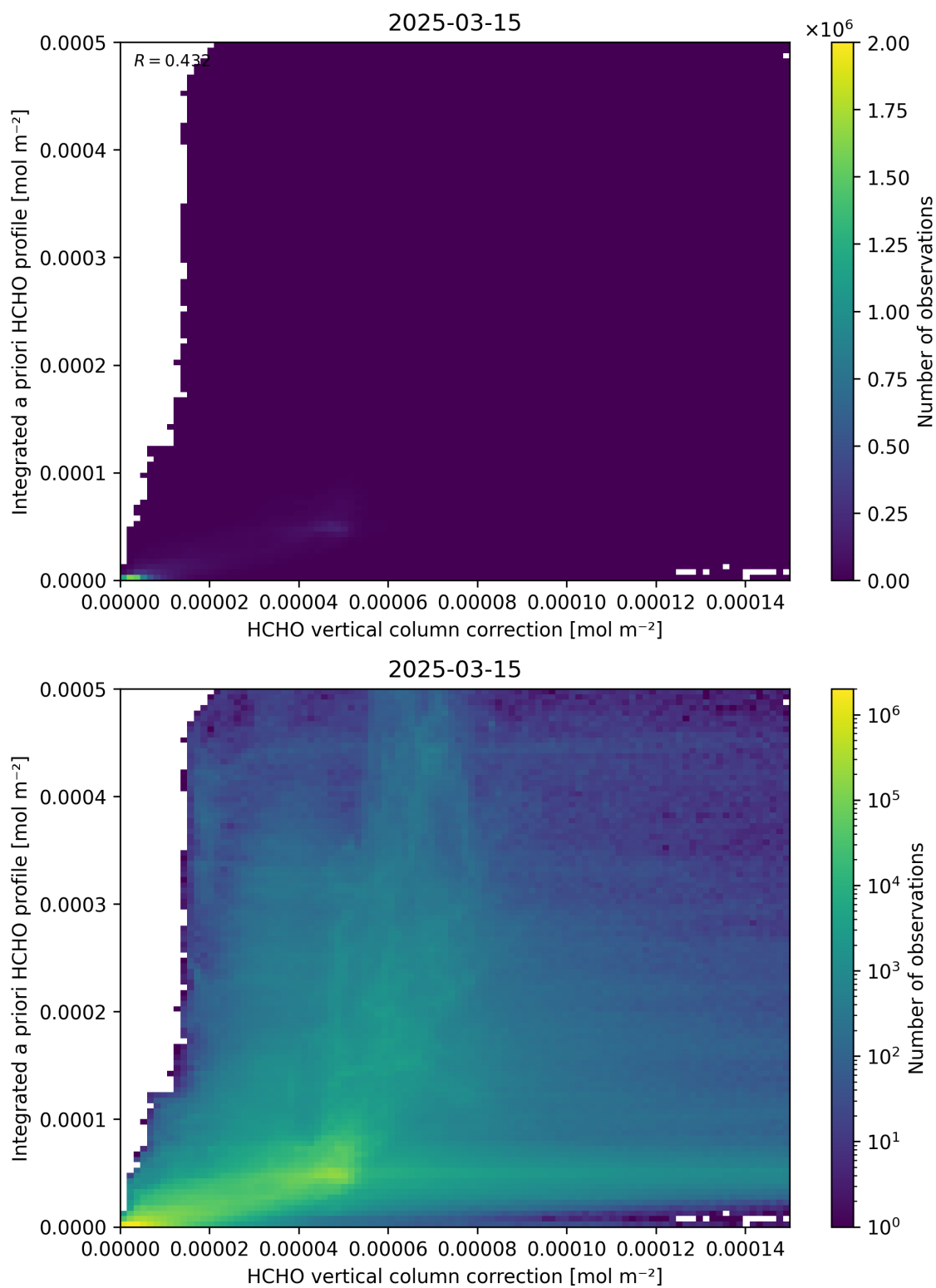
Figure 122: Scatter density plot of “HCHO vertical column correction” against “Integrated a priori HCHO profile” for 2025-03-14 to 2025-03-16.
