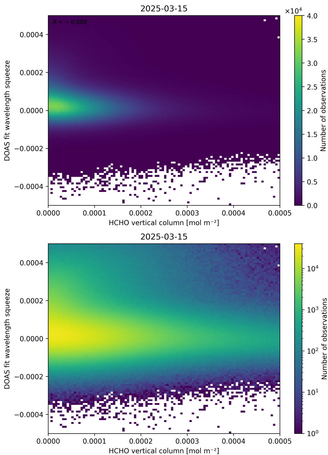
Figure 125: Scatter density plot of “HCHO vertical column” against “DOAS fit wavelength squeeze” for 2025-03-14 to 2025-03-16.
