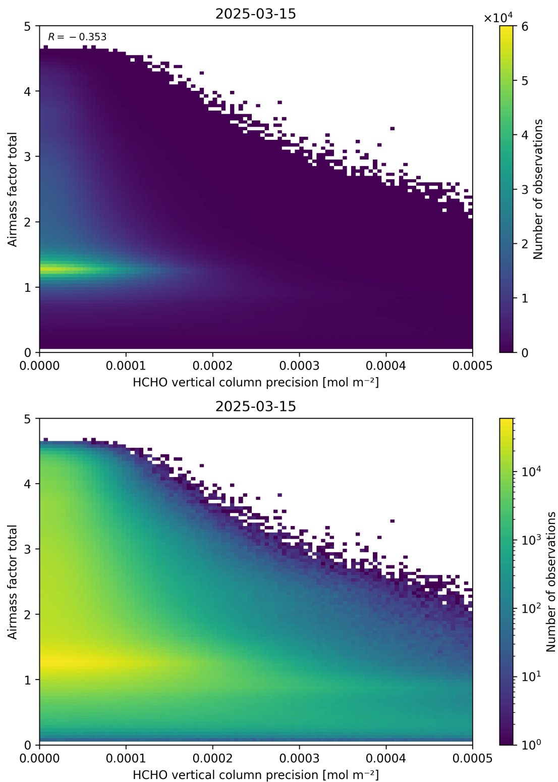
Figure 144: Scatter density plot of “HCHO vertical column precision” against “Airmass factor total” for 2025-03-14 to 2025-03-16.
