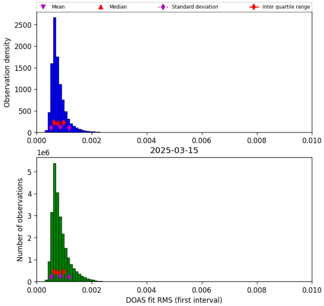
Figure 46: Histogram of “DOAS fit RMS (first interval)” for 2025-03-14 to 2025-03-16
