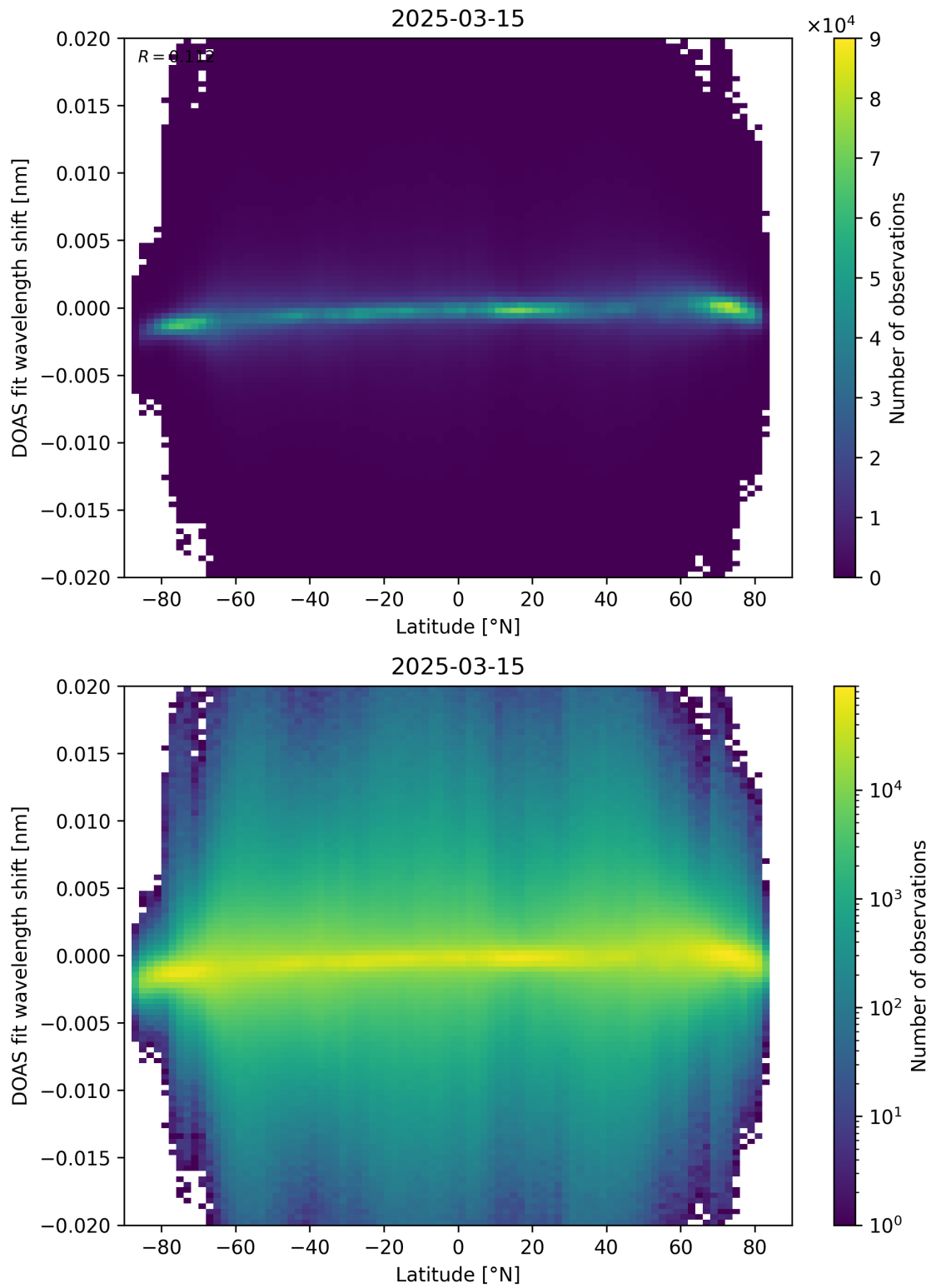
Figure 154: Scatter density plot of “Latitude” against “DOAS fit wavelength shift” for 2025-03-14 to 2025-03-16.
