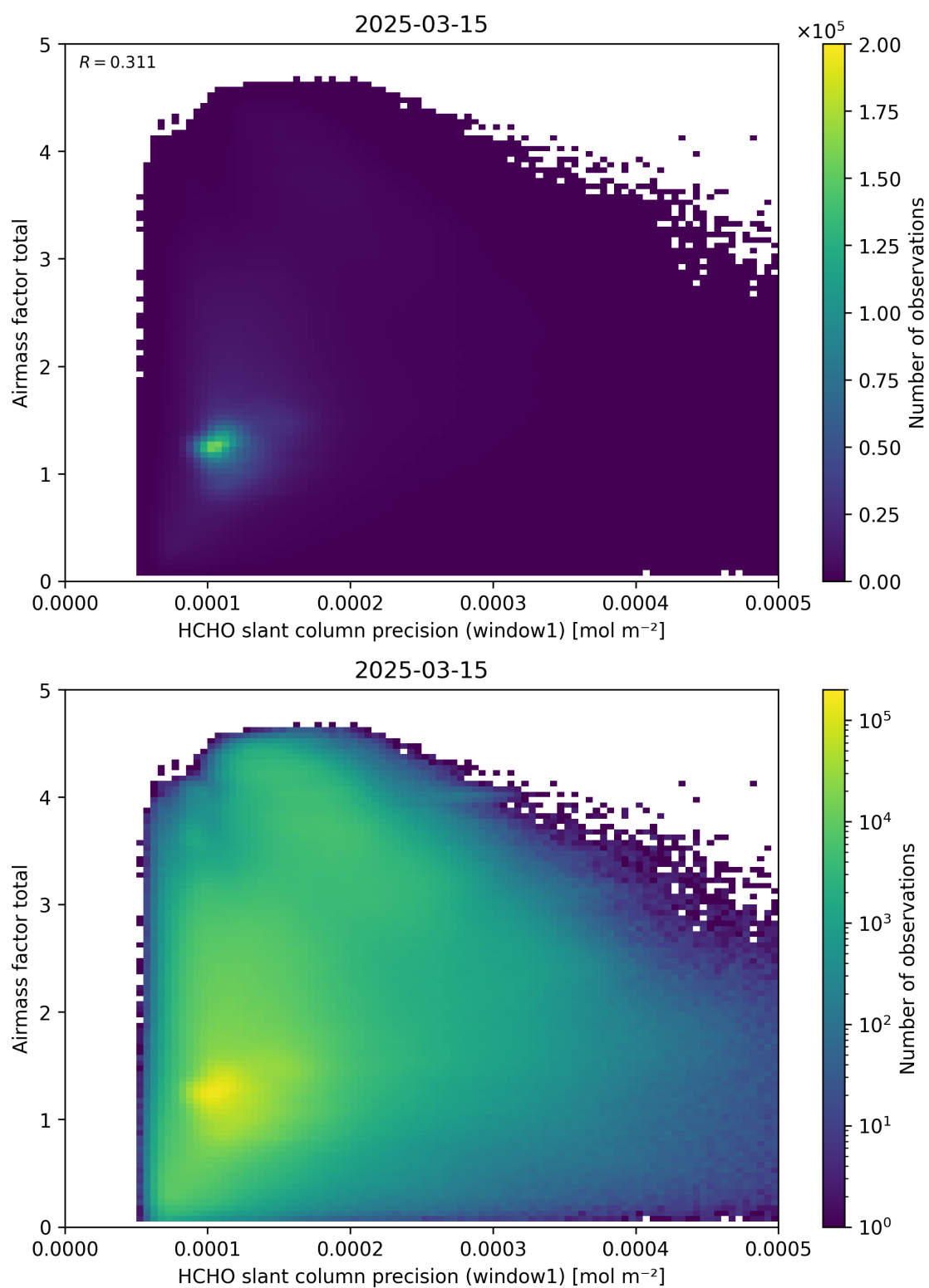
Figure 94: Scatter density plot of “HCHO slant column precision (window1)” against “Airmass factor total” for 2025-03-14 to 2025-03-16.
