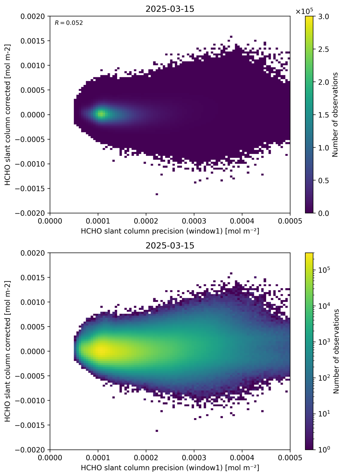
Figure 92: Scatter density plot of “HCHO slant column precision (window1)” against “HCHO slant column corrected” for 2025-03-14 to 2025-03-16.
