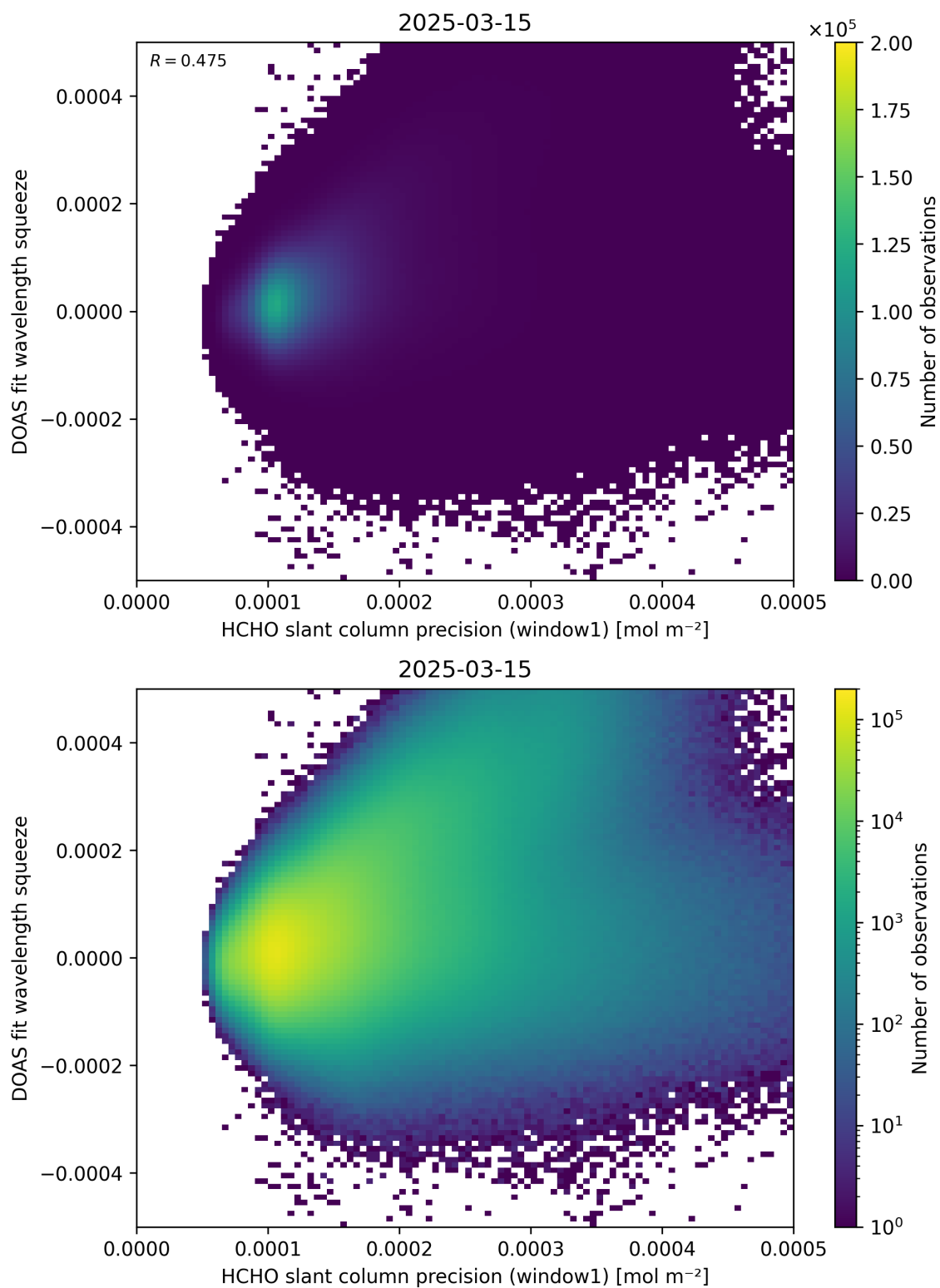
Figure 90: Scatter density plot of “HCHO slant column precision (window1)” against “DOAS fit wavelength squeeze” for 2025-03-14 to 2025-03-16.
