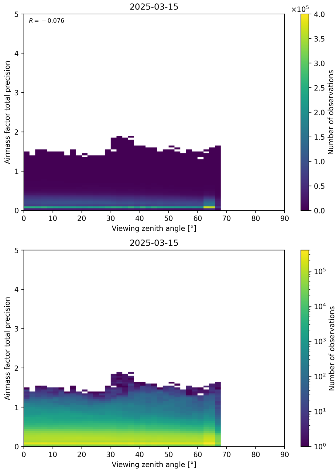
Figure 191: Scatter density plot of “Viewing zenith angle” against “Airmass factor total precision” for 2025-03-14 to 2025-03-16.
