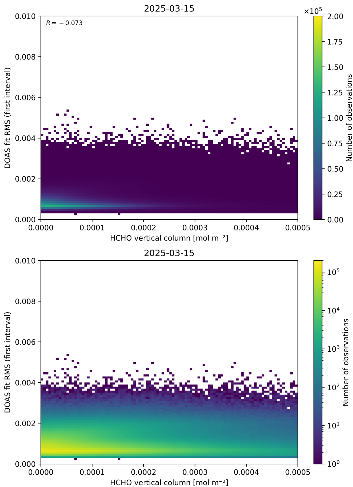
Figure 123: Scatter density plot of “HCHO vertical column” against “DOAS fit RMS (first interval)” for 2025-03-14 to 2025-03-16.
