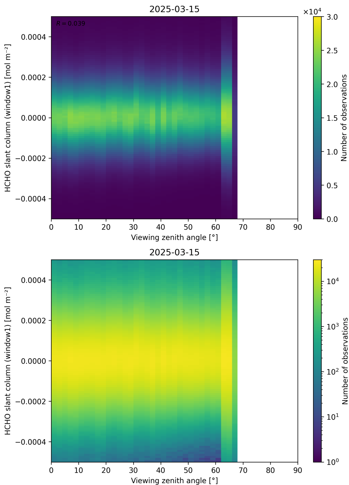
Figure 188: Scatter density plot of “Viewing zenith angle” against “HCHO slant column (window1)” for 2025-03-14 to 2025-03-16.
