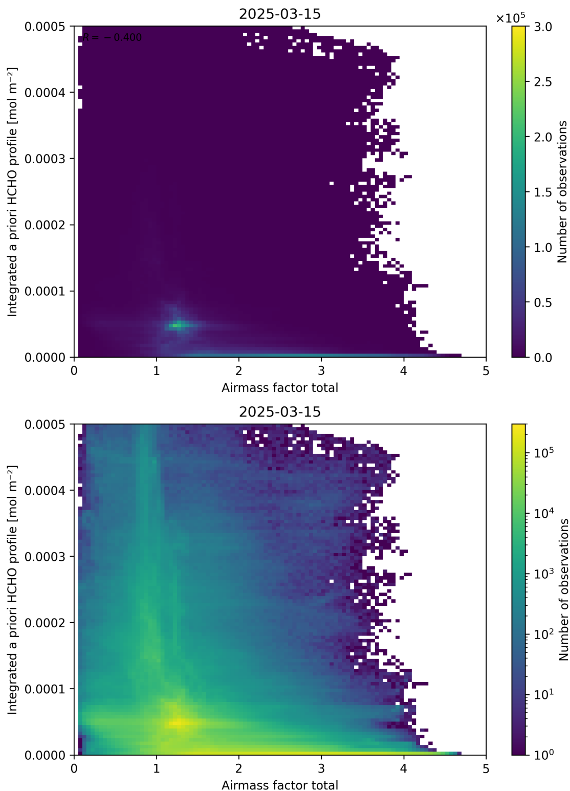
Figure 104: Scatter density plot of “Airmass factor total” against “Integrated a priori HCHO profile” for 2025-03-14 to 2025-03-16.
