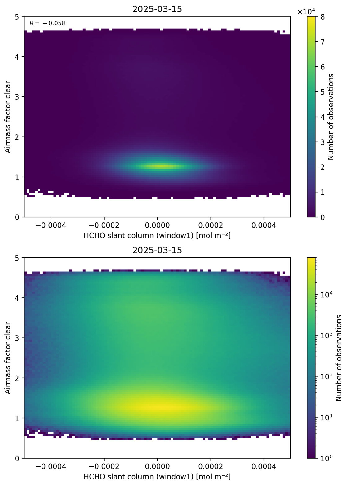
Figure 81: Scatter density plot of “HCHO slant column (window1)” against “Airmass factor clear” for 2025-03-14 to 2025-03-16.
