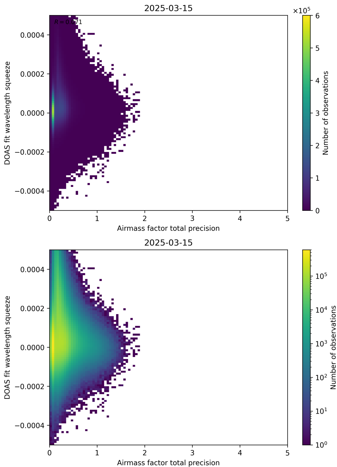
Figure 107: Scatter density plot of “Airmass factor total precision” against “DOAS fit wavelength squeeze” for 2025-03-14 to 2025-03-16.
