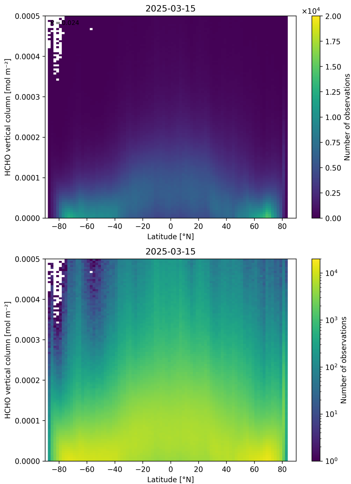
Figure 163: Scatter density plot of “Latitude” against “HCHO vertical column” for 2025-03-14 to 2025-03-16.
