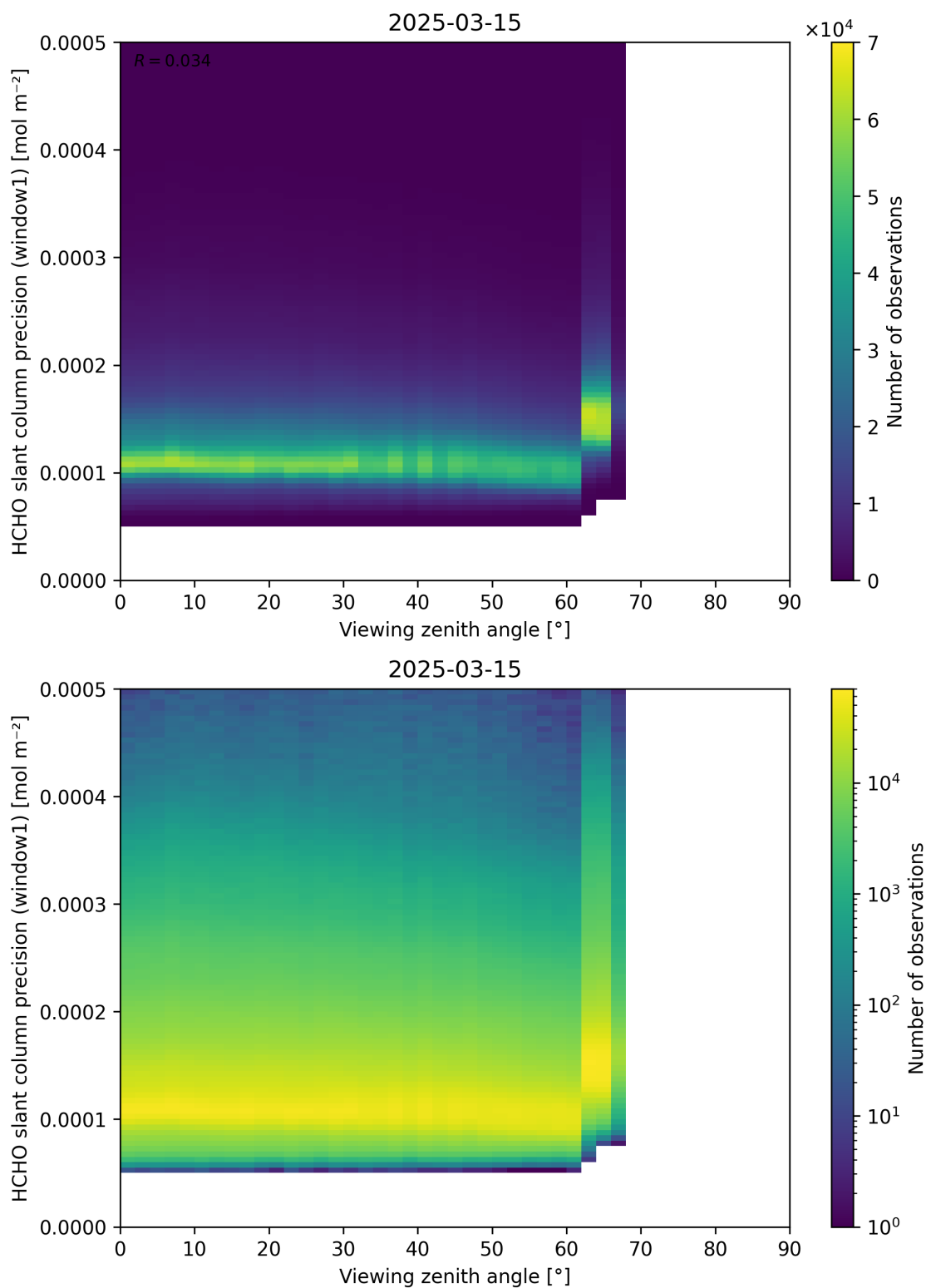
Figure 189: Scatter density plot of “Viewing zenith angle” against “HCHO slant column precision (window1)” for 2025-03-14 to 2025-03-16.
