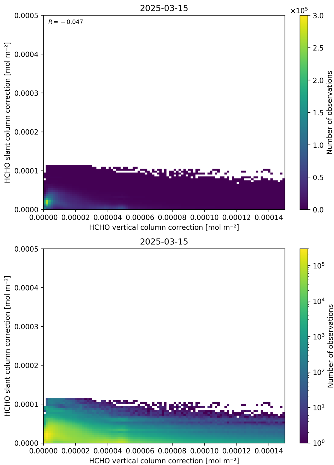
Figure 117: Scatter density plot of “HCHO vertical column correction” against “HCHO slant column correction” for 2025-03-14 to 2025-03-16.
