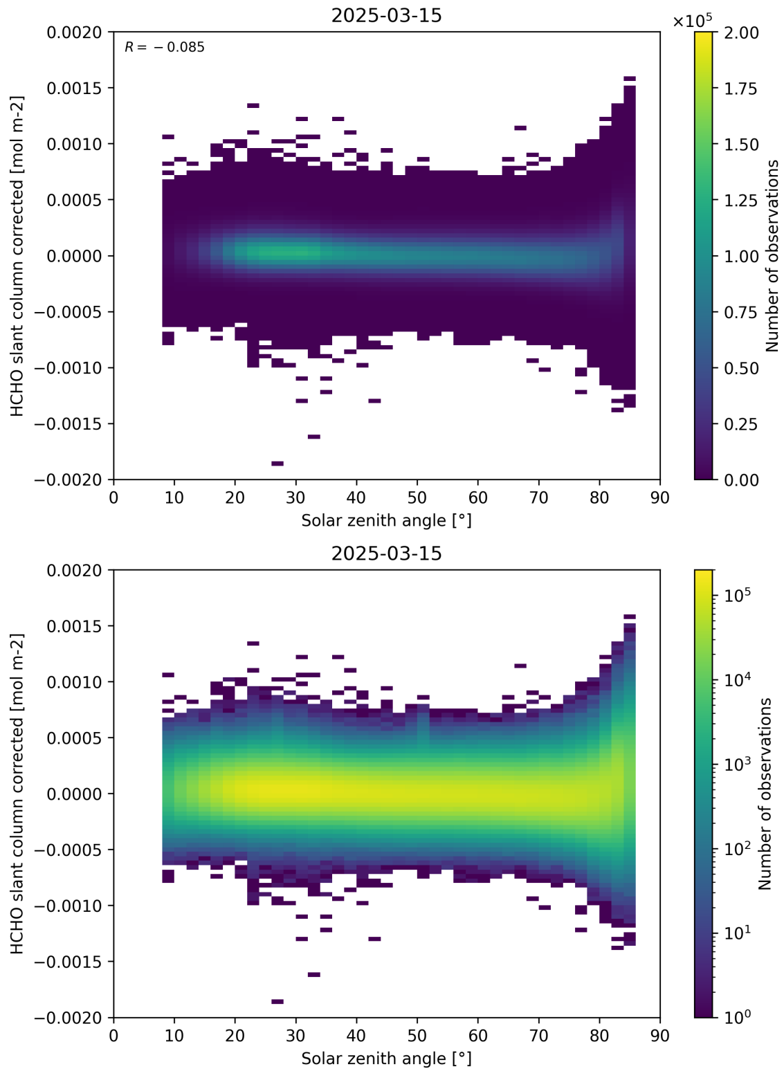
Figure 171: Scatter density plot of “Solar zenith angle” against “HCHO slant column corrected” for 2025-03-14 to 2025-03-16.
