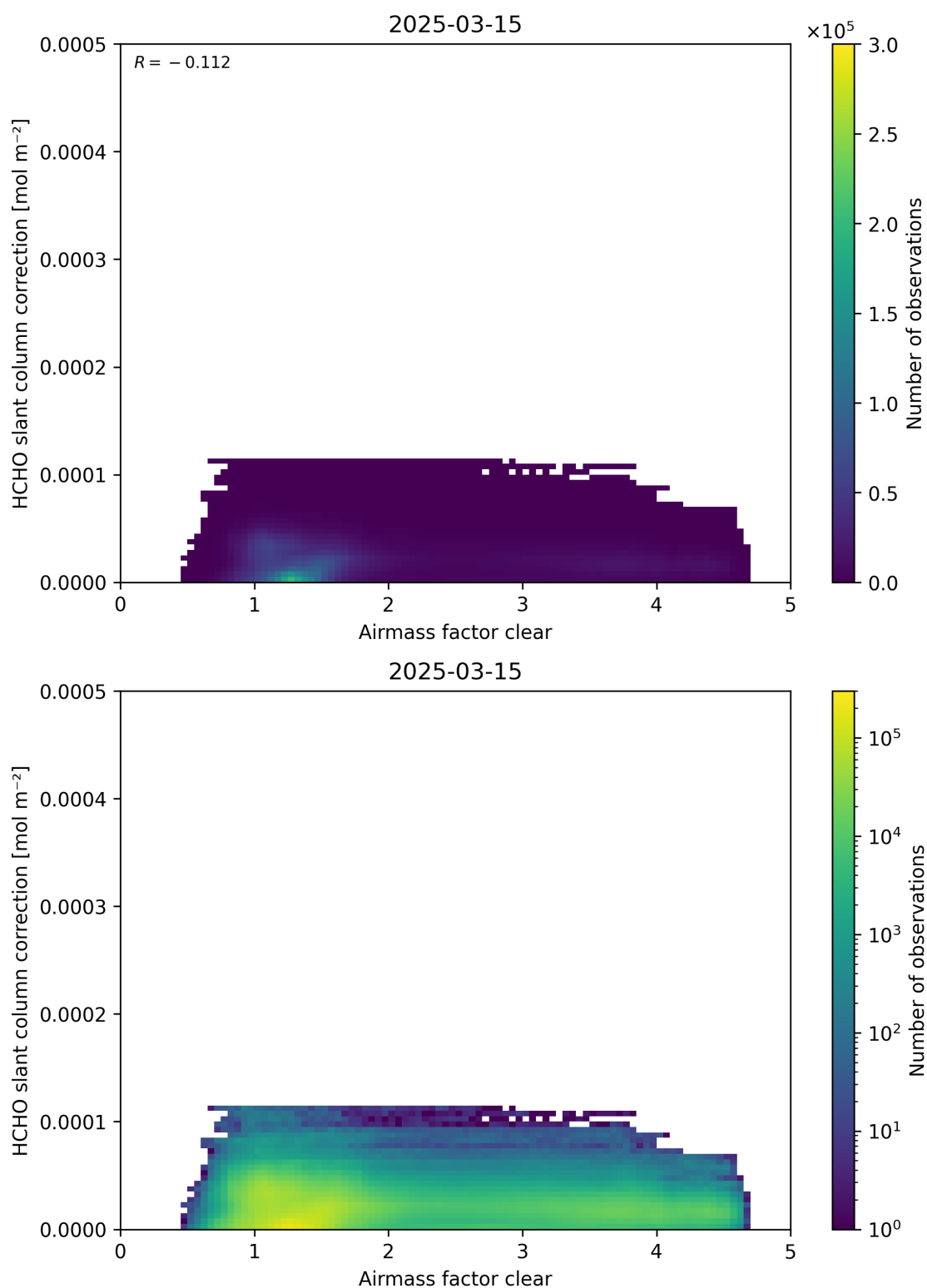
Figure 75: Scatter density plot of “Airmass factor clear” against “HCHO slant column correction” for 2025-03-14 to 2025-03-16.
