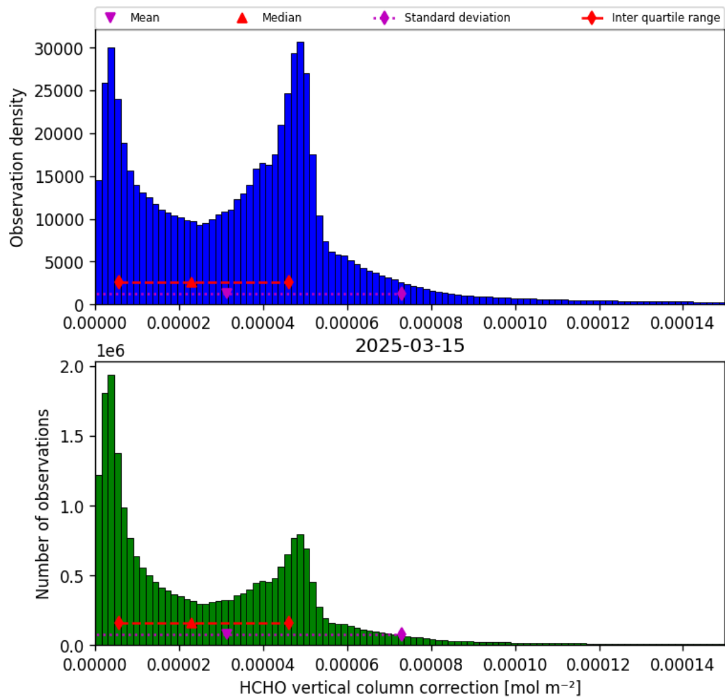
Figure 37: Histogram of “HCHO vertical column correction” for 2025-03-14 to 2025-03-16
