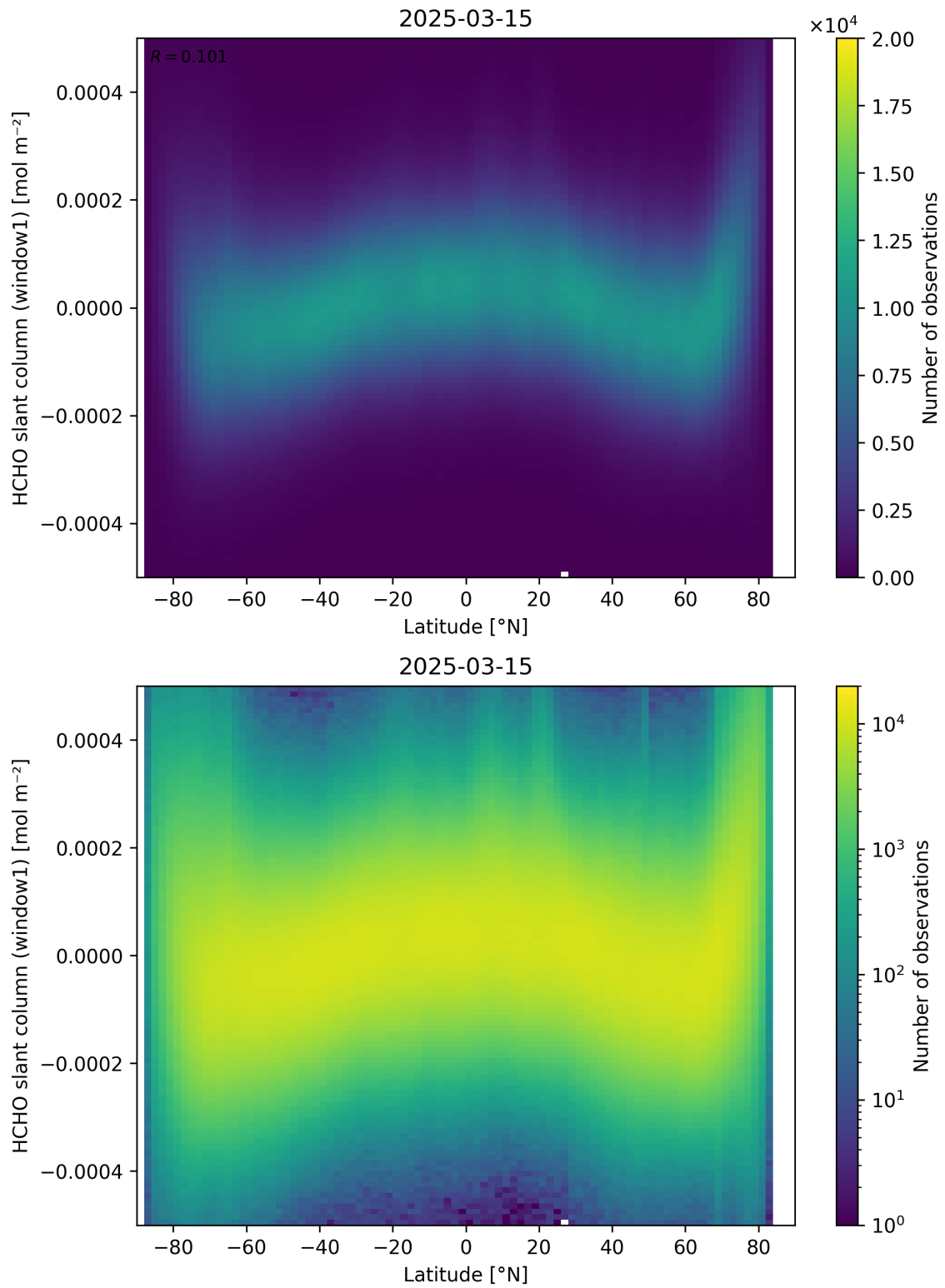
Figure 159: Scatter density plot of “Latitude” against “HCHO slant column (window1)” for 2025-03-14 to 2025-03-16.
