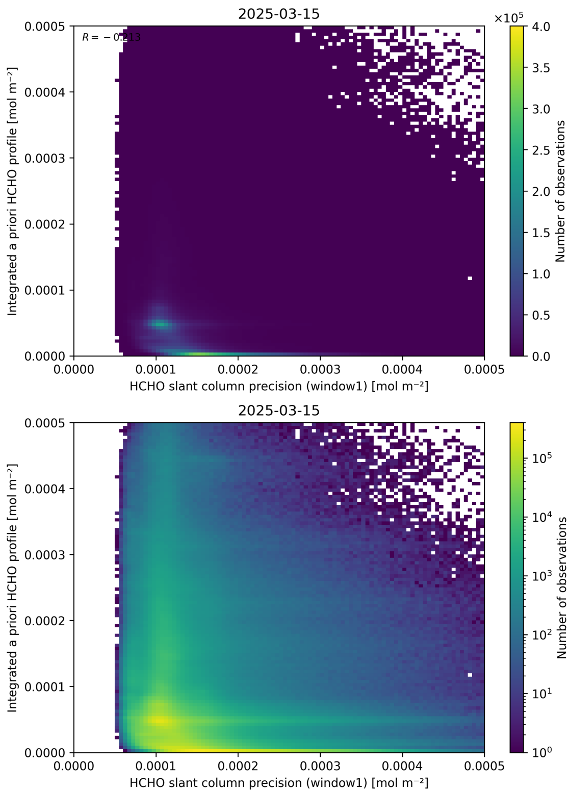
Figure 96: Scatter density plot of “HCHO slant column precision (window1)” against “Integrated a priori HCHO profile” for 2025-03-14 to 2025-03-16.
