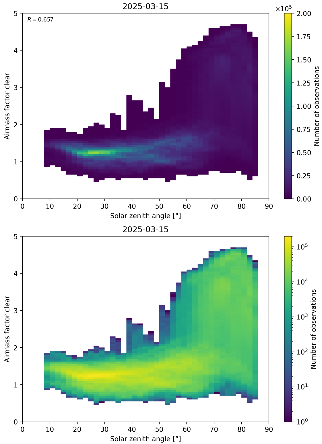
Figure 170: Scatter density plot of “Solar zenith angle” against “Airmass factor clear” for 2025-03-14 to 2025-03-16.
