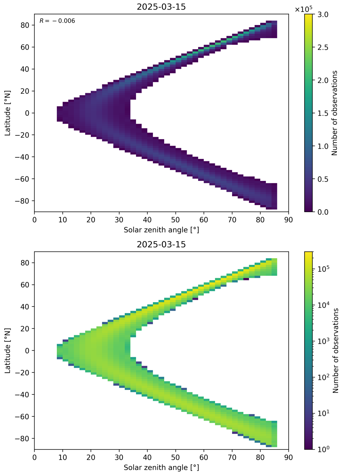
Figure 181: Scatter density plot of “Solar zenith angle” against “Latitude” for 2025-03-14 to 2025-03-16.
