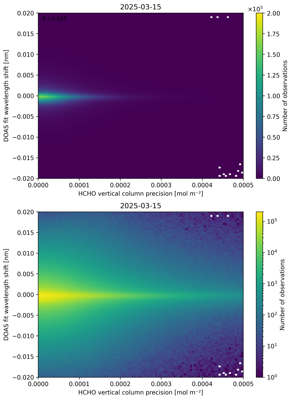
Figure 137: Scatter density plot of “HCHO vertical column precision” against “DOAS fit wavelength shift” for 2025-03-14 to 2025-03-16.
