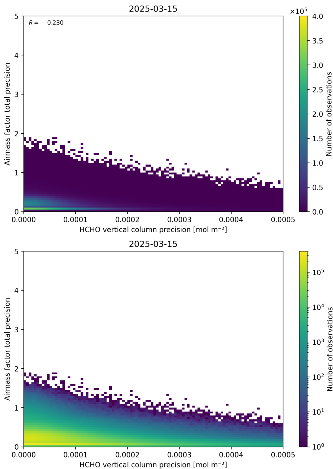
Figure 145: Scatter density plot of “HCHO vertical column precision” against “Airmass factor total precision” for 2025-03-14 to 2025-03-16.
