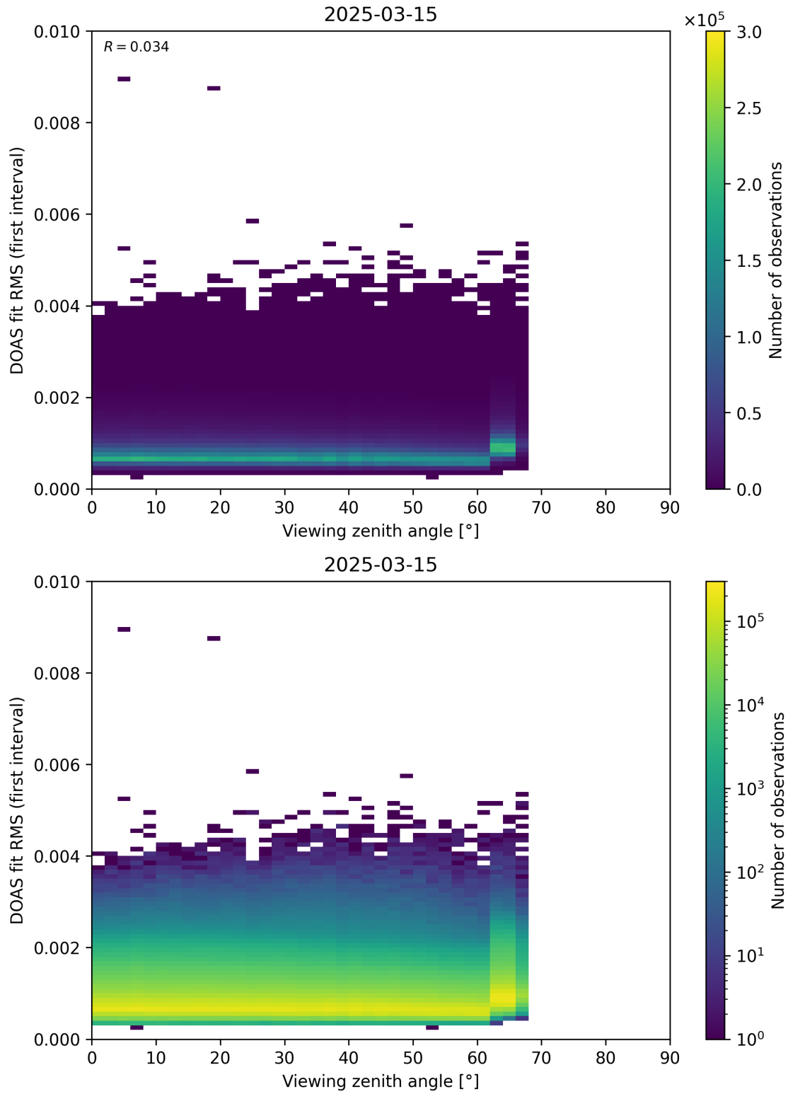
Figure 182: Scatter density plot of “Viewing zenith angle” against “DOAS fit RMS (first interval)” for 2025-03-14 to 2025-03-16.
