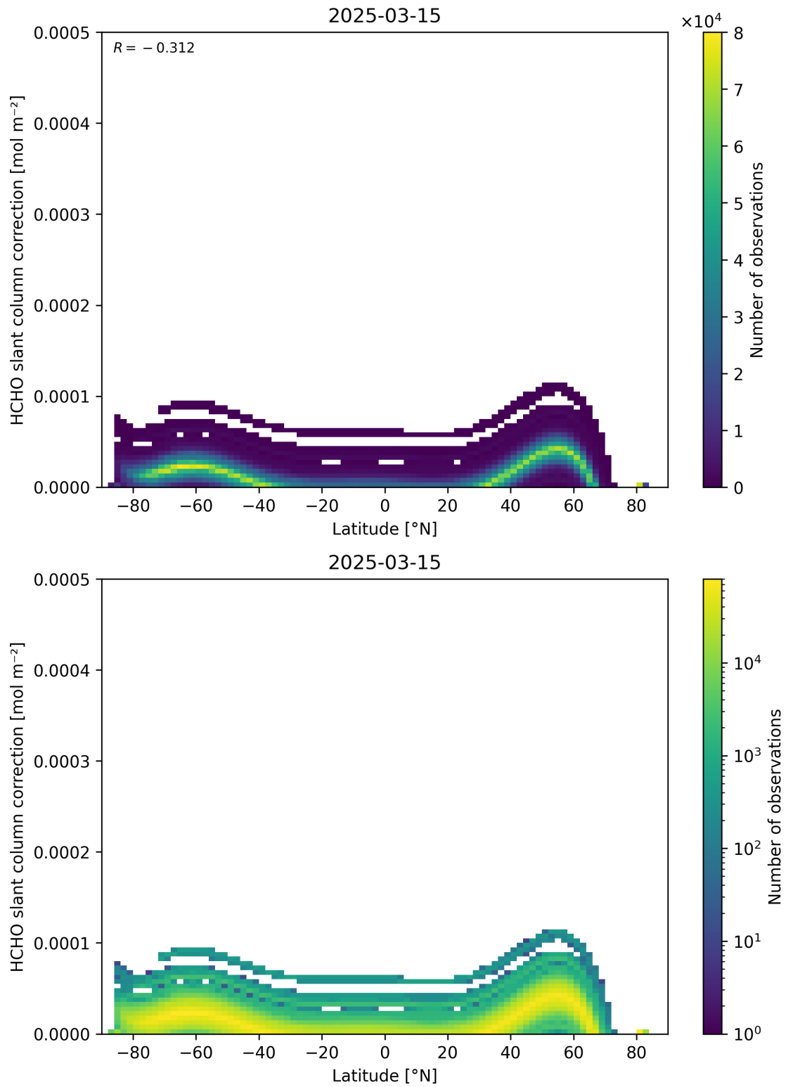
Figure 158: Scatter density plot of “Latitude” against “HCHO slant column correction” for 2025-03-14 to 2025-03-16.
