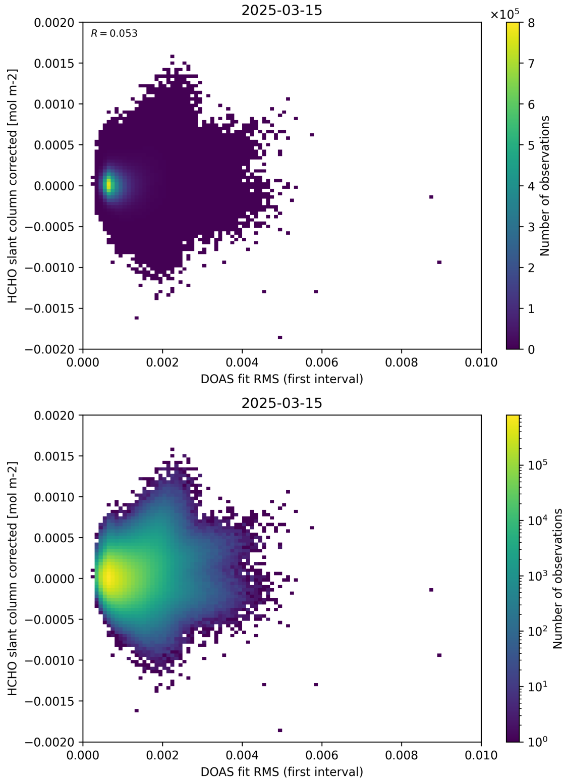
Figure 62: Scatter density plot of “DOAS fit RMS (first interval)” against “HCHO slant column corrected” for 2025-03-14 to 2025-03-16.
