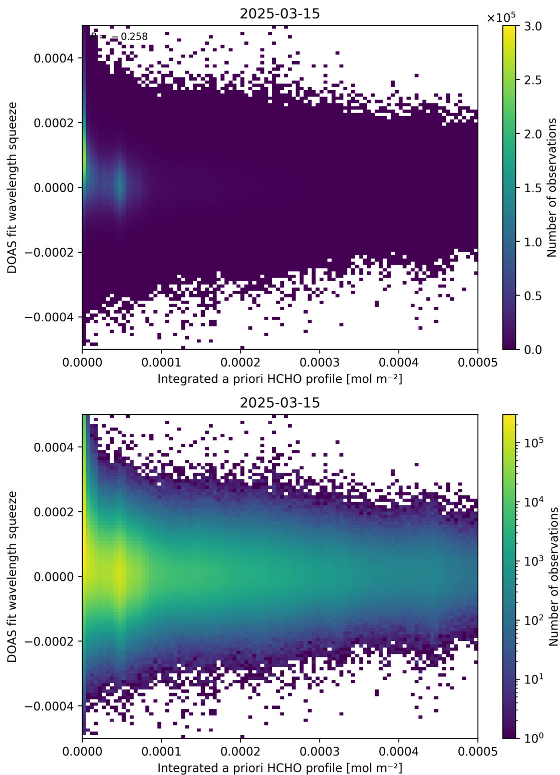
Figure 150: Scatter density plot of “Integrated a priori HCHO profile” against “DOAS fit wavelength squeeze” for 2025-03-14 to 2025-03-16.
