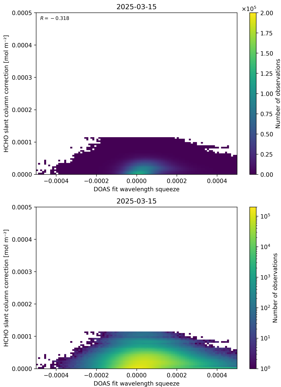
Figure 70: Scatter density plot of “DOAS fit wavelength squeeze” against “HCHO slant column correction” for 2025-03-14 to 2025-03-16.
