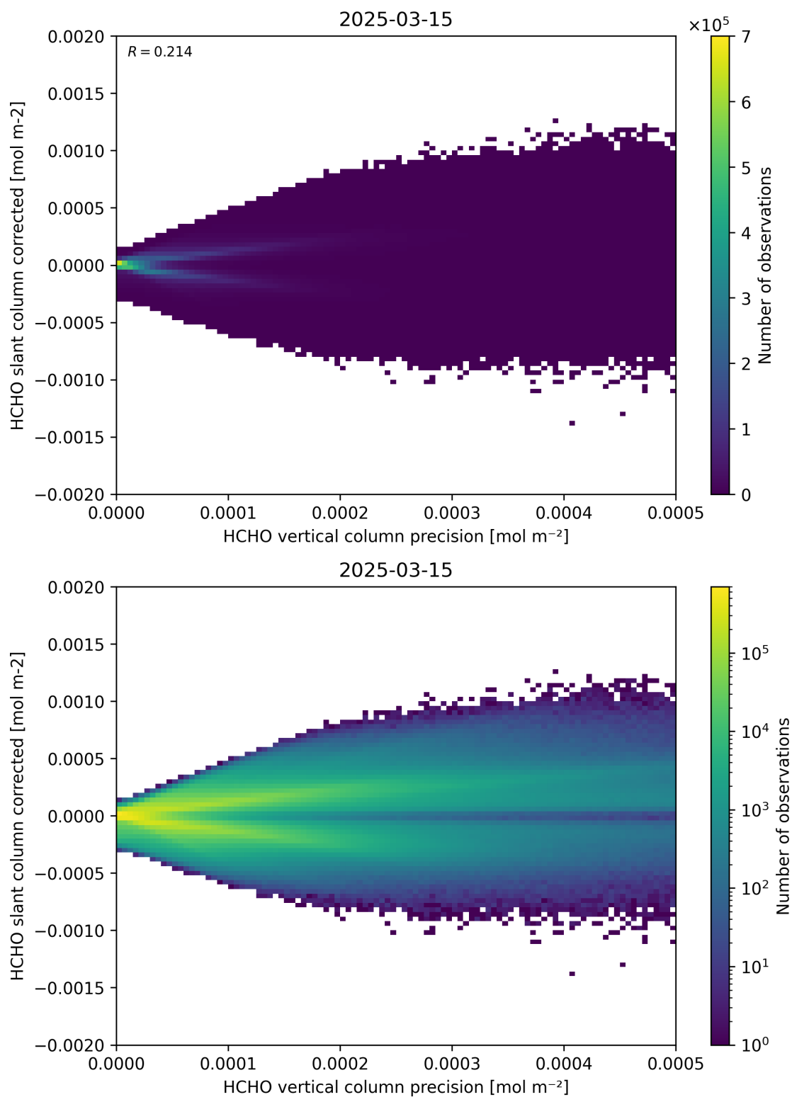
Figure 140: Scatter density plot of “HCHO vertical column precision” against “HCHO slant column corrected” for 2025-03-14 to 2025-03-16.
