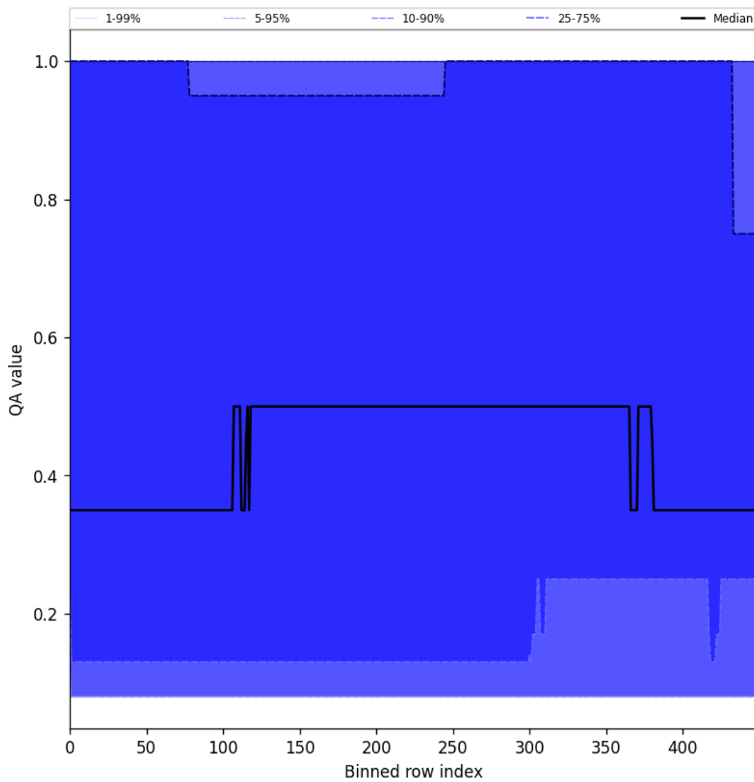
Figure 48: Along track statistics of “QA value” for 2025-03-14 to 2025-03-16
