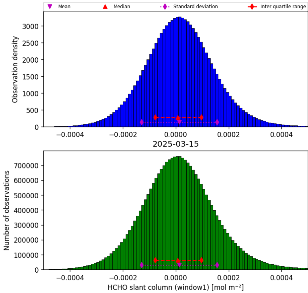
Figure 38: Histogram of “HCHO slant column (window1)” for 2025-03-14 to 2025-03-16
