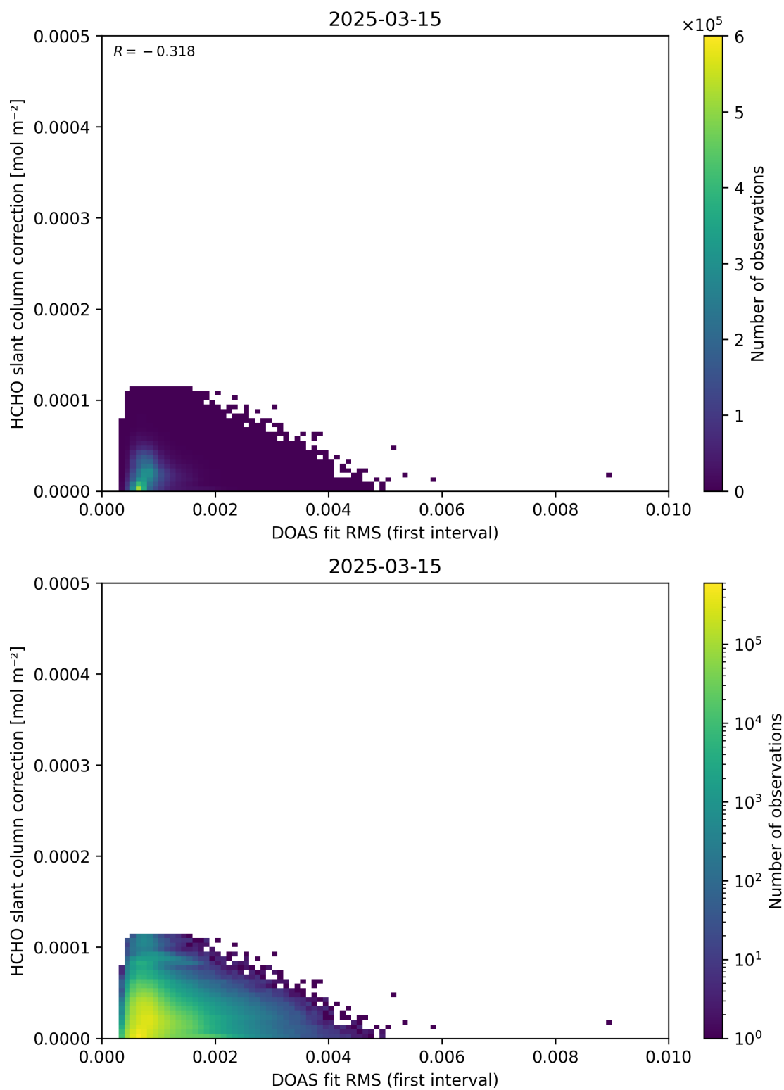
Figure 63: Scatter density plot of “DOAS fit RMS (first interval)” against “HCHO slant column correction” for 2025-03-14 to 2025-03-16.
