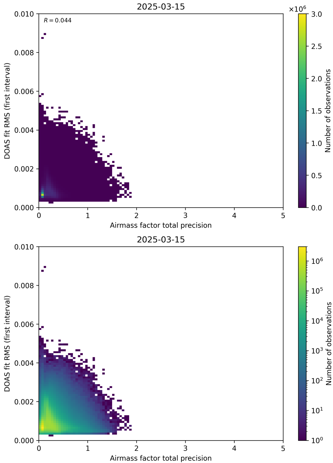
Figure 105: Scatter density plot of “Airmass factor total precision” against “DOAS fit RMS (first interval)” for 2025-03-14 to 2025-03-16.
