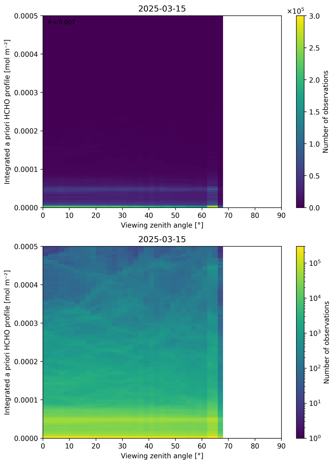
Figure 195: Scatter density plot of “Viewing zenith angle” against “Integrated a priori HCHO profile” for 2025-03-14 to 2025-03-16.
