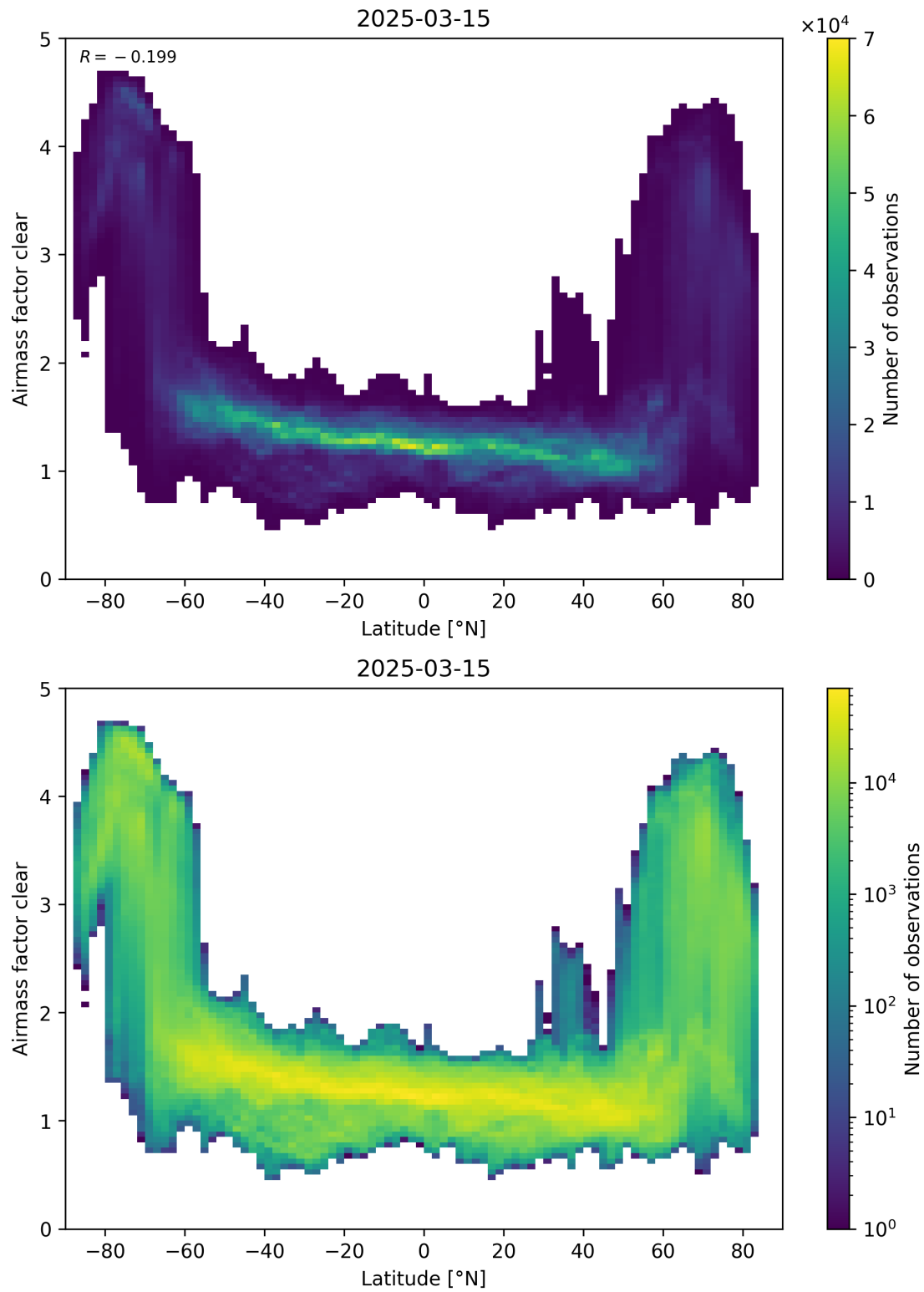
Figure 156: Scatter density plot of “Latitude” against “Airmass factor clear” for 2025-03-14 to 2025-03-16.
