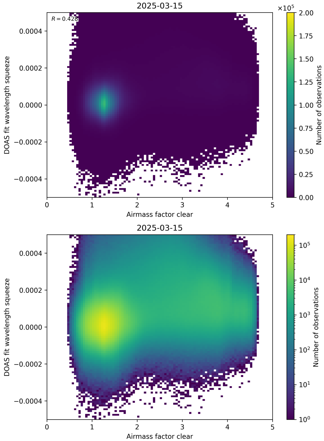
Figure 73: Scatter density plot of “Airmass factor clear” against “DOAS fit wavelength squeeze” for 2025-03-14 to 2025-03-16.
