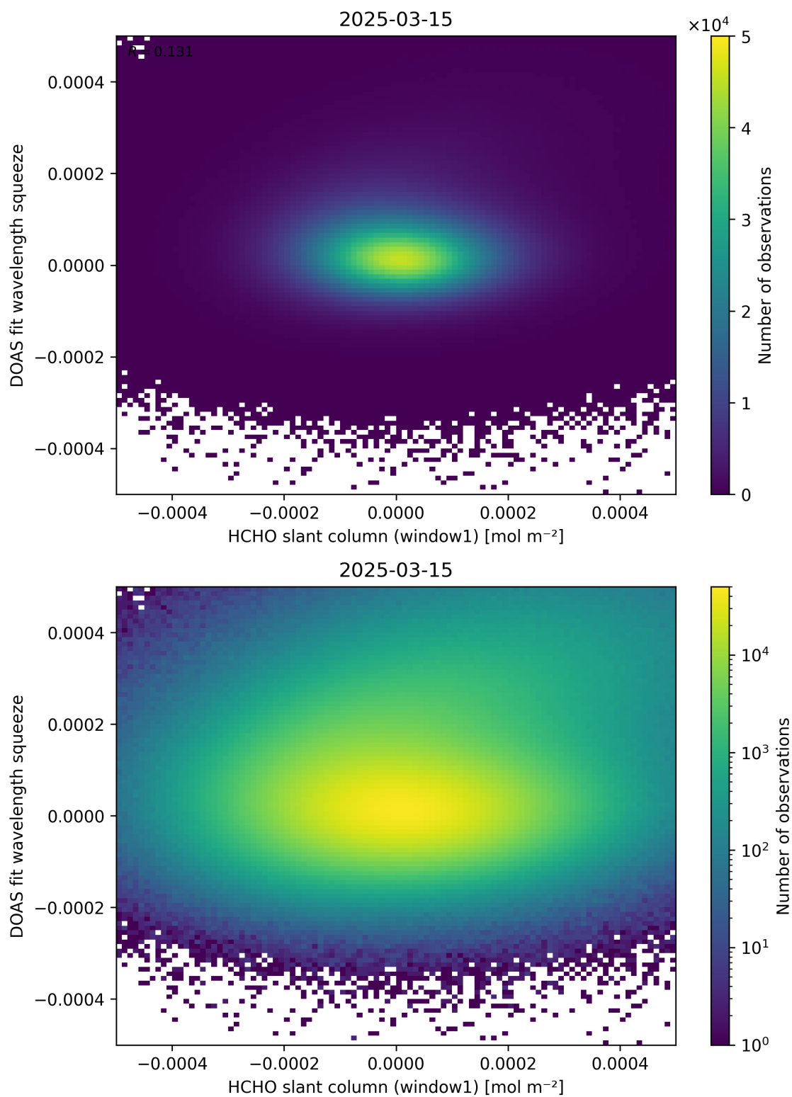
Figure 80: Scatter density plot of “HCHO slant column (window1)” against “DOAS fit wavelength squeeze” for 2025-03-14 to 2025-03-16.
