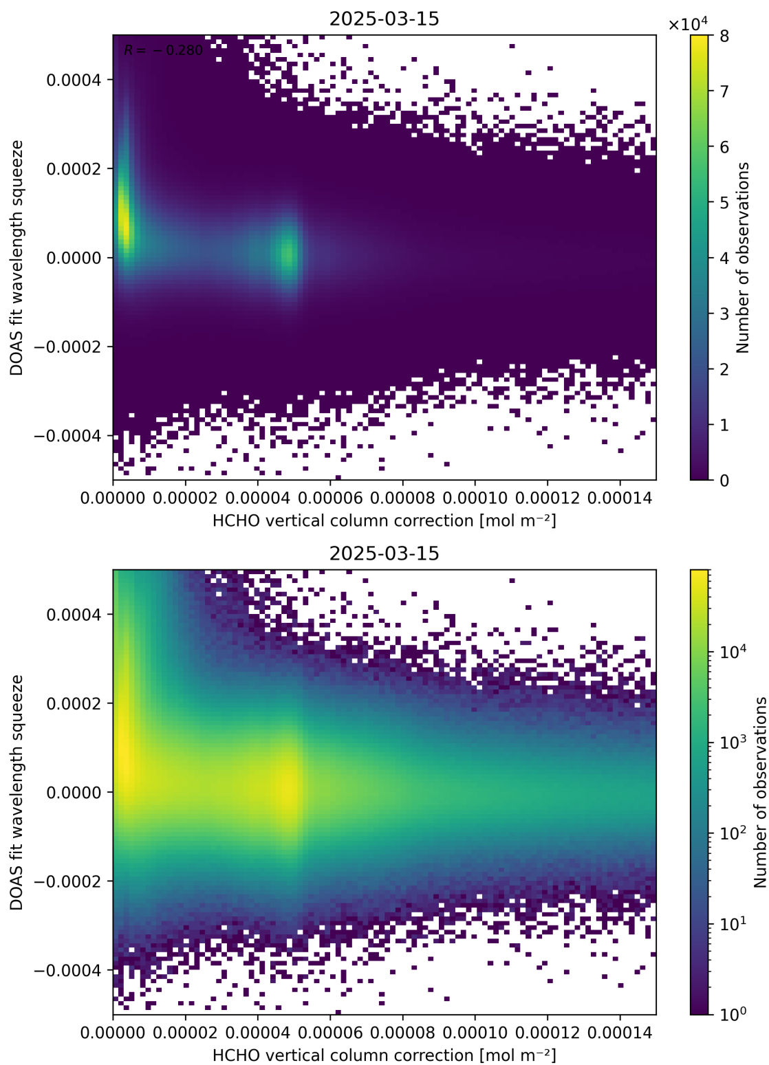
Figure 114: Scatter density plot of “HCHO vertical column correction” against “DOAS fit wavelength squeeze” for 2025-03-14 to 2025-03-16.
