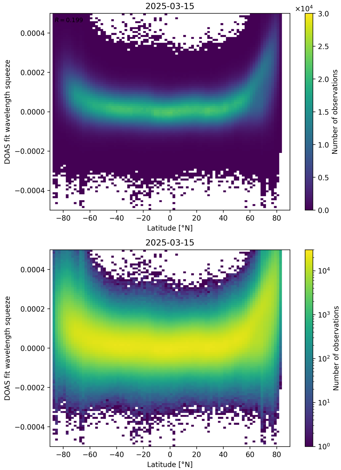
Figure 155: Scatter density plot of “Latitude” against “DOAS fit wavelength squeeze” for 2025-03-14 to 2025-03-16.
