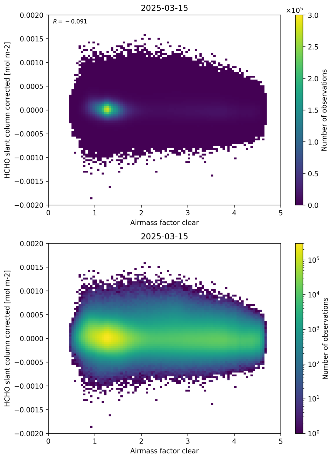
Figure 74: Scatter density plot of “Airmass factor clear” against “HCHO slant column corrected” for 2025-03-14 to 2025-03-16.
