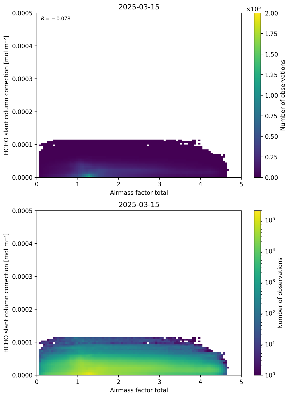
Figure 102: Scatter density plot of “Airmass factor total” against “HCHO slant column correction” for 2025-03-14 to 2025-03-16.
