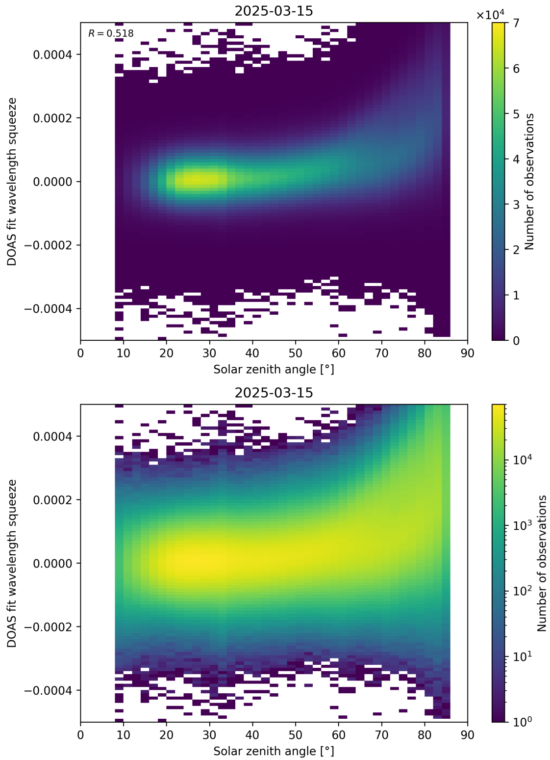
Figure 169: Scatter density plot of “Solar zenith angle” against “DOAS fit wavelength squeeze” for 2025-03-14 to 2025-03-16.
