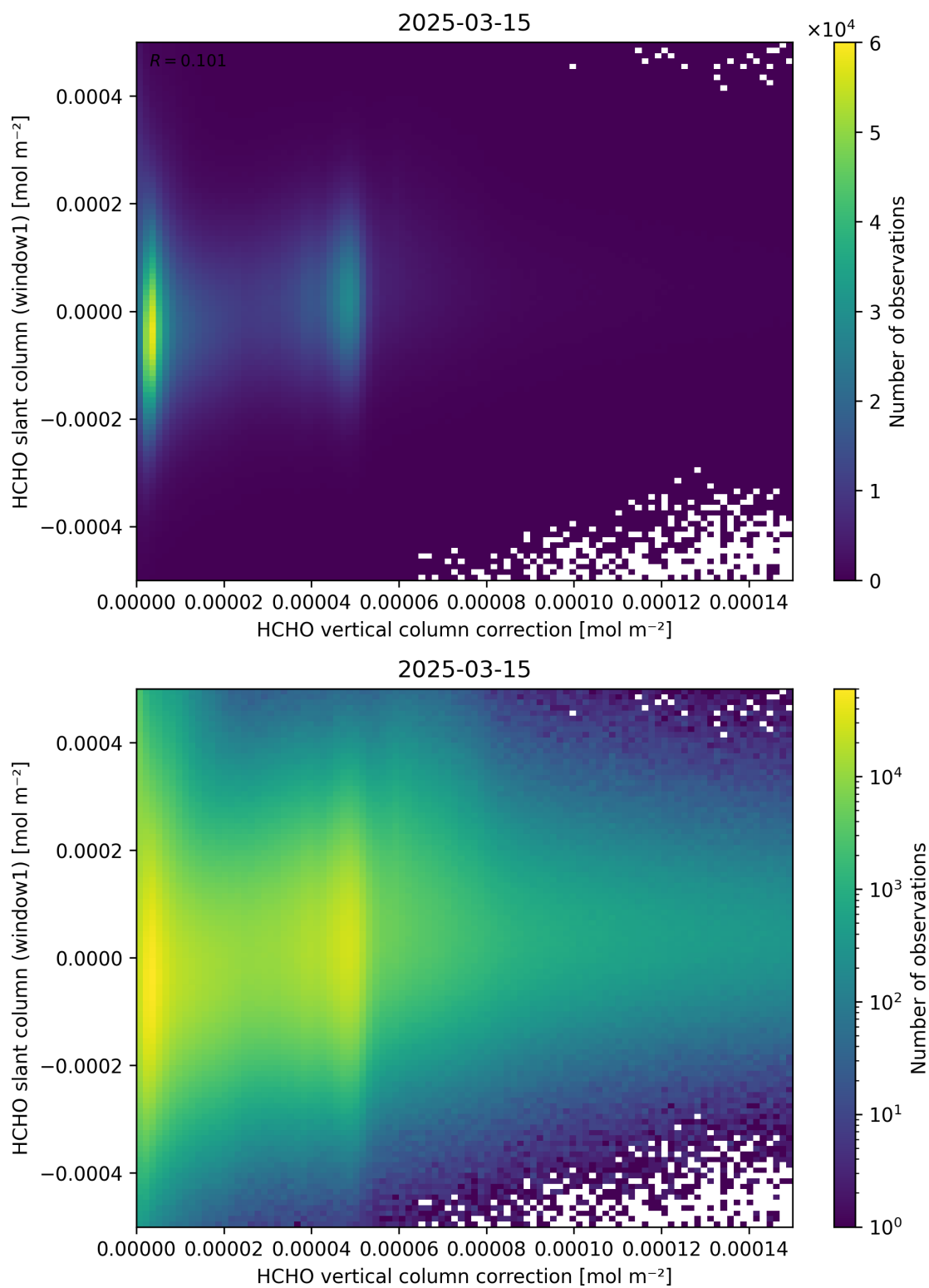
Figure 118: Scatter density plot of “HCHO vertical column correction” against “HCHO slant column (window1)” for 2025-03-14 to 2025-03-16.
