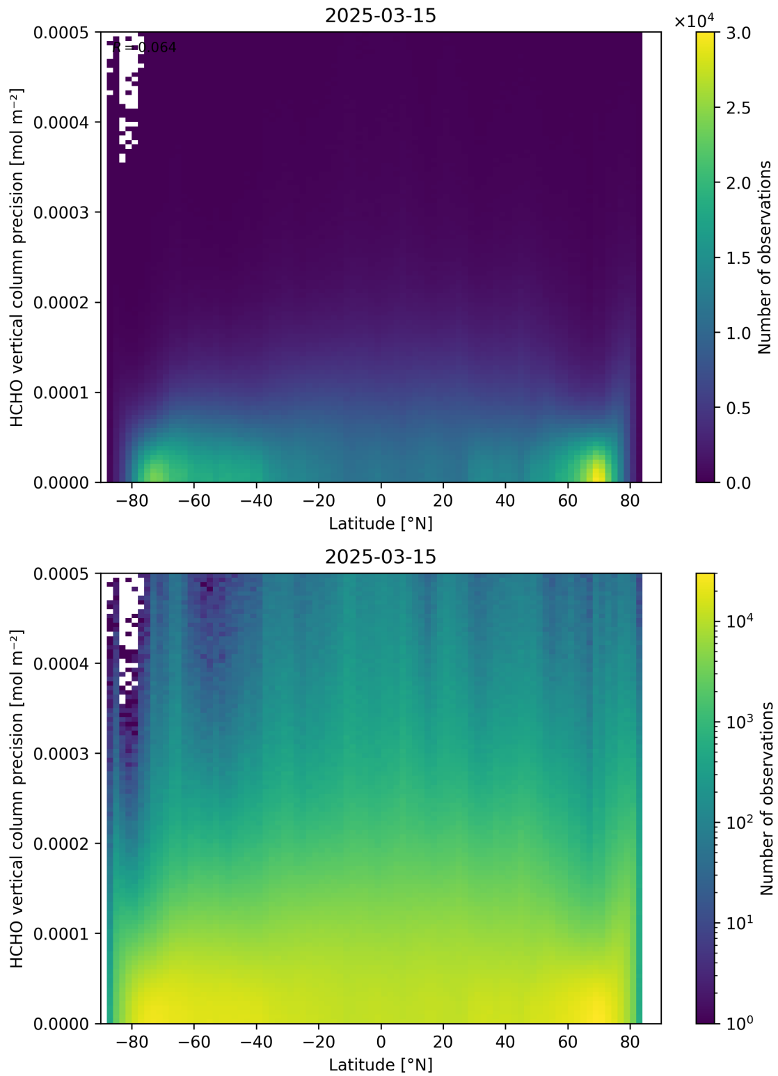
Figure 165: Scatter density plot of “Latitude” against “HCHO vertical column precision” for 2025-03-14 to 2025-03-16.
