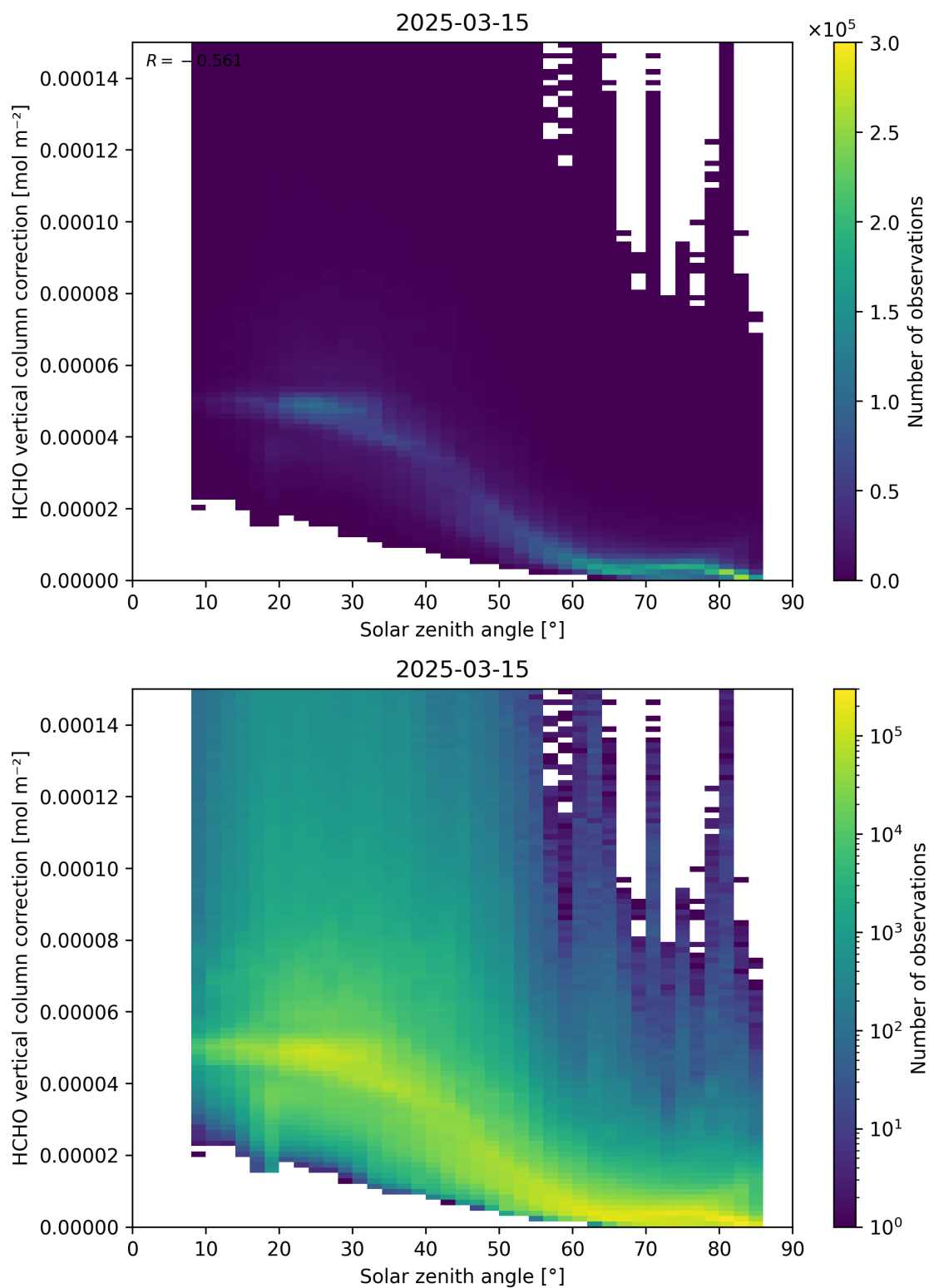
Figure 178: Scatter density plot of “Solar zenith angle” against “HCHO vertical column correction” for 2025-03-14 to 2025-03-16.
