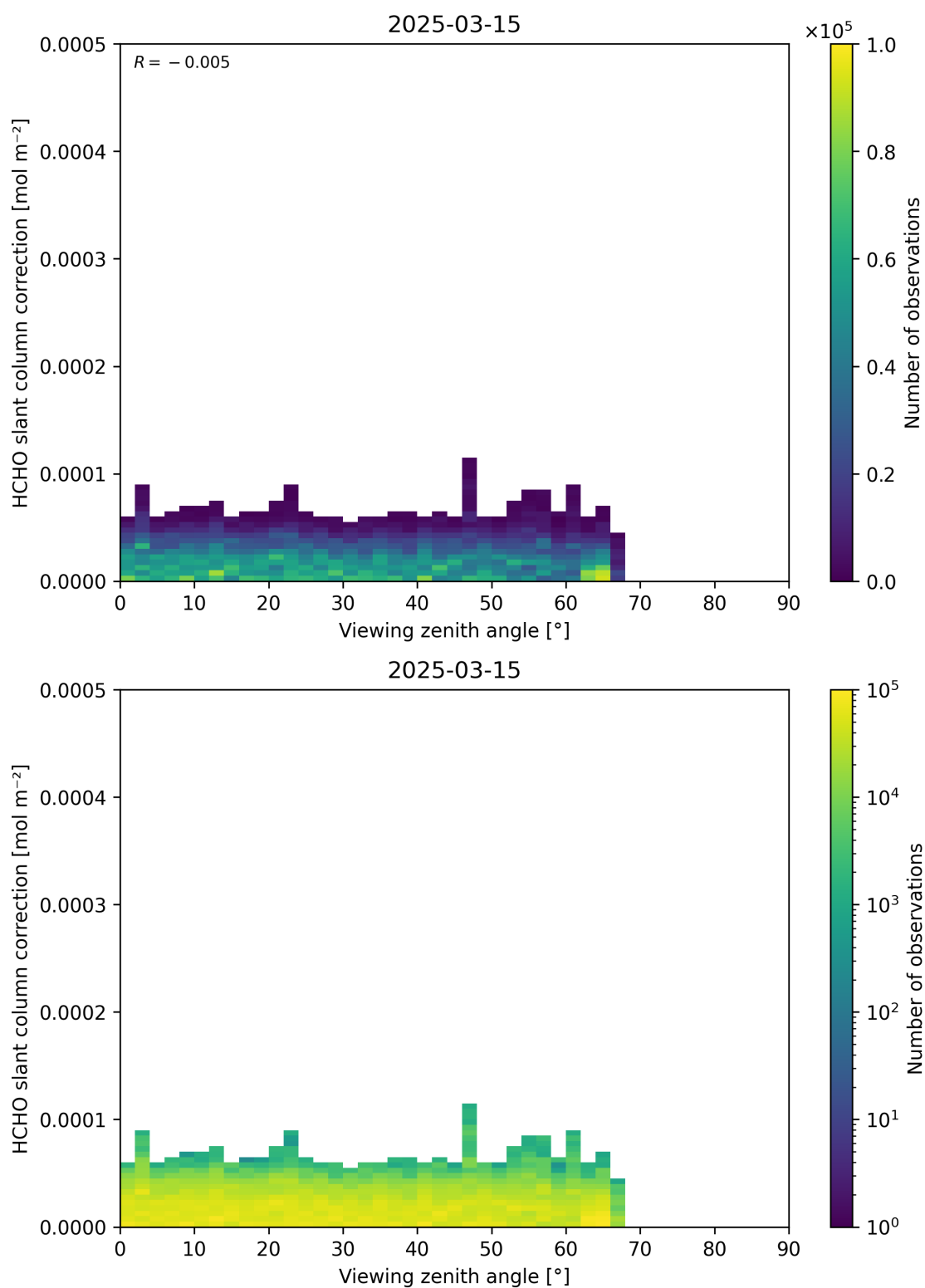
Figure 187: Scatter density plot of “Viewing zenith angle” against “HCHO slant column correction” for 2025-03-14 to 2025-03-16.
