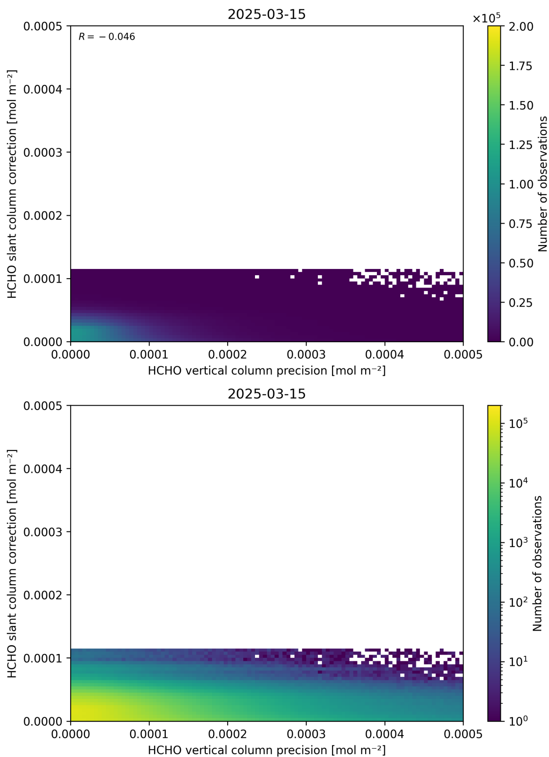
Figure 141: Scatter density plot of “HCHO vertical column precision” against “HCHO slant column correction” for 2025-03-14 to 2025-03-16.
