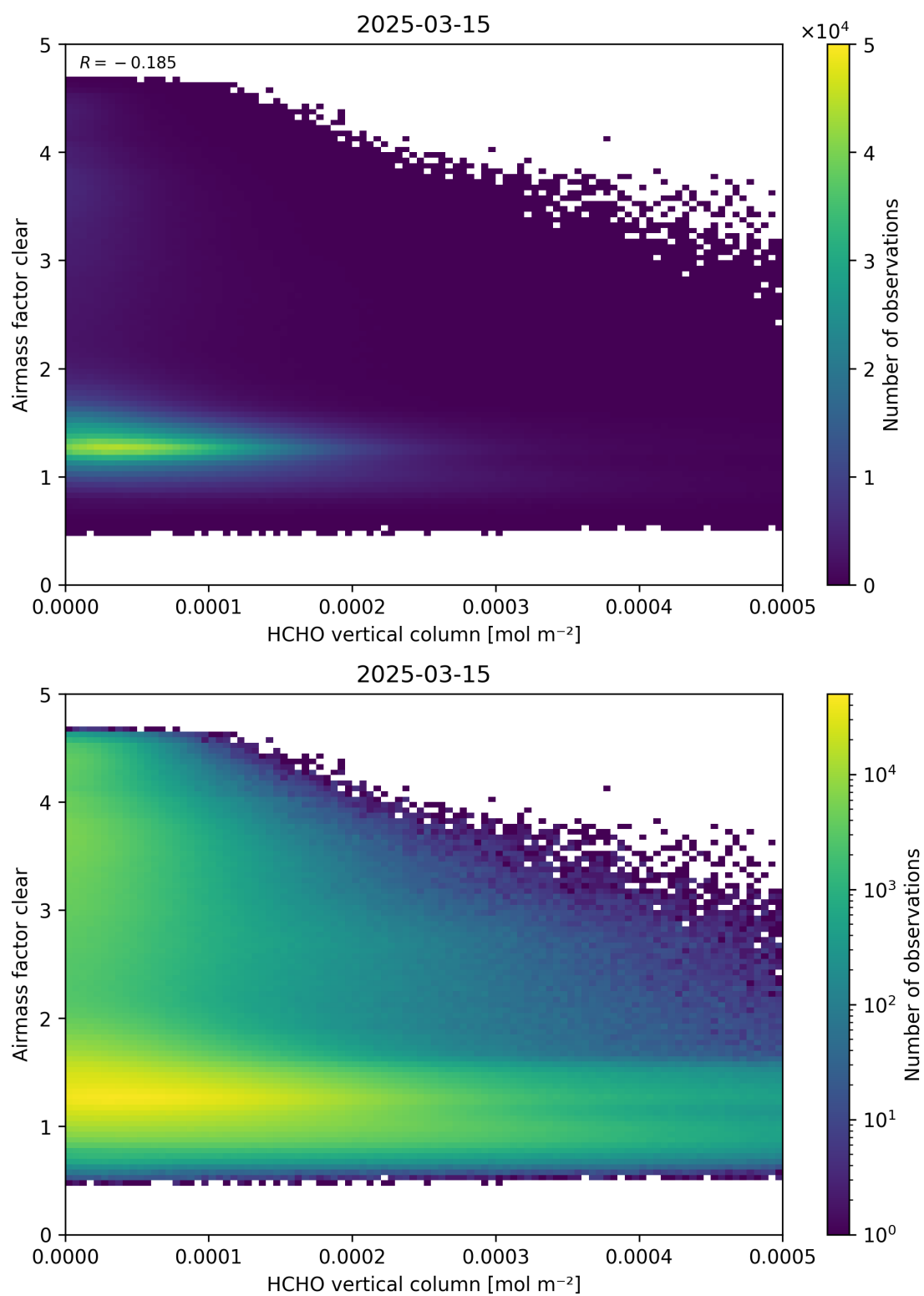
Figure 126: Scatter density plot of “HCHO vertical column” against “Airmass factor clear” for 2025-03-14 to 2025-03-16.
