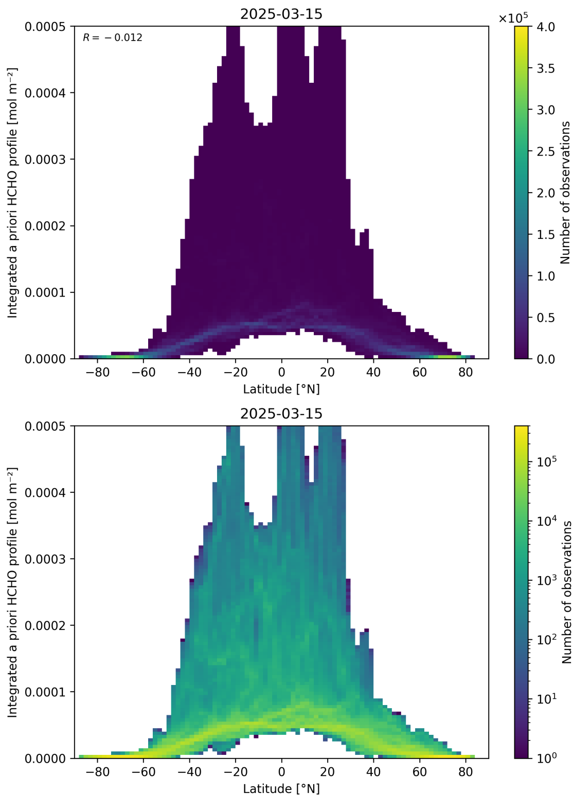
Figure 166: Scatter density plot of “Latitude” against “Integrated a priori HCHO profile” for 2025-03-14 to 2025-03-16.
