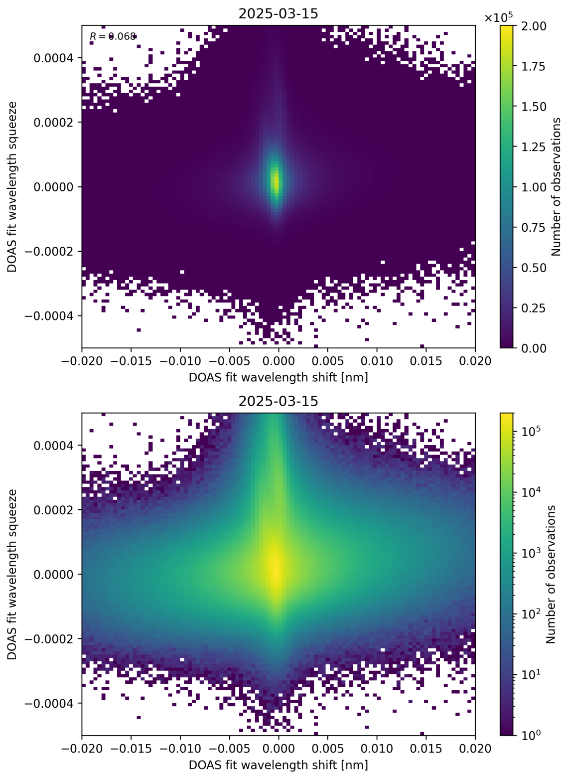
Figure 65: Scatter density plot of “DOAS fit wavelength shift” against “DOAS fit wavelength squeeze” for 2025-03-14 to 2025-03-16.
