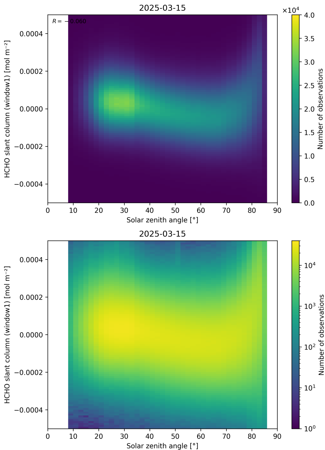
Figure 173: Scatter density plot of “Solar zenith angle” against “HCHO slant column (window1)” for 2025-03-14 to 2025-03-16.
