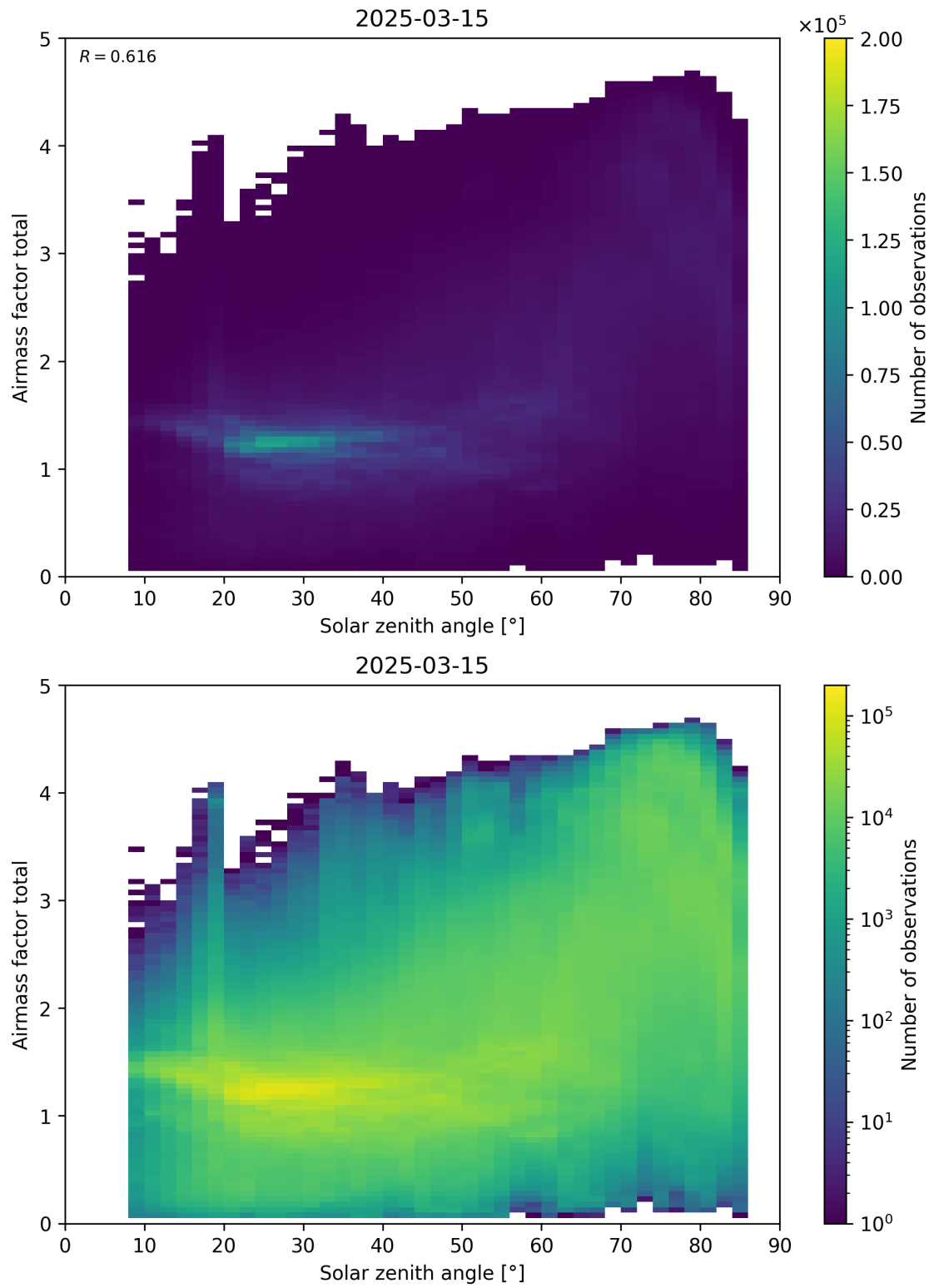
Figure 175: Scatter density plot of “Solar zenith angle” against “Airmass factor total” for 2025-03-14 to 2025-03-16.
