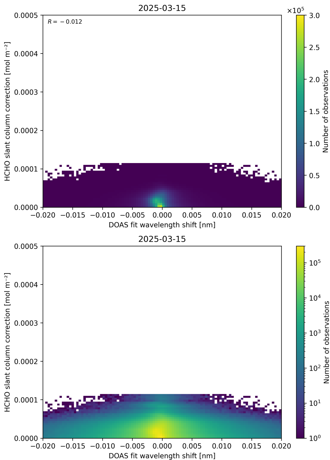
Figure 67: Scatter density plot of “DOAS fit wavelength shift” against “HCHO slant column correction” for 2025-03-14 to 2025-03-16.
