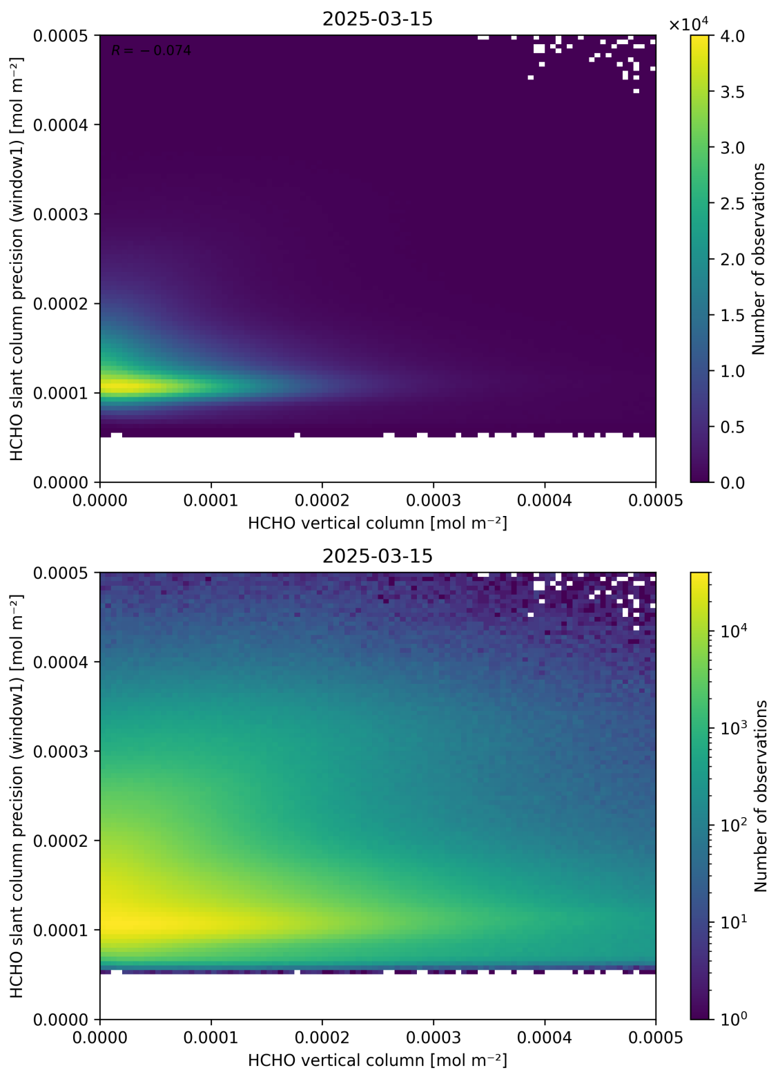
Figure 130: Scatter density plot of “HCHO vertical column” against “HCHO slant column precision (window1)” for 2025-03-14 to 2025-03-16.
