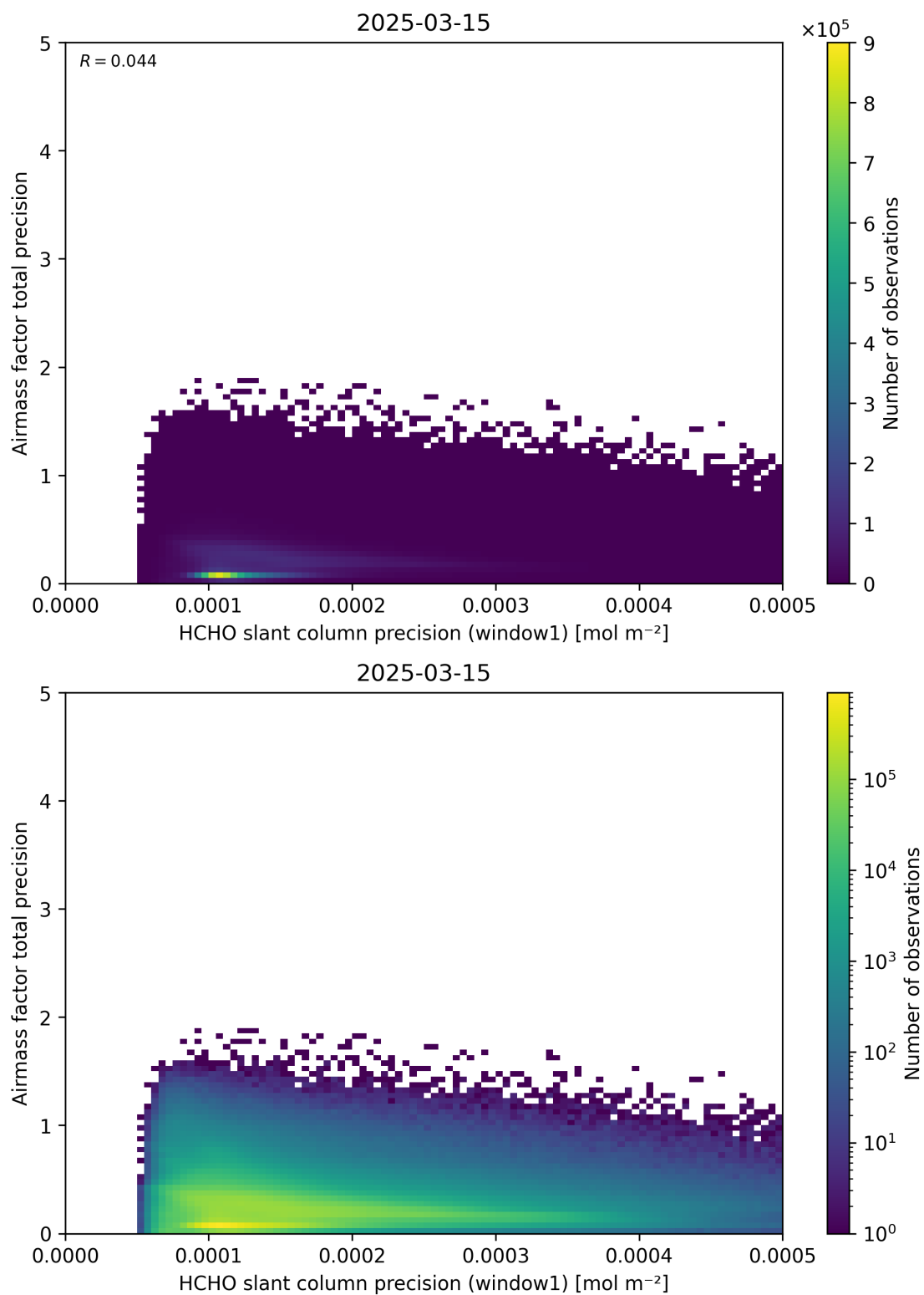
Figure 95: Scatter density plot of “HCHO slant column precision (window1)” against “Airmass factor total precision” for 2025-03-14 to 2025-03-16.
