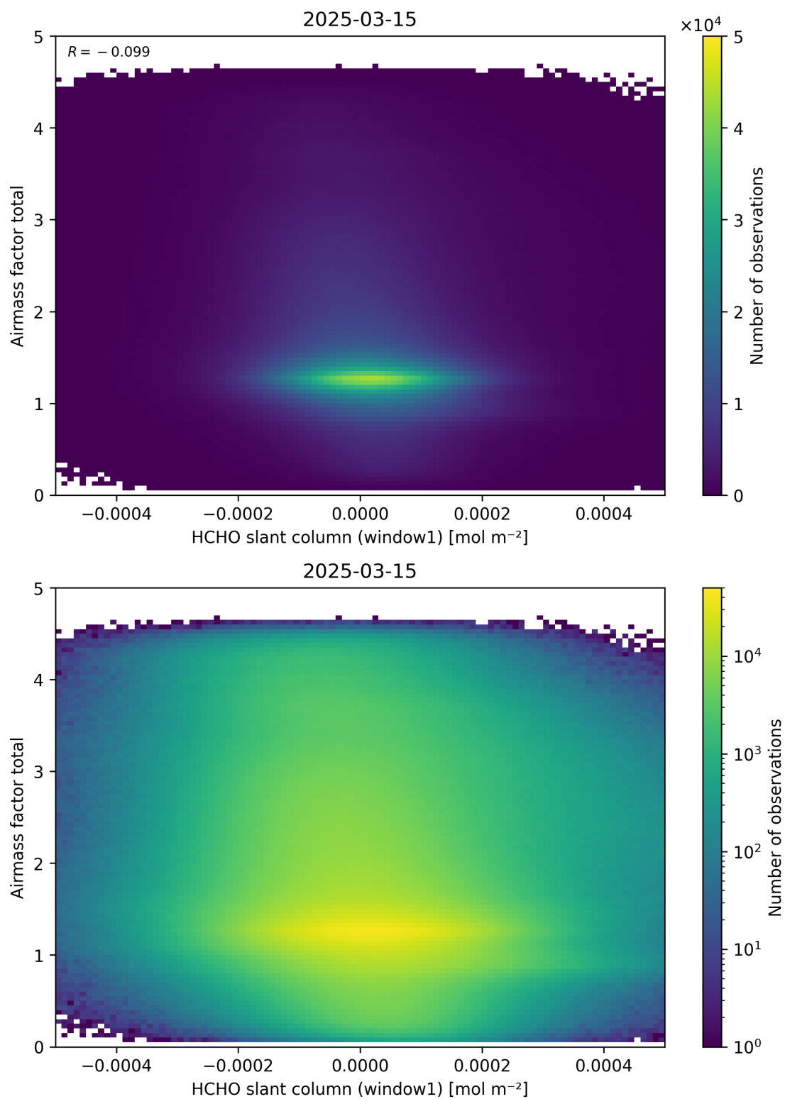
Figure 85: Scatter density plot of “HCHO slant column (window1)” against “Airmass factor total” for 2025-03-14 to 2025-03-16.
