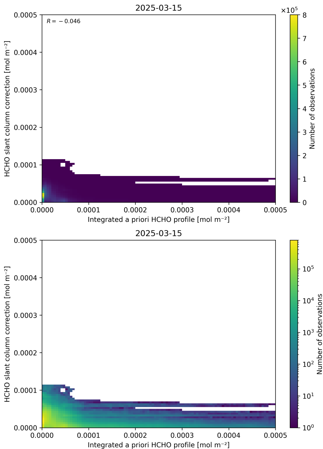
Figure 152: Scatter density plot of “Integrated a priori HCHO profile” against “HCHO slant column correction” for 2025-03-14 to 2025-03-16.
