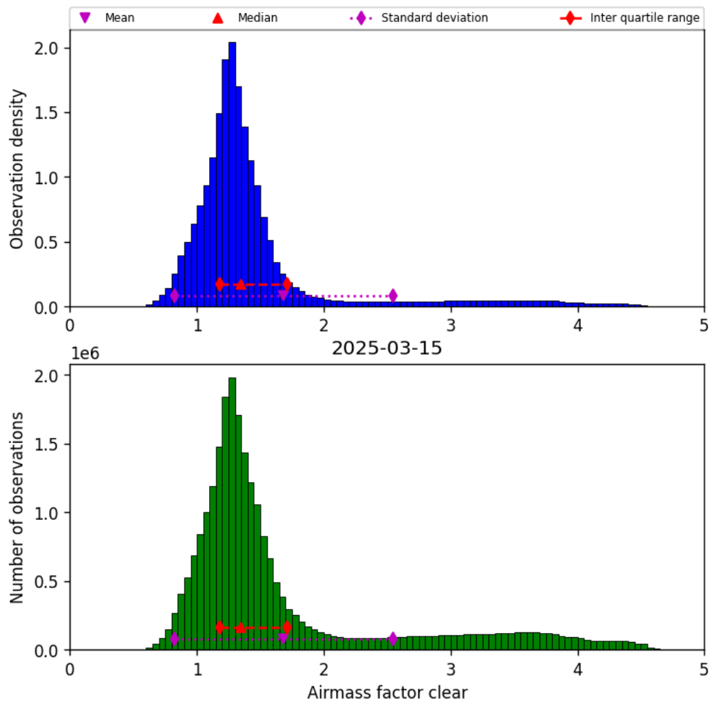
Figure 42: Histogram of “Airmass factor clear” for 2025-03-14 to 2025-03-16
