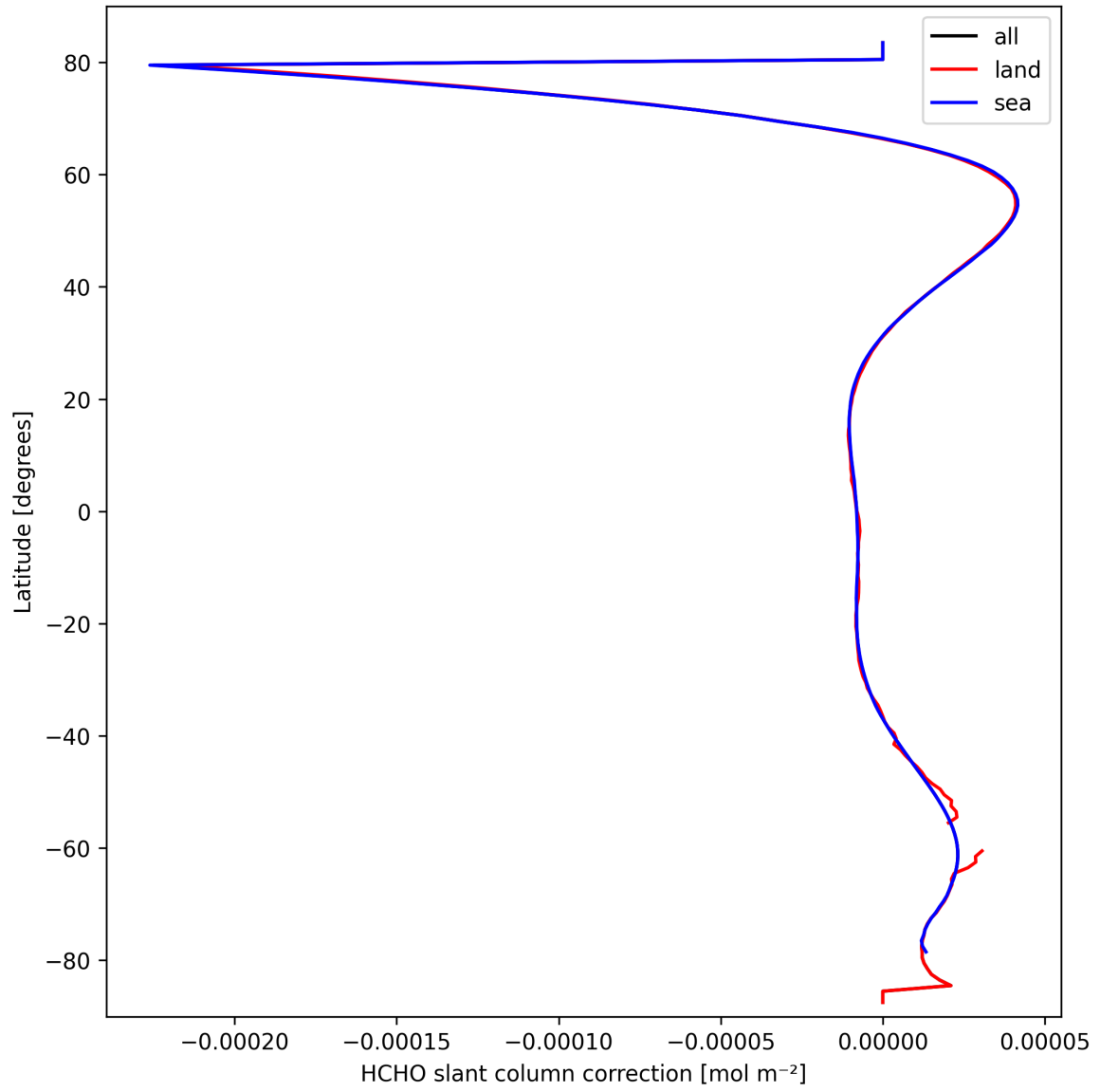
Figure 33: Zonal average of "HCHO slant column correction" for 2025-03-14 to 2025-03-16.
