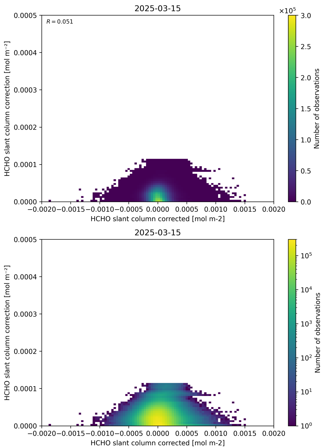
Figure 77: Scatter density plot of “HCHO slant column corrected” against “HCHO slant column correction” for 2025-03-14 to 2025-03-16.
