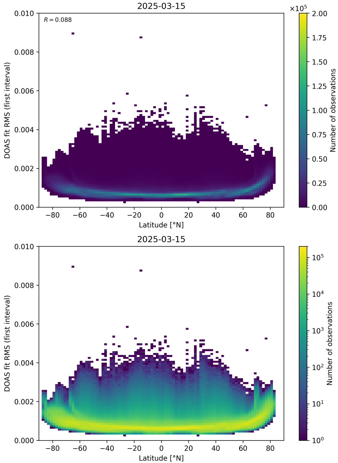
Figure 153: Scatter density plot of “Latitude” against “DOAS fit RMS (first interval)” for 2025-03-14 to 2025-03-16.
