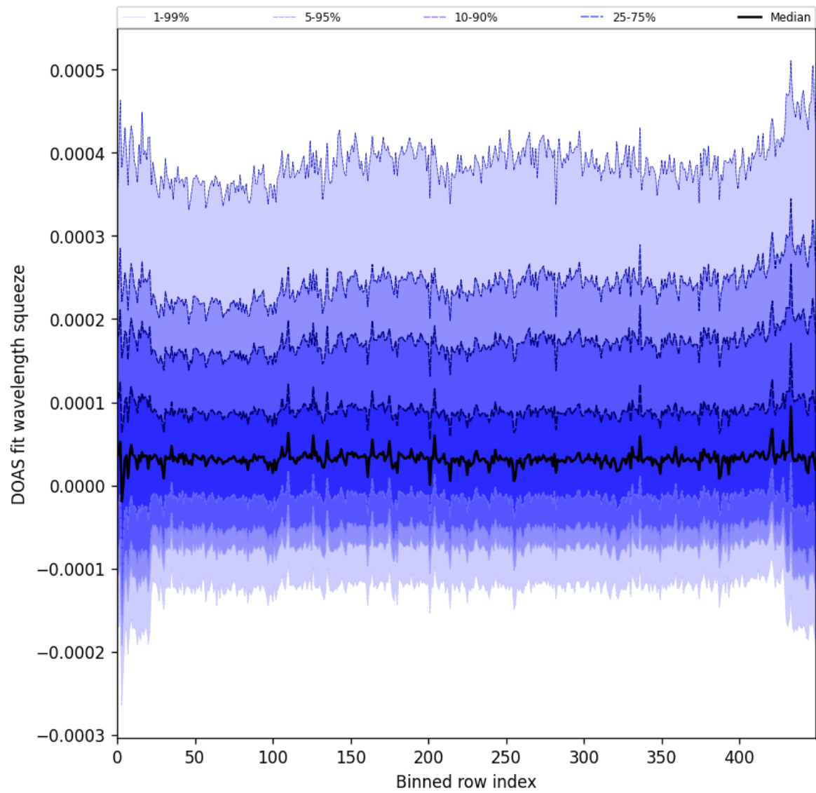
Figure 59: Along track statistics of “DOAS fit wavelength squeeze” for 2025-03-14 to 2025-03-16
