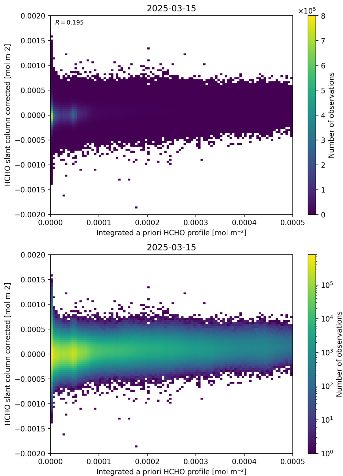
Figure 151: Scatter density plot of “Integrated a priori HCHO profile” against “HCHO slant column corrected” for 2025-03-14 to 2025-03-16.
