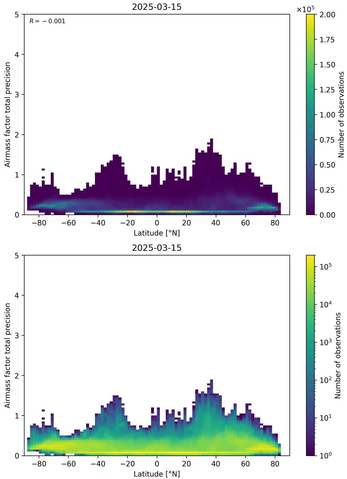
Figure 162: Scatter density plot of “Latitude” against “Airmass factor total precision” for 2025-03-14 to 2025-03-16.
