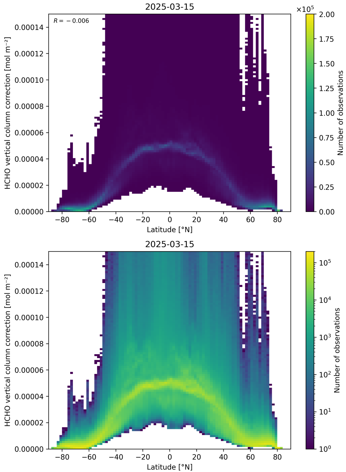
Figure 164: Scatter density plot of “Latitude” against “HCHO vertical column correction” for 2025-03-14 to 2025-03-16.
