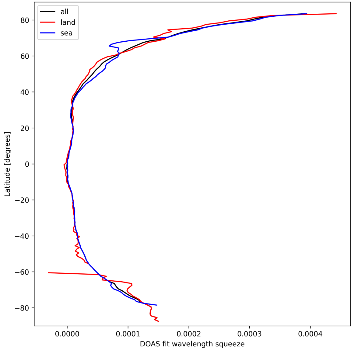
Figure 31: Zonal average of “DOAS fit wavelength squeeze” for 2025-03-14 to 2025-03-16.
