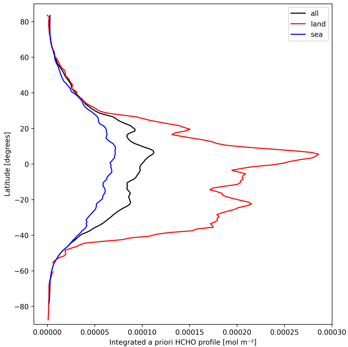
Figure 29: Zonal average of “Integrated a priori HCHO profile” for 2025-03-14 to 2025-03-16.
