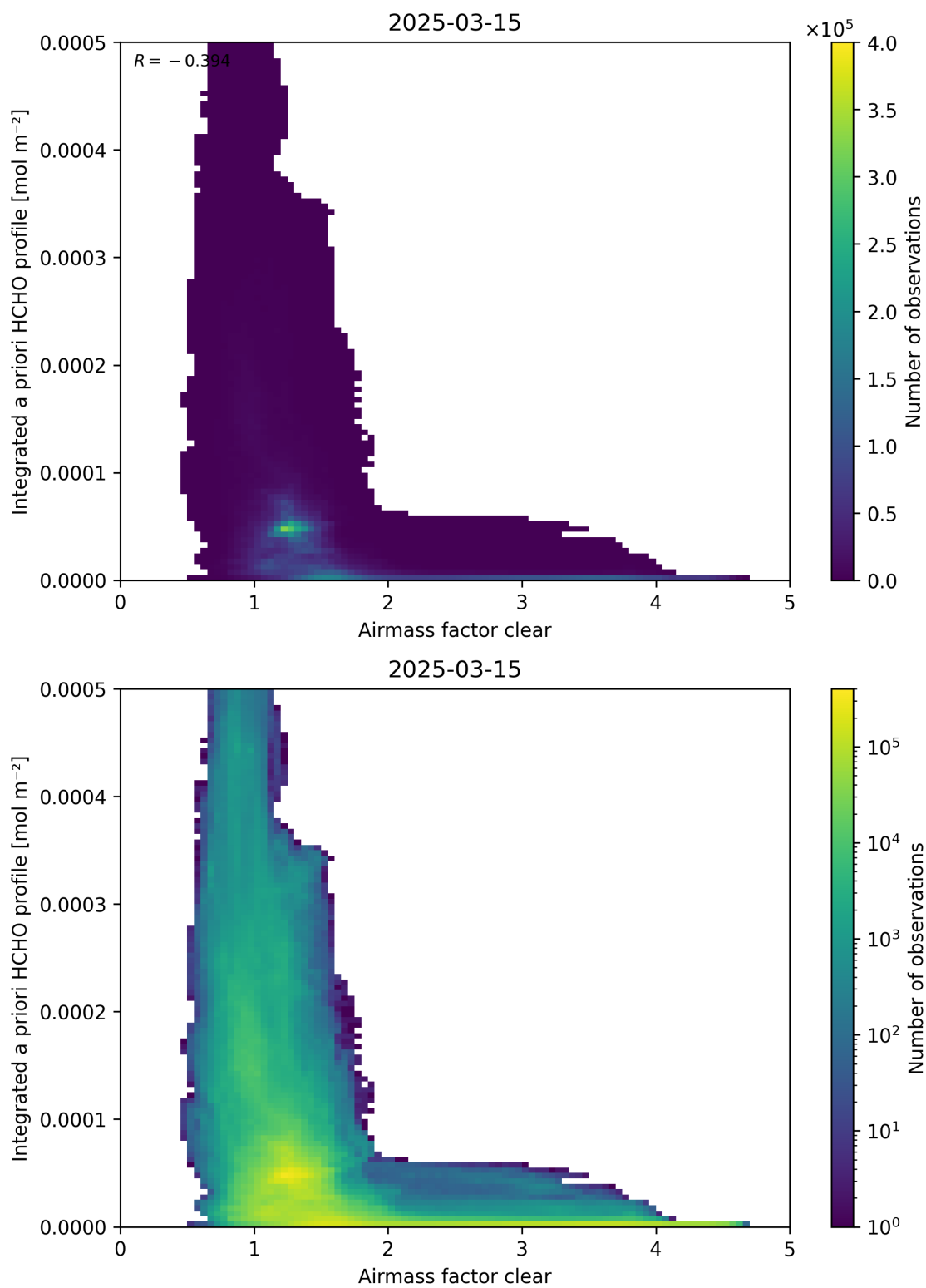
Figure 76: Scatter density plot of “Airmass factor clear” against “Integrated a priori HCHO profile” for 2025-03-14 to 2025-03-16.
