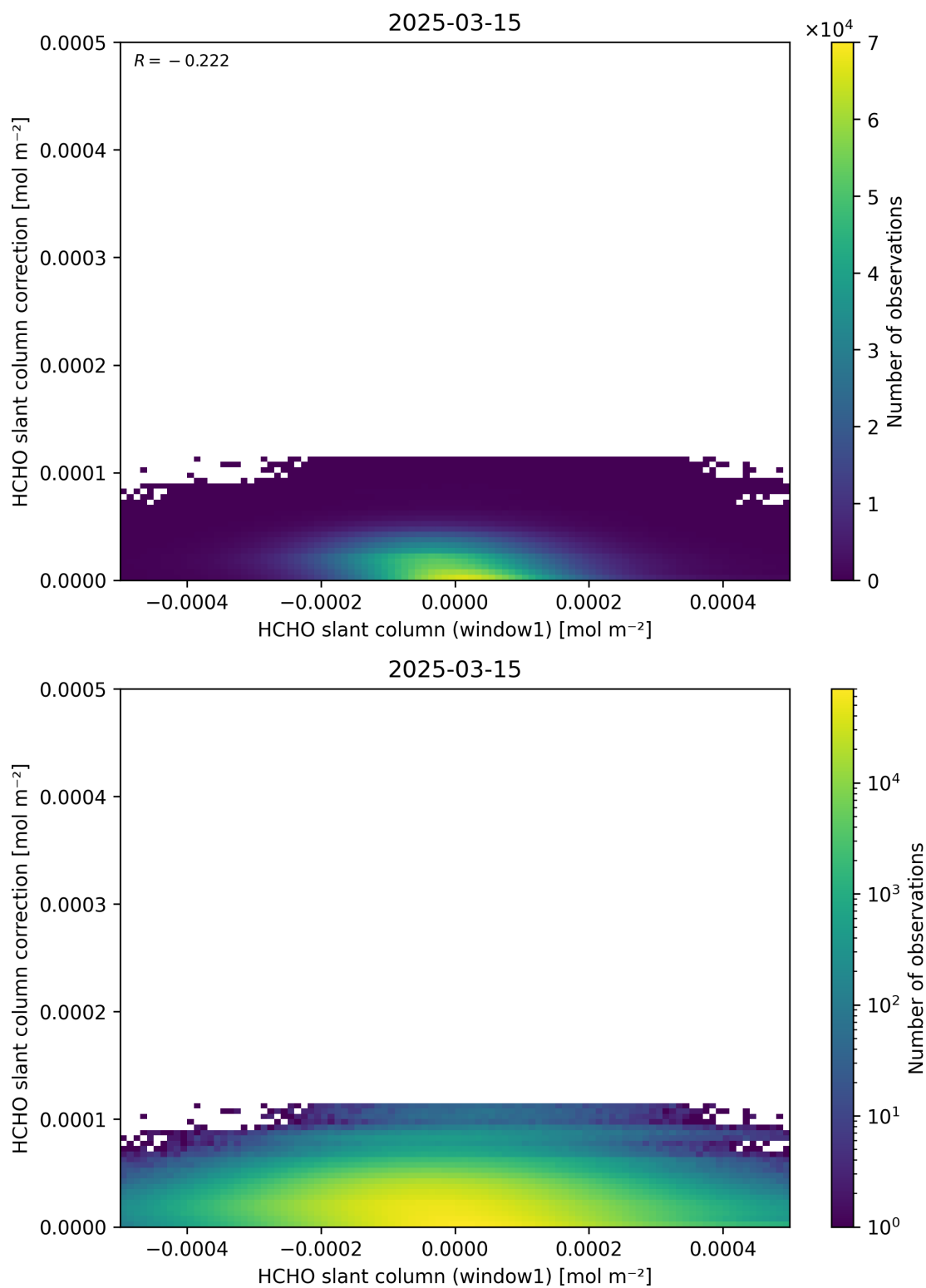
Figure 83: Scatter density plot of “HCHO slant column (window1)” against “HCHO slant column correction” for 2025-03-14 to 2025-03-16.
