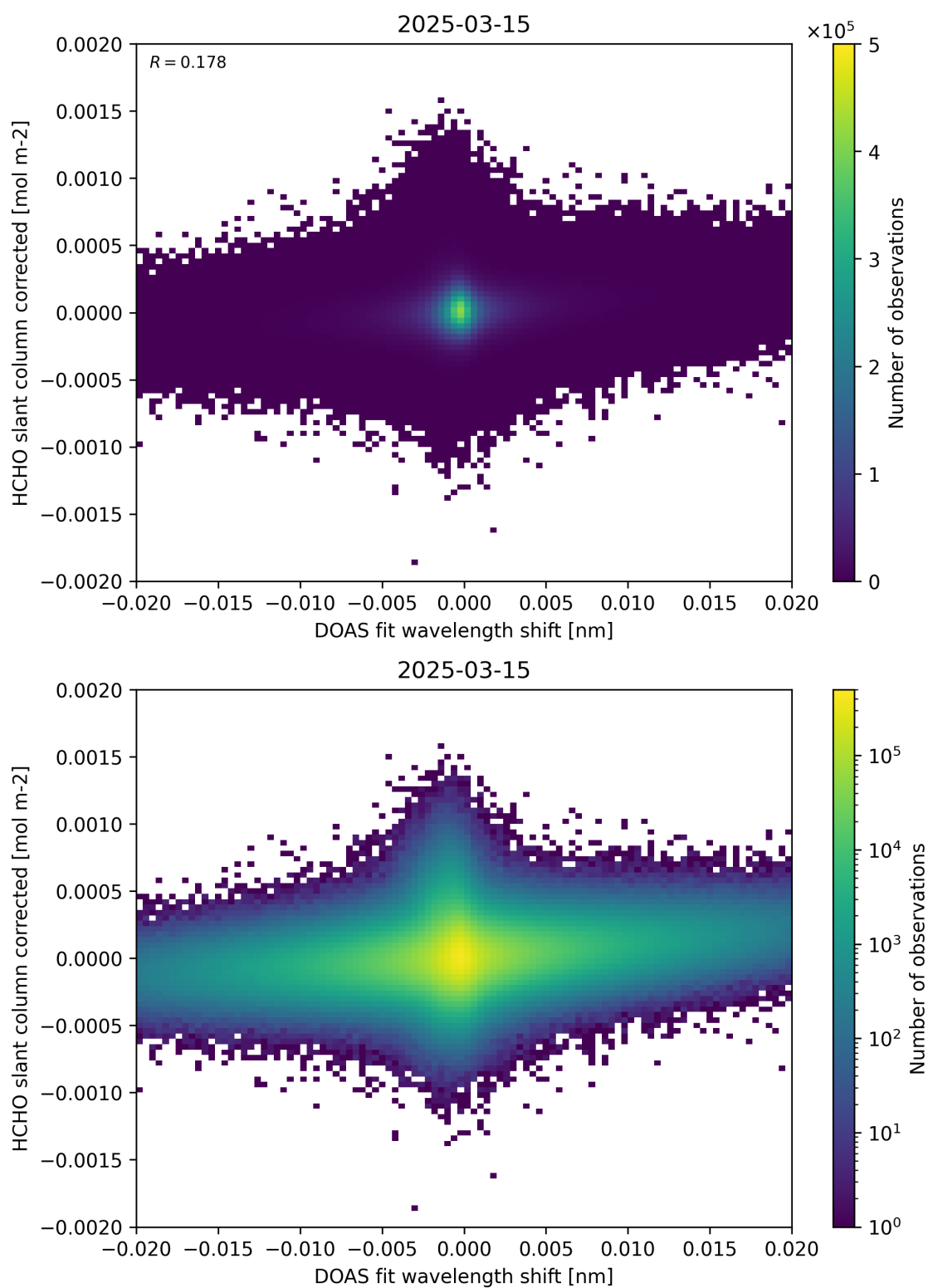
Figure 66: Scatter density plot of “DOAS fit wavelength shift” against “HCHO slant column corrected” for 2025-03-14 to 2025-03-16.
