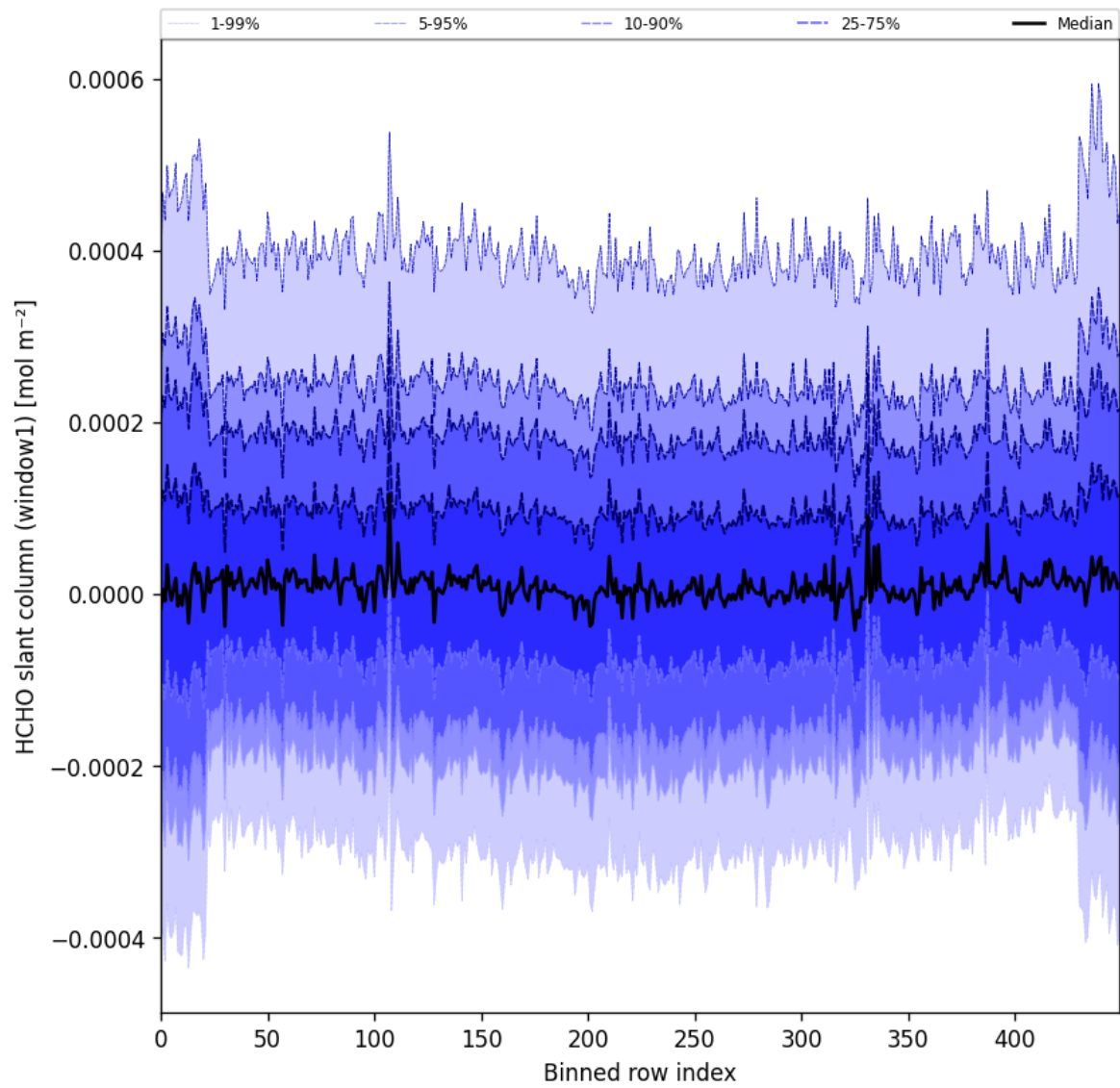
Figure 52: Along track statistics of “HCHO slant column (window1)” for 2025-03-14 to 2025-03-16
