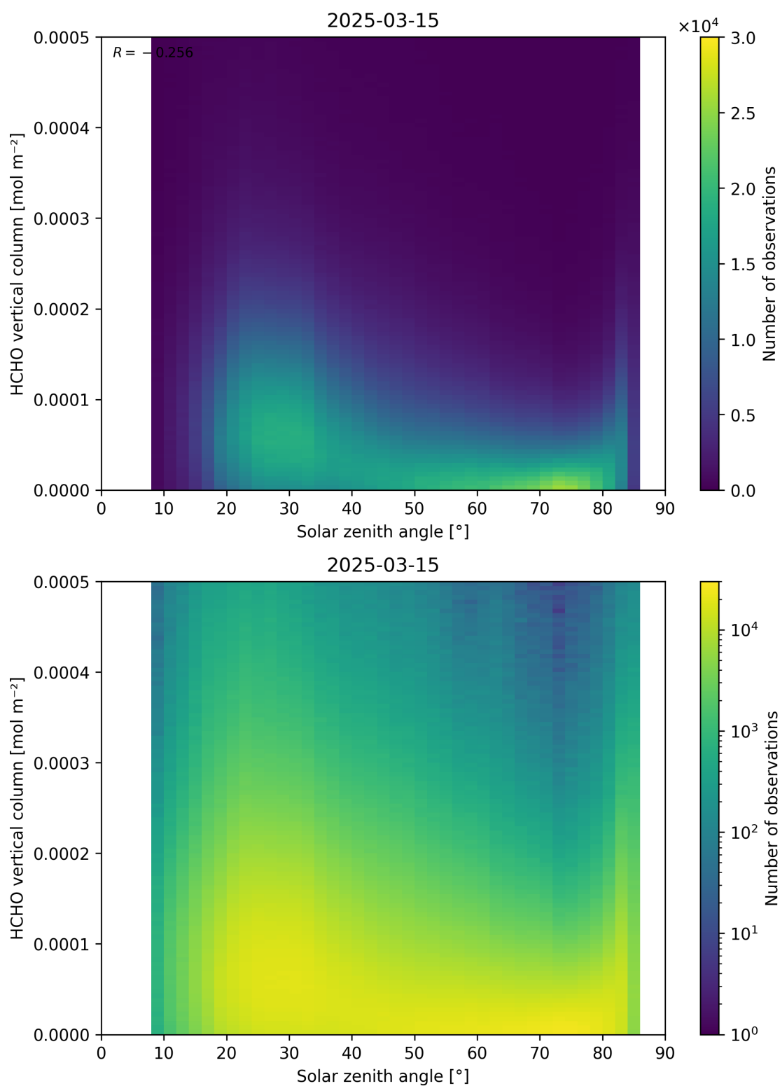
Figure 177: Scatter density plot of “Solar zenith angle” against “HCHO vertical column” for 2025-03-14 to 2025-03-16.
