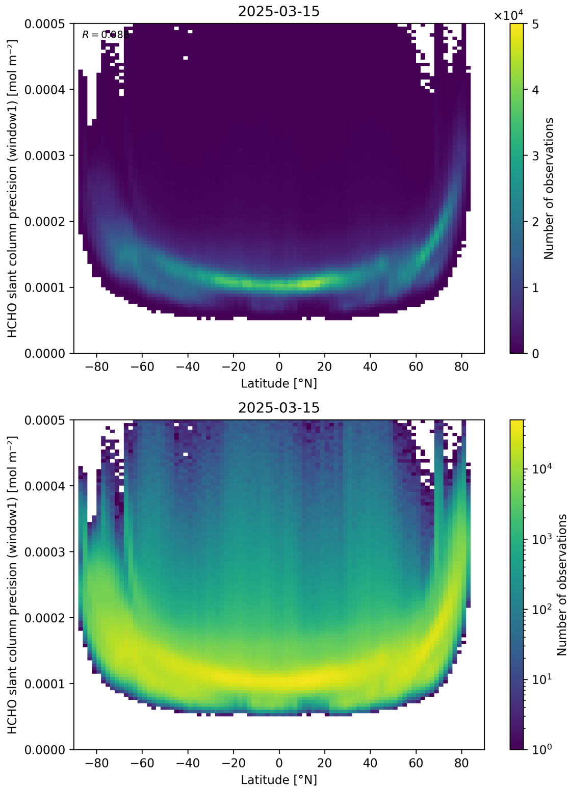
Figure 160: Scatter density plot of “Latitude” against “HCHO slant column precision (window1)” for 2025-03-14 to 2025-03-16.
