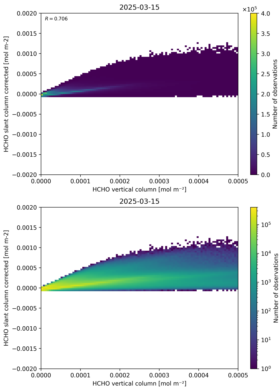
Figure 127: Scatter density plot of “HCHO vertical column” against “HCHO slant column corrected” for 2025-03-14 to 2025-03-16.
