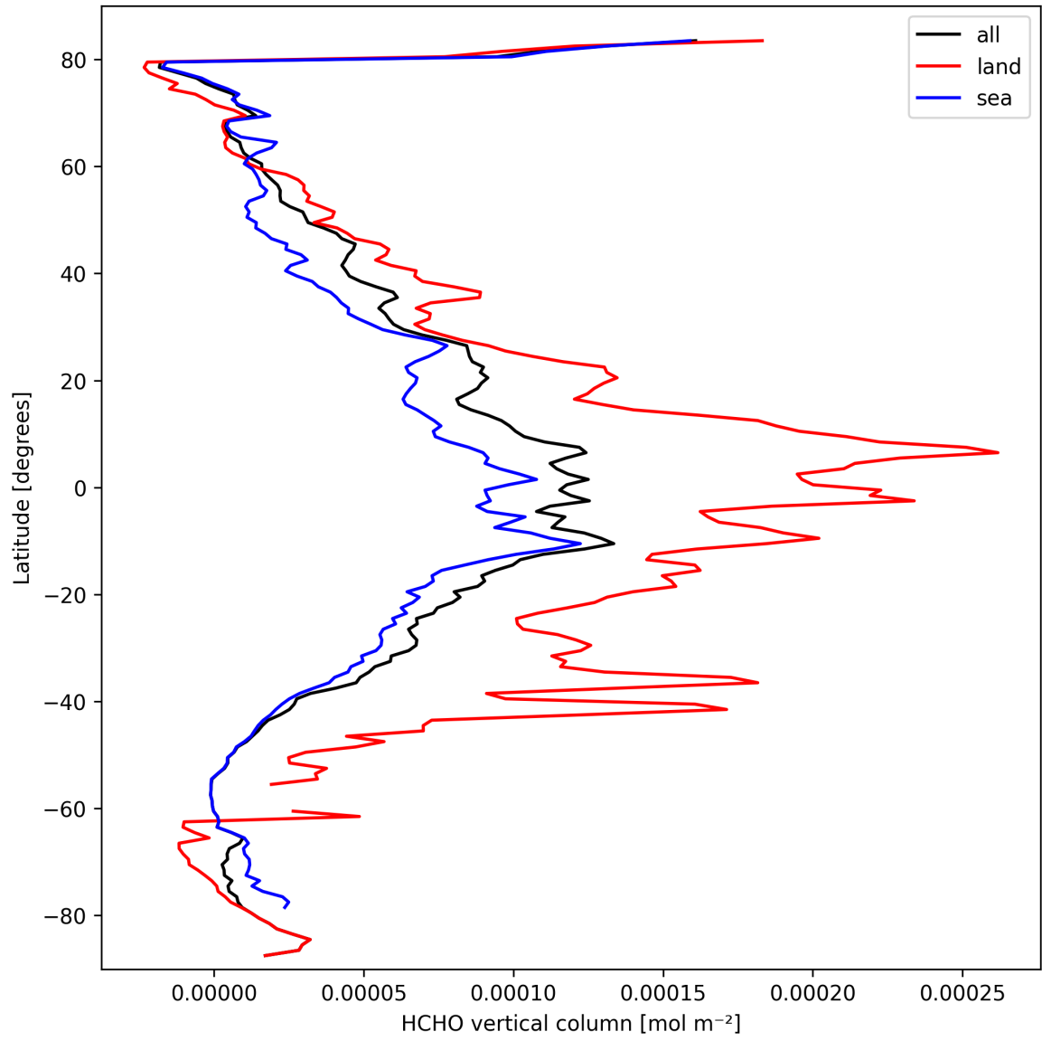
Figure 21: Zonal average of “HCHO vertical column” for 2025-03-14 to 2025-03-16.
