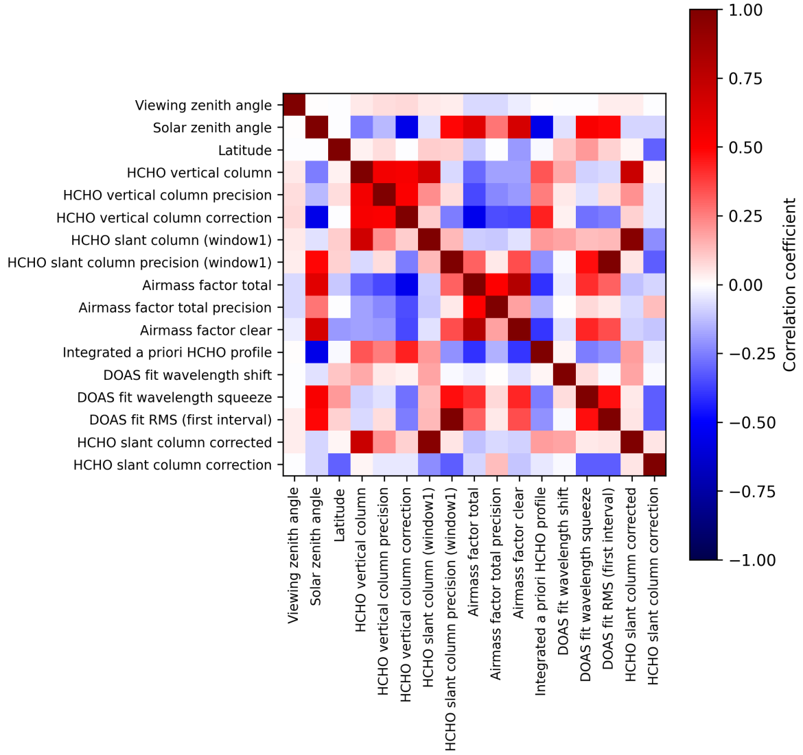
Figure 2: Map of correlation matrix for 2025-03-14 to 2025-03-16.
