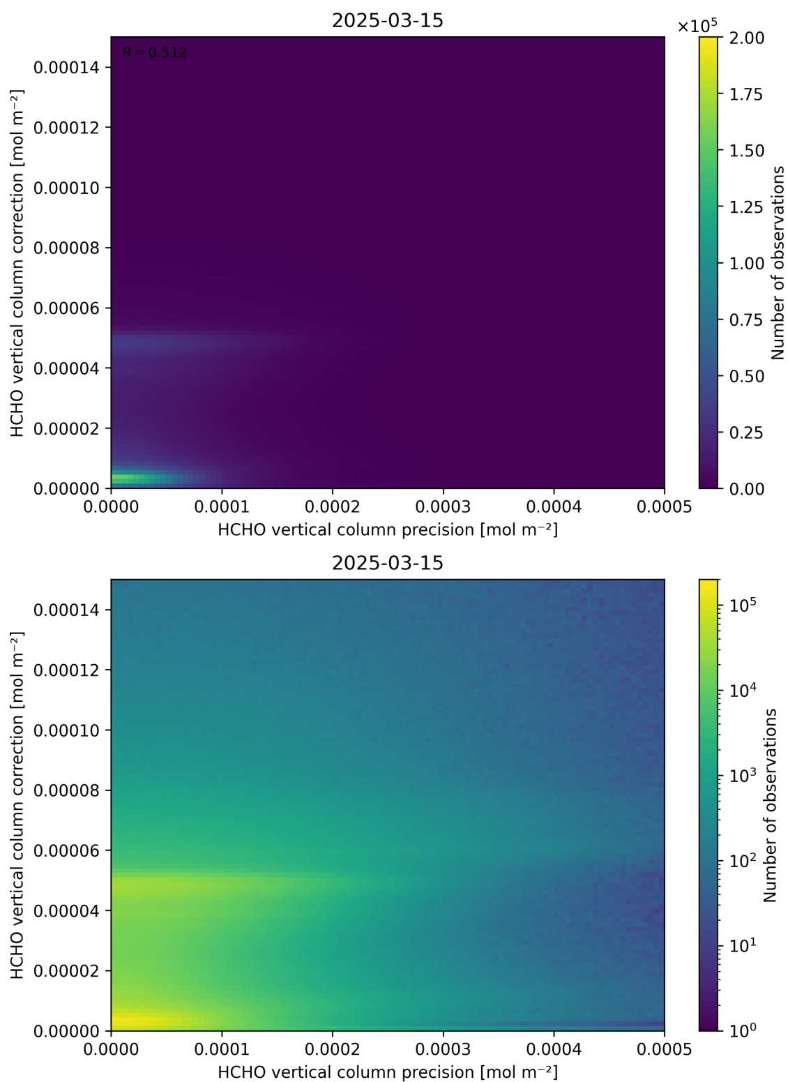
Figure 146: Scatter density plot of “HCHO vertical column precision” against “HCHO vertical column correction” for 2025-03-14 to 2025-03-16.
