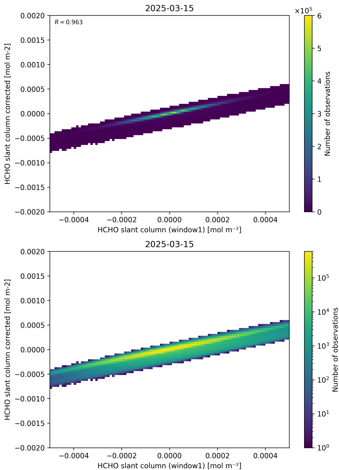
Figure 82: Scatter density plot of “HCHO slant column (window1)” against “HCHO slant column corrected” for 2025-03-14 to 2025-03-16.
