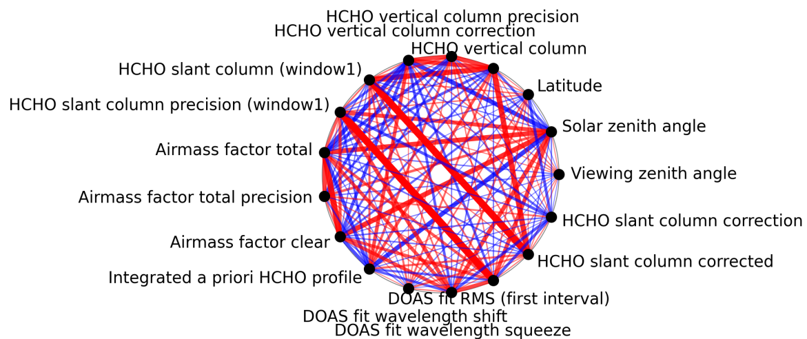
Figure 1: Map of correlation graph for 2025-03-14 to 2025-03-16.
