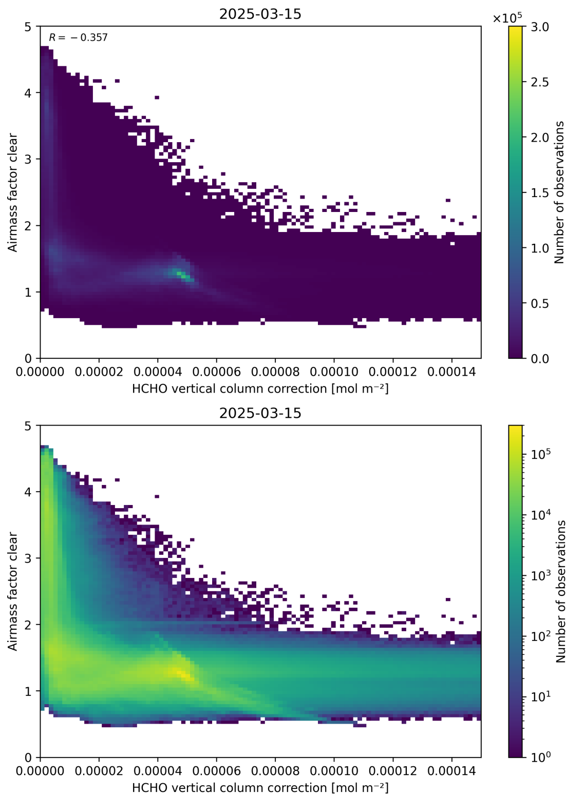
Figure 115: Scatter density plot of “HCHO vertical column correction” against “Airmass factor clear” for 2025-03-14 to 2025-03-16.
