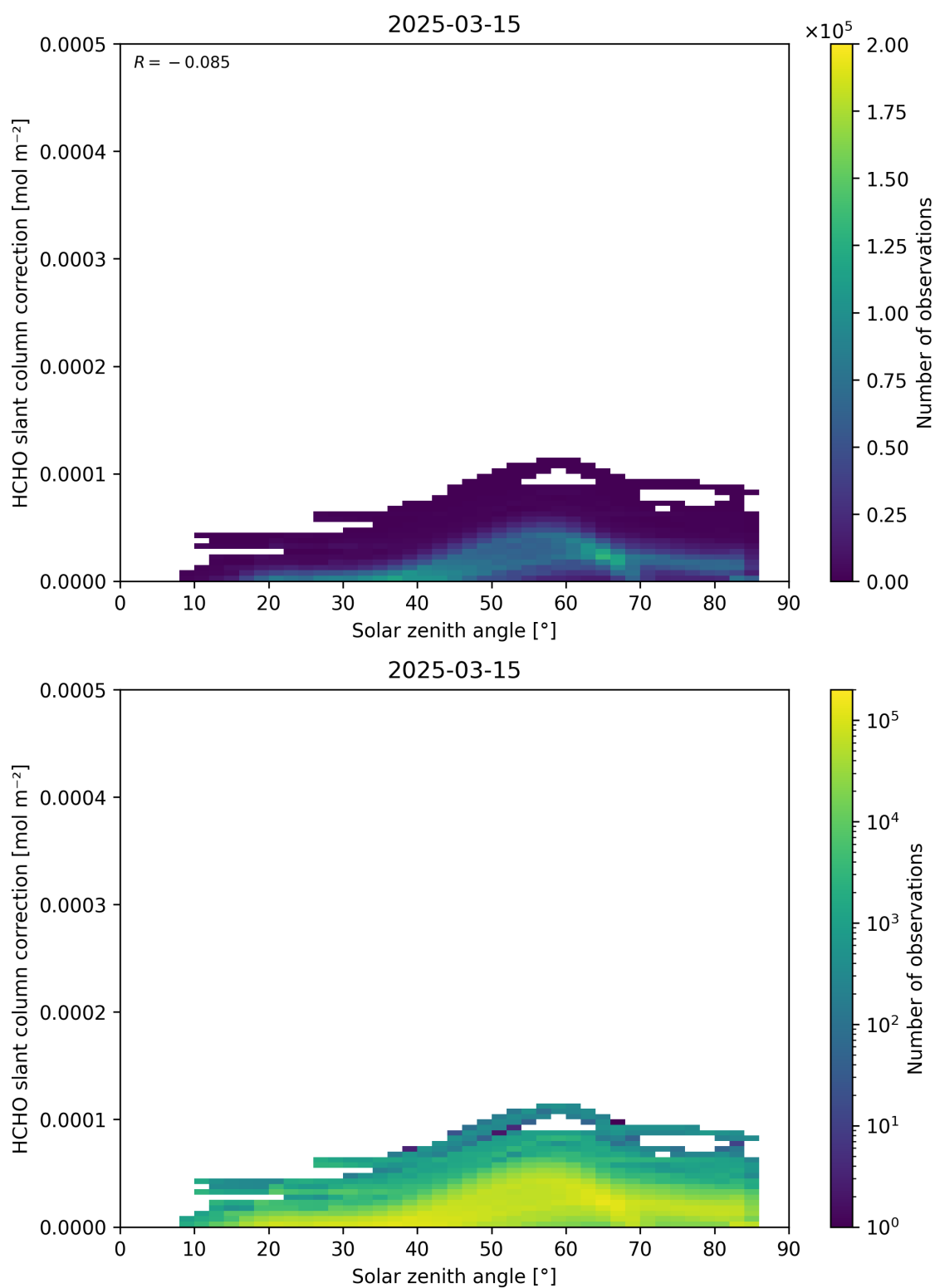
Figure 172: Scatter density plot of “Solar zenith angle” against “HCHO slant column correction” for 2025-03-14 to 2025-03-16.
