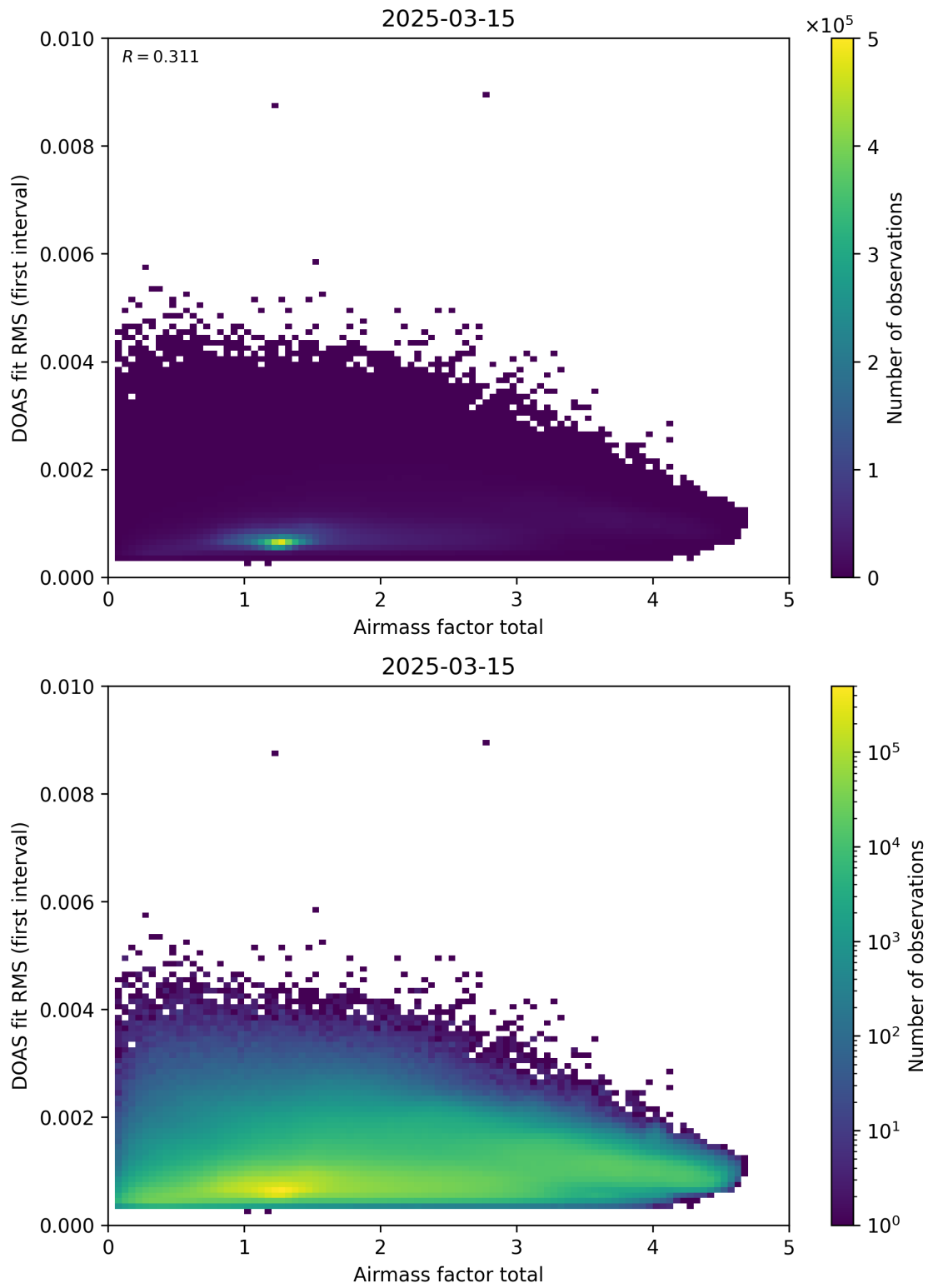
Figure 97: Scatter density plot of “Airmass factor total” against “DOAS fit RMS (first interval)” for 2025-03-14 to 2025-03-16.
