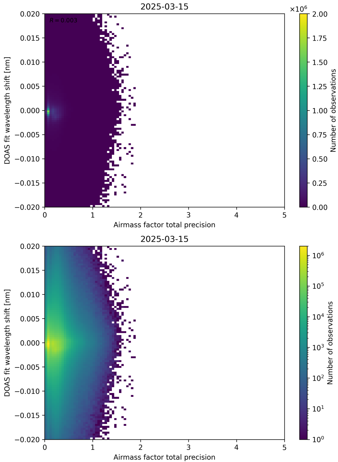
Figure 106: Scatter density plot of “Airmass factor total precision” against “DOAS fit wavelength shift” for 2025-03-14 to 2025-03-16.
