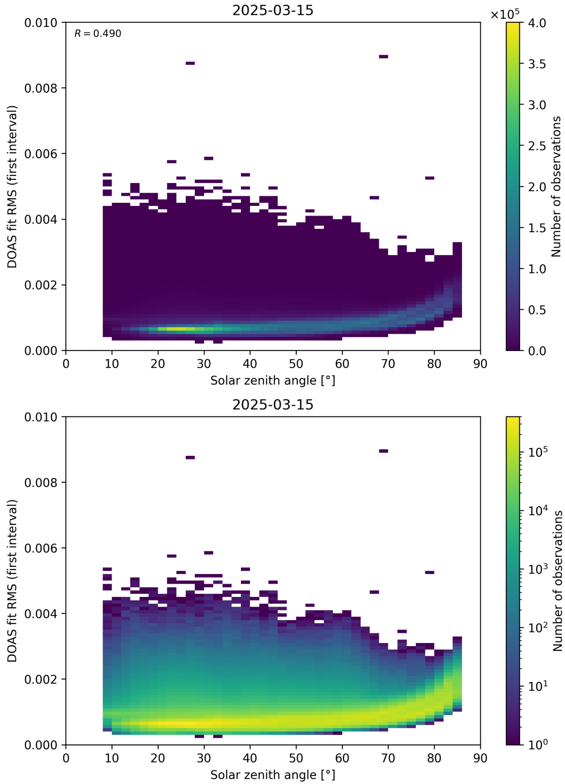
Figure 167: Scatter density plot of “Solar zenith angle” against “DOAS fit RMS (first interval)” for 2025-03-14 to 2025-03-16.
