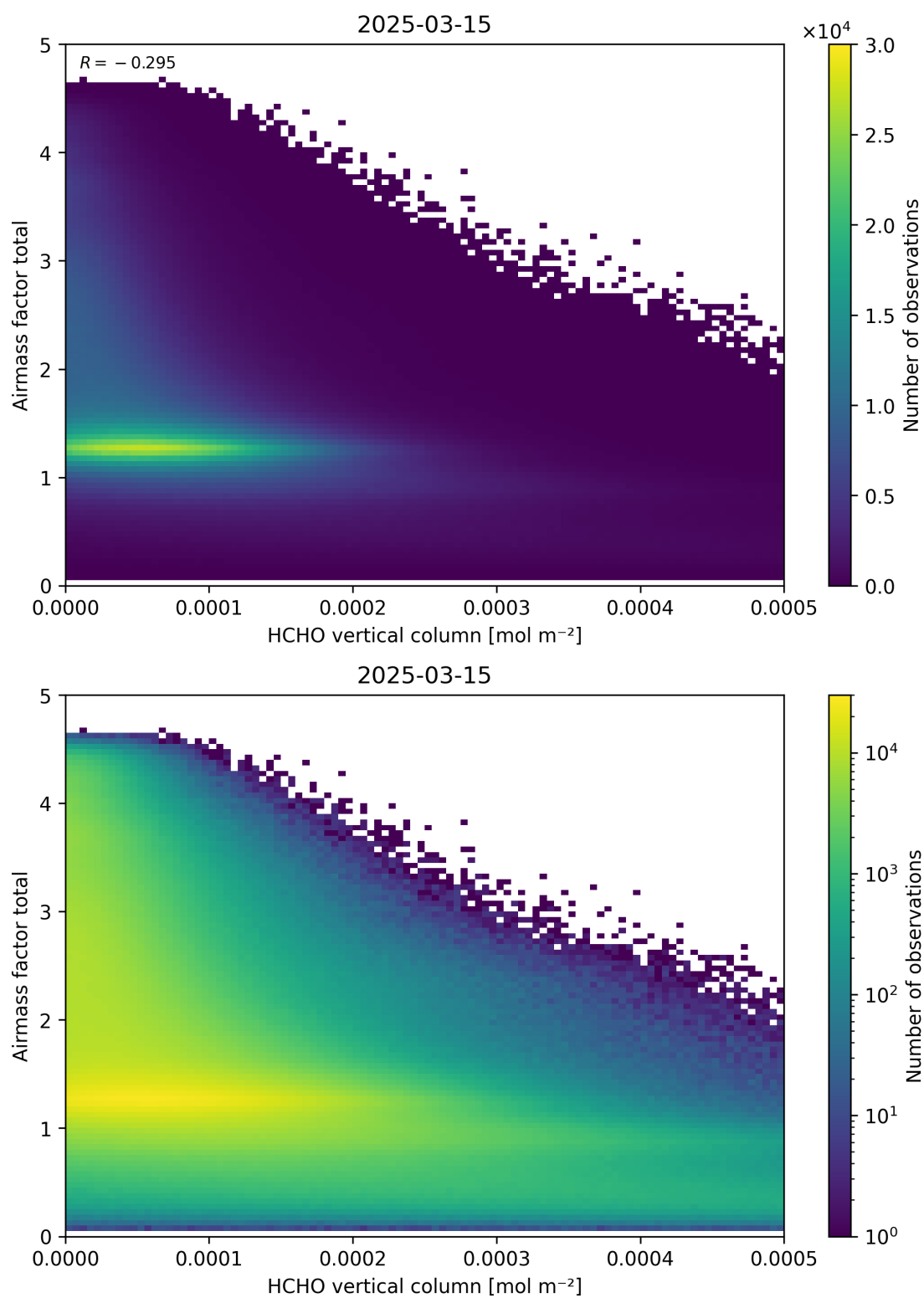
Figure 131: Scatter density plot of “HCHO vertical column” against “Airmass factor total” for 2025-03-14 to 2025-03-16.
