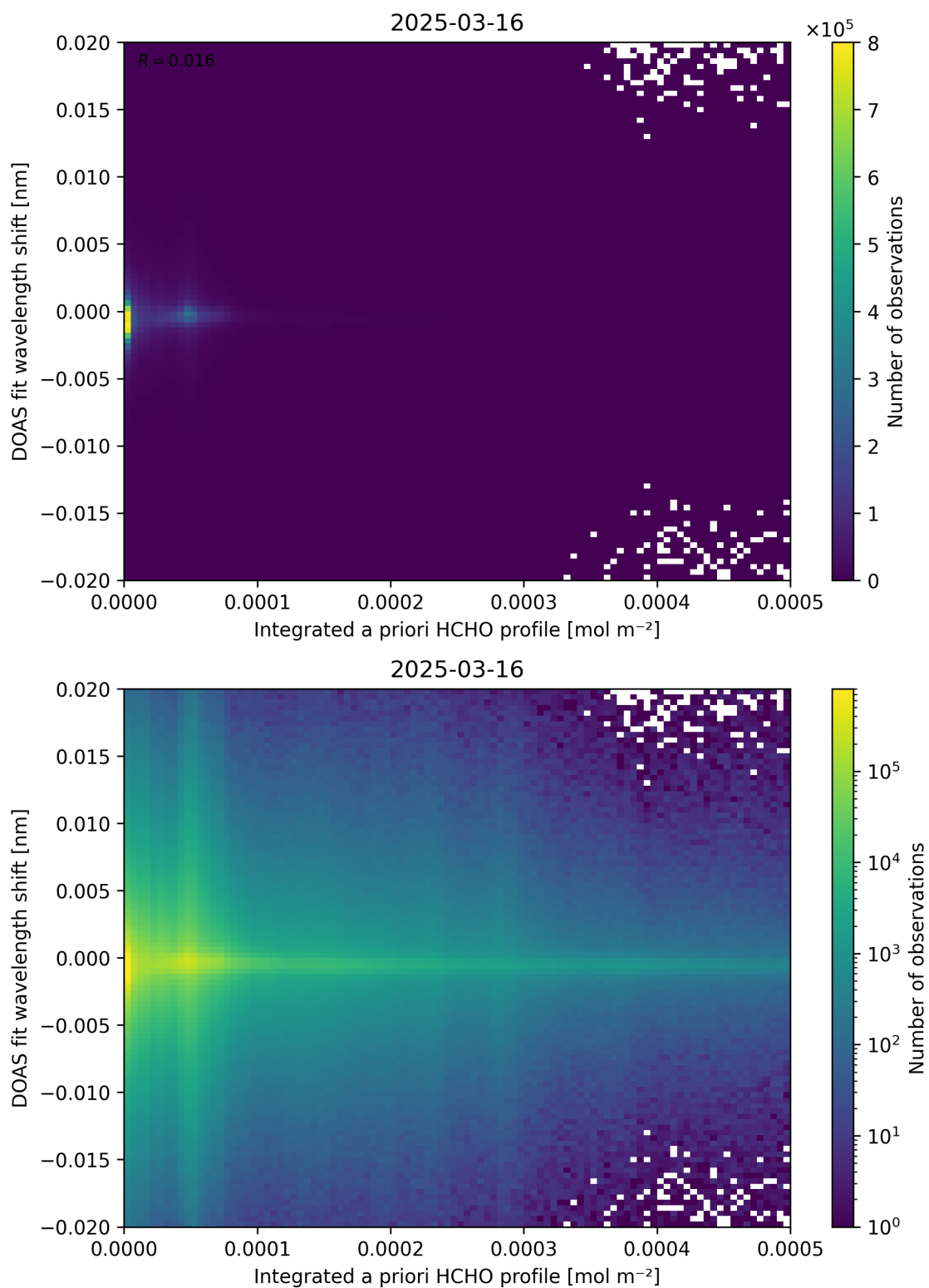
Figure 149: Scatter density plot of “Integrated a priori HCHO profile” against “DOAS fit wavelength shift” for 2025-03-15 to 2025-03-17.
