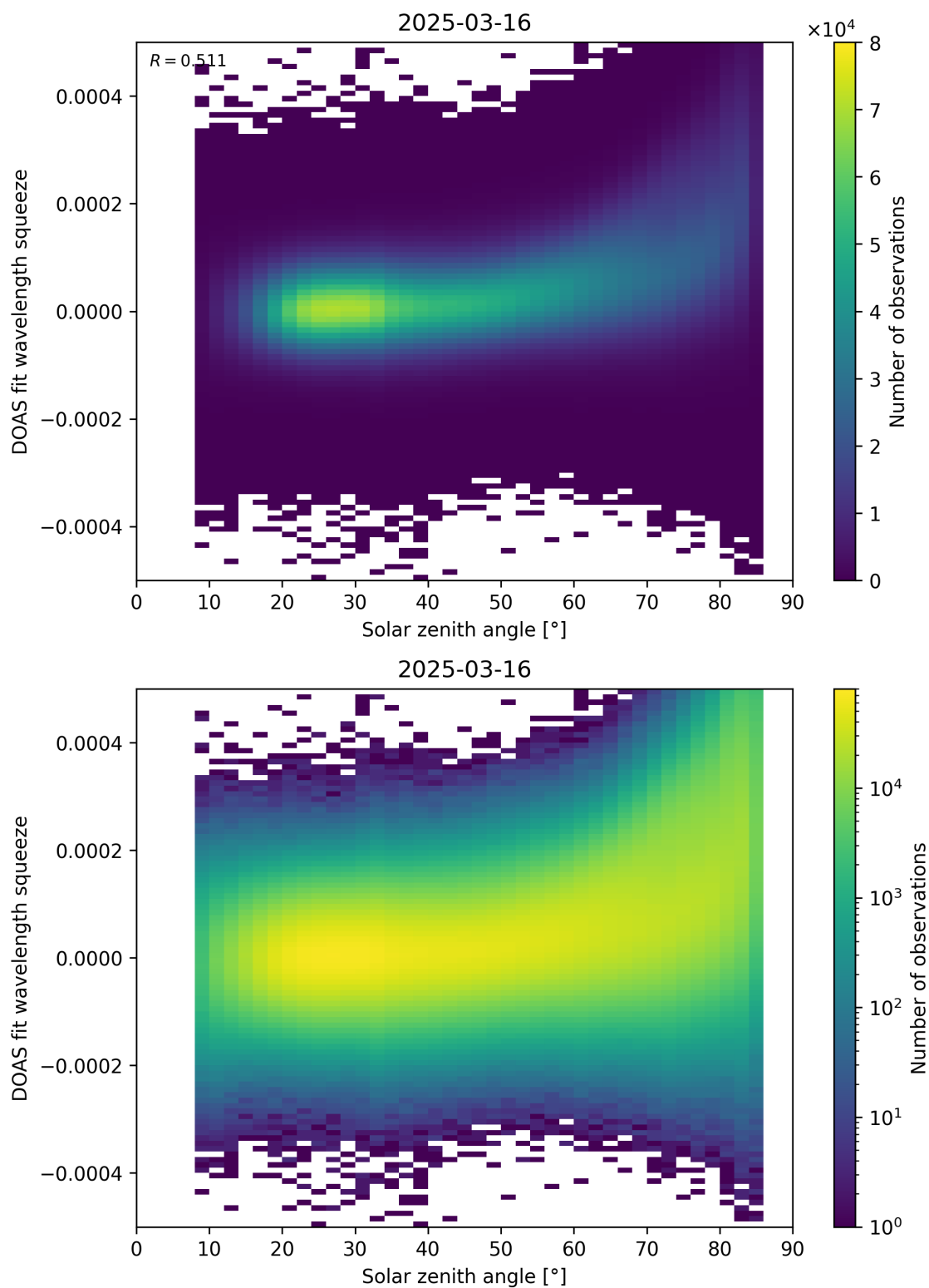
Figure 169: Scatter density plot of “Solar zenith angle” against “DOAS fit wavelength squeeze” for 2025-03-15 to 2025-03-17.
