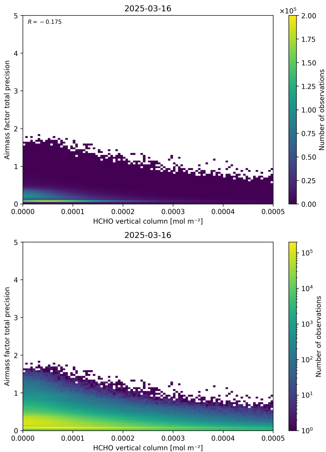
Figure 132: Scatter density plot of “HCHO vertical column” against “Airmass factor total precision” for 2025-03-15 to 2025-03-17.
