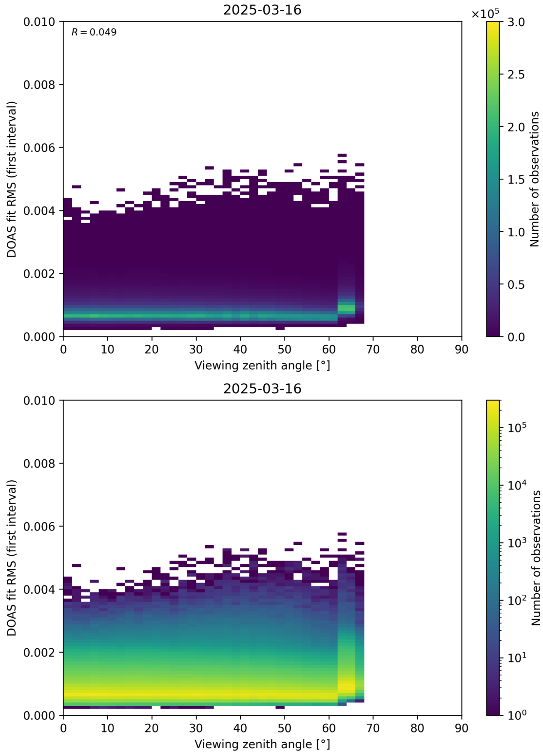
Figure 182: Scatter density plot of “Viewing zenith angle” against “DOAS fit RMS (first interval)” for 2025-03-15 to 2025-03-17.
