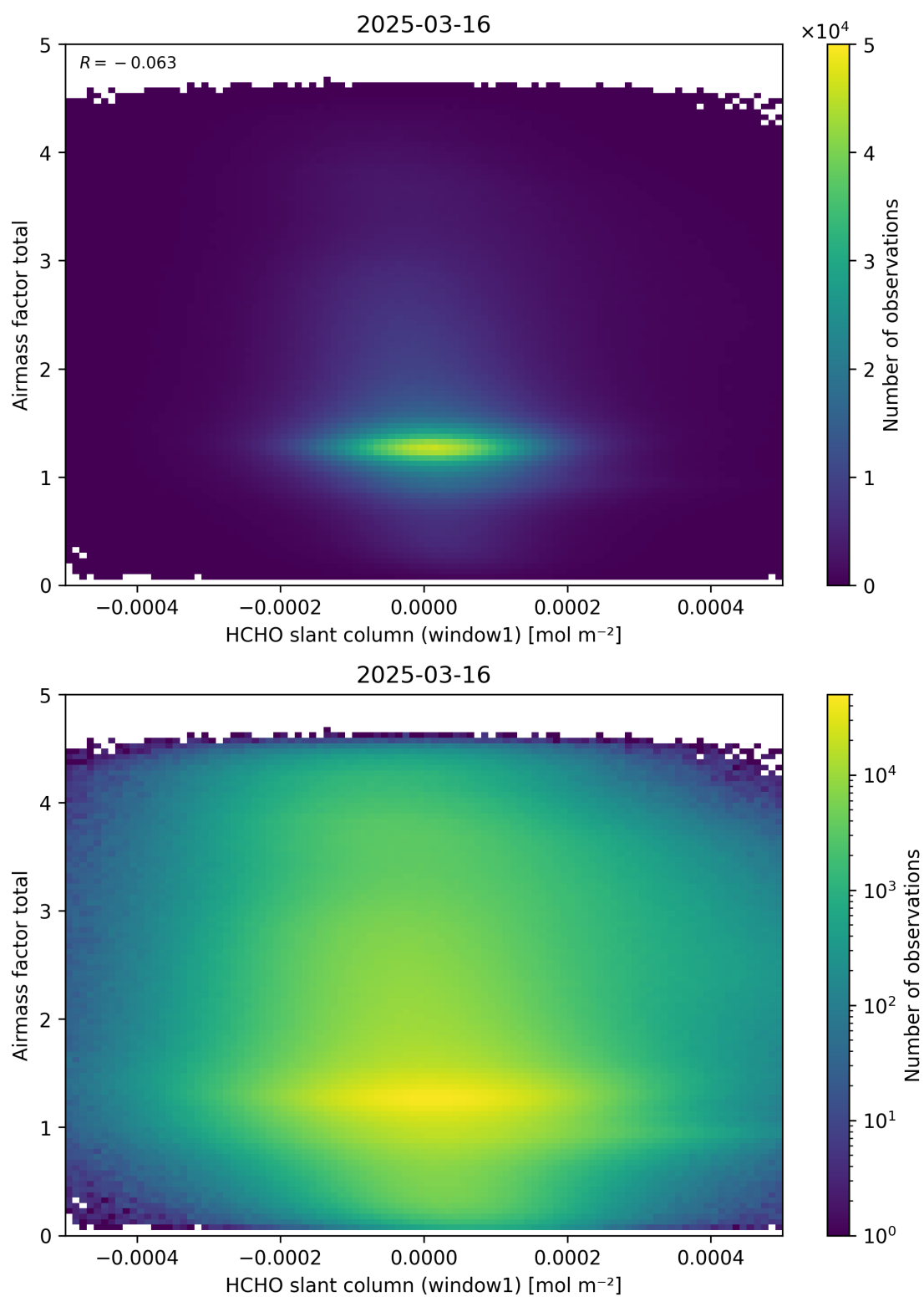
Figure 85: Scatter density plot of “HCHO slant column (window1)” against “Airmass factor total” for 2025-03-15 to 2025-03-17.
