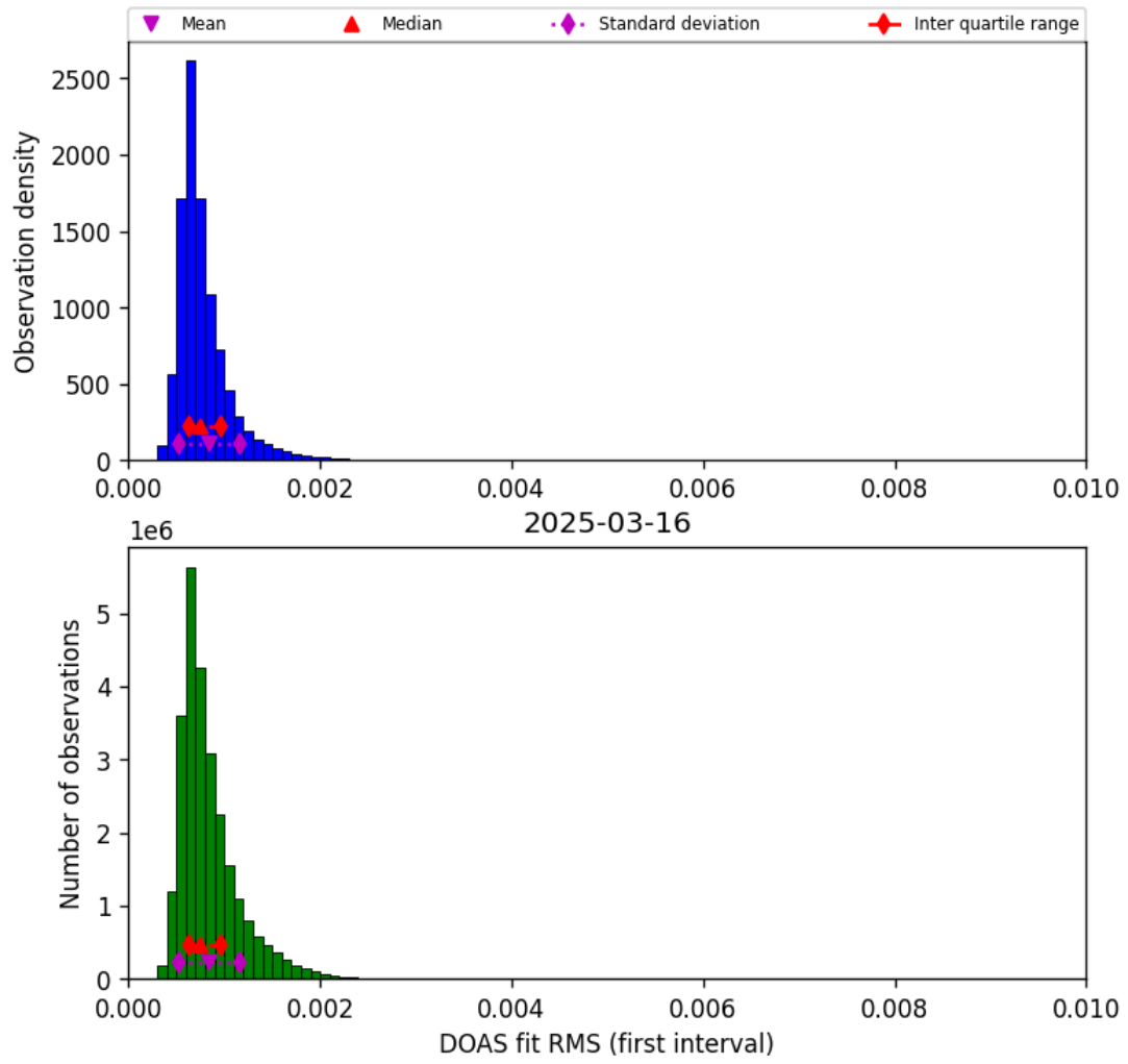
Figure 46: Histogram of “DOAS fit RMS (first interval)” for 2025-03-15 to 2025-03-17
