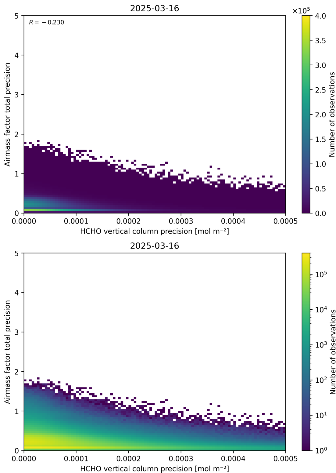
Figure 145: Scatter density plot of “HCHO vertical column precision” against “Airmass factor total precision” for 2025-03-15 to 2025-03-17.
