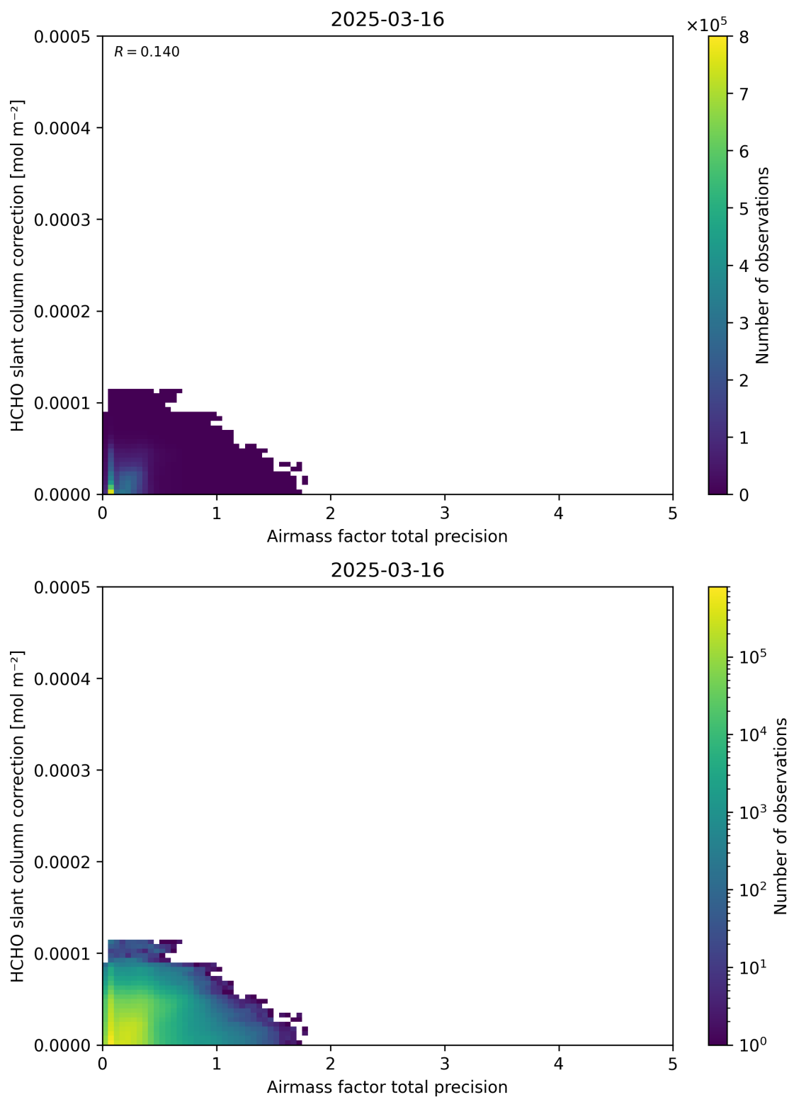
Figure 110: Scatter density plot of “Airmass factor total precision” against “HCHO slant column correction” for 2025-03-15 to 2025-03-17.
