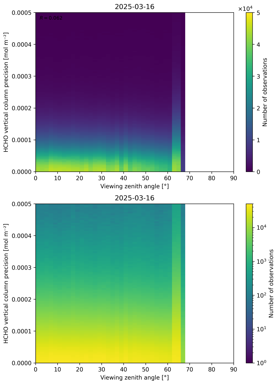
Figure 194: Scatter density plot of “Viewing zenith angle” against “HCHO vertical column precision” for 2025-03-15 to 2025-03-17.
