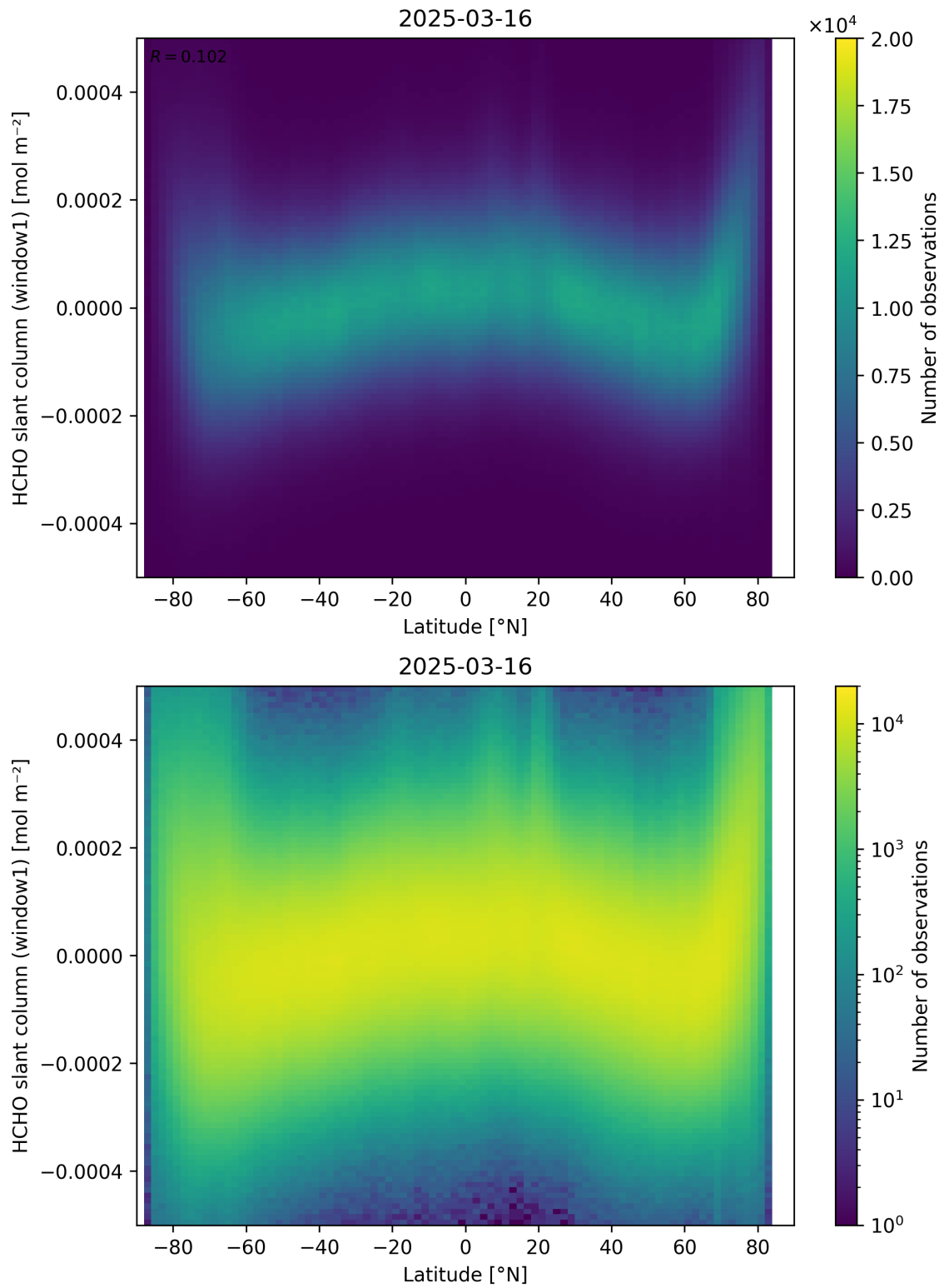
Figure 159: Scatter density plot of “Latitude” against “HCHO slant column (window1)” for 2025-03-15 to 2025-03-17.
