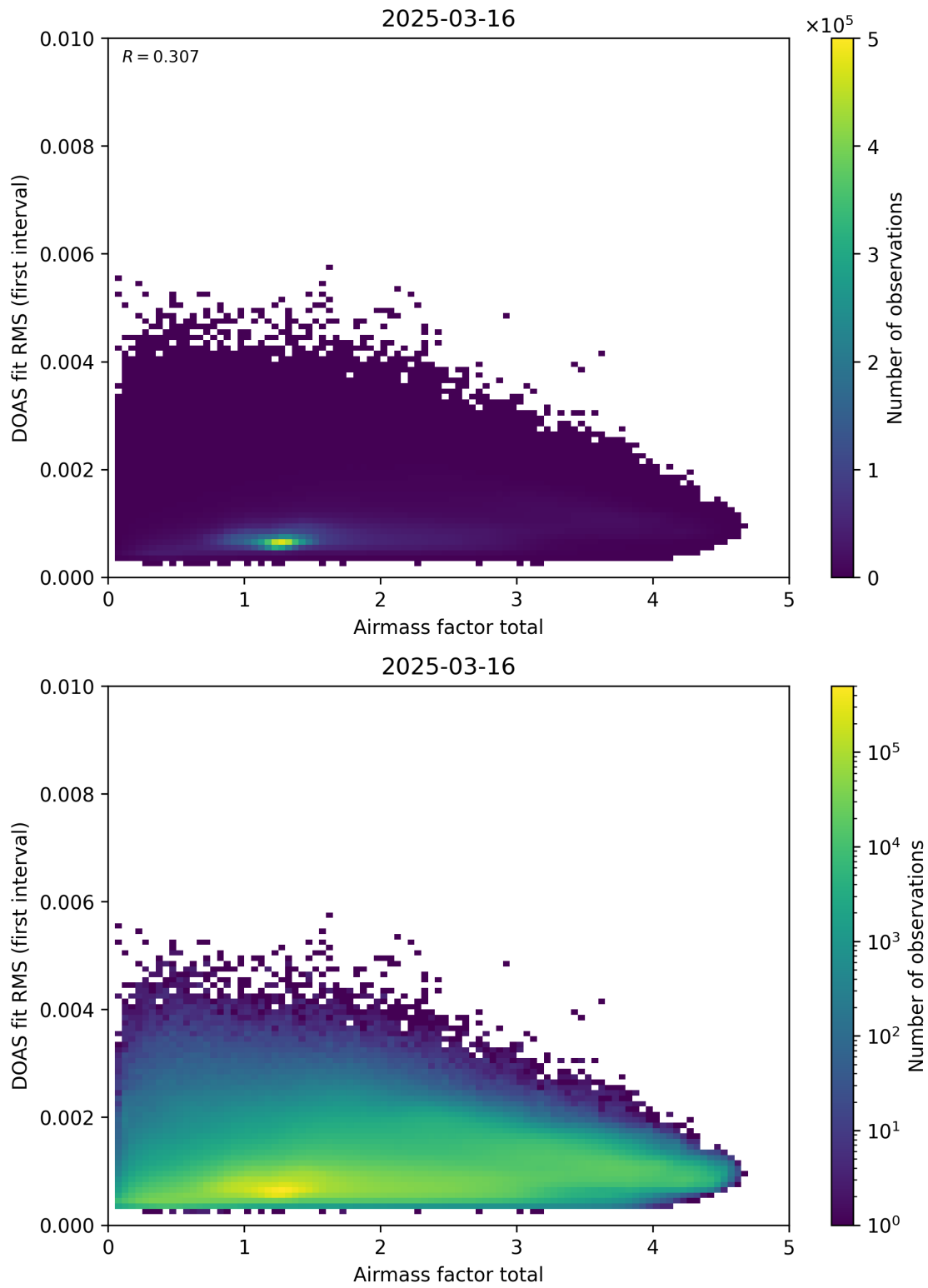
Figure 97: Scatter density plot of “Airmass factor total” against “DOAS fit RMS (first interval)” for 2025-03-15 to 2025-03-17.
