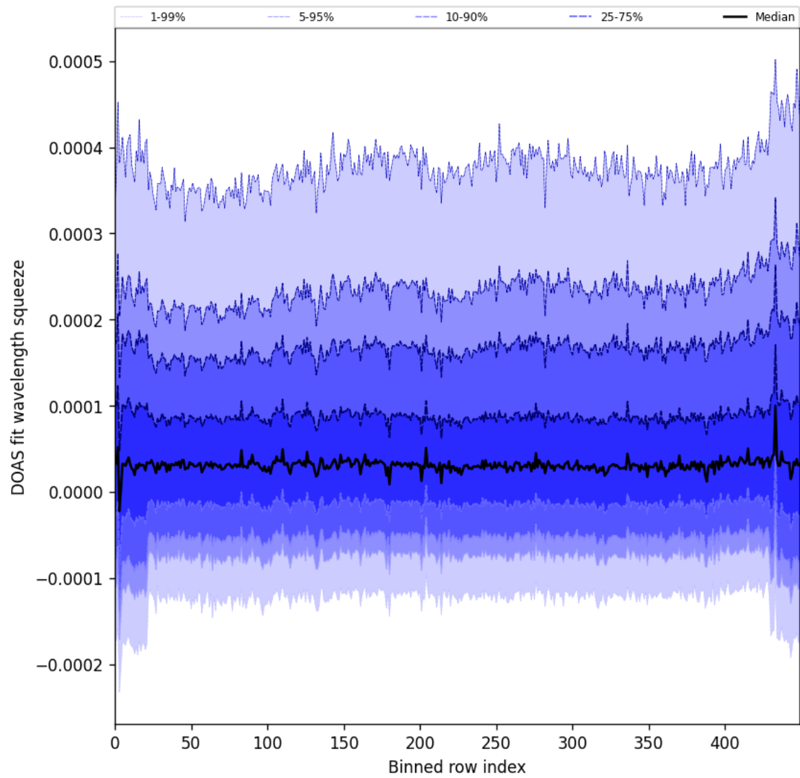
Figure 59: Along track statistics of “DOAS fit wavelength squeeze” for 2025-03-15 to 2025-03-17
