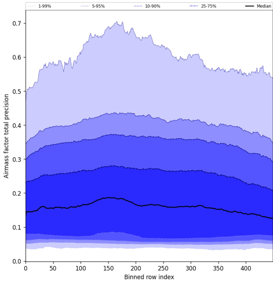
Figure 55: Along track statistics of “Airmass factor total precision” for 2025-03-15 to 2025-03-17
