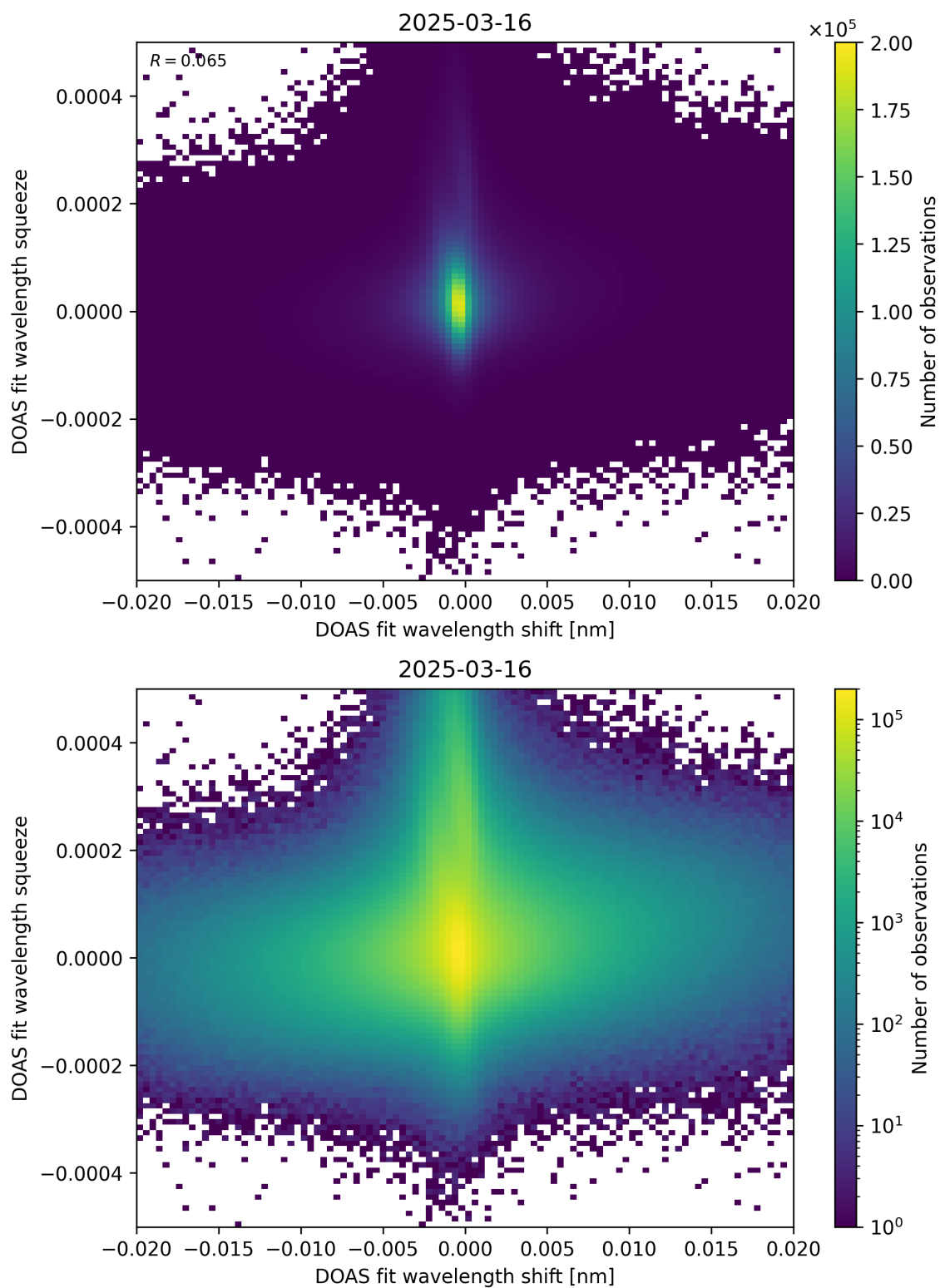
Figure 65: Scatter density plot of “DOAS fit wavelength shift” against “DOAS fit wavelength squeeze” for 2025-03-15 to 2025-03-17.
