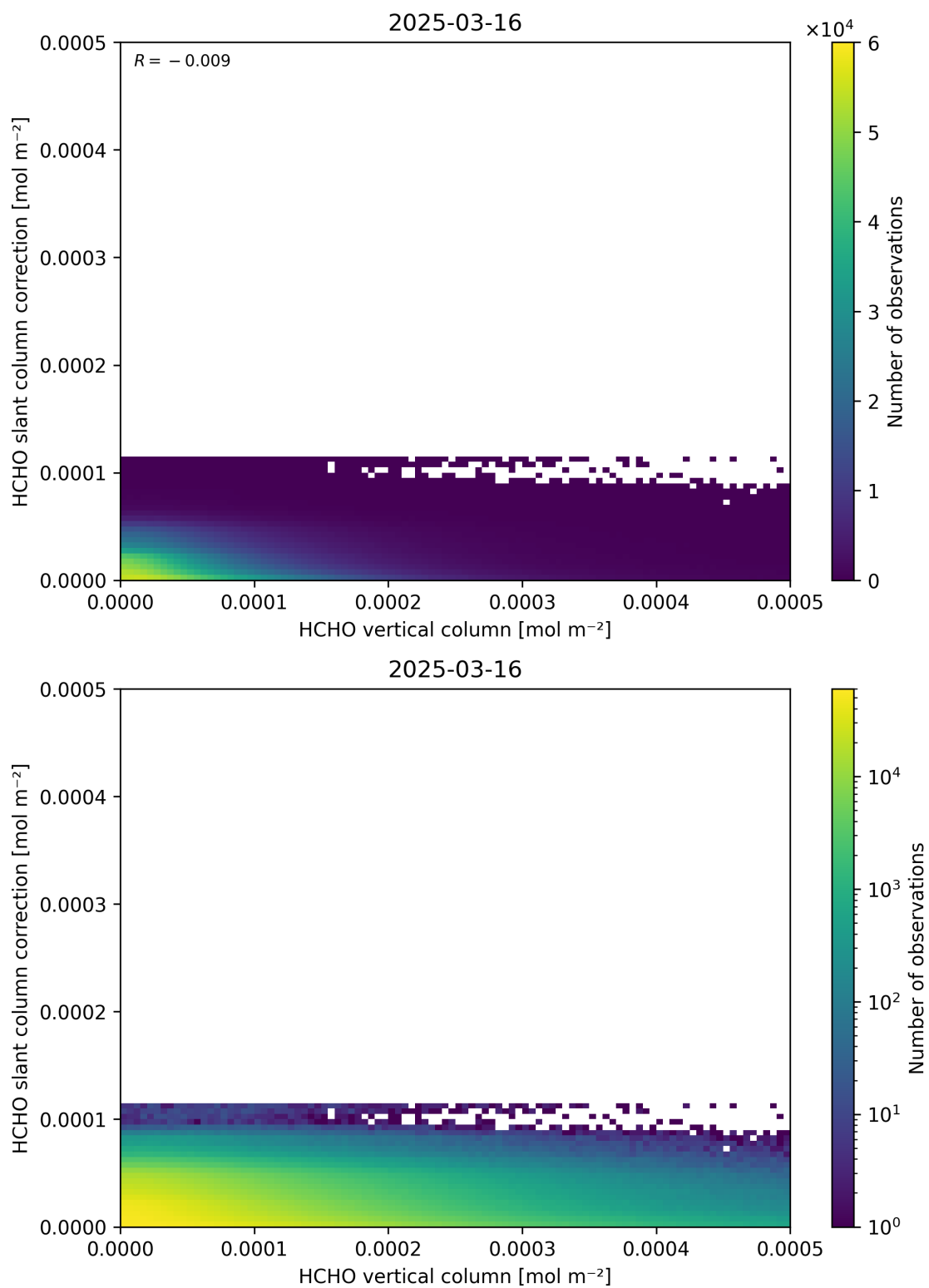
Figure 128: Scatter density plot of “HCHO vertical column” against “HCHO slant column correction” for 2025-03-15 to 2025-03-17.
