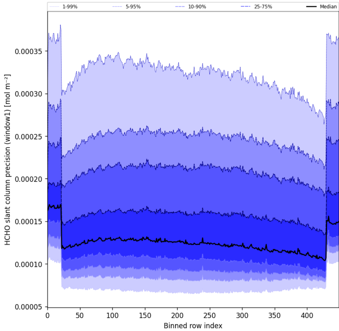
Figure 53: Along track statistics of “HCHO slant column precision (window1)” for 2025-03-15 to 2025-03-17
