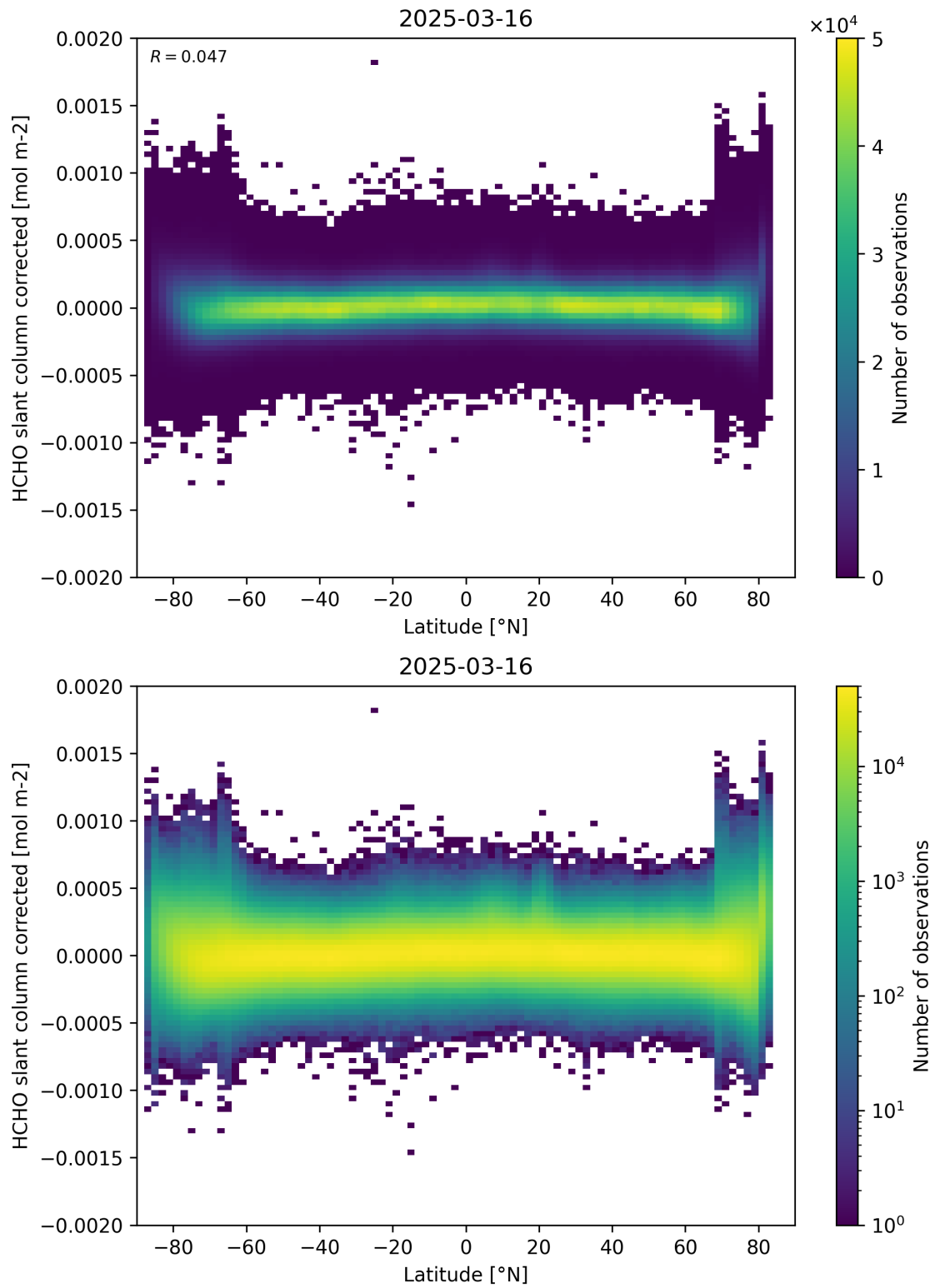
Figure 157: Scatter density plot of “Latitude” against “HCHO slant column corrected” for 2025-03-15 to 2025-03-17.
