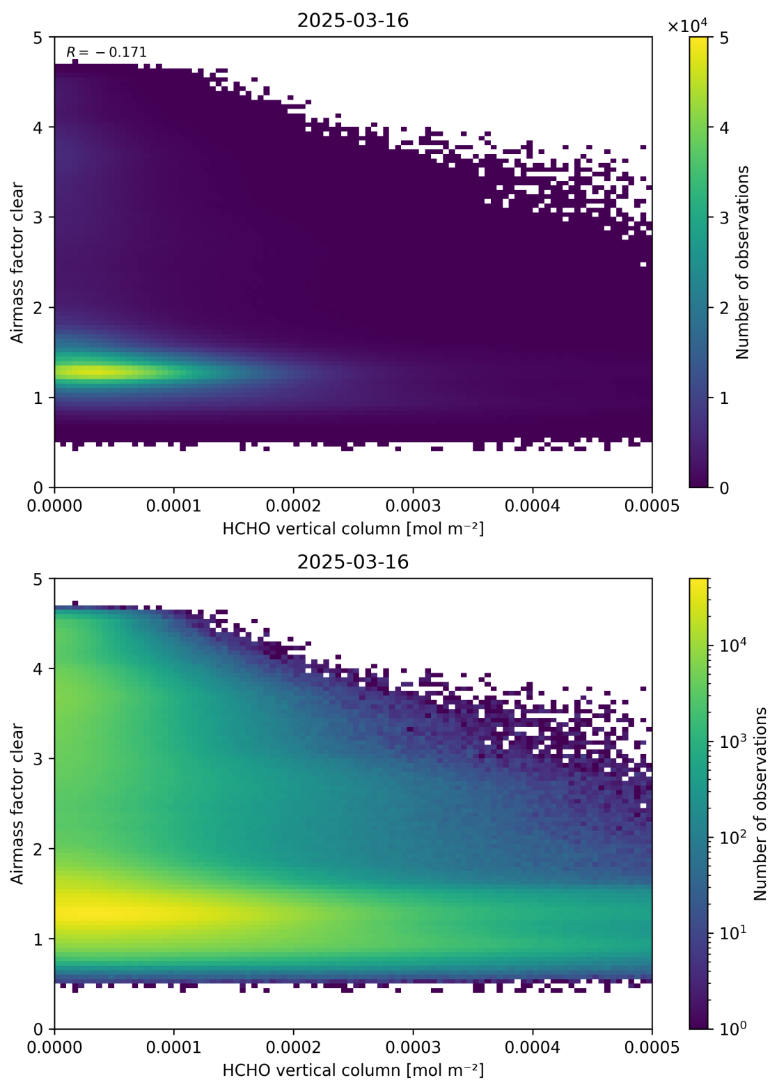
Figure 126: Scatter density plot of “HCHO vertical column” against “Airmass factor clear” for 2025-03-15 to 2025-03-17.
