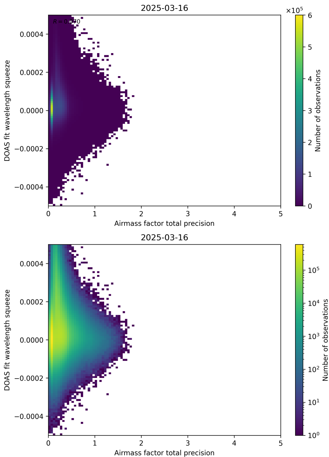
Figure 107: Scatter density plot of “Airmass factor total precision” against “DOAS fit wavelength squeeze” for 2025-03-15 to 2025-03-17.
