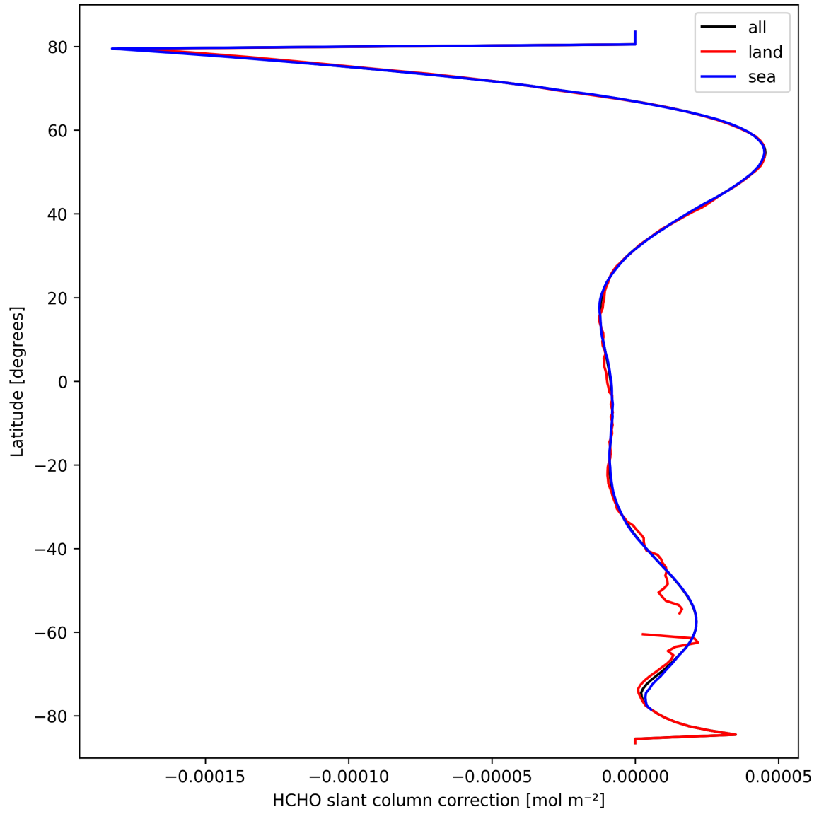
Figure 33: Zonal average of “HCHO slant column correction” for 2025-03-15 to 2025-03-17.
