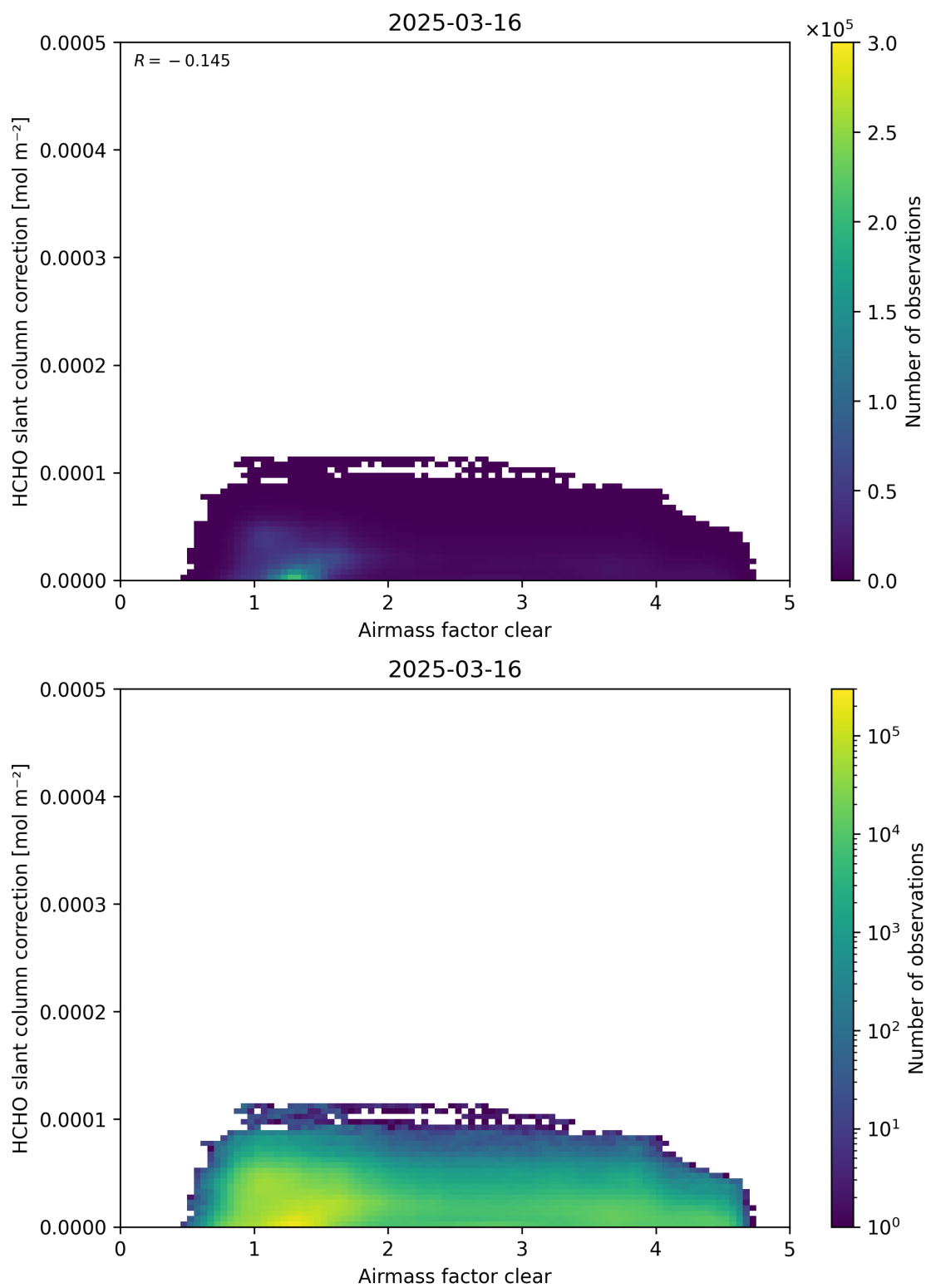
Figure 75: Scatter density plot of “Airmass factor clear” against “HCHO slant column correction” for 2025-03-15 to 2025-03-17.
