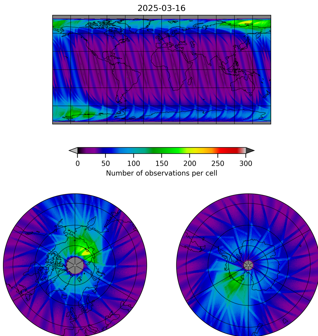
Figure 19: Map of the number of observations for 2025-03-15 to 2025-03-17
