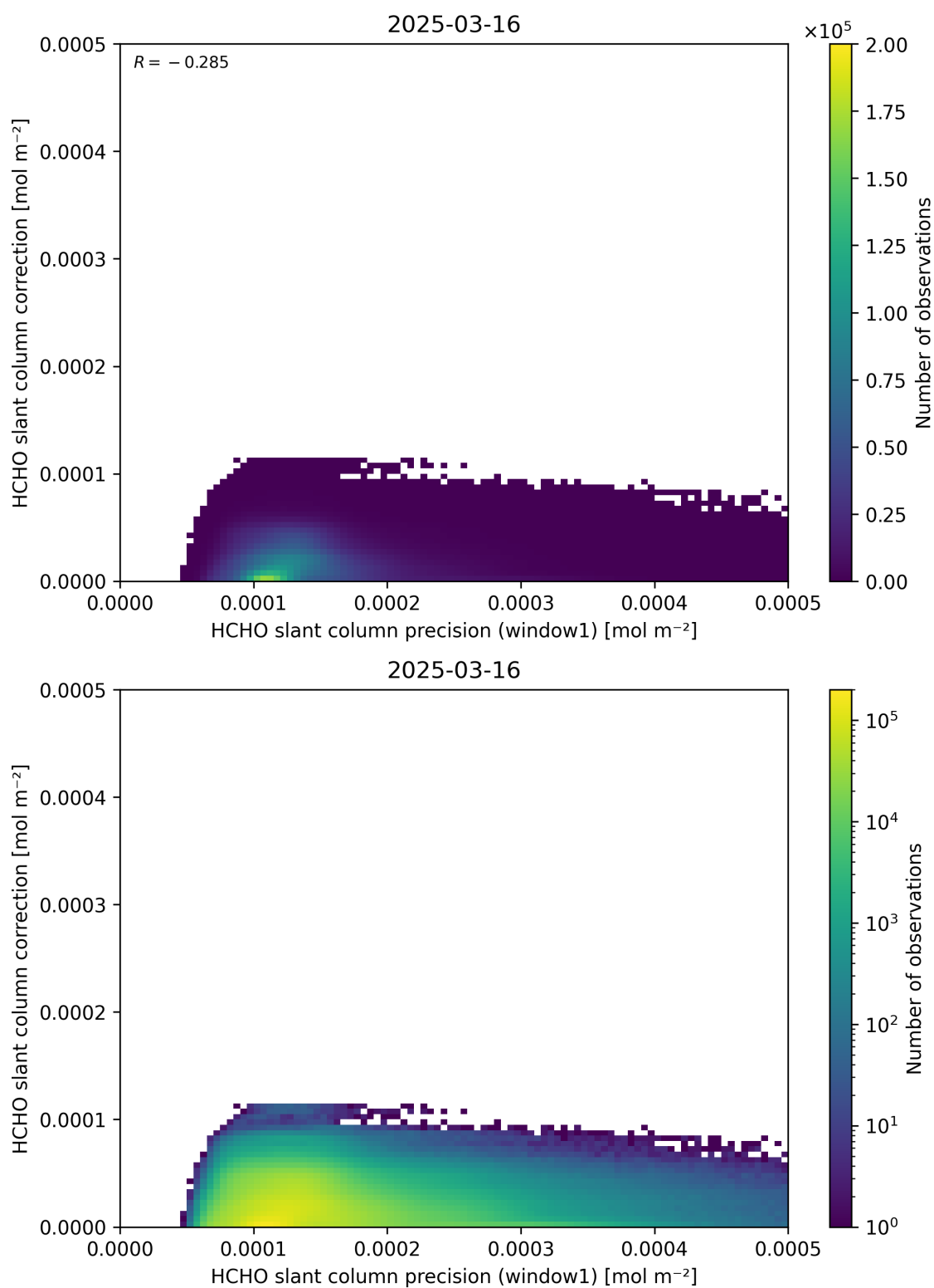
Figure 93: Scatter density plot of “HCHO slant column precision (window1)” against “HCHO slant column correction” for 2025-03-15 to 2025-03-17.
