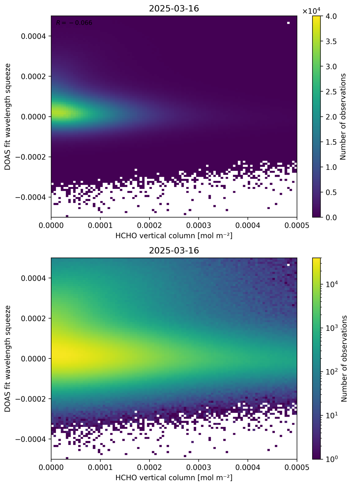
Figure 125: Scatter density plot of “HCHO vertical column” against “DOAS fit wavelength squeeze” for 2025-03-15 to 2025-03-17.
