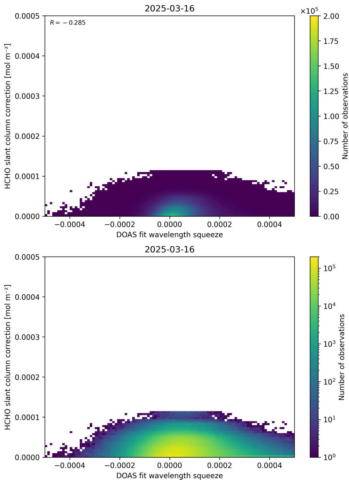
Figure 70: Scatter density plot of “DOAS fit wavelength squeeze” against “HCHO slant column correction” for 2025-03-15 to 2025-03-17.
