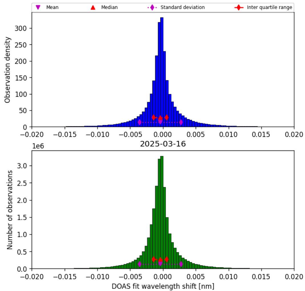
Figure 44: Histogram of “DOAS fit wavelength shift” for 2025-03-15 to 2025-03-17
