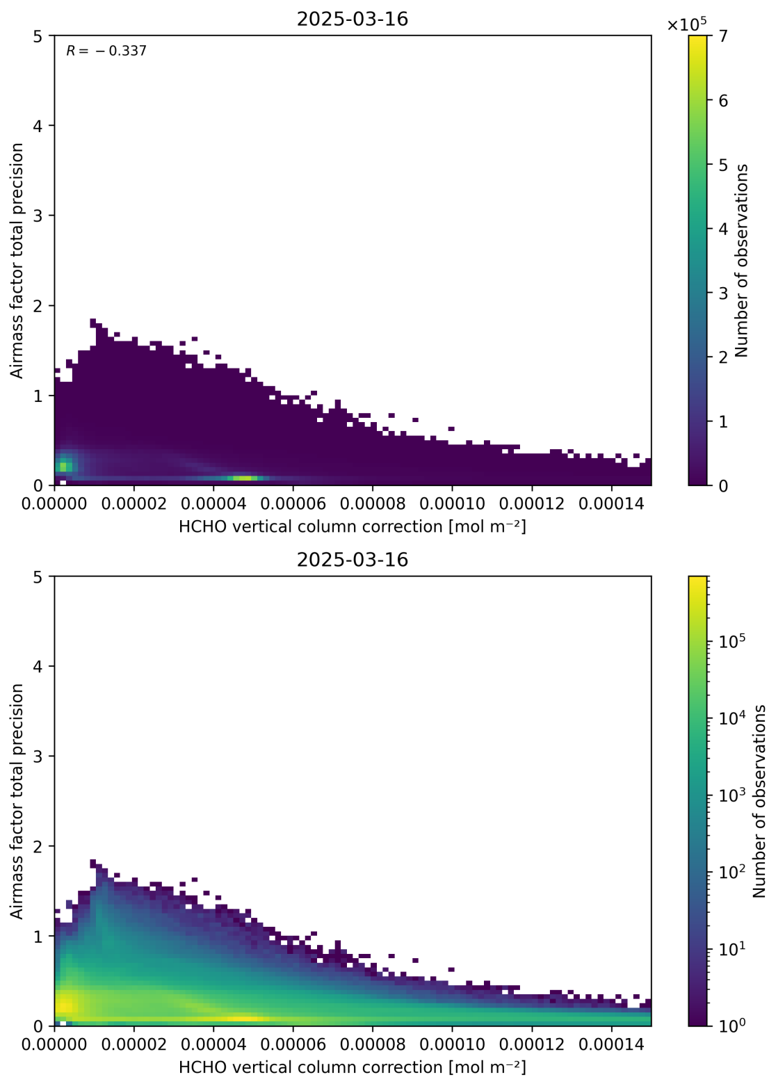
Figure 121: Scatter density plot of “HCHO vertical column correction” against “Airmass factor total precision” for 2025-03-15 to 2025-03-17.
