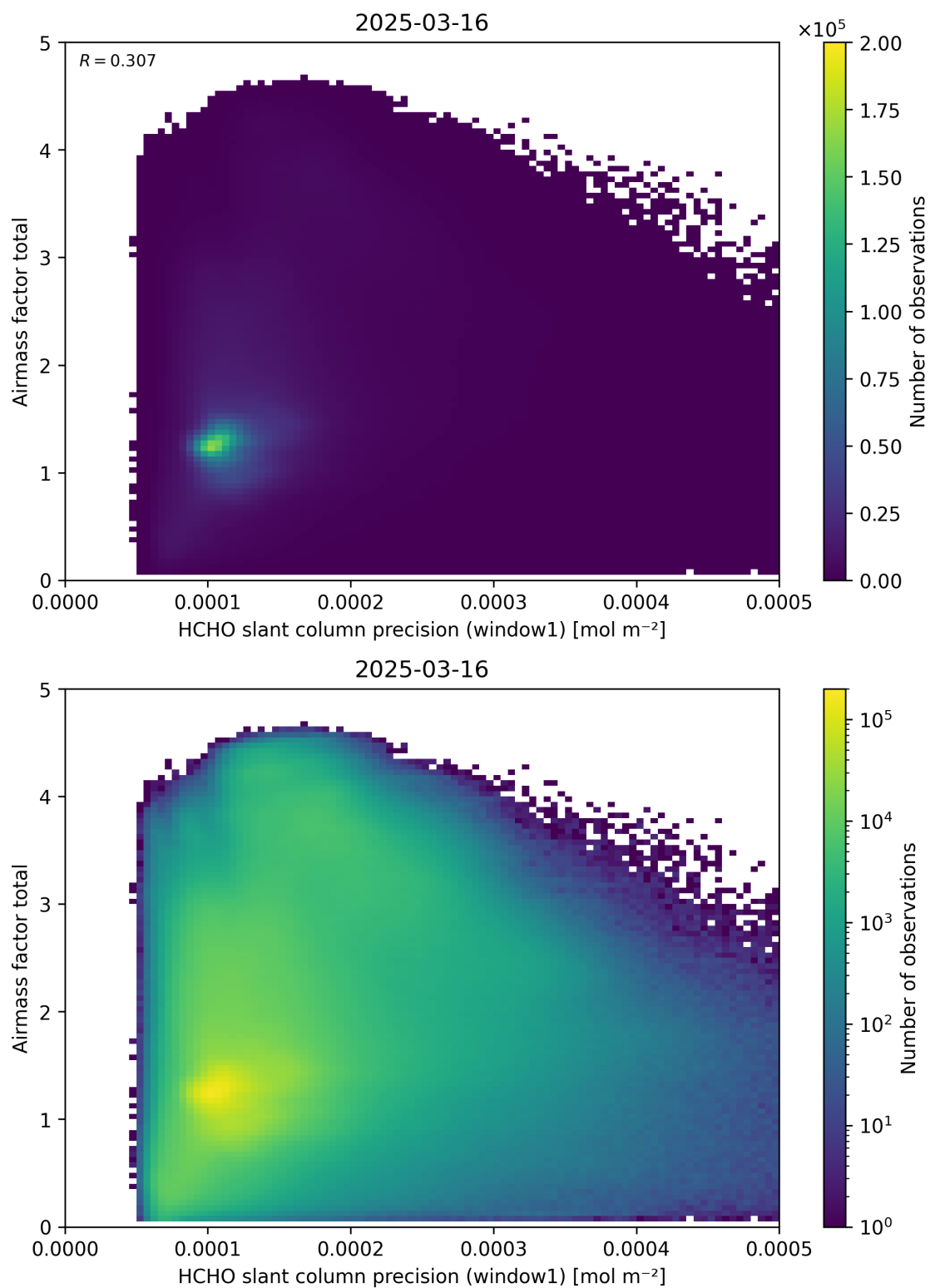
Figure 94: Scatter density plot of “HCHO slant column precision (window1)” against “Airmass factor total” for 2025-03-15 to 2025-03-17.
