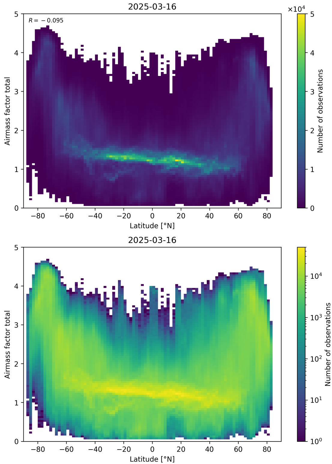
Figure 161: Scatter density plot of “Latitude” against “Airmass factor total” for 2025-03-15 to 2025-03-17.
