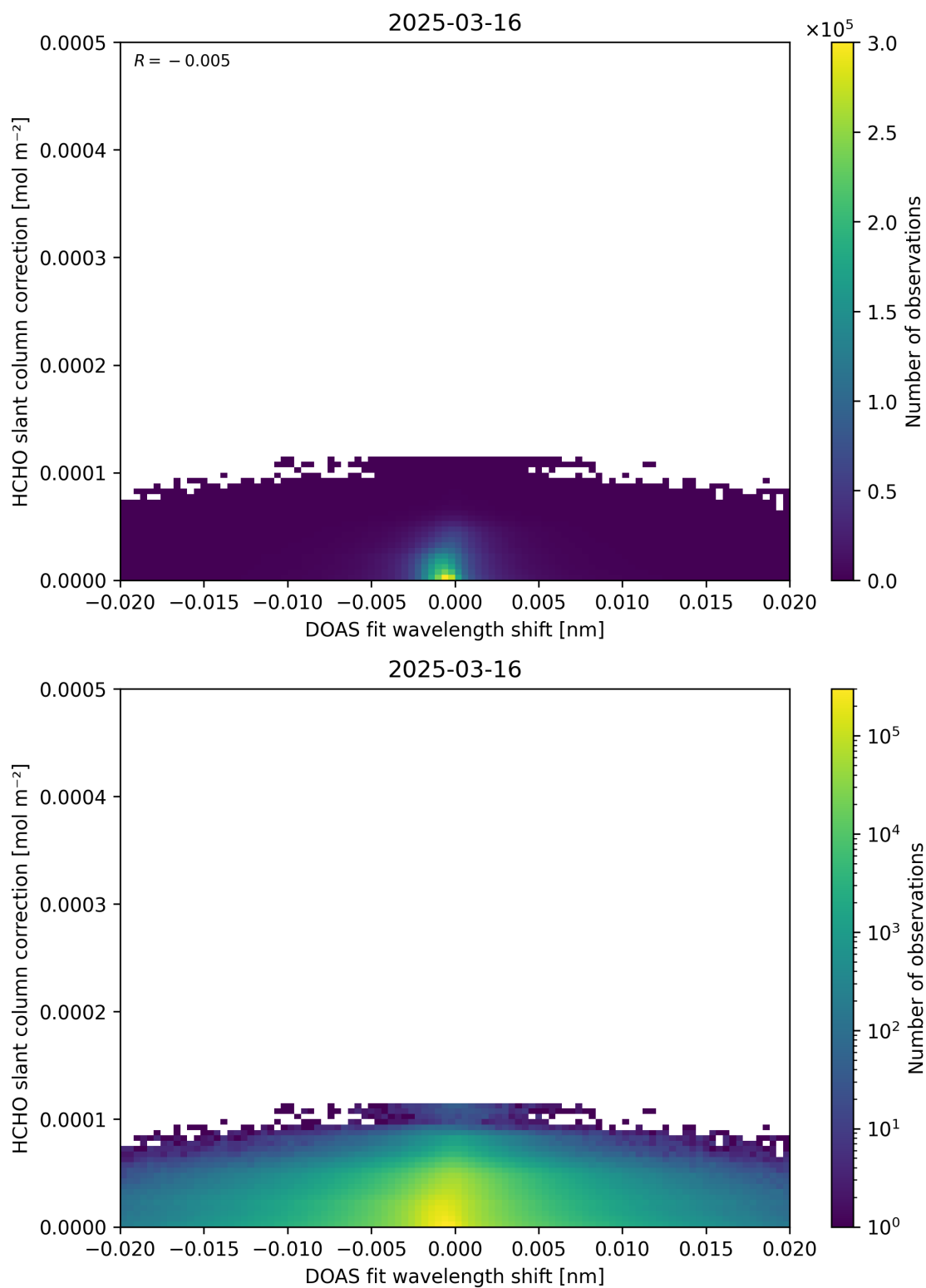
Figure 67: Scatter density plot of “DOAS fit wavelength shift” against “HCHO slant column correction” for 2025-03-15 to 2025-03-17.
