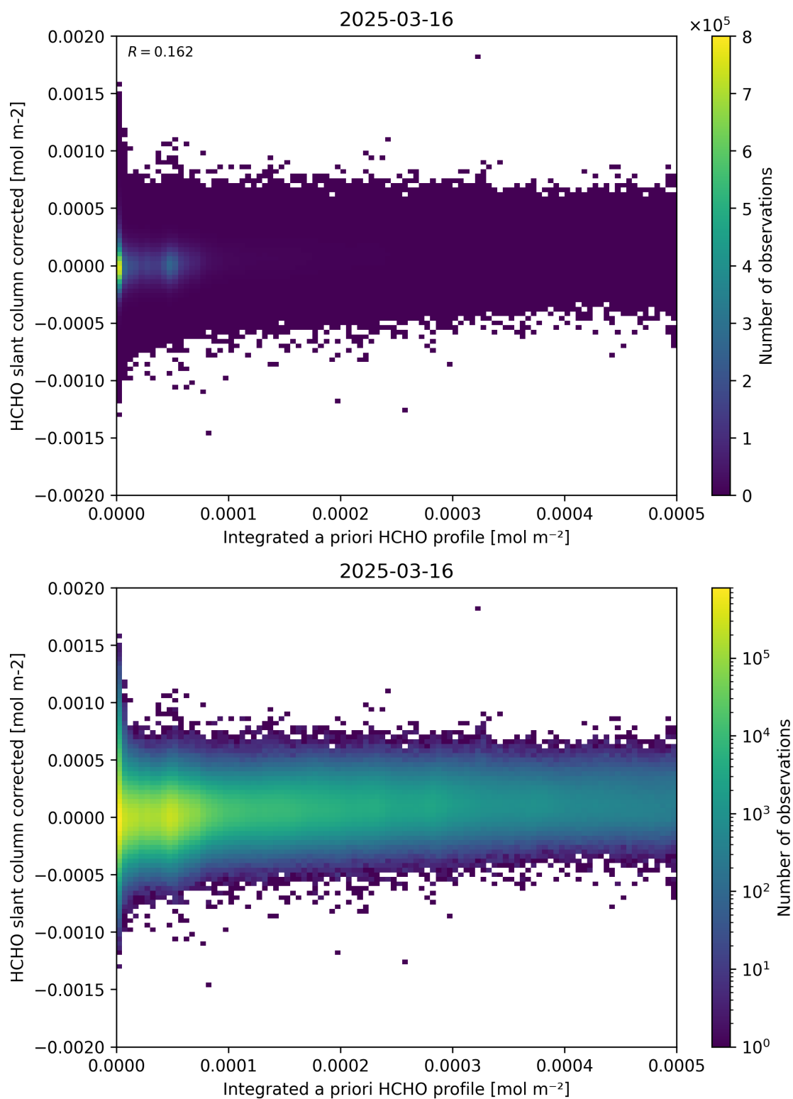
Figure 151: Scatter density plot of “Integrated a priori HCHO profile” against “HCHO slant column corrected” for 2025-03-15 to 2025-03-17.
