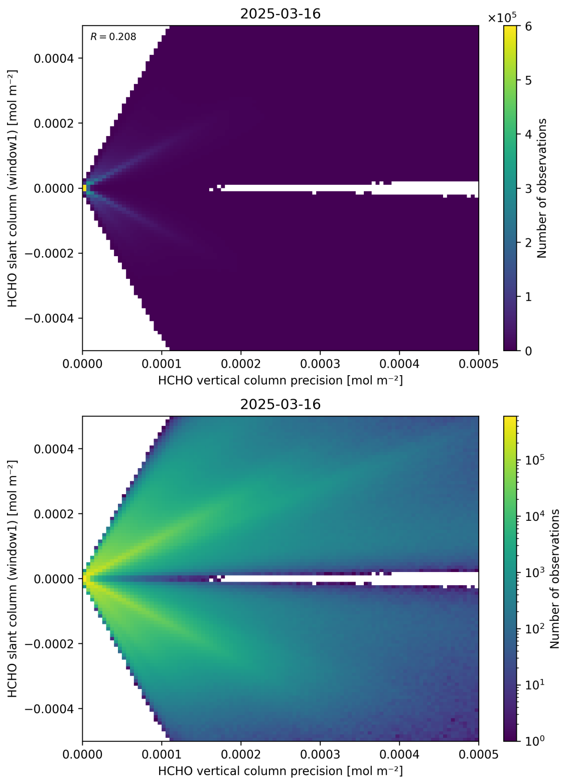
Figure 142: Scatter density plot of “HCHO vertical column precision” against “HCHO slant column (window1)” for 2025-03-15 to 2025-03-17.
