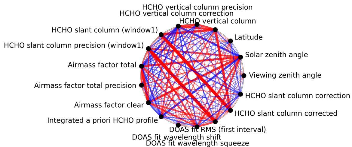
Figure 1: Map of correlation graph for 2025-03-15 to 2025-03-17.
