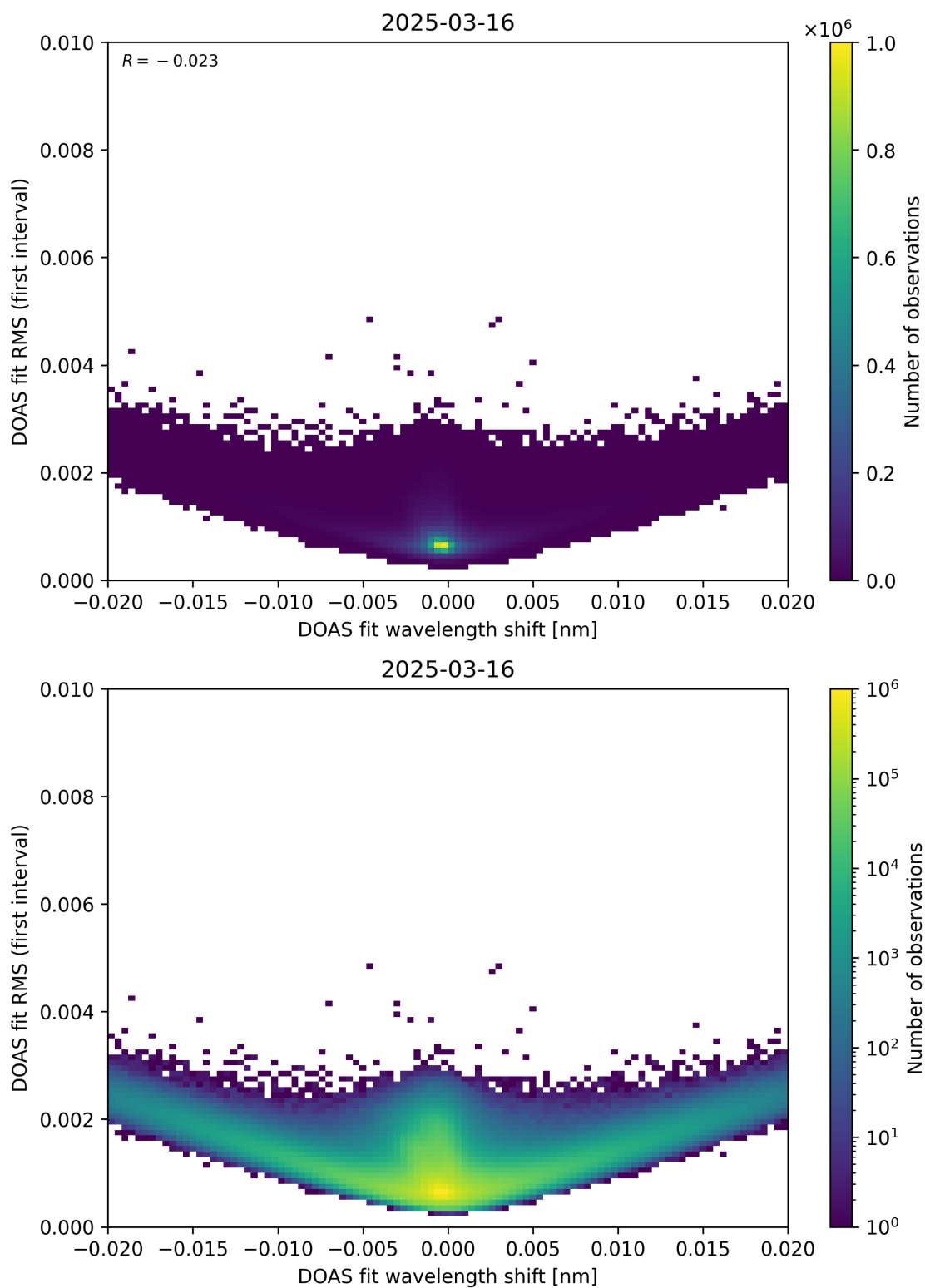
Figure 64: Scatter density plot of “DOAS fit wavelength shift” against “DOAS fit RMS (first interval)” for 2025-03-15 to 2025-03-17.
