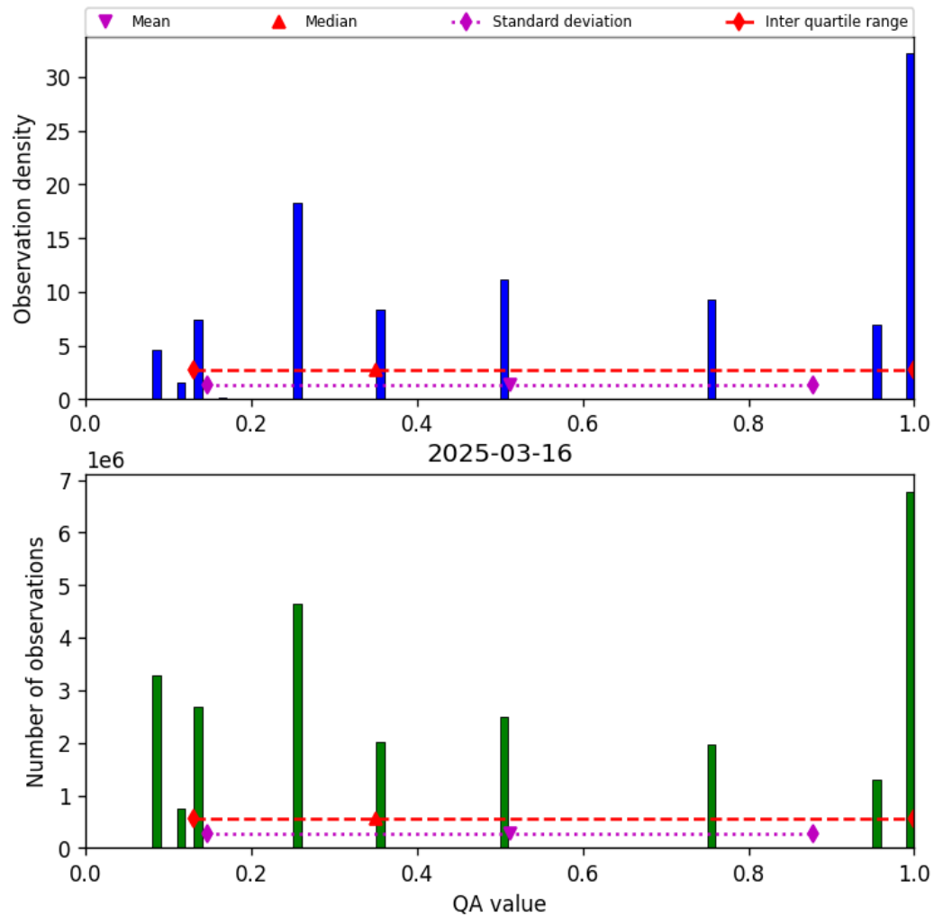
Figure 34: Histogram of “QA value” for 2025-03-15 to 2025-03-17
