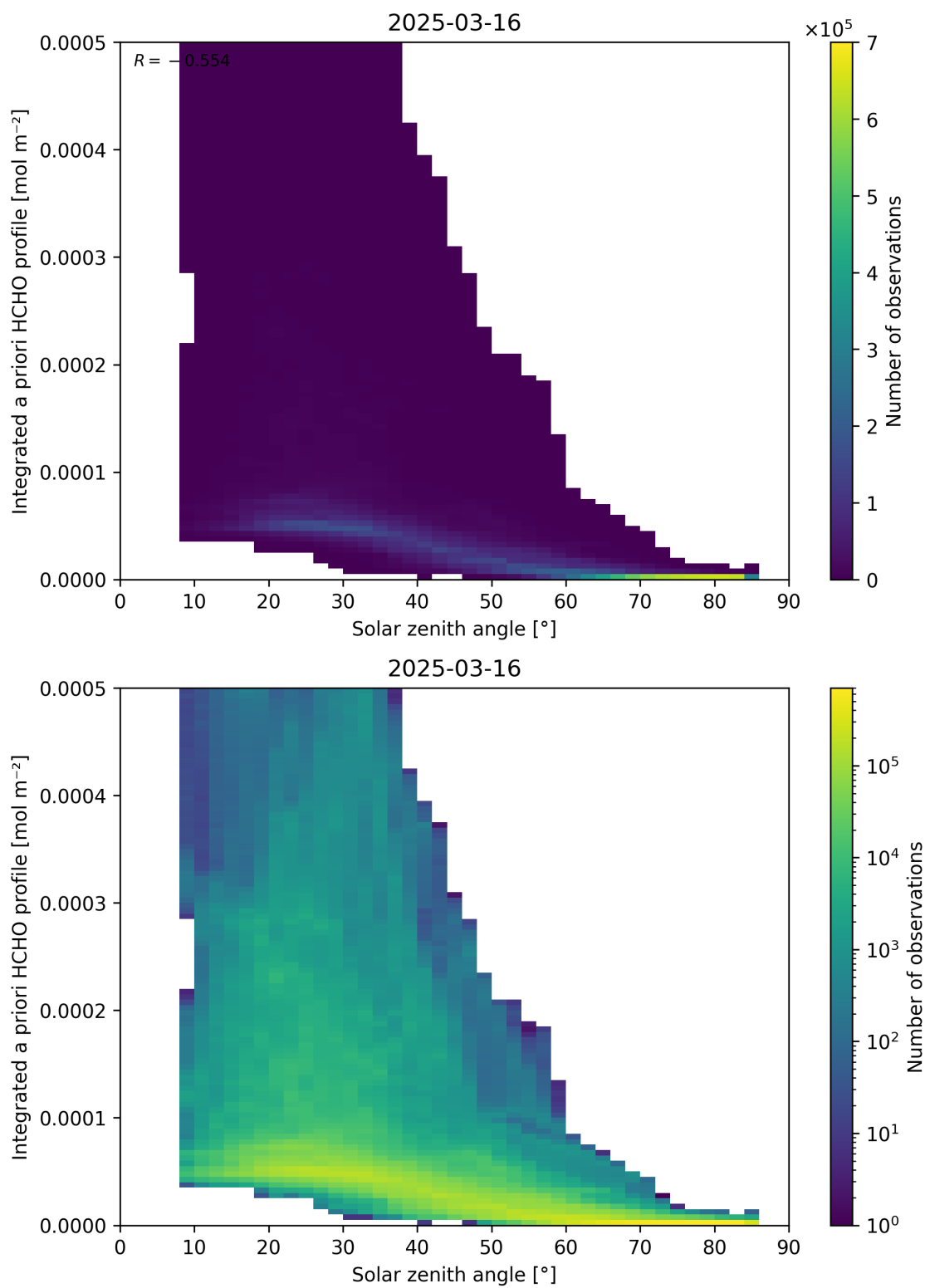
Figure 180: Scatter density plot of “Solar zenith angle” against “Integrated a priori HCHO profile” for 2025-03-15 to 2025-03-17.
