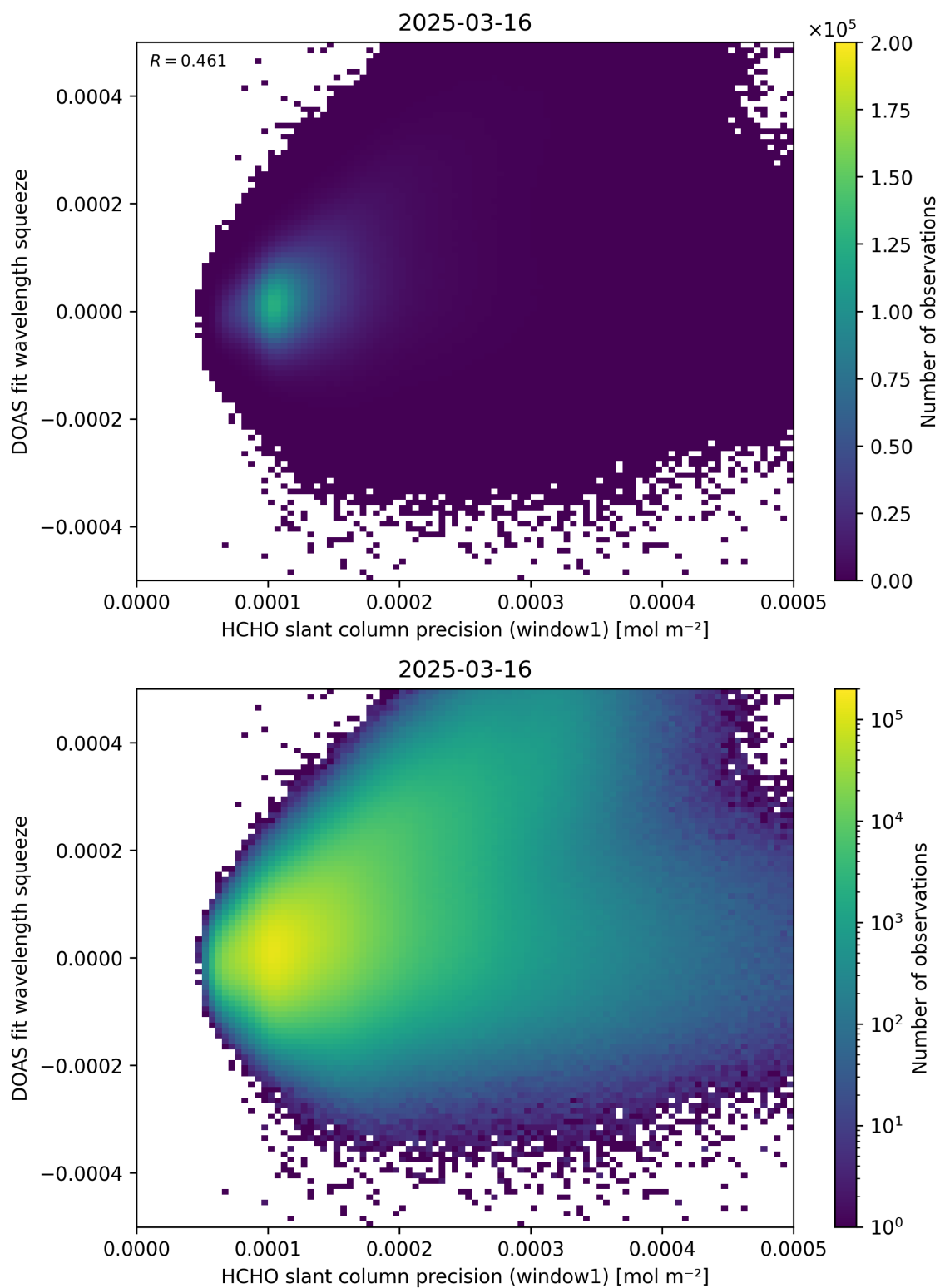
Figure 90: Scatter density plot of “HCHO slant column precision (window1)” against “DOAS fit wavelength squeeze” for 2025-03-15 to 2025-03-17.
