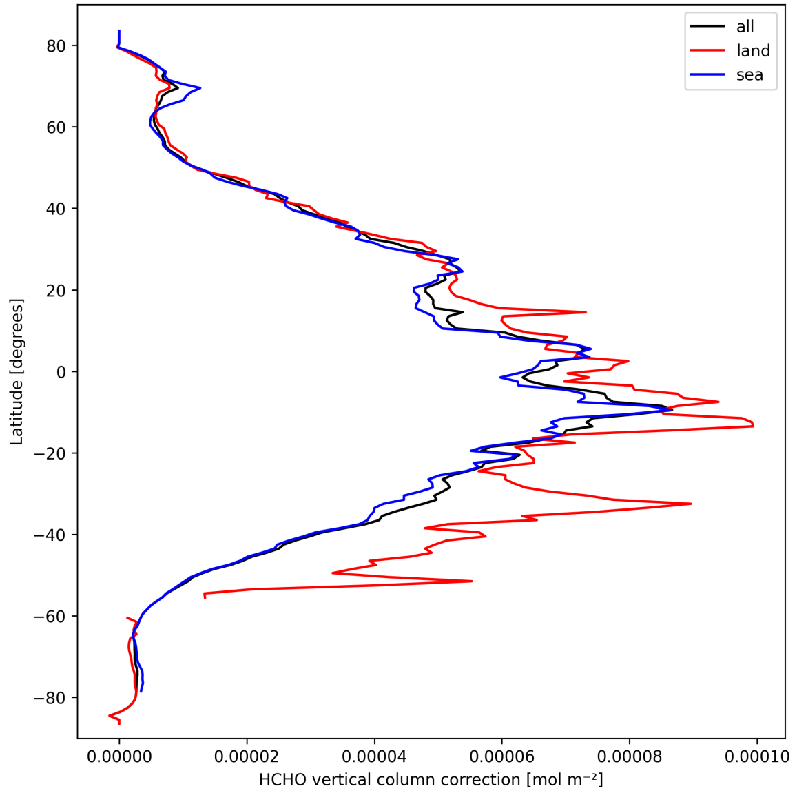
Figure 23: Zonal average of “HCHO vertical column correction” for 2025-03-15 to 2025-03-17.
