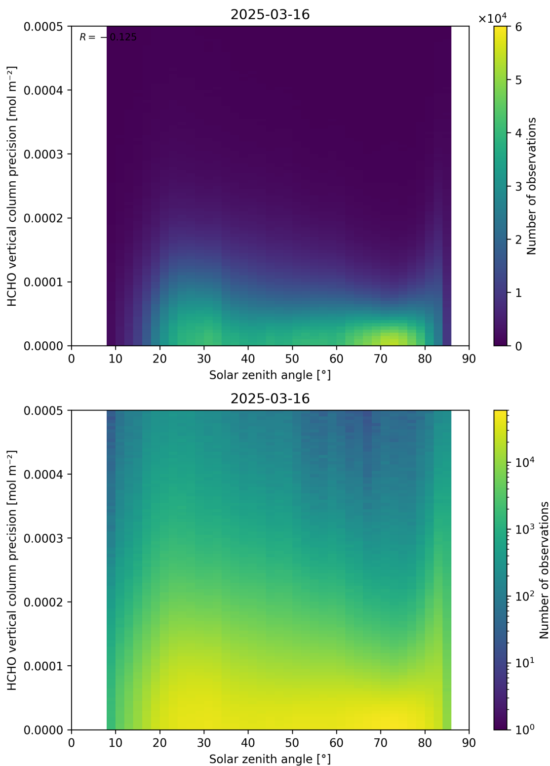
Figure 179: Scatter density plot of “Solar zenith angle” against “HCHO vertical column precision” for 2025-03-15 to 2025-03-17.
