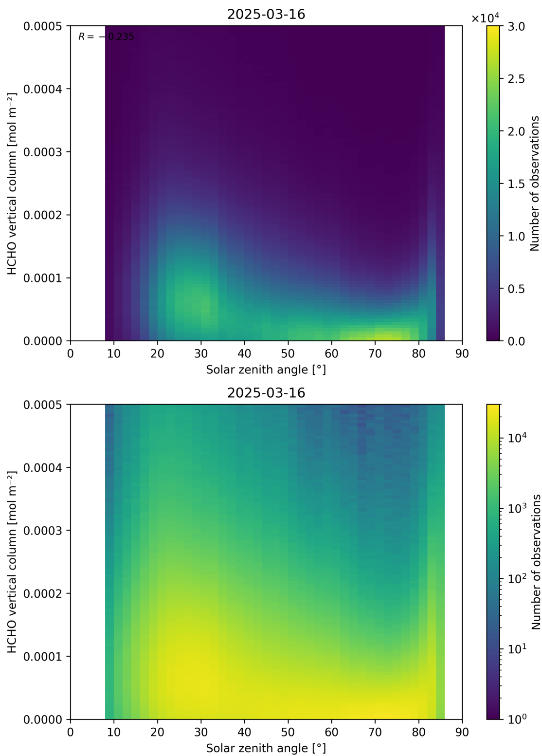
Figure 177: Scatter density plot of “Solar zenith angle” against “HCHO vertical column” for 2025-03-15 to 2025-03-17.
