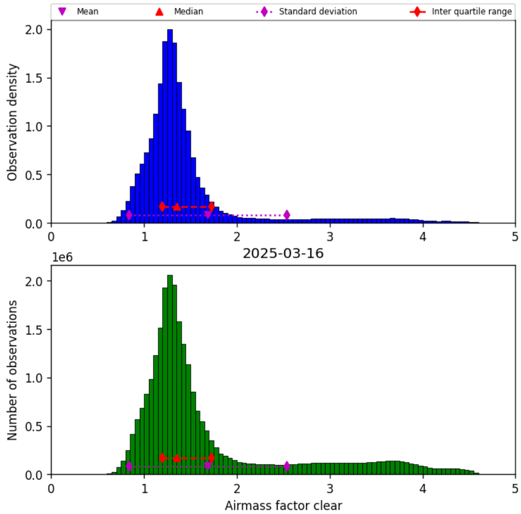
Figure 42: Histogram of “Airmass factor clear” for 2025-03-15 to 2025-03-17
