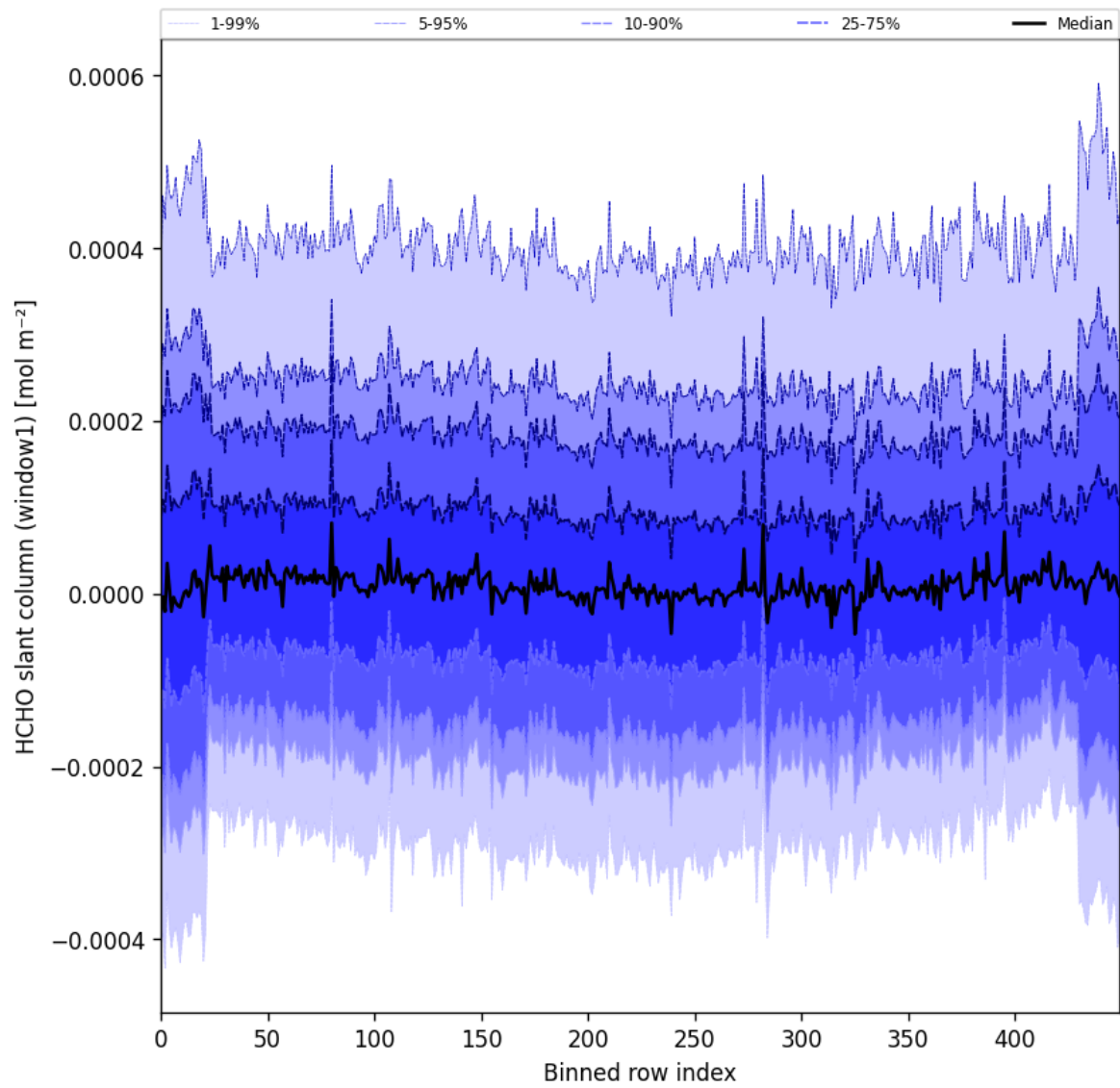
Figure 52: Along track statistics of “HCHO slant column (window1)” for 2025-03-15 to 2025-03-17
