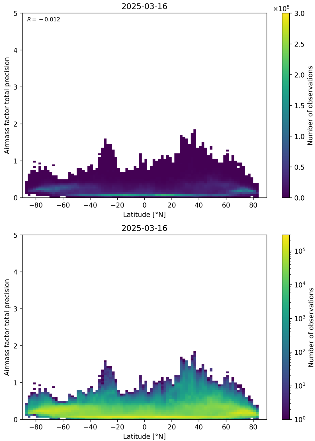
Figure 162: Scatter density plot of “Latitude” against “Airmass factor total precision” for 2025-03-15 to 2025-03-17.
