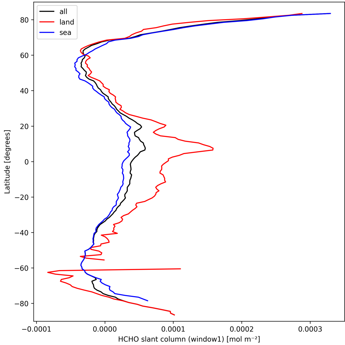
Figure 24: Zonal average of “HCHO slant column (window1)” for 2025-03-15 to 2025-03-17.
