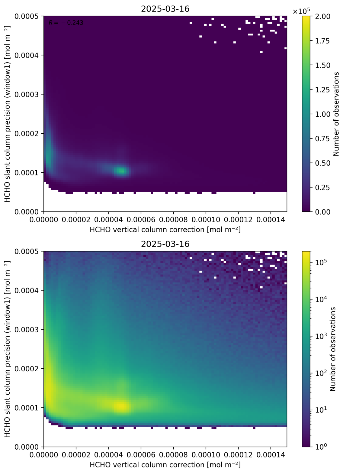
Figure 119: Scatter density plot of “HCHO vertical column correction” against “HCHO slant column precision (window1)” for 2025-03-15 to 2025-03-17.
