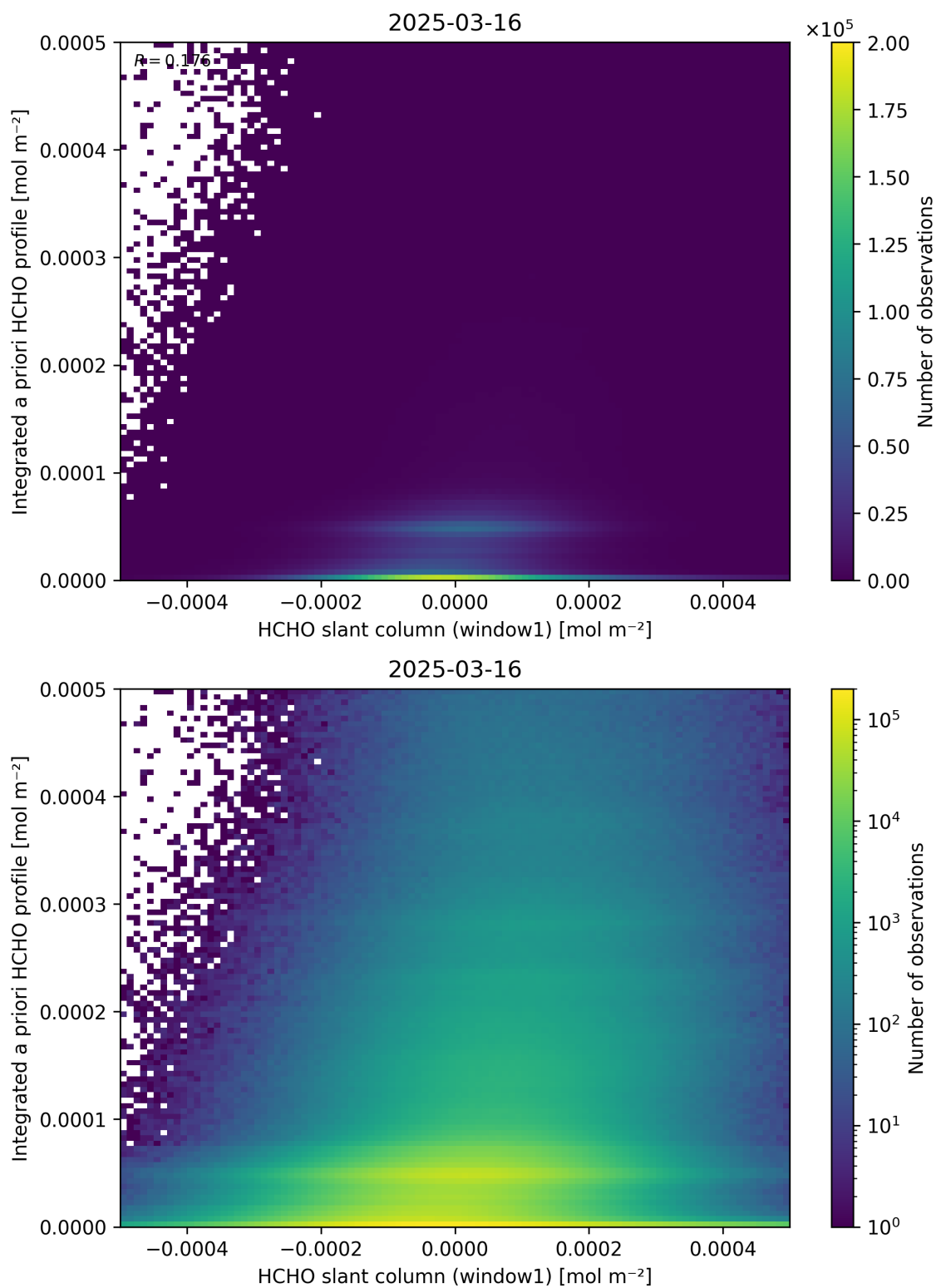
Figure 87: Scatter density plot of “HCHO slant column (window1)” against “Integrated a priori HCHO profile” for 2025-03-15 to 2025-03-17.
