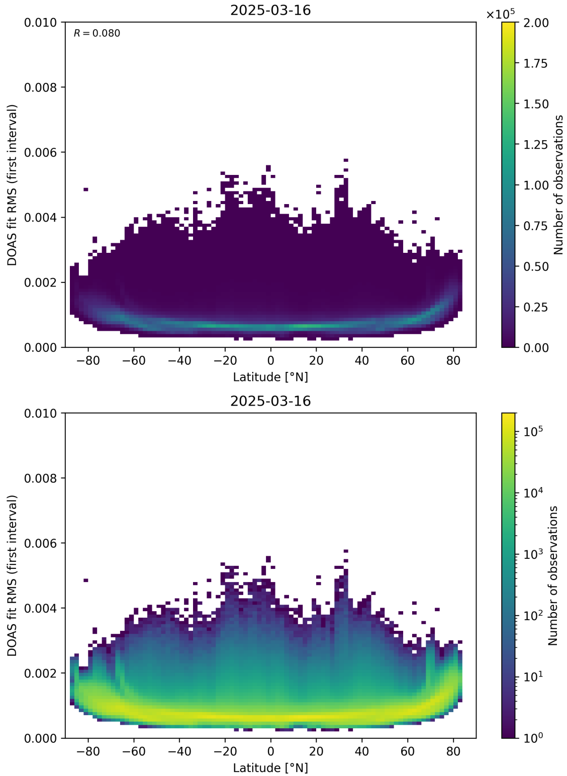
Figure 153: Scatter density plot of “Latitude” against “DOAS fit RMS (first interval)” for 2025-03-15 to 2025-03-17.
