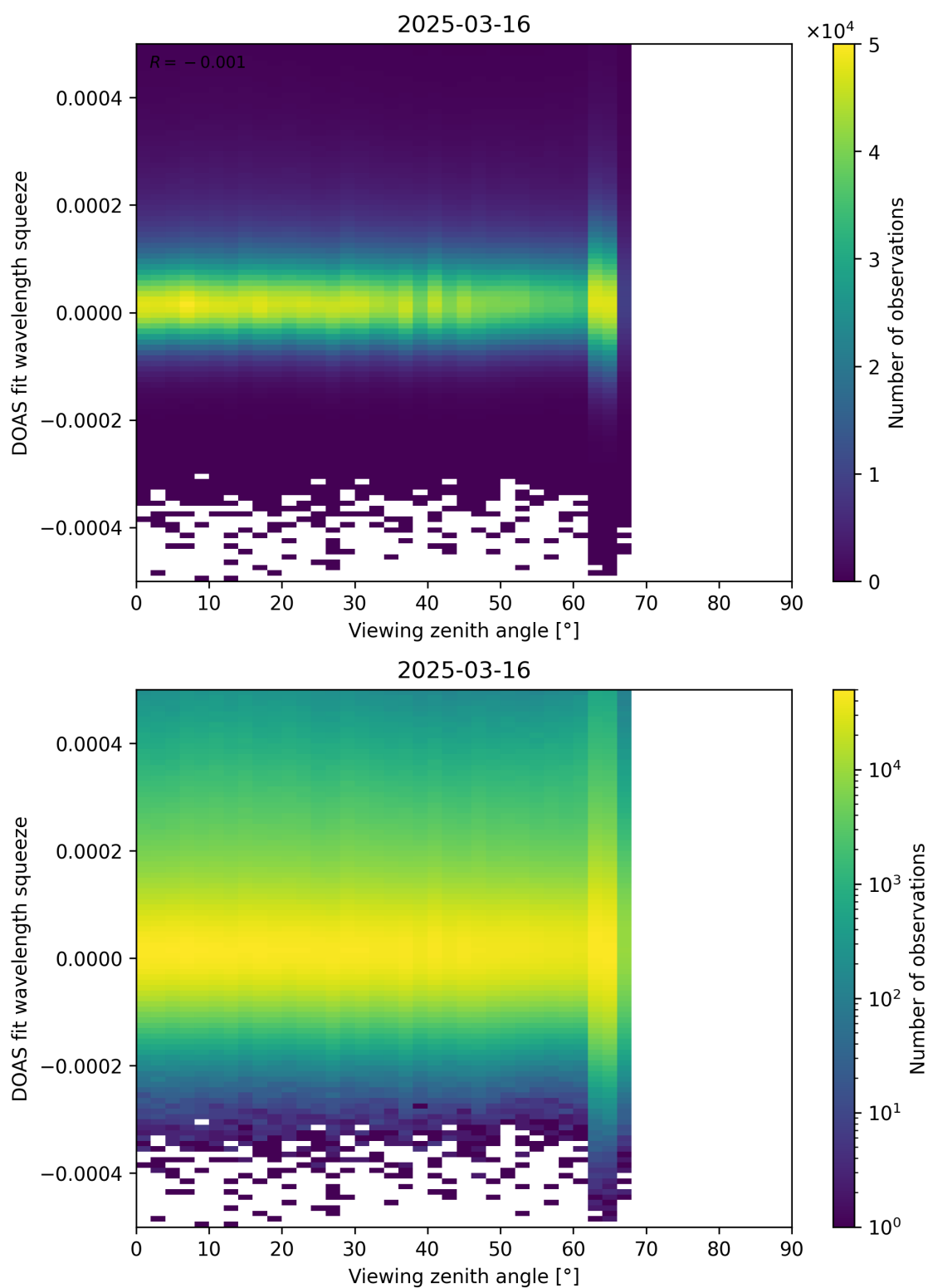
Figure 184: Scatter density plot of “Viewing zenith angle” against “DOAS fit wavelength squeeze” for 2025-03-15 to 2025-03-17.
