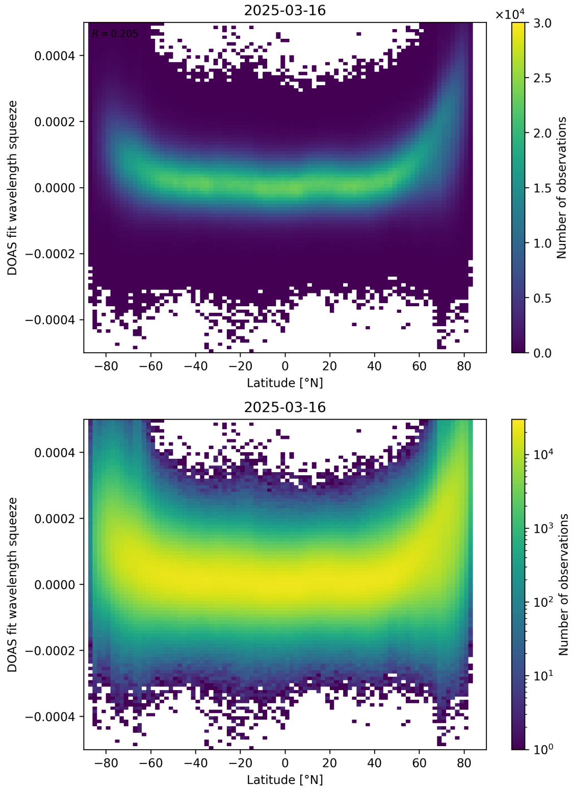
Figure 155: Scatter density plot of “Latitude” against “DOAS fit wavelength squeeze” for 2025-03-15 to 2025-03-17.
