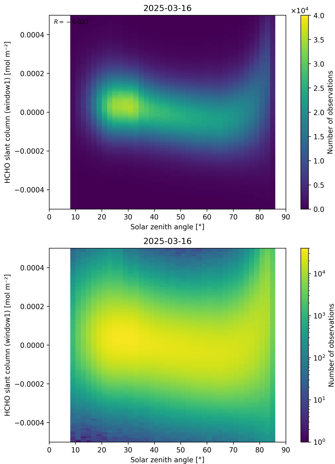
Figure 173: Scatter density plot of “Solar zenith angle” against “HCHO slant column (window1)” for 2025-03-15 to 2025-03-17.
