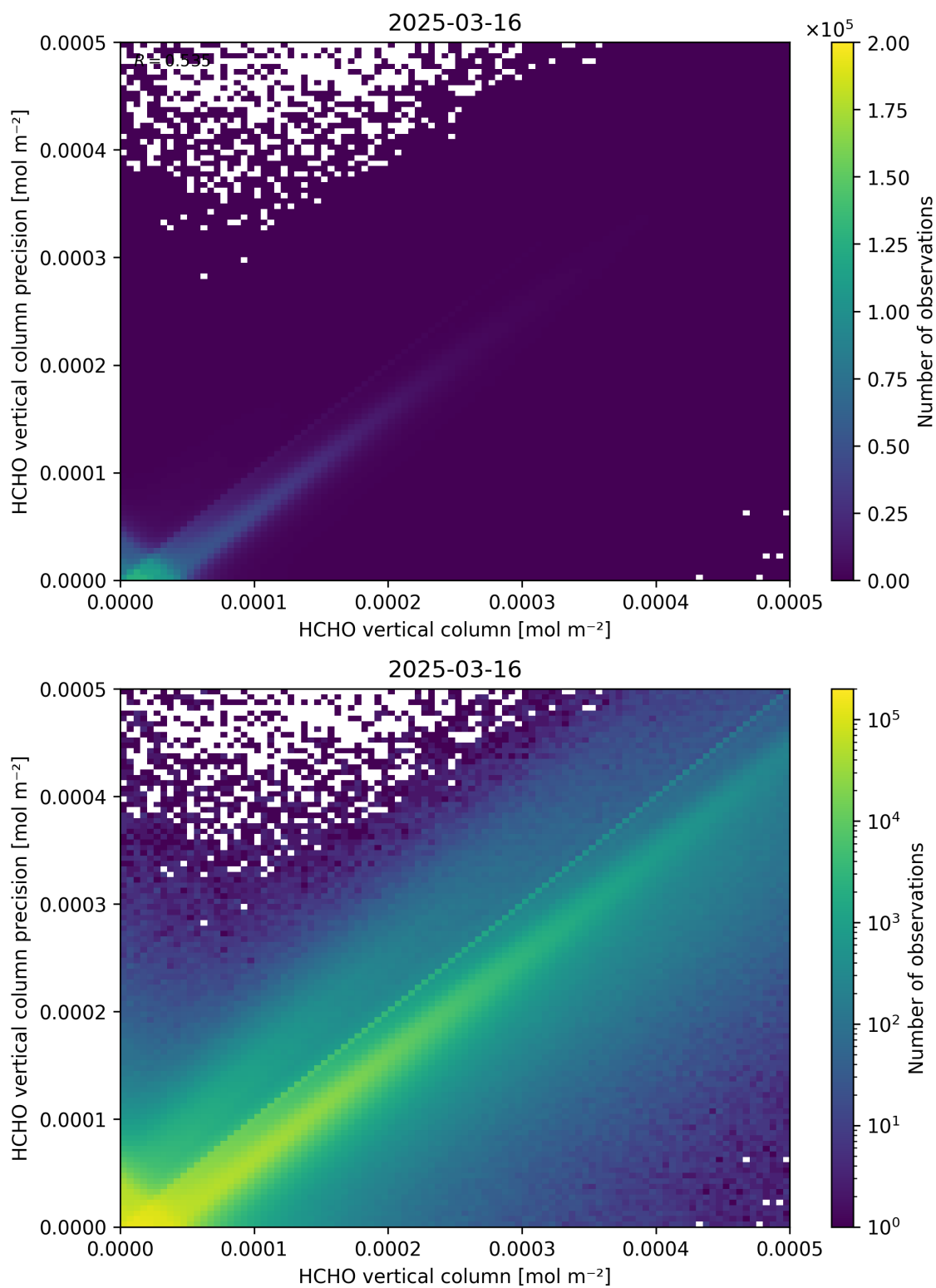
Figure 134: Scatter density plot of “HCHO vertical column” against “HCHO vertical column precision” for 2025-03-15 to 2025-03-17.
