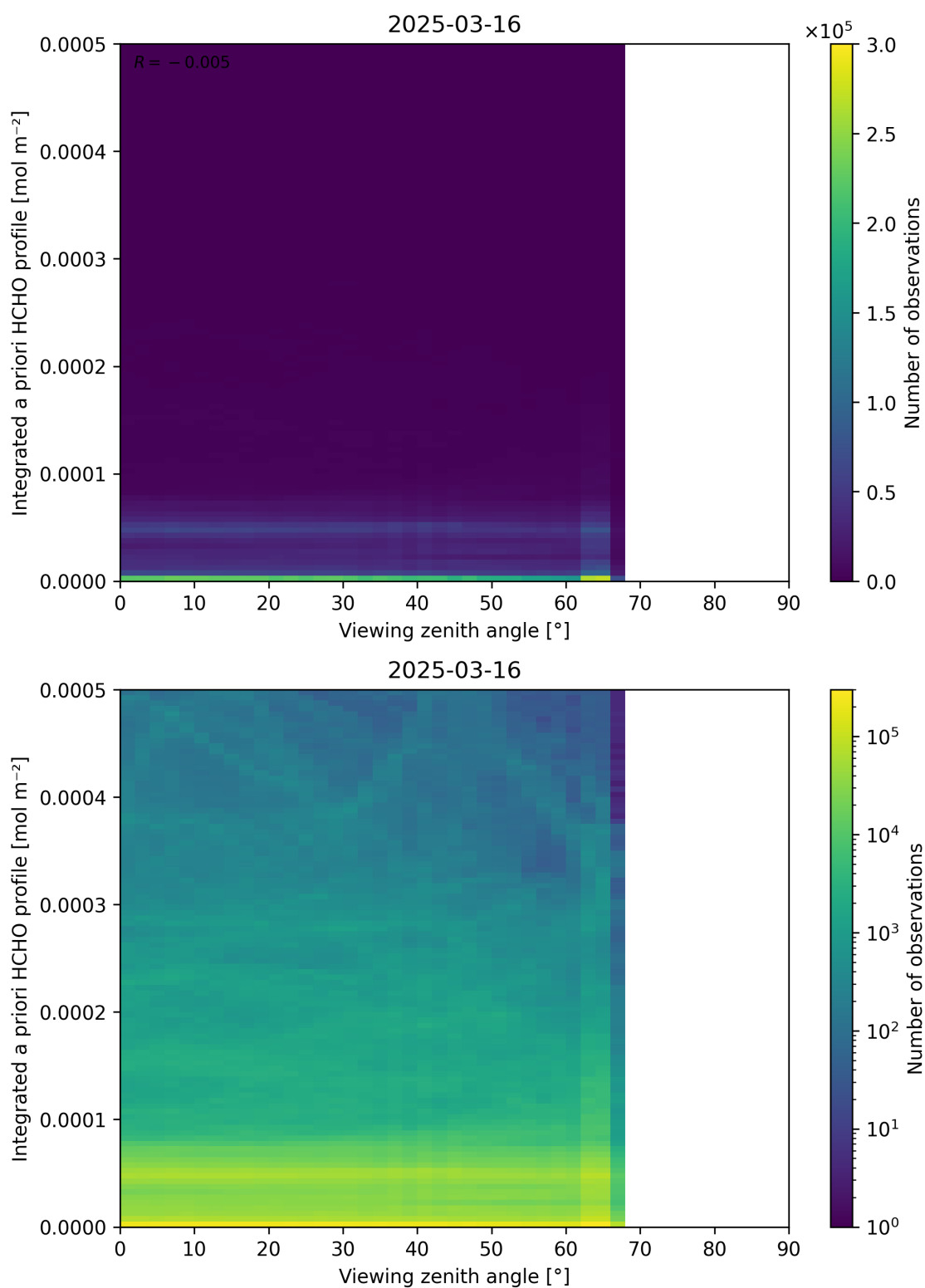
Figure 195: Scatter density plot of “Viewing zenith angle” against “Integrated a priori HCHO profile” for 2025-03-15 to 2025-03-17.
