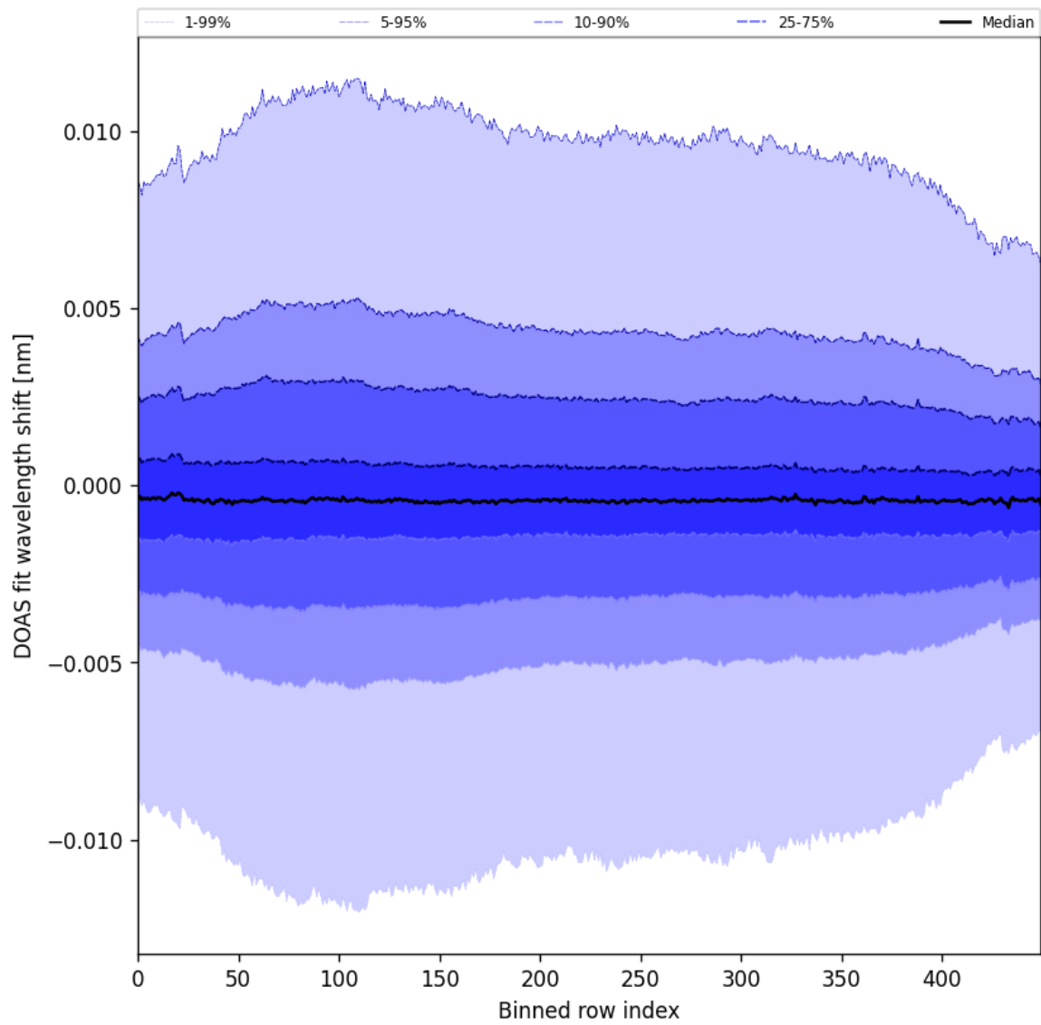
Figure 58: Along track statistics of “DOAS fit wavelength shift” for 2025-03-15 to 2025-03-17
