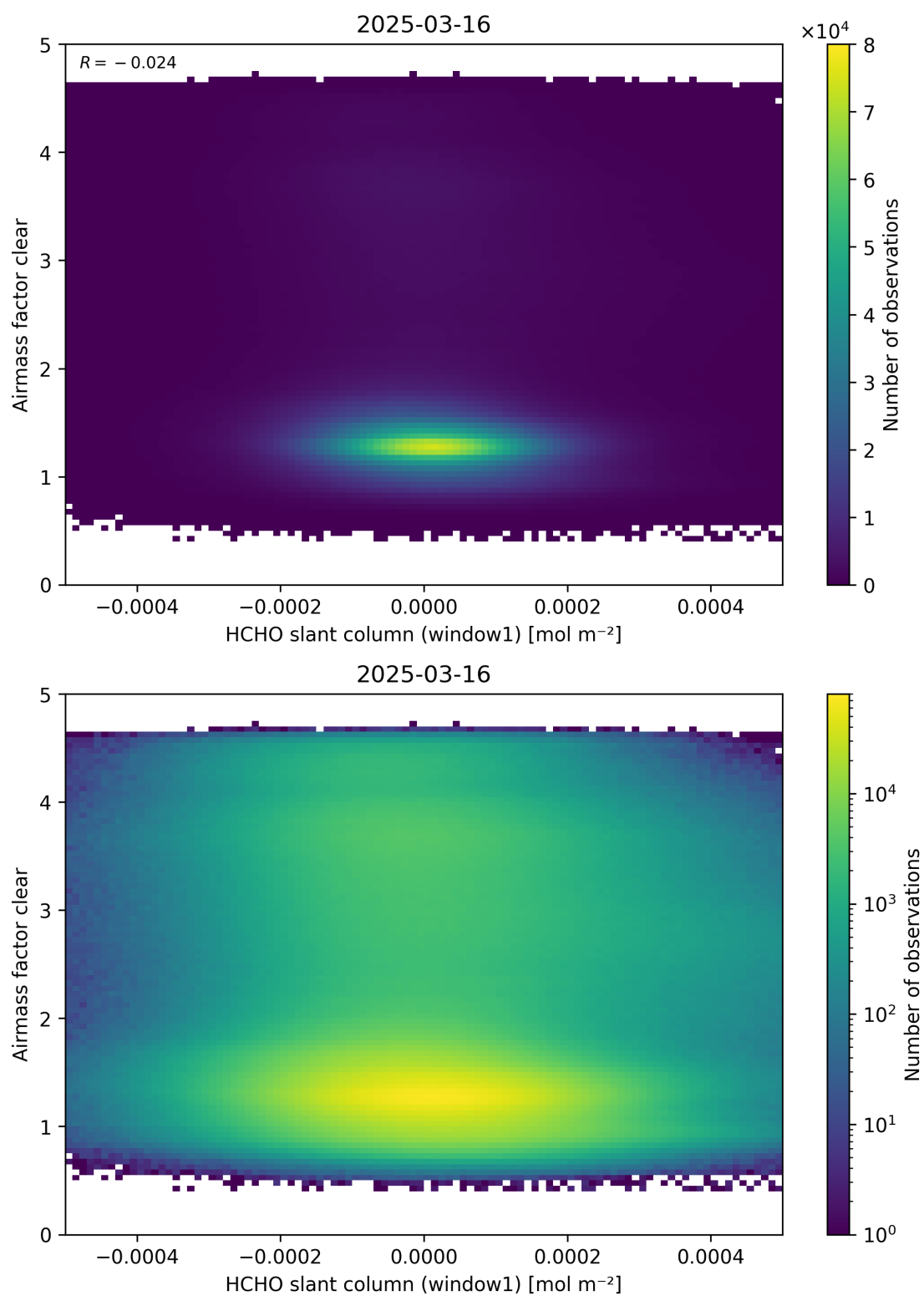
Figure 81: Scatter density plot of “HCHO slant column (window1)” against “Airmass factor clear” for 2025-03-15 to 2025-03-17.
