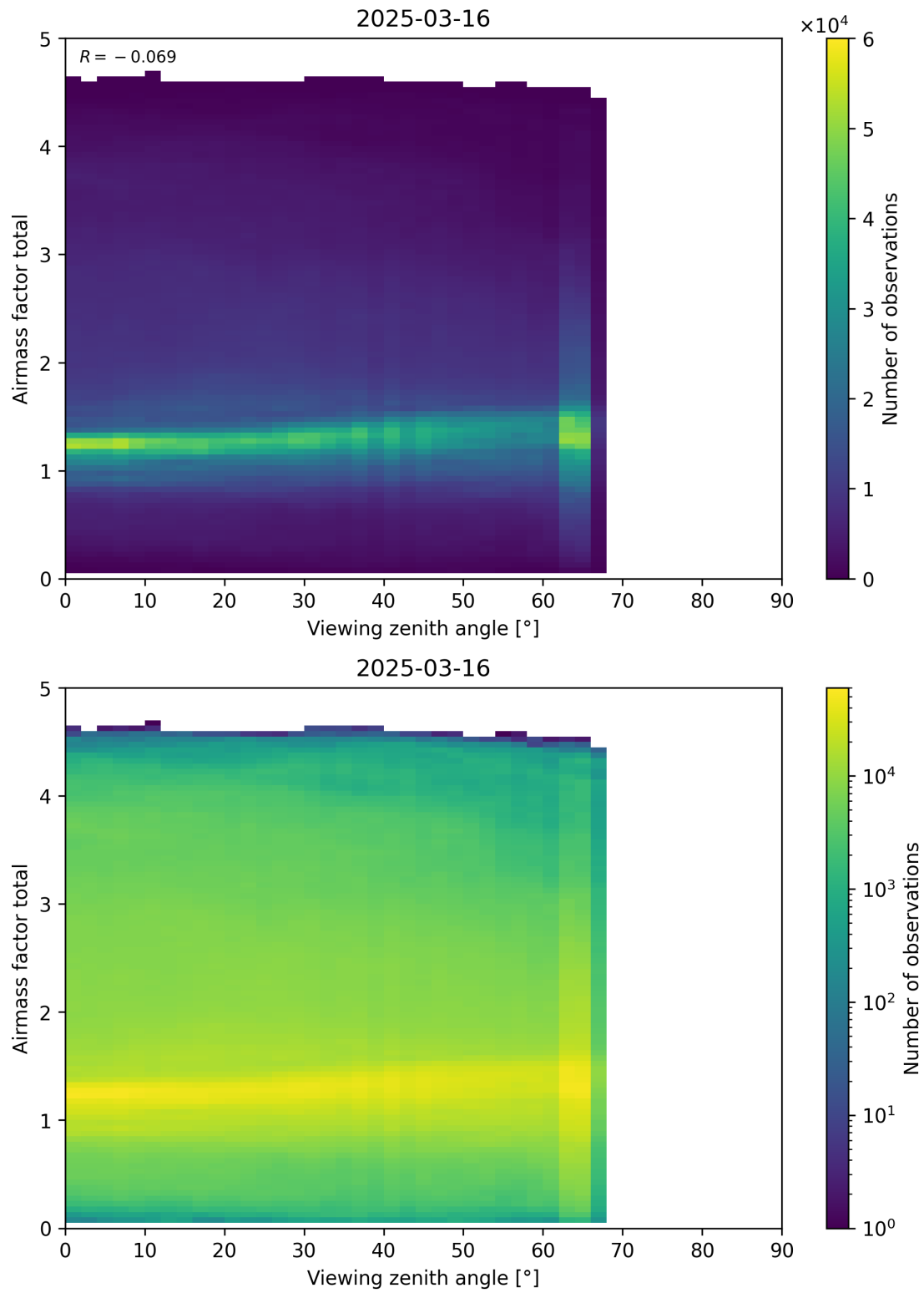
Figure 190: Scatter density plot of “Viewing zenith angle” against “Airmass factor total” for 2025-03-15 to 2025-03-17.
