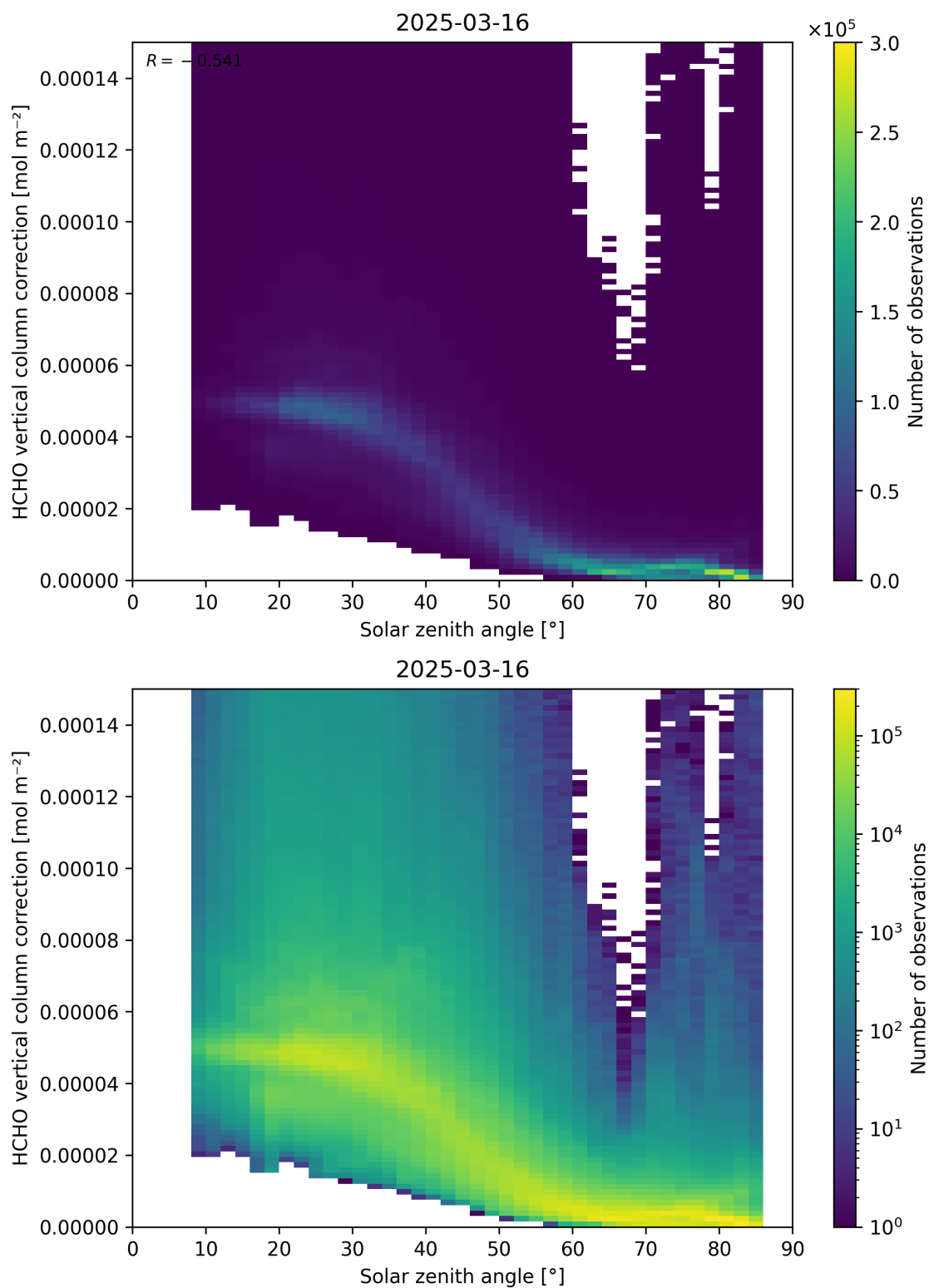
Figure 178: Scatter density plot of “Solar zenith angle” against “HCHO vertical column correction” for 2025-03-15 to 2025-03-17.
