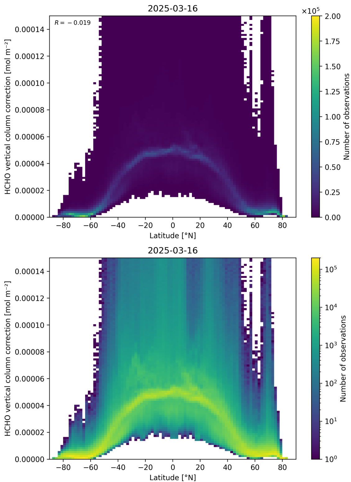
Figure 164: Scatter density plot of “Latitude” against “HCHO vertical column correction” for 2025-03-15 to 2025-03-17.
