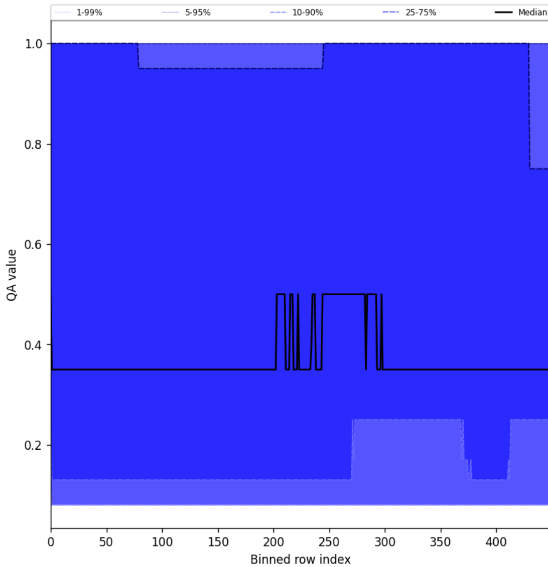
Figure 48: Along track statistics of “QA value” for 2025-03-15 to 2025-03-17
