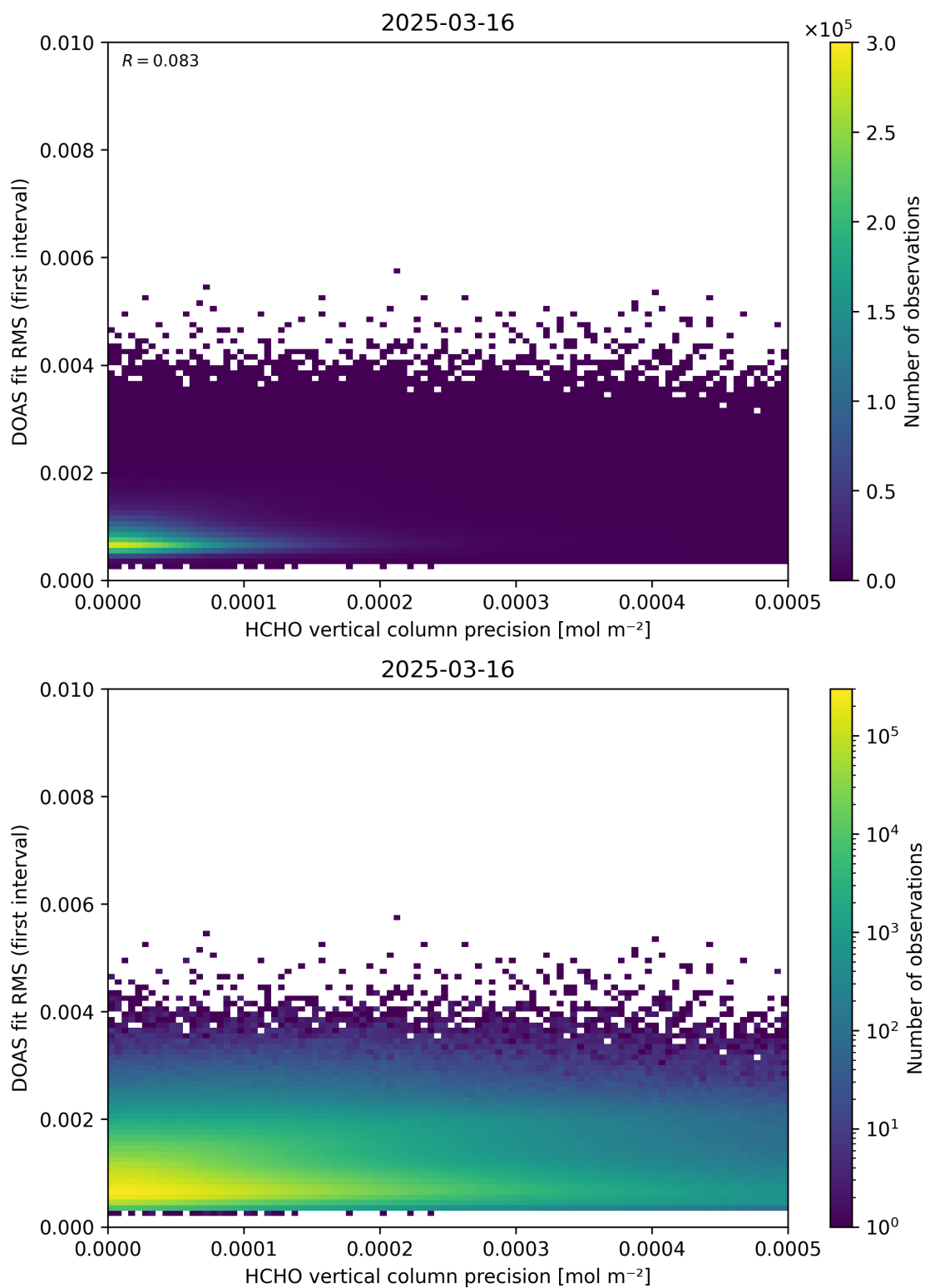
Figure 136: Scatter density plot of “HCHO vertical column precision” against “DOAS fit RMS (first interval)” for 2025-03-15 to 2025-03-17.
