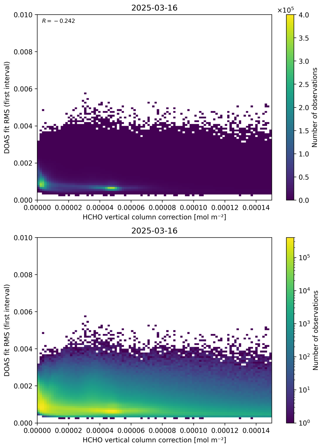
Figure 112: Scatter density plot of “HCHO vertical column correction” against “DOAS fit RMS (first interval)” for 2025-03-15 to 2025-03-17.
