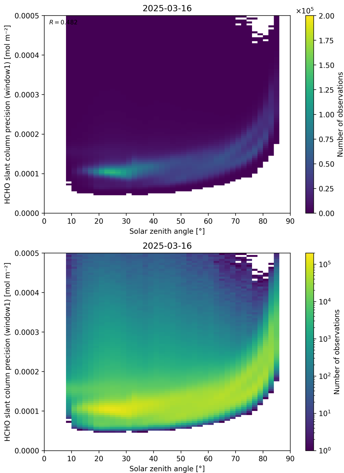
Figure 174: Scatter density plot of “Solar zenith angle” against “HCHO slant column precision (window1)” for 2025-03-15 to 2025-03-17.
