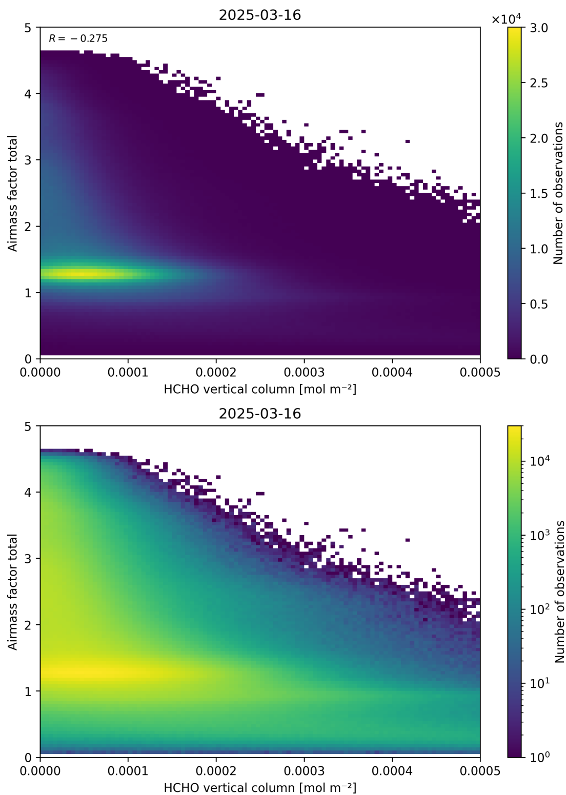
Figure 131: Scatter density plot of “HCHO vertical column” against “Airmass factor total” for 2025-03-15 to 2025-03-17.
