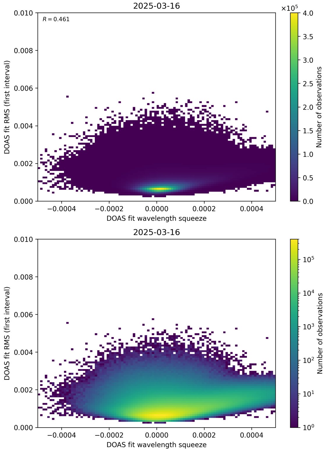
Figure 68: Scatter density plot of “DOAS fit wavelength squeeze” against “DOAS fit RMS (first interval)” for 2025-03-15 to 2025-03-17.
