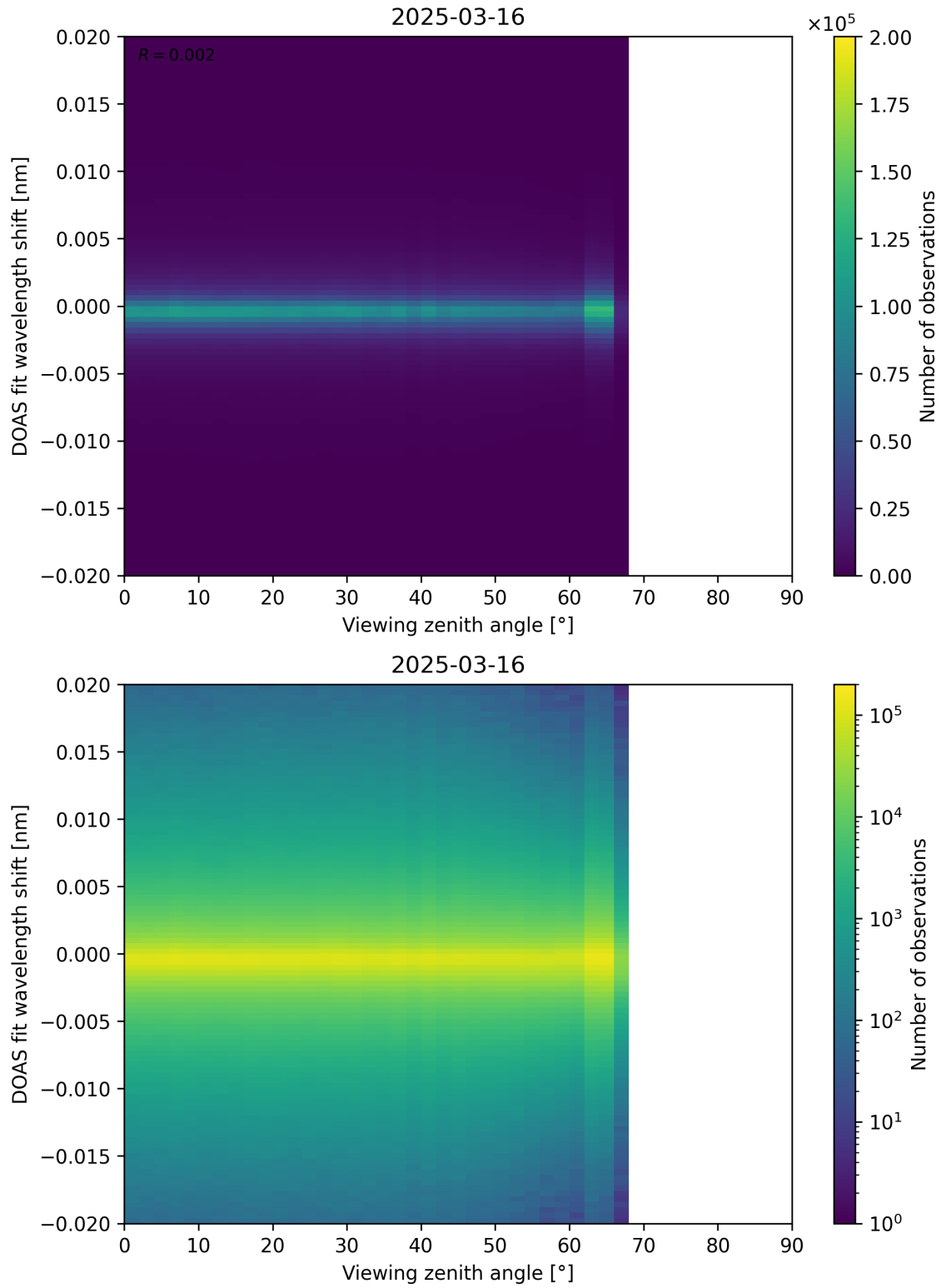
Figure 183: Scatter density plot of “Viewing zenith angle” against “DOAS fit wavelength shift” for 2025-03-15 to 2025-03-17.
