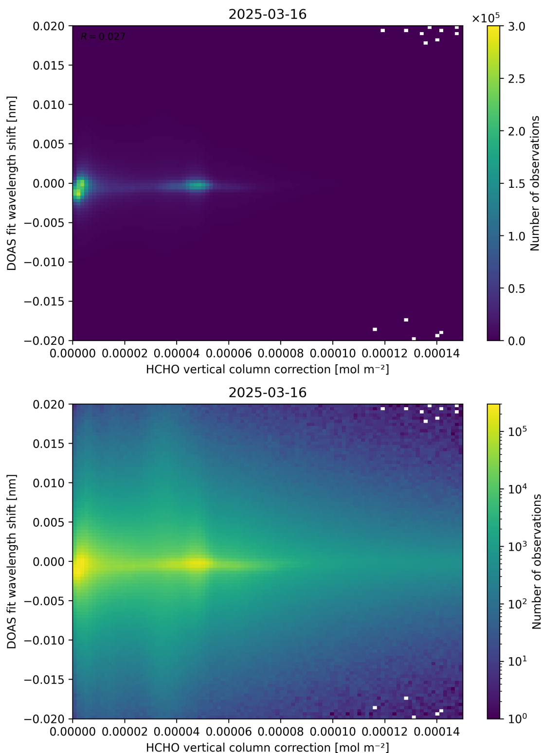
Figure 113: Scatter density plot of “HCHO vertical column correction” against “DOAS fit wavelength shift” for 2025-03-15 to 2025-03-17.
