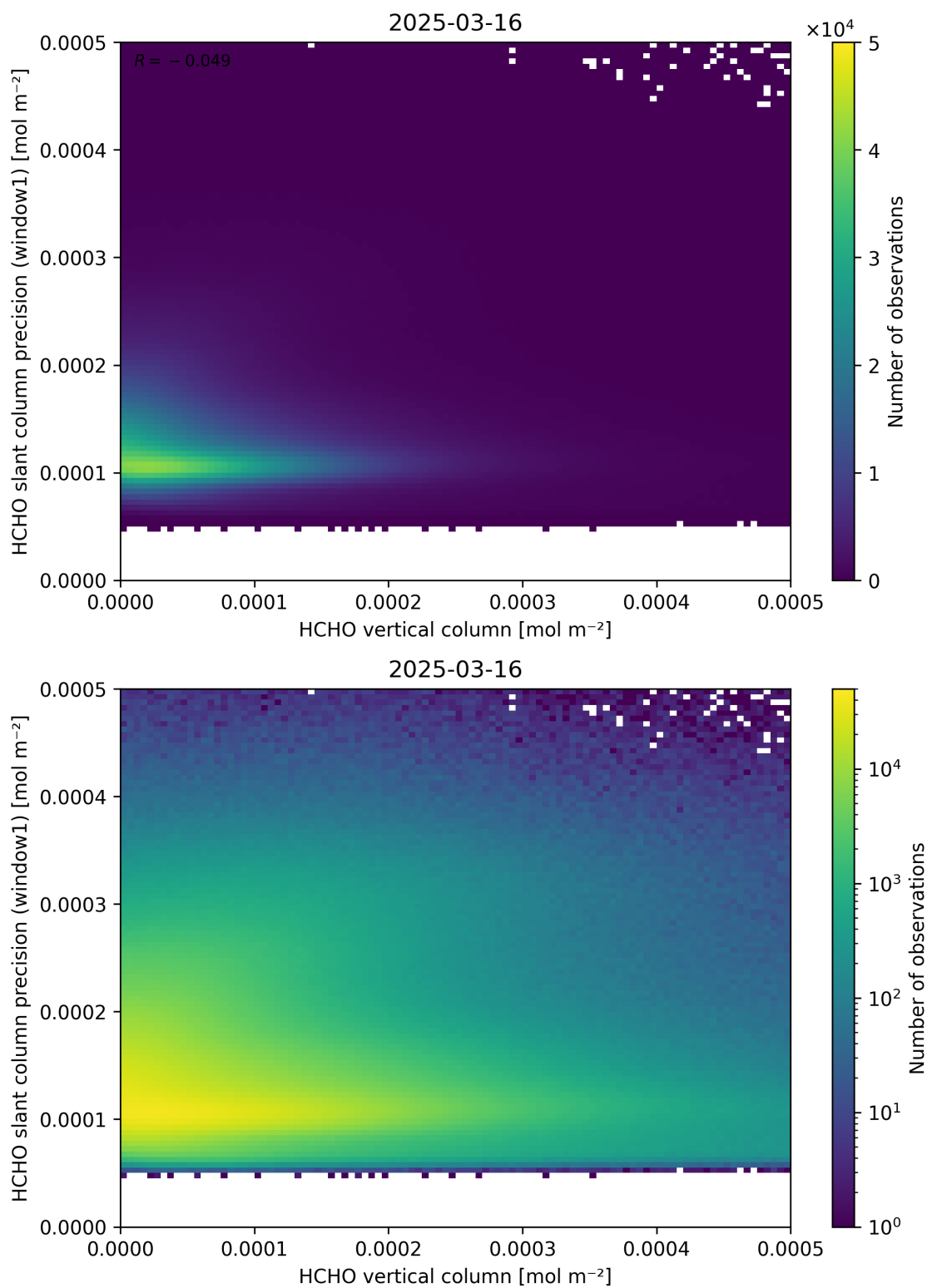
Figure 130: Scatter density plot of “HCHO vertical column” against “HCHO slant column precision (window1)” for 2025-03-15 to 2025-03-17.
