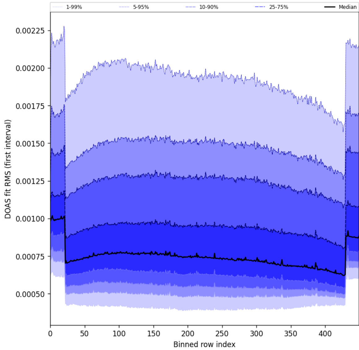
Figure 60: Along track statistics of “DOAS fit RMS (first interval)” for 2025-03-15 to 2025-03-17
