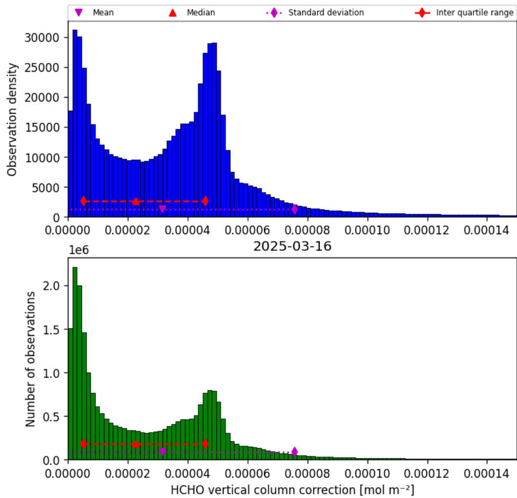
Figure 37: Histogram of “HCHO vertical column correction” for 2025-03-15 to 2025-03-17
