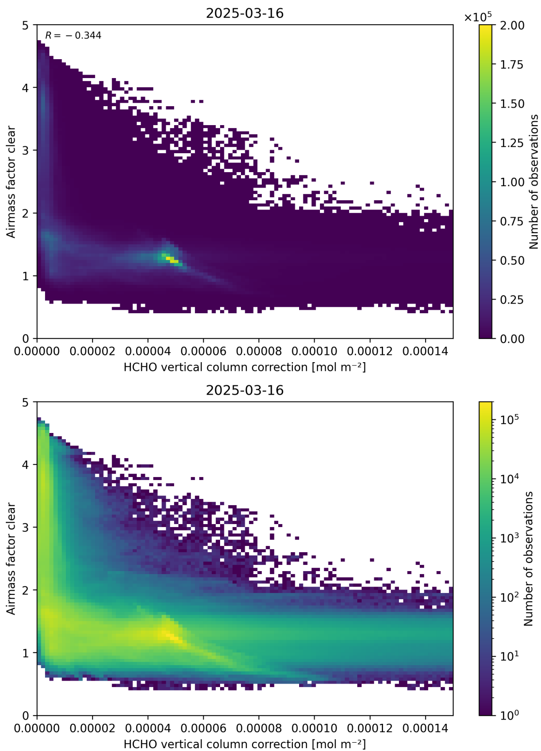
Figure 115: Scatter density plot of “HCHO vertical column correction” against “Airmass factor clear” for 2025-03-15 to 2025-03-17.
