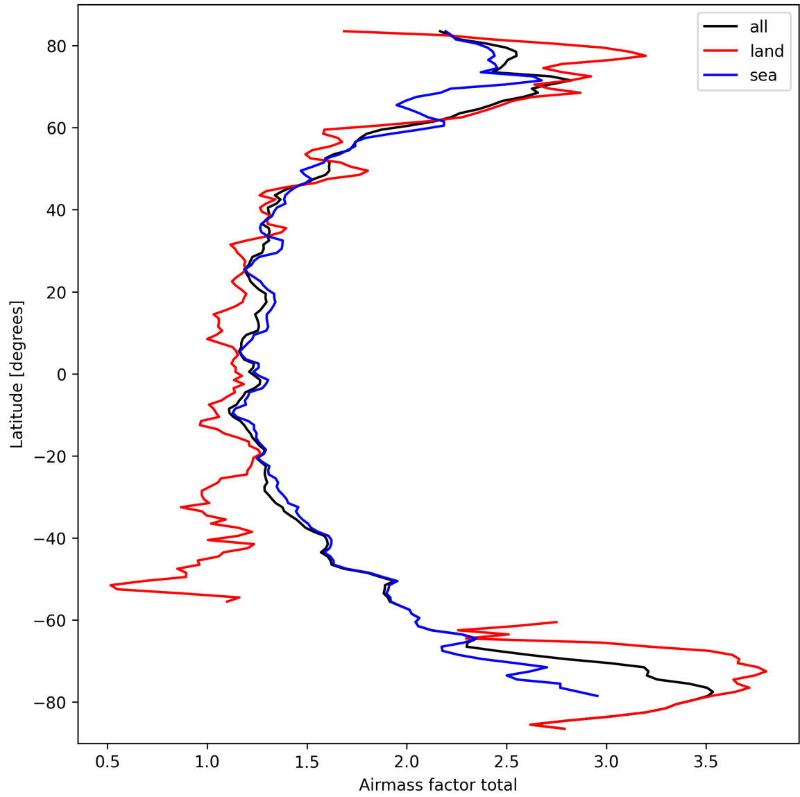
Figure 26: Zonal average of “Airmass factor total” for 2025-03-15 to 2025-03-17.
