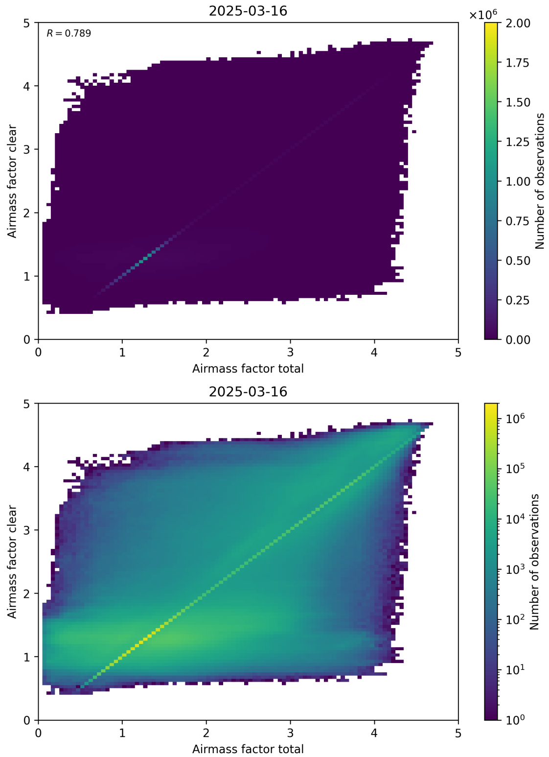
Figure 100: Scatter density plot of “Airmass factor total” against “Airmass factor clear” for 2025-03-15 to 2025-03-17.
