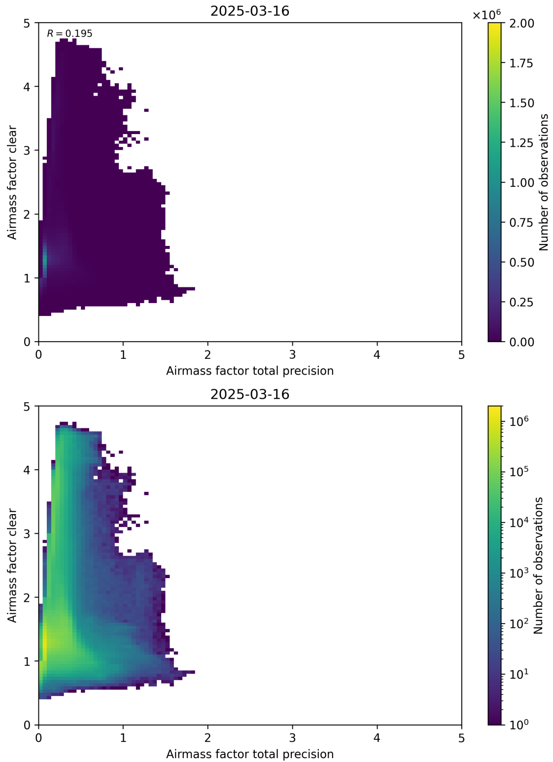
Figure 108: Scatter density plot of “Airmass factor total precision” against “Airmass factor clear” for 2025-03-15 to 2025-03-17.
