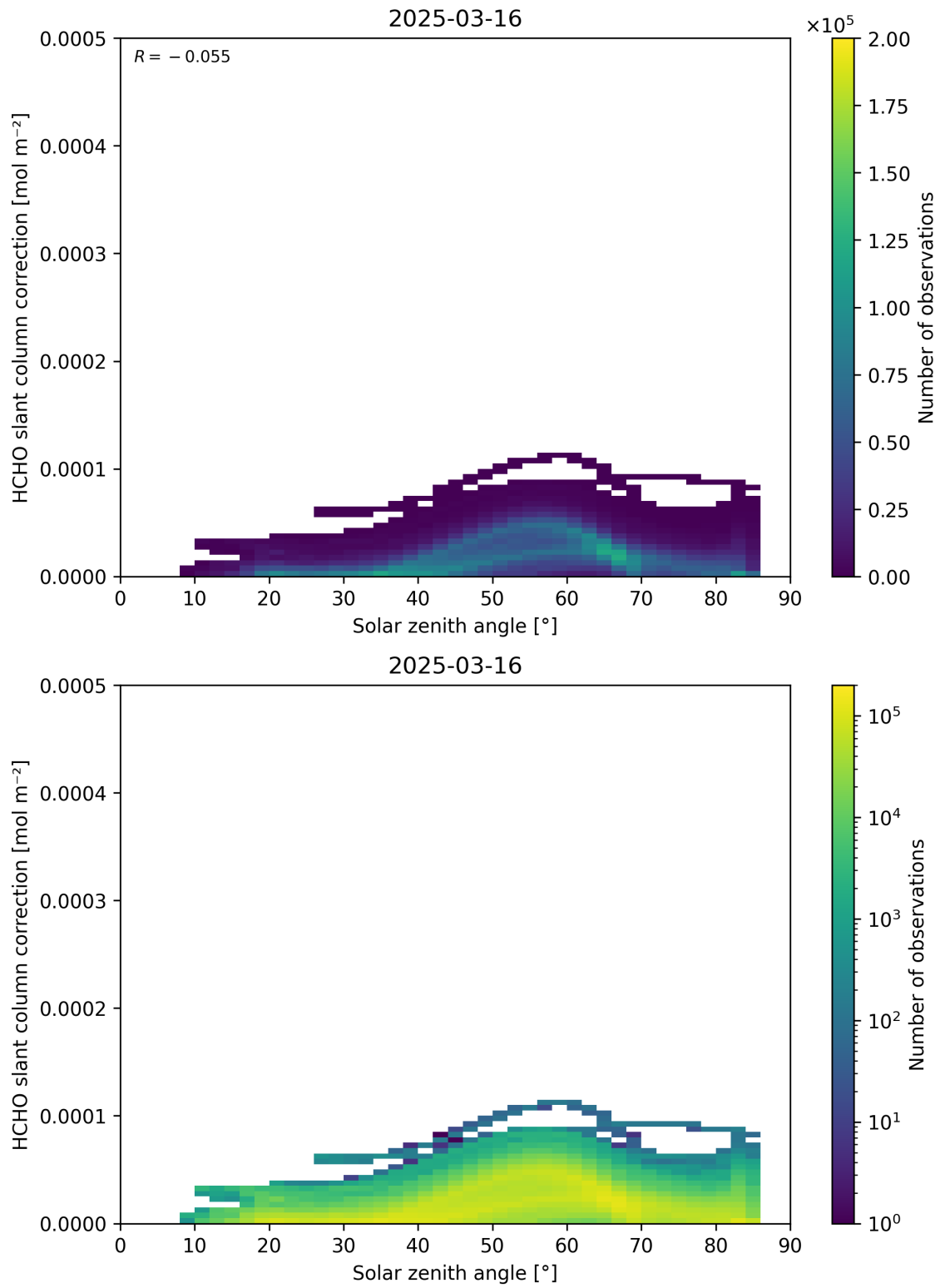
Figure 172: Scatter density plot of “Solar zenith angle” against “HCHO slant column correction” for 2025-03-15 to 2025-03-17.
