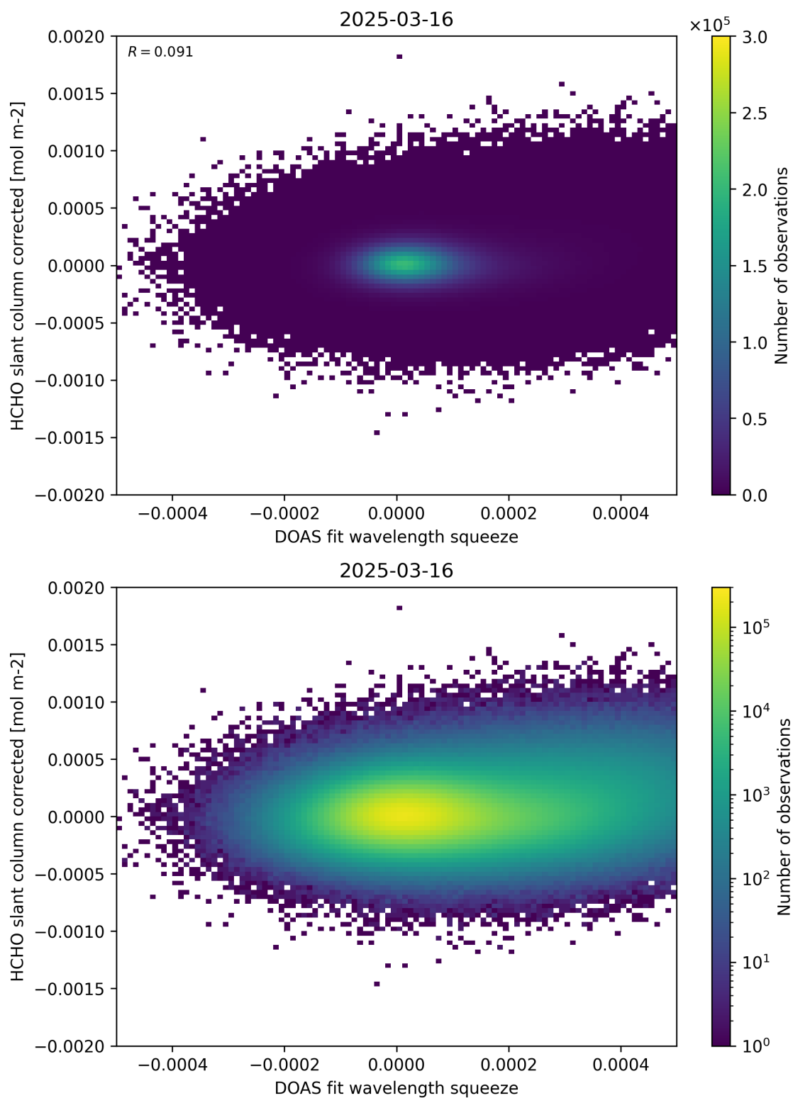
Figure 69: Scatter density plot of “DOAS fit wavelength squeeze” against “HCHO slant column corrected” for 2025-03-15 to 2025-03-17.
