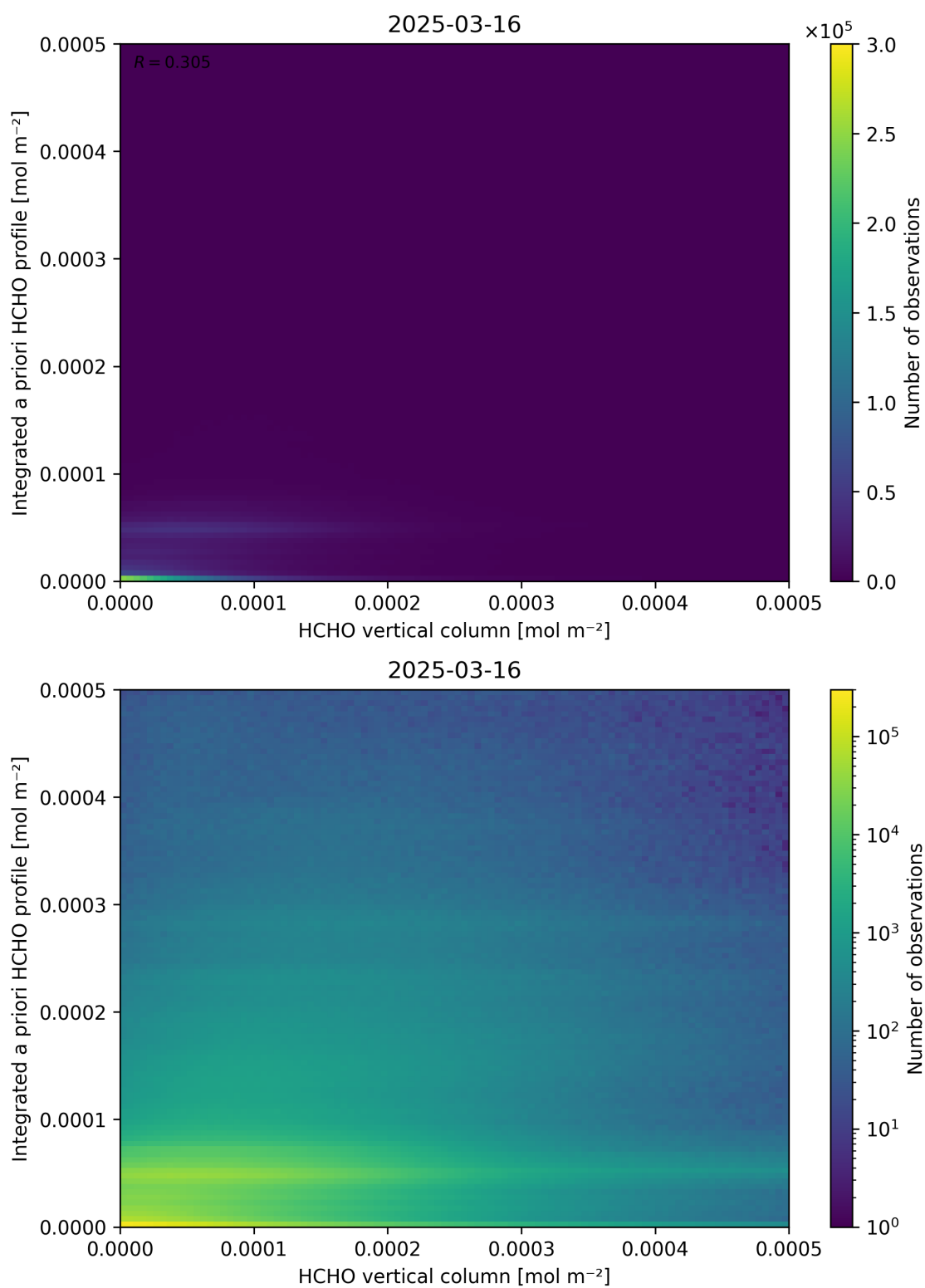
Figure 135: Scatter density plot of “HCHO vertical column” against “Integrated a priori HCHO profile” for 2025-03-15 to 2025-03-17.
