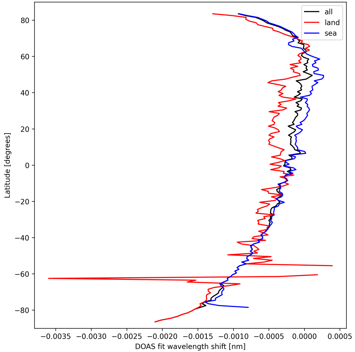
Figure 30: Zonal average of “DOAS fit wavelength shift” for 2025-03-15 to 2025-03-17.
