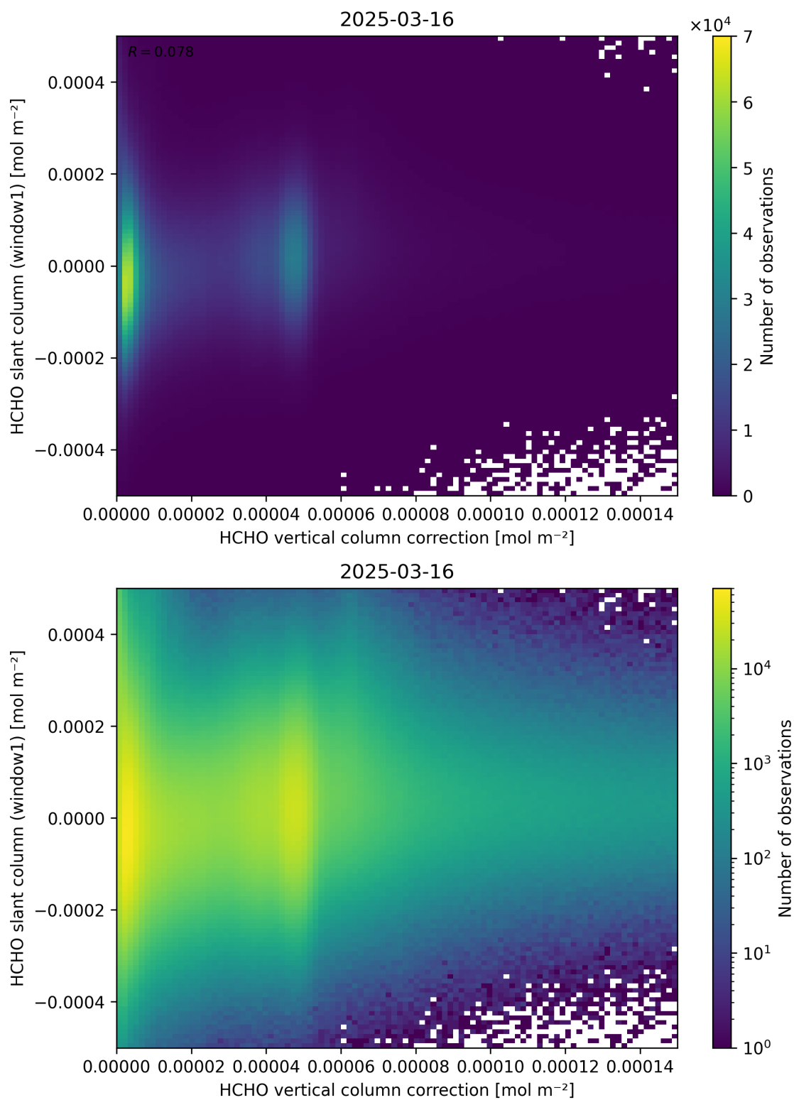
Figure 118: Scatter density plot of “HCHO vertical column correction” against “HCHO slant column (window1)” for 2025-03-15 to 2025-03-17.
