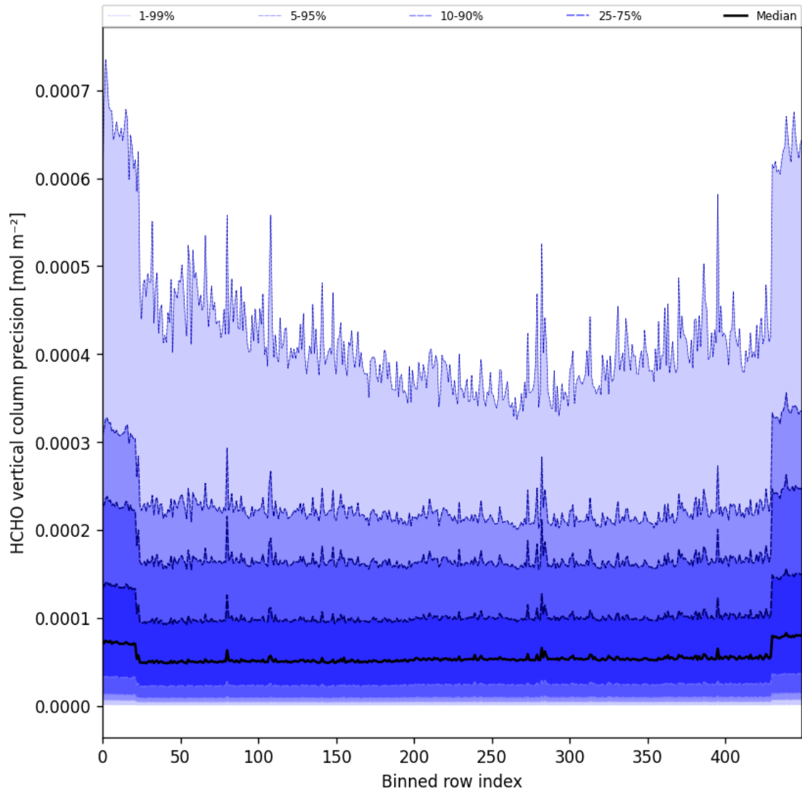
Figure 50: Along track statistics of “HCHO vertical column precision” for 2025-03-15 to 2025-03-17
