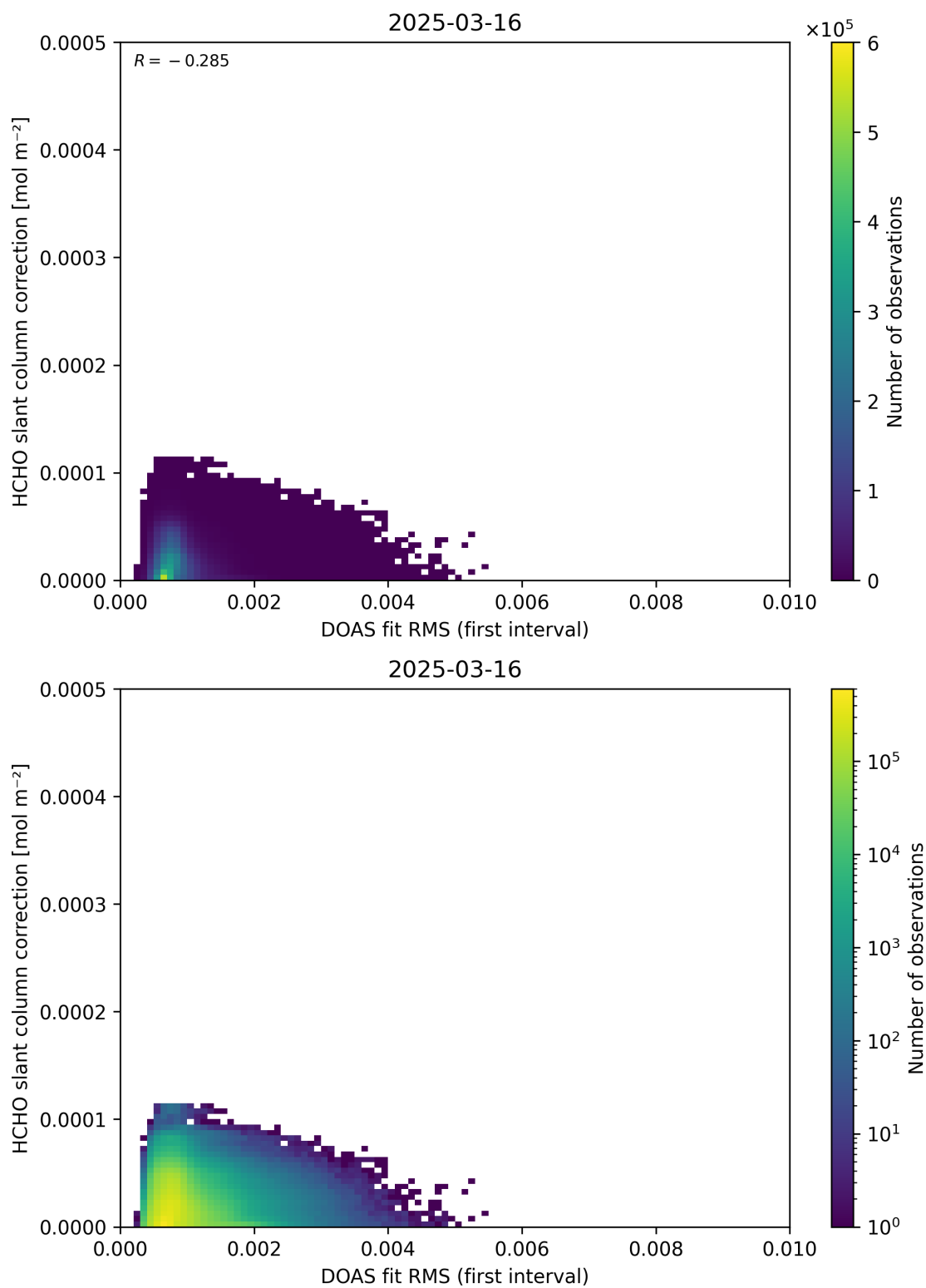
Figure 63: Scatter density plot of “DOAS fit RMS (first interval)” against “HCHO slant column correction” for 2025-03-15 to 2025-03-17.
