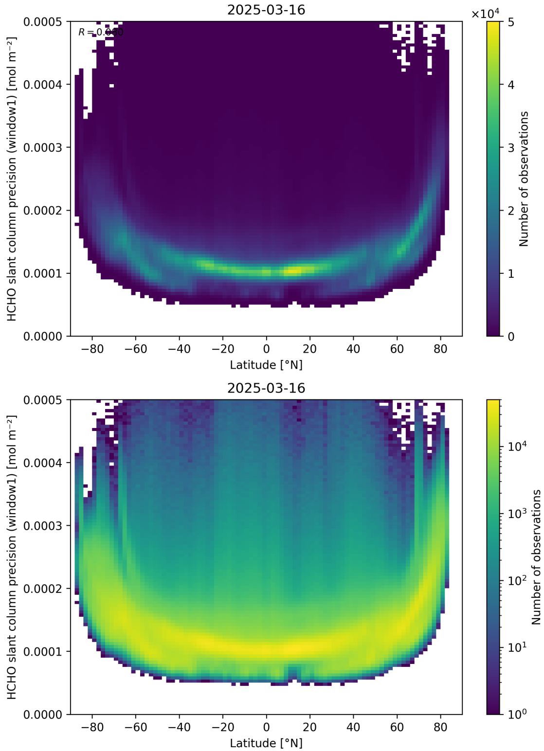
Figure 160: Scatter density plot of “Latitude” against “HCHO slant column precision (window1)” for 2025-03-15 to 2025-03-17.
