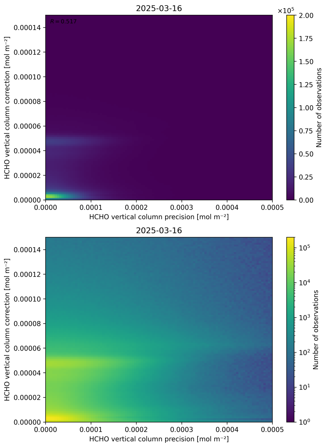
Figure 146: Scatter density plot of “HCHO vertical column precision” against “HCHO vertical column correction” for 2025-03-15 to 2025-03-17.
