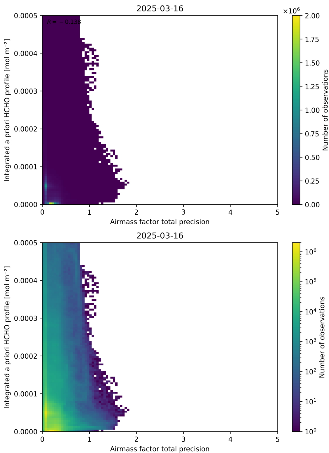
Figure 111: Scatter density plot of “Airmass factor total precision” against “Integrated a priori HCHO profile” for 2025-03-15 to 2025-03-17.
