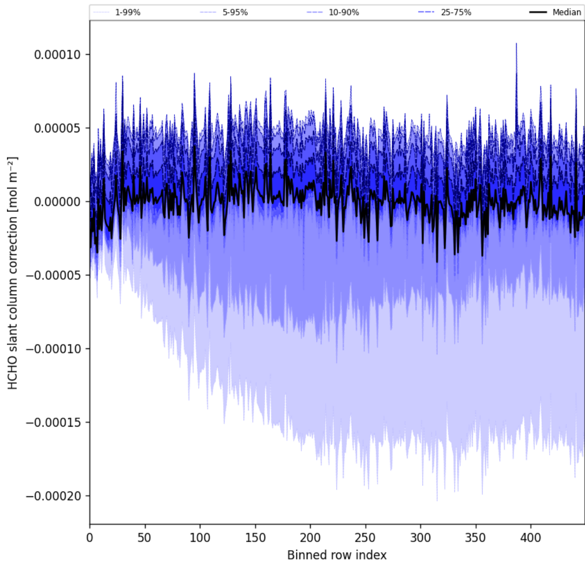
Figure 61: Along track statistics of “HCHO slant column correction” for 2025-03-15 to 2025-03-17
