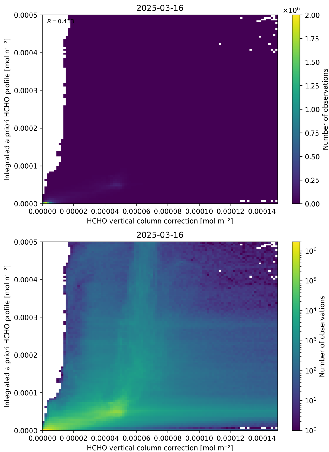
Figure 122: Scatter density plot of “HCHO vertical column correction” against “Integrated a priori HCHO profile” for 2025-03-15 to 2025-03-17.
