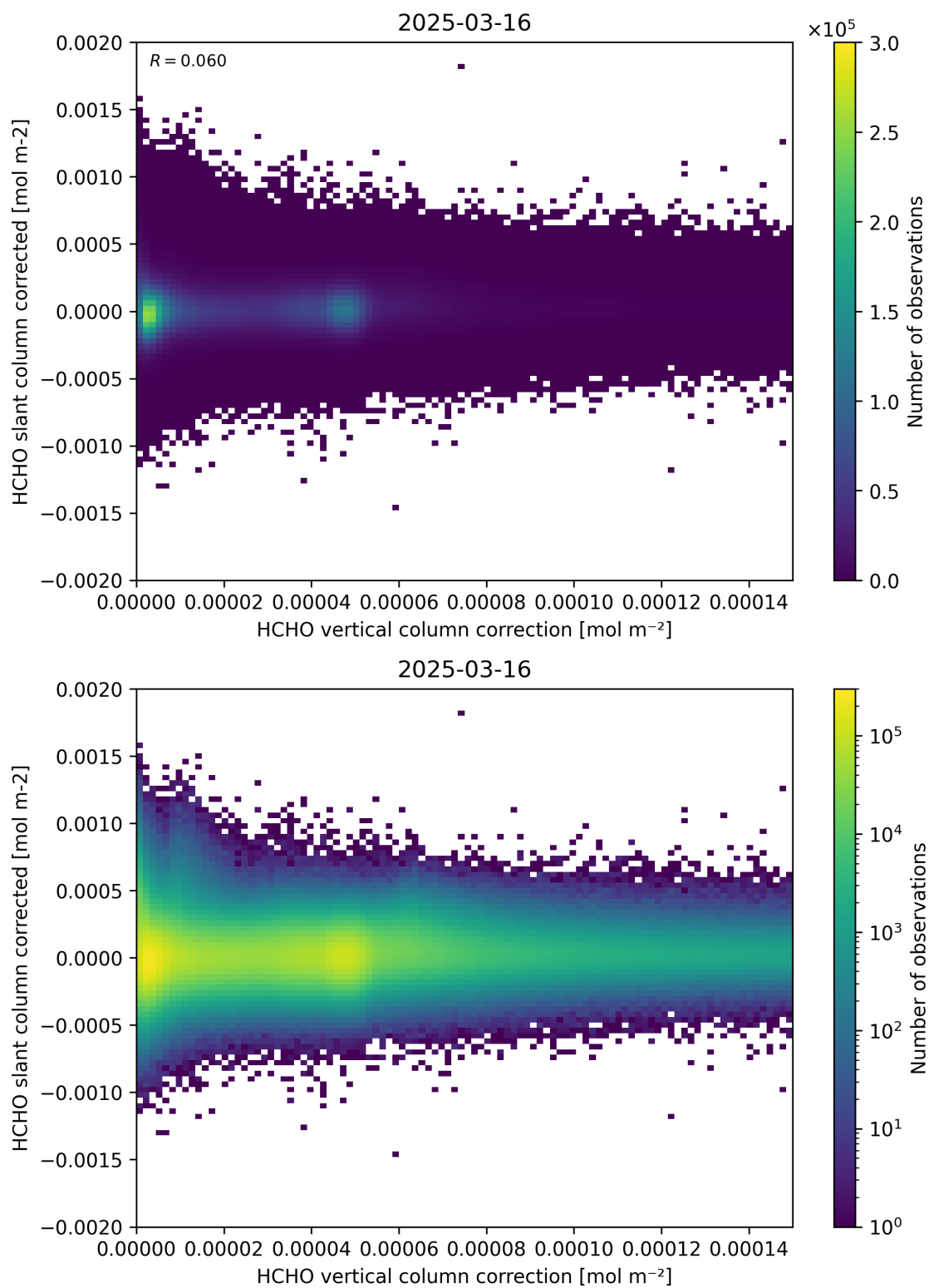
Figure 116: Scatter density plot of “HCHO vertical column correction” against “HCHO slant column corrected” for 2025-03-15 to 2025-03-17.
