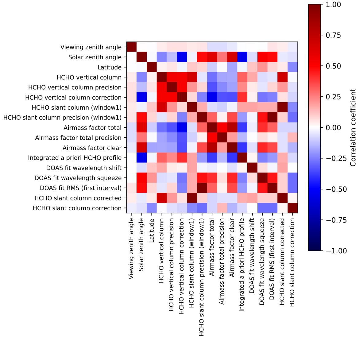
Figure 2: Map of correlation matrix for 2025-03-15 to 2025-03-17.
