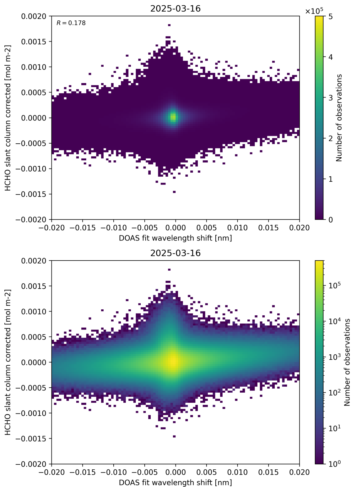
Figure 66: Scatter density plot of “DOAS fit wavelength shift” against “HCHO slant column corrected” for 2025-03-15 to 2025-03-17.
