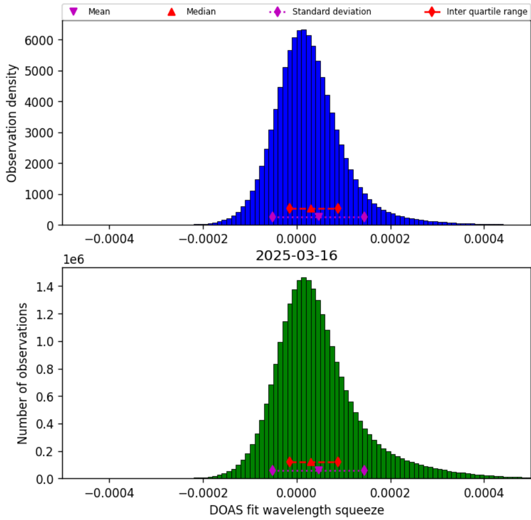
Figure 45: Histogram of “DOAS fit wavelength squeeze” for 2025-03-15 to 2025-03-17
