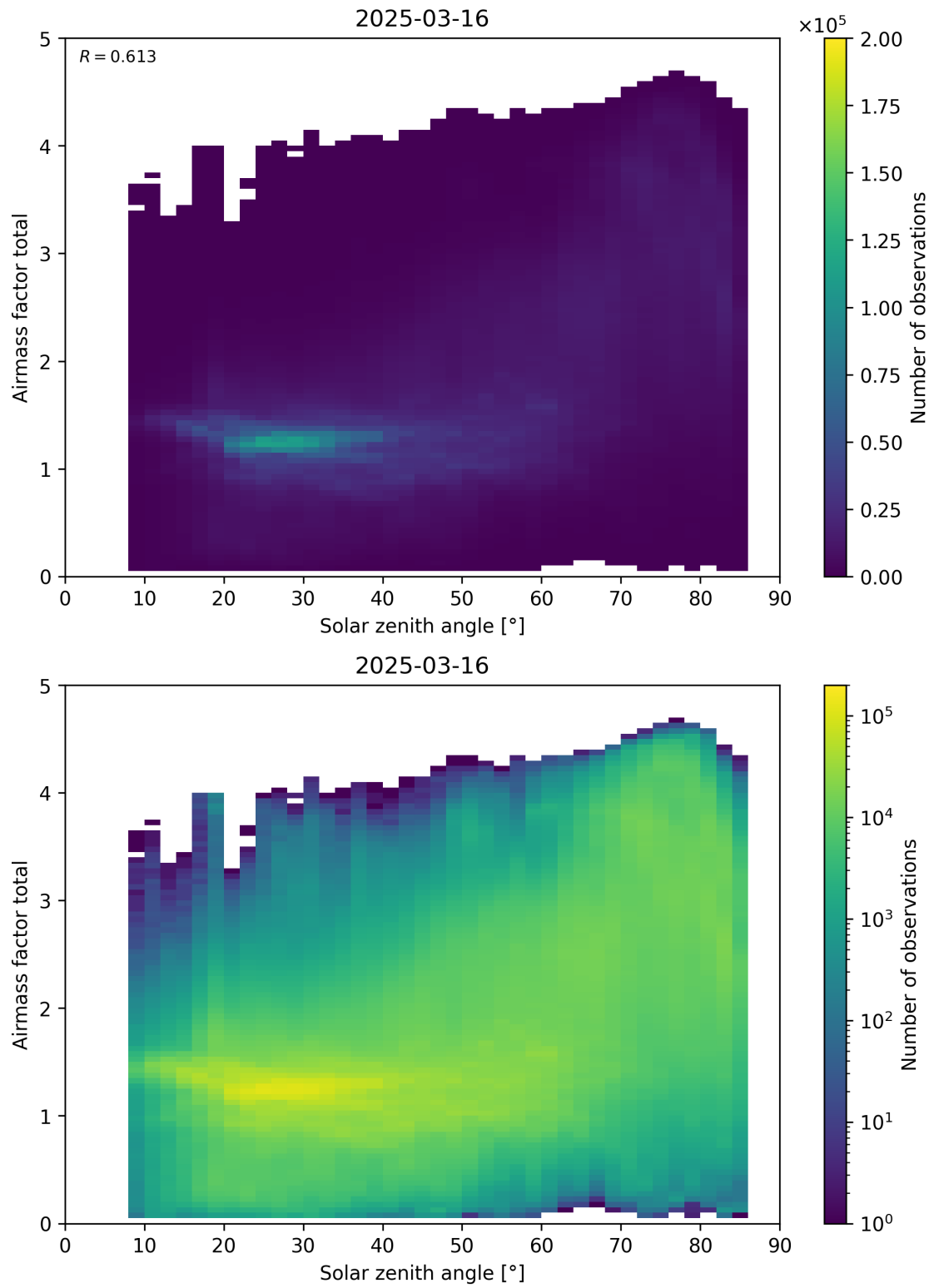
Figure 175: Scatter density plot of “Solar zenith angle” against “Airmass factor total” for 2025-03-15 to 2025-03-17.
