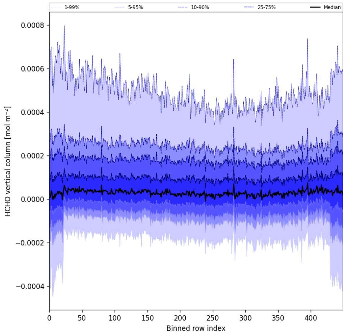
Figure 49: Along track statistics of “HCHO vertical column” for 2025-03-15 to 2025-03-17
