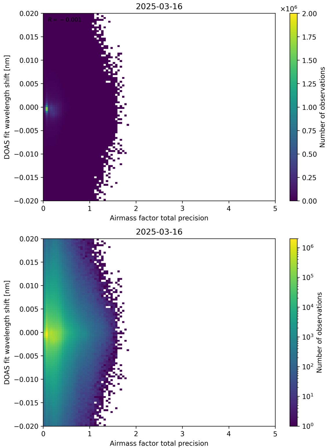
Figure 106: Scatter density plot of “Airmass factor total precision” against “DOAS fit wavelength shift” for 2025-03-15 to 2025-03-17.
