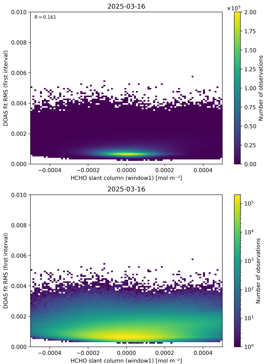
Figure 78: Scatter density plot of “HCHO slant column (window1)” against “DOAS fit RMS (first interval)” for 2025-03-15 to 2025-03-17.
