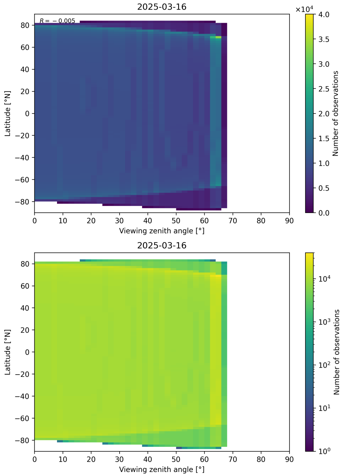
Figure 196: Scatter density plot of “Viewing zenith angle” against “Latitude” for 2025-03-15 to 2025-03-17.
