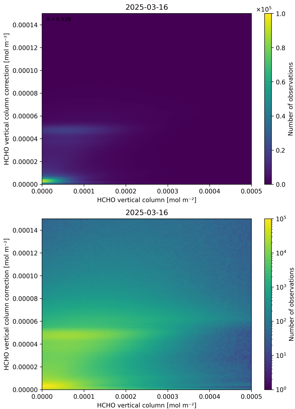
Figure 133: Scatter density plot of “HCHO vertical column” against “HCHO vertical column correction” for 2025-03-15 to 2025-03-17.
