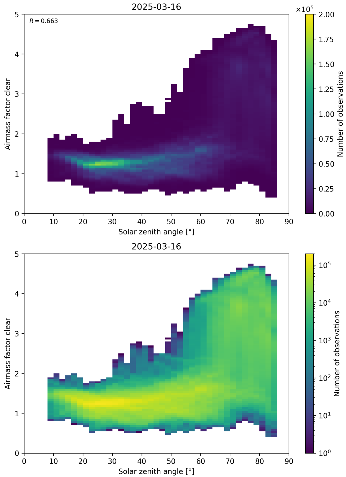
Figure 170: Scatter density plot of “Solar zenith angle” against “Airmass factor clear” for 2025-03-15 to 2025-03-17.
