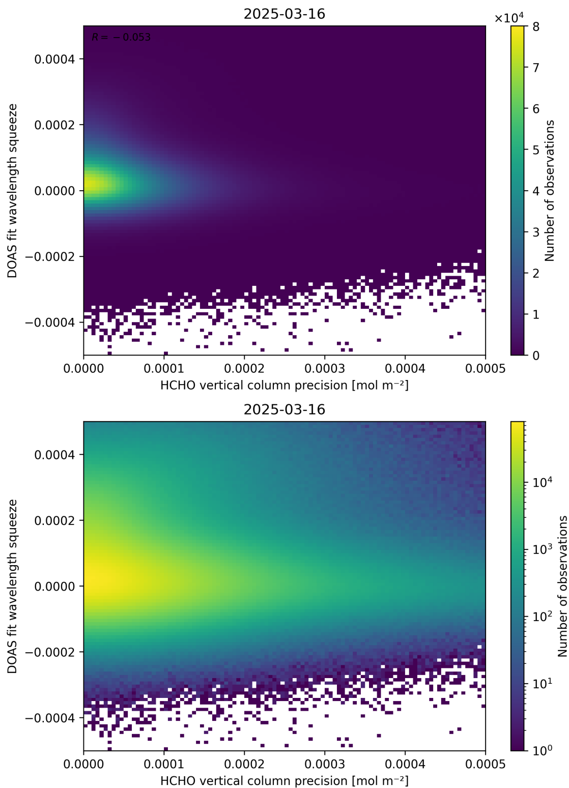
Figure 138: Scatter density plot of “HCHO vertical column precision” against “DOAS fit wavelength squeeze” for 2025-03-15 to 2025-03-17.
