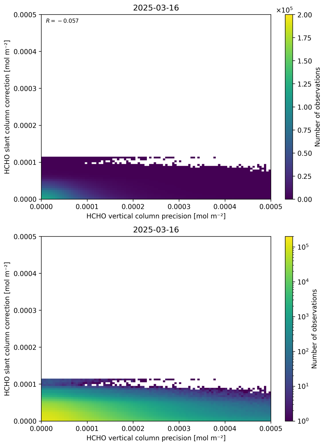
Figure 141: Scatter density plot of “HCHO vertical column precision” against “HCHO slant column correction” for 2025-03-15 to 2025-03-17.
