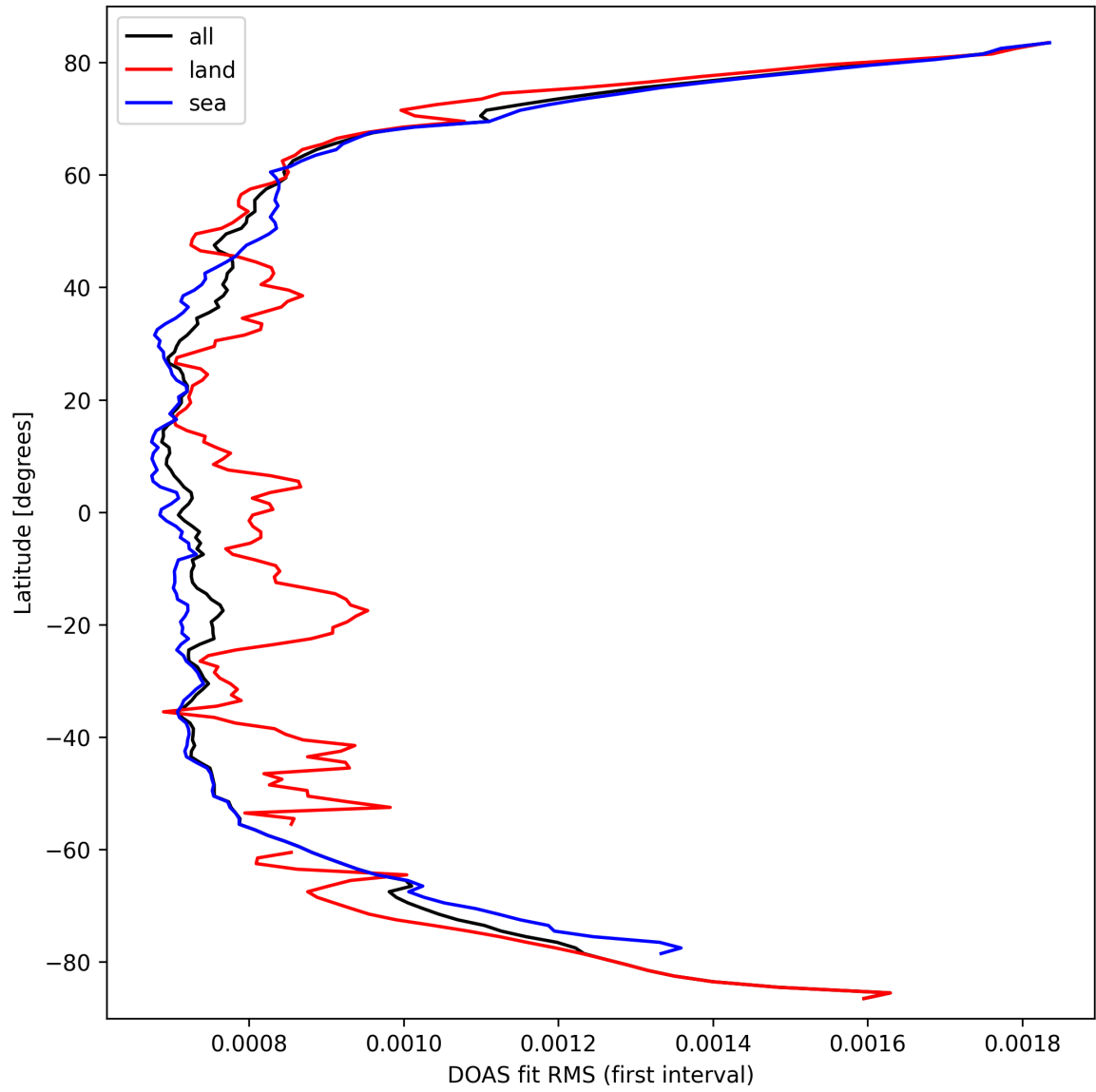
Figure 32: Zonal average of “DOAS fit RMS (first interval)” for 2025-03-15 to 2025-03-17.
