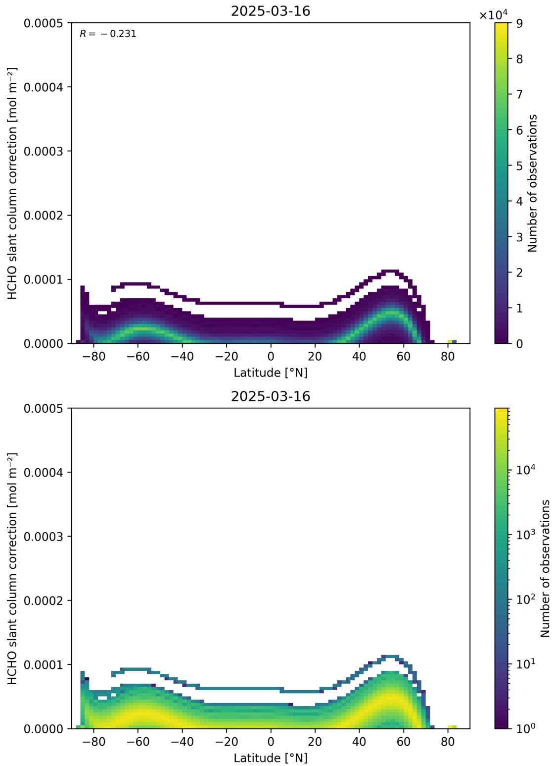
Figure 158: Scatter density plot of “Latitude” against “HCHO slant column correction” for 2025-03-15 to 2025-03-17.
