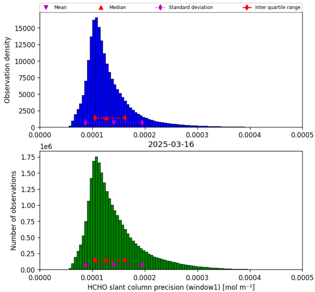
Figure 39: Histogram of “HCHO slant column precision (window1)” for 2025-03-15 to 2025-03-17
