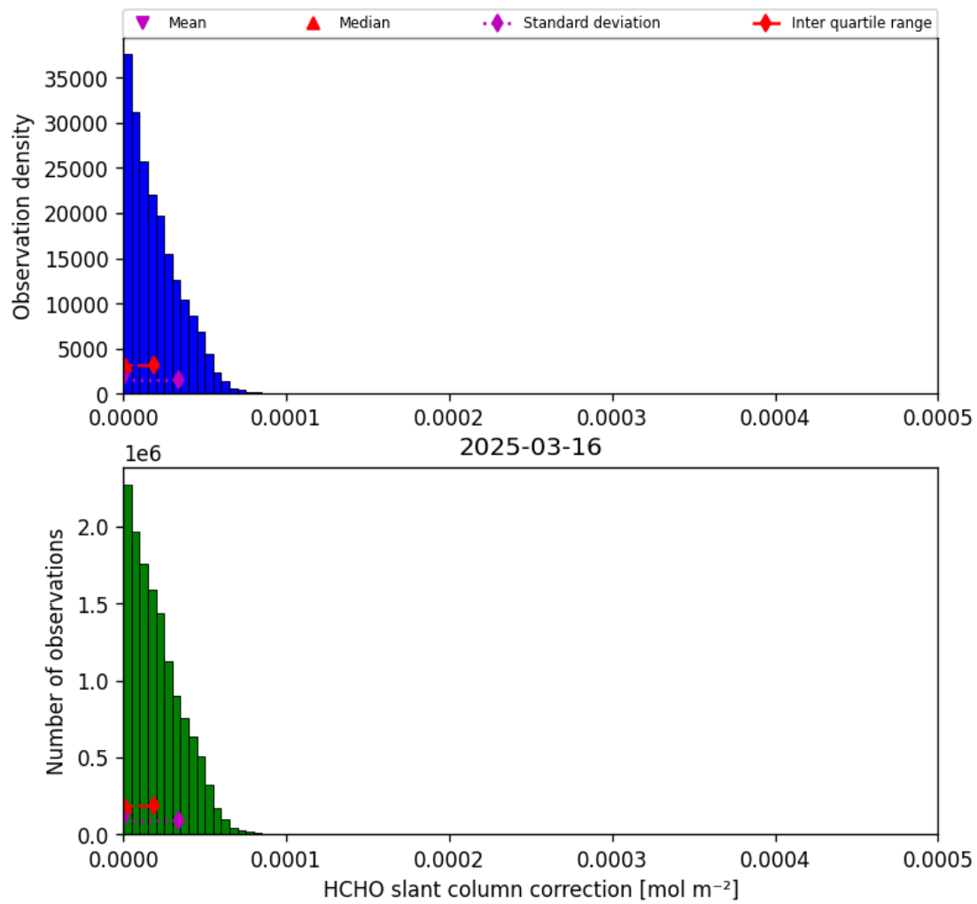
Figure 47: Histogram of “HCHO slant column correction” for 2025-03-15 to 2025-03-17
