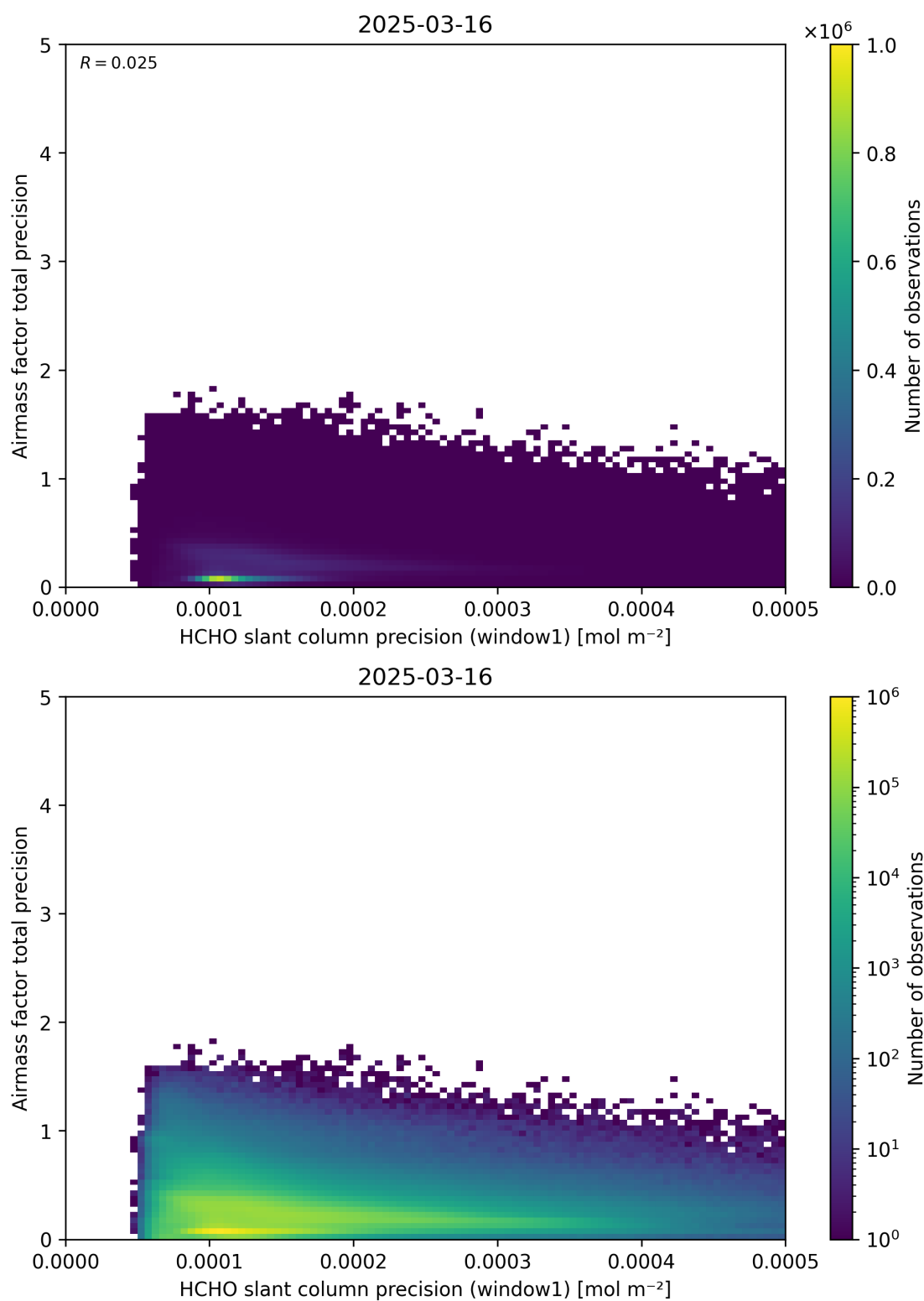
Figure 95: Scatter density plot of “HCHO slant column precision (window1)” against “Airmass factor total precision” for 2025-03-15 to 2025-03-17.
