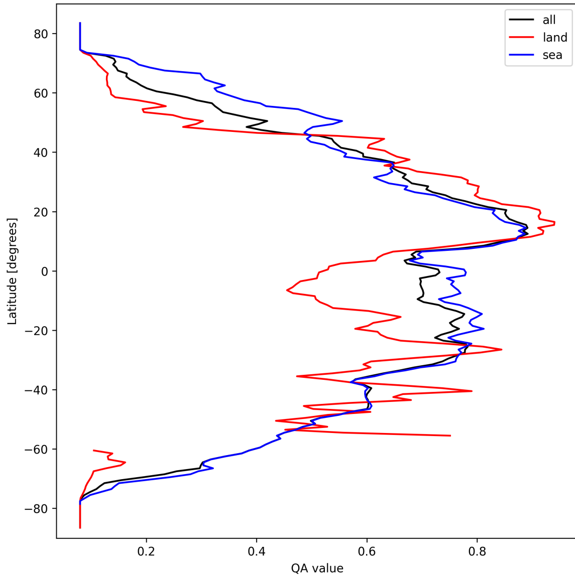
Figure 20: Zonal average of “QA value” for 2025-03-15 to 2025-03-17.
