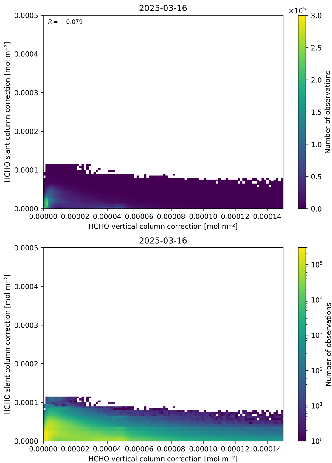
Figure 117: Scatter density plot of “HCHO vertical column correction” against “HCHO slant column correction” for 2025-03-15 to 2025-03-17.
