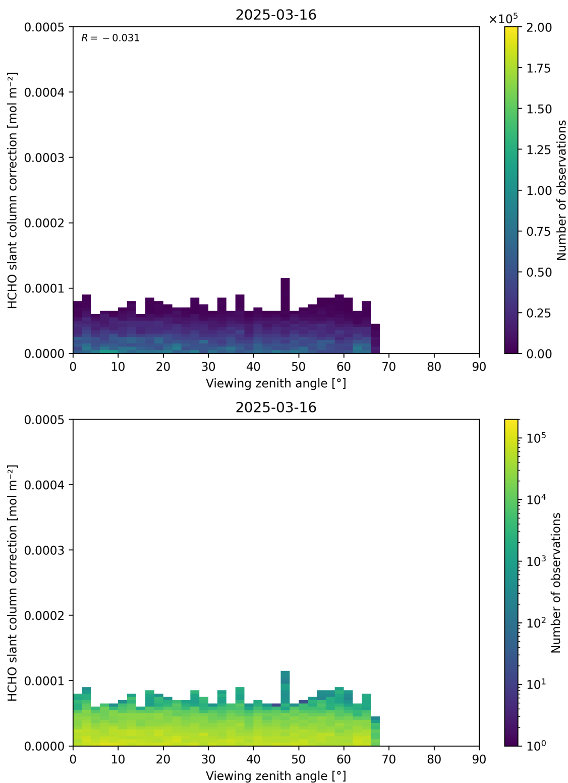
Figure 187: Scatter density plot of “Viewing zenith angle” against “HCHO slant column correction” for 2025-03-15 to 2025-03-17.
