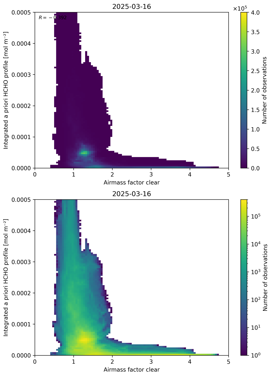
Figure 76: Scatter density plot of “Airmass factor clear” against “Integrated a priori HCHO profile” for 2025-03-15 to 2025-03-17.
