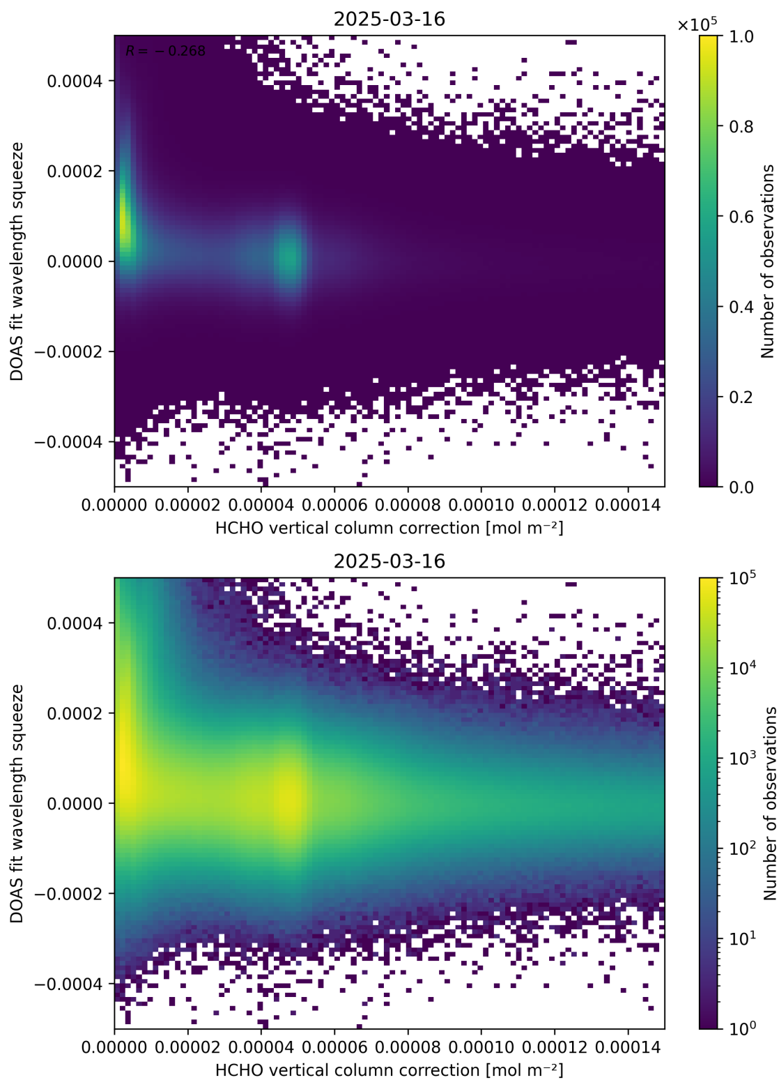
Figure 114: Scatter density plot of “HCHO vertical column correction” against “DOAS fit wavelength squeeze” for 2025-03-15 to 2025-03-17.
