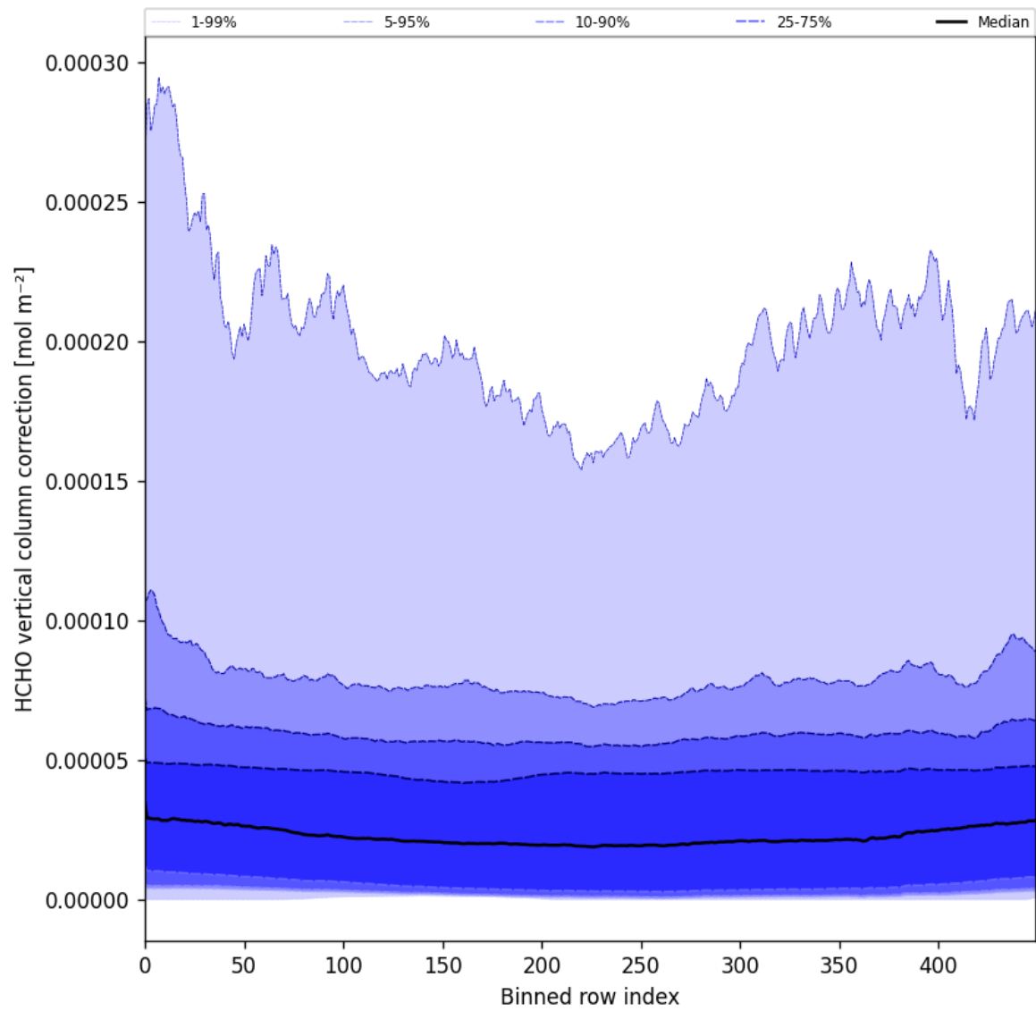
Figure 51: Along track statistics of “HCHO vertical column correction” for 2025-03-15 to 2025-03-17
