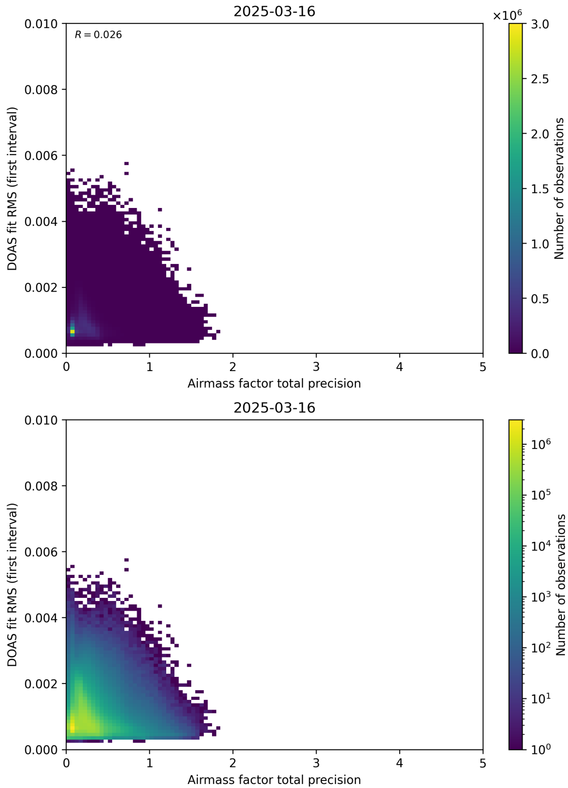
Figure 105: Scatter density plot of “Airmass factor total precision” against “DOAS fit RMS (first interval)” for 2025-03-15 to 2025-03-17.
