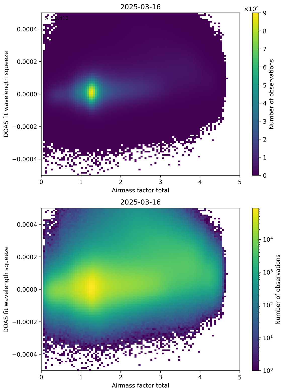
Figure 99: Scatter density plot of “Airmass factor total” against “DOAS fit wavelength squeeze” for 2025-03-15 to 2025-03-17.
