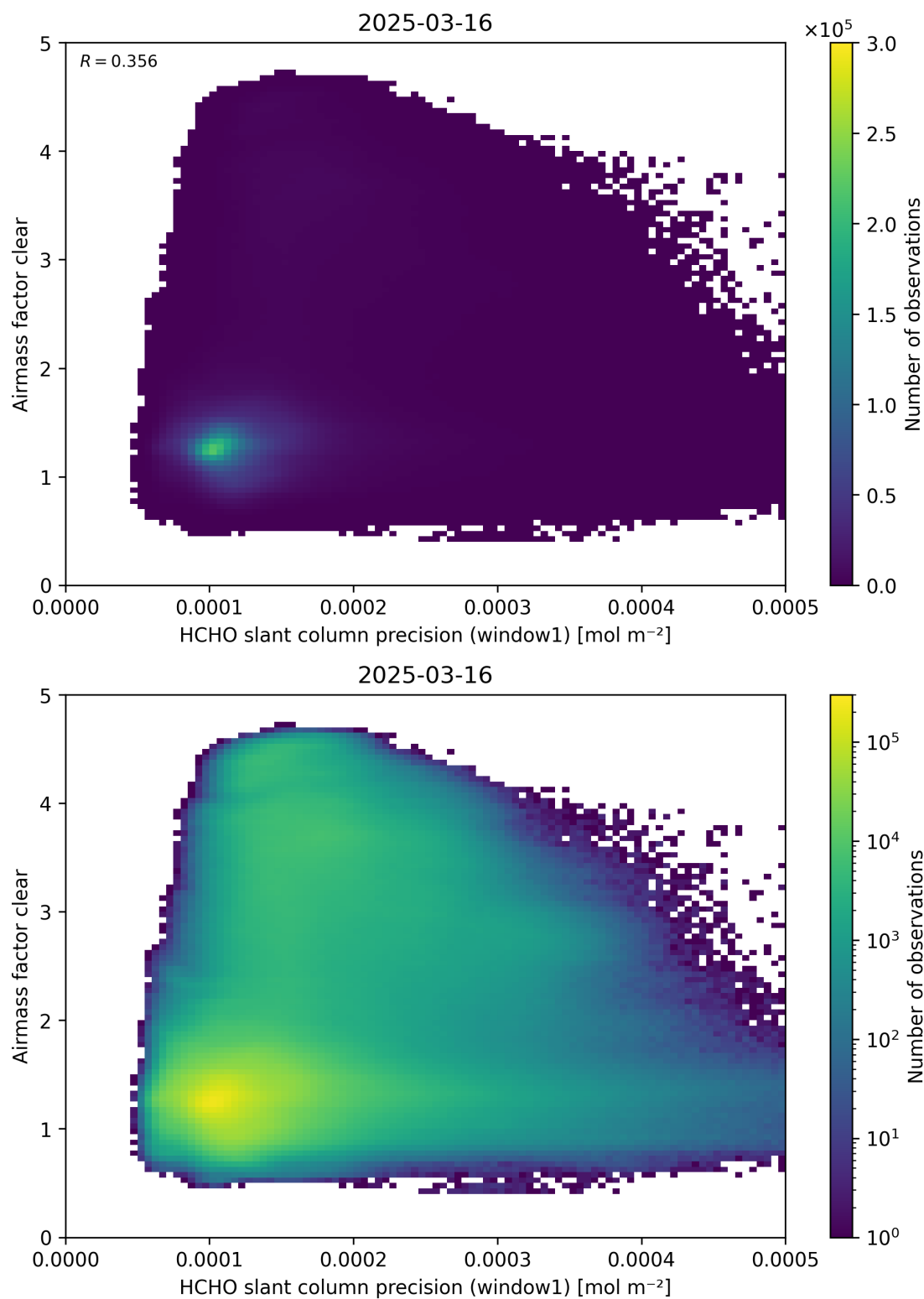
Figure 91: Scatter density plot of “HCHO slant column precision (window1)” against “Airmass factor clear” for 2025-03-15 to 2025-03-17.
