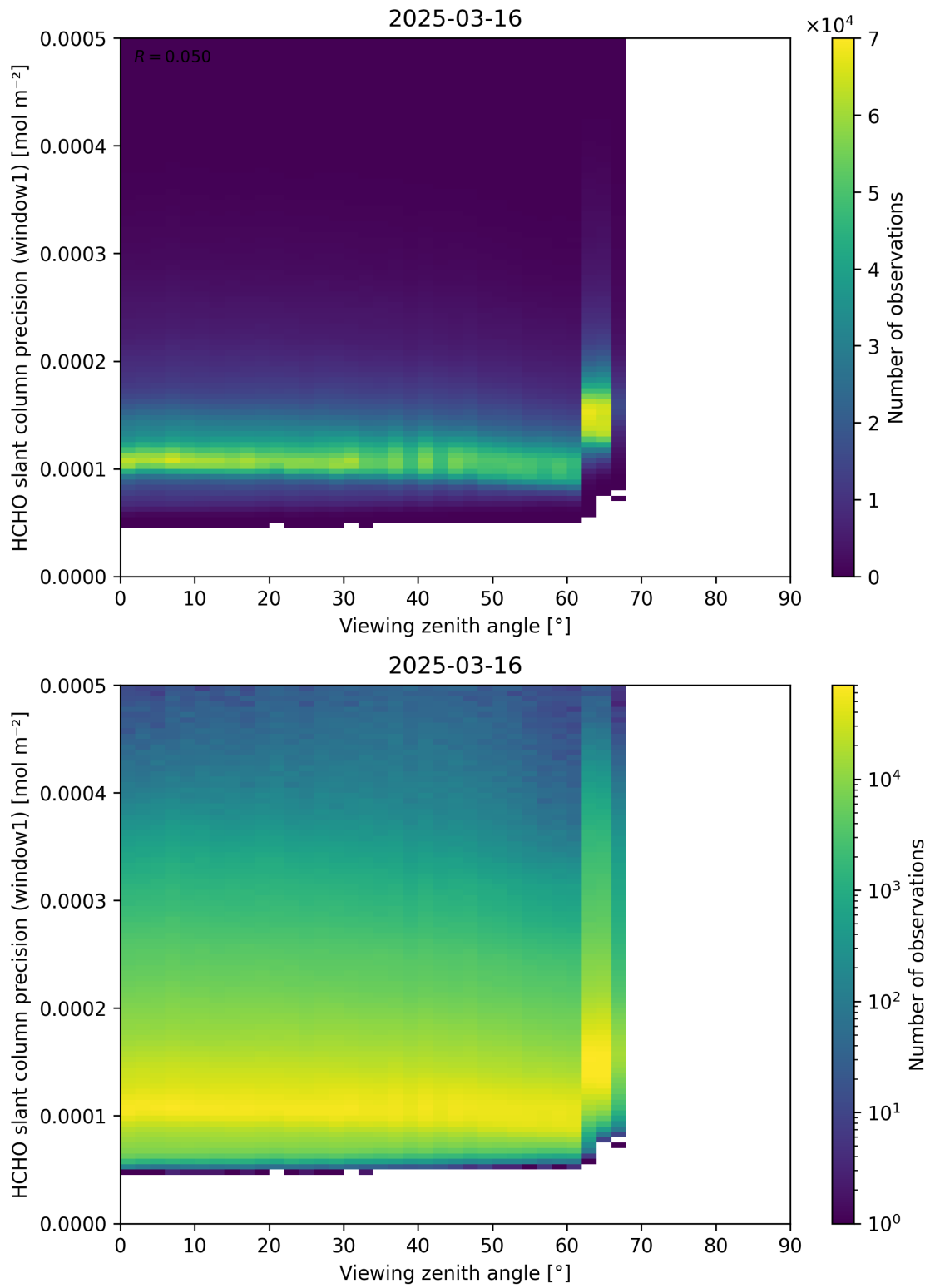
Figure 189: Scatter density plot of “Viewing zenith angle” against “HCHO slant column precision (window1)” for 2025-03-15 to 2025-03-17.
