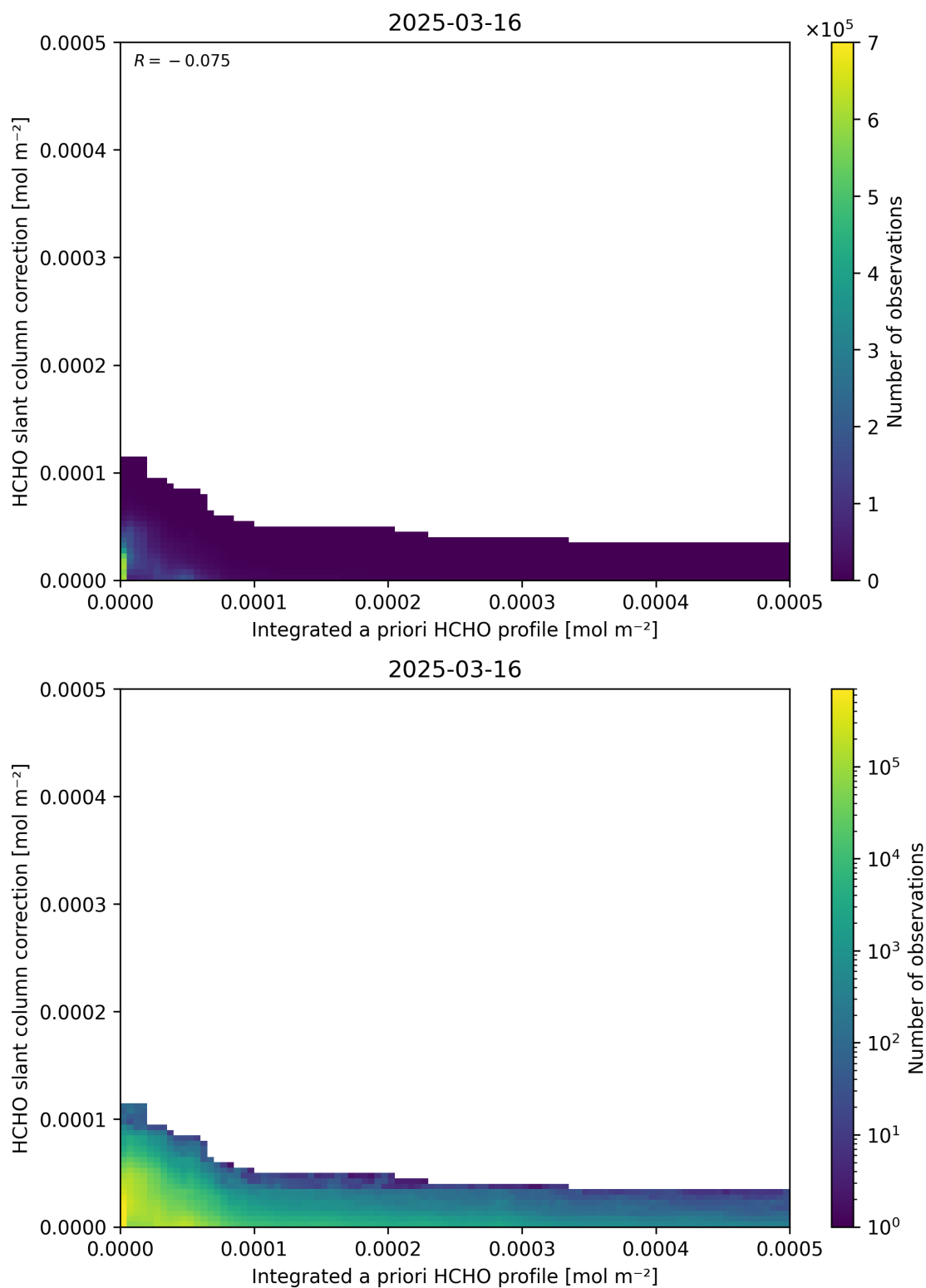
Figure 152: Scatter density plot of “Integrated a priori HCHO profile” against “HCHO slant column correction” for 2025-03-15 to 2025-03-17.
