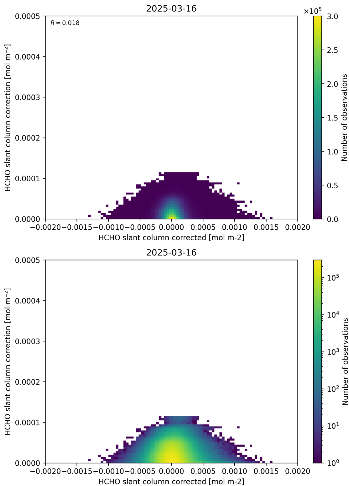
Figure 77: Scatter density plot of “HCHO slant column corrected” against “HCHO slant column correction” for 2025-03-15 to 2025-03-17.
