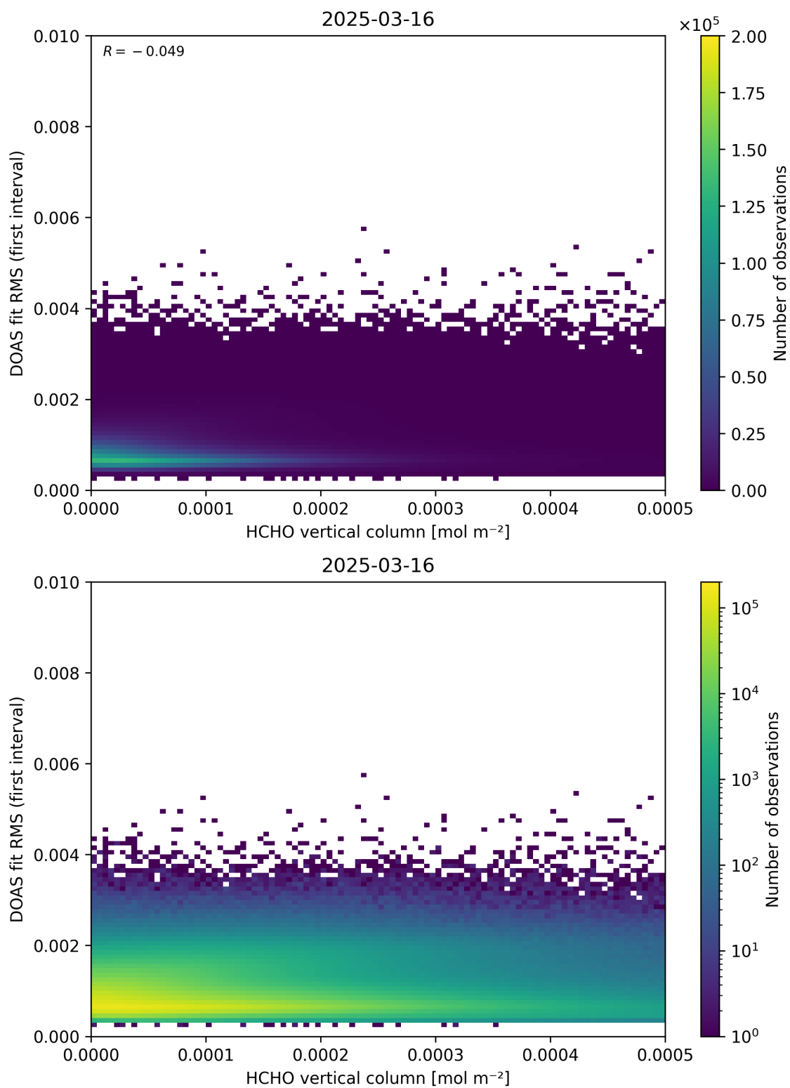
Figure 123: Scatter density plot of “HCHO vertical column” against “DOAS fit RMS (first interval)” for 2025-03-15 to 2025-03-17.
