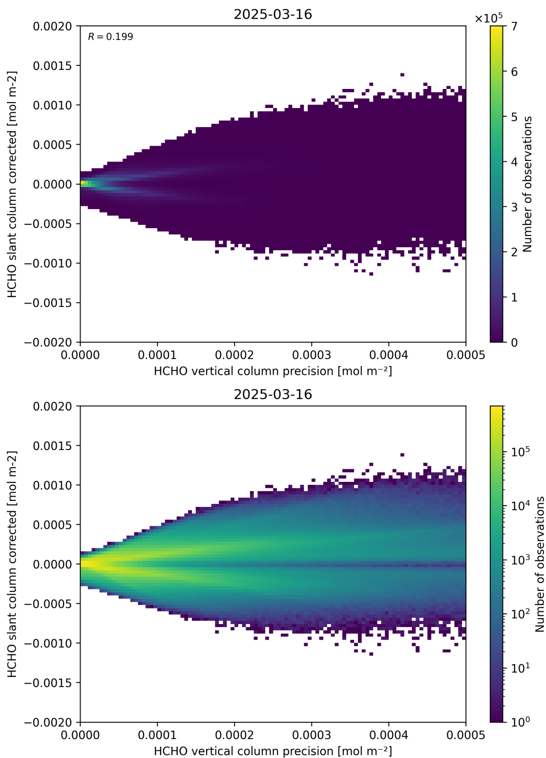
Figure 140: Scatter density plot of “HCHO vertical column precision” against “HCHO slant column corrected” for 2025-03-15 to 2025-03-17.
