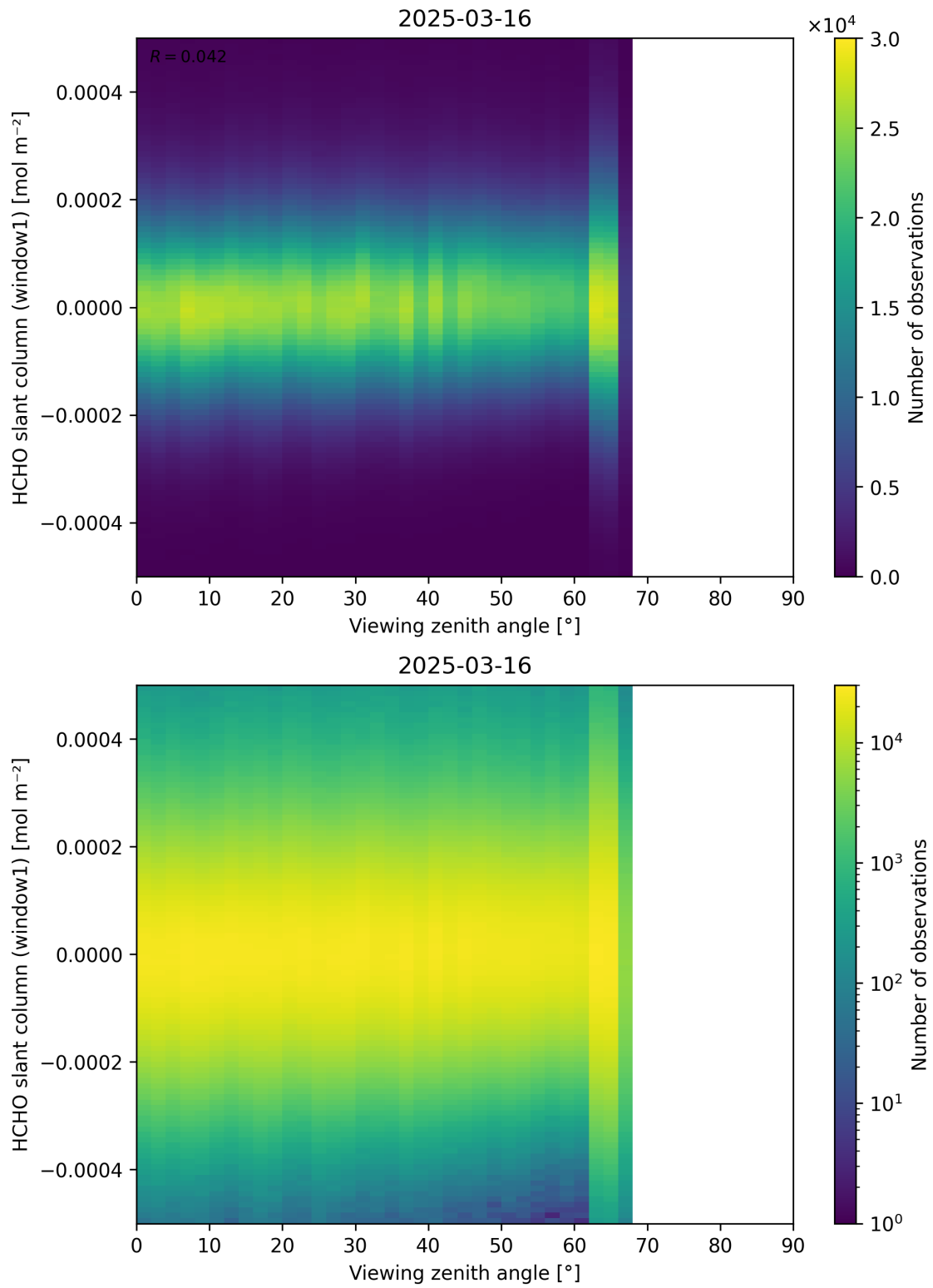
Figure 188: Scatter density plot of “Viewing zenith angle” against “HCHO slant column (window1)” for 2025-03-15 to 2025-03-17.
