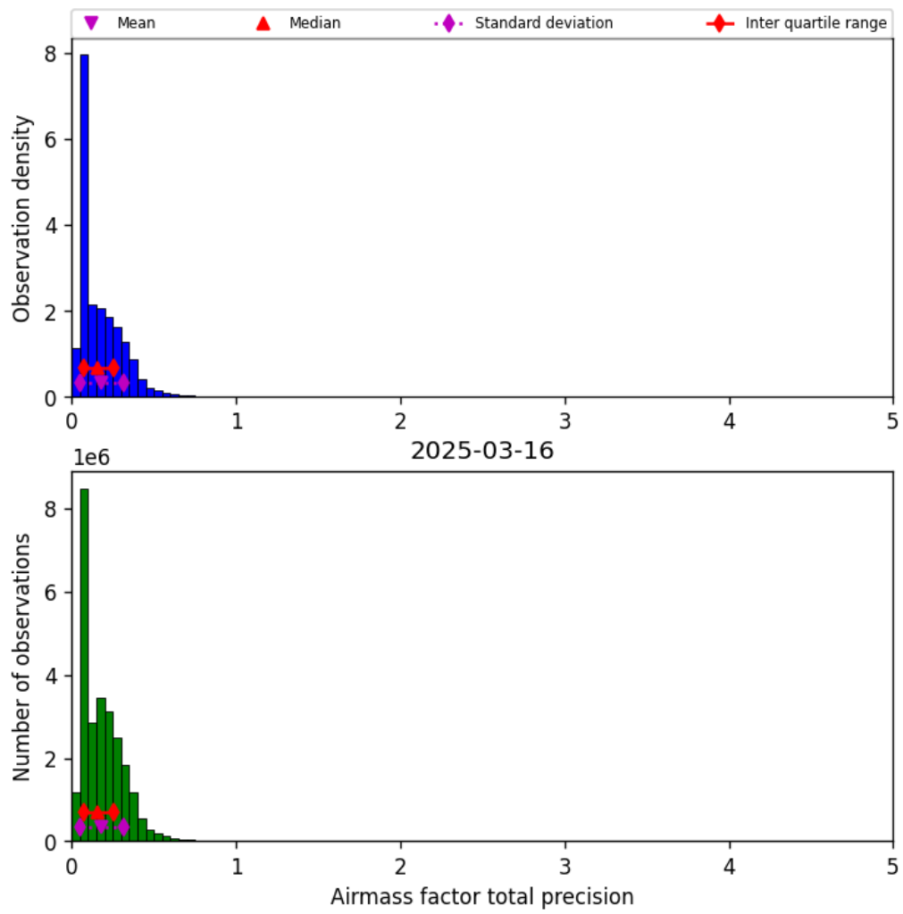
Figure 41: Histogram of “Airmass factor total precision” for 2025-03-15 to 2025-03-17
