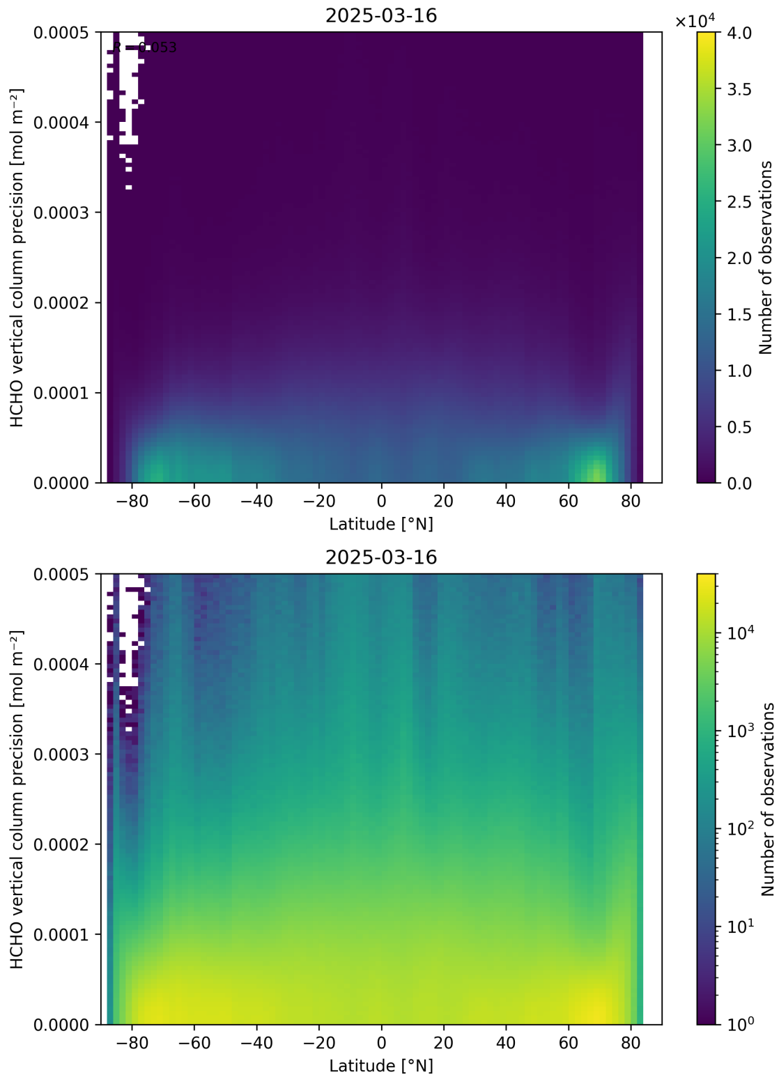
Figure 165: Scatter density plot of “Latitude” against “HCHO vertical column precision” for 2025-03-15 to 2025-03-17.
