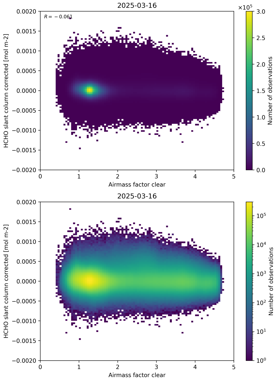
Figure 74: Scatter density plot of “Airmass factor clear” against “HCHO slant column corrected” for 2025-03-15 to 2025-03-17.
