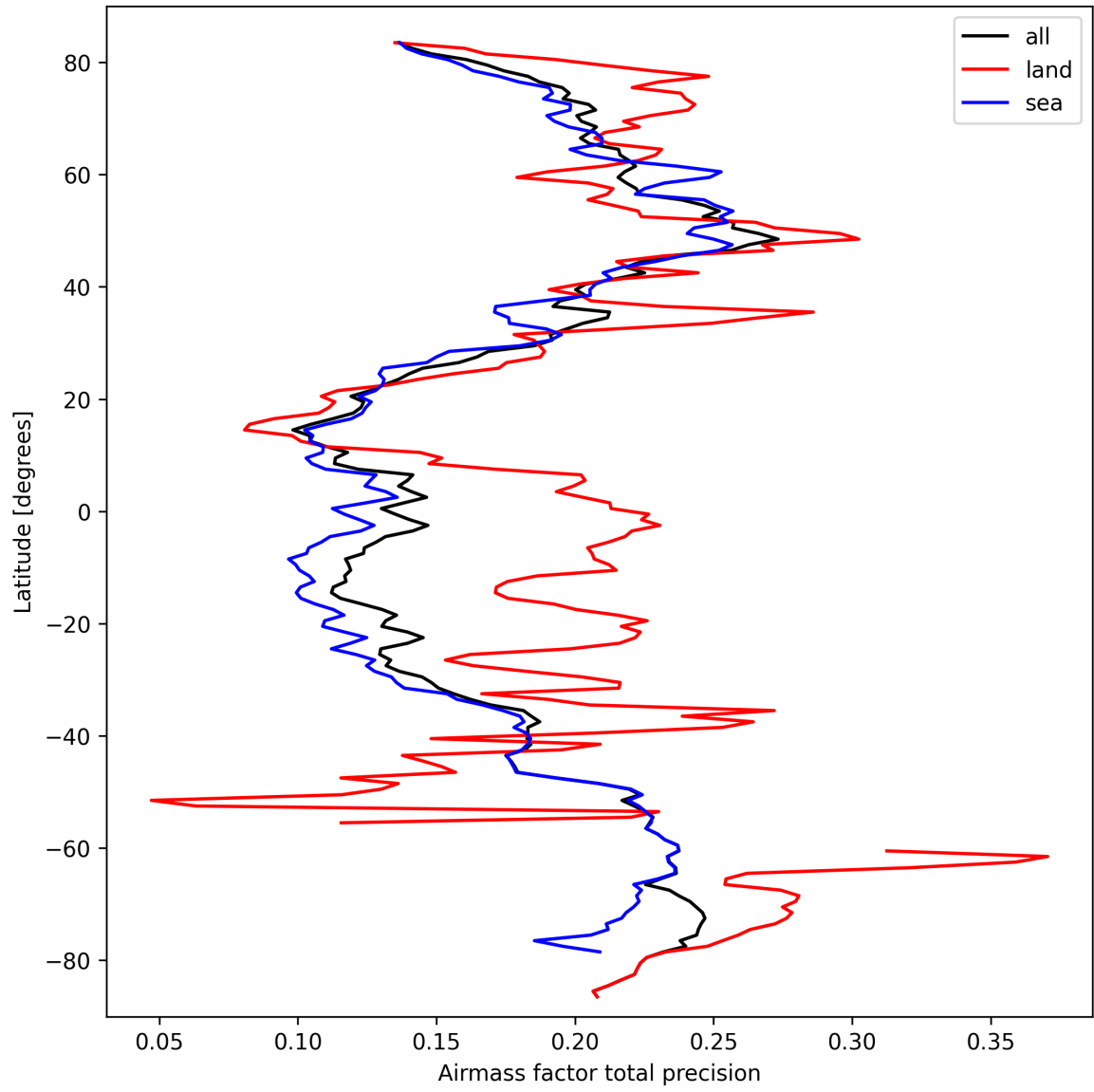
Figure 27: Zonal average of “Airmass factor total precision” for 2025-03-15 to 2025-03-17.
