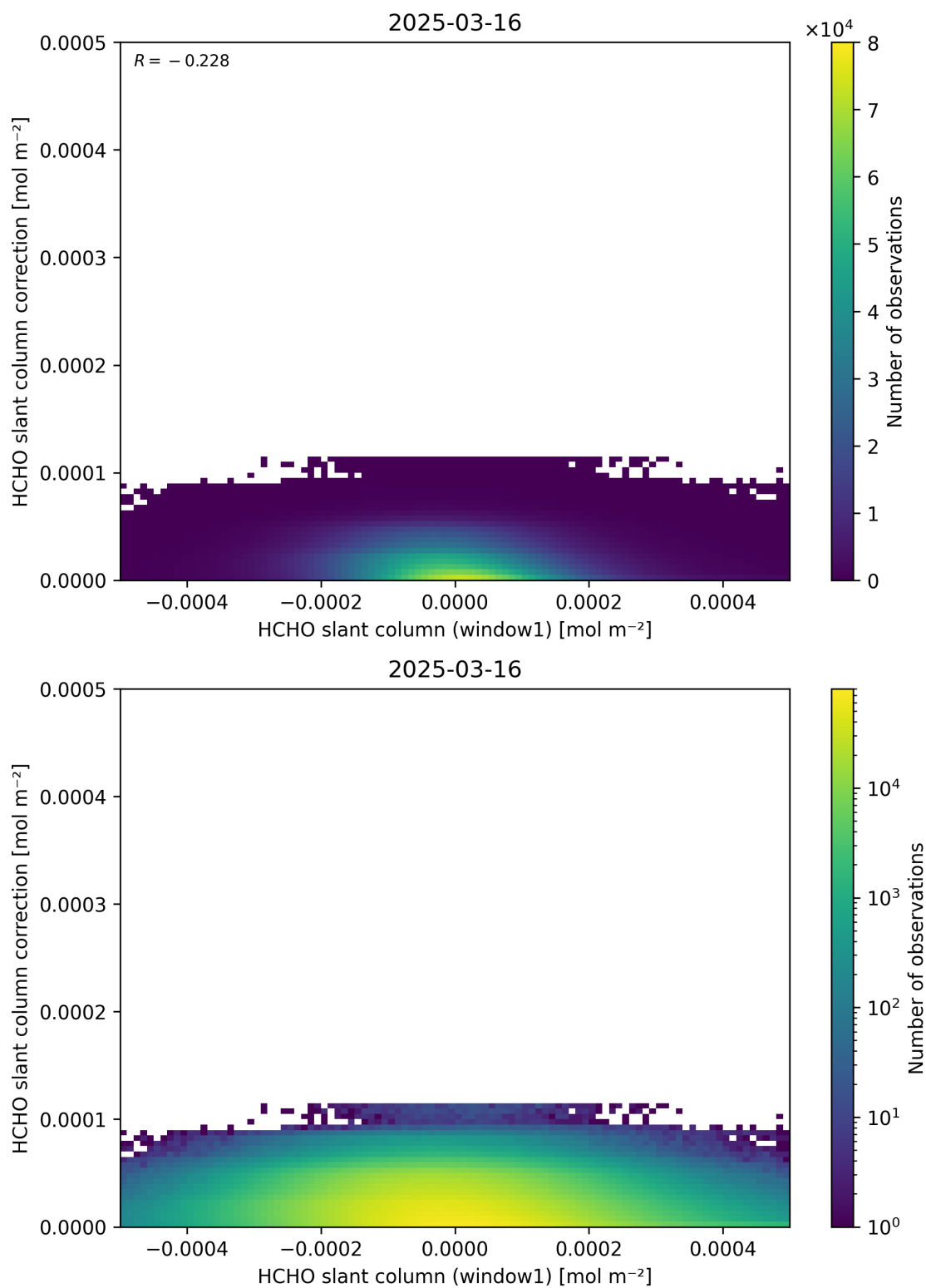
Figure 83: Scatter density plot of “HCHO slant column (window1)” against “HCHO slant column correction” for 2025-03-15 to 2025-03-17.
