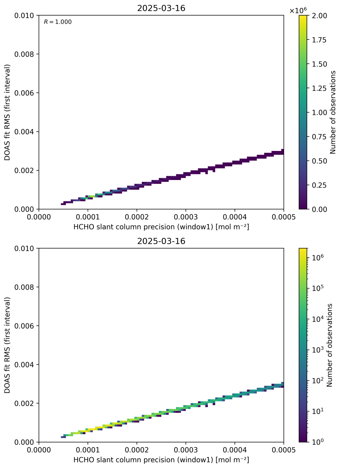
Figure 88: Scatter density plot of “HCHO slant column precision (window1)” against “DOAS fit RMS (first interval)” for 2025-03-15 to 2025-03-17.
