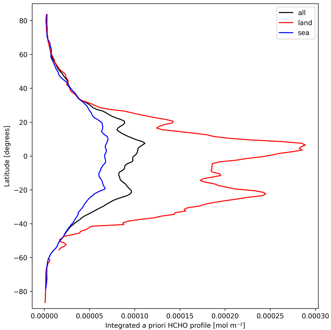
Figure 29: Zonal average of “Integrated a priori HCHO profile” for 2025-03-15 to 2025-03-17.
