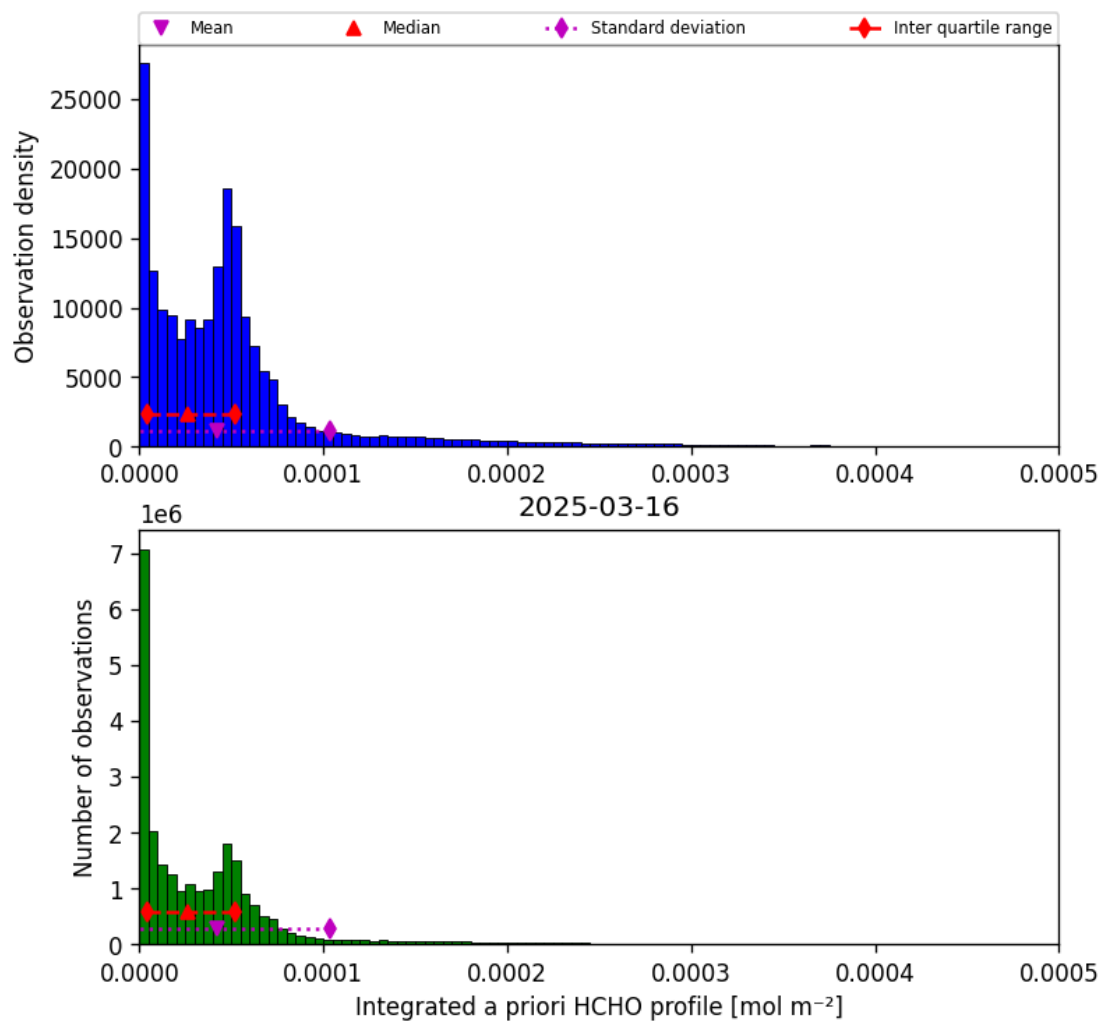
Figure 43: Histogram of “Integrated a priori HCHO profile” for 2025-03-15 to 2025-03-17
