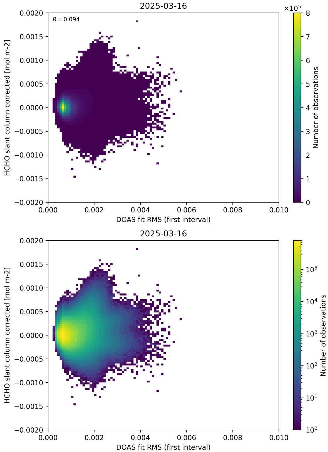
Figure 62: Scatter density plot of “DOAS fit RMS (first interval)” against “HCHO slant column corrected” for 2025-03-15 to 2025-03-17.
