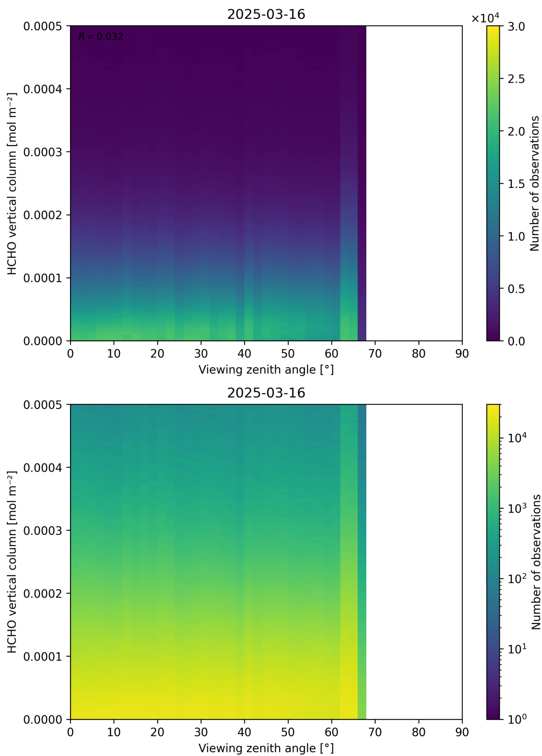
Figure 192: Scatter density plot of “Viewing zenith angle” against “HCHO vertical column” for 2025-03-15 to 2025-03-17.
