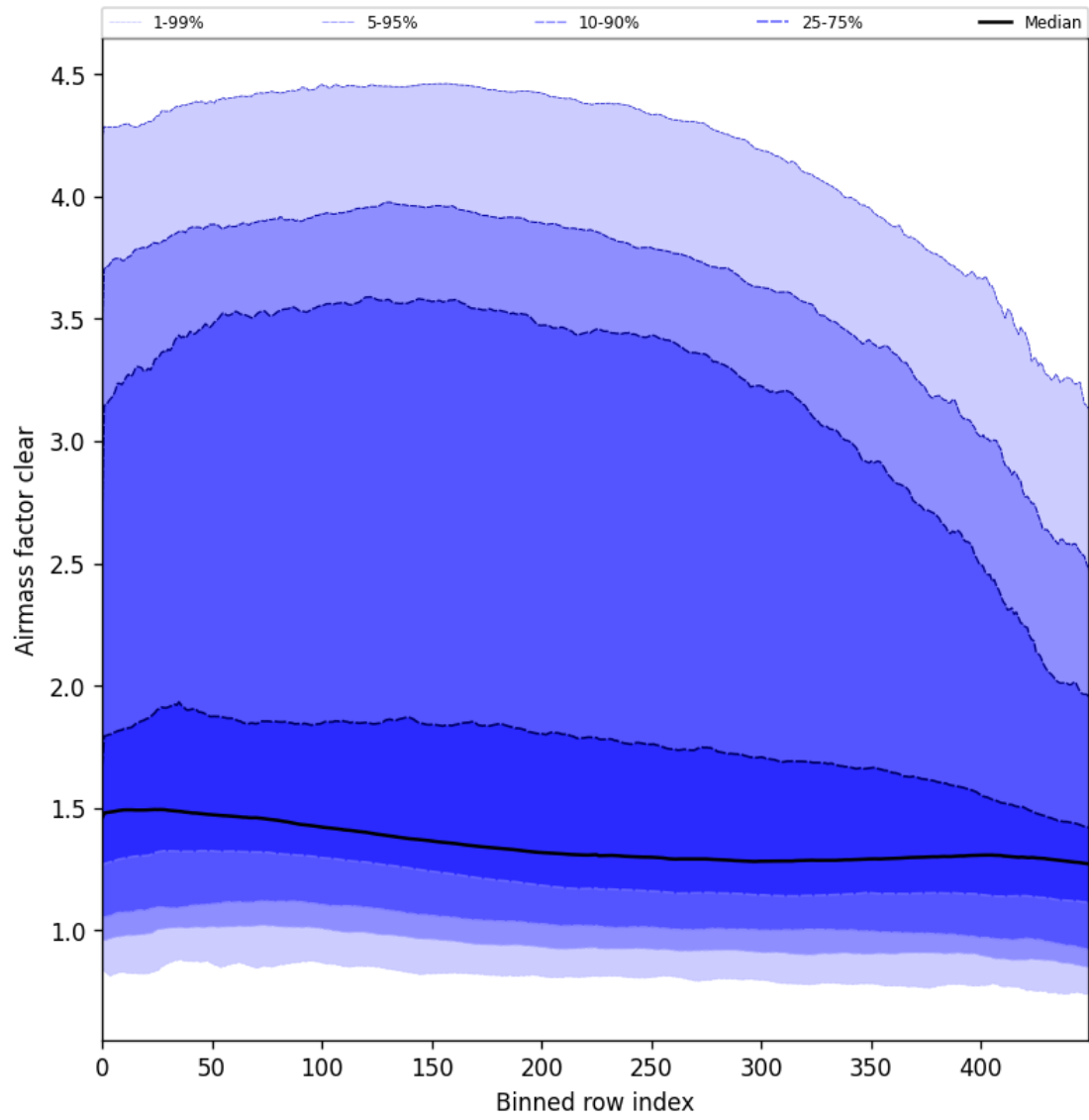
Figure 56: Along track statistics of “Airmass factor clear” for 2025-03-15 to 2025-03-17
