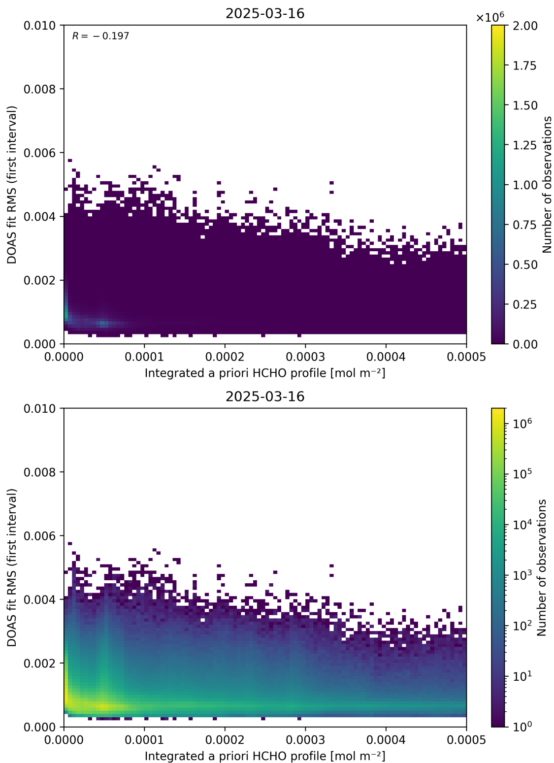
Figure 148: Scatter density plot of “Integrated a priori HCHO profile” against “DOAS fit RMS (first interval)” for 2025-03-15 to 2025-03-17.
