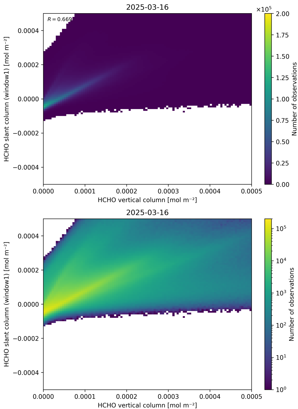
Figure 129: Scatter density plot of “HCHO vertical column” against “HCHO slant column (window1)” for 2025-03-15 to 2025-03-17.
