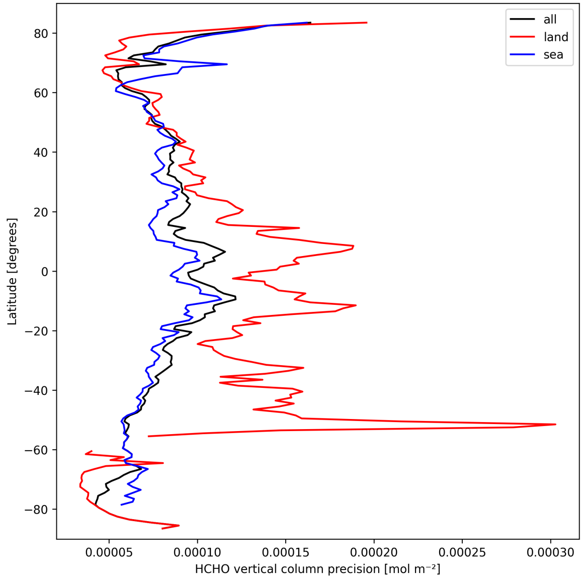
Figure 22: Zonal average of “HCHO vertical column precision” for 2025-03-15 to 2025-03-17.
