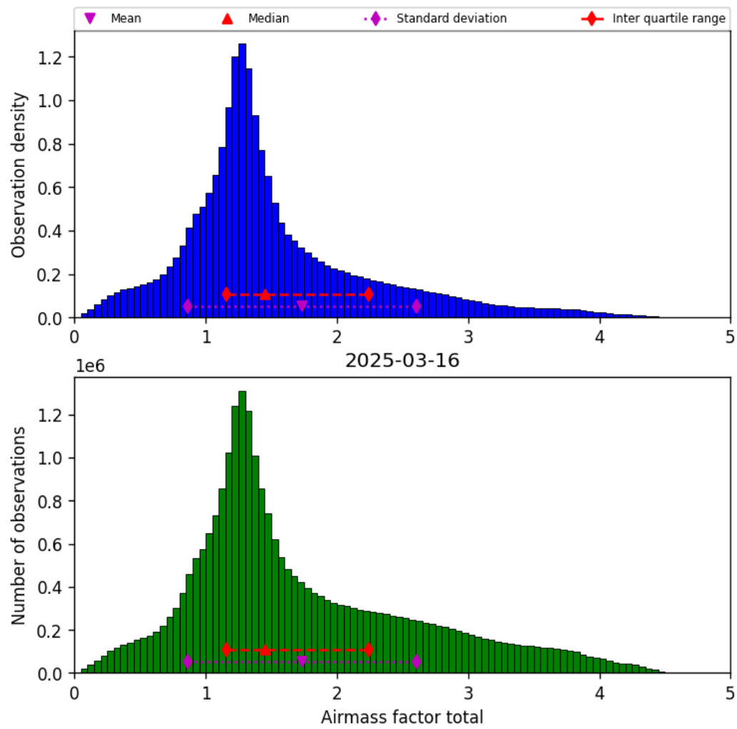
Figure 40: Histogram of “Airmass factor total” for 2025-03-15 to 2025-03-17
