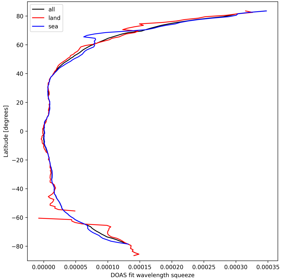
Figure 31: Zonal average of “DOAS fit wavelength squeeze” for 2025-03-15 to 2025-03-17.
