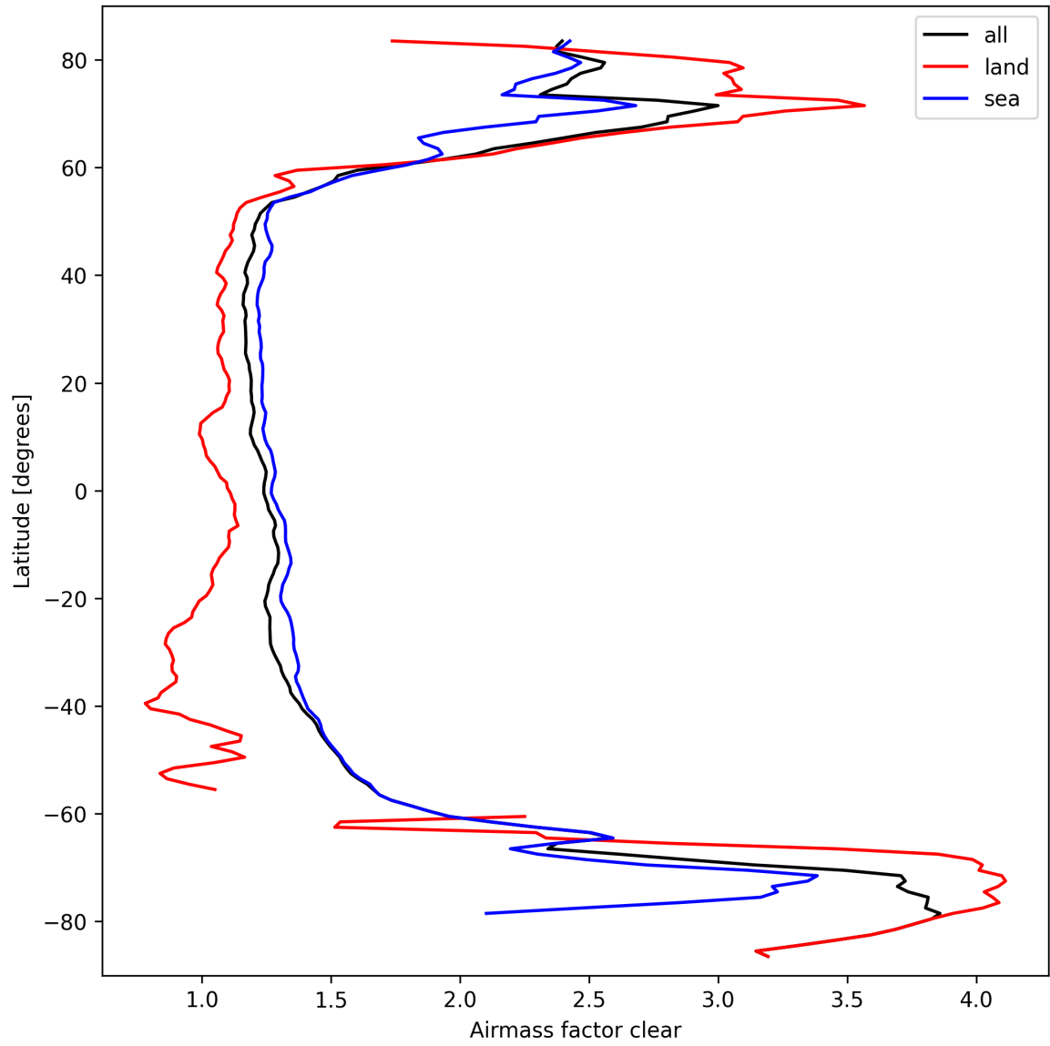
Figure 28: Zonal average of “Airmass factor clear” for 2025-03-15 to 2025-03-17.
