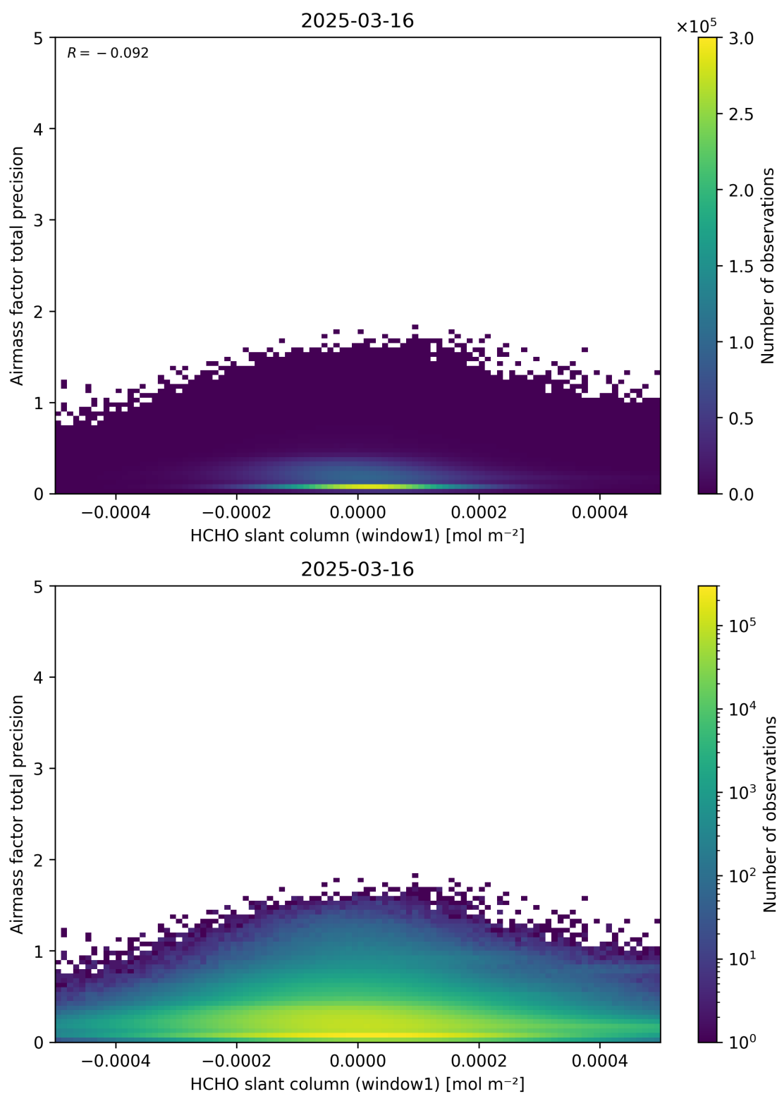
Figure 86: Scatter density plot of “HCHO slant column (window1)” against “Airmass factor total precision” for 2025-03-15 to 2025-03-17.
