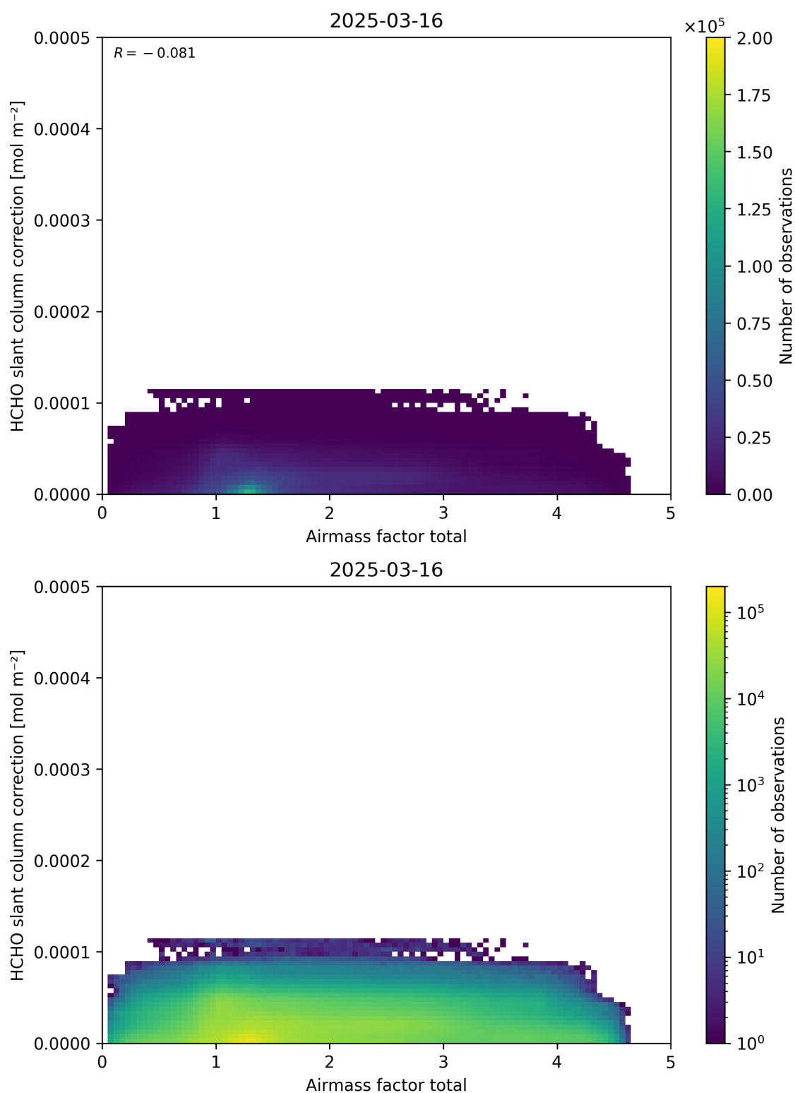
Figure 102: Scatter density plot of “Airmass factor total” against “HCHO slant column correction” for 2025-03-15 to 2025-03-17.
