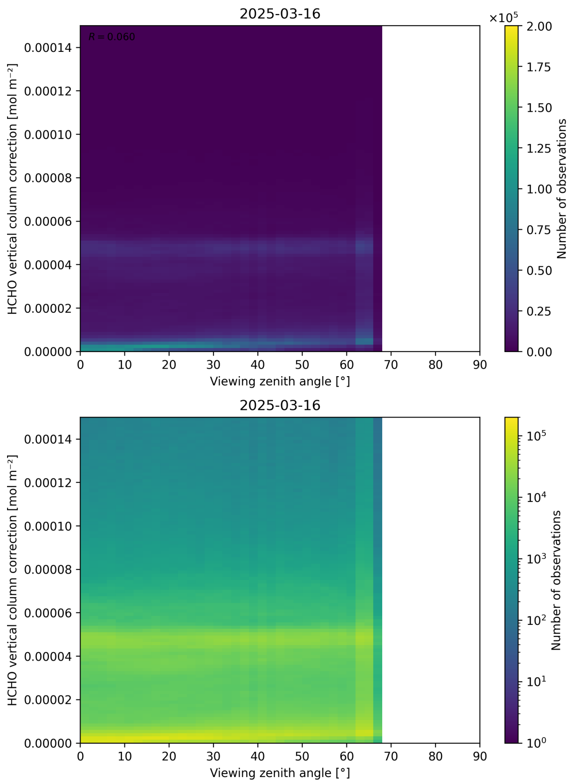
Figure 193: Scatter density plot of “Viewing zenith angle” against “HCHO vertical column correction” for 2025-03-15 to 2025-03-17.
