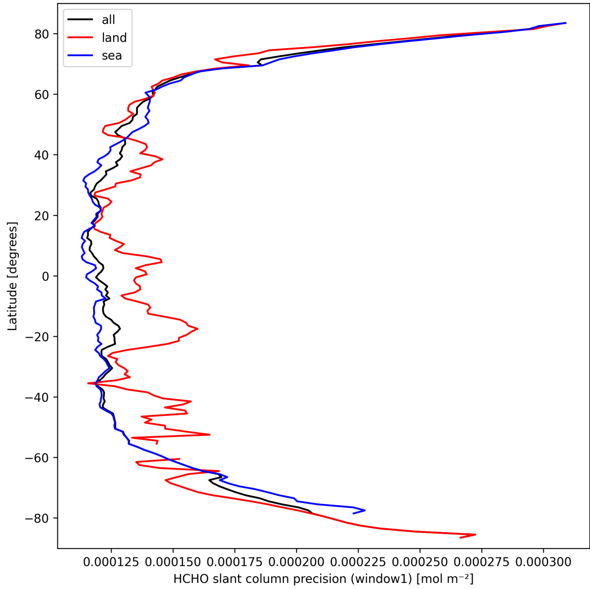
Figure 25: Zonal average of “HCHO slant column precision (window1)” for 2025-03-15 to 2025-03-17.
