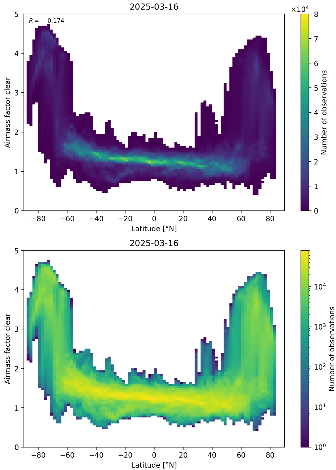
Figure 156: Scatter density plot of “Latitude” against “Airmass factor clear” for 2025-03-15 to 2025-03-17.
