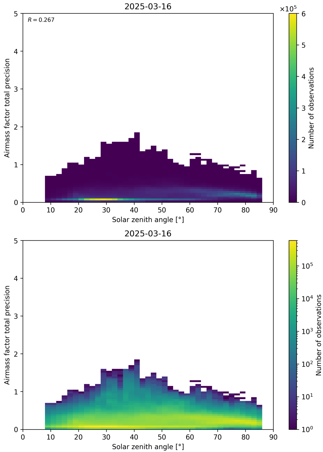
Figure 176: Scatter density plot of “Solar zenith angle” against “Airmass factor total precision” for 2025-03-15 to 2025-03-17.
