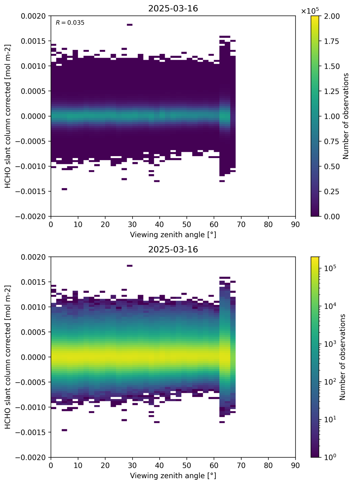
Figure 186: Scatter density plot of “Viewing zenith angle” against “HCHO slant column corrected” for 2025-03-15 to 2025-03-17.
