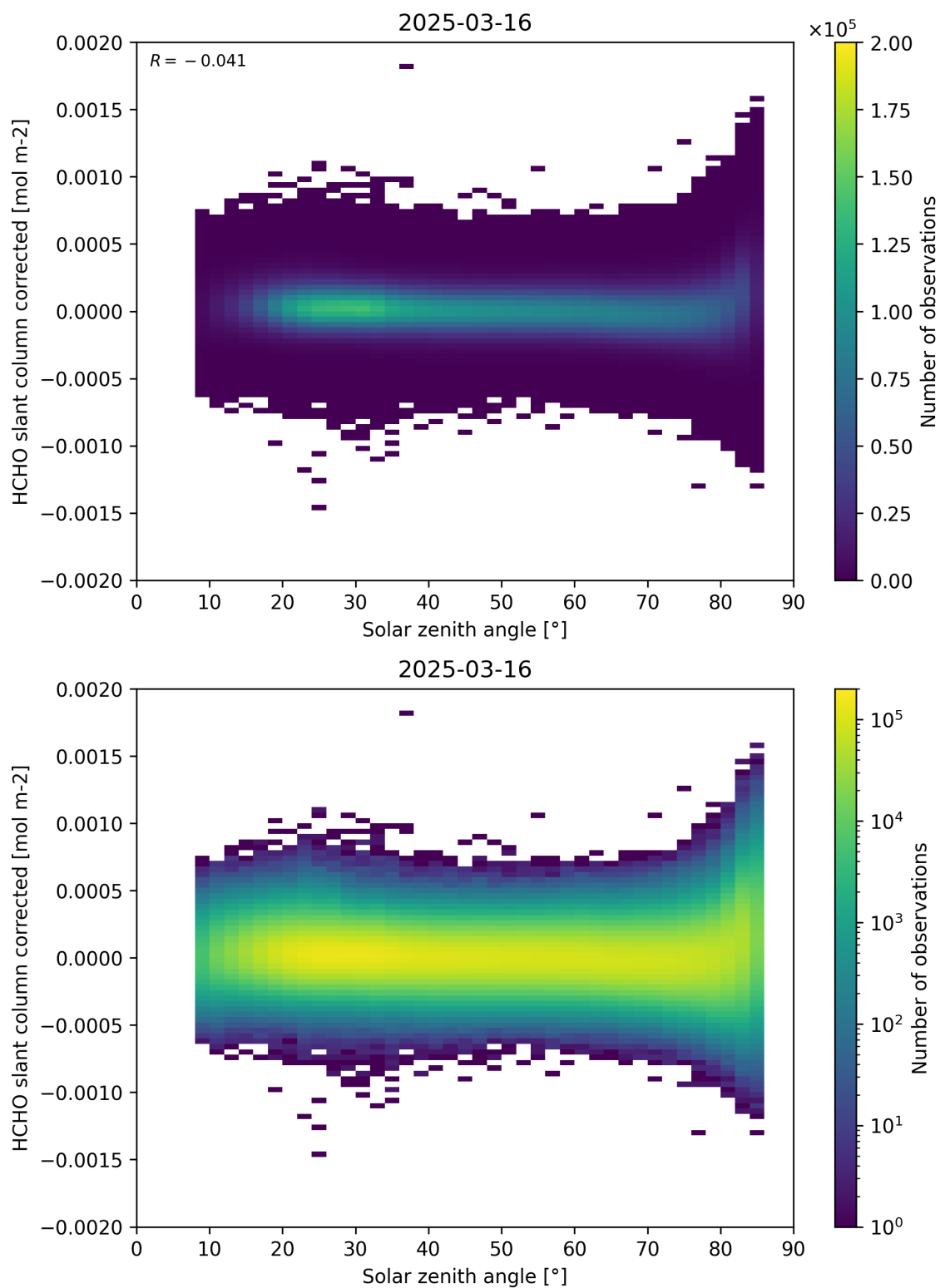
Figure 171: Scatter density plot of “Solar zenith angle” against “HCHO slant column corrected” for 2025-03-15 to 2025-03-17.
