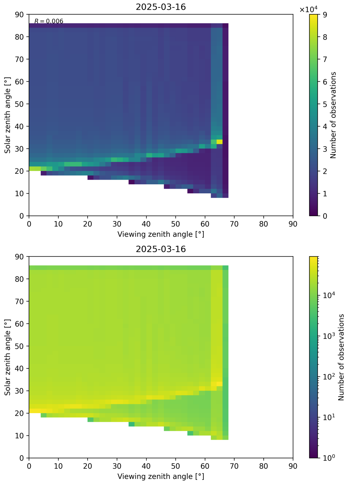
Figure 197: Scatter density plot of “Viewing zenith angle” against “Solar zenith angle” for 2025-03-15 to 2025-03-17.
