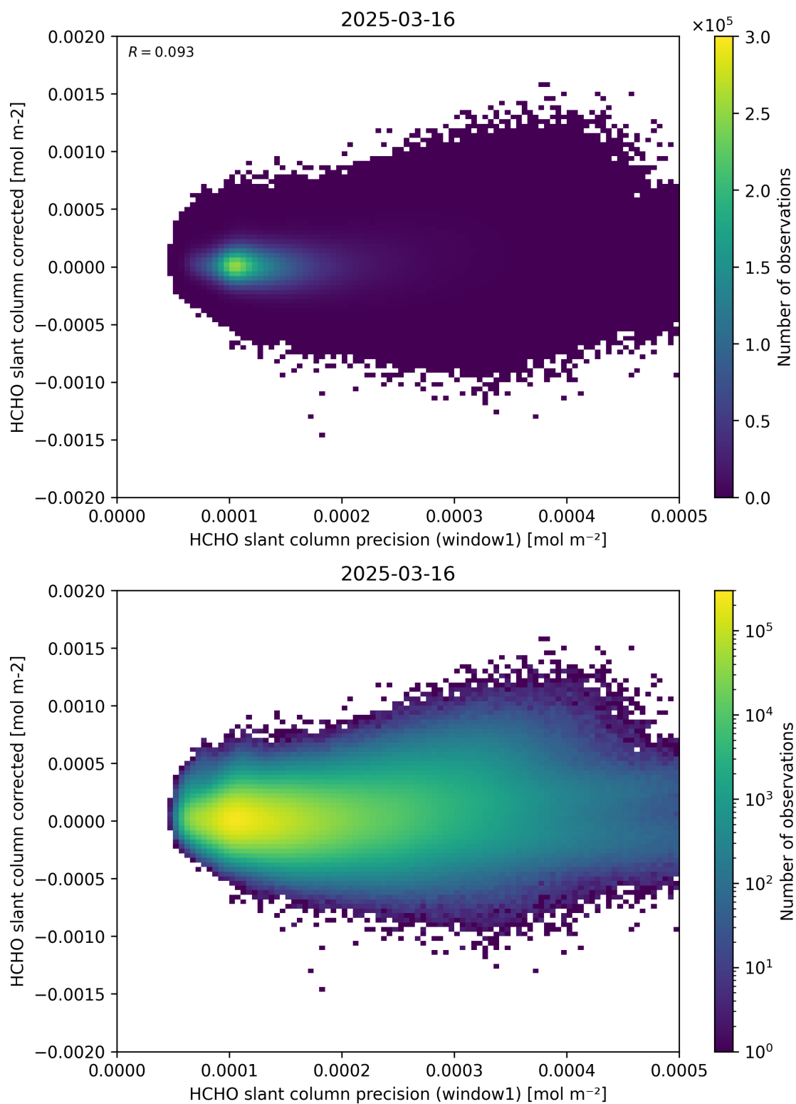
Figure 92: Scatter density plot of “HCHO slant column precision (window1)” against “HCHO slant column corrected” for 2025-03-15 to 2025-03-17.
