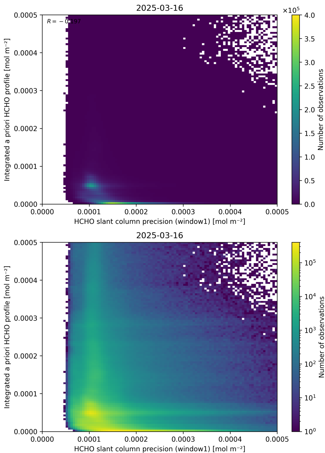
Figure 96: Scatter density plot of “HCHO slant column precision (window1)” against “Integrated a priori HCHO profile” for 2025-03-15 to 2025-03-17.
