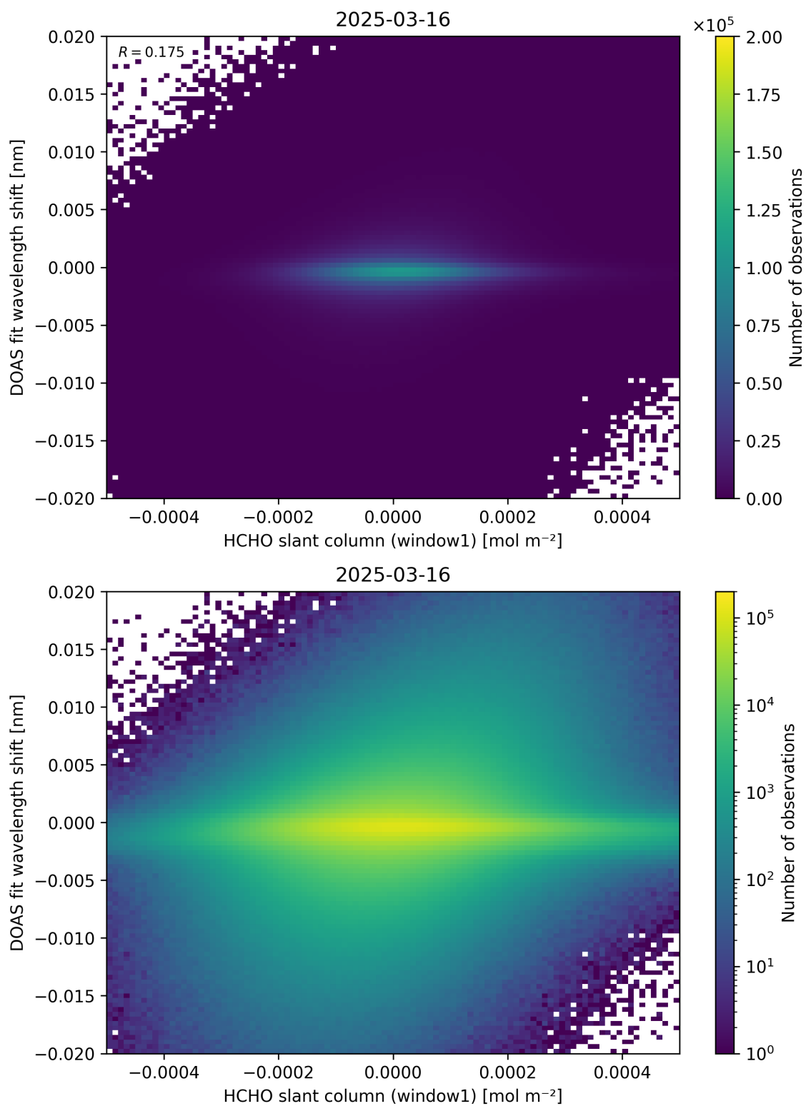
Figure 79: Scatter density plot of “HCHO slant column (window1)” against “DOAS fit wavelength shift” for 2025-03-15 to 2025-03-17.
