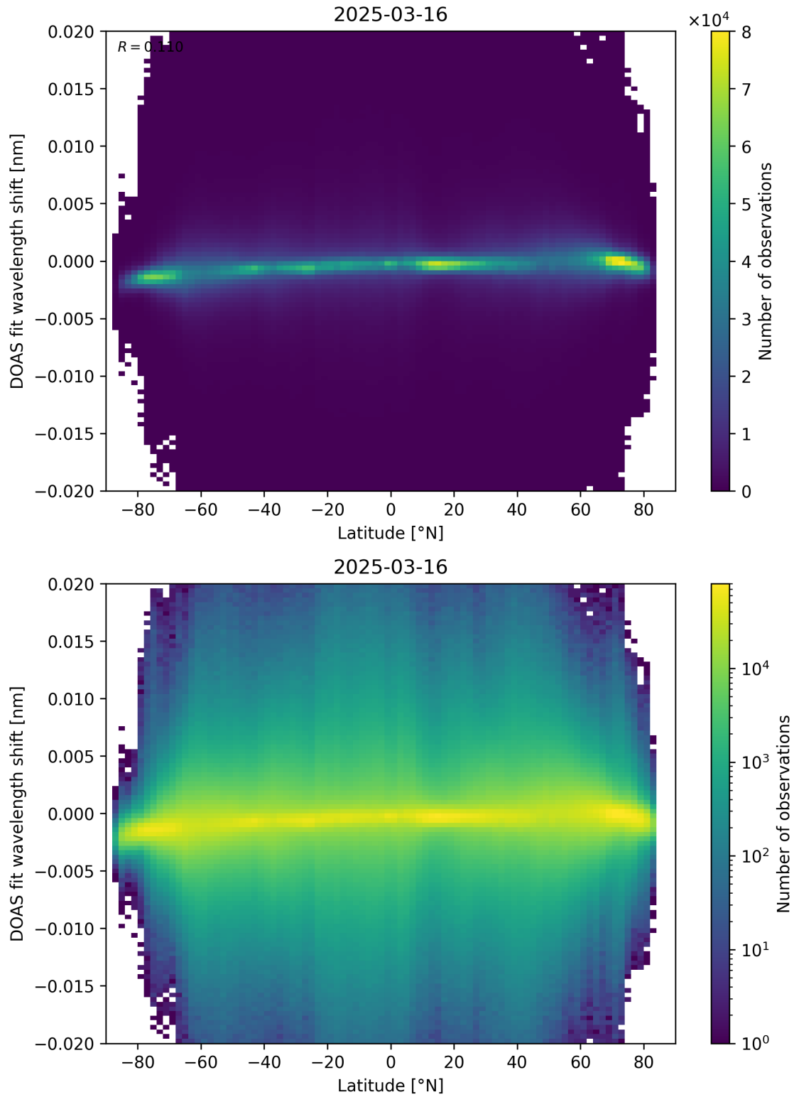
Figure 154: Scatter density plot of “Latitude” against “DOAS fit wavelength shift” for 2025-03-15 to 2025-03-17.
