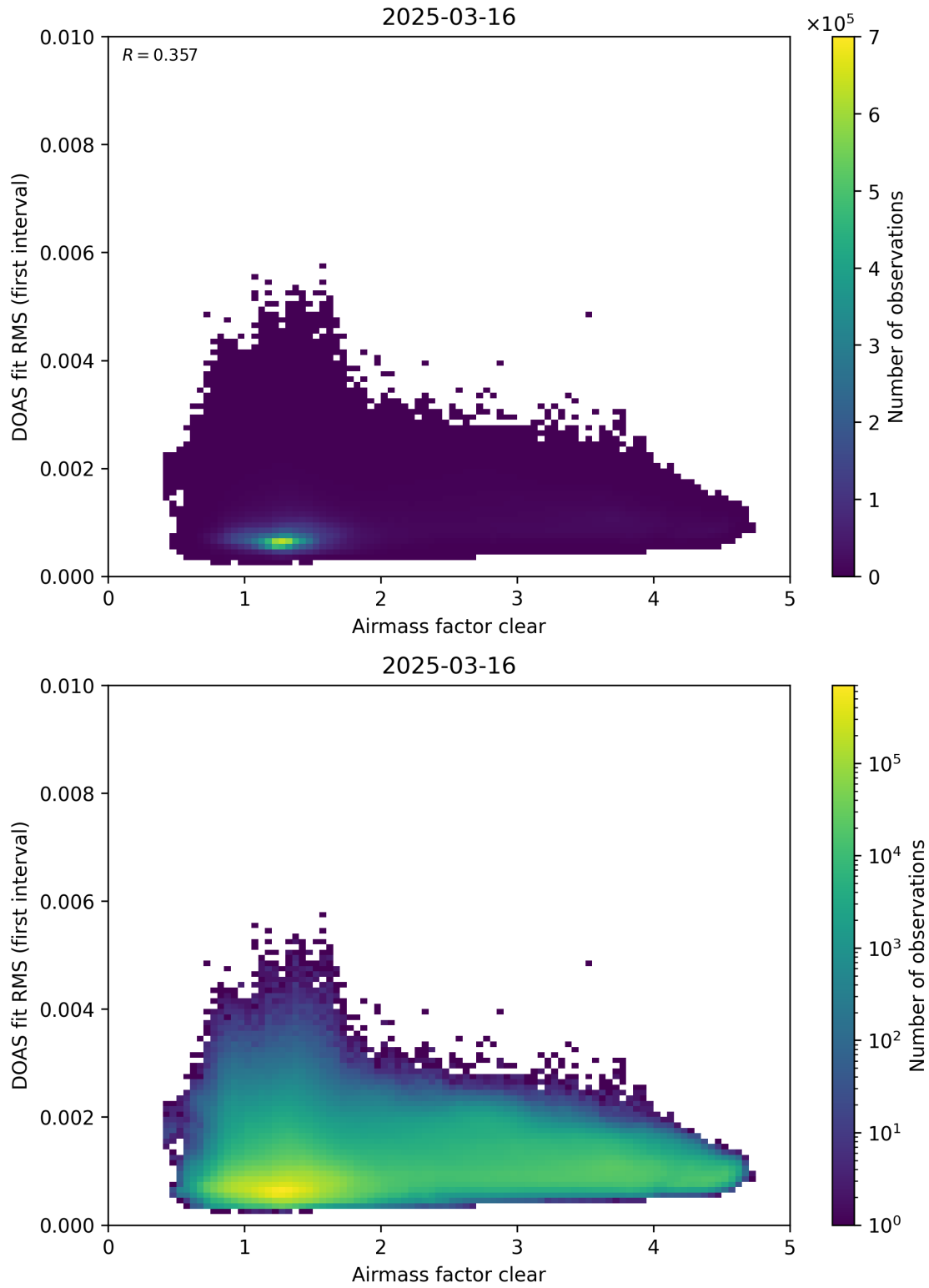
Figure 71: Scatter density plot of “Airmass factor clear” against “DOAS fit RMS (first interval)” for 2025-03-15 to 2025-03-17.
