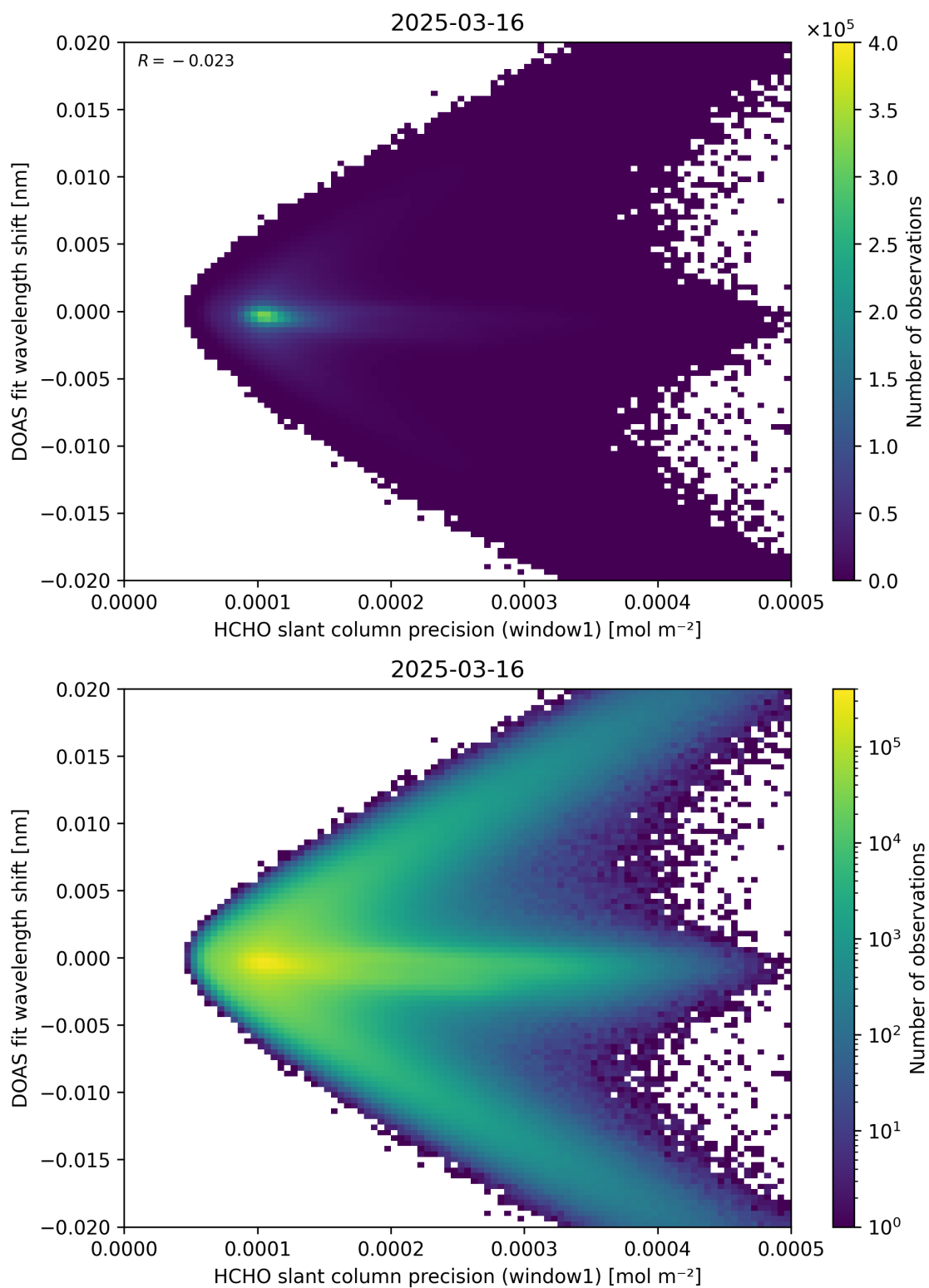
Figure 89: Scatter density plot of “HCHO slant column precision (window1)” against “DOAS fit wavelength shift” for 2025-03-15 to 2025-03-17.
