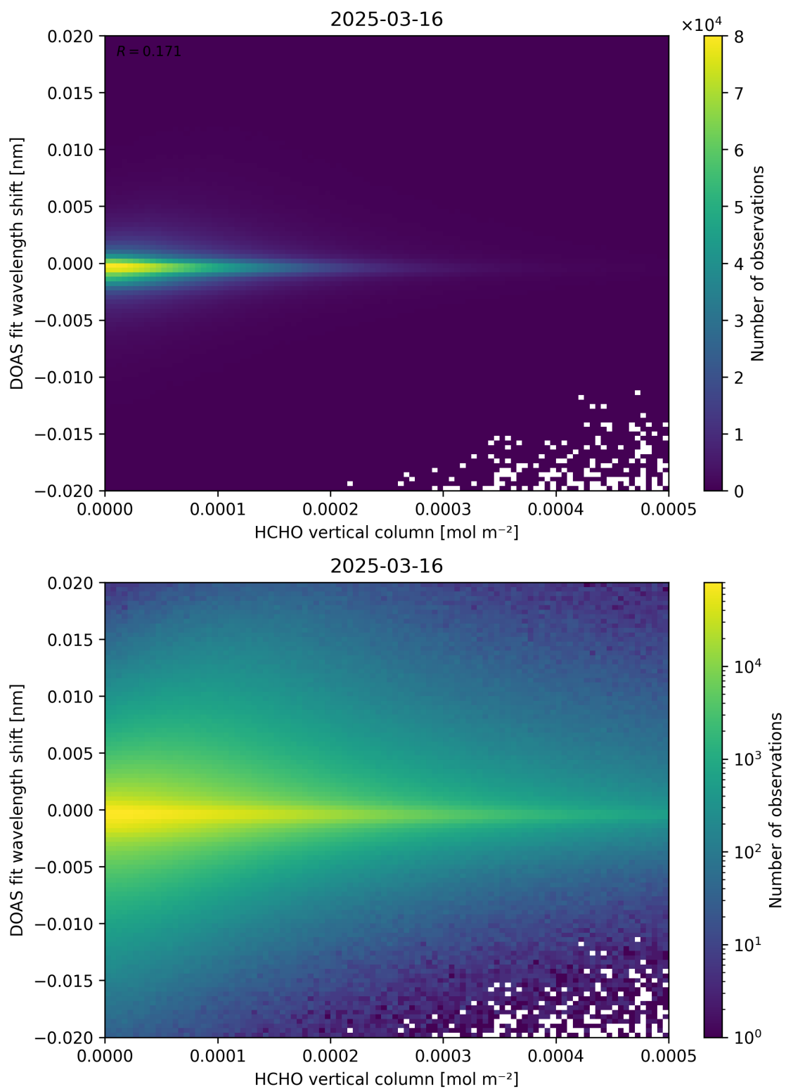
Figure 124: Scatter density plot of “HCHO vertical column” against “DOAS fit wavelength shift” for 2025-03-15 to 2025-03-17.
