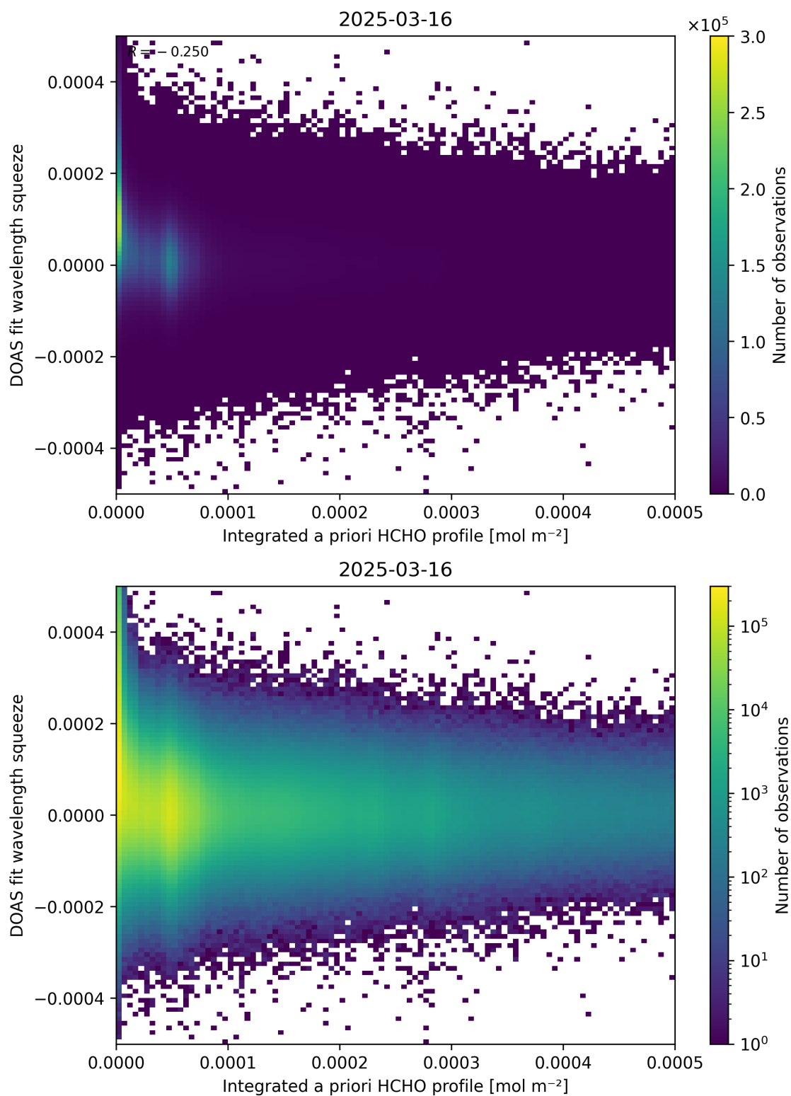
Figure 150: Scatter density plot of “Integrated a priori HCHO profile” against “DOAS fit wavelength squeeze” for 2025-03-15 to 2025-03-17.
