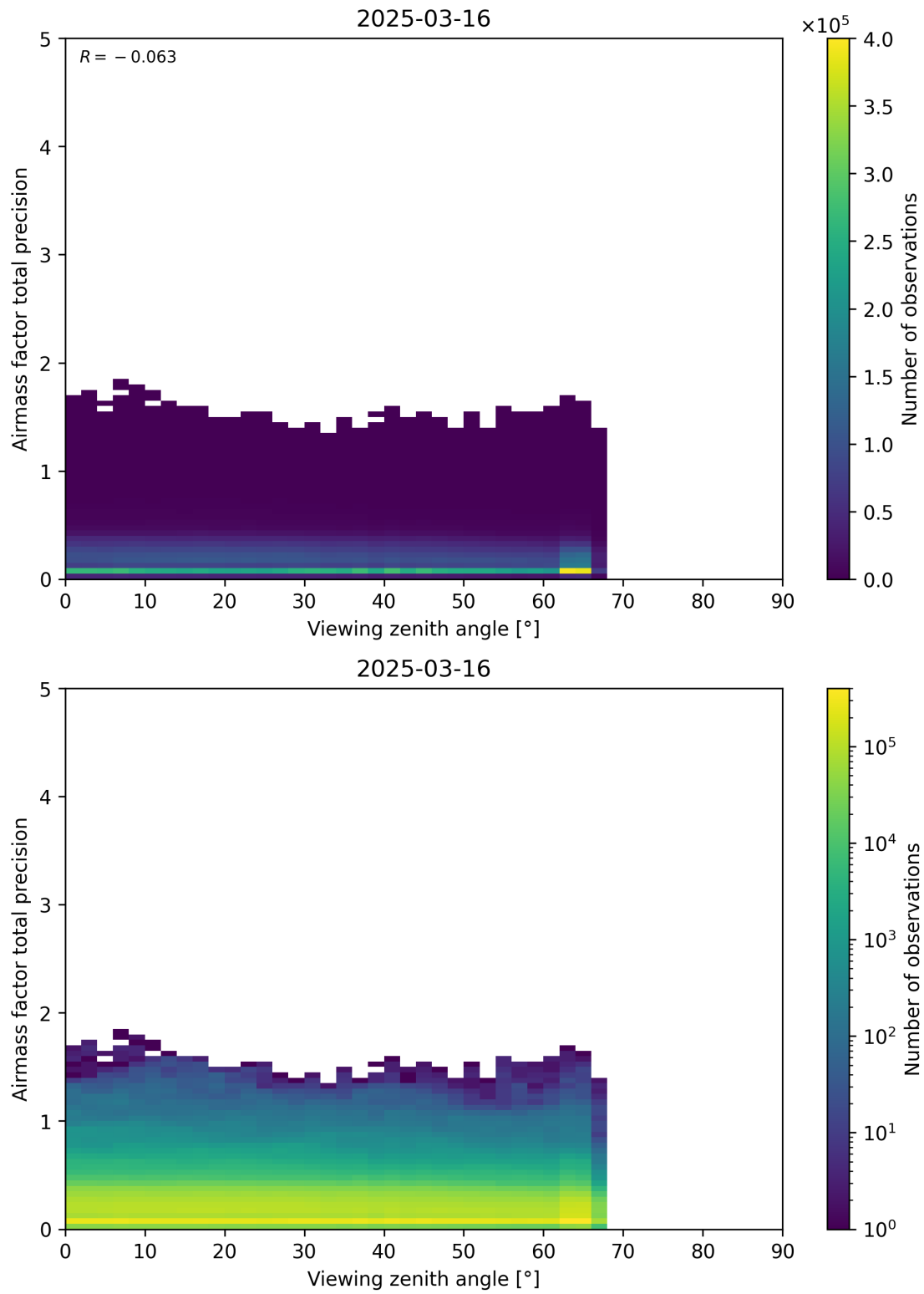
Figure 191: Scatter density plot of “Viewing zenith angle” against “Airmass factor total precision” for 2025-03-15 to 2025-03-17.
