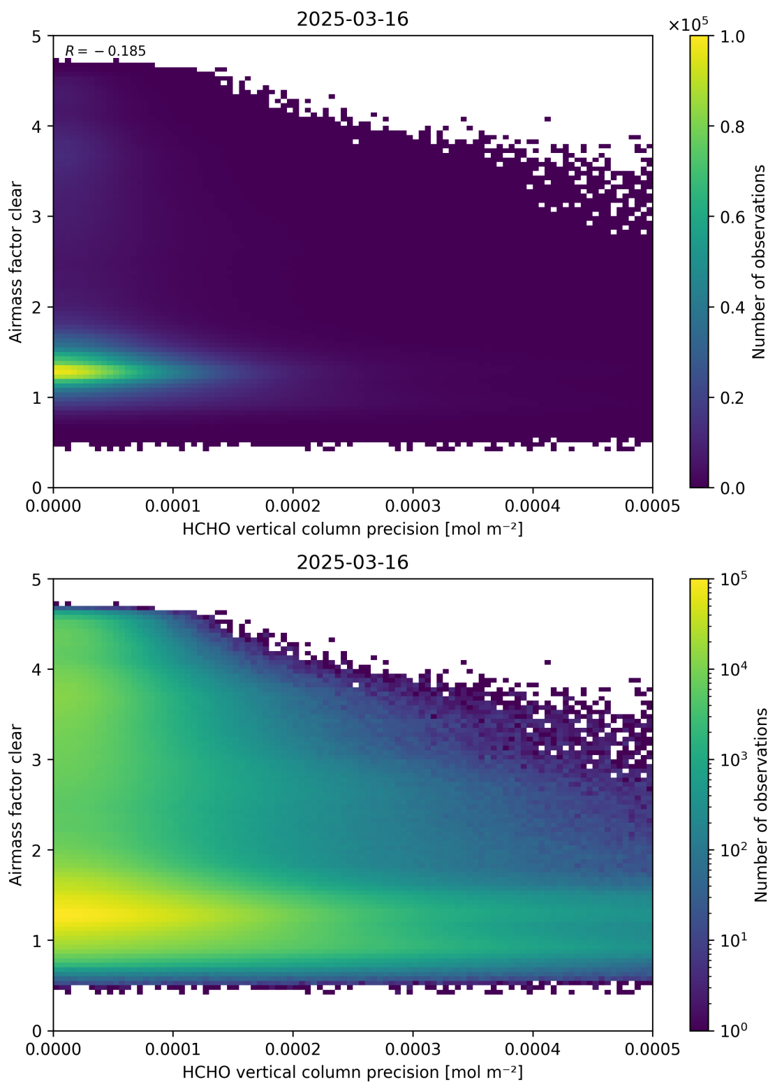
Figure 139: Scatter density plot of “HCHO vertical column precision” against “Airmass factor clear” for 2025-03-15 to 2025-03-17.
