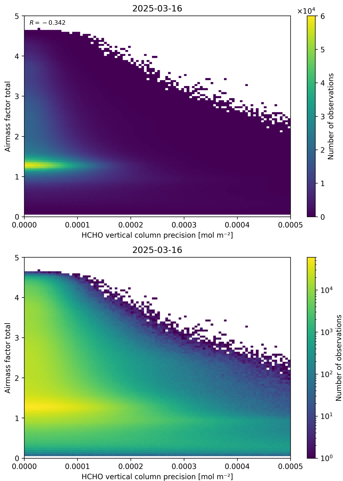
Figure 144: Scatter density plot of “HCHO vertical column precision” against “Airmass factor total” for 2025-03-15 to 2025-03-17.
