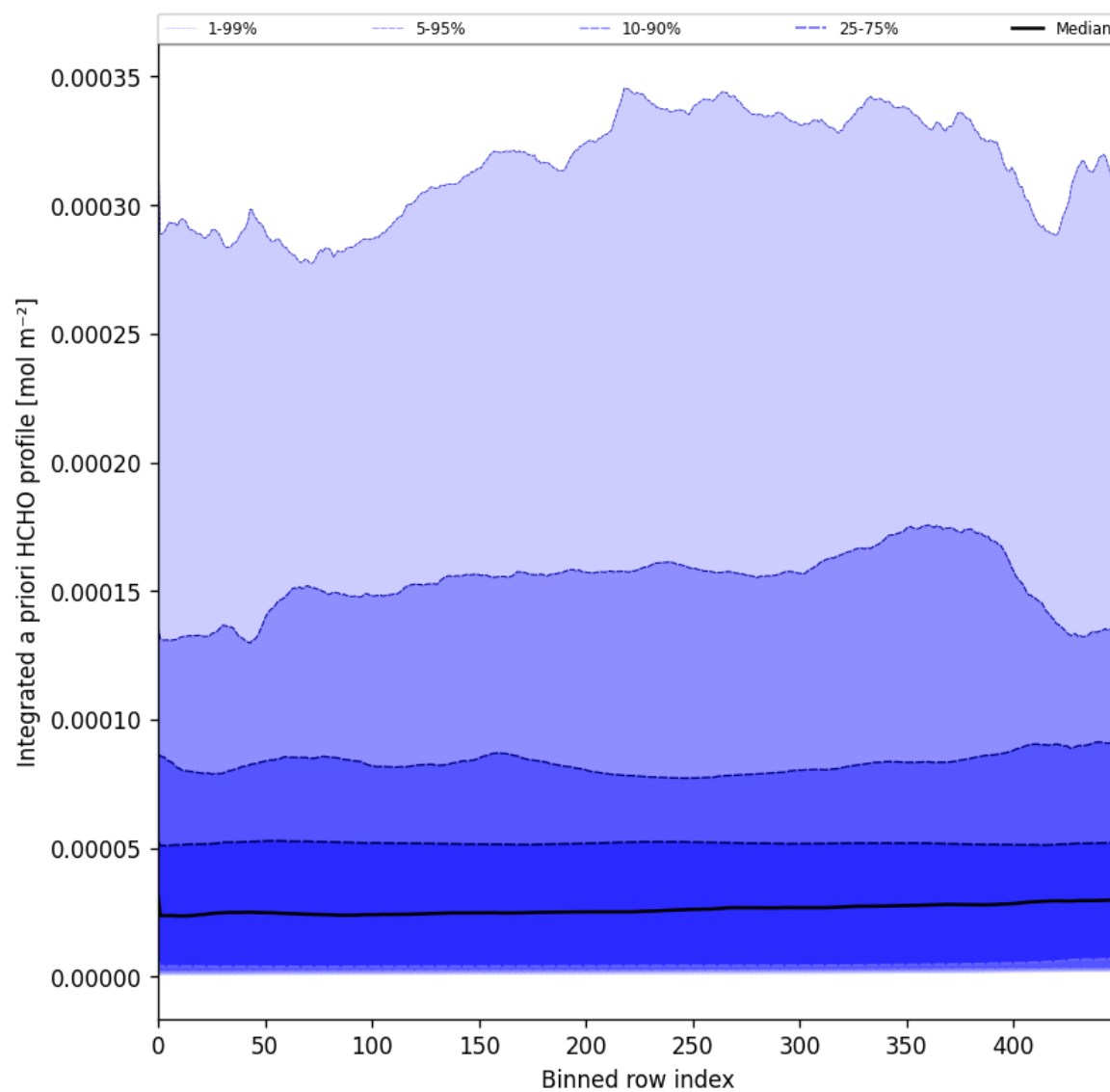
Figure 57: Along track statistics of “Integrated a priori HCHO profile” for 2025-03-15 to 2025-03-17
