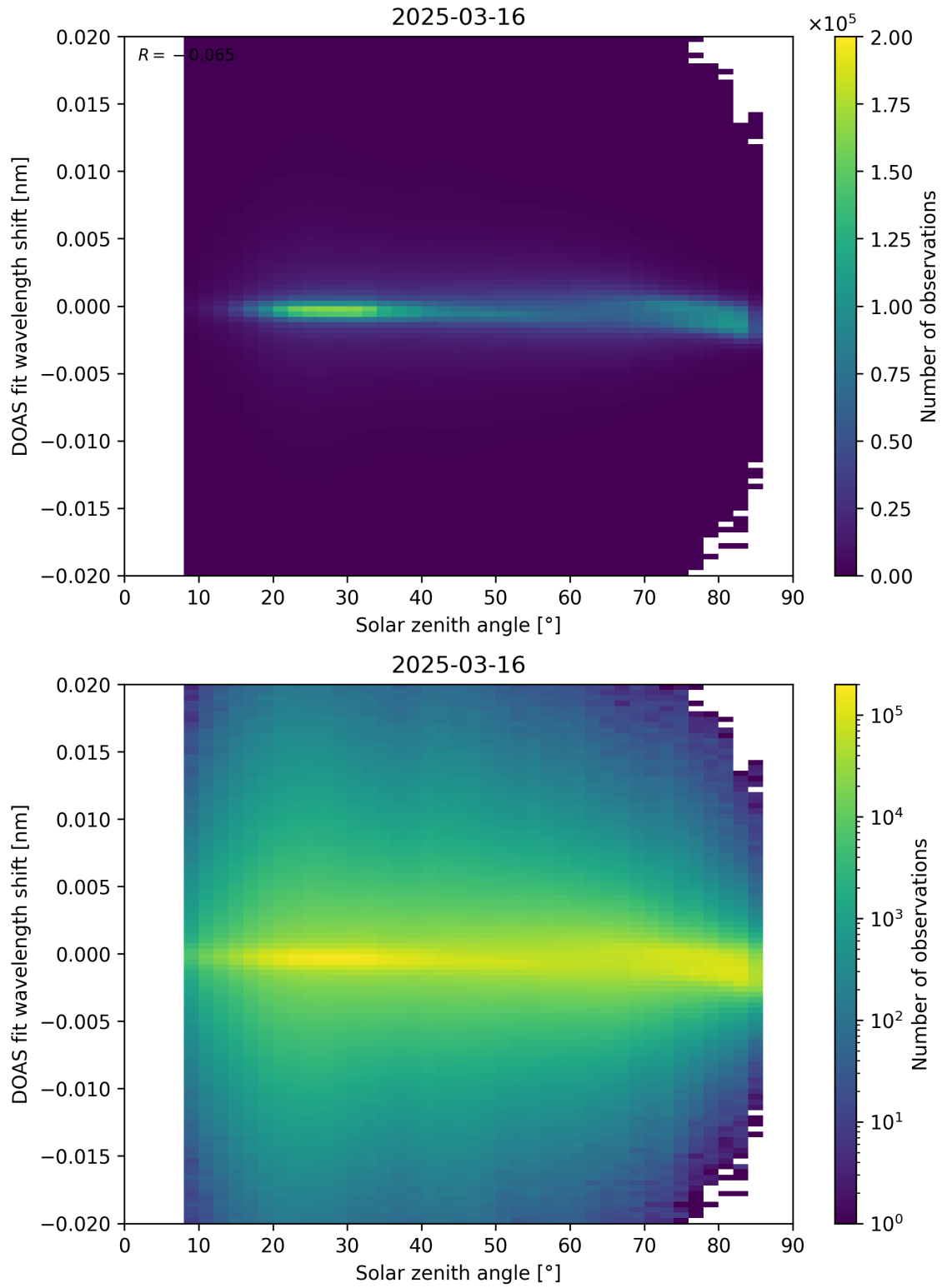
Figure 168: Scatter density plot of “Solar zenith angle” against “DOAS fit wavelength shift” for 2025-03-15 to 2025-03-17.
