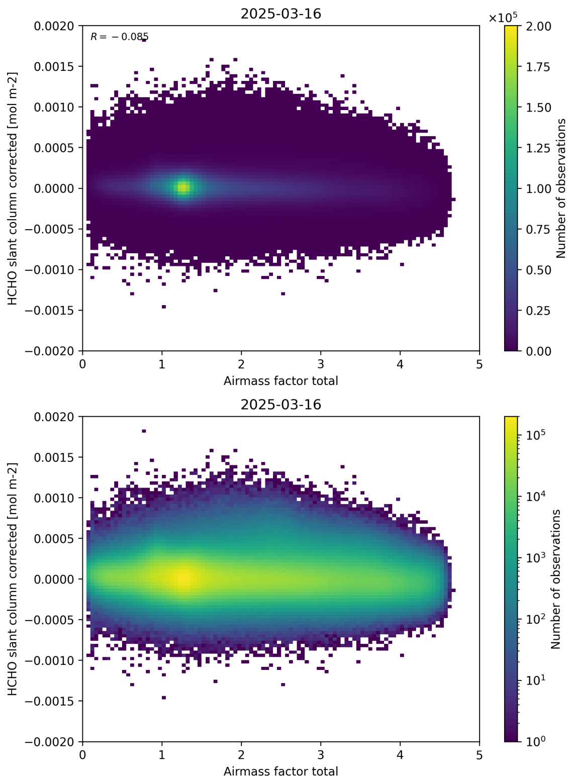
Figure 101: Scatter density plot of “Airmass factor total” against “HCHO slant column corrected” for 2025-03-15 to 2025-03-17.
