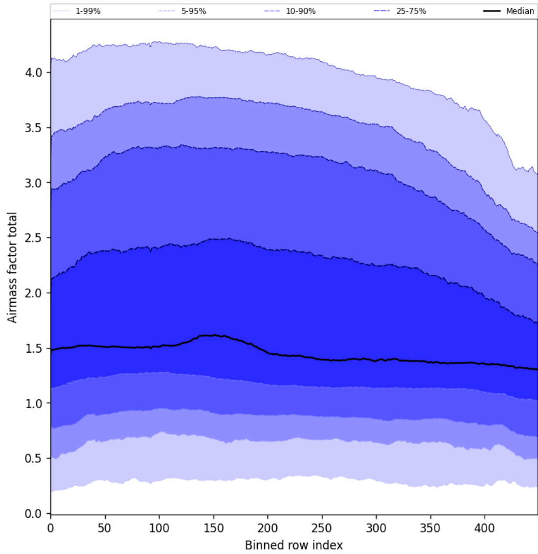
Figure 54: Along track statistics of “Airmass factor total” for 2025-03-15 to 2025-03-17
