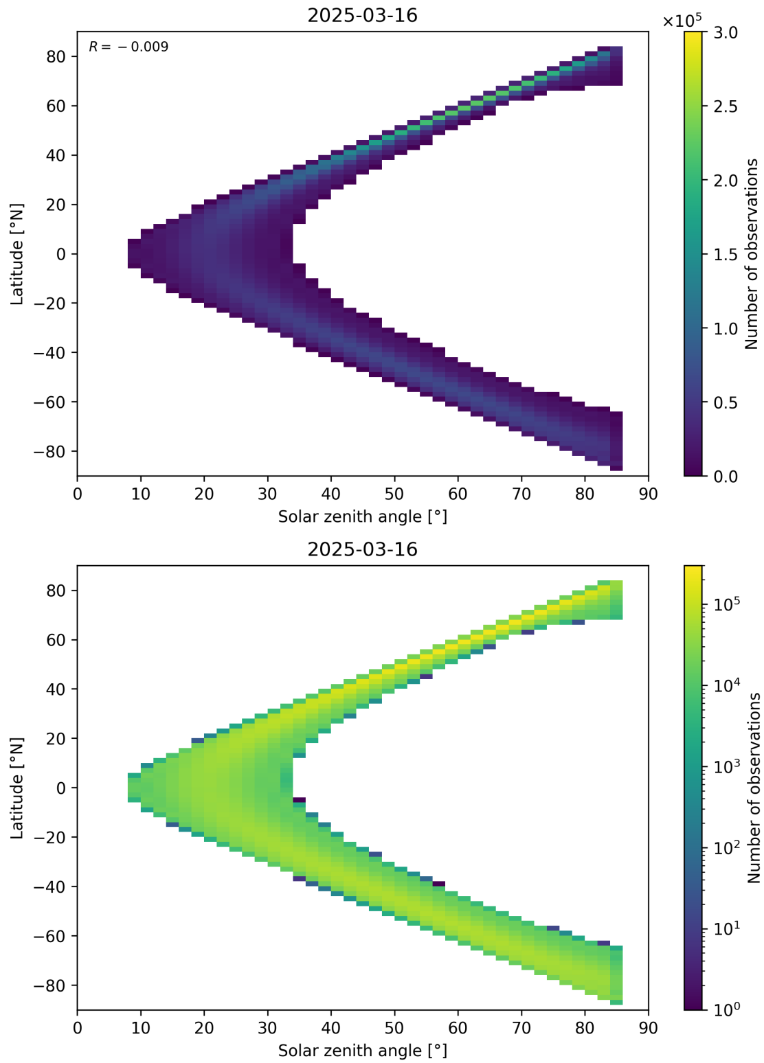
Figure 181: Scatter density plot of “Solar zenith angle” against “Latitude” for 2025-03-15 to 2025-03-17.
