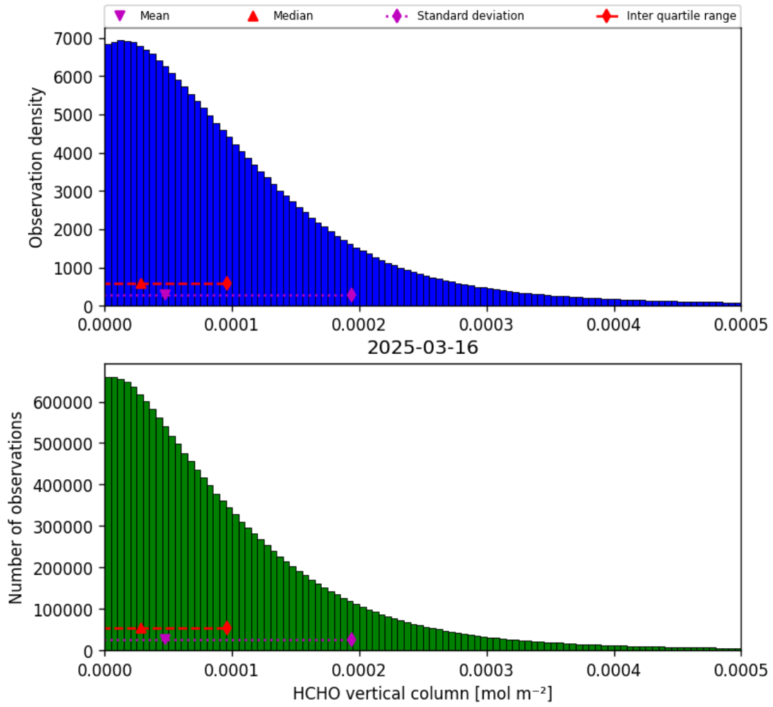
Figure 35: Histogram of “HCHO vertical column” for 2025-03-15 to 2025-03-17
