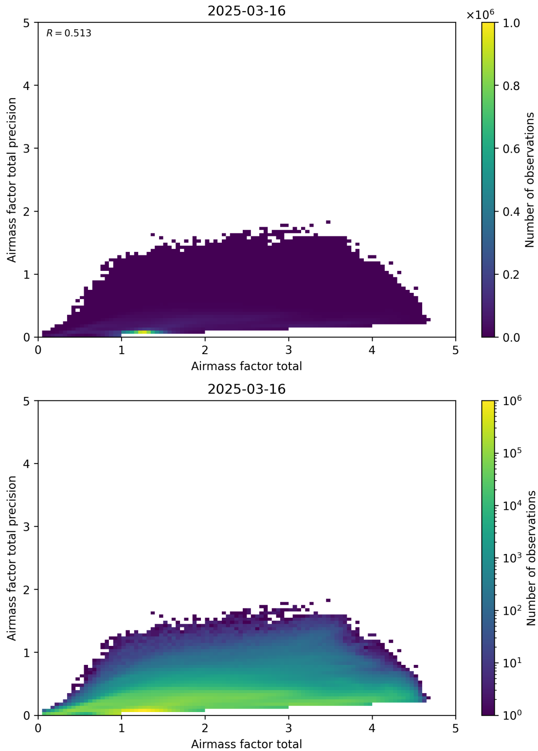
Figure 103: Scatter density plot of “Airmass factor total” against “Airmass factor total precision” for 2025-03-15 to 2025-03-17.
