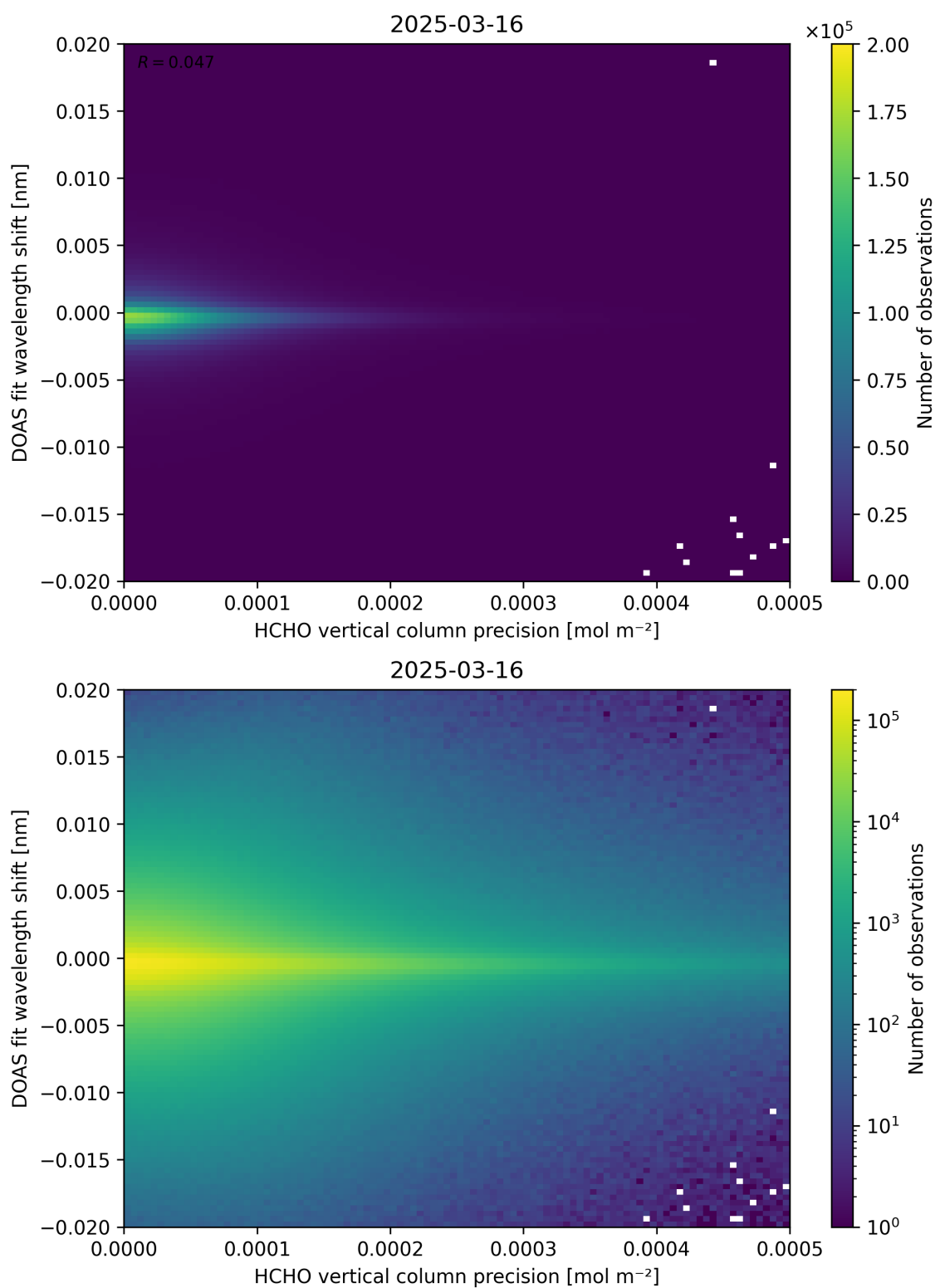
Figure 137: Scatter density plot of “HCHO vertical column precision” against “DOAS fit wavelength shift” for 2025-03-15 to 2025-03-17.
