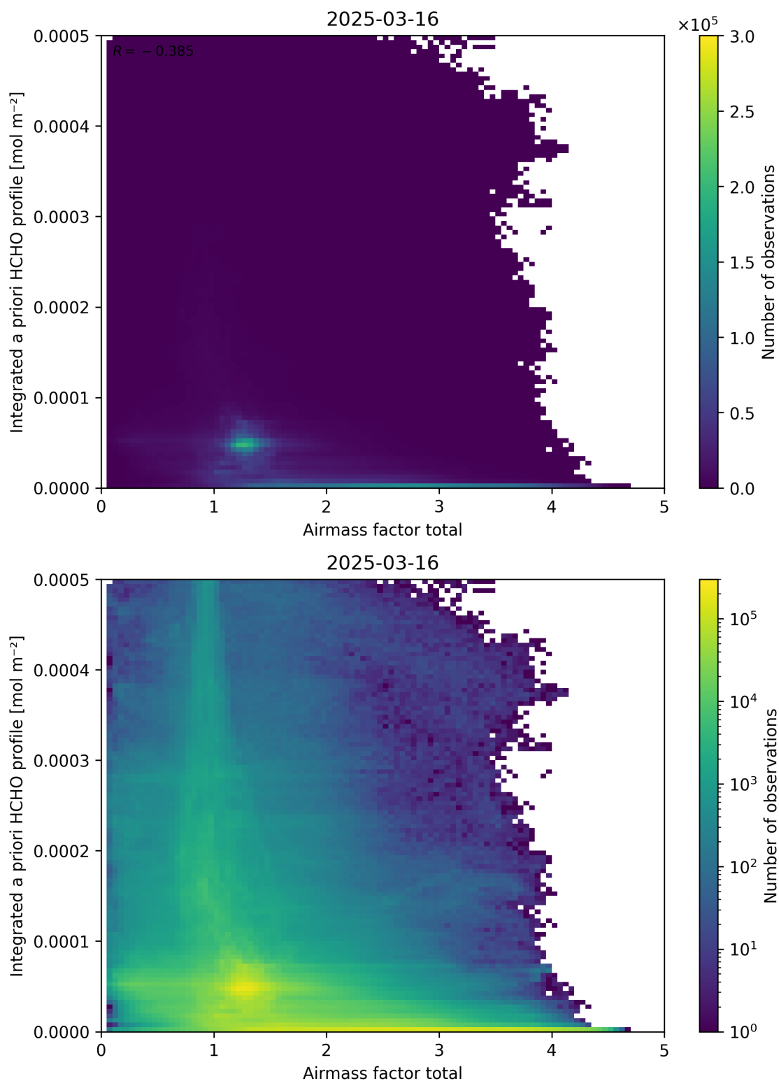
Figure 104: Scatter density plot of “Airmass factor total” against “Integrated a priori HCHO profile” for 2025-03-15 to 2025-03-17.
