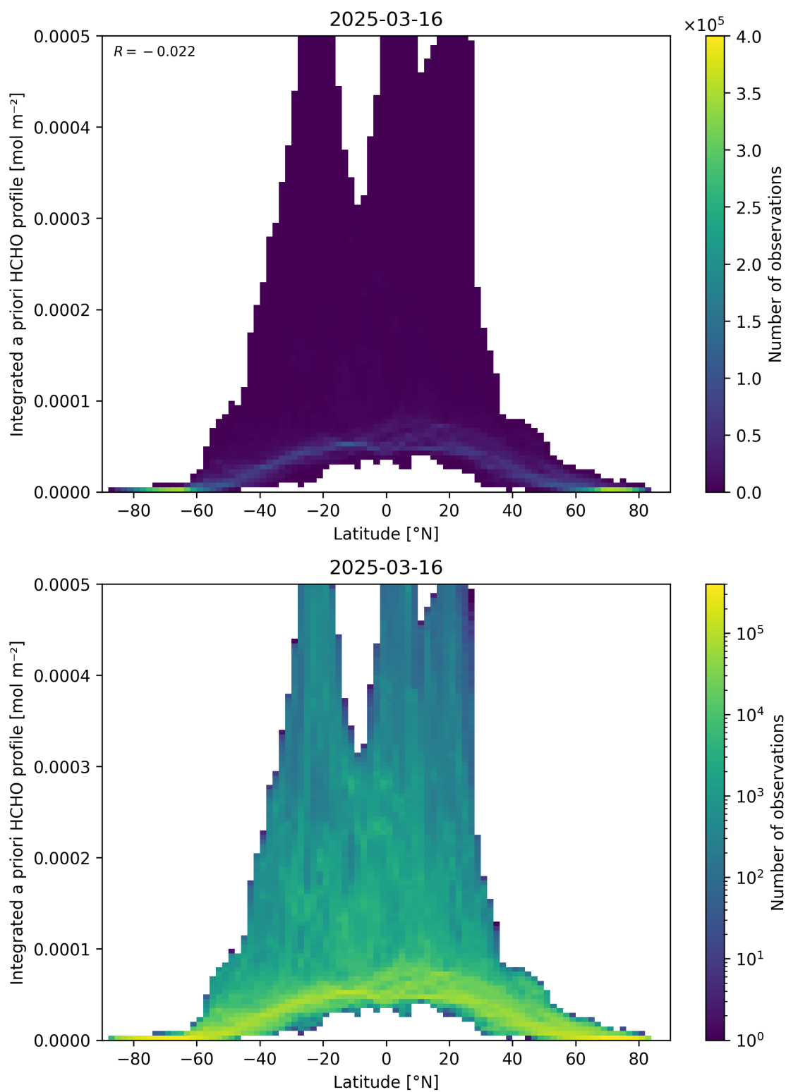
Figure 166: Scatter density plot of “Latitude” against “Integrated a priori HCHO profile” for 2025-03-15 to 2025-03-17.
