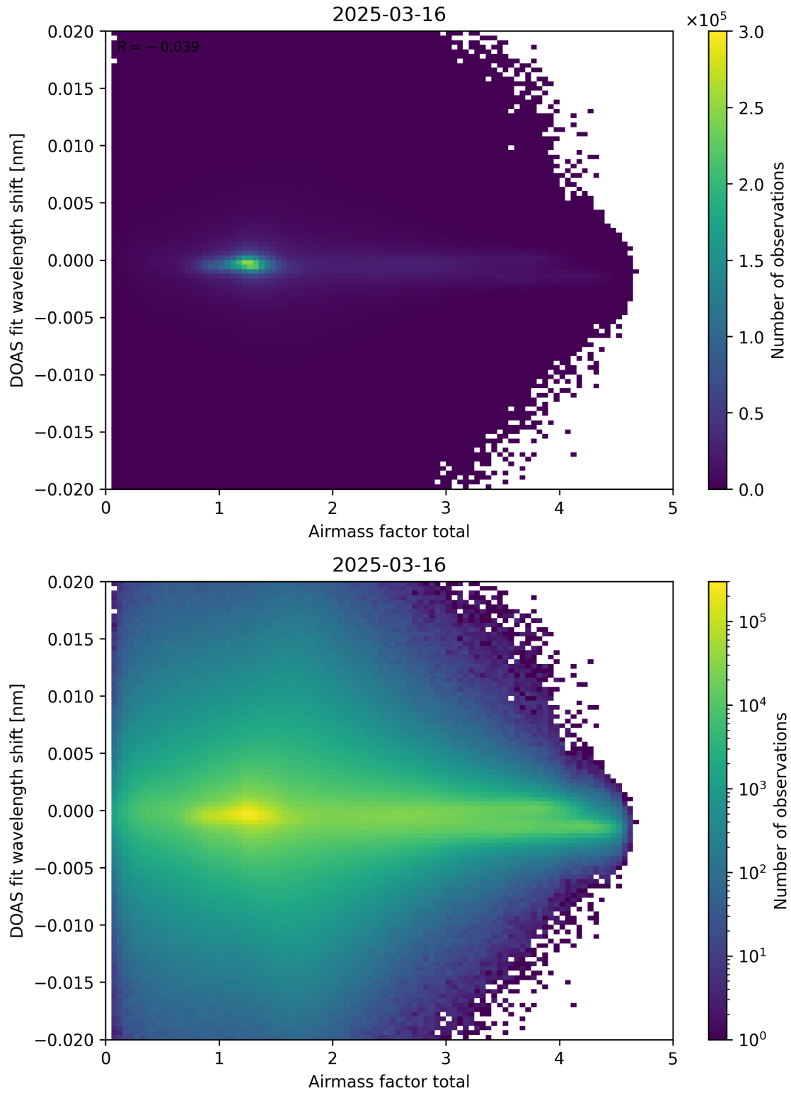
Figure 98: Scatter density plot of “Airmass factor total” against “DOAS fit wavelength shift” for 2025-03-15 to 2025-03-17.
