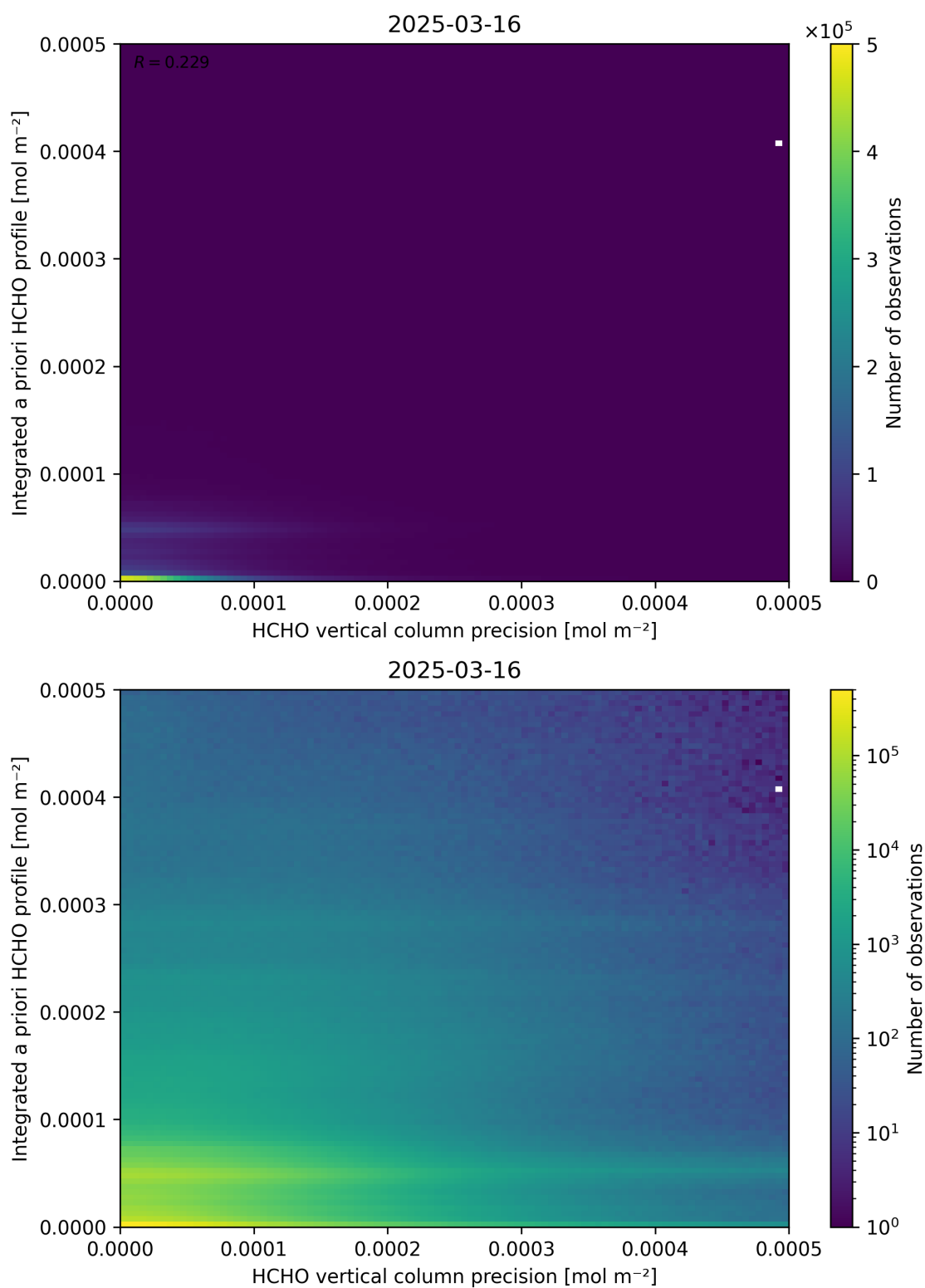
Figure 147: Scatter density plot of “HCHO vertical column precision” against “Integrated a priori HCHO profile” for 2025-03-15 to 2025-03-17.
