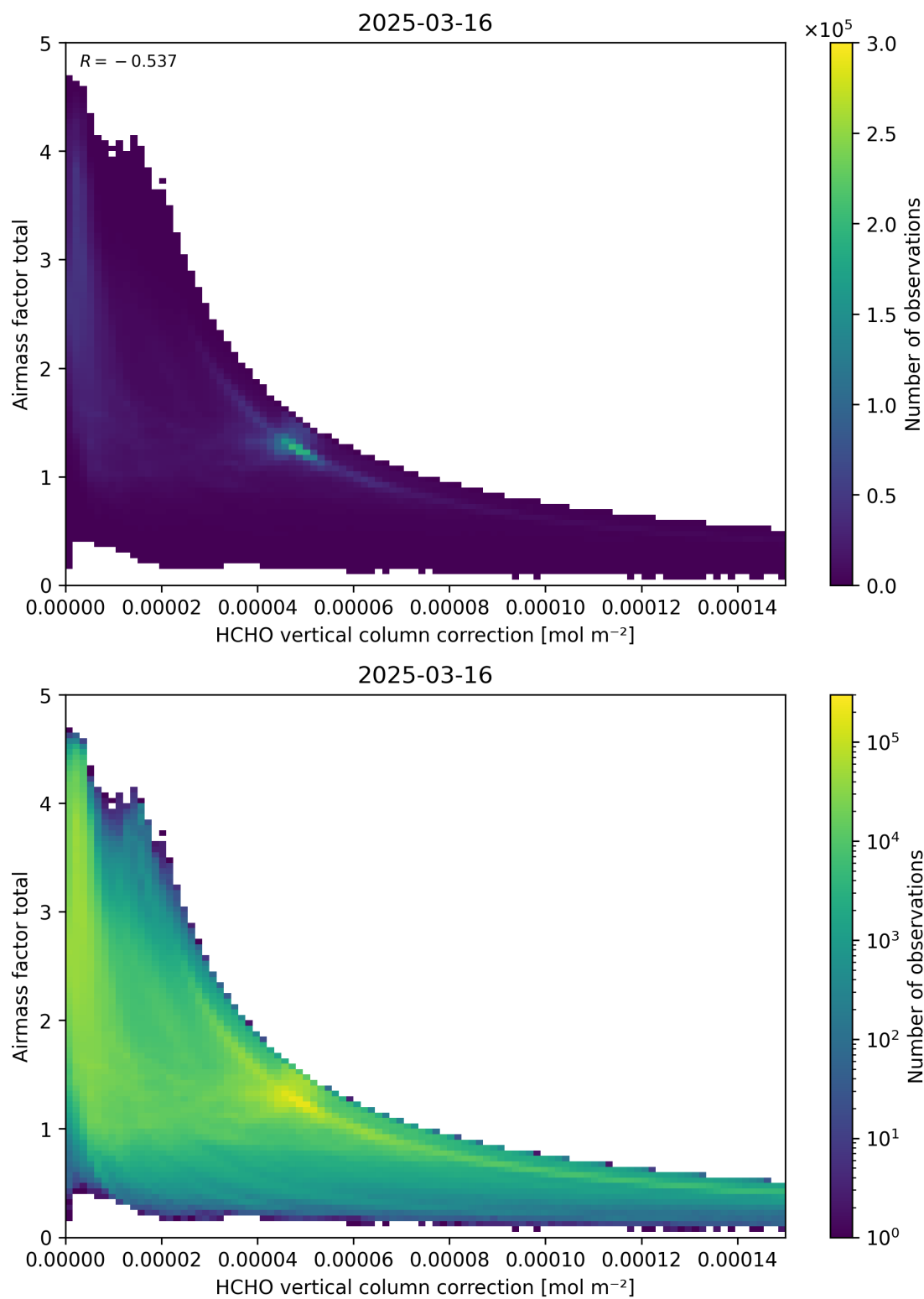
Figure 120: Scatter density plot of “HCHO vertical column correction” against “Airmass factor total” for 2025-03-15 to 2025-03-17.
