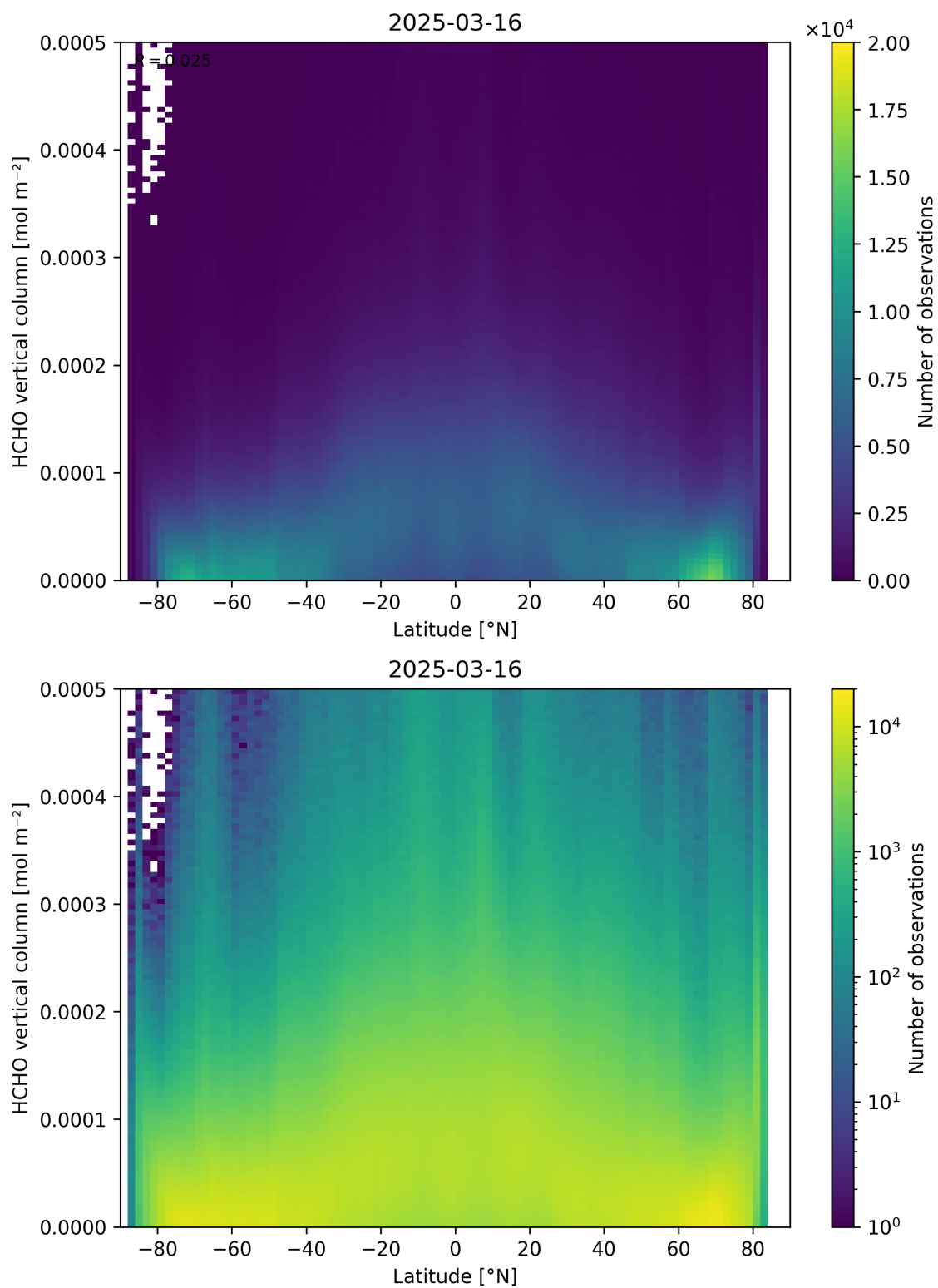
Figure 163: Scatter density plot of “Latitude” against “HCHO vertical column” for 2025-03-15 to 2025-03-17.
