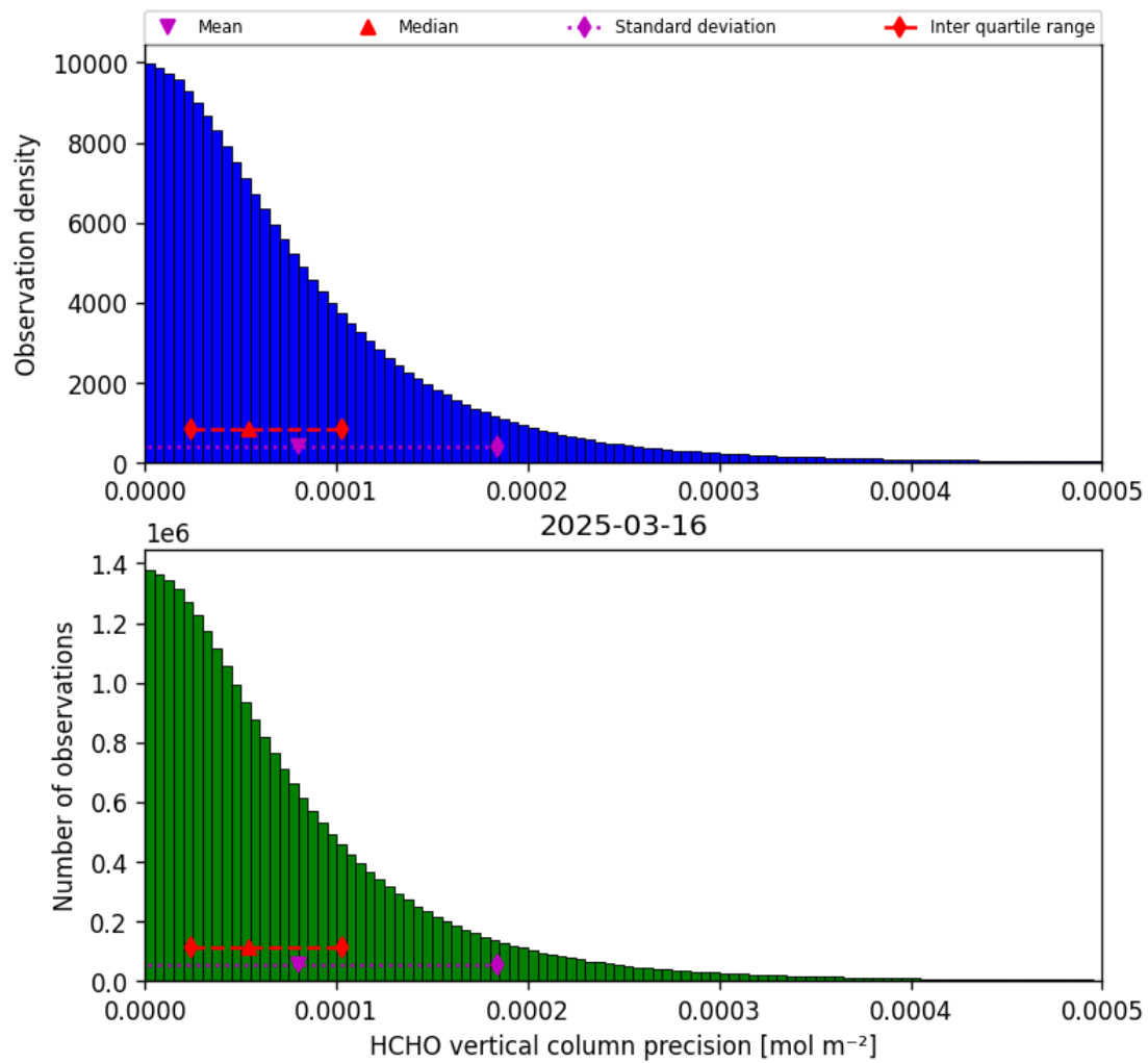
Figure 36: Histogram of “HCHO vertical column precision” for 2025-03-15 to 2025-03-17
