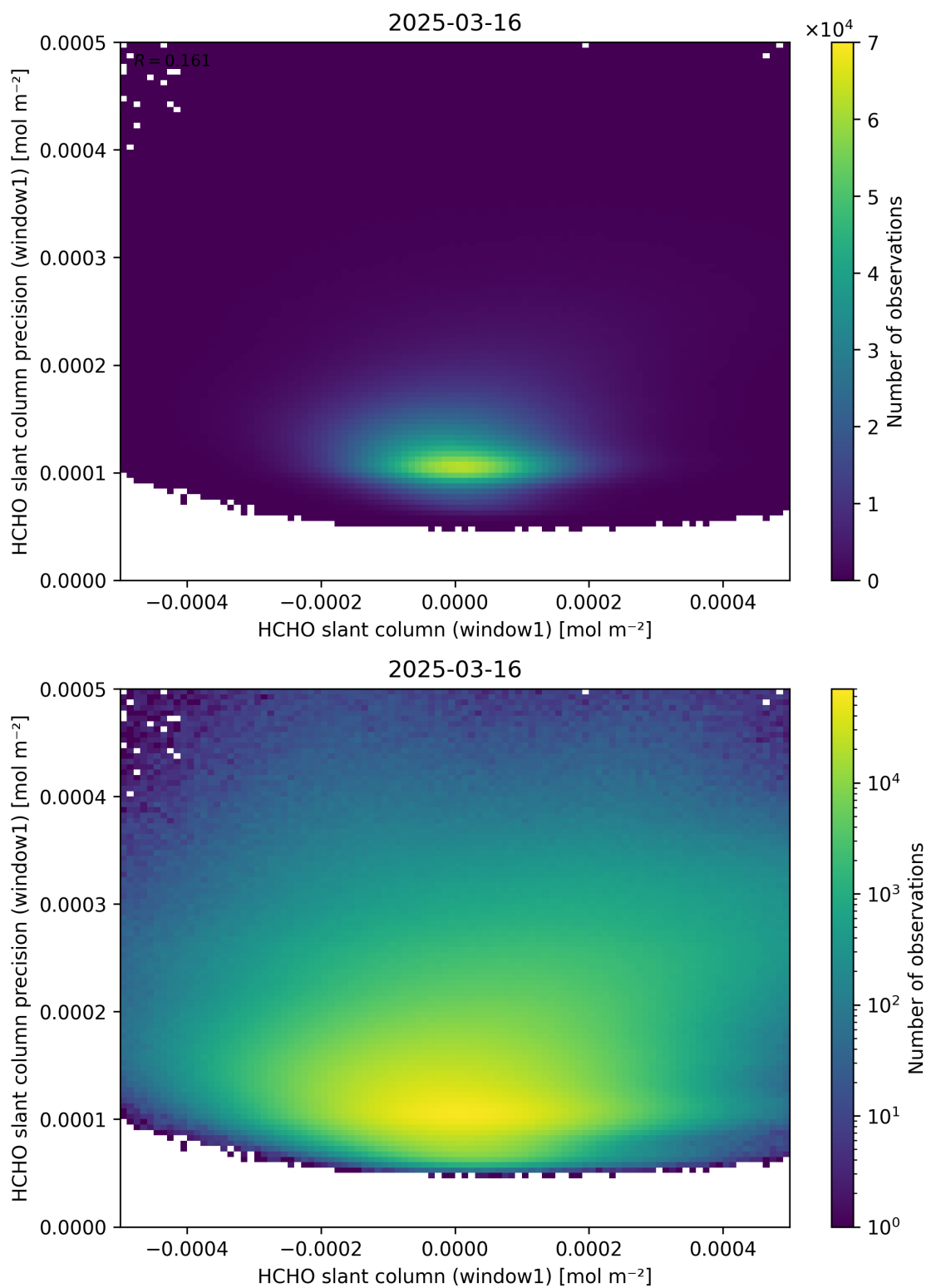
Figure 84: Scatter density plot of “HCHO slant column (window1)” against “HCHO slant column precision (window1)” for 2025-03-15 to 2025-03-17.
