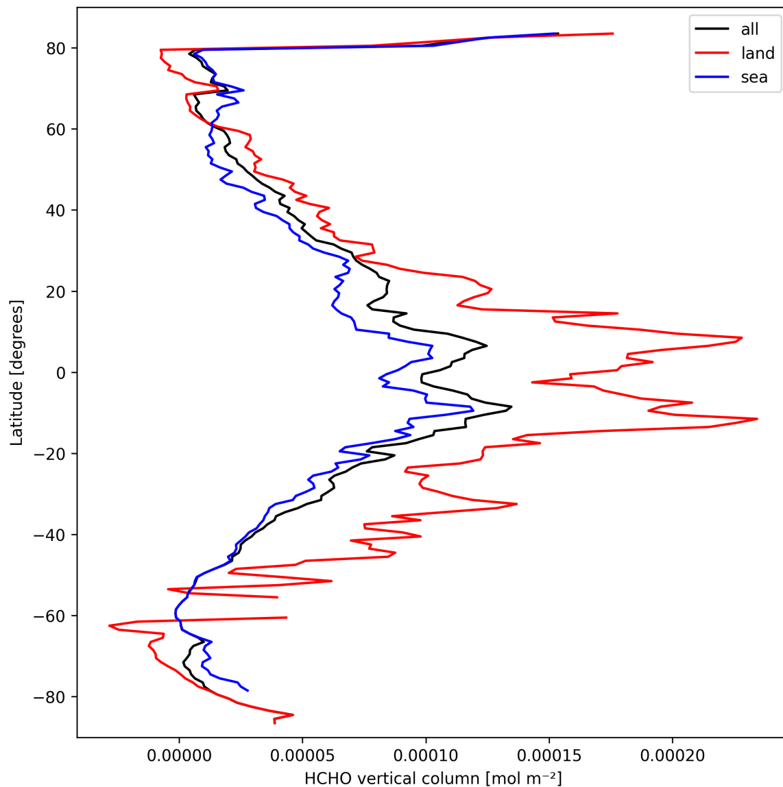
Figure 21: Zonal average of “HCHO vertical column” for 2025-03-15 to 2025-03-17.
