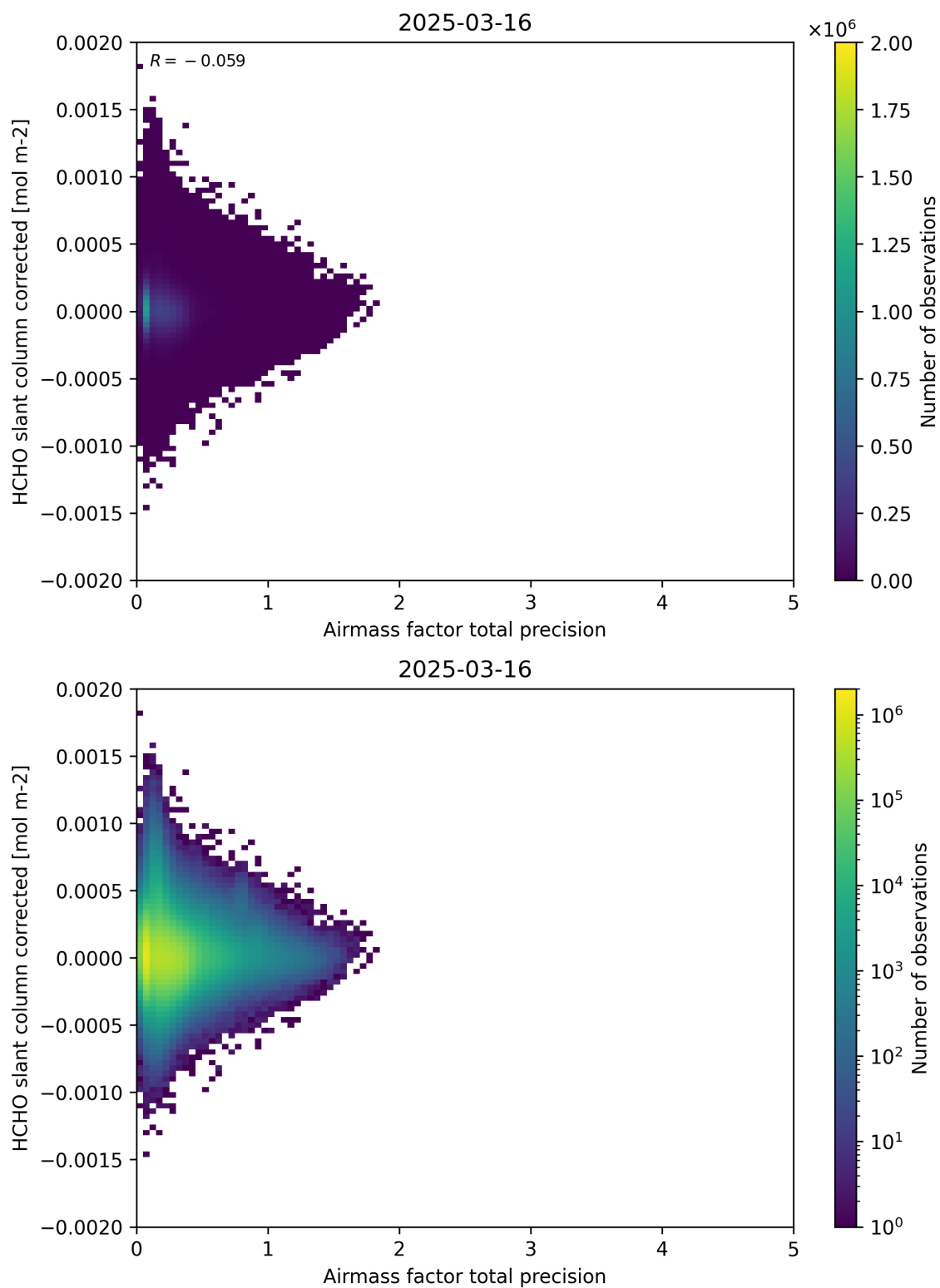
Figure 109: Scatter density plot of “Airmass factor total precision” against “HCHO slant column corrected” for 2025-03-15 to 2025-03-17.
