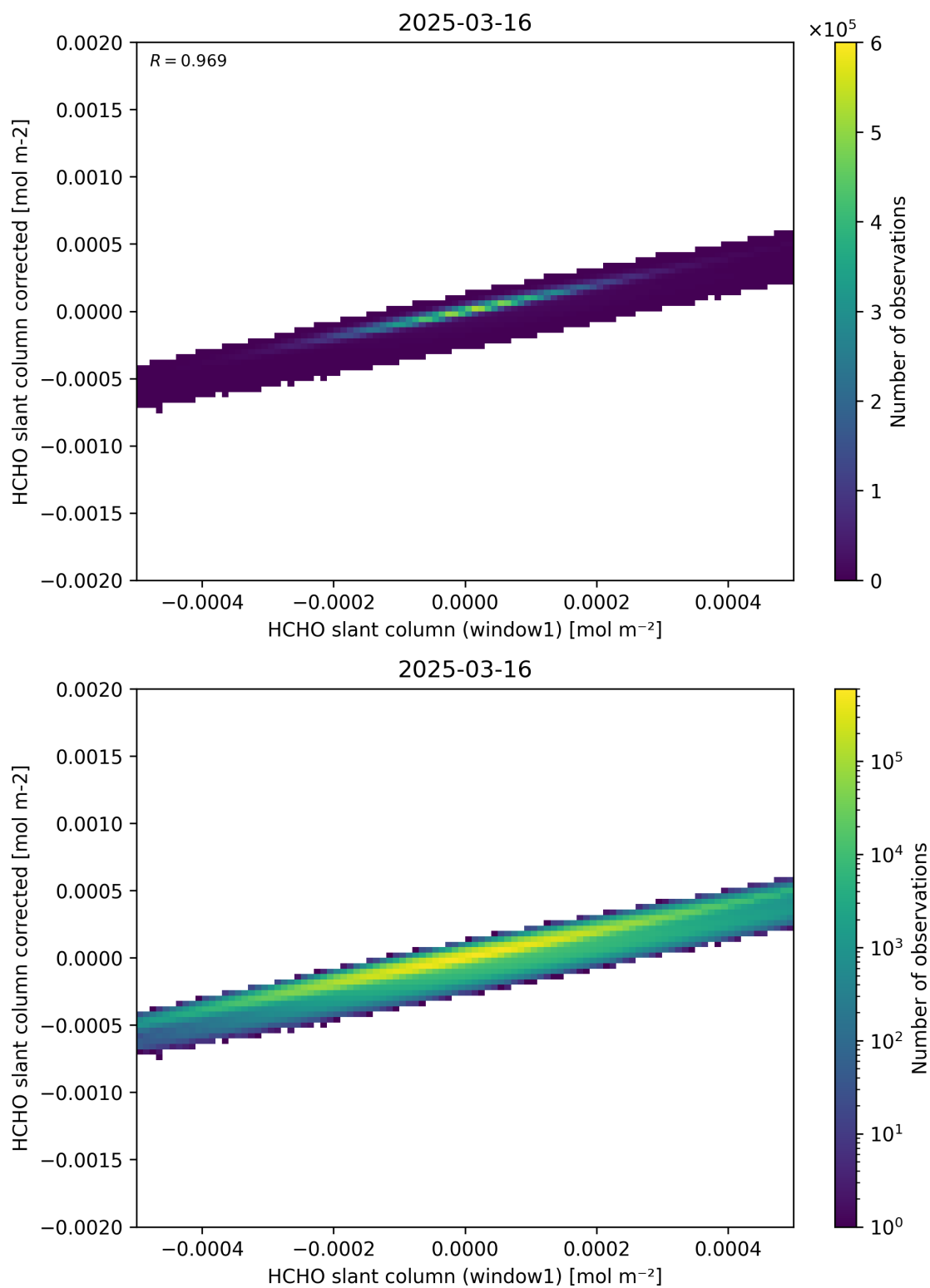
Figure 82: Scatter density plot of “HCHO slant column (window1)” against “HCHO slant column corrected” for 2025-03-15 to 2025-03-17.
