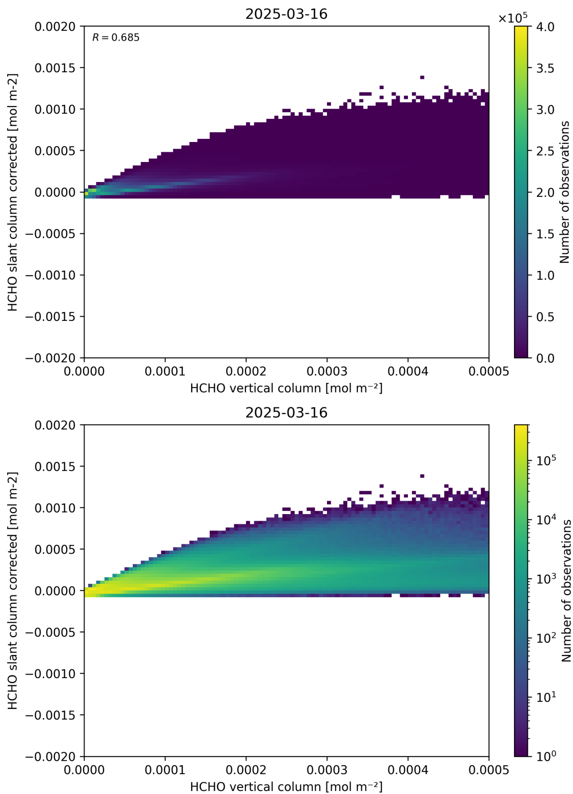
Figure 127: Scatter density plot of “HCHO vertical column” against “HCHO slant column corrected” for 2025-03-15 to 2025-03-17.
