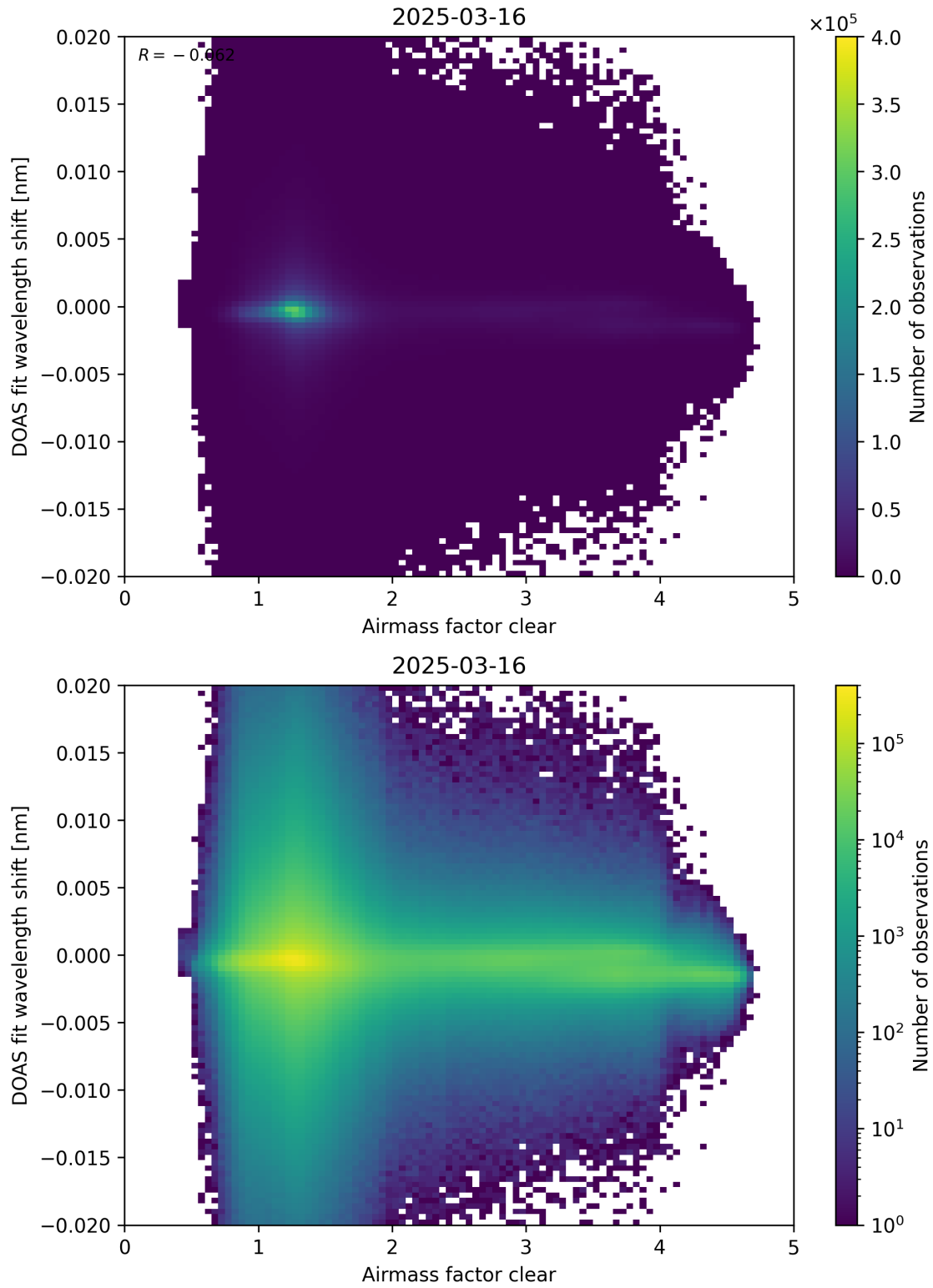
Figure 72: Scatter density plot of “Airmass factor clear” against “DOAS fit wavelength shift” for 2025-03-15 to 2025-03-17.
