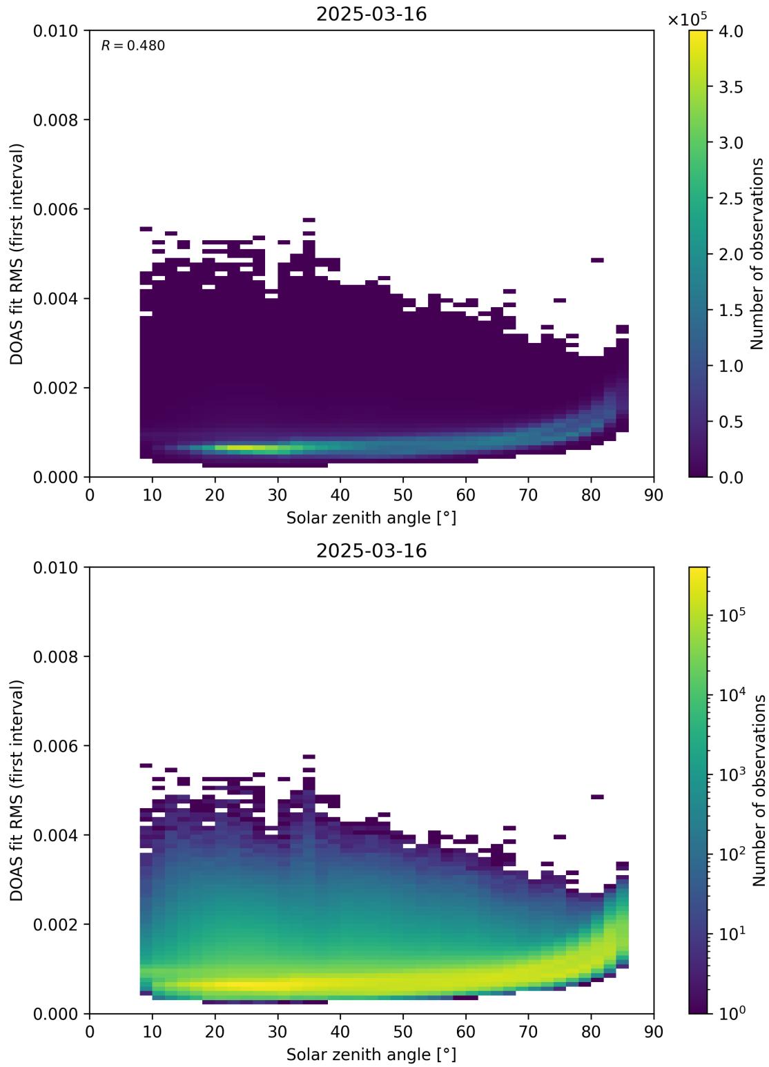
Figure 167: Scatter density plot of “Solar zenith angle” against “DOAS fit RMS (first interval)” for 2025-03-15 to 2025-03-17.
