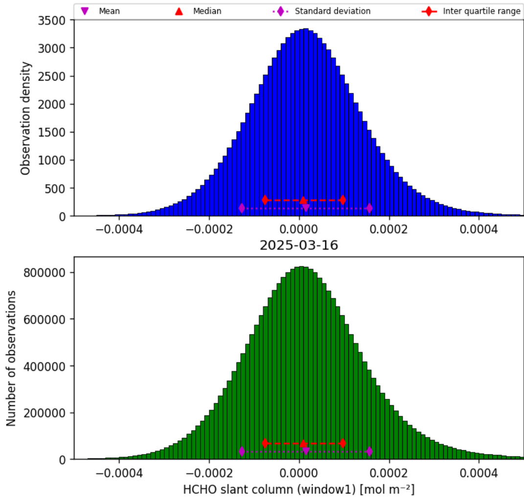
Figure 38: Histogram of “HCHO slant column (window1)” for 2025-03-15 to 2025-03-17
