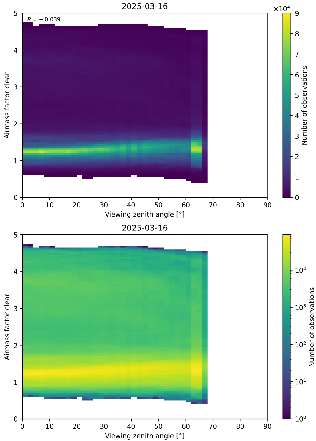
Figure 185: Scatter density plot of “Viewing zenith angle” against “Airmass factor clear” for 2025-03-15 to 2025-03-17.
