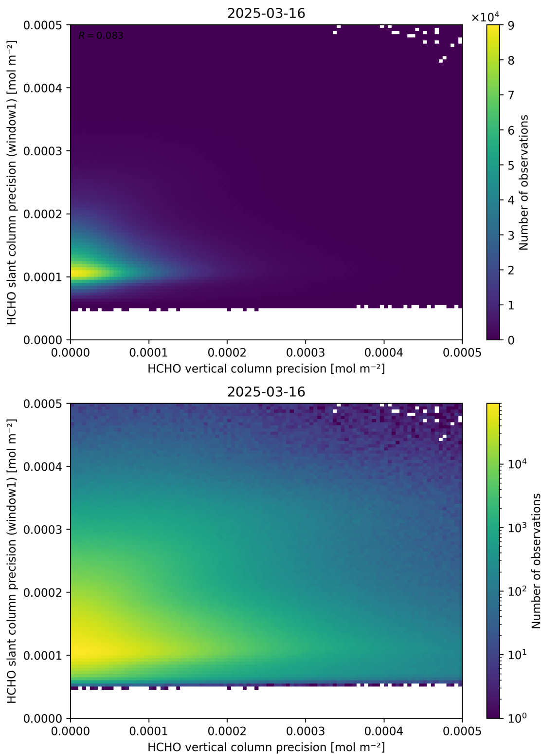
Figure 143: Scatter density plot of “HCHO vertical column precision” against “HCHO slant column precision (window1)” for 2025-03-15 to 2025-03-17.
