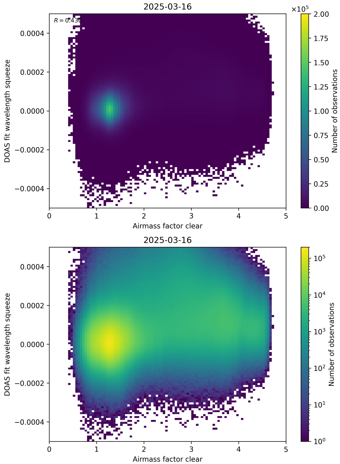
Figure 73: Scatter density plot of “Airmass factor clear” against “DOAS fit wavelength squeeze” for 2025-03-15 to 2025-03-17.
