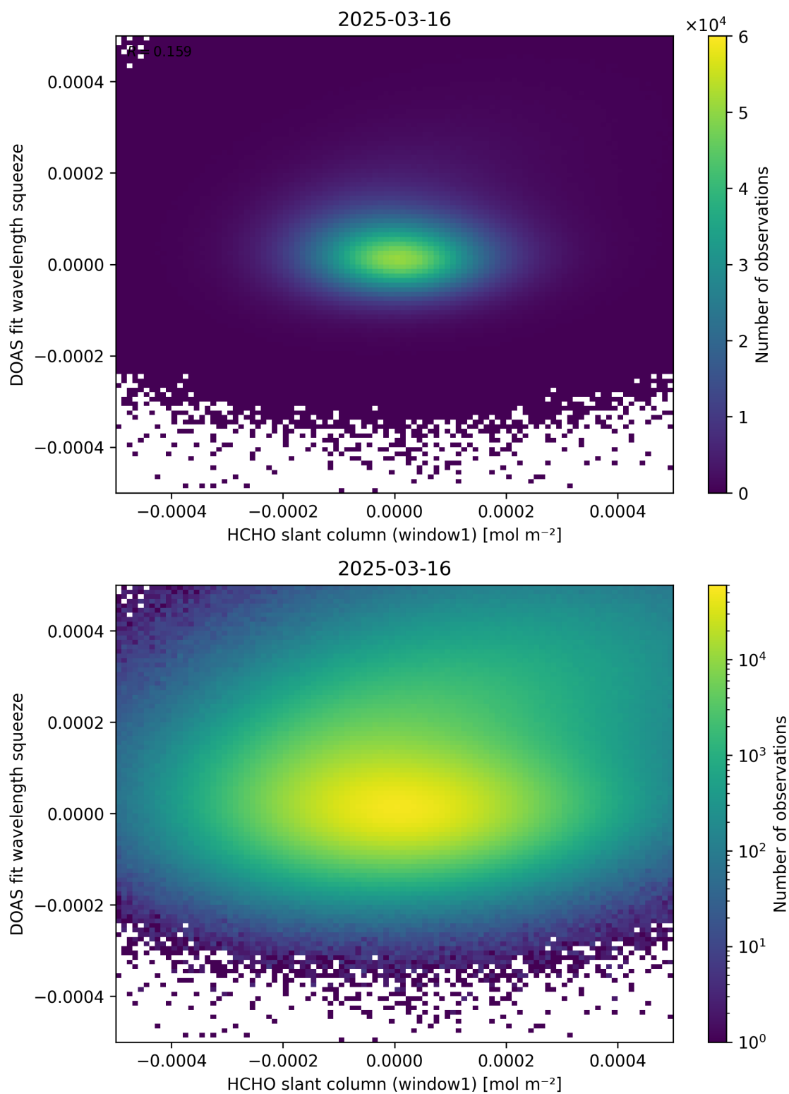
Figure 80: Scatter density plot of “HCHO slant column (window1)” against “DOAS fit wavelength squeeze” for 2025-03-15 to 2025-03-17.
