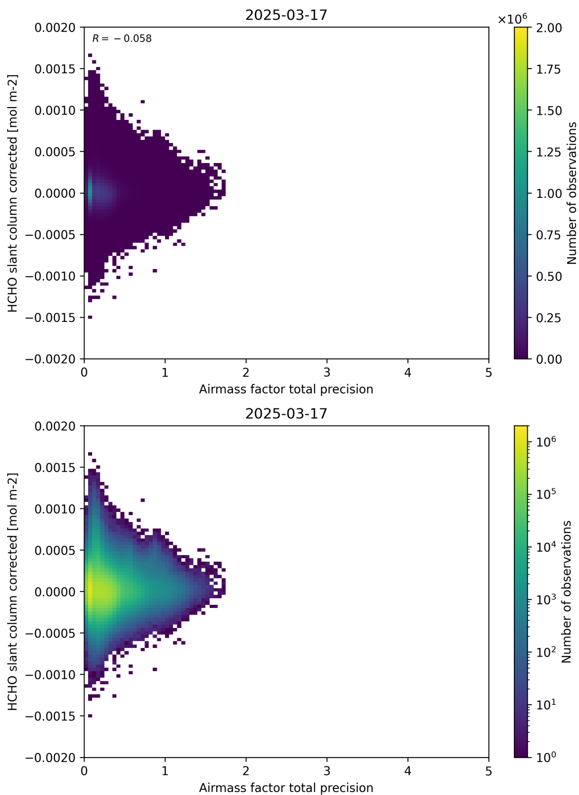
Figure 109: Scatter density plot of “Airmass factor total precision” against “HCHO slant column corrected” for 2025-03-17 to 2025-03-18.
