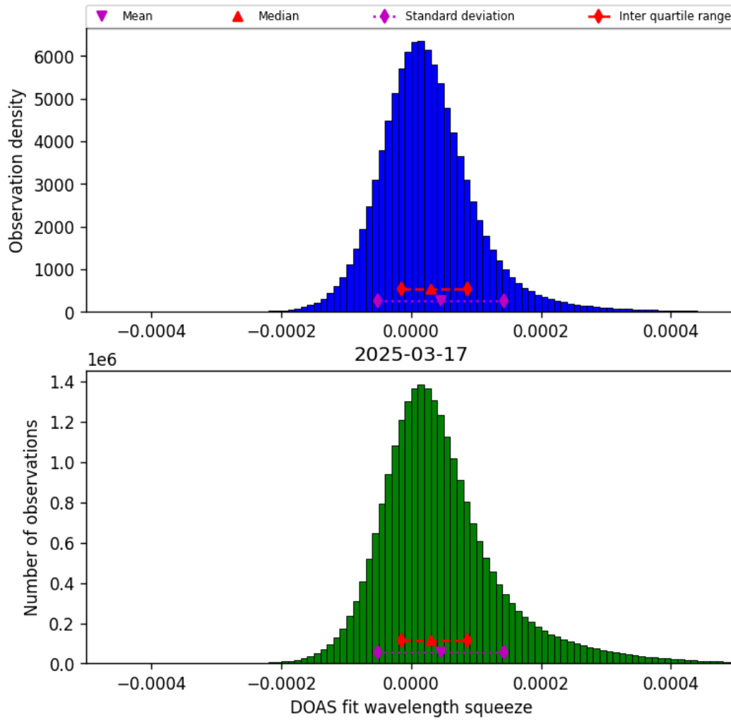
Figure 45: Histogram of “DOAS fit wavelength squeeze” for 2025-03-17 to 2025-03-18
