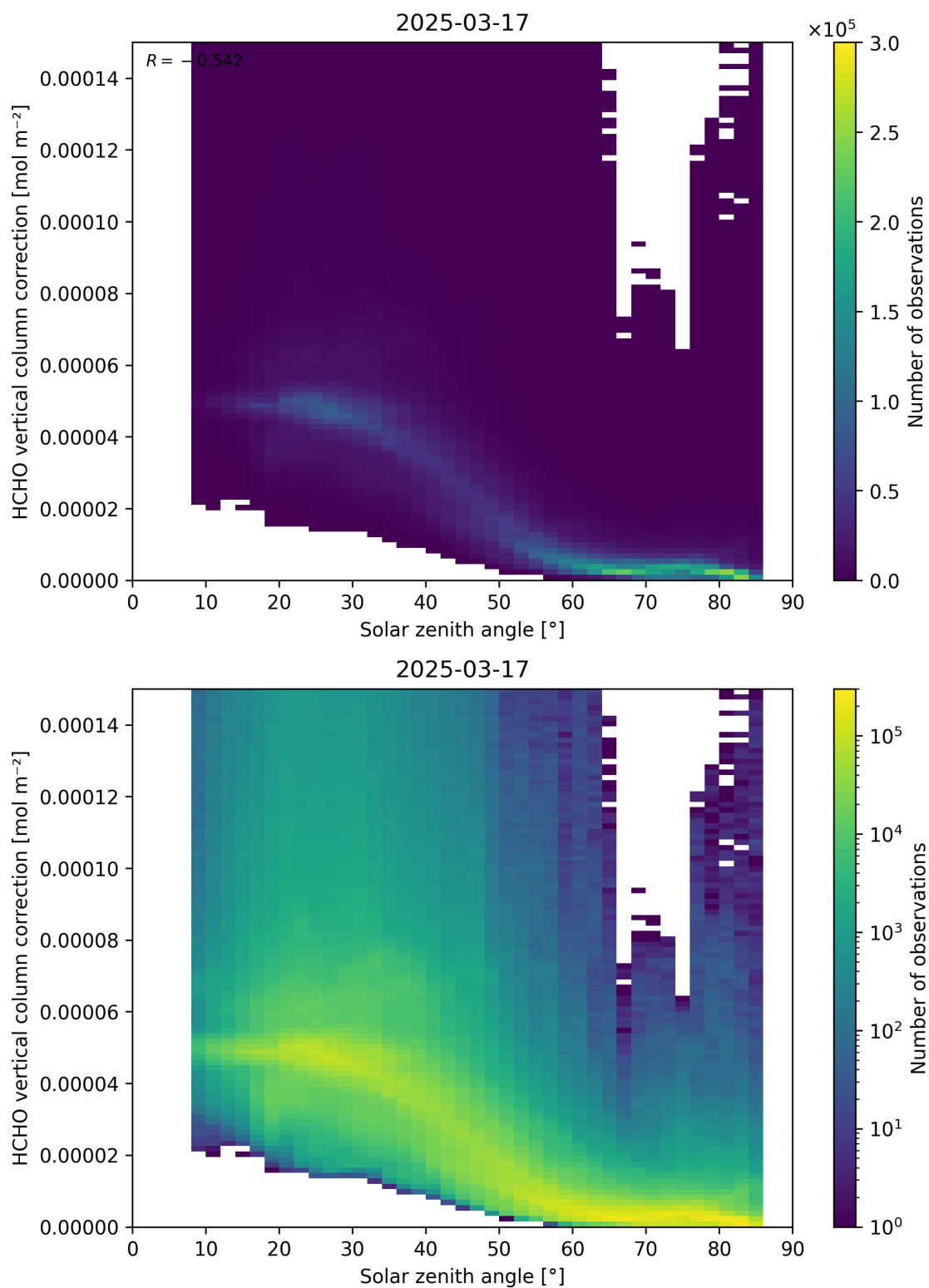
Figure 178: Scatter density plot of “Solar zenith angle” against “HCHO vertical column correction” for 2025-03-17 to 2025-03-18.
