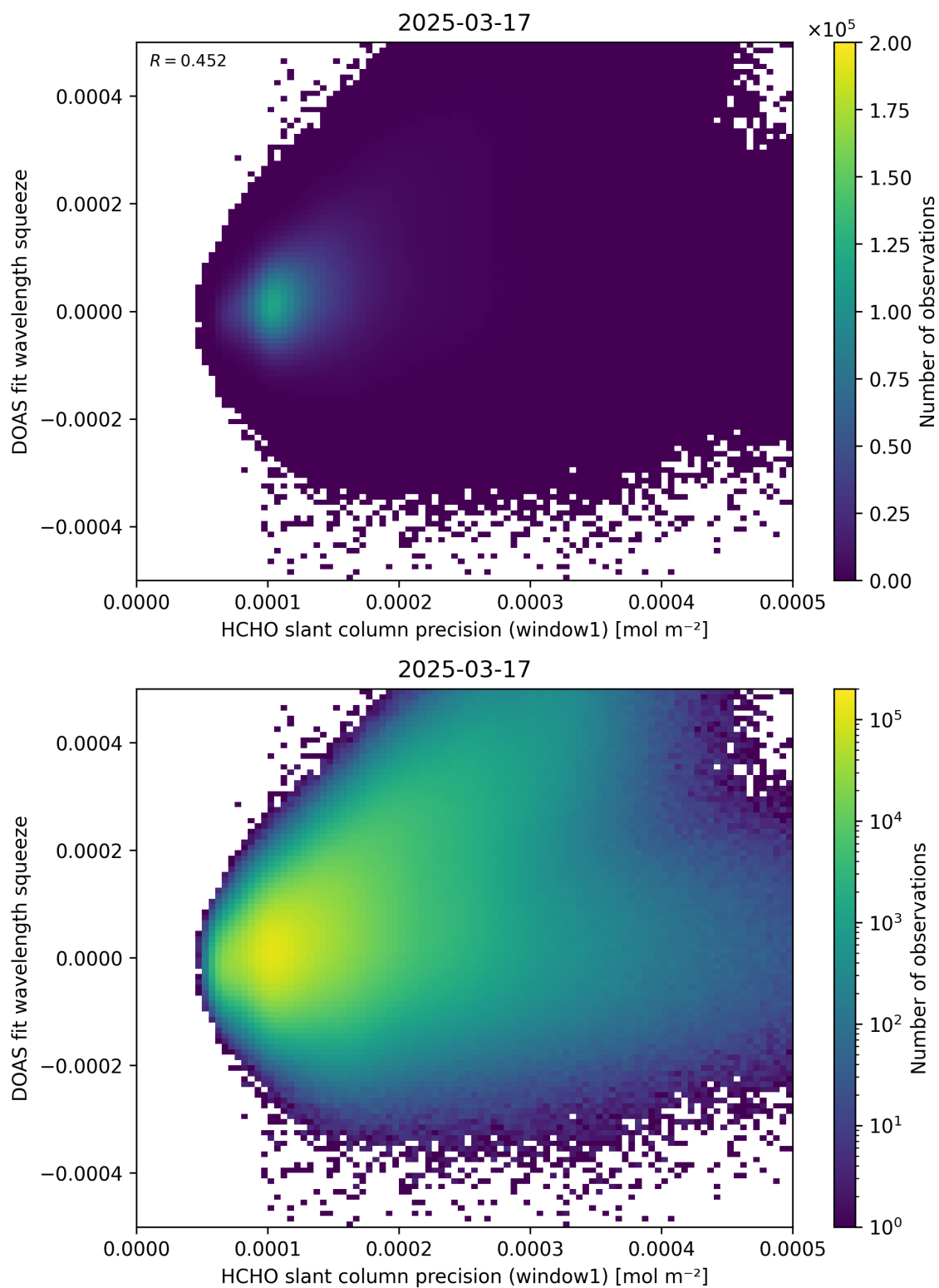
Figure 90: Scatter density plot of “HCHO slant column precision (window1)” against “DOAS fit wavelength squeeze” for 2025-03-17 to 2025-03-18.
