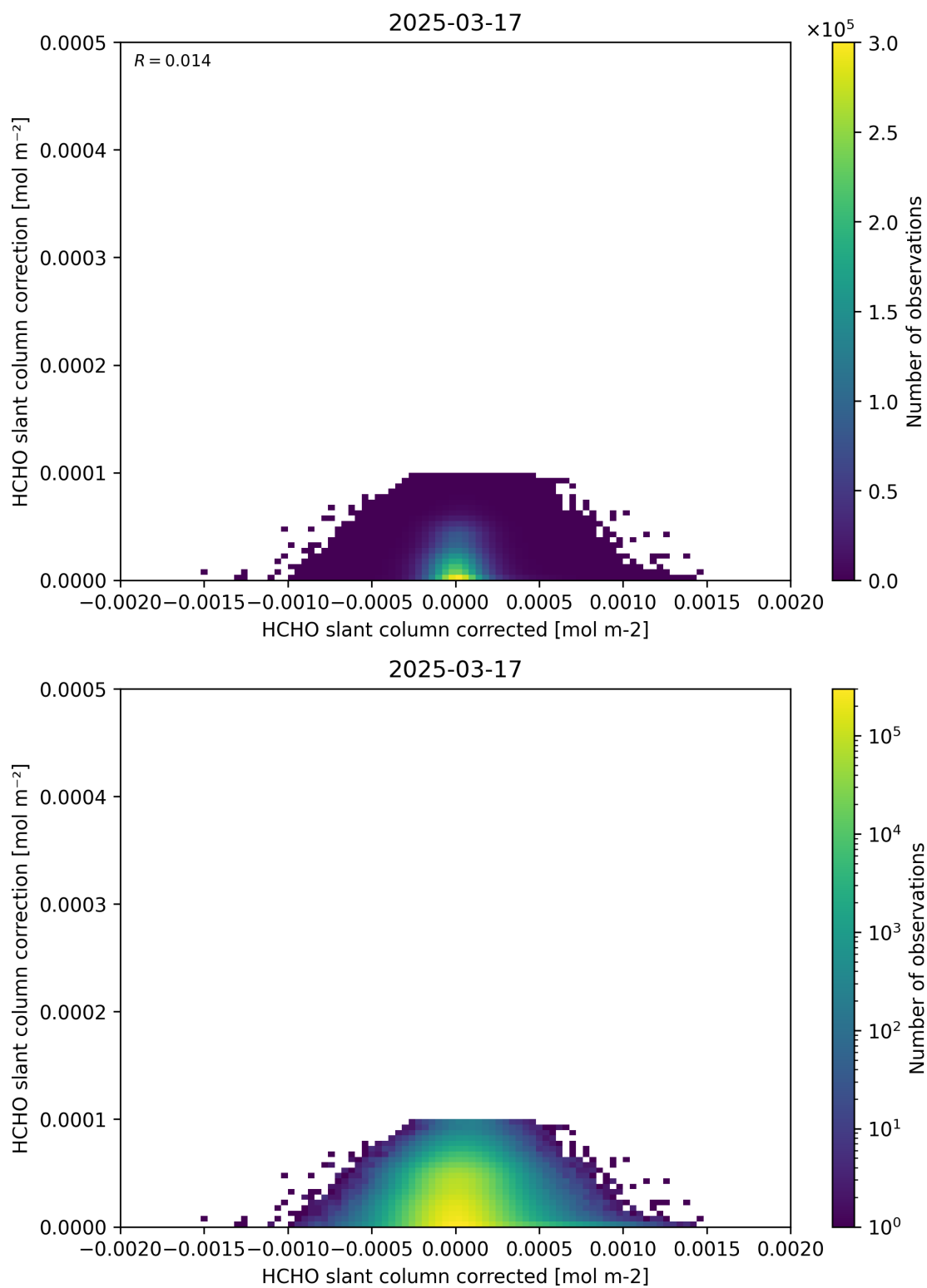
Figure 77: Scatter density plot of “HCHO slant column corrected” against “HCHO slant column correction” for 2025-03-17 to 2025-03-18.
