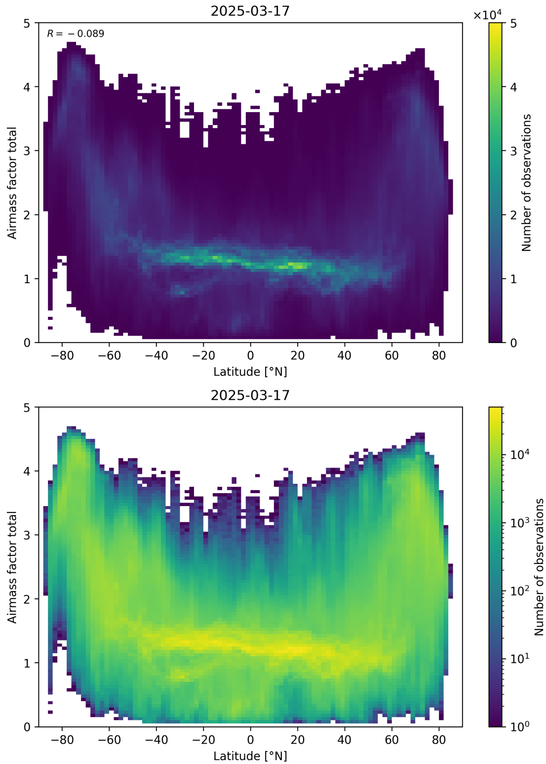
Figure 161: Scatter density plot of “Latitude” against “Airmass factor total” for 2025-03-17 to 2025-03-18.
