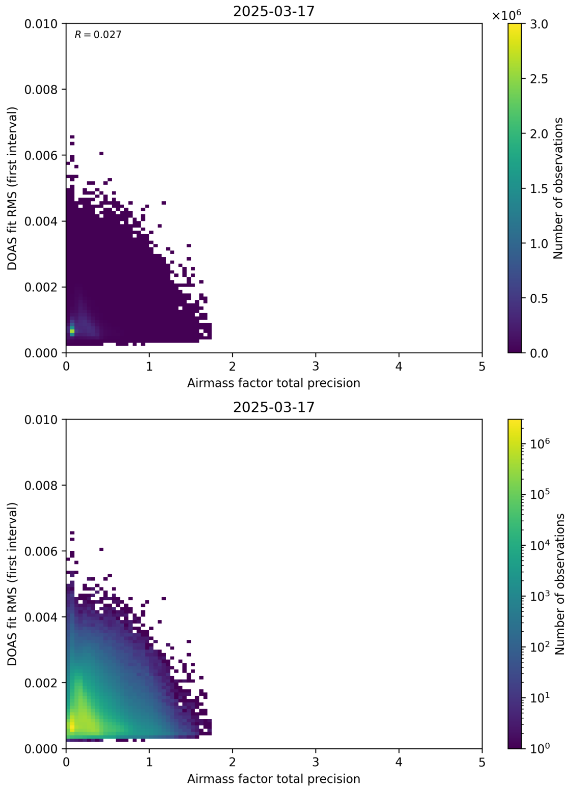
Figure 105: Scatter density plot of “Airmass factor total precision” against “DOAS fit RMS (first interval)” for 2025-03-17 to 2025-03-18.
