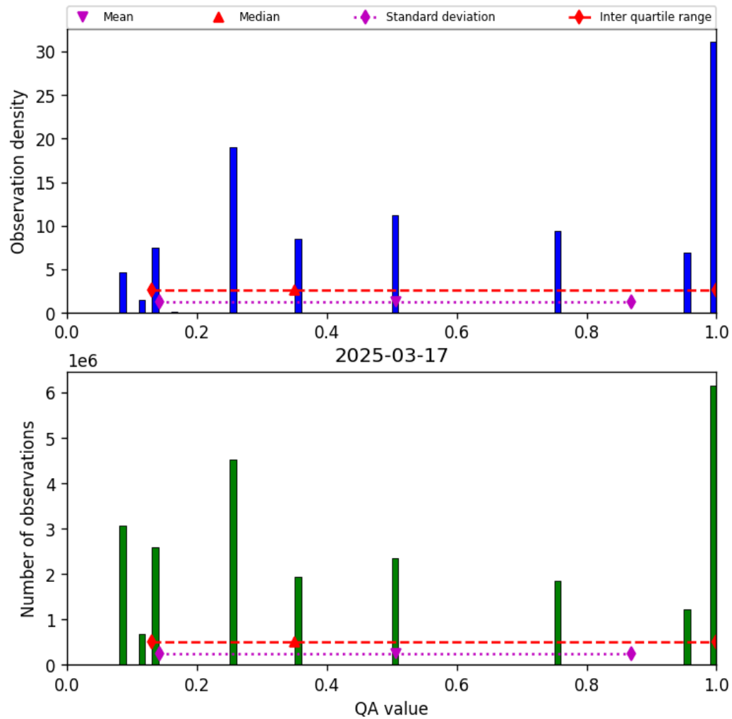
Figure 34: Histogram of “QA value” for 2025-03-17 to 2025-03-18
