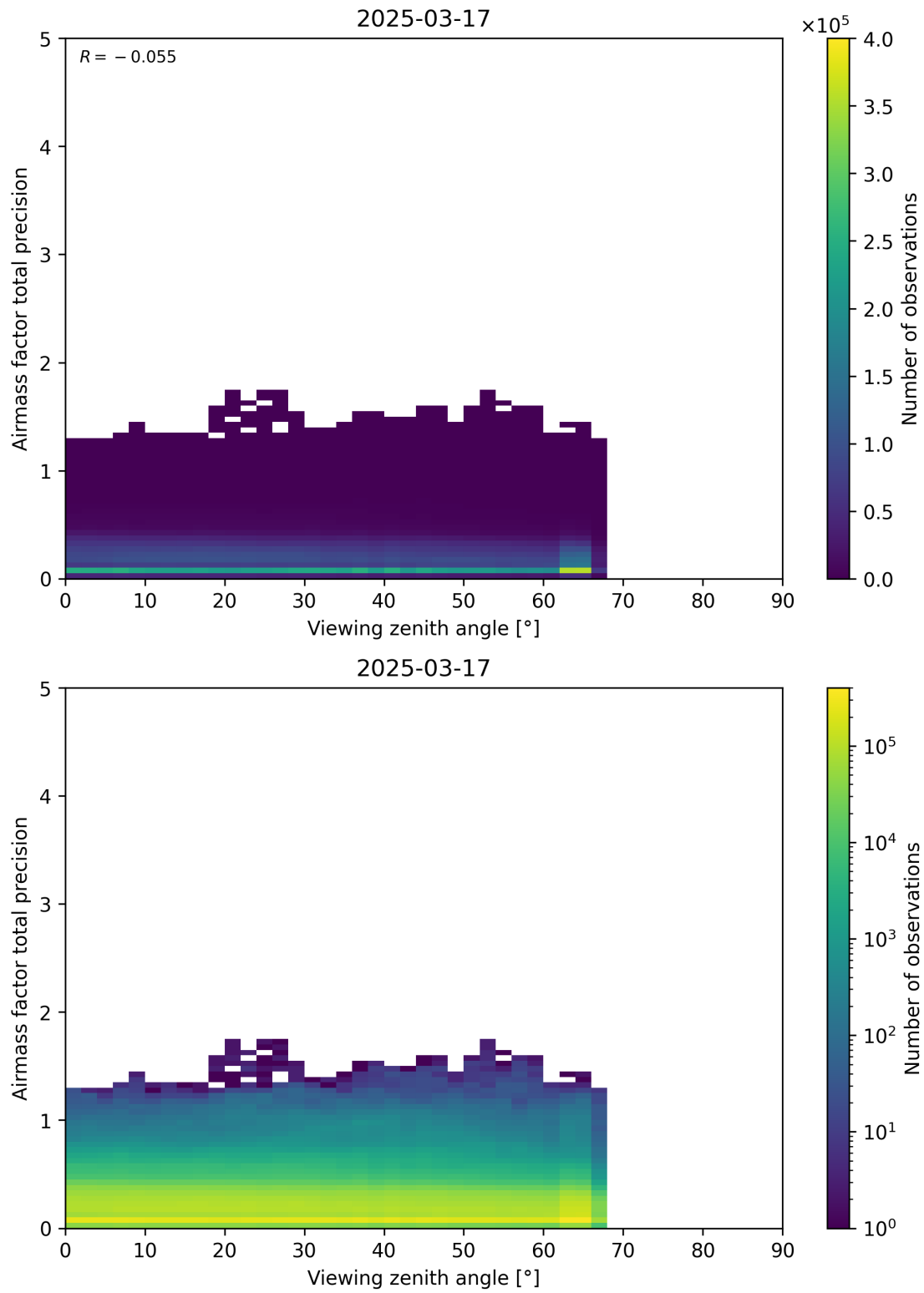
Figure 191: Scatter density plot of “Viewing zenith angle” against “Airmass factor total precision” for 2025-03-17 to 2025-03-18.
