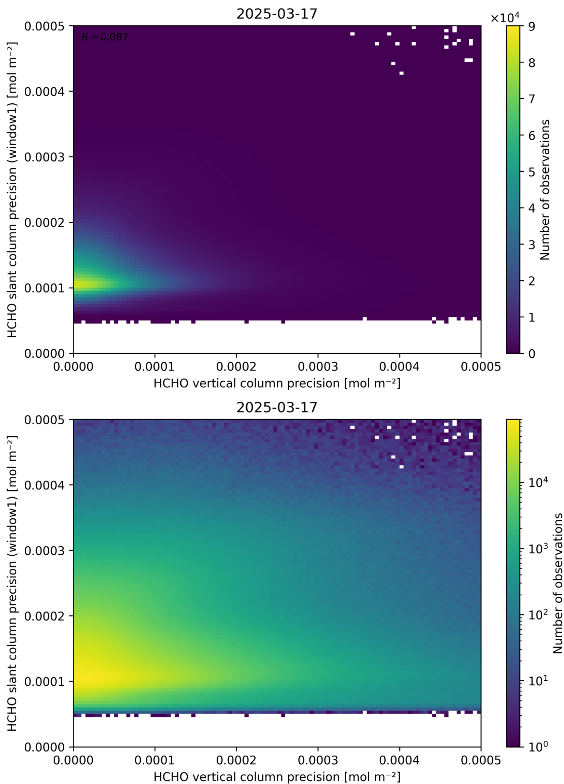
Figure 143: Scatter density plot of “HCHO vertical column precision” against “HCHO slant column precision (window1)” for 2025-03-17 to 2025-03-18.
