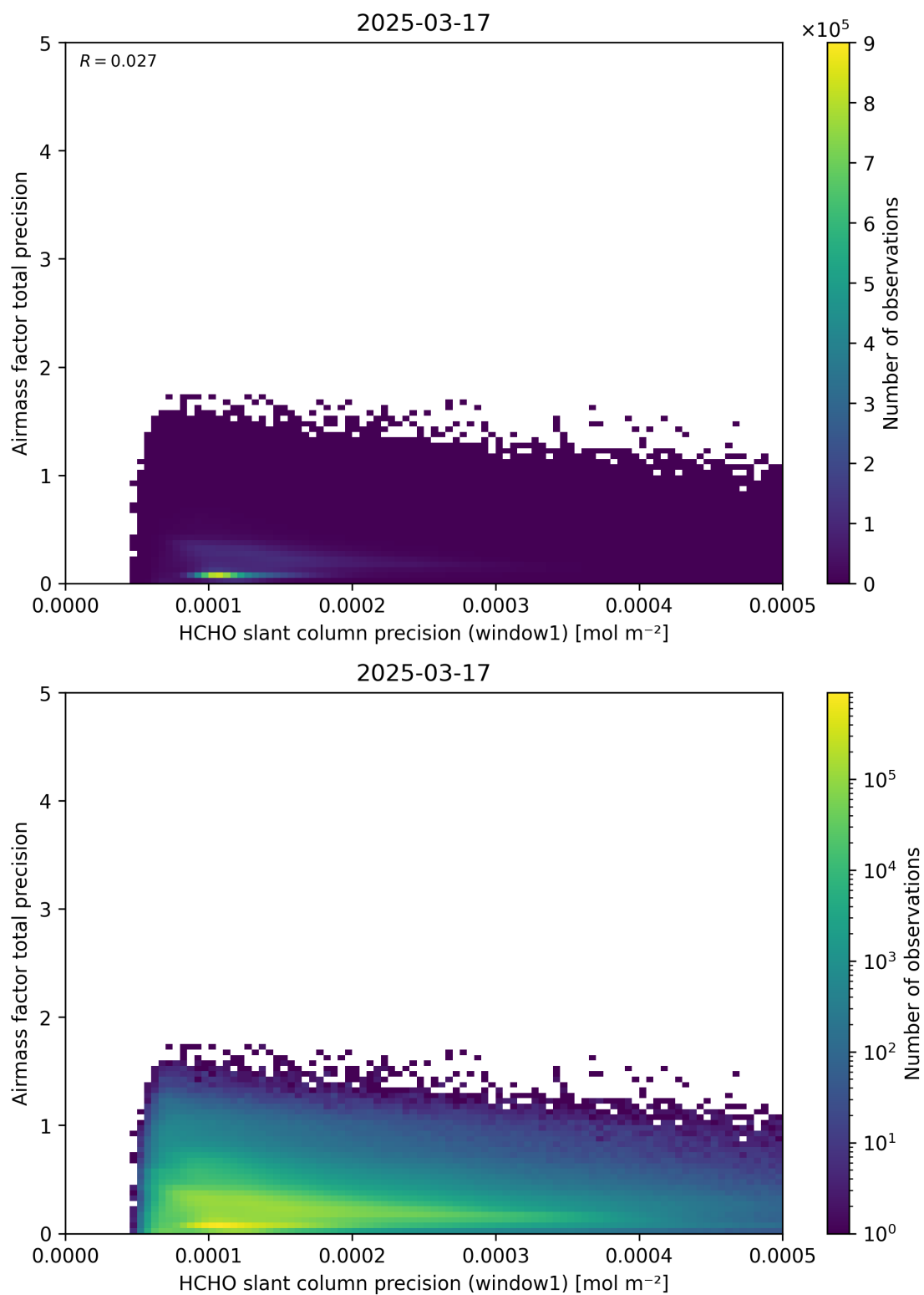
Figure 95: Scatter density plot of “HCHO slant column precision (window1)” against “Airmass factor total precision” for 2025-03-17 to 2025-03-18.
