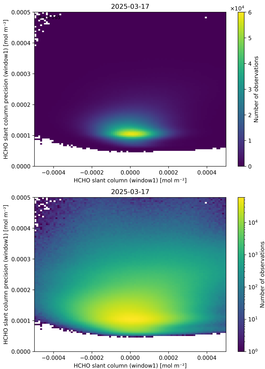
Figure 84: Scatter density plot of “HCHO slant column (window1)” against “HCHO slant column precision (window1)” for 2025-03-17 to 2025-03-18.
