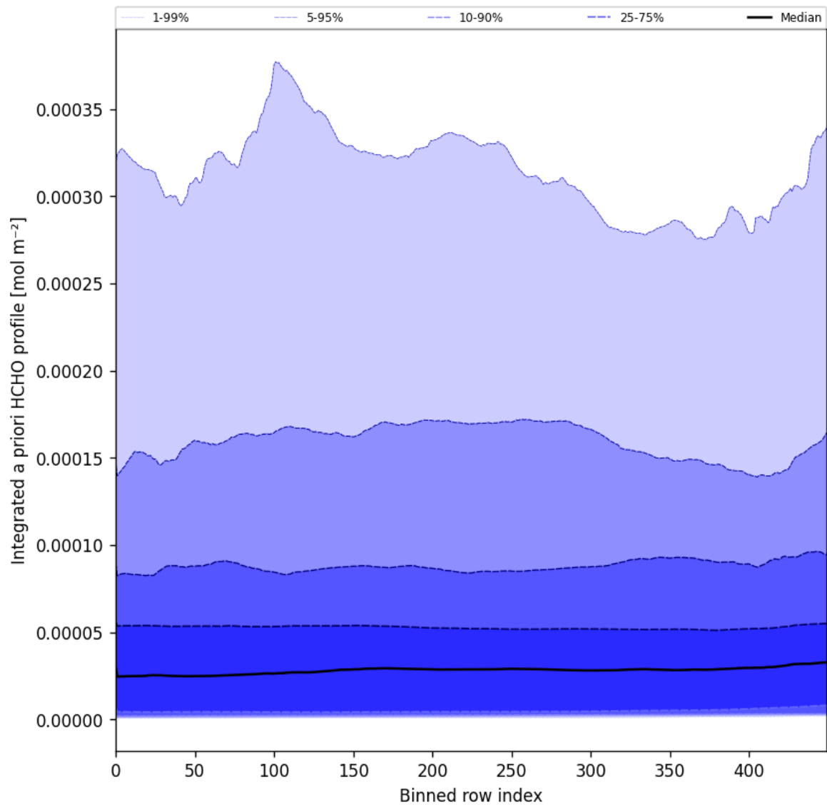
Figure 57: Along track statistics of “Integrated a priori HCHO profile” for 2025-03-17 to 2025-03-18
