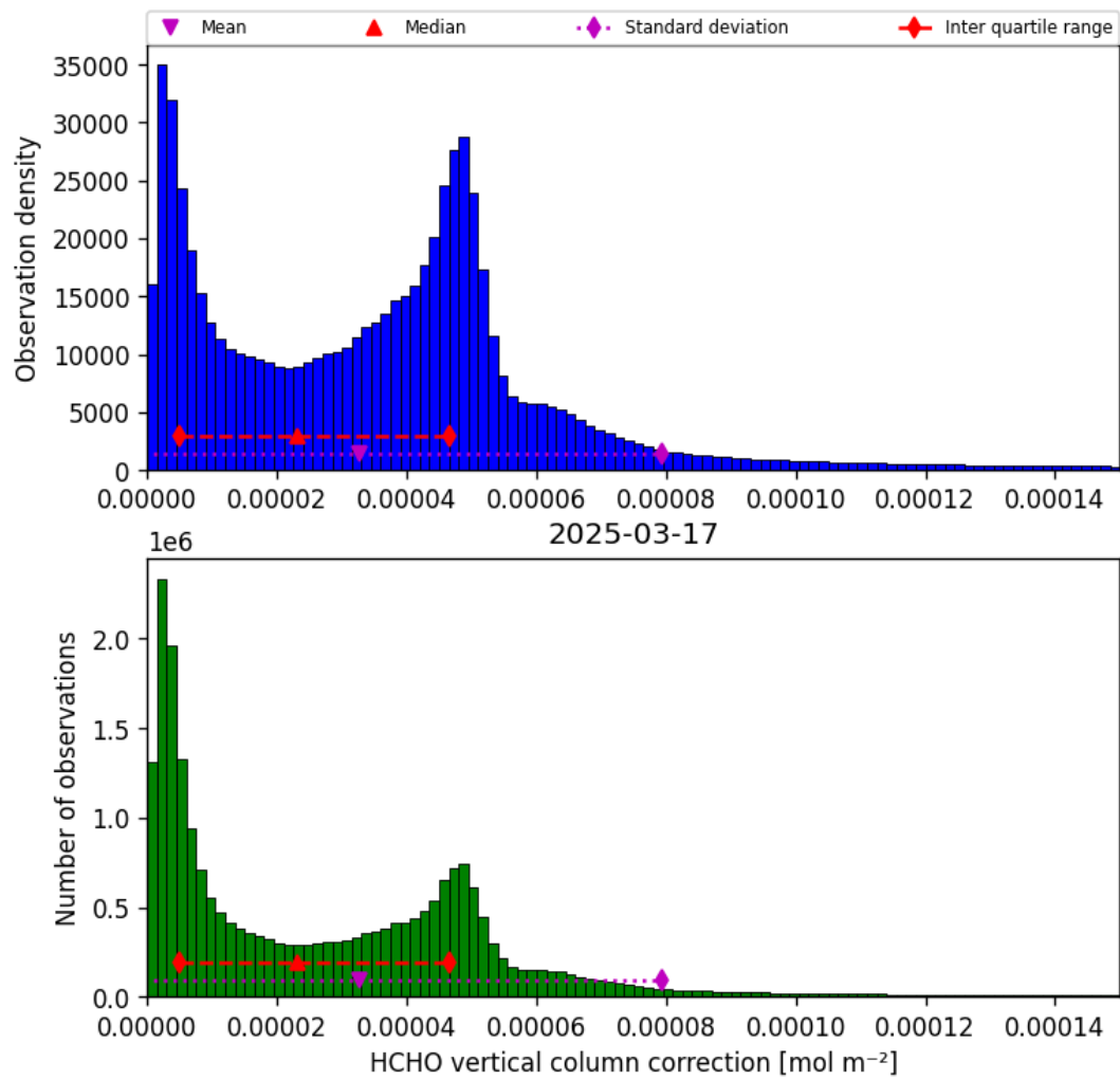
Figure 37: Histogram of “HCHO vertical column correction” for 2025-03-17 to 2025-03-18
