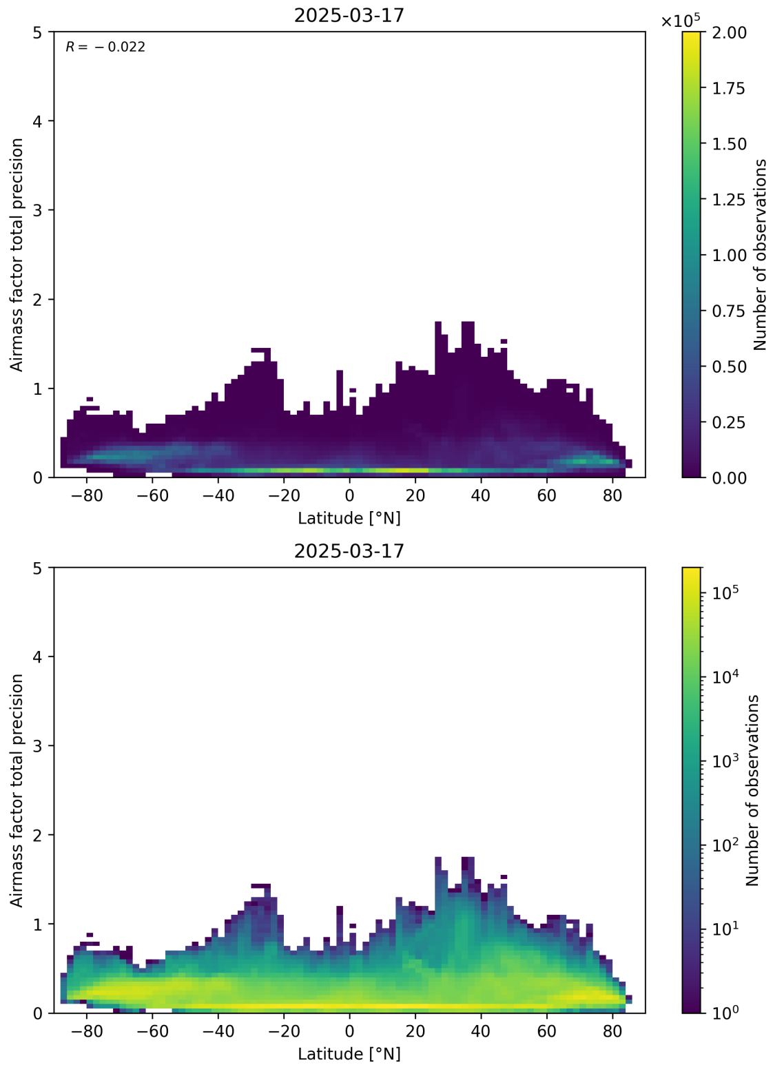
Figure 162: Scatter density plot of “Latitude” against “Airmass factor total precision” for 2025-03-17 to 2025-03-18.
