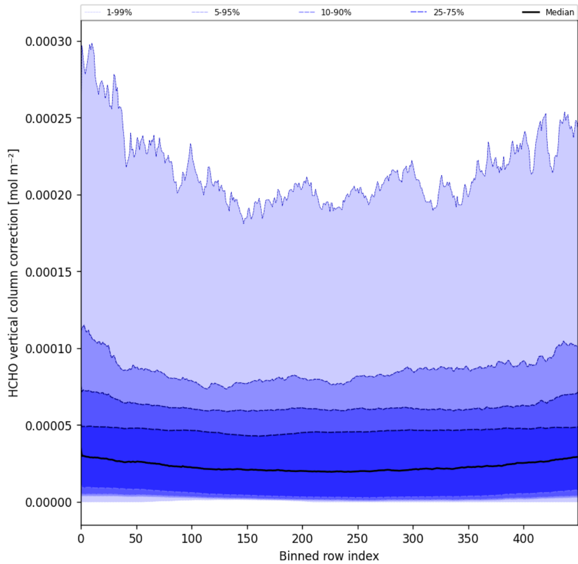
Figure 51: Along track statistics of “HCHO vertical column correction” for 2025-03-17 to 2025-03-18
