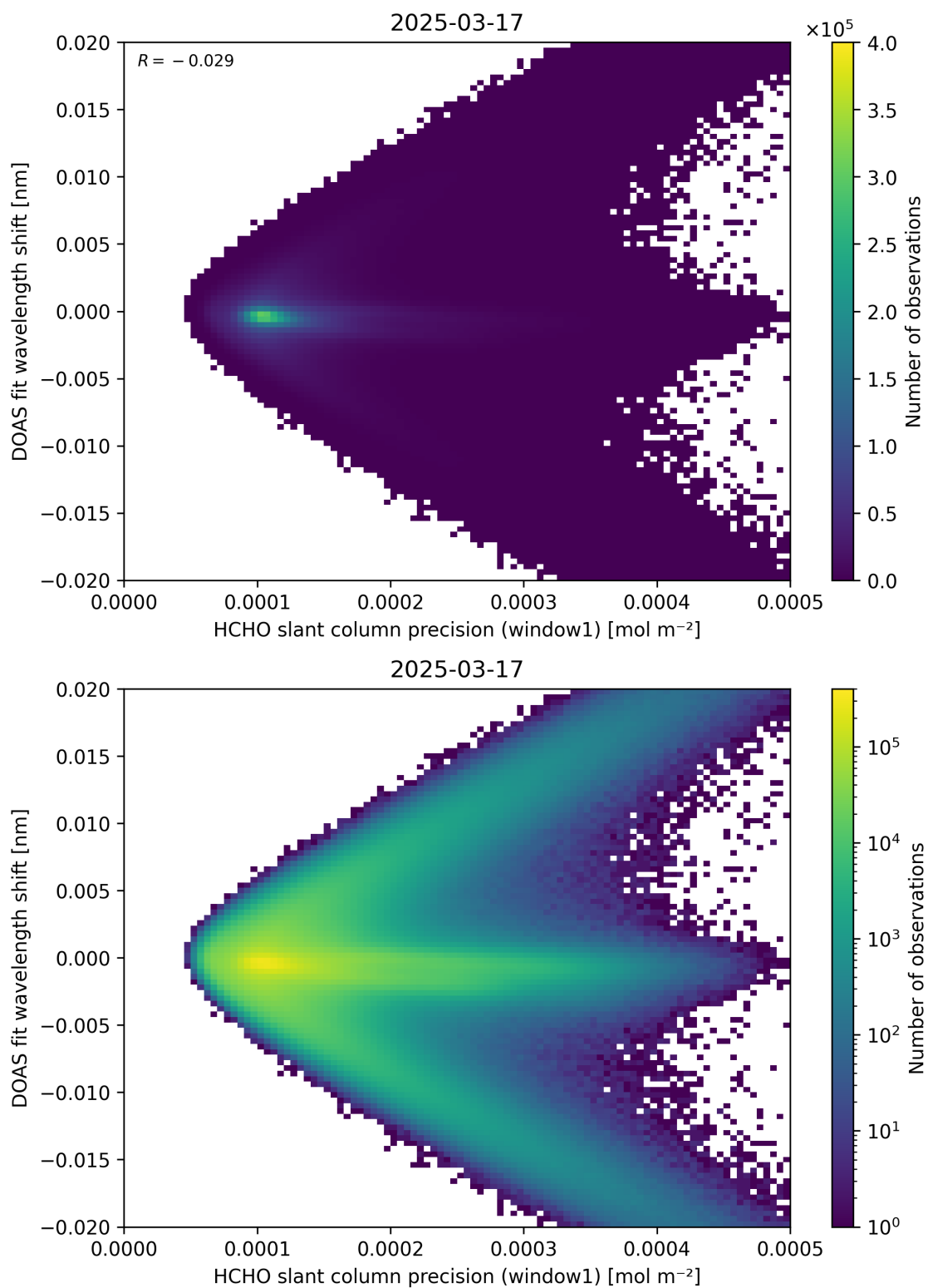
Figure 89: Scatter density plot of “HCHO slant column precision (window1)” against “DOAS fit wavelength shift” for 2025-03-17 to 2025-03-18.
