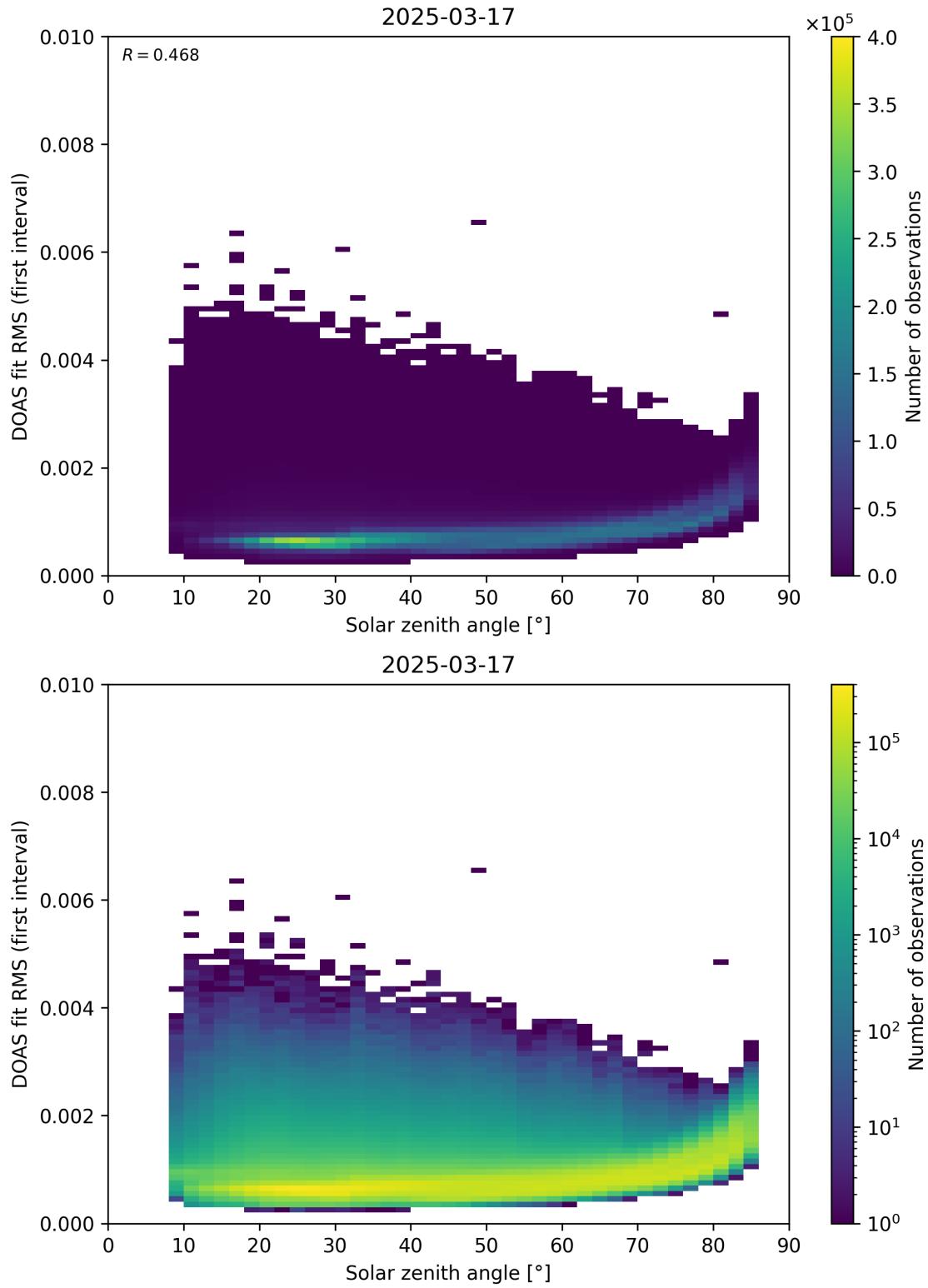
Figure 167: Scatter density plot of “Solar zenith angle” against “DOAS fit RMS (first interval)” for 2025-03-17 to 2025-03-18.
