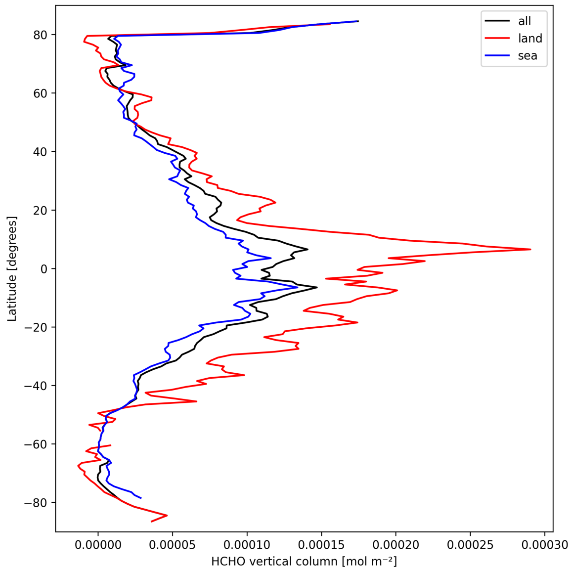
Figure 21: Zonal average of “HCHO vertical column” for 2025-03-17 to 2025-03-18.
