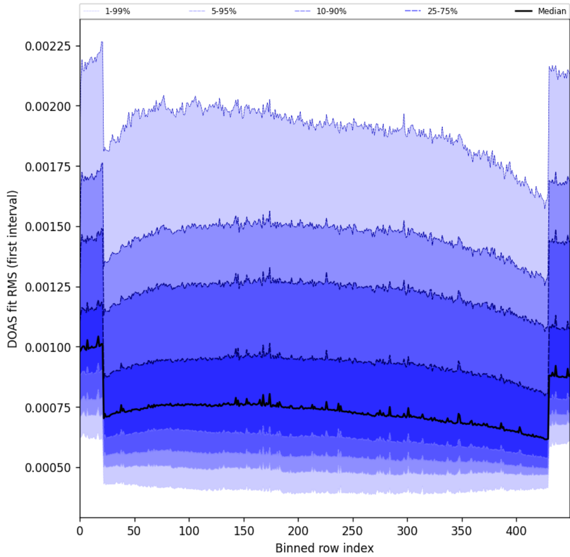
Figure 60: Along track statistics of “DOAS fit RMS (first interval)” for 2025-03-17 to 2025-03-18
