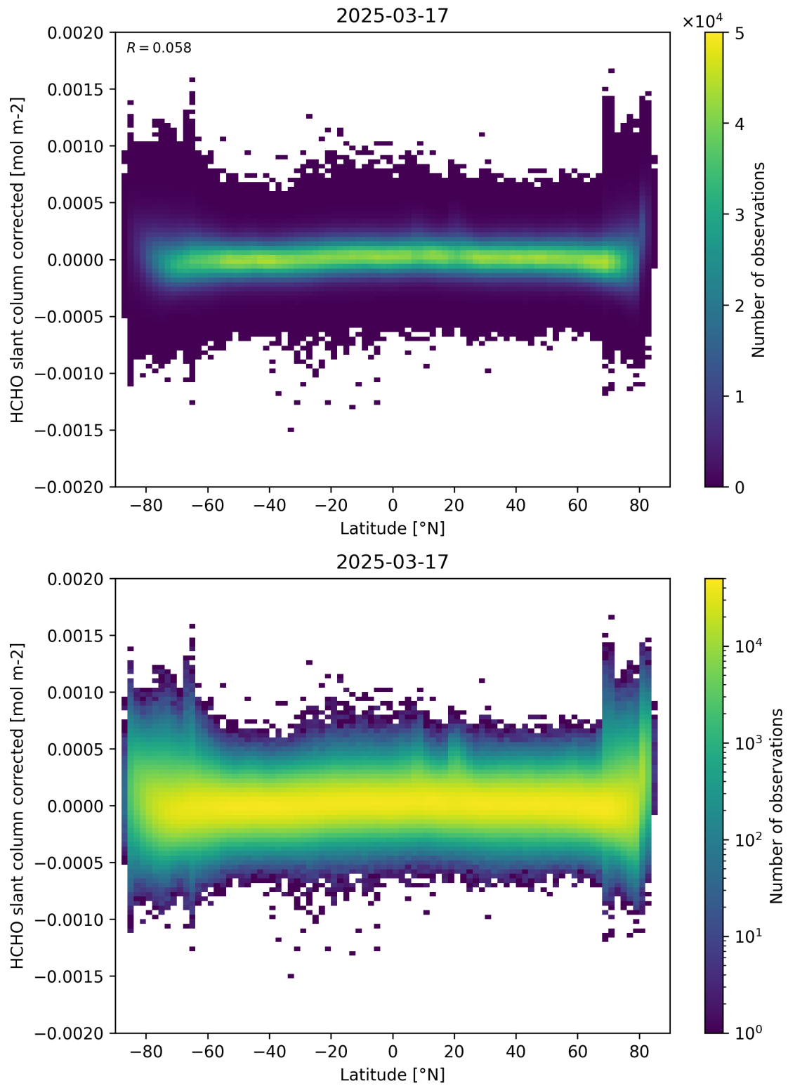
Figure 157: Scatter density plot of “Latitude” against “HCHO slant column corrected” for 2025-03-17 to 2025-03-18.
