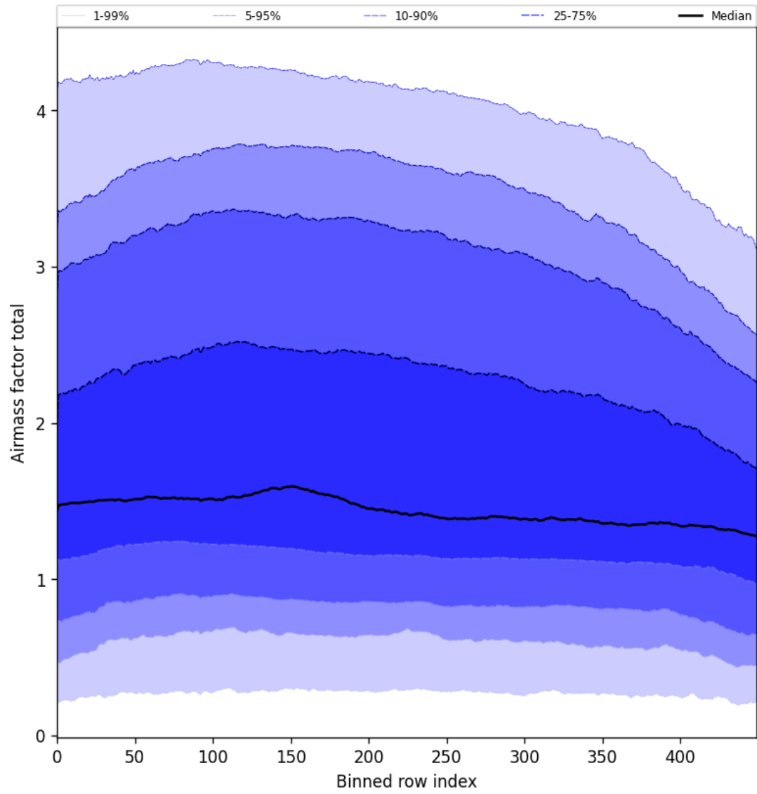
Figure 54: Along track statistics of “Airmass factor total” for 2025-03-17 to 2025-03-18
