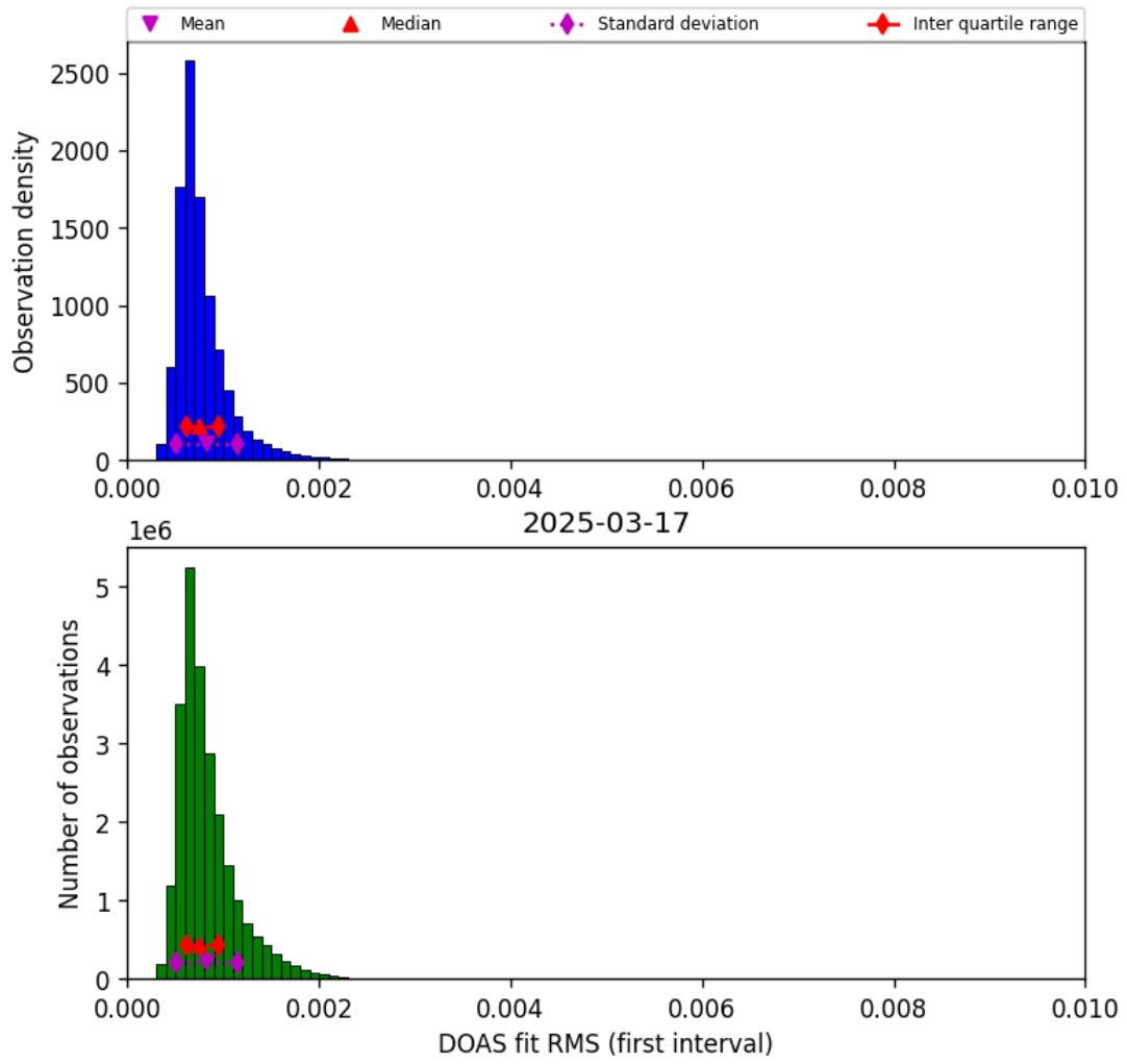
Figure 46: Histogram of “DOAS fit RMS (first interval)” for 2025-03-17 to 2025-03-18
