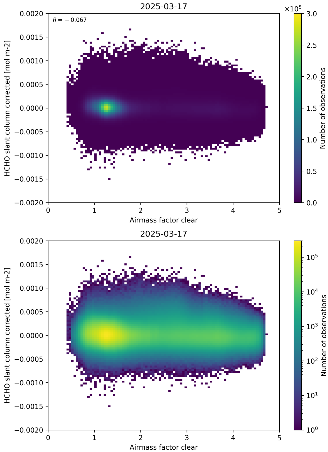
Figure 74: Scatter density plot of “Airmass factor clear” against “HCHO slant column corrected” for 2025-03-17 to 2025-03-18.
