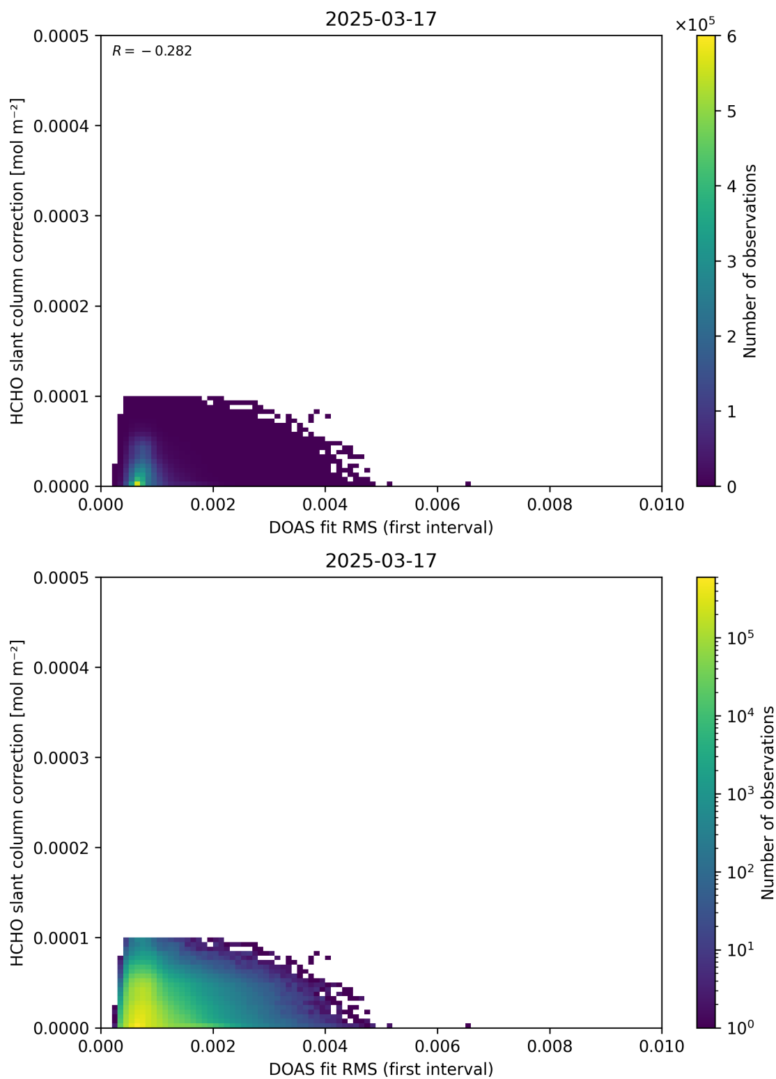
Figure 63: Scatter density plot of “DOAS fit RMS (first interval)” against “HCHO slant column correction” for 2025-03-17 to 2025-03-18.
