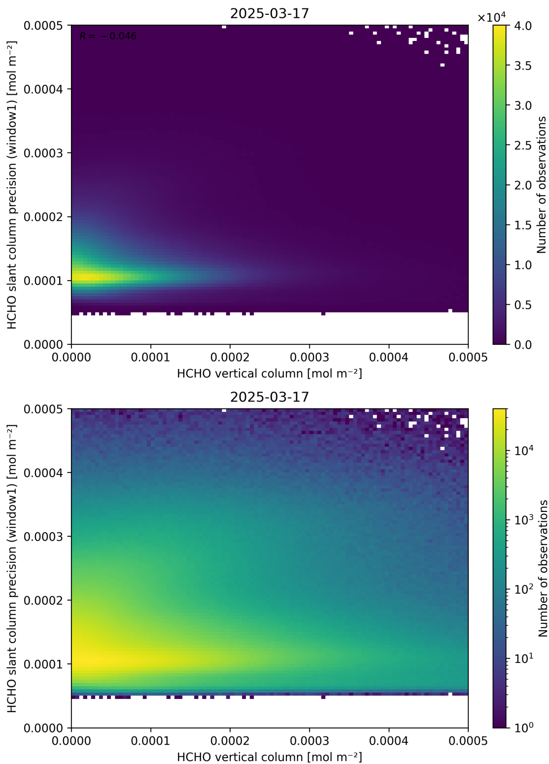
Figure 130: Scatter density plot of “HCHO vertical column” against “HCHO slant column precision (window1)” for 2025-03-17 to 2025-03-18.
