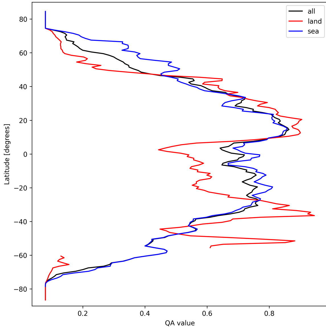
Figure 20: Zonal average of “QA value” for 2025-03-17 to 2025-03-18.
