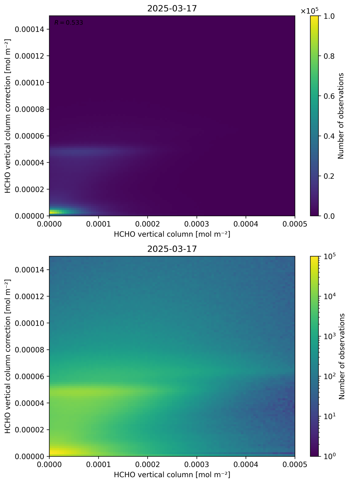
Figure 133: Scatter density plot of “HCHO vertical column” against “HCHO vertical column correction” for 2025-03-17 to 2025-03-18.
