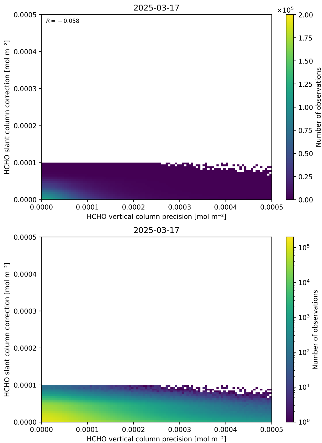
Figure 141: Scatter density plot of “HCHO vertical column precision” against “HCHO slant column correction” for 2025-03-17 to 2025-03-18.
