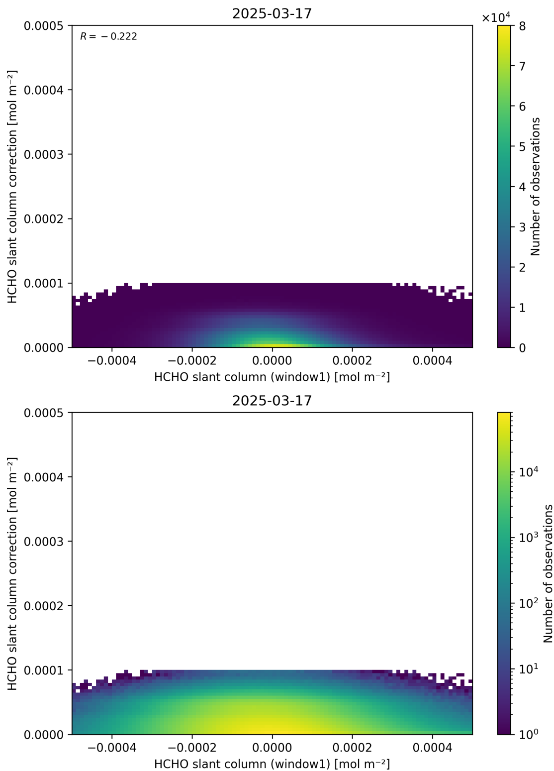
Figure 83: Scatter density plot of “HCHO slant column (window1)” against “HCHO slant column correction” for 2025-03-17 to 2025-03-18.
