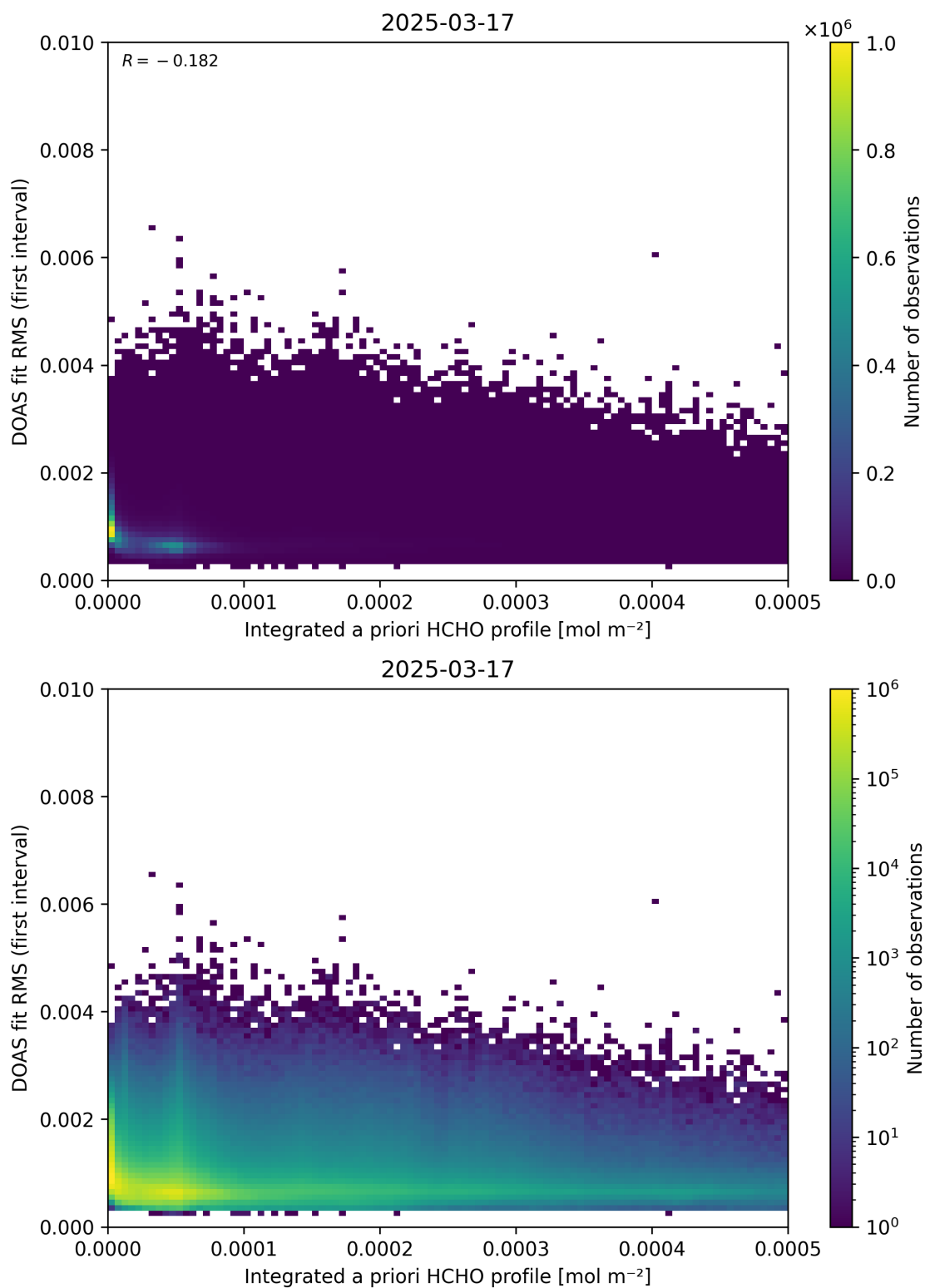
Figure 148: Scatter density plot of “Integrated a priori HCHO profile” against “DOAS fit RMS (first interval)” for 2025-03-17 to 2025-03-18.
