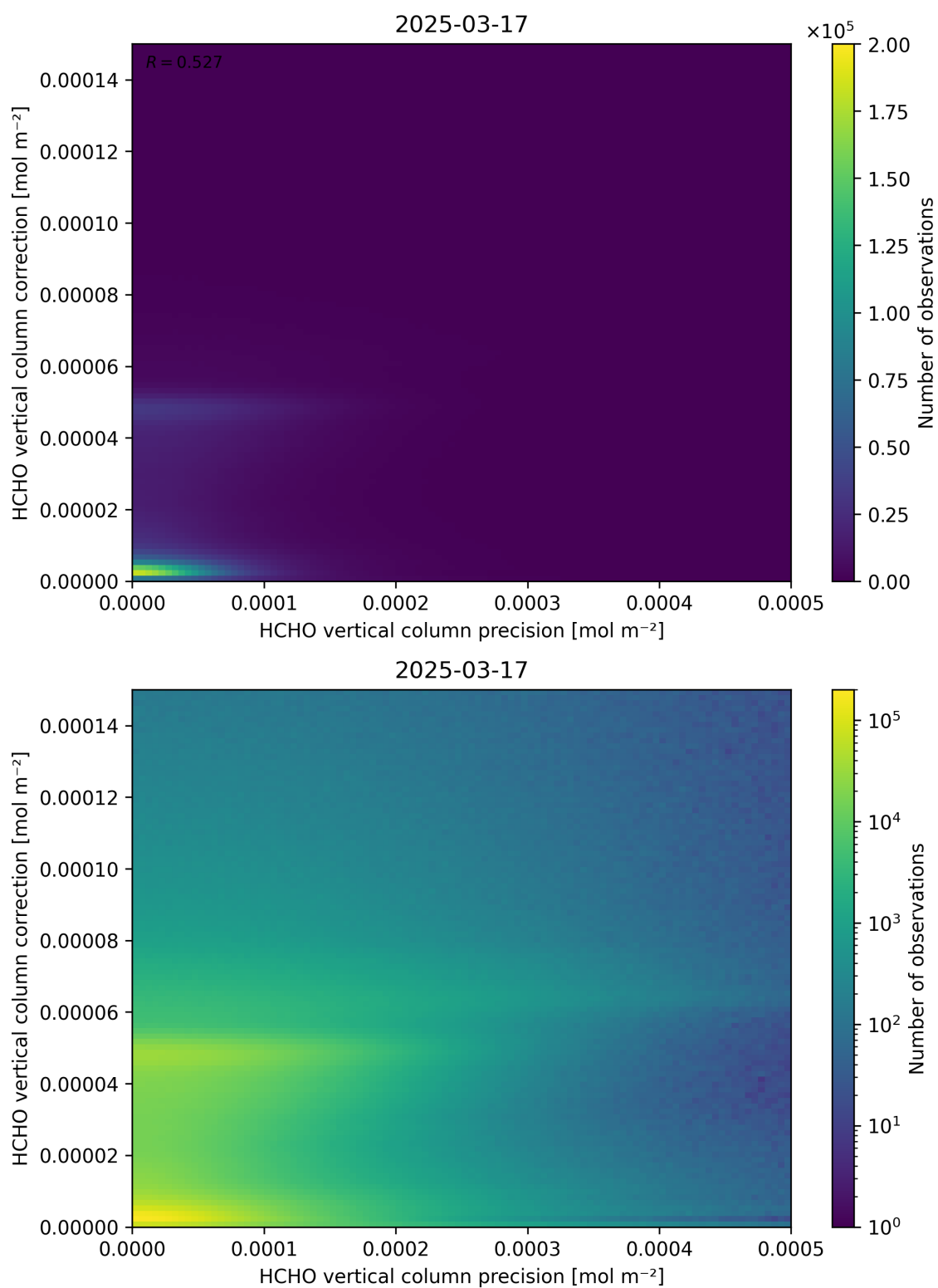
Figure 146: Scatter density plot of “HCHO vertical column precision” against “HCHO vertical column correction” for 2025-03-17 to 2025-03-18.
