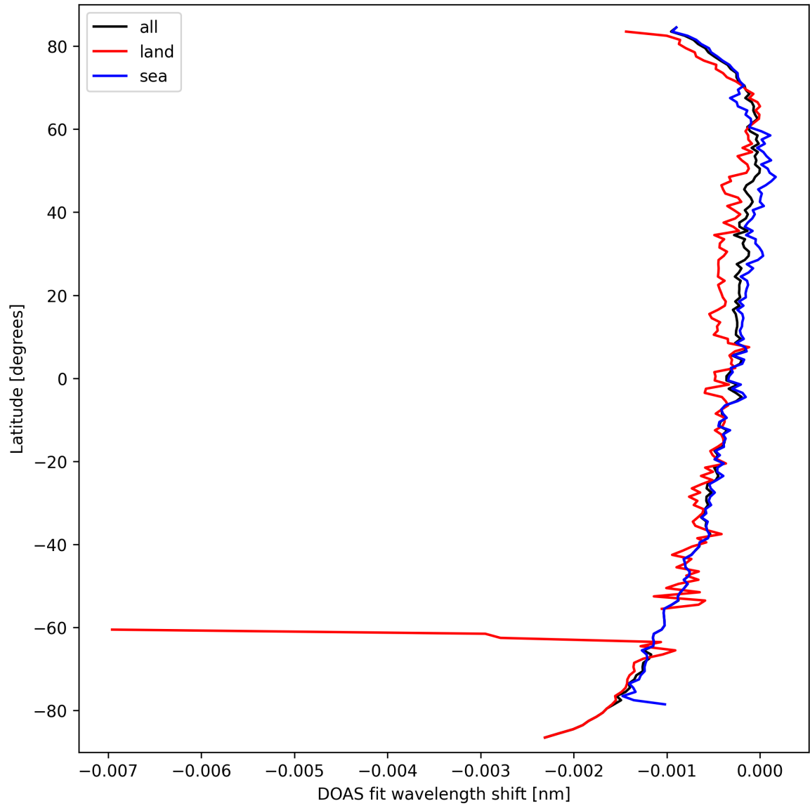
Figure 30: Zonal average of “DOAS fit wavelength shift” for 2025-03-17 to 2025-03-18.
