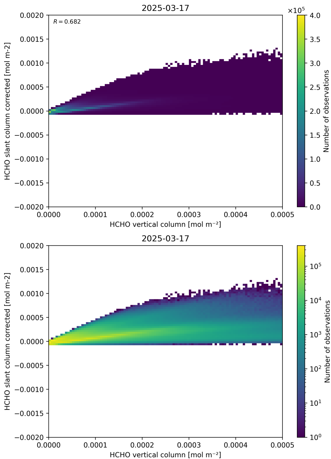
Figure 127: Scatter density plot of “HCHO vertical column” against “HCHO slant column corrected” for 2025-03-17 to 2025-03-18.
