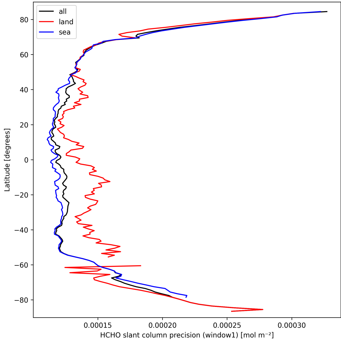
Figure 25: Zonal average of "HCHO slant column precision (window1)" for 2025-03-17 to 2025-03-18.
