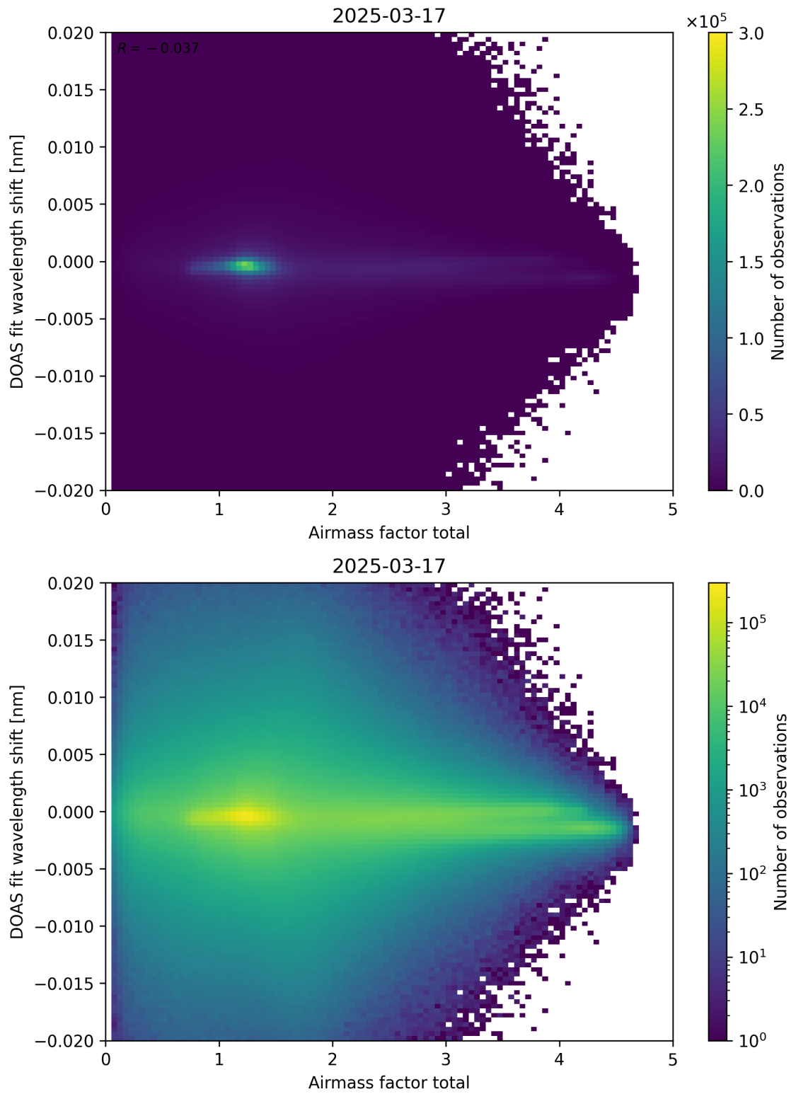
Figure 98: Scatter density plot of “Airmass factor total” against “DOAS fit wavelength shift” for 2025-03-17 to 2025-03-18.
