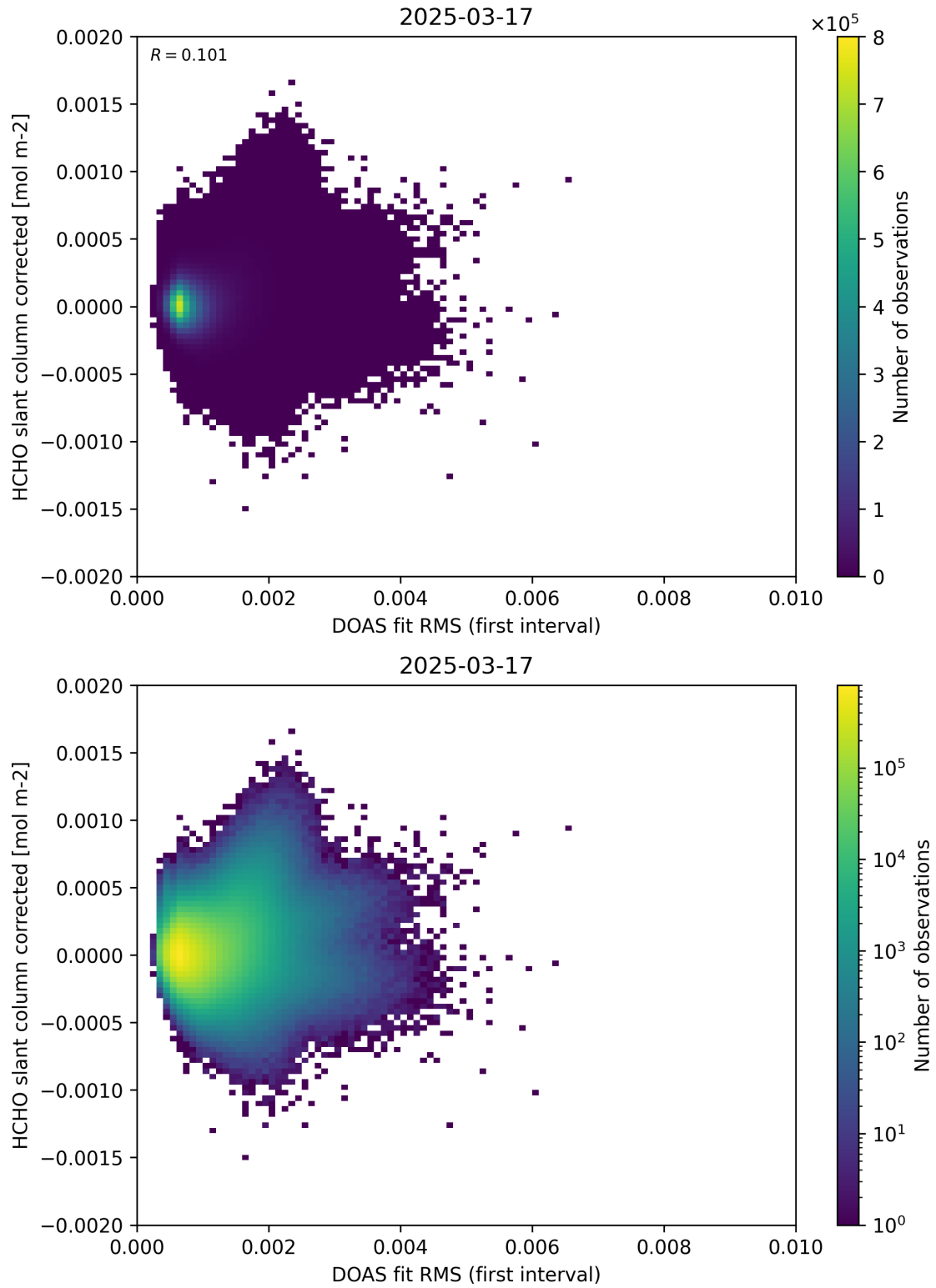
Figure 62: Scatter density plot of “DOAS fit RMS (first interval)” against “HCHO slant column corrected” for 2025-03-17 to 2025-03-18.
