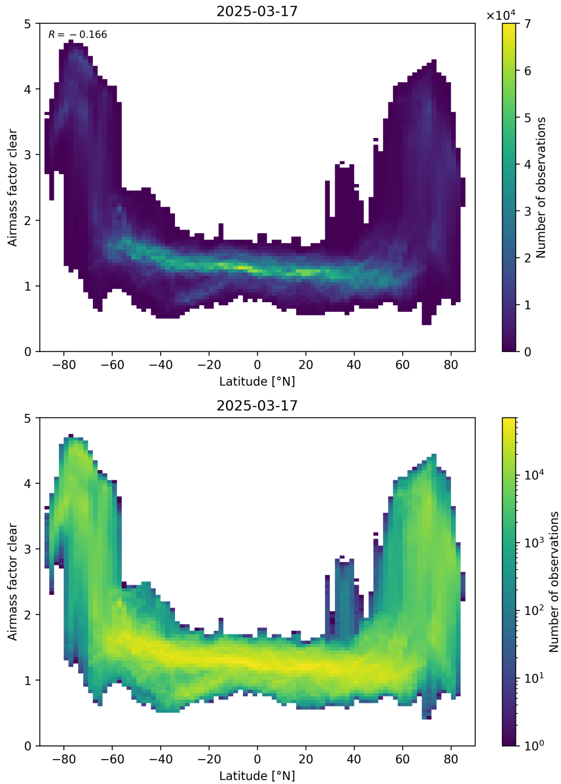
Figure 156: Scatter density plot of “Latitude” against “Airmass factor clear” for 2025-03-17 to 2025-03-18.
