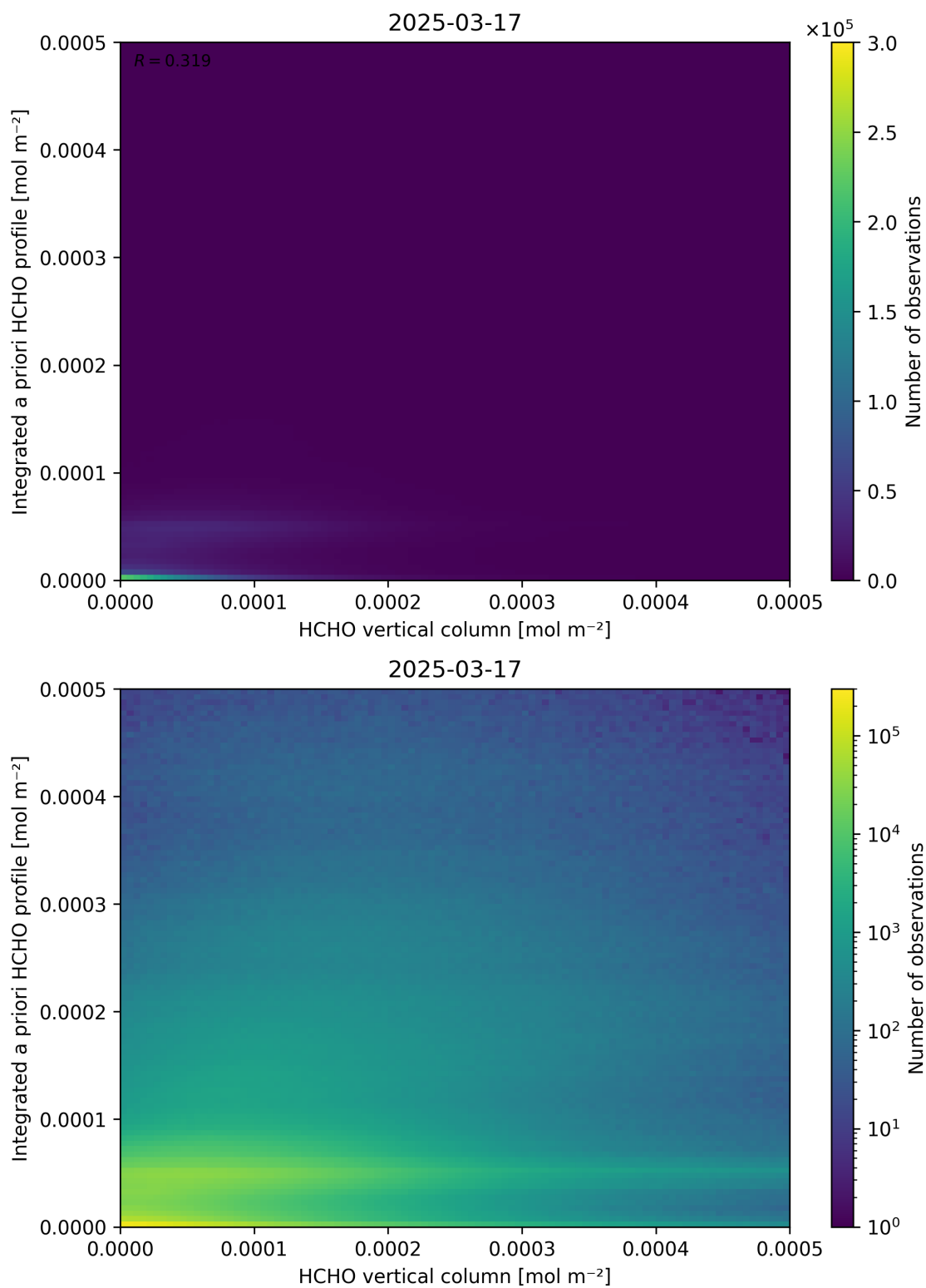
Figure 135: Scatter density plot of “HCHO vertical column” against “Integrated a priori HCHO profile” for 2025-03-17 to 2025-03-18.
