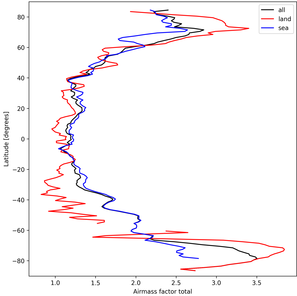
Figure 26: Zonal average of “Airmass factor total” for 2025-03-17 to 2025-03-18.
