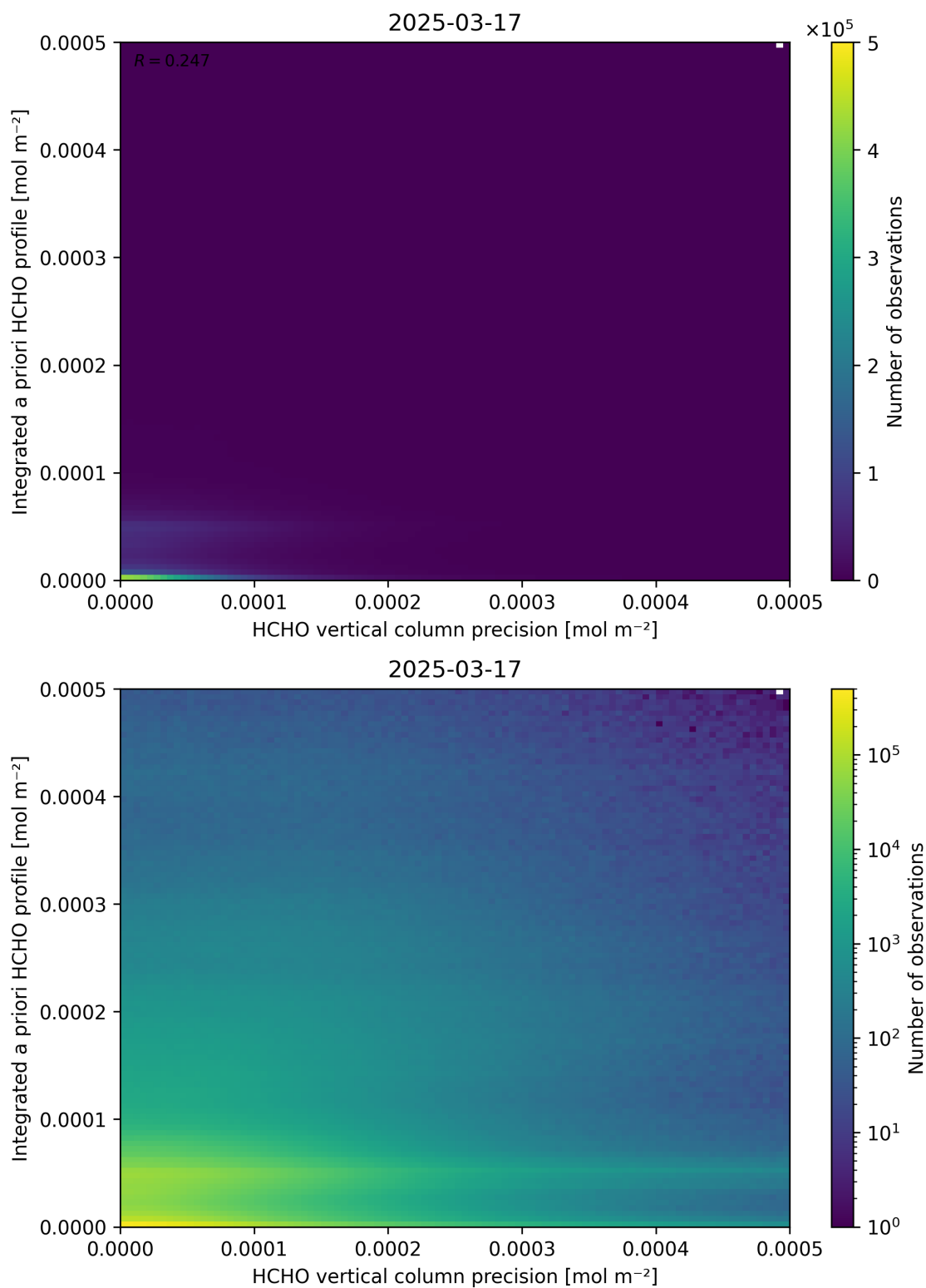
Figure 147: Scatter density plot of “HCHO vertical column precision” against “Integrated a priori HCHO profile” for 2025-03-17 to 2025-03-18.
