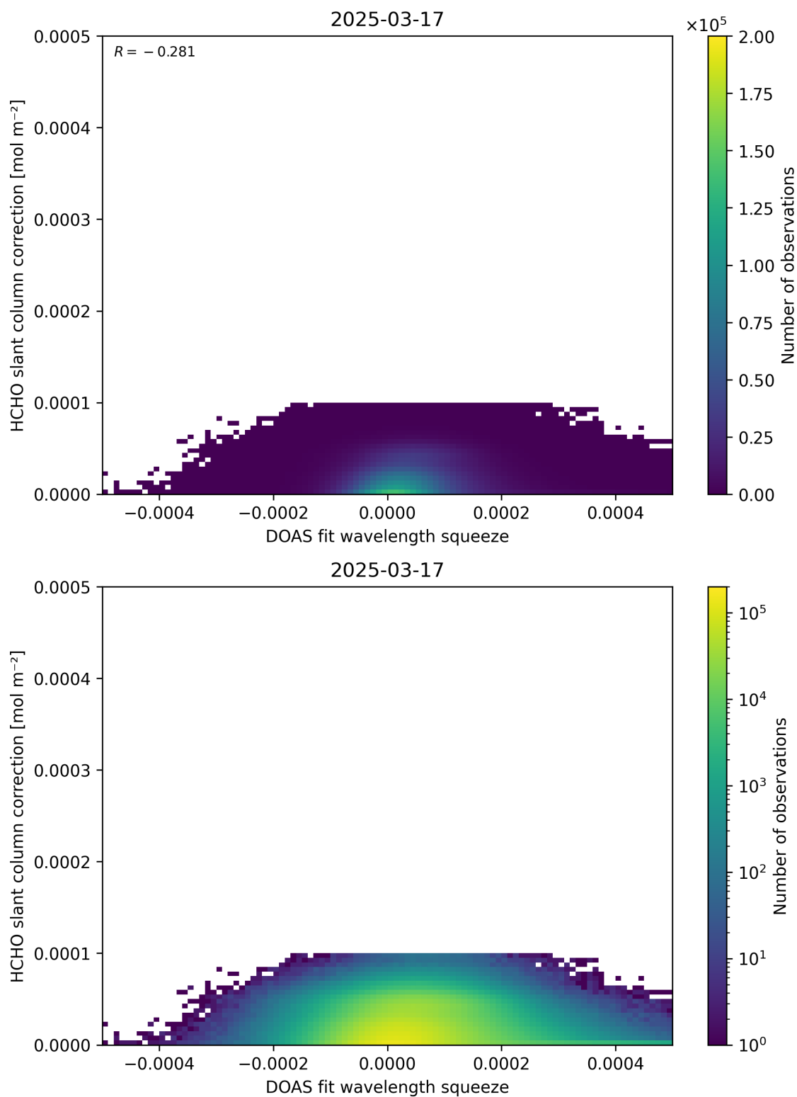
Figure 70: Scatter density plot of “DOAS fit wavelength squeeze” against “HCHO slant column correction” for 2025-03-17 to 2025-03-18.
