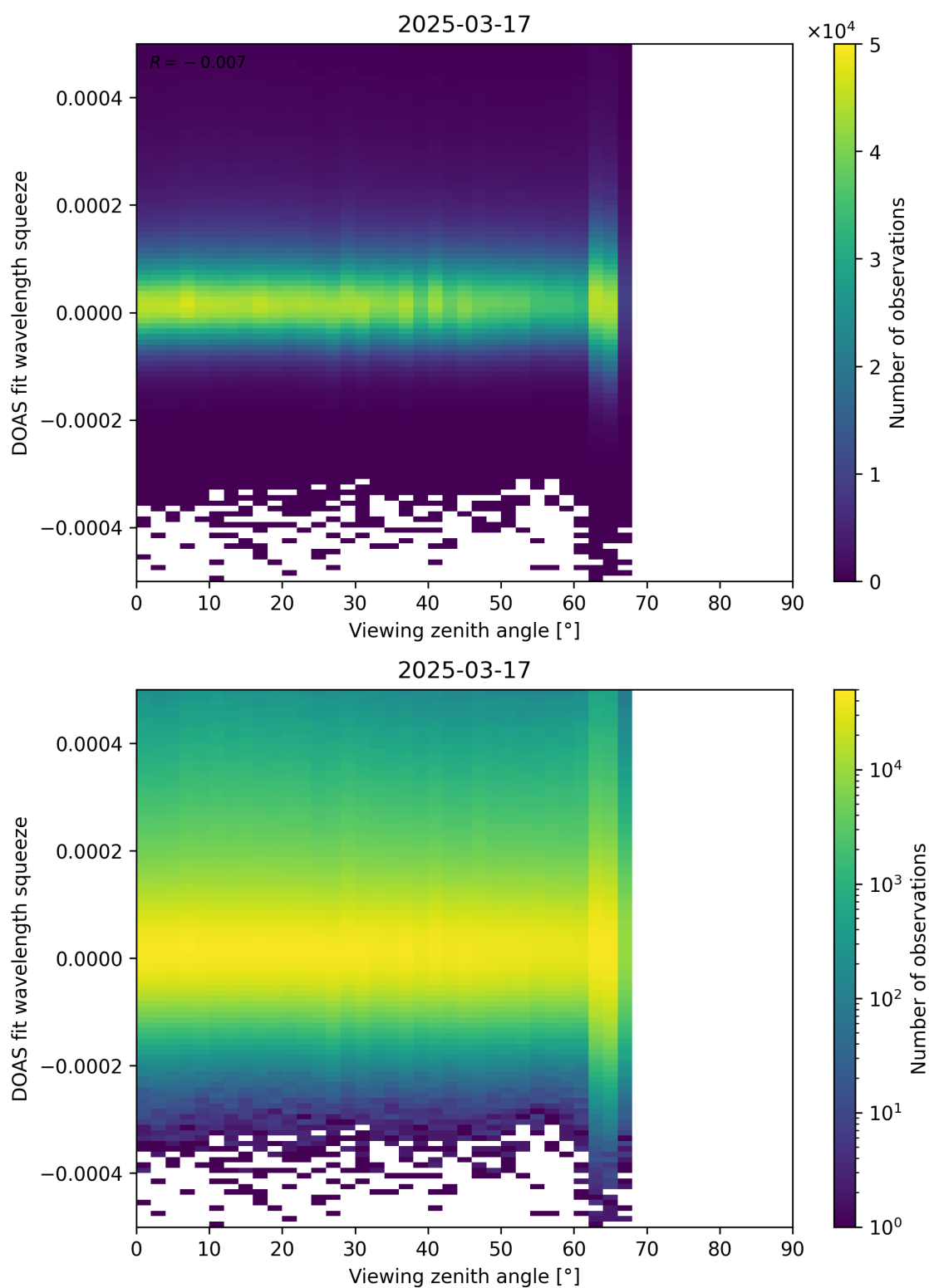
Figure 184: Scatter density plot of “Viewing zenith angle” against “DOAS fit wavelength squeeze” for 2025-03-17 to 2025-03-18.
