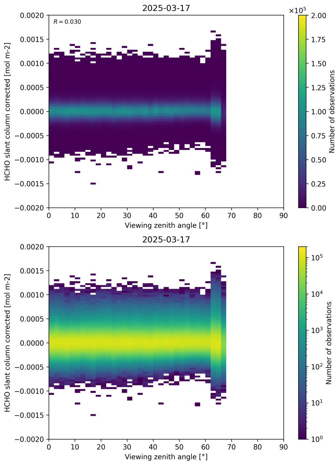
Figure 186: Scatter density plot of “Viewing zenith angle” against “HCHO slant column corrected” for 2025-03-17 to 2025-03-18.
