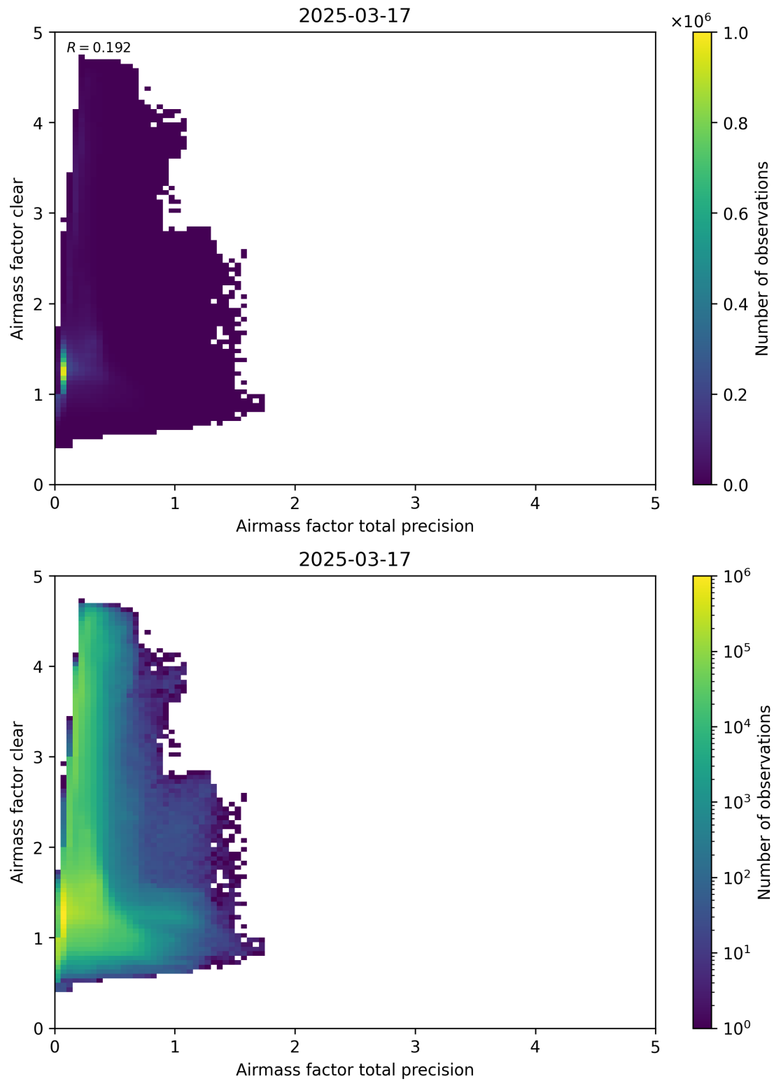
Figure 108: Scatter density plot of “Airmass factor total precision” against “Airmass factor clear” for 2025-03-17 to 2025-03-18.
