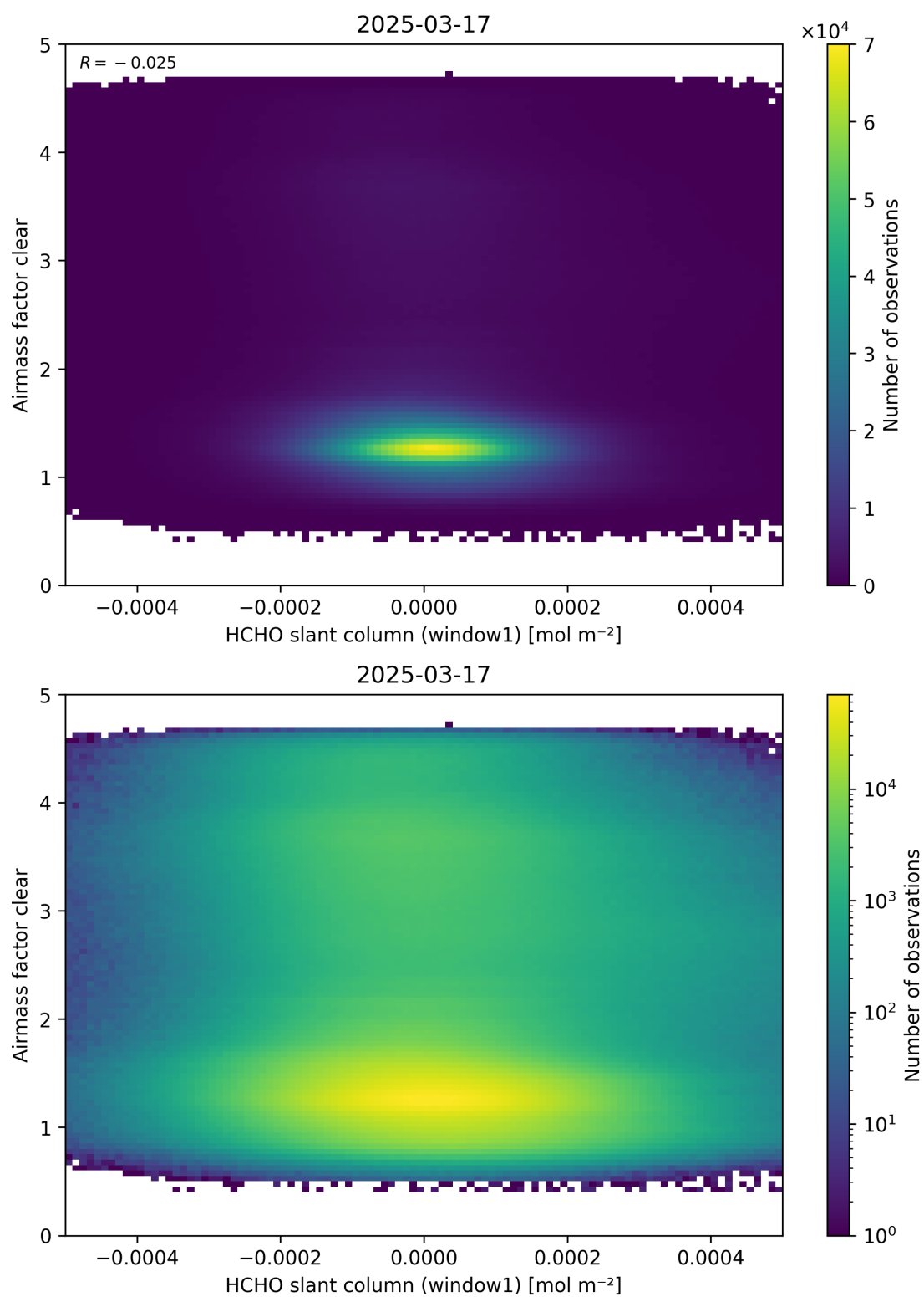
Figure 81: Scatter density plot of “HCHO slant column (window1)” against “Airmass factor clear” for 2025-03-17 to 2025-03-18.
