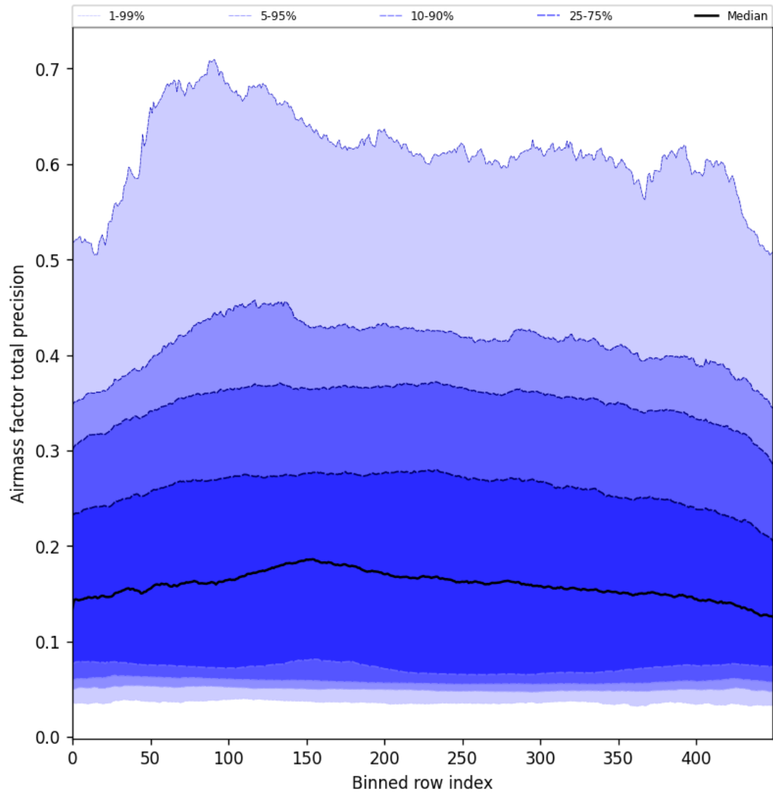
Figure 55: Along track statistics of “Airmass factor total precision” for 2025-03-17 to 2025-03-18
