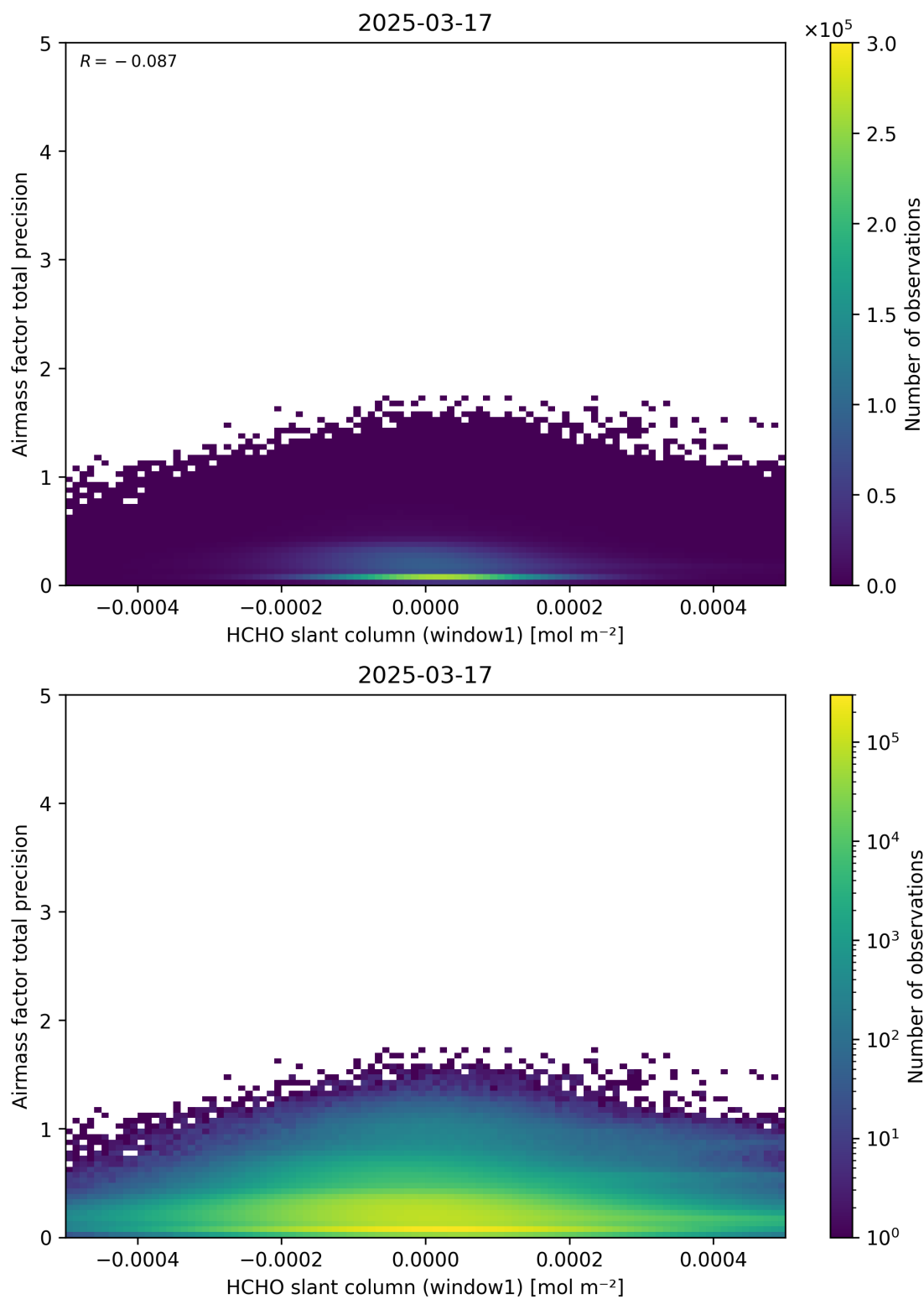
Figure 86: Scatter density plot of “HCHO slant column (window1)” against “Airmass factor total precision” for 2025-03-17 to 2025-03-18.
