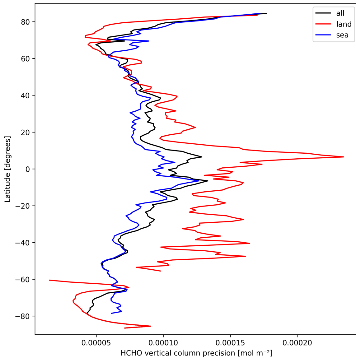
Figure 22: Zonal average of “HCHO vertical column precision” for 2025-03-17 to 2025-03-18.
