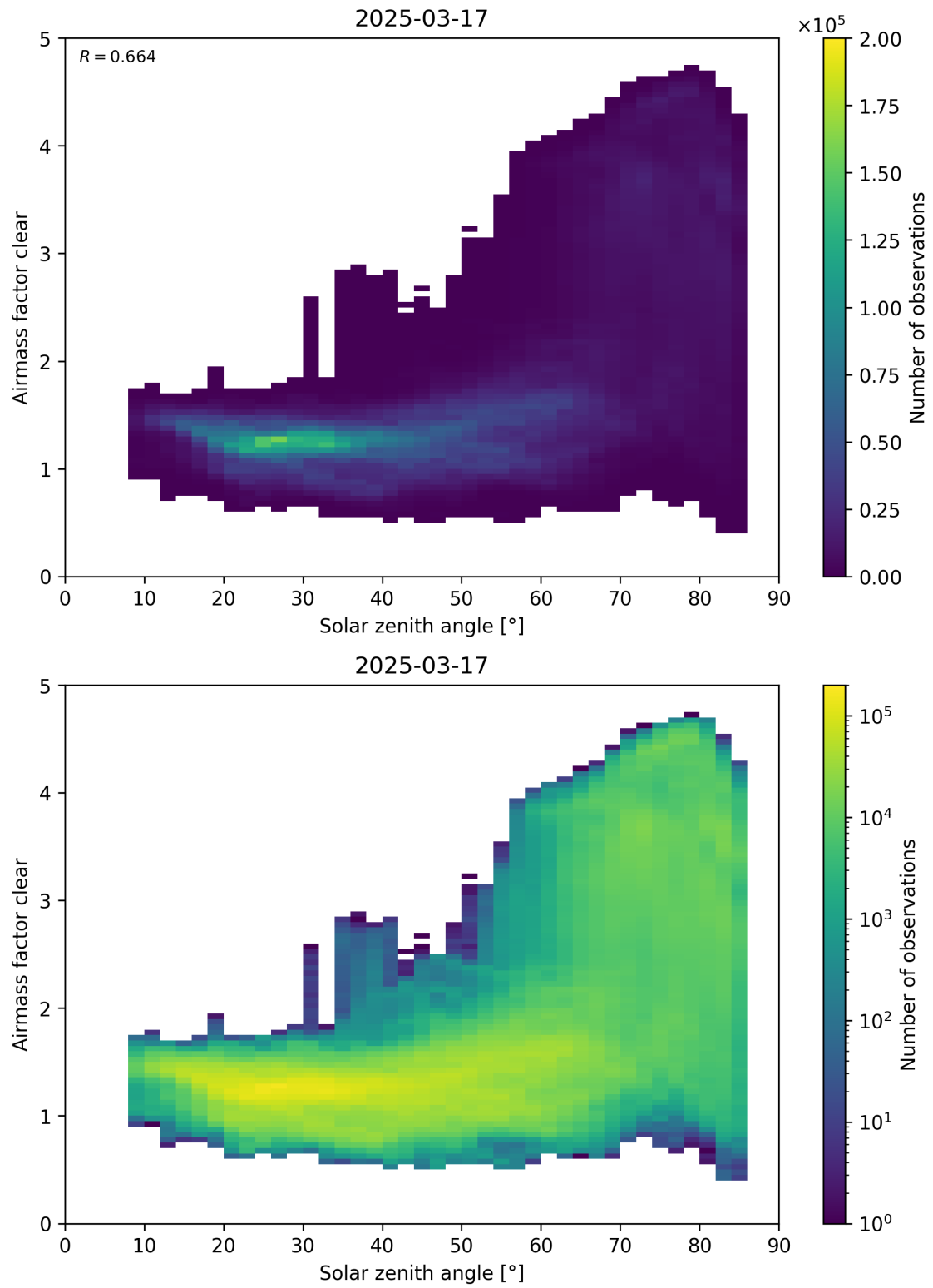
Figure 170: Scatter density plot of “Solar zenith angle” against “Airmass factor clear” for 2025-03-17 to 2025-03-18.
