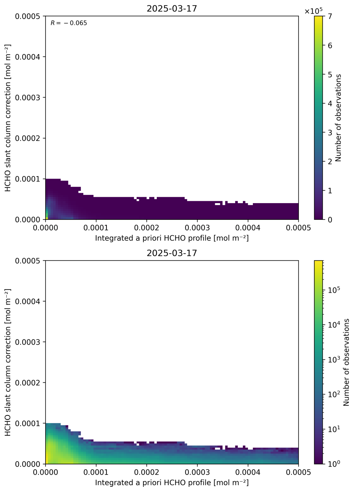
Figure 152: Scatter density plot of “Integrated a priori HCHO profile” against “HCHO slant column correction” for 2025-03-17 to 2025-03-18.
