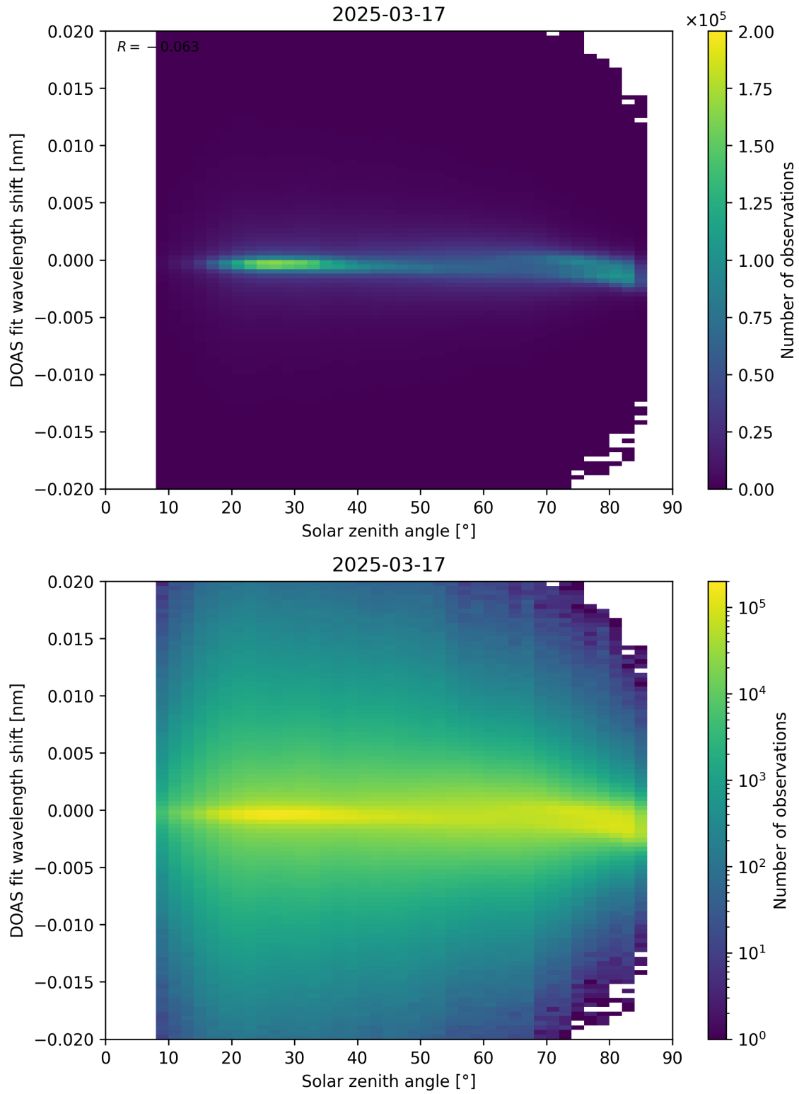
Figure 168: Scatter density plot of “Solar zenith angle” against “DOAS fit wavelength shift” for 2025-03-17 to 2025-03-18.
