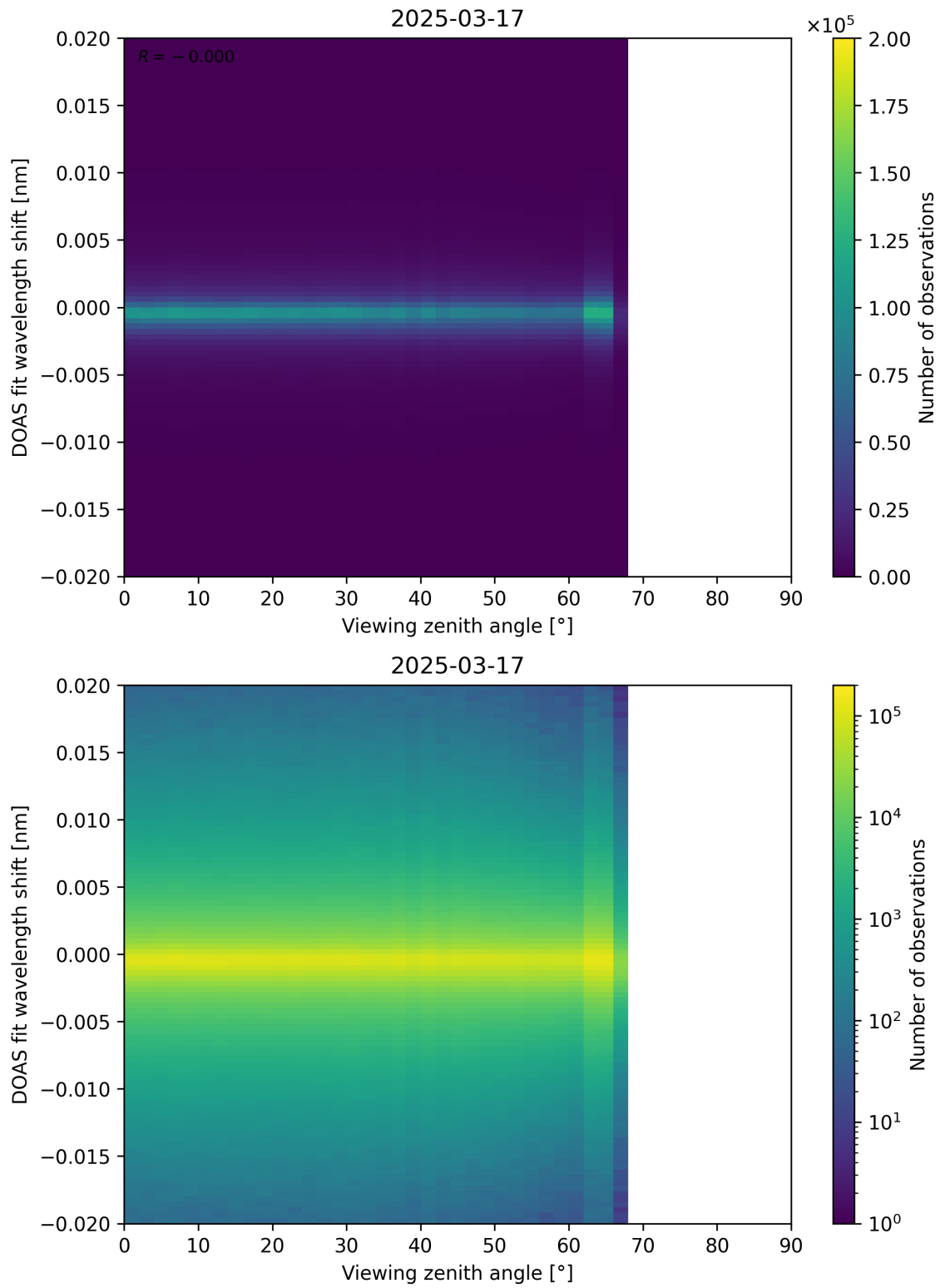
Figure 183: Scatter density plot of “Viewing zenith angle” against “DOAS fit wavelength shift” for 2025-03-17 to 2025-03-18.
