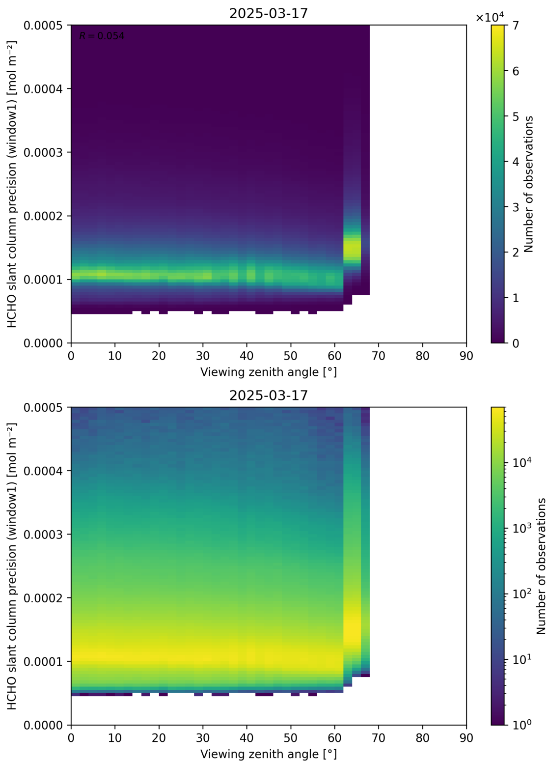
Figure 189: Scatter density plot of “Viewing zenith angle” against “HCHO slant column precision (window1)” for 2025-03-17 to 2025-03-18.
