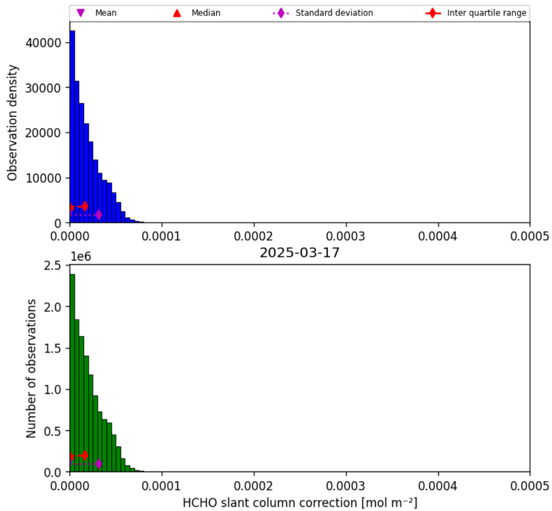
Figure 47: Histogram of “HCHO slant column correction” for 2025-03-17 to 2025-03-18
