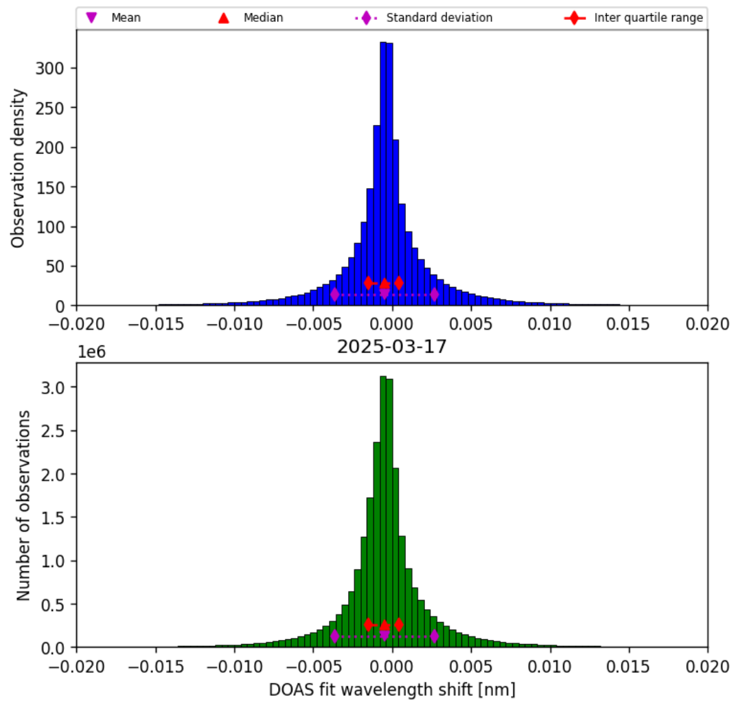
Figure 44: Histogram of “DOAS fit wavelength shift” for 2025-03-17 to 2025-03-18
