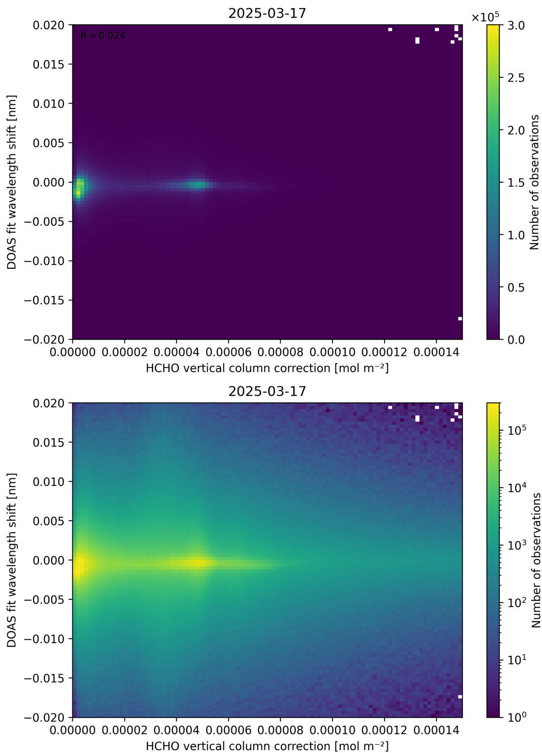
Figure 113: Scatter density plot of “HCHO vertical column correction” against “DOAS fit wavelength shift” for 2025-03-17 to 2025-03-18.
