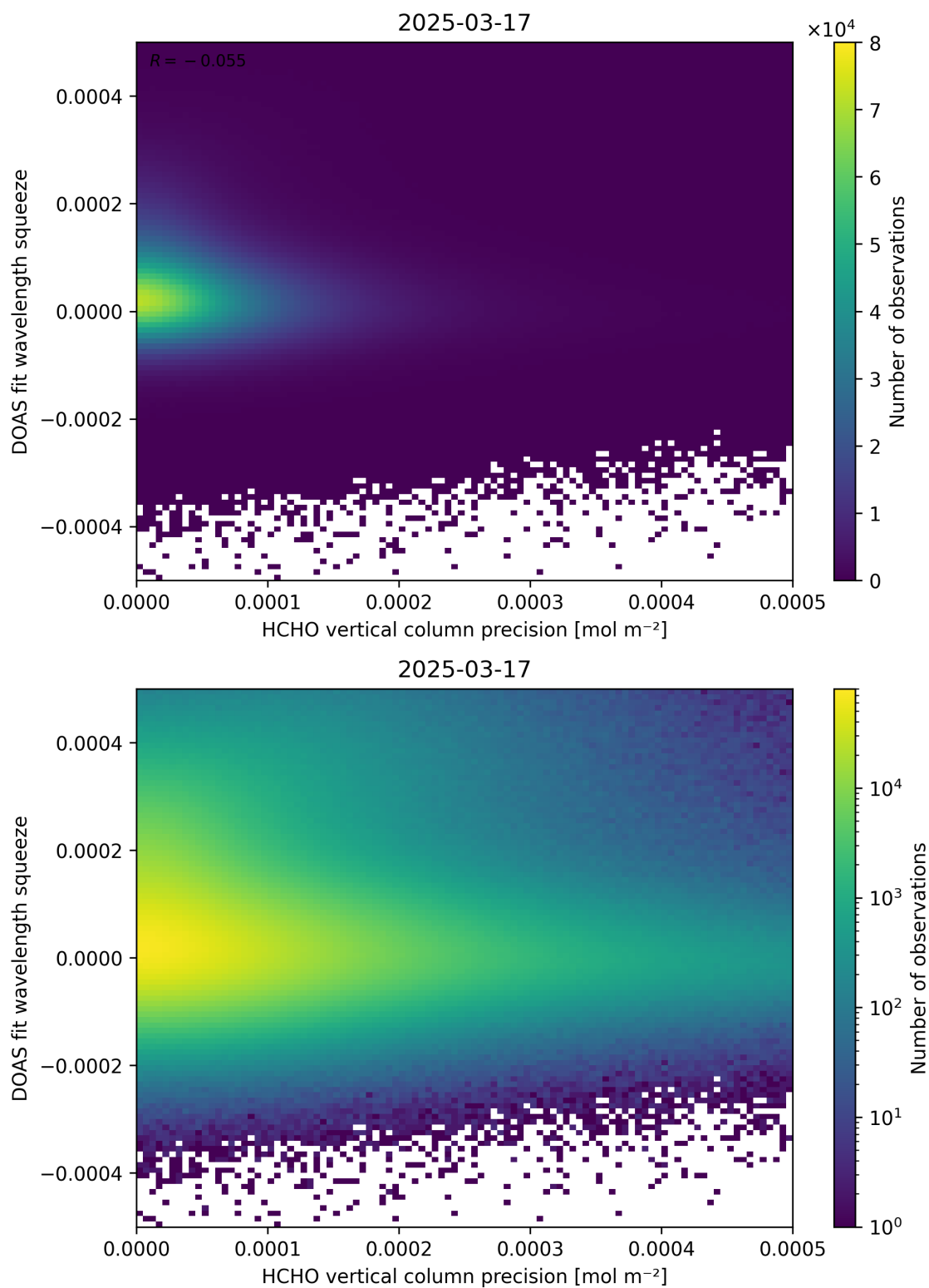
Figure 138: Scatter density plot of “HCHO vertical column precision” against “DOAS fit wavelength squeeze” for 2025-03-17 to 2025-03-18.
