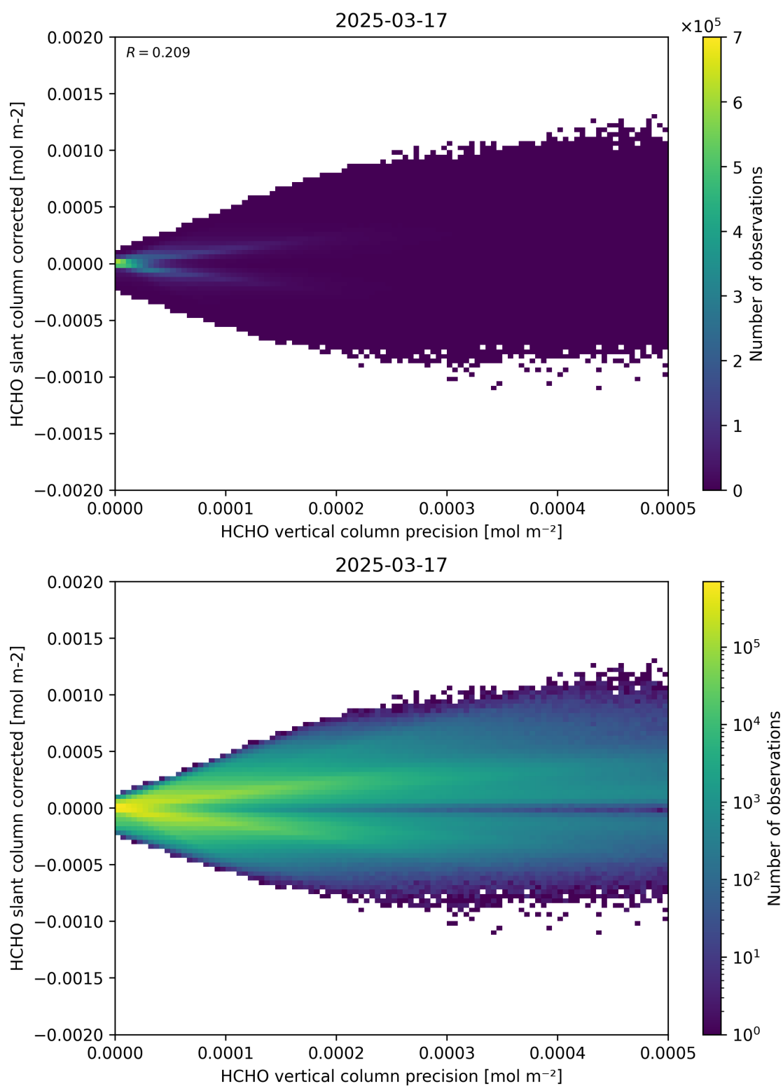
Figure 140: Scatter density plot of “HCHO vertical column precision” against “HCHO slant column corrected” for 2025-03-17 to 2025-03-18.
