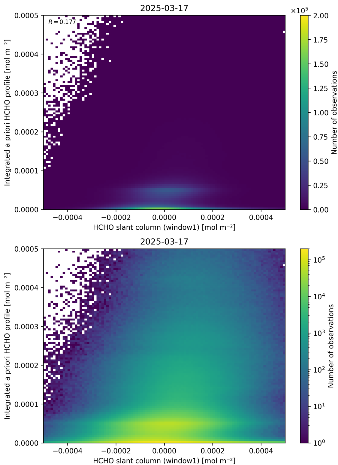
Figure 87: Scatter density plot of “HCHO slant column (window1)” against “Integrated a priori HCHO profile” for 2025-03-17 to 2025-03-18.
