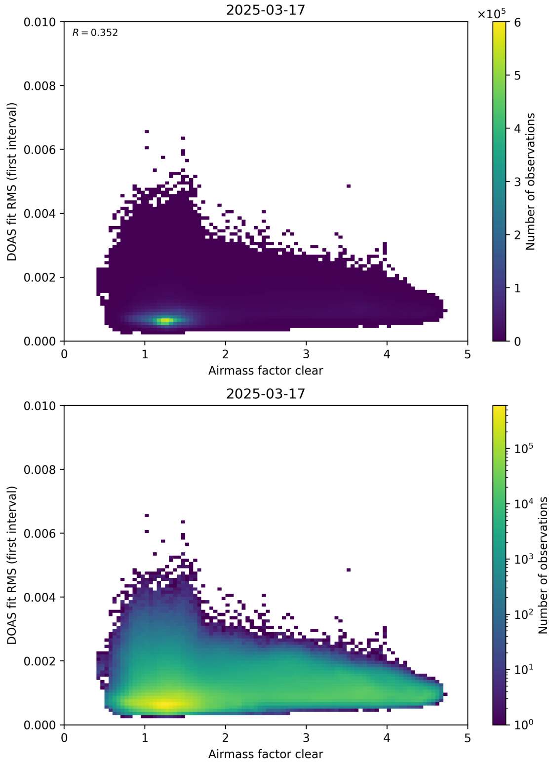
Figure 71: Scatter density plot of “Airmass factor clear” against “DOAS fit RMS (first interval)” for 2025-03-17 to 2025-03-18.
