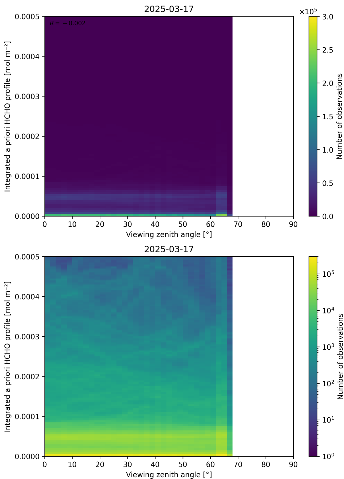
Figure 195: Scatter density plot of “Viewing zenith angle” against “Integrated a priori HCHO profile” for 2025-03-17 to 2025-03-18.
