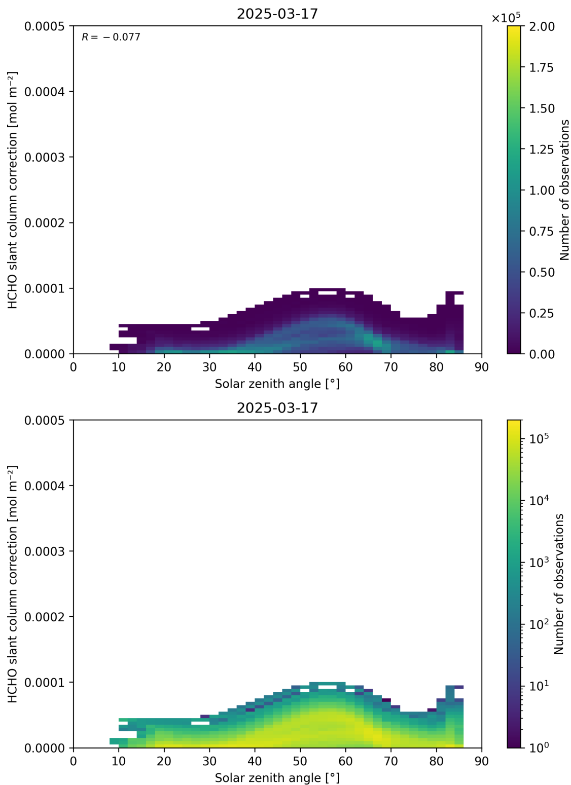
Figure 172: Scatter density plot of “Solar zenith angle” against “HCHO slant column correction” for 2025-03-17 to 2025-03-18.
