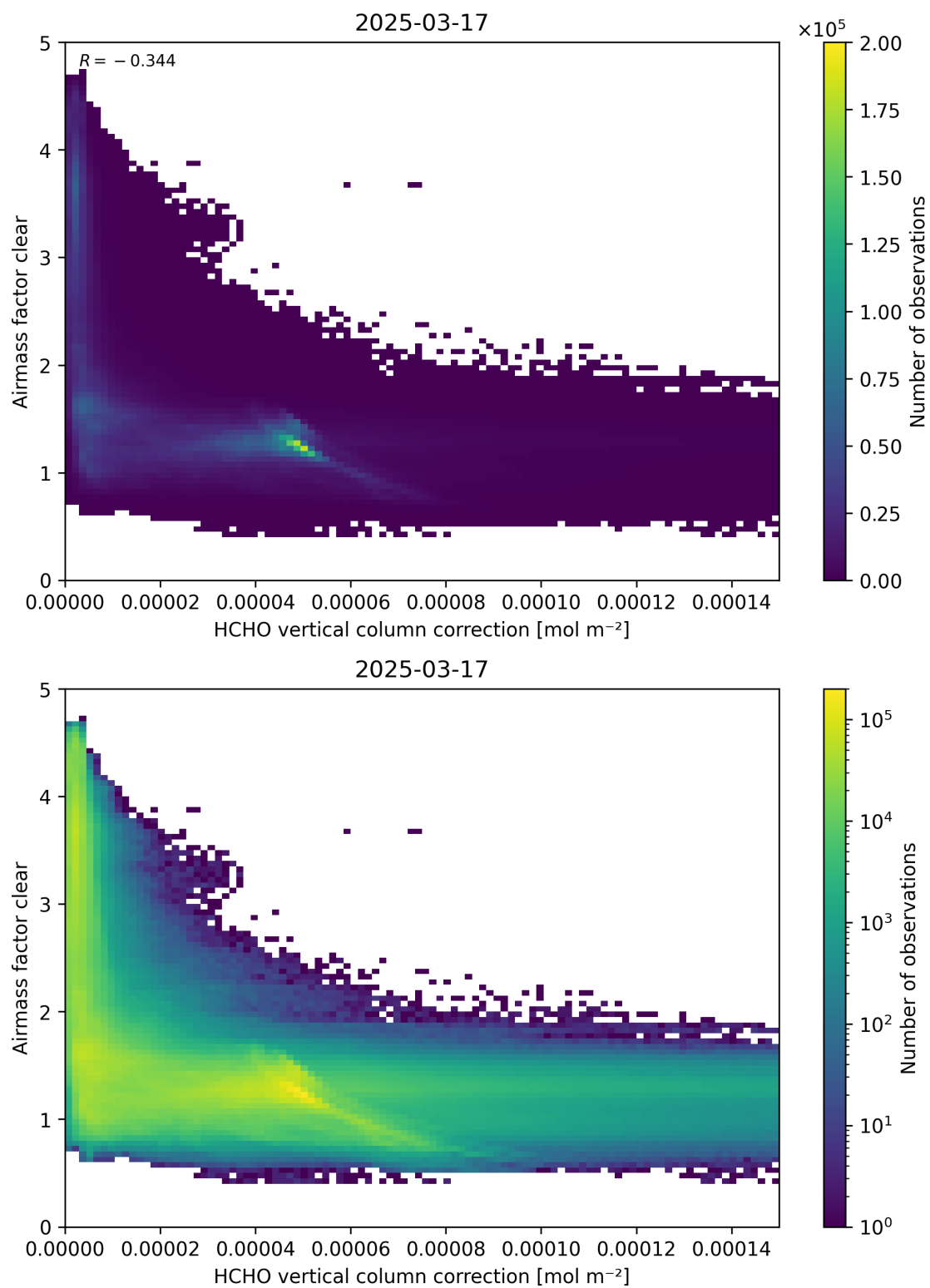
Figure 115: Scatter density plot of “HCHO vertical column correction” against “Airmass factor clear” for 2025-03-17 to 2025-03-18.
