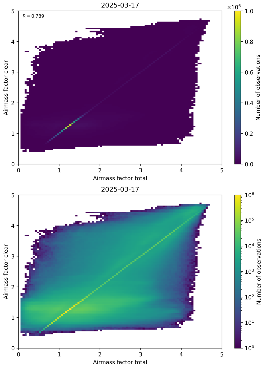
Figure 100: Scatter density plot of “Airmass factor total” against “Airmass factor clear” for 2025-03-17 to 2025-03-18.
