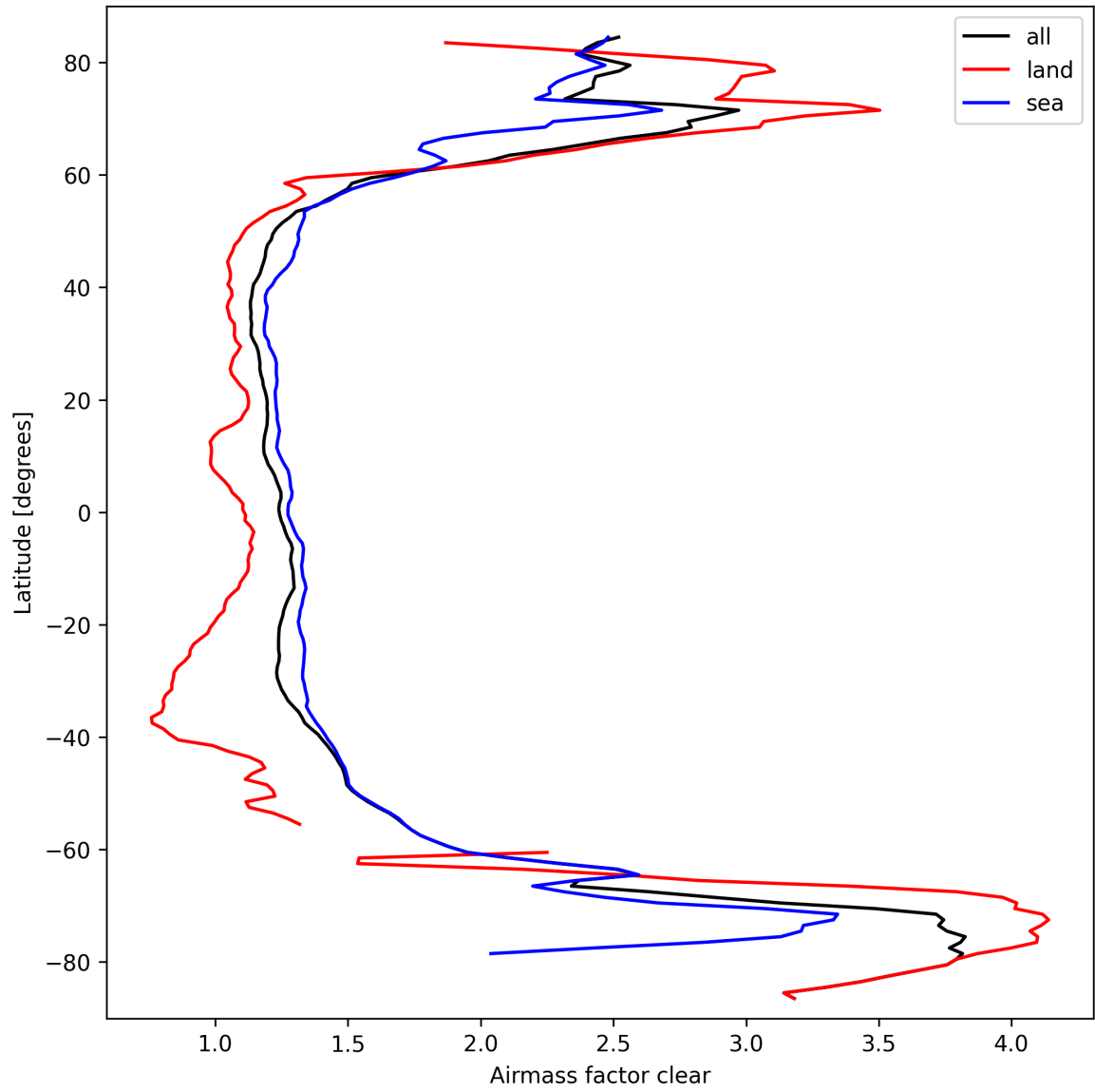
Figure 28: Zonal average of “Airmass factor clear” for 2025-03-17 to 2025-03-18.
