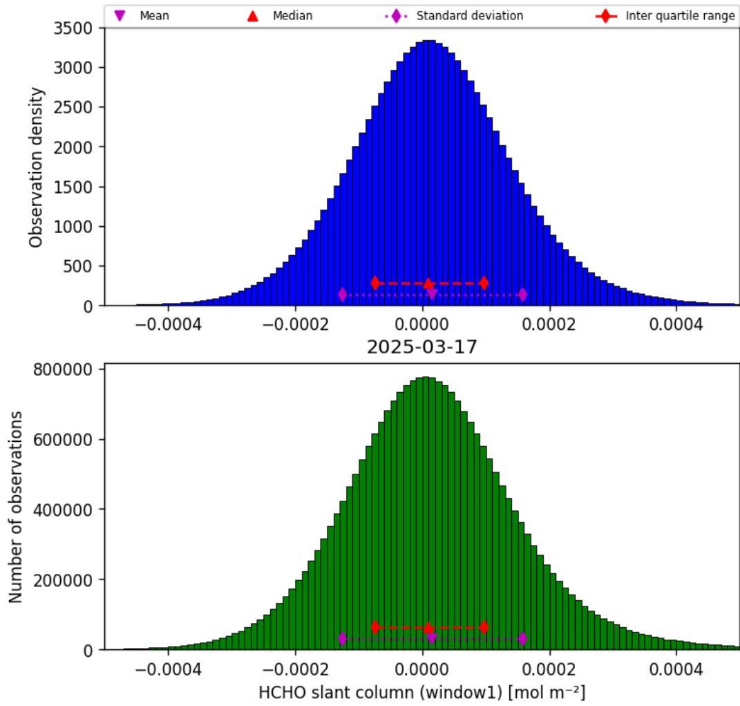
Figure 38: Histogram of “HCHO slant column (window1)” for 2025-03-17 to 2025-03-18
