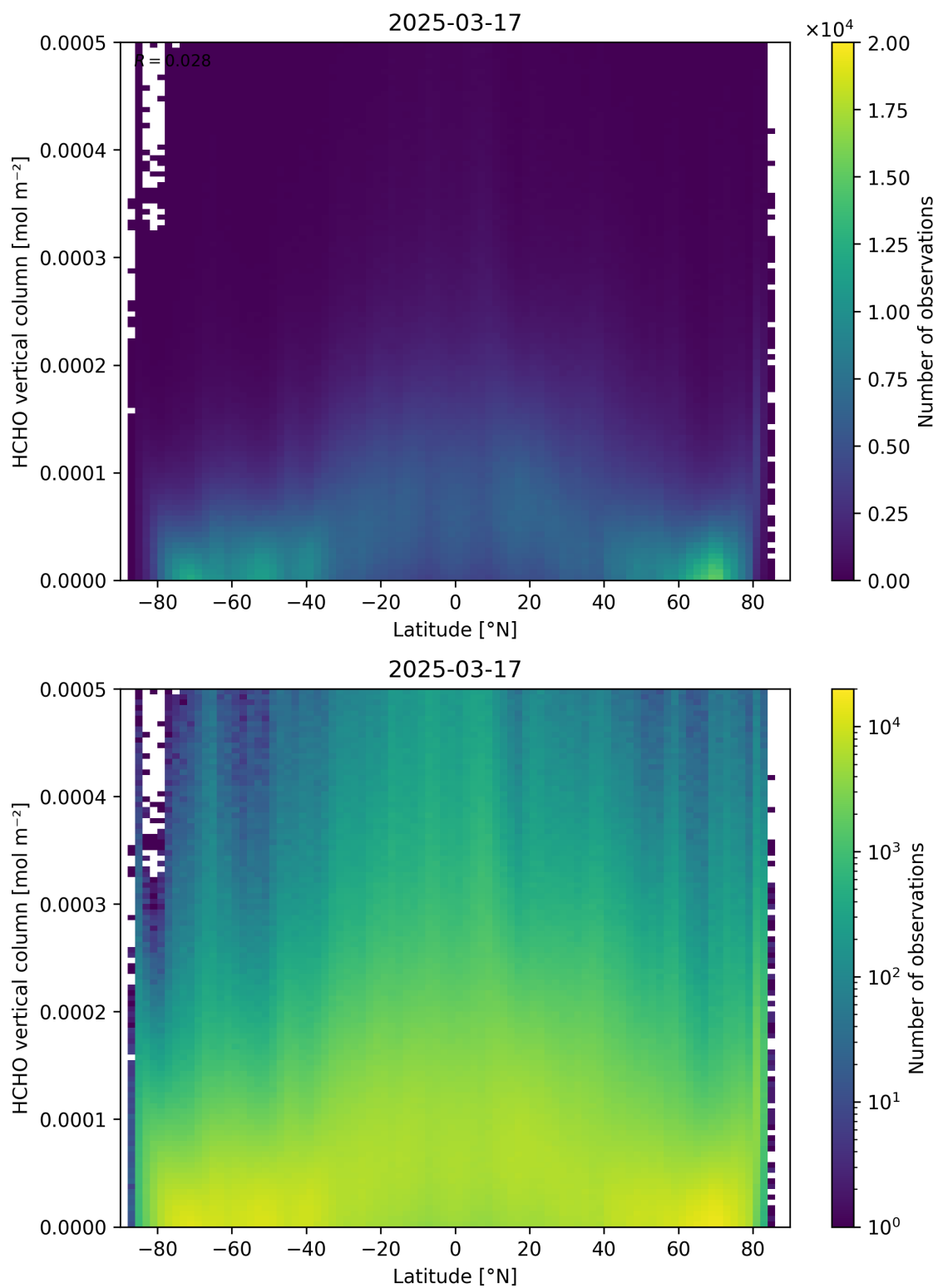
Figure 163: Scatter density plot of “Latitude” against “HCHO vertical column” for 2025-03-17 to 2025-03-18.
