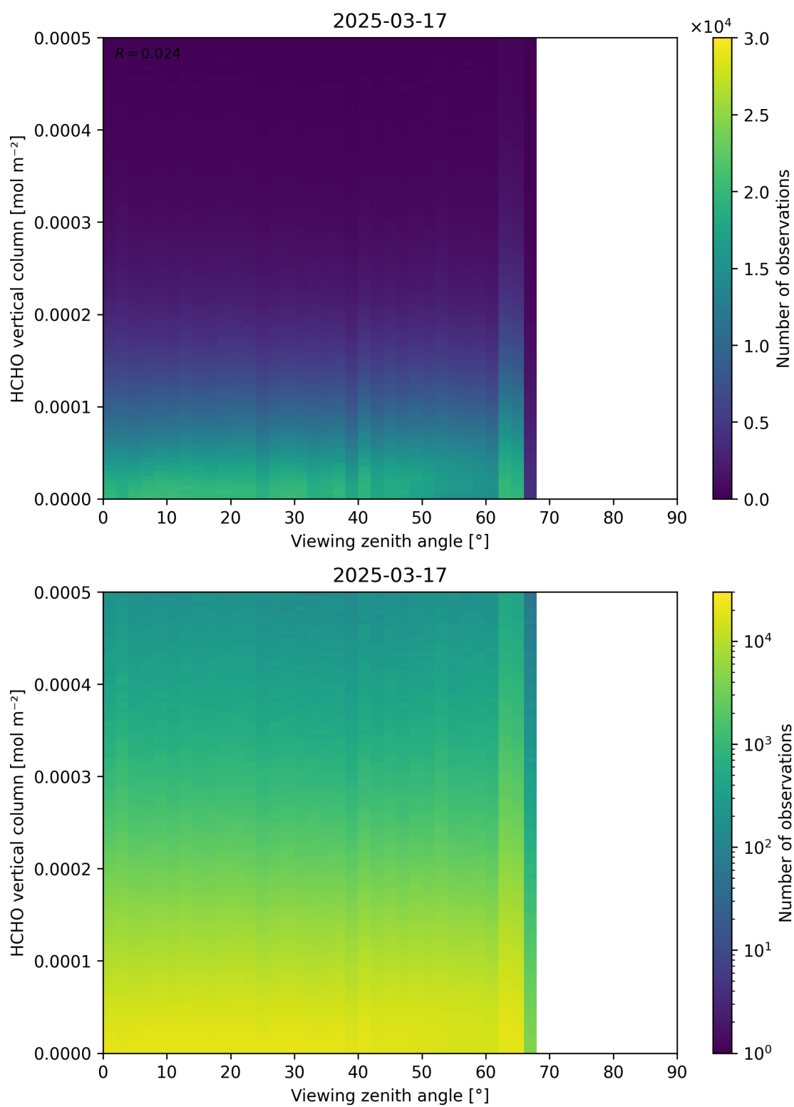
Figure 192: Scatter density plot of “Viewing zenith angle” against “HCHO vertical column” for 2025-03-17 to 2025-03-18.
