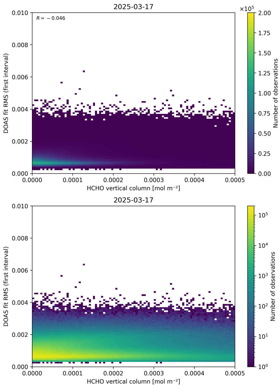
Figure 123: Scatter density plot of “HCHO vertical column” against “DOAS fit RMS (first interval)” for 2025-03-17 to 2025-03-18.
