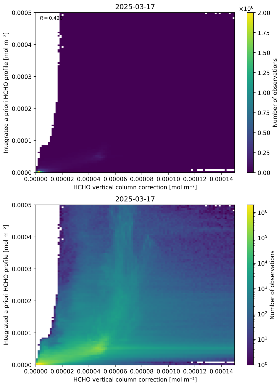
Figure 122: Scatter density plot of “HCHO vertical column correction” against “Integrated a priori HCHO profile” for 2025-03-17 to 2025-03-18.
