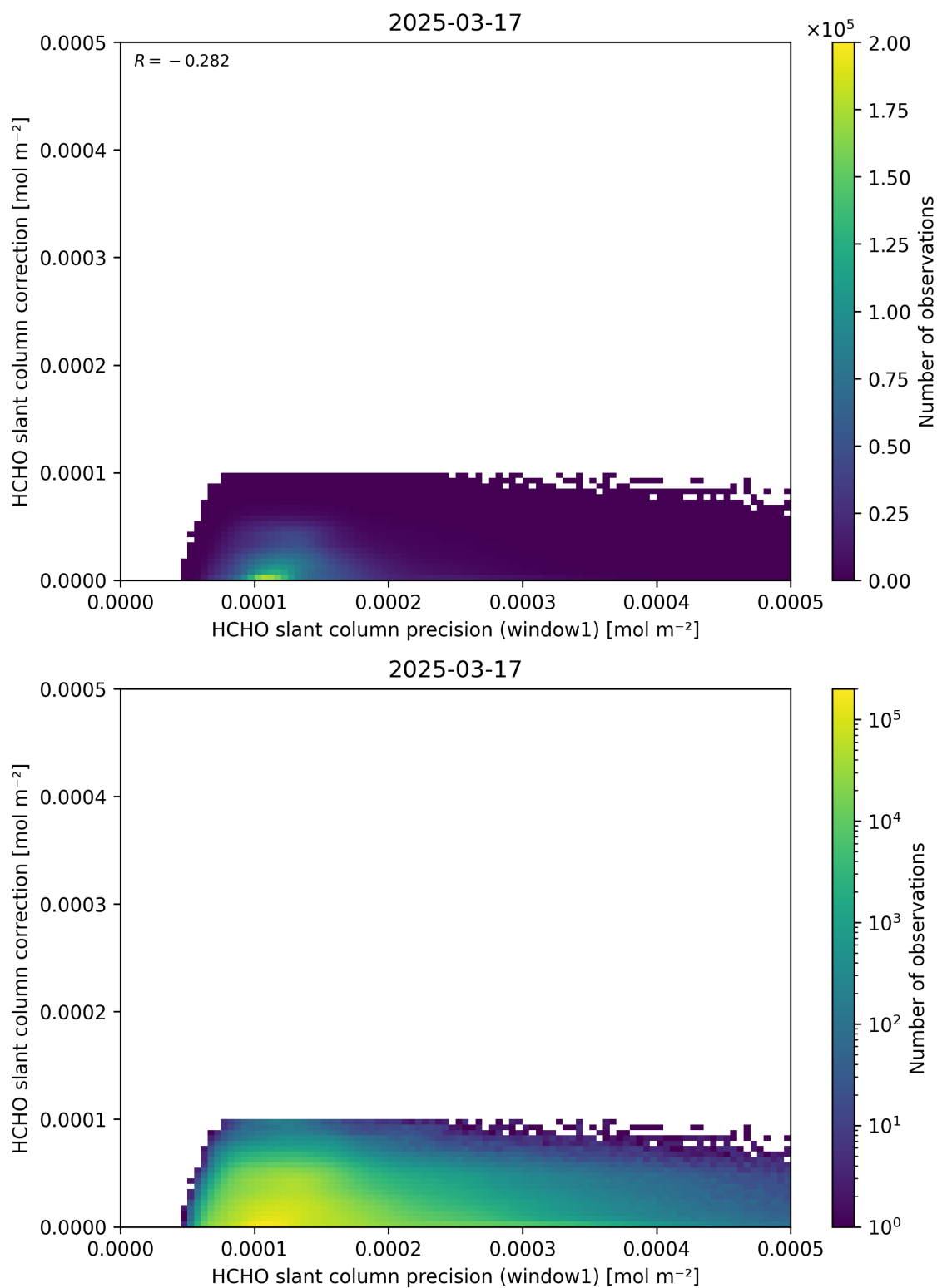
Figure 93: Scatter density plot of “HCHO slant column precision (window1)” against “HCHO slant column correction” for 2025-03-17 to 2025-03-18.
