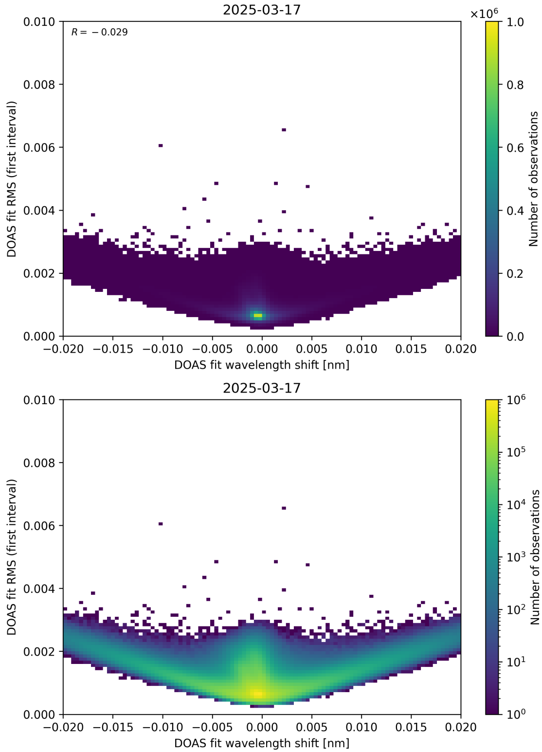
Figure 64: Scatter density plot of “DOAS fit wavelength shift” against “DOAS fit RMS (first interval)” for 2025-03-17 to 2025-03-18.
