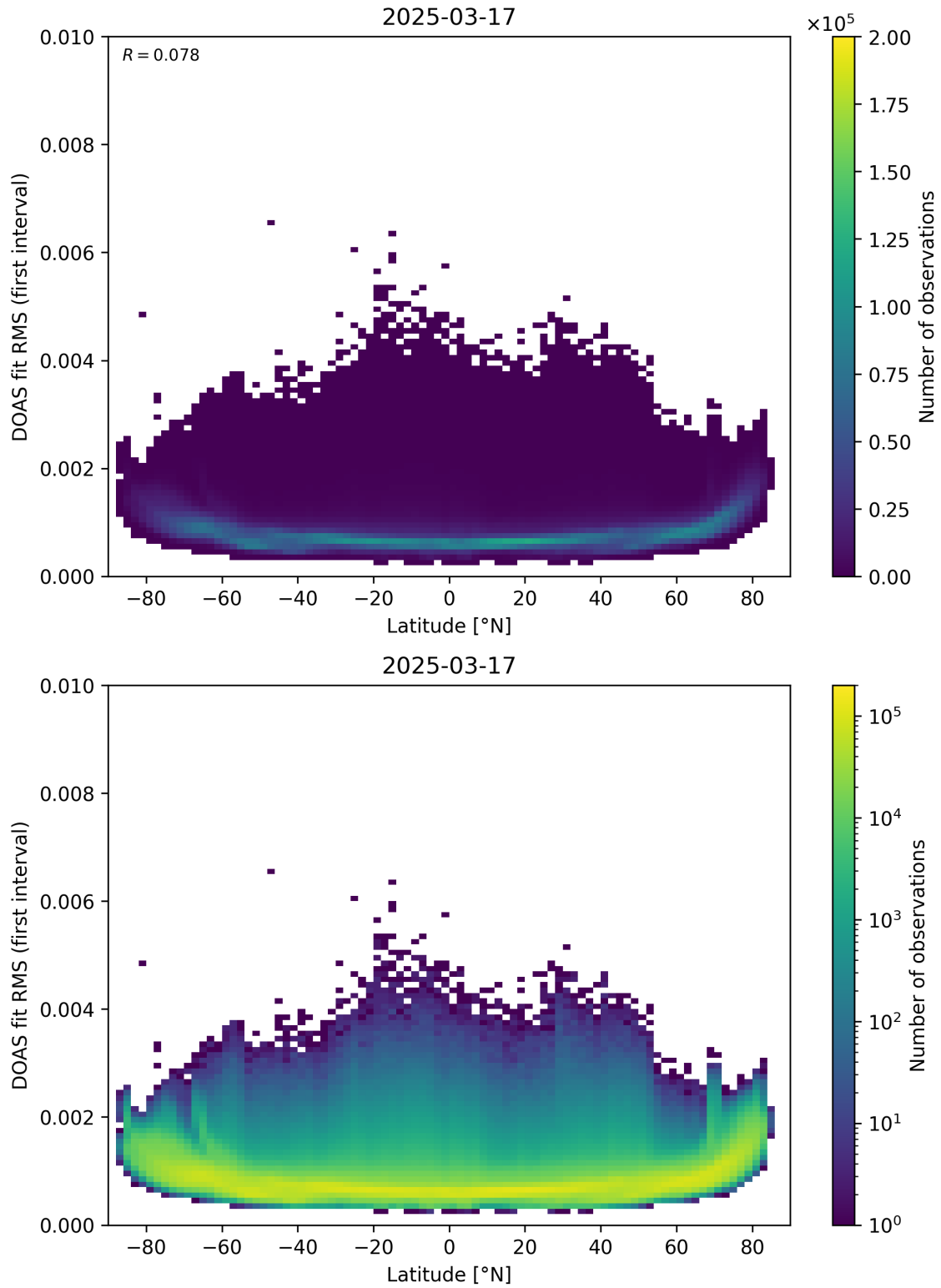
Figure 153: Scatter density plot of “Latitude” against “DOAS fit RMS (first interval)” for 2025-03-17 to 2025-03-18.
