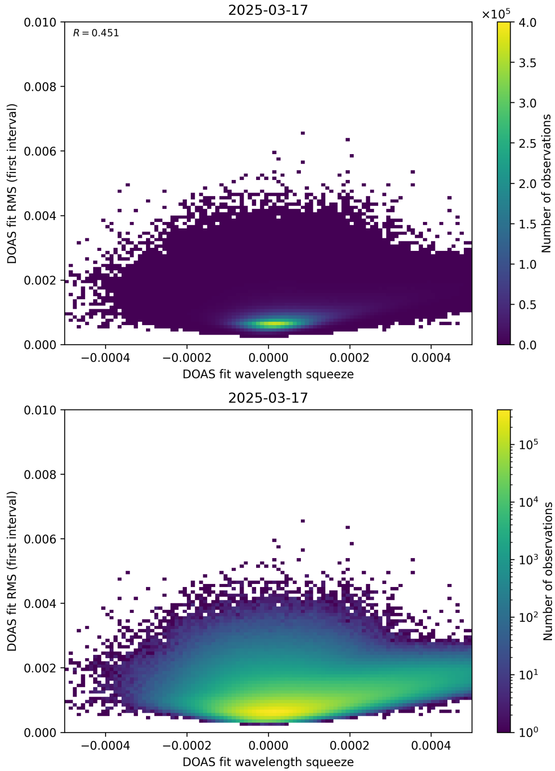
Figure 68: Scatter density plot of “DOAS fit wavelength squeeze” against “DOAS fit RMS (first interval)” for 2025-03-17 to 2025-03-18.
