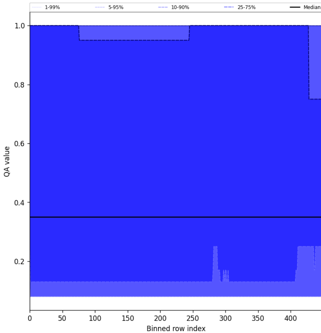
Figure 48: Along track statistics of “QA value” for 2025-03-17 to 2025-03-18
