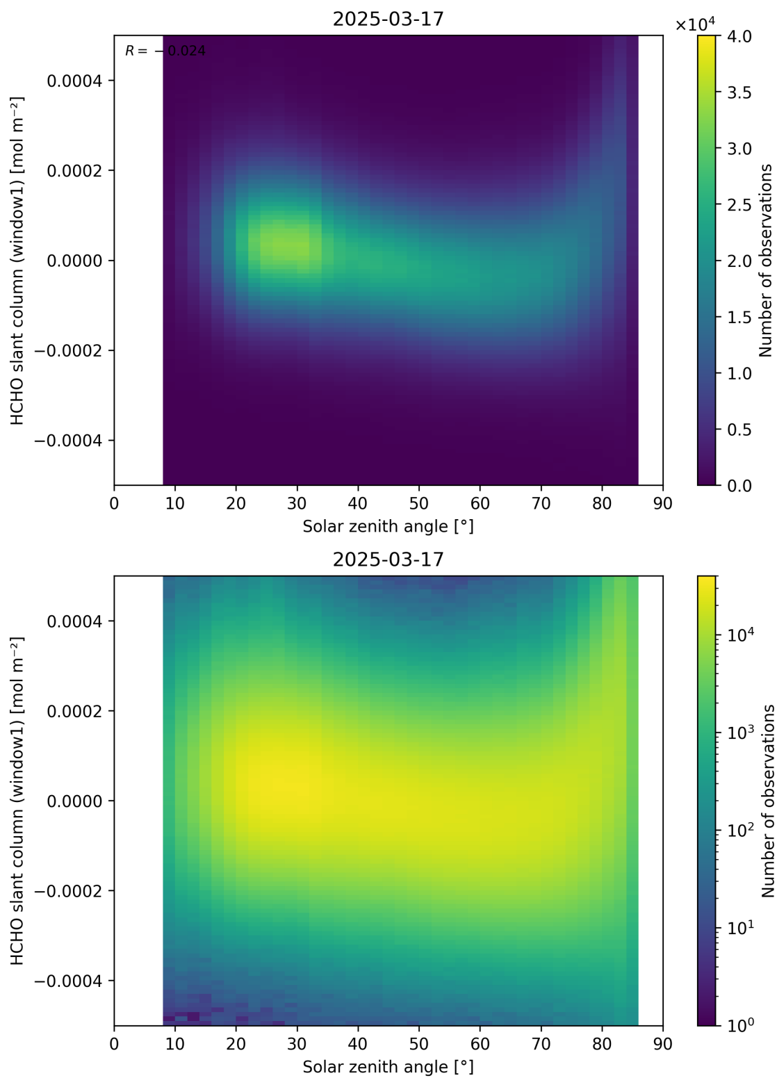
Figure 173: Scatter density plot of “Solar zenith angle” against “HCHO slant column (window1)” for 2025-03-17 to 2025-03-18.
