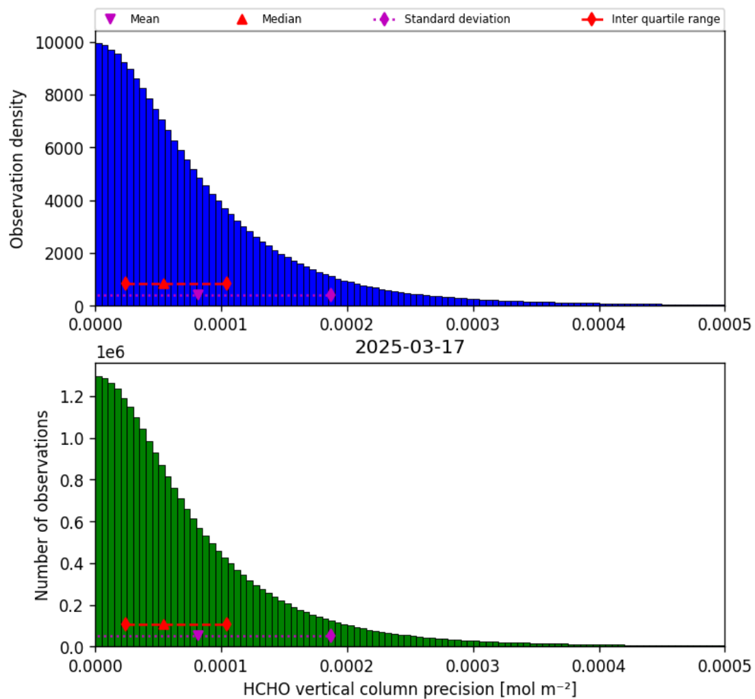
Figure 36: Histogram of “HCHO vertical column precision” for 2025-03-17 to 2025-03-18
