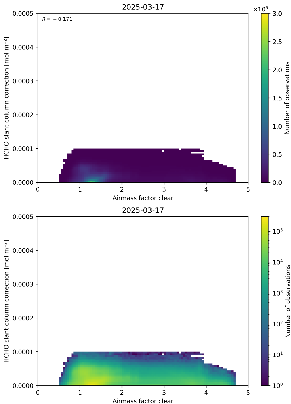
Figure 75: Scatter density plot of “Airmass factor clear” against “HCHO slant column correction” for 2025-03-17 to 2025-03-18.
