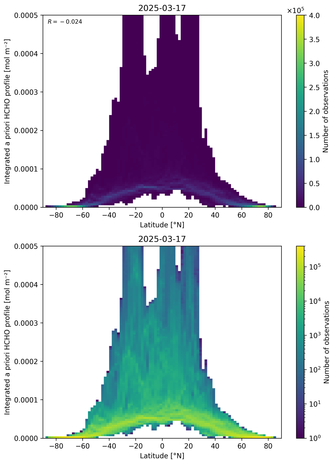
Figure 166: Scatter density plot of “Latitude” against “Integrated a priori HCHO profile” for 2025-03-17 to 2025-03-18.
