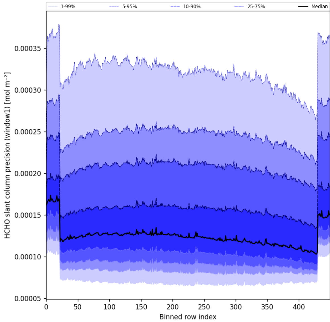
Figure 53: Along track statistics of “HCHO slant column precision (window1)” for 2025-03-17 to 2025-03-18
