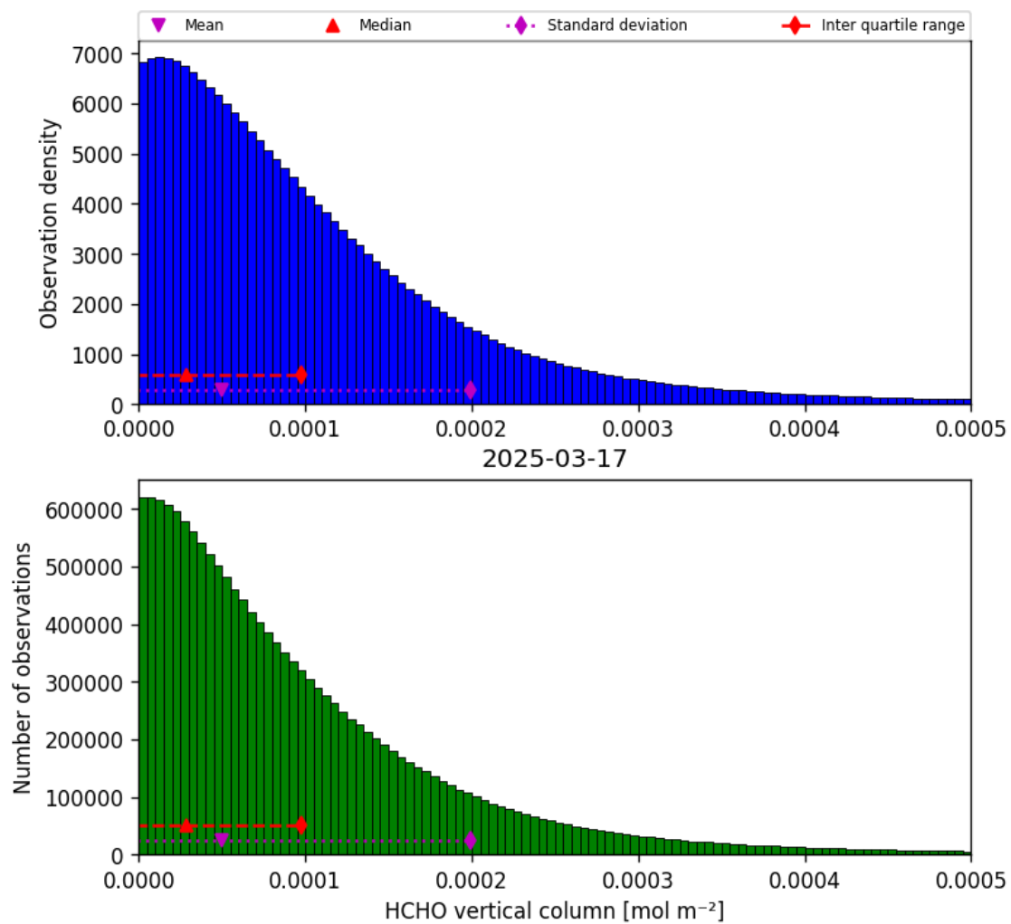
Figure 35: Histogram of “HCHO vertical column” for 2025-03-17 to 2025-03-18
