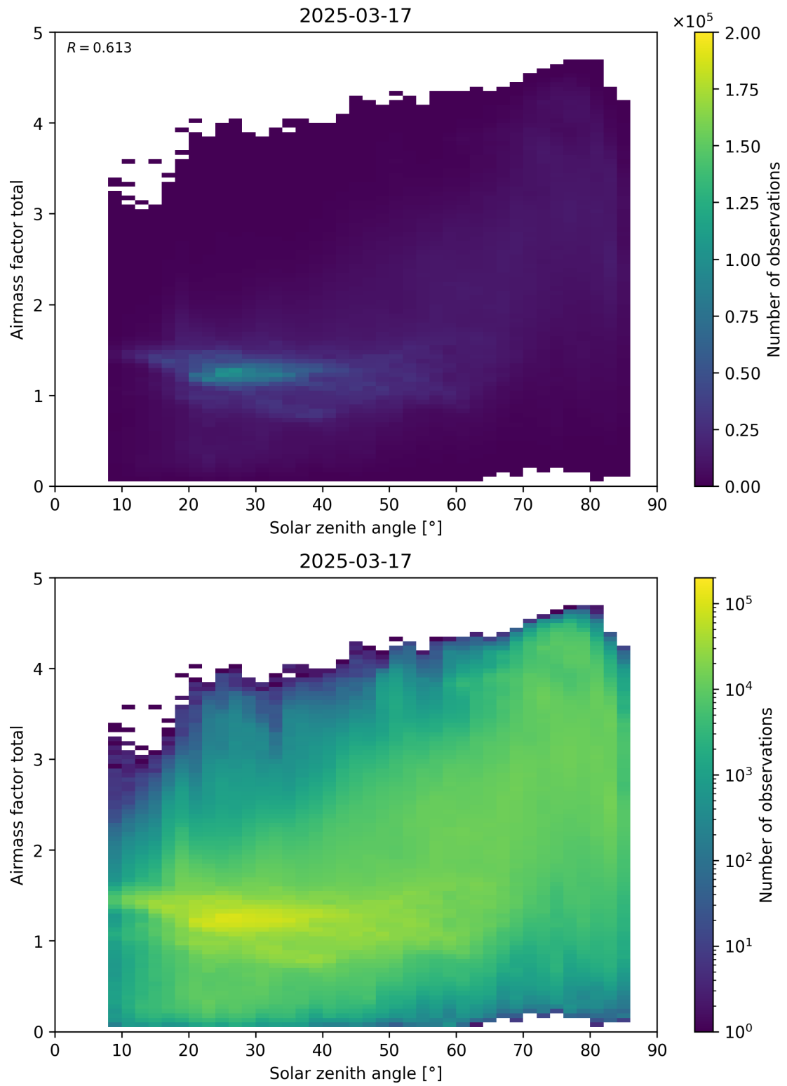
Figure 175: Scatter density plot of “Solar zenith angle” against “Airmass factor total” for 2025-03-17 to 2025-03-18.
