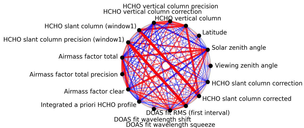
Figure 1: Map of correlation graph for 2025-03-17 to 2025-03-18.
