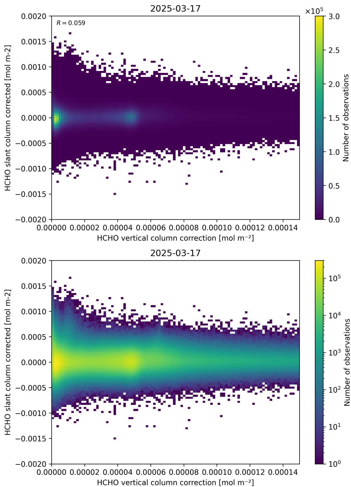
Figure 116: Scatter density plot of “HCHO vertical column correction” against “HCHO slant column corrected” for 2025-03-17 to 2025-03-18.
