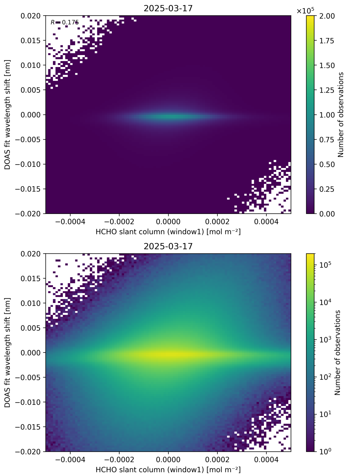
Figure 79: Scatter density plot of “HCHO slant column (window1)” against “DOAS fit wavelength shift” for 2025-03-17 to 2025-03-18.
