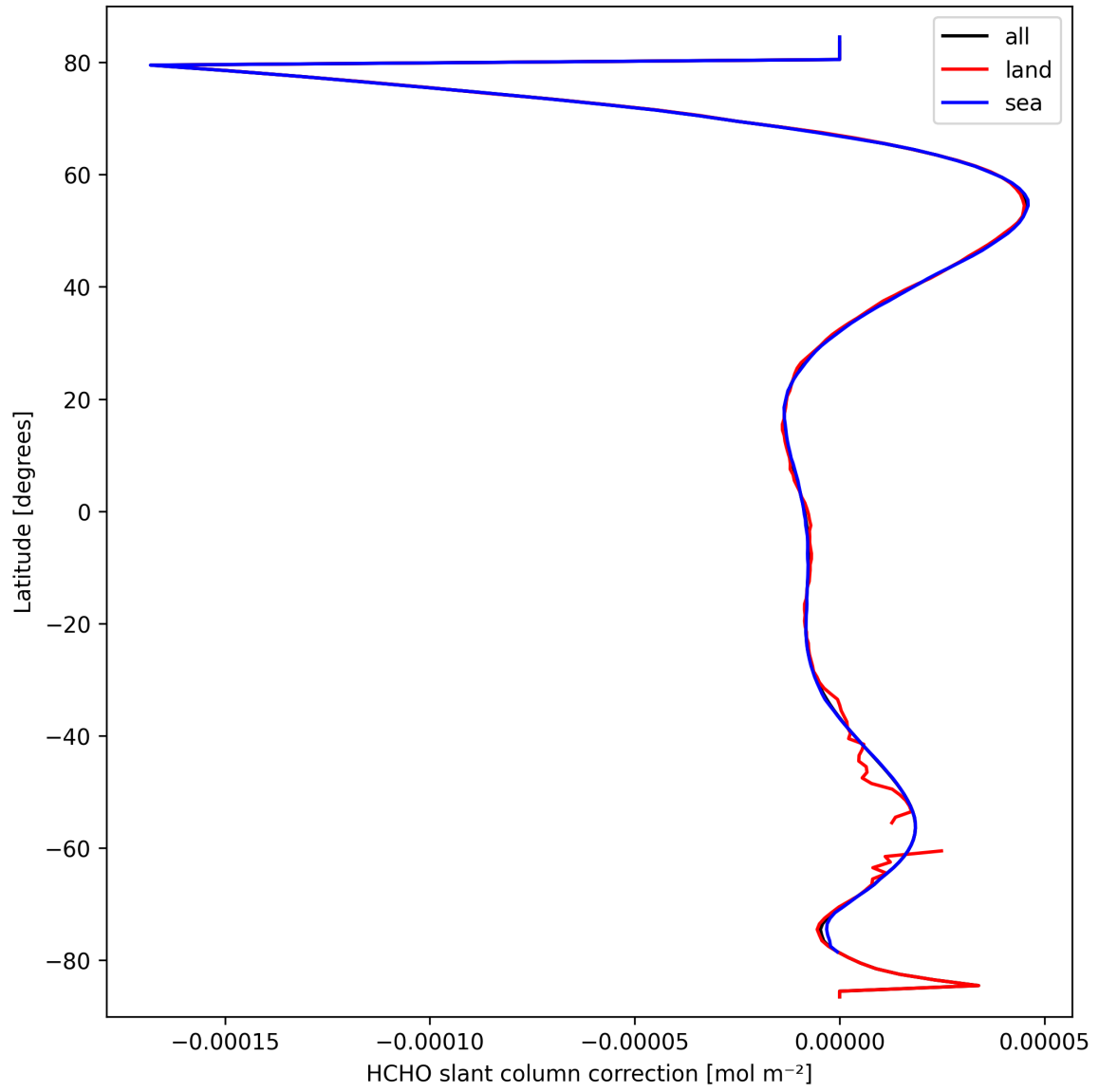
Figure 33: Zonal average of "HCHO slant column correction" for 2025-03-17 to 2025-03-18.
