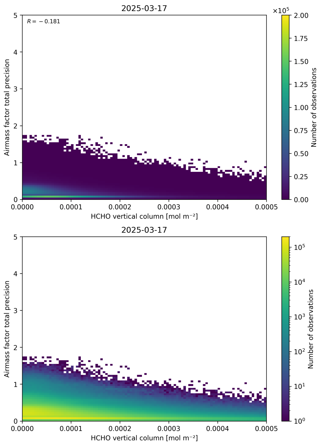
Figure 132: Scatter density plot of “HCHO vertical column” against “Airmass factor total precision” for 2025-03-17 to 2025-03-18.
