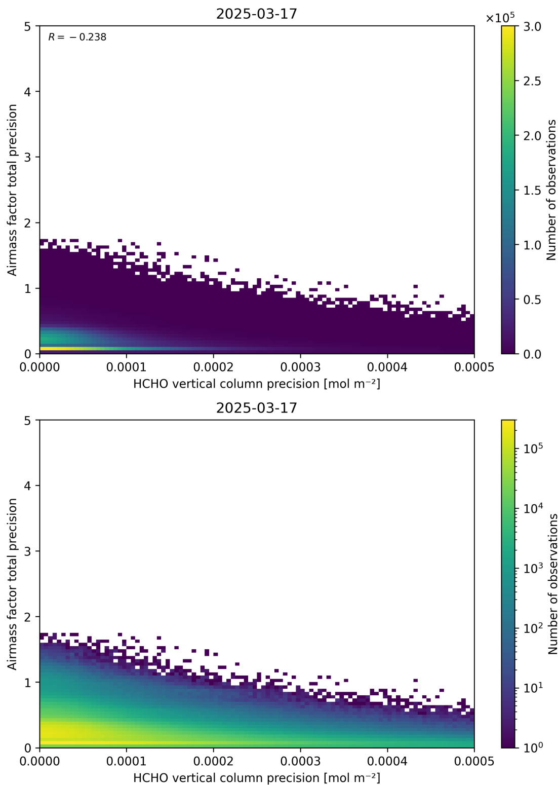
Figure 145: Scatter density plot of “HCHO vertical column precision” against “Airmass factor total precision” for 2025-03-17 to 2025-03-18.
