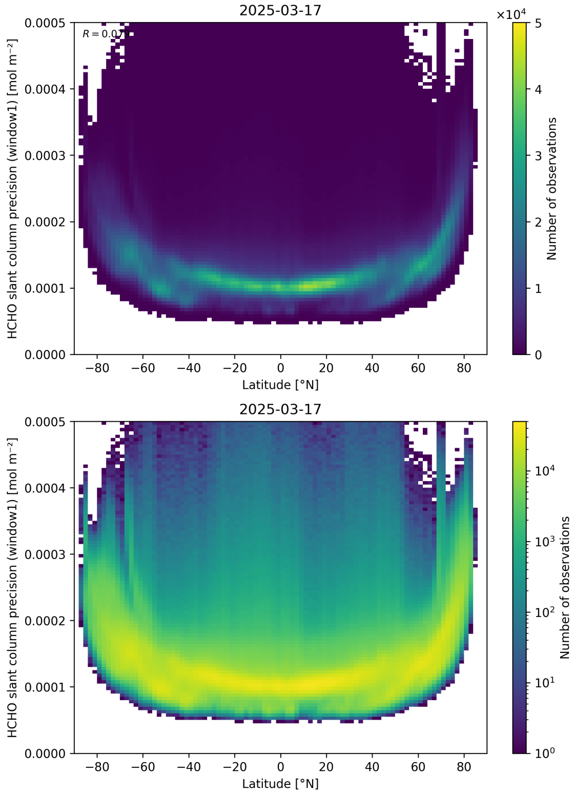
Figure 160: Scatter density plot of “Latitude” against “HCHO slant column precision (window1)” for 2025-03-17 to 2025-03-18.
