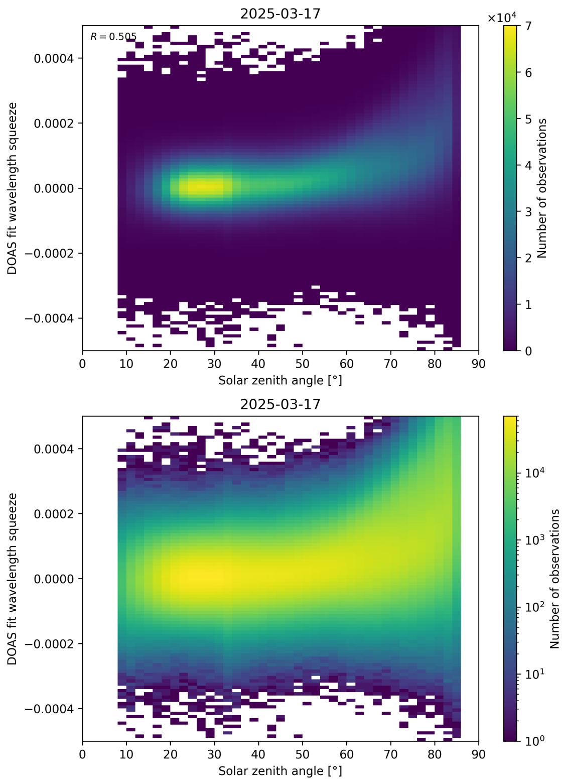
Figure 169: Scatter density plot of “Solar zenith angle” against “DOAS fit wavelength squeeze” for 2025-03-17 to 2025-03-18.
