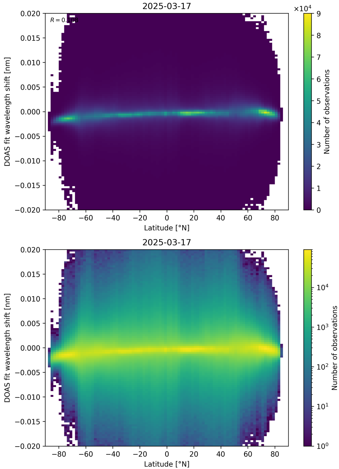
Figure 154: Scatter density plot of “Latitude” against “DOAS fit wavelength shift” for 2025-03-17 to 2025-03-18.
