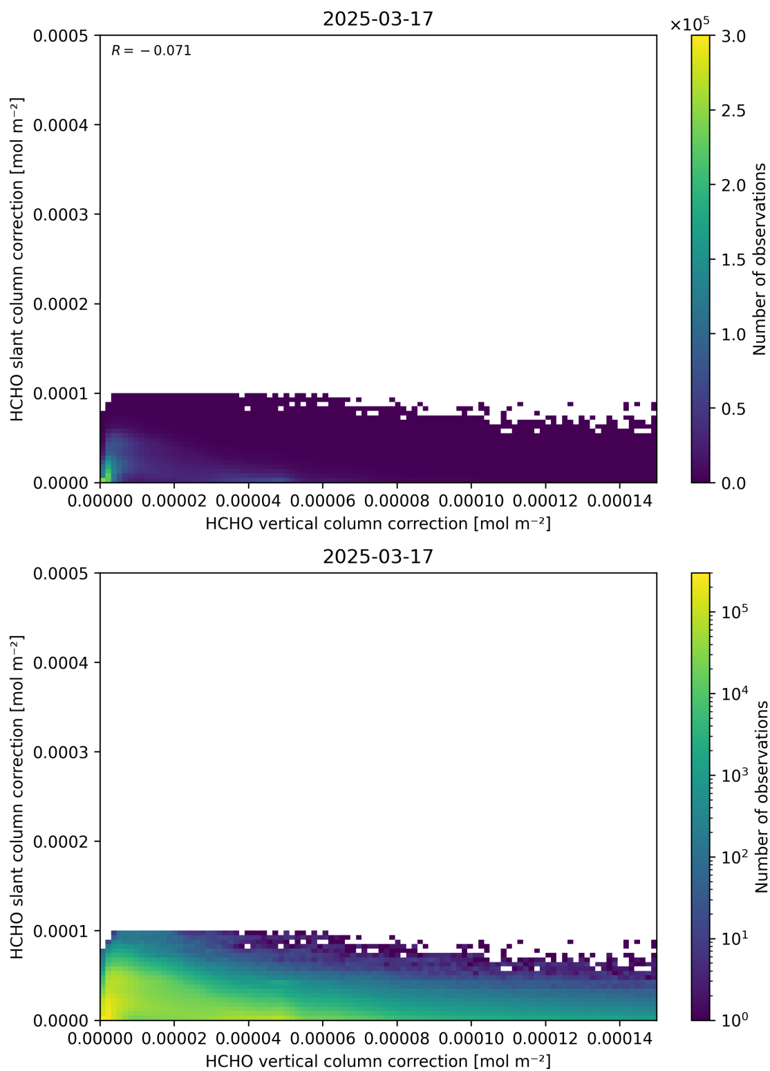
Figure 117: Scatter density plot of “HCHO vertical column correction” against “HCHO slant column correction” for 2025-03-17 to 2025-03-18.
