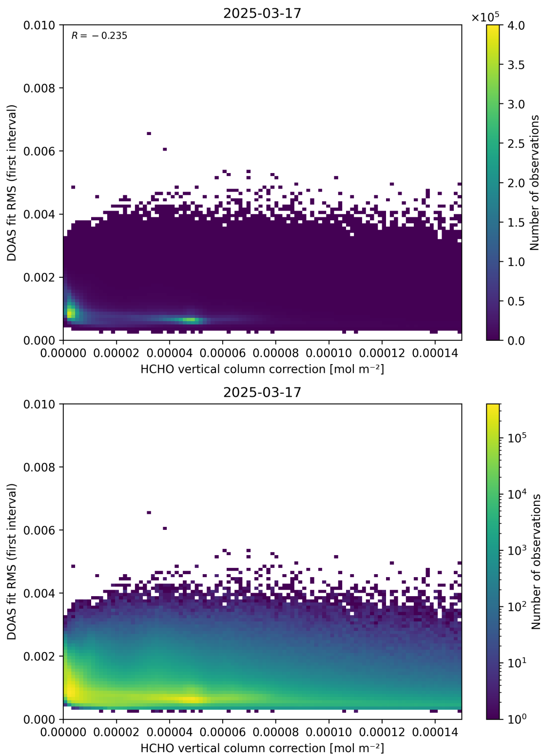
Figure 112: Scatter density plot of “HCHO vertical column correction” against “DOAS fit RMS (first interval)” for 2025-03-17 to 2025-03-18.
