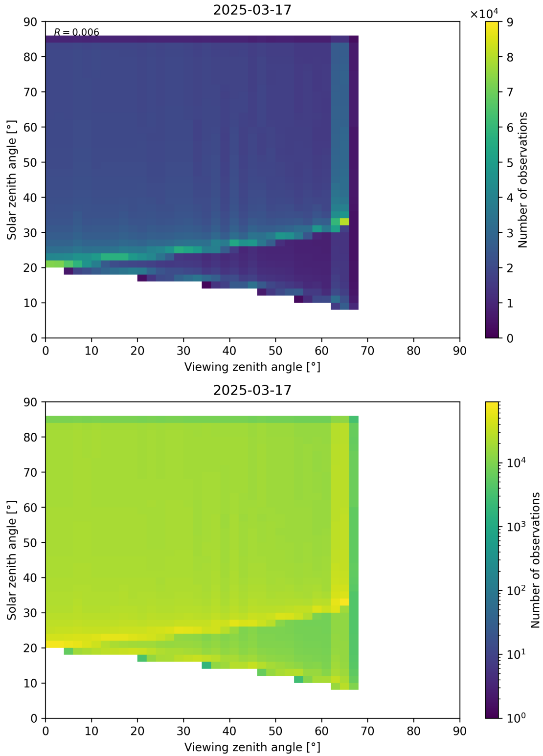
Figure 197: Scatter density plot of “Viewing zenith angle” against “Solar zenith angle” for 2025-03-17 to 2025-03-18.
