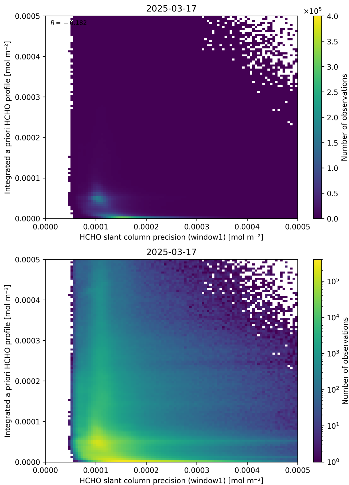
Figure 96: Scatter density plot of “HCHO slant column precision (window1)” against “Integrated a priori HCHO profile” for 2025-03-17 to 2025-03-18.
