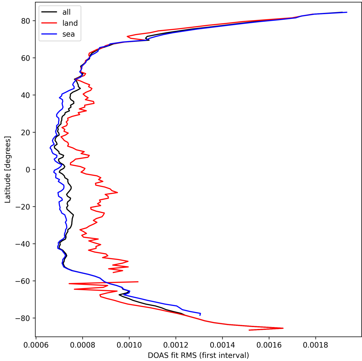
Figure 32: Zonal average of “DOAS fit RMS (first interval)” for 2025-03-17 to 2025-03-18.
