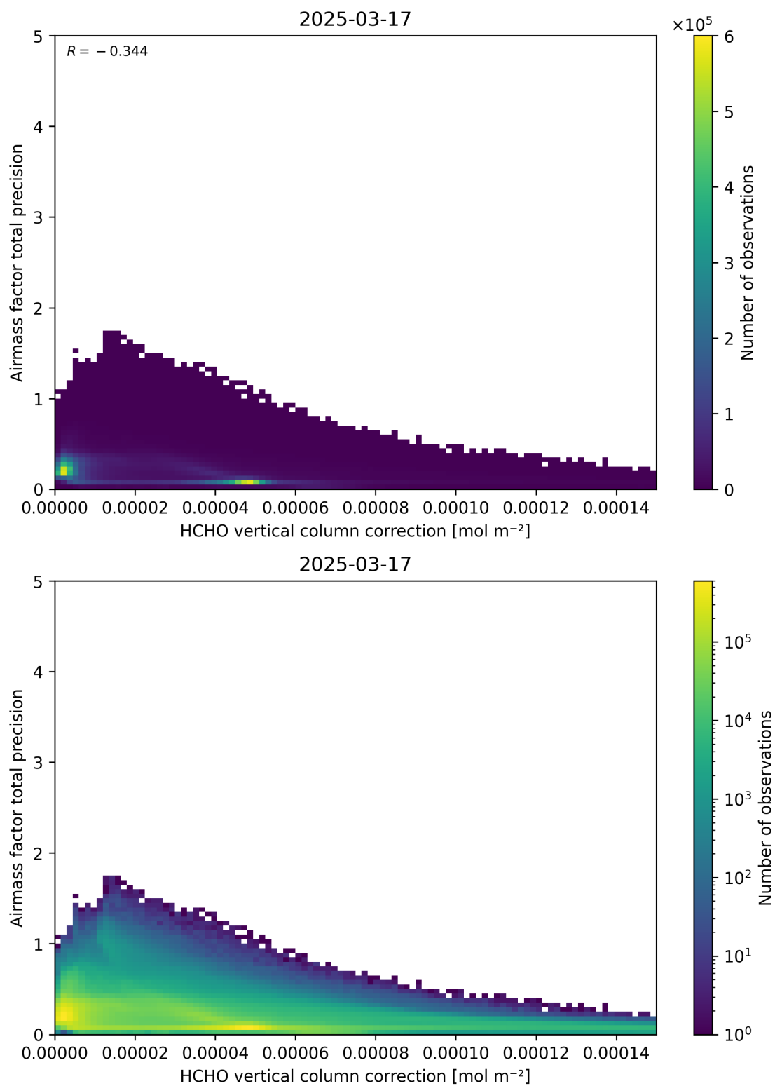
Figure 121: Scatter density plot of “HCHO vertical column correction” against “Airmass factor total precision” for 2025-03-17 to 2025-03-18.
