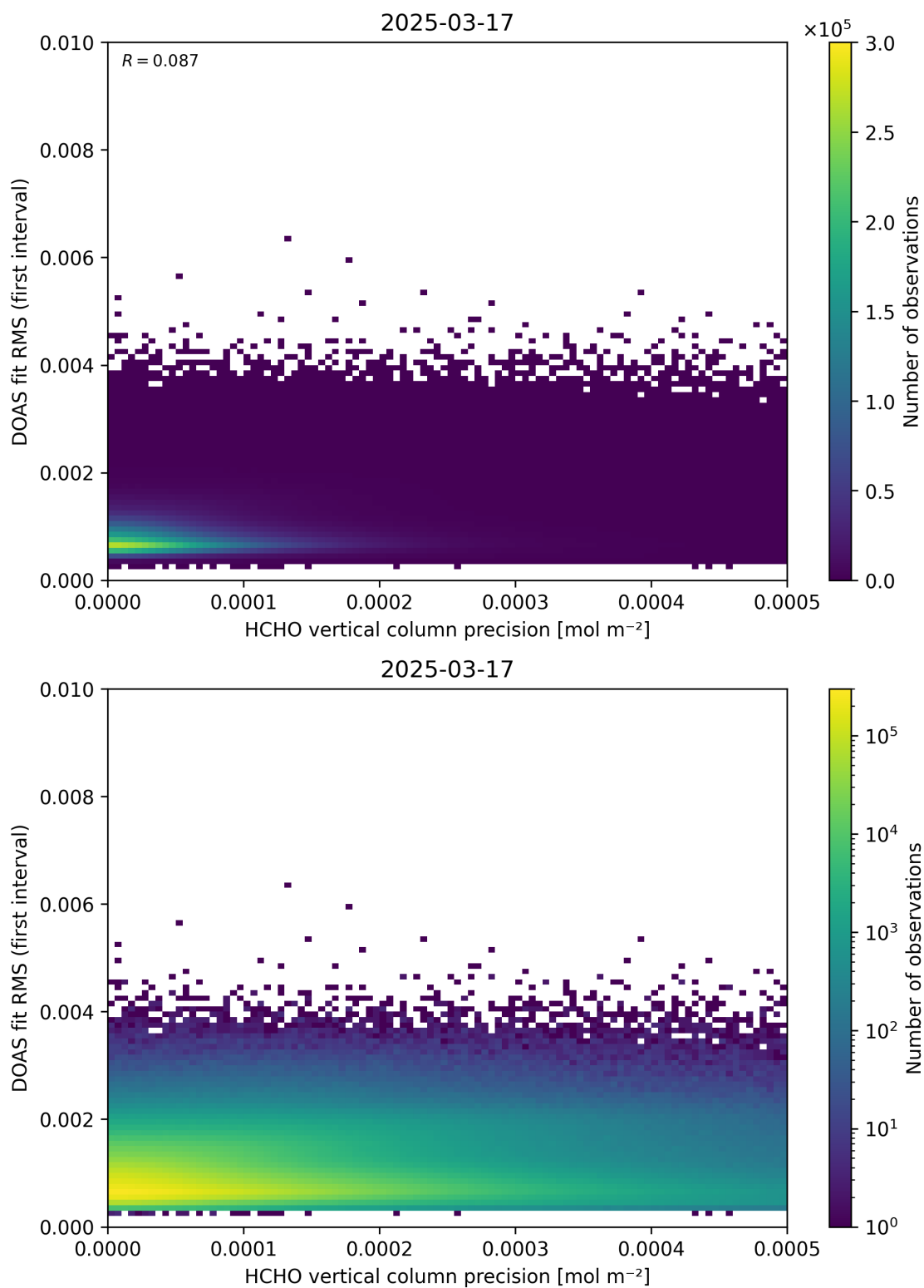
Figure 136: Scatter density plot of “HCHO vertical column precision” against “DOAS fit RMS (first interval)” for 2025-03-17 to 2025-03-18.
