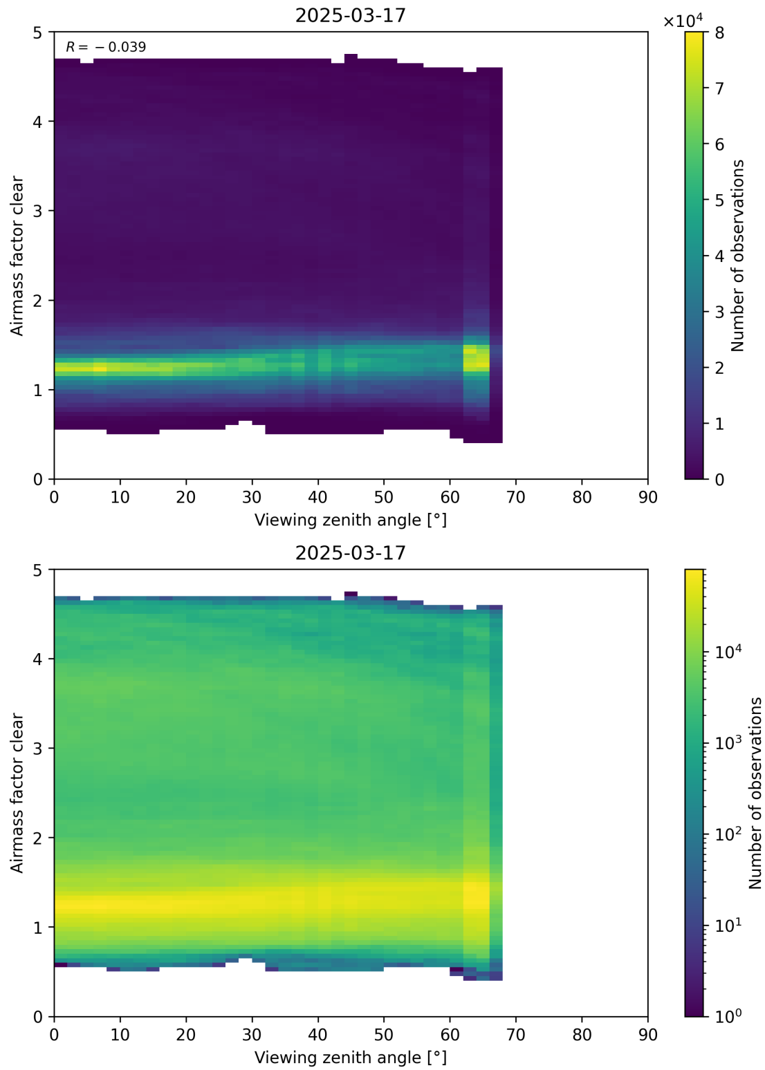
Figure 185: Scatter density plot of “Viewing zenith angle” against “Airmass factor clear” for 2025-03-17 to 2025-03-18.
