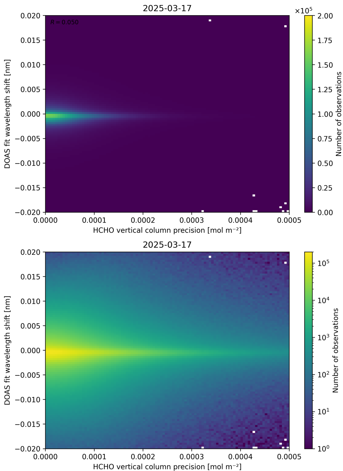
Figure 137: Scatter density plot of “HCHO vertical column precision” against “DOAS fit wavelength shift” for 2025-03-17 to 2025-03-18.
