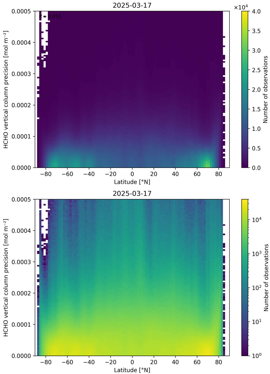
Figure 165: Scatter density plot of “Latitude” against “HCHO vertical column precision” for 2025-03-17 to 2025-03-18.
