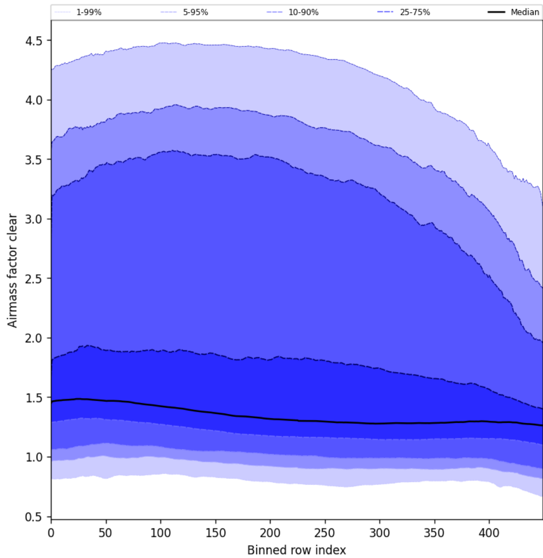
Figure 56: Along track statistics of “Airmass factor clear” for 2025-03-17 to 2025-03-18
