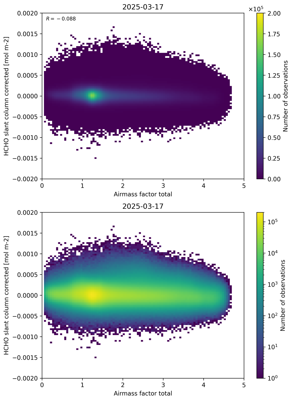
Figure 101: Scatter density plot of “Airmass factor total” against “HCHO slant column corrected” for 2025-03-17 to 2025-03-18.
