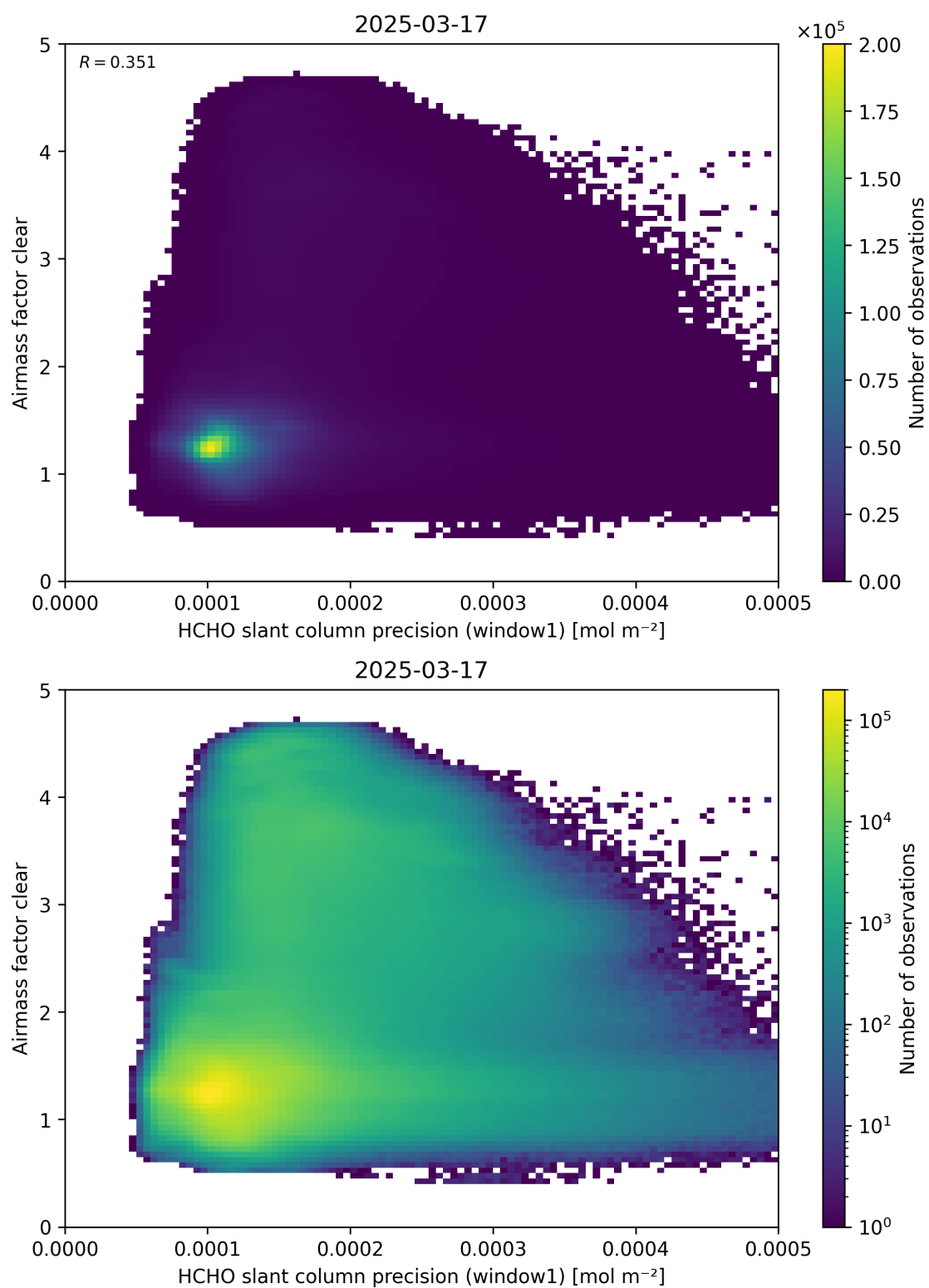
Figure 91: Scatter density plot of “HCHO slant column precision (window1)” against “Airmass factor clear” for 2025-03-17 to 2025-03-18.
