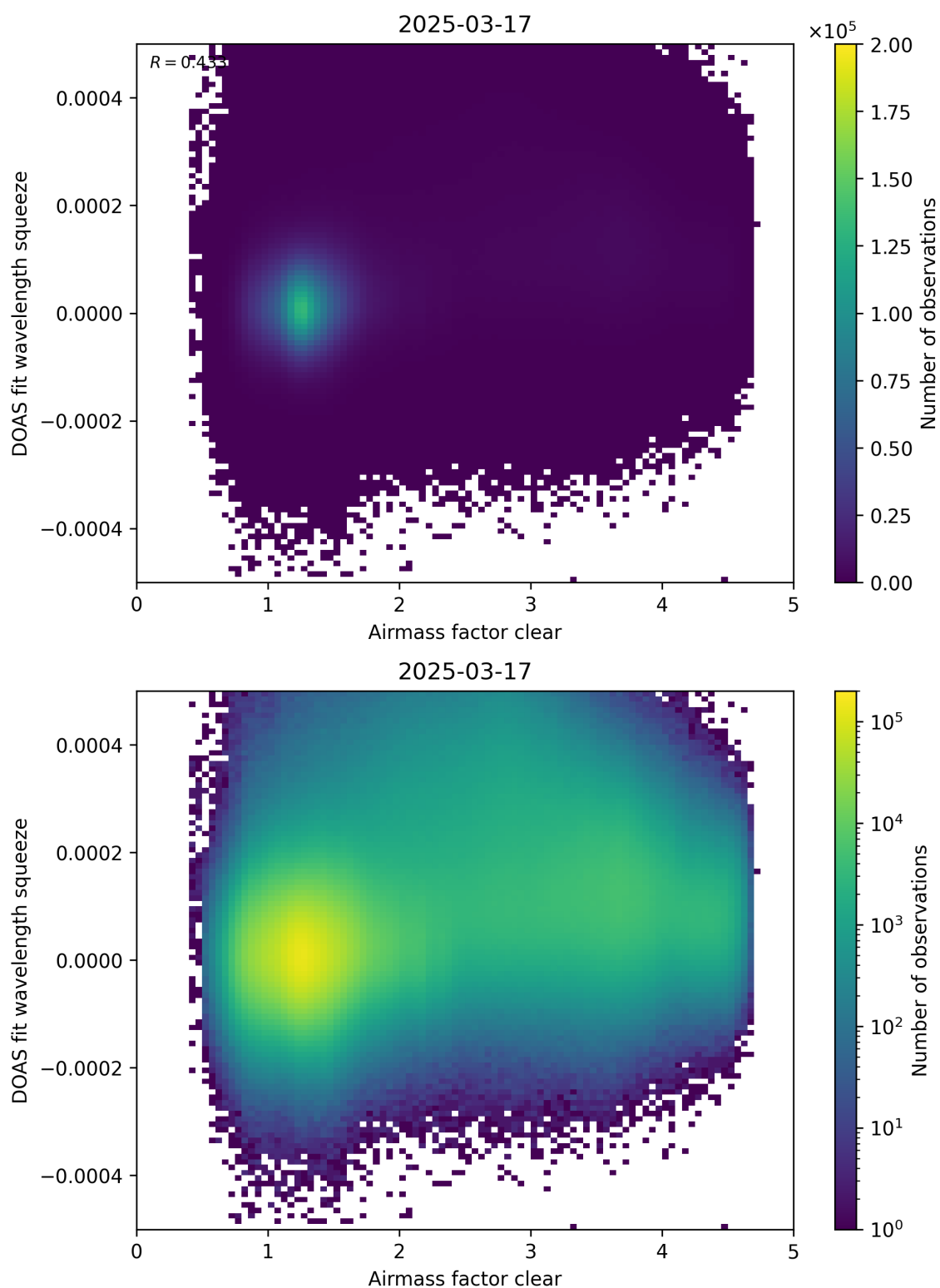
Figure 73: Scatter density plot of “Airmass factor clear” against “DOAS fit wavelength squeeze” for 2025-03-17 to 2025-03-18.
