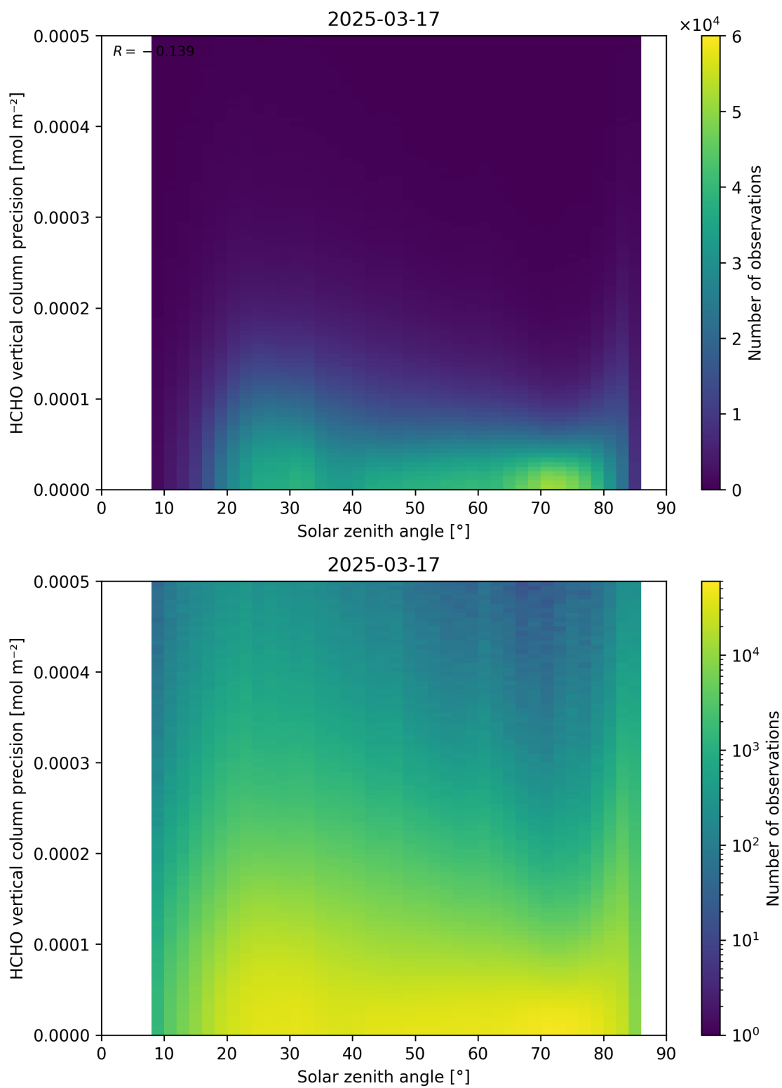
Figure 179: Scatter density plot of “Solar zenith angle” against “HCHO vertical column precision” for 2025-03-17 to 2025-03-18.
