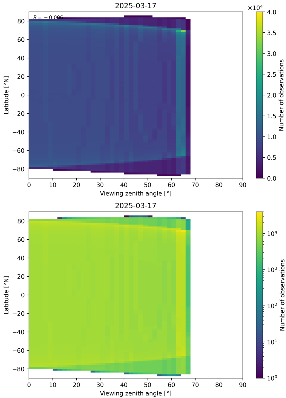
Figure 196: Scatter density plot of “Viewing zenith angle” against “Latitude” for 2025-03-17 to 2025-03-18.
