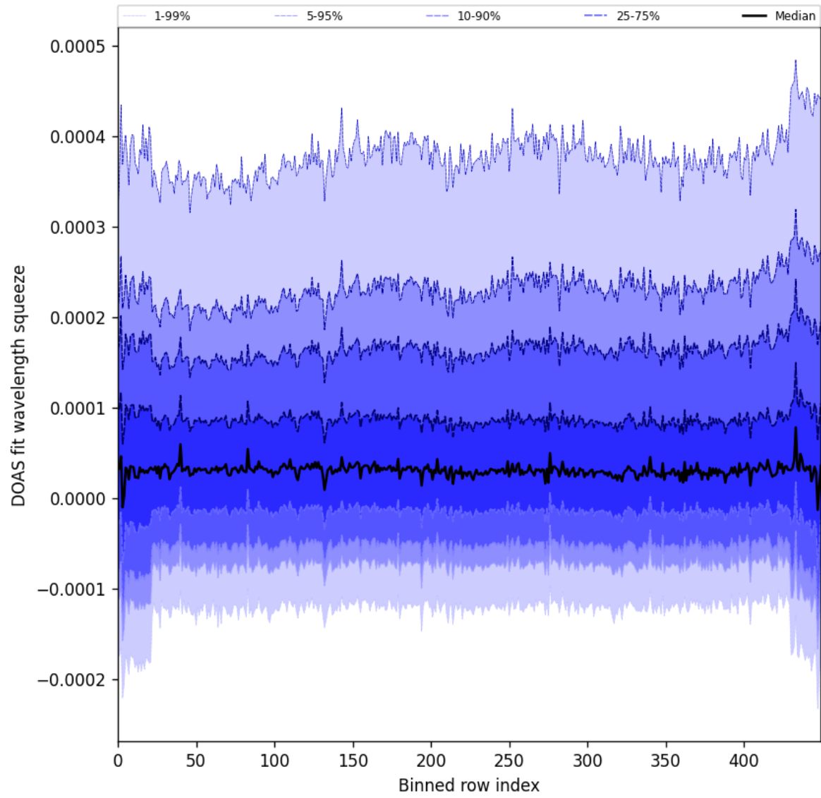
Figure 59: Along track statistics of “DOAS fit wavelength squeeze” for 2025-03-17 to 2025-03-18
