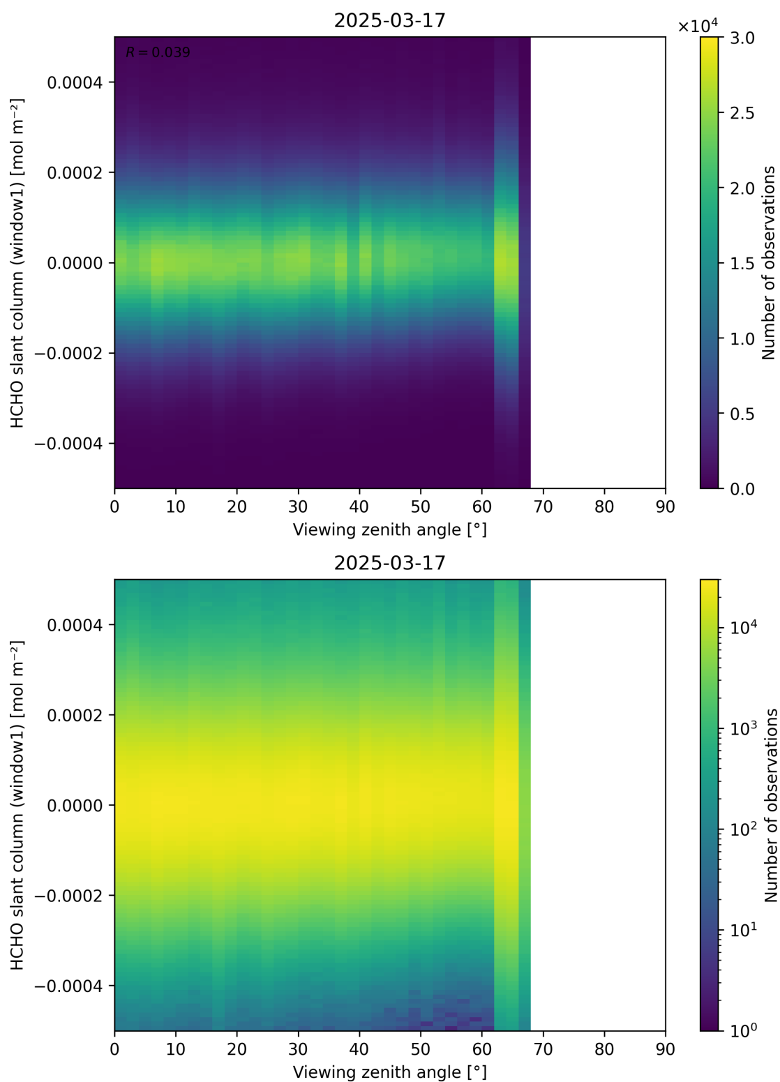
Figure 188: Scatter density plot of “Viewing zenith angle” against “HCHO slant column (window1)” for 2025-03-17 to 2025-03-18.
