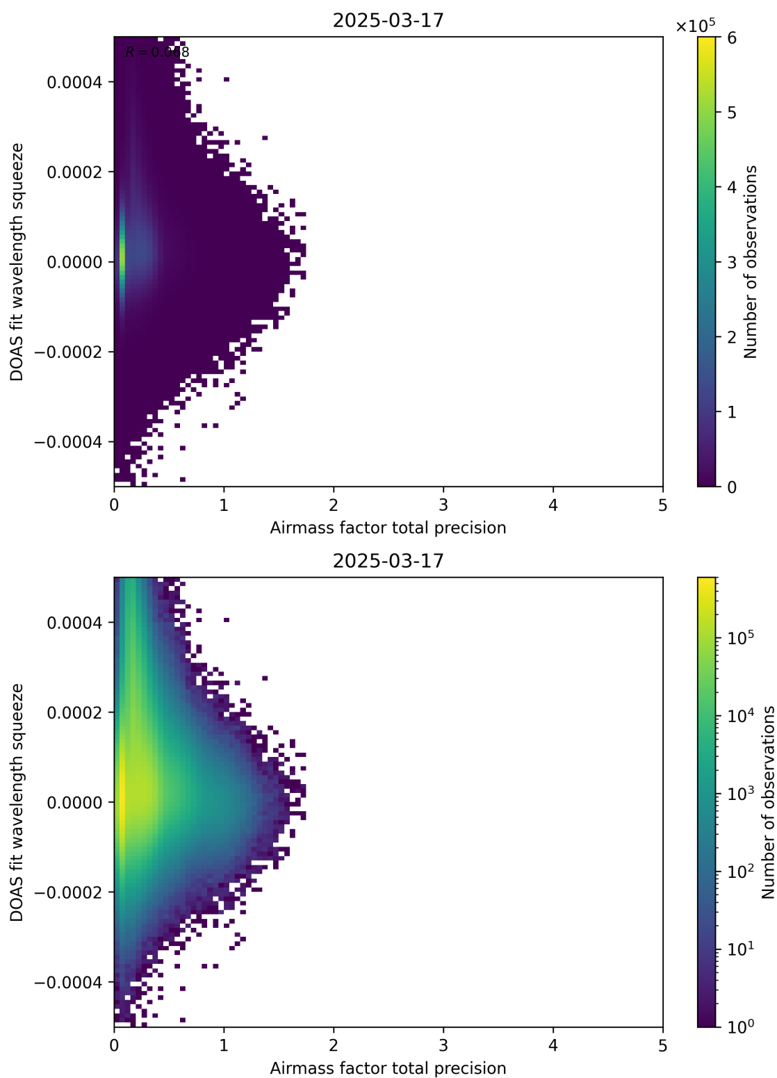
Figure 107: Scatter density plot of “Airmass factor total precision” against “DOAS fit wavelength squeeze” for 2025-03-17 to 2025-03-18.
