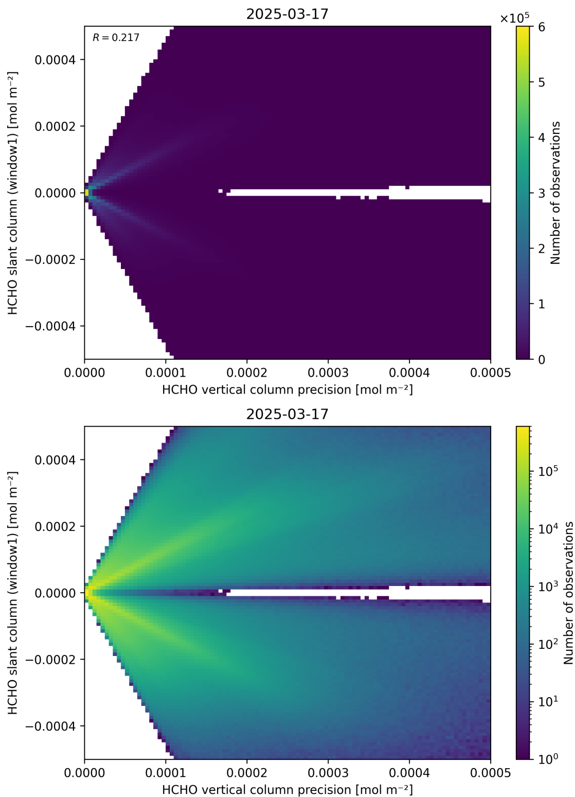
Figure 142: Scatter density plot of “HCHO vertical column precision” against “HCHO slant column (window1)” for 2025-03-17 to 2025-03-18.
