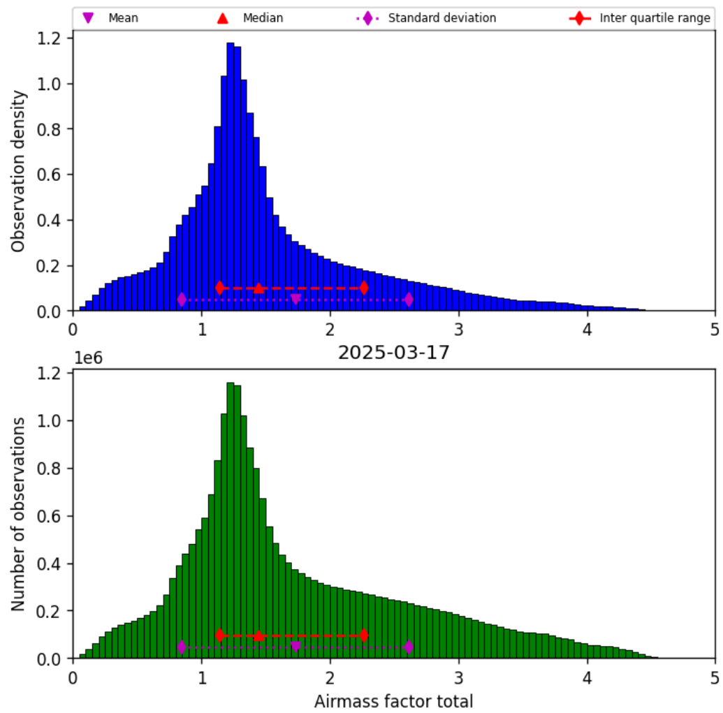
Figure 40: Histogram of “Airmass factor total” for 2025-03-17 to 2025-03-18
