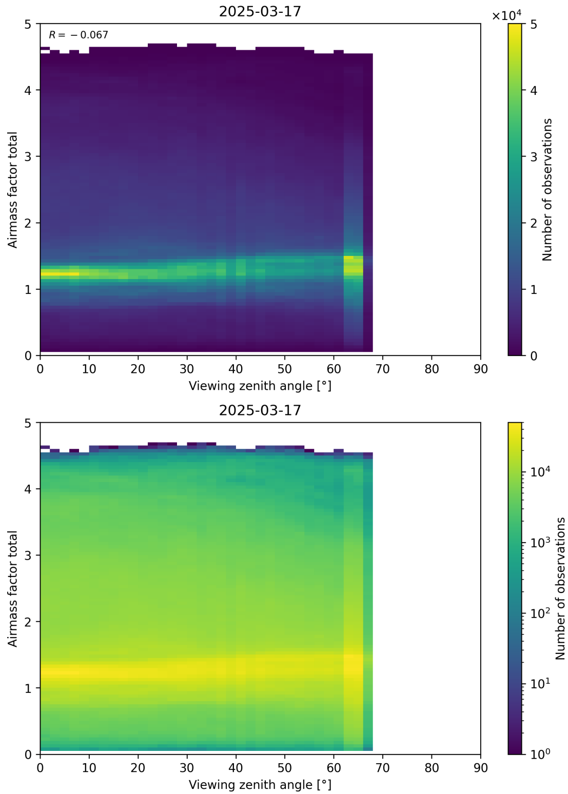
Figure 190: Scatter density plot of “Viewing zenith angle” against “Airmass factor total” for 2025-03-17 to 2025-03-18.
