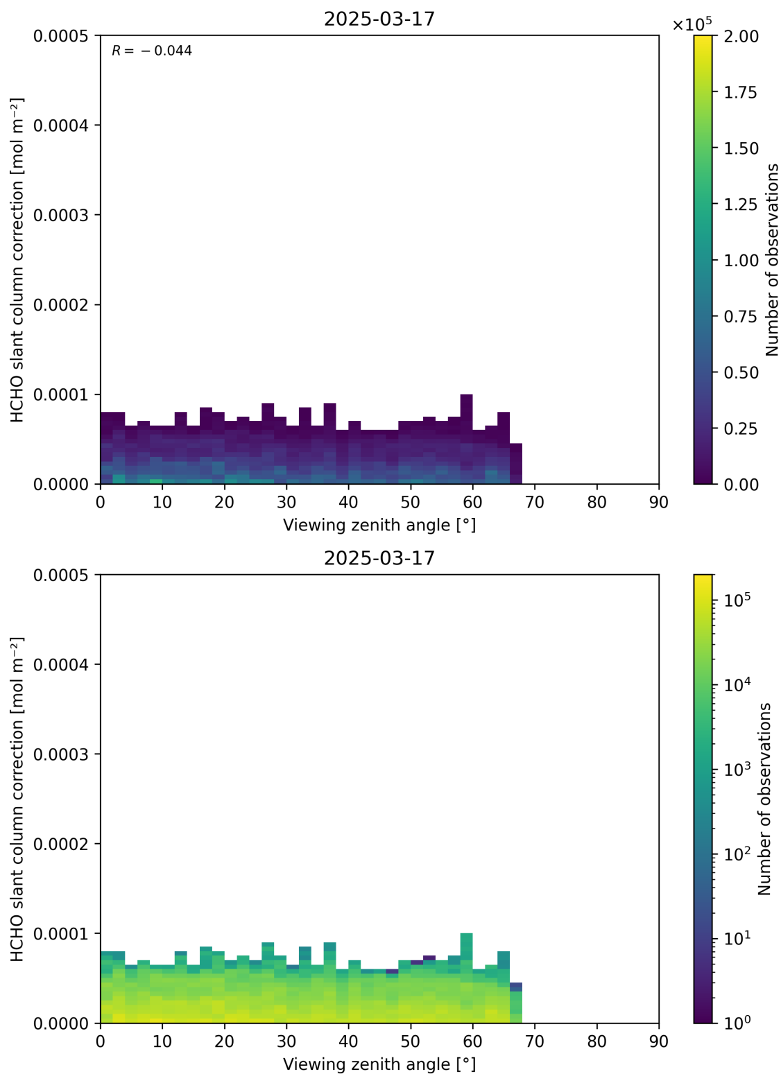
Figure 187: Scatter density plot of “Viewing zenith angle” against “HCHO slant column correction” for 2025-03-17 to 2025-03-18.
