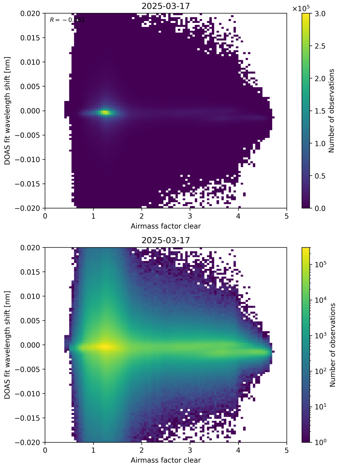
Figure 72: Scatter density plot of “Airmass factor clear” against “DOAS fit wavelength shift” for 2025-03-17 to 2025-03-18.
