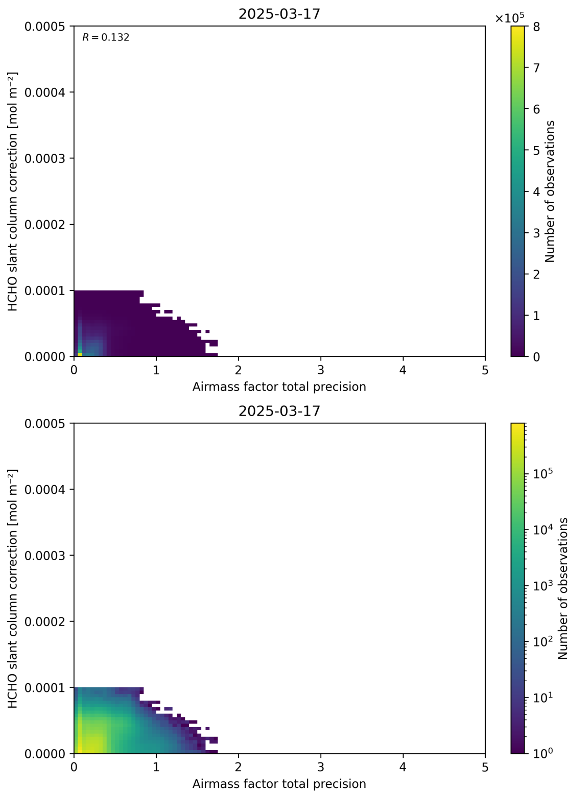
Figure 110: Scatter density plot of “Airmass factor total precision” against “HCHO slant column correction” for 2025-03-17 to 2025-03-18.
