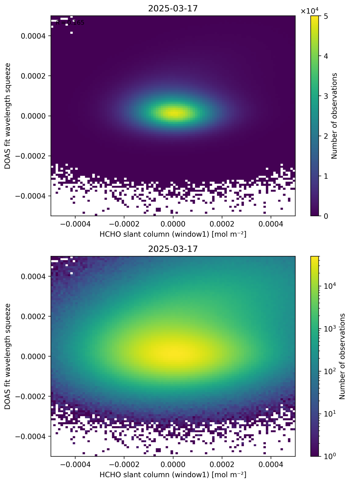
Figure 80: Scatter density plot of “HCHO slant column (window1)” against “DOAS fit wavelength squeeze” for 2025-03-17 to 2025-03-18.
