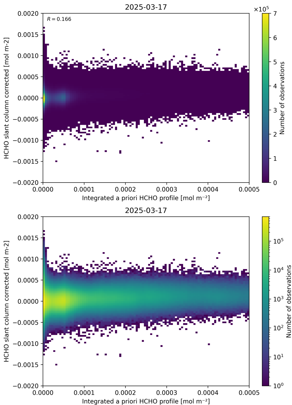
Figure 151: Scatter density plot of “Integrated a priori HCHO profile” against “HCHO slant column corrected” for 2025-03-17 to 2025-03-18.
