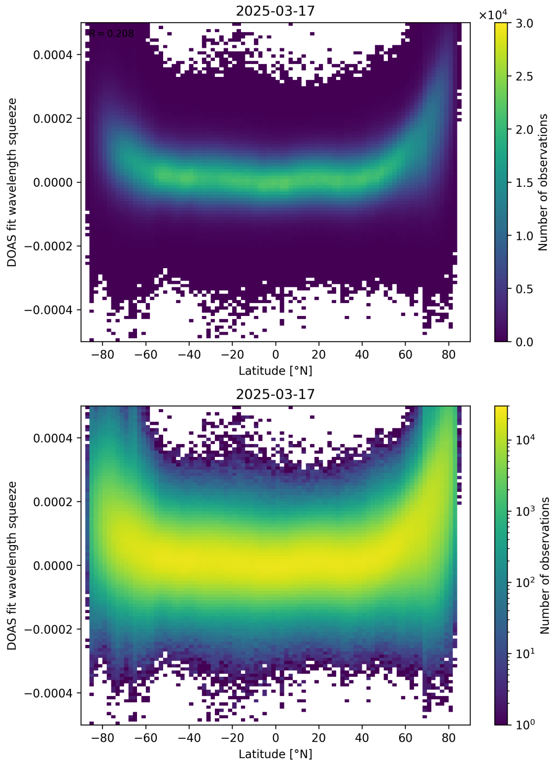
Figure 155: Scatter density plot of “Latitude” against “DOAS fit wavelength squeeze” for 2025-03-17 to 2025-03-18.
