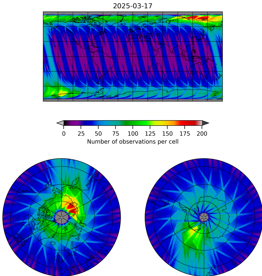
Figure 19: Map of the number of observations for 2025-03-17 to 2025-03-18
