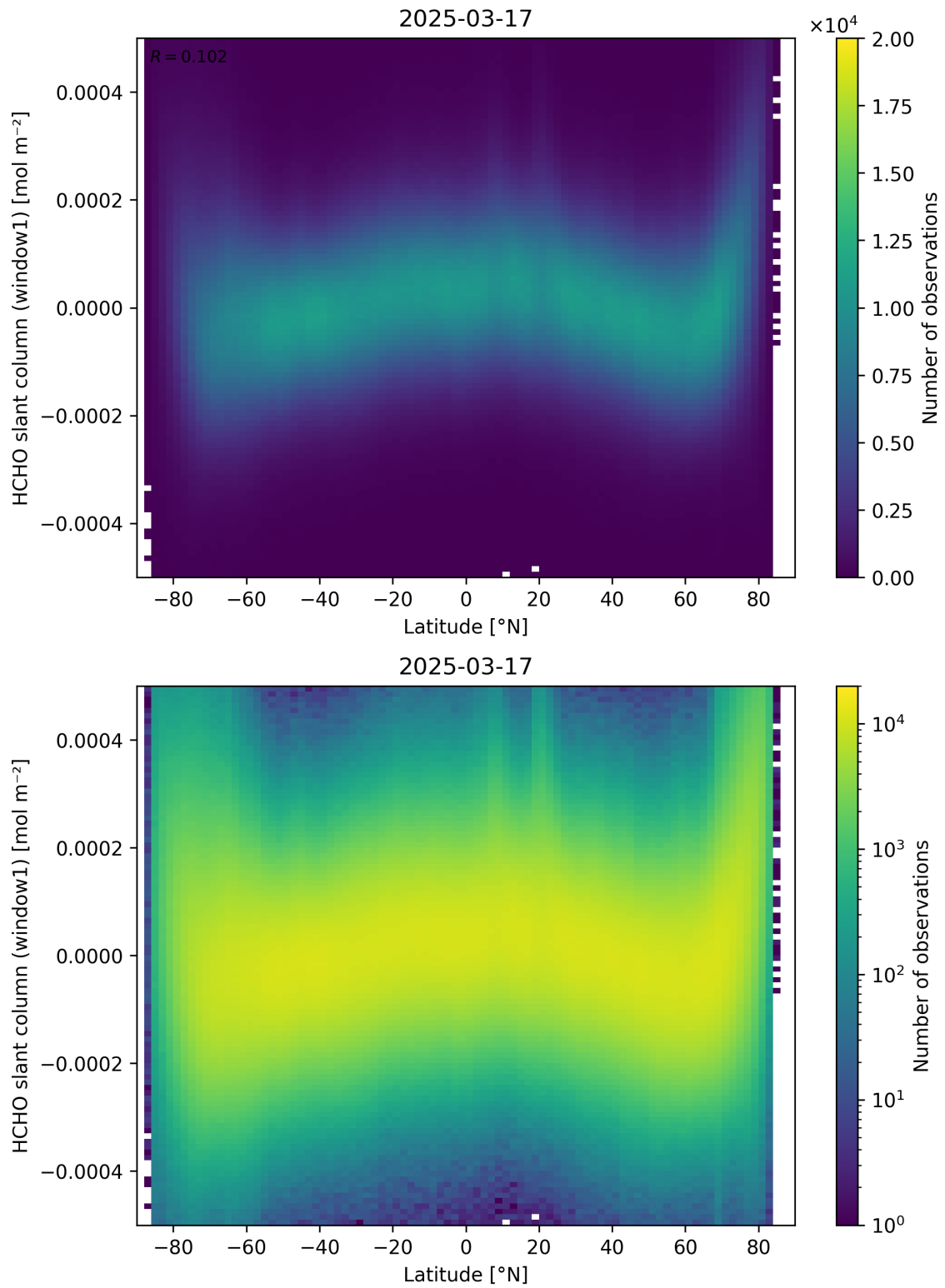
Figure 159: Scatter density plot of “Latitude” against “HCHO slant column (window1)” for 2025-03-17 to 2025-03-18.
