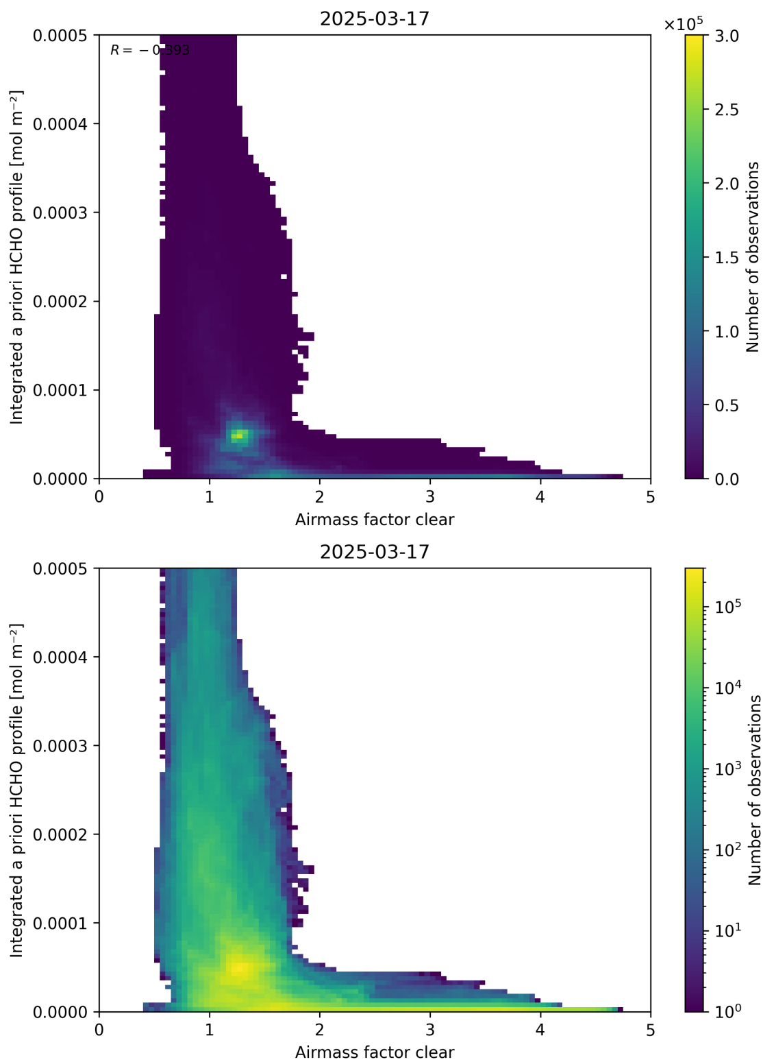
Figure 76: Scatter density plot of “Airmass factor clear” against “Integrated a priori HCHO profile” for 2025-03-17 to 2025-03-18.
