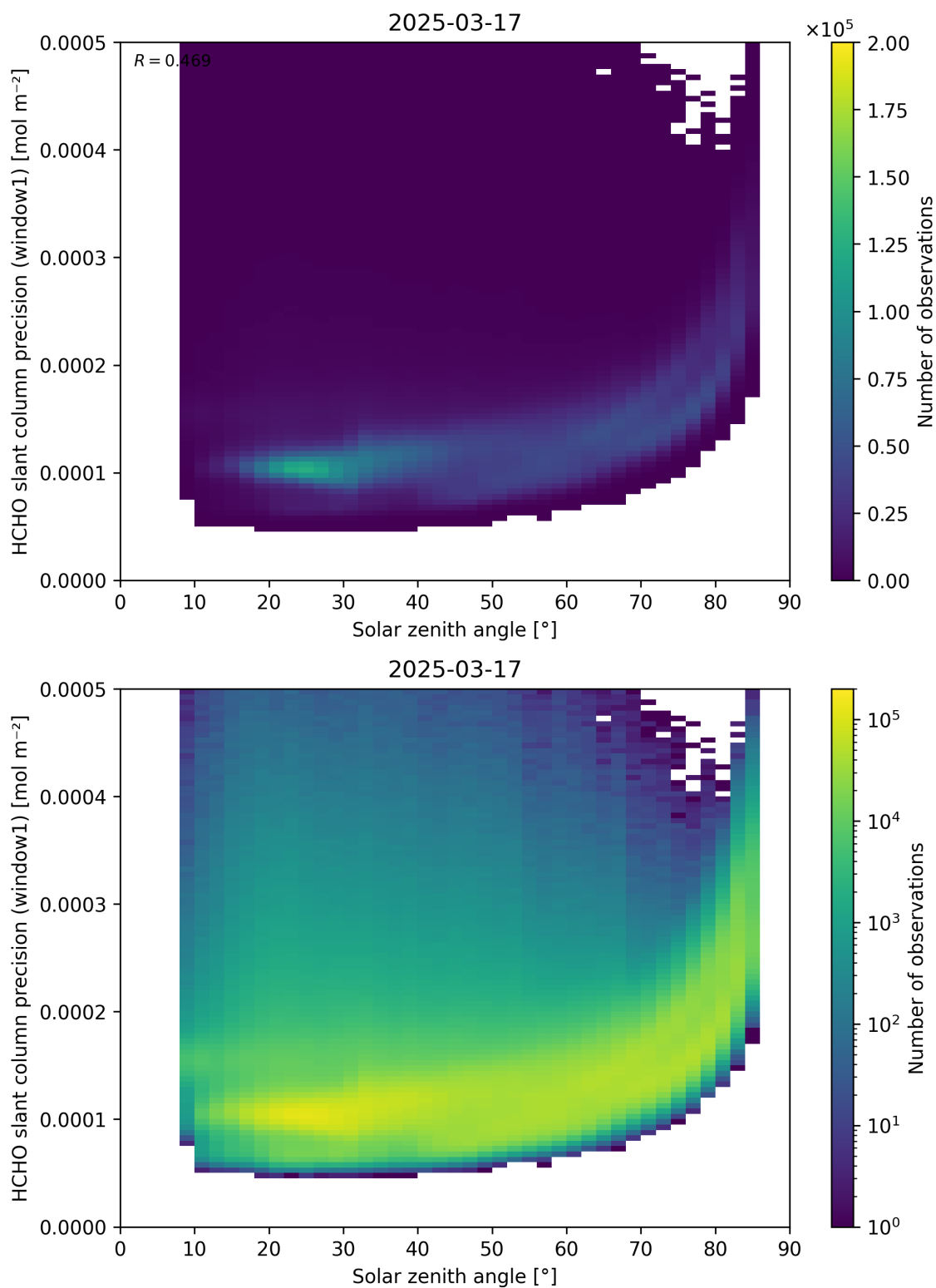
Figure 174: Scatter density plot of “Solar zenith angle” against “HCHO slant column precision (window1)” for 2025-03-17 to 2025-03-18.
