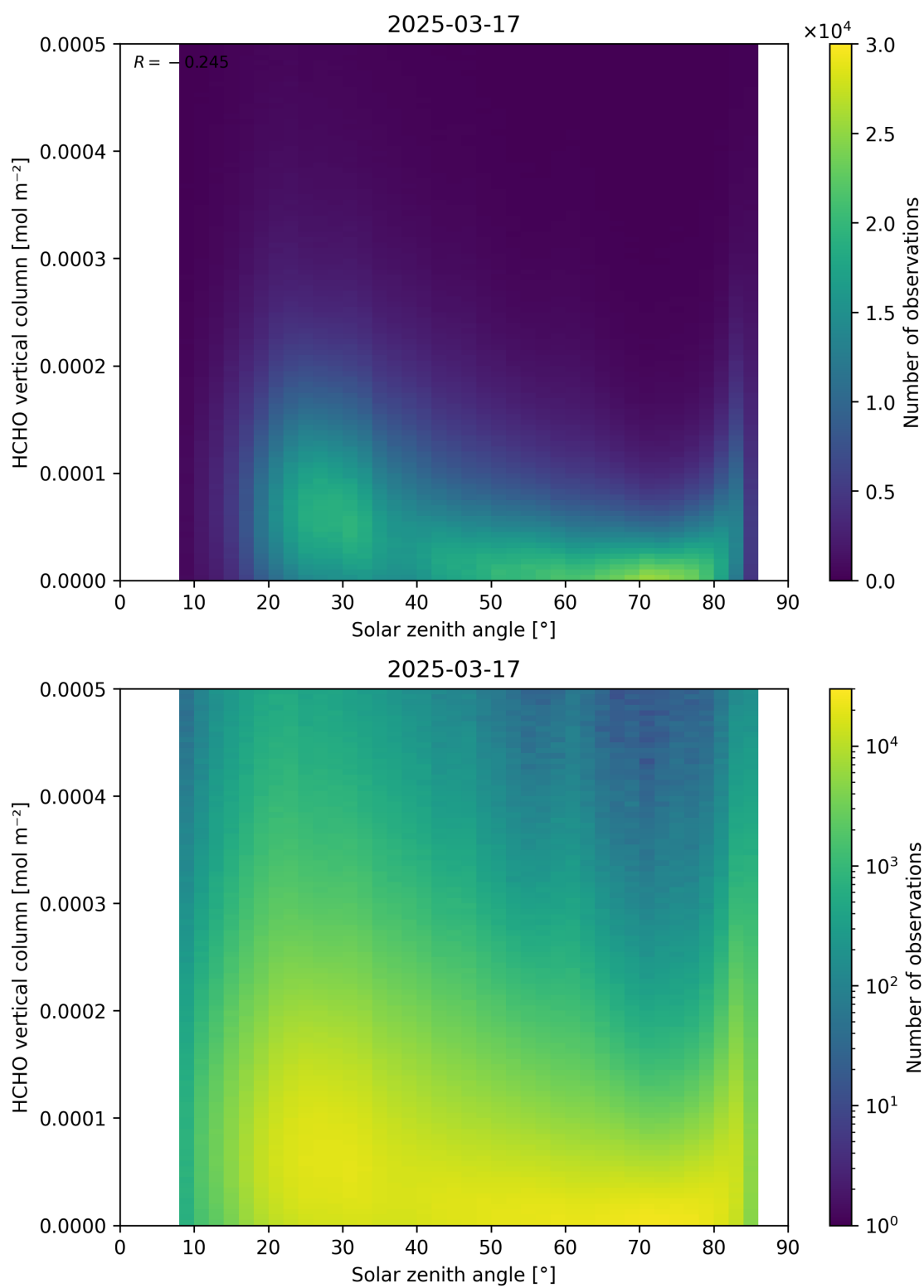
Figure 177: Scatter density plot of “Solar zenith angle” against “HCHO vertical column” for 2025-03-17 to 2025-03-18.
