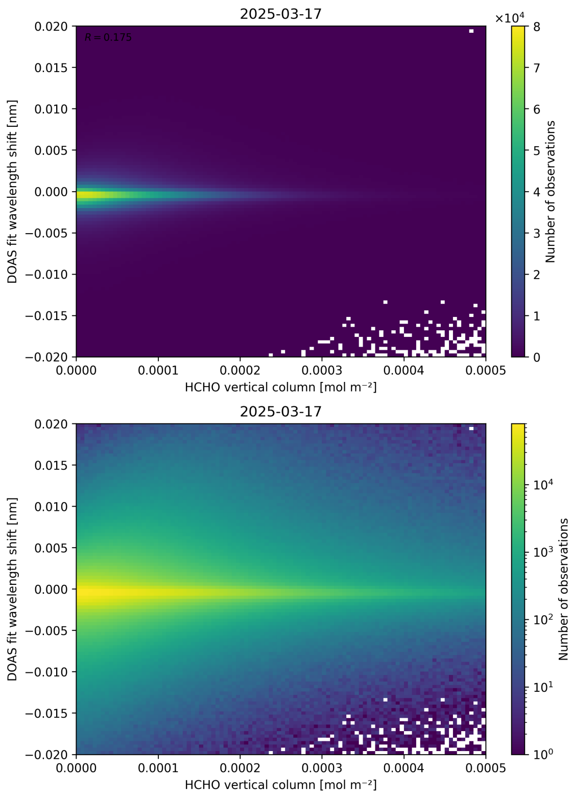
Figure 124: Scatter density plot of “HCHO vertical column” against “DOAS fit wavelength shift” for 2025-03-17 to 2025-03-18.
