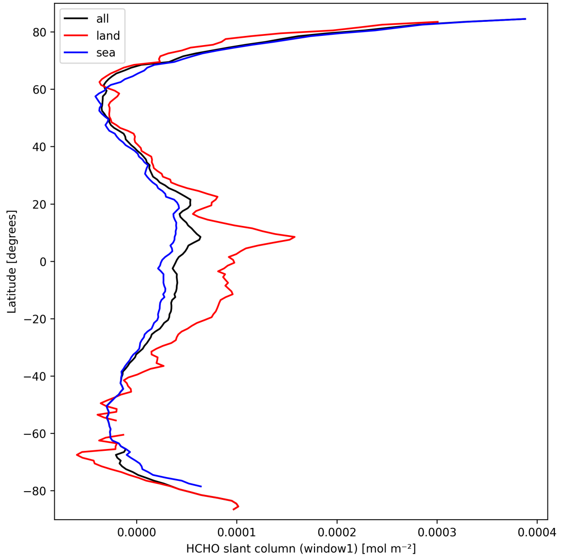
Figure 24: Zonal average of “HCHO slant column (window1)” for 2025-03-17 to 2025-03-18.
