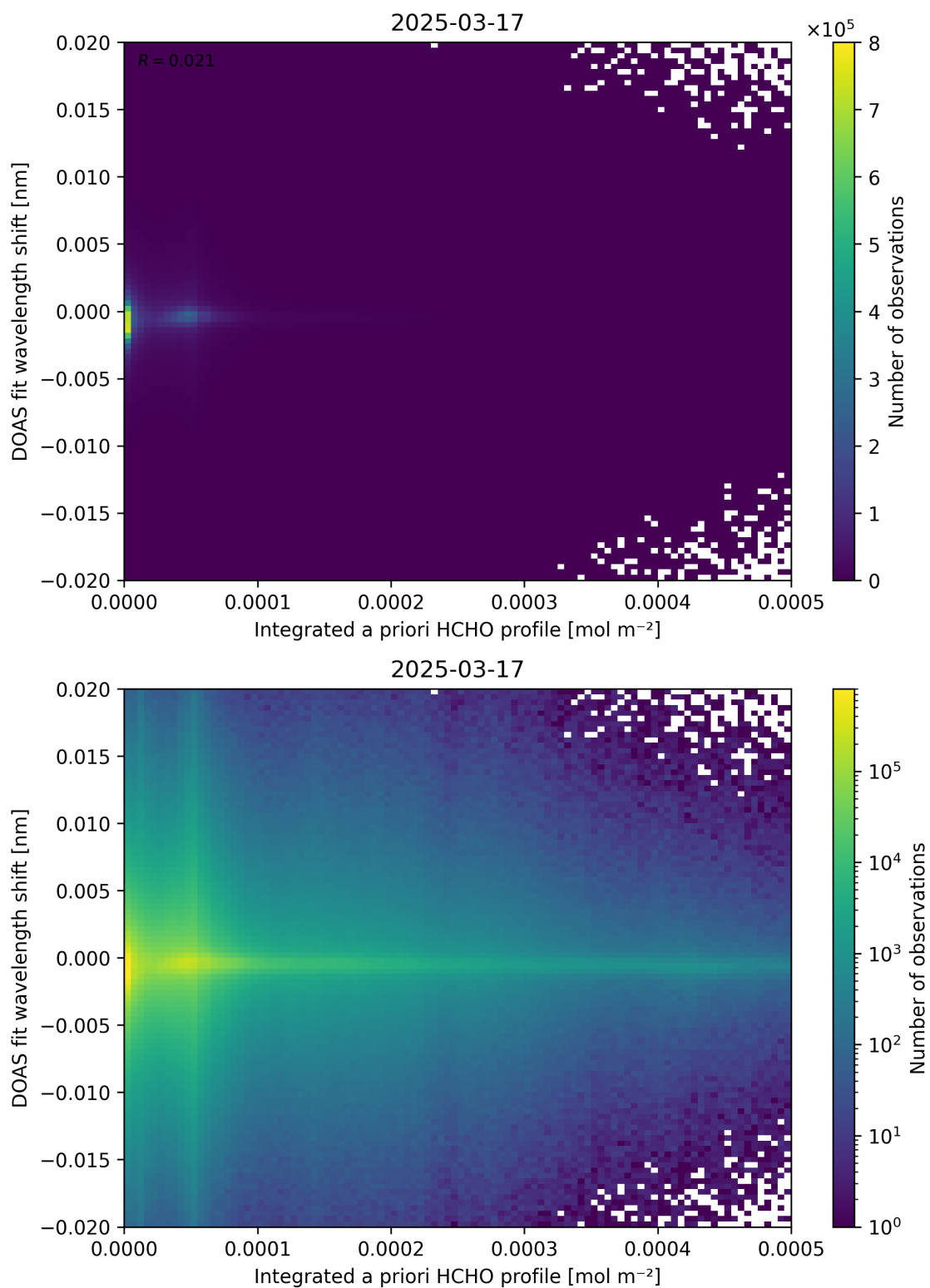
Figure 149: Scatter density plot of “Integrated a priori HCHO profile” against “DOAS fit wavelength shift” for 2025-03-17 to 2025-03-18.
