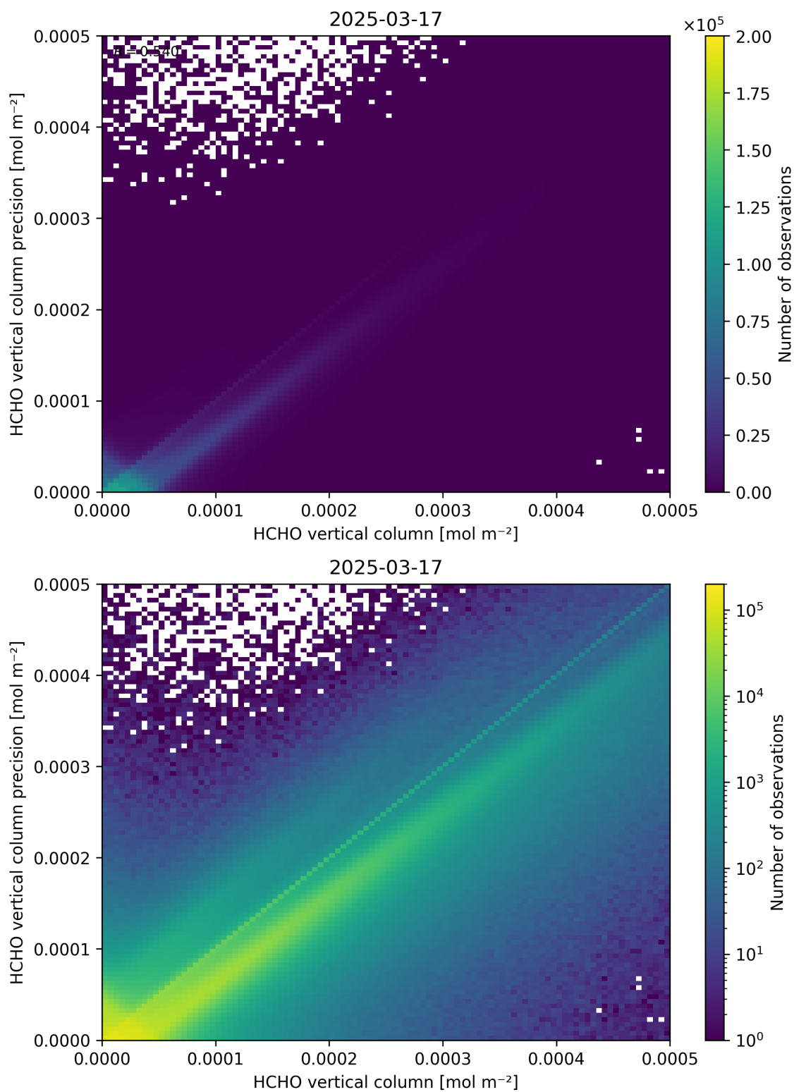
Figure 134: Scatter density plot of “HCHO vertical column” against “HCHO vertical column precision” for 2025-03-17 to 2025-03-18.
