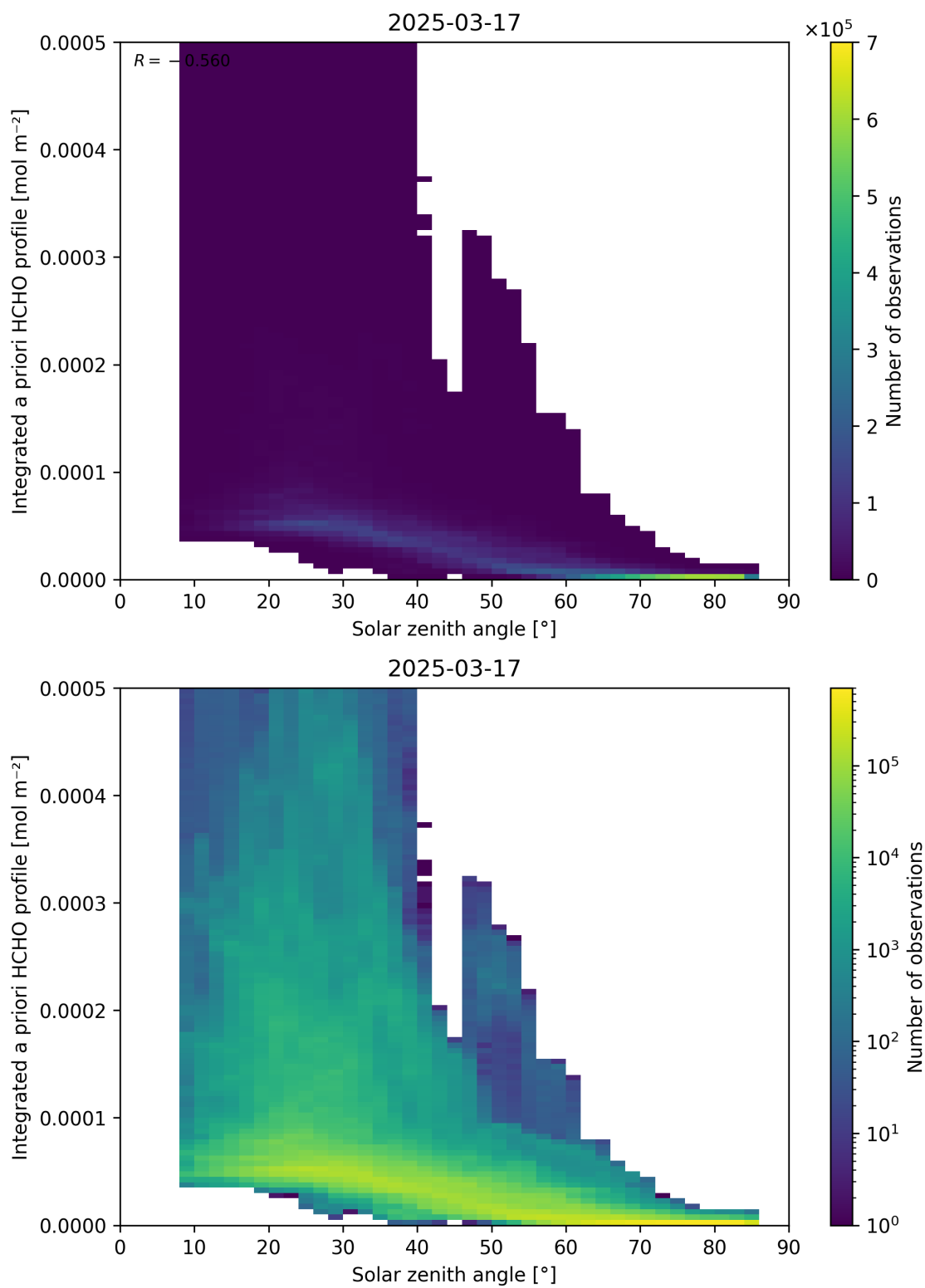
Figure 180: Scatter density plot of “Solar zenith angle” against “Integrated a priori HCHO profile” for 2025-03-17 to 2025-03-18.
