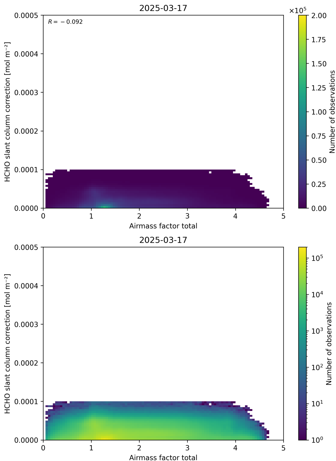
Figure 102: Scatter density plot of “Airmass factor total” against “HCHO slant column correction” for 2025-03-17 to 2025-03-18.
