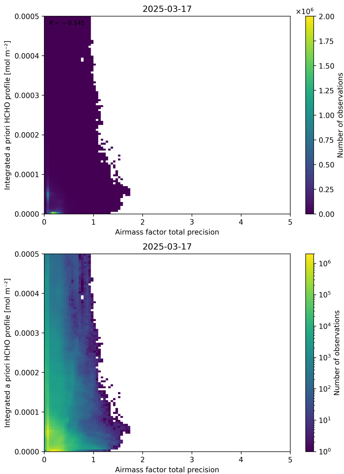
Figure 111: Scatter density plot of “Airmass factor total precision” against “Integrated a priori HCHO profile” for 2025-03-17 to 2025-03-18.
