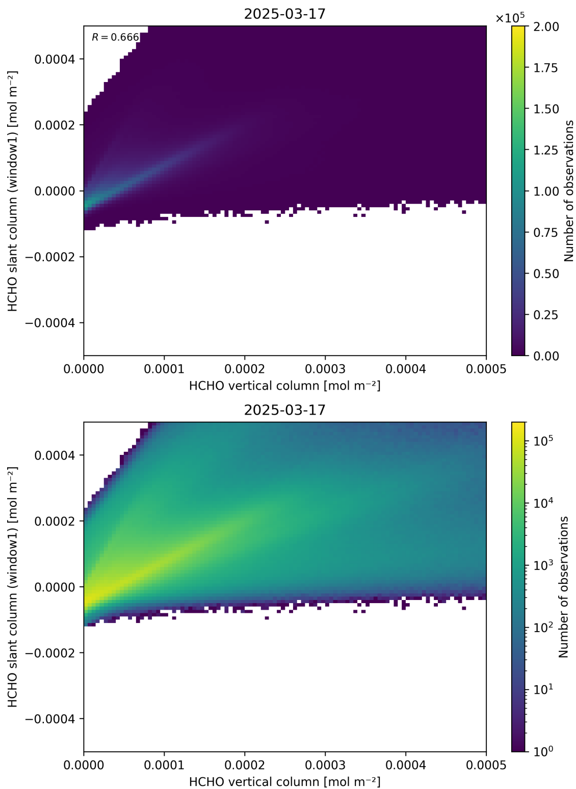
Figure 129: Scatter density plot of “HCHO vertical column” against “HCHO slant column (window1)” for 2025-03-17 to 2025-03-18.
