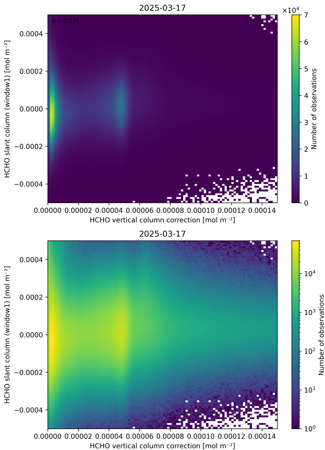
Figure 118: Scatter density plot of “HCHO vertical column correction” against “HCHO slant column (window1)” for 2025-03-17 to 2025-03-18.
