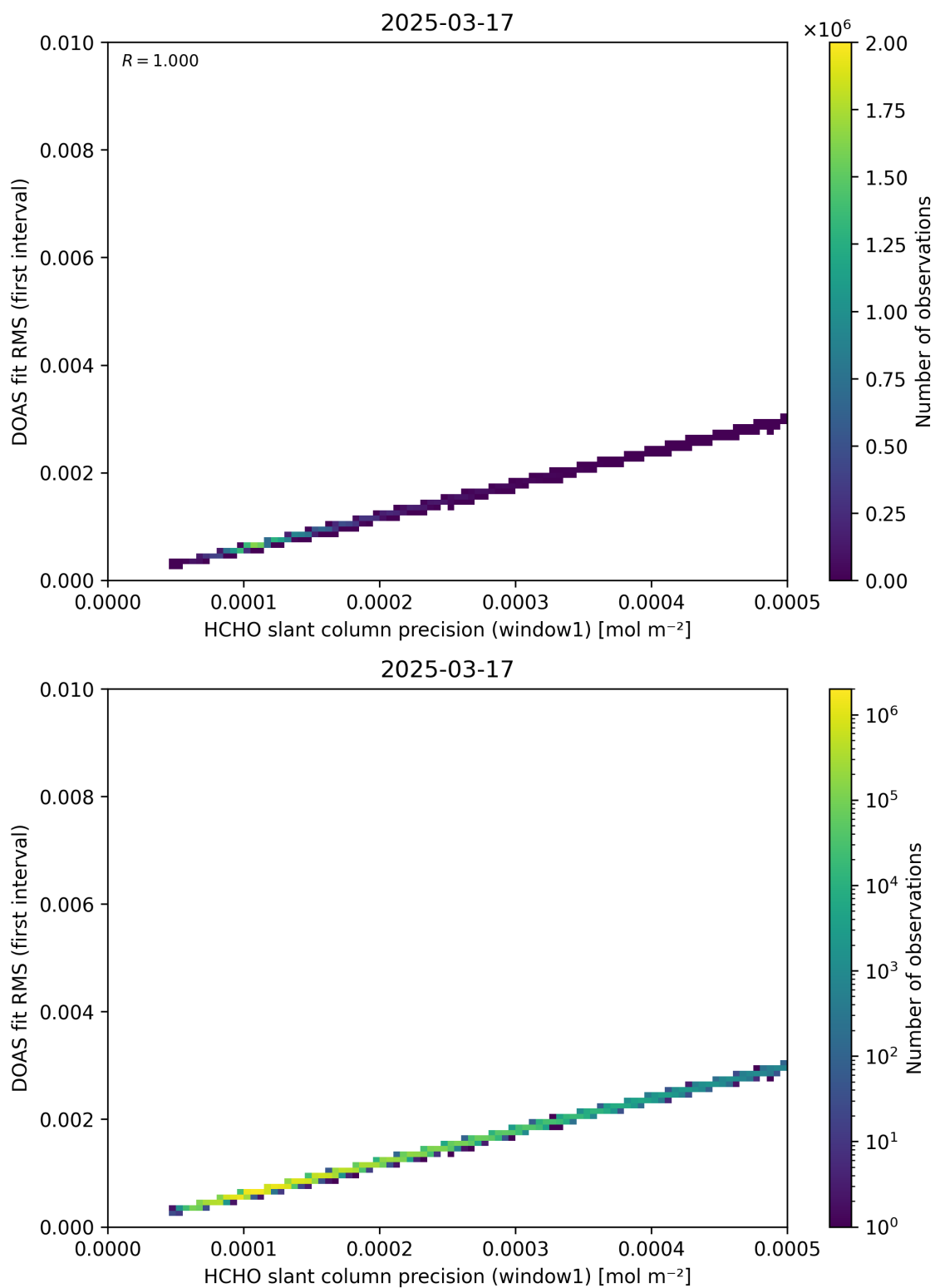
Figure 88: Scatter density plot of “HCHO slant column precision (window1)” against “DOAS fit RMS (first interval)” for 2025-03-17 to 2025-03-18.
