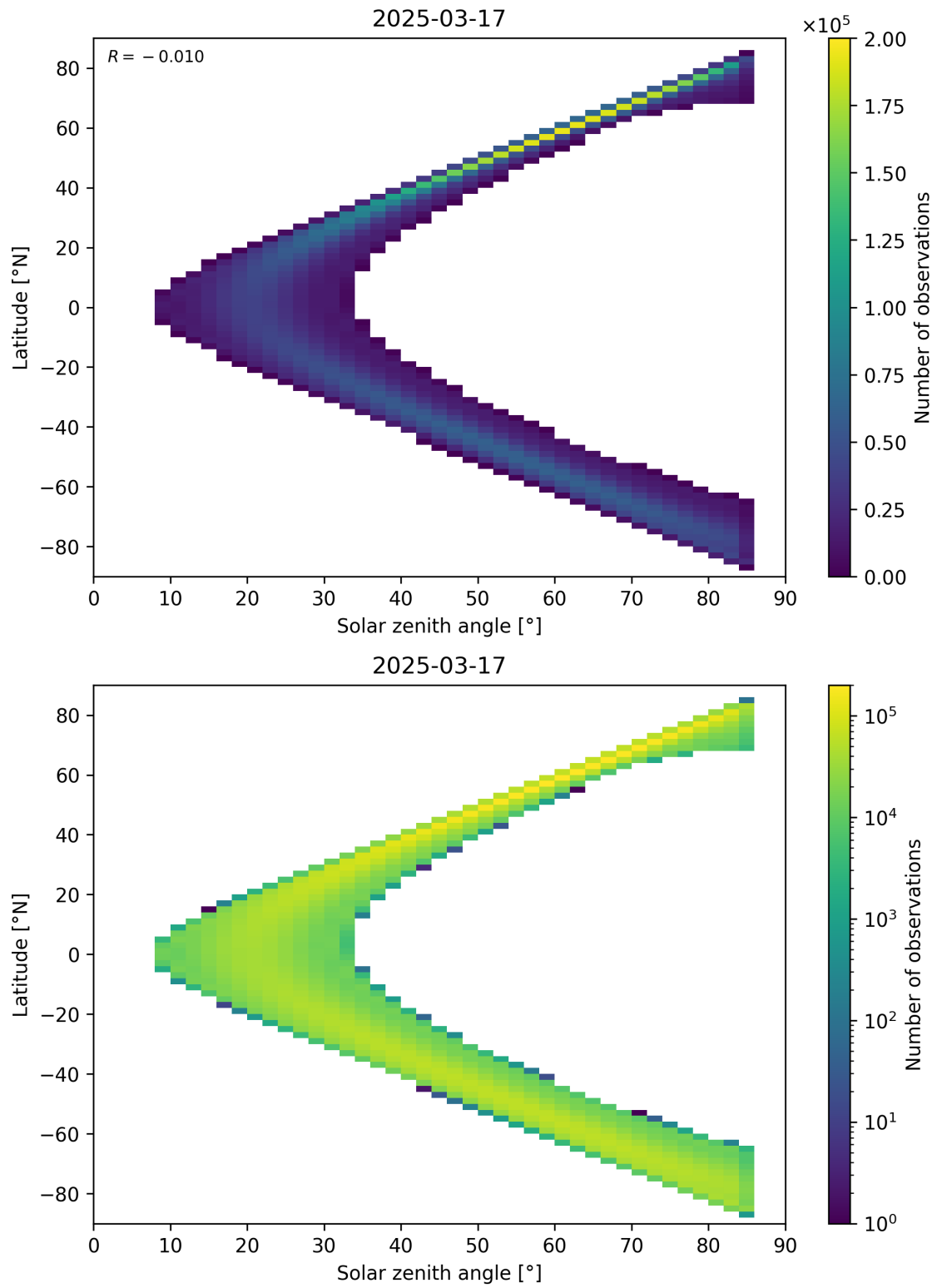
Figure 181: Scatter density plot of “Solar zenith angle” against “Latitude” for 2025-03-17 to 2025-03-18.
