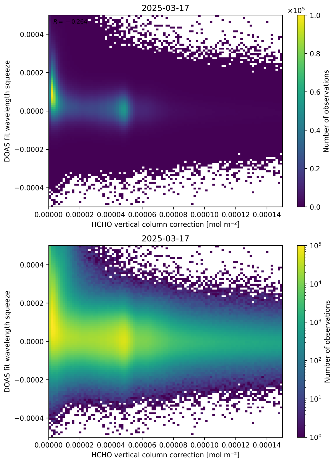
Figure 114: Scatter density plot of “HCHO vertical column correction” against “DOAS fit wavelength squeeze” for 2025-03-17 to 2025-03-18.
