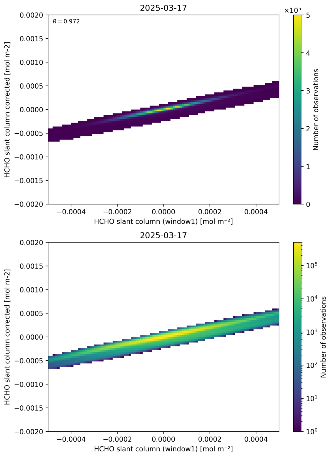
Figure 82: Scatter density plot of “HCHO slant column (window1)” against “HCHO slant column corrected” for 2025-03-17 to 2025-03-18.
