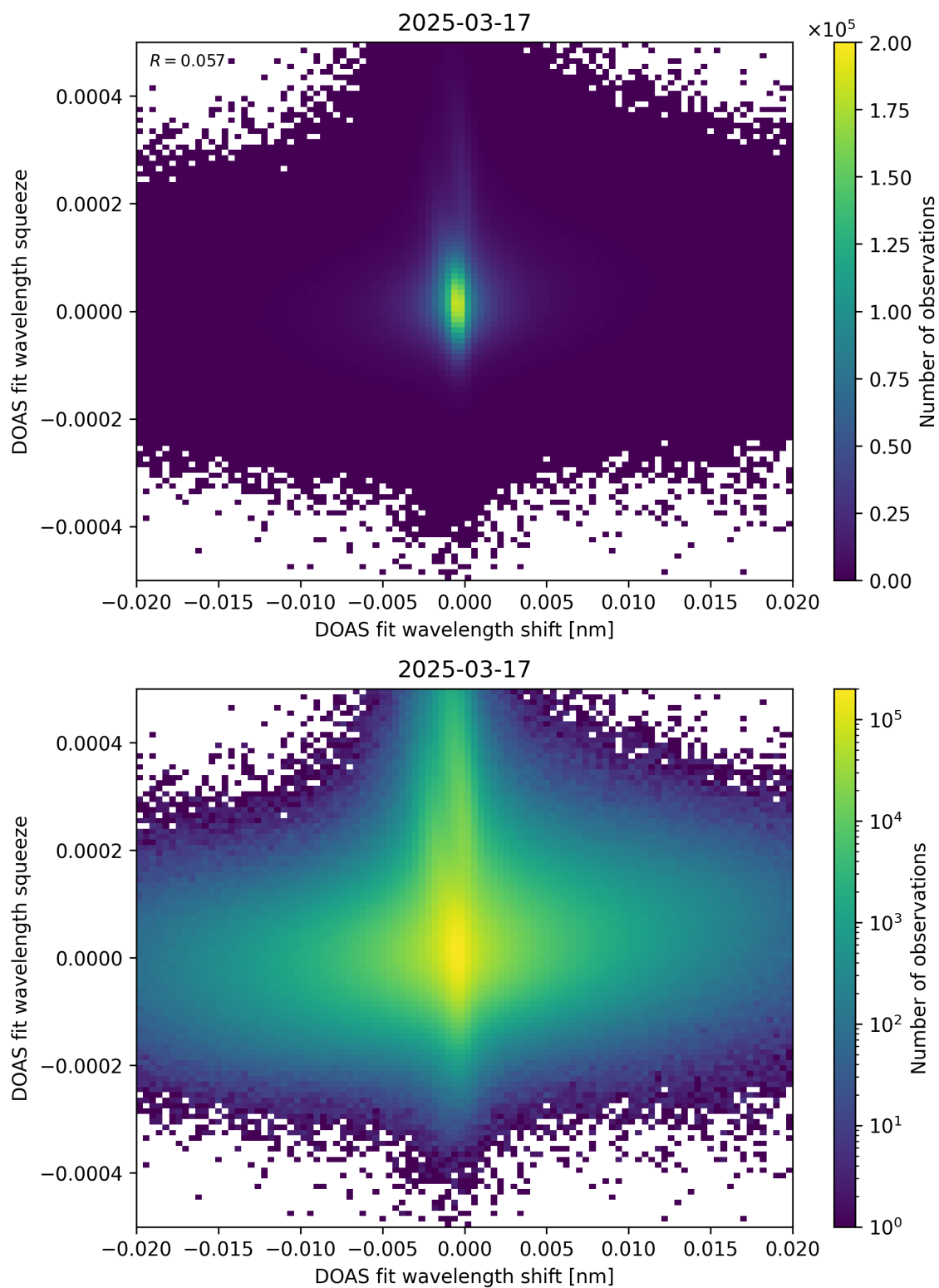
Figure 65: Scatter density plot of “DOAS fit wavelength shift” against “DOAS fit wavelength squeeze” for 2025-03-17 to 2025-03-18.
