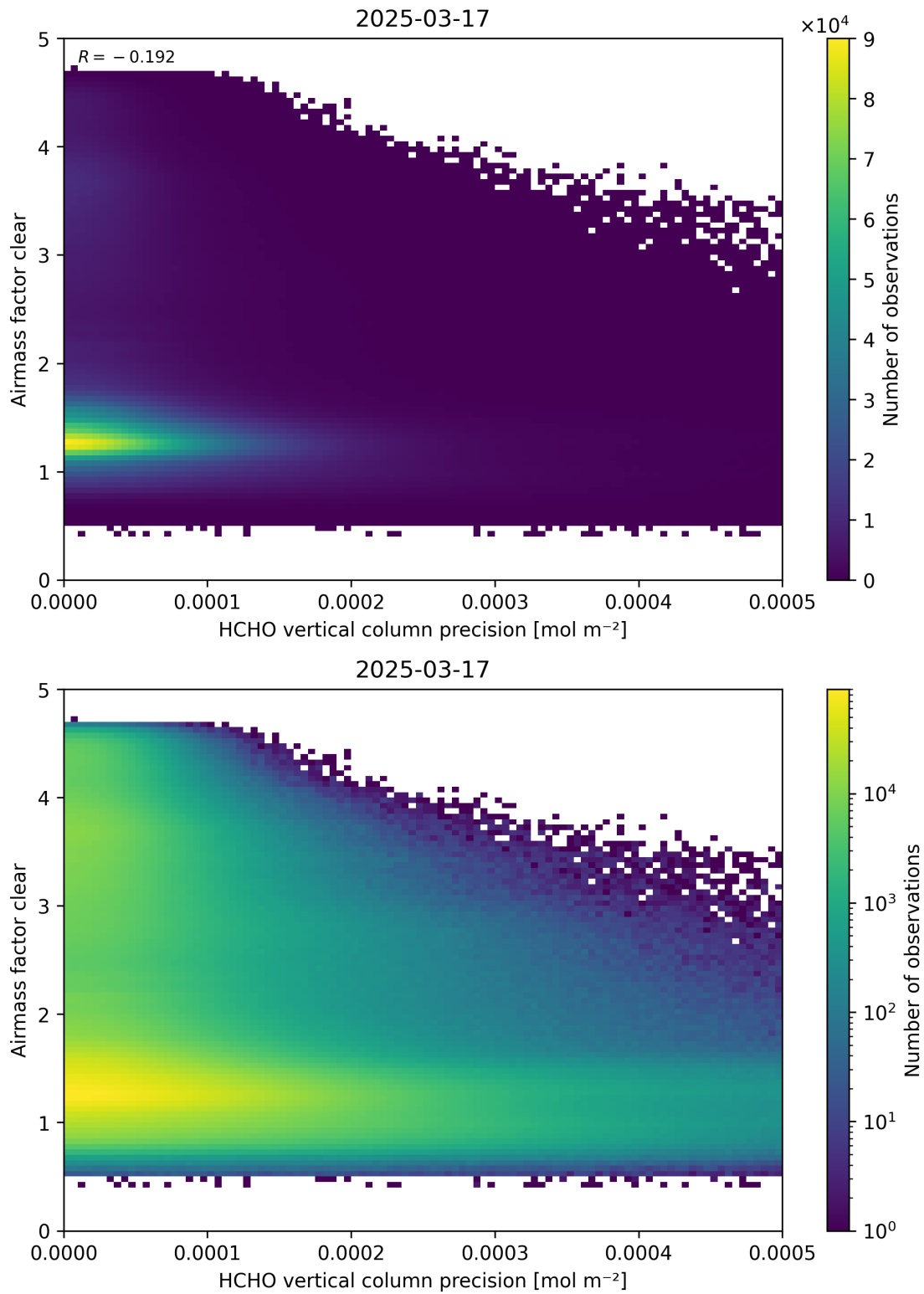
Figure 139: Scatter density plot of “HCHO vertical column precision” against “Airmass factor clear” for 2025-03-17 to 2025-03-18.
