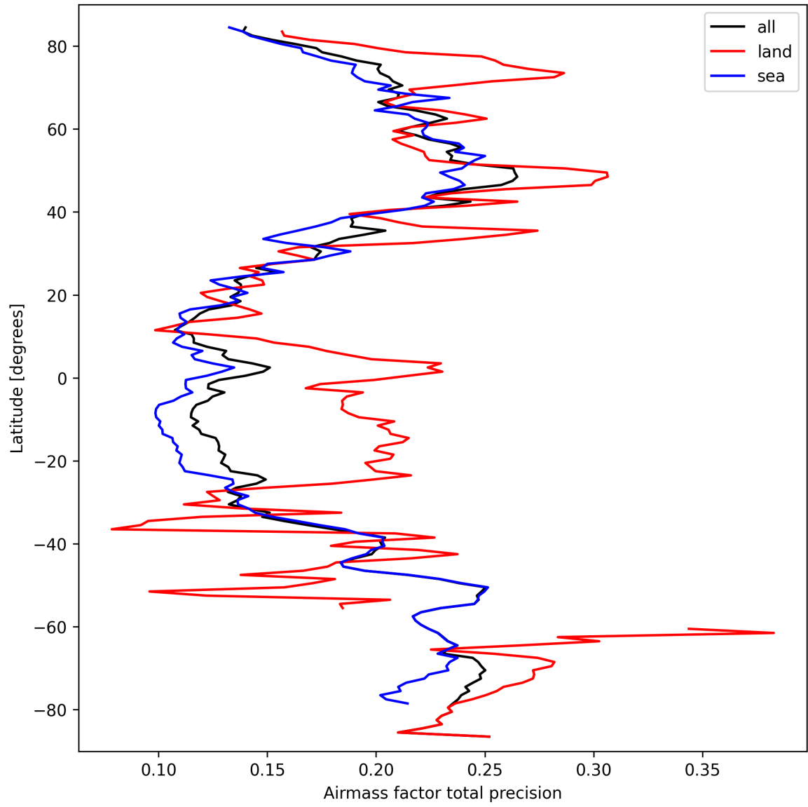
Figure 27: Zonal average of “Airmass factor total precision” for 2025-03-17 to 2025-03-18.
