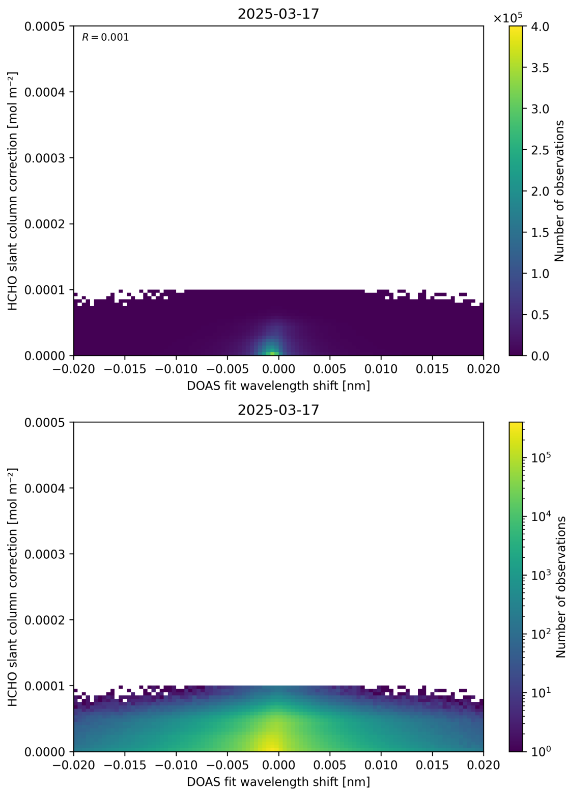
Figure 67: Scatter density plot of “DOAS fit wavelength shift” against “HCHO slant column correction” for 2025-03-17 to 2025-03-18.
