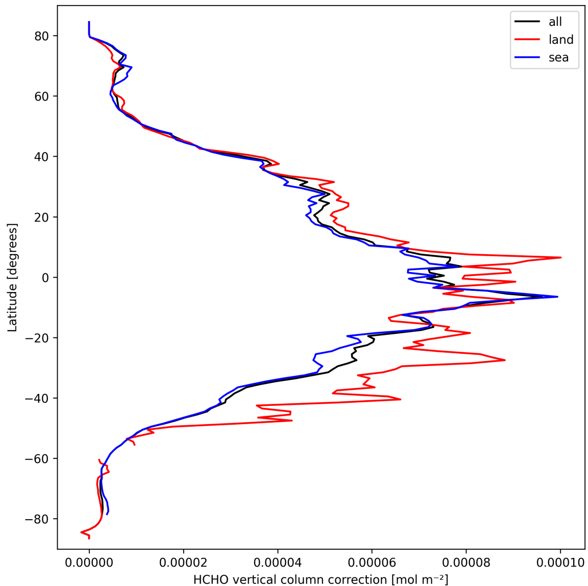
Figure 23: Zonal average of “HCHO vertical column correction” for 2025-03-17 to 2025-03-18.
