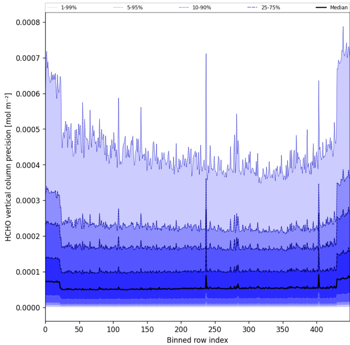
Figure 50: Along track statistics of “HCHO vertical column precision” for 2025-03-17 to 2025-03-18
