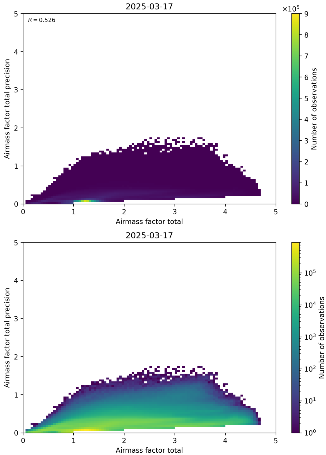
Figure 103: Scatter density plot of “Airmass factor total” against “Airmass factor total precision” for 2025-03-17 to 2025-03-18.
