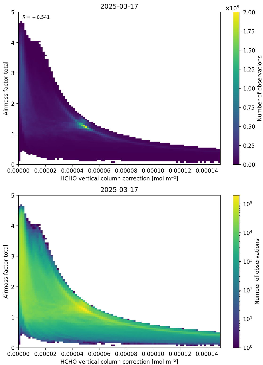
Figure 120: Scatter density plot of “HCHO vertical column correction” against “Airmass factor total” for 2025-03-17 to 2025-03-18.
