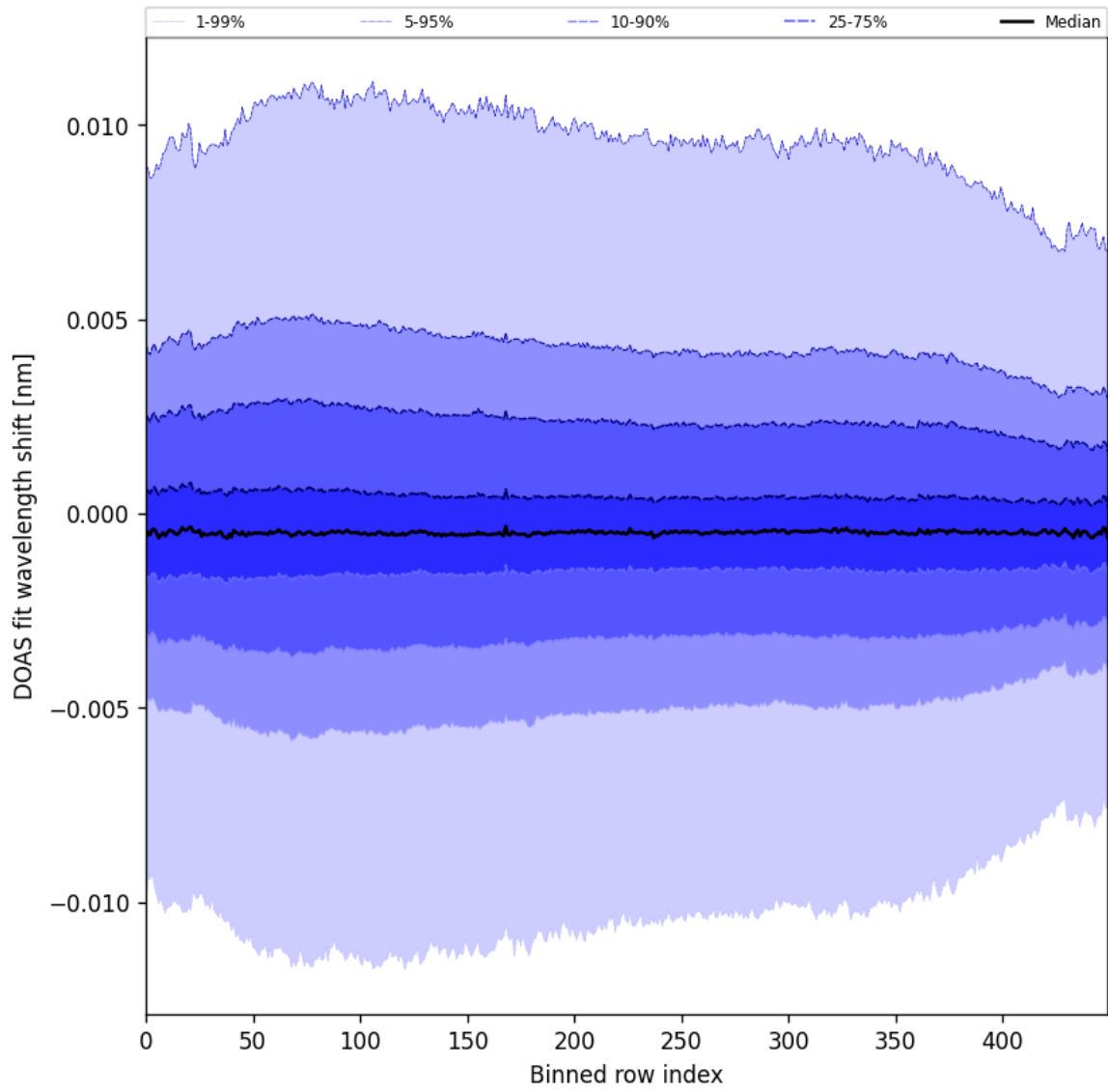
Figure 58: Along track statistics of “DOAS fit wavelength shift” for 2025-03-17 to 2025-03-18
