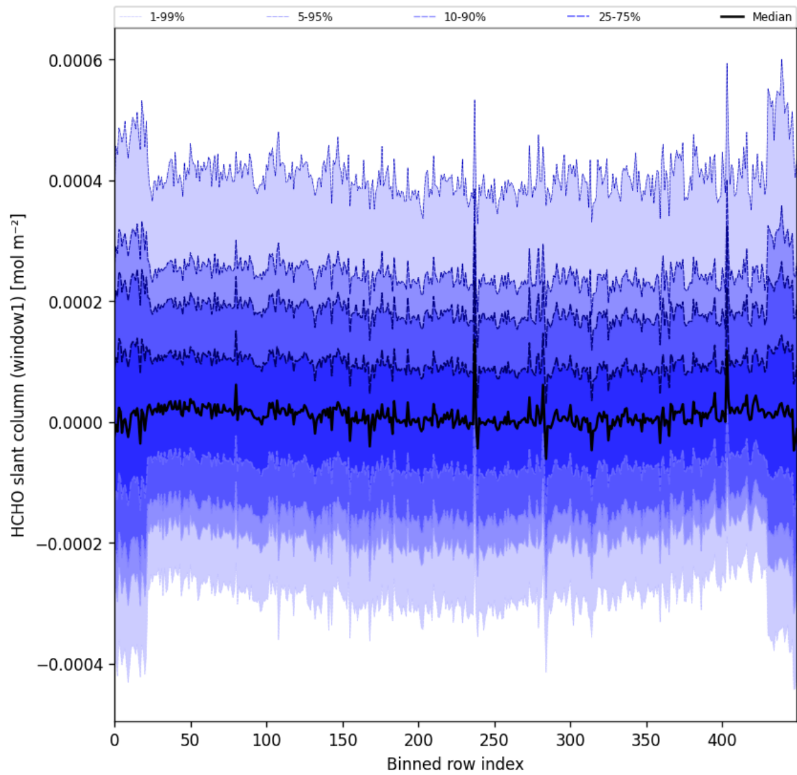
Figure 52: Along track statistics of “HCHO slant column (window1)” for 2025-03-17 to 2025-03-18
