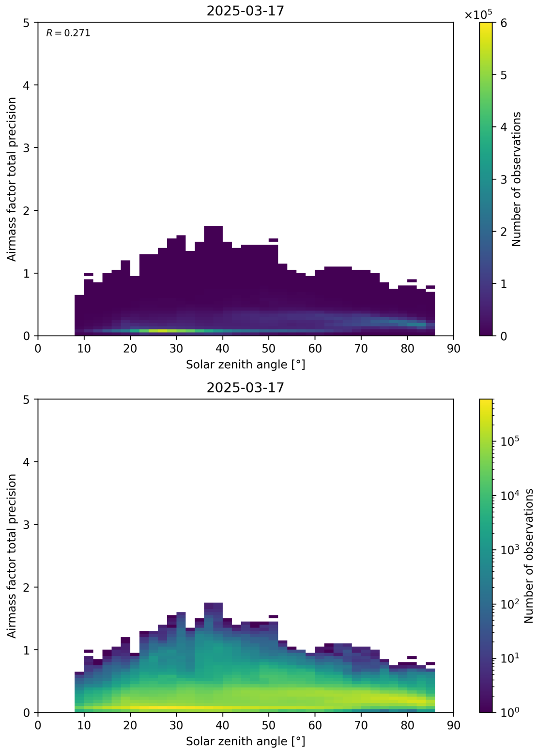
Figure 176: Scatter density plot of “Solar zenith angle” against “Airmass factor total precision” for 2025-03-17 to 2025-03-18.
