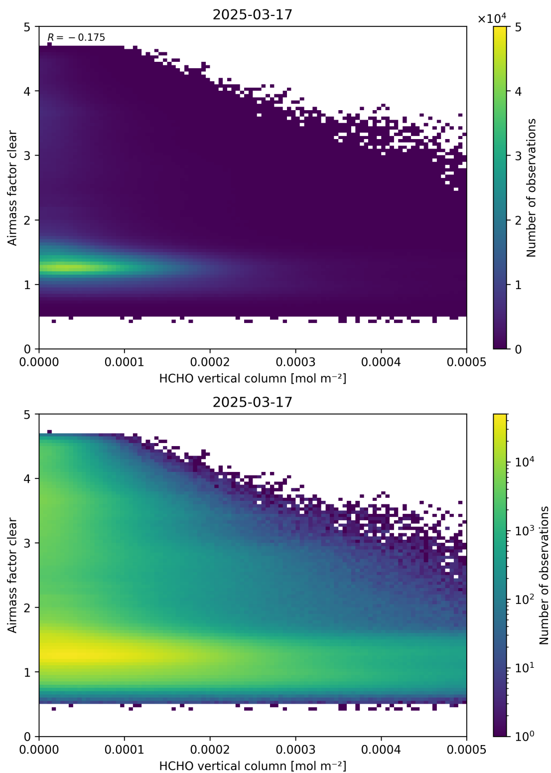
Figure 126: Scatter density plot of “HCHO vertical column” against “Airmass factor clear” for 2025-03-17 to 2025-03-18.
