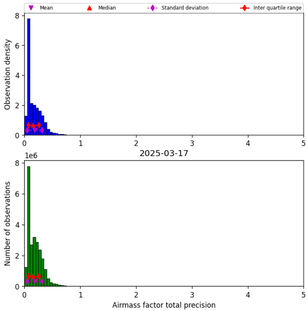
Figure 41: Histogram of “Airmass factor total precision” for 2025-03-17 to 2025-03-18
