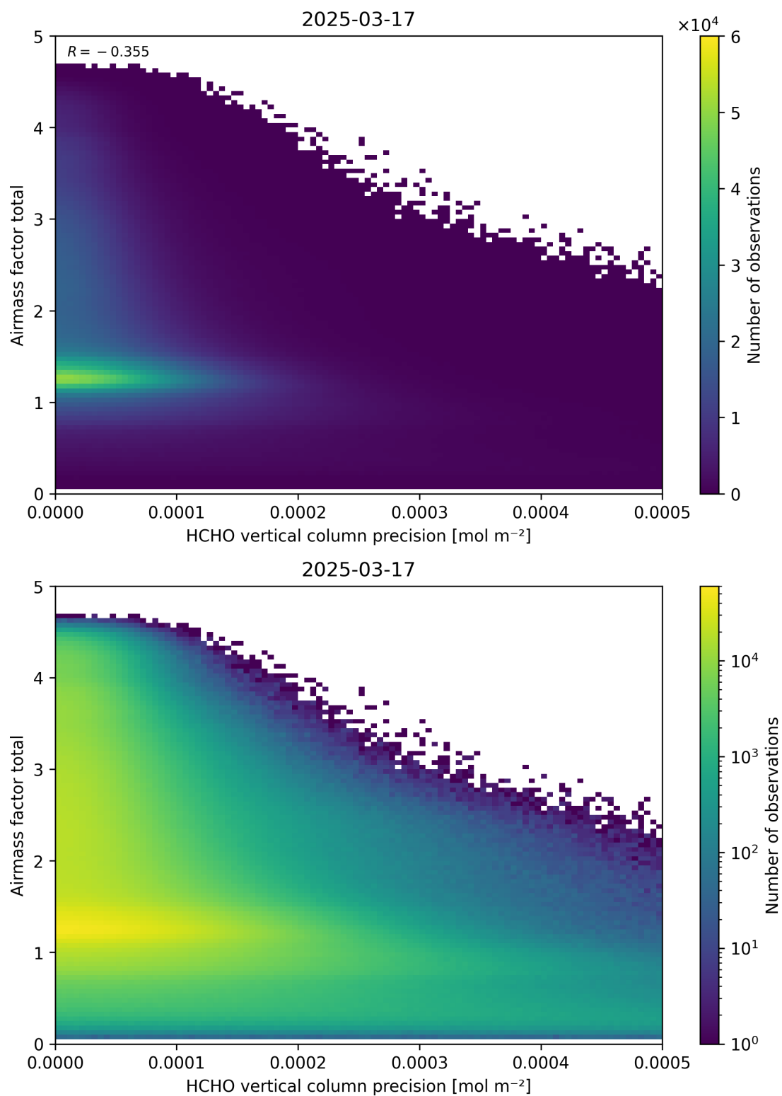
Figure 144: Scatter density plot of “HCHO vertical column precision” against “Airmass factor total” for 2025-03-17 to 2025-03-18.
