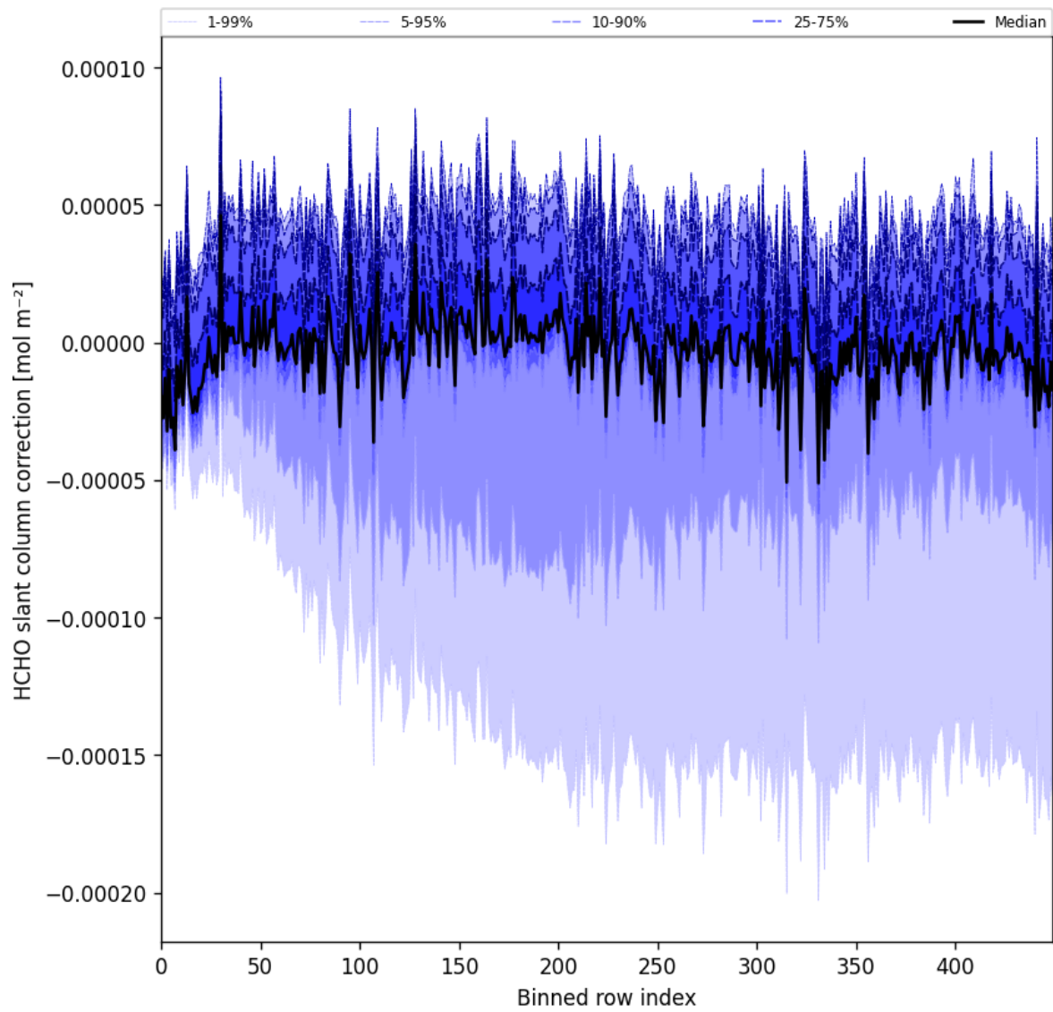
Figure 61: Along track statistics of “HCHO slant column correction” for 2025-03-17 to 2025-03-18
