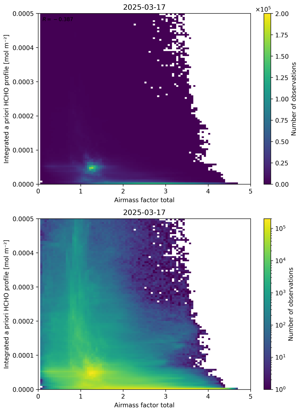
Figure 104: Scatter density plot of “Airmass factor total” against “Integrated a priori HCHO profile” for 2025-03-17 to 2025-03-18.
