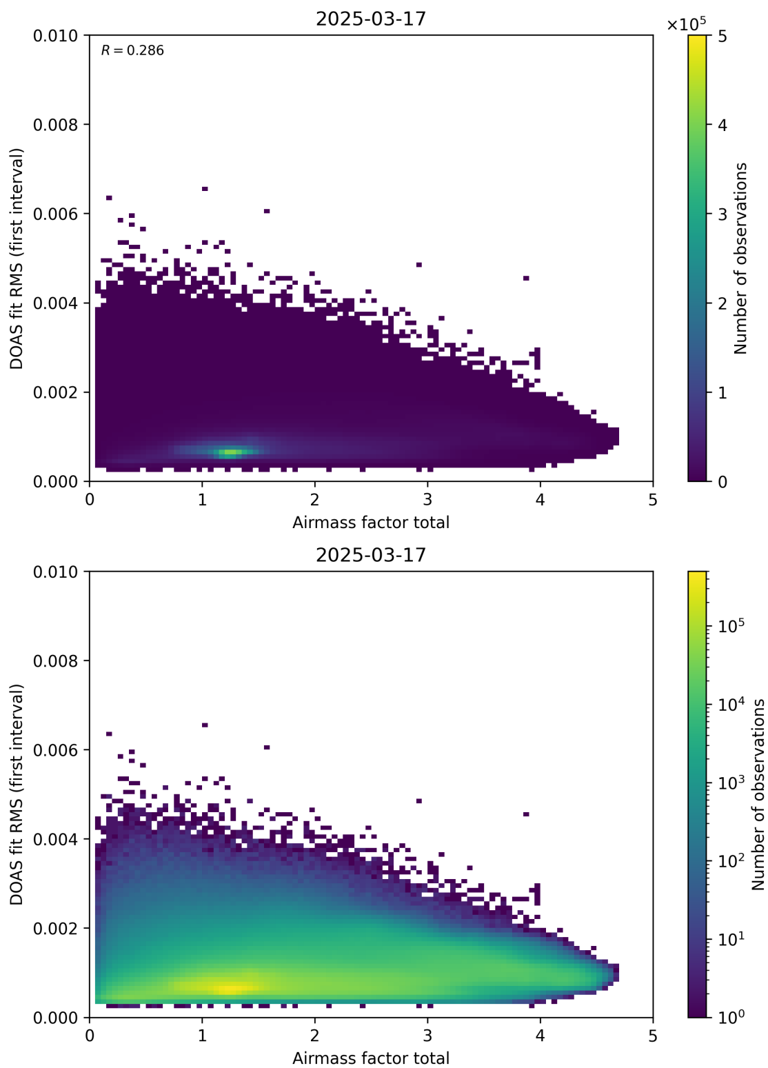
Figure 97: Scatter density plot of “Airmass factor total” against “DOAS fit RMS (first interval)” for 2025-03-17 to 2025-03-18.
