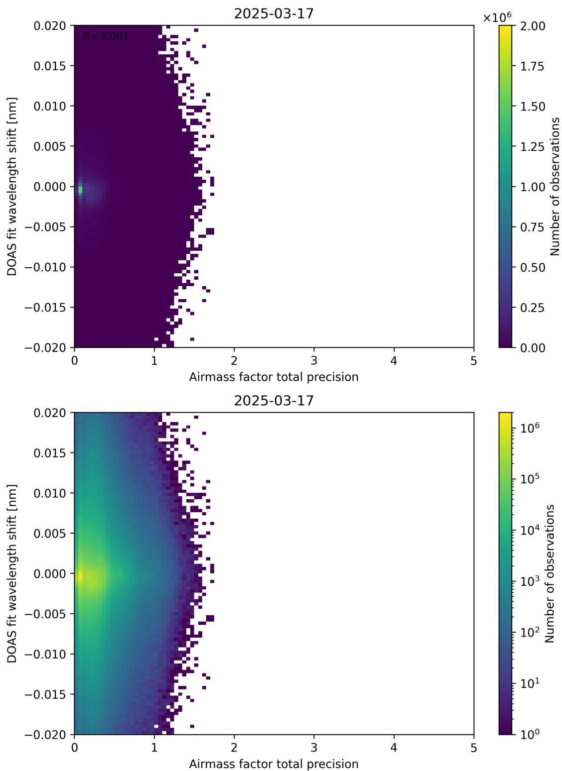
Figure 106: Scatter density plot of “Airmass factor total precision” against “DOAS fit wavelength shift” for 2025-03-17 to 2025-03-18.
