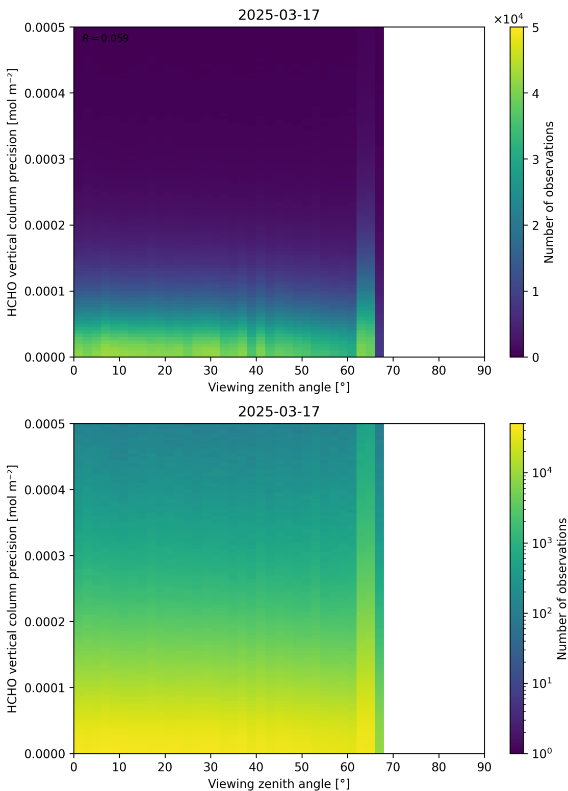
Figure 194: Scatter density plot of “Viewing zenith angle” against “HCHO vertical column precision” for 2025-03-17 to 2025-03-18.
