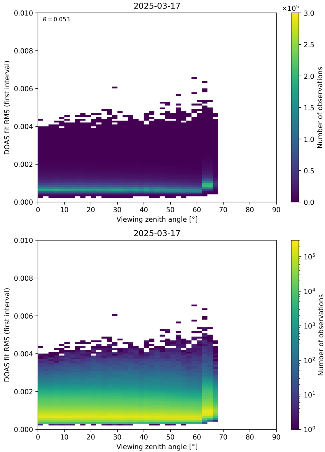
Figure 182: Scatter density plot of “Viewing zenith angle” against “DOAS fit RMS (first interval)” for 2025-03-17 to 2025-03-18.
