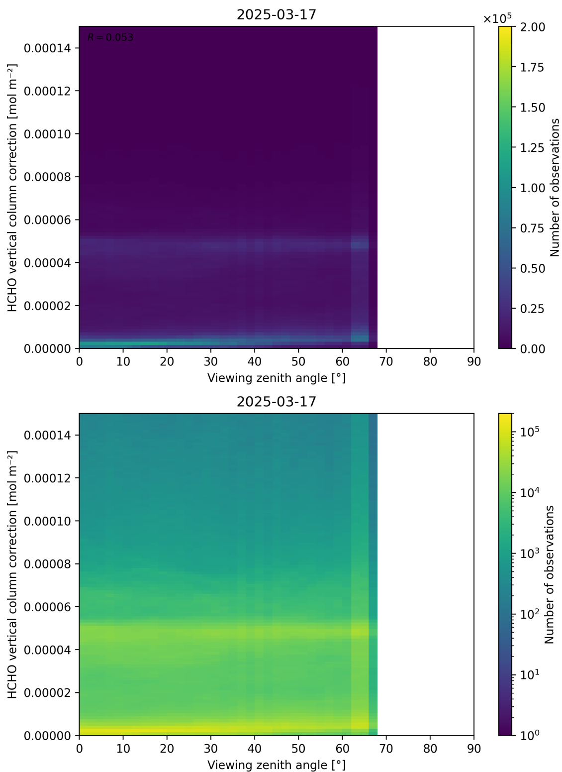
Figure 193: Scatter density plot of “Viewing zenith angle” against “HCHO vertical column correction” for 2025-03-17 to 2025-03-18.
