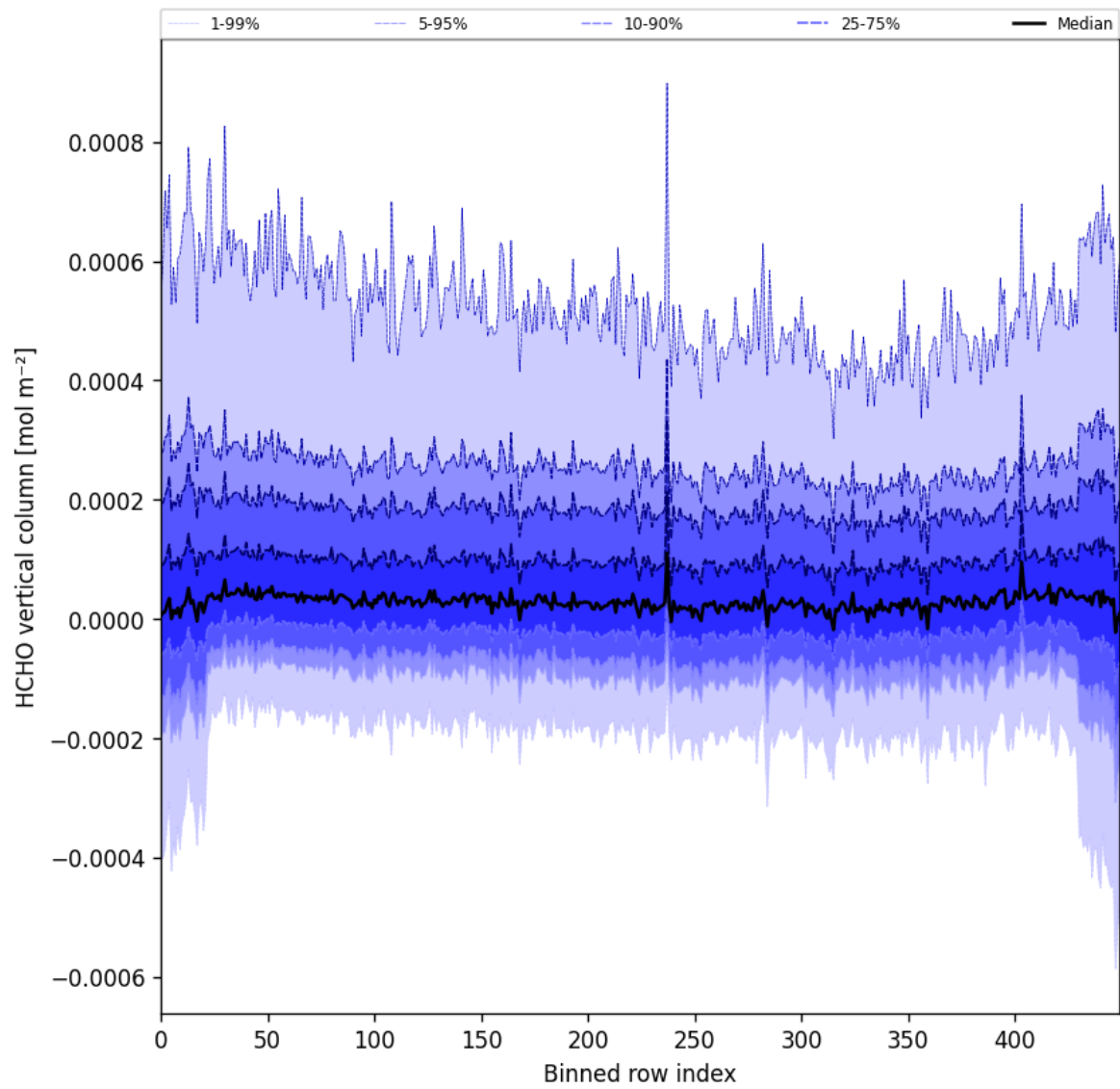
Figure 49: Along track statistics of “HCHO vertical column” for 2025-03-17 to 2025-03-18
