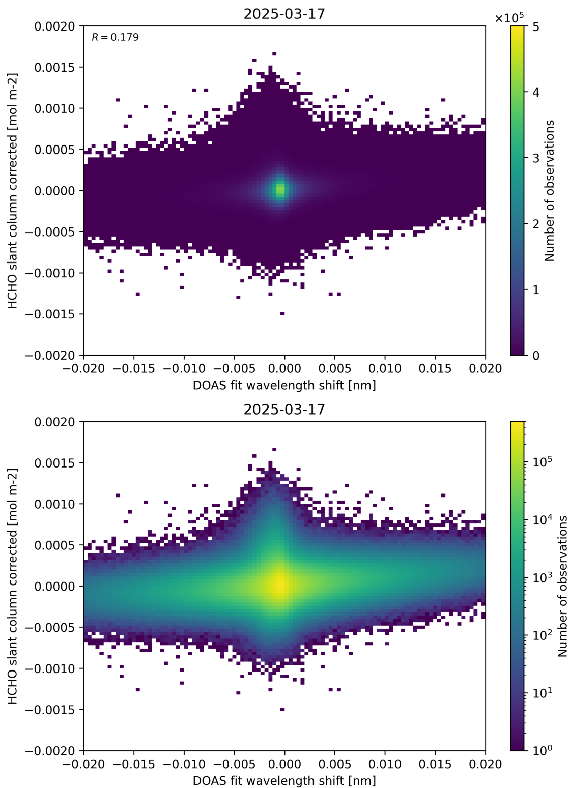
Figure 66: Scatter density plot of “DOAS fit wavelength shift” against “HCHO slant column corrected” for 2025-03-17 to 2025-03-18.
