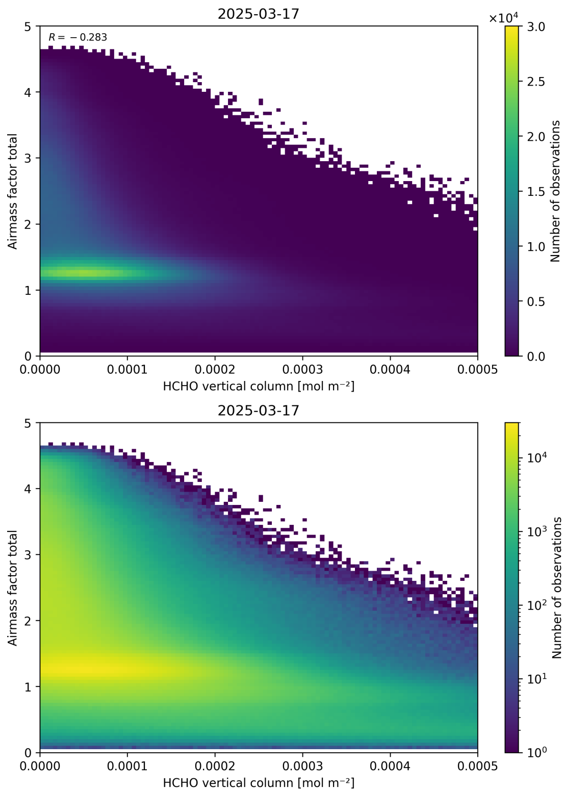
Figure 131: Scatter density plot of “HCHO vertical column” against “Airmass factor total” for 2025-03-17 to 2025-03-18.
