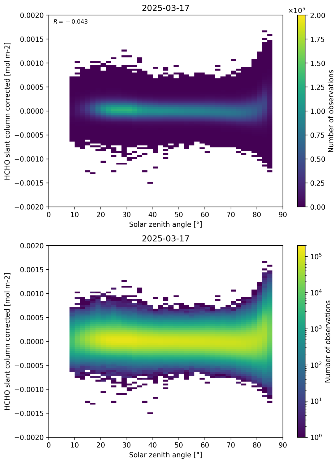
Figure 171: Scatter density plot of “Solar zenith angle” against “HCHO slant column corrected” for 2025-03-17 to 2025-03-18.
