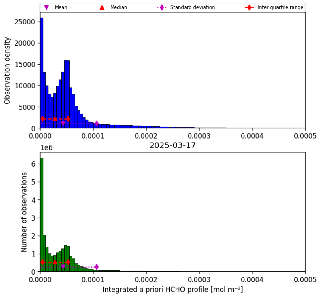
Figure 43: Histogram of “Integrated a priori HCHO profile” for 2025-03-17 to 2025-03-18
