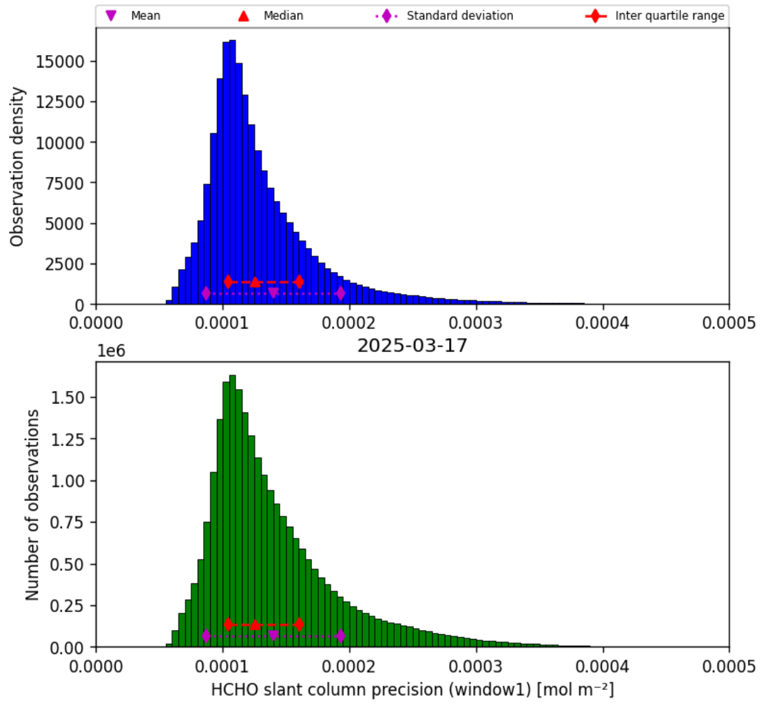
Figure 39: Histogram of “HCHO slant column precision (window1)” for 2025-03-17 to 2025-03-18
