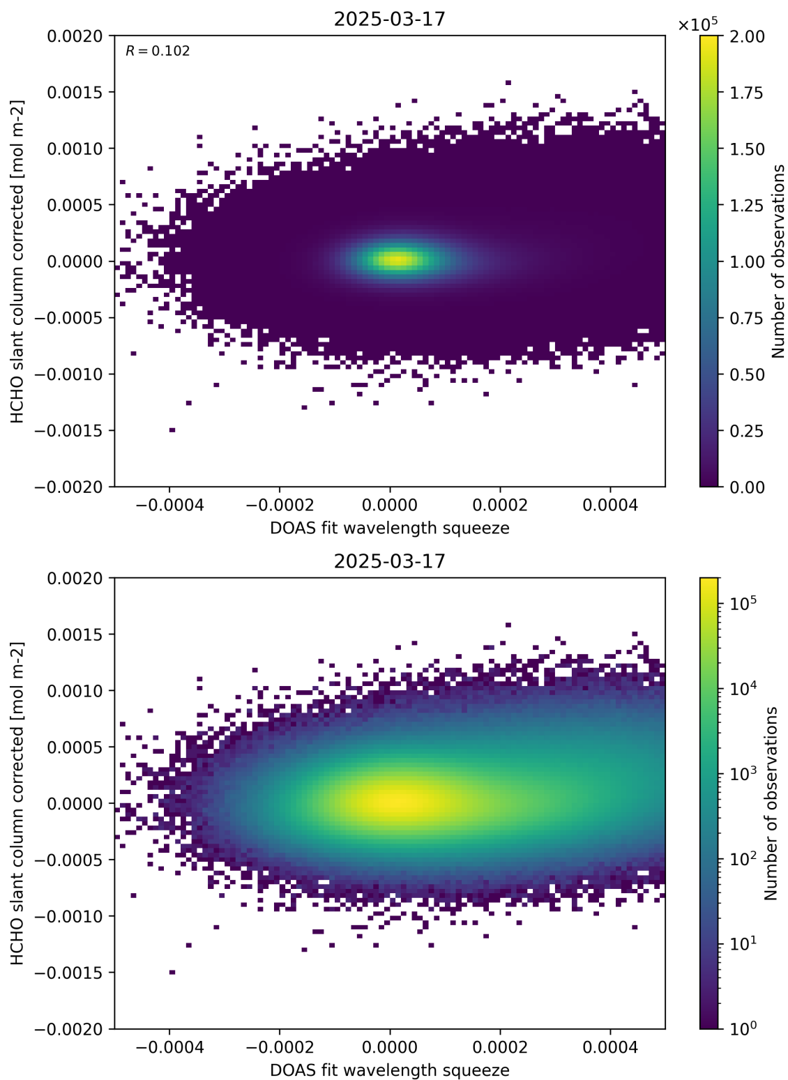
Figure 69: Scatter density plot of “DOAS fit wavelength squeeze” against “HCHO slant column corrected” for 2025-03-17 to 2025-03-18.
