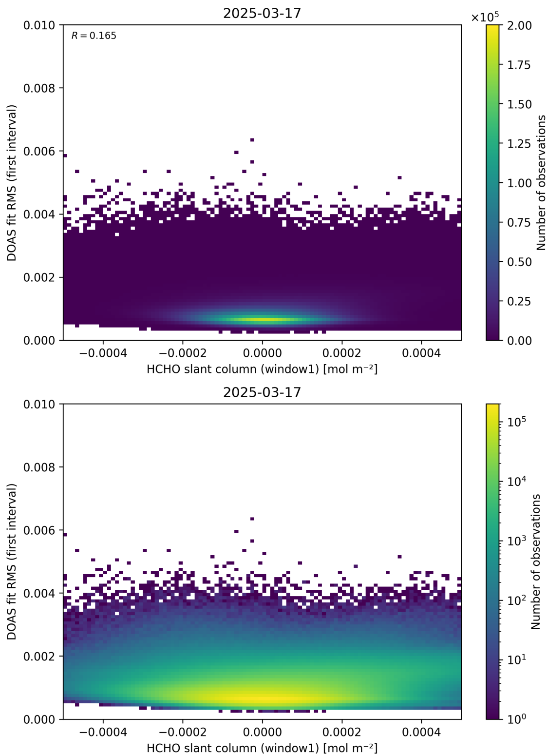
Figure 78: Scatter density plot of “HCHO slant column (window1)” against “DOAS fit RMS (first interval)” for 2025-03-17 to 2025-03-18.
