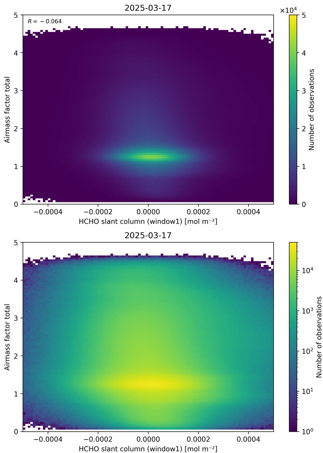
Figure 85: Scatter density plot of “HCHO slant column (window1)” against “Airmass factor total” for 2025-03-17 to 2025-03-18.
