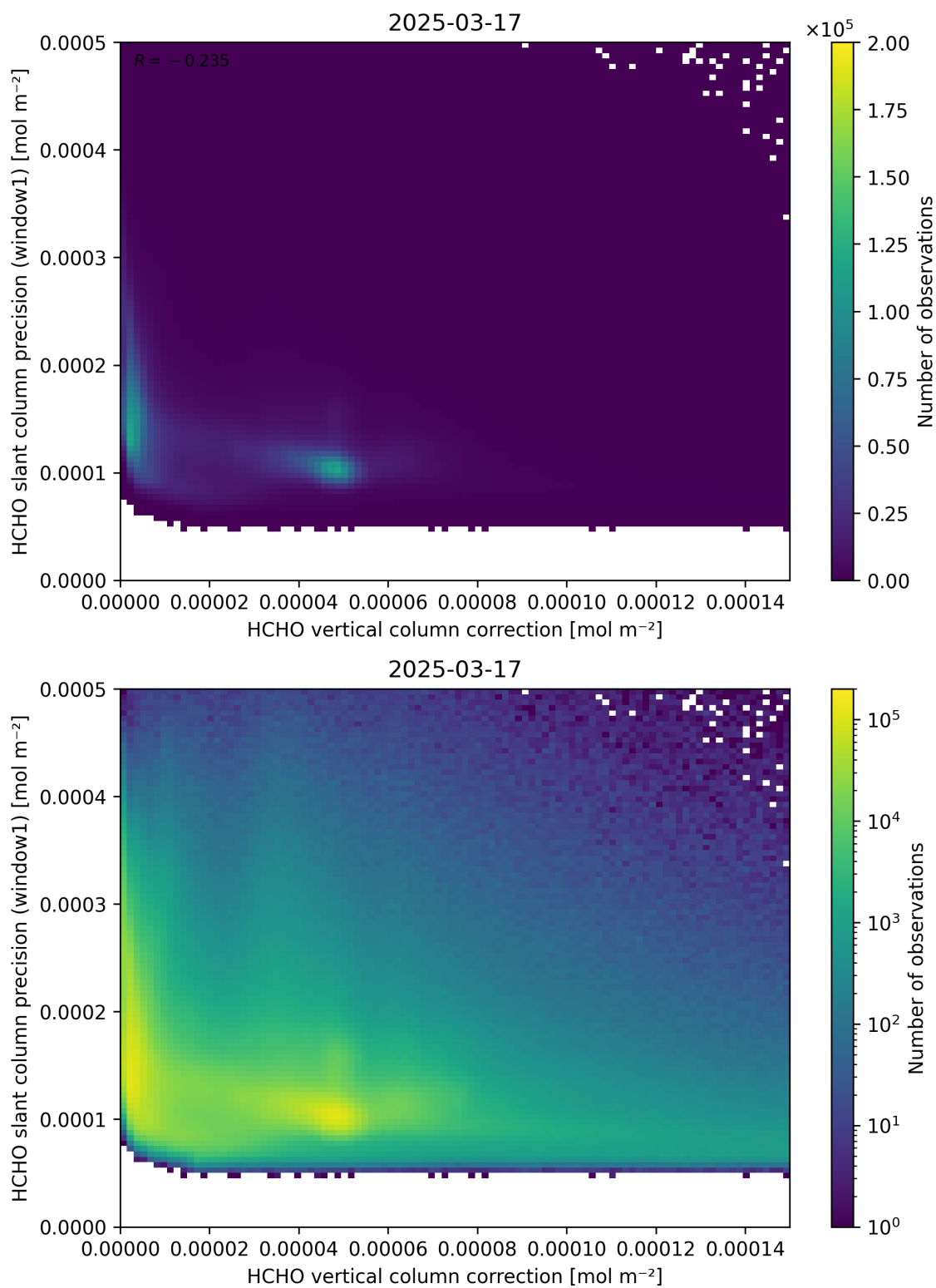
Figure 119: Scatter density plot of “HCHO vertical column correction” against “HCHO slant column precision (window1)” for 2025-03-17 to 2025-03-18.
