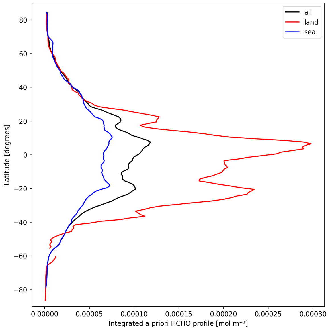
Figure 29: Zonal average of “Integrated a priori HCHO profile” for 2025-03-17 to 2025-03-18.
