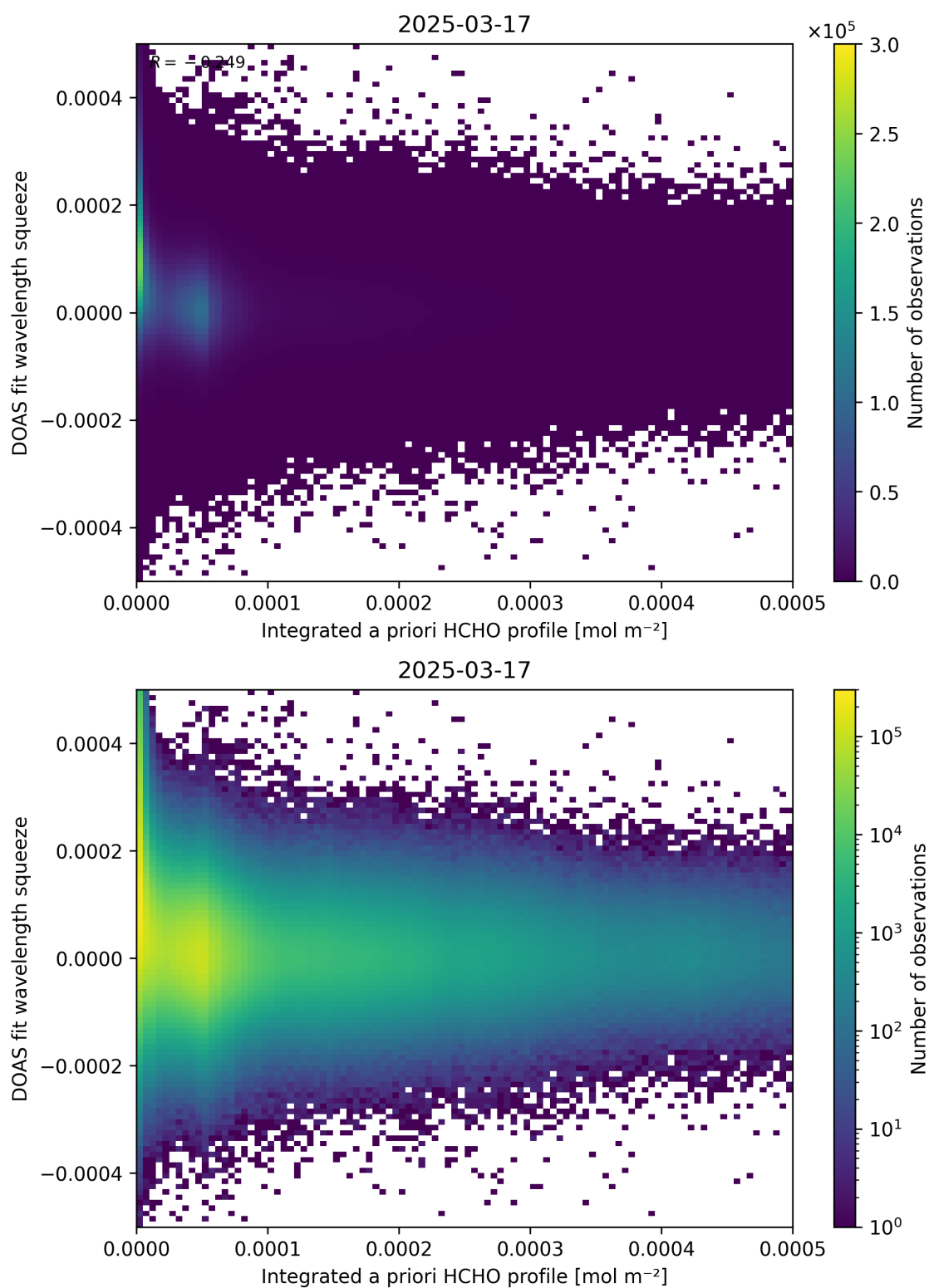
Figure 150: Scatter density plot of “Integrated a priori HCHO profile” against “DOAS fit wavelength squeeze” for 2025-03-17 to 2025-03-18.
