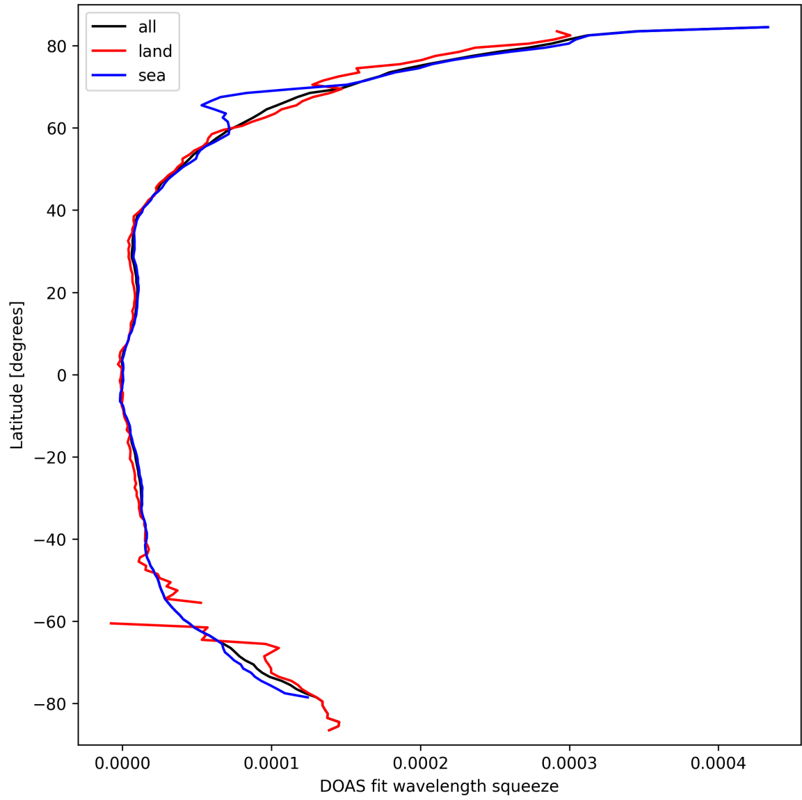
Figure 31: Zonal average of “DOAS fit wavelength squeeze” for 2025-03-17 to 2025-03-18.
