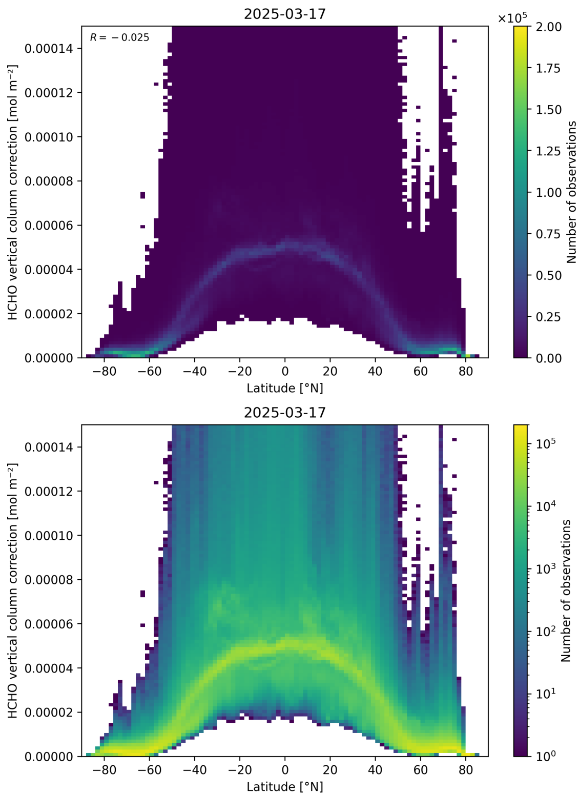
Figure 164: Scatter density plot of “Latitude” against “HCHO vertical column correction” for 2025-03-17 to 2025-03-18.
