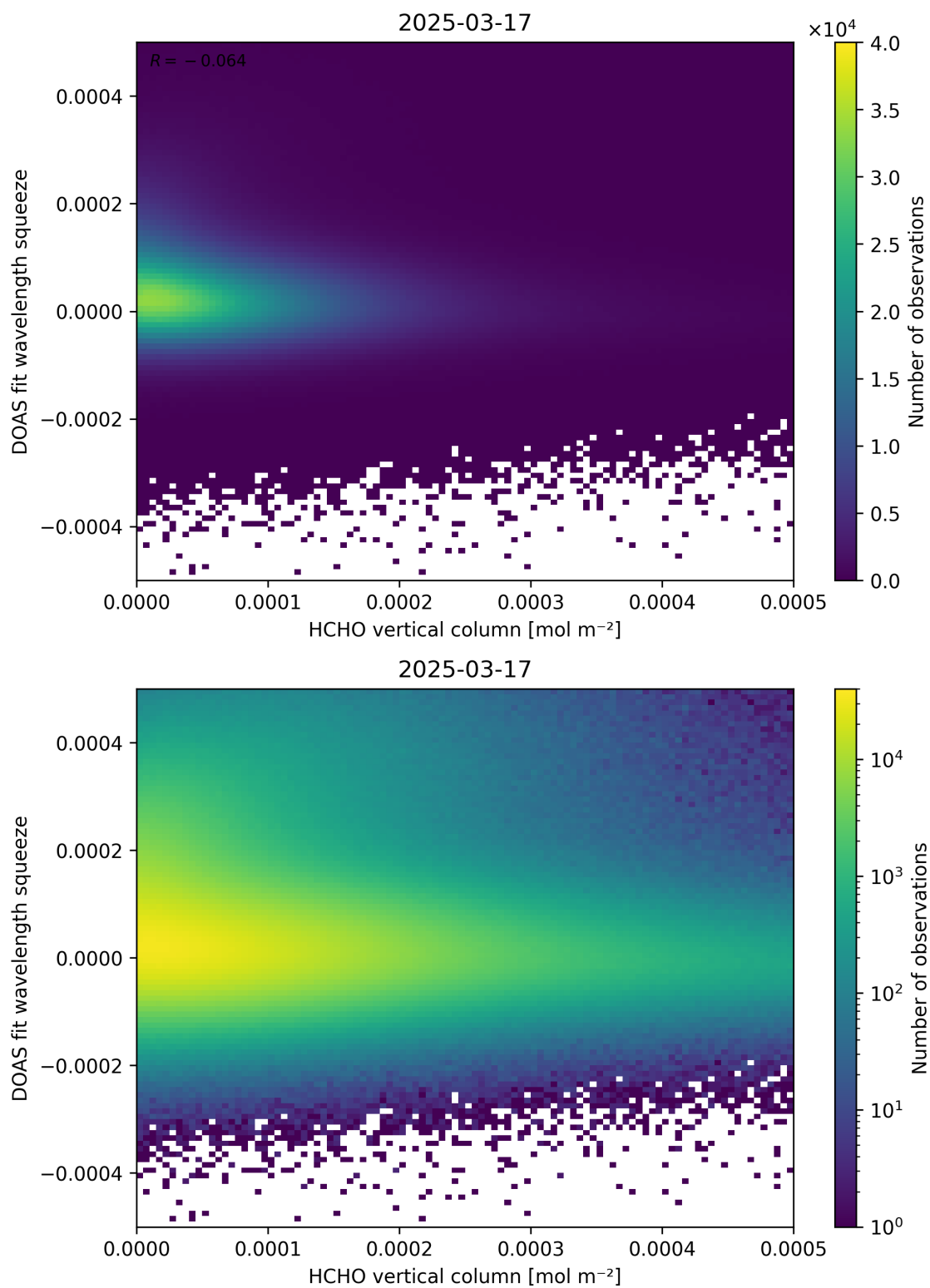
Figure 125: Scatter density plot of “HCHO vertical column” against “DOAS fit wavelength squeeze” for 2025-03-17 to 2025-03-18.
