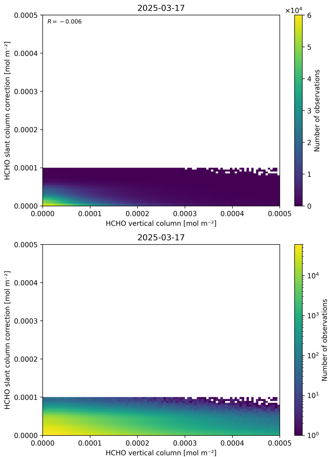
Figure 128: Scatter density plot of “HCHO vertical column” against “HCHO slant column correction” for 2025-03-17 to 2025-03-18.
