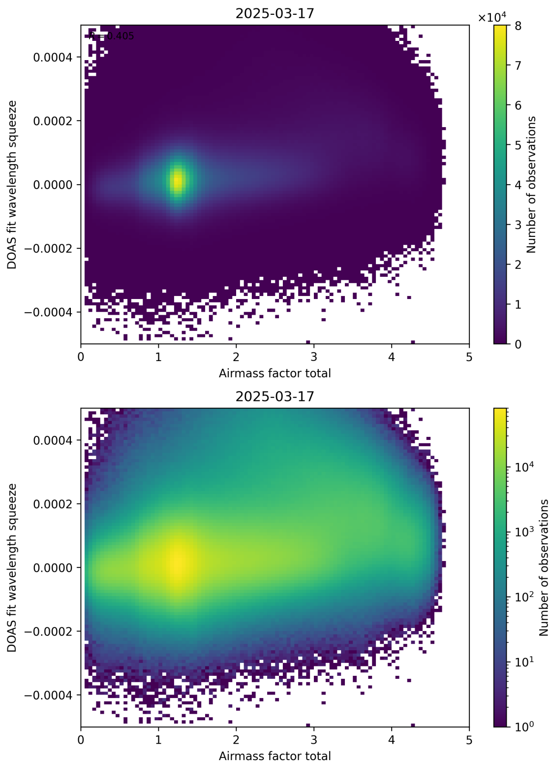
Figure 99: Scatter density plot of “Airmass factor total” against “DOAS fit wavelength squeeze” for 2025-03-17 to 2025-03-18.
