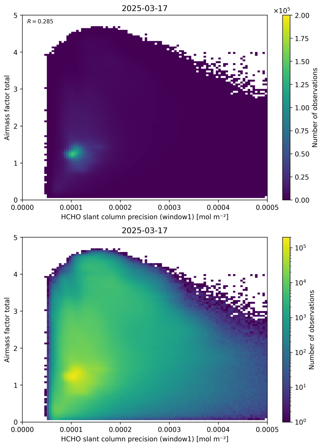
Figure 94: Scatter density plot of “HCHO slant column precision (window1)” against “Airmass factor total” for 2025-03-17 to 2025-03-18.
