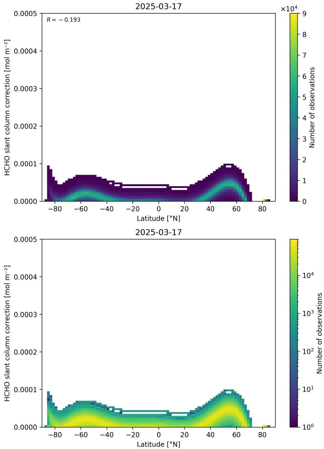
Figure 158: Scatter density plot of “Latitude” against “HCHO slant column correction” for 2025-03-17 to 2025-03-18.
