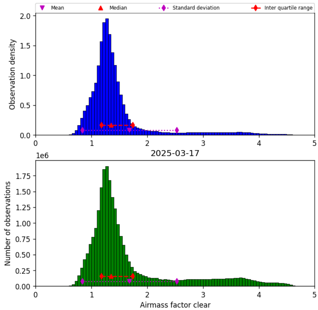
Figure 42: Histogram of “Airmass factor clear” for 2025-03-17 to 2025-03-18
