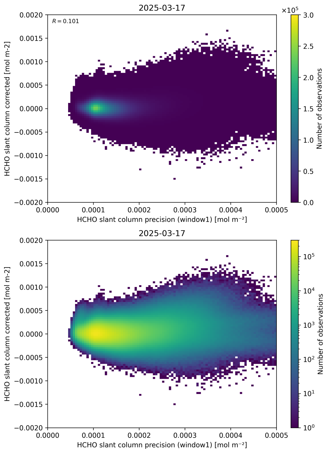
Figure 92: Scatter density plot of “HCHO slant column precision (window1)” against “HCHO slant column corrected” for 2025-03-17 to 2025-03-18.
