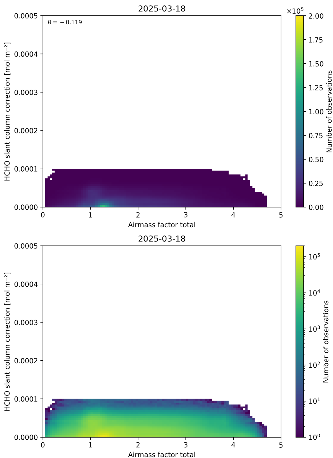
Figure 102: Scatter density plot of “Airmass factor total” against “HCHO slant column correction” for 2025-03-17 to 2025-03-19.
