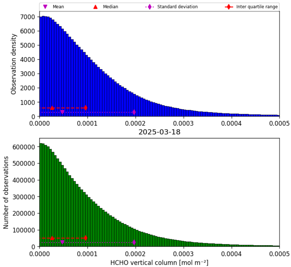
Figure 35: Histogram of “HCHO vertical column” for 2025-03-17 to 2025-03-19
