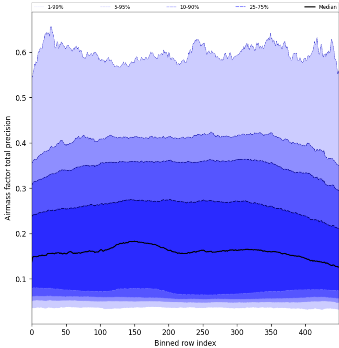
Figure 55: Along track statistics of “Airmass factor total precision” for 2025-03-17 to 2025-03-19
