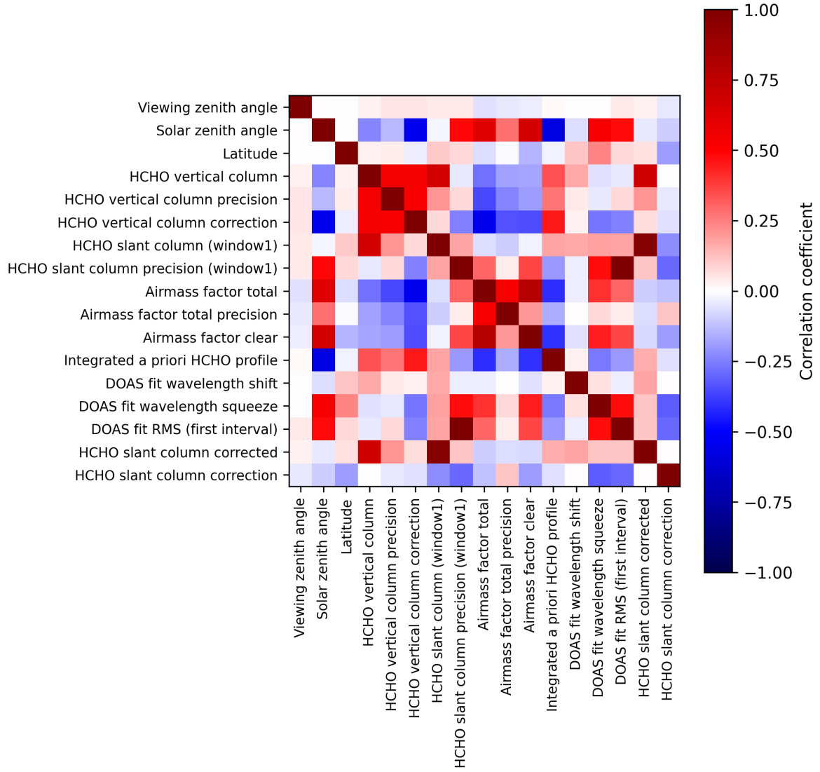
Figure 2: Map of correlation matrix for 2025-03-17 to 2025-03-19.
