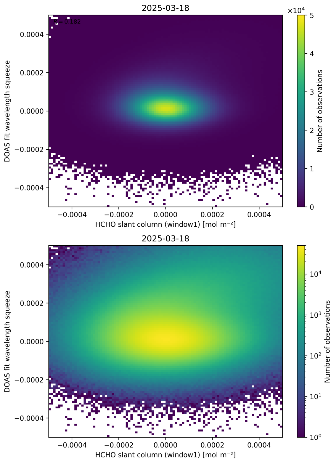
Figure 80: Scatter density plot of “HCHO slant column (window1)” against “DOAS fit wavelength squeeze” for 2025-03-17 to 2025-03-19.
