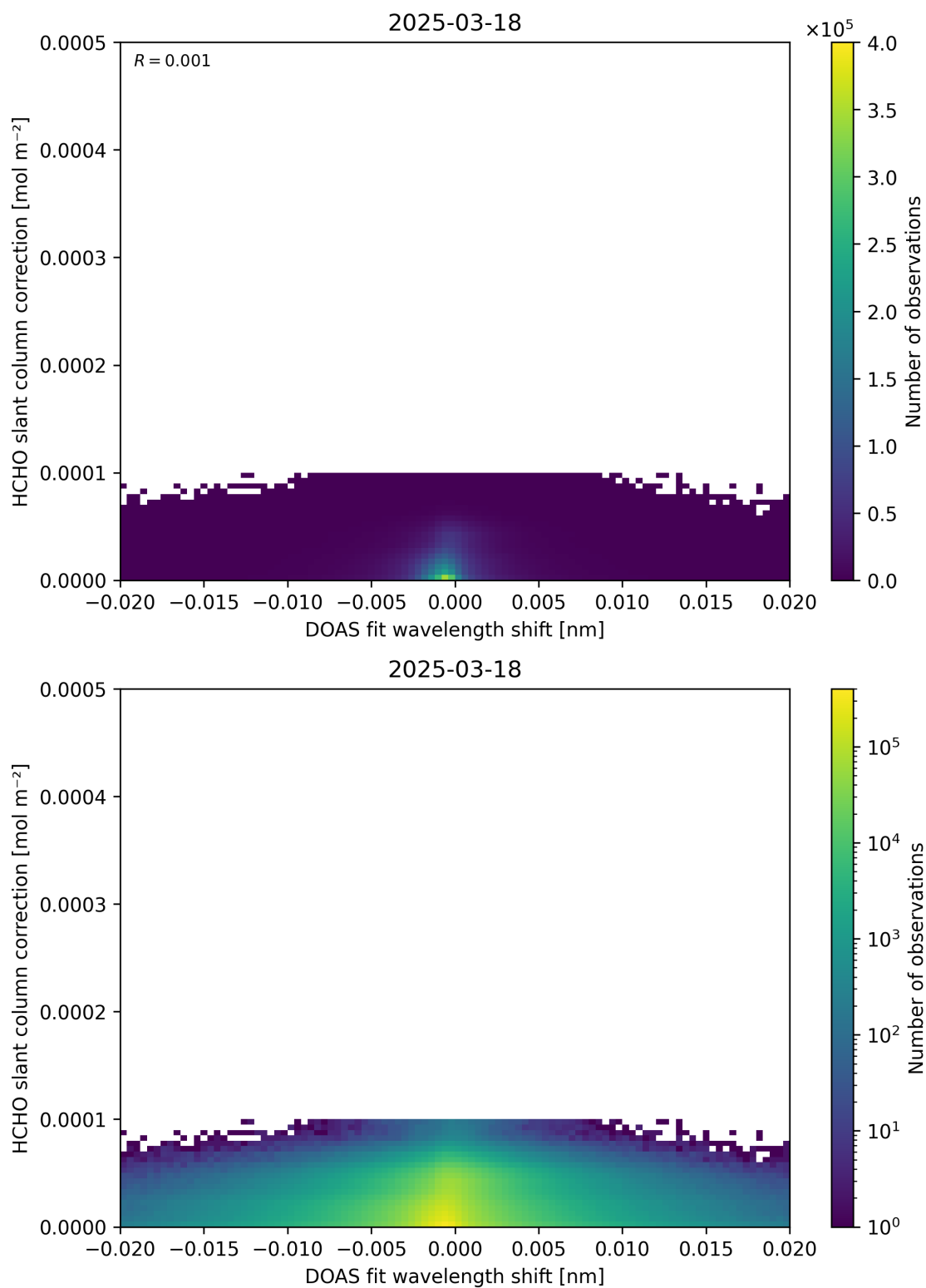
Figure 67: Scatter density plot of “DOAS fit wavelength shift” against “HCHO slant column correction” for 2025-03-17 to 2025-03-19.
