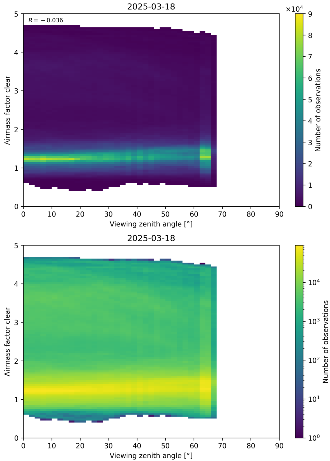
Figure 185: Scatter density plot of “Viewing zenith angle” against “Airmass factor clear” for 2025-03-17 to 2025-03-19.
