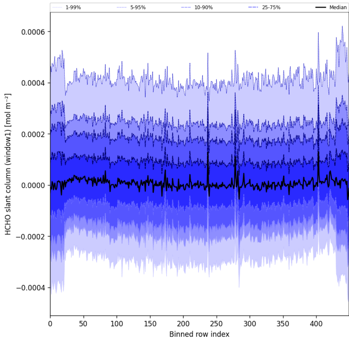
Figure 52: Along track statistics of “HCHO slant column (window1)” for 2025-03-17 to 2025-03-19
