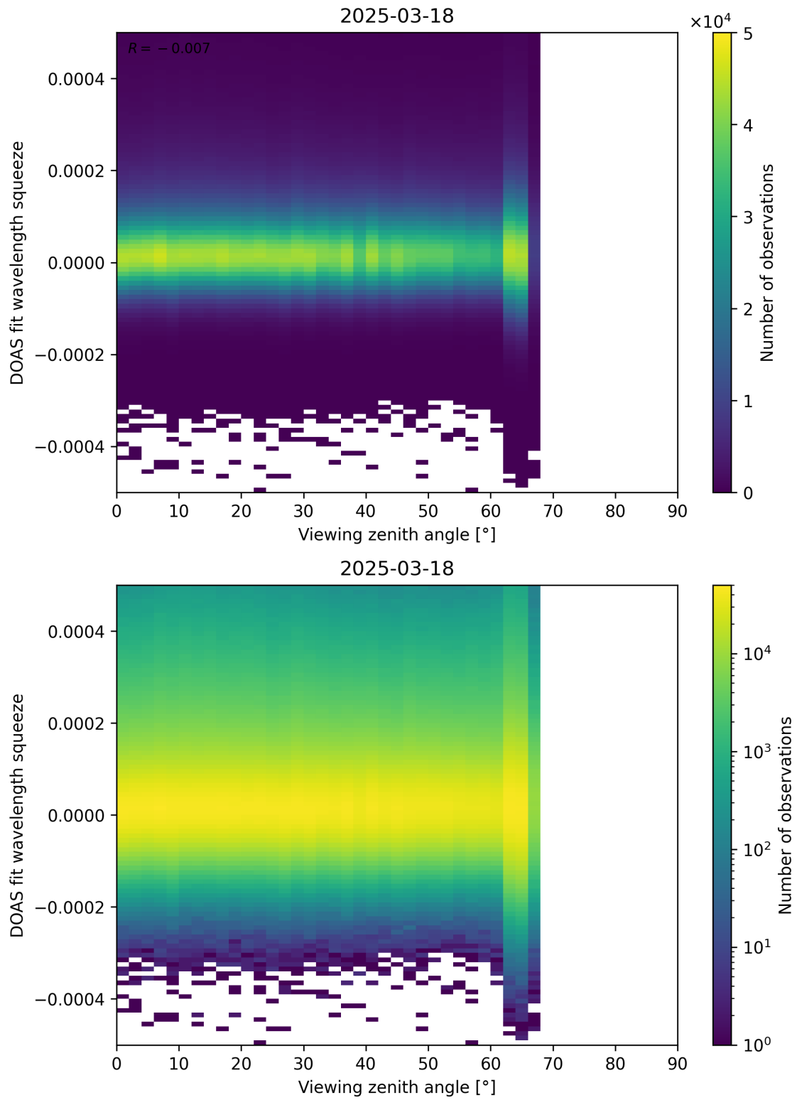
Figure 184: Scatter density plot of “Viewing zenith angle” against “DOAS fit wavelength squeeze” for 2025-03-17 to 2025-03-19.
