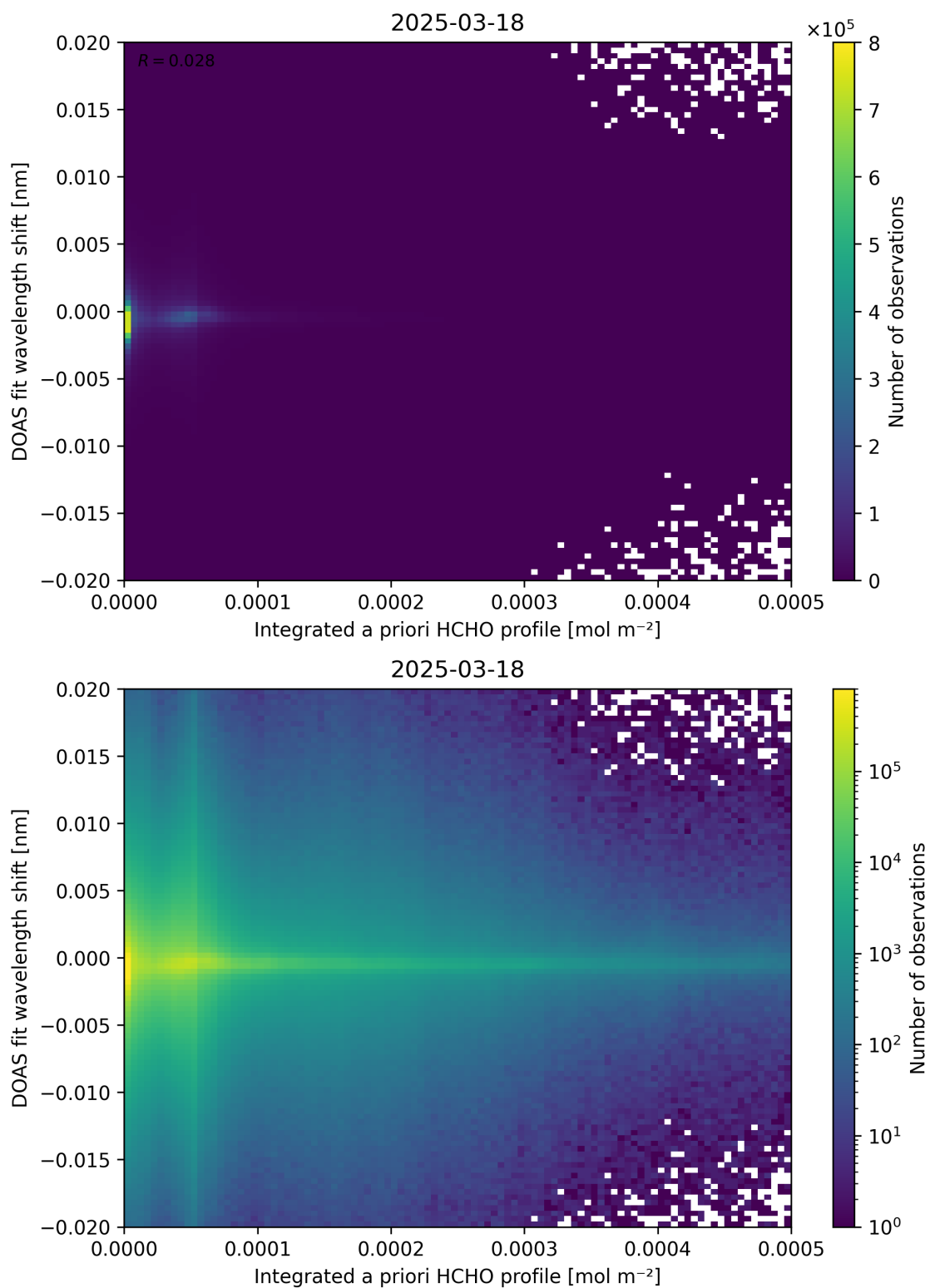
Figure 149: Scatter density plot of “Integrated a priori HCHO profile” against “DOAS fit wavelength shift” for 2025-03-17 to 2025-03-19.
