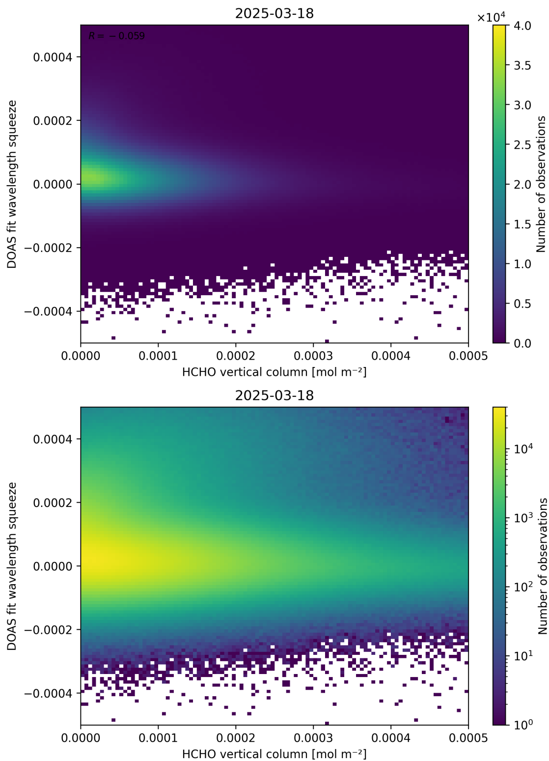
Figure 125: Scatter density plot of “HCHO vertical column” against “DOAS fit wavelength squeeze” for 2025-03-17 to 2025-03-19.
