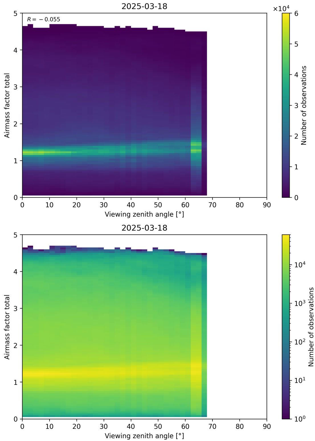
Figure 190: Scatter density plot of “Viewing zenith angle” against “Airmass factor total” for 2025-03-17 to 2025-03-19.
