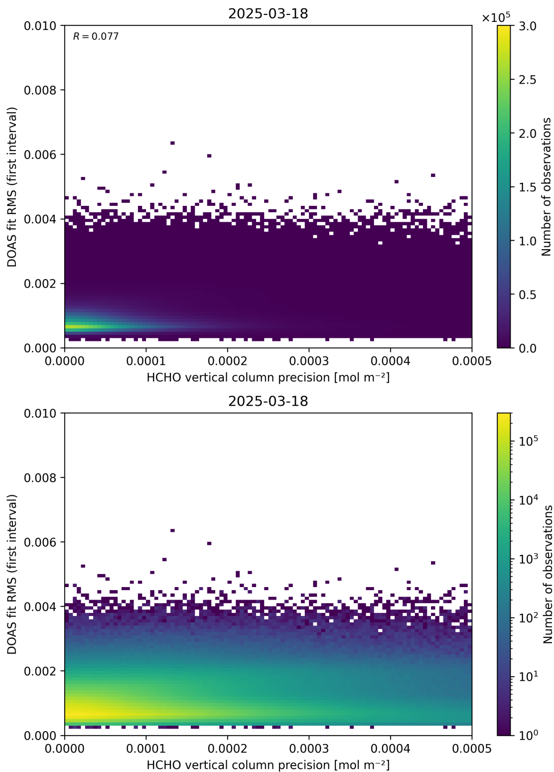
Figure 136: Scatter density plot of “HCHO vertical column precision” against “DOAS fit RMS (first interval)” for 2025-03-17 to 2025-03-19.
