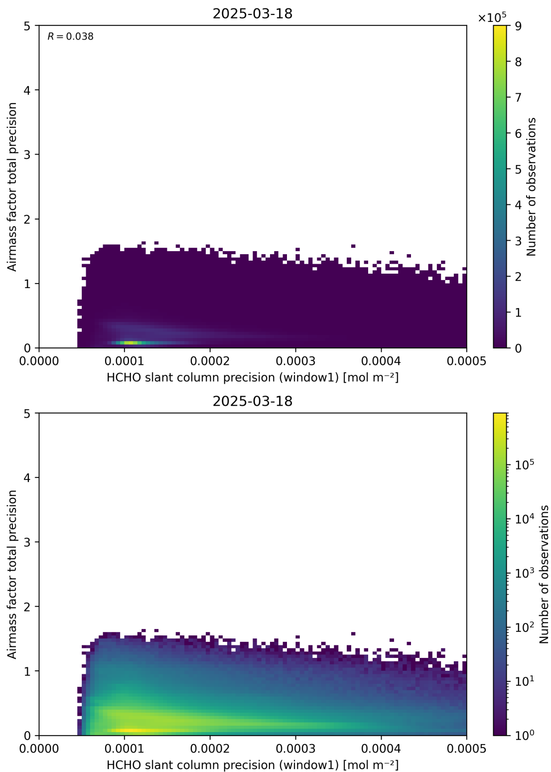
Figure 95: Scatter density plot of “HCHO slant column precision (window1)” against “Airmass factor total precision” for 2025-03-17 to 2025-03-19.
