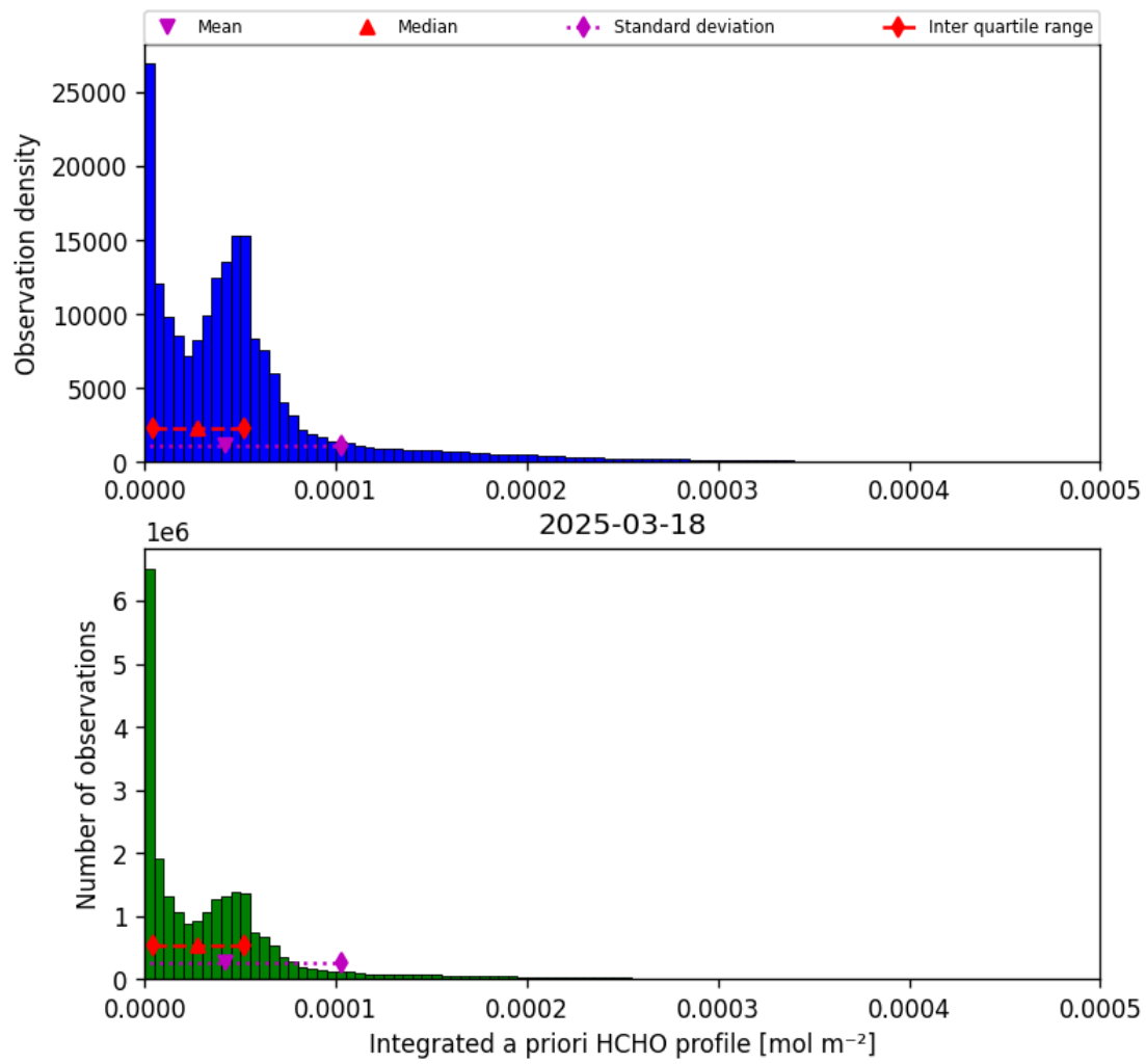
Figure 43: Histogram of “Integrated a priori HCHO profile” for 2025-03-17 to 2025-03-19
