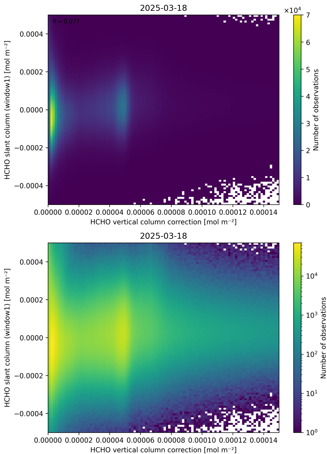
Figure 118: Scatter density plot of “HCHO vertical column correction” against “HCHO slant column (window1)” for 2025-03-17 to 2025-03-19.
