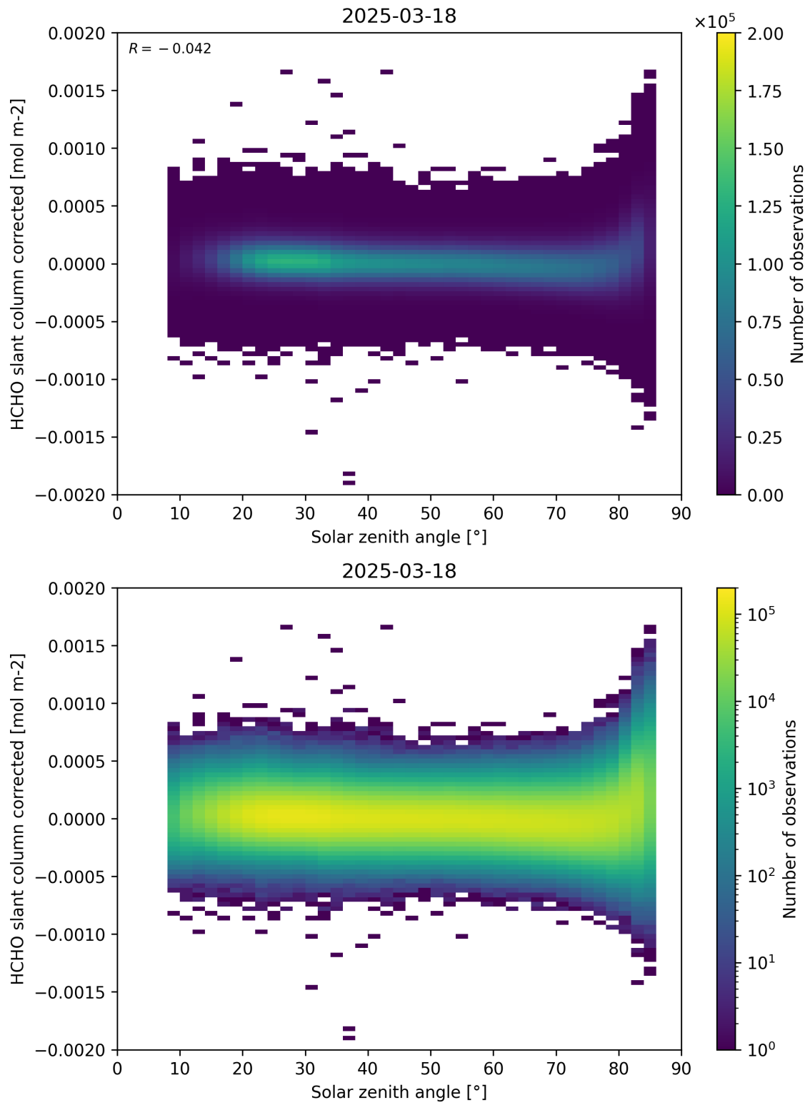
Figure 171: Scatter density plot of “Solar zenith angle” against “HCHO slant column corrected” for 2025-03-17 to 2025-03-19.
