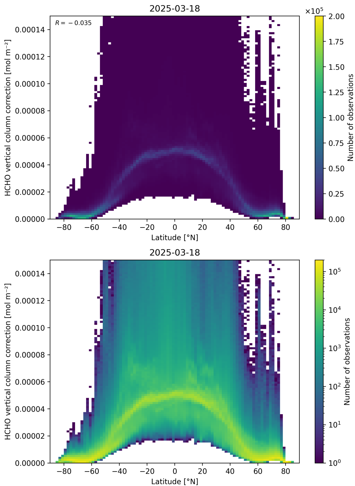
Figure 164: Scatter density plot of “Latitude” against “HCHO vertical column correction” for 2025-03-17 to 2025-03-19.
