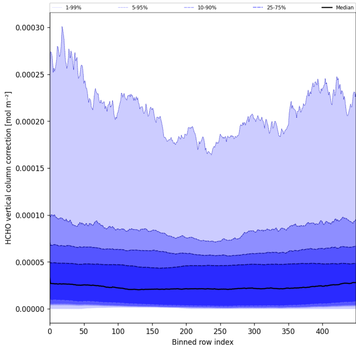
Figure 51: Along track statistics of “HCHO vertical column correction” for 2025-03-17 to 2025-03-19
