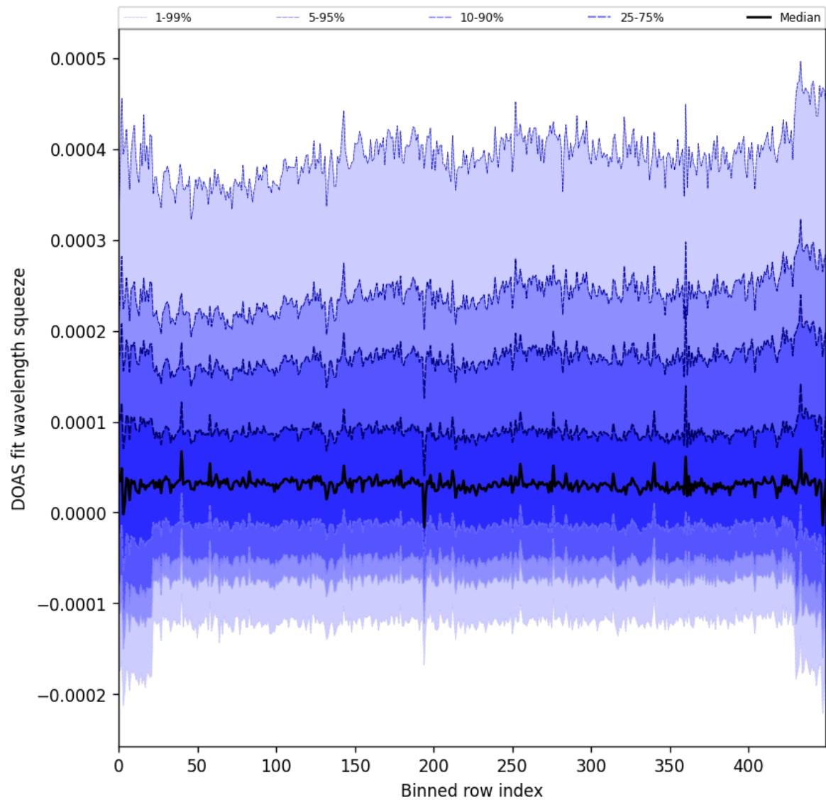
Figure 59: Along track statistics of “DOAS fit wavelength squeeze” for 2025-03-17 to 2025-03-19
