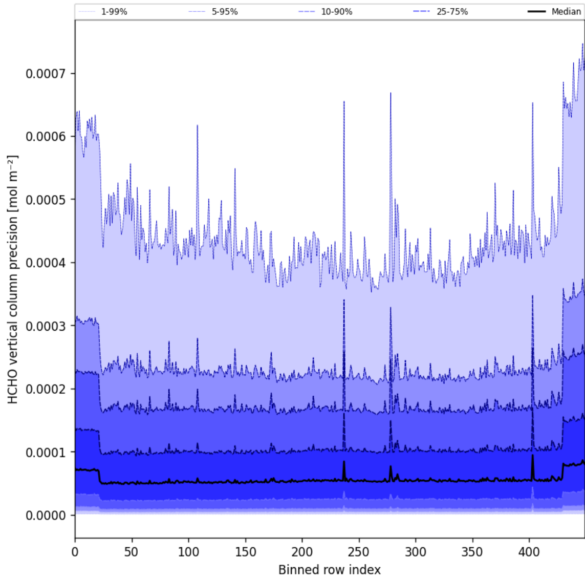
Figure 50: Along track statistics of “HCHO vertical column precision” for 2025-03-17 to 2025-03-19
