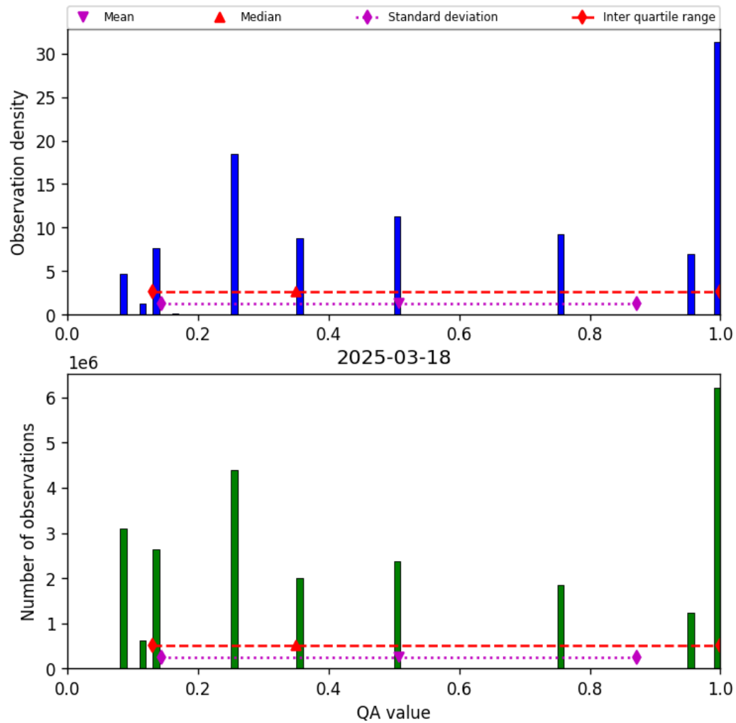
Figure 34: Histogram of “QA value” for 2025-03-17 to 2025-03-19
