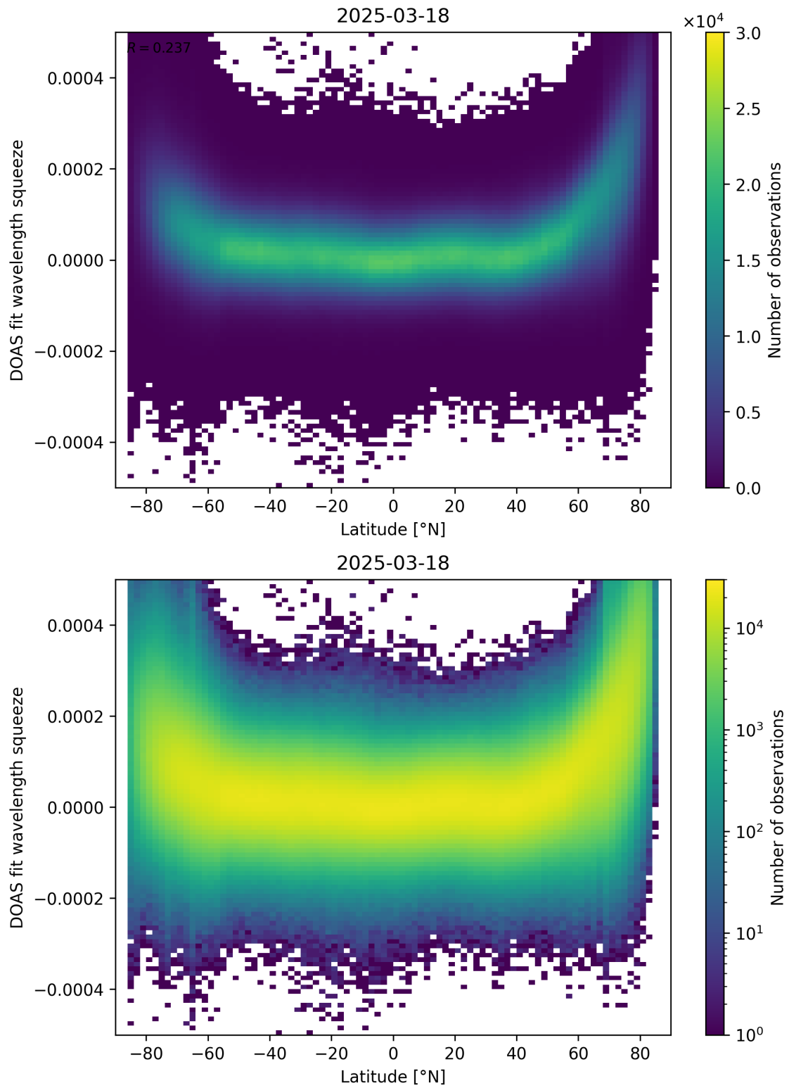
Figure 155: Scatter density plot of “Latitude” against “DOAS fit wavelength squeeze” for 2025-03-17 to 2025-03-19.
