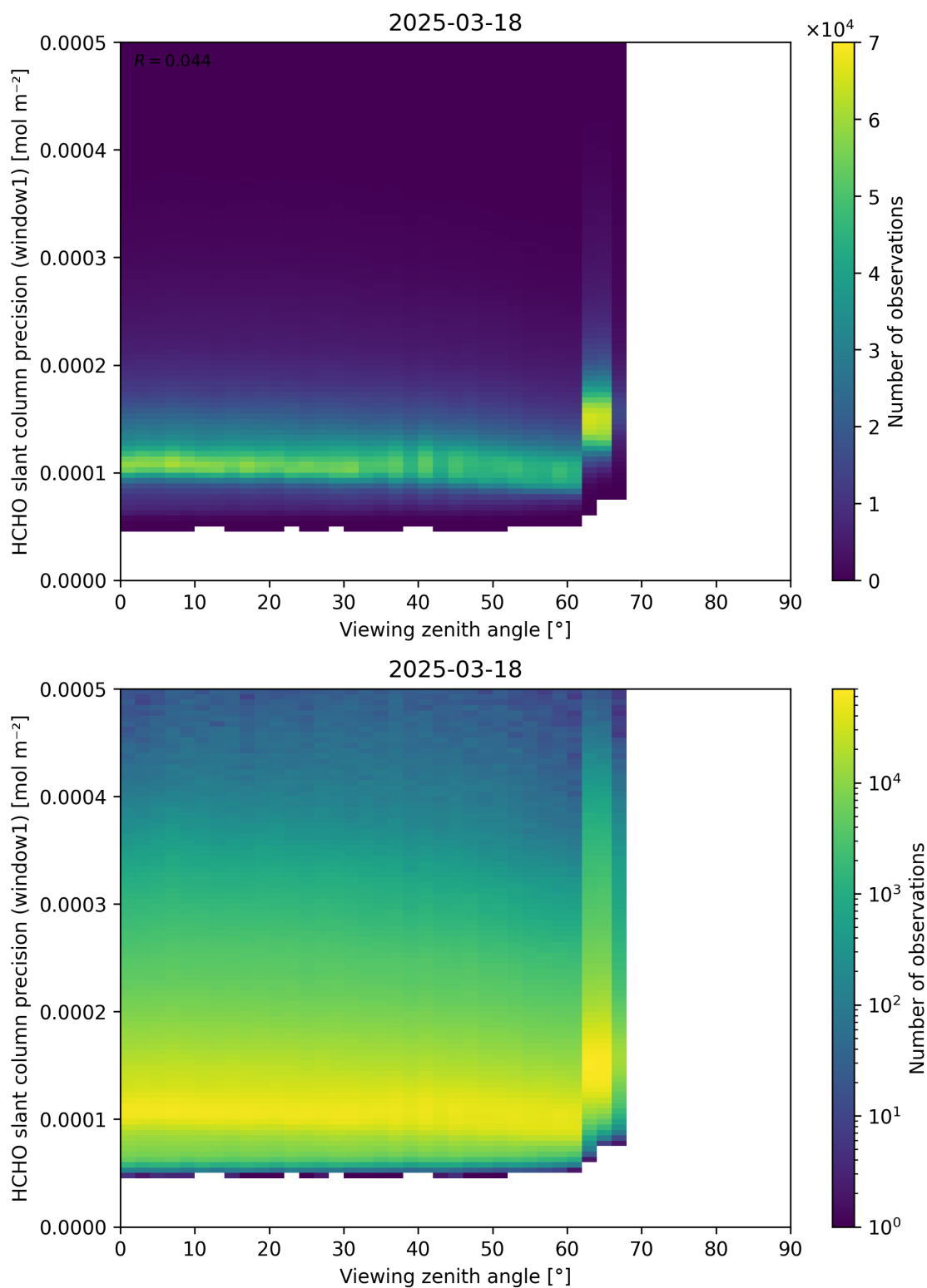
Figure 189: Scatter density plot of “Viewing zenith angle” against “HCHO slant column precision (window1)” for 2025-03-17 to 2025-03-19.
