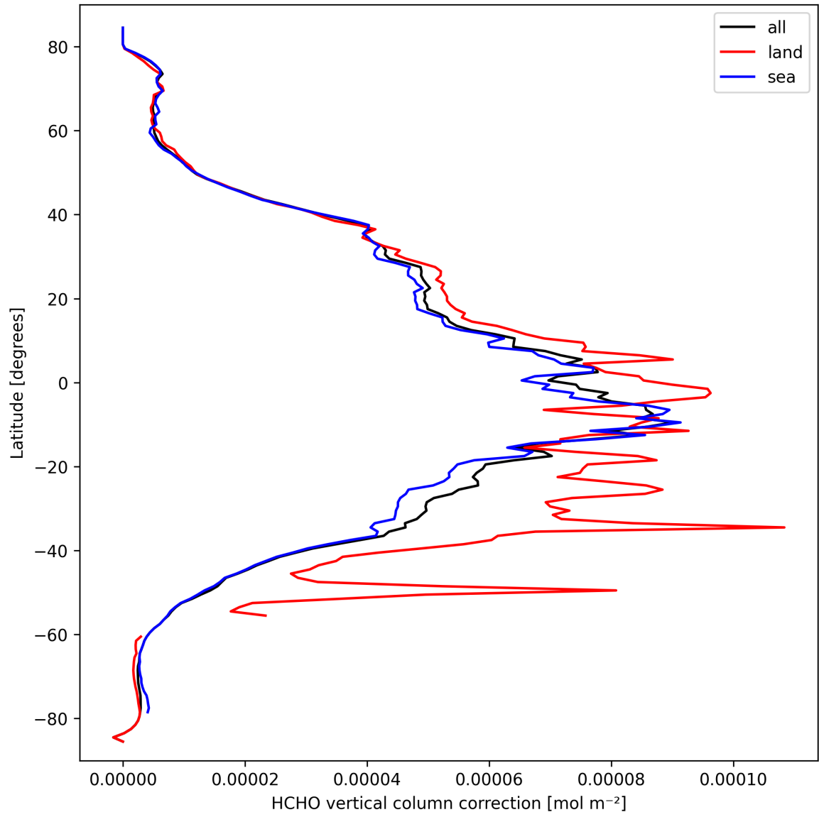
Figure 23: Zonal average of “HCHO vertical column correction” for 2025-03-17 to 2025-03-19.
