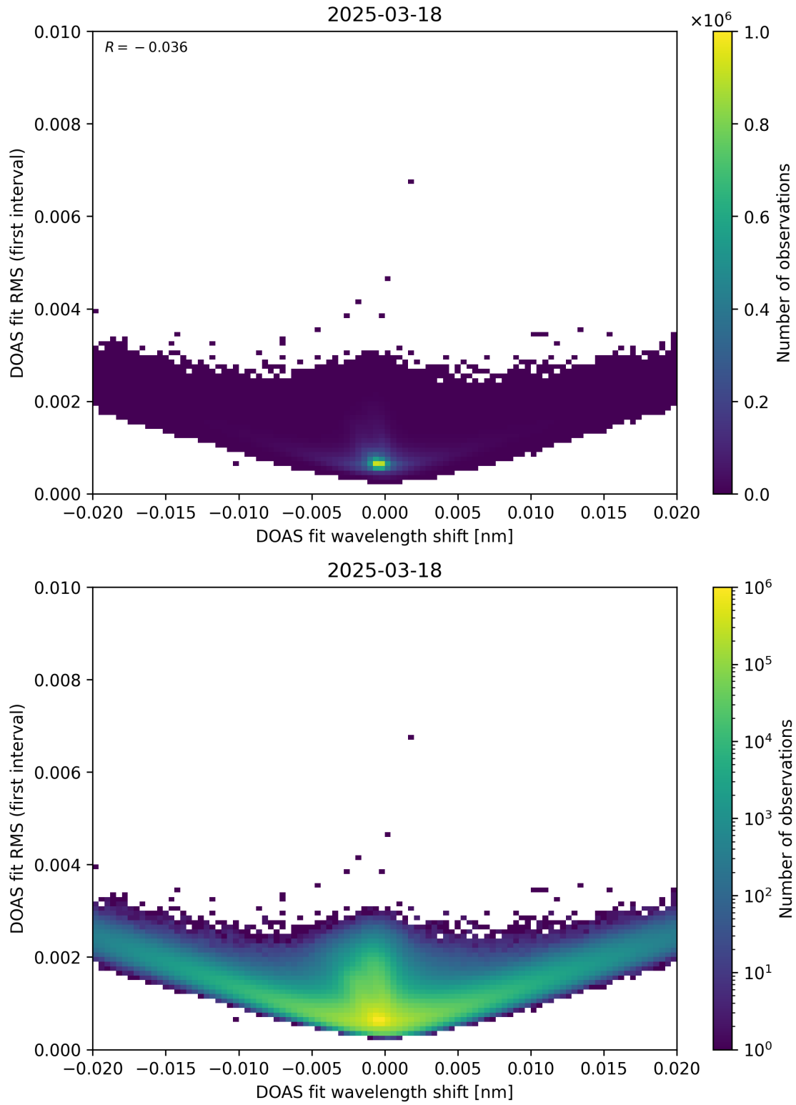
Figure 64: Scatter density plot of “DOAS fit wavelength shift” against “DOAS fit RMS (first interval)” for 2025-03-17 to 2025-03-19.
