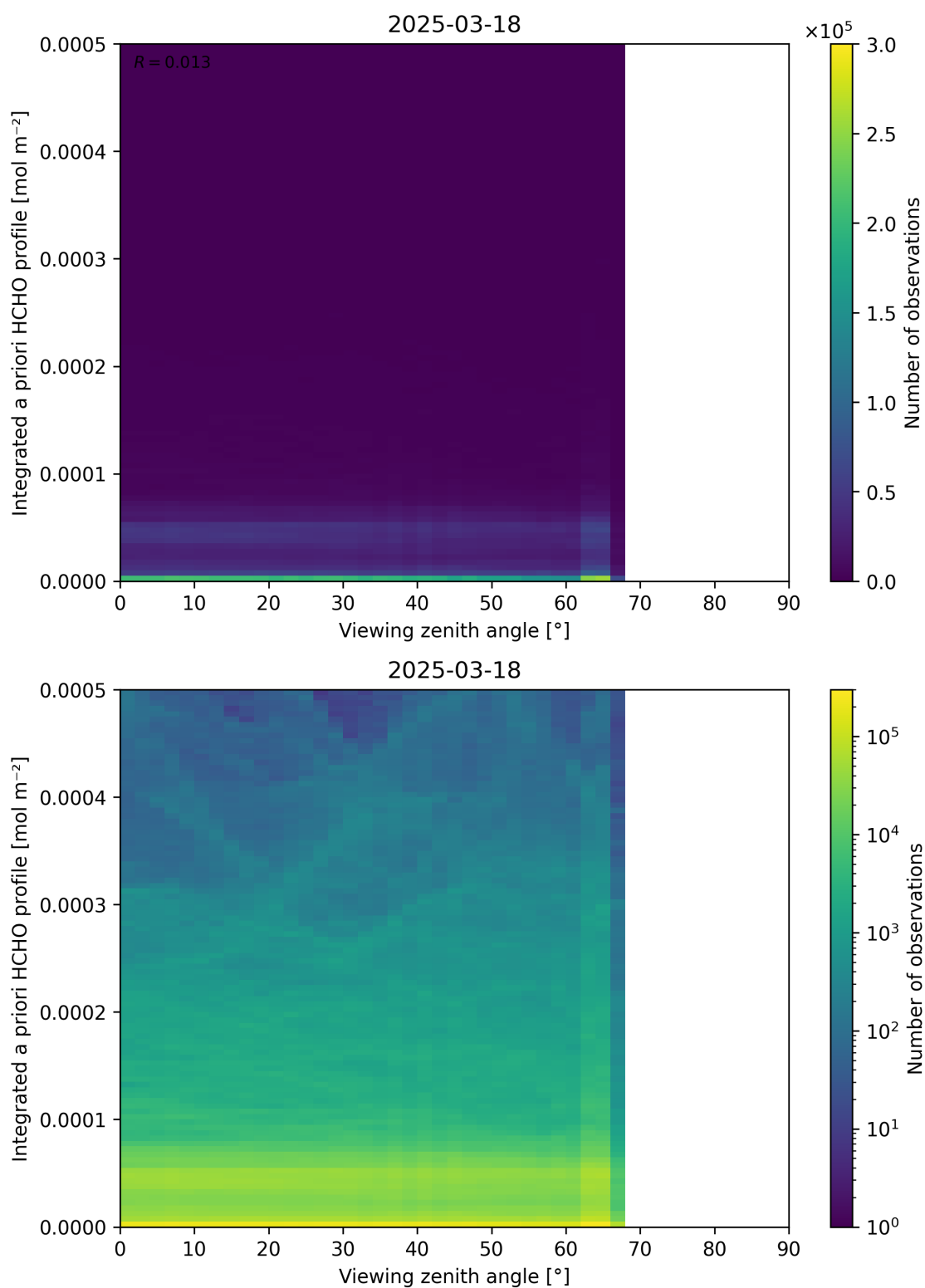
Figure 195: Scatter density plot of “Viewing zenith angle” against “Integrated a priori HCHO profile” for 2025-03-17 to 2025-03-19.
