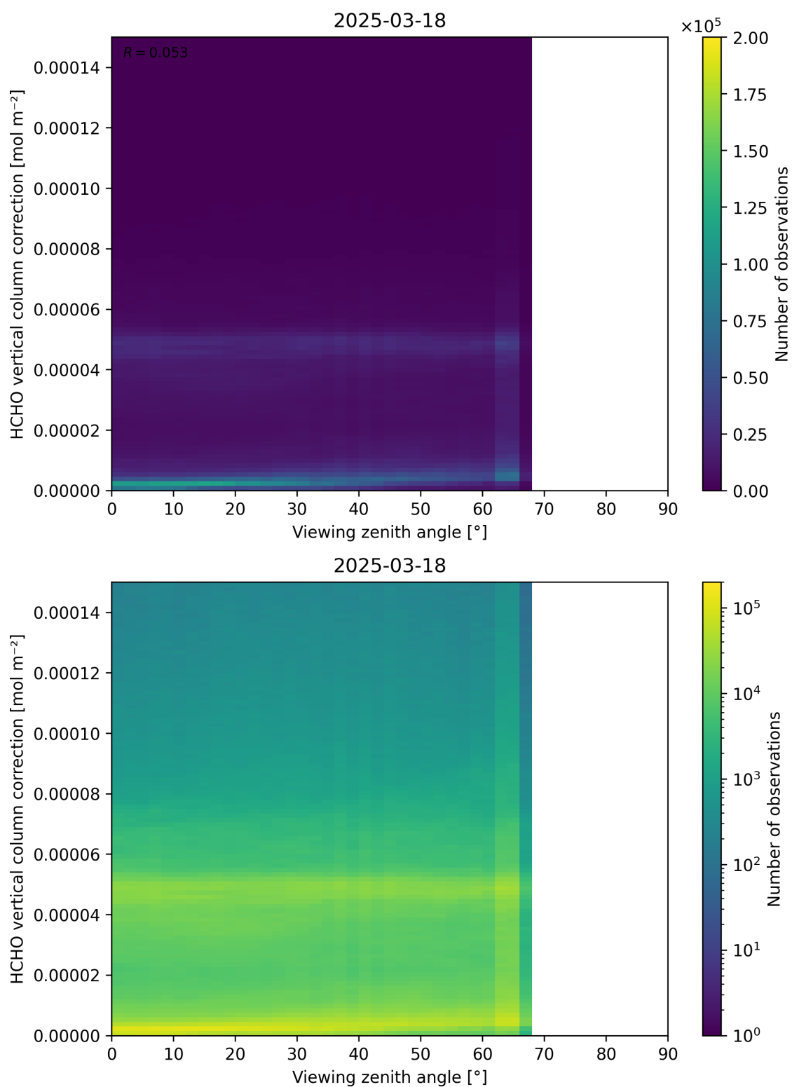
Figure 193: Scatter density plot of “Viewing zenith angle” against “HCHO vertical column correction” for 2025-03-17 to 2025-03-19.
