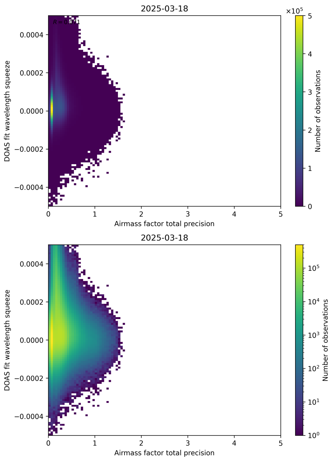
Figure 107: Scatter density plot of “Airmass factor total precision” against “DOAS fit wavelength squeeze” for 2025-03-17 to 2025-03-19.
