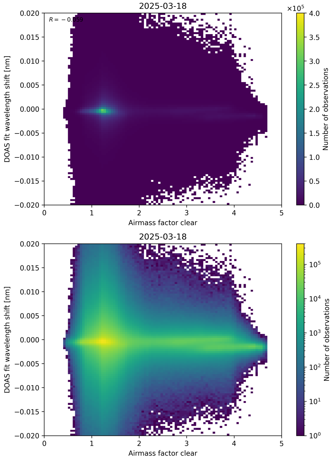
Figure 72: Scatter density plot of “Airmass factor clear” against “DOAS fit wavelength shift” for 2025-03-17 to 2025-03-19.
