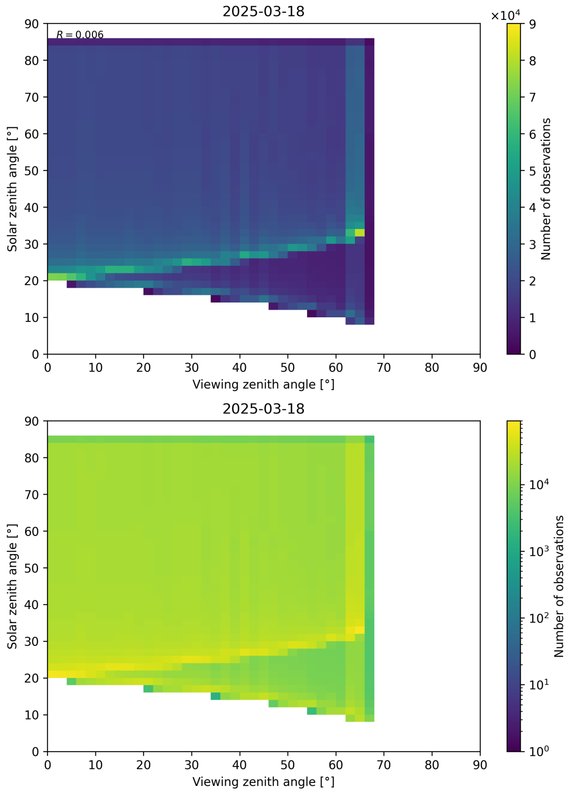
Figure 197: Scatter density plot of “Viewing zenith angle” against “Solar zenith angle” for 2025-03-17 to 2025-03-19.
