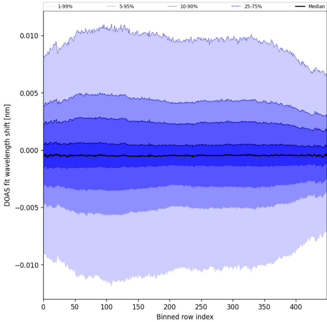
Figure 58: Along track statistics of “DOAS fit wavelength shift” for 2025-03-17 to 2025-03-19
