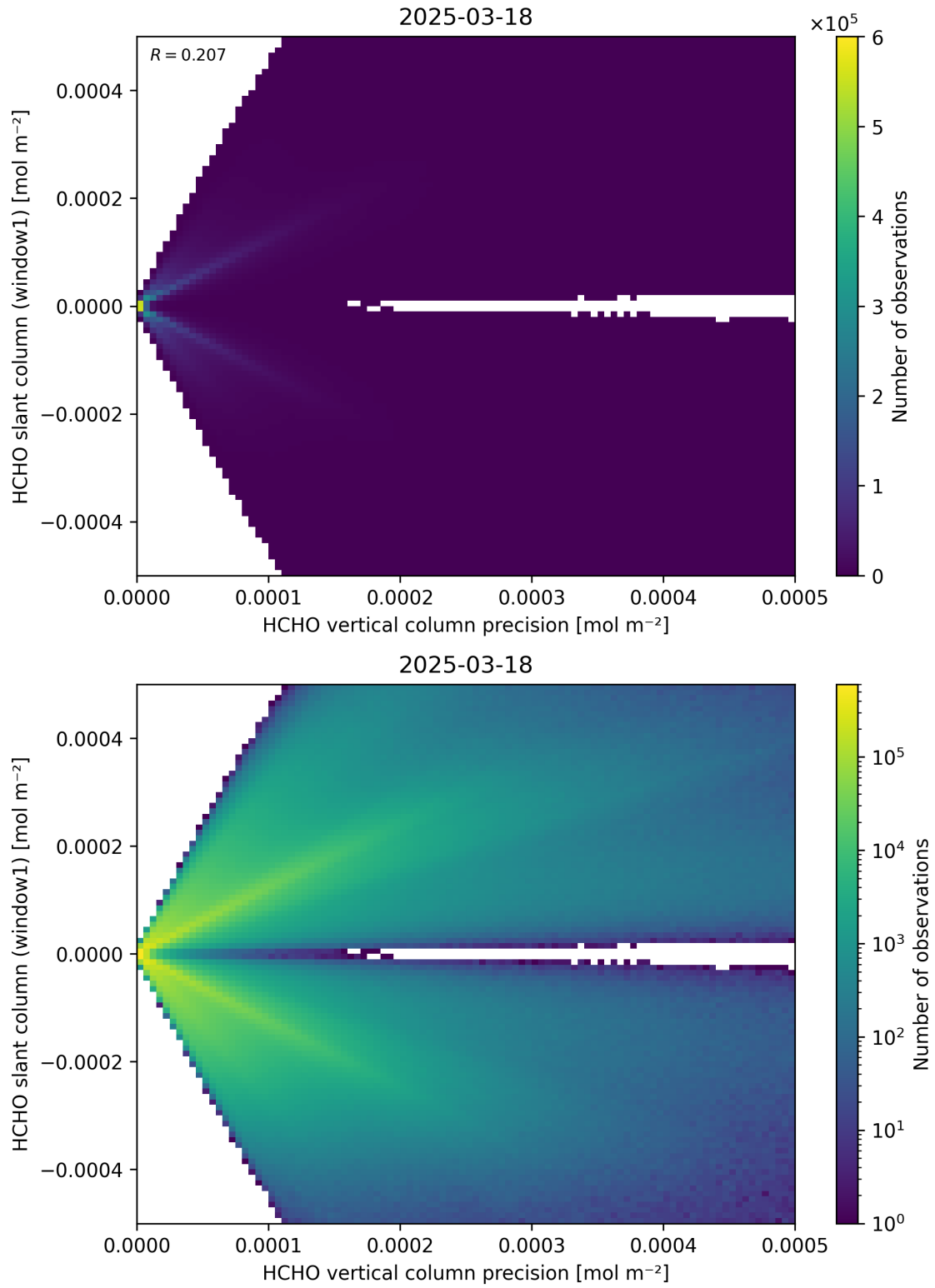
Figure 142: Scatter density plot of “HCHO vertical column precision” against “HCHO slant column (window1)” for 2025-03-17 to 2025-03-19.
