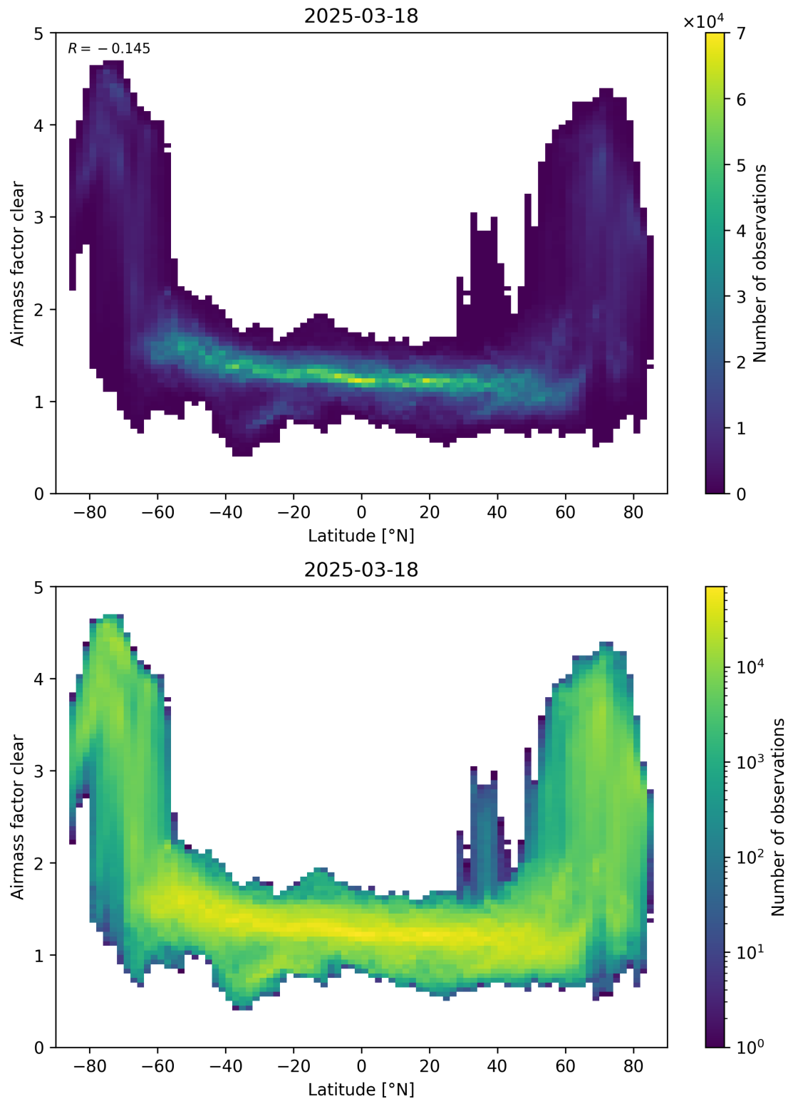
Figure 156: Scatter density plot of “Latitude” against “Airmass factor clear” for 2025-03-17 to 2025-03-19.
