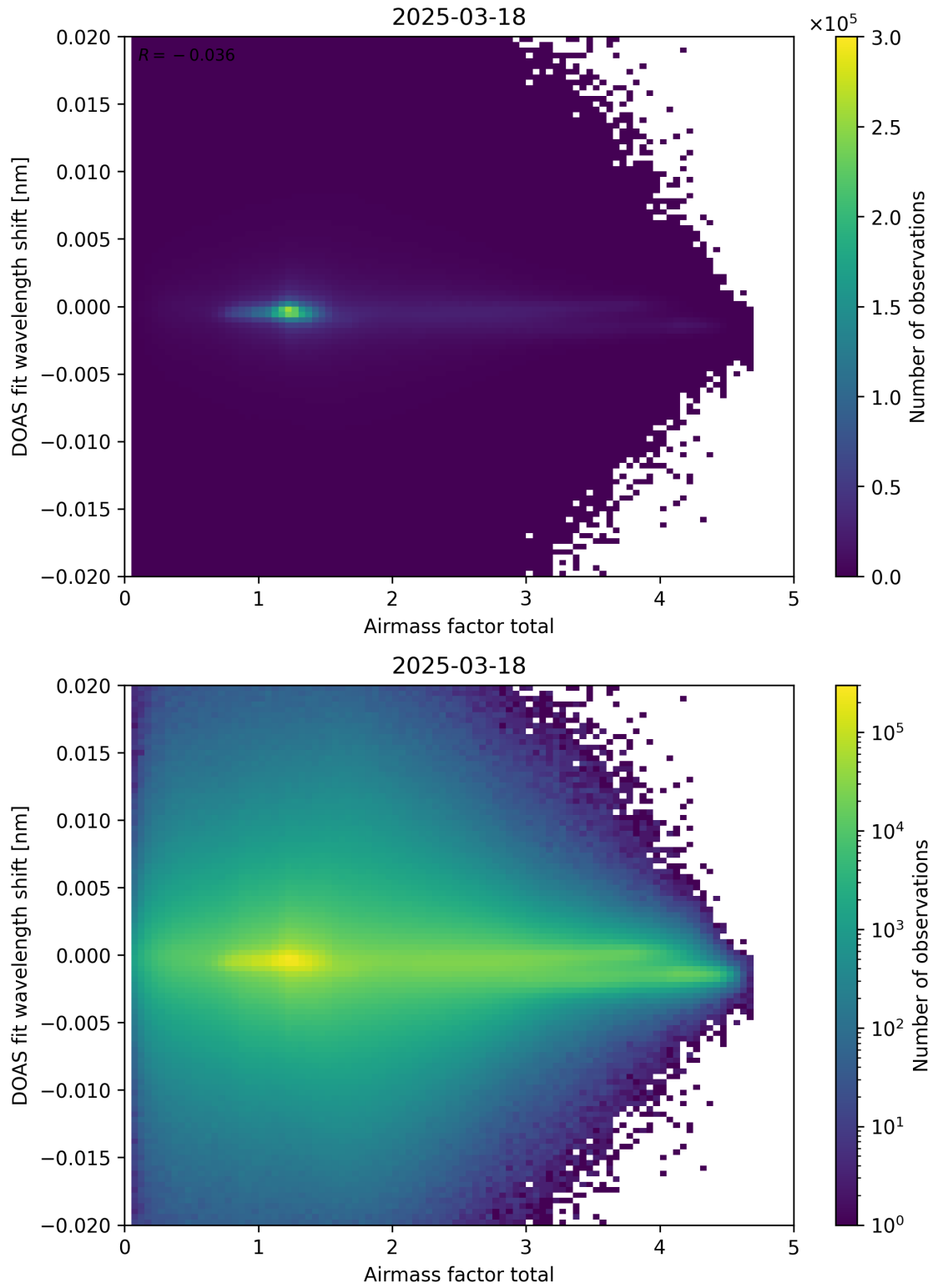
Figure 98: Scatter density plot of “Airmass factor total” against “DOAS fit wavelength shift” for 2025-03-17 to 2025-03-19.
