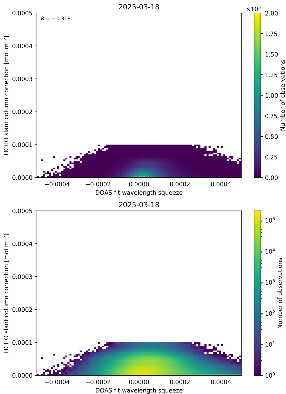
Figure 70: Scatter density plot of “DOAS fit wavelength squeeze” against “HCHO slant column correction” for 2025-03-17 to 2025-03-19.
