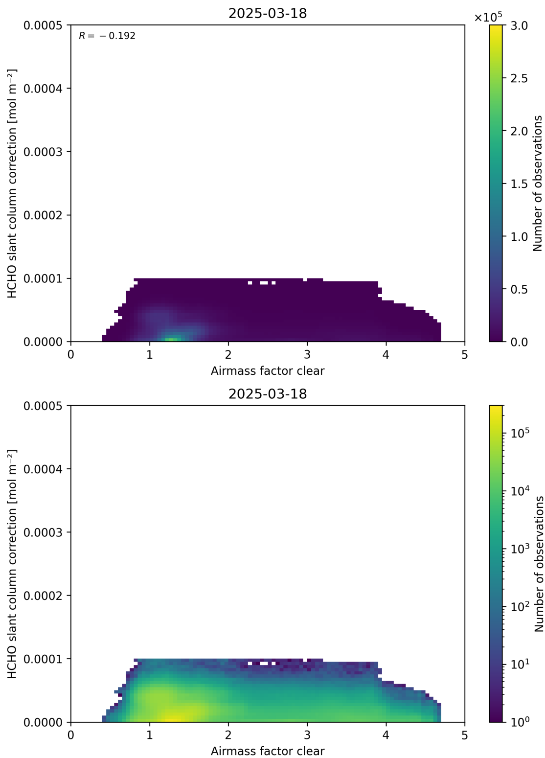
Figure 75: Scatter density plot of “Airmass factor clear” against “HCHO slant column correction” for 2025-03-17 to 2025-03-19.
