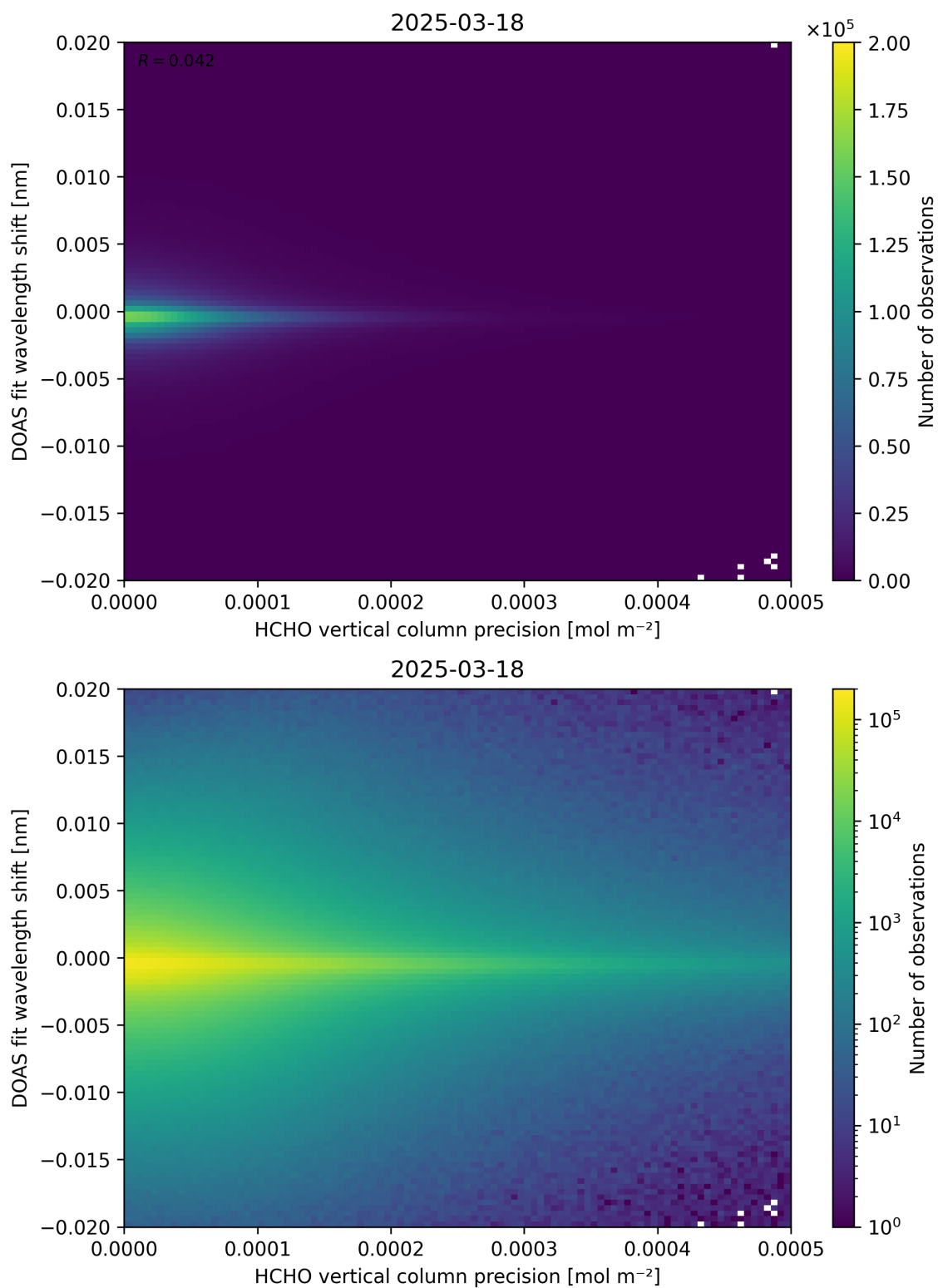
Figure 137: Scatter density plot of “HCHO vertical column precision” against “DOAS fit wavelength shift” for 2025-03-17 to 2025-03-19.
