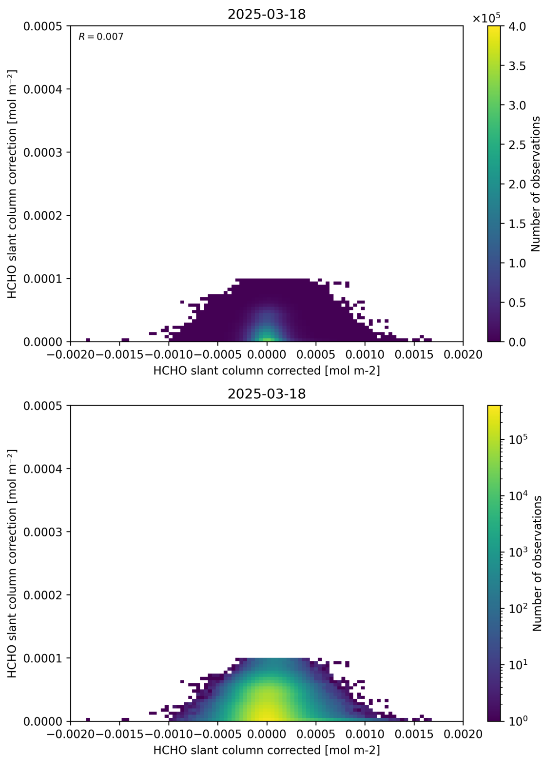
Figure 77: Scatter density plot of “HCHO slant column corrected” against “HCHO slant column correction” for 2025-03-17 to 2025-03-19.
