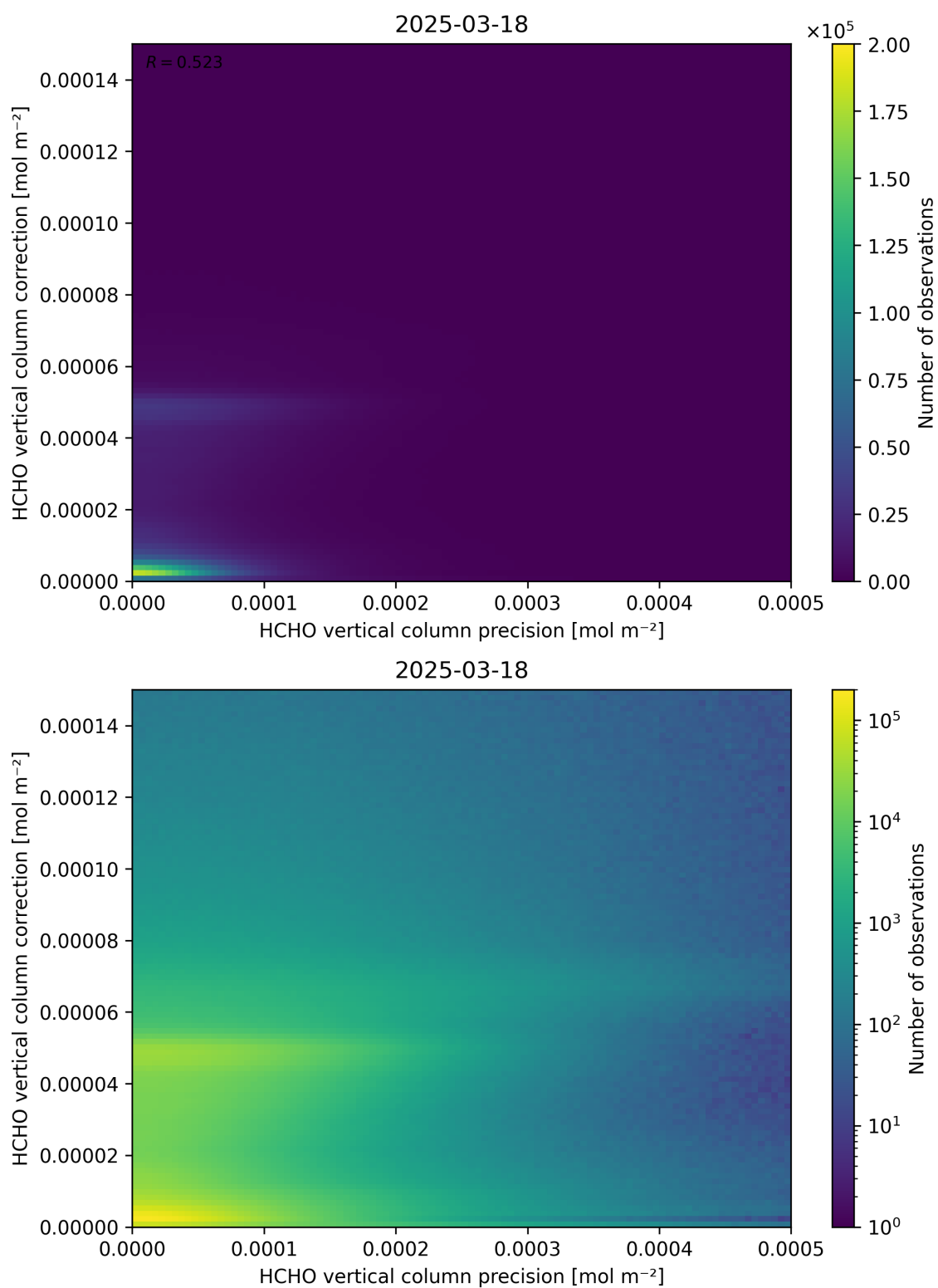
Figure 146: Scatter density plot of “HCHO vertical column precision” against “HCHO vertical column correction” for 2025-03-17 to 2025-03-19.
