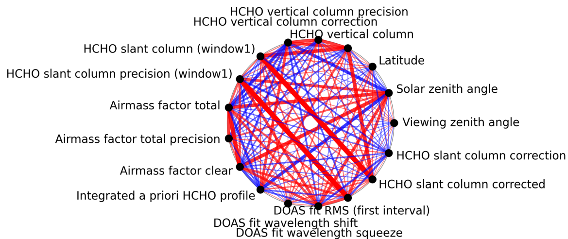
Figure 1: Map of correlation graph for 2025-03-17 to 2025-03-19.
