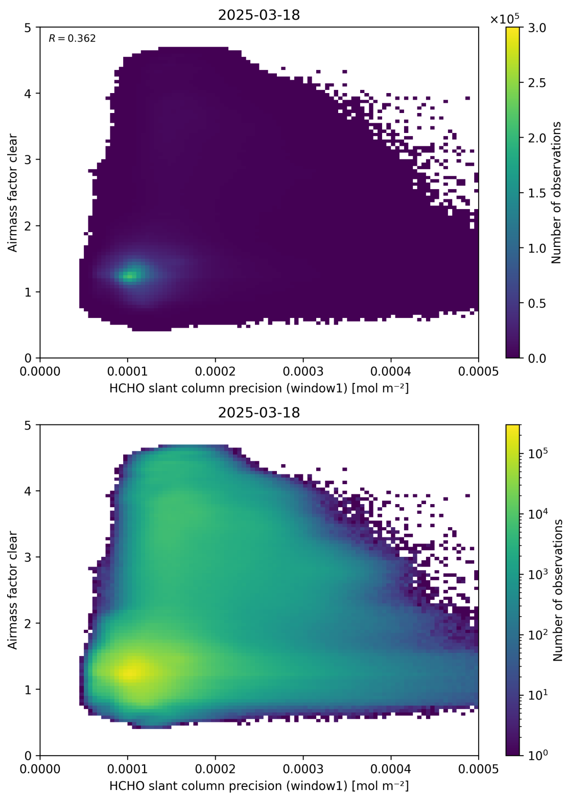
Figure 91: Scatter density plot of “HCHO slant column precision (window1)” against “Airmass factor clear” for 2025-03-17 to 2025-03-19.
