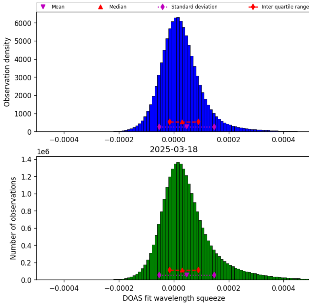
Figure 45: Histogram of “DOAS fit wavelength squeeze” for 2025-03-17 to 2025-03-19
