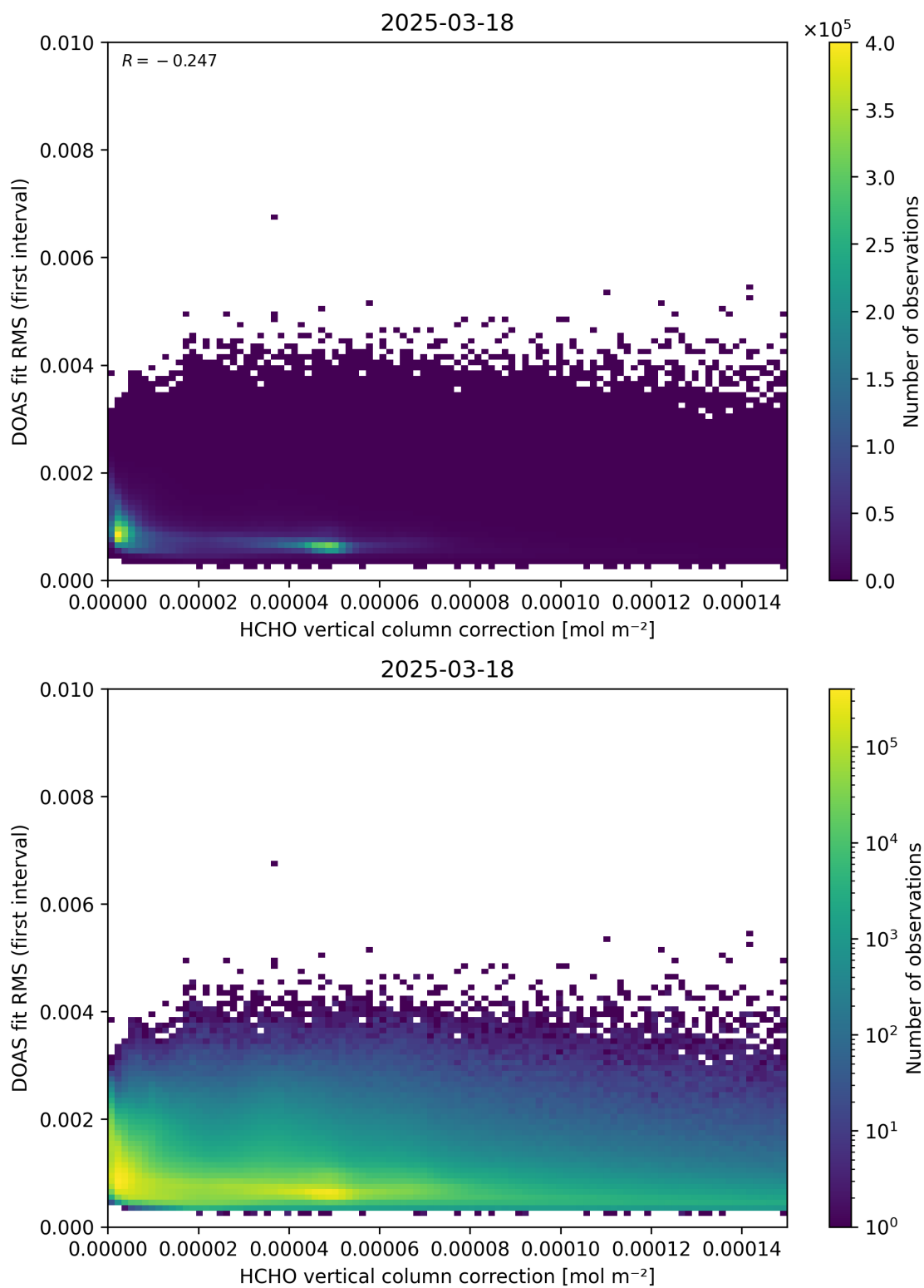
Figure 112: Scatter density plot of “HCHO vertical column correction” against “DOAS fit RMS (first interval)” for 2025-03-17 to 2025-03-19.
