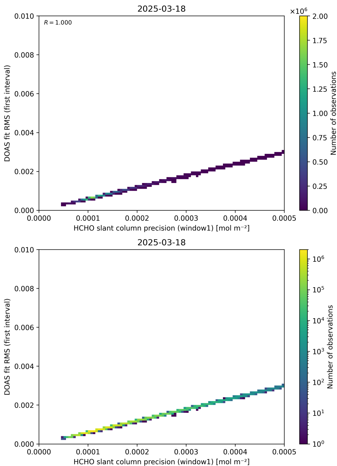
Figure 88: Scatter density plot of “HCHO slant column precision (window1)” against “DOAS fit RMS (first interval)” for 2025-03-17 to 2025-03-19.
