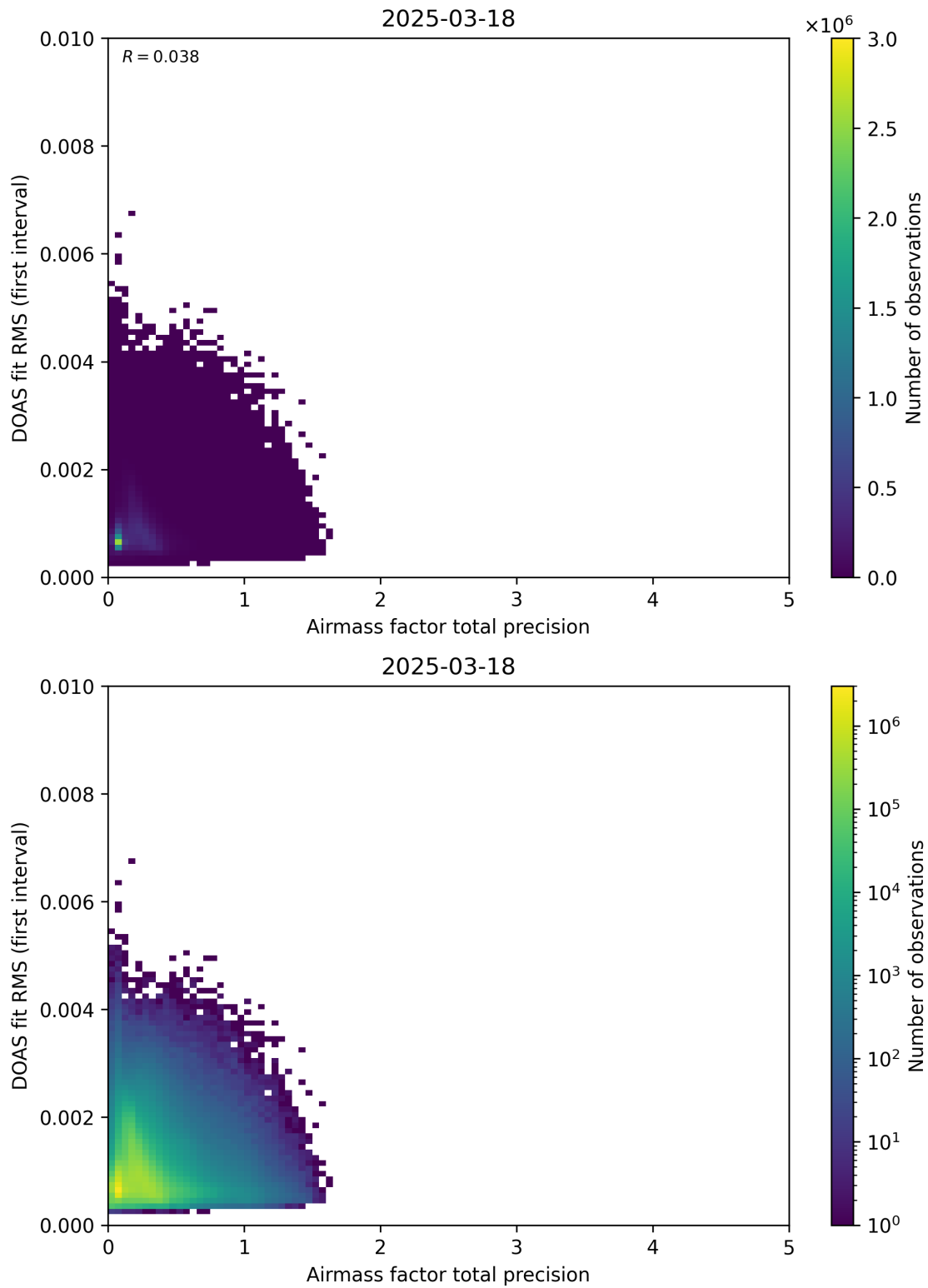
Figure 105: Scatter density plot of “Airmass factor total precision” against “DOAS fit RMS (first interval)” for 2025-03-17 to 2025-03-19.
