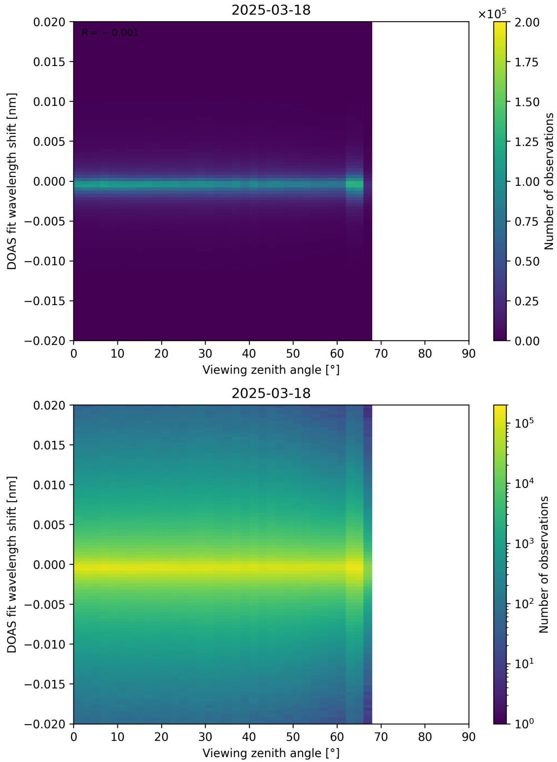
Figure 183: Scatter density plot of “Viewing zenith angle” against “DOAS fit wavelength shift” for 2025-03-17 to 2025-03-19.
