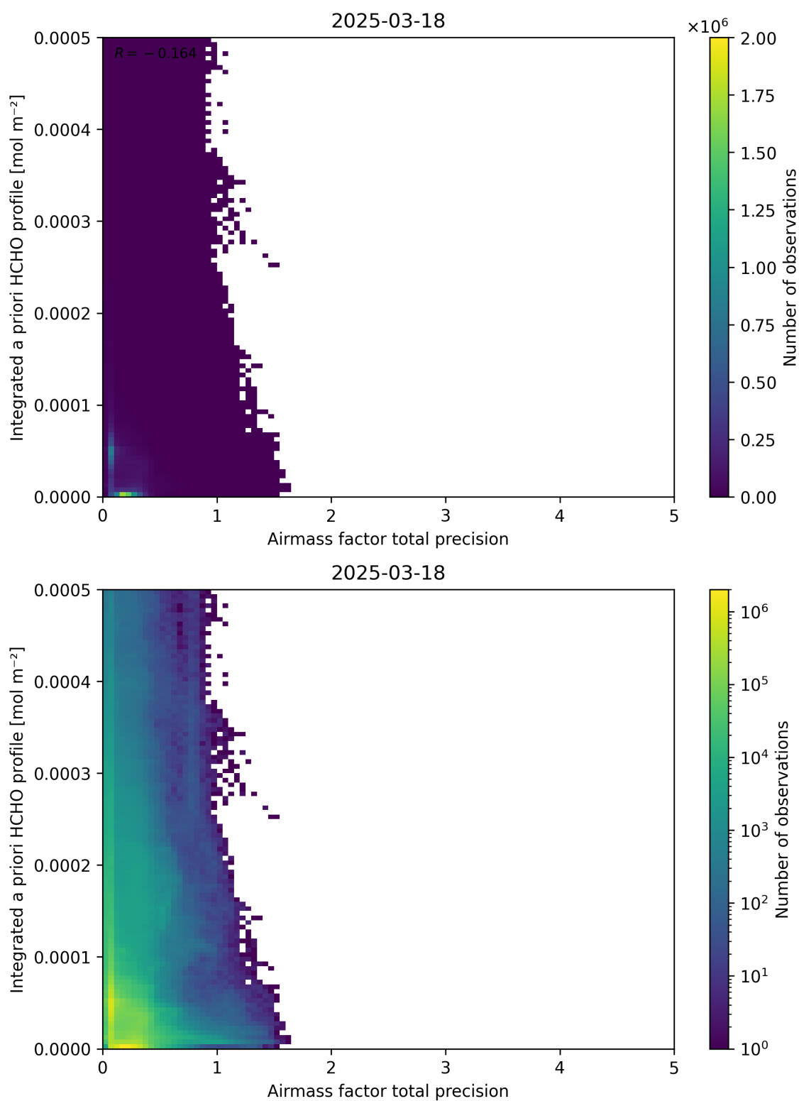
Figure 111: Scatter density plot of “Airmass factor total precision” against “Integrated a priori HCHO profile” for 2025-03-17 to 2025-03-19.
