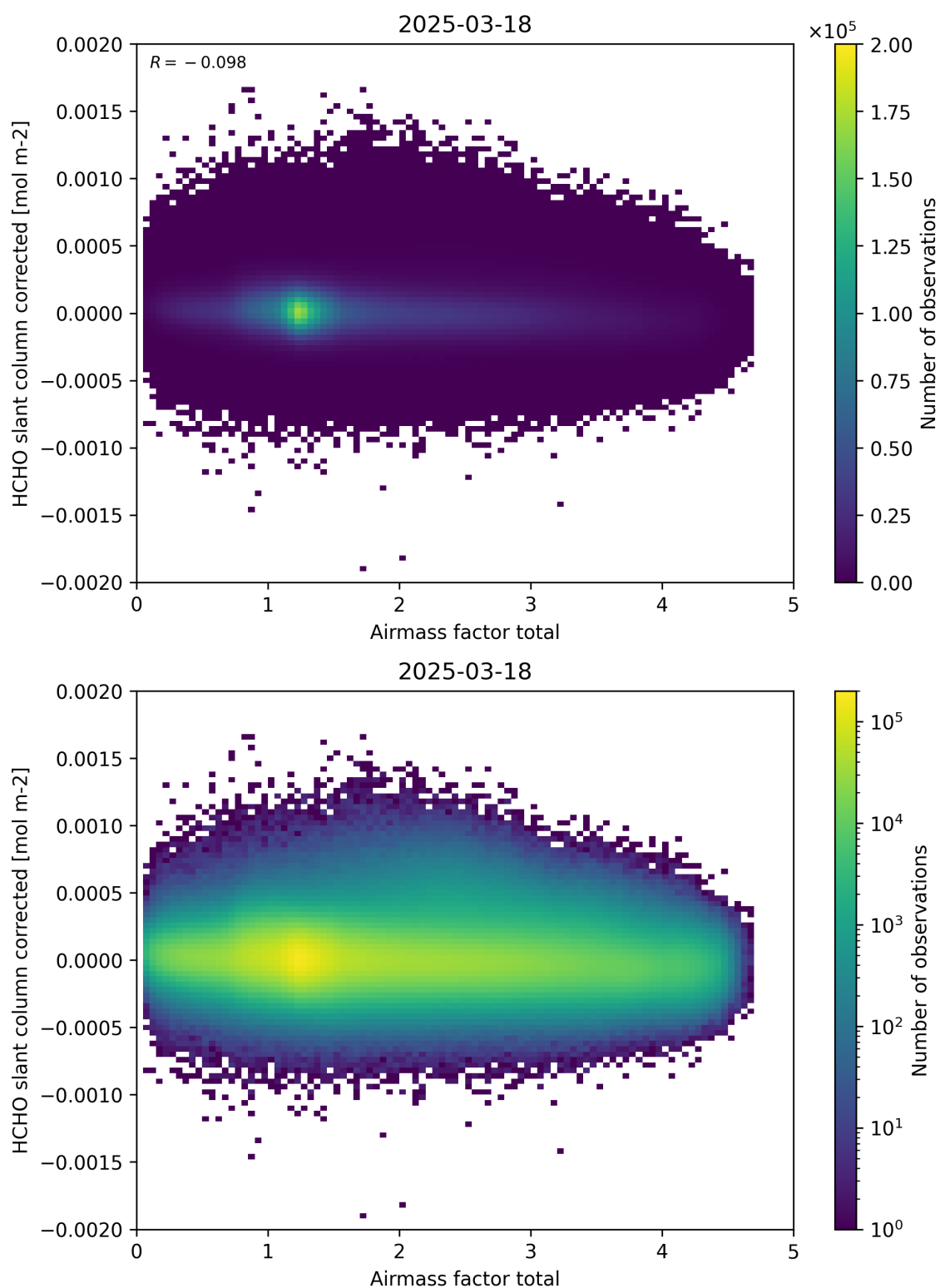
Figure 101: Scatter density plot of “Airmass factor total” against “HCHO slant column corrected” for 2025-03-17 to 2025-03-19.
