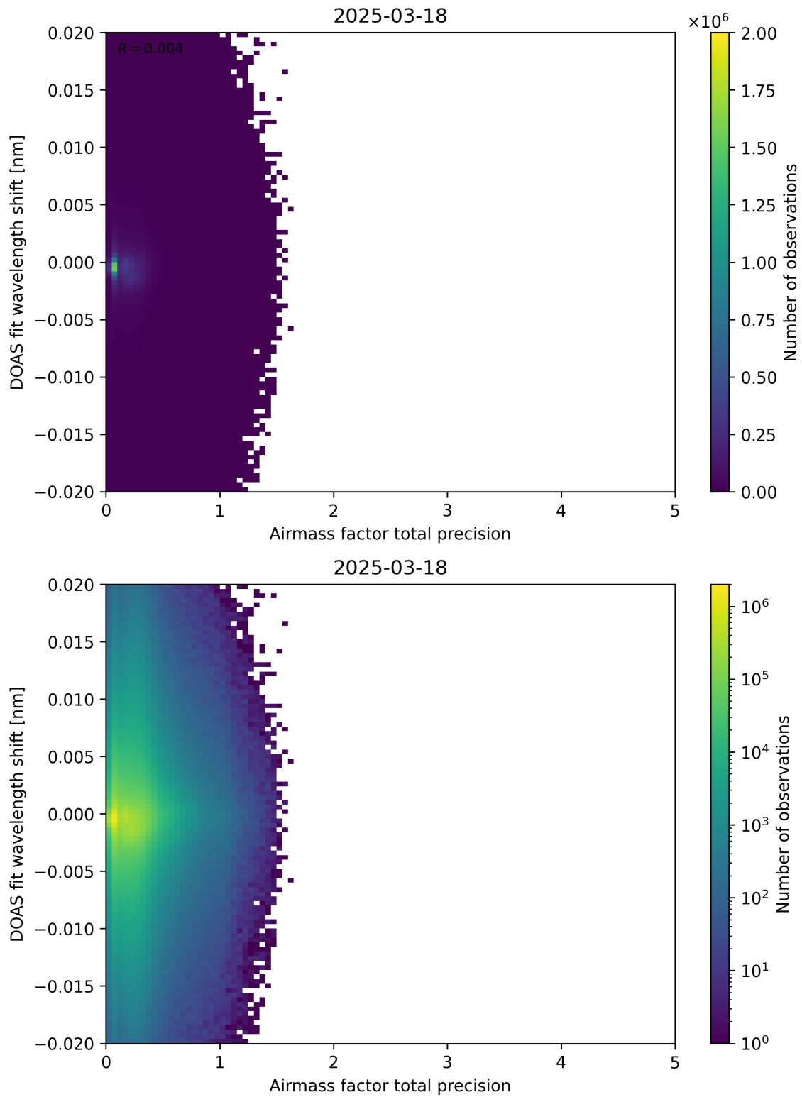
Figure 106: Scatter density plot of “Airmass factor total precision” against “DOAS fit wavelength shift” for 2025-03-17 to 2025-03-19.
