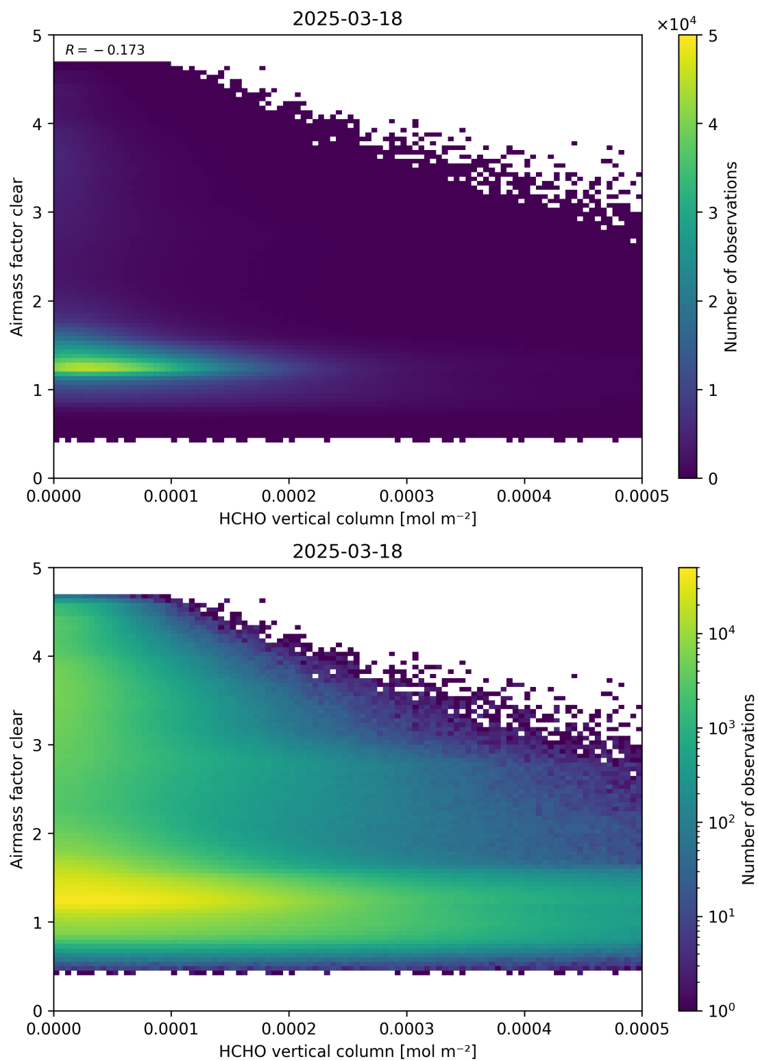
Figure 126: Scatter density plot of “HCHO vertical column” against “Airmass factor clear” for 2025-03-17 to 2025-03-19.
