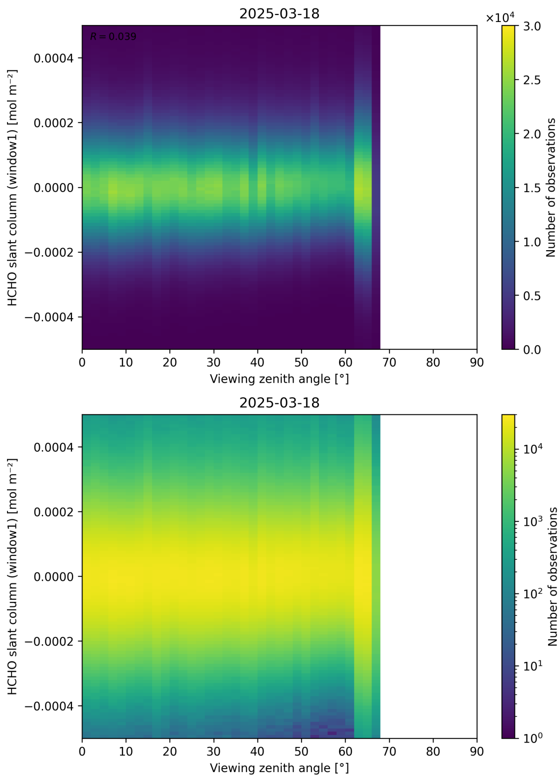
Figure 188: Scatter density plot of “Viewing zenith angle” against “HCHO slant column (window1)” for 2025-03-17 to 2025-03-19.
