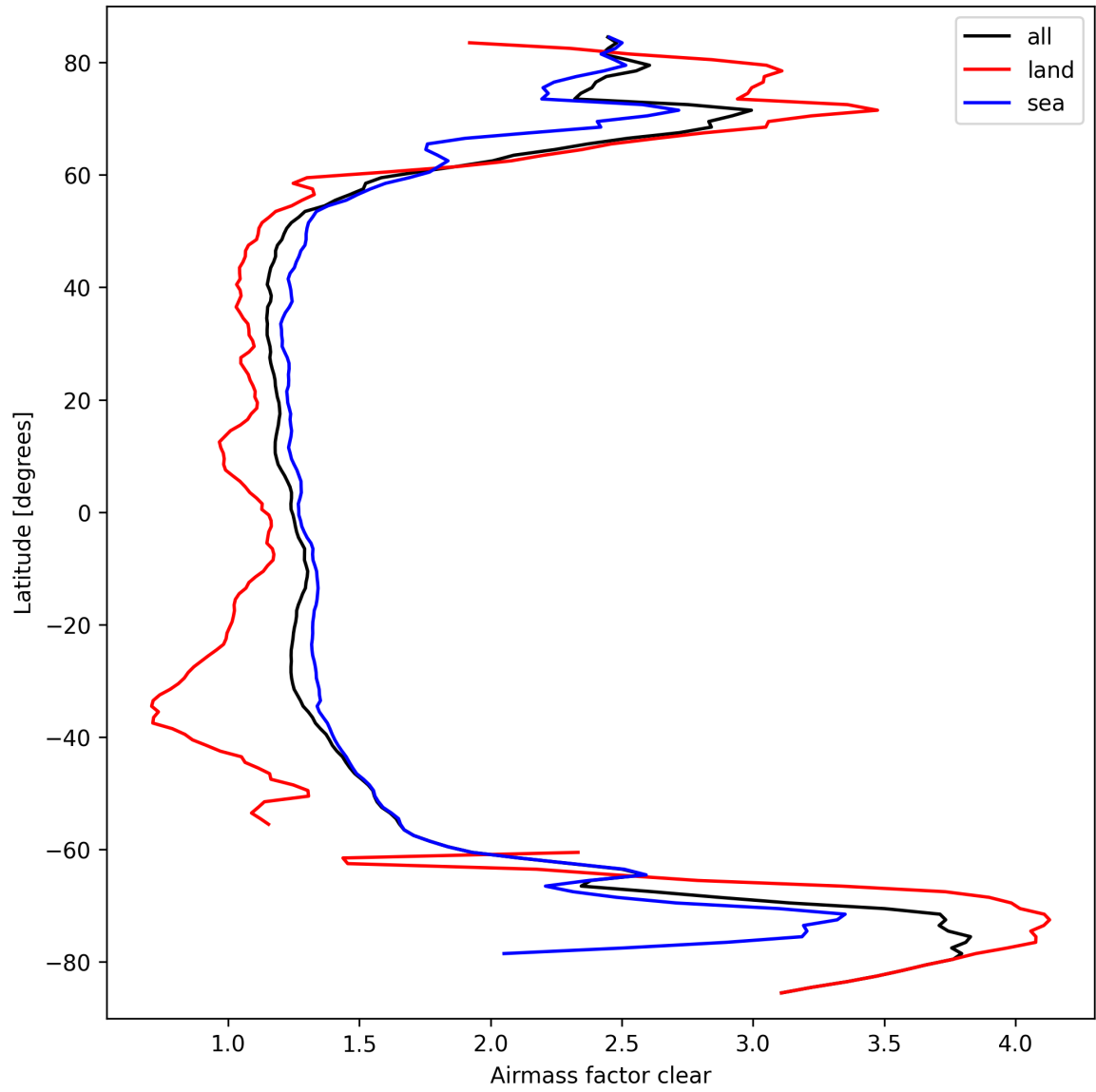
Figure 28: Zonal average of “Airmass factor clear” for 2025-03-17 to 2025-03-19.
