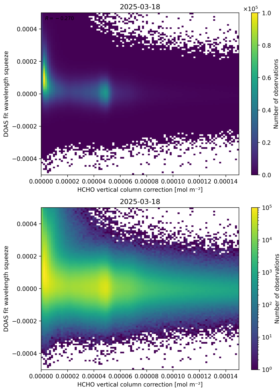
Figure 114: Scatter density plot of “HCHO vertical column correction” against “DOAS fit wavelength squeeze” for 2025-03-17 to 2025-03-19.
