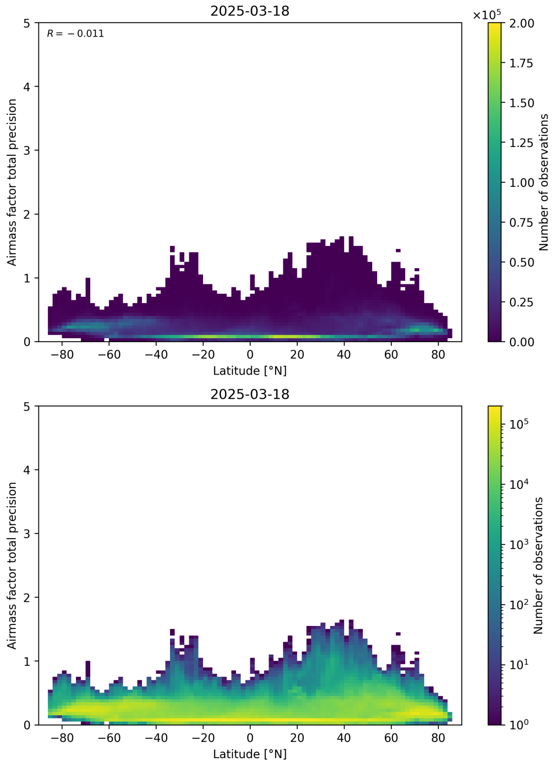
Figure 162: Scatter density plot of “Latitude” against “Airmass factor total precision” for 2025-03-17 to 2025-03-19.
