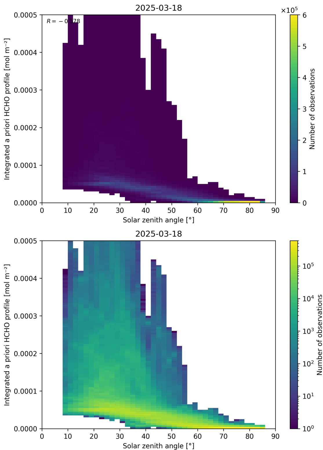
Figure 180: Scatter density plot of “Solar zenith angle” against “Integrated a priori HCHO profile” for 2025-03-17 to 2025-03-19.
