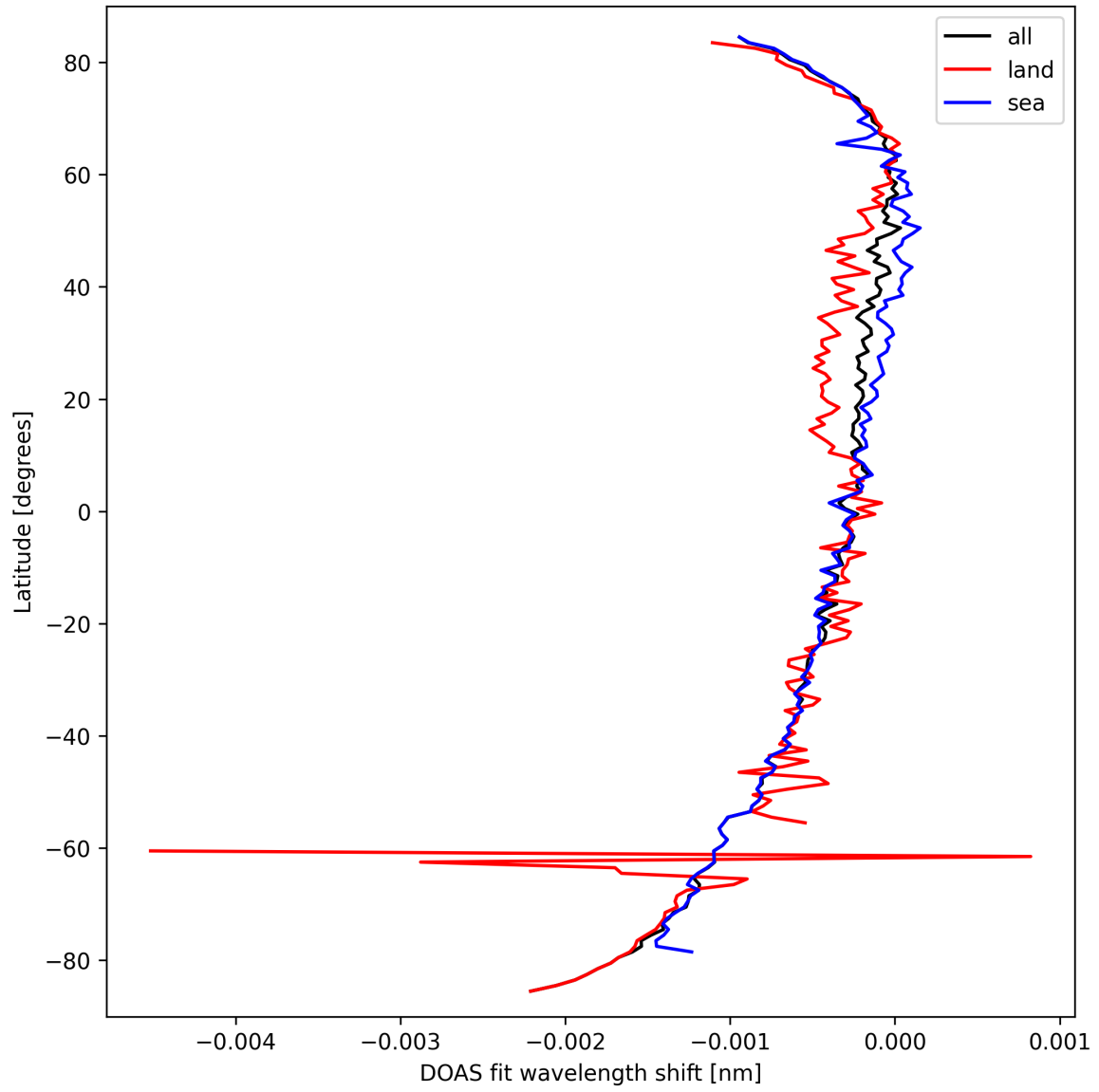
Figure 30: Zonal average of “DOAS fit wavelength shift” for 2025-03-17 to 2025-03-19.
