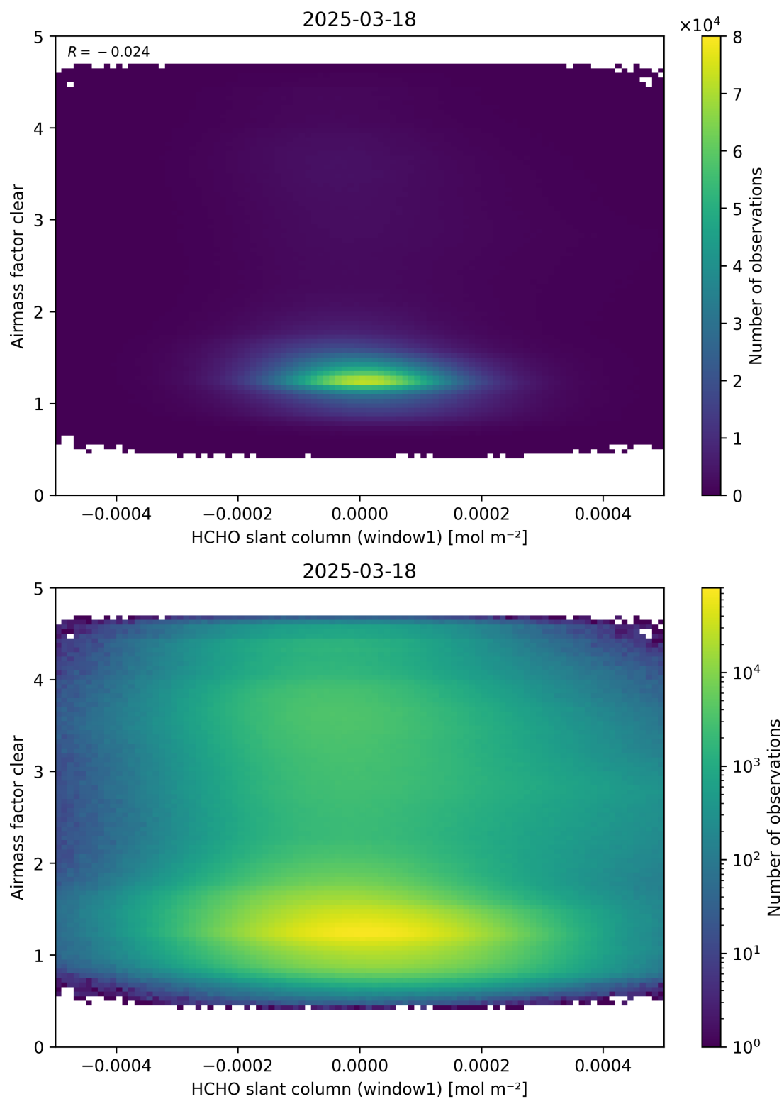
Figure 81: Scatter density plot of “HCHO slant column (window1)” against “Airmass factor clear” for 2025-03-17 to 2025-03-19.
