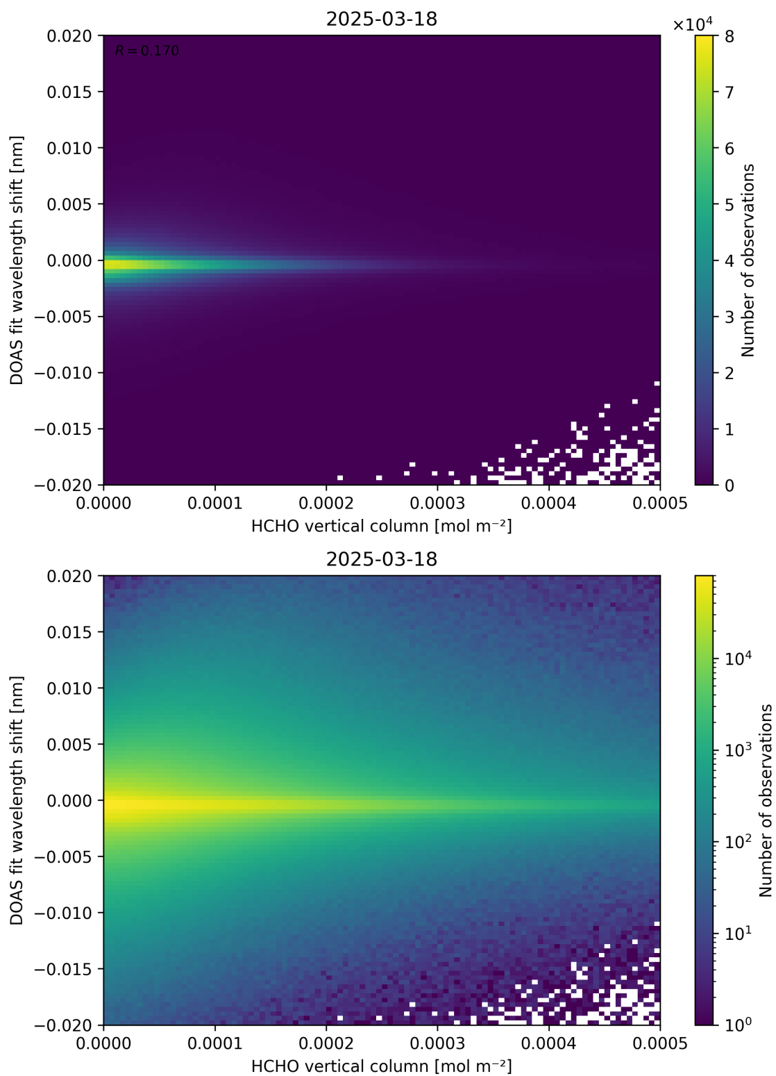
Figure 124: Scatter density plot of “HCHO vertical column” against “DOAS fit wavelength shift” for 2025-03-17 to 2025-03-19.
