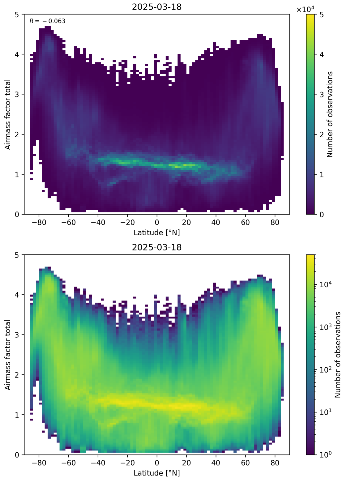
Figure 161: Scatter density plot of “Latitude” against “Airmass factor total” for 2025-03-17 to 2025-03-19.
