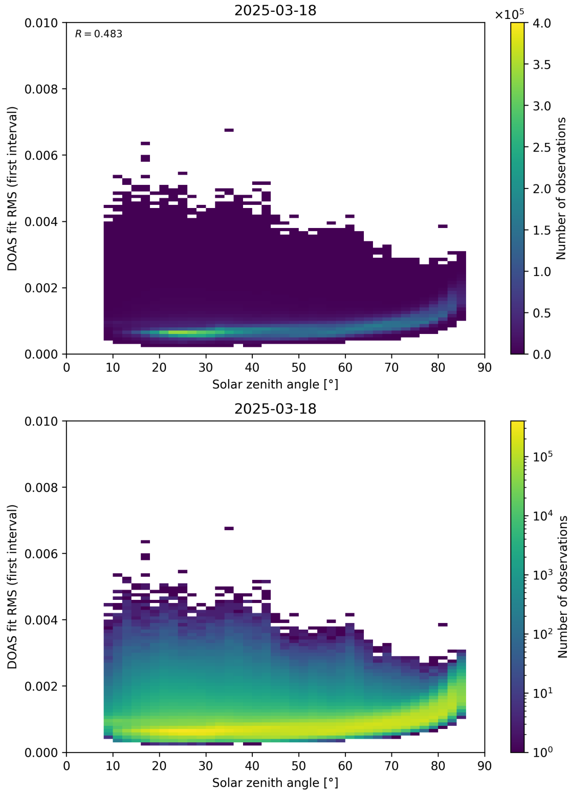
Figure 167: Scatter density plot of “Solar zenith angle” against “DOAS fit RMS (first interval)” for 2025-03-17 to 2025-03-19.
