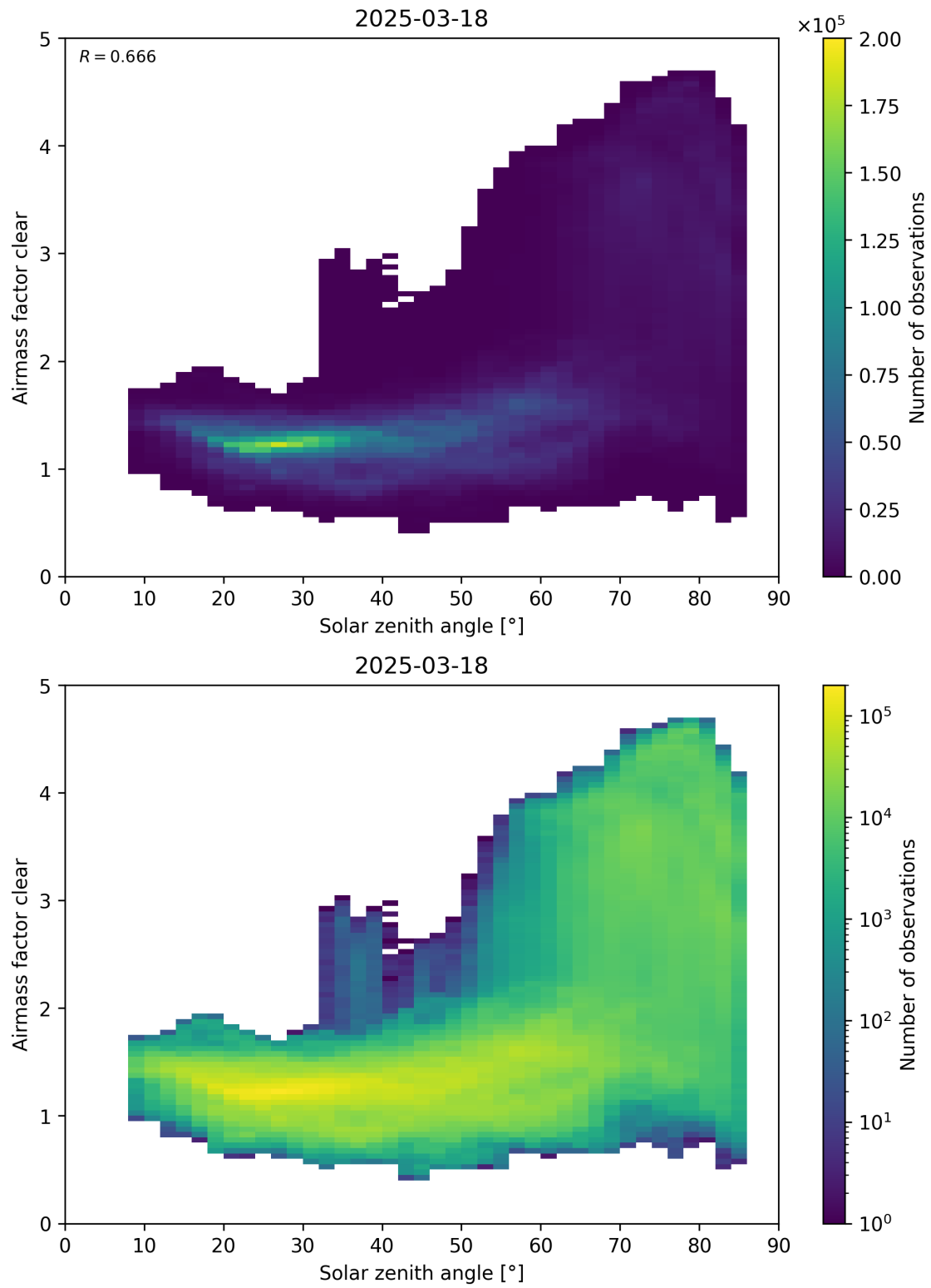
Figure 170: Scatter density plot of “Solar zenith angle” against “Airmass factor clear” for 2025-03-17 to 2025-03-19.
