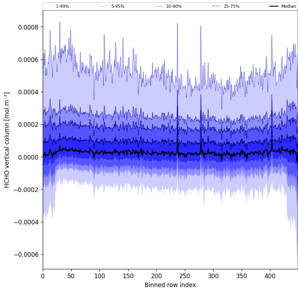
Figure 49: Along track statistics of “HCHO vertical column” for 2025-03-17 to 2025-03-19
