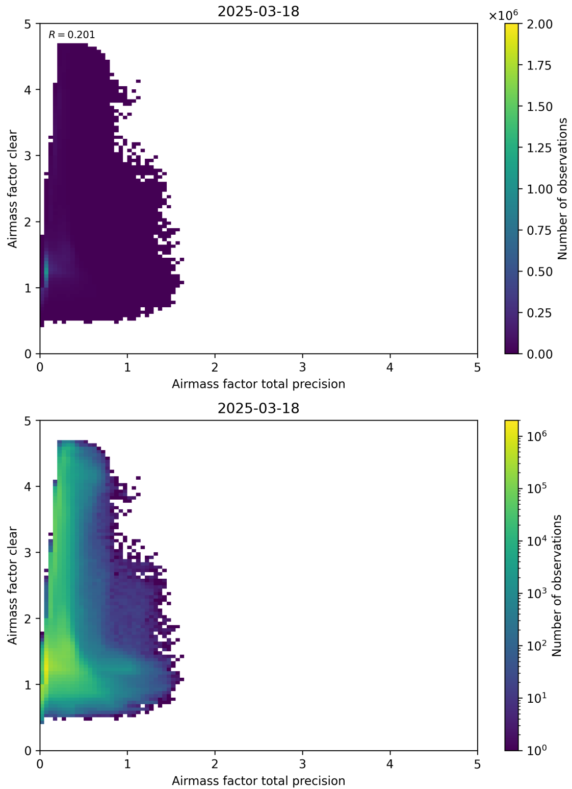
Figure 108: Scatter density plot of “Airmass factor total precision” against “Airmass factor clear” for 2025-03-17 to 2025-03-19.
