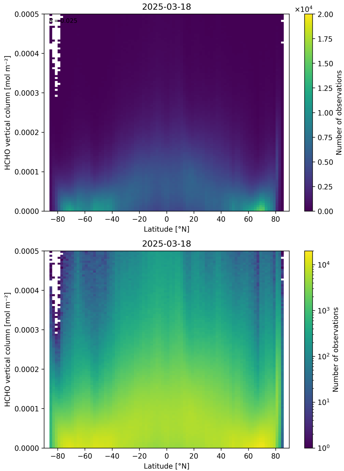
Figure 163: Scatter density plot of “Latitude” against “HCHO vertical column” for 2025-03-17 to 2025-03-19.
