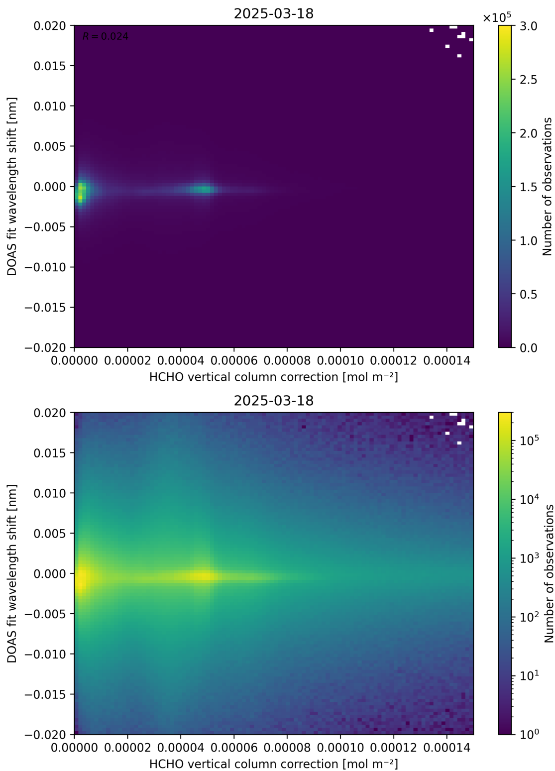
Figure 113: Scatter density plot of “HCHO vertical column correction” against “DOAS fit wavelength shift” for 2025-03-17 to 2025-03-19.
