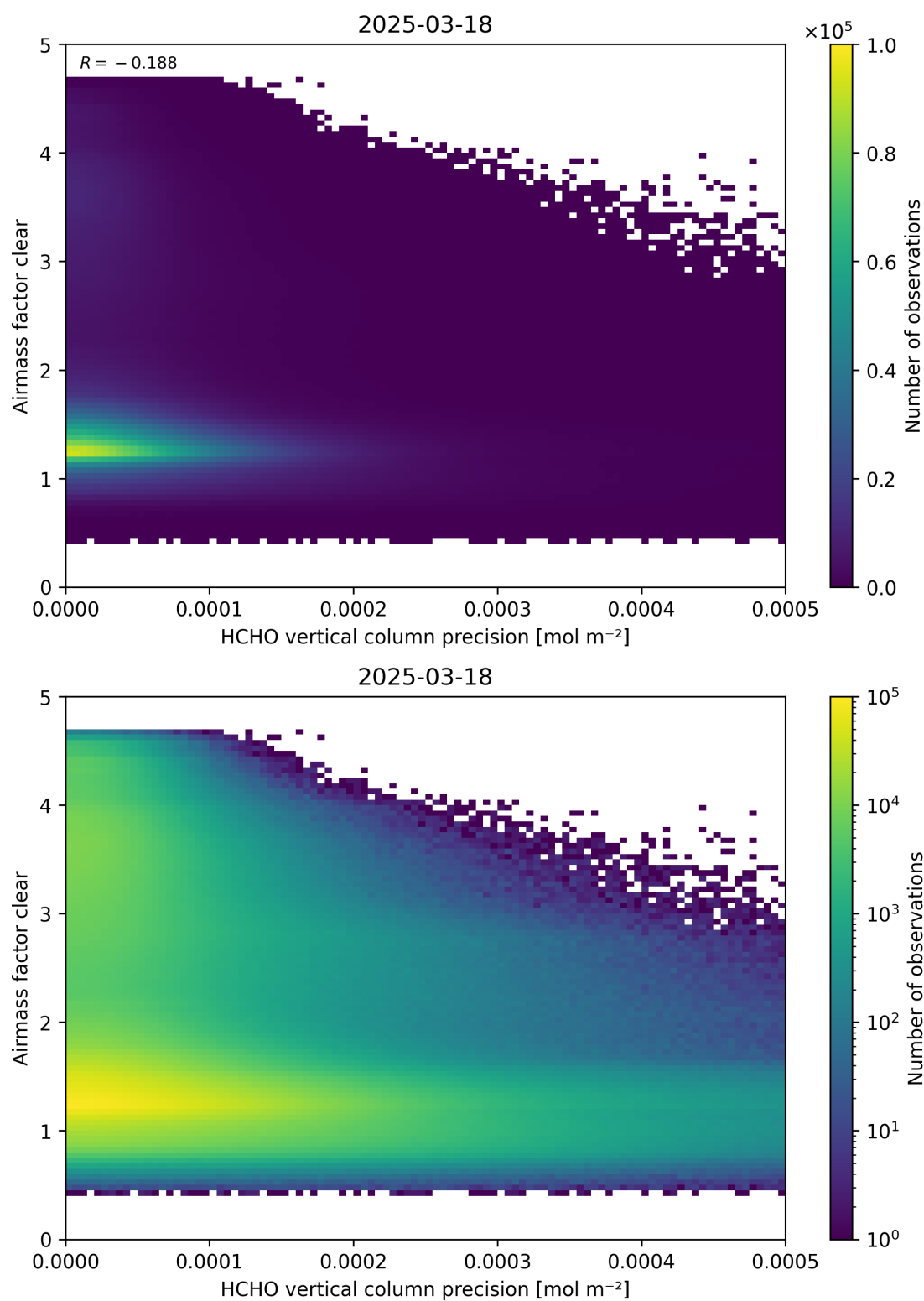
Figure 139: Scatter density plot of “HCHO vertical column precision” against “Airmass factor clear” for 2025-03-17 to 2025-03-19.
