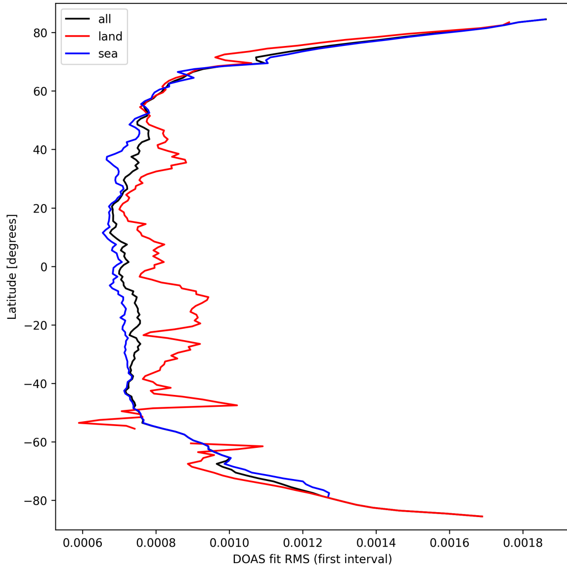
Figure 32: Zonal average of “DOAS fit RMS (first interval)” for 2025-03-17 to 2025-03-19.
