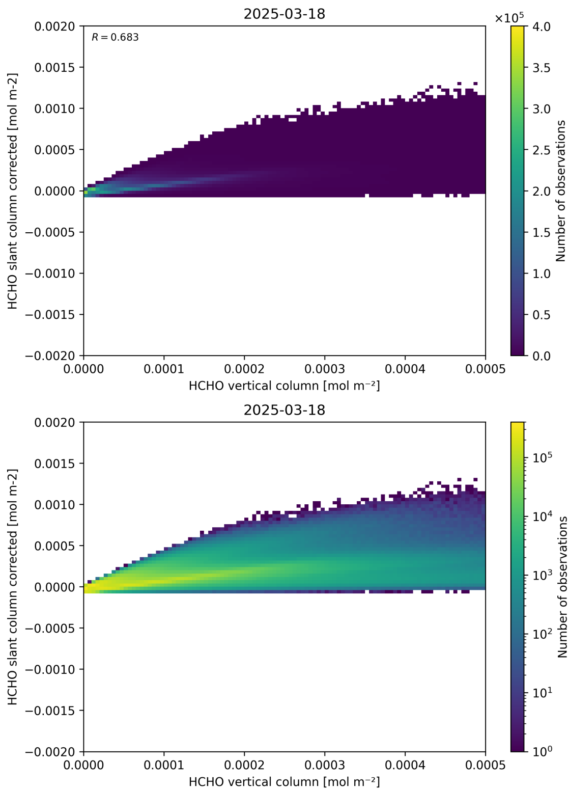
Figure 127: Scatter density plot of “HCHO vertical column” against “HCHO slant column corrected” for 2025-03-17 to 2025-03-19.
