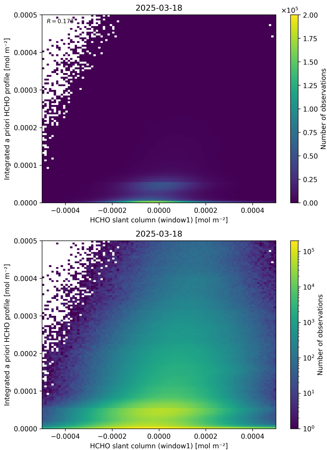
Figure 87: Scatter density plot of “HCHO slant column (window1)” against “Integrated a priori HCHO profile” for 2025-03-17 to 2025-03-19.
