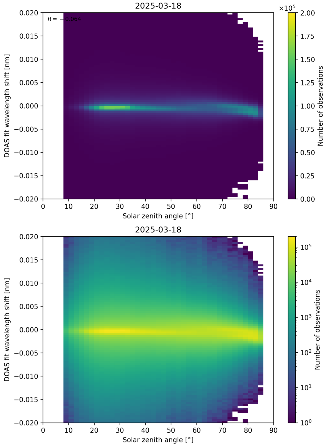
Figure 168: Scatter density plot of “Solar zenith angle” against “DOAS fit wavelength shift” for 2025-03-17 to 2025-03-19.
