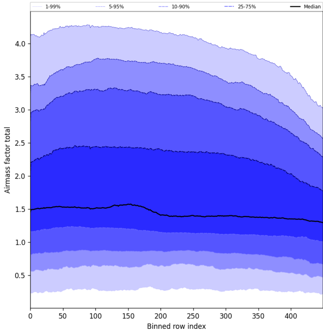
Figure 54: Along track statistics of “Airmass factor total” for 2025-03-17 to 2025-03-19
