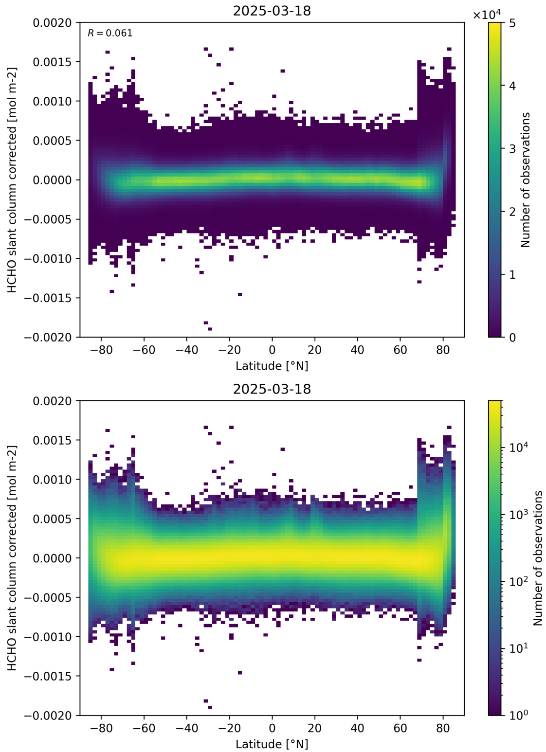
Figure 157: Scatter density plot of “Latitude” against “HCHO slant column corrected” for 2025-03-17 to 2025-03-19.
