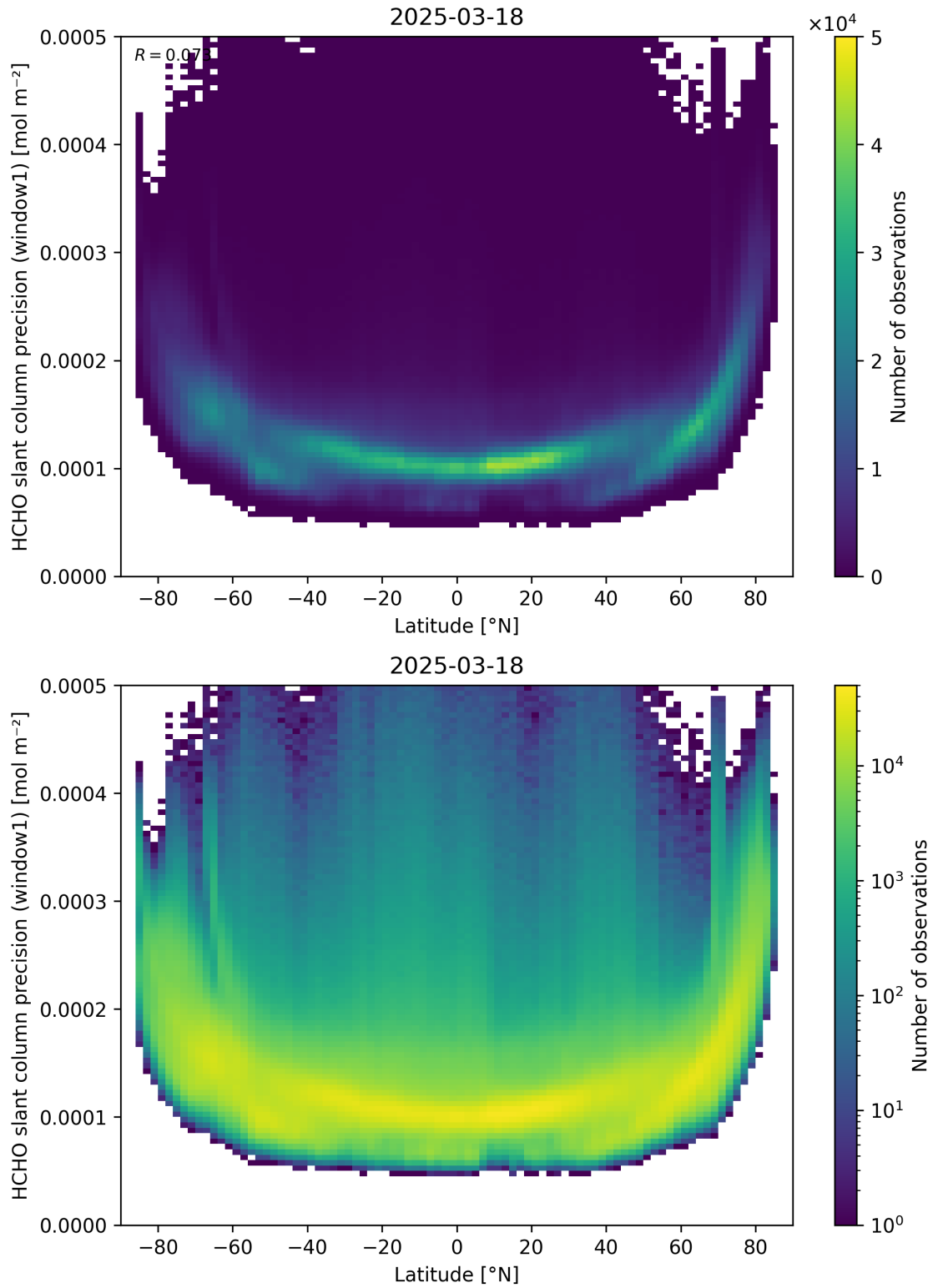
Figure 160: Scatter density plot of “Latitude” against “HCHO slant column precision (window1)” for 2025-03-17 to 2025-03-19.
