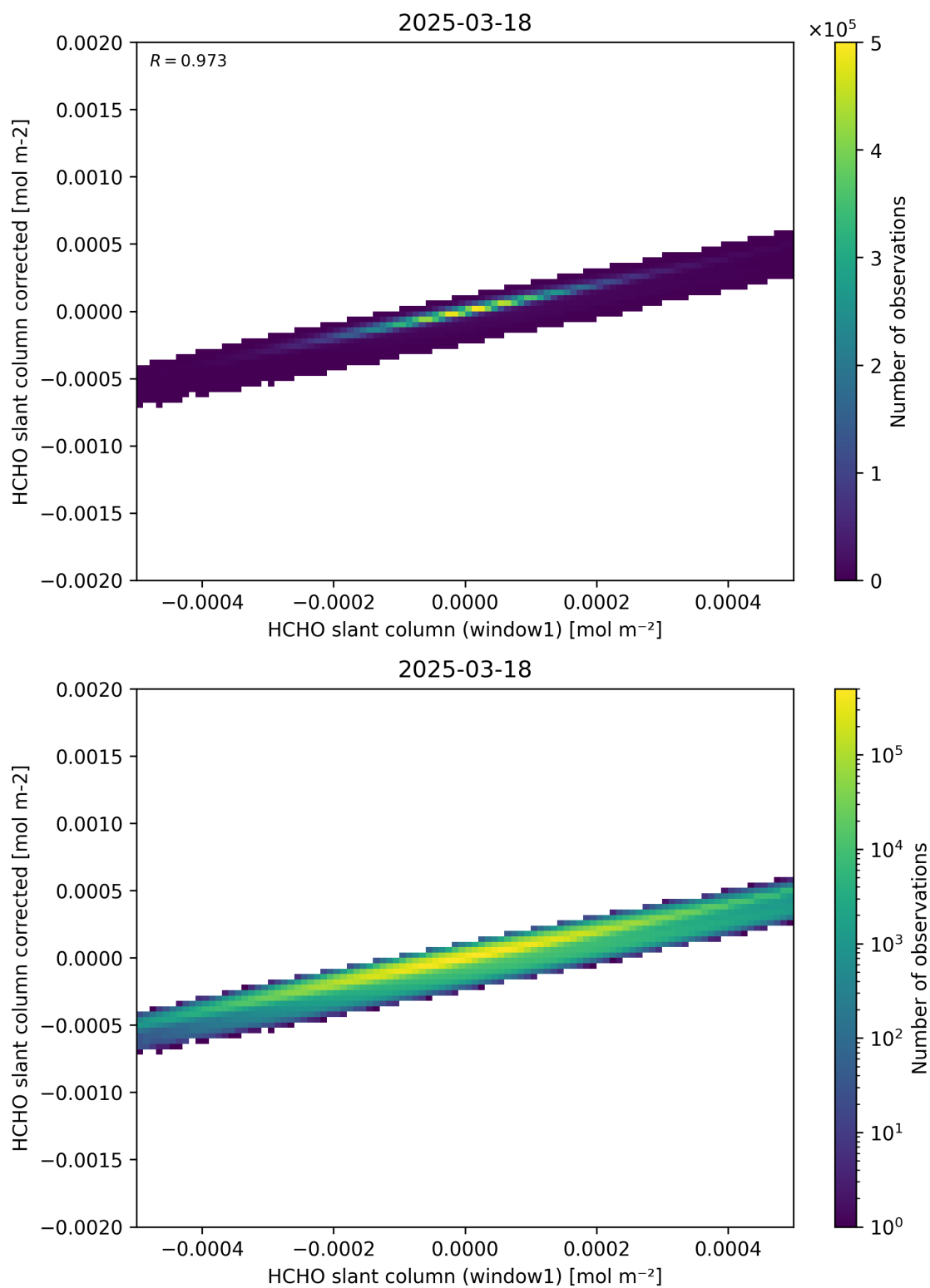
Figure 82: Scatter density plot of “HCHO slant column (window1)” against “HCHO slant column corrected” for 2025-03-17 to 2025-03-19.
