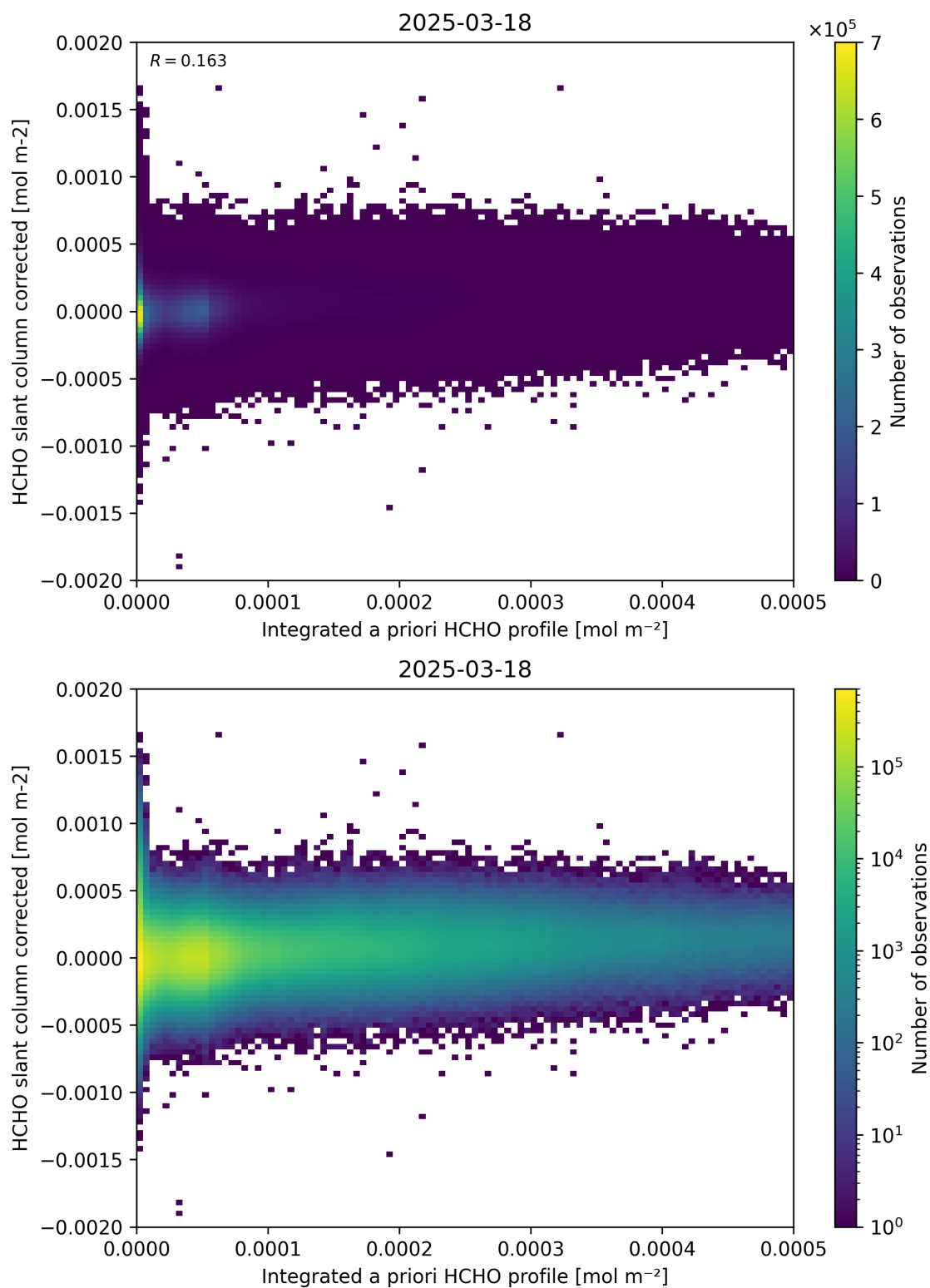
Figure 151: Scatter density plot of “Integrated a priori HCHO profile” against “HCHO slant column corrected” for 2025-03-17 to 2025-03-19.
