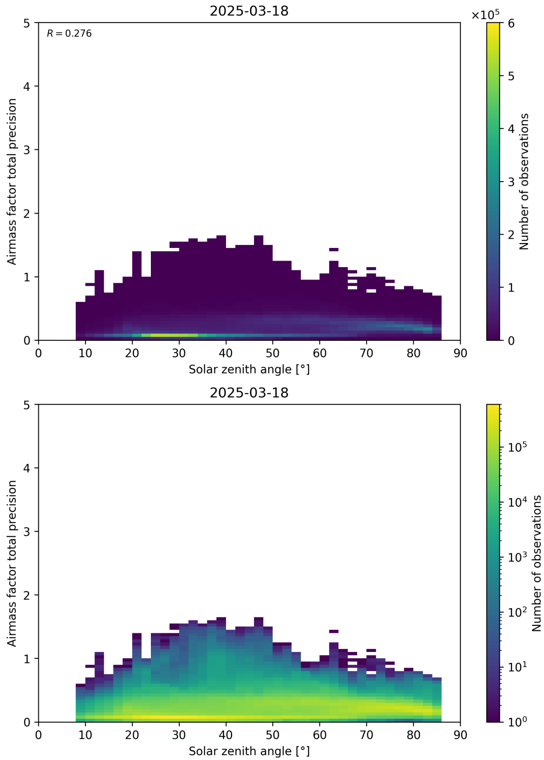
Figure 176: Scatter density plot of “Solar zenith angle” against “Airmass factor total precision” for 2025-03-17 to 2025-03-19.
