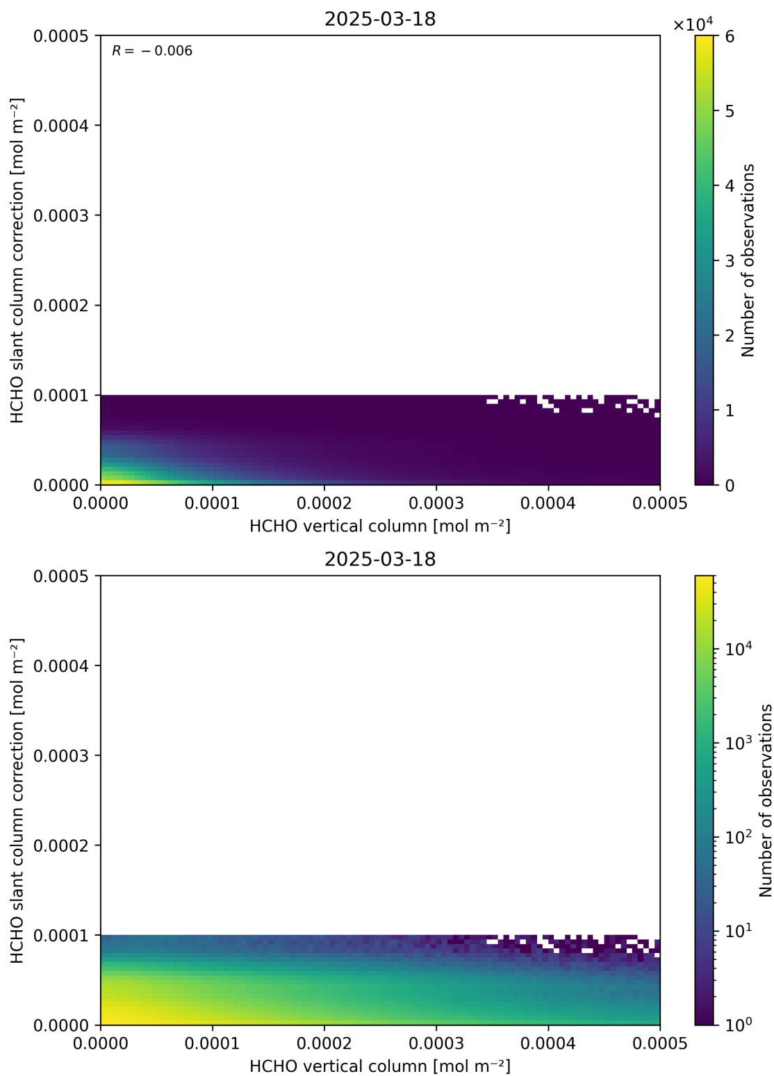
Figure 128: Scatter density plot of “HCHO vertical column” against “HCHO slant column correction” for 2025-03-17 to 2025-03-19.
