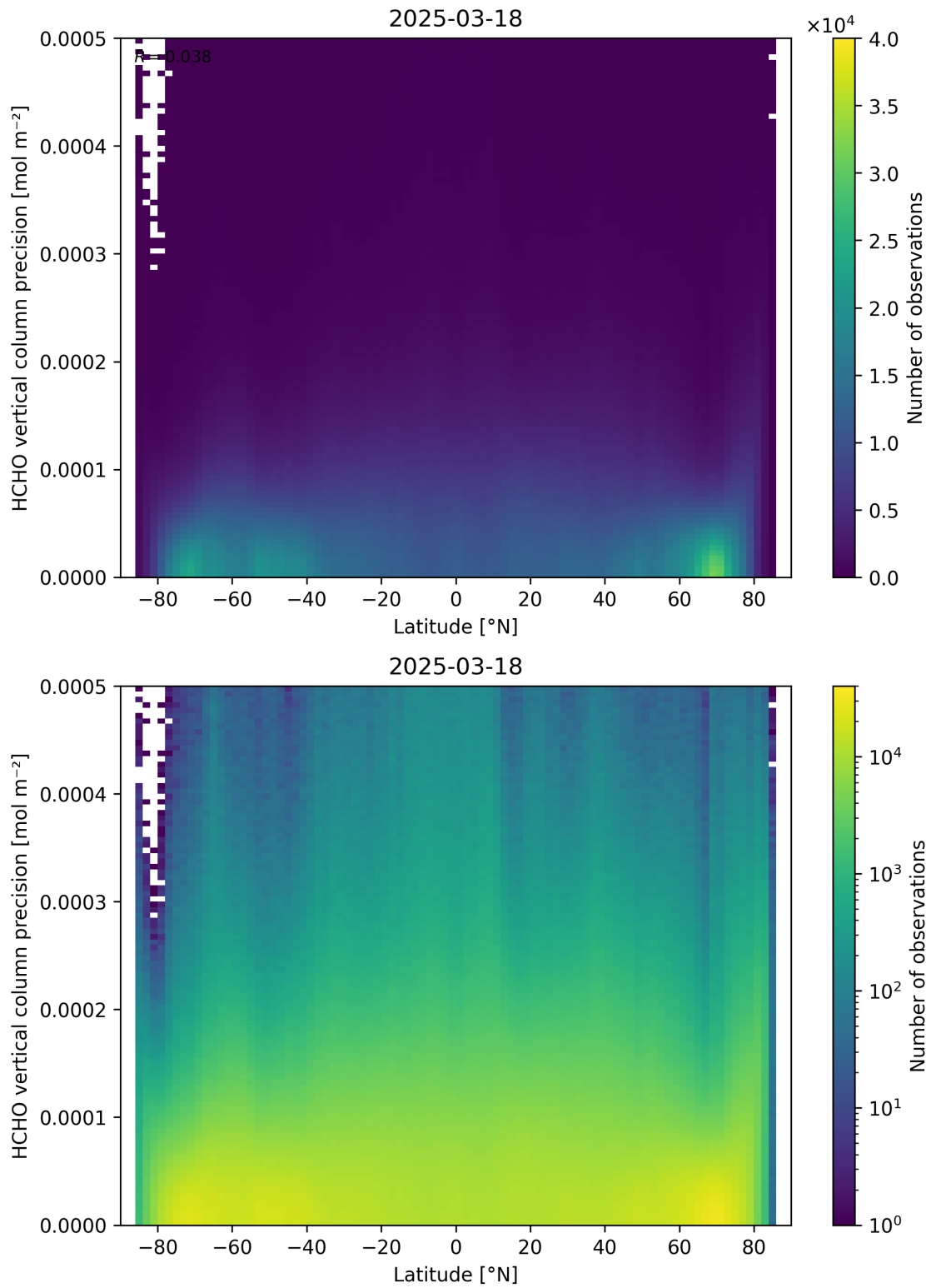
Figure 165: Scatter density plot of “Latitude” against “HCHO vertical column precision” for 2025-03-17 to 2025-03-19.
