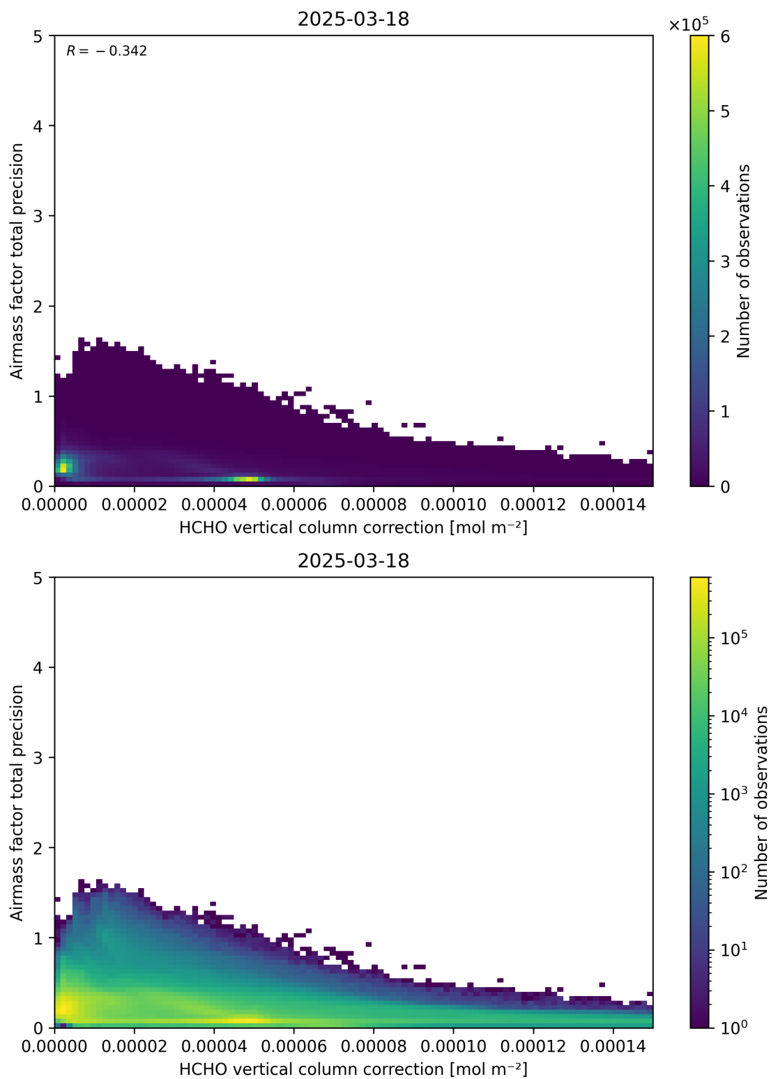
Figure 121: Scatter density plot of “HCHO vertical column correction” against “Airmass factor total precision” for 2025-03-17 to 2025-03-19.
