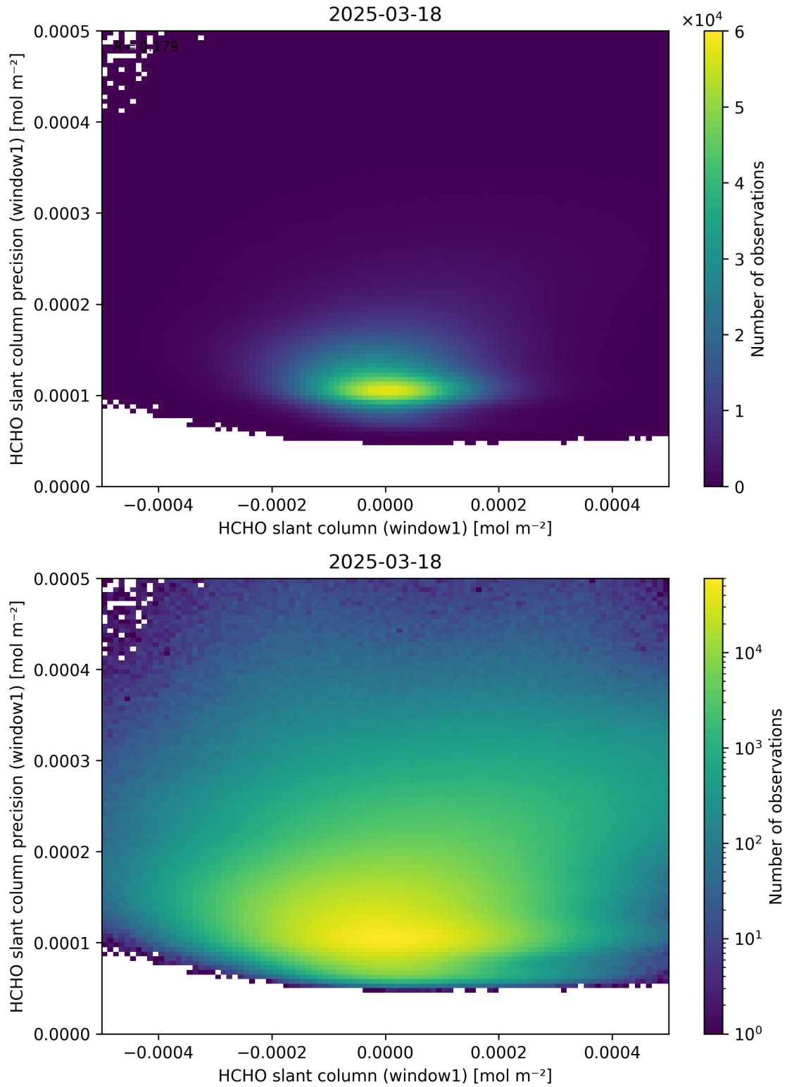
Figure 84: Scatter density plot of “HCHO slant column (window1)” against “HCHO slant column precision (window1)” for 2025-03-17 to 2025-03-19.
