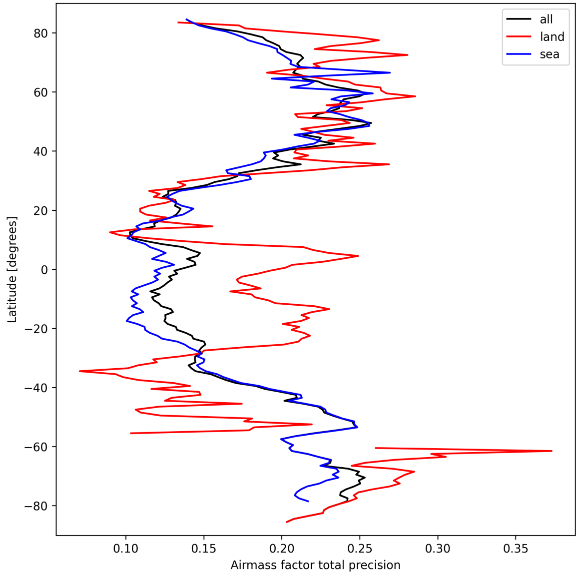
Figure 27: Zonal average of “Airmass factor total precision” for 2025-03-17 to 2025-03-19.
