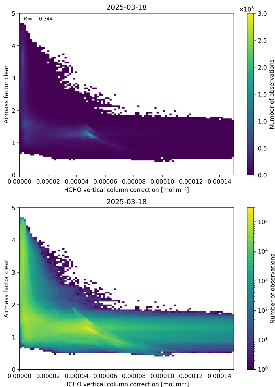
Figure 115: Scatter density plot of “HCHO vertical column correction” against “Airmass factor clear” for 2025-03-17 to 2025-03-19.
