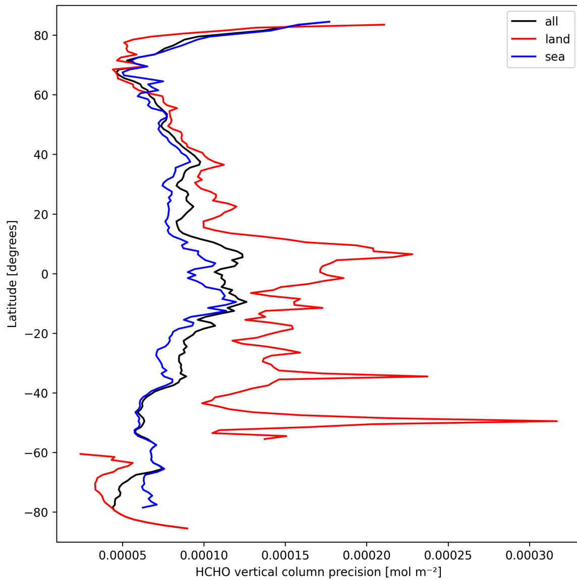
Figure 22: Zonal average of “HCHO vertical column precision” for 2025-03-17 to 2025-03-19.
