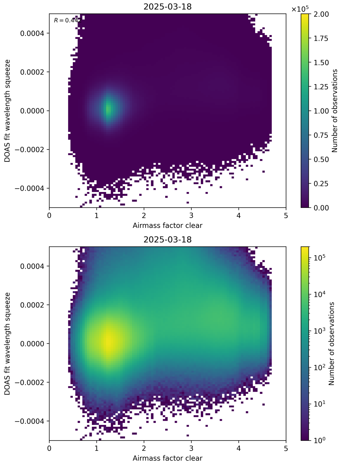
Figure 73: Scatter density plot of “Airmass factor clear” against “DOAS fit wavelength squeeze” for 2025-03-17 to 2025-03-19.
