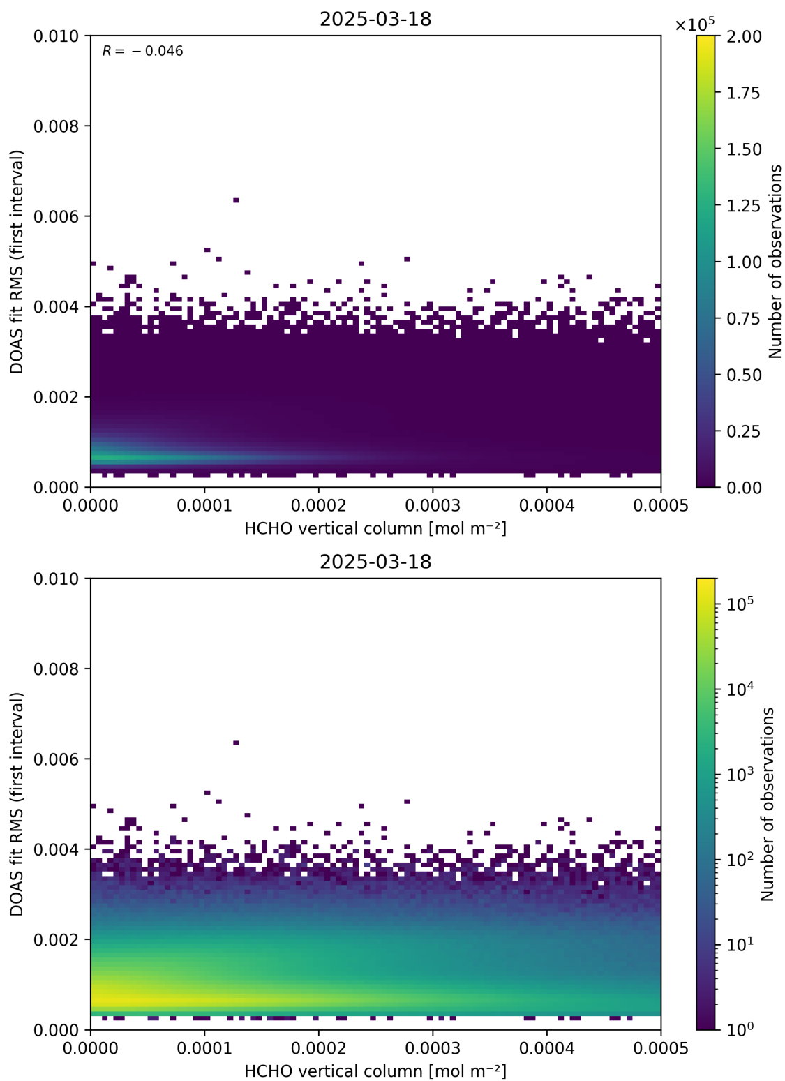
Figure 123: Scatter density plot of “HCHO vertical column” against “DOAS fit RMS (first interval)” for 2025-03-17 to 2025-03-19.
