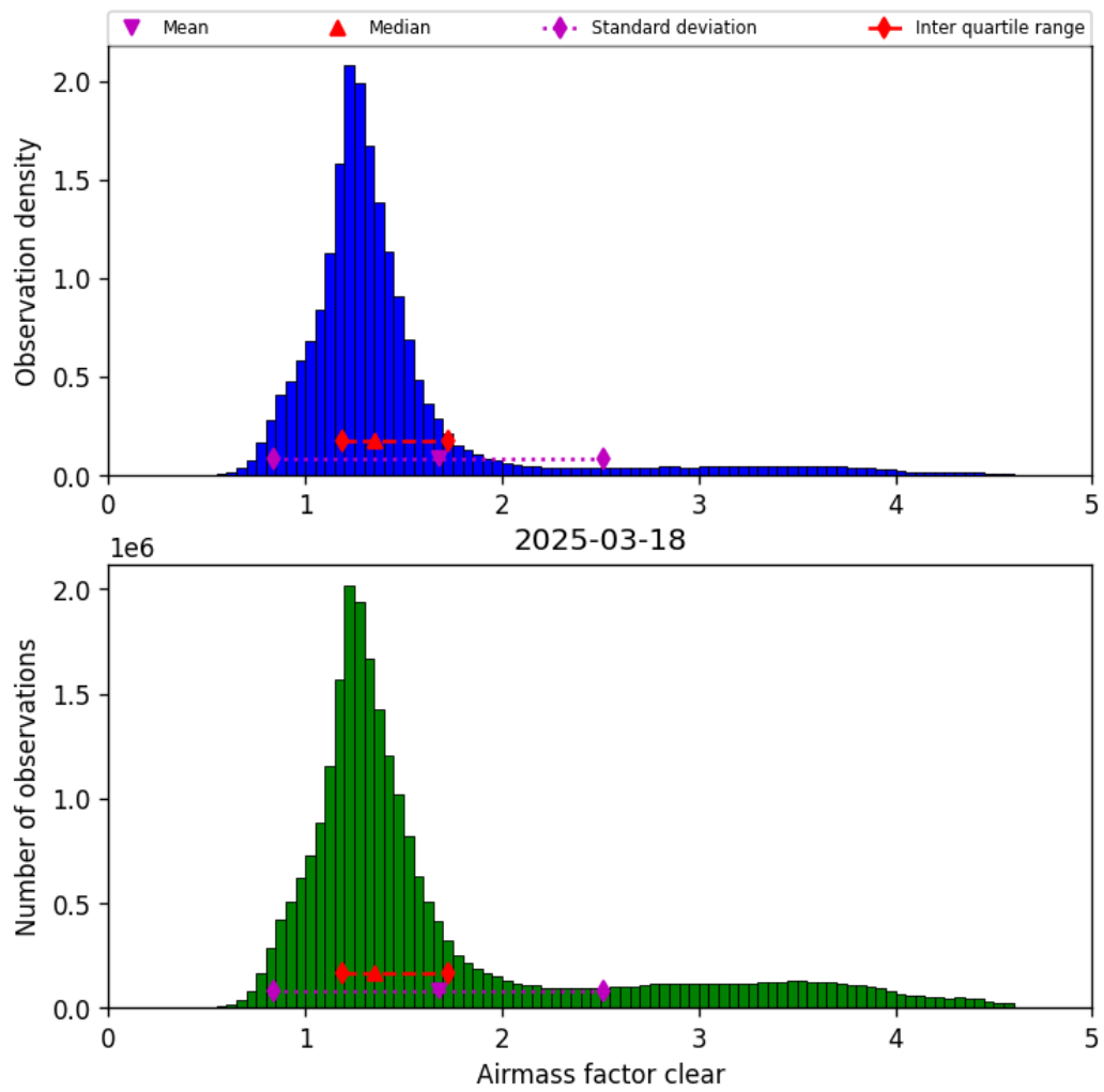
Figure 42: Histogram of “Airmass factor clear” for 2025-03-17 to 2025-03-19
