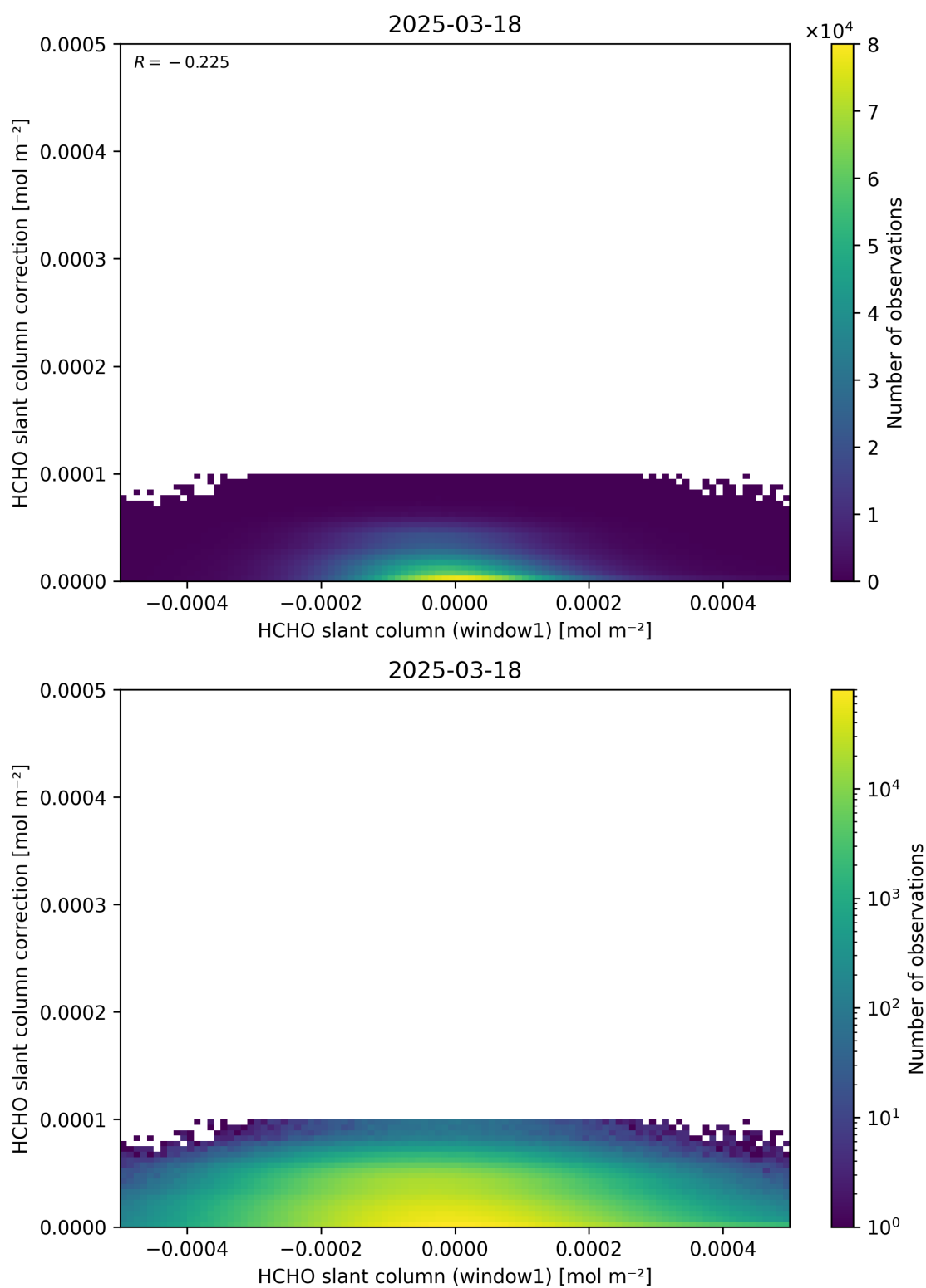
Figure 83: Scatter density plot of “HCHO slant column (window1)” against “HCHO slant column correction” for 2025-03-17 to 2025-03-19.
