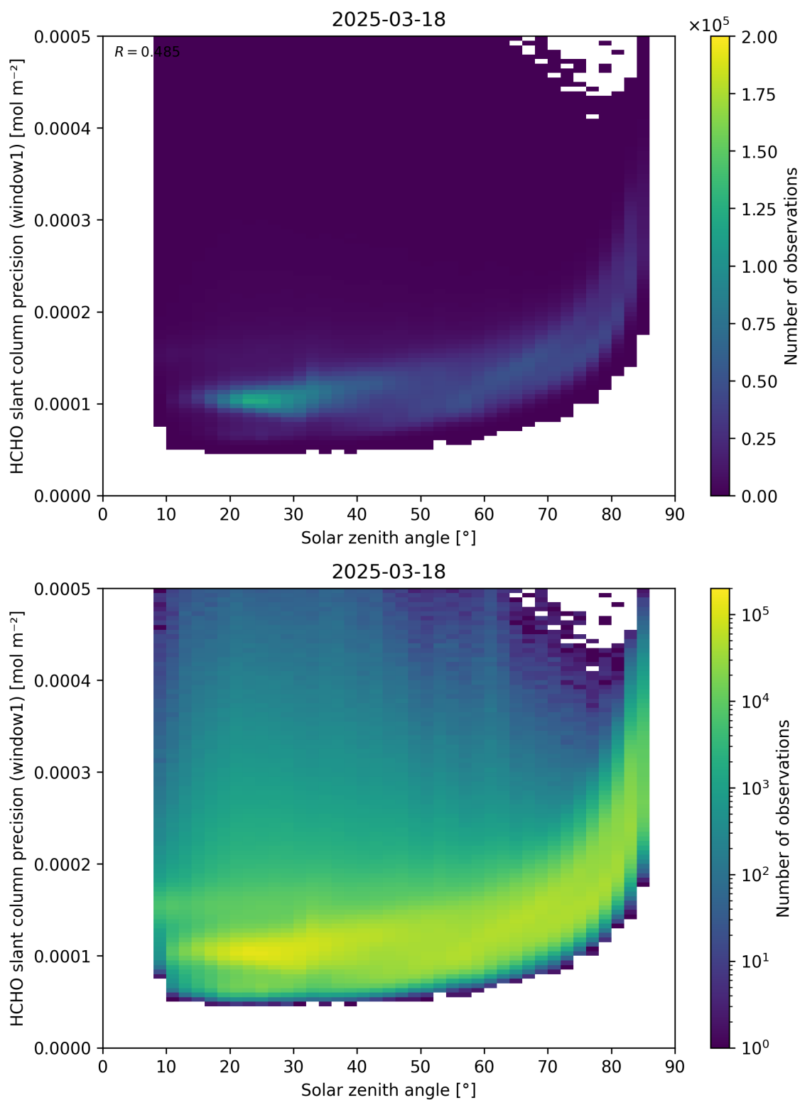
Figure 174: Scatter density plot of “Solar zenith angle” against “HCHO slant column precision (window1)” for 2025-03-17 to 2025-03-19.
