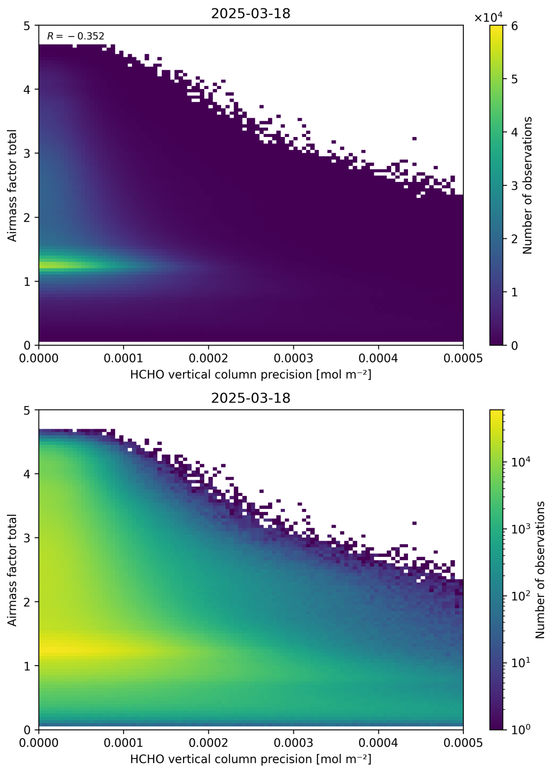
Figure 144: Scatter density plot of “HCHO vertical column precision” against “Airmass factor total” for 2025-03-17 to 2025-03-19.
