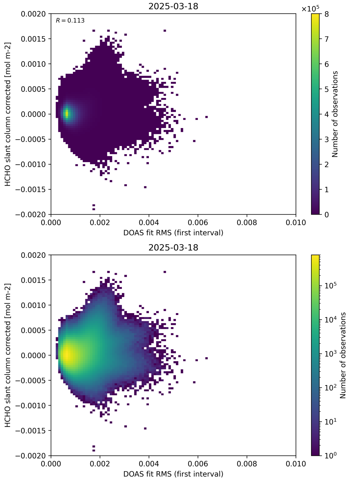
Figure 62: Scatter density plot of “DOAS fit RMS (first interval)” against “HCHO slant column corrected” for 2025-03-17 to 2025-03-19.
