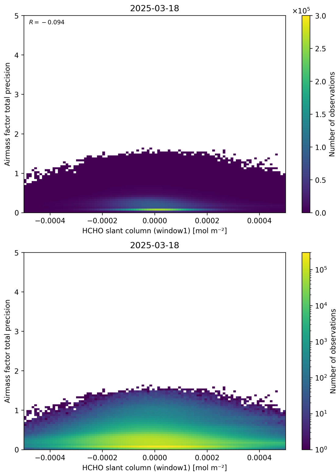
Figure 86: Scatter density plot of “HCHO slant column (window1)” against “Airmass factor total precision” for 2025-03-17 to 2025-03-19.
