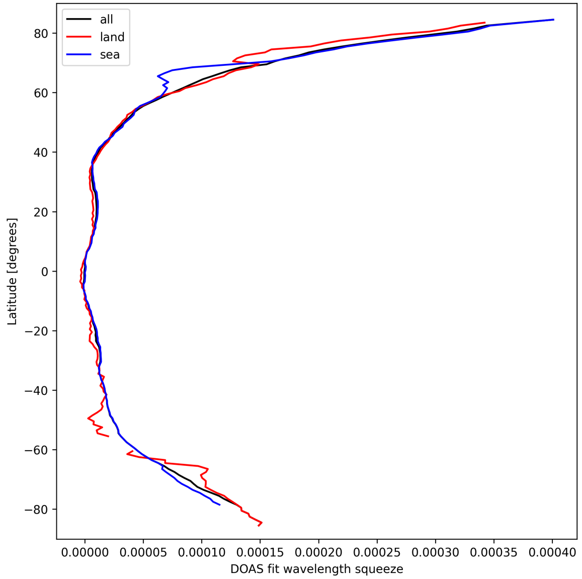
Figure 31: Zonal average of “DOAS fit wavelength squeeze” for 2025-03-17 to 2025-03-19.
