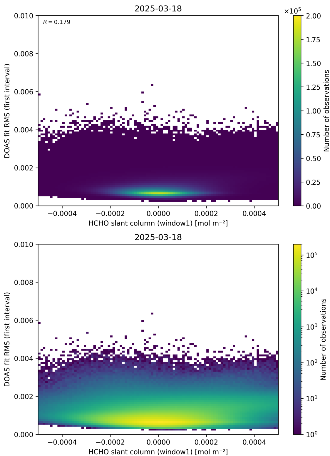
Figure 78: Scatter density plot of “HCHO slant column (window1)” against “DOAS fit RMS (first interval)” for 2025-03-17 to 2025-03-19.
