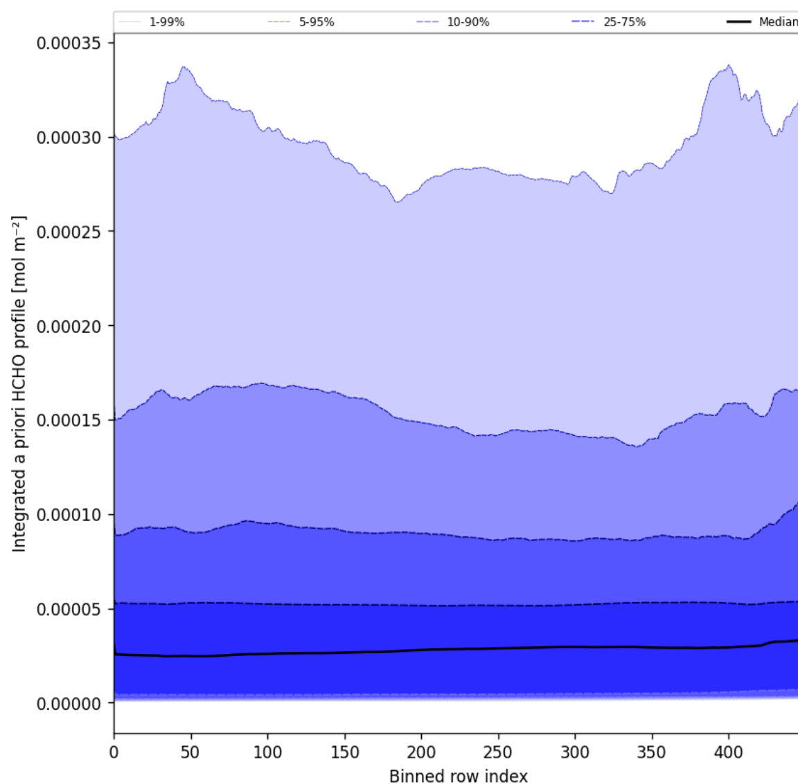
Figure 57: Along track statistics of "Integrated a priori HCHO profile" for 2025-03-17 to 2025-03-19
