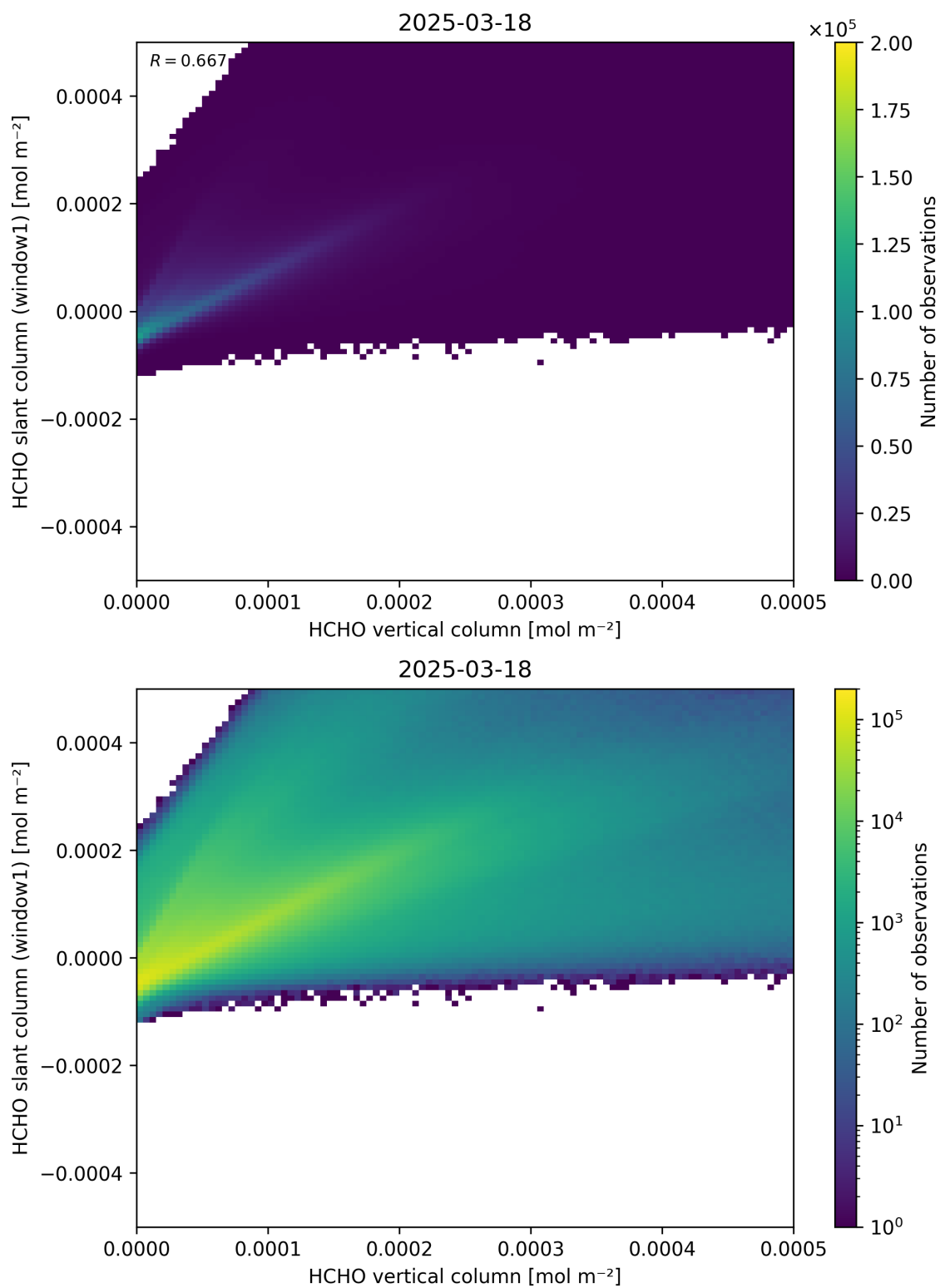
Figure 129: Scatter density plot of “HCHO vertical column” against “HCHO slant column (window1)” for 2025-03-17 to 2025-03-19.
