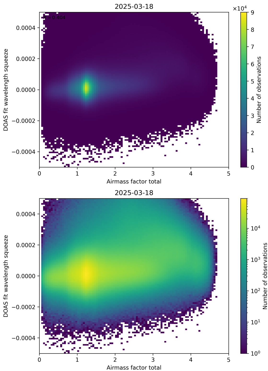
Figure 99: Scatter density plot of “Airmass factor total” against “DOAS fit wavelength squeeze” for 2025-03-17 to 2025-03-19.
