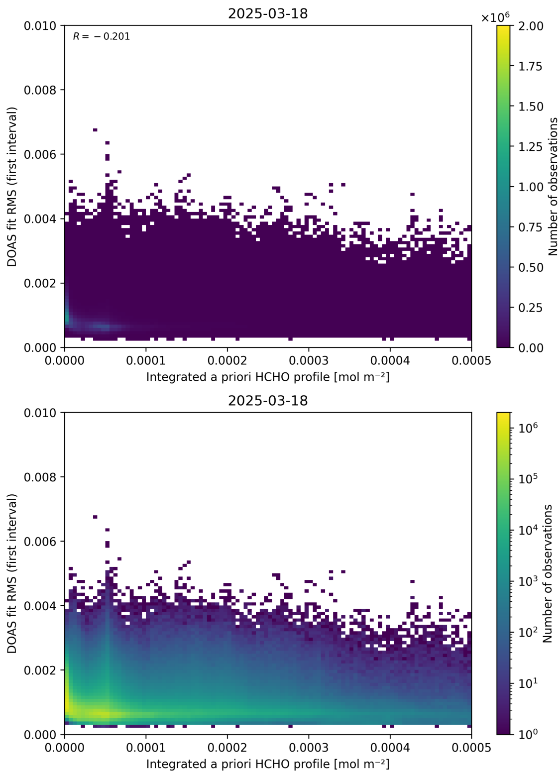
Figure 148: Scatter density plot of “Integrated a priori HCHO profile” against “DOAS fit RMS (first interval)” for 2025-03-17 to 2025-03-19.
