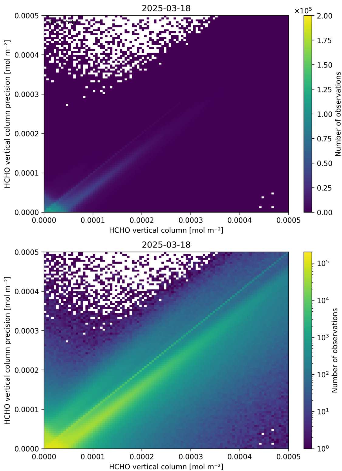
Figure 134: Scatter density plot of “HCHO vertical column” against “HCHO vertical column precision” for 2025-03-17 to 2025-03-19.
