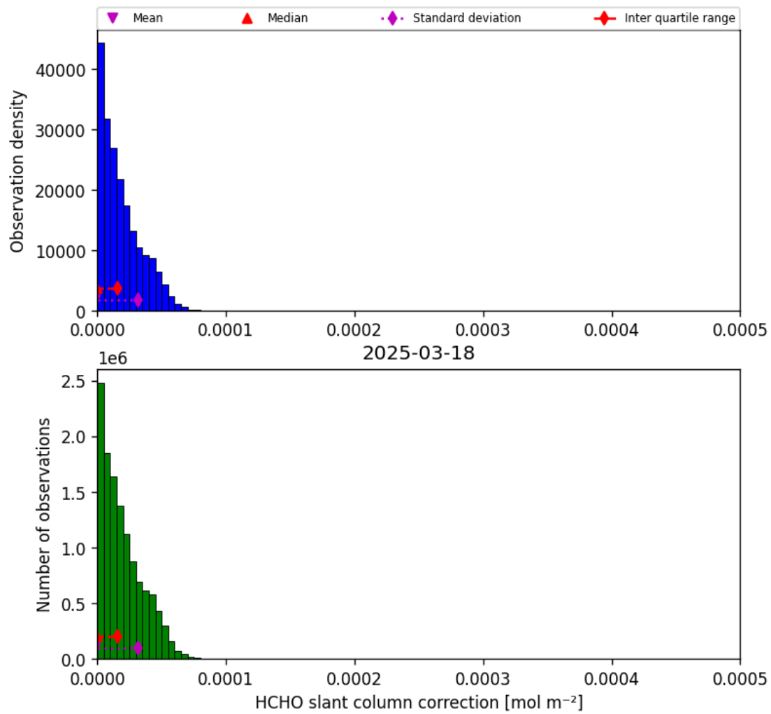
Figure 47: Histogram of “HCHO slant column correction” for 2025-03-17 to 2025-03-19
