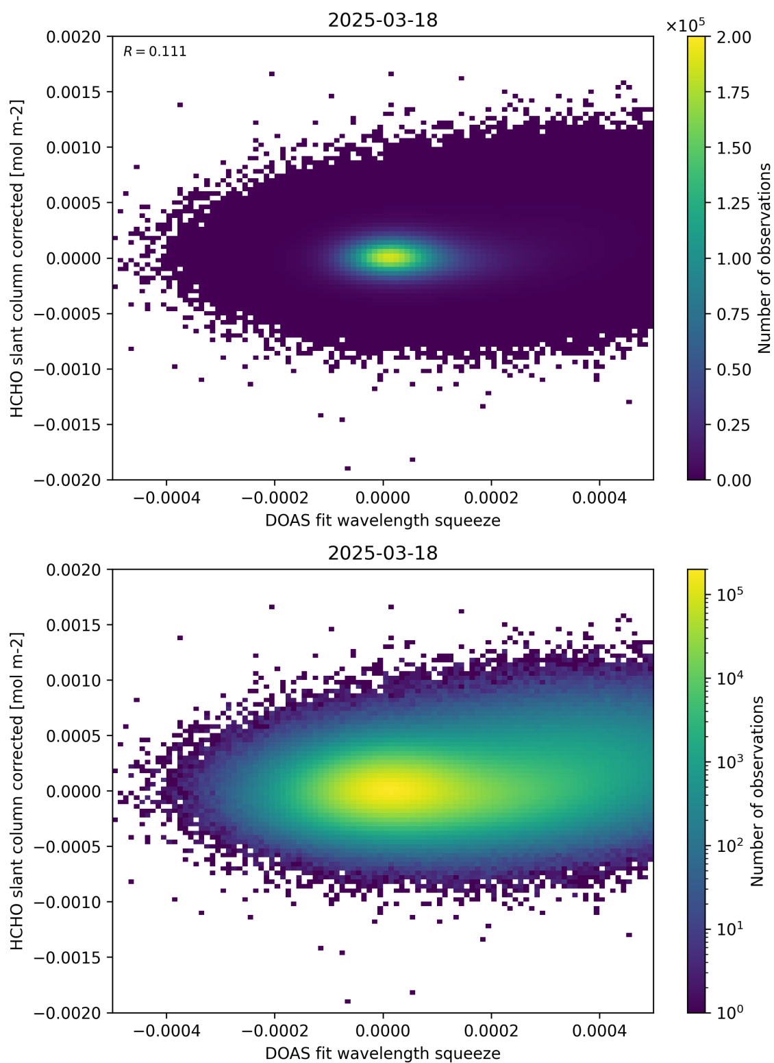
Figure 69: Scatter density plot of “DOAS fit wavelength squeeze” against “HCHO slant column corrected” for 2025-03-17 to 2025-03-19.
