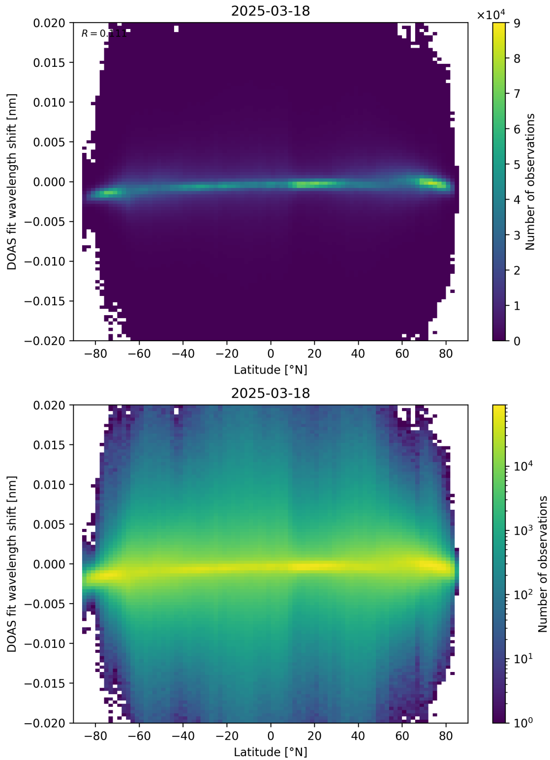
Figure 154: Scatter density plot of “Latitude” against “DOAS fit wavelength shift” for 2025-03-17 to 2025-03-19.
