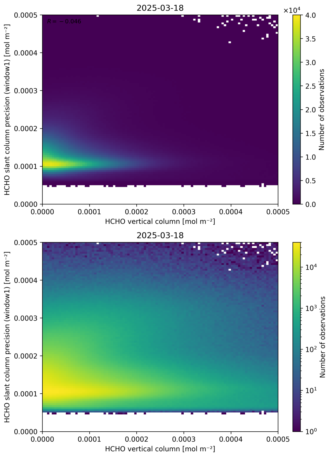
Figure 130: Scatter density plot of “HCHO vertical column” against “HCHO slant column precision (window1)” for 2025-03-17 to 2025-03-19.
