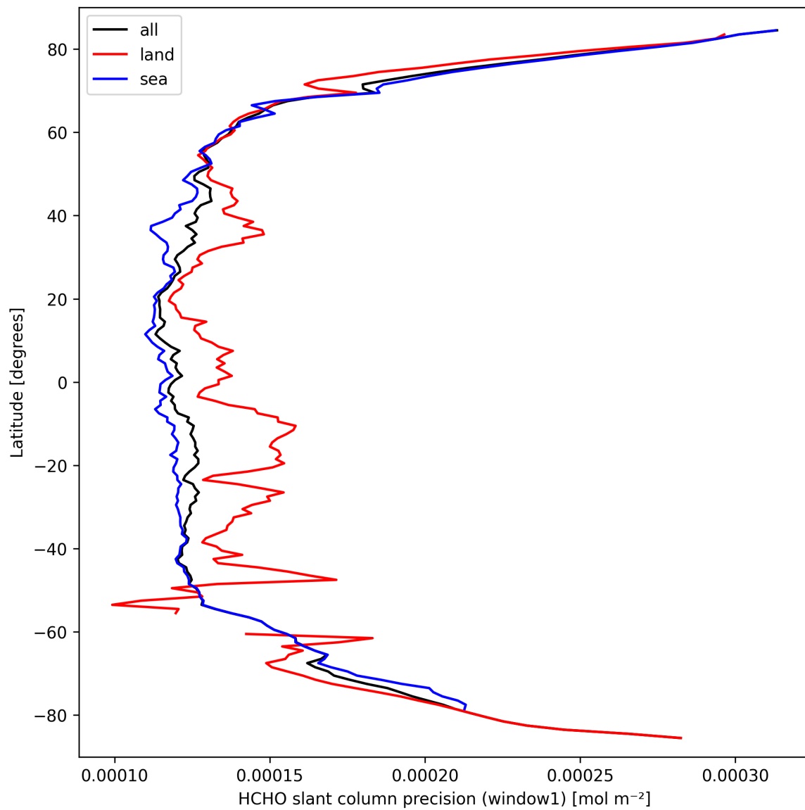
Figure 25: Zonal average of “HCHO slant column precision (window1)” for 2025-03-17 to 2025-03-19.
