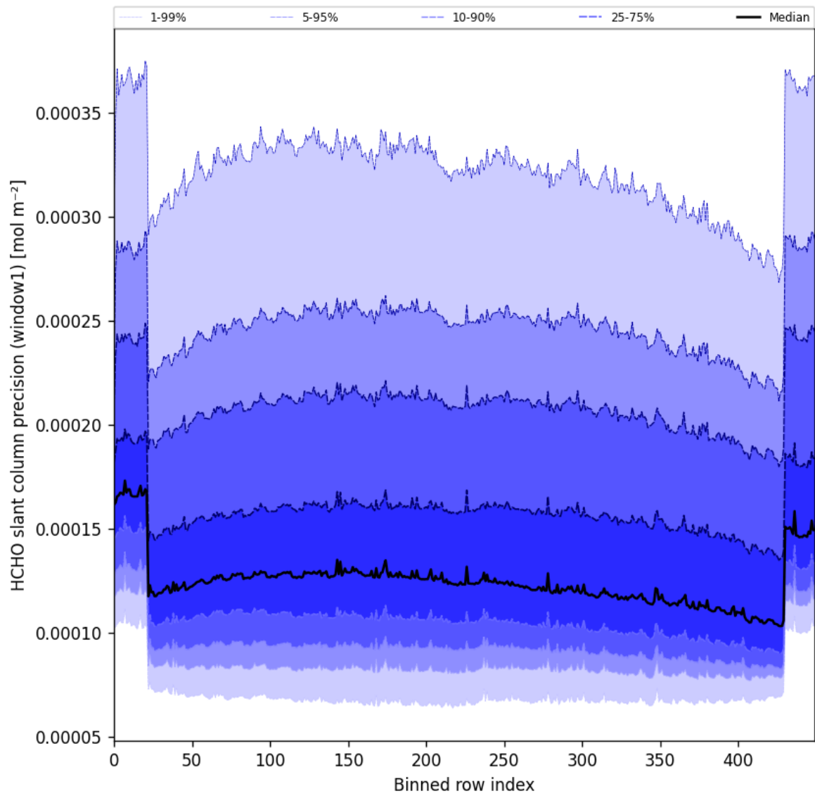
Figure 53: Along track statistics of “HCHO slant column precision (window1)” for 2025-03-17 to 2025-03-19
