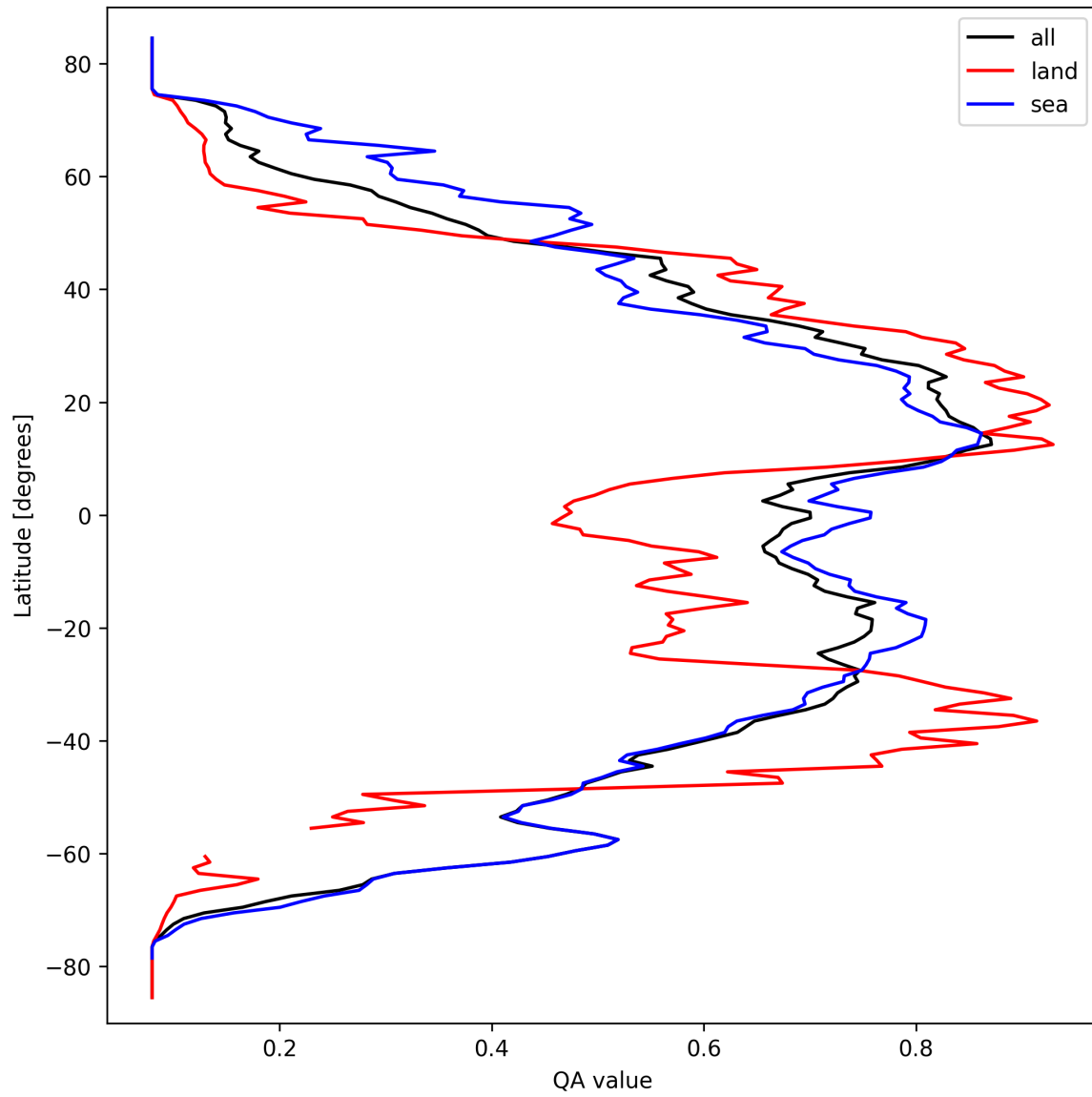
Figure 20: Zonal average of “QA value” for 2025-03-17 to 2025-03-19.
