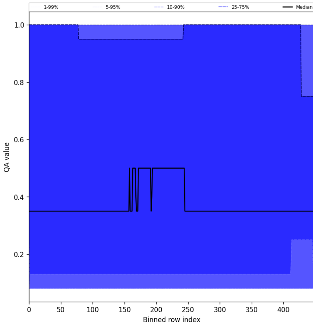
Figure 48: Along track statistics of “QA value” for 2025-03-17 to 2025-03-19
