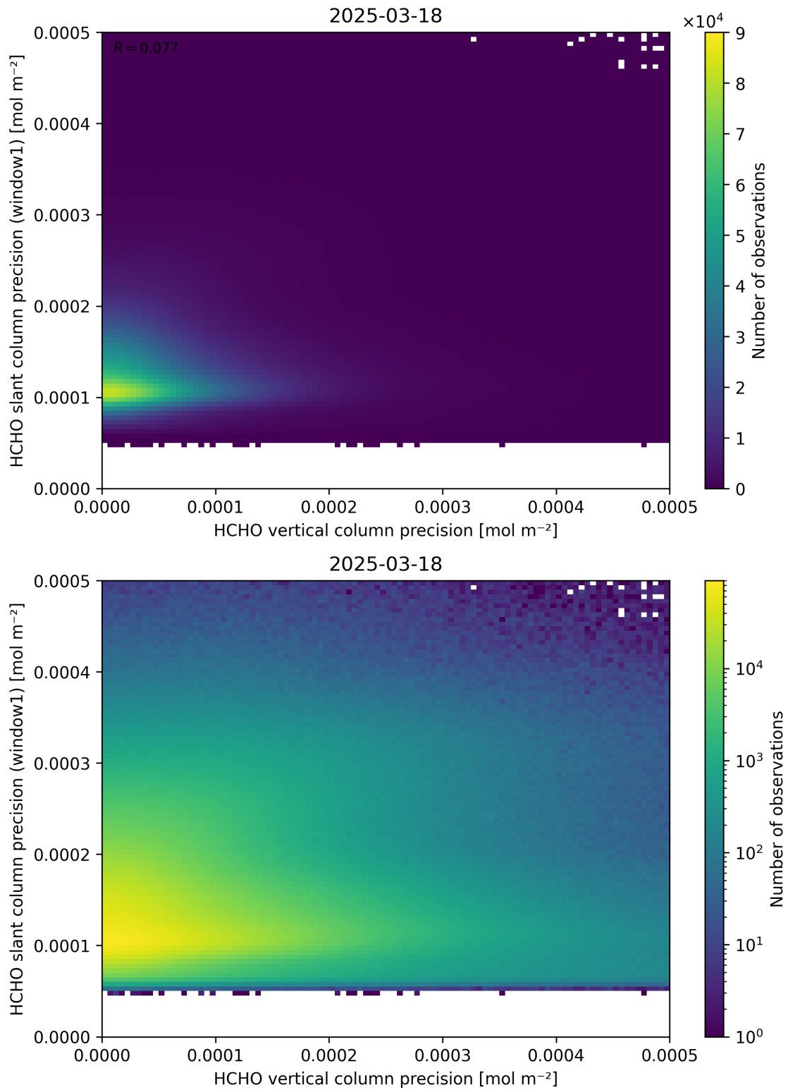
Figure 143: Scatter density plot of “HCHO vertical column precision” against “HCHO slant column precision (window1)” for 2025-03-17 to 2025-03-19.
