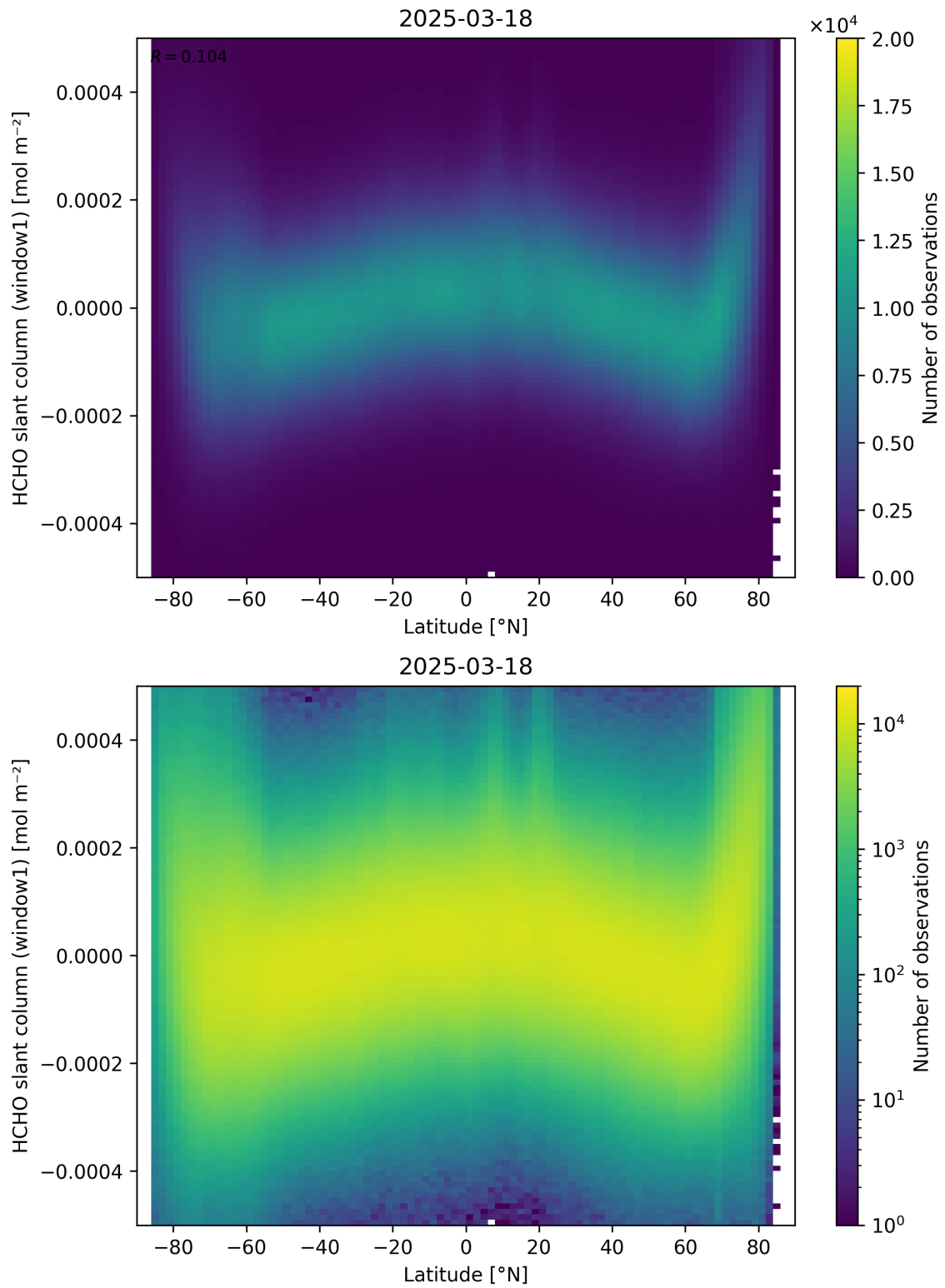
Figure 159: Scatter density plot of “Latitude” against “HCHO slant column (window1)” for 2025-03-17 to 2025-03-19.
