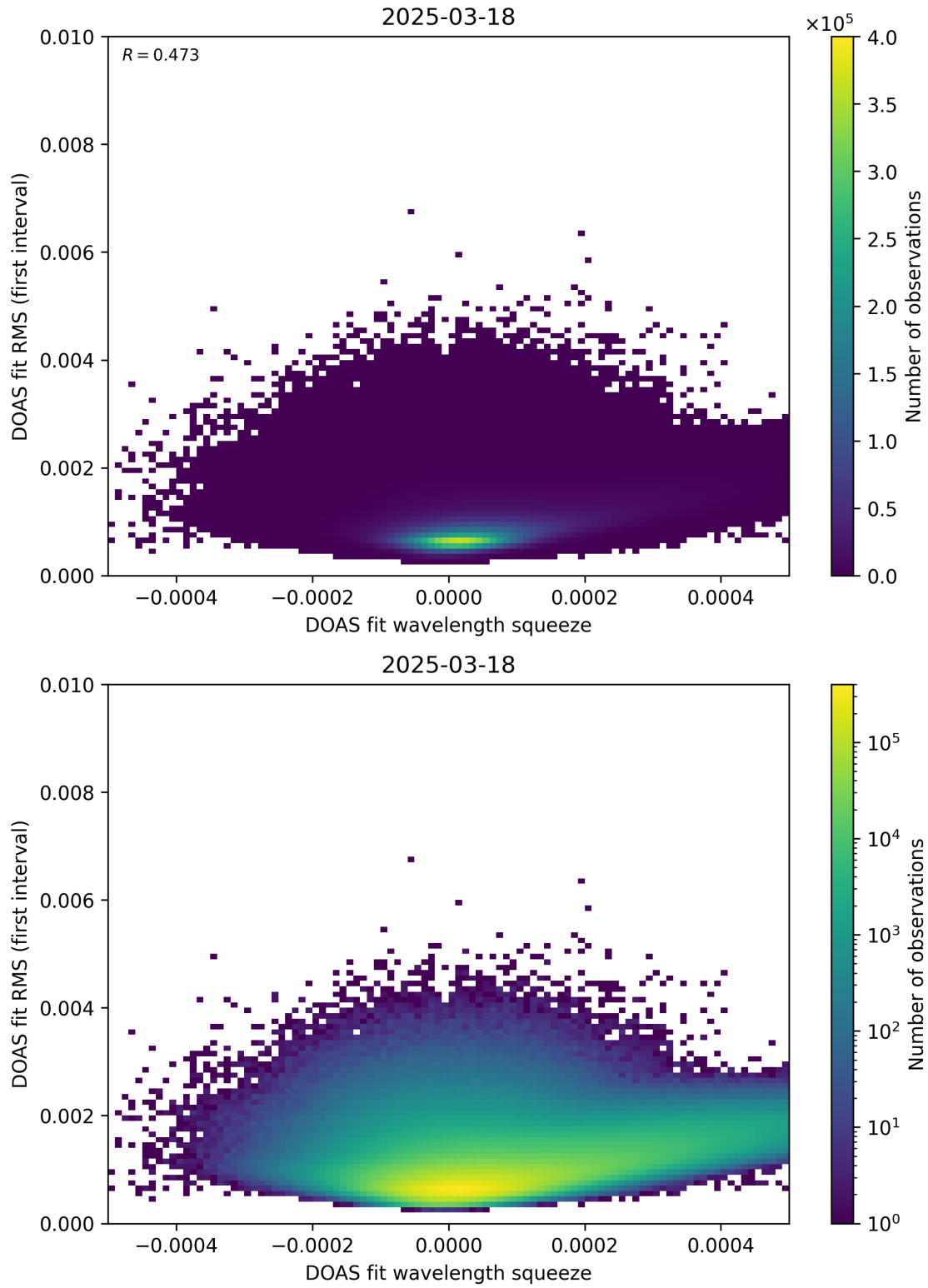
Figure 68: Scatter density plot of “DOAS fit wavelength squeeze” against “DOAS fit RMS (first interval)” for 2025-03-17 to 2025-03-19.
