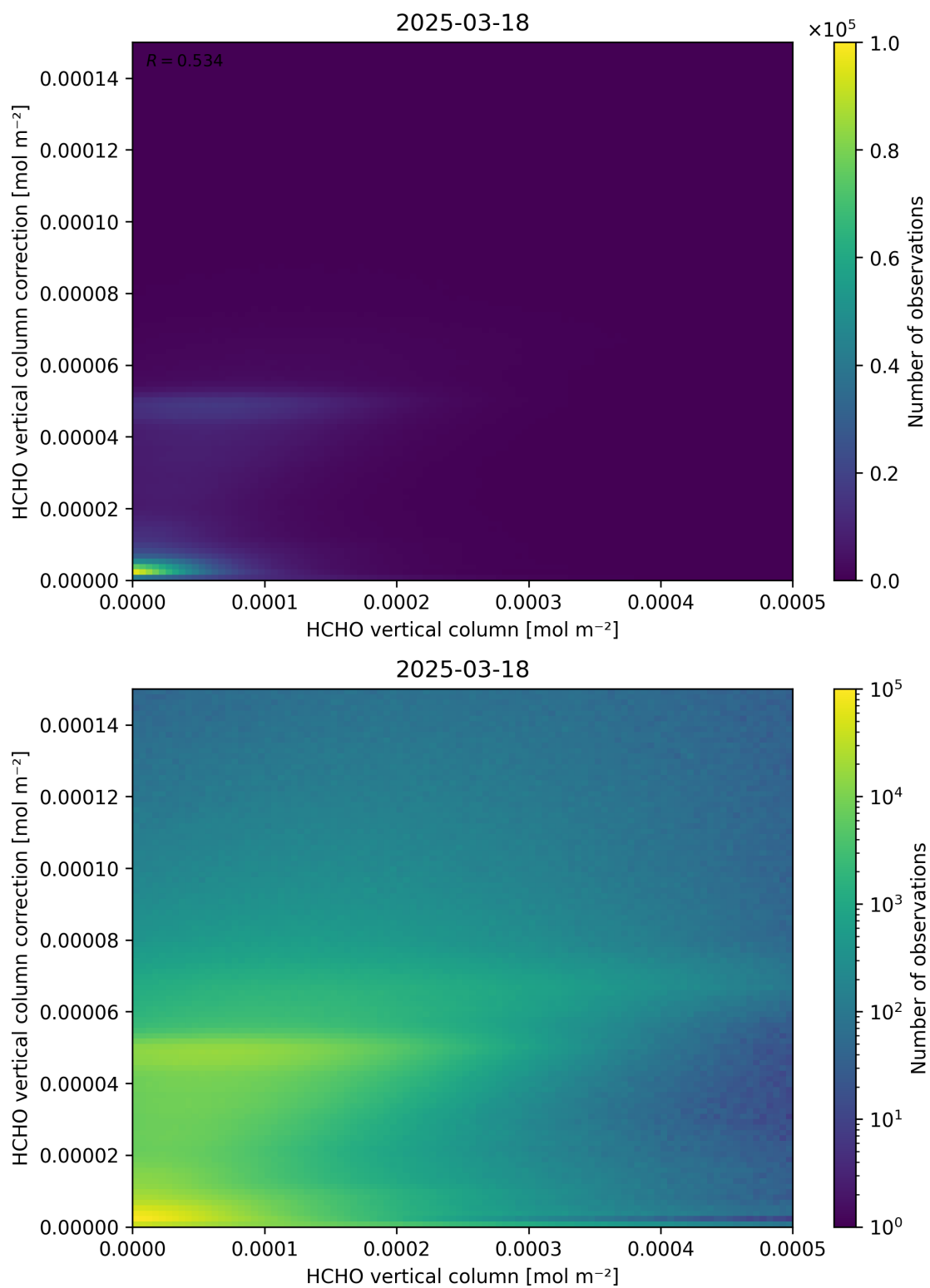
Figure 133: Scatter density plot of “HCHO vertical column” against “HCHO vertical column correction” for 2025-03-17 to 2025-03-19.
