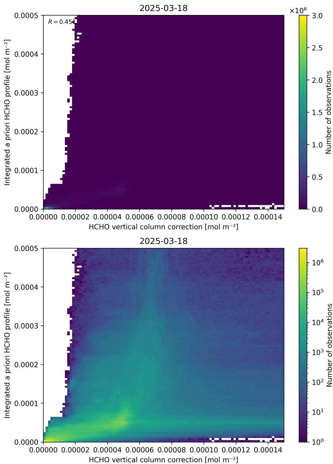
Figure 122: Scatter density plot of “HCHO vertical column correction” against “Integrated a priori HCHO profile” for 2025-03-17 to 2025-03-19.
