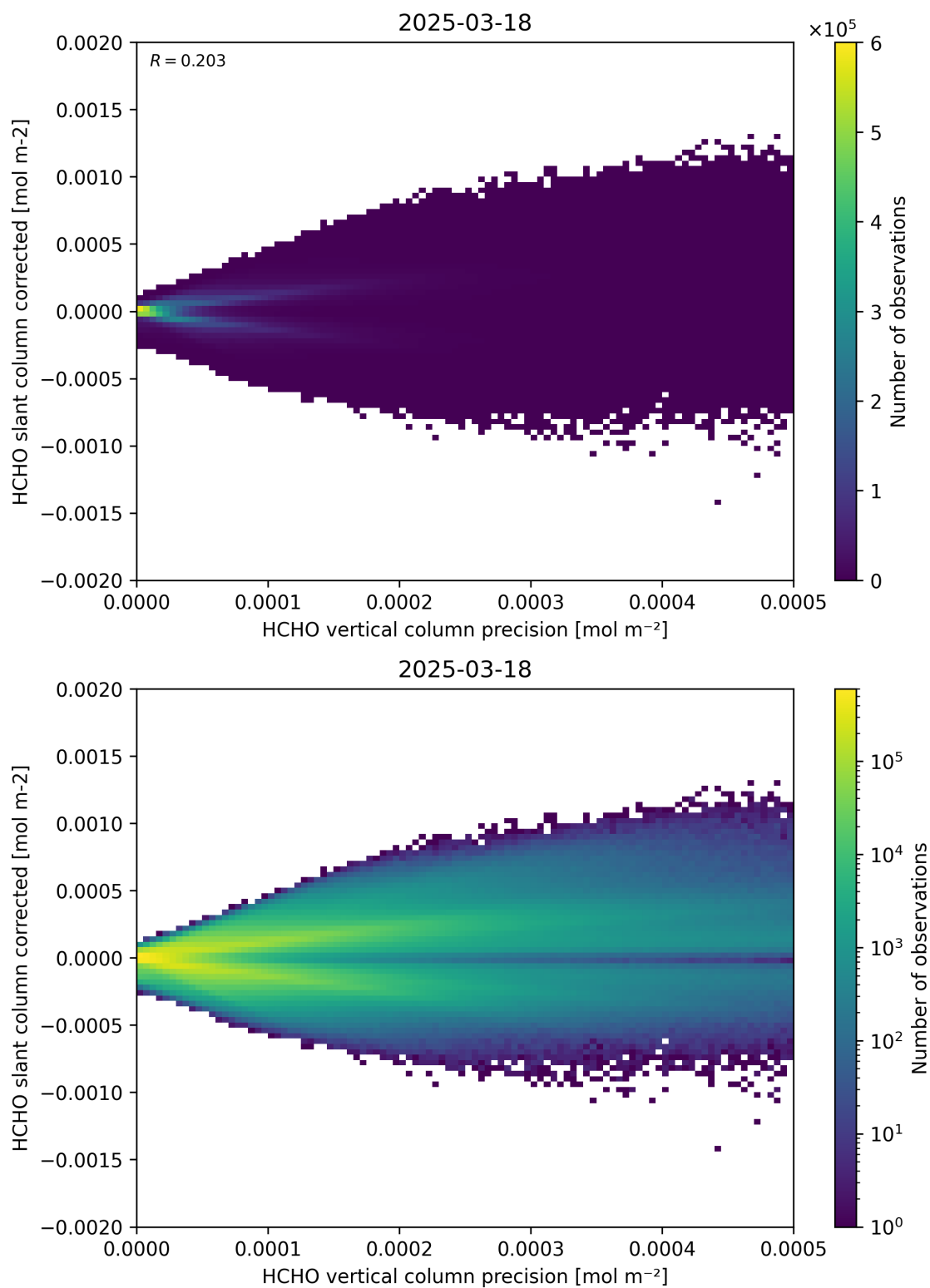
Figure 140: Scatter density plot of “HCHO vertical column precision” against “HCHO slant column corrected” for 2025-03-17 to 2025-03-19.
