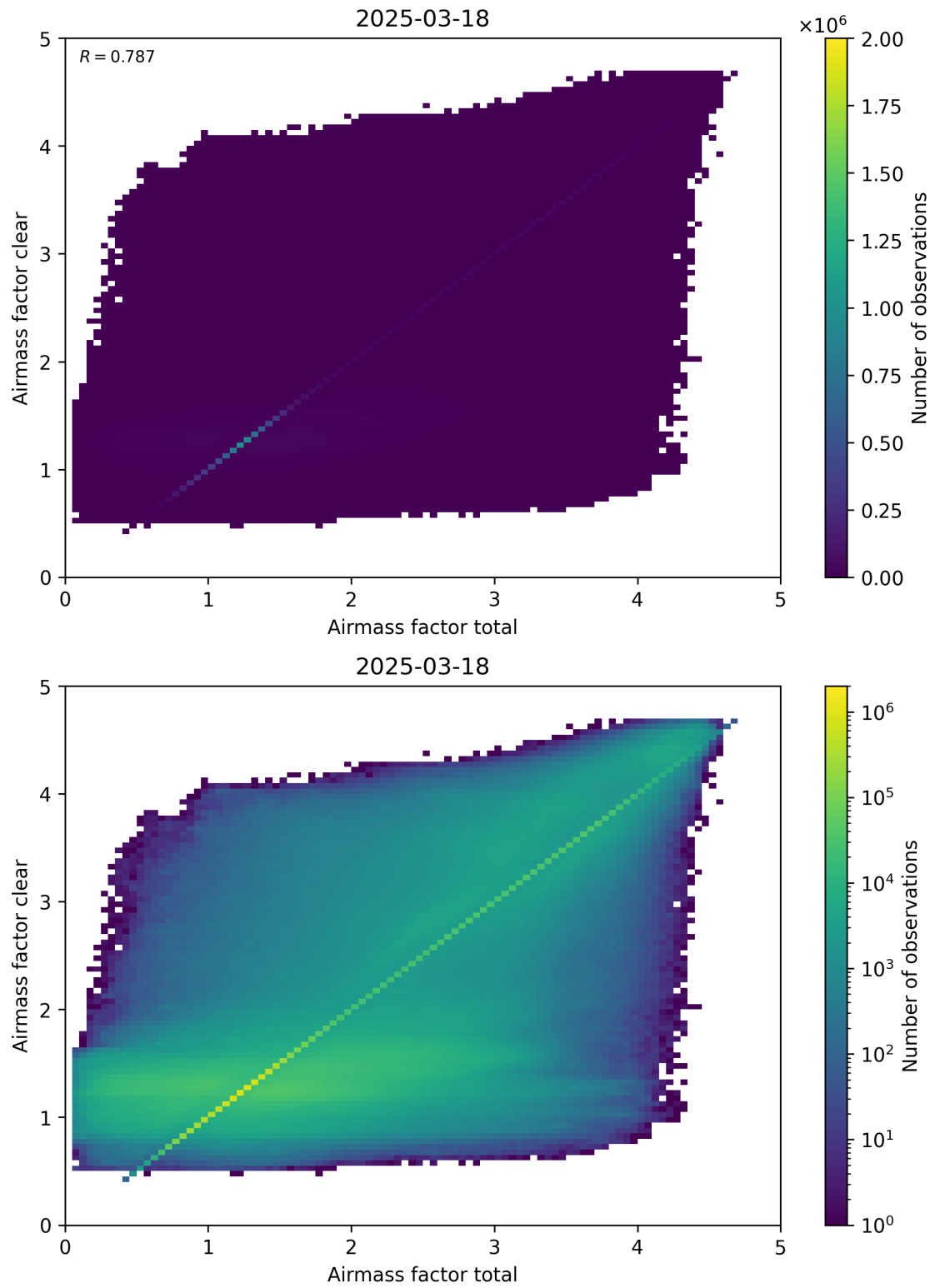
Figure 100: Scatter density plot of “Airmass factor total” against “Airmass factor clear” for 2025-03-17 to 2025-03-19.
