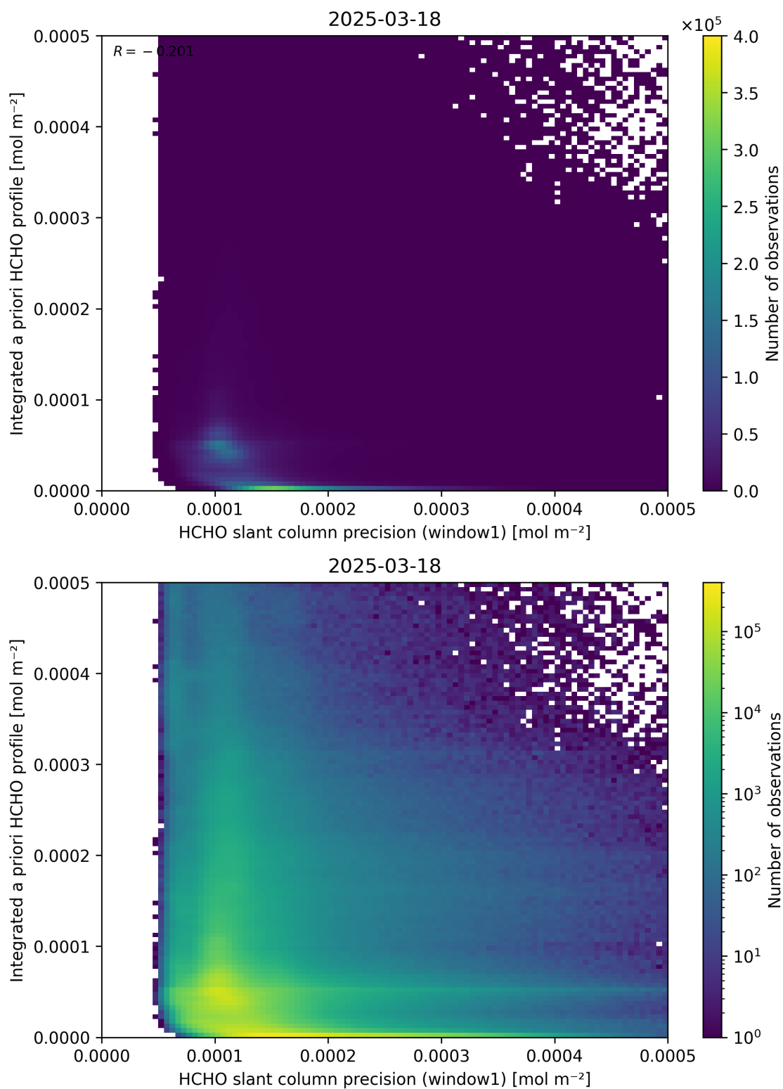
Figure 96: Scatter density plot of “HCHO slant column precision (window1)” against “Integrated a priori HCHO profile” for 2025-03-17 to 2025-03-19.
