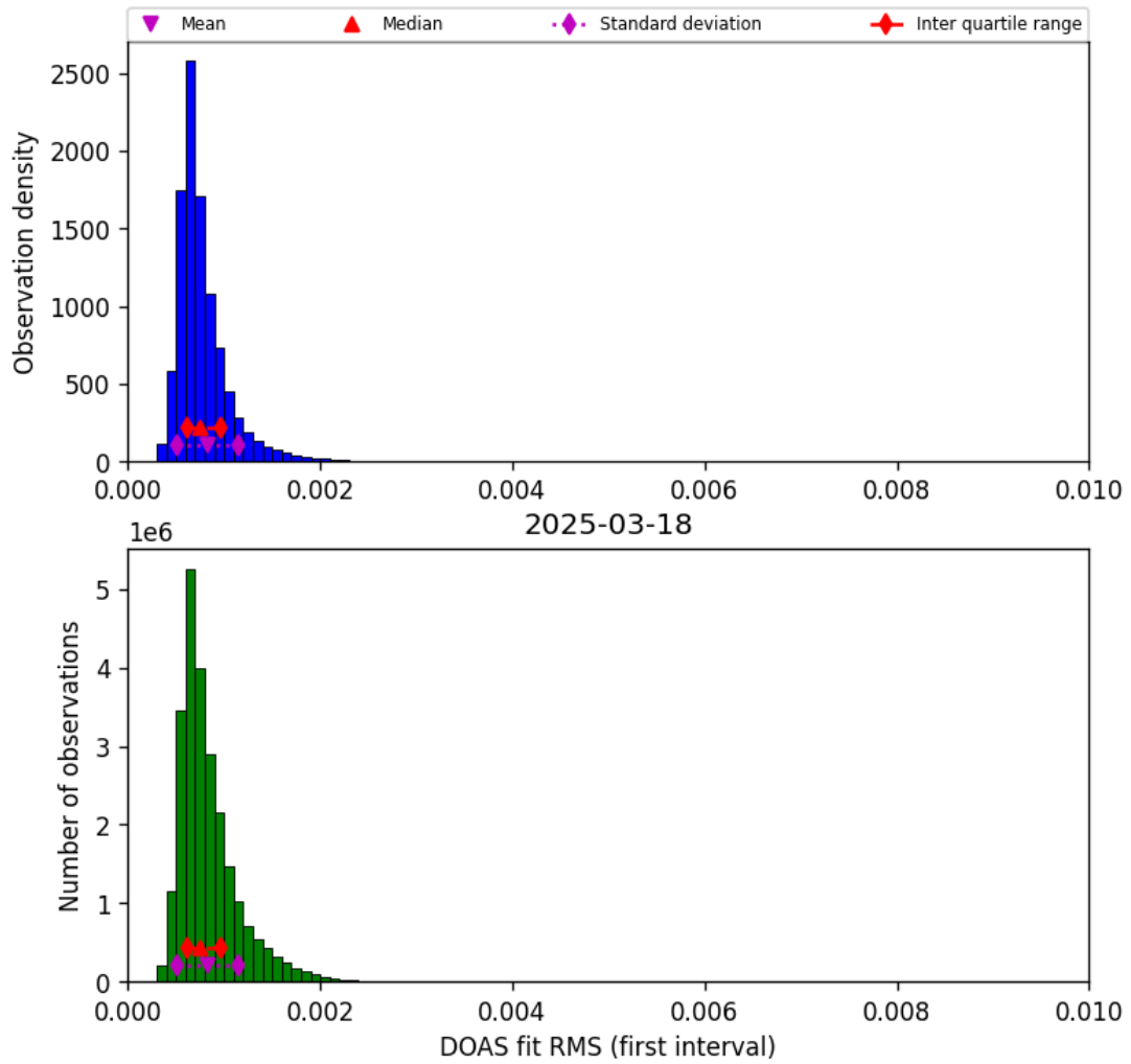
Figure 46: Histogram of “DOAS fit RMS (first interval)” for 2025-03-17 to 2025-03-19
