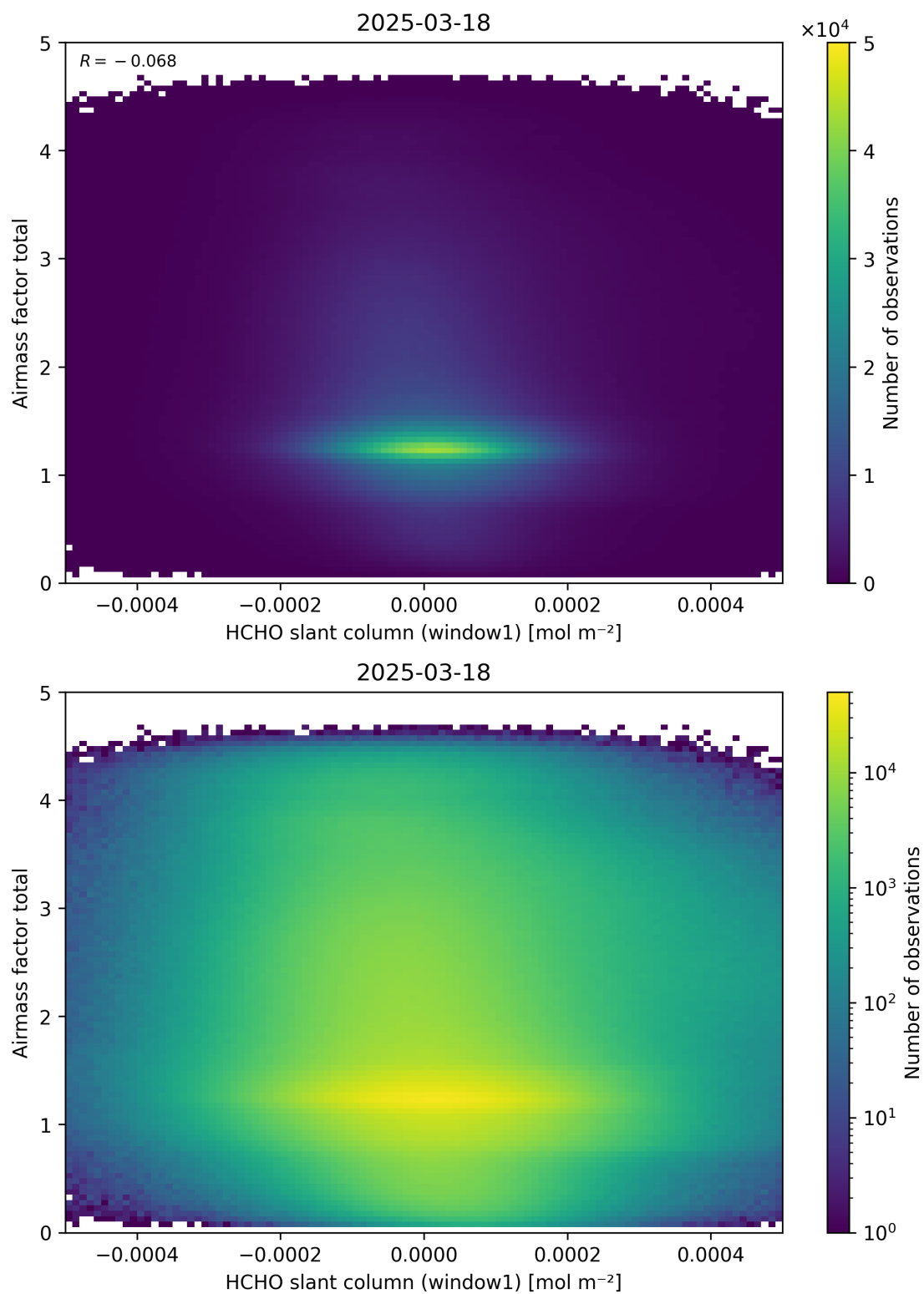
Figure 85: Scatter density plot of “HCHO slant column (window1)” against “Airmass factor total” for 2025-03-17 to 2025-03-19.
