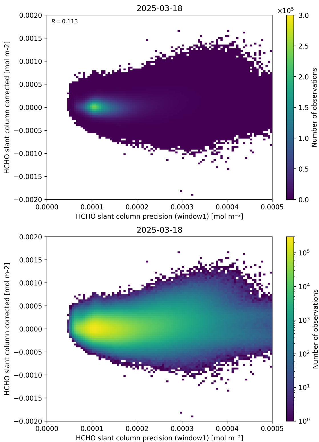
Figure 92: Scatter density plot of “HCHO slant column precision (window1)” against “HCHO slant column corrected” for 2025-03-17 to 2025-03-19.
