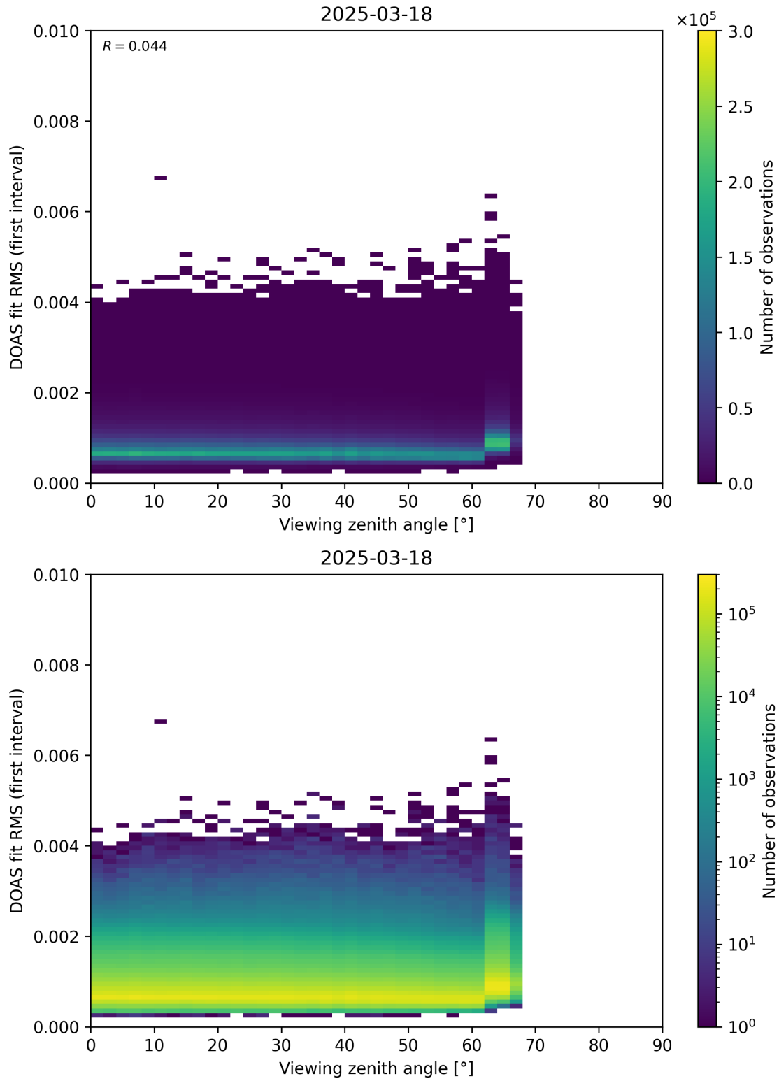
Figure 182: Scatter density plot of “Viewing zenith angle” against “DOAS fit RMS (first interval)” for 2025-03-17 to 2025-03-19.
