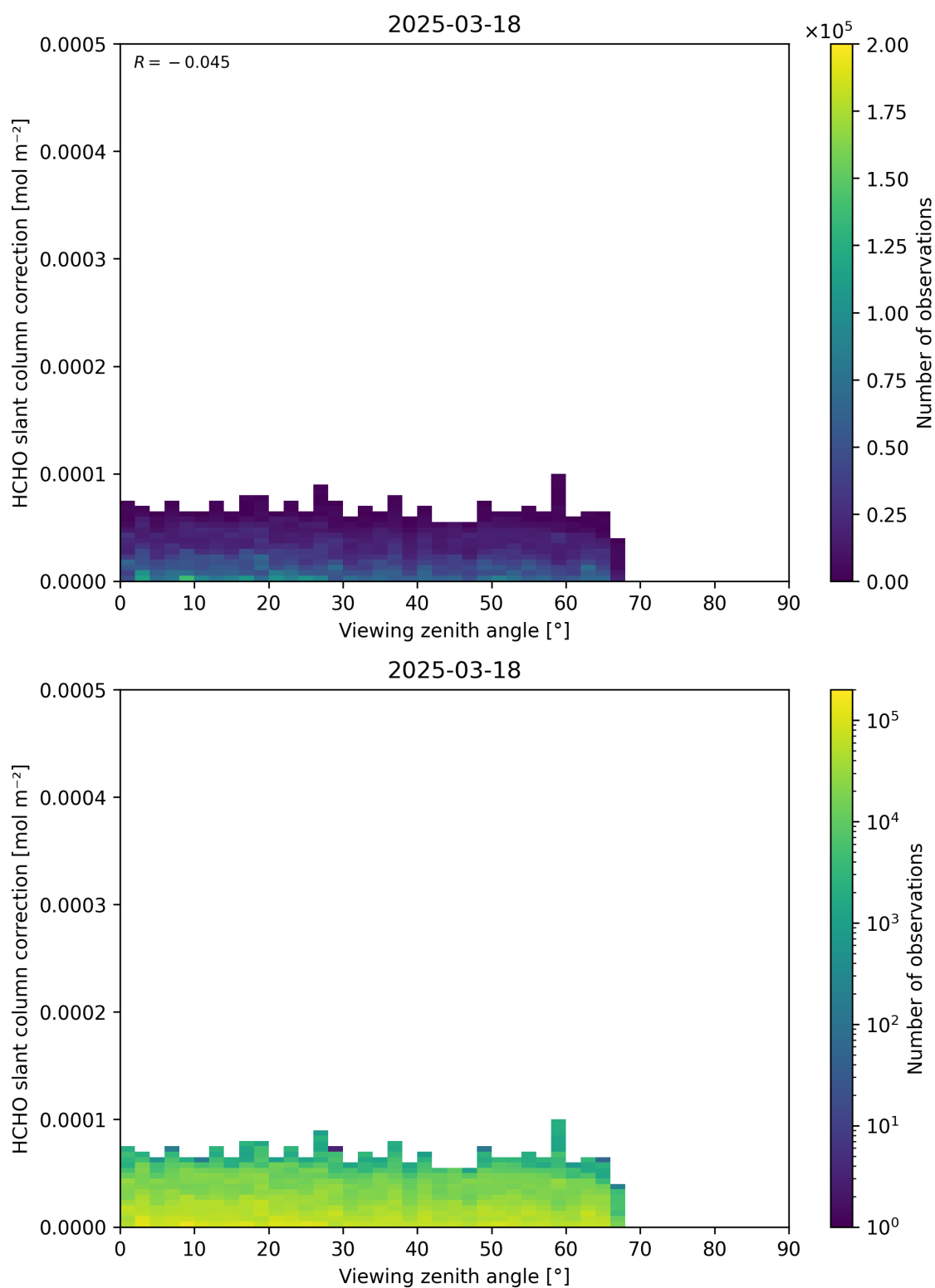
Figure 187: Scatter density plot of “Viewing zenith angle” against “HCHO slant column correction” for 2025-03-17 to 2025-03-19.
