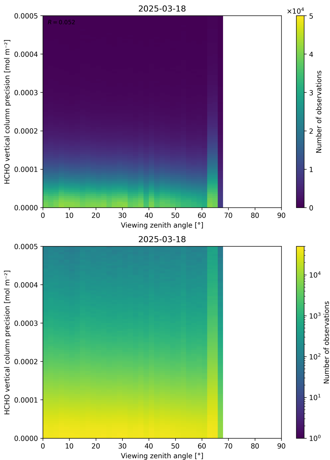
Figure 194: Scatter density plot of “Viewing zenith angle” against “HCHO vertical column precision” for 2025-03-17 to 2025-03-19.
