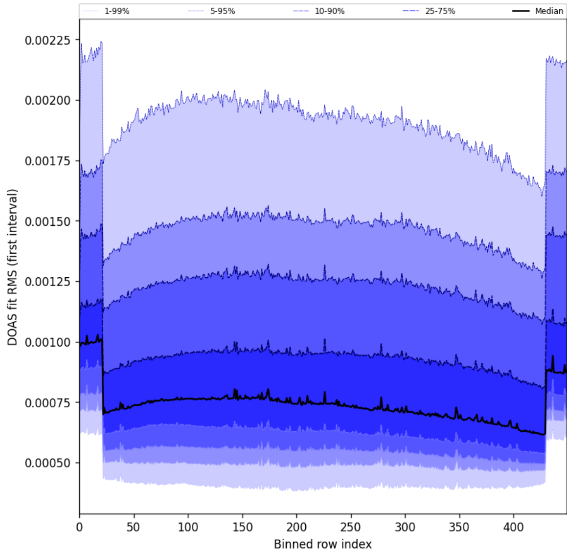
Figure 60: Along track statistics of “DOAS fit RMS (first interval)” for 2025-03-17 to 2025-03-19
