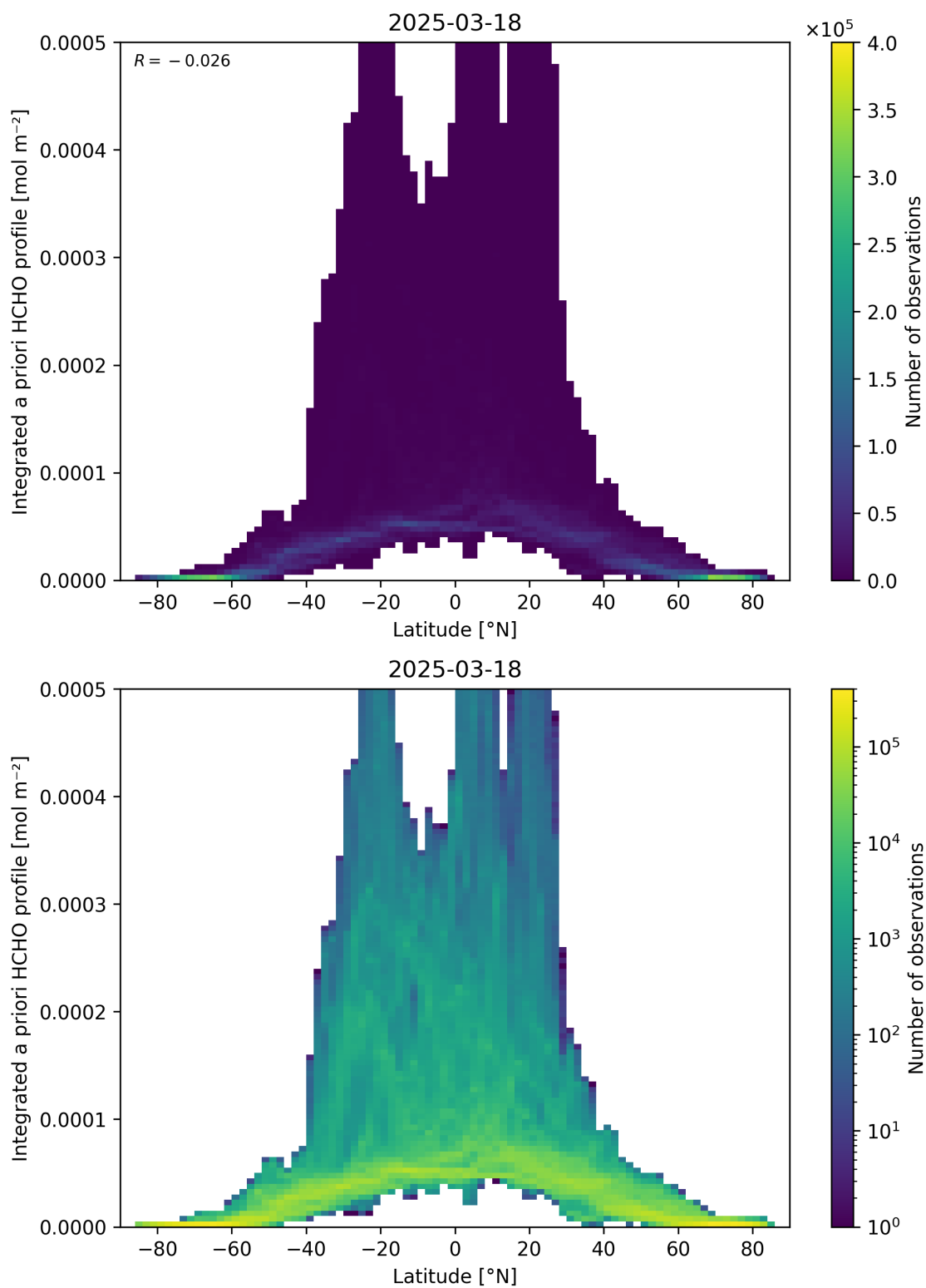
Figure 166: Scatter density plot of “Latitude” against “Integrated a priori HCHO profile” for 2025-03-17 to 2025-03-19.
