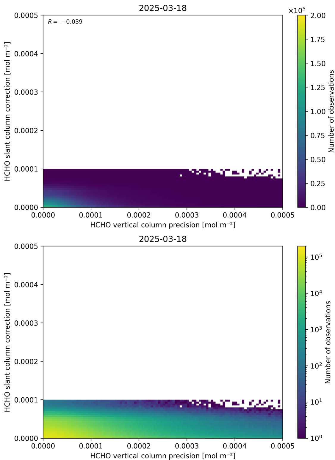
Figure 141: Scatter density plot of “HCHO vertical column precision” against “HCHO slant column correction” for 2025-03-17 to 2025-03-19.
