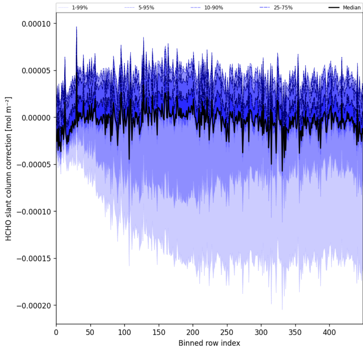
Figure 61: Along track statistics of “HCHO slant column correction” for 2025-03-17 to 2025-03-19
