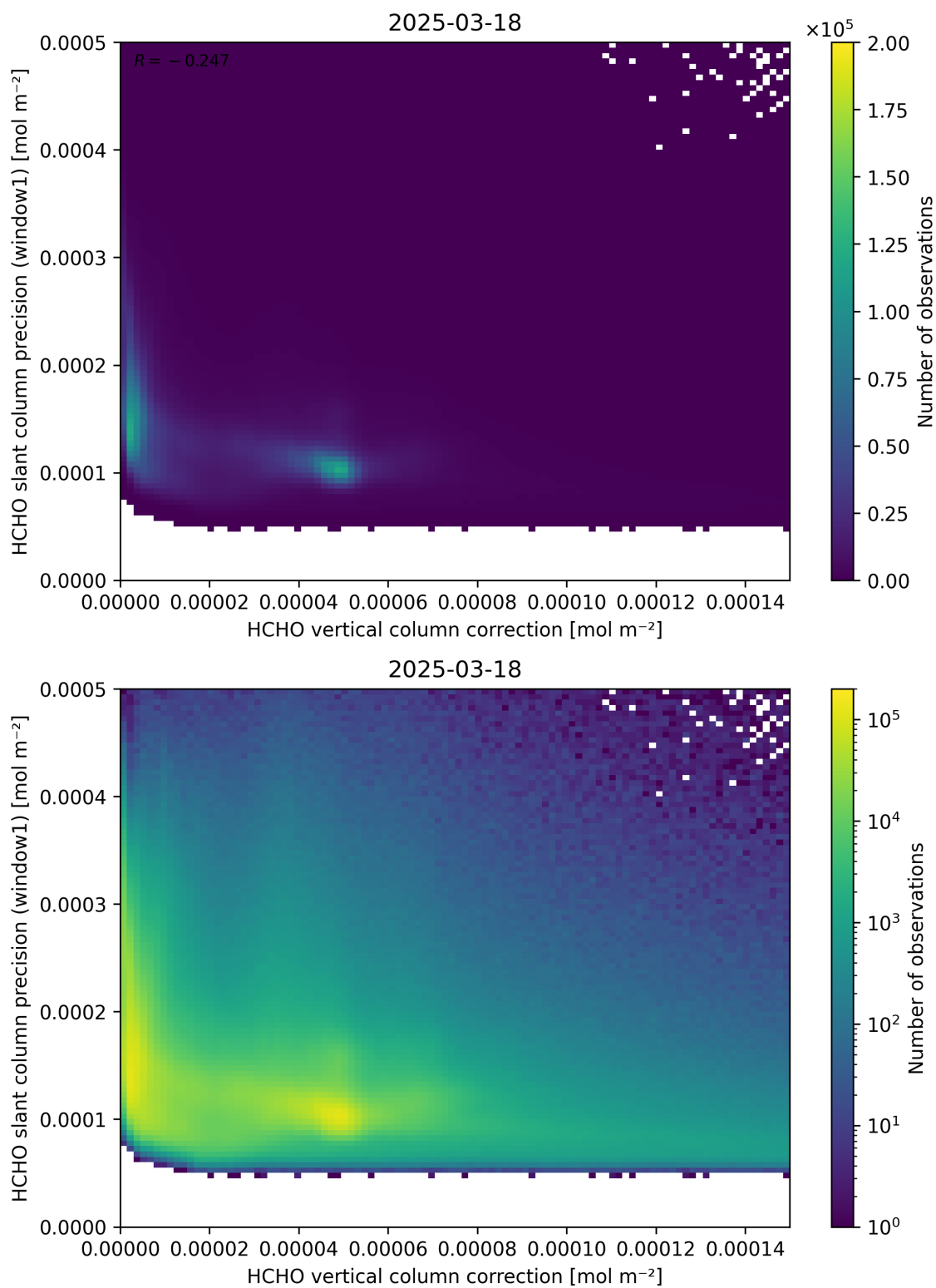
Figure 119: Scatter density plot of “HCHO vertical column correction” against “HCHO slant column precision (window1)” for 2025-03-17 to 2025-03-19.
