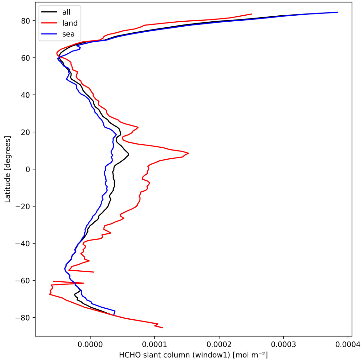
Figure 24: Zonal average of “HCHO slant column (window1)” for 2025-03-17 to 2025-03-19.
