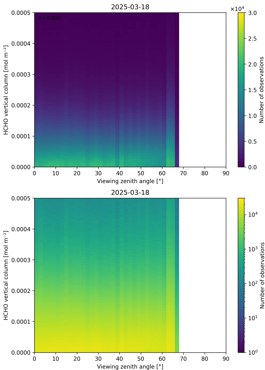
Figure 192: Scatter density plot of “Viewing zenith angle” against “HCHO vertical column” for 2025-03-17 to 2025-03-19.
