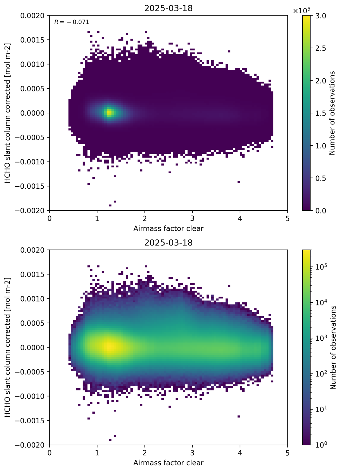
Figure 74: Scatter density plot of “Airmass factor clear” against “HCHO slant column corrected” for 2025-03-17 to 2025-03-19.
