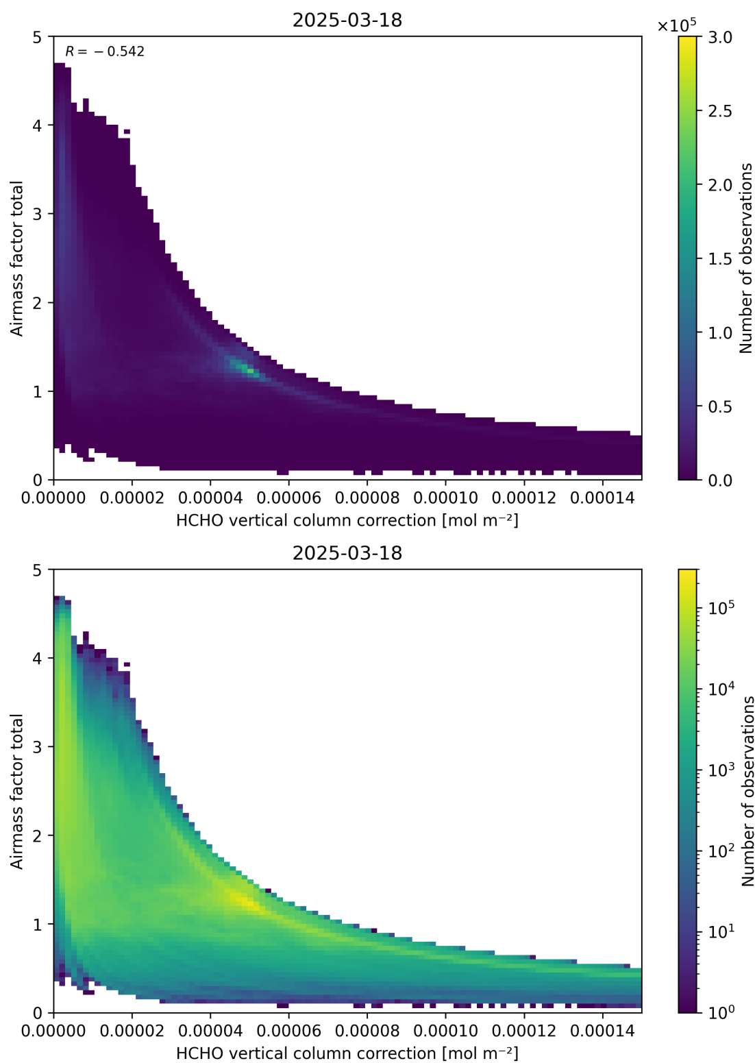
Figure 120: Scatter density plot of “HCHO vertical column correction” against “Airmass factor total” for 2025-03-17 to 2025-03-19.
