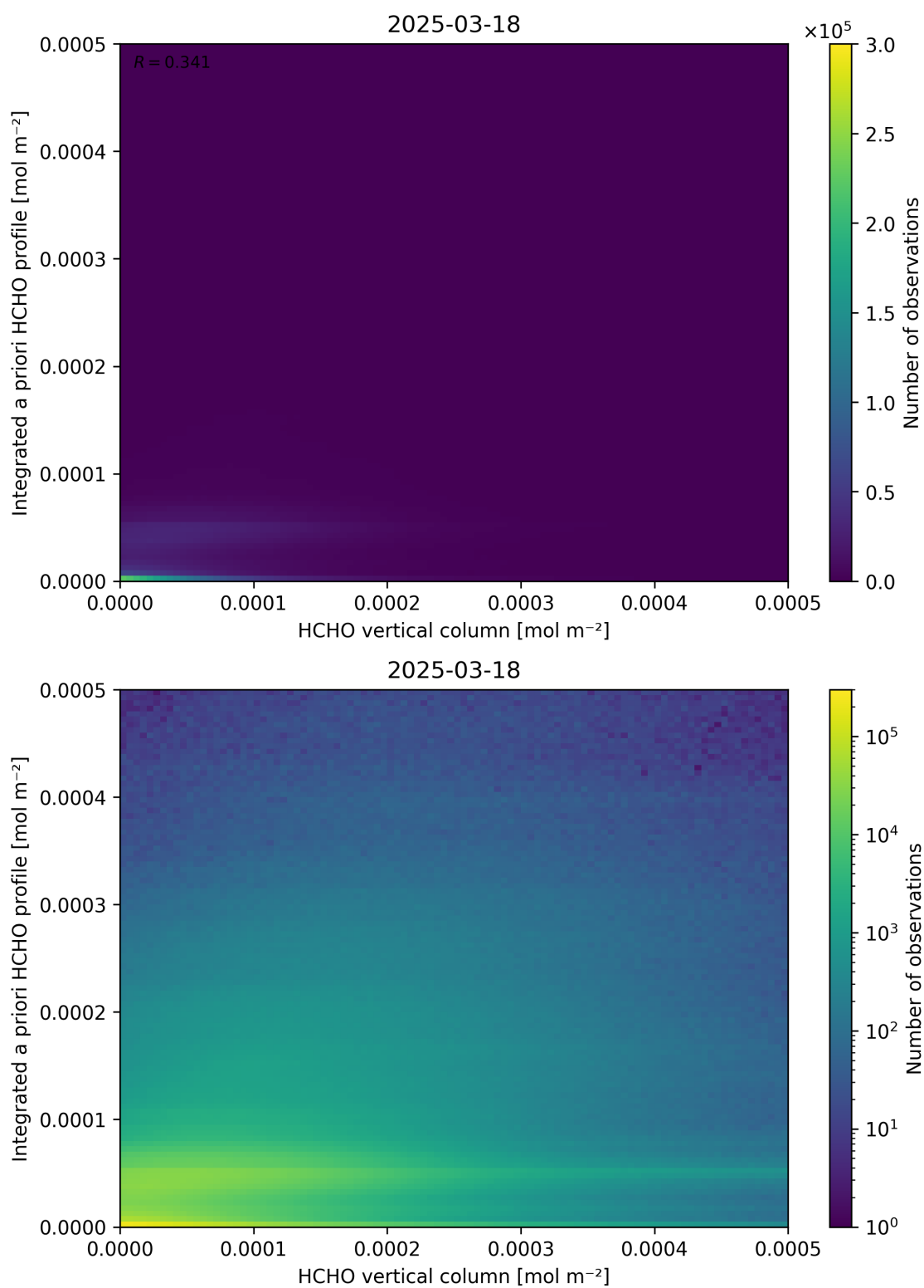
Figure 135: Scatter density plot of “HCHO vertical column” against “Integrated a priori HCHO profile” for 2025-03-17 to 2025-03-19.
