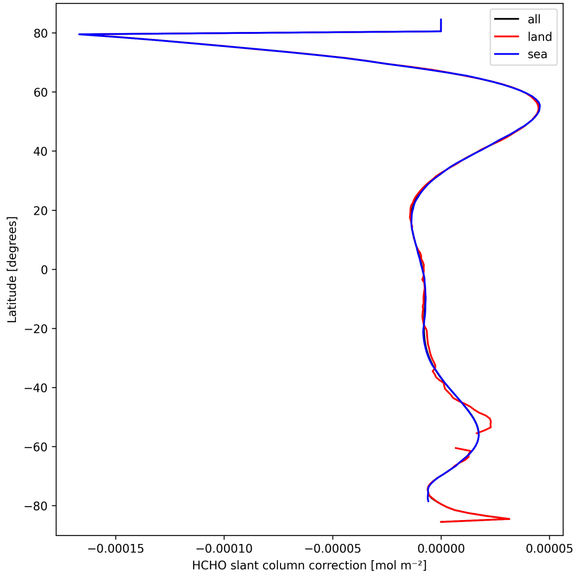
Figure 33: Zonal average of “HCHO slant column correction” for 2025-03-17 to 2025-03-19.
