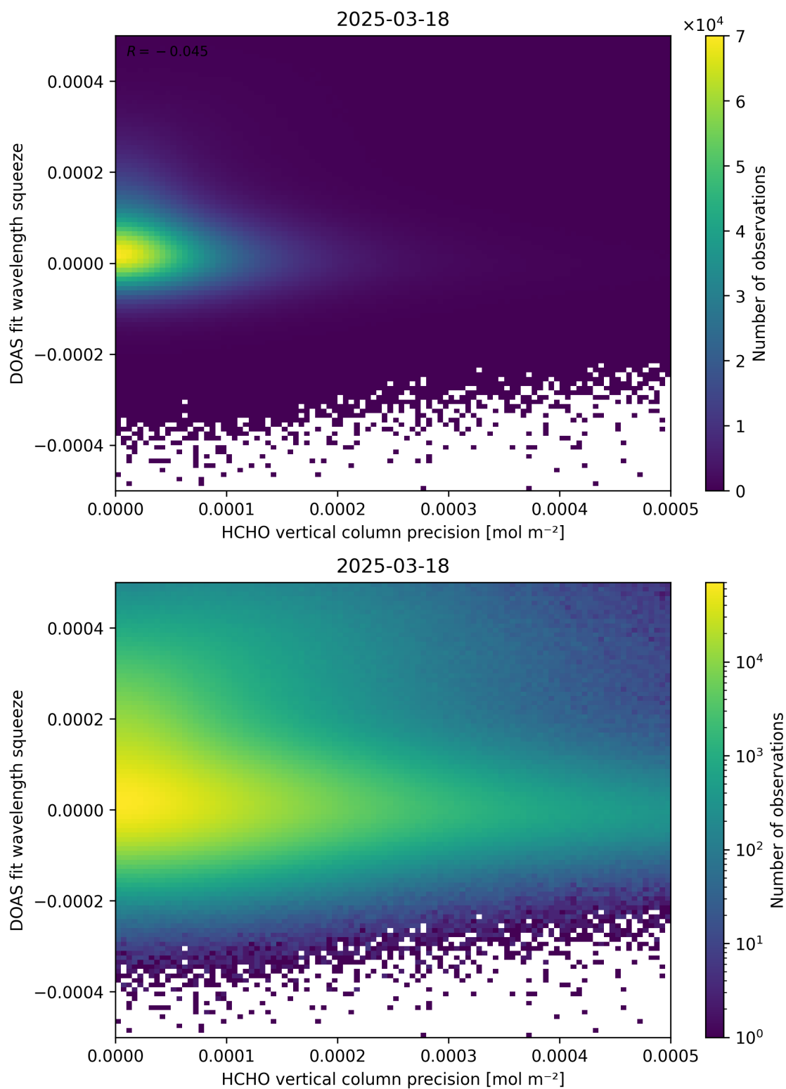
Figure 138: Scatter density plot of “HCHO vertical column precision” against “DOAS fit wavelength squeeze” for 2025-03-17 to 2025-03-19.
