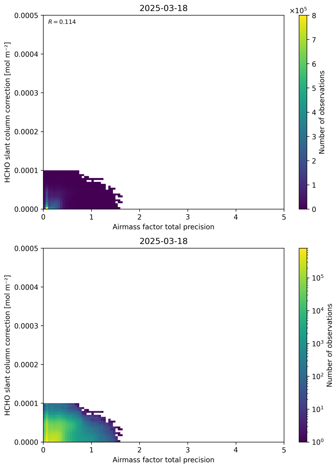
Figure 110: Scatter density plot of “Airmass factor total precision” against “HCHO slant column correction” for 2025-03-17 to 2025-03-19.
