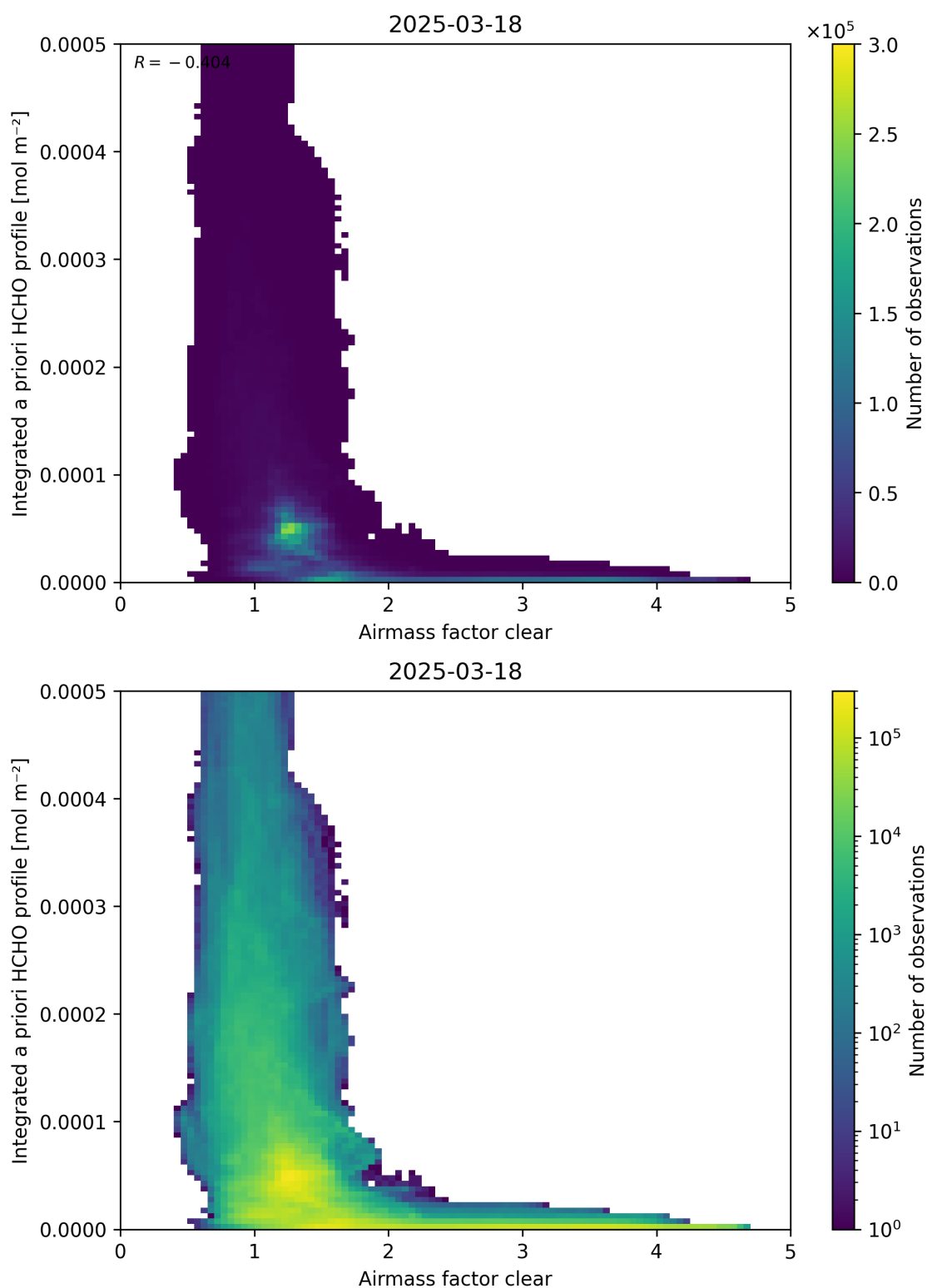
Figure 76: Scatter density plot of “Airmass factor clear” against “Integrated a priori HCHO profile” for 2025-03-17 to 2025-03-19.
