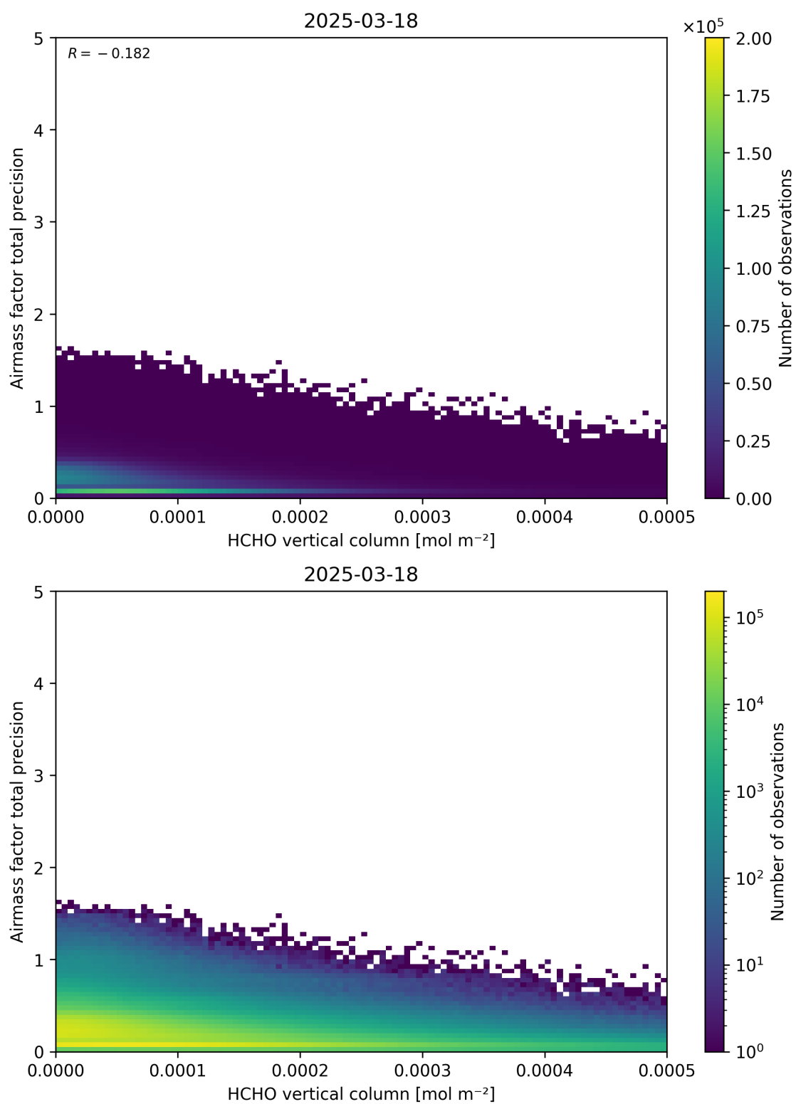
Figure 132: Scatter density plot of “HCHO vertical column” against “Airmass factor total precision” for 2025-03-17 to 2025-03-19.
