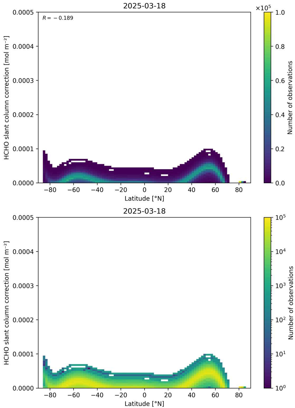
Figure 158: Scatter density plot of “Latitude” against “HCHO slant column correction” for 2025-03-17 to 2025-03-19.
