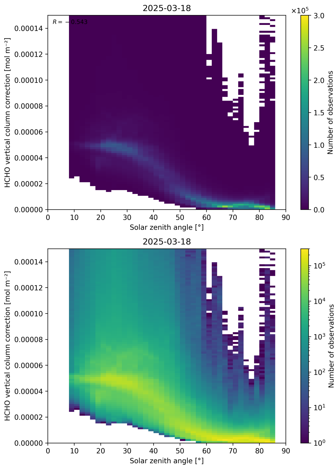
Figure 178: Scatter density plot of “Solar zenith angle” against “HCHO vertical column correction” for 2025-03-17 to 2025-03-19.
