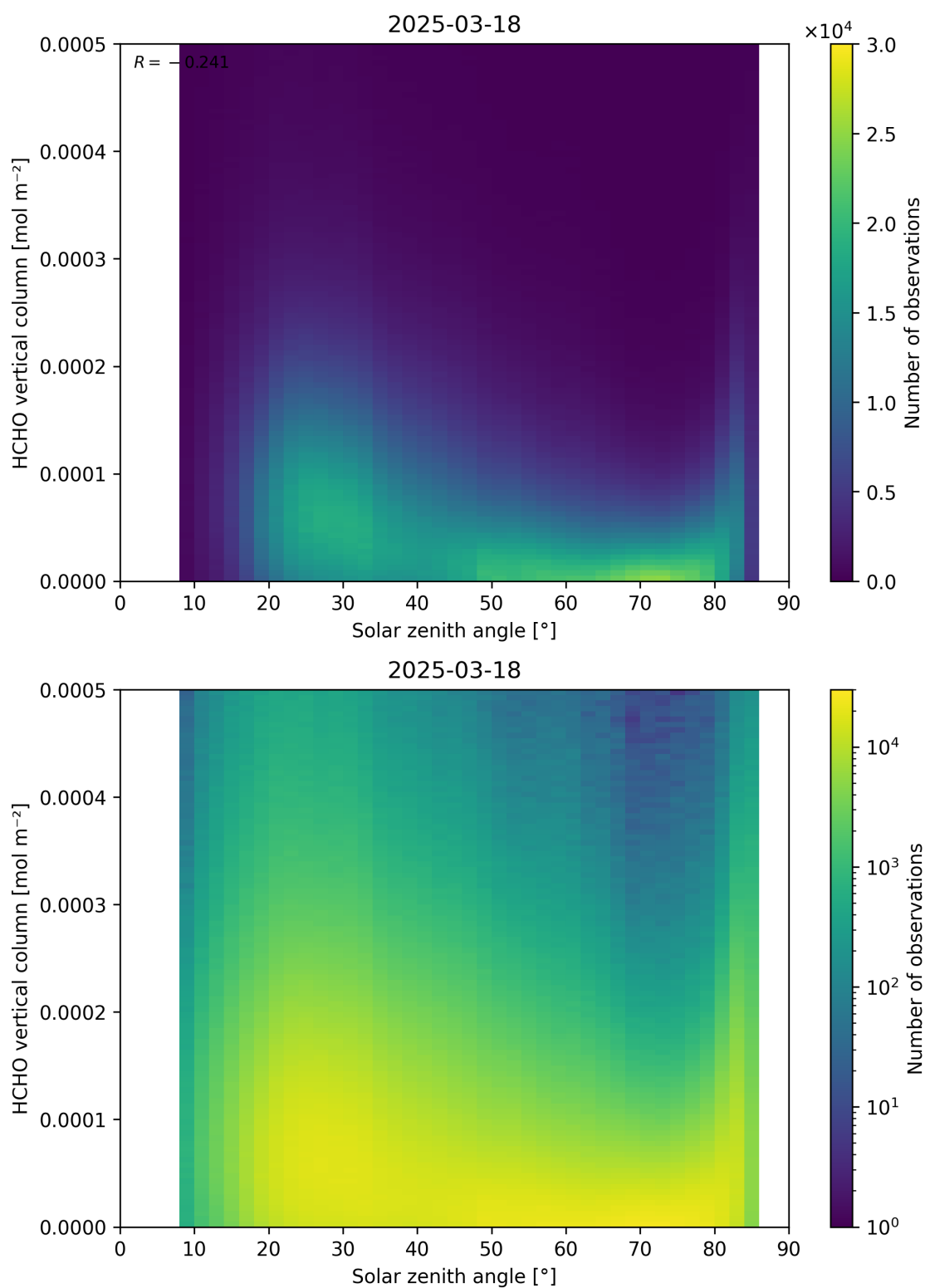
Figure 177: Scatter density plot of “Solar zenith angle” against “HCHO vertical column” for 2025-03-17 to 2025-03-19.
