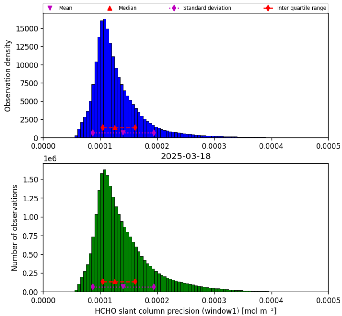
Figure 39: Histogram of “HCHO slant column precision (window1)” for 2025-03-17 to 2025-03-19
