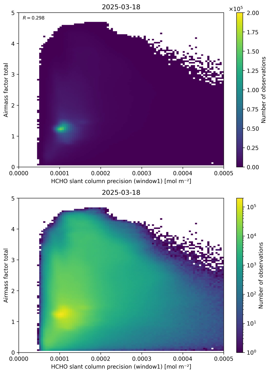
Figure 94: Scatter density plot of “HCHO slant column precision (window1)” against “Airmass factor total” for 2025-03-17 to 2025-03-19.
