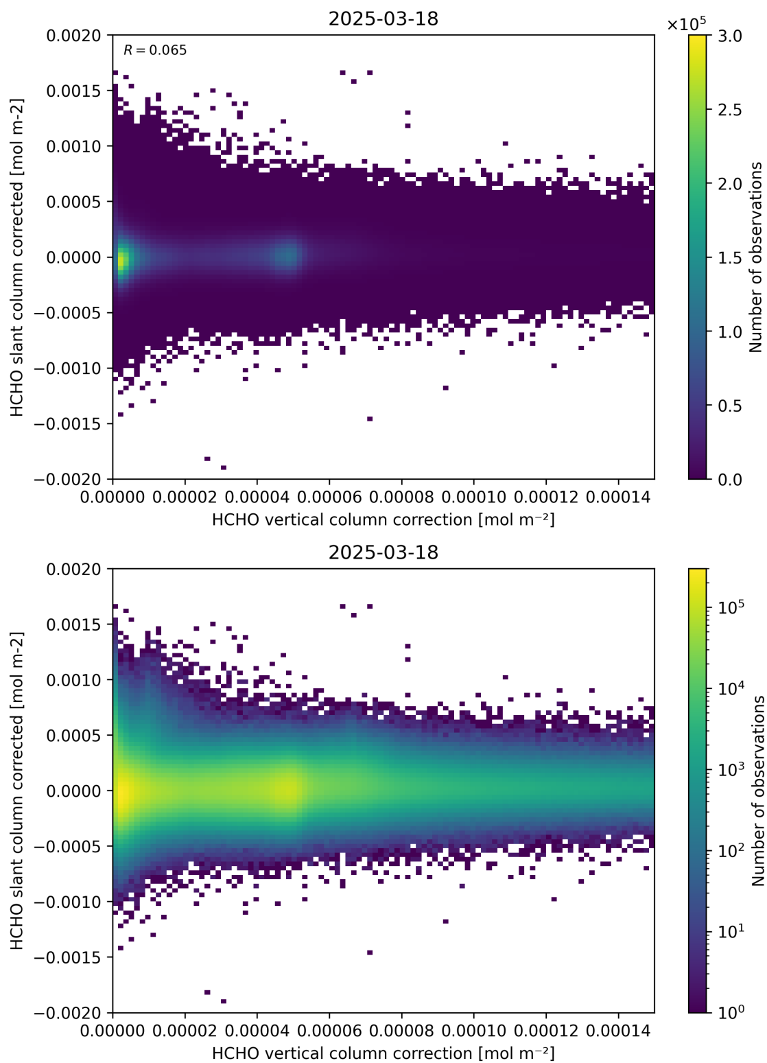
Figure 116: Scatter density plot of “HCHO vertical column correction” against “HCHO slant column corrected” for 2025-03-17 to 2025-03-19.
