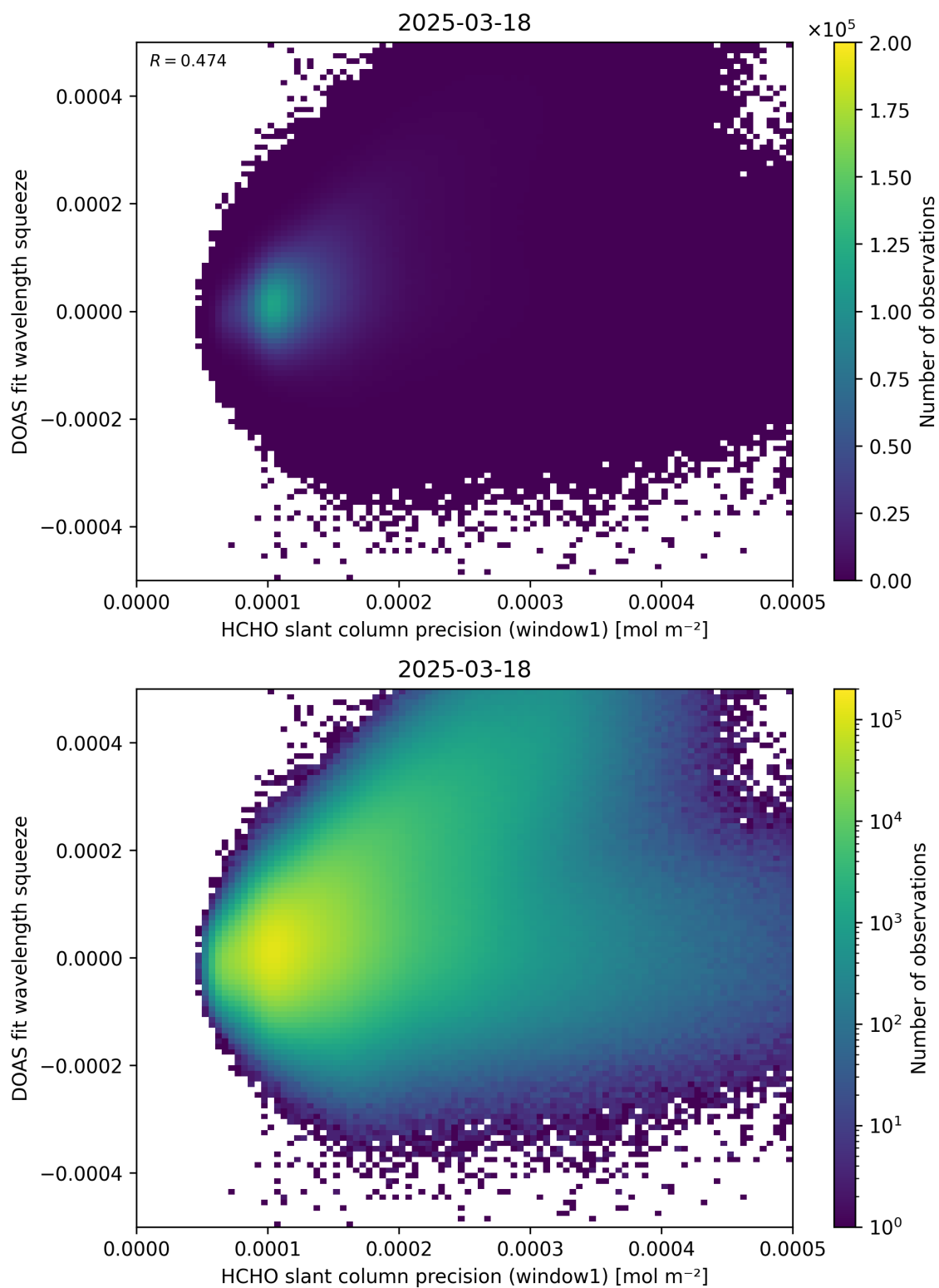
Figure 90: Scatter density plot of “HCHO slant column precision (window1)” against “DOAS fit wavelength squeeze” for 2025-03-17 to 2025-03-19.
