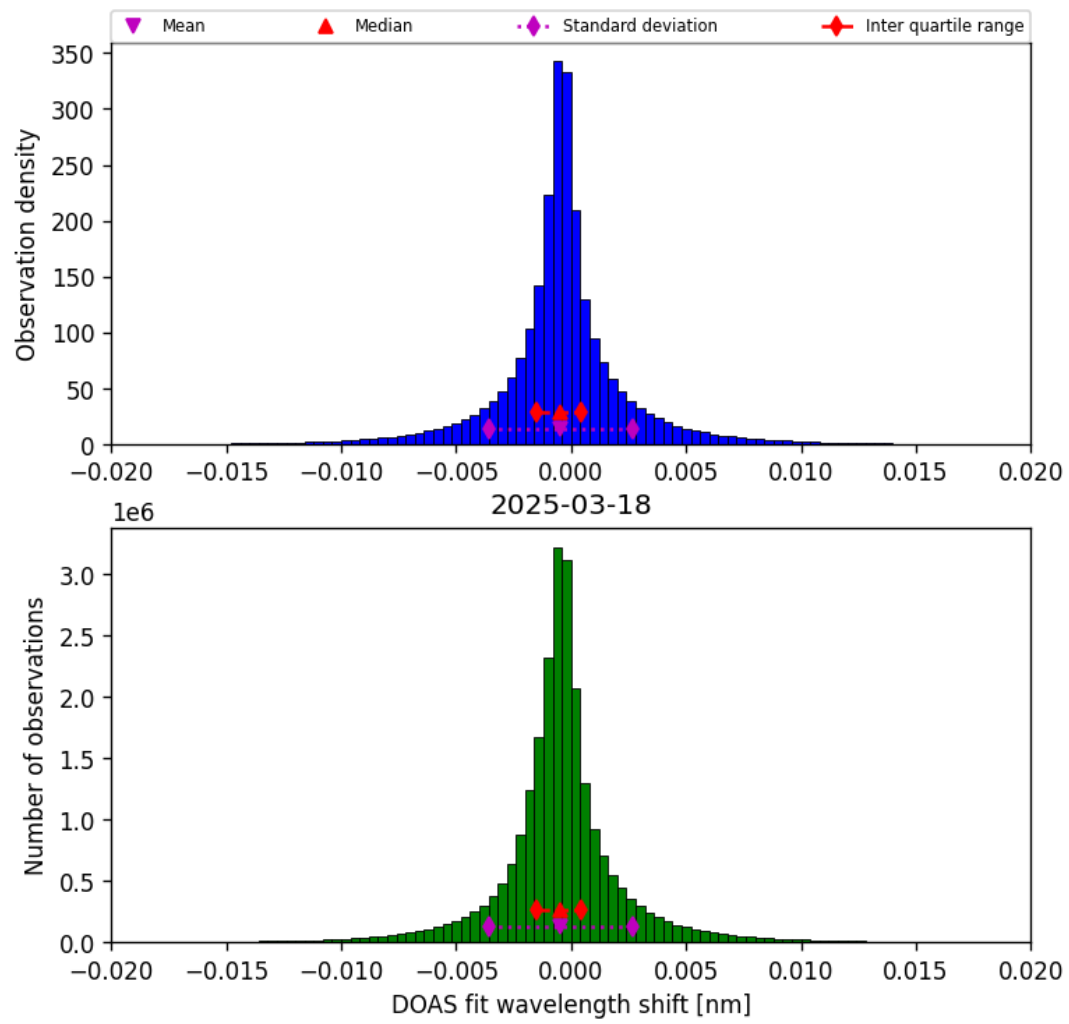
Figure 44: Histogram of “DOAS fit wavelength shift” for 2025-03-17 to 2025-03-19
