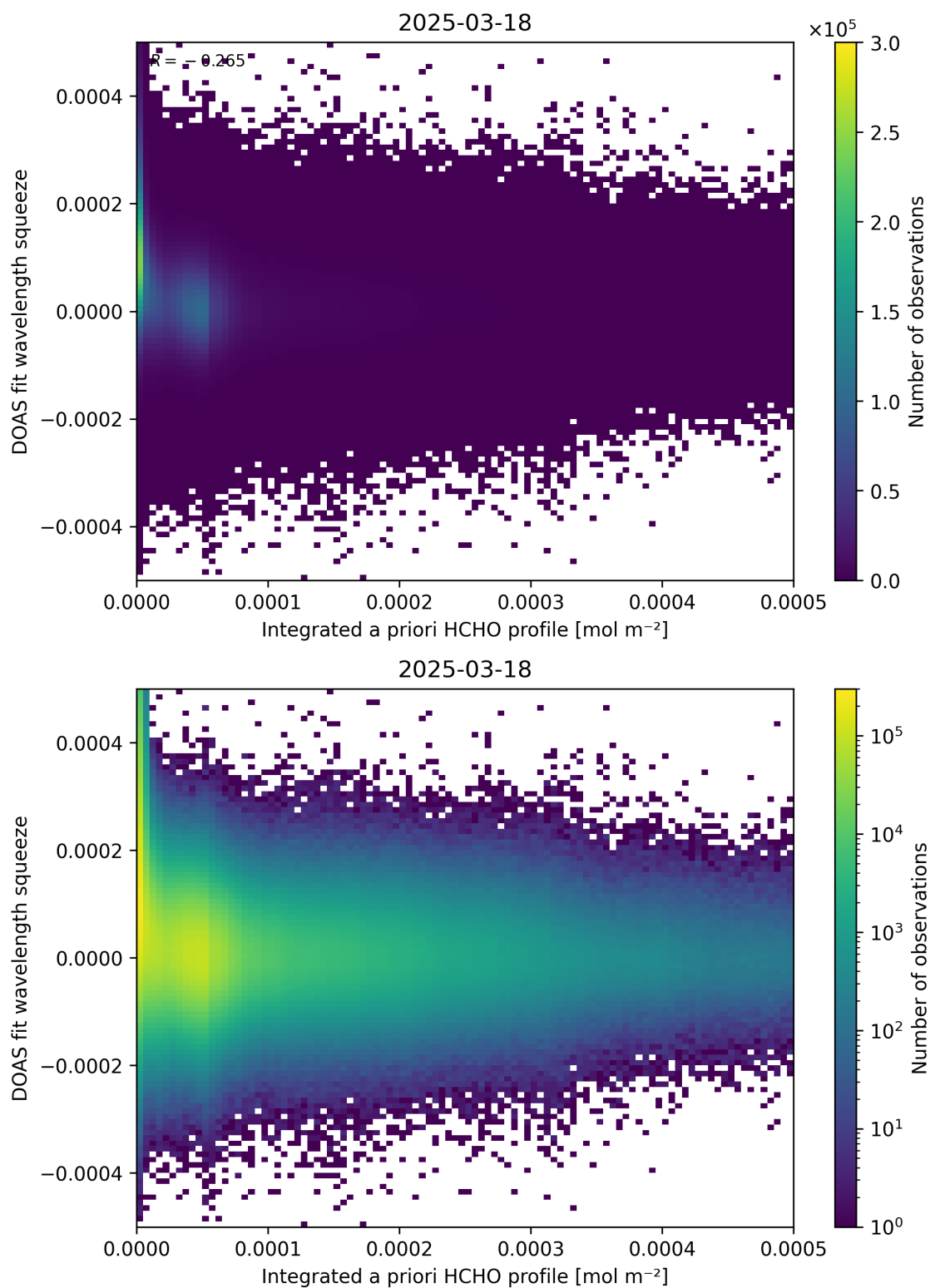
Figure 150: Scatter density plot of “Integrated a priori HCHO profile” against “DOAS fit wavelength squeeze” for 2025-03-17 to 2025-03-19.
