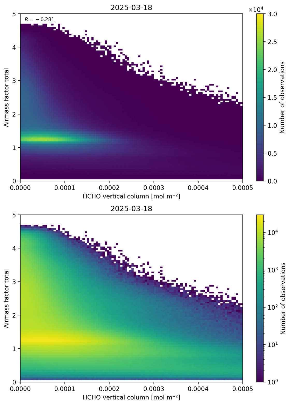
Figure 131: Scatter density plot of “HCHO vertical column” against “Airmass factor total” for 2025-03-17 to 2025-03-19.
