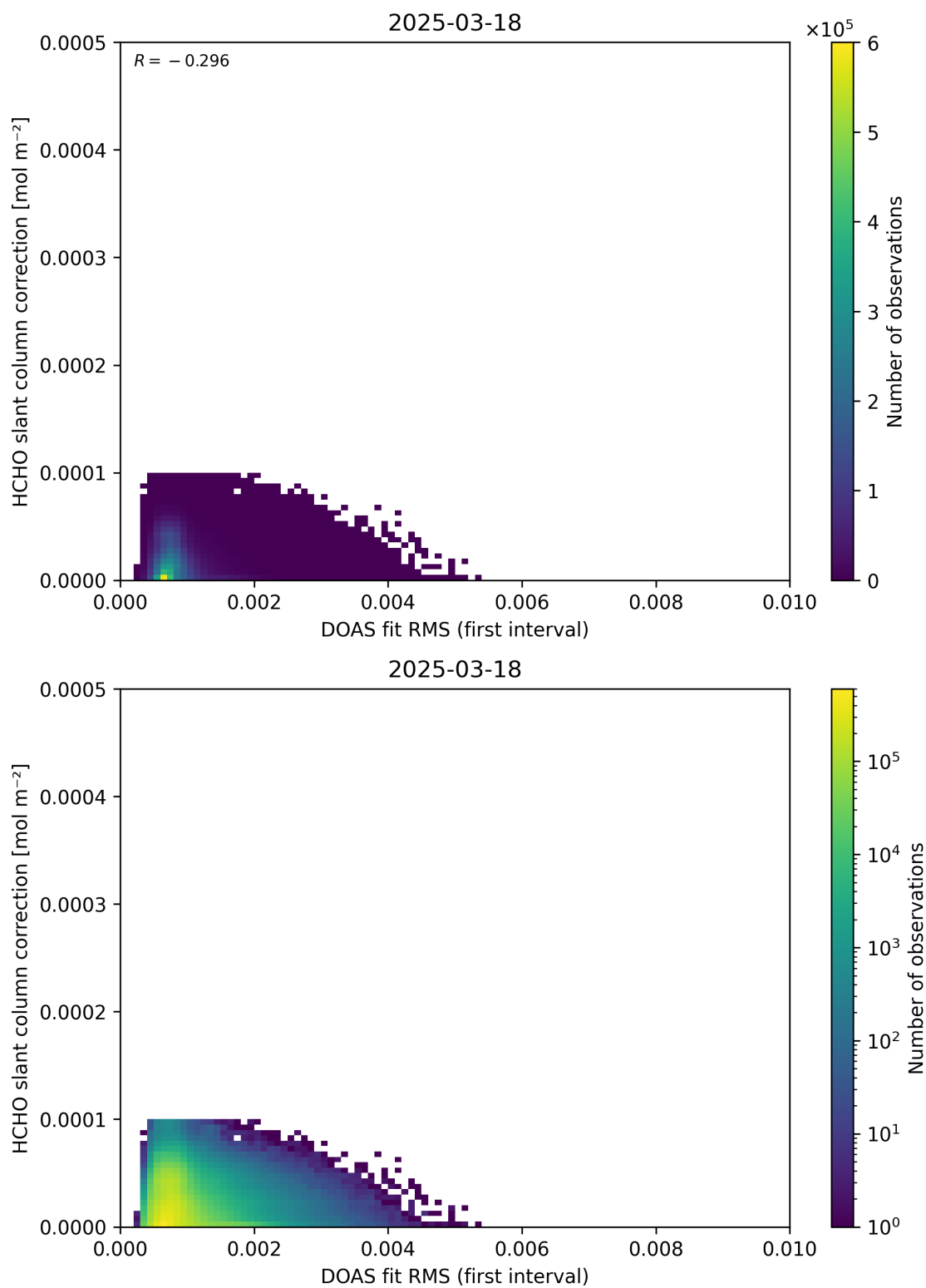
Figure 63: Scatter density plot of “DOAS fit RMS (first interval)” against “HCHO slant column correction” for 2025-03-17 to 2025-03-19.
