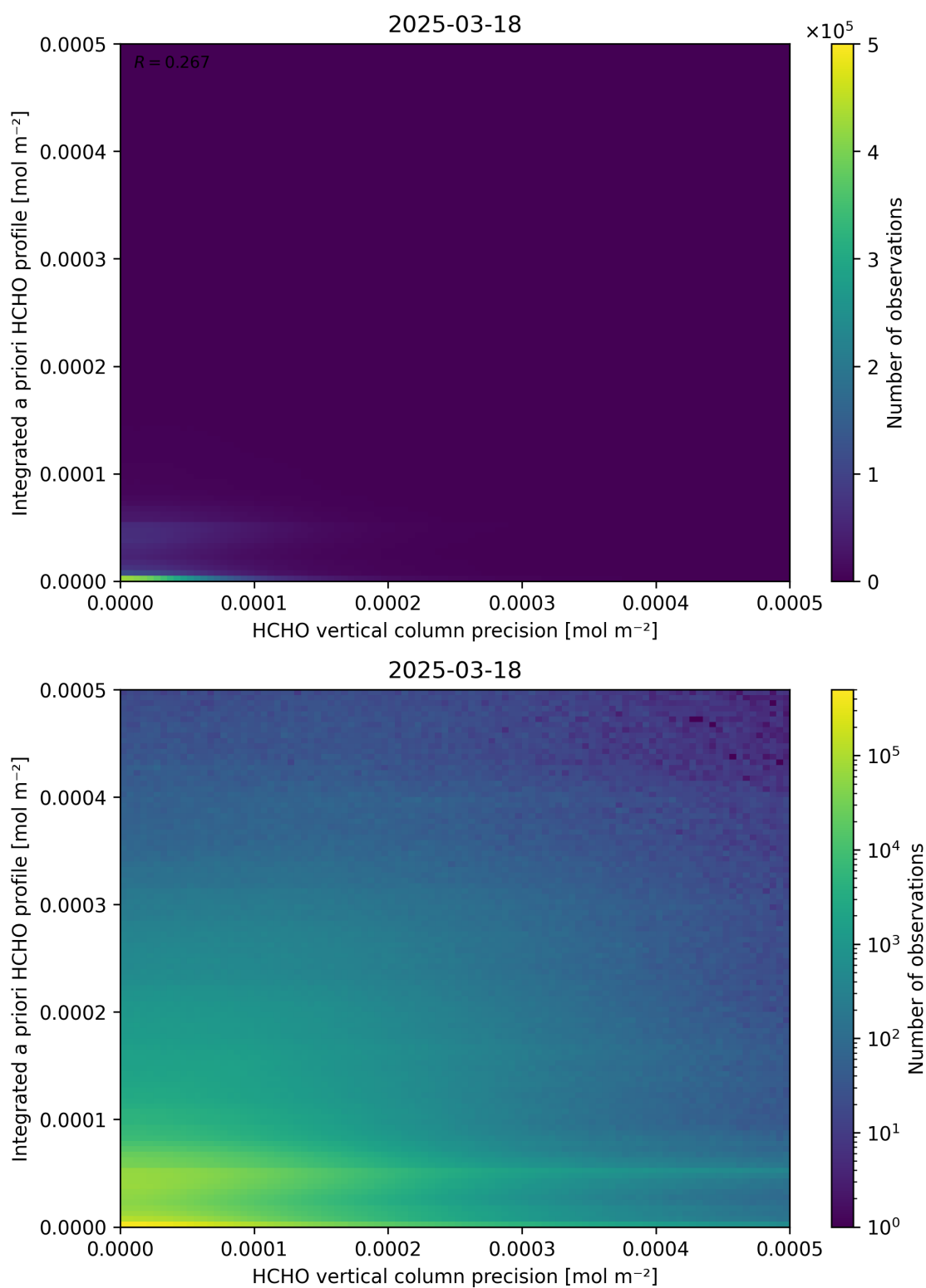
Figure 147: Scatter density plot of “HCHO vertical column precision” against “Integrated a priori HCHO profile” for 2025-03-17 to 2025-03-19.
