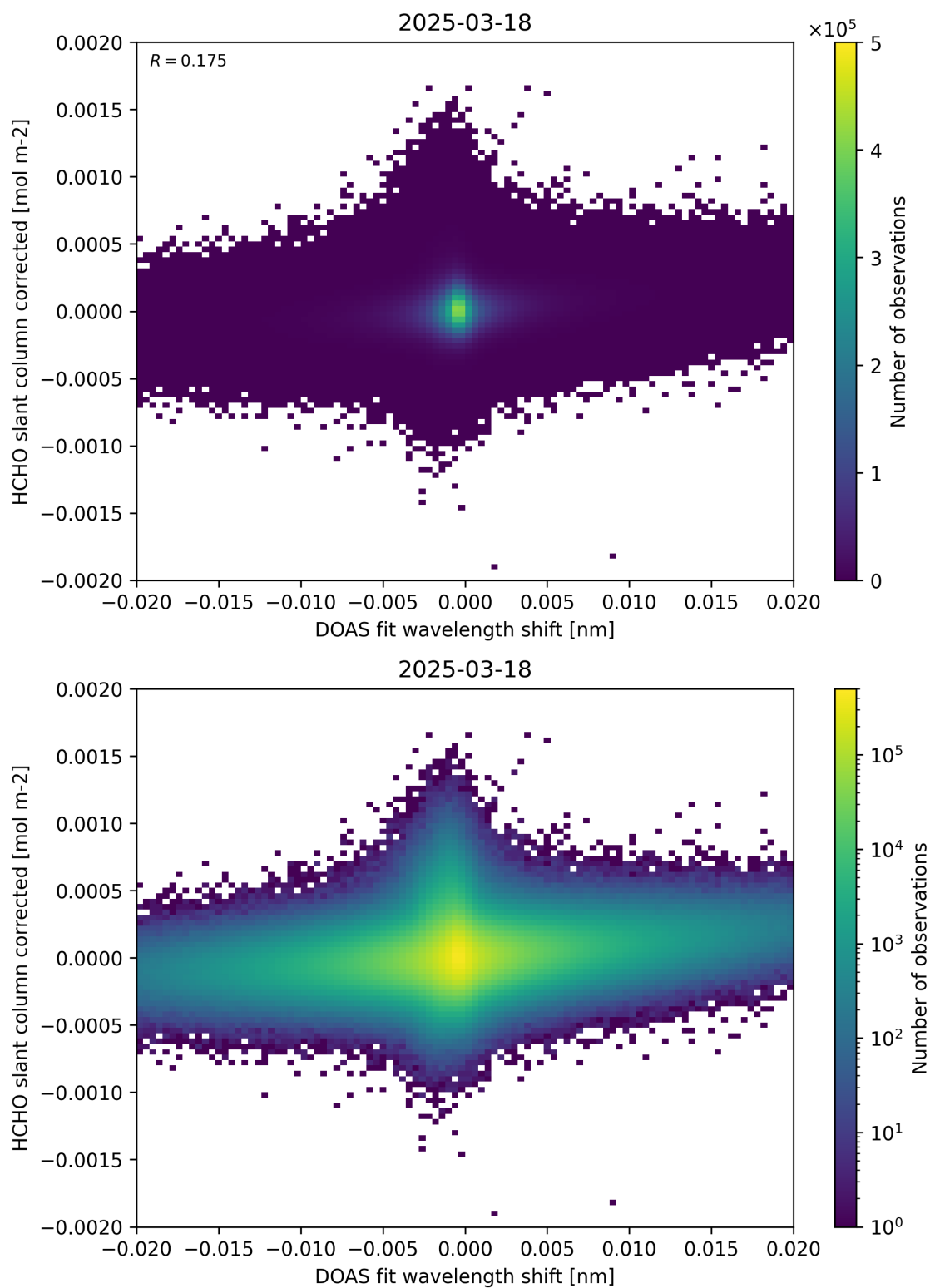
Figure 66: Scatter density plot of “DOAS fit wavelength shift” against “HCHO slant column corrected” for 2025-03-17 to 2025-03-19.
