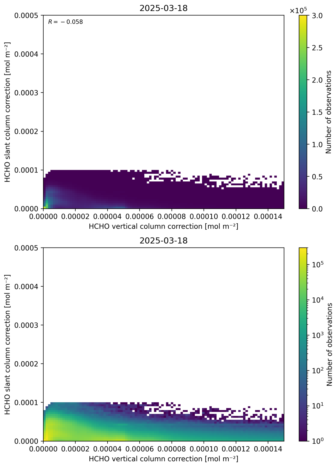
Figure 117: Scatter density plot of “HCHO vertical column correction” against “HCHO slant column correction” for 2025-03-17 to 2025-03-19.
