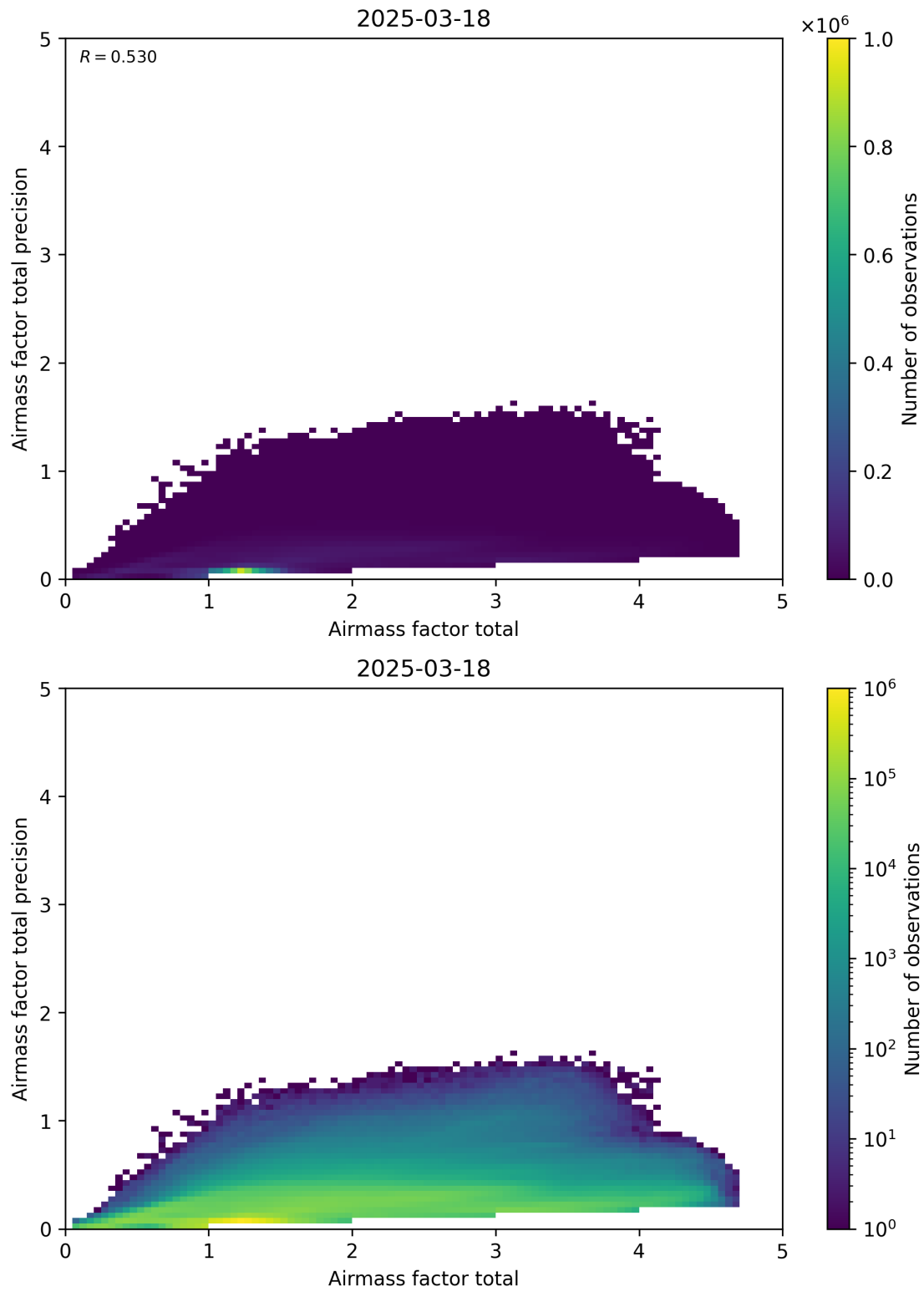
Figure 103: Scatter density plot of “Airmass factor total” against “Airmass factor total precision” for 2025-03-17 to 2025-03-19.
