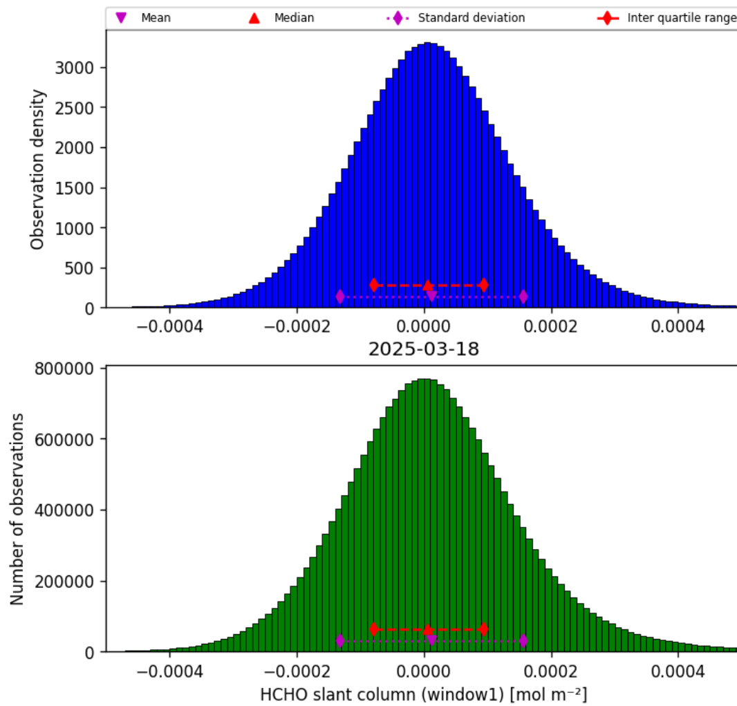
Figure 38: Histogram of “HCHO slant column (window1)” for 2025-03-17 to 2025-03-19
