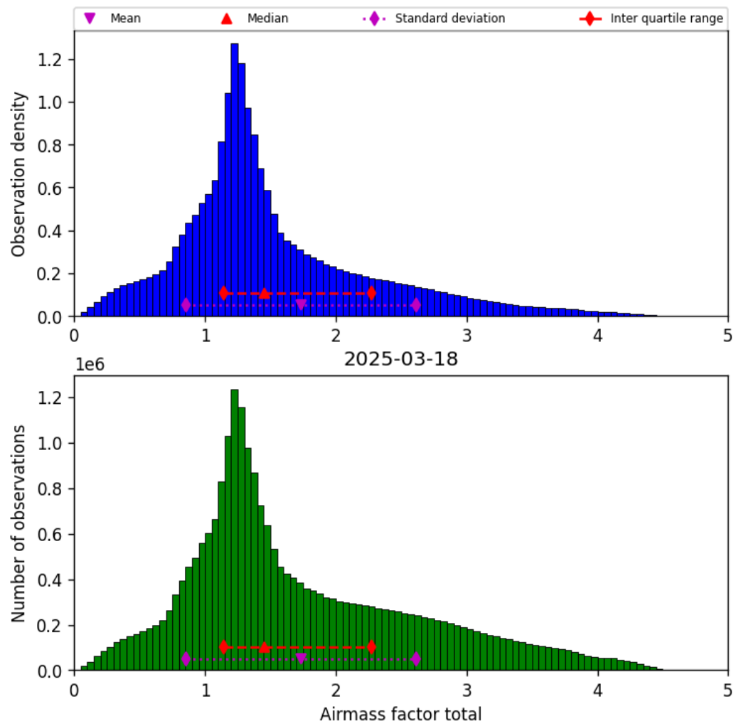
Figure 40: Histogram of “Airmass factor total” for 2025-03-17 to 2025-03-19
