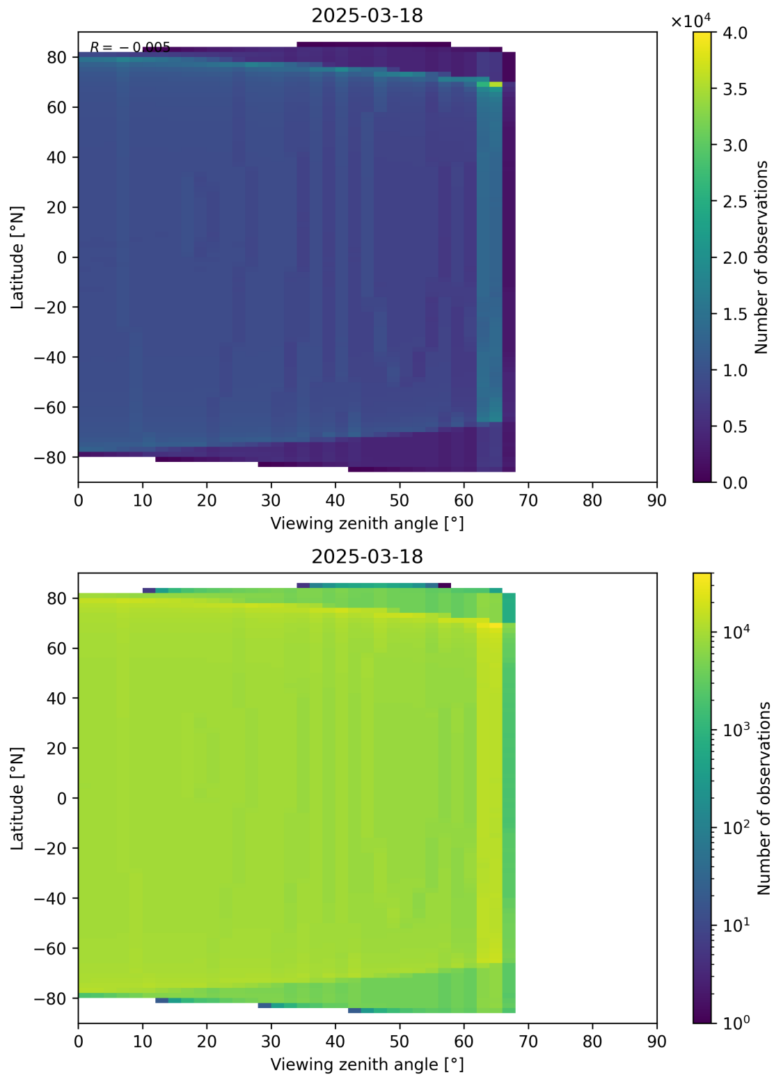
Figure 196: Scatter density plot of “Viewing zenith angle” against “Latitude” for 2025-03-17 to 2025-03-19.
