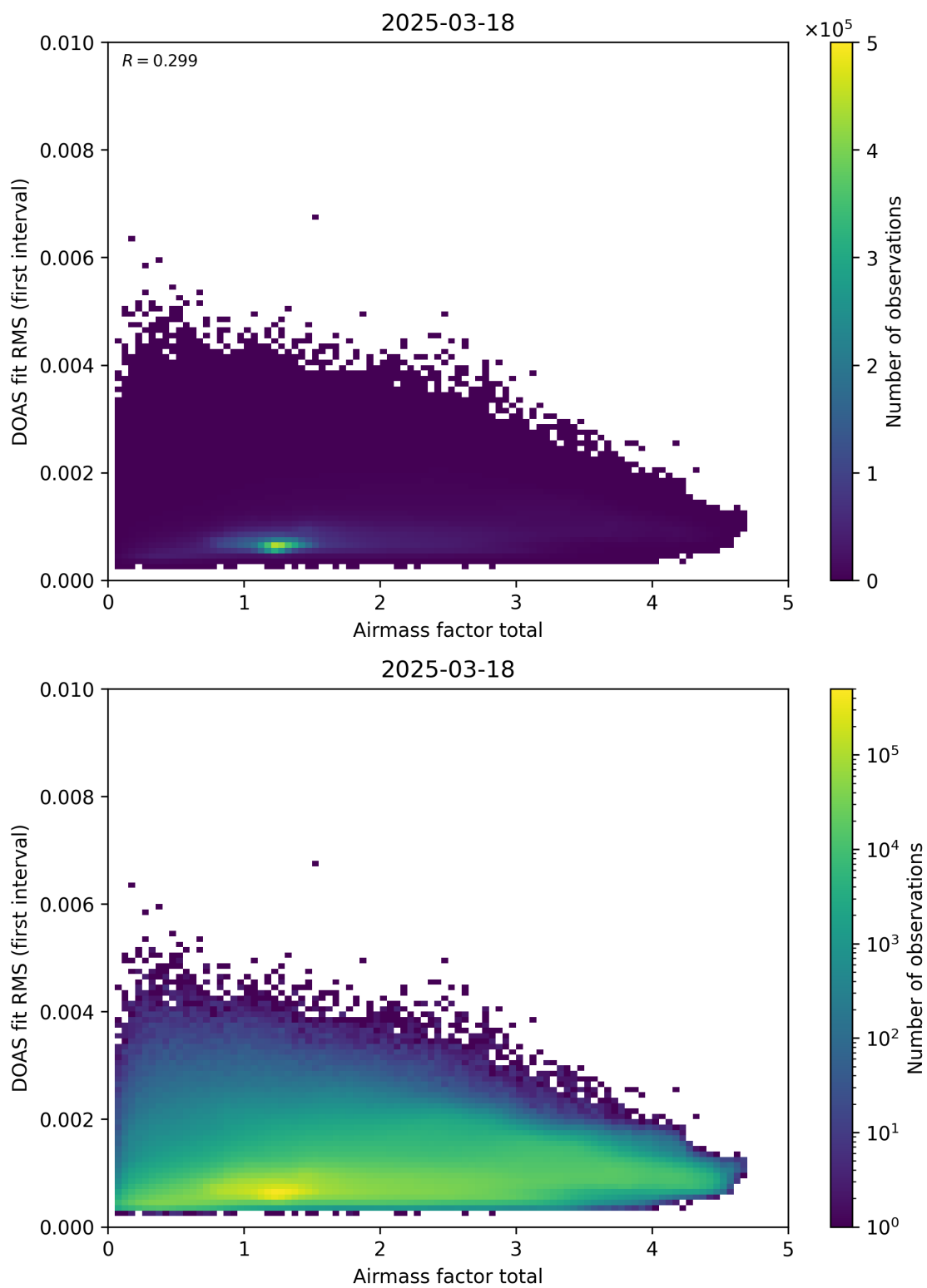
Figure 97: Scatter density plot of “Airmass factor total” against “DOAS fit RMS (first interval)” for 2025-03-17 to 2025-03-19.
