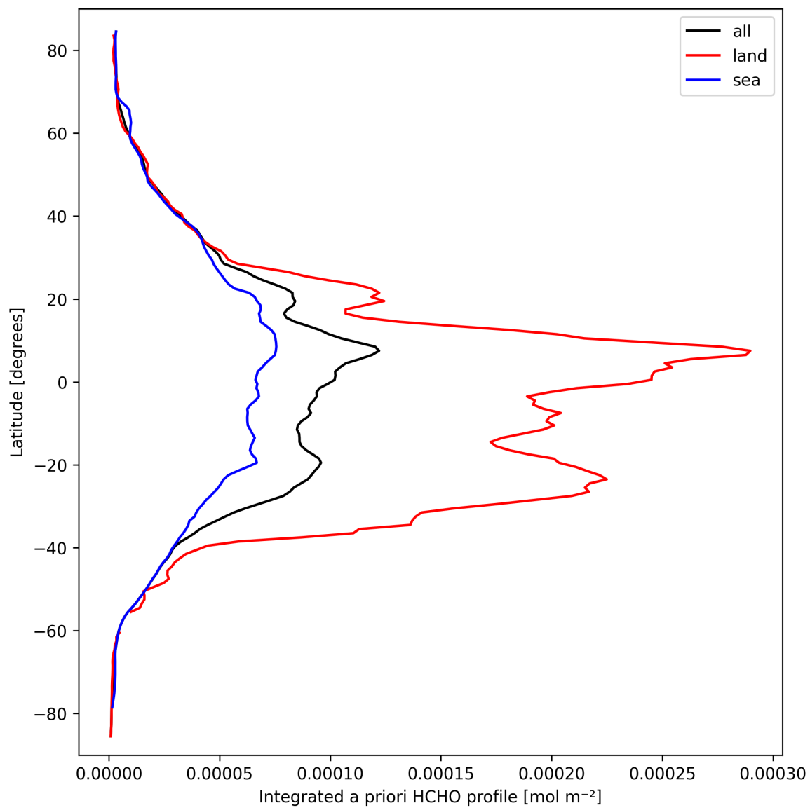
Figure 29: Zonal average of “Integrated a priori HCHO profile” for 2025-03-17 to 2025-03-19.
