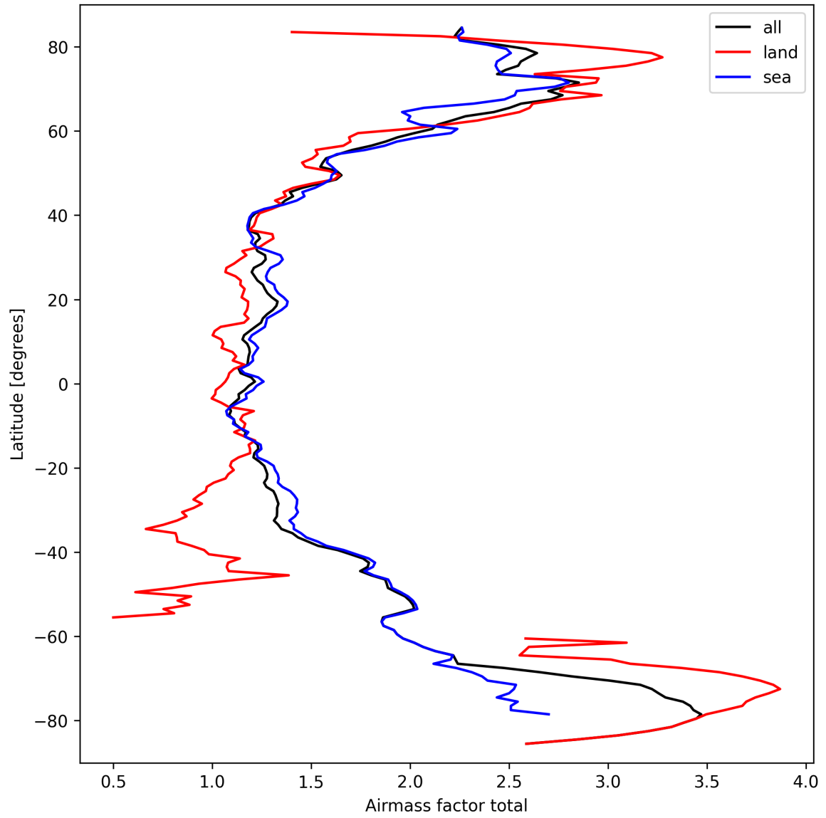
Figure 26: Zonal average of “Airmass factor total” for 2025-03-17 to 2025-03-19.
