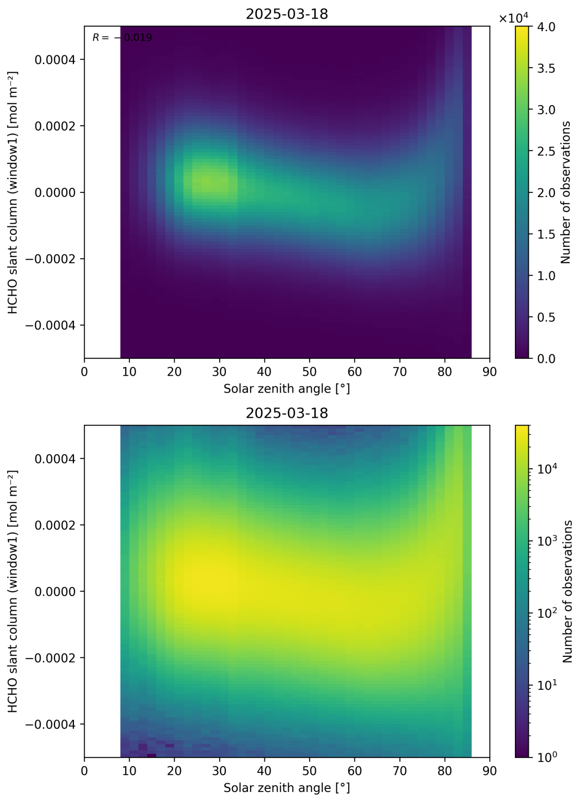
Figure 173: Scatter density plot of “Solar zenith angle” against “HCHO slant column (window1)” for 2025-03-17 to 2025-03-19.
