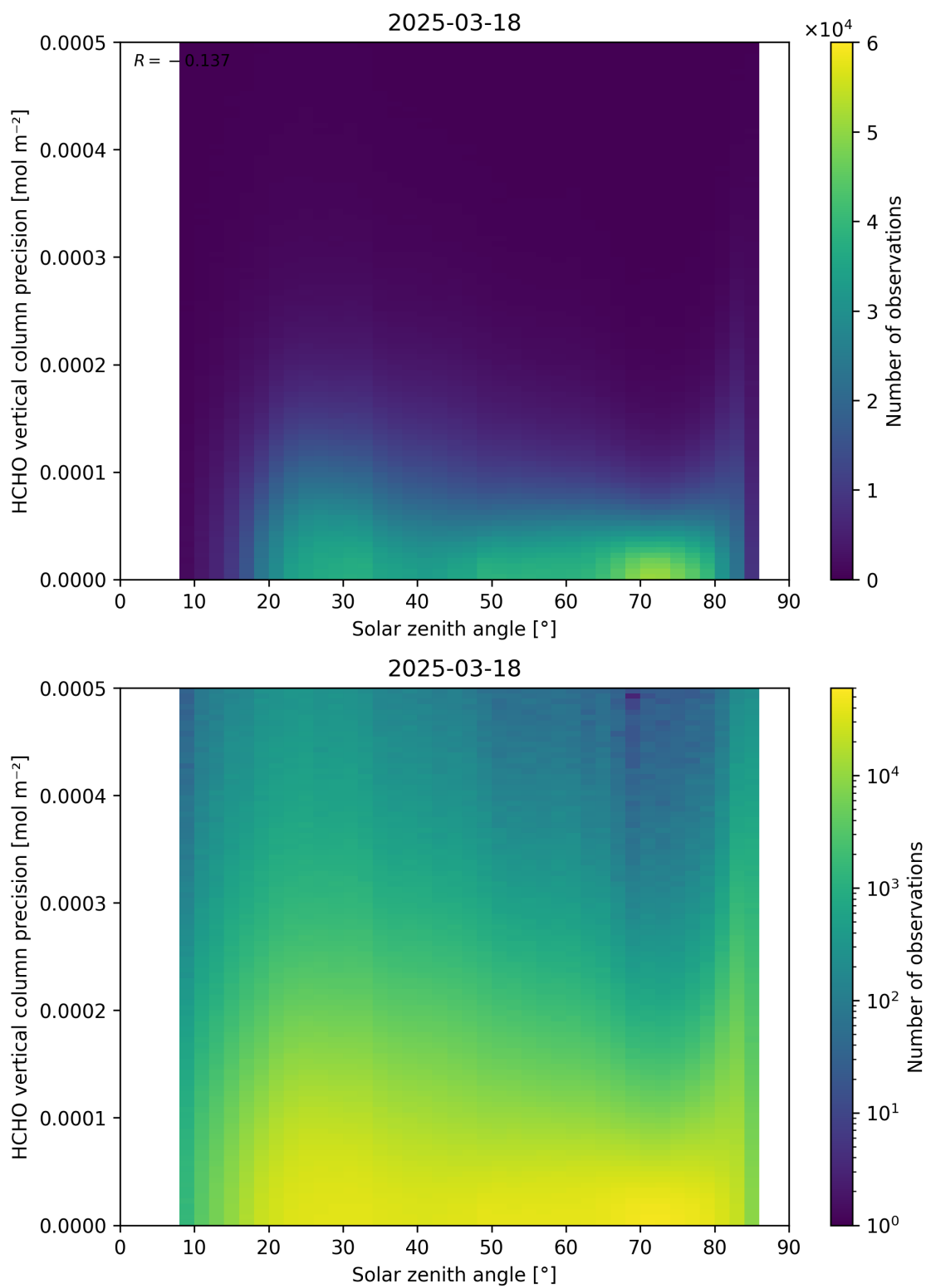
Figure 179: Scatter density plot of “Solar zenith angle” against “HCHO vertical column precision” for 2025-03-17 to 2025-03-19.
