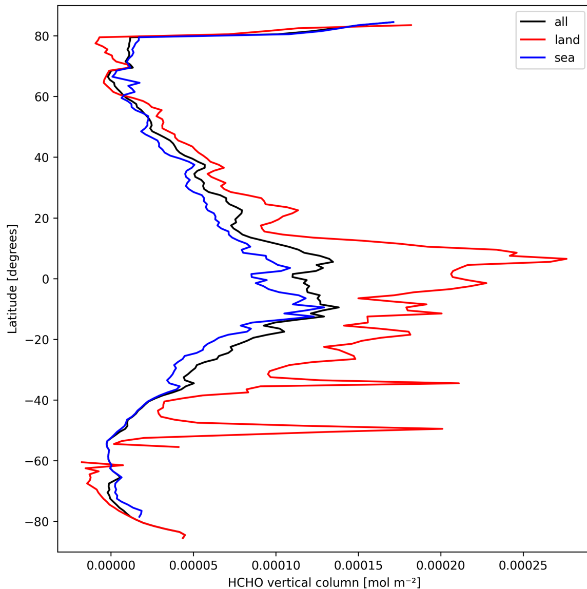
Figure 21: Zonal average of “HCHO vertical column” for 2025-03-17 to 2025-03-19.
