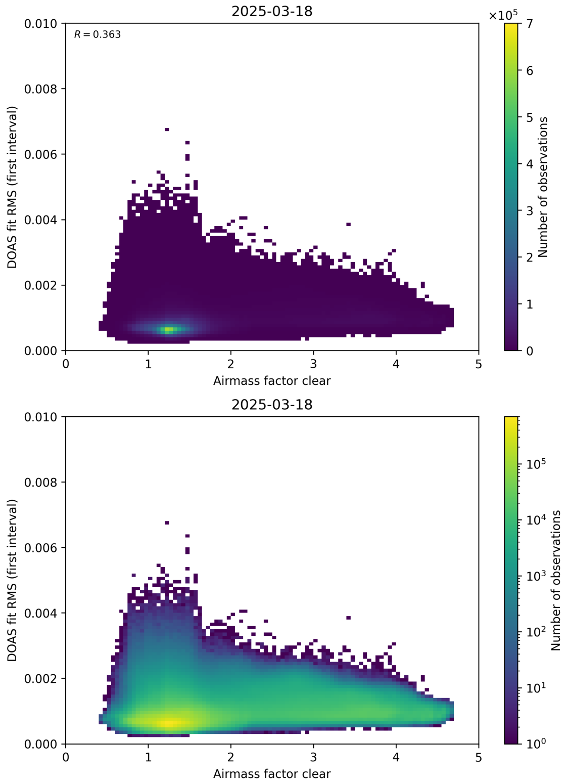
Figure 71: Scatter density plot of “Airmass factor clear” against “DOAS fit RMS (first interval)” for 2025-03-17 to 2025-03-19.
