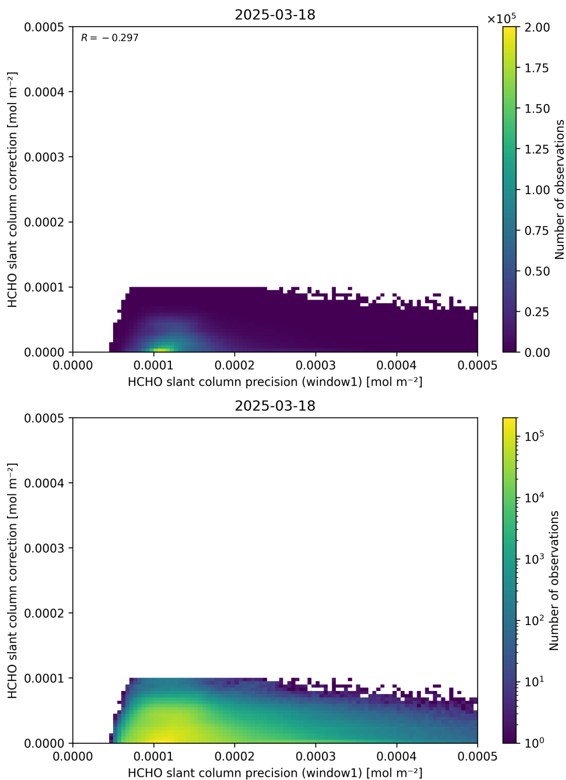
Figure 93: Scatter density plot of “HCHO slant column precision (window1)” against “HCHO slant column correction” for 2025-03-17 to 2025-03-19.
