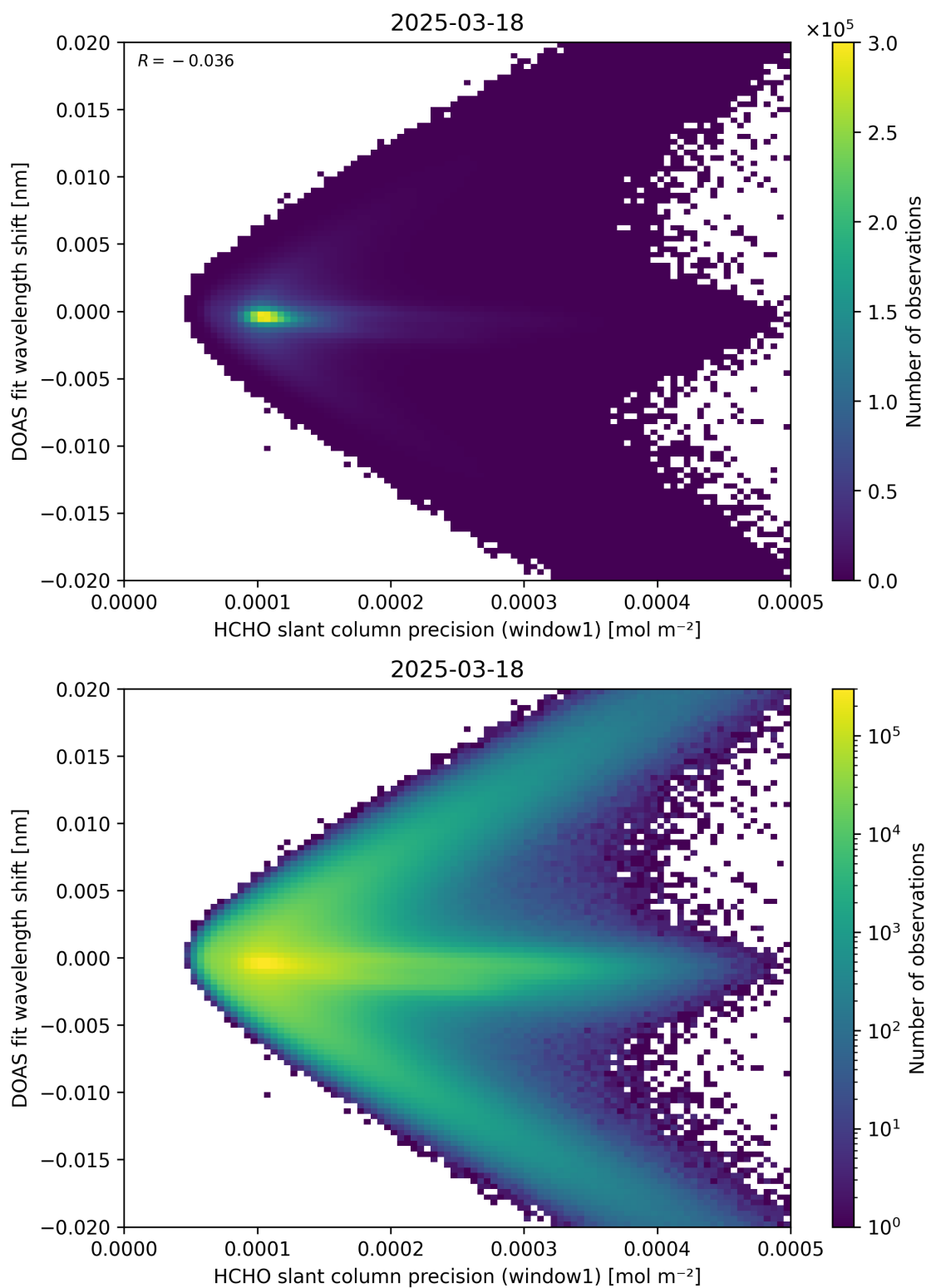
Figure 89: Scatter density plot of “HCHO slant column precision (window1)” against “DOAS fit wavelength shift” for 2025-03-17 to 2025-03-19.
