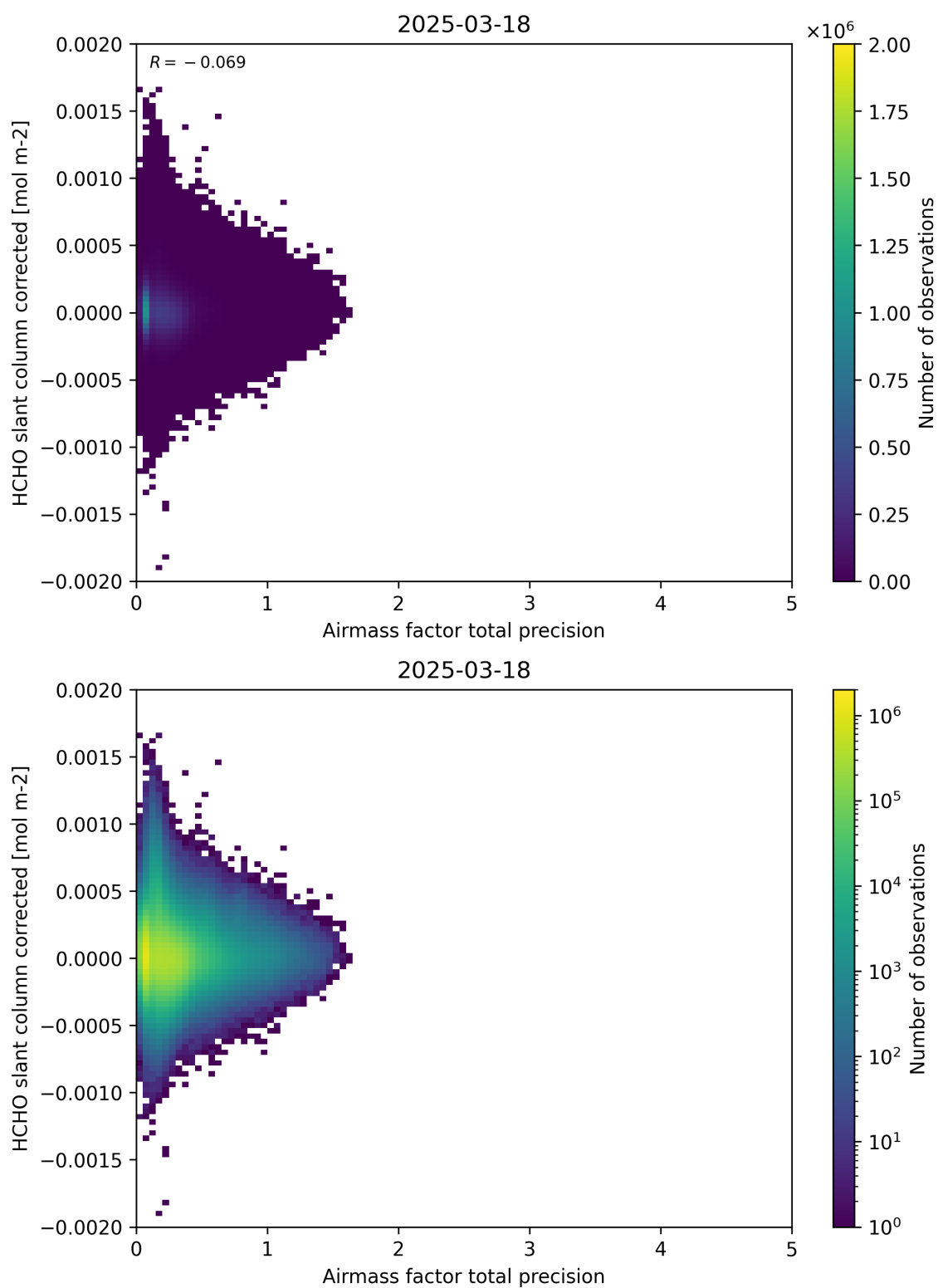
Figure 109: Scatter density plot of “Airmass factor total precision” against “HCHO slant column corrected” for 2025-03-17 to 2025-03-19.
