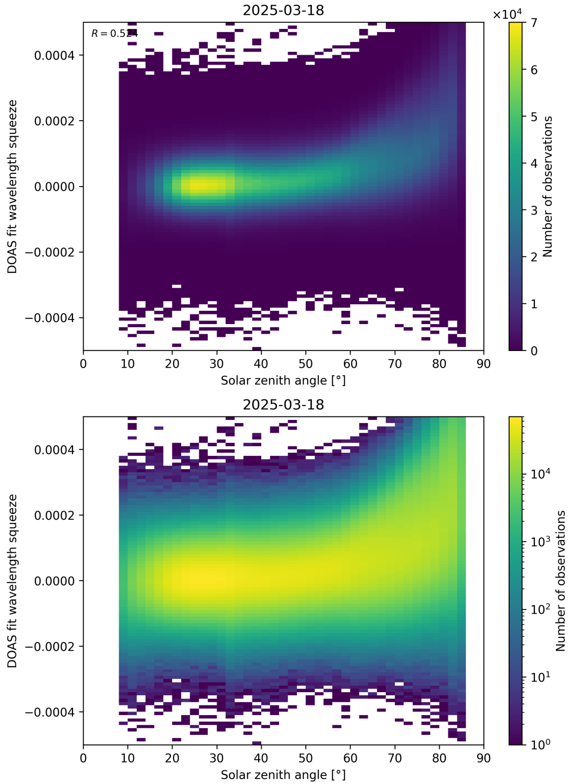
Figure 169: Scatter density plot of “Solar zenith angle” against “DOAS fit wavelength squeeze” for 2025-03-17 to 2025-03-19.
