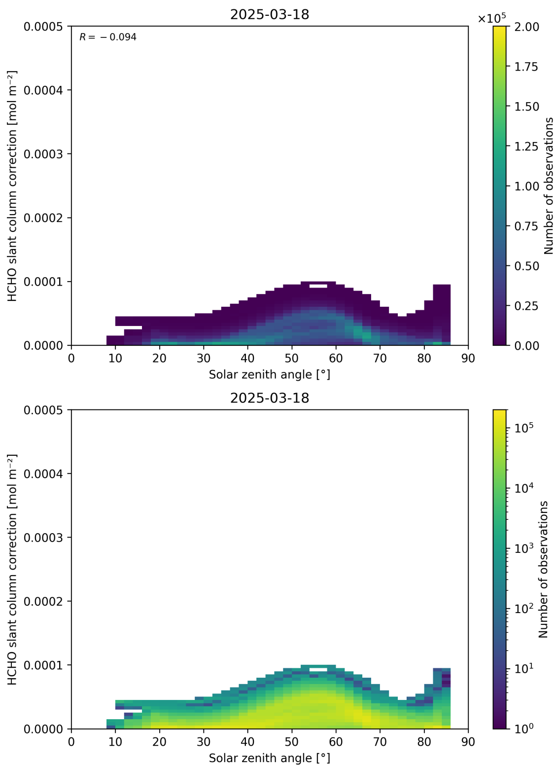
Figure 172: Scatter density plot of “Solar zenith angle” against “HCHO slant column correction” for 2025-03-17 to 2025-03-19.
