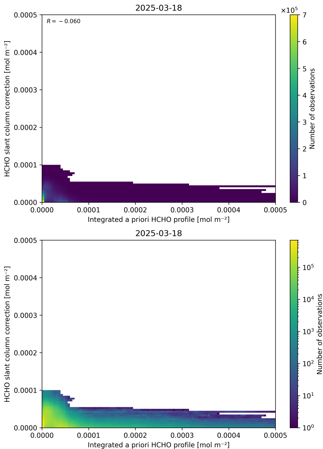
Figure 152: Scatter density plot of “Integrated a priori HCHO profile” against “HCHO slant column correction” for 2025-03-17 to 2025-03-19.
