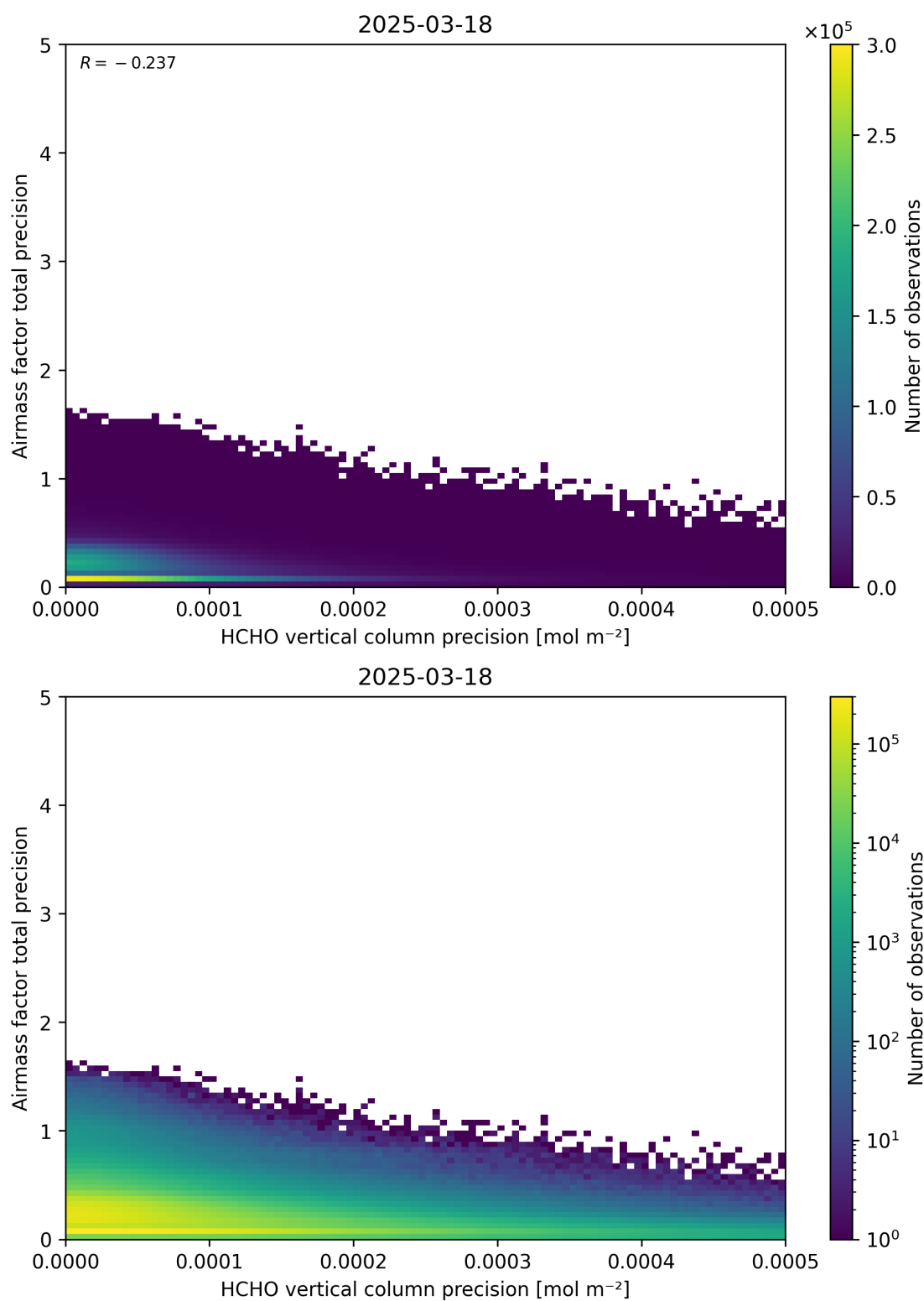
Figure 145: Scatter density plot of “HCHO vertical column precision” against “Airmass factor total precision” for 2025-03-17 to 2025-03-19.
