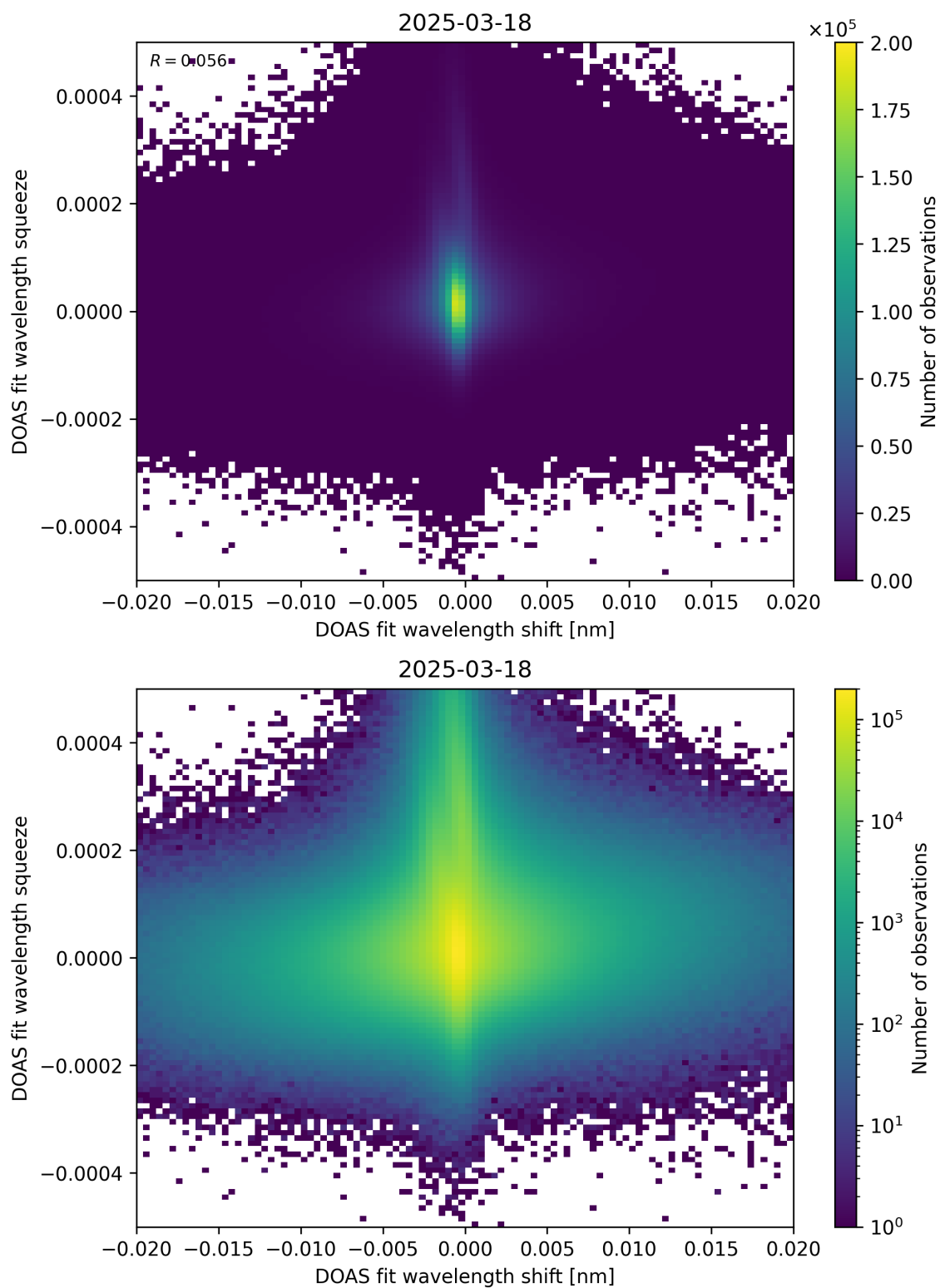
Figure 65: Scatter density plot of “DOAS fit wavelength shift” against “DOAS fit wavelength squeeze” for 2025-03-17 to 2025-03-19.
