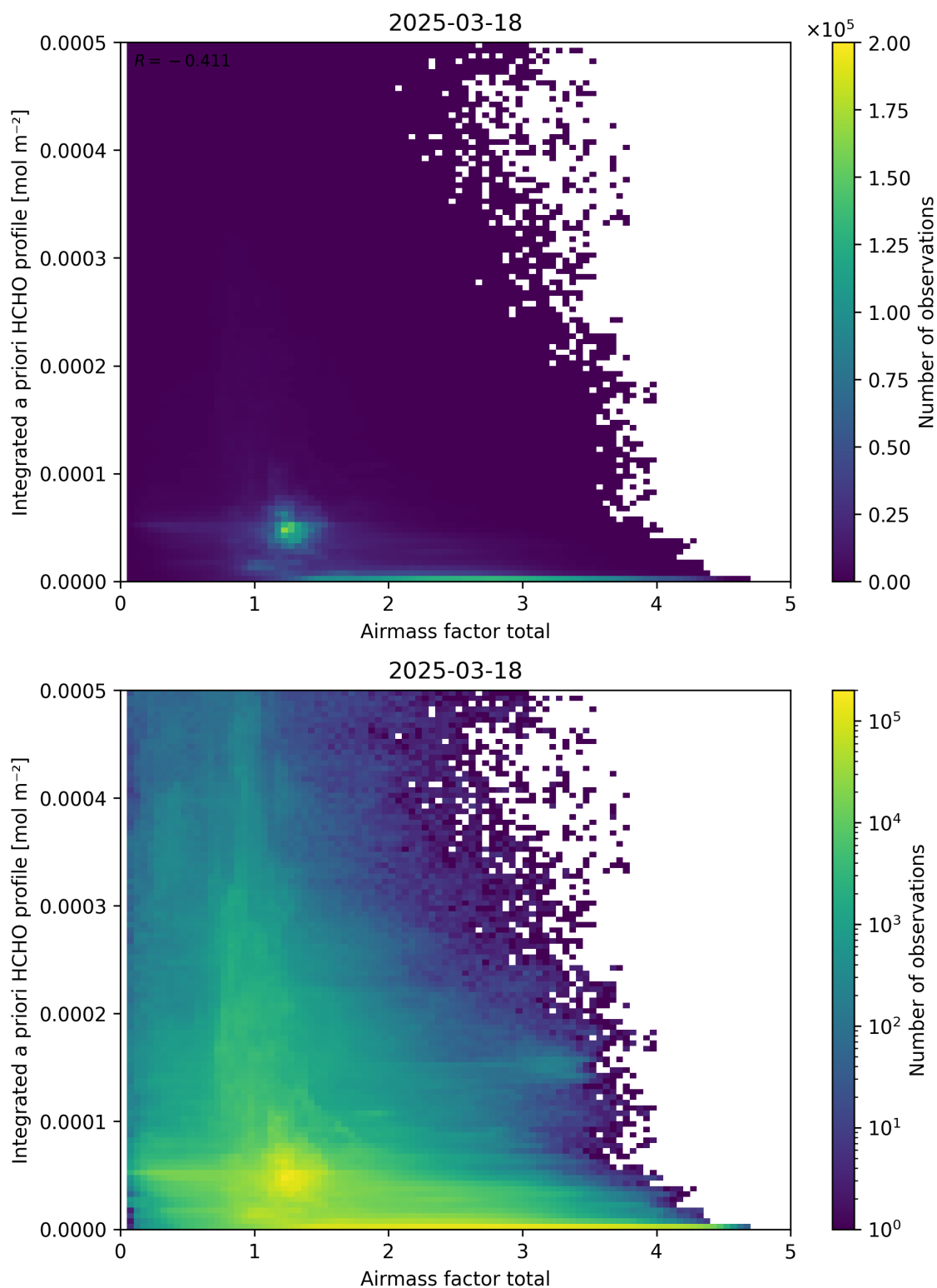
Figure 104: Scatter density plot of “Airmass factor total” against “Integrated a priori HCHO profile” for 2025-03-17 to 2025-03-19.
