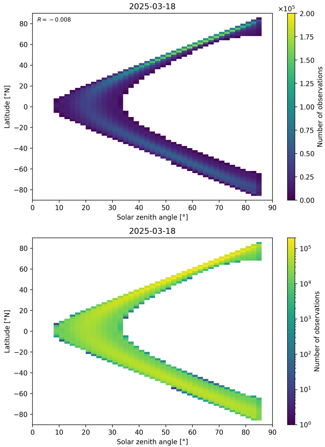
Figure 181: Scatter density plot of “Solar zenith angle” against “Latitude” for 2025-03-17 to 2025-03-19.
