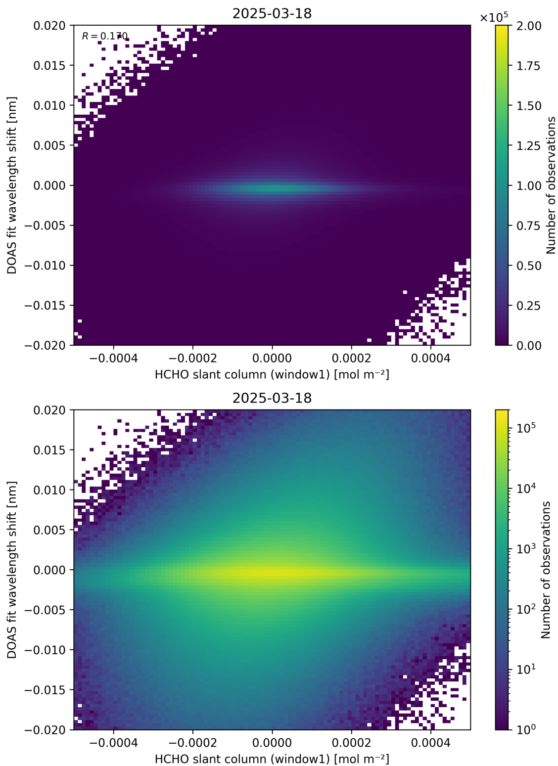
Figure 79: Scatter density plot of “HCHO slant column (window1)” against “DOAS fit wavelength shift” for 2025-03-17 to 2025-03-19.
