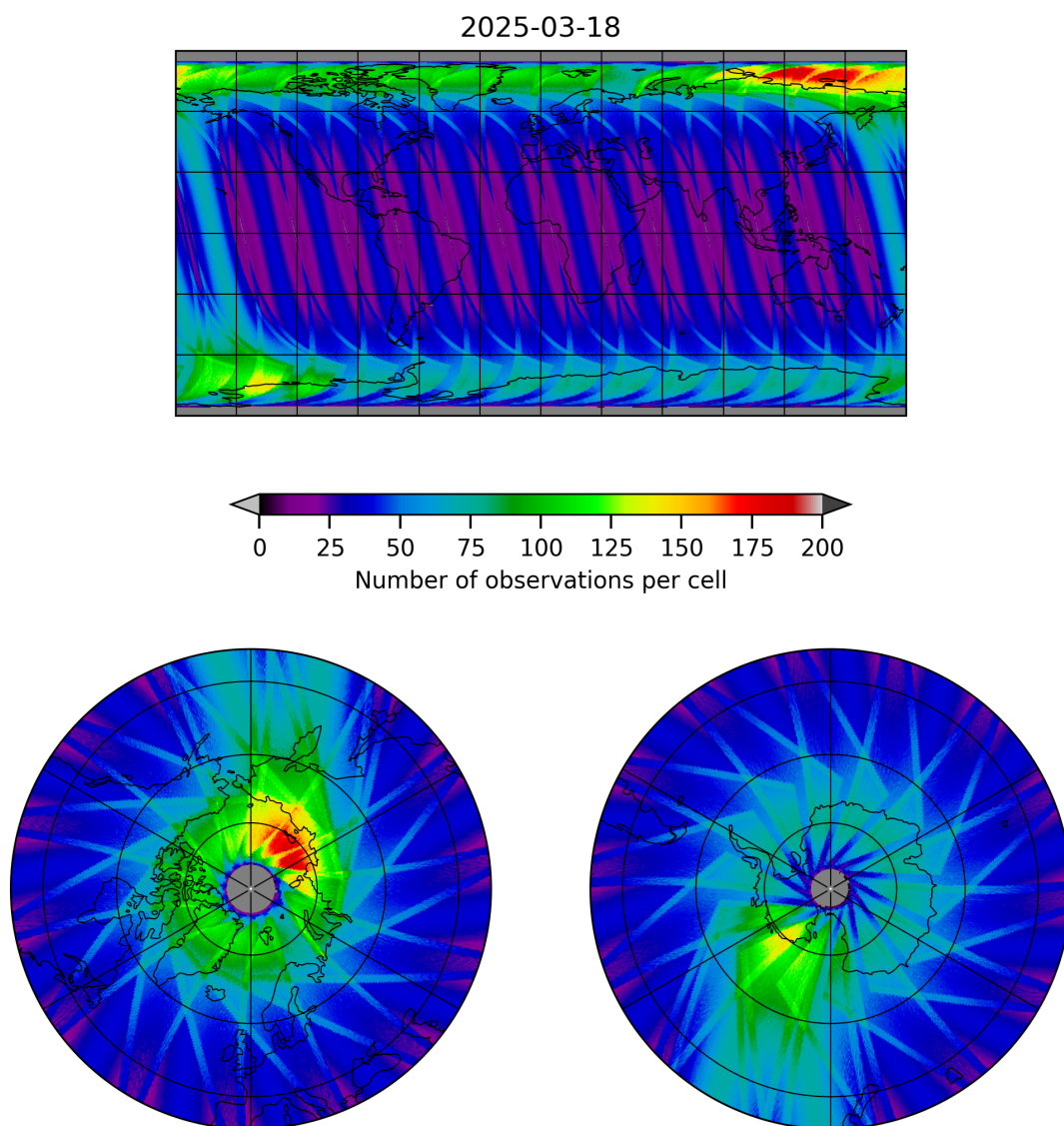
Figure 19: Map of the number of observations for 2025-03-17 to 2025-03-19
