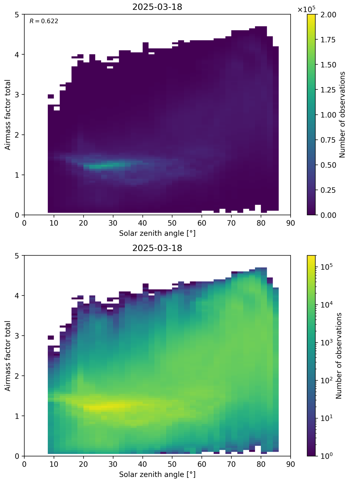
Figure 175: Scatter density plot of “Solar zenith angle” against “Airmass factor total” for 2025-03-17 to 2025-03-19.
