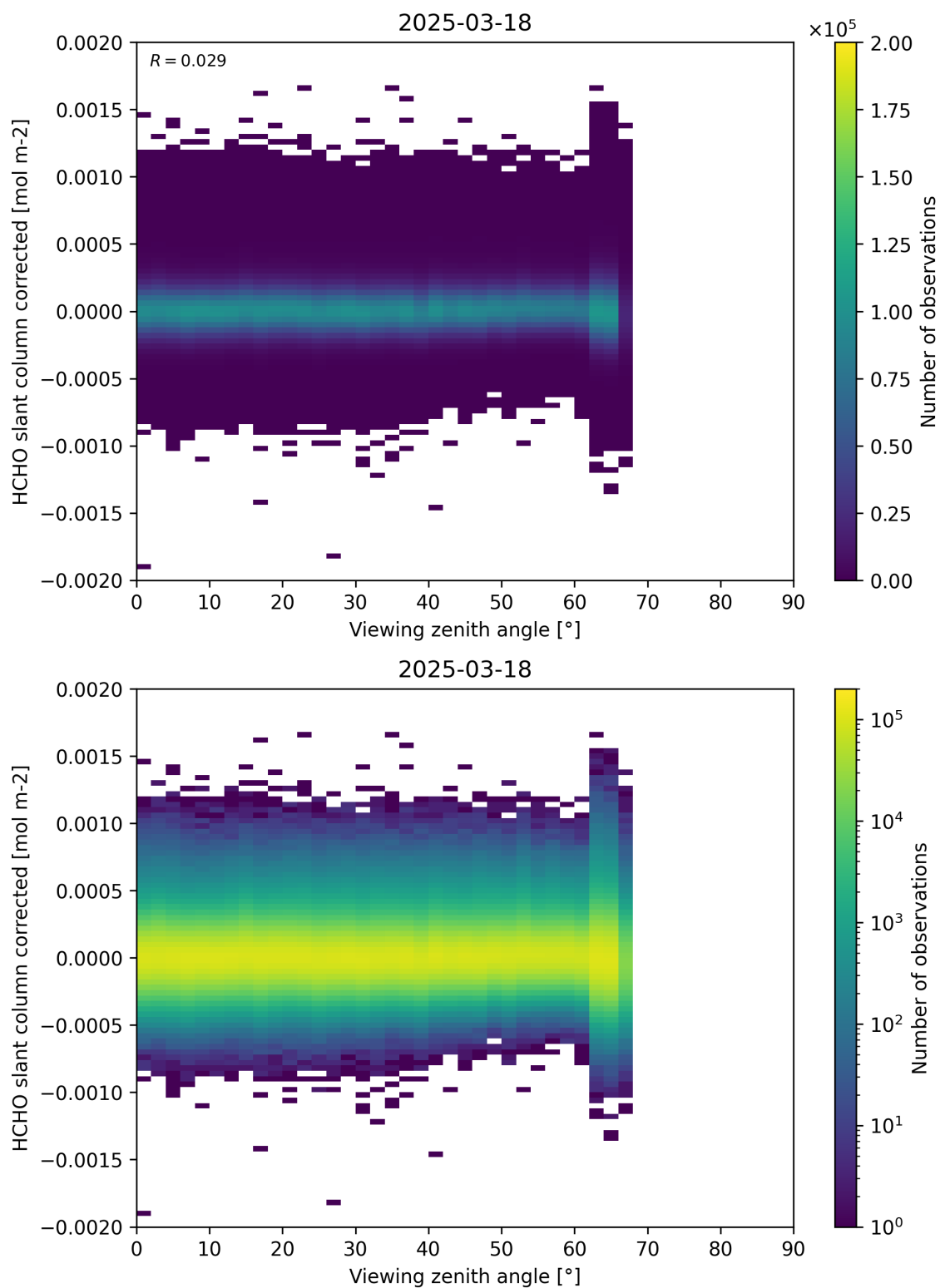
Figure 186: Scatter density plot of “Viewing zenith angle” against “HCHO slant column corrected” for 2025-03-17 to 2025-03-19.
