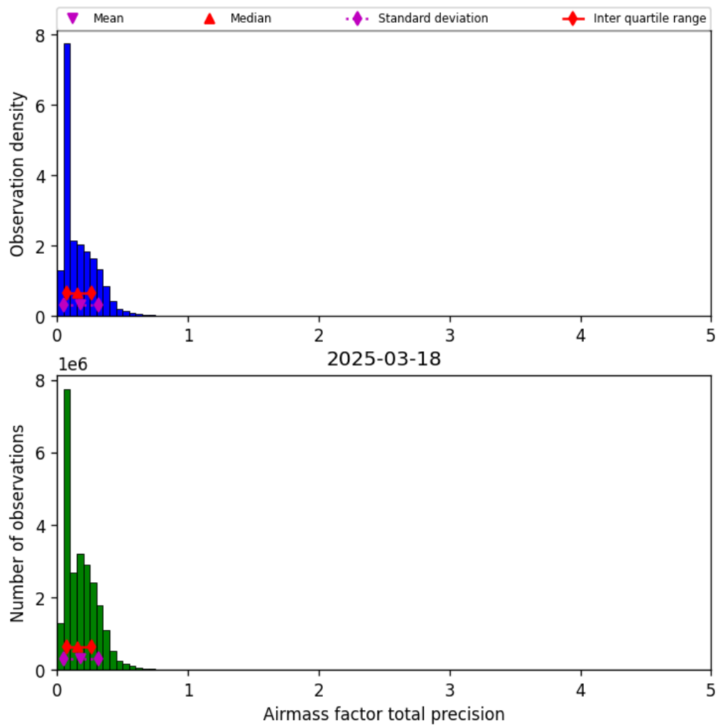
Figure 41: Histogram of “Airmass factor total precision” for 2025-03-17 to 2025-03-19
