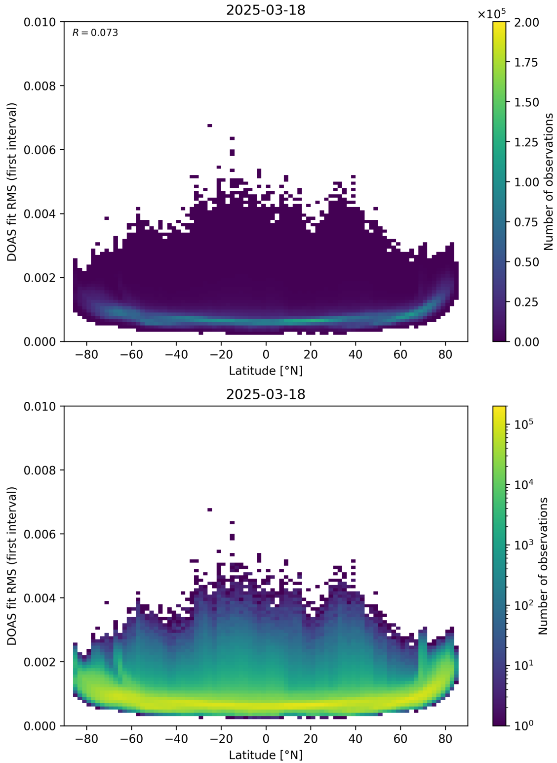
Figure 153: Scatter density plot of “Latitude” against “DOAS fit RMS (first interval)” for 2025-03-17 to 2025-03-19.
