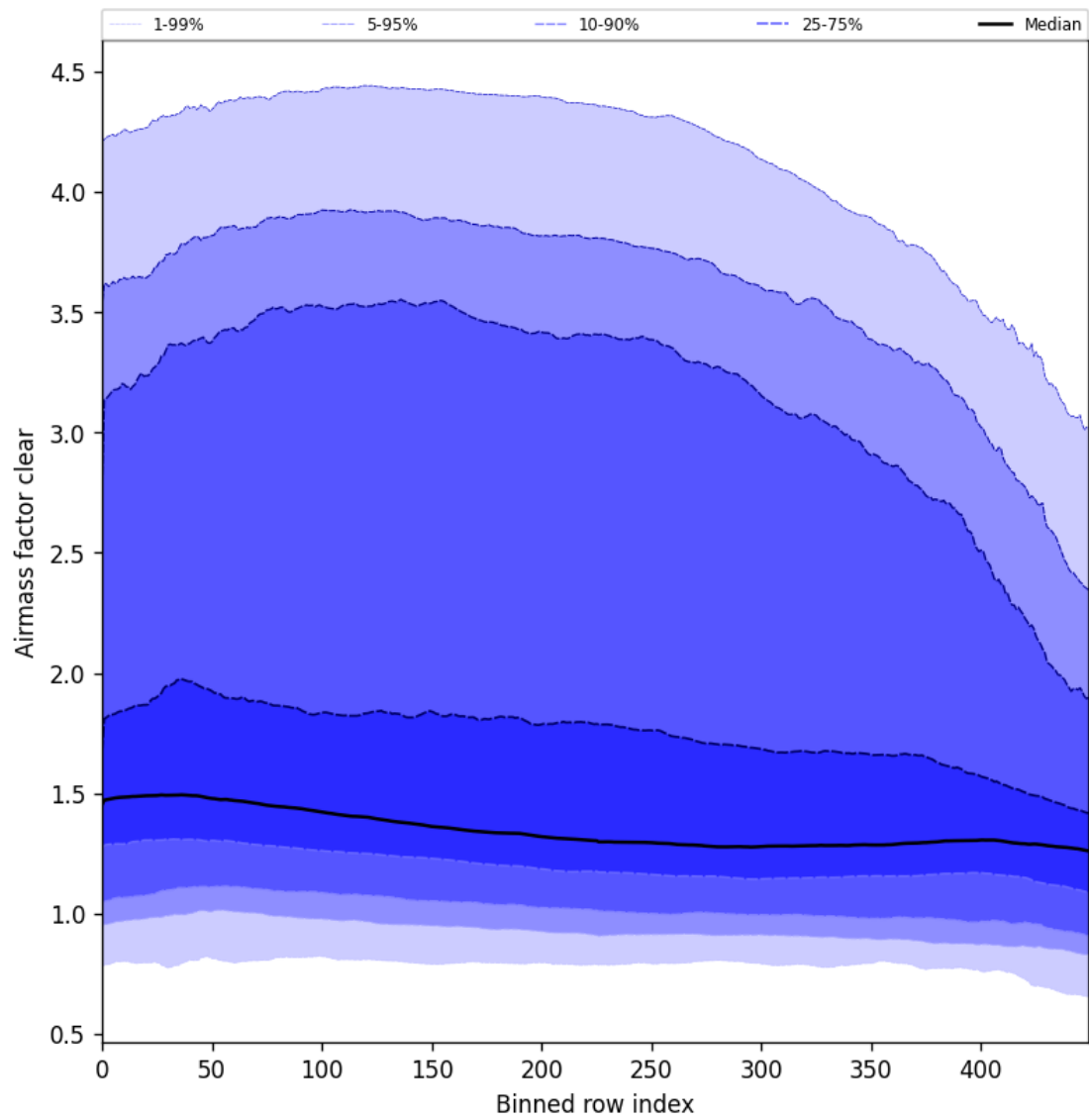
Figure 56: Along track statistics of “Air mass factor clear” for 2025-03-17 to 2025-03-19
