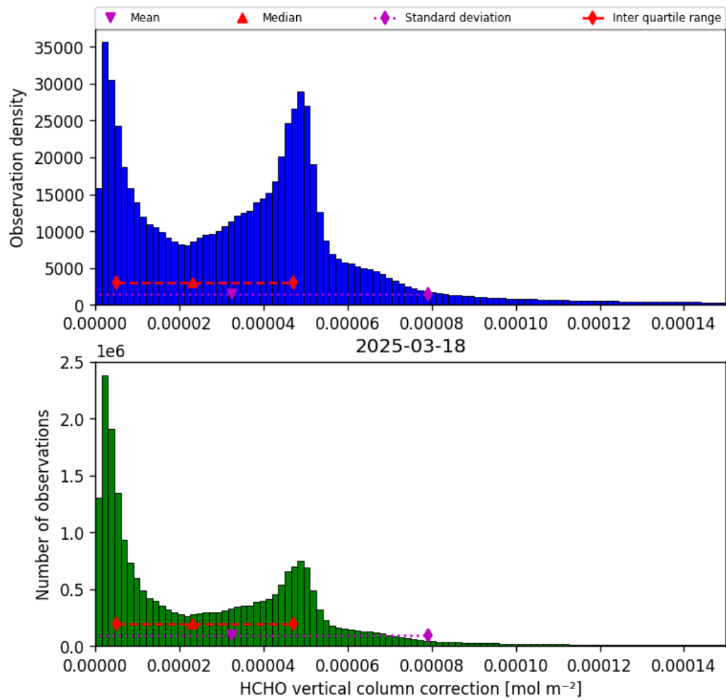
Figure 37: Histogram of “HCHO vertical column correction” for 2025-03-17 to 2025-03-19
