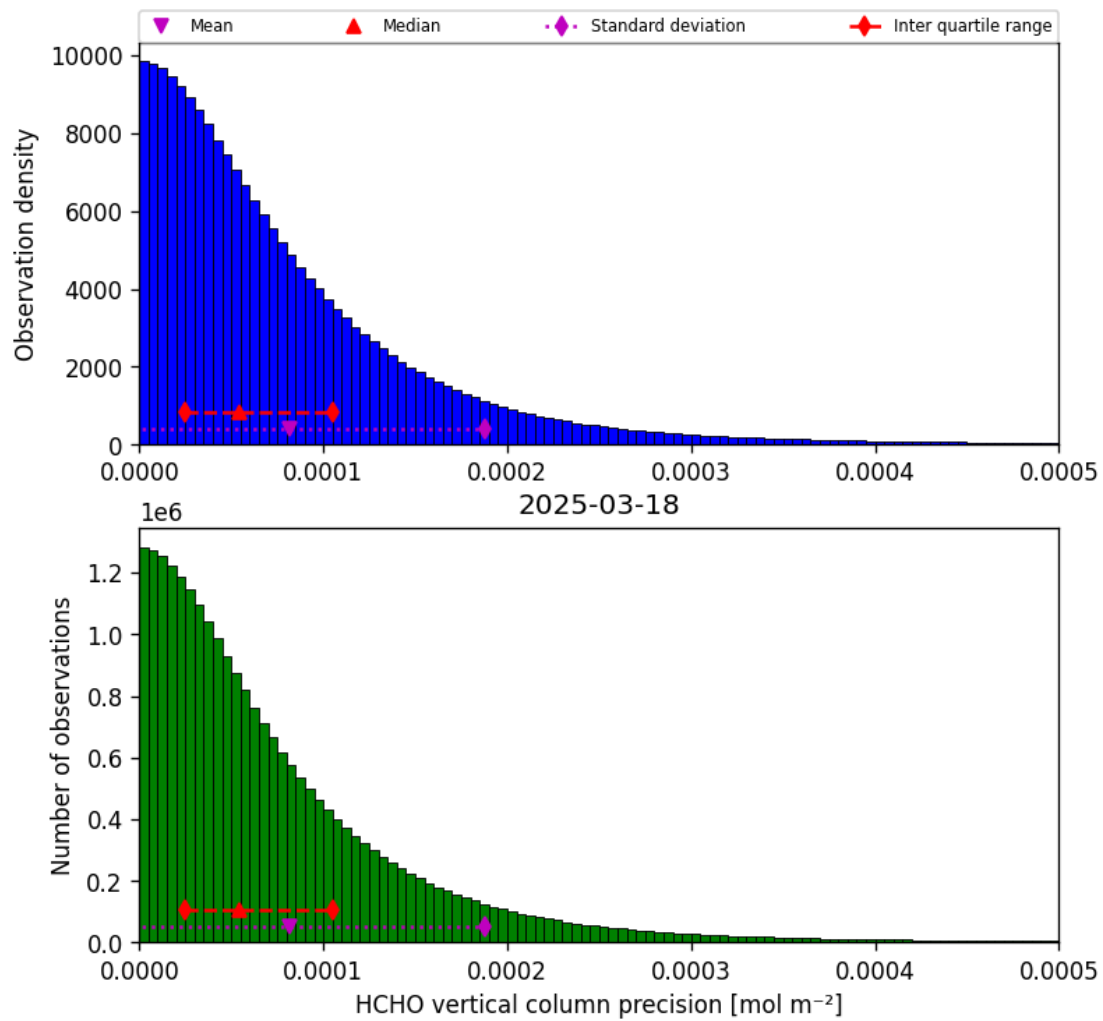
Figure 36: Histogram of “HCHO vertical column precision” for 2025-03-17 to 2025-03-19
