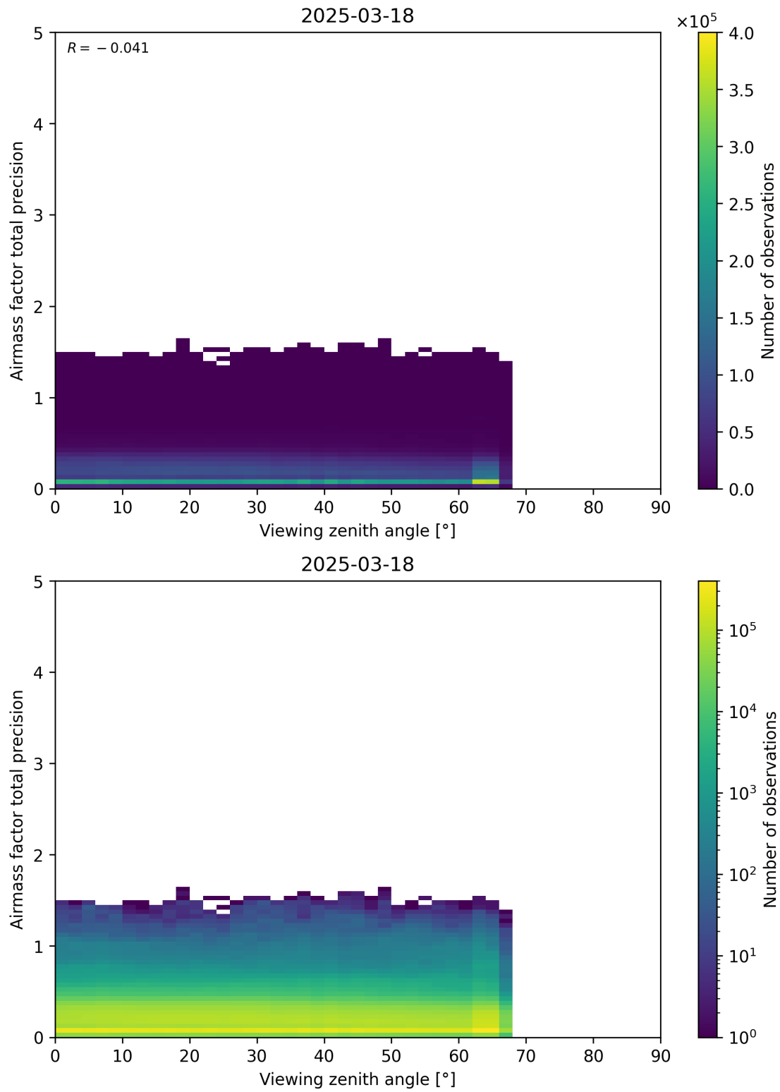
Figure 191: Scatter density plot of “Viewing zenith angle” against “Airmass factor total precision” for 2025-03-17 to 2025-03-19.
