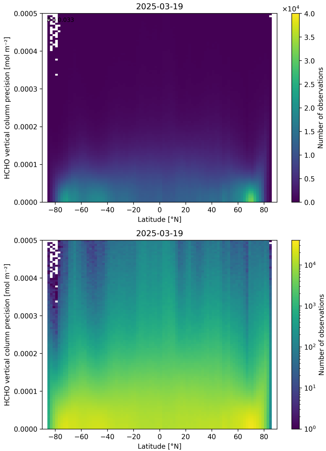
Figure 165: Scatter density plot of “Latitude” against “HCHO vertical column precision” for 2025-03-18 to 2025-03-20.
