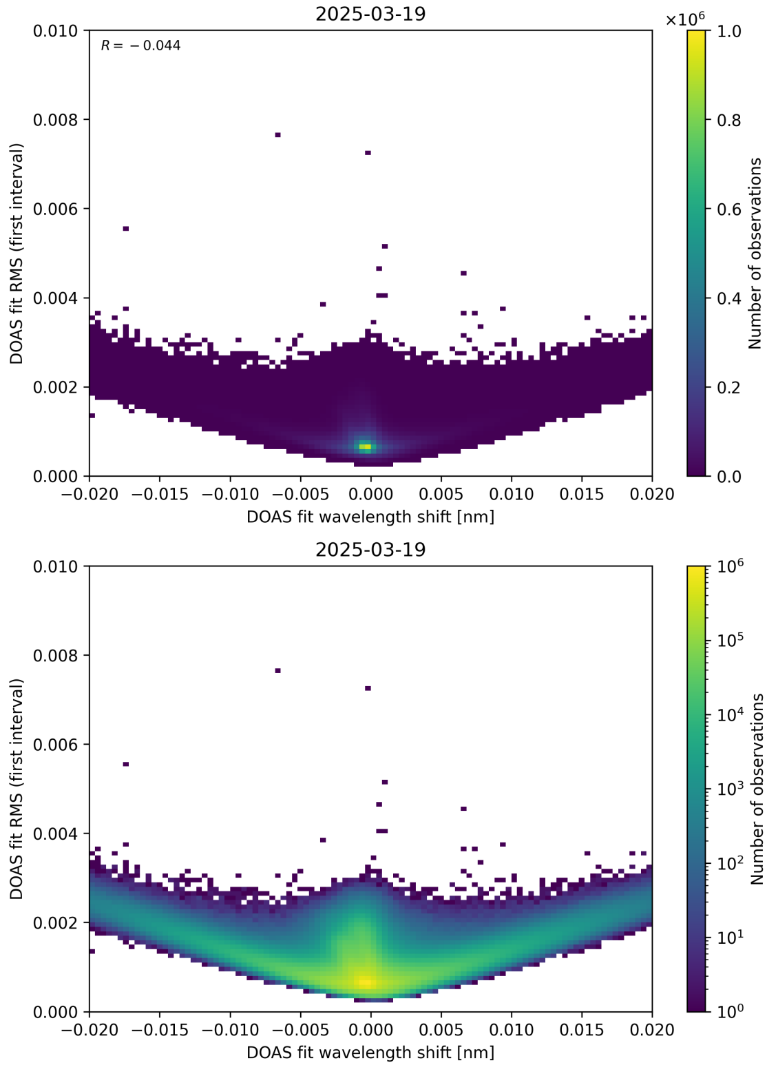
Figure 64: Scatter density plot of “DOAS fit wavelength shift” against “DOAS fit RMS (first interval)” for 2025-03-18 to 2025-03-20.
