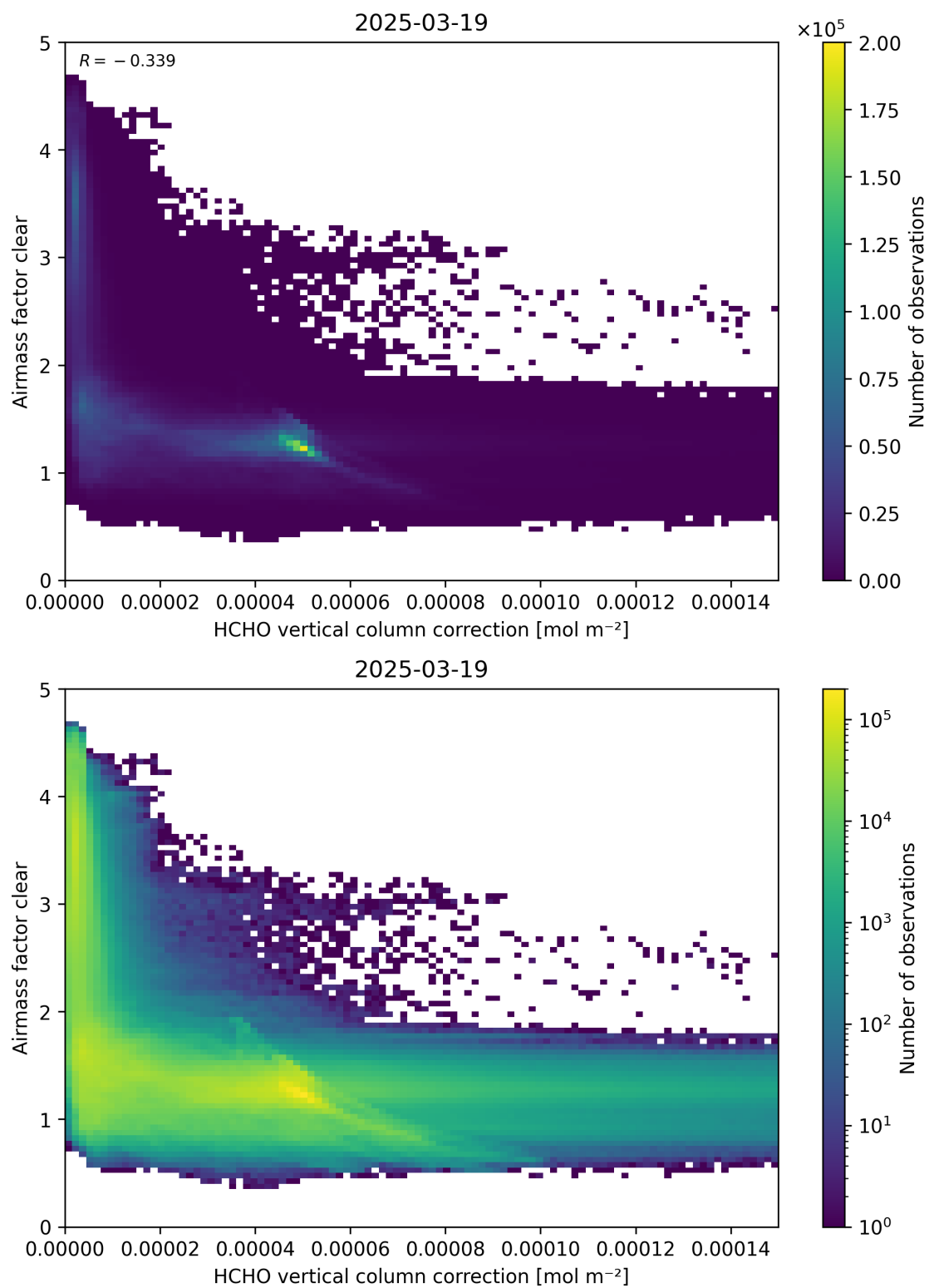
Figure 115: Scatter density plot of “HCHO vertical column correction” against “Airmass factor clear” for 2025-03-18 to 2025-03-20.
