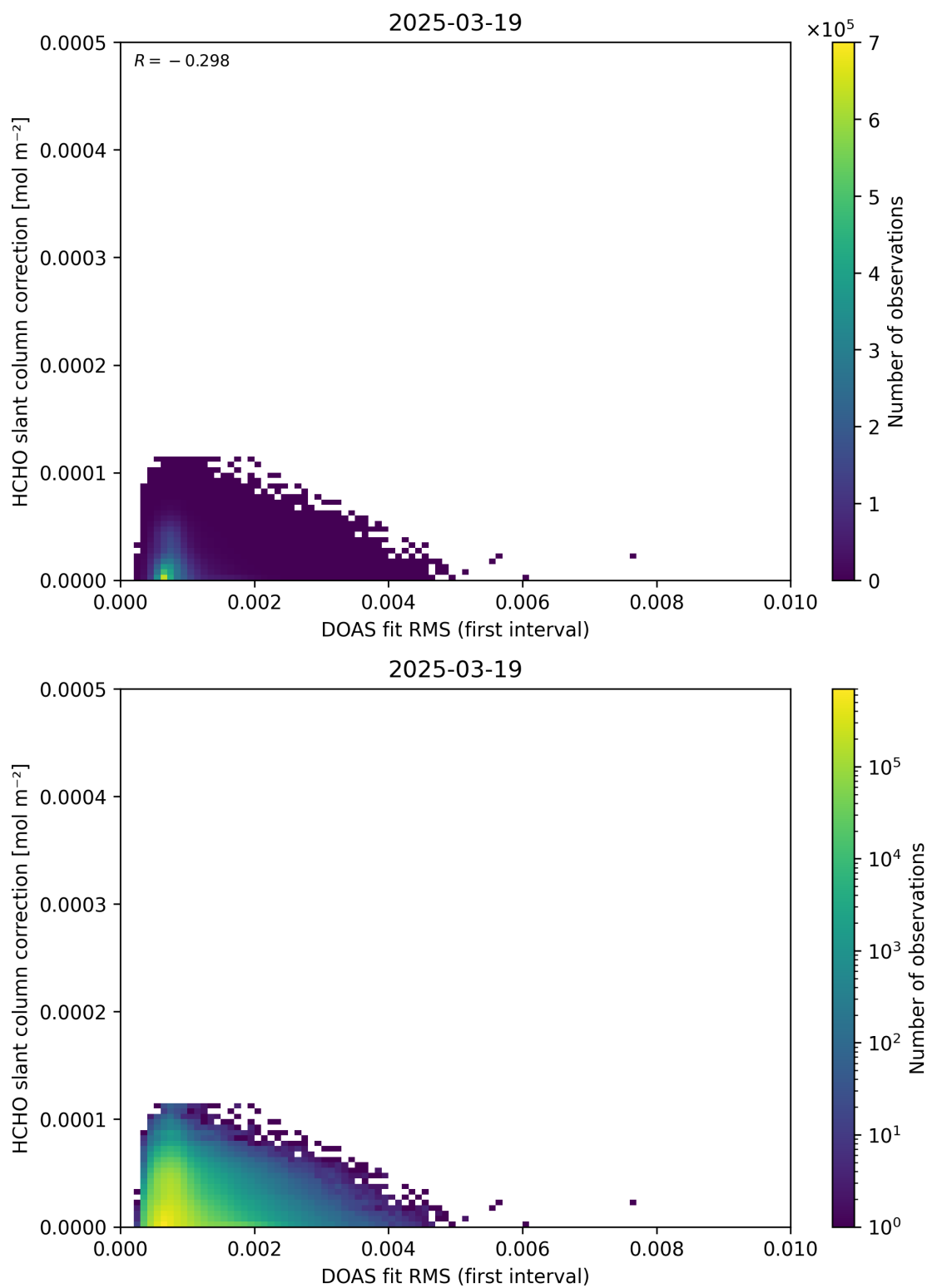
Figure 63: Scatter density plot of “DOAS fit RMS (first interval)” against “HCHO slant column correction” for 2025-03-18 to 2025-03-20.
