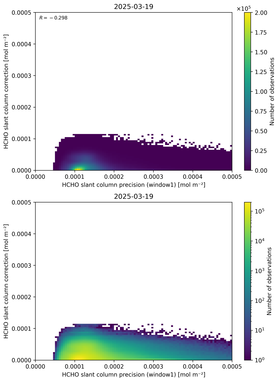
Figure 93: Scatter density plot of “HCHO slant column precision (window1)” against “HCHO slant column correction” for 2025-03-18 to 2025-03-20.
