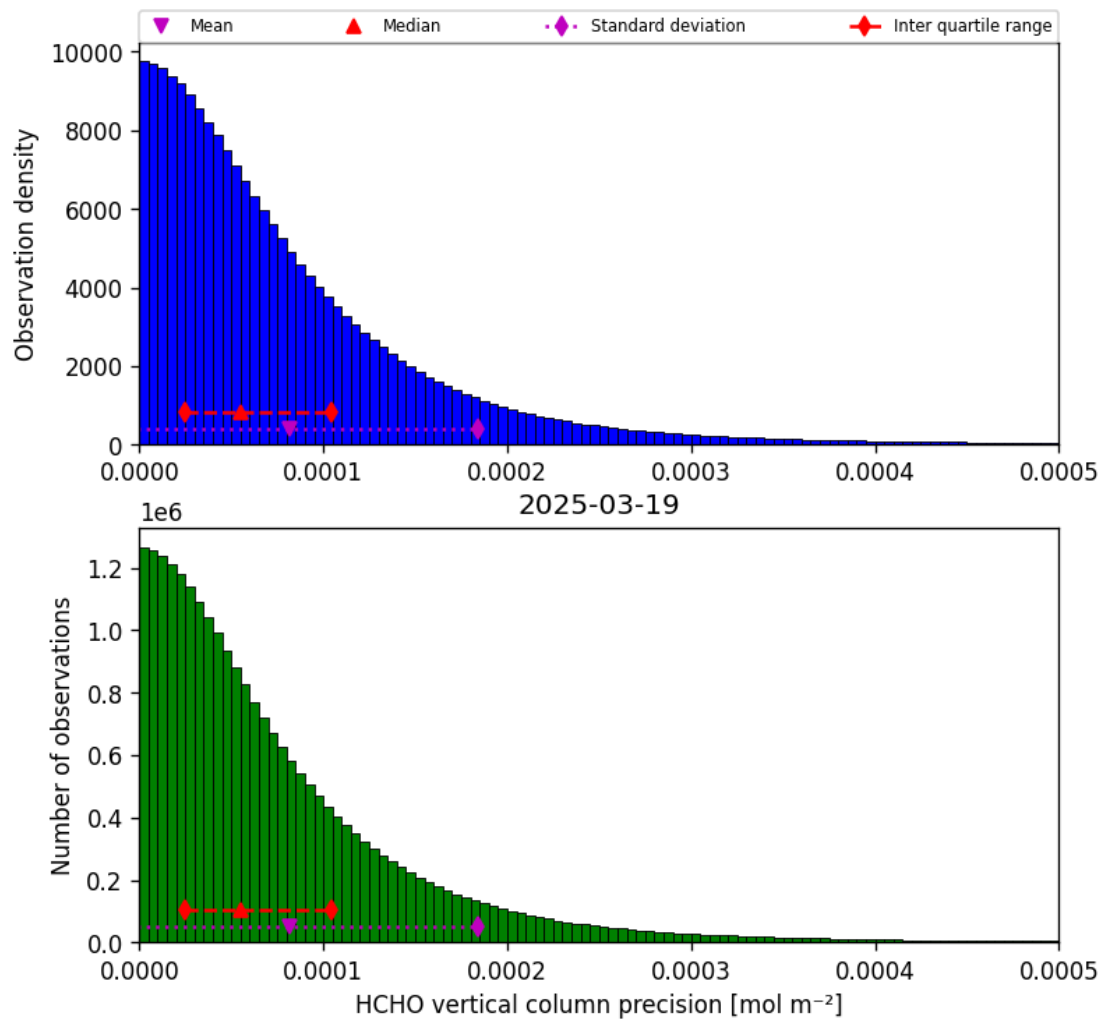
Figure 36: Histogram of “HCHO vertical column precision” for 2025-03-18 to 2025-03-20
