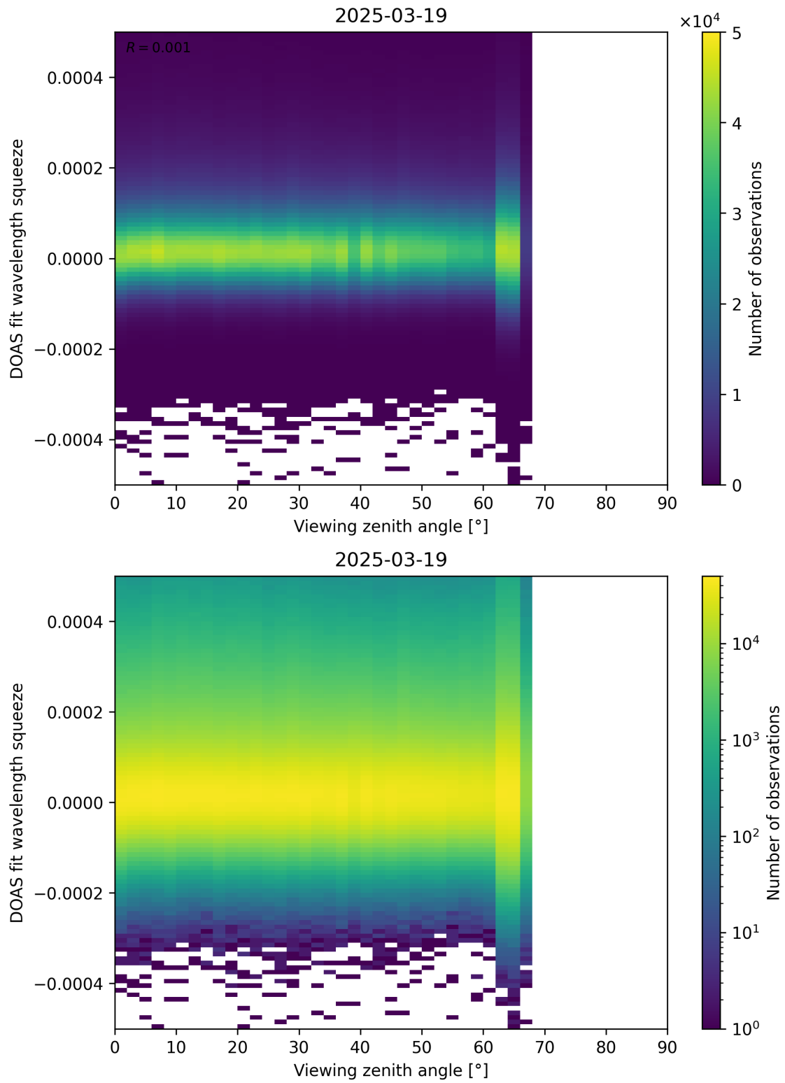
Figure 184: Scatter density plot of “Viewing zenith angle” against “DOAS fit wavelength squeeze” for 2025-03-18 to 2025-03-20.
