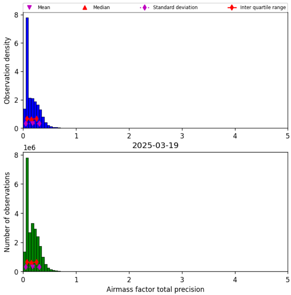
Figure 41: Histogram of “Airmass factor total precision” for 2025-03-18 to 2025-03-20
