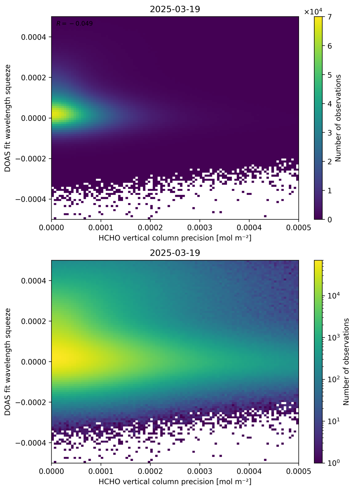
Figure 138: Scatter density plot of “HCHO vertical column precision” against “DOAS fit wavelength squeeze” for 2025-03-18 to 2025-03-20.
