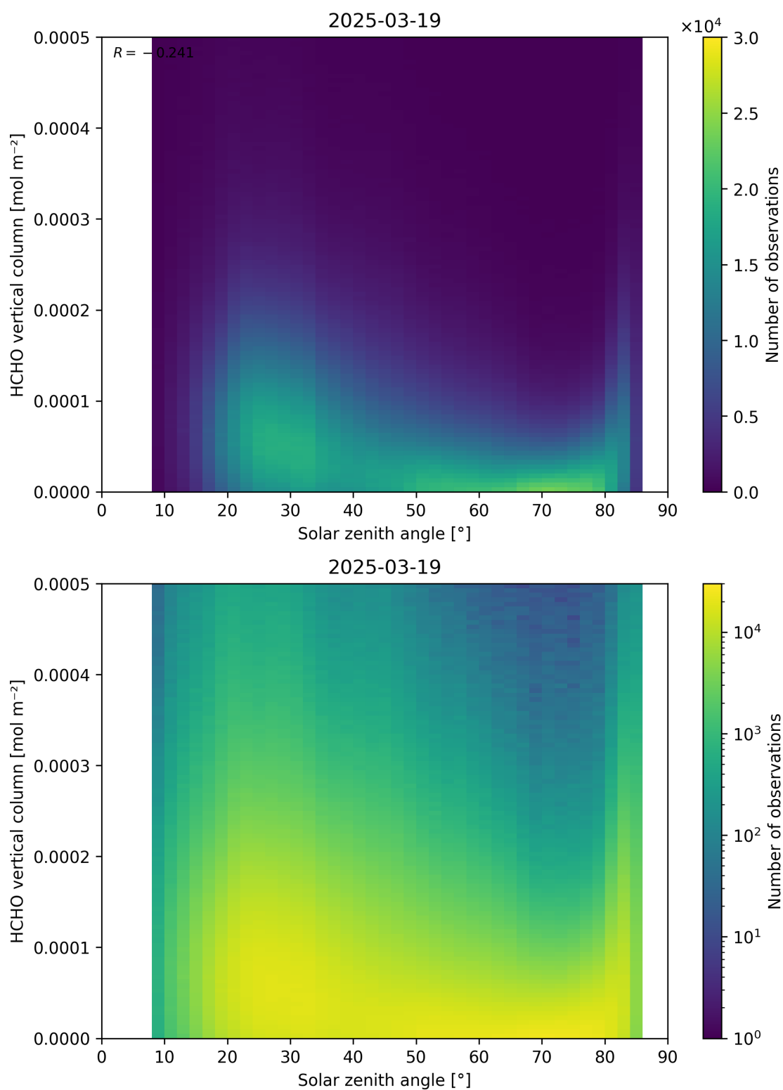
Figure 177: Scatter density plot of “Solar zenith angle” against “HCHO vertical column” for 2025-03-18 to 2025-03-20.
