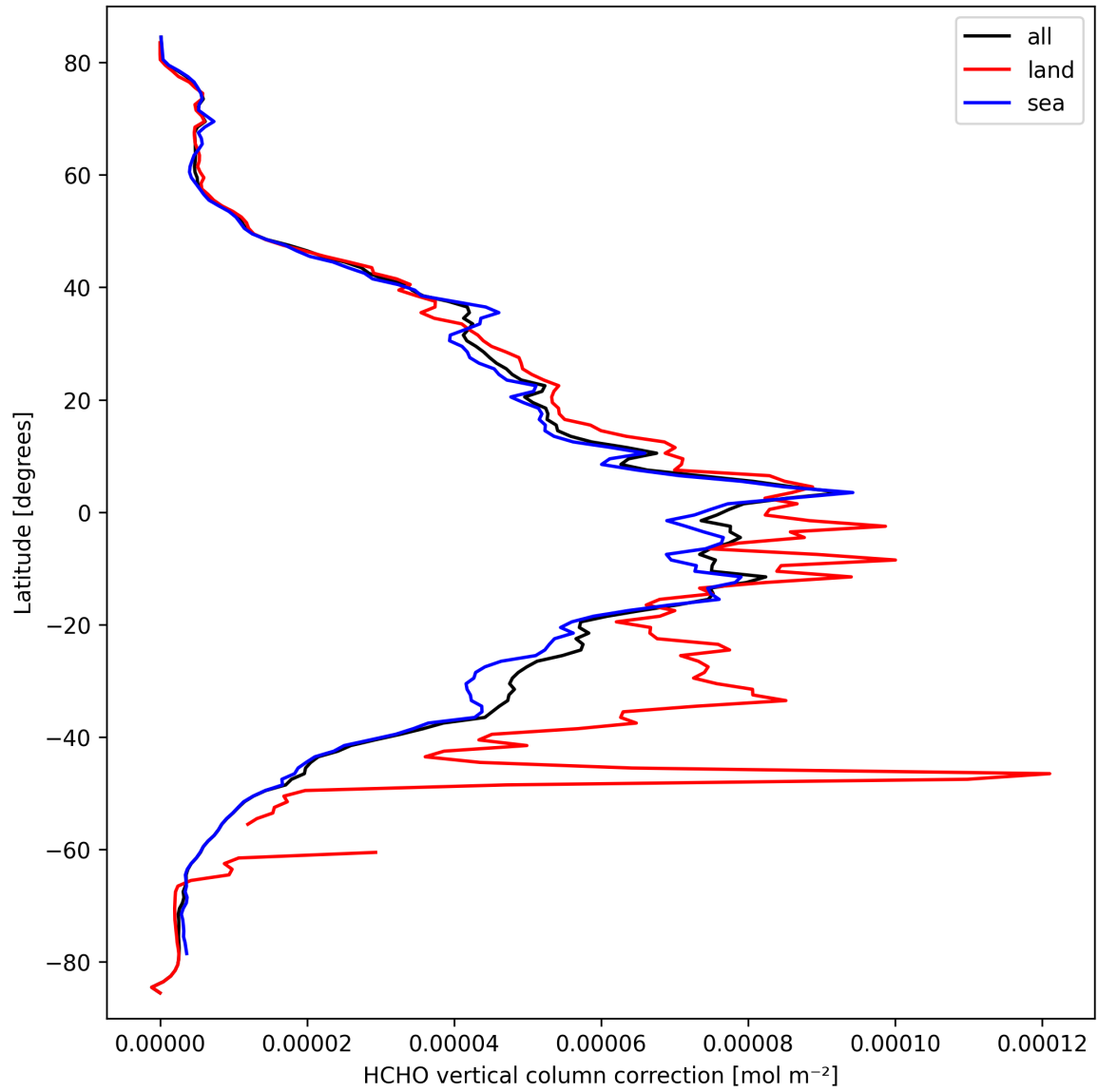
Figure 23: Zonal average of “HCHO vertical column correction” for 2025-03-18 to 2025-03-20.
