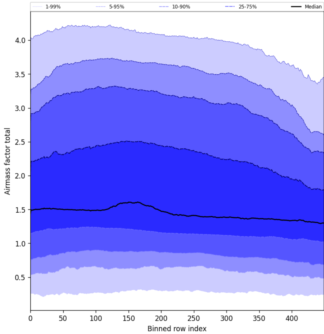
Figure 54: Along track statistics of “Airmass factor total” for 2025-03-18 to 2025-03-20
