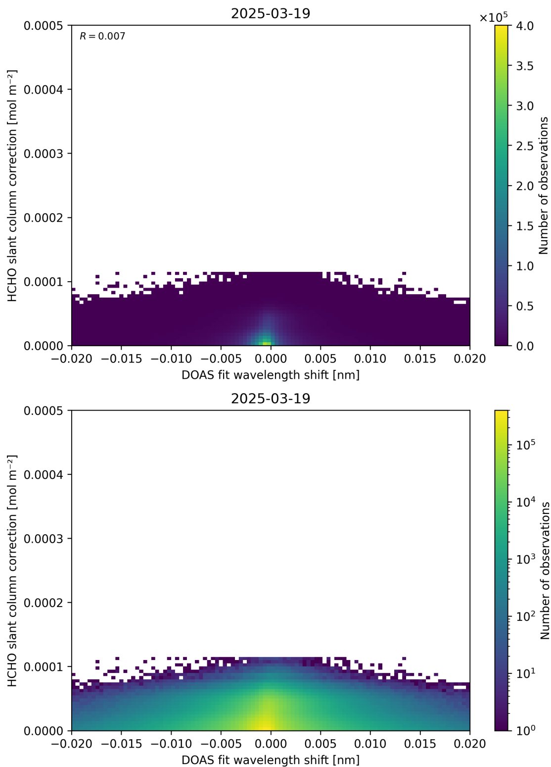
Figure 67: Scatter density plot of “DOAS fit wavelength shift” against “HCHO slant column correction” for 2025-03-18 to 2025-03-20.
