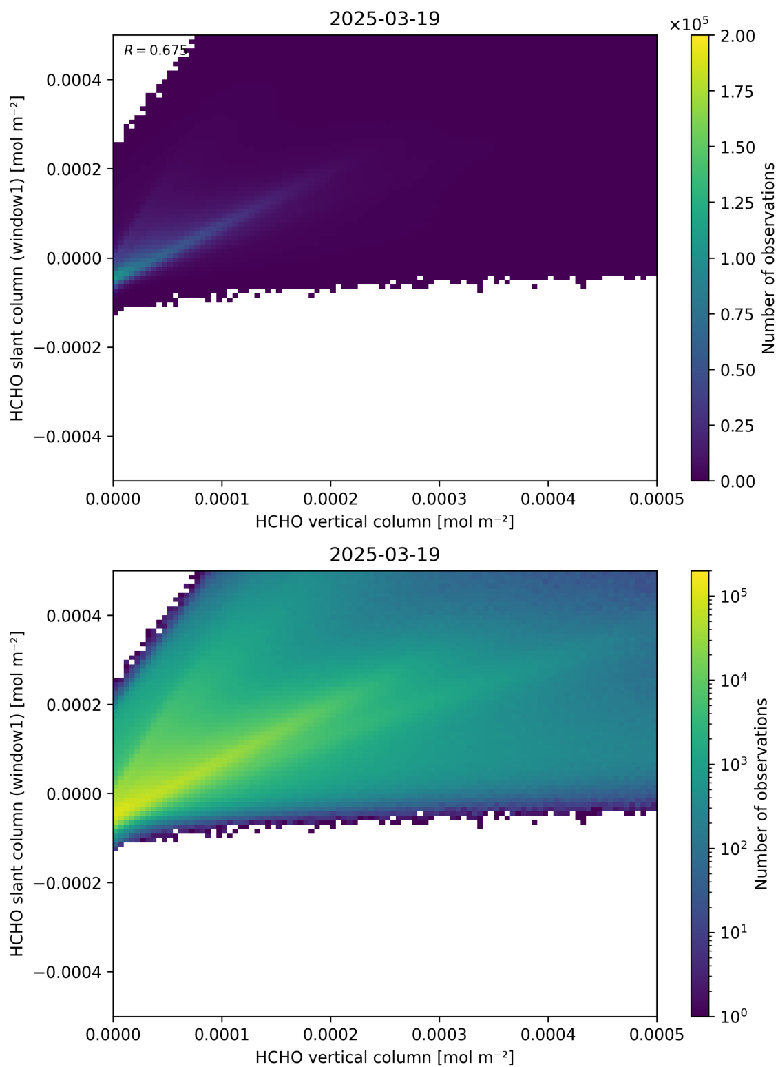
Figure 129: Scatter density plot of “HCHO vertical column” against “HCHO slant column (window1)” for 2025-03-18 to 2025-03-20.
