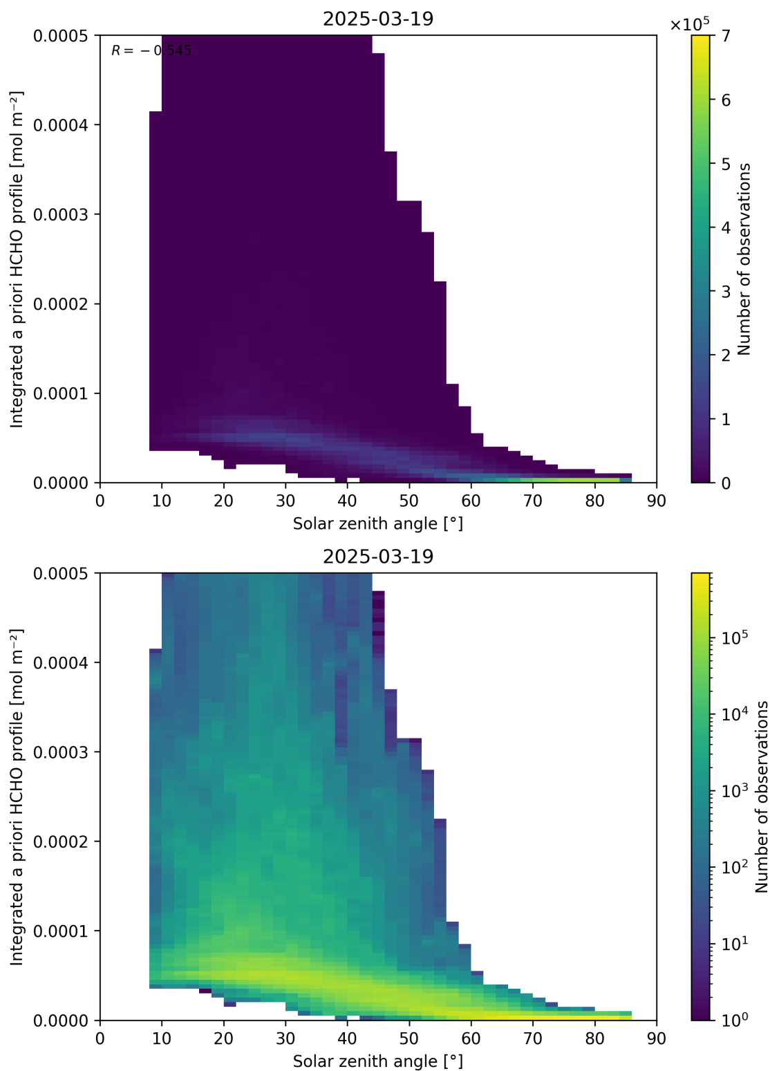
Figure 180: Scatter density plot of “Solar zenith angle” against “Integrated a priori HCHO profile” for 2025-03-18 to 2025-03-20.
