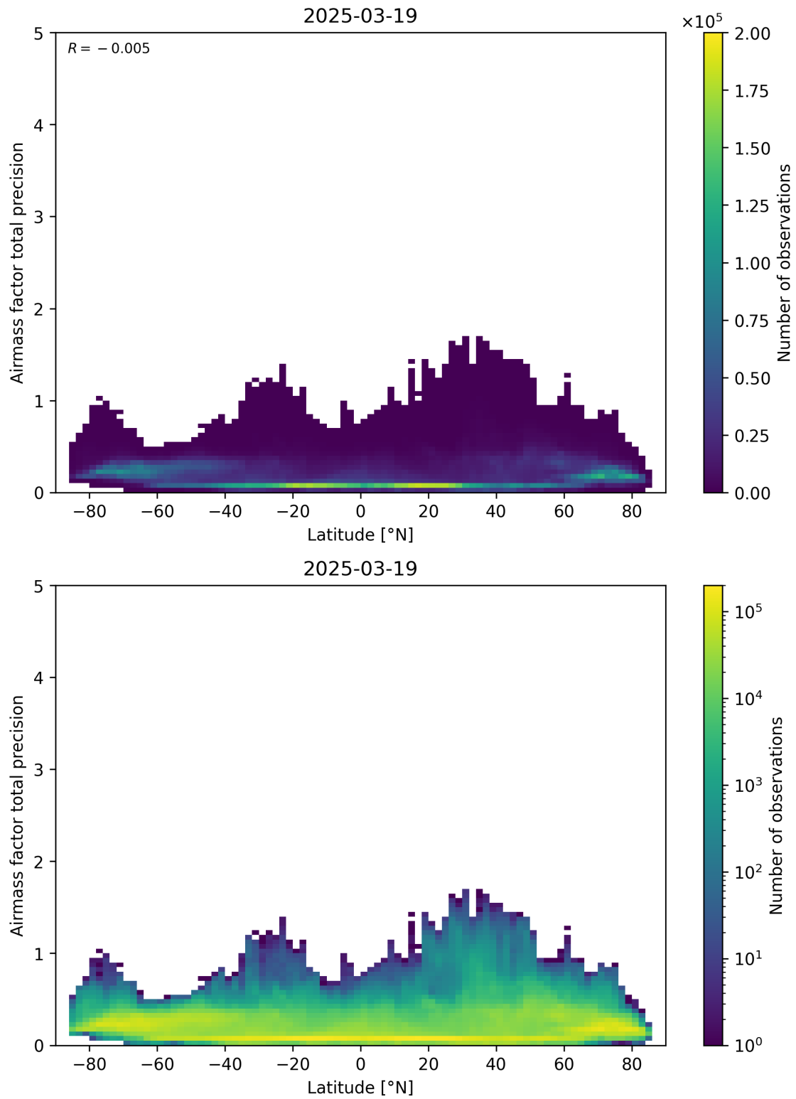
Figure 162: Scatter density plot of “Latitude” against “Airmass factor total precision” for 2025-03-18 to 2025-03-20.
