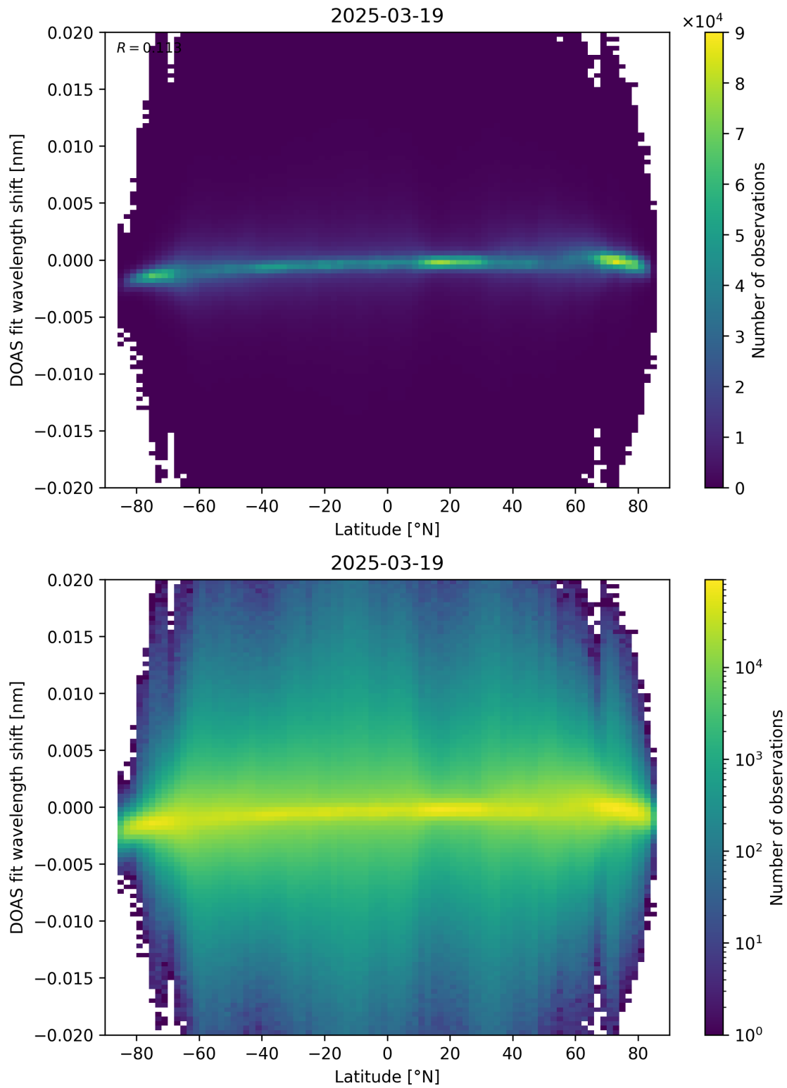
Figure 154: Scatter density plot of “Latitude” against “DOAS fit wavelength shift” for 2025-03-18 to 2025-03-20.
