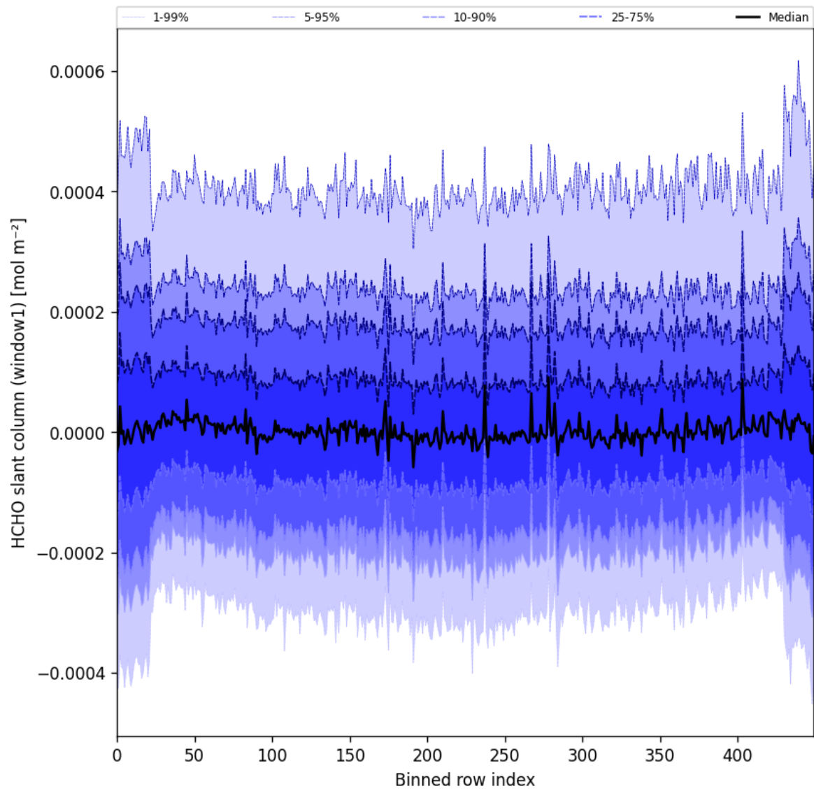
Figure 52: Along track statistics of “HCHO slant column (window1)” for 2025-03-18 to 2025-03-20
