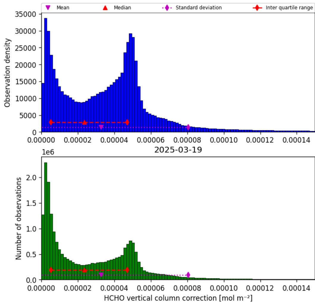
Figure 37: Histogram of “HCHO vertical column correction” for 2025-03-18 to 2025-03-20
