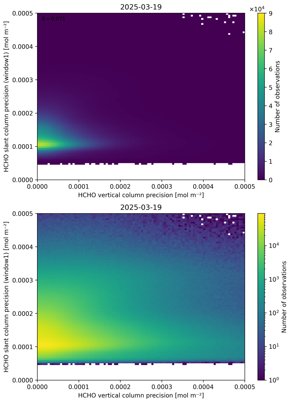
Figure 143: Scatter density plot of “HCHO vertical column precision” against “HCHO slant column precision (window1)” for 2025-03-18 to 2025-03-20.
