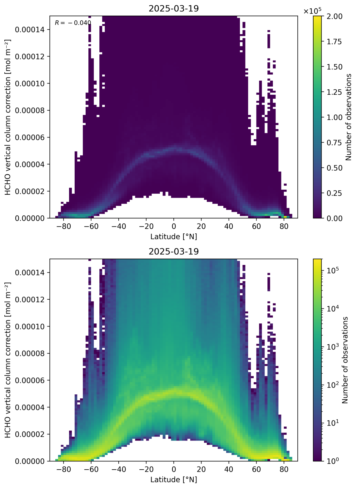
Figure 164: Scatter density plot of “Latitude” against “HCHO vertical column correction” for 2025-03-18 to 2025-03-20.
