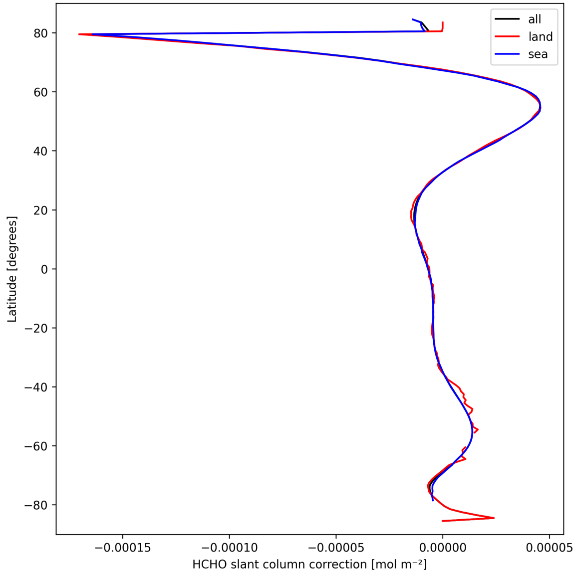
Figure 33: Zonal average of “HCHO slant column correction” for 2025-03-18 to 2025-03-20.
