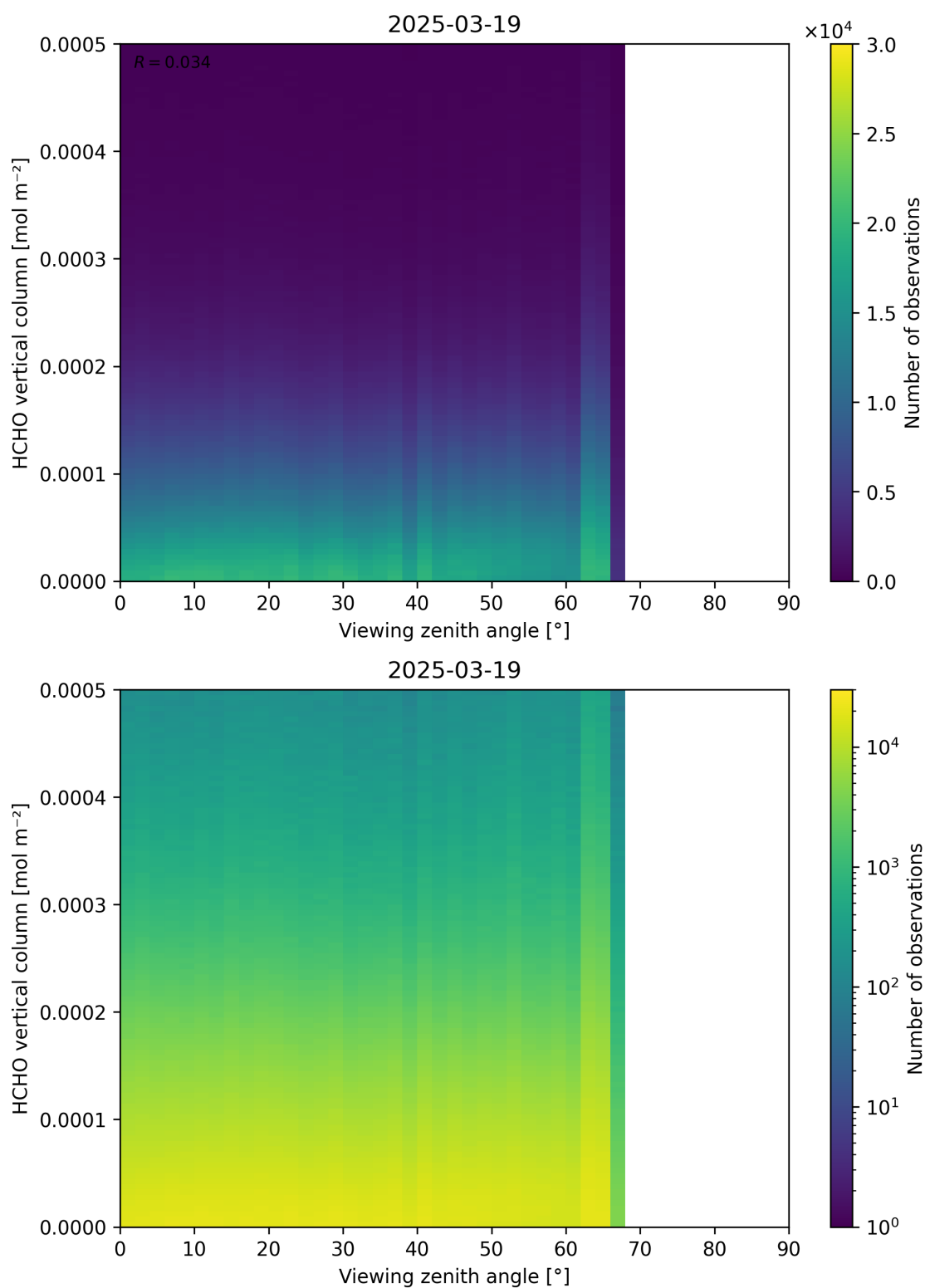
Figure 192: Scatter density plot of “Viewing zenith angle” against “HCHO vertical column” for 2025-03-18 to 2025-03-20.
