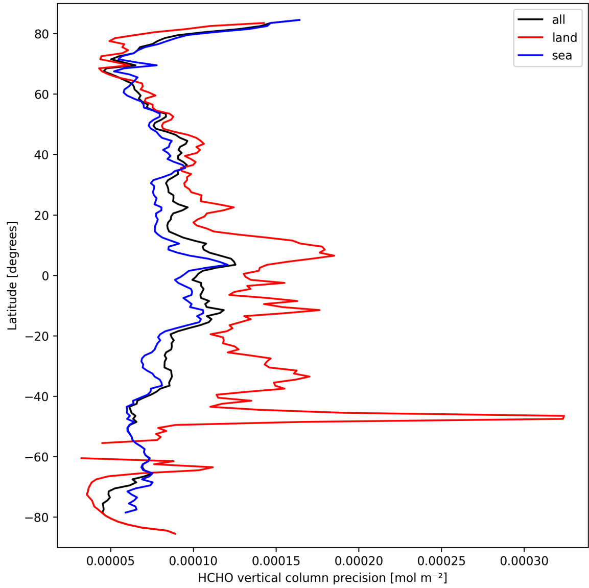
Figure 22: Zonal average of “HCHO vertical column precision” for 2025-03-18 to 2025-03-20.
