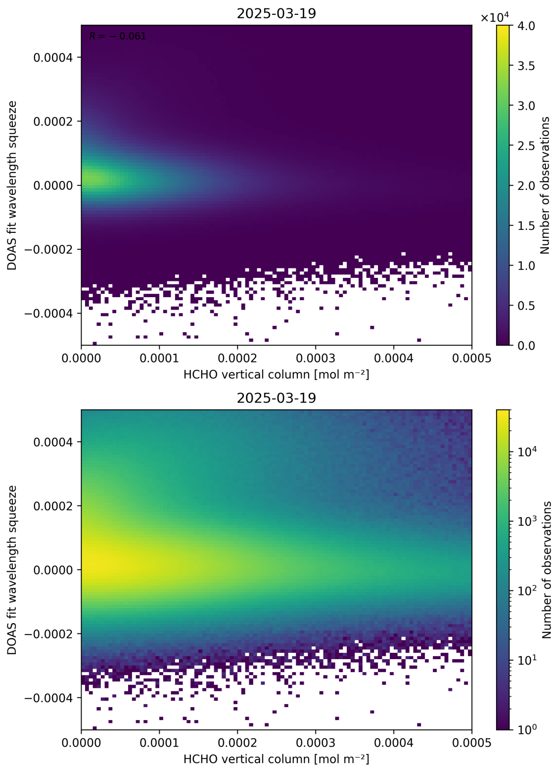
Figure 125: Scatter density plot of “HCHO vertical column” against “DOAS fit wavelength squeeze” for 2025-03-18 to 2025-03-20.
