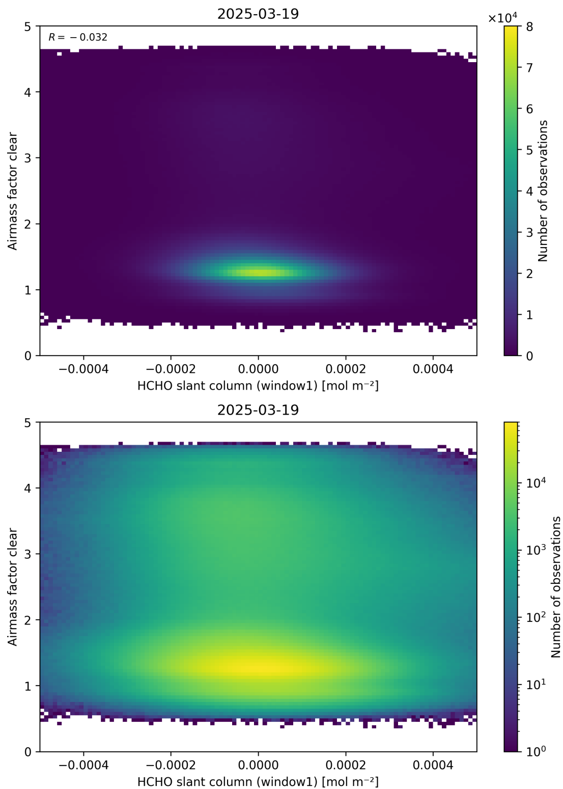
Figure 81: Scatter density plot of “HCHO slant column (window1)” against “Airmass factor clear” for 2025-03-18 to 2025-03-20.
