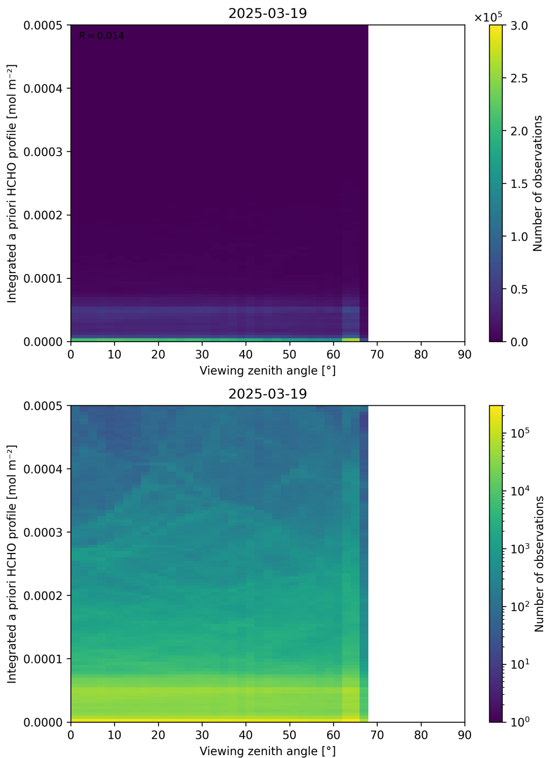
Figure 195: Scatter density plot of “Viewing zenith angle” against “Integrated a priori HCHO profile” for 2025-03-18 to 2025-03-20.
