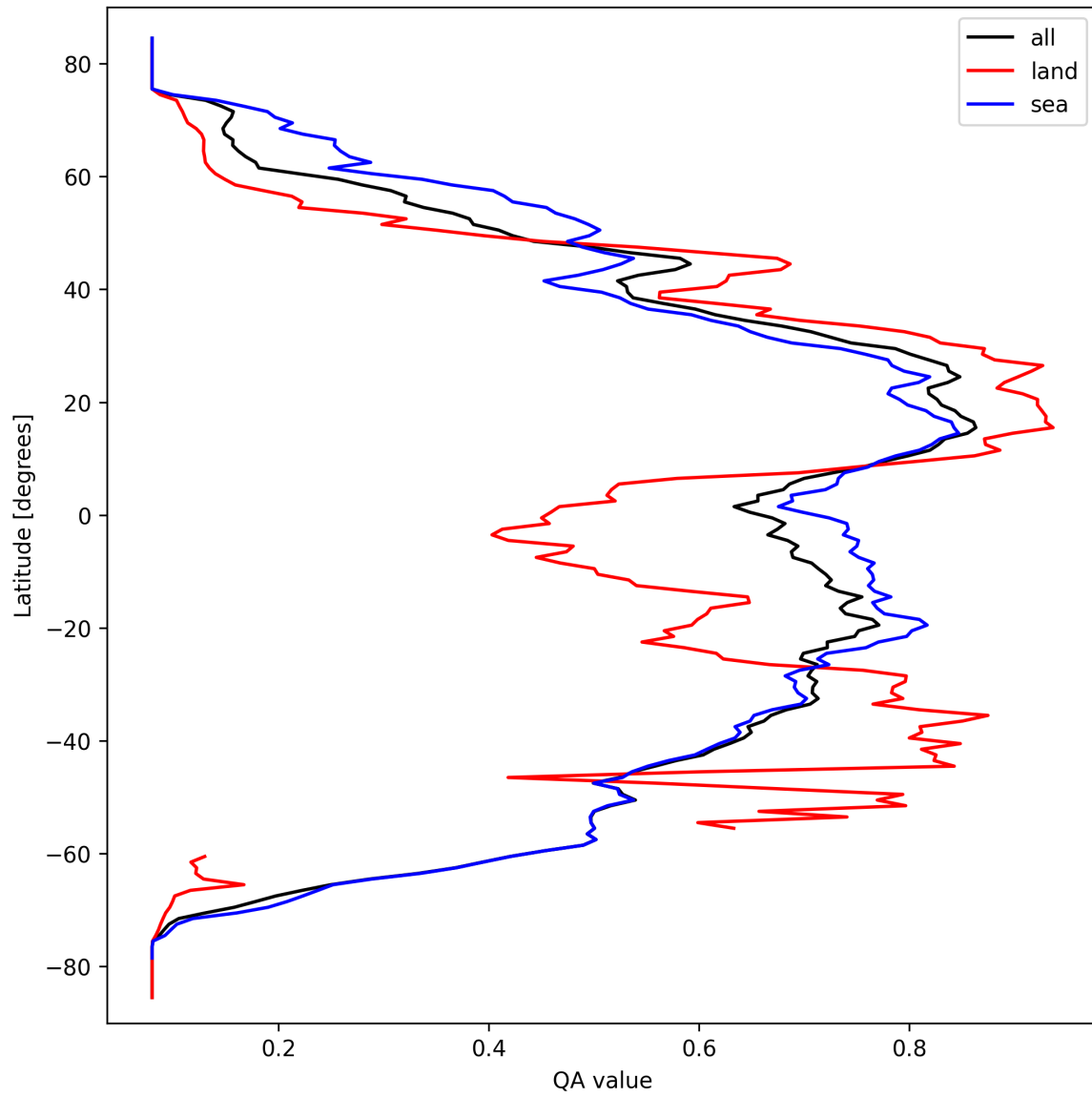
Figure 20: Zonal average of “QA value” for 2025-03-18 to 2025-03-20.
