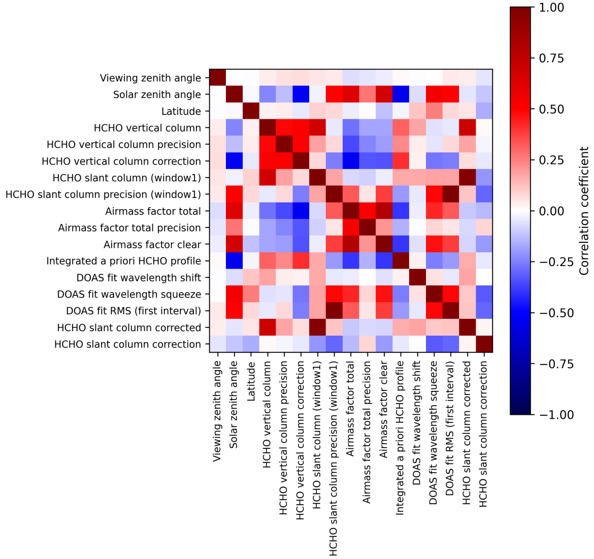
Figure 2: Map of correlation matrix for 2025-03-18 to 2025-03-20.
