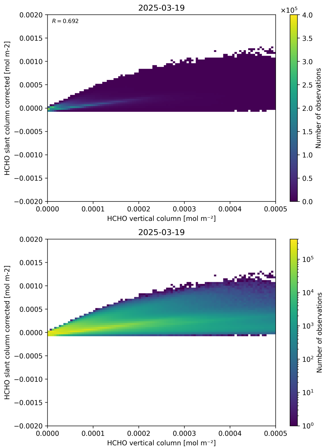
Figure 127: Scatter density plot of “HCHO vertical column” against “HCHO slant column corrected” for 2025-03-18 to 2025-03-20.
