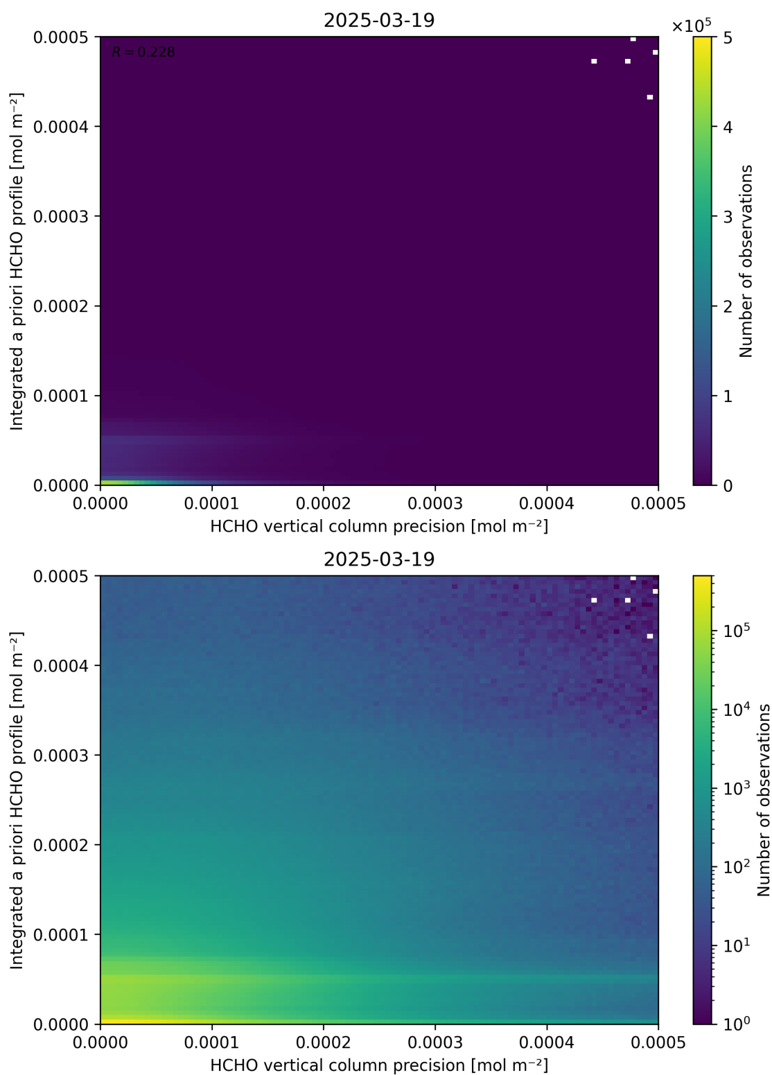
Figure 147: Scatter density plot of “HCHO vertical column precision” against “Integrated a priori HCHO profile” for 2025-03-18 to 2025-03-20.
