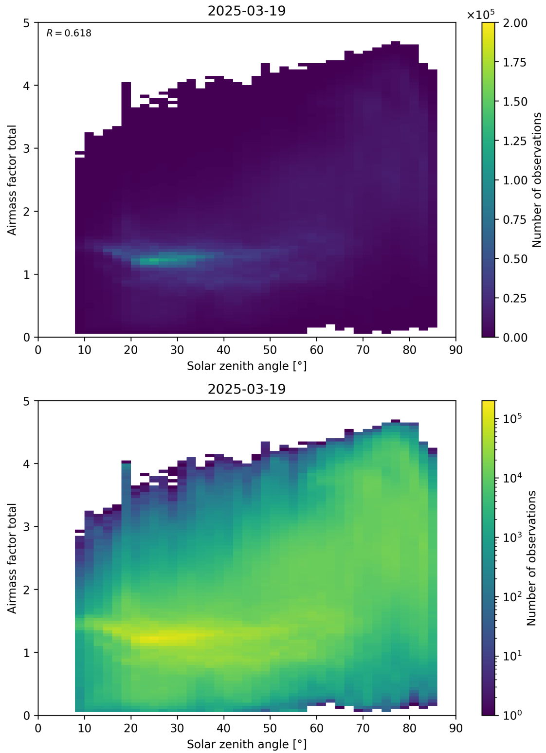
Figure 175: Scatter density plot of “Solar zenith angle” against “Airmass factor total” for 2025-03-18 to 2025-03-20.
