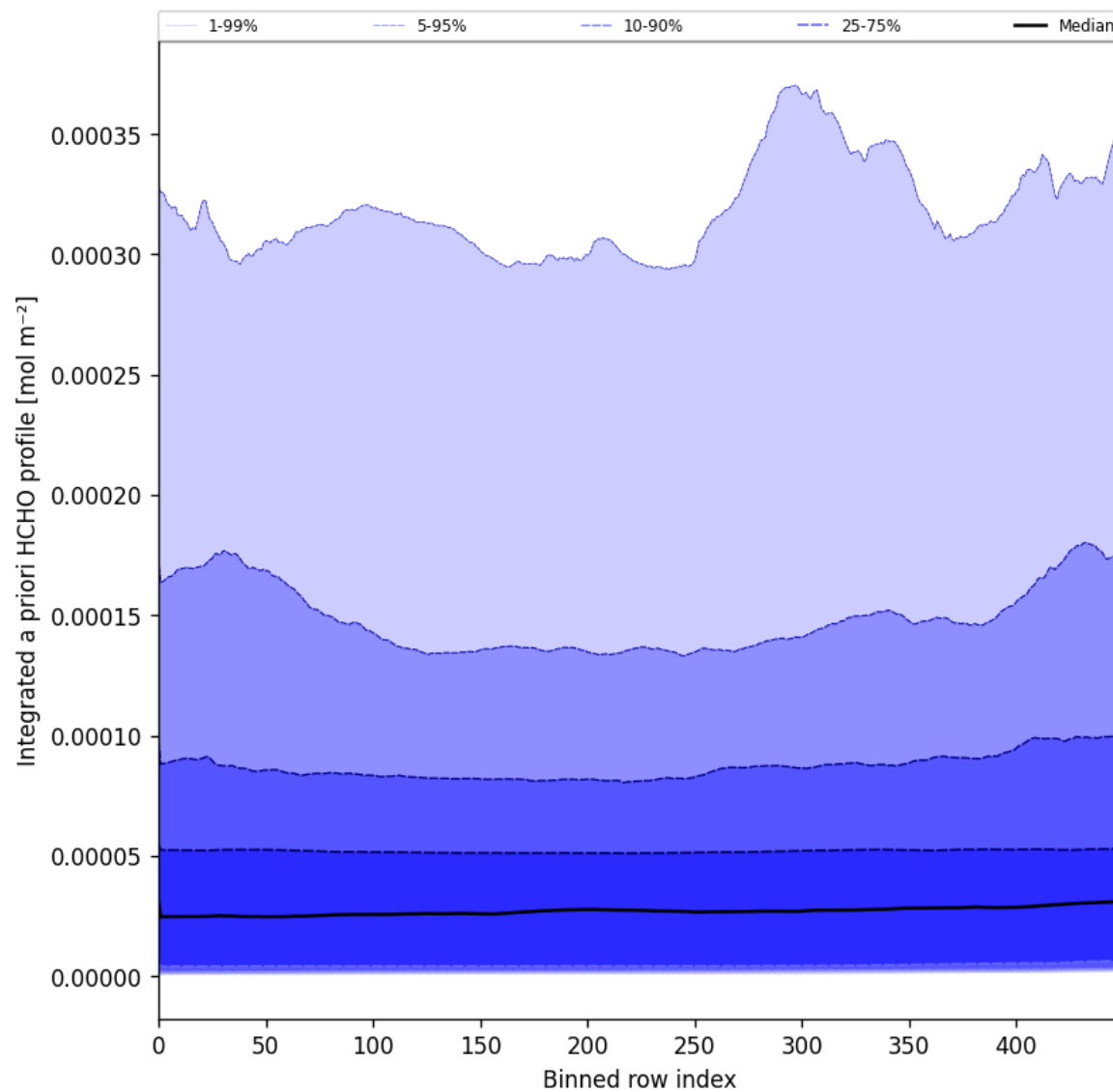
Figure 57: Along track statistics of “Integrated a priori HCHO profile” for 2025-03-18 to 2025-03-20
