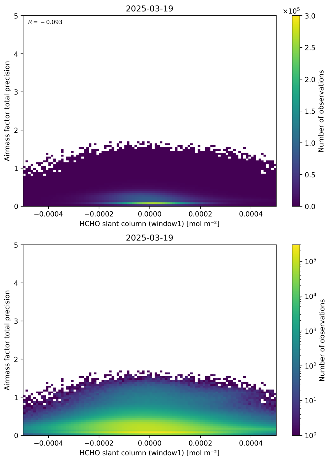
Figure 86: Scatter density plot of “HCHO slant column (window1)” against “Airmass factor total precision” for 2025-03-18 to 2025-03-20.
