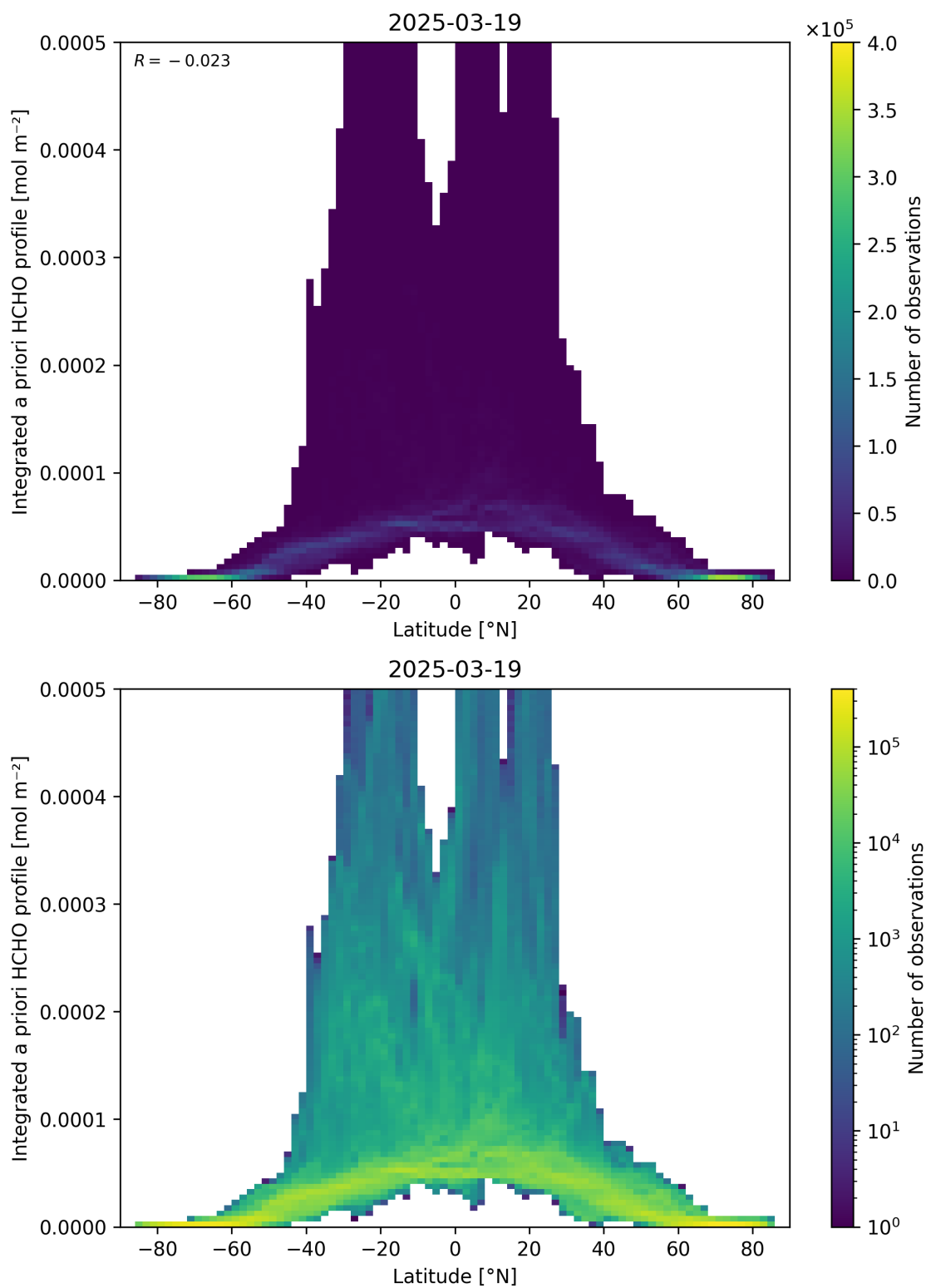
Figure 166: Scatter density plot of “Latitude” against “Integrated a priori HCHO profile” for 2025-03-18 to 2025-03-20.
