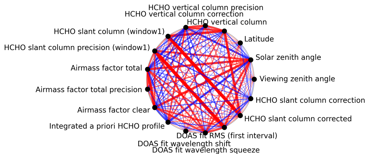
Figure 1: Map of correlation graph for 2025-03-18 to 2025-03-20.
