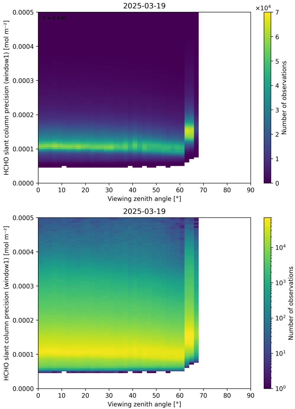
Figure 189: Scatter density plot of “Viewing zenith angle” against “HCHO slant column precision (window1)” for 2025-03-18 to 2025-03-20.
