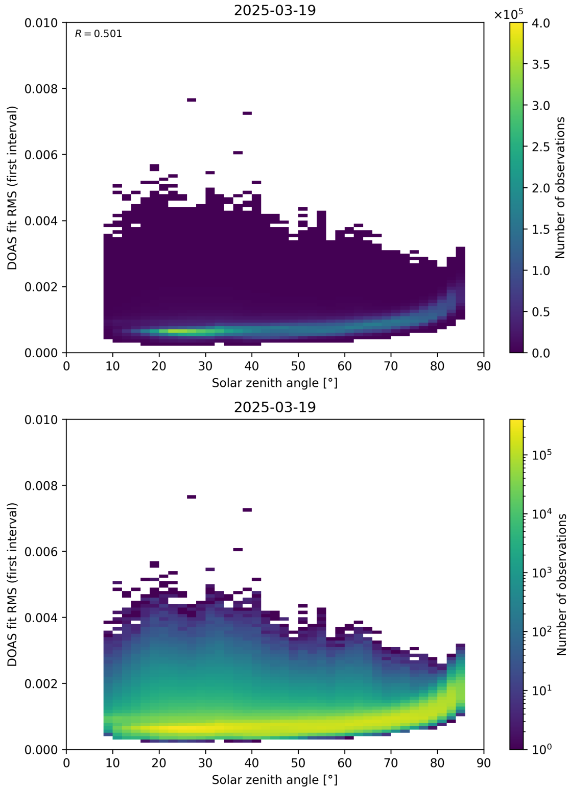
Figure 167: Scatter density plot of “Solar zenith angle” against “DOAS fit RMS (first interval)” for 2025-03-18 to 2025-03-20.
