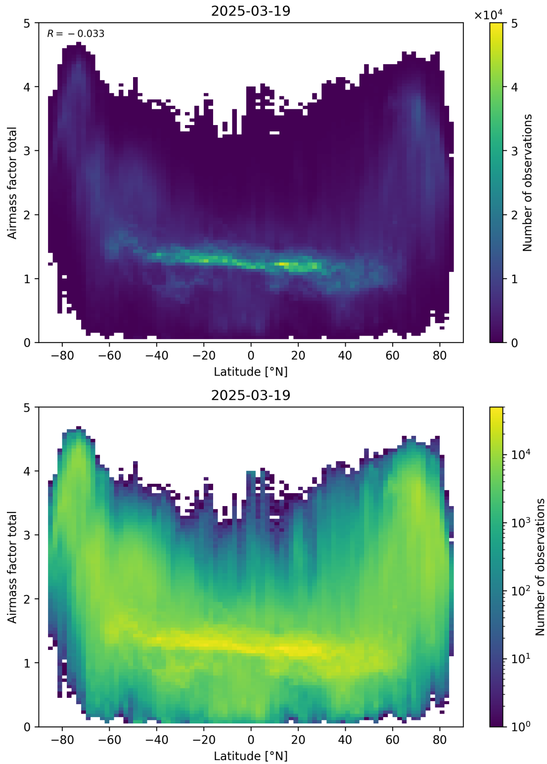
Figure 161: Scatter density plot of “Latitude” against “Airmass factor total” for 2025-03-18 to 2025-03-20.
