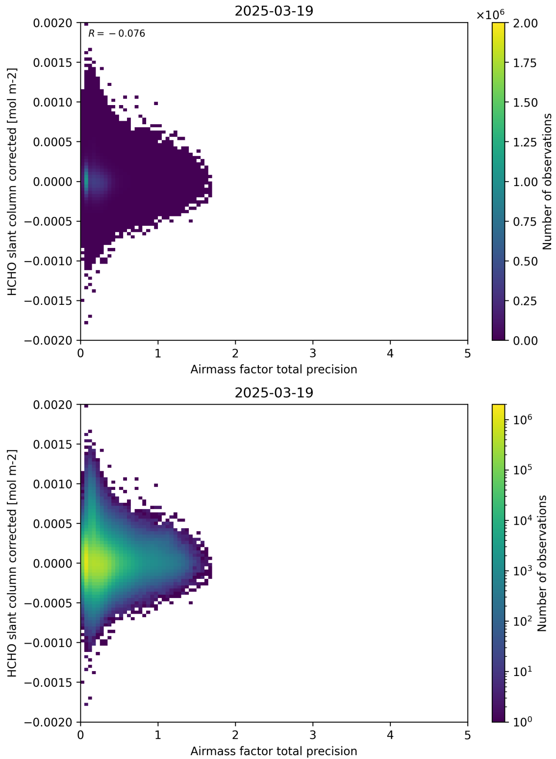
Figure 109: Scatter density plot of “Airmass factor total precision” against “HCHO slant column corrected” for 2025-03-18 to 2025-03-20.
