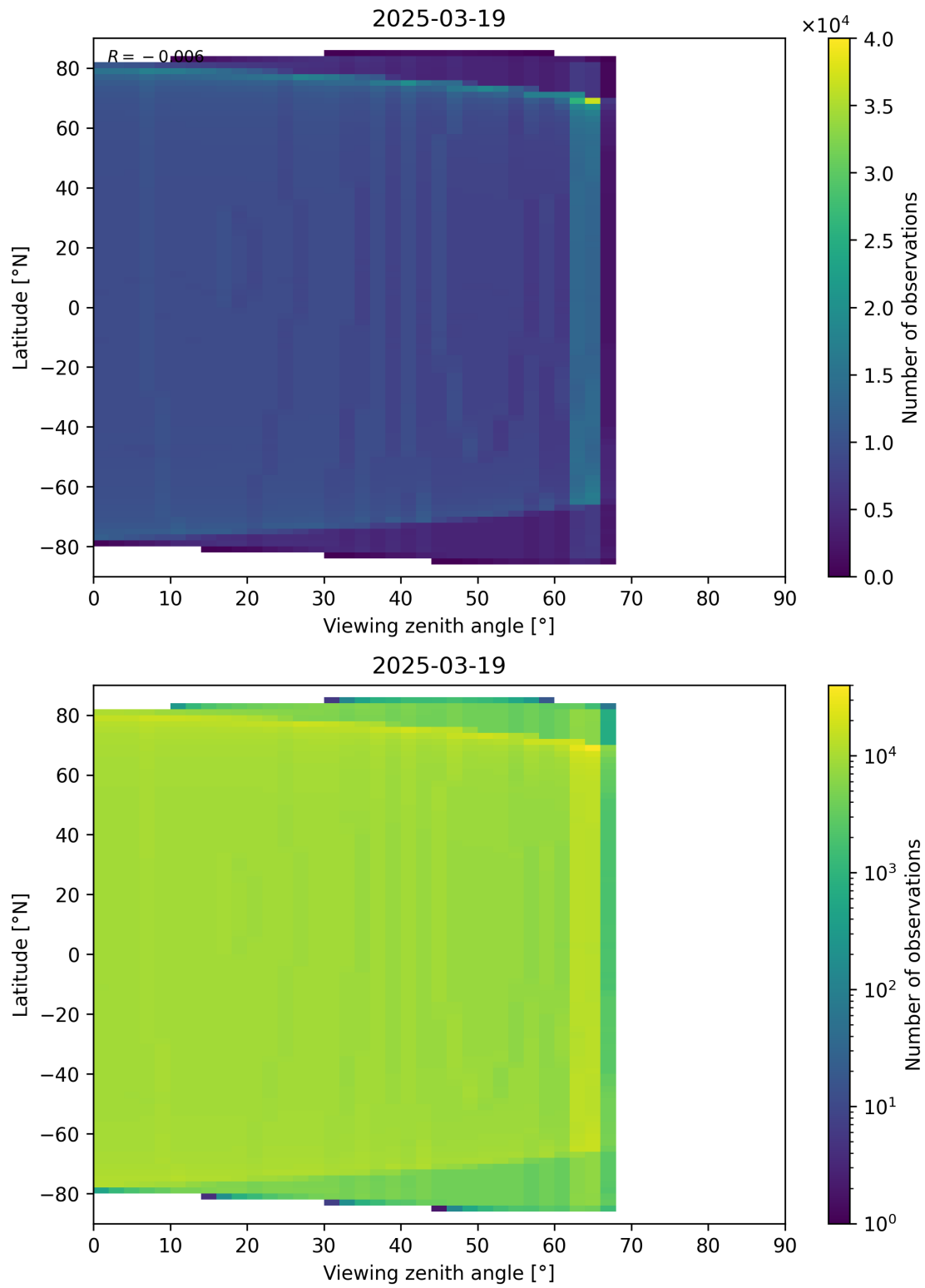
Figure 196: Scatter density plot of “Viewing zenith angle” against “Latitude” for 2025-03-18 to 2025-03-20.
