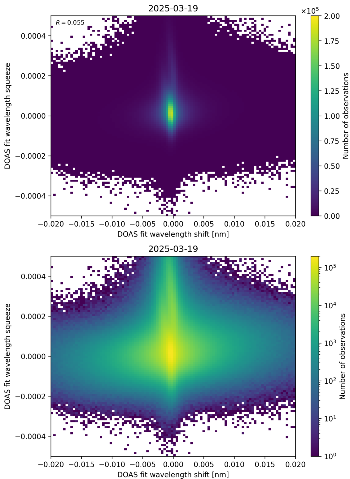
Figure 65: Scatter density plot of “DOAS fit wavelength shift” against “DOAS fit wavelength squeeze” for 2025-03-18 to 2025-03-20.
