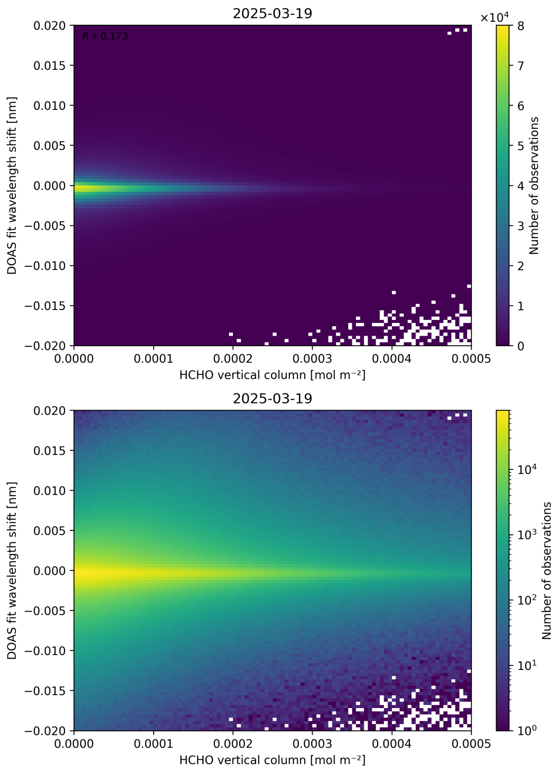
Figure 124: Scatter density plot of “HCHO vertical column” against “DOAS fit wavelength shift” for 2025-03-18 to 2025-03-20.
