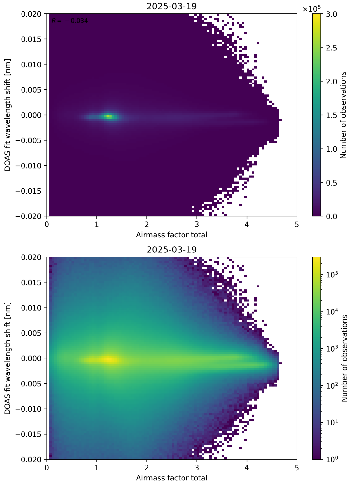
Figure 98: Scatter density plot of “Airmass factor total” against “DOAS fit wavelength shift” for 2025-03-18 to 2025-03-20.
