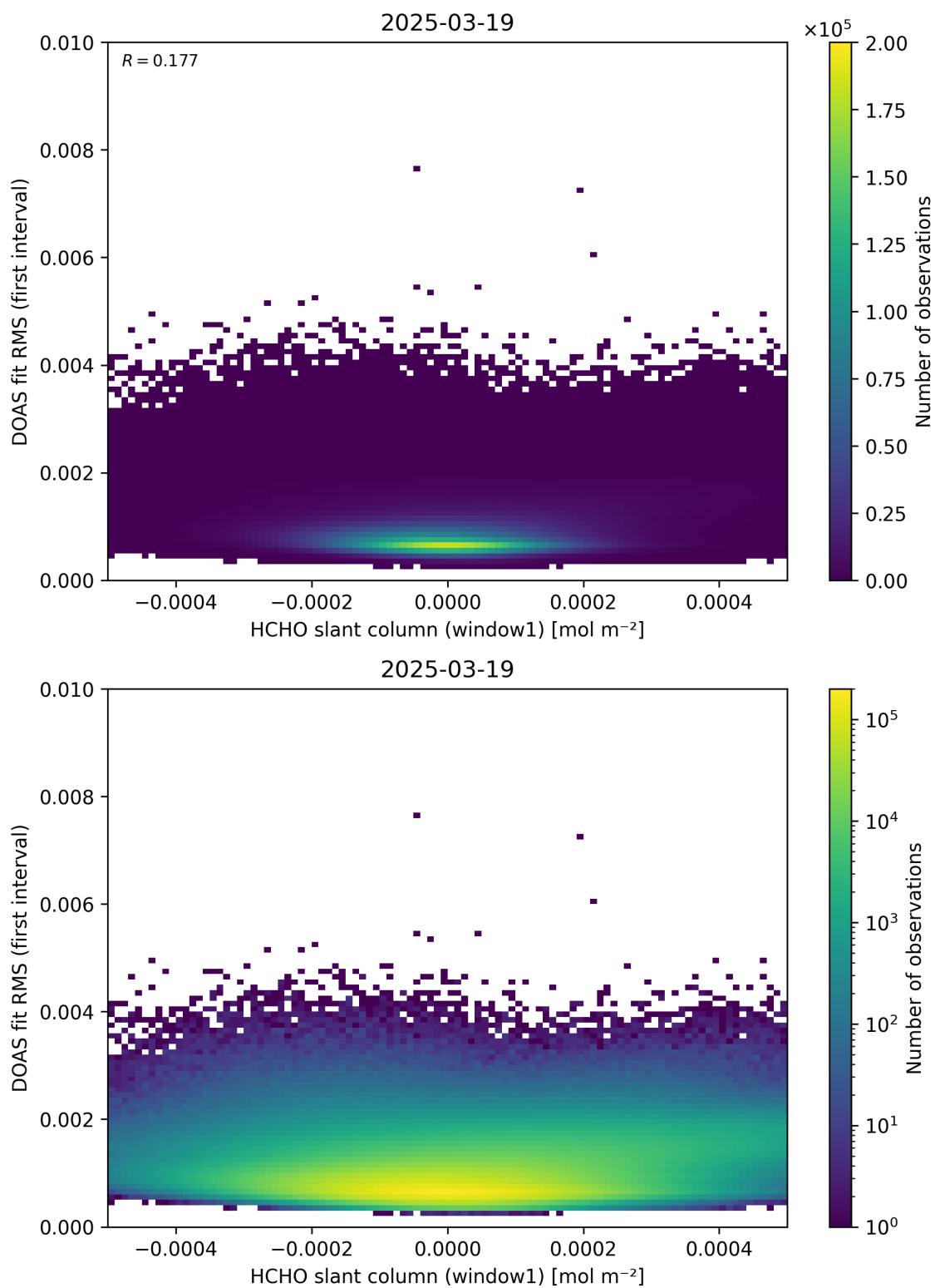
Figure 78: Scatter density plot of “HCHO slant column (window1)” against “DOAS fit RMS (first interval)” for 2025-03-18 to 2025-03-20.
