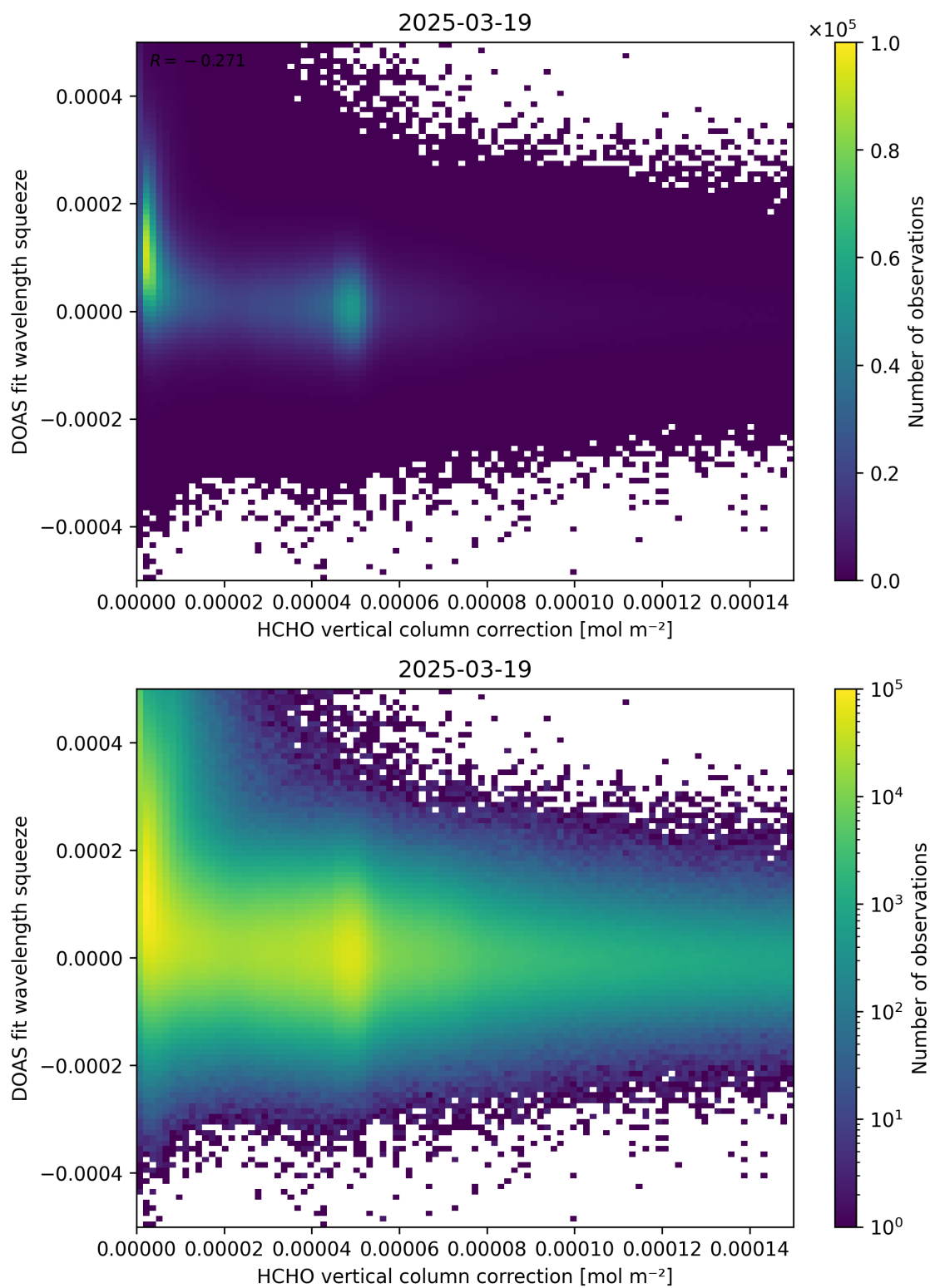
Figure 114: Scatter density plot of “HCHO vertical column correction” against “DOAS fit wavelength squeeze” for 2025-03-18 to 2025-03-20.
