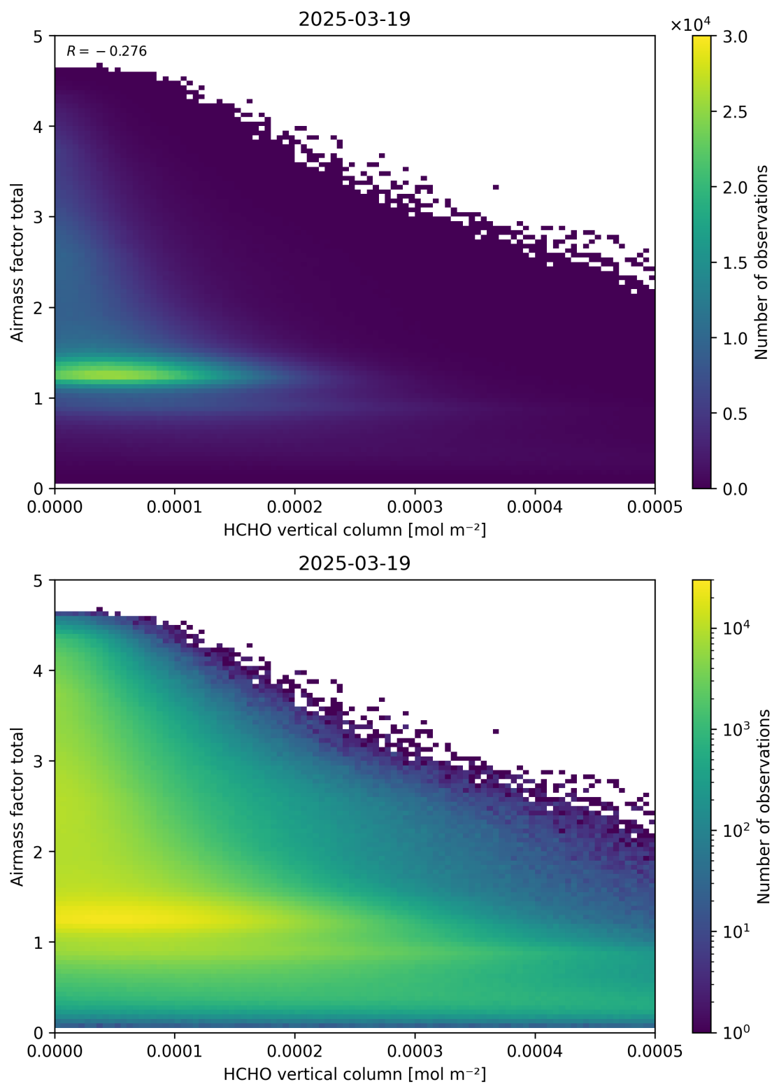
Figure 131: Scatter density plot of “HCHO vertical column” against “Airmass factor total” for 2025-03-18 to 2025-03-20.
