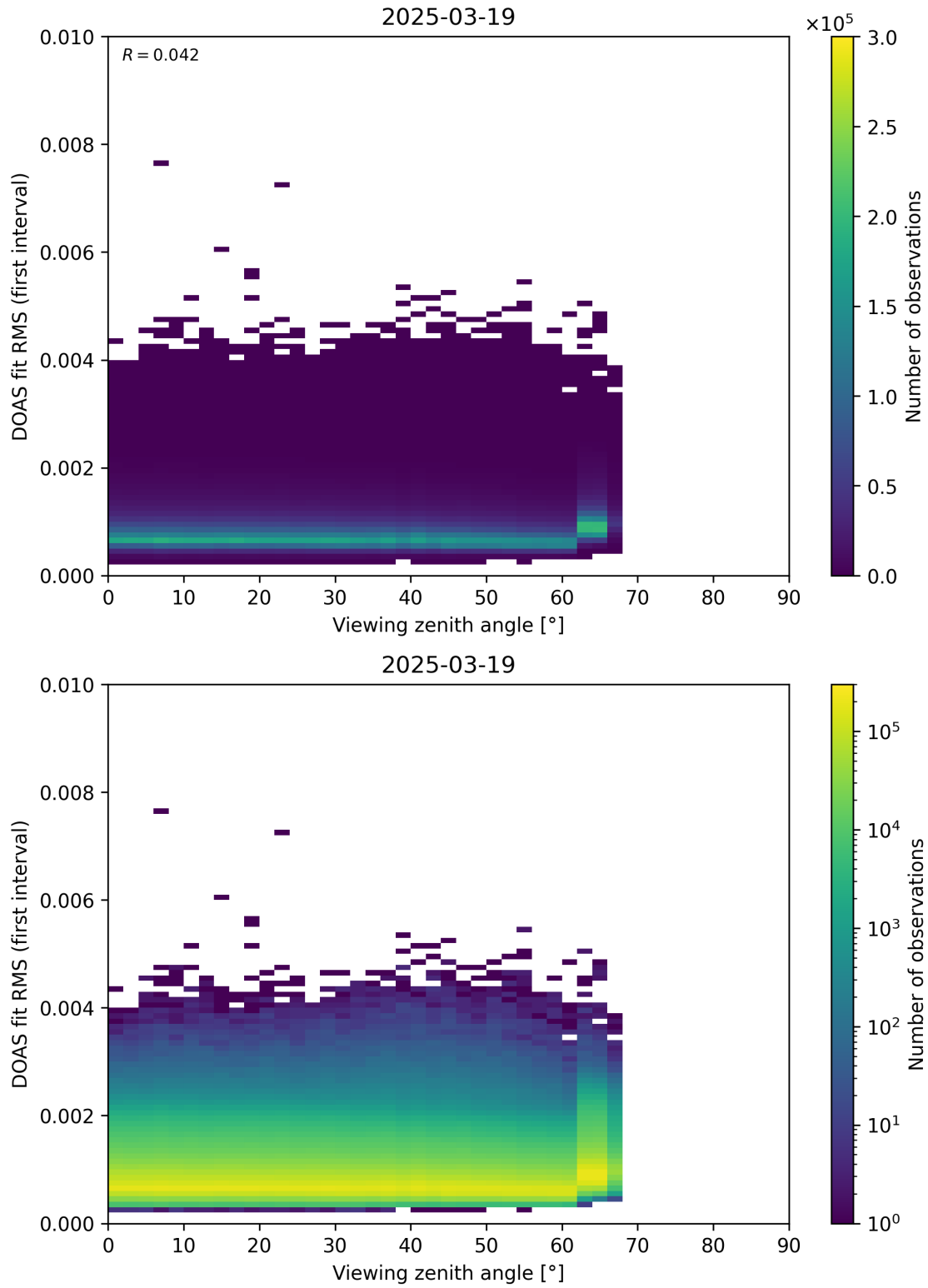
Figure 182: Scatter density plot of “Viewing zenith angle” against “DOAS fit RMS (first interval)” for 2025-03-18 to 2025-03-20.
