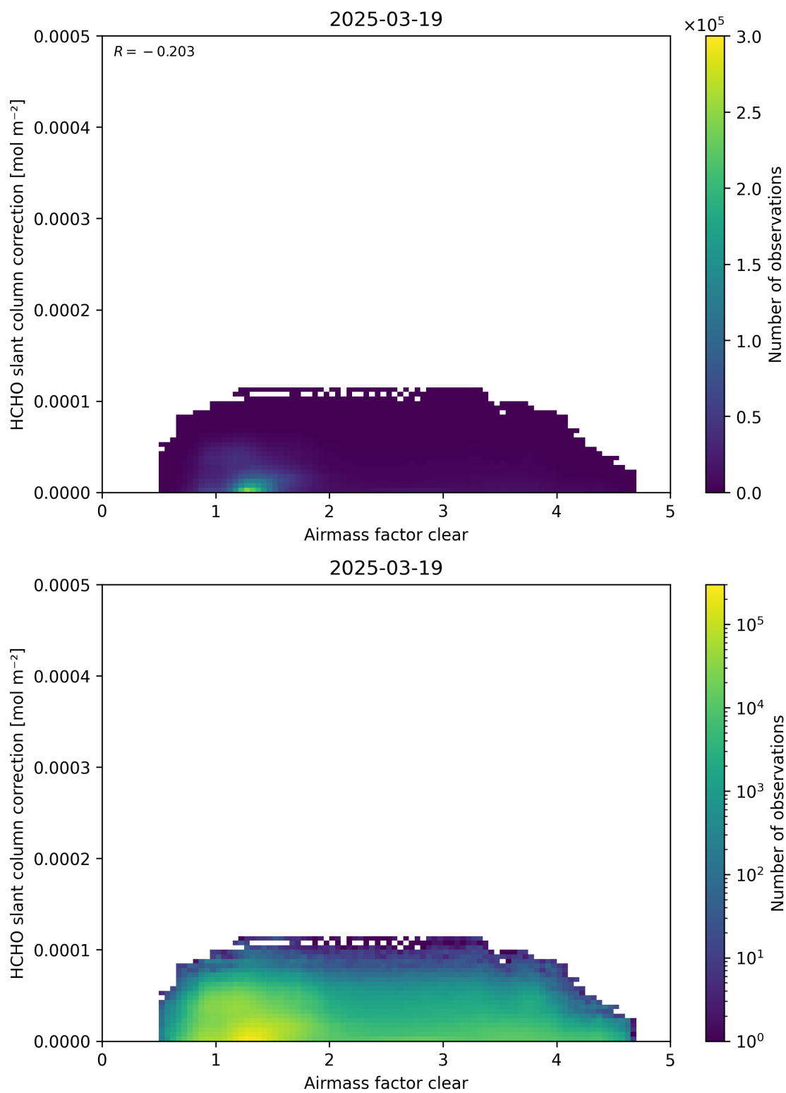
Figure 75: Scatter density plot of “Airmass factor clear” against “HCHO slant column correction” for 2025-03-18 to 2025-03-20.
