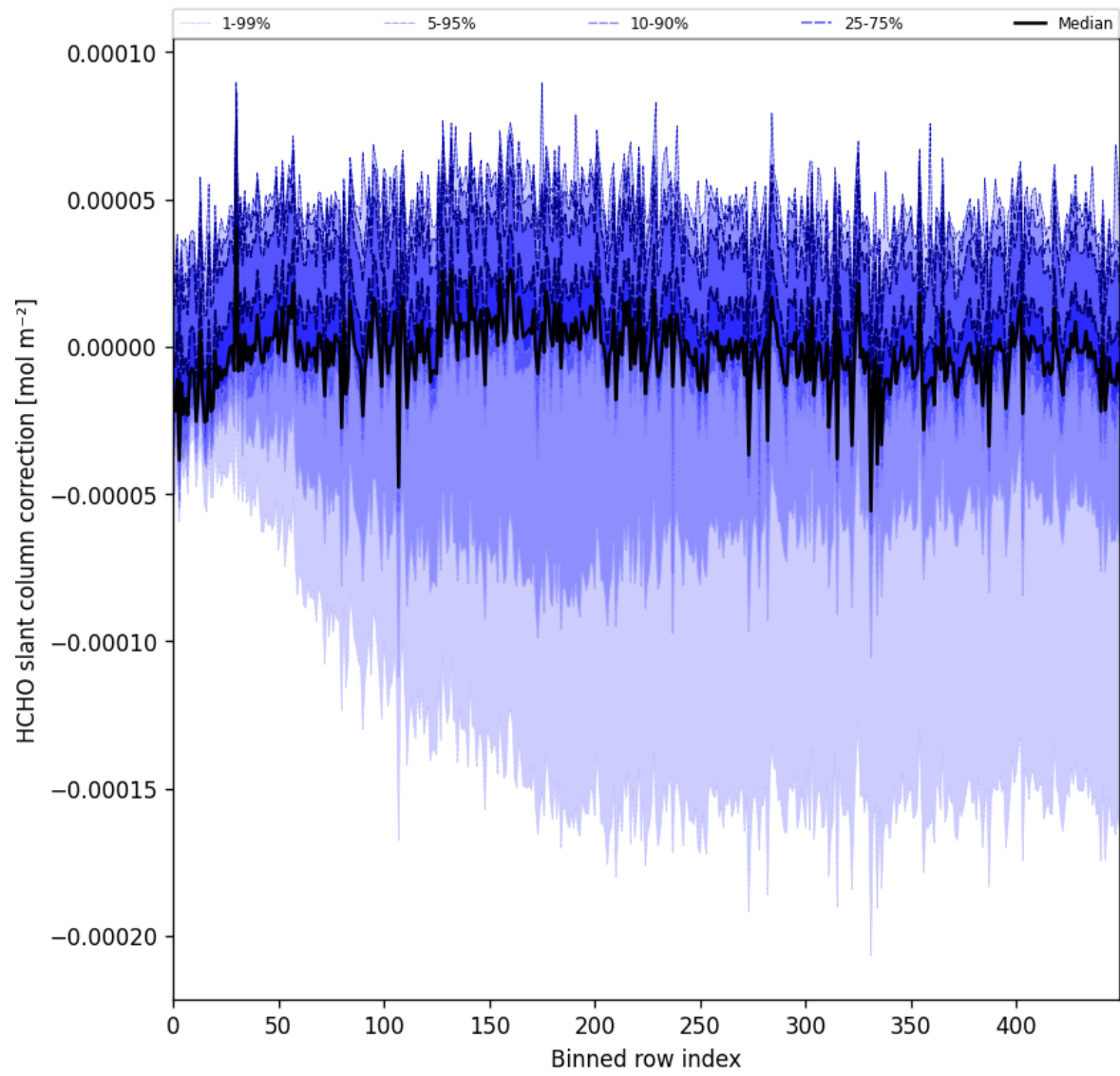
Figure 61: Along track statistics of “HCHO slant column correction” for 2025-03-18 to 2025-03-20
