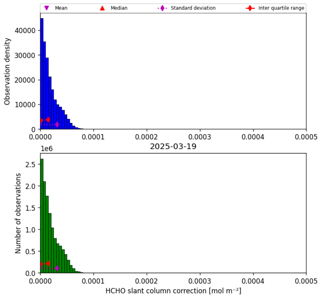
Figure 47: Histogram of “HCHO slant column correction” for 2025-03-18 to 2025-03-20
