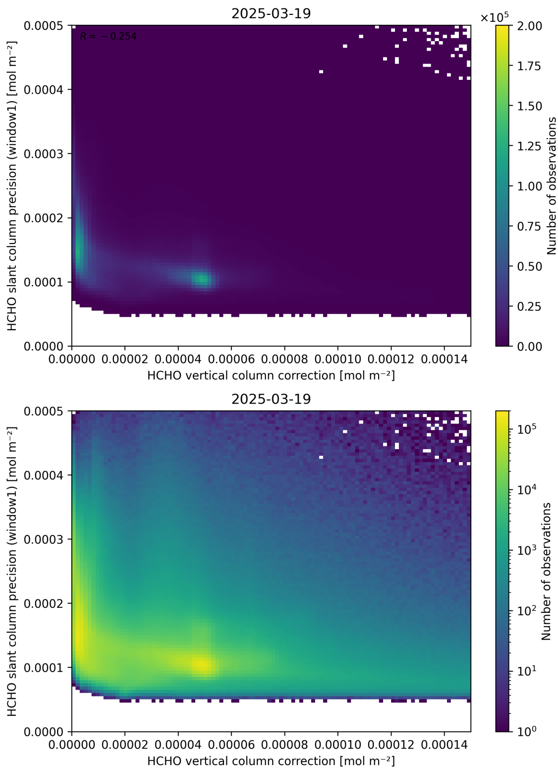
Figure 119: Scatter density plot of “HCHO vertical column correction” against “HCHO slant column precision (window1)” for 2025-03-18 to 2025-03-20.
