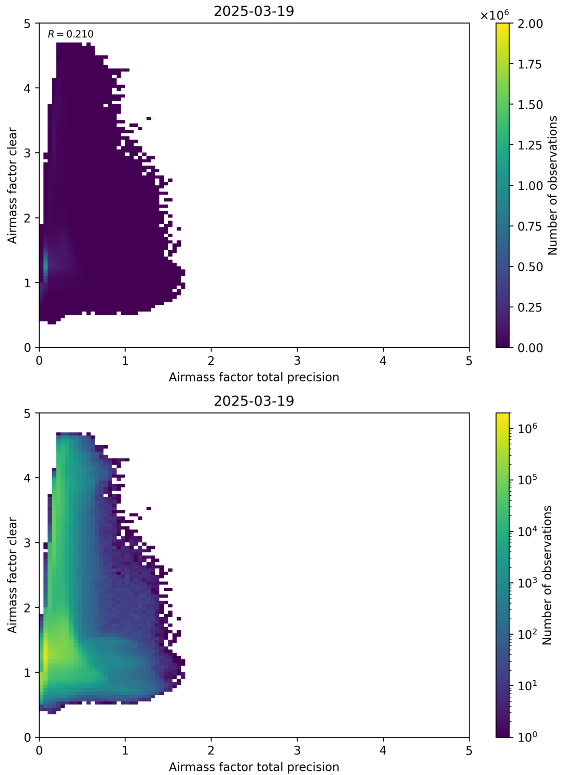
Figure 108: Scatter density plot of “Airmass factor total precision” against “Airmass factor clear” for 2025-03-18 to 2025-03-20.
