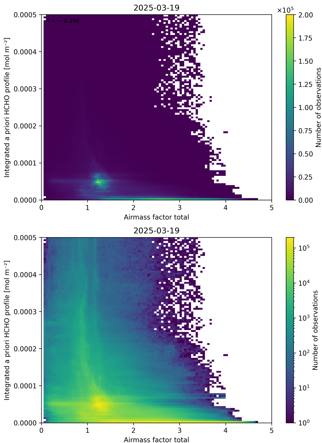
Figure 104: Scatter density plot of “Airmass factor total” against “Integrated a priori HCHO profile” for 2025-03-18 to 2025-03-20.
