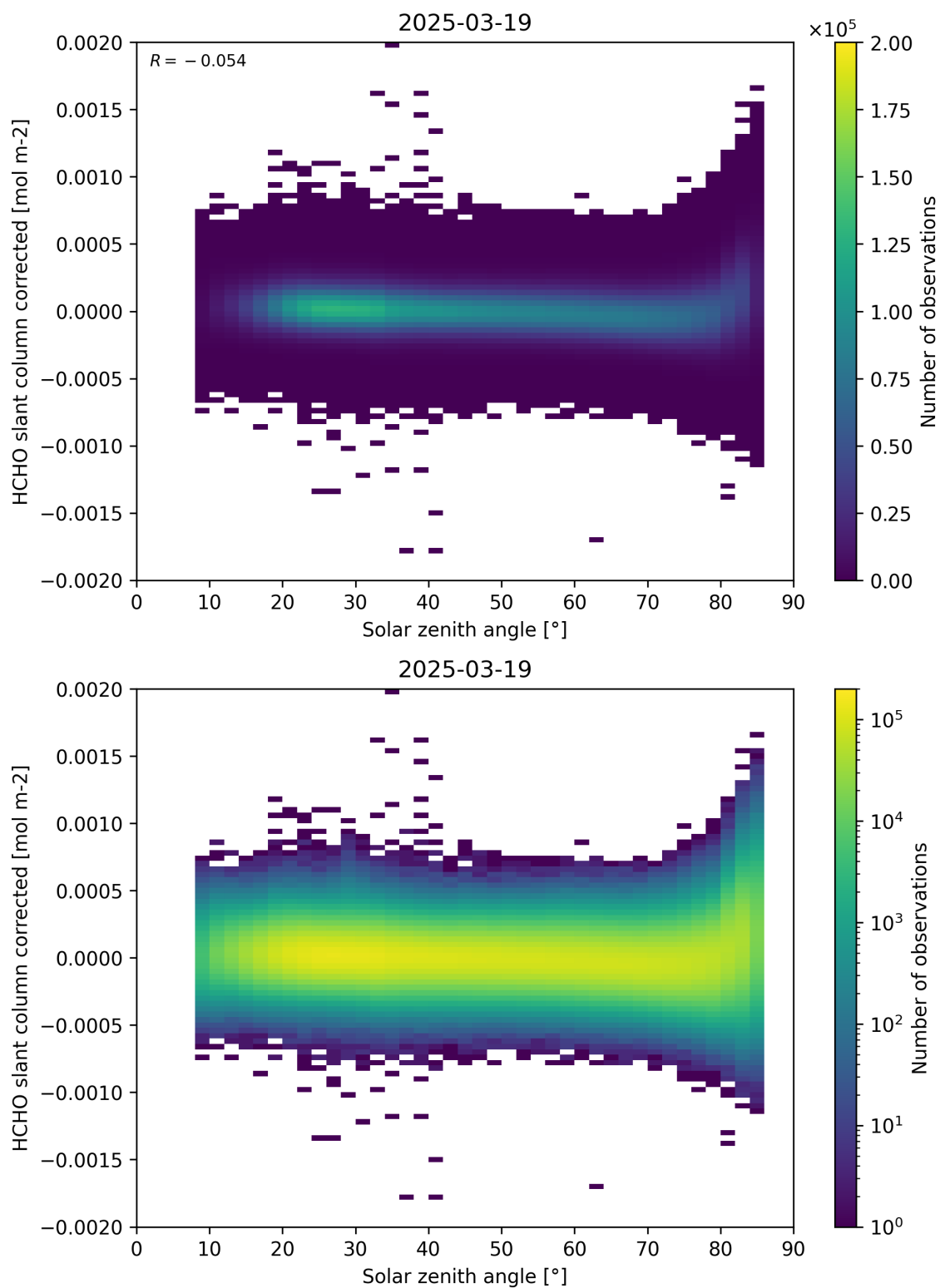
Figure 171: Scatter density plot of “Solar zenith angle” against “HCHO slant column corrected” for 2025-03-18 to 2025-03-20.
