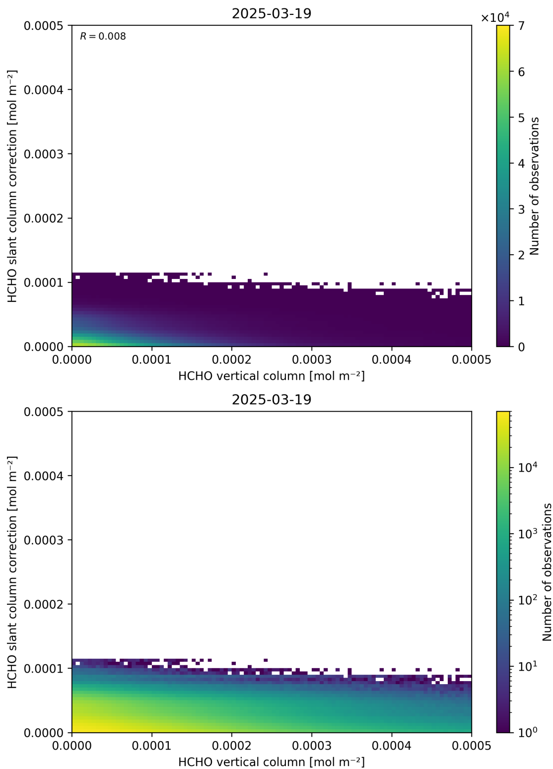
Figure 128: Scatter density plot of “HCHO vertical column” against “HCHO slant column correction” for 2025-03-18 to 2025-03-20.
