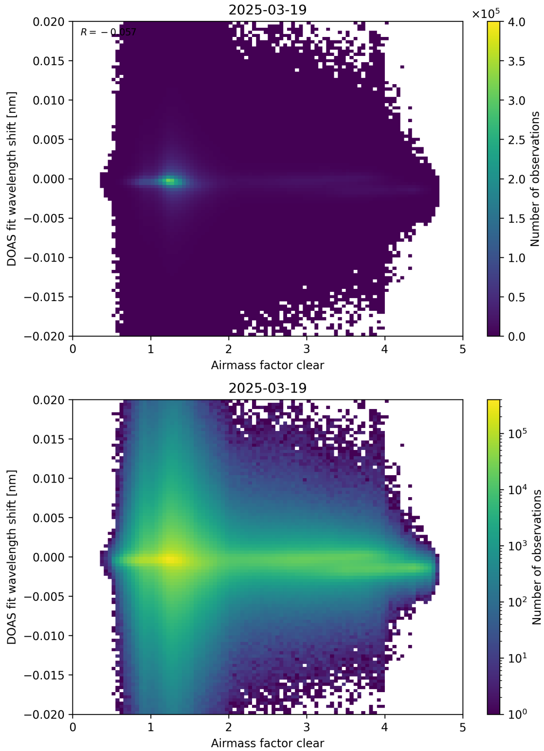
Figure 72: Scatter density plot of “Airmass factor clear” against “DOAS fit wavelength shift” for 2025-03-18 to 2025-03-20.
