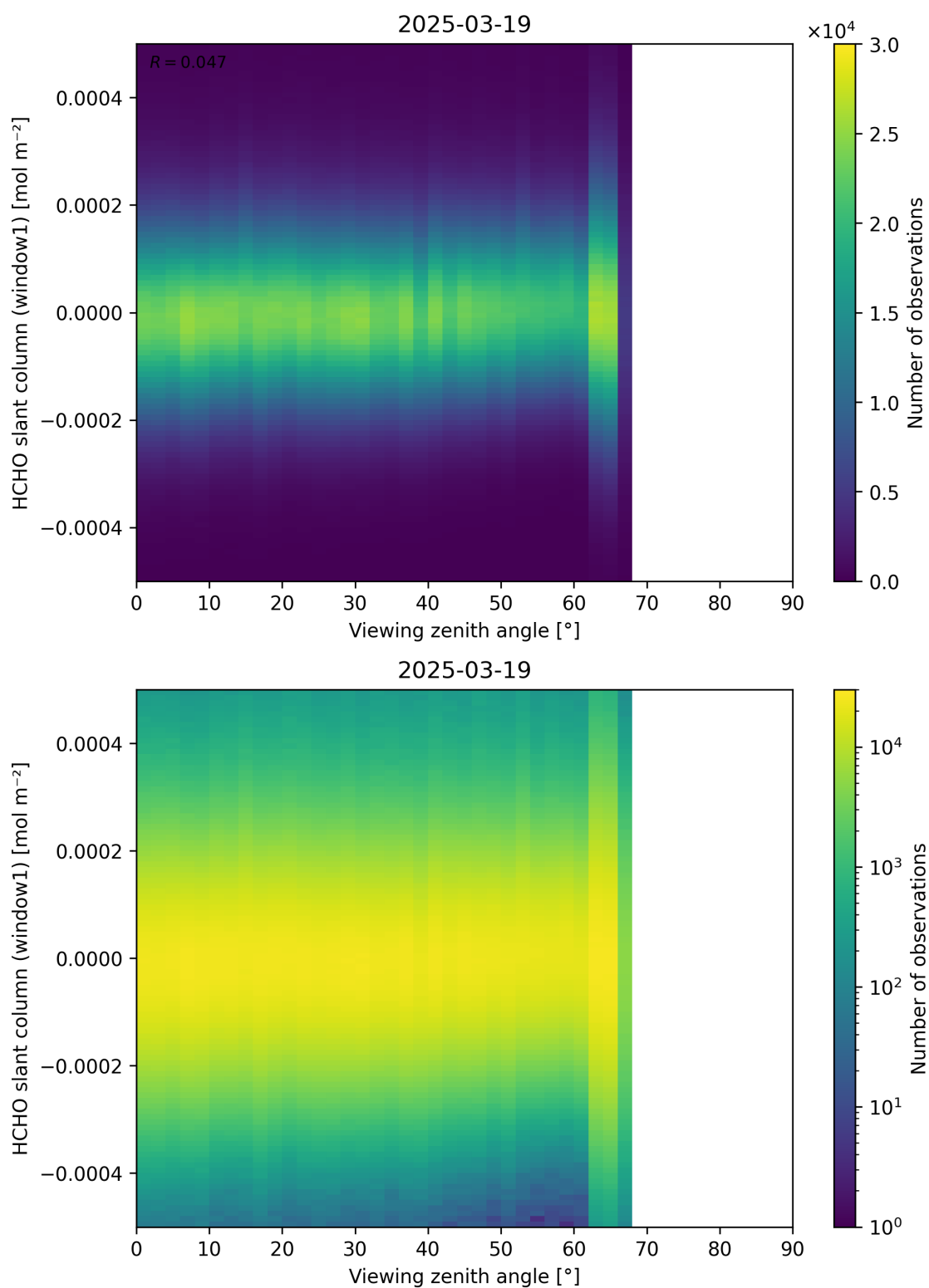
Figure 188: Scatter density plot of “Viewing zenith angle” against “HCHO slant column (window1)” for 2025-03-18 to 2025-03-20.
