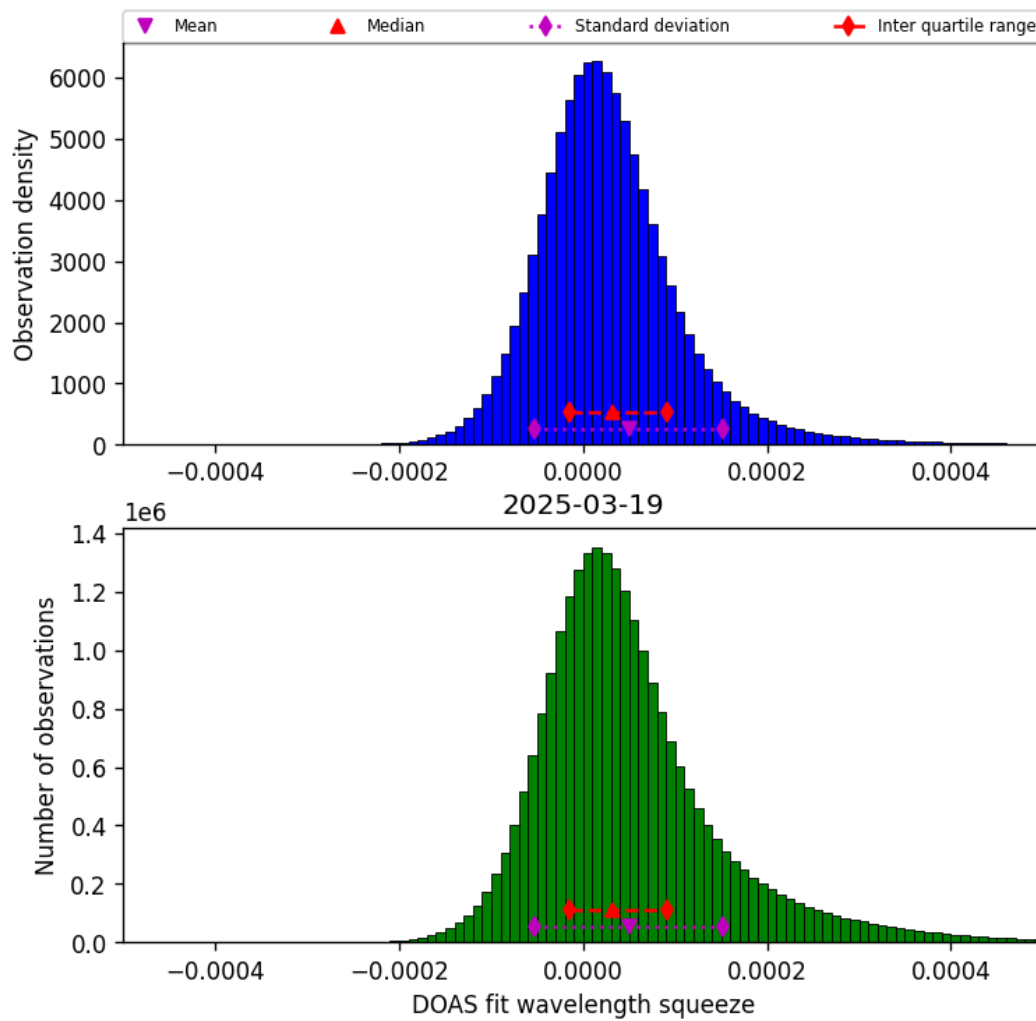
Figure 45: Histogram of “DOAS fit wavelength squeeze” for 2025-03-18 to 2025-03-20
