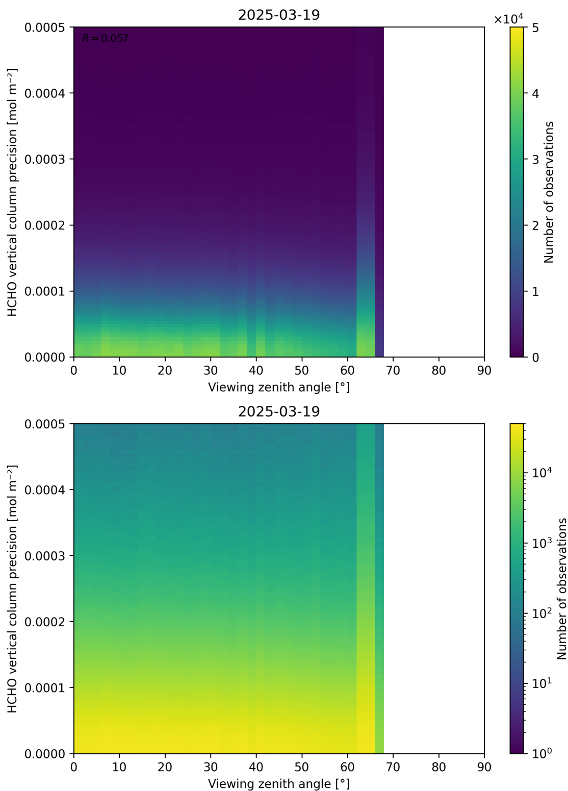
Figure 194: Scatter density plot of “Viewing zenith angle” against “HCHO vertical column precision” for 2025-03-18 to 2025-03-20.
