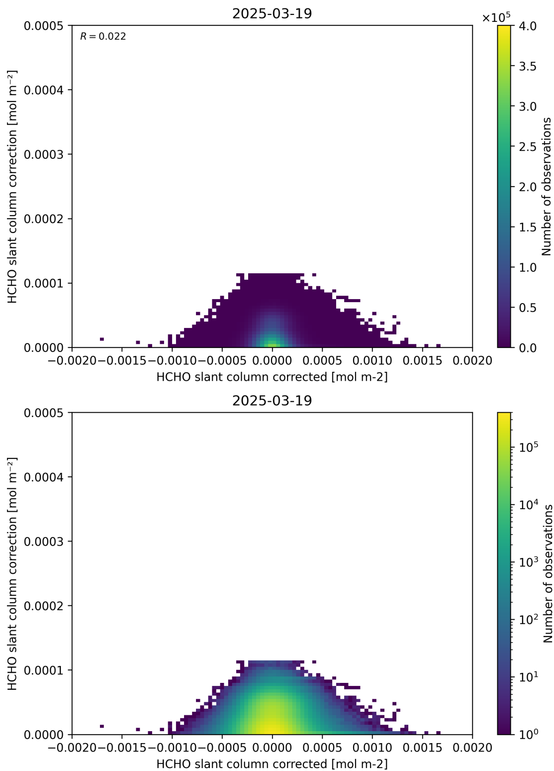
Figure 77: Scatter density plot of “HCHO slant column corrected” against “HCHO slant column correction” for 2025-03-18 to 2025-03-20.
