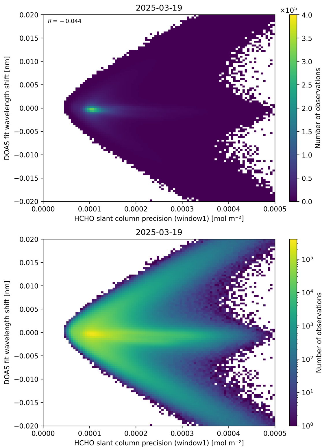
Figure 89: Scatter density plot of “HCHO slant column precision (window1)” against “DOAS fit wavelength shift” for 2025-03-18 to 2025-03-20.
