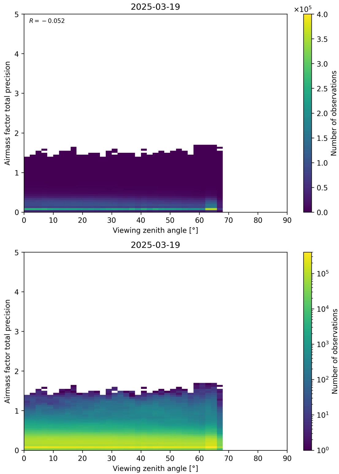
Figure 191: Scatter density plot of “Viewing zenith angle” against “Airmass factor total precision” for 2025-03-18 to 2025-03-20.
