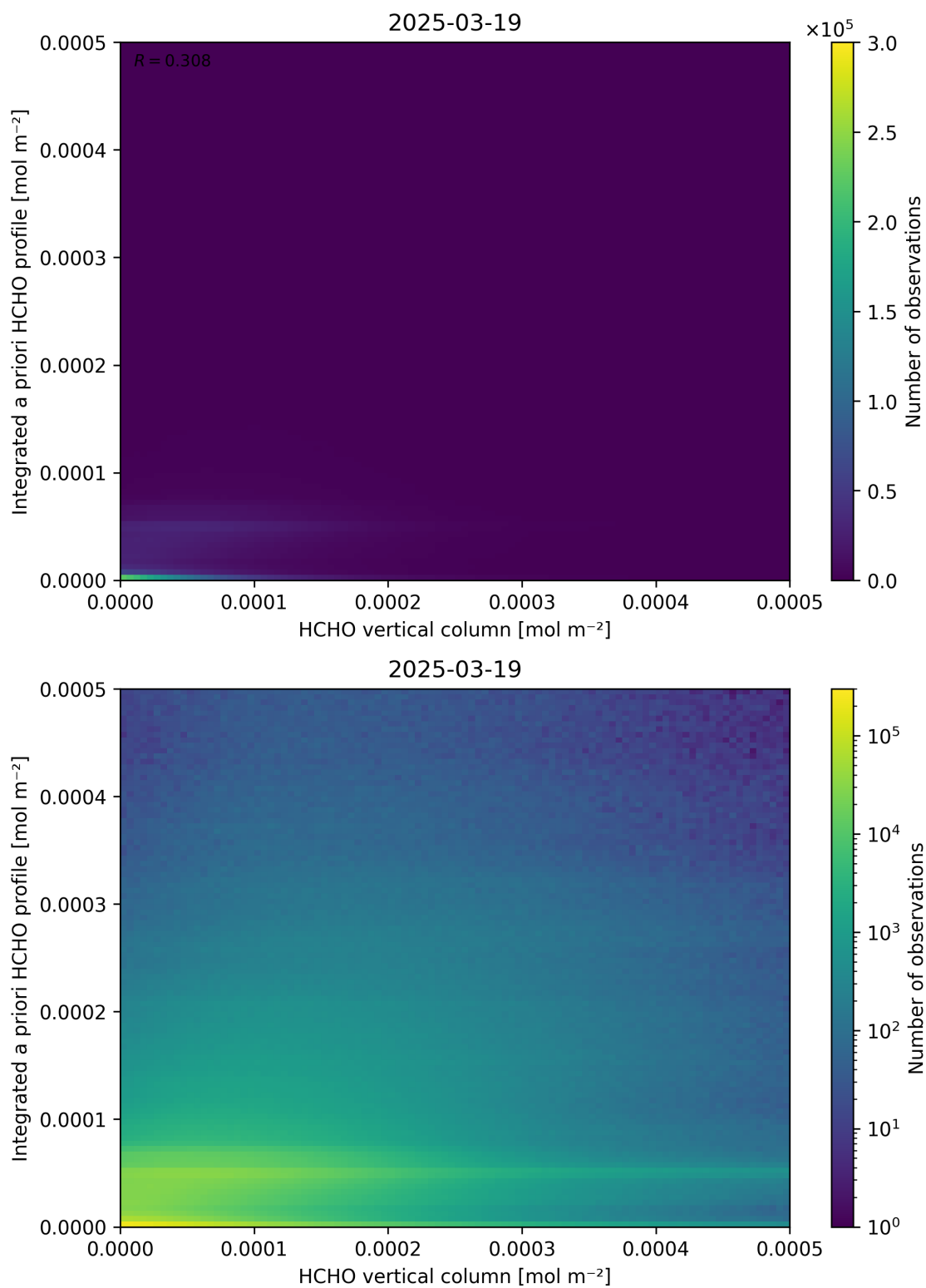
Figure 135: Scatter density plot of “HCHO vertical column” against “Integrated a priori HCHO profile” for 2025-03-18 to 2025-03-20.
