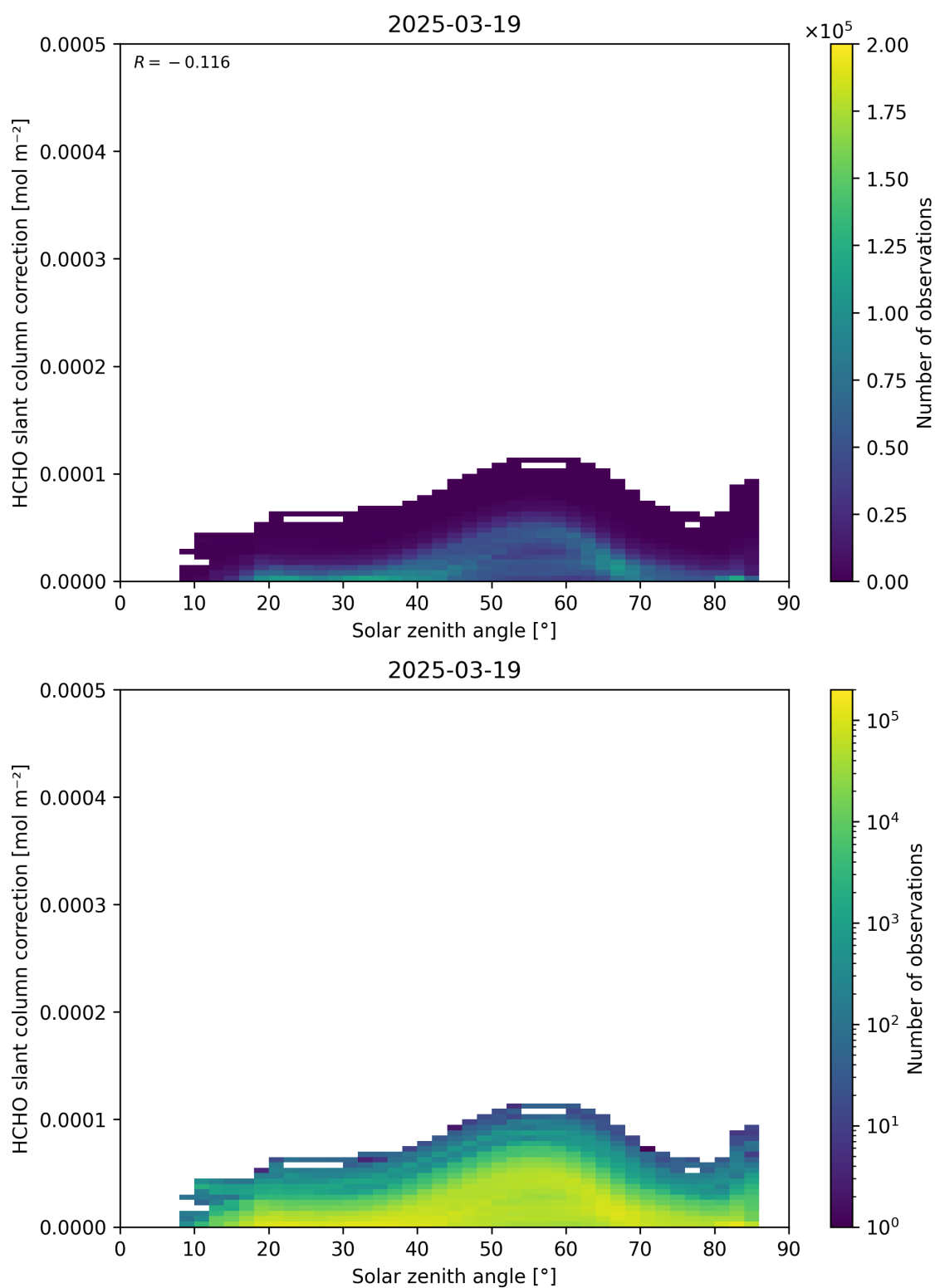
Figure 172: Scatter density plot of “Solar zenith angle” against “HCHO slant column correction” for 2025-03-18 to 2025-03-20.
