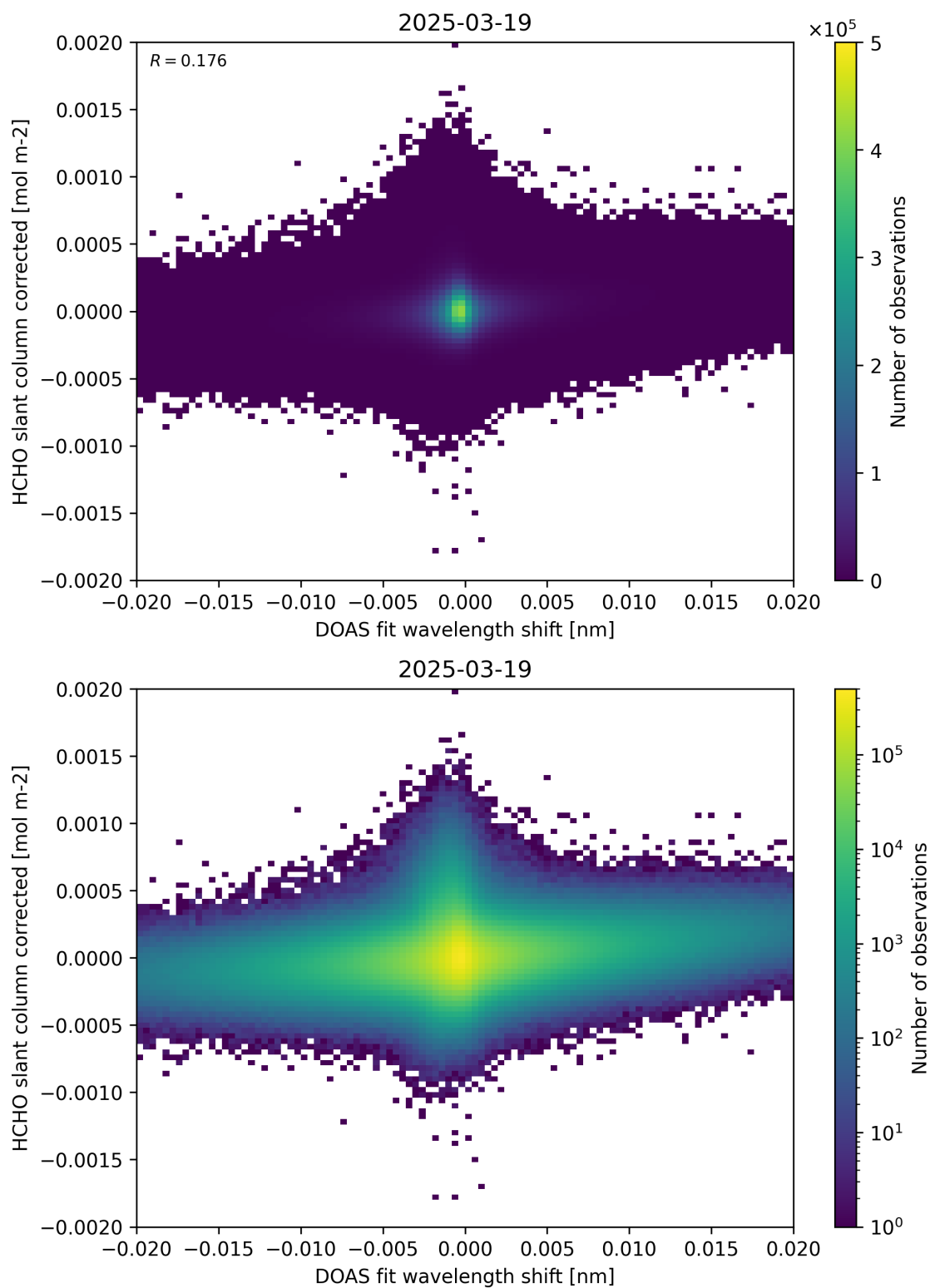
Figure 66: Scatter density plot of “DOAS fit wavelength shift” against “HCHO slant column corrected” for 2025-03-18 to 2025-03-20.
