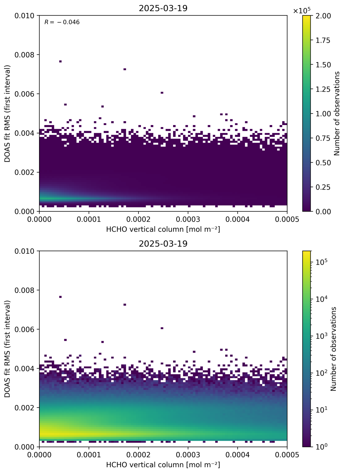
Figure 123: Scatter density plot of “HCHO vertical column” against “DOAS fit RMS (first interval)” for 2025-03-18 to 2025-03-20.
