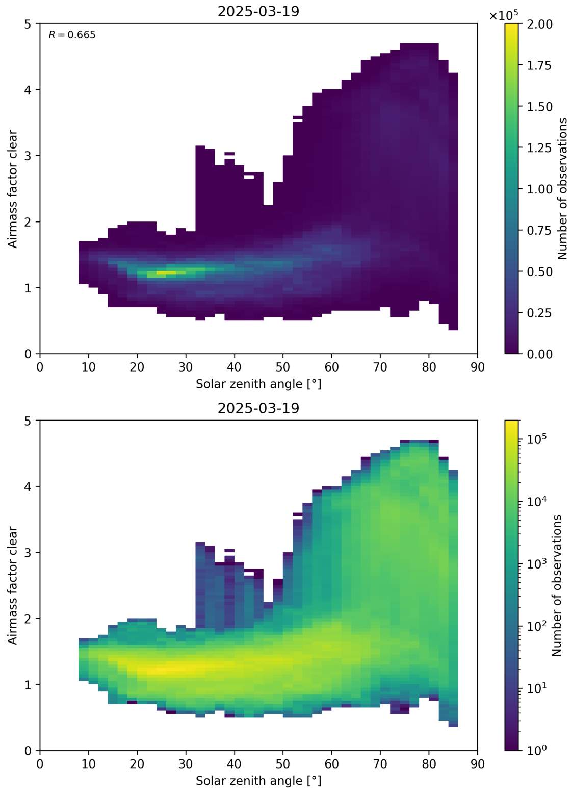
Figure 170: Scatter density plot of “Solar zenith angle” against “Airmass factor clear” for 2025-03-18 to 2025-03-20.
