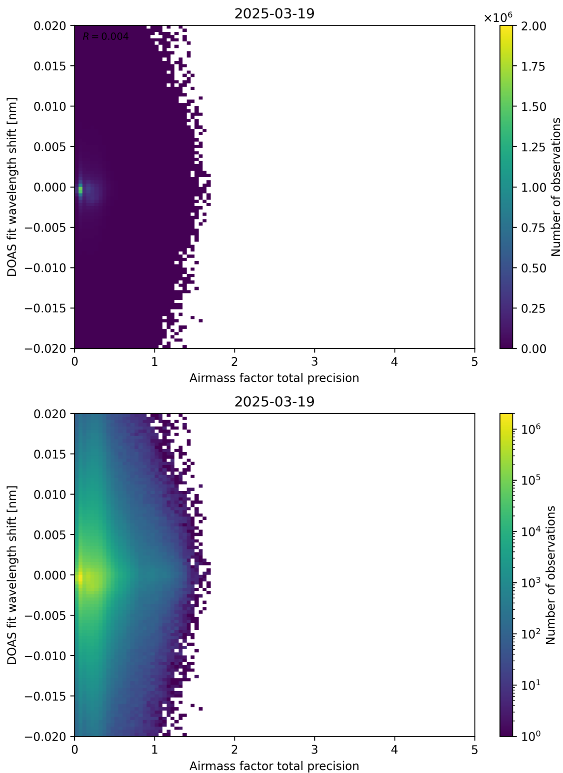
Figure 106: Scatter density plot of “Airmass factor total precision” against “DOAS fit wavelength shift” for 2025-03-18 to 2025-03-20.
