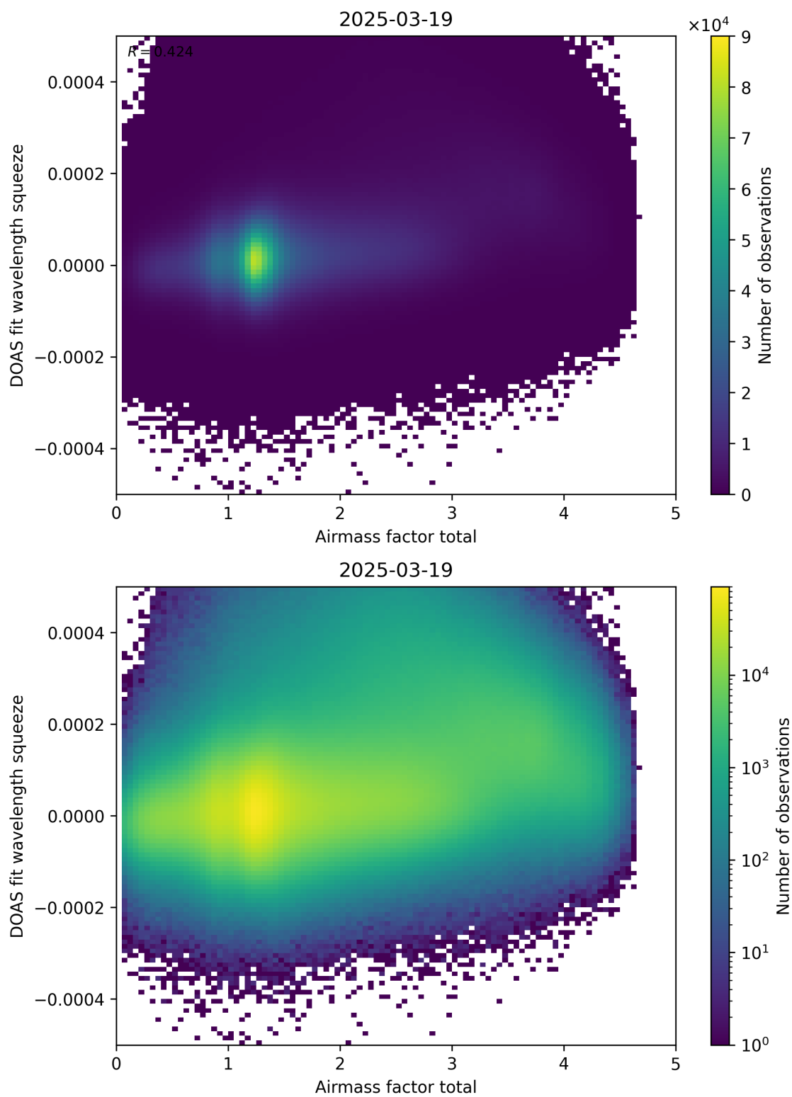
Figure 99: Scatter density plot of “Airmass factor total” against “DOAS fit wavelength squeeze” for 2025-03-18 to 2025-03-20.
