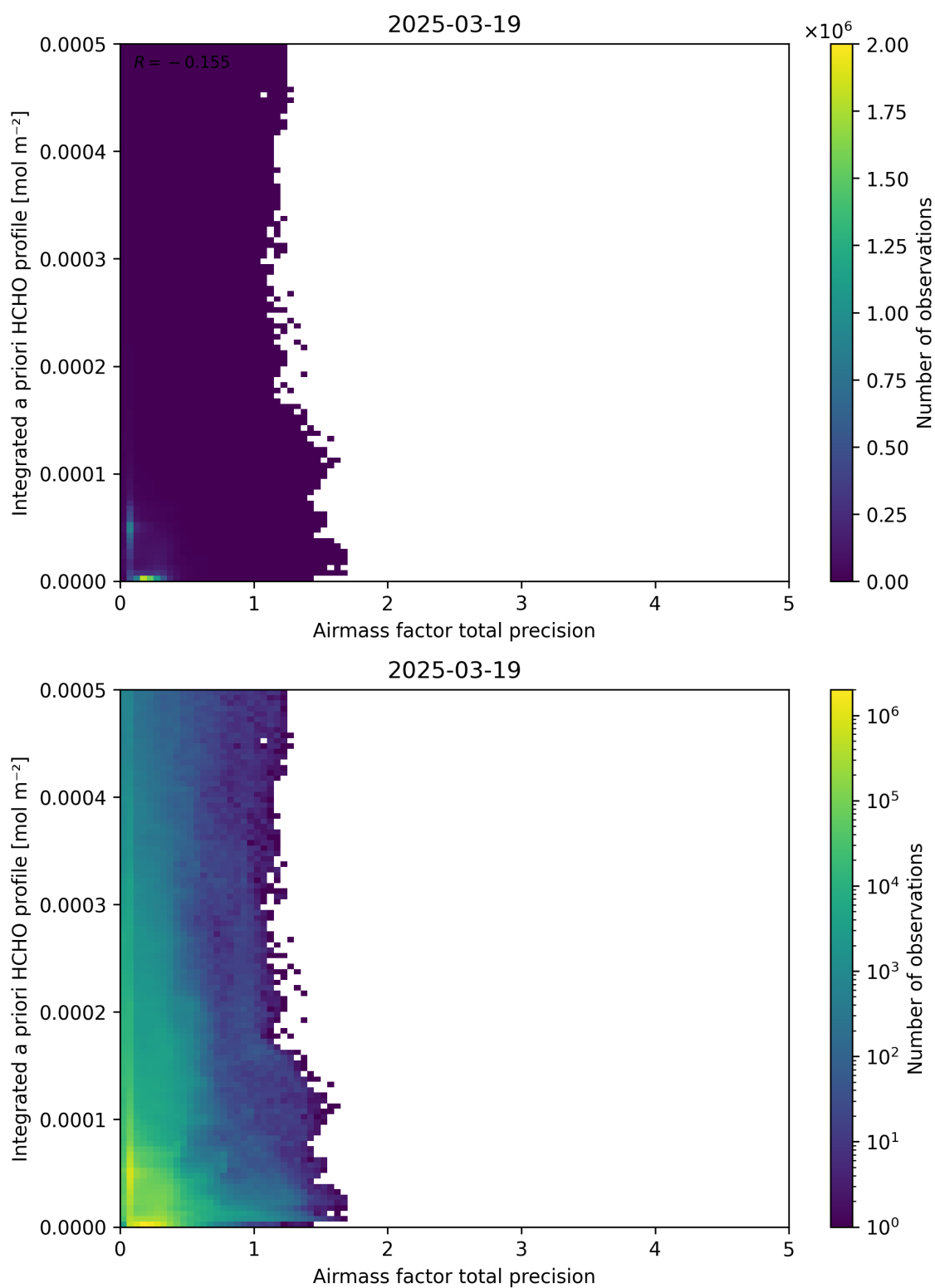
Figure 111: Scatter density plot of “Airmass factor total precision” against “Integrated a priori HCHO profile” for 2025-03-18 to 2025-03-20.
