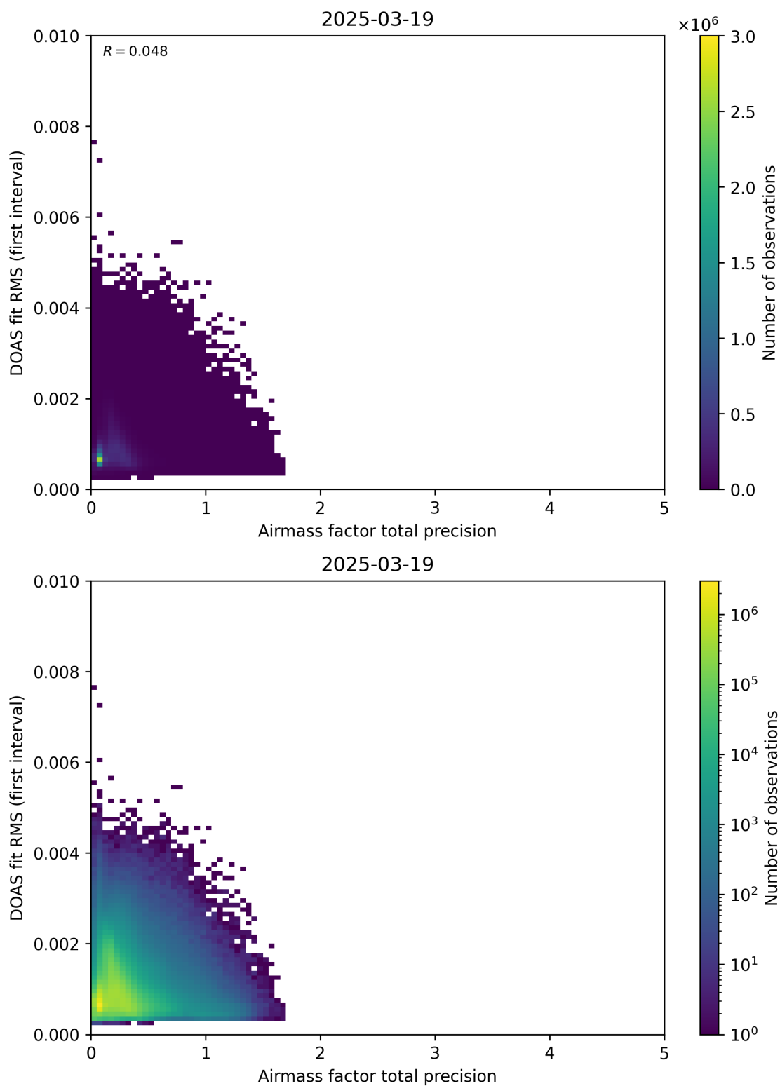
Figure 105: Scatter density plot of “Airmass factor total precision” against “DOAS fit RMS (first interval)” for 2025-03-18 to 2025-03-20.
