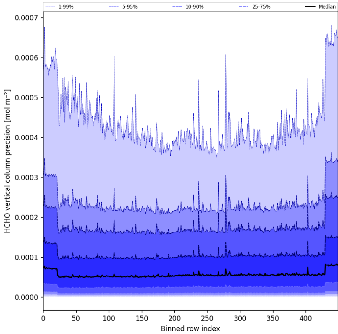
Figure 50: Along track statistics of “HCHO vertical column precision” for 2025-03-18 to 2025-03-20
