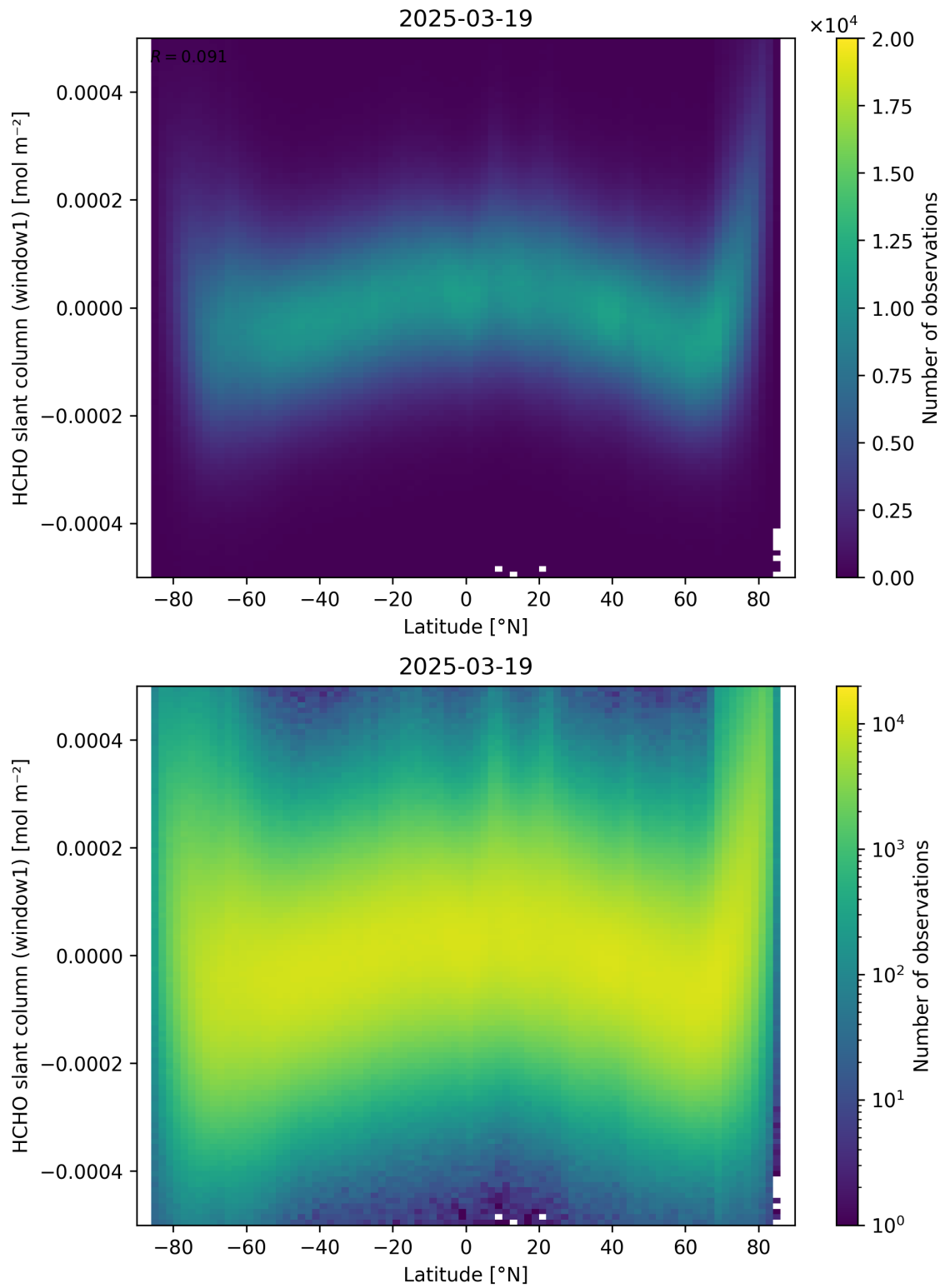
Figure 159: Scatter density plot of “Latitude” against “HCHO slant column (window1)” for 2025-03-18 to 2025-03-20.
