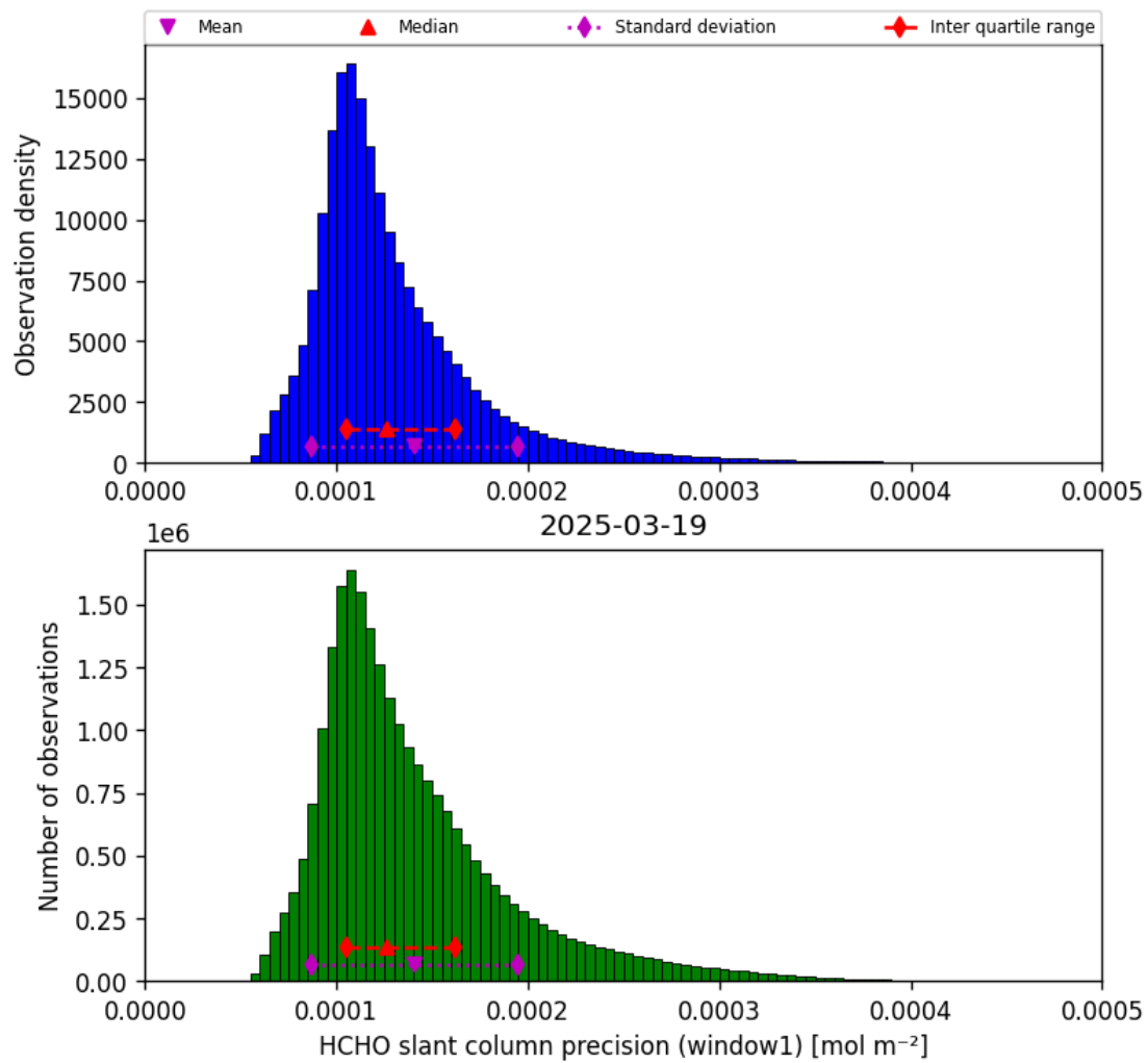
Figure 39: Histogram of “HCHO slant column precision (window1)” for 2025-03-18 to 2025-03-20
