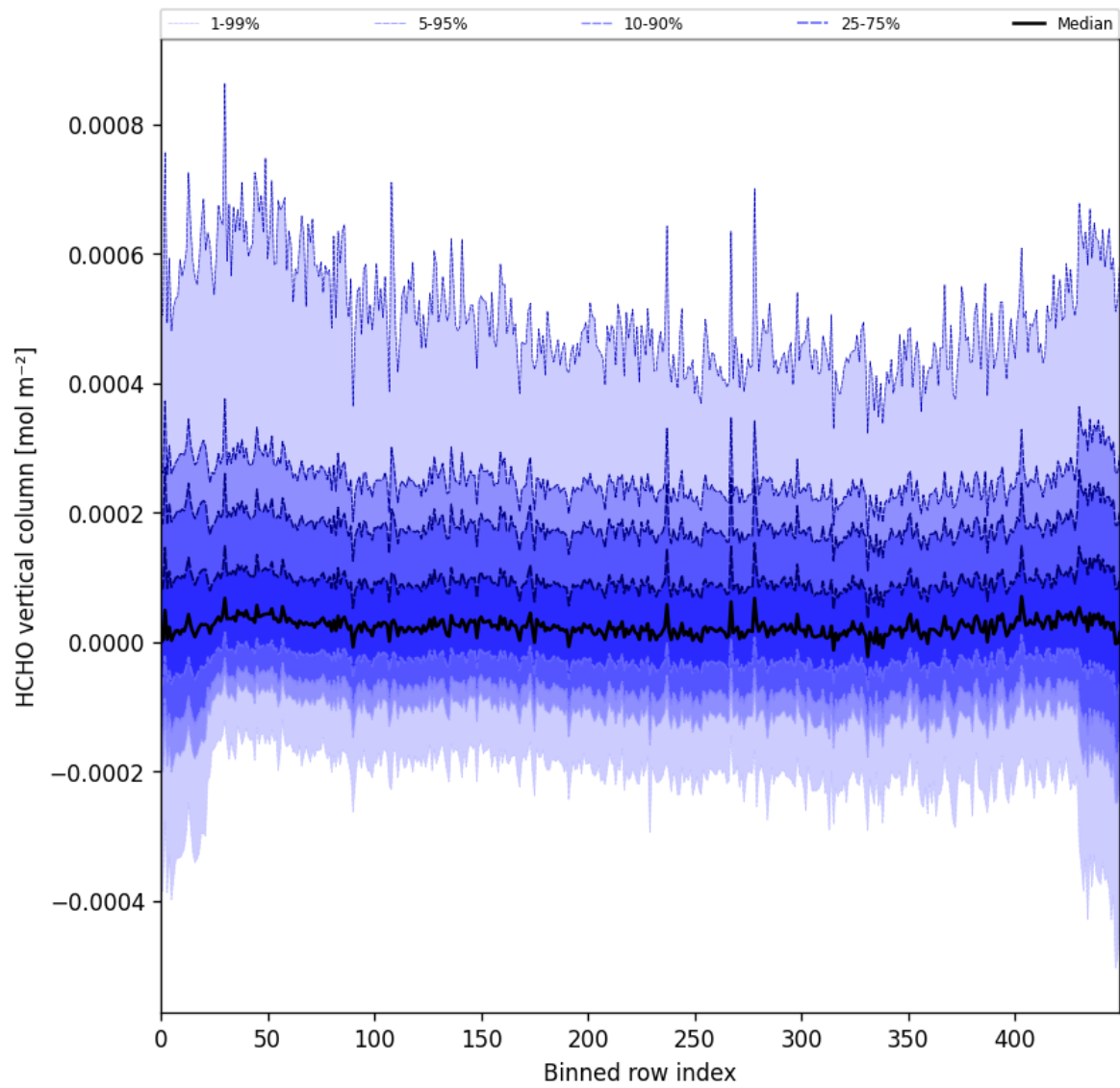
Figure 49: Along track statistics of “HCHO vertical column” for 2025-03-18 to 2025-03-20
