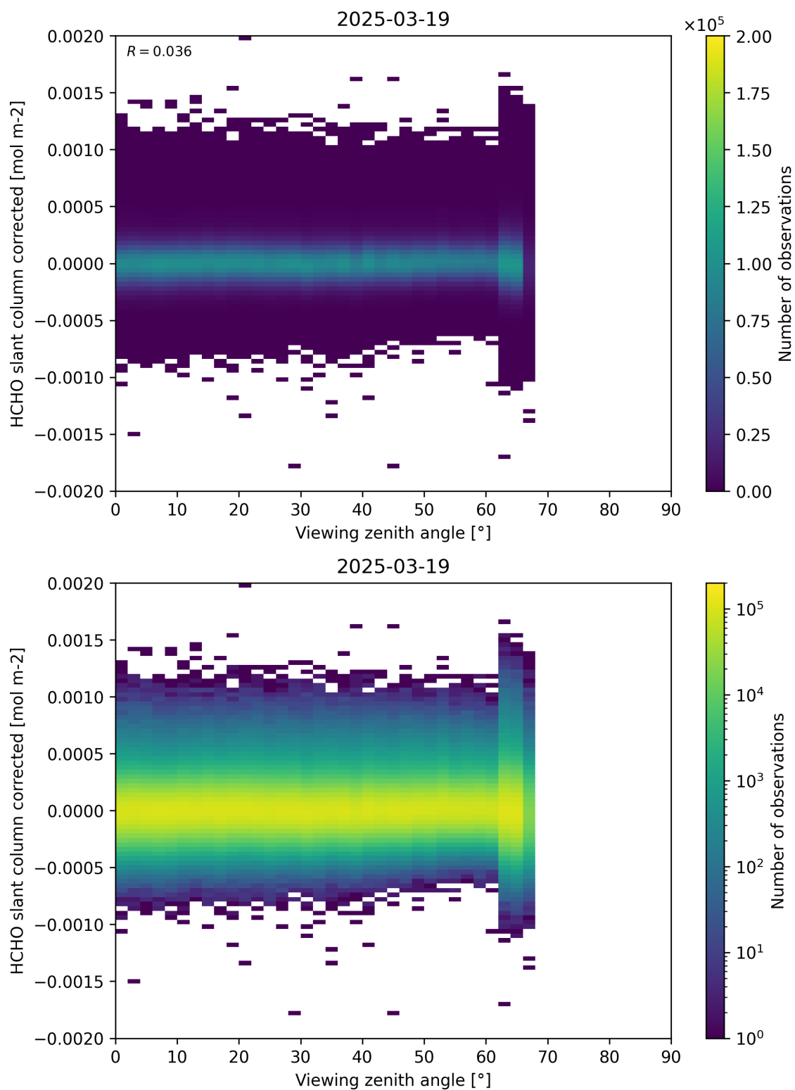
Figure 186: Scatter density plot of “Viewing zenith angle” against “HCHO slant column corrected” for 2025-03-18 to 2025-03-20.
