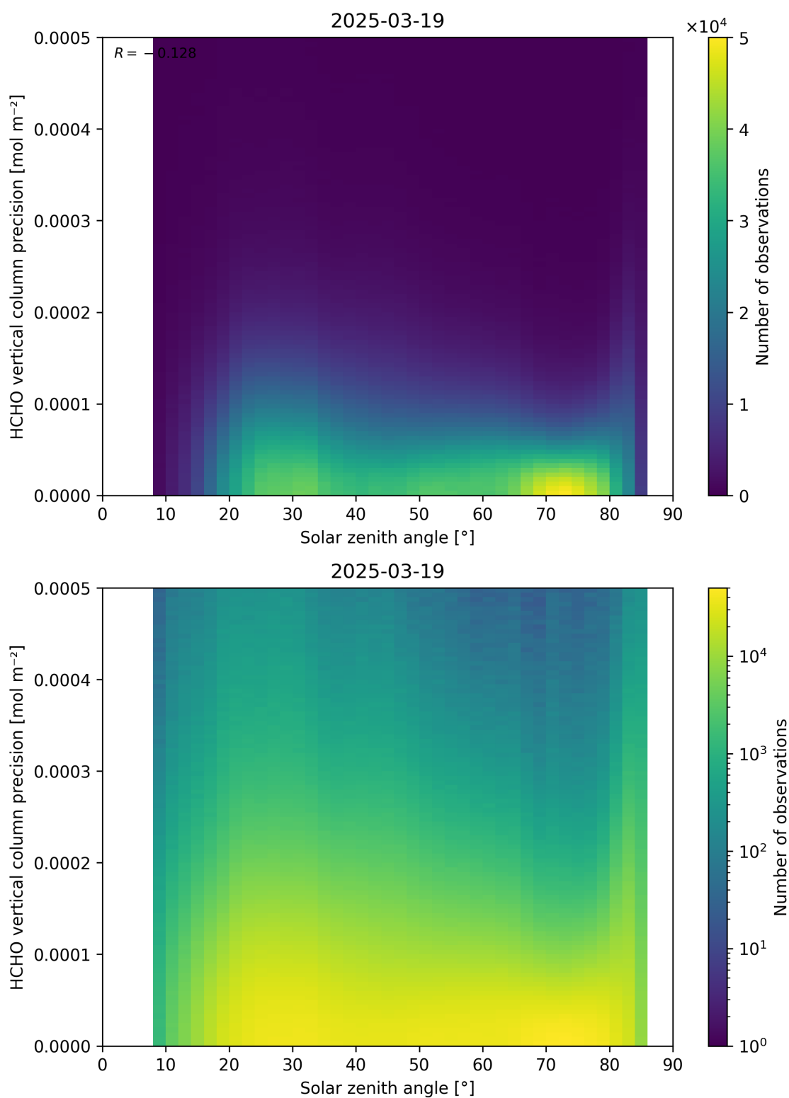
Figure 179: Scatter density plot of “Solar zenith angle” against “HCHO vertical column precision” for 2025-03-18 to 2025-03-20.
