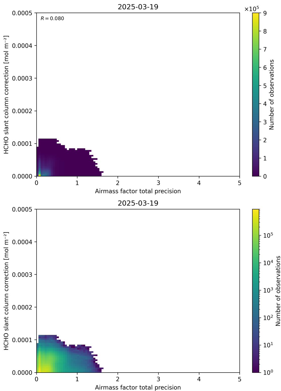
Figure 110: Scatter density plot of “Airmass factor total precision” against “HCHO slant column correction” for 2025-03-18 to 2025-03-20.
