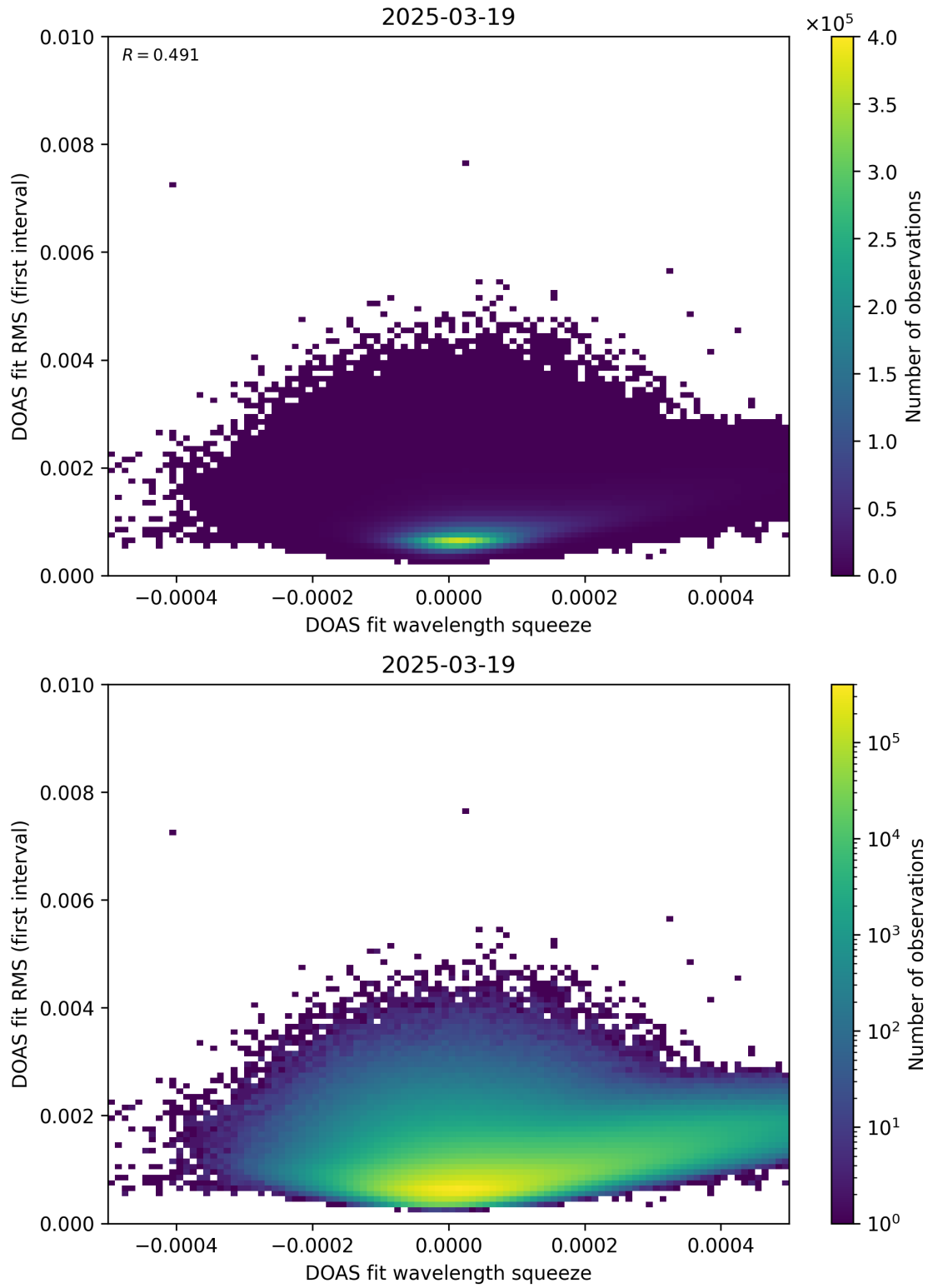
Figure 68: Scatter density plot of “DOAS fit wavelength squeeze” against “DOAS fit RMS (first interval)” for 2025-03-18 to 2025-03-20.
