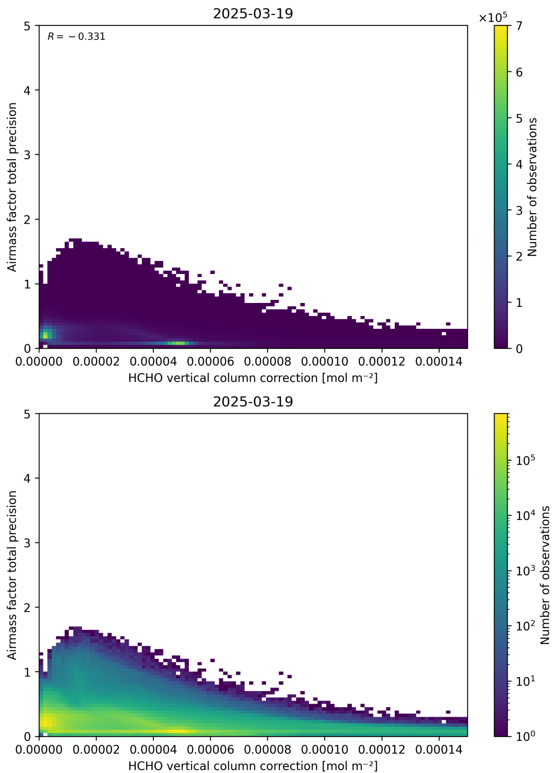
Figure 121: Scatter density plot of “HCHO vertical column correction” against “Airmass factor total precision” for 2025-03-18 to 2025-03-20.
