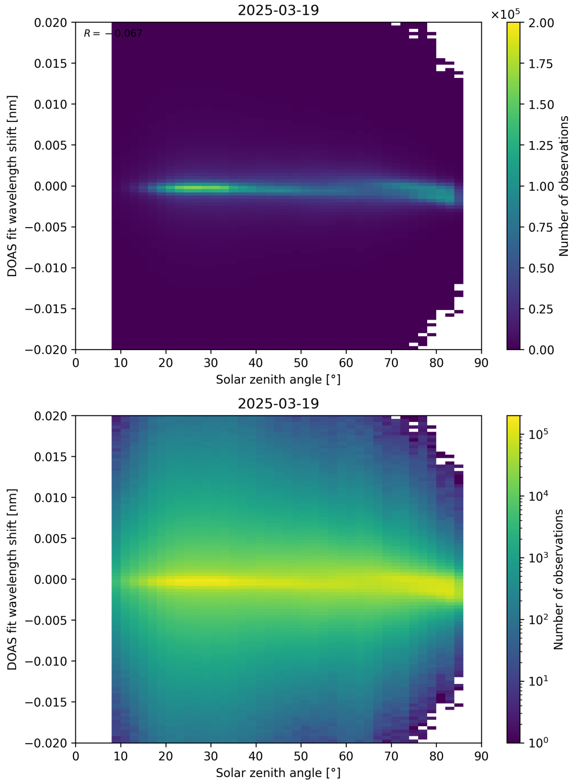
Figure 168: Scatter density plot of “Solar zenith angle” against “DOAS fit wavelength shift” for 2025-03-18 to 2025-03-20.
