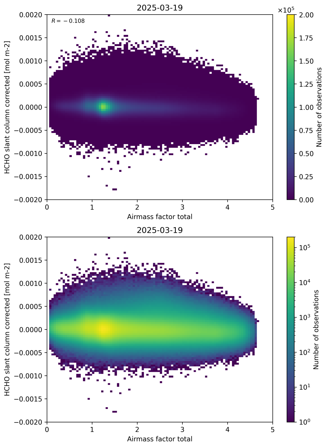
Figure 101: Scatter density plot of “Airmass factor total” against “HCHO slant column corrected” for 2025-03-18 to 2025-03-20.
