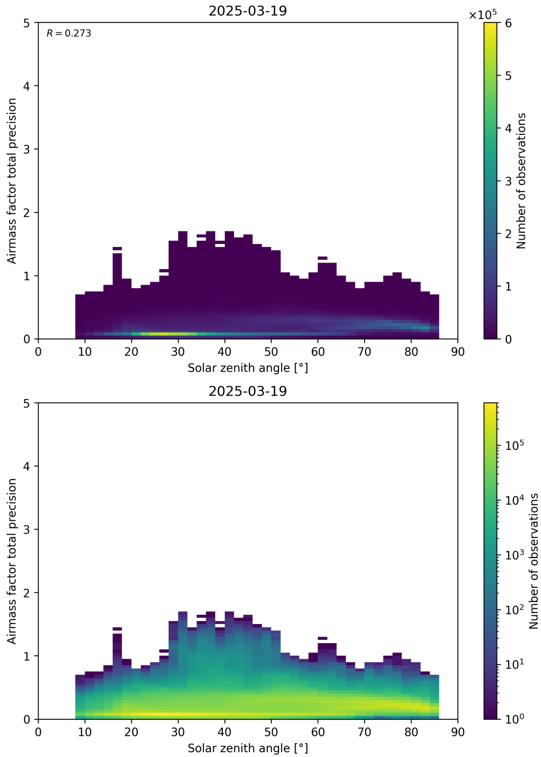
Figure 176: Scatter density plot of “Solar zenith angle” against “Airmass factor total precision” for 2025-03-18 to 2025-03-20.
