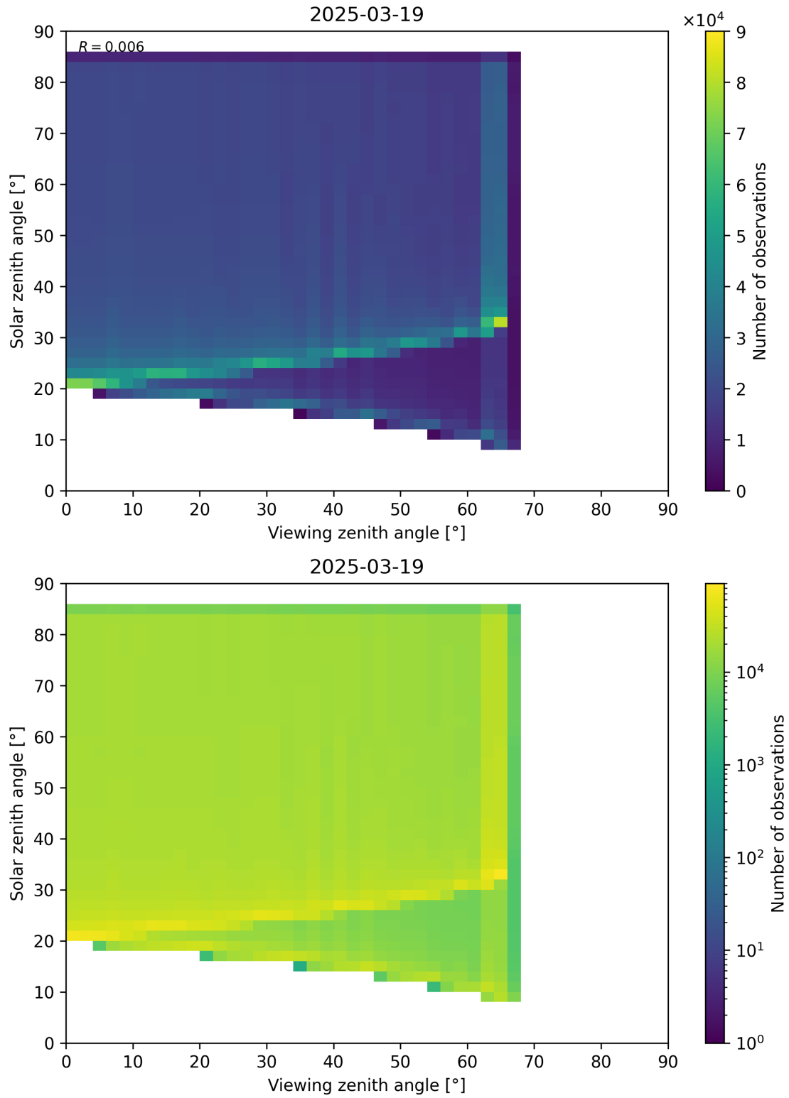
Figure 197: Scatter density plot of “Viewing zenith angle” against “Solar zenith angle” for 2025-03-18 to 2025-03-20.
