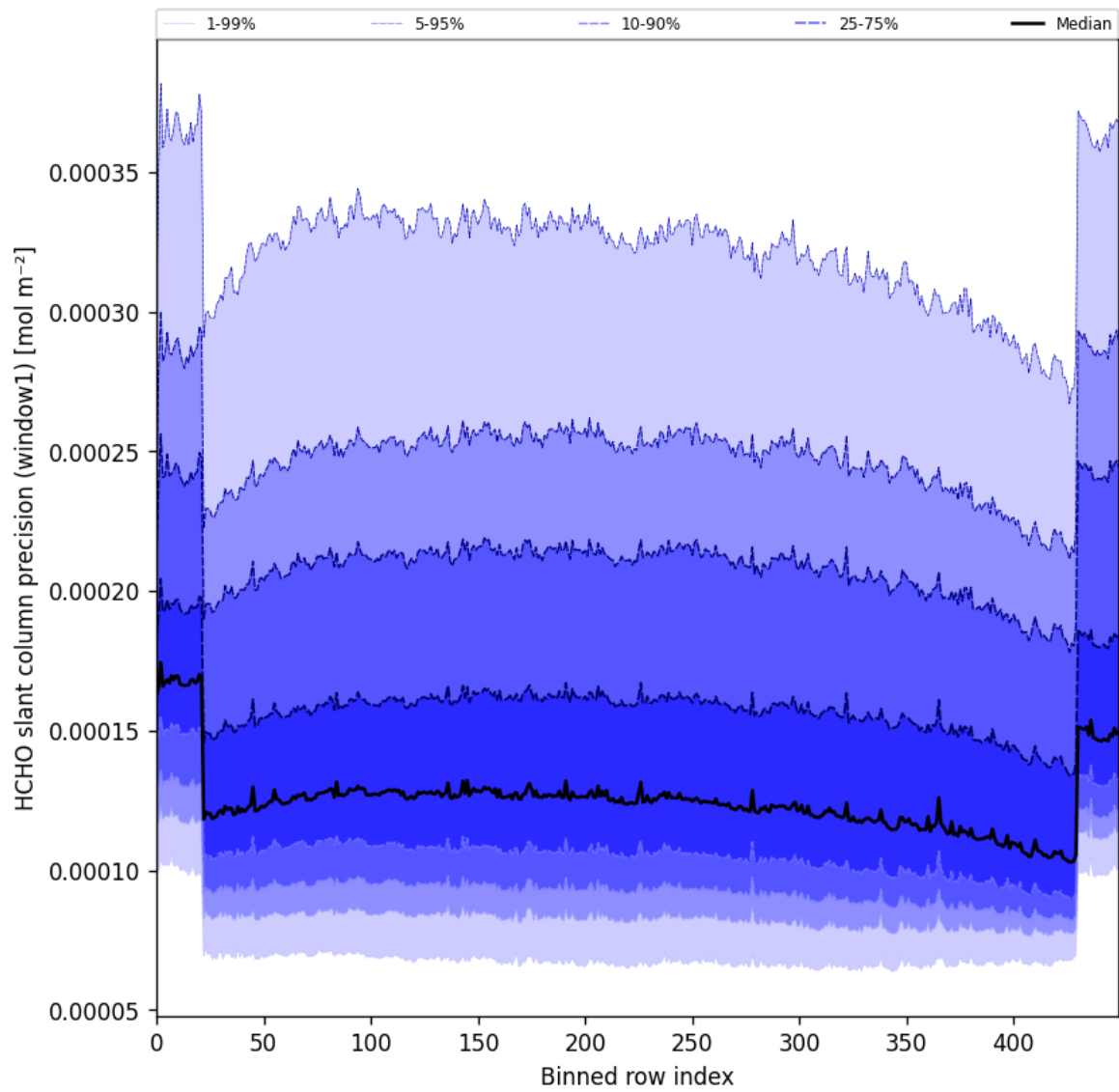
Figure 53: Along track statistics of “HCHO slant column precision (window1)” for 2025-03-18 to 2025-03-20
