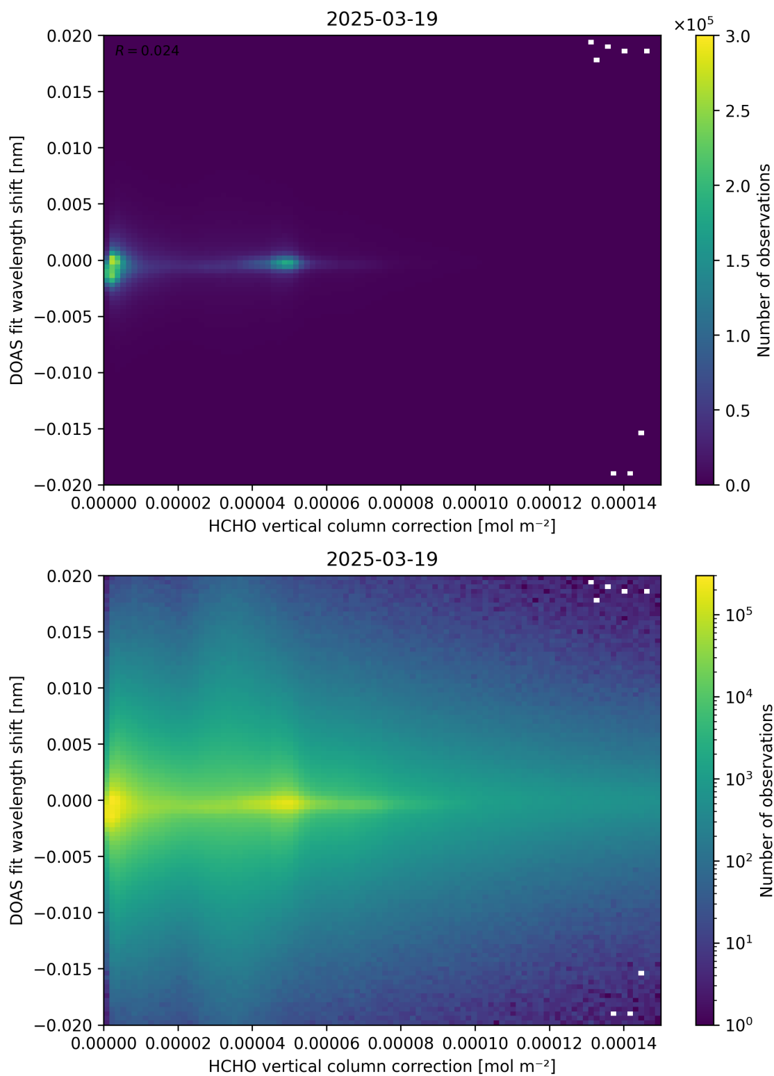
Figure 113: Scatter density plot of “HCHO vertical column correction” against “DOAS fit wavelength shift” for 2025-03-18 to 2025-03-20.
