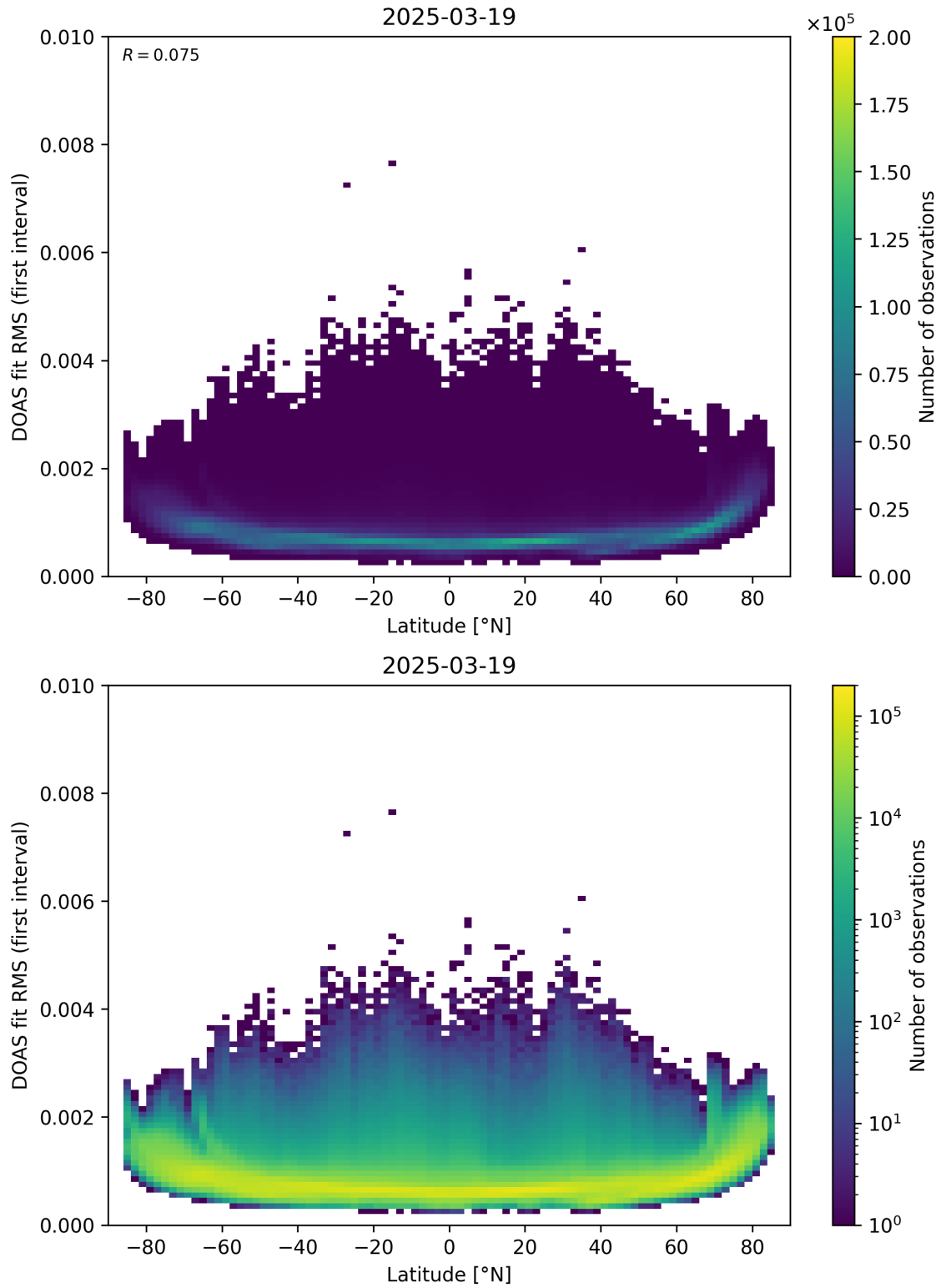
Figure 153: Scatter density plot of “Latitude” against “DOAS fit RMS (first interval)” for 2025-03-18 to 2025-03-20.
