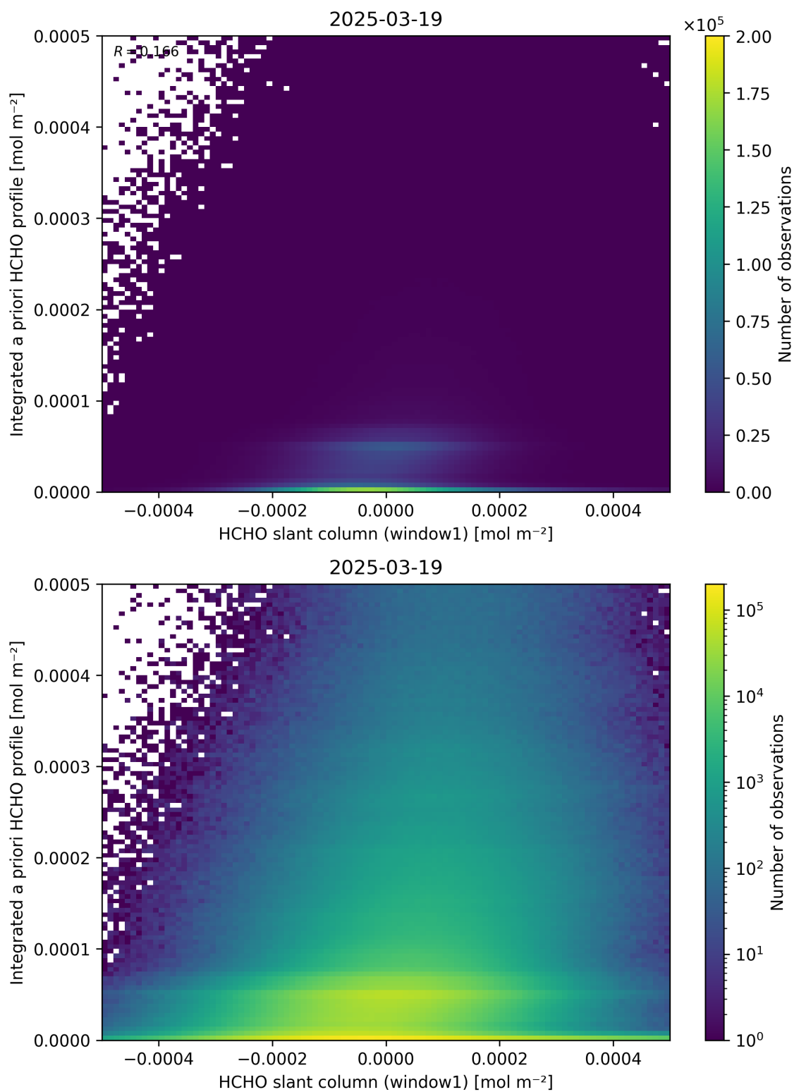
Figure 87: Scatter density plot of “HCHO slant column (window1)” against “Integrated a priori HCHO profile” for 2025-03-18 to 2025-03-20.
