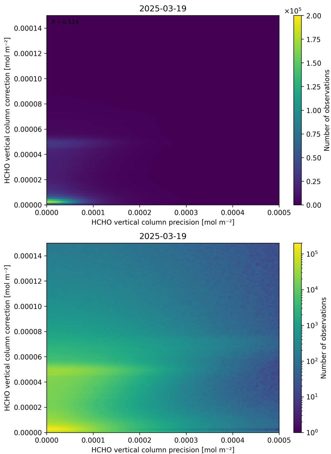
Figure 146: Scatter density plot of “HCHO vertical column precision” against “HCHO vertical column correction” for 2025-03-18 to 2025-03-20.
