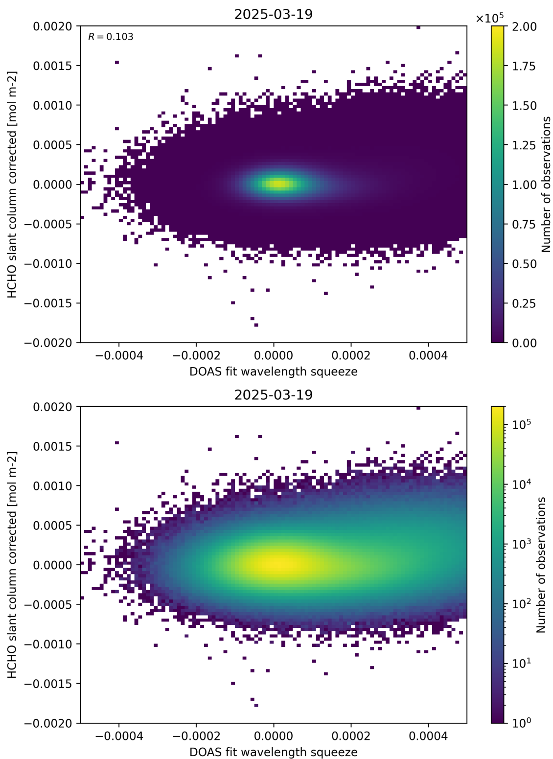
Figure 69: Scatter density plot of “DOAS fit wavelength squeeze” against “HCHO slant column corrected” for 2025-03-18 to 2025-03-20.
