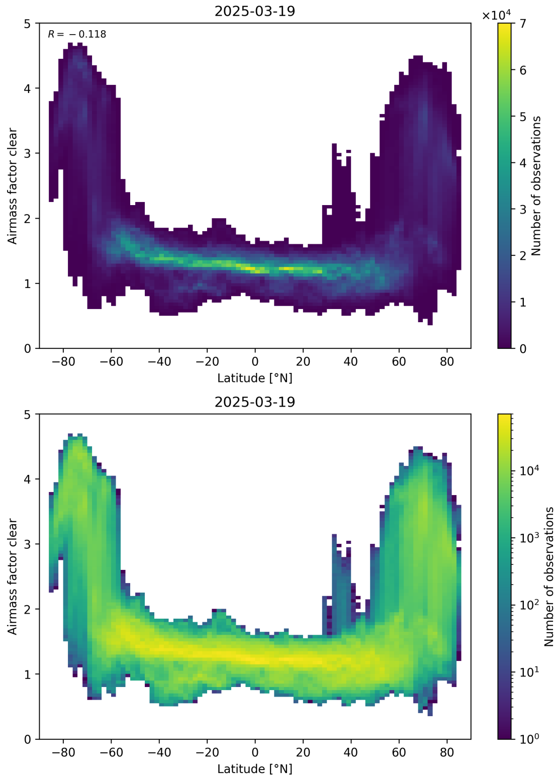
Figure 156: Scatter density plot of “Latitude” against “Airmass factor clear” for 2025-03-18 to 2025-03-20.
