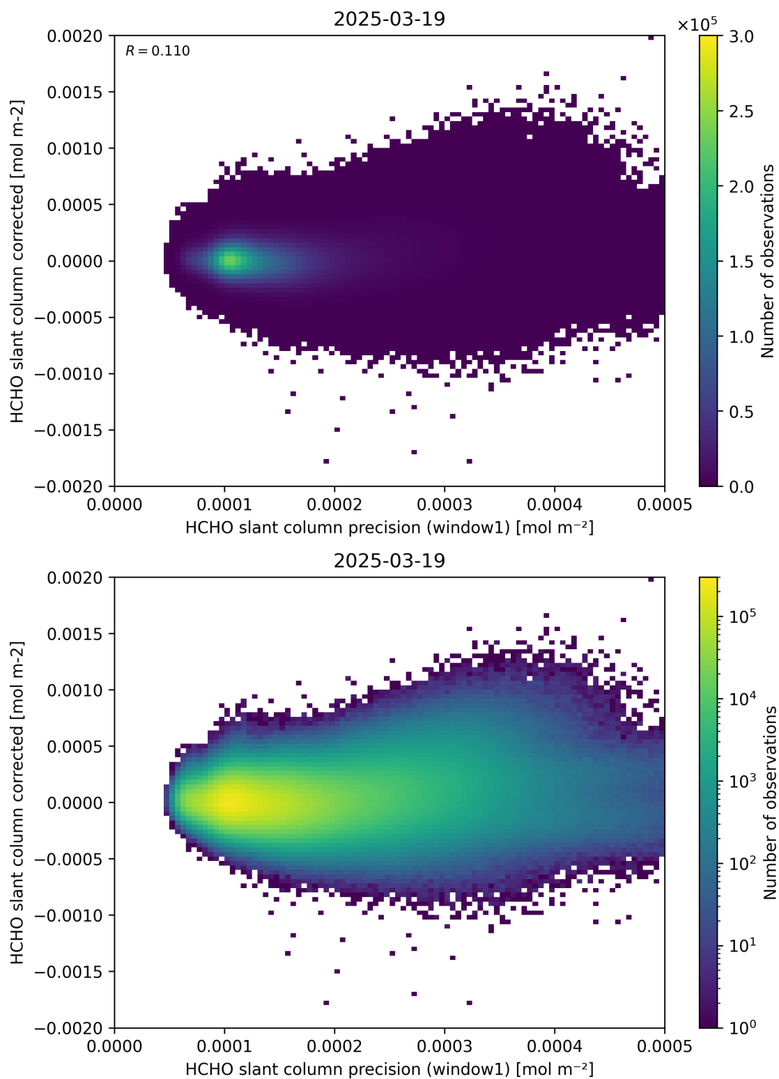
Figure 92: Scatter density plot of “HCHO slant column precision (window1)” against “HCHO slant column corrected” for 2025-03-18 to 2025-03-20.
