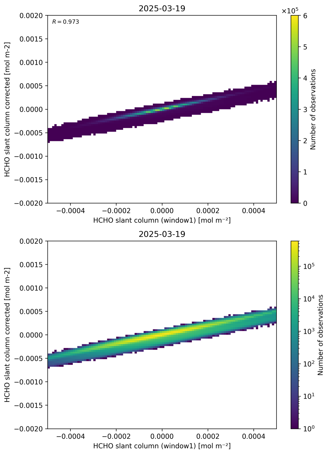
Figure 82: Scatter density plot of “HCHO slant column (window1)” against “HCHO slant column corrected” for 2025-03-18 to 2025-03-20.
