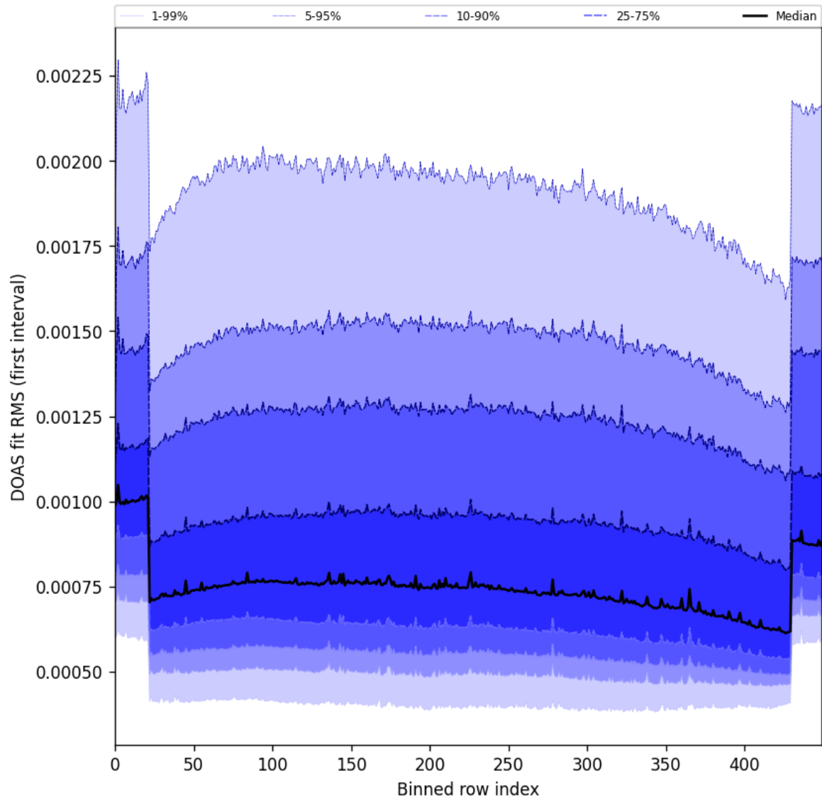
Figure 60: Along track statistics of “DOAS fit RMS (first interval)” for 2025-03-18 to 2025-03-20
