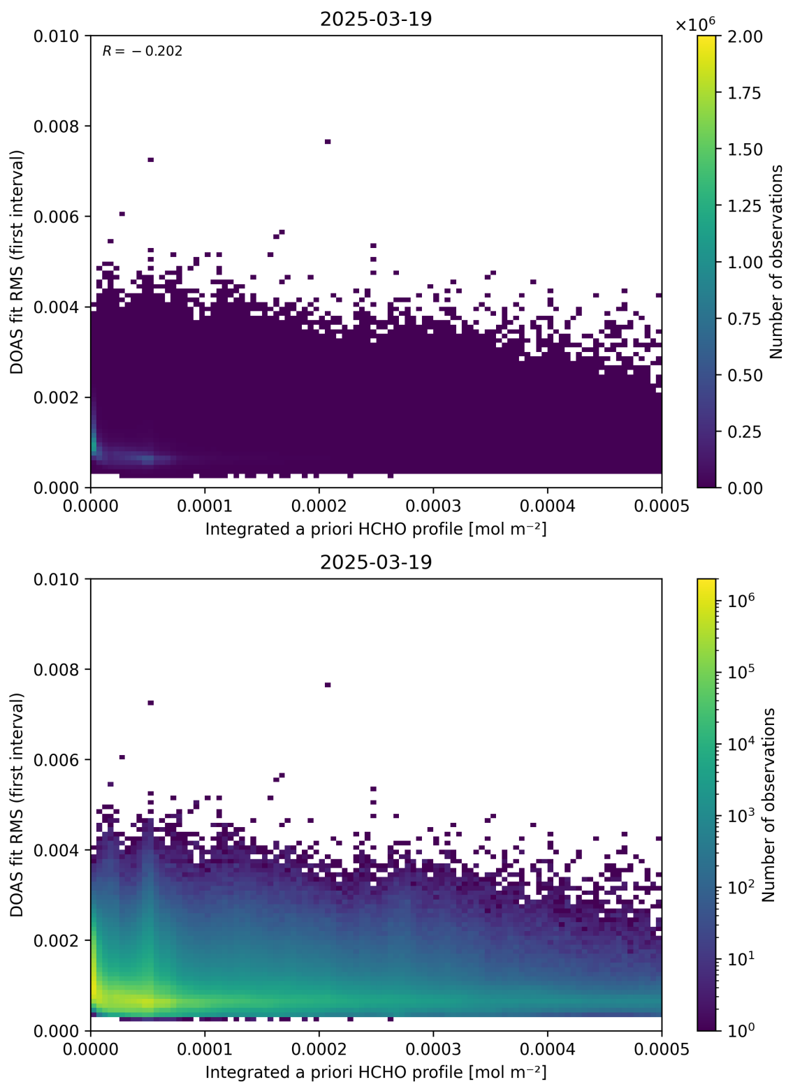
Figure 148: Scatter density plot of “Integrated a priori HCHO profile” against “DOAS fit RMS (first interval)” for 2025-03-18 to 2025-03-20.
