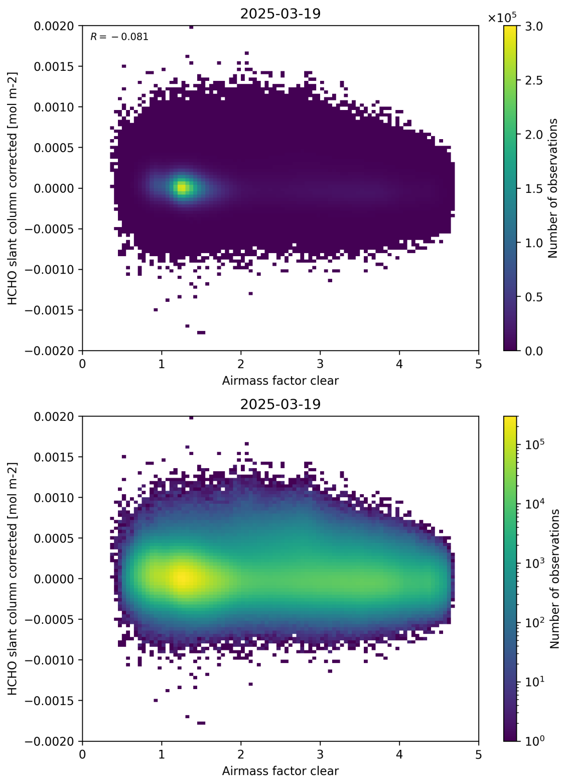
Figure 74: Scatter density plot of “Airmass factor clear” against “HCHO slant column corrected” for 2025-03-18 to 2025-03-20.
