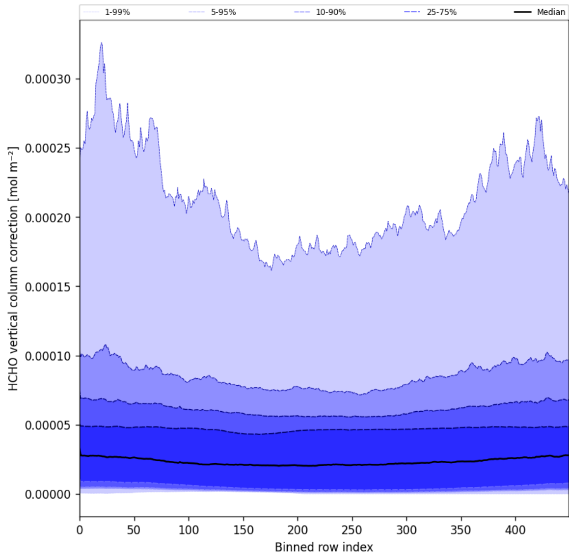
Figure 51: Along track statistics of “HCHO vertical column correction” for 2025-03-18 to 2025-03-20
