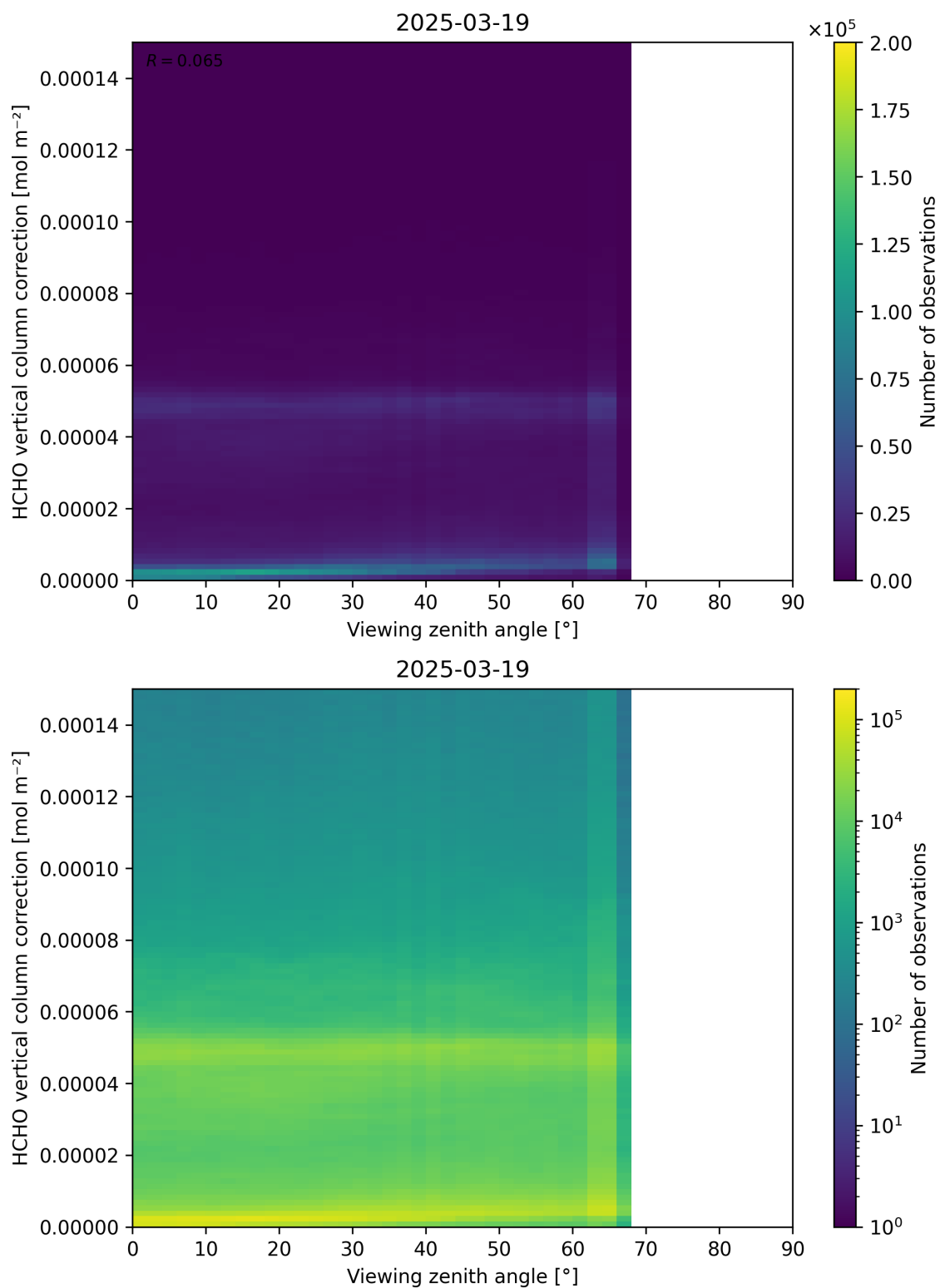
Figure 193: Scatter density plot of “Viewing zenith angle” against “HCHO vertical column correction” for 2025-03-18 to 2025-03-20.
