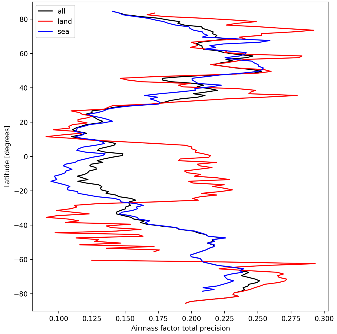
Figure 27: Zonal average of “Airmass factor total precision” for 2025-03-18 to 2025-03-20.
