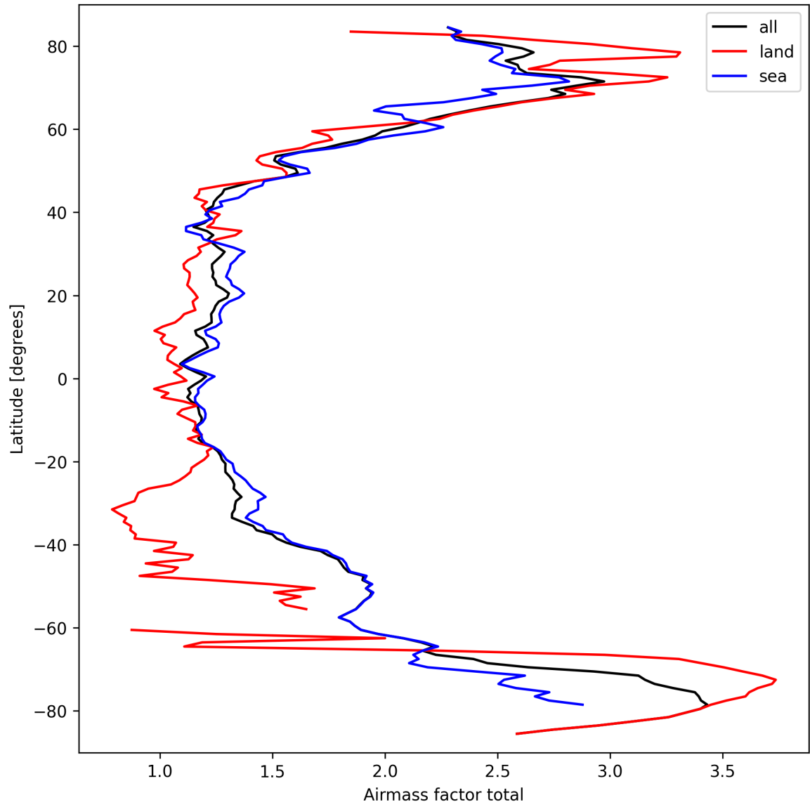
Figure 26: Zonal average of “Airmass factor total” for 2025-03-18 to 2025-03-20.
