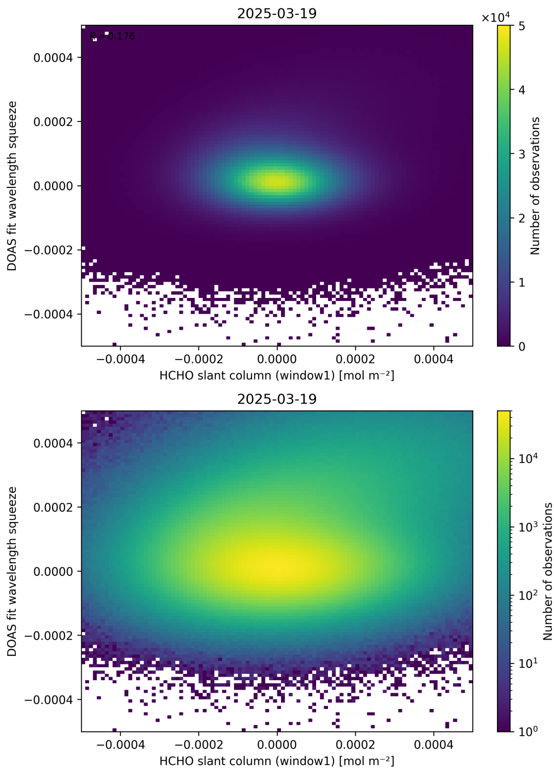
Figure 80: Scatter density plot of “HCHO slant column (window1)” against “DOAS fit wavelength squeeze” for 2025-03-18 to 2025-03-20.
