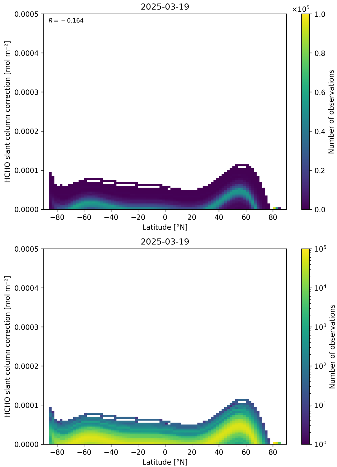
Figure 158: Scatter density plot of “Latitude” against “HCHO slant column correction” for 2025-03-18 to 2025-03-20.
