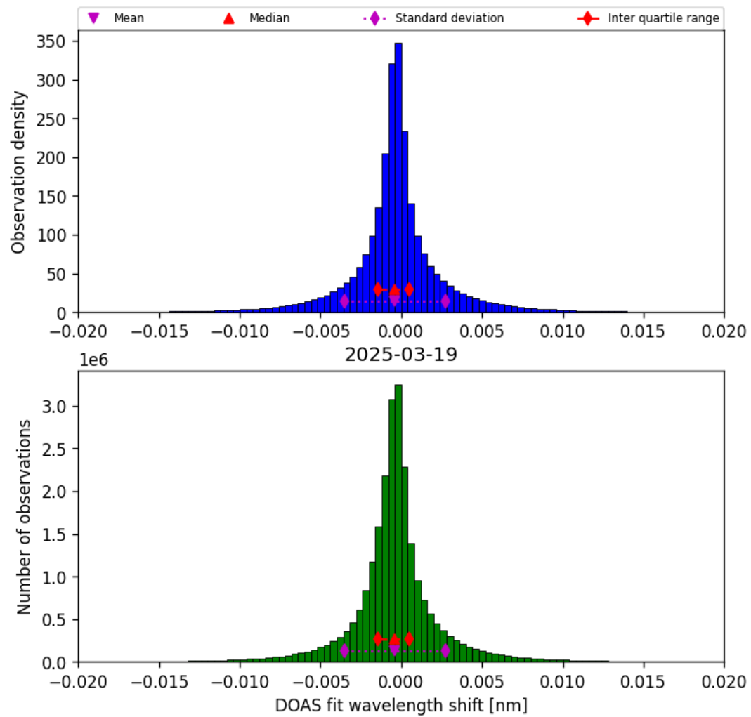
Figure 44: Histogram of “DOAS fit wavelength shift” for 2025-03-18 to 2025-03-20
