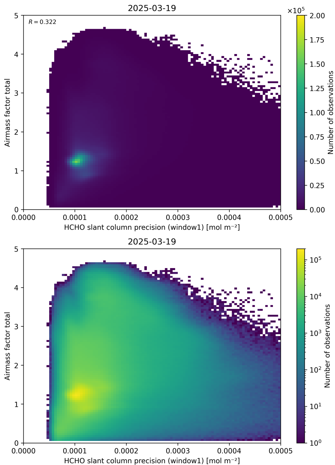
Figure 94: Scatter density plot of “HCHO slant column precision (window1)” against “Airmass factor total” for 2025-03-18 to 2025-03-20.
