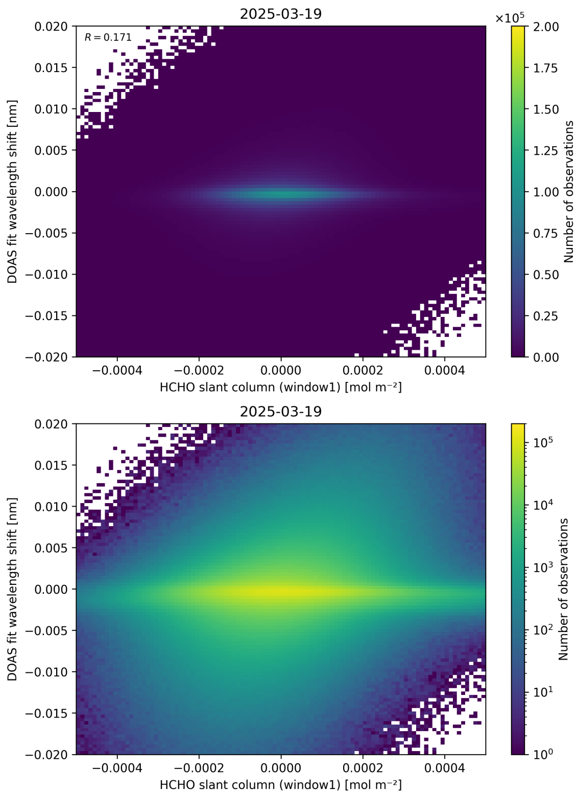
Figure 79: Scatter density plot of “HCHO slant column (window1)” against “DOAS fit wavelength shift” for 2025-03-18 to 2025-03-20.
