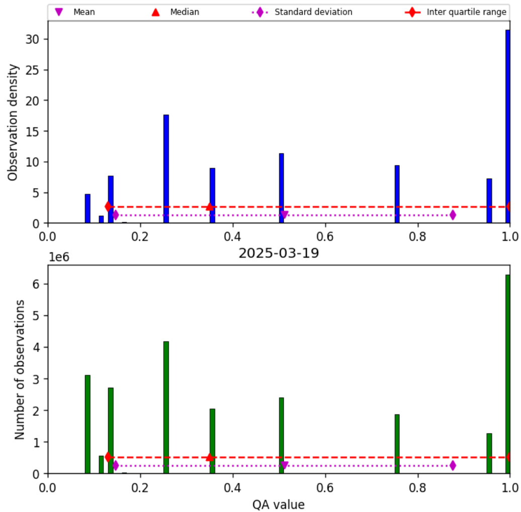
Figure 34: Histogram of “QA value” for 2025-03-18 to 2025-03-20
