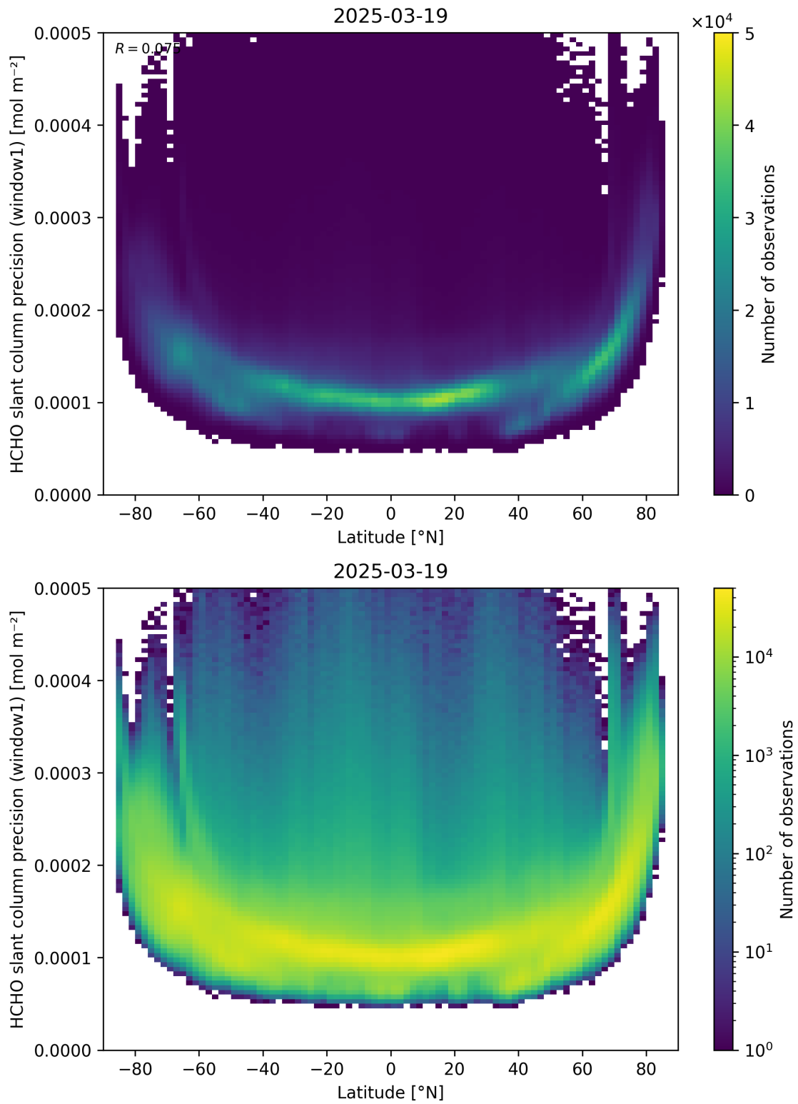
Figure 160: Scatter density plot of “Latitude” against “HCHO slant column precision (window1)” for 2025-03-18 to 2025-03-20.
