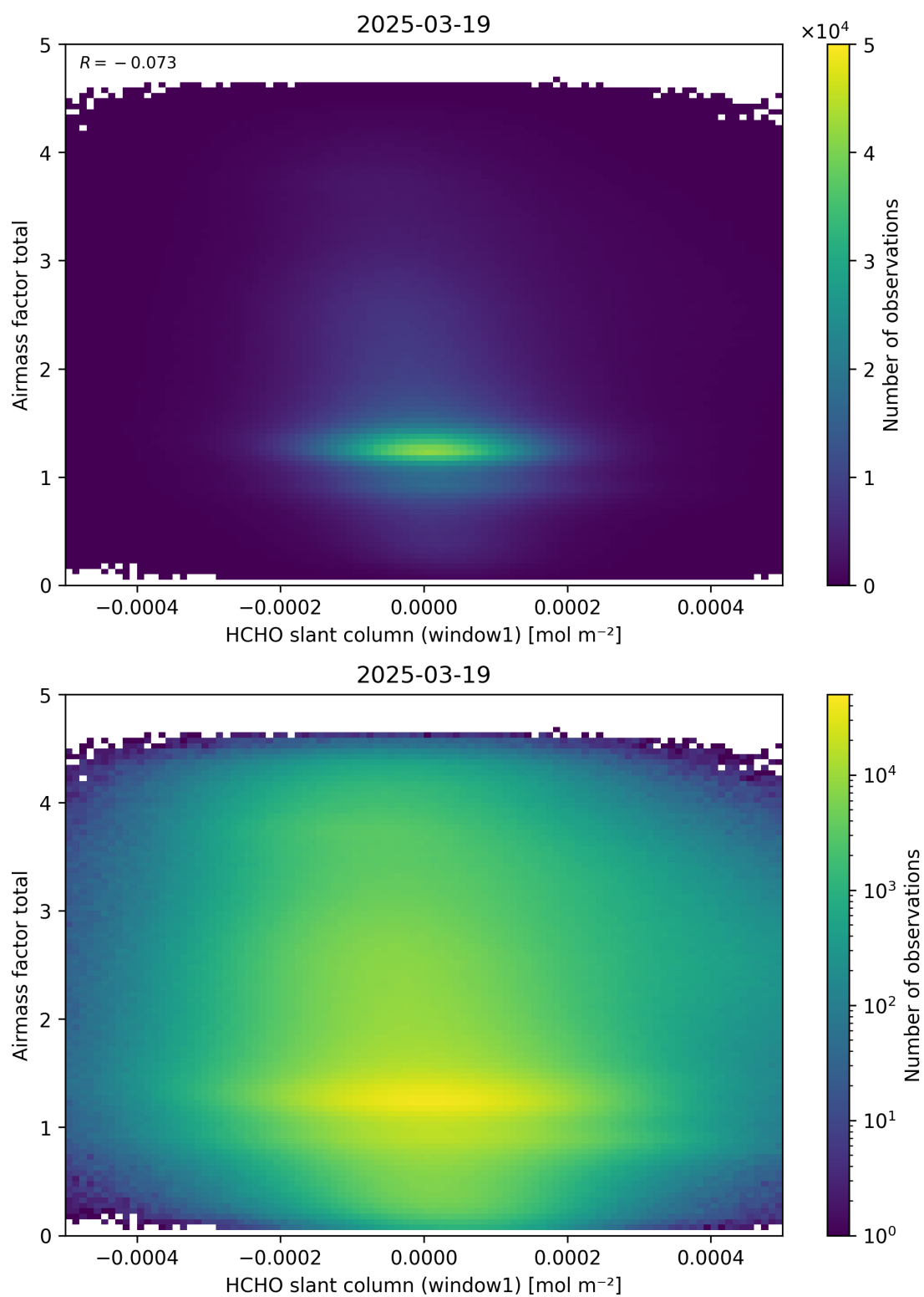
Figure 85: Scatter density plot of “HCHO slant column (window1)” against “Airmass factor total” for 2025-03-18 to 2025-03-20.
