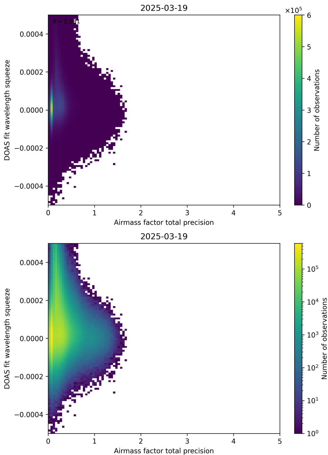
Figure 107: Scatter density plot of “Airmass factor total precision” against “DOAS fit wavelength squeeze” for 2025-03-18 to 2025-03-20.
