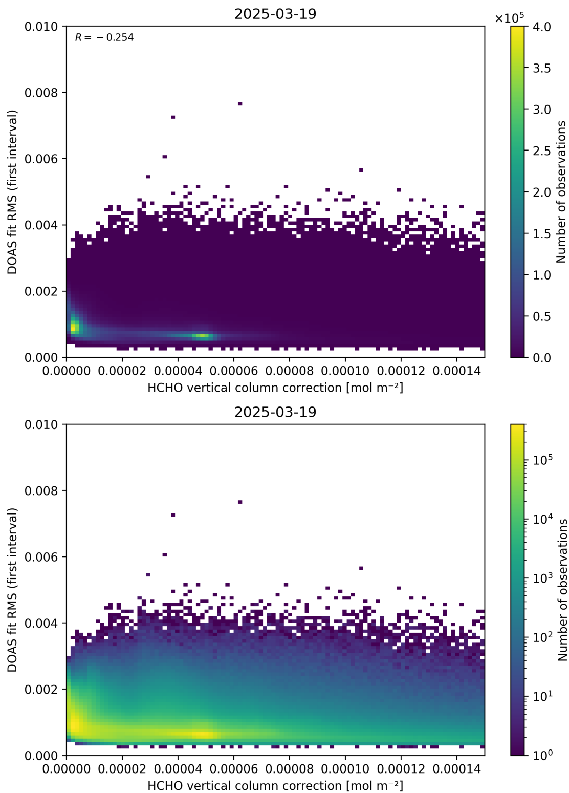
Figure 112: Scatter density plot of “HCHO vertical column correction” against “DOAS fit RMS (first interval)” for 2025-03-18 to 2025-03-20.
