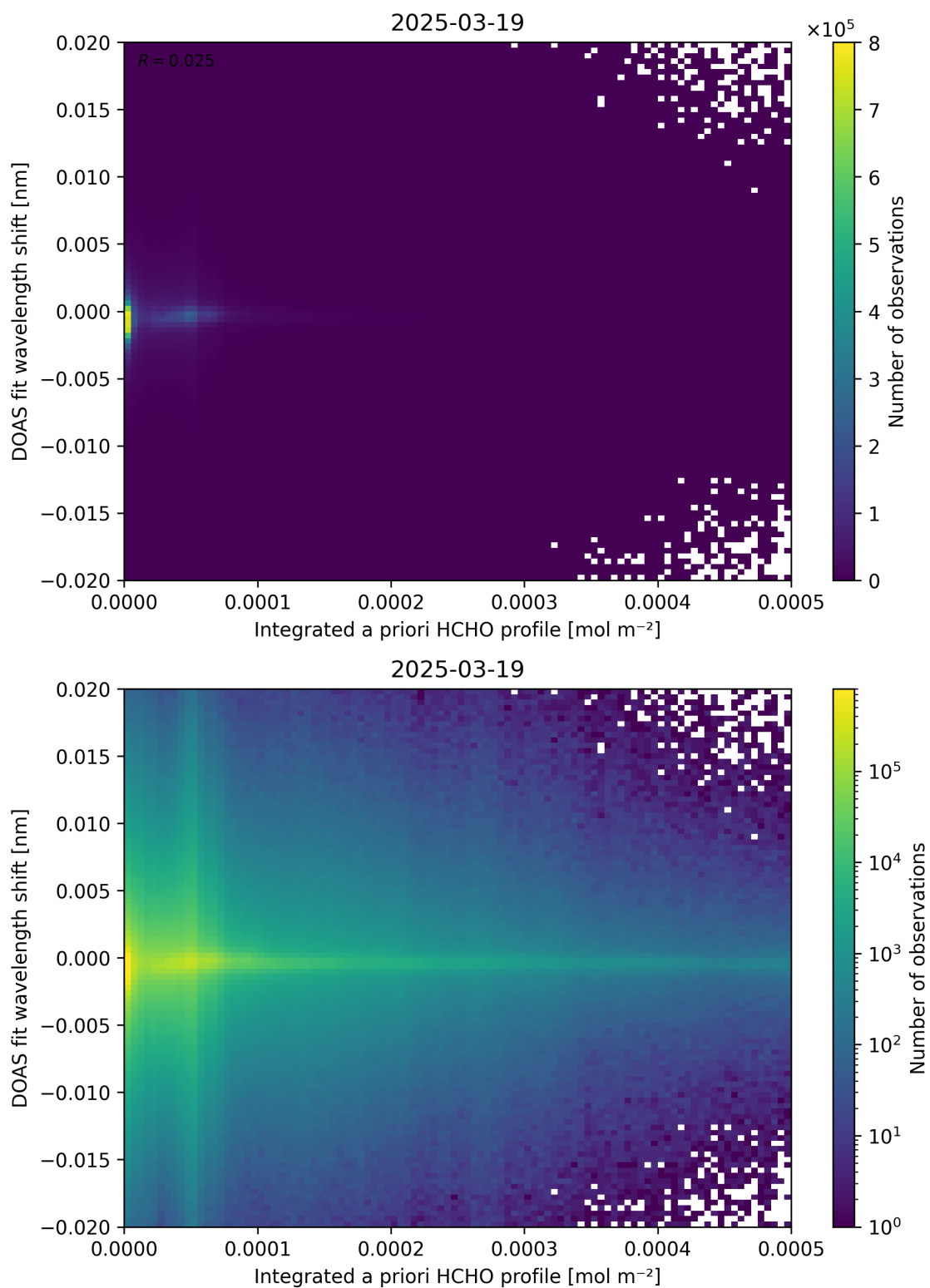
Figure 149: Scatter density plot of “Integrated a priori HCHO profile” against “DOAS fit wavelength shift” for 2025-03-18 to 2025-03-20.
