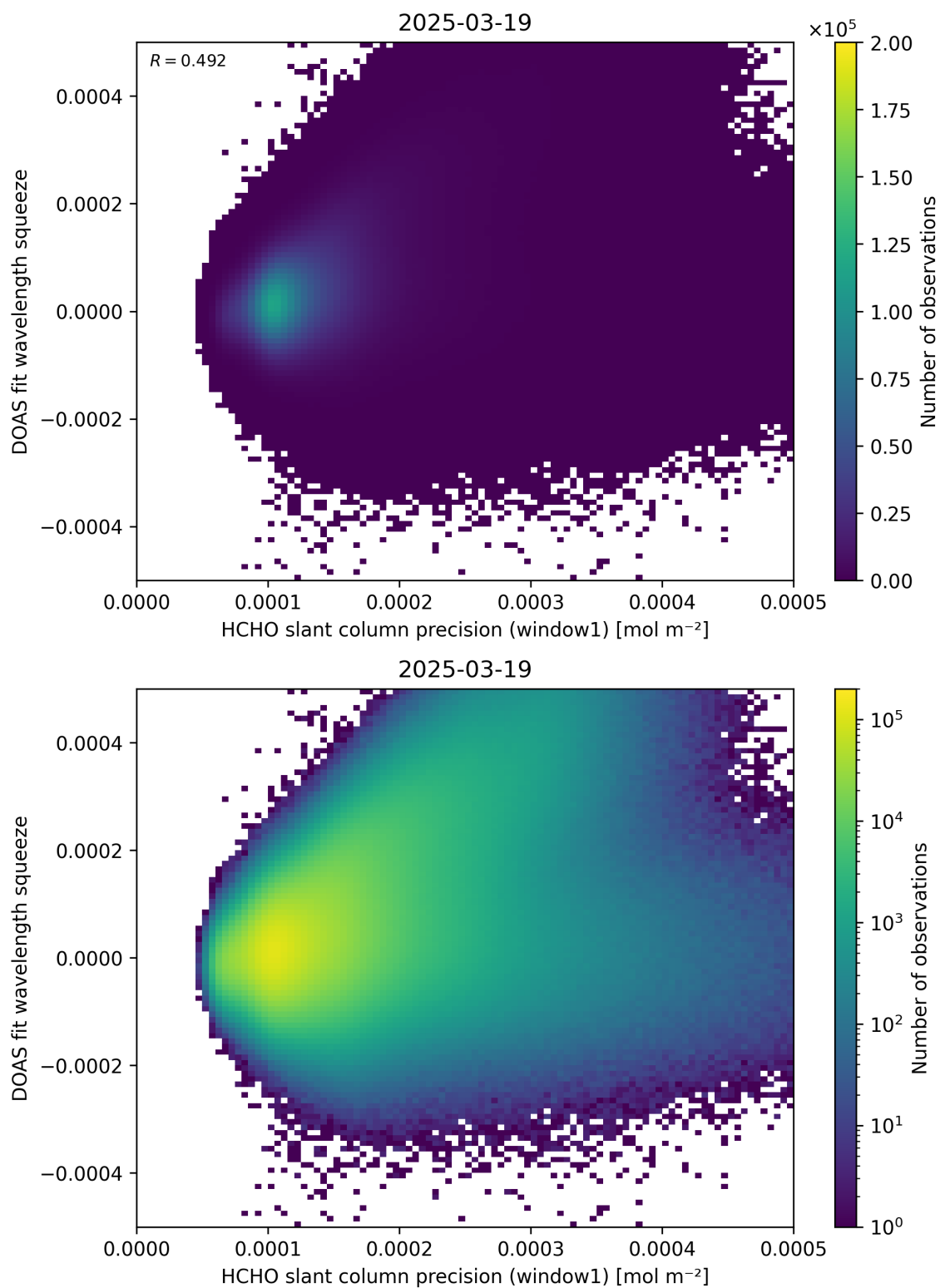
Figure 90: Scatter density plot of “HCHO slant column precision (window1)” against “DOAS fit wavelength squeeze” for 2025-03-18 to 2025-03-20.
