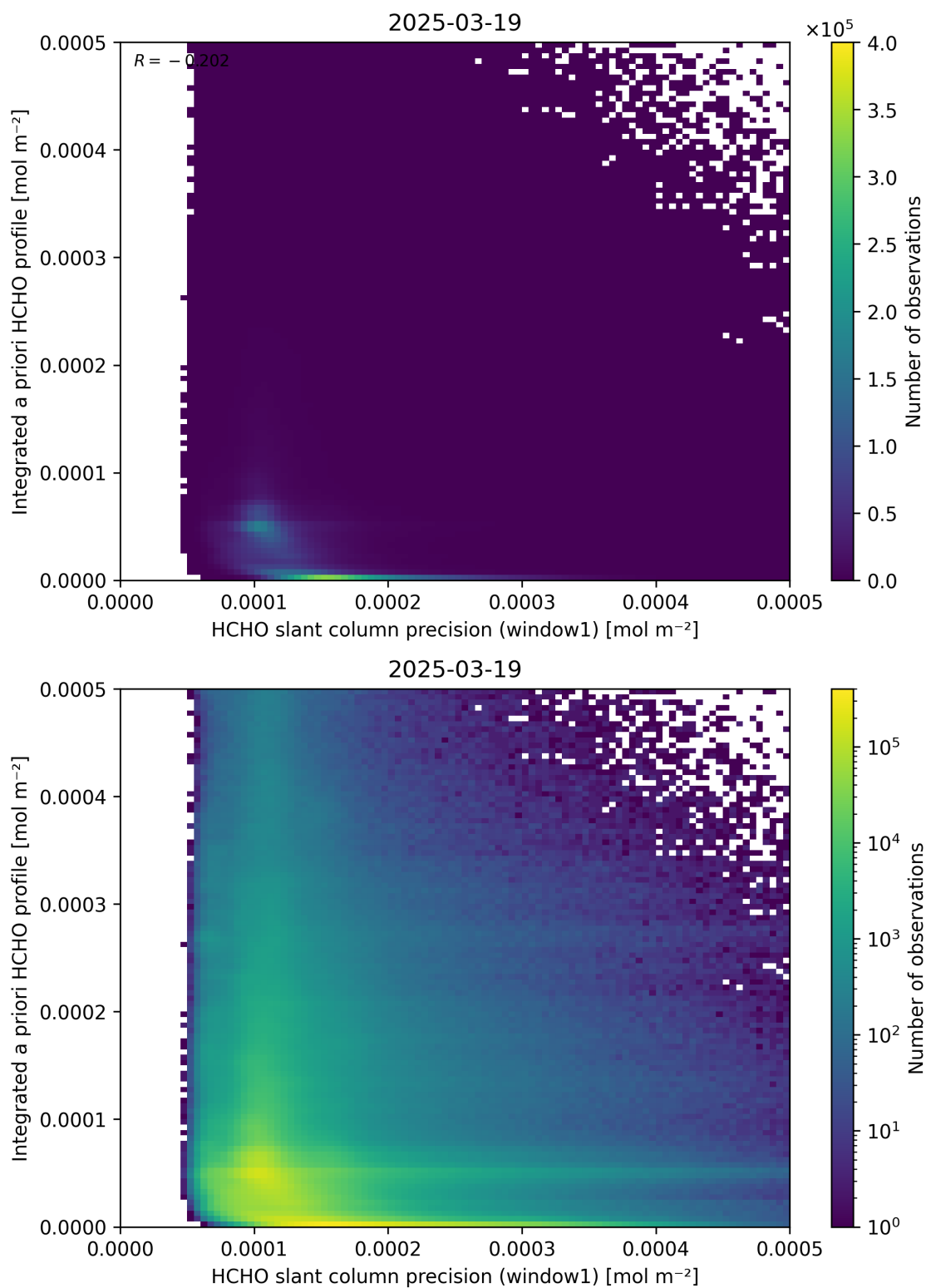
Figure 96: Scatter density plot of “HCHO slant column precision (window1)” against “Integrated a priori HCHO profile” for 2025-03-18 to 2025-03-20.
