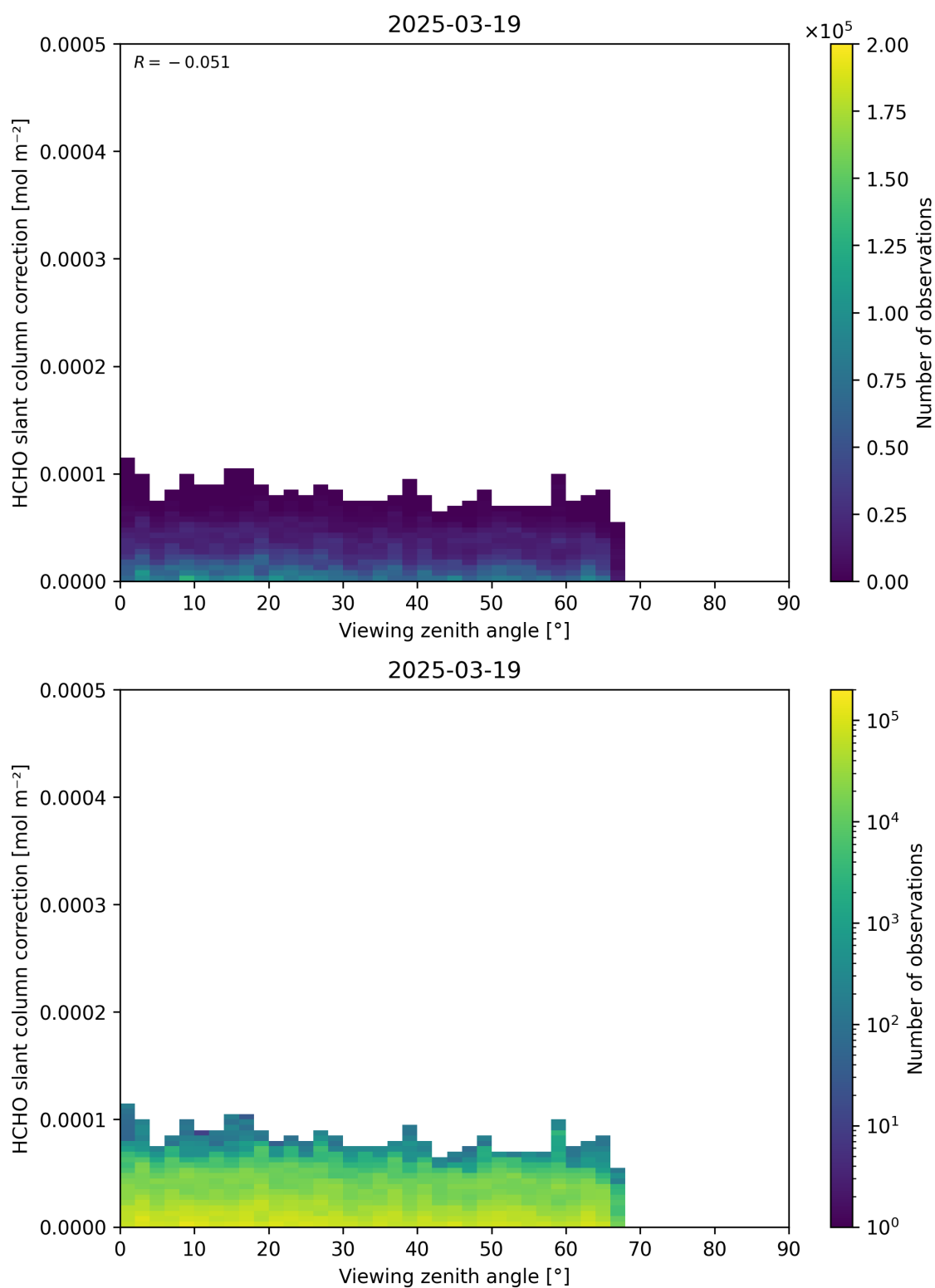
Figure 187: Scatter density plot of “Viewing zenith angle” against “HCHO slant column correction” for 2025-03-18 to 2025-03-20.
