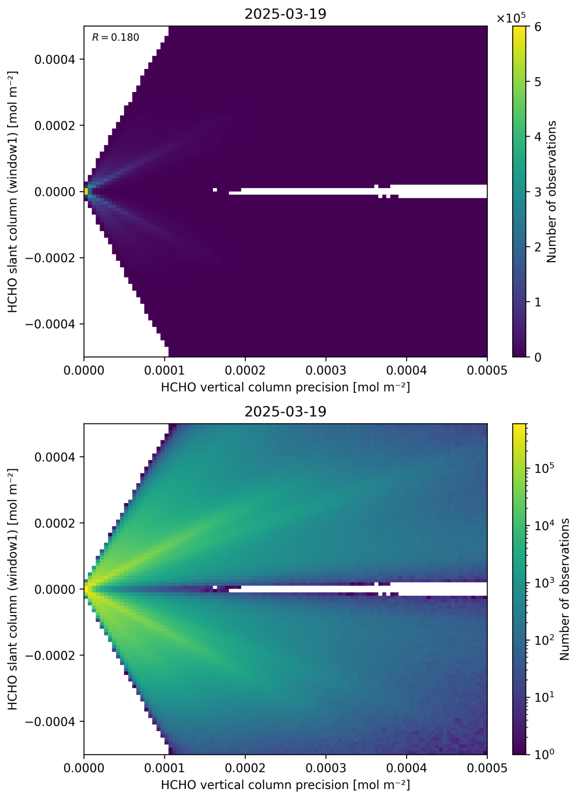
Figure 142: Scatter density plot of “HCHO vertical column precision” against “HCHO slant column (window1)” for 2025-03-18 to 2025-03-20.
