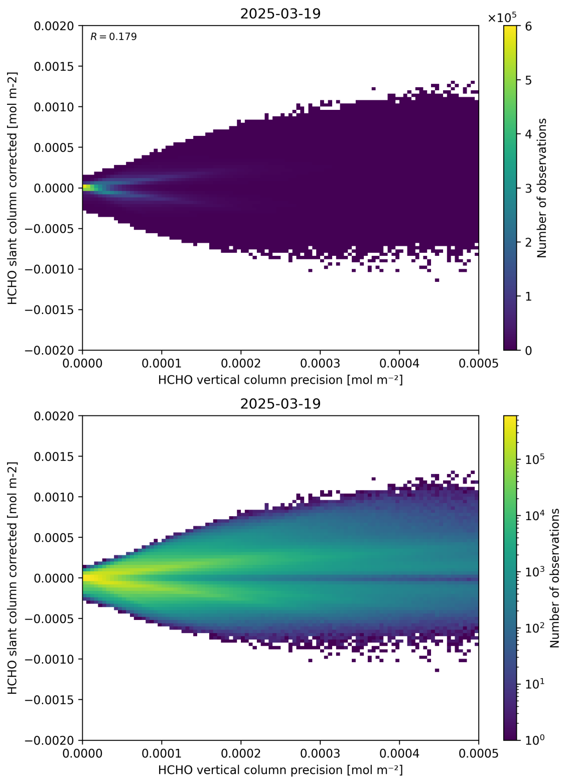
Figure 140: Scatter density plot of “HCHO vertical column precision” against “HCHO slant column corrected” for 2025-03-18 to 2025-03-20.
