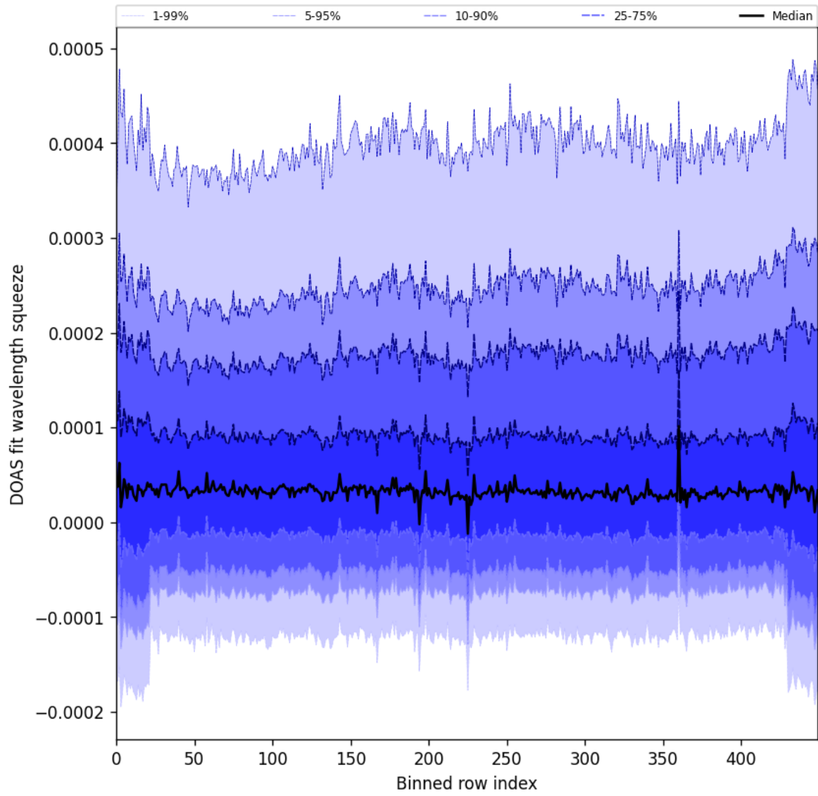
Figure 59: Along track statistics of “DOAS fit wavelength squeeze” for 2025-03-18 to 2025-03-20
