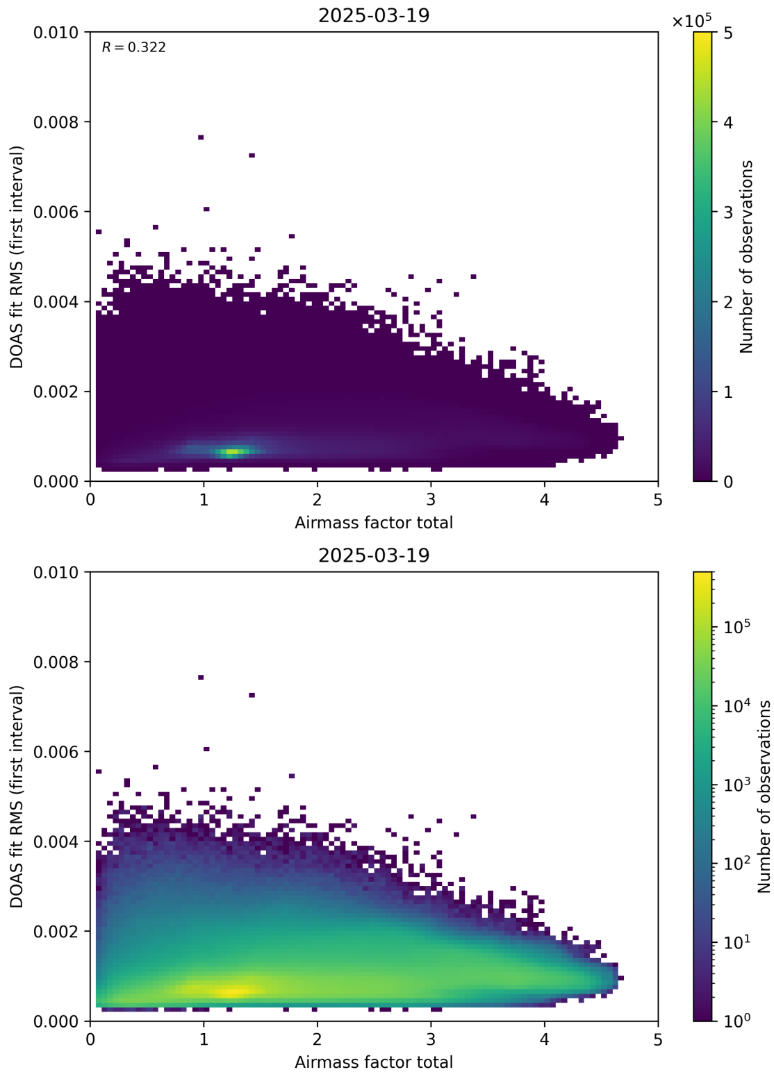
Figure 97: Scatter density plot of “Airmass factor total” against “DOAS fit RMS (first interval)” for 2025-03-18 to 2025-03-20.
