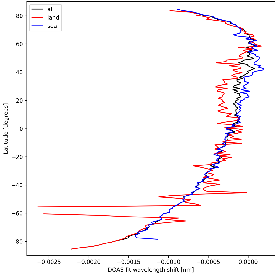
Figure 30: Zonal average of “DOAS fit wavelength shift” for 2025-03-18 to 2025-03-20.
