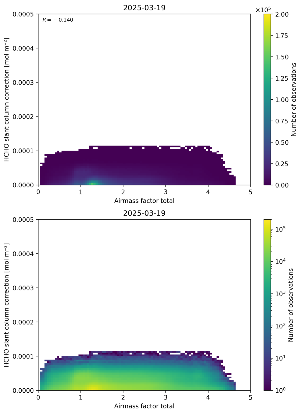
Figure 102: Scatter density plot of “Airmass factor total” against “HCHO slant column correction” for 2025-03-18 to 2025-03-20.
