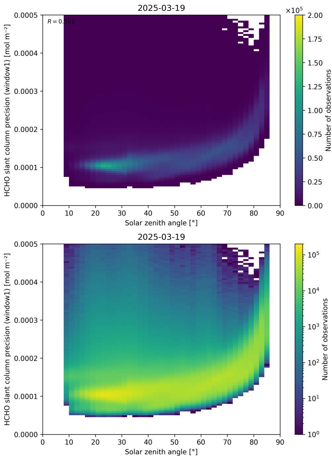
Figure 174: Scatter density plot of “Solar zenith angle” against “HCHO slant column precision (window1)” for 2025-03-18 to 2025-03-20.
