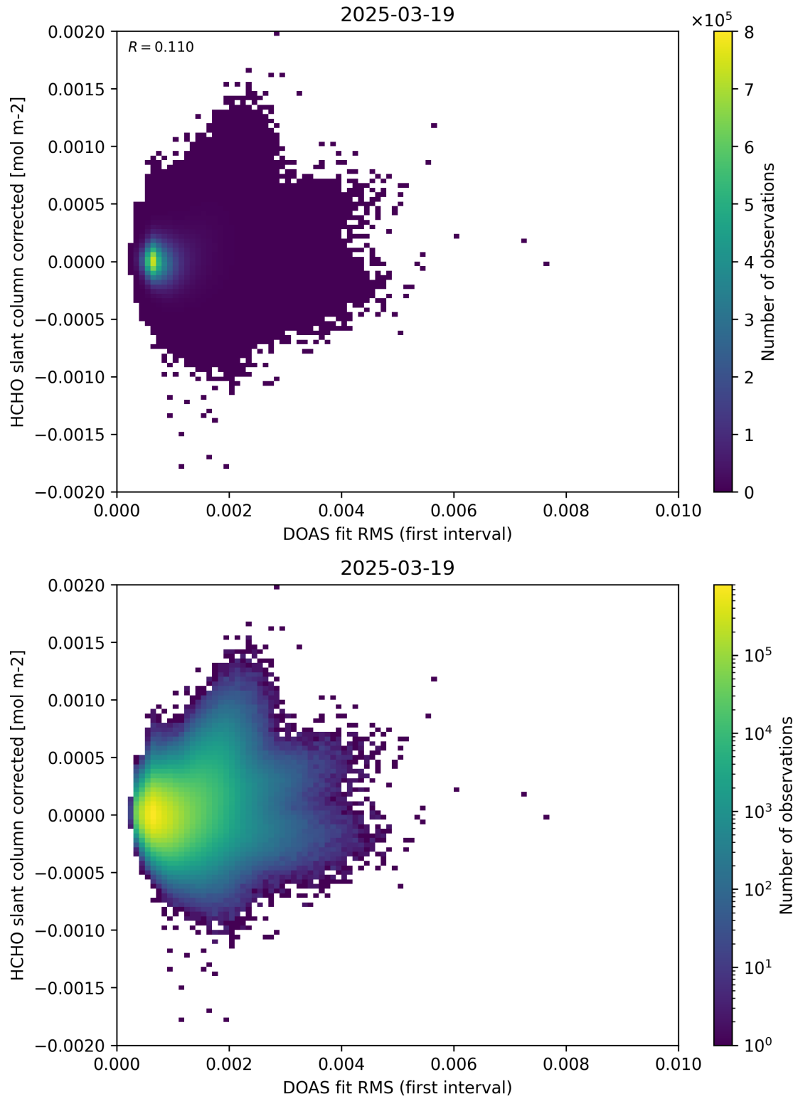
Figure 62: Scatter density plot of “DOAS fit RMS (first interval)” against “HCHO slant column corrected” for 2025-03-18 to 2025-03-20.
