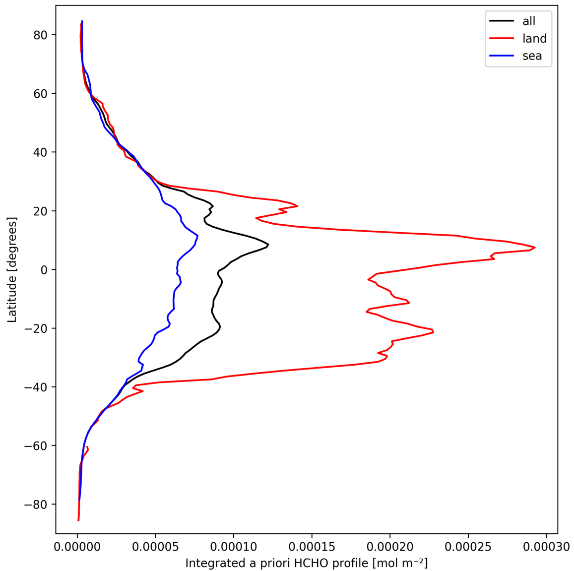
Figure 29: Zonal average of “Integrated a priori HCHO profile” for 2025-03-18 to 2025-03-20.
