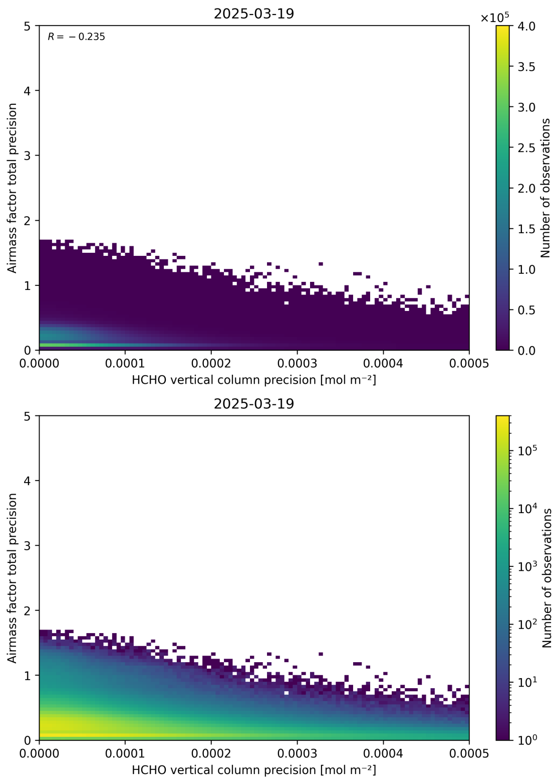
Figure 145: Scatter density plot of “HCHO vertical column precision” against “Airmass factor total precision” for 2025-03-18 to 2025-03-20.
