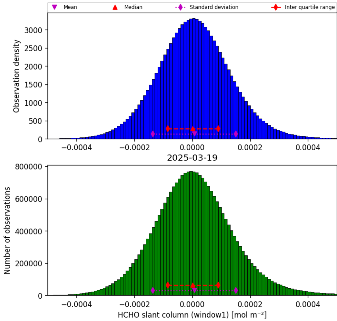
Figure 38: Histogram of “HCHO slant column (window1)” for 2025-03-18 to 2025-03-20
