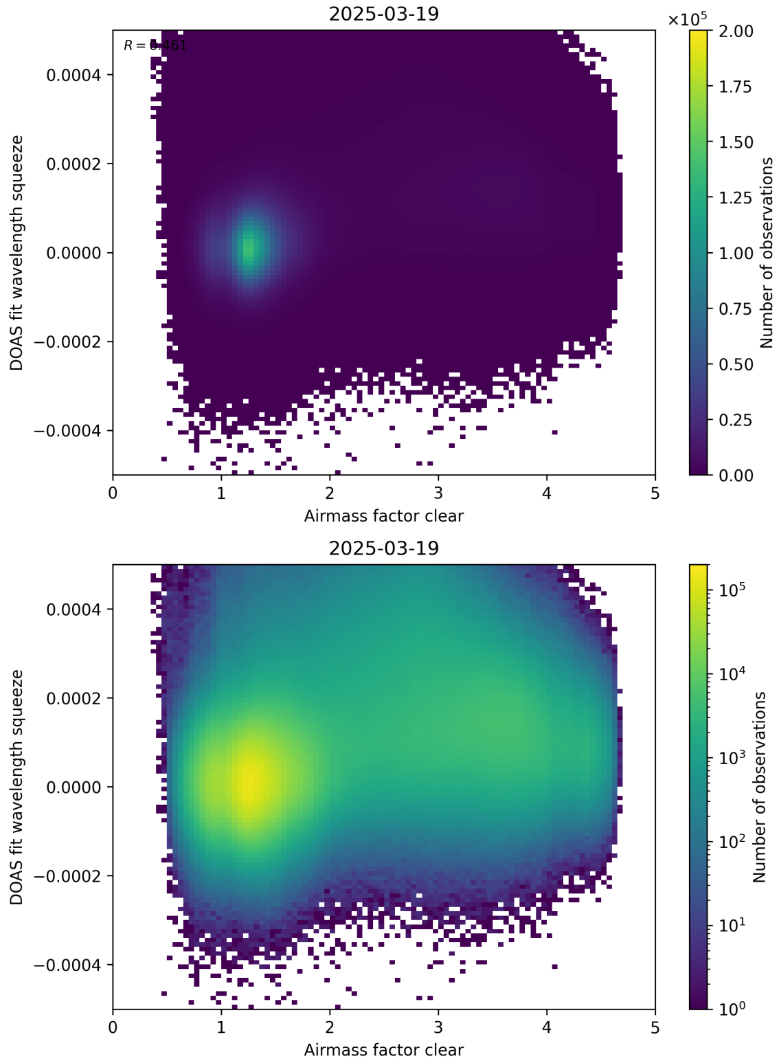
Figure 73: Scatter density plot of “Airmass factor clear” against “DOAS fit wavelength squeeze” for 2025-03-18 to 2025-03-20.
