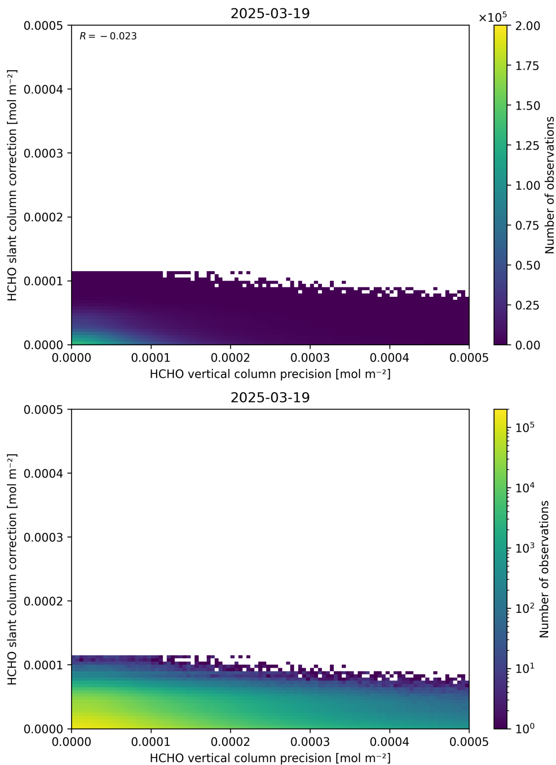
Figure 141: Scatter density plot of “HCHO vertical column precision” against “HCHO slant column correction” for 2025-03-18 to 2025-03-20.
