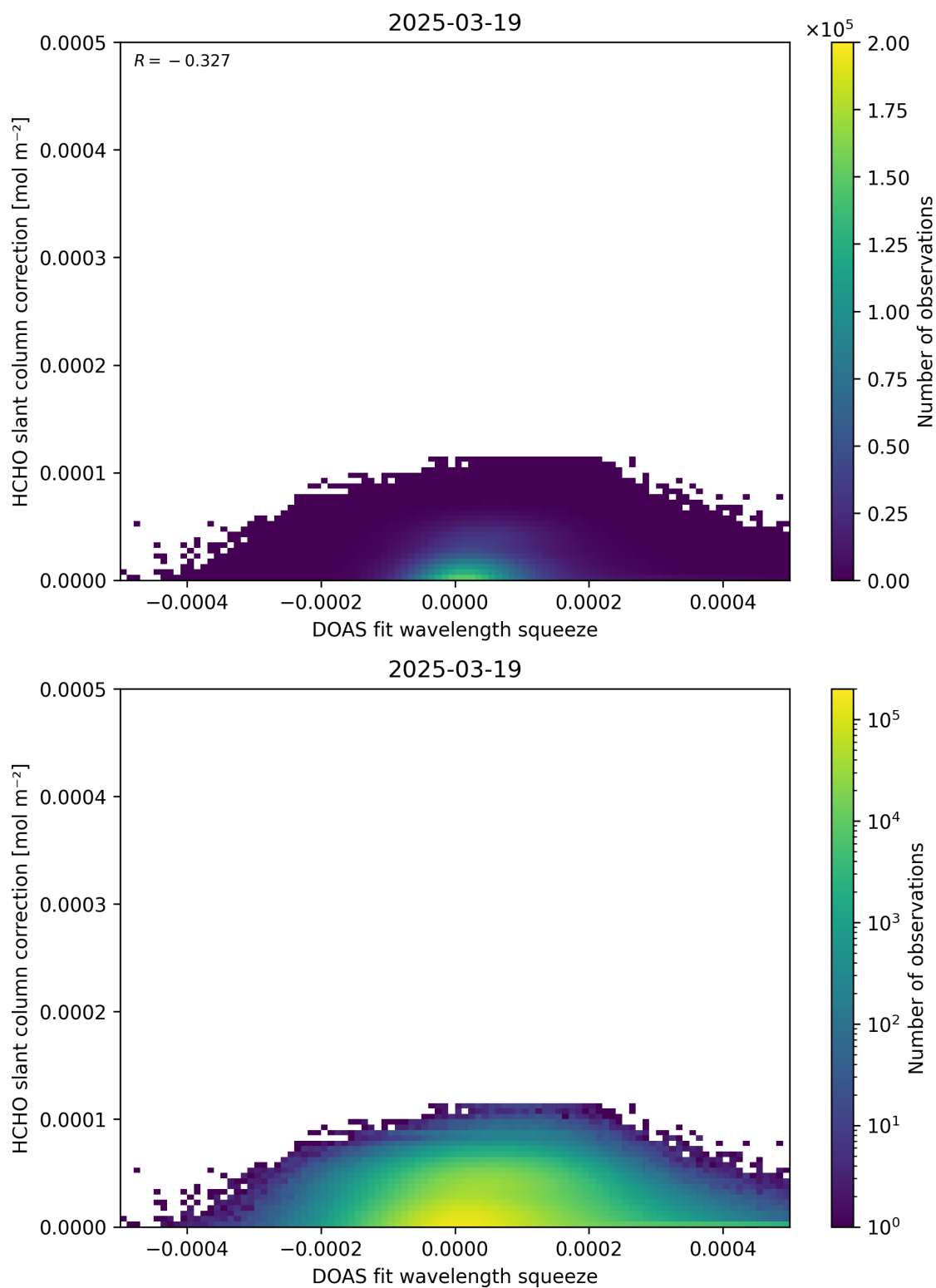
Figure 70: Scatter density plot of “DOAS fit wavelength squeeze” against “HCHO slant column correction” for 2025-03-18 to 2025-03-20.
