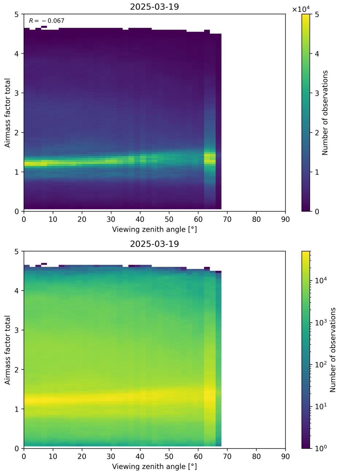
Figure 190: Scatter density plot of “Viewing zenith angle” against “Airmass factor total” for 2025-03-18 to 2025-03-20.
