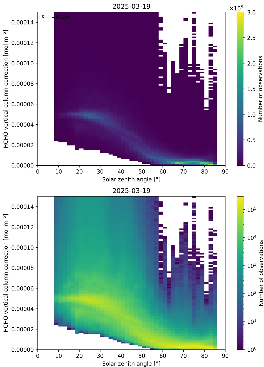
Figure 178: Scatter density plot of “Solar zenith angle” against “HCHO vertical column correction” for 2025-03-18 to 2025-03-20.
