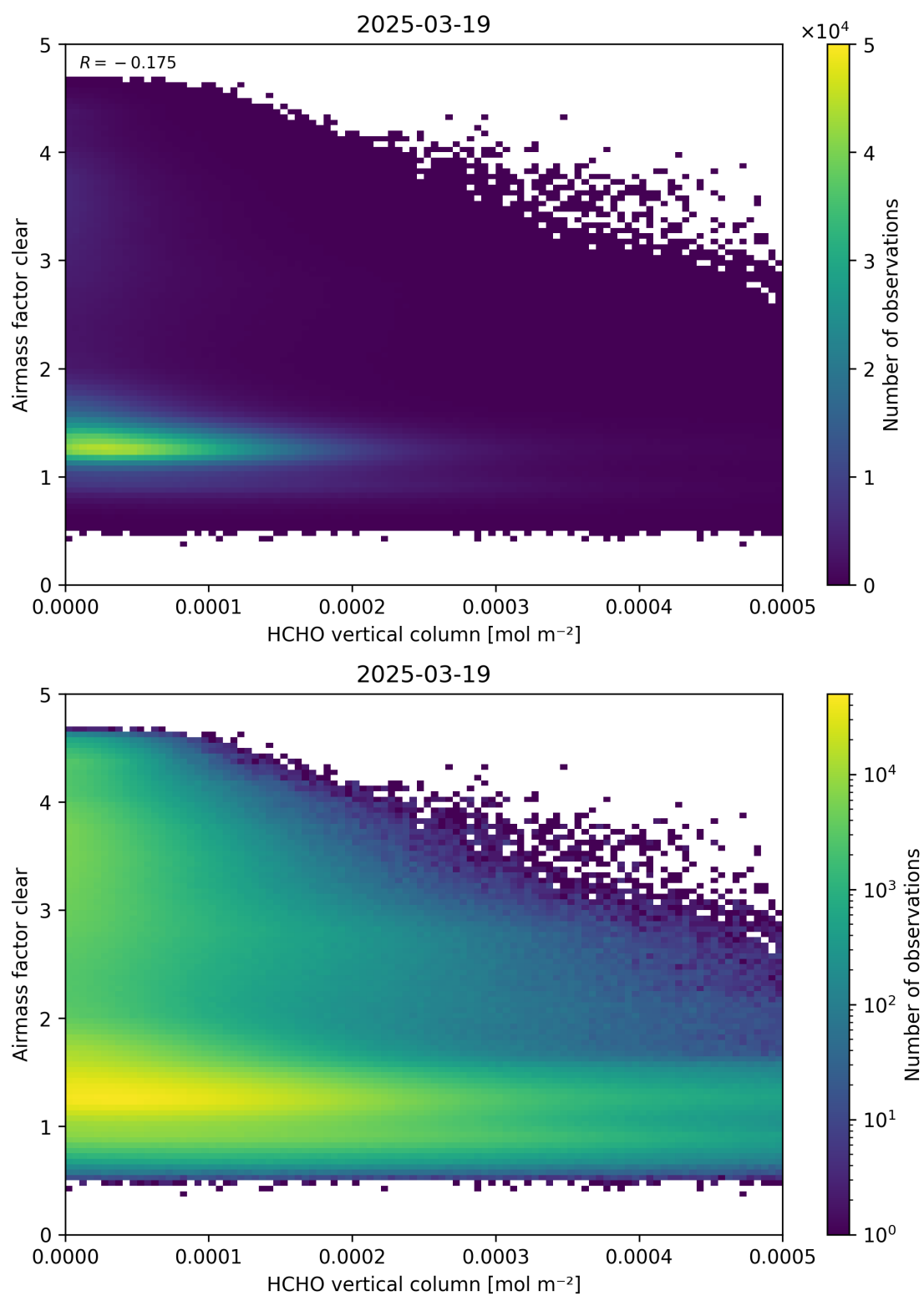
Figure 126: Scatter density plot of “HCHO vertical column” against “Airmass factor clear” for 2025-03-18 to 2025-03-20.
