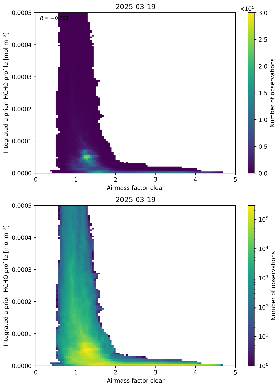
Figure 76: Scatter density plot of “Airmass factor clear” against “Integrated a priori HCHO profile” for 2025-03-18 to 2025-03-20.
