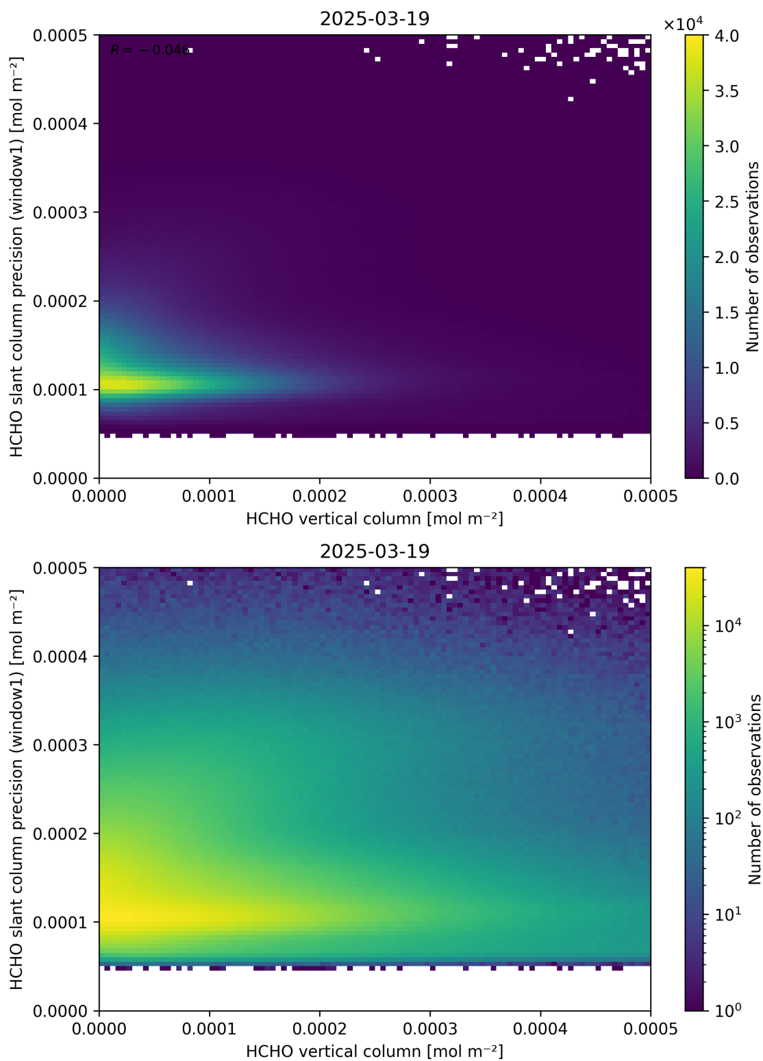
Figure 130: Scatter density plot of “HCHO vertical column” against “HCHO slant column precision (window1)” for 2025-03-18 to 2025-03-20.
