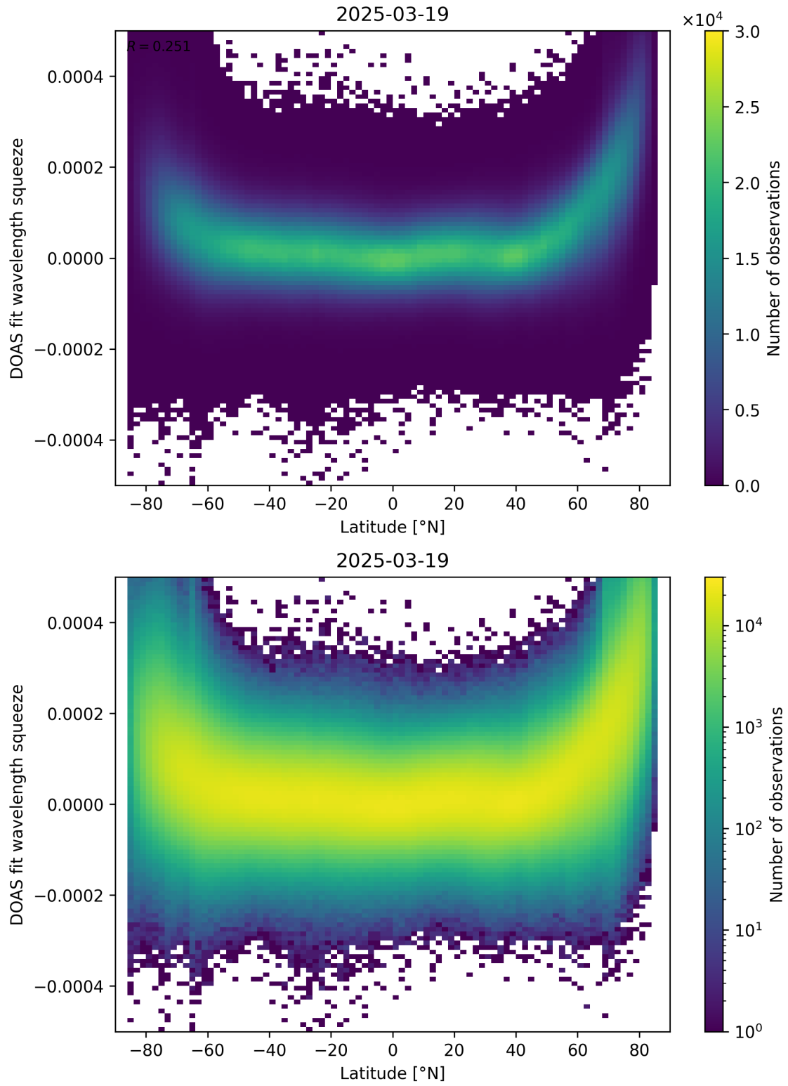
Figure 155: Scatter density plot of “Latitude” against “DOAS fit wavelength squeeze” for 2025-03-18 to 2025-03-20.
