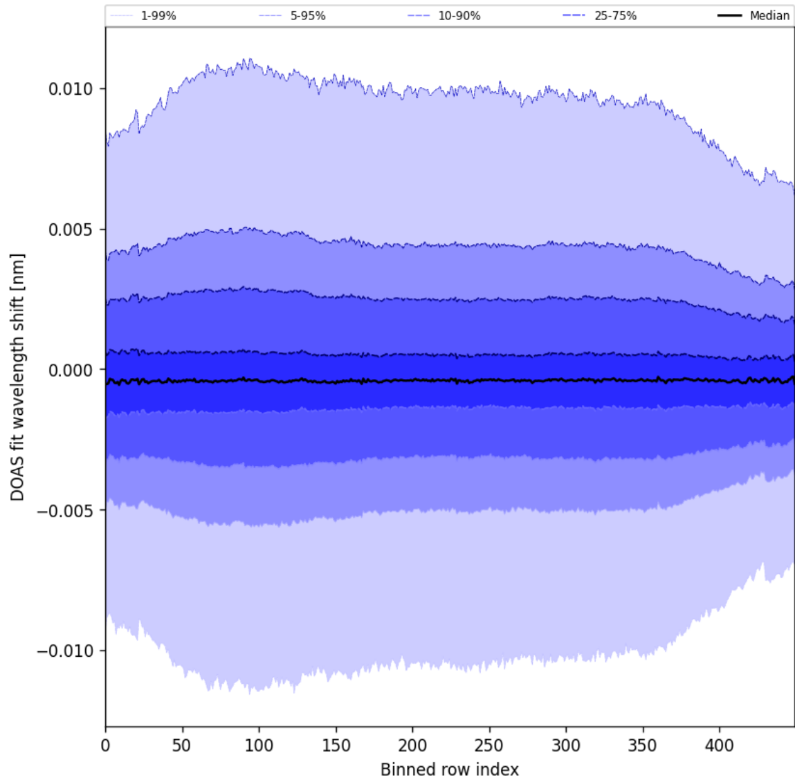
Figure 58: Along track statistics of “DOAS fit wavelength shift” for 2025-03-18 to 2025-03-20
