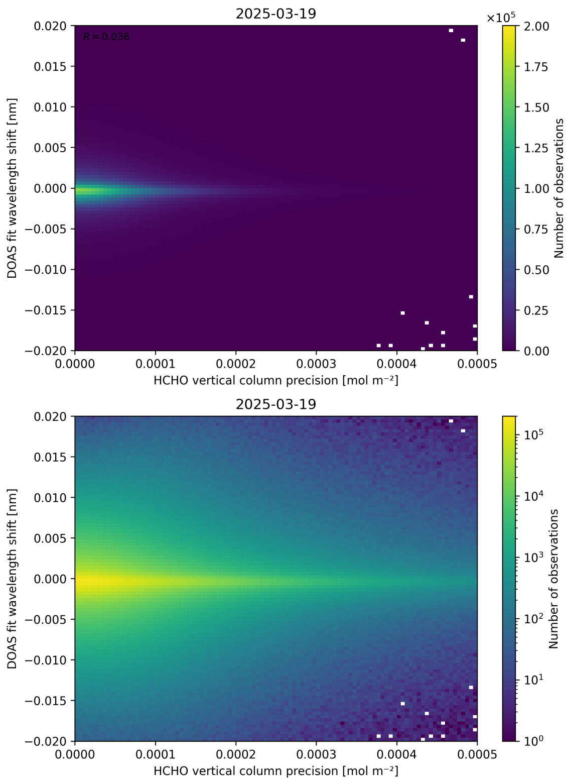
Figure 137: Scatter density plot of “HCHO vertical column precision” against “DOAS fit wavelength shift” for 2025-03-18 to 2025-03-20.
