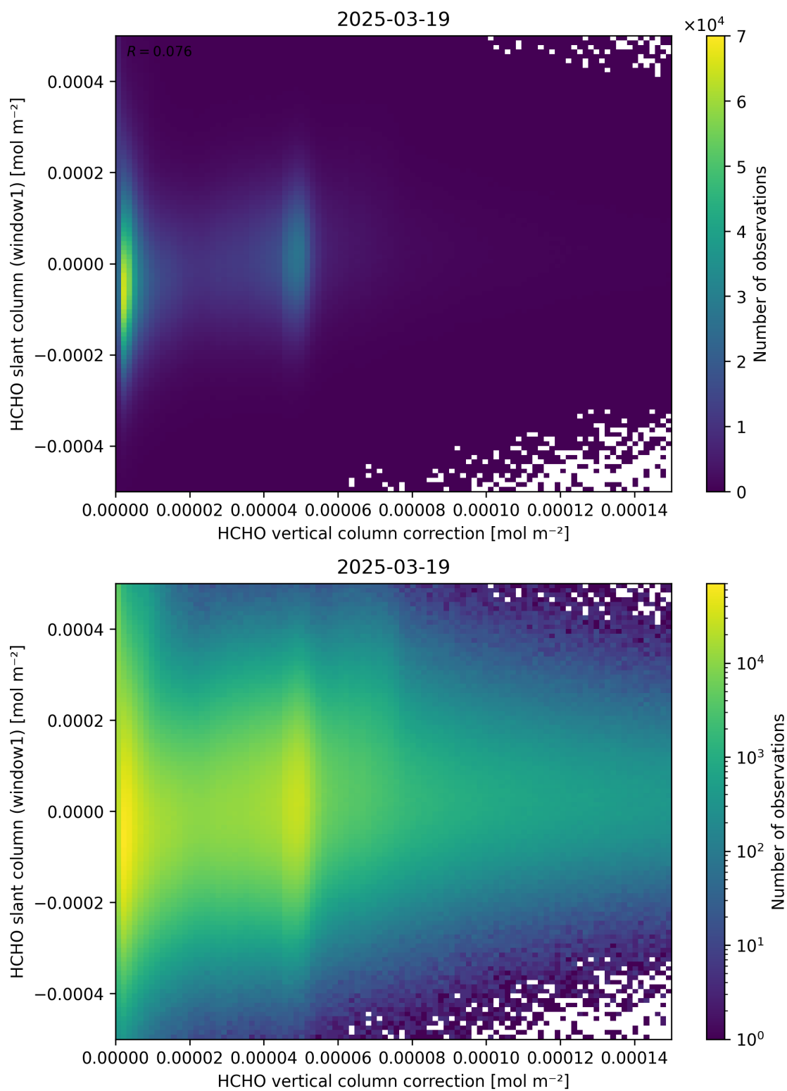
Figure 118: Scatter density plot of “HCHO vertical column correction” against “HCHO slant column (window1)” for 2025-03-18 to 2025-03-20.
