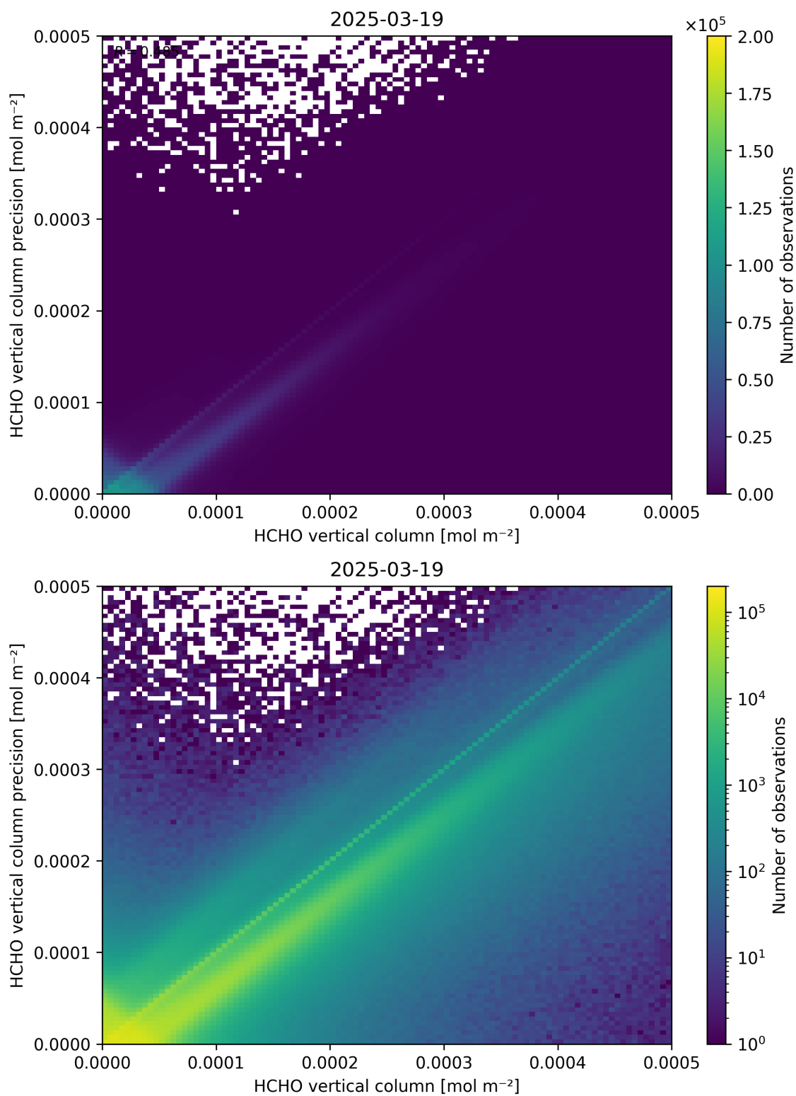
Figure 134: Scatter density plot of “HCHO vertical column” against “HCHO vertical column precision” for 2025-03-18 to 2025-03-20.
