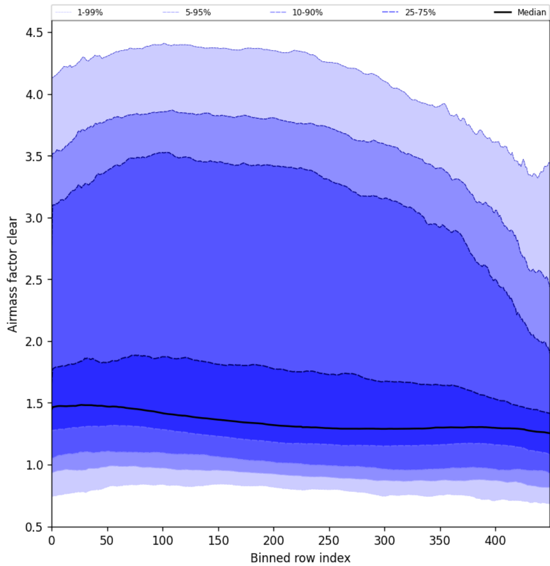
Figure 56: Along track statistics of “Airmass factor clear” for 2025-03-18 to 2025-03-20
