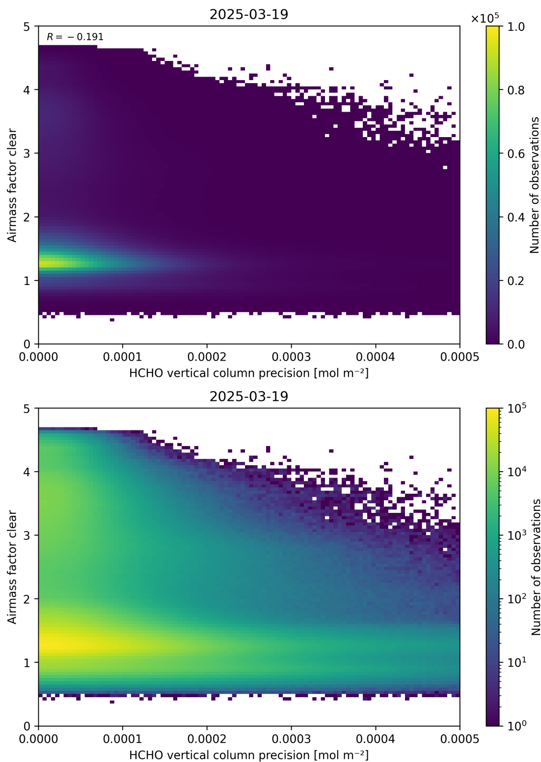
Figure 139: Scatter density plot of “HCHO vertical column precision” against “Airmass factor clear” for 2025-03-18 to 2025-03-20.
