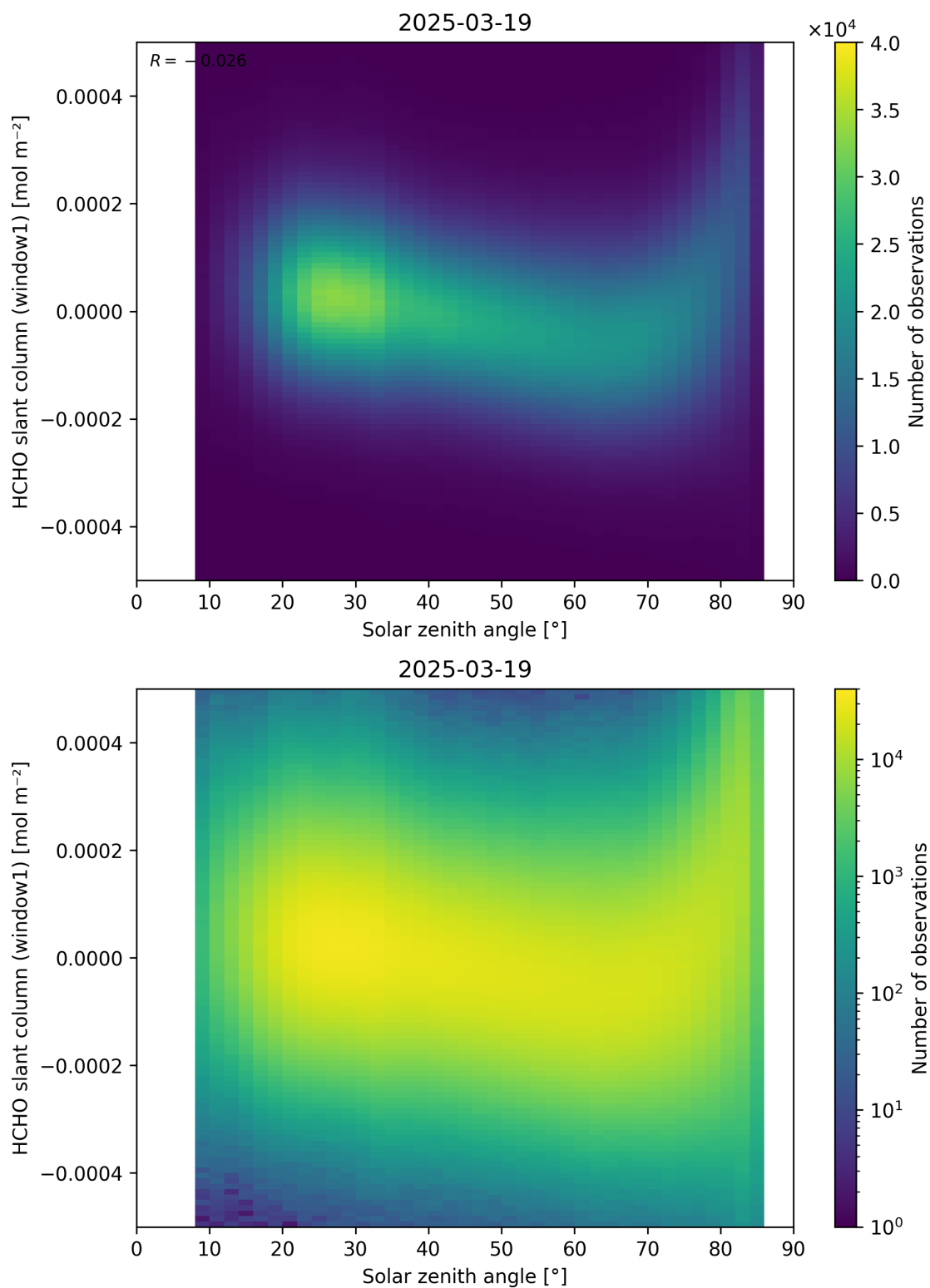
Figure 173: Scatter density plot of “Solar zenith angle” against “HCHO slant column (window1)” for 2025-03-18 to 2025-03-20.
