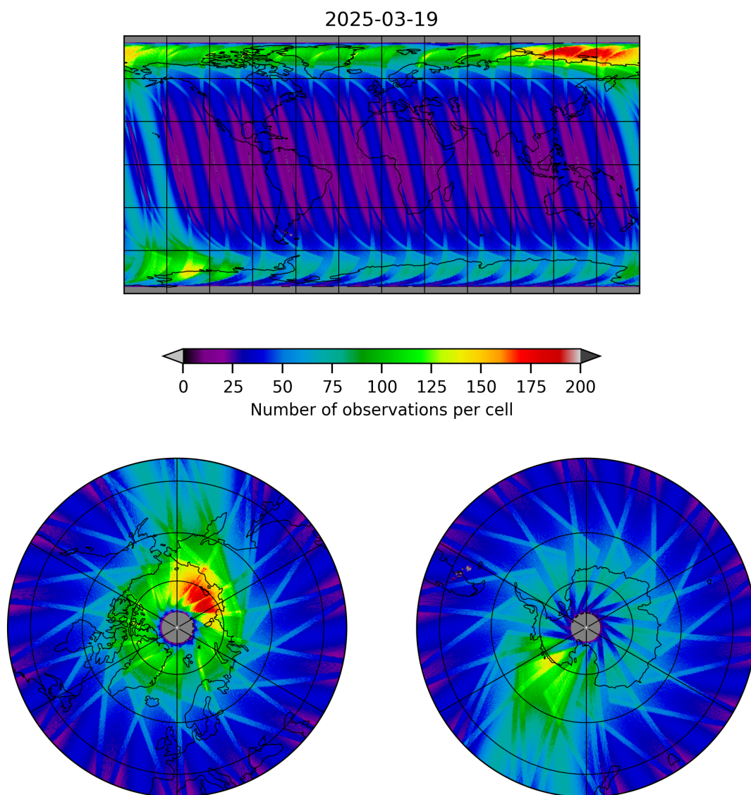
Figure 19: Map of the number of observations for 2025-03-18 to 2025-03-20
