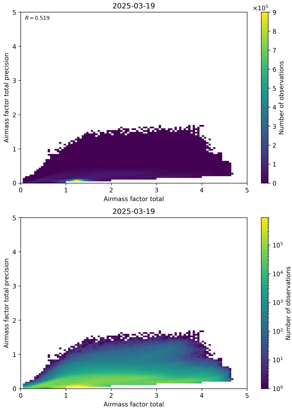
Figure 103: Scatter density plot of “Airmass factor total” against “Airmass factor total precision” for 2025-03-18 to 2025-03-20.
