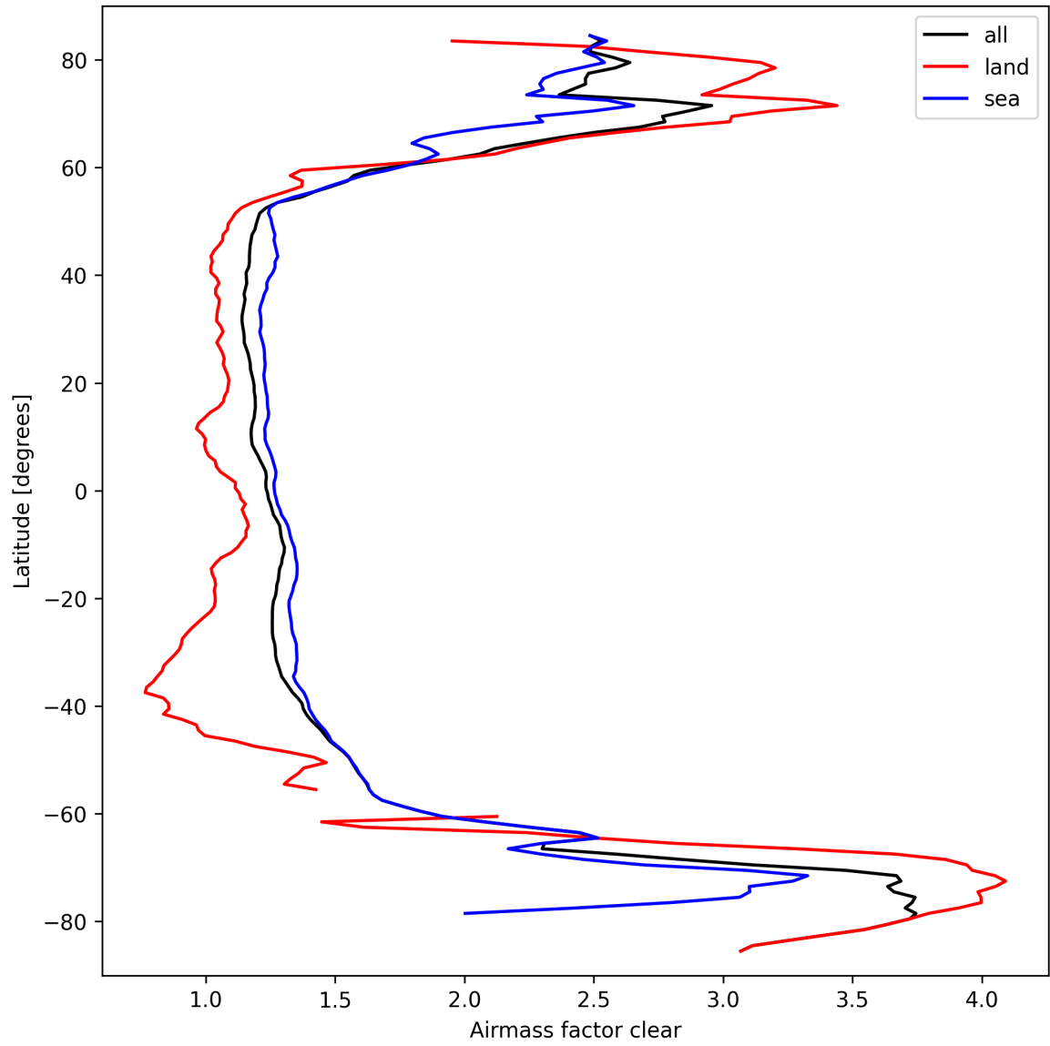
Figure 28: Zonal average of “Airmass factor clear” for 2025-03-18 to 2025-03-20.
