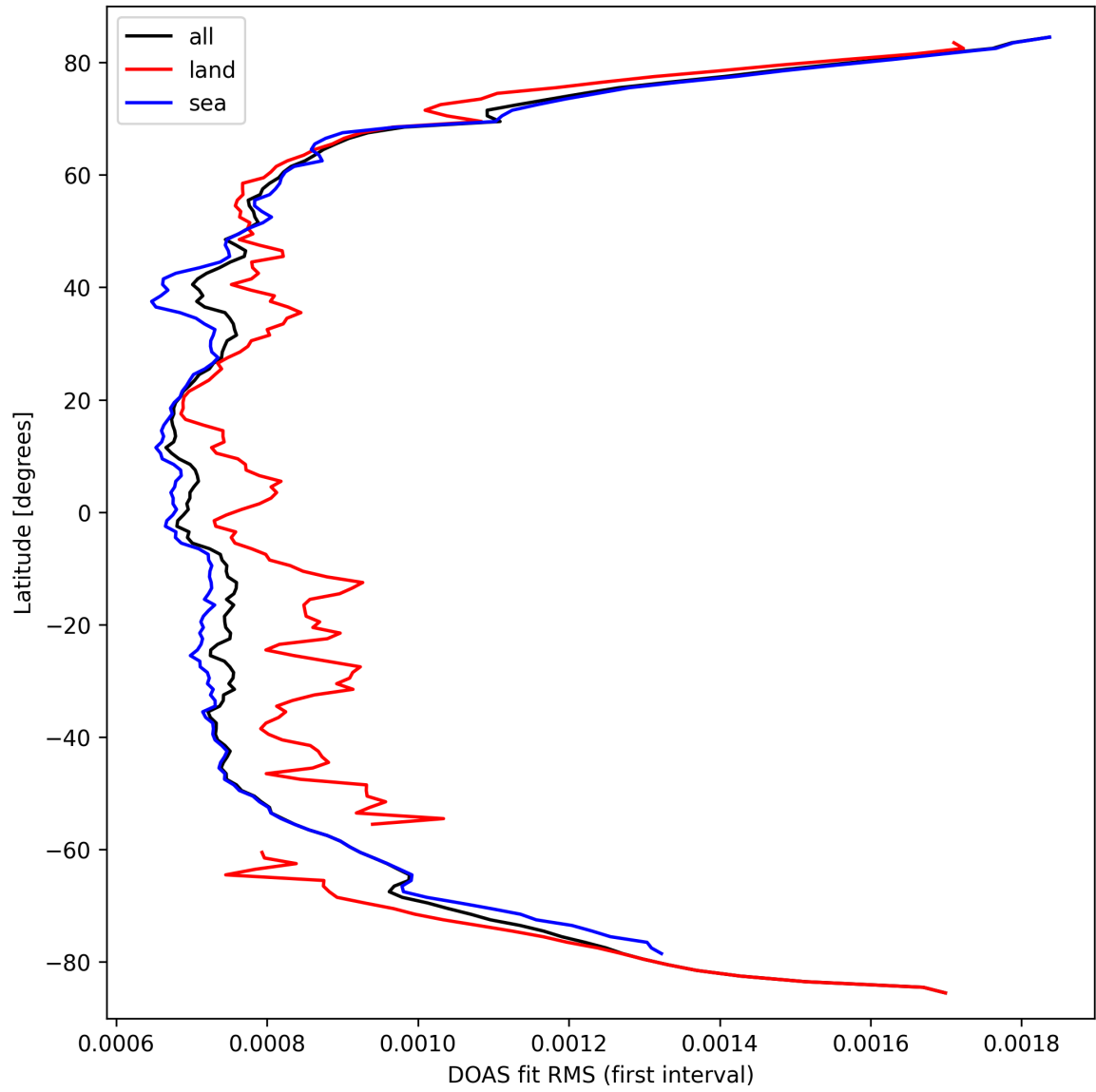
Figure 32: Zonal average of “DOAS fit RMS (first interval)” for 2025-03-18 to 2025-03-20.
