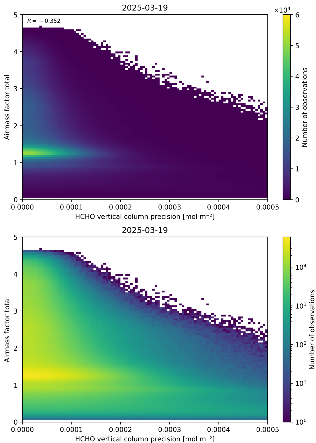
Figure 144: Scatter density plot of “HCHO vertical column precision” against “Airmass factor total” for 2025-03-18 to 2025-03-20.
