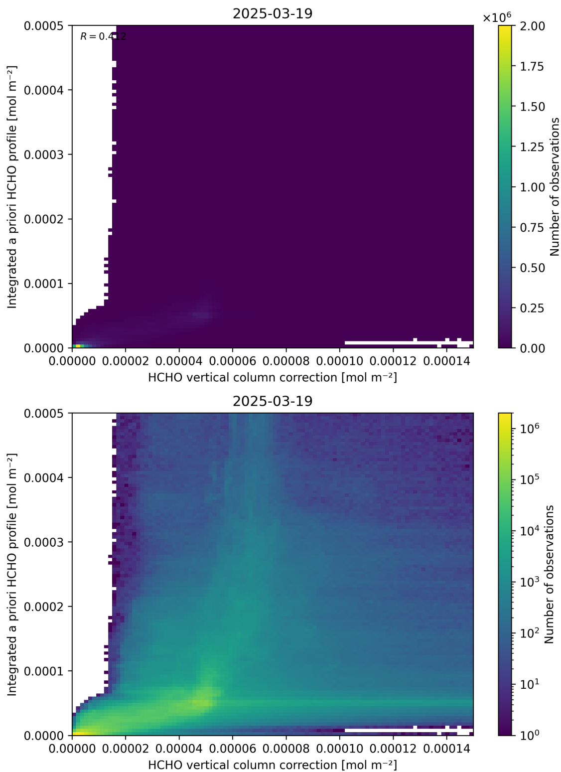
Figure 122: Scatter density plot of “HCHO vertical column correction” against “Integrated a priori HCHO profile” for 2025-03-18 to 2025-03-20.
