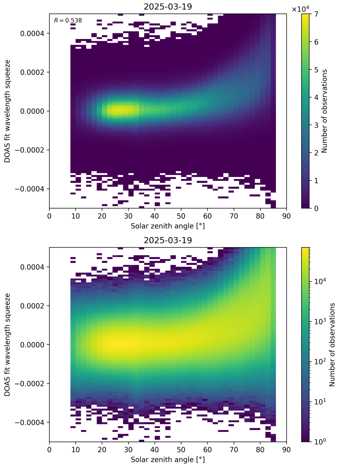
Figure 169: Scatter density plot of “Solar zenith angle” against “DOAS fit wavelength squeeze” for 2025-03-18 to 2025-03-20.
