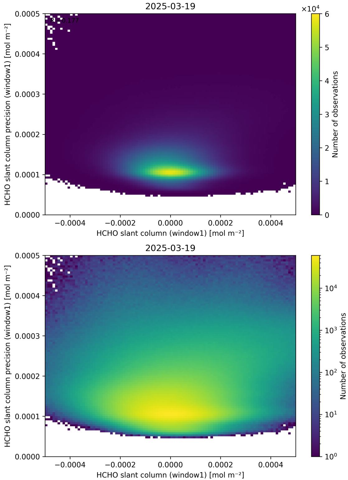
Figure 84: Scatter density plot of “HCHO slant column (window1)” against “HCHO slant column precision (window1)” for 2025-03-18 to 2025-03-20.
