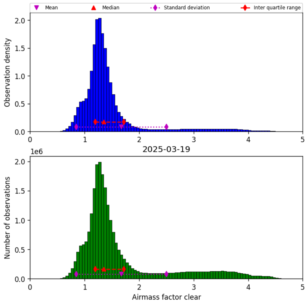
Figure 42: Histogram of “Airmass factor clear” for 2025-03-18 to 2025-03-20
