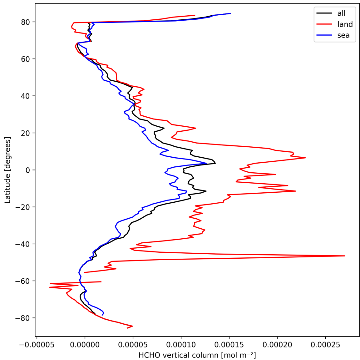
Figure 21: Zonal average of “HCHO vertical column” for 2025-03-18 to 2025-03-20.
