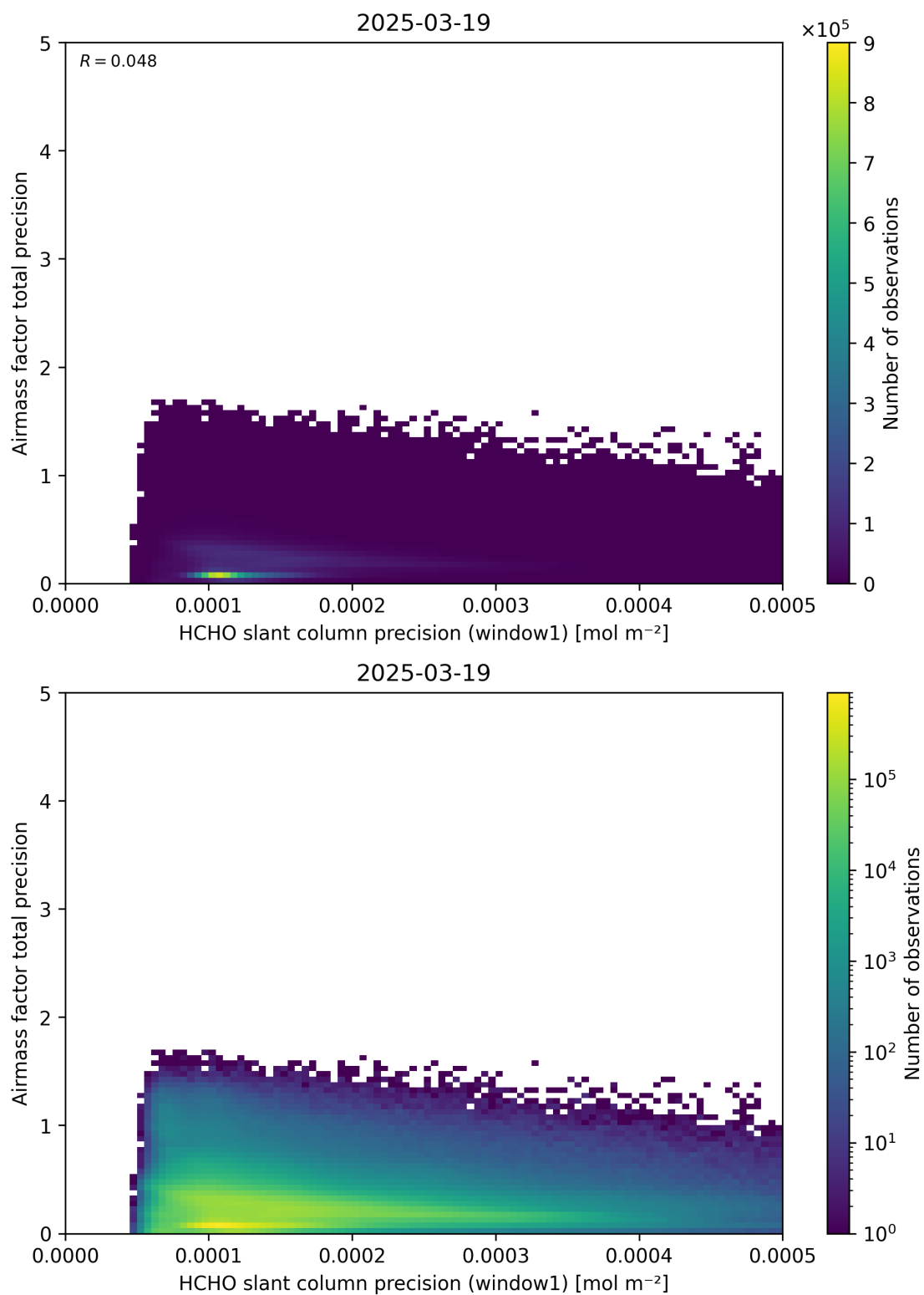
Figure 95: Scatter density plot of “HCHO slant column precision (window1)” against “Airmass factor total precision” for 2025-03-18 to 2025-03-20.
