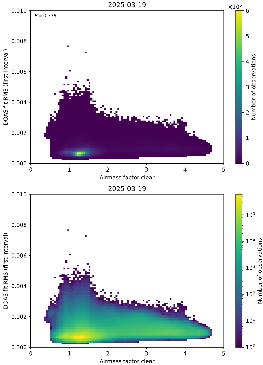
Figure 71: Scatter density plot of “Airmass factor clear” against “DOAS fit RMS (first interval)” for 2025-03-18 to 2025-03-20.
