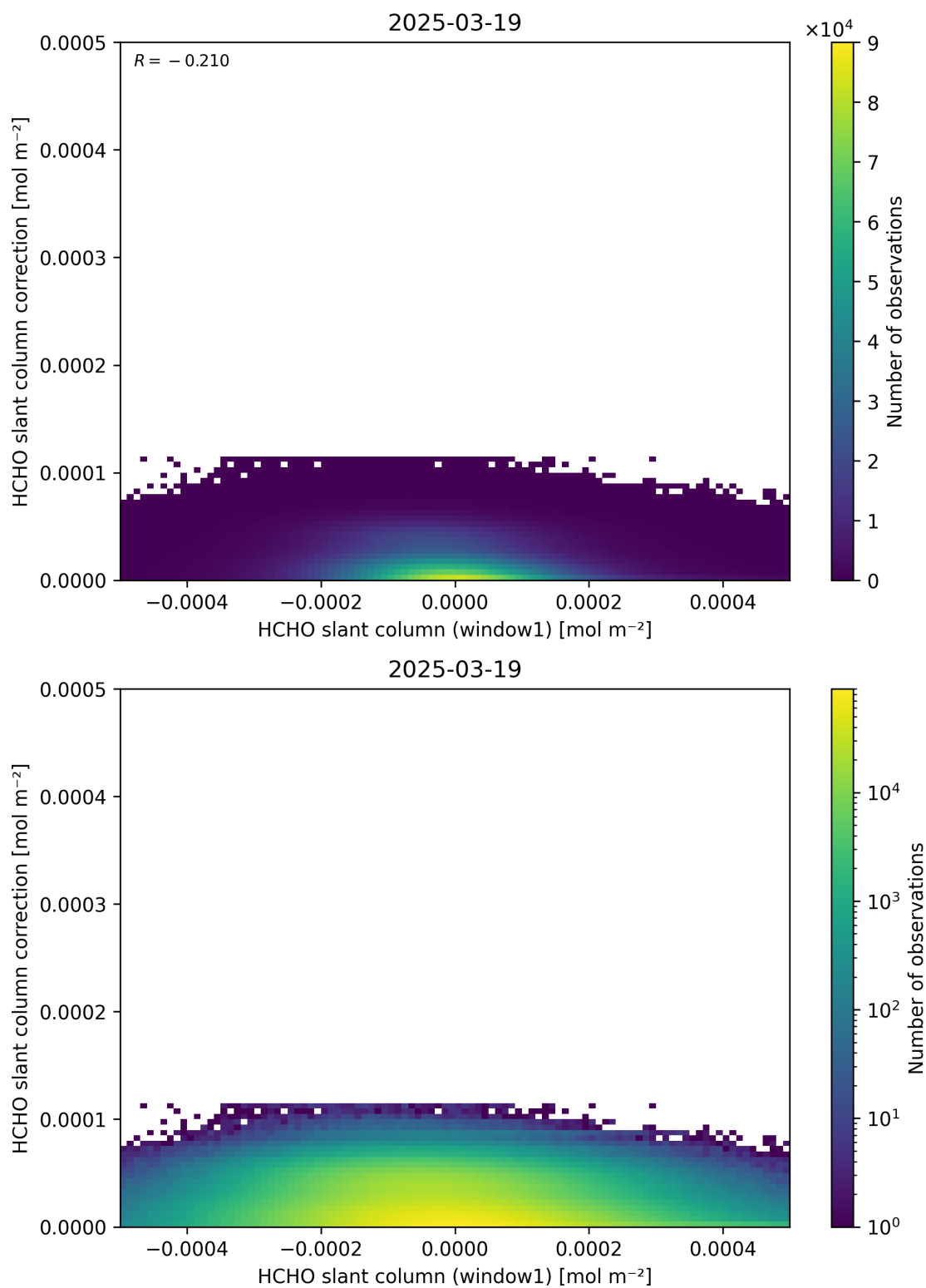
Figure 83: Scatter density plot of “HCHO slant column (window1)” against “HCHO slant column correction” for 2025-03-18 to 2025-03-20.
