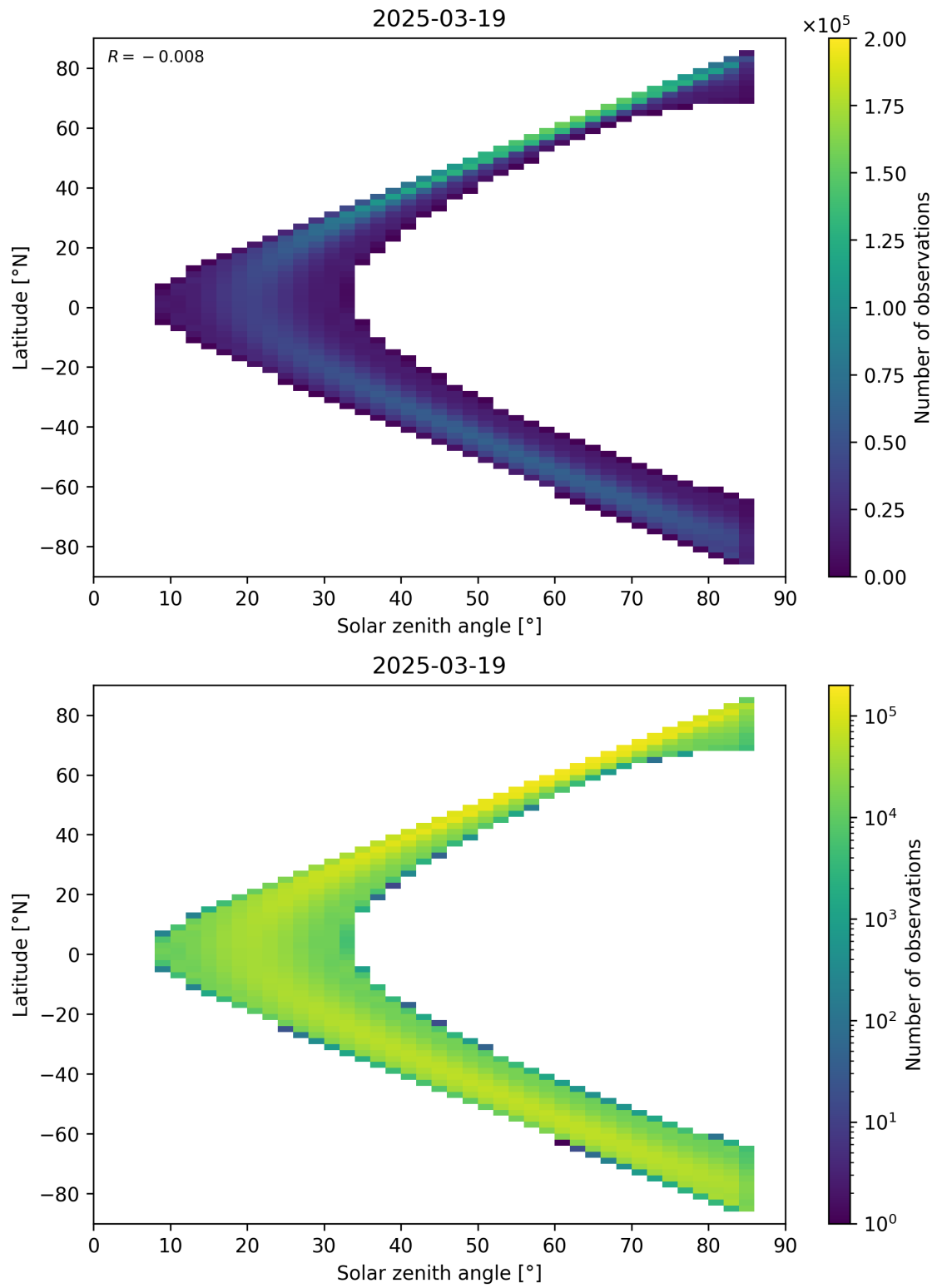
Figure 181: Scatter density plot of “Solar zenith angle” against “Latitude” for 2025-03-18 to 2025-03-20.
