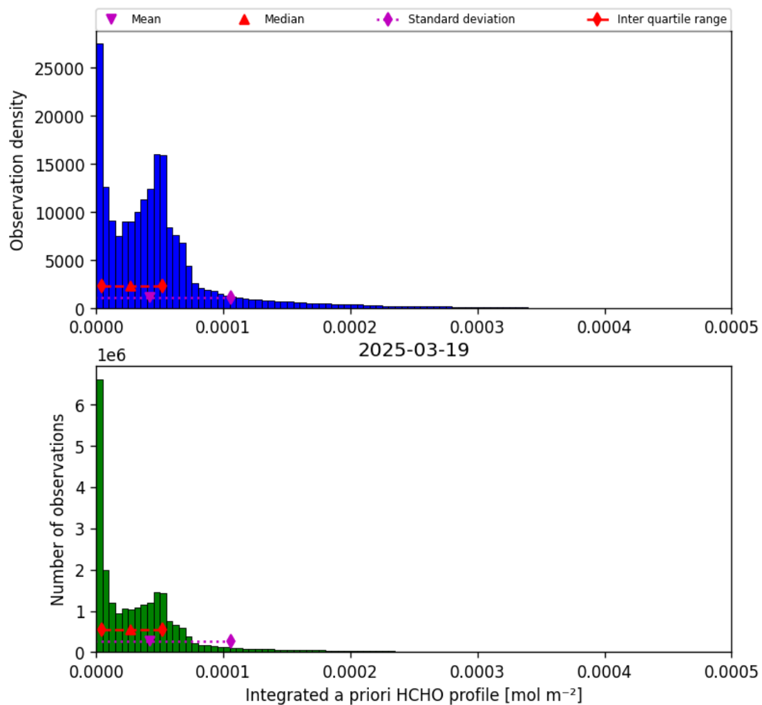
Figure 43: Histogram of “Integrated a priori HCHO profile” for 2025-03-18 to 2025-03-20
