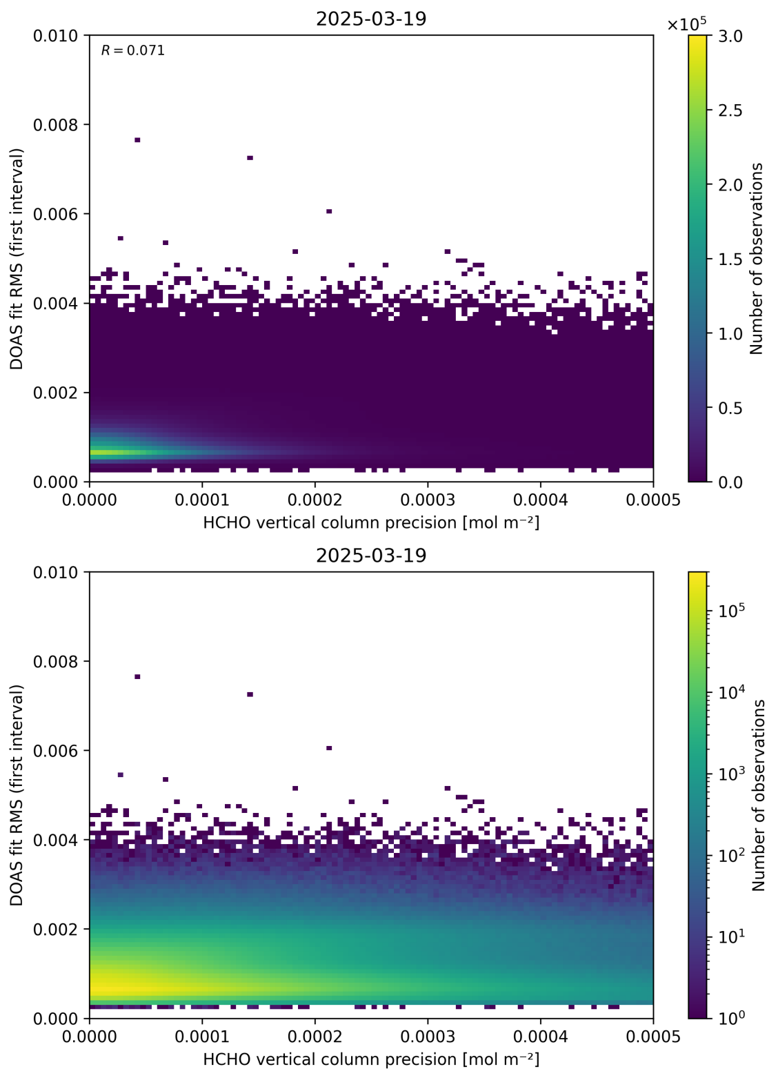
Figure 136: Scatter density plot of “HCHO vertical column precision” against “DOAS fit RMS (first interval)” for 2025-03-18 to 2025-03-20.
