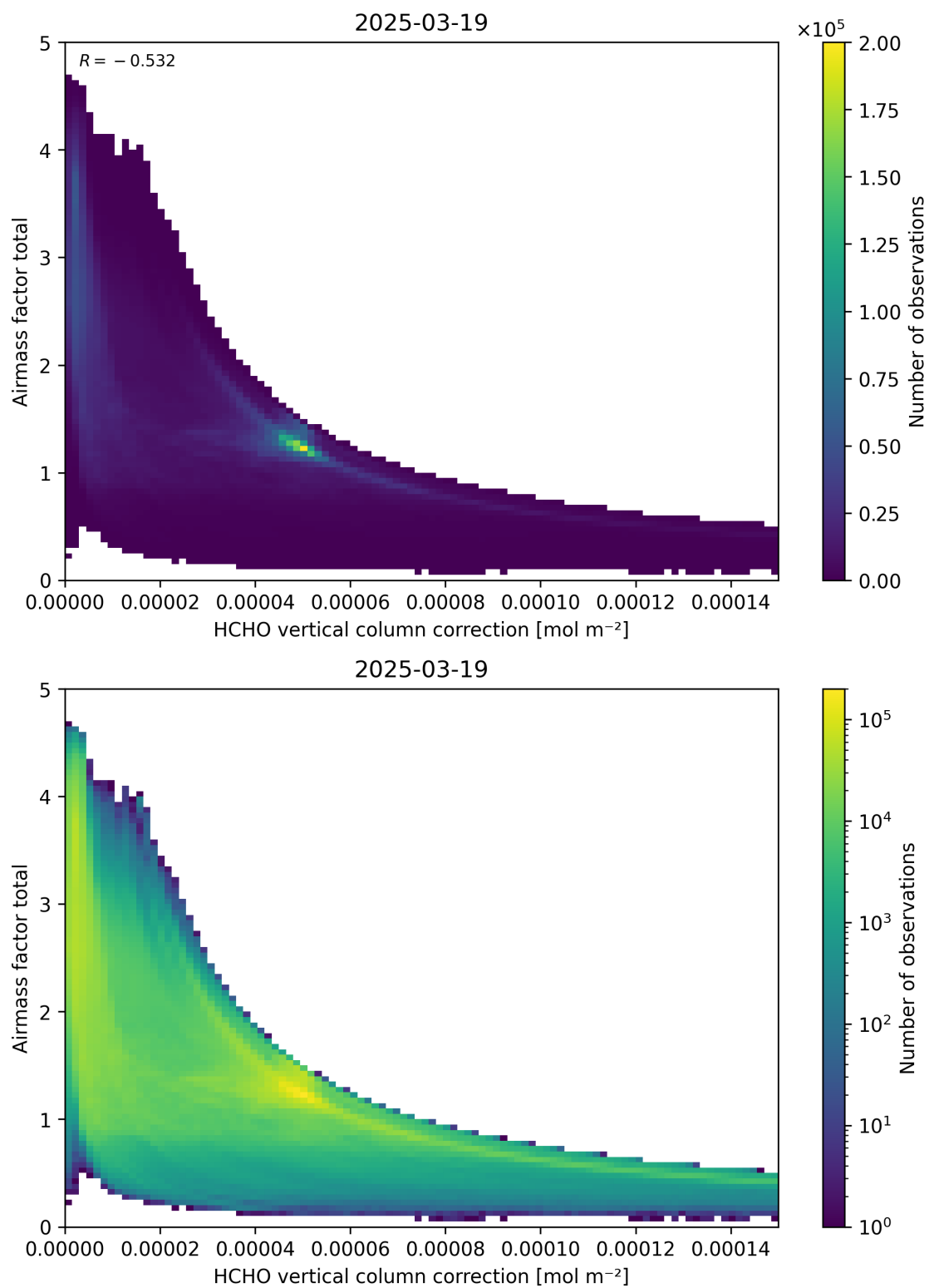
Figure 120: Scatter density plot of “HCHO vertical column correction” against “Airmass factor total” for 2025-03-18 to 2025-03-20.
