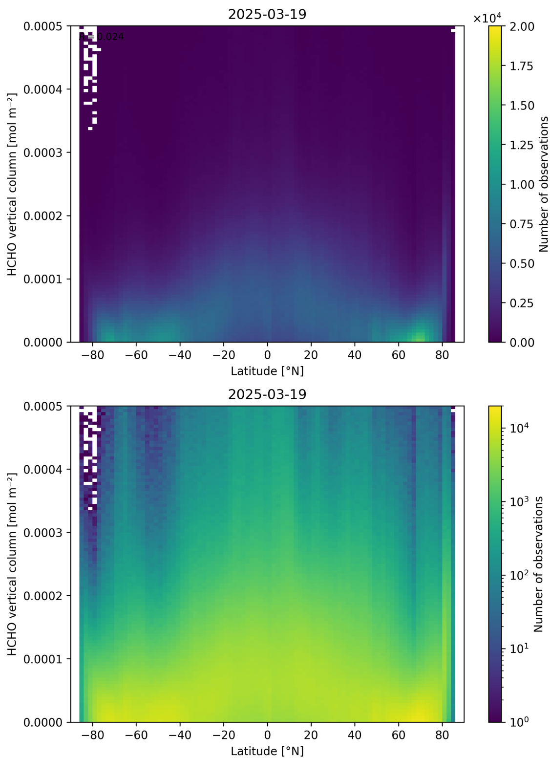
Figure 163: Scatter density plot of “Latitude” against “HCHO vertical column” for 2025-03-18 to 2025-03-20.
