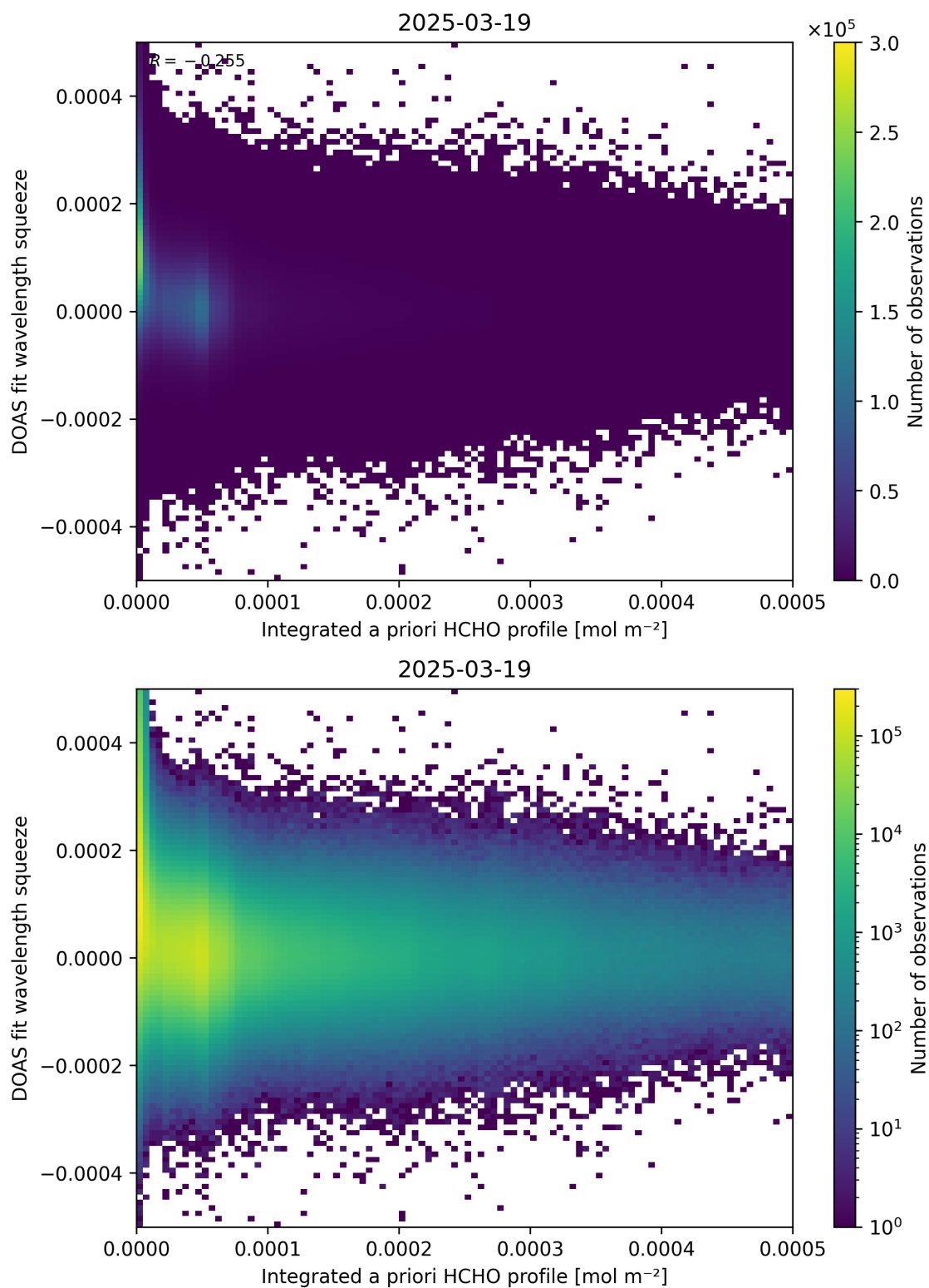
Figure 150: Scatter density plot of “Integrated a priori HCHO profile” against “DOAS fit wavelength squeeze” for 2025-03-18 to 2025-03-20.
