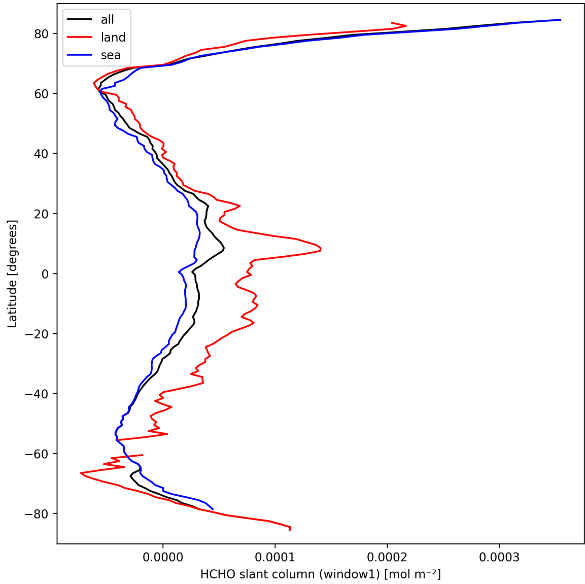
Figure 24: Zonal average of “HCHO slant column (window1)” for 2025-03-18 to 2025-03-20.
