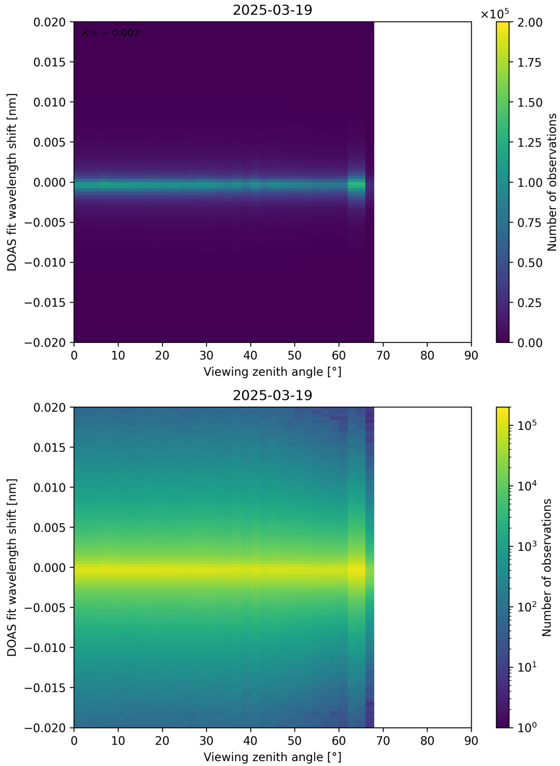
Figure 183: Scatter density plot of “Viewing zenith angle” against “DOAS fit wavelength shift” for 2025-03-18 to 2025-03-20.
