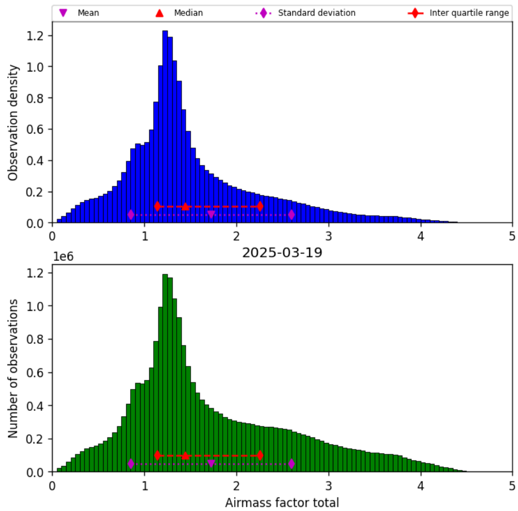
Figure 40: Histogram of “Airmass factor total” for 2025-03-18 to 2025-03-20
