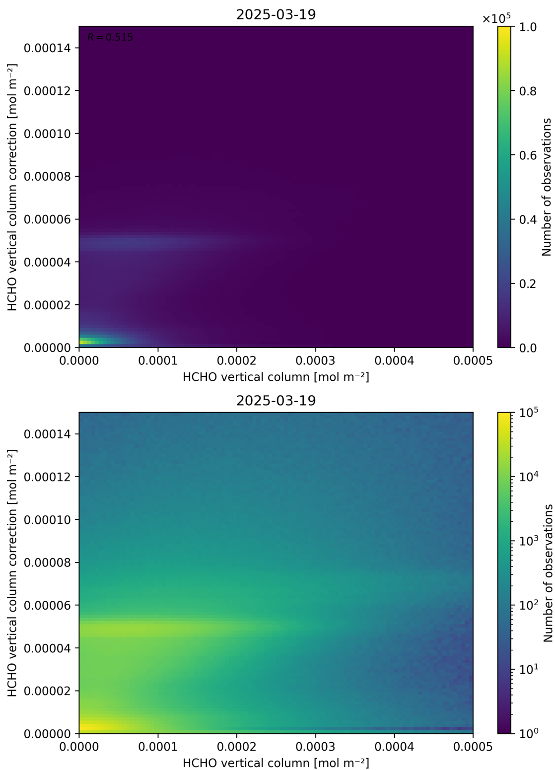
Figure 133: Scatter density plot of “HCHO vertical column” against “HCHO vertical column correction” for 2025-03-18 to 2025-03-20.
