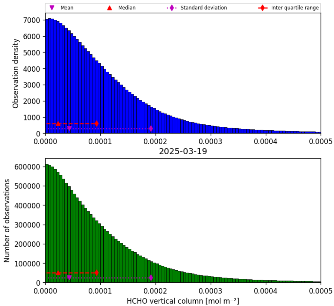
Figure 35: Histogram of “HCHO vertical column” for 2025-03-18 to 2025-03-20
