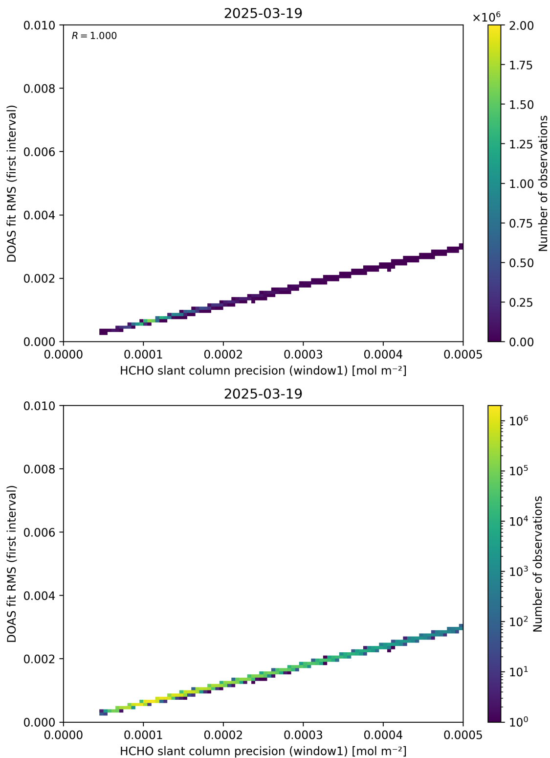
Figure 88: Scatter density plot of “HCHO slant column precision (window1)” against “DOAS fit RMS (first interval)” for 2025-03-18 to 2025-03-20.
