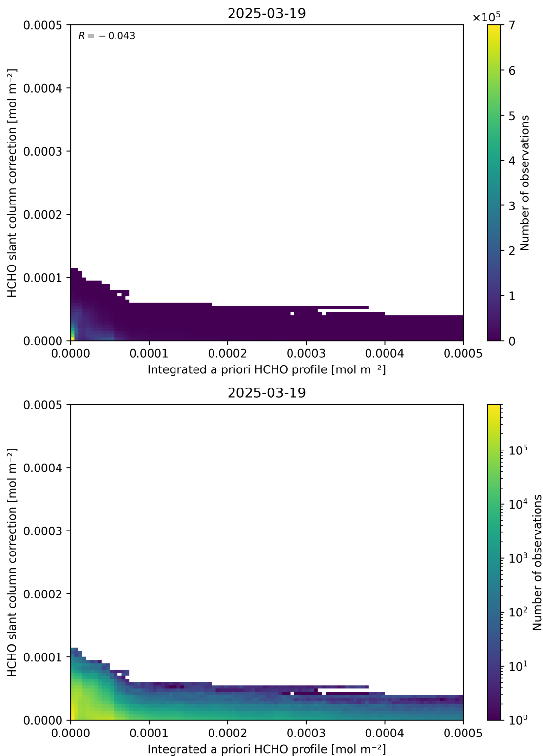
Figure 152: Scatter density plot of “Integrated a priori HCHO profile” against “HCHO slant column correction” for 2025-03-18 to 2025-03-20.
