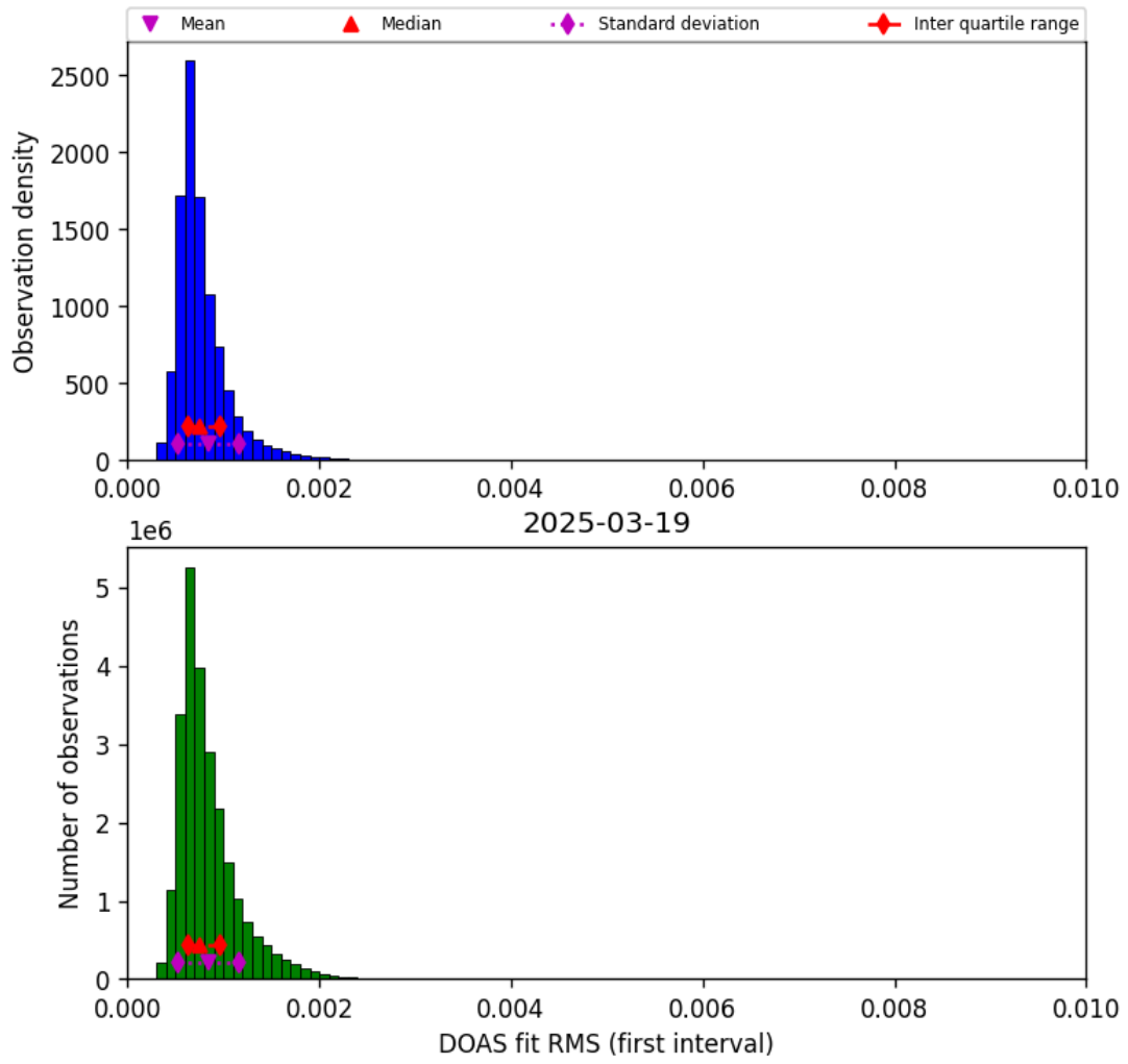
Figure 46: Histogram of “DOAS fit RMS (first interval)” for 2025-03-18 to 2025-03-20
