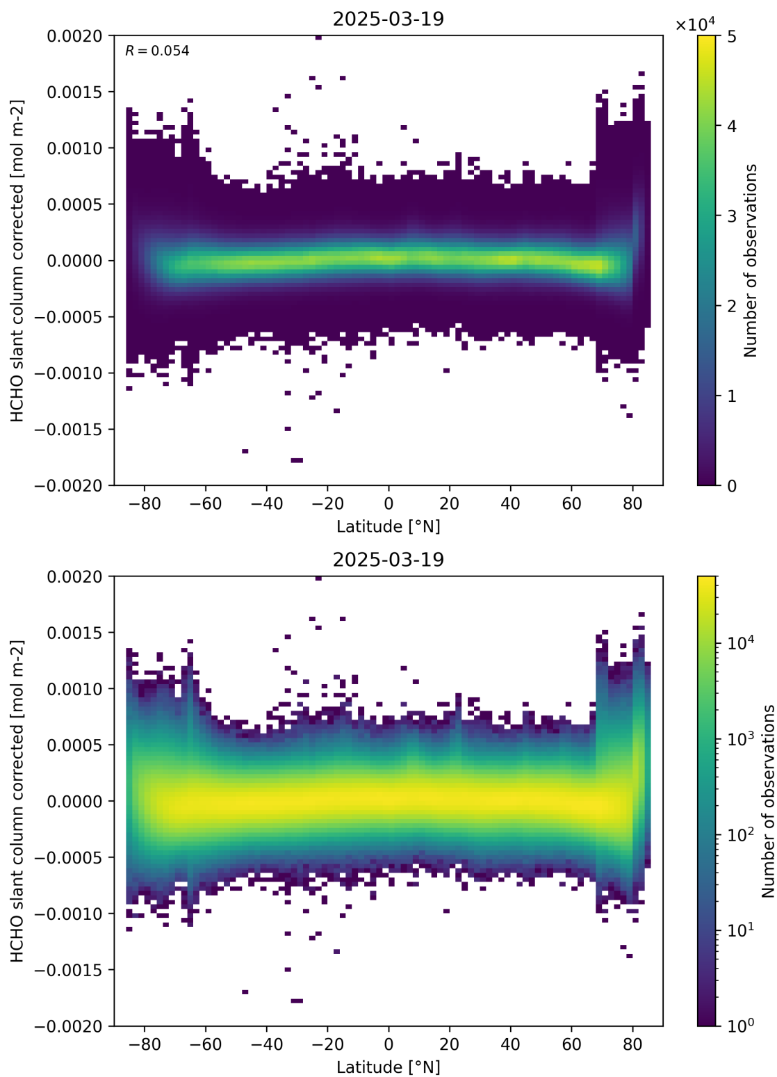
Figure 157: Scatter density plot of “Latitude” against “HCHO slant column corrected” for 2025-03-18 to 2025-03-20.
