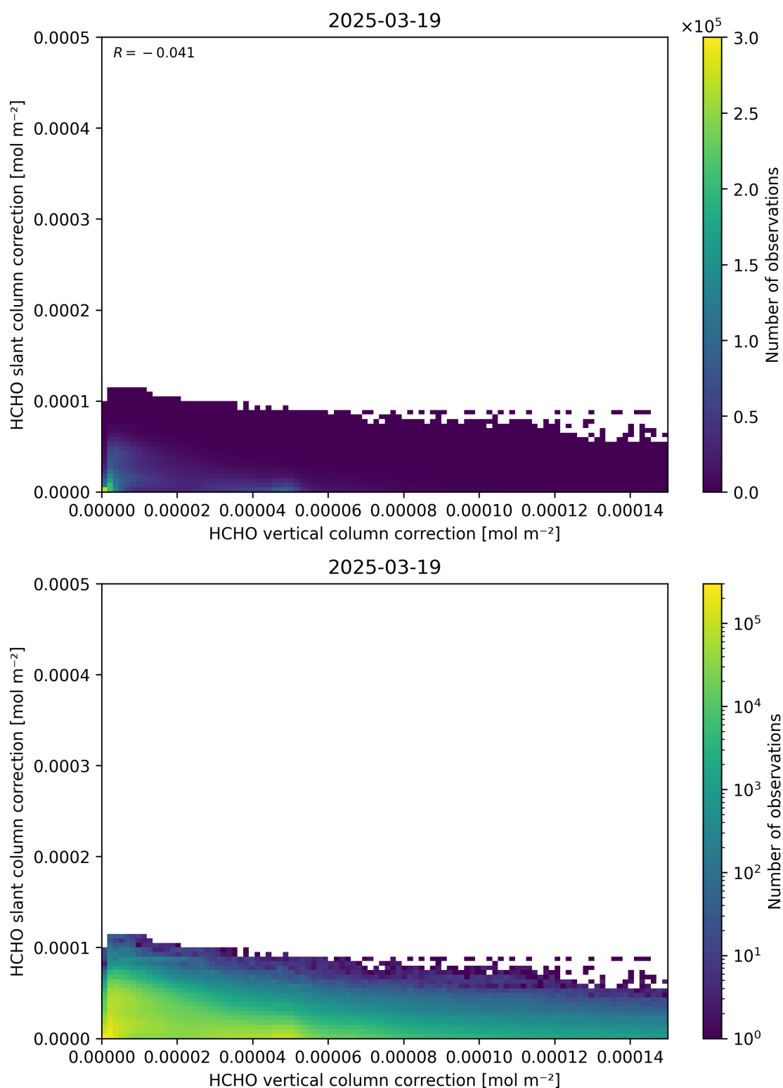
Figure 117: Scatter density plot of “HCHO vertical column correction” against “HCHO slant column correction” for 2025-03-18 to 2025-03-20.
