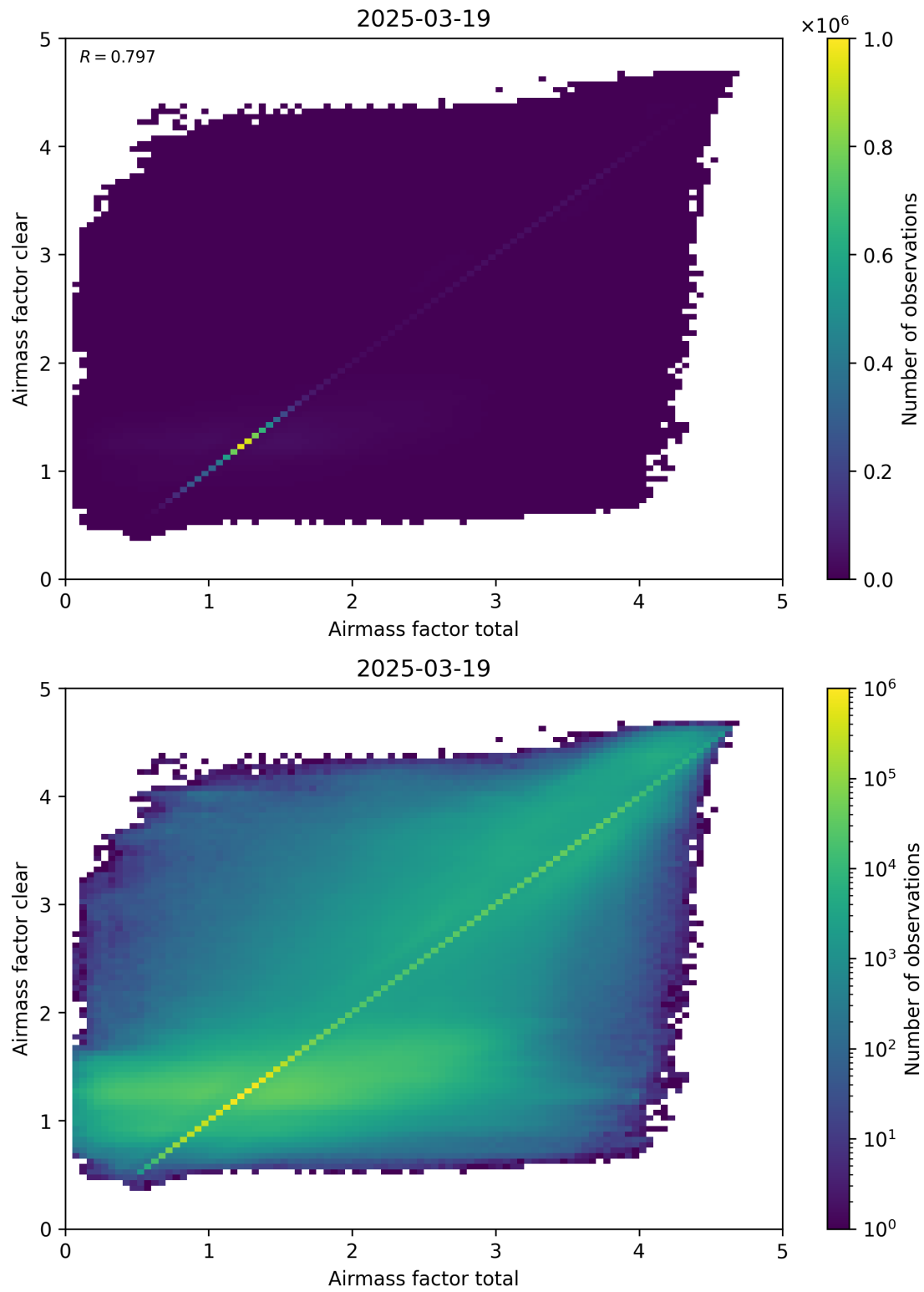
Figure 100: Scatter density plot of “Airmass factor total” against “Airmass factor clear” for 2025-03-18 to 2025-03-20.
