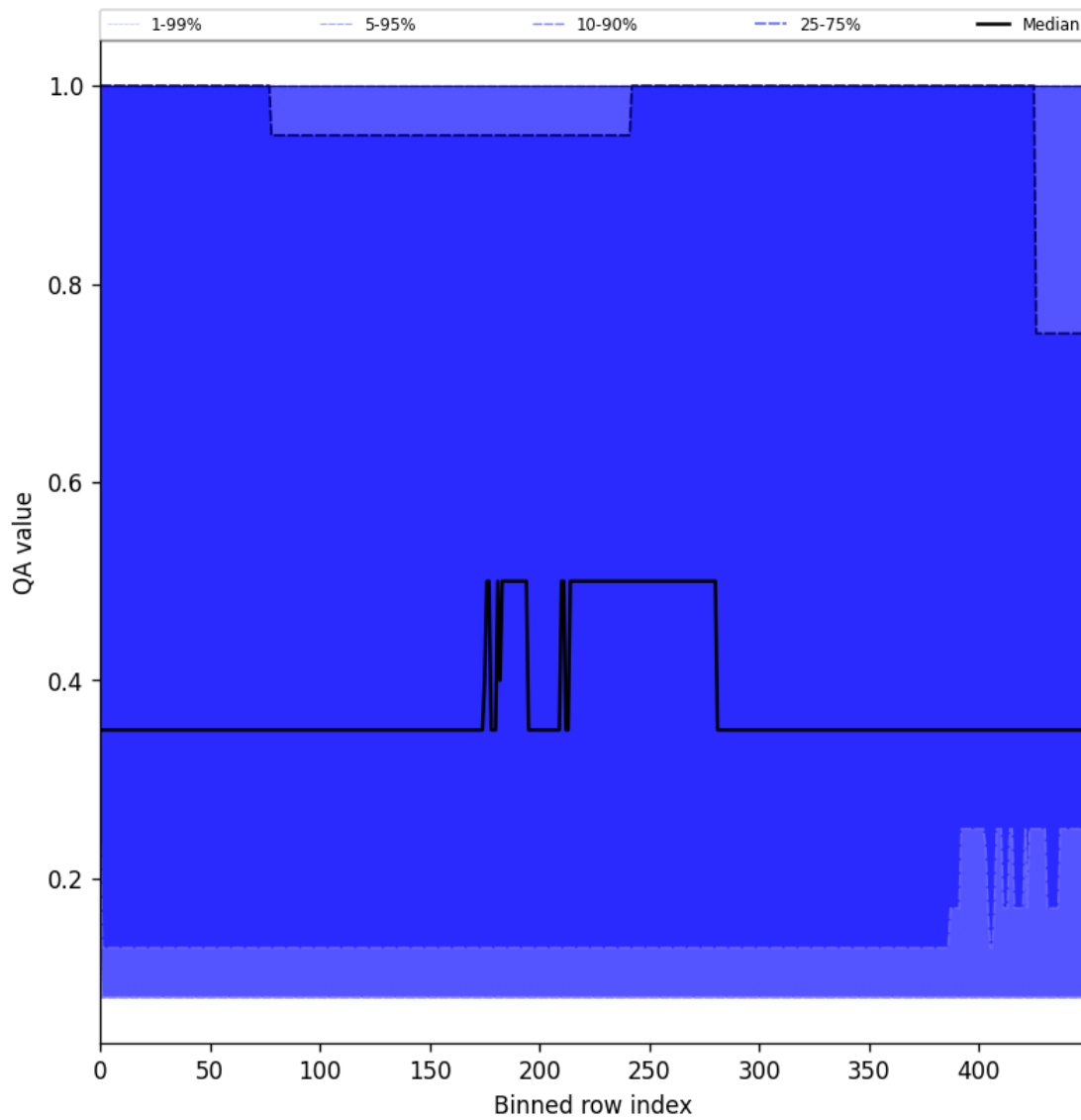
Figure 48: Along track statistics of “QA value” for 2025-03-18 to 2025-03-20
