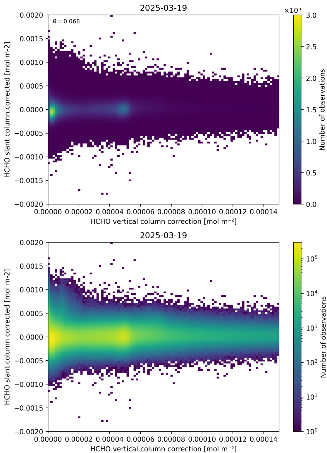
Figure 116: Scatter density plot of “HCHO vertical column correction” against “HCHO slant column corrected” for 2025-03-18 to 2025-03-20.
