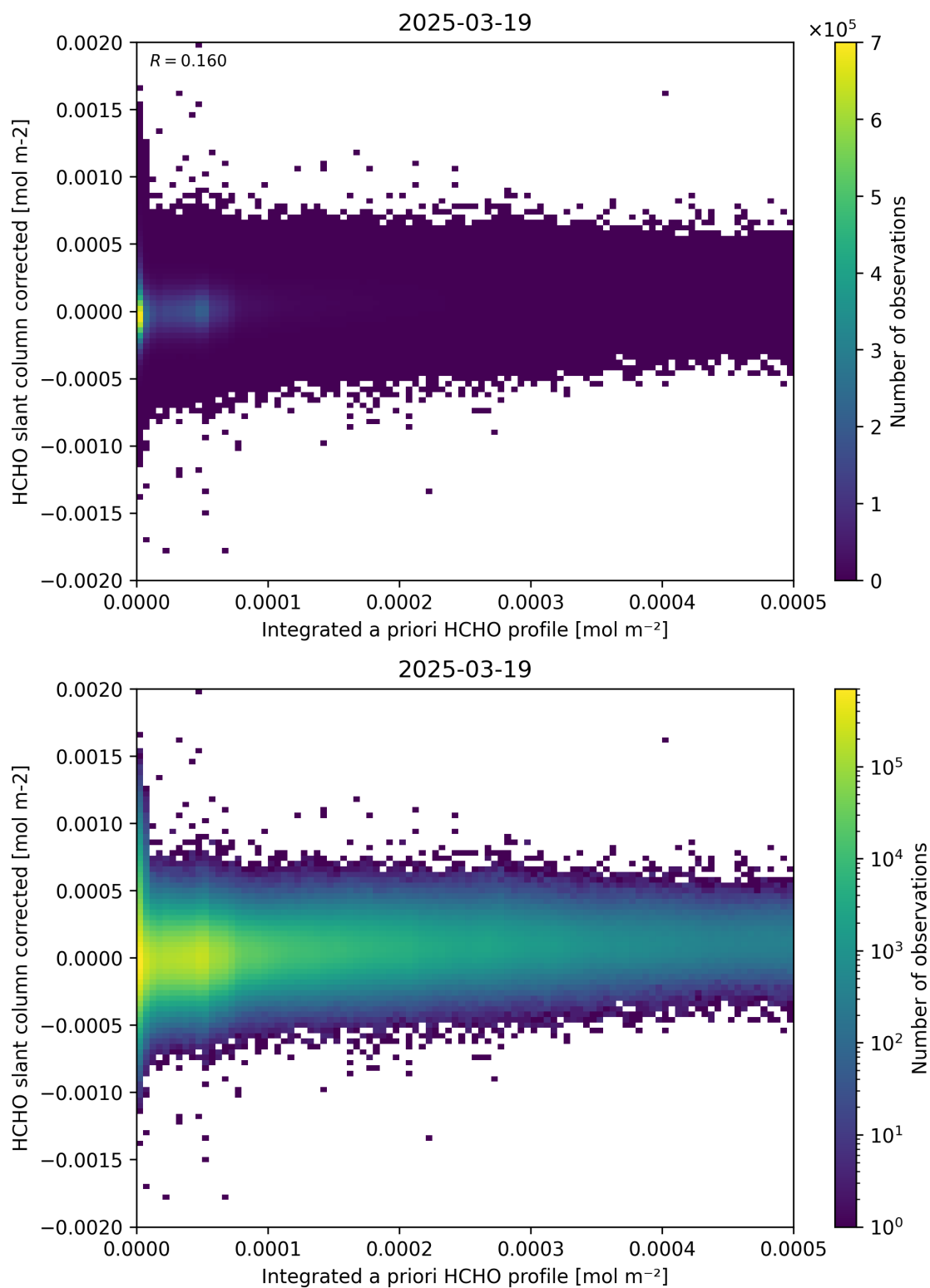
Figure 151: Scatter density plot of “Integrated a priori HCHO profile” against “HCHO slant column corrected” for 2025-03-18 to 2025-03-20.
