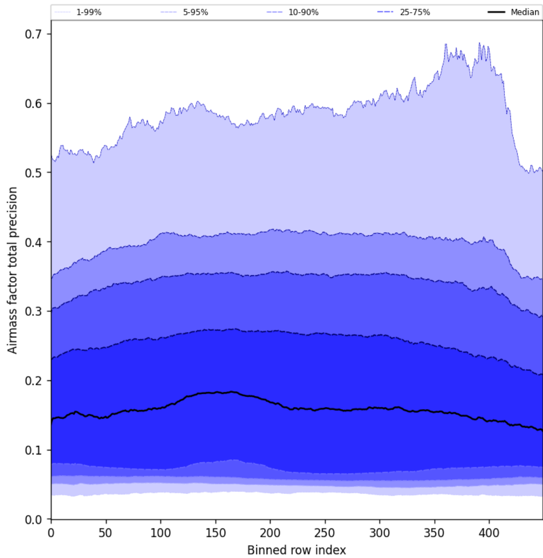
Figure 55: Along track statistics of “Airmass factor total precision” for 2025-03-18 to 2025-03-20
