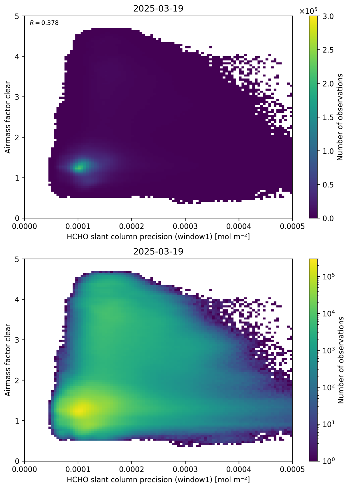
Figure 91: Scatter density plot of “HCHO slant column precision (window1)” against “Airmass factor clear” for 2025-03-18 to 2025-03-20.
