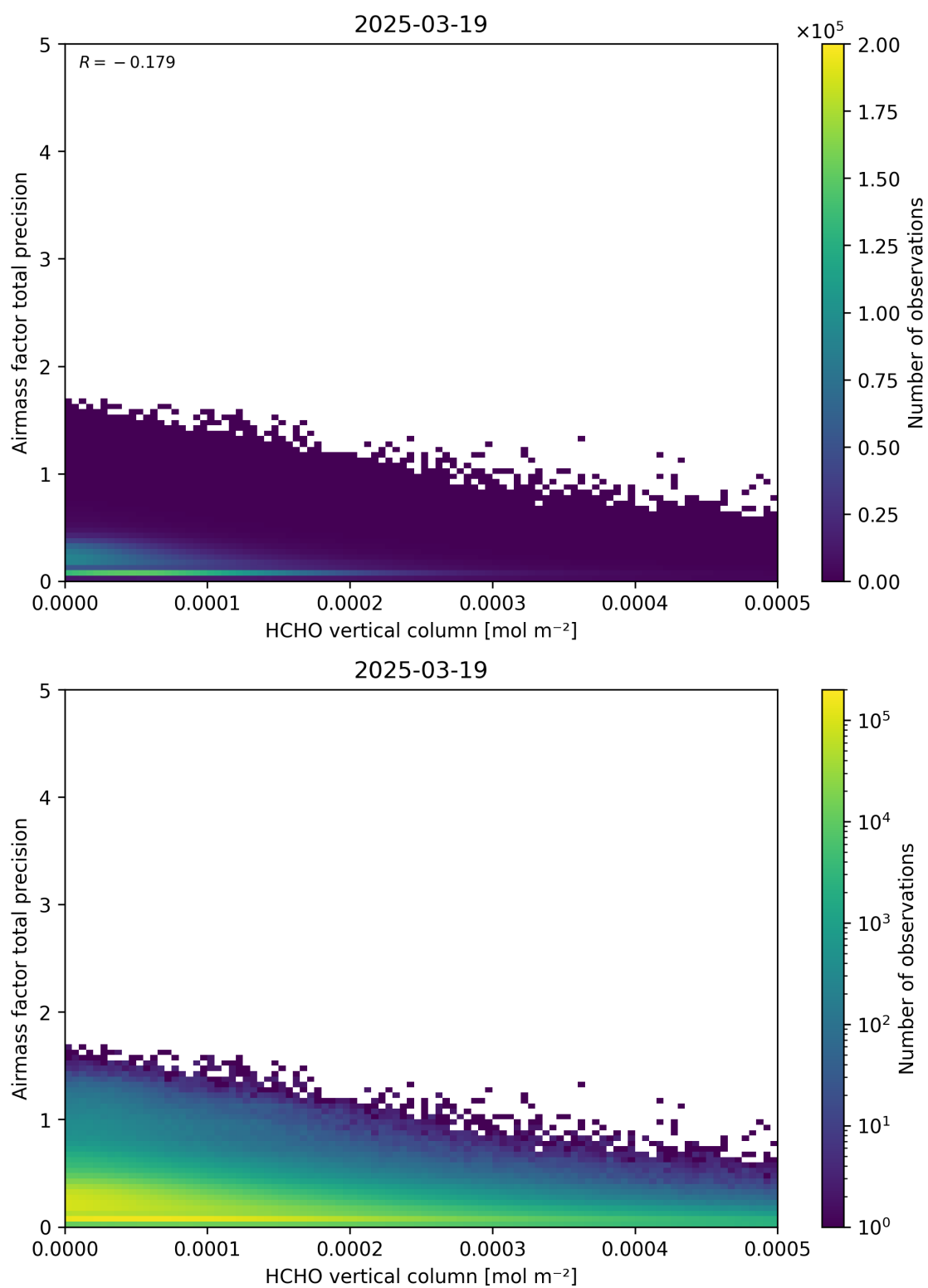
Figure 132: Scatter density plot of “HCHO vertical column” against “Airmass factor total precision” for 2025-03-18 to 2025-03-20.
