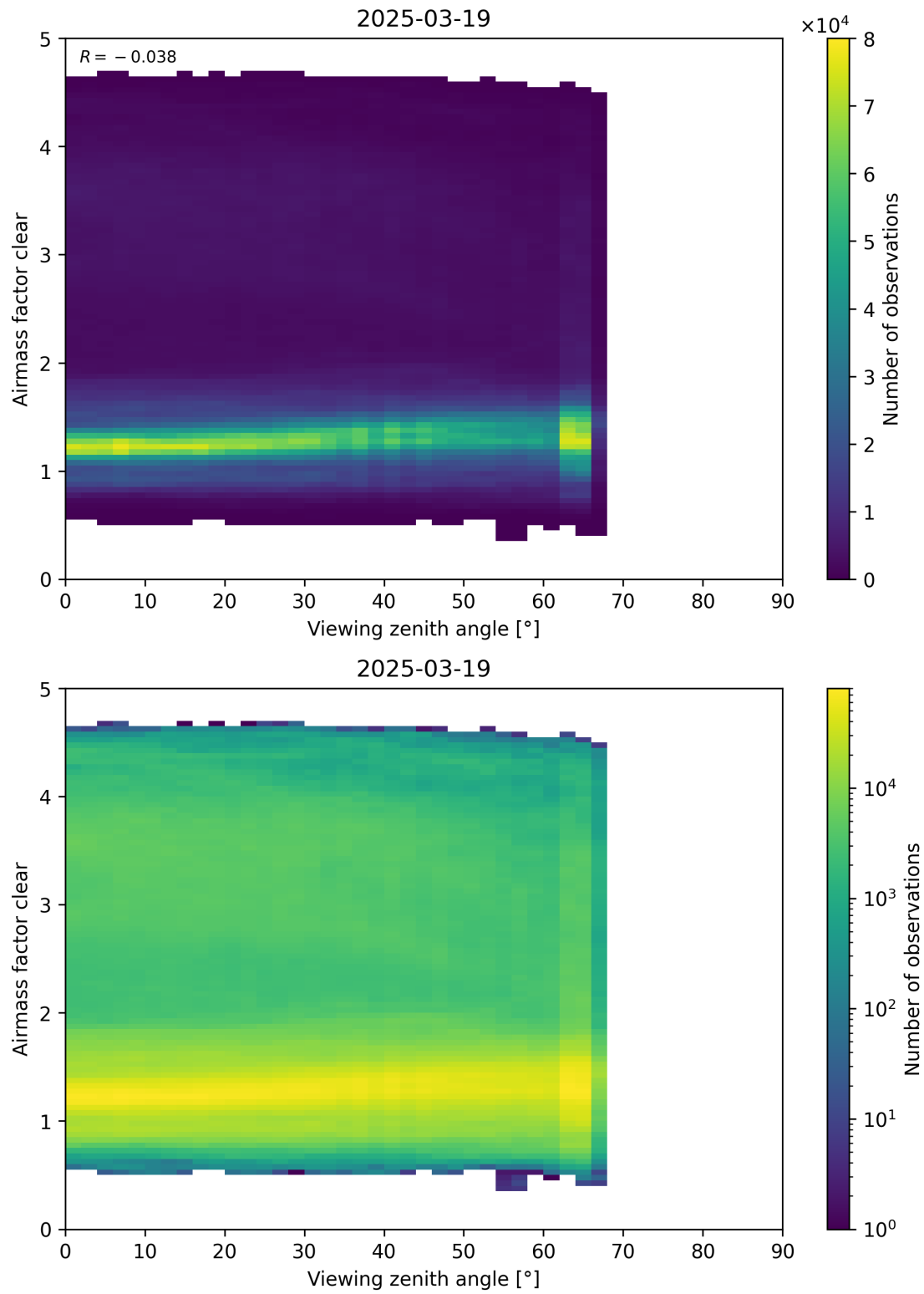
Figure 185: Scatter density plot of “Viewing zenith angle” against “Airmass factor clear” for 2025-03-18 to 2025-03-20.
