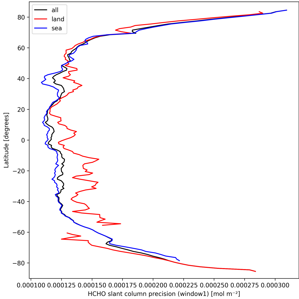
Figure 25: Zonal average of “HCHO slant column precision (window1)” for 2025-03-18 to 2025-03-20.
