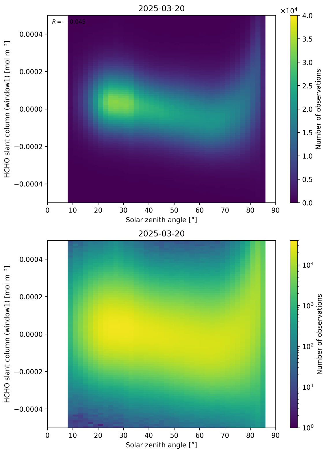
Figure 173: Scatter density plot of “Solar zenith angle” against “HCHO slant column (window1)” for 2025-03-19 to 2025-03-21.
