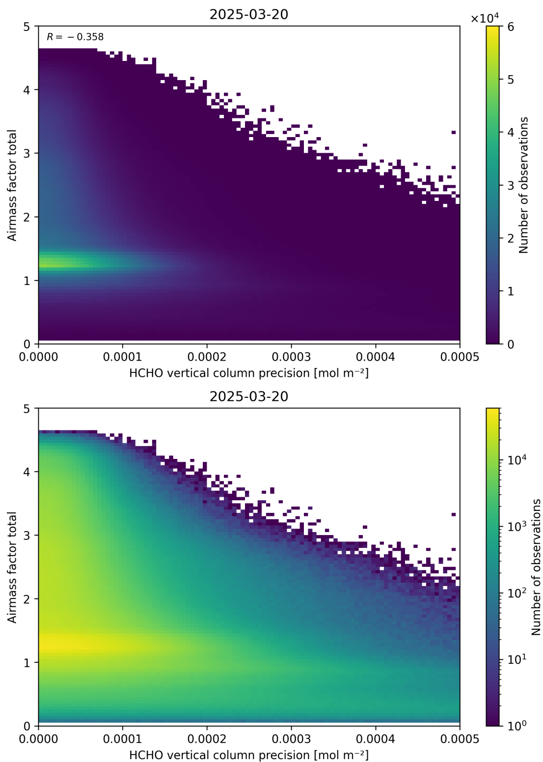
Figure 144: Scatter density plot of “HCHO vertical column precision” against “Airmass factor total” for 2025-03-19 to 2025-03-21.
