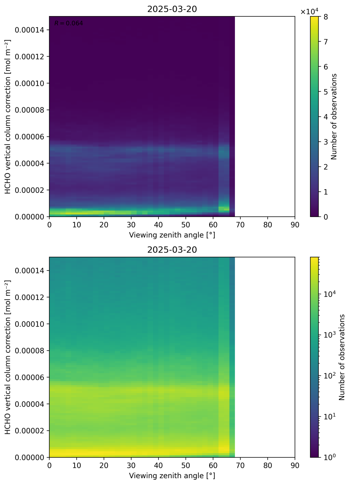
Figure 193: Scatter density plot of “Viewing zenith angle” against “HCHO vertical column correction” for 2025-03-19 to 2025-03-21.
