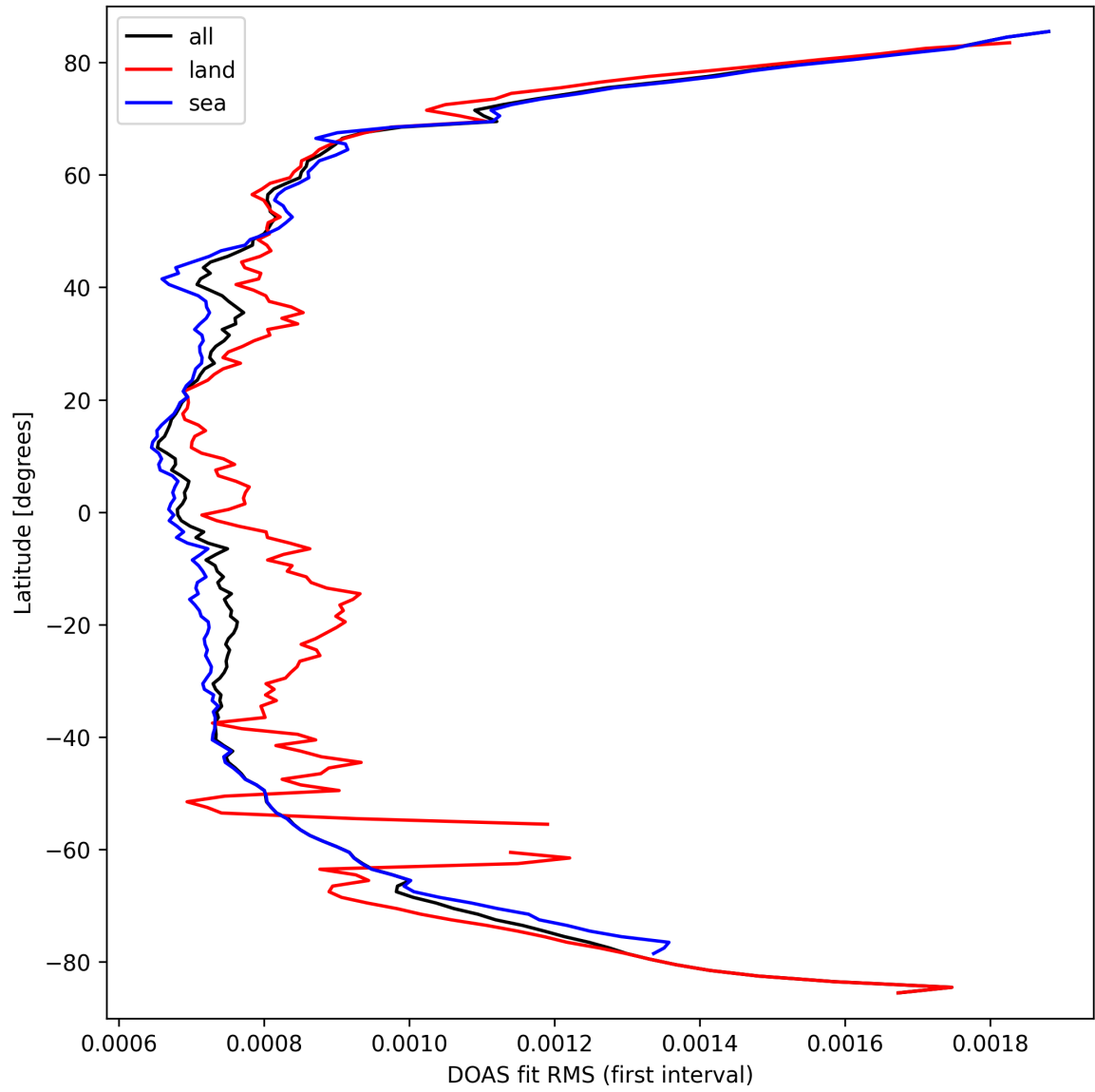
Figure 32: Zonal average of “DOAS fit RMS (first interval)” for 2025-03-19 to 2025-03-21.
