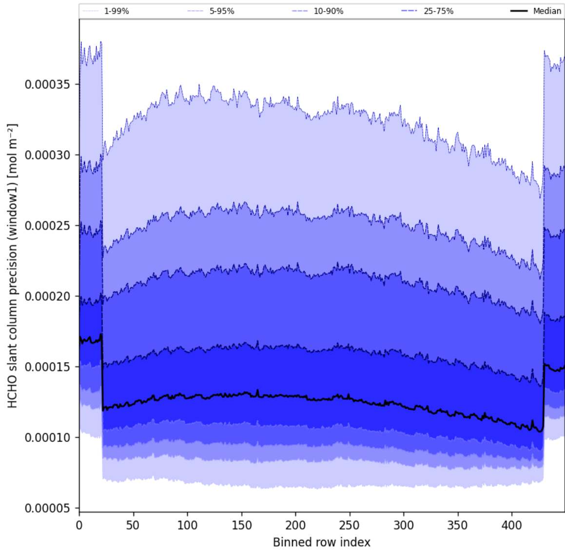
Figure 53: Along track statistics of “HCHO slant column precision (window1)” for 2025-03-19 to 2025-03-21
