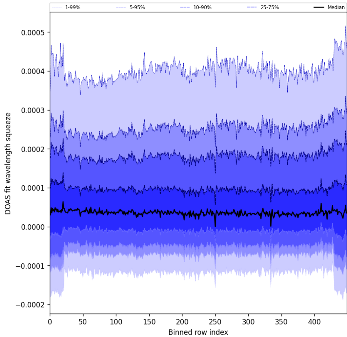
Figure 59: Along track statistics of “DOAS fit wavelength squeeze” for 2025-03-19 to 2025-03-21
