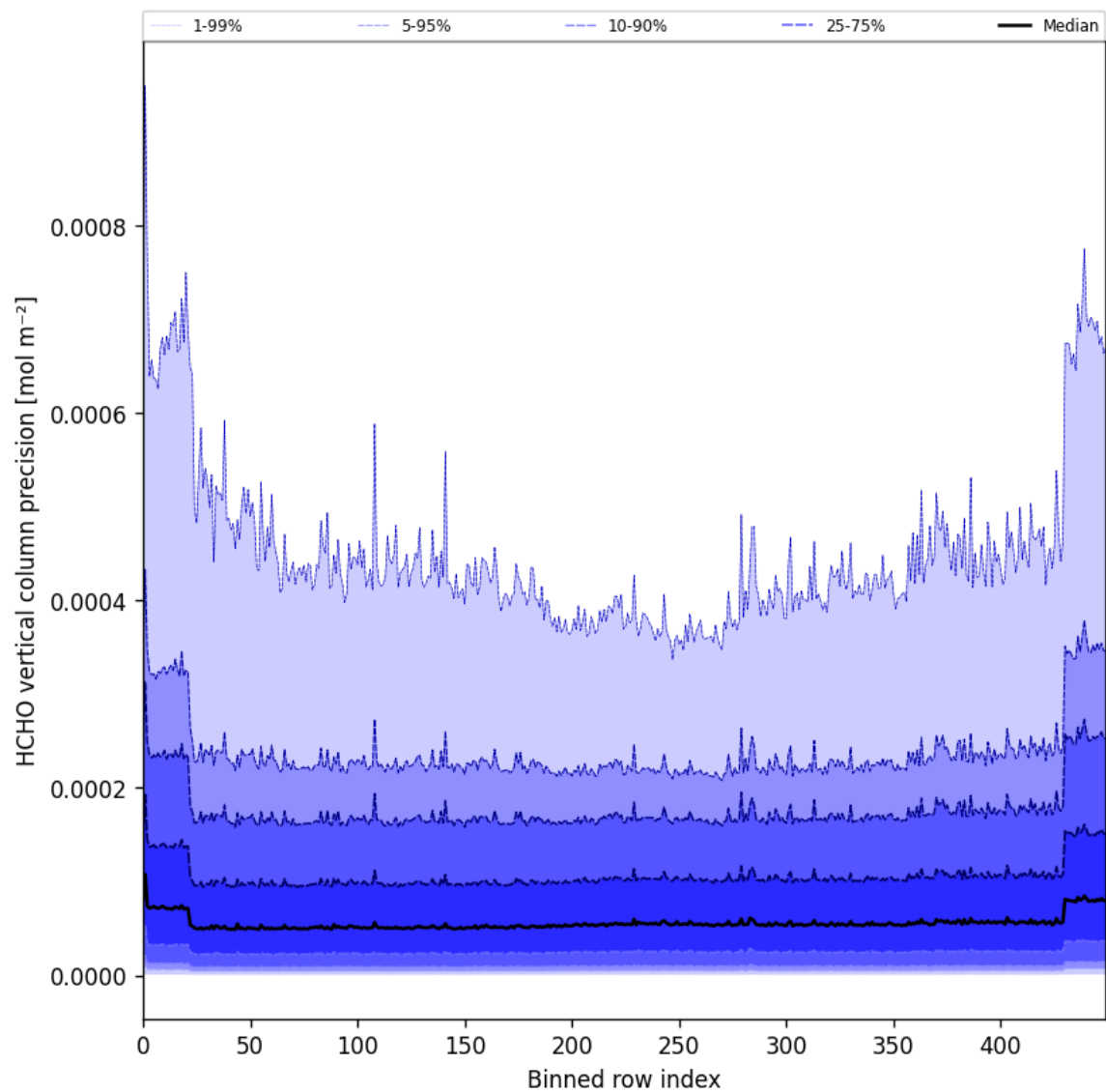
Figure 50: Along track statistics of “HCHO vertical column precision” for 2025-03-19 to 2025-03-21
