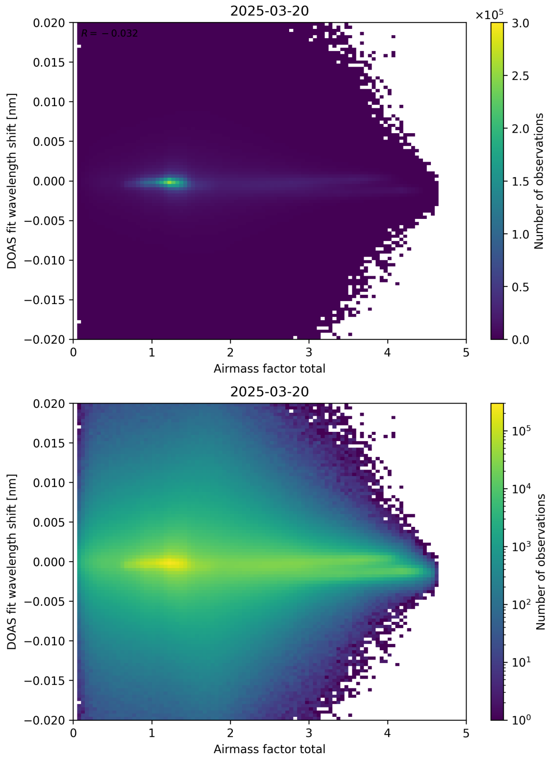
Figure 98: Scatter density plot of “Airmass factor total” against “DOAS fit wavelength shift” for 2025-03-19 to 2025-03-21.
