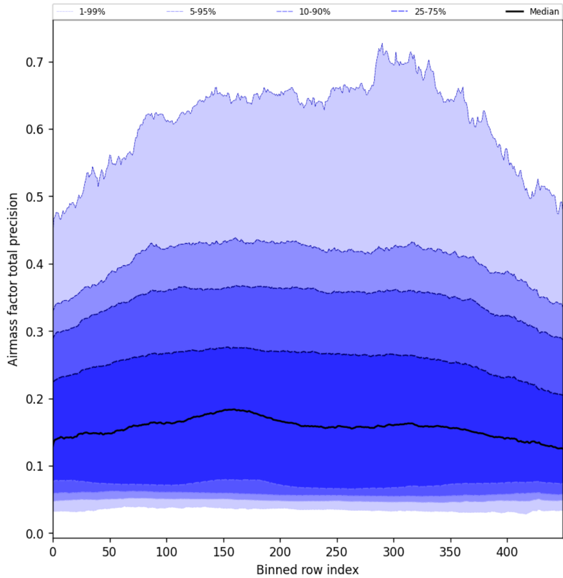
Figure 55: Along track statistics of “Airmass factor total precision” for 2025-03-19 to 2025-03-21
