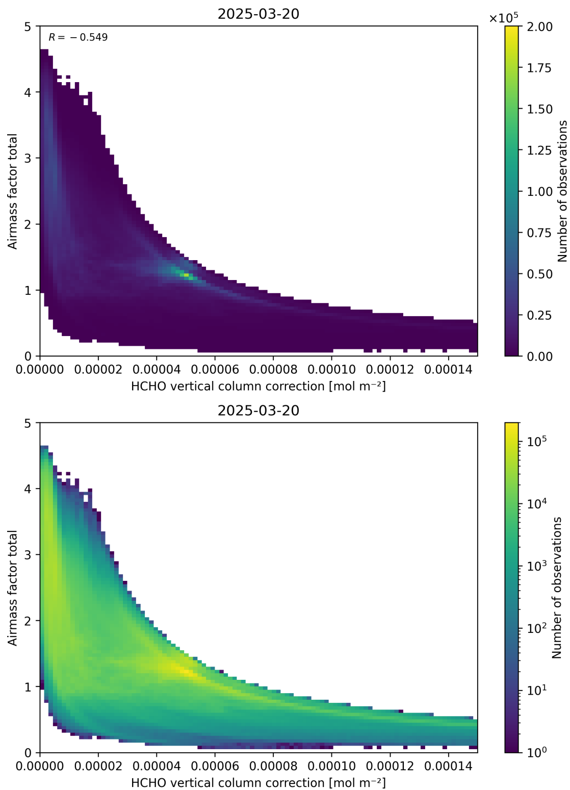
Figure 120: Scatter density plot of “HCHO vertical column correction” against “Airmass factor total” for 2025-03-19 to 2025-03-21.
