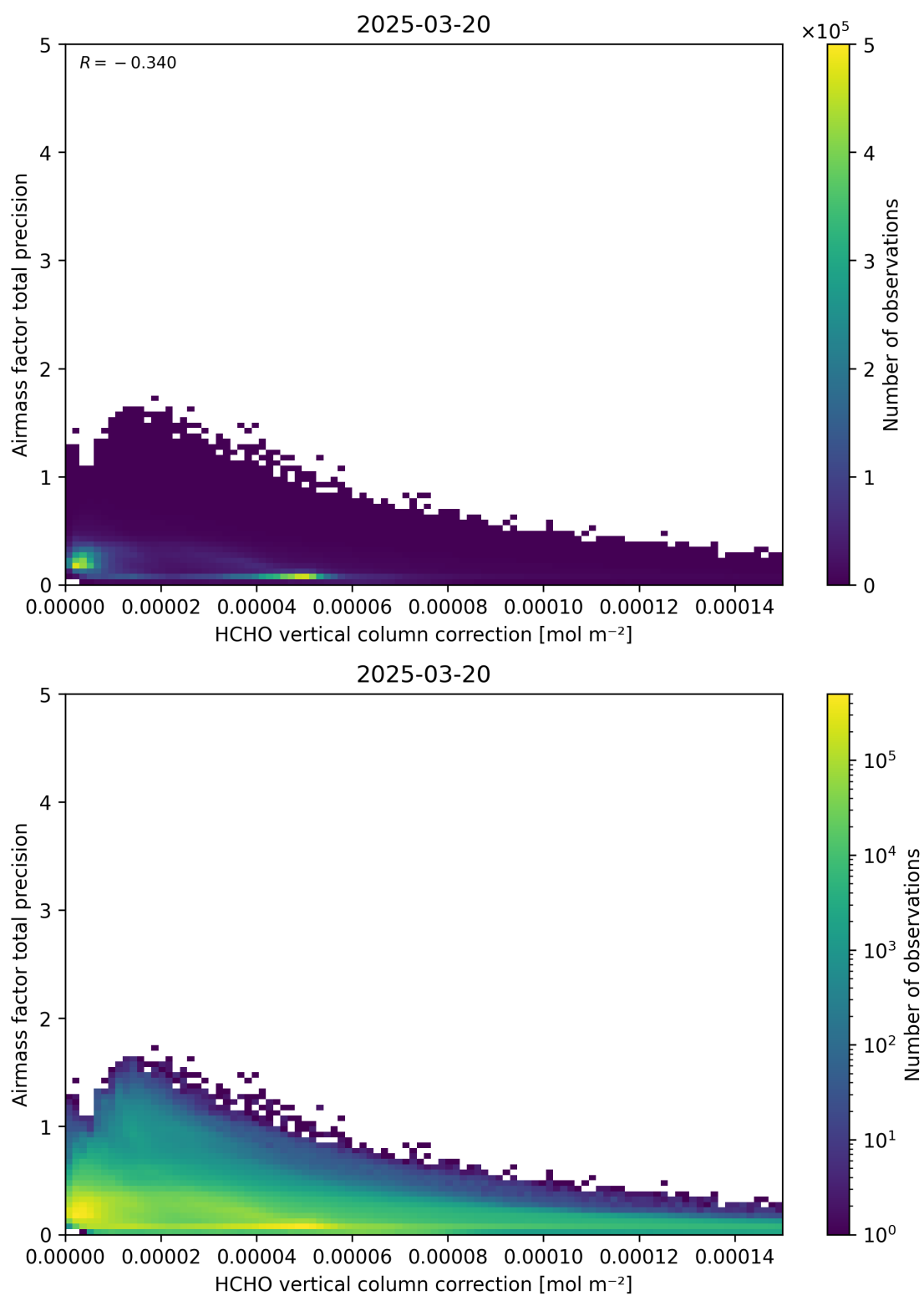
Figure 121: Scatter density plot of “HCHO vertical column correction” against “Airmass factor total precision” for 2025-03-19 to 2025-03-21.
