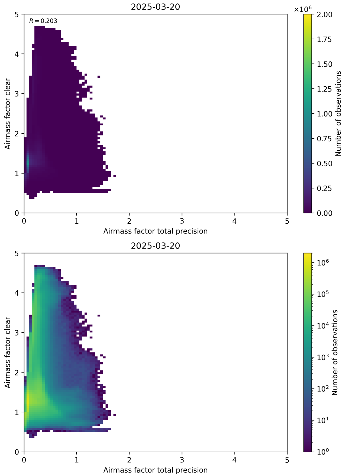
Figure 108: Scatter density plot of “Airmass factor total precision” against “Airmass factor clear” for 2025-03-19 to 2025-03-21.
