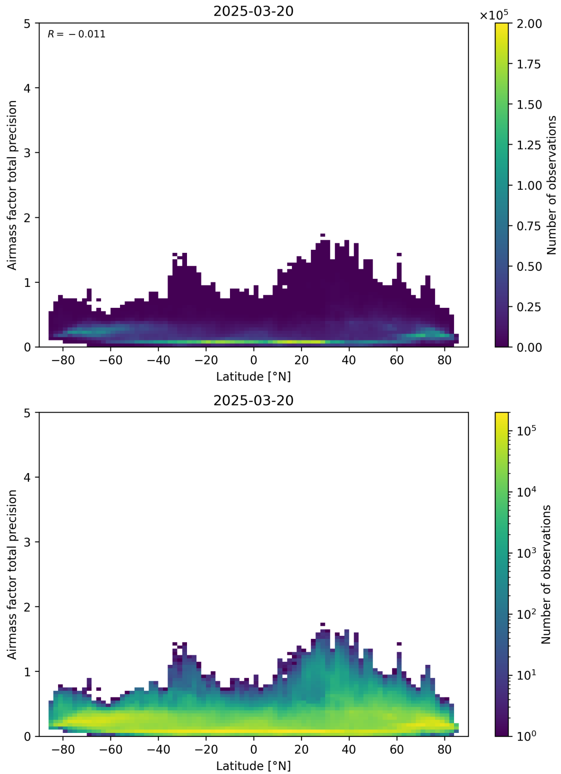
Figure 162: Scatter density plot of “Latitude” against “Airmass factor total precision” for 2025-03-19 to 2025-03-21.
