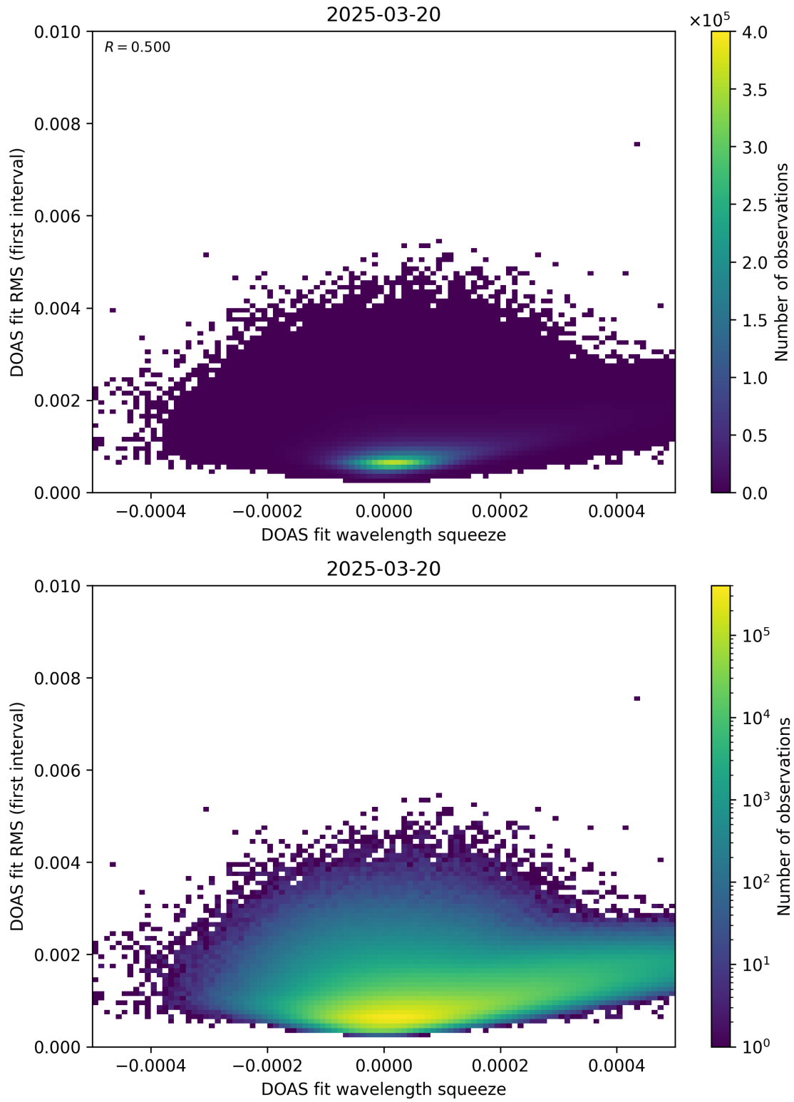
Figure 68: Scatter density plot of “DOAS fit wavelength squeeze” against “DOAS fit RMS (first interval)” for 2025-03-19 to 2025-03-21.
