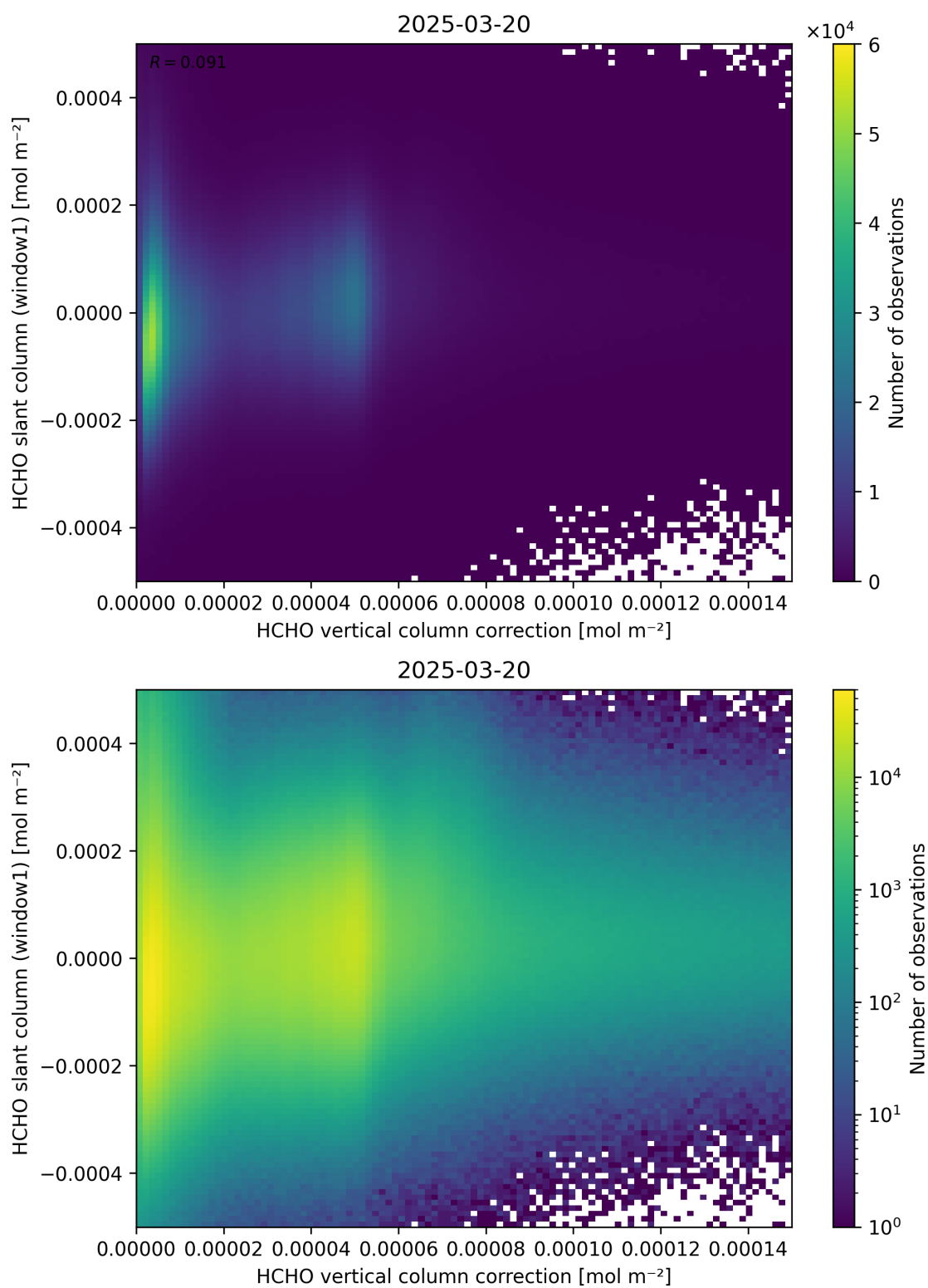
Figure 118: Scatter density plot of “HCHO vertical column correction” against “HCHO slant column (window1)” for 2025-03-19 to 2025-03-21.
