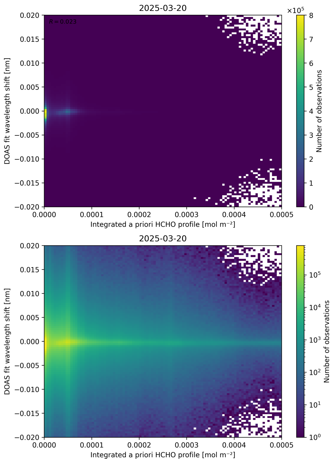
Figure 149: Scatter density plot of “Integrated a priori HCHO profile” against “DOAS fit wavelength shift” for 2025-03-19 to 2025-03-21.
