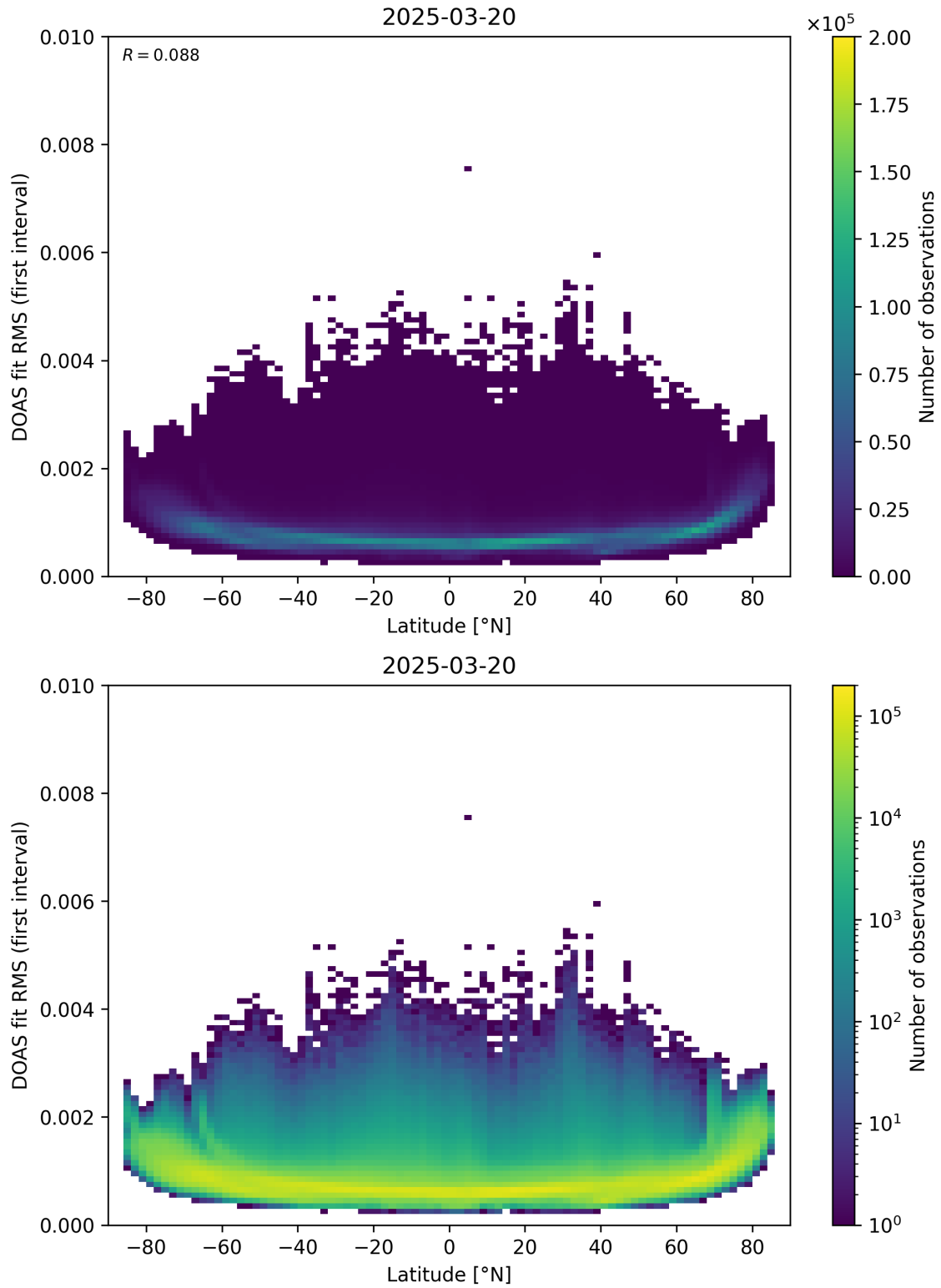
Figure 153: Scatter density plot of “Latitude” against “DOAS fit RMS (first interval)” for 2025-03-19 to 2025-03-21.
