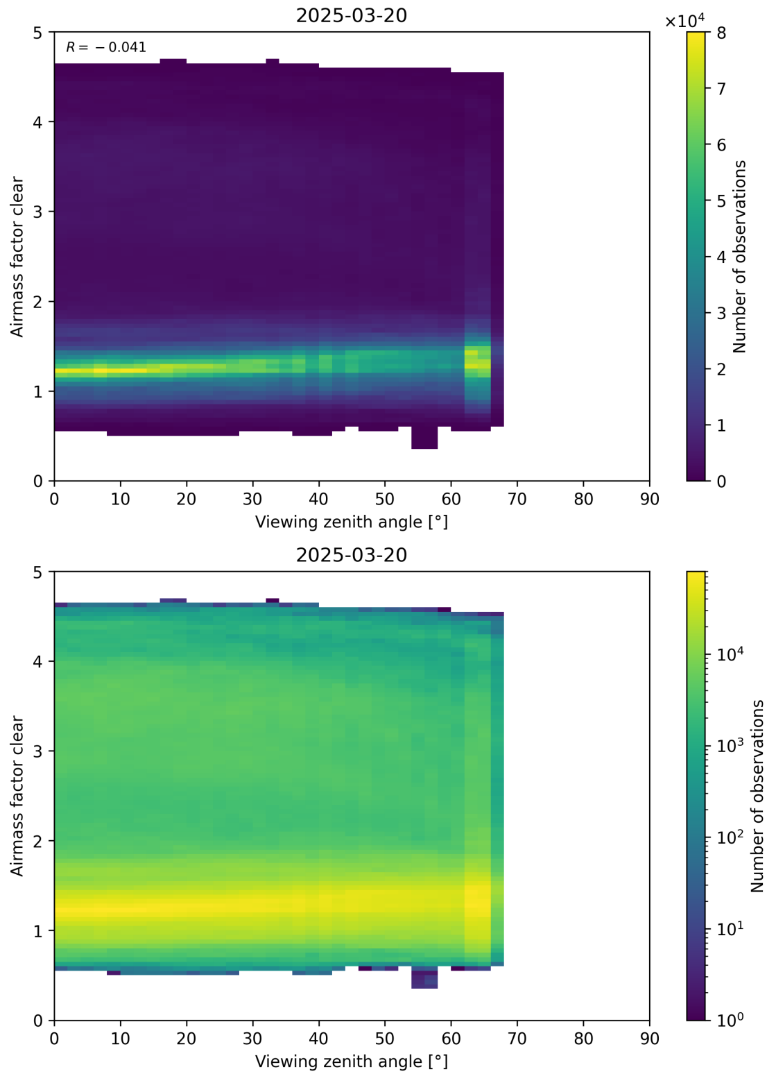
Figure 185: Scatter density plot of “Viewing zenith angle” against “Airmass factor clear” for 2025-03-19 to 2025-03-21.
