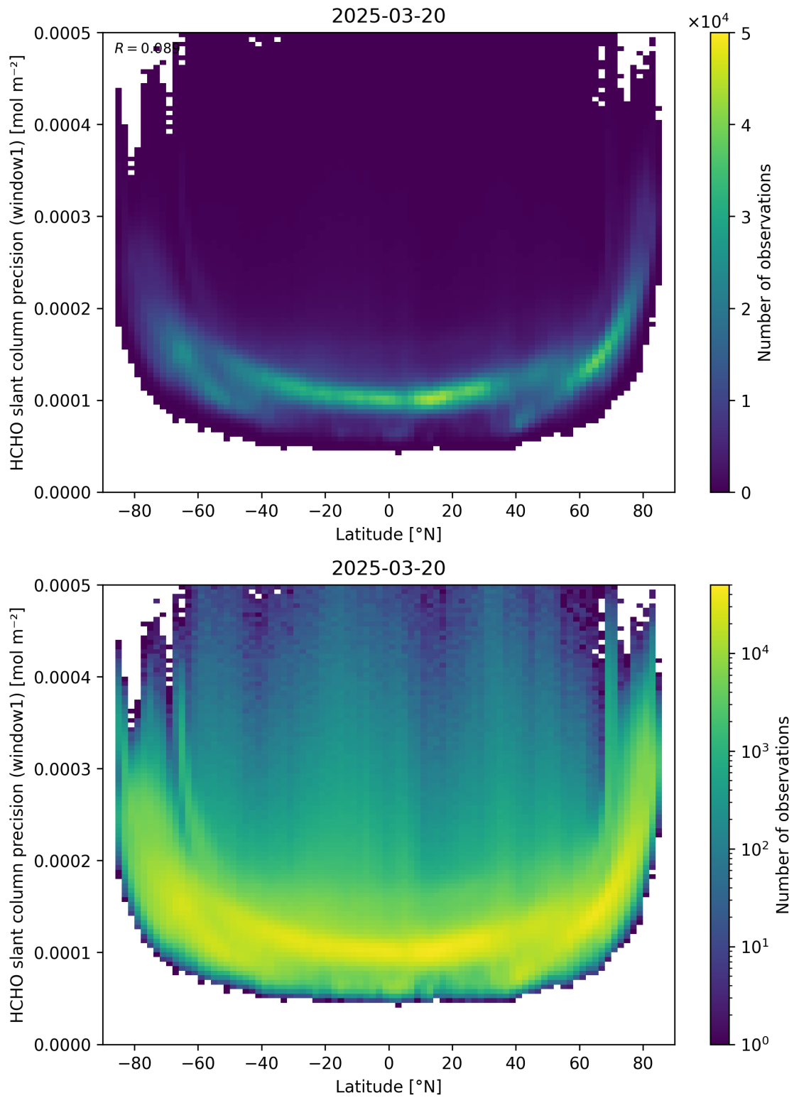
Figure 160: Scatter density plot of “Latitude” against “HCHO slant column precision (window1)” for 2025-03-19 to 2025-03-21.
