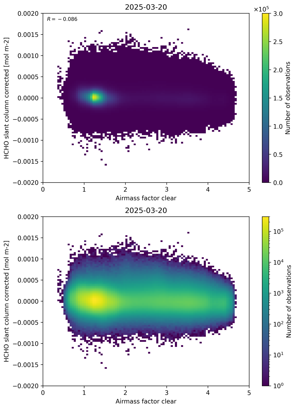
Figure 74: Scatter density plot of “Airmass factor clear” against “HCHO slant column corrected” for 2025-03-19 to 2025-03-21.
