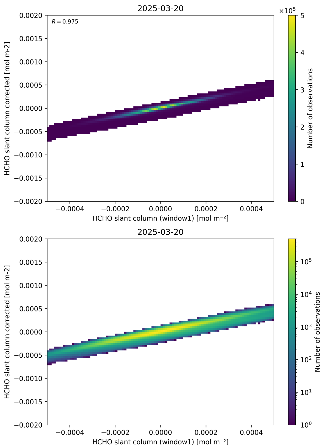
Figure 82: Scatter density plot of “HCHO slant column (window1)” against “HCHO slant column corrected” for 2025-03-19 to 2025-03-21.
