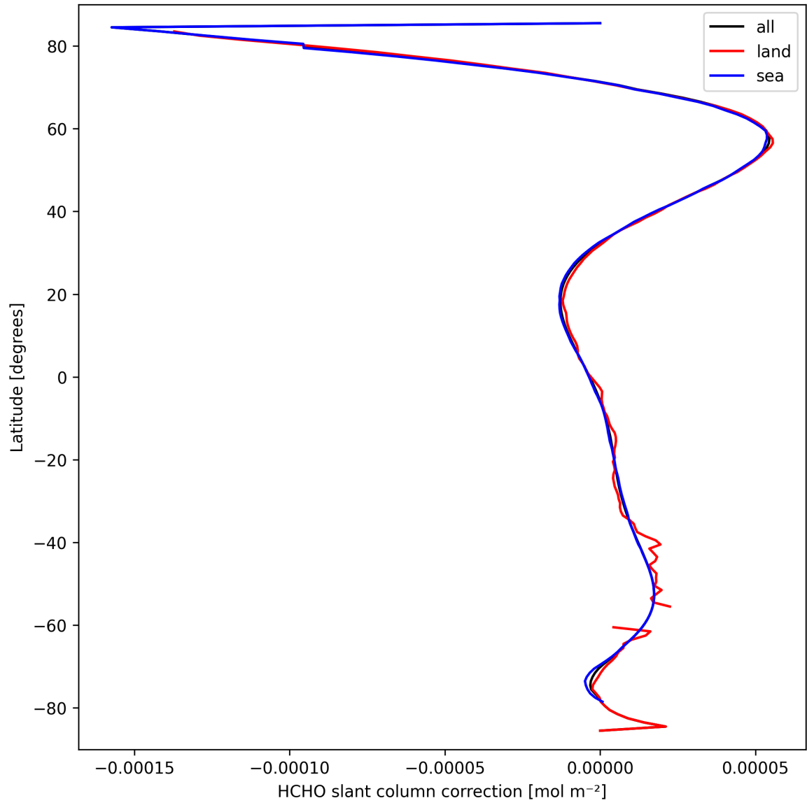
Figure 33: Zonal average of "HCHO slant column correction" for 2025-03-19 to 2025-03-21.
