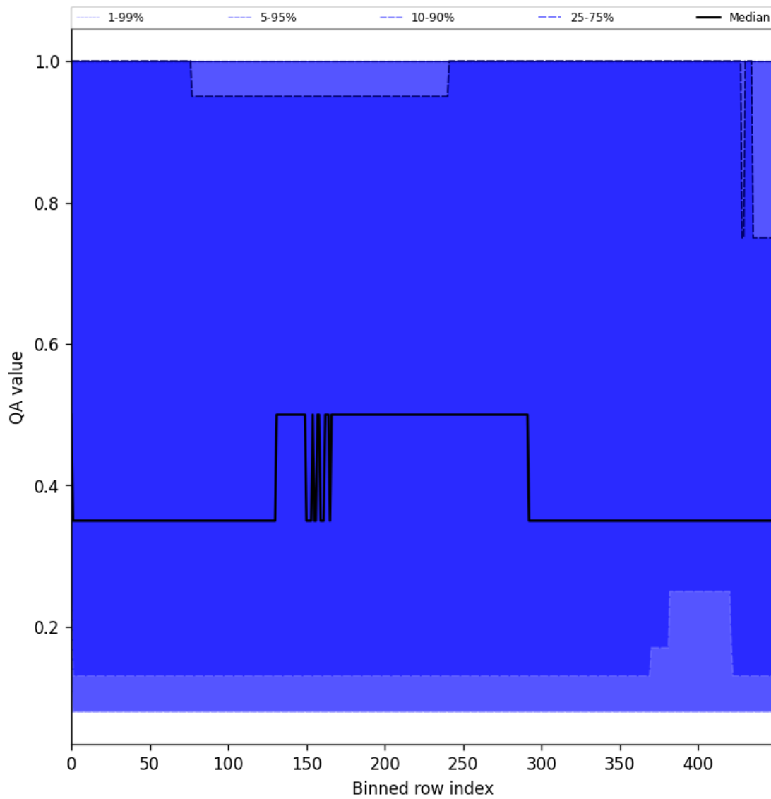
Figure 48: Along track statistics of “QA value” for 2025-03-19 to 2025-03-21
