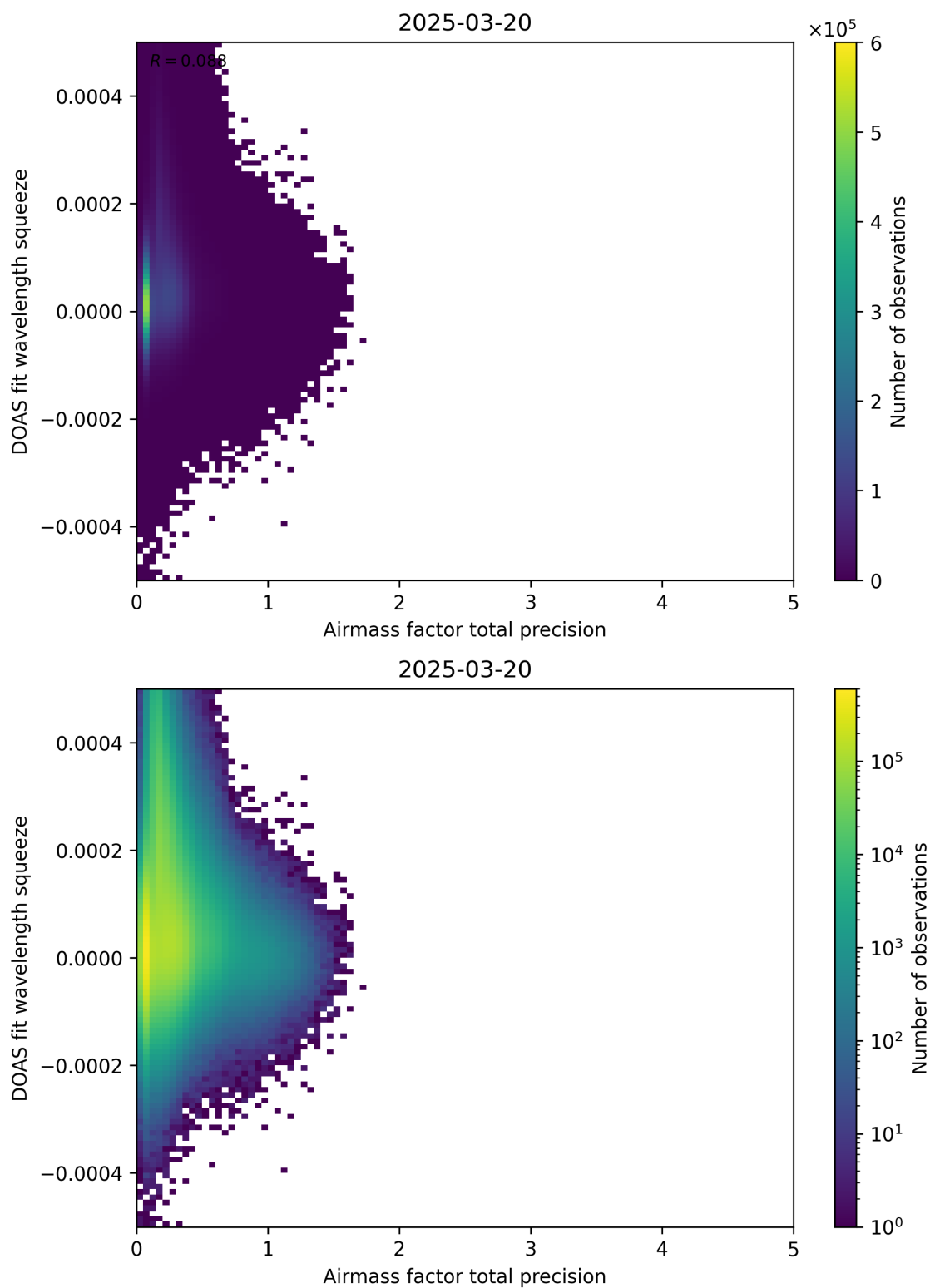
Figure 107: Scatter density plot of “Airmass factor total precision” against “DOAS fit wavelength squeeze” for 2025-03-19 to 2025-03-21.
