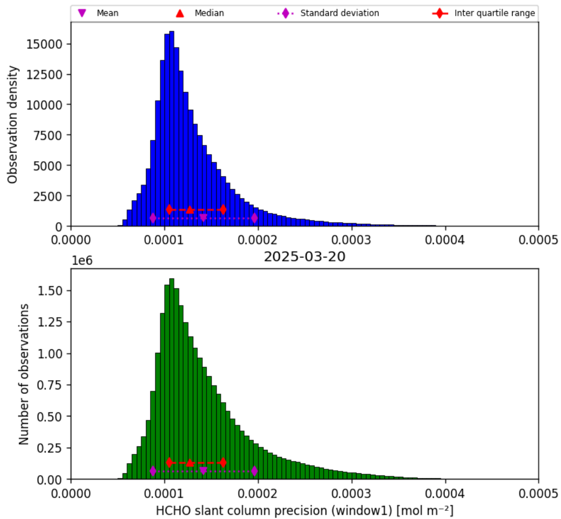
Figure 39: Histogram of “HCHO slant column precision (window1)” for 2025-03-19 to 2025-03-21
