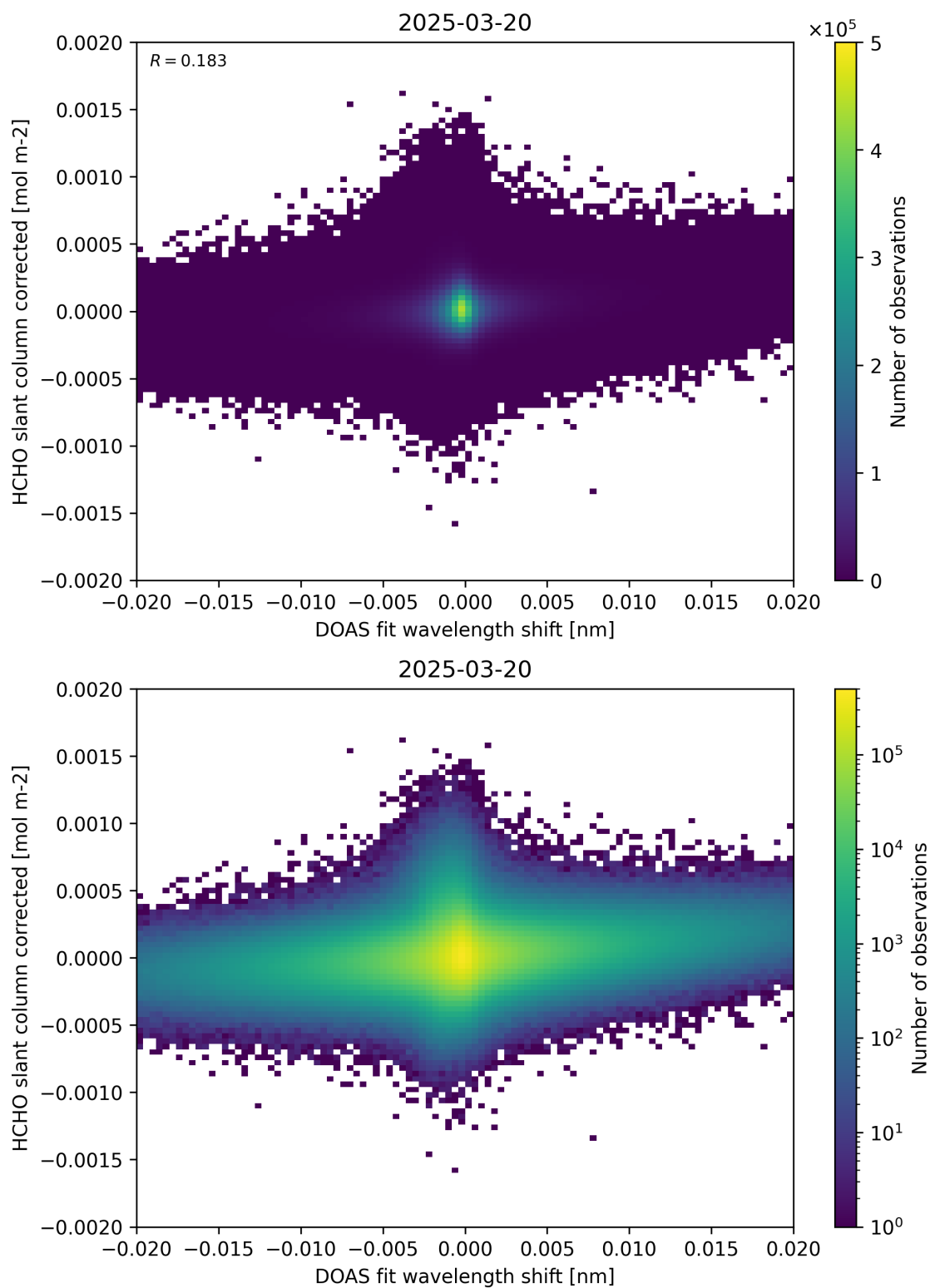
Figure 66: Scatter density plot of “DOAS fit wavelength shift” against “HCHO slant column corrected” for 2025-03-19 to 2025-03-21.
