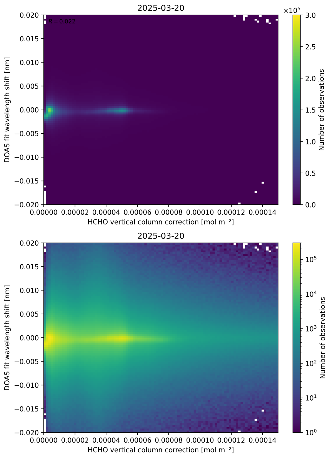
Figure 113: Scatter density plot of “HCHO vertical column correction” against “DOAS fit wavelength shift” for 2025-03-19 to 2025-03-21.
