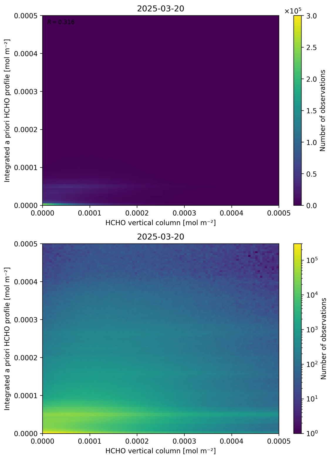
Figure 135: Scatter density plot of “HCHO vertical column” against “Integrated a priori HCHO profile” for 2025-03-19 to 2025-03-21.
