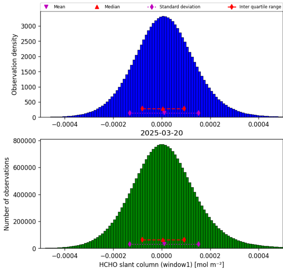
Figure 38: Histogram of “HCHO slant column (window1)” for 2025-03-19 to 2025-03-21
