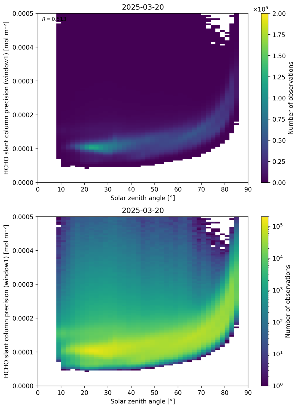
Figure 174: Scatter density plot of “Solar zenith angle” against “HCHO slant column precision (window1)” for 2025-03-19 to 2025-03-21.
