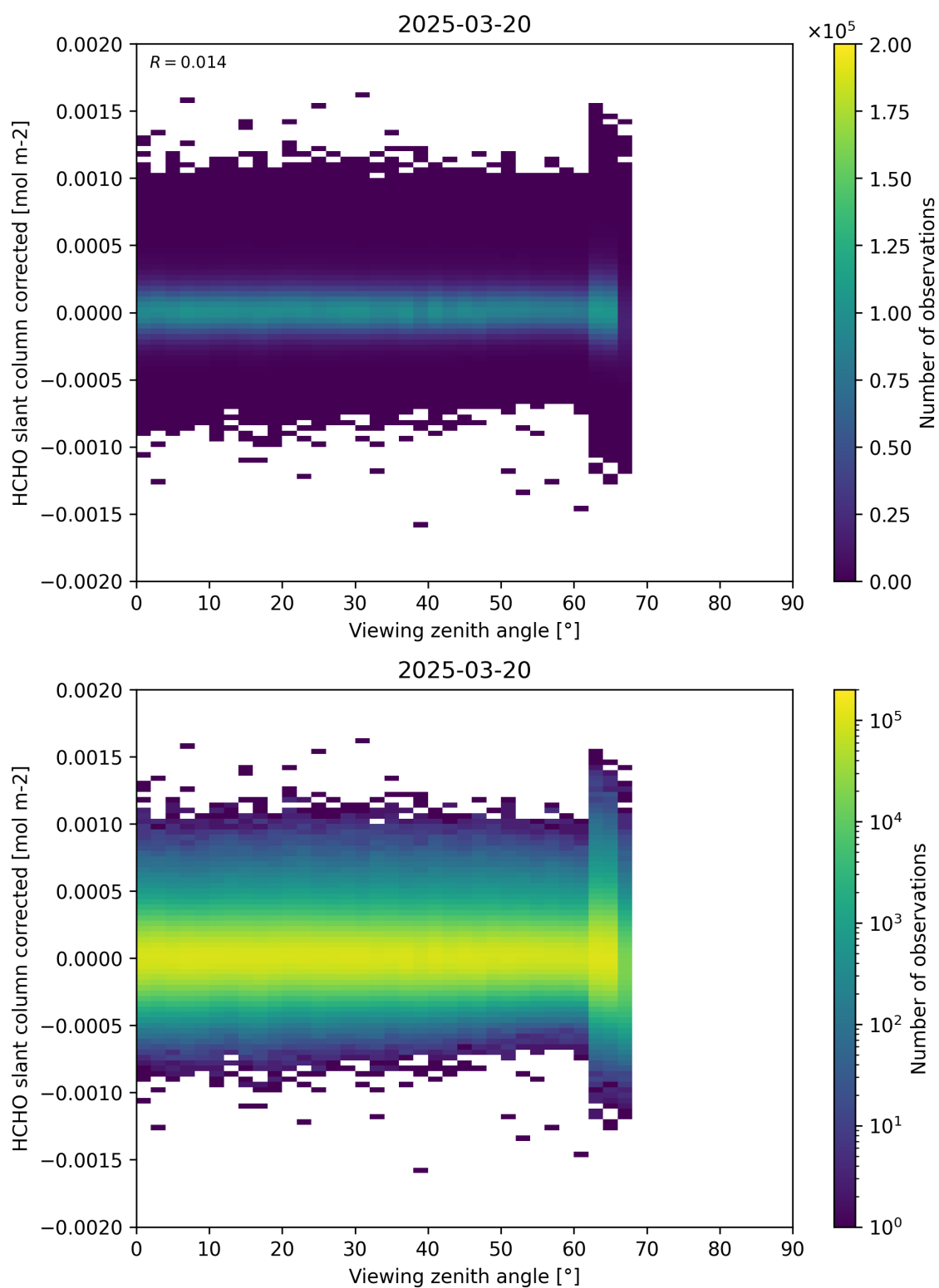
Figure 186: Scatter density plot of “Viewing zenith angle” against “HCHO slant column corrected” for 2025-03-19 to 2025-03-21.
