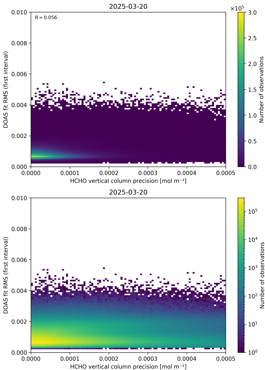
Figure 136: Scatter density plot of “HCHO vertical column precision” against “DOAS fit RMS (first interval)” for 2025-03-19 to 2025-03-21.
