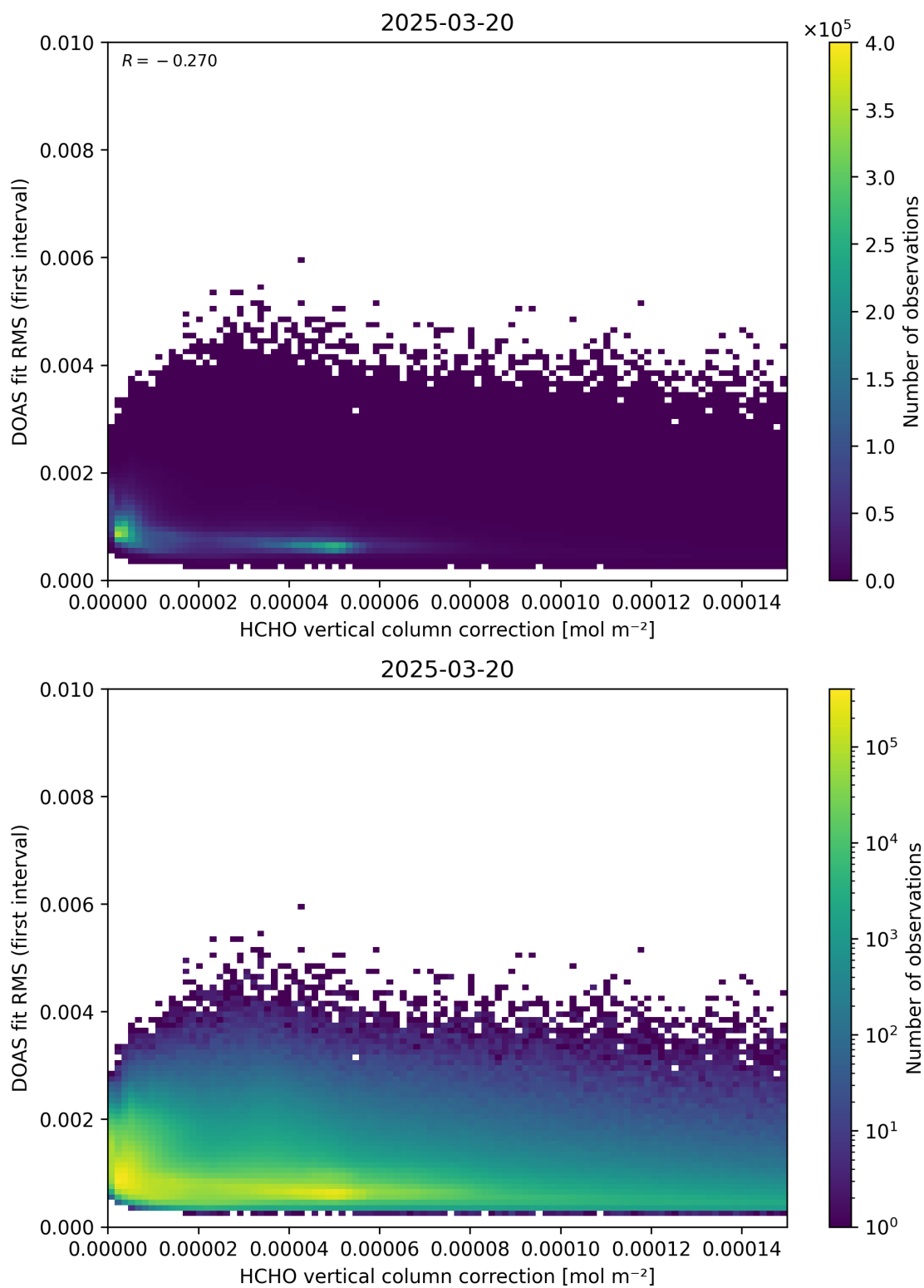
Figure 112: Scatter density plot of “HCHO vertical column correction” against “DOAS fit RMS (first interval)” for 2025-03-19 to 2025-03-21.
