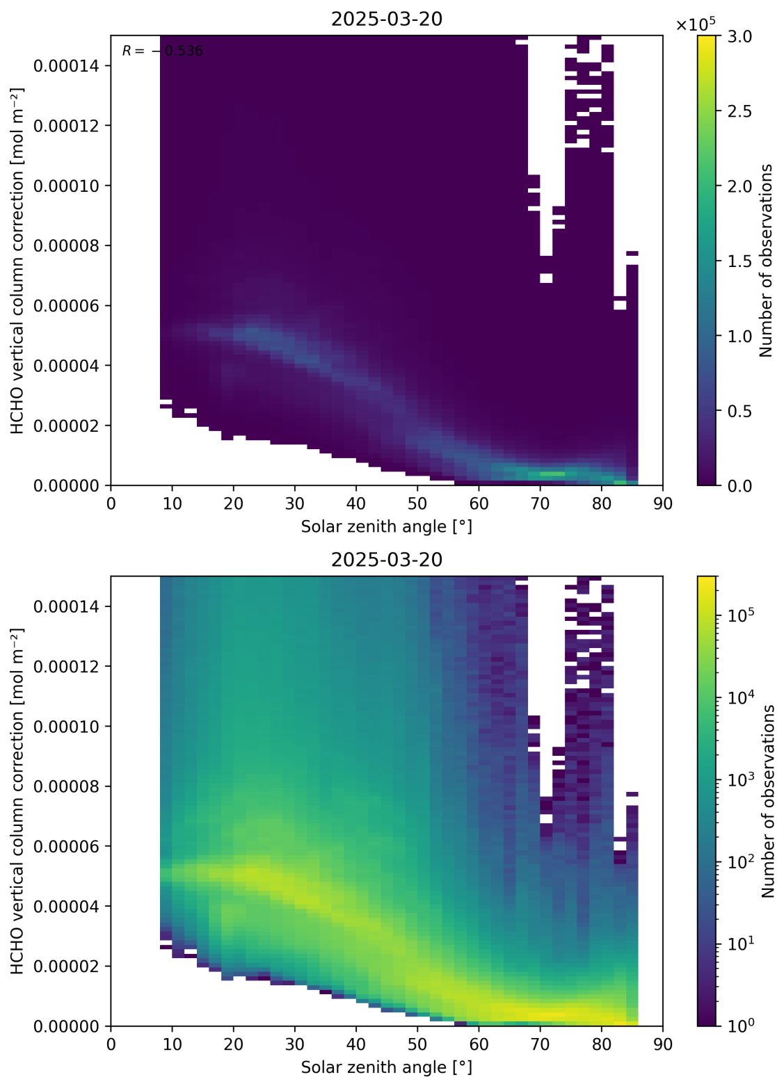
Figure 178: Scatter density plot of “Solar zenith angle” against “HCHO vertical column correction” for 2025-03-19 to 2025-03-21.
