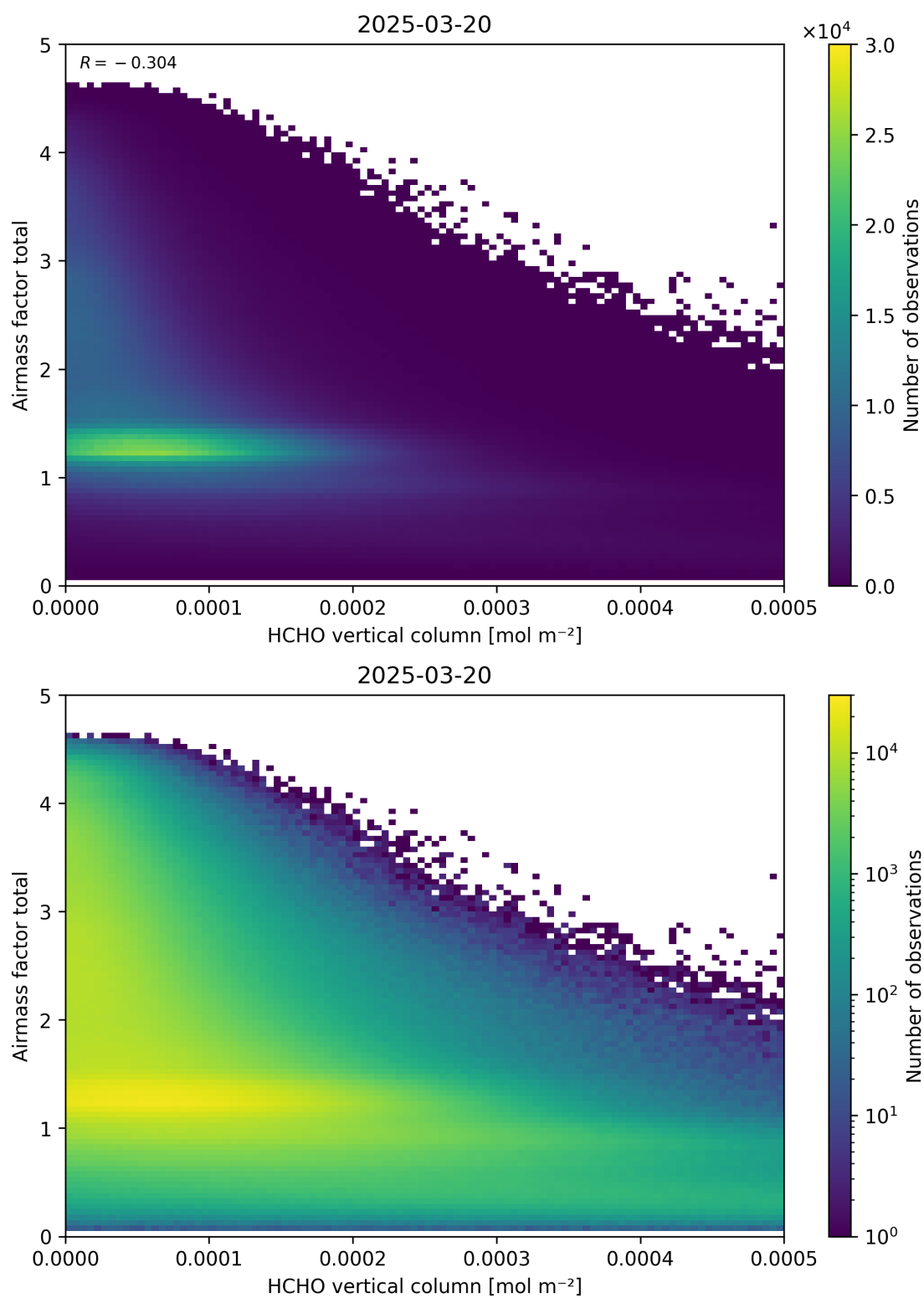
Figure 131: Scatter density plot of “HCHO vertical column” against “Airmass factor total” for 2025-03-19 to 2025-03-21.
