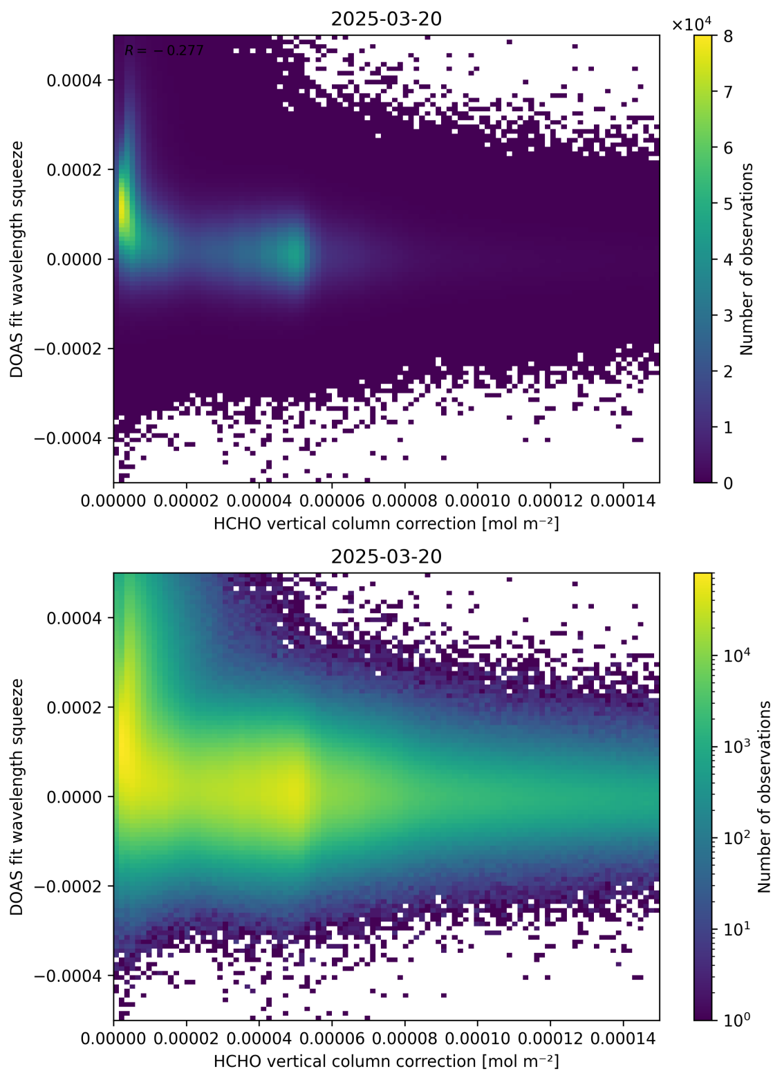
Figure 114: Scatter density plot of “HCHO vertical column correction” against “DOAS fit wavelength squeeze” for 2025-03-19 to 2025-03-21.
