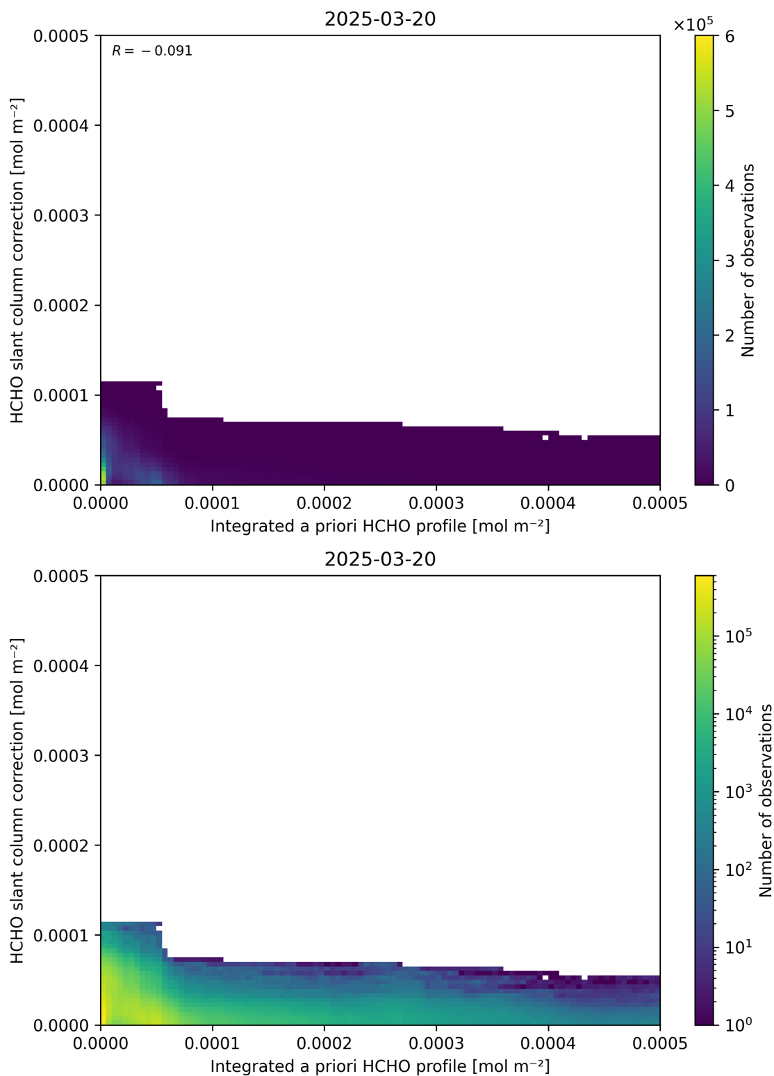
Figure 152: Scatter density plot of “Integrated a priori HCHO profile” against “HCHO slant column correction” for 2025-03-19 to 2025-03-21.
