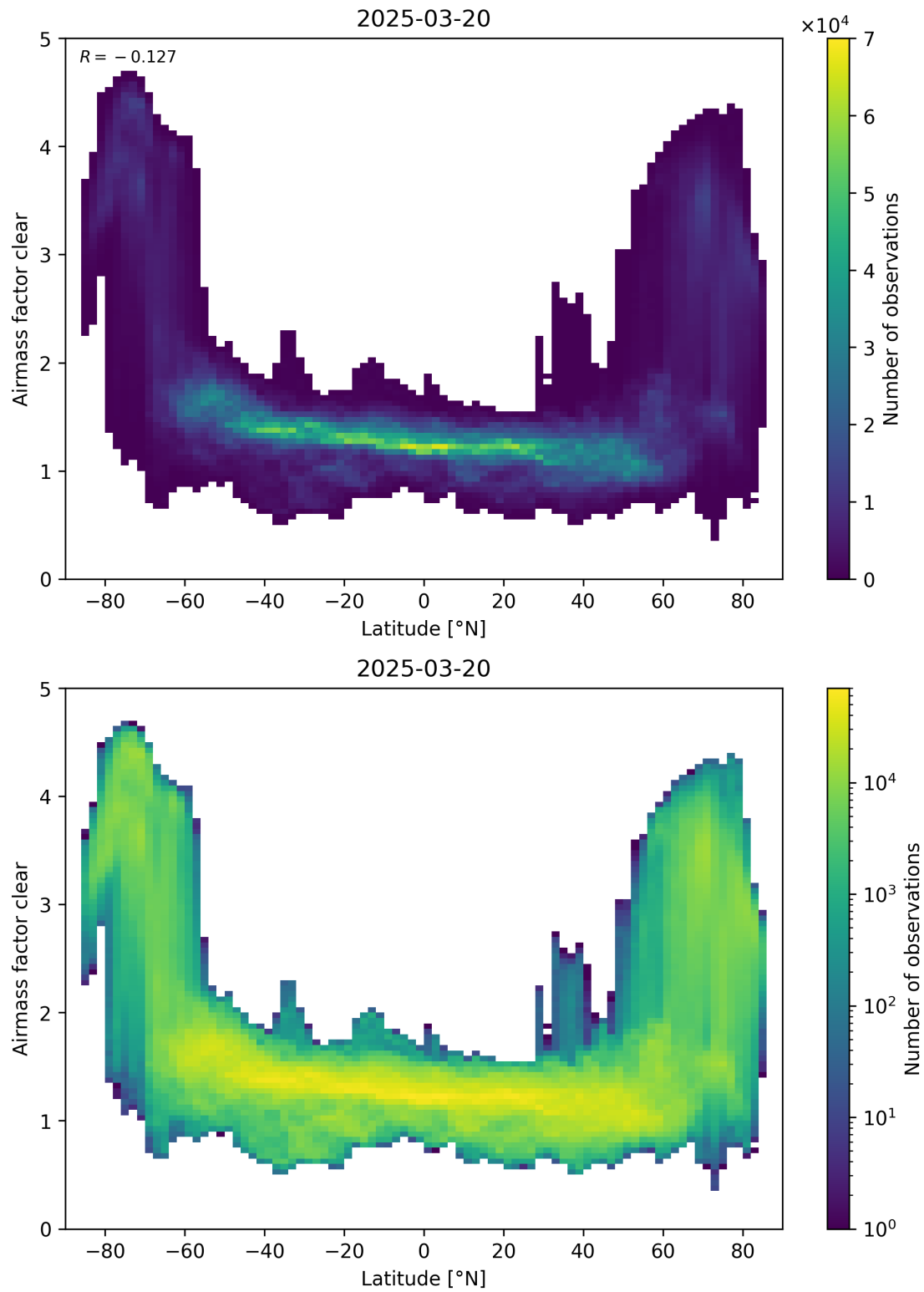
Figure 156: Scatter density plot of “Latitude” against “Airmass factor clear” for 2025-03-19 to 2025-03-21.
