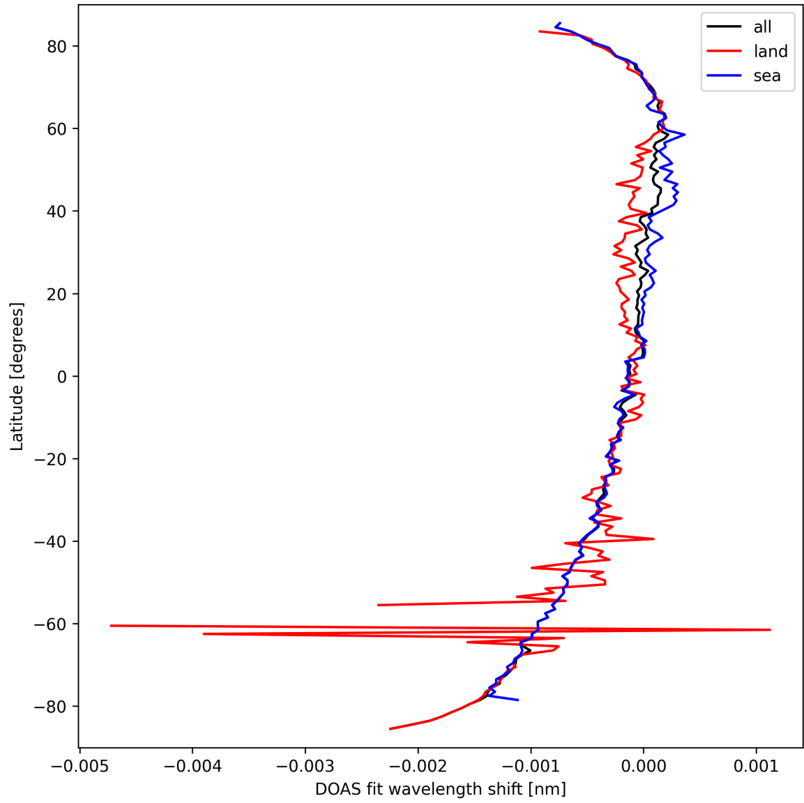
Figure 30: Zonal average of “DOAS fit wavelength shift” for 2025-03-19 to 2025-03-21.
