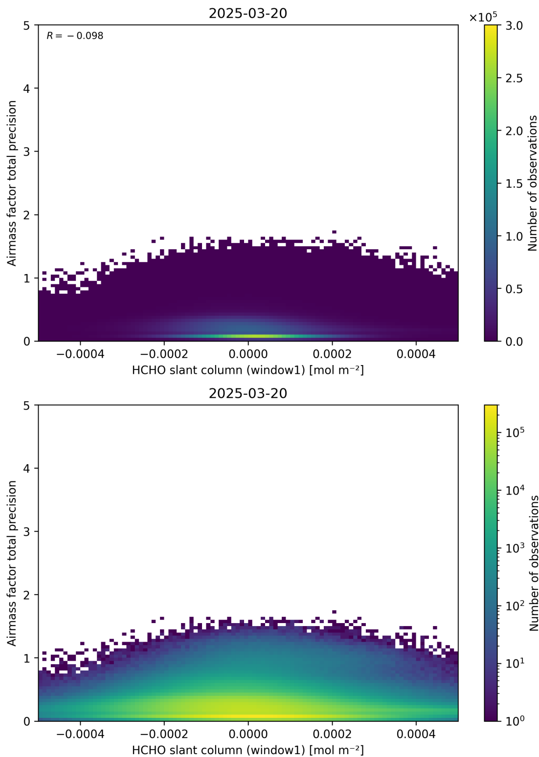
Figure 86: Scatter density plot of “HCHO slant column (window1)” against “Airmass factor total precision” for 2025-03-19 to 2025-03-21.
