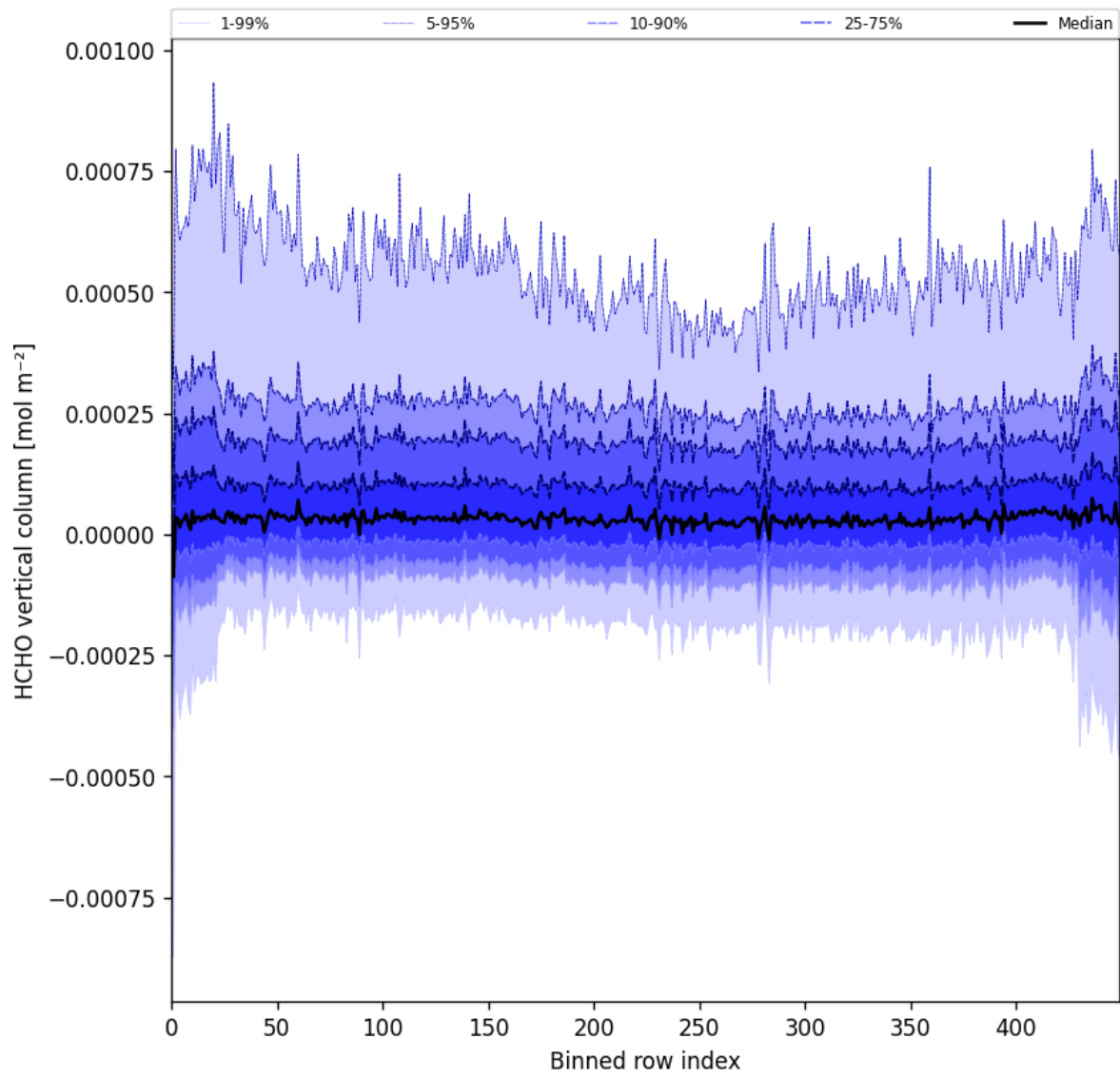
Figure 49: Along track statistics of “HCHO vertical column” for 2025-03-19 to 2025-03-21
