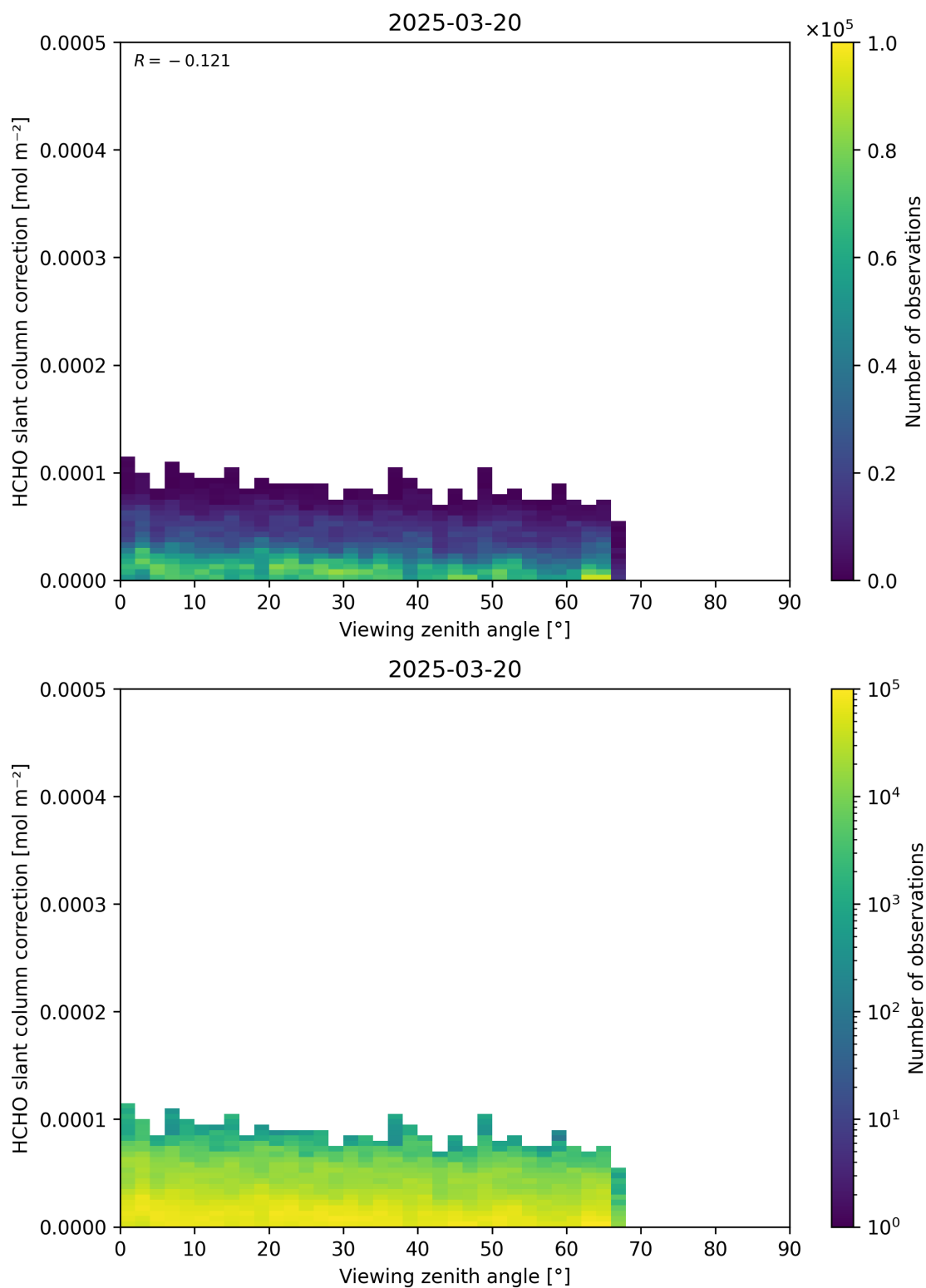
Figure 187: Scatter density plot of “Viewing zenith angle” against “HCHO slant column correction” for 2025-03-19 to 2025-03-21.
