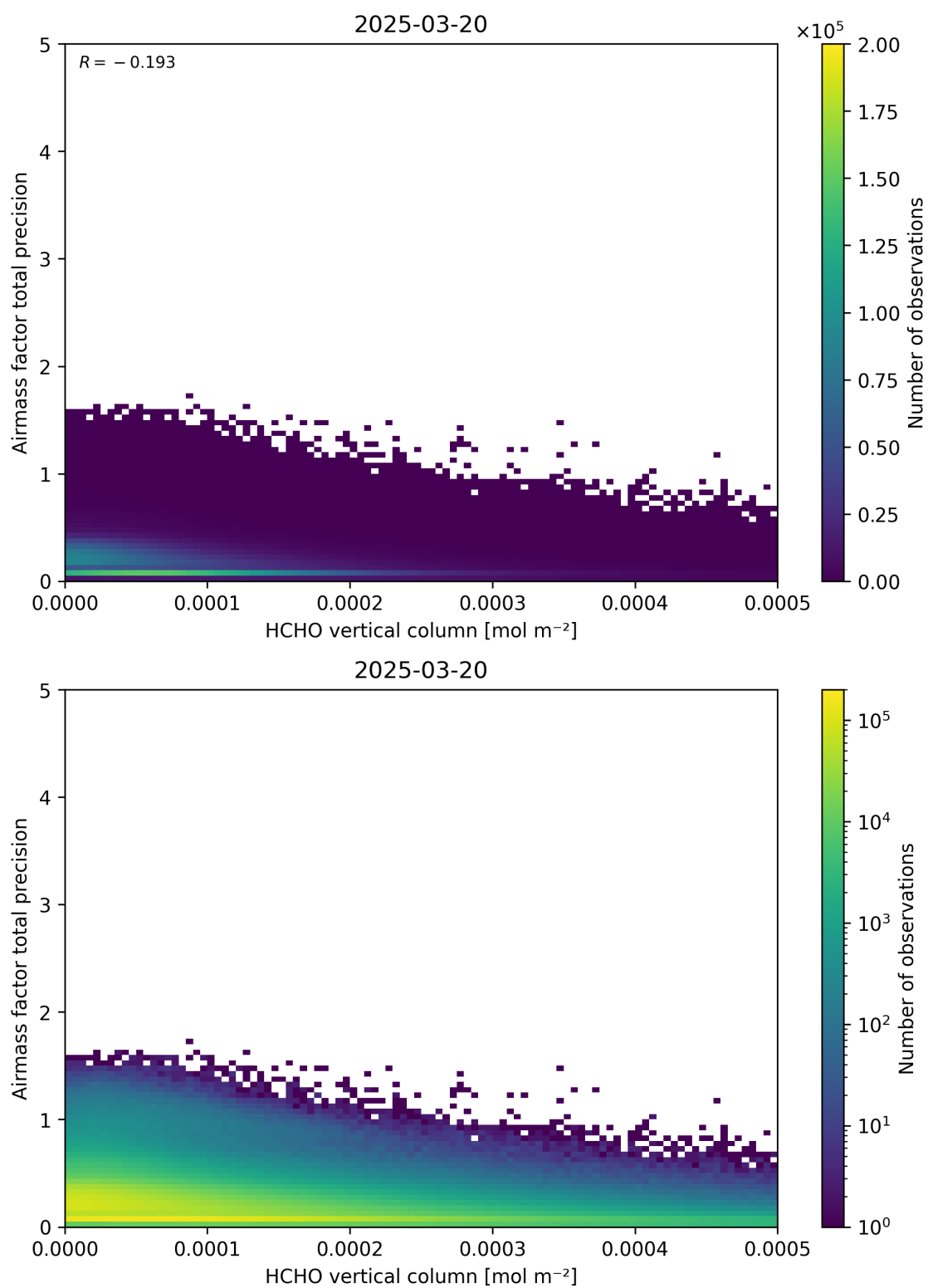
Figure 132: Scatter density plot of “HCHO vertical column” against “Airmass factor total precision” for 2025-03-19 to 2025-03-21.
