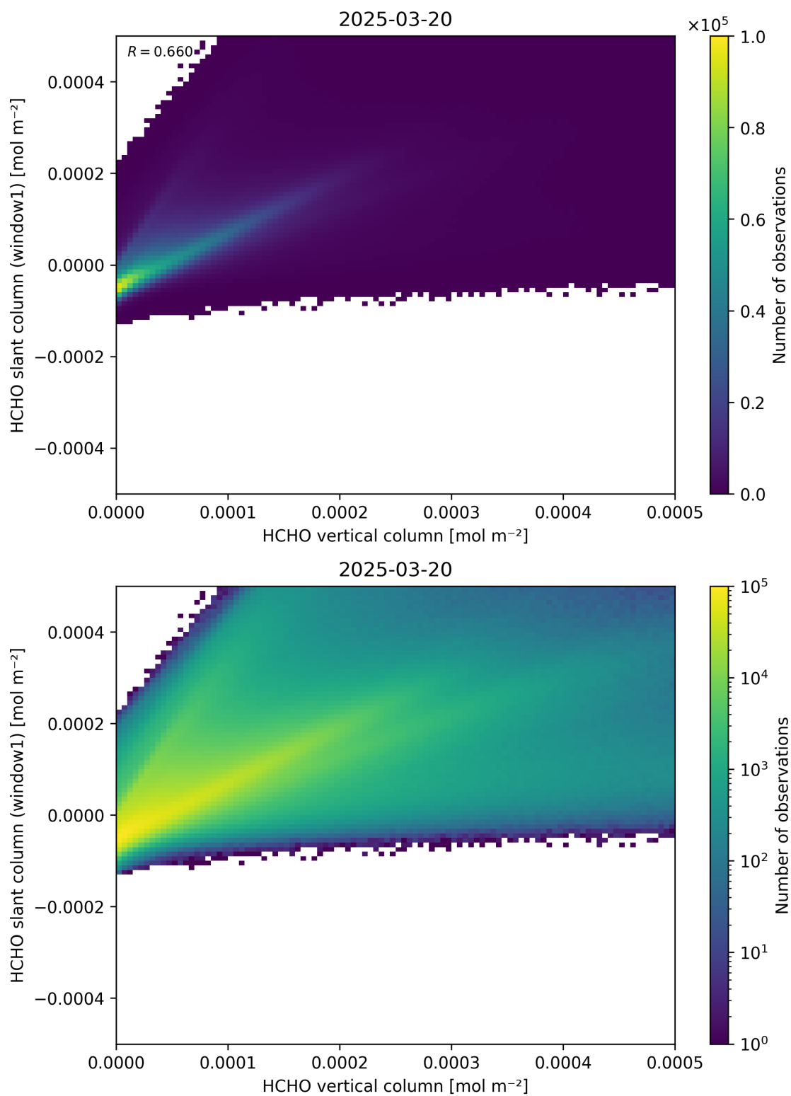
Figure 129: Scatter density plot of “HCHO vertical column” against “HCHO slant column (window1)” for 2025-03-19 to 2025-03-21.
