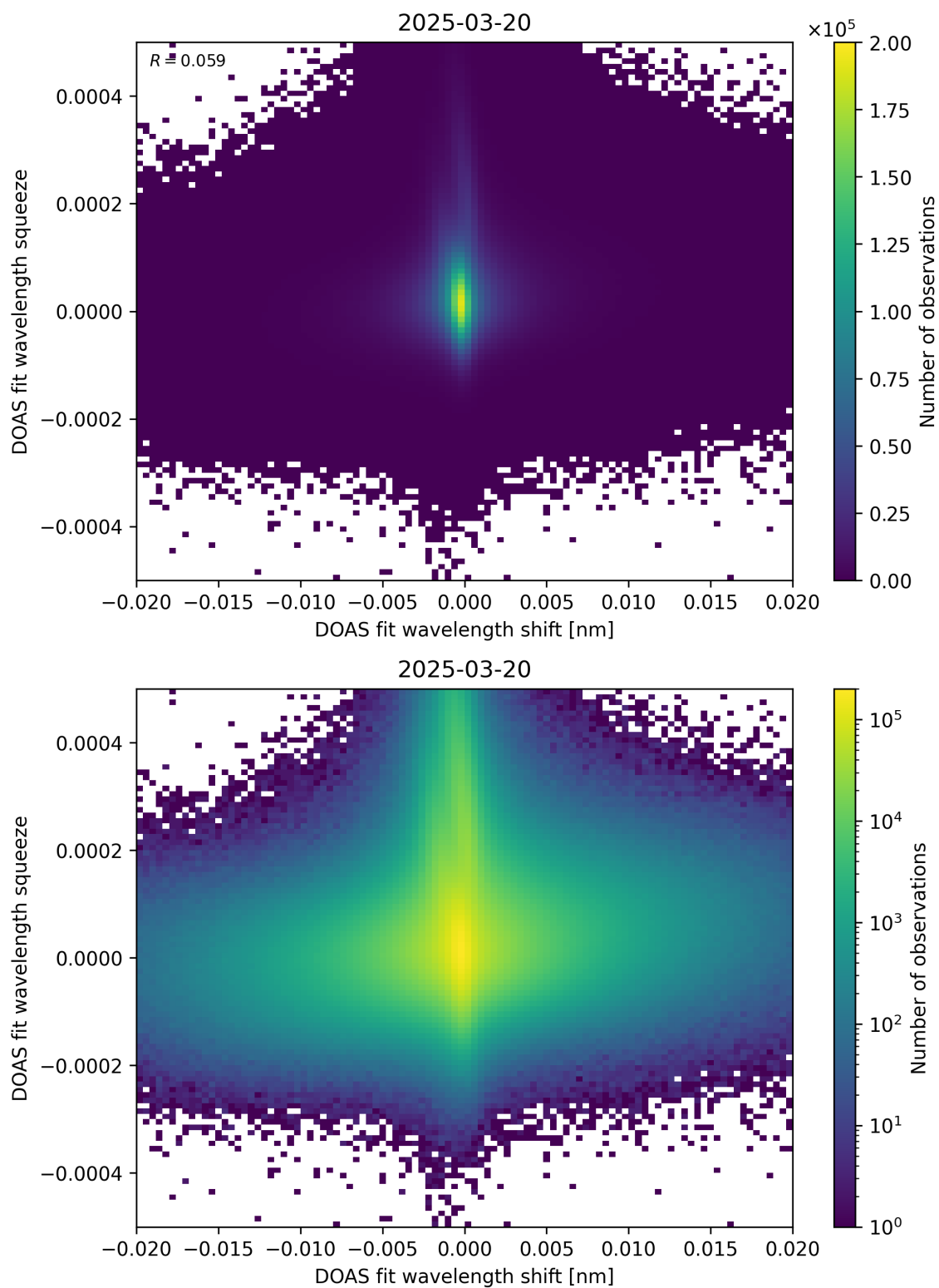
Figure 65: Scatter density plot of “DOAS fit wavelength shift” against “DOAS fit wavelength squeeze” for 2025-03-19 to 2025-03-21.
