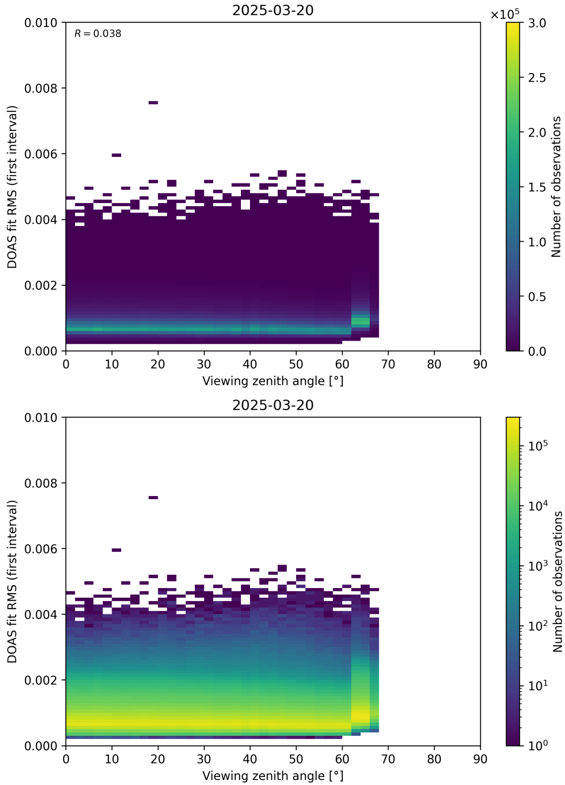
Figure 182: Scatter density plot of “Viewing zenith angle” against “DOAS fit RMS (first interval)” for 2025-03-19 to 2025-03-21.
