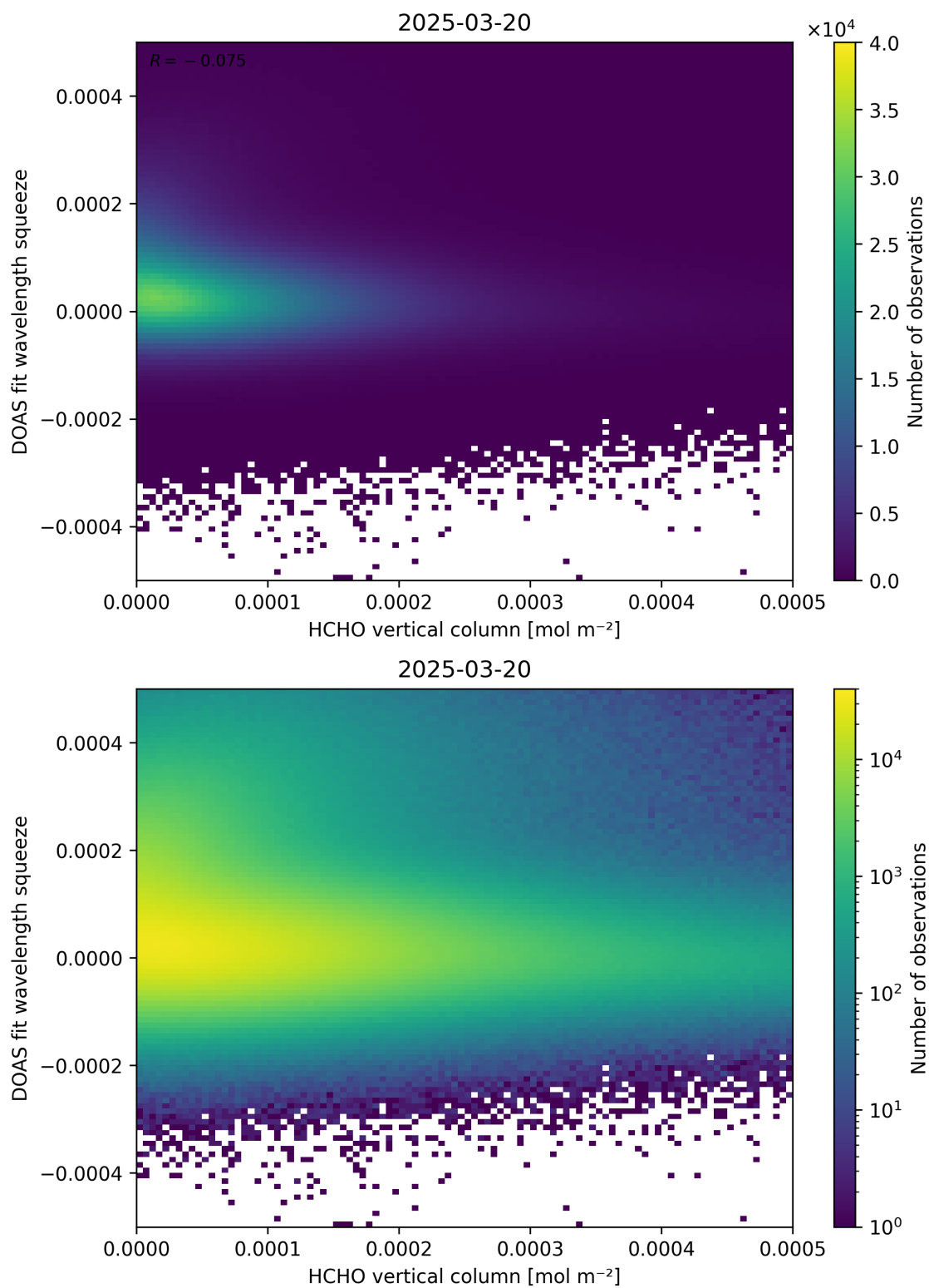
Figure 125: Scatter density plot of “HCHO vertical column” against “DOAS fit wavelength squeeze” for 2025-03-19 to 2025-03-21.
