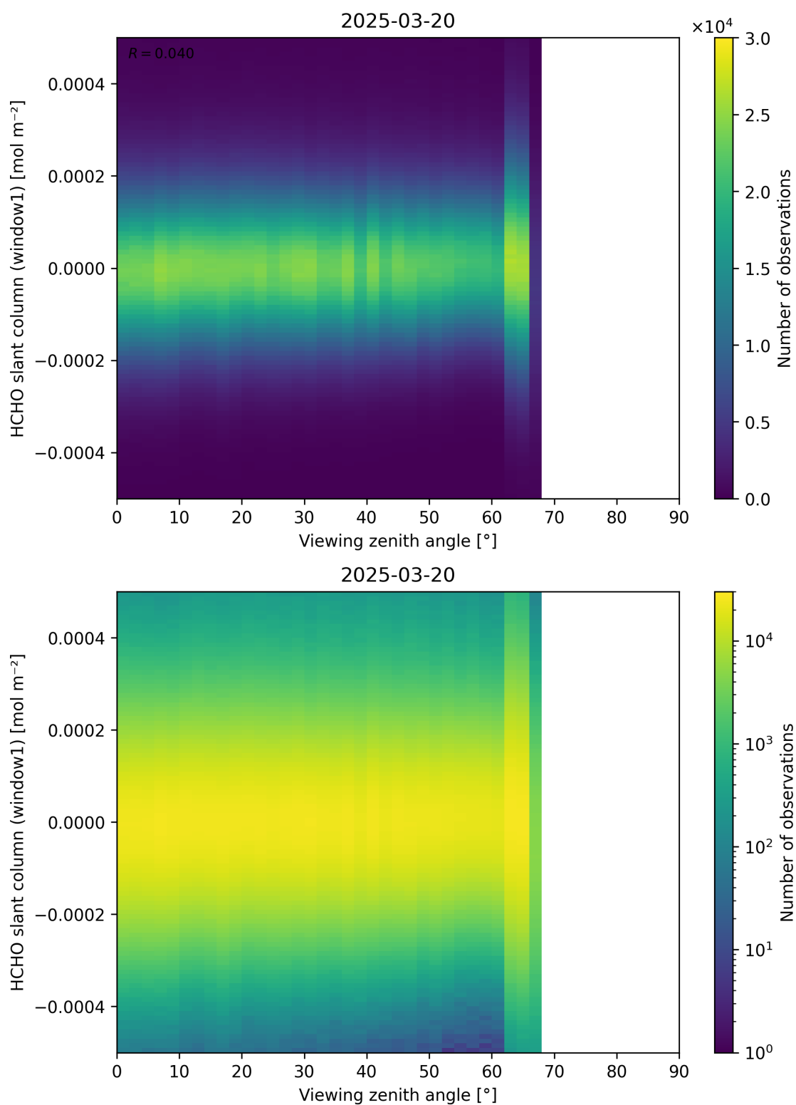
Figure 188: Scatter density plot of “Viewing zenith angle” against “HCHO slant column (window1)” for 2025-03-19 to 2025-03-21.
