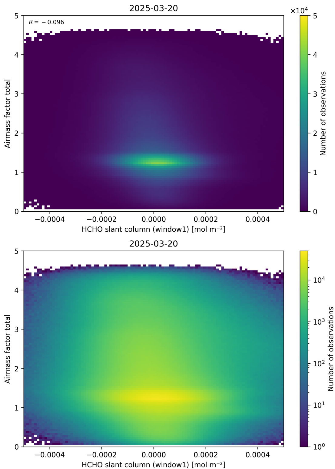
Figure 85: Scatter density plot of “HCHO slant column (window1)” against “Airmass factor total” for 2025-03-19 to 2025-03-21.
