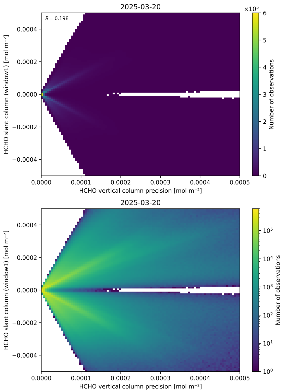
Figure 142: Scatter density plot of “HCHO vertical column precision” against “HCHO slant column (window1)” for 2025-03-19 to 2025-03-21.
