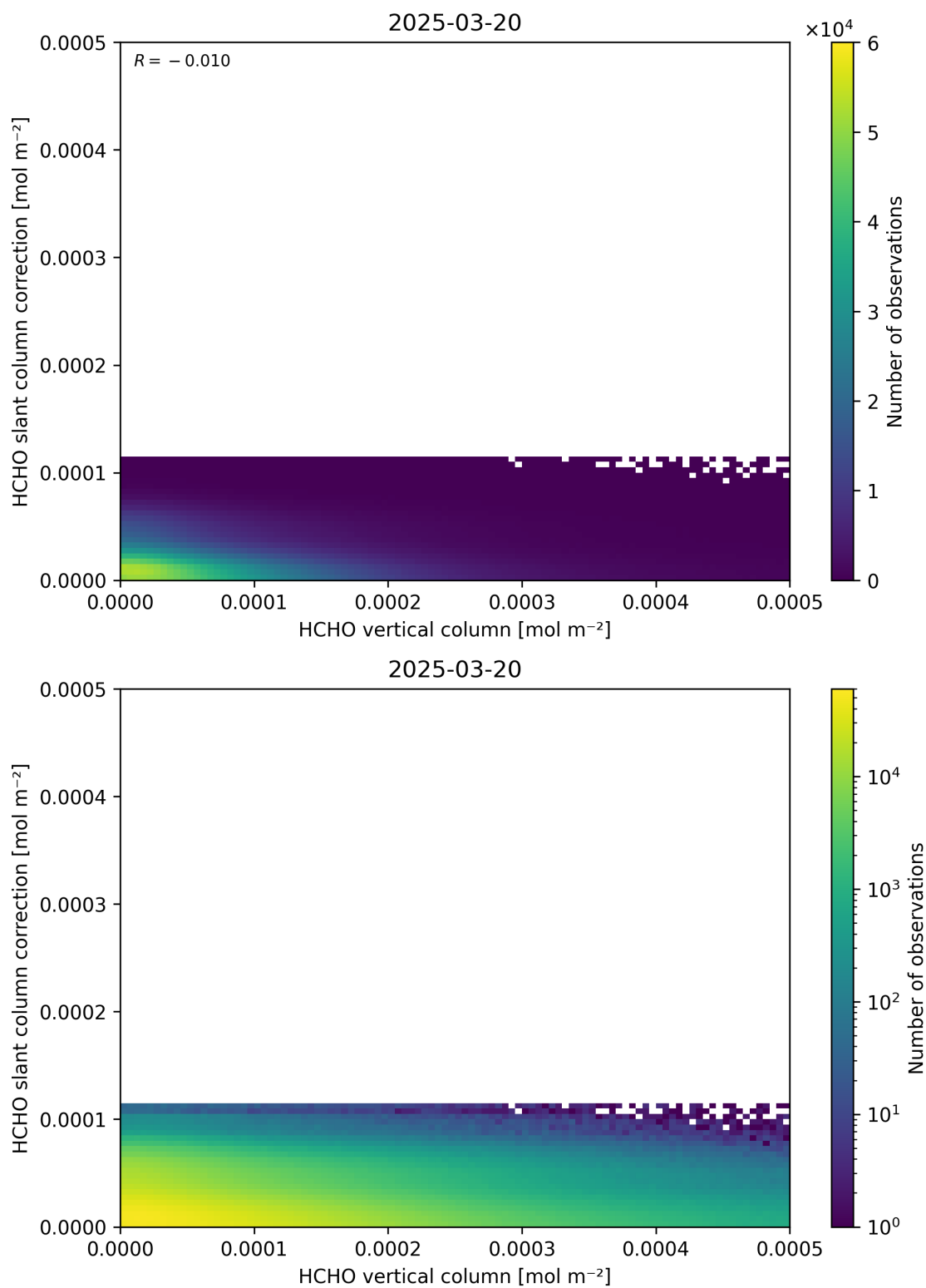
Figure 128: Scatter density plot of “HCHO vertical column” against “HCHO slant column correction” for 2025-03-19 to 2025-03-21.
