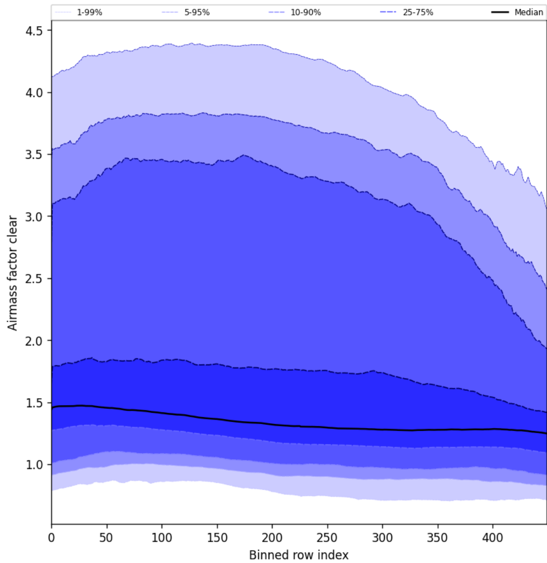
Figure 56: Along track statistics of “Airmass factor clear” for 2025-03-19 to 2025-03-21
