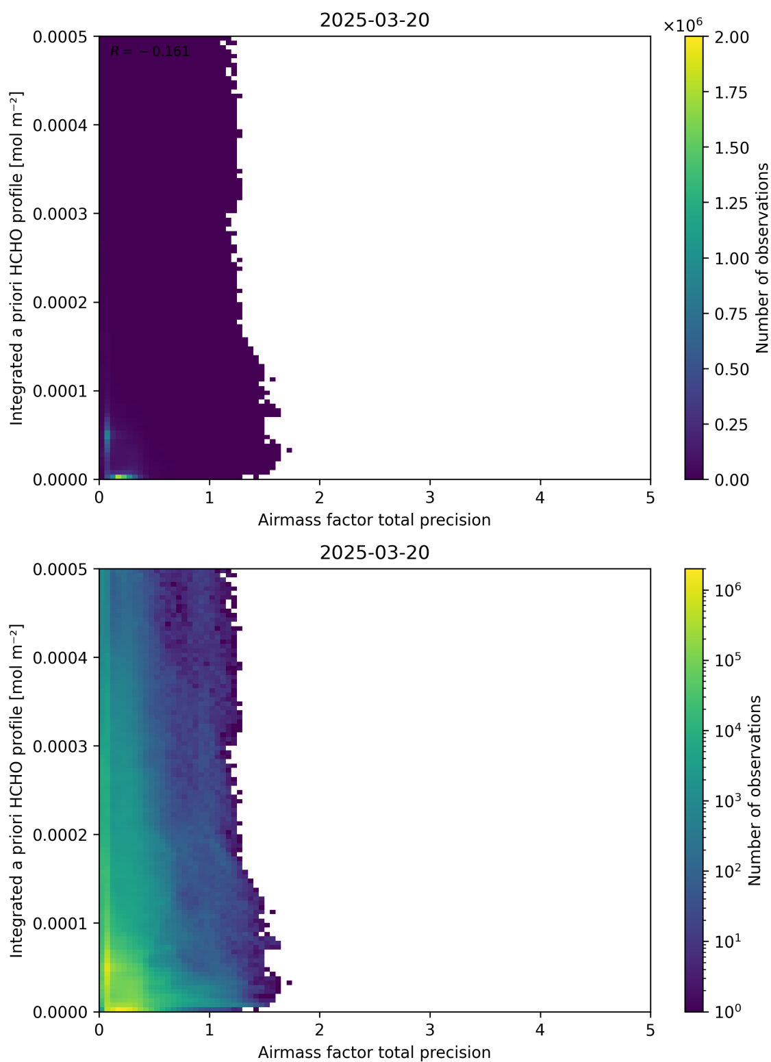
Figure 111: Scatter density plot of “Airmass factor total precision” against “Integrated a priori HCHO profile” for 2025-03-19 to 2025-03-21.
