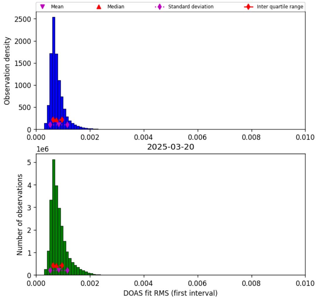
Figure 46: Histogram of “DOAS fit RMS (first interval)” for 2025-03-19 to 2025-03-21
