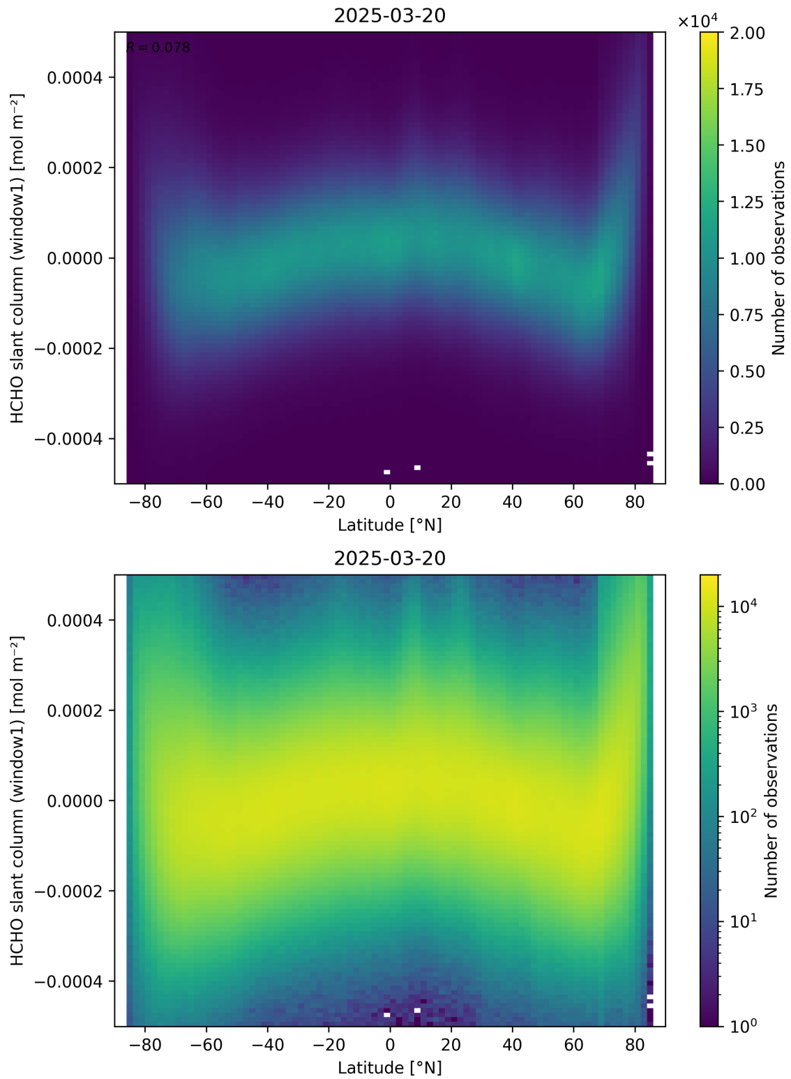
Figure 159: Scatter density plot of “Latitude” against “HCHO slant column (window1)” for 2025-03-19 to 2025-03-21.
