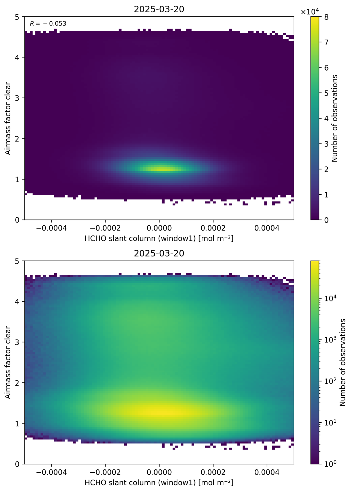
Figure 81: Scatter density plot of “HCHO slant column (window1)” against “Airmass factor clear” for 2025-03-19 to 2025-03-21.
