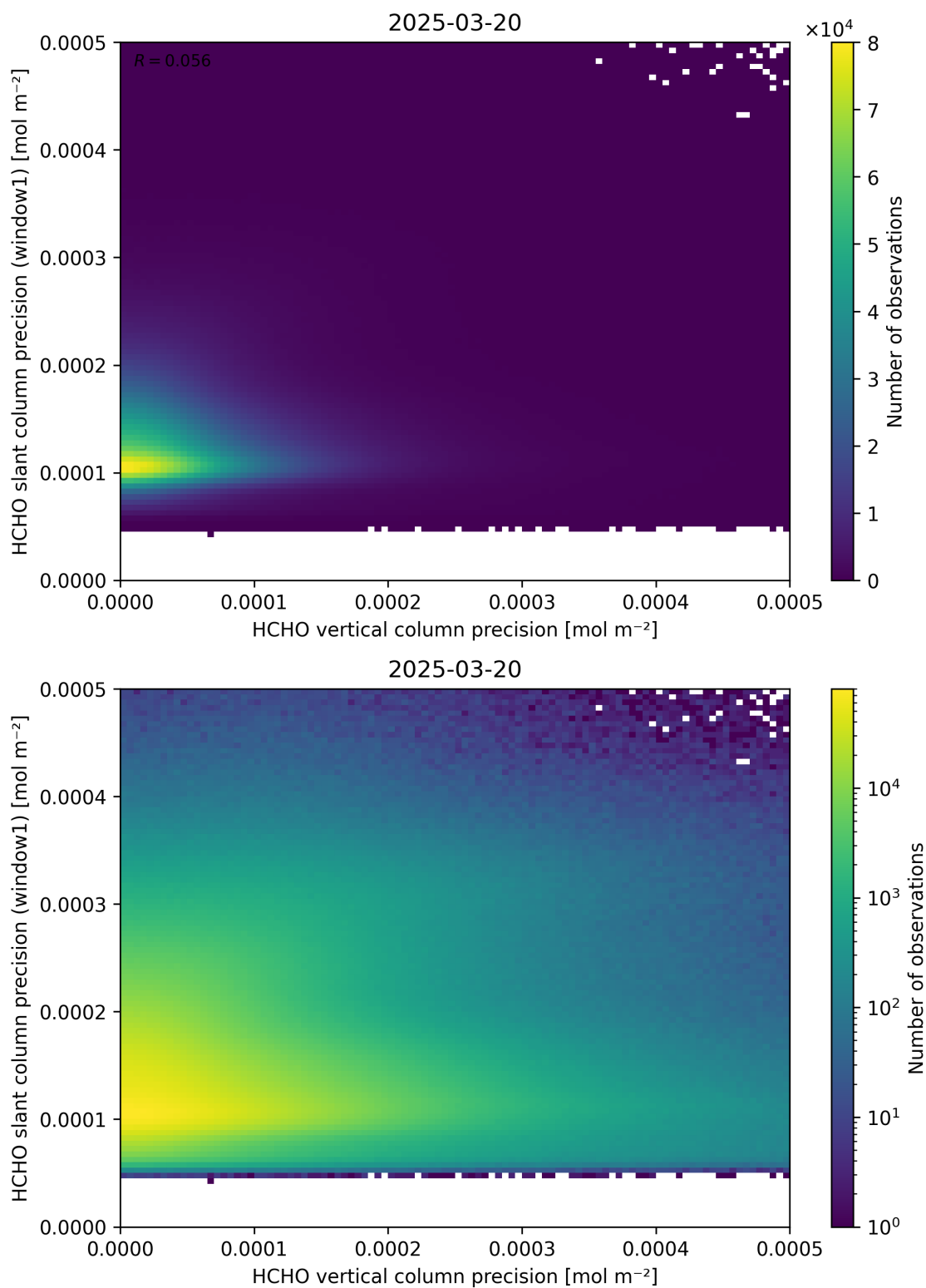
Figure 143: Scatter density plot of “HCHO vertical column precision” against “HCHO slant column precision (window1)” for 2025-03-19 to 2025-03-21.
