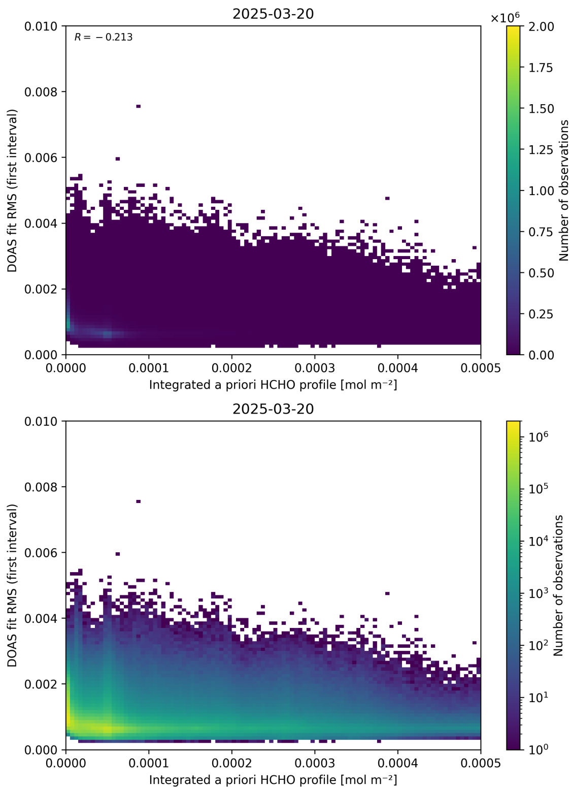
Figure 148: Scatter density plot of “Integrated a priori HCHO profile” against “DOAS fit RMS (first interval)” for 2025-03-19 to 2025-03-21.
