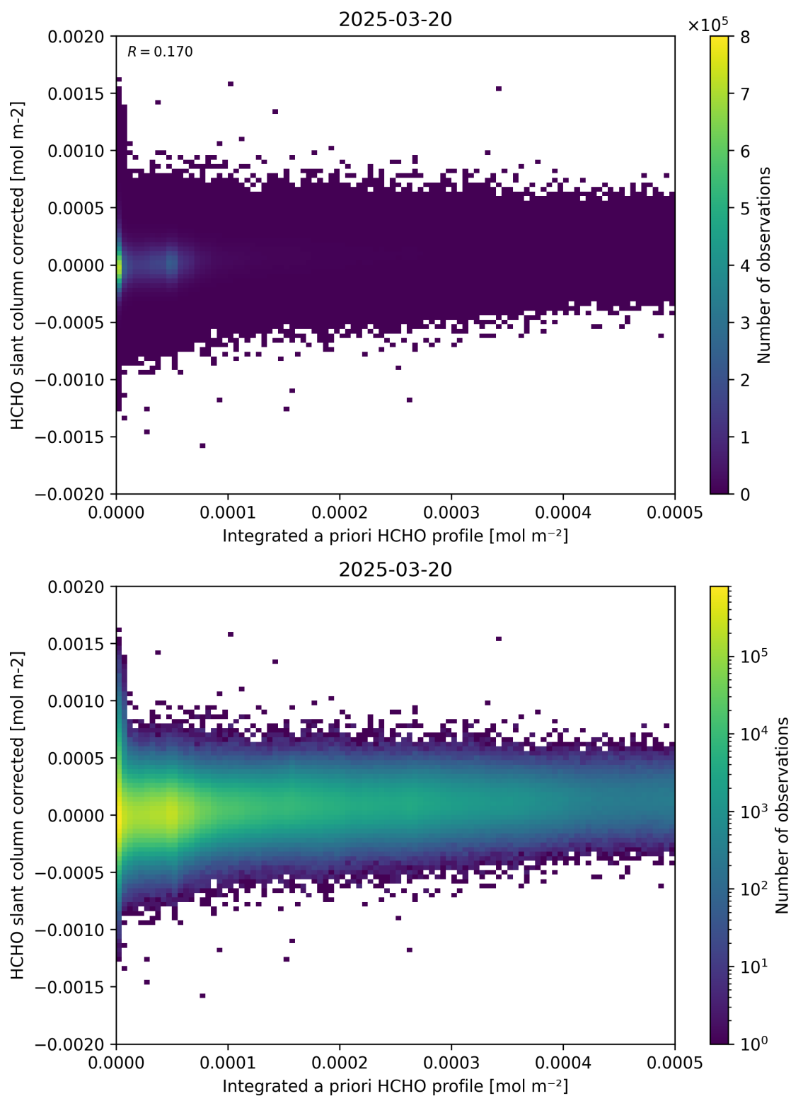
Figure 151: Scatter density plot of “Integrated a priori HCHO profile” against “HCHO slant column corrected” for 2025-03-19 to 2025-03-21.
