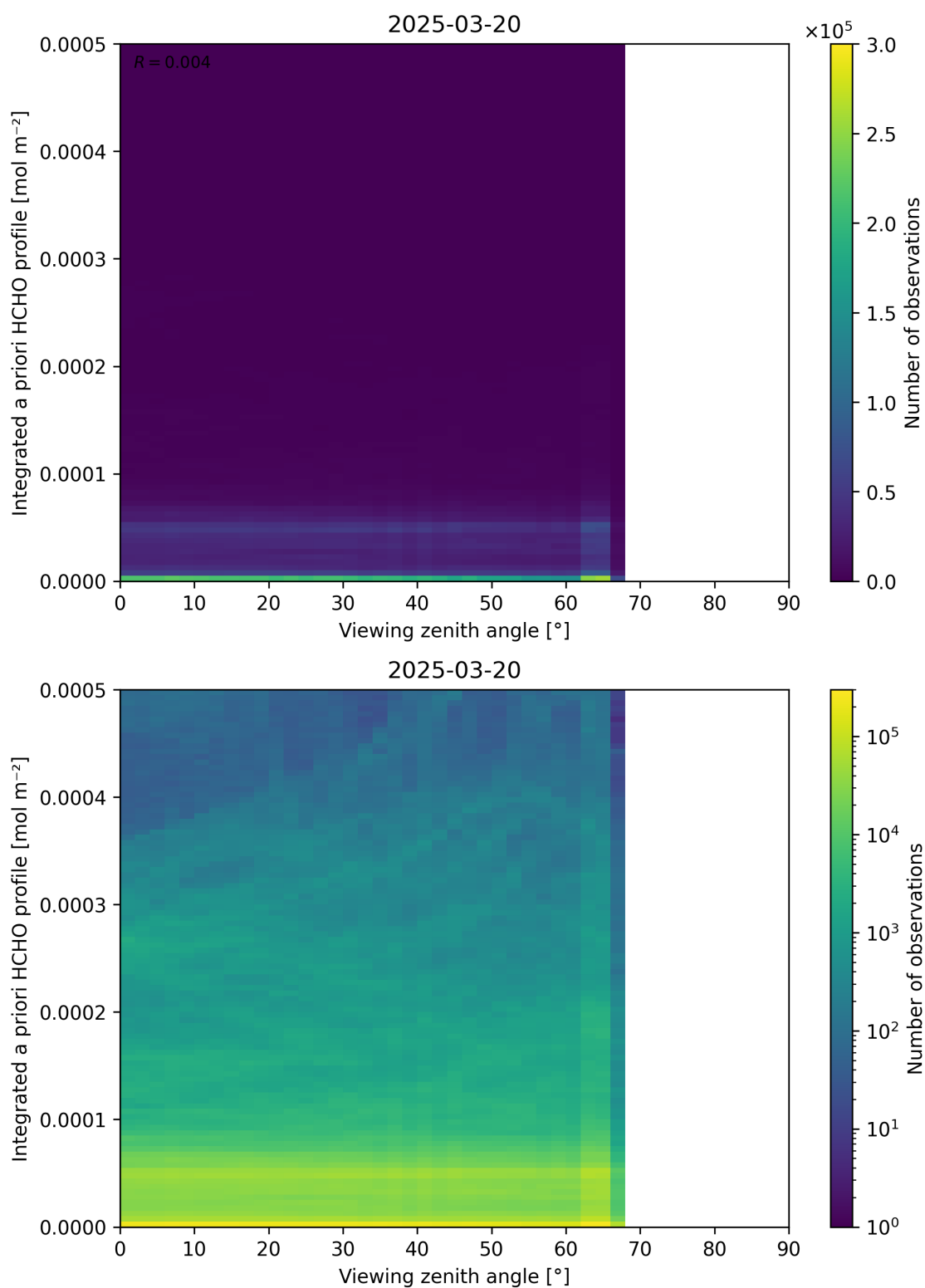
Figure 195: Scatter density plot of “Viewing zenith angle” against “Integrated a priori HCHO profile” for 2025-03-19 to 2025-03-21.
