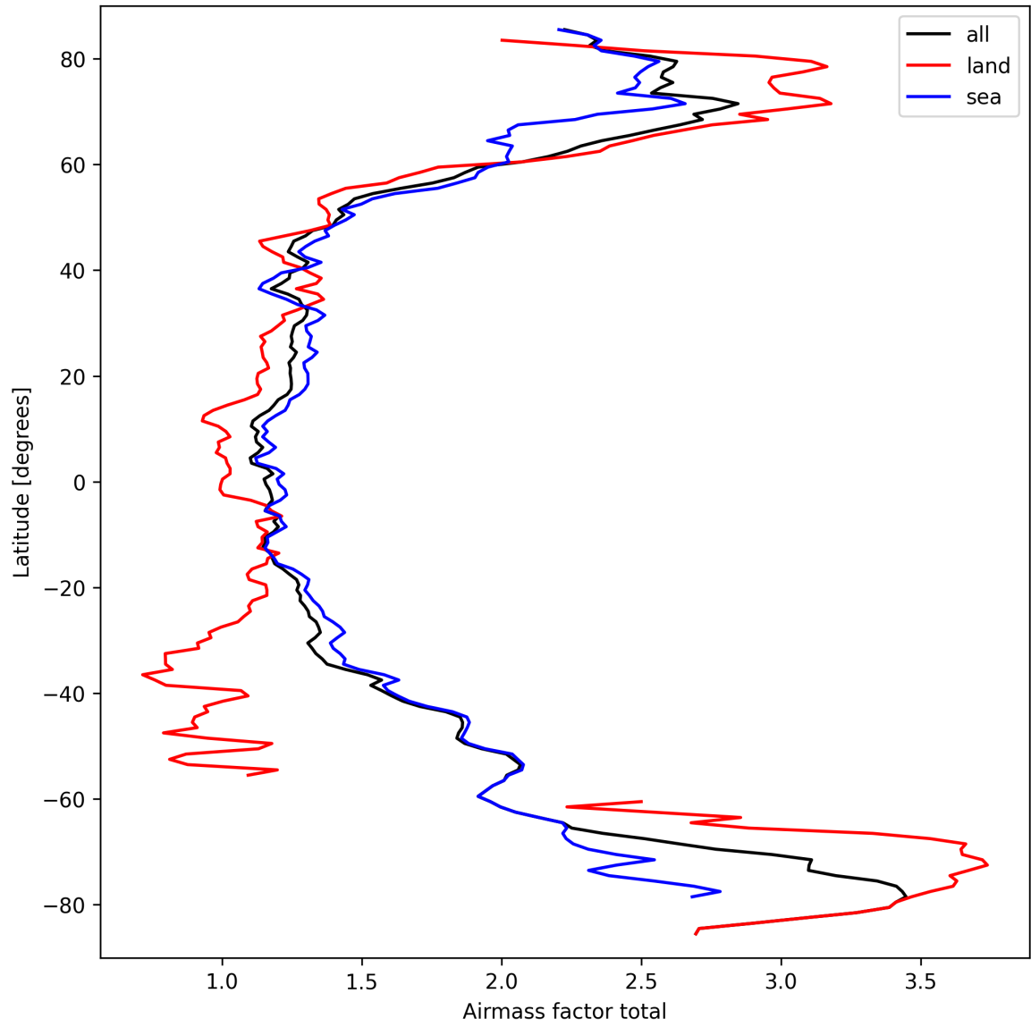
Figure 26: Zonal average of “Airmass factor total” for 2025-03-19 to 2025-03-21.
