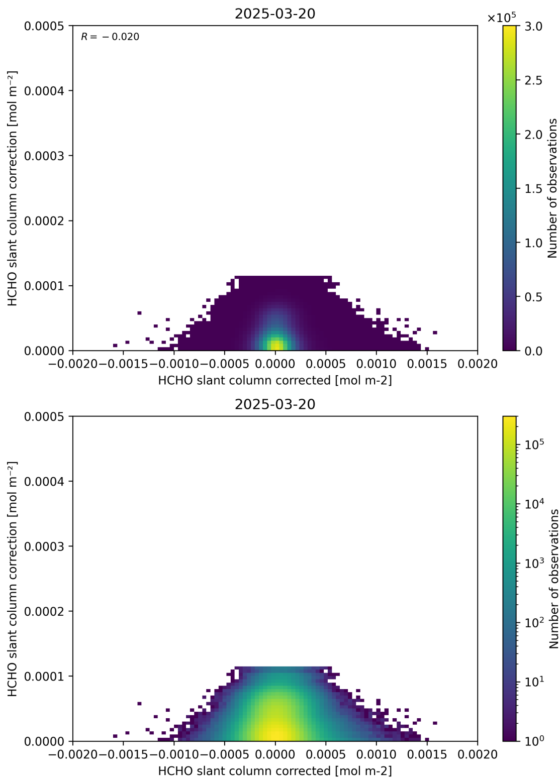
Figure 77: Scatter density plot of “HCHO slant column corrected” against “HCHO slant column correction” for 2025-03-19 to 2025-03-21.
