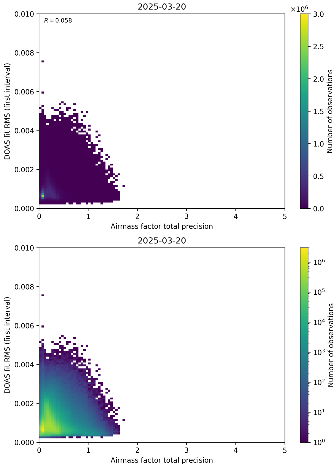
Figure 105: Scatter density plot of “Airmass factor total precision” against “DOAS fit RMS (first interval)” for 2025-03-19 to 2025-03-21.
