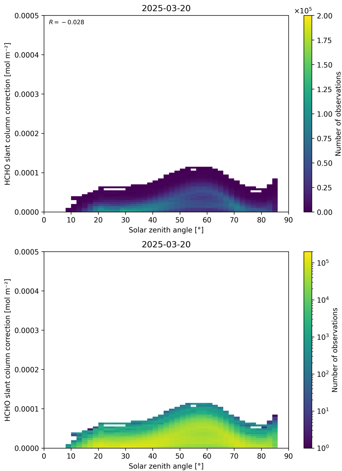
Figure 172: Scatter density plot of “Solar zenith angle” against “HCHO slant column correction” for 2025-03-19 to 2025-03-21.
