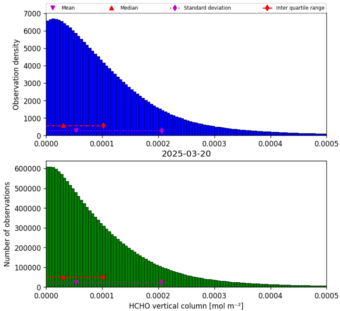
Figure 35: Histogram of “HCHO vertical column” for 2025-03-19 to 2025-03-21
