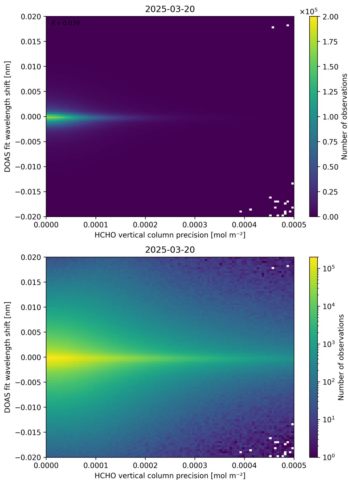
Figure 137: Scatter density plot of “HCHO vertical column precision” against “DOAS fit wavelength shift” for 2025-03-19 to 2025-03-21.
