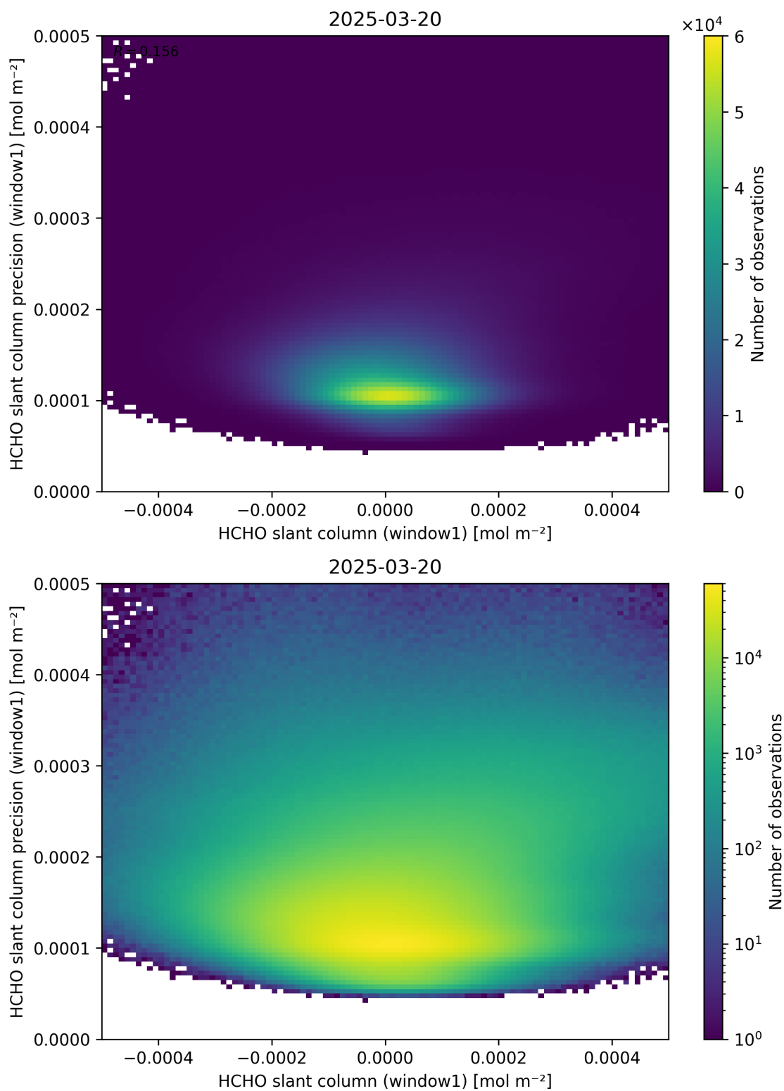
Figure 84: Scatter density plot of “HCHO slant column (window1)” against “HCHO slant column precision (window1)” for 2025-03-19 to 2025-03-21.
