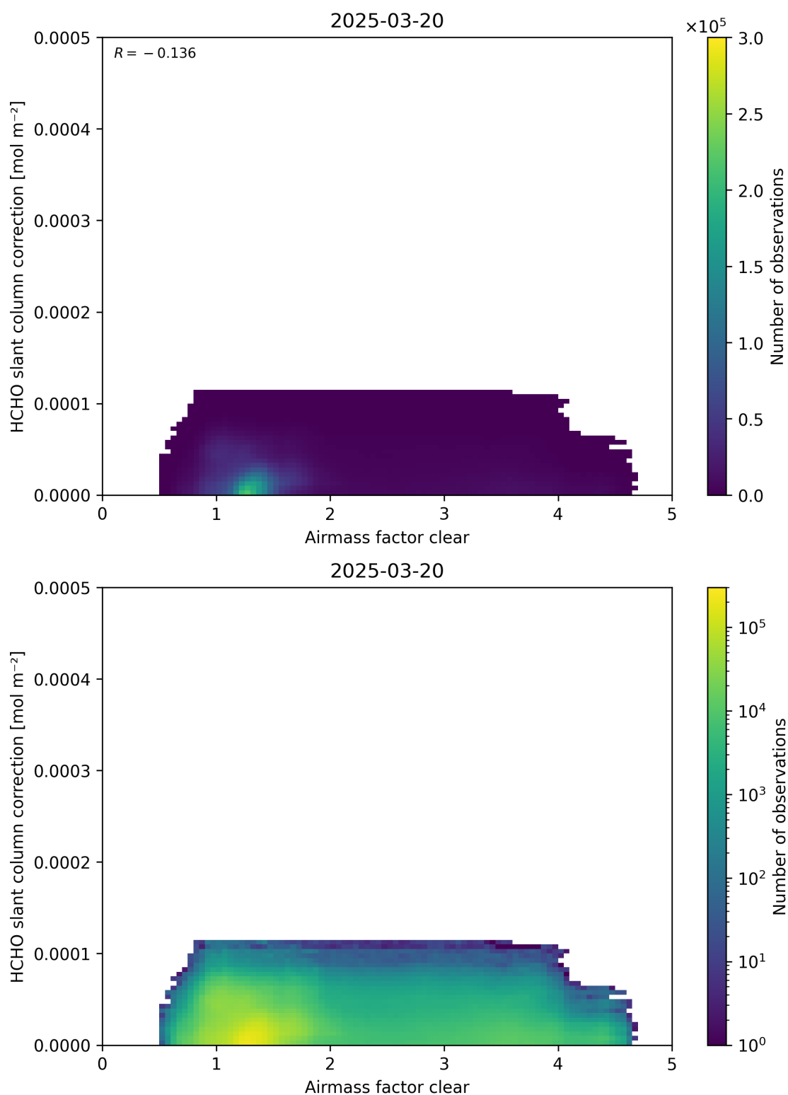
Figure 75: Scatter density plot of “Airmass factor clear” against “HCHO slant column correction” for 2025-03-19 to 2025-03-21.
