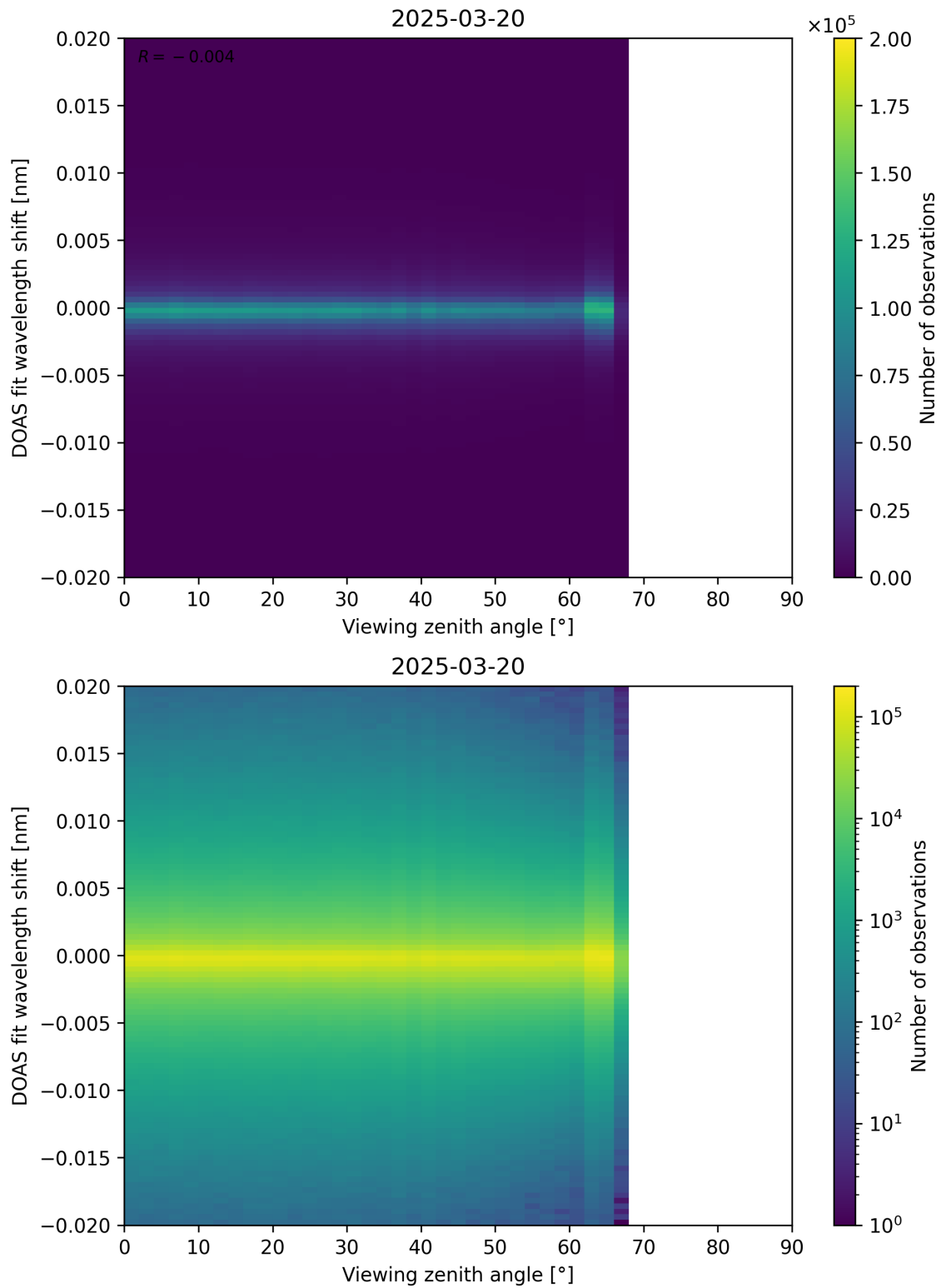
Figure 183: Scatter density plot of “Viewing zenith angle” against “DOAS fit wavelength shift” for 2025-03-19 to 2025-03-21.
