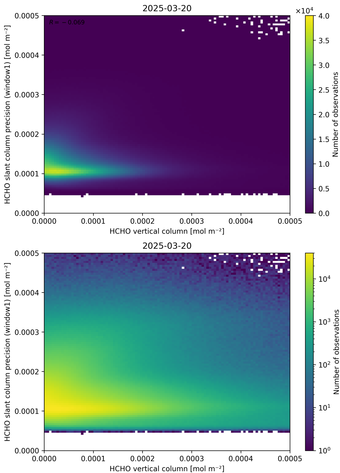
Figure 130: Scatter density plot of “HCHO vertical column” against “HCHO slant column precision (window1)” for 2025-03-19 to 2025-03-21.
