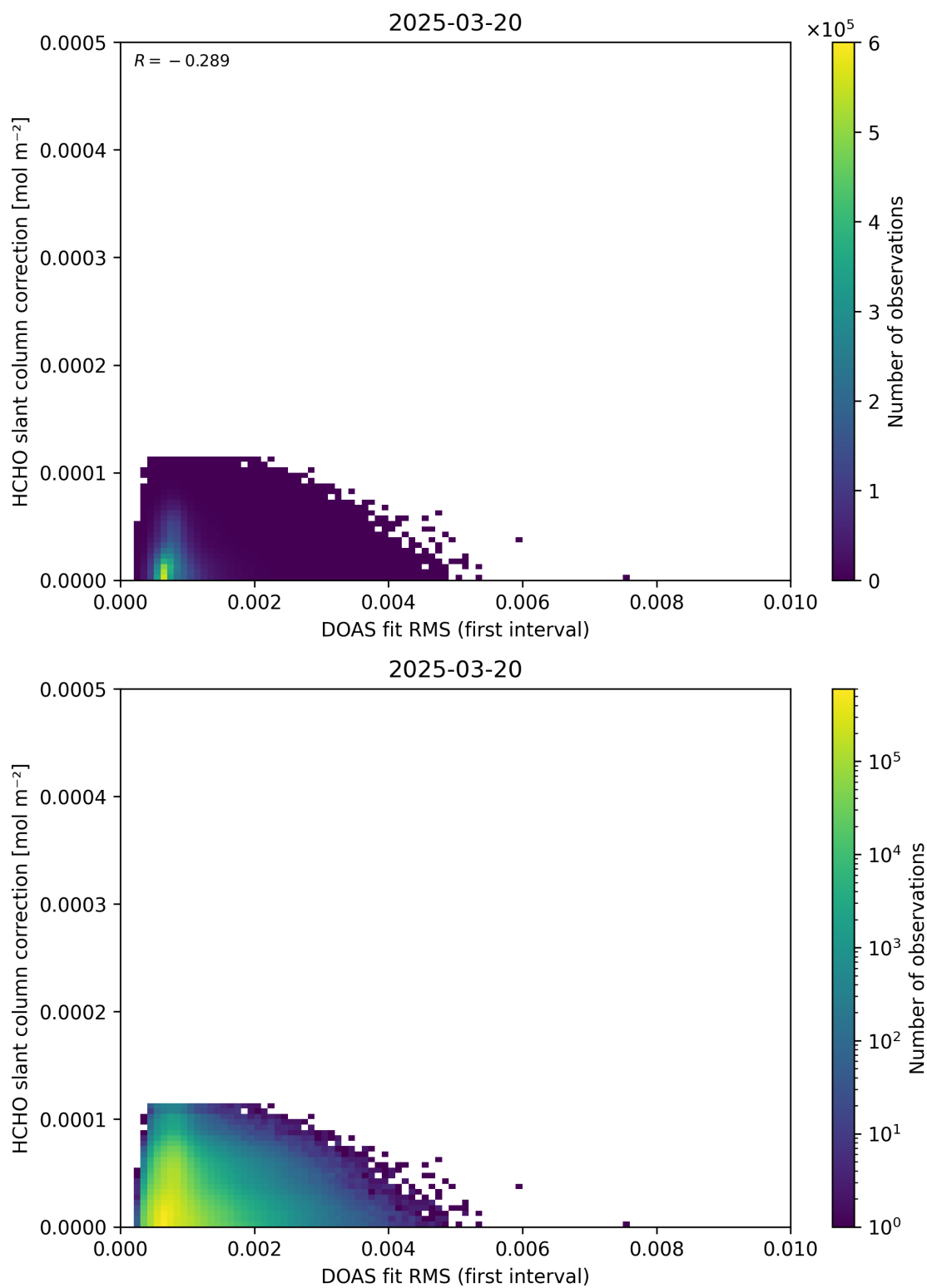
Figure 63: Scatter density plot of “DOAS fit RMS (first interval)” against “HCHO slant column correction” for 2025-03-19 to 2025-03-21.
