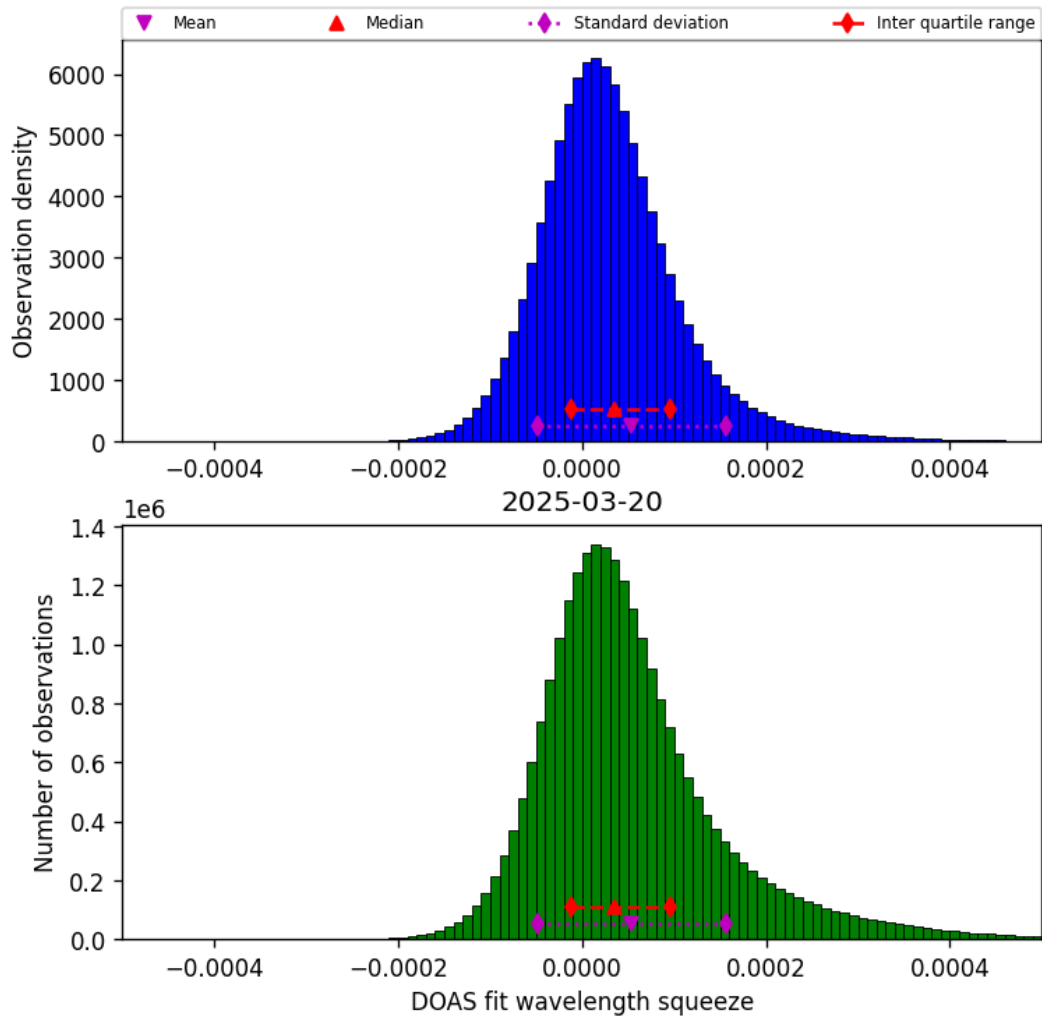
Figure 45: Histogram of “DOAS fit wavelength squeeze” for 2025-03-19 to 2025-03-21
