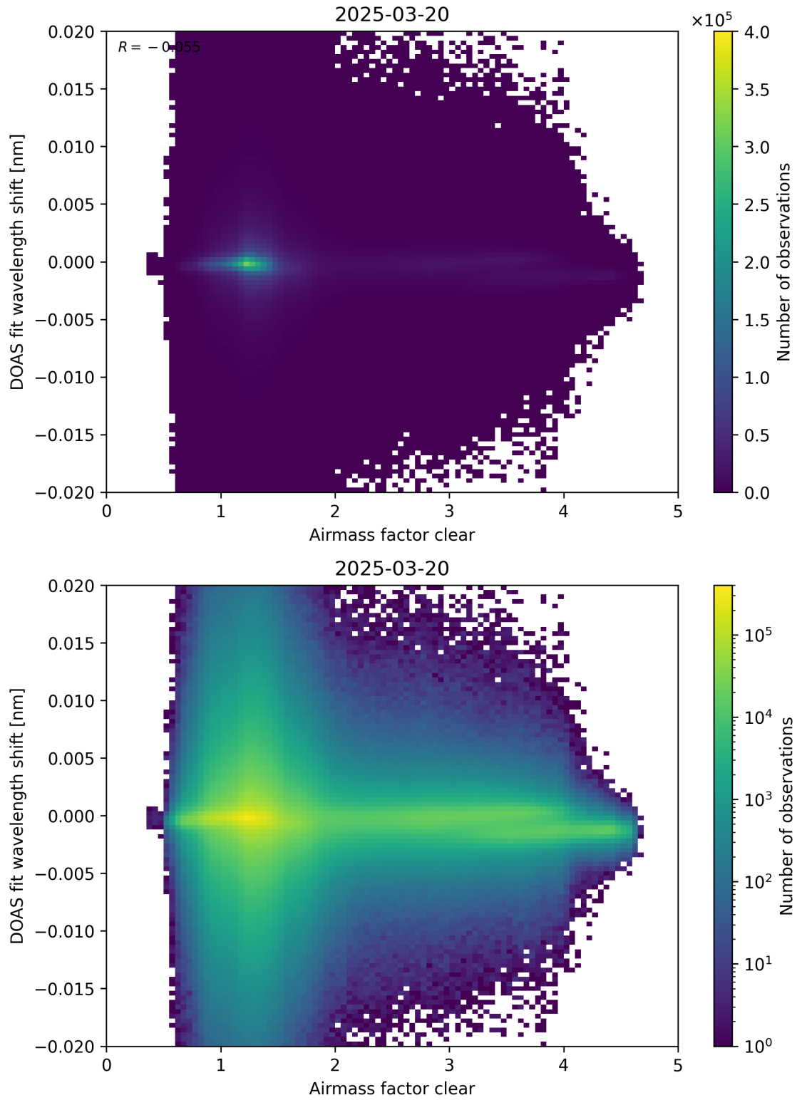
Figure 72: Scatter density plot of “Airmass factor clear” against “DOAS fit wavelength shift” for 2025-03-19 to 2025-03-21.
