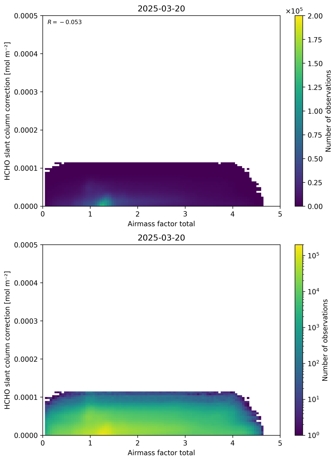
Figure 102: Scatter density plot of “Airmass factor total” against “HCHO slant column correction” for 2025-03-19 to 2025-03-21.
