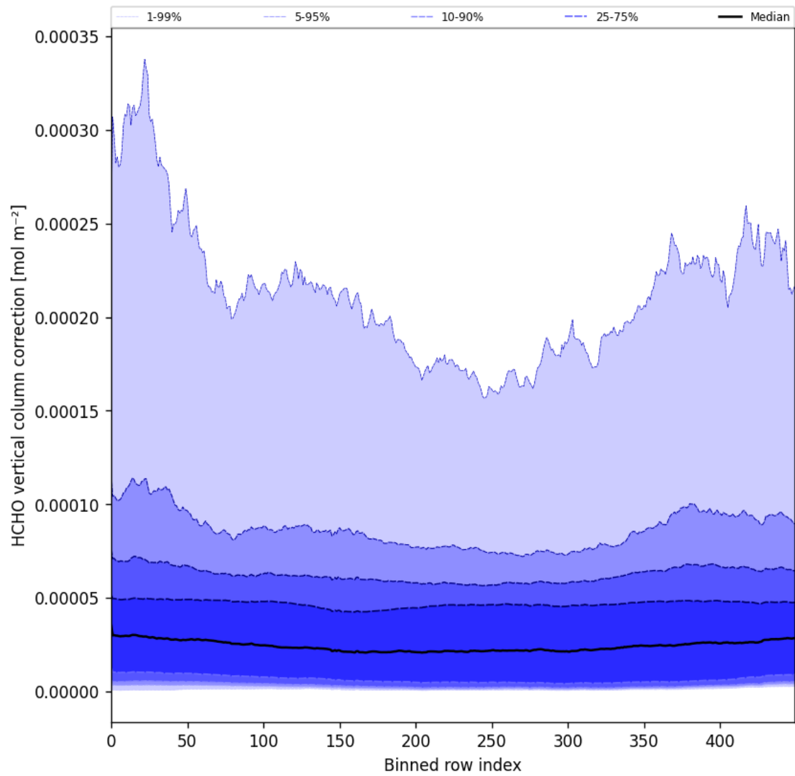
Figure 51: Along track statistics of “HCHO vertical column correction” for 2025-03-19 to 2025-03-21
