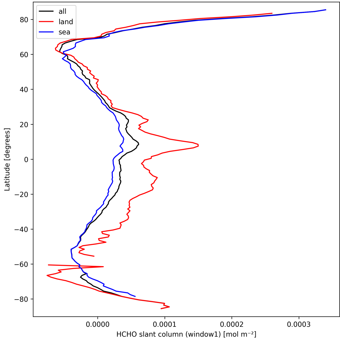
Figure 24: Zonal average of “HCHO slant column (window1)” for 2025-03-19 to 2025-03-21.
