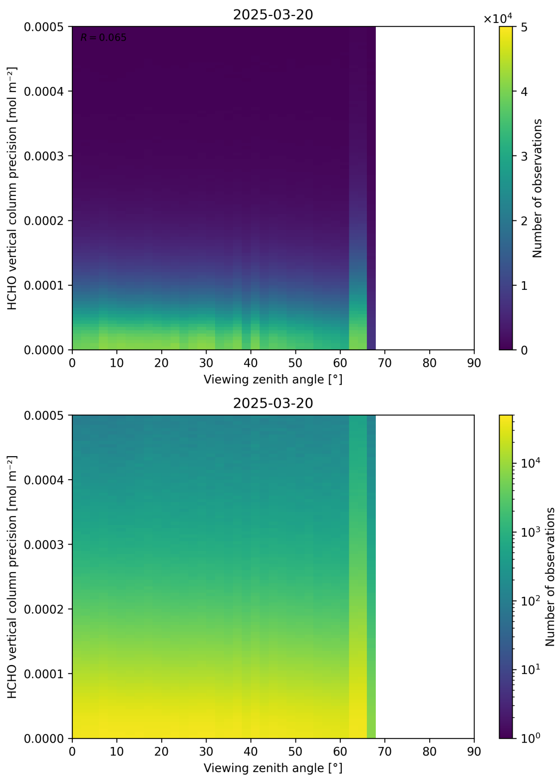
Figure 194: Scatter density plot of “Viewing zenith angle” against “HCHO vertical column precision” for 2025-03-19 to 2025-03-21.
