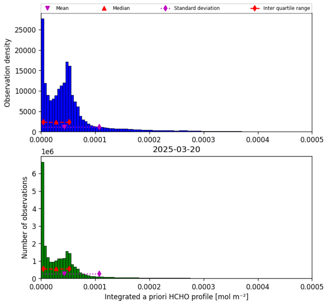
Figure 43: Histogram of “Integrated a priori HCHO profile” for 2025-03-19 to 2025-03-21
