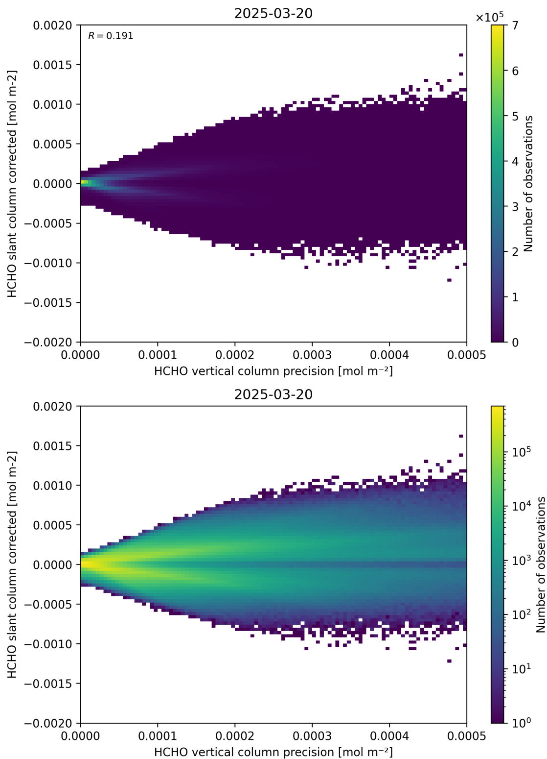
Figure 140: Scatter density plot of “HCHO vertical column precision” against “HCHO slant column corrected” for 2025-03-19 to 2025-03-21.
