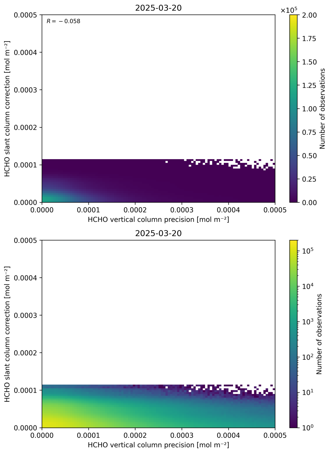
Figure 141: Scatter density plot of “HCHO vertical column precision” against “HCHO slant column correction” for 2025-03-19 to 2025-03-21.
