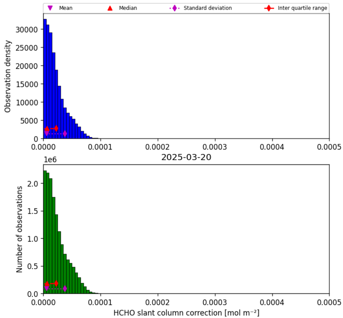
Figure 47: Histogram of “HCHO slant column correction” for 2025-03-19 to 2025-03-21
