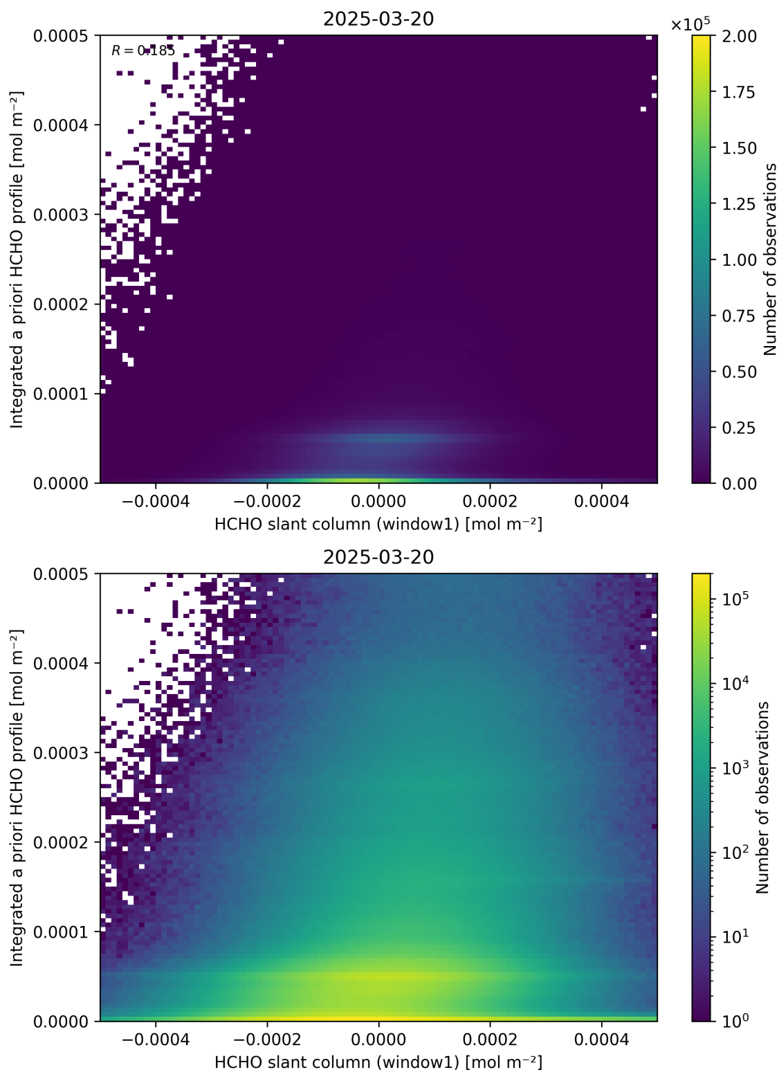
Figure 87: Scatter density plot of “HCHO slant column (window1)” against “Integrated a priori HCHO profile” for 2025-03-19 to 2025-03-21.
