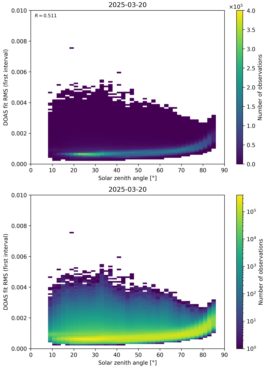
Figure 167: Scatter density plot of “Solar zenith angle” against “DOAS fit RMS (first interval)” for 2025-03-19 to 2025-03-21.
