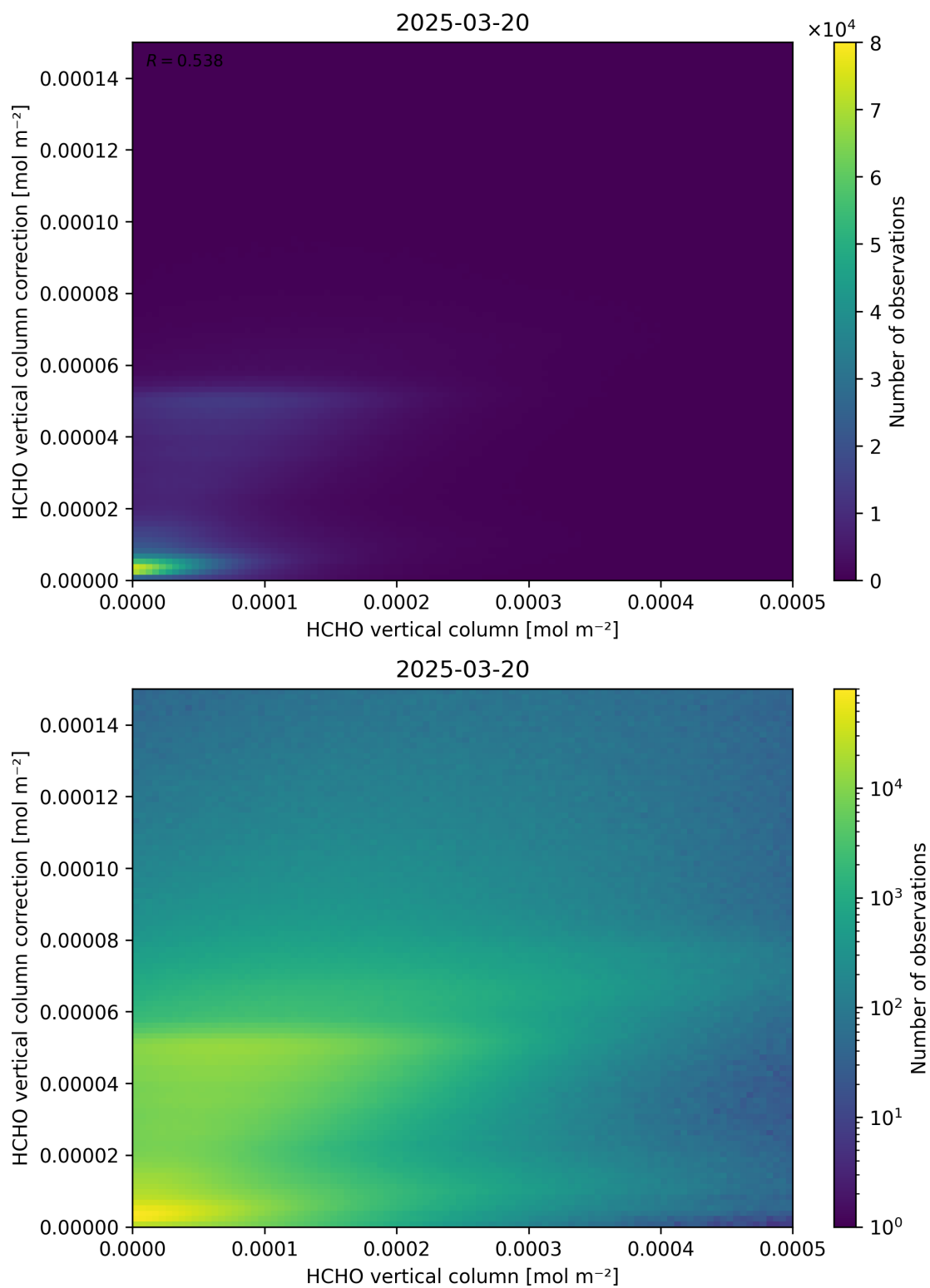
Figure 133: Scatter density plot of “HCHO vertical column” against “HCHO vertical column correction” for 2025-03-19 to 2025-03-21.
