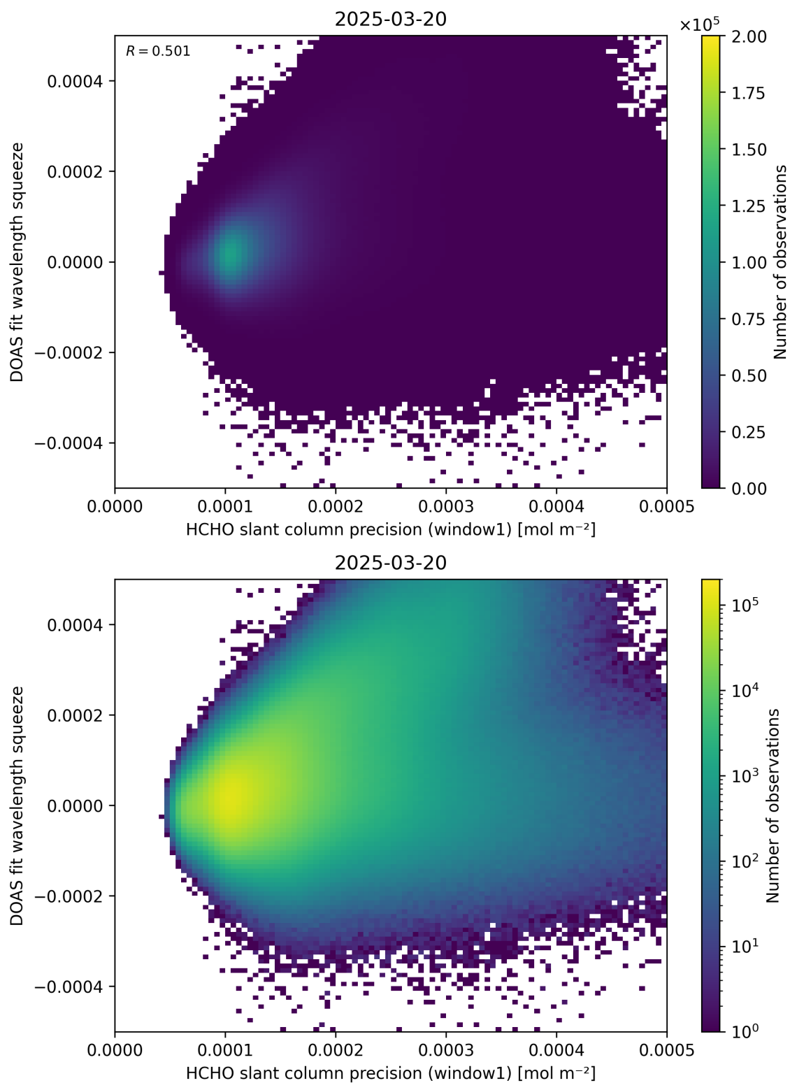
Figure 90: Scatter density plot of “HCHO slant column precision (window1)” against “DOAS fit wavelength squeeze” for 2025-03-19 to 2025-03-21.
