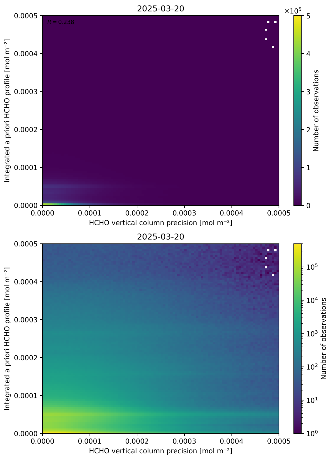
Figure 147: Scatter density plot of “HCHO vertical column precision” against “Integrated a priori HCHO profile” for 2025-03-19 to 2025-03-21.
