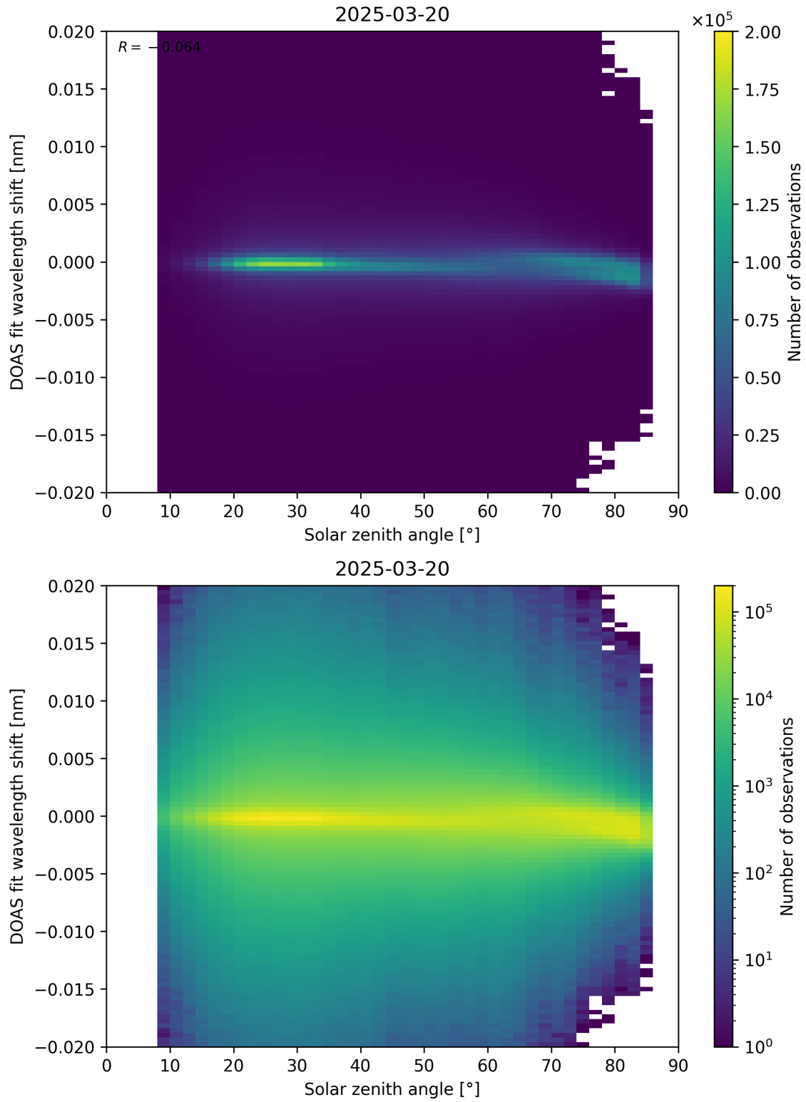
Figure 168: Scatter density plot of “Solar zenith angle” against “DOAS fit wavelength shift” for 2025-03-19 to 2025-03-21.
