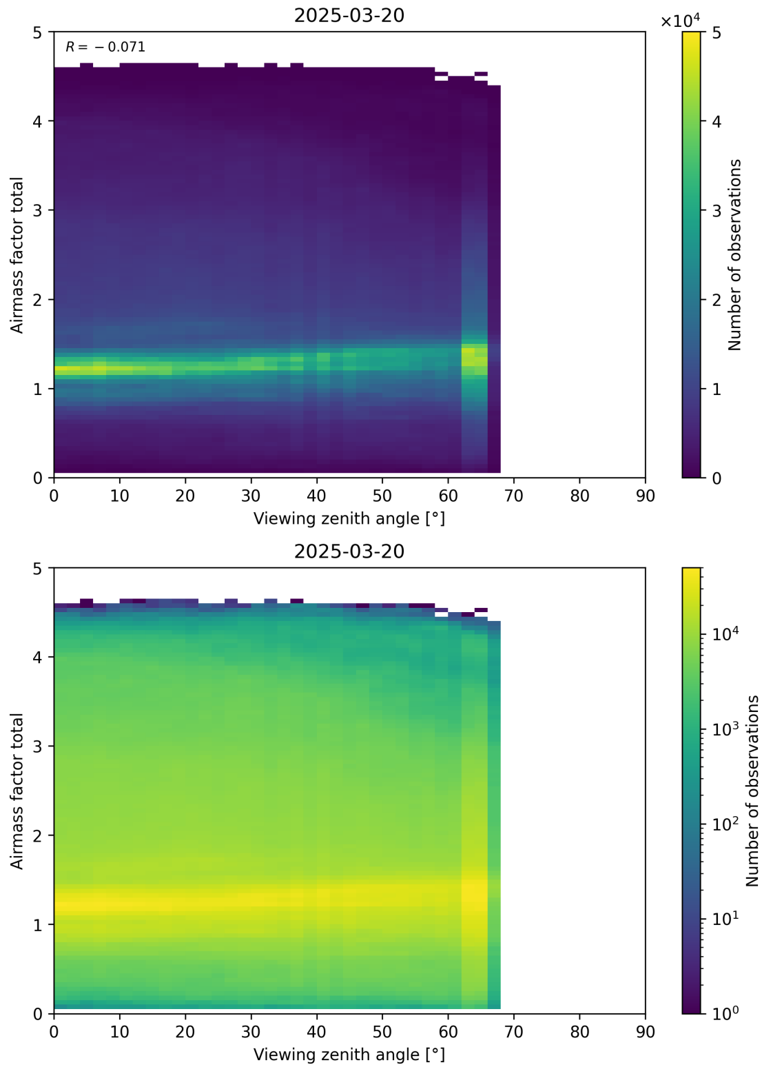
Figure 190: Scatter density plot of “Viewing zenith angle” against “Airmass factor total” for 2025-03-19 to 2025-03-21.
