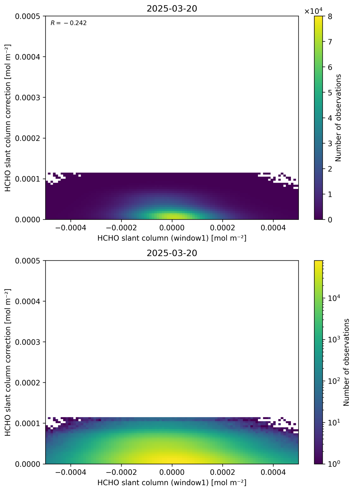
Figure 83: Scatter density plot of “HCHO slant column (window1)” against “HCHO slant column correction” for 2025-03-19 to 2025-03-21.
