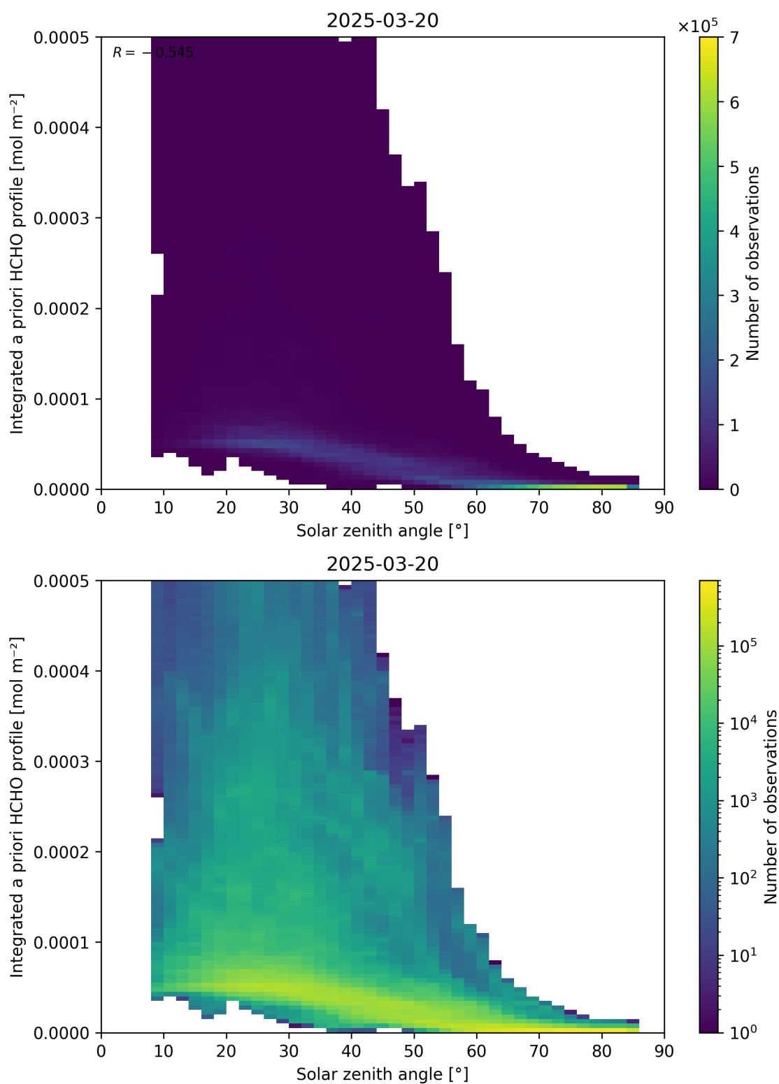
Figure 180: Scatter density plot of “Solar zenith angle” against “Integrated a priori HCHO profile” for 2025-03-19 to 2025-03-21.
