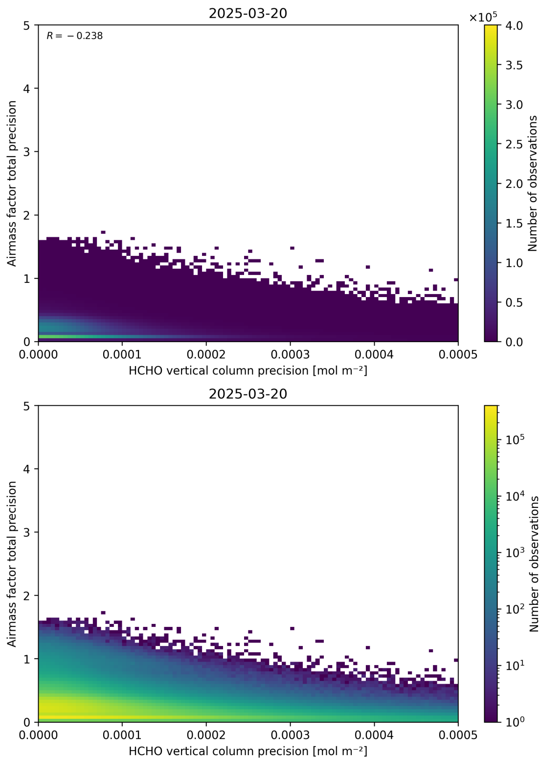
Figure 145: Scatter density plot of “HCHO vertical column precision” against “Airmass factor total precision” for 2025-03-19 to 2025-03-21.
