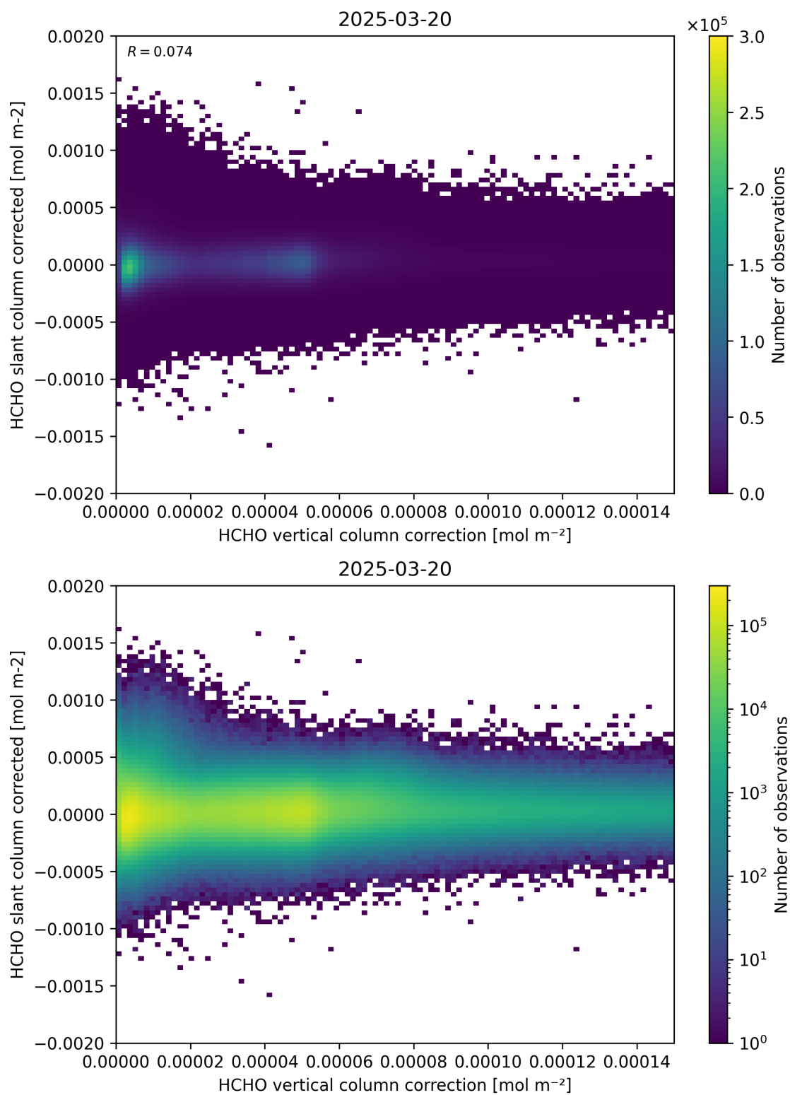
Figure 116: Scatter density plot of “HCHO vertical column correction” against “HCHO slant column corrected” for 2025-03-19 to 2025-03-21.
