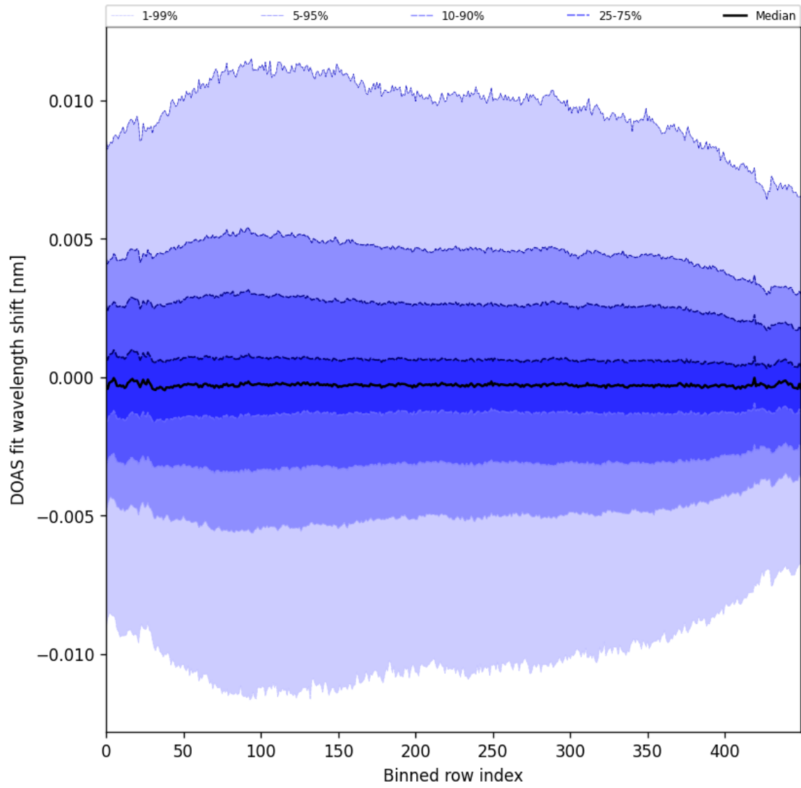
Figure 58: Along track statistics of “DOAS fit wavelength shift” for 2025-03-19 to 2025-03-21
