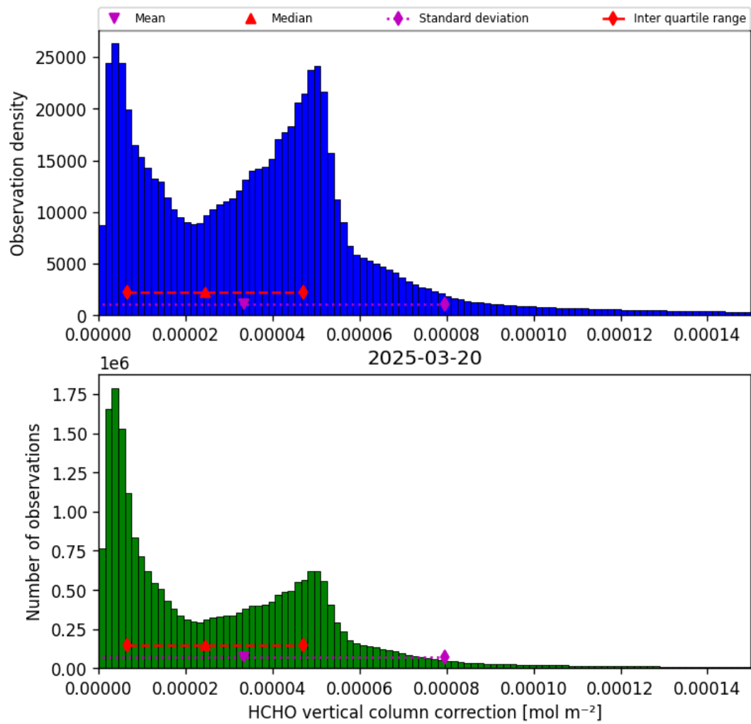
Figure 37: Histogram of “HCHO vertical column correction” for 2025-03-19 to 2025-03-21
