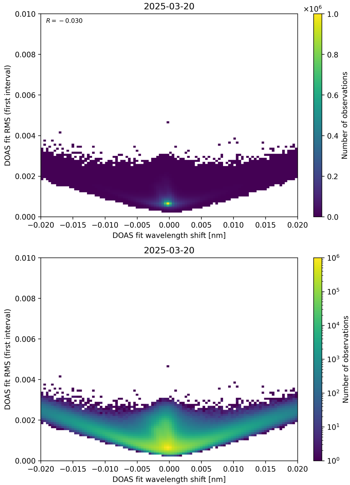
Figure 64: Scatter density plot of “DOAS fit wavelength shift” against “DOAS fit RMS (first interval)” for 2025-03-19 to 2025-03-21.
