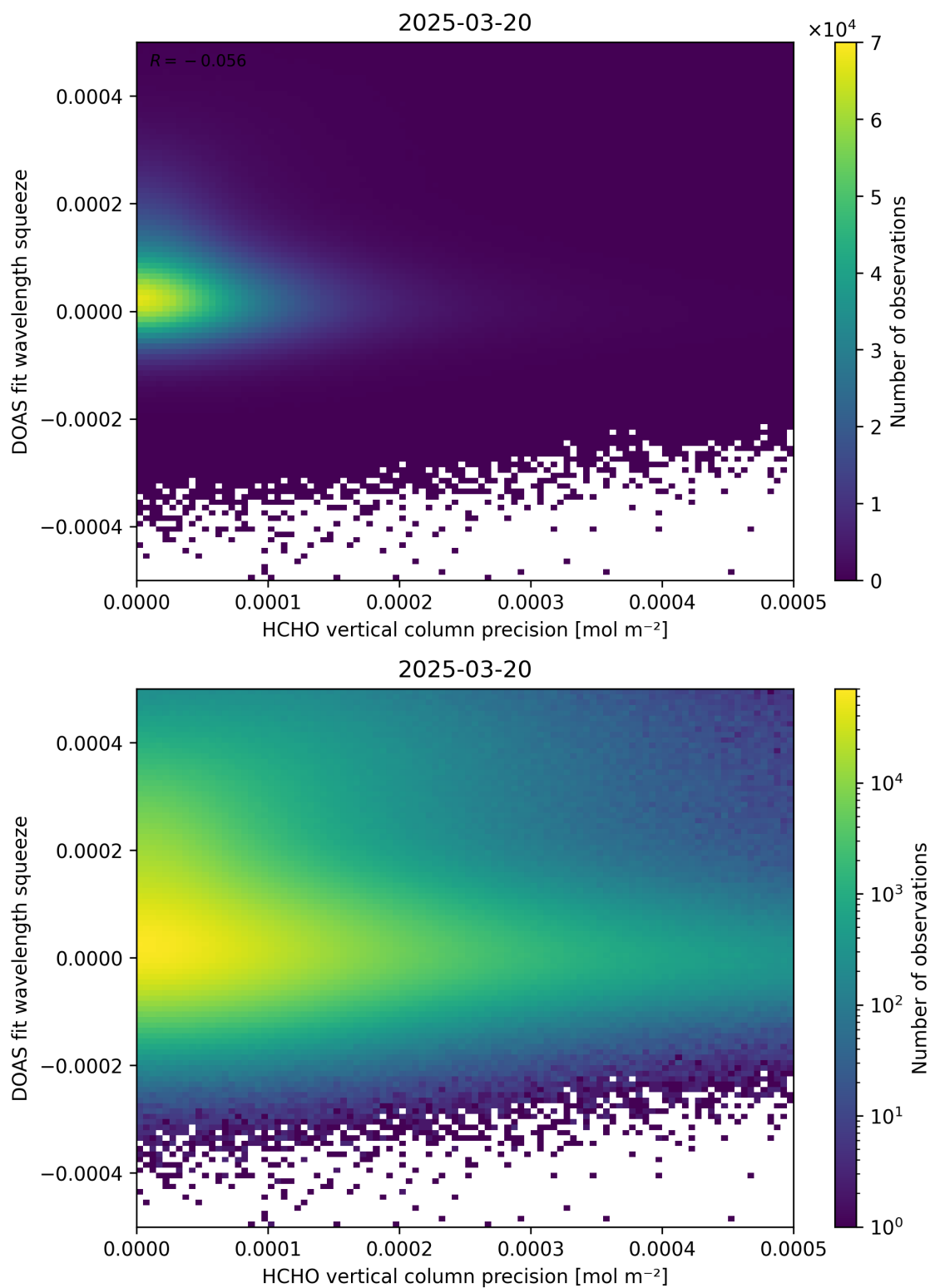
Figure 138: Scatter density plot of “HCHO vertical column precision” against “DOAS fit wavelength squeeze” for 2025-03-19 to 2025-03-21.
