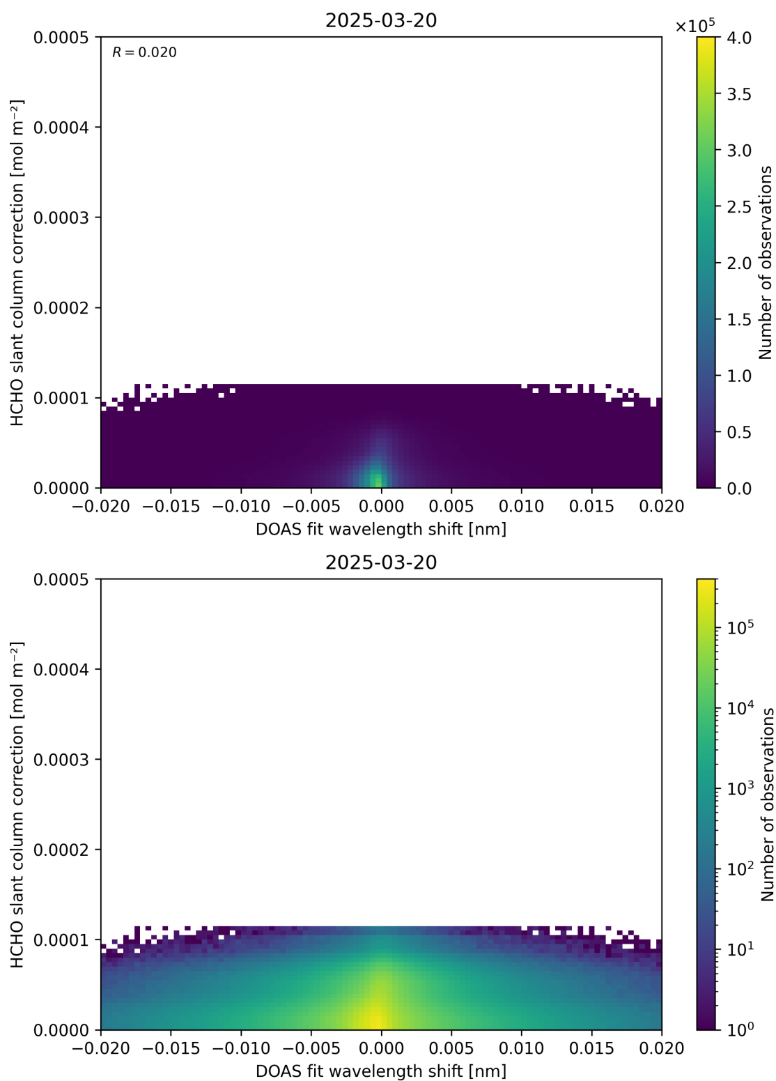
Figure 67: Scatter density plot of “DOAS fit wavelength shift” against “HCHO slant column correction” for 2025-03-19 to 2025-03-21.
