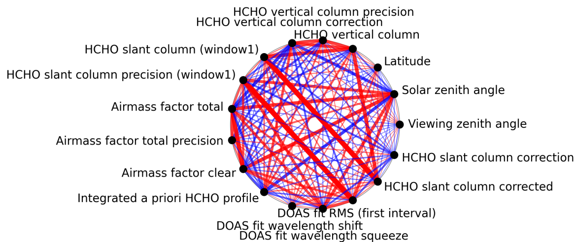
Figure 1: Map of correlation graph for 2025-03-20 to 2025-03-22.
