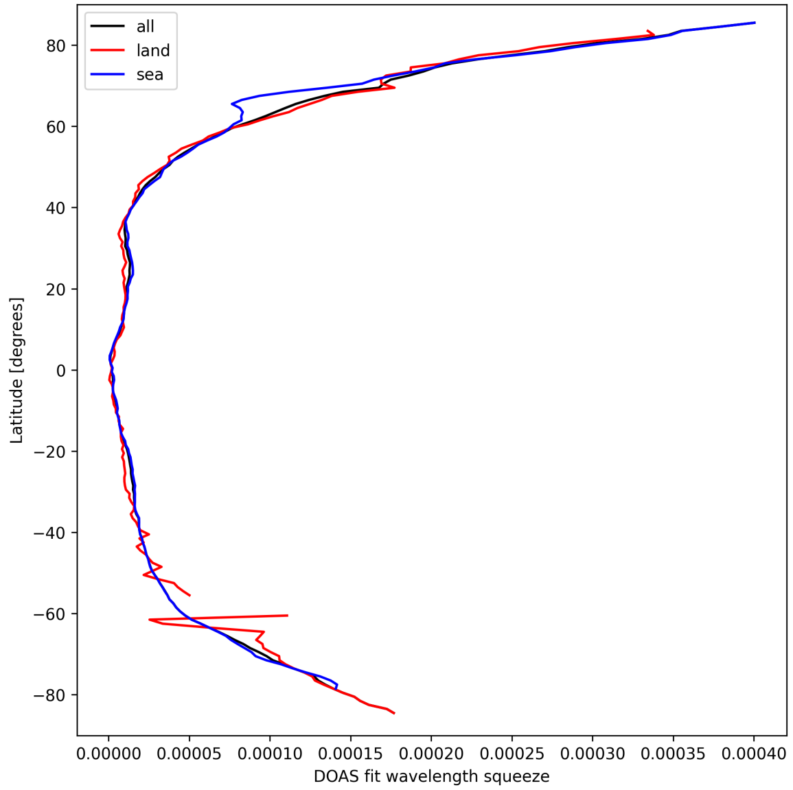
Figure 31: Zonal average of “DOAS fit wavelength squeeze” for 2025-03-20 to 2025-03-22.
