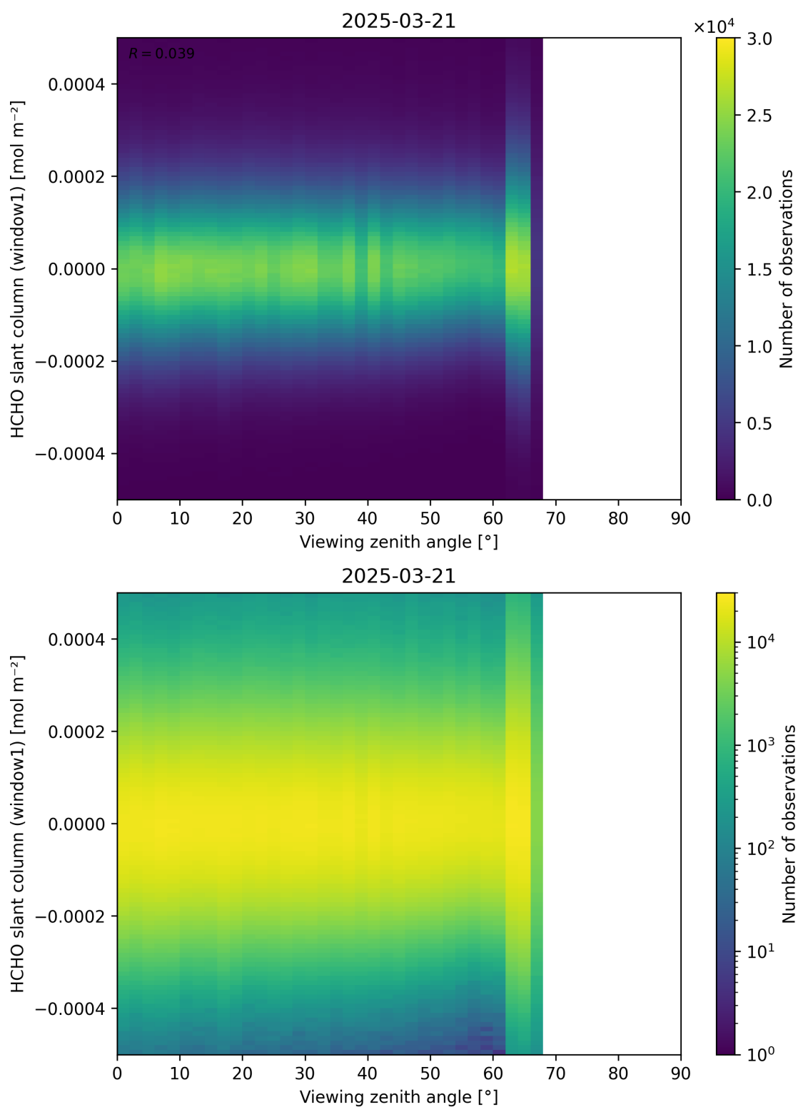
Figure 188: Scatter density plot of “Viewing zenith angle” against “HCHO slant column (window1)” for 2025-03-20 to 2025-03-22.
