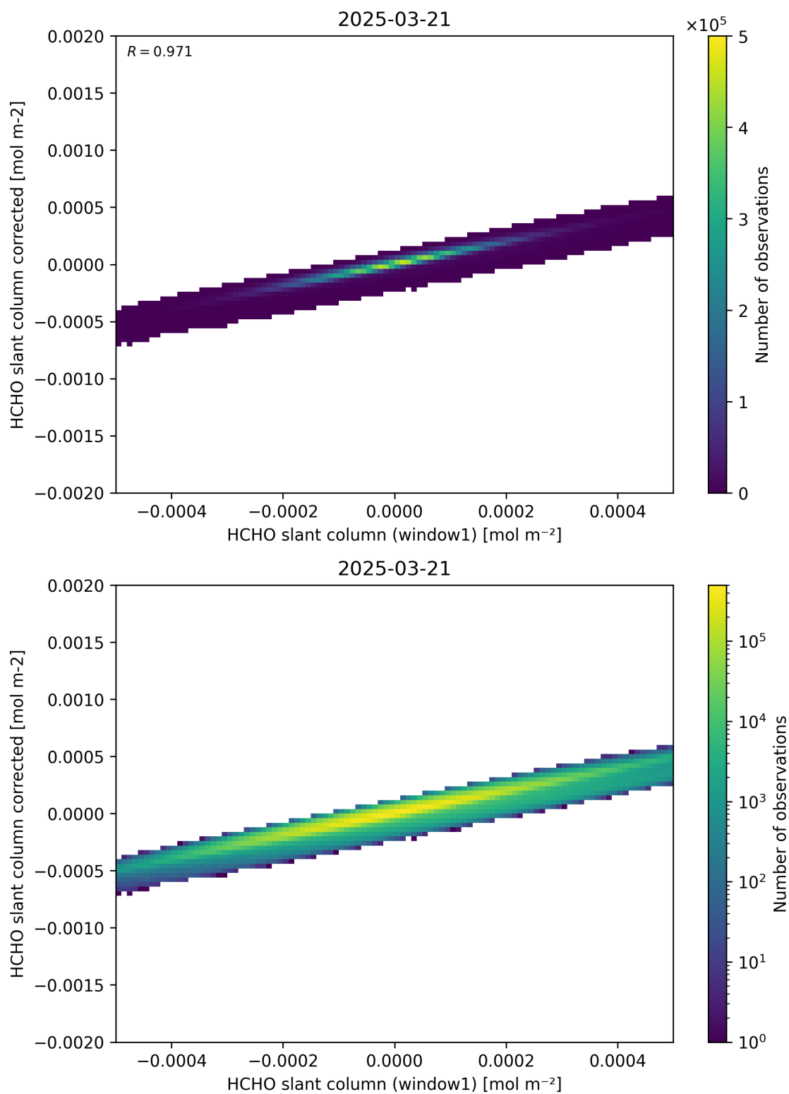
Figure 82: Scatter density plot of “HCHO slant column (window1)” against “HCHO slant column corrected” for 2025-03-20 to 2025-03-22.
