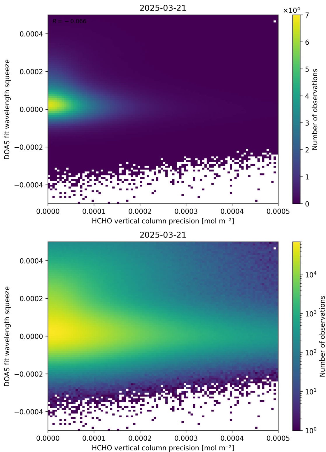
Figure 138: Scatter density plot of “HCHO vertical column precision” against “DOAS fit wavelength squeeze” for 2025-03-20 to 2025-03-22.
