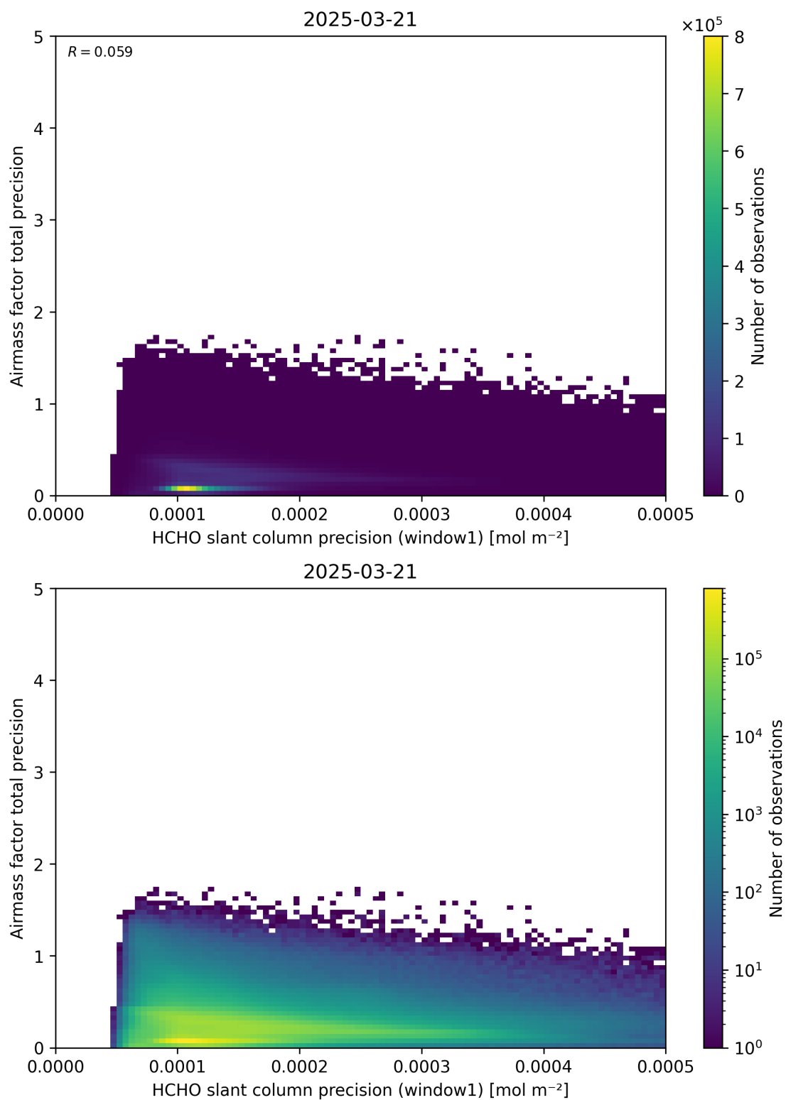
Figure 95: Scatter density plot of “HCHO slant column precision (window1)” against “Airmass factor total precision” for 2025-03-20 to 2025-03-22.
