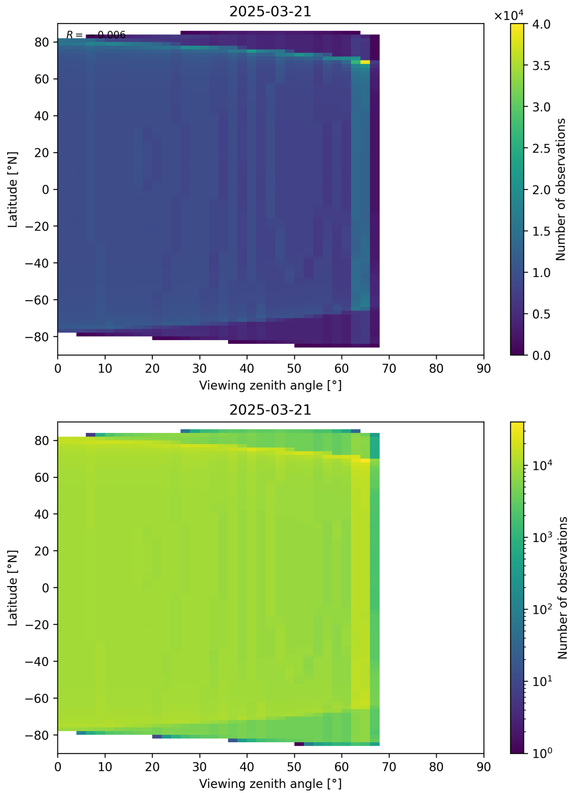
Figure 196: Scatter density plot of “Viewing zenith angle” against “Latitude” for 2025-03-20 to 2025-03-22.
