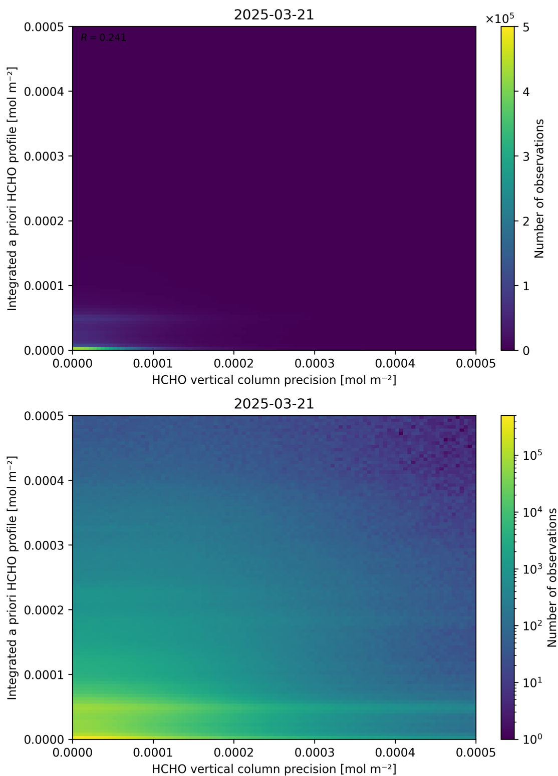
Figure 147: Scatter density plot of “HCHO vertical column precision” against “Integrated a priori HCHO profile” for 2025-03-20 to 2025-03-22.
