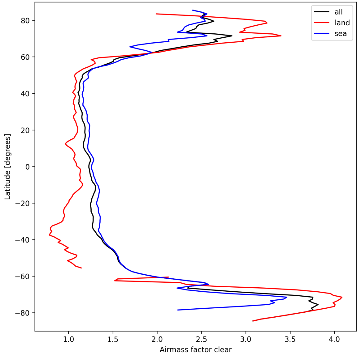
Figure 28: Zonal average of “Airmass factor clear” for 2025-03-20 to 2025-03-22.
