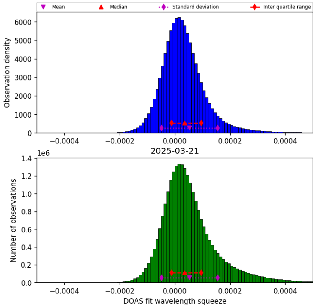
Figure 45: Histogram of “DOAS fit wavelength squeeze” for 2025-03-20 to 2025-03-22
