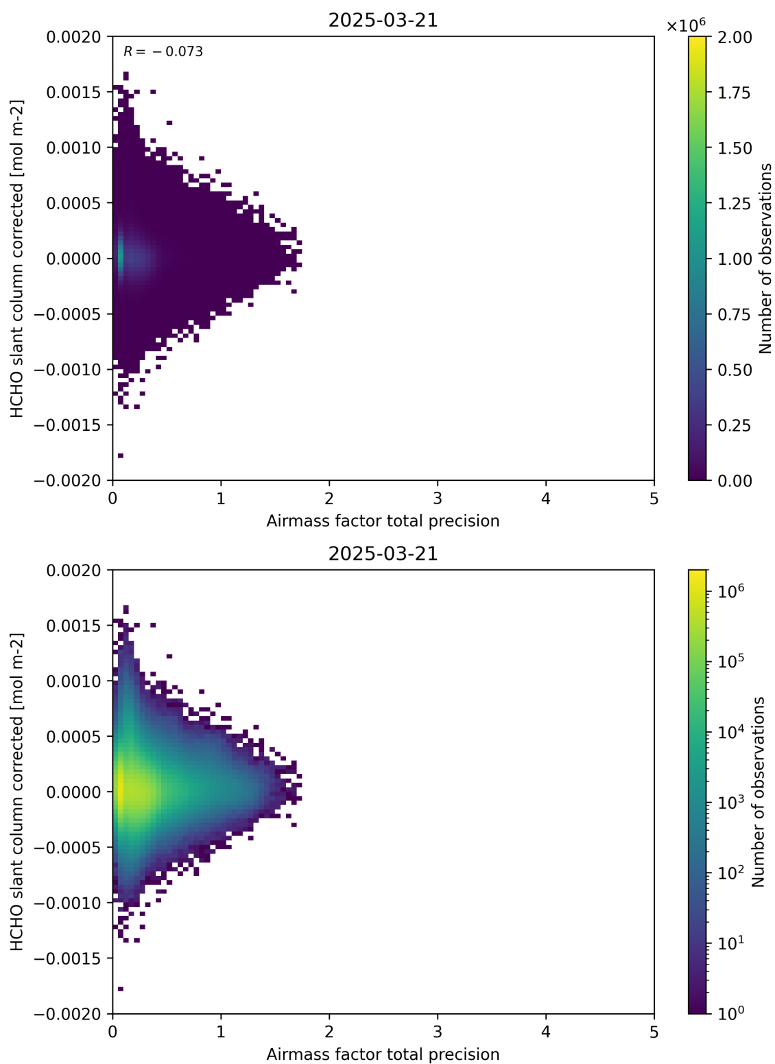
Figure 109: Scatter density plot of “Airmass factor total precision” against “HCHO slant column corrected” for 2025-03-20 to 2025-03-22.
