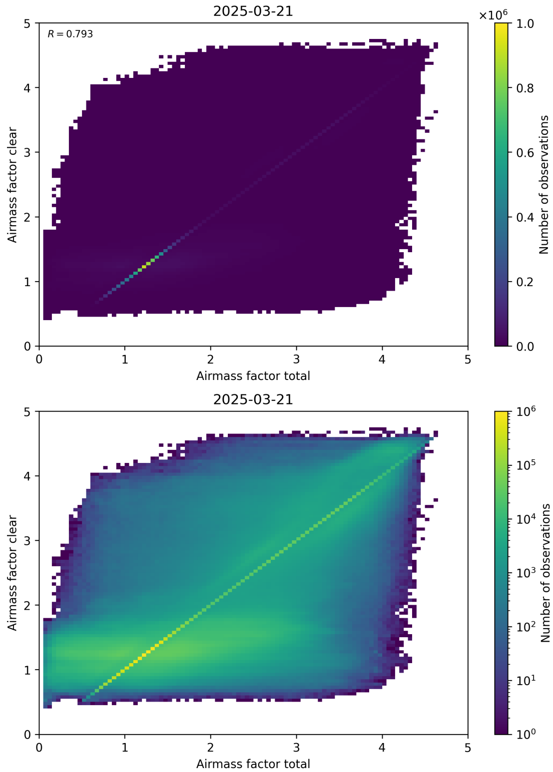
Figure 100: Scatter density plot of “Airmass factor total” against “Airmass factor clear” for 2025-03-20 to 2025-03-22.
