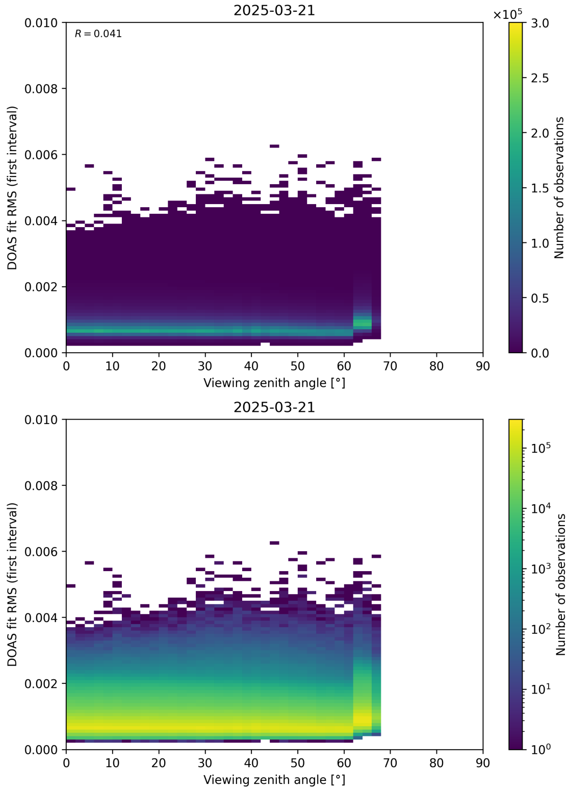
Figure 182: Scatter density plot of “Viewing zenith angle” against “DOAS fit RMS (first interval)” for 2025-03-20 to 2025-03-22.
