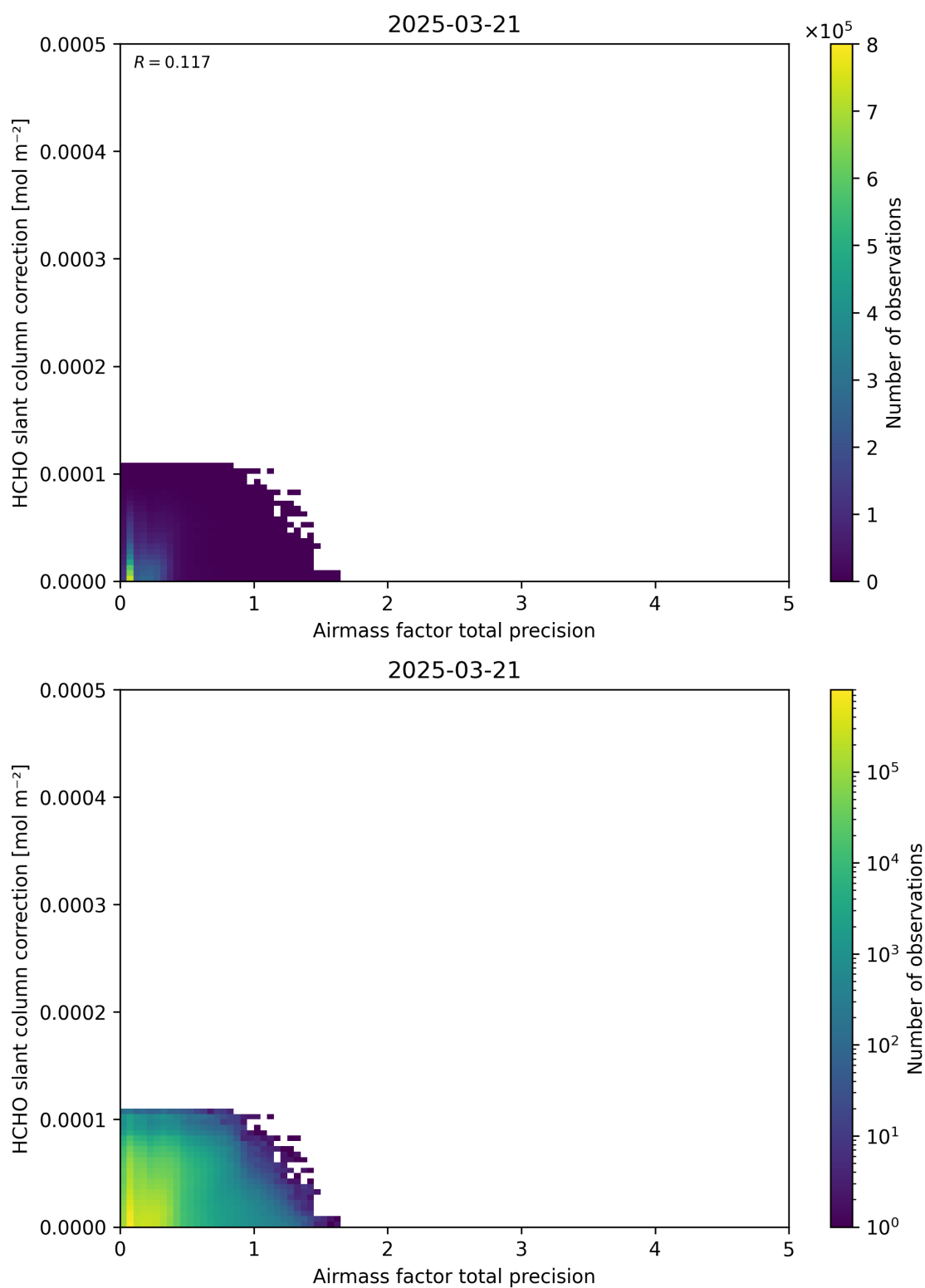
Figure 110: Scatter density plot of “Airmass factor total precision” against “HCHO slant column correction” for 2025-03-20 to 2025-03-22.
