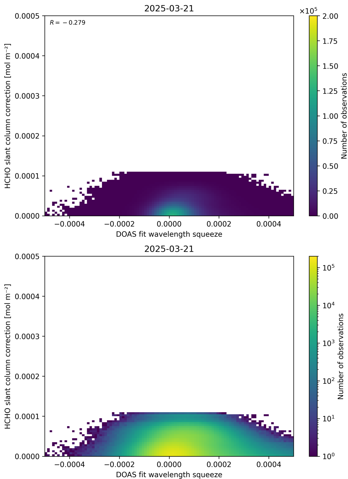
Figure 70: Scatter density plot of “DOAS fit wavelength squeeze” against “HCHO slant column correction” for 2025-03-20 to 2025-03-22.
