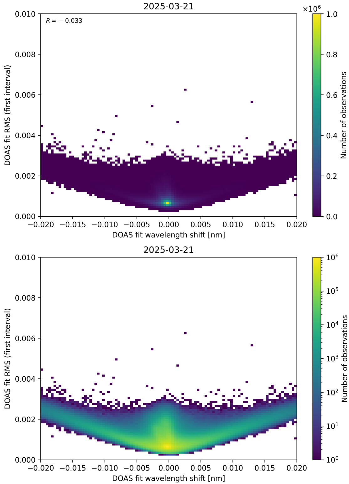
Figure 64: Scatter density plot of “DOAS fit wavelength shift” against “DOAS fit RMS (first interval)” for 2025-03-20 to 2025-03-22.
