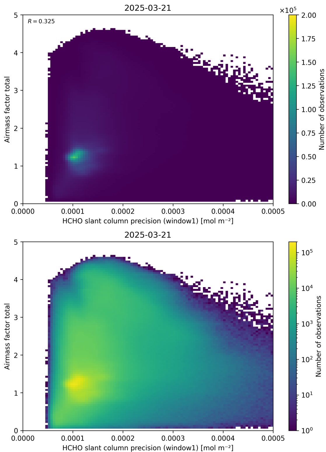
Figure 94: Scatter density plot of “HCHO slant column precision (window1)” against “Airmass factor total” for 2025-03-20 to 2025-03-22.
