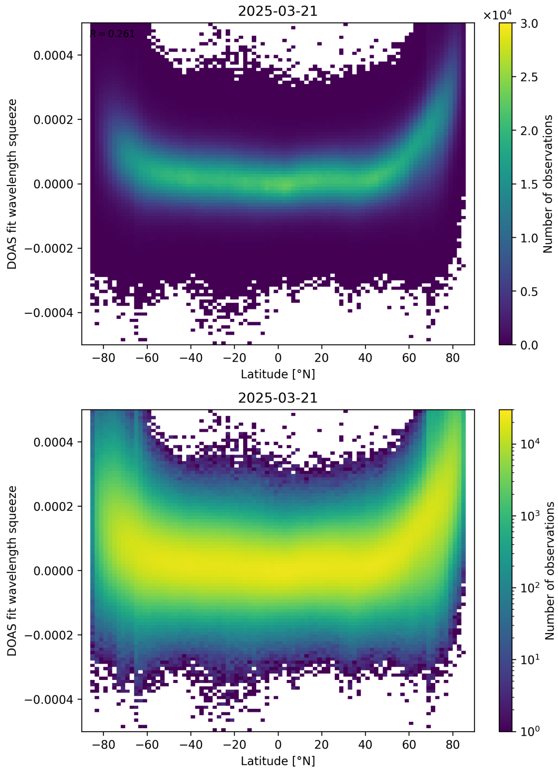
Figure 155: Scatter density plot of “Latitude” against “DOAS fit wavelength squeeze” for 2025-03-20 to 2025-03-22.
