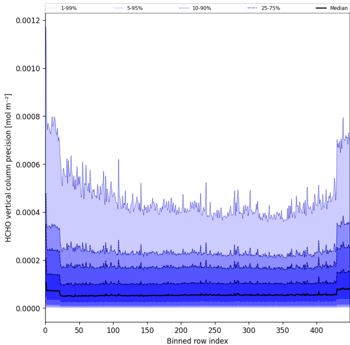
Figure 50: Along track statistics of “HCHO vertical column precision” for 2025-03-20 to 2025-03-22
