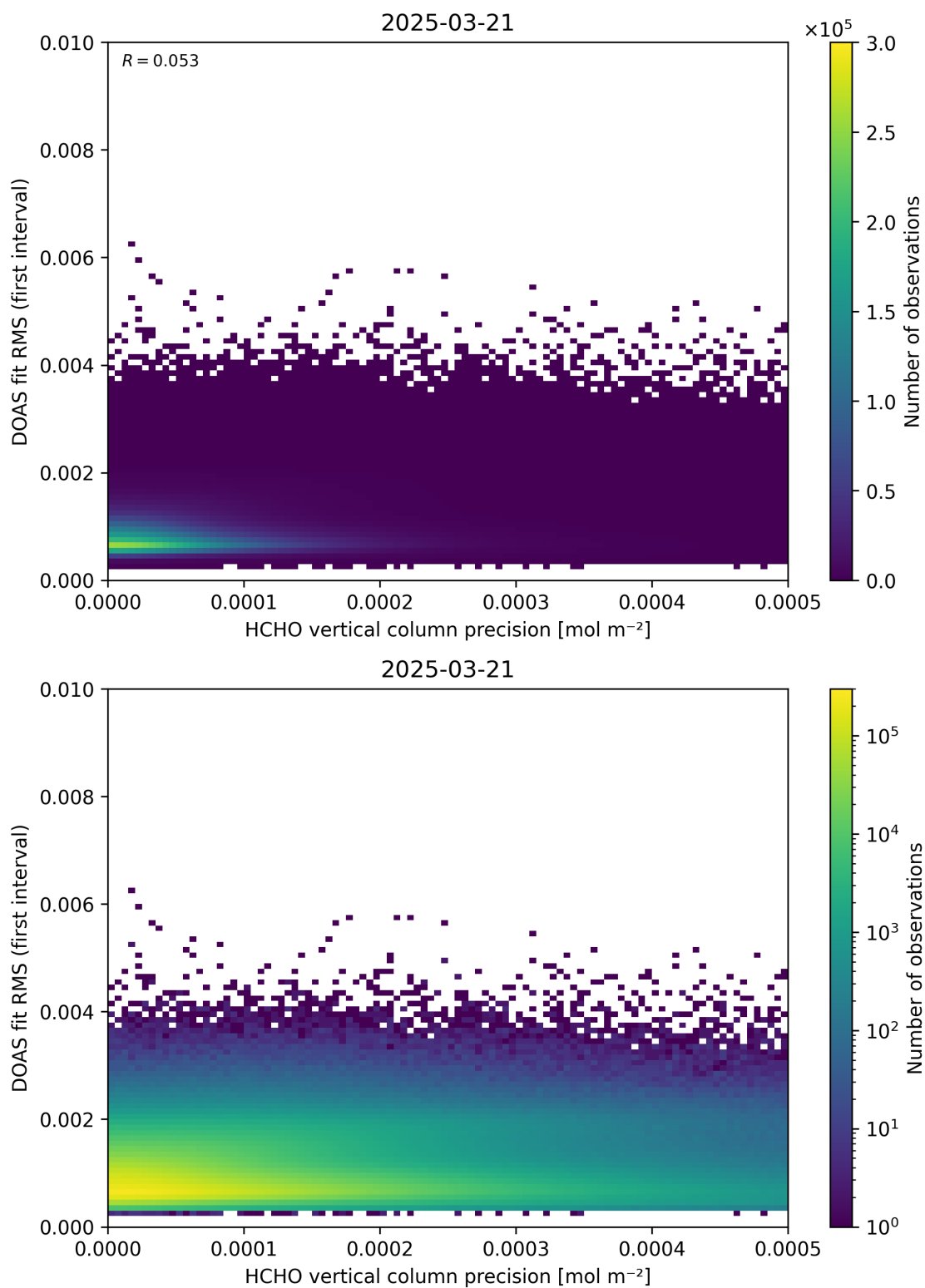
Figure 136: Scatter density plot of “HCHO vertical column precision” against “DOAS fit RMS (first interval)” for 2025-03-20 to 2025-03-22.
