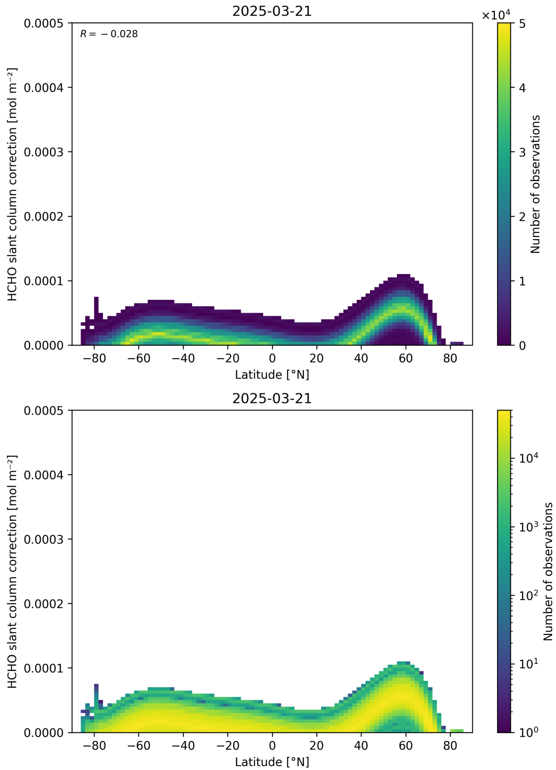
Figure 158: Scatter density plot of “Latitude” against “HCHO slant column correction” for 2025-03-20 to 2025-03-22.
