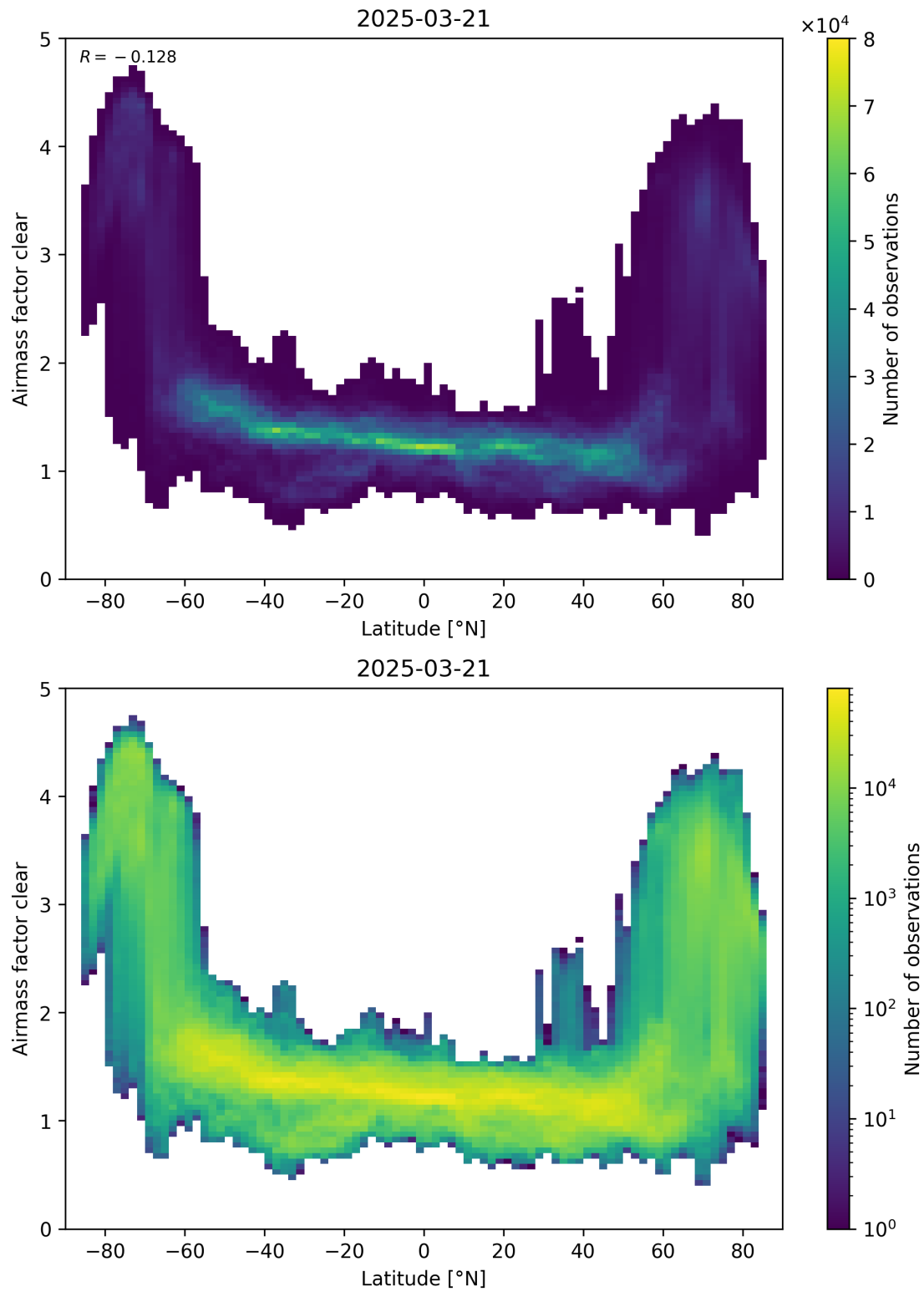
Figure 156: Scatter density plot of “Latitude” against “Airmass factor clear” for 2025-03-20 to 2025-03-22.
