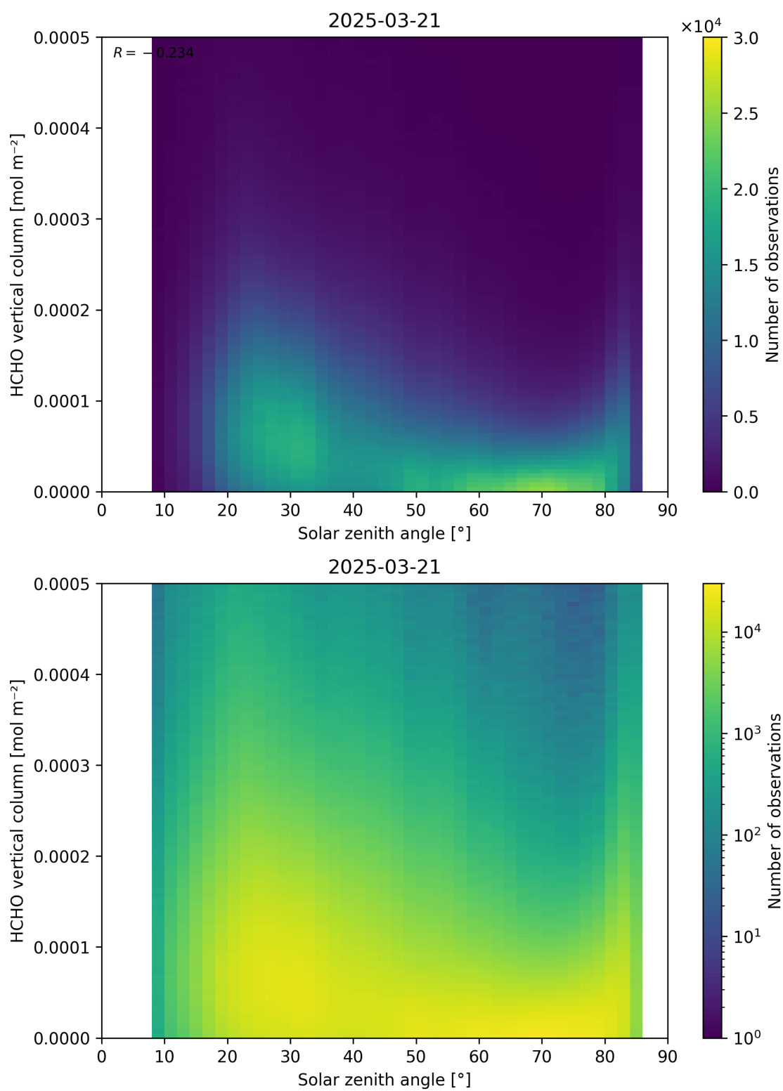
Figure 177: Scatter density plot of “Solar zenith angle” against “HCHO vertical column” for 2025-03-20 to 2025-03-22.
