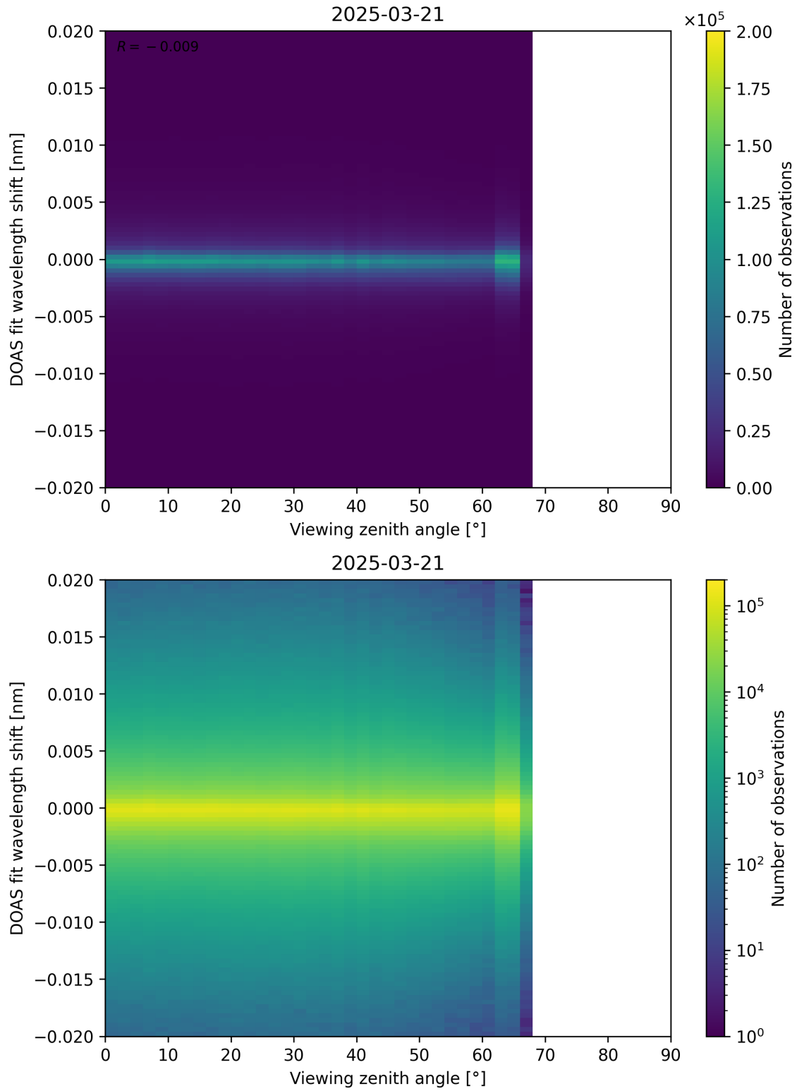
Figure 183: Scatter density plot of “Viewing zenith angle” against “DOAS fit wavelength shift” for 2025-03-20 to 2025-03-22.
