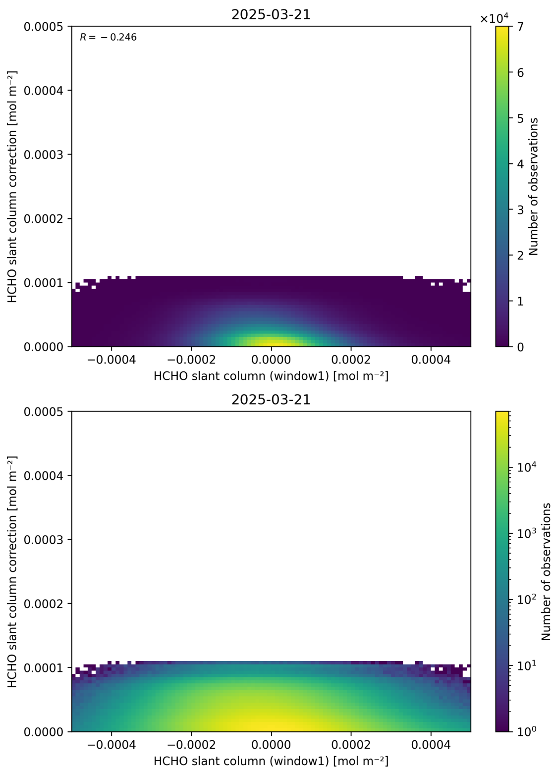
Figure 83: Scatter density plot of “HCHO slant column (window1)” against “HCHO slant column correction” for 2025-03-20 to 2025-03-22.
