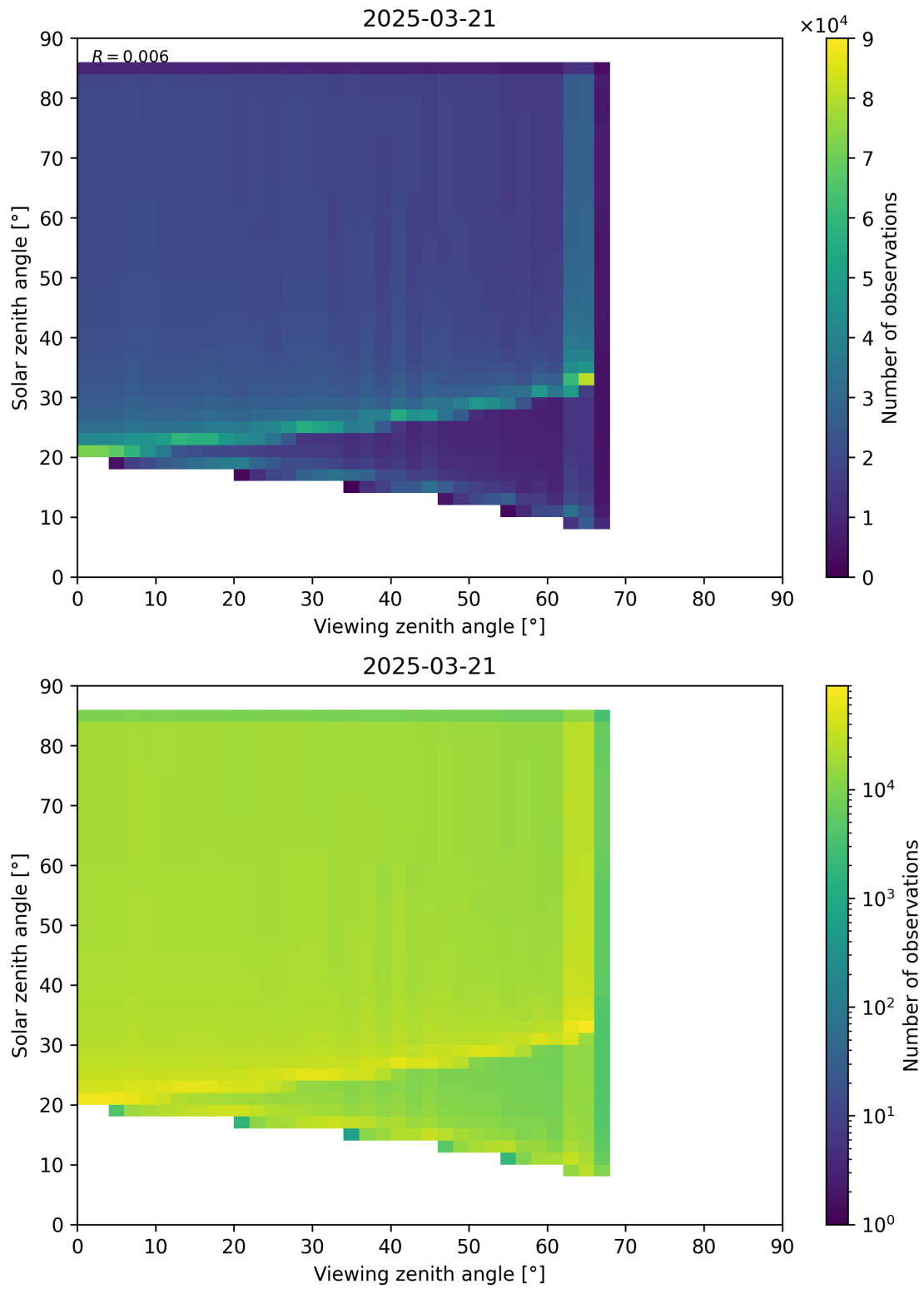
Figure 197: Scatter density plot of “Viewing zenith angle” against “Solar zenith angle” for 2025-03-20 to 2025-03-22.
