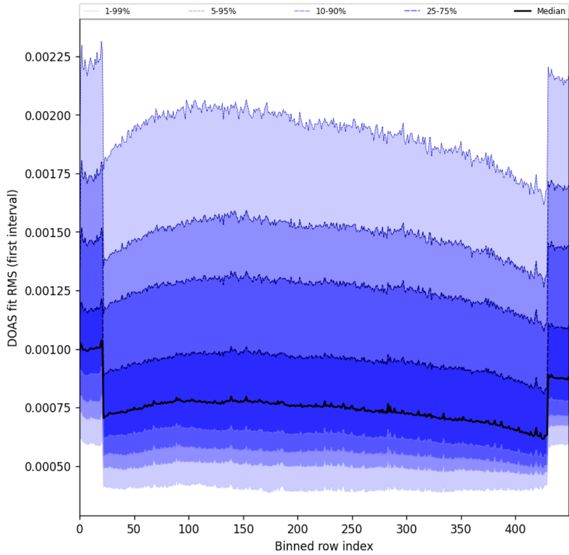
Figure 60: Along track statistics of “DOAS fit RMS (first interval)” for 2025-03-20 to 2025-03-22
