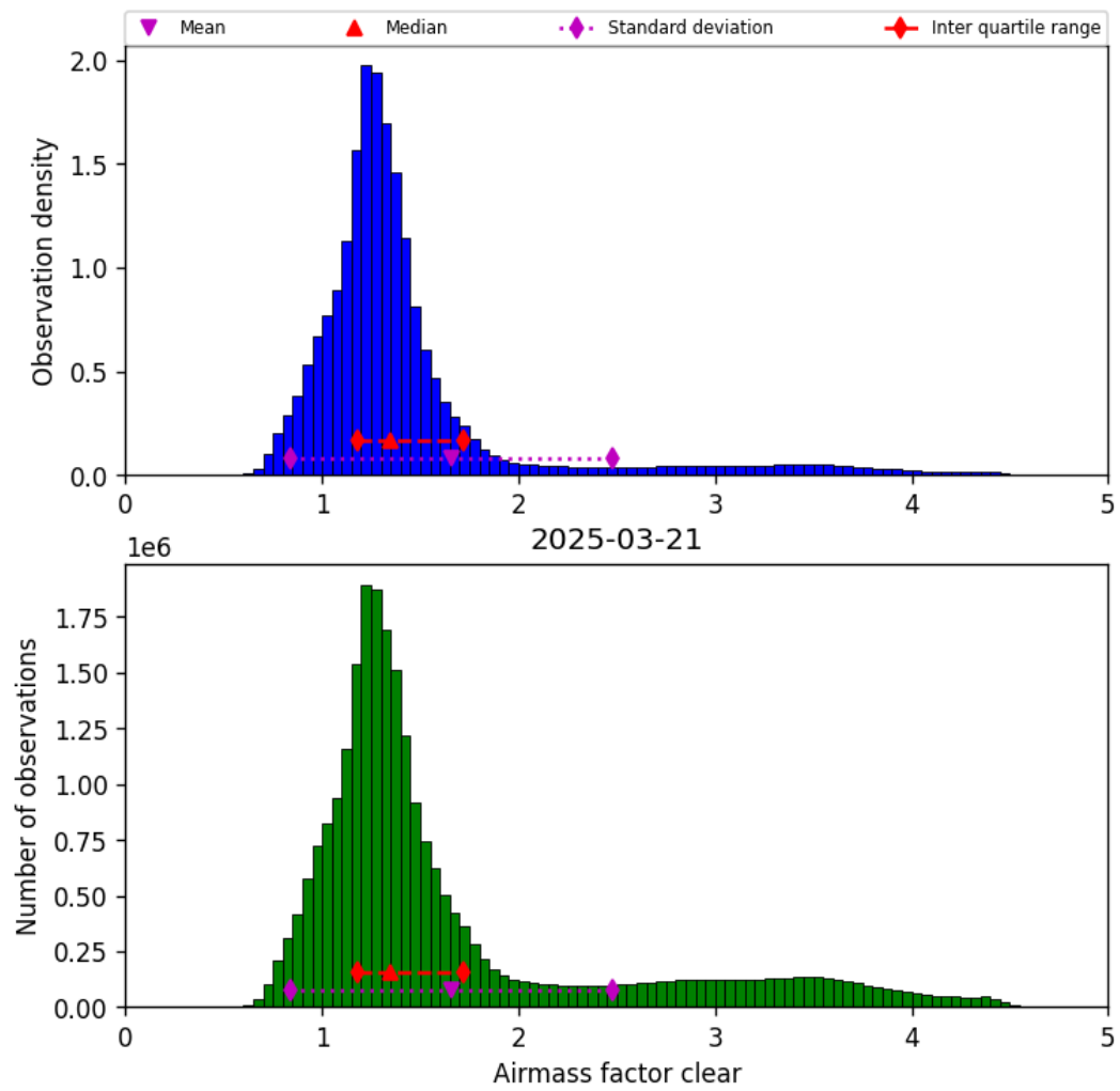
Figure 42: Histogram of “Airmass factor clear” for 2025-03-20 to 2025-03-22
