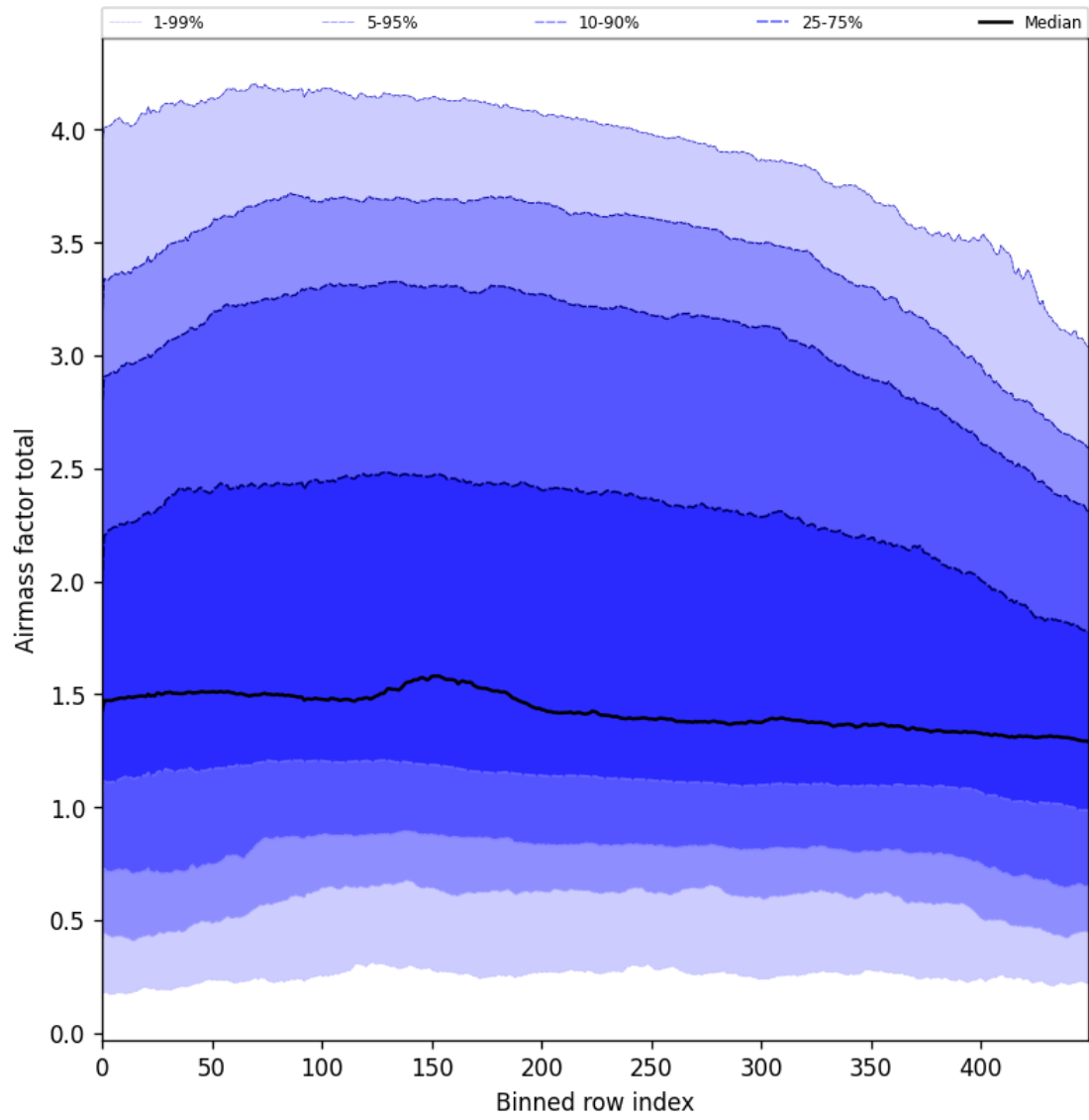
Figure 54: Along track statistics of “Airmass factor total” for 2025-03-20 to 2025-03-22
