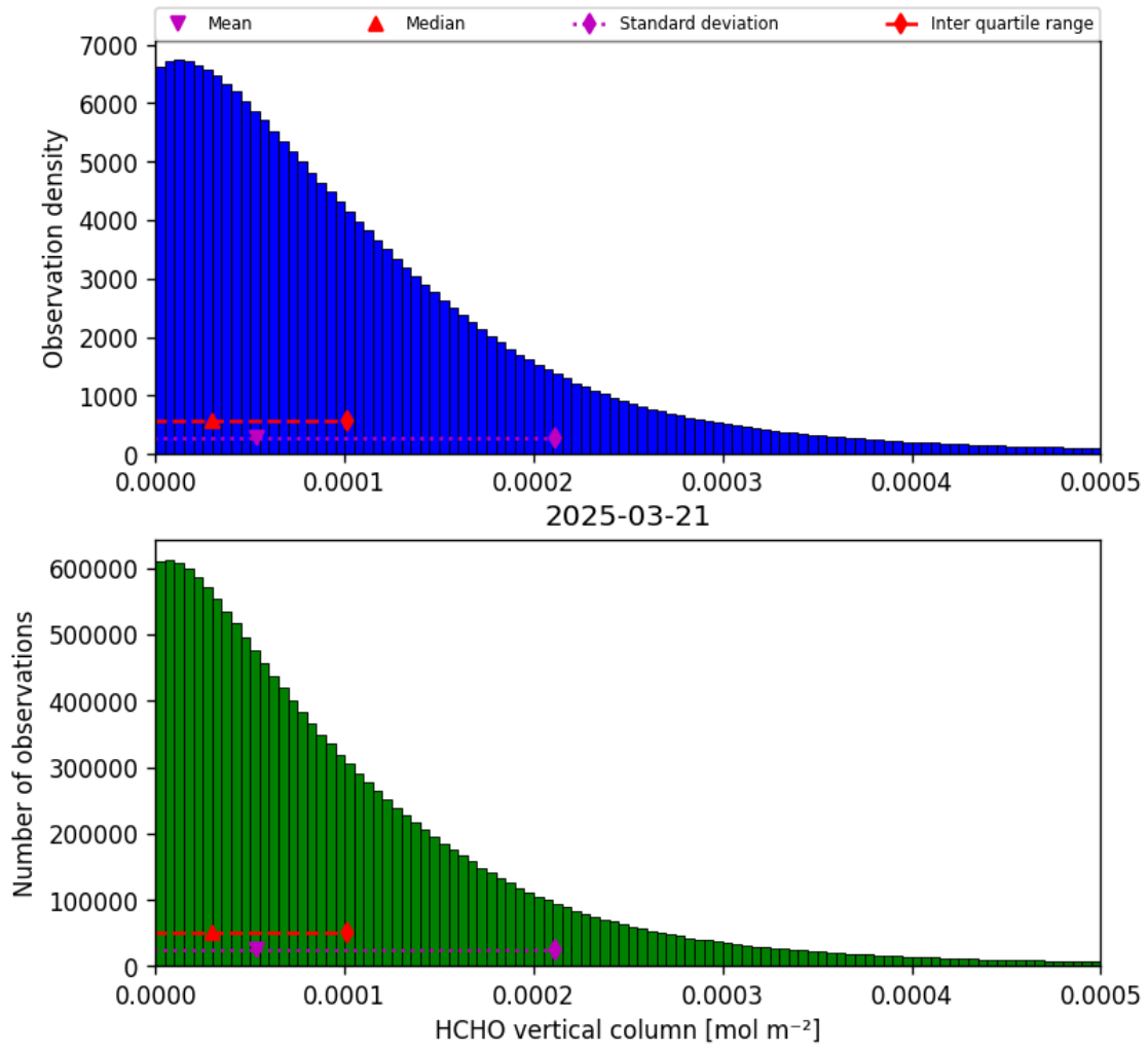
Figure 35: Histogram of “HCHO vertical column” for 2025-03-20 to 2025-03-22
