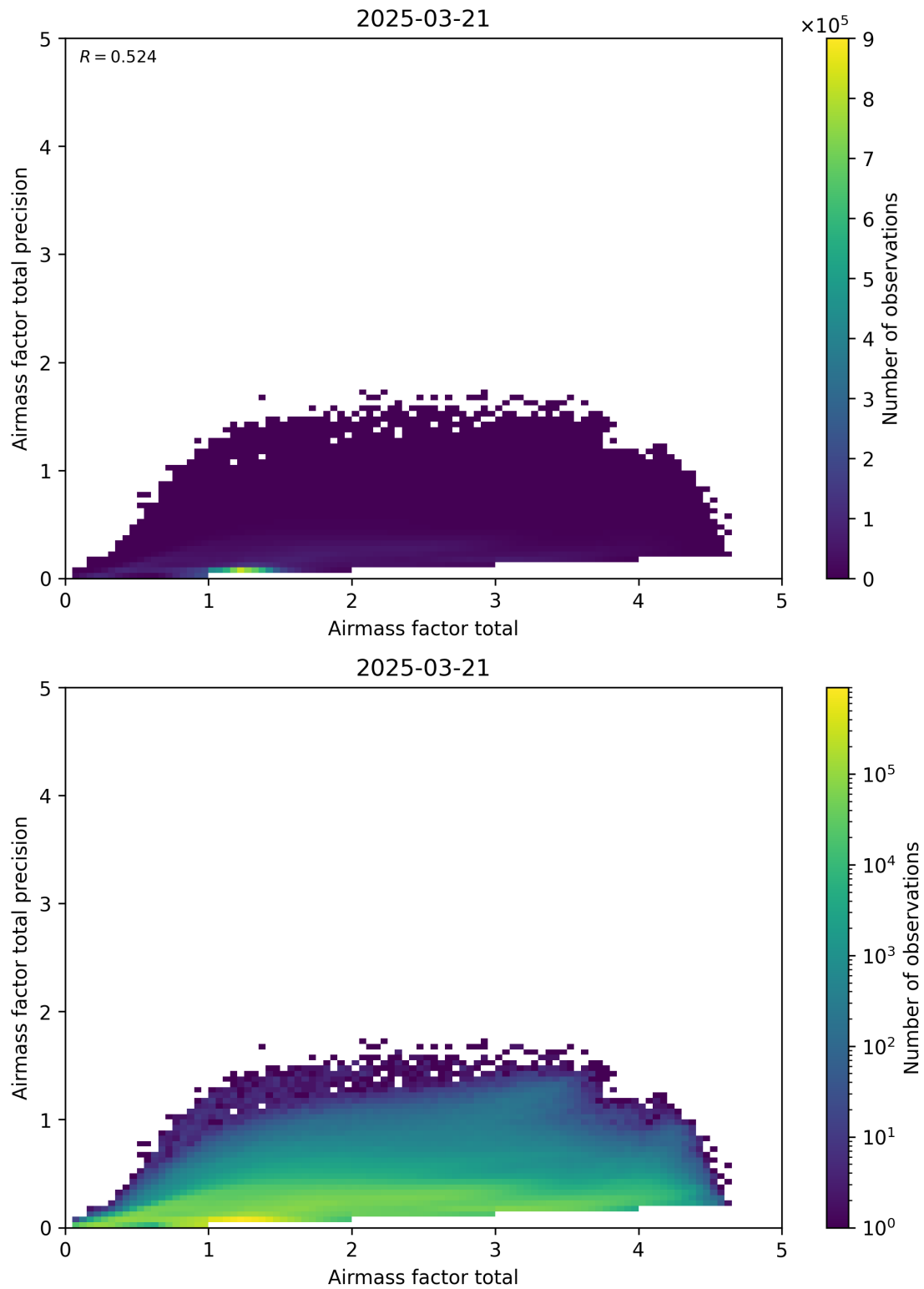
Figure 103: Scatter density plot of “Airmass factor total” against “Airmass factor total precision” for 2025-03-20 to 2025-03-22.
