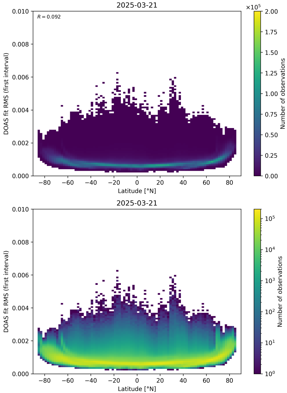
Figure 153: Scatter density plot of “Latitude” against “DOAS fit RMS (first interval)” for 2025-03-20 to 2025-03-22.
