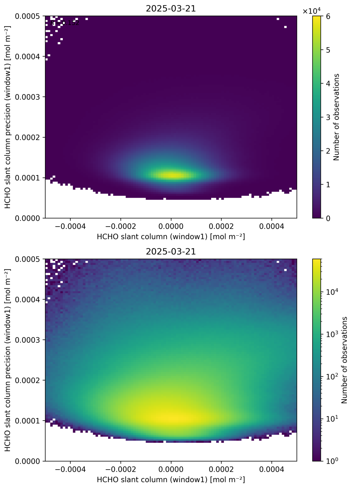
Figure 84: Scatter density plot of “HCHO slant column (window1)” against “HCHO slant column precision (window1)” for 2025-03-20 to 2025-03-22.
