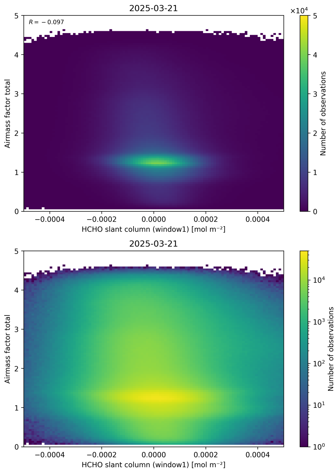
Figure 85: Scatter density plot of “HCHO slant column (window1)” against “Airmass factor total” for 2025-03-20 to 2025-03-22.
