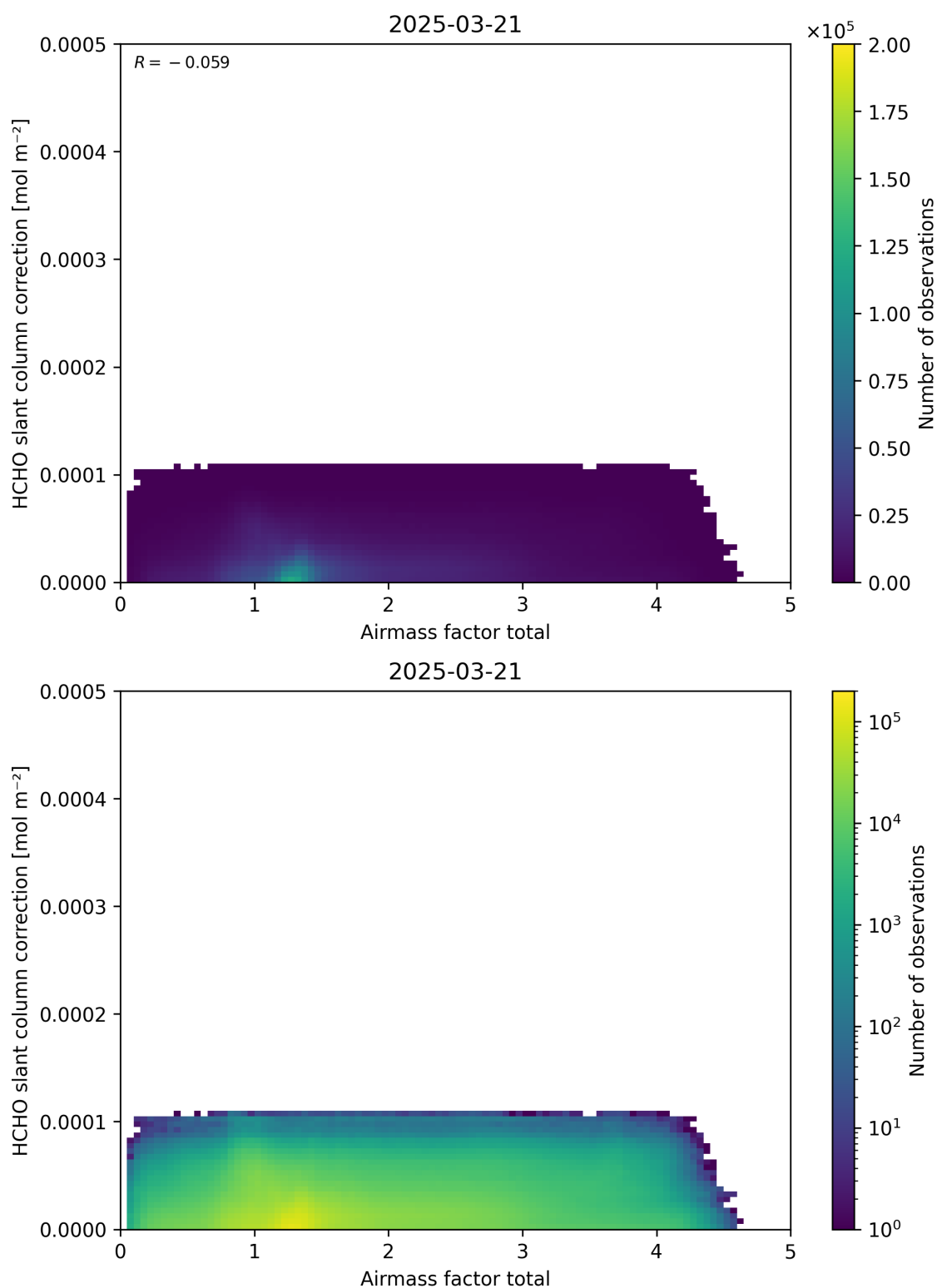
Figure 102: Scatter density plot of “Airmass factor total” against “HCHO slant column correction” for 2025-03-20 to 2025-03-22.
