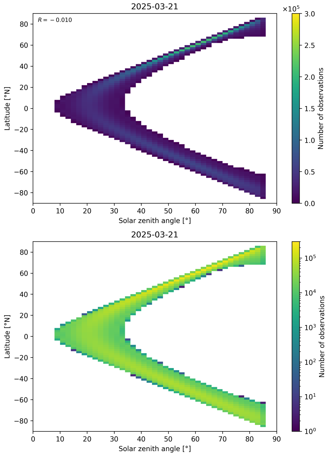
Figure 181: Scatter density plot of “Solar zenith angle” against “Latitude” for 2025-03-20 to 2025-03-22.
