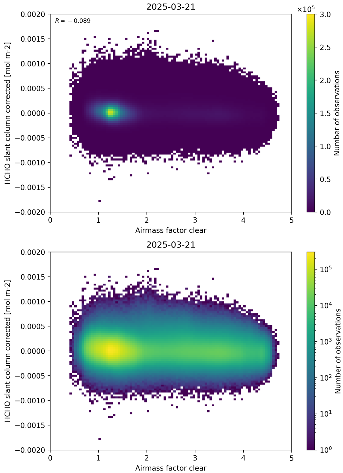
Figure 74: Scatter density plot of “Airmass factor clear” against “HCHO slant column corrected” for 2025-03-20 to 2025-03-22.
