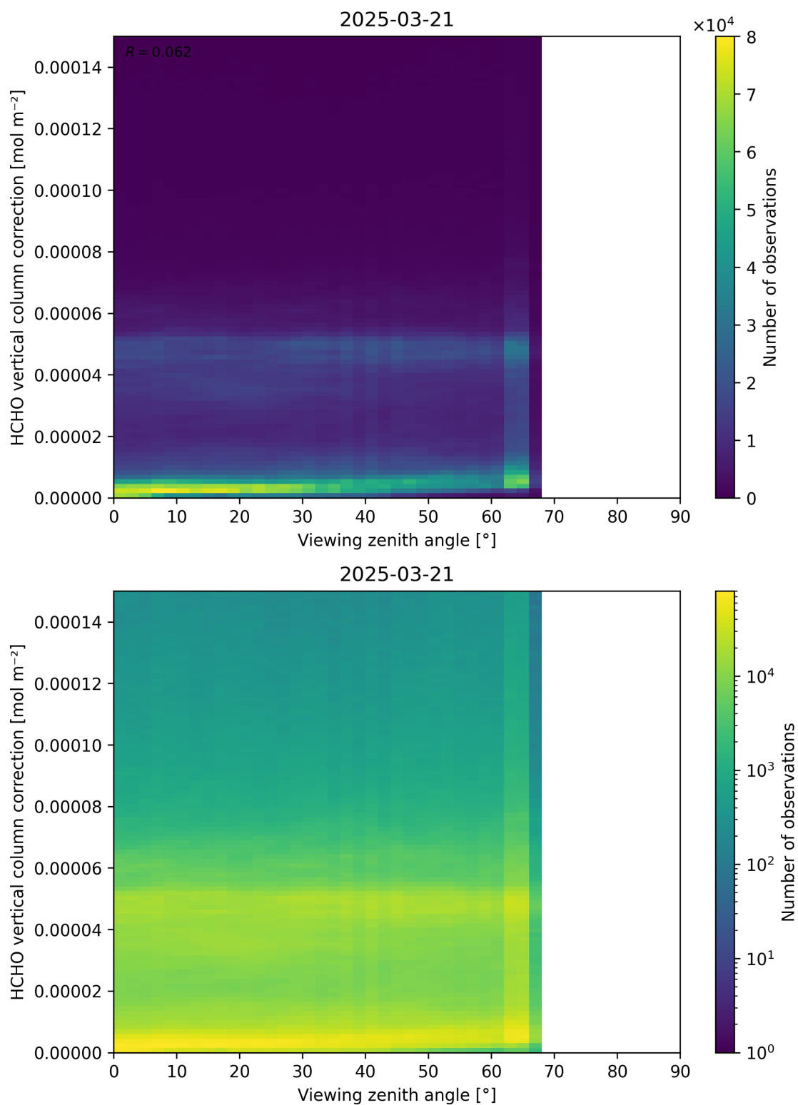
Figure 193: Scatter density plot of “Viewing zenith angle” against “HCHO vertical column correction” for 2025-03-20 to 2025-03-22.
