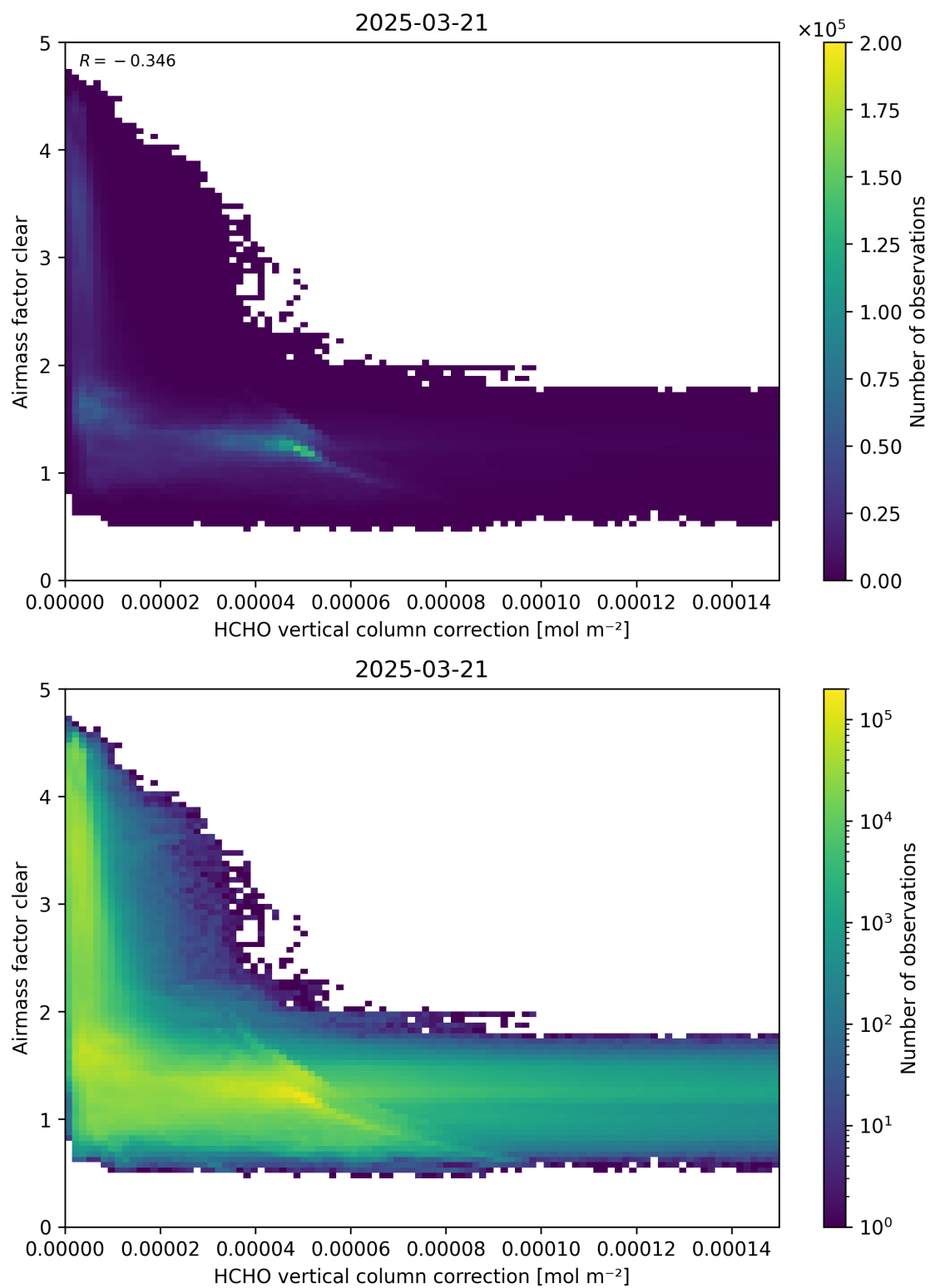
Figure 115: Scatter density plot of “HCHO vertical column correction” against “Airmass factor clear” for 2025-03-20 to 2025-03-22.
