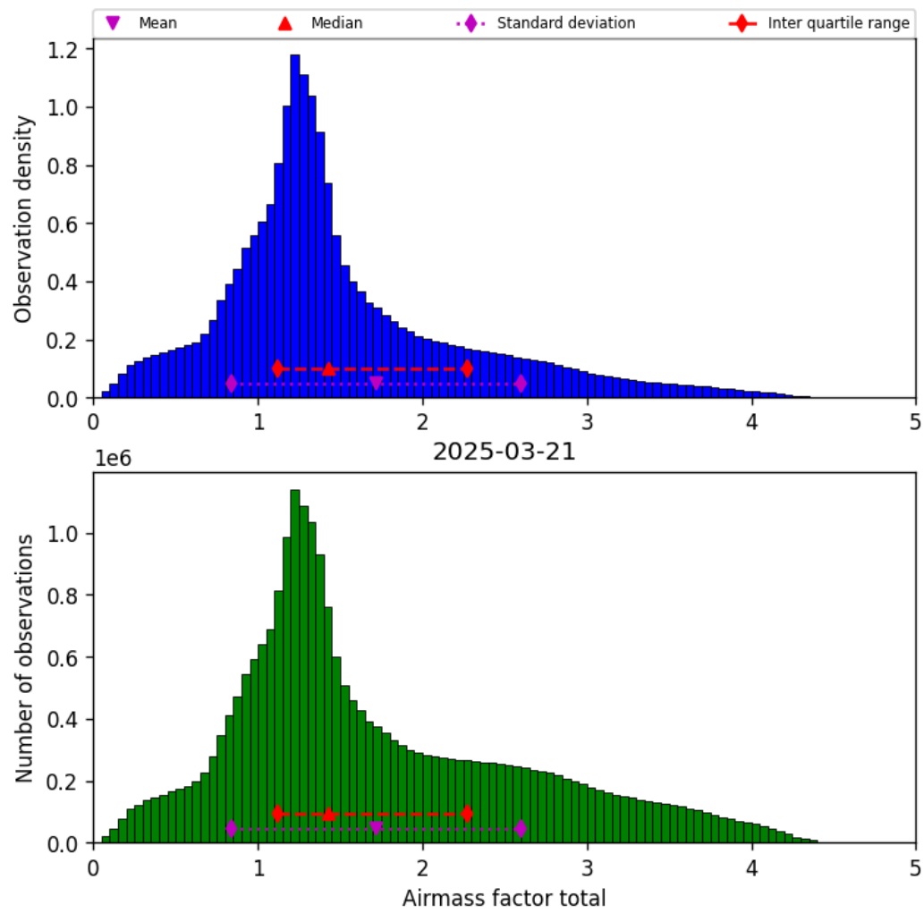
Figure 40: Histogram of “Airmass factor total” for 2025-03-20 to 2025-03-22
