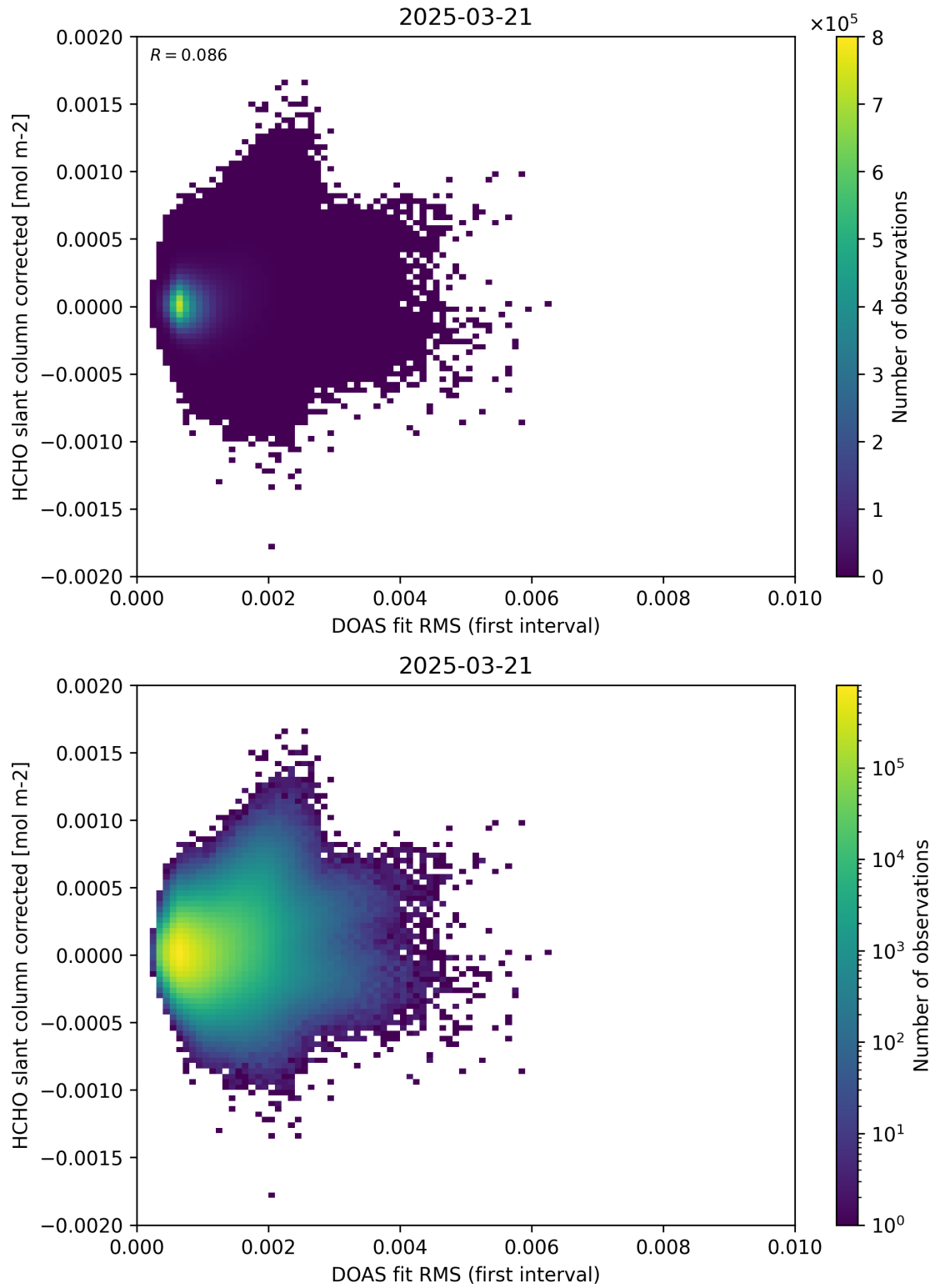
Figure 62: Scatter density plot of “DOAS fit RMS (first interval)” against “HCHO slant column corrected” for 2025-03-20 to 2025-03-22.
