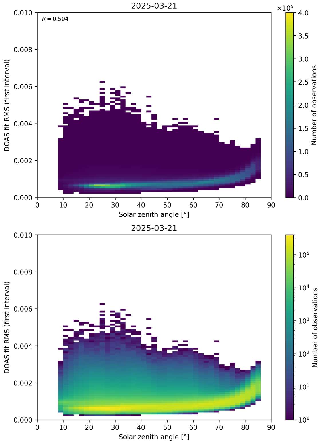
Figure 167: Scatter density plot of “Solar zenith angle” against “DOAS fit RMS (first interval)” for 2025-03-20 to 2025-03-22.
