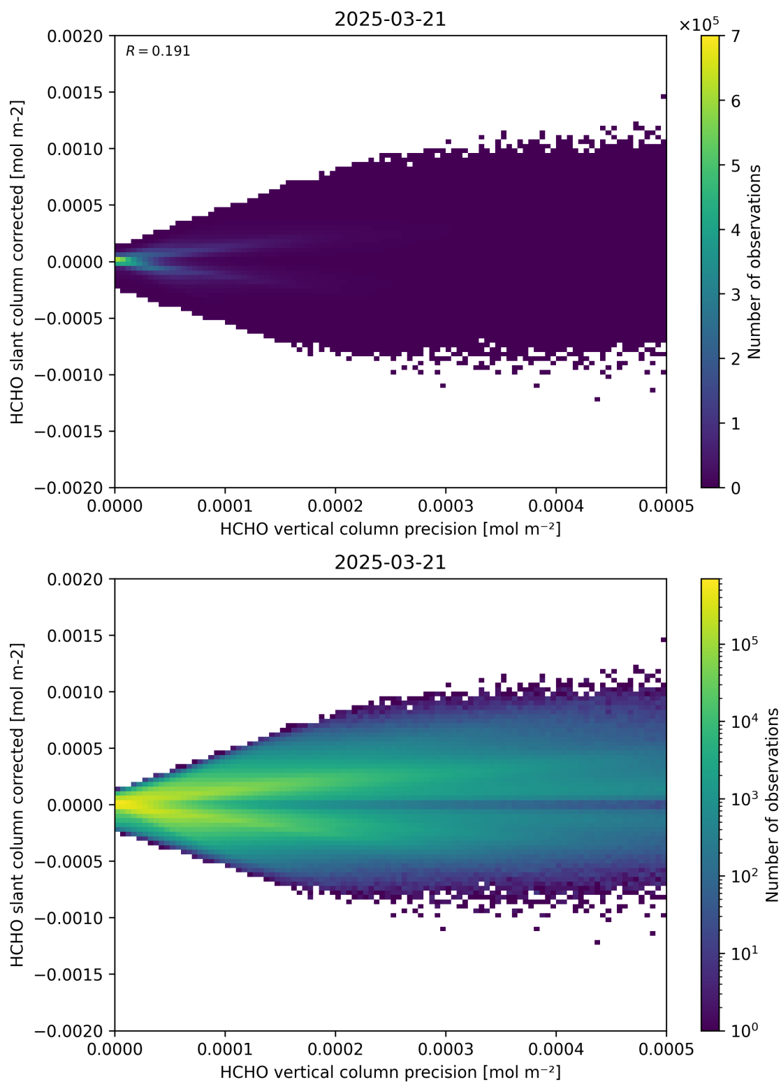
Figure 140: Scatter density plot of “HCHO vertical column precision” against “HCHO slant column corrected” for 2025-03-20 to 2025-03-22.
