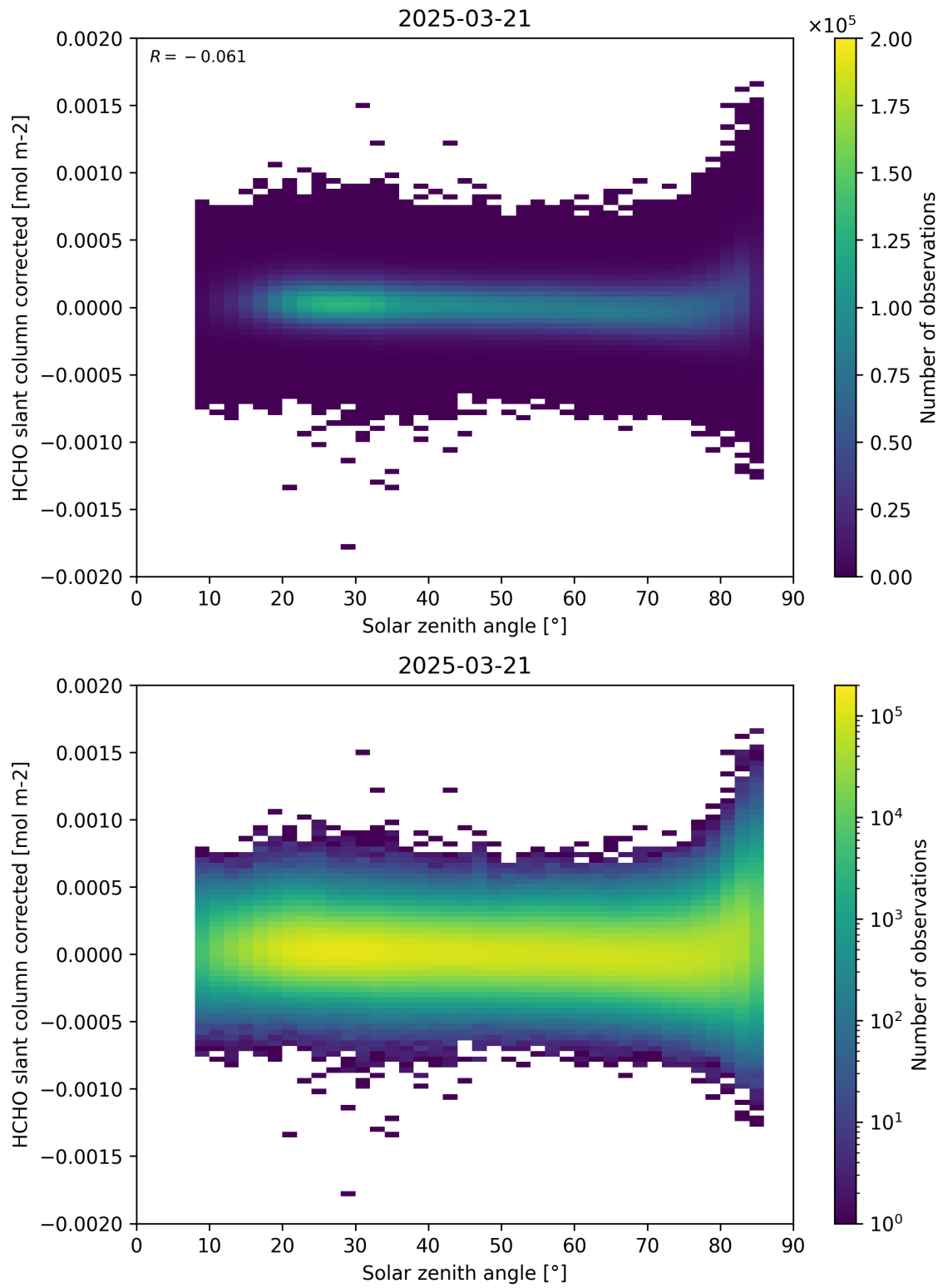
Figure 171: Scatter density plot of “Solar zenith angle” against “HCHO slant column corrected” for 2025-03-20 to 2025-03-22.
