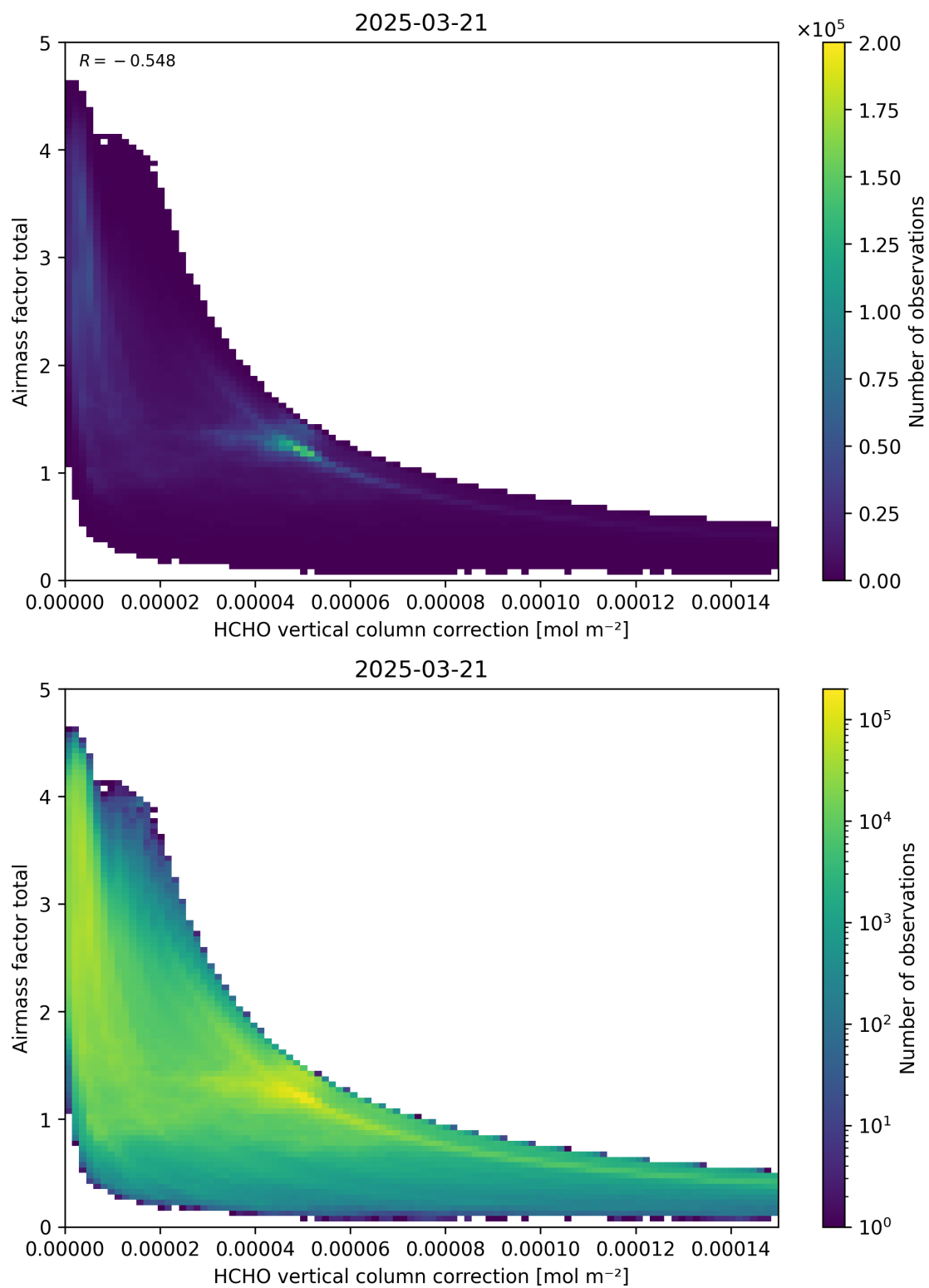
Figure 120: Scatter density plot of “HCHO vertical column correction” against “Airmass factor total” for 2025-03-20 to 2025-03-22.
