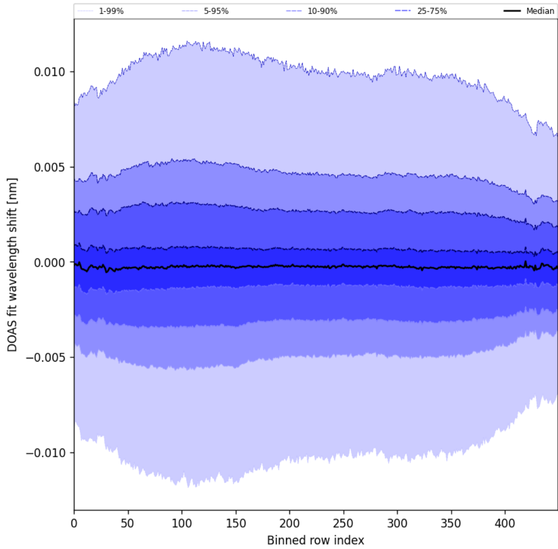
Figure 58: Along track statistics of “DOAS fit wavelength shift” for 2025-03-20 to 2025-03-22
