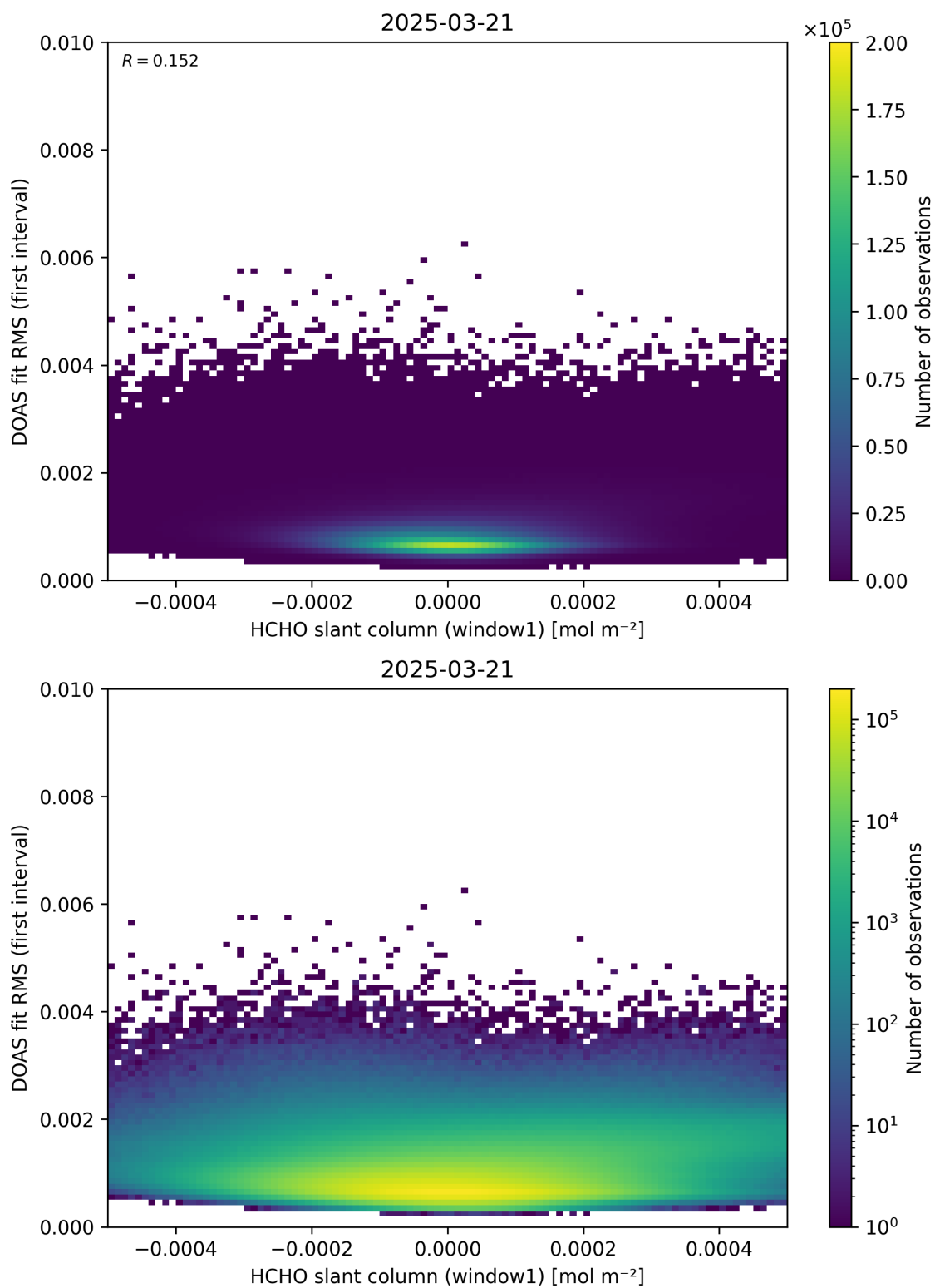
Figure 78: Scatter density plot of “HCHO slant column (window1)” against “DOAS fit RMS (first interval)” for 2025-03-20 to 2025-03-22.
