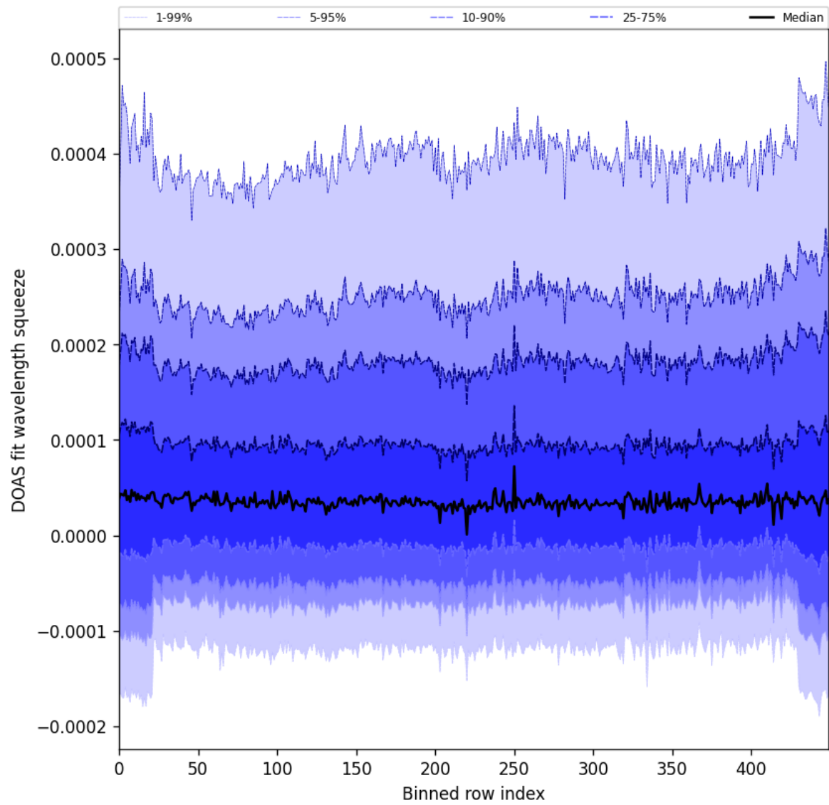
Figure 59: Along track statistics of “DOAS fit wavelength squeeze” for 2025-03-20 to 2025-03-22
