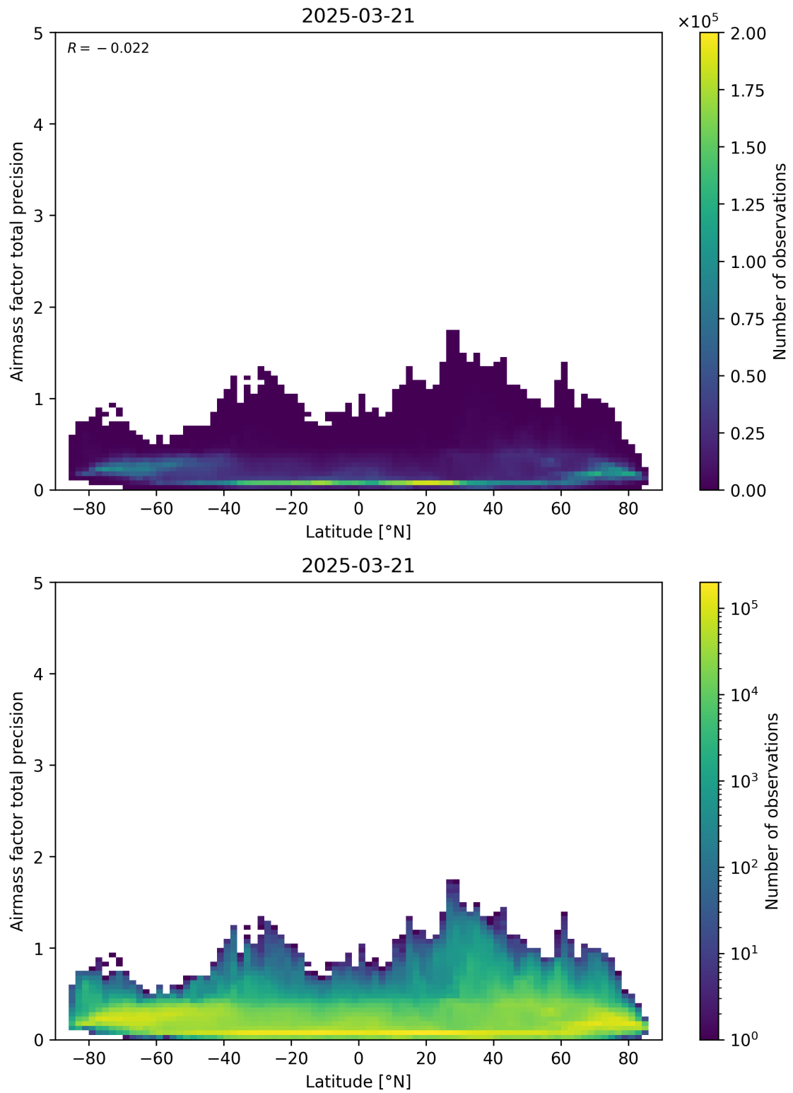
Figure 162: Scatter density plot of “Latitude” against “Airmass factor total precision” for 2025-03-20 to 2025-03-22.
