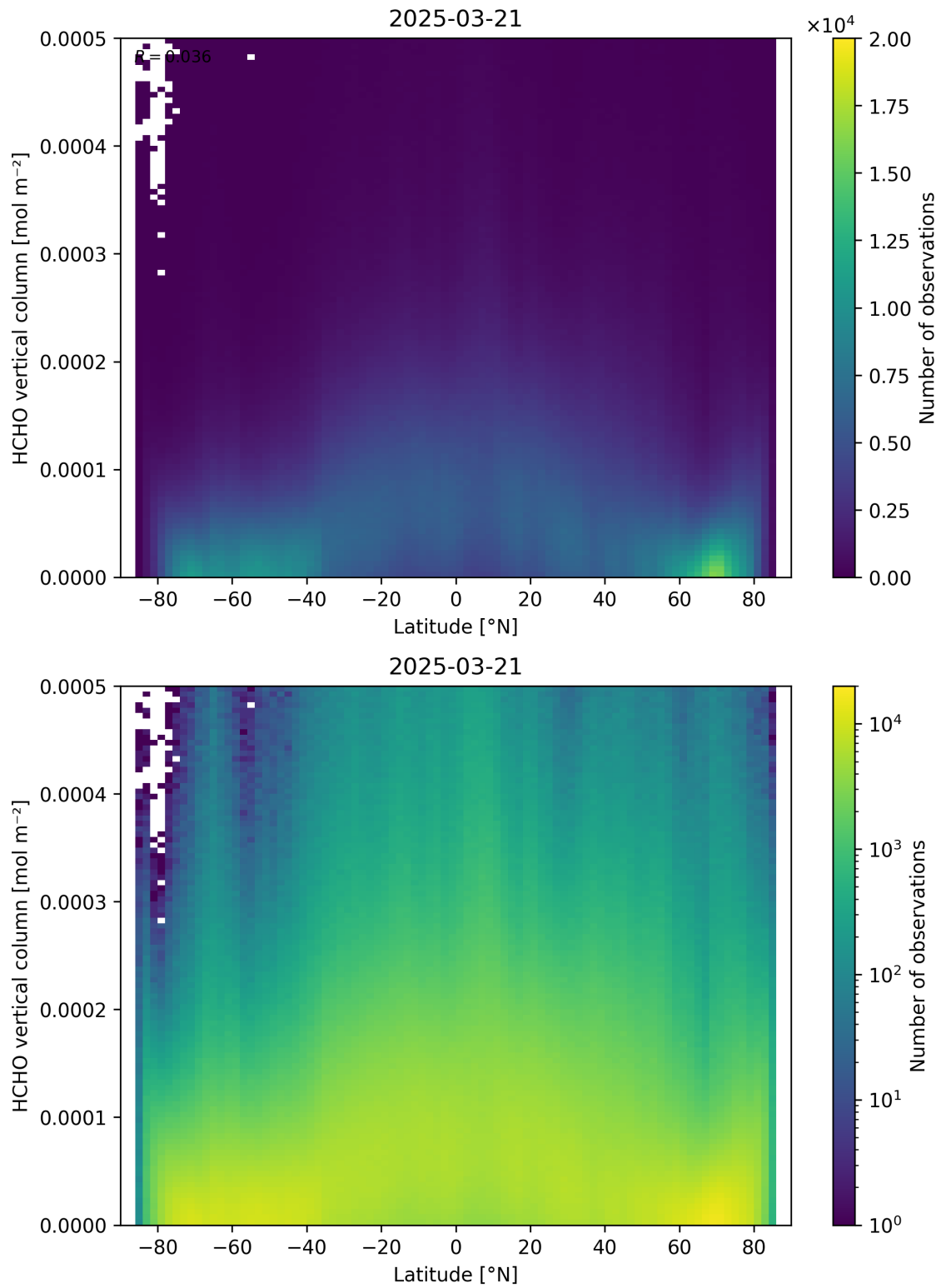
Figure 163: Scatter density plot of “Latitude” against “HCHO vertical column” for 2025-03-20 to 2025-03-22.
