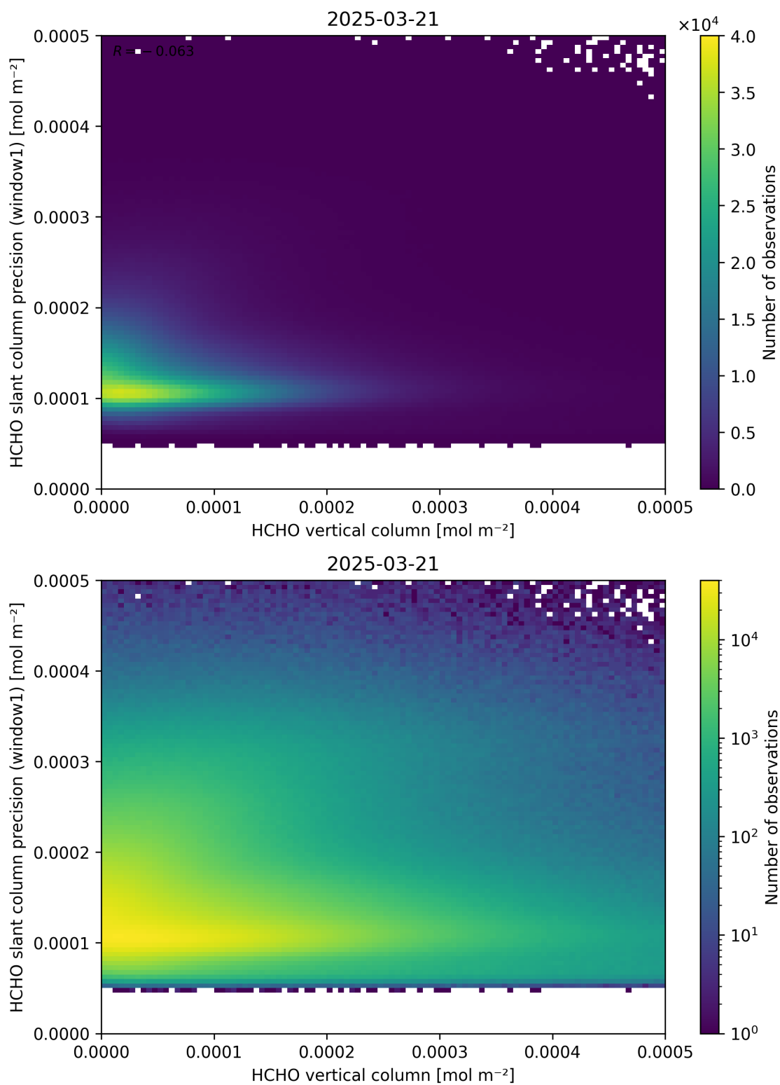
Figure 130: Scatter density plot of “HCHO vertical column” against “HCHO slant column precision (window1)” for 2025-03-20 to 2025-03-22.
