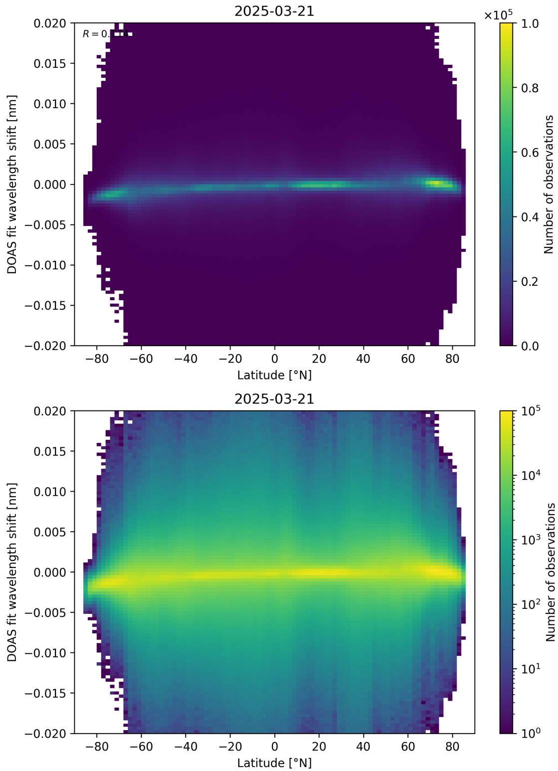
Figure 154: Scatter density plot of “Latitude” against “DOAS fit wavelength shift” for 2025-03-20 to 2025-03-22.
