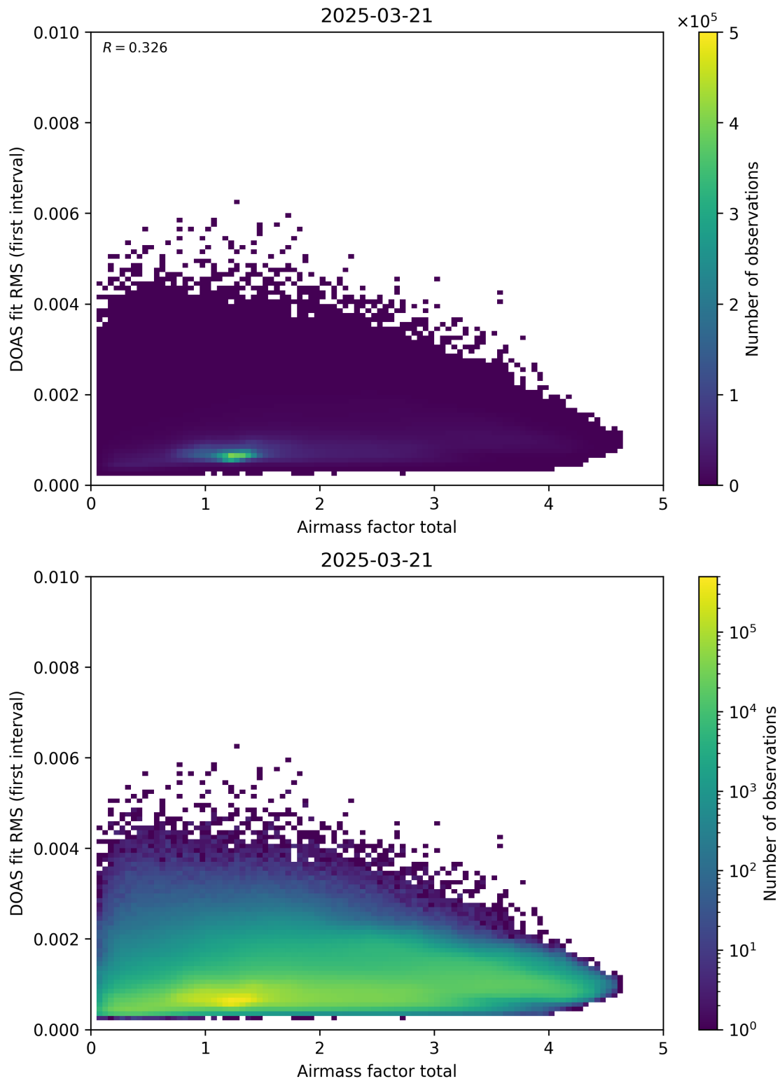
Figure 97: Scatter density plot of “Airmass factor total” against “DOAS fit RMS (first interval)” for 2025-03-20 to 2025-03-22.
