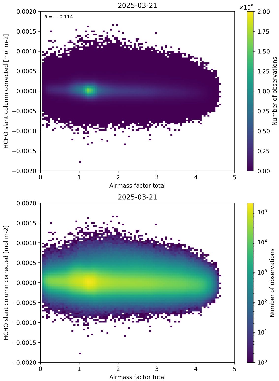
Figure 101: Scatter density plot of “Airmass factor total” against “HCHO slant column corrected” for 2025-03-20 to 2025-03-22.
