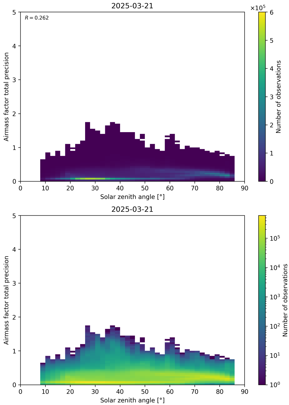
Figure 176: Scatter density plot of “Solar zenith angle” against “Airmass factor total precision” for 2025-03-20 to 2025-03-22.
