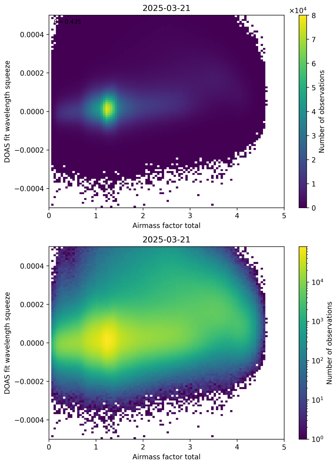
Figure 99: Scatter density plot of “Airmass factor total” against “DOAS fit wavelength squeeze” for 2025-03-20 to 2025-03-22.
