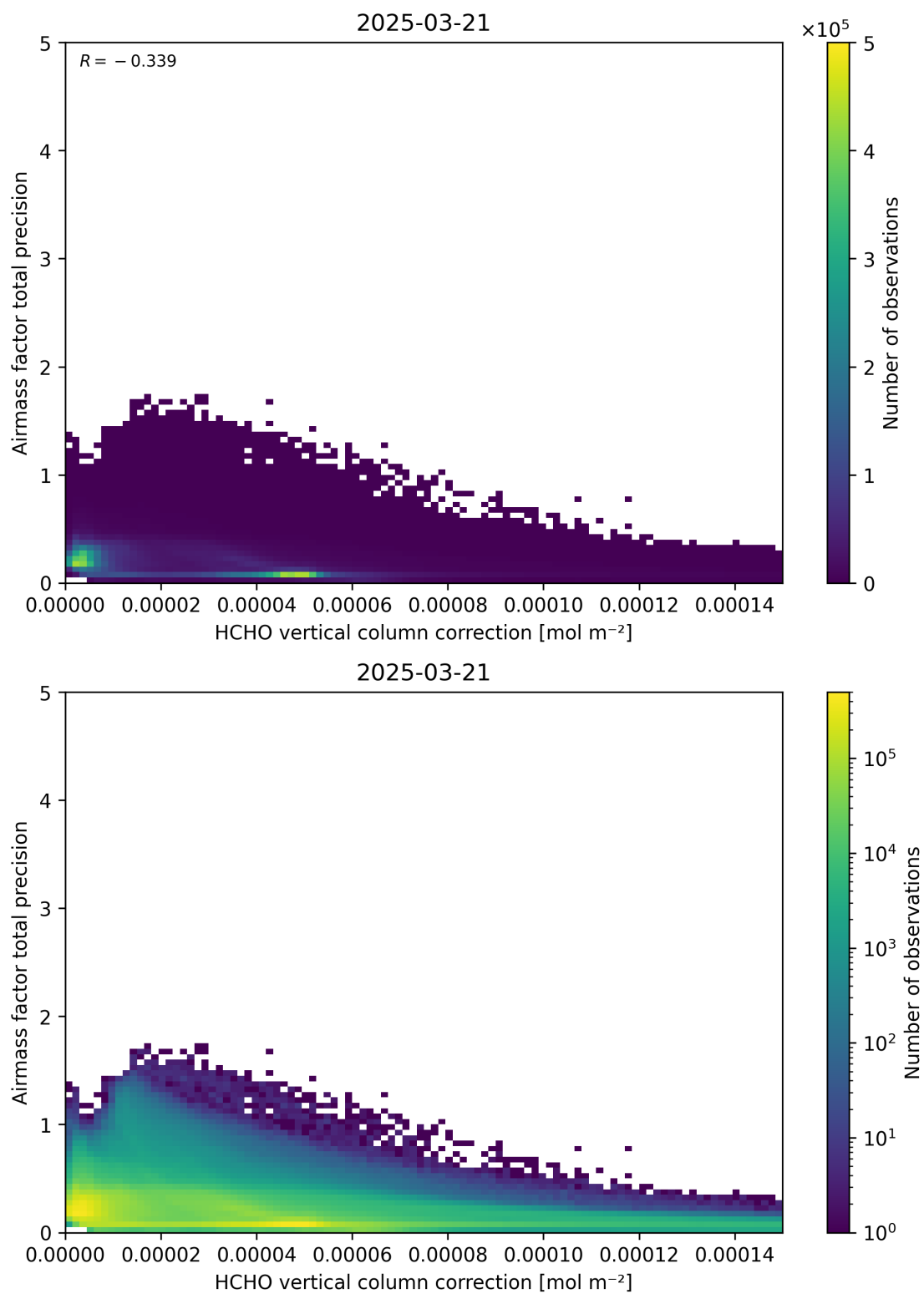
Figure 121: Scatter density plot of “HCHO vertical column correction” against “Airmass factor total precision” for 2025-03-20 to 2025-03-22.
