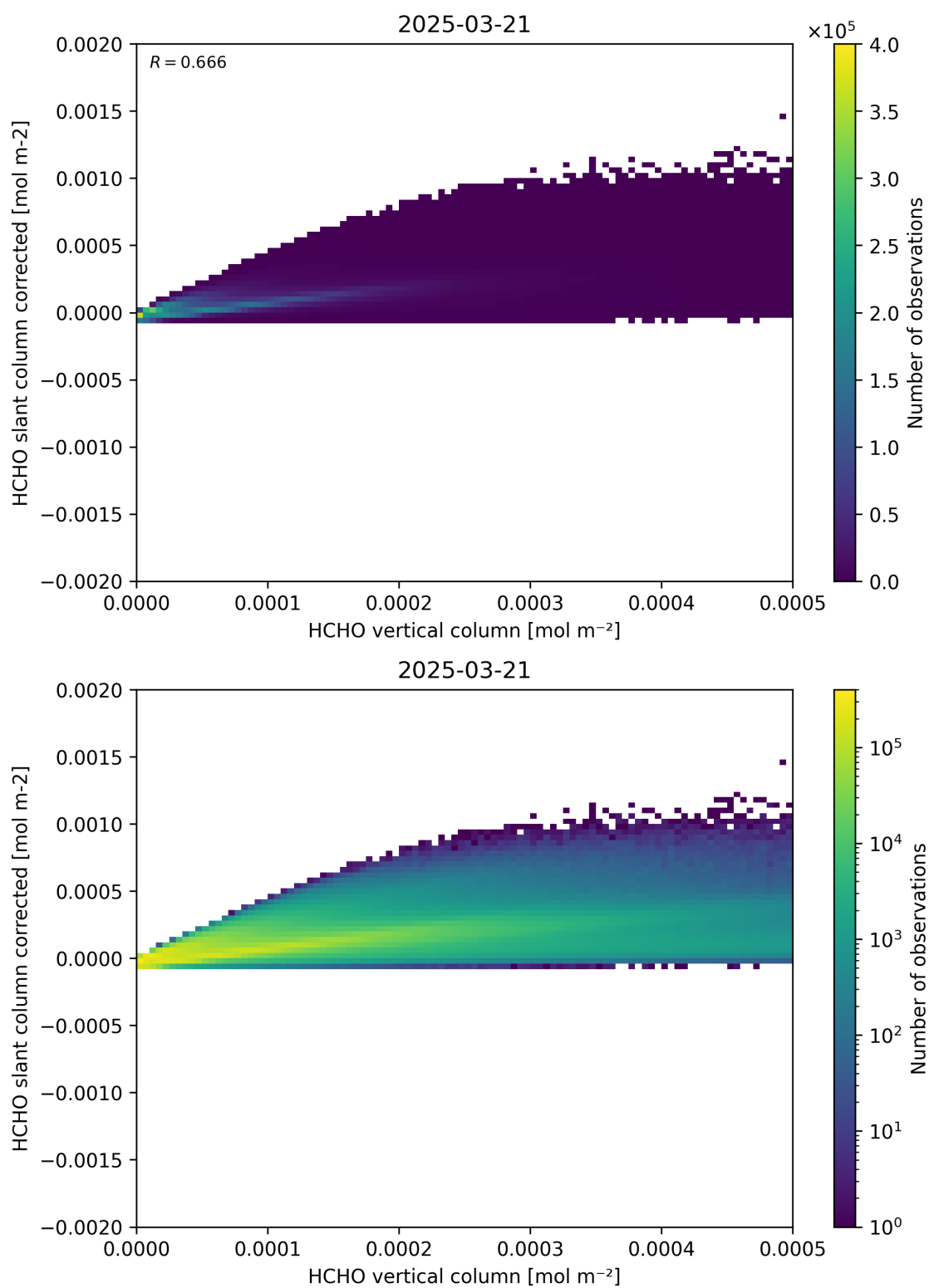
Figure 127: Scatter density plot of “HCHO vertical column” against “HCHO slant column corrected” for 2025-03-20 to 2025-03-22.
