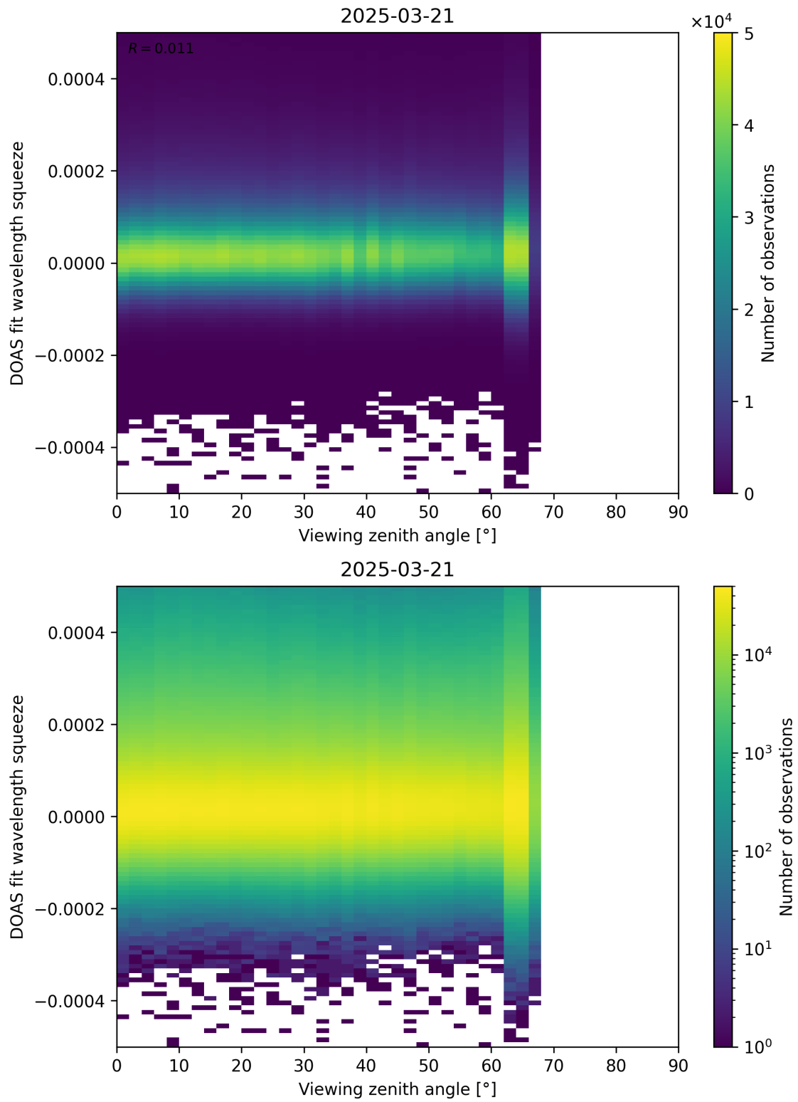
Figure 184: Scatter density plot of “Viewing zenith angle” against “DOAS fit wavelength squeeze” for 2025-03-20 to 2025-03-22.
