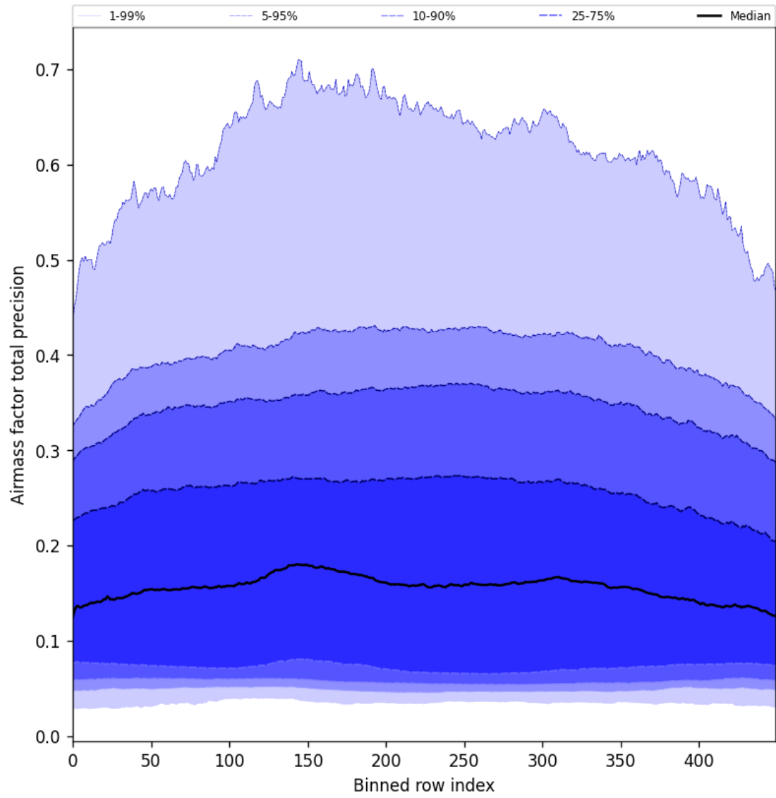
Figure 55: Along track statistics of “Airmass factor total precision” for 2025-03-20 to 2025-03-22
