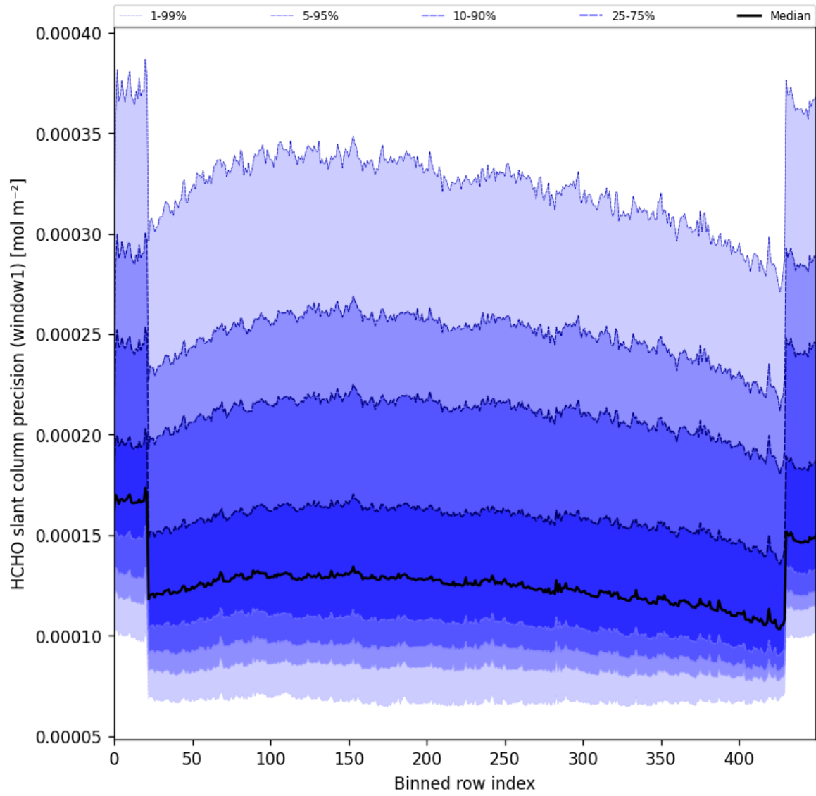
Figure 53: Along track statistics of “HCHO slant column precision (window1)” for 2025-03-20 to 2025-03-22
