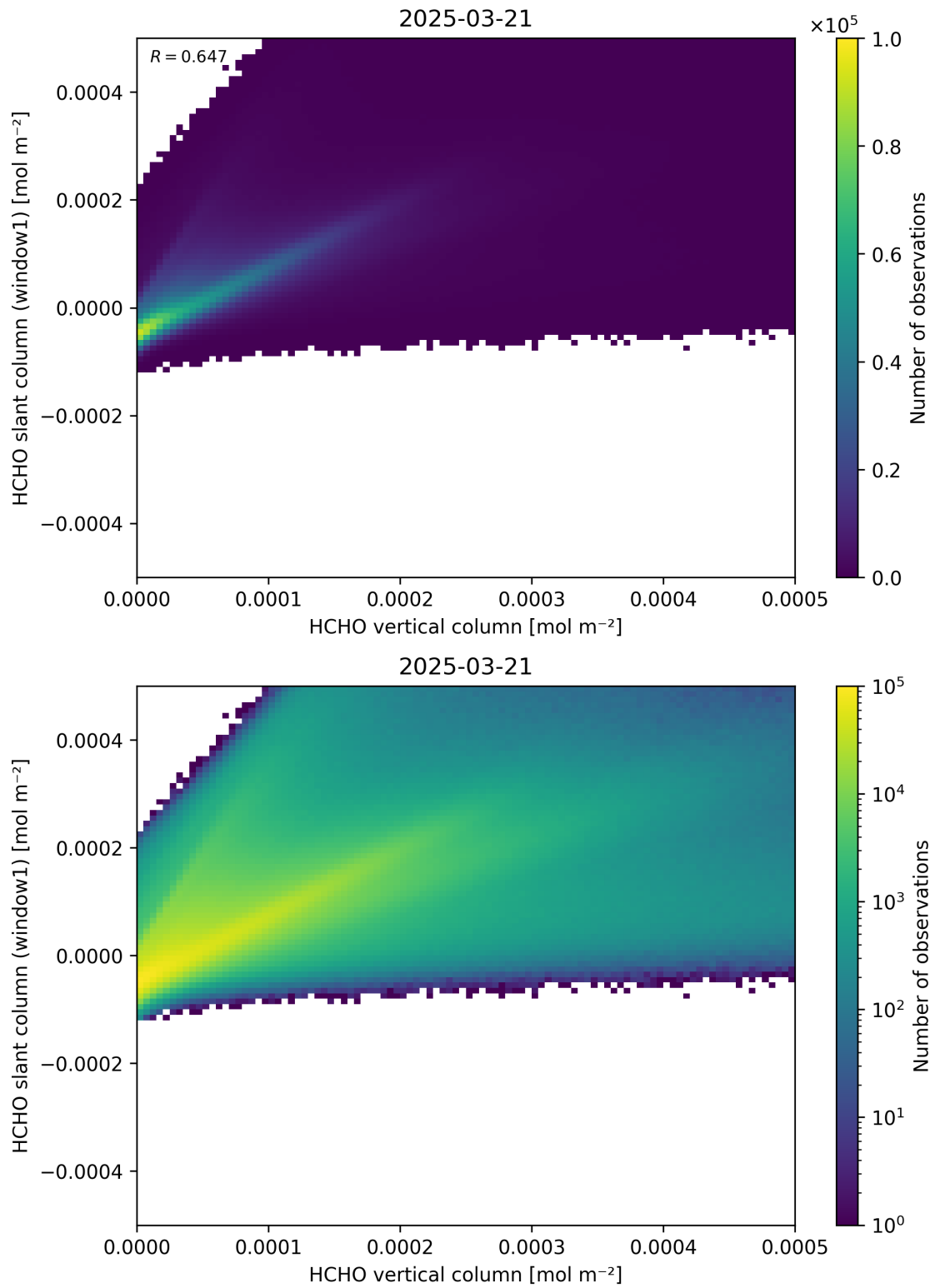
Figure 129: Scatter density plot of “HCHO vertical column” against “HCHO slant column (window1)” for 2025-03-20 to 2025-03-22.
