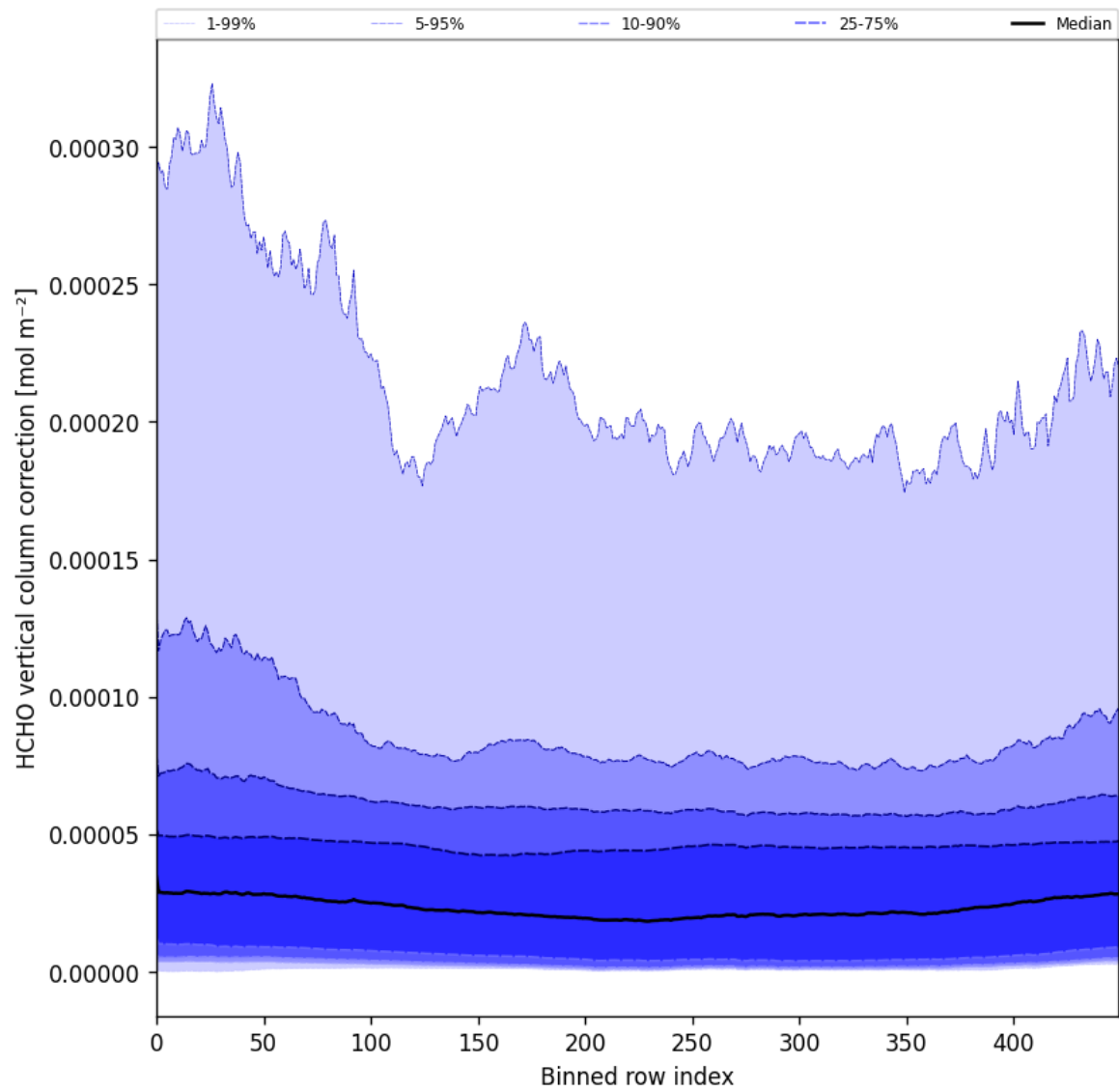
Figure 51: Along track statistics of “HCHO vertical column correction” for 2025-03-20 to 2025-03-22
