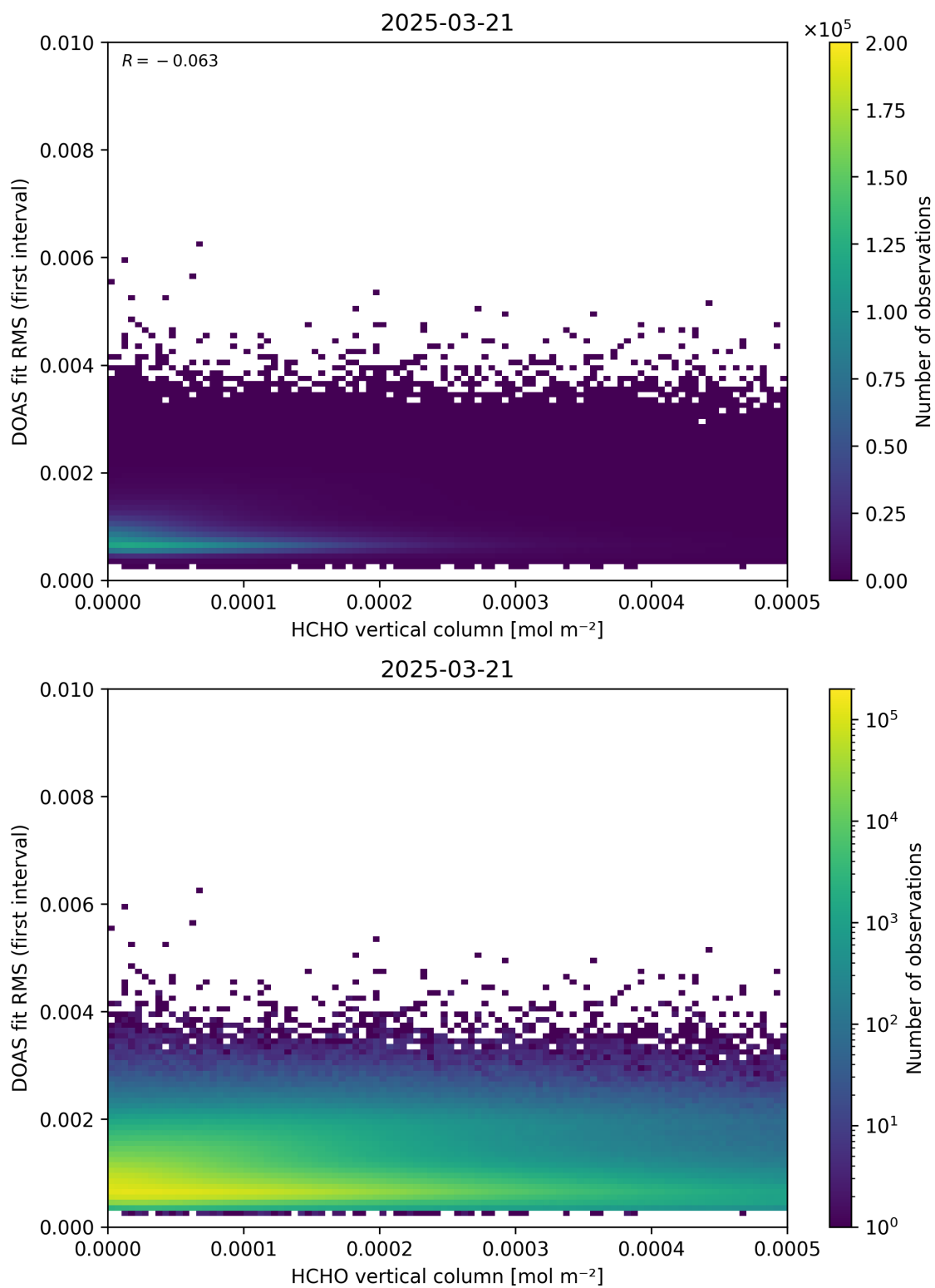
Figure 123: Scatter density plot of “HCHO vertical column” against “DOAS fit RMS (first interval)” for 2025-03-20 to 2025-03-22.
