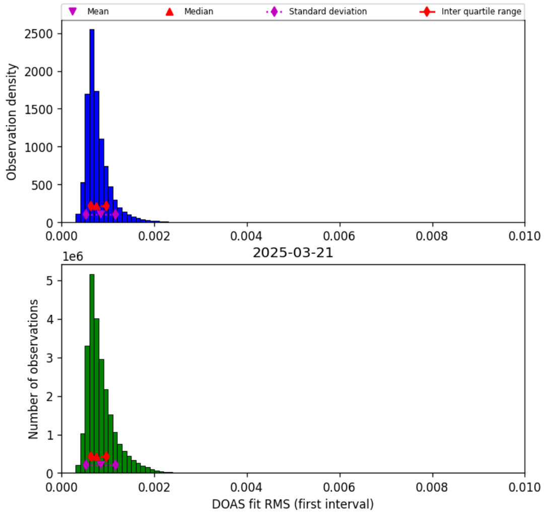
Figure 46: Histogram of “DOAS fit RMS (first interval)” for 2025-03-20 to 2025-03-22
