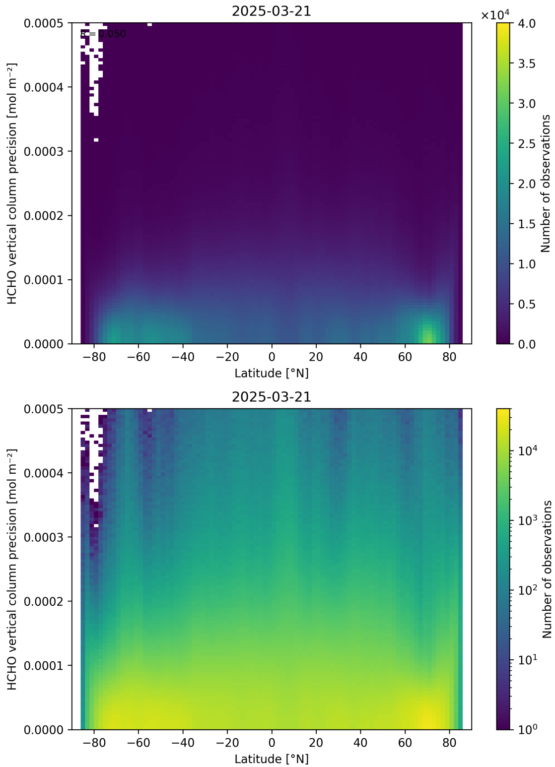
Figure 165: Scatter density plot of “Latitude” against “HCHO vertical column precision” for 2025-03-20 to 2025-03-22.
