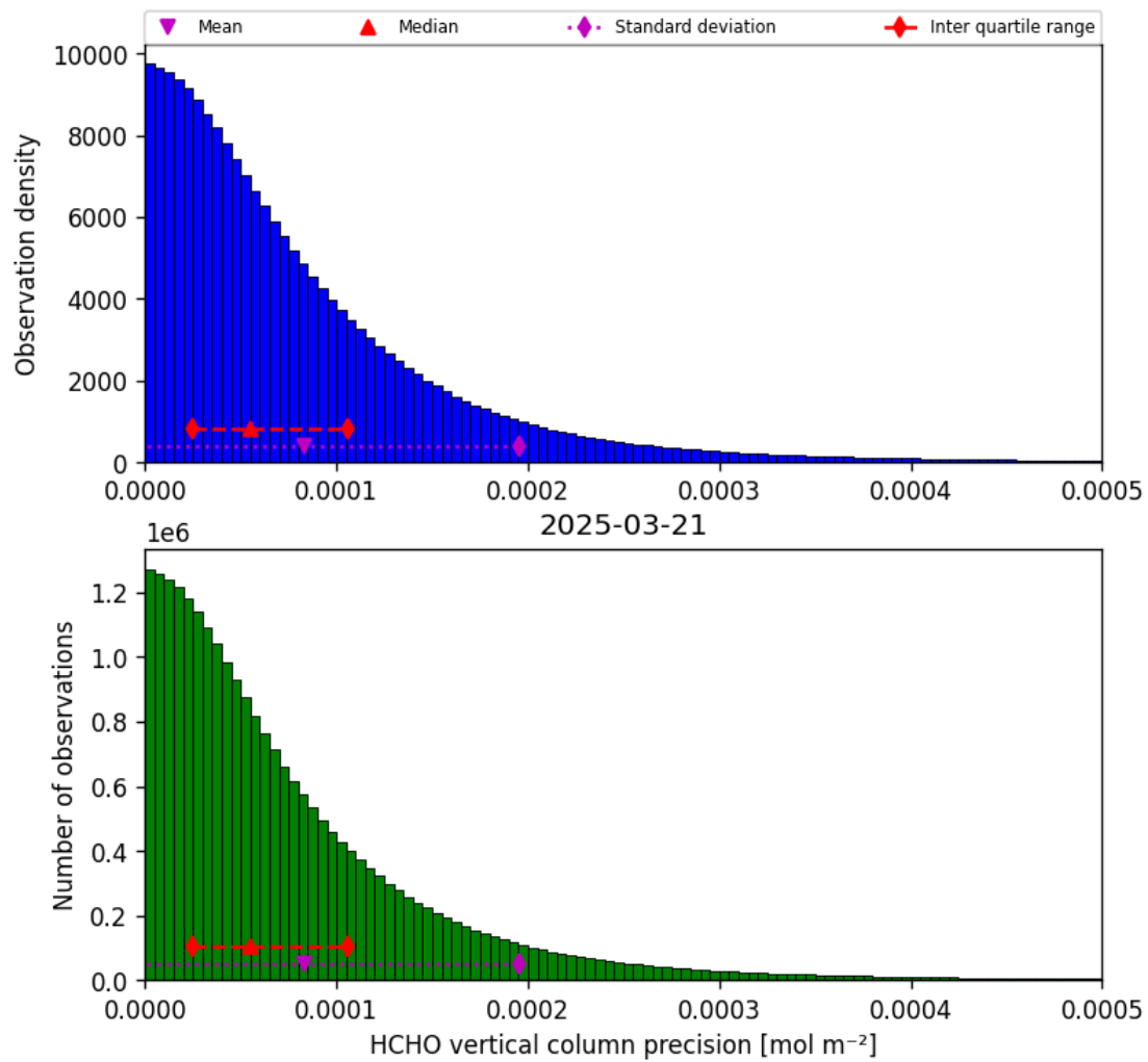
Figure 36: Histogram of “HCHO vertical column precision” for 2025-03-20 to 2025-03-22
