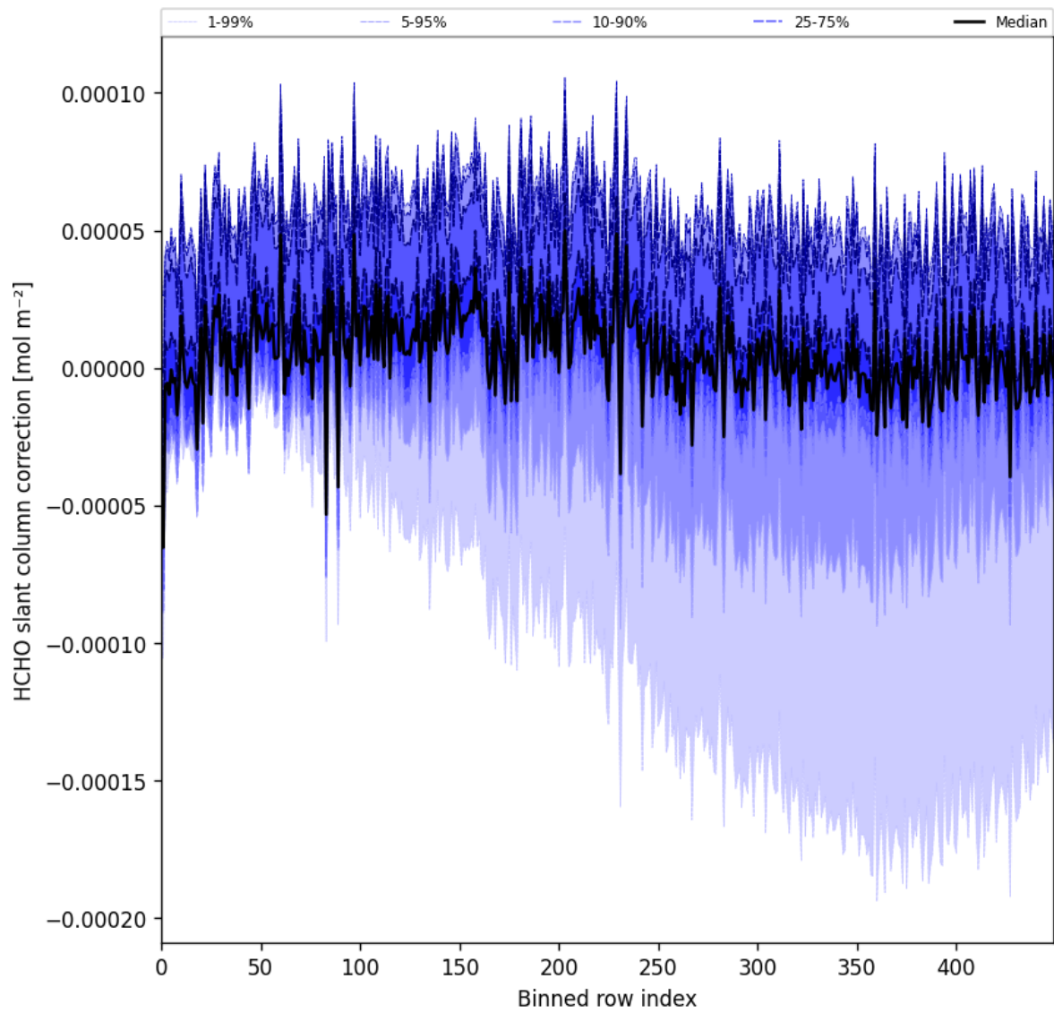
Figure 61: Along track statistics of “HCHO slant column correction” for 2025-03-20 to 2025-03-22
