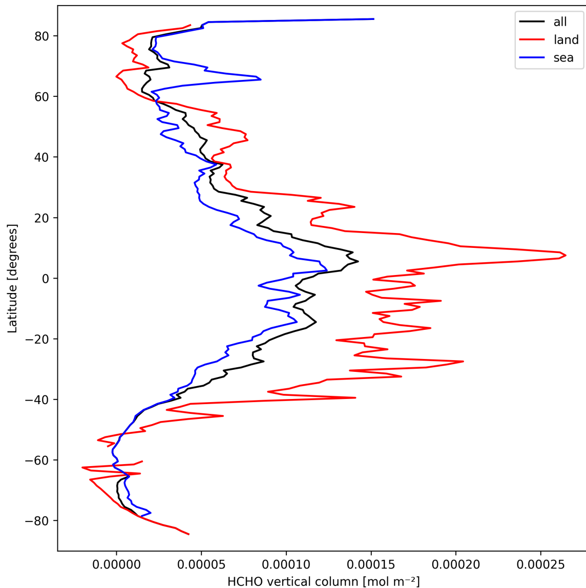
Figure 21: Zonal average of “HCHO vertical column” for 2025-03-20 to 2025-03-22.
