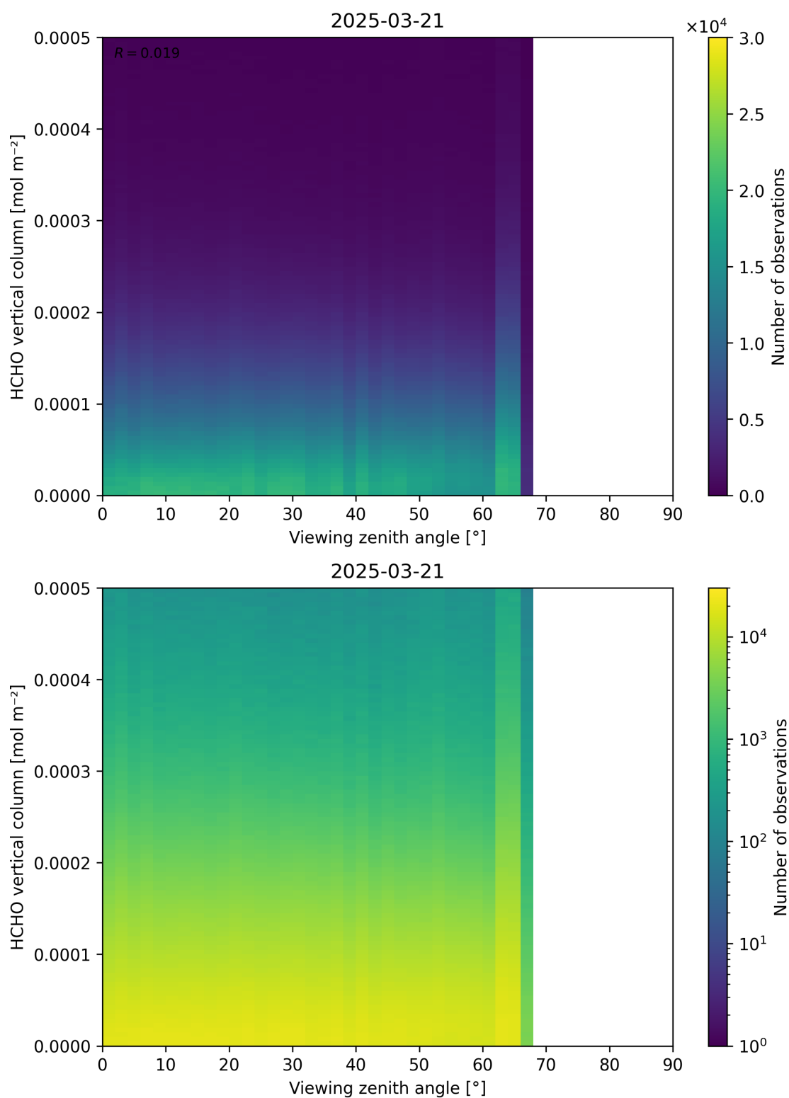
Figure 192: Scatter density plot of “Viewing zenith angle” against “HCHO vertical column” for 2025-03-20 to 2025-03-22.
