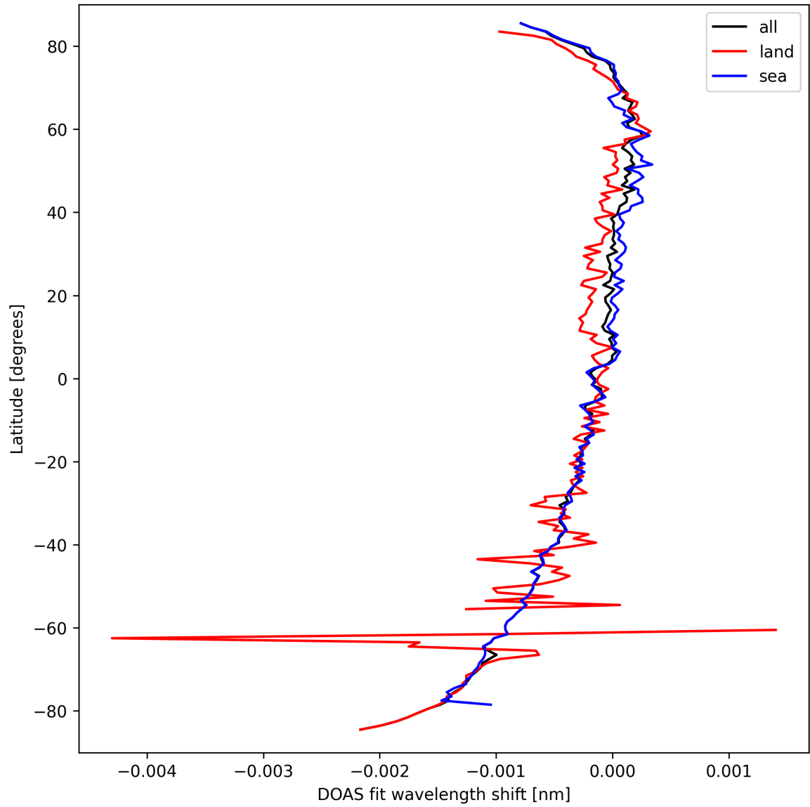
Figure 30: Zonal average of "DOAS fit wavelength shift" for 2025-03-20 to 2025-03-22.
