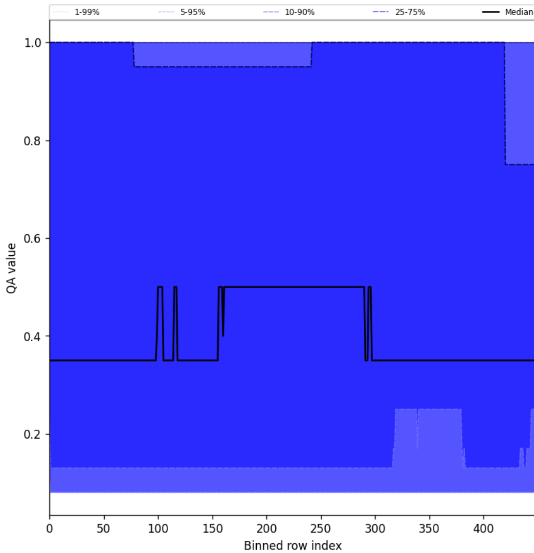
Figure 48: Along track statistics of “QA value” for 2025-03-20 to 2025-03-22
