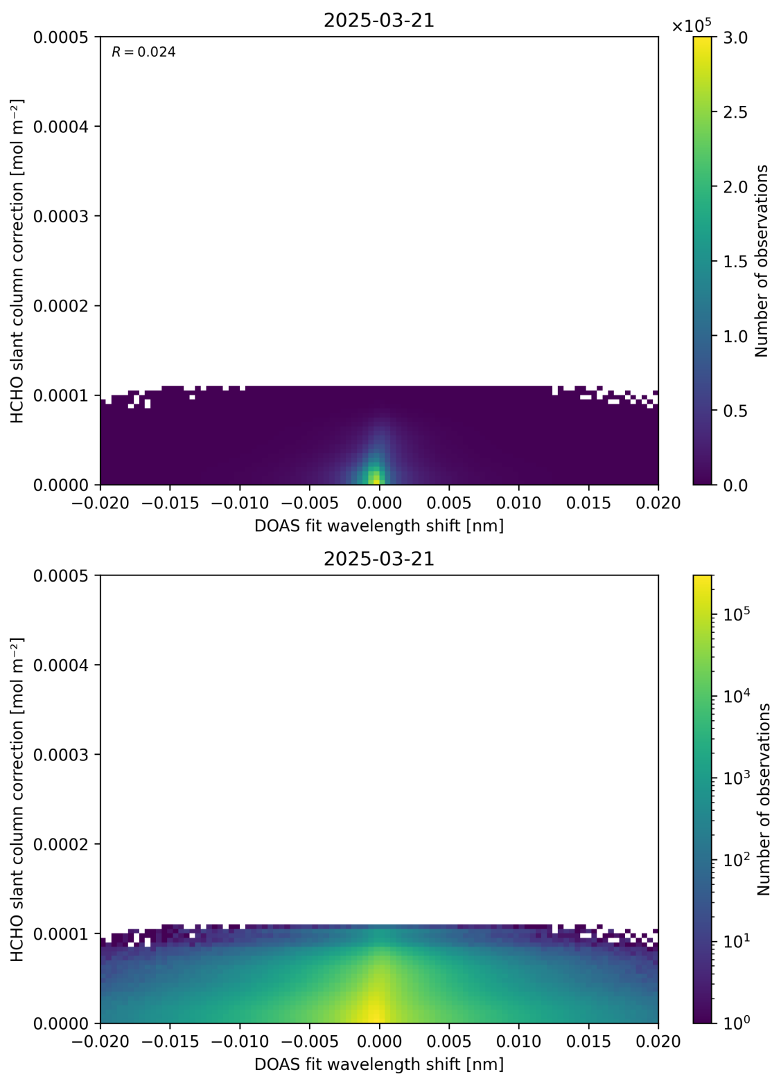
Figure 67: Scatter density plot of “DOAS fit wavelength shift” against “HCHO slant column correction” for 2025-03-20 to 2025-03-22.
