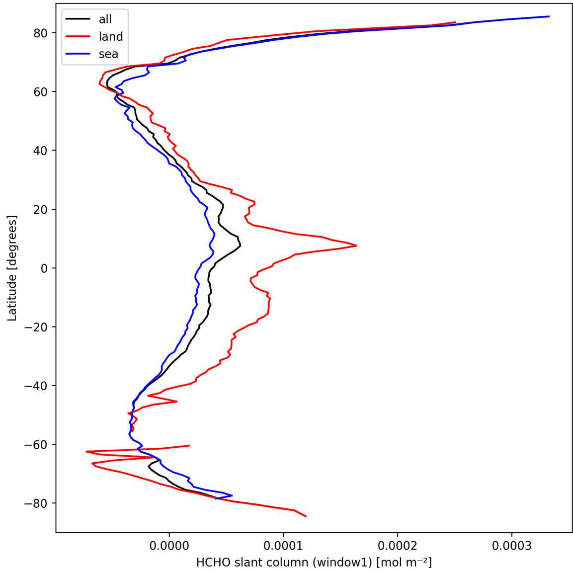
Figure 24: Zonal average of “HCHO slant column (window1)” for 2025-03-20 to 2025-03-22.
