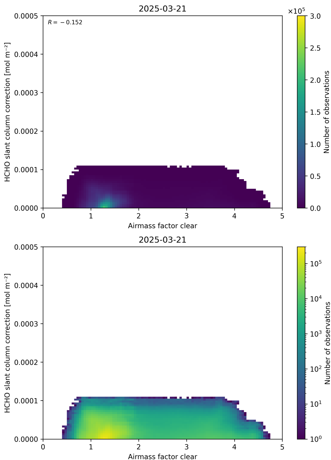
Figure 75: Scatter density plot of “Airmass factor clear” against “HCHO slant column correction” for 2025-03-20 to 2025-03-22.
