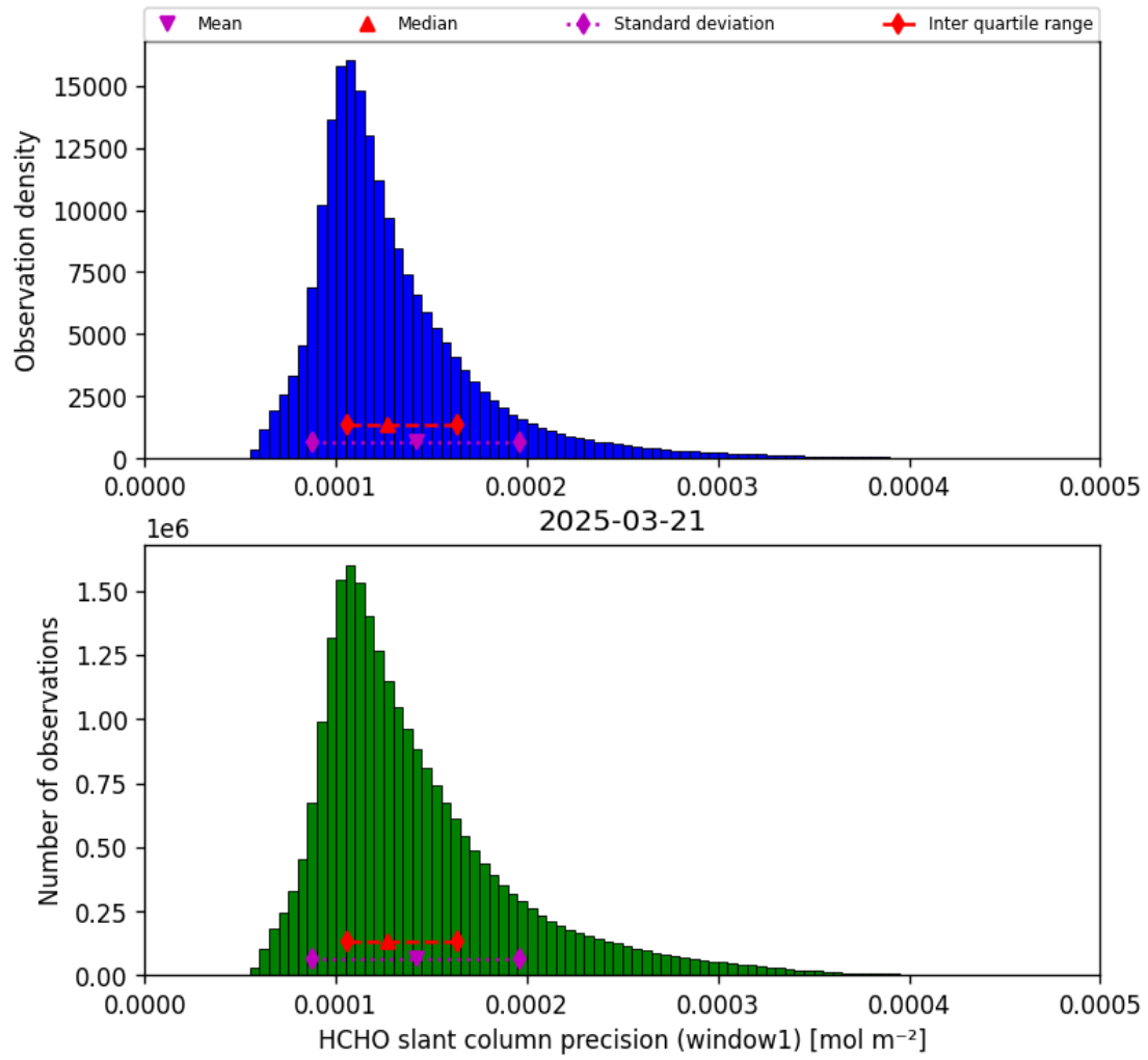
Figure 39: Histogram of “HCHO slant column precision (window1)” for 2025-03-20 to 2025-03-22
