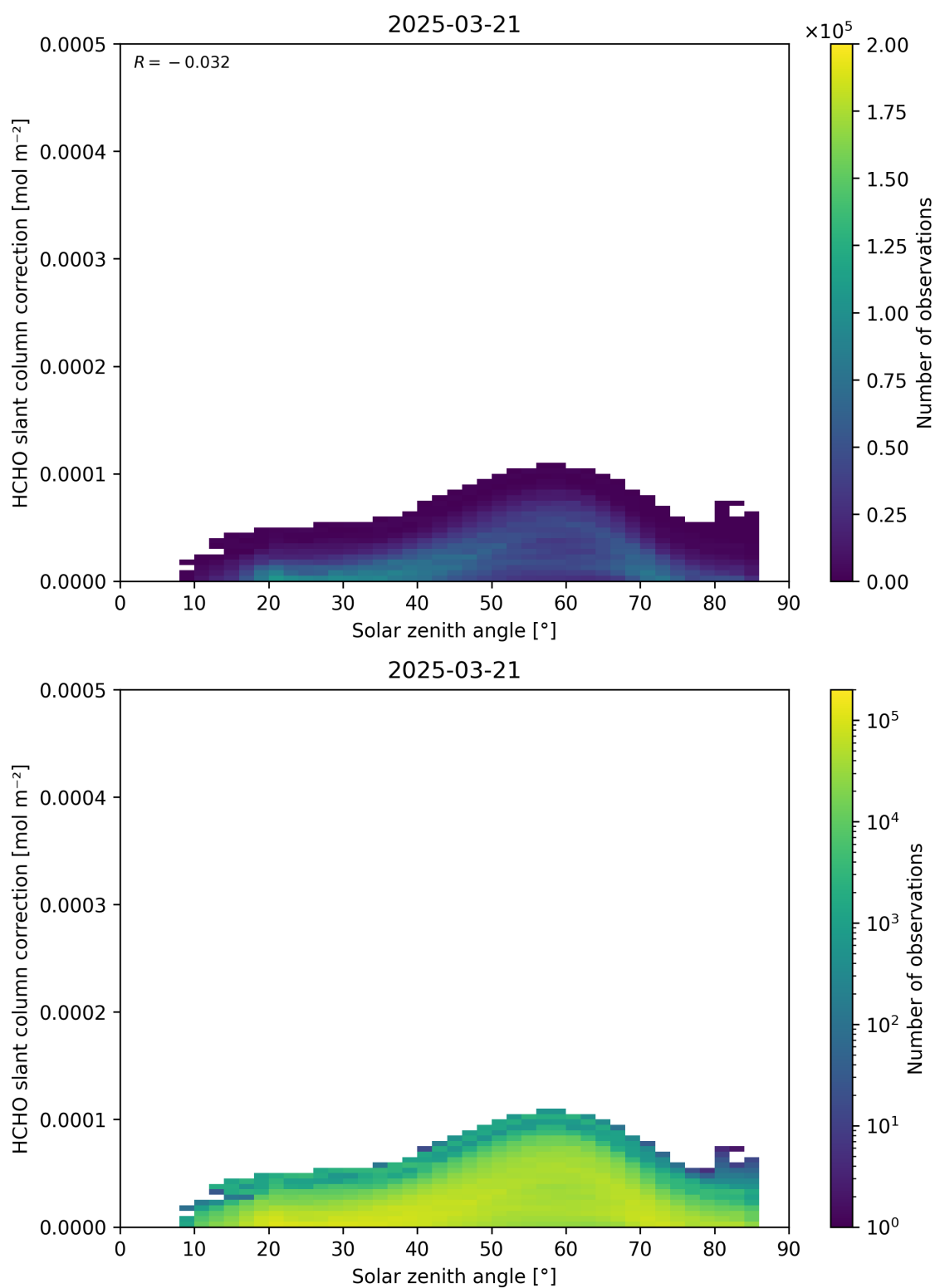
Figure 172: Scatter density plot of “Solar zenith angle” against “HCHO slant column correction” for 2025-03-20 to 2025-03-22.
