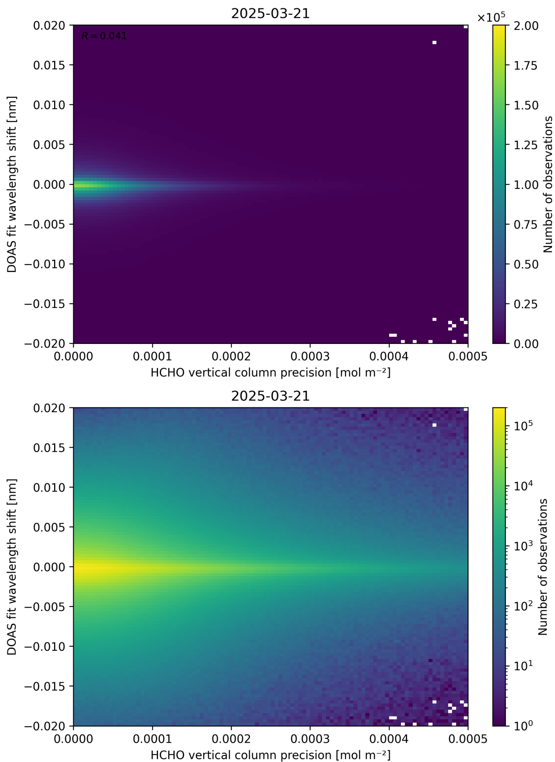
Figure 137: Scatter density plot of “HCHO vertical column precision” against “DOAS fit wavelength shift” for 2025-03-20 to 2025-03-22.
