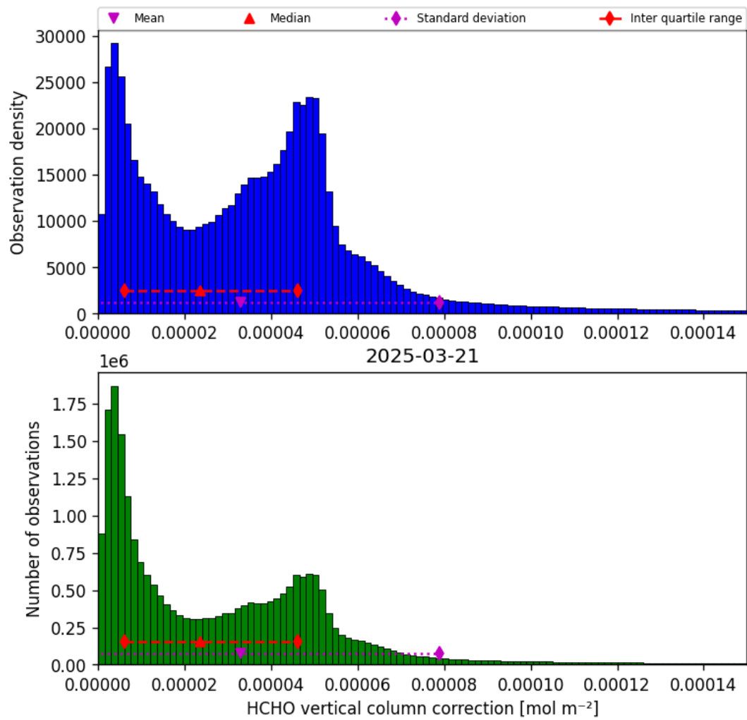
Figure 37: Histogram of “HCHO vertical column correction” for 2025-03-20 to 2025-03-22
