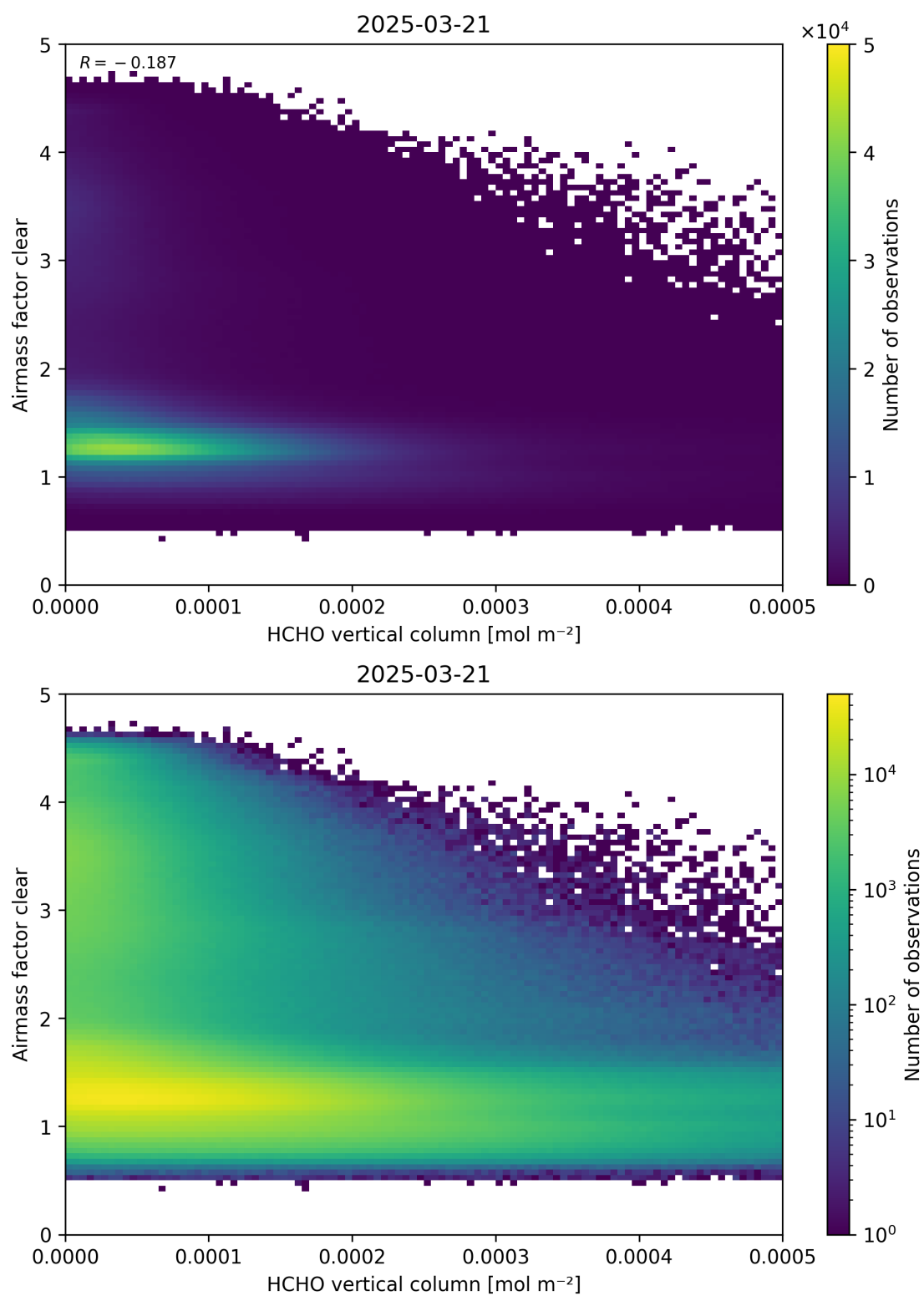
Figure 126: Scatter density plot of “HCHO vertical column” against “Airmass factor clear” for 2025-03-20 to 2025-03-22.
