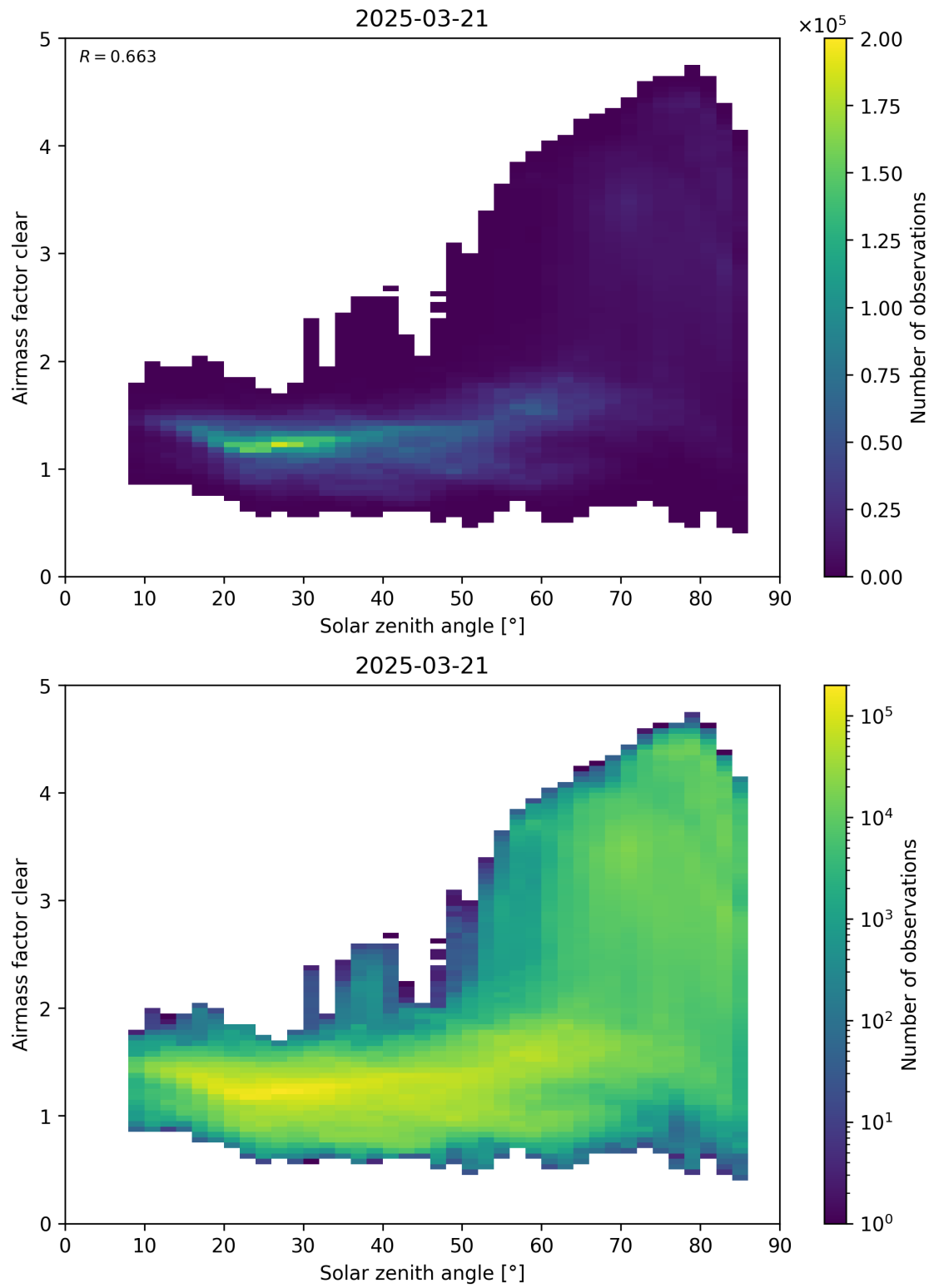
Figure 170: Scatter density plot of “Solar zenith angle” against “Airmass factor clear” for 2025-03-20 to 2025-03-22.
