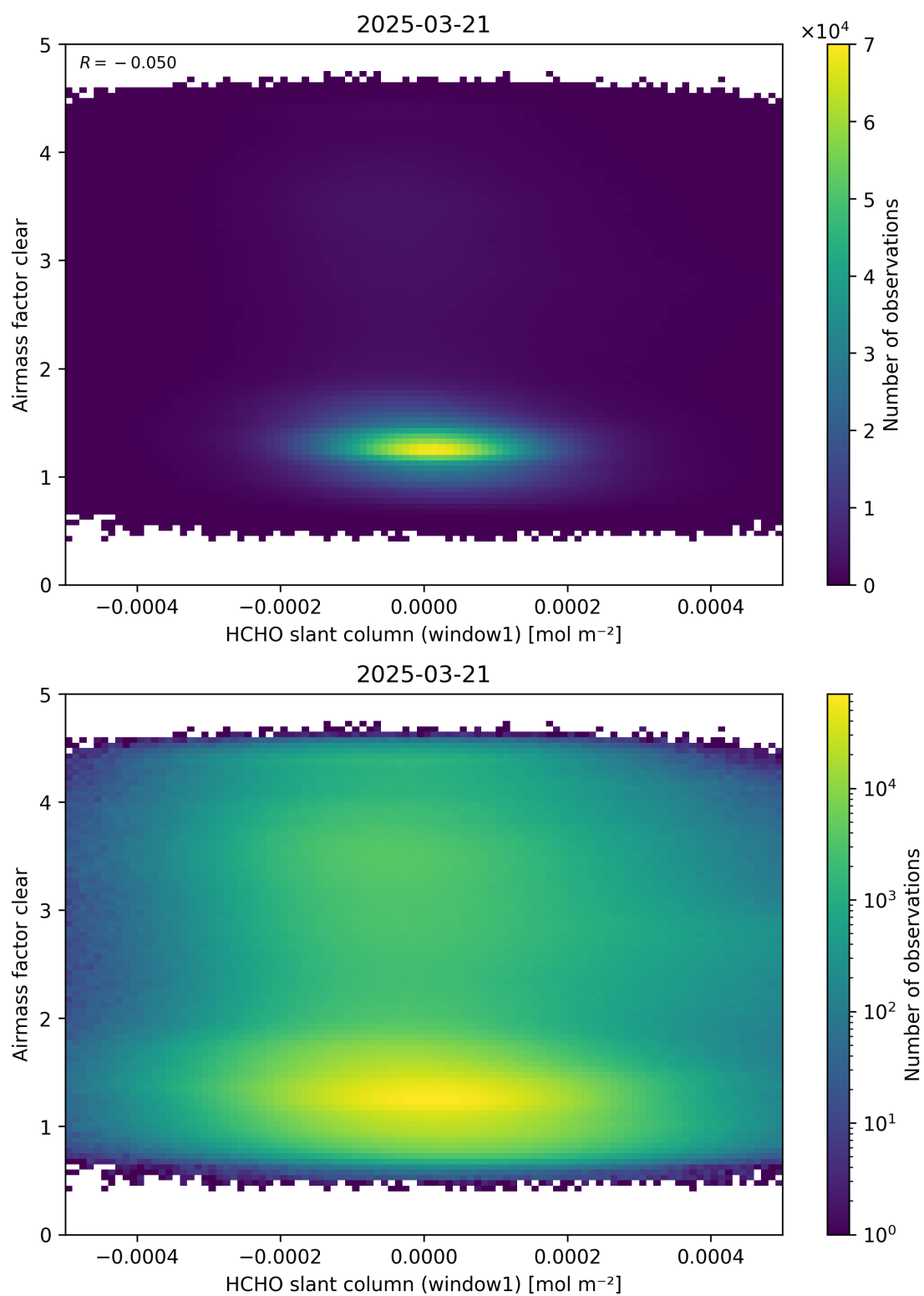
Figure 81: Scatter density plot of “HCHO slant column (window1)” against “Airmass factor clear” for 2025-03-20 to 2025-03-22.
