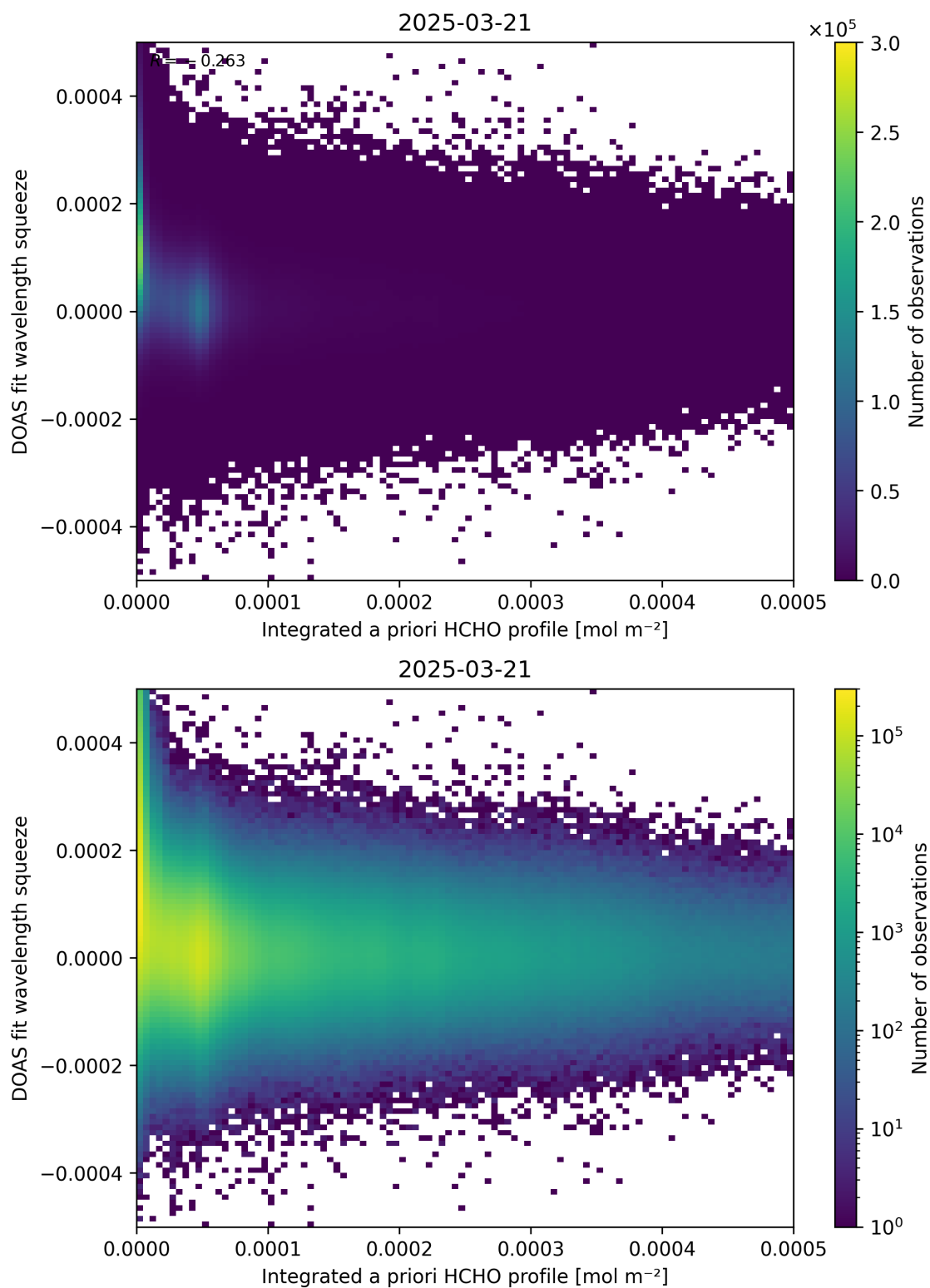
Figure 150: Scatter density plot of “Integrated a priori HCHO profile” against “DOAS fit wavelength squeeze” for 2025-03-20 to 2025-03-22.
