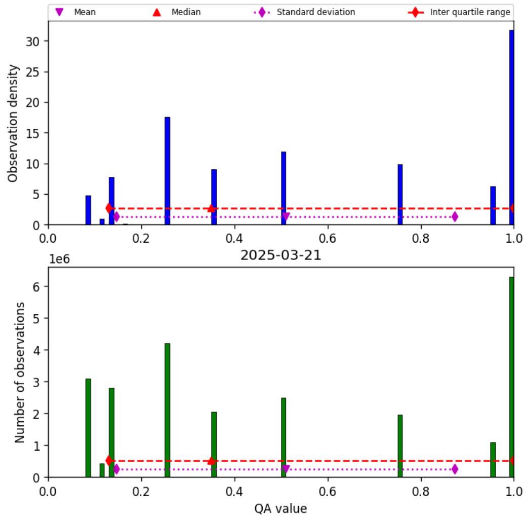
Figure 34: Histogram of “QA value” for 2025-03-20 to 2025-03-22
