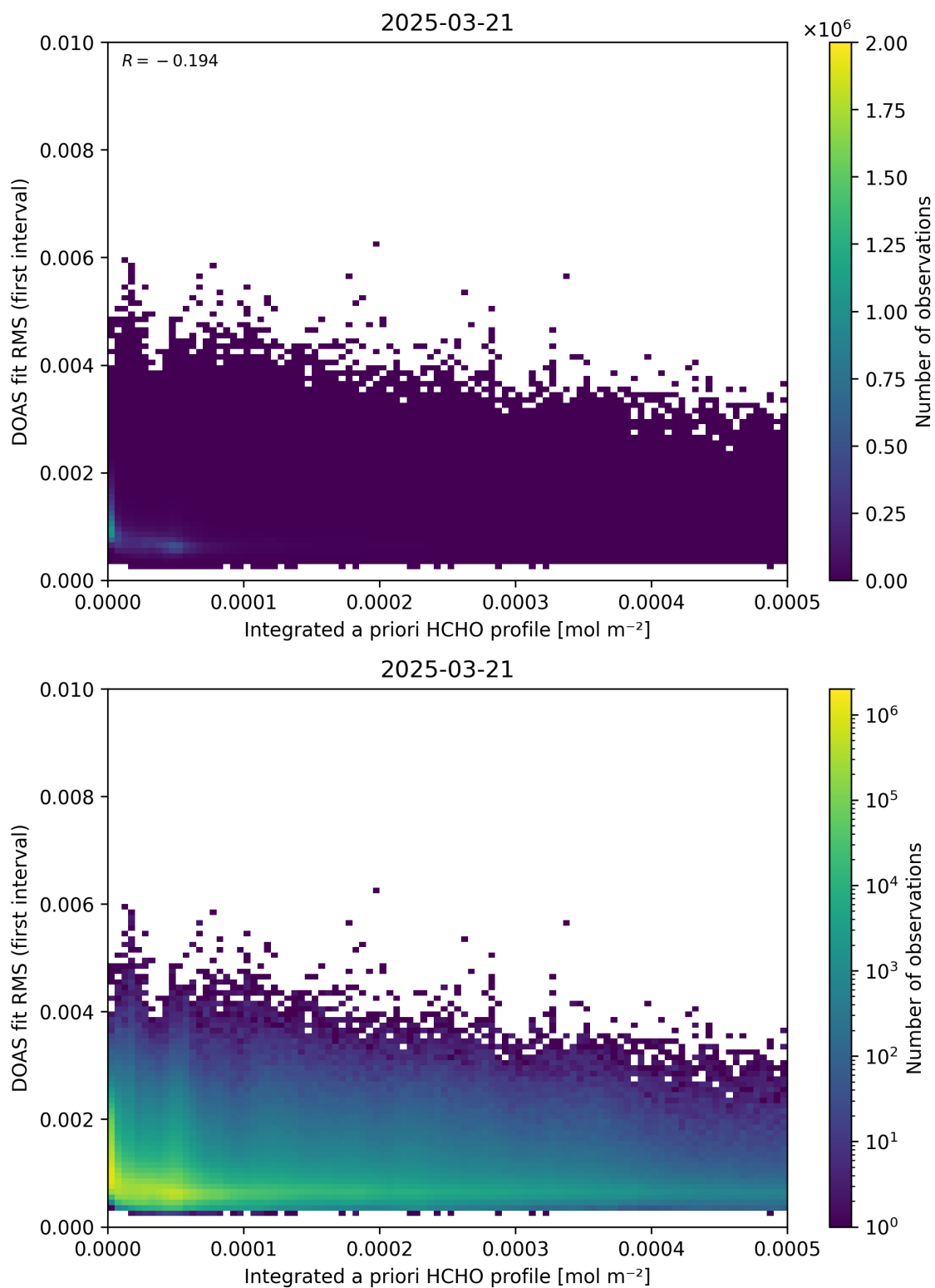
Figure 148: Scatter density plot of “Integrated a priori HCHO profile” against “DOAS fit RMS (first interval)” for 2025-03-20 to 2025-03-22.
