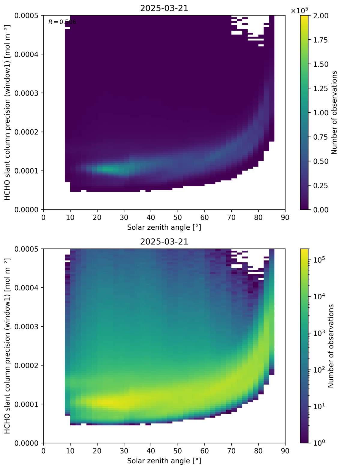
Figure 174: Scatter density plot of “Solar zenith angle” against “HCHO slant column precision (window1)” for 2025-03-20 to 2025-03-22.
