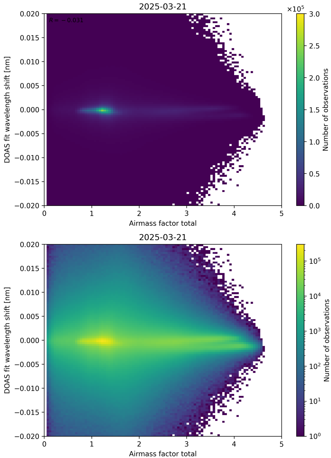
Figure 98: Scatter density plot of “Airmass factor total” against “DOAS fit wavelength shift” for 2025-03-20 to 2025-03-22.
