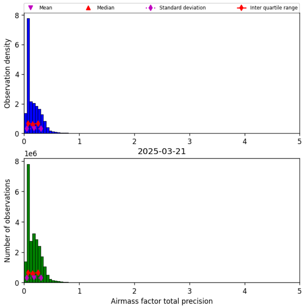
Figure 41: Histogram of “Airmass factor total precision” for 2025-03-20 to 2025-03-22
