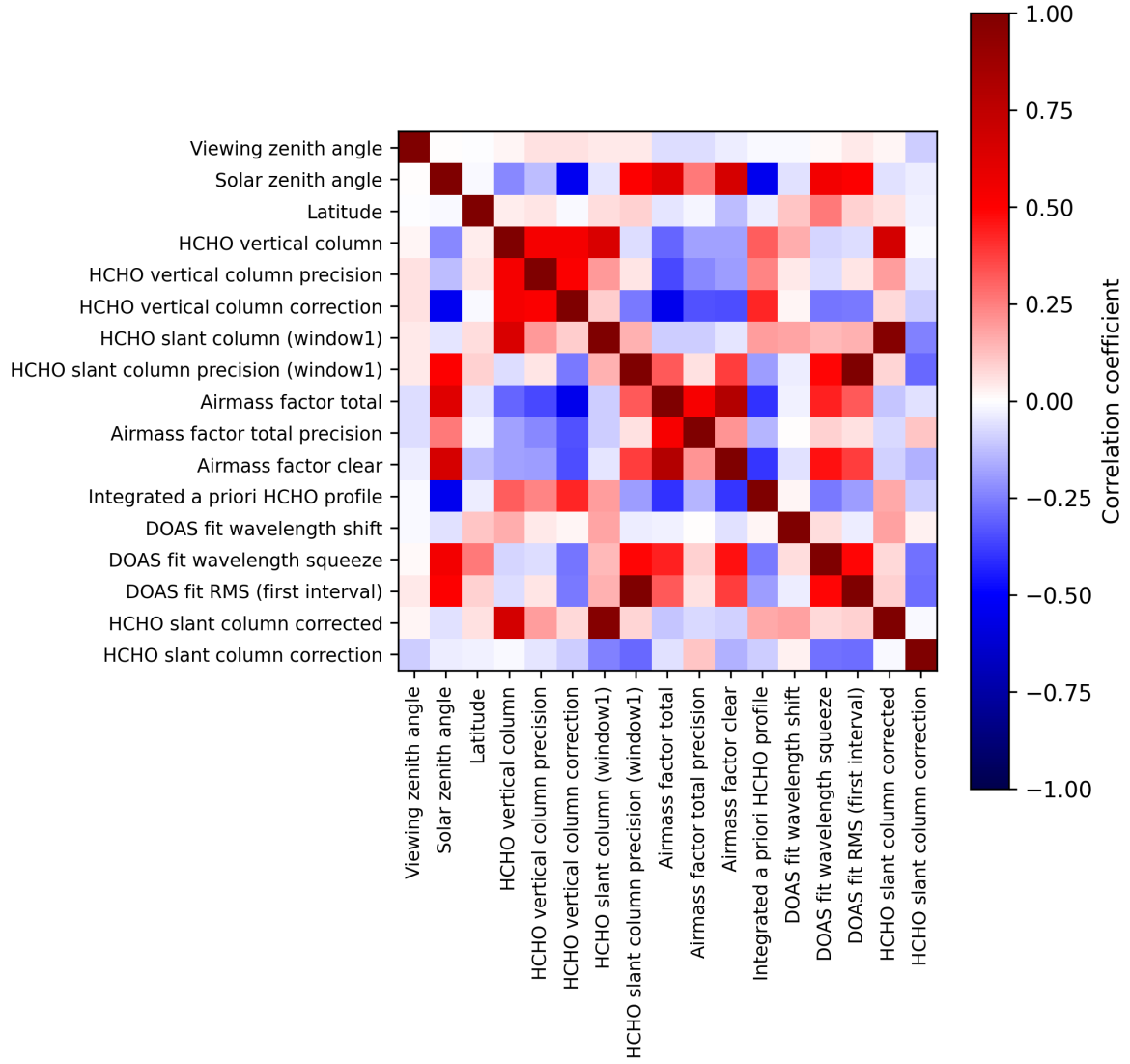
Figure 2: Map of correlation matrix for 2025-03-20 to 2025-03-22.
