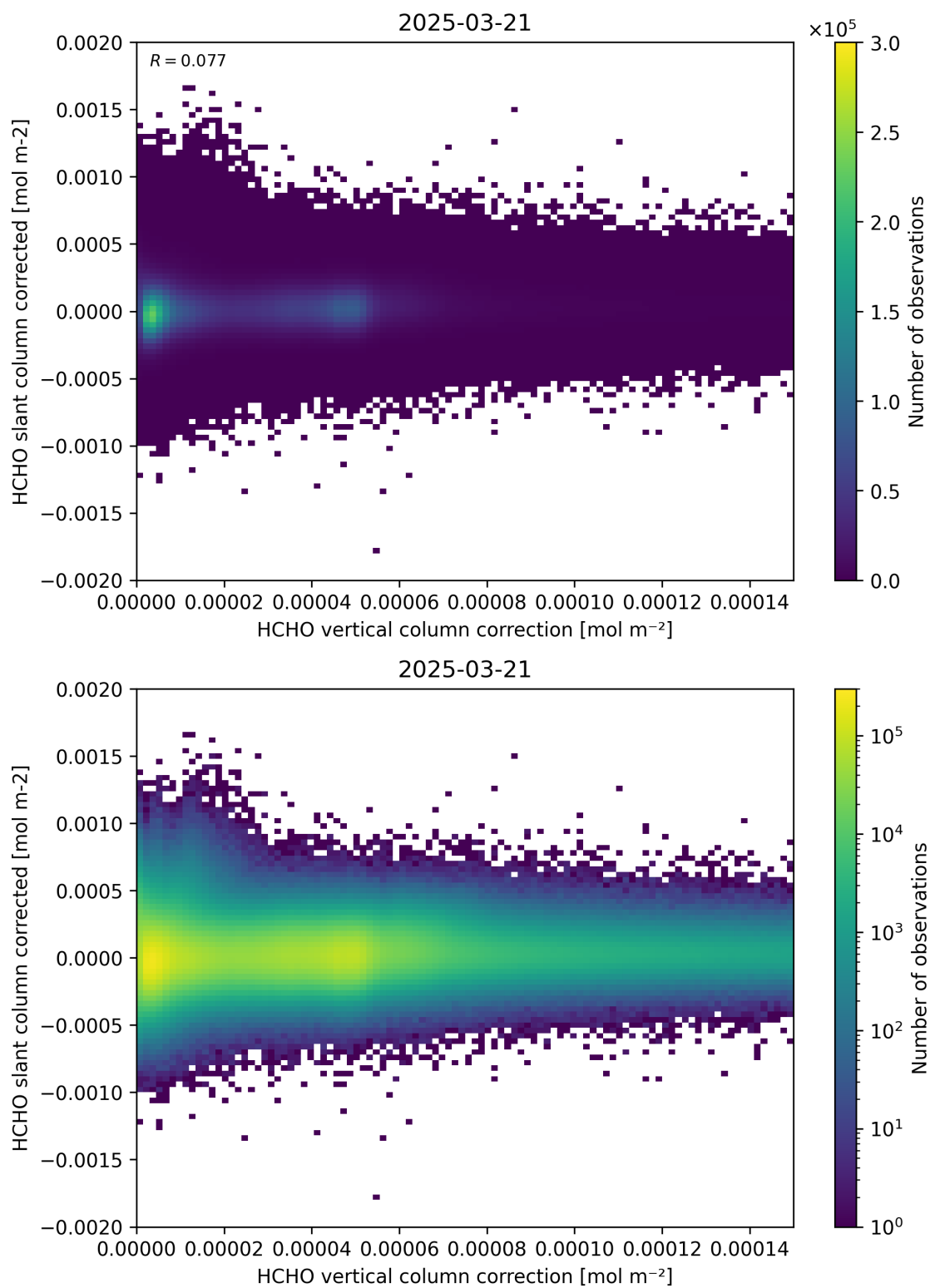
Figure 116: Scatter density plot of “HCHO vertical column correction” against “HCHO slant column corrected” for 2025-03-20 to 2025-03-22.
