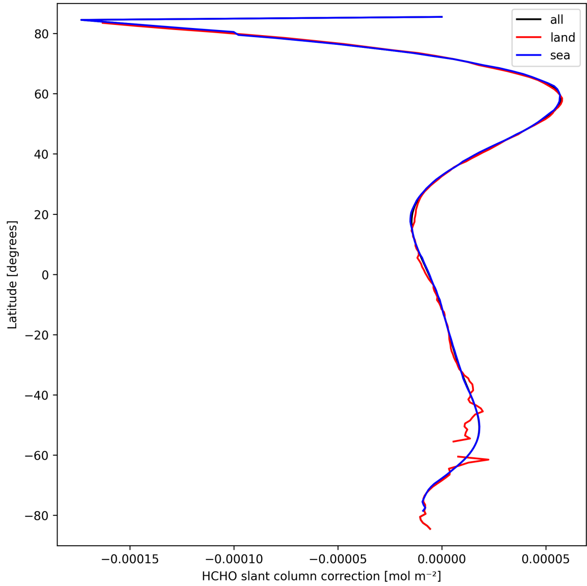
Figure 33: Zonal average of “HCHO slant column correction” for 2025-03-20 to 2025-03-22.
