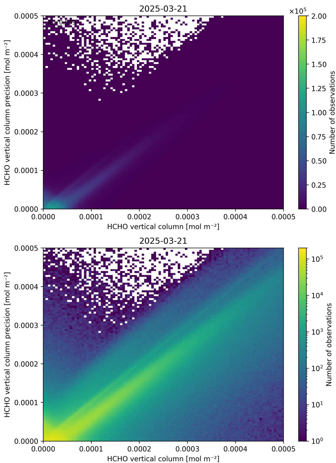
Figure 134: Scatter density plot of “HCHO vertical column” against “HCHO vertical column precision” for 2025-03-20 to 2025-03-22.
