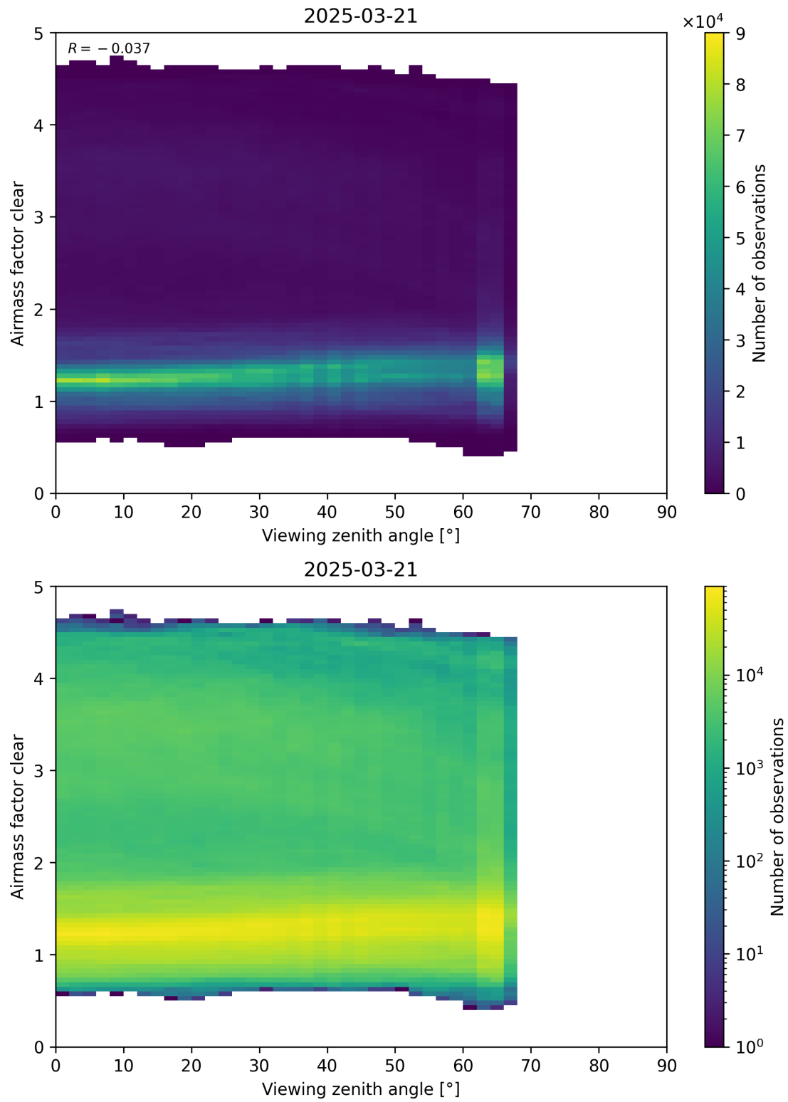
Figure 185: Scatter density plot of “Viewing zenith angle” against “Airmass factor clear” for 2025-03-20 to 2025-03-22.
