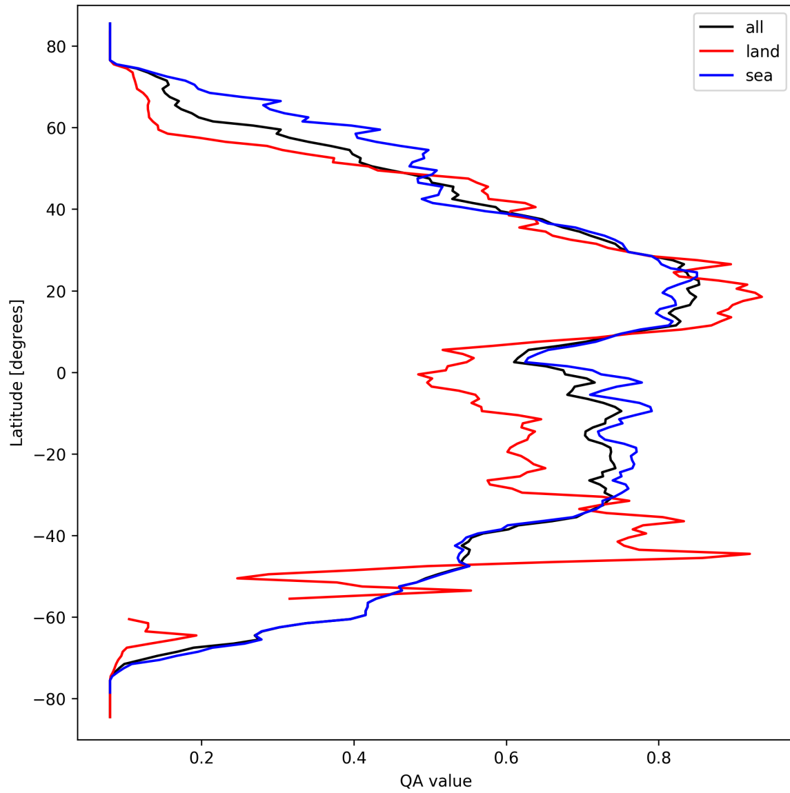
Figure 20: Zonal average of “QA value” for 2025-03-20 to 2025-03-22.
