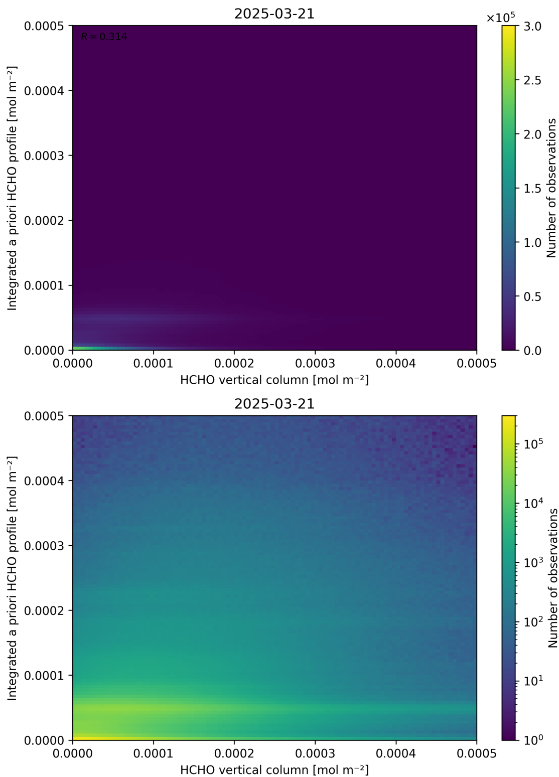
Figure 135: Scatter density plot of “HCHO vertical column” against “Integrated a priori HCHO profile” for 2025-03-20 to 2025-03-22.
