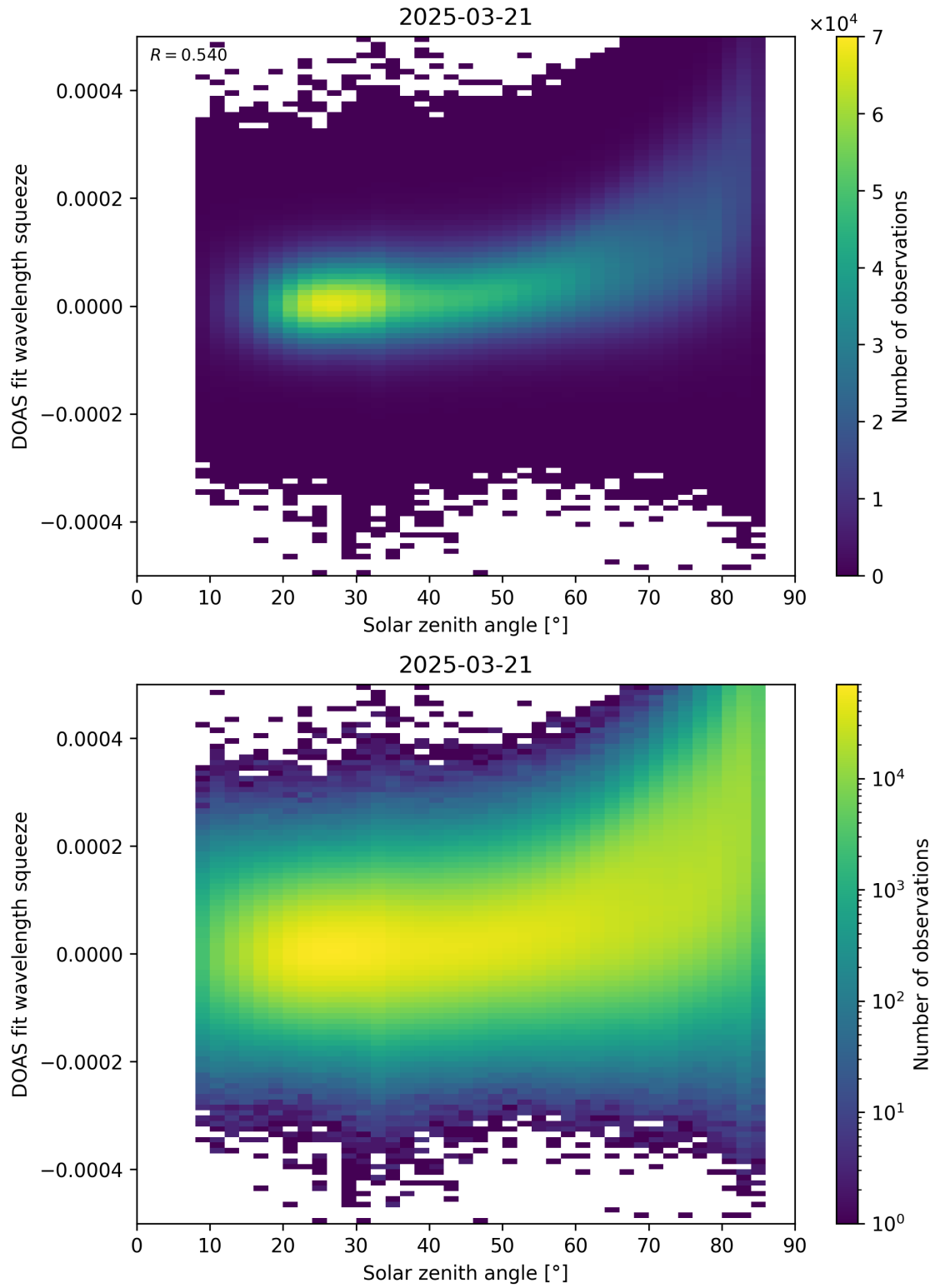
Figure 169: Scatter density plot of “Solar zenith angle” against “DOAS fit wavelength squeeze” for 2025-03-20 to 2025-03-22.
