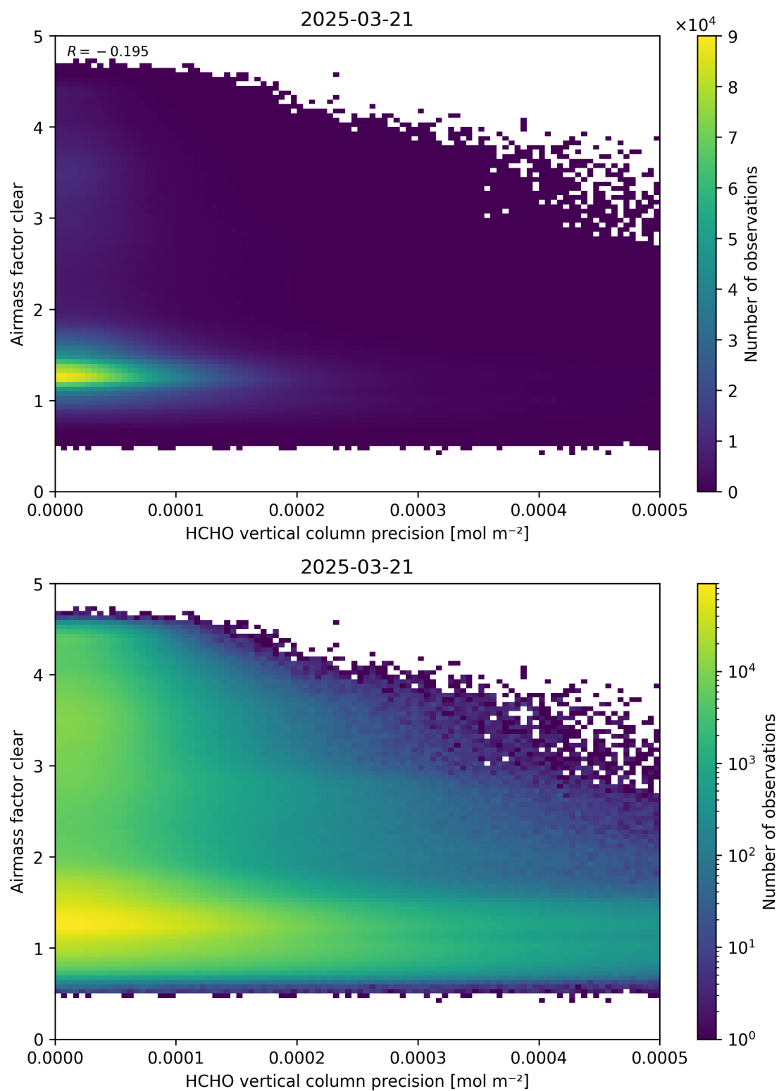
Figure 139: Scatter density plot of “HCHO vertical column precision” against “Airmass factor clear” for 2025-03-20 to 2025-03-22.
