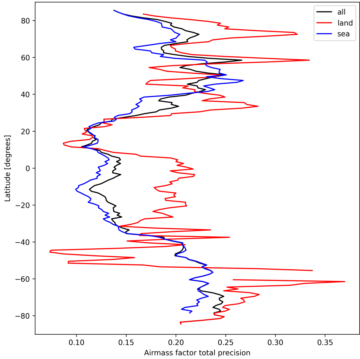
Figure 27: Zonal average of “Airmass factor total precision” for 2025-03-20 to 2025-03-22.
