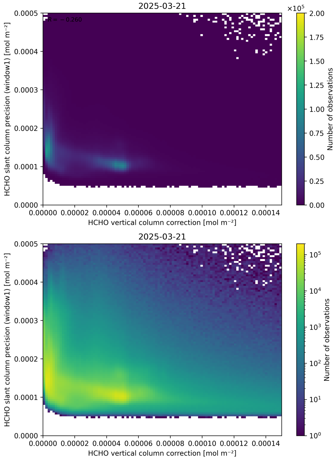
Figure 119: Scatter density plot of “HCHO vertical column correction” against “HCHO slant column precision (window1)” for 2025-03-20 to 2025-03-22.
