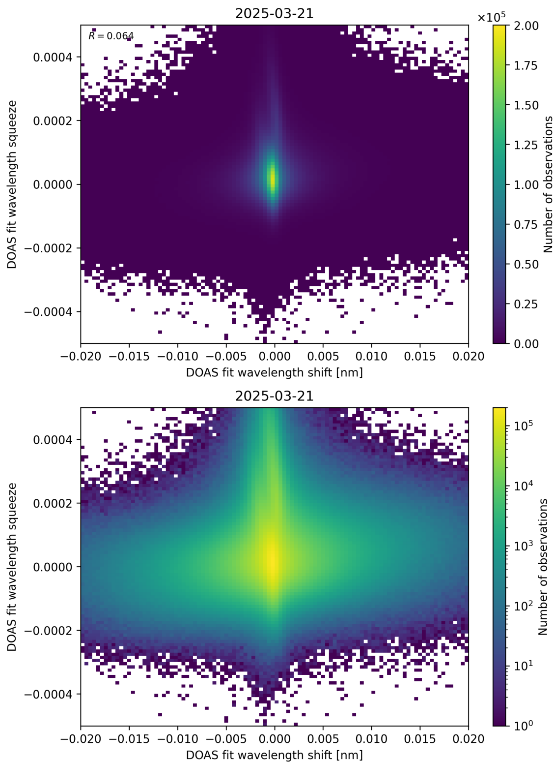
Figure 65: Scatter density plot of “DOAS fit wavelength shift” against “DOAS fit wavelength squeeze” for 2025-03-20 to 2025-03-22.
