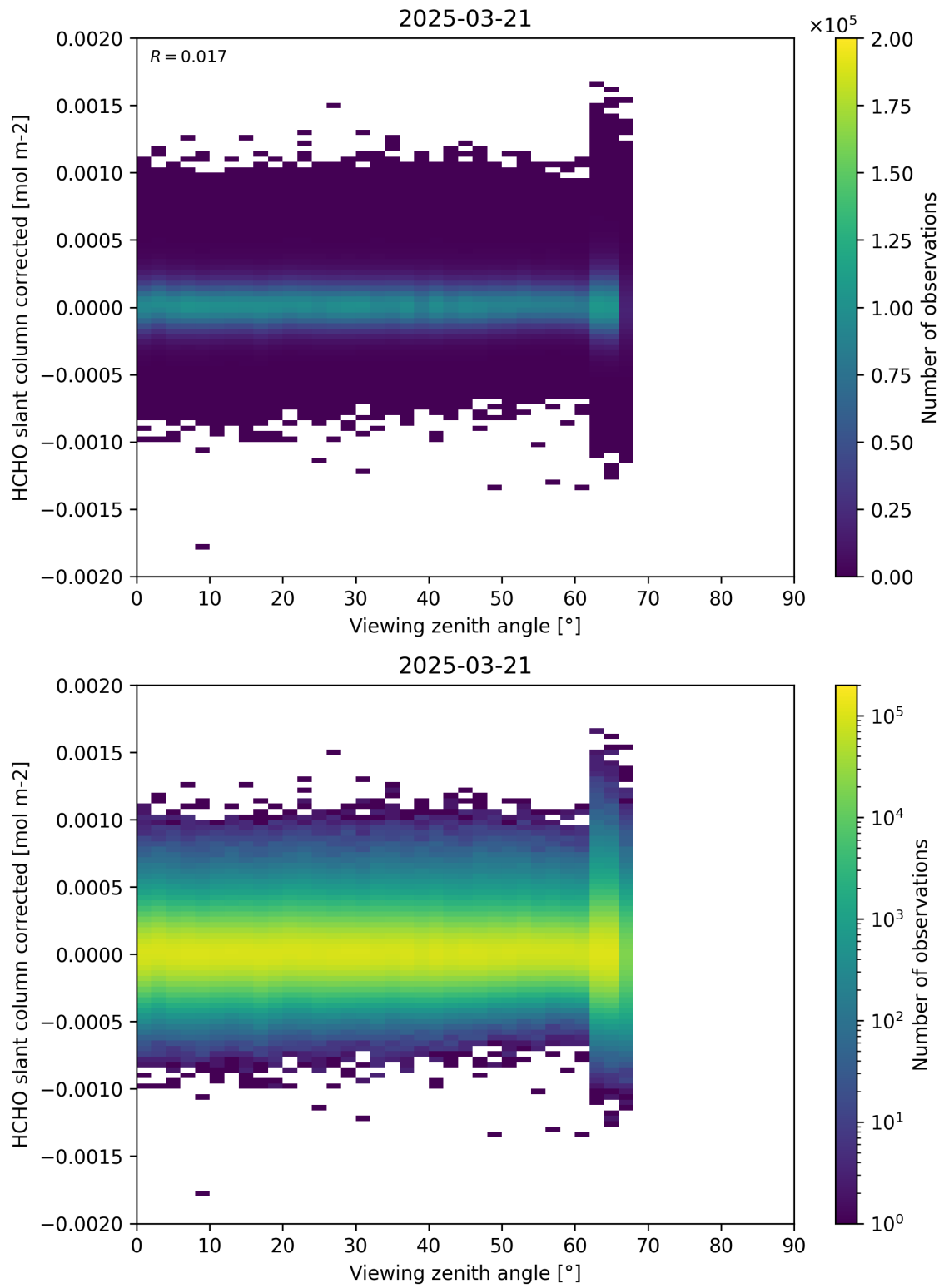
Figure 186: Scatter density plot of “Viewing zenith angle” against “HCHO slant column corrected” for 2025-03-20 to 2025-03-22.
