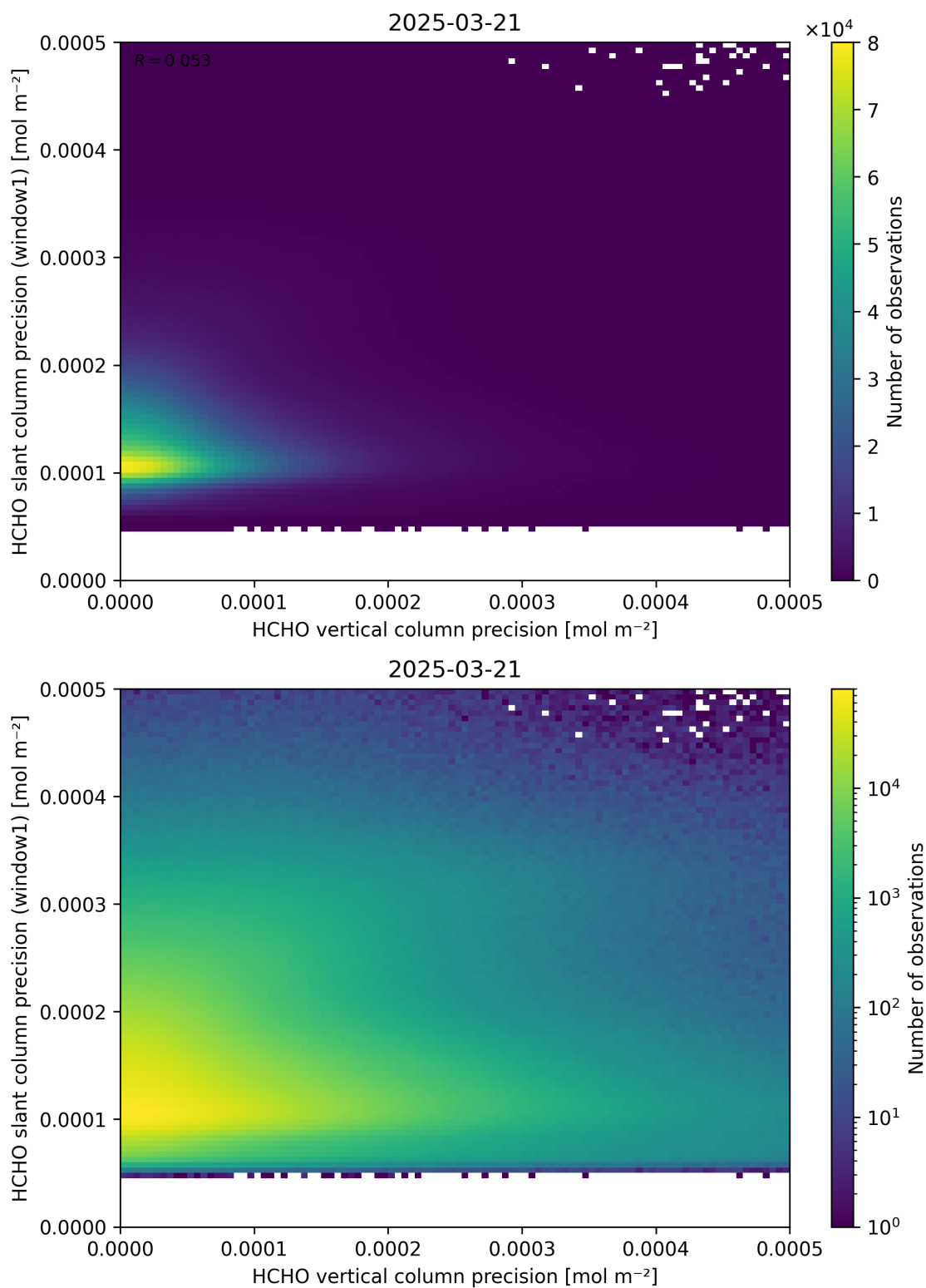
Figure 143: Scatter density plot of “HCHO vertical column precision” against “HCHO slant column precision (window1)” for 2025-03-20 to 2025-03-22.
