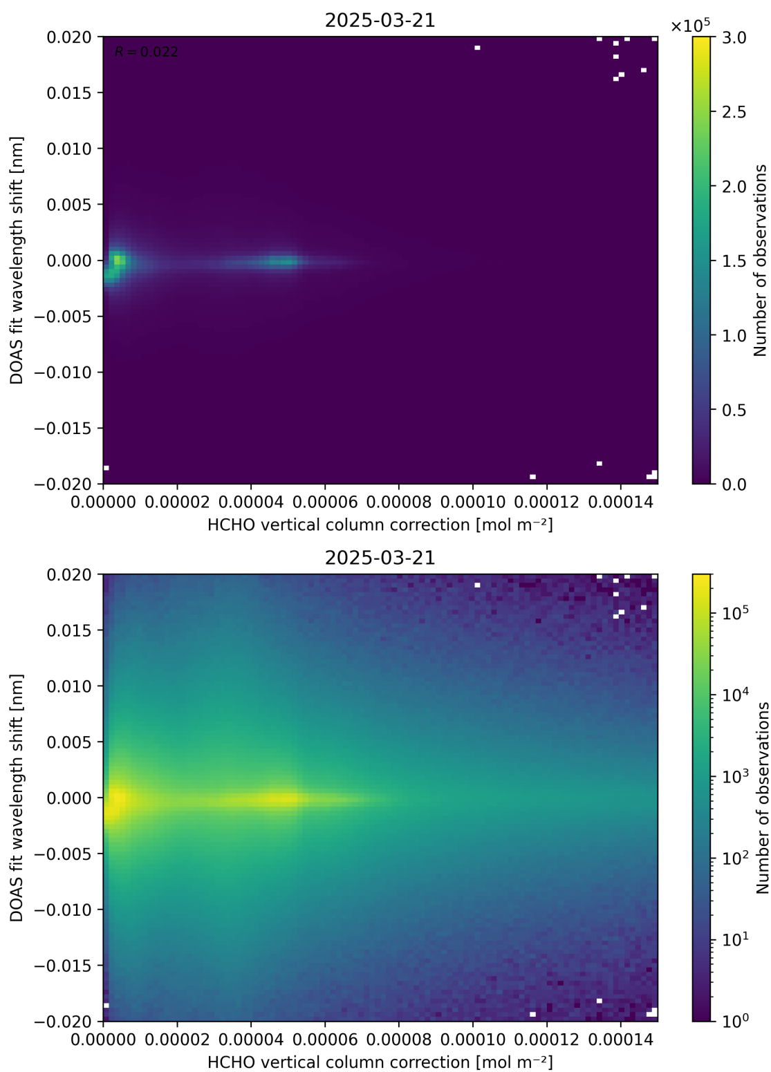
Figure 113: Scatter density plot of “HCHO vertical column correction” against “DOAS fit wavelength shift” for 2025-03-20 to 2025-03-22.
