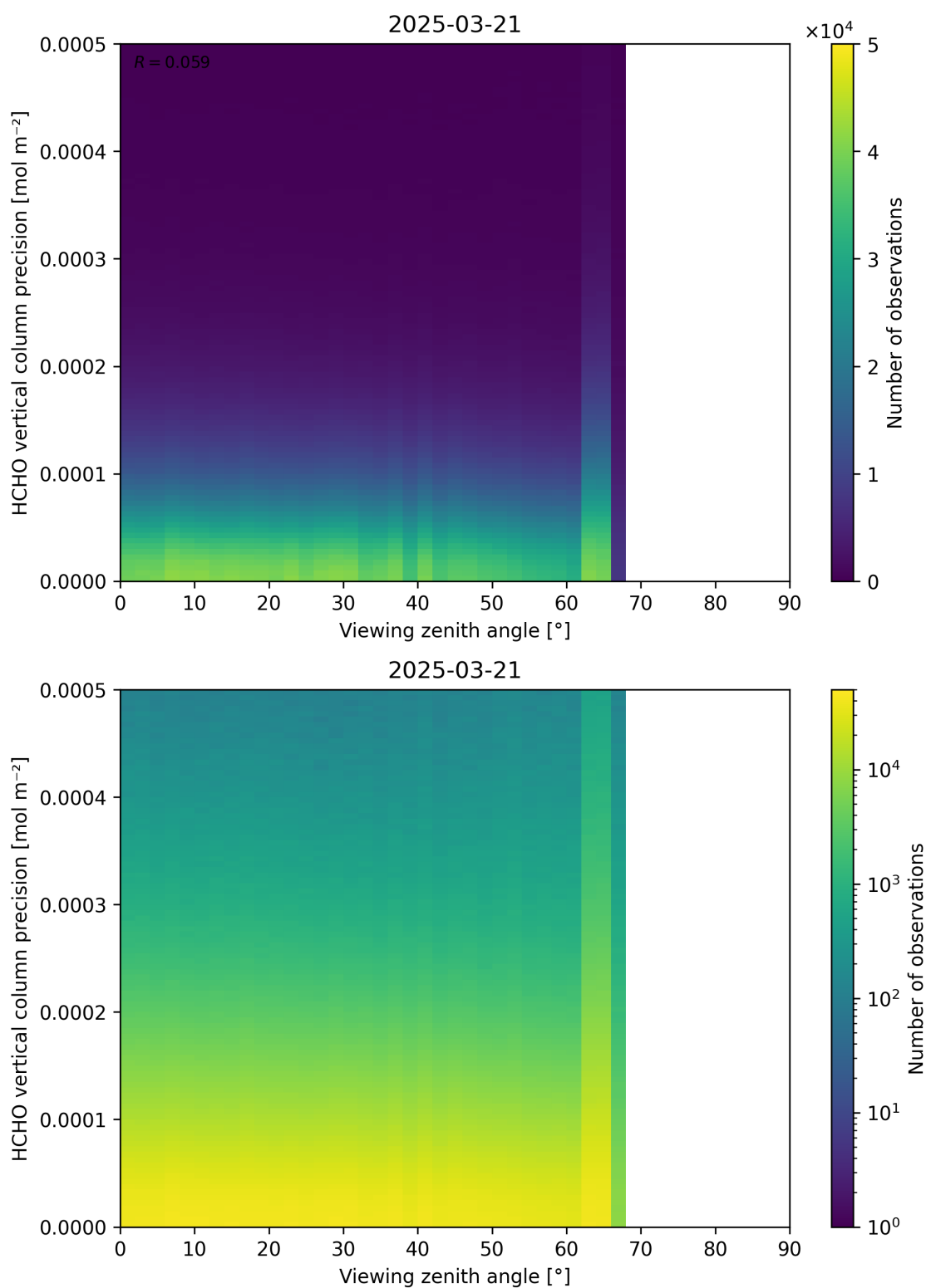
Figure 194: Scatter density plot of “Viewing zenith angle” against “HCHO vertical column precision” for 2025-03-20 to 2025-03-22.
