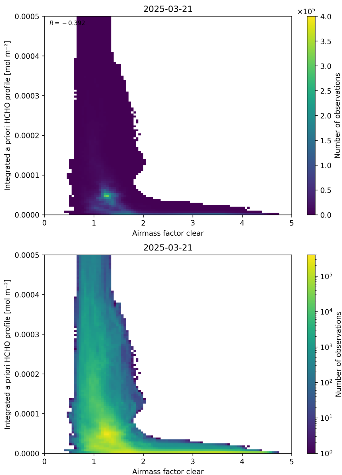
Figure 76: Scatter density plot of “Airmass factor clear” against “Integrated a priori HCHO profile” for 2025-03-20 to 2025-03-22.
