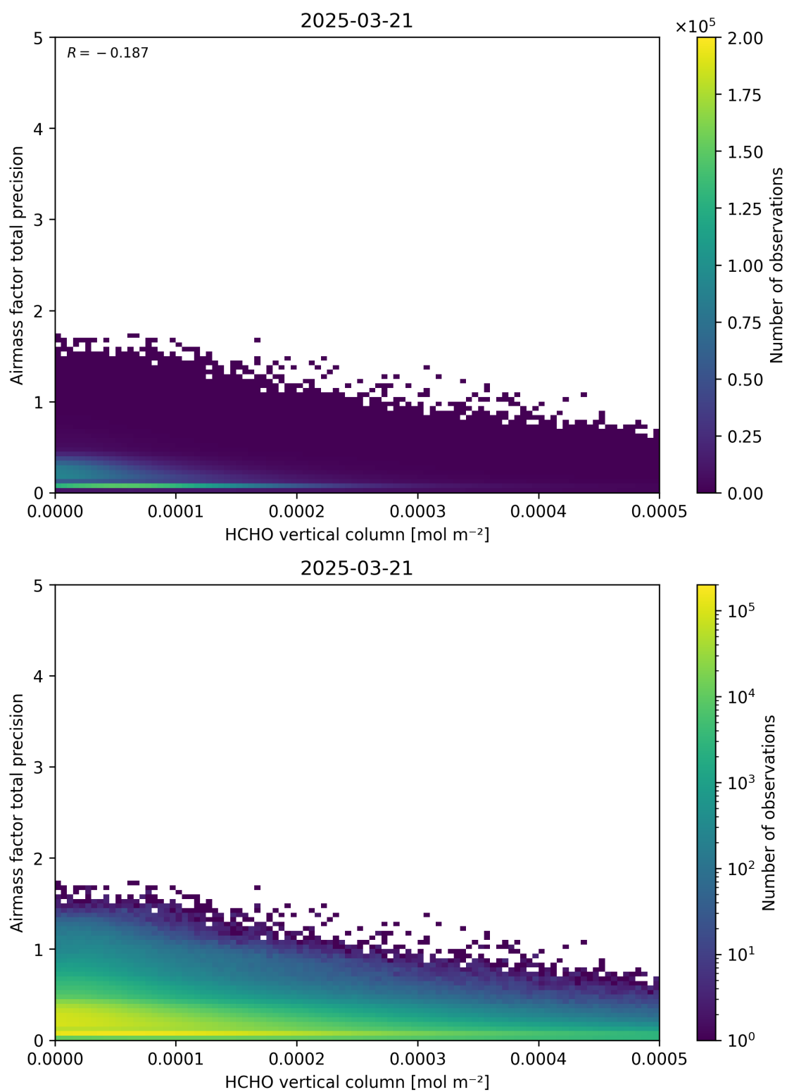
Figure 132: Scatter density plot of “HCHO vertical column” against “Airmass factor total precision” for 2025-03-20 to 2025-03-22.
