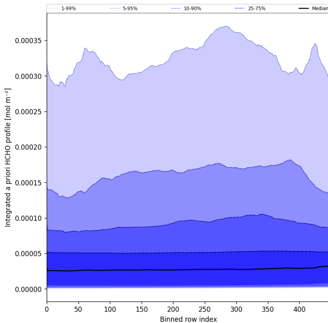
Figure 57: Along track statistics of “Integrated a priori HCHO profile” for 2025-03-20 to 2025-03-22
