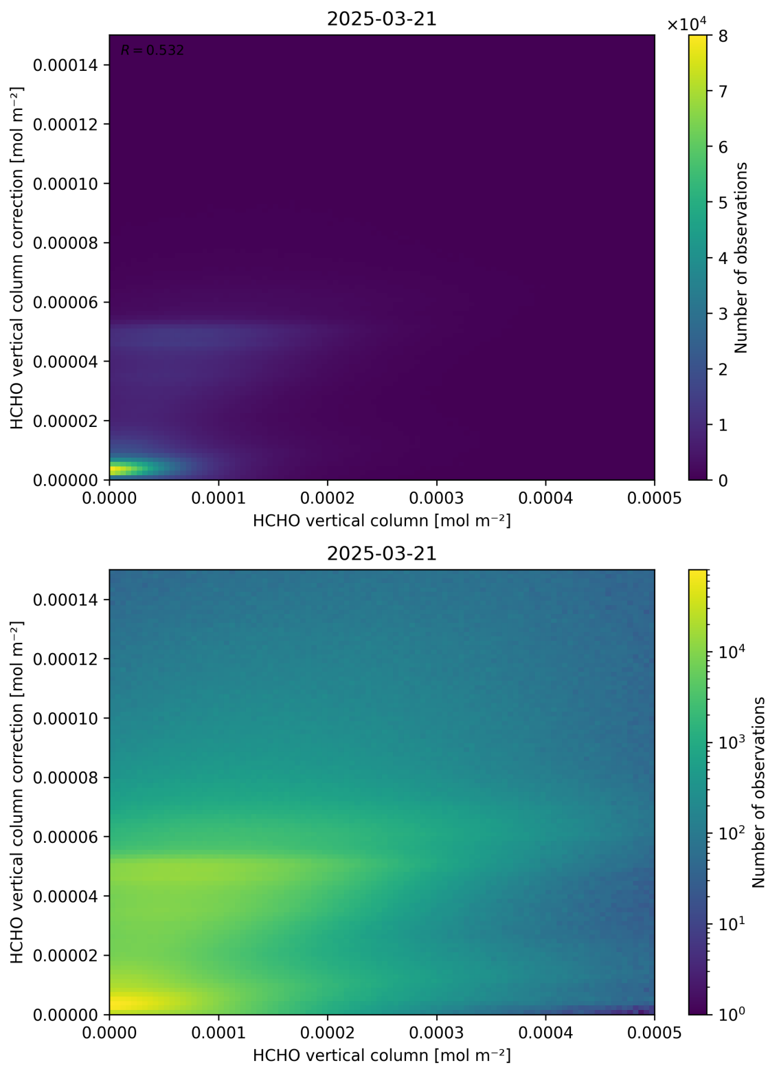
Figure 133: Scatter density plot of “HCHO vertical column” against “HCHO vertical column correction” for 2025-03-20 to 2025-03-22.
