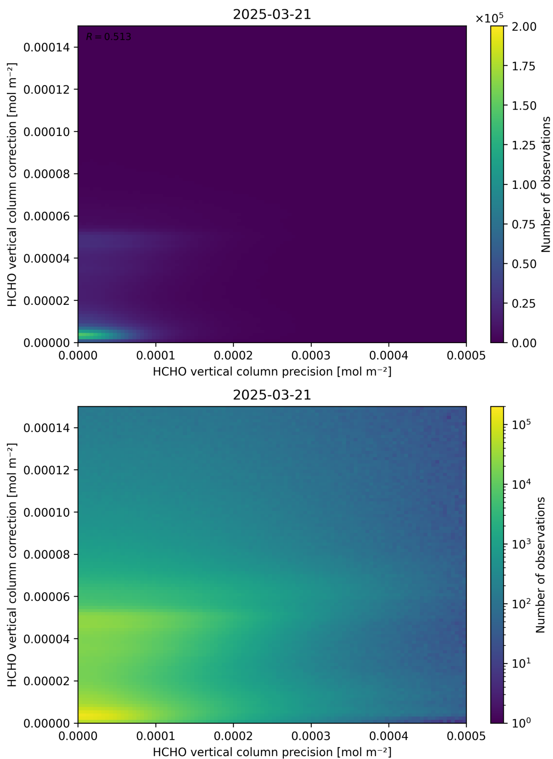
Figure 146: Scatter density plot of “HCHO vertical column precision” against “HCHO vertical column correction” for 2025-03-20 to 2025-03-22.
