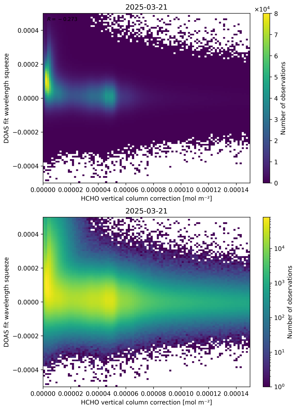
Figure 114: Scatter density plot of “HCHO vertical column correction” against “DOAS fit wavelength squeeze” for 2025-03-20 to 2025-03-22.
