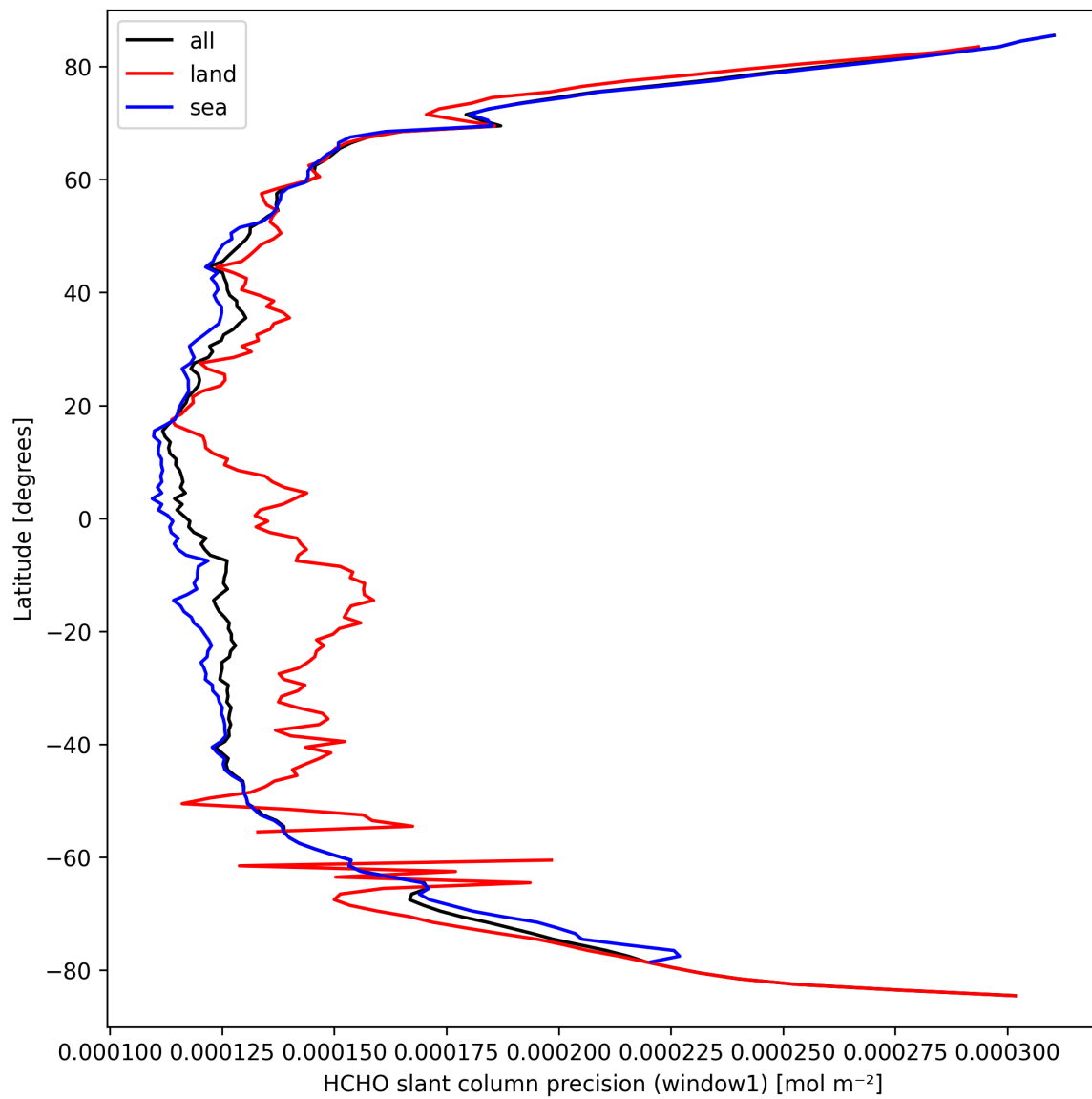
Figure 25: Zonal average of “HCHO slant column precision (window1)” for 2025-03-20 to 2025-03-22.
