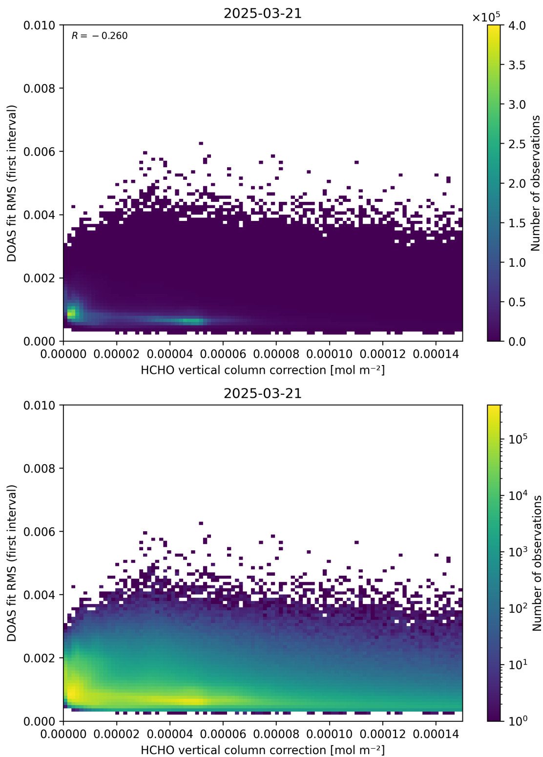
Figure 112: Scatter density plot of “HCHO vertical column correction” against “DOAS fit RMS (first interval)” for 2025-03-20 to 2025-03-22.
