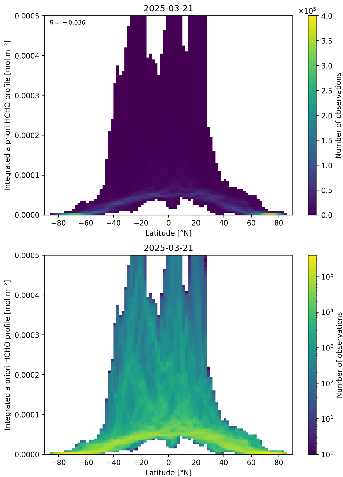
Figure 166: Scatter density plot of “Latitude” against “Integrated a priori HCHO profile” for 2025-03-20 to 2025-03-22.
