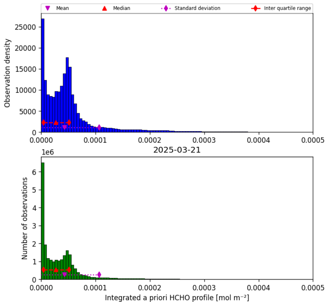
Figure 43: Histogram of “Integrated a priori HCHO profile” for 2025-03-20 to 2025-03-22
