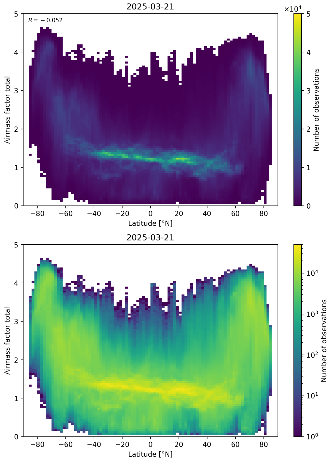
Figure 161: Scatter density plot of “Latitude” against “Airmass factor total” for 2025-03-20 to 2025-03-22.
