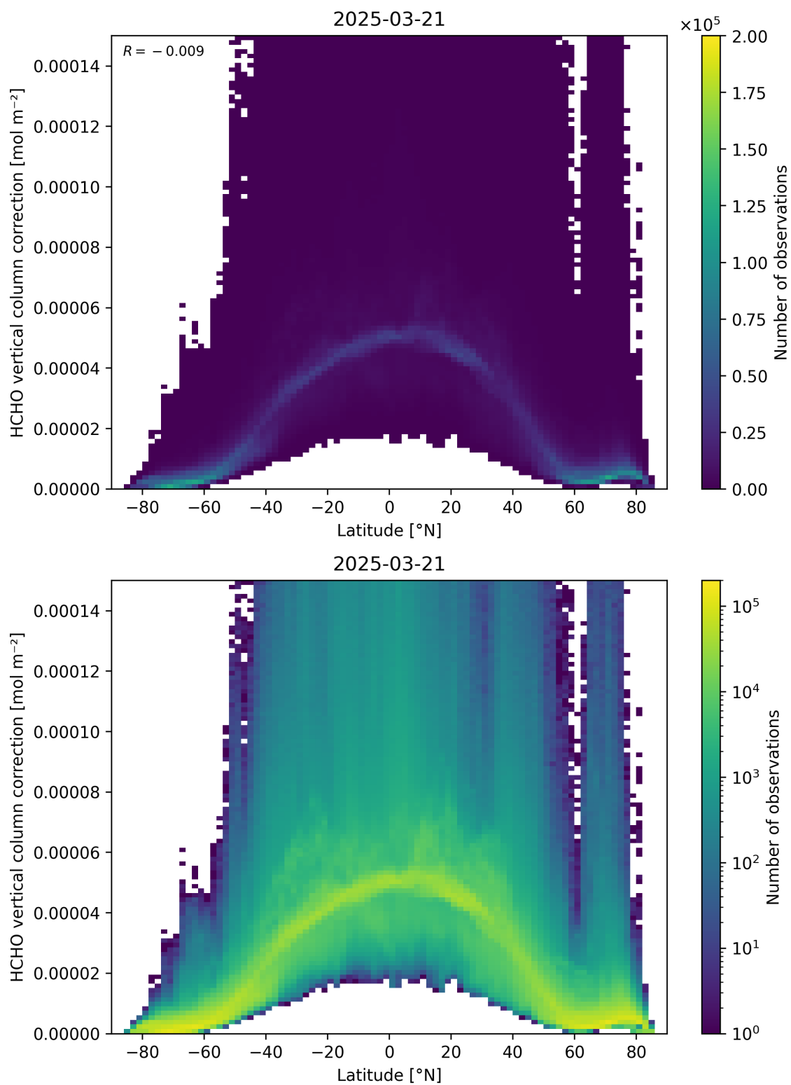
Figure 164: Scatter density plot of “Latitude” against “HCHO vertical column correction” for 2025-03-20 to 2025-03-22.
