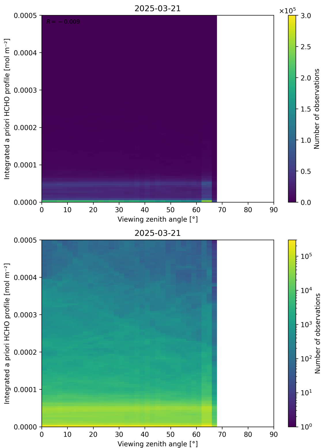
Figure 195: Scatter density plot of “Viewing zenith angle” against “Integrated a priori HCHO profile” for 2025-03-20 to 2025-03-22.
