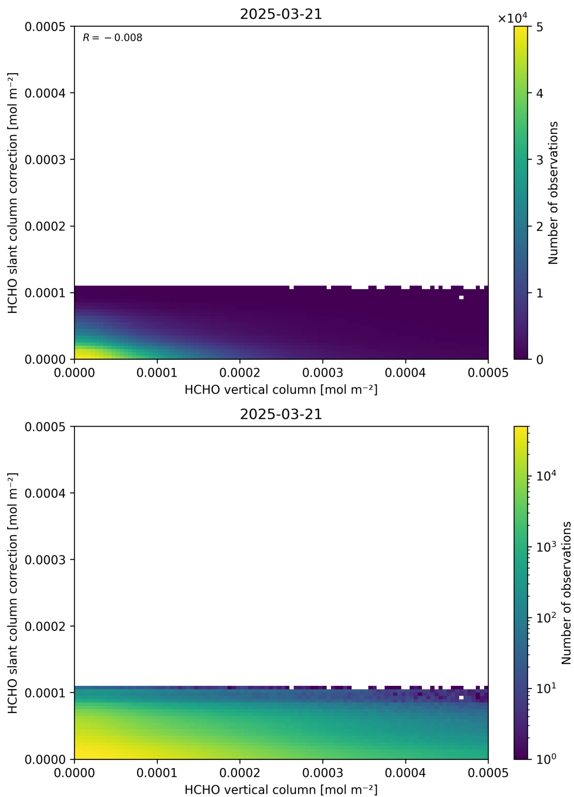
Figure 128: Scatter density plot of “HCHO vertical column” against “HCHO slant column correction” for 2025-03-20 to 2025-03-22.
