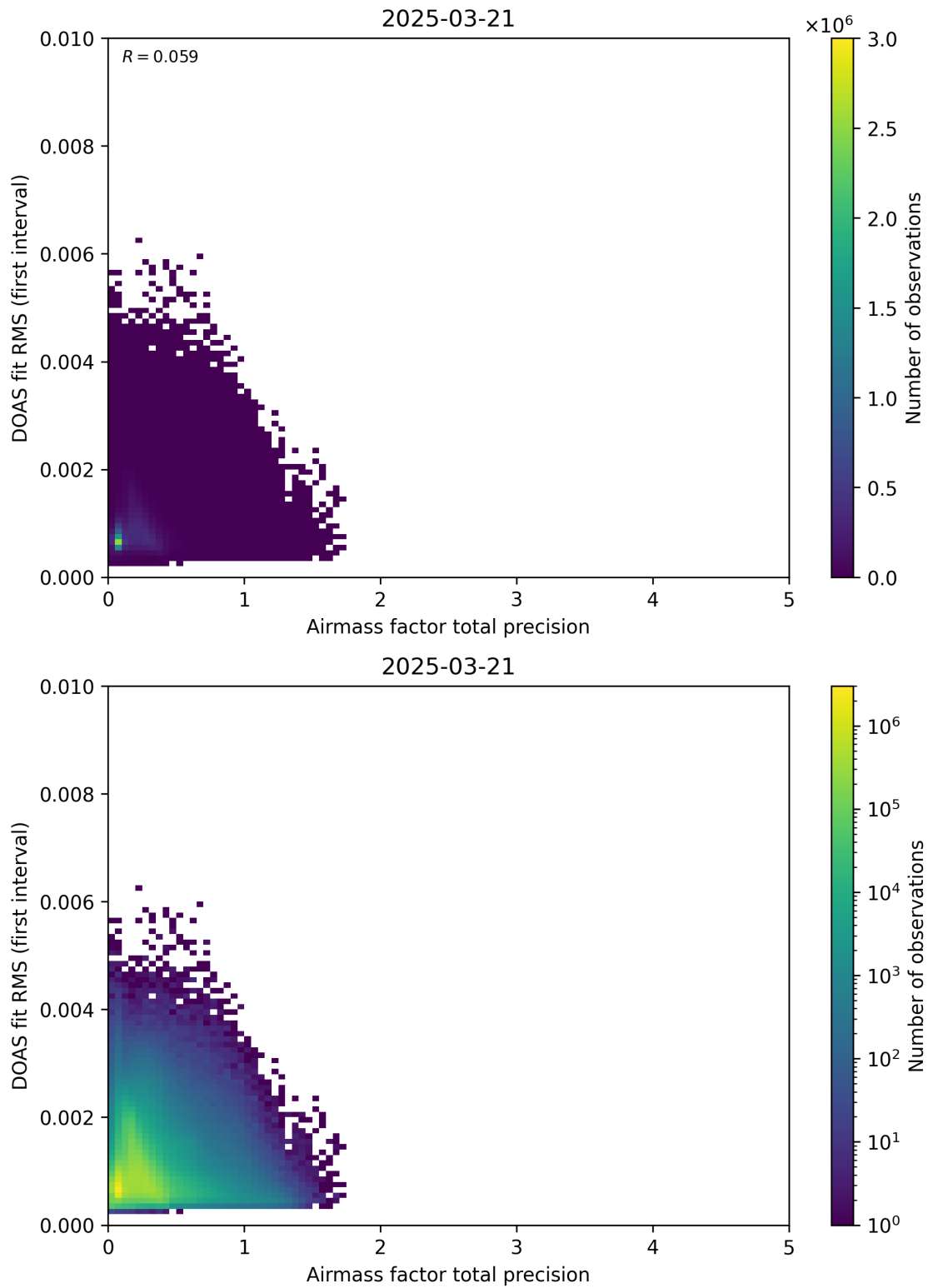
Figure 105: Scatter density plot of “Airmass factor total precision” against “DOAS fit RMS (first interval)” for 2025-03-20 to 2025-03-22.
