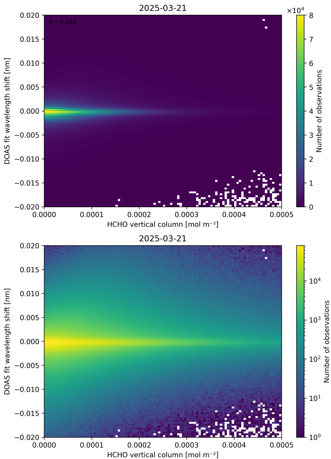
Figure 124: Scatter density plot of “HCHO vertical column” against “DOAS fit wavelength shift” for 2025-03-20 to 2025-03-22.
