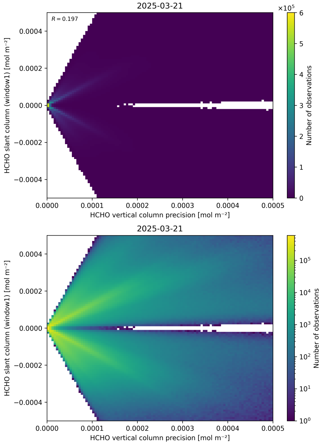
Figure 142: Scatter density plot of “HCHO vertical column precision” against “HCHO slant column (window1)” for 2025-03-20 to 2025-03-22.
