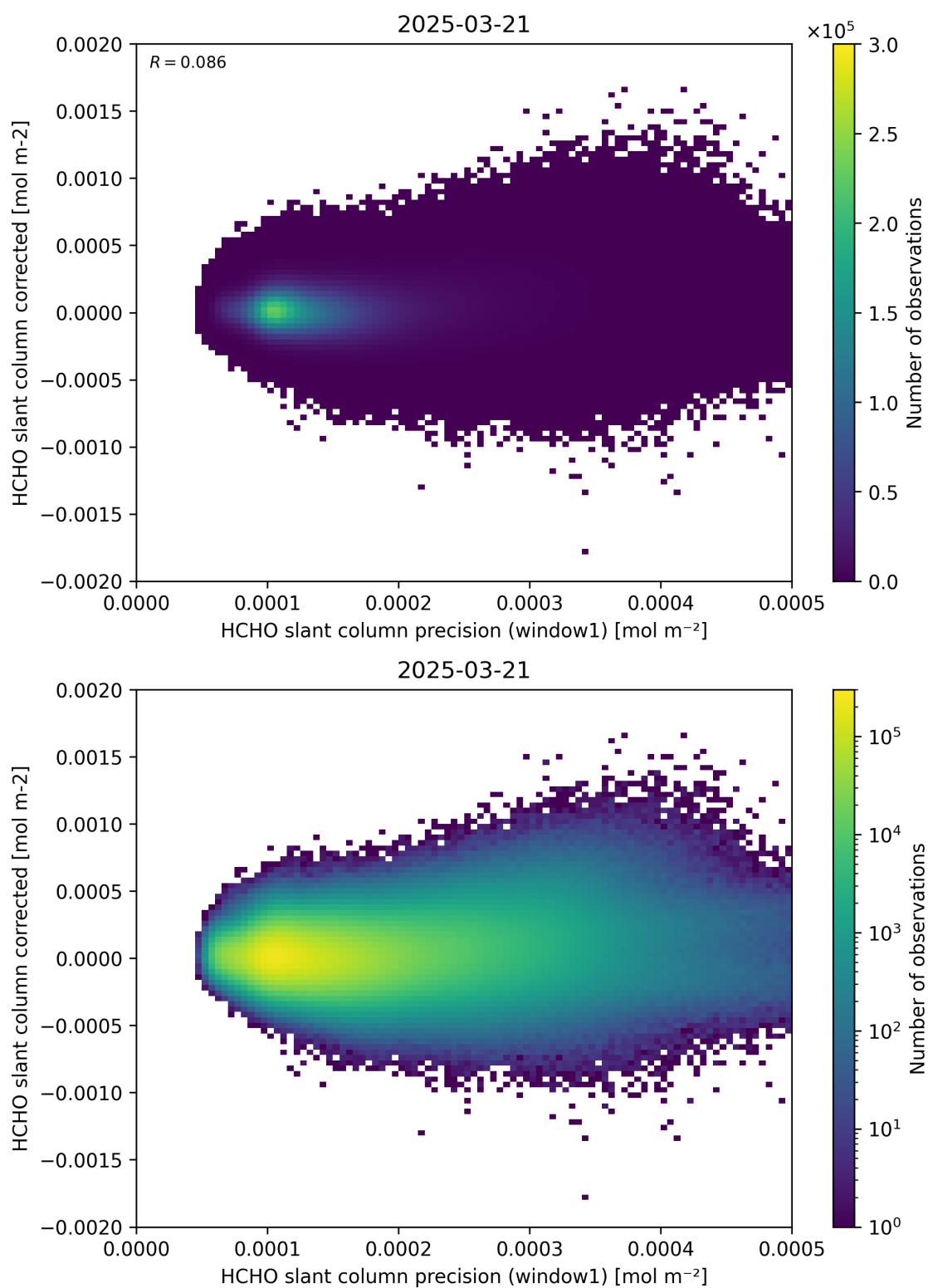
Figure 92: Scatter density plot of “HCHO slant column precision (window1)” against “HCHO slant column corrected” for 2025-03-20 to 2025-03-22.
