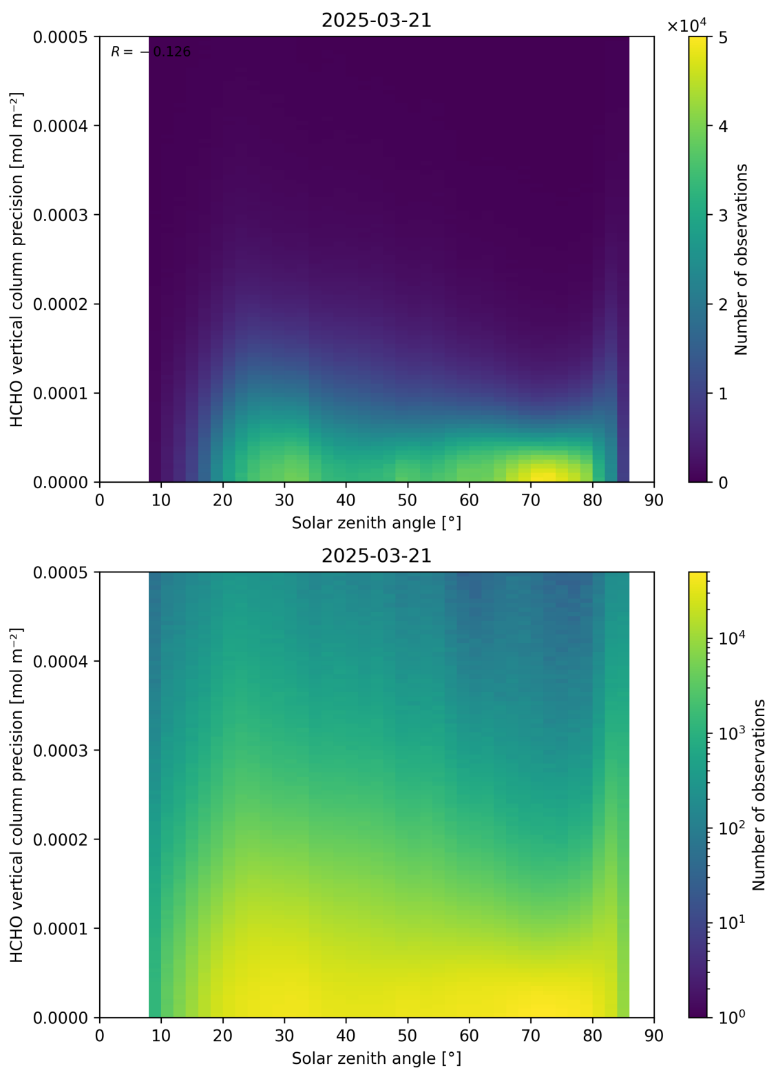
Figure 179: Scatter density plot of “Solar zenith angle” against “HCHO vertical column precision” for 2025-03-20 to 2025-03-22.
