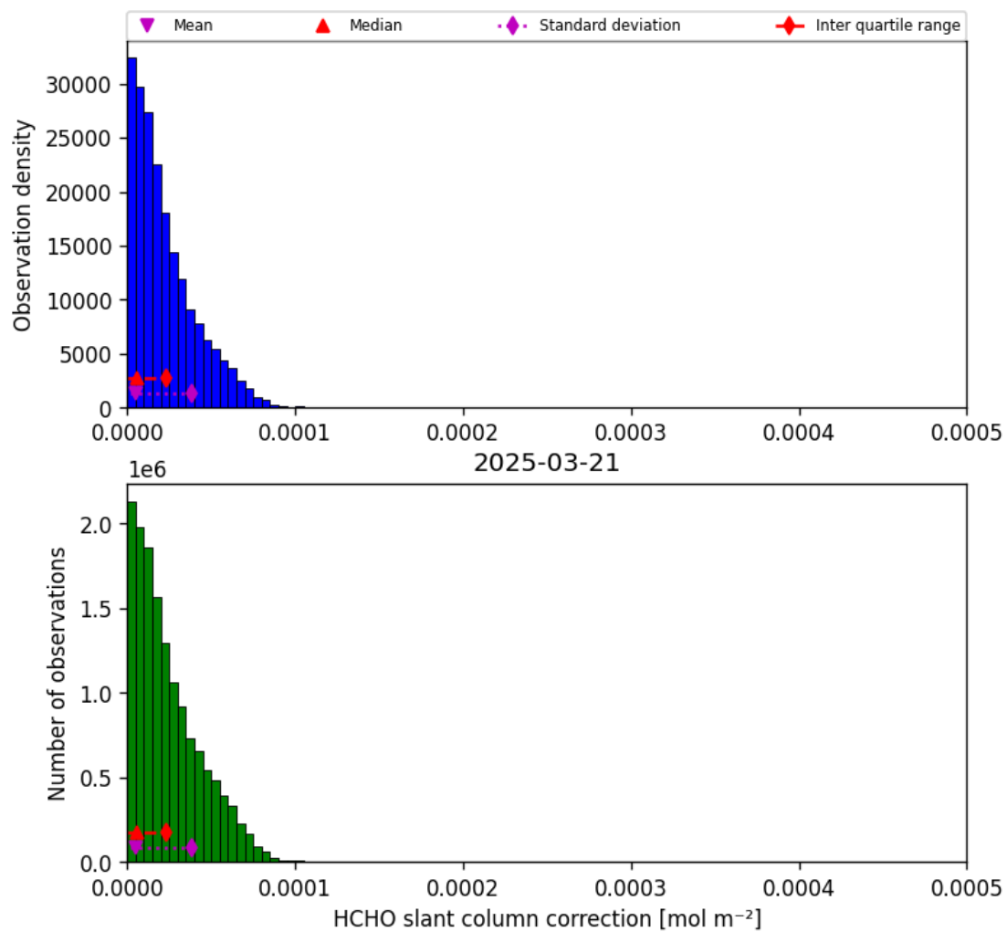
Figure 47: Histogram of “HCHO slant column correction” for 2025-03-20 to 2025-03-22
