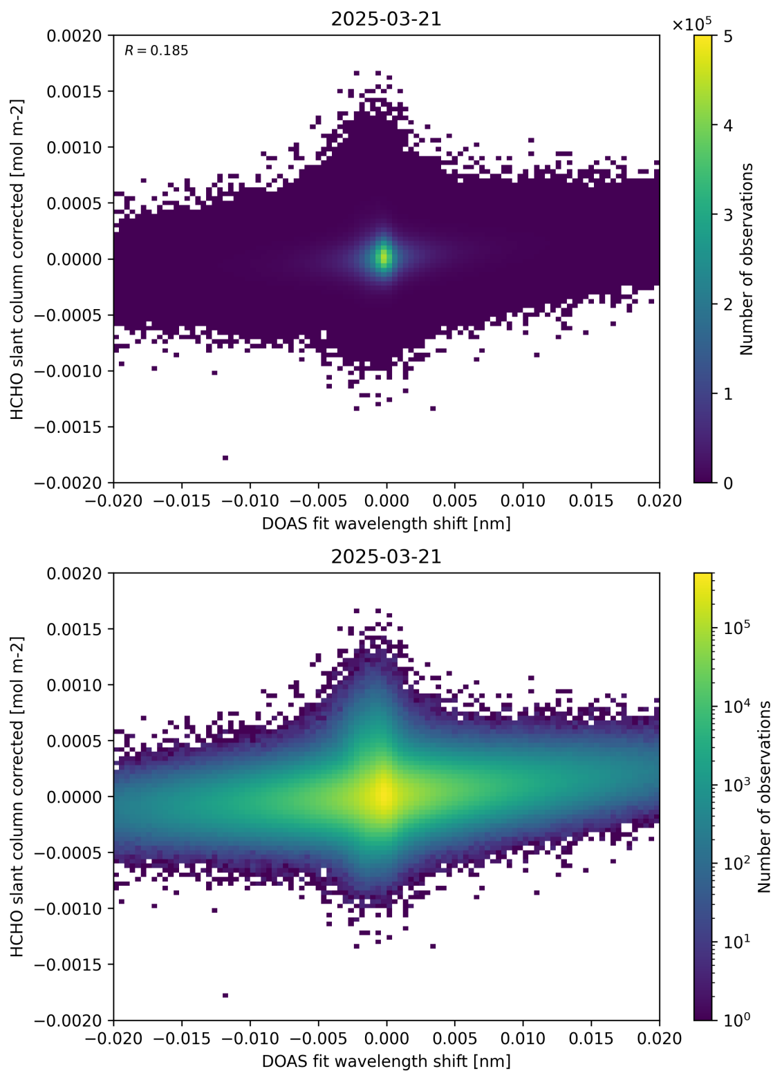
Figure 66: Scatter density plot of “DOAS fit wavelength shift” against “HCHO slant column corrected” for 2025-03-20 to 2025-03-22.
