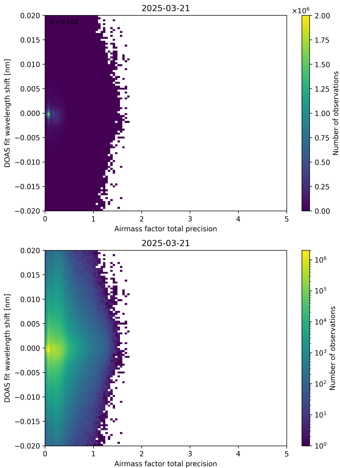
Figure 106: Scatter density plot of “Airmass factor total precision” against “DOAS fit wavelength shift” for 2025-03-20 to 2025-03-22.
