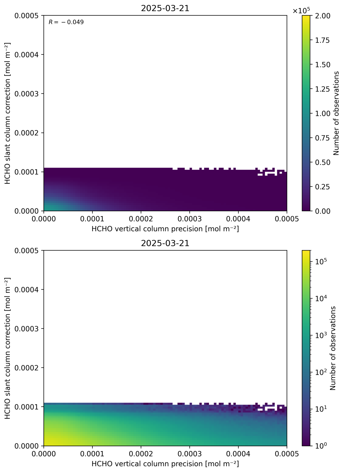
Figure 141: Scatter density plot of “HCHO vertical column precision” against “HCHO slant column correction” for 2025-03-20 to 2025-03-22.
