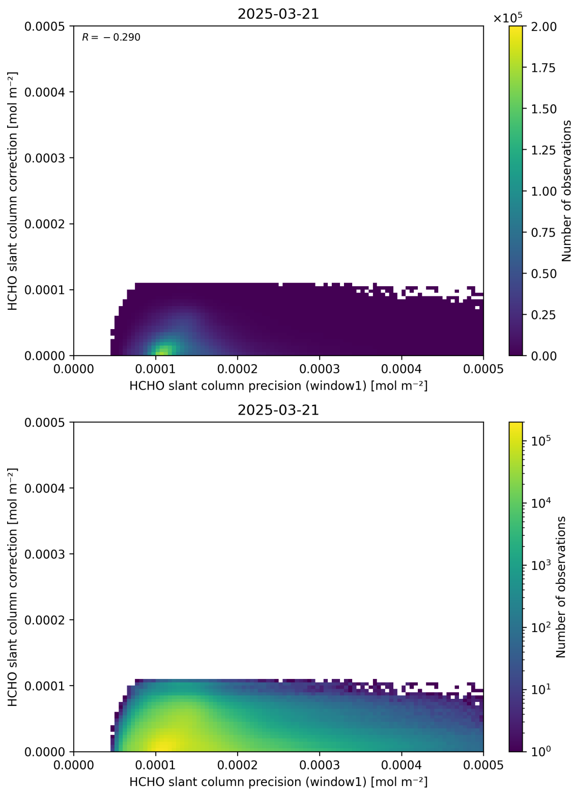
Figure 93: Scatter density plot of “HCHO slant column precision (window1)” against “HCHO slant column correction” for 2025-03-20 to 2025-03-22.
