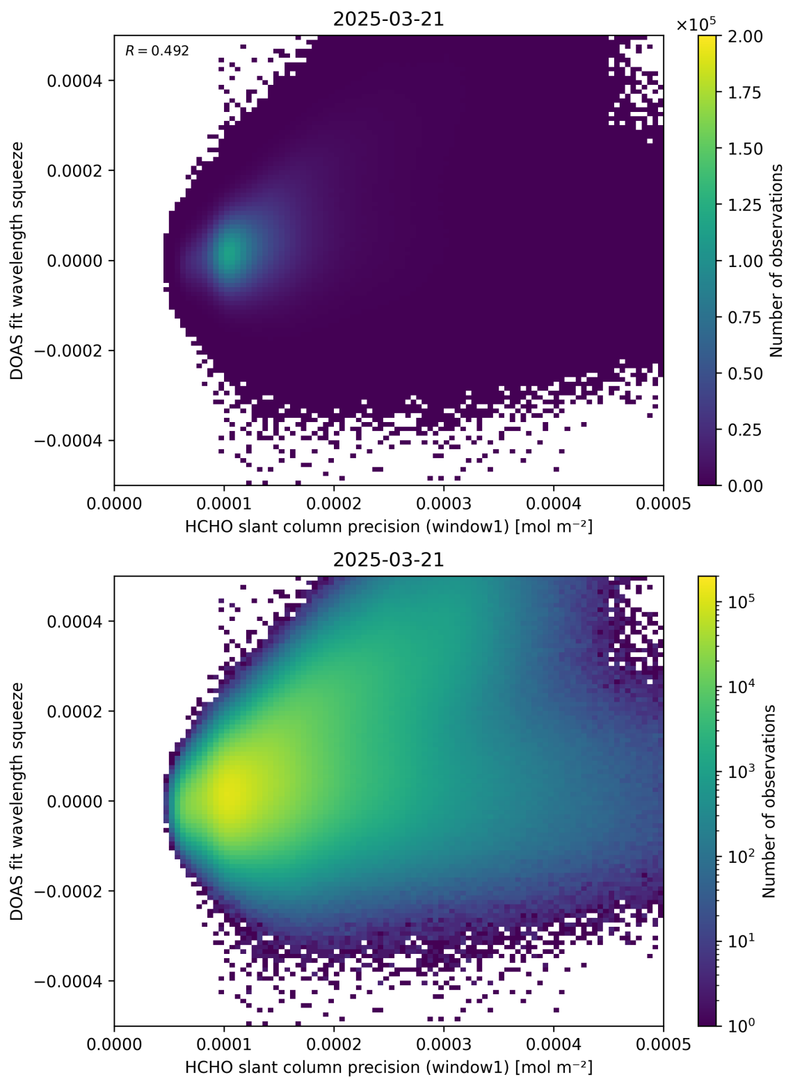
Figure 90: Scatter density plot of “HCHO slant column precision (window1)” against “DOAS fit wavelength squeeze” for 2025-03-20 to 2025-03-22.
