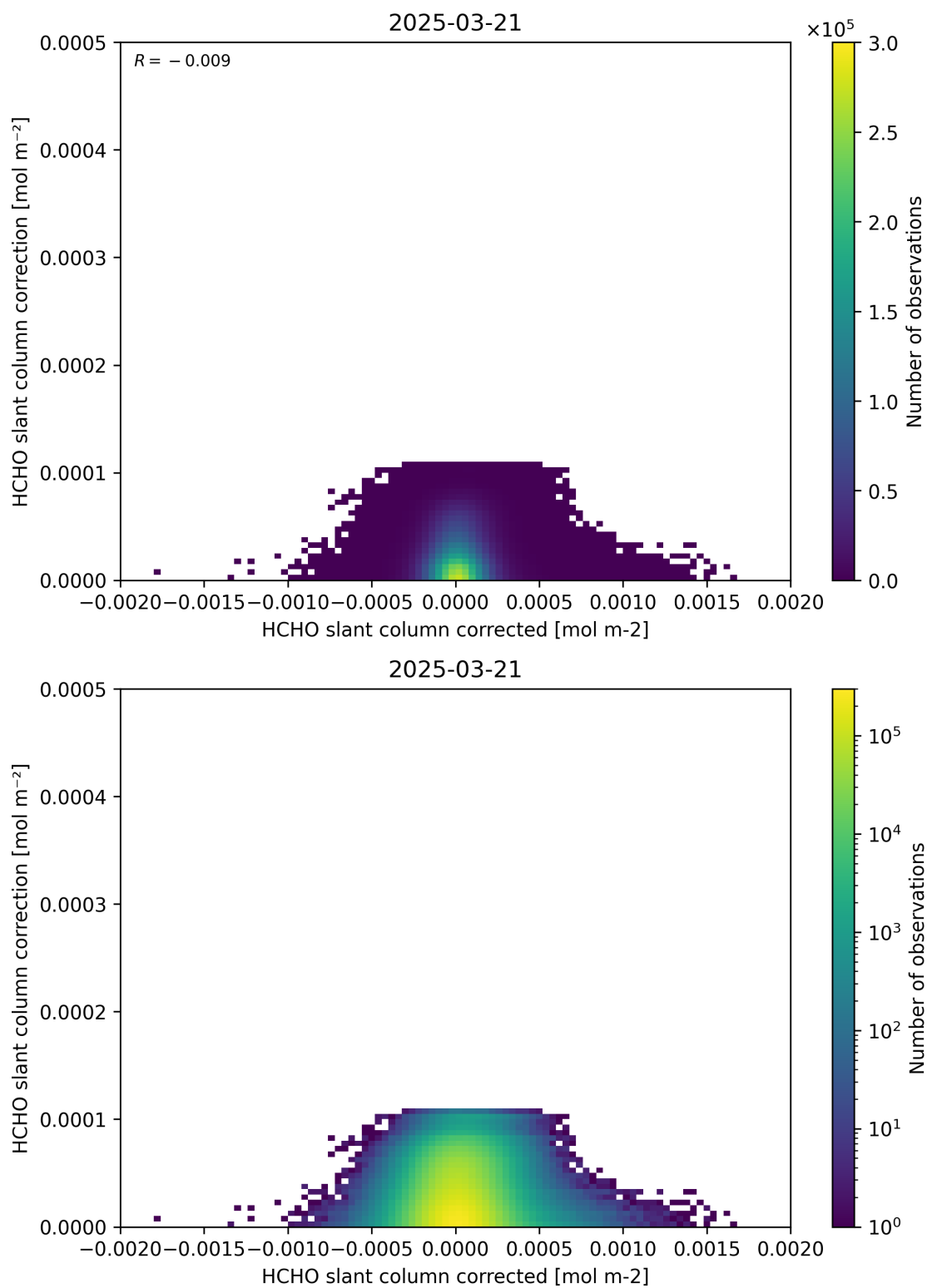
Figure 77: Scatter density plot of “HCHO slant column corrected” against “HCHO slant column correction” for 2025-03-20 to 2025-03-22.
