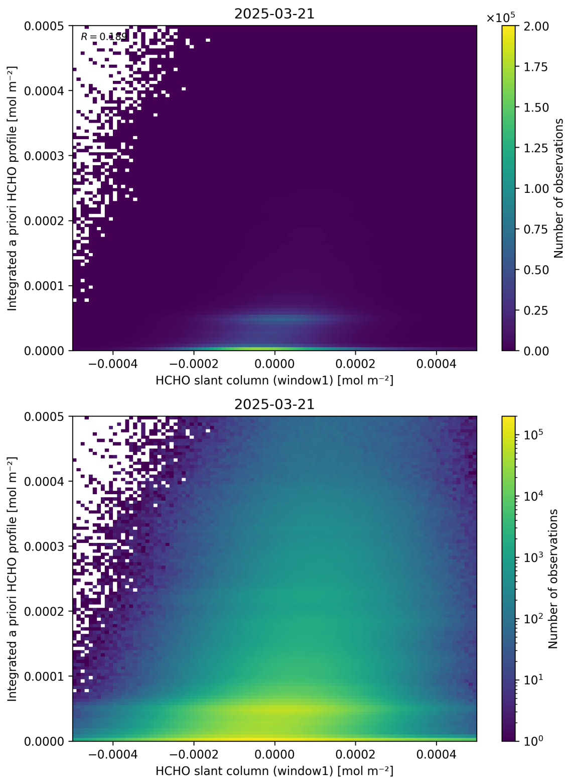
Figure 87: Scatter density plot of “HCHO slant column (window1)” against “Integrated a priori HCHO profile” for 2025-03-20 to 2025-03-22.
