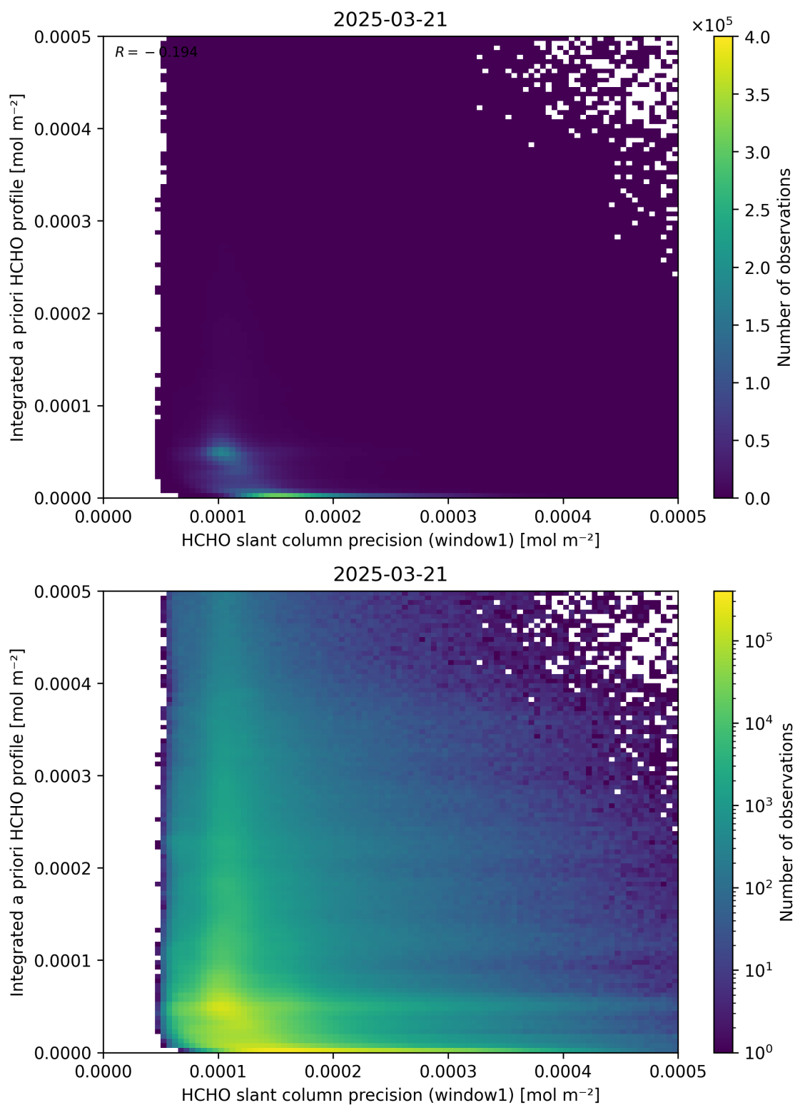
Figure 96: Scatter density plot of “HCHO slant column precision (window1)” against “Integrated a priori HCHO profile” for 2025-03-20 to 2025-03-22.
