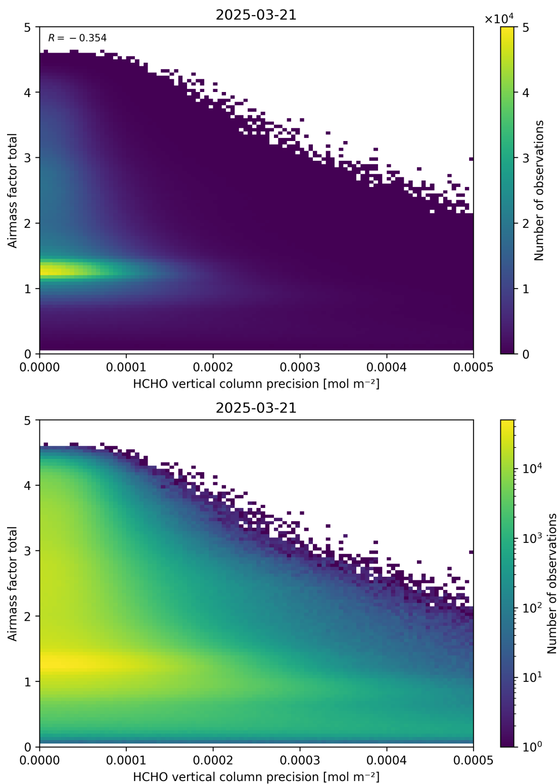
Figure 144: Scatter density plot of “HCHO vertical column precision” against “Airmass factor total” for 2025-03-20 to 2025-03-22.
