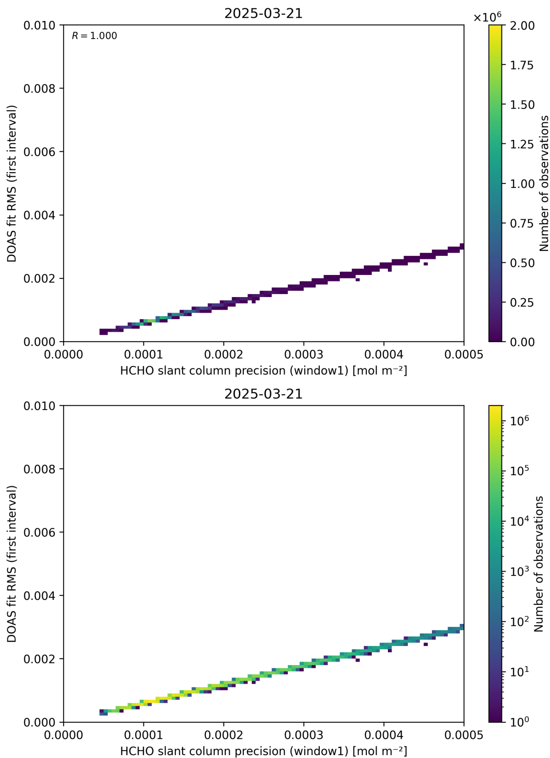
Figure 88: Scatter density plot of “HCHO slant column precision (window1)” against “DOAS fit RMS (first interval)” for 2025-03-20 to 2025-03-22.
