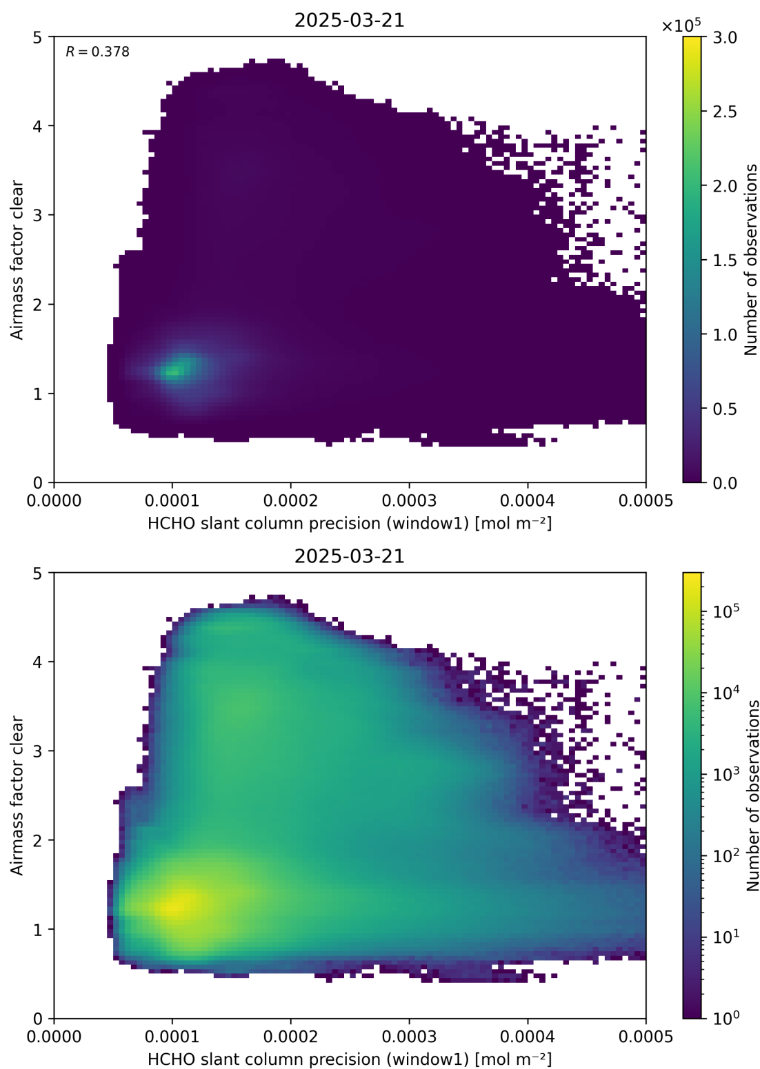
Figure 91: Scatter density plot of “HCHO slant column precision (window1)” against “Airmass factor clear” for 2025-03-20 to 2025-03-22.
