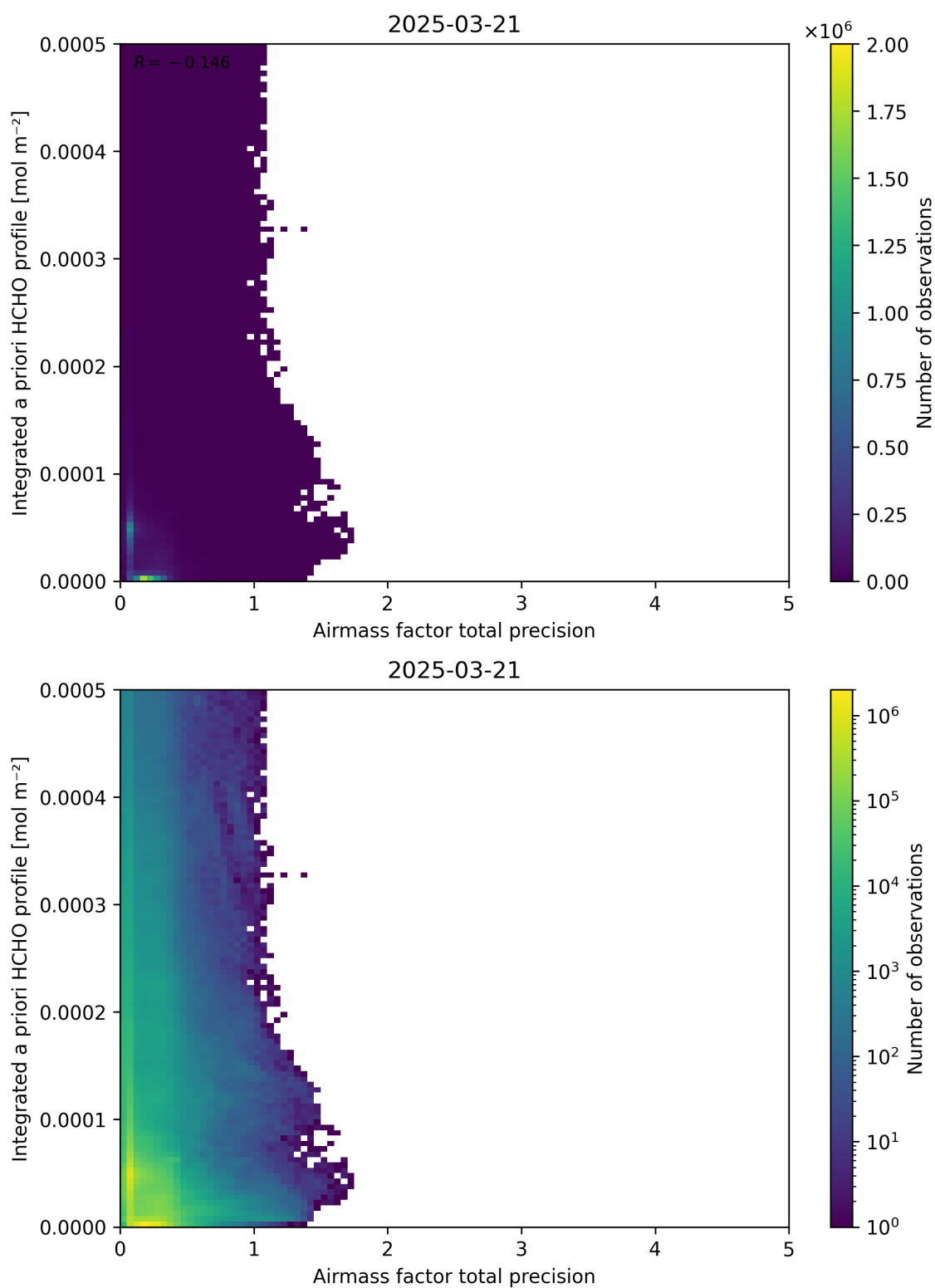
Figure 111: Scatter density plot of “Airmass factor total precision” against “Integrated a priori HCHO profile” for 2025-03-20 to 2025-03-22.
