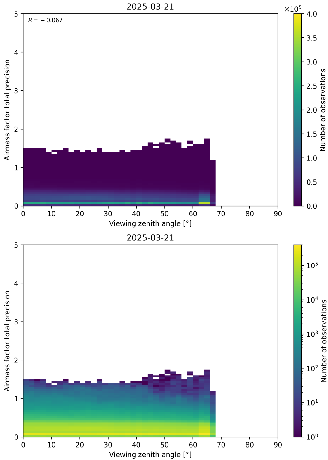
Figure 191: Scatter density plot of “Viewing zenith angle” against “Airmass factor total precision” for 2025-03-20 to 2025-03-22.
