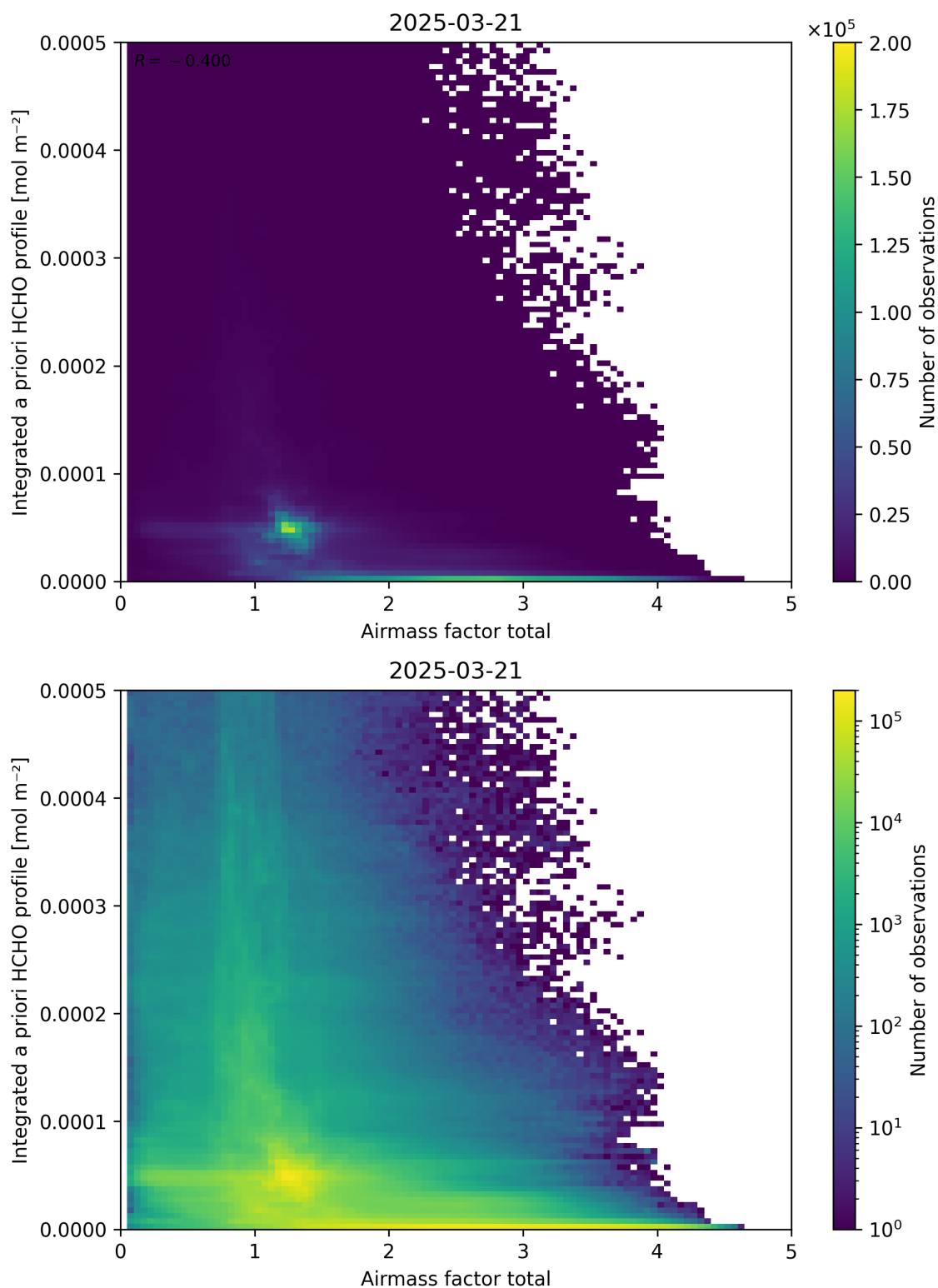
Figure 104: Scatter density plot of “Airmass factor total” against “Integrated a priori HCHO profile” for 2025-03-20 to 2025-03-22.
