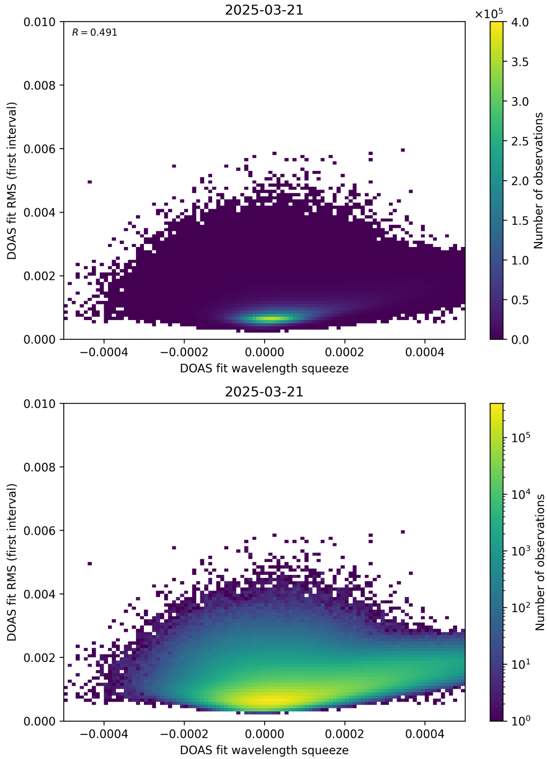
Figure 68: Scatter density plot of “DOAS fit wavelength squeeze” against “DOAS fit RMS (first interval)” for 2025-03-20 to 2025-03-22.
