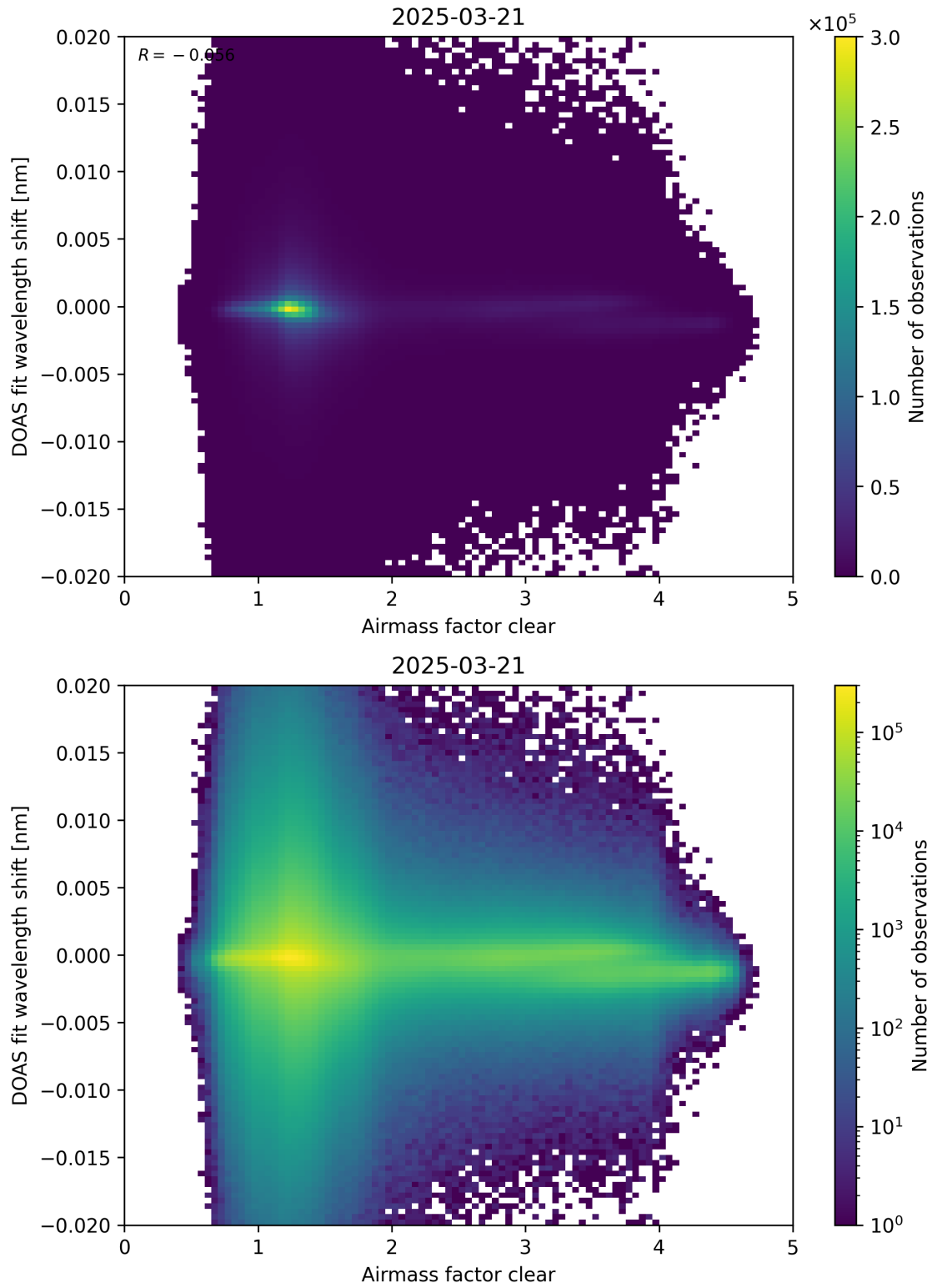
Figure 72: Scatter density plot of “Airmass factor clear” against “DOAS fit wavelength shift” for 2025-03-20 to 2025-03-22.
