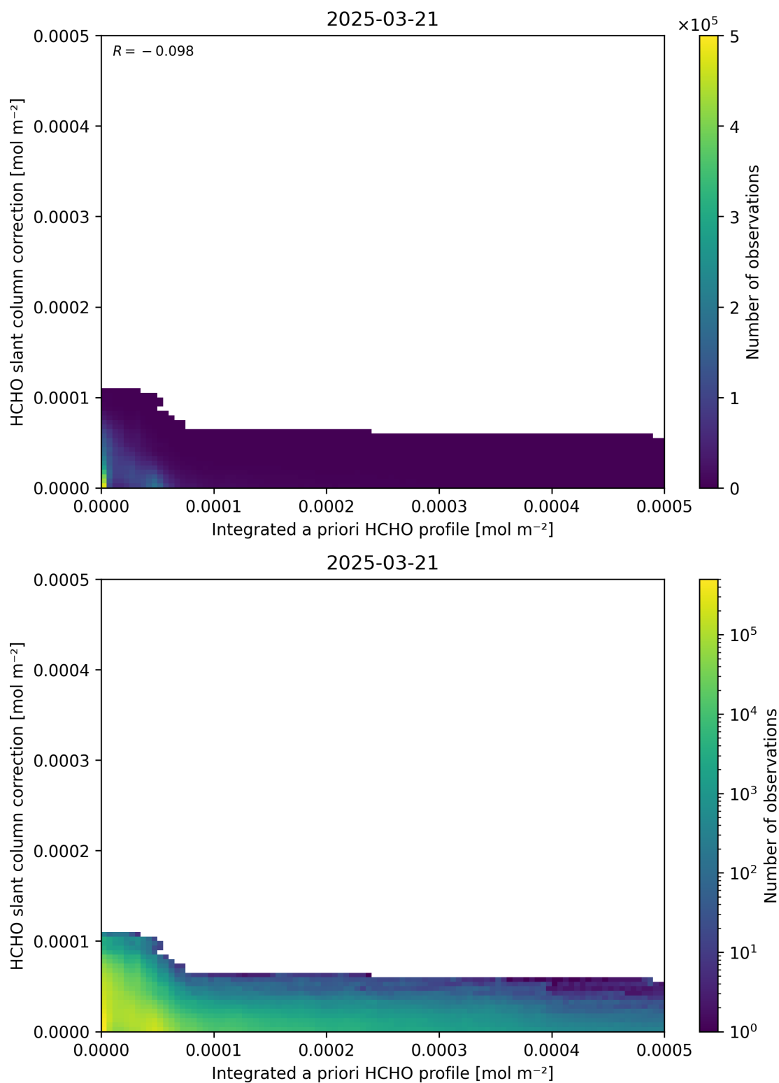
Figure 152: Scatter density plot of “Integrated a priori HCHO profile” against “HCHO slant column correction” for 2025-03-20 to 2025-03-22.
