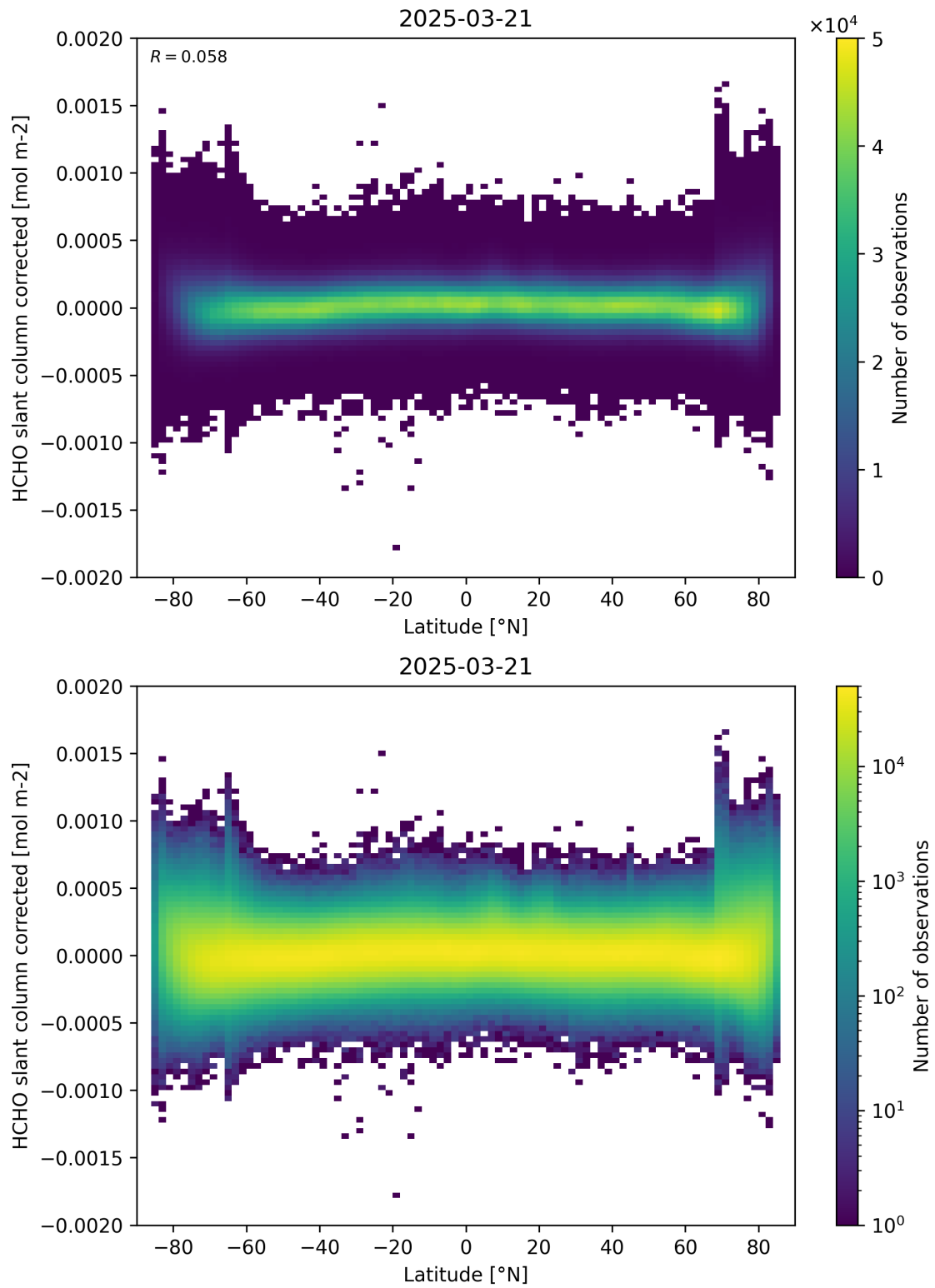
Figure 157: Scatter density plot of “Latitude” against “HCHO slant column corrected” for 2025-03-20 to 2025-03-22.
