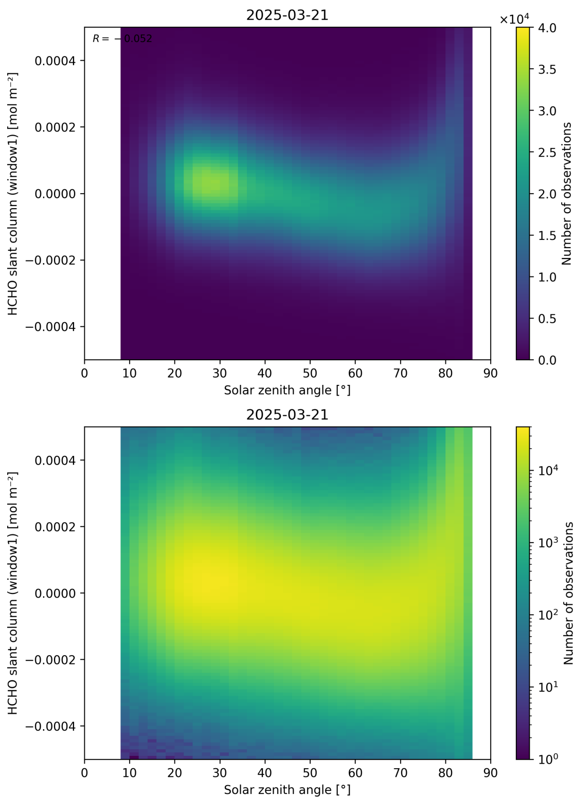
Figure 173: Scatter density plot of “Solar zenith angle” against “HCHO slant column (window1)” for 2025-03-20 to 2025-03-22.
