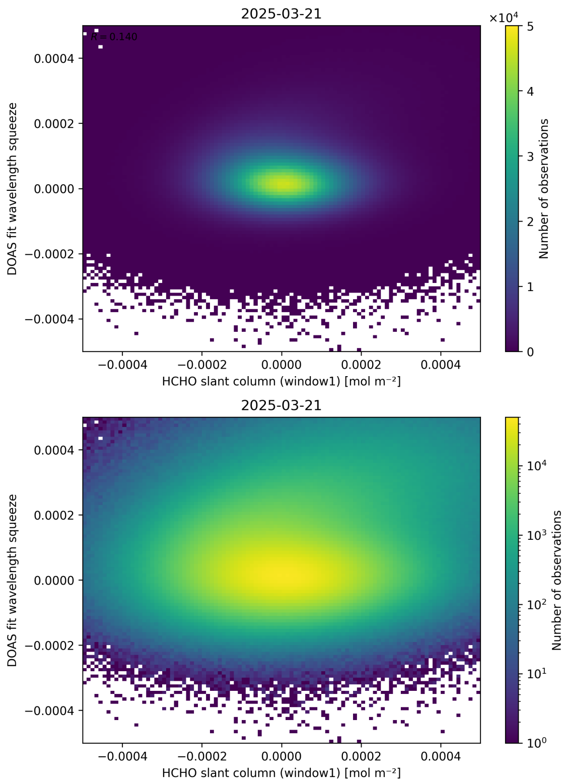
Figure 80: Scatter density plot of “HCHO slant column (window1)” against “DOAS fit wavelength squeeze” for 2025-03-20 to 2025-03-22.
