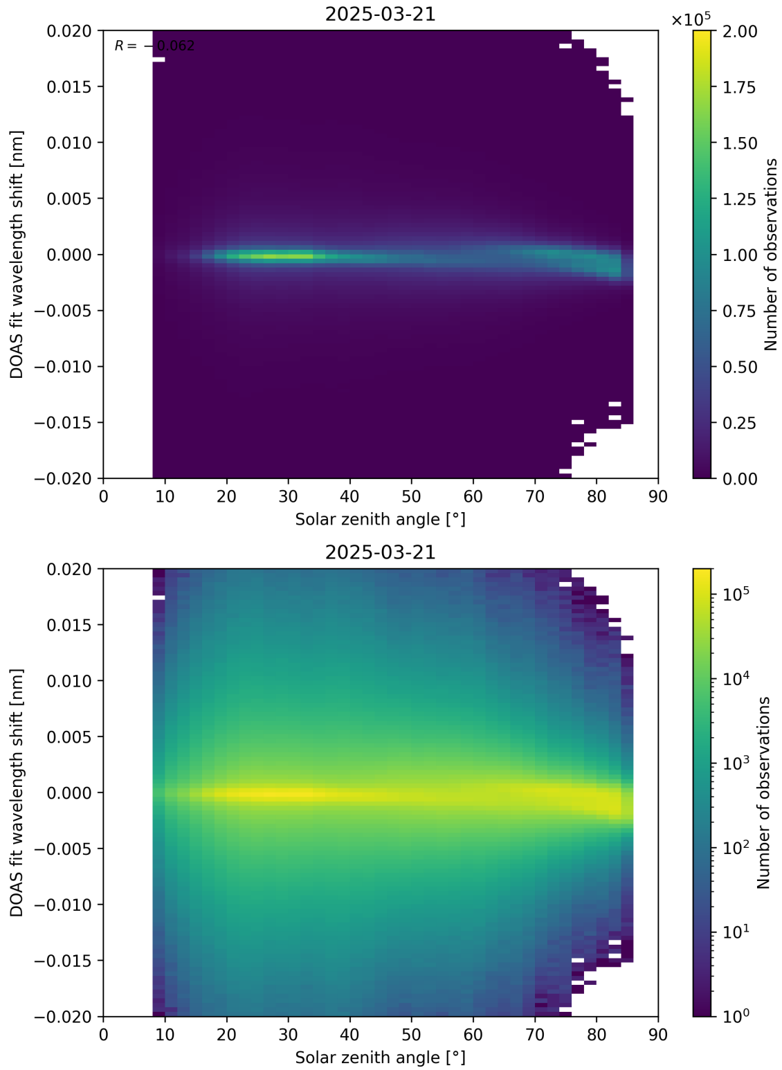
Figure 168: Scatter density plot of “Solar zenith angle” against “DOAS fit wavelength shift” for 2025-03-20 to 2025-03-22.
