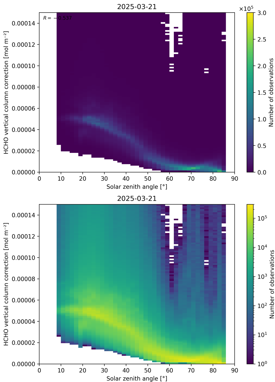
Figure 178: Scatter density plot of “Solar zenith angle” against “HCHO vertical column correction” for 2025-03-20 to 2025-03-22.
