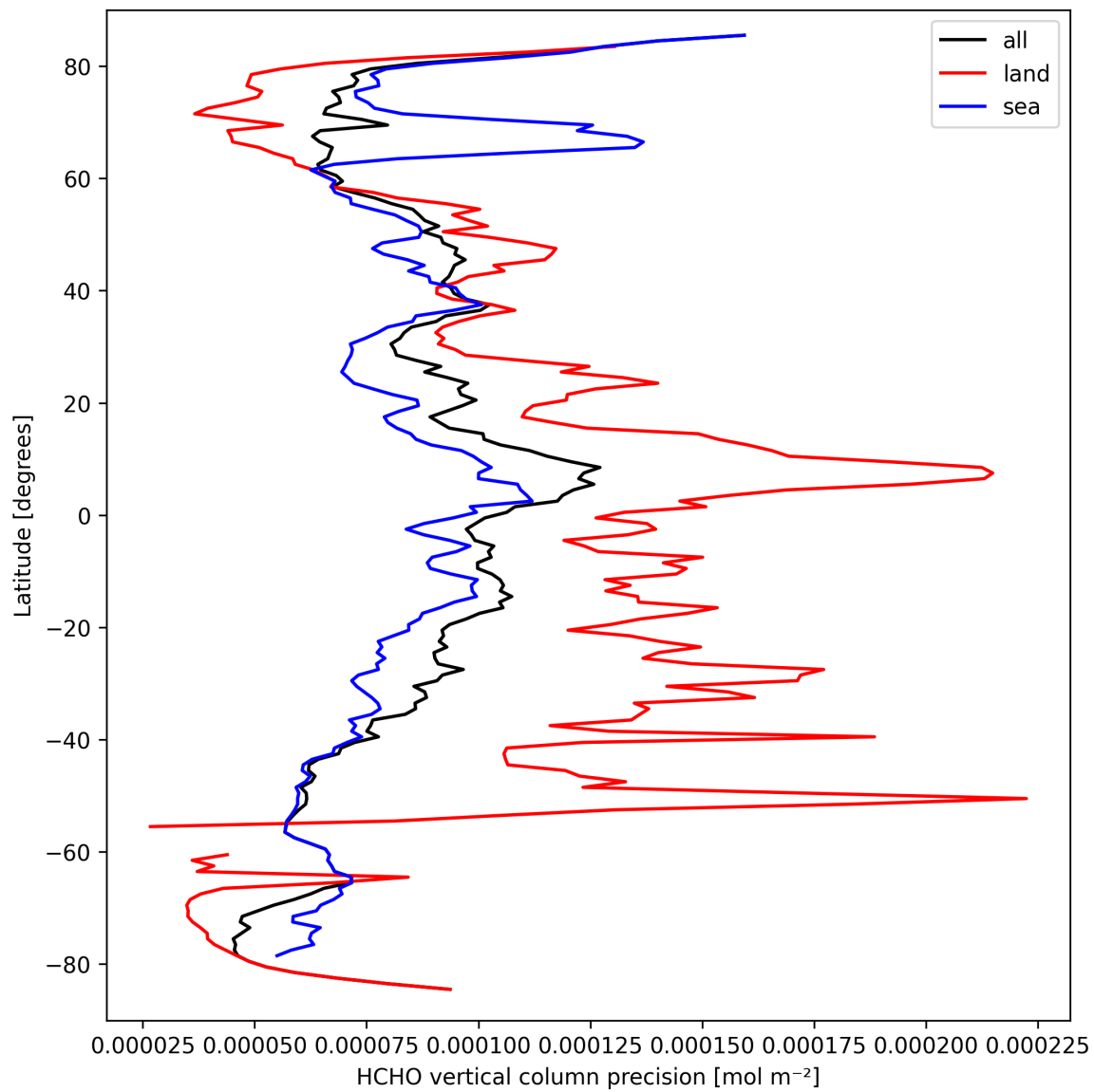
Figure 22: Zonal average of “HCHO vertical column precision” for 2025-03-20 to 2025-03-22.
