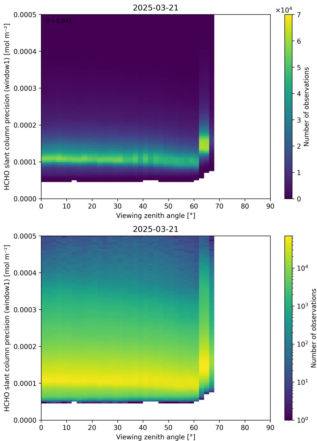
Figure 189: Scatter density plot of “Viewing zenith angle” against “HCHO slant column precision (window1)” for 2025-03-20 to 2025-03-22.
