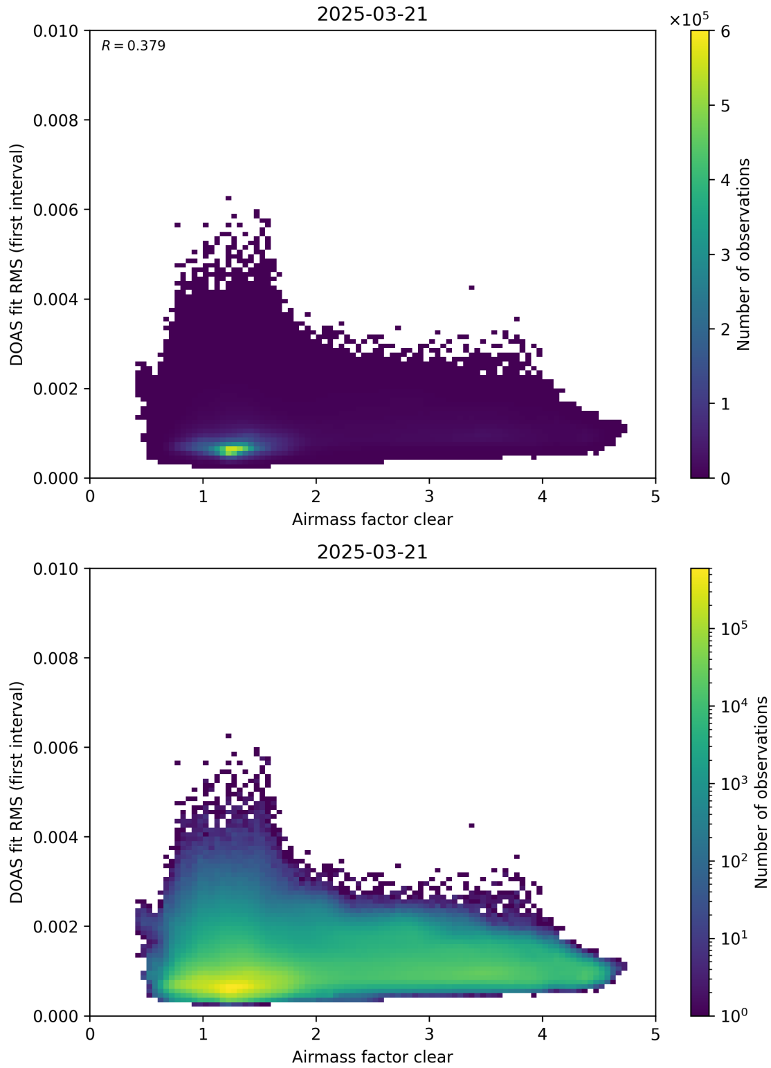
Figure 71: Scatter density plot of “Airmass factor clear” against “DOAS fit RMS (first interval)” for 2025-03-20 to 2025-03-22.
