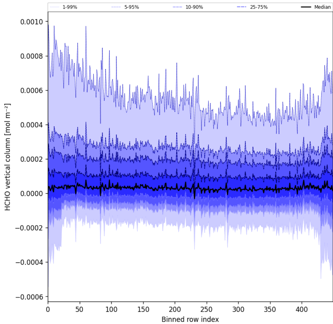
Figure 49: Along track statistics of “HCHO vertical column” for 2025-03-20 to 2025-03-22
