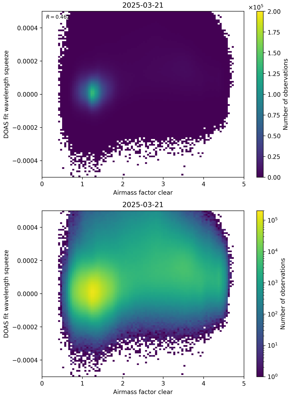
Figure 73: Scatter density plot of “Airmass factor clear” against “DOAS fit wavelength squeeze” for 2025-03-20 to 2025-03-22.
