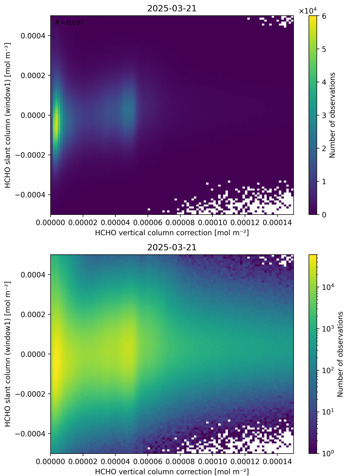
Figure 118: Scatter density plot of “HCHO vertical column correction” against “HCHO slant column (window1)” for 2025-03-20 to 2025-03-22.
