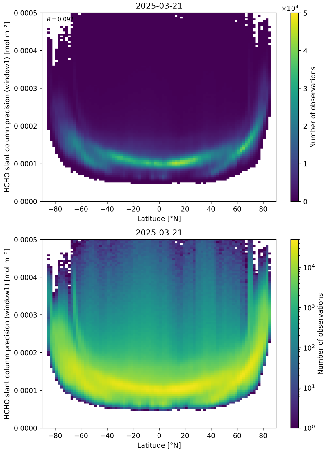
Figure 160: Scatter density plot of “Latitude” against “HCHO slant column precision (window1)” for 2025-03-20 to 2025-03-22.
