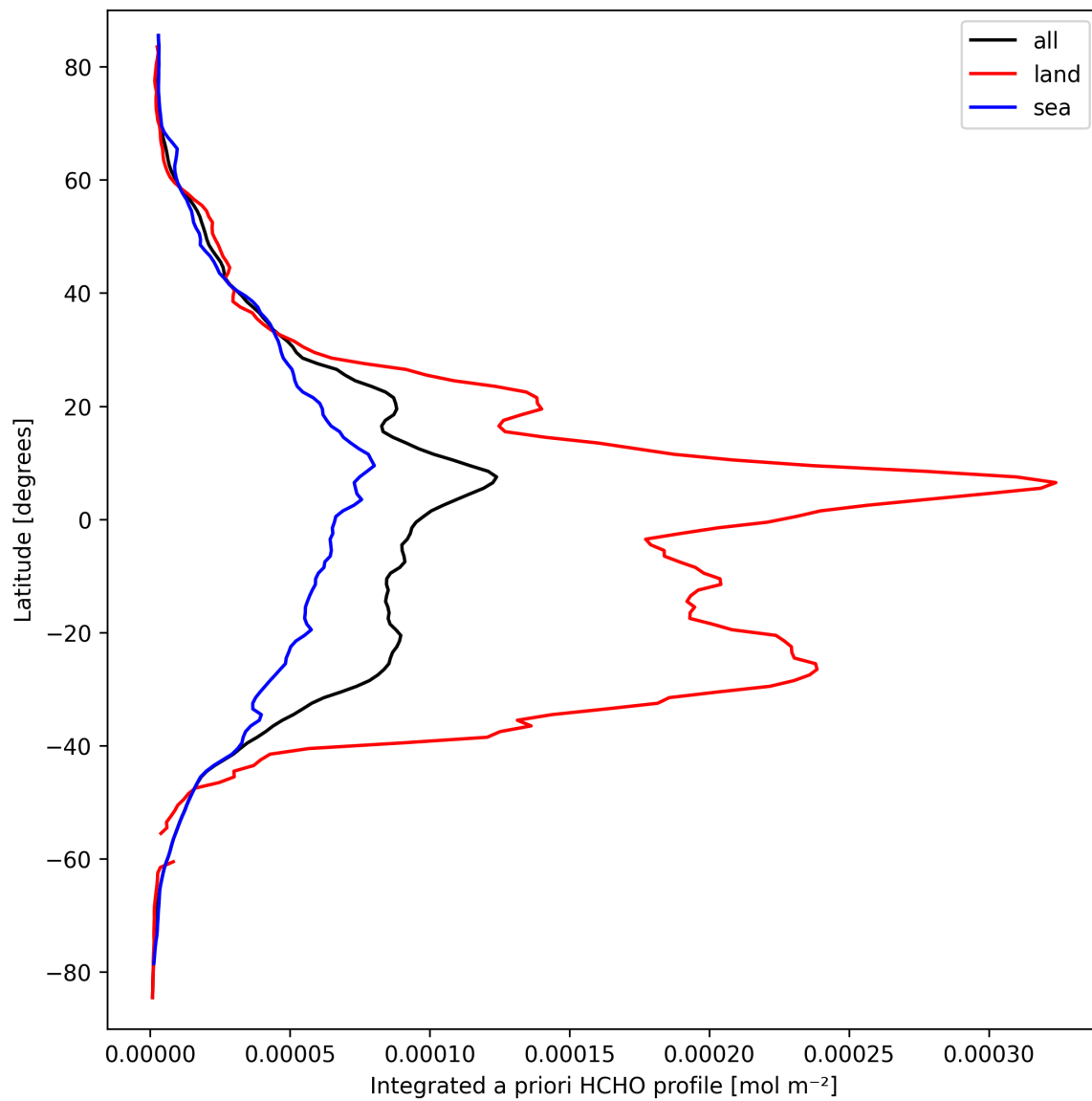
Figure 29: Zonal average of “Integrated a priori HCHO profile” for 2025-03-20 to 2025-03-22.
