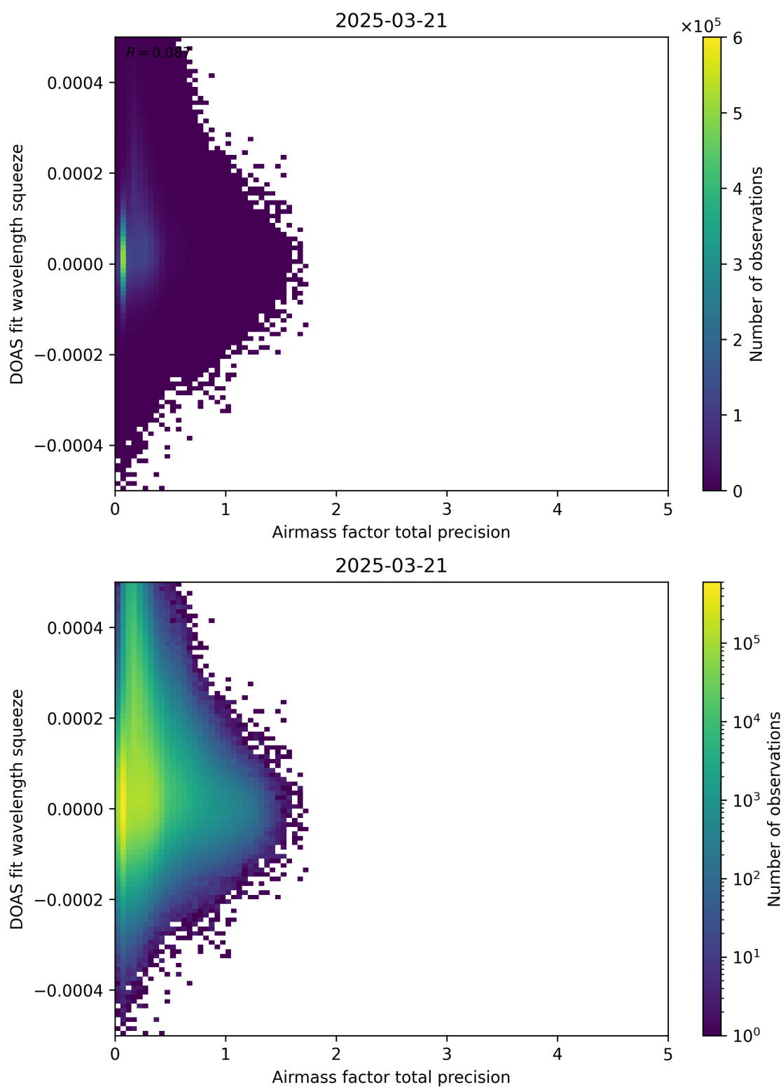
Figure 107: Scatter density plot of “Airmass factor total precision” against “DOAS fit wavelength squeeze” for 2025-03-20 to 2025-03-22.
