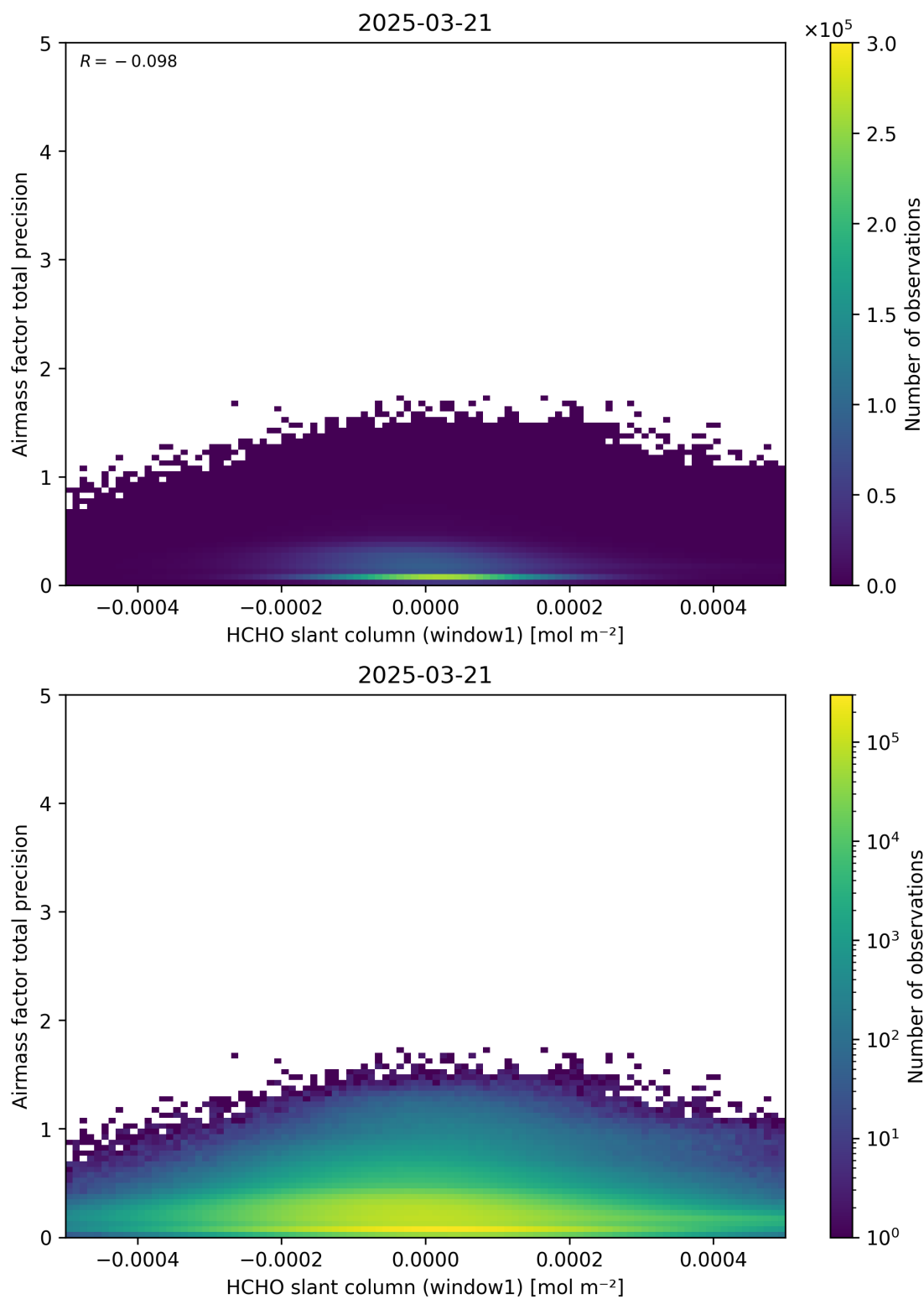
Figure 86: Scatter density plot of “HCHO slant column (window1)” against “Airmass factor total precision” for 2025-03-20 to 2025-03-22.
