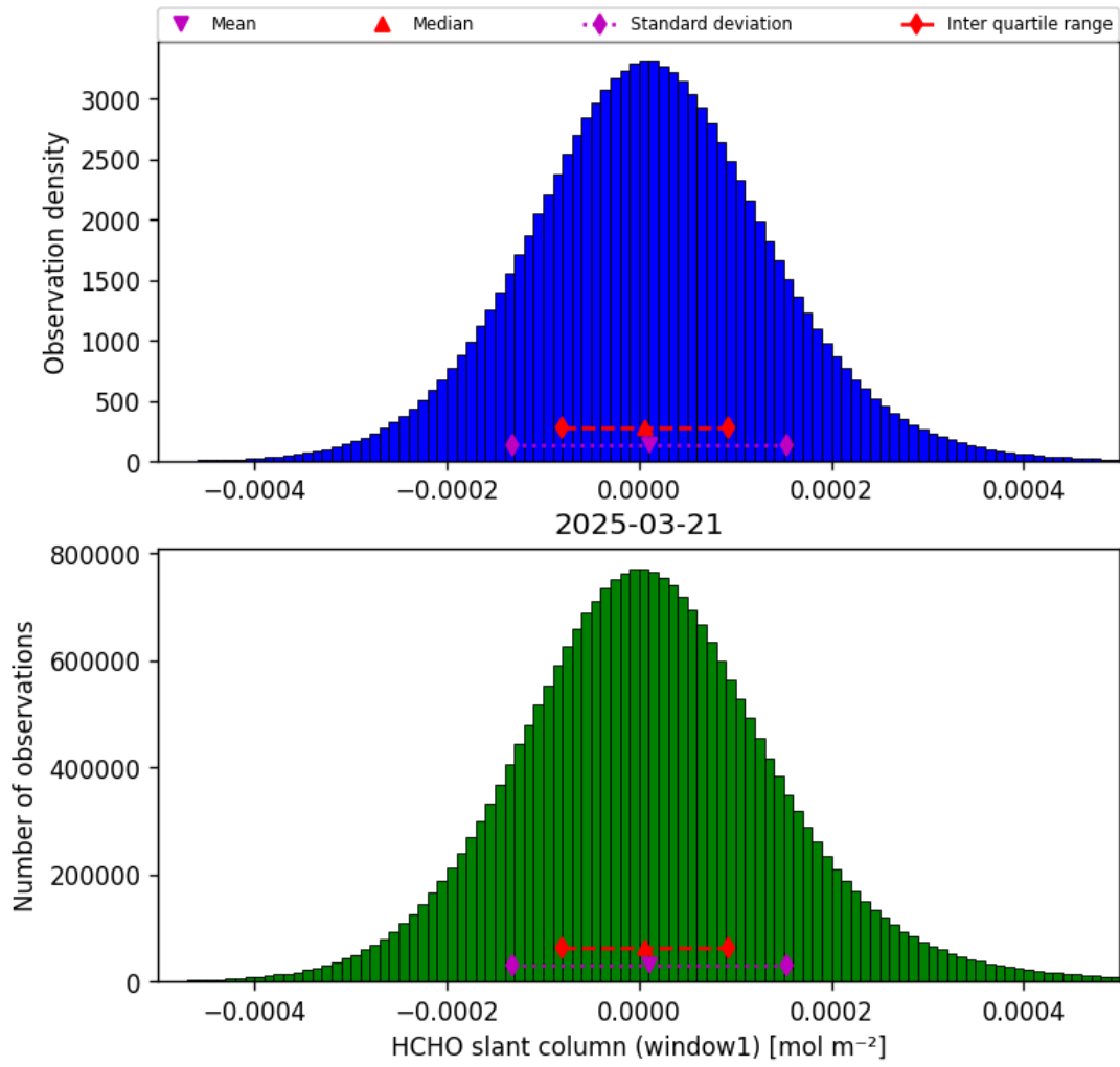
Figure 38: Histogram of “HCHO slant column (window1)” for 2025-03-20 to 2025-03-22
