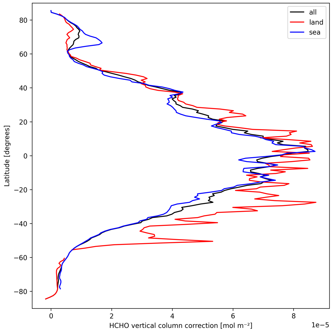
Figure 23: Zonal average of “HCHO vertical column correction” for 2025-03-20 to 2025-03-22.
