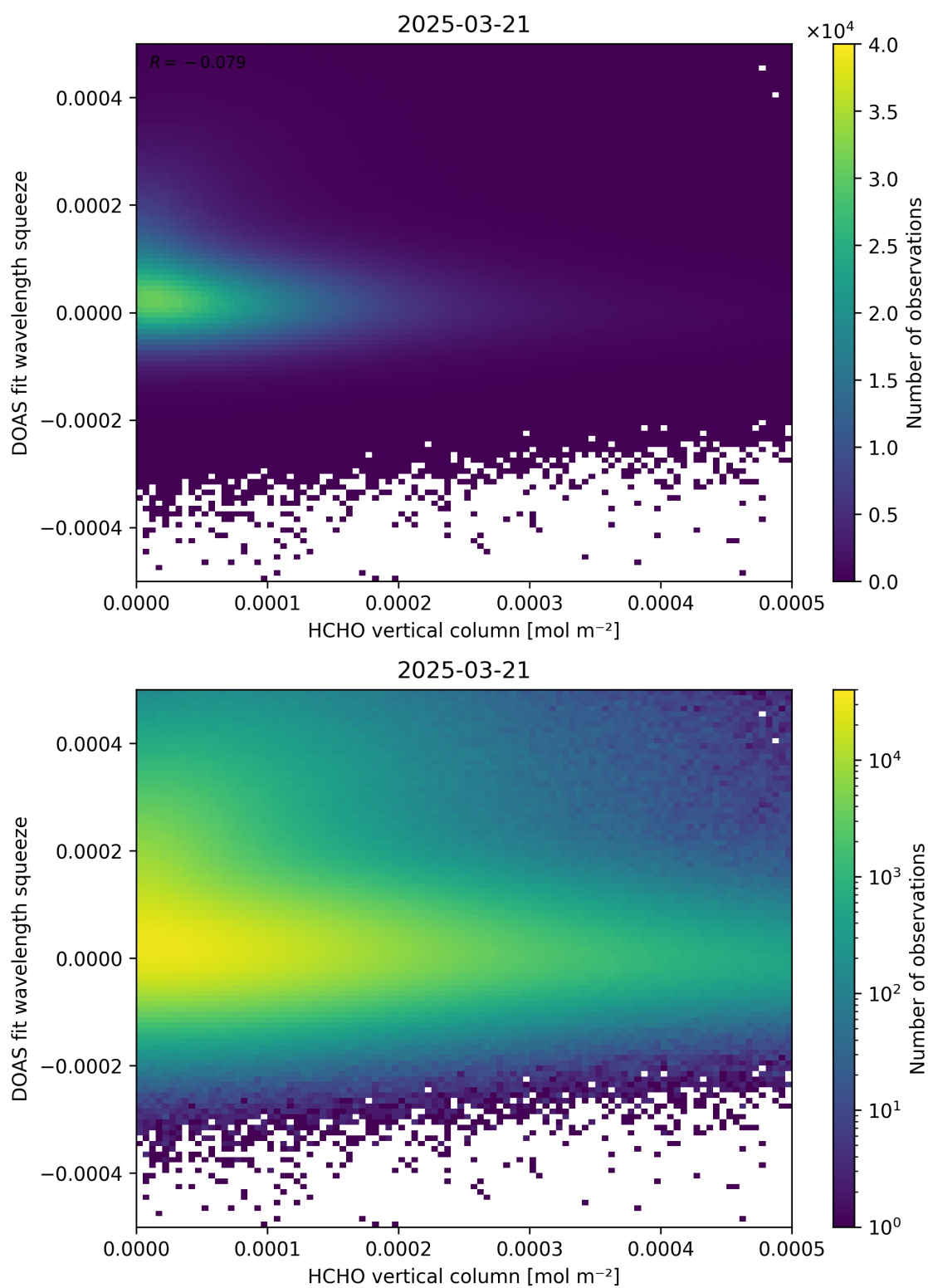
Figure 125: Scatter density plot of “HCHO vertical column” against “DOAS fit wavelength squeeze” for 2025-03-20 to 2025-03-22.
