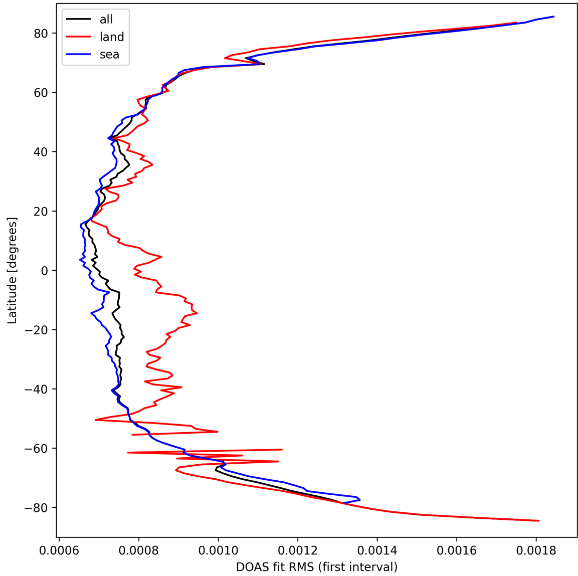
Figure 32: Zonal average of “DOAS fit RMS (first interval)” for 2025-03-20 to 2025-03-22.
