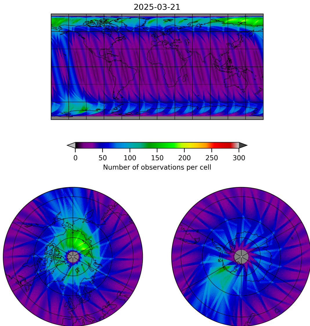
Figure 19: Map of the number of observations for 2025-03-20 to 2025-03-22
