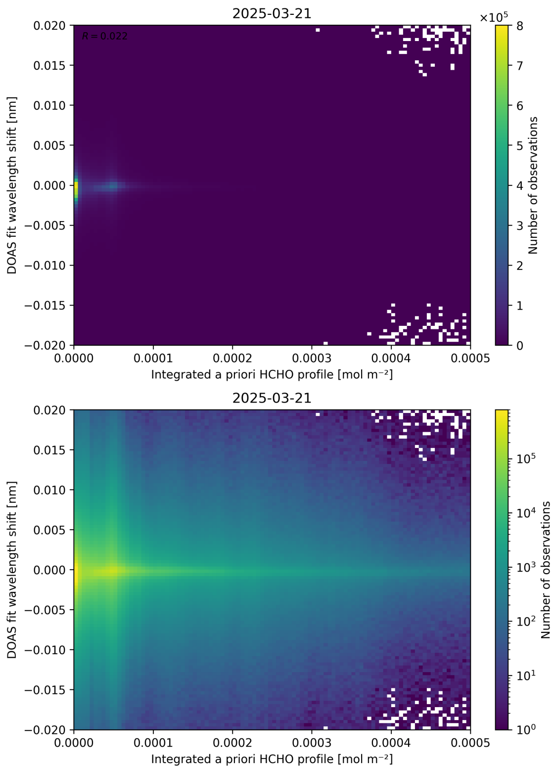
Figure 149: Scatter density plot of “Integrated a priori HCHO profile” against “DOAS fit wavelength shift” for 2025-03-20 to 2025-03-22.
