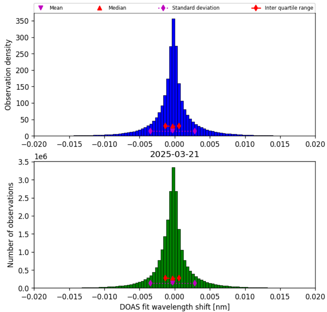
Figure 44: Histogram of “DOAS fit wavelength shift” for 2025-03-20 to 2025-03-22
