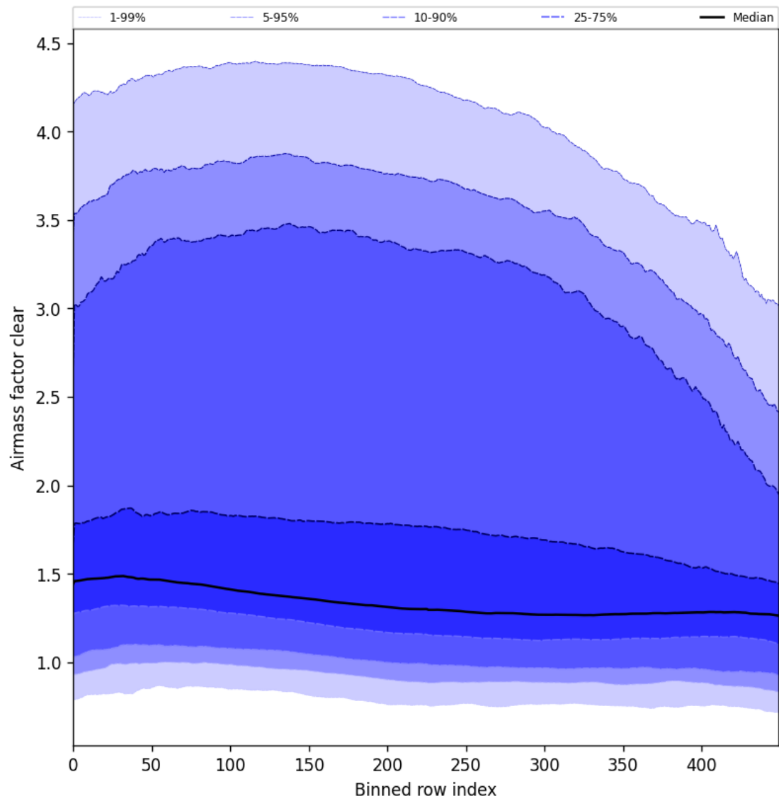
Figure 56: Along track statistics of “Airmass factor clear” for 2025-03-20 to 2025-03-22
