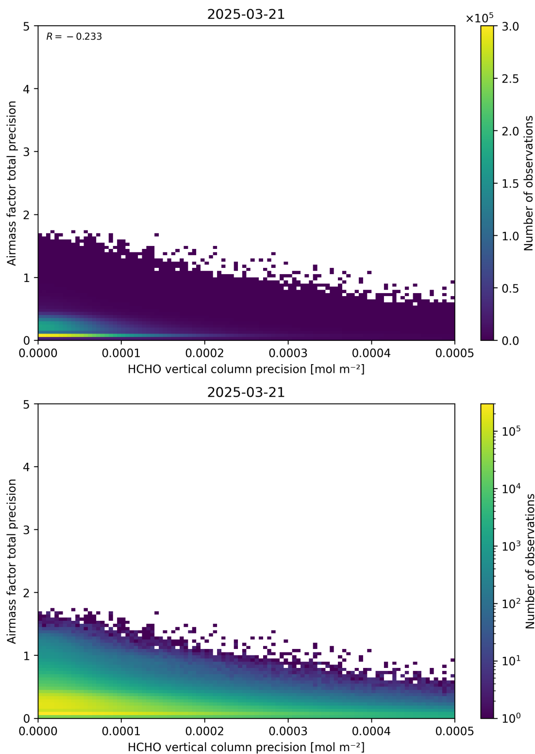
Figure 145: Scatter density plot of “HCHO vertical column precision” against “Airmass factor total precision” for 2025-03-20 to 2025-03-22.
