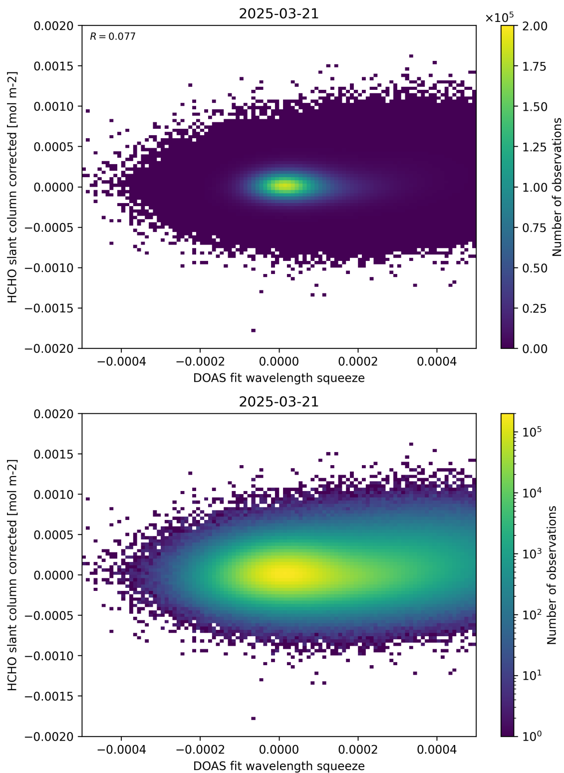
Figure 69: Scatter density plot of “DOAS fit wavelength squeeze” against “HCHO slant column corrected” for 2025-03-20 to 2025-03-22.
