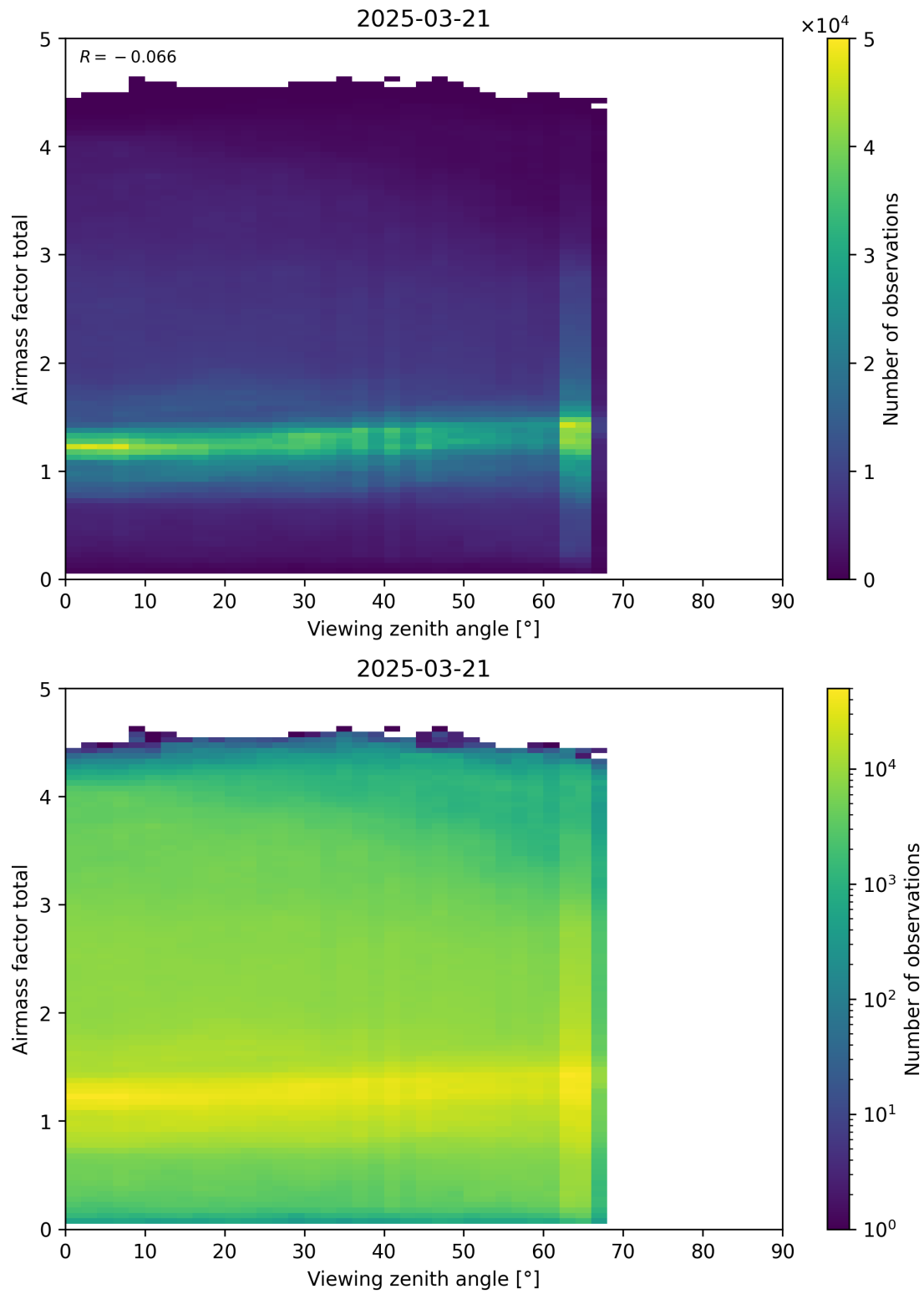
Figure 190: Scatter density plot of “Viewing zenith angle” against “Airmass factor total” for 2025-03-20 to 2025-03-22.
