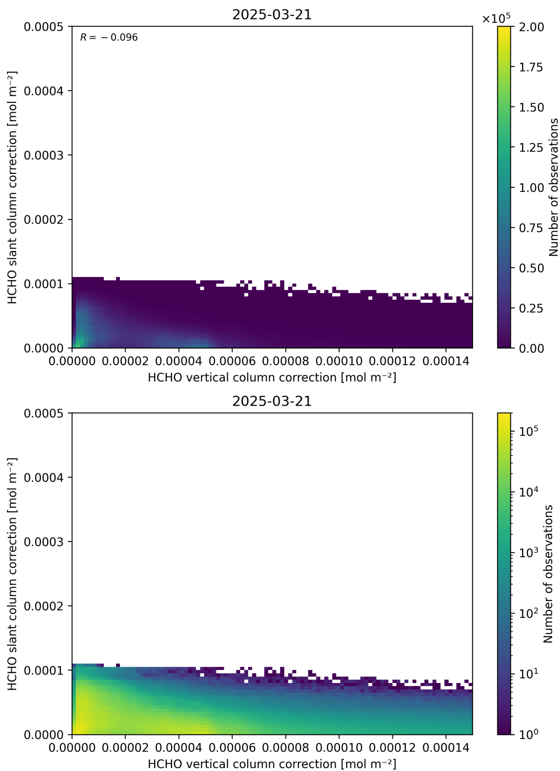
Figure 117: Scatter density plot of “HCHO vertical column correction” against “HCHO slant column correction” for 2025-03-20 to 2025-03-22.
