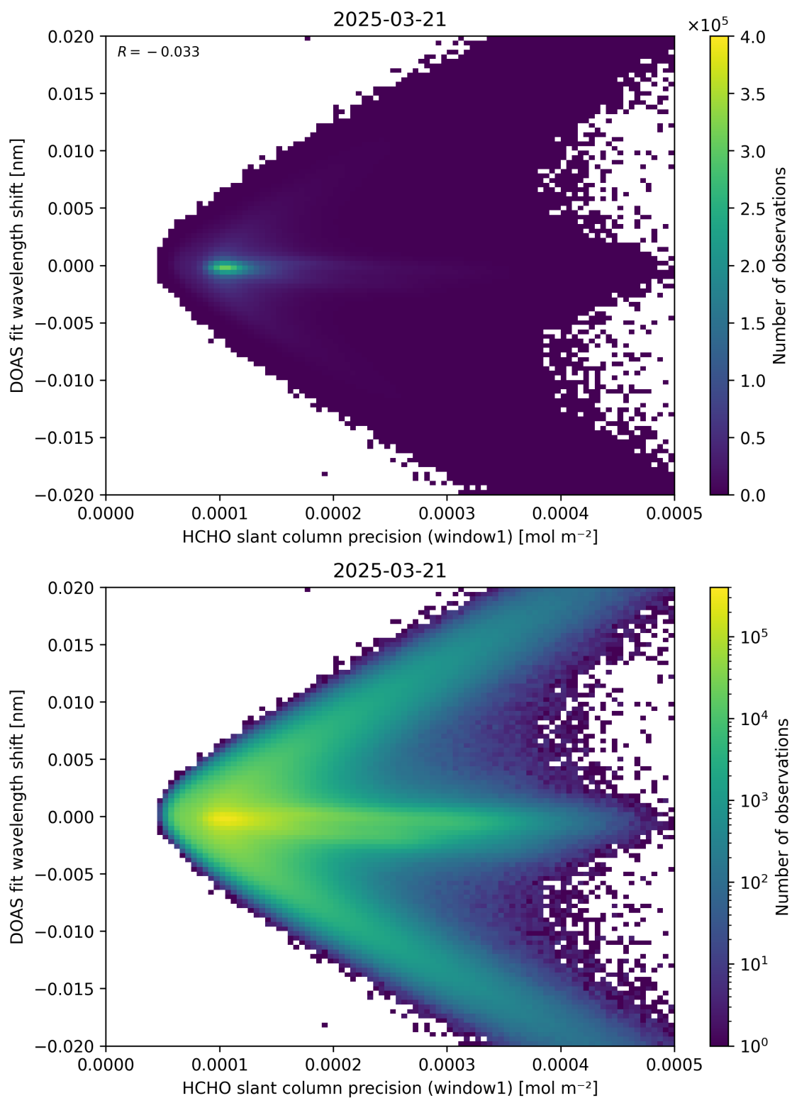
Figure 89: Scatter density plot of “HCHO slant column precision (window1)” against “DOAS fit wavelength shift” for 2025-03-20 to 2025-03-22.
