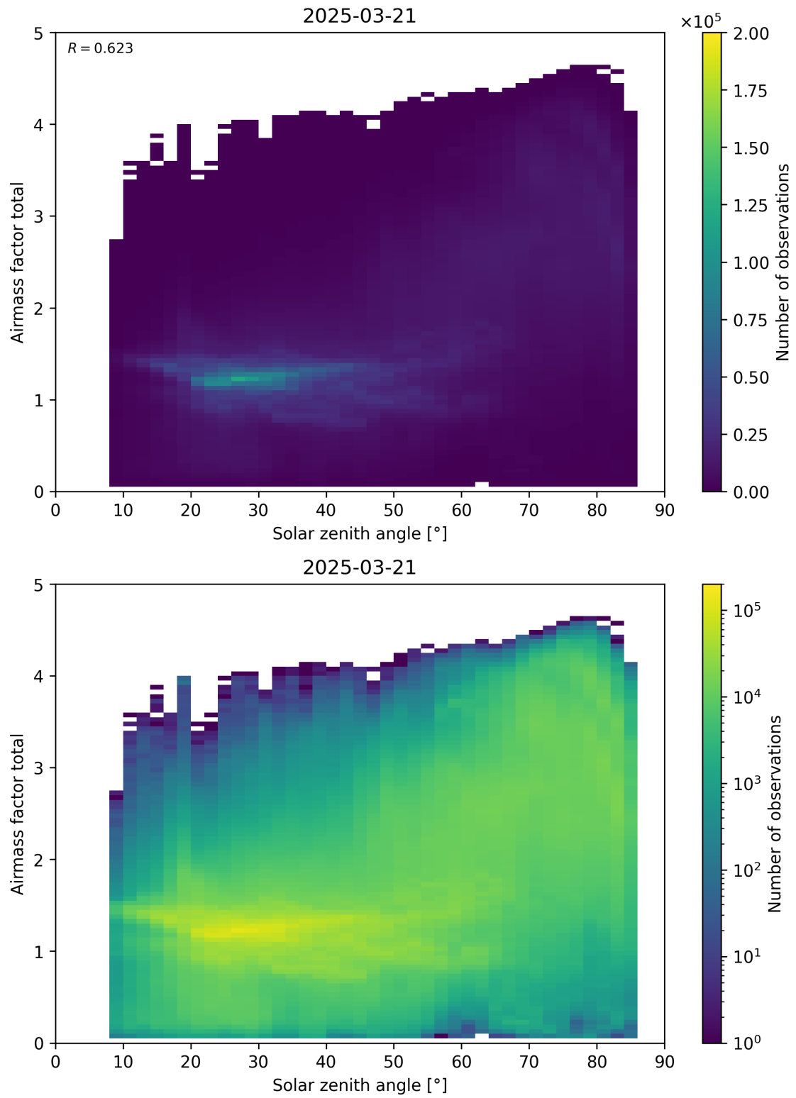
Figure 175: Scatter density plot of “Solar zenith angle” against “Airmass factor total” for 2025-03-20 to 2025-03-22.
