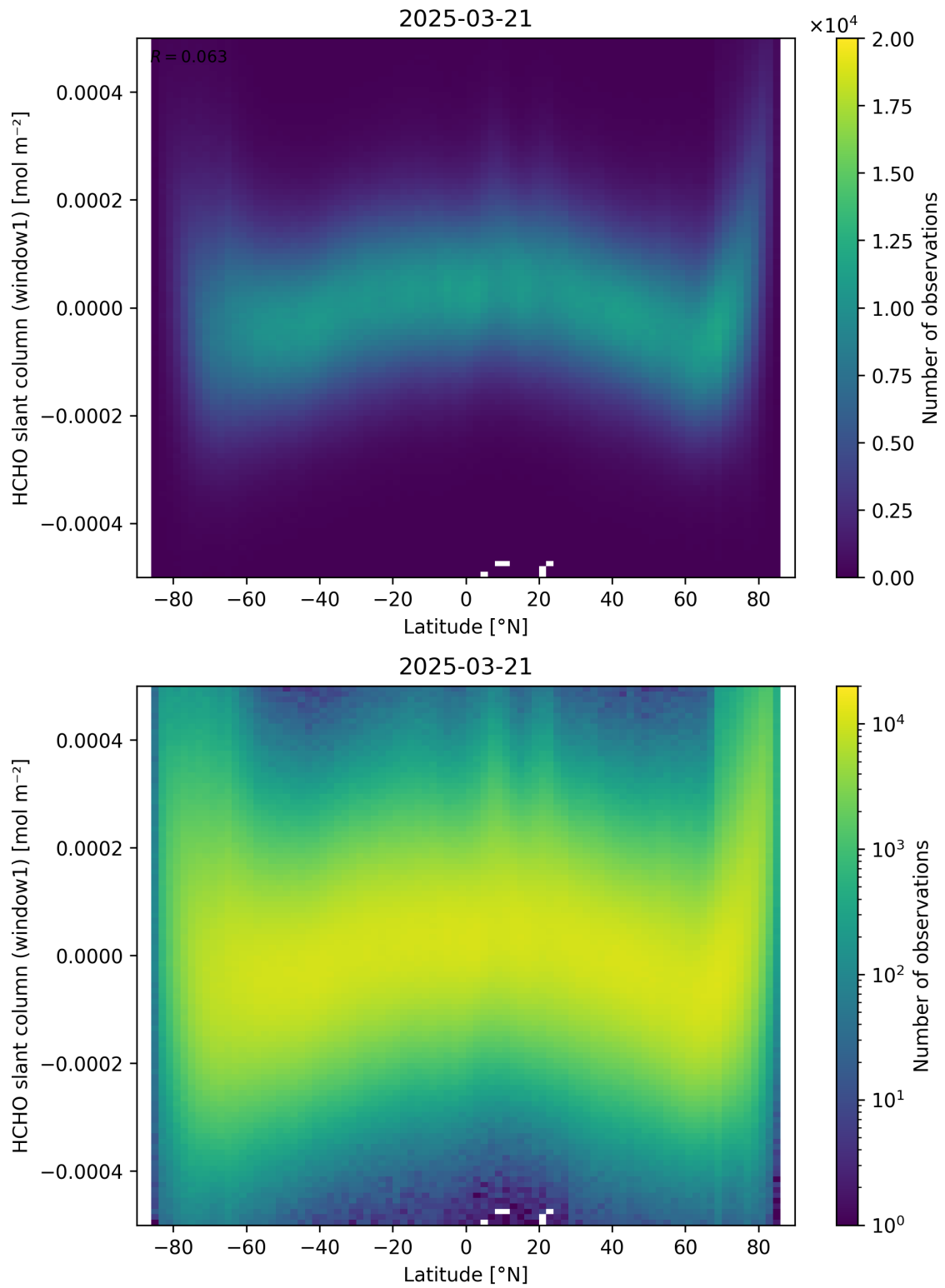
Figure 159: Scatter density plot of “Latitude” against “HCHO slant column (window1)” for 2025-03-20 to 2025-03-22.
