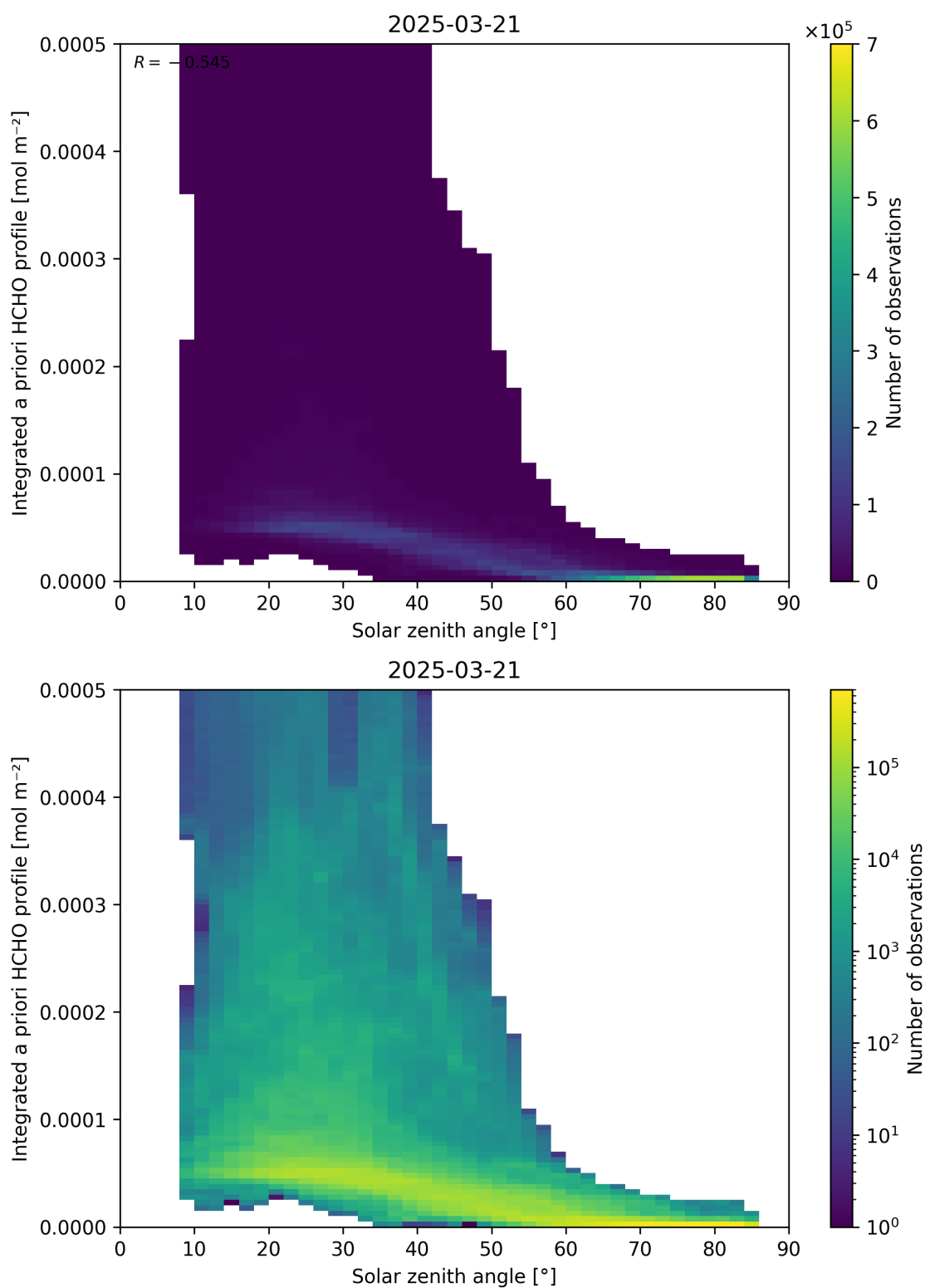
Figure 180: Scatter density plot of “Solar zenith angle” against “Integrated a priori HCHO profile” for 2025-03-20 to 2025-03-22.
