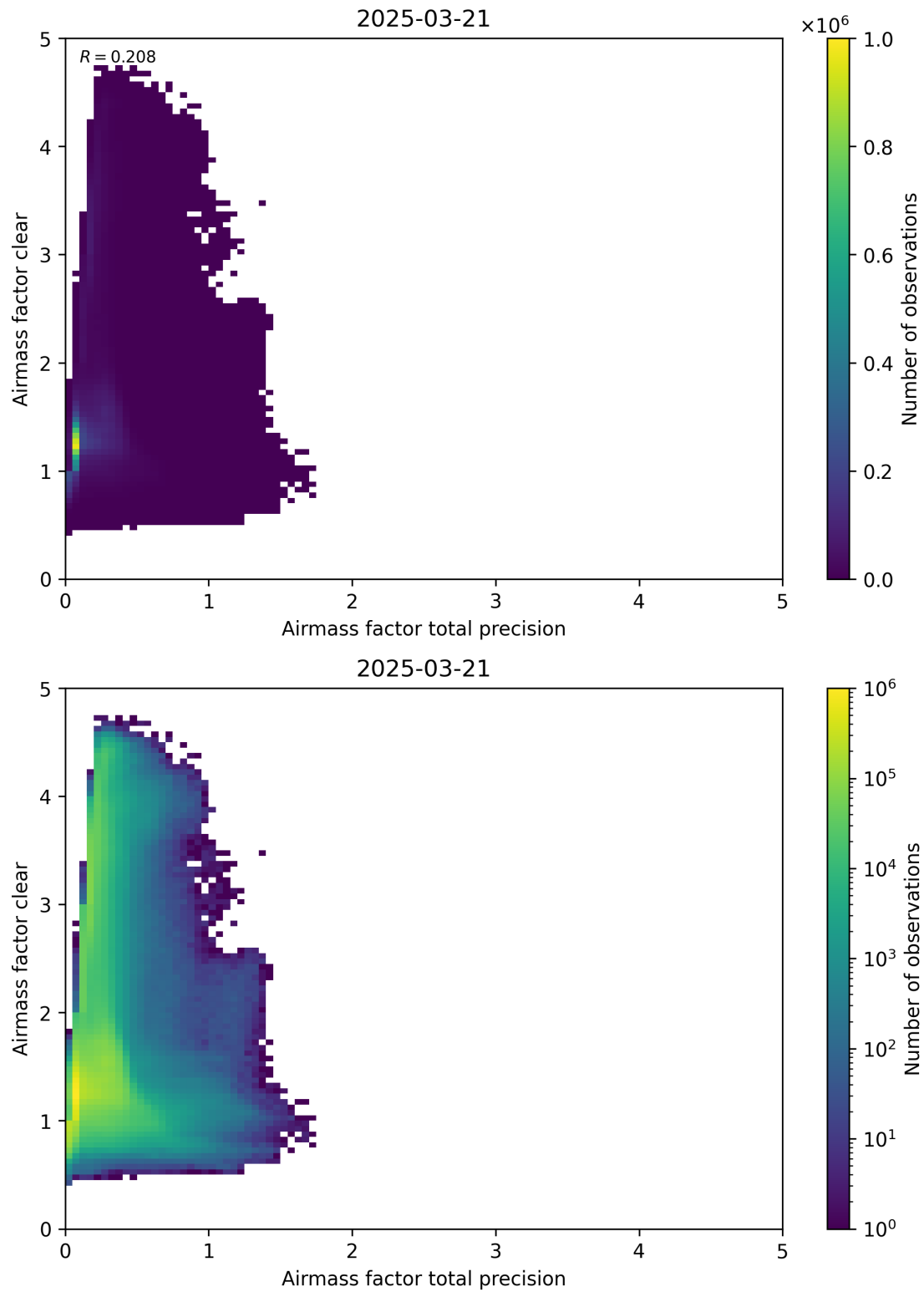
Figure 108: Scatter density plot of “Airmass factor total precision” against “Airmass factor clear” for 2025-03-20 to 2025-03-22.
