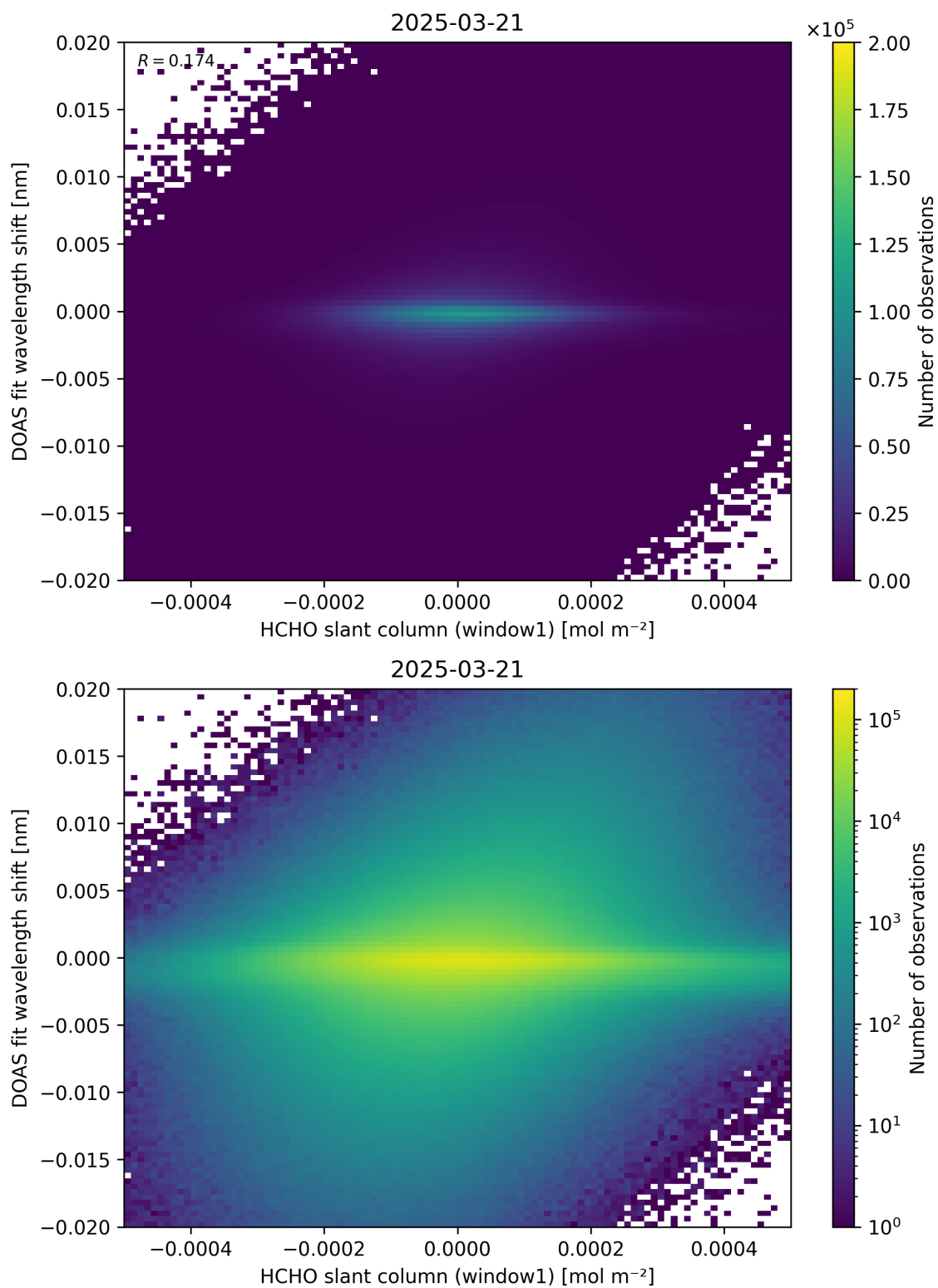
Figure 79: Scatter density plot of “HCHO slant column (window1)” against “DOAS fit wavelength shift” for 2025-03-20 to 2025-03-22.
