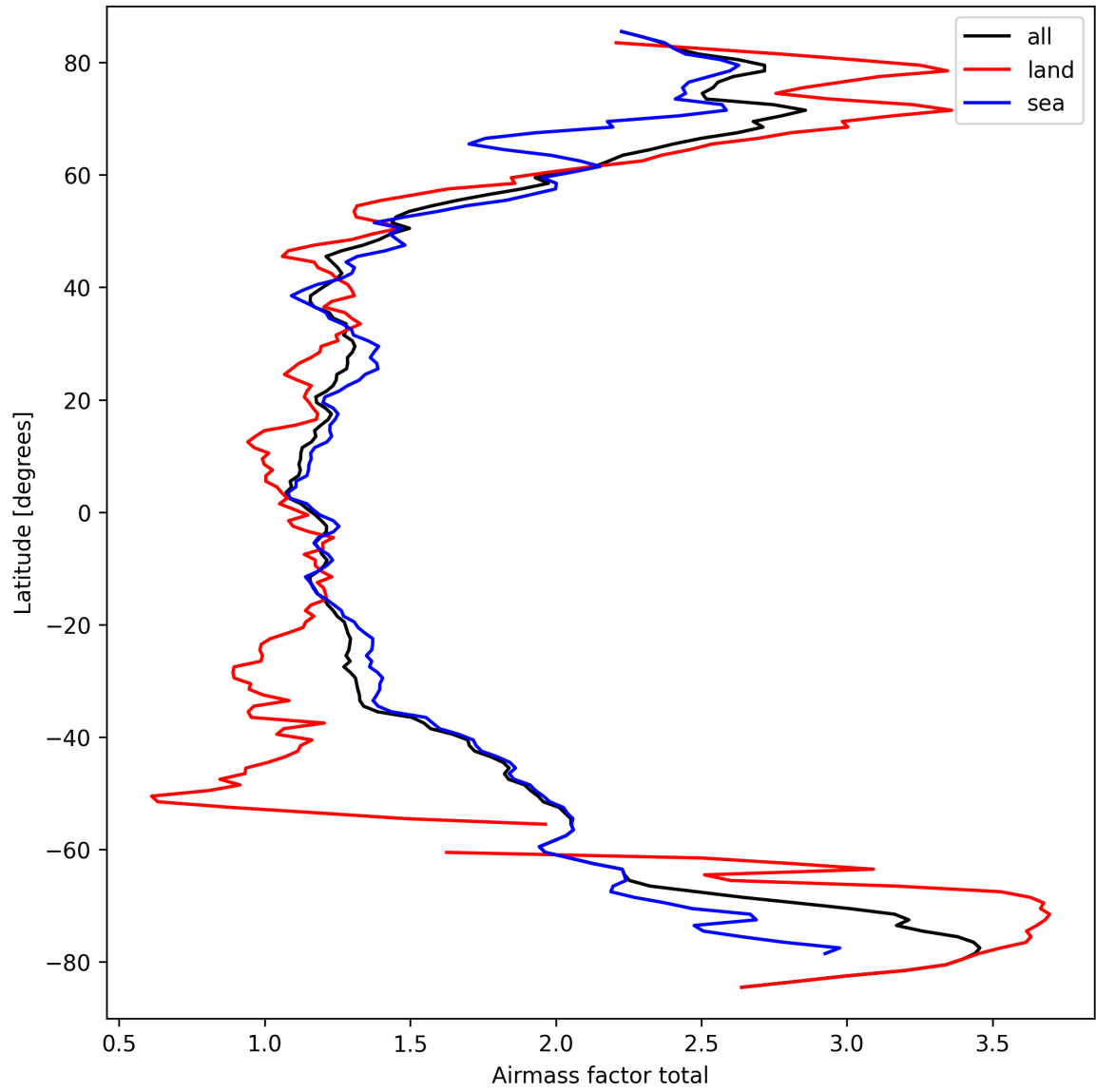
Figure 26: Zonal average of “Airmass factor total” for 2025-03-20 to 2025-03-22.
