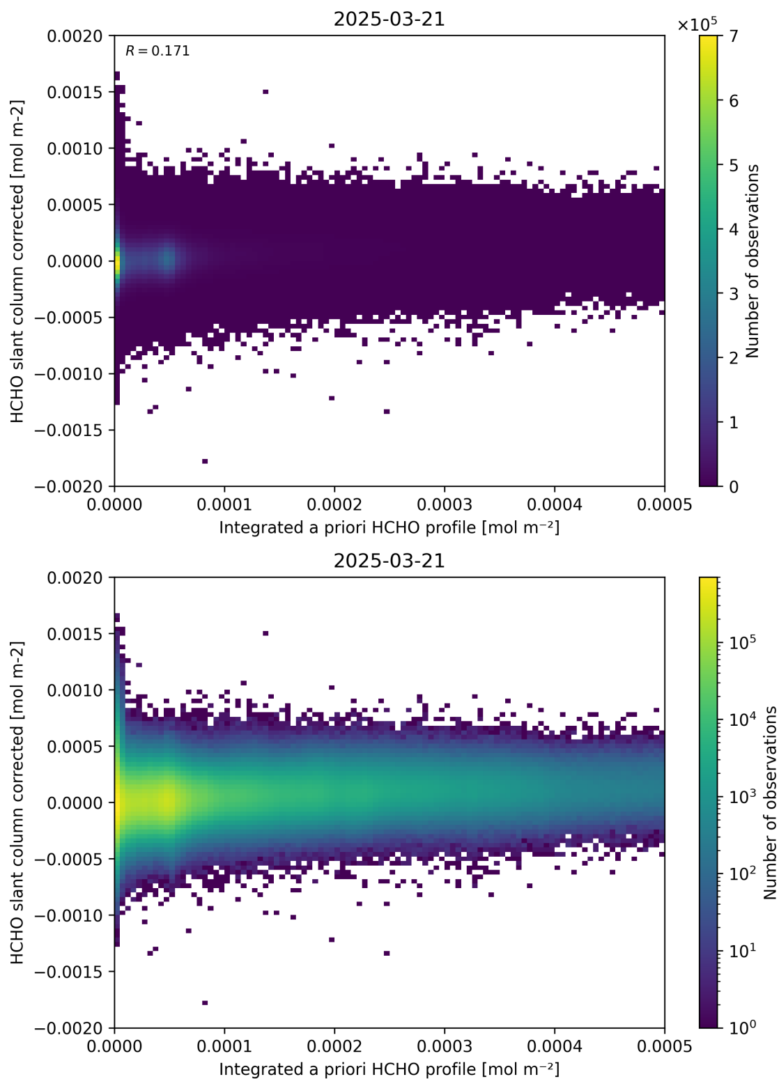
Figure 151: Scatter density plot of “Integrated a priori HCHO profile” against “HCHO slant column corrected” for 2025-03-20 to 2025-03-22.
