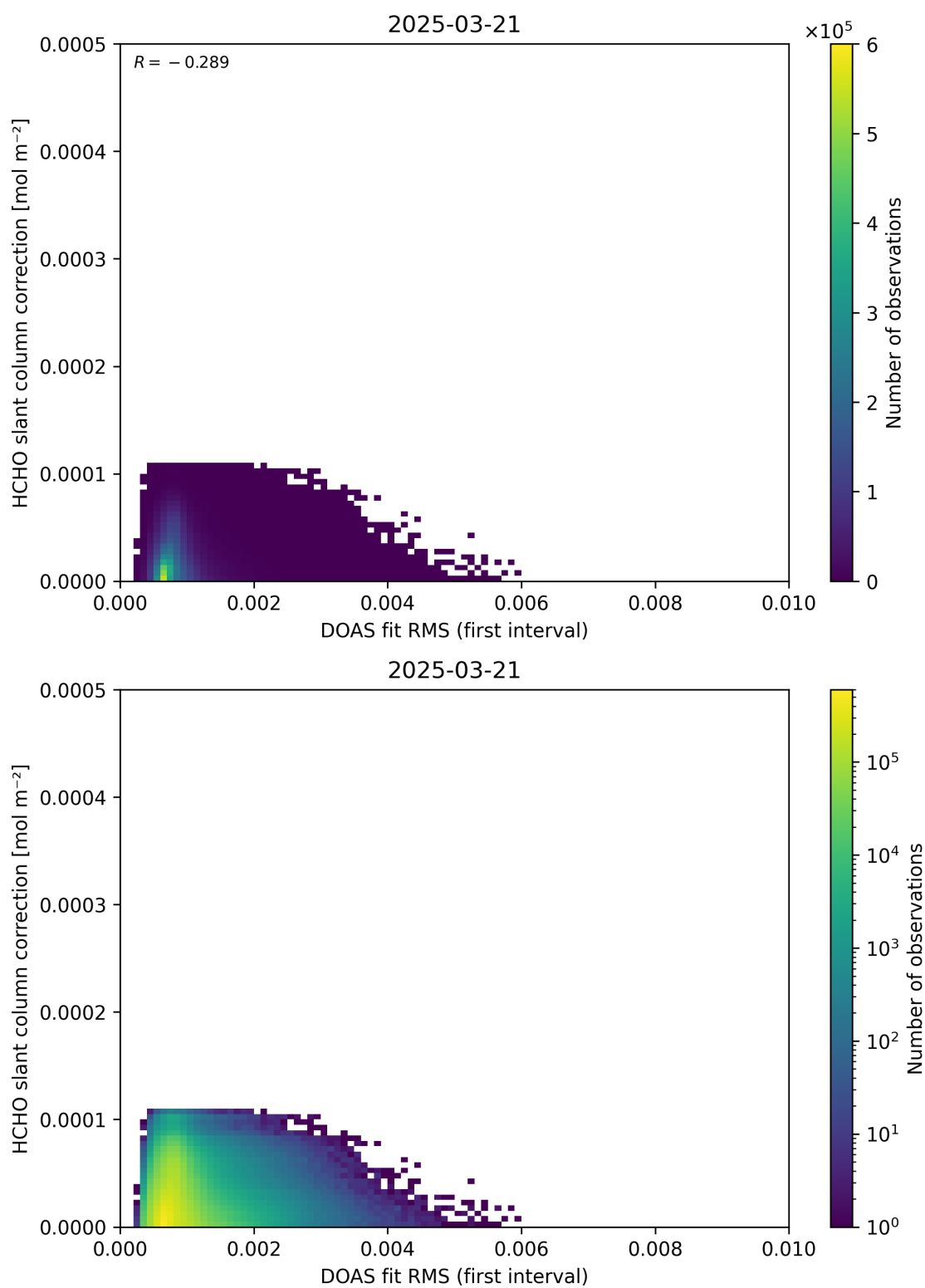
Figure 63: Scatter density plot of “DOAS fit RMS (first interval)” against “HCHO slant column correction” for 2025-03-20 to 2025-03-22.
