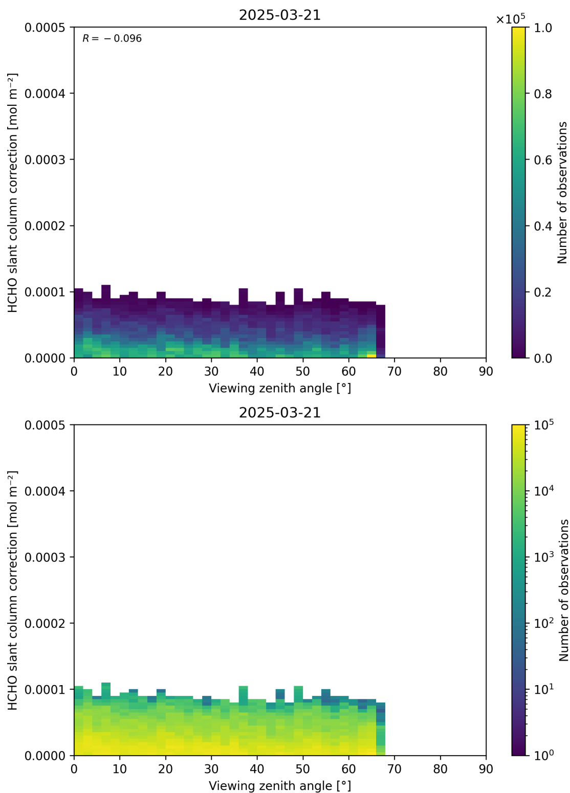
Figure 187: Scatter density plot of “Viewing zenith angle” against “HCHO slant column correction” for 2025-03-20 to 2025-03-22.
