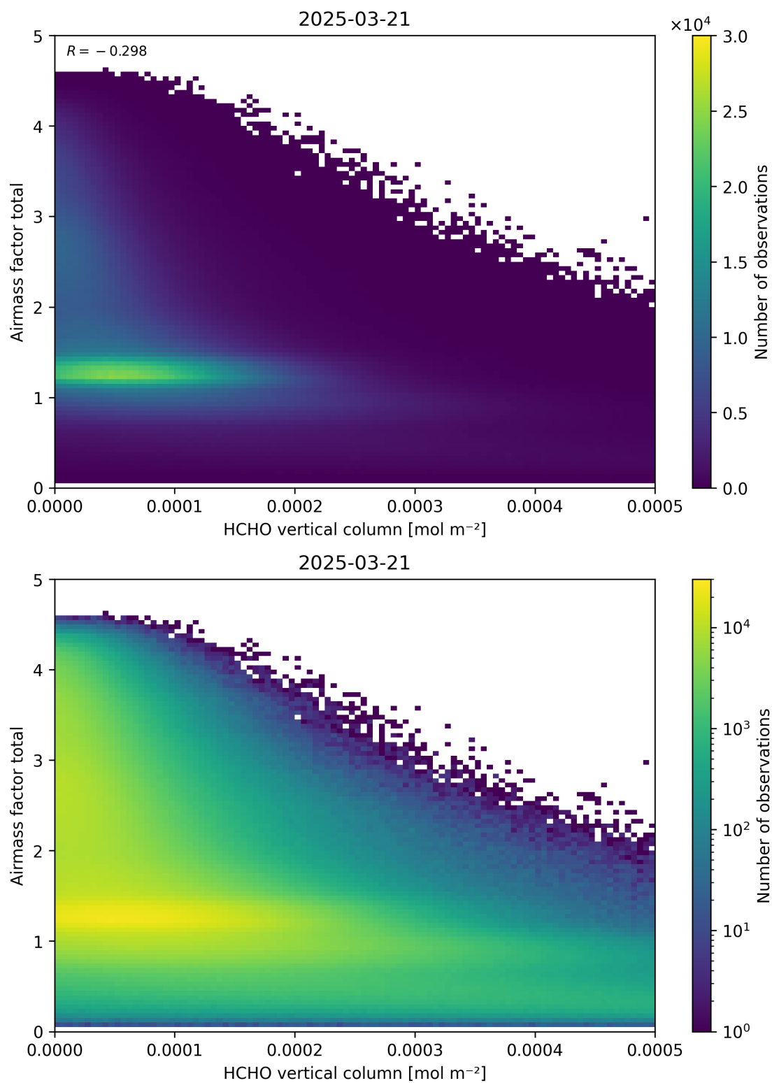
Figure 131: Scatter density plot of “HCHO vertical column” against “Airmass factor total” for 2025-03-20 to 2025-03-22.
