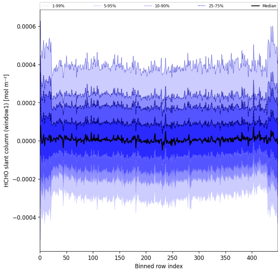
Figure 52: Along track statistics of “HCHO slant column (window1)” for 2025-03-20 to 2025-03-22
