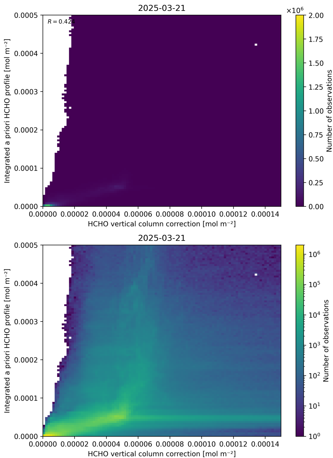
Figure 122: Scatter density plot of “HCHO vertical column correction” against “Integrated a priori HCHO profile” for 2025-03-20 to 2025-03-22.
