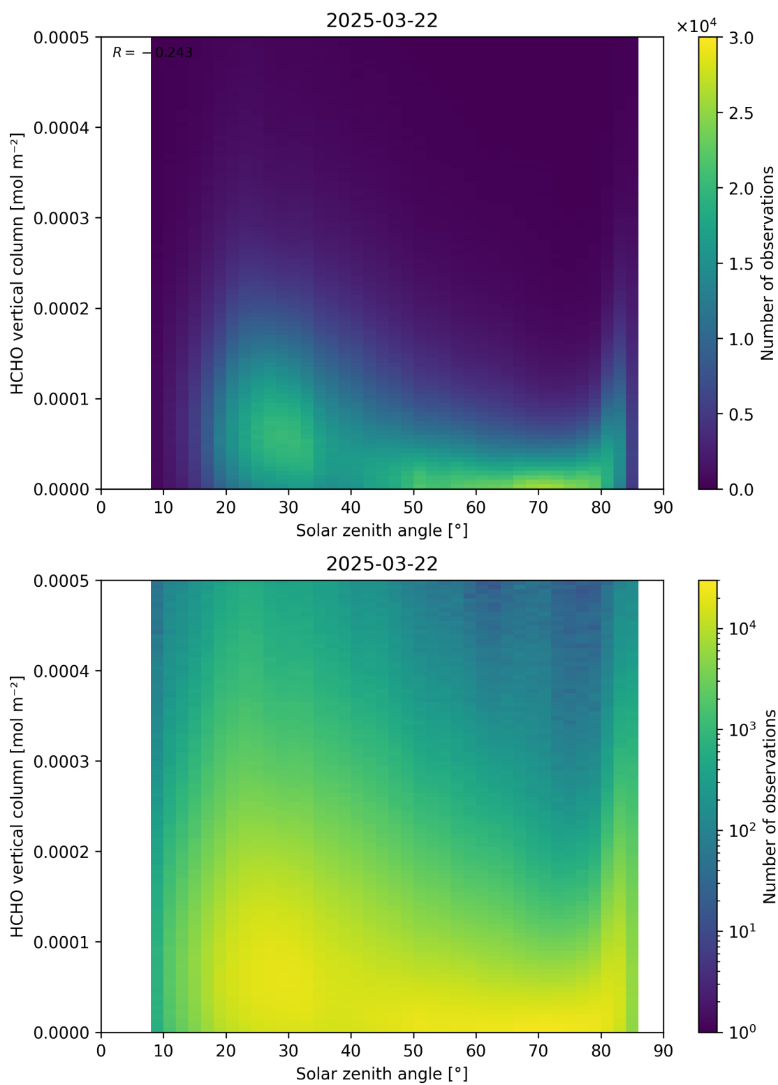
Figure 177: Scatter density plot of “Solar zenith angle” against “HCHO vertical column” for 2025-03-21 to 2025-03-23.
