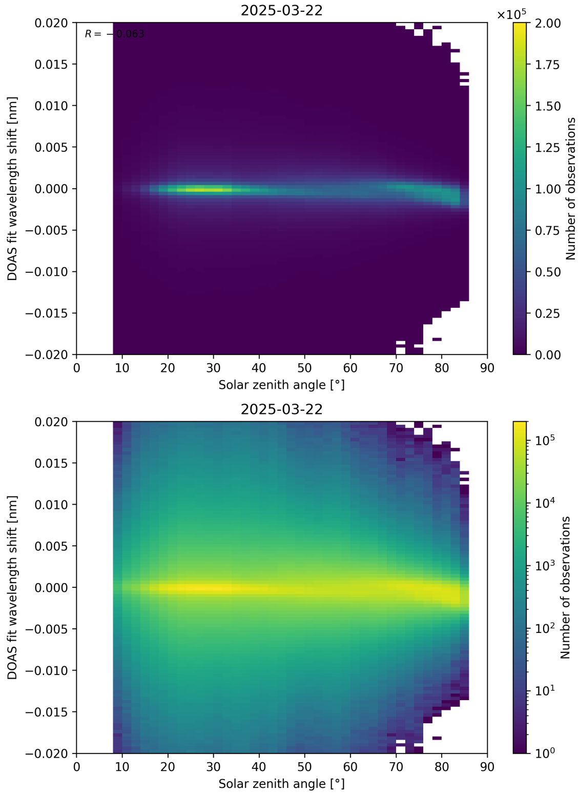
Figure 168: Scatter density plot of “Solar zenith angle” against “DOAS fit wavelength shift” for 2025-03-21 to 2025-03-23.
