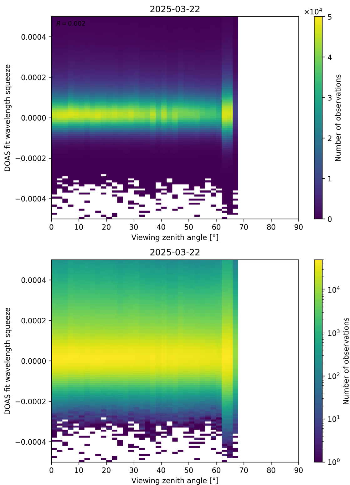
Figure 184: Scatter density plot of “Viewing zenith angle” against “DOAS fit wavelength squeeze” for 2025-03-21 to 2025-03-23.
