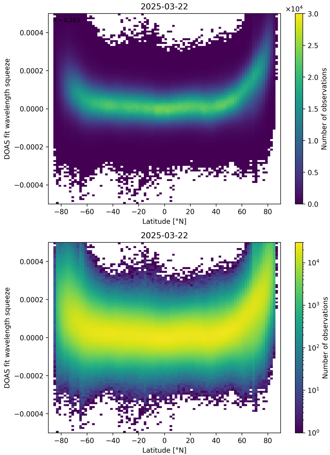
Figure 155: Scatter density plot of “Latitude” against “DOAS fit wavelength squeeze” for 2025-03-21 to 2025-03-23.
