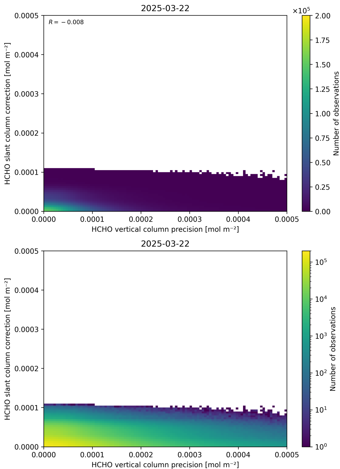
Figure 141: Scatter density plot of “HCHO vertical column precision” against “HCHO slant column correction” for 2025-03-21 to 2025-03-23.
