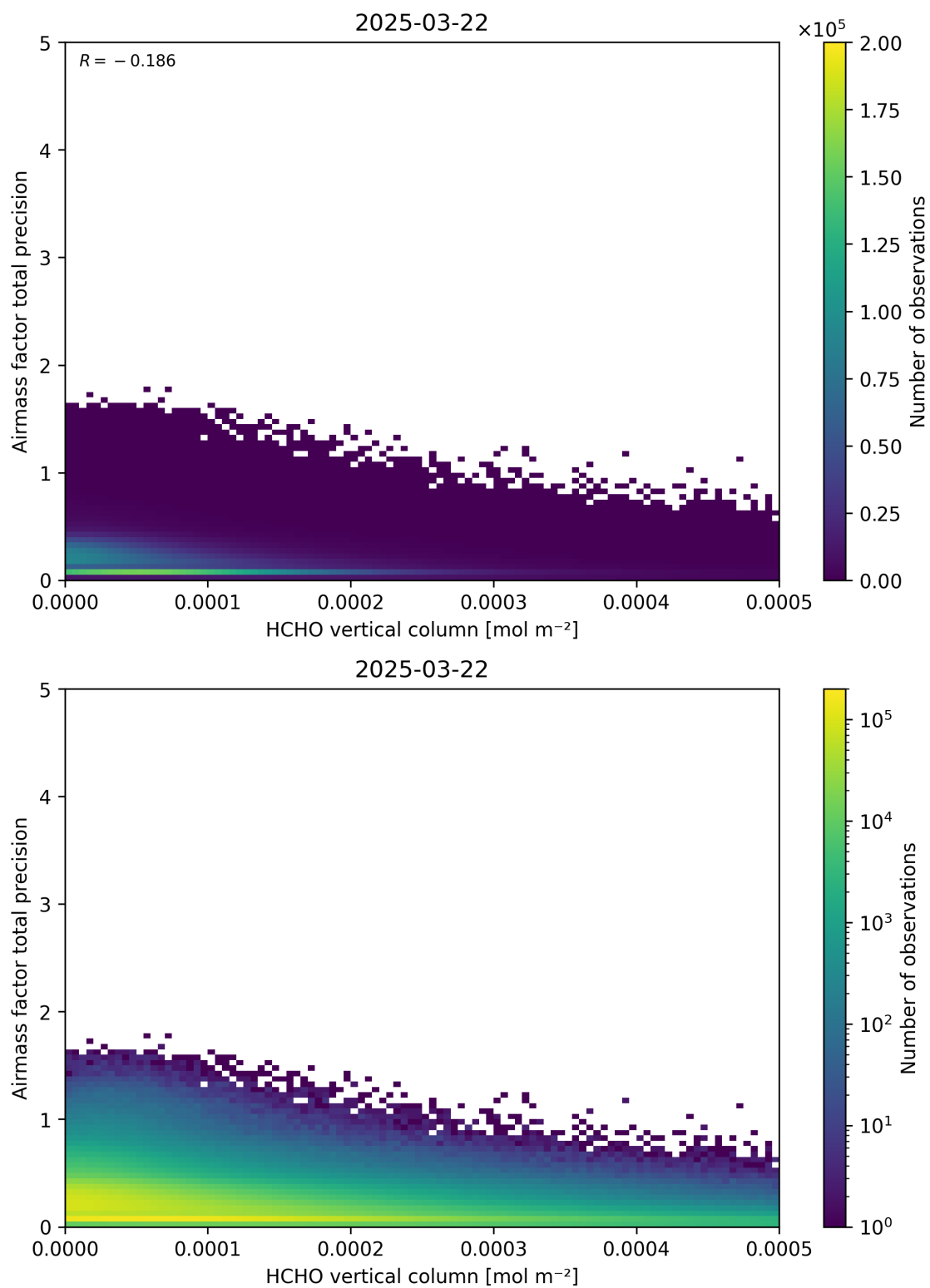
Figure 132: Scatter density plot of “HCHO vertical column” against “Airmass factor total precision” for 2025-03-21 to 2025-03-23.
