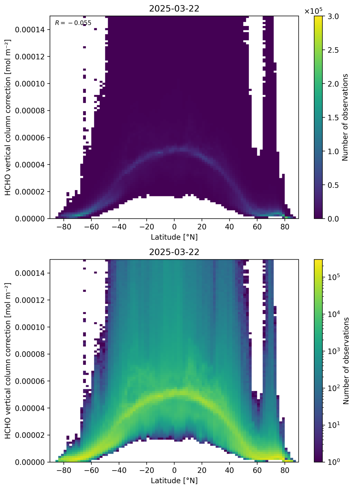
Figure 164: Scatter density plot of “Latitude” against “HCHO vertical column correction” for 2025-03-21 to 2025-03-23.
