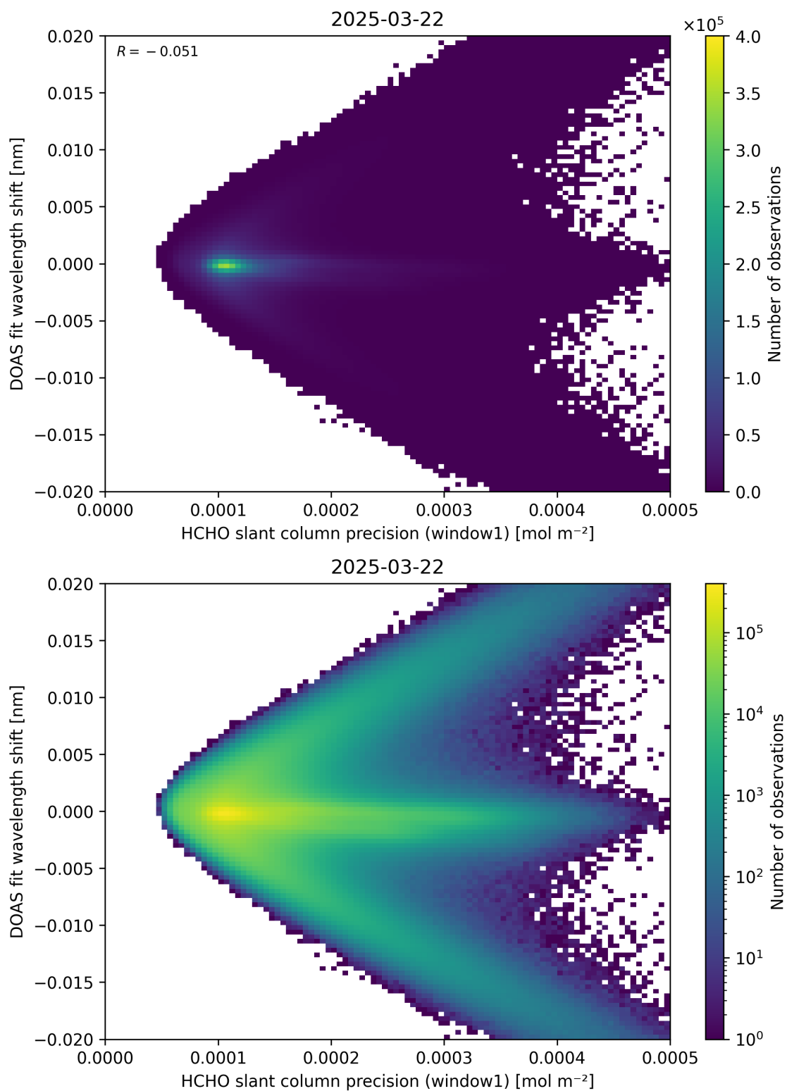
Figure 89: Scatter density plot of “HCHO slant column precision (window1)” against “DOAS fit wavelength shift” for 2025-03-21 to 2025-03-23.
