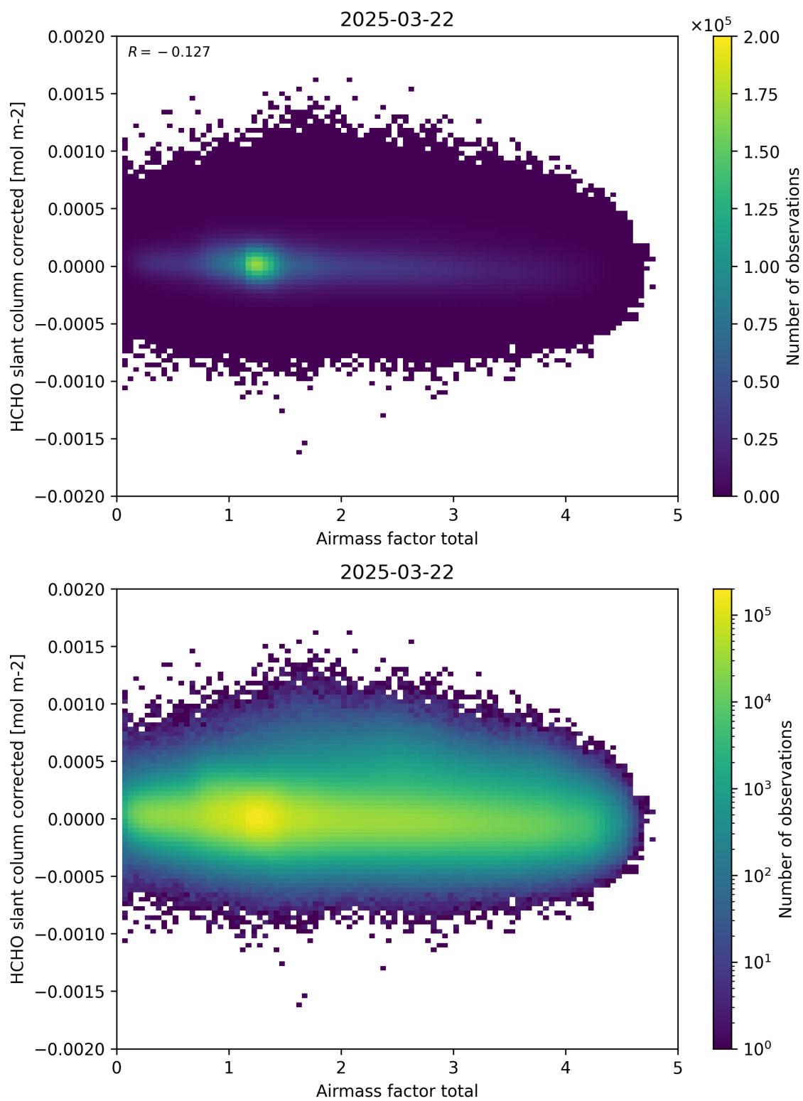
Figure 101: Scatter density plot of “Airmass factor total” against “HCHO slant column corrected” for 2025-03-21 to 2025-03-23.
