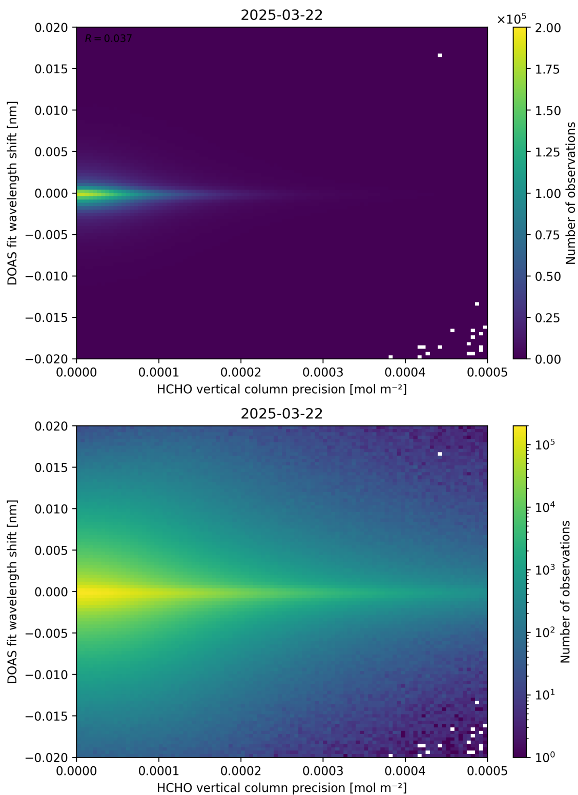
Figure 137: Scatter density plot of “HCHO vertical column precision” against “DOAS fit wavelength shift” for 2025-03-21 to 2025-03-23.
