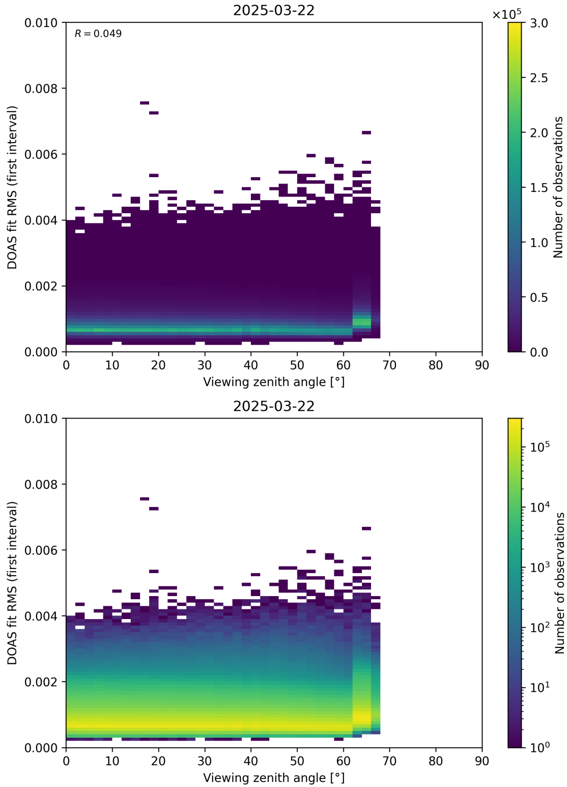
Figure 182: Scatter density plot of “Viewing zenith angle” against “DOAS fit RMS (first interval)” for 2025-03-21 to 2025-03-23.
