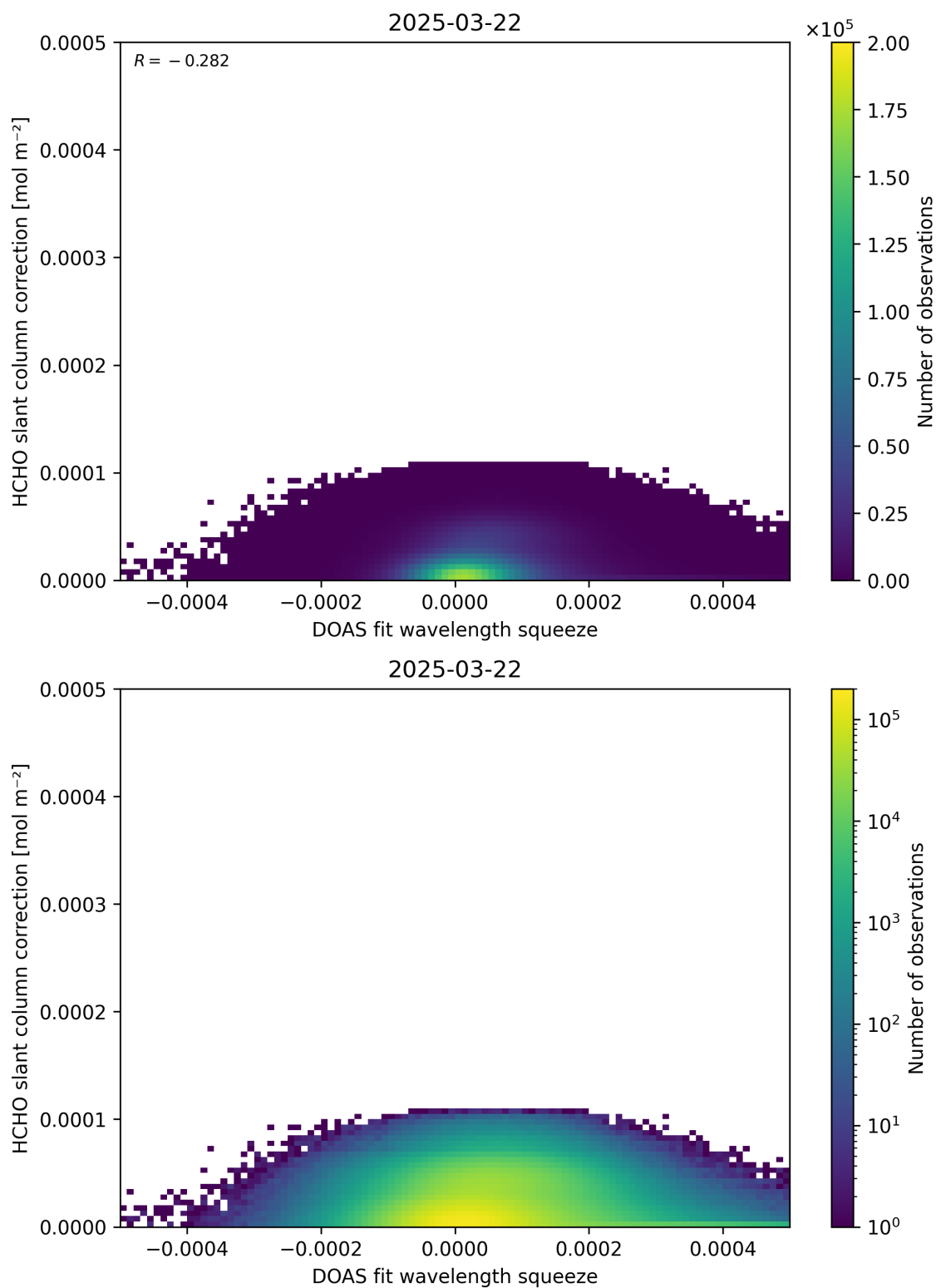
Figure 70: Scatter density plot of “DOAS fit wavelength squeeze” against “HCHO slant column correction” for 2025-03-21 to 2025-03-23.
