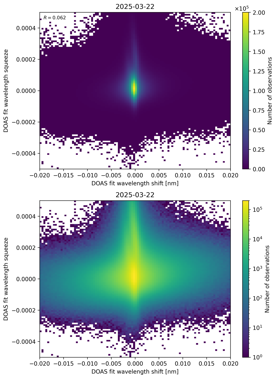
Figure 65: Scatter density plot of “DOAS fit wavelength shift” against “DOAS fit wavelength squeeze” for 2025-03-21 to 2025-03-23.
