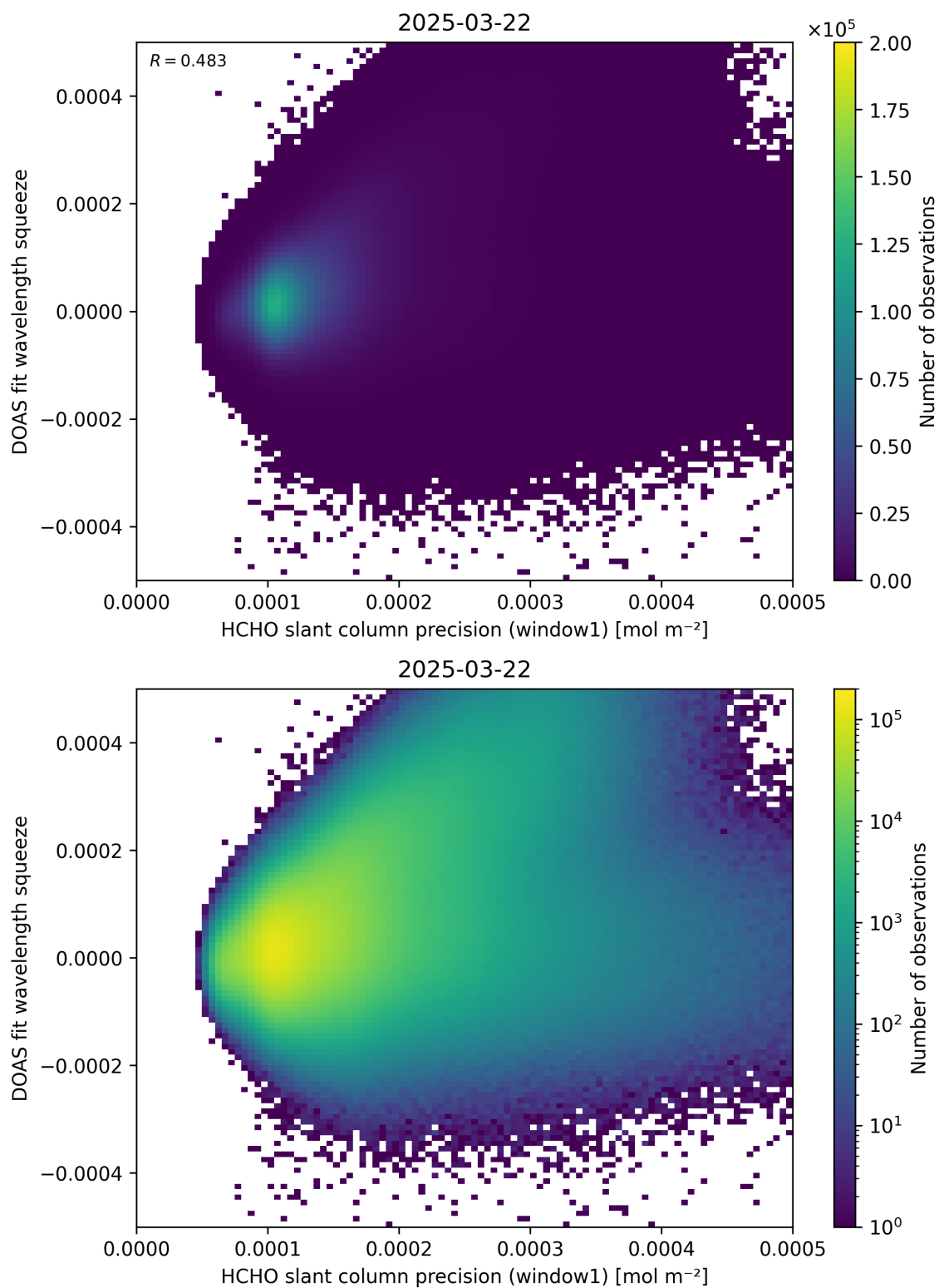
Figure 90: Scatter density plot of “HCHO slant column precision (window1)” against “DOAS fit wavelength squeeze” for 2025-03-21 to 2025-03-23.
