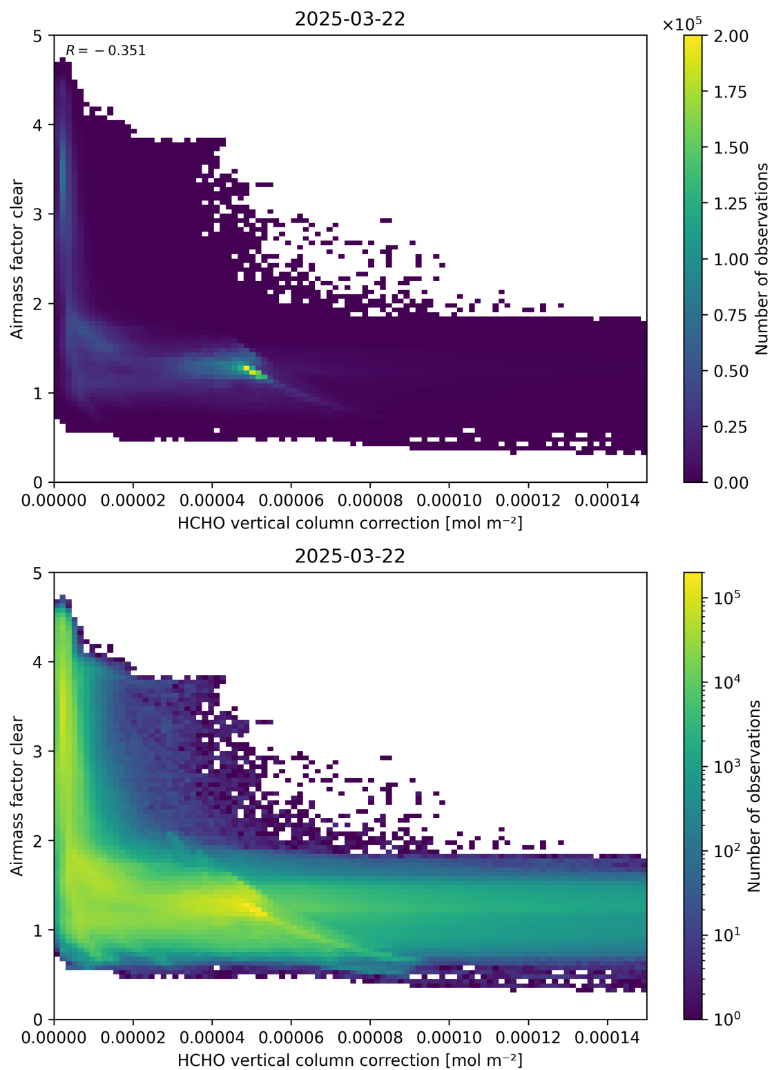
Figure 115: Scatter density plot of “HCHO vertical column correction” against “Airmass factor clear” for 2025-03-21 to 2025-03-23.
