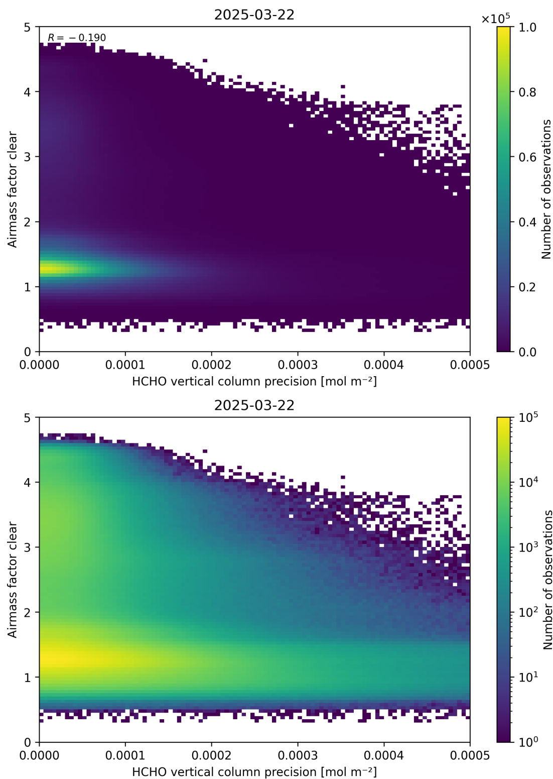
Figure 139: Scatter density plot of “HCHO vertical column precision” against “Airmass factor clear” for 2025-03-21 to 2025-03-23.
