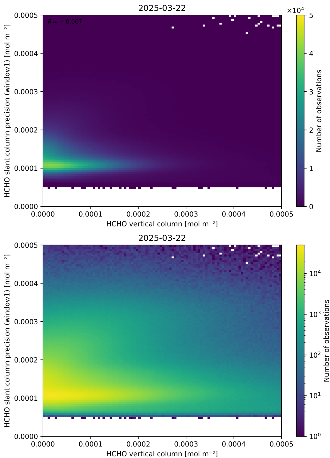
Figure 130: Scatter density plot of “HCHO vertical column” against “HCHO slant column precision (window1)” for 2025-03-21 to 2025-03-23.
