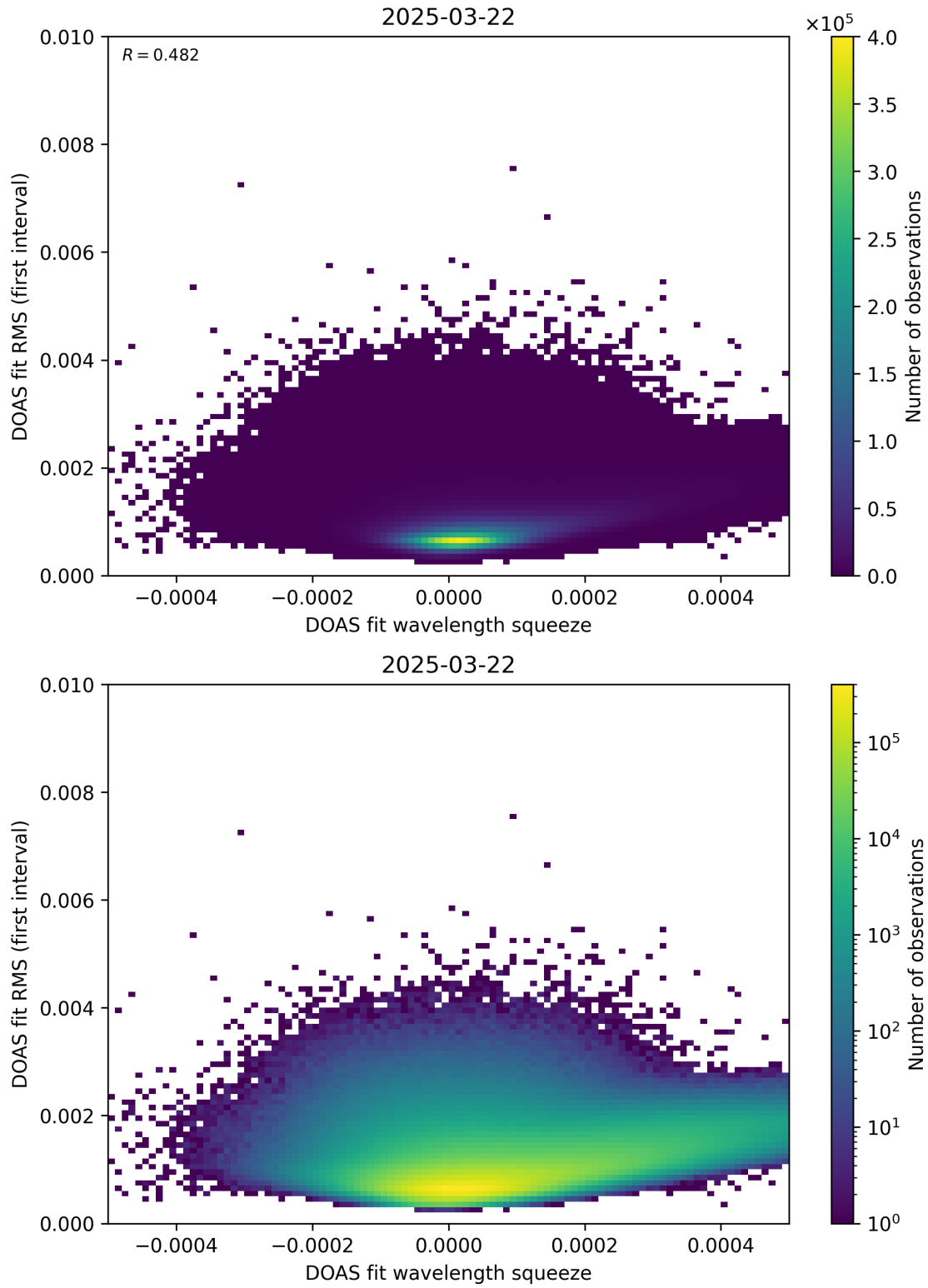
Figure 68: Scatter density plot of “DOAS fit wavelength squeeze” against “DOAS fit RMS (first interval)” for 2025-03-21 to 2025-03-23.
