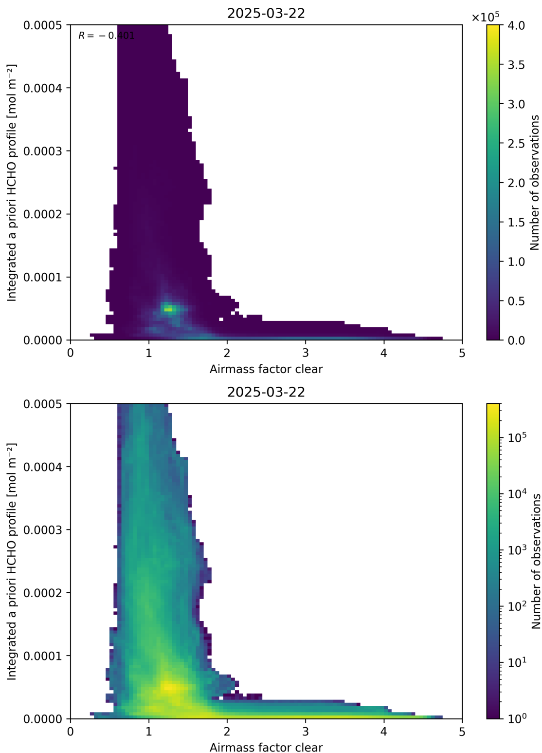
Figure 76: Scatter density plot of “Airmass factor clear” against “Integrated a priori HCHO profile” for 2025-03-21 to 2025-03-23.
