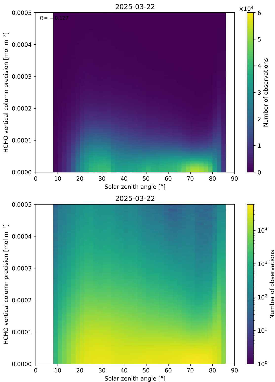
Figure 179: Scatter density plot of “Solar zenith angle” against “HCHO vertical column precision” for 2025-03-21 to 2025-03-23.
