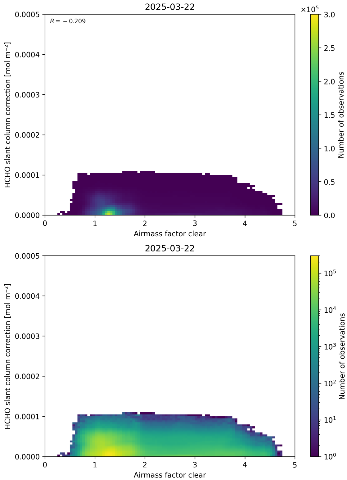
Figure 75: Scatter density plot of “Airmass factor clear” against “HCHO slant column correction” for 2025-03-21 to 2025-03-23.
