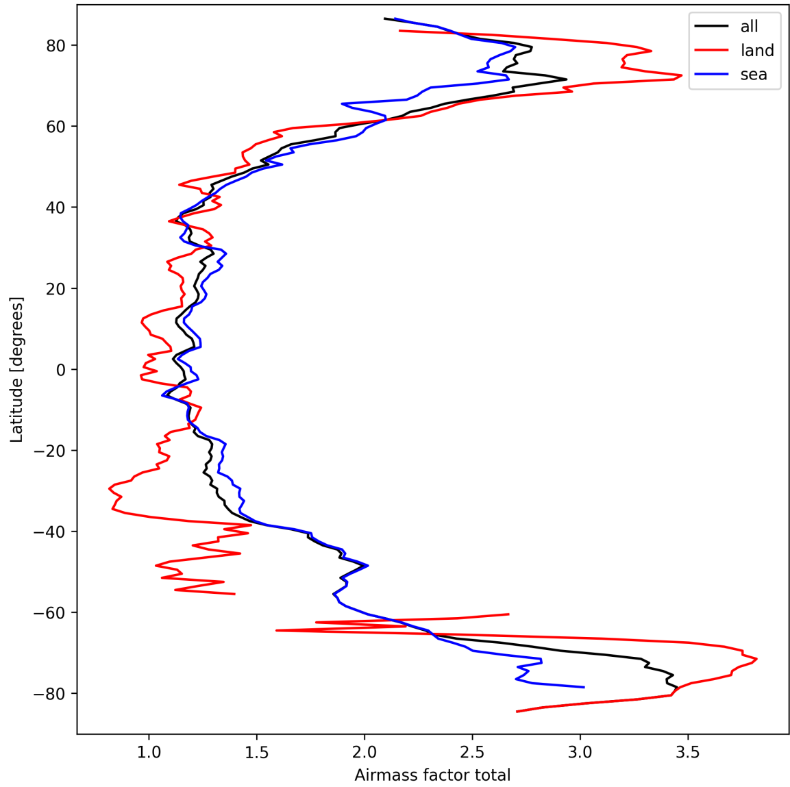
Figure 26: Zonal average of “Airmass factor total” for 2025-03-21 to 2025-03-23.
