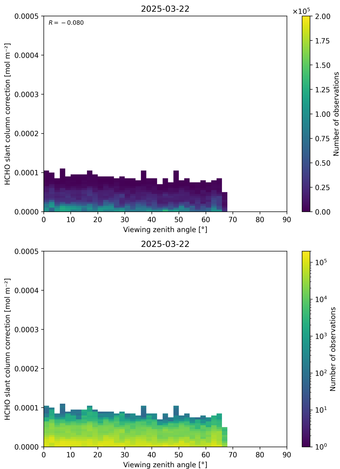
Figure 187: Scatter density plot of “Viewing zenith angle” against “HCHO slant column correction” for 2025-03-21 to 2025-03-23.
