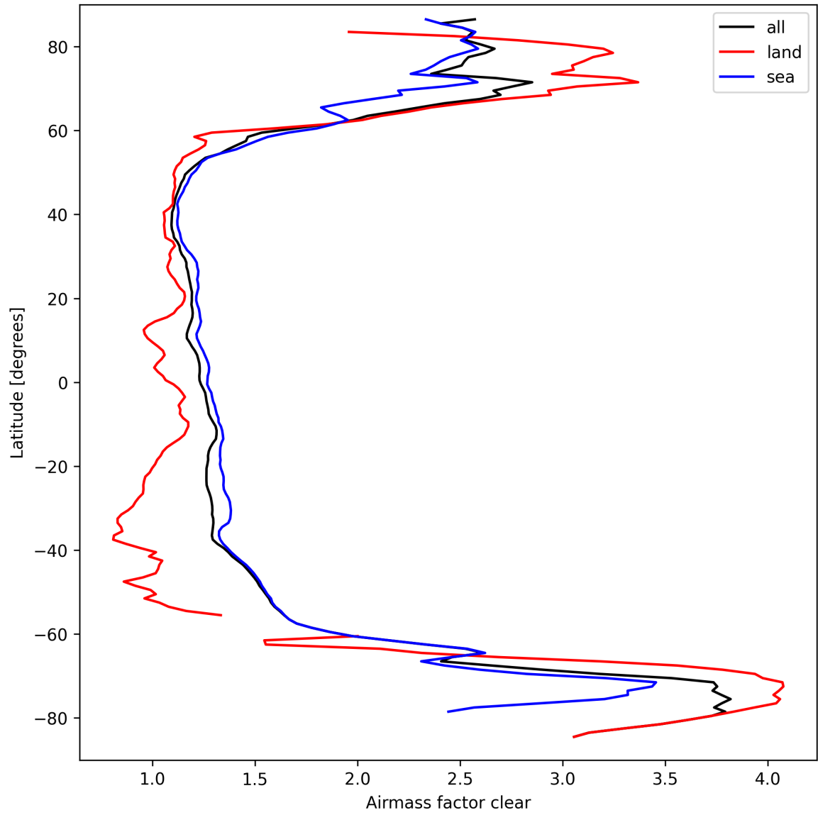
Figure 28: Zonal average of “Airmass factor clear” for 2025-03-21 to 2025-03-23.
