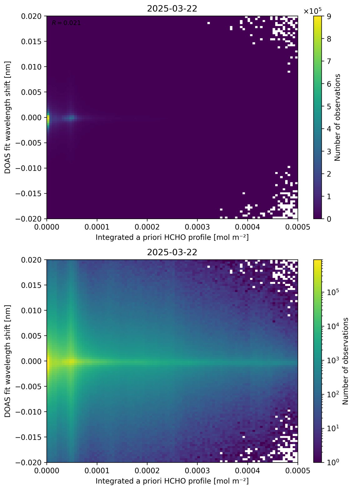
Figure 149: Scatter density plot of “Integrated a priori HCHO profile” against “DOAS fit wavelength shift” for 2025-03-21 to 2025-03-23.
