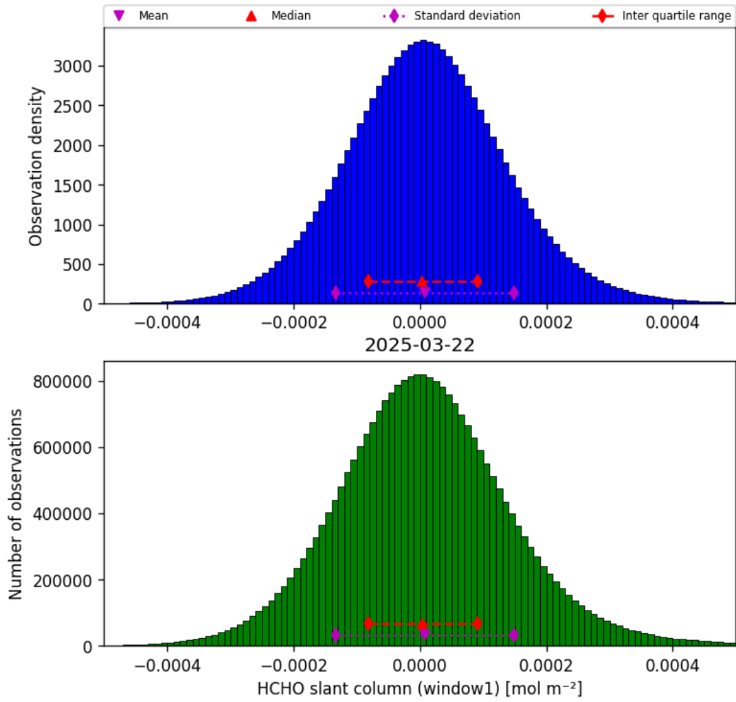
Figure 38: Histogram of “HCHO slant column (window1)” for 2025-03-21 to 2025-03-23
