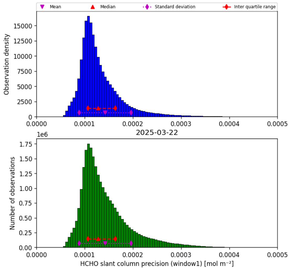
Figure 39: Histogram of “HCHO slant column precision (window1)” for 2025-03-21 to 2025-03-23
