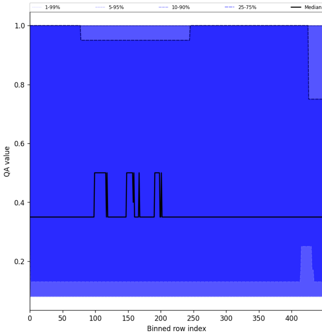
Figure 48: Along track statistics of “QA value” for 2025-03-21 to 2025-03-23
