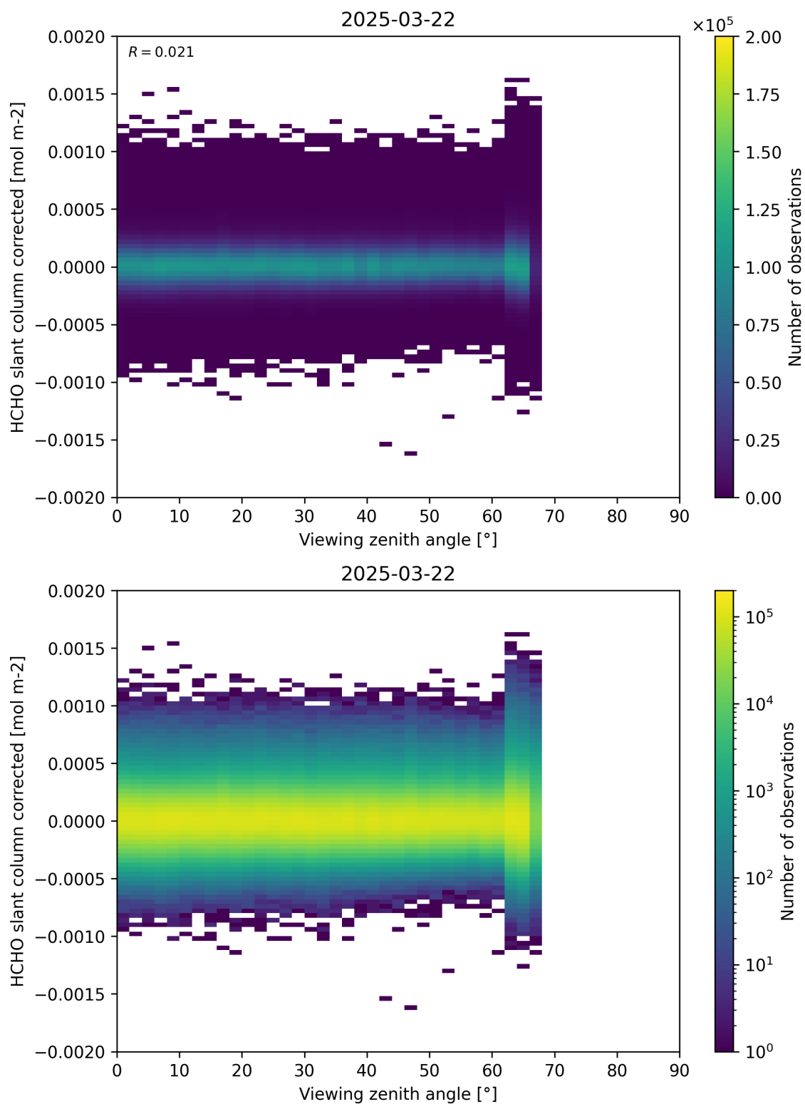
Figure 186: Scatter density plot of “Viewing zenith angle” against “HCHO slant column corrected” for 2025-03-21 to 2025-03-23.
