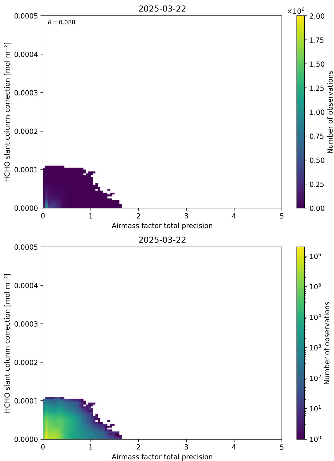
Figure 110: Scatter density plot of “Airmass factor total precision” against “HCHO slant column correction” for 2025-03-21 to 2025-03-23.
