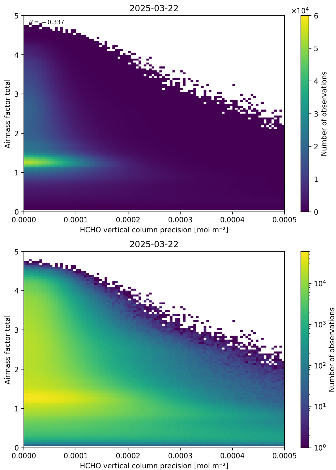
Figure 144: Scatter density plot of “HCHO vertical column precision” against “Airmass factor total” for 2025-03-21 to 2025-03-23.
