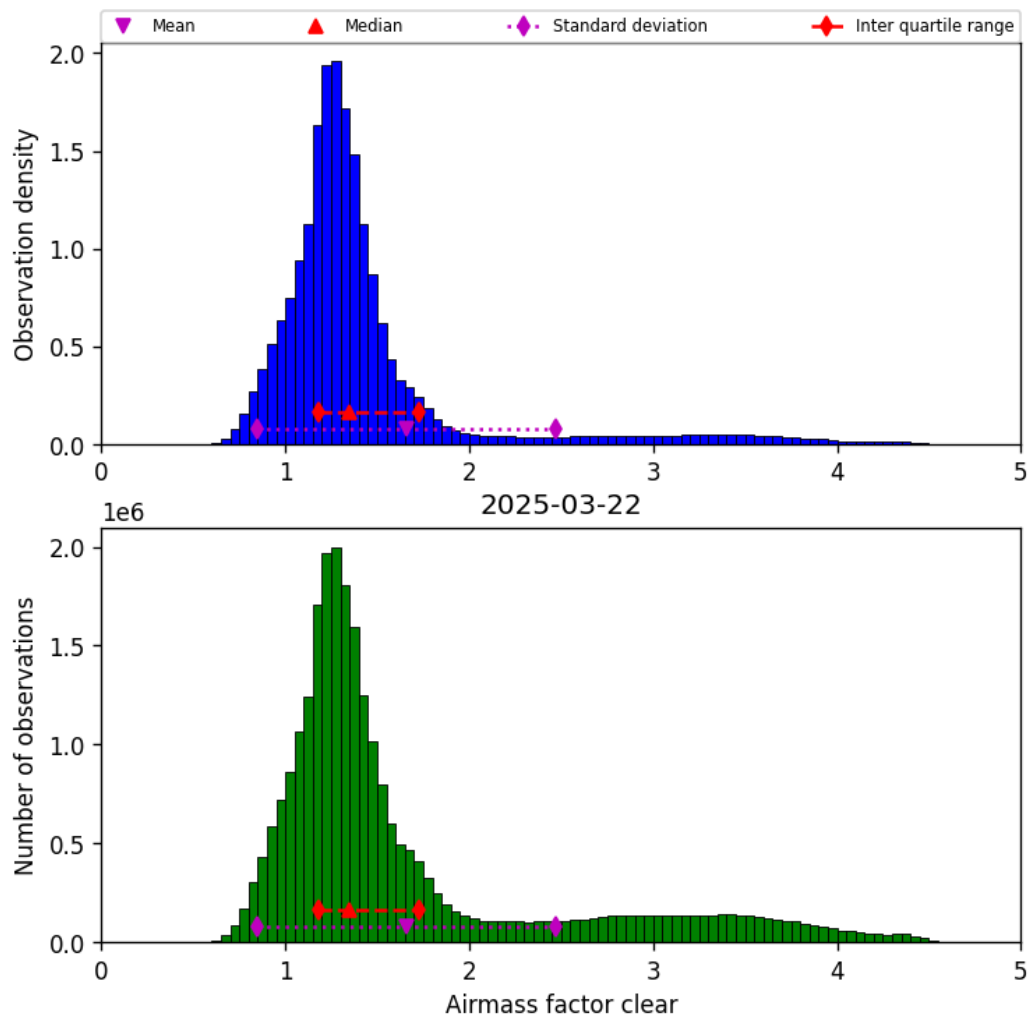
Figure 42: Histogram of “Airmass factor clear” for 2025-03-21 to 2025-03-23
