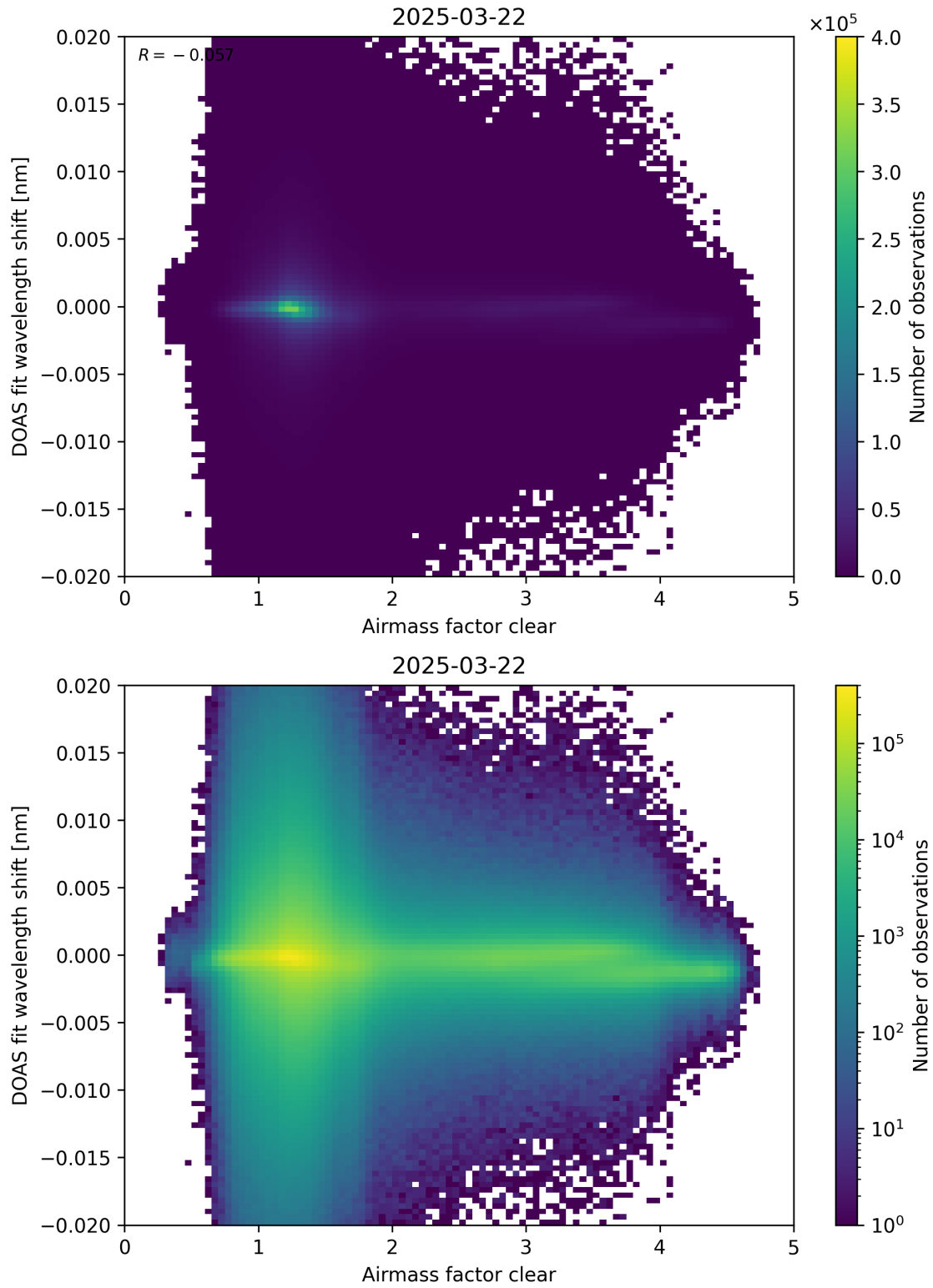
Figure 72: Scatter density plot of “Airmass factor clear” against “DOAS fit wavelength shift” for 2025-03-21 to 2025-03-23.
