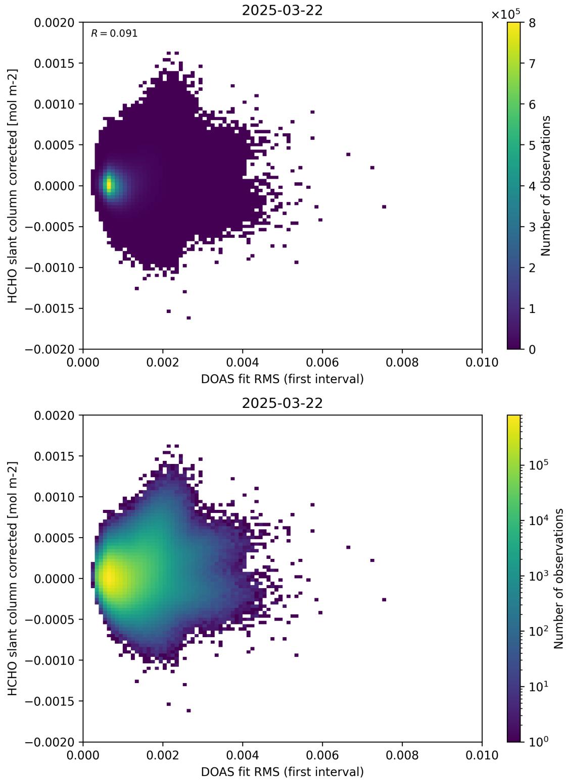
Figure 62: Scatter density plot of “DOAS fit RMS (first interval)” against “HCHO slant column corrected” for 2025-03-21 to 2025-03-23.
