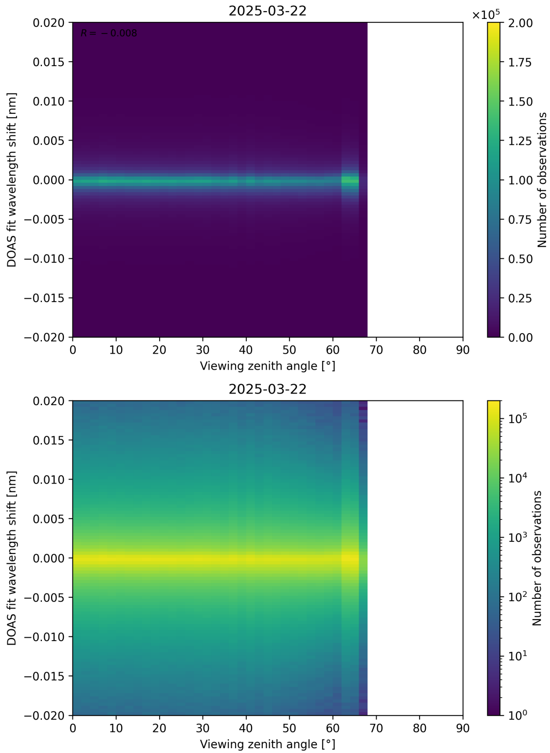
Figure 183: Scatter density plot of “Viewing zenith angle” against “DOAS fit wavelength shift” for 2025-03-21 to 2025-03-23.
