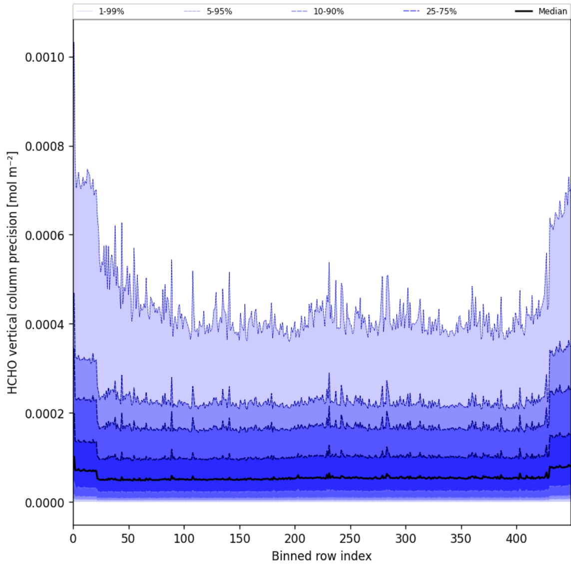
Figure 50: Along track statistics of “HCHO vertical column precision” for 2025-03-21 to 2025-03-23
