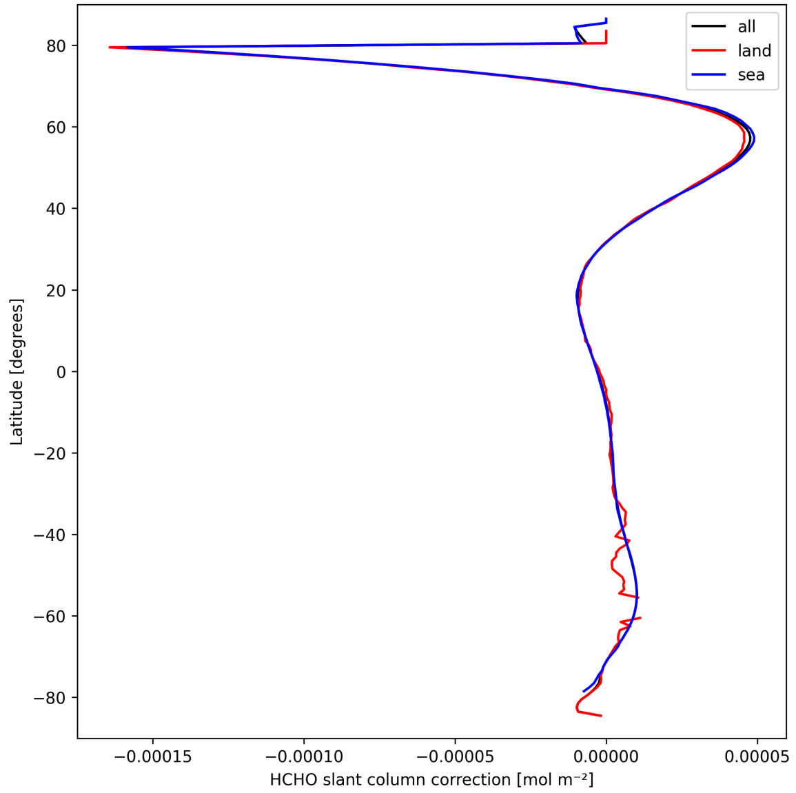
Figure 33: Zonal average of "HCHO slant column correction" for 2025-03-21 to 2025-03-23.
