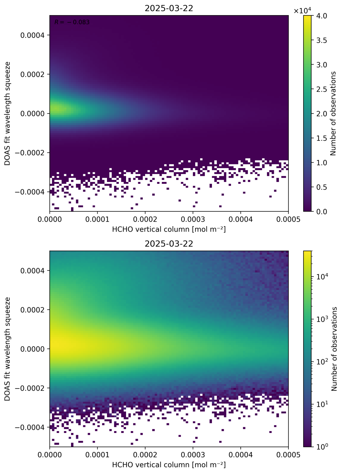
Figure 125: Scatter density plot of “HCHO vertical column” against “DOAS fit wavelength squeeze” for 2025-03-21 to 2025-03-23.
