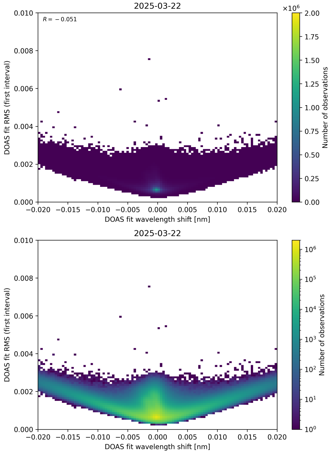
Figure 64: Scatter density plot of “DOAS fit wavelength shift” against “DOAS fit RMS (first interval)” for 2025-03-21 to 2025-03-23.
