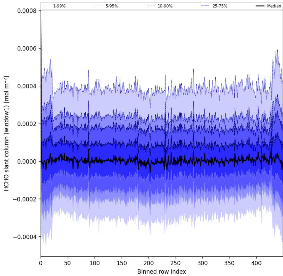
Figure 52: Along track statistics of “HCHO slant column (window1)” for 2025-03-21 to 2025-03-23
