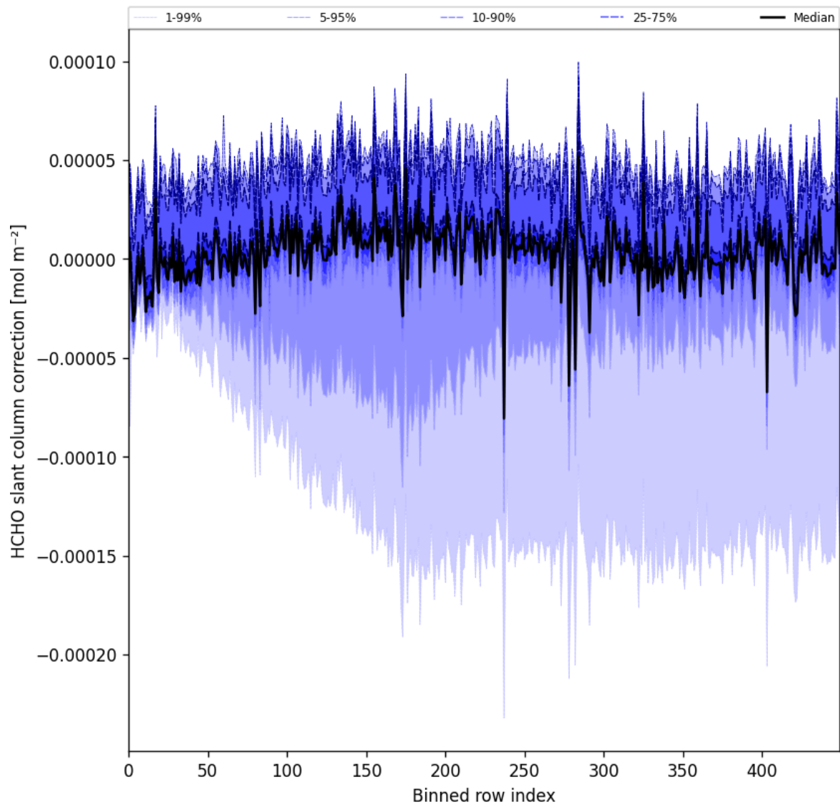
Figure 61: Along track statistics of “HCHO slant column correction” for 2025-03-21 to 2025-03-23
