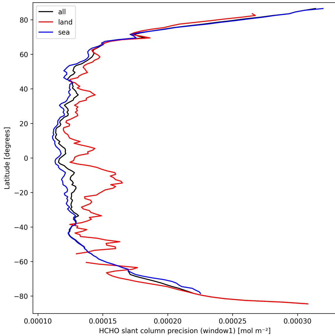
Figure 25: Zonal average of "HCHO slant column precision (window1)" for 2025-03-21 to 2025-03-23.
