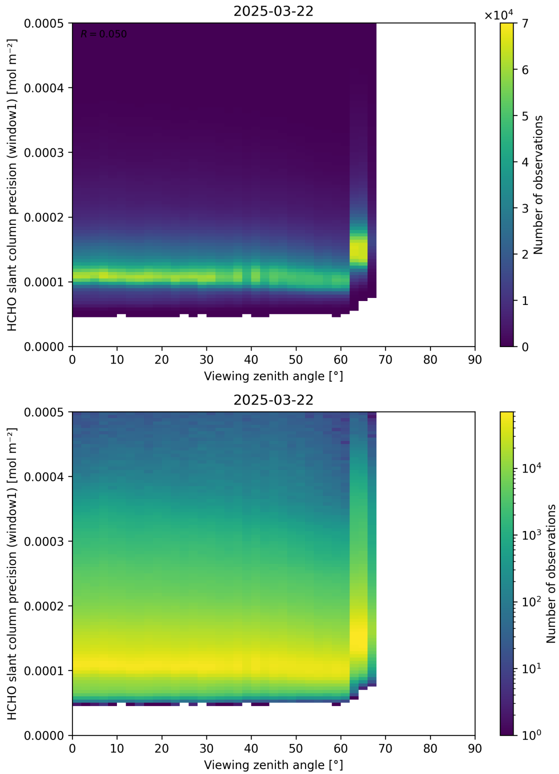
Figure 189: Scatter density plot of “Viewing zenith angle” against “HCHO slant column precision (window1)” for 2025-03-21 to 2025-03-23.
