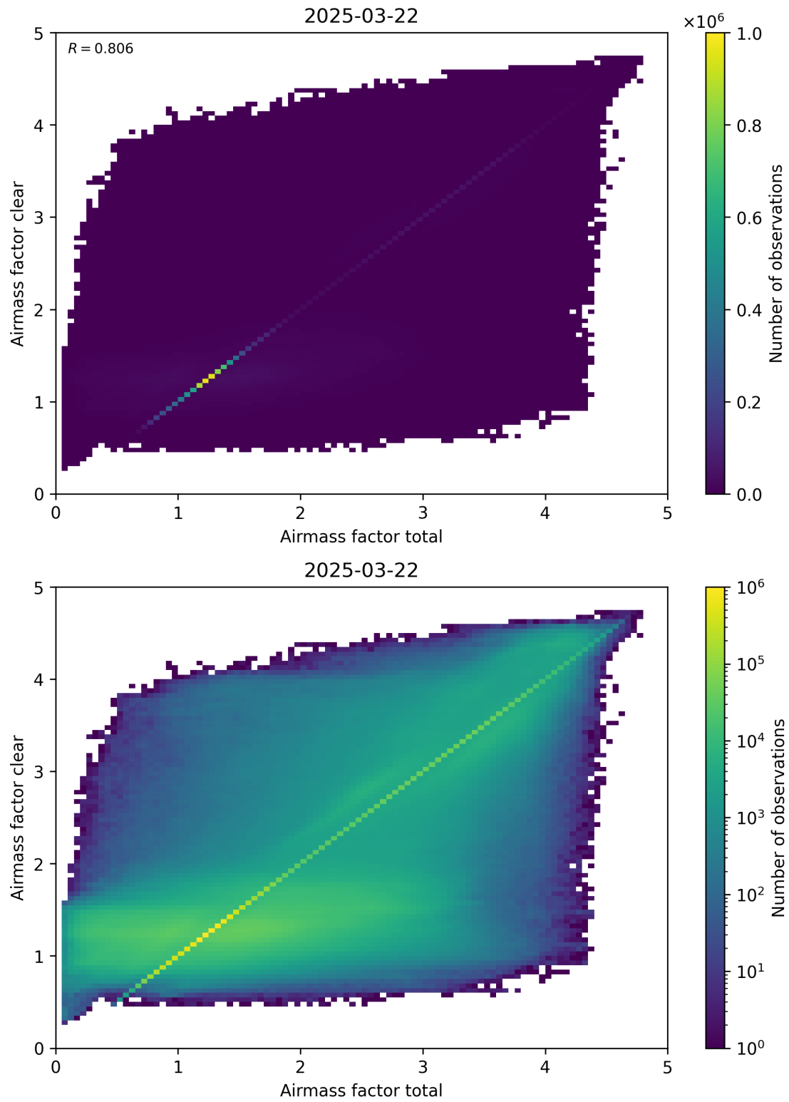
Figure 100: Scatter density plot of “Airmass factor total” against “Airmass factor clear” for 2025-03-21 to 2025-03-23.
