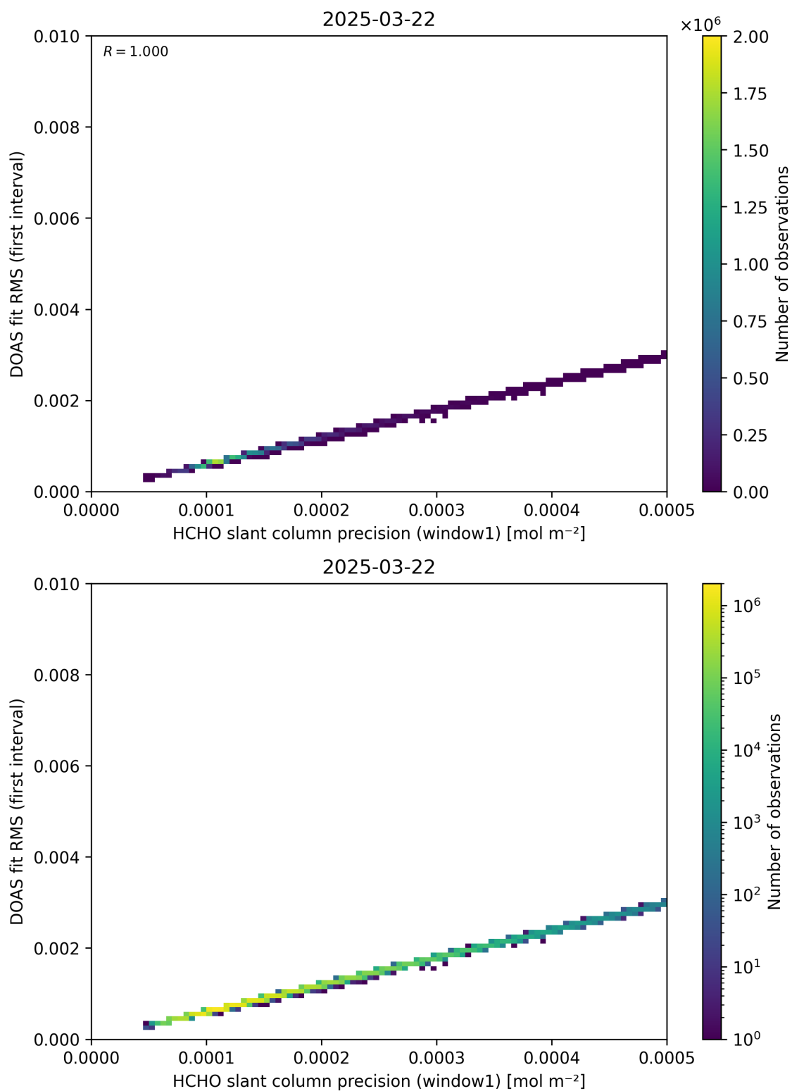
Figure 88: Scatter density plot of “HCHO slant column precision (window1)” against “DOAS fit RMS (first interval)” for 2025-03-21 to 2025-03-23.
