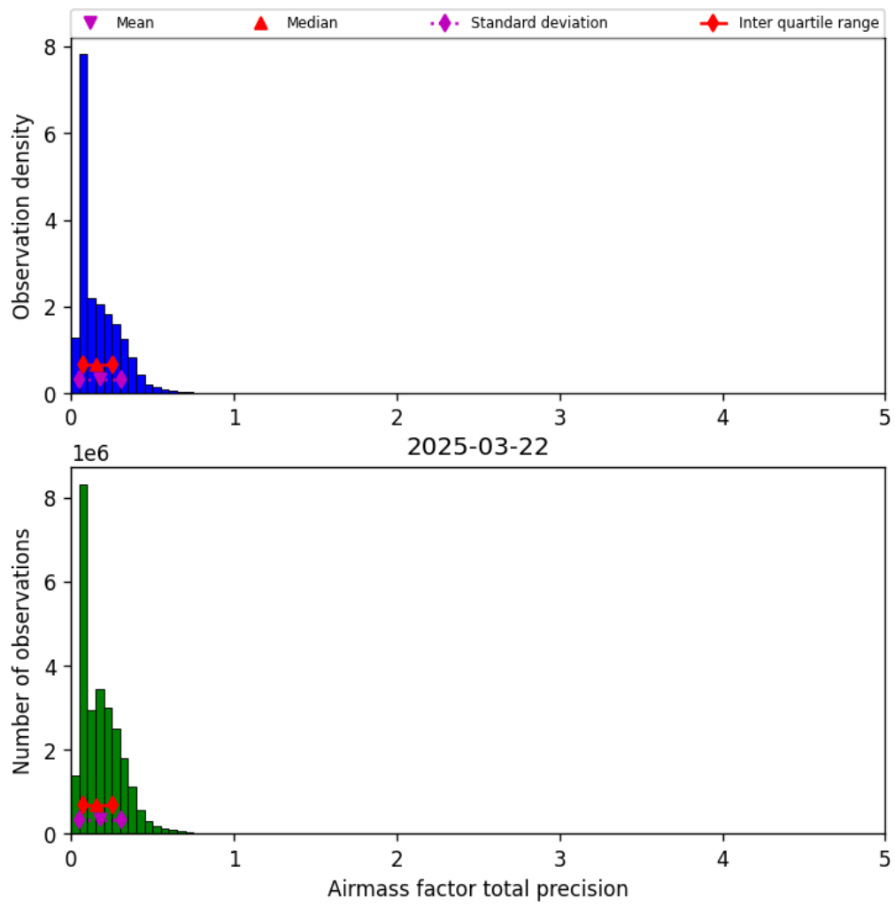
Figure 41: Histogram of “Airmass factor total precision” for 2025-03-21 to 2025-03-23
