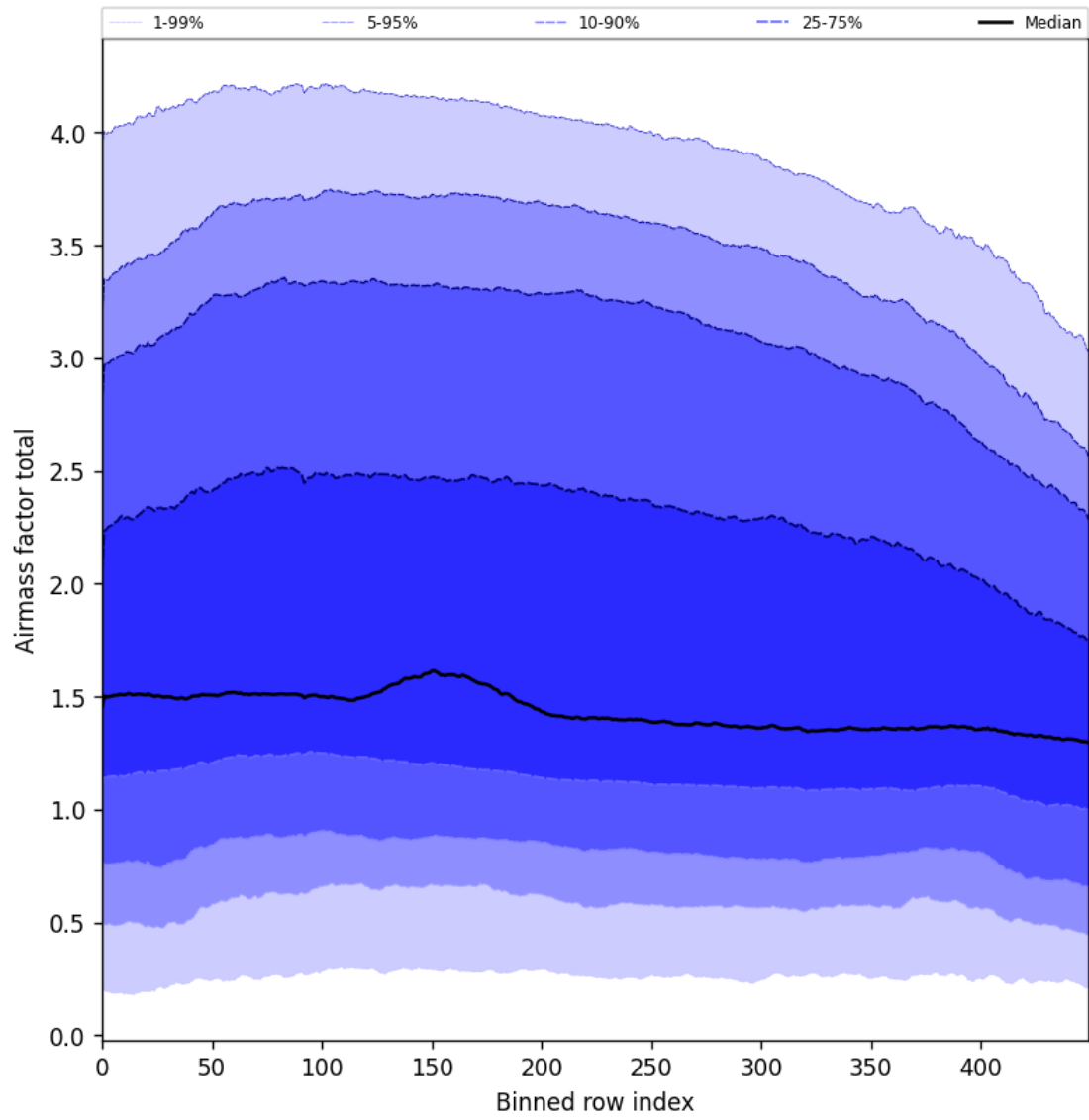
Figure 54: Along track statistics of “Airmass factor total” for 2025-03-21 to 2025-03-23
