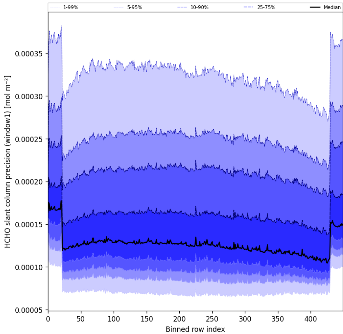
Figure 53: Along track statistics of “HCHO slant column precision (window1)” for 2025-03-21 to 2025-03-23
