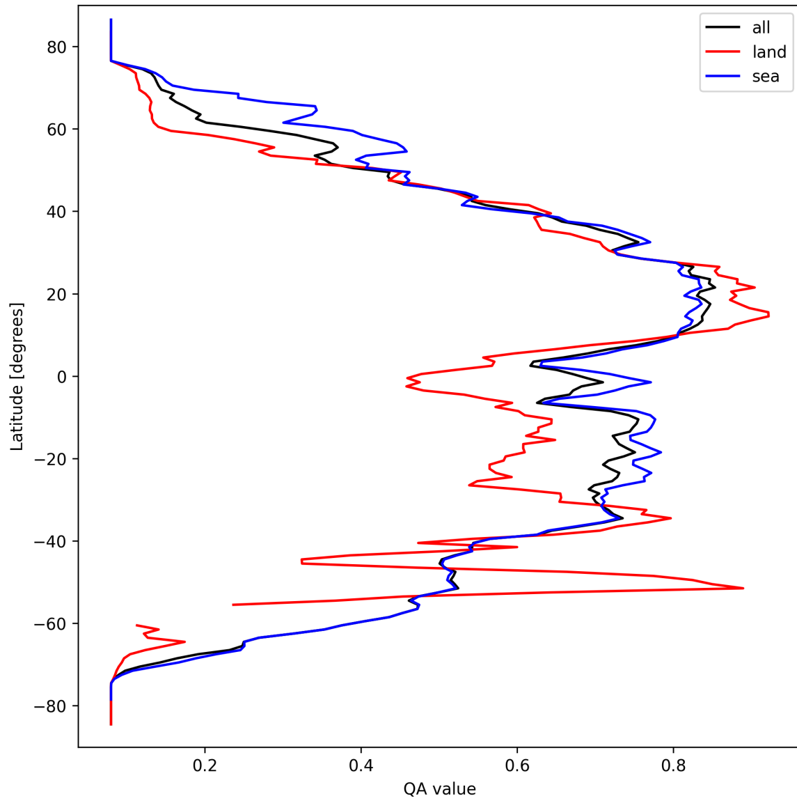
Figure 20: Zonal average of “QA value” for 2025-03-21 to 2025-03-23.
