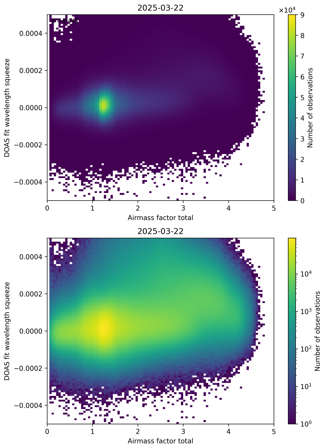
Figure 99: Scatter density plot of “Airmass factor total” against “DOAS fit wavelength squeeze” for 2025-03-21 to 2025-03-23.
