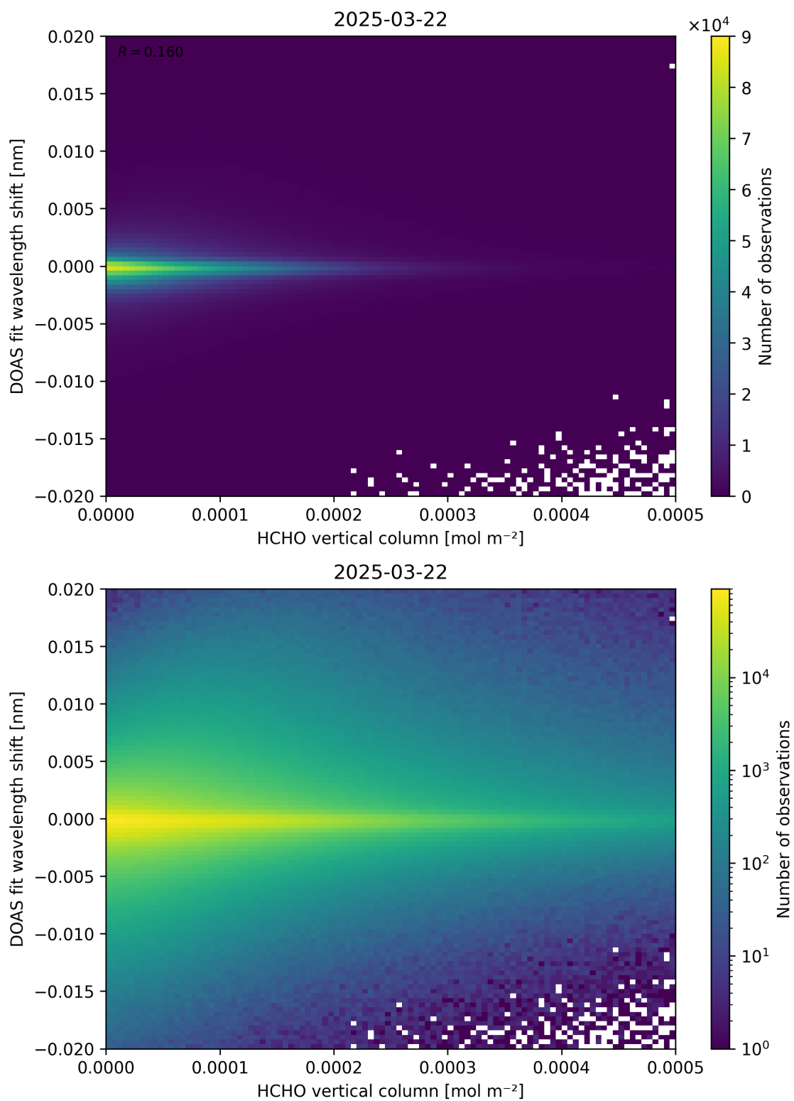
Figure 124: Scatter density plot of “HCHO vertical column” against “DOAS fit wavelength shift” for 2025-03-21 to 2025-03-23.
