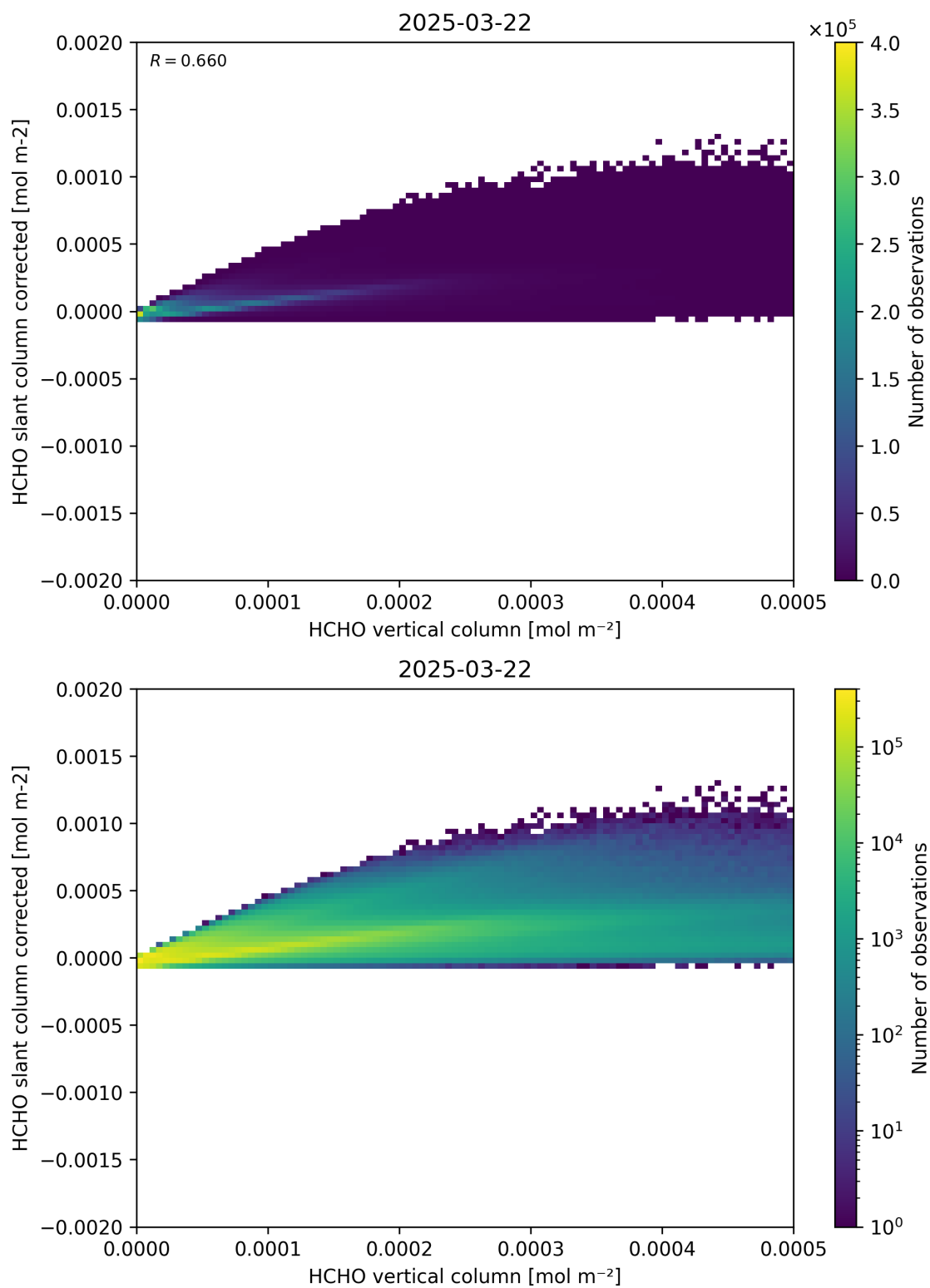
Figure 127: Scatter density plot of “HCHO vertical column” against “HCHO slant column corrected” for 2025-03-21 to 2025-03-23.
