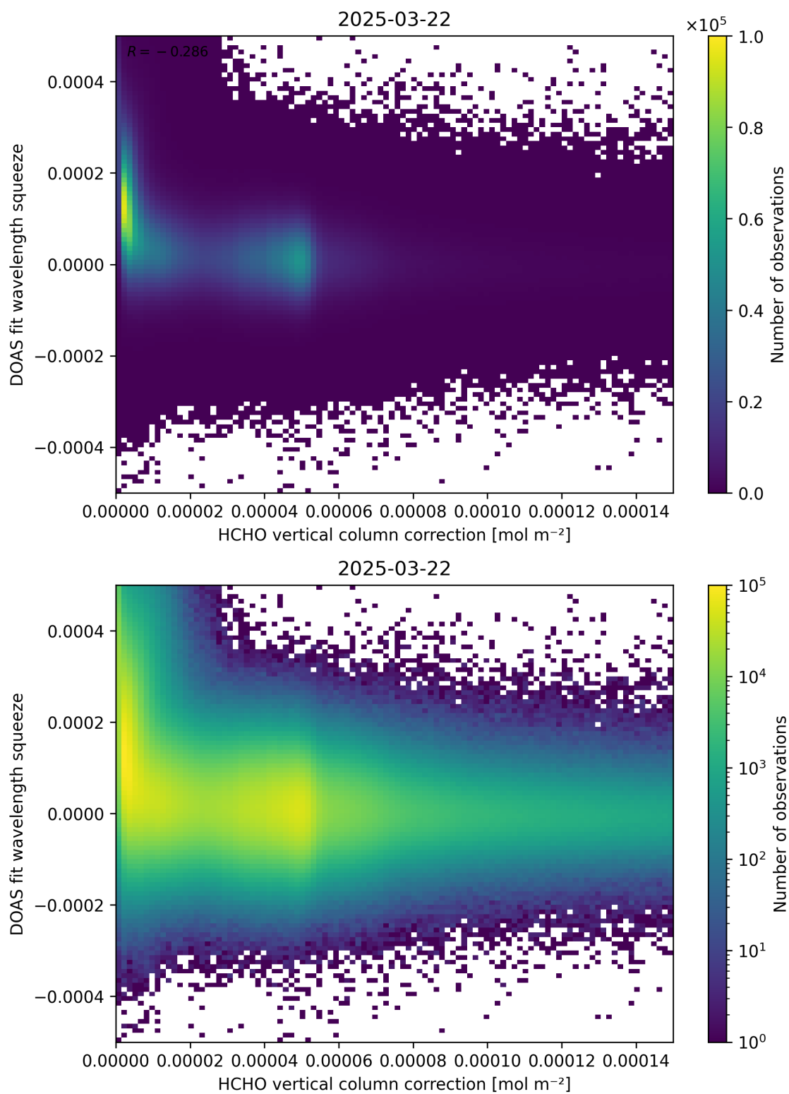
Figure 114: Scatter density plot of “HCHO vertical column correction” against “DOAS fit wavelength squeeze” for 2025-03-21 to 2025-03-23.
