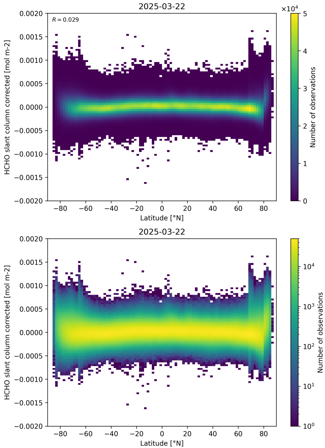
Figure 157: Scatter density plot of “Latitude” against “HCHO slant column corrected” for 2025-03-21 to 2025-03-23.
