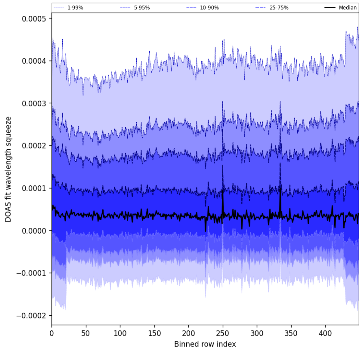
Figure 59: Along track statistics of “DOAS fit wavelength squeeze” for 2025-03-21 to 2025-03-23
