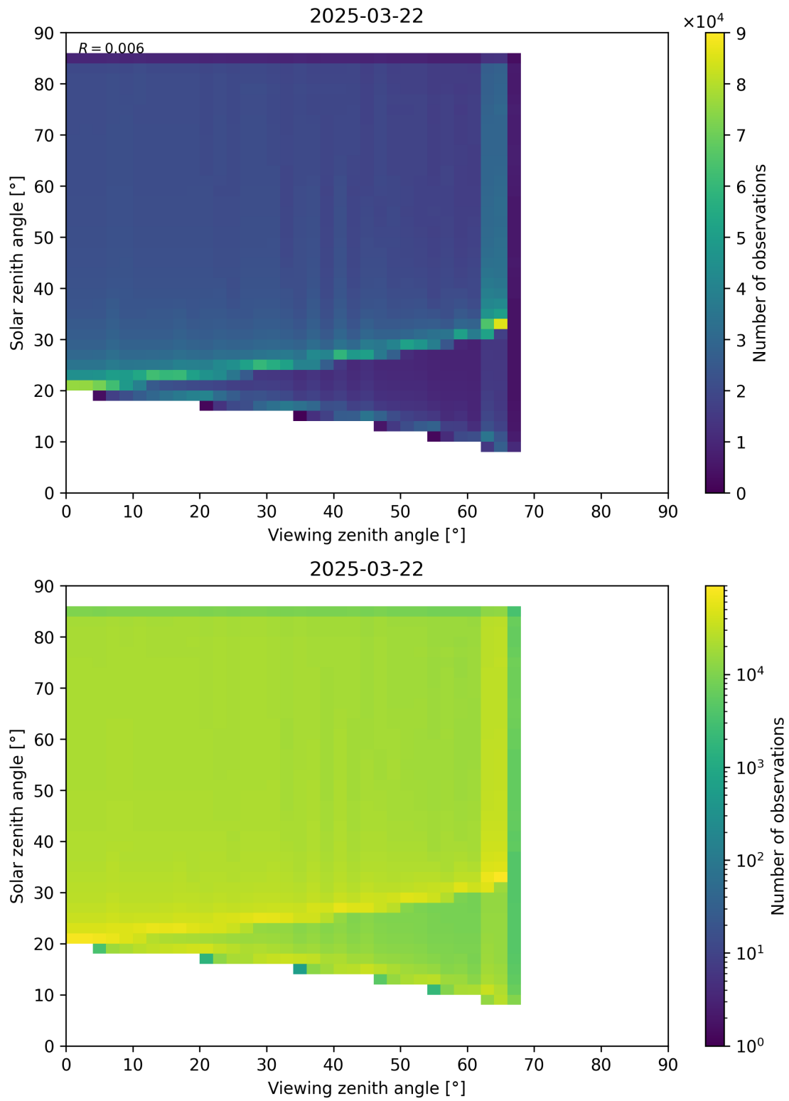
Figure 197: Scatter density plot of “Viewing zenith angle” against “Solar zenith angle” for 2025-03-21 to 2025-03-23.
