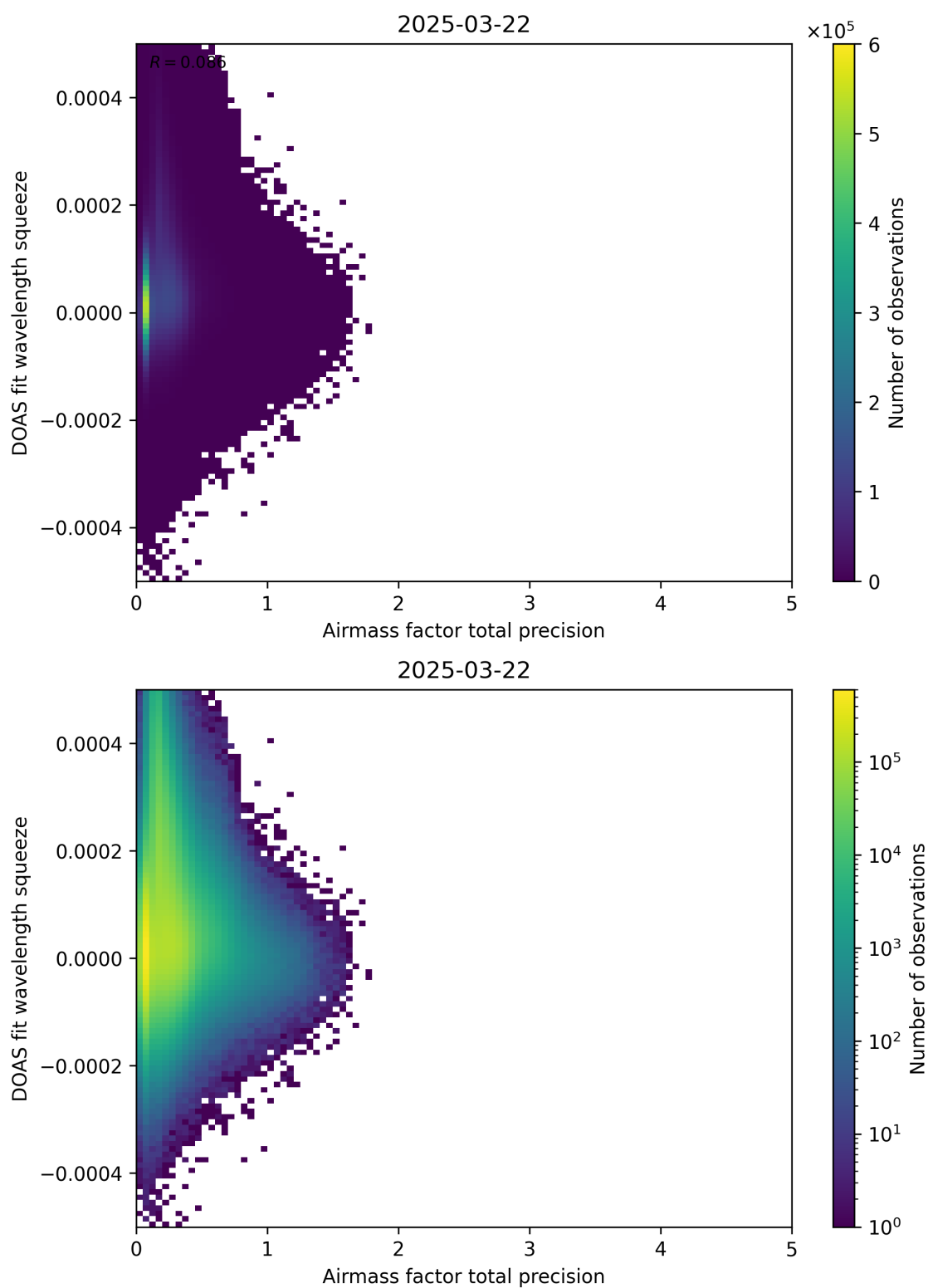
Figure 107: Scatter density plot of “Airmass factor total precision” against “DOAS fit wavelength squeeze” for 2025-03-21 to 2025-03-23.
