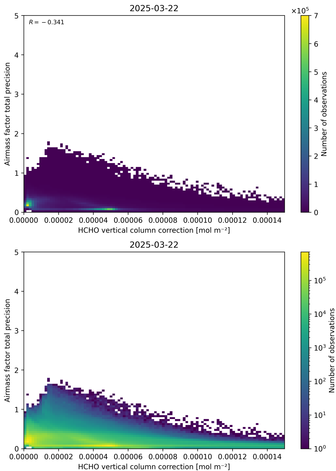
Figure 121: Scatter density plot of “HCHO vertical column correction” against “Airmass factor total precision” for 2025-03-21 to 2025-03-23.
