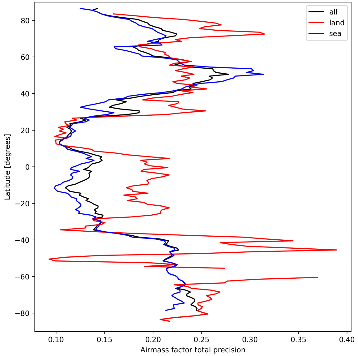
Figure 27: Zonal average of “Airmass factor total precision” for 2025-03-21 to 2025-03-23.
