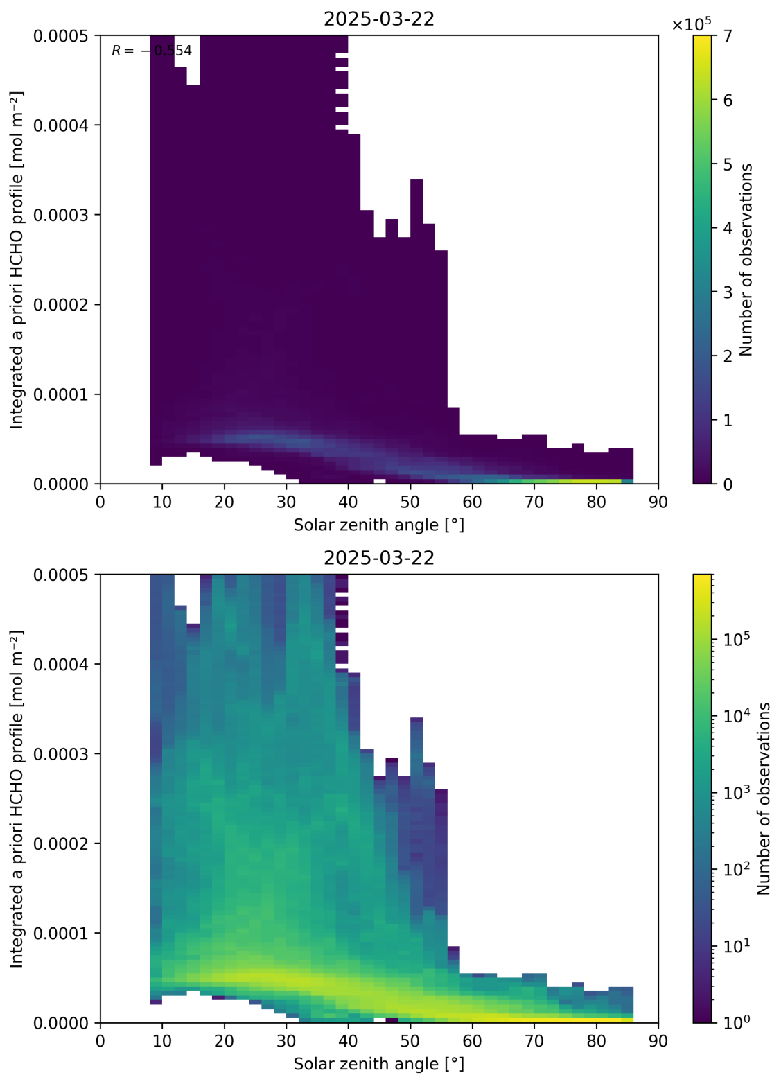
Figure 180: Scatter density plot of “Solar zenith angle” against “Integrated a priori HCHO profile” for 2025-03-21 to 2025-03-23.
