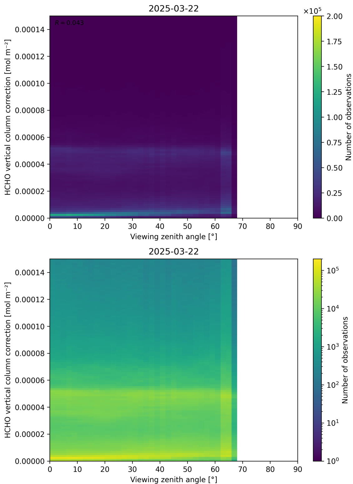
Figure 193: Scatter density plot of “Viewing zenith angle” against “HCHO vertical column correction” for 2025-03-21 to 2025-03-23.
