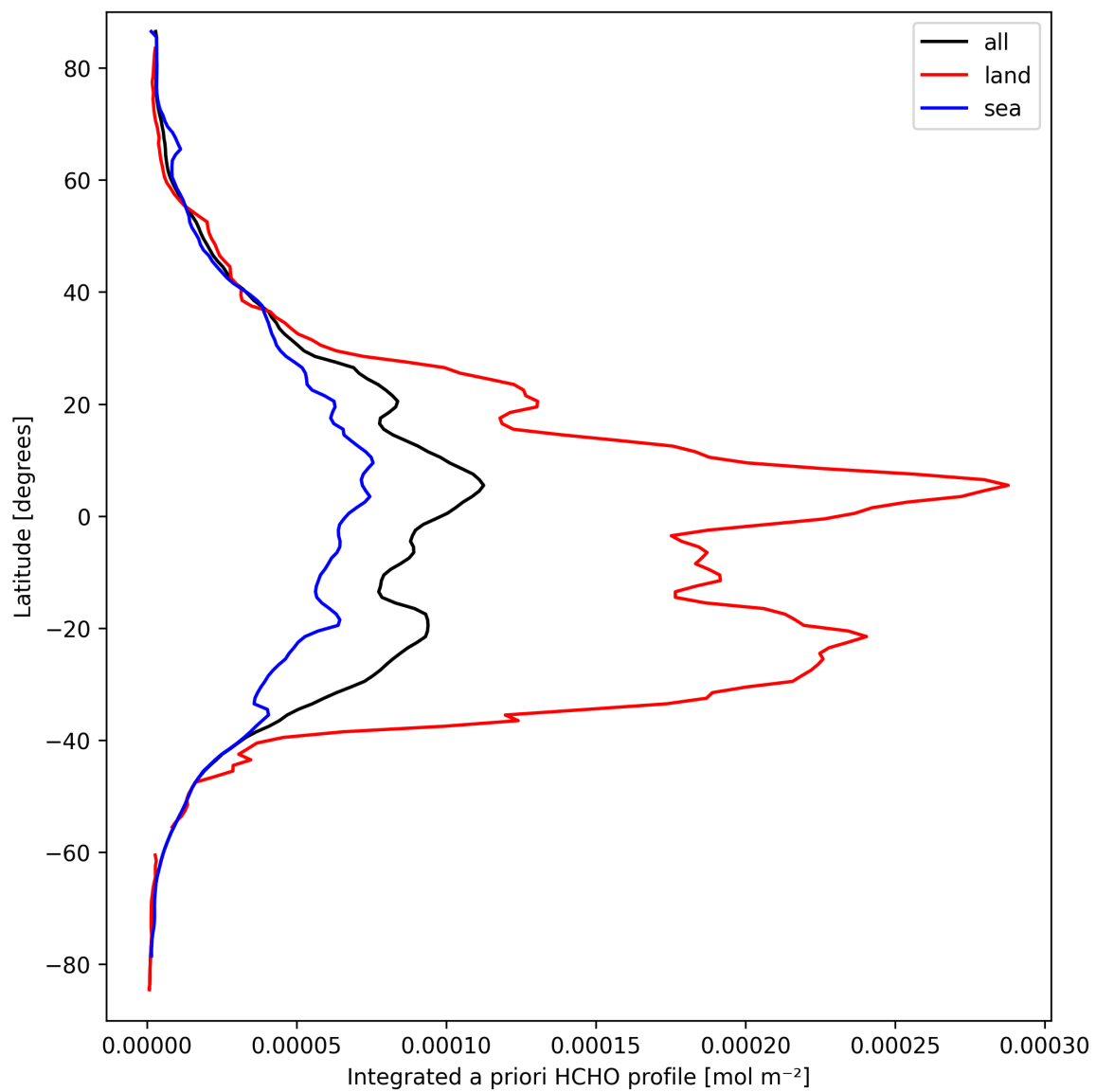
Figure 29: Zonal average of “Integrated a priori HCHO profile” for 2025-03-21 to 2025-03-23.
