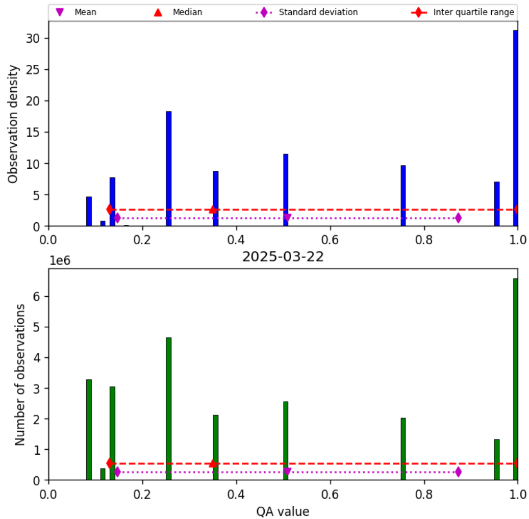
Figure 34: Histogram of “QA value” for 2025-03-21 to 2025-03-23
