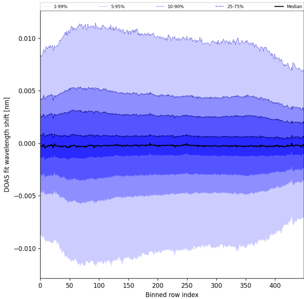
Figure 58: Along track statistics of “DOAS fit wavelength shift” for 2025-03-21 to 2025-03-23
