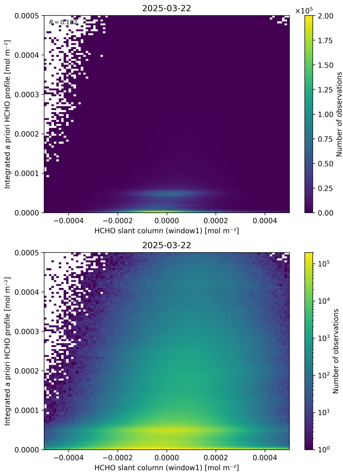
Figure 87: Scatter density plot of “HCHO slant column (window1)” against “Integrated a priori HCHO profile” for 2025-03-21 to 2025-03-23.
