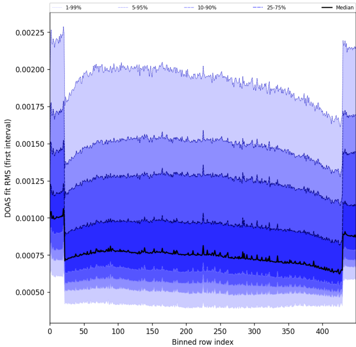
Figure 60: Along track statistics of “DOAS fit RMS (first interval)” for 2025-03-21 to 2025-03-23
