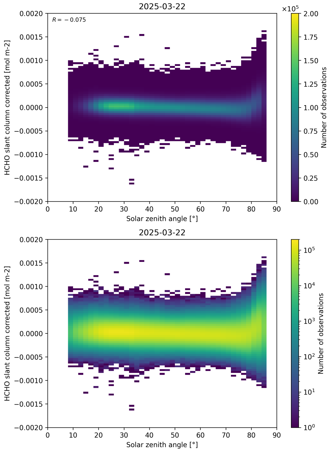
Figure 171: Scatter density plot of “Solar zenith angle” against “HCHO slant column corrected” for 2025-03-21 to 2025-03-23.
