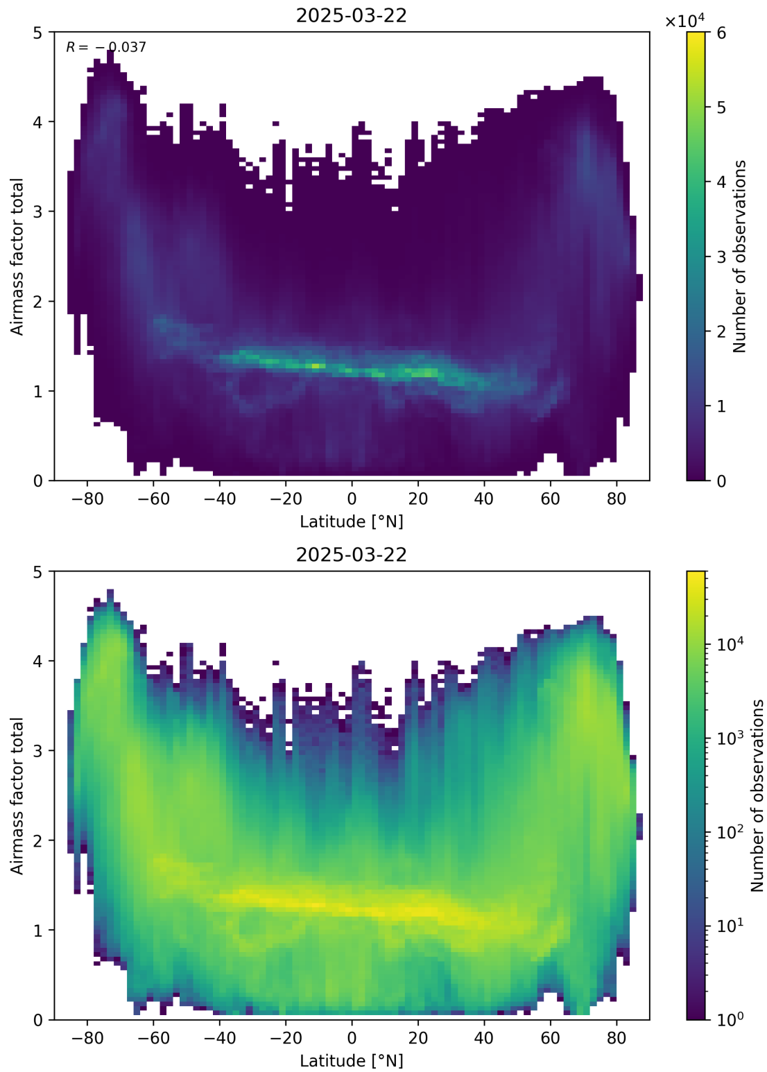
Figure 161: Scatter density plot of “Latitude” against “Airmass factor total” for 2025-03-21 to 2025-03-23.
