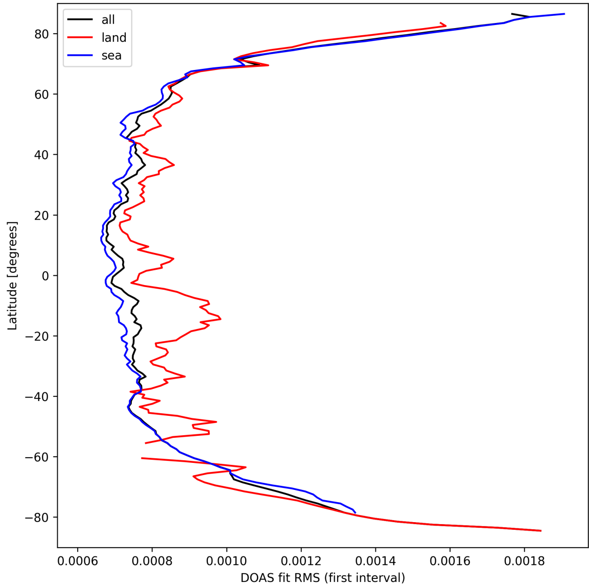
Figure 32: Zonal average of “DOAS fit RMS (first interval)” for 2025-03-21 to 2025-03-23.
