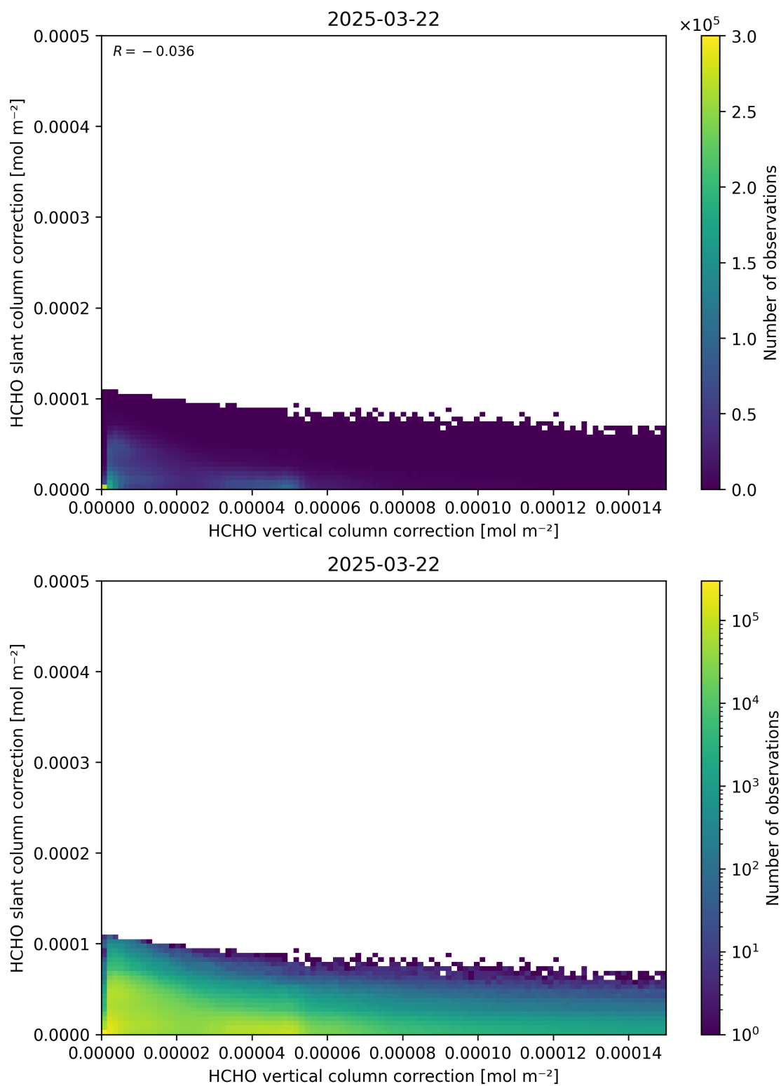
Figure 117: Scatter density plot of “HCHO vertical column correction” against “HCHO slant column correction” for 2025-03-21 to 2025-03-23.
