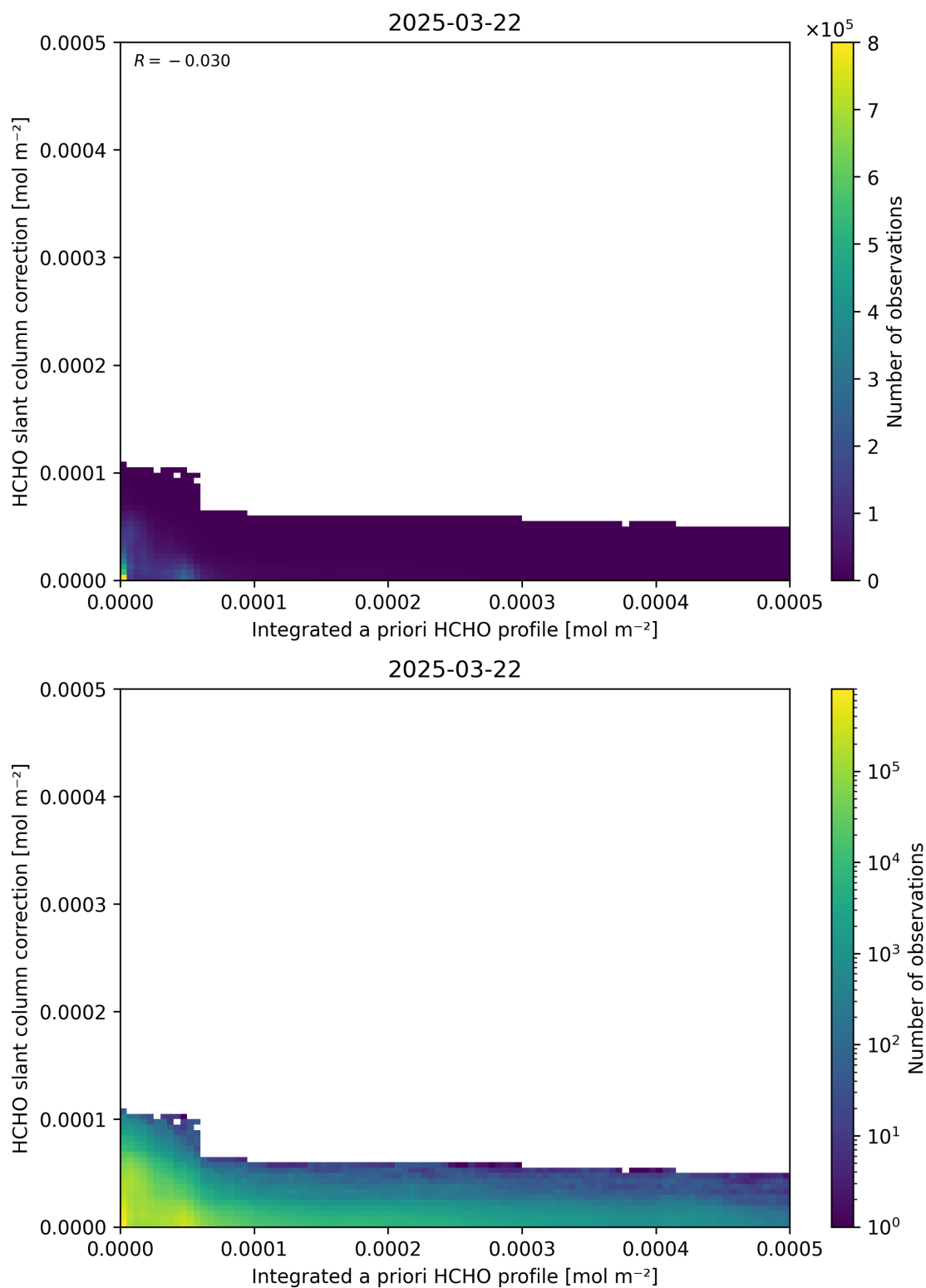
Figure 152: Scatter density plot of “Integrated a priori HCHO profile” against “HCHO slant column correction” for 2025-03-21 to 2025-03-23.
