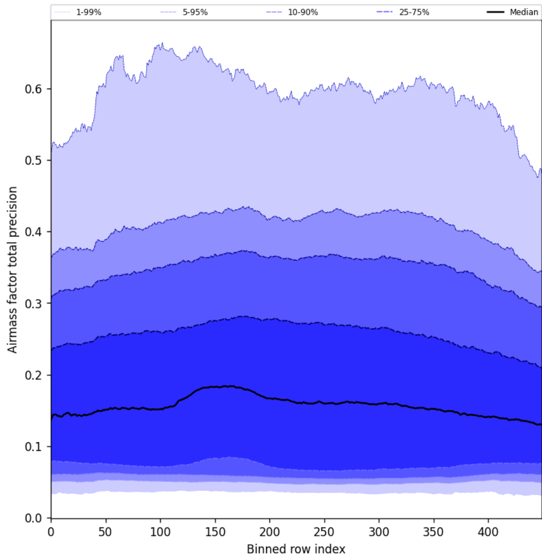
Figure 55: Along track statistics of “Airmass factor total precision” for 2025-03-21 to 2025-03-23
