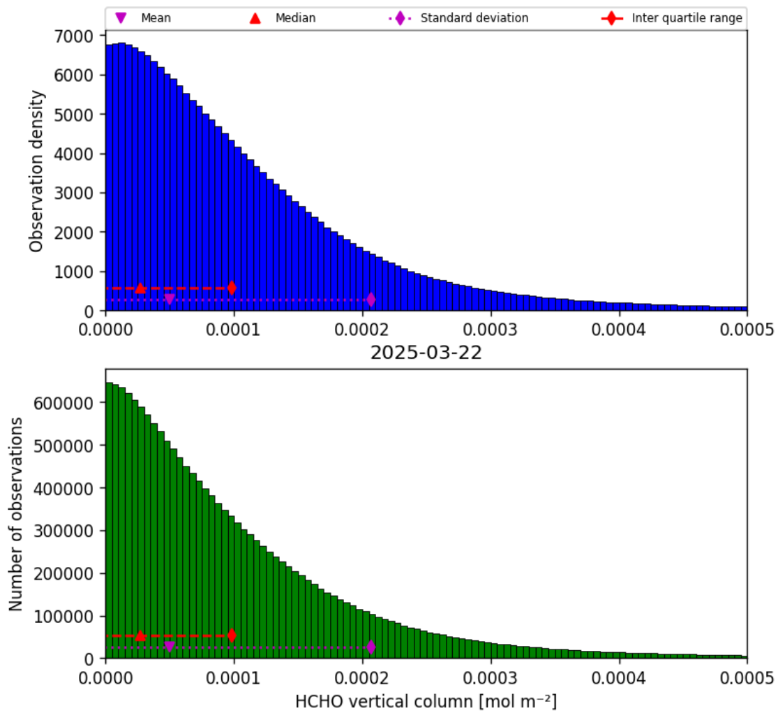
Figure 35: Histogram of “HCHO vertical column” for 2025-03-21 to 2025-03-23
