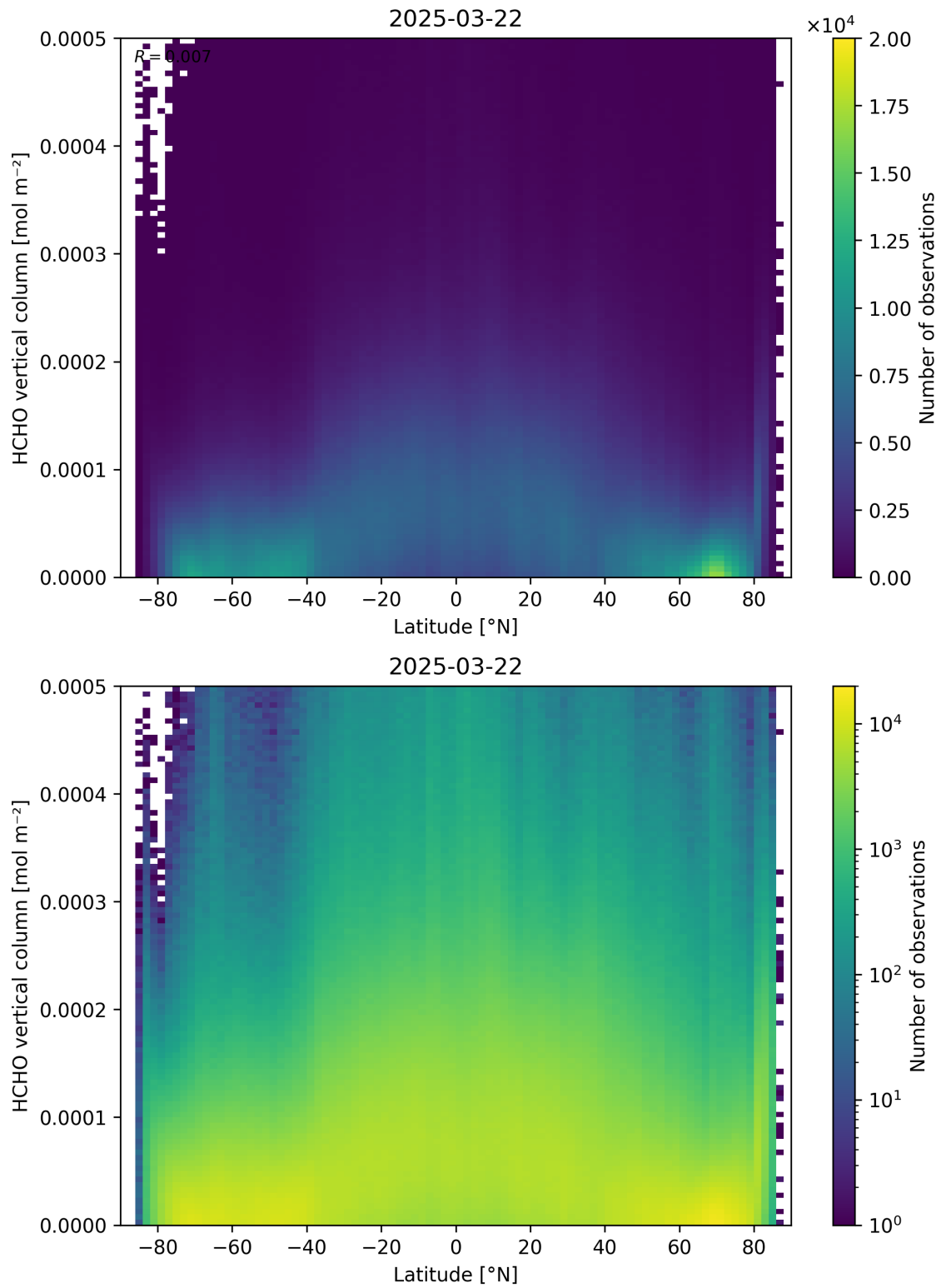
Figure 163: Scatter density plot of “Latitude” against “HCHO vertical column” for 2025-03-21 to 2025-03-23.
