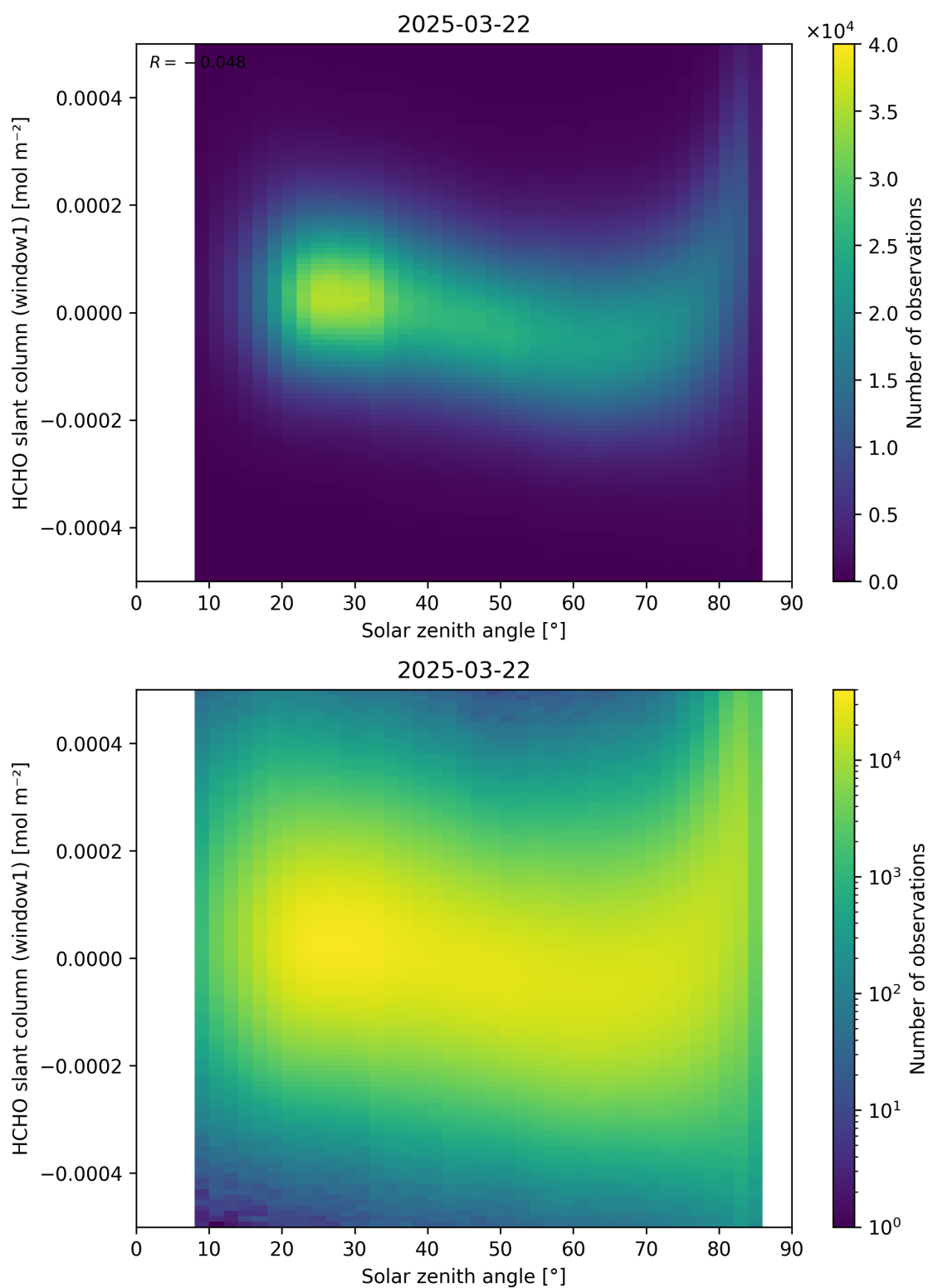
Figure 173: Scatter density plot of “Solar zenith angle” against “HCHO slant column (window1)” for 2025-03-21 to 2025-03-23.
