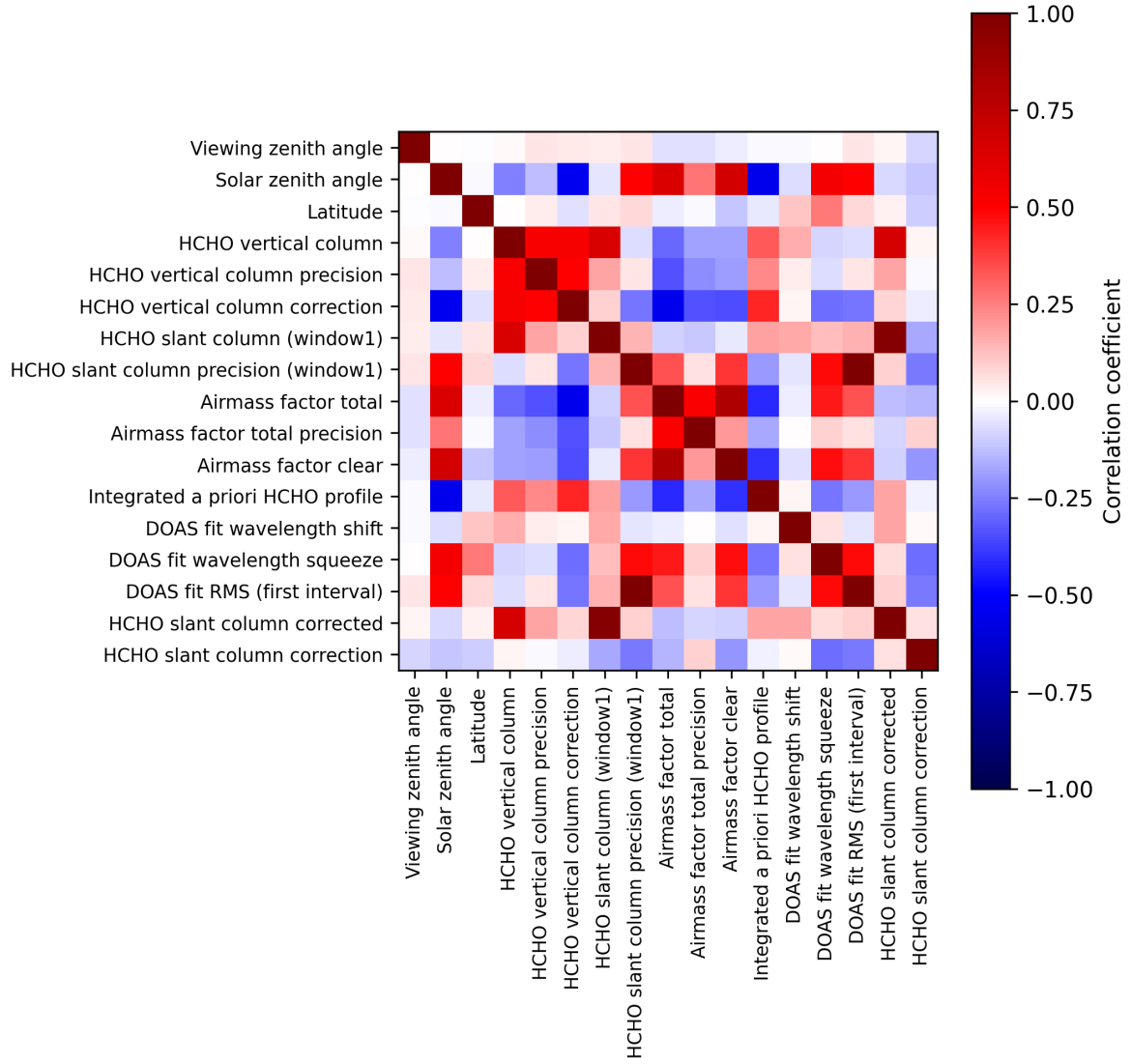
Figure 2: Map of correlation matrix for 2025-03-21 to 2025-03-23.
