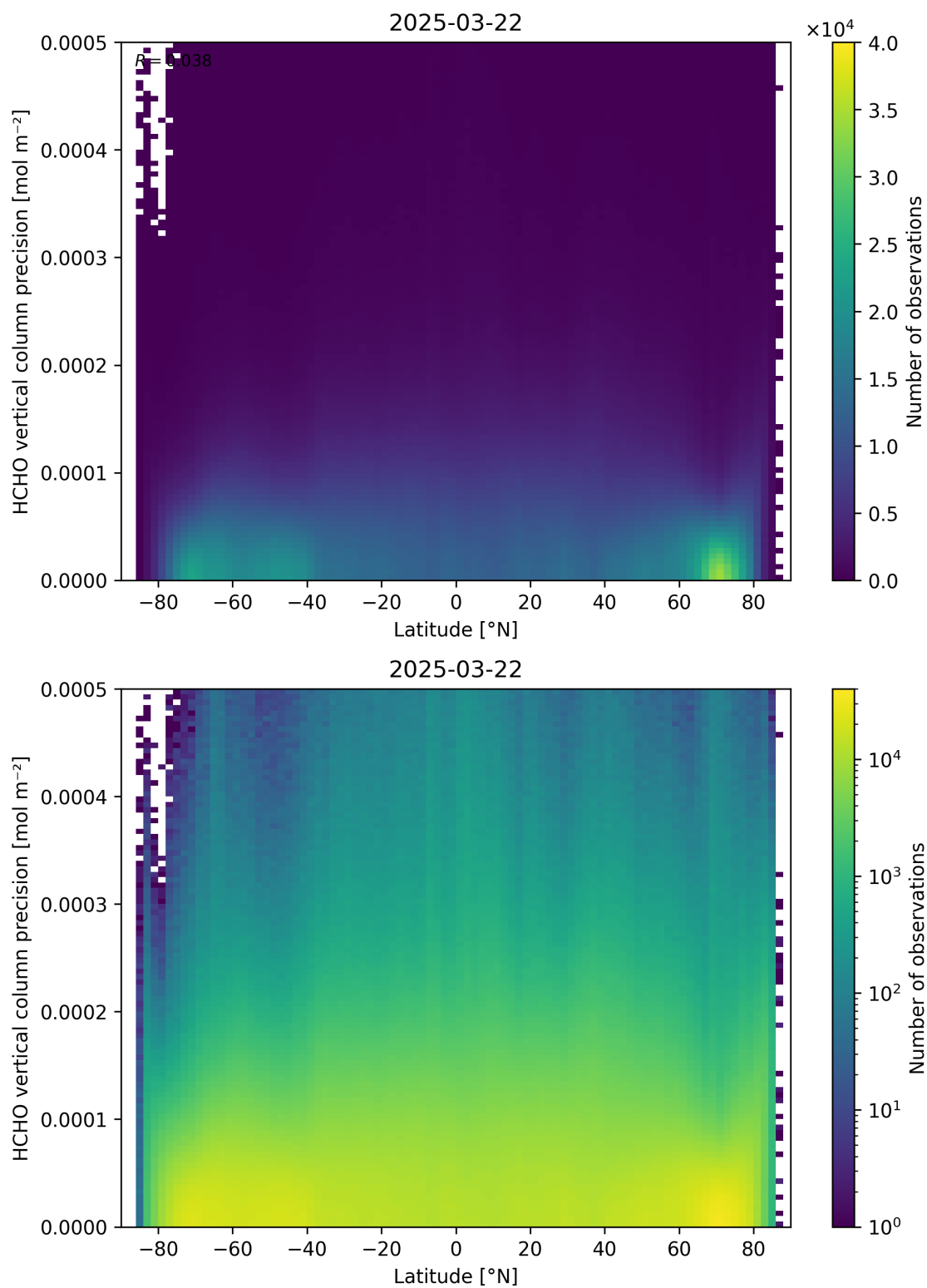
Figure 165: Scatter density plot of “Latitude” against “HCHO vertical column precision” for 2025-03-21 to 2025-03-23.
