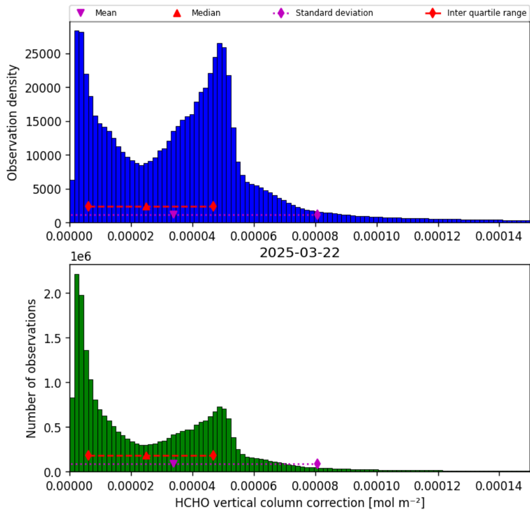
Figure 37: Histogram of “HCHO vertical column correction” for 2025-03-21 to 2025-03-23
