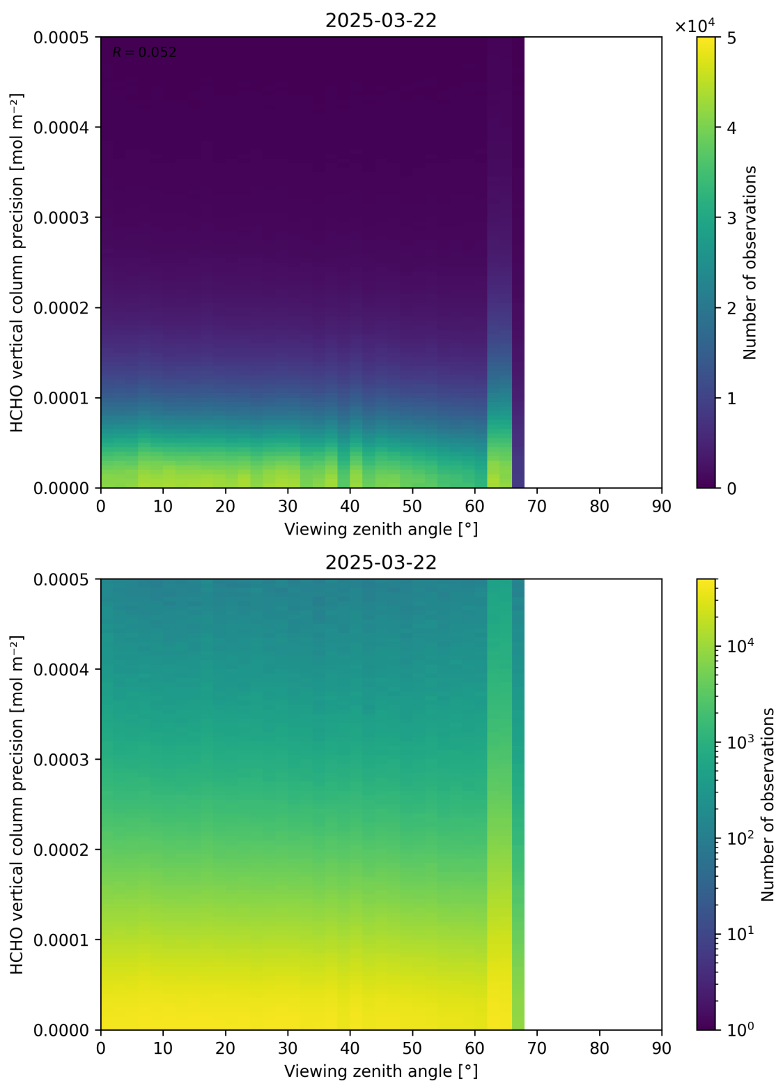
Figure 194: Scatter density plot of “Viewing zenith angle” against “HCHO vertical column precision” for 2025-03-21 to 2025-03-23.
