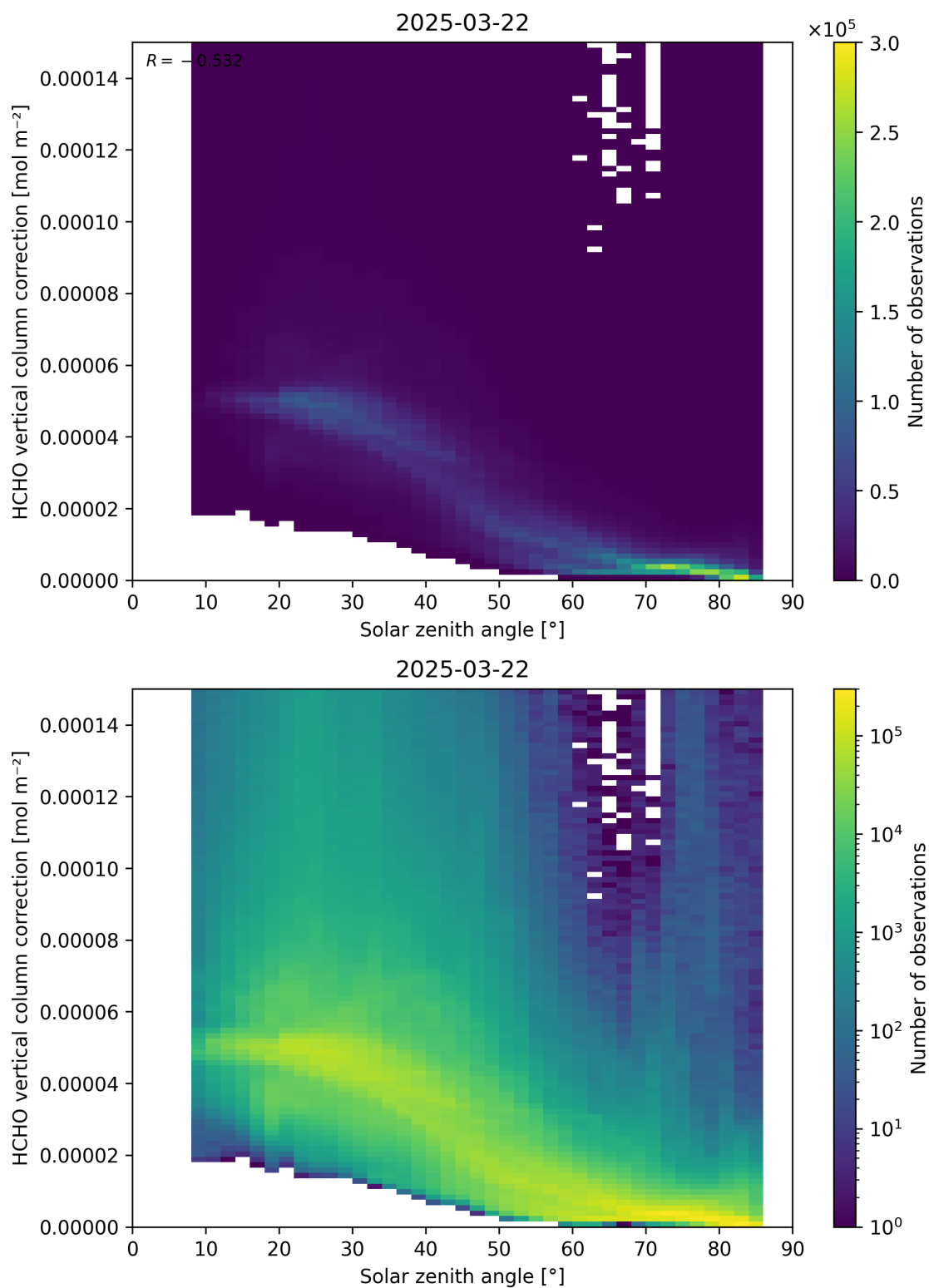
Figure 178: Scatter density plot of “Solar zenith angle” against “HCHO vertical column correction” for 2025-03-21 to 2025-03-23.
