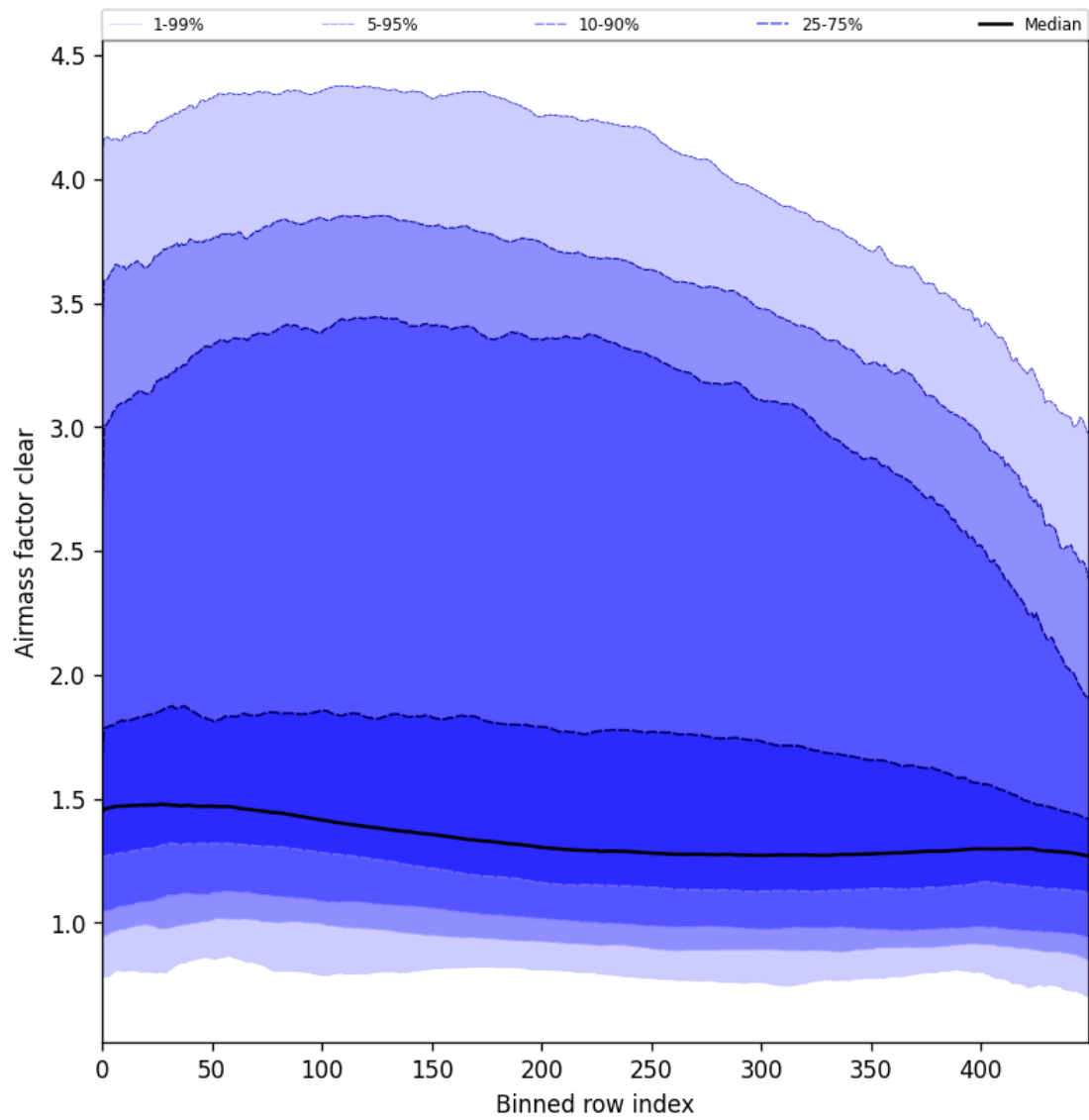
Figure 56: Along track statistics of “Airmass factor clear” for 2025-03-21 to 2025-03-23
