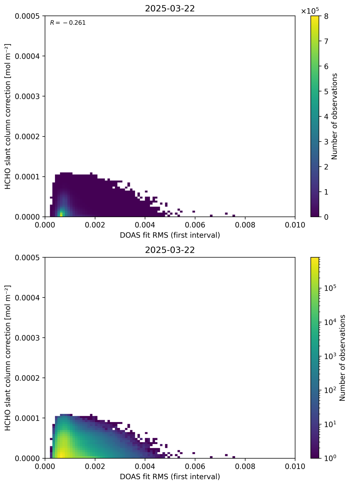
Figure 63: Scatter density plot of “DOAS fit RMS (first interval)” against “HCHO slant column correction” for 2025-03-21 to 2025-03-23.
