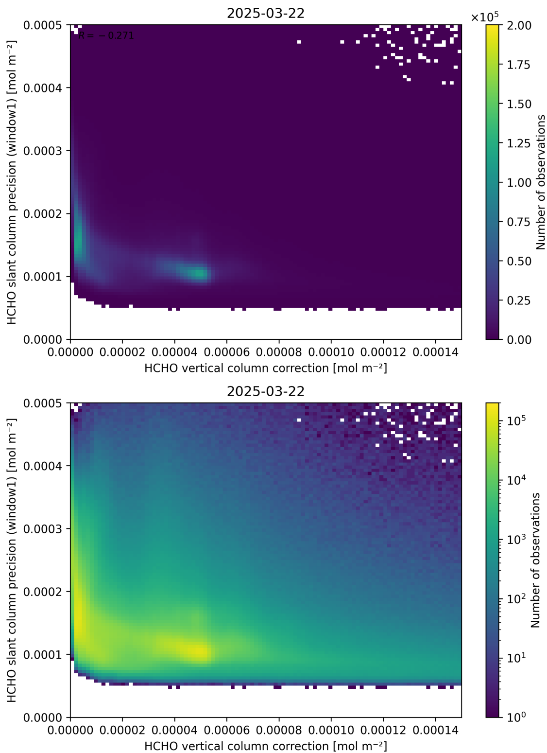
Figure 119: Scatter density plot of “HCHO vertical column correction” against “HCHO slant column precision (window1)” for 2025-03-21 to 2025-03-23.
