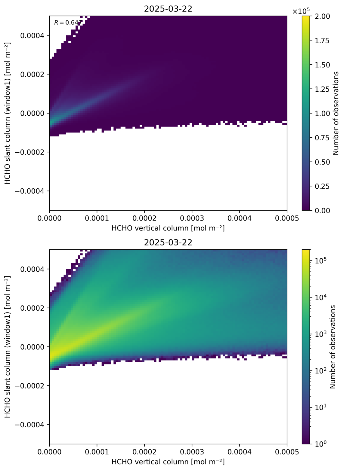
Figure 129: Scatter density plot of “HCHO vertical column” against “HCHO slant column (window1)” for 2025-03-21 to 2025-03-23.
