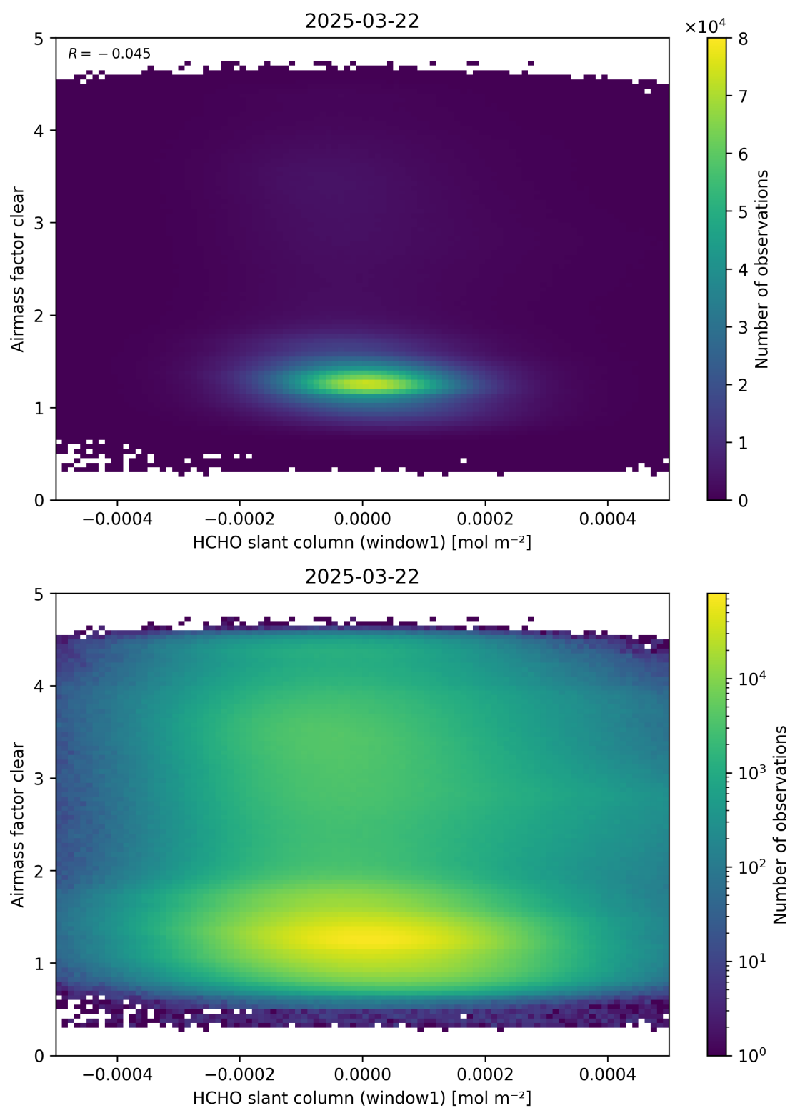
Figure 81: Scatter density plot of “HCHO slant column (window1)” against “Airmass factor clear” for 2025-03-21 to 2025-03-23.
