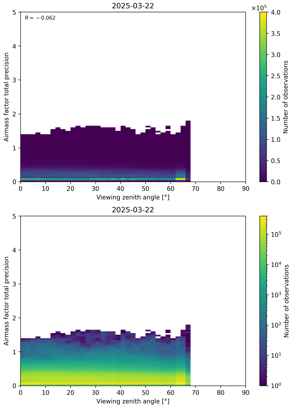
Figure 191: Scatter density plot of “Viewing zenith angle” against “Airmass factor total precision” for 2025-03-21 to 2025-03-23.
