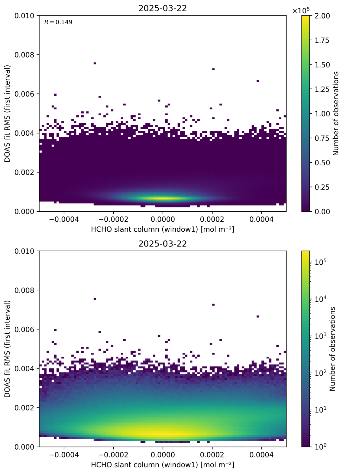
Figure 78: Scatter density plot of “HCHO slant column (window1)” against “DOAS fit RMS (first interval)” for 2025-03-21 to 2025-03-23.
