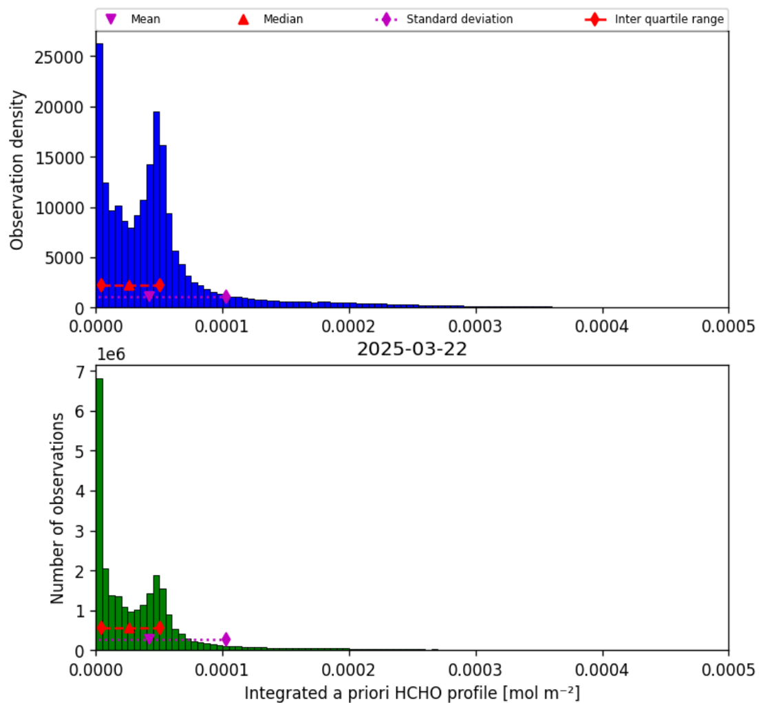
Figure 43: Histogram of “Integrated a priori HCHO profile” for 2025-03-21 to 2025-03-23
