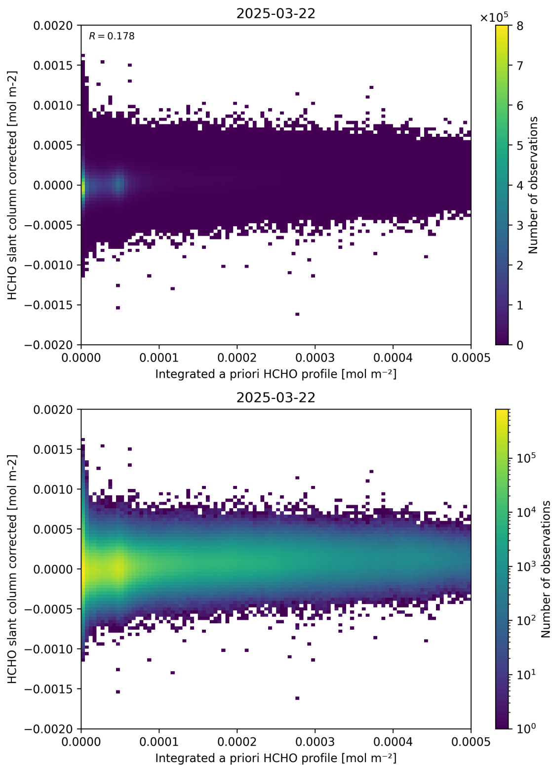
Figure 151: Scatter density plot of “Integrated a priori HCHO profile” against “HCHO slant column corrected” for 2025-03-21 to 2025-03-23.
