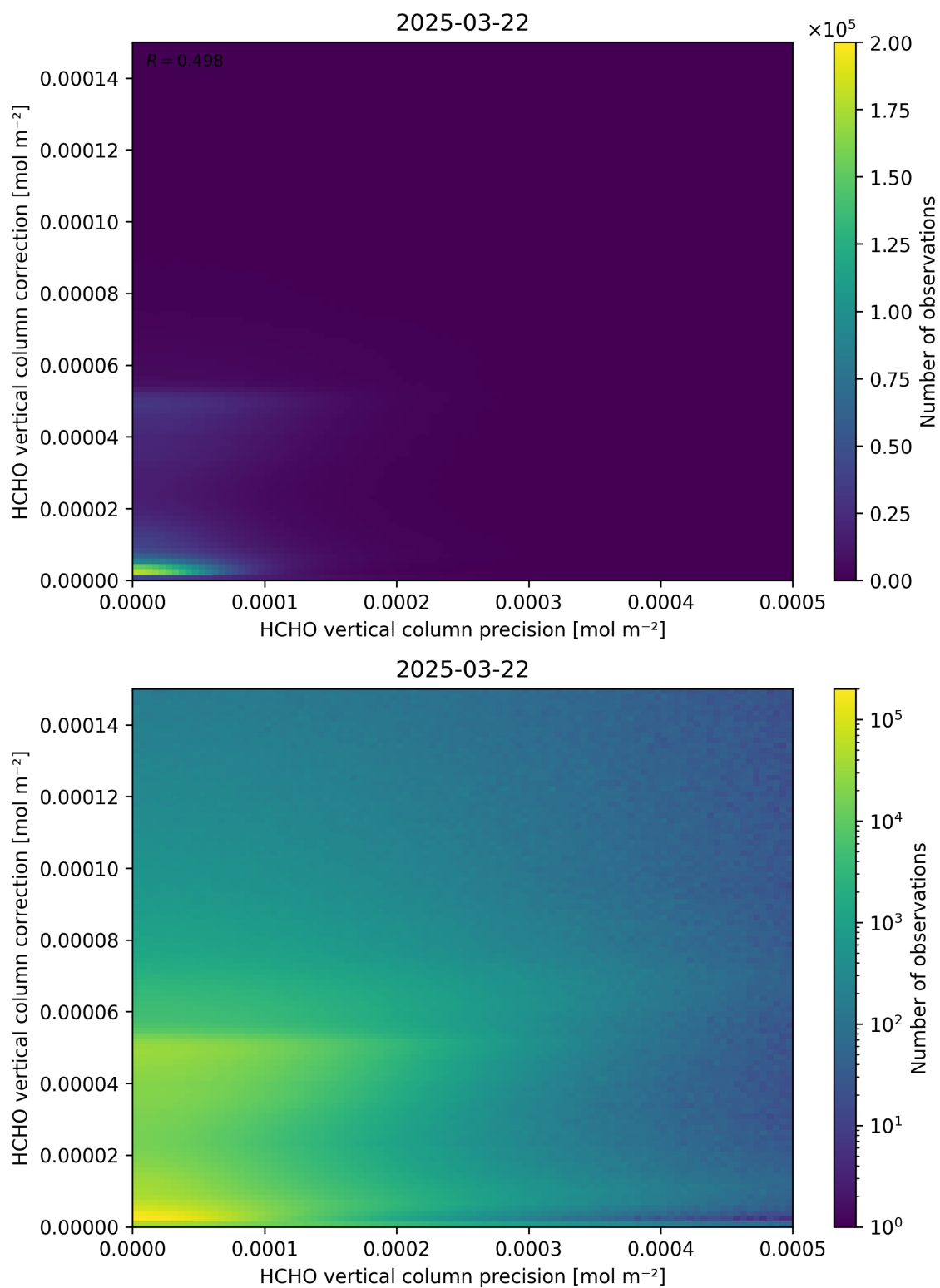
Figure 146: Scatter density plot of “HCHO vertical column precision” against “HCHO vertical column correction” for 2025-03-21 to 2025-03-23.
