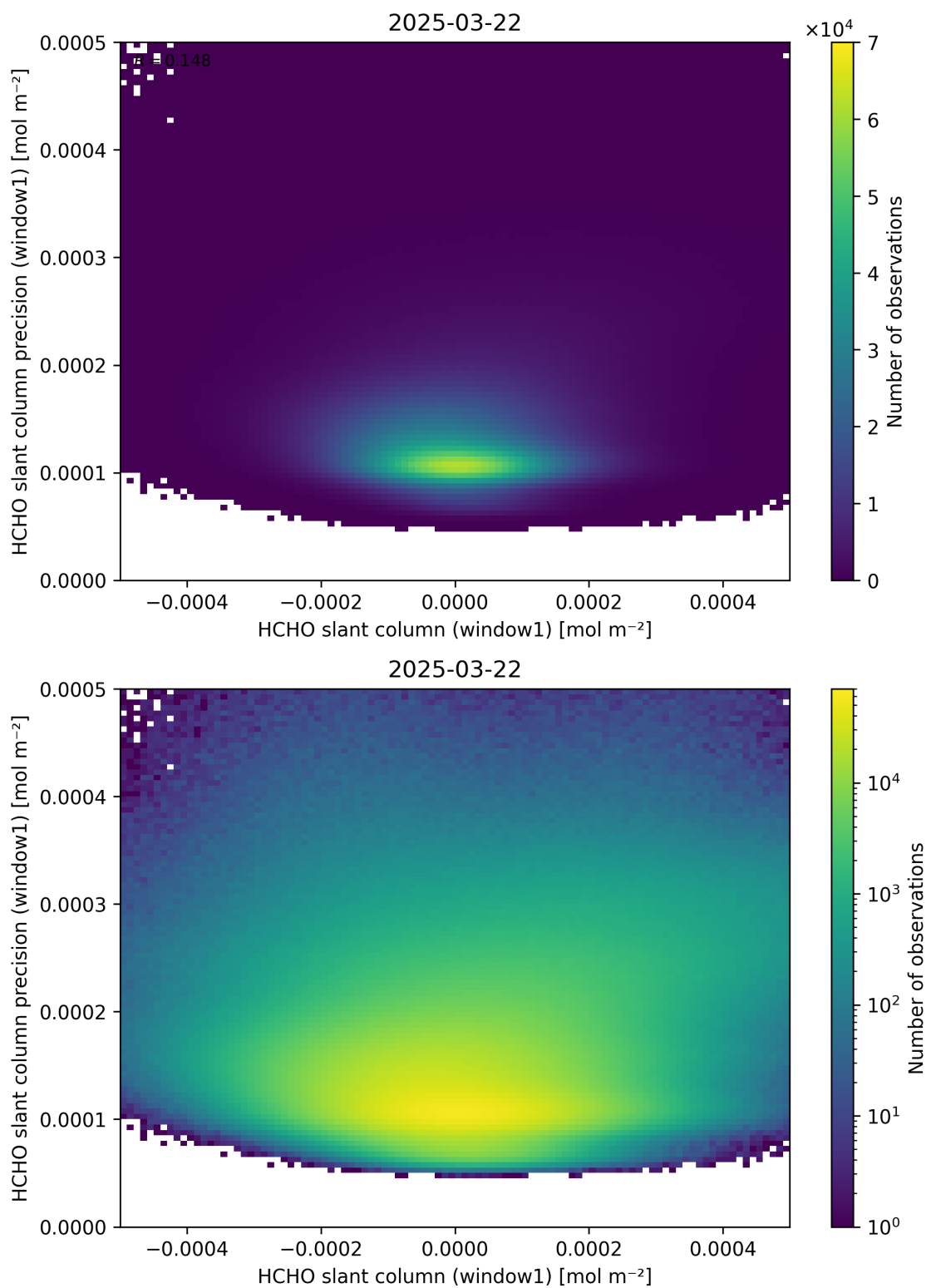
Figure 84: Scatter density plot of “HCHO slant column (window1)” against “HCHO slant column precision (window1)” for 2025-03-21 to 2025-03-23.
