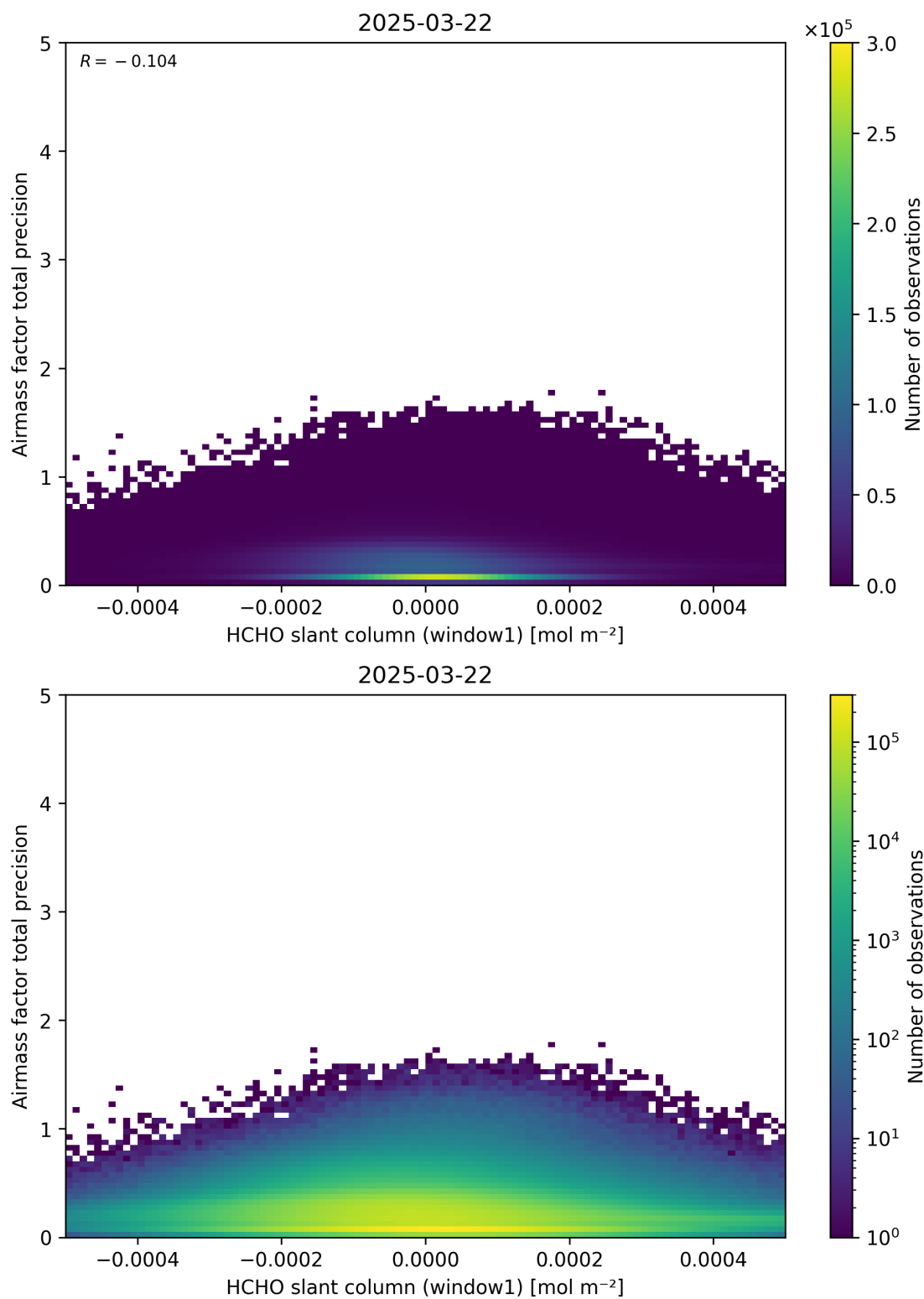
Figure 86: Scatter density plot of “HCHO slant column (window1)” against “Airmass factor total precision” for 2025-03-21 to 2025-03-23.
