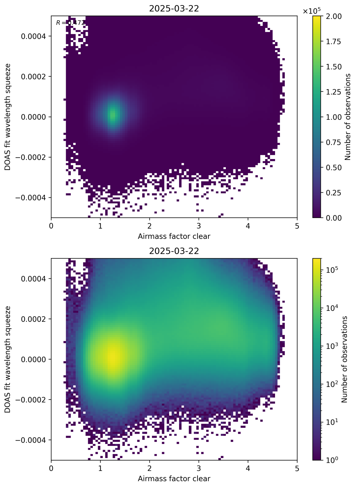
Figure 73: Scatter density plot of “Airmass factor clear” against “DOAS fit wavelength squeeze” for 2025-03-21 to 2025-03-23.
