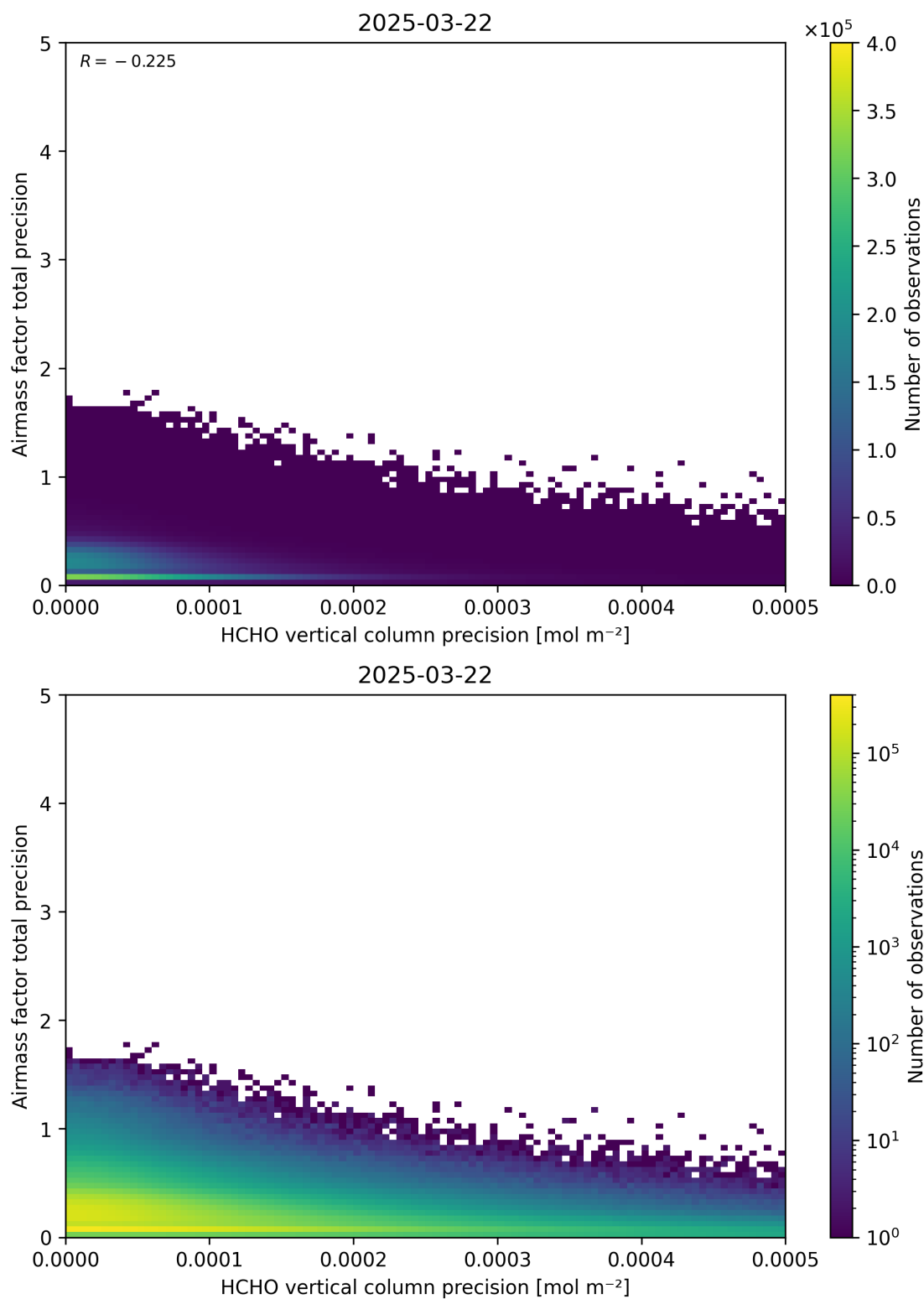
Figure 145: Scatter density plot of “HCHO vertical column precision” against “Airmass factor total precision” for 2025-03-21 to 2025-03-23.
