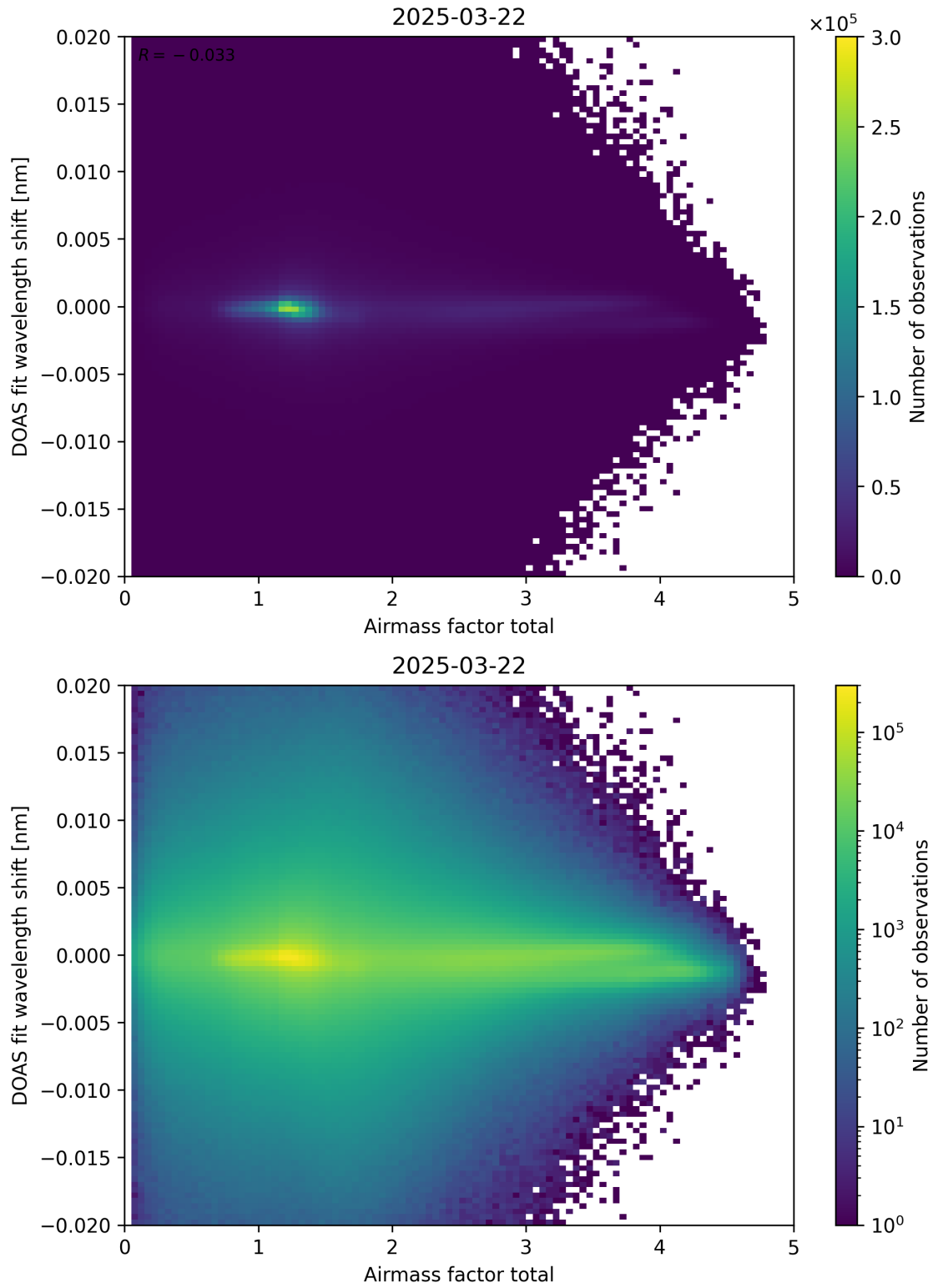
Figure 98: Scatter density plot of “Airmass factor total” against “DOAS fit wavelength shift” for 2025-03-21 to 2025-03-23.
