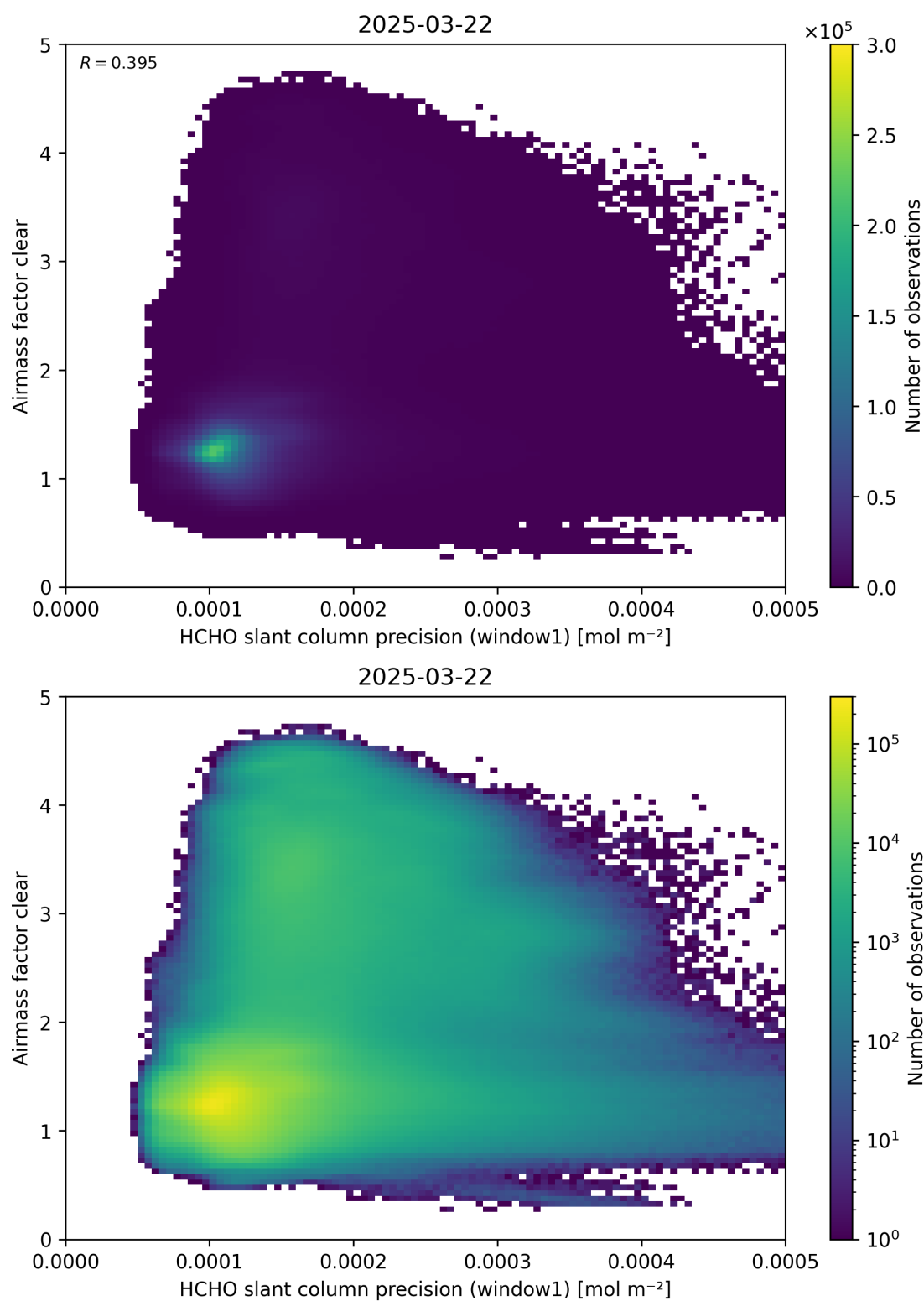
Figure 91: Scatter density plot of “HCHO slant column precision (window1)” against “Airmass factor clear” for 2025-03-21 to 2025-03-23.
