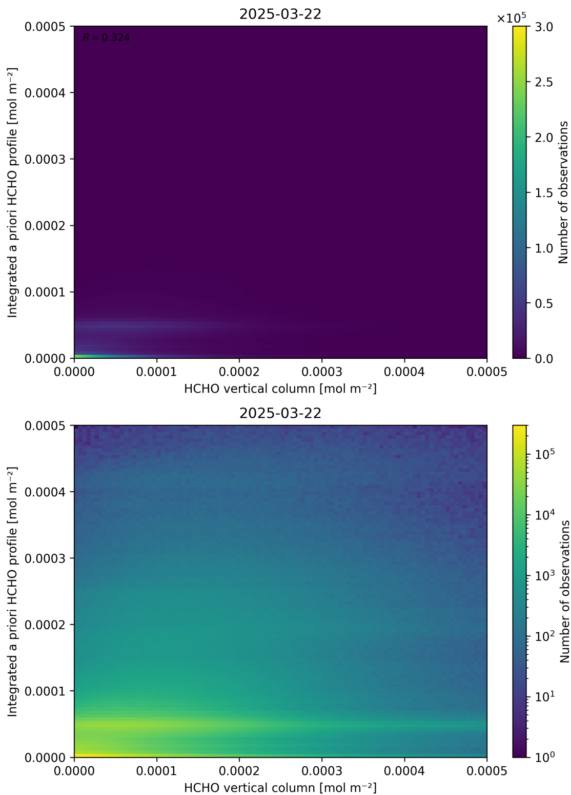
Figure 135: Scatter density plot of “HCHO vertical column” against “Integrated a priori HCHO profile” for 2025-03-21 to 2025-03-23.
