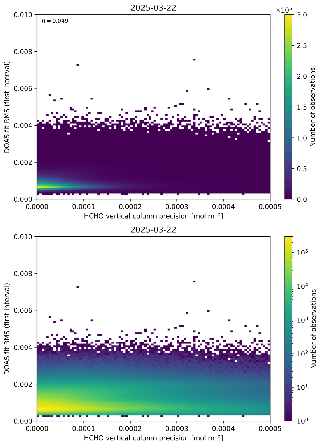
Figure 136: Scatter density plot of “HCHO vertical column precision” against “DOAS fit RMS (first interval)” for 2025-03-21 to 2025-03-23.
