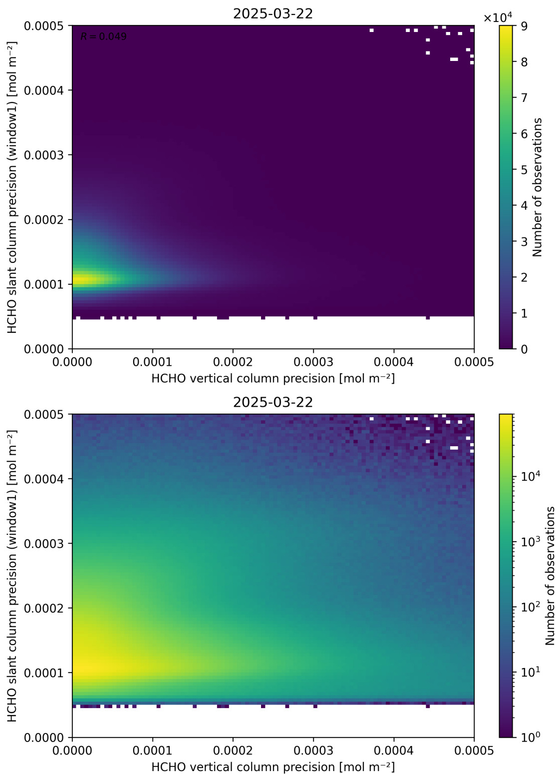
Figure 143: Scatter density plot of “HCHO vertical column precision” against “HCHO slant column precision (window1)” for 2025-03-21 to 2025-03-23.
