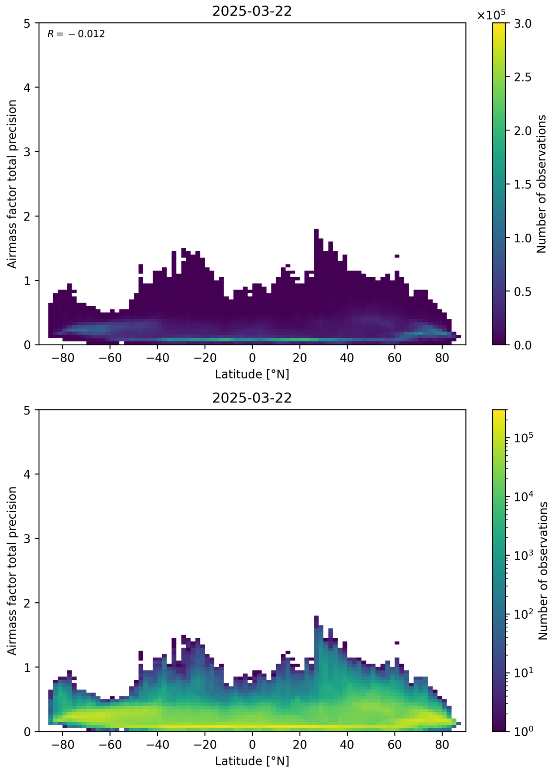
Figure 162: Scatter density plot of “Latitude” against “Airmass factor total precision” for 2025-03-21 to 2025-03-23.
