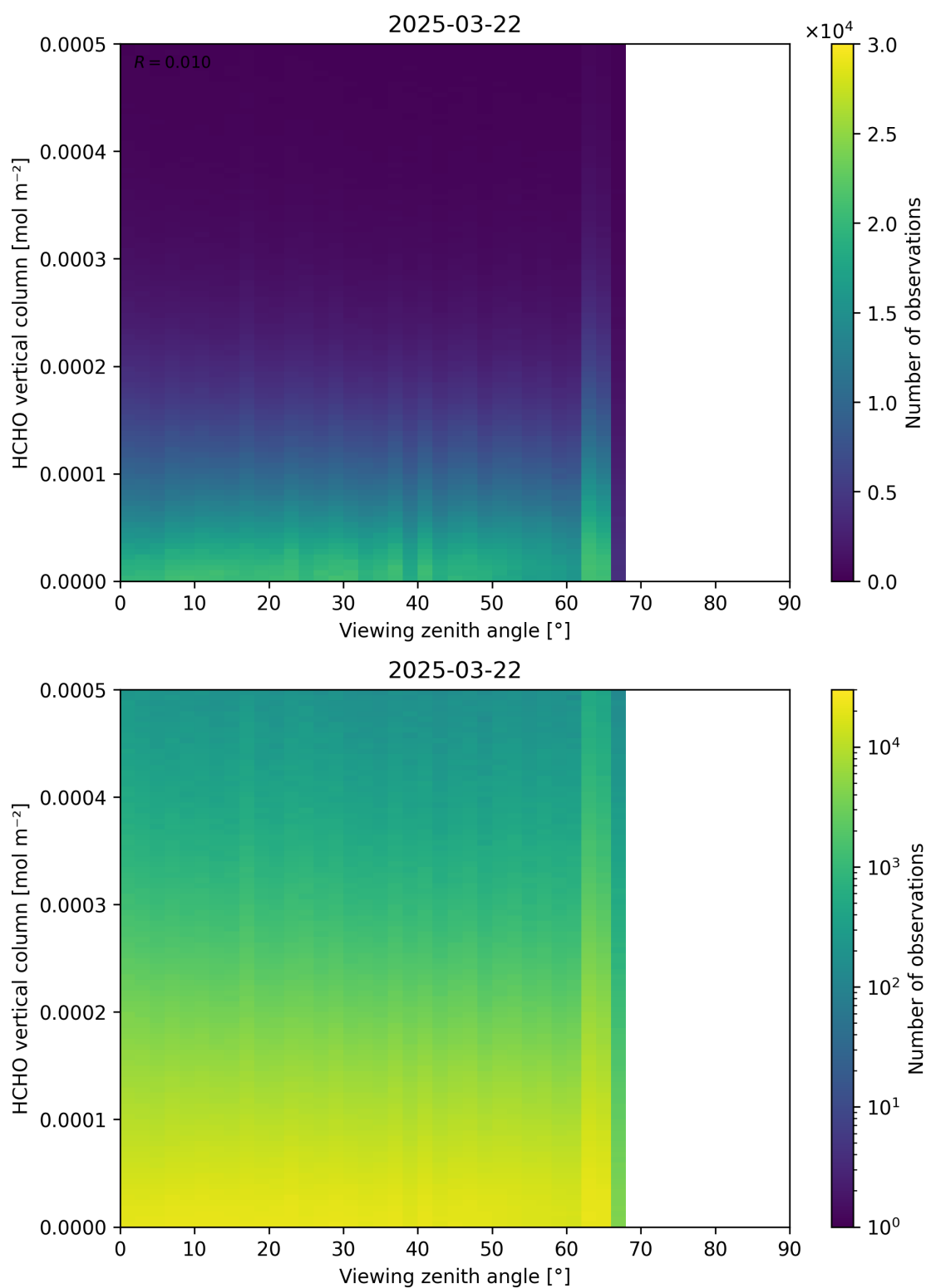
Figure 192: Scatter density plot of “Viewing zenith angle” against “HCHO vertical column” for 2025-03-21 to 2025-03-23.
