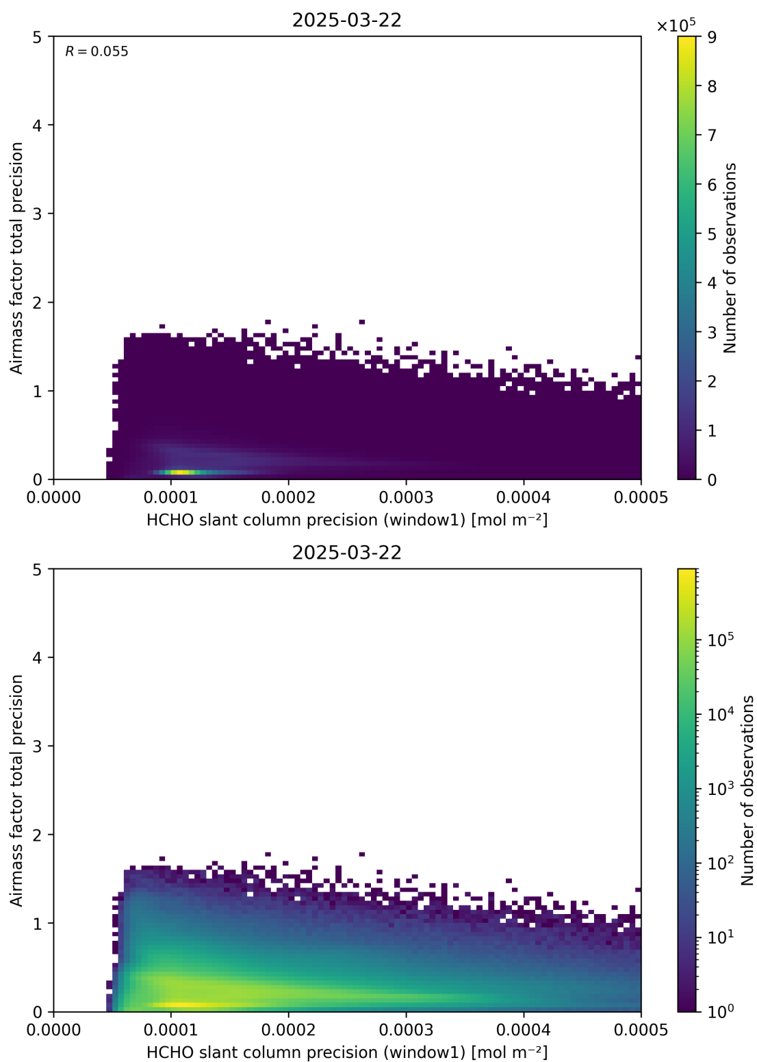
Figure 95: Scatter density plot of “HCHO slant column precision (window1)” against “Airmass factor total precision” for 2025-03-21 to 2025-03-23.
