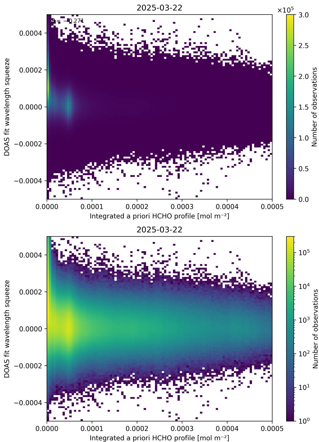
Figure 150: Scatter density plot of “Integrated a priori HCHO profile” against “DOAS fit wavelength squeeze” for 2025-03-21 to 2025-03-23.
