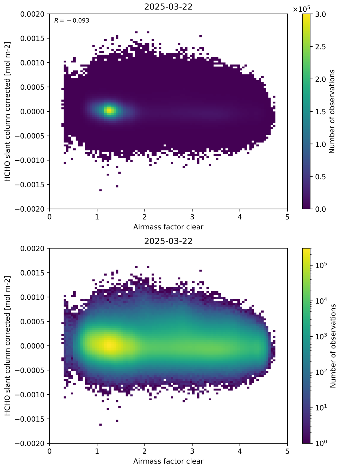
Figure 74: Scatter density plot of “Airmass factor clear” against “HCHO slant column corrected” for 2025-03-21 to 2025-03-23.
