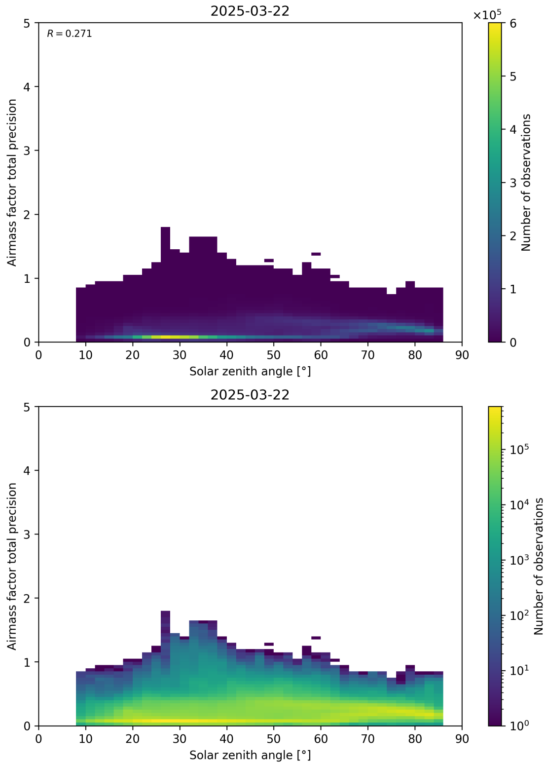
Figure 176: Scatter density plot of “Solar zenith angle” against “Airmass factor total precision” for 2025-03-21 to 2025-03-23.
