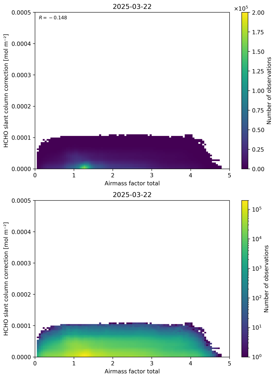
Figure 102: Scatter density plot of “Airmass factor total” against “HCHO slant column correction” for 2025-03-21 to 2025-03-23.
