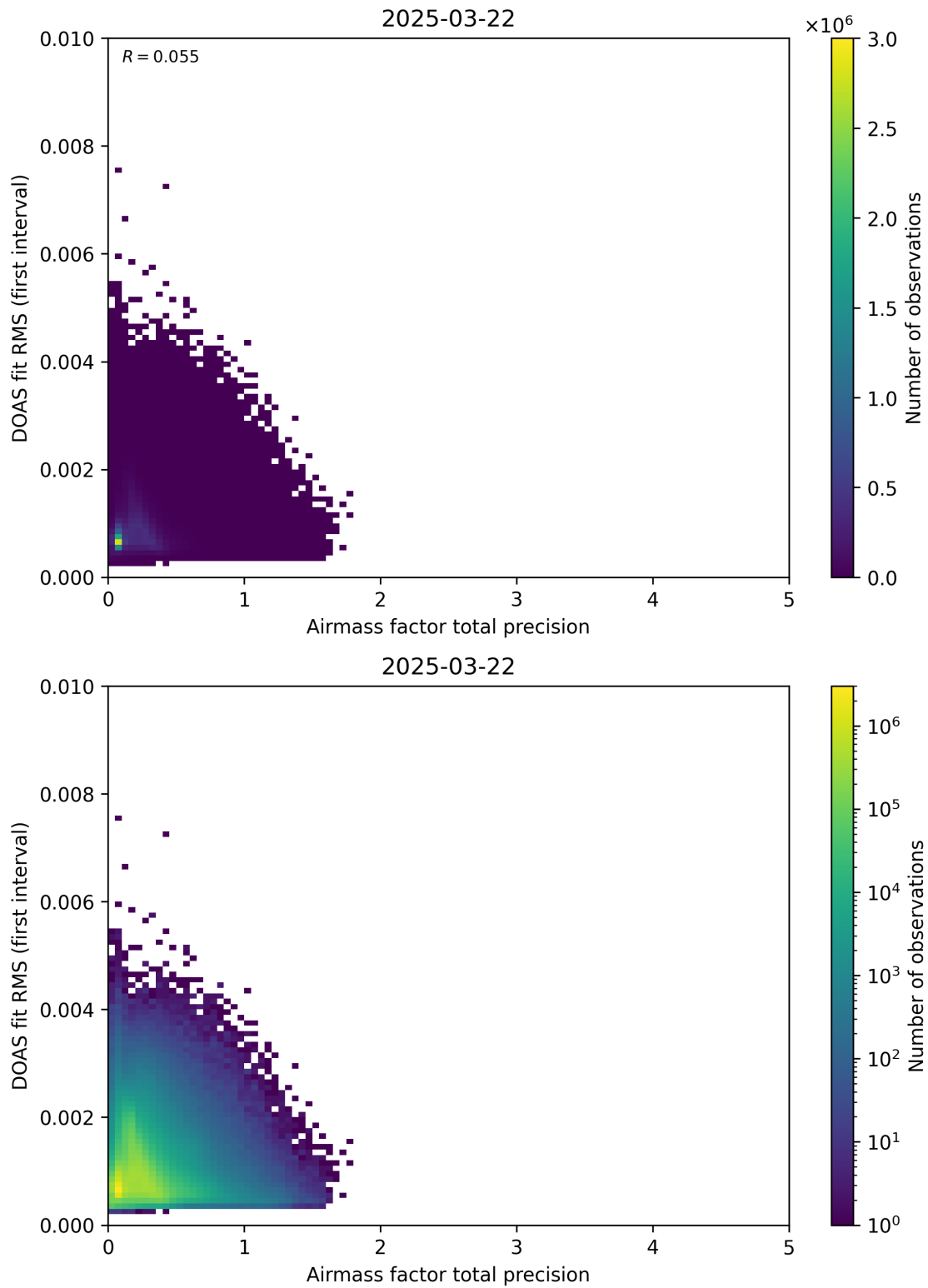
Figure 105: Scatter density plot of “Airmass factor total precision” against “DOAS fit RMS (first interval)” for 2025-03-21 to 2025-03-23.
