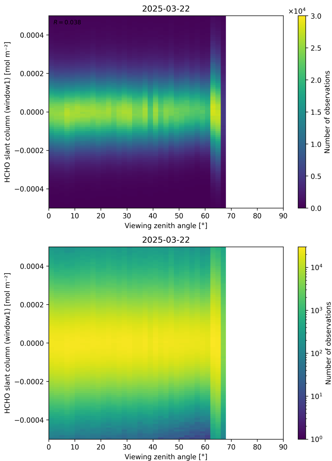
Figure 188: Scatter density plot of “Viewing zenith angle” against “HCHO slant column (window1)” for 2025-03-21 to 2025-03-23.
