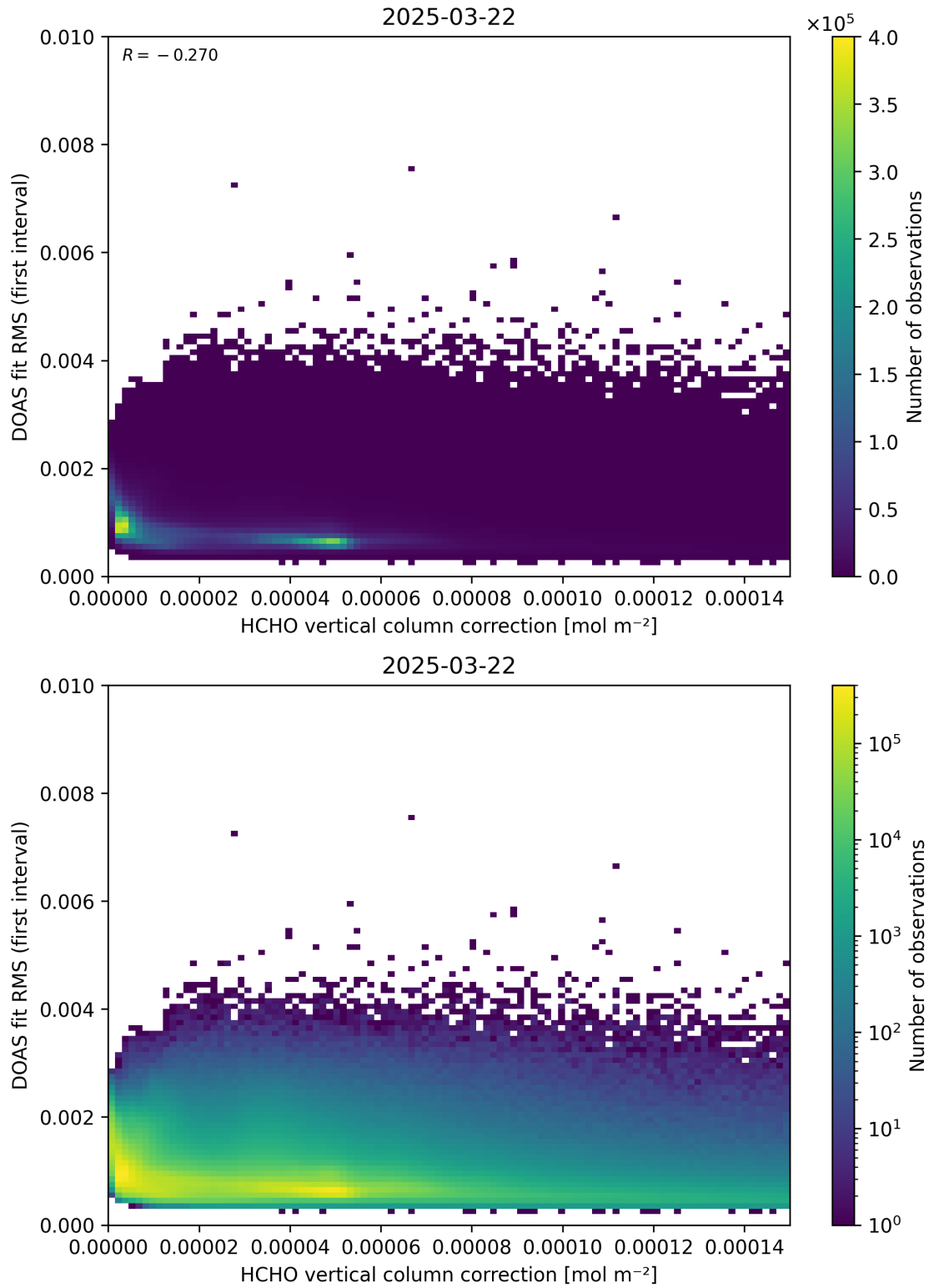
Figure 112: Scatter density plot of “HCHO vertical column correction” against “DOAS fit RMS (first interval)” for 2025-03-21 to 2025-03-23.
