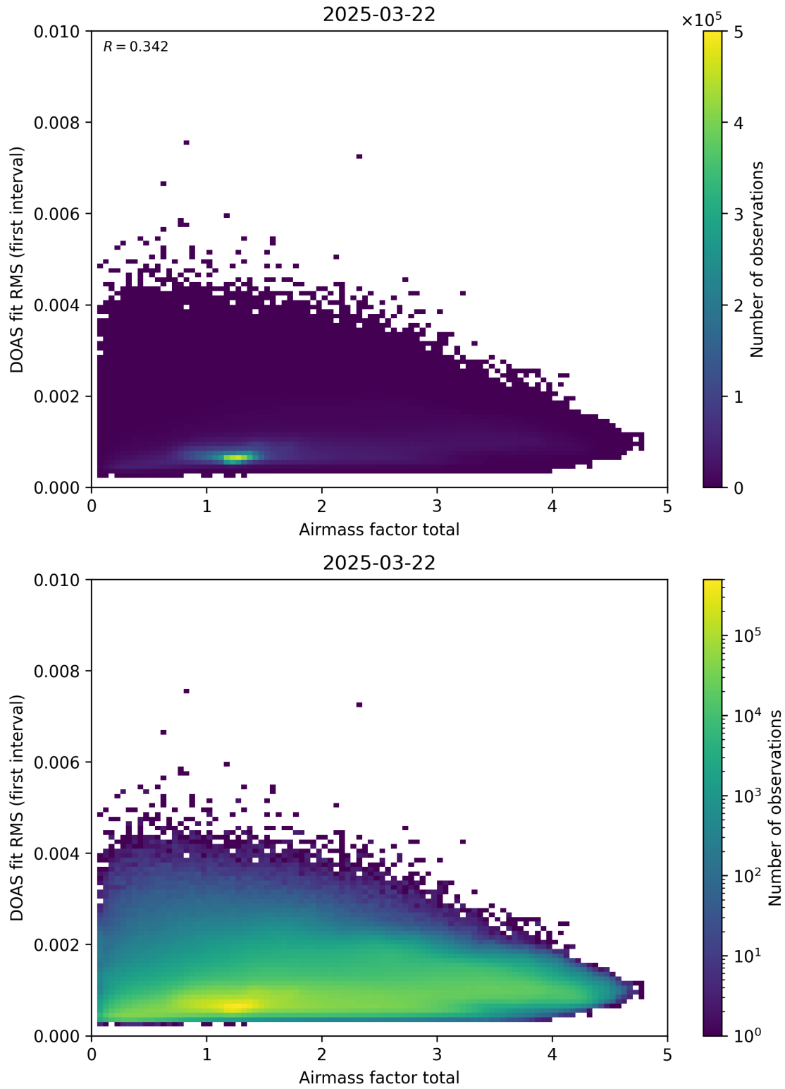
Figure 97: Scatter density plot of “Airmass factor total” against “DOAS fit RMS (first interval)” for 2025-03-21 to 2025-03-23.
