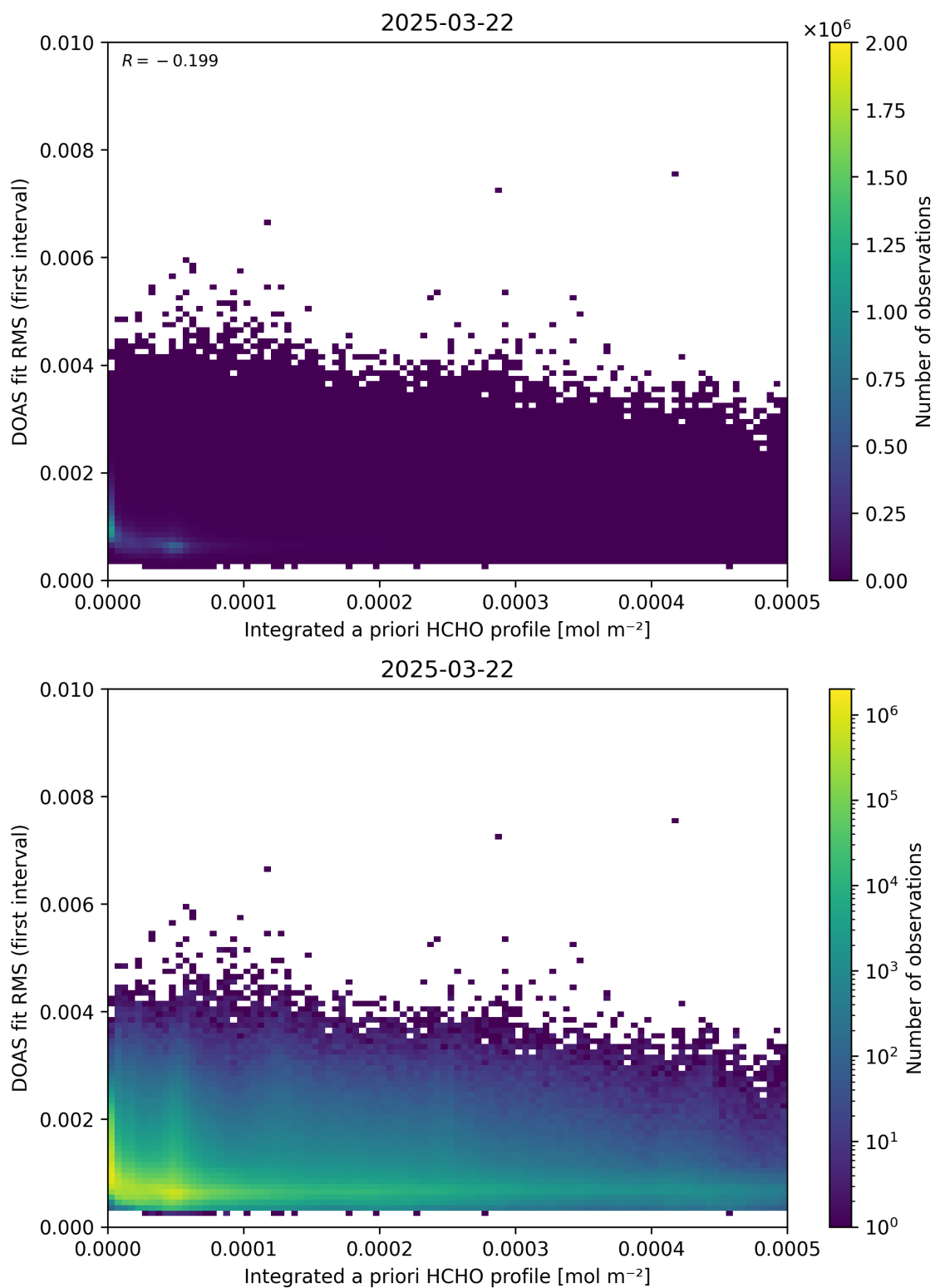
Figure 148: Scatter density plot of “Integrated a priori HCHO profile” against “DOAS fit RMS (first interval)” for 2025-03-21 to 2025-03-23.
