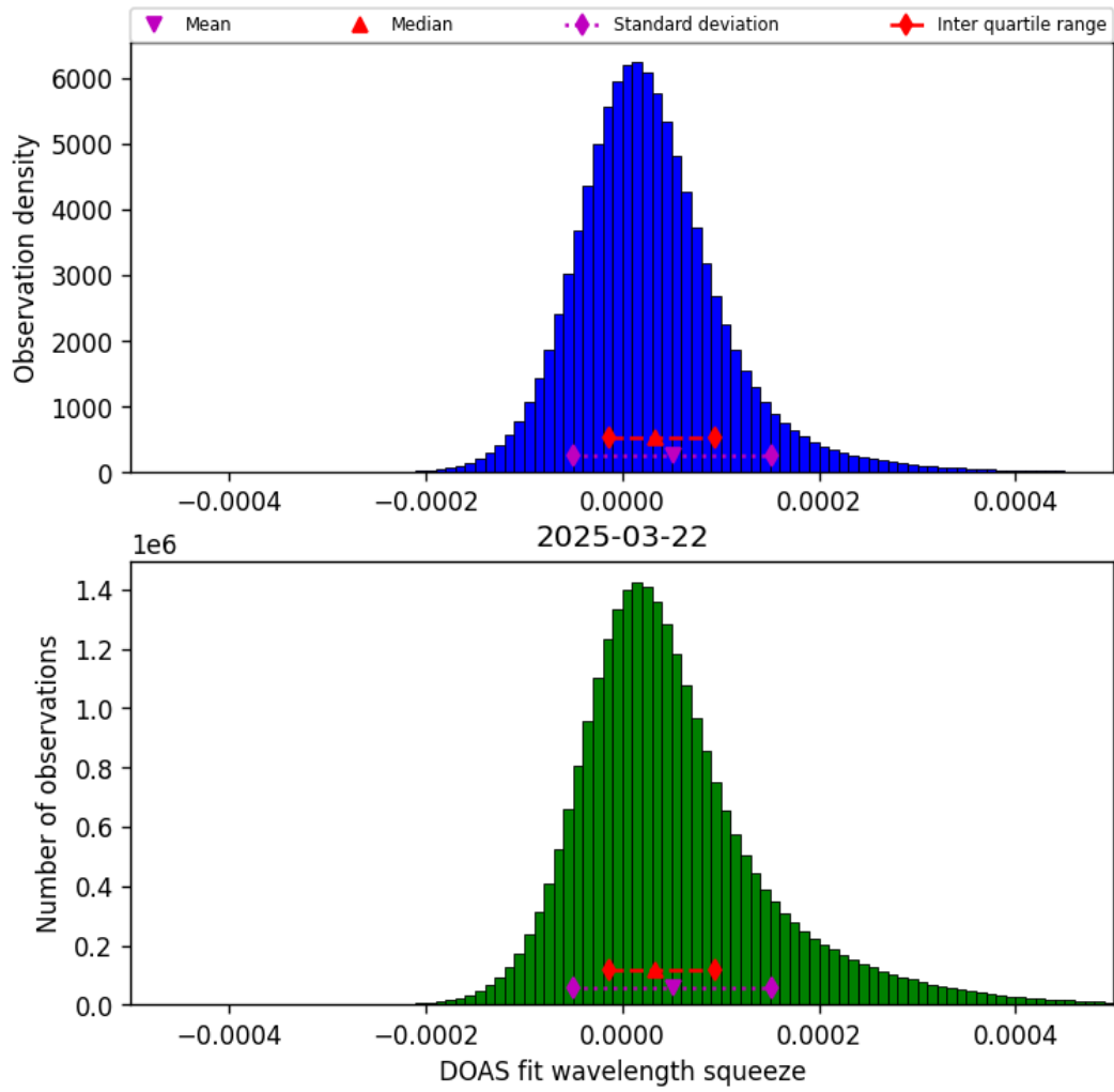
Figure 45: Histogram of “DOAS fit wavelength squeeze” for 2025-03-21 to 2025-03-23
