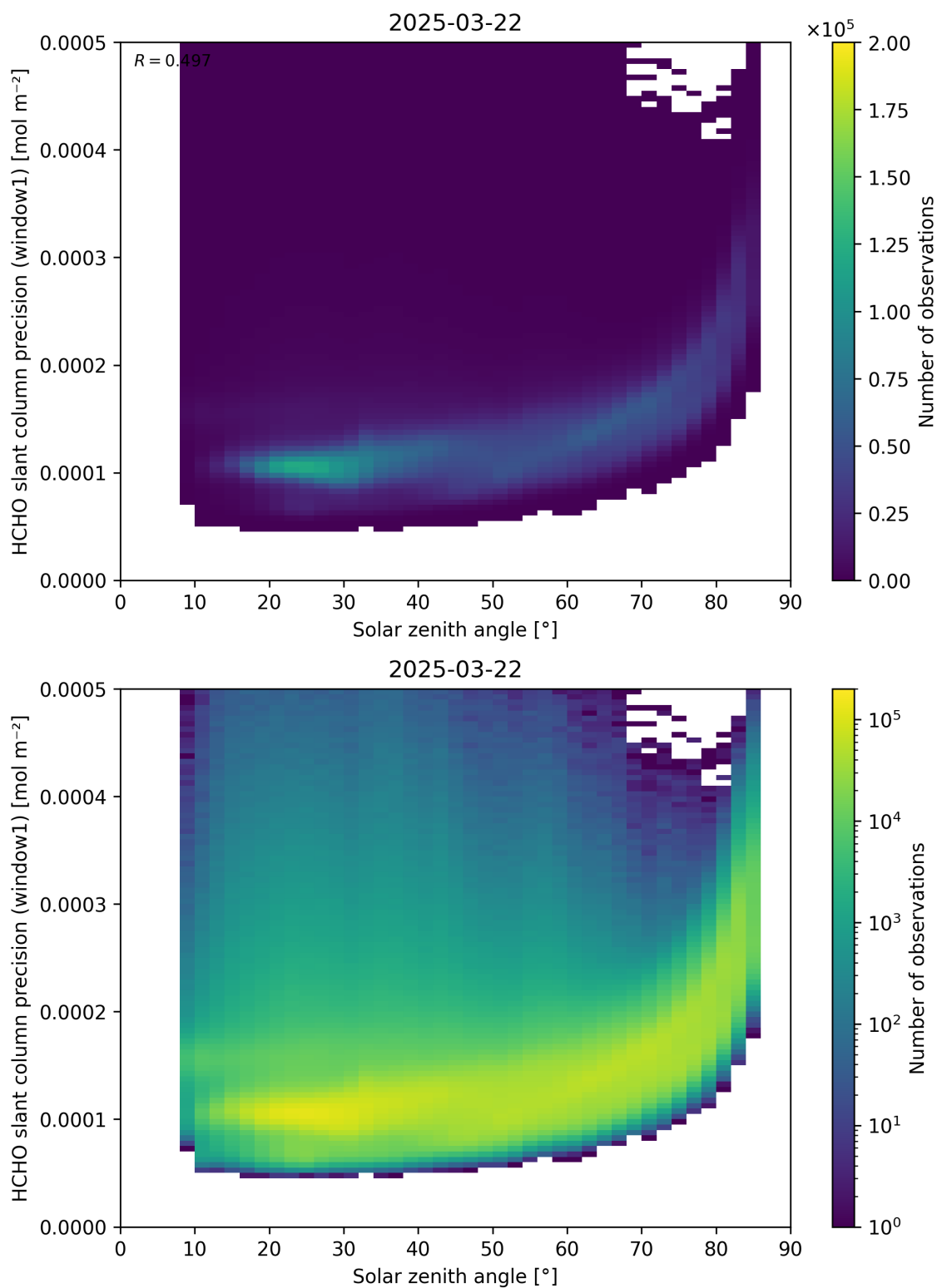
Figure 174: Scatter density plot of “Solar zenith angle” against “HCHO slant column precision (window1)” for 2025-03-21 to 2025-03-23.
