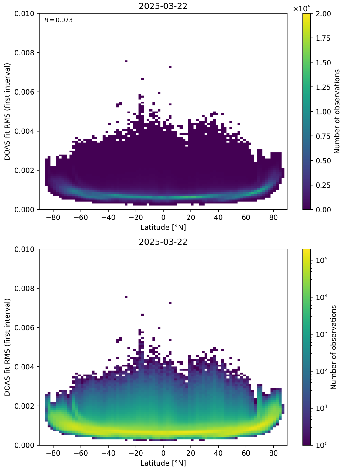
Figure 153: Scatter density plot of “Latitude” against “DOAS fit RMS (first interval)” for 2025-03-21 to 2025-03-23.
