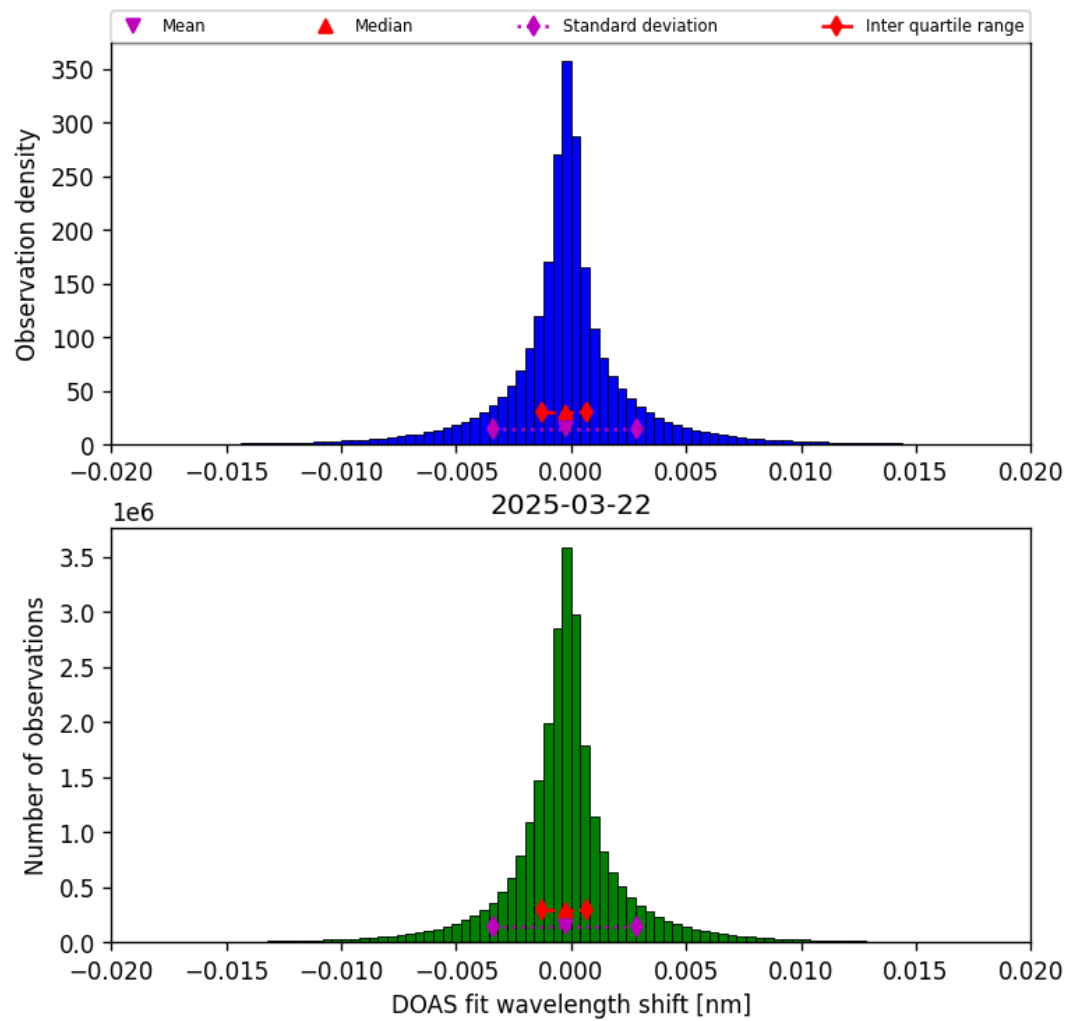
Figure 44: Histogram of “DOAS fit wavelength shift” for 2025-03-21 to 2025-03-23
