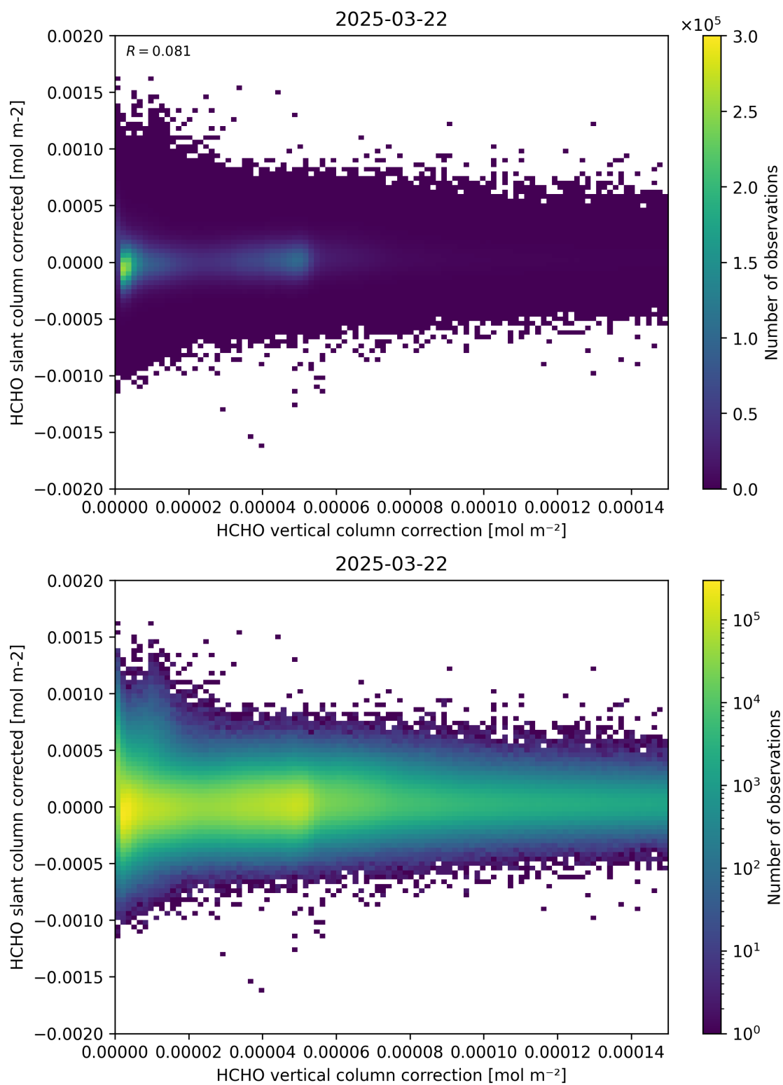
Figure 116: Scatter density plot of “HCHO vertical column correction” against “HCHO slant column corrected” for 2025-03-21 to 2025-03-23.
