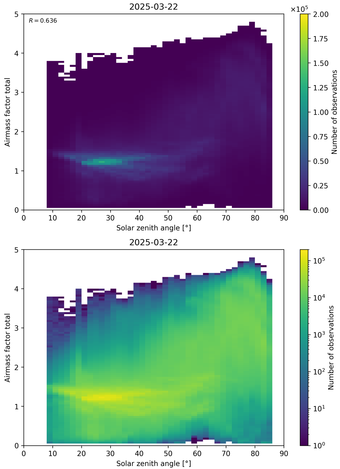
Figure 175: Scatter density plot of “Solar zenith angle” against “Airmass factor total” for 2025-03-21 to 2025-03-23.
