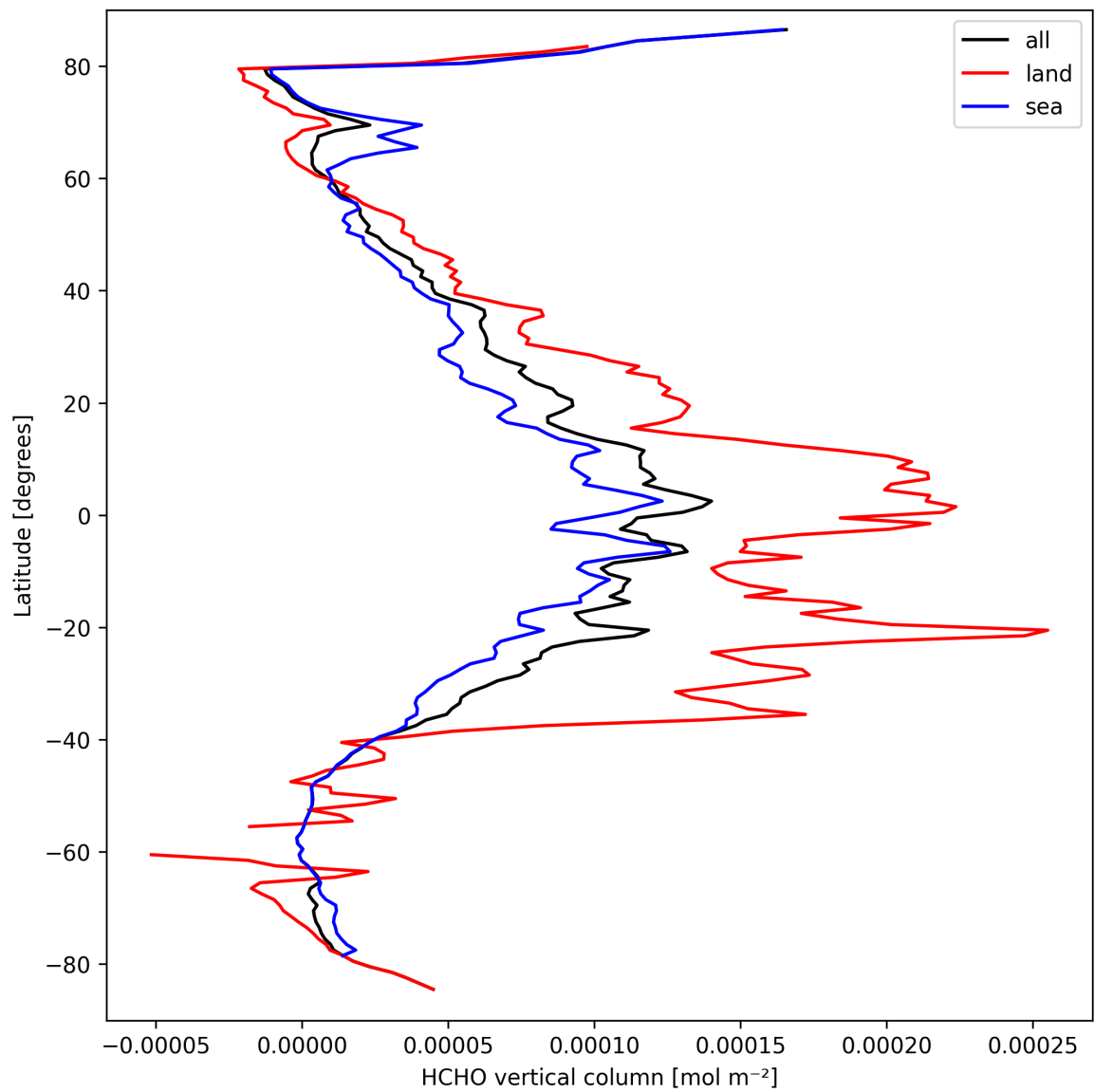
Figure 21: Zonal average of “HCHO vertical column” for 2025-03-21 to 2025-03-23.
