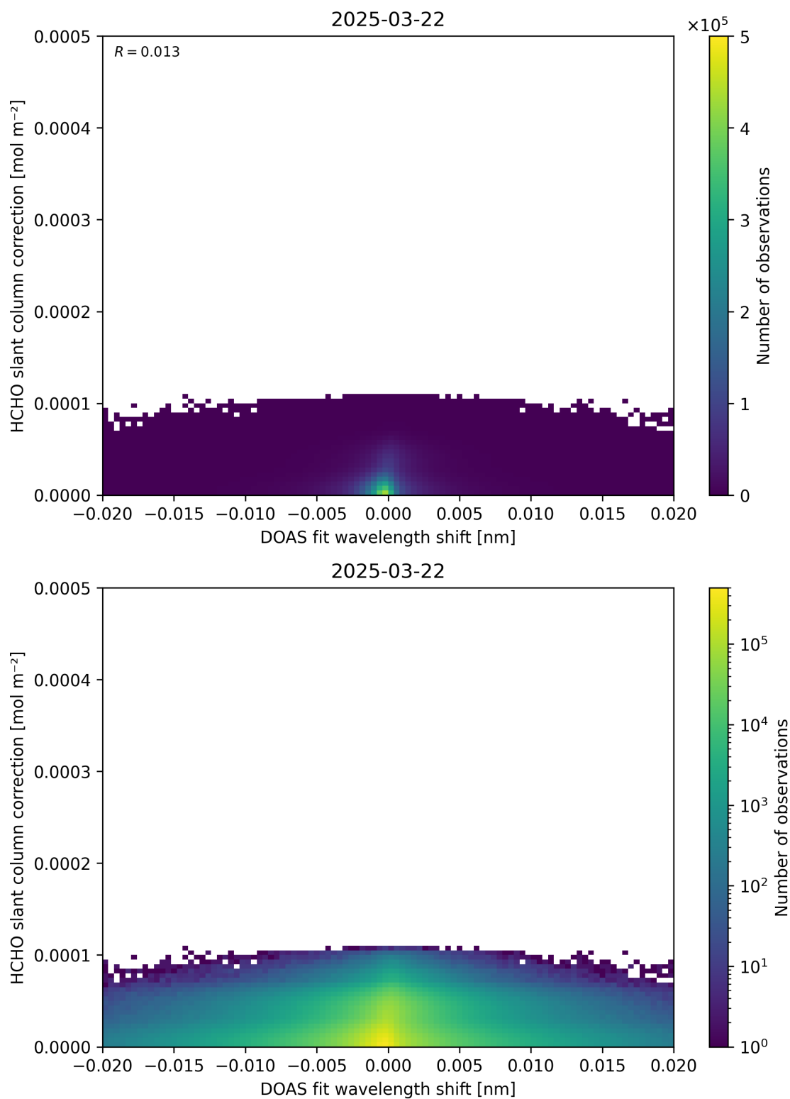
Figure 67: Scatter density plot of “DOAS fit wavelength shift” against “HCHO slant column correction” for 2025-03-21 to 2025-03-23.
