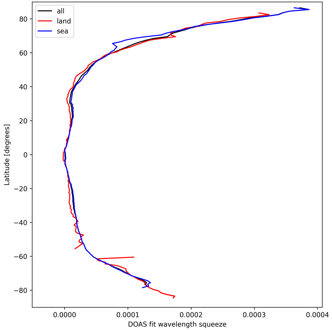
Figure 31: Zonal average of “DOAS fit wavelength squeeze” for 2025-03-21 to 2025-03-23.
