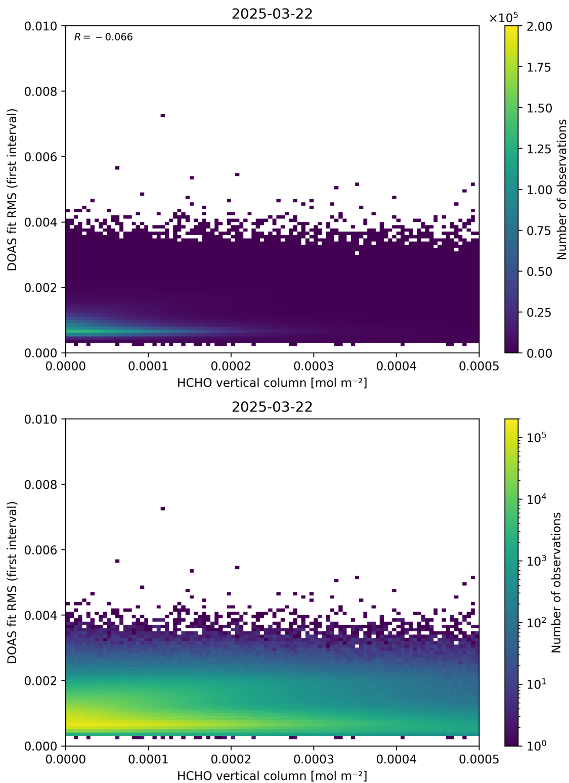
Figure 123: Scatter density plot of “HCHO vertical column” against “DOAS fit RMS (first interval)” for 2025-03-21 to 2025-03-23.
