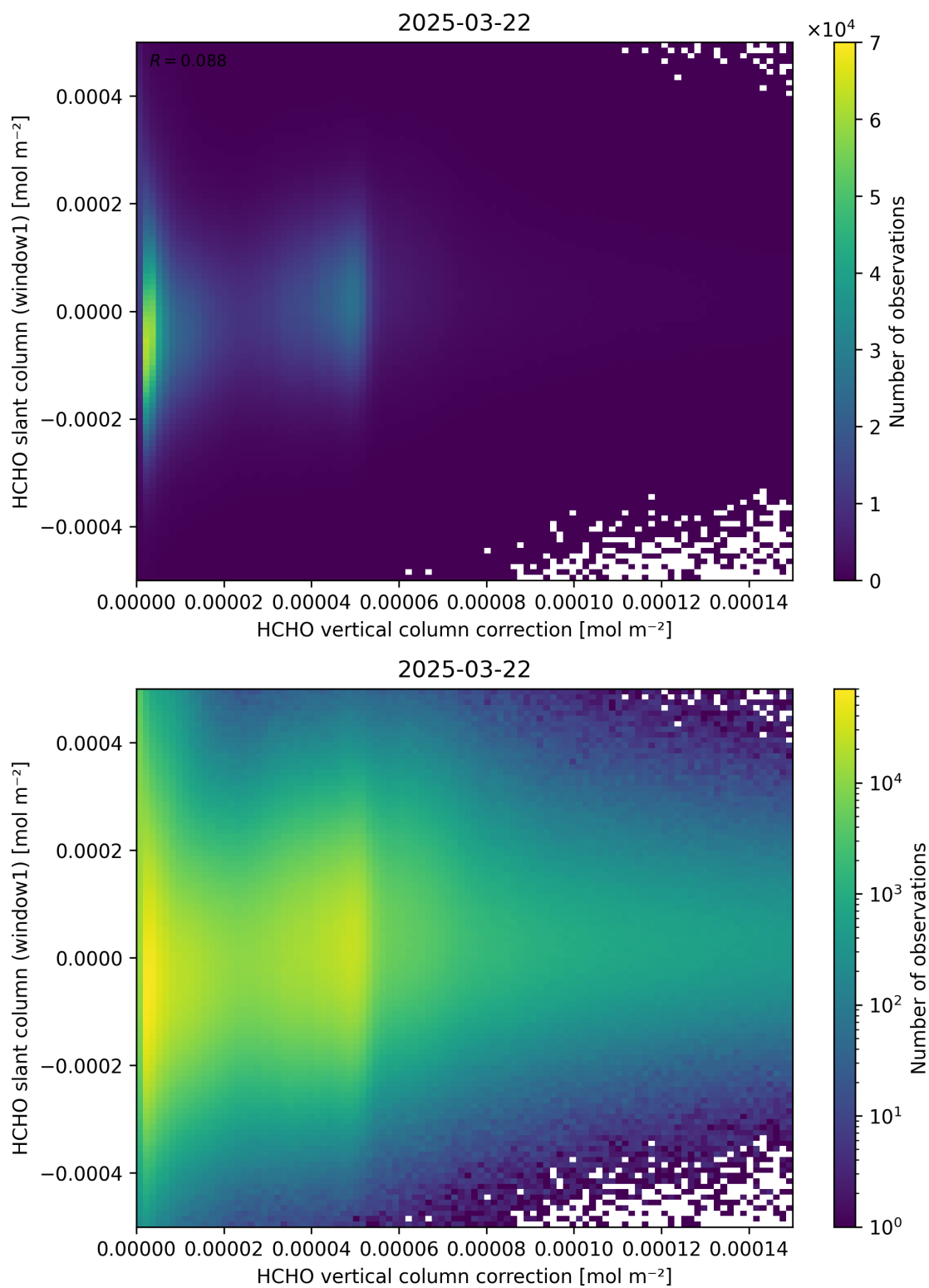
Figure 118: Scatter density plot of “HCHO vertical column correction” against “HCHO slant column (window1)” for 2025-03-21 to 2025-03-23.
