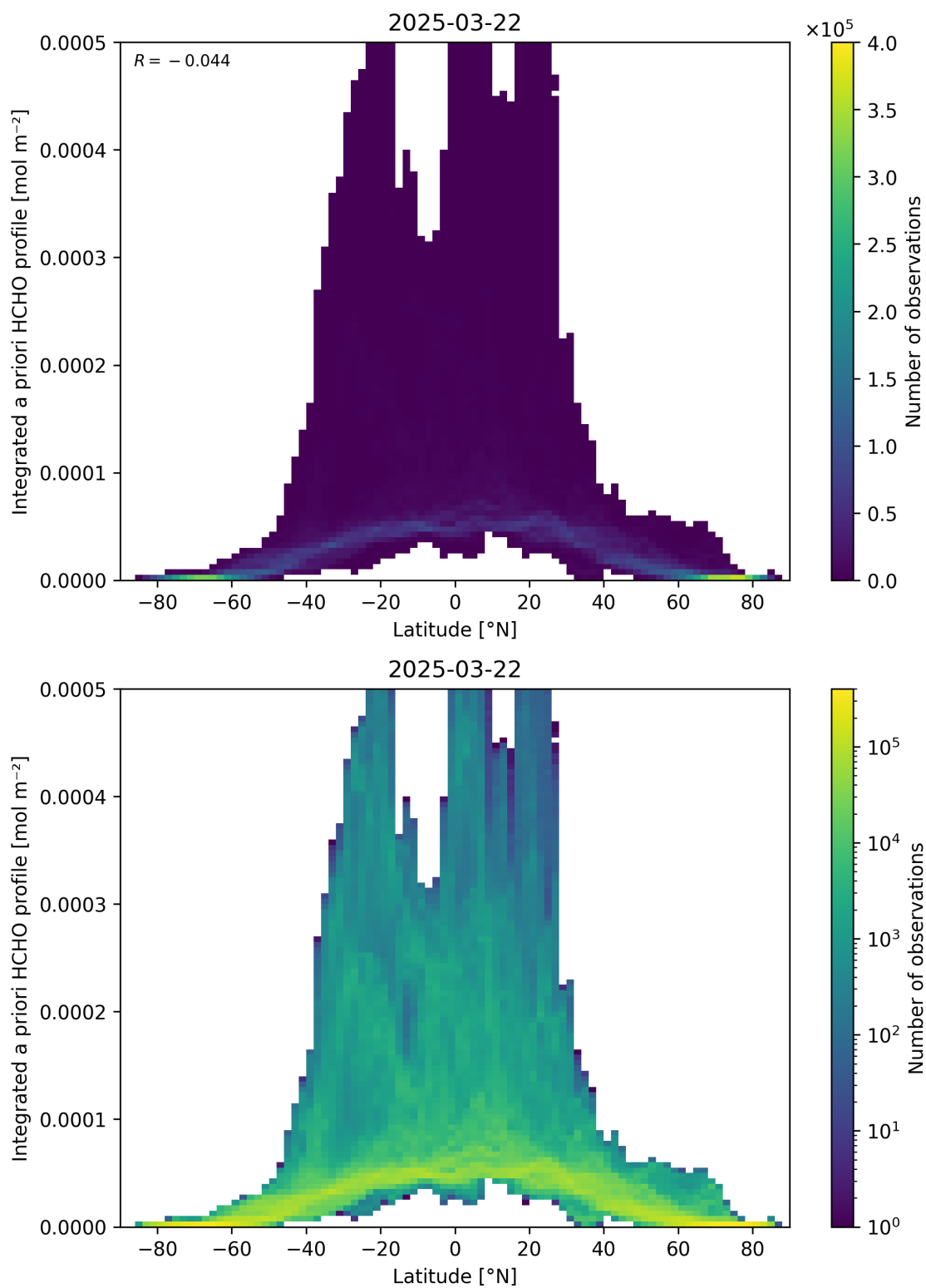
Figure 166: Scatter density plot of “Latitude” against “Integrated a priori HCHO profile” for 2025-03-21 to 2025-03-23.
