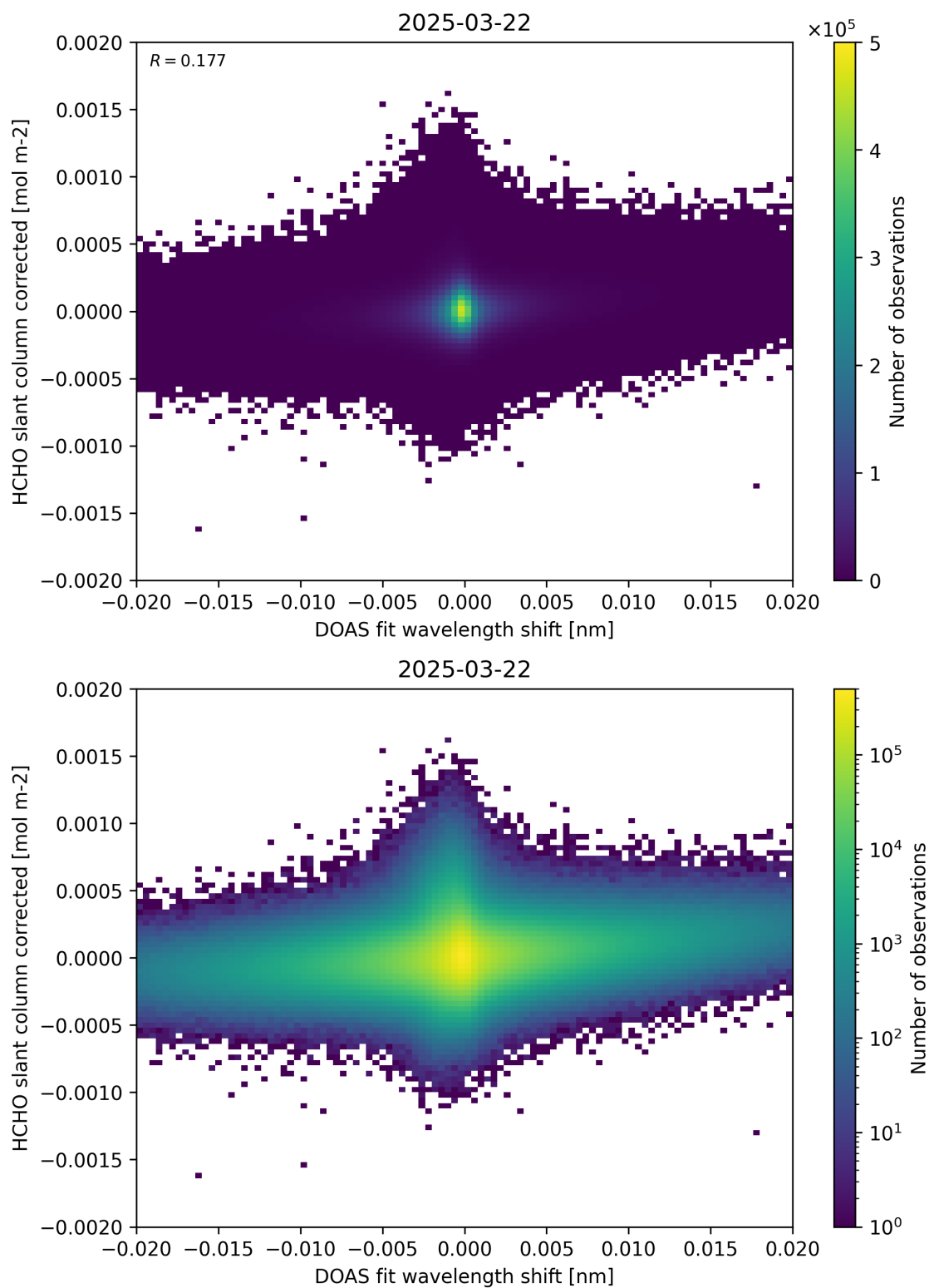
Figure 66: Scatter density plot of “DOAS fit wavelength shift” against “HCHO slant column corrected” for 2025-03-21 to 2025-03-23.
