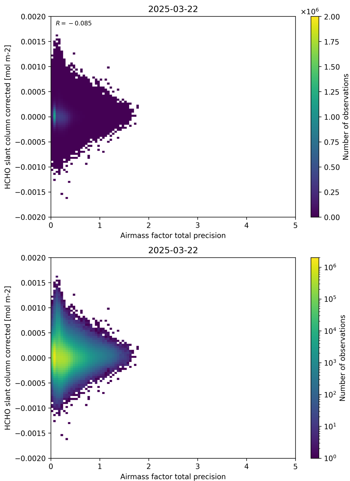
Figure 109: Scatter density plot of “Airmass factor total precision” against “HCHO slant column corrected” for 2025-03-21 to 2025-03-23.
