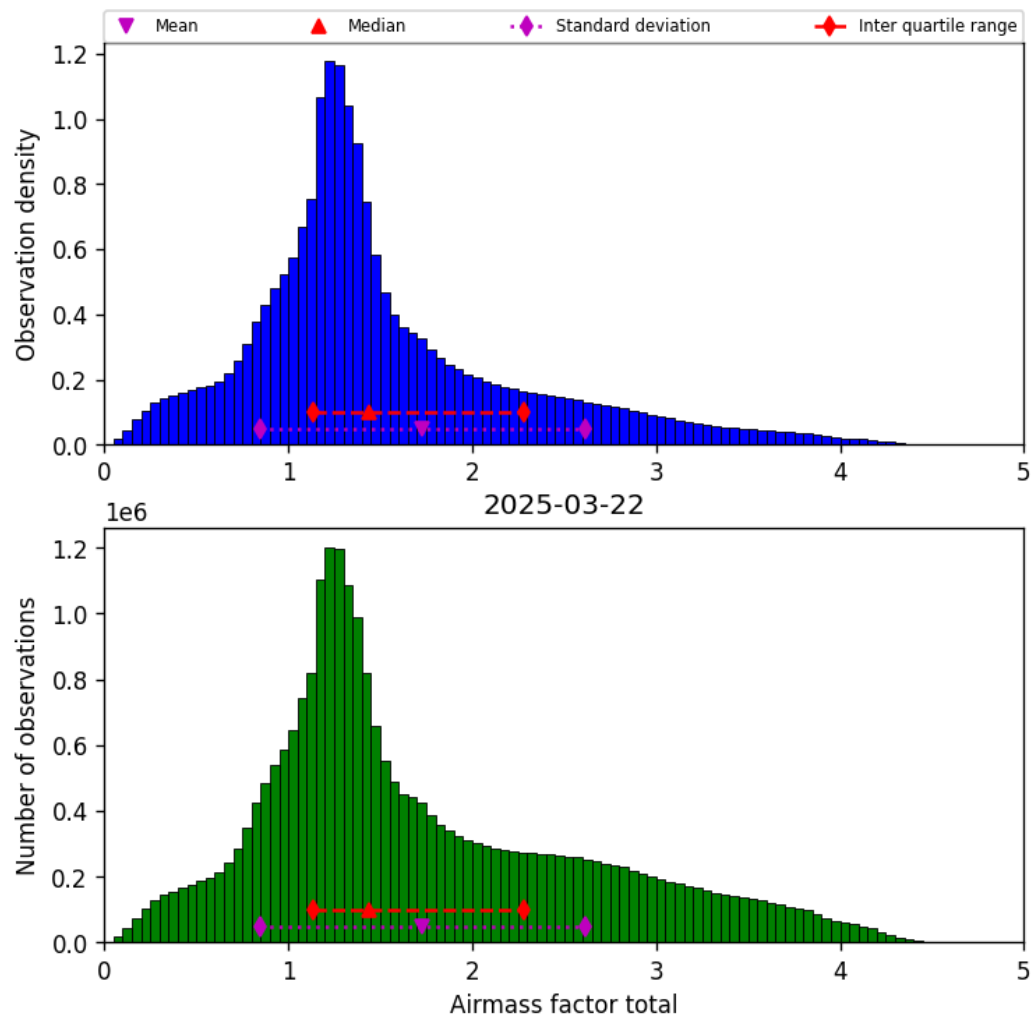
Figure 40: Histogram of “Airmass factor total” for 2025-03-21 to 2025-03-23
