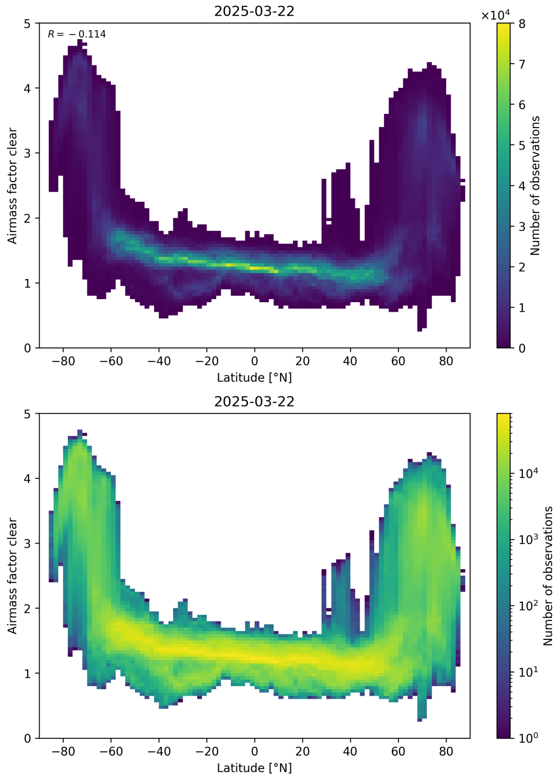
Figure 156: Scatter density plot of “Latitude” against “Airmass factor clear” for 2025-03-21 to 2025-03-23.
