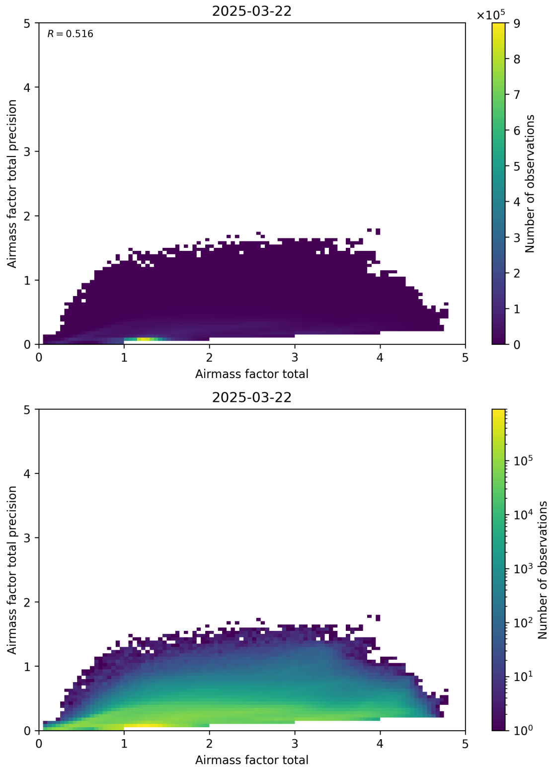
Figure 103: Scatter density plot of “Airmass factor total” against “Airmass factor total precision” for 2025-03-21 to 2025-03-23.
