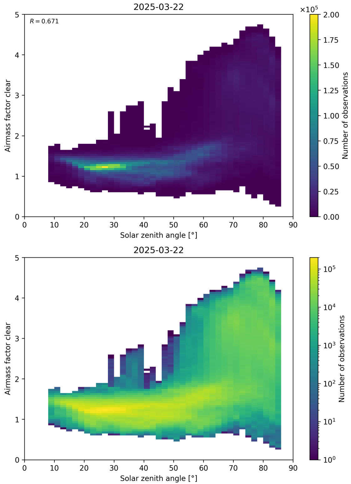
Figure 170: Scatter density plot of “Solar zenith angle” against “Airmass factor clear” for 2025-03-21 to 2025-03-23.
