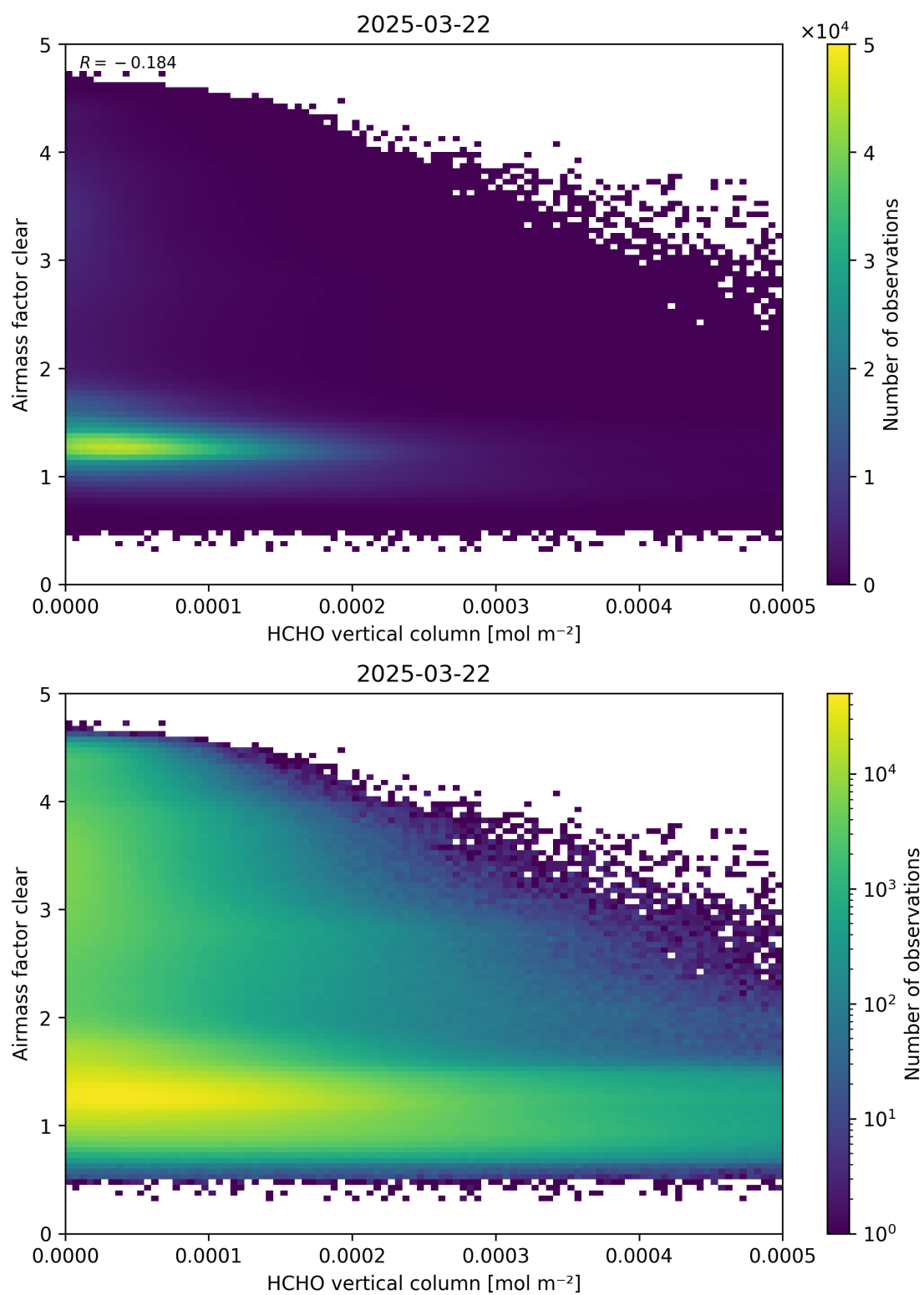
Figure 126: Scatter density plot of “HCHO vertical column” against “Airmass factor clear” for 2025-03-21 to 2025-03-23.
