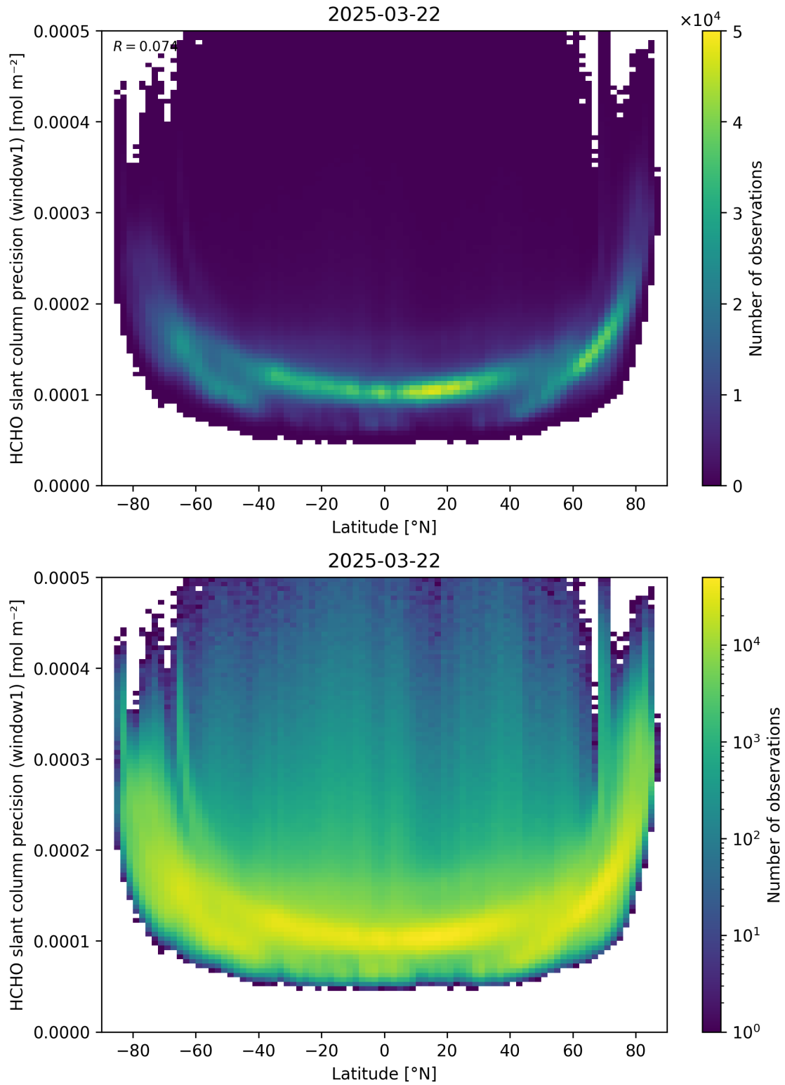
Figure 160: Scatter density plot of “Latitude” against “HCHO slant column precision (window1)” for 2025-03-21 to 2025-03-23.
