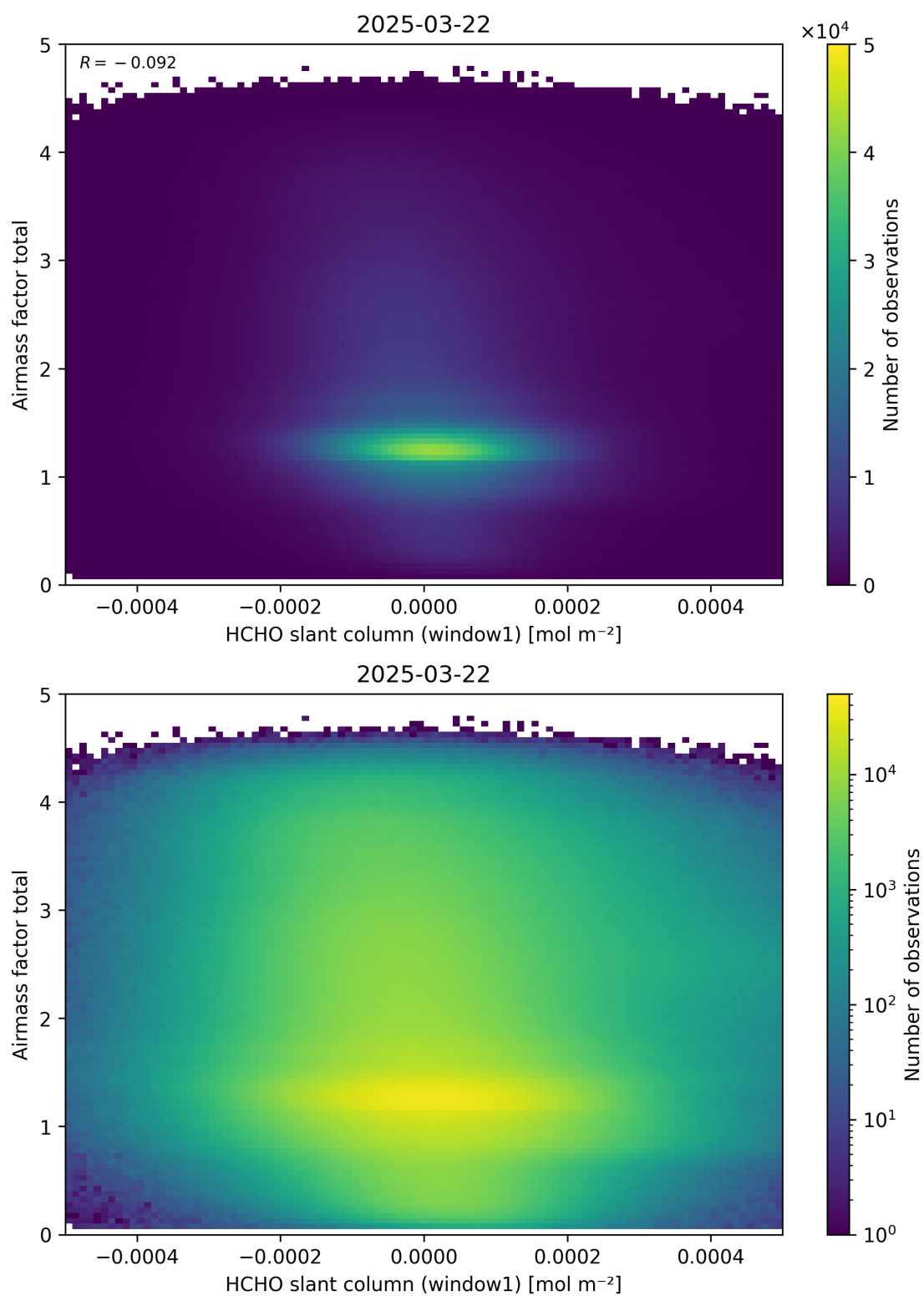
Figure 85: Scatter density plot of “HCHO slant column (window1)” against “Airmass factor total” for 2025-03-21 to 2025-03-23.
