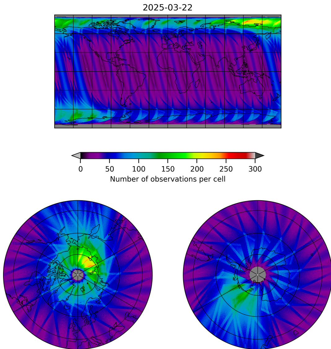
Figure 19: Map of the number of observations for 2025-03-21 to 2025-03-23
