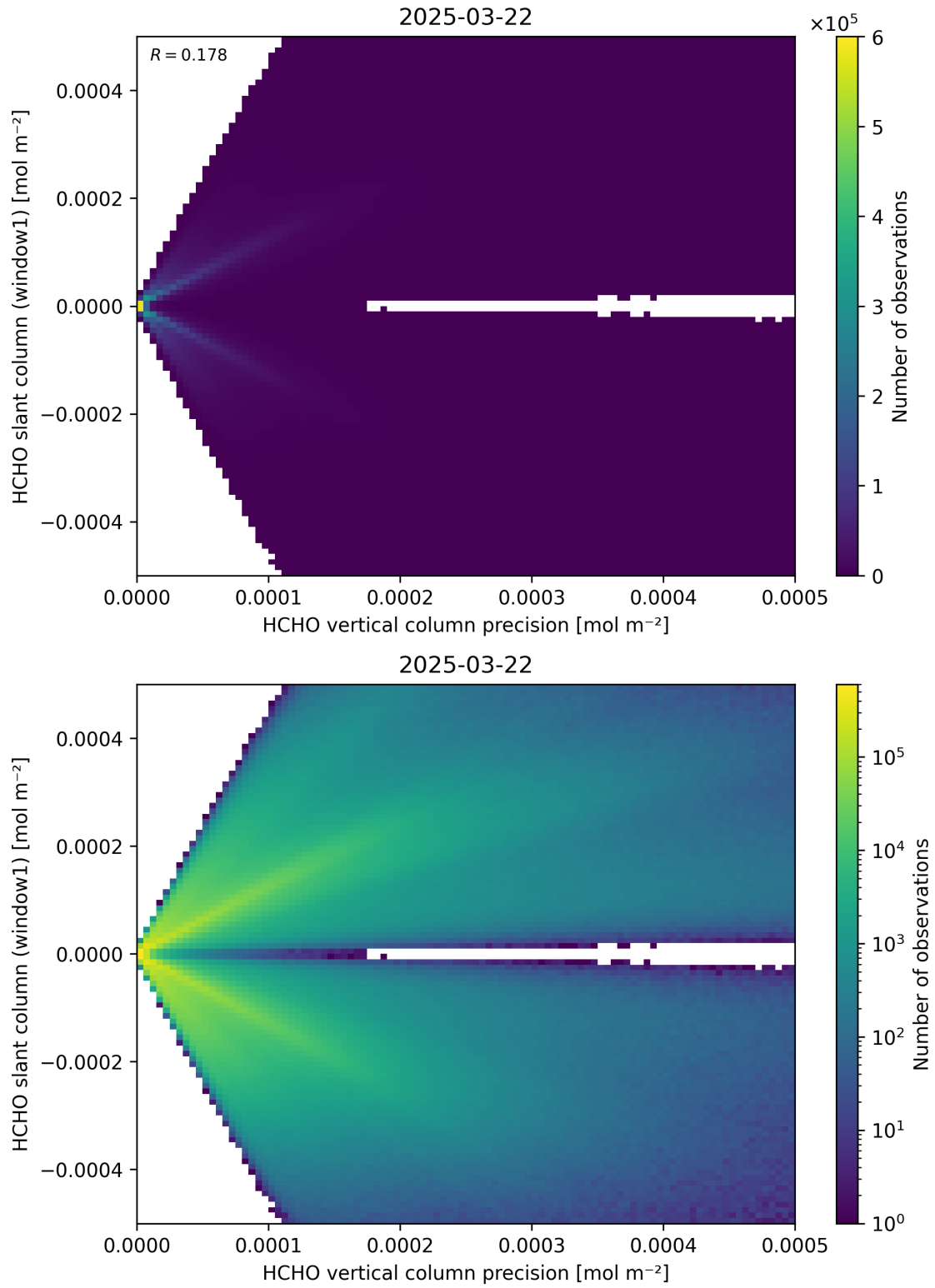
Figure 142: Scatter density plot of “HCHO vertical column precision” against “HCHO slant column (window1)” for 2025-03-21 to 2025-03-23.
