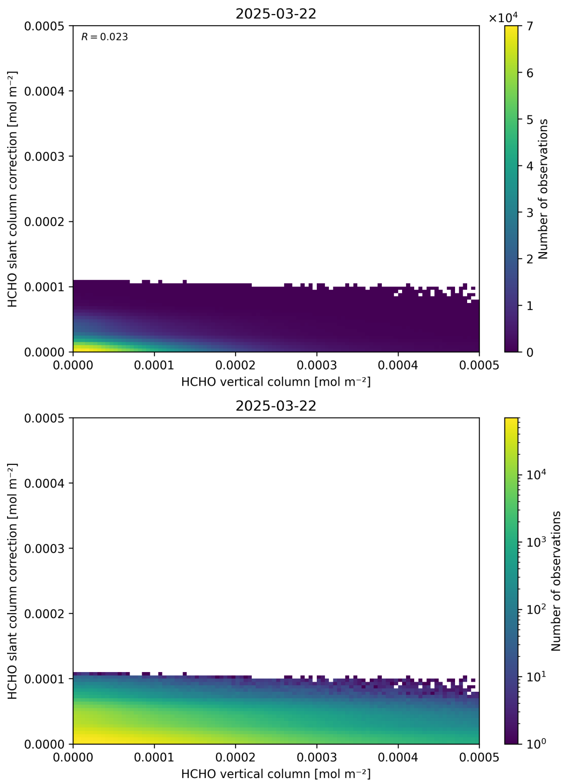
Figure 128: Scatter density plot of “HCHO vertical column” against “HCHO slant column correction” for 2025-03-21 to 2025-03-23.
