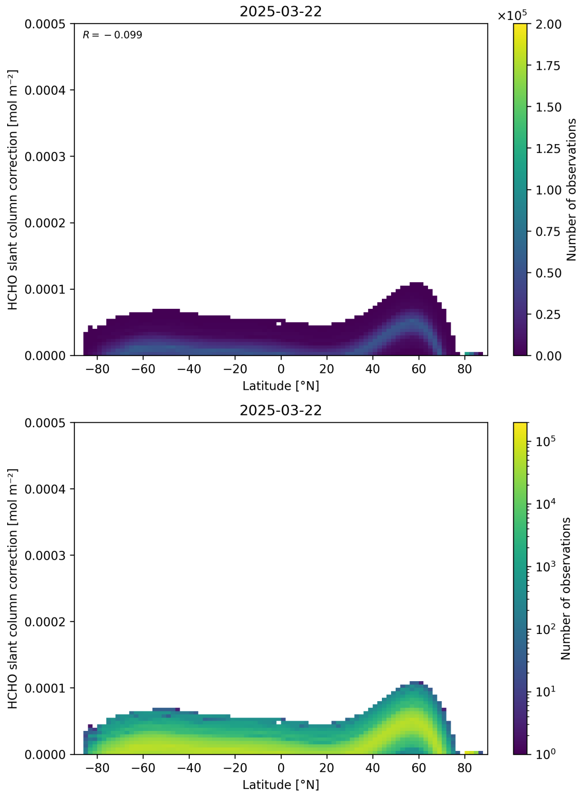
Figure 158: Scatter density plot of “Latitude” against “HCHO slant column correction” for 2025-03-21 to 2025-03-23.
