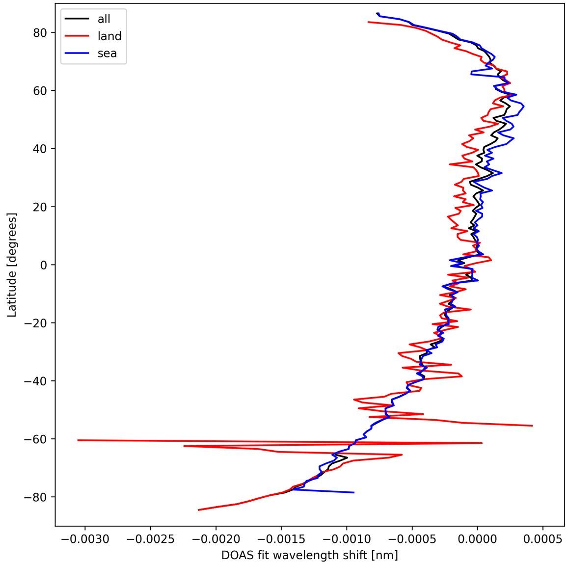
Figure 30: Zonal average of “DOAS fit wavelength shift” for 2025-03-21 to 2025-03-23.
