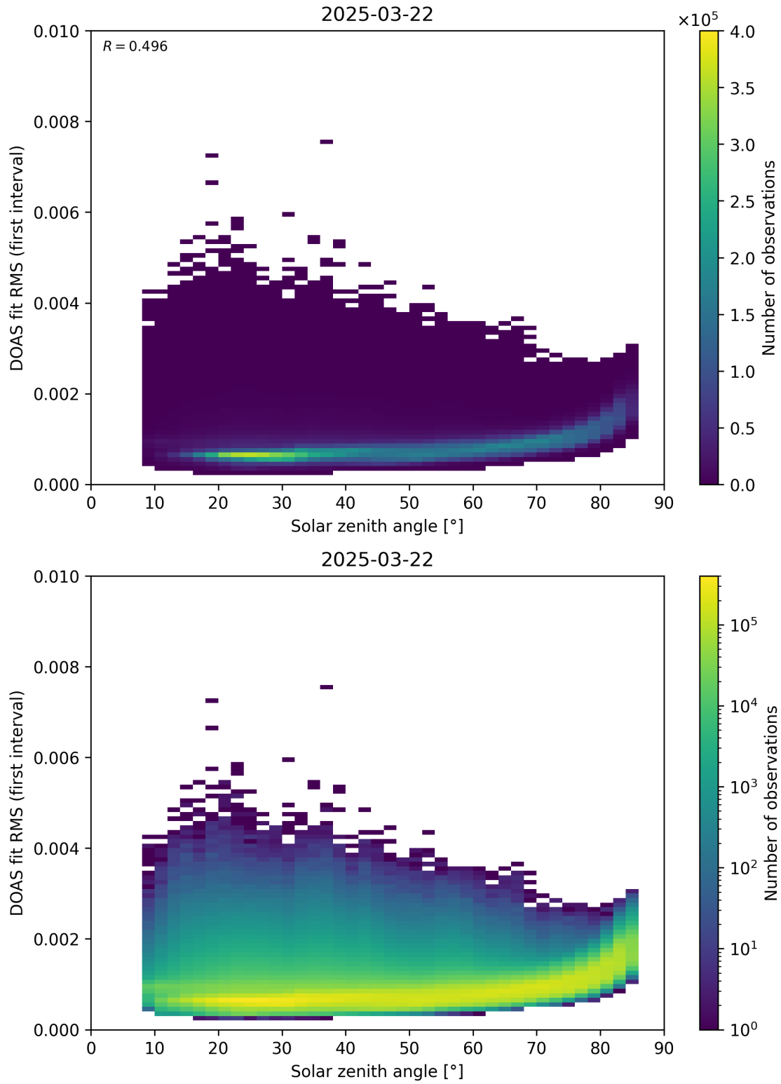
Figure 167: Scatter density plot of “Solar zenith angle” against “DOAS fit RMS (first interval)” for 2025-03-21 to 2025-03-23.
