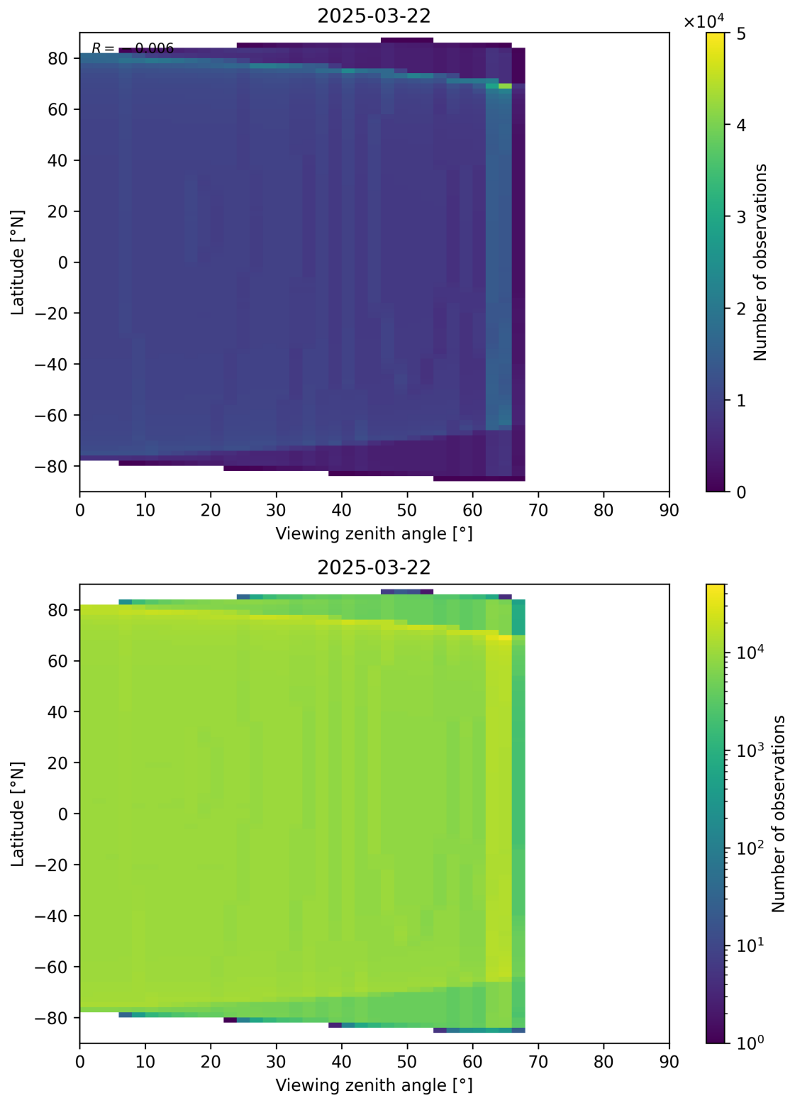
Figure 196: Scatter density plot of “Viewing zenith angle” against “Latitude” for 2025-03-21 to 2025-03-23.
