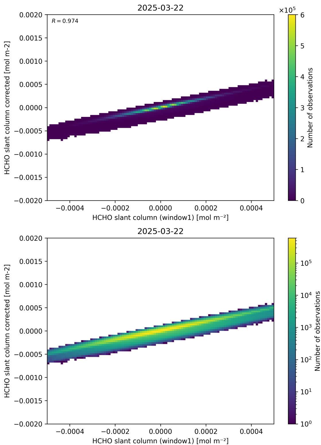
Figure 82: Scatter density plot of “HCHO slant column (window1)” against “HCHO slant column corrected” for 2025-03-21 to 2025-03-23.
