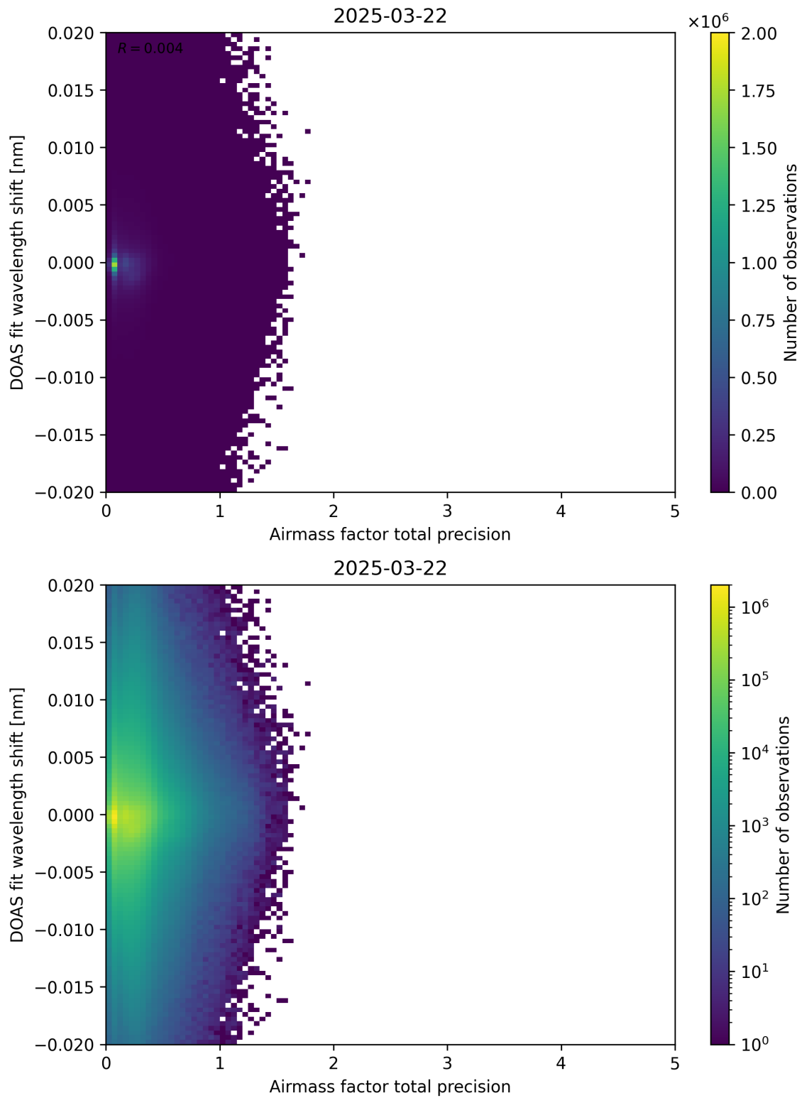
Figure 106: Scatter density plot of “Airmass factor total precision” against “DOAS fit wavelength shift” for 2025-03-21 to 2025-03-23.
