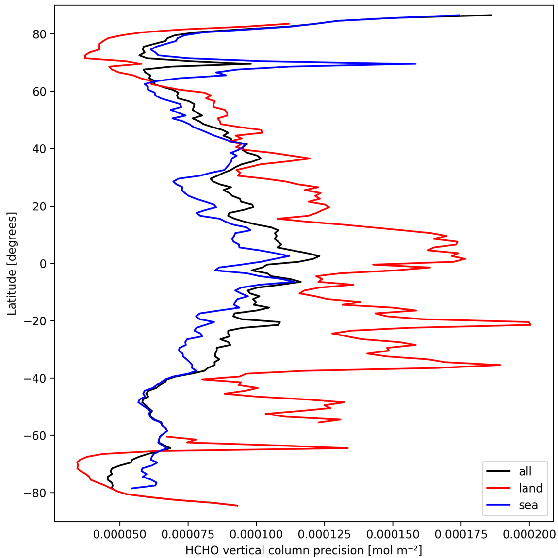
Figure 22: Zonal average of “HCHO vertical column precision” for 2025-03-21 to 2025-03-23.
