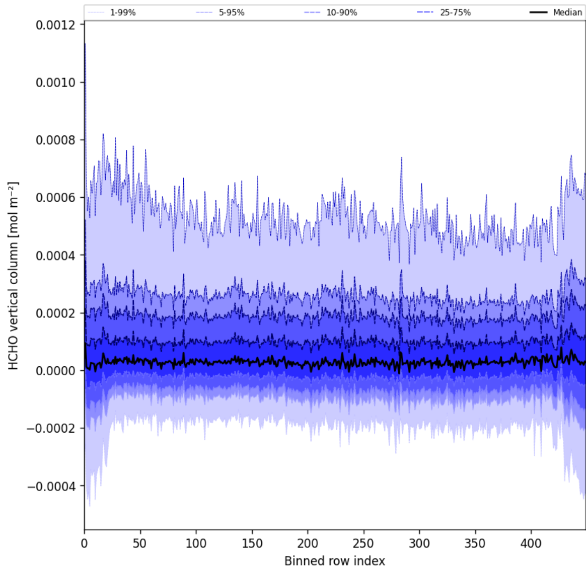
Figure 49: Along track statistics of “HCHO vertical column” for 2025-03-21 to 2025-03-23
