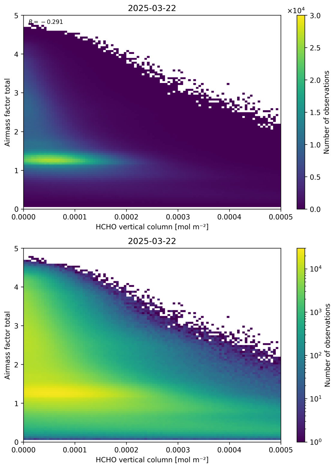
Figure 131: Scatter density plot of “HCHO vertical column” against “Airmass factor total” for 2025-03-21 to 2025-03-23.
