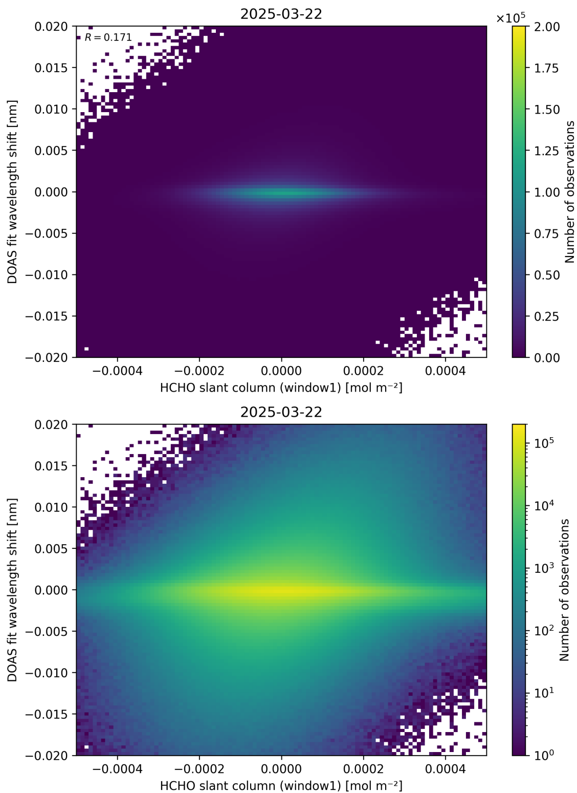
Figure 79: Scatter density plot of “HCHO slant column (window1)” against “DOAS fit wavelength shift” for 2025-03-21 to 2025-03-23.
