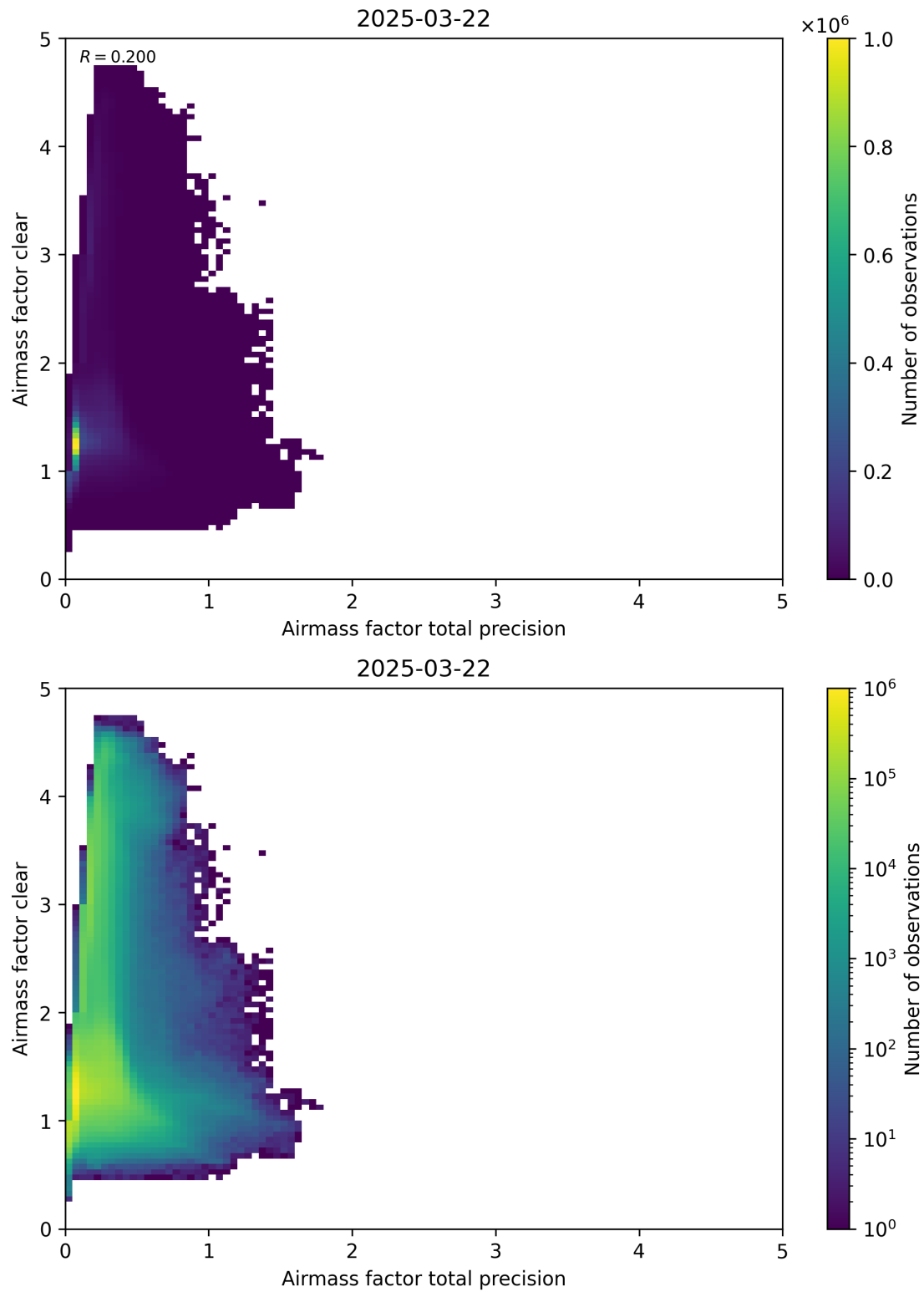
Figure 108: Scatter density plot of “Airmass factor total precision” against “Airmass factor clear” for 2025-03-21 to 2025-03-23.
