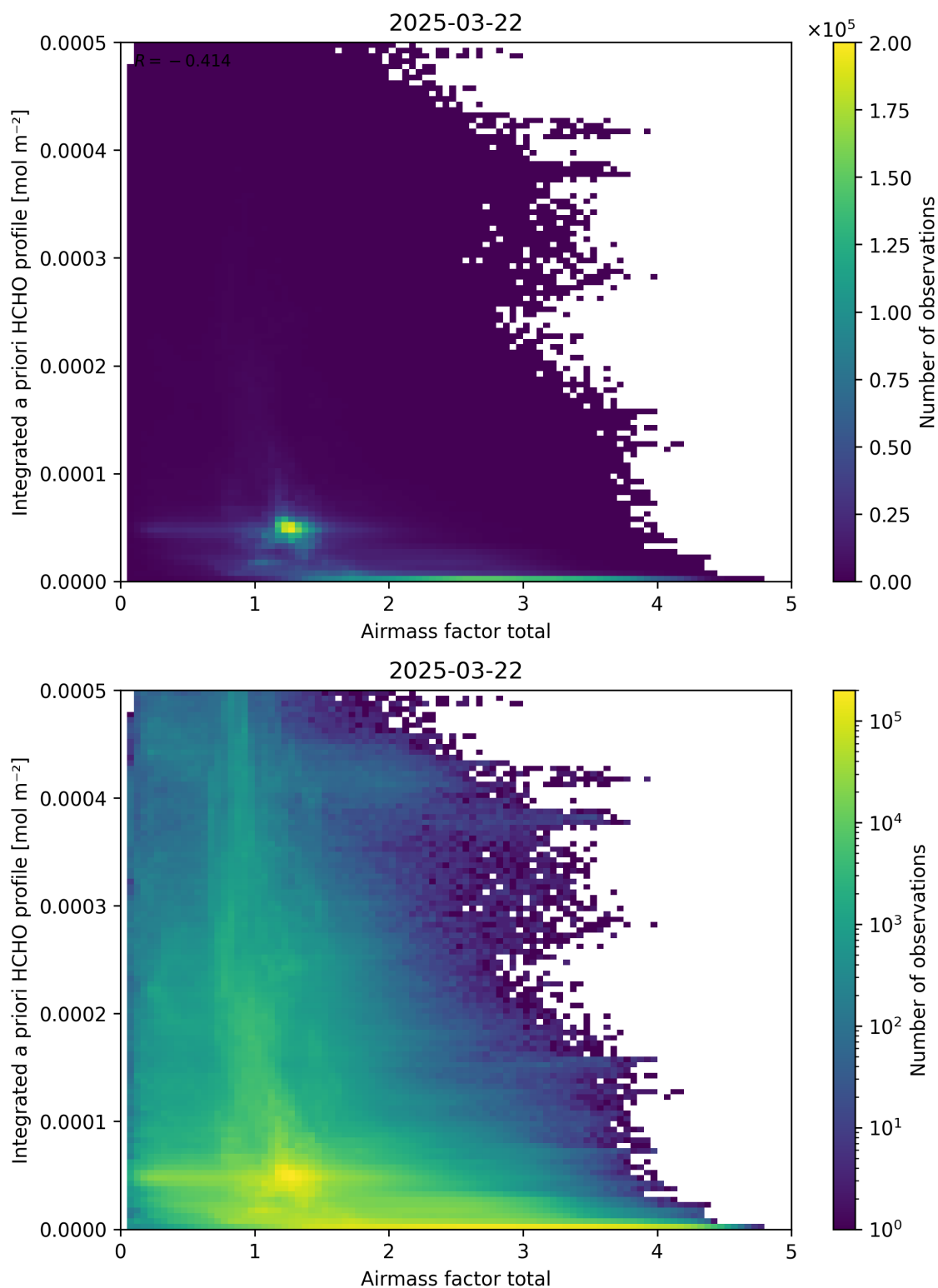
Figure 104: Scatter density plot of “Airmass factor total” against “Integrated a priori HCHO profile” for 2025-03-21 to 2025-03-23.
