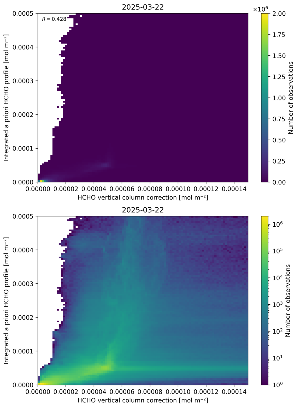
Figure 122: Scatter density plot of “HCHO vertical column correction” against “Integrated a priori HCHO profile” for 2025-03-21 to 2025-03-23.
