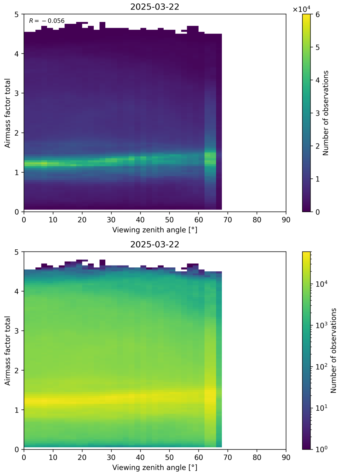
Figure 190: Scatter density plot of “Viewing zenith angle” against “Airmass factor total” for 2025-03-21 to 2025-03-23.
