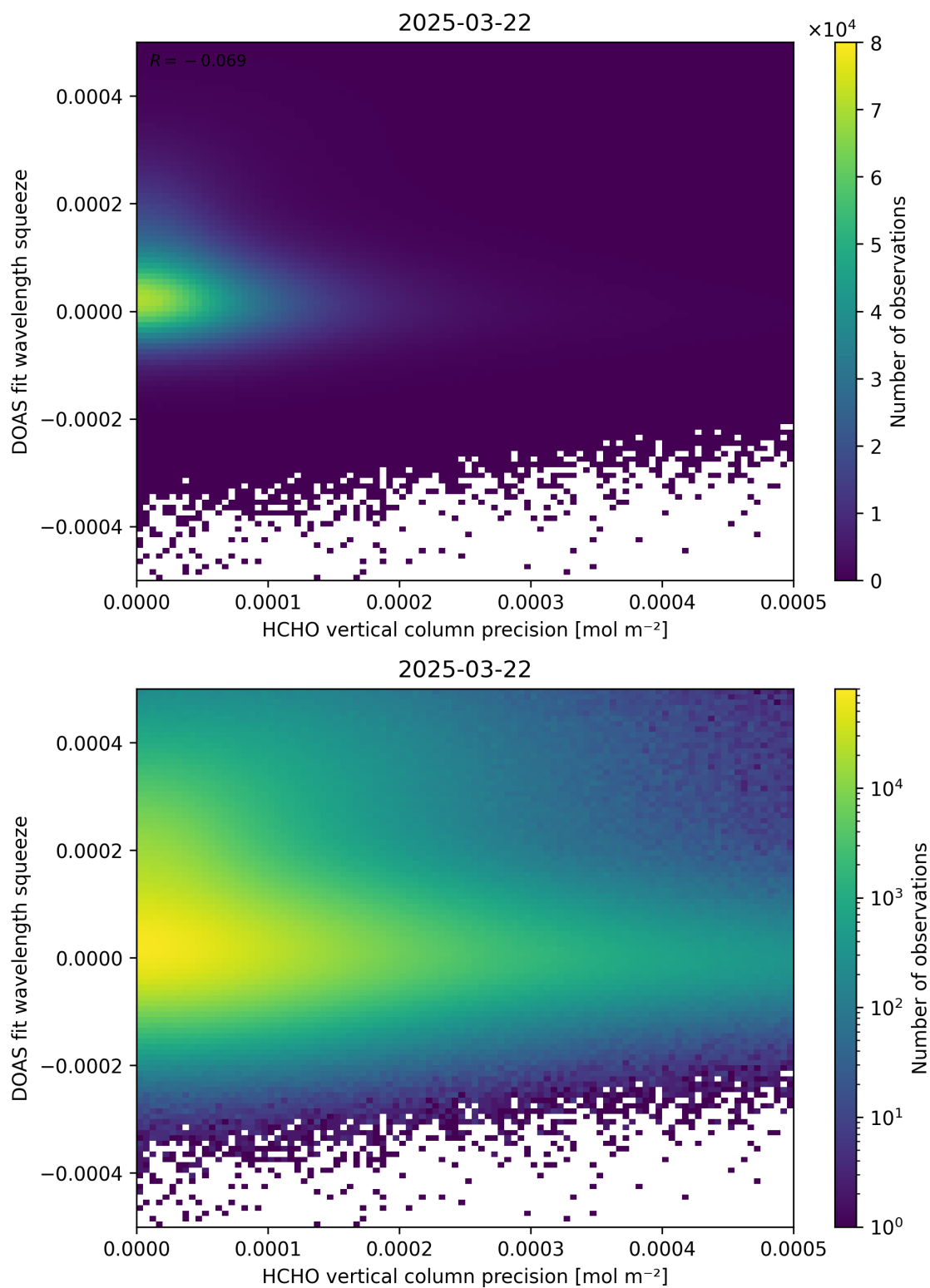
Figure 138: Scatter density plot of “HCHO vertical column precision” against “DOAS fit wavelength squeeze” for 2025-03-21 to 2025-03-23.
