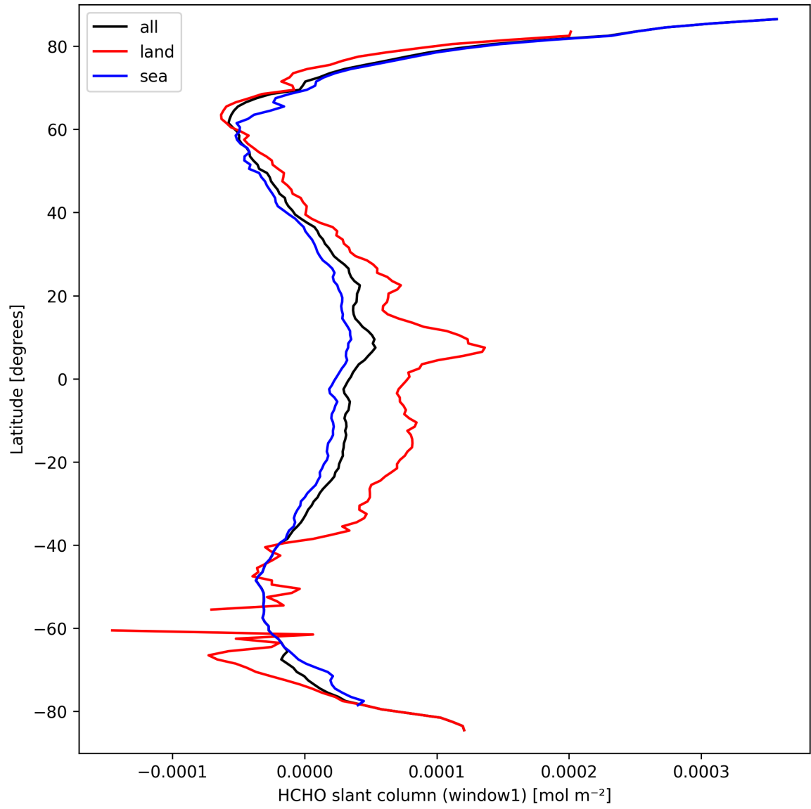
Figure 24: Zonal average of “HCHO slant column (window1)” for 2025-03-21 to 2025-03-23.
