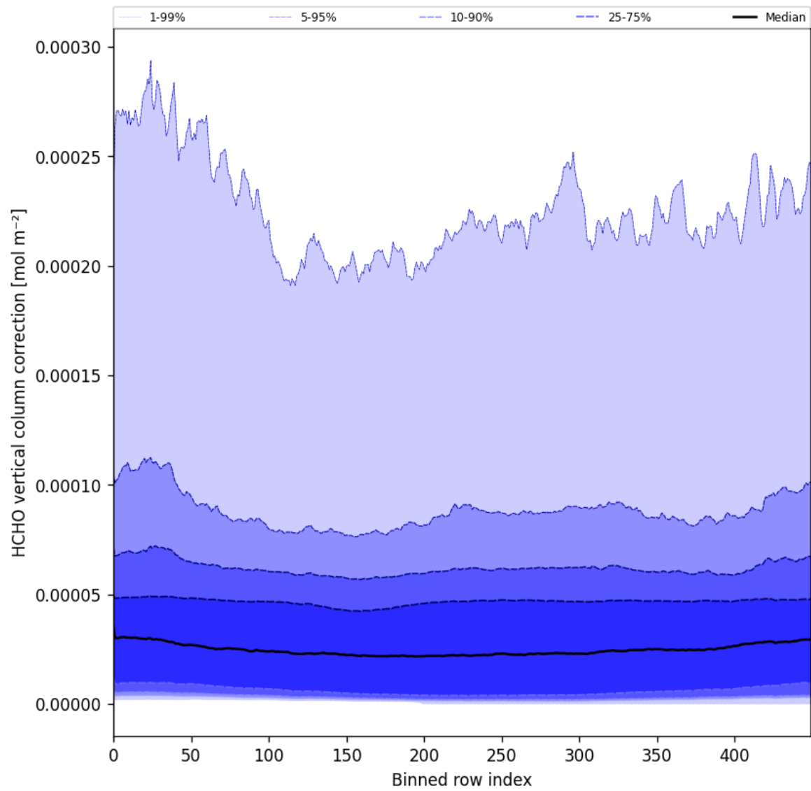
Figure 51: Along track statistics of “HCHO vertical column correction” for 2025-03-21 to 2025-03-23
