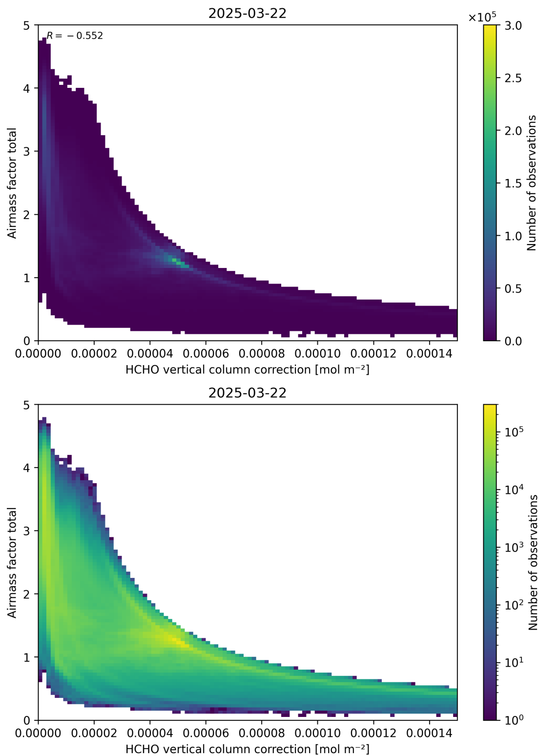
Figure 120: Scatter density plot of “HCHO vertical column correction” against “Airmass factor total” for 2025-03-21 to 2025-03-23.
