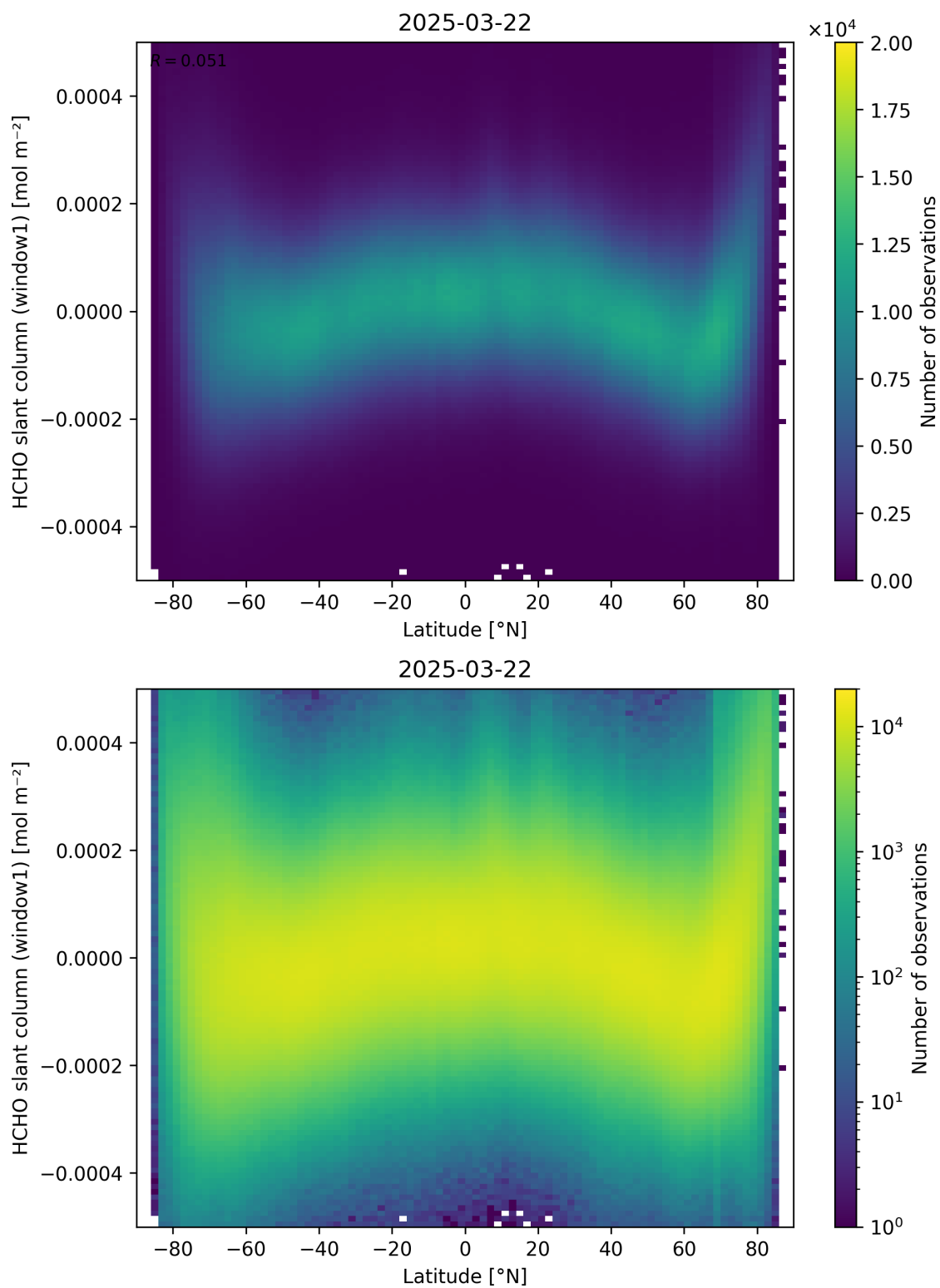
Figure 159: Scatter density plot of “Latitude” against “HCHO slant column (window1)” for 2025-03-21 to 2025-03-23.
