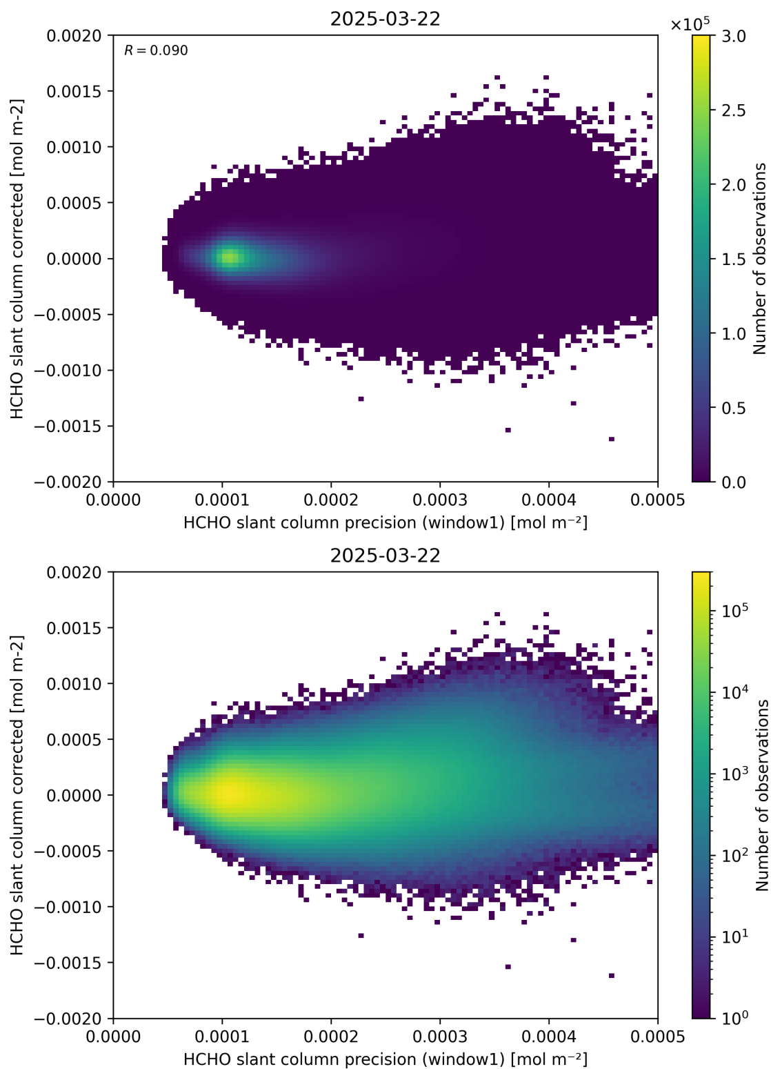
Figure 92: Scatter density plot of “HCHO slant column precision (window1)” against “HCHO slant column corrected” for 2025-03-21 to 2025-03-23.
