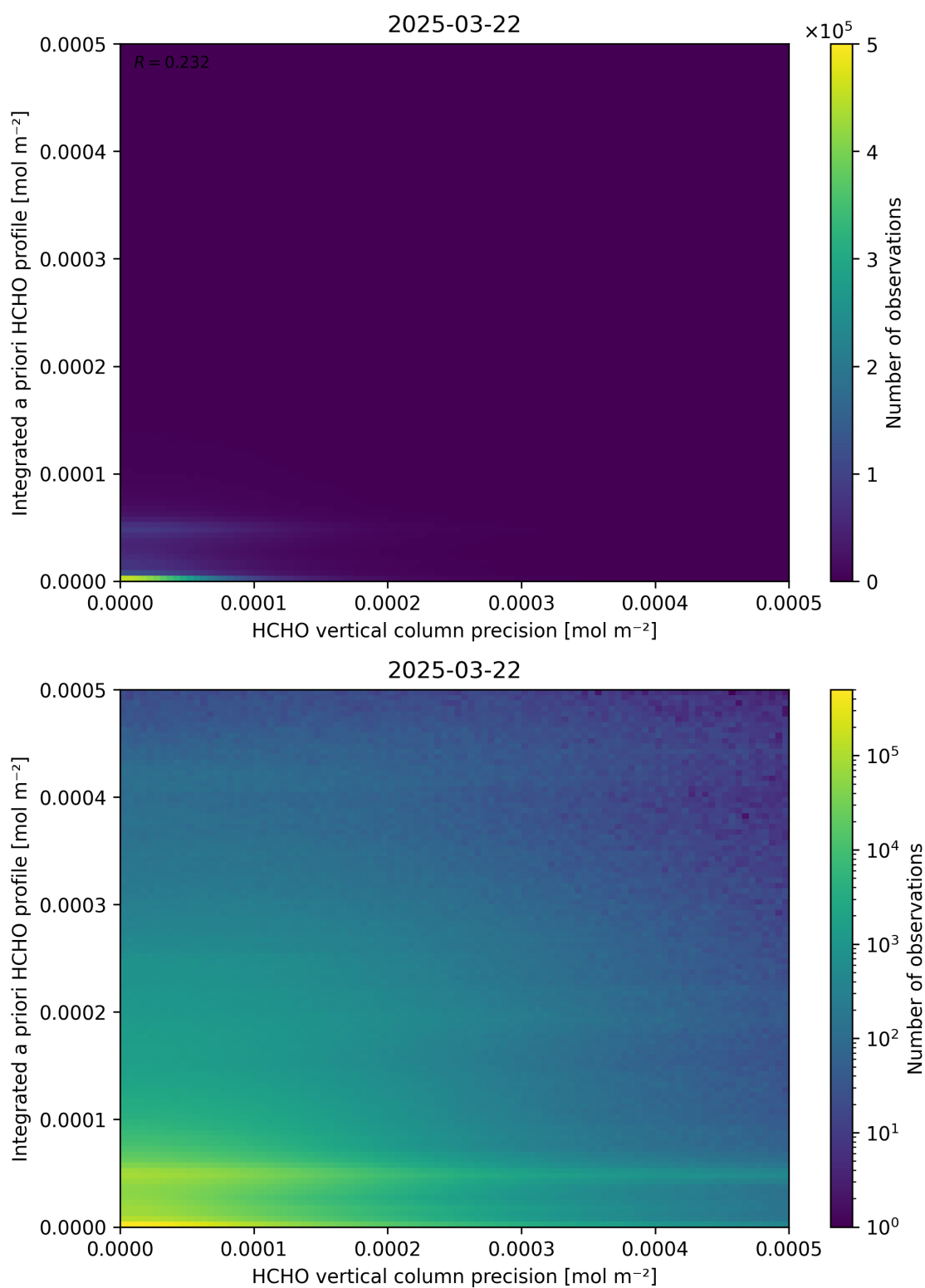
Figure 147: Scatter density plot of “HCHO vertical column precision” against “Integrated a priori HCHO profile” for 2025-03-21 to 2025-03-23.
