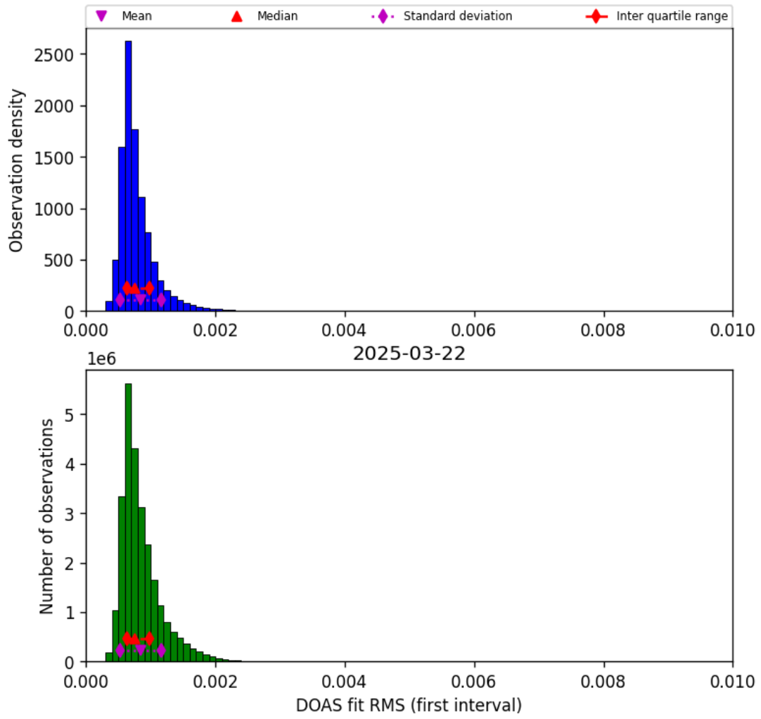
Figure 46: Histogram of “DOAS fit RMS (first interval)” for 2025-03-21 to 2025-03-23
