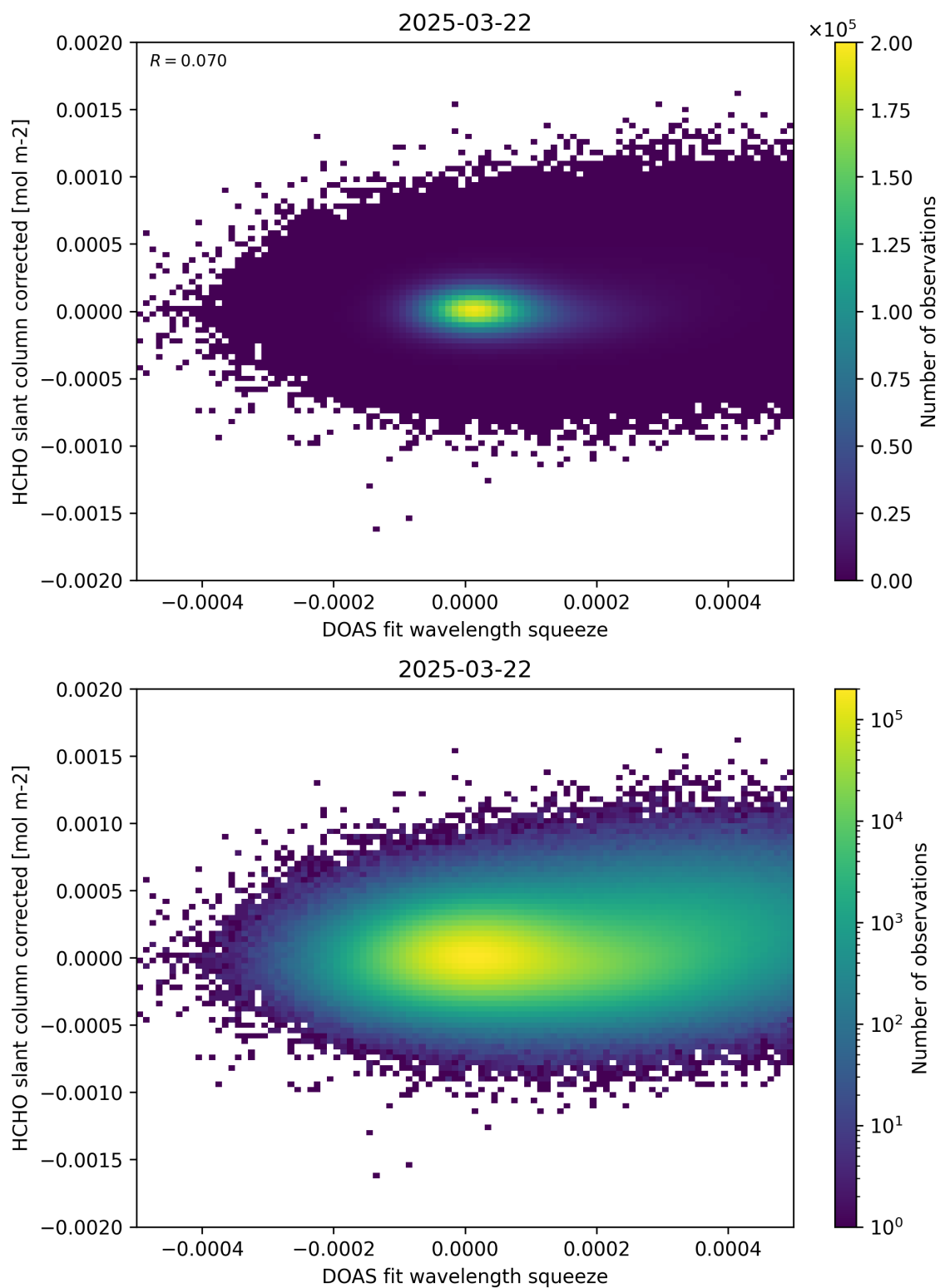
Figure 69: Scatter density plot of “DOAS fit wavelength squeeze” against “HCHO slant column corrected” for 2025-03-21 to 2025-03-23.
