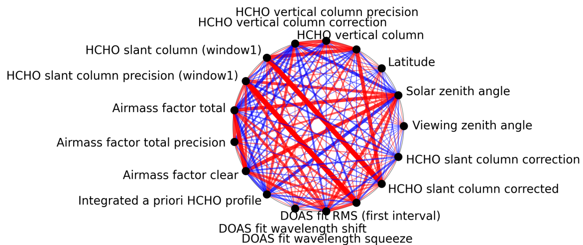
Figure 1: Map of correlation graph for 2025-03-21 to 2025-03-23.
