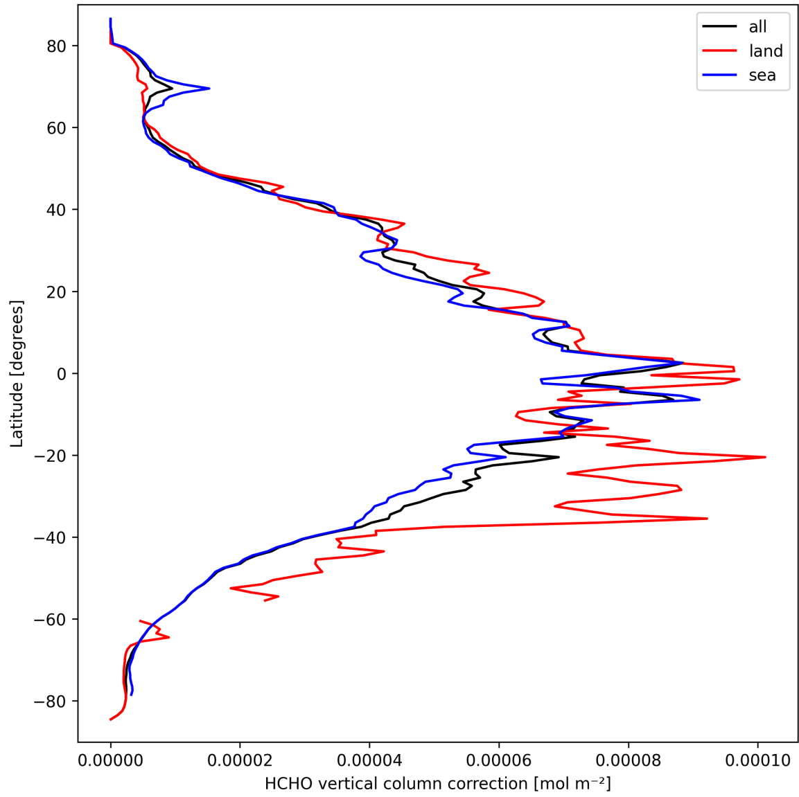
Figure 23: Zonal average of “HCHO vertical column correction” for 2025-03-21 to 2025-03-23.
