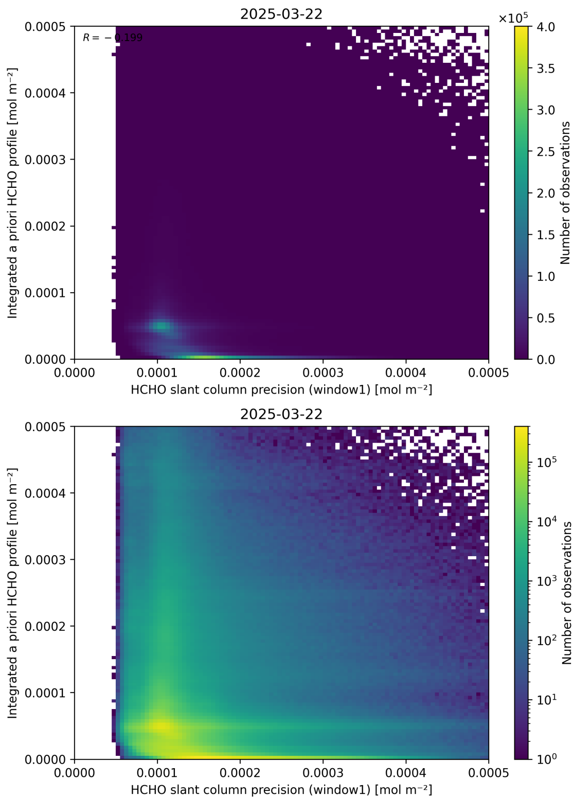
Figure 96: Scatter density plot of “HCHO slant column precision (window1)” against “Integrated a priori HCHO profile” for 2025-03-21 to 2025-03-23.
