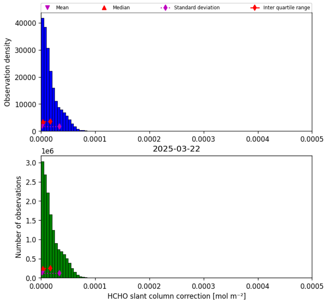
Figure 47: Histogram of “HCHO slant column correction” for 2025-03-21 to 2025-03-23
