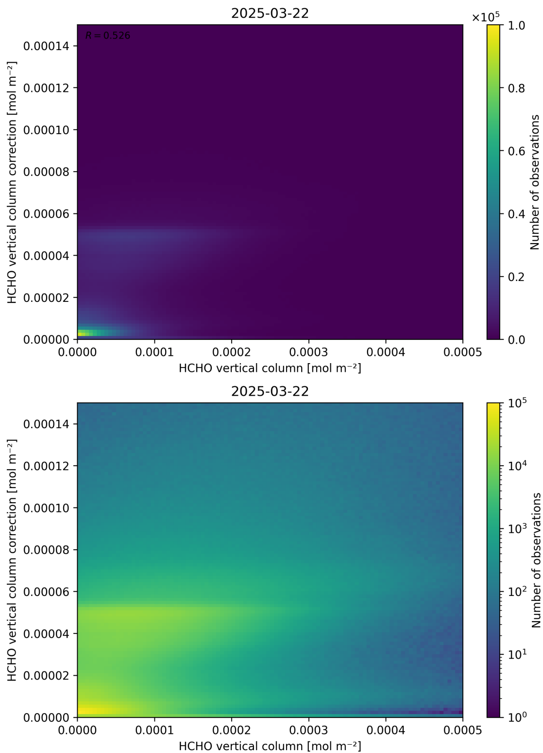
Figure 133: Scatter density plot of “HCHO vertical column” against “HCHO vertical column correction” for 2025-03-21 to 2025-03-23.
