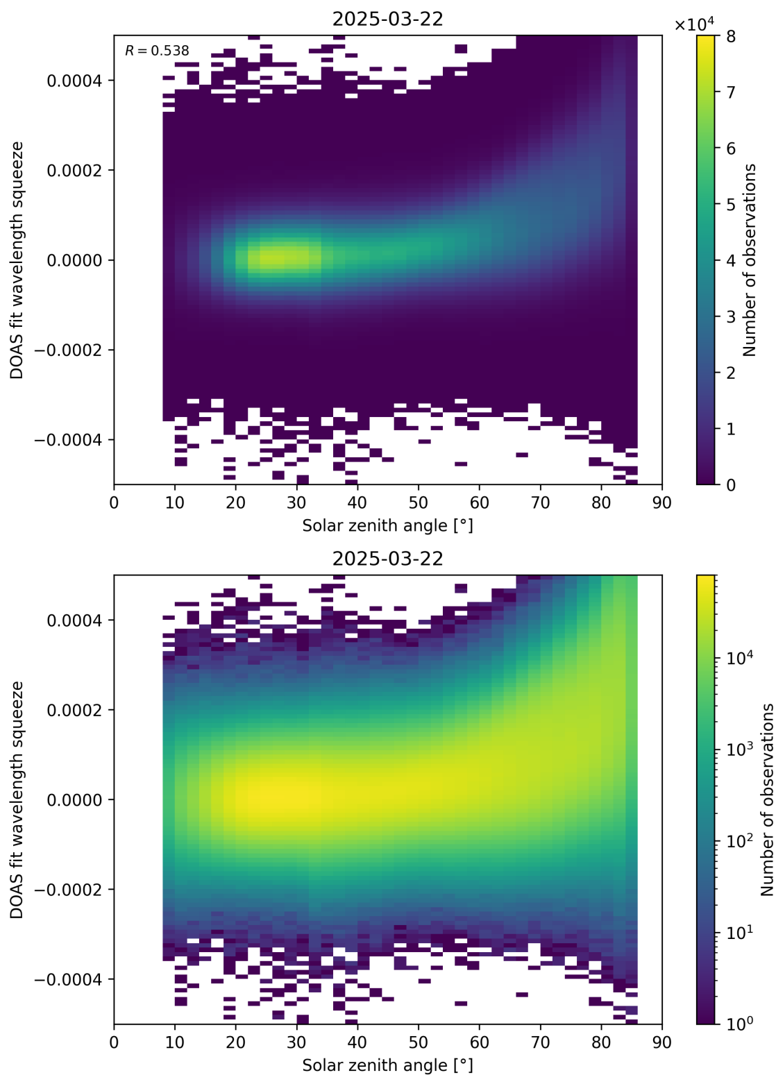
Figure 169: Scatter density plot of “Solar zenith angle” against “DOAS fit wavelength squeeze” for 2025-03-21 to 2025-03-23.
