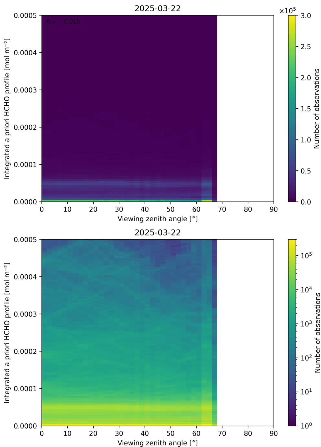
Figure 195: Scatter density plot of “Viewing zenith angle” against “Integrated a priori HCHO profile” for 2025-03-21 to 2025-03-23.
