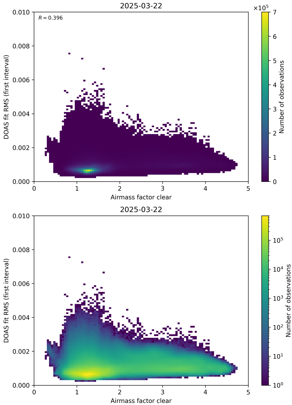
Figure 71: Scatter density plot of “Airmass factor clear” against “DOAS fit RMS (first interval)” for 2025-03-21 to 2025-03-23.
