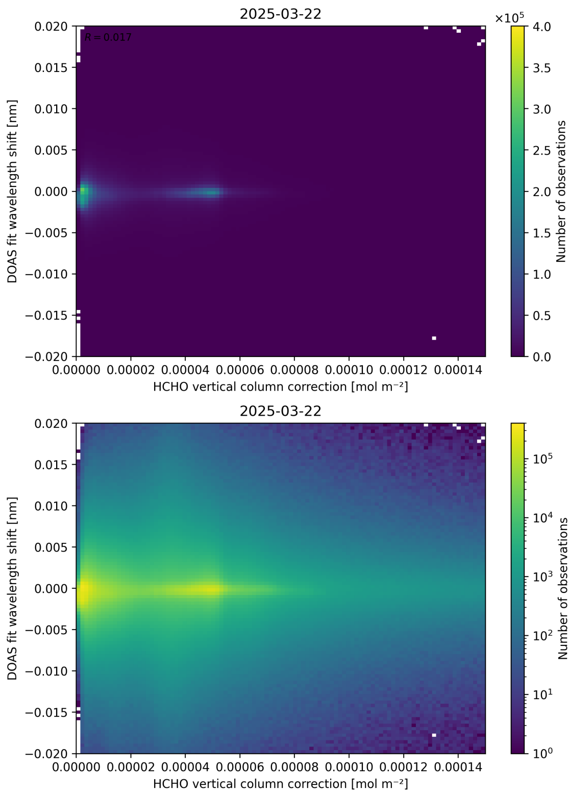
Figure 113: Scatter density plot of “HCHO vertical column correction” against “DOAS fit wavelength shift” for 2025-03-21 to 2025-03-23.
