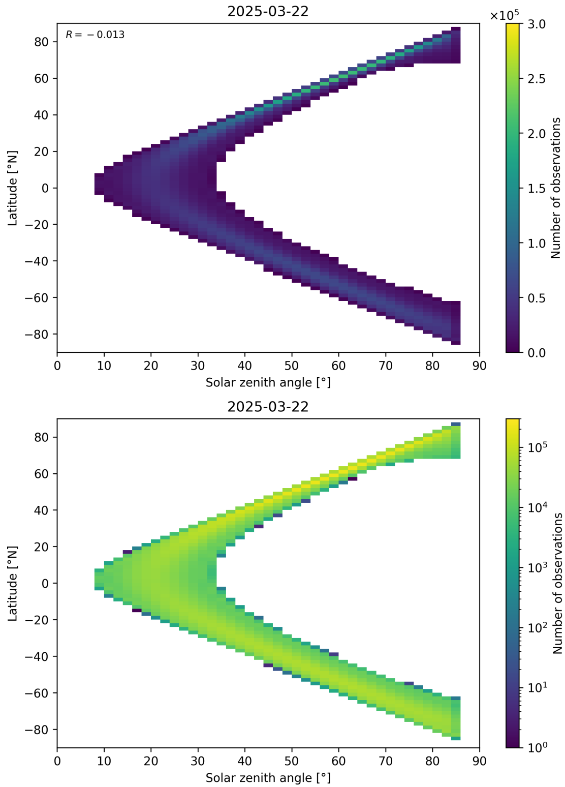
Figure 181: Scatter density plot of “Solar zenith angle” against “Latitude” for 2025-03-21 to 2025-03-23.
