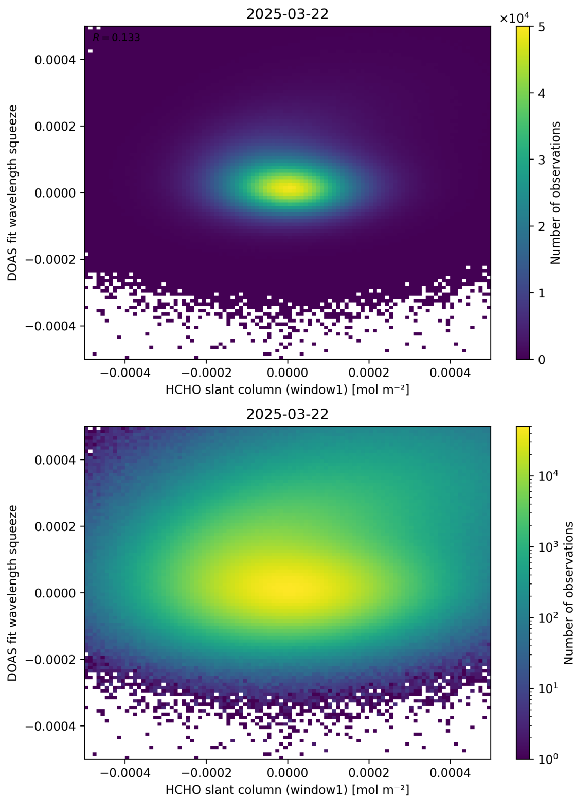
Figure 80: Scatter density plot of “HCHO slant column (window1)” against “DOAS fit wavelength squeeze” for 2025-03-21 to 2025-03-23.
