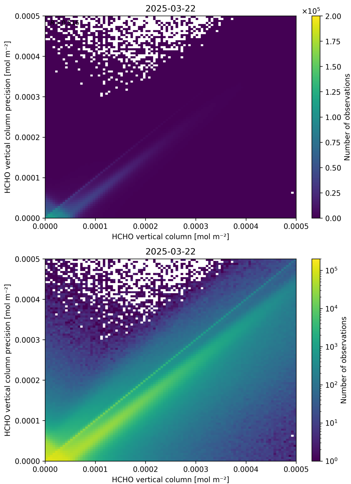
Figure 134: Scatter density plot of “HCHO vertical column” against “HCHO vertical column precision” for 2025-03-21 to 2025-03-23.
