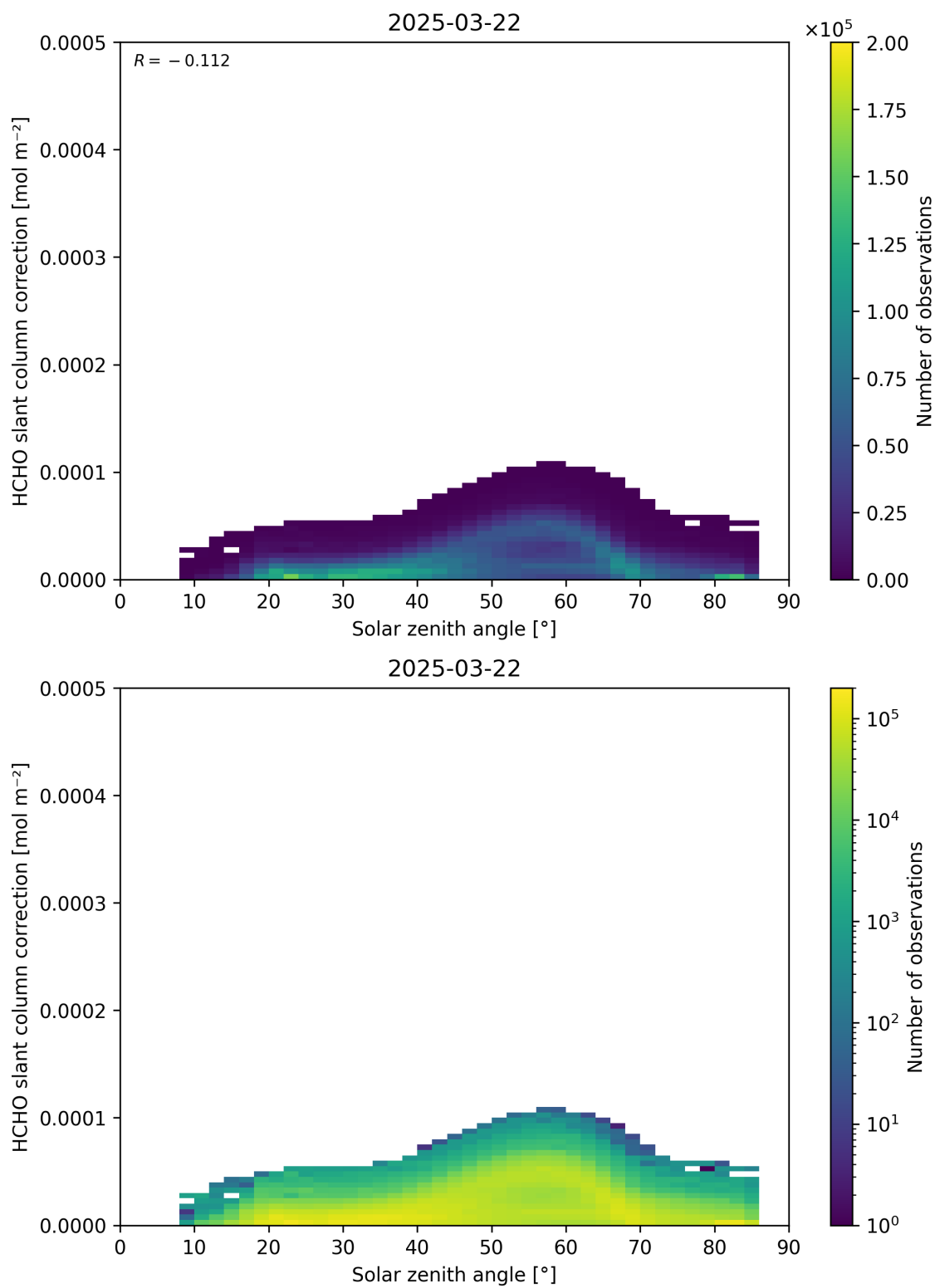
Figure 172: Scatter density plot of “Solar zenith angle” against “HCHO slant column correction” for 2025-03-21 to 2025-03-23.
