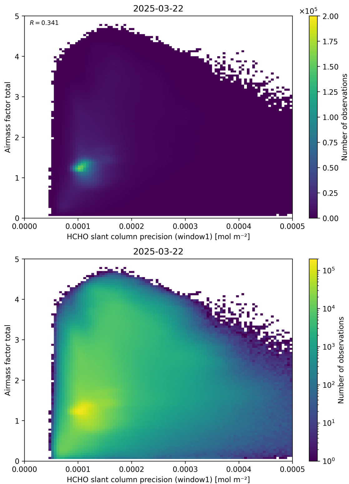
Figure 94: Scatter density plot of “HCHO slant column precision (window1)” against “Airmass factor total” for 2025-03-21 to 2025-03-23.
