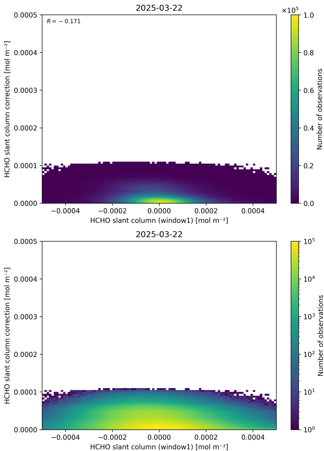
Figure 83: Scatter density plot of “HCHO slant column (window1)” against “HCHO slant column correction” for 2025-03-21 to 2025-03-23.
