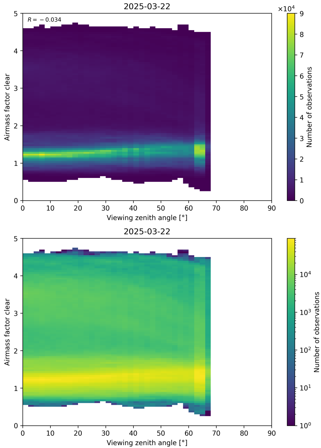
Figure 185: Scatter density plot of “Viewing zenith angle” against “Airmass factor clear” for 2025-03-21 to 2025-03-23.
