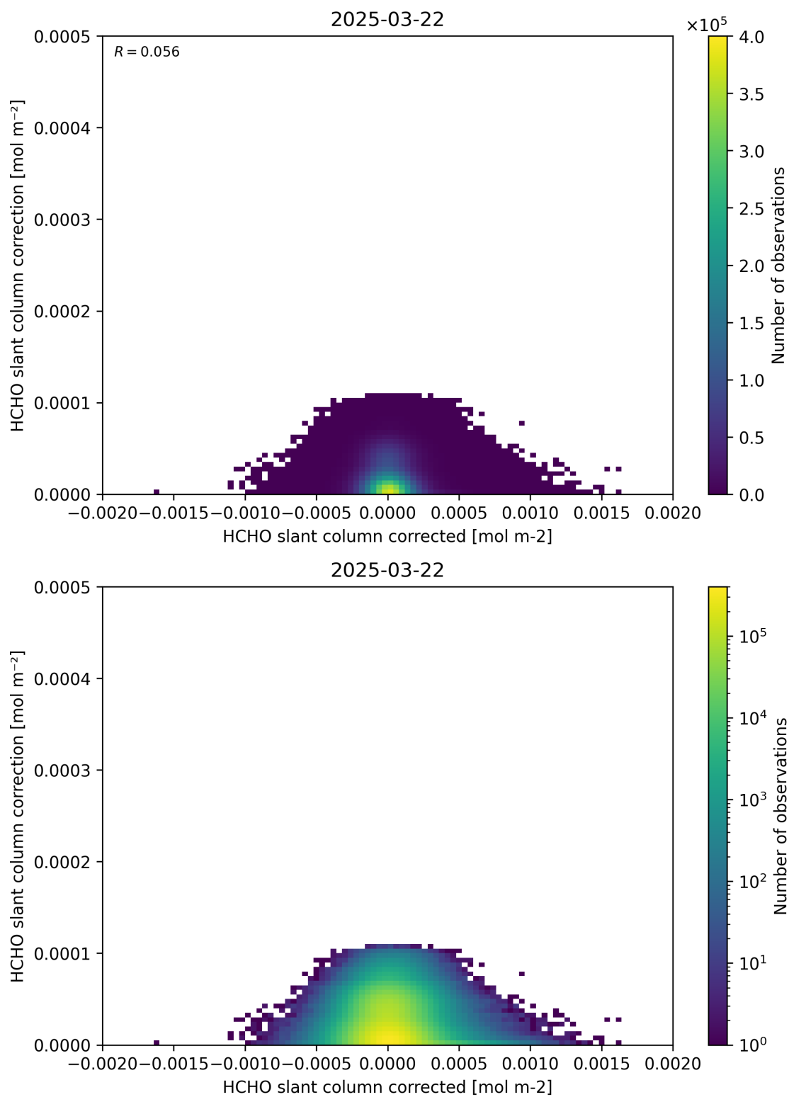
Figure 77: Scatter density plot of “HCHO slant column corrected” against “HCHO slant column correction” for 2025-03-21 to 2025-03-23.
