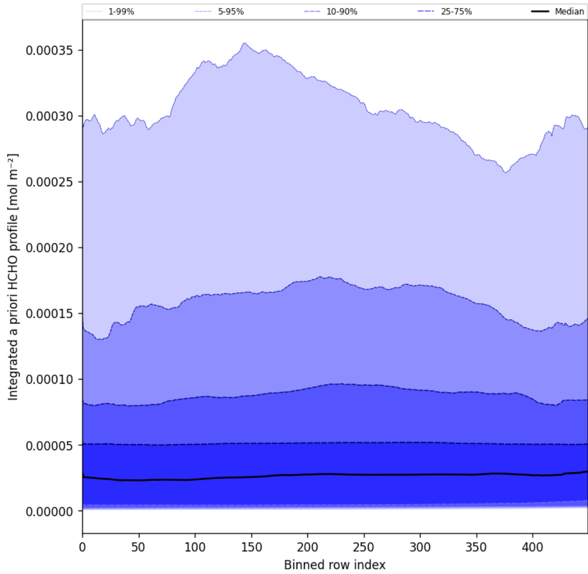
Figure 57: Along track statistics of "Integrated a priori HCHO profile" for 2025-03-21 to 2025-03-23
