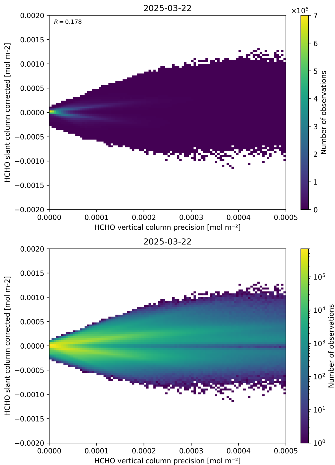
Figure 140: Scatter density plot of “HCHO vertical column precision” against “HCHO slant column corrected” for 2025-03-21 to 2025-03-23.
