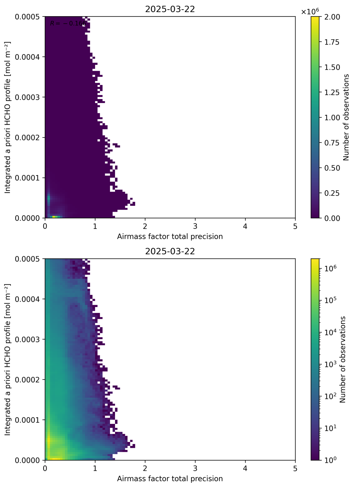
Figure 111: Scatter density plot of “Airmass factor total precision” against “Integrated a priori HCHO profile” for 2025-03-21 to 2025-03-23.
