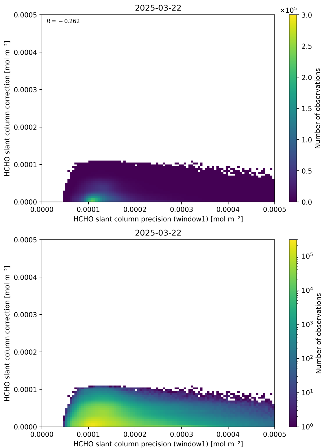
Figure 93: Scatter density plot of “HCHO slant column precision (window1)” against “HCHO slant column correction” for 2025-03-21 to 2025-03-23.
