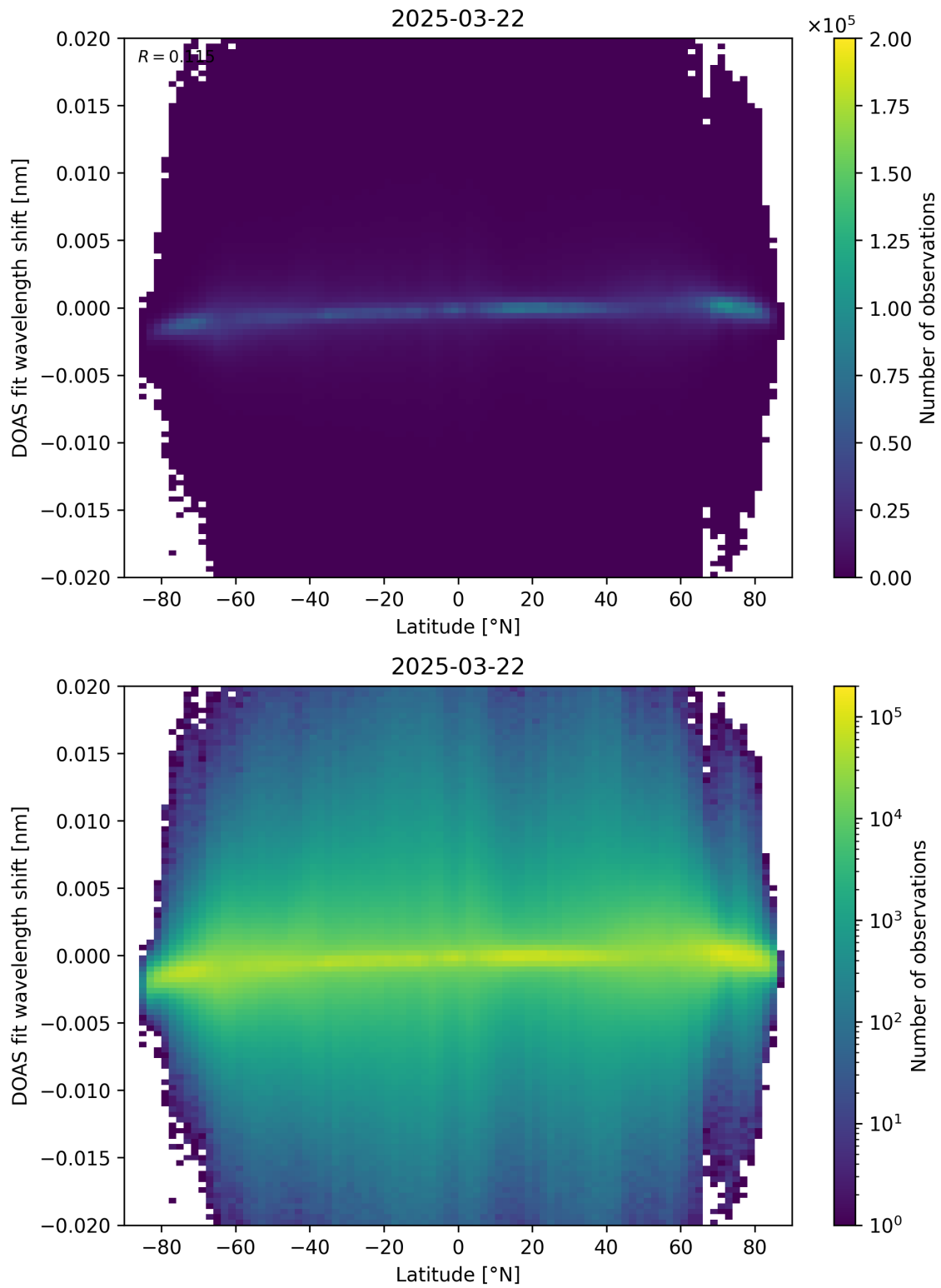
Figure 154: Scatter density plot of “Latitude” against “DOAS fit wavelength shift” for 2025-03-21 to 2025-03-23.
