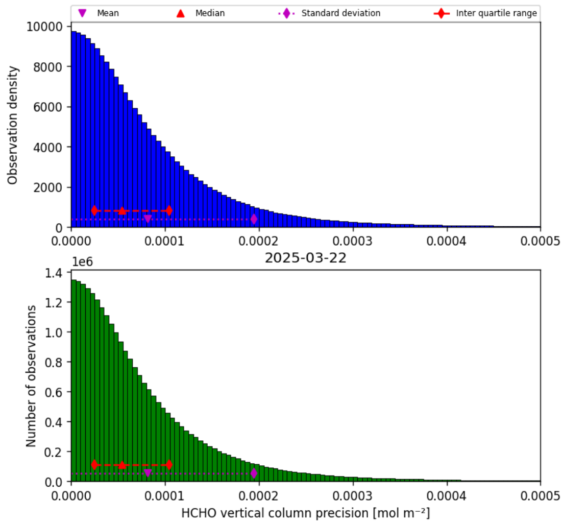
Figure 36: Histogram of “HCHO vertical column precision” for 2025-03-21 to 2025-03-23
