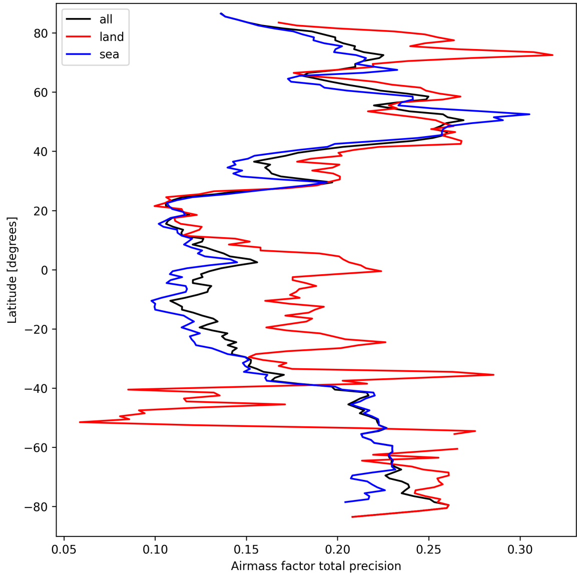
Figure 27: Zonal average of “Airmass factor total precision” for 2025-03-23 to 2025-03-24.
