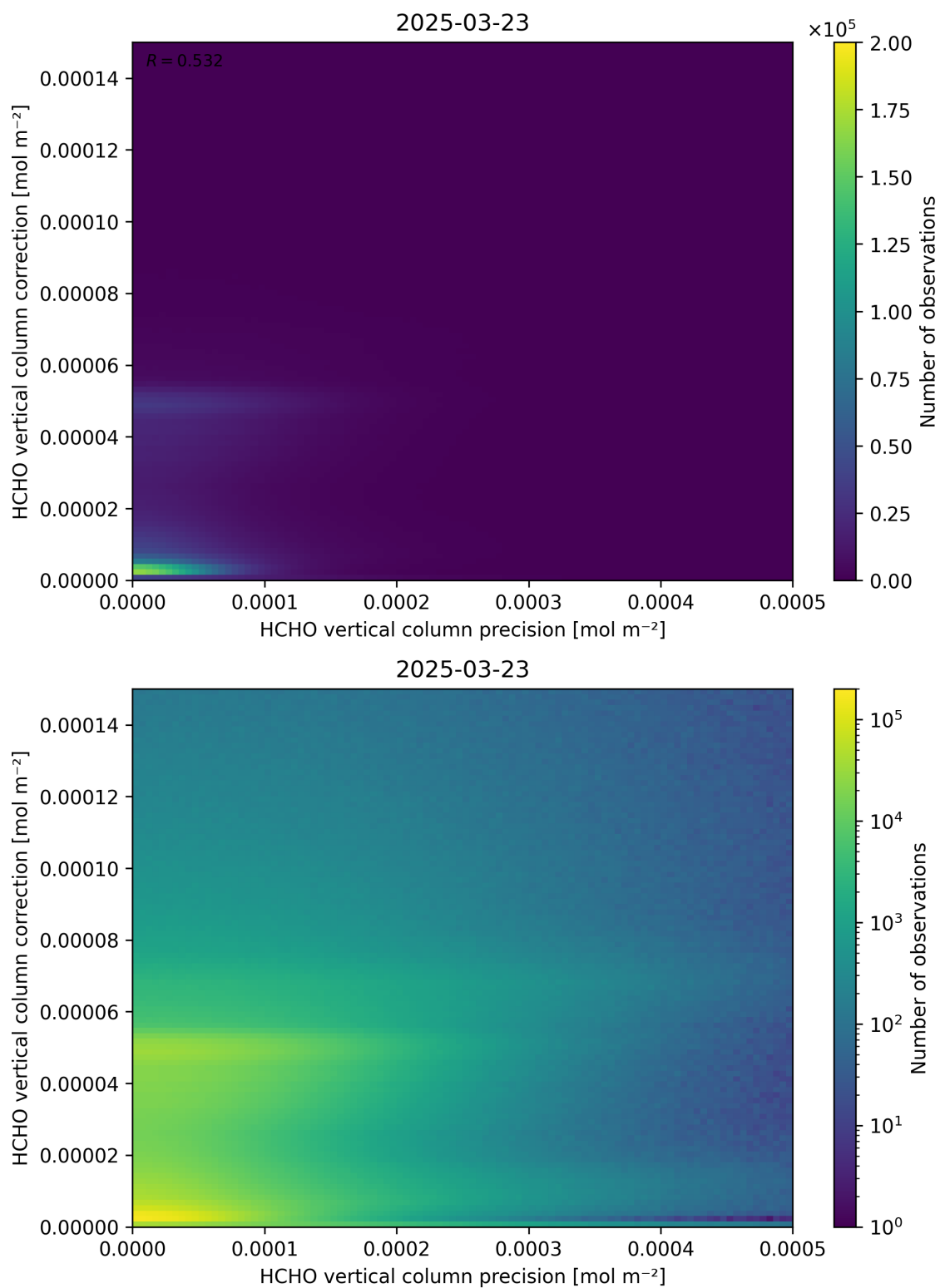
Figure 146: Scatter density plot of “HCHO vertical column precision” against “HCHO vertical column correction” for 2025-03-23 to 2025-03-24.
