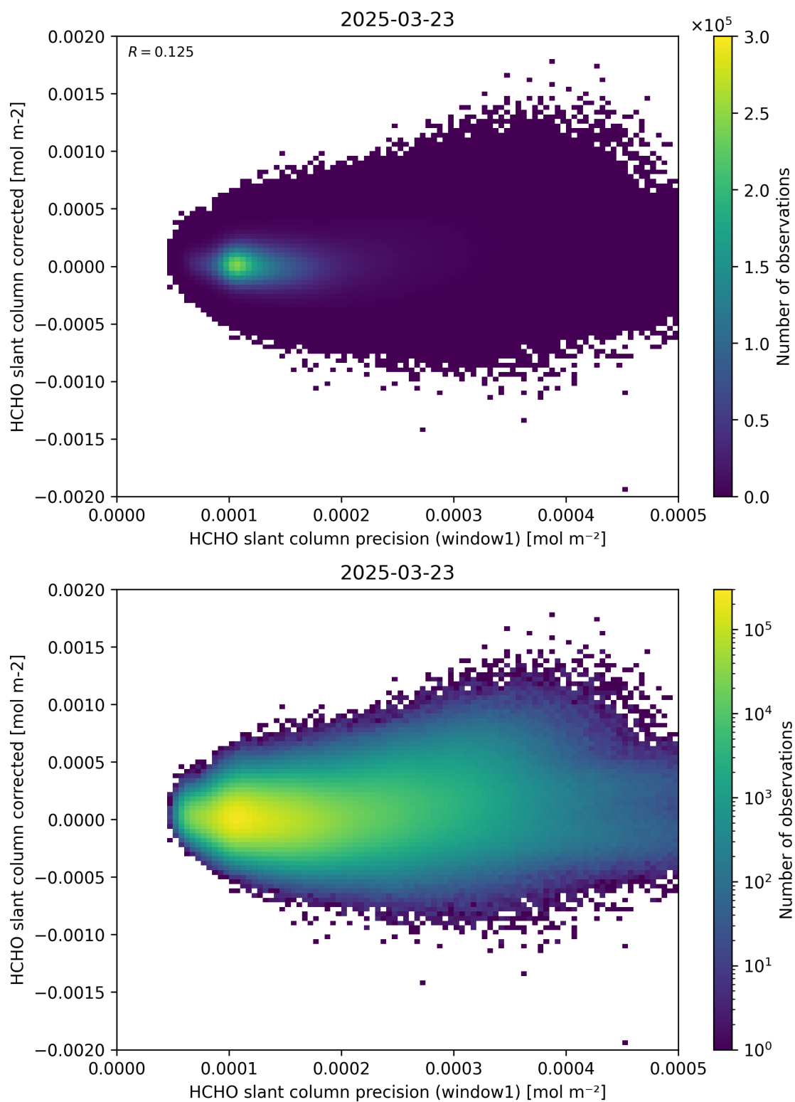
Figure 92: Scatter density plot of “HCHO slant column precision (window1)” against “HCHO slant column corrected” for 2025-03-23 to 2025-03-24.
