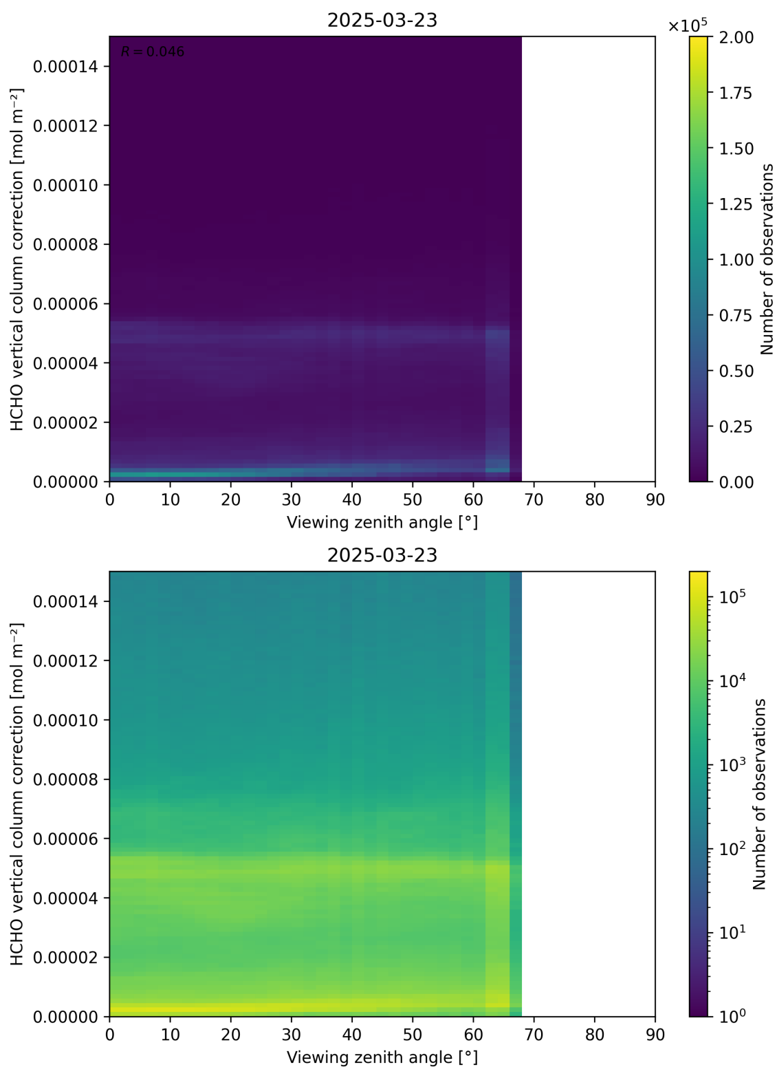
Figure 193: Scatter density plot of “Viewing zenith angle” against “HCHO vertical column correction” for 2025-03-23 to 2025-03-24.
