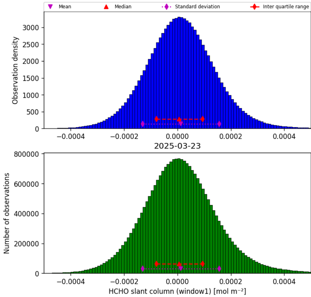
Figure 38: Histogram of “HCHO slant column (window1)” for 2025-03-23 to 2025-03-24
