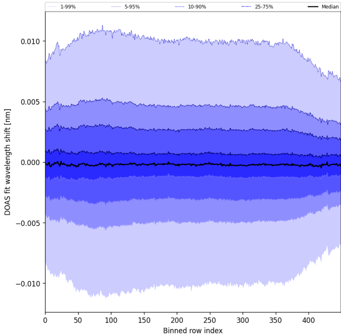
Figure 58: Along track statistics of “DOAS fit wavelength shift” for 2025-03-23 to 2025-03-24
