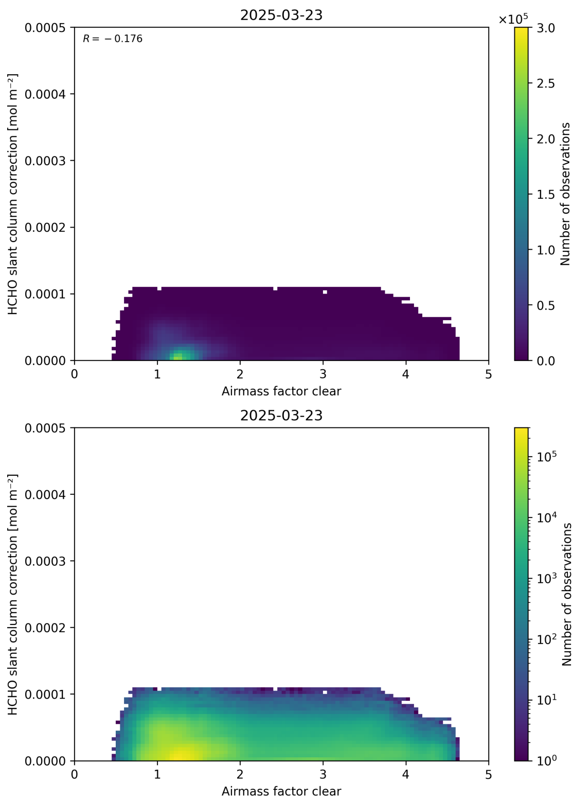
Figure 75: Scatter density plot of “Airmass factor clear” against “HCHO slant column correction” for 2025-03-23 to 2025-03-24.
