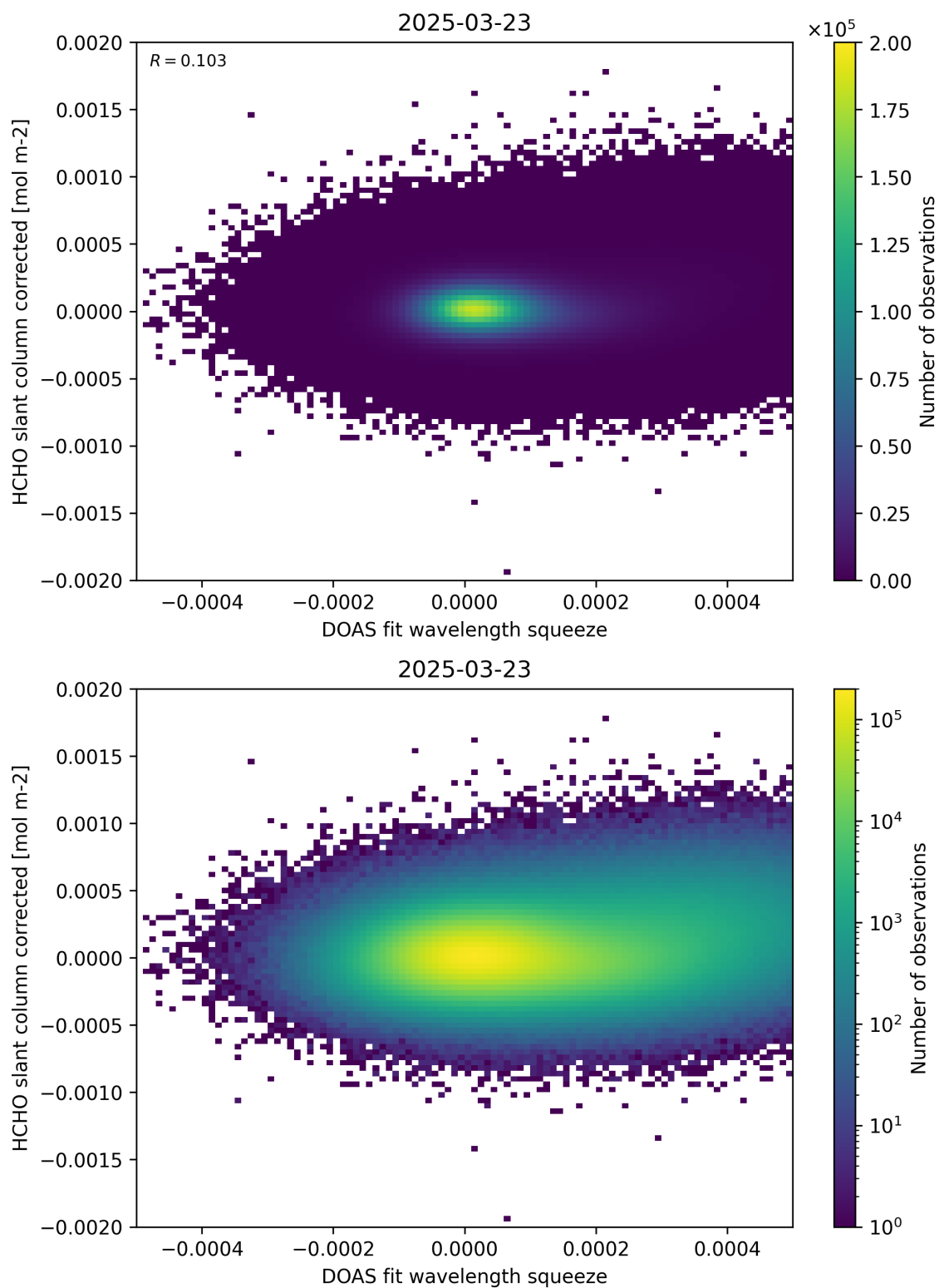
Figure 69: Scatter density plot of “DOAS fit wavelength squeeze” against “HCHO slant column corrected” for 2025-03-23 to 2025-03-24.
