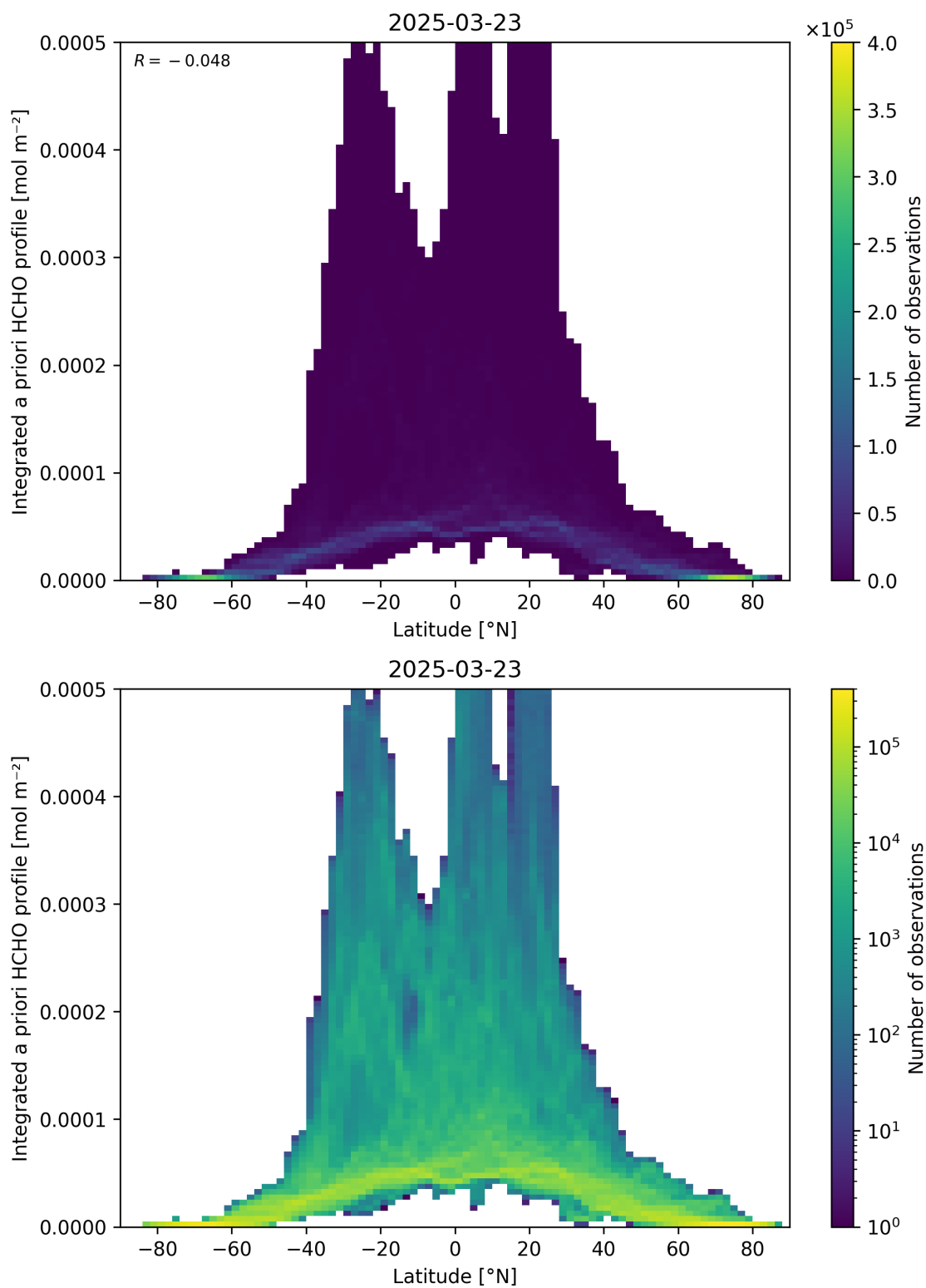
Figure 166: Scatter density plot of “Latitude” against “Integrated a priori HCHO profile” for 2025-03-23 to 2025-03-24.
