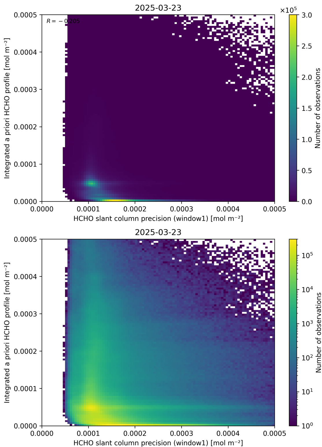
Figure 96: Scatter density plot of “HCHO slant column precision (window1)” against “Integrated a priori HCHO profile” for 2025-03-23 to 2025-03-24.
