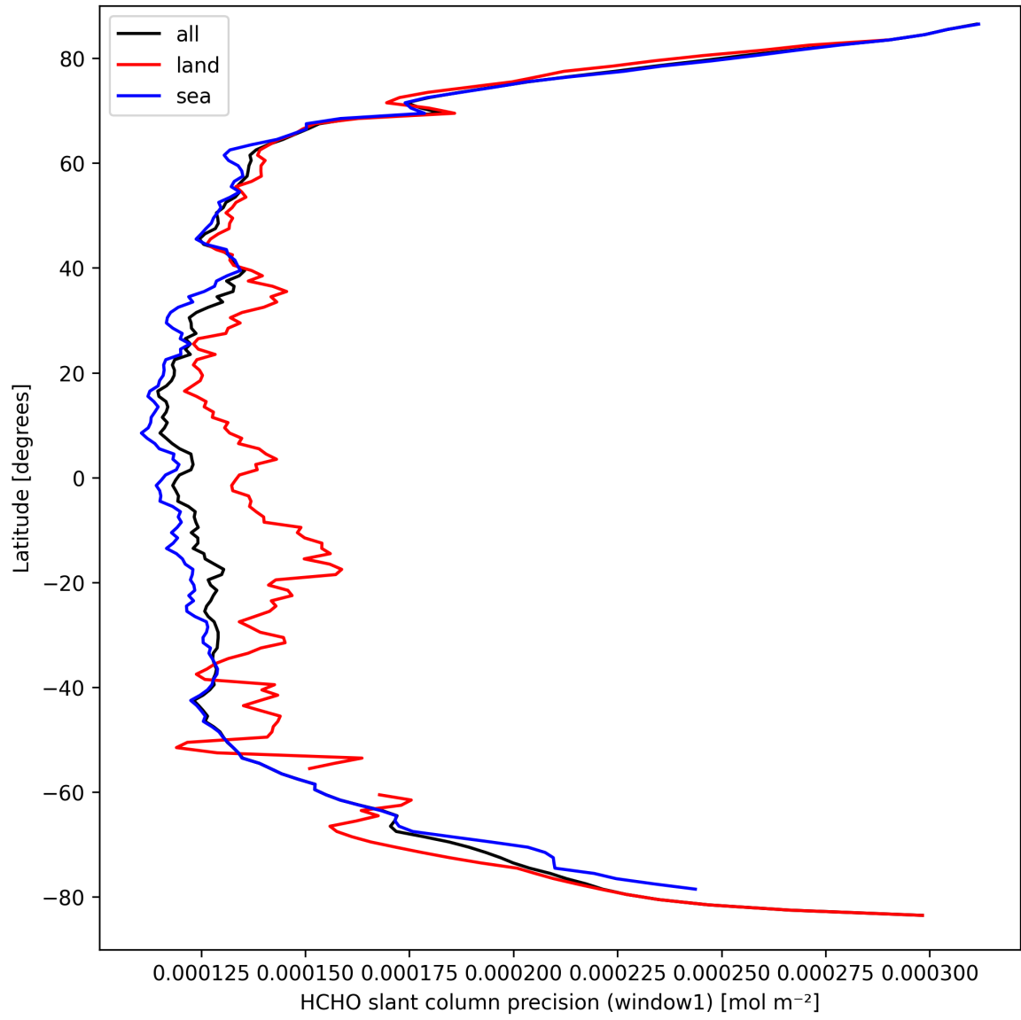
Figure 25: Zonal average of “HCHO slant column precision (window1)” for 2025-03-23 to 2025-03-24.
