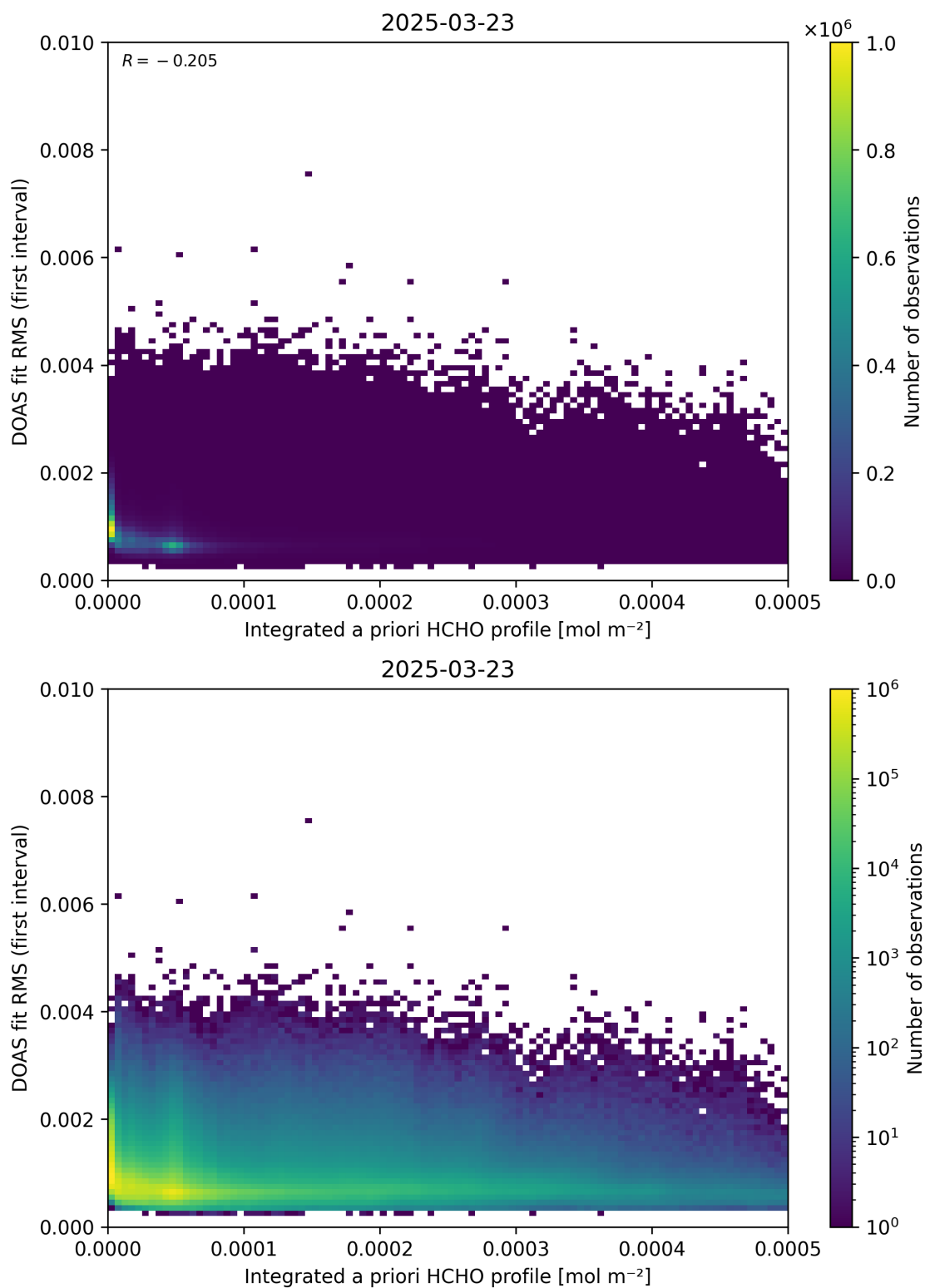
Figure 148: Scatter density plot of “Integrated a priori HCHO profile” against “DOAS fit RMS (first interval)” for 2025-03-23 to 2025-03-24.
