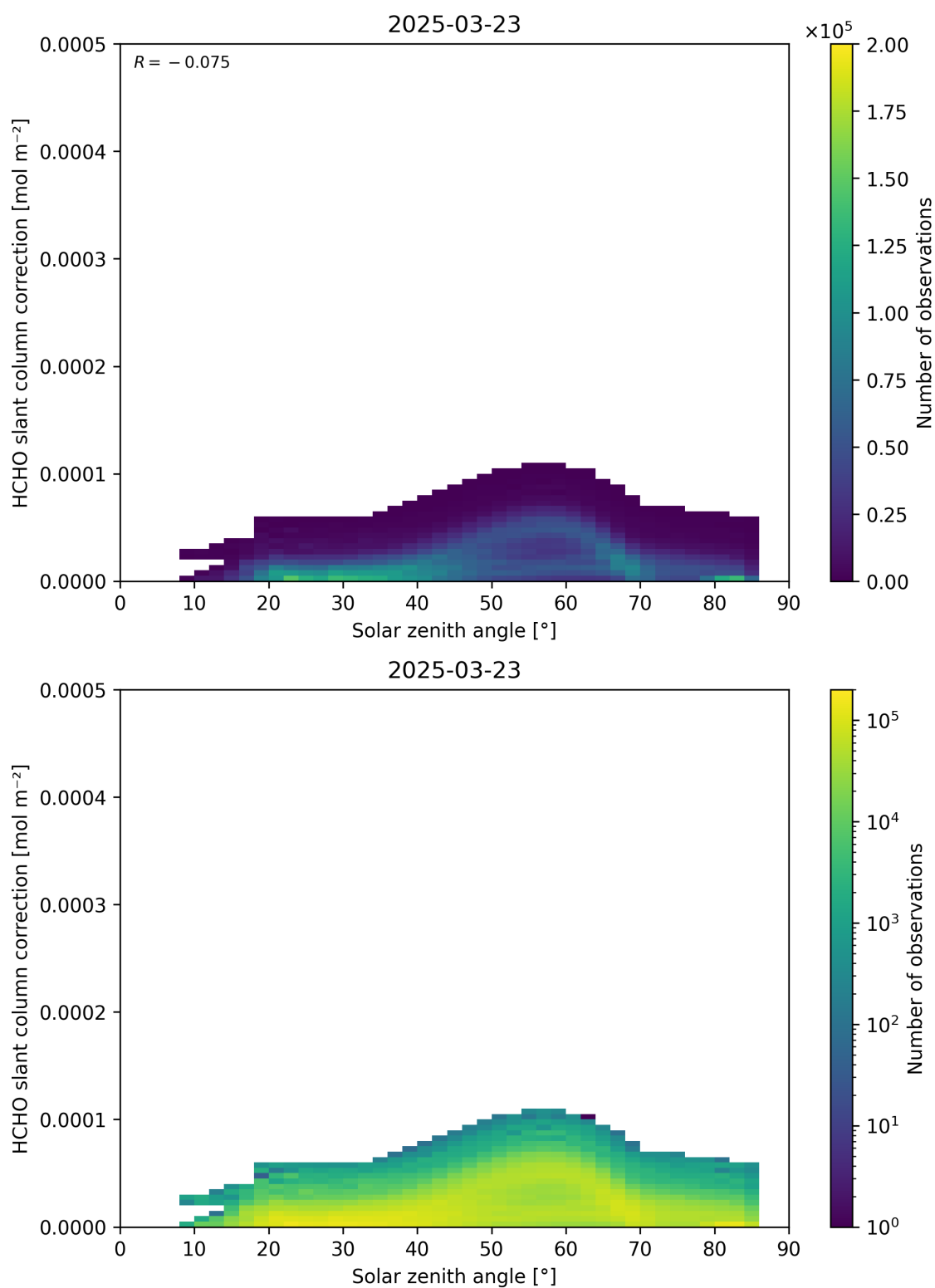
Figure 172: Scatter density plot of “Solar zenith angle” against “HCHO slant column correction” for 2025-03-23 to 2025-03-24.
