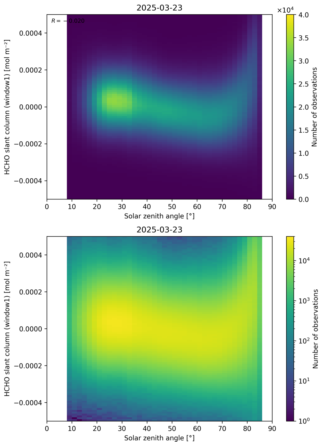
Figure 173: Scatter density plot of “Solar zenith angle” against “HCHO slant column (window1)” for 2025-03-23 to 2025-03-24.
