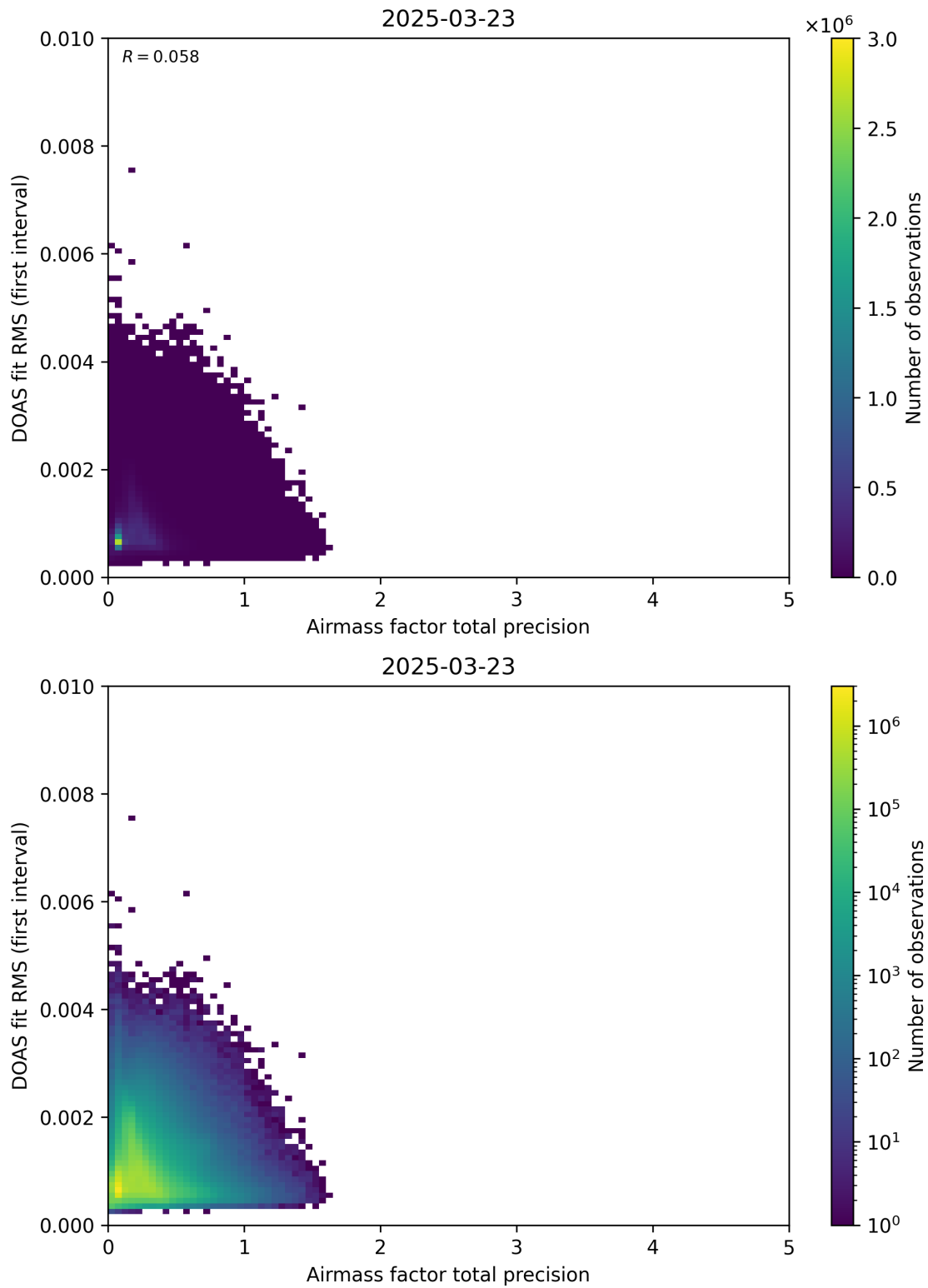
Figure 105: Scatter density plot of “Airmass factor total precision” against “DOAS fit RMS (first interval)” for 2025-03-23 to 2025-03-24.
