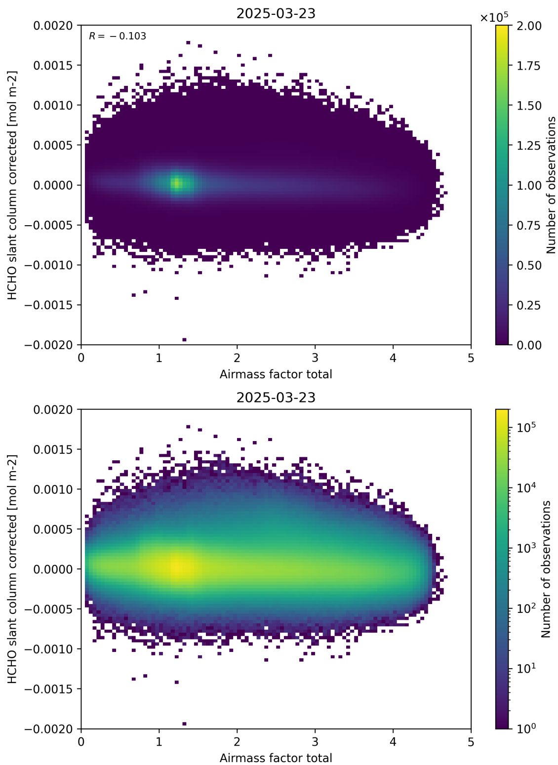
Figure 101: Scatter density plot of “Airmass factor total” against “HCHO slant column corrected” for 2025-03-23 to 2025-03-24.
