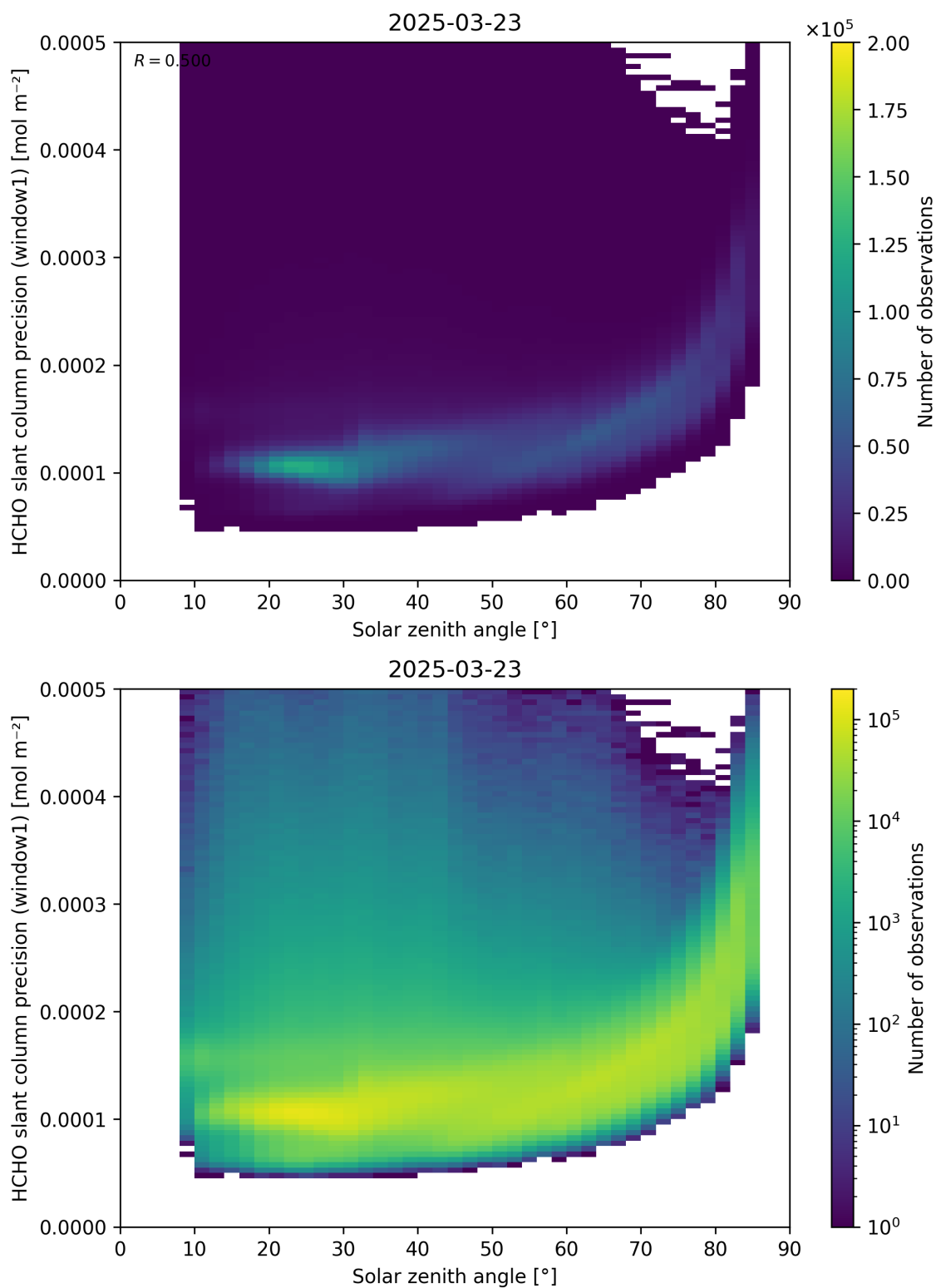
Figure 174: Scatter density plot of “Solar zenith angle” against “HCHO slant column precision (window1)” for 2025-03-23 to 2025-03-24.
