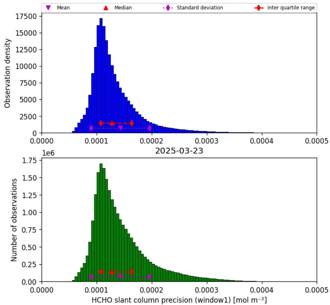
Figure 39: Histogram of “HCHO slant column precision (window1)” for 2025-03-23 to 2025-03-24
