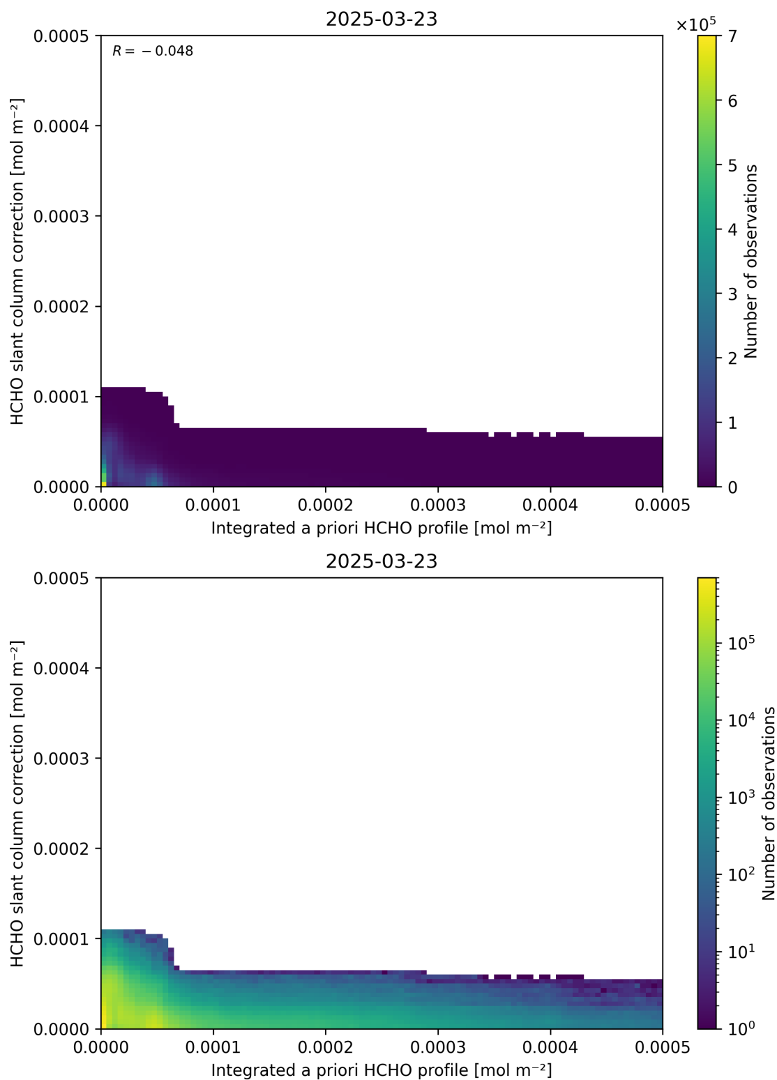
Figure 152: Scatter density plot of “Integrated a priori HCHO profile” against “HCHO slant column correction” for 2025-03-23 to 2025-03-24.
