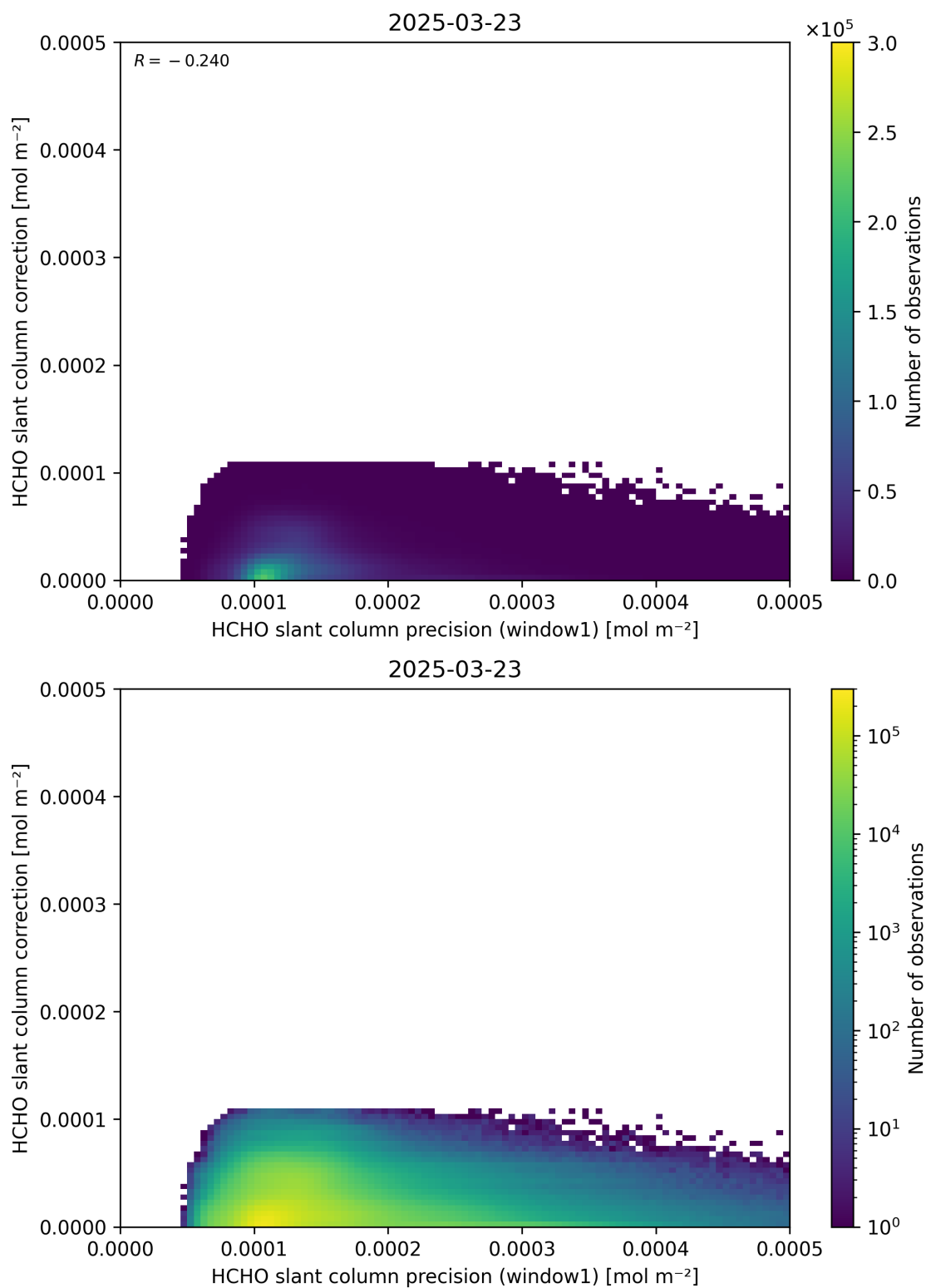
Figure 93: Scatter density plot of “HCHO slant column precision (window1)” against “HCHO slant column correction” for 2025-03-23 to 2025-03-24.
