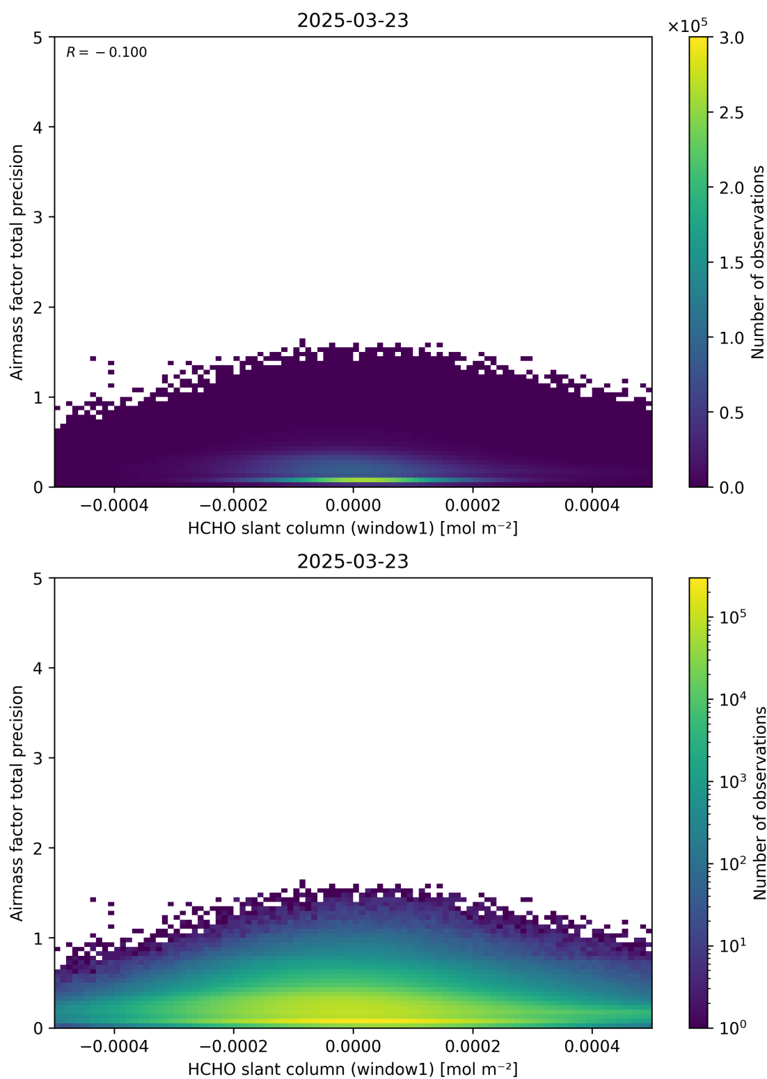
Figure 86: Scatter density plot of “HCHO slant column (window1)” against “Airmass factor total precision” for 2025-03-23 to 2025-03-24.
