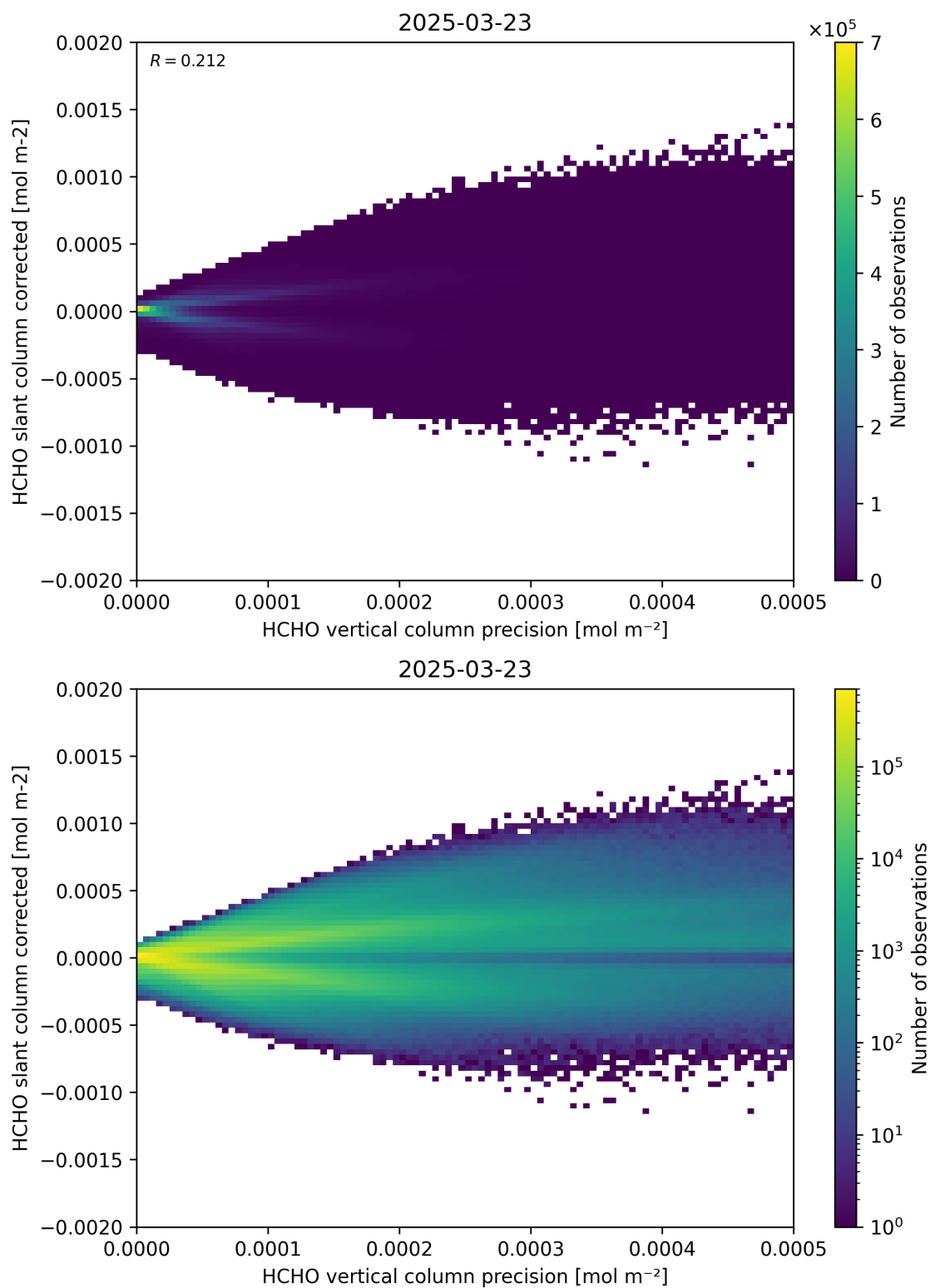
Figure 140: Scatter density plot of “HCHO vertical column precision” against “HCHO slant column corrected” for 2025-03-23 to 2025-03-24.
