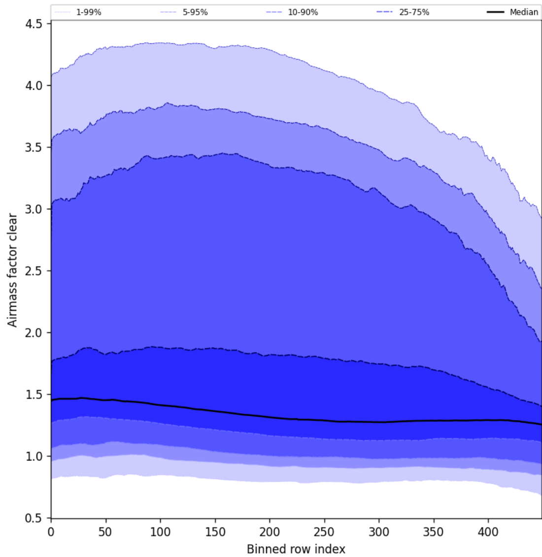
Figure 56: Along track statistics of “Air mass factor clear” for 2025-03-23 to 2025-03-24
