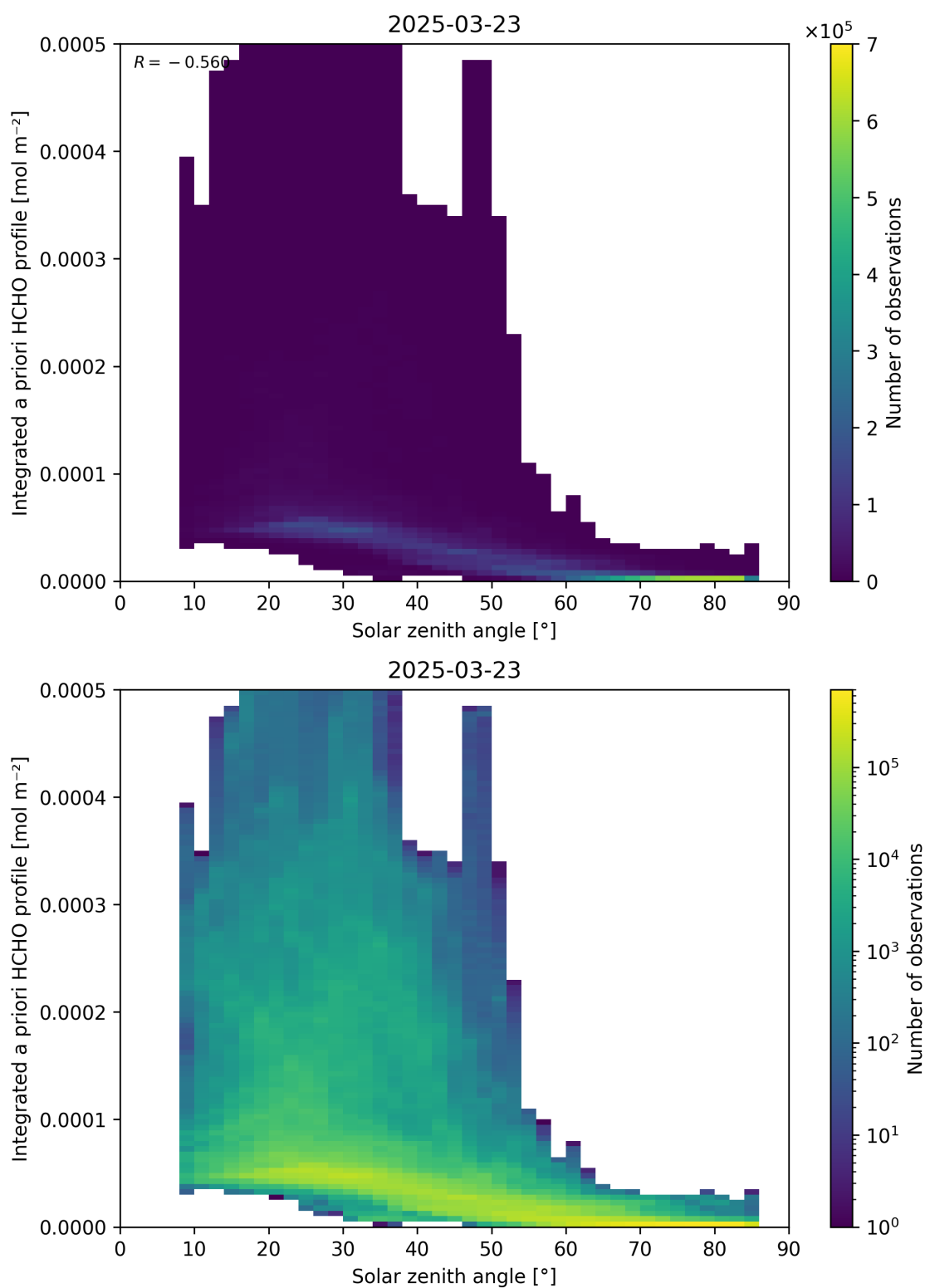
Figure 180: Scatter density plot of “Solar zenith angle” against “Integrated a priori HCHO profile” for 2025-03-23 to 2025-03-24.
