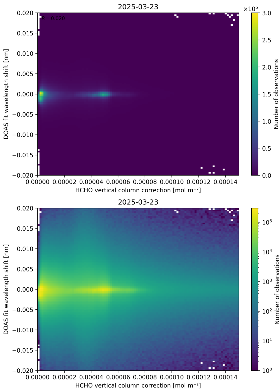
Figure 113: Scatter density plot of “HCHO vertical column correction” against “DOAS fit wavelength shift” for 2025-03-23 to 2025-03-24.
