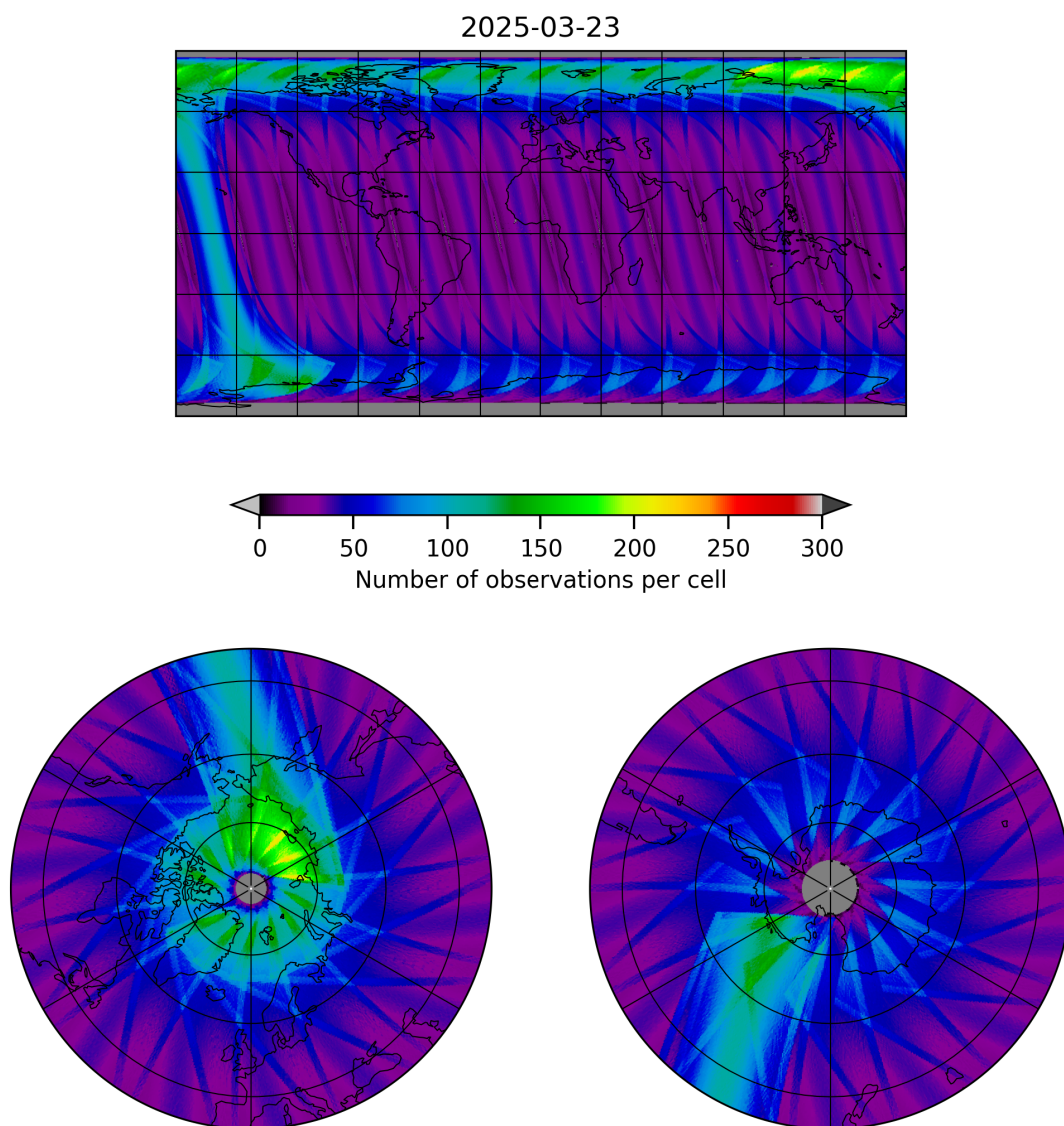
Figure 19: Map of the number of observations for 2025-03-23 to 2025-03-24
