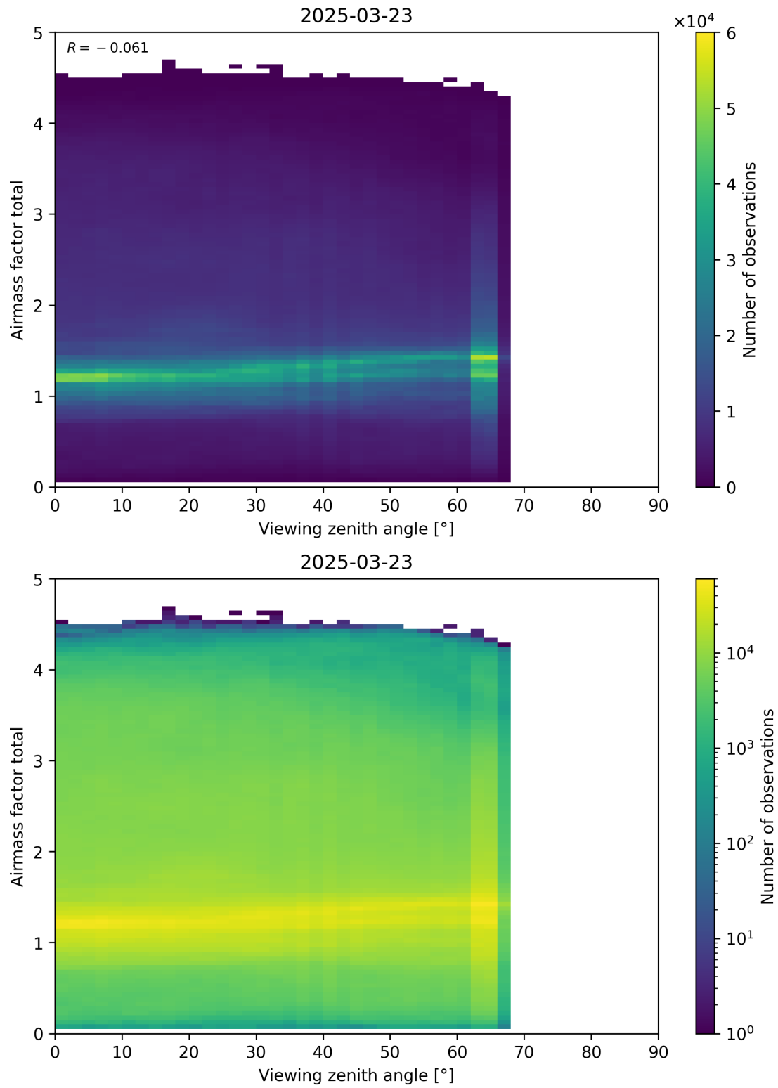
Figure 190: Scatter density plot of “Viewing zenith angle” against “Airmass factor total” for 2025-03-23 to 2025-03-24.
