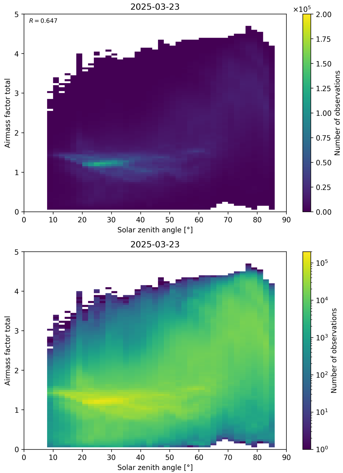
Figure 175: Scatter density plot of “Solar zenith angle” against “Airmass factor total” for 2025-03-23 to 2025-03-24.
