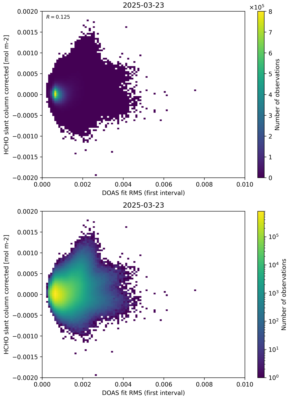
Figure 62: Scatter density plot of “DOAS fit RMS (first interval)” against “HCHO slant column corrected” for 2025-03-23 to 2025-03-24.
