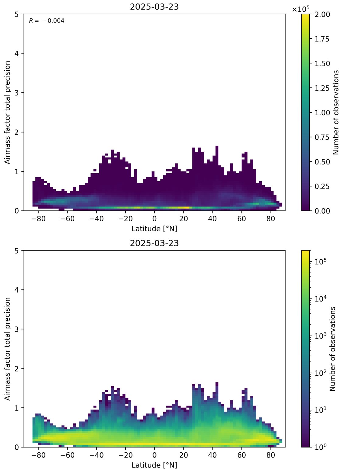
Figure 162: Scatter density plot of “Latitude” against “Airmass factor total precision” for 2025-03-23 to 2025-03-24.
