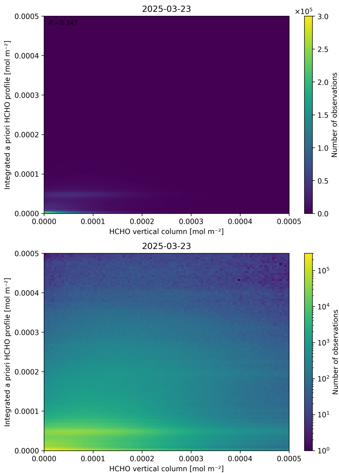
Figure 135: Scatter density plot of “HCHO vertical column” against “Integrated a priori HCHO profile” for 2025-03-23 to 2025-03-24.
