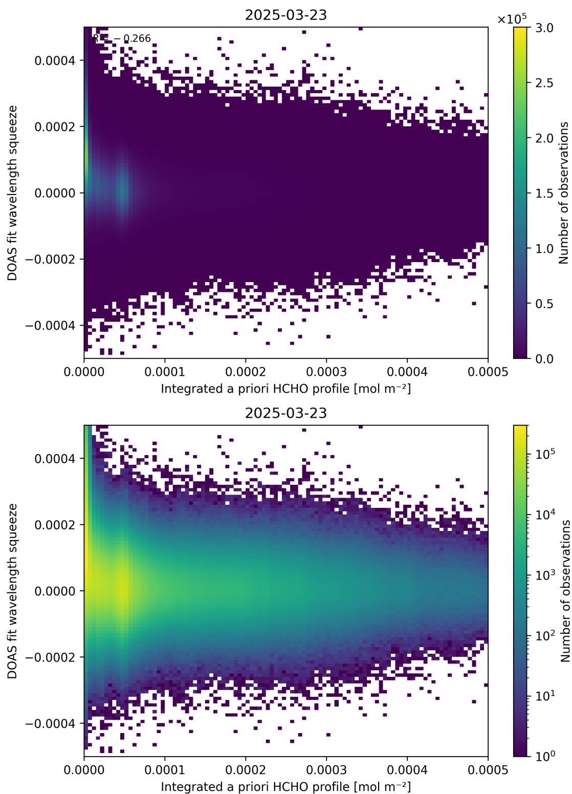
Figure 150: Scatter density plot of “Integrated a priori HCHO profile” against “DOAS fit wavelength squeeze” for 2025-03-23 to 2025-03-24.
