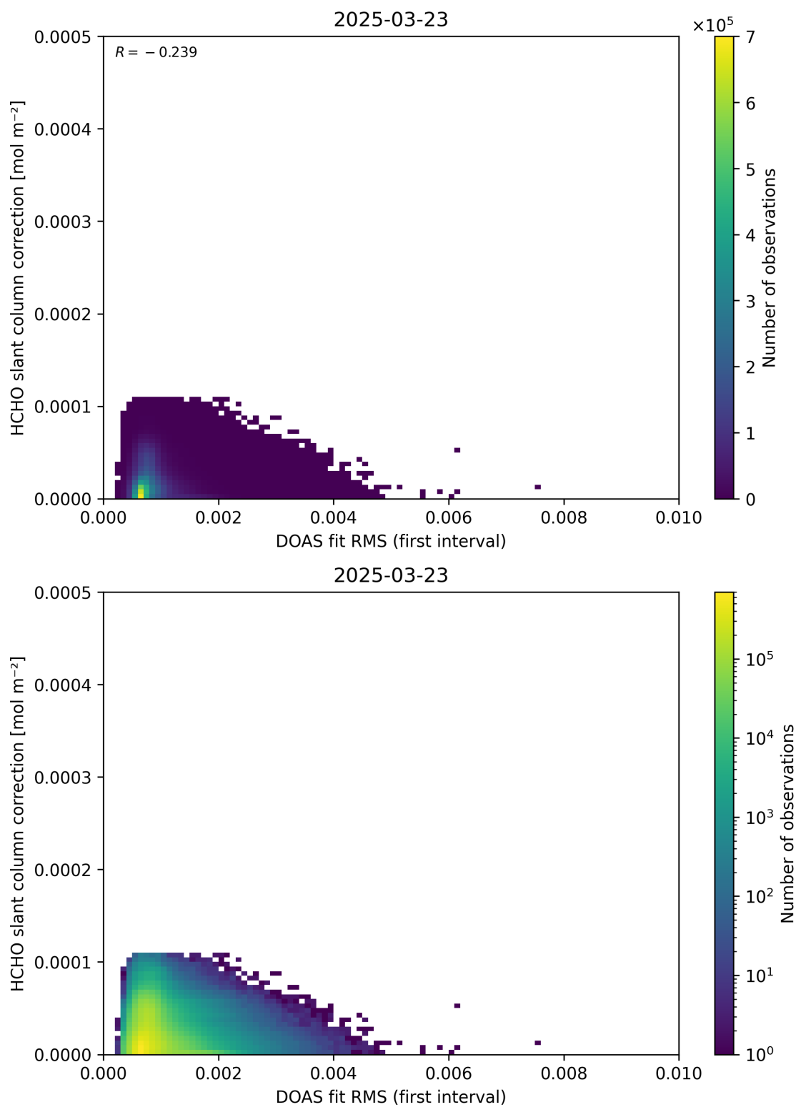
Figure 63: Scatter density plot of “DOAS fit RMS (first interval)” against “HCHO slant column correction” for 2025-03-23 to 2025-03-24.
