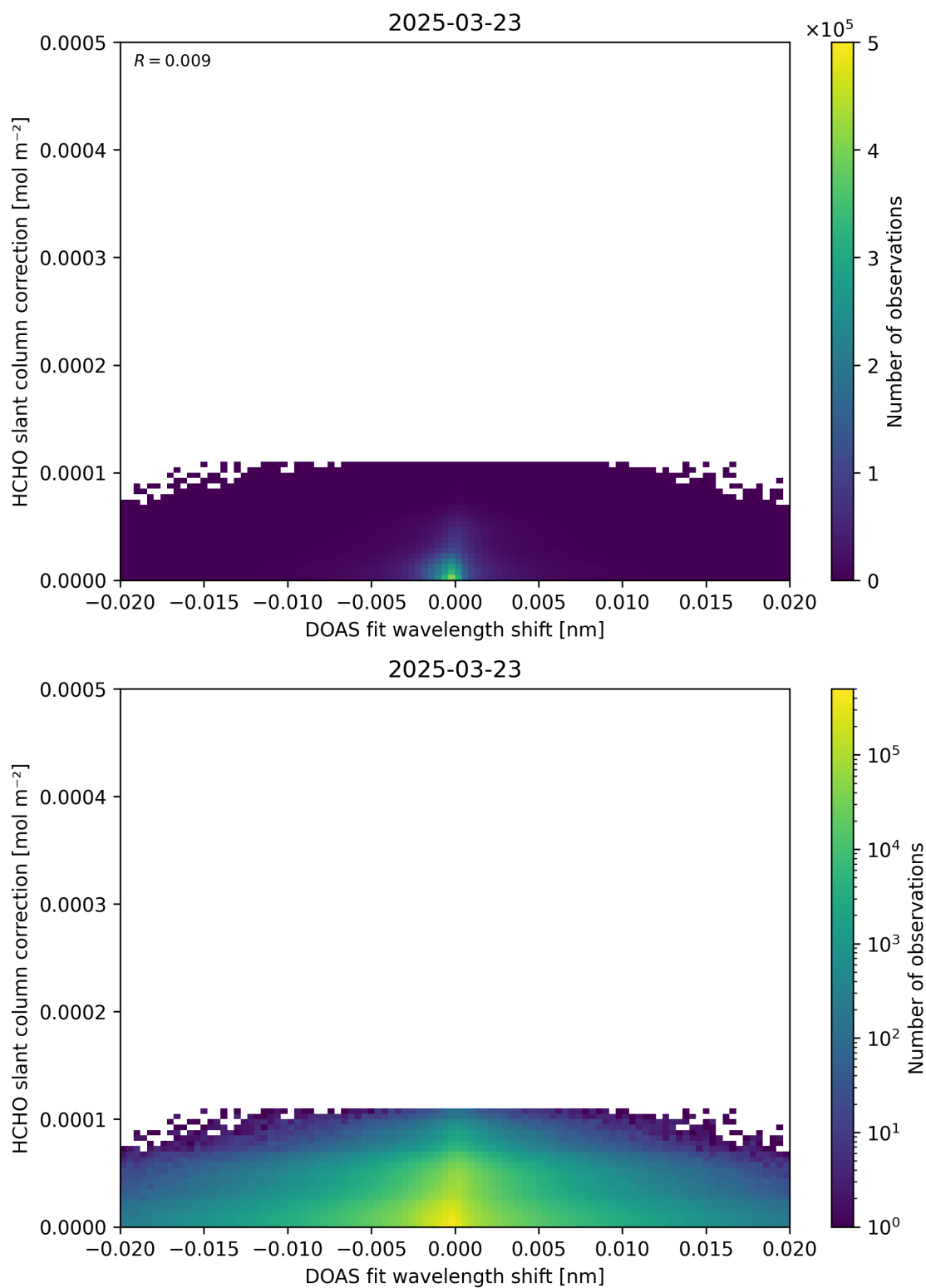
Figure 67: Scatter density plot of “DOAS fit wavelength shift” against “HCHO slant column correction” for 2025-03-23 to 2025-03-24.
