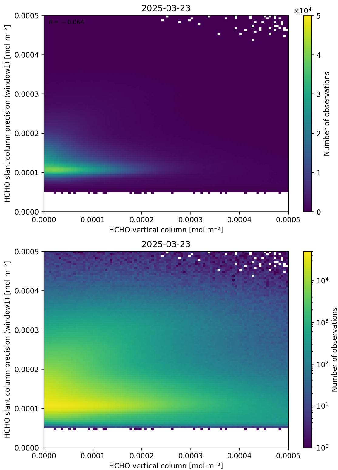
Figure 130: Scatter density plot of “HCHO vertical column” against “HCHO slant column precision (window1)” for 2025-03-23 to 2025-03-24.
