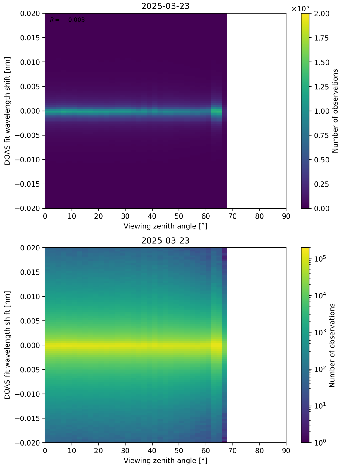
Figure 183: Scatter density plot of “Viewing zenith angle” against “DOAS fit wavelength shift” for 2025-03-23 to 2025-03-24.
