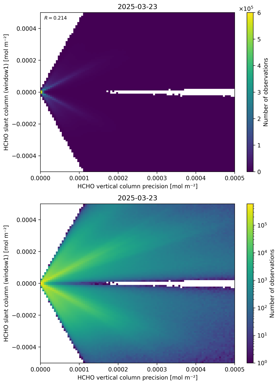
Figure 142: Scatter density plot of “HCHO vertical column precision” against “HCHO slant column (window1)” for 2025-03-23 to 2025-03-24.
