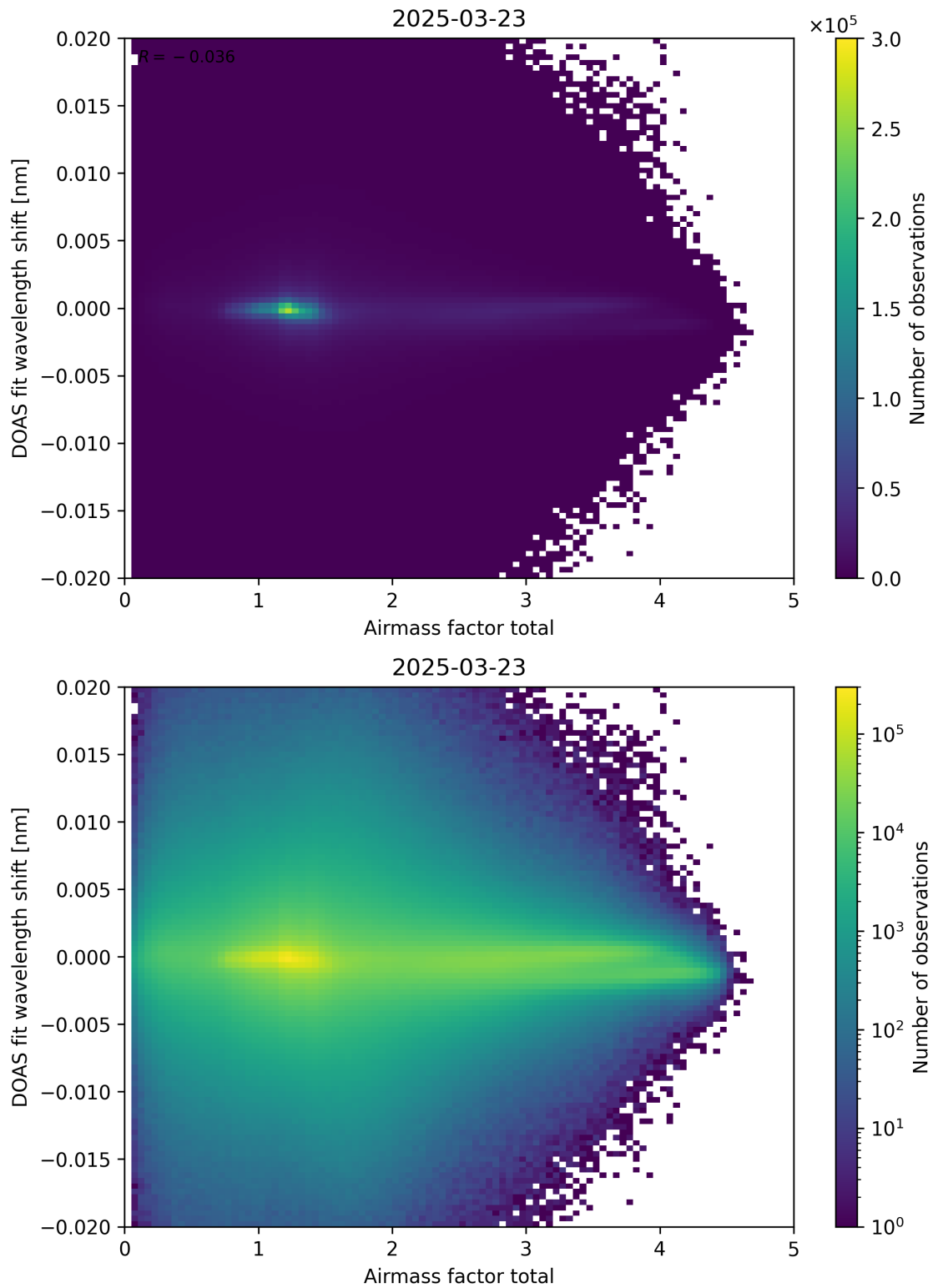
Figure 98: Scatter density plot of “Airmass factor total” against “DOAS fit wavelength shift” for 2025-03-23 to 2025-03-24.
