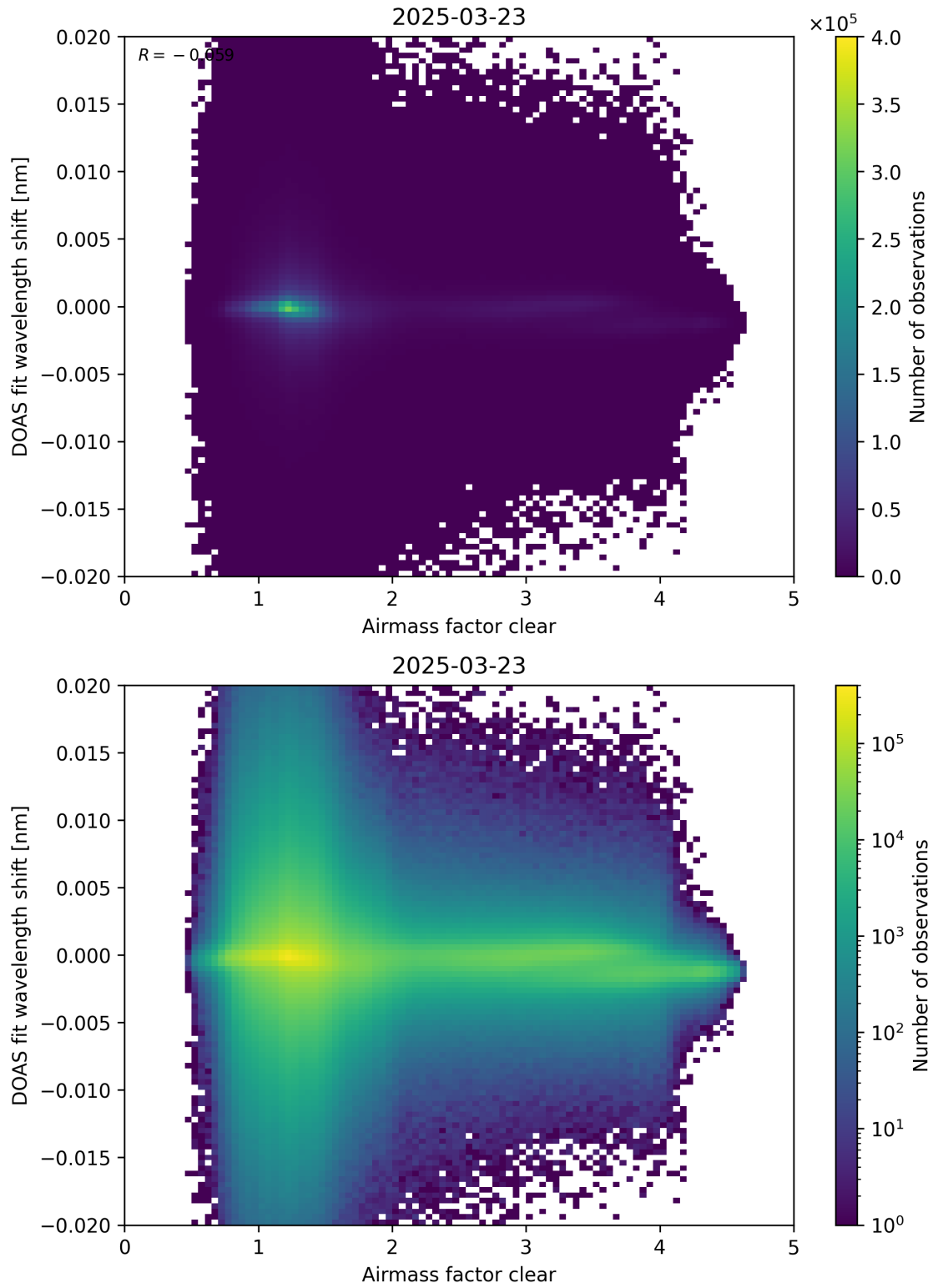
Figure 72: Scatter density plot of “Airmass factor clear” against “DOAS fit wavelength shift” for 2025-03-23 to 2025-03-24.
