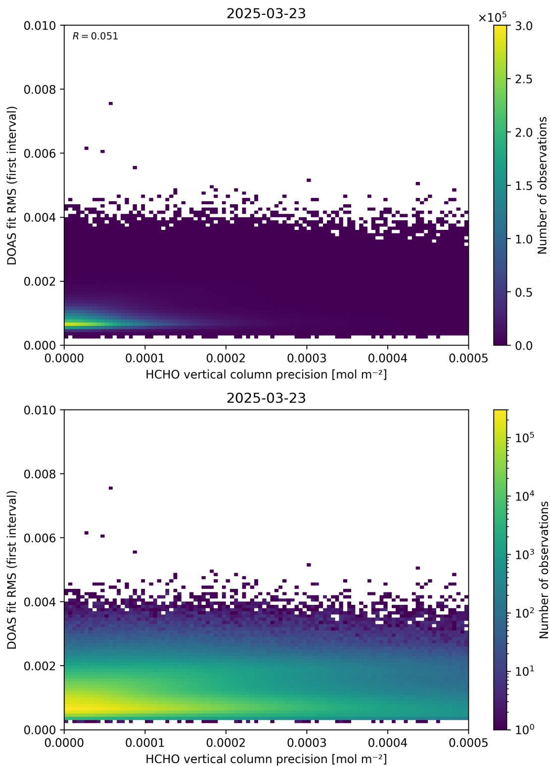
Figure 136: Scatter density plot of “HCHO vertical column precision” against “DOAS fit RMS (first interval)” for 2025-03-23 to 2025-03-24.
