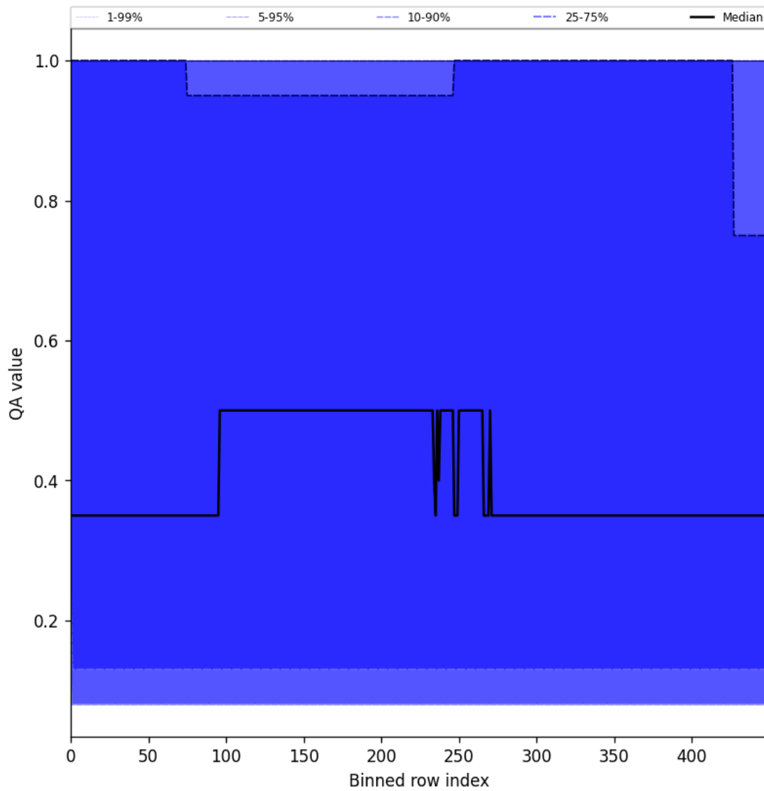
Figure 48: Along track statistics of “QA value” for 2025-03-23 to 2025-03-24
