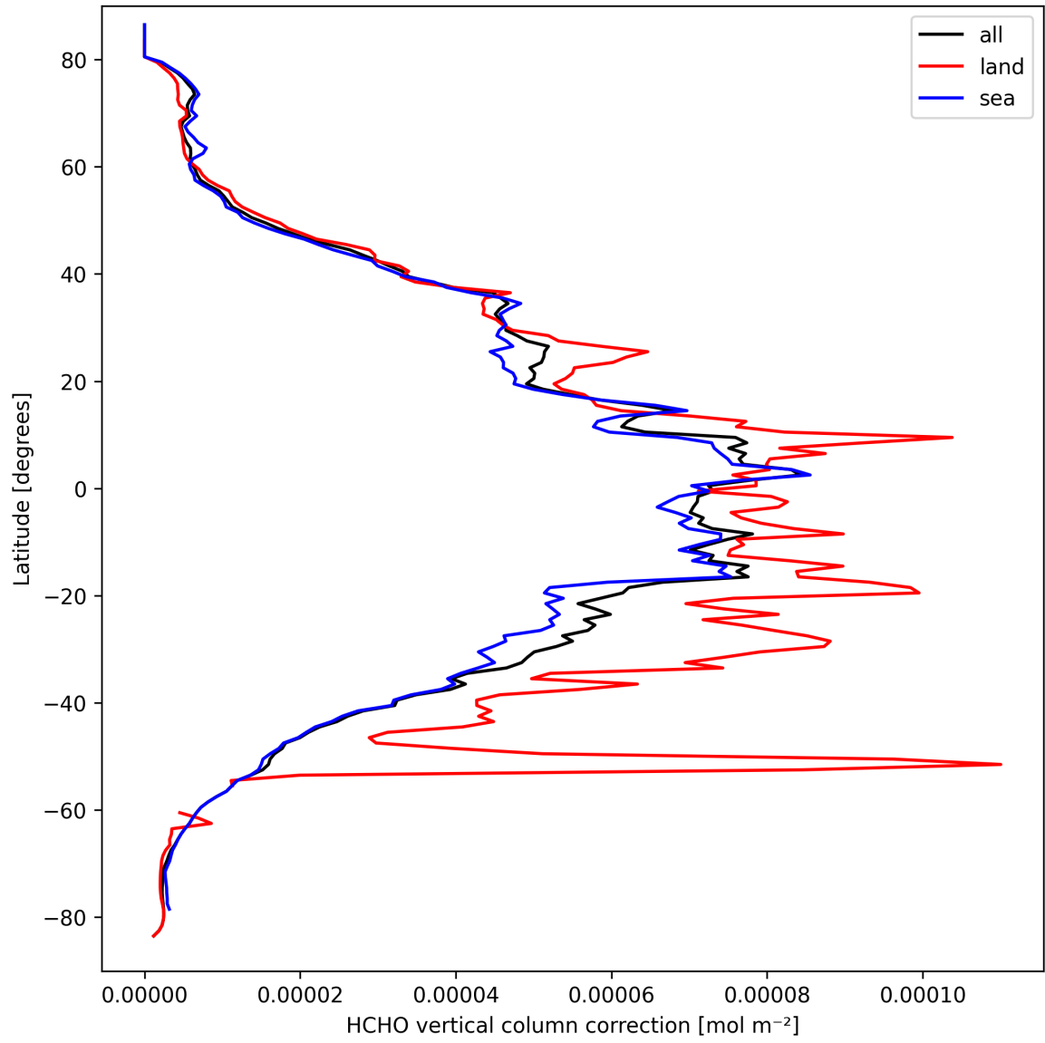
Figure 23: Zonal average of “HCHO vertical column correction” for 2025-03-23 to 2025-03-24.
