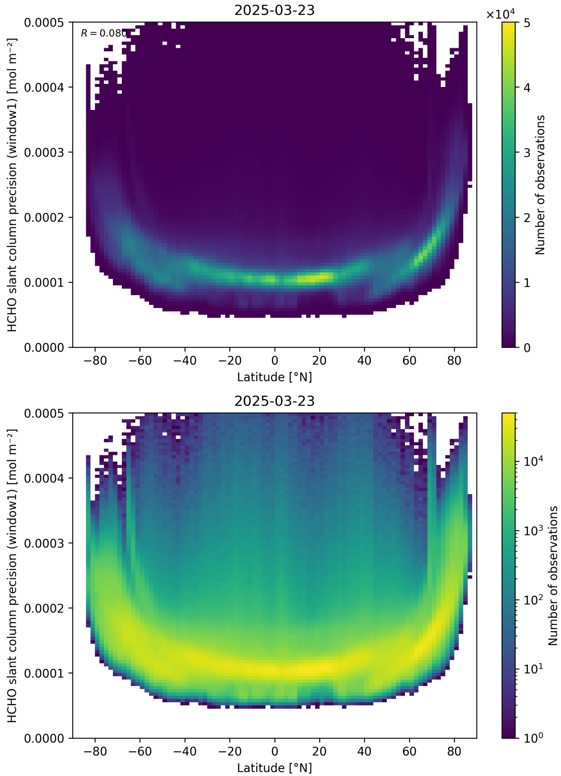
Figure 160: Scatter density plot of “Latitude” against “HCHO slant column precision (window1)” for 2025-03-23 to 2025-03-24.
