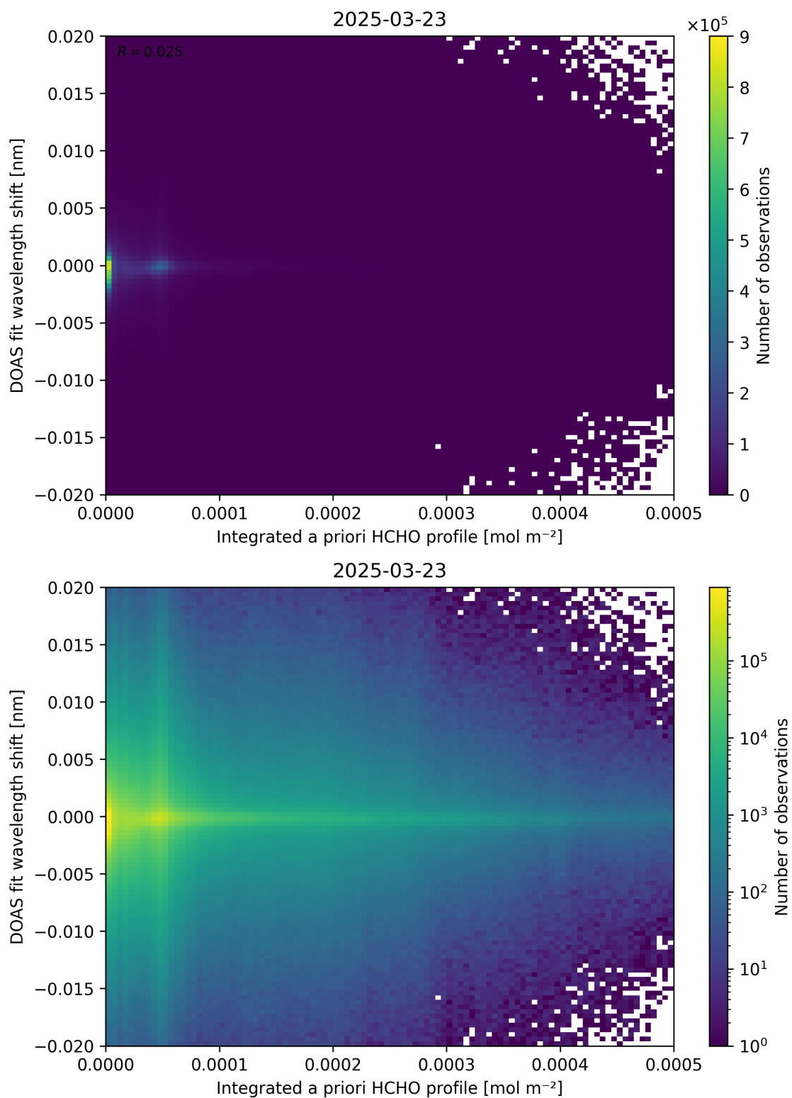
Figure 149: Scatter density plot of “Integrated a priori HCHO profile” against “DOAS fit wavelength shift” for 2025-03-23 to 2025-03-24.
