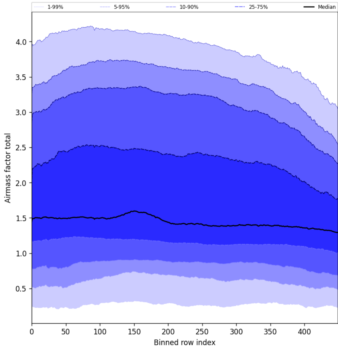
Figure 54: Along track statistics of “Airmass factor total” for 2025-03-23 to 2025-03-24
