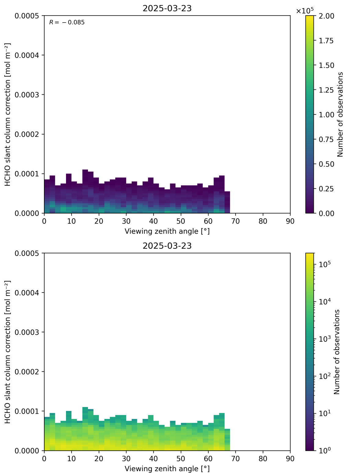
Figure 187: Scatter density plot of “Viewing zenith angle” against “HCHO slant column correction” for 2025-03-23 to 2025-03-24.
