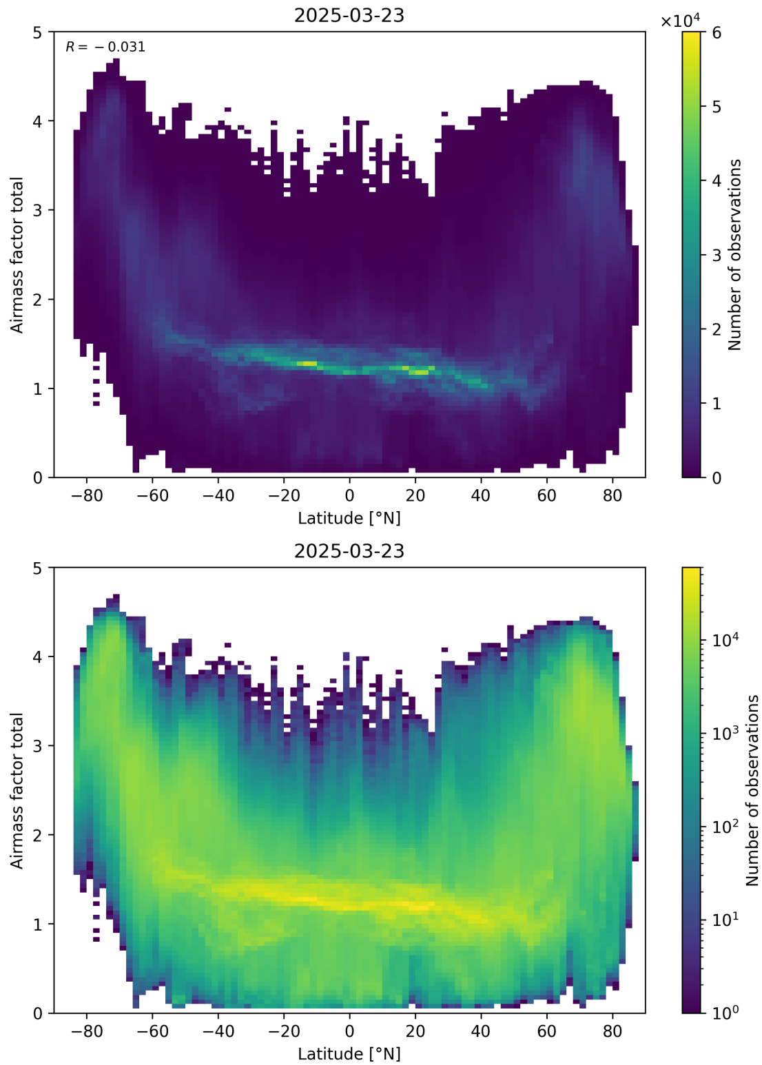
Figure 161: Scatter density plot of “Latitude” against “Airmass factor total” for 2025-03-23 to 2025-03-24.
