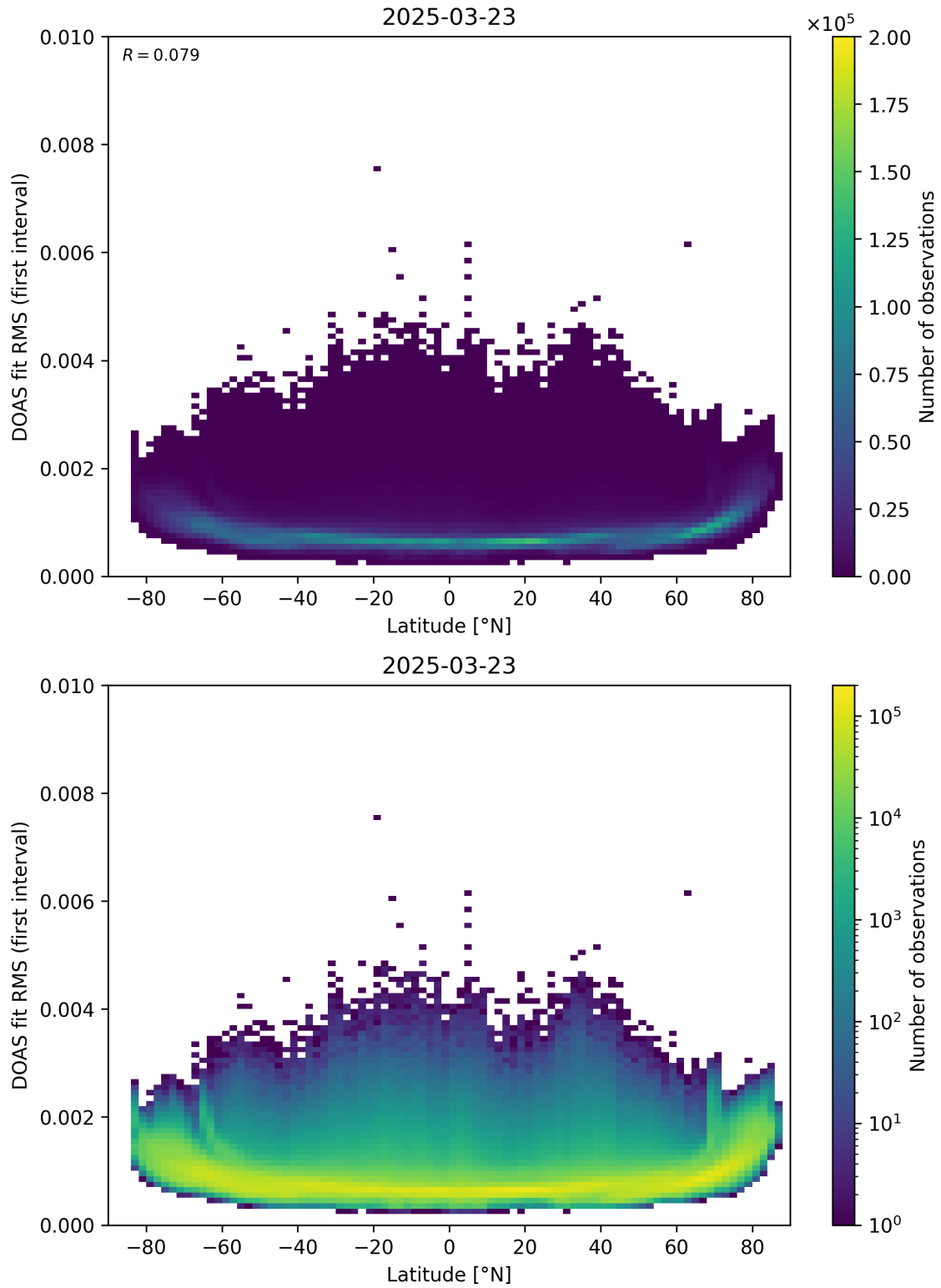
Figure 153: Scatter density plot of “Latitude” against “DOAS fit RMS (first interval)” for 2025-03-23 to 2025-03-24.
