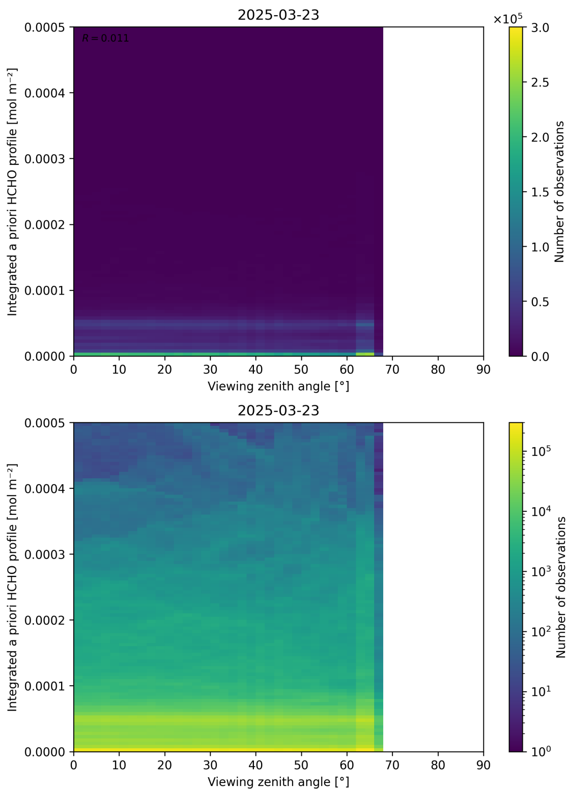
Figure 195: Scatter density plot of “Viewing zenith angle” against “Integrated a priori HCHO profile” for 2025-03-23 to 2025-03-24.
