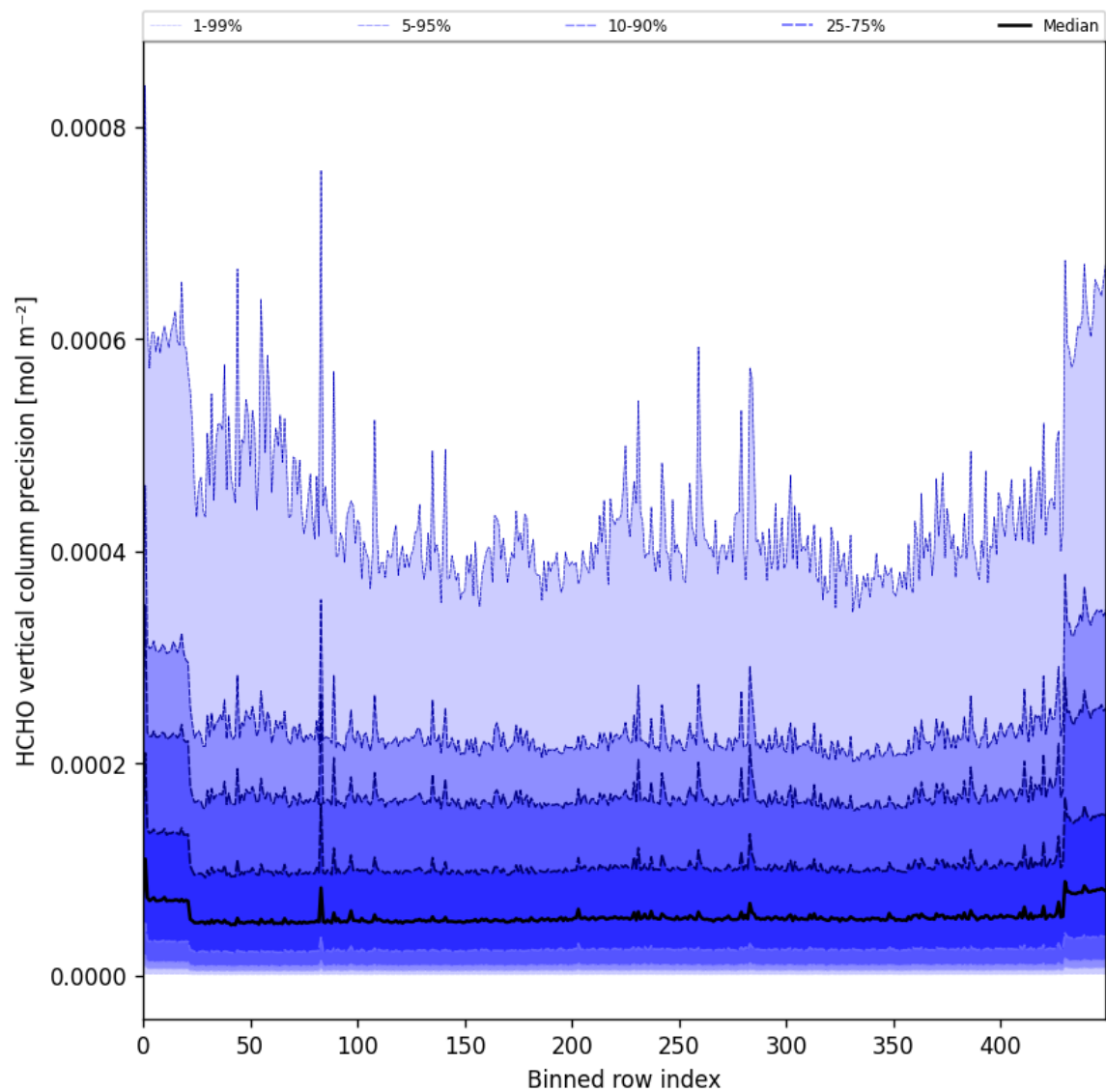
Figure 50: Along track statistics of “HCHO vertical column precision” for 2025-03-23 to 2025-03-24
