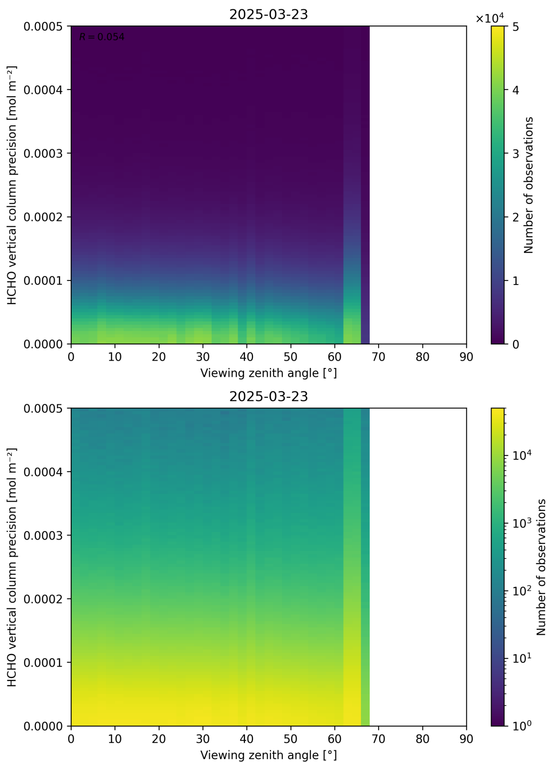
Figure 194: Scatter density plot of “Viewing zenith angle” against “HCHO vertical column precision” for 2025-03-23 to 2025-03-24.
