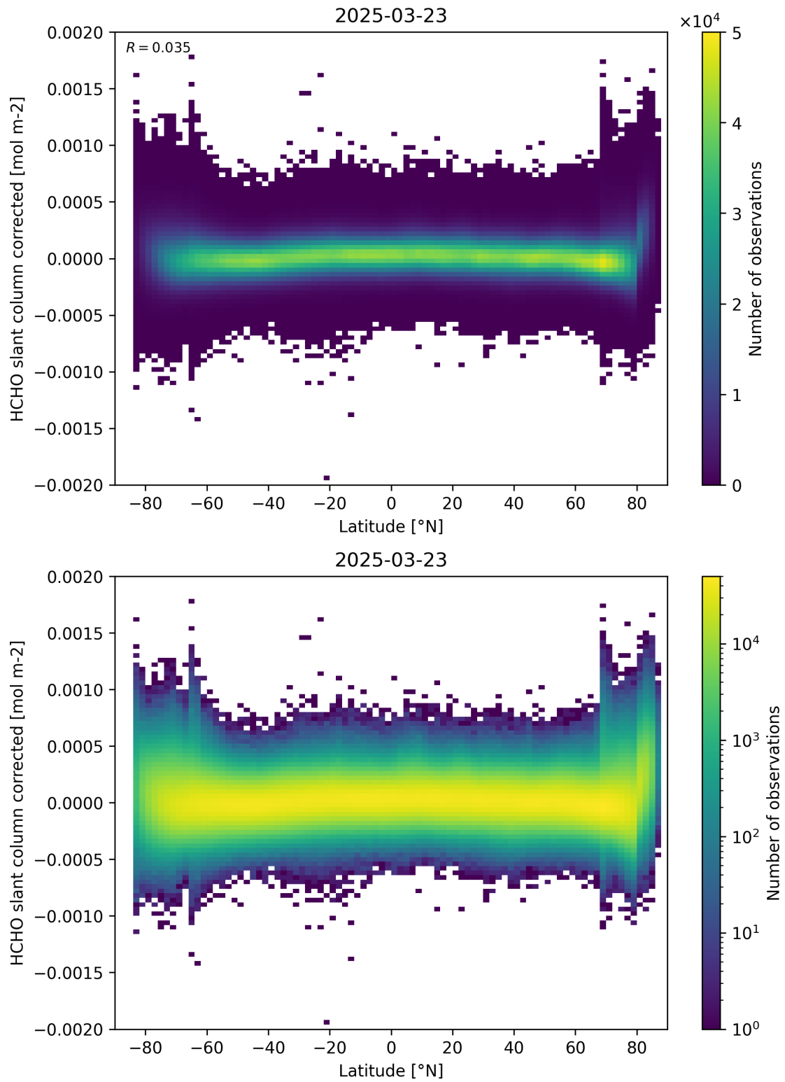
Figure 157: Scatter density plot of “Latitude” against “HCHO slant column corrected” for 2025-03-23 to 2025-03-24.
