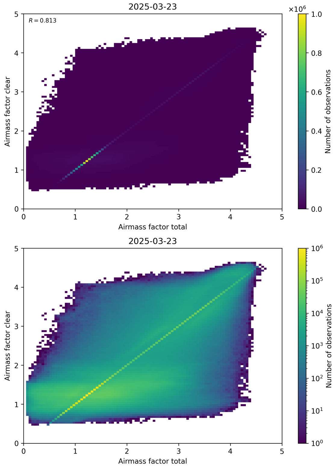
Figure 100: Scatter density plot of “Airmass factor total” against “Airmass factor clear” for 2025-03-23 to 2025-03-24.
