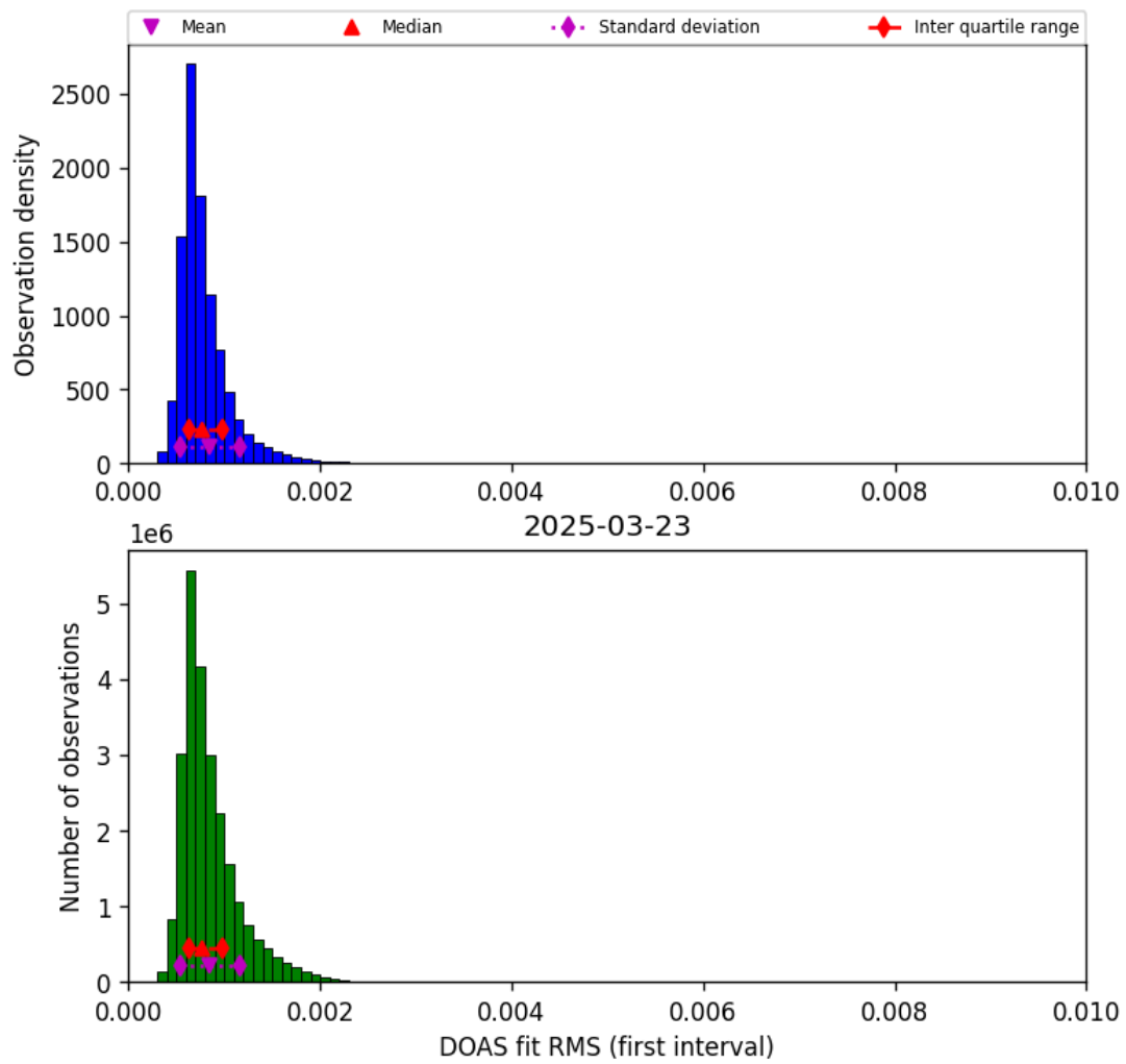
Figure 46: Histogram of “DOAS fit RMS (first interval)” for 2025-03-23 to 2025-03-24
