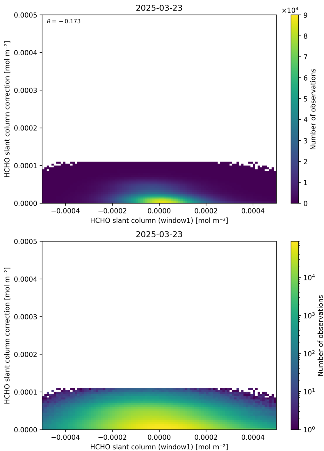
Figure 83: Scatter density plot of “HCHO slant column (window1)” against “HCHO slant column correction” for 2025-03-23 to 2025-03-24.
