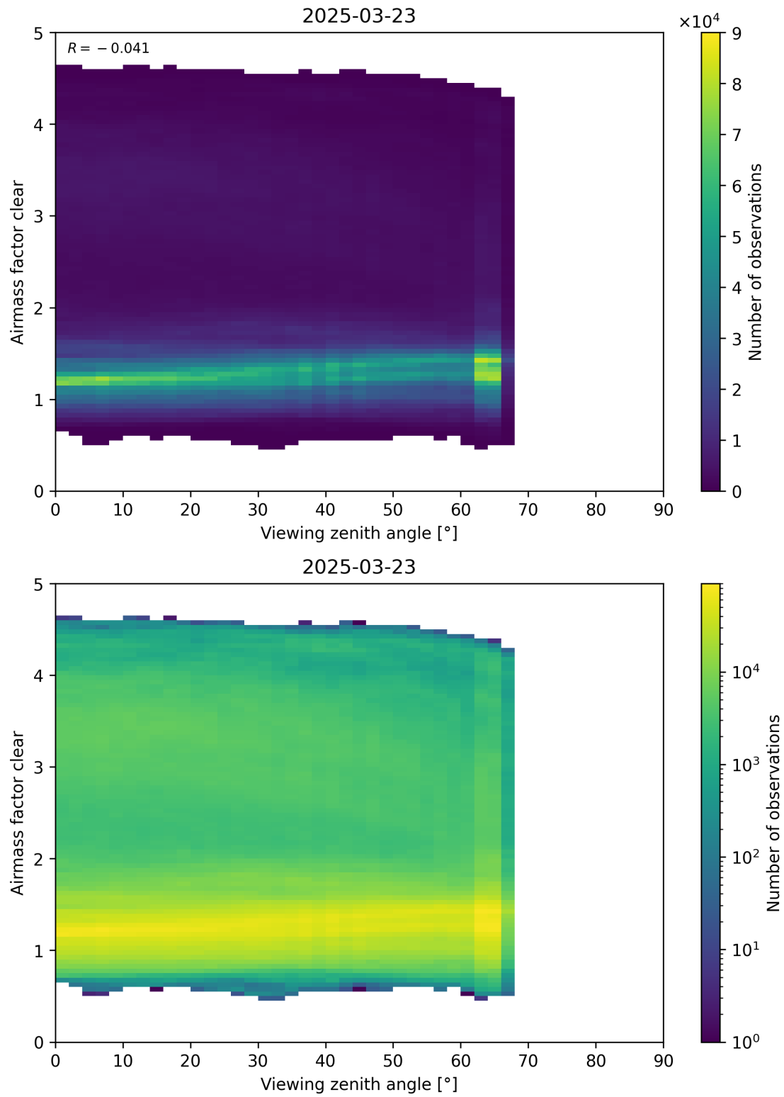
Figure 185: Scatter density plot of “Viewing zenith angle” against “Airmass factor clear” for 2025-03-23 to 2025-03-24.
