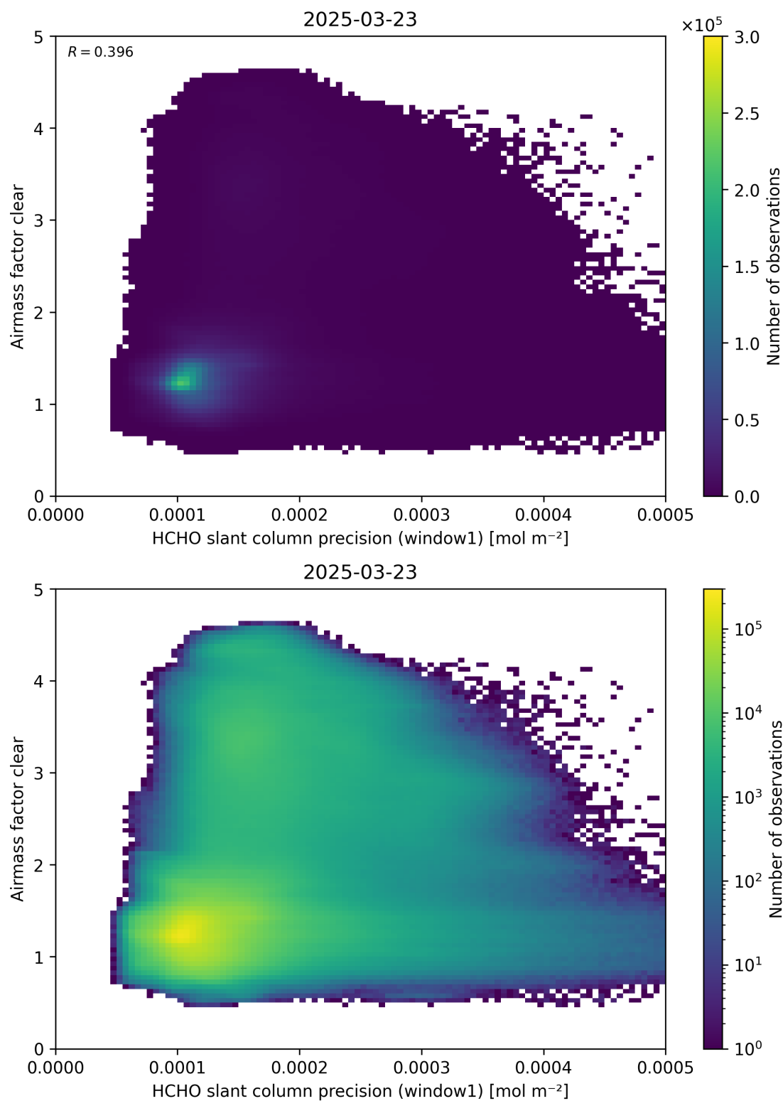
Figure 91: Scatter density plot of “HCHO slant column precision (window1)” against “Airmass factor clear” for 2025-03-23 to 2025-03-24.
