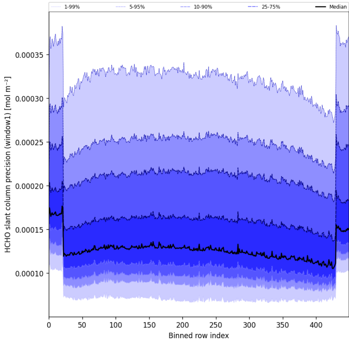
Figure 53: Along track statistics of “HCHO slant column precision (window1)” for 2025-03-23 to 2025-03-24
