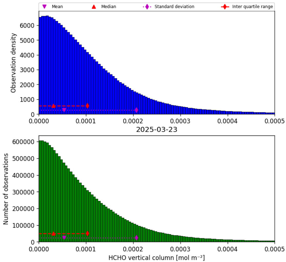
Figure 35: Histogram of “HCHO vertical column” for 2025-03-23 to 2025-03-24
