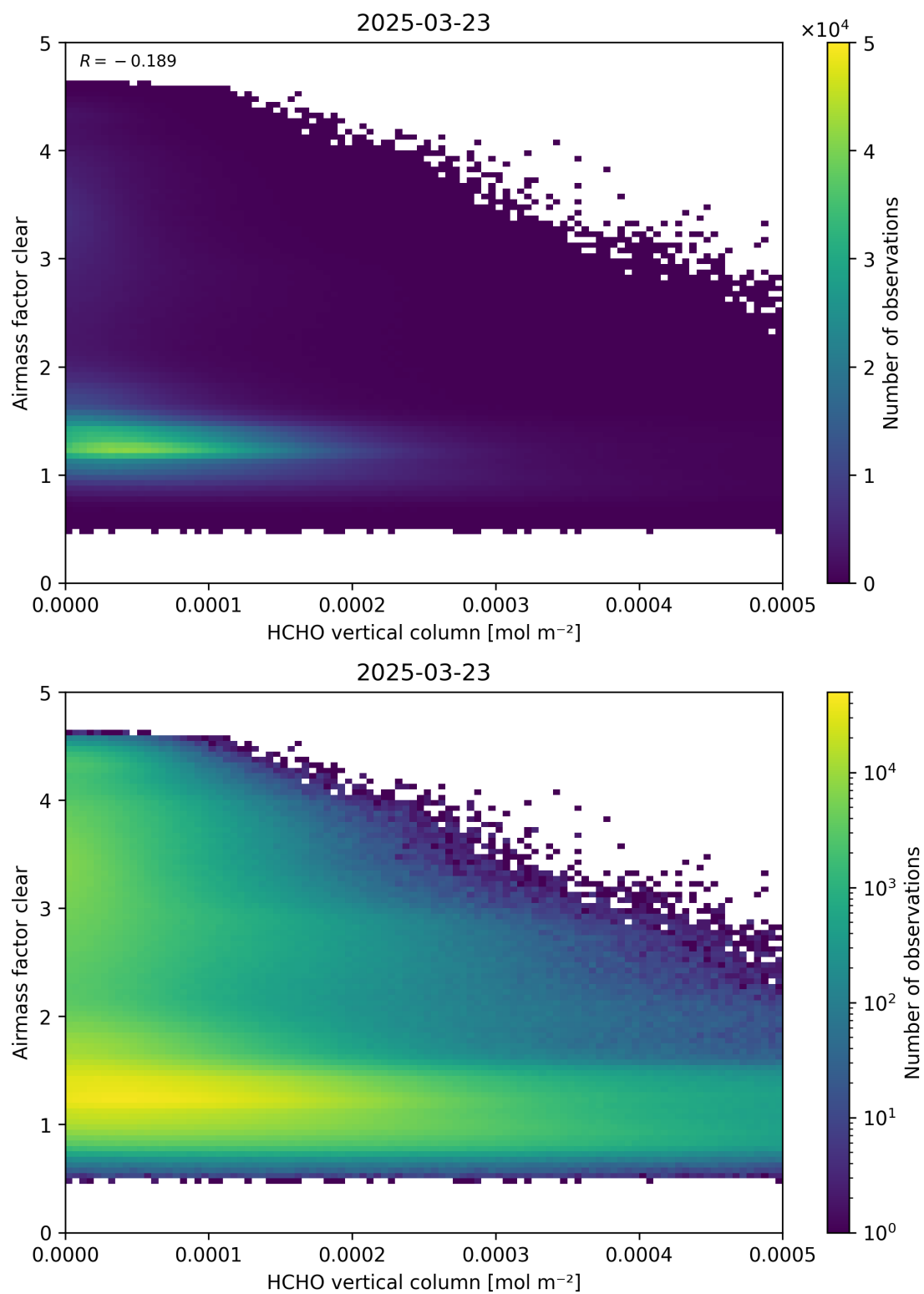
Figure 126: Scatter density plot of “HCHO vertical column” against “Airmass factor clear” for 2025-03-23 to 2025-03-24.
