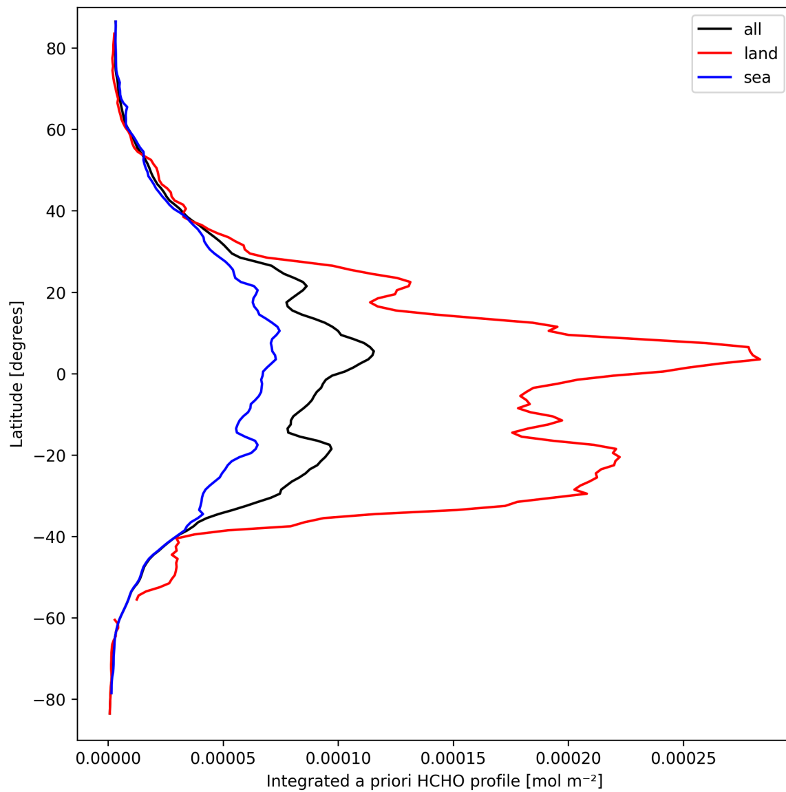
Figure 29: Zonal average of “Integrated a priori HCHO profile” for 2025-03-23 to 2025-03-24.
