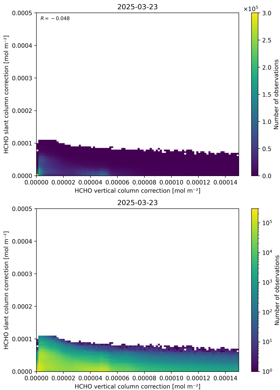
Figure 117: Scatter density plot of “HCHO vertical column correction” against “HCHO slant column correction” for 2025-03-23 to 2025-03-24.
