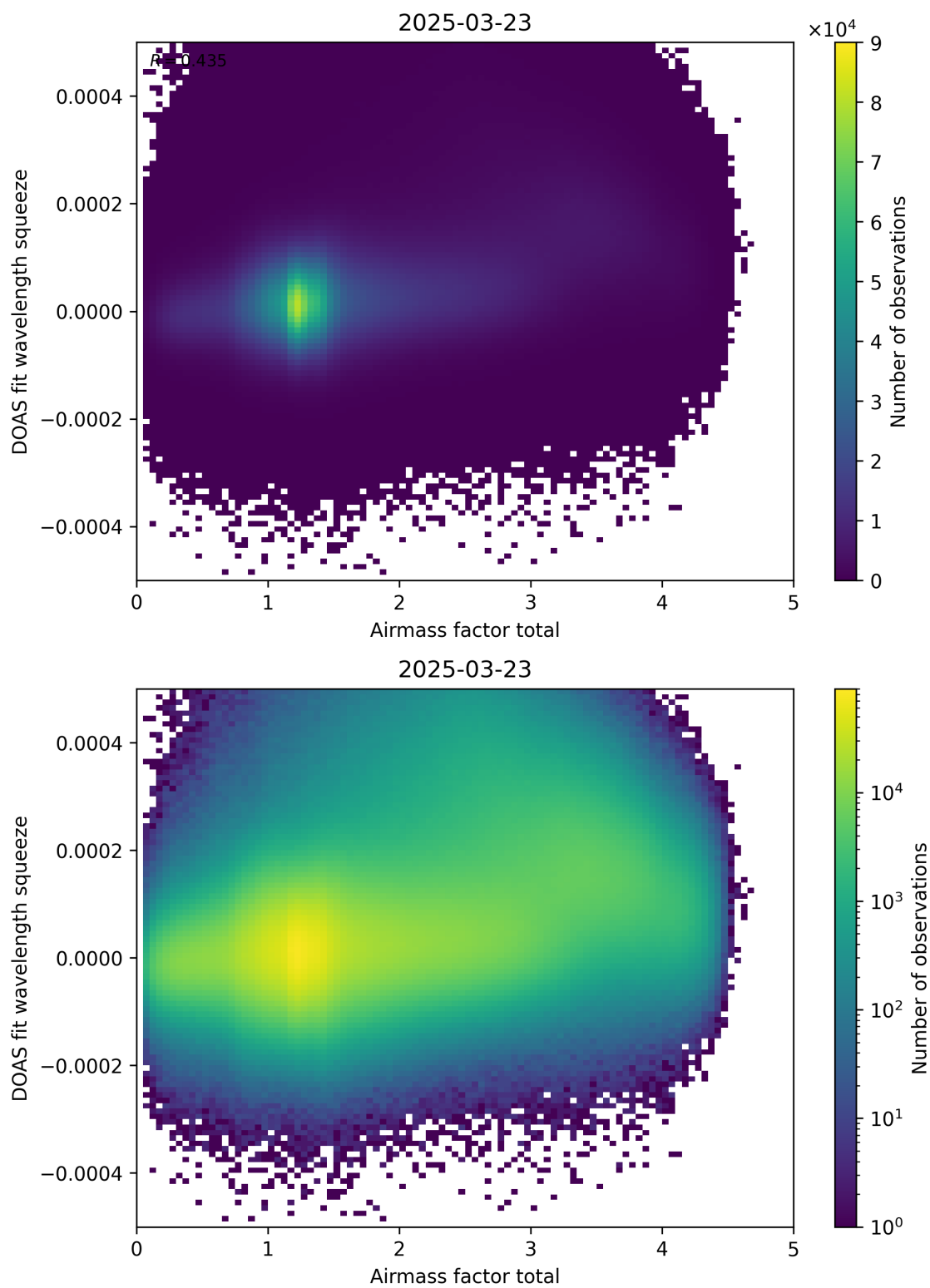
Figure 99: Scatter density plot of “Airmass factor total” against “DOAS fit wavelength squeeze” for 2025-03-23 to 2025-03-24.
