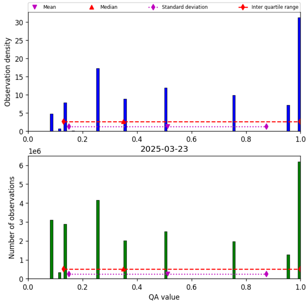
Figure 34: Histogram of “QA value” for 2025-03-23 to 2025-03-24
