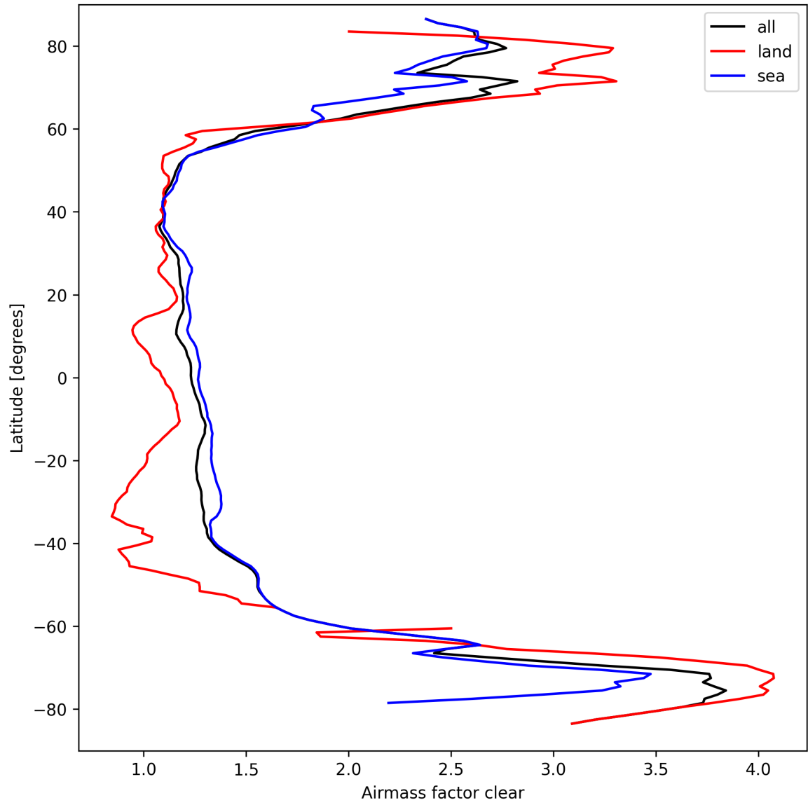
Figure 28: Zonal average of “Airmass factor clear” for 2025-03-23 to 2025-03-24.
