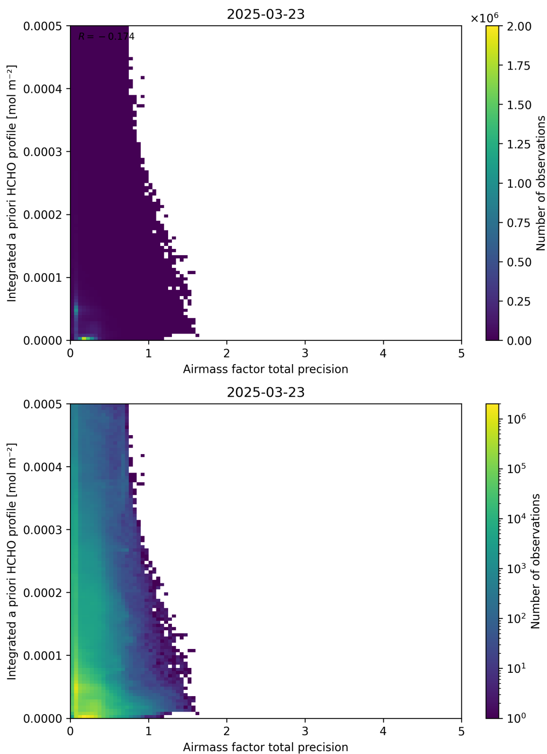
Figure 111: Scatter density plot of “Airmass factor total precision” against “Integrated a priori HCHO profile” for 2025-03-23 to 2025-03-24.
