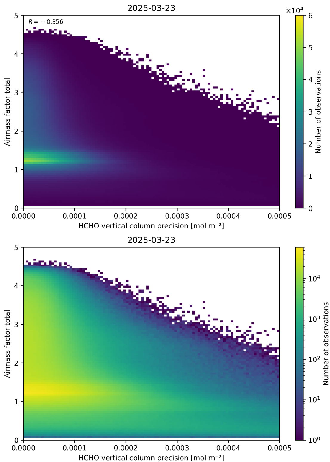
Figure 144: Scatter density plot of “HCHO vertical column precision” against “Airmass factor total” for 2025-03-23 to 2025-03-24.
