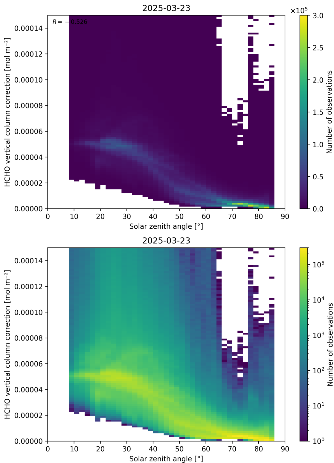
Figure 178: Scatter density plot of “Solar zenith angle” against “HCHO vertical column correction” for 2025-03-23 to 2025-03-24.
