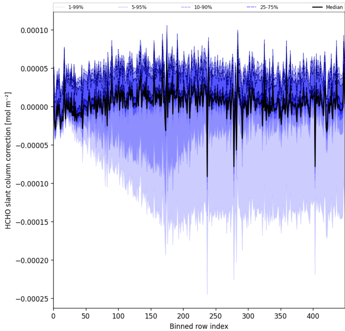
Figure 61: Along track statistics of “HCHO slant column correction” for 2025-03-23 to 2025-03-24
