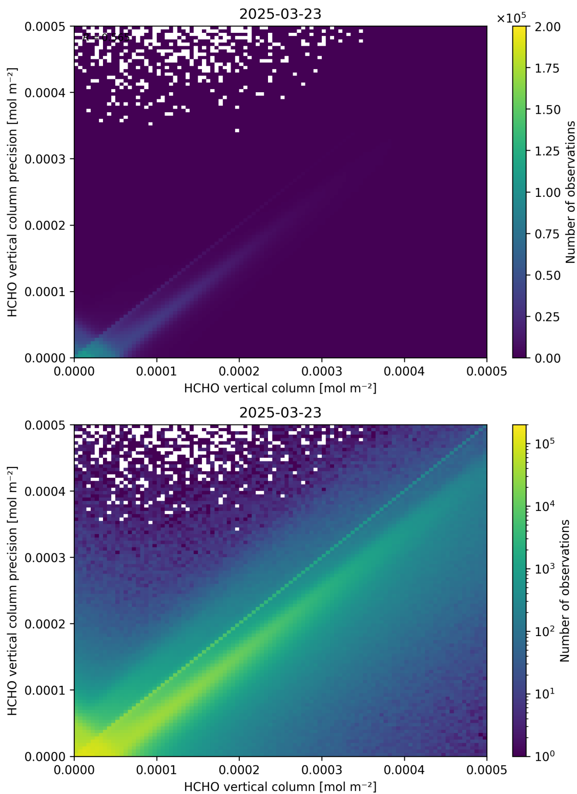
Figure 134: Scatter density plot of “HCHO vertical column” against “HCHO vertical column precision” for 2025-03-23 to 2025-03-24.
