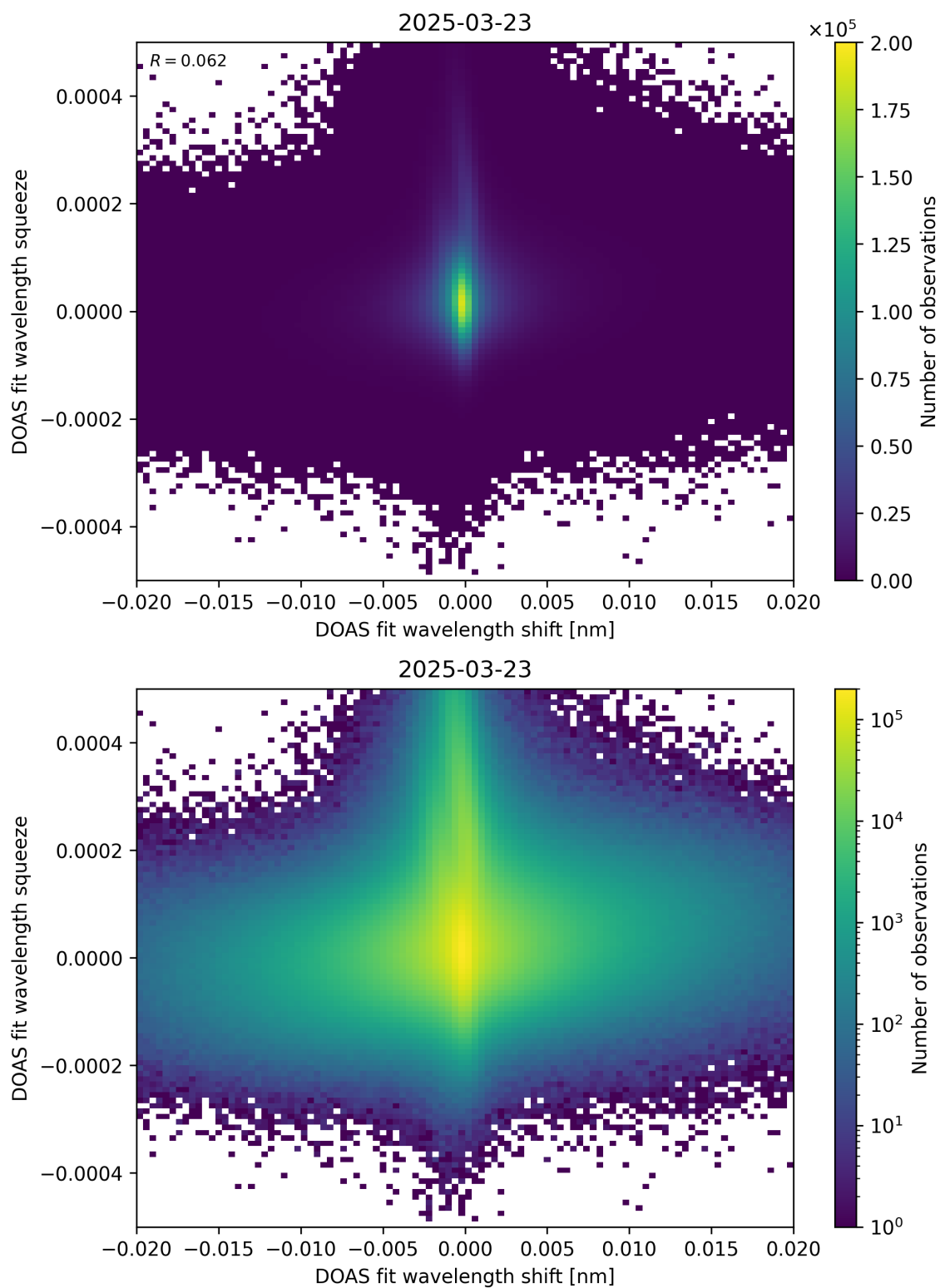
Figure 65: Scatter density plot of “DOAS fit wavelength shift” against “DOAS fit wavelength squeeze” for 2025-03-23 to 2025-03-24.
