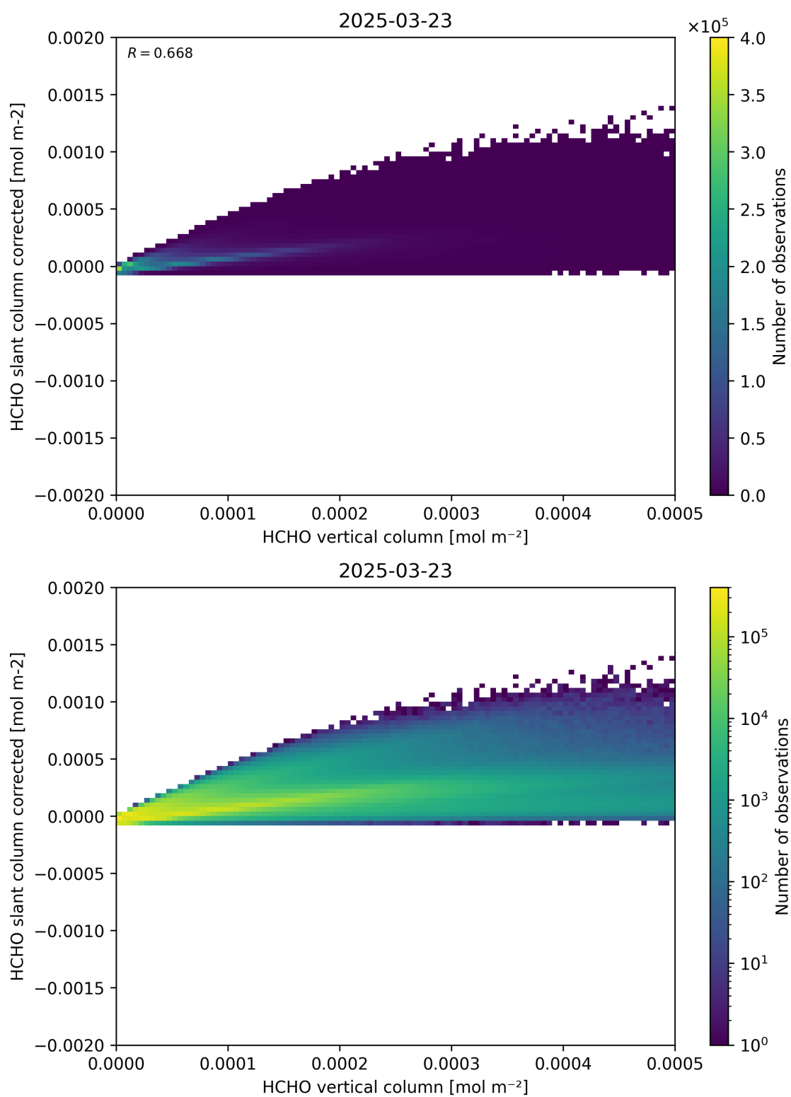
Figure 127: Scatter density plot of “HCHO vertical column” against “HCHO slant column corrected” for 2025-03-23 to 2025-03-24.
