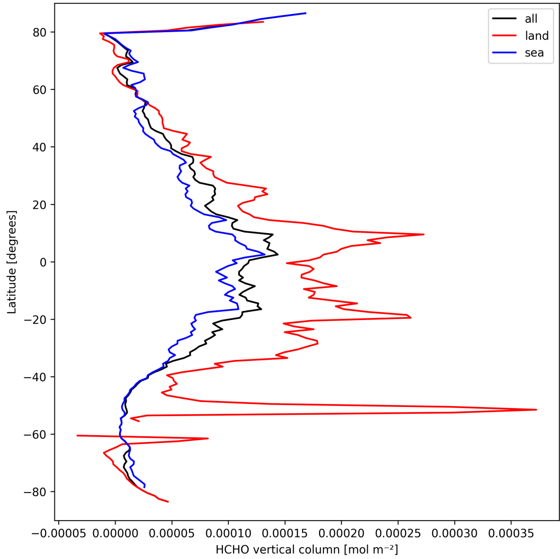
Figure 21: Zonal average of “HCHO vertical column” for 2025-03-23 to 2025-03-24.
