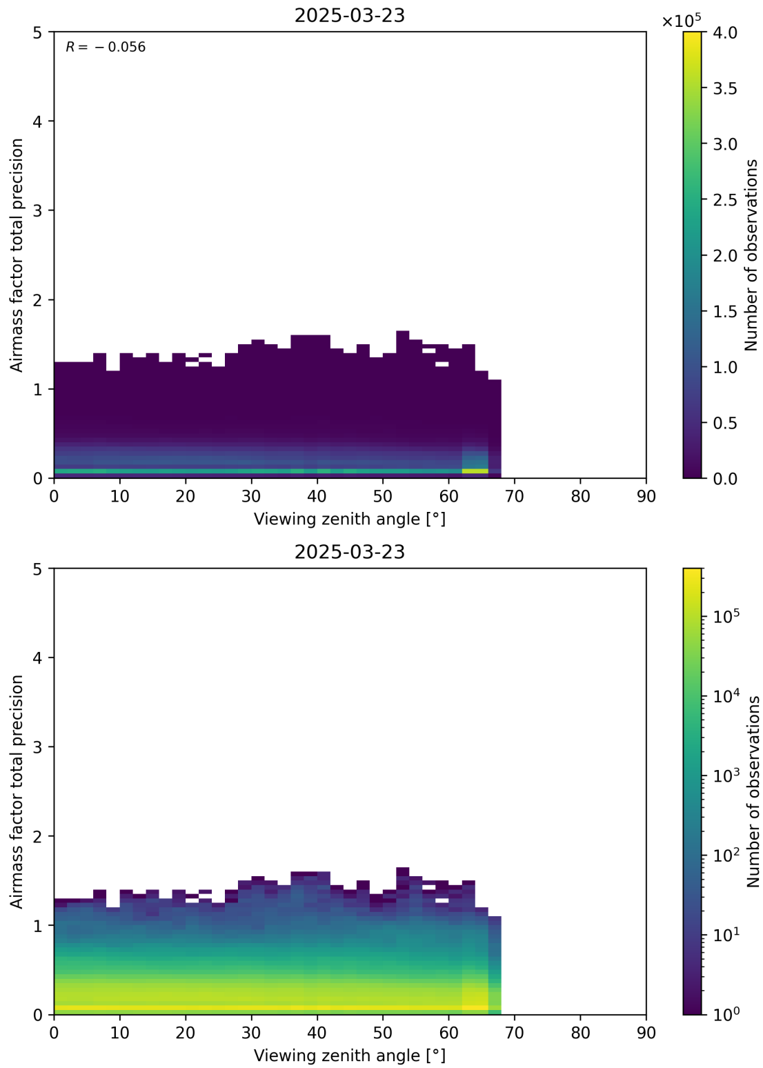
Figure 191: Scatter density plot of “Viewing zenith angle” against “Airmass factor total precision” for 2025-03-23 to 2025-03-24.
