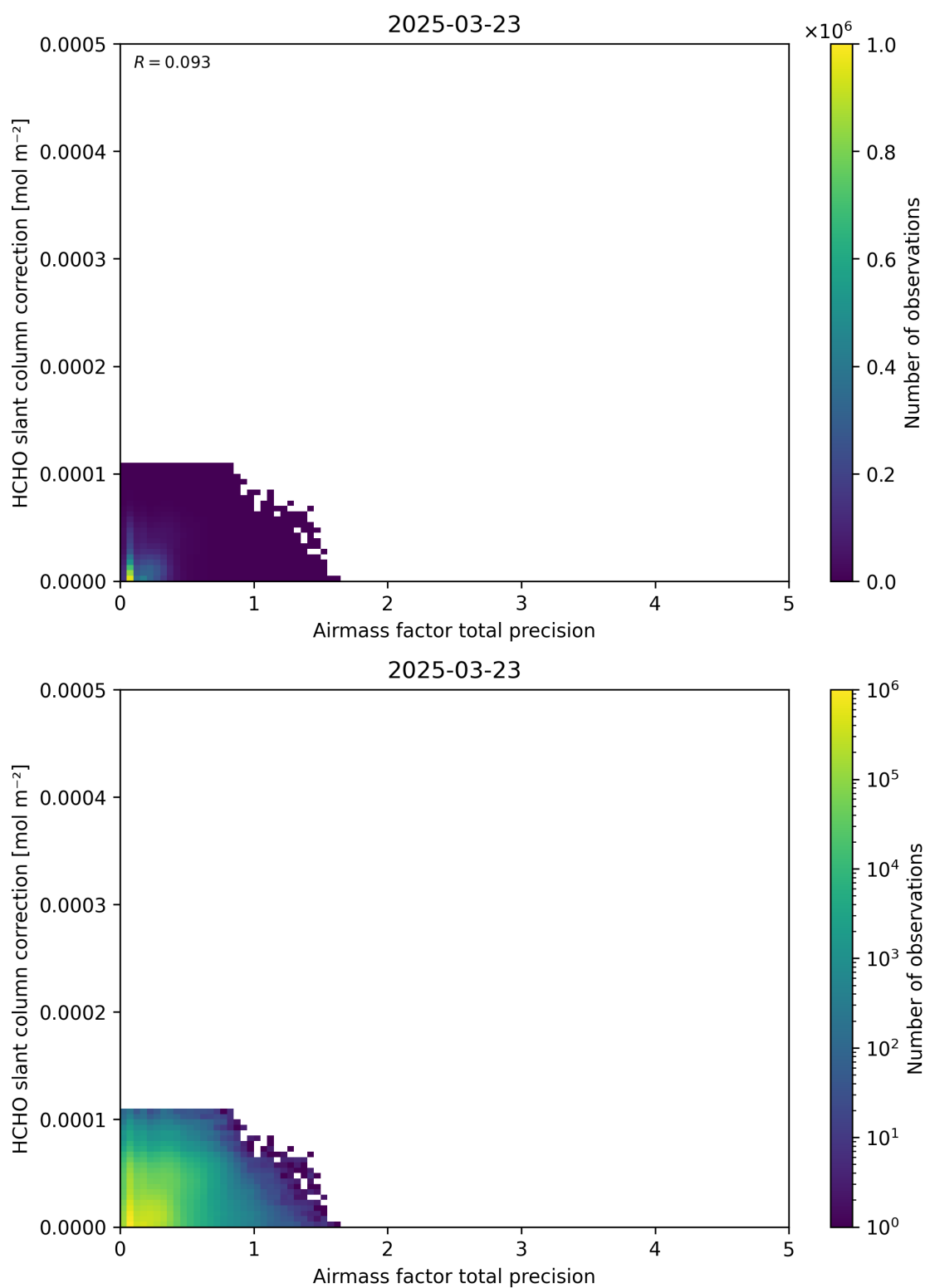
Figure 110: Scatter density plot of “Airmass factor total precision” against “HCHO slant column correction” for 2025-03-23 to 2025-03-24.
