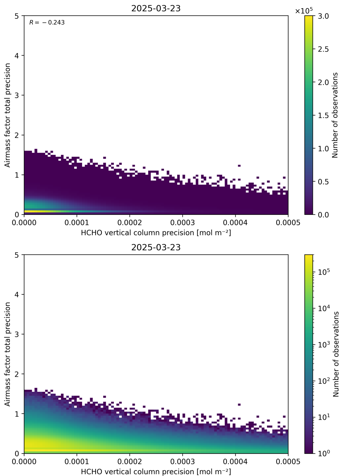
Figure 145: Scatter density plot of “HCHO vertical column precision” against “Airmass factor total precision” for 2025-03-23 to 2025-03-24.
