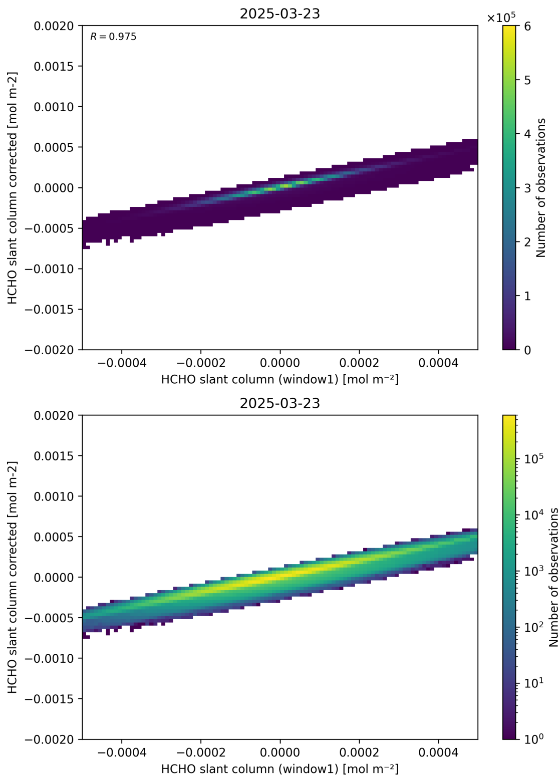
Figure 82: Scatter density plot of “HCHO slant column (window1)” against “HCHO slant column corrected” for 2025-03-23 to 2025-03-24.
