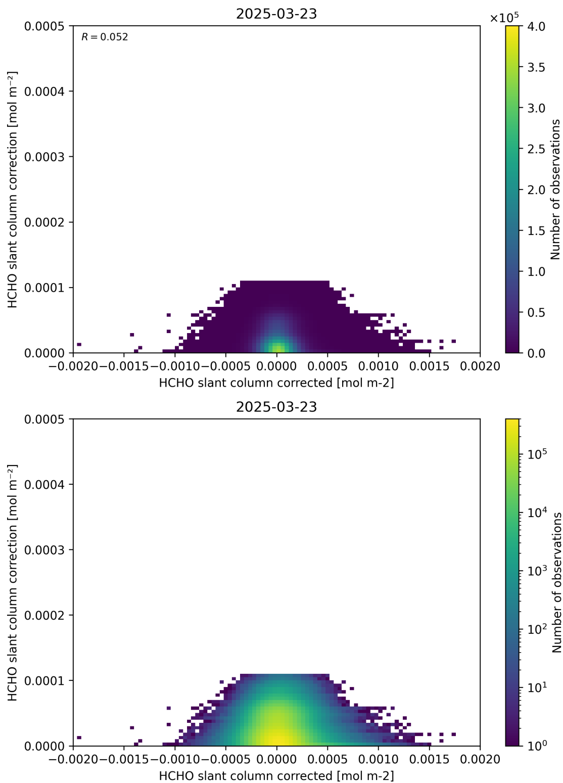
Figure 77: Scatter density plot of “HCHO slant column corrected” against “HCHO slant column correction” for 2025-03-23 to 2025-03-24.
