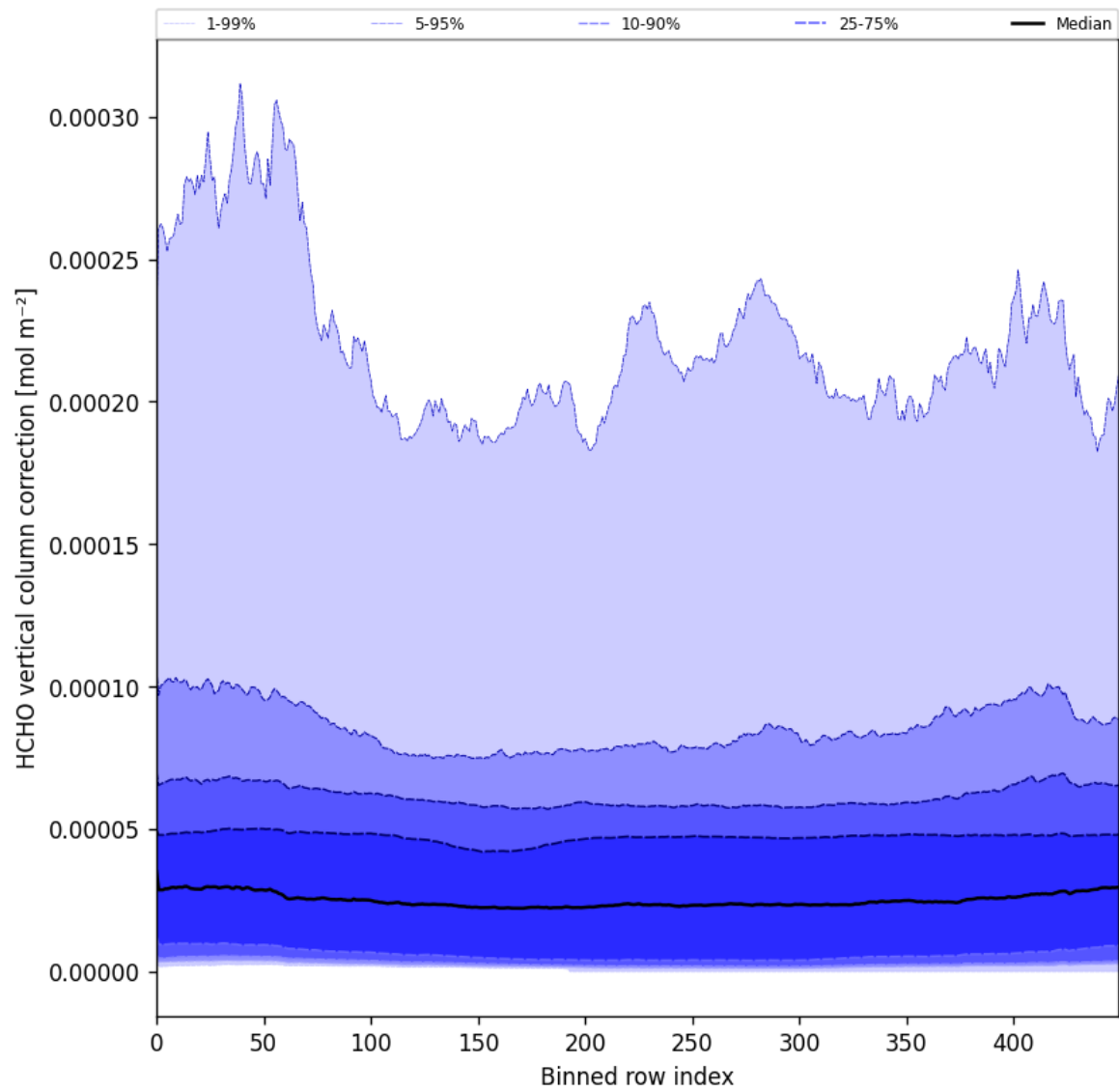
Figure 51: Along track statistics of “HCHO vertical column correction” for 2025-03-23 to 2025-03-24
