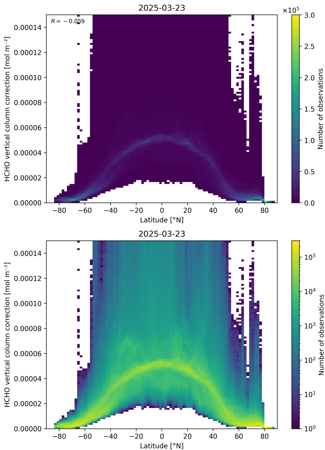
Figure 164: Scatter density plot of “Latitude” against “HCHO vertical column correction” for 2025-03-23 to 2025-03-24.
