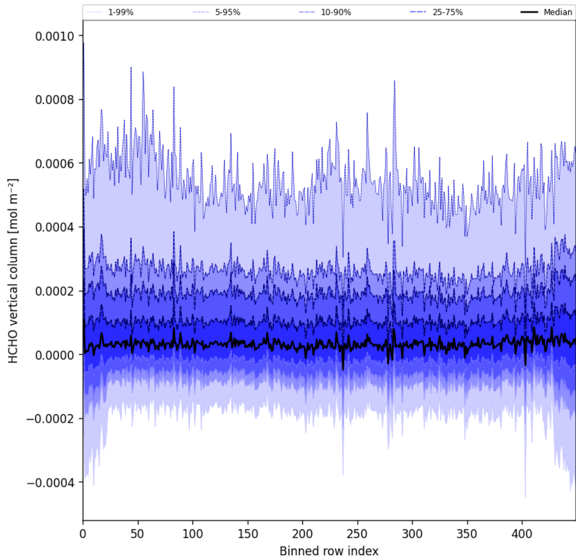
Figure 49: Along track statistics of “HCHO vertical column” for 2025-03-23 to 2025-03-24
