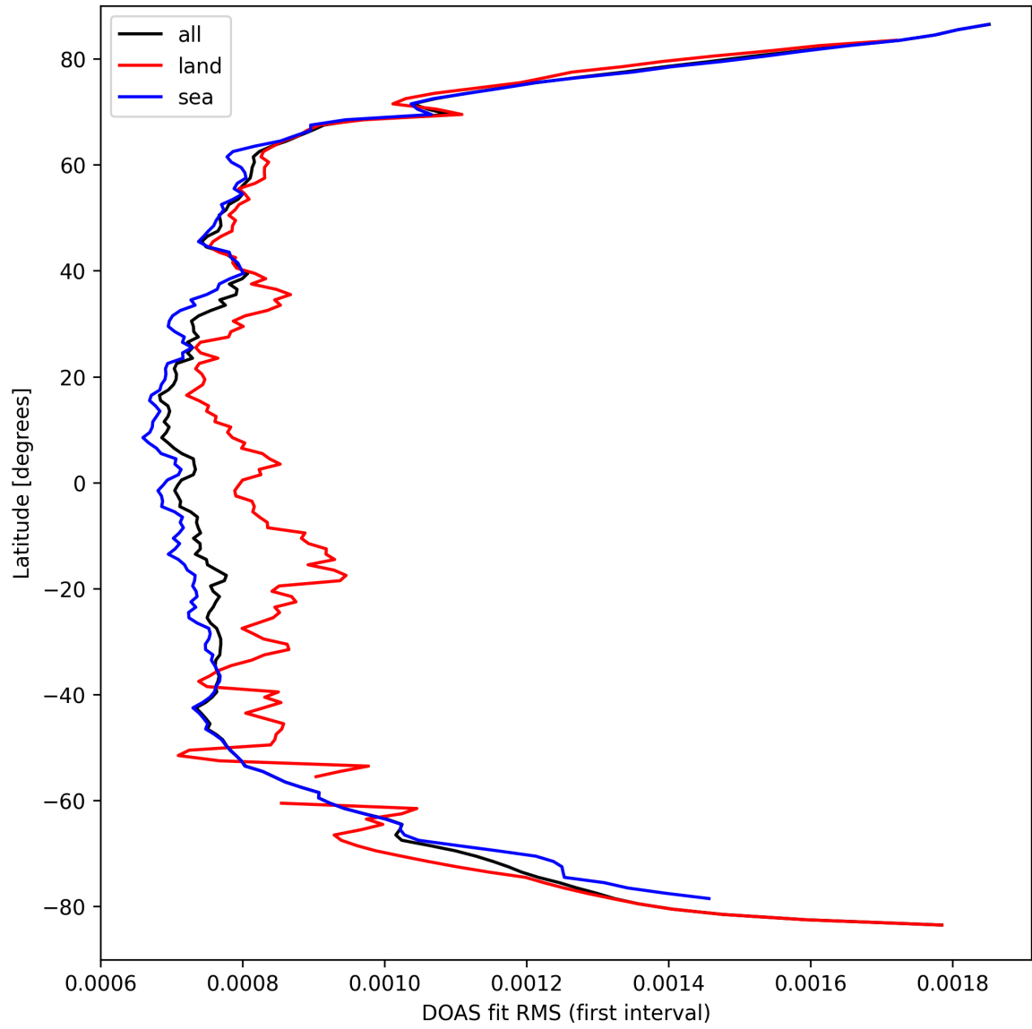
Figure 32: Zonal average of “DOAS fit RMS (first interval)” for 2025-03-23 to 2025-03-24.
