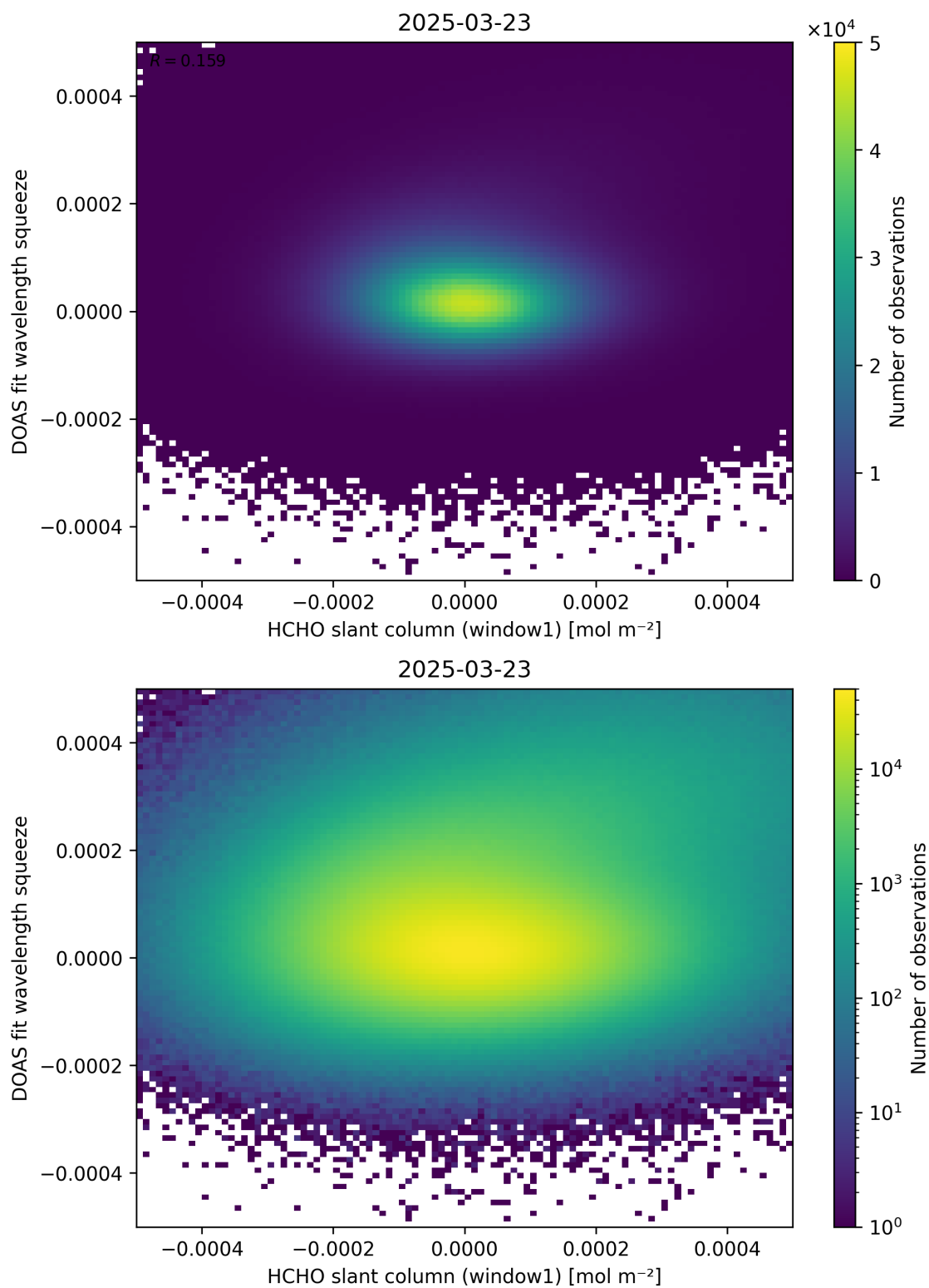
Figure 80: Scatter density plot of “HCHO slant column (window1)” against “DOAS fit wavelength squeeze” for 2025-03-23 to 2025-03-24.
