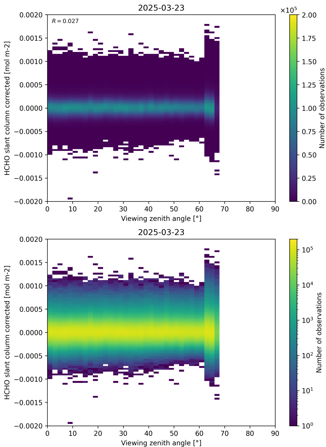
Figure 186: Scatter density plot of “Viewing zenith angle” against “HCHO slant column corrected” for 2025-03-23 to 2025-03-24.
