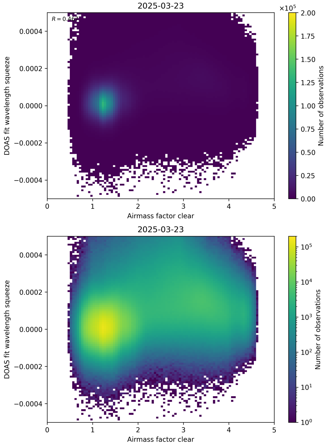
Figure 73: Scatter density plot of “Airmass factor clear” against “DOAS fit wavelength squeeze” for 2025-03-23 to 2025-03-24.
