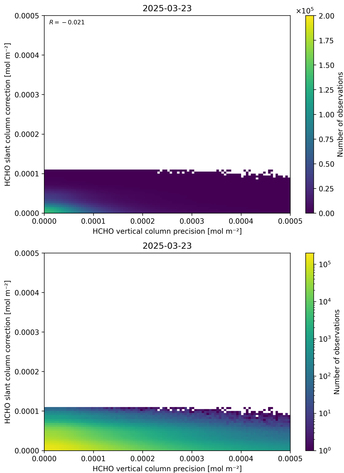
Figure 141: Scatter density plot of “HCHO vertical column precision” against “HCHO slant column correction” for 2025-03-23 to 2025-03-24.
