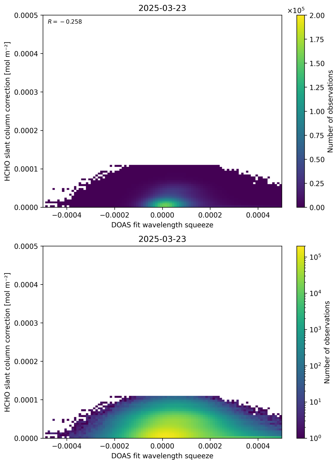
Figure 70: Scatter density plot of “DOAS fit wavelength squeeze” against “HCHO slant column correction” for 2025-03-23 to 2025-03-24.
