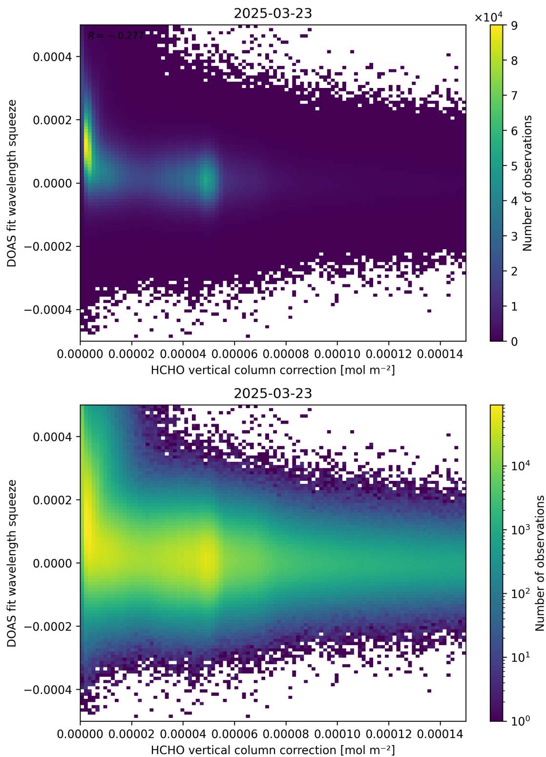
Figure 114: Scatter density plot of “HCHO vertical column correction” against “DOAS fit wavelength squeeze” for 2025-03-23 to 2025-03-24.
