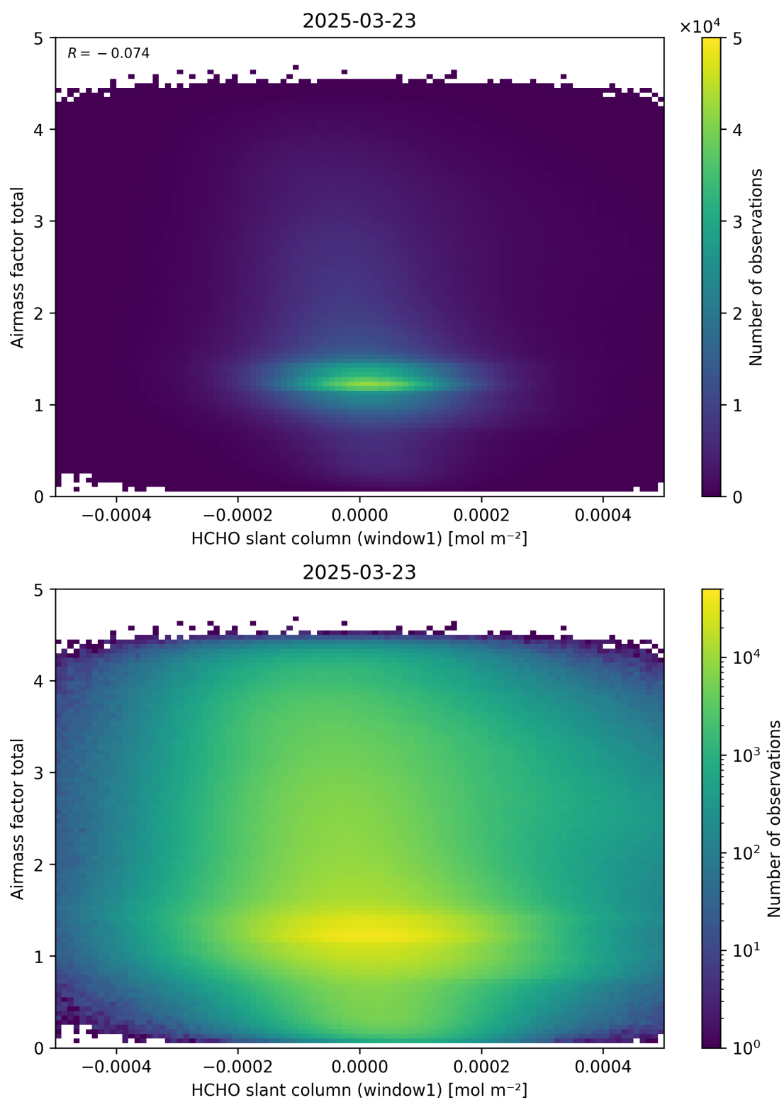
Figure 85: Scatter density plot of “HCHO slant column (window1)” against “Airmass factor total” for 2025-03-23 to 2025-03-24.
