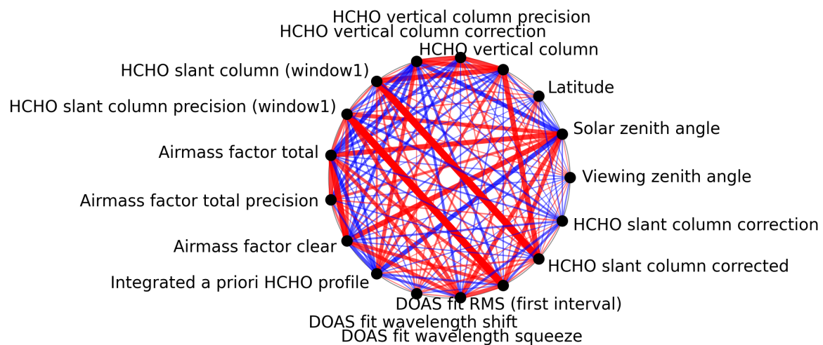
Figure 1: Map of correlation graph for 2025-03-23 to 2025-03-24.
