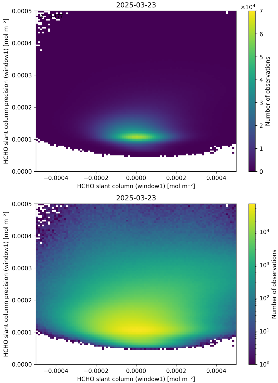
Figure 84: Scatter density plot of “HCHO slant column (window1)” against “HCHO slant column precision (window1)” for 2025-03-23 to 2025-03-24.
