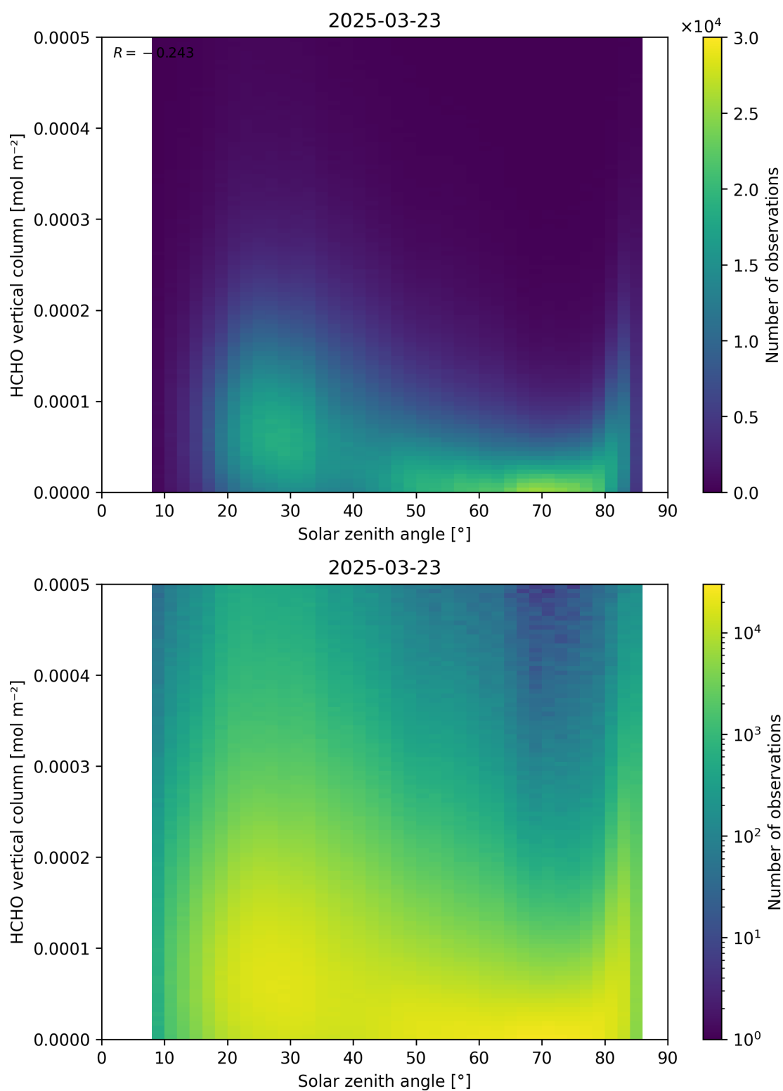
Figure 177: Scatter density plot of “Solar zenith angle” against “HCHO vertical column” for 2025-03-23 to 2025-03-24.
