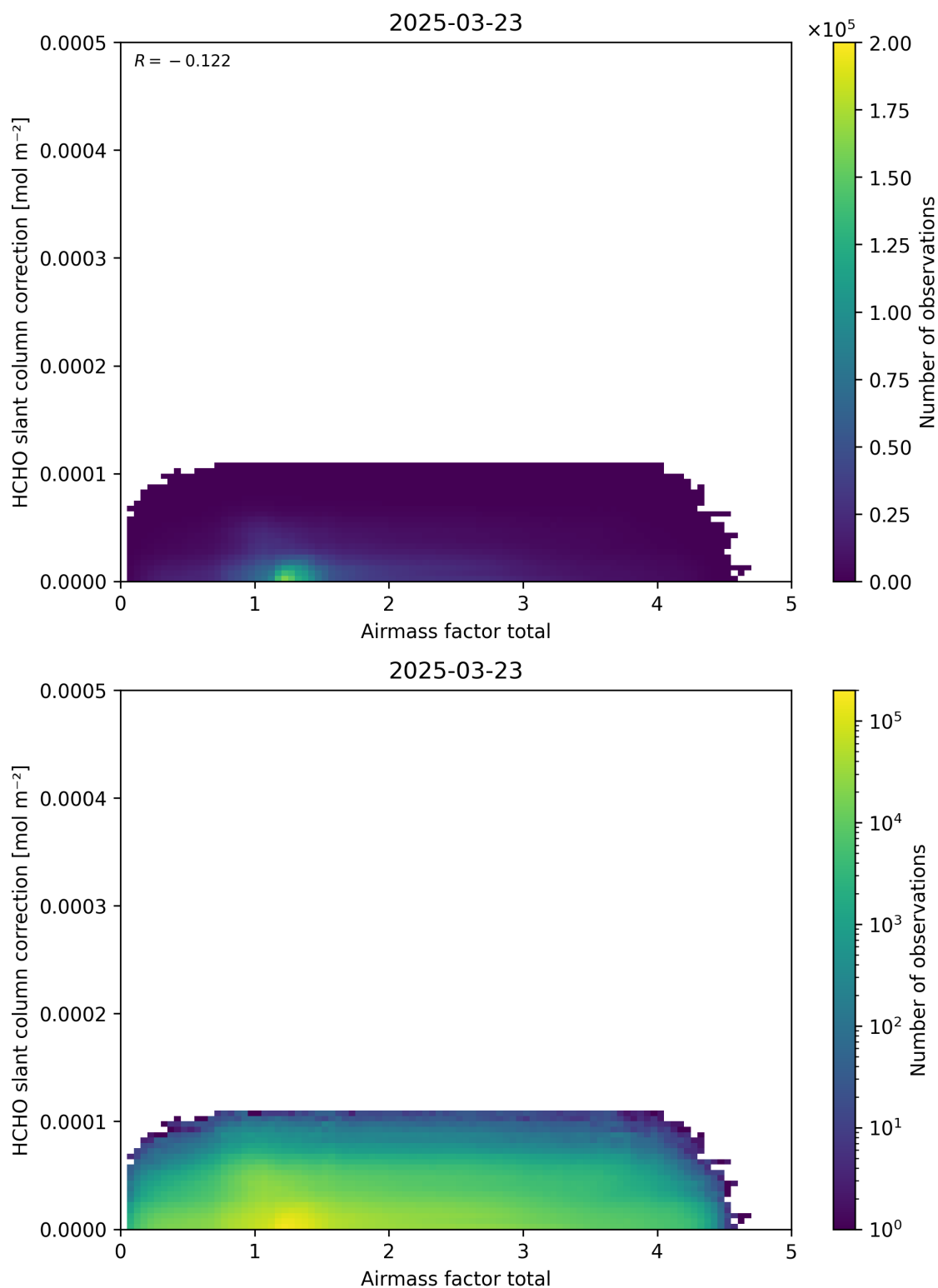
Figure 102: Scatter density plot of “Airmass factor total” against “HCHO slant column correction” for 2025-03-23 to 2025-03-24.
