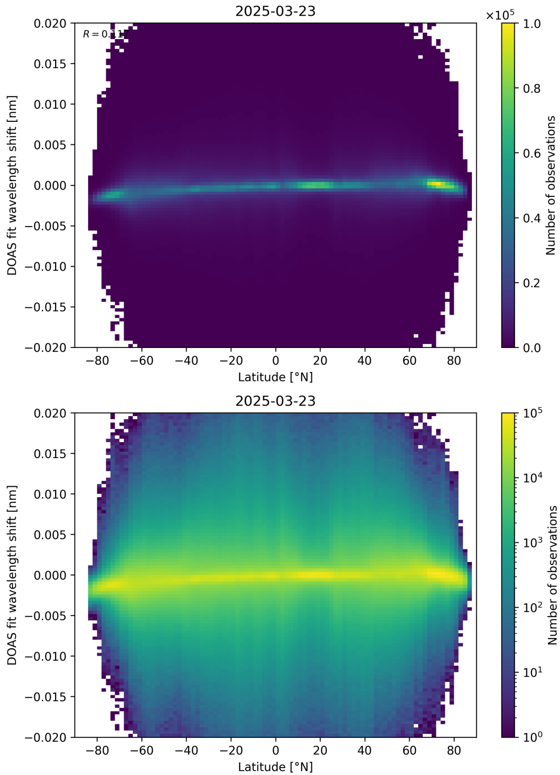
Figure 154: Scatter density plot of “Latitude” against “DOAS fit wavelength shift” for 2025-03-23 to 2025-03-24.
