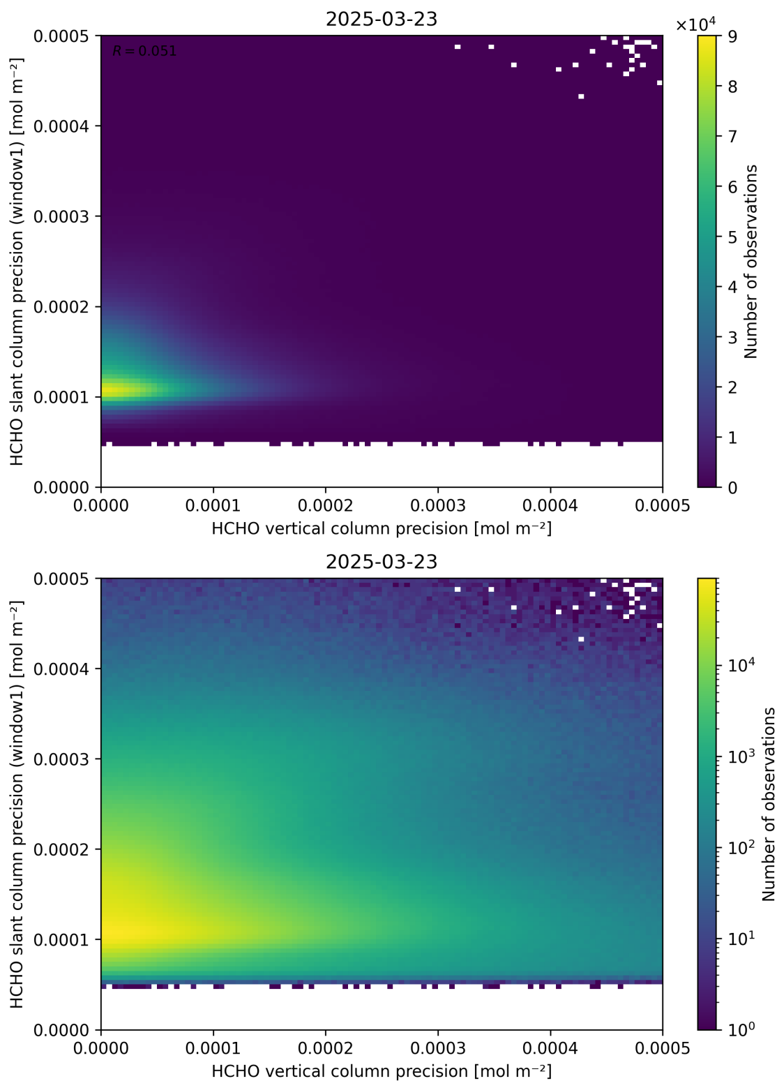
Figure 143: Scatter density plot of “HCHO vertical column precision” against “HCHO slant column precision (window1)” for 2025-03-23 to 2025-03-24.
