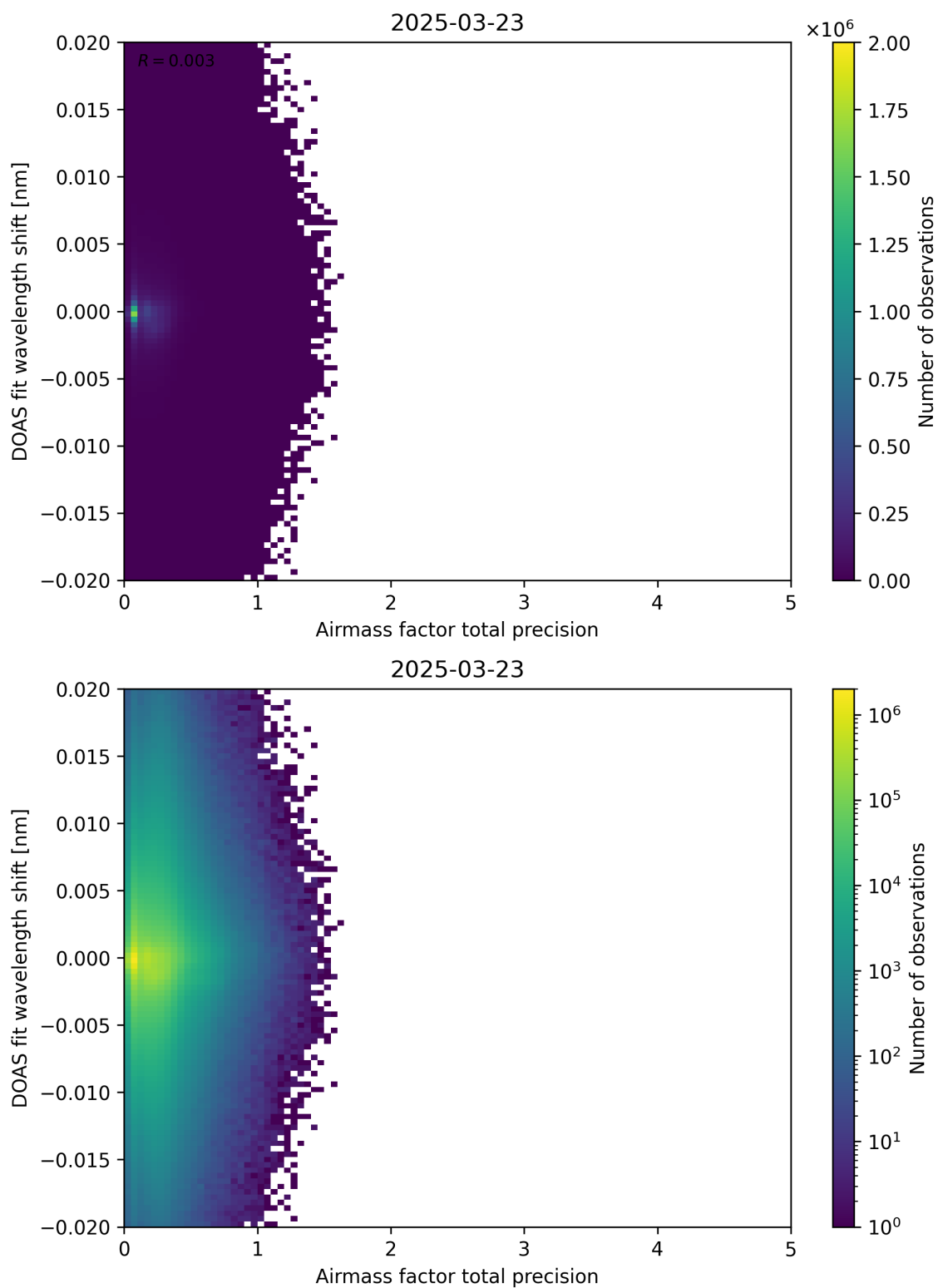
Figure 106: Scatter density plot of “Airmass factor total precision” against “DOAS fit wavelength shift” for 2025-03-23 to 2025-03-24.
