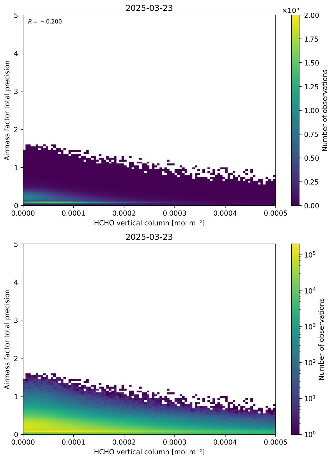
Figure 132: Scatter density plot of “HCHO vertical column” against “Airmass factor total precision” for 2025-03-23 to 2025-03-24.
