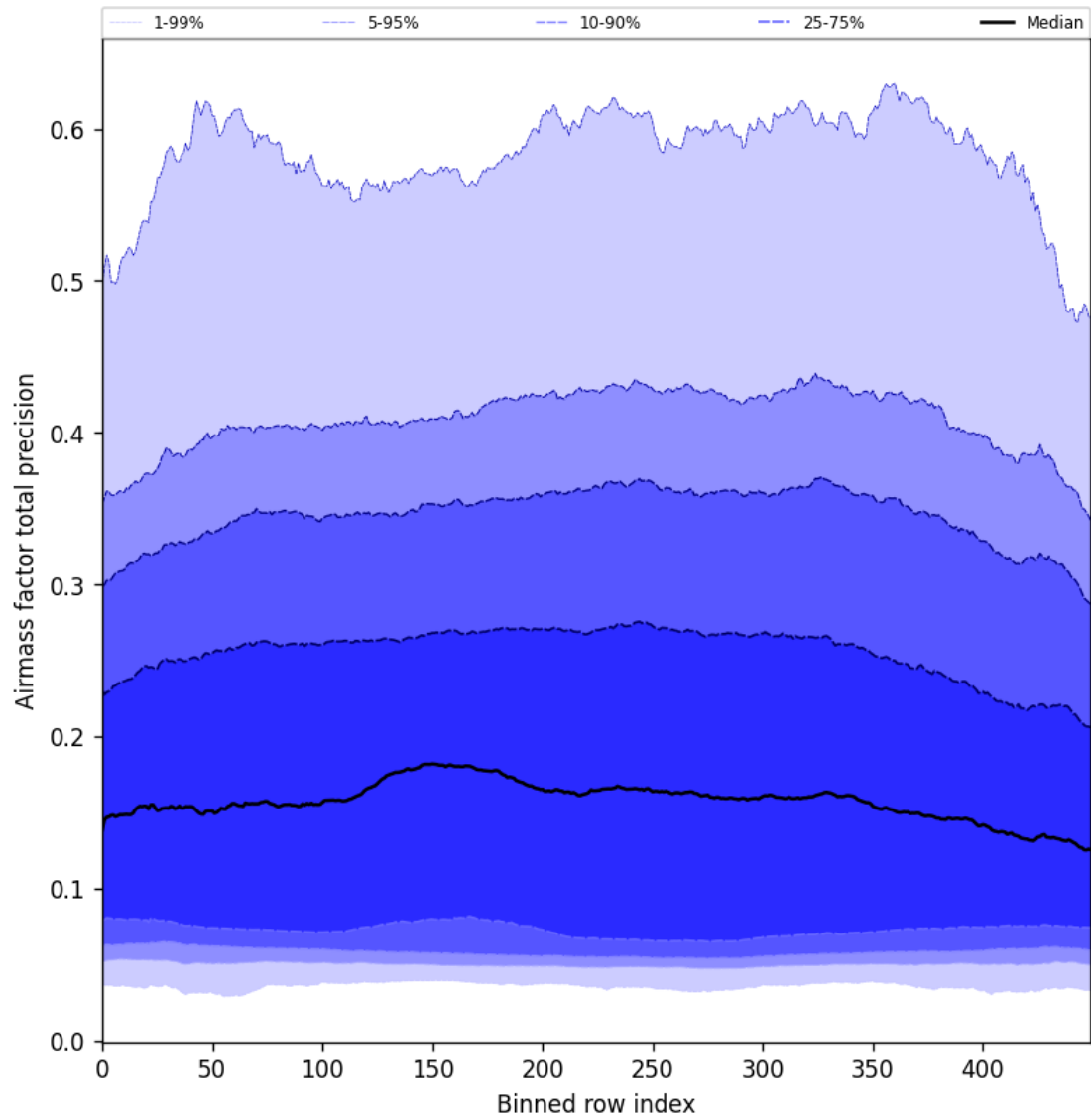
Figure 55: Along track statistics of “Airmass factor total precision” for 2025-03-23 to 2025-03-24
