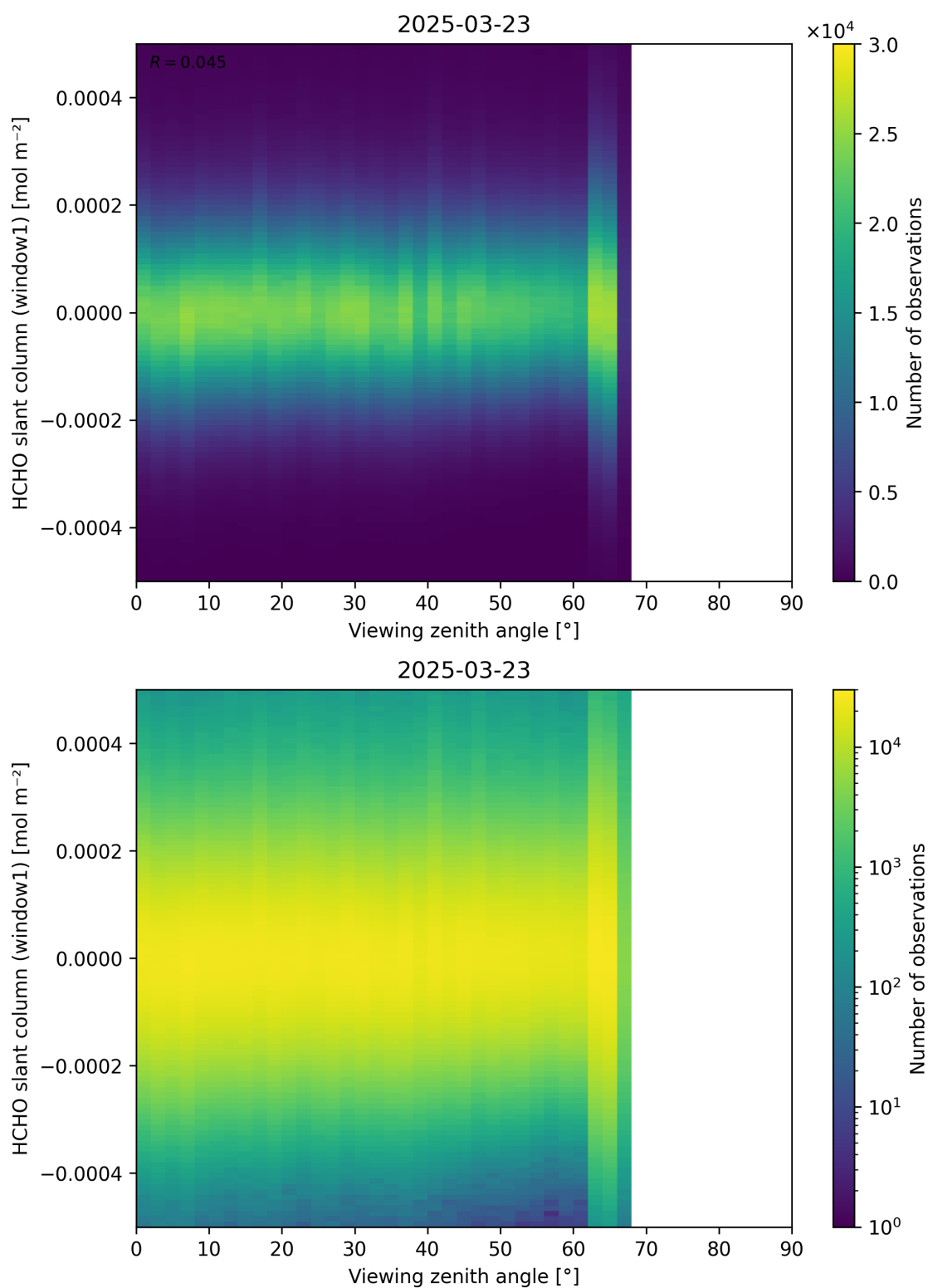
Figure 188: Scatter density plot of “Viewing zenith angle” against “HCHO slant column (window1)” for 2025-03-23 to 2025-03-24.
