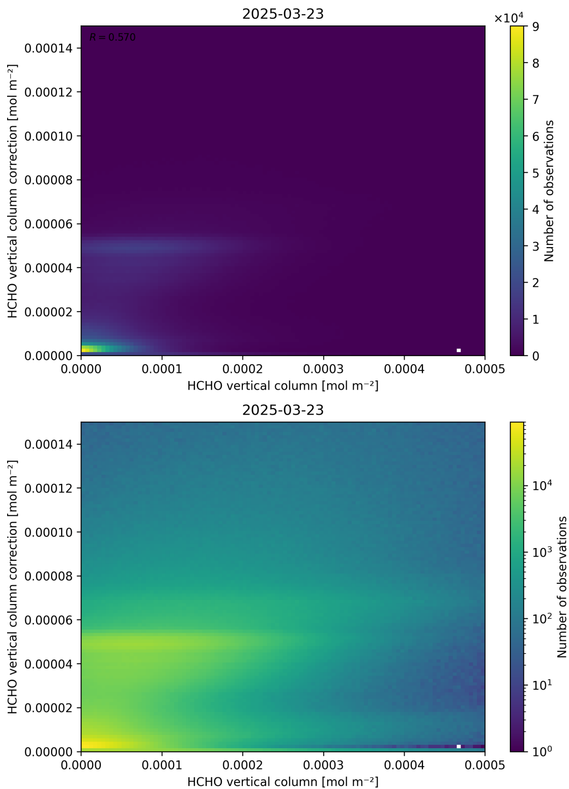
Figure 133: Scatter density plot of “HCHO vertical column” against “HCHO vertical column correction” for 2025-03-23 to 2025-03-24.
