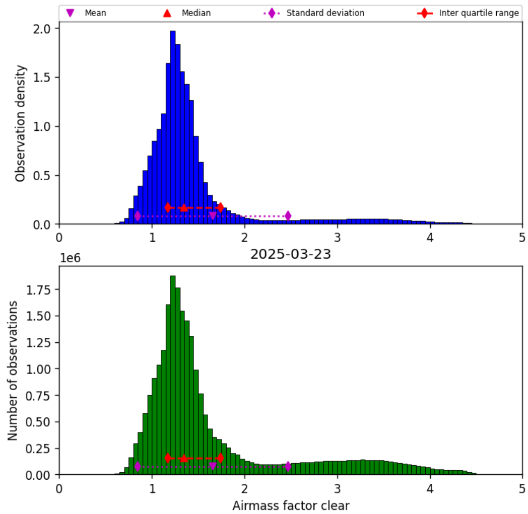
Figure 42: Histogram of “Airmass factor clear” for 2025-03-23 to 2025-03-24
