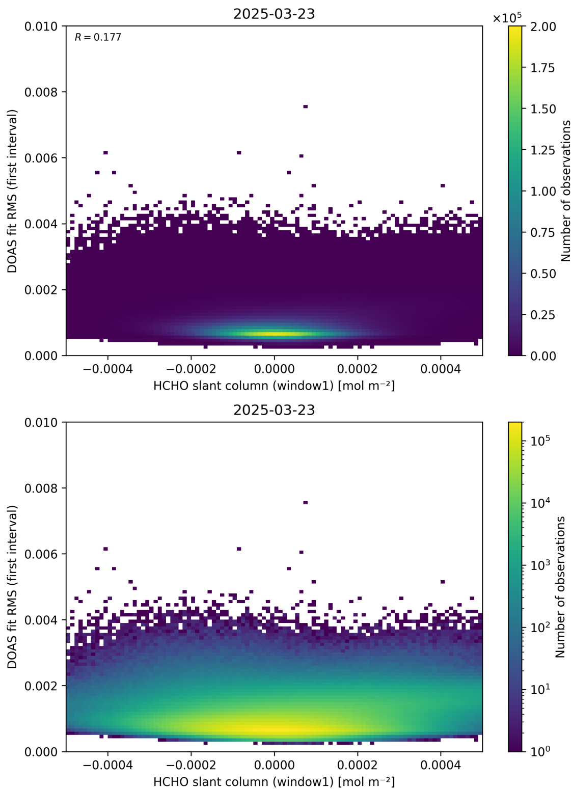
Figure 78: Scatter density plot of “HCHO slant column (window1)” against “DOAS fit RMS (first interval)” for 2025-03-23 to 2025-03-24.
