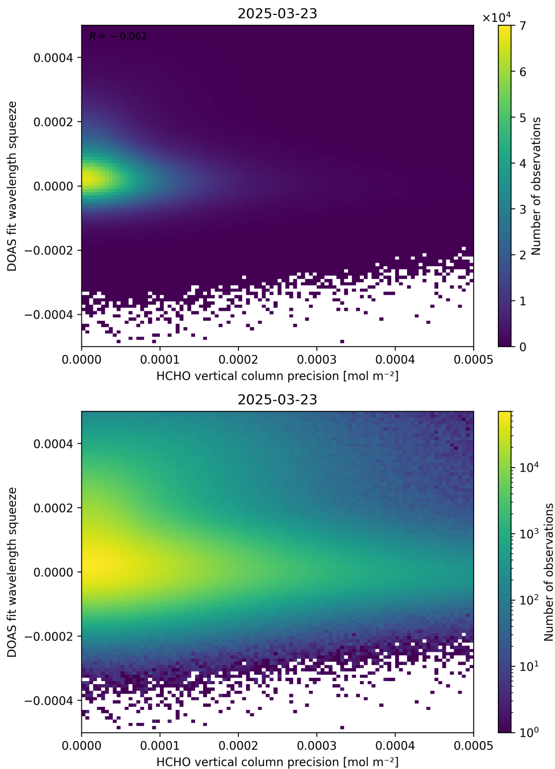
Figure 138: Scatter density plot of “HCHO vertical column precision” against “DOAS fit wavelength squeeze” for 2025-03-23 to 2025-03-24.
