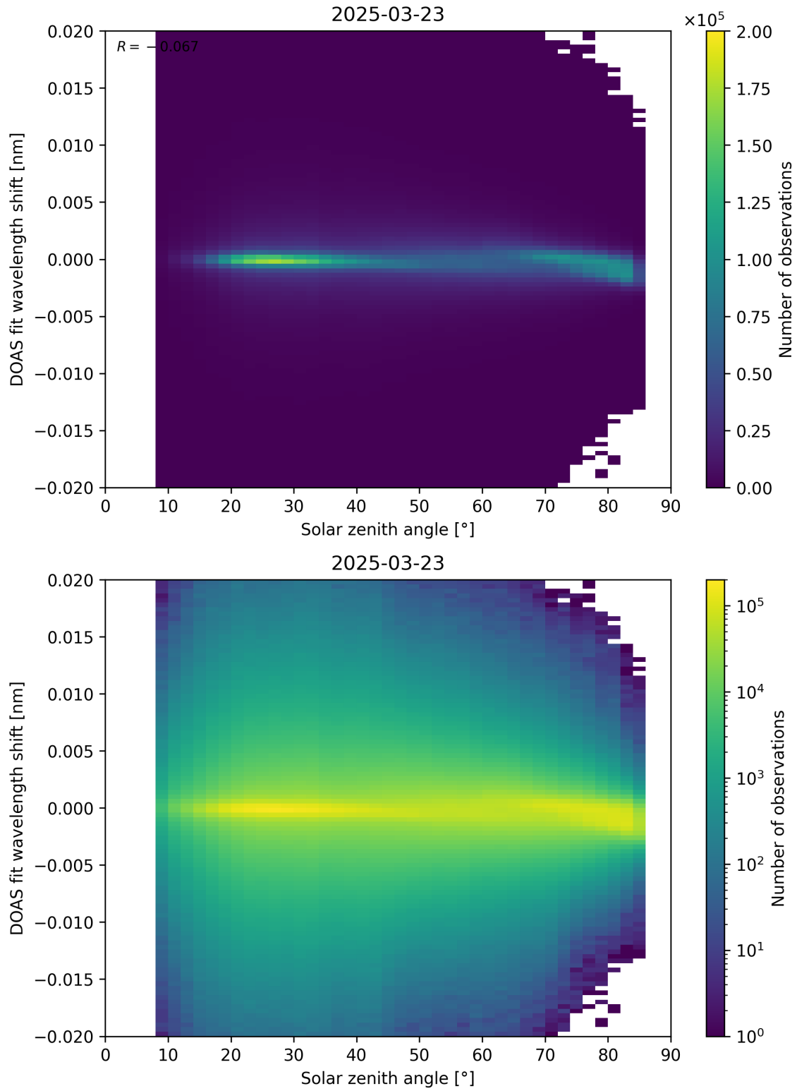
Figure 168: Scatter density plot of “Solar zenith angle” against “DOAS fit wavelength shift” for 2025-03-23 to 2025-03-24.
