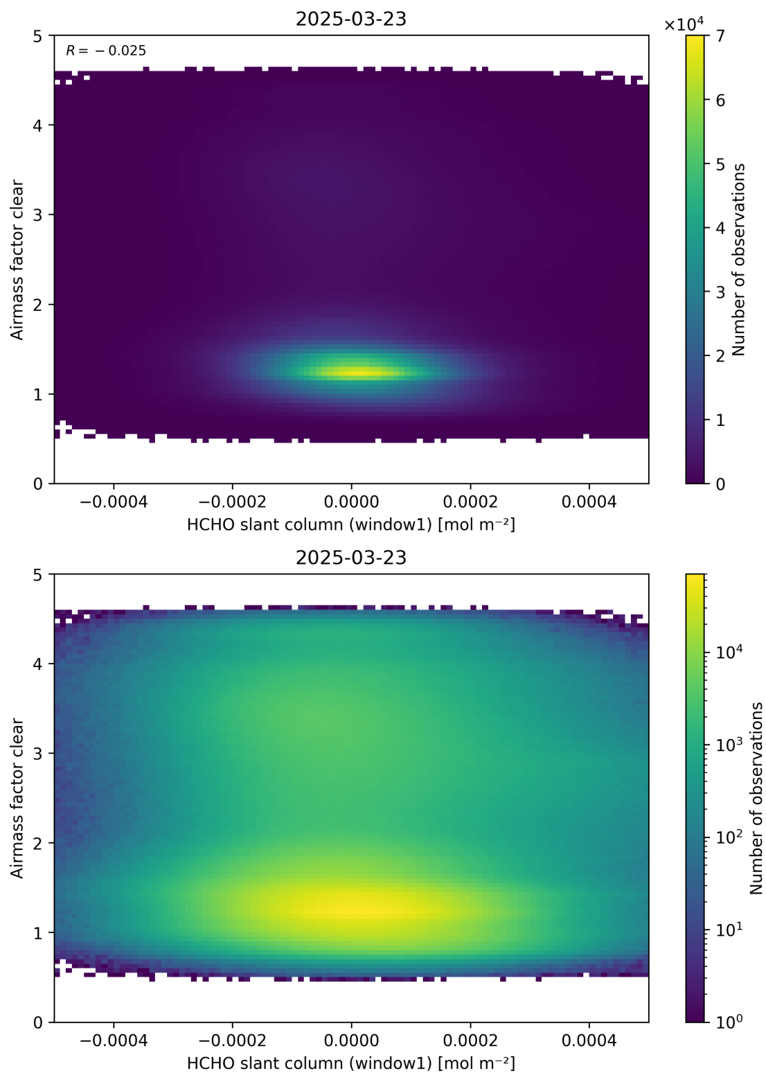
Figure 81: Scatter density plot of “HCHO slant column (window1)” against “Airmass factor clear” for 2025-03-23 to 2025-03-24.
