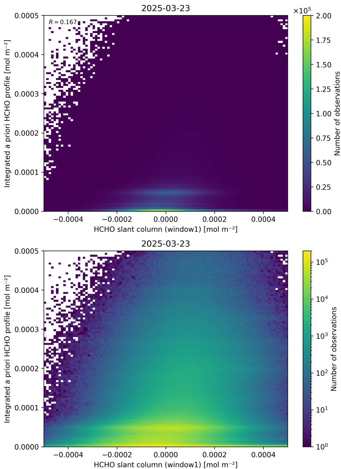
Figure 87: Scatter density plot of “HCHO slant column (window1)” against “Integrated a priori HCHO profile” for 2025-03-23 to 2025-03-24.
