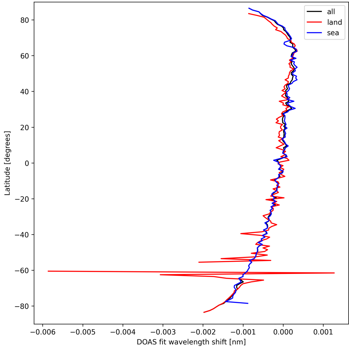
Figure 30: Zonal average of “DOAS fit wavelength shift” for 2025-03-23 to 2025-03-24.
