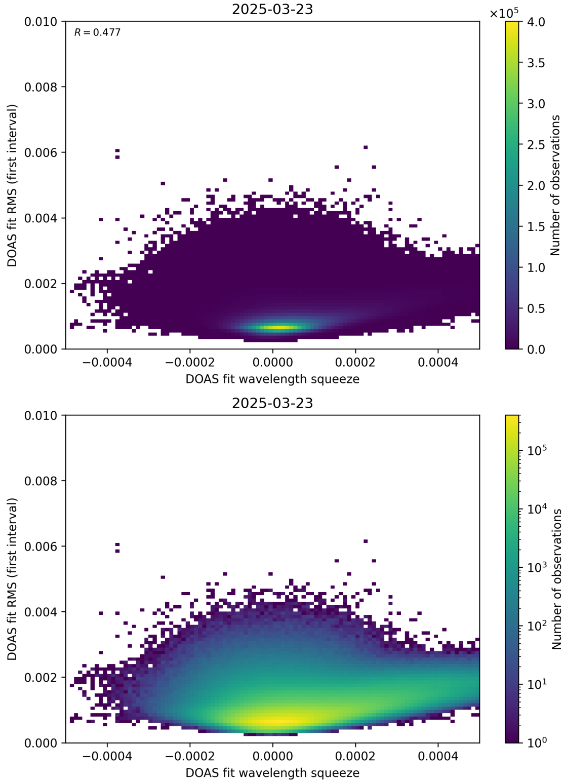
Figure 68: Scatter density plot of “DOAS fit wavelength squeeze” against “DOAS fit RMS (first interval)” for 2025-03-23 to 2025-03-24.
