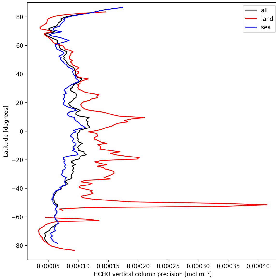
Figure 22: Zonal average of “HCHO vertical column precision” for 2025-03-23 to 2025-03-24.
