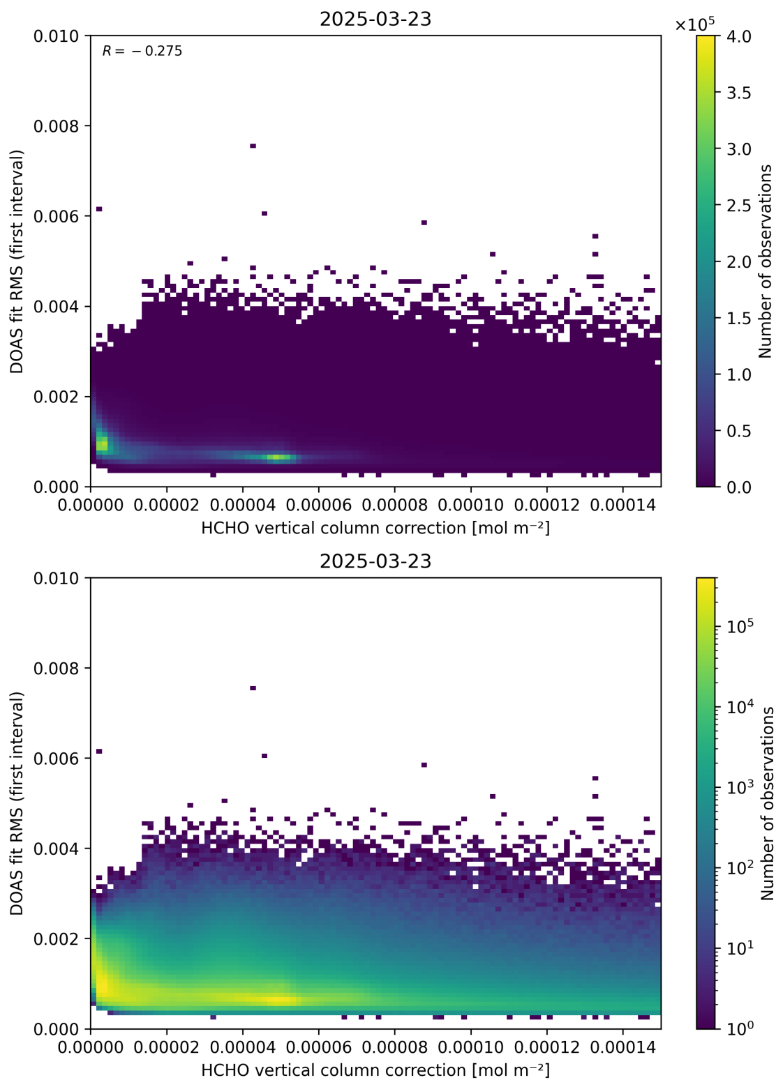
Figure 112: Scatter density plot of “HCHO vertical column correction” against “DOAS fit RMS (first interval)” for 2025-03-23 to 2025-03-24.
