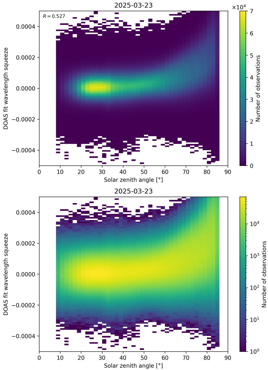
Figure 169: Scatter density plot of “Solar zenith angle” against “DOAS fit wavelength squeeze” for 2025-03-23 to 2025-03-24.
