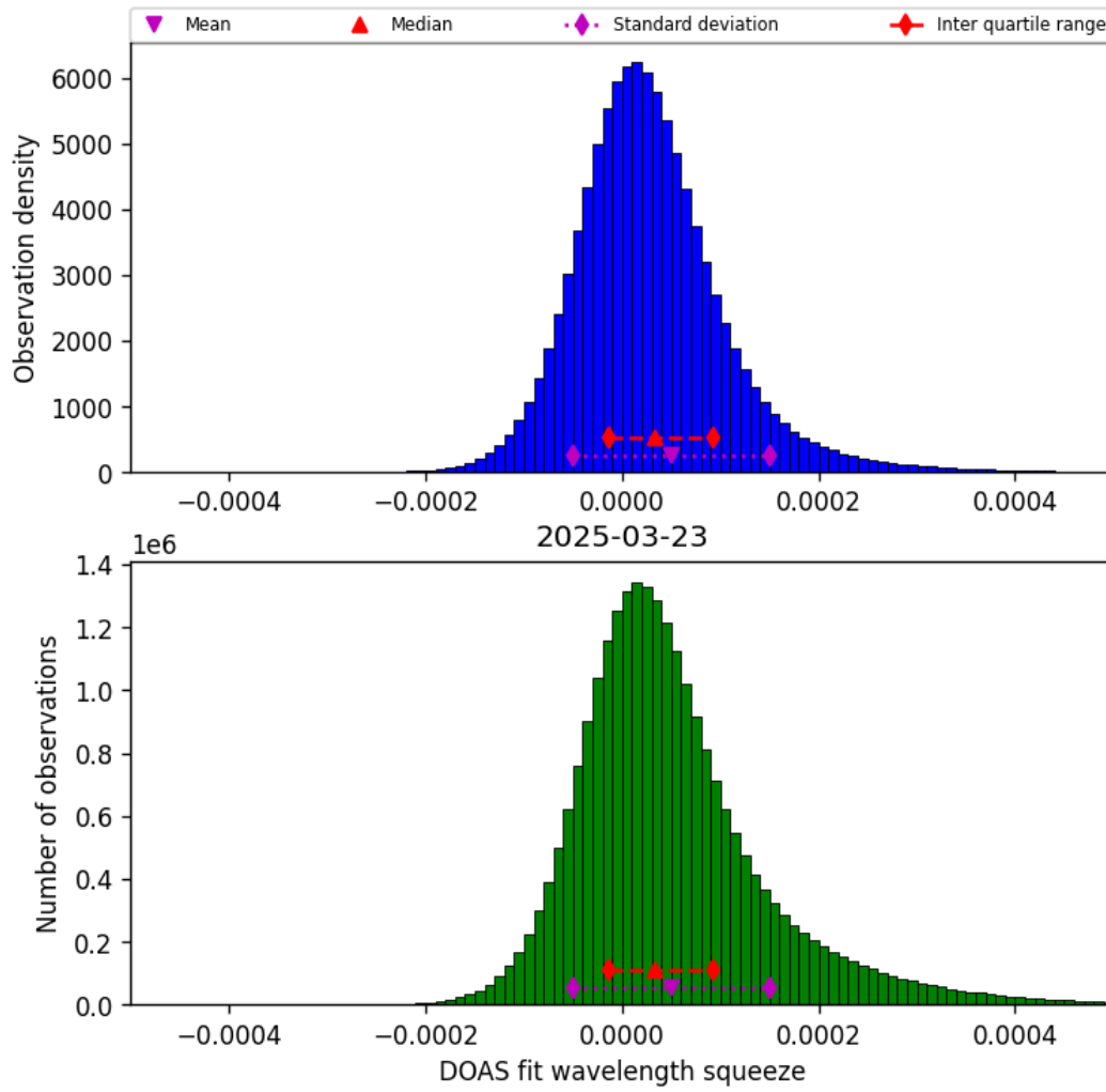
Figure 45: Histogram of “DOAS fit wavelength squeeze” for 2025-03-23 to 2025-03-24
