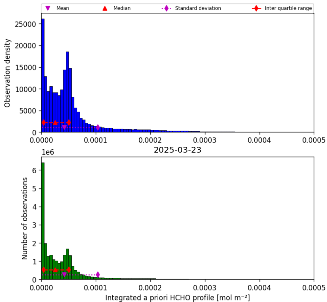
Figure 43: Histogram of “Integrated a priori HCHO profile” for 2025-03-23 to 2025-03-24
