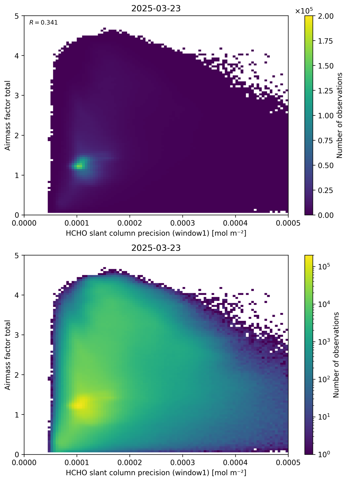
Figure 94: Scatter density plot of “HCHO slant column precision (window1)” against “Airmass factor total” for 2025-03-23 to 2025-03-24.
