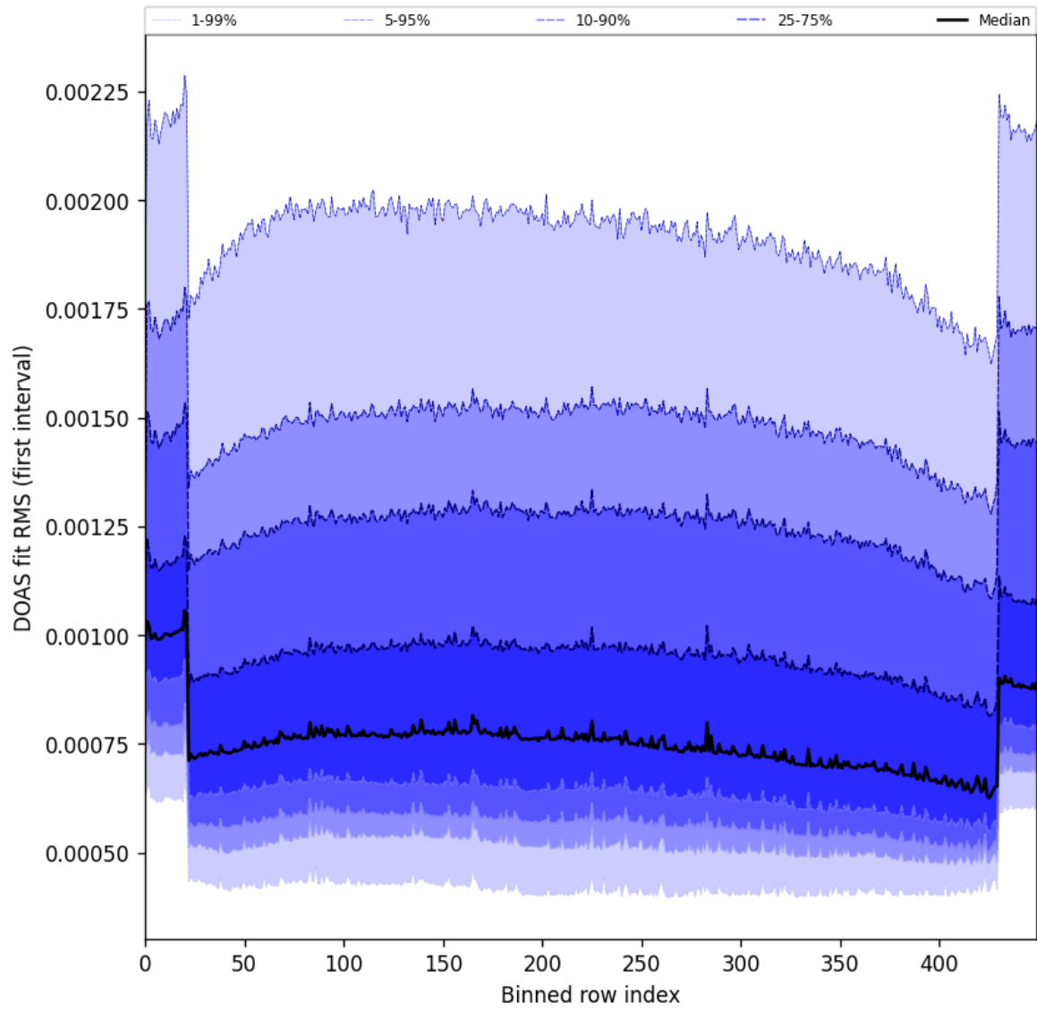
Figure 60: Along track statistics of “DOAS fit RMS (first interval)” for 2025-03-23 to 2025-03-24
