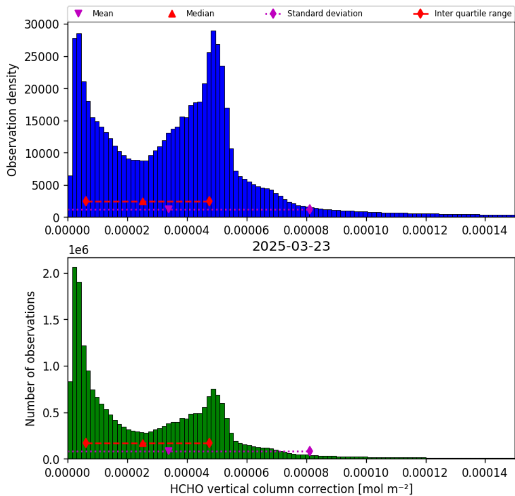
Figure 37: Histogram of “HCHO vertical column correction” for 2025-03-23 to 2025-03-24
