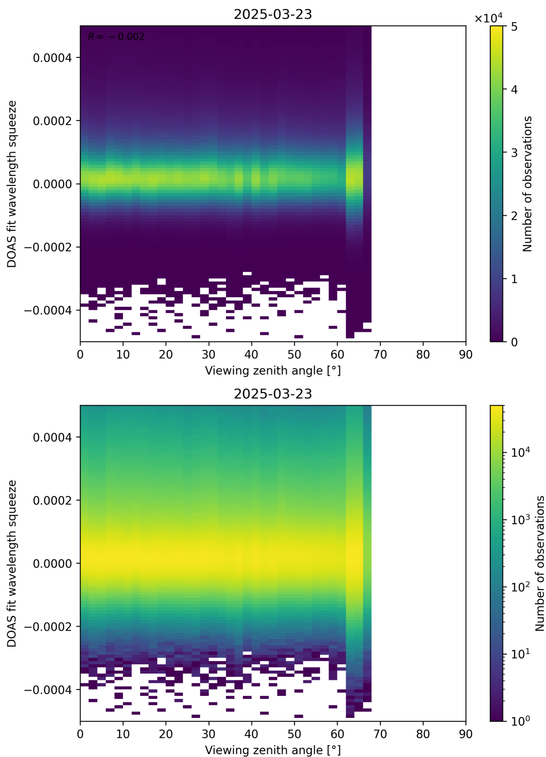
Figure 184: Scatter density plot of “Viewing zenith angle” against “DOAS fit wavelength squeeze” for 2025-03-23 to 2025-03-24.
