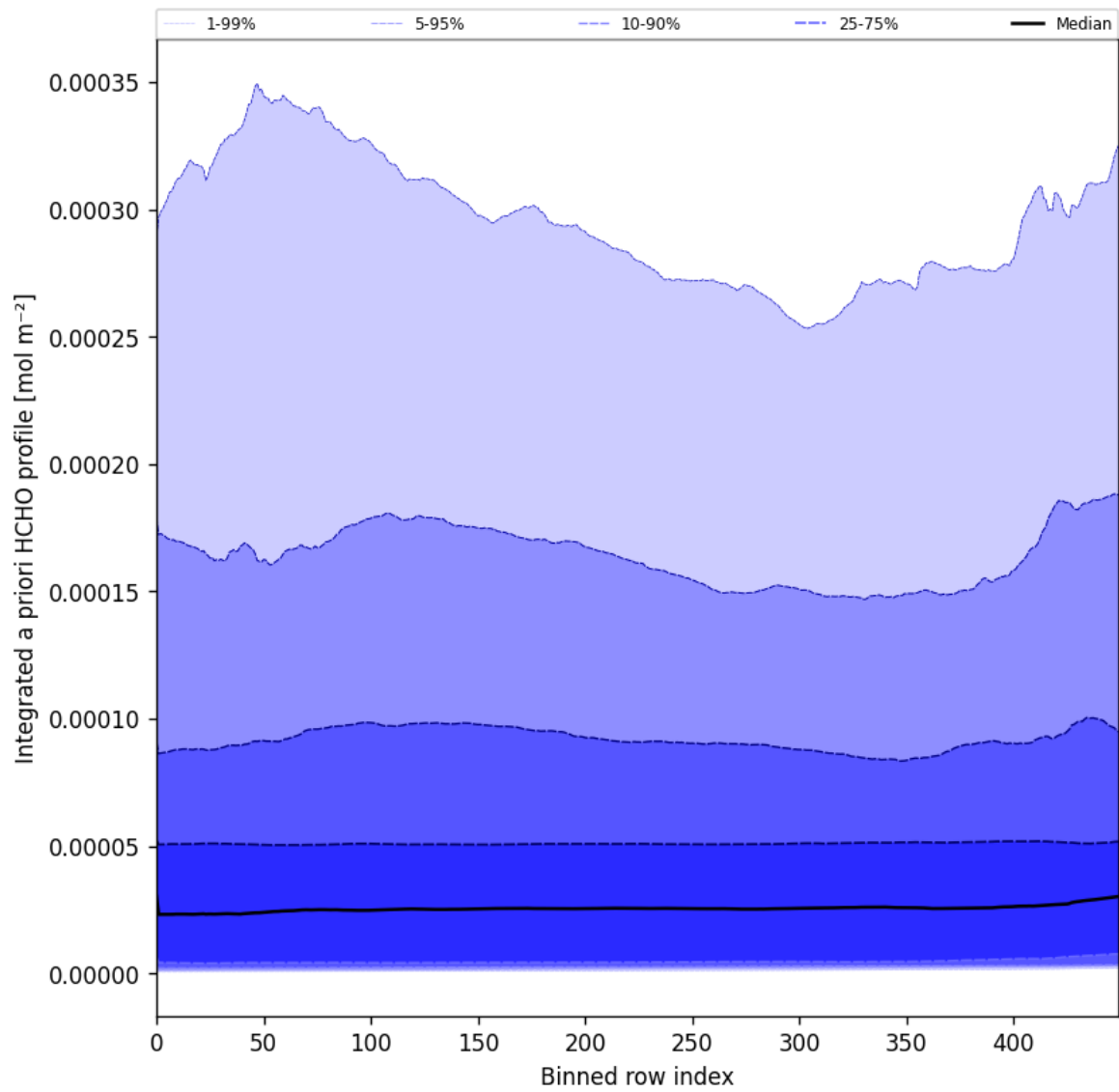
Figure 57: Along track statistics of “Integrated a priori HCHO profile” for 2025-03-23 to 2025-03-24
