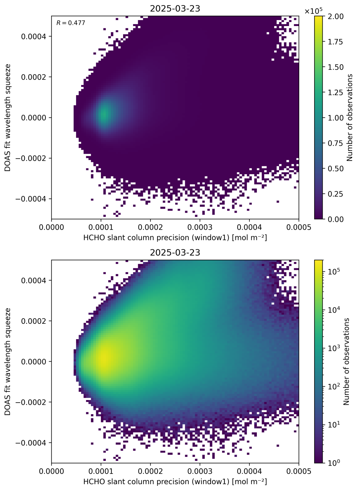
Figure 90: Scatter density plot of “HCHO slant column precision (window1)” against “DOAS fit wavelength squeeze” for 2025-03-23 to 2025-03-24.
