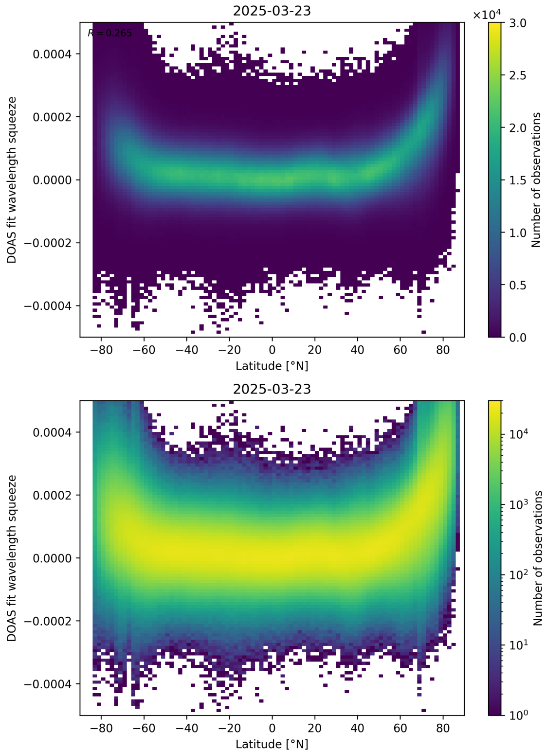
Figure 155: Scatter density plot of “Latitude” against “DOAS fit wavelength squeeze” for 2025-03-23 to 2025-03-24.
