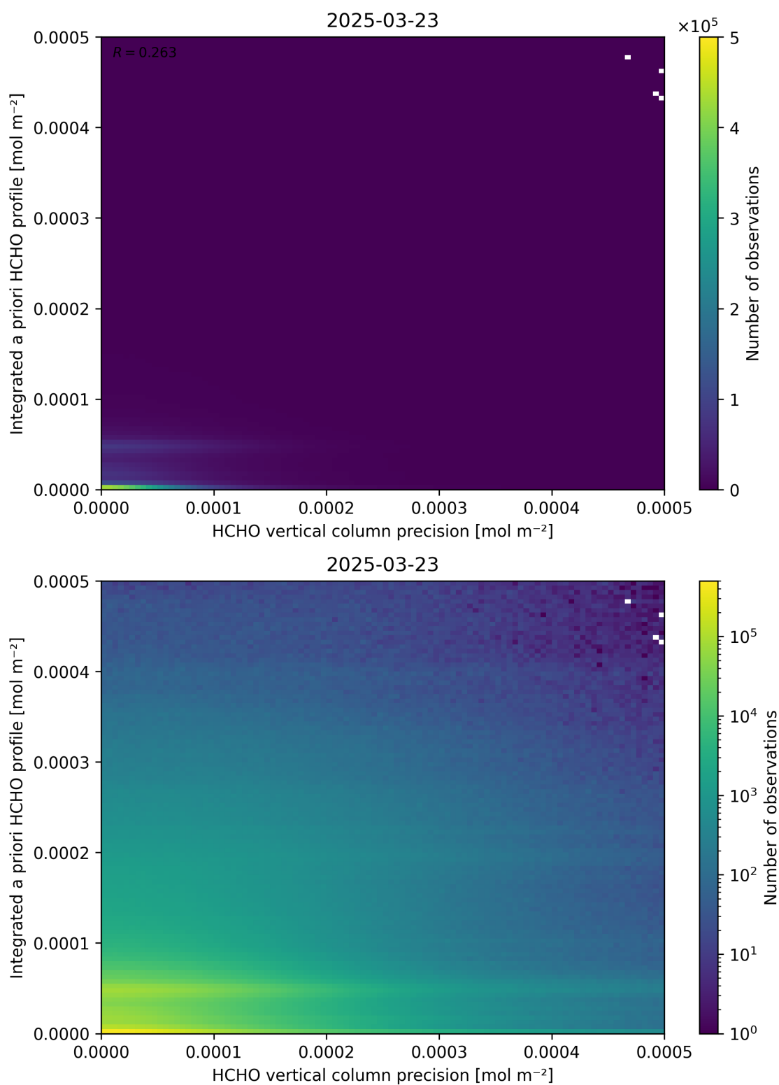
Figure 147: Scatter density plot of “HCHO vertical column precision” against “Integrated a priori HCHO profile” for 2025-03-23 to 2025-03-24.
