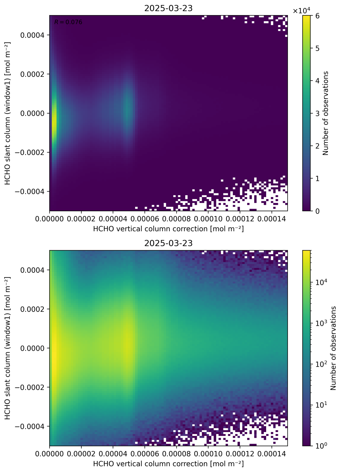
Figure 118: Scatter density plot of “HCHO vertical column correction” against “HCHO slant column (window1)” for 2025-03-23 to 2025-03-24.
