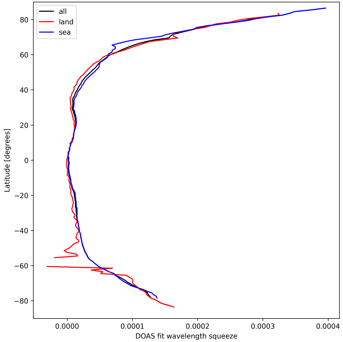
Figure 31: Zonal average of “DOAS fit wavelength squeeze” for 2025-03-23 to 2025-03-24.
