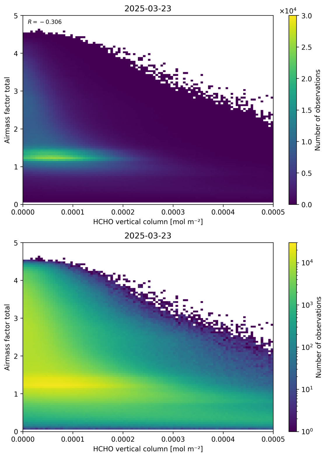
Figure 131: Scatter density plot of “HCHO vertical column” against “Airmass factor total” for 2025-03-23 to 2025-03-24.
