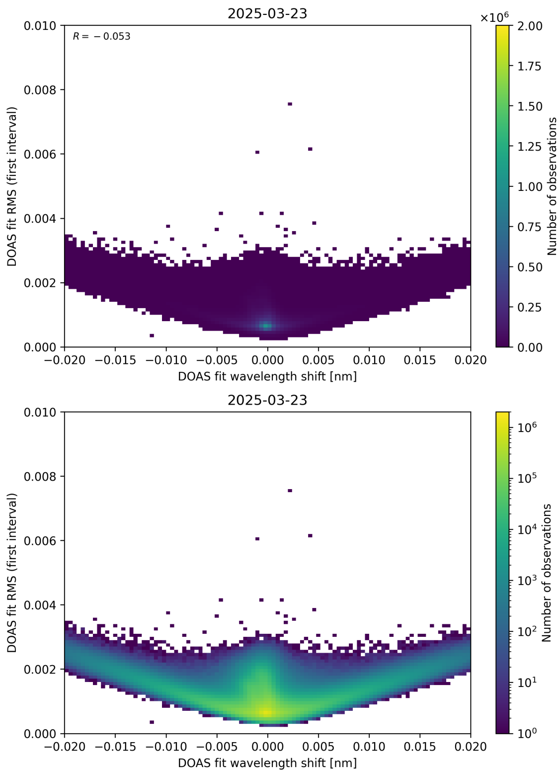
Figure 64: Scatter density plot of “DOAS fit wavelength shift” against “DOAS fit RMS (first interval)” for 2025-03-23 to 2025-03-24.
