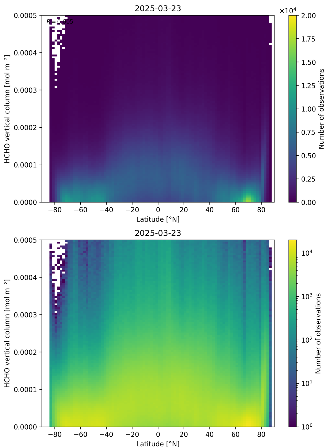
Figure 163: Scatter density plot of “Latitude” against “HCHO vertical column” for 2025-03-23 to 2025-03-24.
