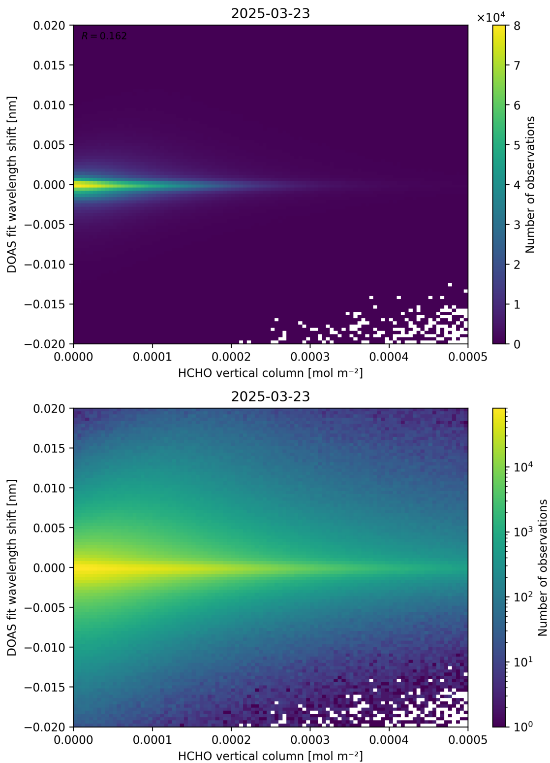
Figure 124: Scatter density plot of “HCHO vertical column” against “DOAS fit wavelength shift” for 2025-03-23 to 2025-03-24.
