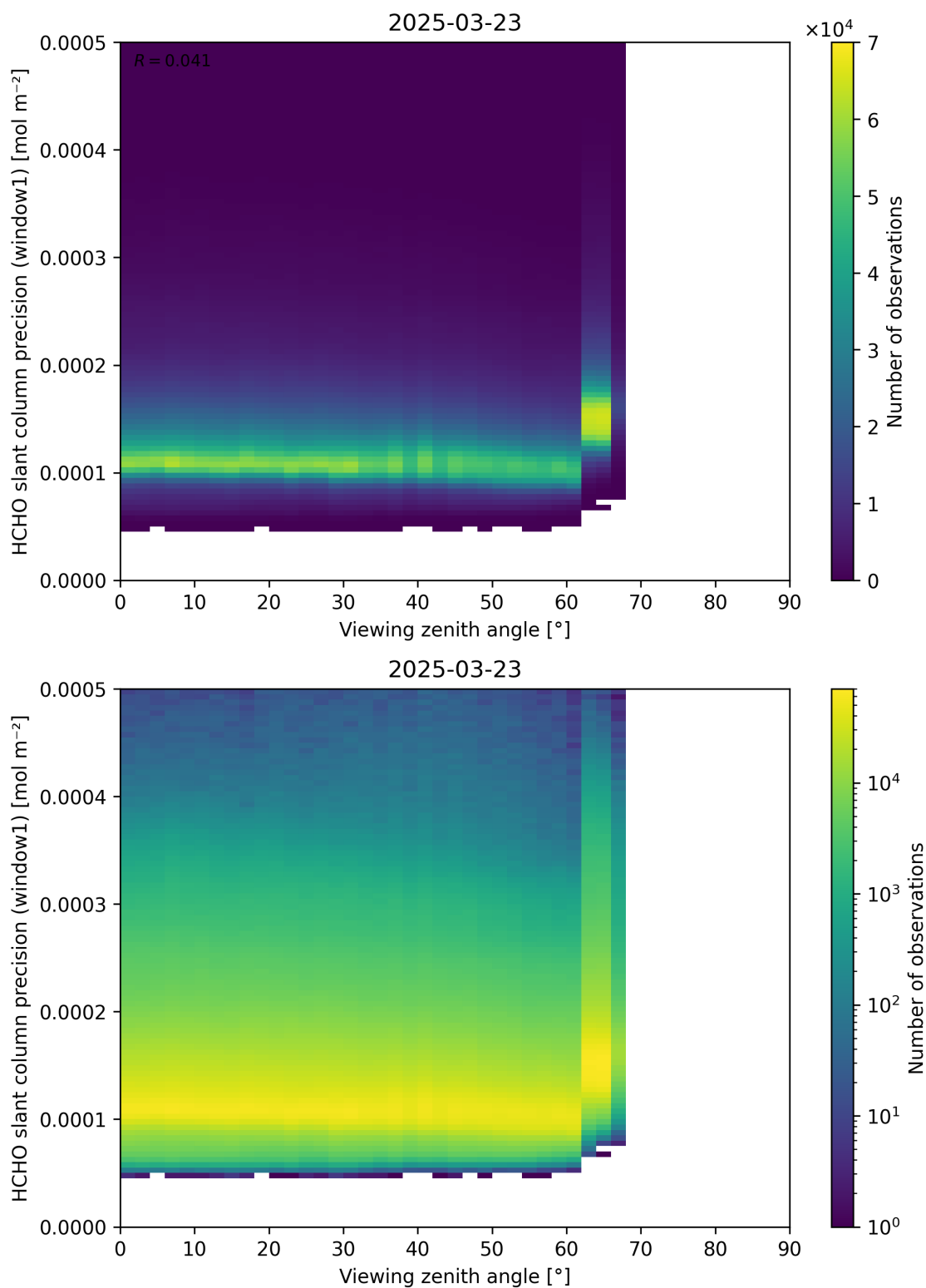
Figure 189: Scatter density plot of “Viewing zenith angle” against “HCHO slant column precision (window1)” for 2025-03-23 to 2025-03-24.
