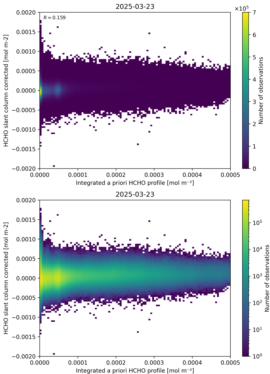
Figure 151: Scatter density plot of “Integrated a priori HCHO profile” against “HCHO slant column corrected” for 2025-03-23 to 2025-03-24.
