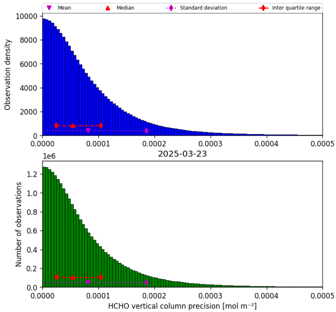
Figure 36: Histogram of “HCHO vertical column precision” for 2025-03-23 to 2025-03-24
