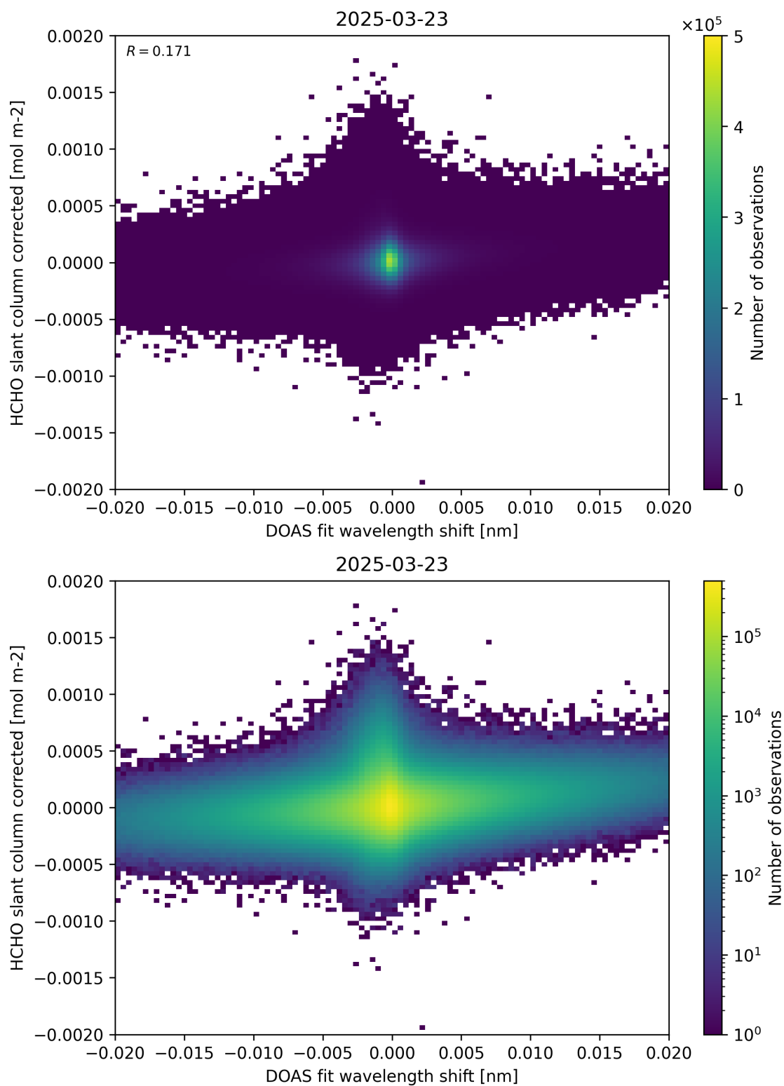
Figure 66: Scatter density plot of “DOAS fit wavelength shift” against “HCHO slant column corrected” for 2025-03-23 to 2025-03-24.
