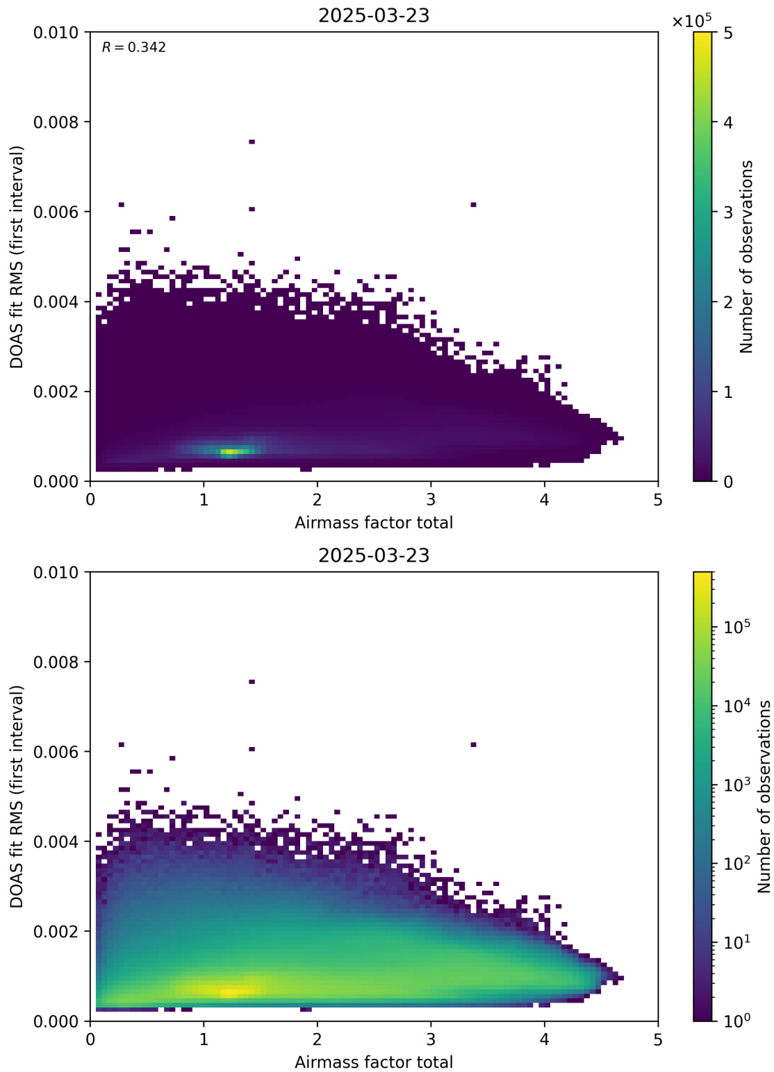
Figure 97: Scatter density plot of “Airmass factor total” against “DOAS fit RMS (first interval)” for 2025-03-23 to 2025-03-24.
