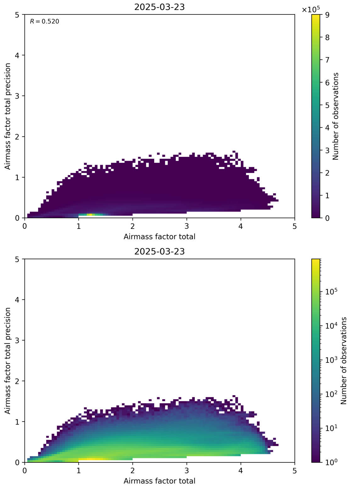
Figure 103: Scatter density plot of “Airmass factor total” against “Airmass factor total precision” for 2025-03-23 to 2025-03-24.
