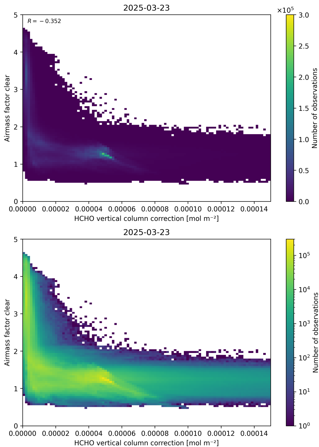
Figure 115: Scatter density plot of “HCHO vertical column correction” against “Airmass factor clear” for 2025-03-23 to 2025-03-24.
