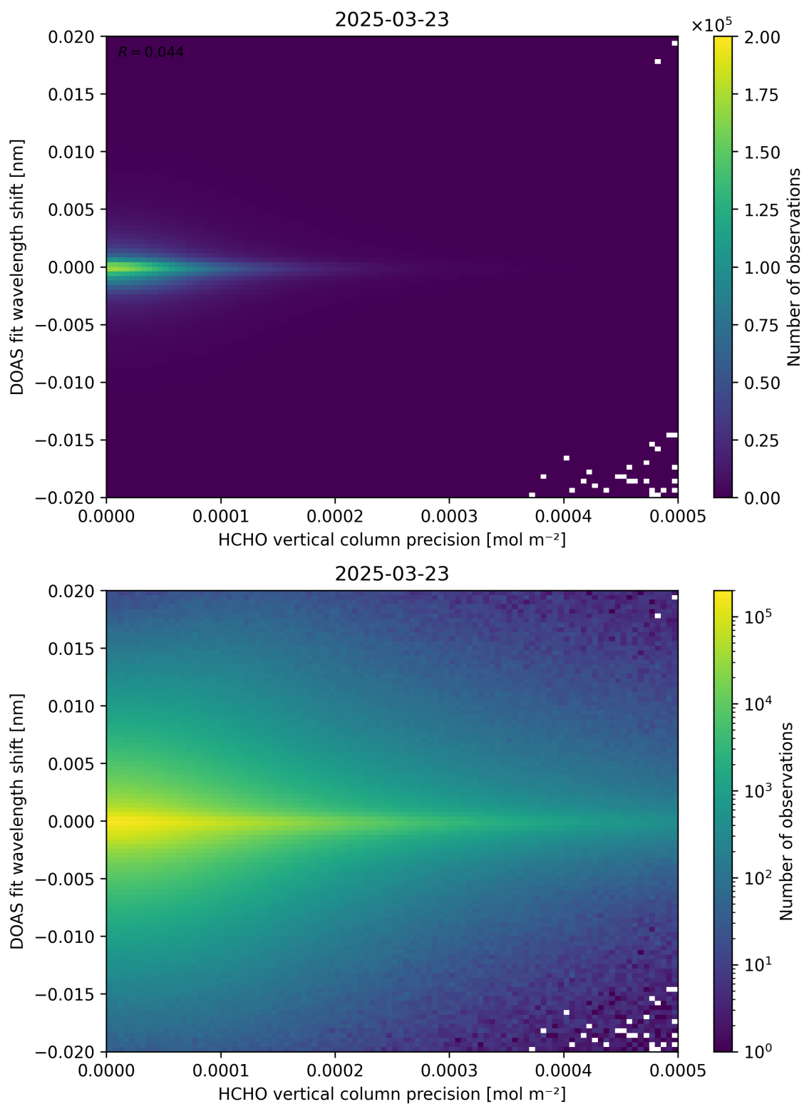
Figure 137: Scatter density plot of “HCHO vertical column precision” against “DOAS fit wavelength shift” for 2025-03-23 to 2025-03-24.
