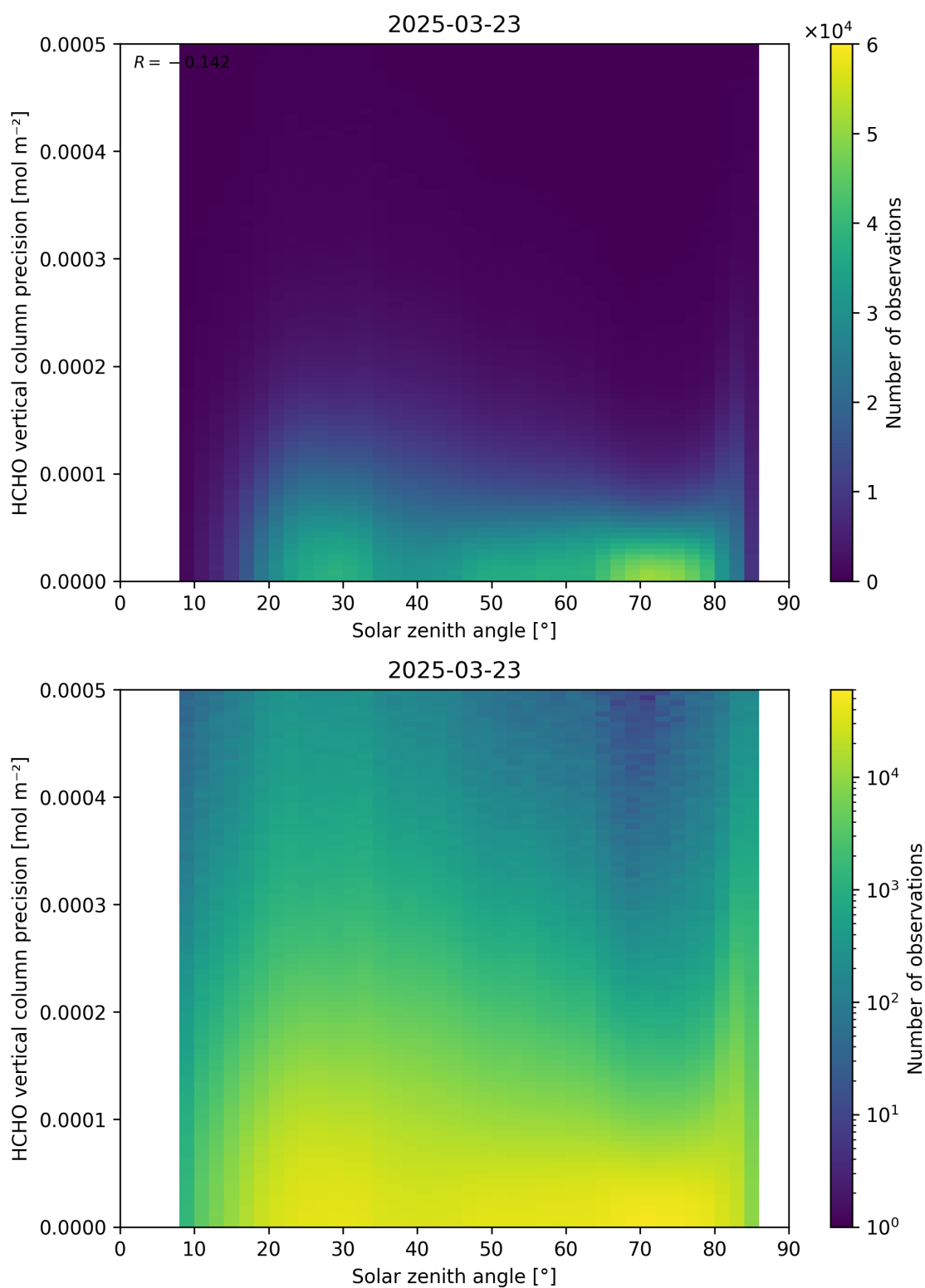
Figure 179: Scatter density plot of “Solar zenith angle” against “HCHO vertical column precision” for 2025-03-23 to 2025-03-24.
