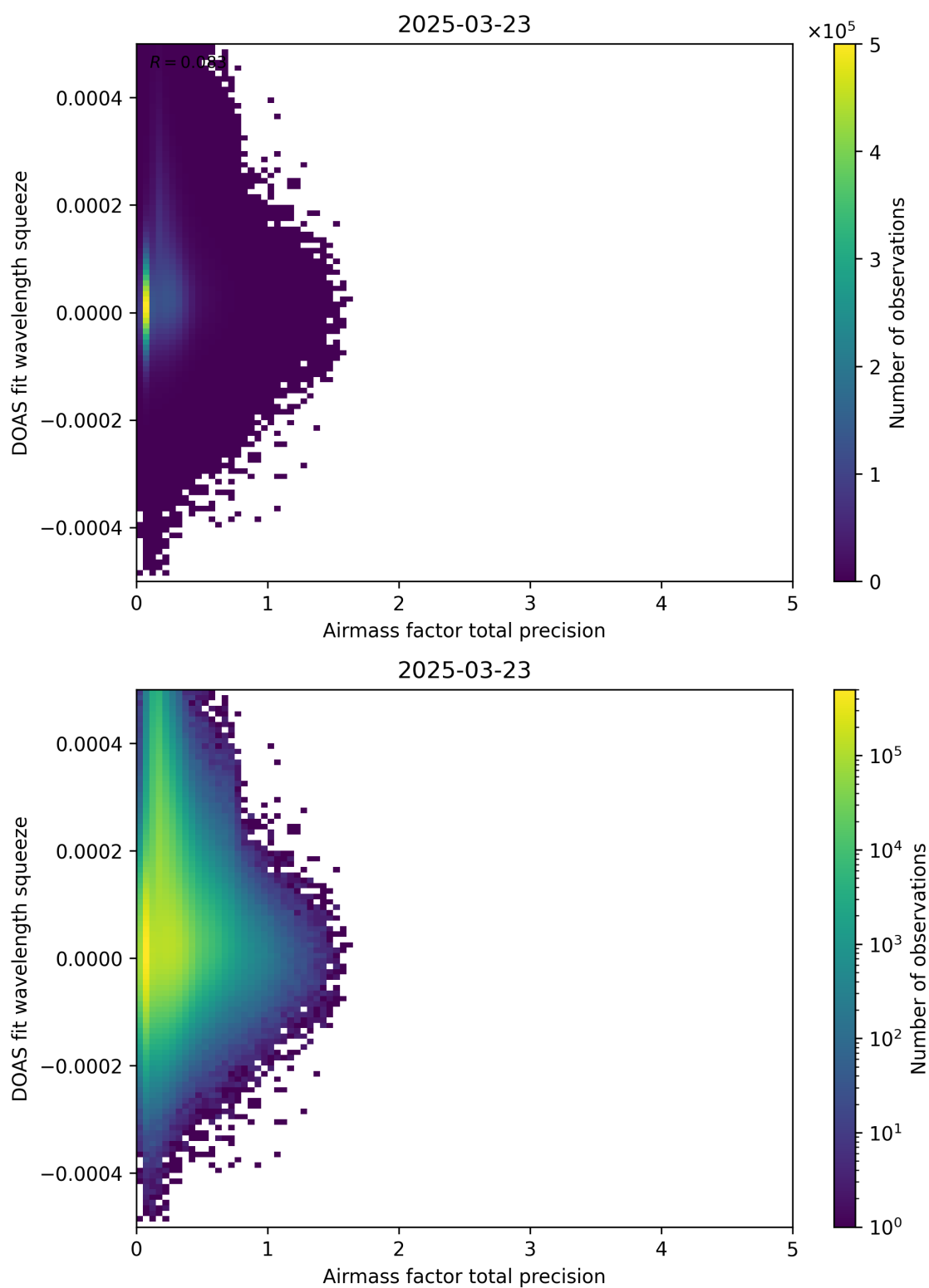
Figure 107: Scatter density plot of “Airmass factor total precision” against “DOAS fit wavelength squeeze” for 2025-03-23 to 2025-03-24.
