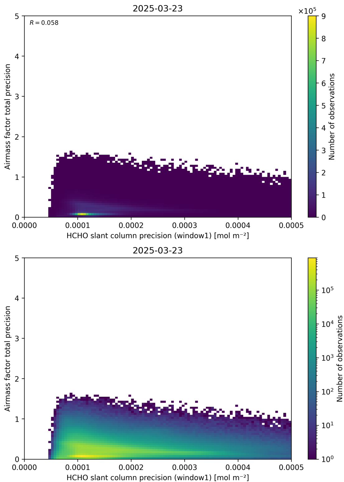
Figure 95: Scatter density plot of “HCHO slant column precision (window1)” against “Airmass factor total precision” for 2025-03-23 to 2025-03-24.
