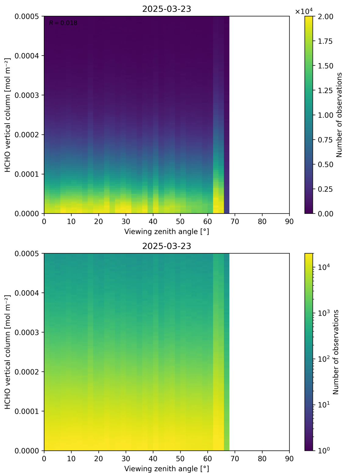
Figure 192: Scatter density plot of “Viewing zenith angle” against “HCHO vertical column” for 2025-03-23 to 2025-03-24.
