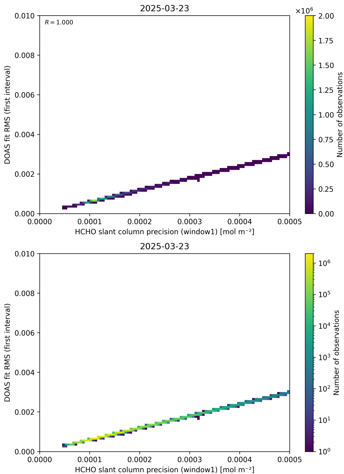
Figure 88: Scatter density plot of “HCHO slant column precision (window1)” against “DOAS fit RMS (first interval)” for 2025-03-23 to 2025-03-24.
