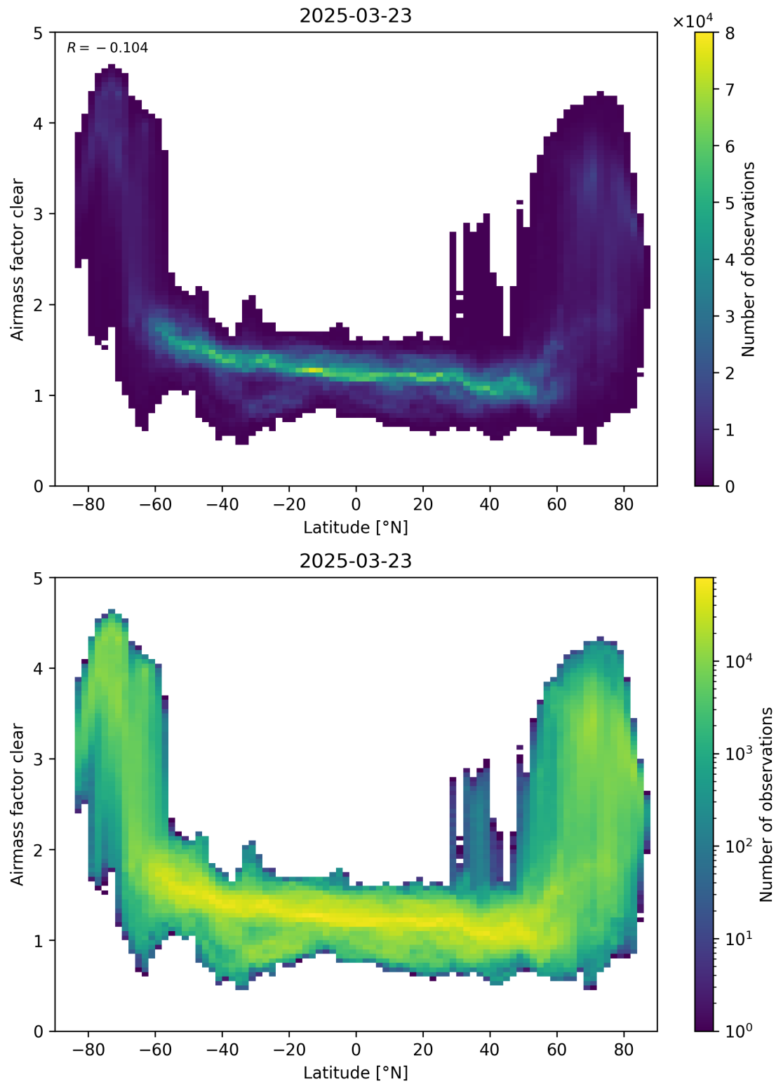
Figure 156: Scatter density plot of “Latitude” against “Airmass factor clear” for 2025-03-23 to 2025-03-24.
