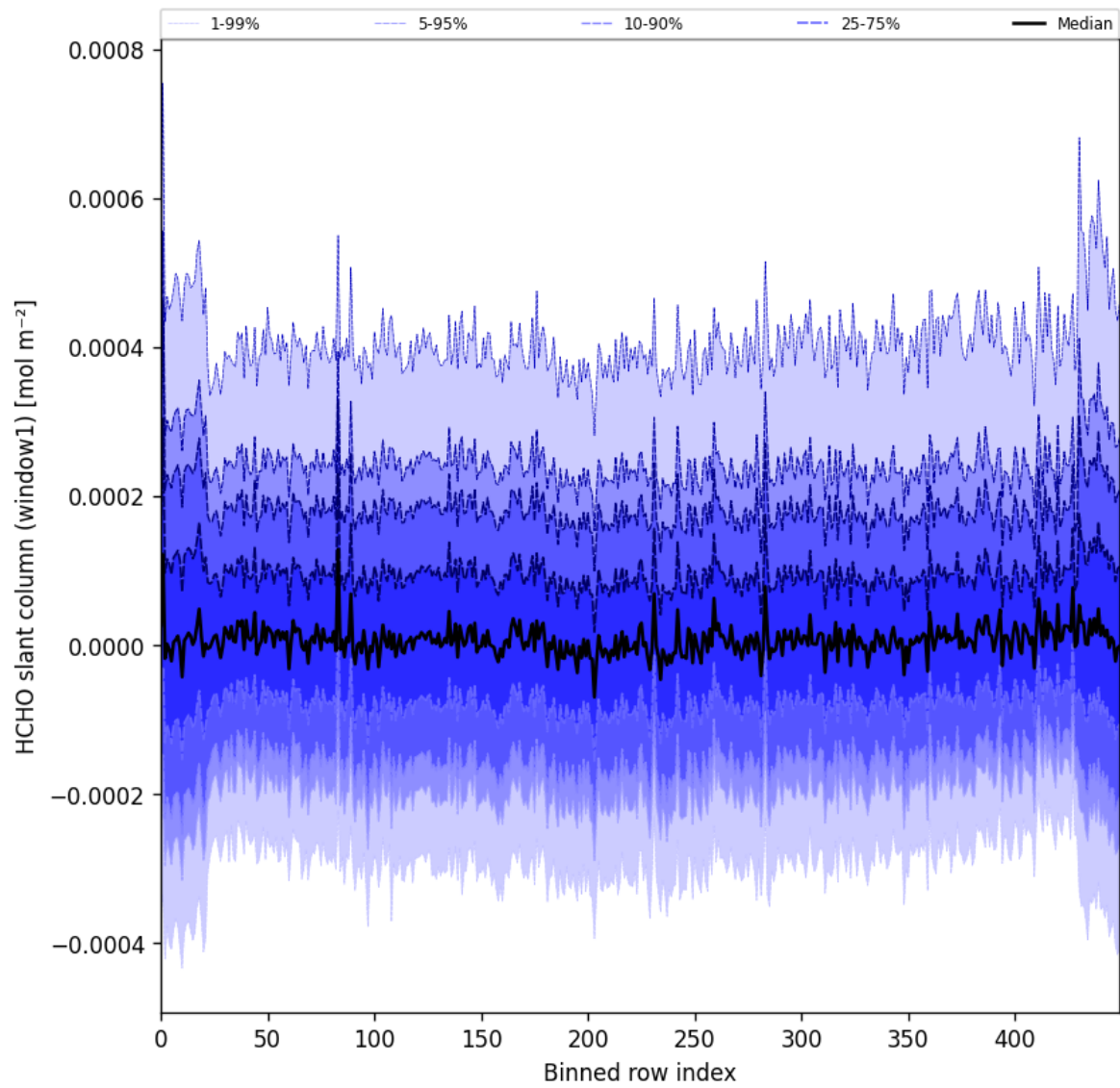
Figure 52: Along track statistics of “HCHO slant column (window1)” for 2025-03-23 to 2025-03-24
