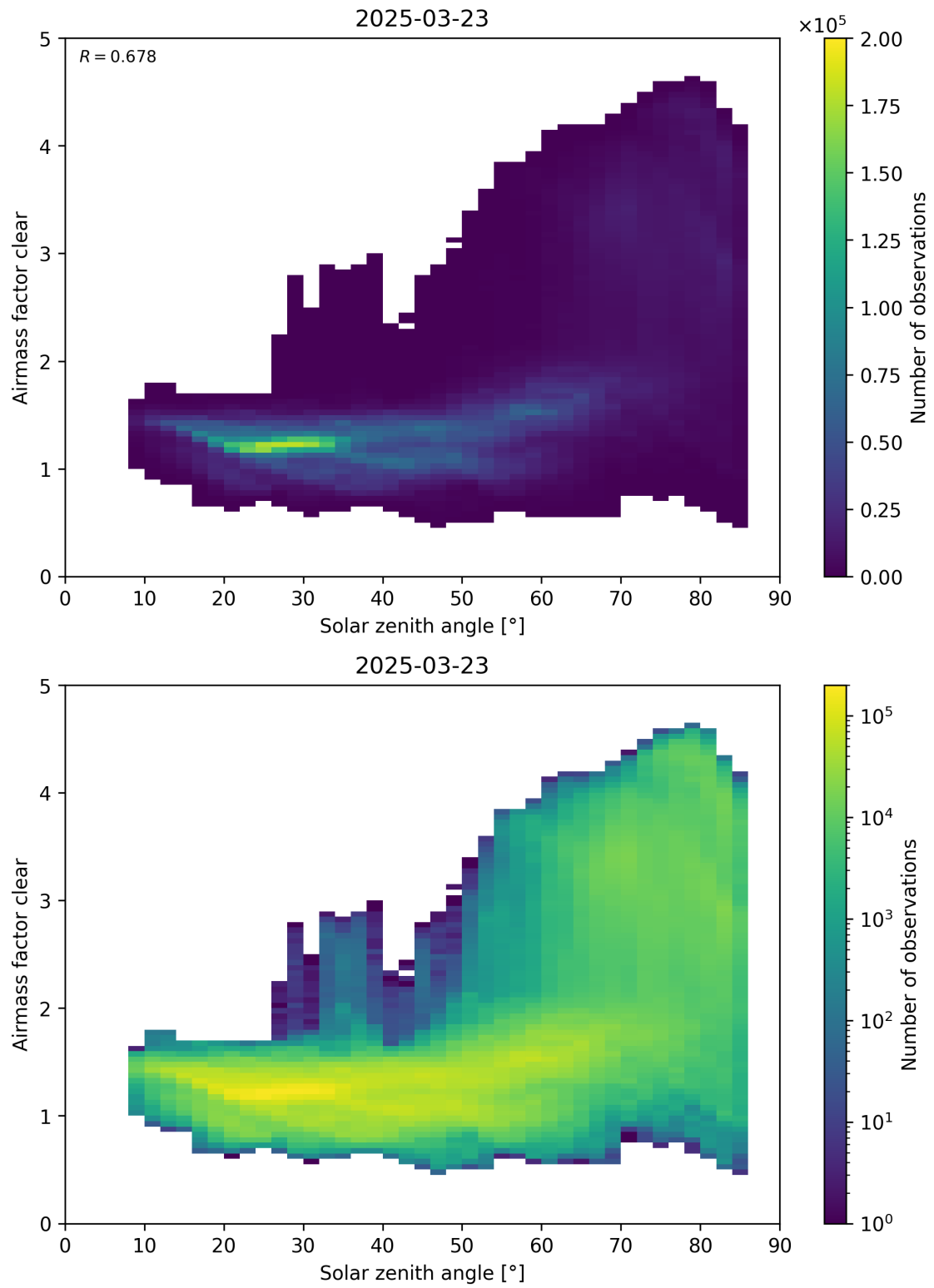
Figure 170: Scatter density plot of “Solar zenith angle” against “Airmass factor clear” for 2025-03-23 to 2025-03-24.
