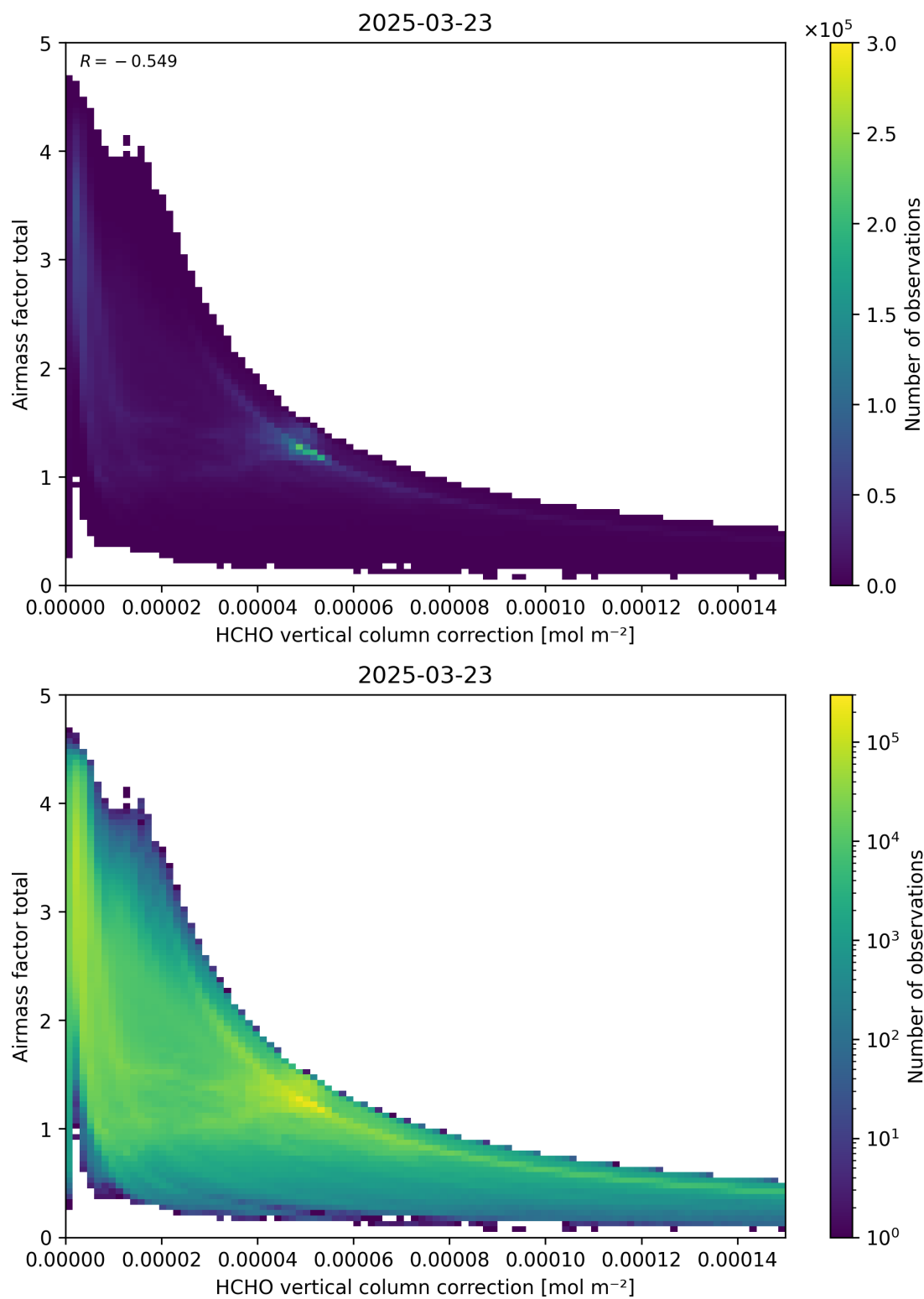
Figure 120: Scatter density plot of “HCHO vertical column correction” against “Airmass factor total” for 2025-03-23 to 2025-03-24.
