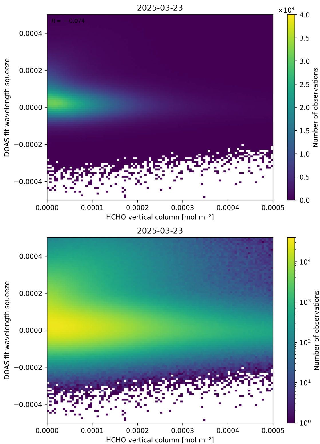
Figure 125: Scatter density plot of “HCHO vertical column” against “DOAS fit wavelength squeeze” for 2025-03-23 to 2025-03-24.
