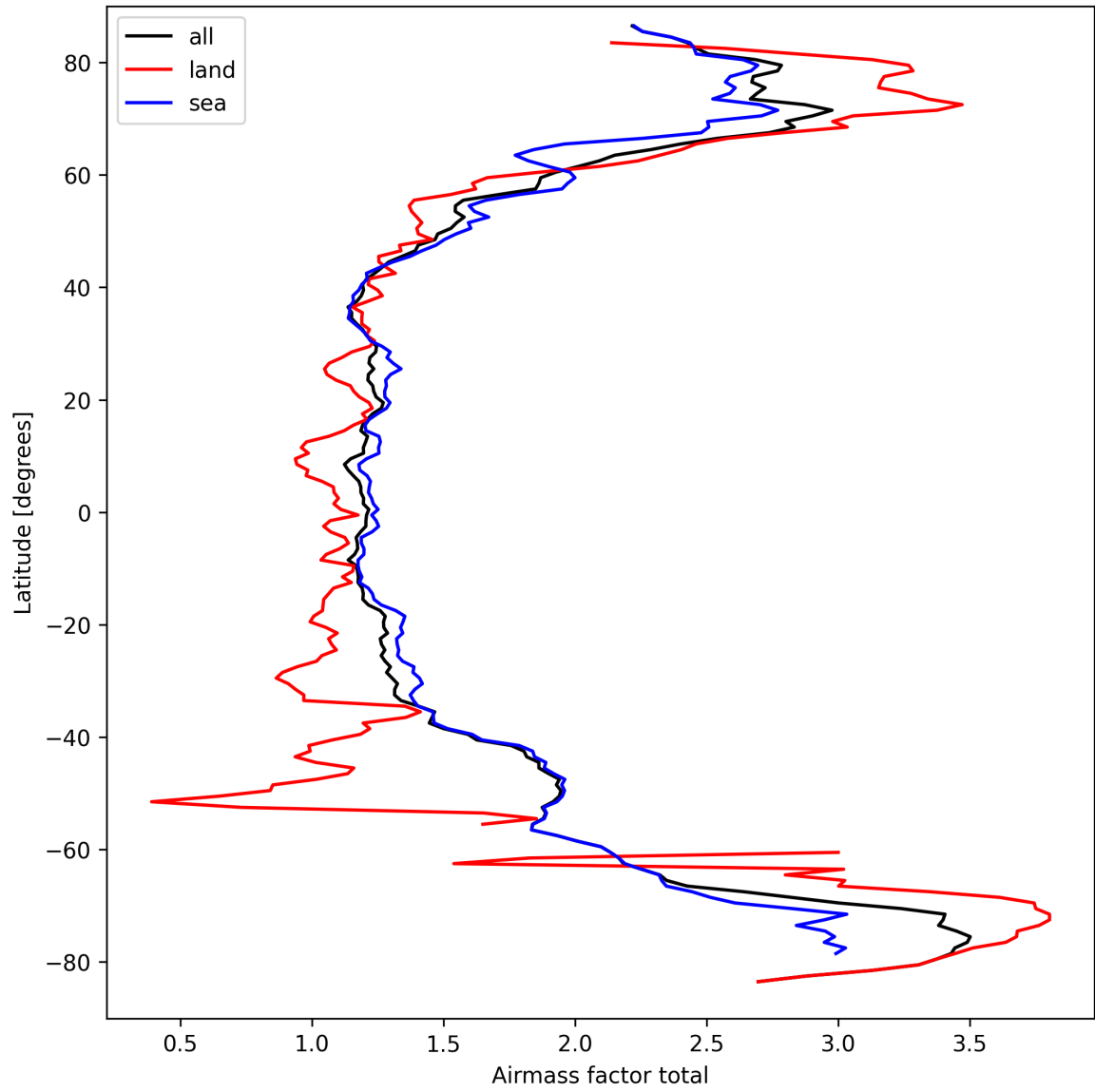
Figure 26: Zonal average of “Airmass factor total” for 2025-03-23 to 2025-03-24.
