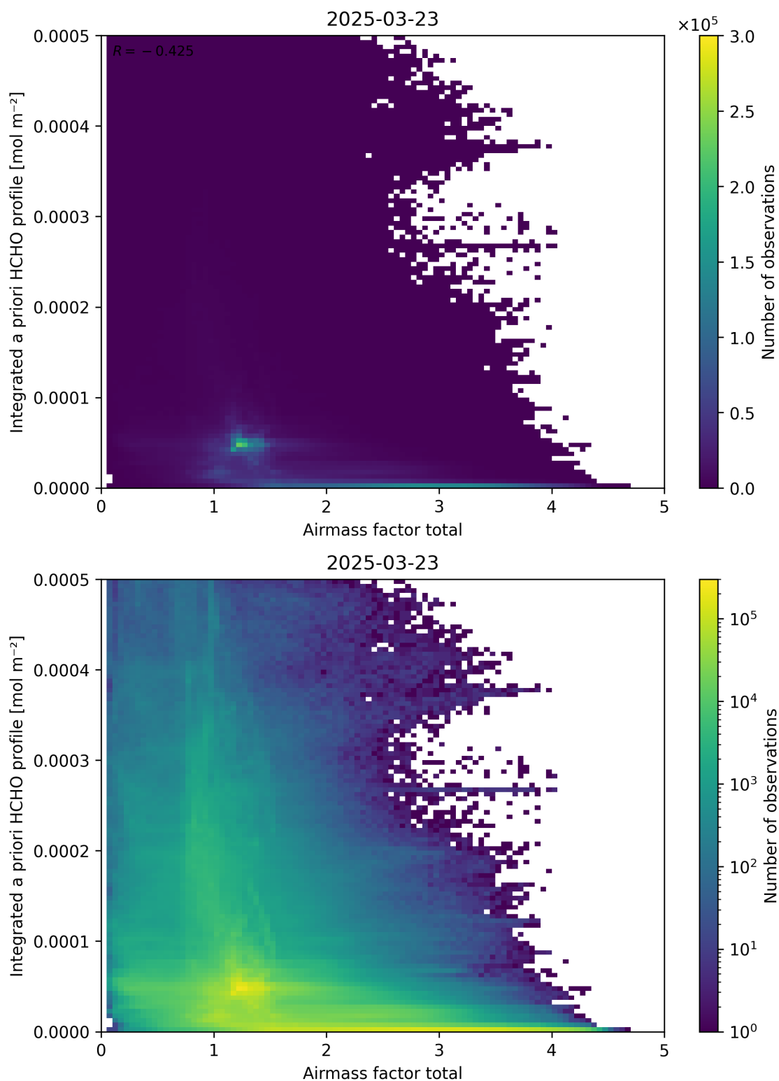
Figure 104: Scatter density plot of “Airmass factor total” against “Integrated a priori HCHO profile” for 2025-03-23 to 2025-03-24.
