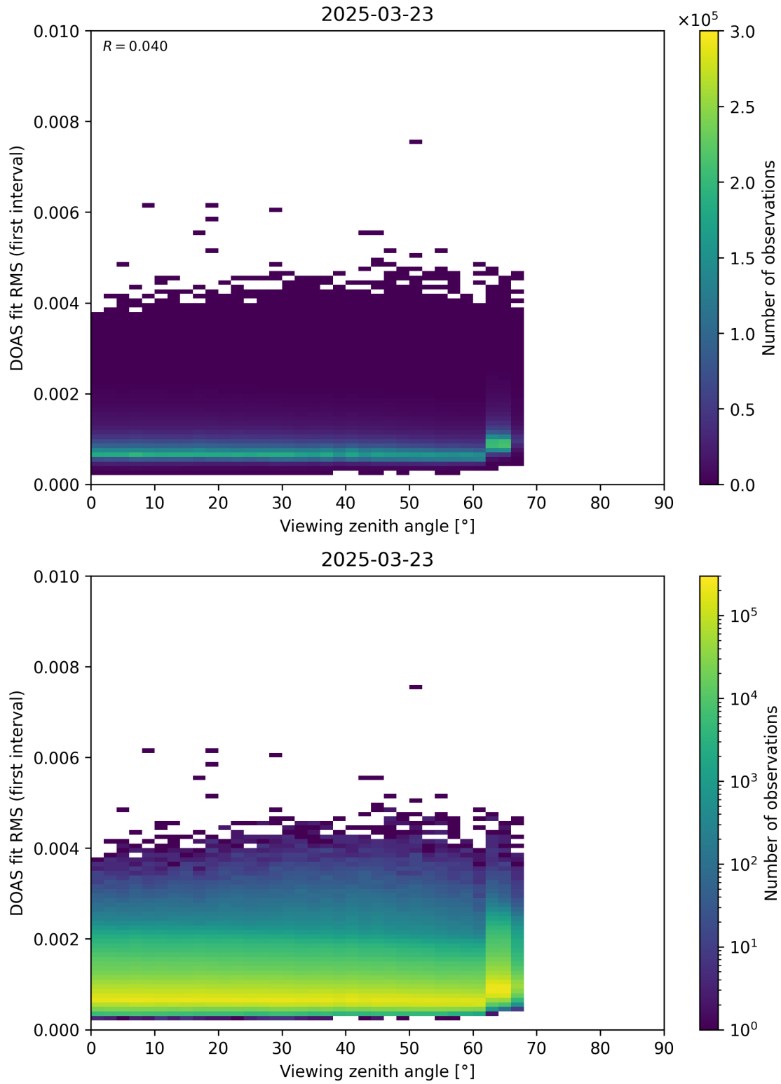
Figure 182: Scatter density plot of “Viewing zenith angle” against “DOAS fit RMS (first interval)” for 2025-03-23 to 2025-03-24.
