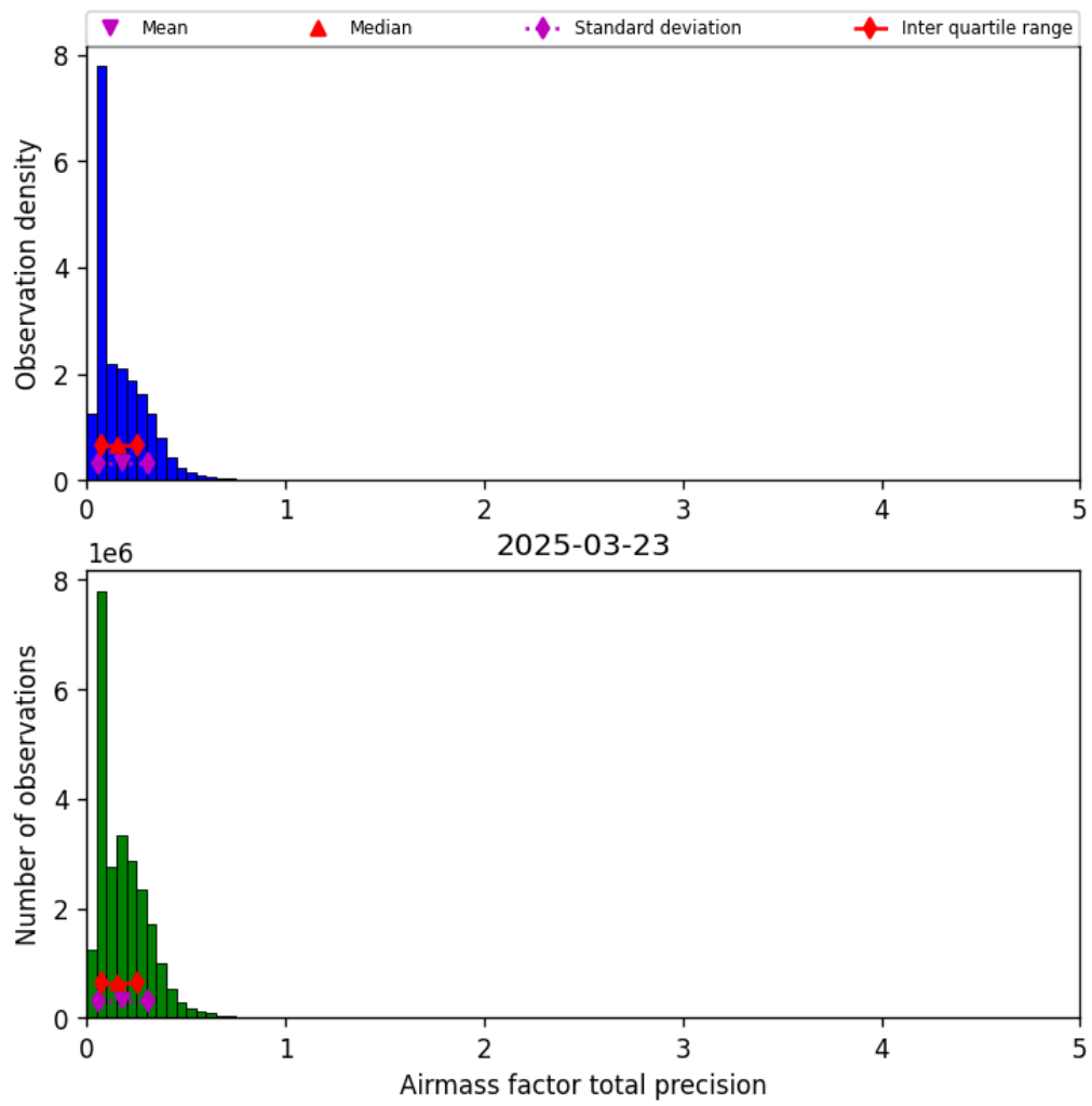
Figure 41: Histogram of “Airmass factor total precision” for 2025-03-23 to 2025-03-24
