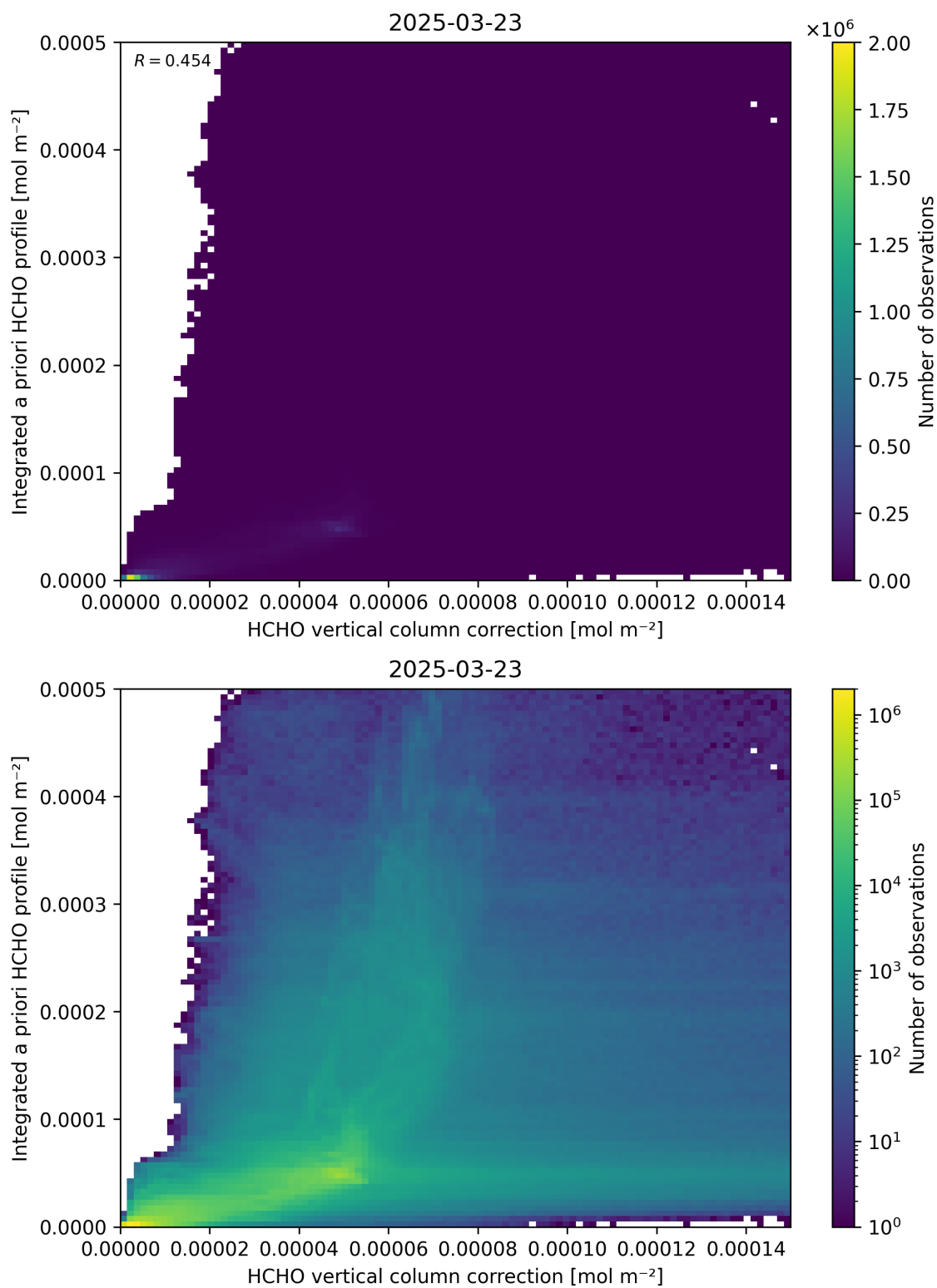
Figure 122: Scatter density plot of “HCHO vertical column correction” against “Integrated a priori HCHO profile” for 2025-03-23 to 2025-03-24.
