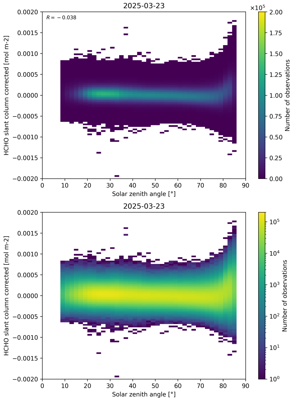
Figure 171: Scatter density plot of “Solar zenith angle” against “HCHO slant column corrected” for 2025-03-23 to 2025-03-24.
