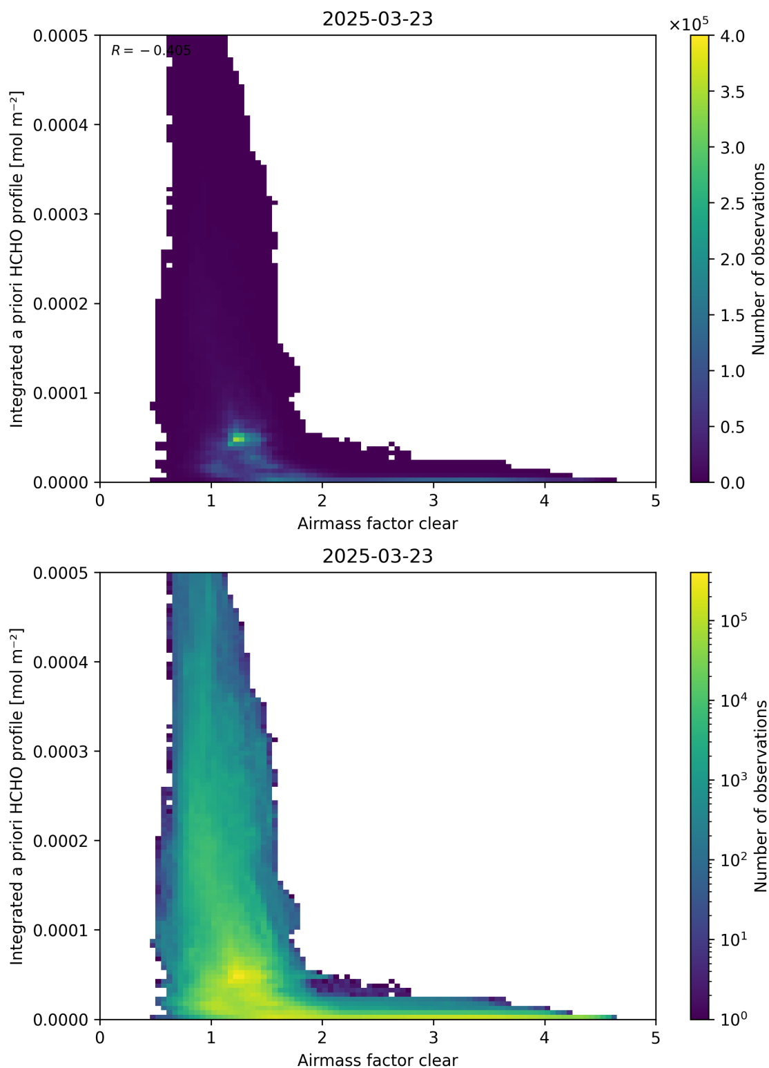
Figure 76: Scatter density plot of “Airmass factor clear” against “Integrated a priori HCHO profile” for 2025-03-23 to 2025-03-24.
