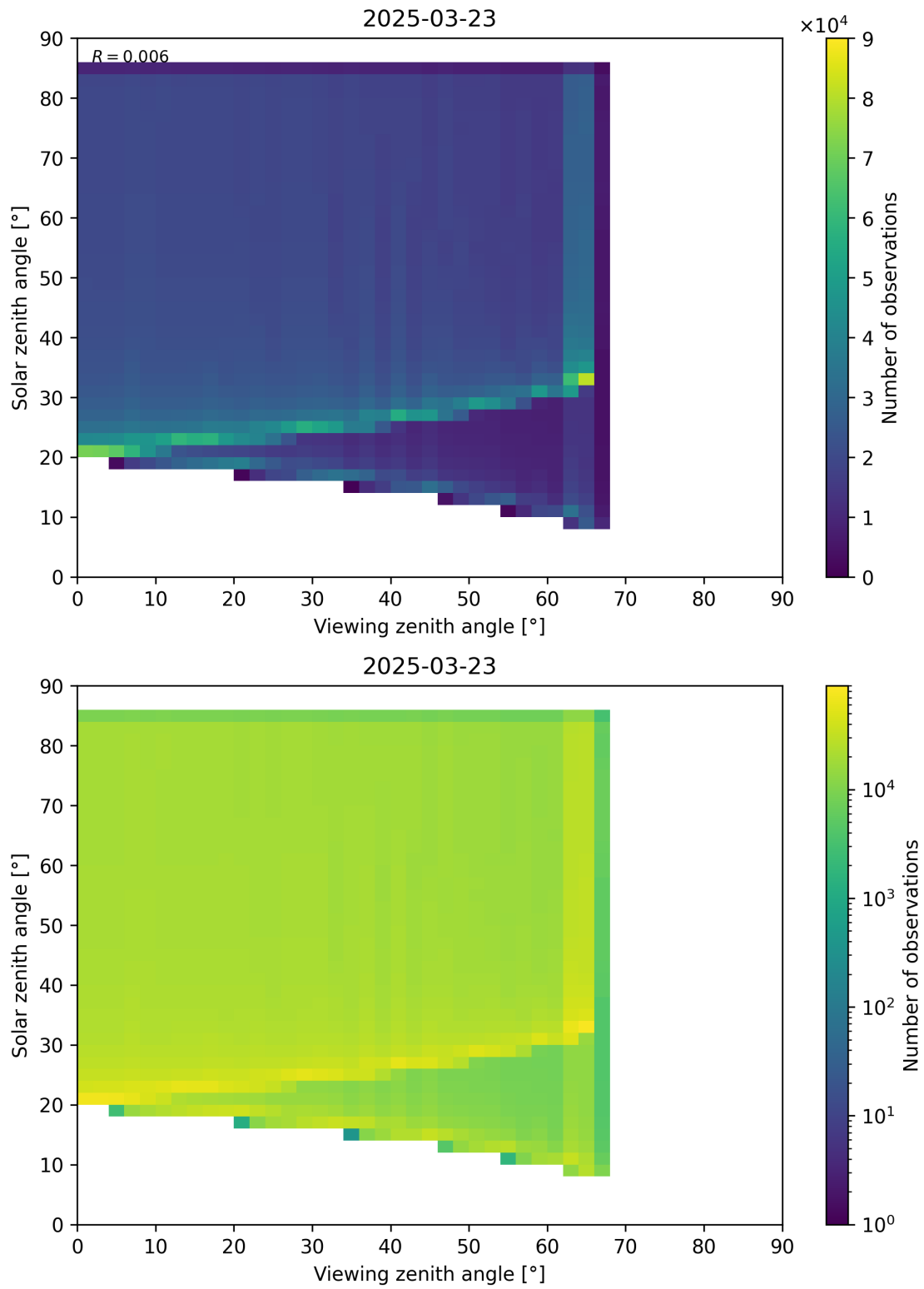
Figure 197: Scatter density plot of “Viewing zenith angle” against “Solar zenith angle” for 2025-03-23 to 2025-03-24.
