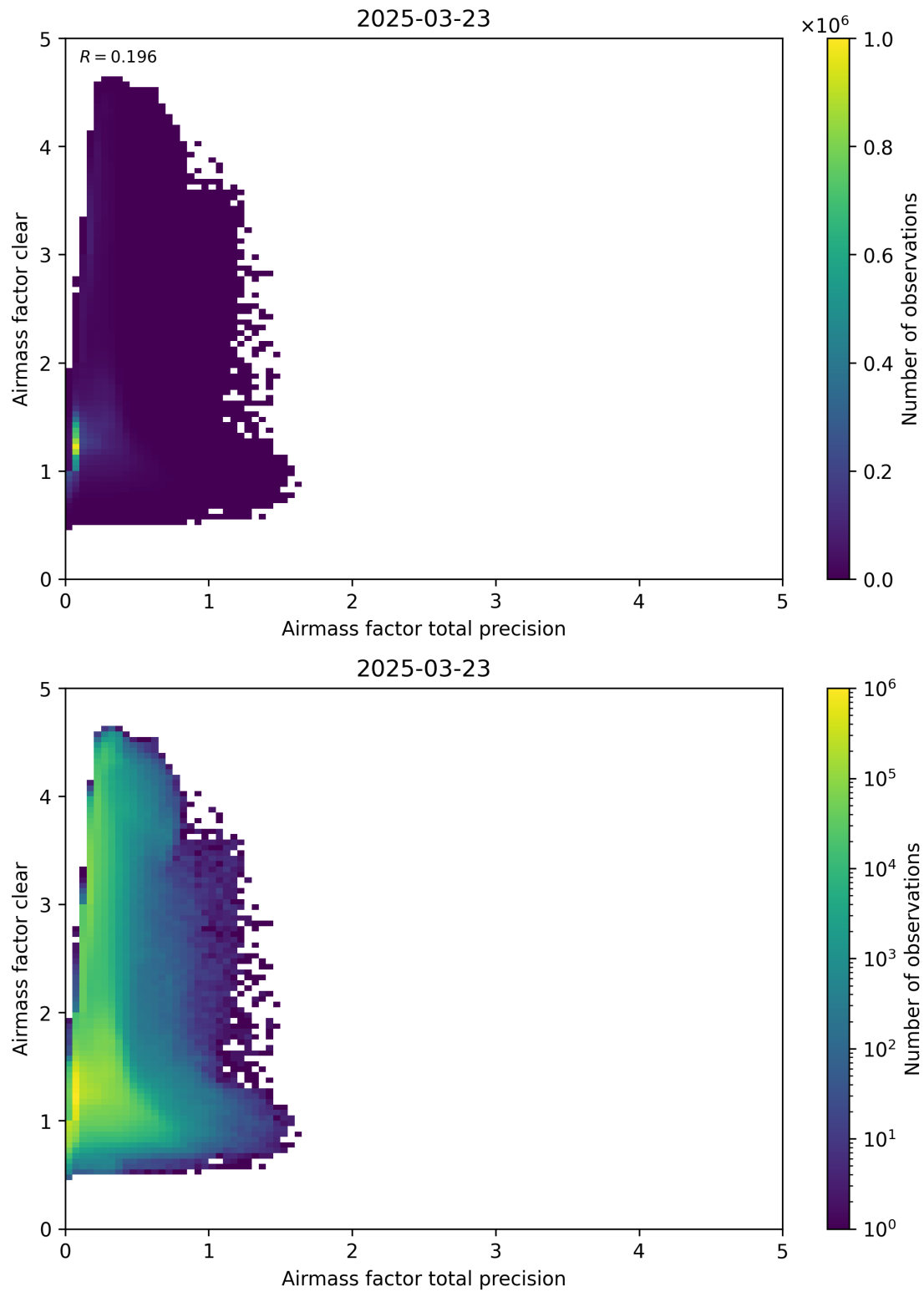
Figure 108: Scatter density plot of “Airmass factor total precision” against “Airmass factor clear” for 2025-03-23 to 2025-03-24.
