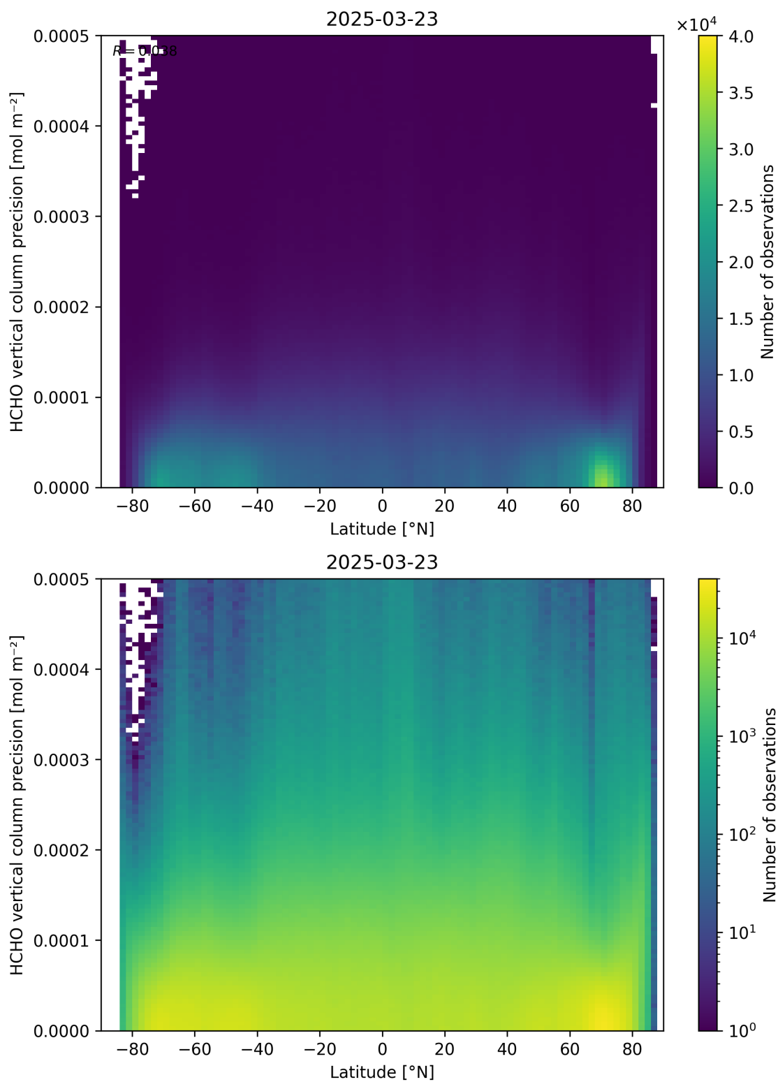
Figure 165: Scatter density plot of “Latitude” against “HCHO vertical column precision” for 2025-03-23 to 2025-03-24.
