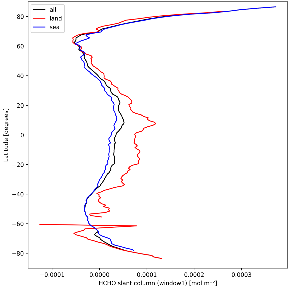
Figure 24: Zonal average of “HCHO slant column (window1)” for 2025-03-23 to 2025-03-24.
