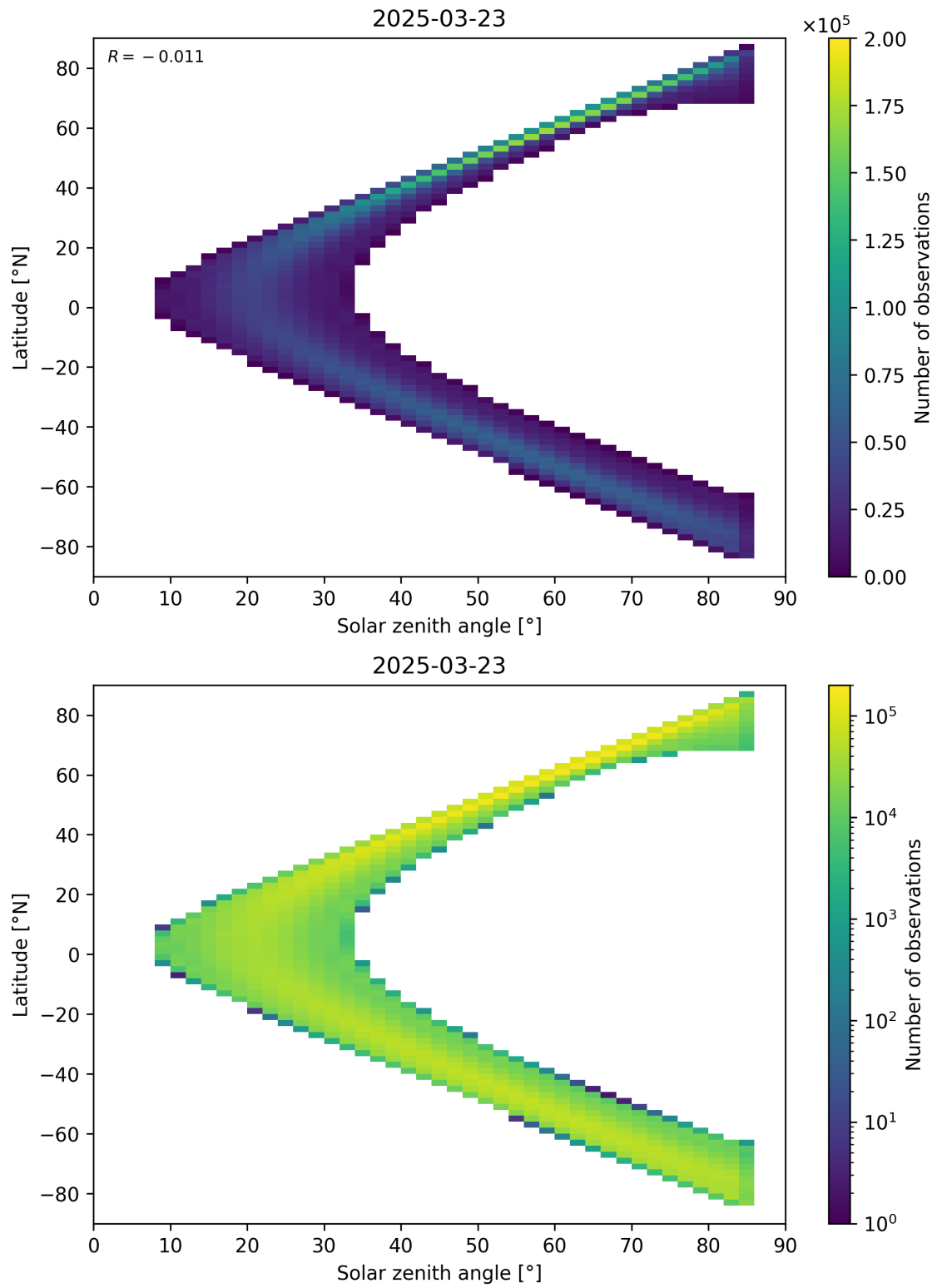
Figure 181: Scatter density plot of “Solar zenith angle” against “Latitude” for 2025-03-23 to 2025-03-24.
