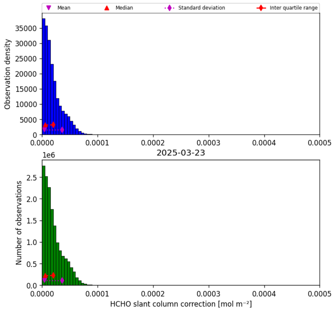
Figure 47: Histogram of “HCHO slant column correction” for 2025-03-23 to 2025-03-24
