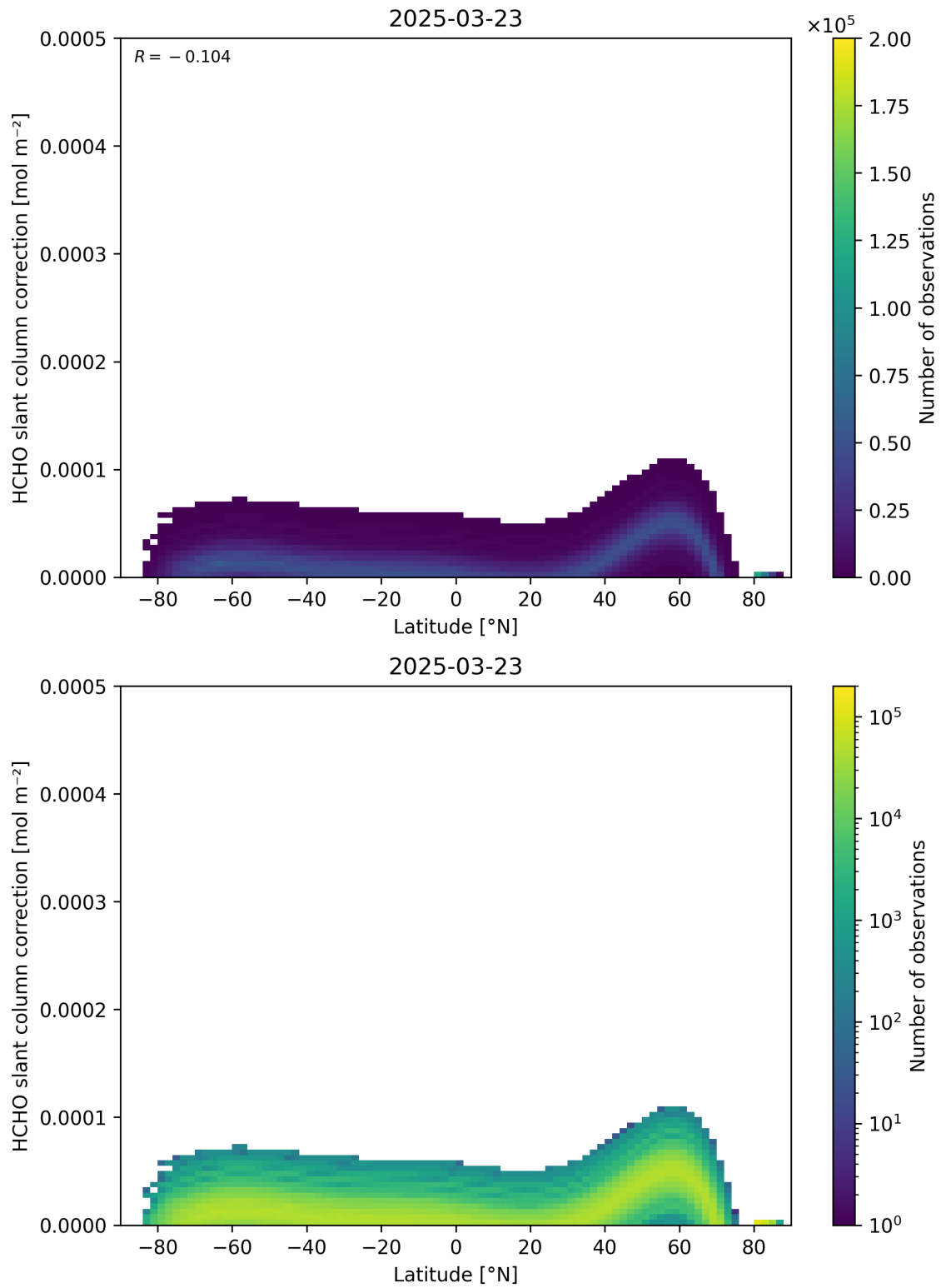
Figure 158: Scatter density plot of “Latitude” against “HCHO slant column correction” for 2025-03-23 to 2025-03-24.
