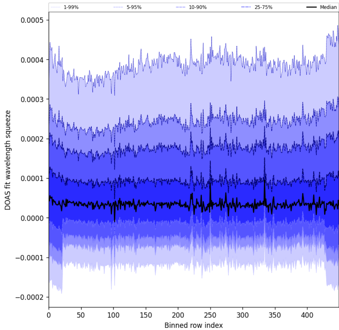
Figure 59: Along track statistics of “DOAS fit wavelength squeeze” for 2025-03-23 to 2025-03-24
