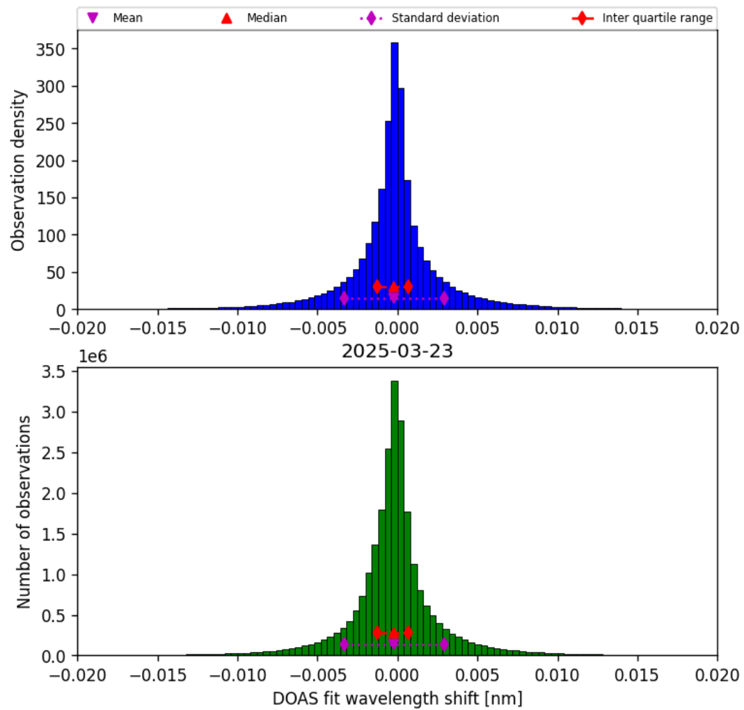
Figure 44: Histogram of “DOAS fit wavelength shift” for 2025-03-23 to 2025-03-24
