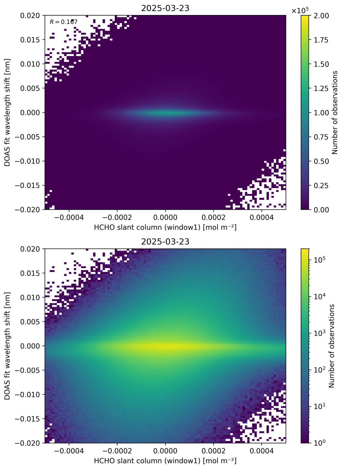
Figure 79: Scatter density plot of “HCHO slant column (window1)” against “DOAS fit wavelength shift” for 2025-03-23 to 2025-03-24.
