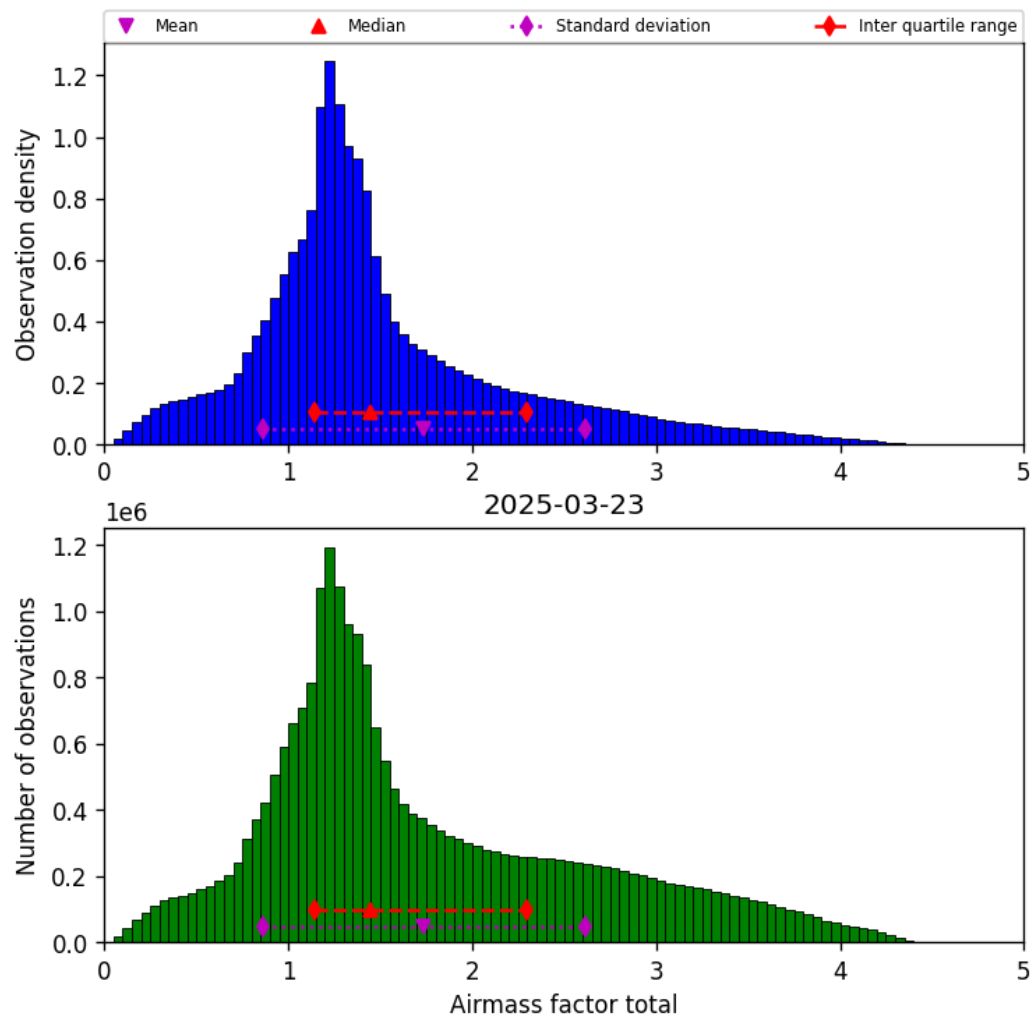
Figure 40: Histogram of “Airmass factor total” for 2025-03-23 to 2025-03-24
