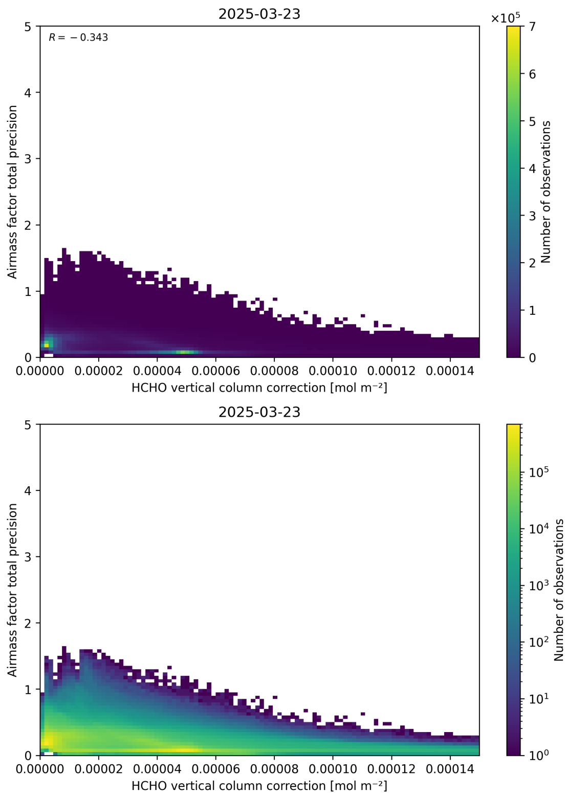
Figure 121: Scatter density plot of “HCHO vertical column correction” against “Airmass factor total precision” for 2025-03-23 to 2025-03-24.
