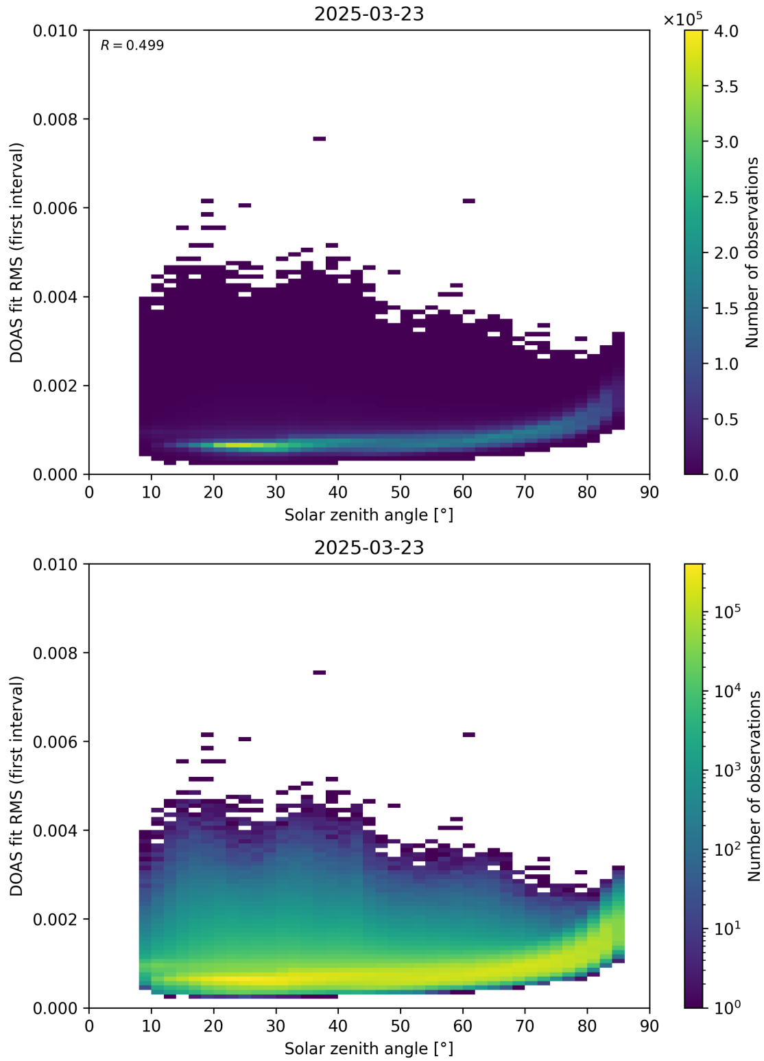
Figure 167: Scatter density plot of “Solar zenith angle” against “DOAS fit RMS (first interval)” for 2025-03-23 to 2025-03-24.
