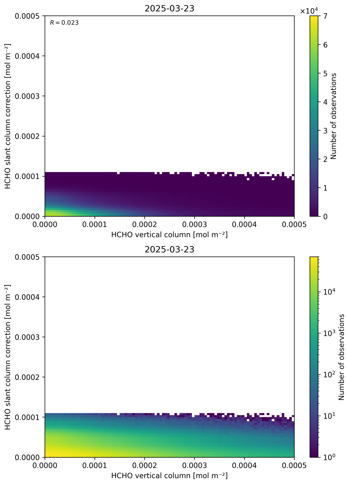
Figure 128: Scatter density plot of “HCHO vertical column” against “HCHO slant column correction” for 2025-03-23 to 2025-03-24.
