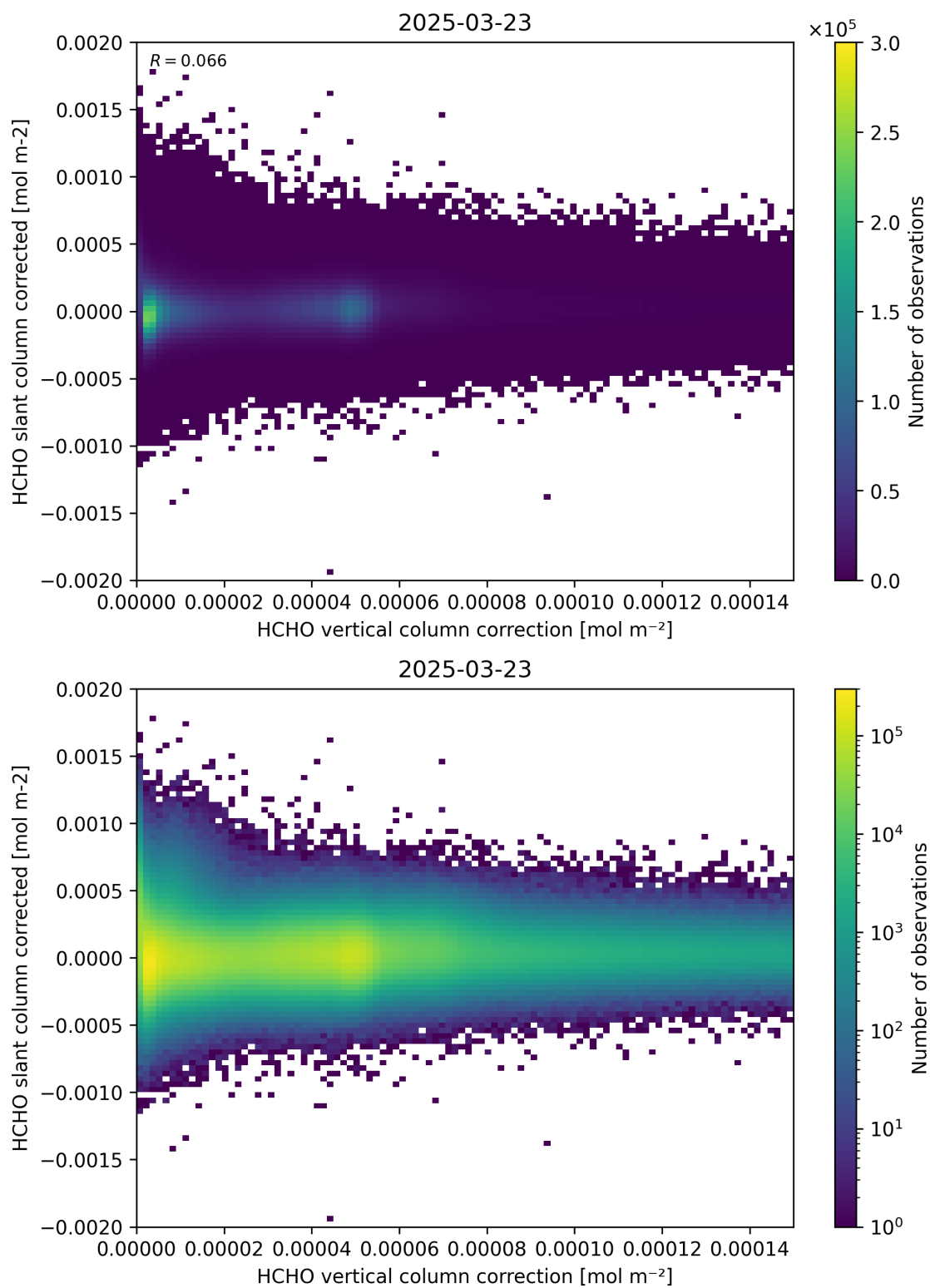
Figure 116: Scatter density plot of “HCHO vertical column correction” against “HCHO slant column corrected” for 2025-03-23 to 2025-03-24.
