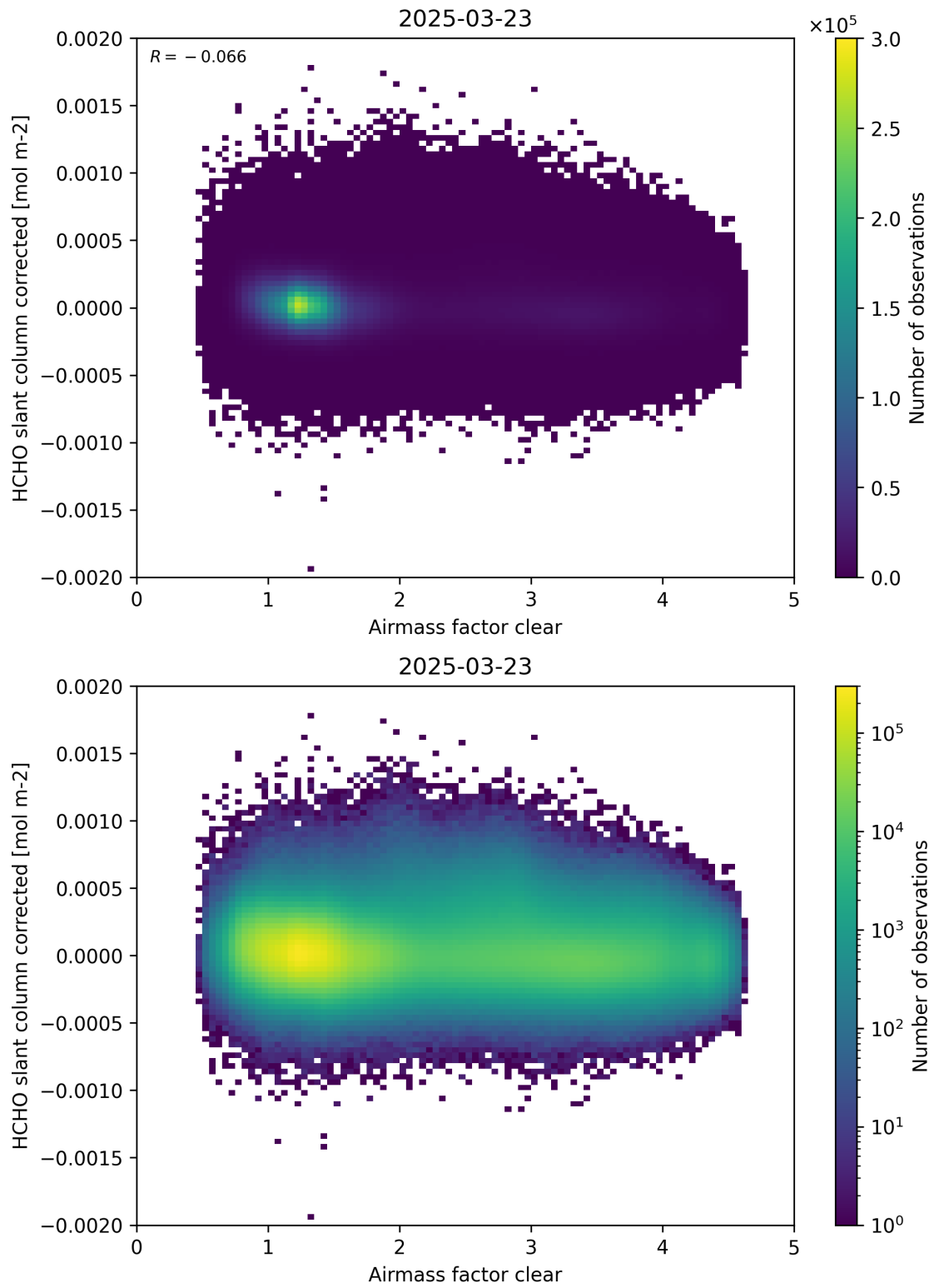
Figure 74: Scatter density plot of “Airmass factor clear” against “HCHO slant column corrected” for 2025-03-23 to 2025-03-24.
