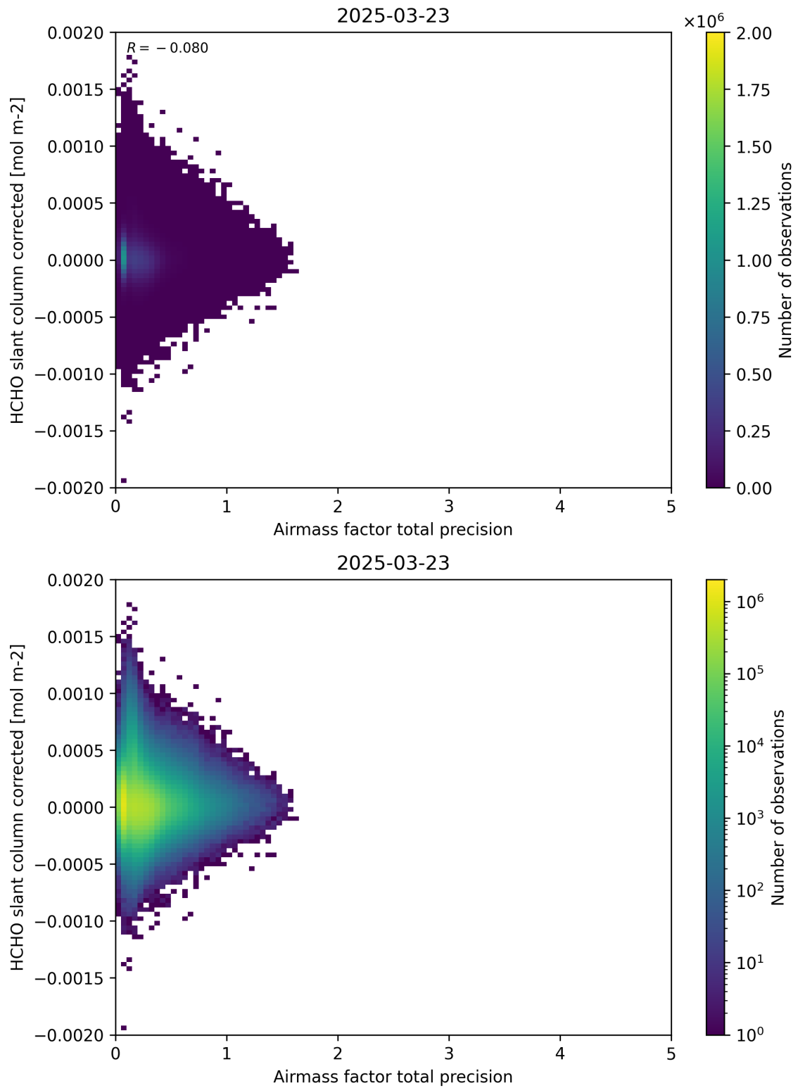
Figure 109: Scatter density plot of “Airmass factor total precision” against “HCHO slant column corrected” for 2025-03-23 to 2025-03-24.
