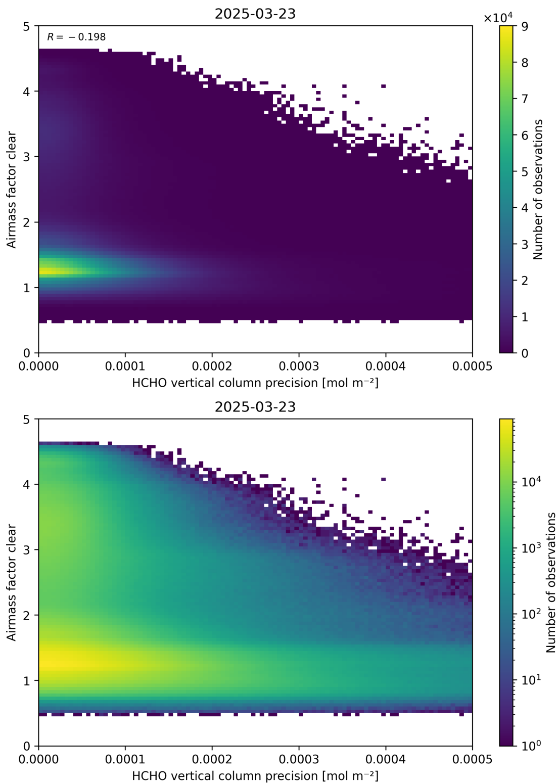
Figure 139: Scatter density plot of “HCHO vertical column precision” against “Airmass factor clear” for 2025-03-23 to 2025-03-24.
