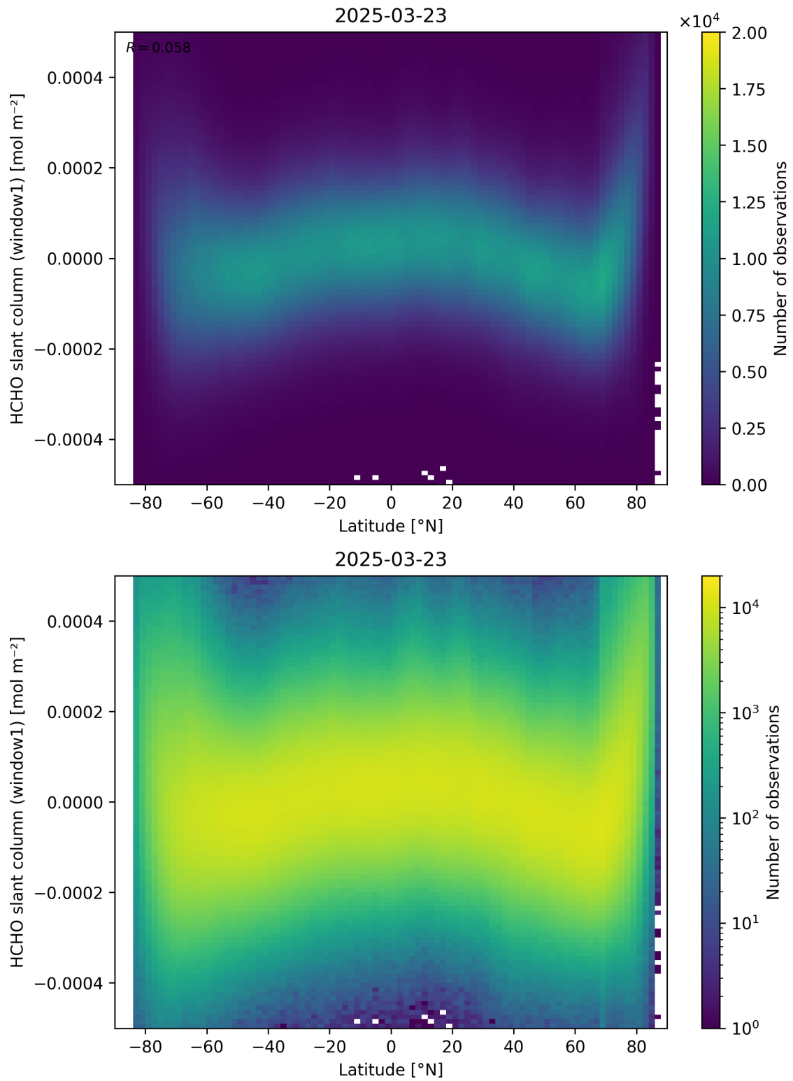
Figure 159: Scatter density plot of “Latitude” against “HCHO slant column (window1)” for 2025-03-23 to 2025-03-24.
