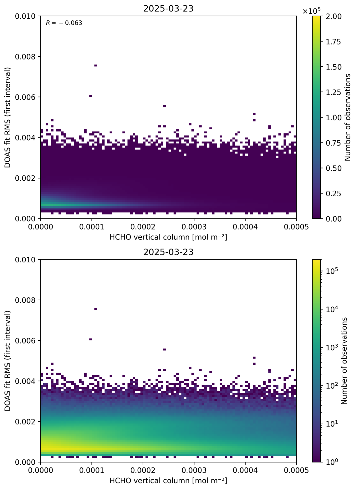
Figure 123: Scatter density plot of “HCHO vertical column” against “DOAS fit RMS (first interval)” for 2025-03-23 to 2025-03-24.
