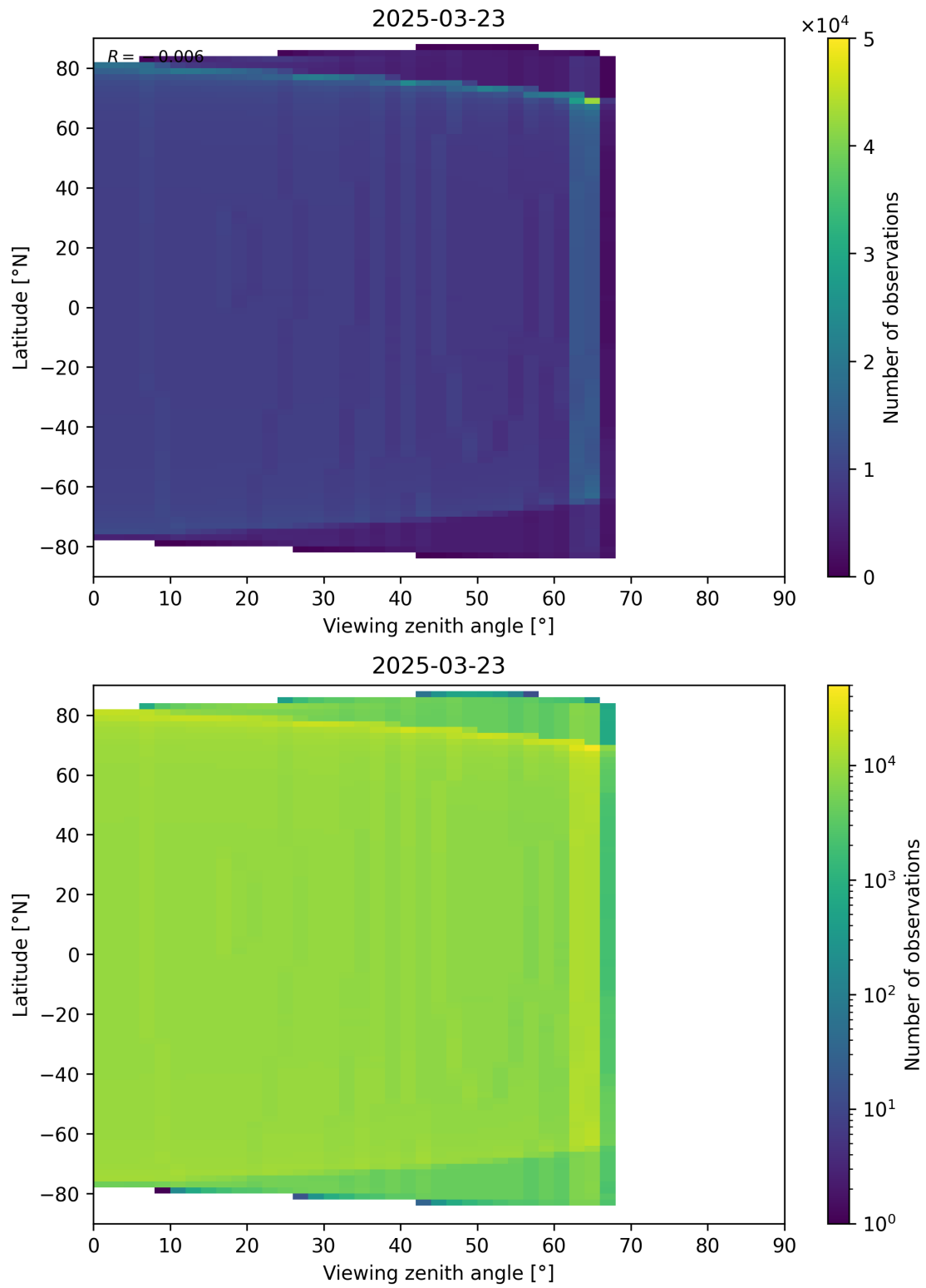
Figure 196: Scatter density plot of “Viewing zenith angle” against “Latitude” for 2025-03-23 to 2025-03-24.
