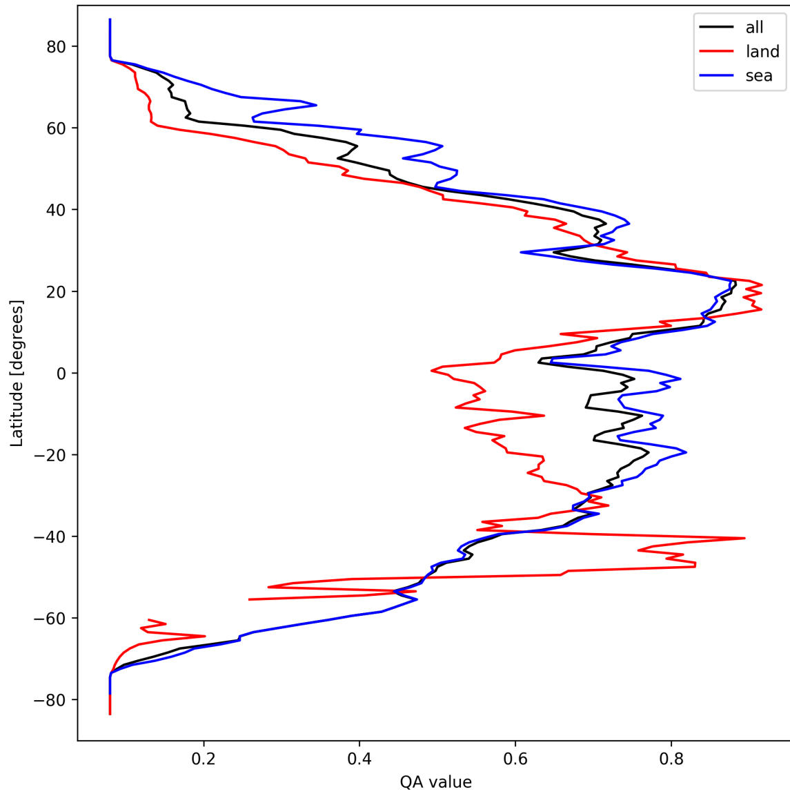
Figure 20: Zonal average of “QA value” for 2025-03-23 to 2025-03-24.
