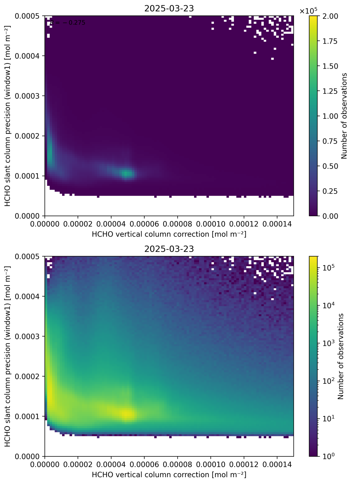
Figure 119: Scatter density plot of “HCHO vertical column correction” against “HCHO slant column precision (window1)” for 2025-03-23 to 2025-03-24.
