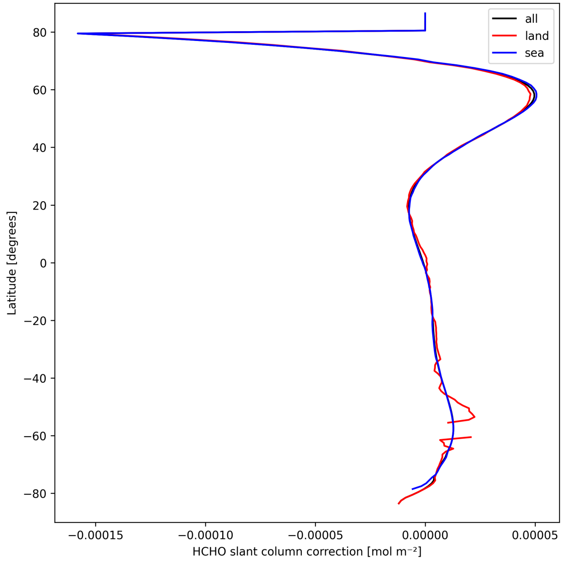
Figure 33: Zonal average of "HCHO slant column correction" for 2025-03-23 to 2025-03-24.
