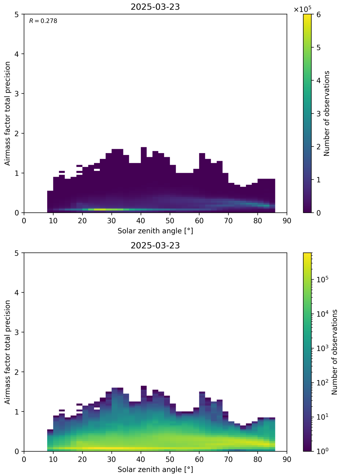
Figure 176: Scatter density plot of “Solar zenith angle” against “Airmass factor total precision” for 2025-03-23 to 2025-03-24.
