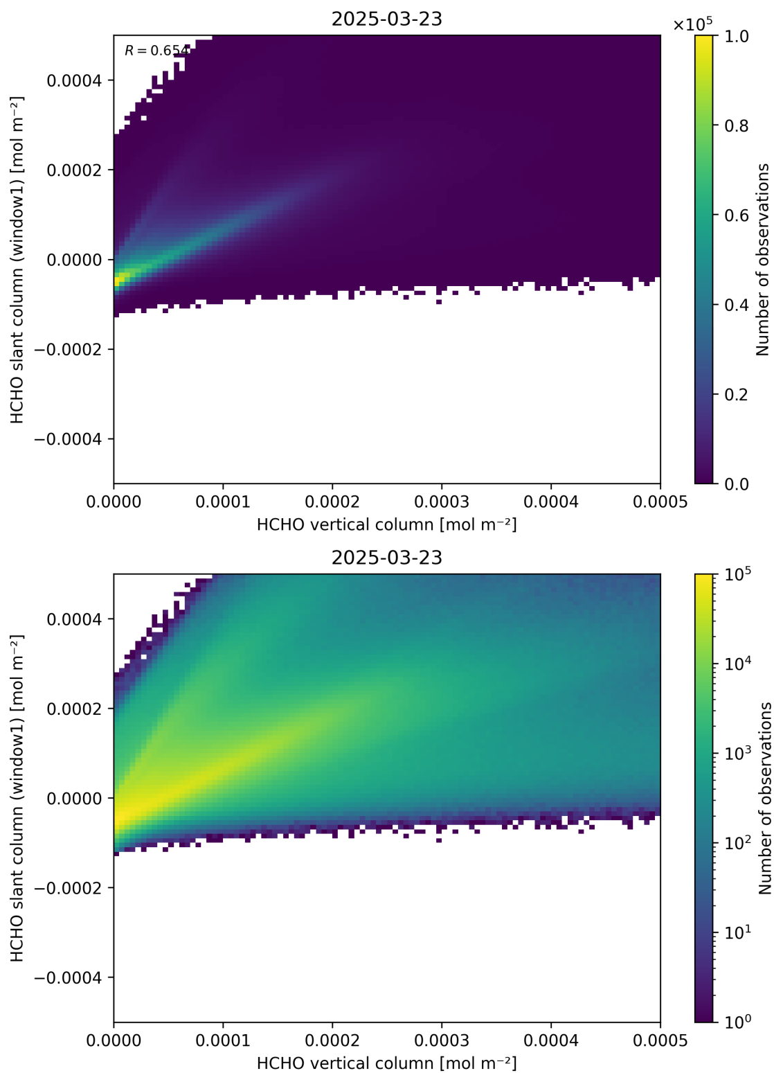
Figure 129: Scatter density plot of “HCHO vertical column” against “HCHO slant column (window1)” for 2025-03-23 to 2025-03-24.
