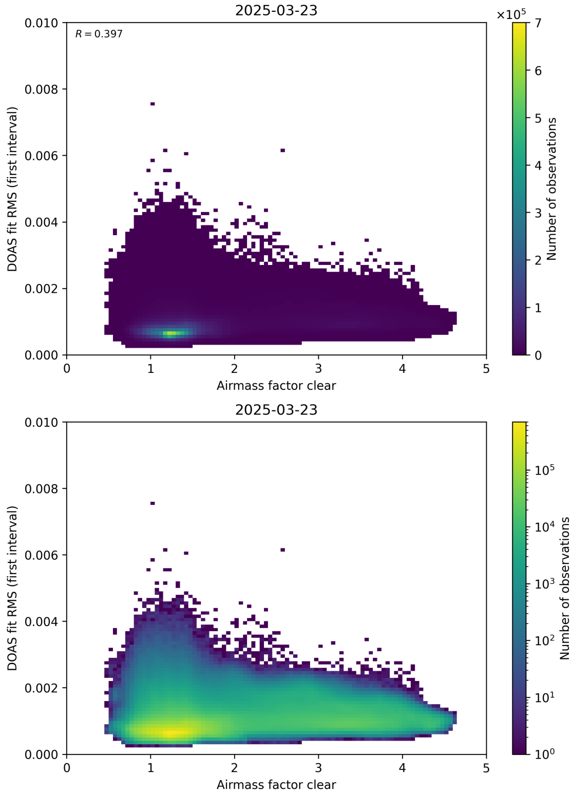
Figure 71: Scatter density plot of “Airmass factor clear” against “DOAS fit RMS (first interval)” for 2025-03-23 to 2025-03-24.
