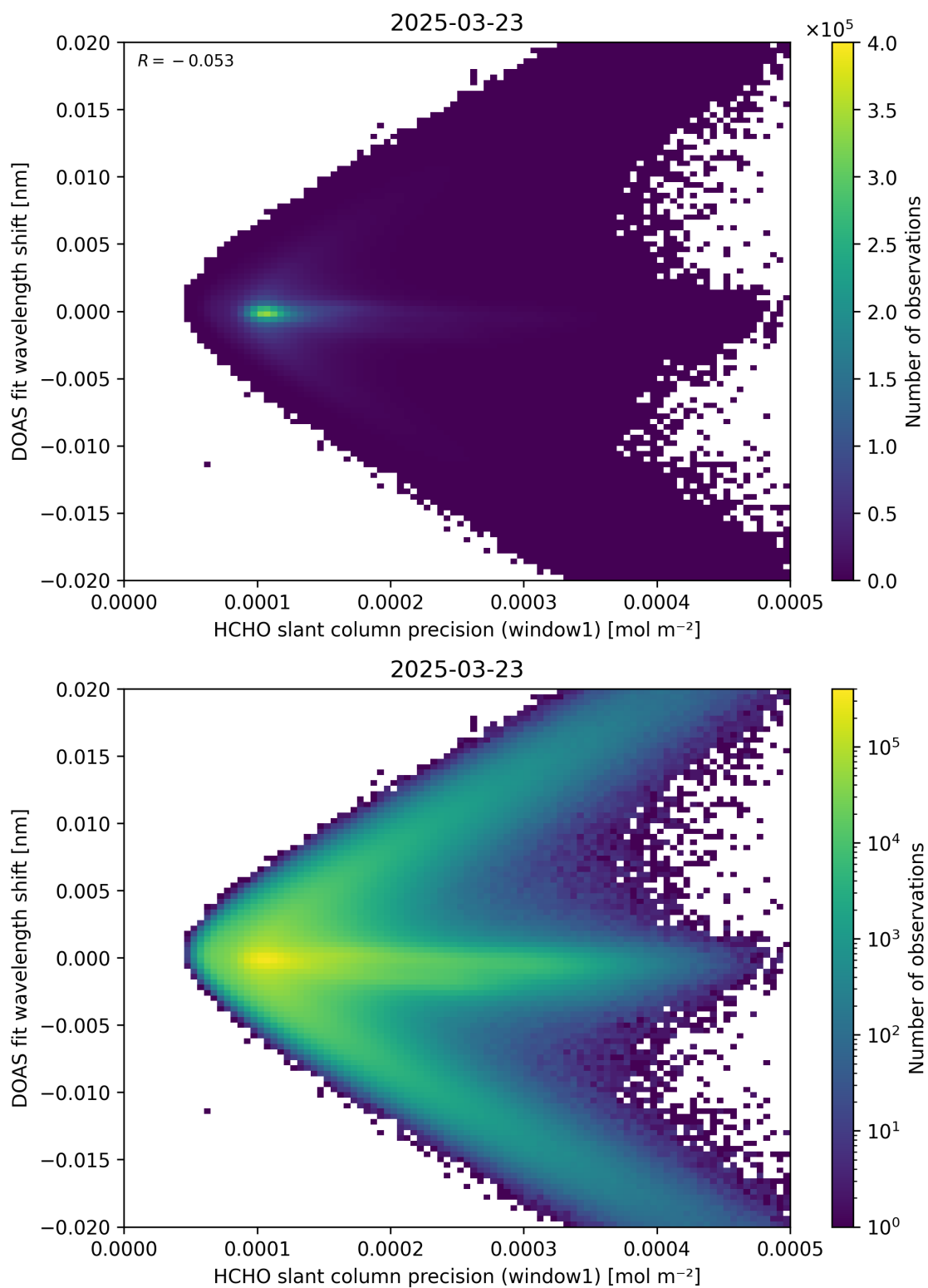
Figure 89: Scatter density plot of “HCHO slant column precision (window1)” against “DOAS fit wavelength shift” for 2025-03-23 to 2025-03-24.
