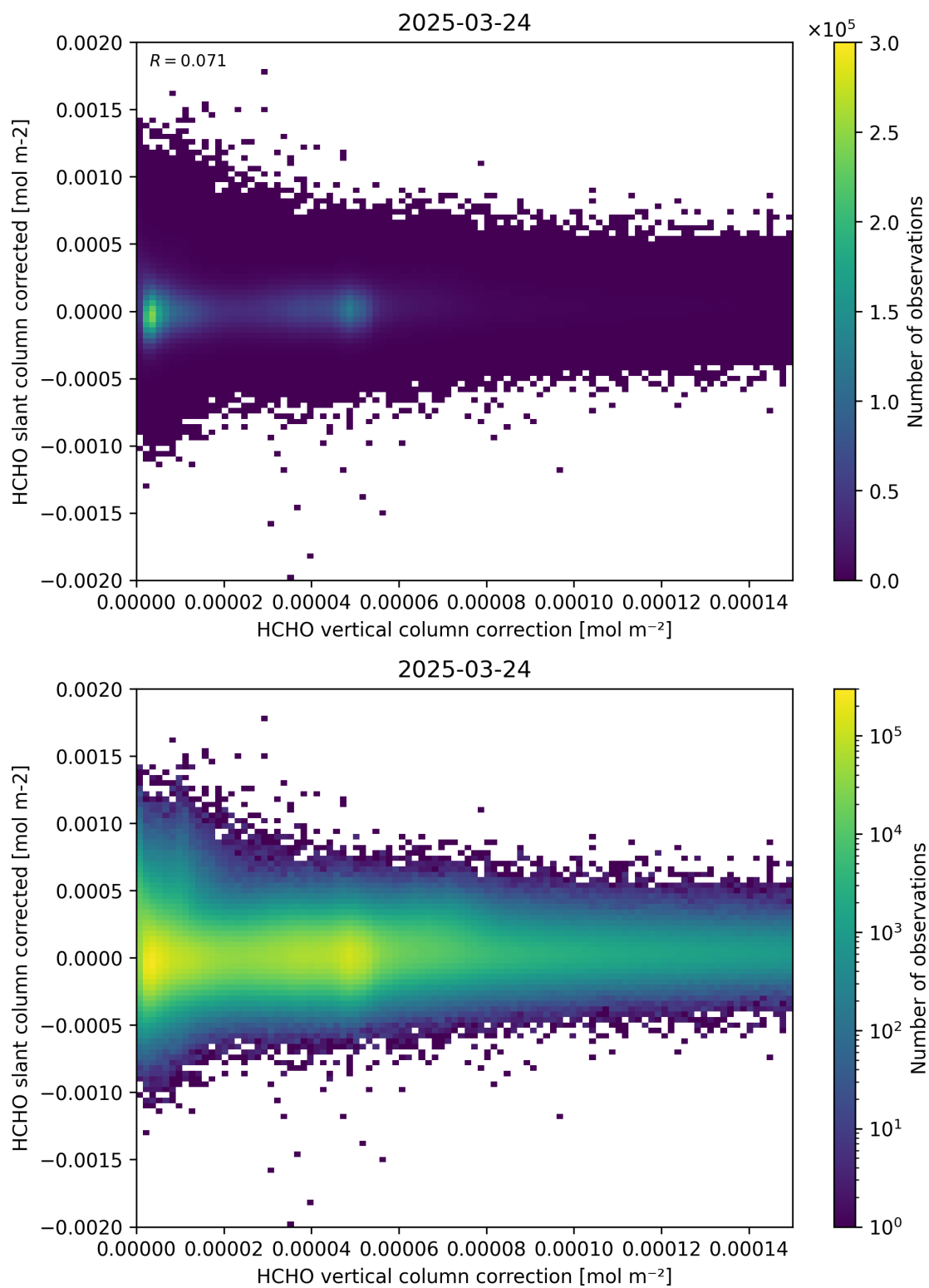
Figure 116: Scatter density plot of “HCHO vertical column correction” against “HCHO slant column corrected” for 2025-03-23 to 2025-03-25.
