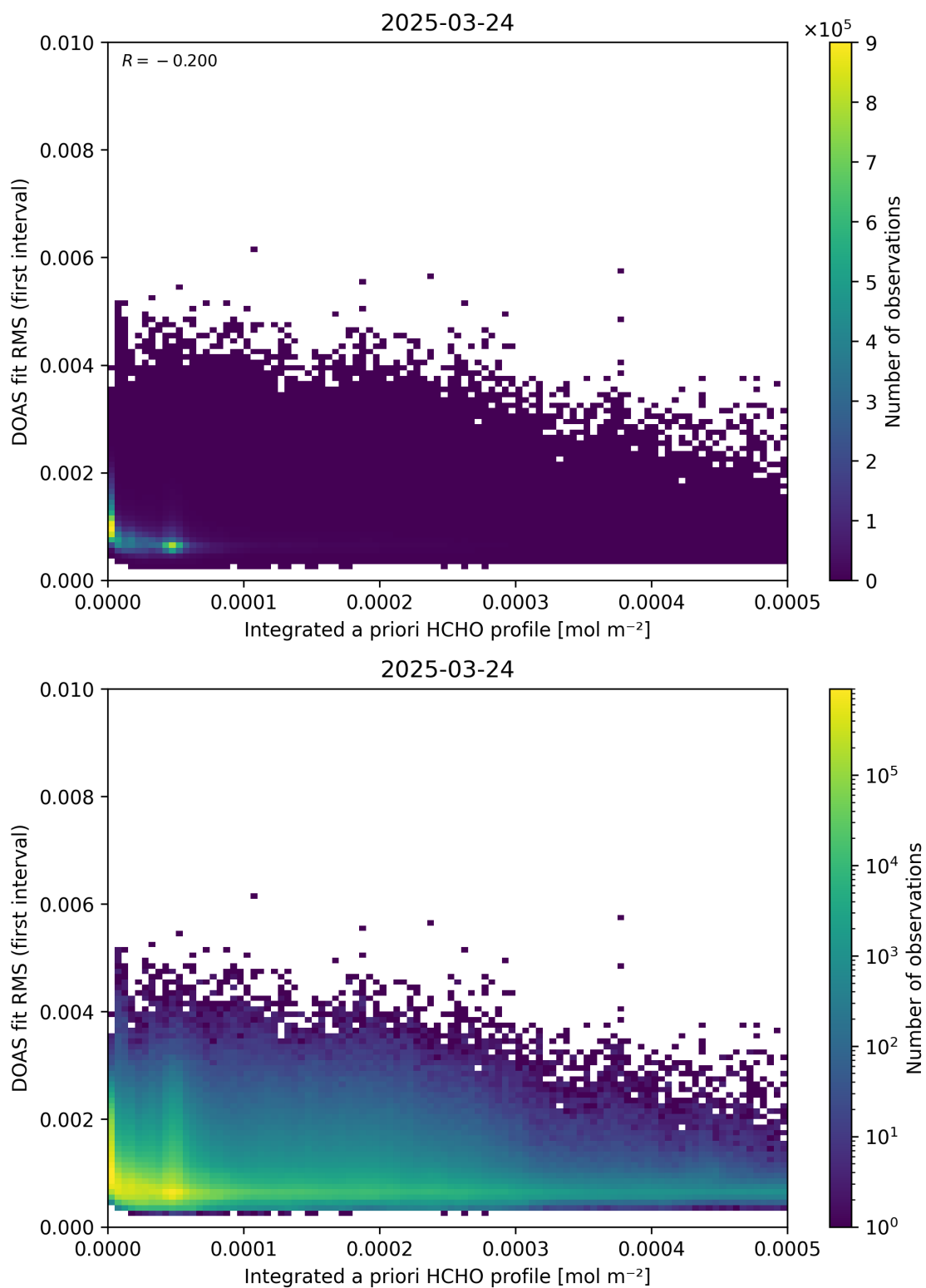
Figure 148: Scatter density plot of “Integrated a priori HCHO profile” against “DOAS fit RMS (first interval)” for 2025-03-23 to 2025-03-25.
