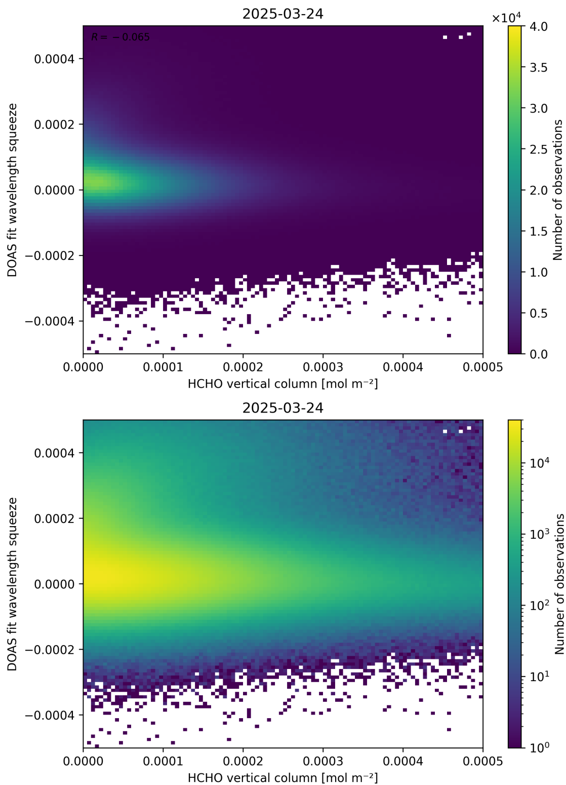
Figure 125: Scatter density plot of “HCHO vertical column” against “DOAS fit wavelength squeeze” for 2025-03-23 to 2025-03-25.
