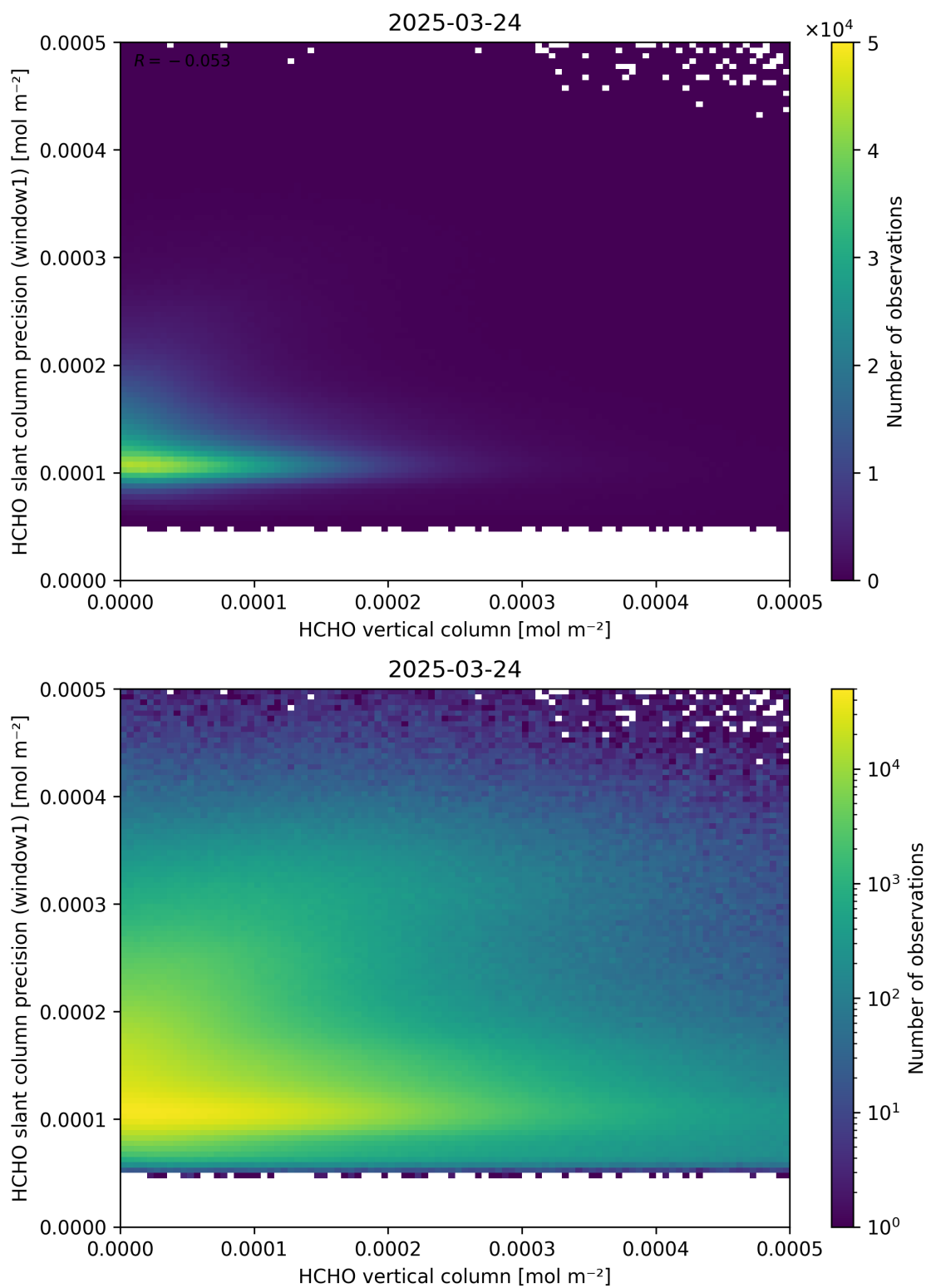
Figure 130: Scatter density plot of “HCHO vertical column” against “HCHO slant column precision (window1)” for 2025-03-23 to 2025-03-25.
