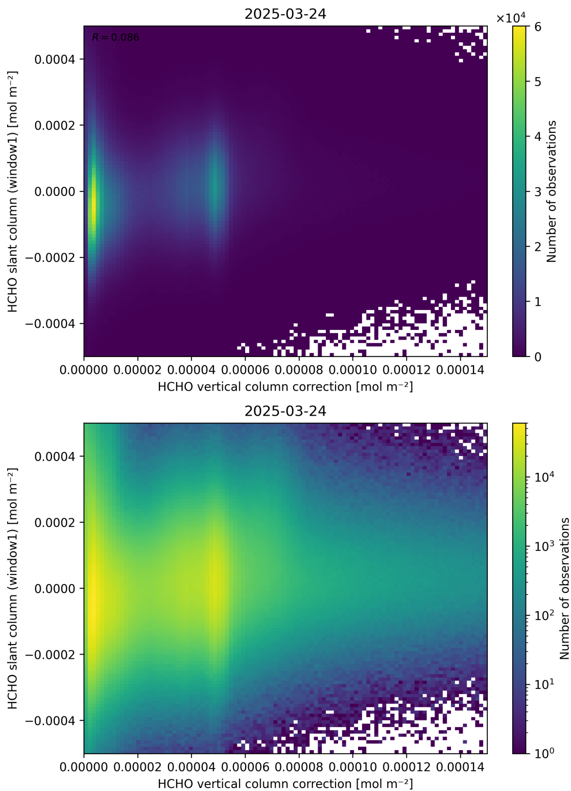
Figure 118: Scatter density plot of “HCHO vertical column correction” against “HCHO slant column (window1)” for 2025-03-23 to 2025-03-25.
