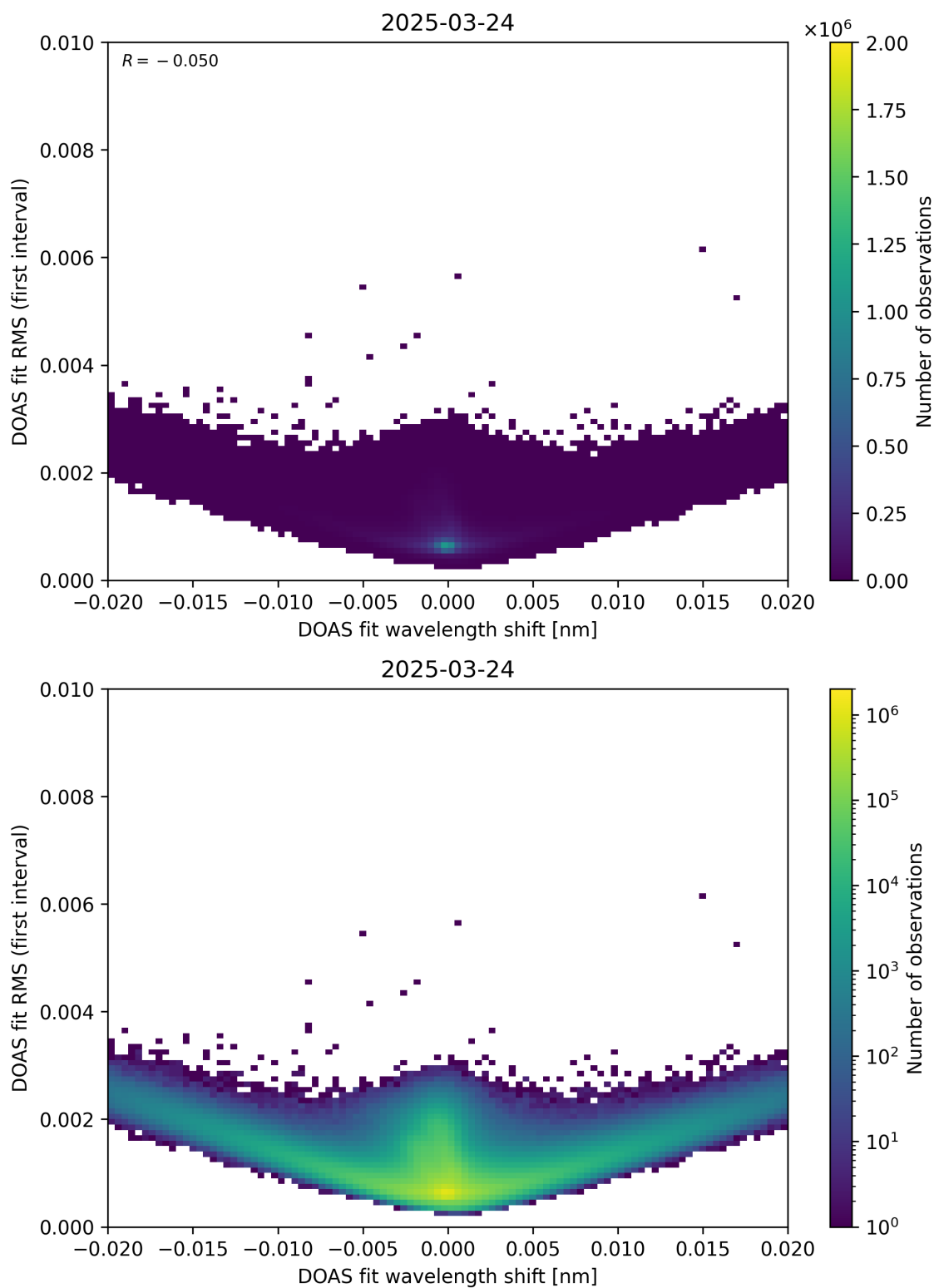
Figure 64: Scatter density plot of “DOAS fit wavelength shift” against “DOAS fit RMS (first interval)” for 2025-03-23 to 2025-03-25.
