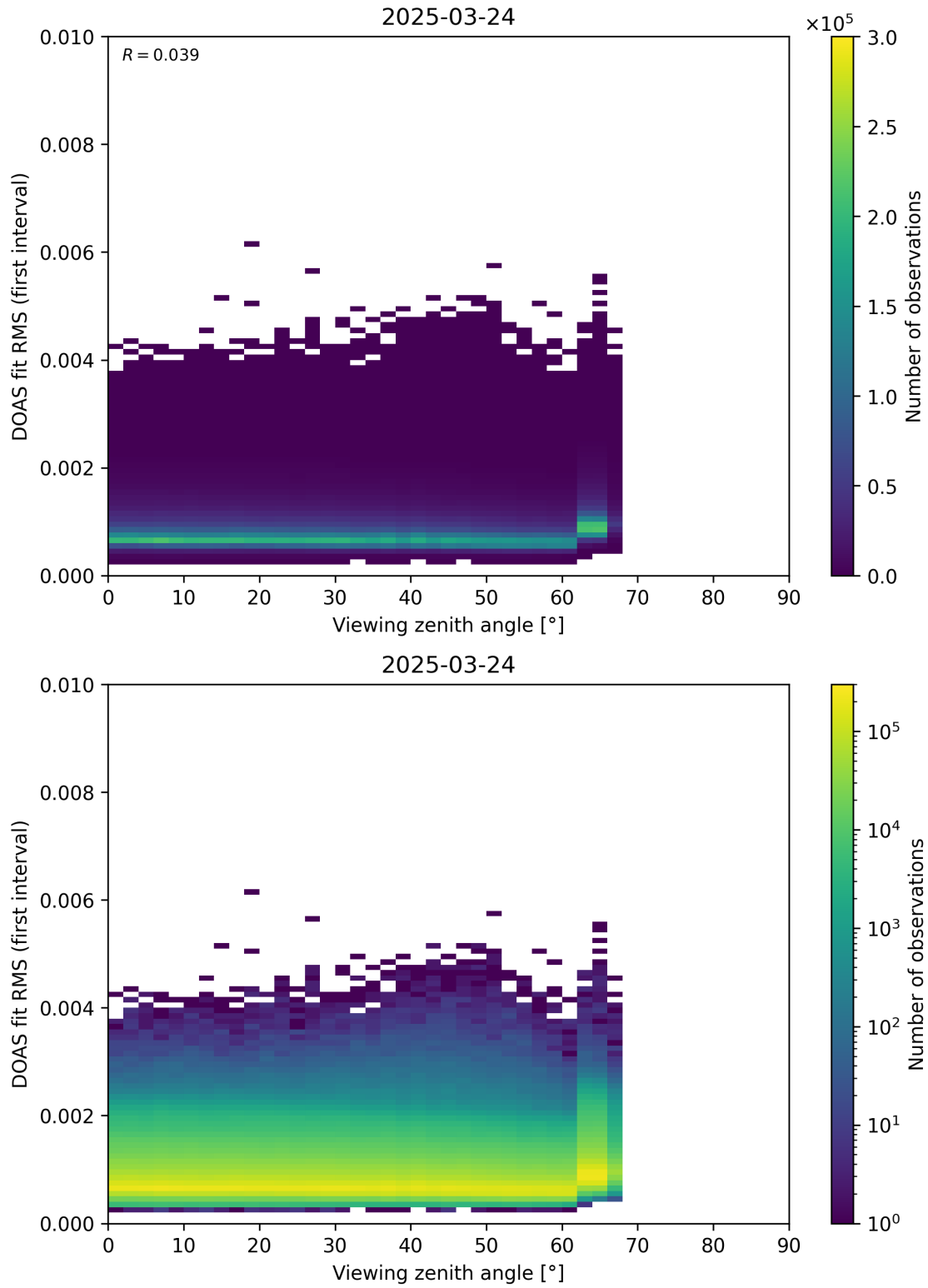
Figure 182: Scatter density plot of “Viewing zenith angle” against “DOAS fit RMS (first interval)” for 2025-03-23 to 2025-03-25.
