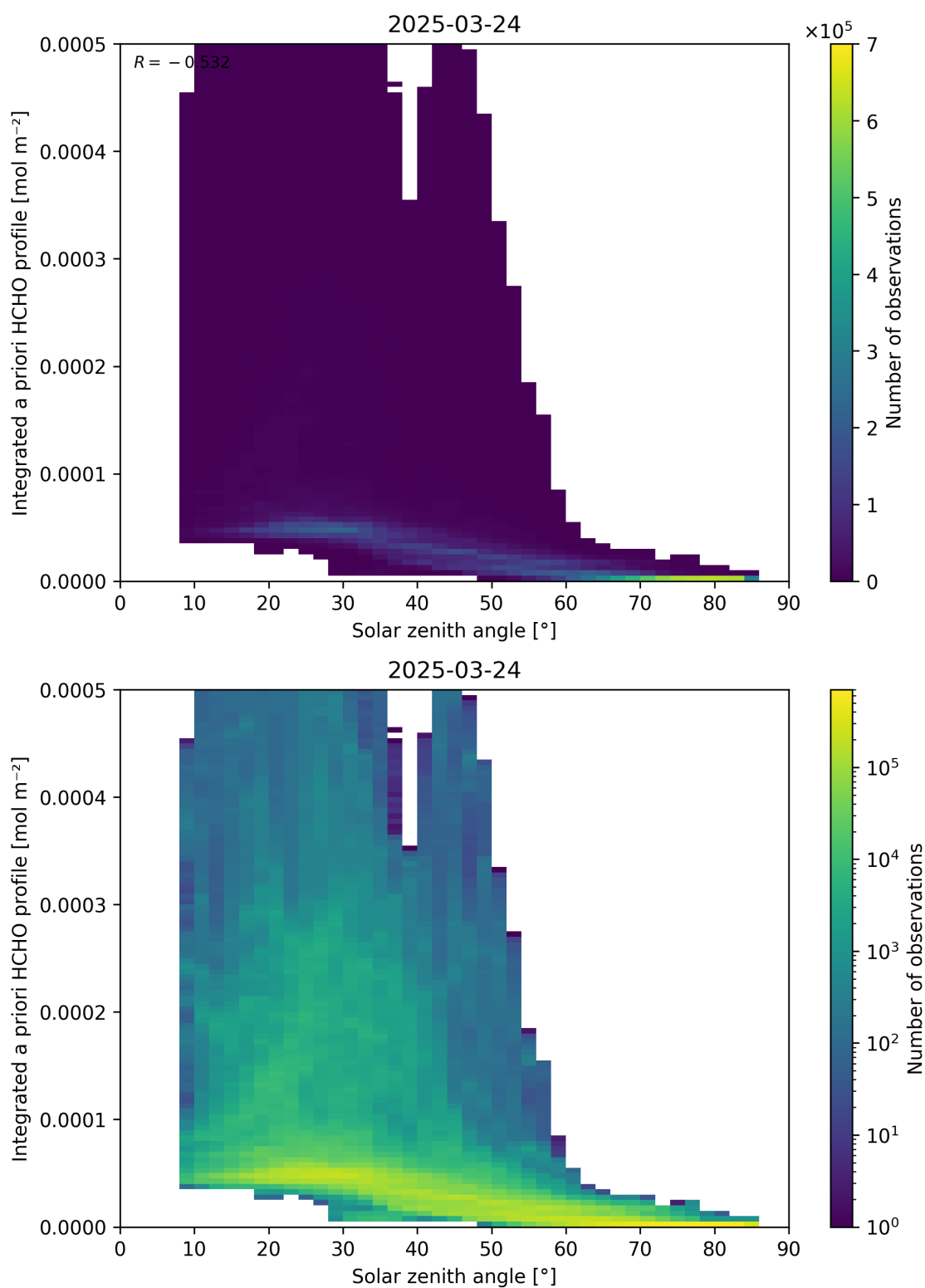
Figure 180: Scatter density plot of “Solar zenith angle” against “Integrated a priori HCHO profile” for 2025-03-23 to 2025-03-25.
