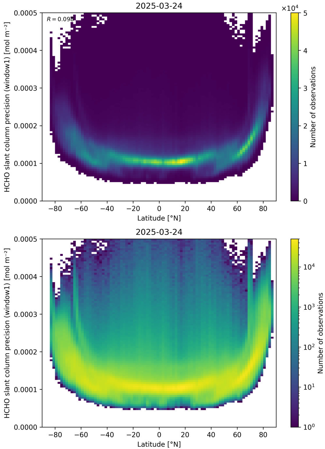
Figure 160: Scatter density plot of “Latitude” against “HCHO slant column precision (window1)” for 2025-03-23 to 2025-03-25.
