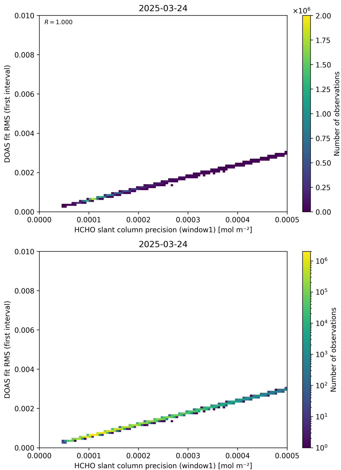
Figure 88: Scatter density plot of “HCHO slant column precision (window1)” against “DOAS fit RMS (first interval)” for 2025-03-23 to 2025-03-25.
