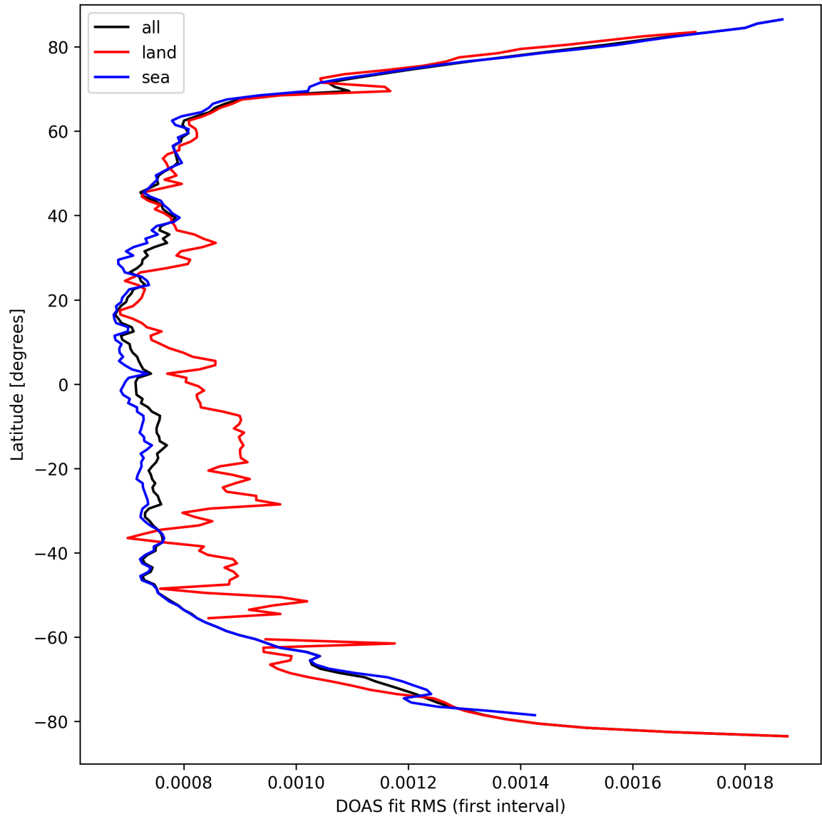
Figure 32: Zonal average of “DOAS fit RMS (first interval)” for 2025-03-23 to 2025-03-25.
