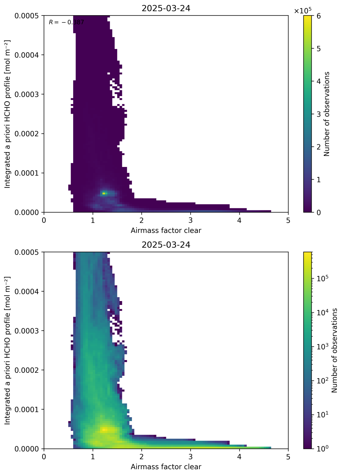
Figure 76: Scatter density plot of “Airmass factor clear” against “Integrated a priori HCHO profile” for 2025-03-23 to 2025-03-25.
