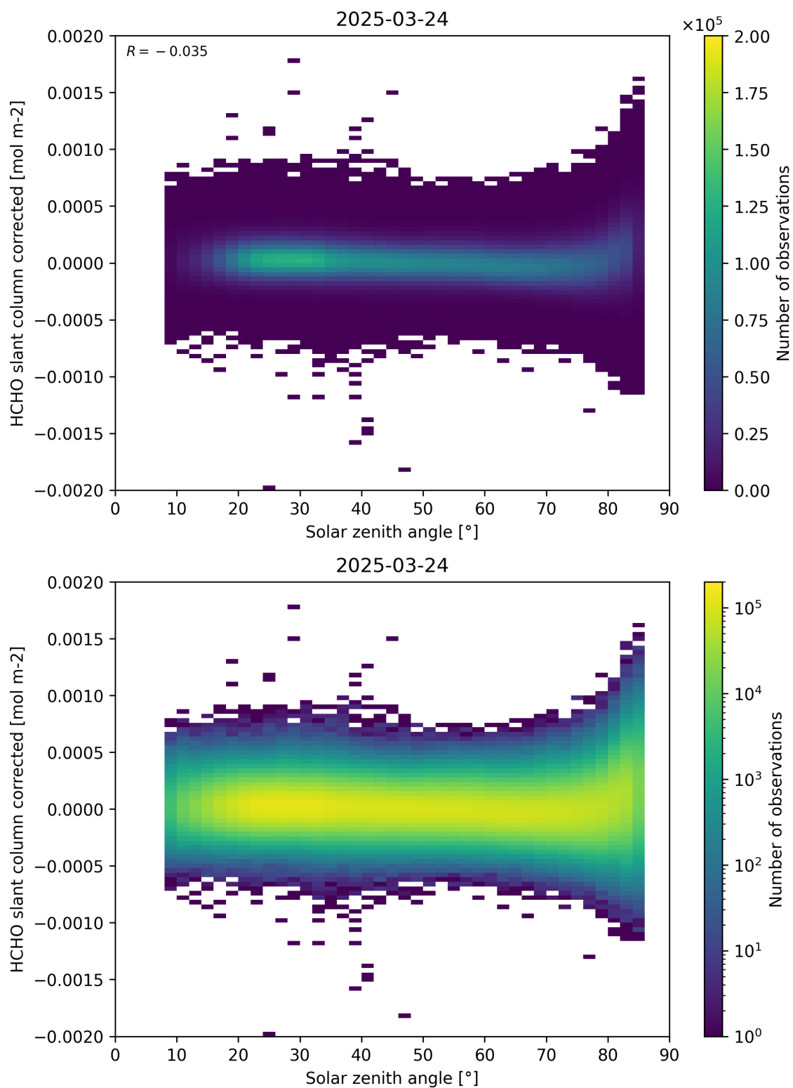
Figure 171: Scatter density plot of “Solar zenith angle” against “HCHO slant column corrected” for 2025-03-23 to 2025-03-25.
