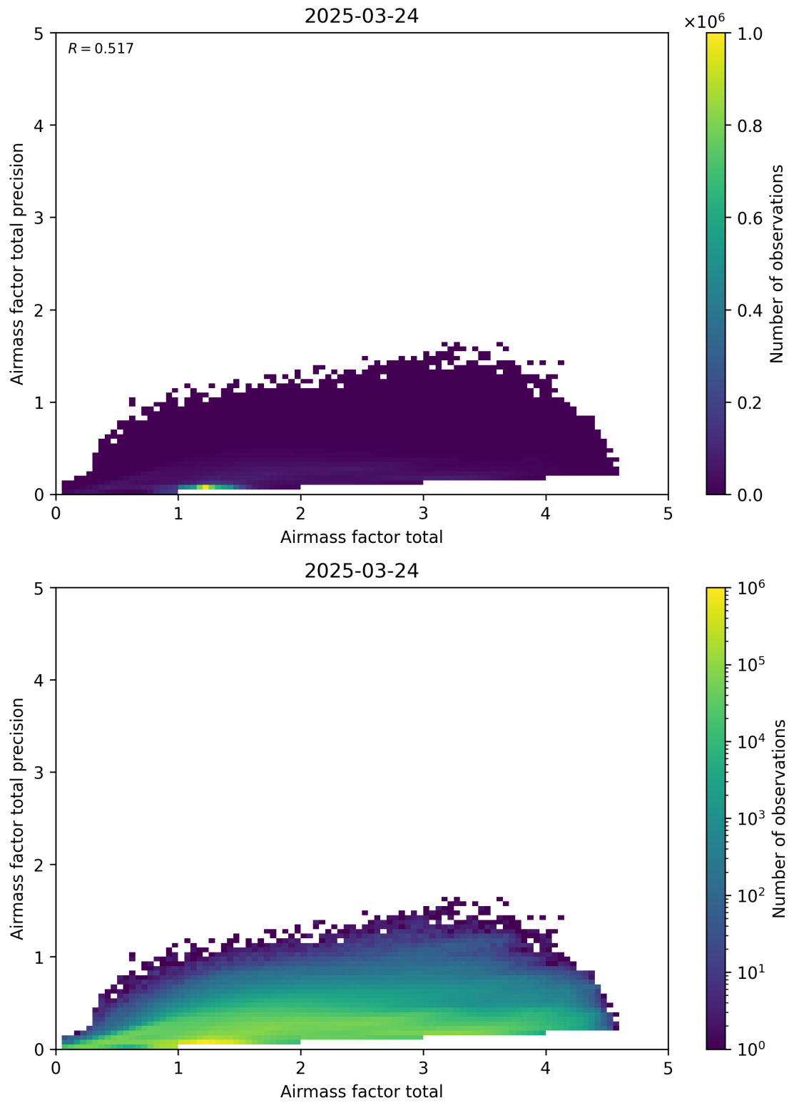
Figure 103: Scatter density plot of “Airmass factor total” against “Airmass factor total precision” for 2025-03-23 to 2025-03-25.
