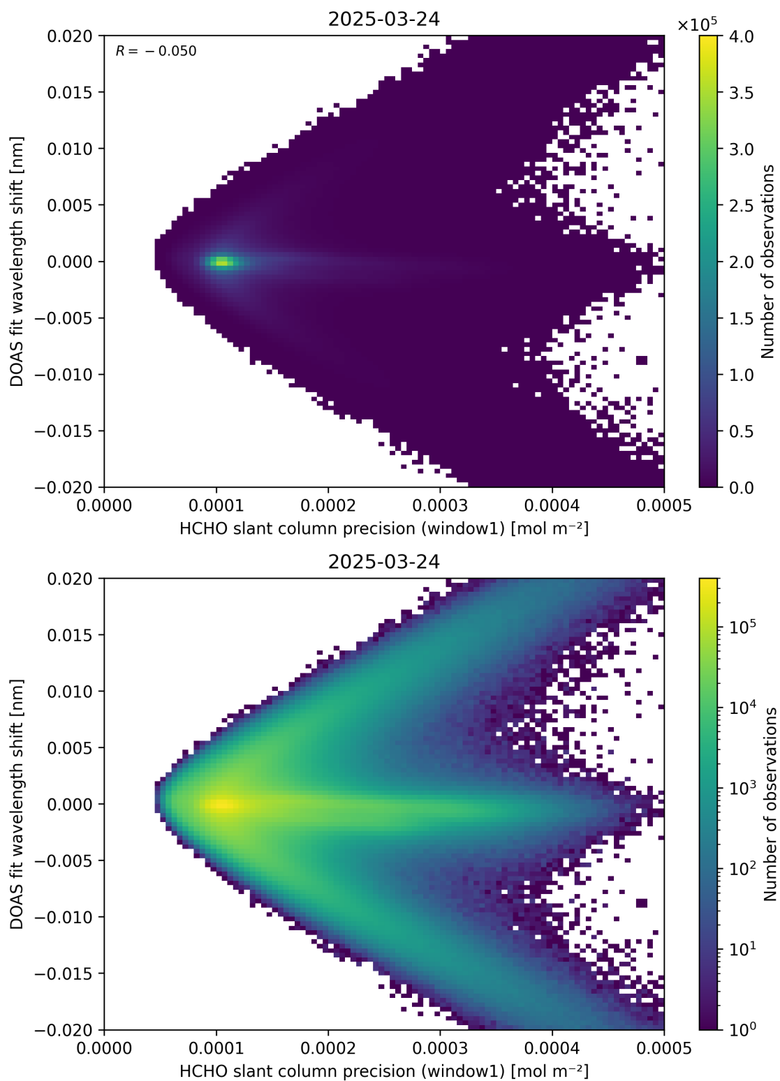
Figure 89: Scatter density plot of “HCHO slant column precision (window1)” against “DOAS fit wavelength shift” for 2025-03-23 to 2025-03-25.
