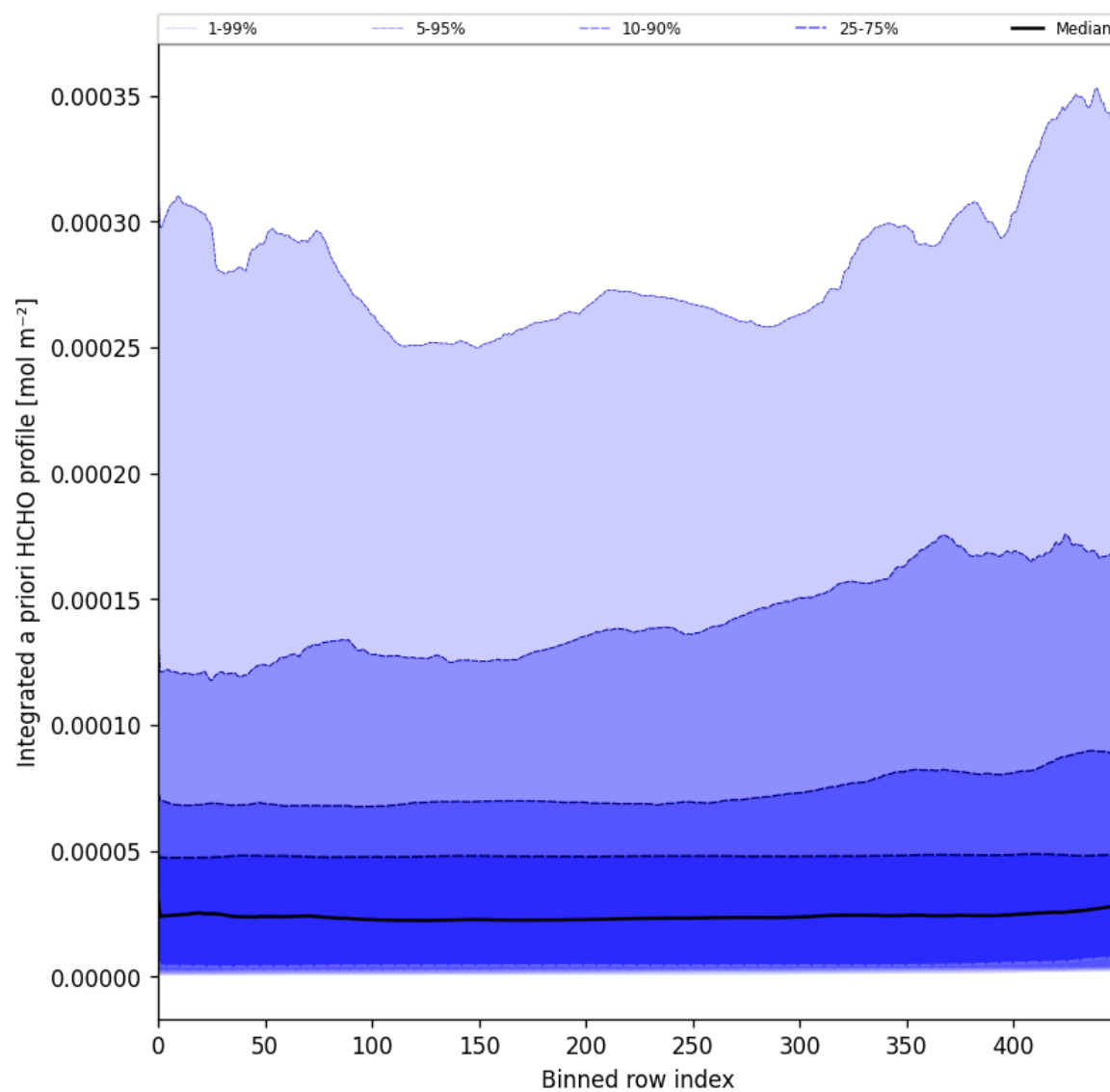
Figure 57: Along track statistics of “Integrated a priori HCHO profile” for 2025-03-23 to 2025-03-25
