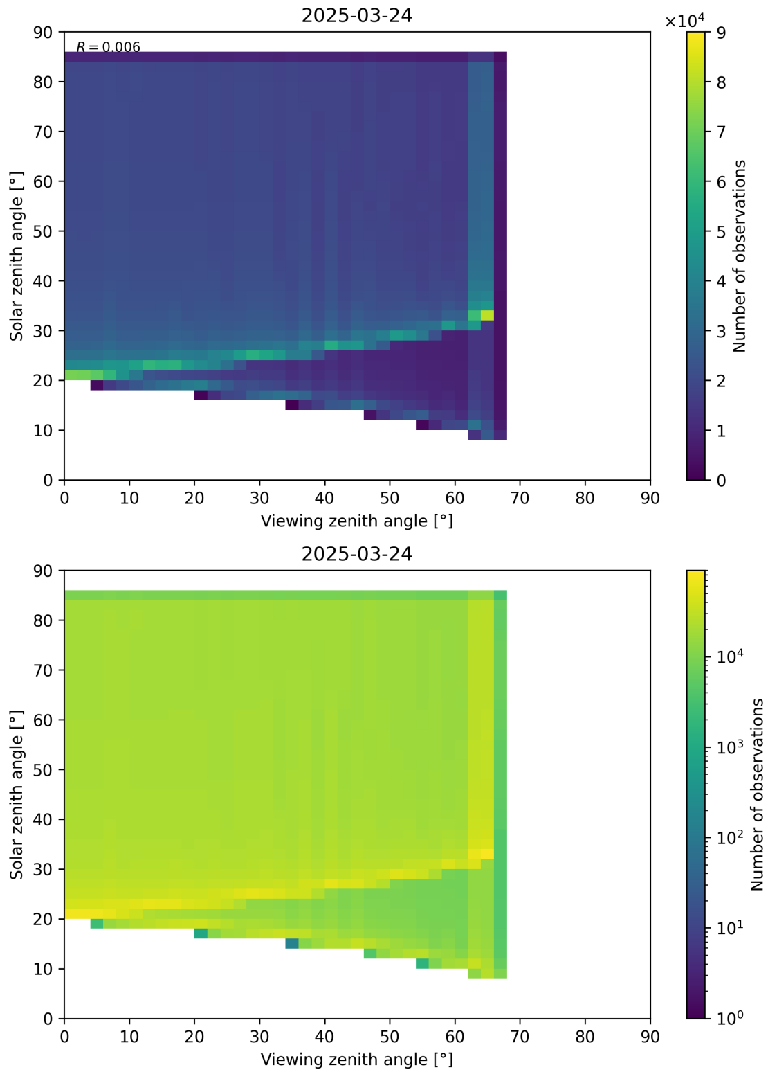
Figure 197: Scatter density plot of “Viewing zenith angle” against “Solar zenith angle” for 2025-03-23 to 2025-03-25.
