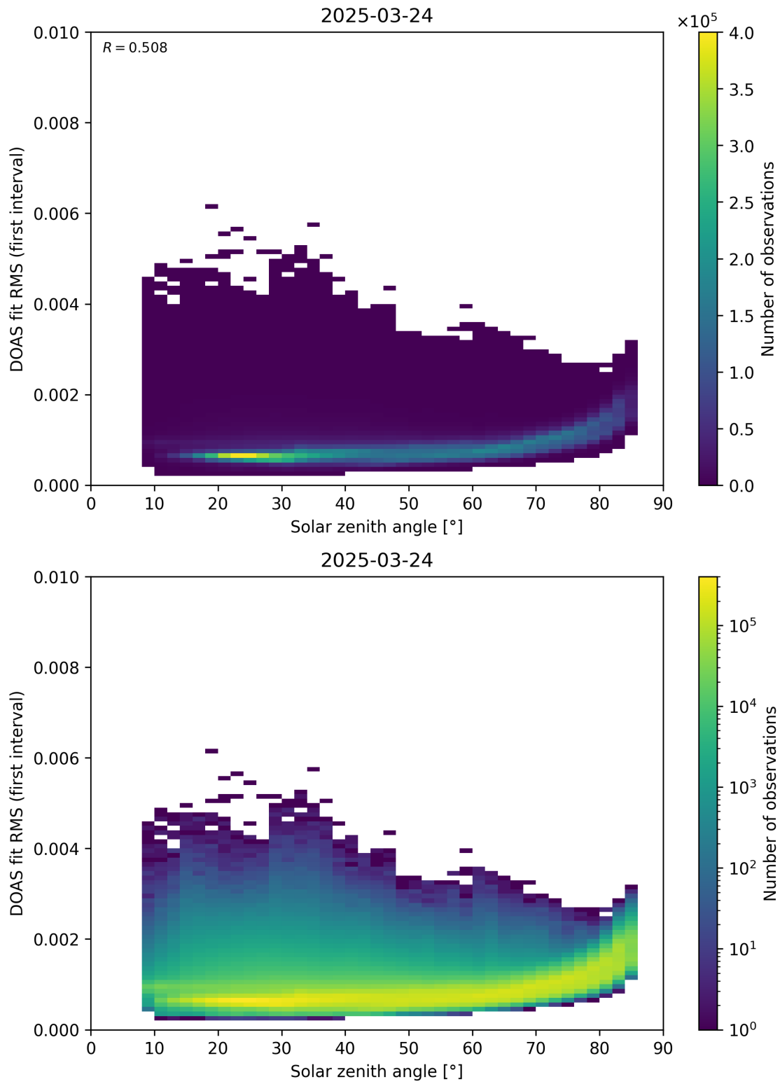
Figure 167: Scatter density plot of “Solar zenith angle” against “DOAS fit RMS (first interval)” for 2025-03-23 to 2025-03-25.
