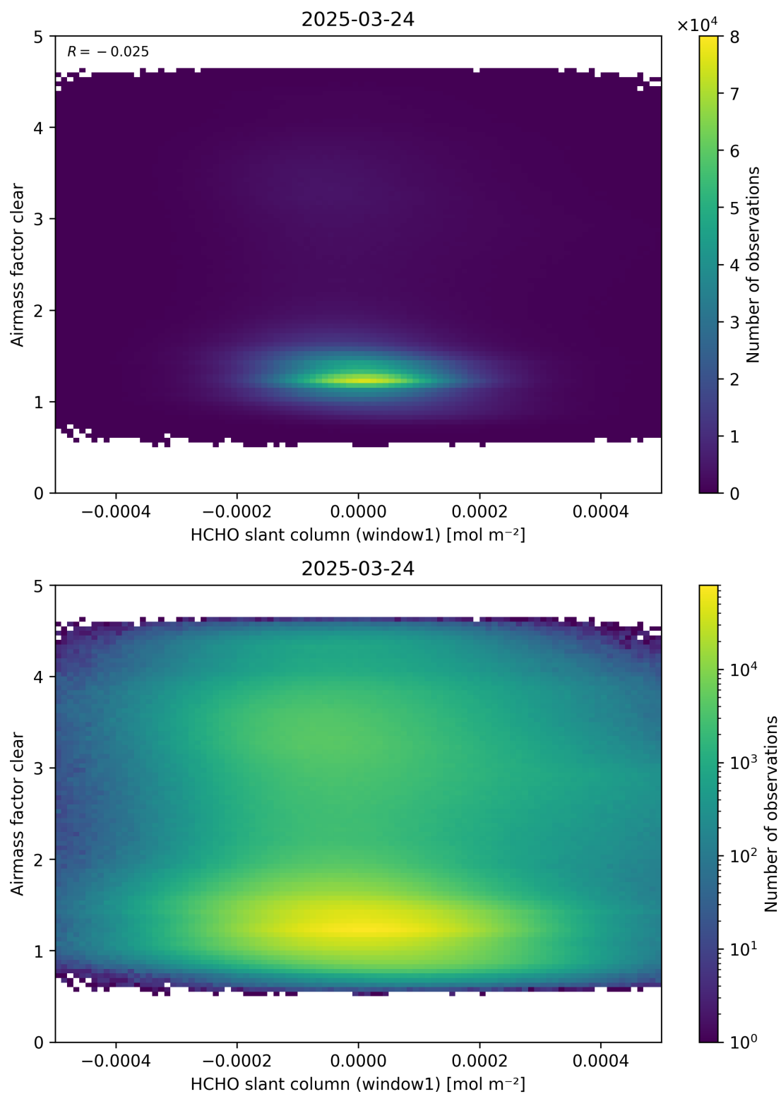
Figure 81: Scatter density plot of “HCHO slant column (window1)” against “Airmass factor clear” for 2025-03-23 to 2025-03-25.
