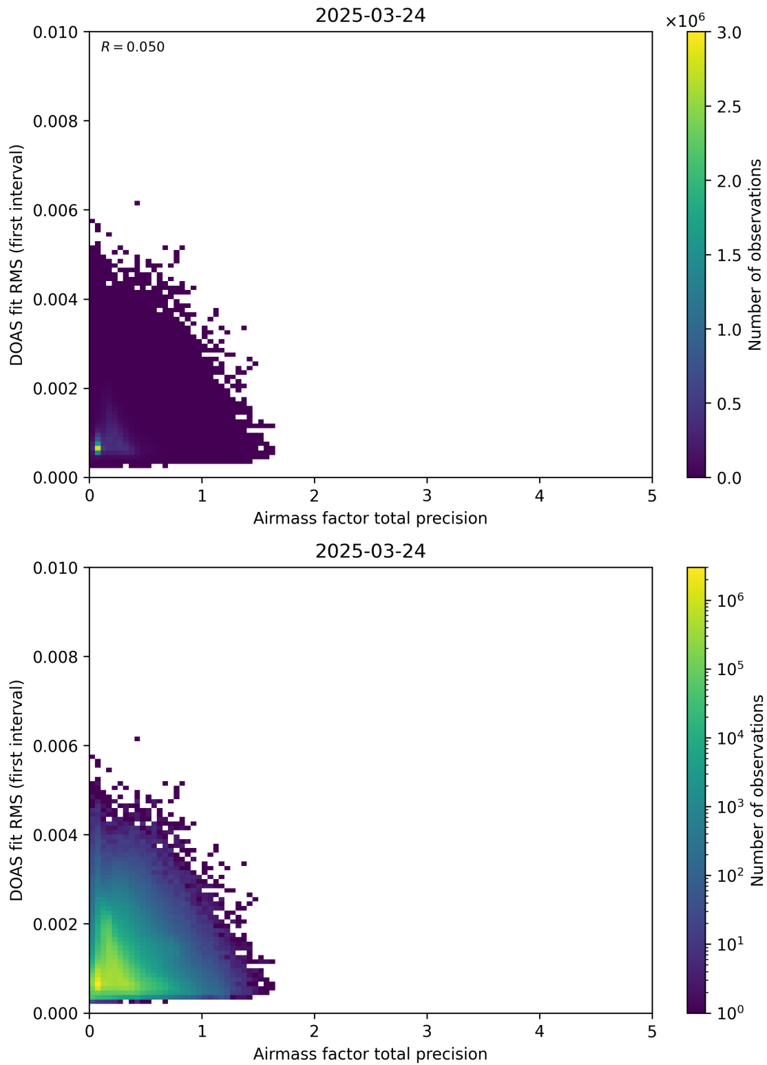
Figure 105: Scatter density plot of “Airmass factor total precision” against “DOAS fit RMS (first interval)” for 2025-03-23 to 2025-03-25.
