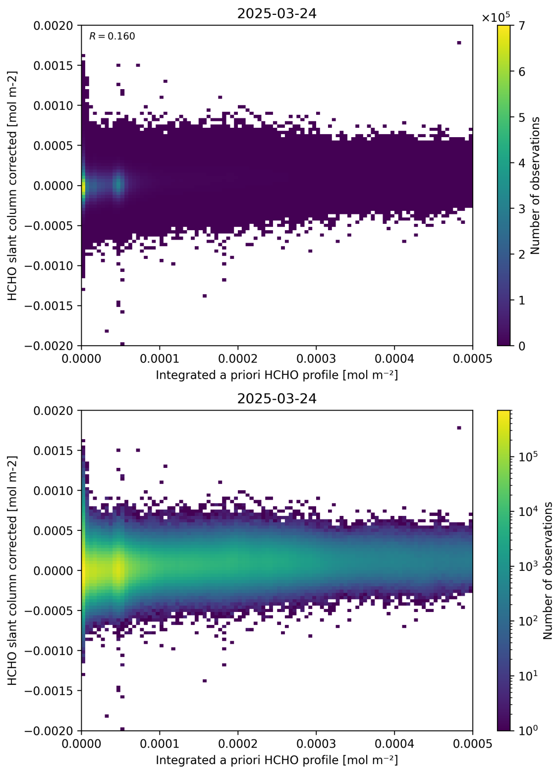
Figure 151: Scatter density plot of “Integrated a priori HCHO profile” against “HCHO slant column corrected” for 2025-03-23 to 2025-03-25.
