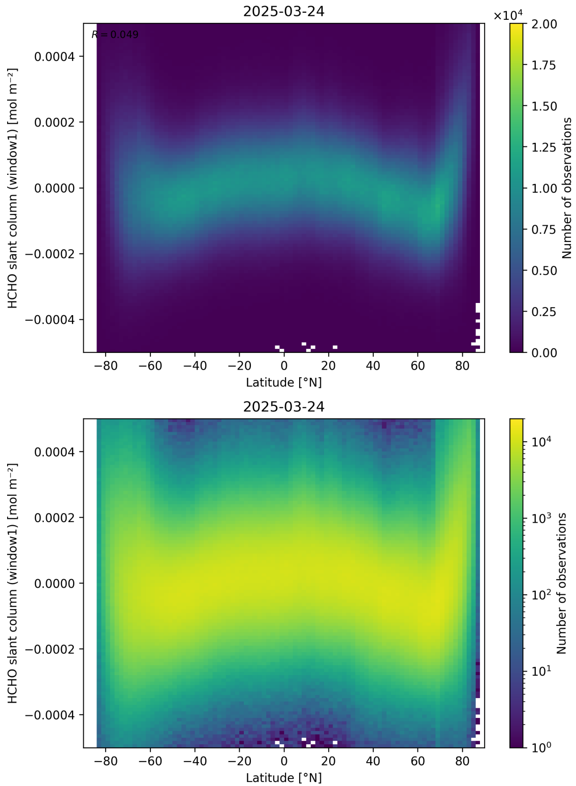
Figure 159: Scatter density plot of “Latitude” against “HCHO slant column (window1)” for 2025-03-23 to 2025-03-25.
