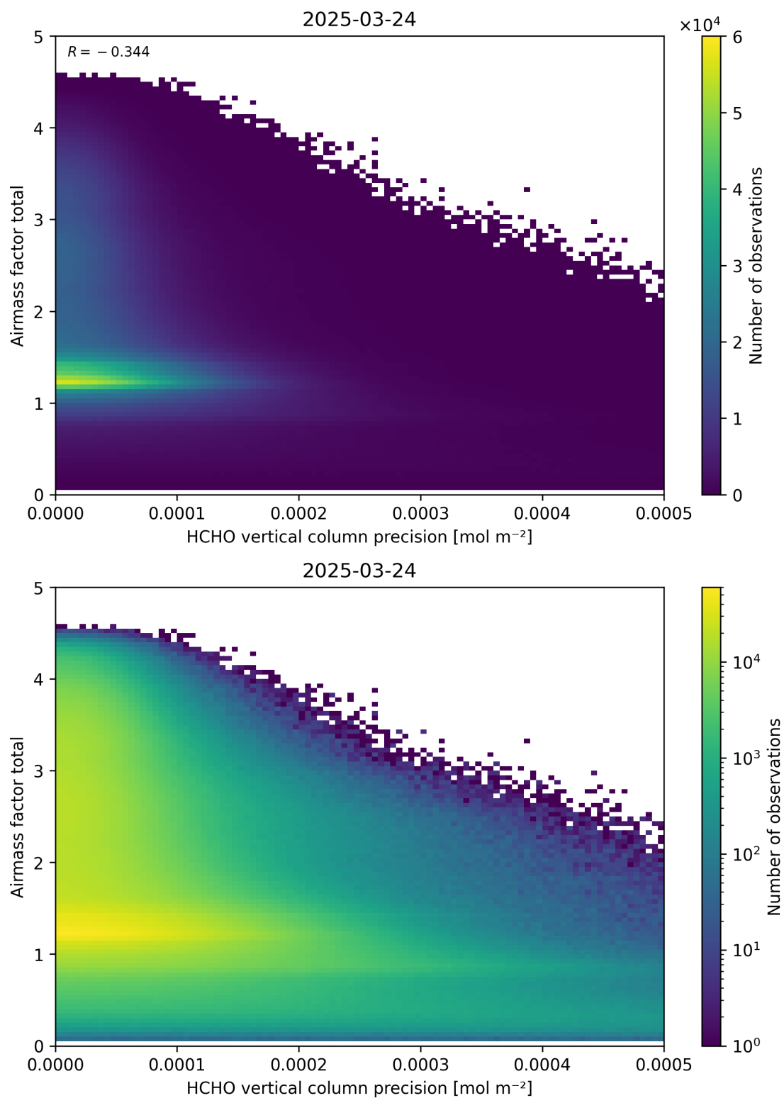
Figure 144: Scatter density plot of “HCHO vertical column precision” against “Airmass factor total” for 2025-03-23 to 2025-03-25.
