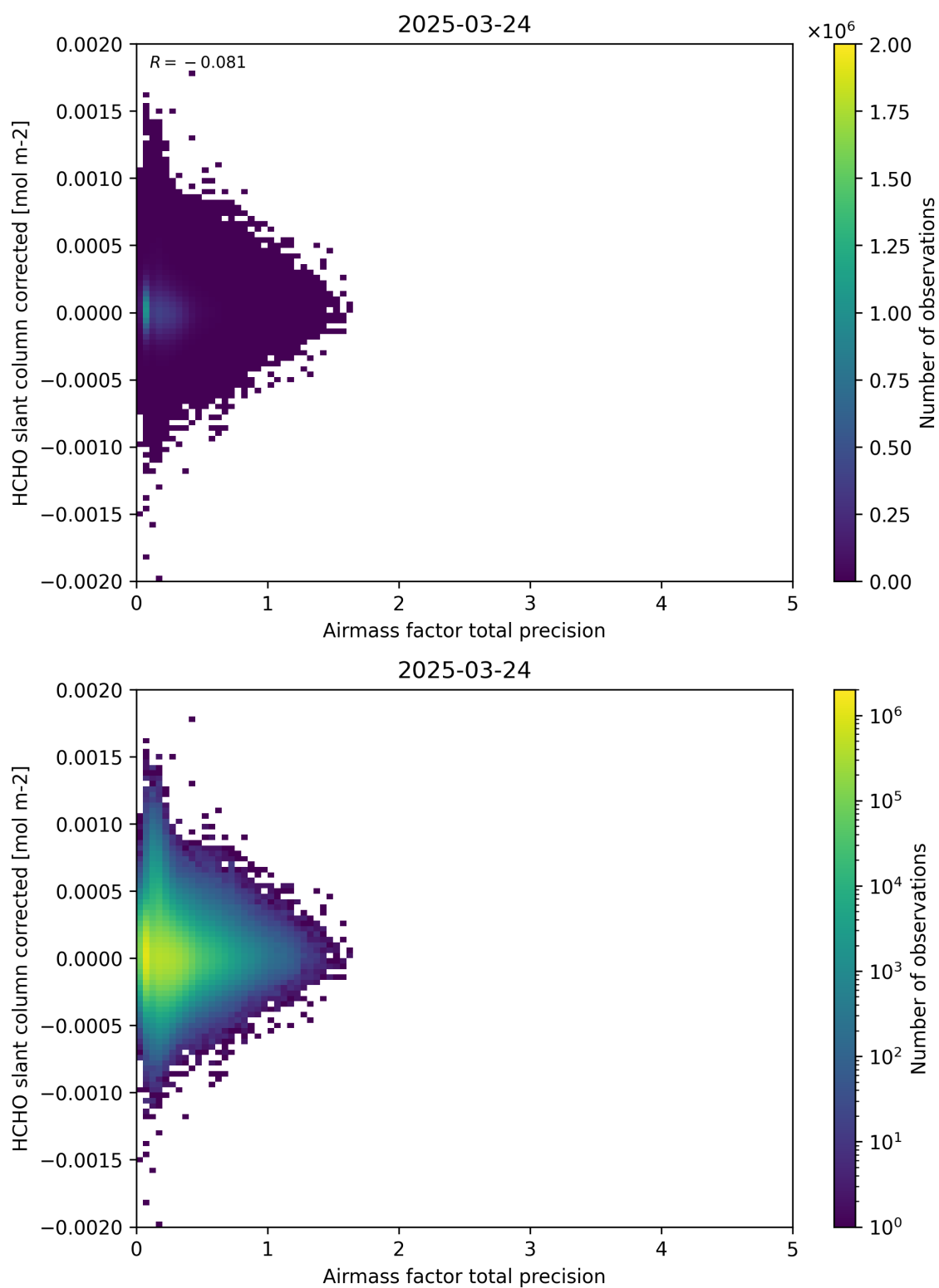
Figure 109: Scatter density plot of “Airmass factor total precision” against “HCHO slant column corrected” for 2025-03-23 to 2025-03-25.
