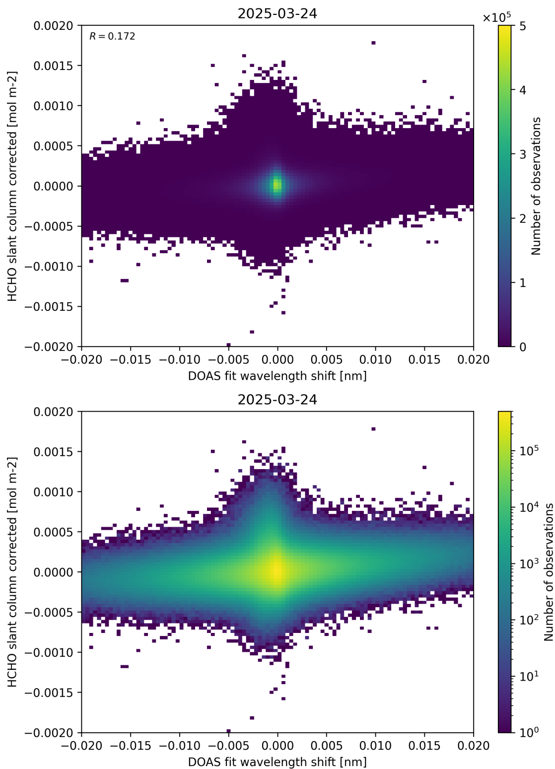
Figure 66: Scatter density plot of “DOAS fit wavelength shift” against “HCHO slant column corrected” for 2025-03-23 to 2025-03-25.
