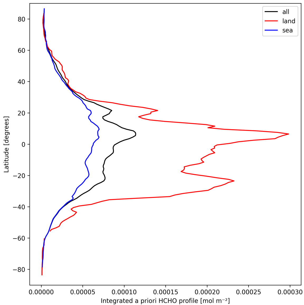
Figure 29: Zonal average of “Integrated a priori HCHO profile” for 2025-03-23 to 2025-03-25.
