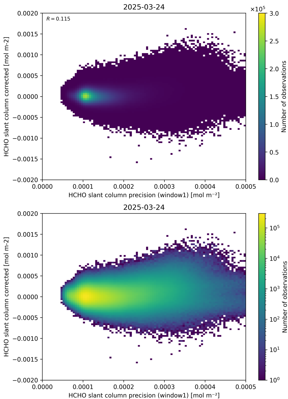
Figure 92: Scatter density plot of “HCHO slant column precision (window1)” against “HCHO slant column corrected” for 2025-03-23 to 2025-03-25.
