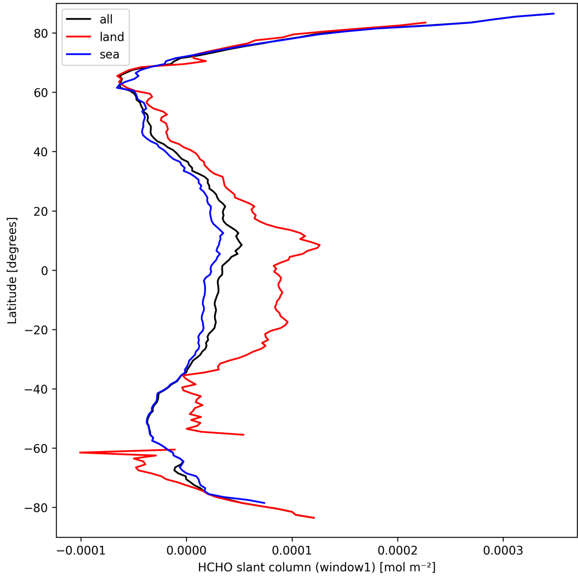
Figure 24: Zonal average of “HCHO slant column (window1)” for 2025-03-23 to 2025-03-25.
