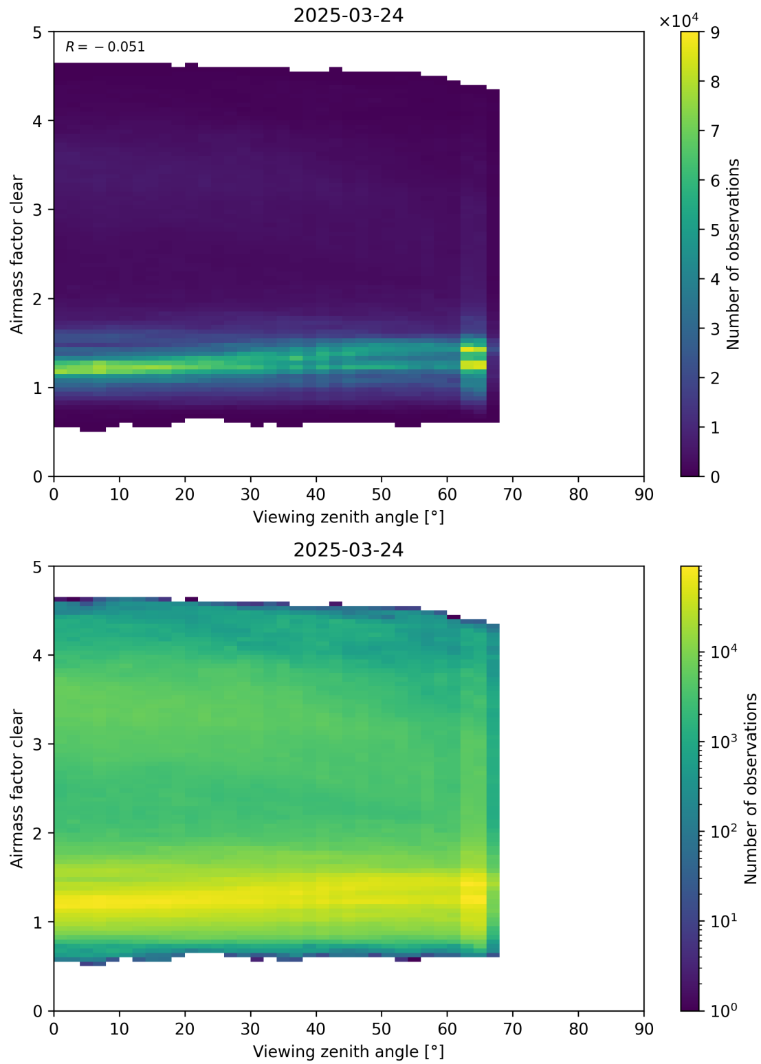
Figure 185: Scatter density plot of “Viewing zenith angle” against “Airmass factor clear” for 2025-03-23 to 2025-03-25.
