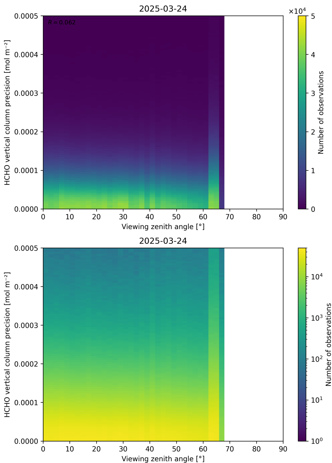
Figure 194: Scatter density plot of “Viewing zenith angle” against “HCHO vertical column precision” for 2025-03-23 to 2025-03-25.
