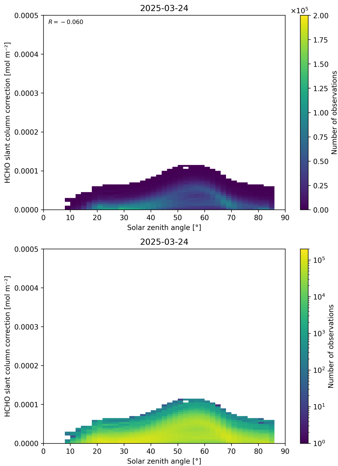
Figure 172: Scatter density plot of “Solar zenith angle” against “HCHO slant column correction” for 2025-03-23 to 2025-03-25.
