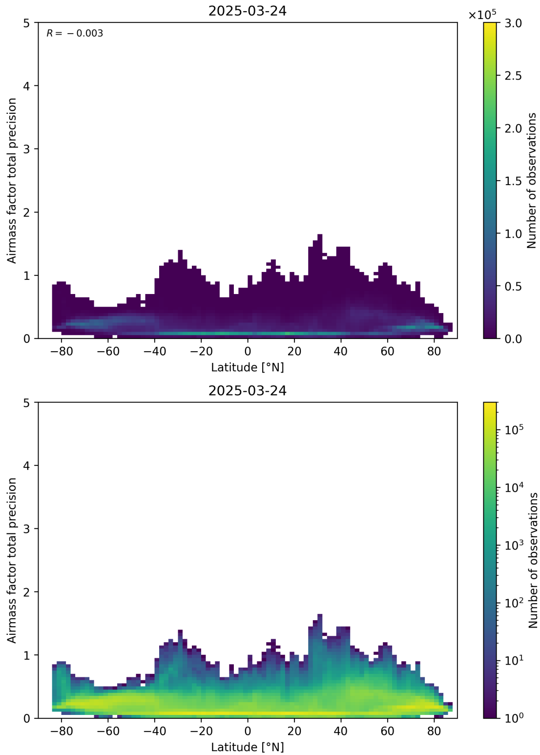
Figure 162: Scatter density plot of “Latitude” against “Airmass factor total precision” for 2025-03-23 to 2025-03-25.
