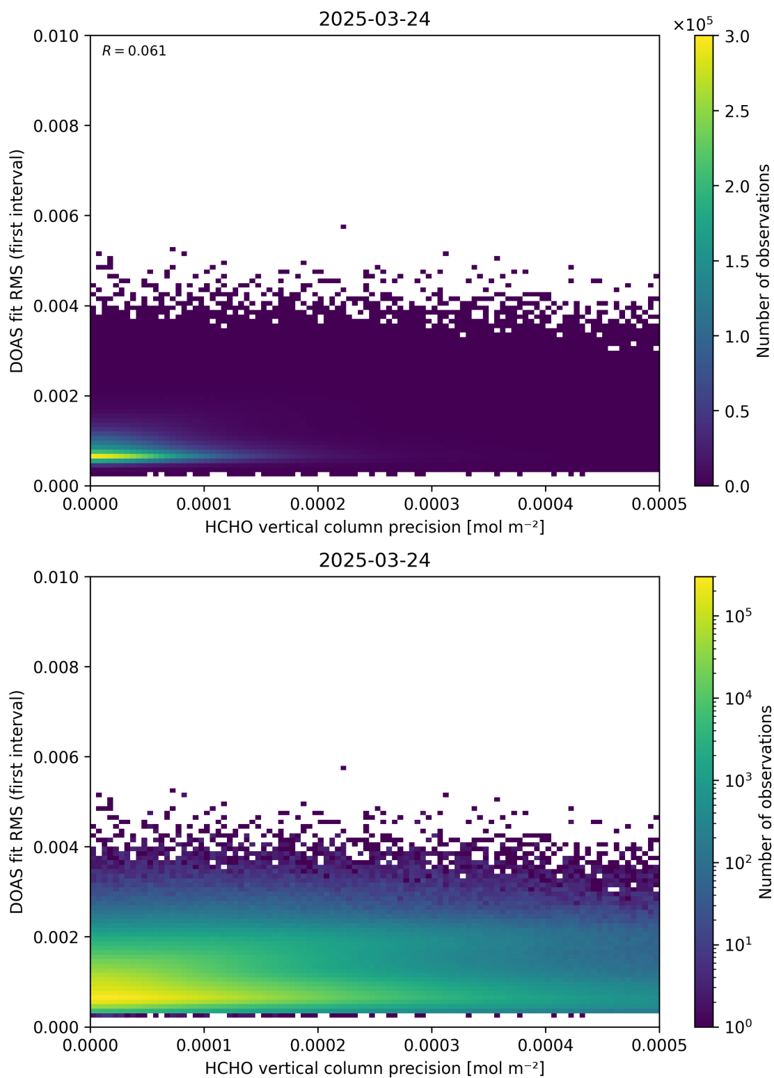
Figure 136: Scatter density plot of “HCHO vertical column precision” against “DOAS fit RMS (first interval)” for 2025-03-23 to 2025-03-25.
