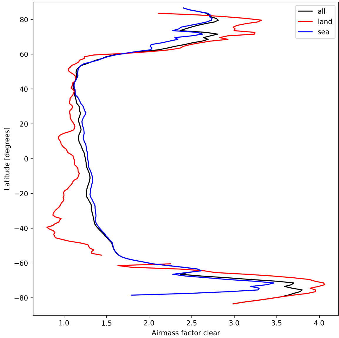
Figure 28: Zonal average of “Airmass factor clear” for 2025-03-23 to 2025-03-25.
