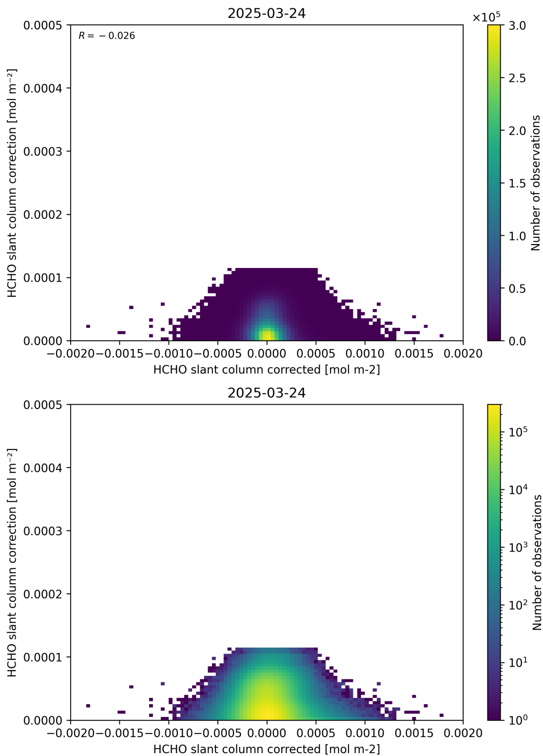
Figure 77: Scatter density plot of “HCHO slant column corrected” against “HCHO slant column correction” for 2025-03-23 to 2025-03-25.
