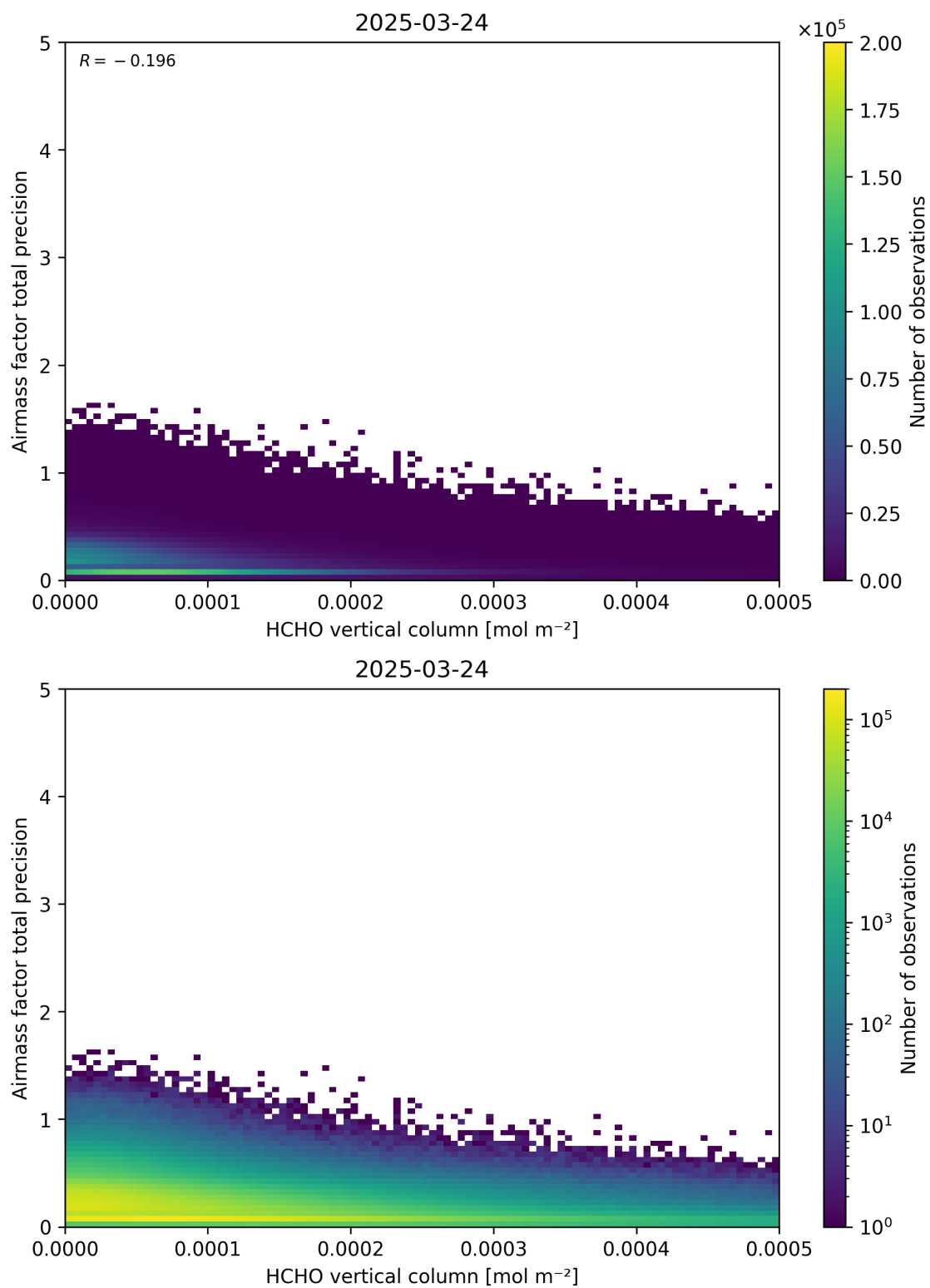
Figure 132: Scatter density plot of “HCHO vertical column” against “Airmass factor total precision” for 2025-03-23 to 2025-03-25.
