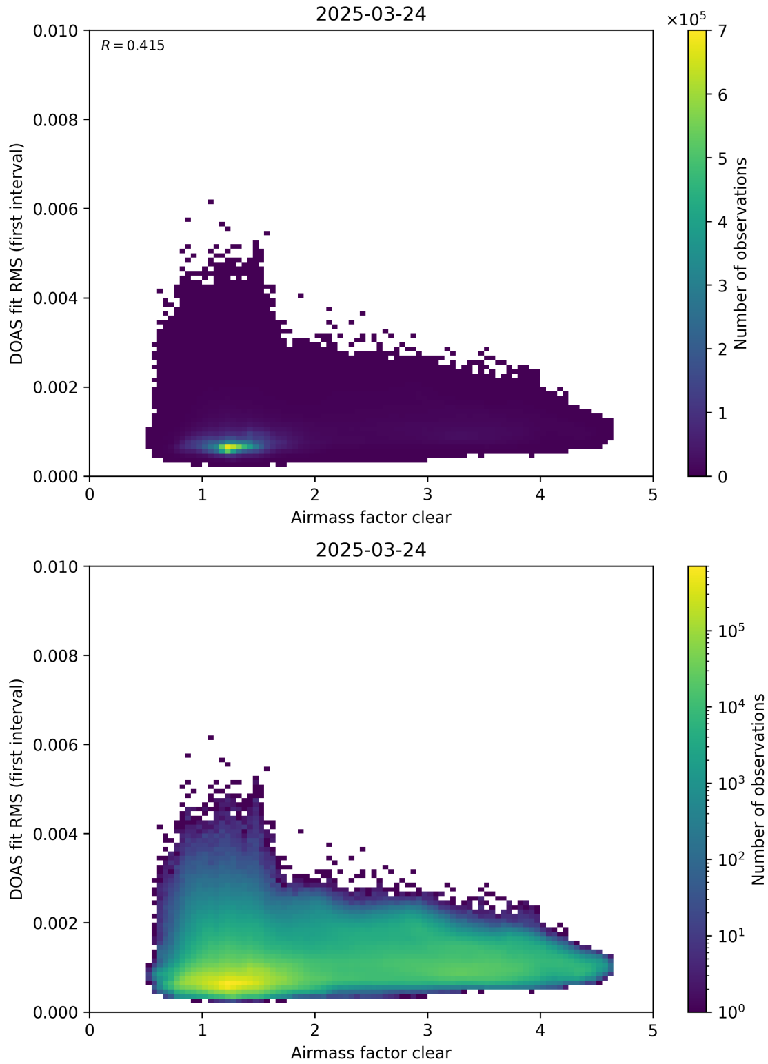
Figure 71: Scatter density plot of “Airmass factor clear” against “DOAS fit RMS (first interval)” for 2025-03-23 to 2025-03-25.
