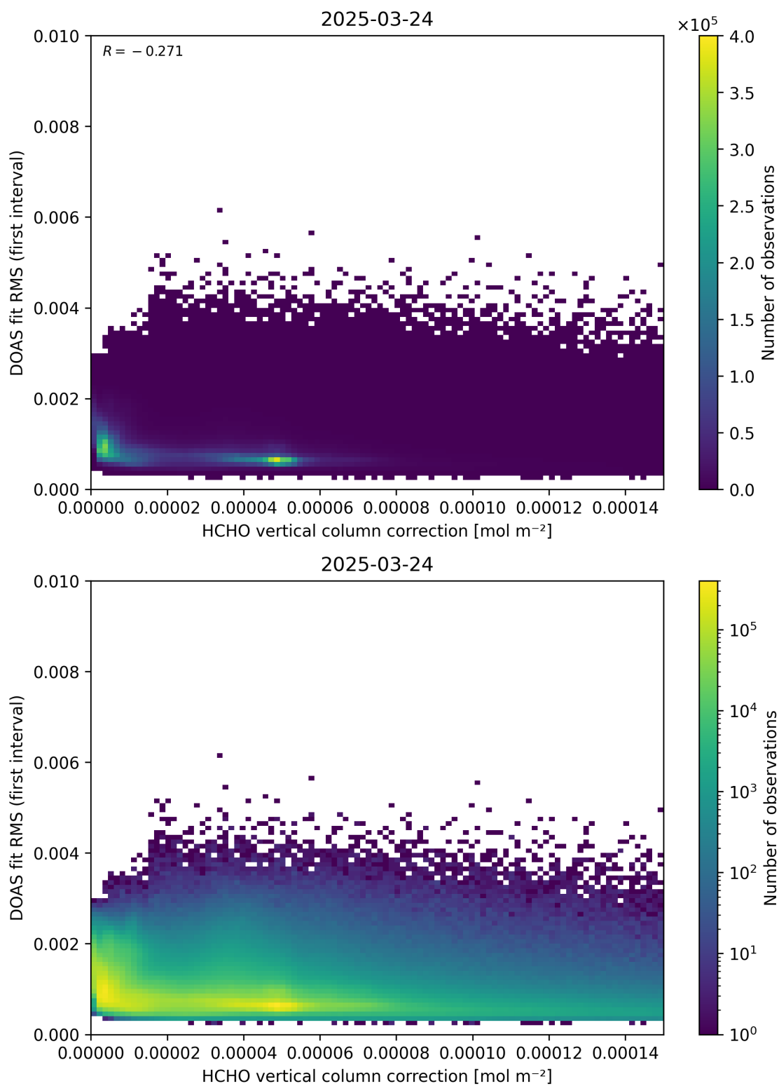
Figure 112: Scatter density plot of “HCHO vertical column correction” against “DOAS fit RMS (first interval)” for 2025-03-23 to 2025-03-25.
