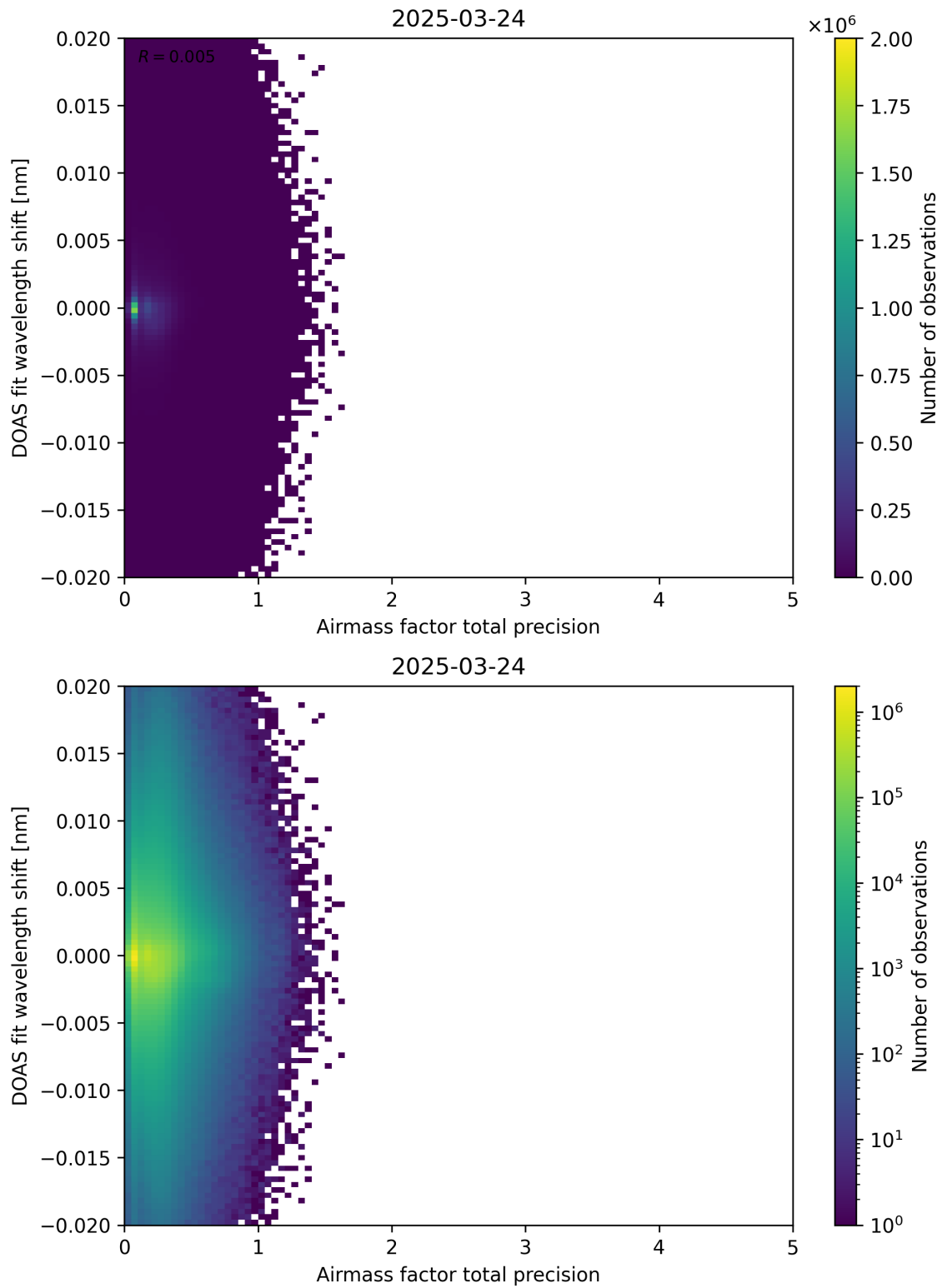
Figure 106: Scatter density plot of “Airmass factor total precision” against “DOAS fit wavelength shift” for 2025-03-23 to 2025-03-25.
