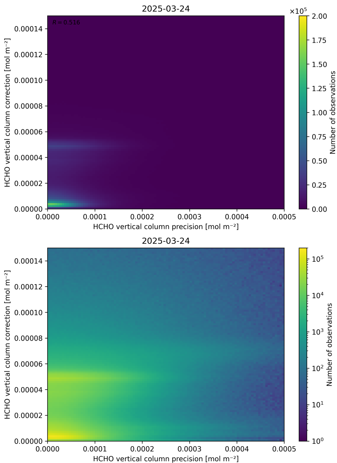
Figure 146: Scatter density plot of “HCHO vertical column precision” against “HCHO vertical column correction” for 2025-03-23 to 2025-03-25.
