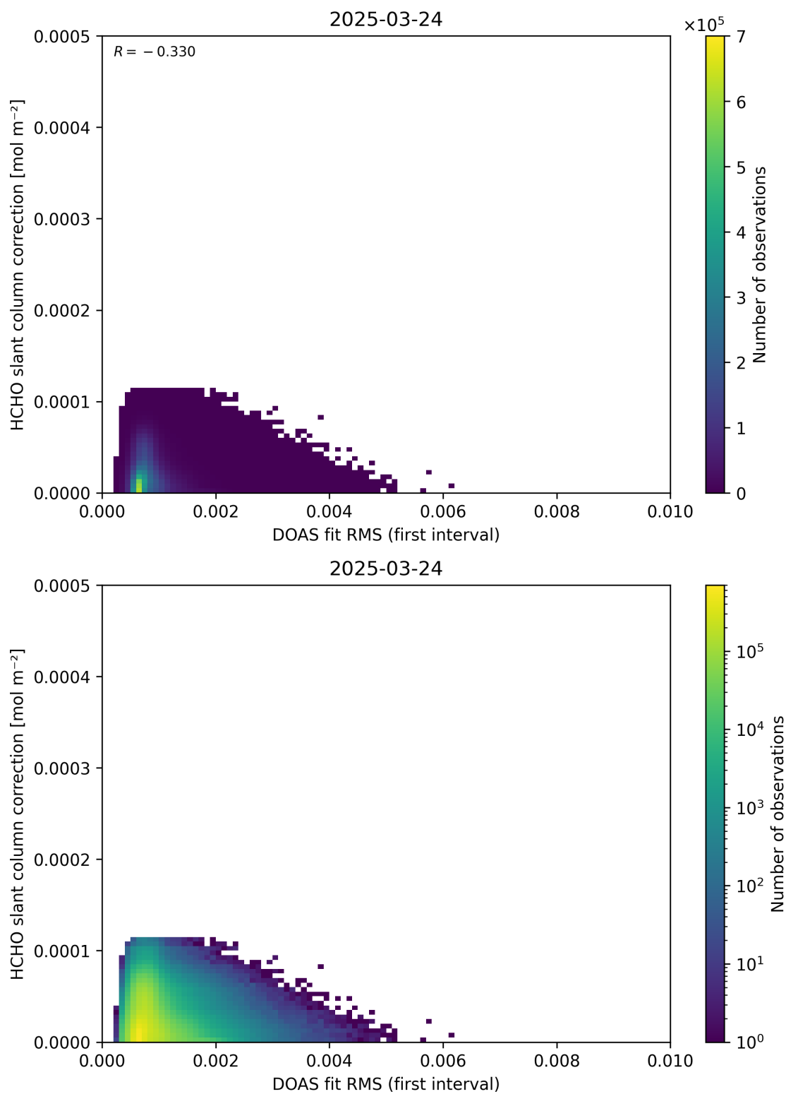
Figure 63: Scatter density plot of “DOAS fit RMS (first interval)” against “HCHO slant column correction” for 2025-03-23 to 2025-03-25.
