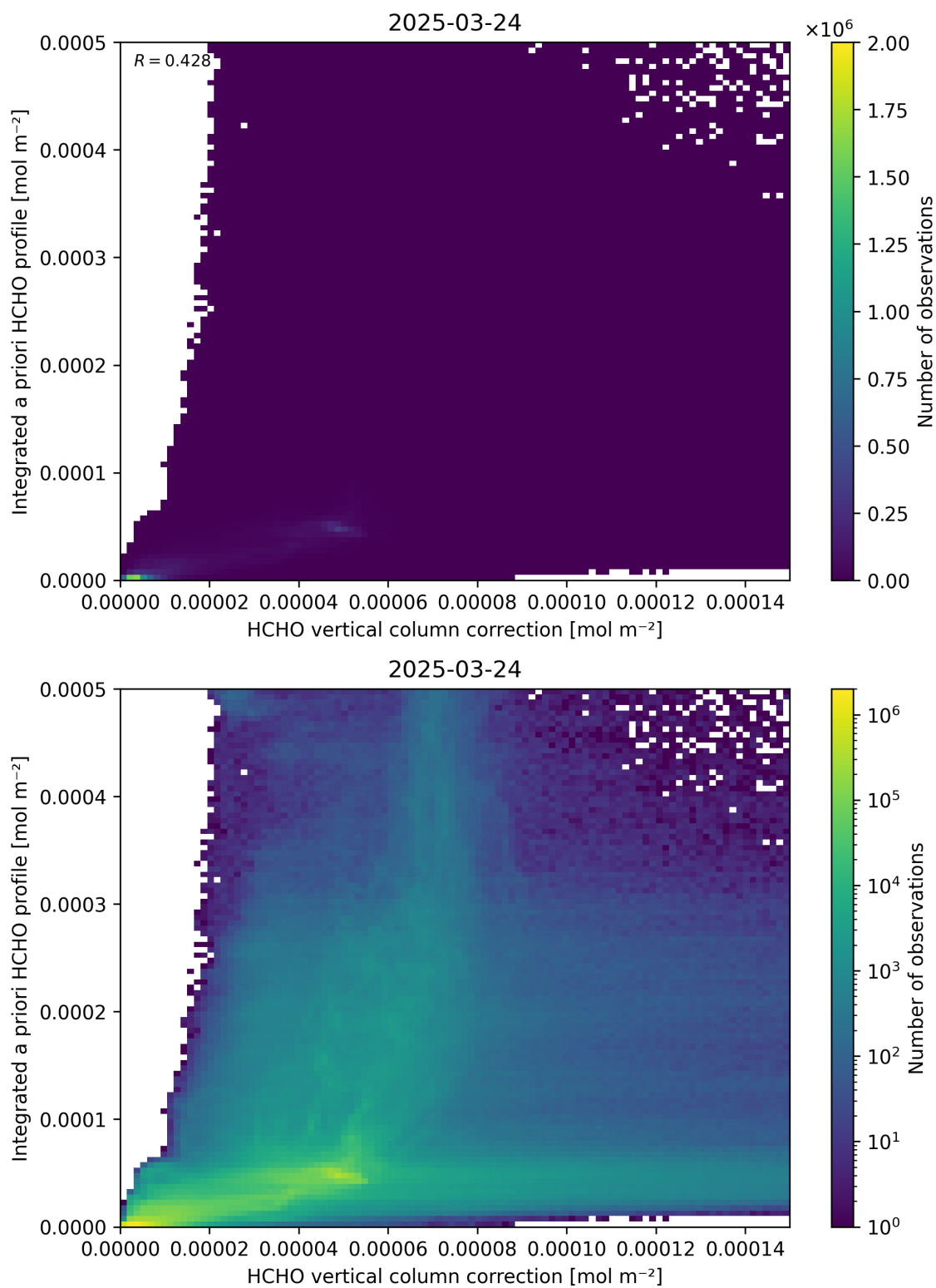
Figure 122: Scatter density plot of “HCHO vertical column correction” against “Integrated a priori HCHO profile” for 2025-03-23 to 2025-03-25.
