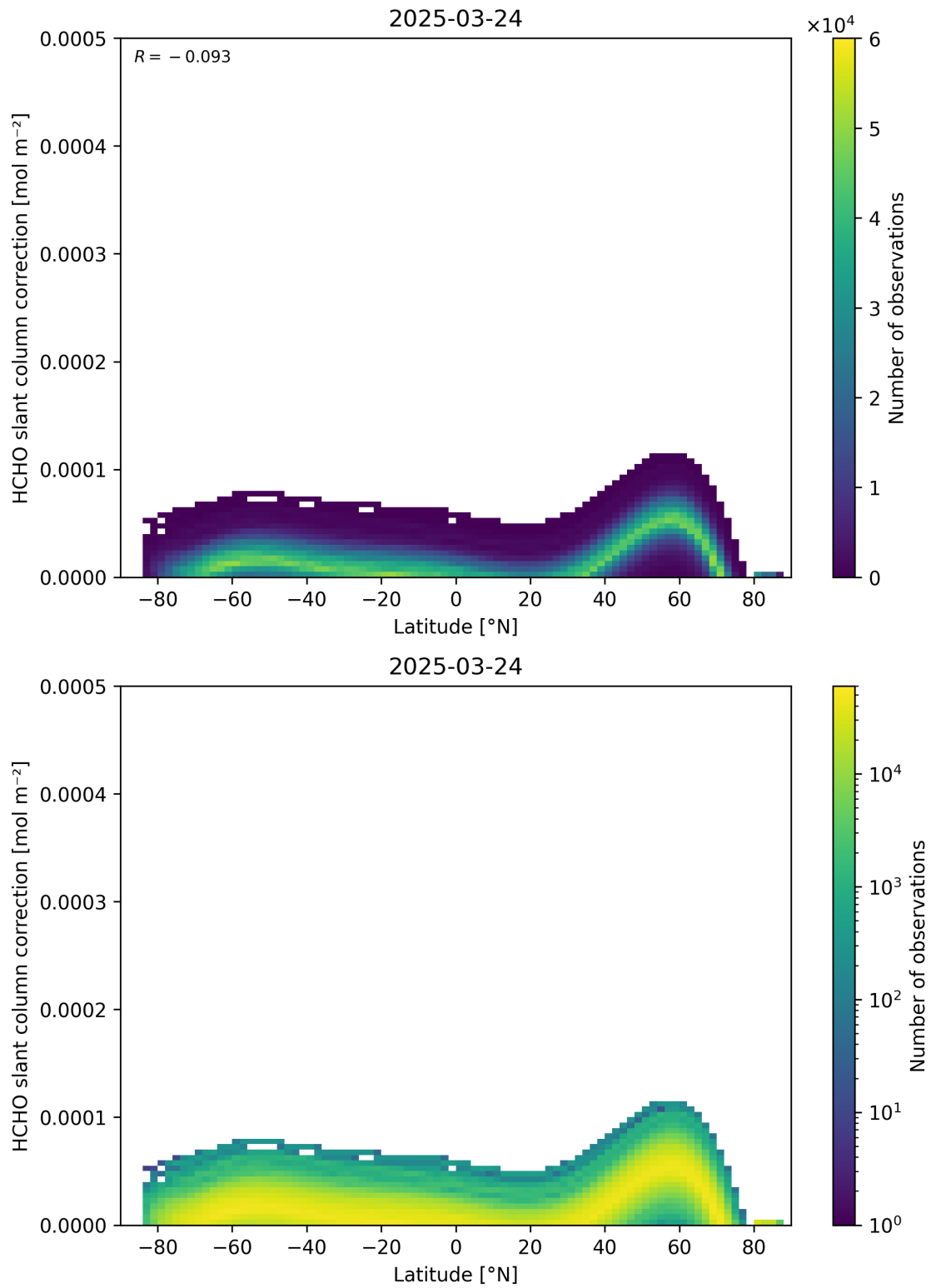
Figure 158: Scatter density plot of “Latitude” against “HCHO slant column correction” for 2025-03-23 to 2025-03-25.
