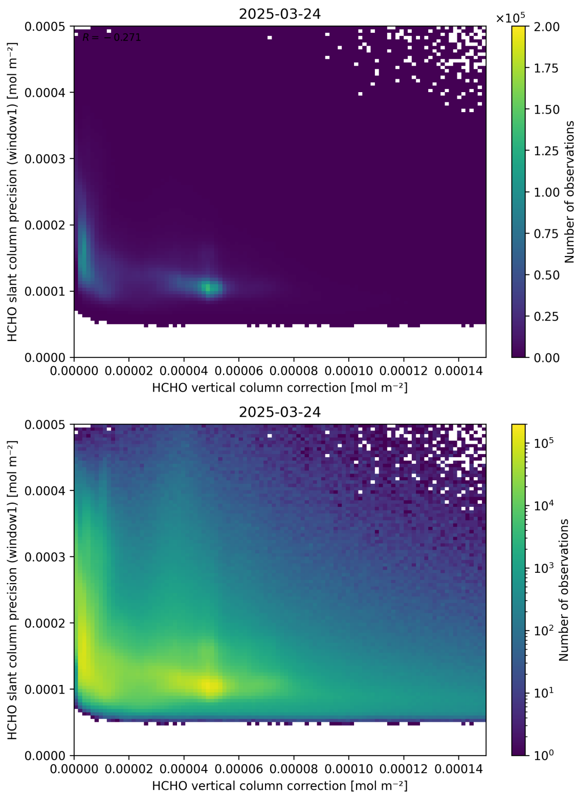
Figure 119: Scatter density plot of “HCHO vertical column correction” against “HCHO slant column precision (window1)” for 2025-03-23 to 2025-03-25.
