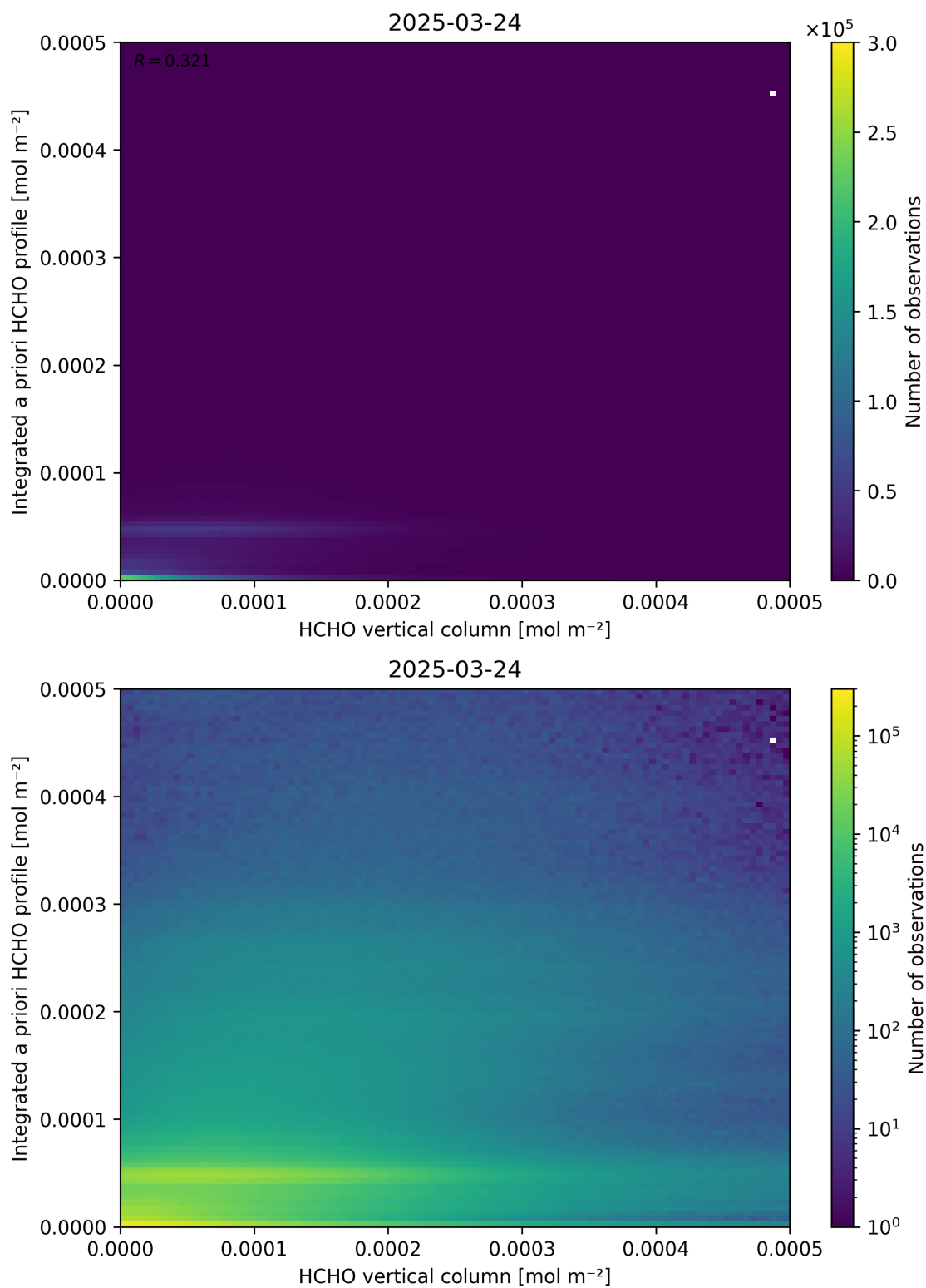
Figure 135: Scatter density plot of “HCHO vertical column” against “Integrated a priori HCHO profile” for 2025-03-23 to 2025-03-25.
