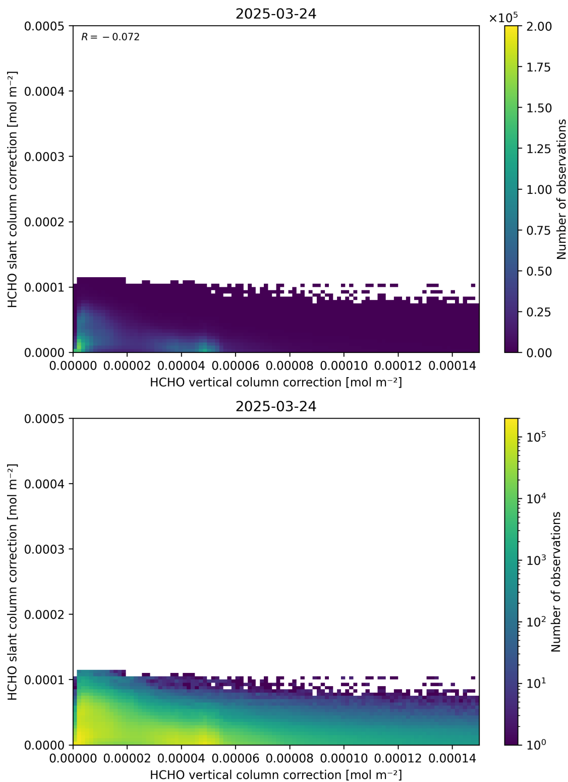
Figure 117: Scatter density plot of “HCHO vertical column correction” against “HCHO slant column correction” for 2025-03-23 to 2025-03-25.
