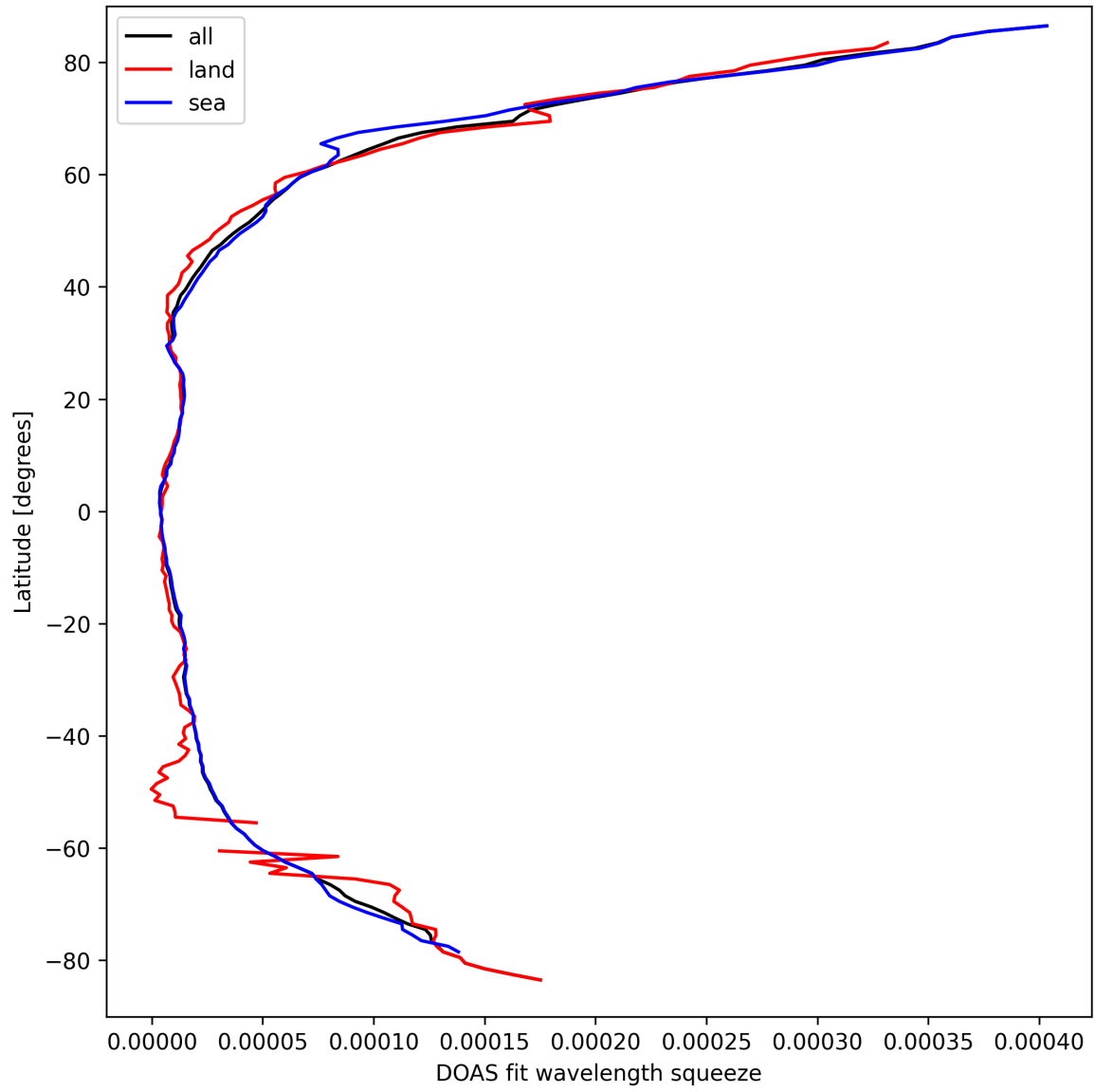
Figure 31: Zonal average of “DOAS fit wavelength squeeze” for 2025-03-23 to 2025-03-25.
