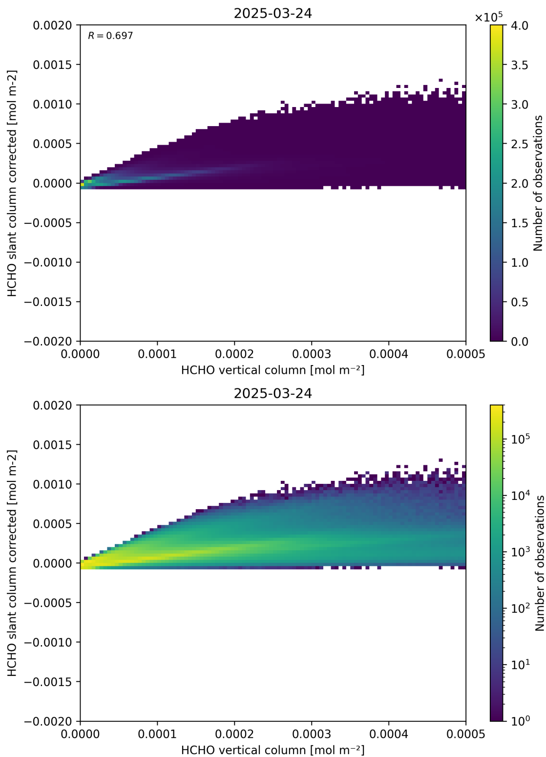
Figure 127: Scatter density plot of “HCHO vertical column” against “HCHO slant column corrected” for 2025-03-23 to 2025-03-25.
