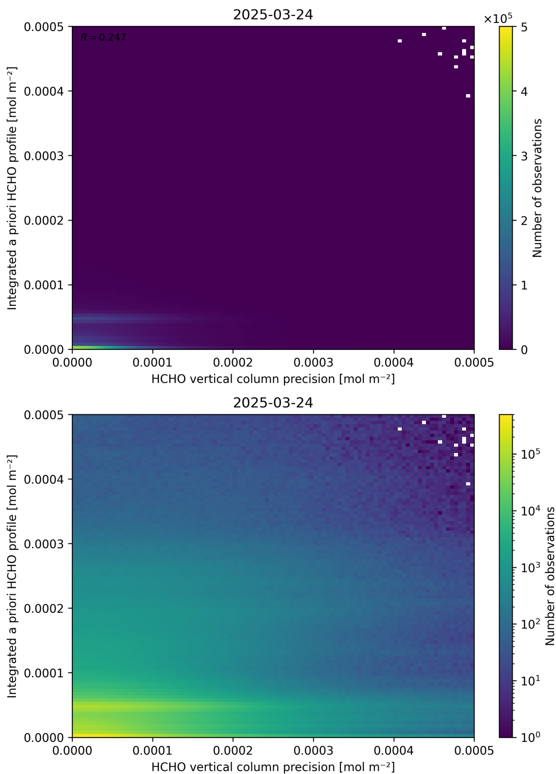
Figure 147: Scatter density plot of “HCHO vertical column precision” against “Integrated a priori HCHO profile” for 2025-03-23 to 2025-03-25.
