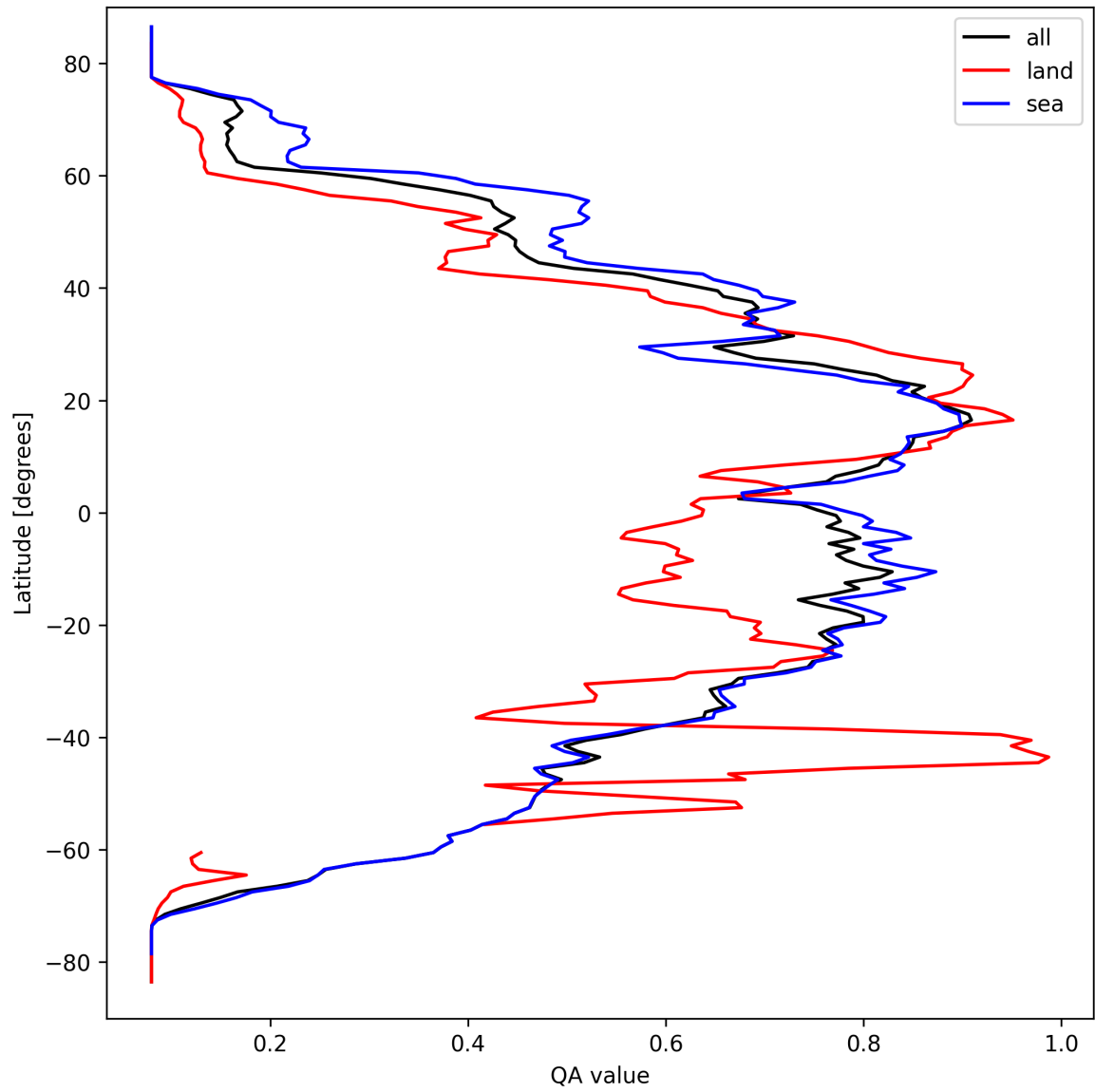
Figure 20: Zonal average of “QA value” for 2025-03-23 to 2025-03-25.
