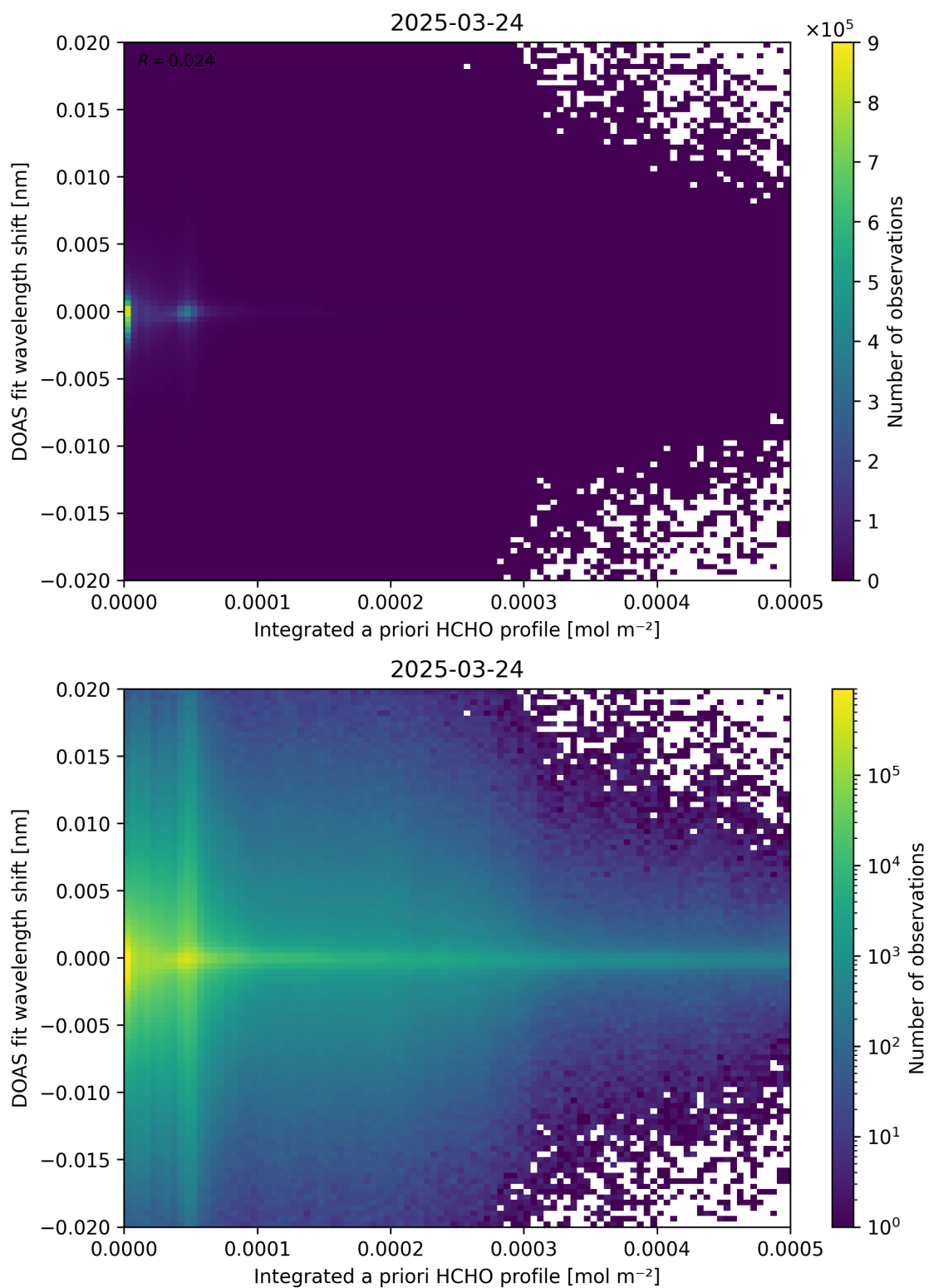
Figure 149: Scatter density plot of “Integrated a priori HCHO profile” against “DOAS fit wavelength shift” for 2025-03-23 to 2025-03-25.
