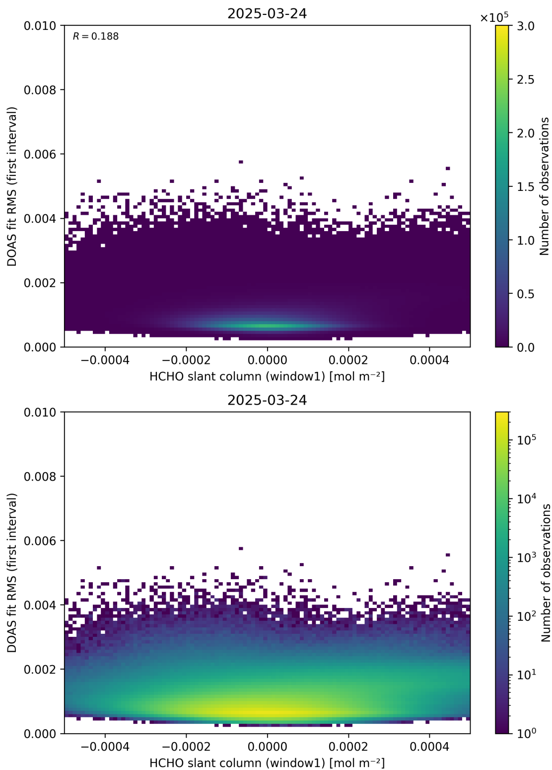
Figure 78: Scatter density plot of “HCHO slant column (window1)” against “DOAS fit RMS (first interval)” for 2025-03-23 to 2025-03-25.
