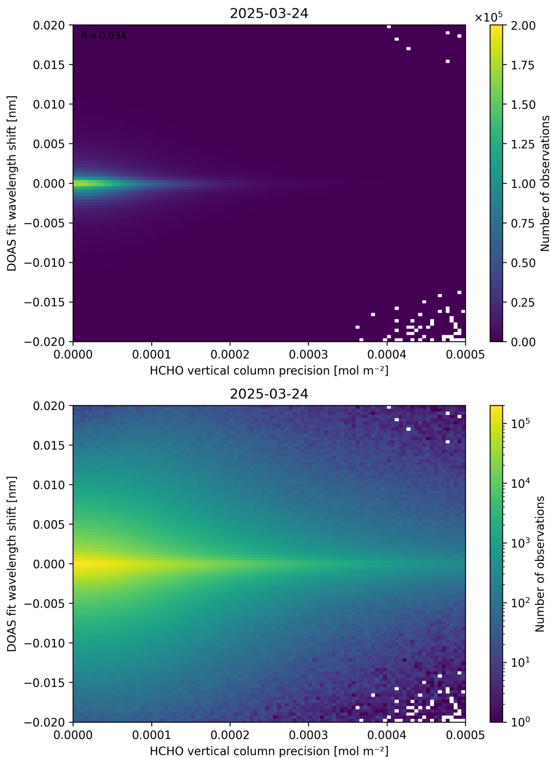
Figure 137: Scatter density plot of “HCHO vertical column precision” against “DOAS fit wavelength shift” for 2025-03-23 to 2025-03-25.
