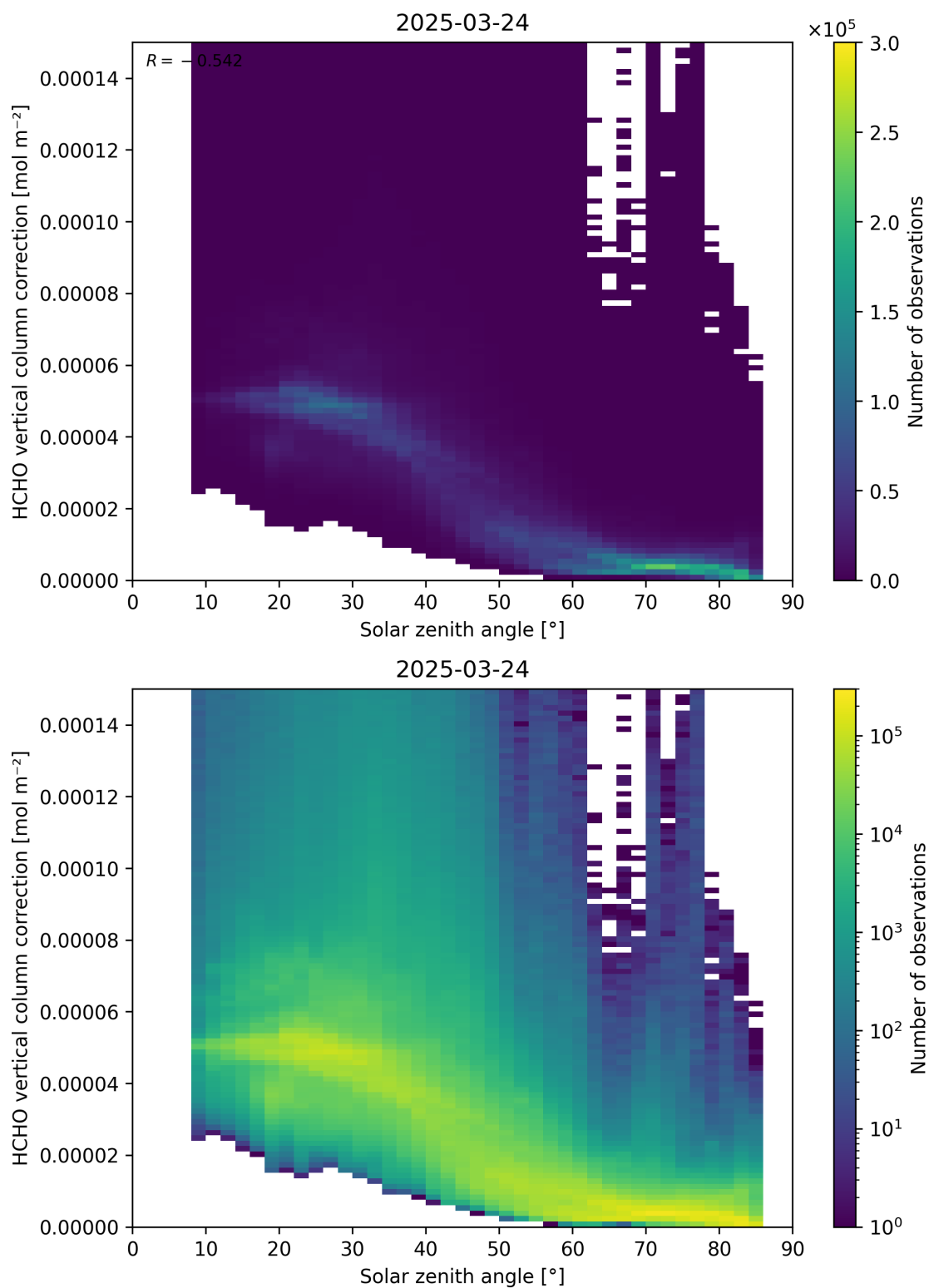
Figure 178: Scatter density plot of “Solar zenith angle” against “HCHO vertical column correction” for 2025-03-23 to 2025-03-25.
