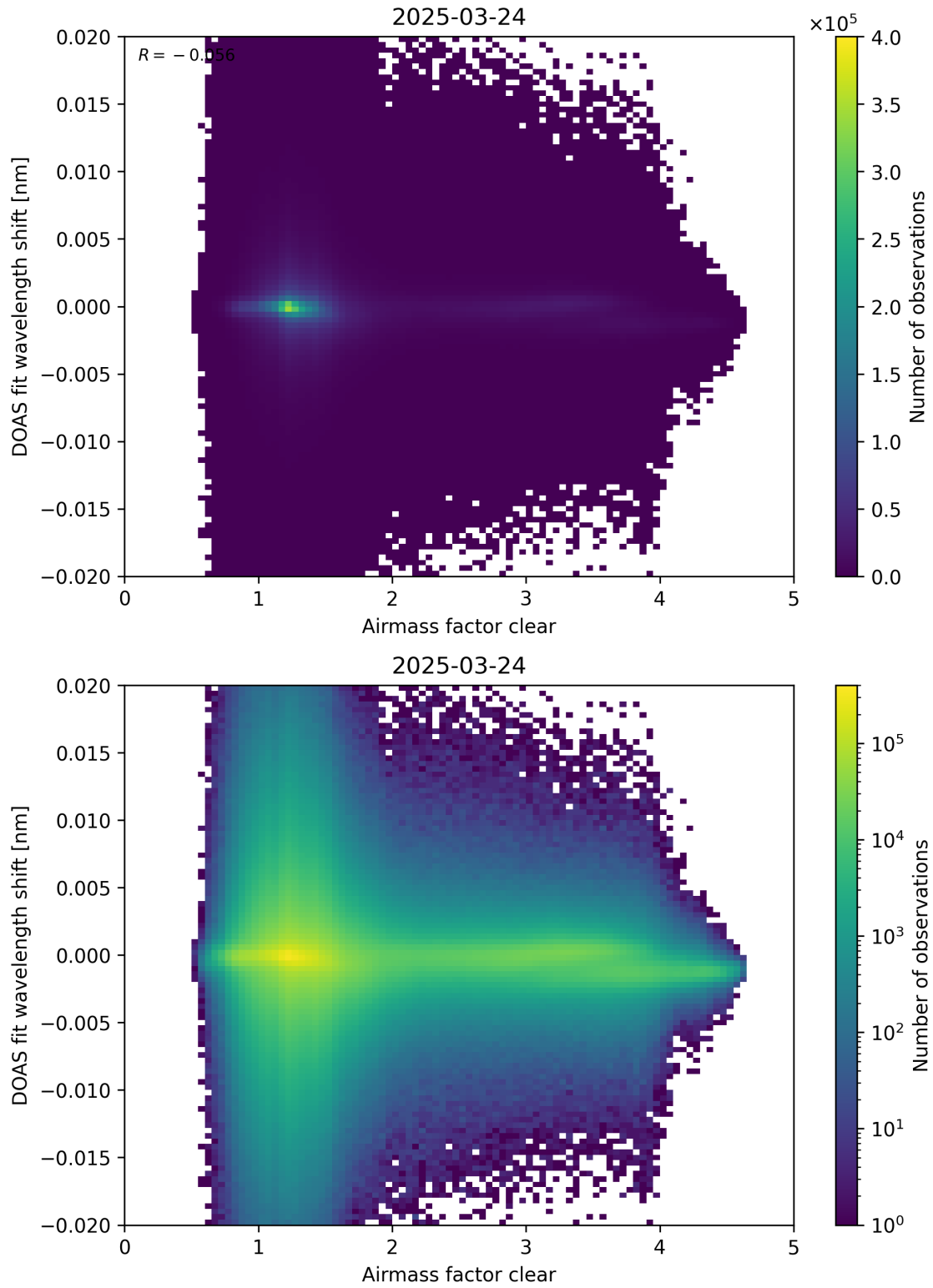
Figure 72: Scatter density plot of “Airmass factor clear” against “DOAS fit wavelength shift” for 2025-03-23 to 2025-03-25.
