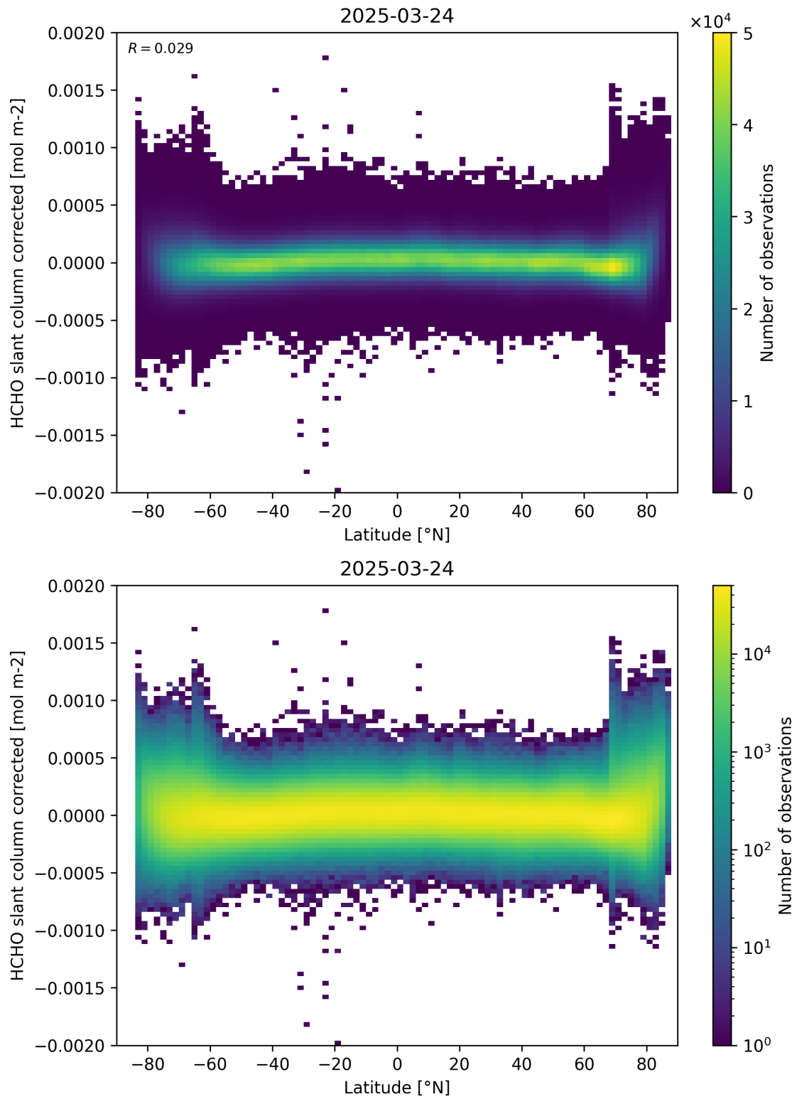
Figure 157: Scatter density plot of “Latitude” against “HCHO slant column corrected” for 2025-03-23 to 2025-03-25.
