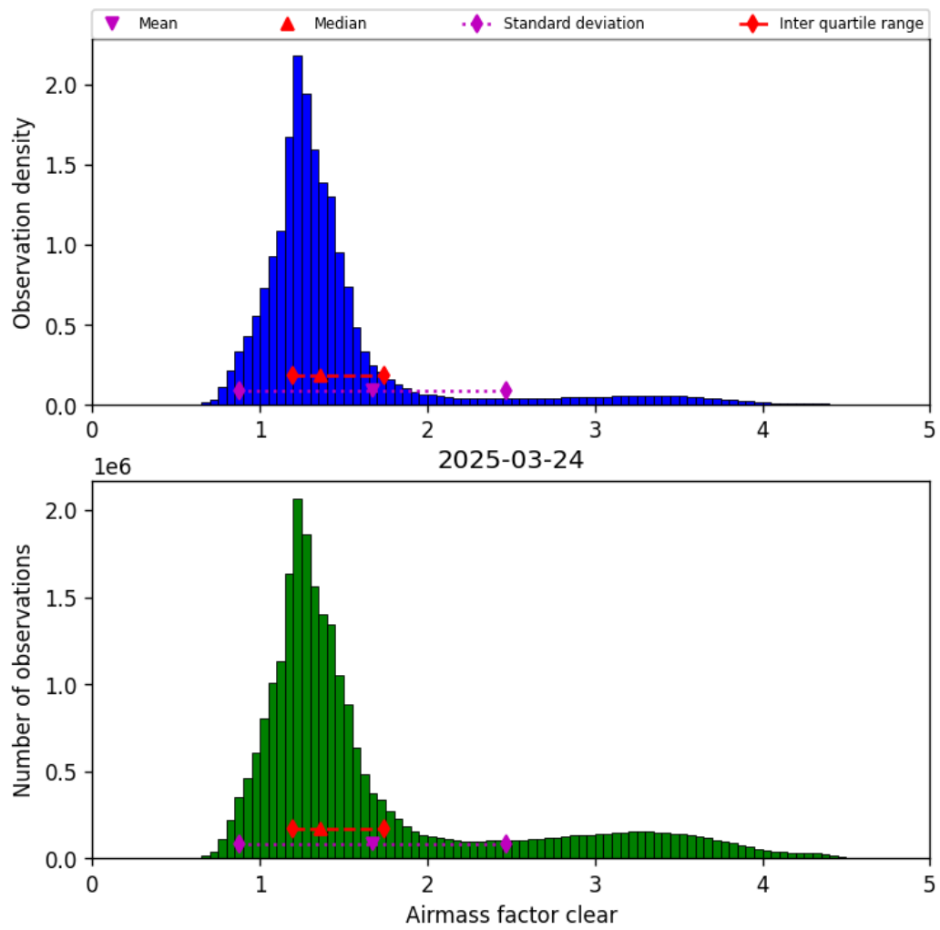
Figure 42: Histogram of “Airmass factor clear” for 2025-03-23 to 2025-03-25
