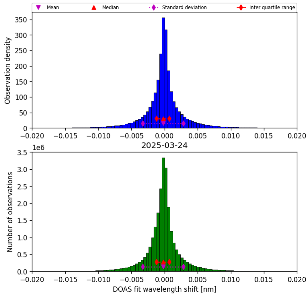
Figure 44: Histogram of “DOAS fit wavelength shift” for 2025-03-23 to 2025-03-25
