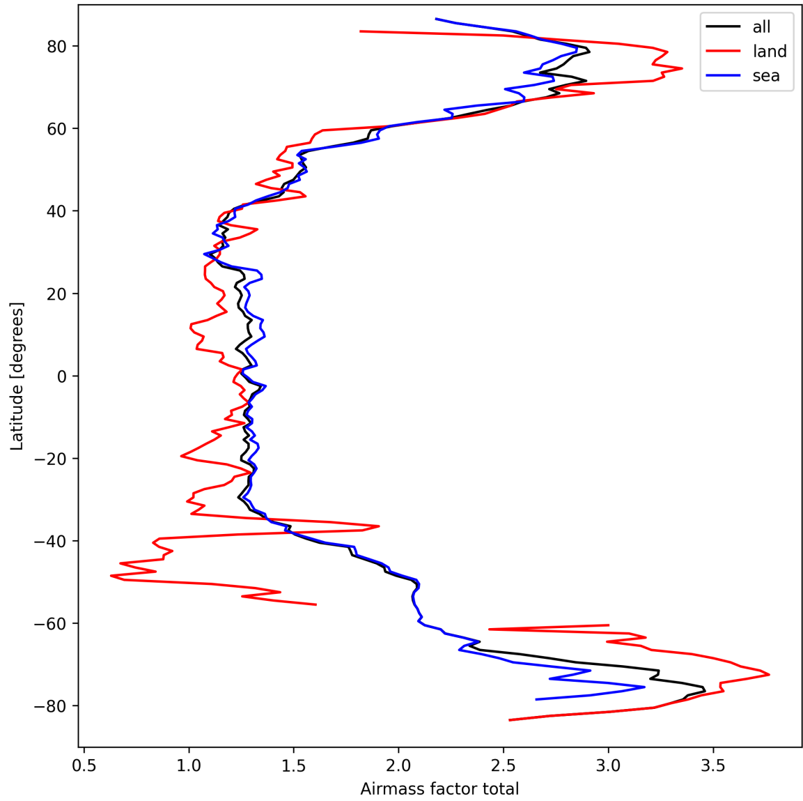
Figure 26: Zonal average of “Airmass factor total” for 2025-03-23 to 2025-03-25.
