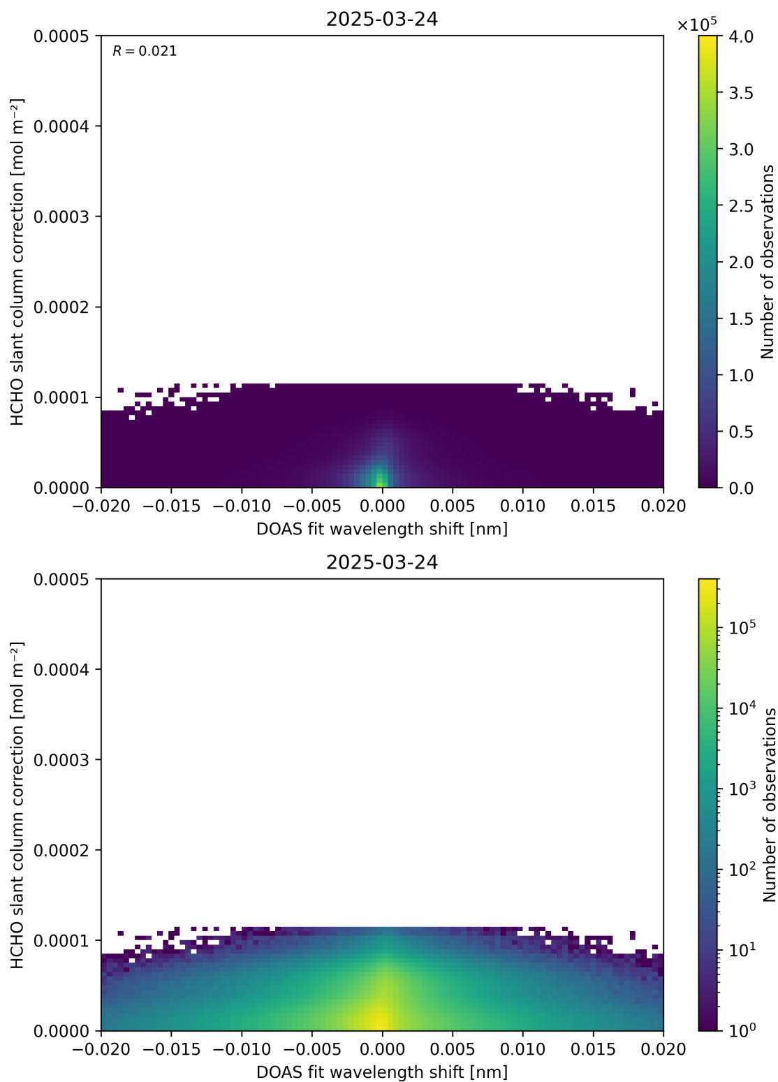
Figure 67: Scatter density plot of “DOAS fit wavelength shift” against “HCHO slant column correction” for 2025-03-23 to 2025-03-25.
