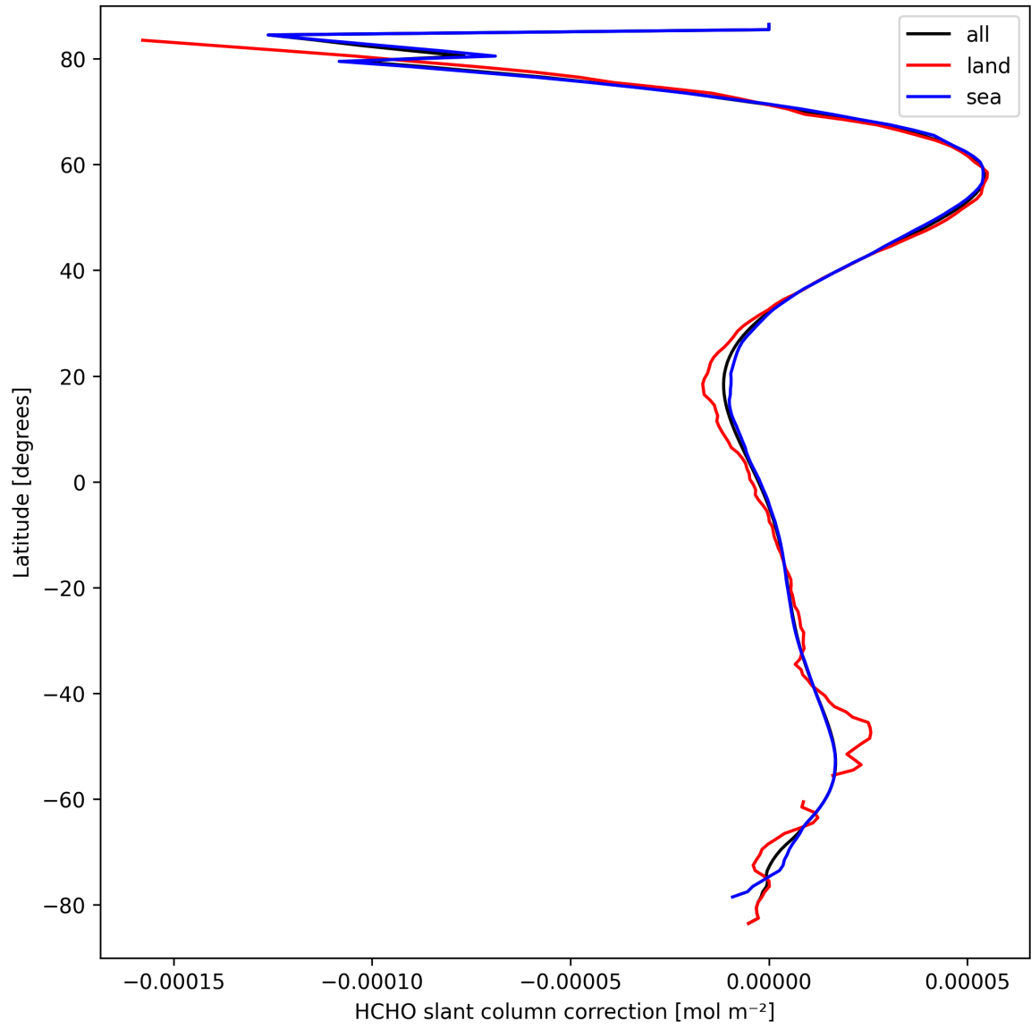
Figure 33: Zonal average of “HCHO slant column correction” for 2025-03-23 to 2025-03-25.
