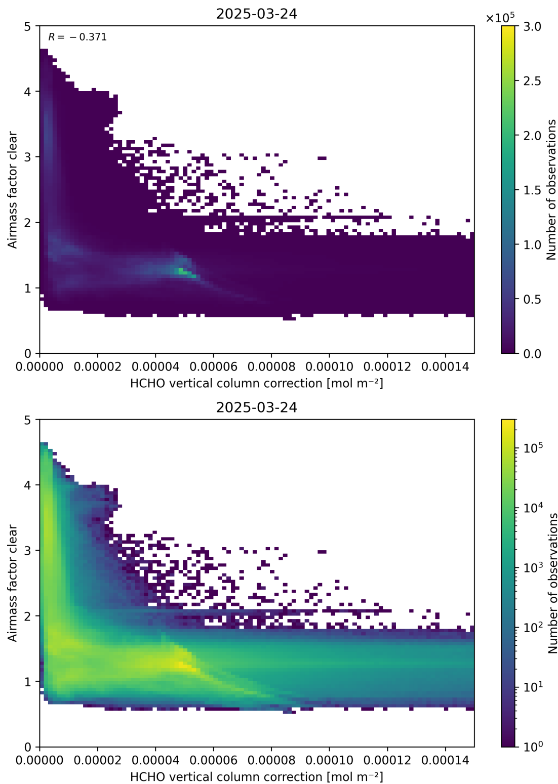
Figure 115: Scatter density plot of “HCHO vertical column correction” against “Airmass factor clear” for 2025-03-23 to 2025-03-25.
