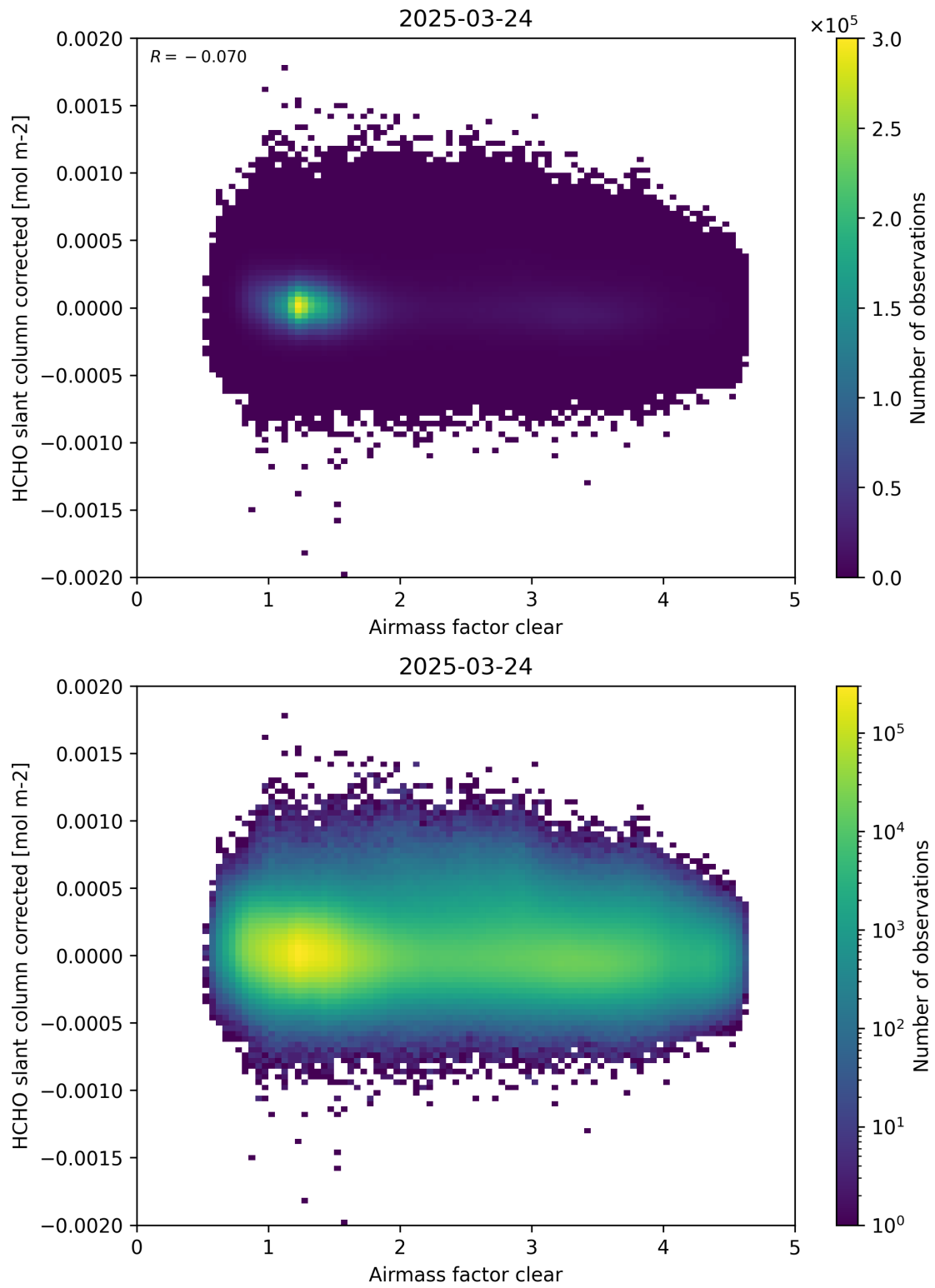
Figure 74: Scatter density plot of “Airmass factor clear” against “HCHO slant column corrected” for 2025-03-23 to 2025-03-25.
