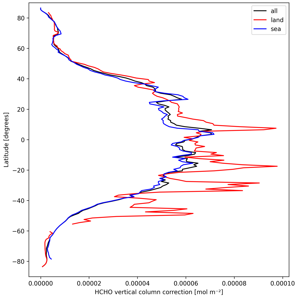
Figure 23: Zonal average of “HCHO vertical column correction” for 2025-03-23 to 2025-03-25.
