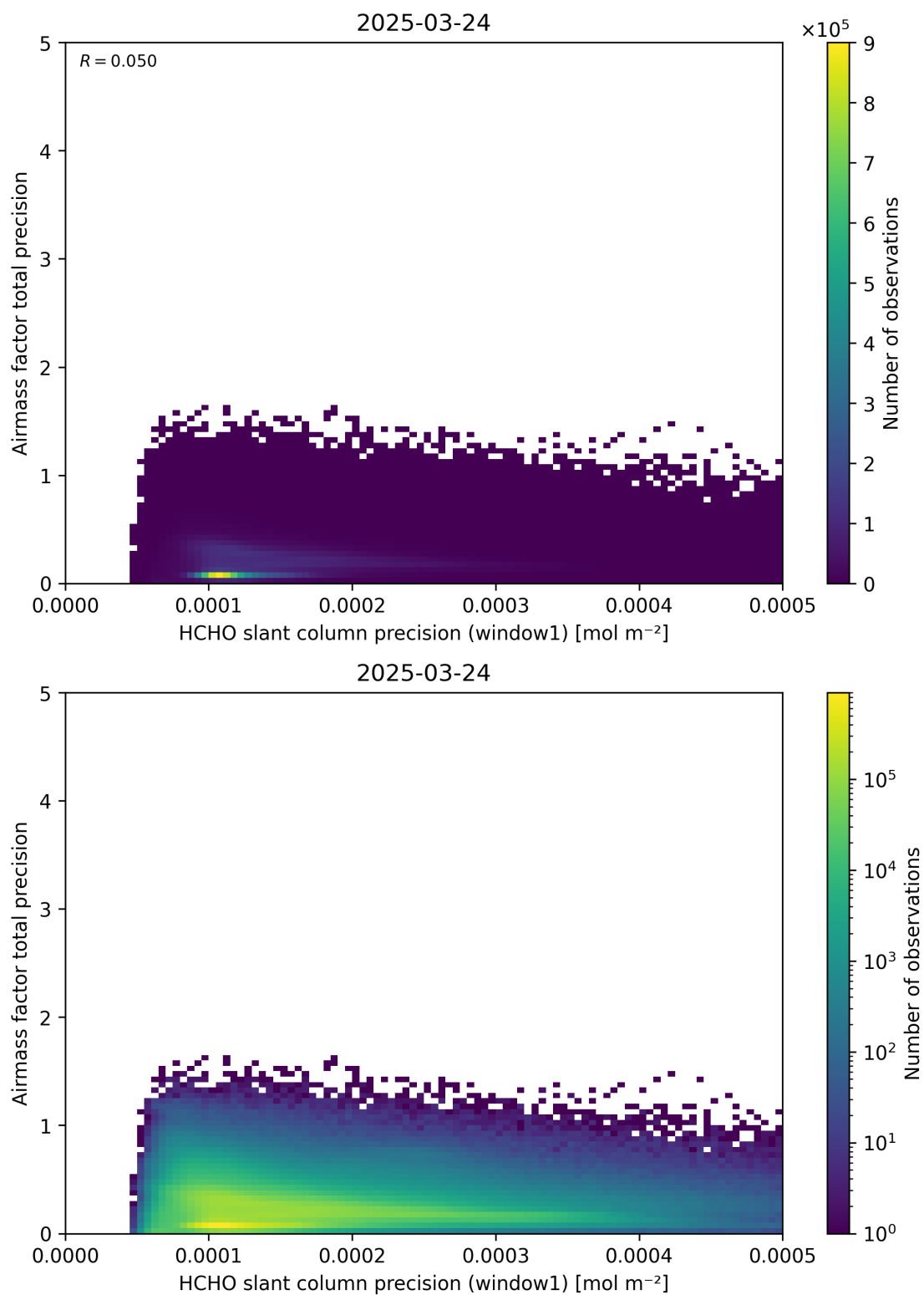
Figure 95: Scatter density plot of “HCHO slant column precision (window1)” against “Airmass factor total precision” for 2025-03-23 to 2025-03-25.
