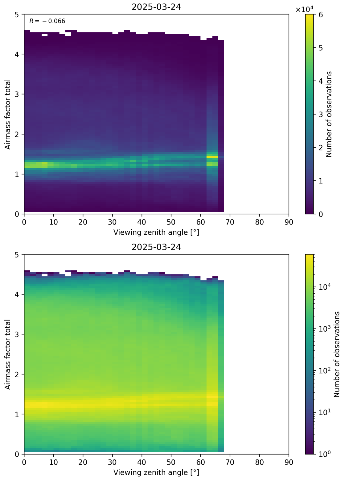
Figure 190: Scatter density plot of “Viewing zenith angle” against “Airmass factor total” for 2025-03-23 to 2025-03-25.
