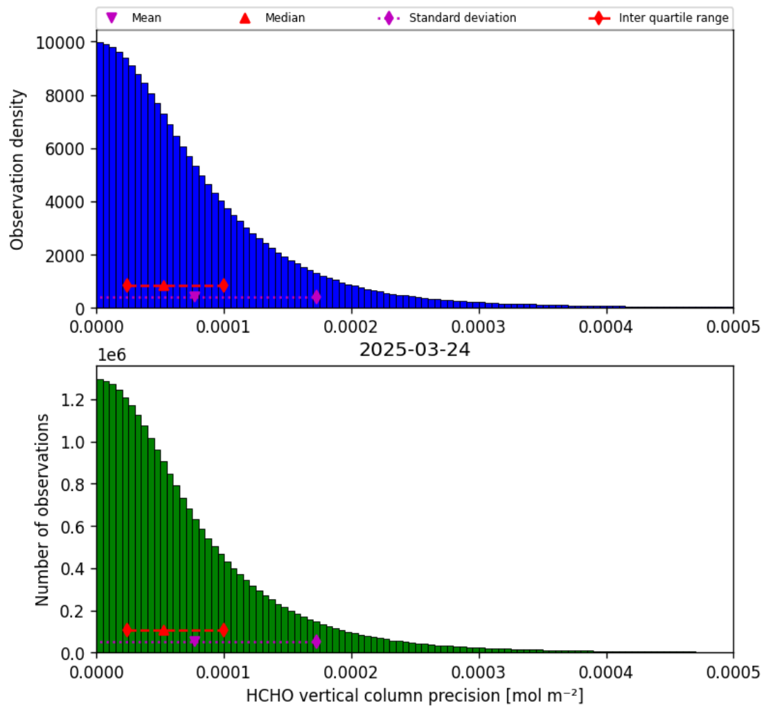
Figure 36: Histogram of “HCHO vertical column precision” for 2025-03-23 to 2025-03-25
