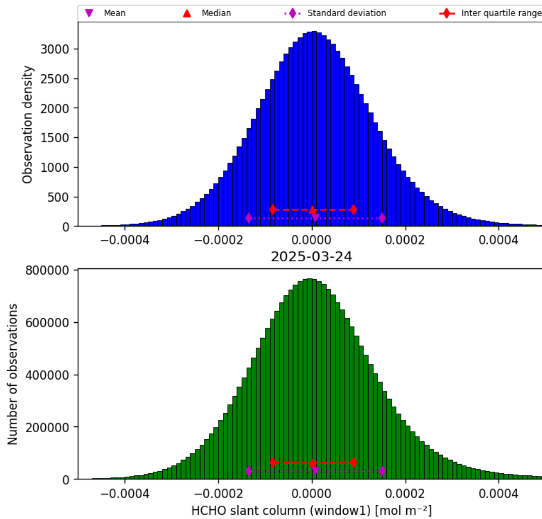
Figure 38: Histogram of “HCHO slant column (window1)” for 2025-03-23 to 2025-03-25
