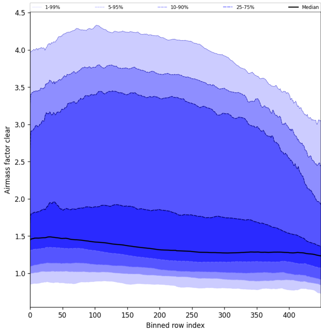
Figure 56: Along track statistics of “Airmass factor clear” for 2025-03-23 to 2025-03-25
