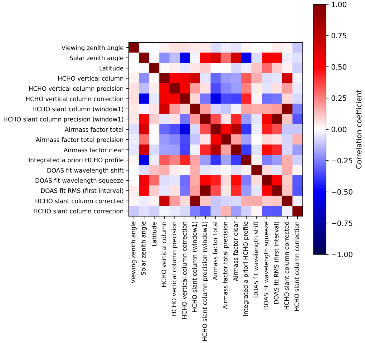
Figure 2: Map of correlation matrix for 2025-03-23 to 2025-03-25.
