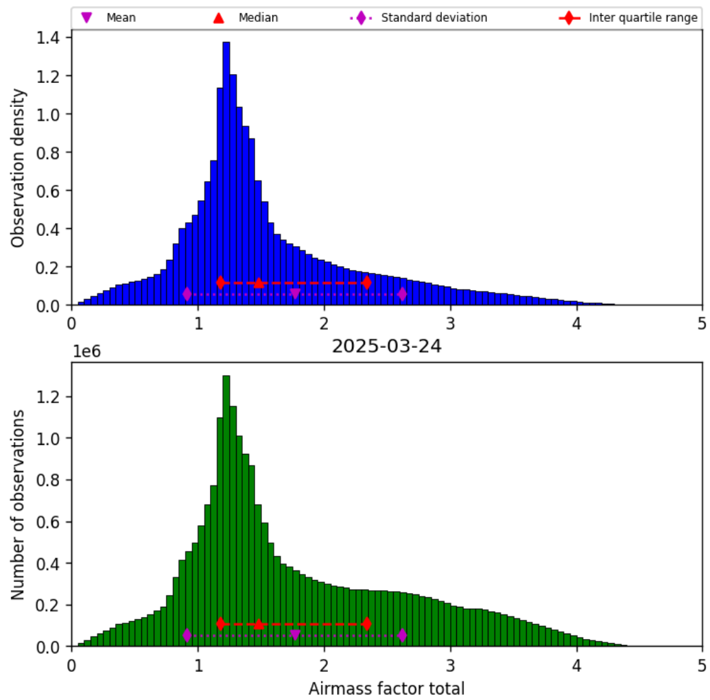
Figure 40: Histogram of “Airmass factor total” for 2025-03-23 to 2025-03-25
