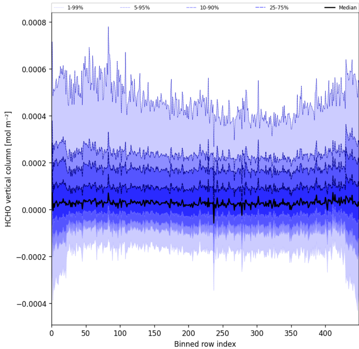
Figure 49: Along track statistics of “HCHO vertical column” for 2025-03-23 to 2025-03-25
