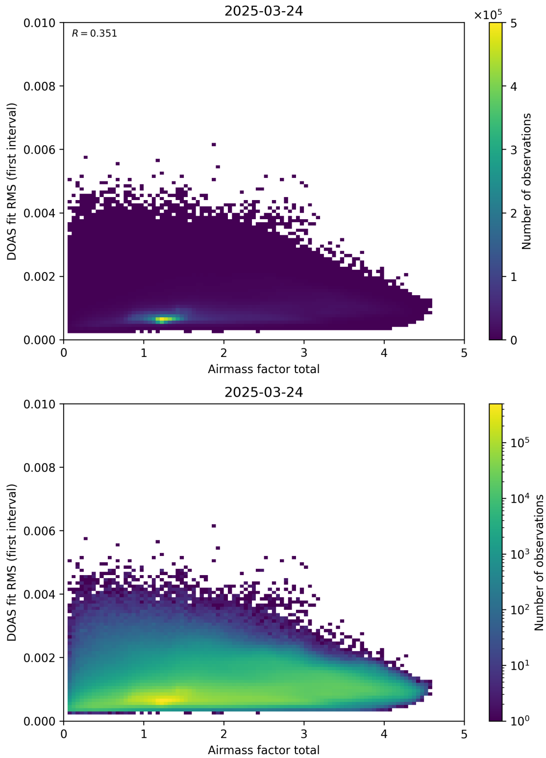
Figure 97: Scatter density plot of “Airmass factor total” against “DOAS fit RMS (first interval)” for 2025-03-23 to 2025-03-25.
