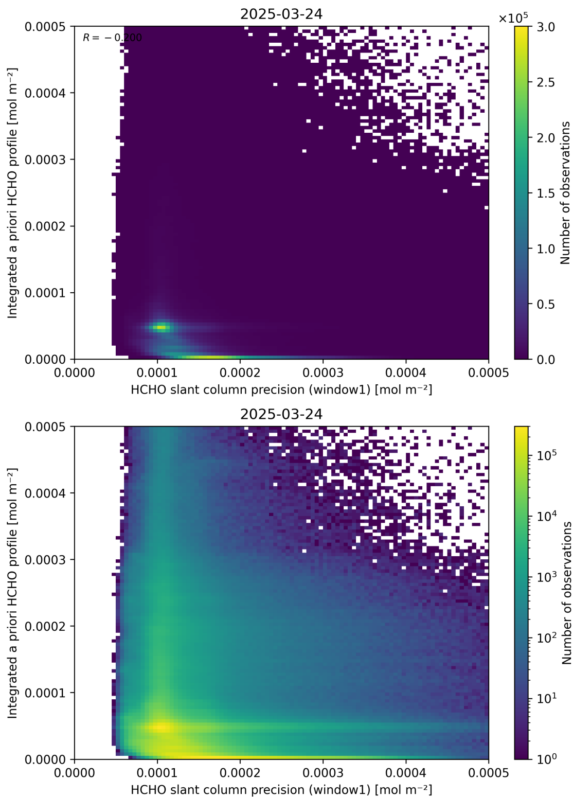
Figure 96: Scatter density plot of “HCHO slant column precision (window1)” against “Integrated a priori HCHO profile” for 2025-03-23 to 2025-03-25.
