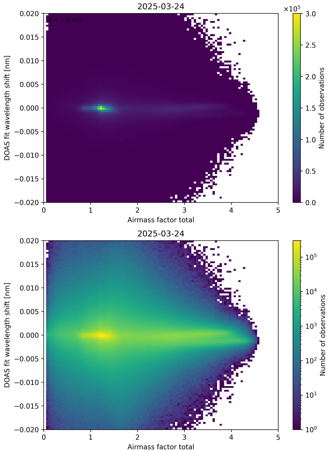
Figure 98: Scatter density plot of “Airmass factor total” against “DOAS fit wavelength shift” for 2025-03-23 to 2025-03-25.
