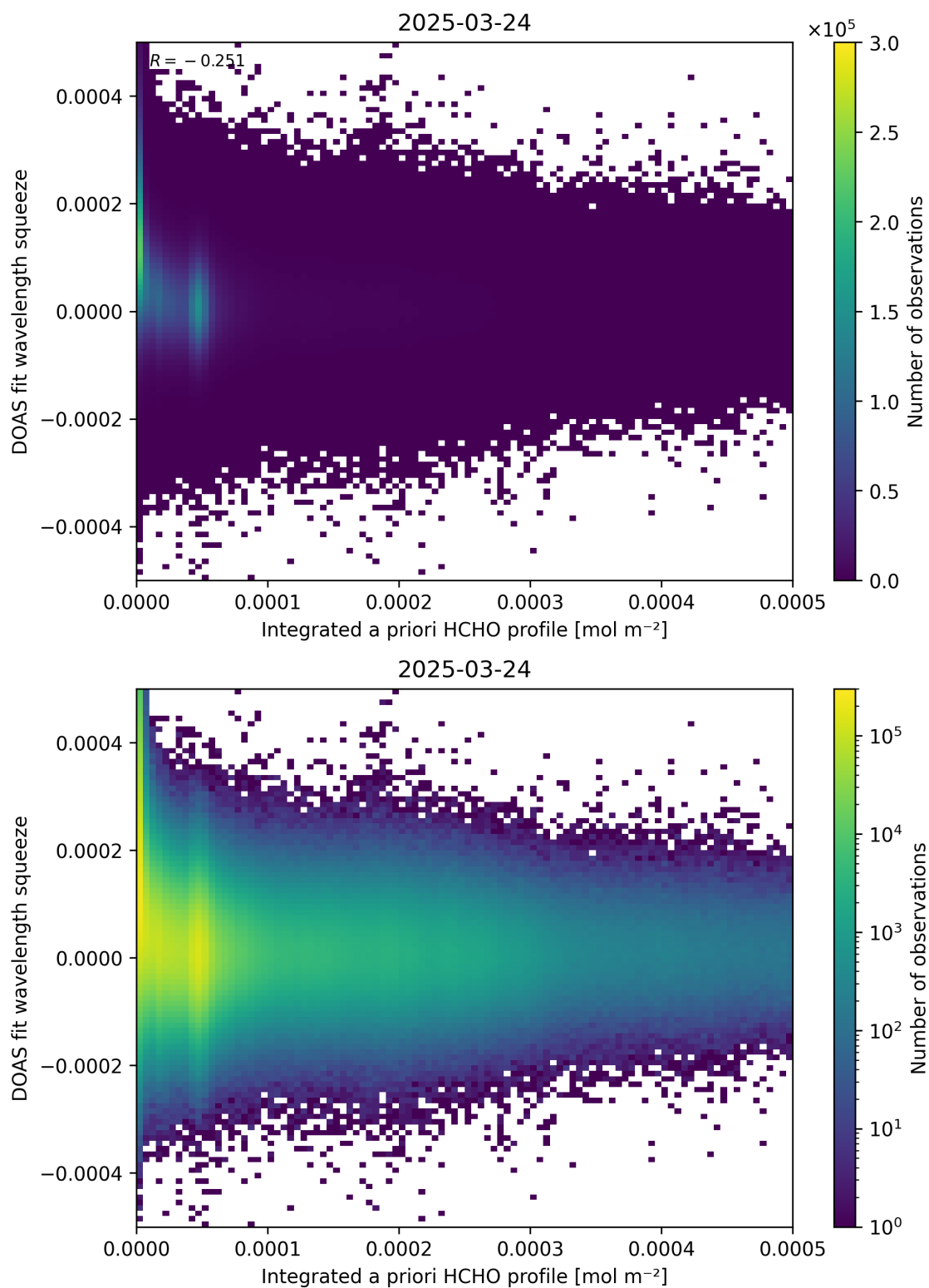
Figure 150: Scatter density plot of “Integrated a priori HCHO profile” against “DOAS fit wavelength squeeze” for 2025-03-23 to 2025-03-25.
