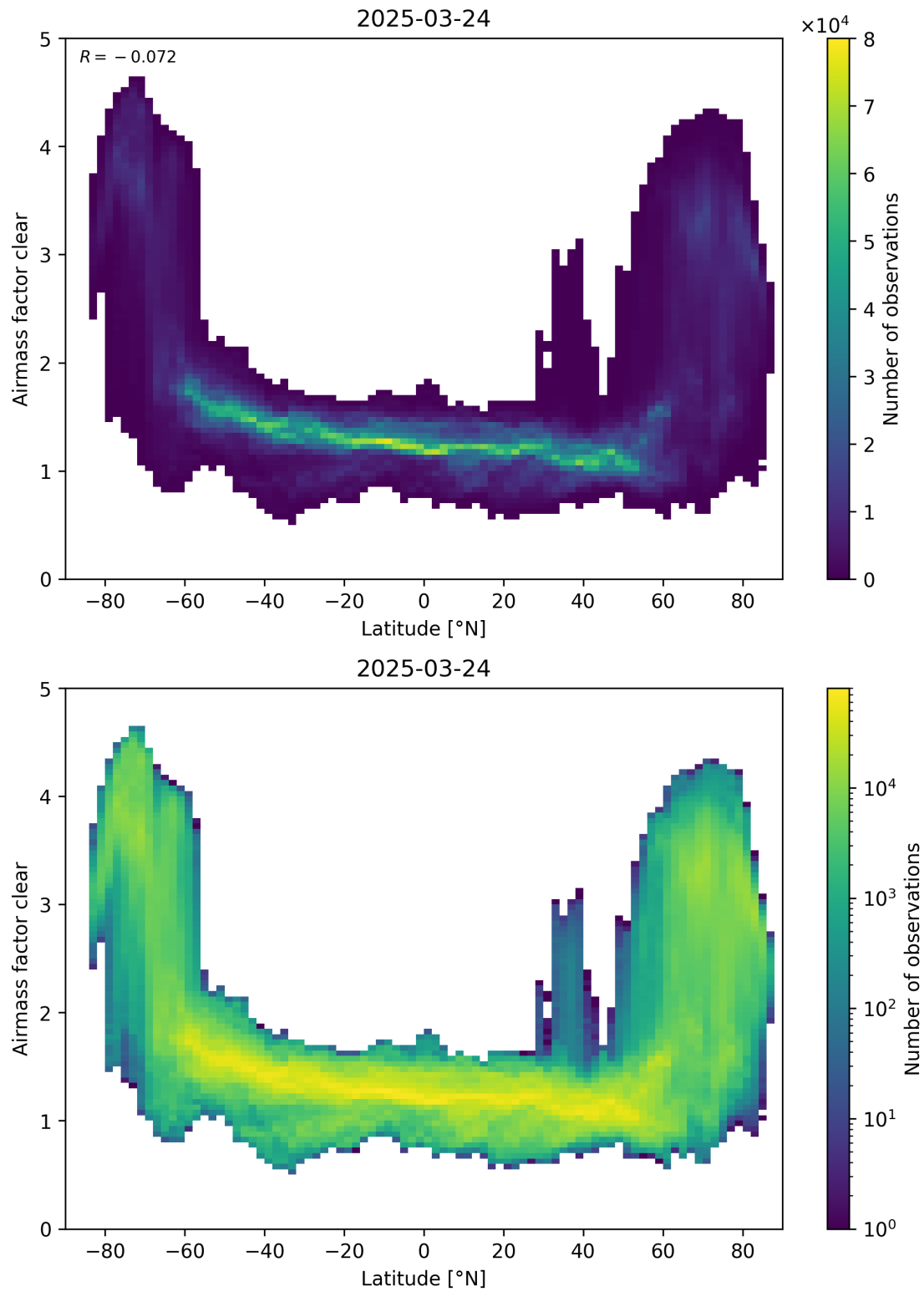
Figure 156: Scatter density plot of “Latitude” against “Airmass factor clear” for 2025-03-23 to 2025-03-25.
