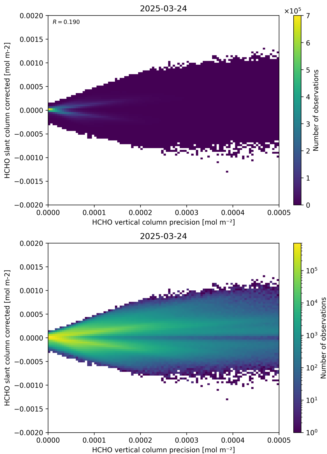
Figure 140: Scatter density plot of “HCHO vertical column precision” against “HCHO slant column corrected” for 2025-03-23 to 2025-03-25.
