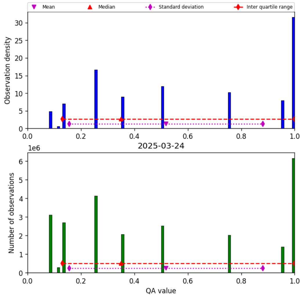
Figure 34: Histogram of “QA value” for 2025-03-23 to 2025-03-25
