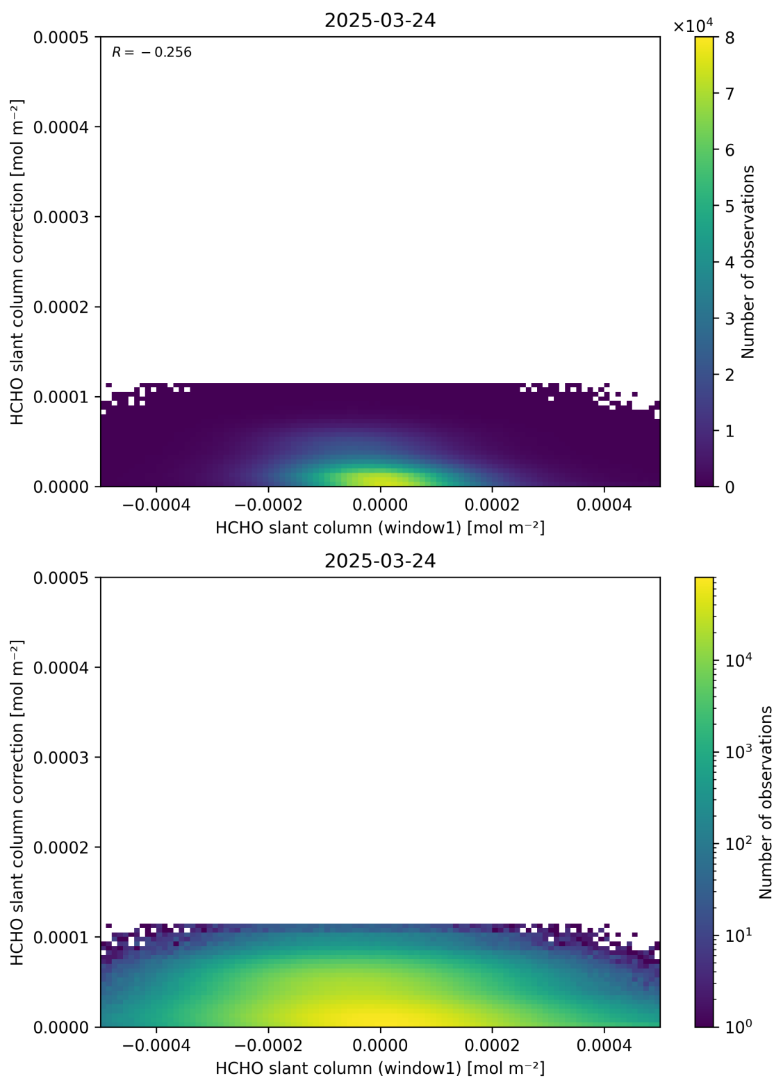
Figure 83: Scatter density plot of “HCHO slant column (window1)” against “HCHO slant column correction” for 2025-03-23 to 2025-03-25.
