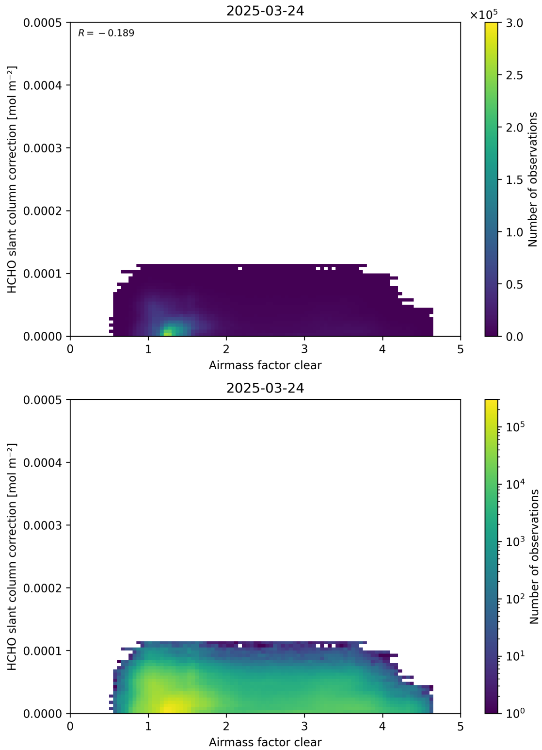
Figure 75: Scatter density plot of “Airmass factor clear” against “HCHO slant column correction” for 2025-03-23 to 2025-03-25.
