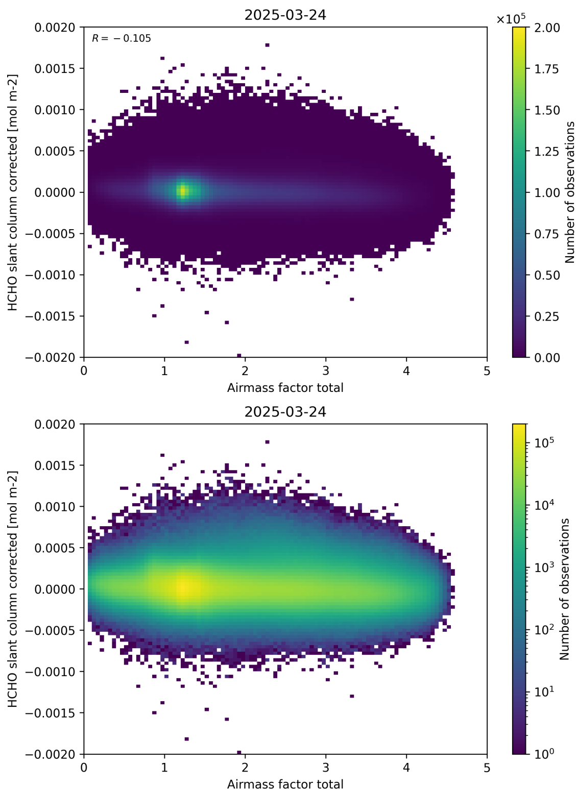
Figure 101: Scatter density plot of “Airmass factor total” against “HCHO slant column corrected” for 2025-03-23 to 2025-03-25.
