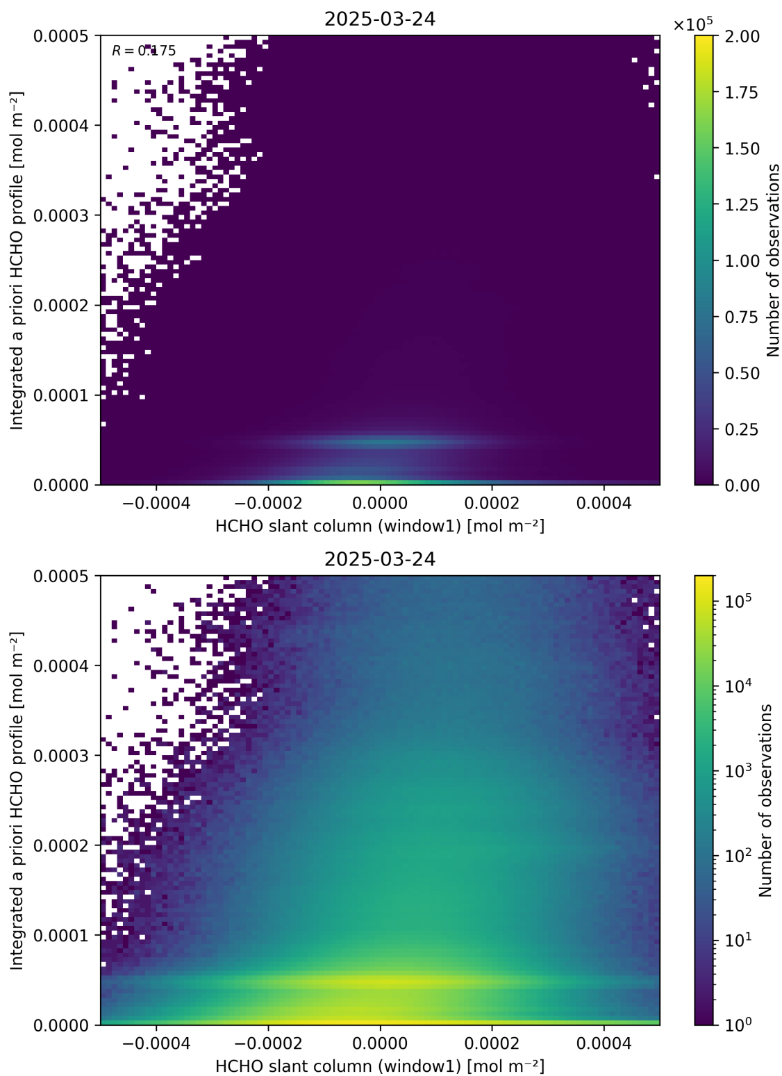
Figure 87: Scatter density plot of “HCHO slant column (window1)” against “Integrated a priori HCHO profile” for 2025-03-23 to 2025-03-25.
