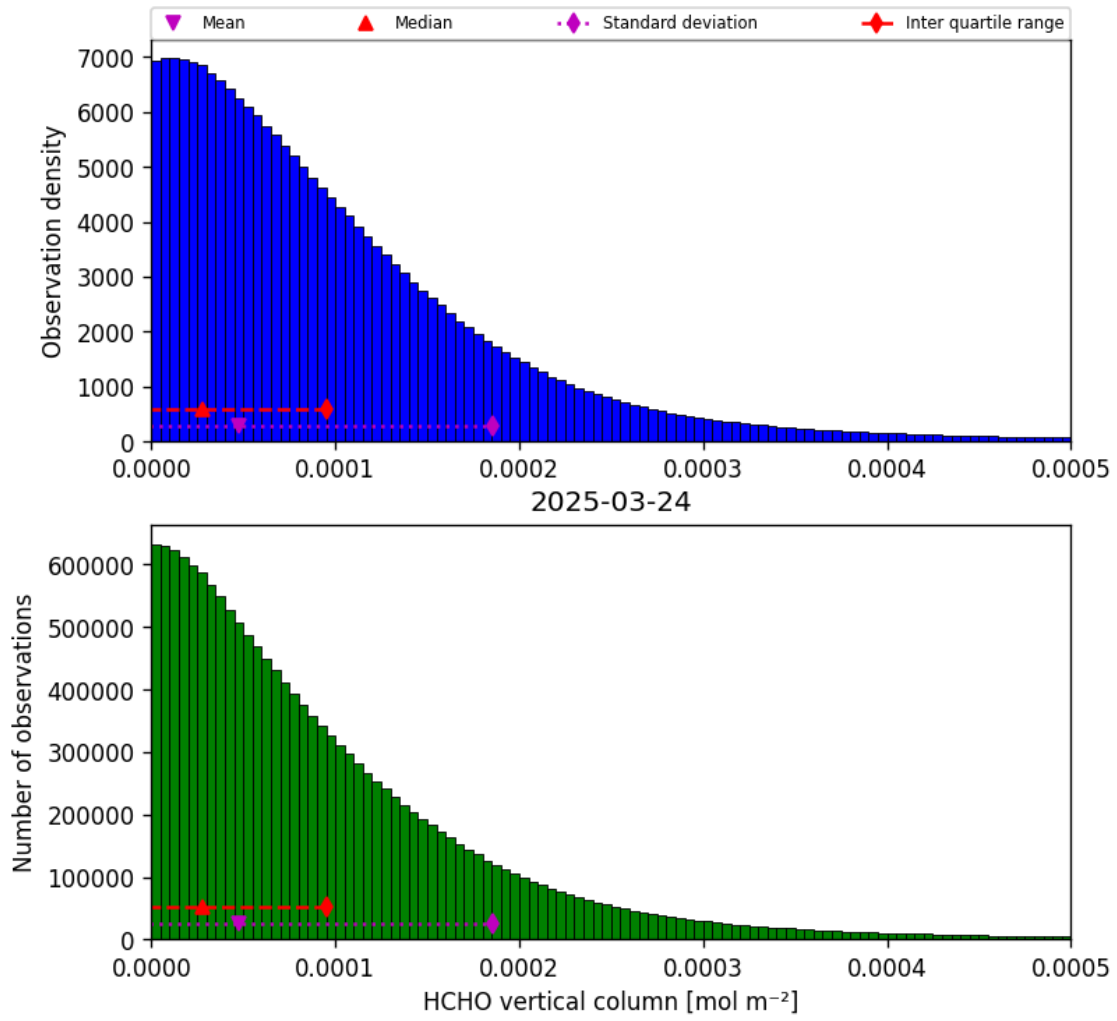
Figure 35: Histogram of “HCHO vertical column” for 2025-03-23 to 2025-03-25
