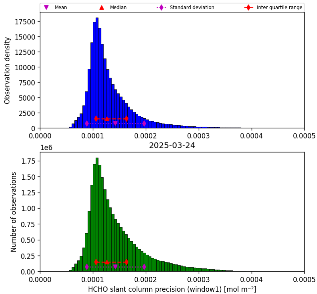
Figure 39: Histogram of “HCHO slant column precision (window1)” for 2025-03-23 to 2025-03-25
