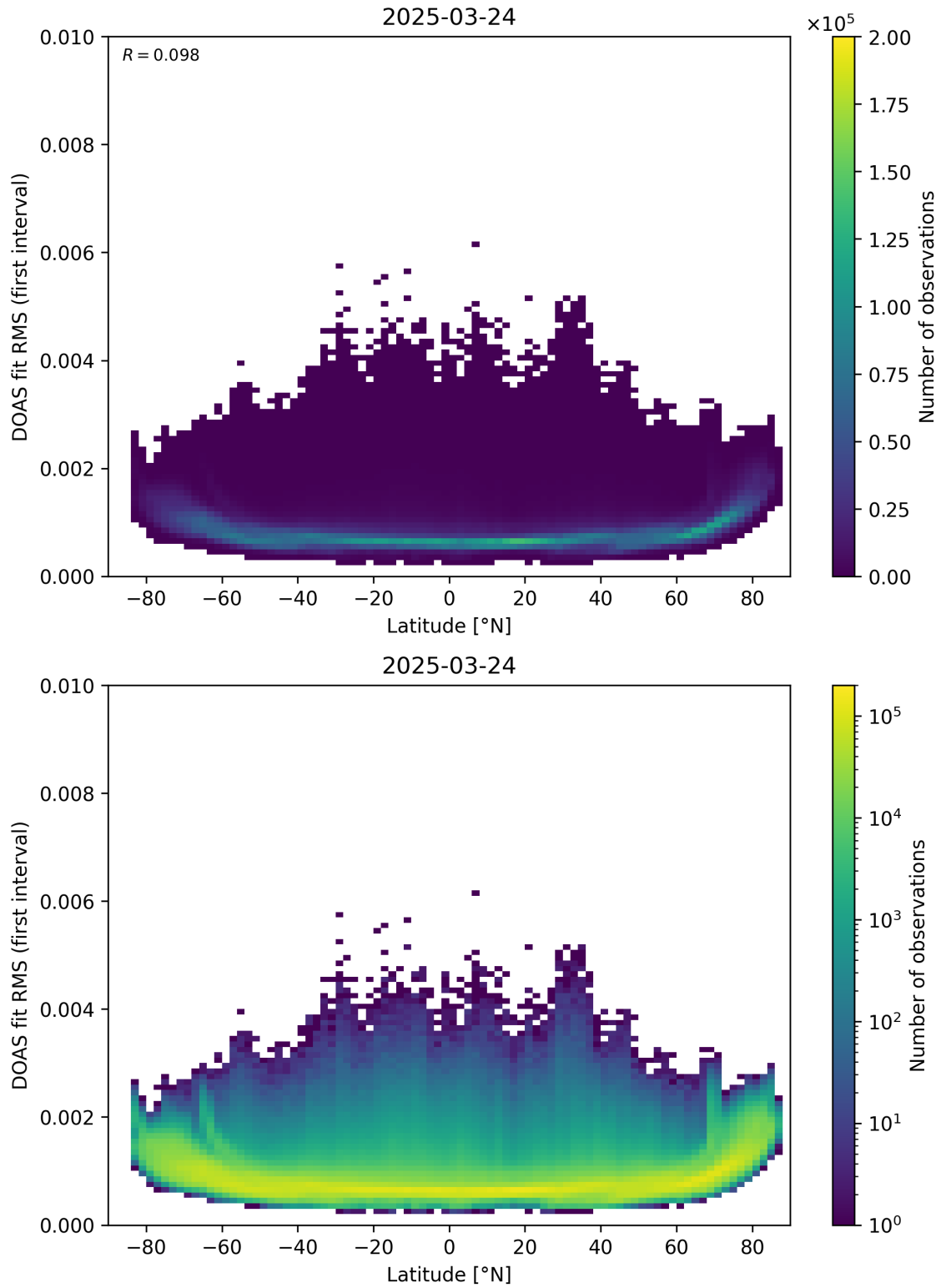
Figure 153: Scatter density plot of “Latitude” against “DOAS fit RMS (first interval)” for 2025-03-23 to 2025-03-25.
