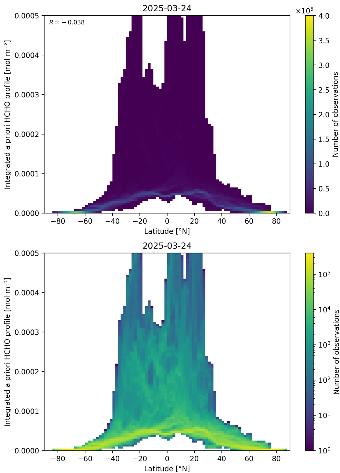
Figure 166: Scatter density plot of “Latitude” against “Integrated a priori HCHO profile” for 2025-03-23 to 2025-03-25.
