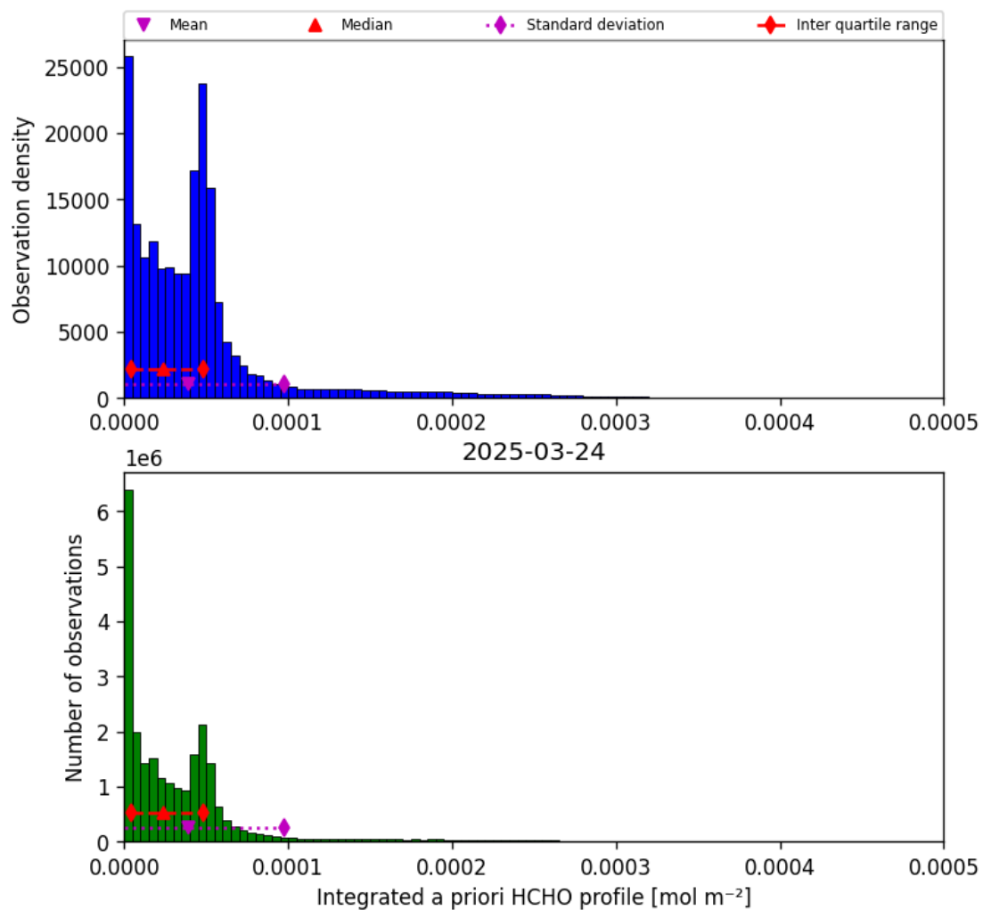
Figure 43: Histogram of “Integrated a priori HCHO profile” for 2025-03-23 to 2025-03-25
