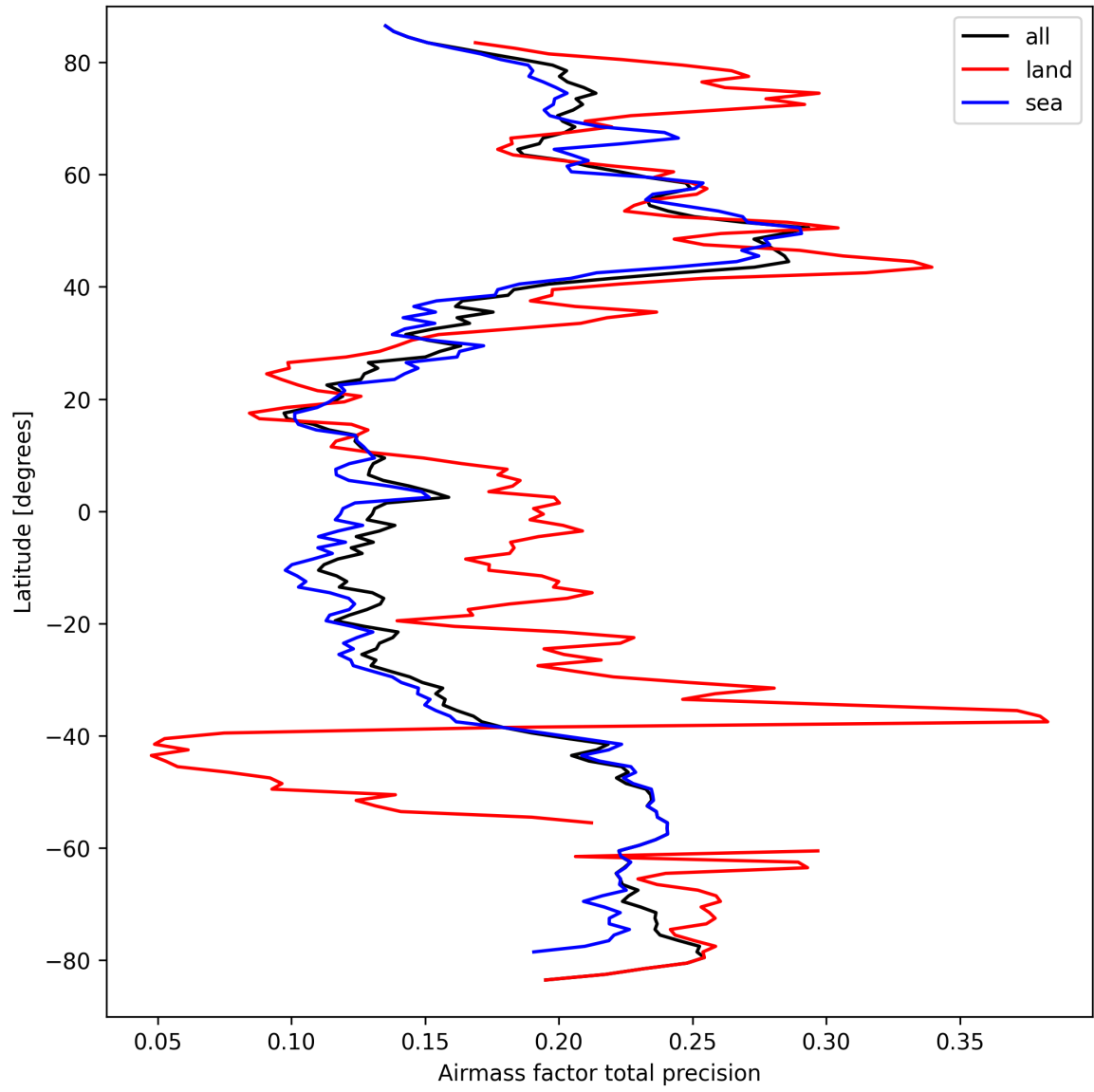
Figure 27: Zonal average of “Airmass factor total precision” for 2025-03-23 to 2025-03-25.
