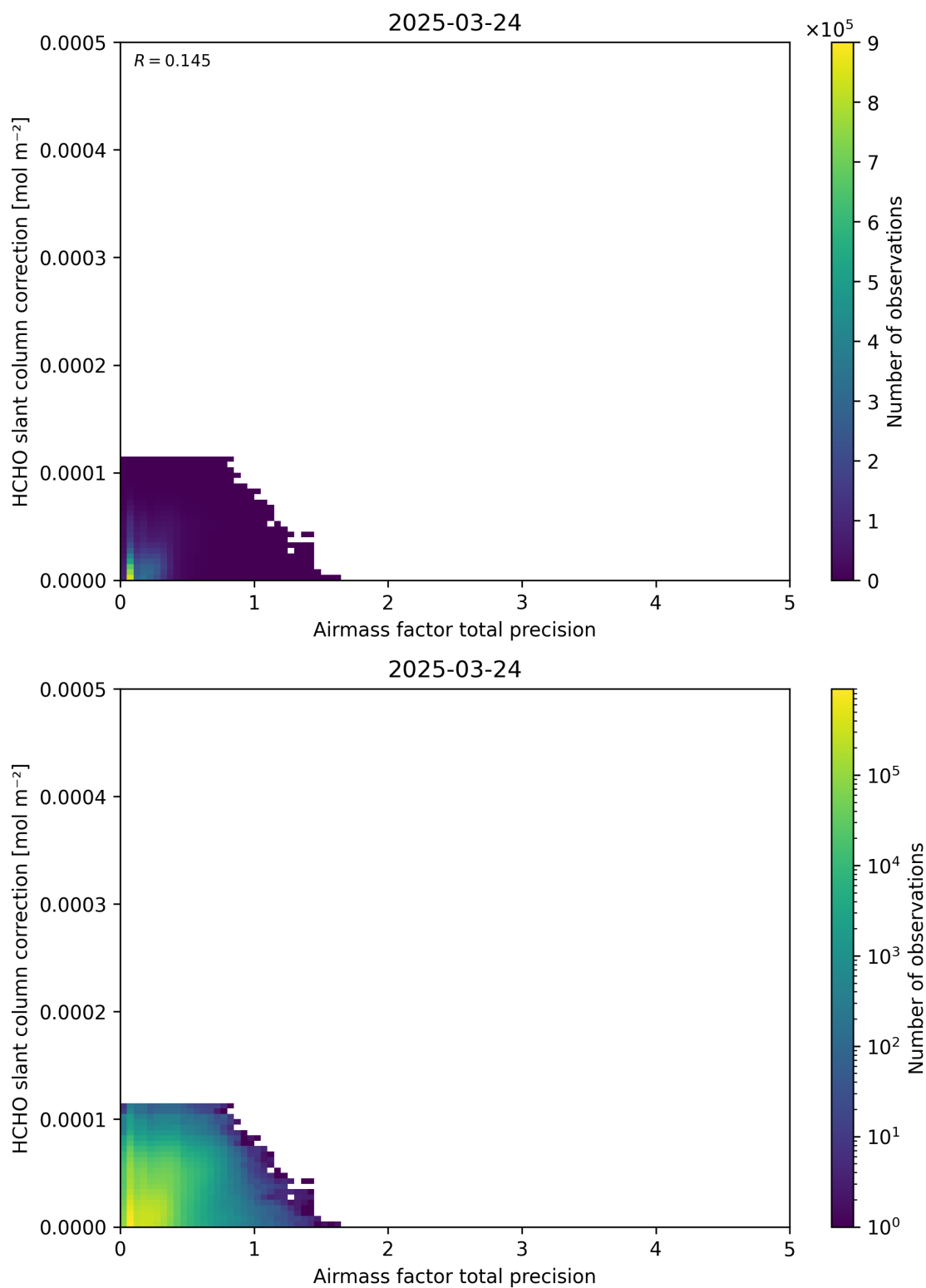
Figure 110: Scatter density plot of “Airmass factor total precision” against “HCHO slant column correction” for 2025-03-23 to 2025-03-25.
