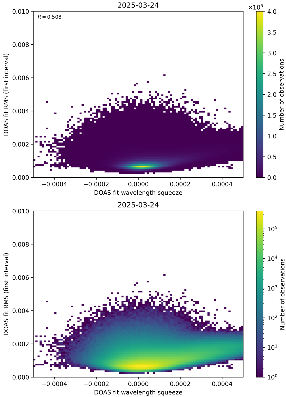
Figure 68: Scatter density plot of “DOAS fit wavelength squeeze” against “DOAS fit RMS (first interval)” for 2025-03-23 to 2025-03-25.
