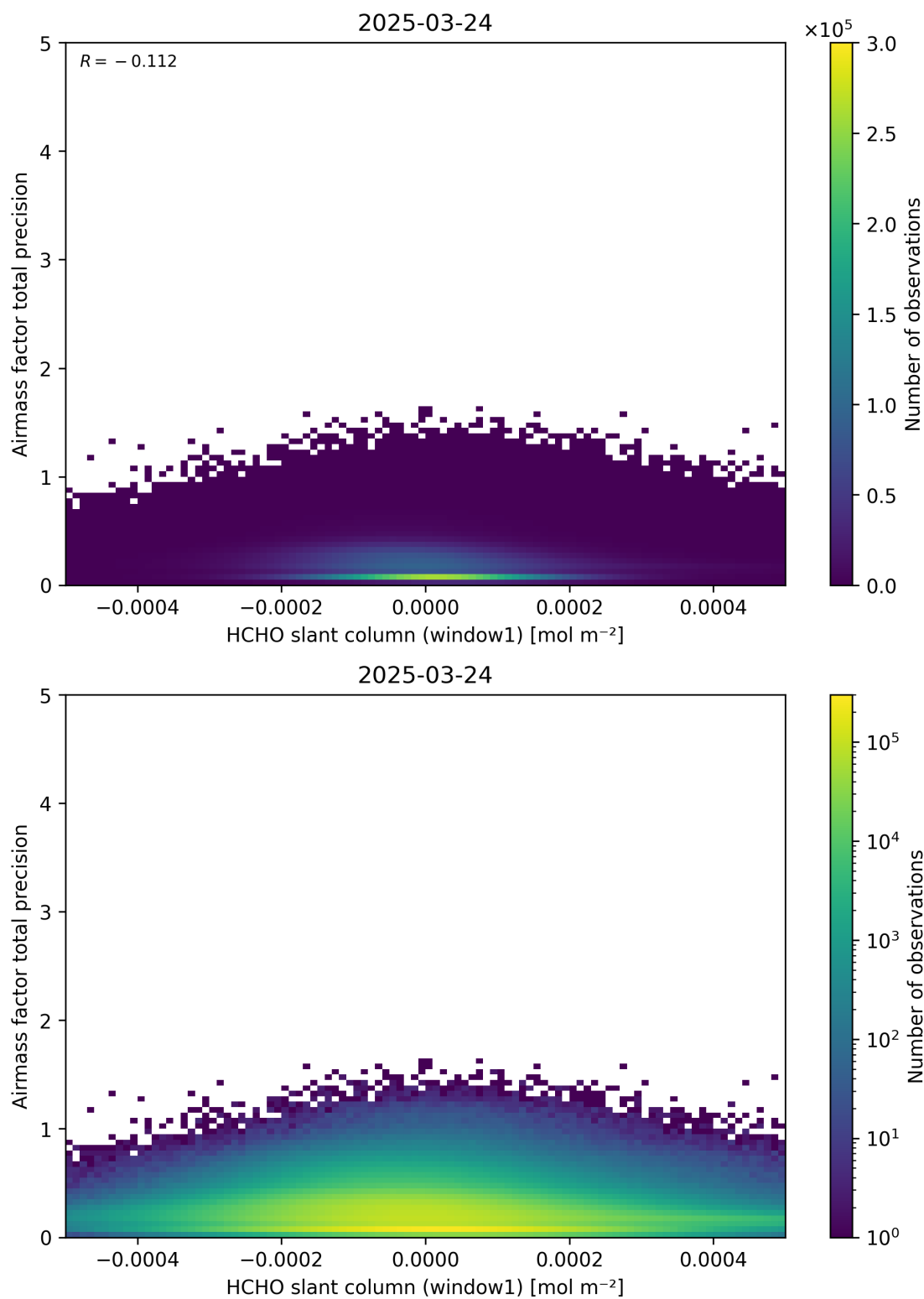
Figure 86: Scatter density plot of “HCHO slant column (window1)” against “Airmass factor total precision” for 2025-03-23 to 2025-03-25.
