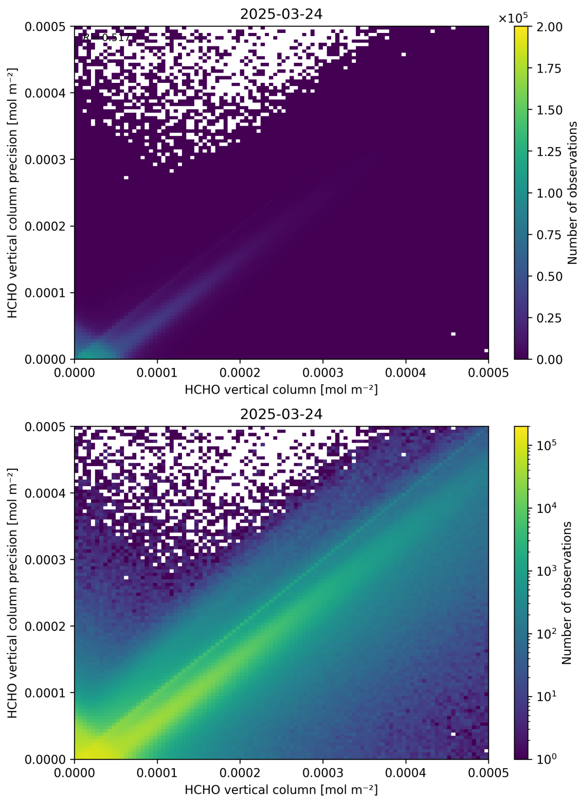
Figure 134: Scatter density plot of “HCHO vertical column” against “HCHO vertical column precision” for 2025-03-23 to 2025-03-25.
