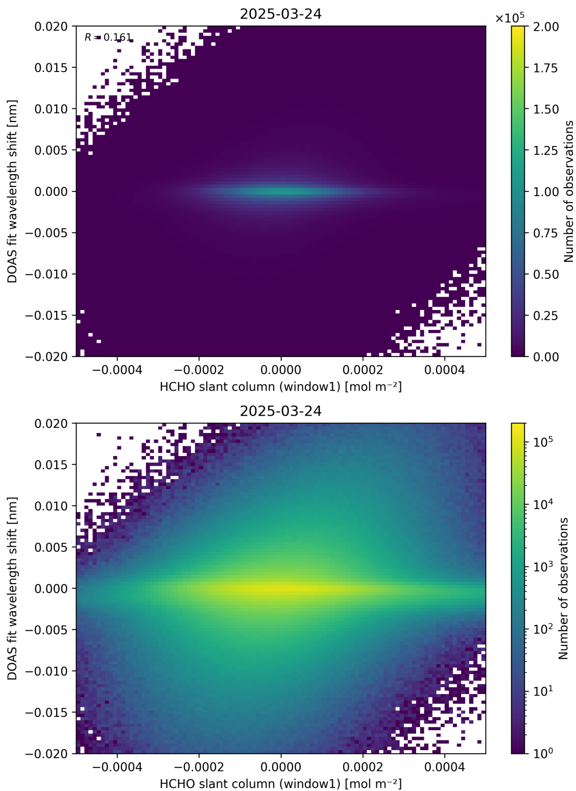
Figure 79: Scatter density plot of “HCHO slant column (window1)” against “DOAS fit wavelength shift” for 2025-03-23 to 2025-03-25.
