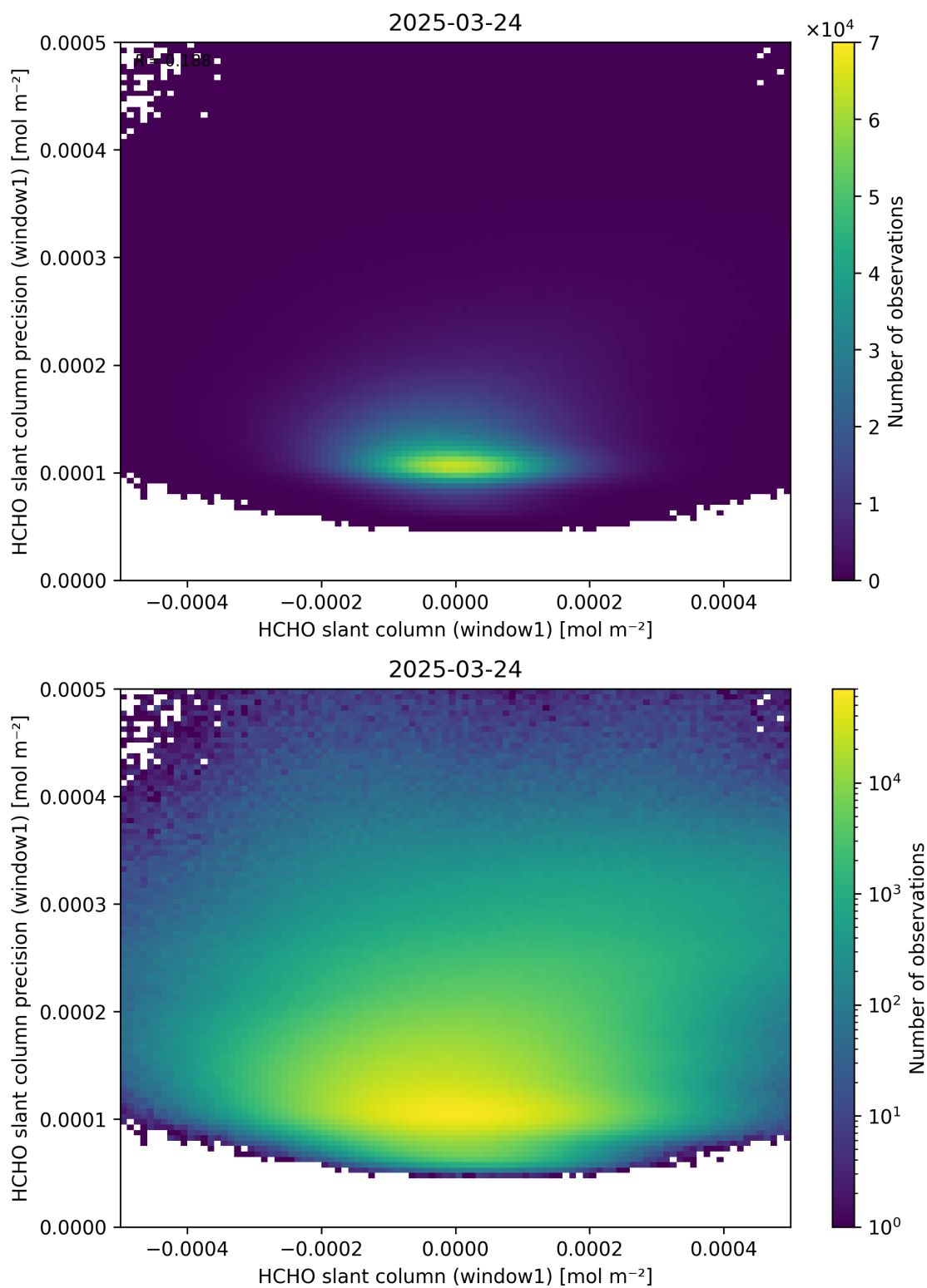
Figure 84: Scatter density plot of “HCHO slant column (window1)” against “HCHO slant column precision (window1)” for 2025-03-23 to 2025-03-25.
