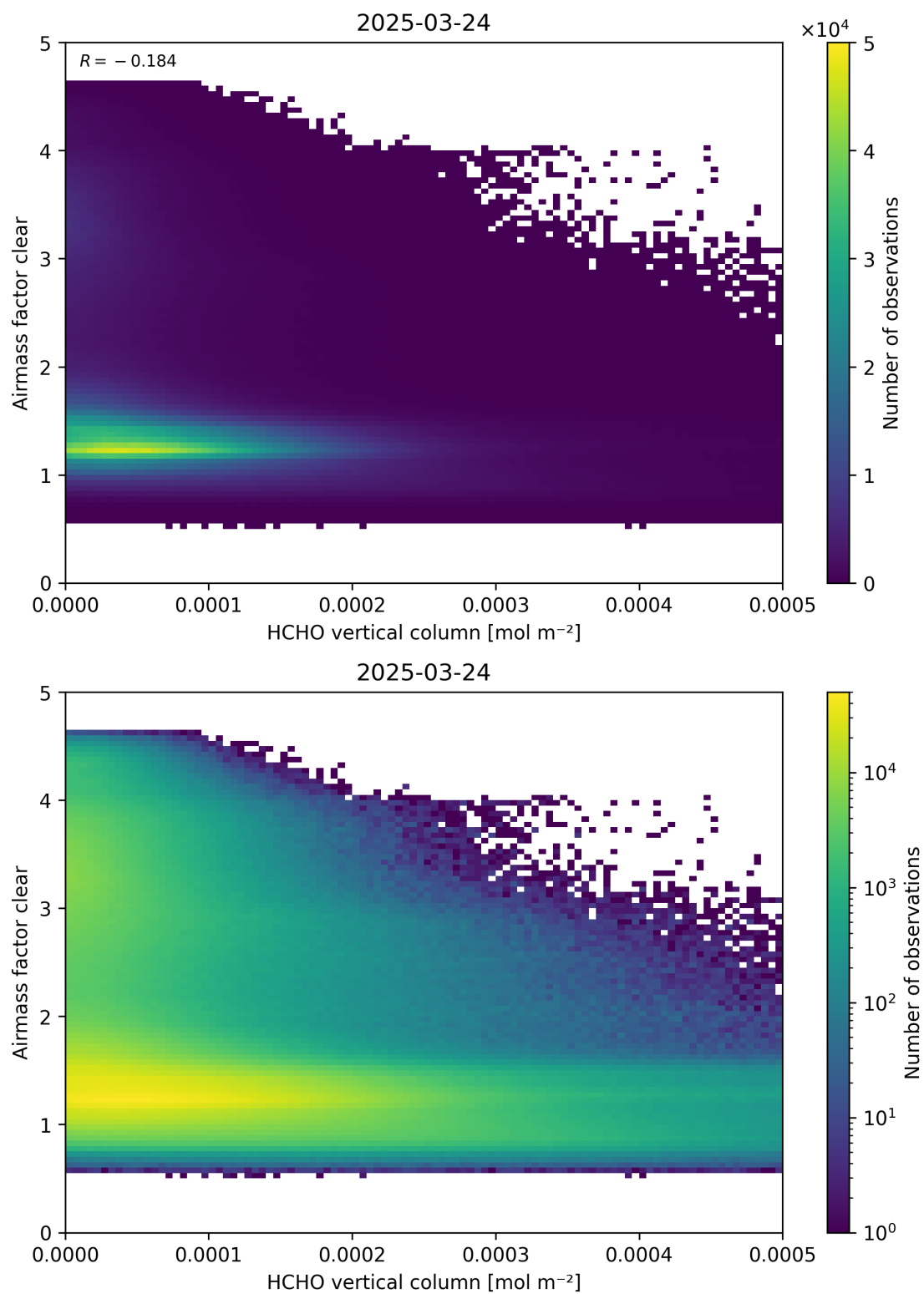
Figure 126: Scatter density plot of “HCHO vertical column” against “Airmass factor clear” for 2025-03-23 to 2025-03-25.
