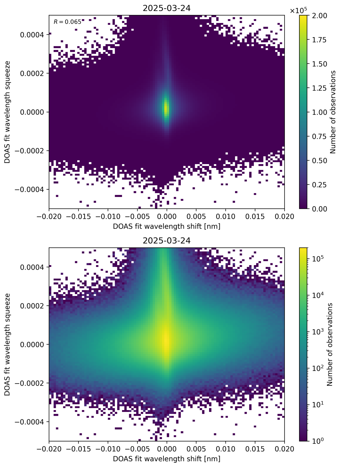
Figure 65: Scatter density plot of “DOAS fit wavelength shift” against “DOAS fit wavelength squeeze” for 2025-03-23 to 2025-03-25.
