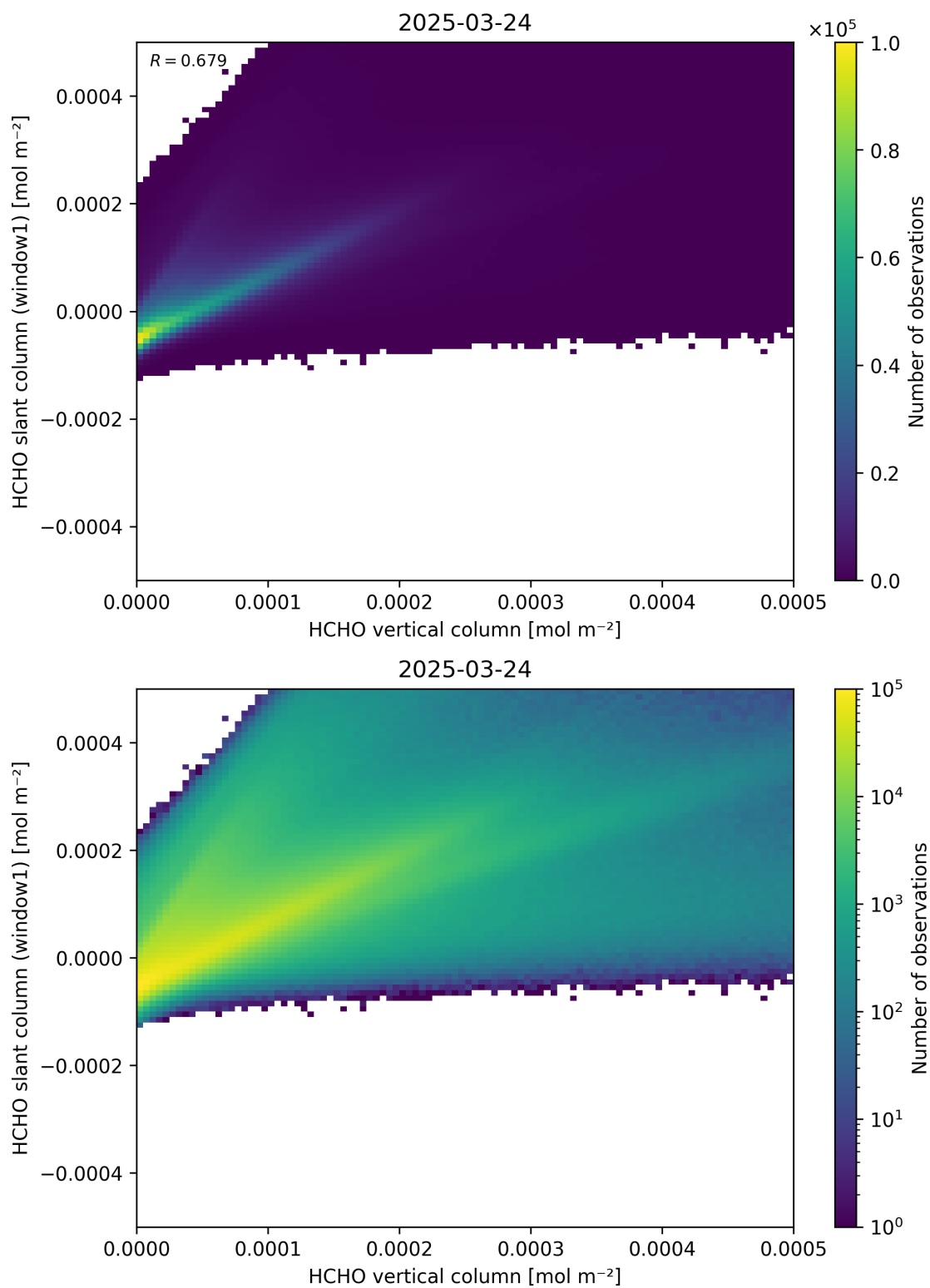
Figure 129: Scatter density plot of “HCHO vertical column” against “HCHO slant column (window1)” for 2025-03-23 to 2025-03-25.
