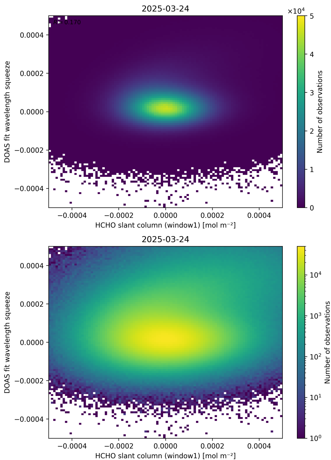
Figure 80: Scatter density plot of “HCHO slant column (window1)” against “DOAS fit wavelength squeeze” for 2025-03-23 to 2025-03-25.
