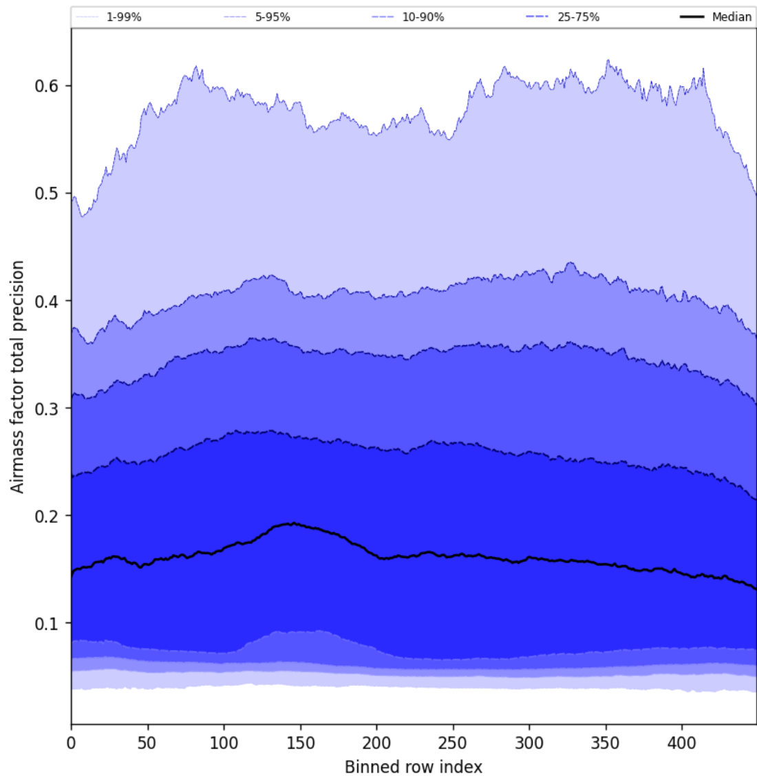
Figure 55: Along track statistics of “Airmass factor total precision” for 2025-03-23 to 2025-03-25
