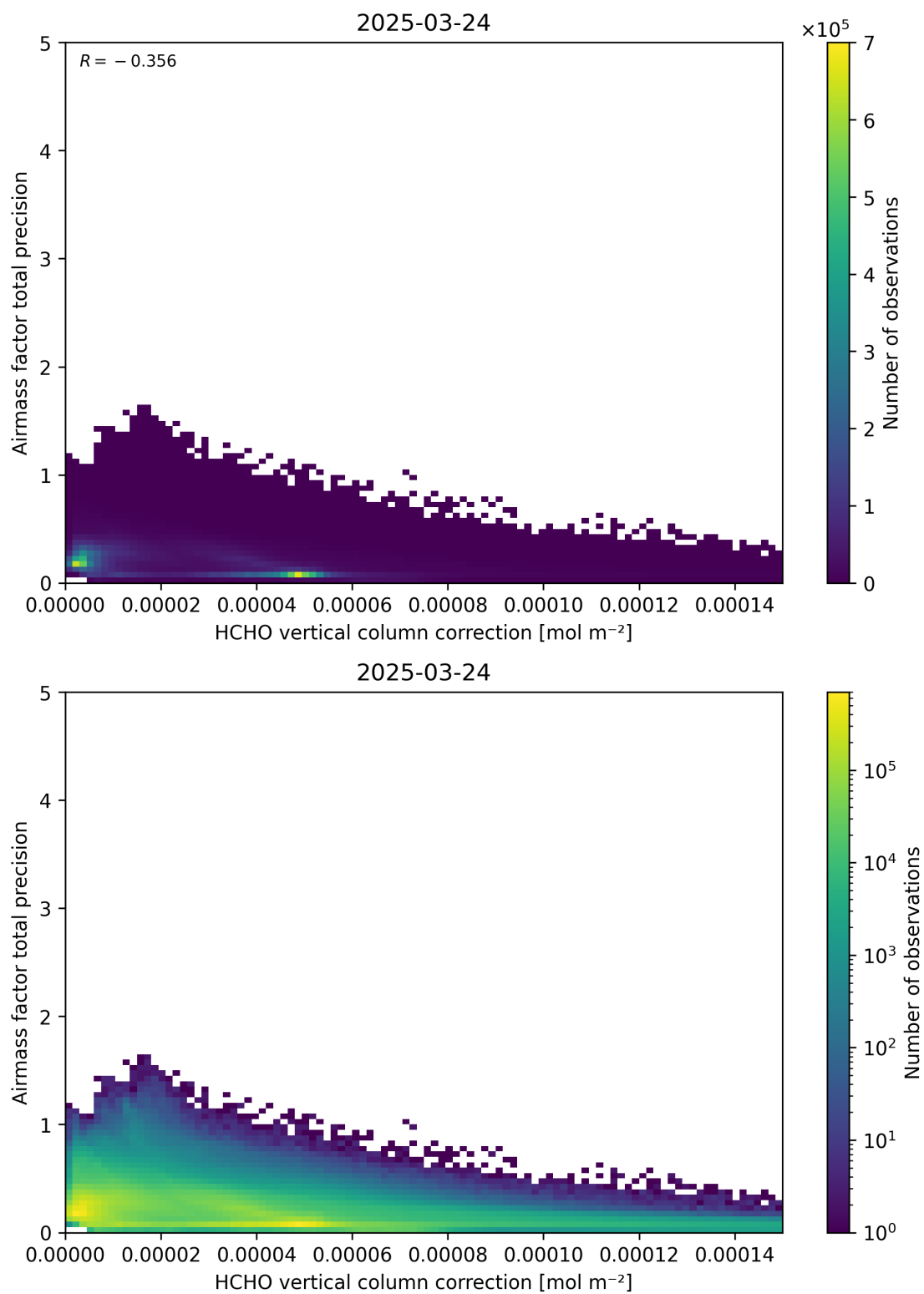
Figure 121: Scatter density plot of “HCHO vertical column correction” against “Airmass factor total precision” for 2025-03-23 to 2025-03-25.
