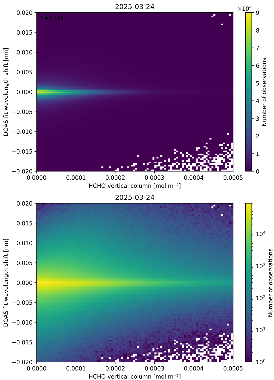
Figure 124: Scatter density plot of “HCHO vertical column” against “DOAS fit wavelength shift” for 2025-03-23 to 2025-03-25.
