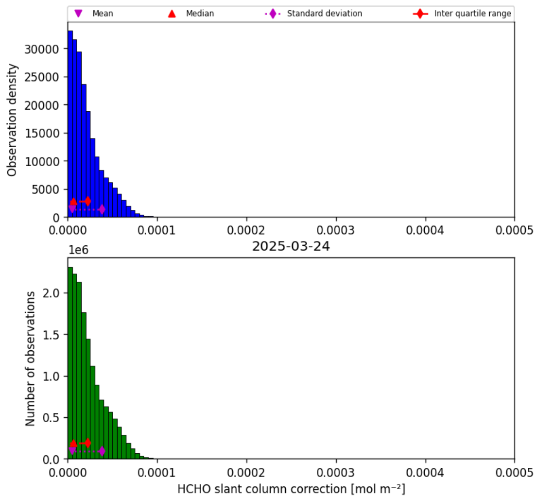
Figure 47: Histogram of “HCHO slant column correction” for 2025-03-23 to 2025-03-25
