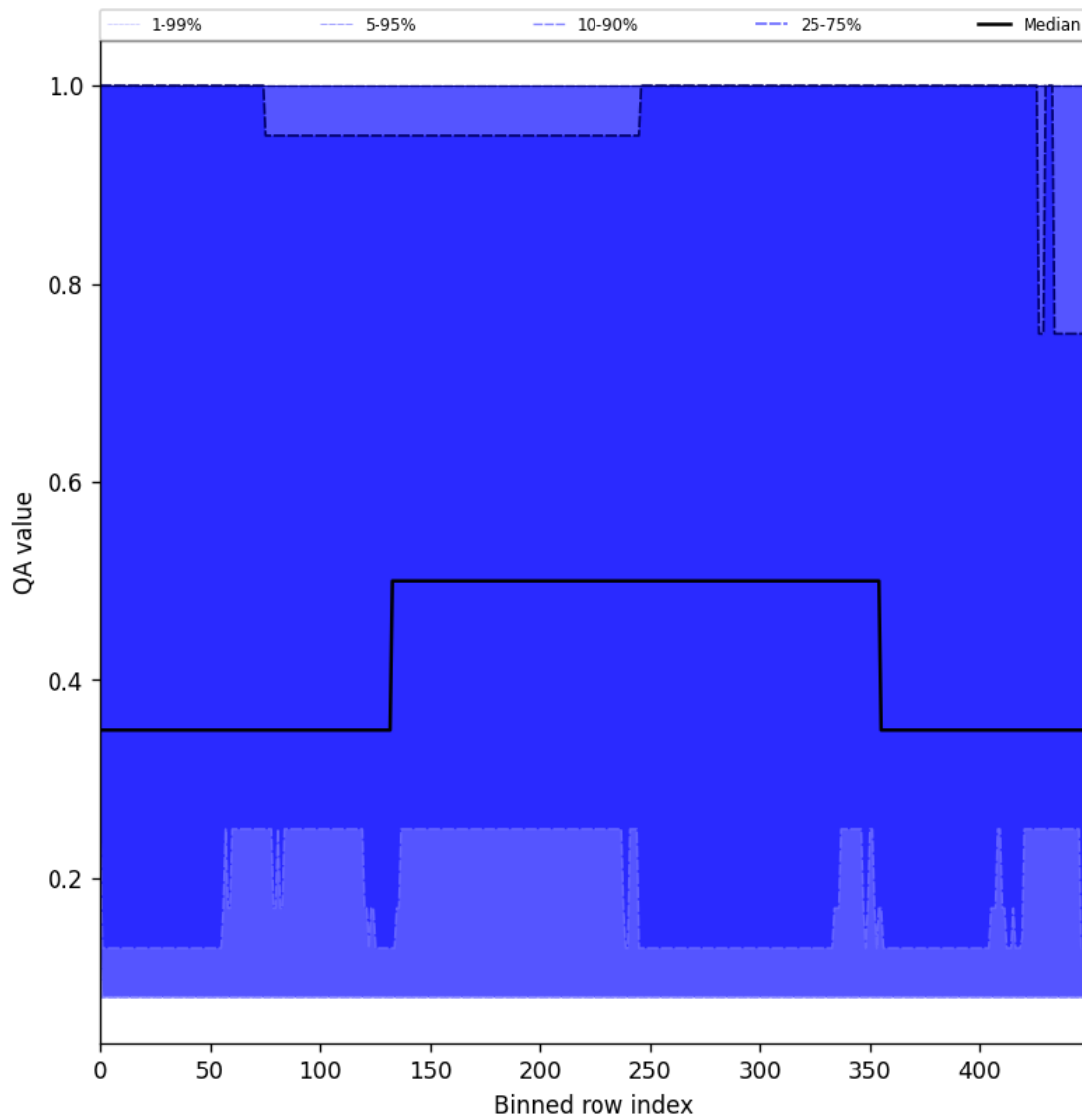
Figure 48: Along track statistics of “QA value” for 2025-03-23 to 2025-03-25
