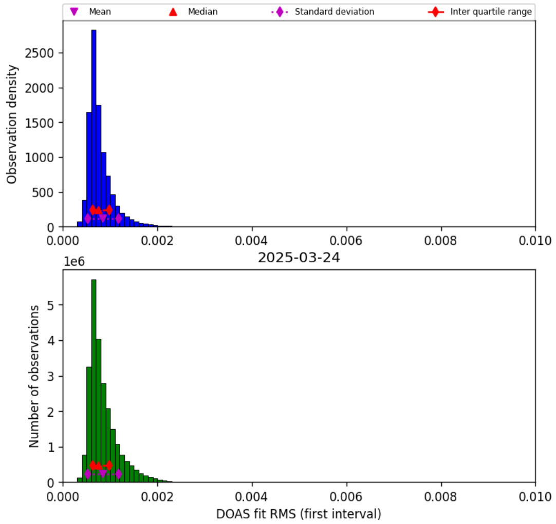
Figure 46: Histogram of “DOAS fit RMS (first interval)” for 2025-03-23 to 2025-03-25
