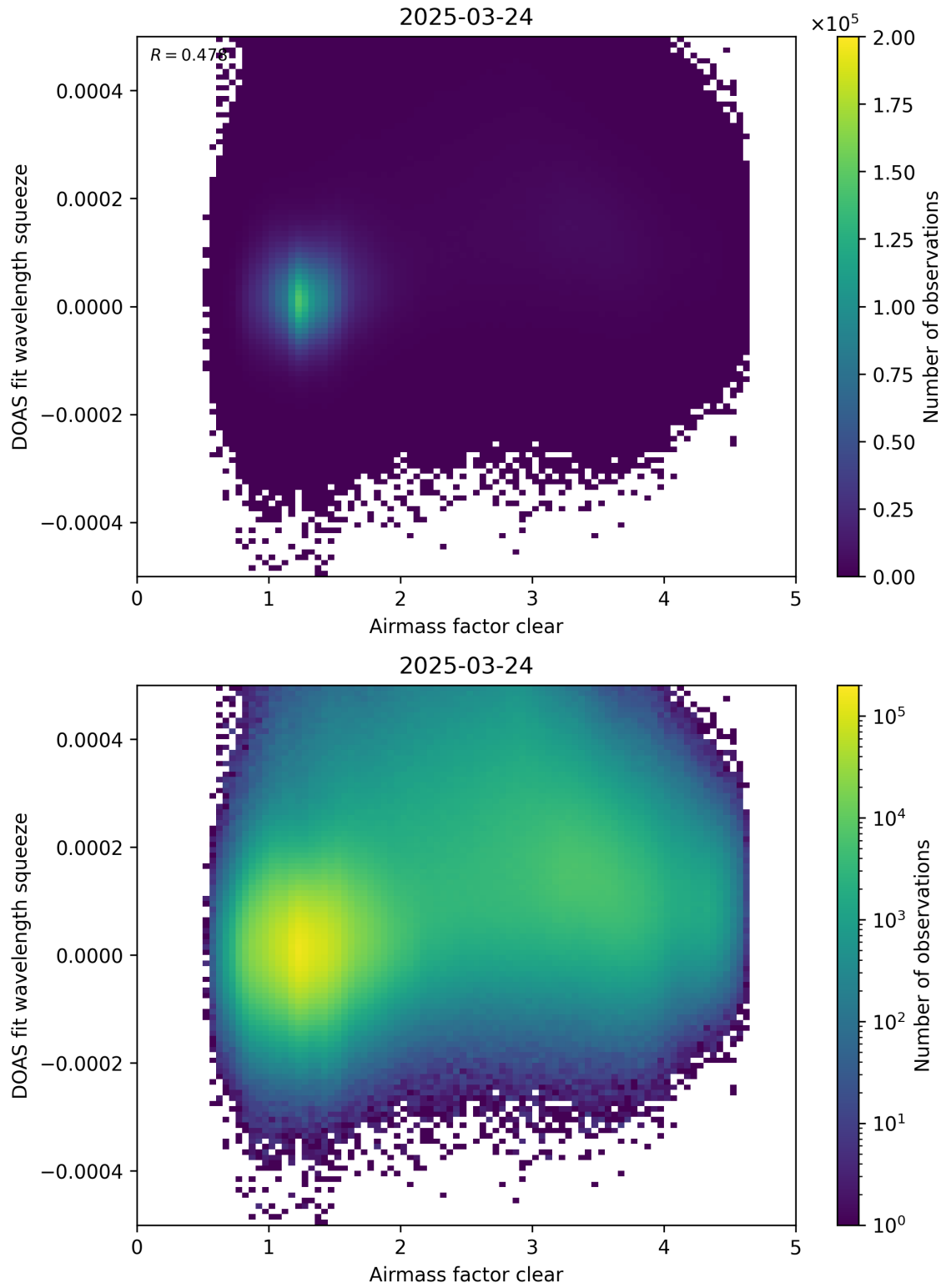
Figure 73: Scatter density plot of “Airmass factor clear” against “DOAS fit wavelength squeeze” for 2025-03-23 to 2025-03-25.
