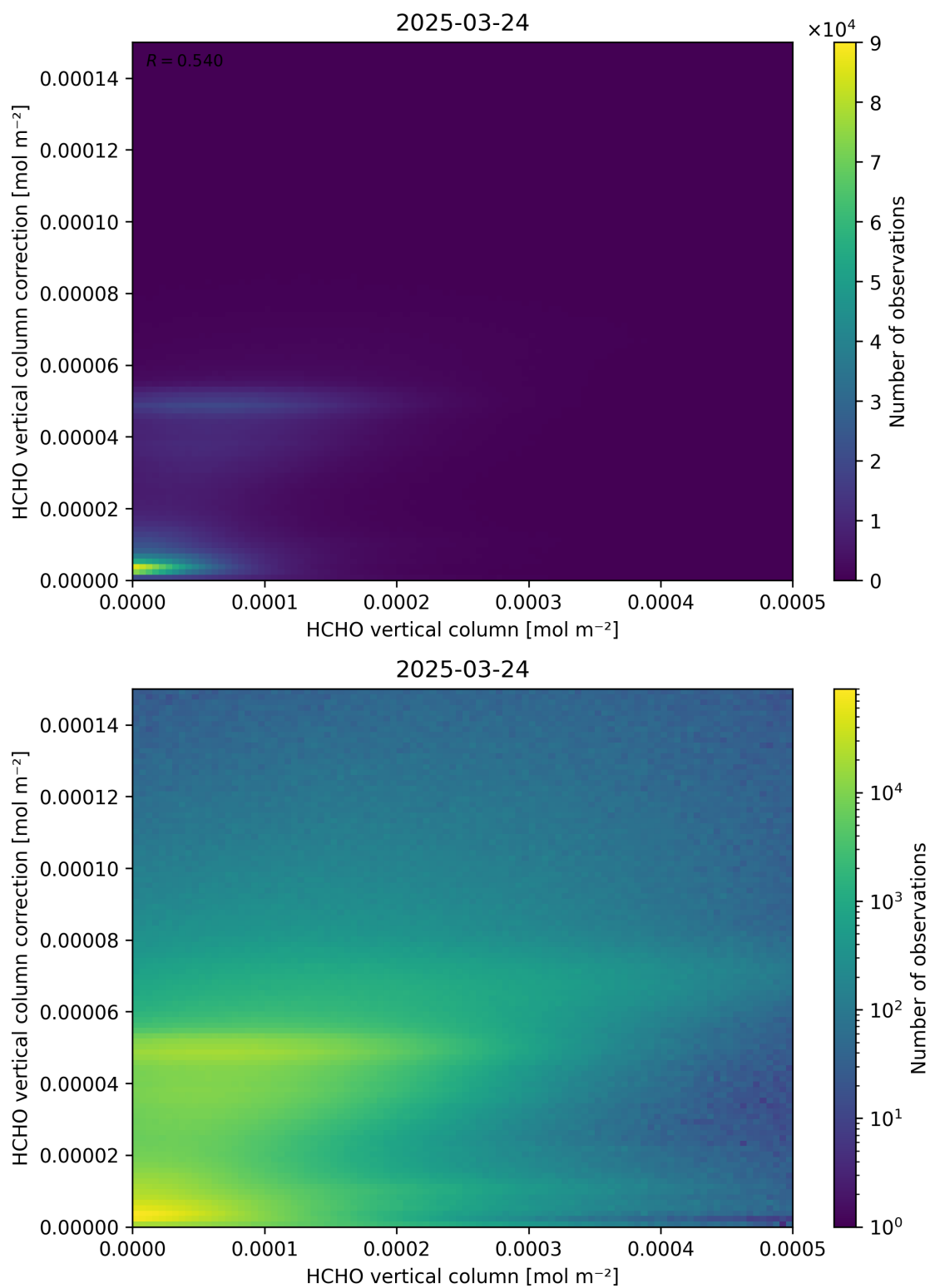
Figure 133: Scatter density plot of “HCHO vertical column” against “HCHO vertical column correction” for 2025-03-23 to 2025-03-25.
