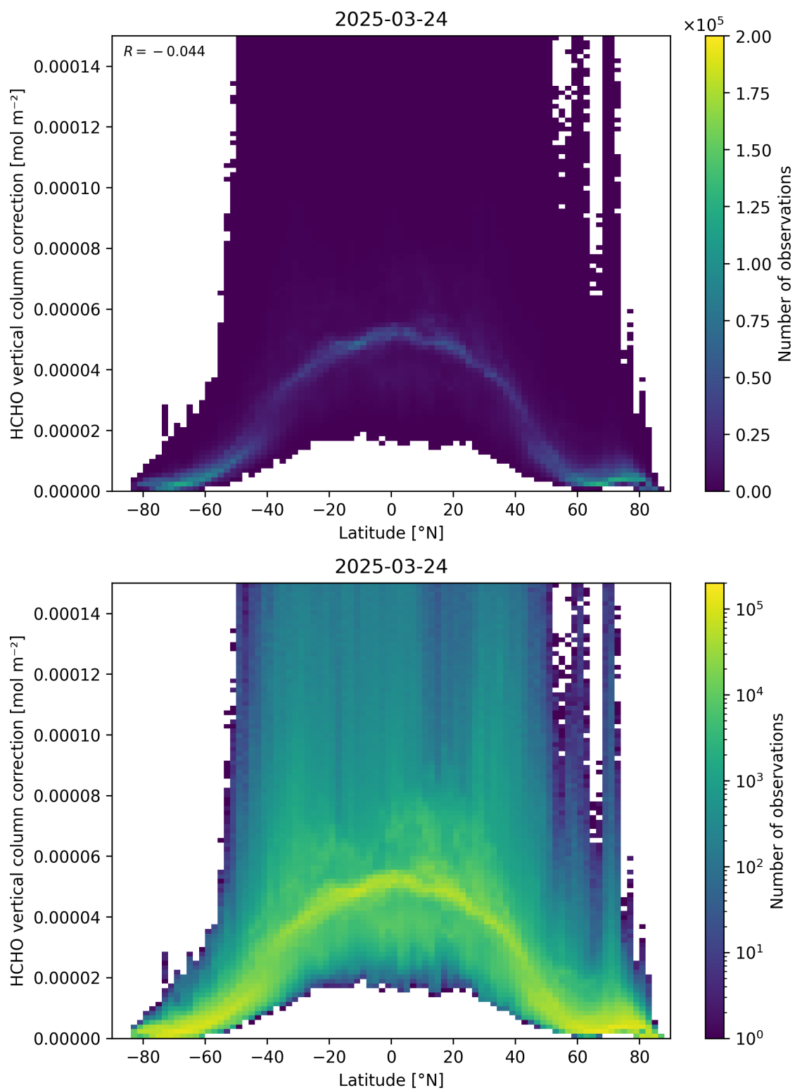
Figure 164: Scatter density plot of “Latitude” against “HCHO vertical column correction” for 2025-03-23 to 2025-03-25.
