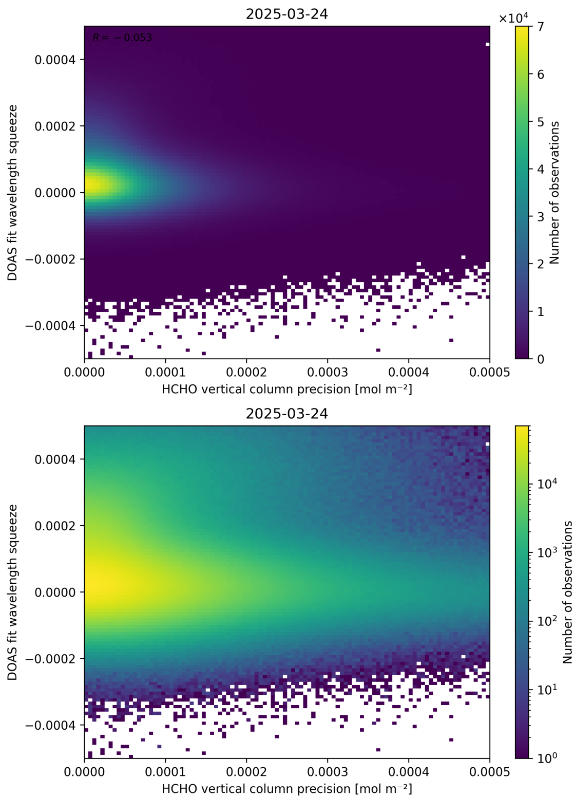
Figure 138: Scatter density plot of “HCHO vertical column precision” against “DOAS fit wavelength squeeze” for 2025-03-23 to 2025-03-25.
