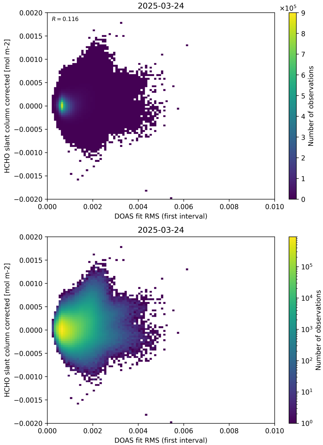
Figure 62: Scatter density plot of “DOAS fit RMS (first interval)” against “HCHO slant column corrected” for 2025-03-23 to 2025-03-25.
