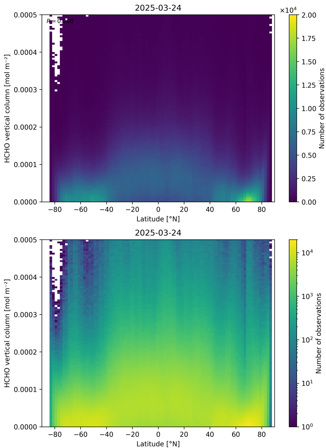
Figure 163: Scatter density plot of “Latitude” against “HCHO vertical column” for 2025-03-23 to 2025-03-25.
