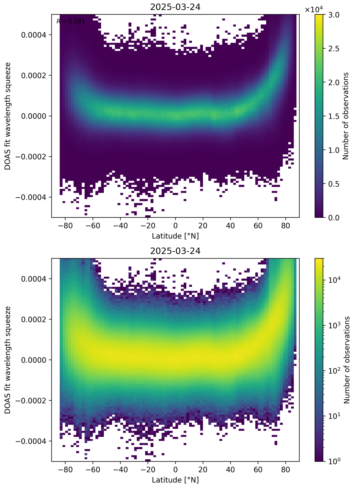
Figure 155: Scatter density plot of “Latitude” against “DOAS fit wavelength squeeze” for 2025-03-23 to 2025-03-25.
