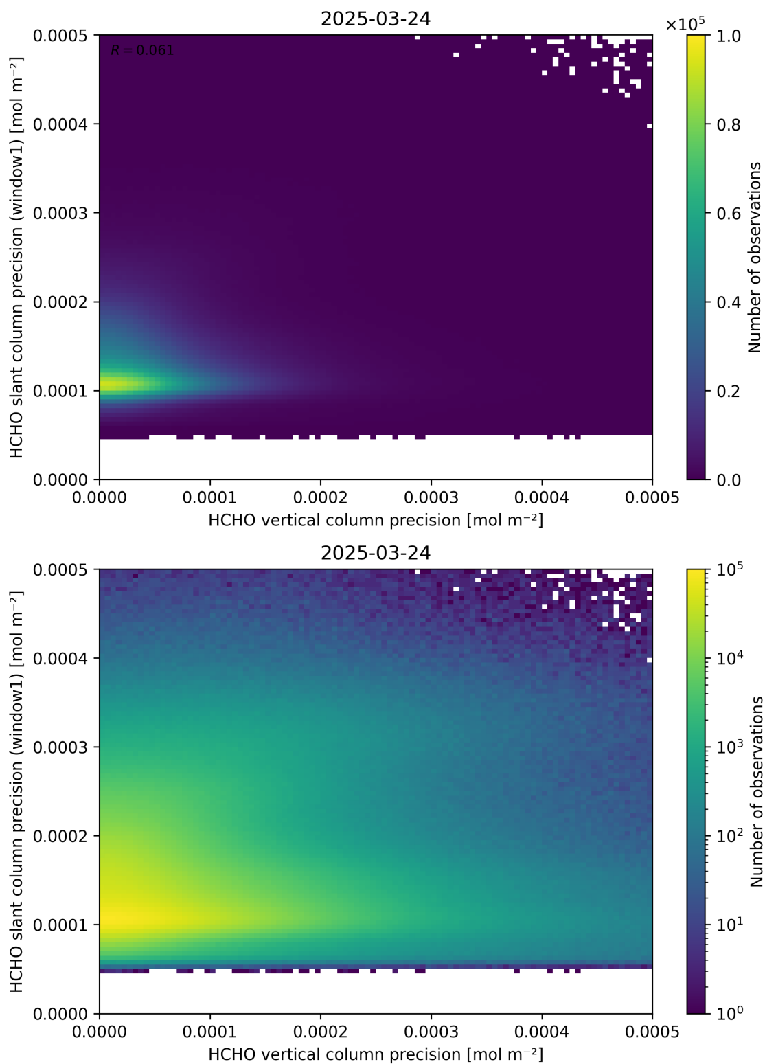
Figure 143: Scatter density plot of “HCHO vertical column precision” against “HCHO slant column precision (window1)” for 2025-03-23 to 2025-03-25.
