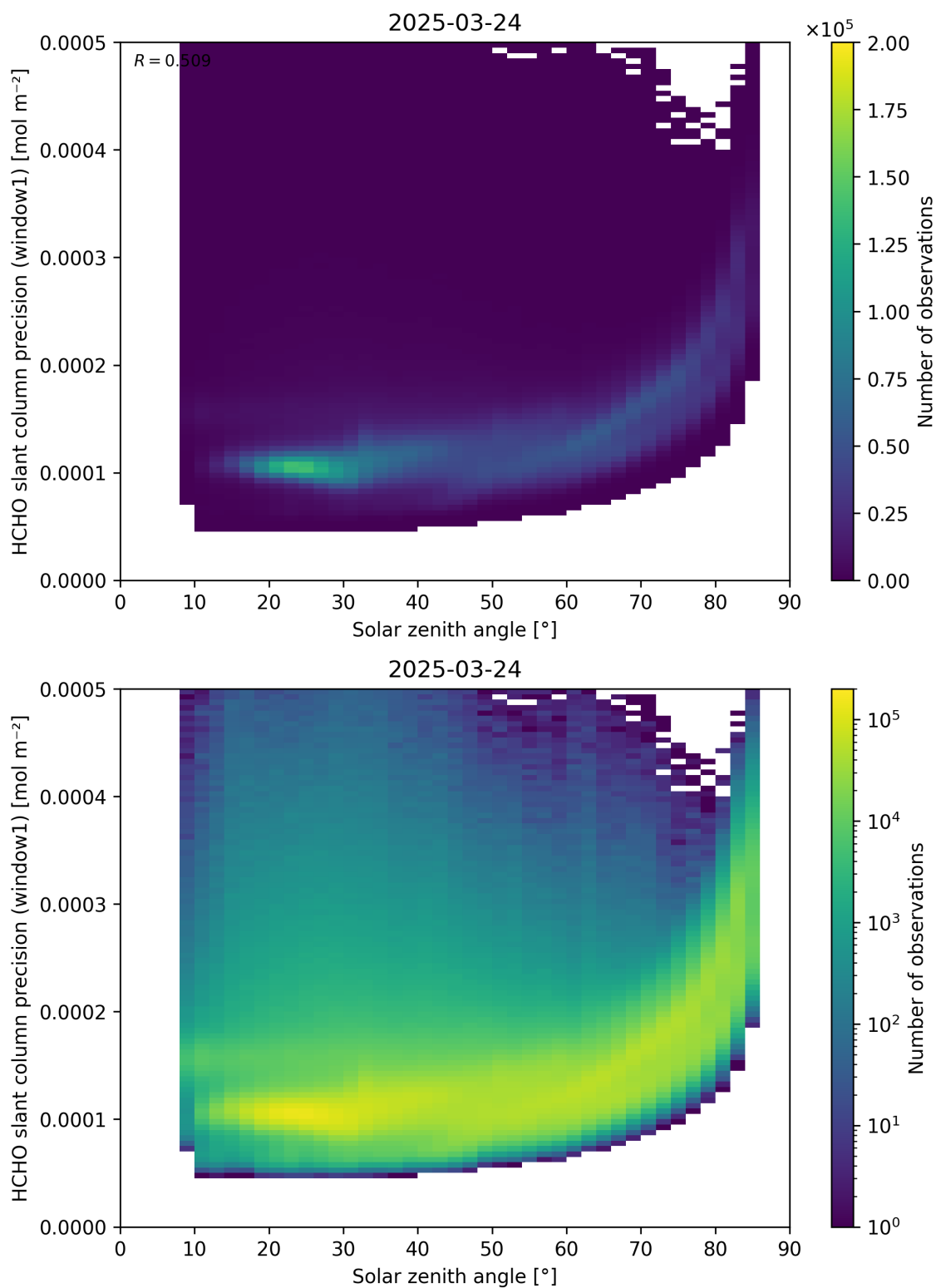
Figure 174: Scatter density plot of “Solar zenith angle” against “HCHO slant column precision (window1)” for 2025-03-23 to 2025-03-25.
