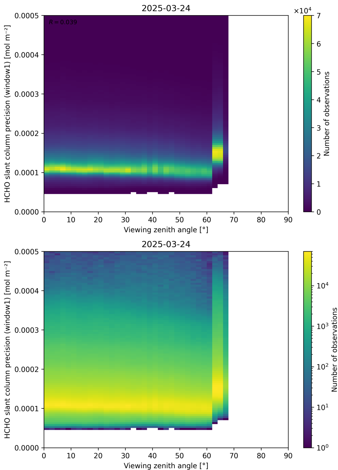
Figure 189: Scatter density plot of “Viewing zenith angle” against “HCHO slant column precision (window1)” for 2025-03-23 to 2025-03-25.
