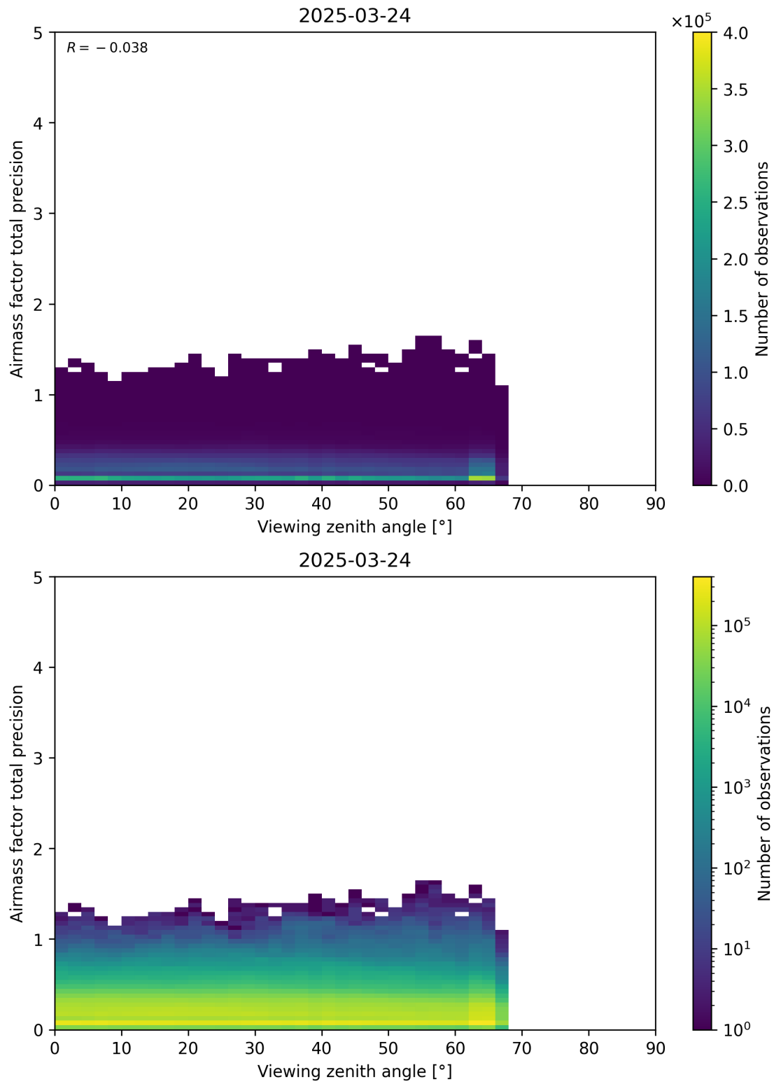
Figure 191: Scatter density plot of “Viewing zenith angle” against “Airmass factor total precision” for 2025-03-23 to 2025-03-25.
