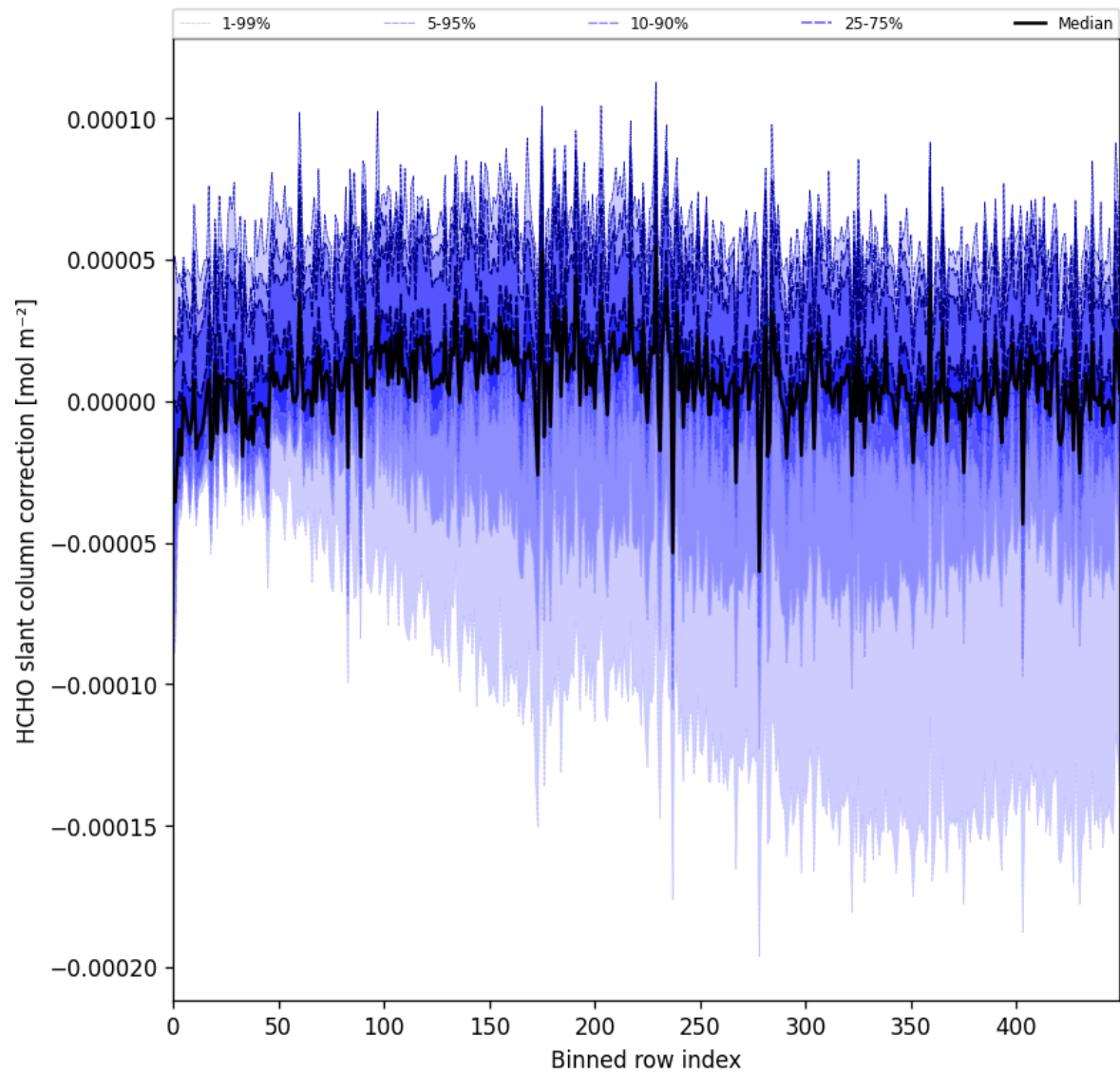
Figure 61: Along track statistics of “HCHO slant column correction” for 2025-03-23 to 2025-03-25
