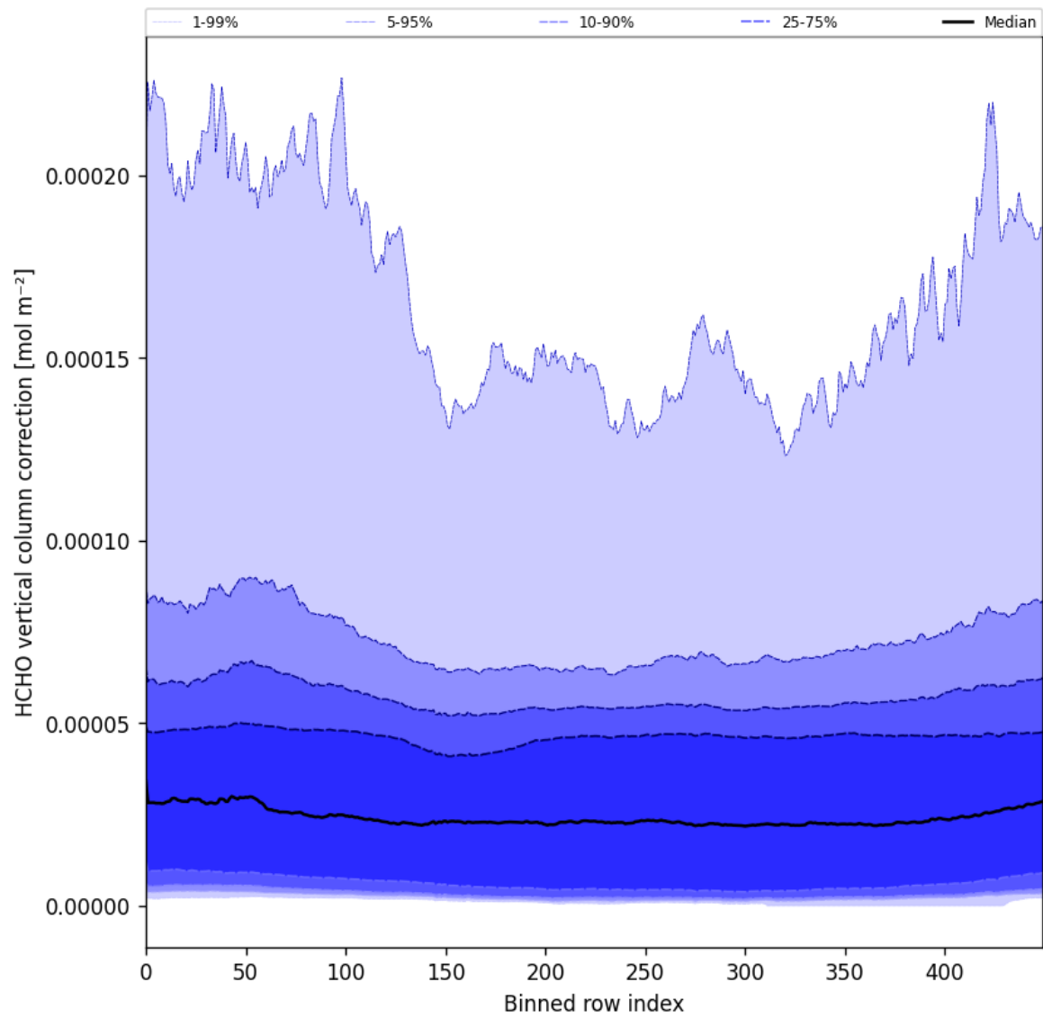
Figure 51: Along track statistics of “HCHO vertical column correction” for 2025-03-23 to 2025-03-25
