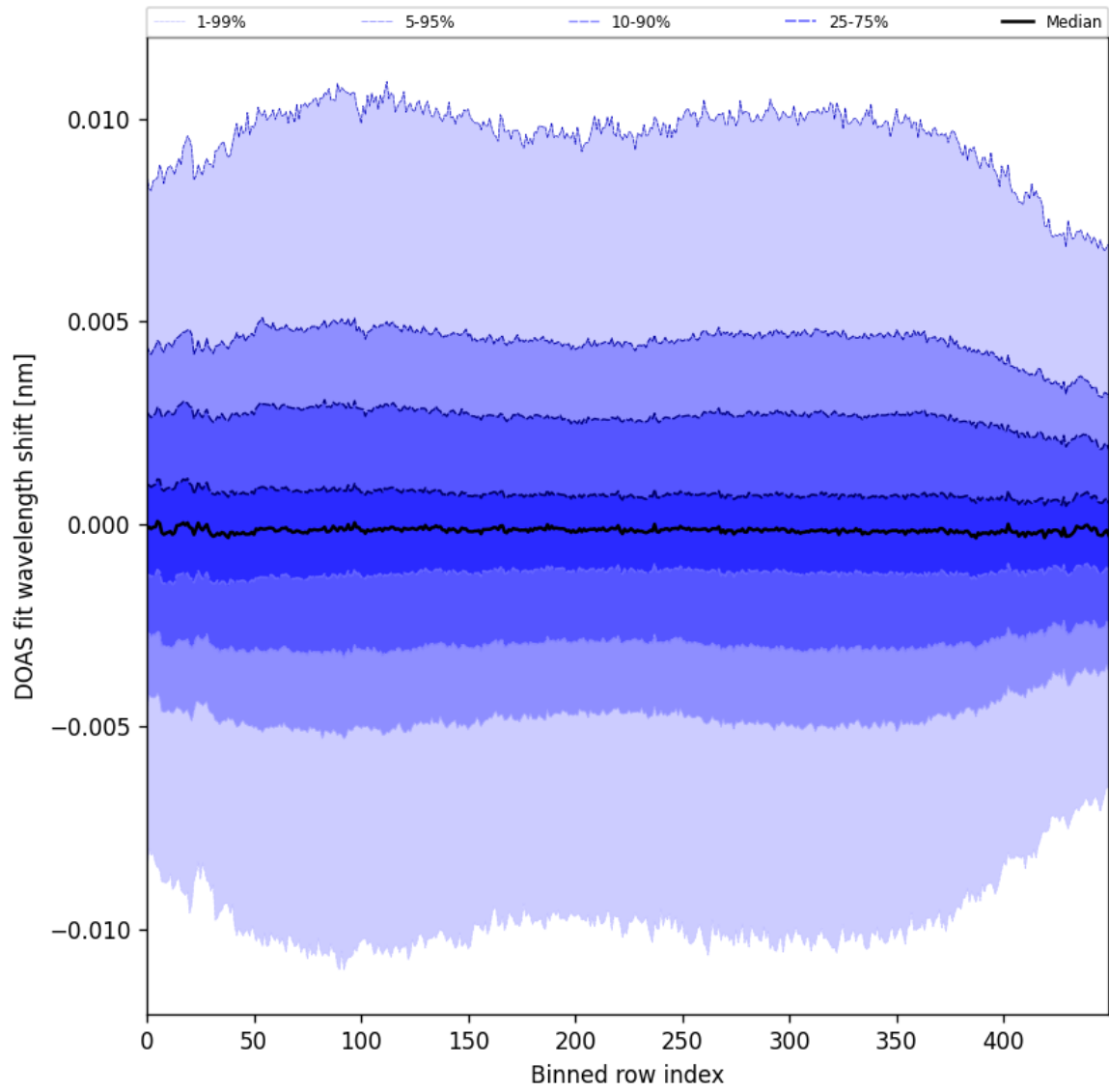
Figure 58: Along track statistics of “DOAS fit wavelength shift” for 2025-03-23 to 2025-03-25
