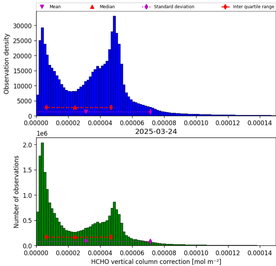
Figure 37: Histogram of “HCHO vertical column correction” for 2025-03-23 to 2025-03-25
