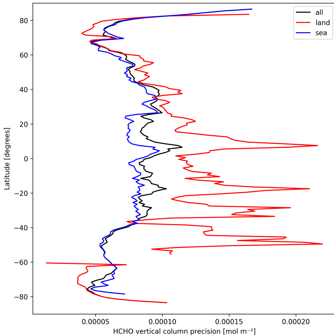
Figure 22: Zonal average of “HCHO vertical column precision” for 2025-03-23 to 2025-03-25.
