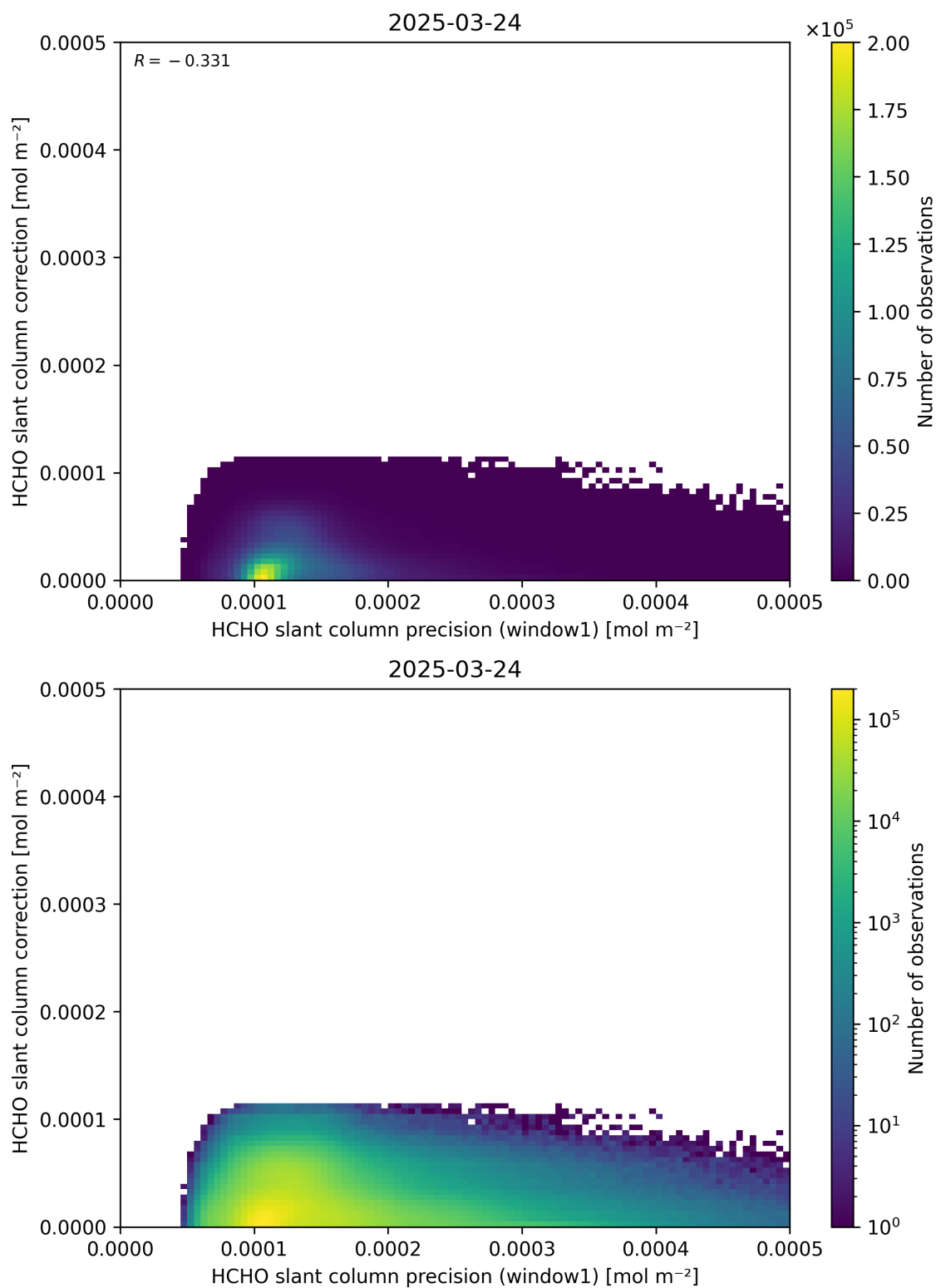
Figure 93: Scatter density plot of “HCHO slant column precision (window1)” against “HCHO slant column correction” for 2025-03-23 to 2025-03-25.
