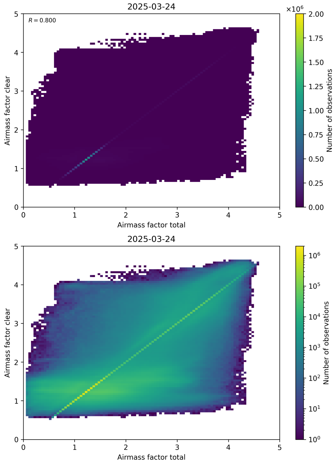
Figure 100: Scatter density plot of “Airmass factor total” against “Airmass factor clear” for 2025-03-23 to 2025-03-25.
