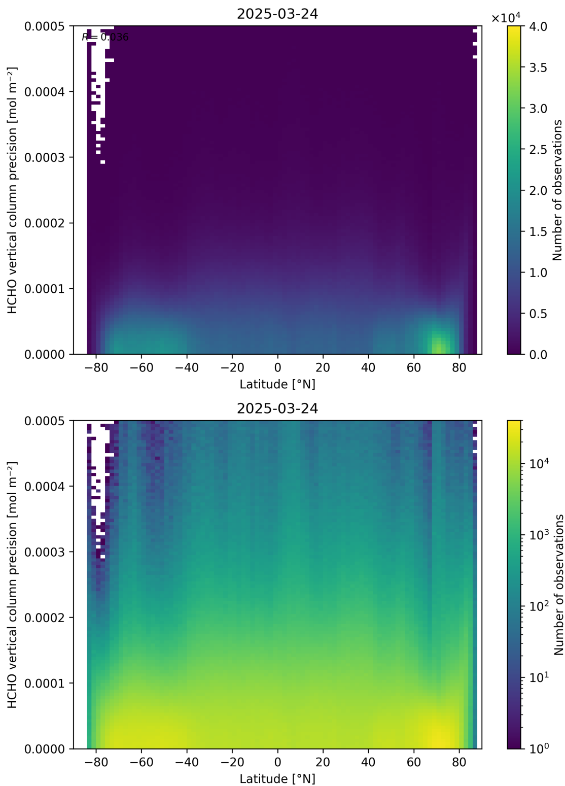
Figure 165: Scatter density plot of “Latitude” against “HCHO vertical column precision” for 2025-03-23 to 2025-03-25.
