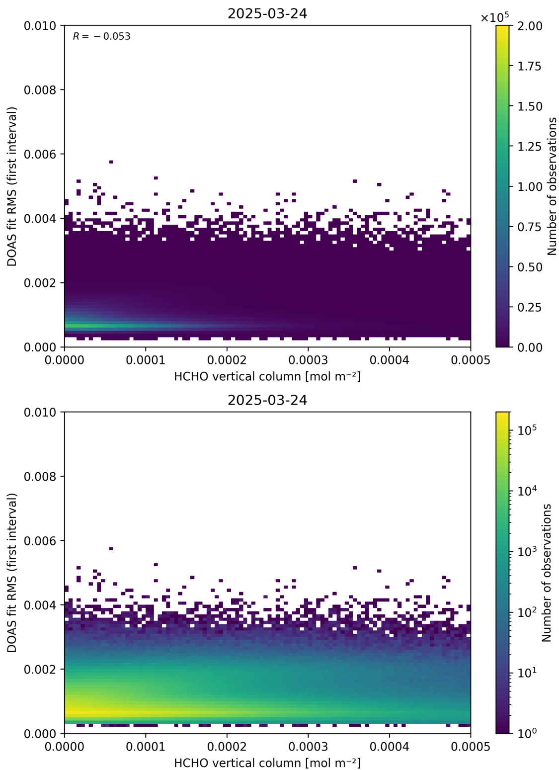
Figure 123: Scatter density plot of “HCHO vertical column” against “DOAS fit RMS (first interval)” for 2025-03-23 to 2025-03-25.
