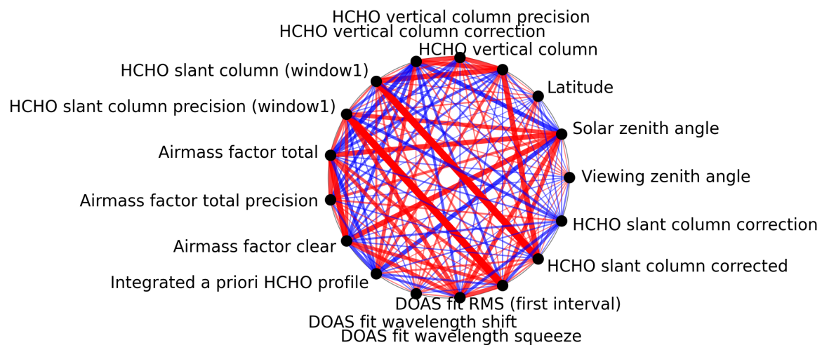
Figure 1: Map of correlation graph for 2025-03-23 to 2025-03-25.
