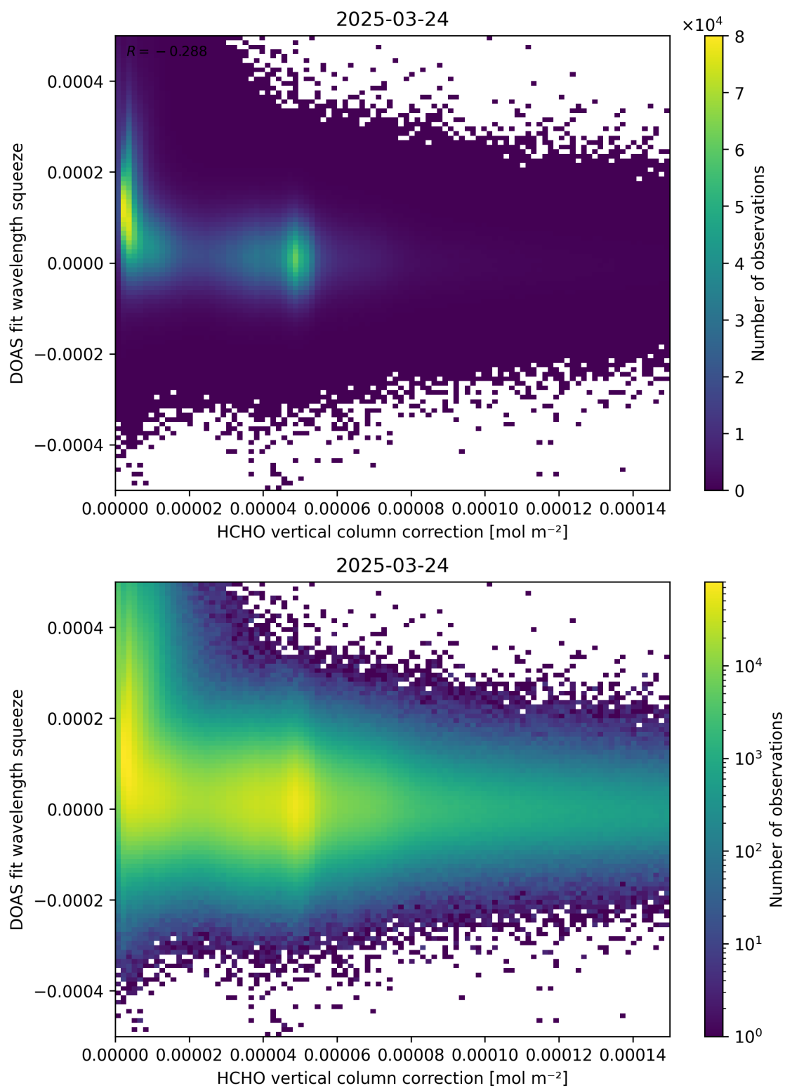
Figure 114: Scatter density plot of “HCHO vertical column correction” against “DOAS fit wavelength squeeze” for 2025-03-23 to 2025-03-25.
