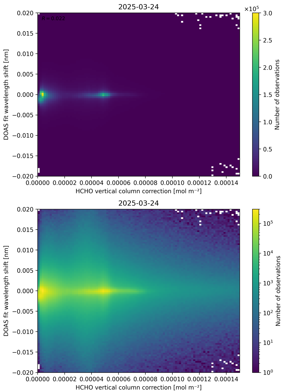
Figure 113: Scatter density plot of “HCHO vertical column correction” against “DOAS fit wavelength shift” for 2025-03-23 to 2025-03-25.
