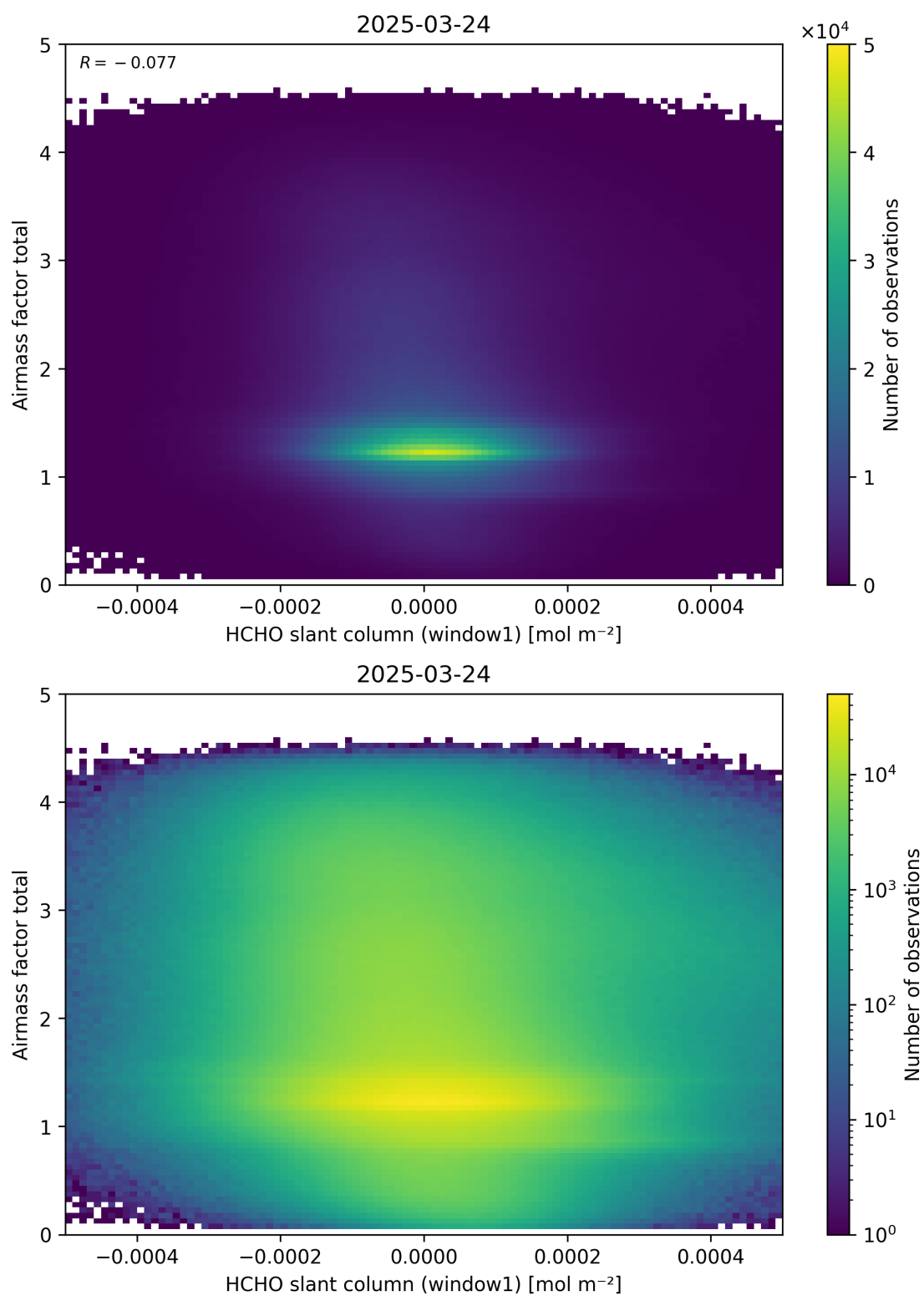
Figure 85: Scatter density plot of “HCHO slant column (window1)” against “Airmass factor total” for 2025-03-23 to 2025-03-25.
