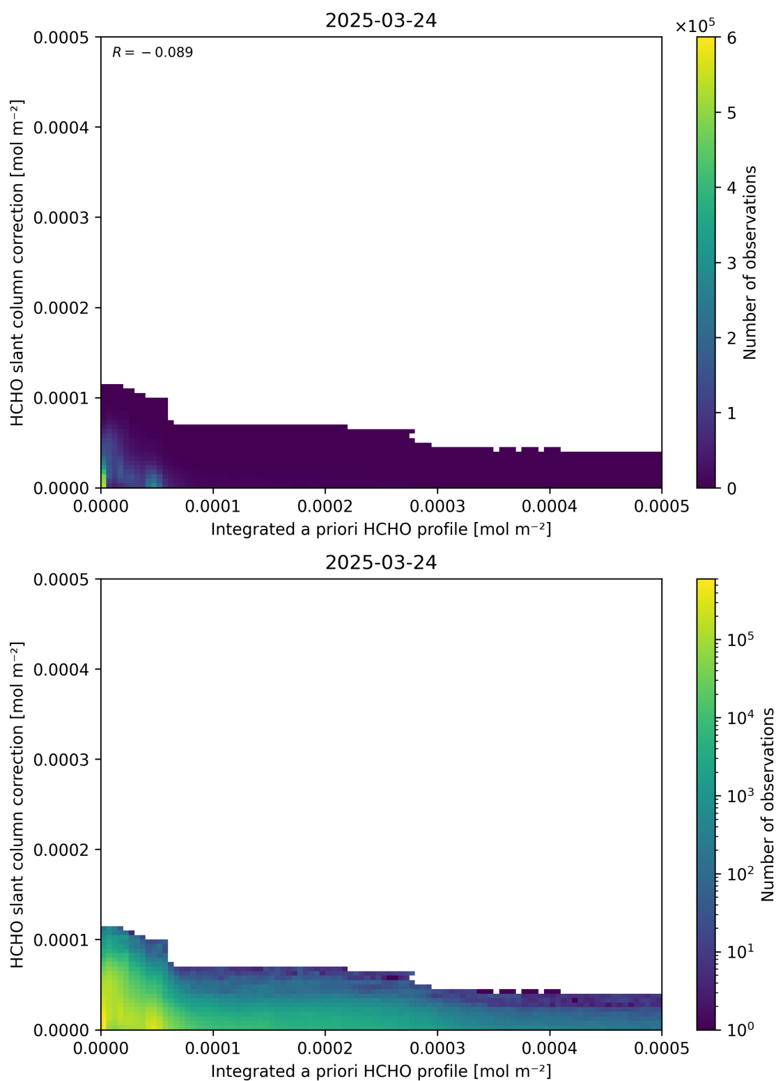
Figure 152: Scatter density plot of “Integrated a priori HCHO profile” against “HCHO slant column correction” for 2025-03-23 to 2025-03-25.
