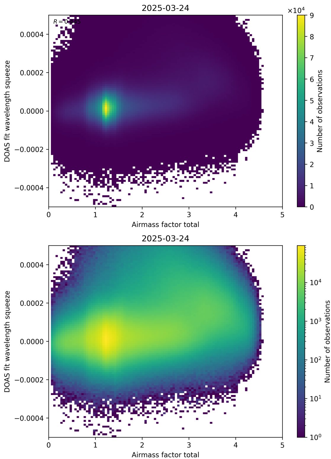
Figure 99: Scatter density plot of “Airmass factor total” against “DOAS fit wavelength squeeze” for 2025-03-23 to 2025-03-25.
