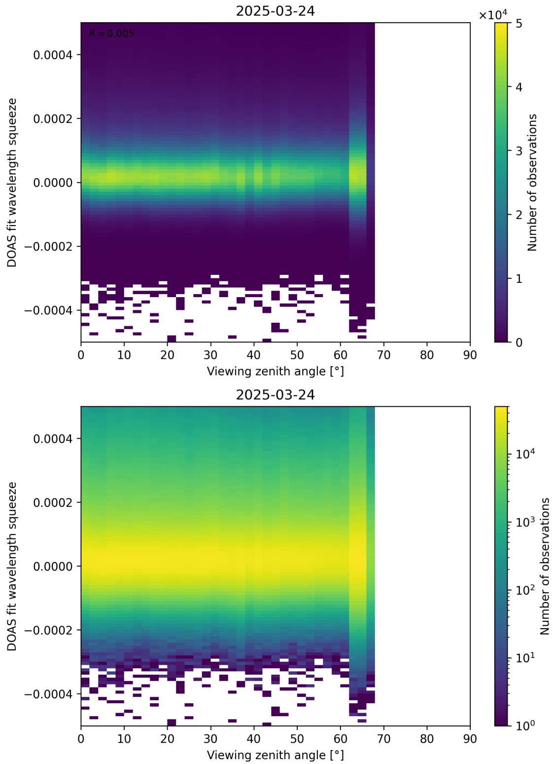
Figure 184: Scatter density plot of “Viewing zenith angle” against “DOAS fit wavelength squeeze” for 2025-03-23 to 2025-03-25.
