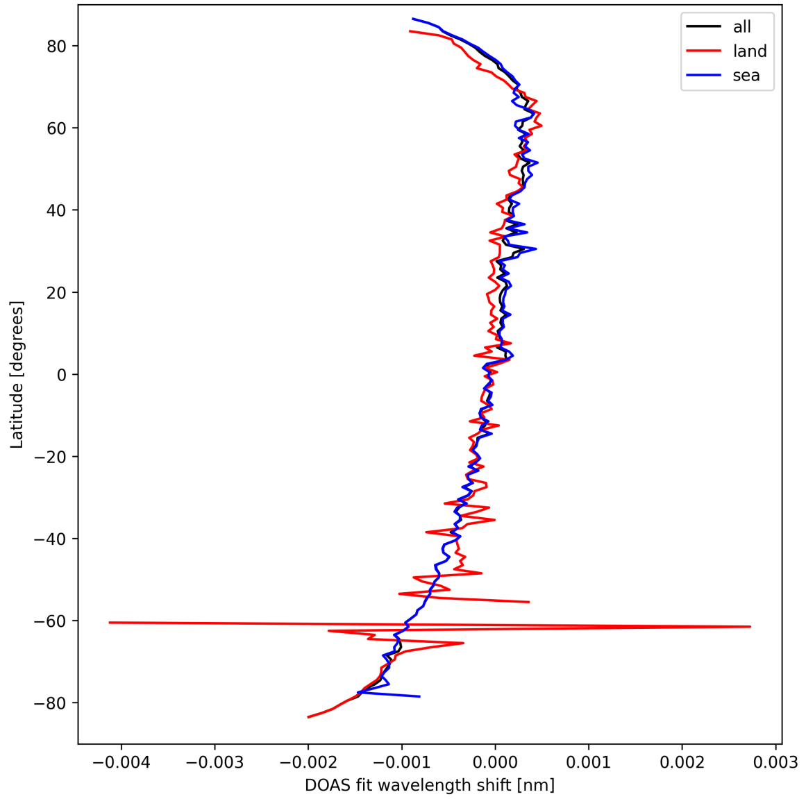
Figure 30: Zonal average of "DOAS fit wavelength shift" for 2025-03-23 to 2025-03-25.
