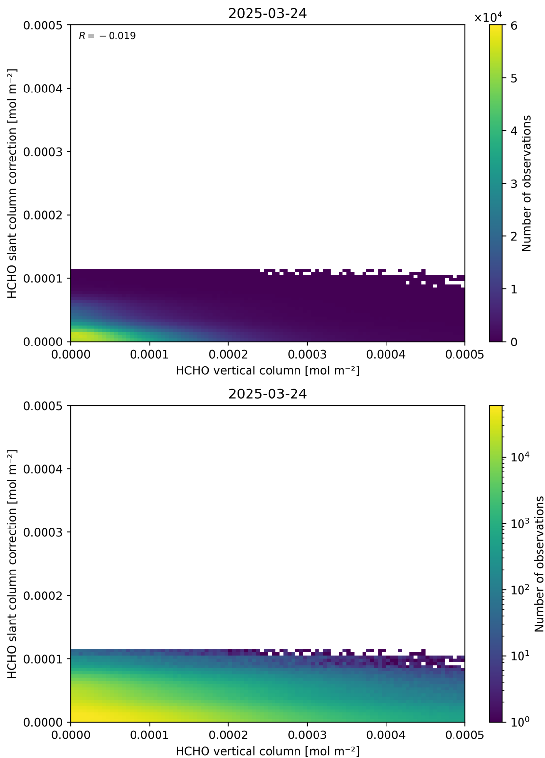
Figure 128: Scatter density plot of “HCHO vertical column” against “HCHO slant column correction” for 2025-03-23 to 2025-03-25.
