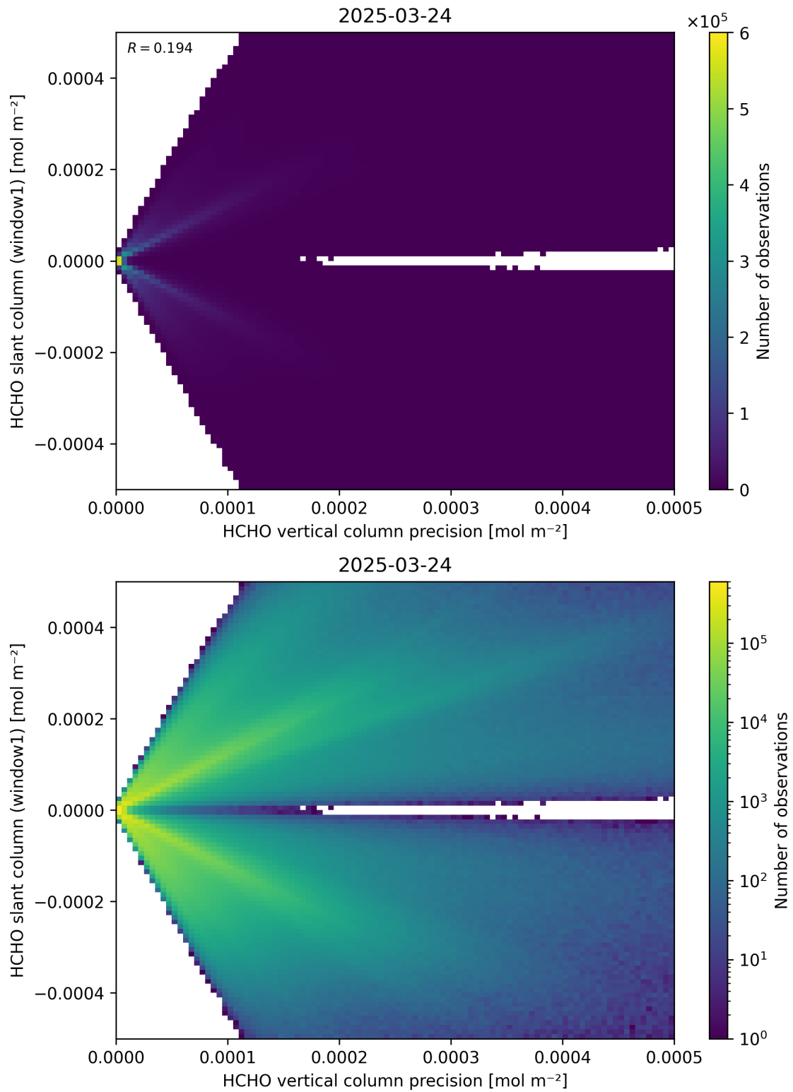
Figure 142: Scatter density plot of “HCHO vertical column precision” against “HCHO slant column (window1)” for 2025-03-23 to 2025-03-25.
