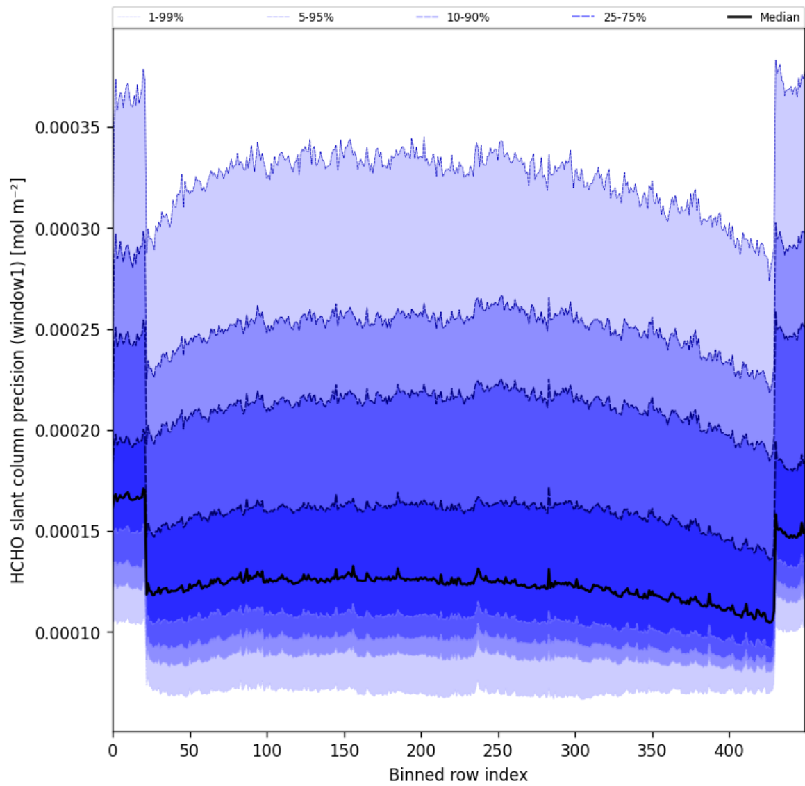
Figure 53: Along track statistics of “HCHO slant column precision (window1)” for 2025-03-23 to 2025-03-25
