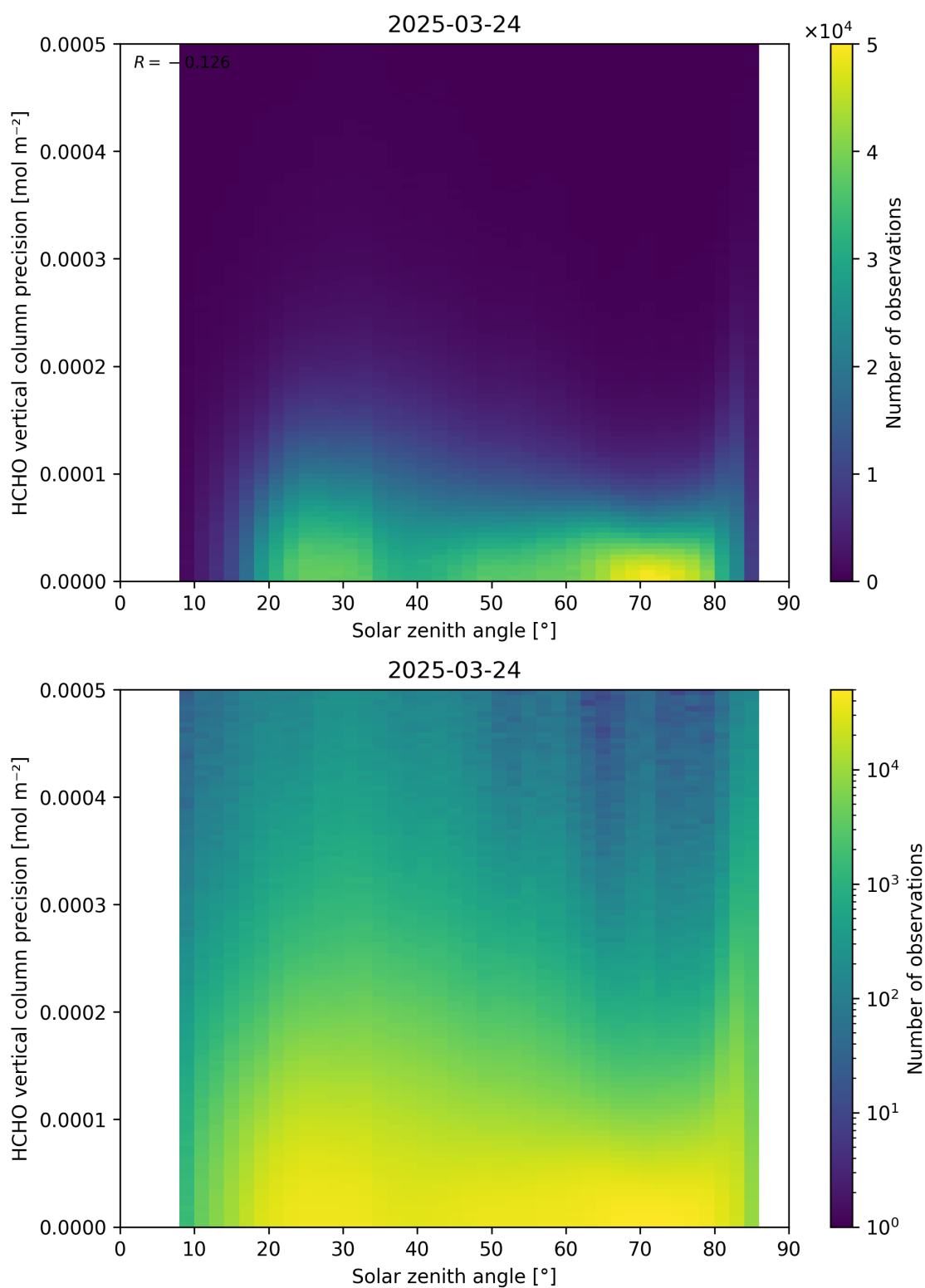
Figure 179: Scatter density plot of “Solar zenith angle” against “HCHO vertical column precision” for 2025-03-23 to 2025-03-25.
