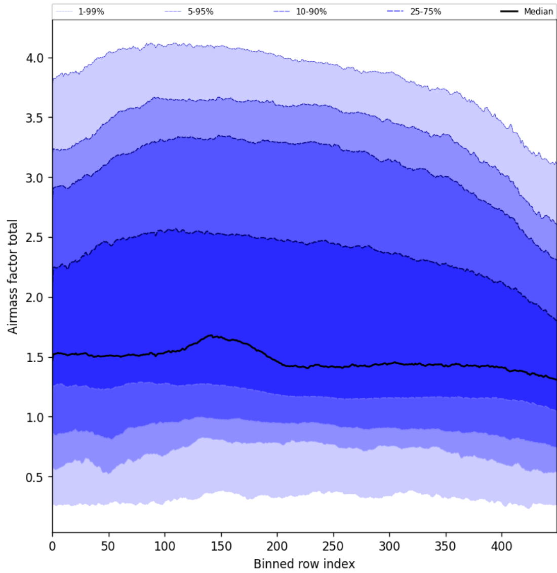
Figure 54: Along track statistics of “Airmass factor total” for 2025-03-23 to 2025-03-25
