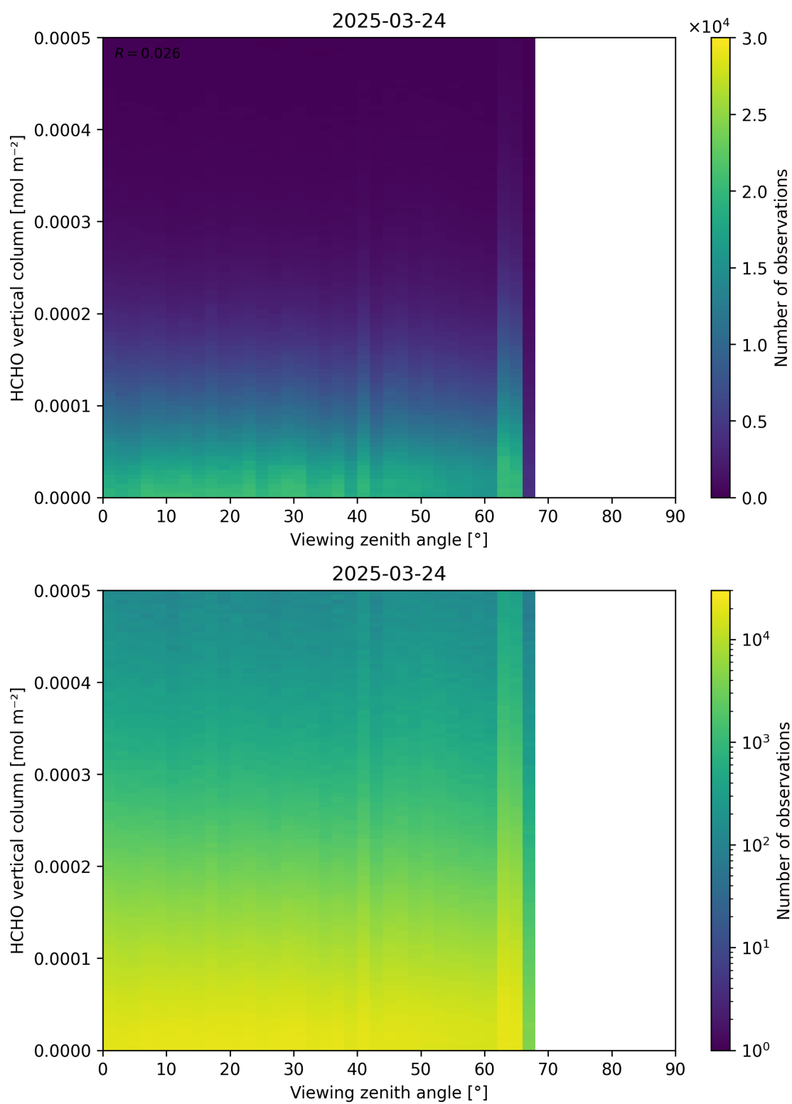
Figure 192: Scatter density plot of “Viewing zenith angle” against “HCHO vertical column” for 2025-03-23 to 2025-03-25.
