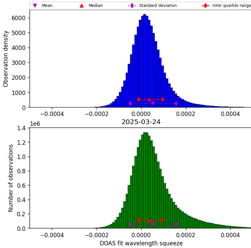
Figure 45: Histogram of “DOAS fit wavelength squeeze” for 2025-03-23 to 2025-03-25
