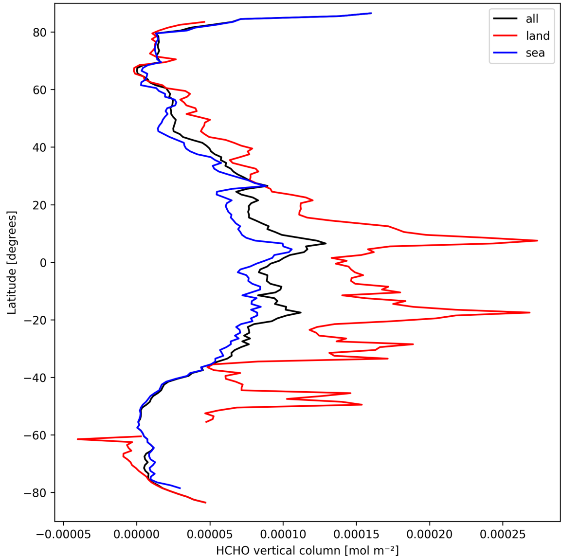
Figure 21: Zonal average of “HCHO vertical column” for 2025-03-23 to 2025-03-25.
