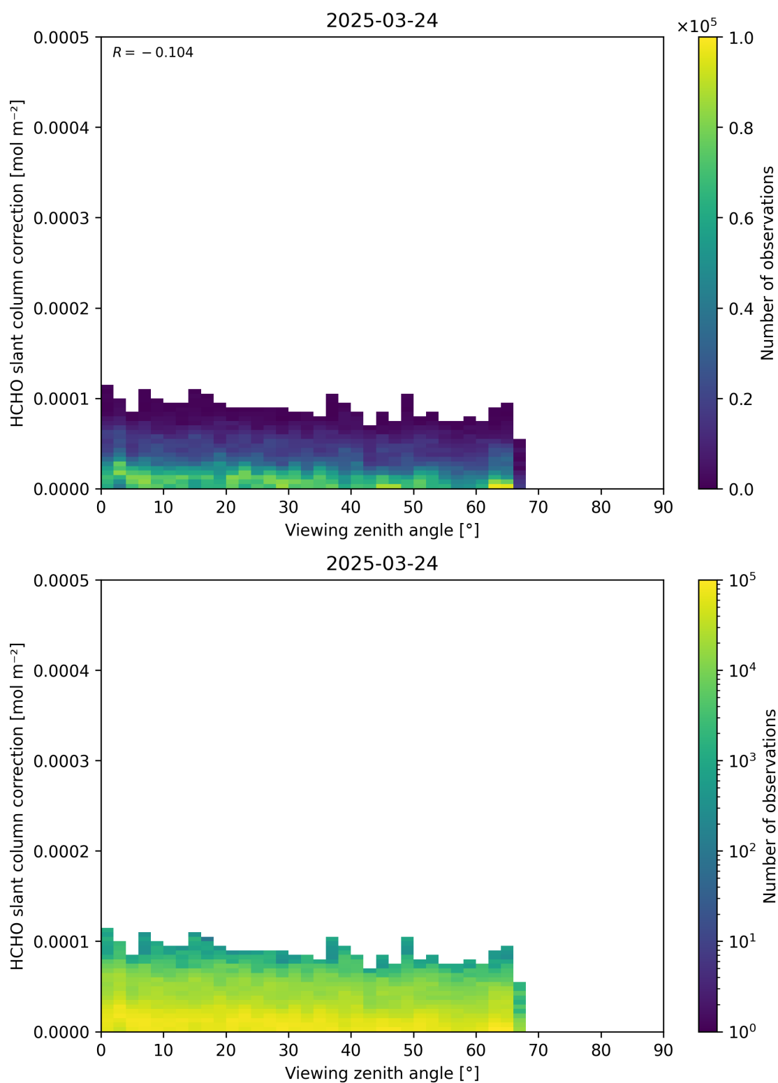
Figure 187: Scatter density plot of “Viewing zenith angle” against “HCHO slant column correction” for 2025-03-23 to 2025-03-25.
