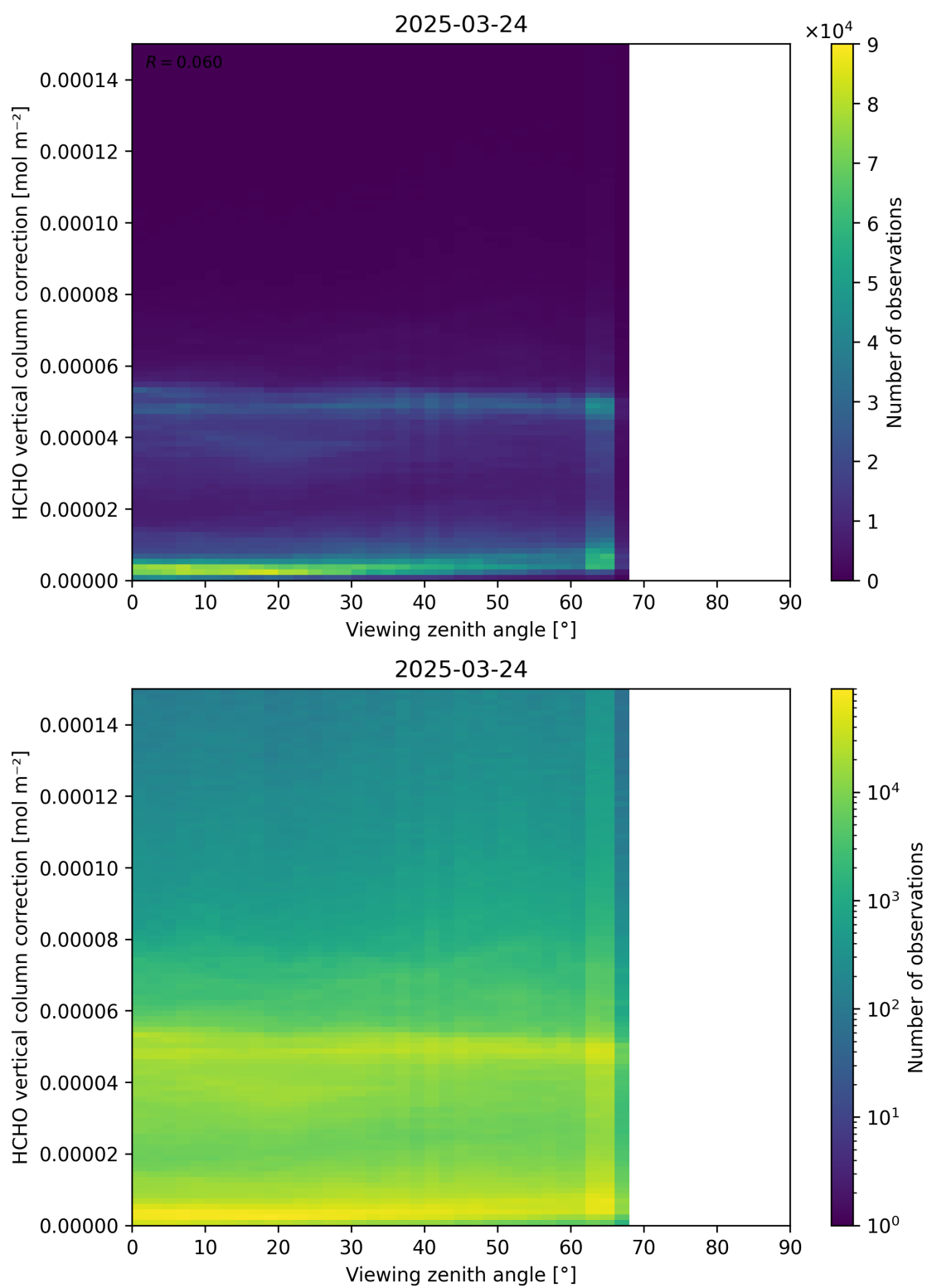
Figure 193: Scatter density plot of “Viewing zenith angle” against “HCHO vertical column correction” for 2025-03-23 to 2025-03-25.
