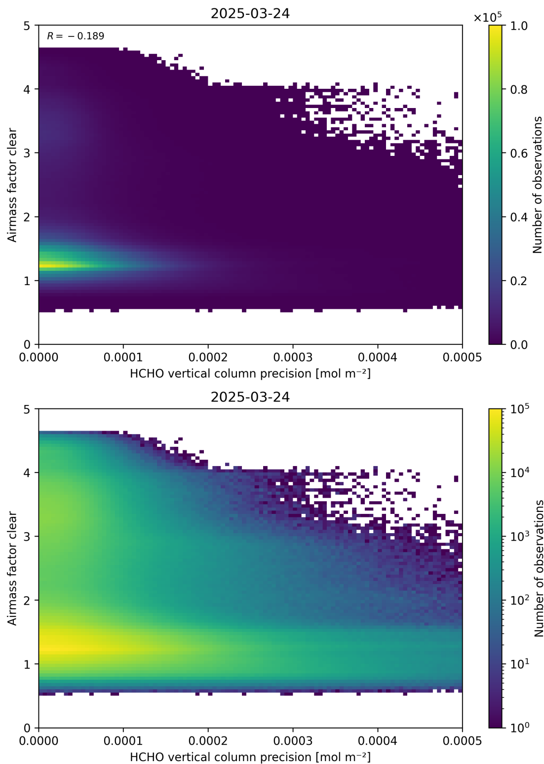
Figure 139: Scatter density plot of “HCHO vertical column precision” against “Airmass factor clear” for 2025-03-23 to 2025-03-25.
