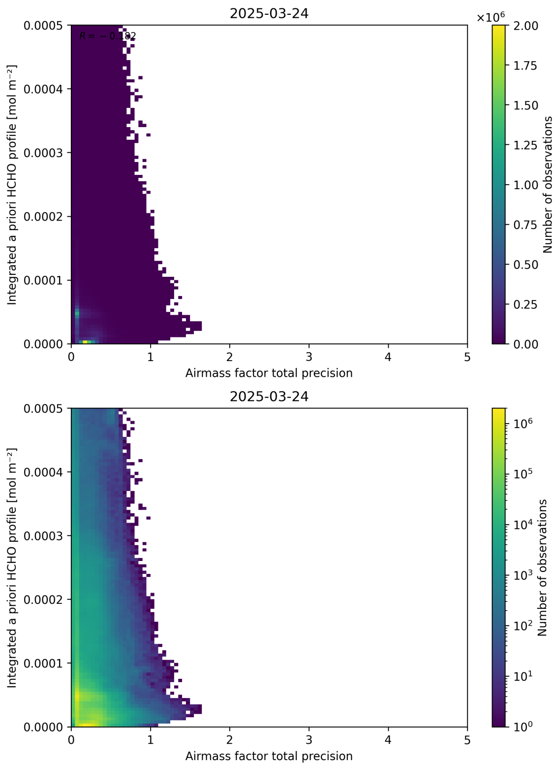
Figure 111: Scatter density plot of “Airmass factor total precision” against “Integrated a priori HCHO profile” for 2025-03-23 to 2025-03-25.
