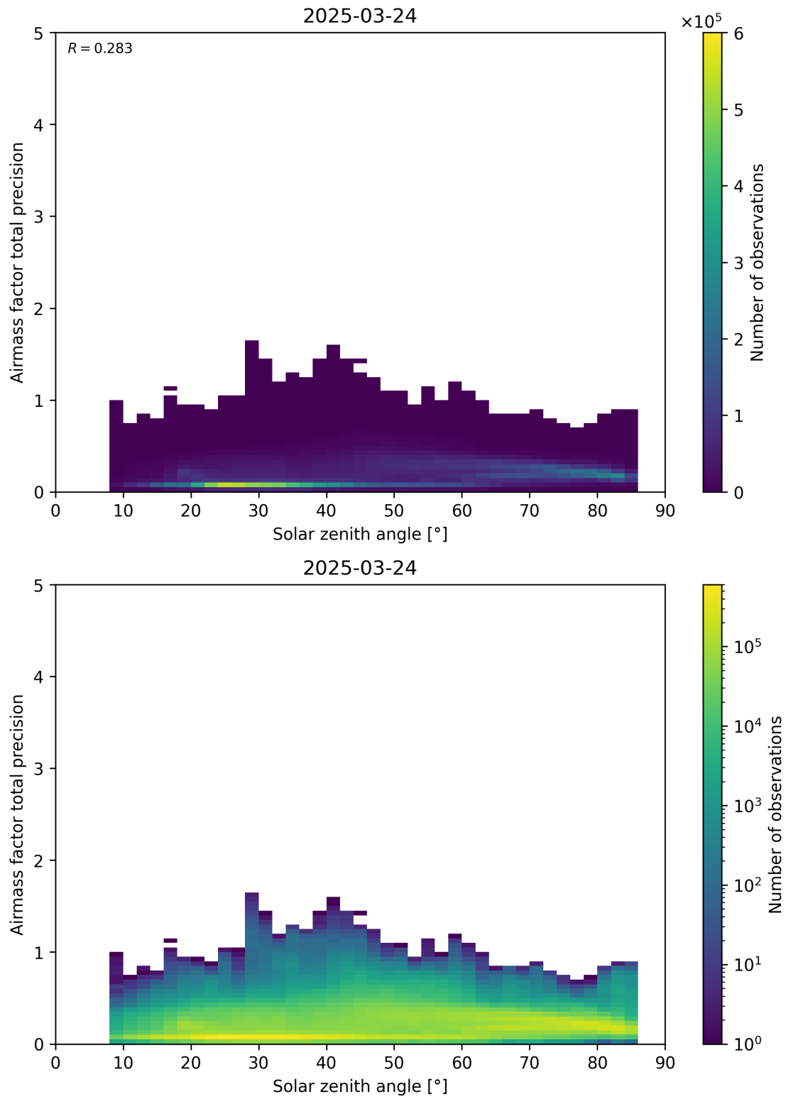
Figure 176: Scatter density plot of “Solar zenith angle” against “Airmass factor total precision” for 2025-03-23 to 2025-03-25.
