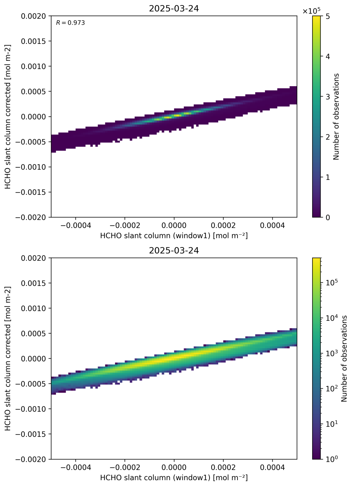
Figure 82: Scatter density plot of “HCHO slant column (window1)” against “HCHO slant column corrected” for 2025-03-23 to 2025-03-25.
