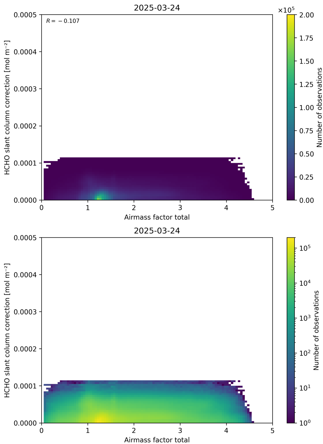
Figure 102: Scatter density plot of “Airmass factor total” against “HCHO slant column correction” for 2025-03-23 to 2025-03-25.
