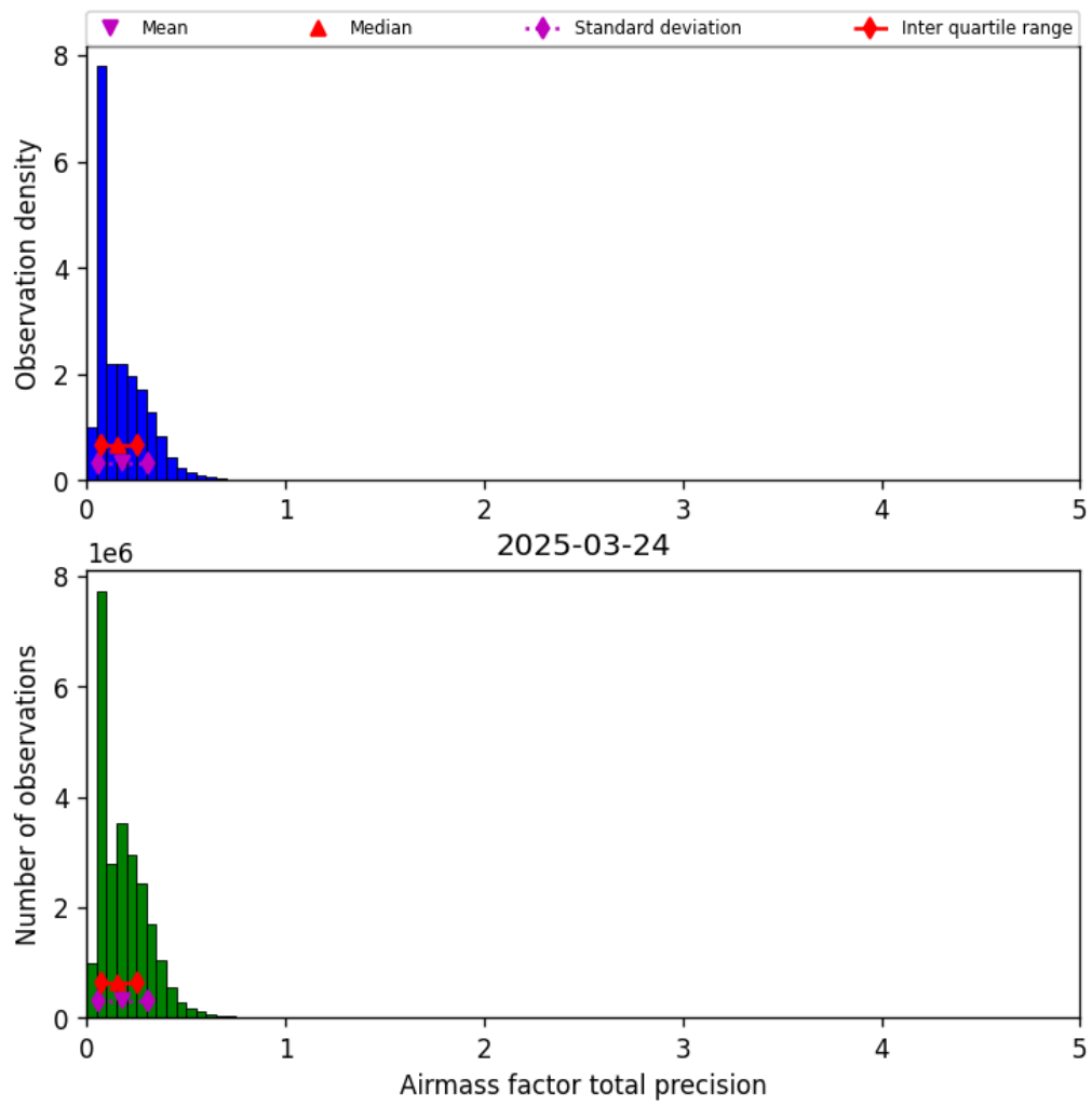
Figure 41: Histogram of “Airmass factor total precision” for 2025-03-23 to 2025-03-25
