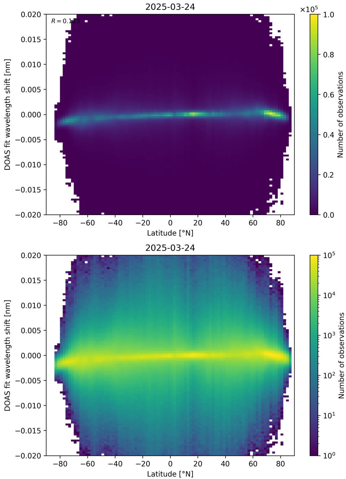
Figure 154: Scatter density plot of “Latitude” against “DOAS fit wavelength shift” for 2025-03-23 to 2025-03-25.
