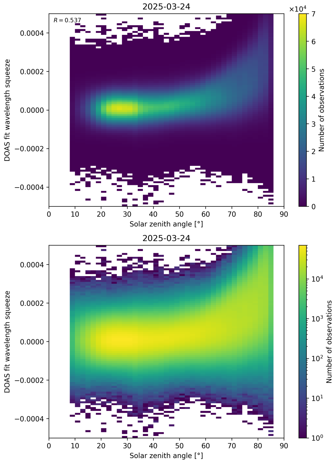
Figure 169: Scatter density plot of “Solar zenith angle” against “DOAS fit wavelength squeeze” for 2025-03-23 to 2025-03-25.
