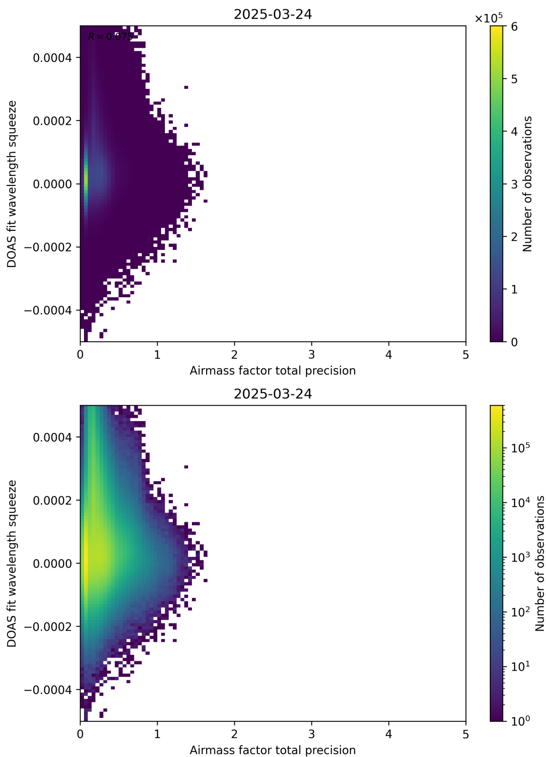
Figure 107: Scatter density plot of “Airmass factor total precision” against “DOAS fit wavelength squeeze” for 2025-03-23 to 2025-03-25.
