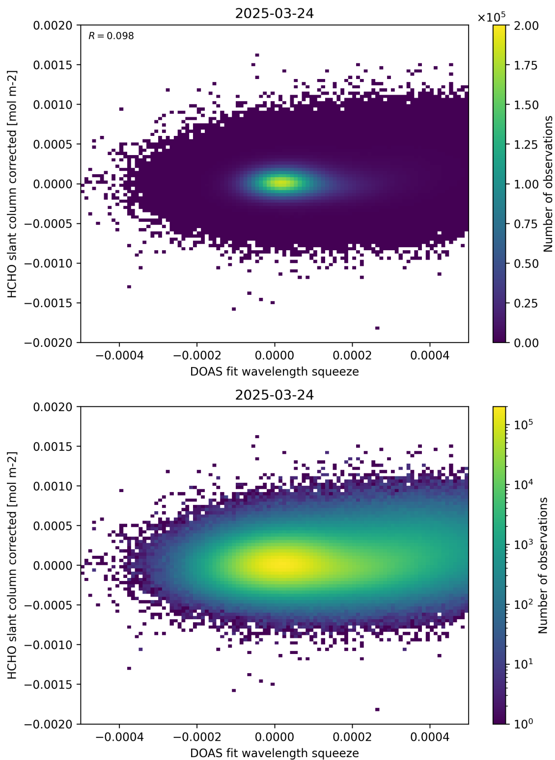
Figure 69: Scatter density plot of “DOAS fit wavelength squeeze” against “HCHO slant column corrected” for 2025-03-23 to 2025-03-25.
