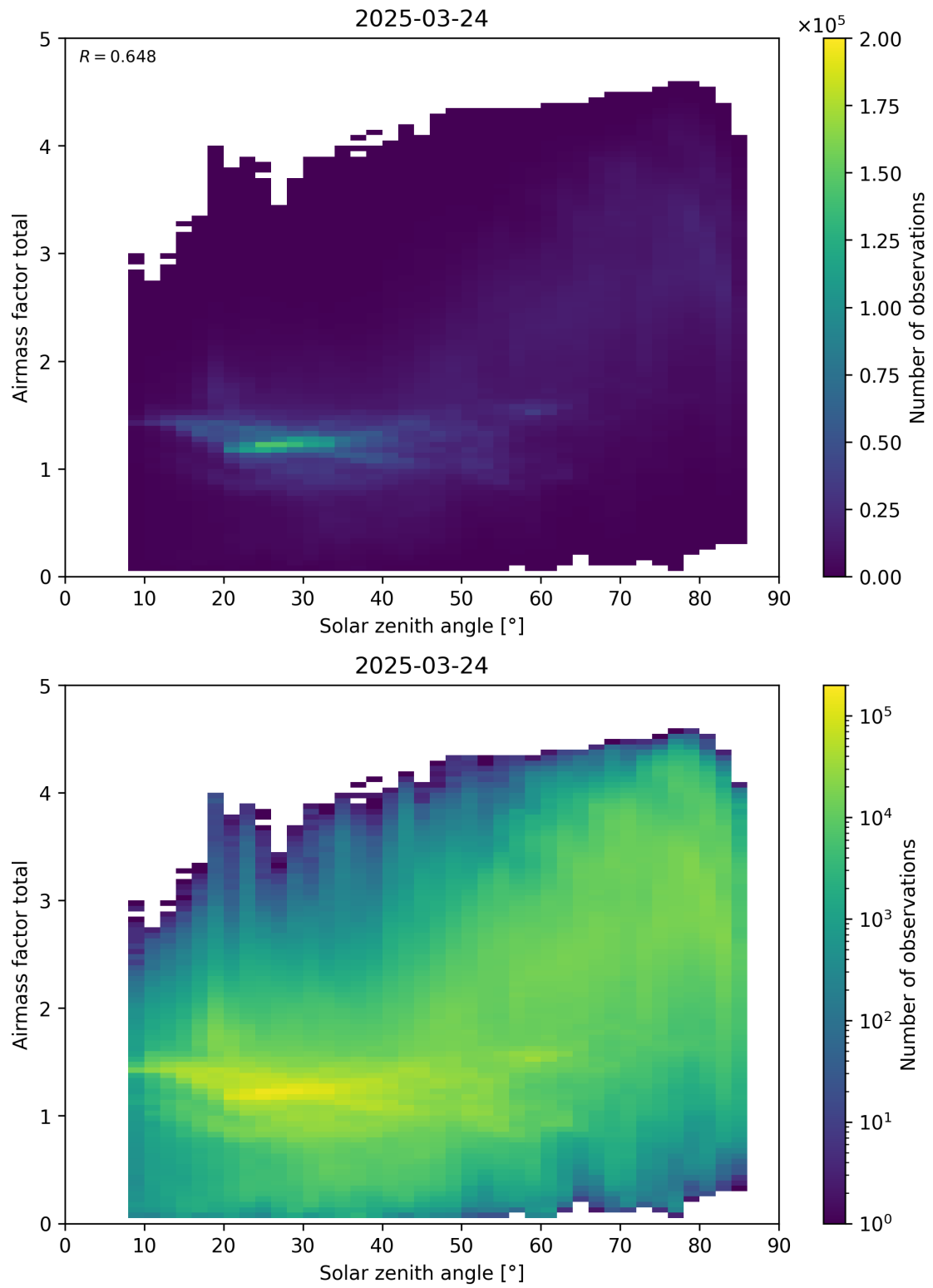
Figure 175: Scatter density plot of “Solar zenith angle” against “Airmass factor total” for 2025-03-23 to 2025-03-25.
