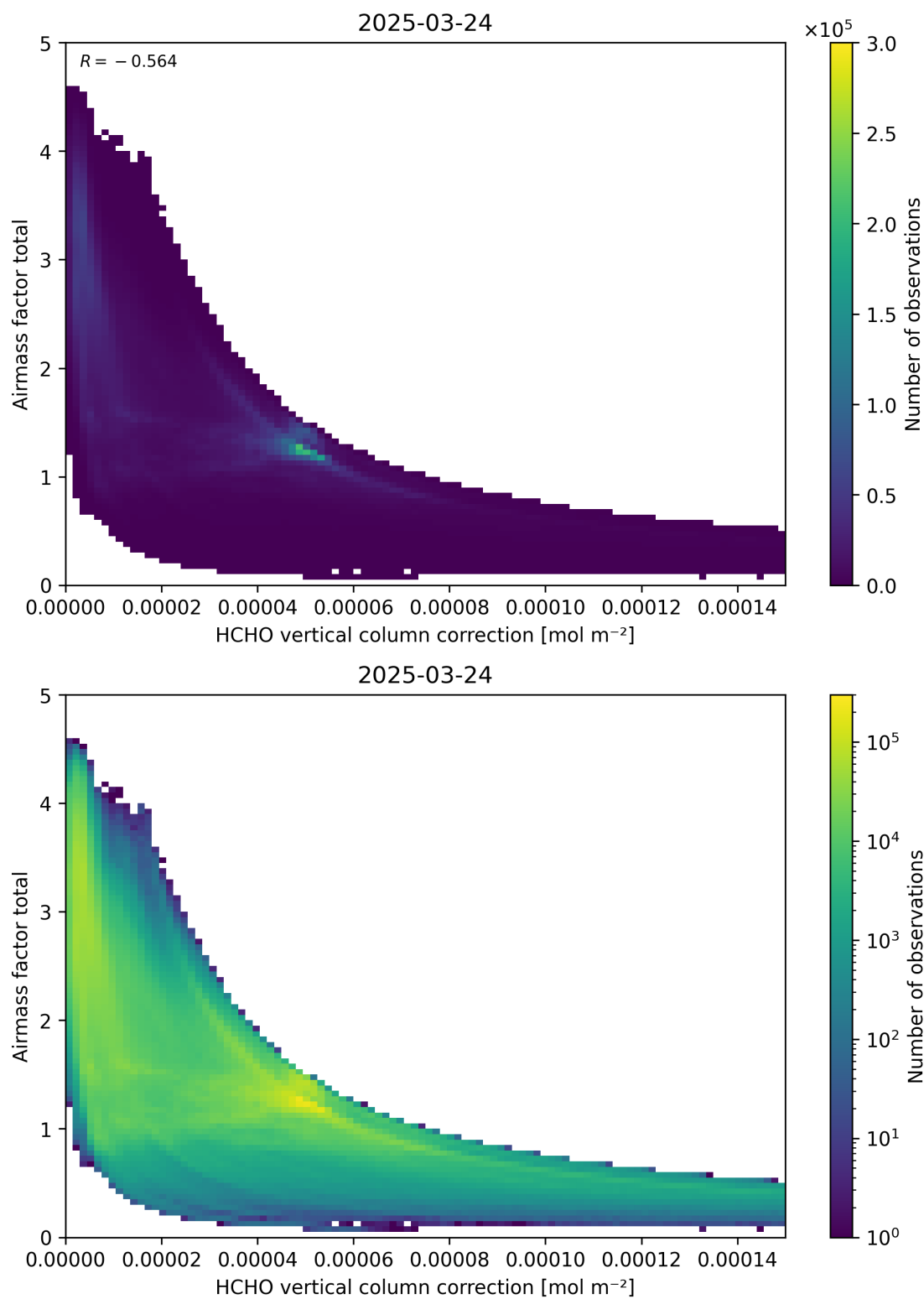
Figure 120: Scatter density plot of “HCHO vertical column correction” against “Airmass factor total” for 2025-03-23 to 2025-03-25.
