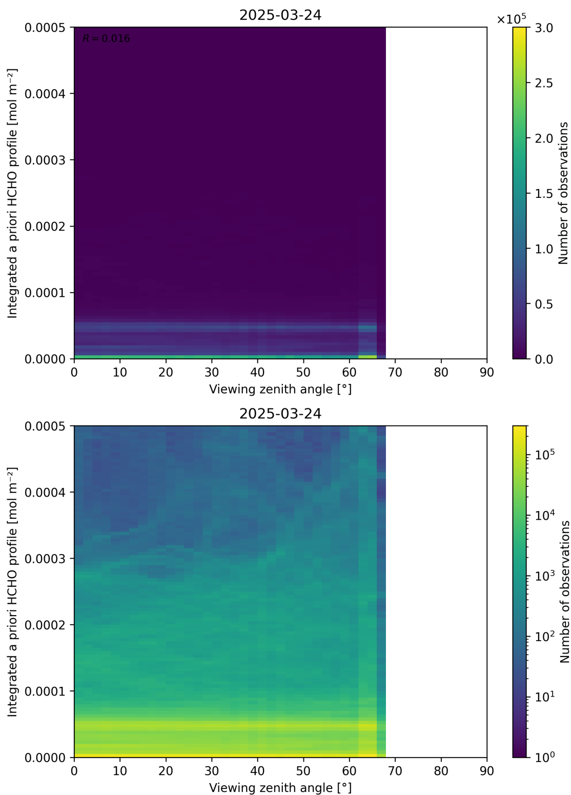
Figure 195: Scatter density plot of “Viewing zenith angle” against “Integrated a priori HCHO profile” for 2025-03-23 to 2025-03-25.
