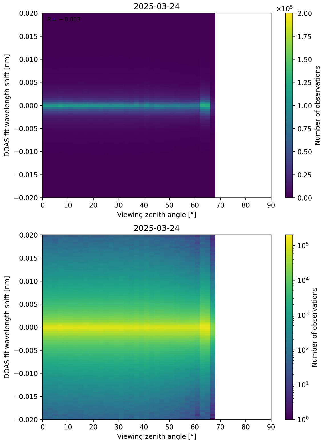
Figure 183: Scatter density plot of “Viewing zenith angle” against “DOAS fit wavelength shift” for 2025-03-23 to 2025-03-25.
