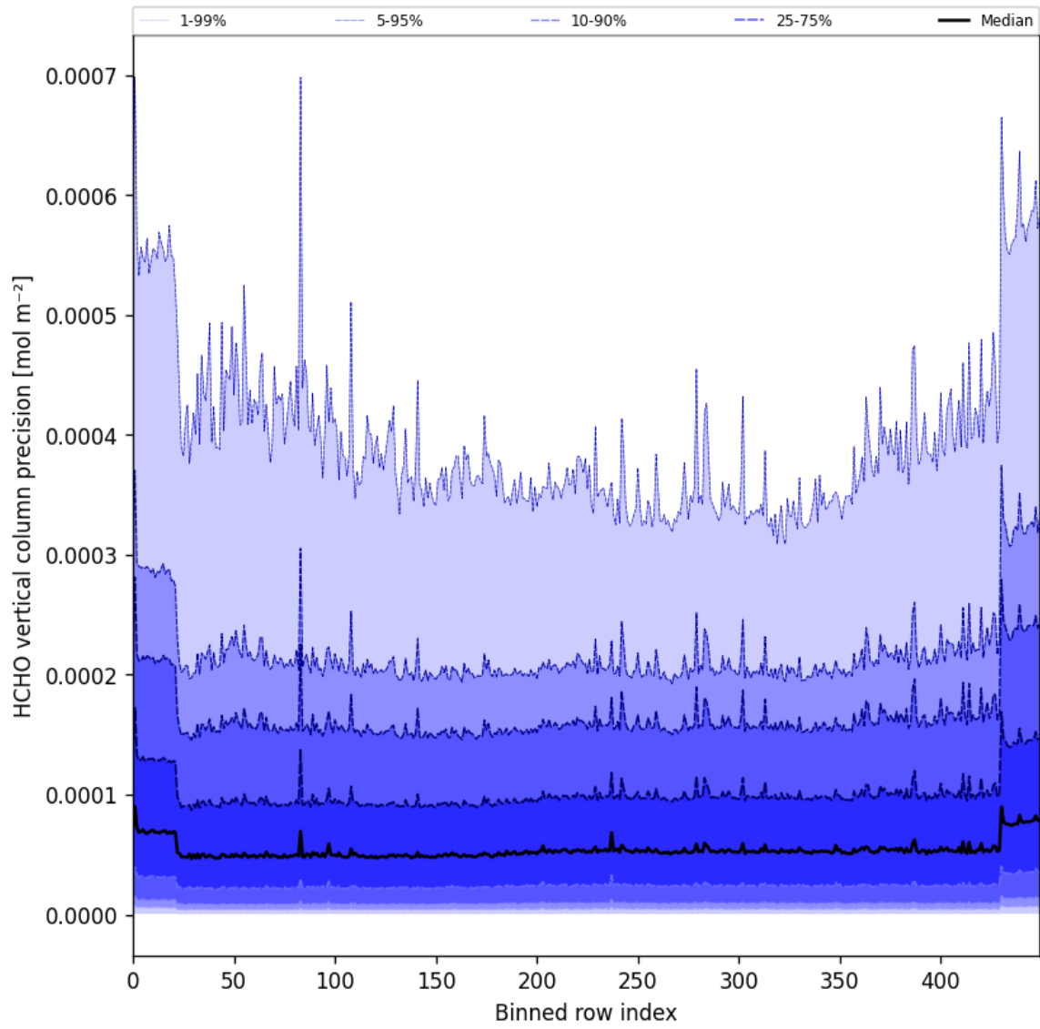
Figure 50: Along track statistics of “HCHO vertical column precision” for 2025-03-23 to 2025-03-25
