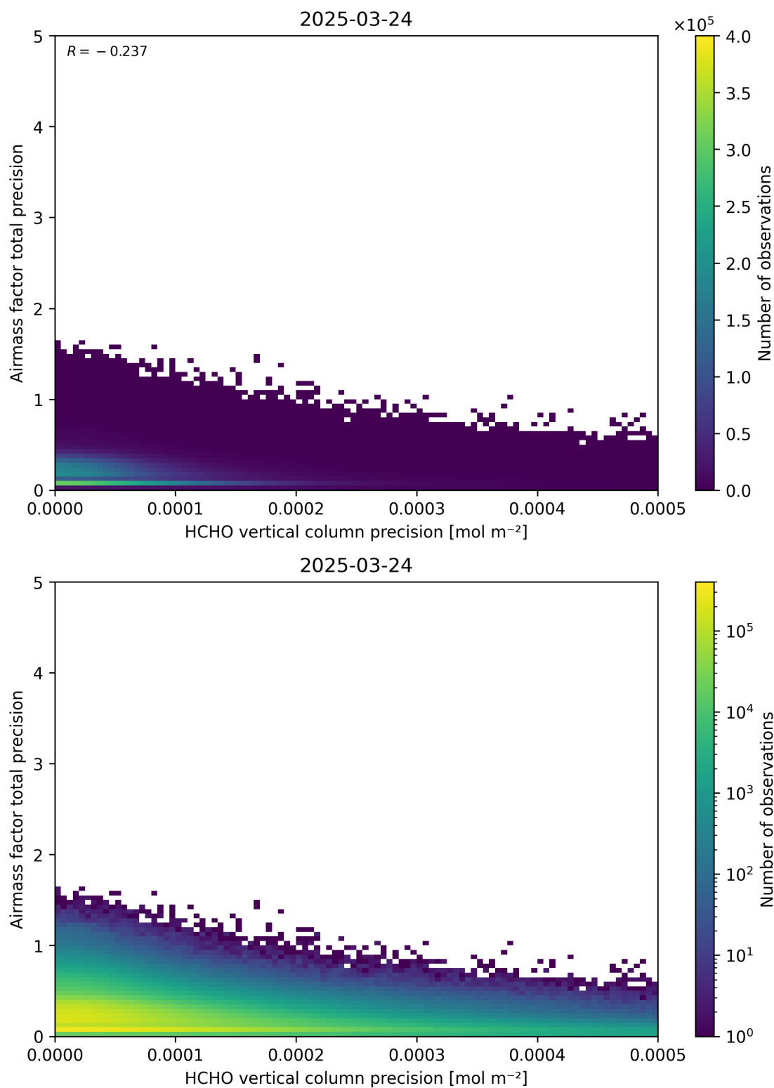
Figure 145: Scatter density plot of “HCHO vertical column precision” against “Airmass factor total precision” for 2025-03-23 to 2025-03-25.
