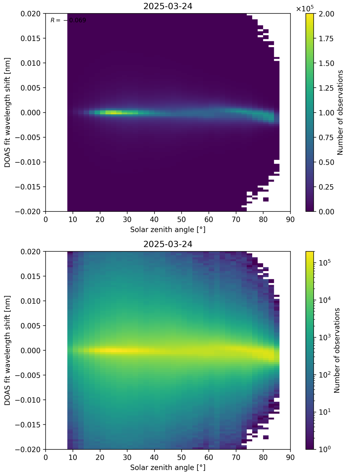
Figure 168: Scatter density plot of “Solar zenith angle” against “DOAS fit wavelength shift” for 2025-03-23 to 2025-03-25.
