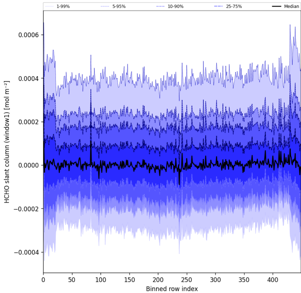
Figure 52: Along track statistics of “HCHO slant column (window1)” for 2025-03-23 to 2025-03-25
