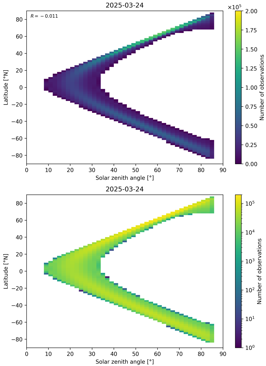
Figure 181: Scatter density plot of “Solar zenith angle” against “Latitude” for 2025-03-23 to 2025-03-25.
