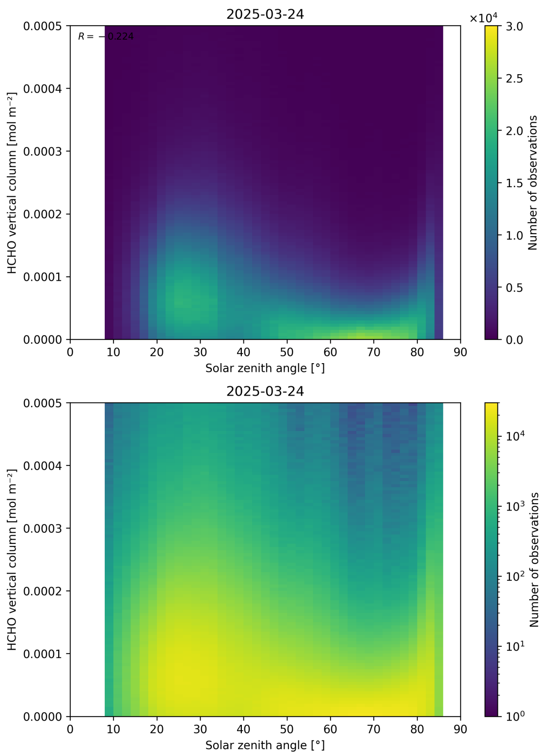
Figure 177: Scatter density plot of “Solar zenith angle” against “HCHO vertical column” for 2025-03-23 to 2025-03-25.
