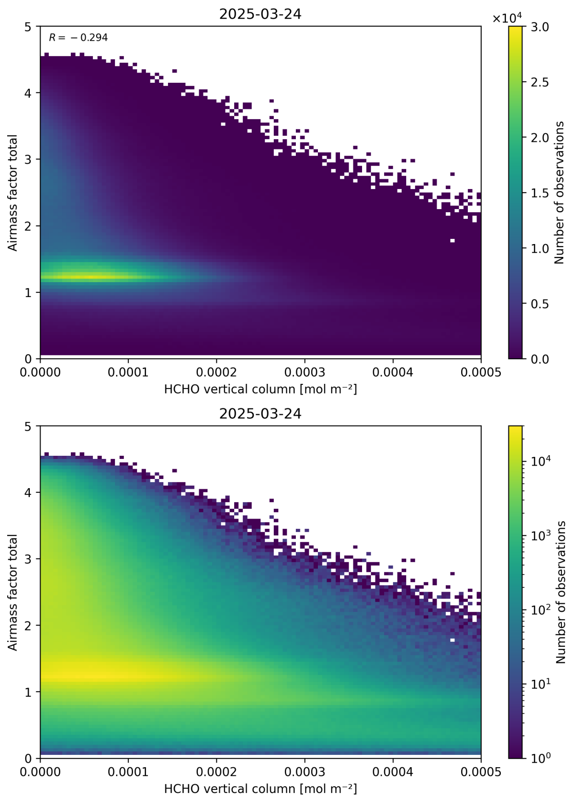
Figure 131: Scatter density plot of “HCHO vertical column” against “Airmass factor total” for 2025-03-23 to 2025-03-25.
