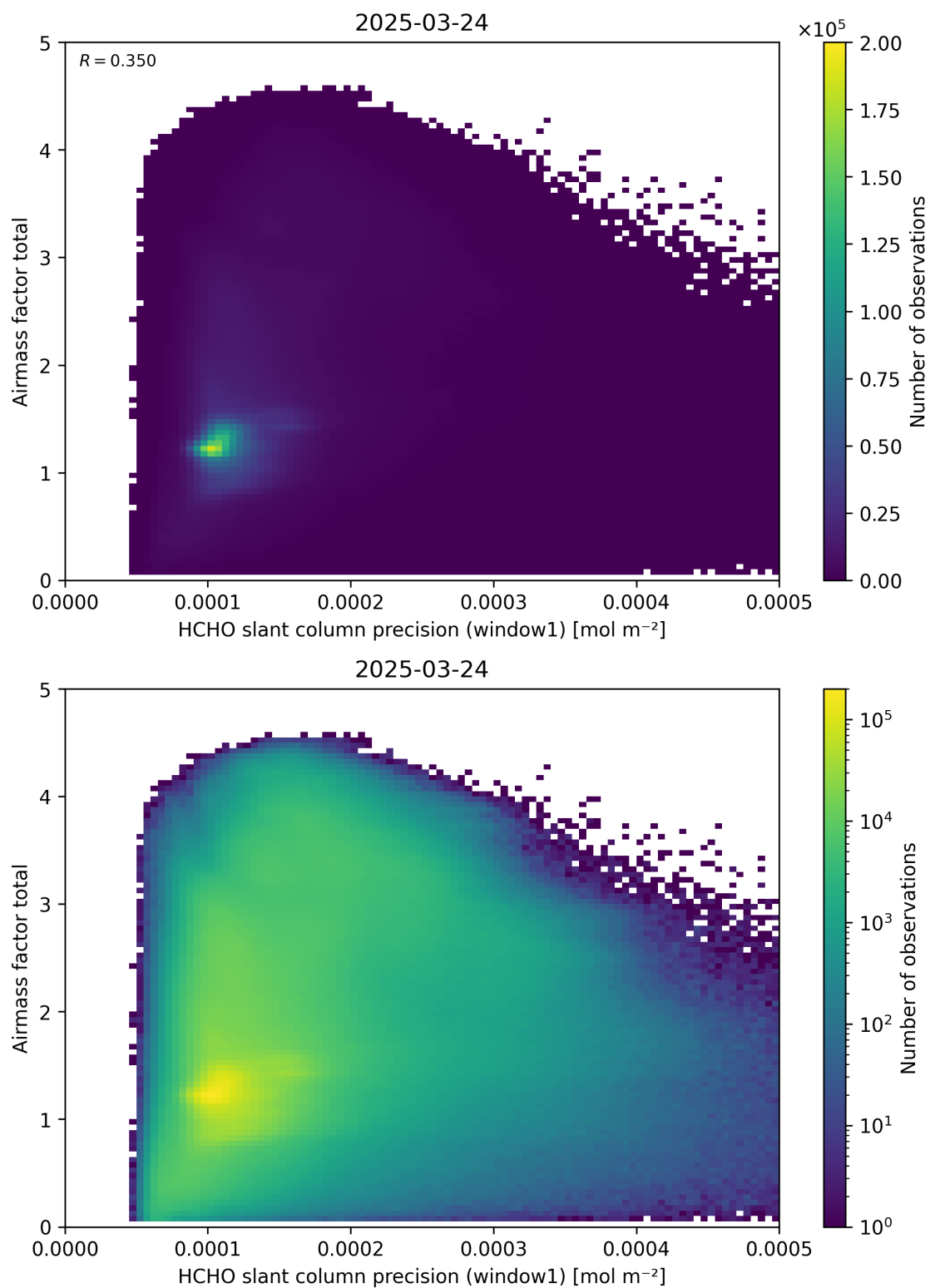
Figure 94: Scatter density plot of “HCHO slant column precision (window1)” against “Airmass factor total” for 2025-03-23 to 2025-03-25.
