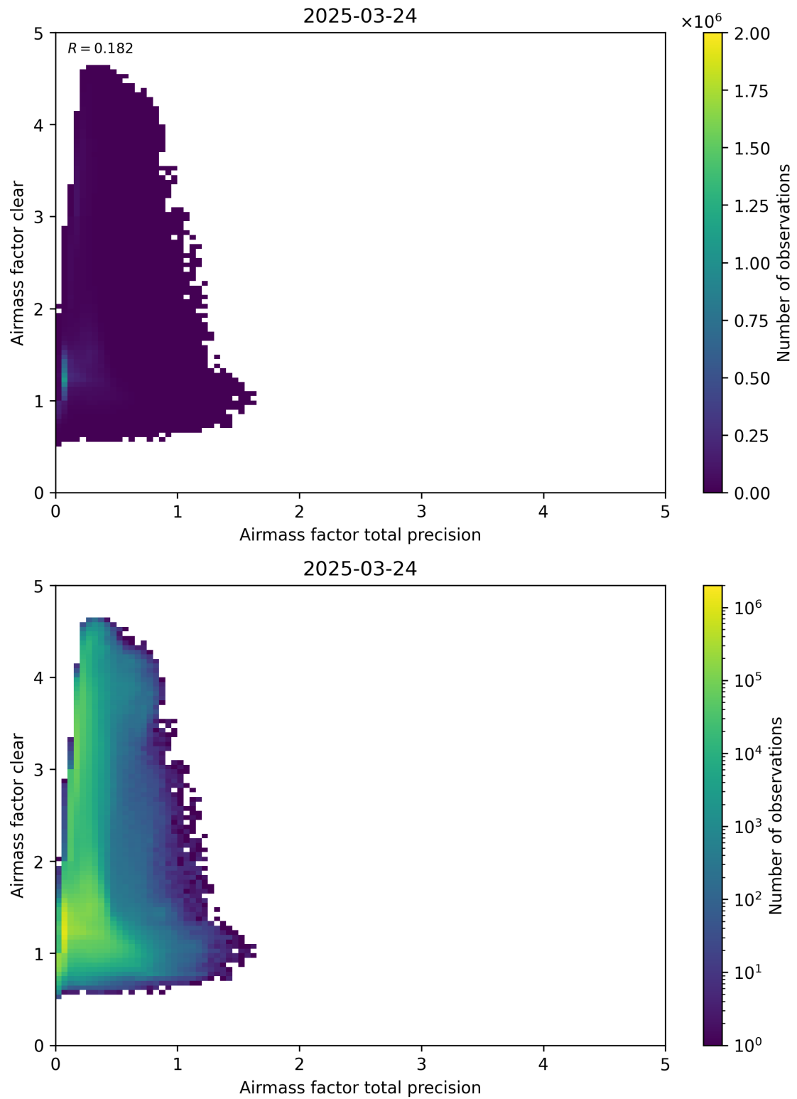
Figure 108: Scatter density plot of “Airmass factor total precision” against “Airmass factor clear” for 2025-03-23 to 2025-03-25.
