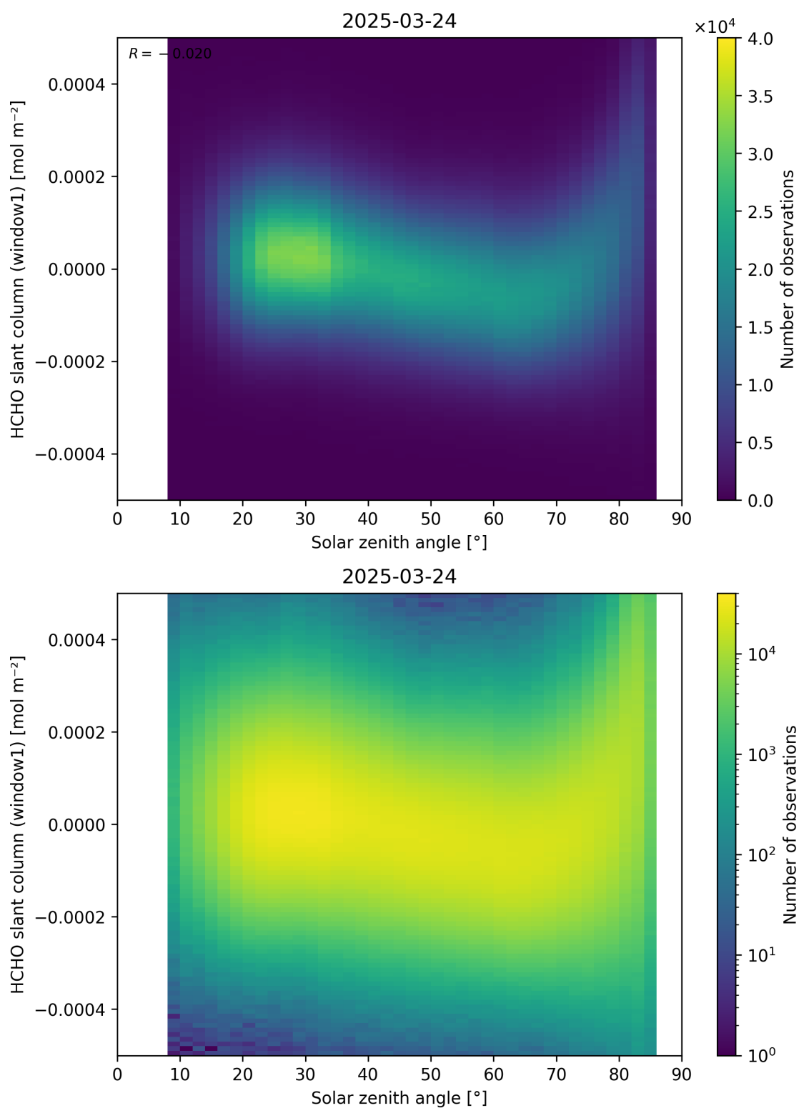
Figure 173: Scatter density plot of “Solar zenith angle” against “HCHO slant column (window1)” for 2025-03-23 to 2025-03-25.
