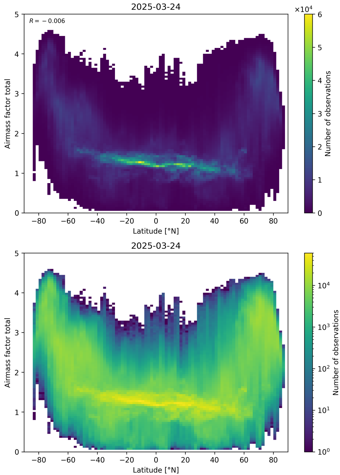
Figure 161: Scatter density plot of “Latitude” against “Airmass factor total” for 2025-03-23 to 2025-03-25.
