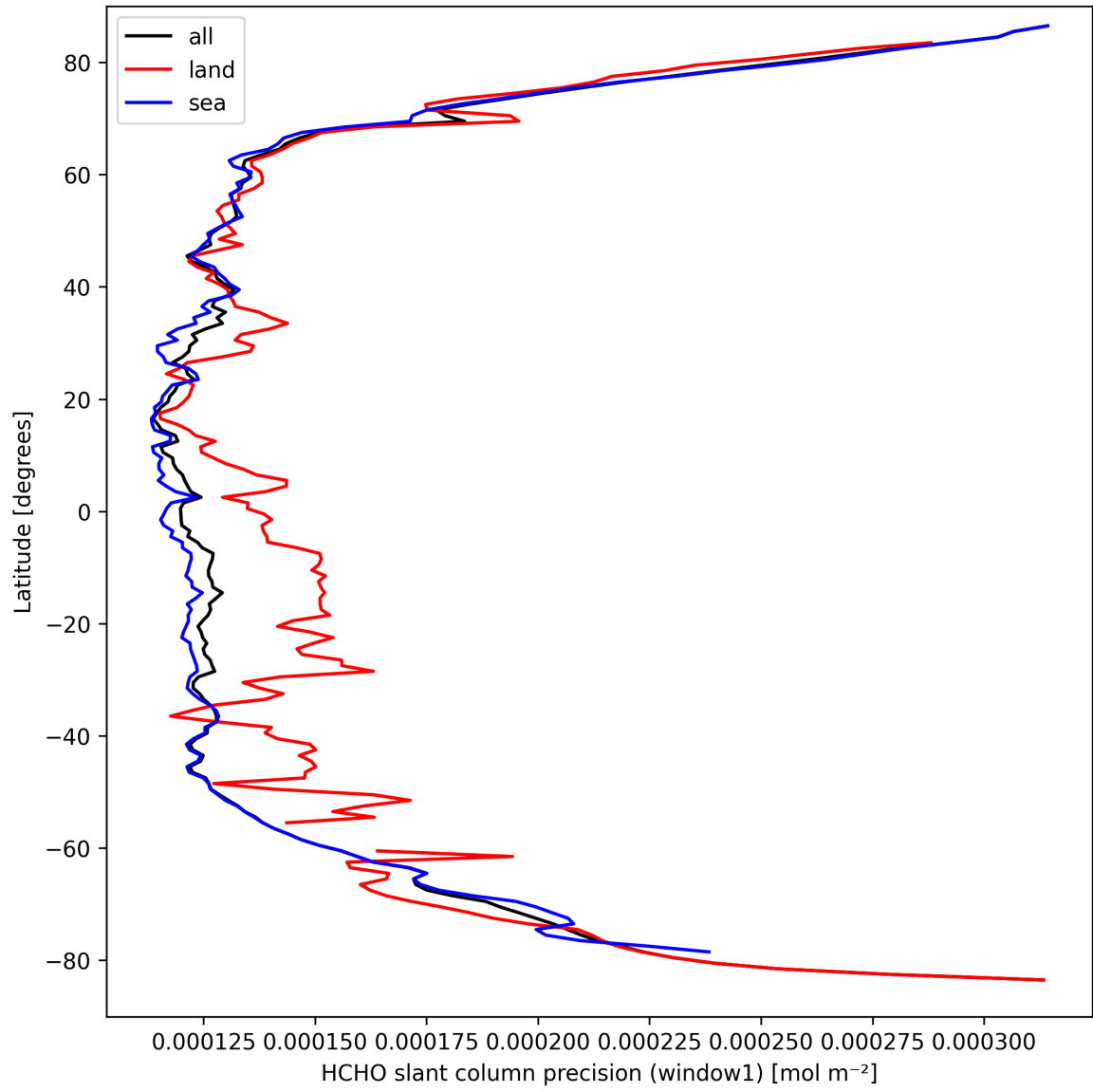
Figure 25: Zonal average of “HCHO slant column precision (window1)” for 2025-03-23 to 2025-03-25.
