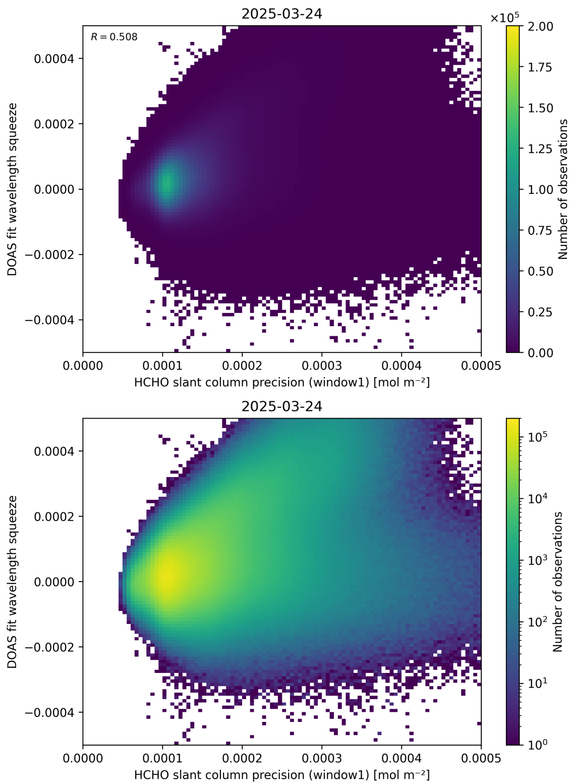
Figure 90: Scatter density plot of “HCHO slant column precision (window1)” against “DOAS fit wavelength squeeze” for 2025-03-23 to 2025-03-25.
