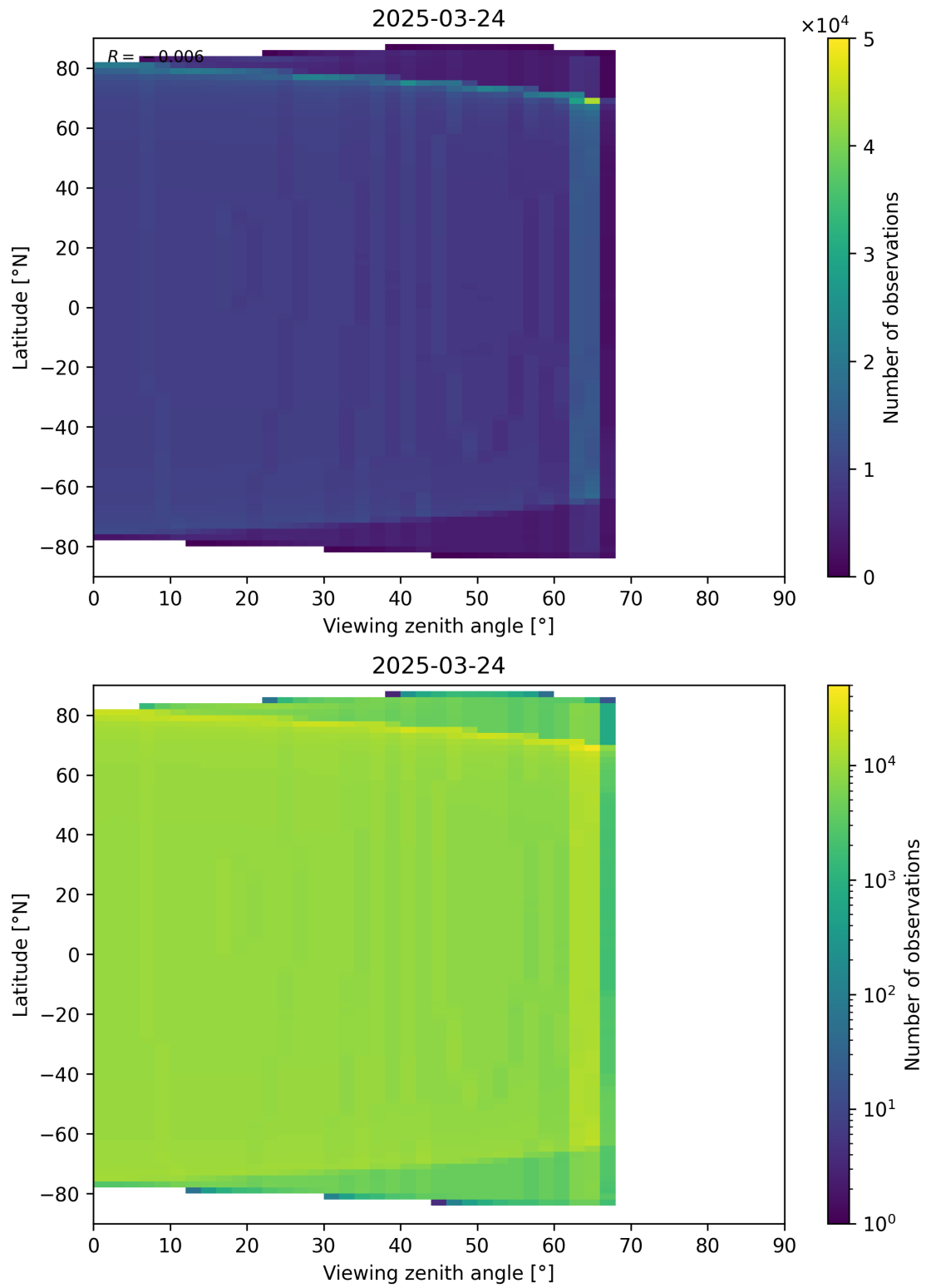
Figure 196: Scatter density plot of “Viewing zenith angle” against “Latitude” for 2025-03-23 to 2025-03-25.
