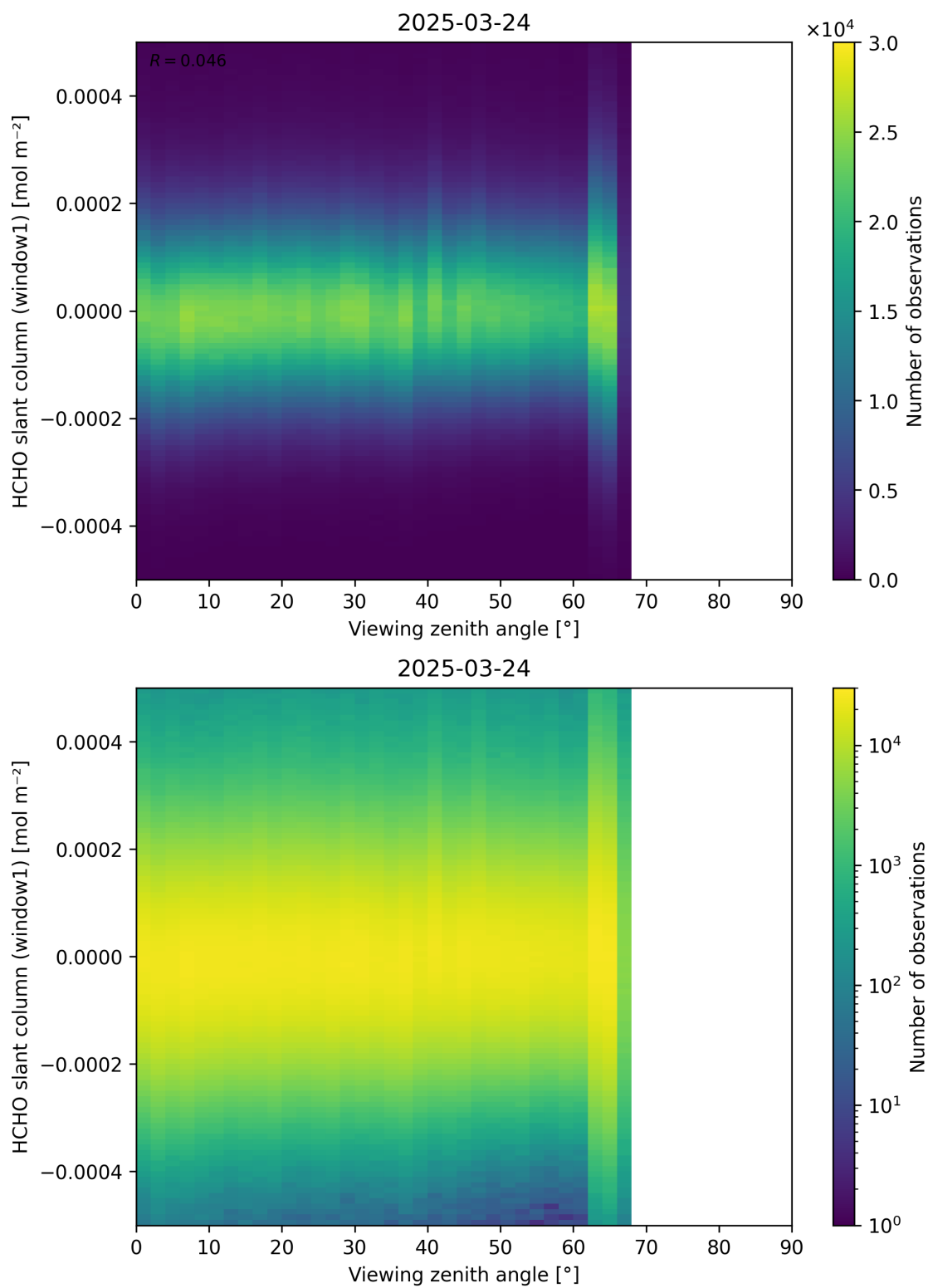
Figure 188: Scatter density plot of “Viewing zenith angle” against “HCHO slant column (window1)” for 2025-03-23 to 2025-03-25.
