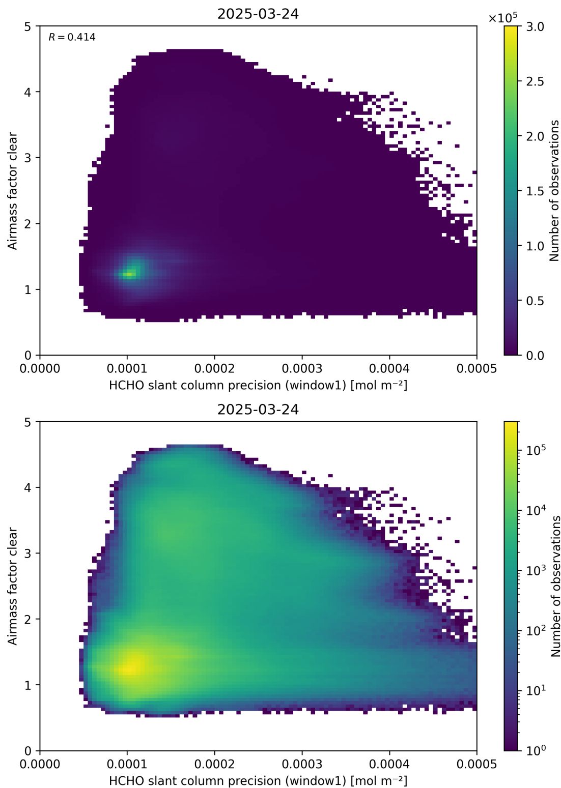
Figure 91: Scatter density plot of “HCHO slant column precision (window1)” against “Airmass factor clear” for 2025-03-23 to 2025-03-25.
