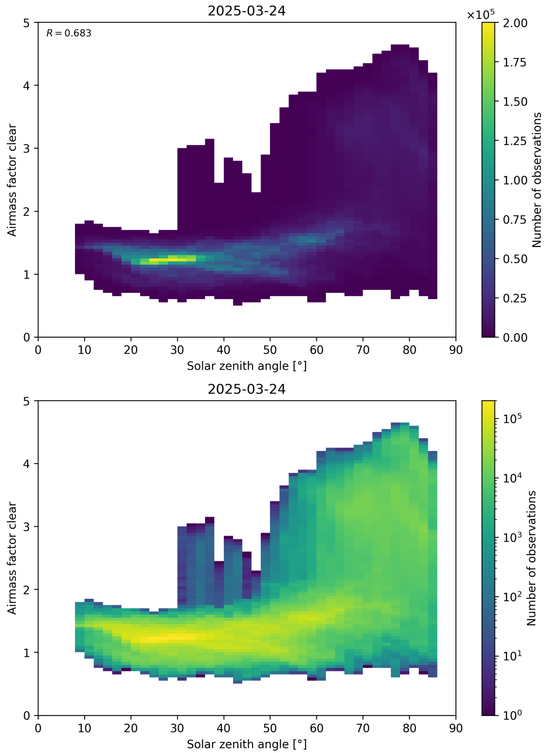
Figure 170: Scatter density plot of “Solar zenith angle” against “Airmass factor clear” for 2025-03-23 to 2025-03-25.
