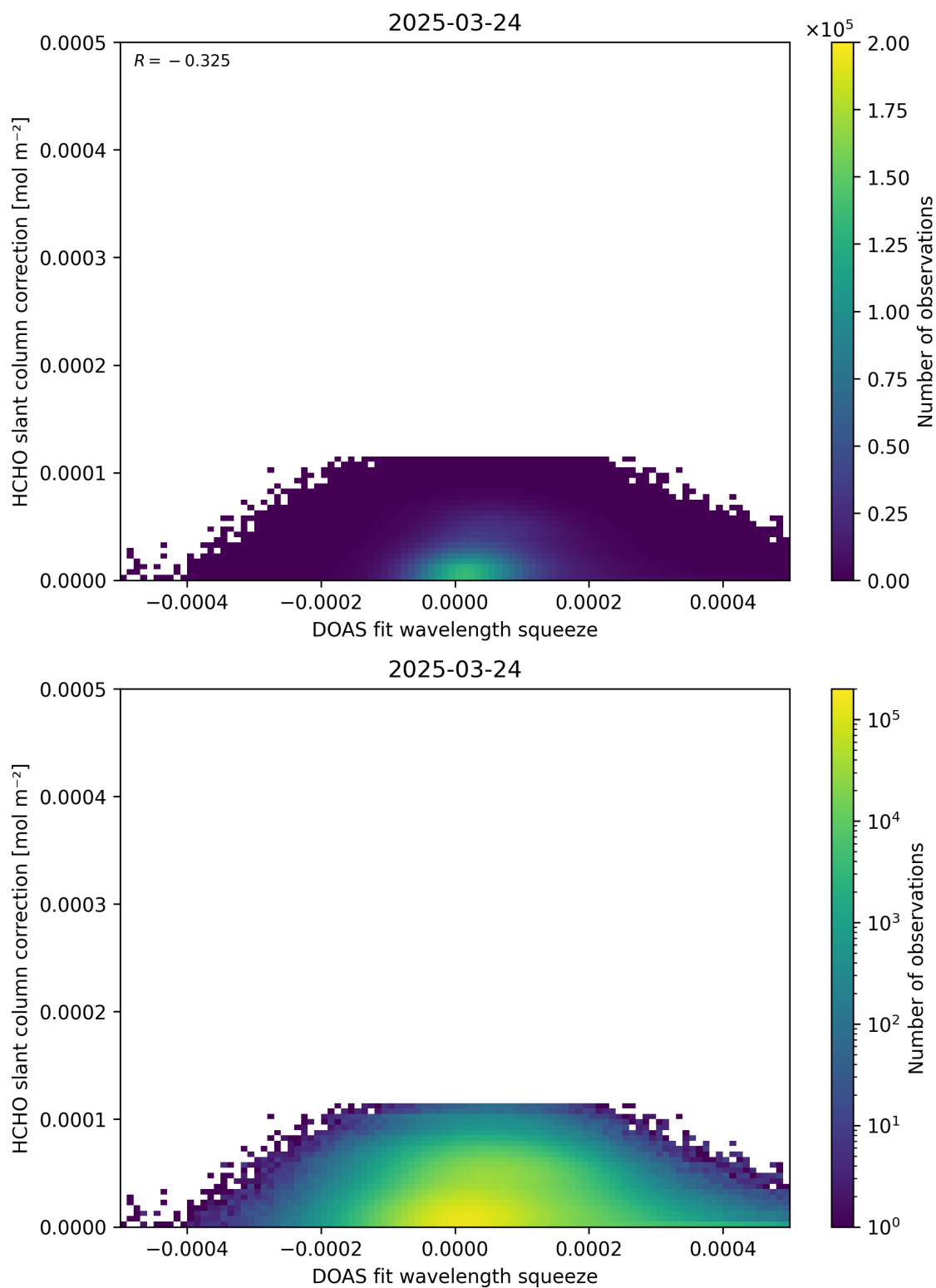
Figure 70: Scatter density plot of “DOAS fit wavelength squeeze” against “HCHO slant column correction” for 2025-03-23 to 2025-03-25.
