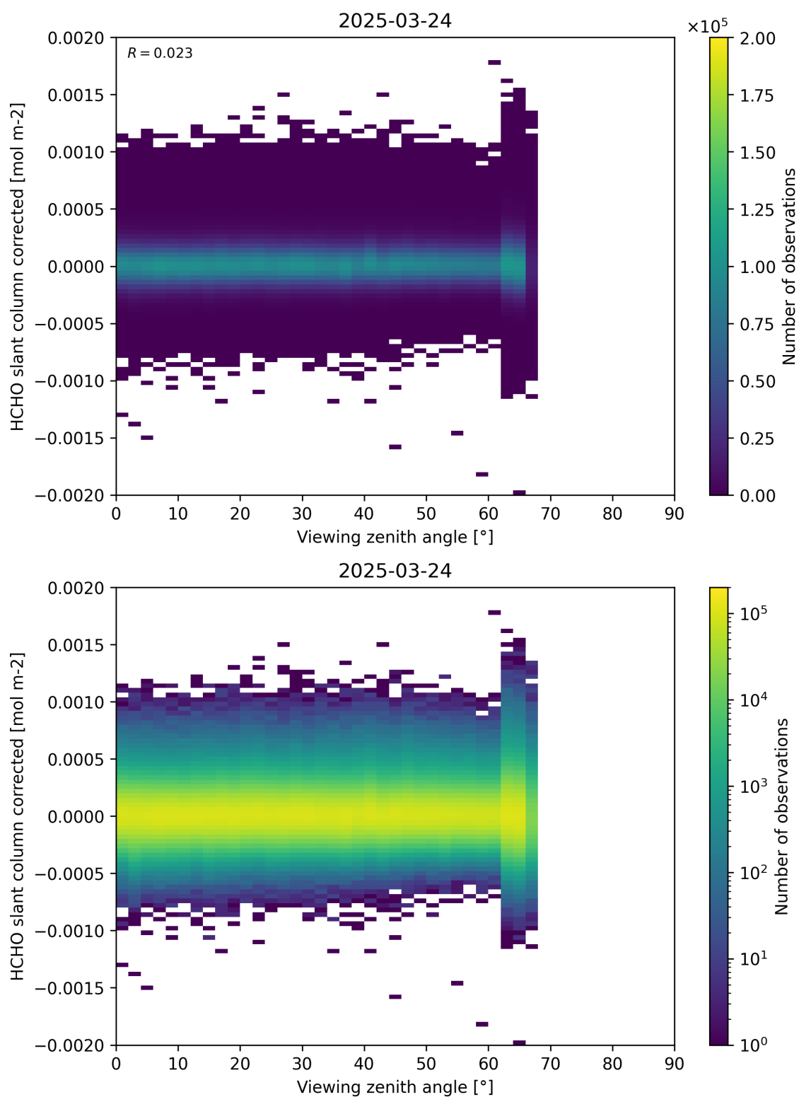
Figure 186: Scatter density plot of “Viewing zenith angle” against “HCHO slant column corrected” for 2025-03-23 to 2025-03-25.
