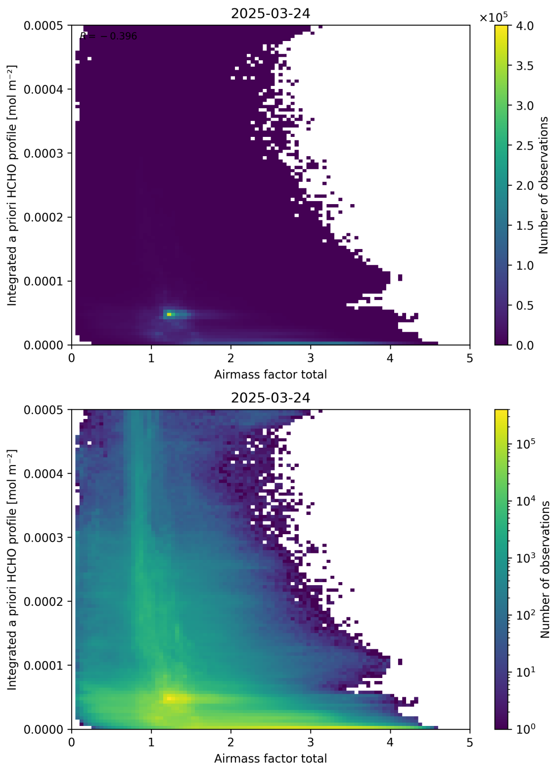
Figure 104: Scatter density plot of “Airmass factor total” against “Integrated a priori HCHO profile” for 2025-03-23 to 2025-03-25.
