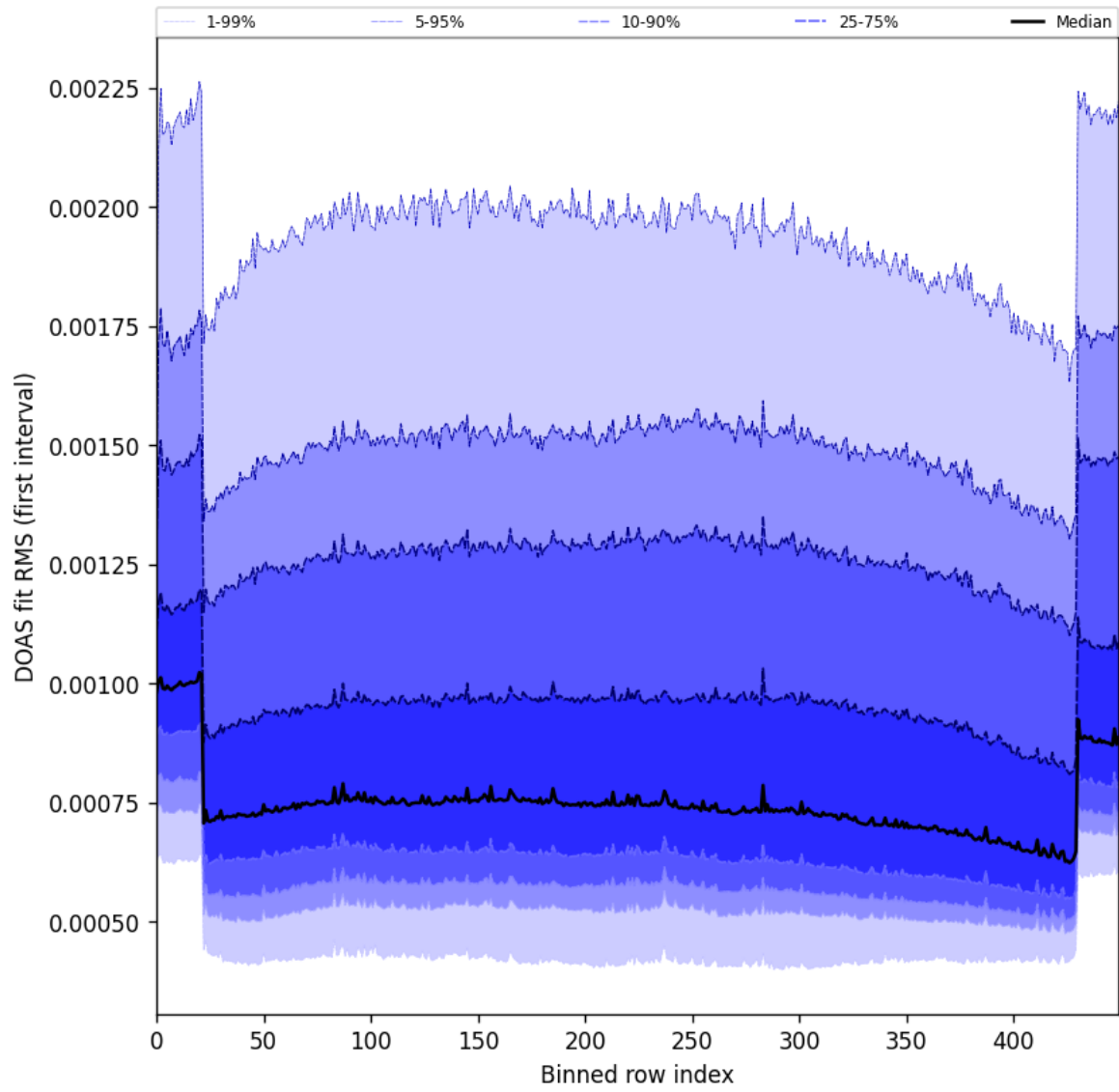
Figure 60: Along track statistics of “DOAS fit RMS (first interval)” for 2025-03-23 to 2025-03-25
