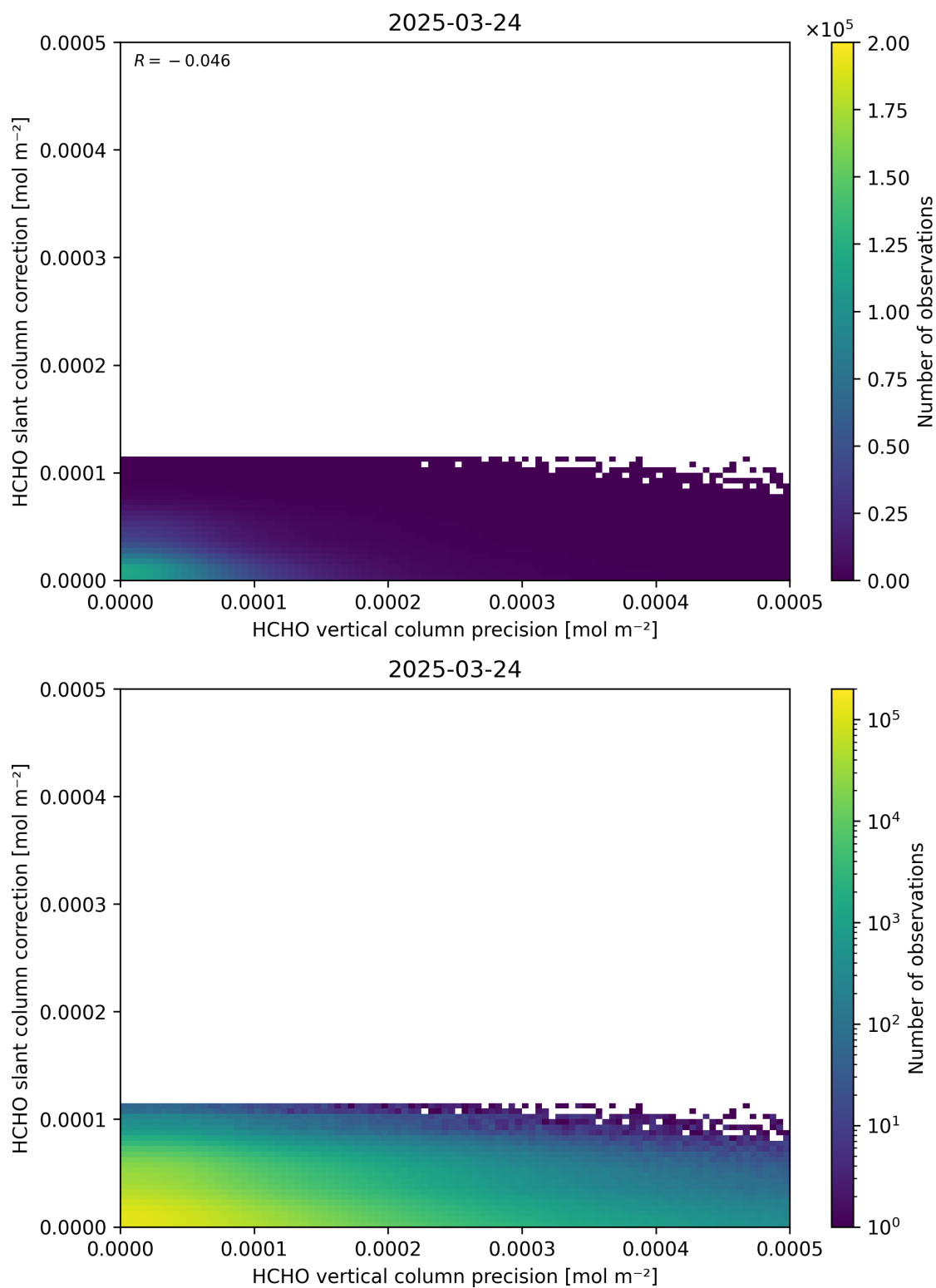
Figure 141: Scatter density plot of “HCHO vertical column precision” against “HCHO slant column correction” for 2025-03-23 to 2025-03-25.
