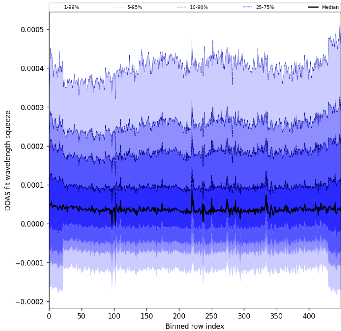
Figure 59: Along track statistics of “DOAS fit wavelength squeeze” for 2025-03-23 to 2025-03-25
