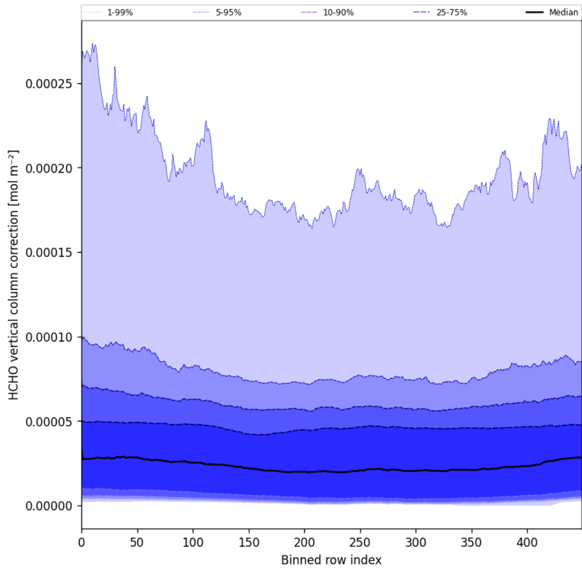
Figure 51: Along track statistics of “HCHO vertical column correction” for 2025-03-24 to 2025-03-26
