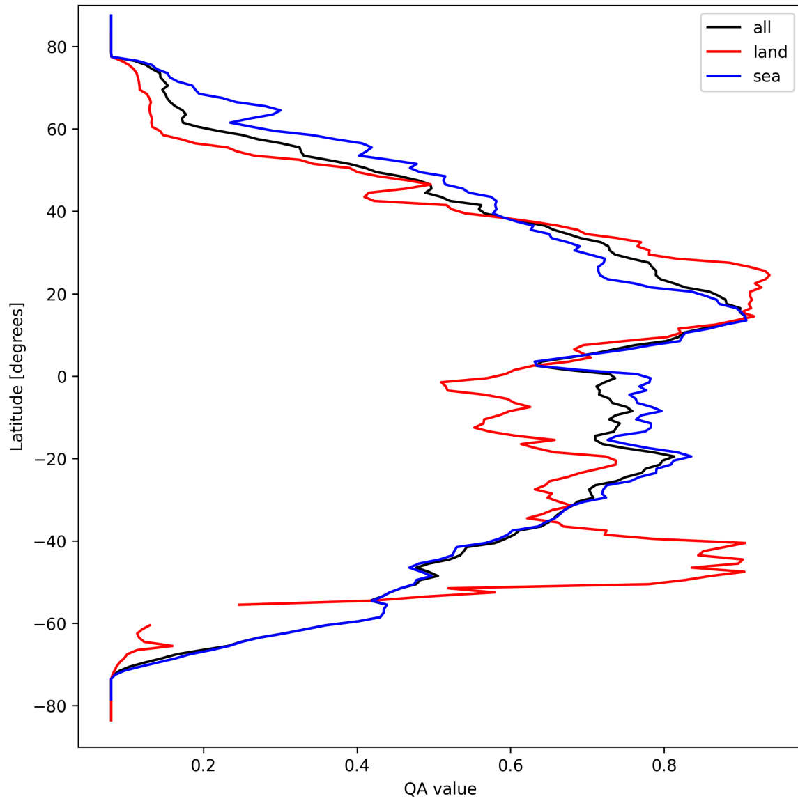
Figure 20: Zonal average of “QA value” for 2025-03-24 to 2025-03-26.
