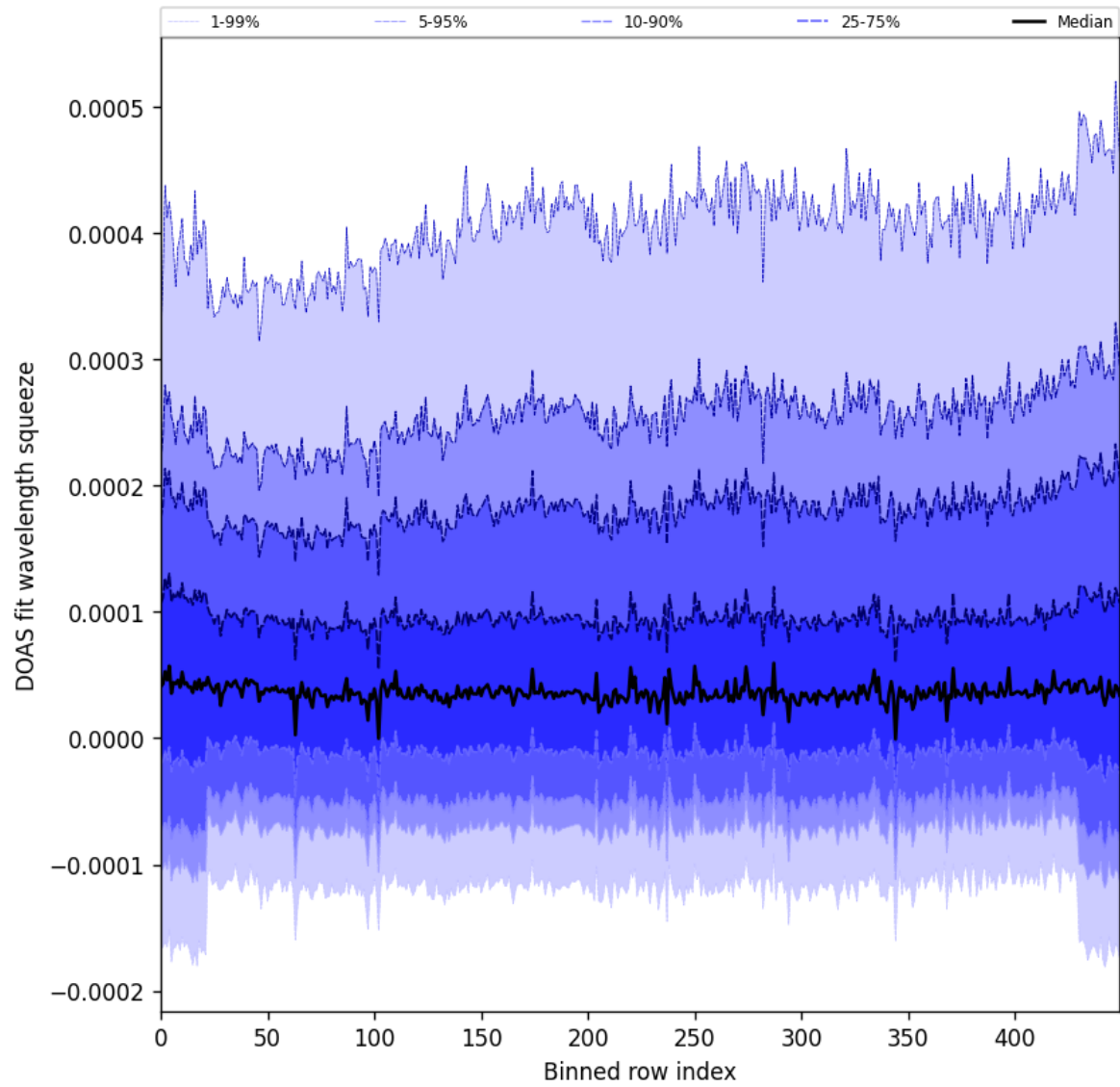
Figure 59: Along track statistics of “DOAS fit wavelength squeeze” for 2025-03-24 to 2025-03-26
