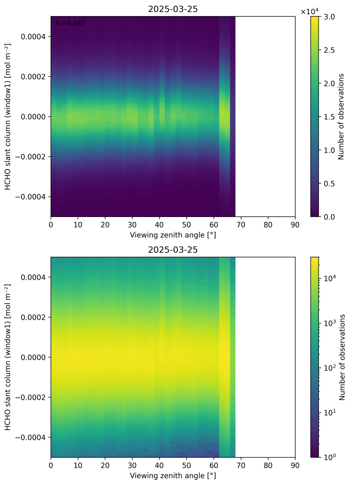
Figure 188: Scatter density plot of “Viewing zenith angle” against “HCHO slant column (window1)” for 2025-03-24 to 2025-03-26.
