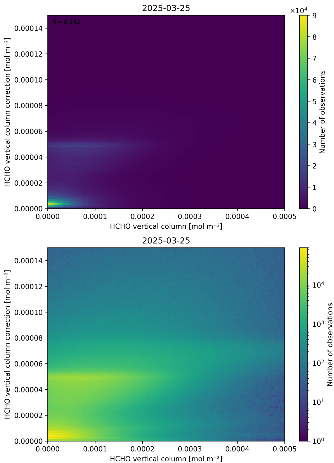
Figure 133: Scatter density plot of “HCHO vertical column” against “HCHO vertical column correction” for 2025-03-24 to 2025-03-26.
