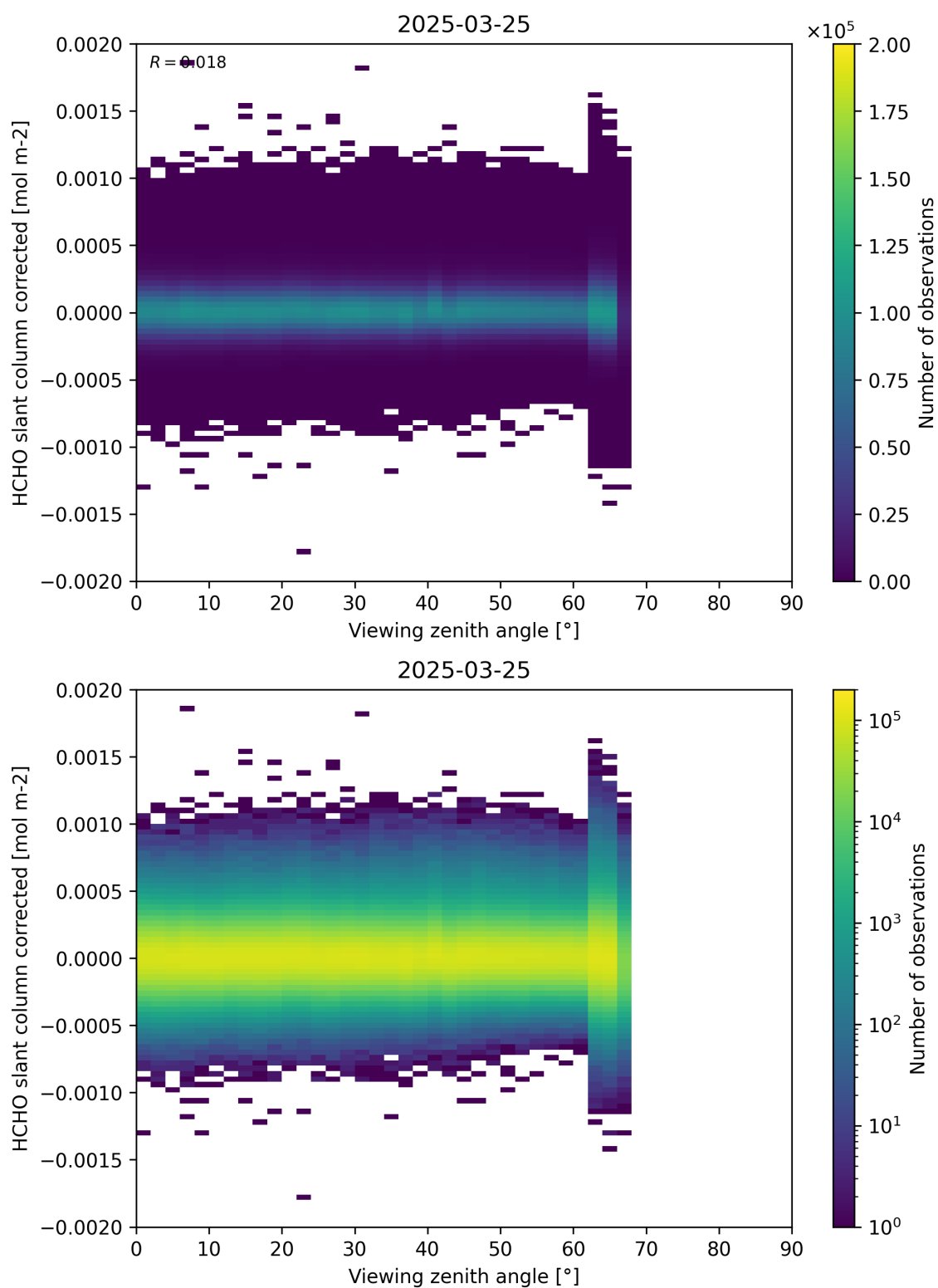
Figure 186: Scatter density plot of “Viewing zenith angle” against “HCHO slant column corrected” for 2025-03-24 to 2025-03-26.
