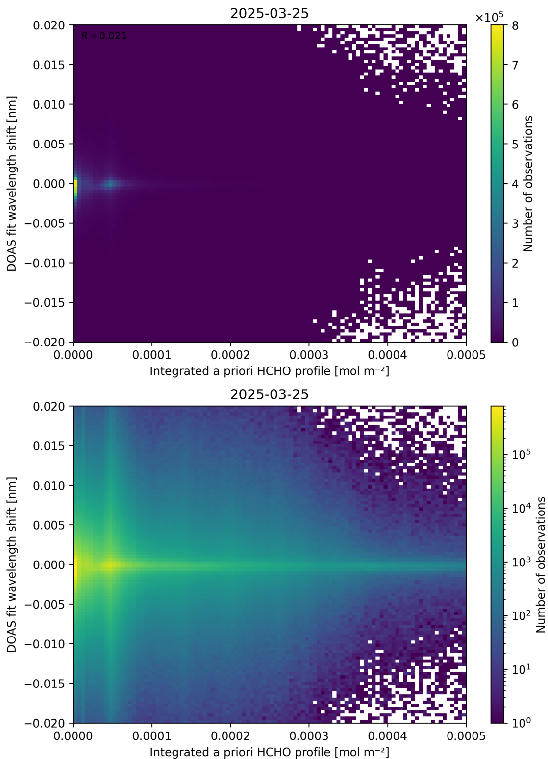
Figure 149: Scatter density plot of “Integrated a priori HCHO profile” against “DOAS fit wavelength shift” for 2025-03-24 to 2025-03-26.
