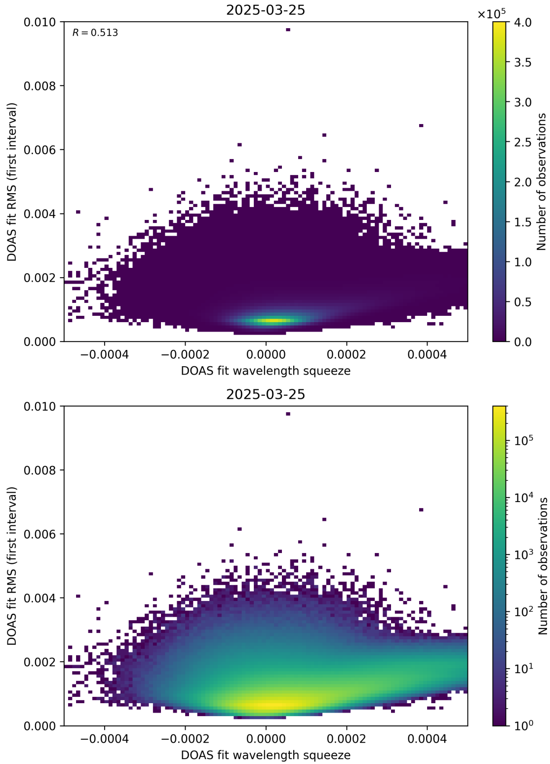
Figure 68: Scatter density plot of “DOAS fit wavelength squeeze” against “DOAS fit RMS (first interval)” for 2025-03-24 to 2025-03-26.
