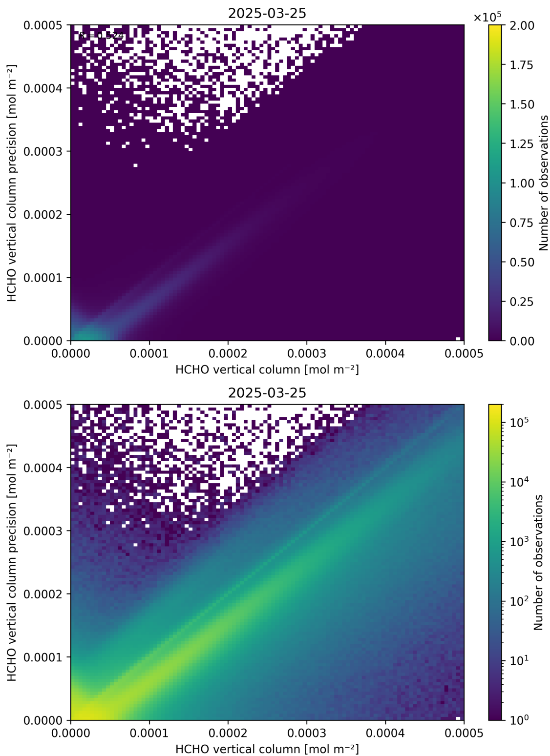
Figure 134: Scatter density plot of “HCHO vertical column” against “HCHO vertical column precision” for 2025-03-24 to 2025-03-26.
