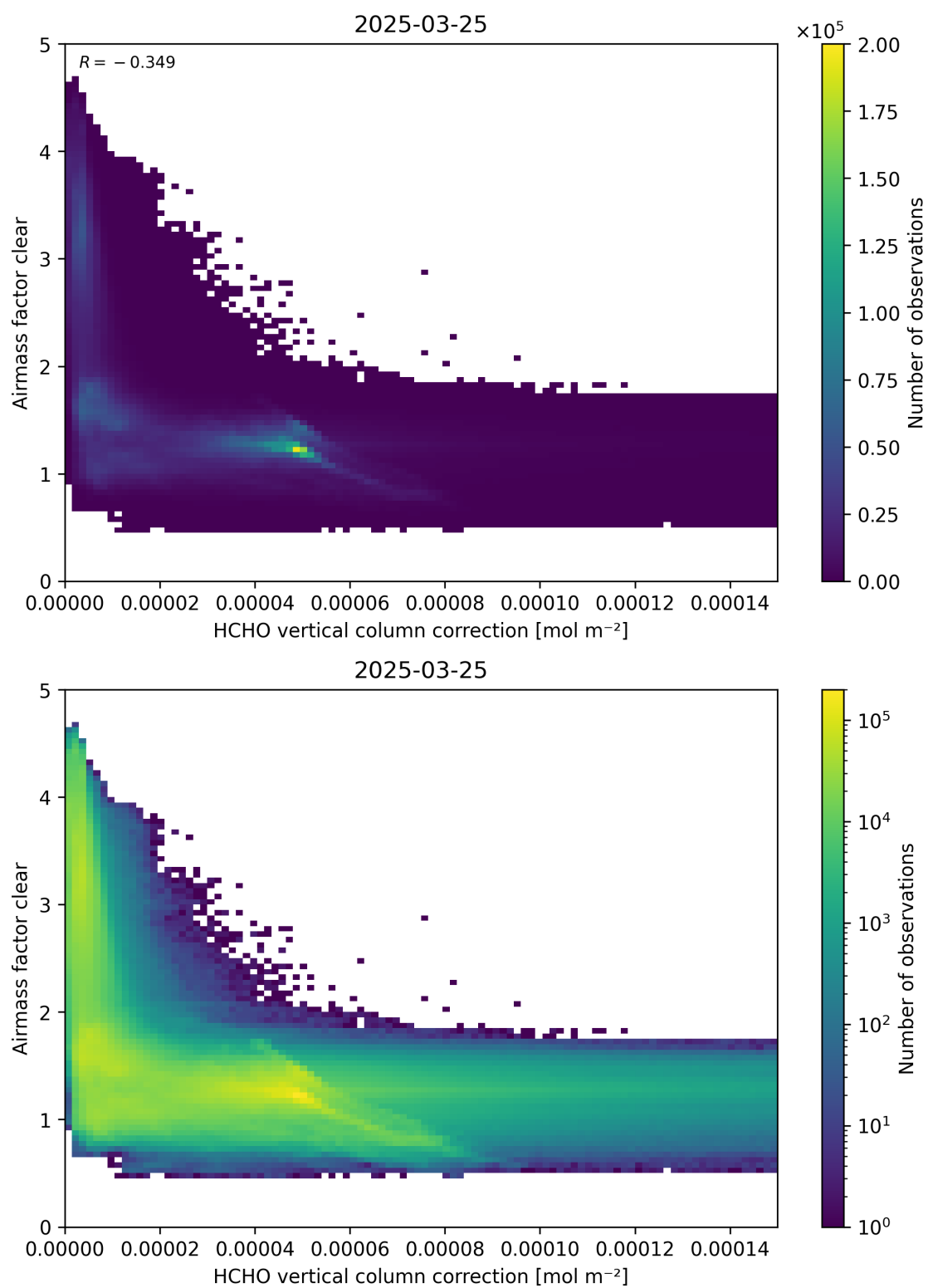
Figure 115: Scatter density plot of “HCHO vertical column correction” against “Airmass factor clear” for 2025-03-24 to 2025-03-26.
