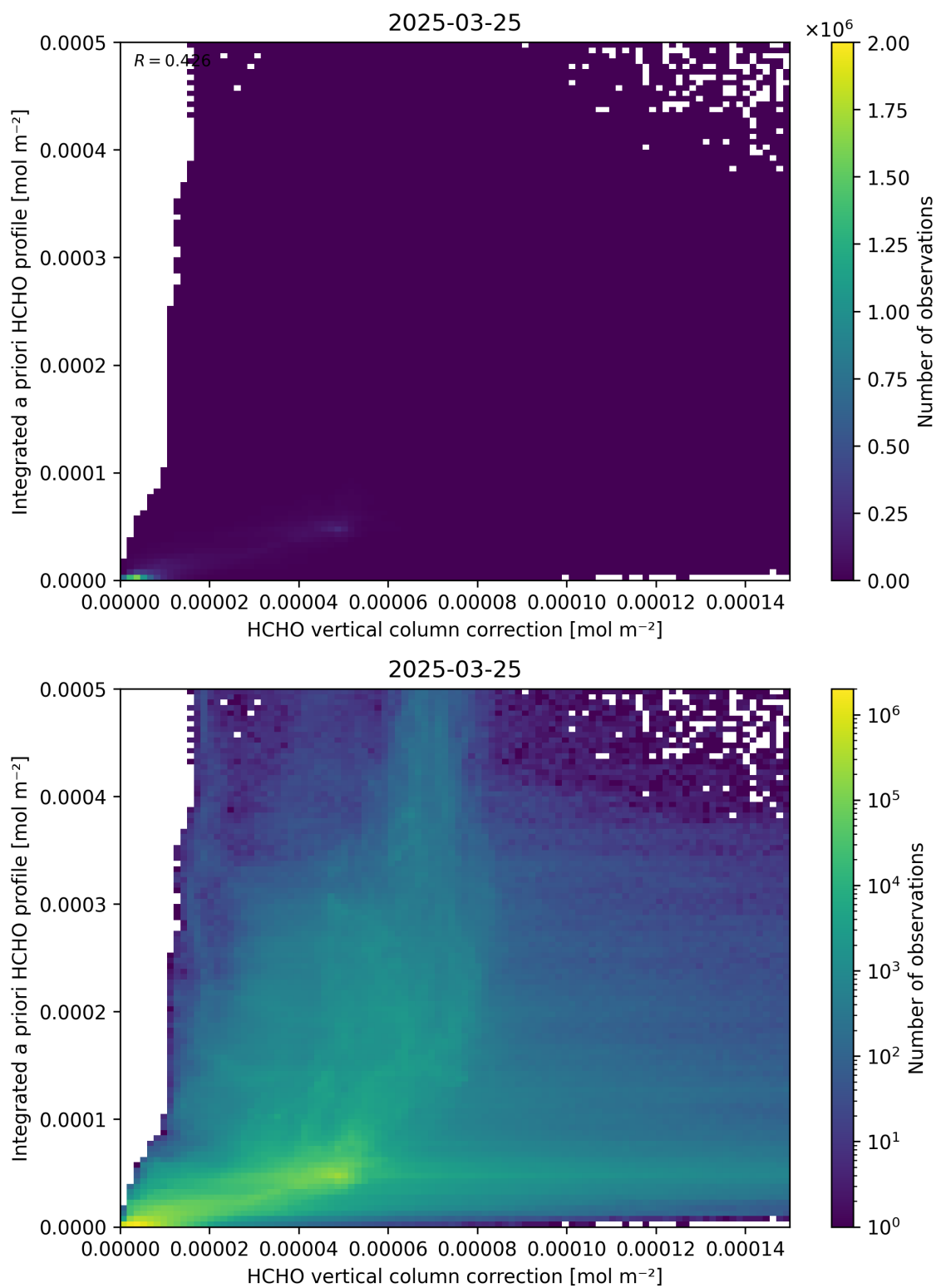
Figure 122: Scatter density plot of “HCHO vertical column correction” against “Integrated a priori HCHO profile” for 2025-03-24 to 2025-03-26.
