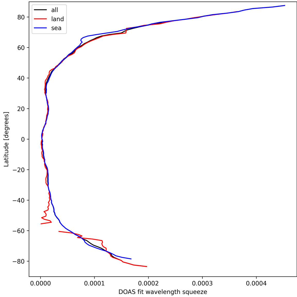
Figure 31: Zonal average of “DOAS fit wavelength squeeze” for 2025-03-24 to 2025-03-26.
