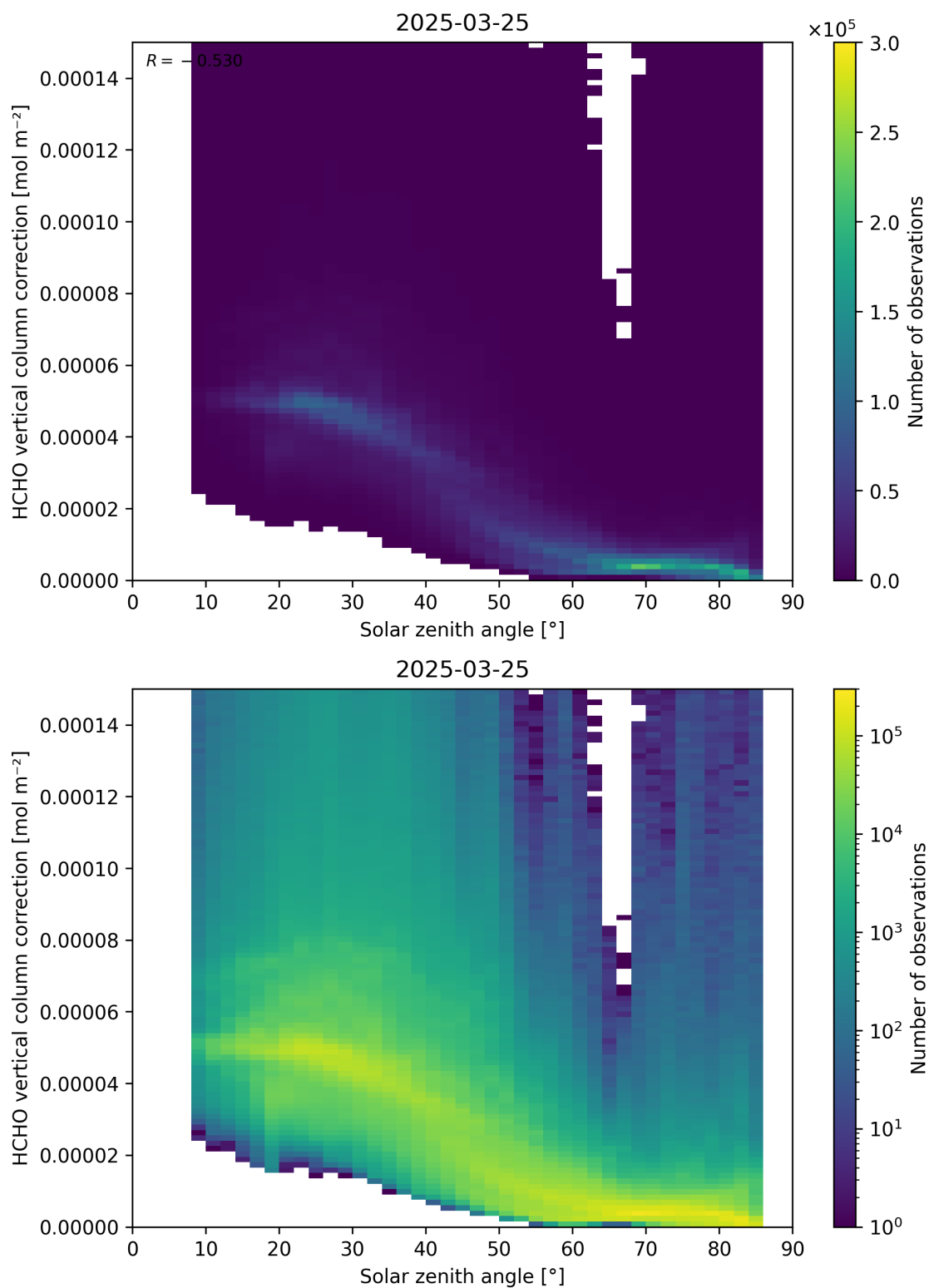
Figure 178: Scatter density plot of “Solar zenith angle” against “HCHO vertical column correction” for 2025-03-24 to 2025-03-26.
