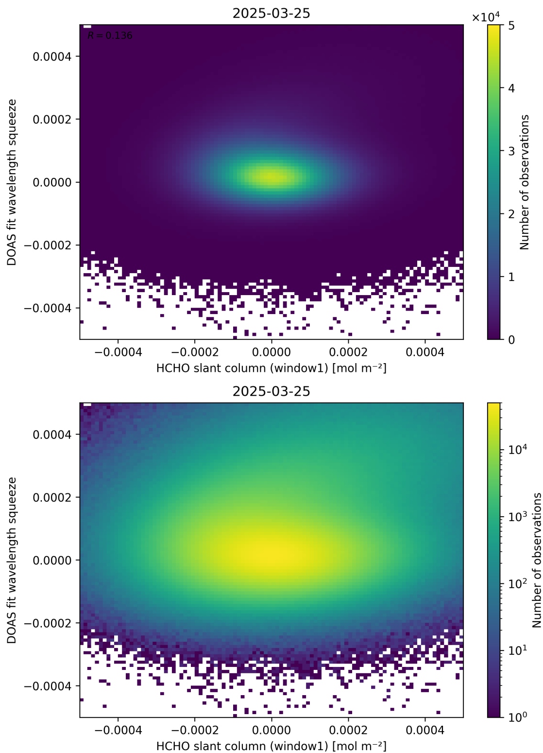
Figure 80: Scatter density plot of “HCHO slant column (window1)” against “DOAS fit wavelength squeeze” for 2025-03-24 to 2025-03-26.
