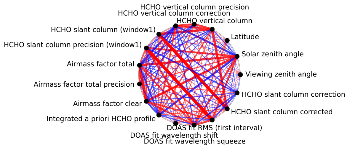
Figure 1: Map of correlation graph for 2025-03-24 to 2025-03-26.
