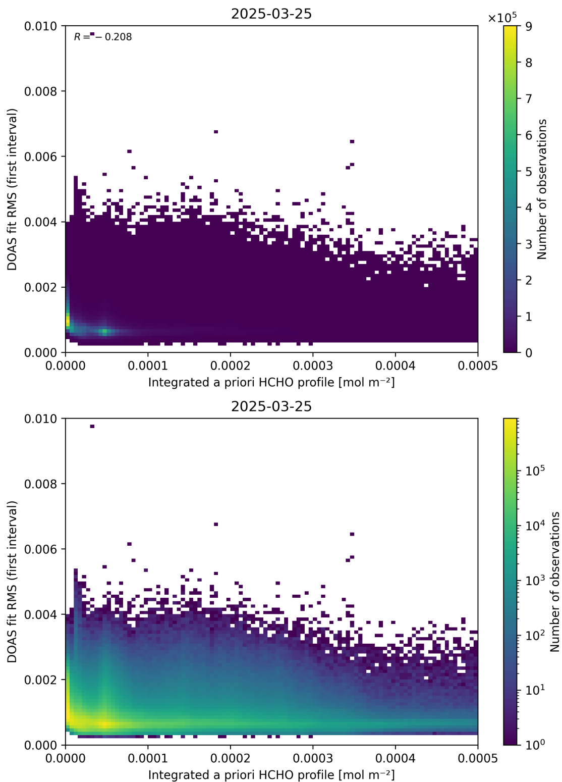
Figure 148: Scatter density plot of “Integrated a priori HCHO profile” against “DOAS fit RMS (first interval)” for 2025-03-24 to 2025-03-26.
