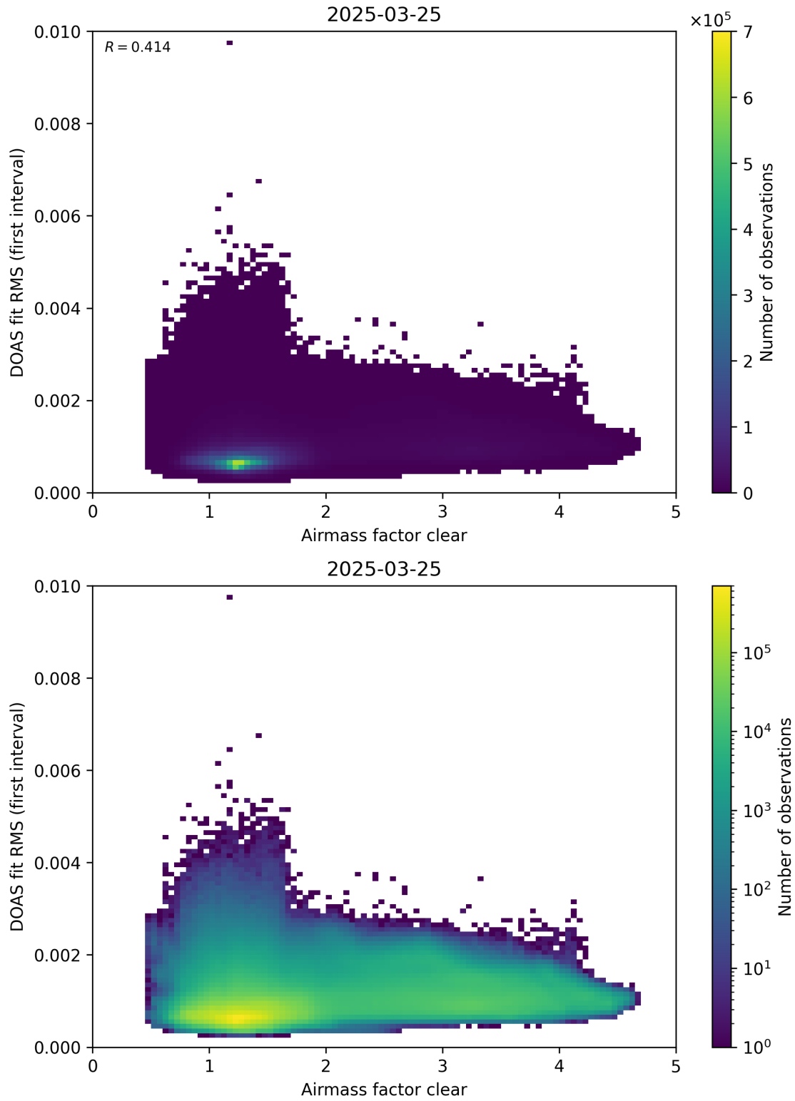
Figure 71: Scatter density plot of “Airmass factor clear” against “DOAS fit RMS (first interval)” for 2025-03-24 to 2025-03-26.
