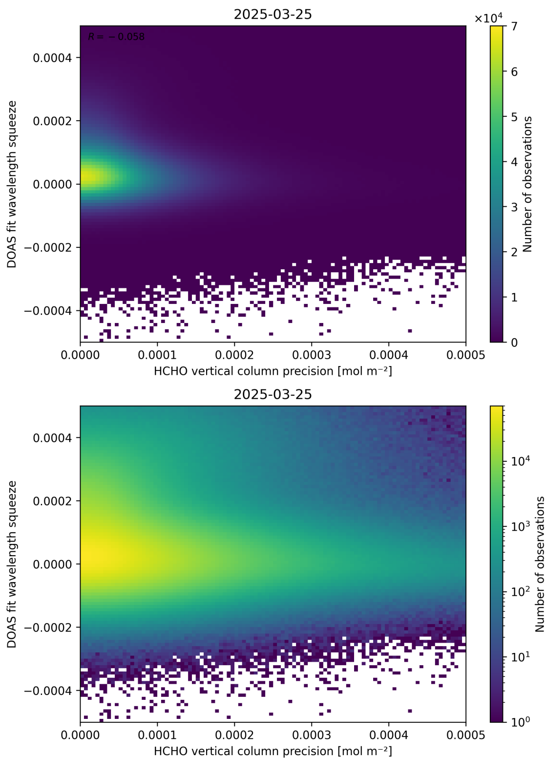
Figure 138: Scatter density plot of “HCHO vertical column precision” against “DOAS fit wavelength squeeze” for 2025-03-24 to 2025-03-26.
