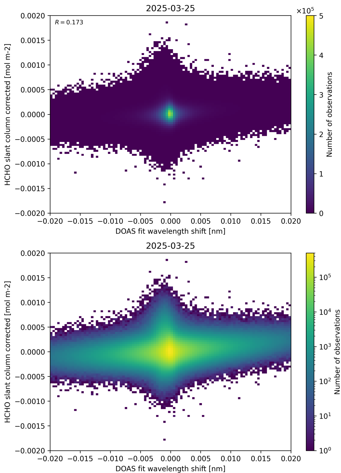
Figure 66: Scatter density plot of “DOAS fit wavelength shift” against “HCHO slant column corrected” for 2025-03-24 to 2025-03-26.
