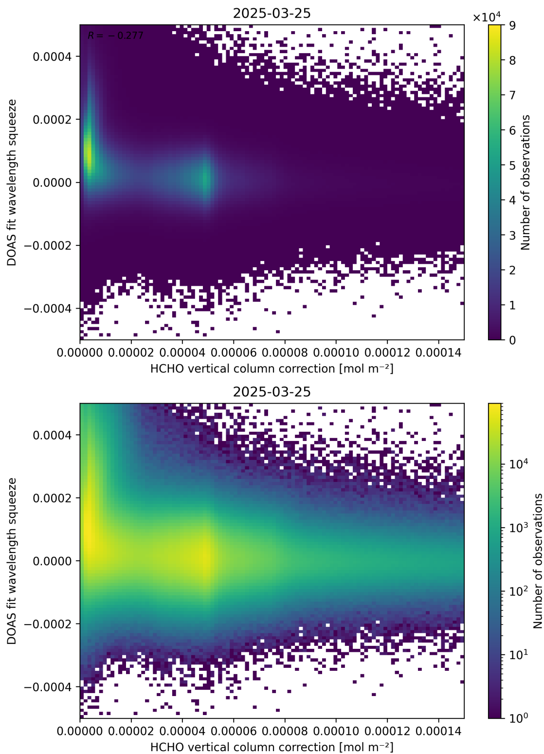
Figure 114: Scatter density plot of “HCHO vertical column correction” against “DOAS fit wavelength squeeze” for 2025-03-24 to 2025-03-26.
