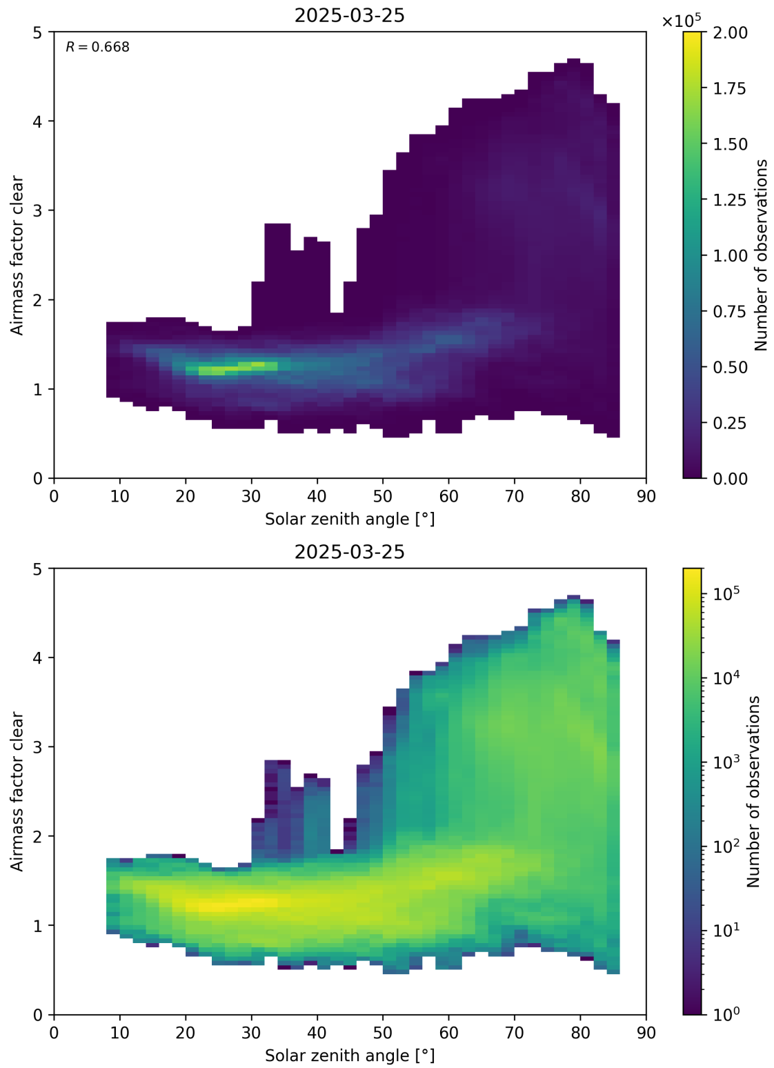
Figure 170: Scatter density plot of “Solar zenith angle” against “Airmass factor clear” for 2025-03-24 to 2025-03-26.
