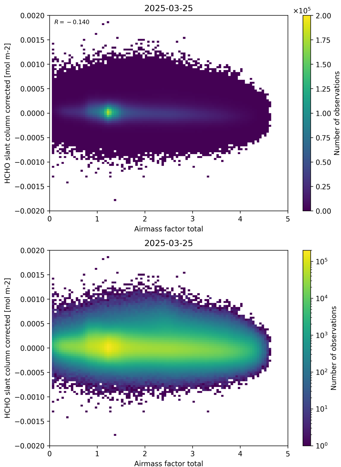
Figure 101: Scatter density plot of “Airmass factor total” against “HCHO slant column corrected” for 2025-03-24 to 2025-03-26.
