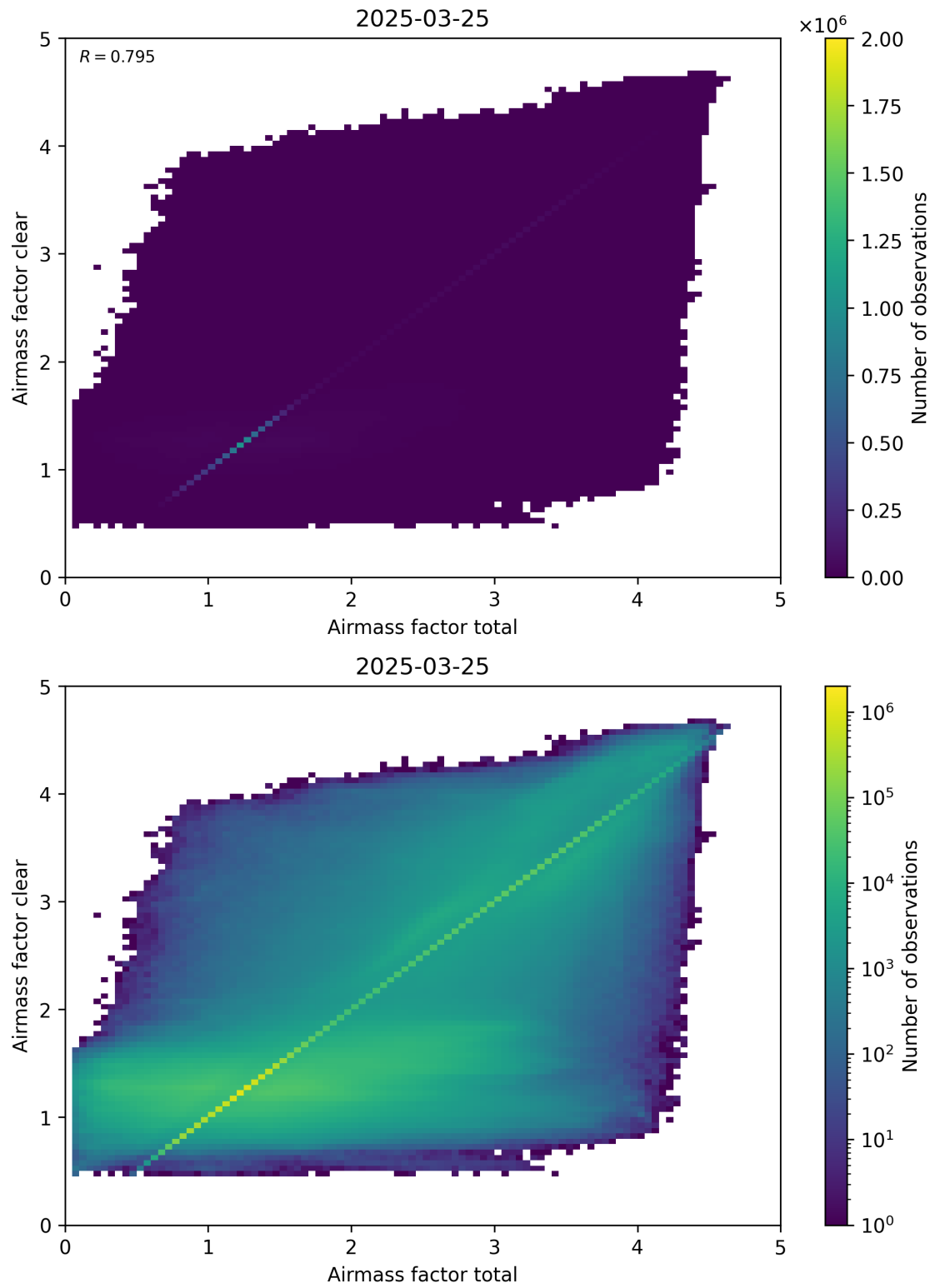
Figure 100: Scatter density plot of “Airmass factor total” against “Airmass factor clear” for 2025-03-24 to 2025-03-26.
