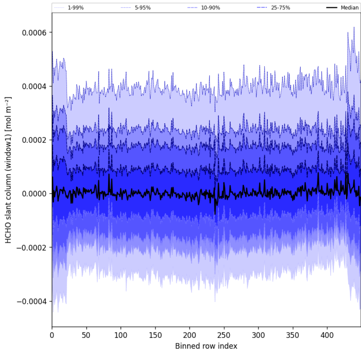
Figure 52: Along track statistics of “HCHO slant column (window1)” for 2025-03-24 to 2025-03-26
