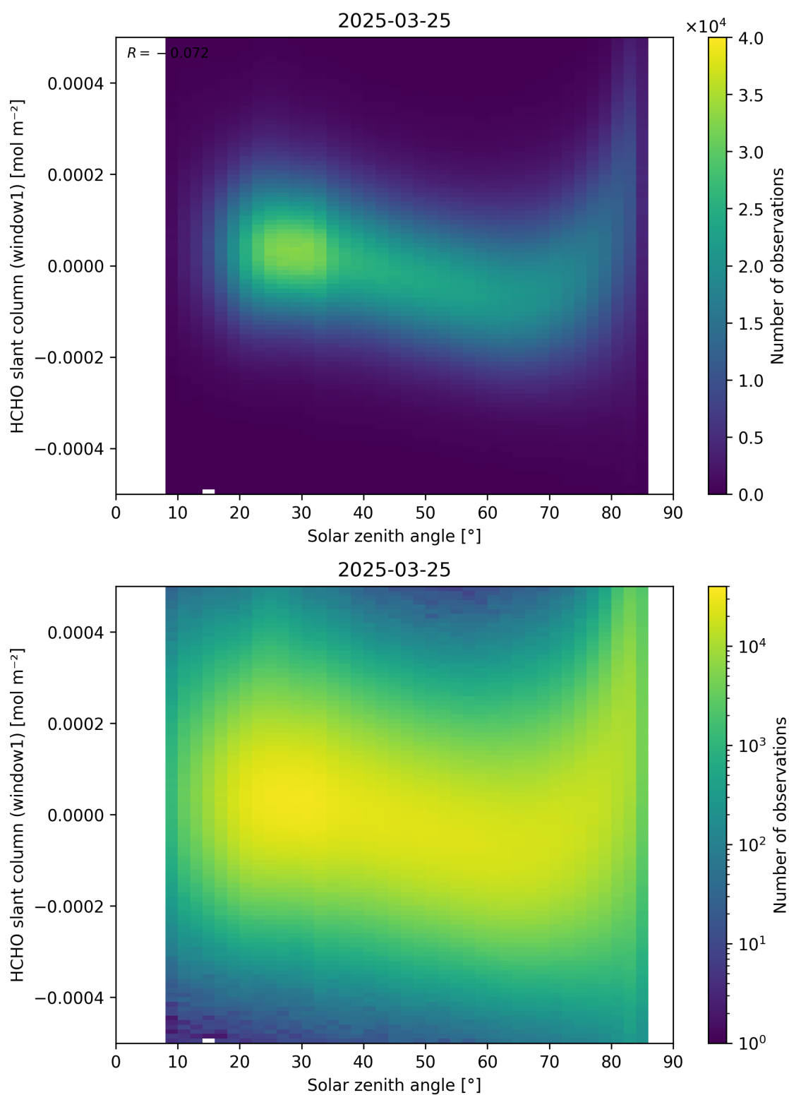
Figure 173: Scatter density plot of “Solar zenith angle” against “HCHO slant column (window1)” for 2025-03-24 to 2025-03-26.
