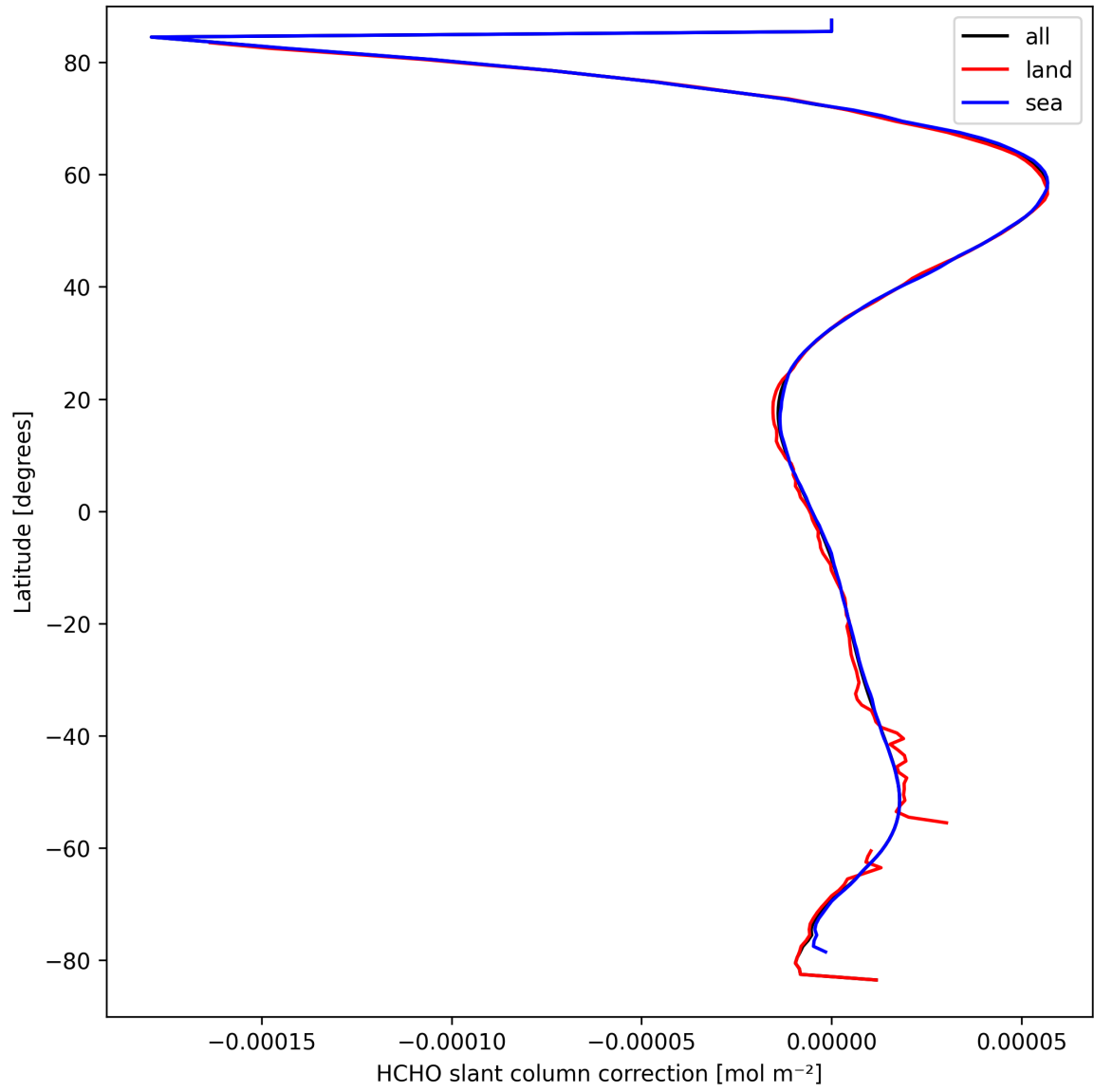
Figure 33: Zonal average of “HCHO slant column correction” for 2025-03-24 to 2025-03-26.
