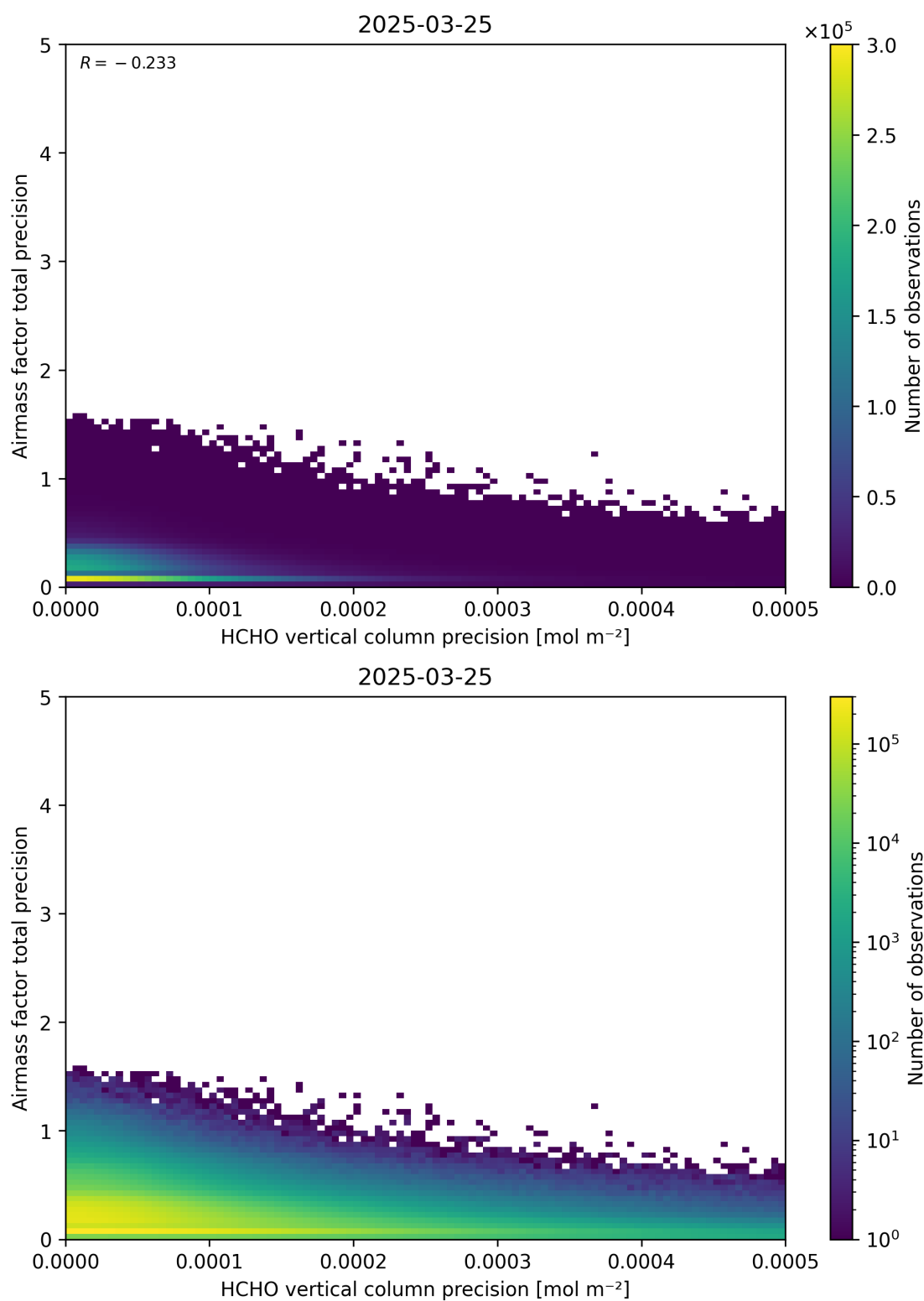
Figure 145: Scatter density plot of “HCHO vertical column precision” against “Airmass factor total precision” for 2025-03-24 to 2025-03-26.
