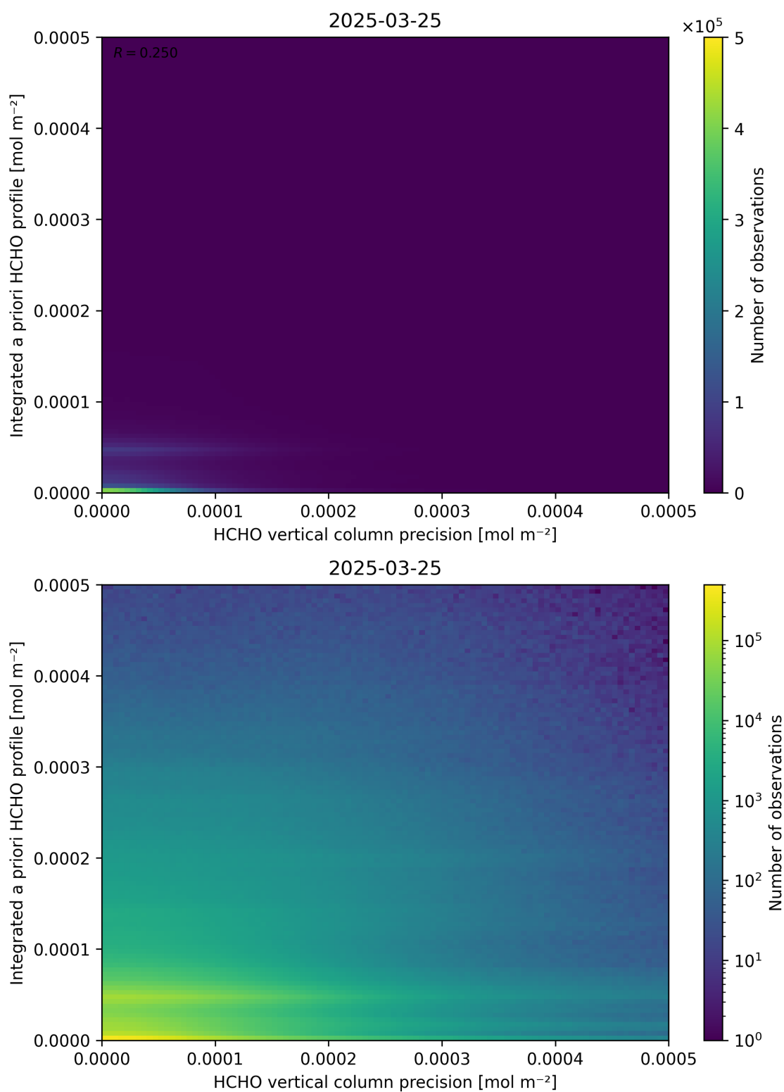
Figure 147: Scatter density plot of “HCHO vertical column precision” against “Integrated a priori HCHO profile” for 2025-03-24 to 2025-03-26.
