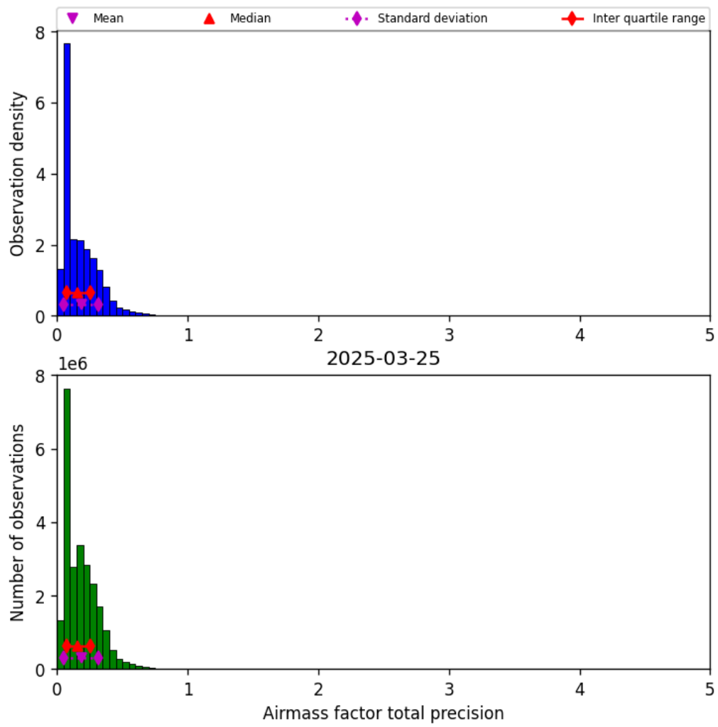
Figure 41: Histogram of “Airmass factor total precision” for 2025-03-24 to 2025-03-26
