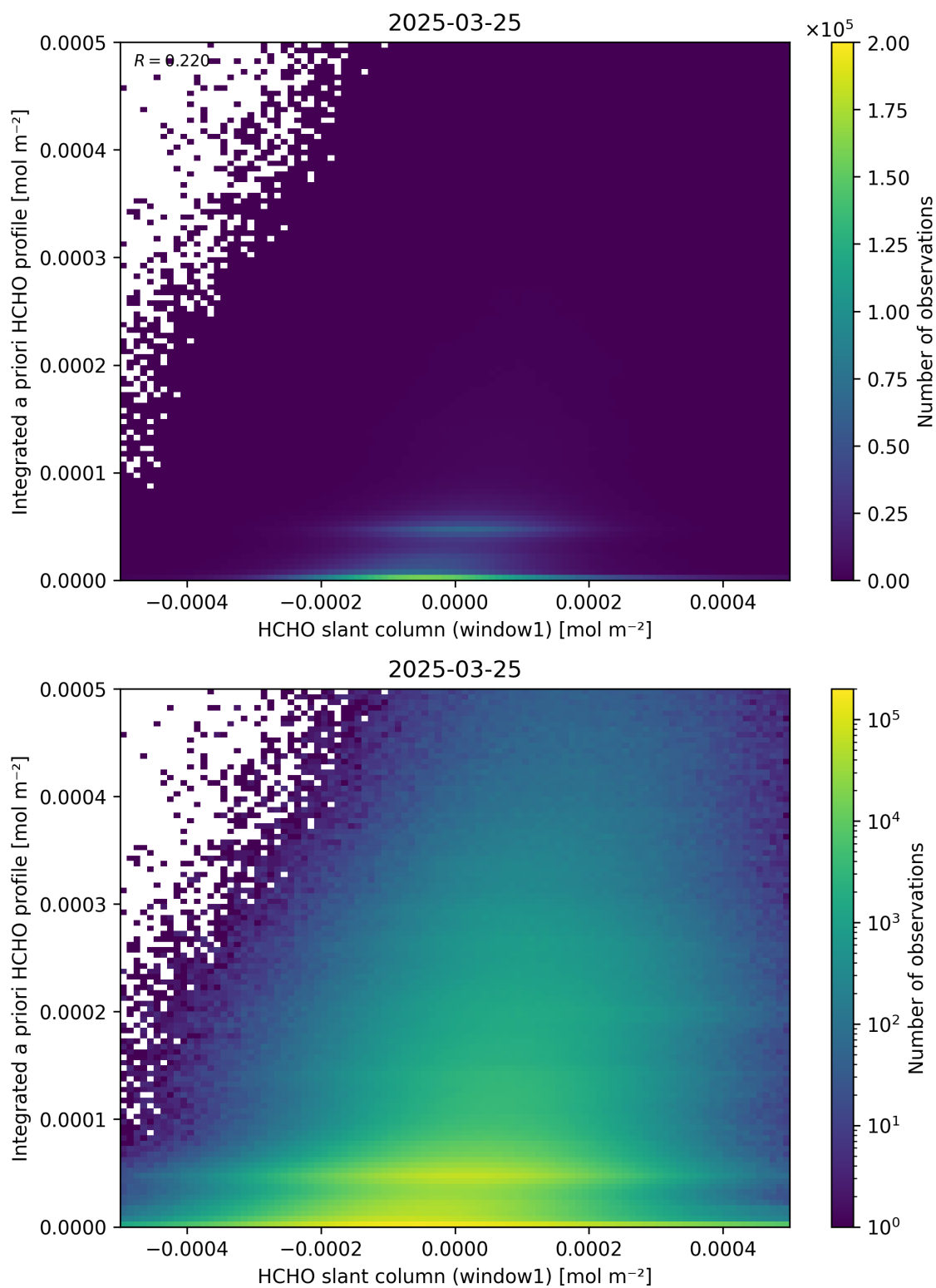
Figure 87: Scatter density plot of “HCHO slant column (window1)” against “Integrated a priori HCHO profile” for 2025-03-24 to 2025-03-26.
