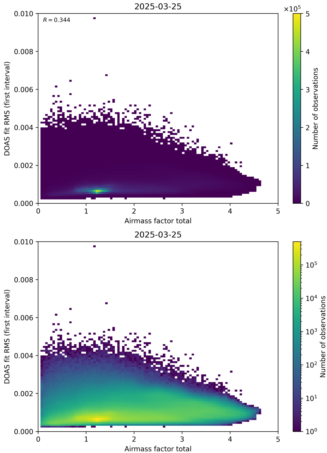
Figure 97: Scatter density plot of “Airmass factor total” against “DOAS fit RMS (first interval)” for 2025-03-24 to 2025-03-26.
