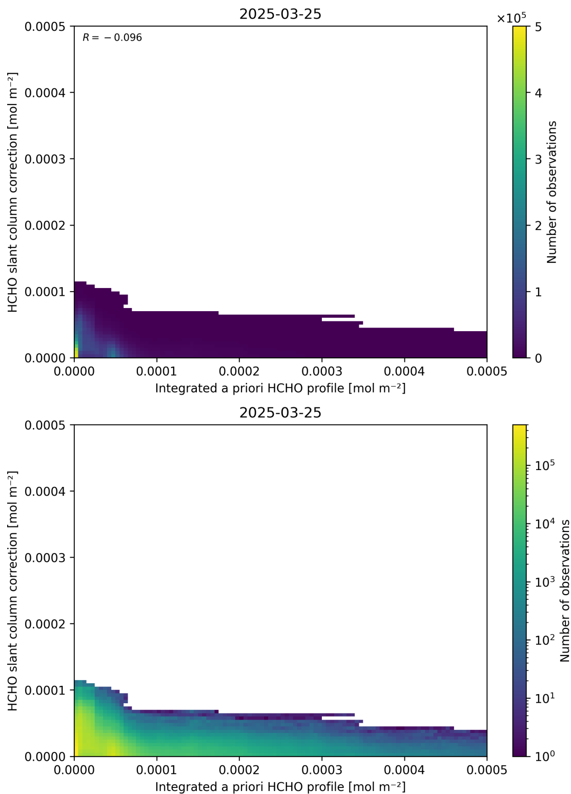
Figure 152: Scatter density plot of “Integrated a priori HCHO profile” against “HCHO slant column correction” for 2025-03-24 to 2025-03-26.
