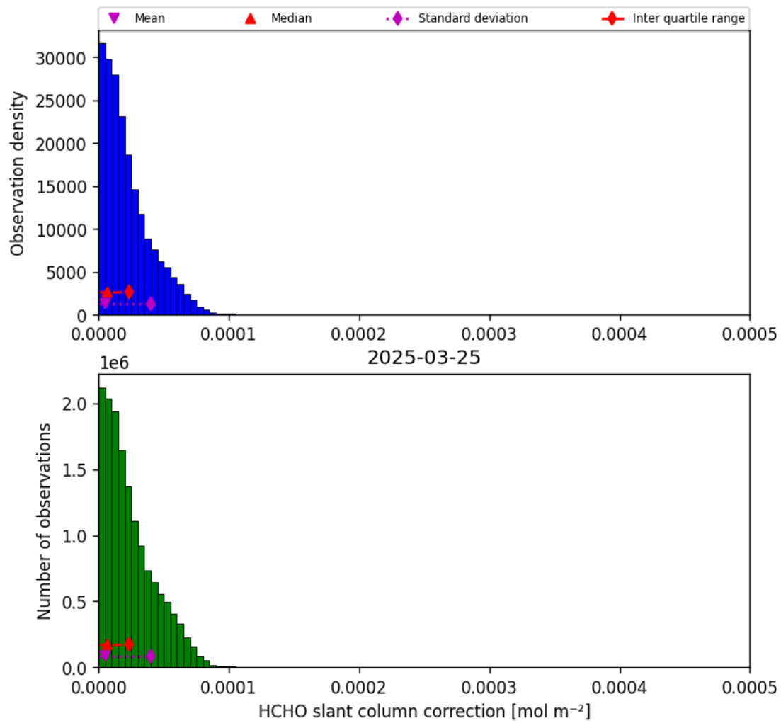
Figure 47: Histogram of “HCHO slant column correction” for 2025-03-24 to 2025-03-26
