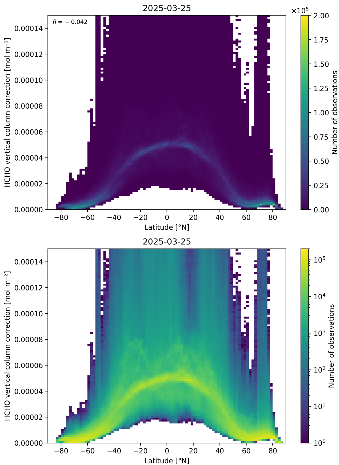
Figure 164: Scatter density plot of “Latitude” against “HCHO vertical column correction” for 2025-03-24 to 2025-03-26.
