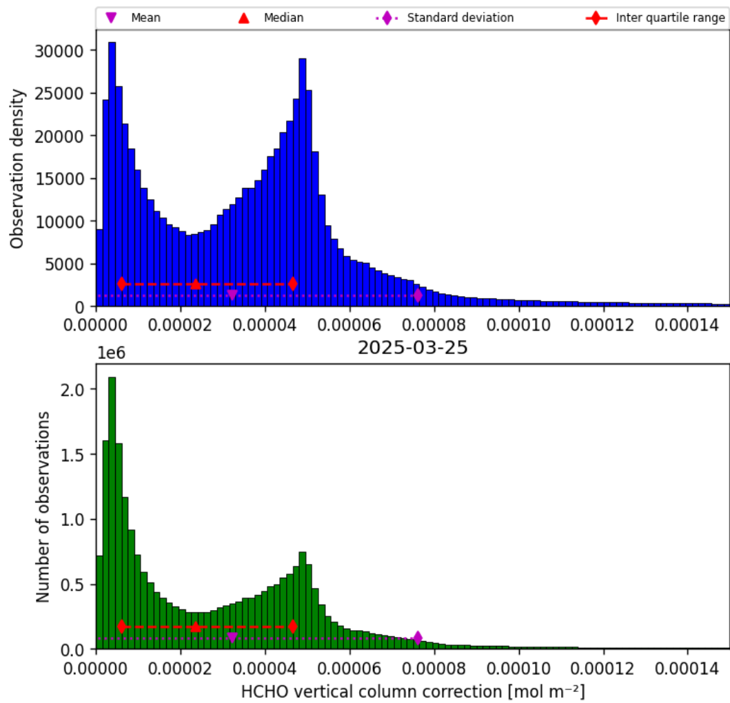
Figure 37: Histogram of “HCHO vertical column correction” for 2025-03-24 to 2025-03-26
