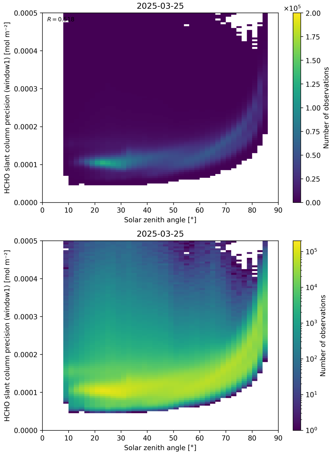
Figure 174: Scatter density plot of “Solar zenith angle” against “HCHO slant column precision (window1)” for 2025-03-24 to 2025-03-26.
