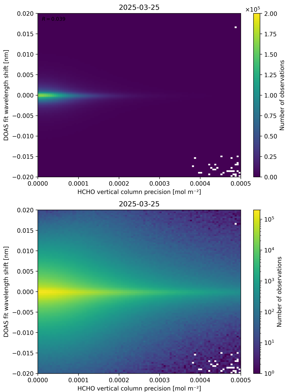
Figure 137: Scatter density plot of “HCHO vertical column precision” against “DOAS fit wavelength shift” for 2025-03-24 to 2025-03-26.
