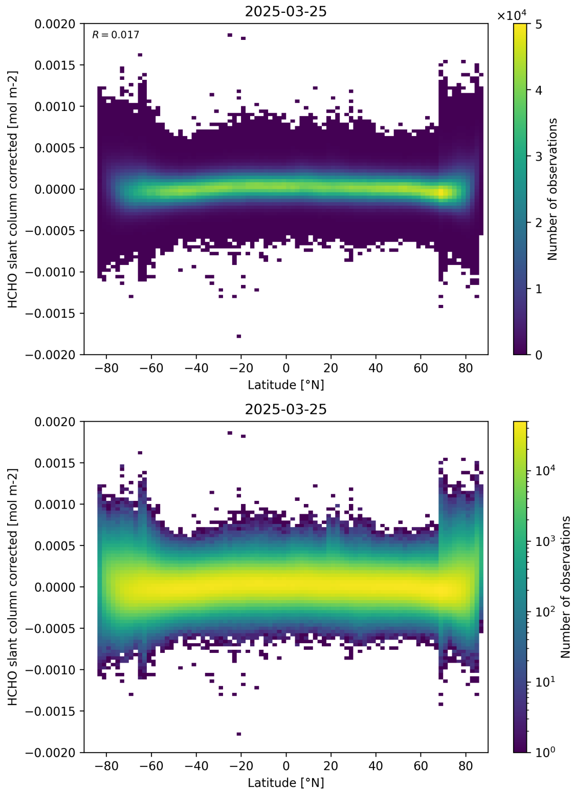
Figure 157: Scatter density plot of “Latitude” against “HCHO slant column corrected” for 2025-03-24 to 2025-03-26.
