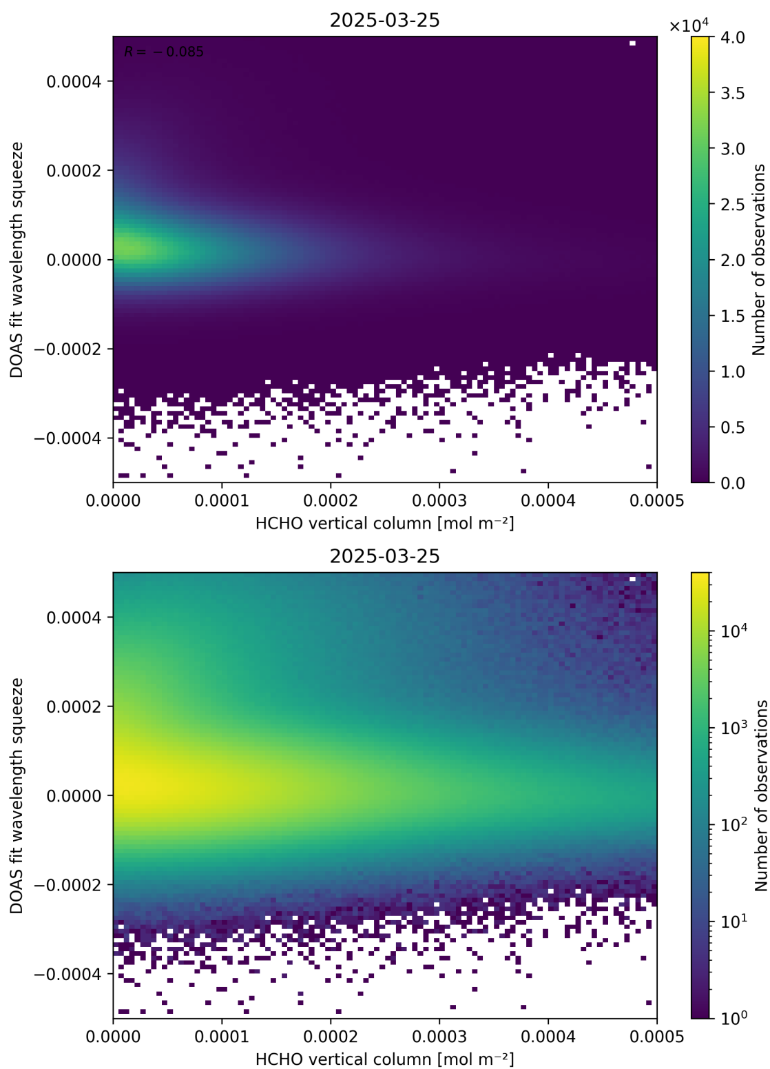
Figure 125: Scatter density plot of “HCHO vertical column” against “DOAS fit wavelength squeeze” for 2025-03-24 to 2025-03-26.
