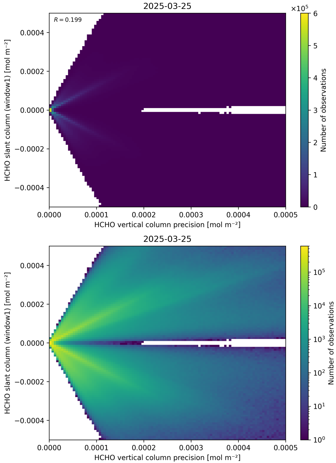
Figure 142: Scatter density plot of “HCHO vertical column precision” against “HCHO slant column (window1)” for 2025-03-24 to 2025-03-26.
