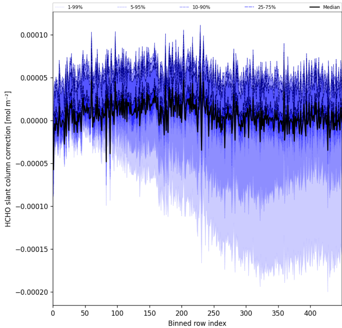
Figure 61: Along track statistics of “HCHO slant column correction” for 2025-03-24 to 2025-03-26
