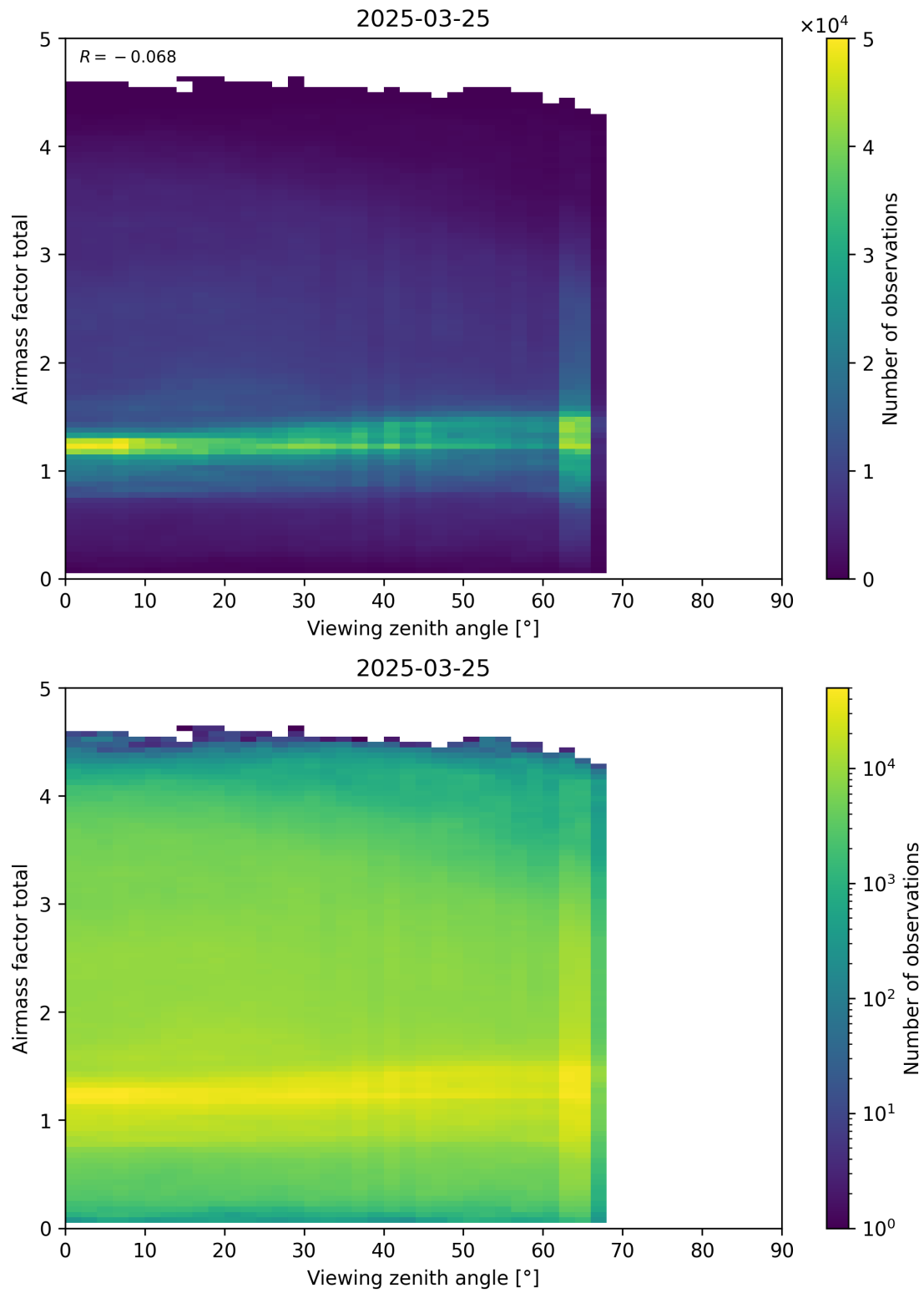
Figure 190: Scatter density plot of “Viewing zenith angle” against “Airmass factor total” for 2025-03-24 to 2025-03-26.
