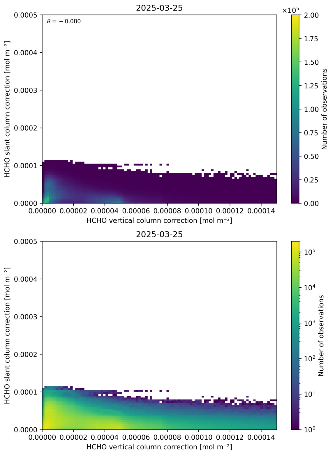
Figure 117: Scatter density plot of “HCHO vertical column correction” against “HCHO slant column correction” for 2025-03-24 to 2025-03-26.
