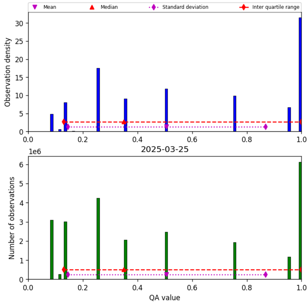
Figure 34: Histogram of “QA value” for 2025-03-24 to 2025-03-26
