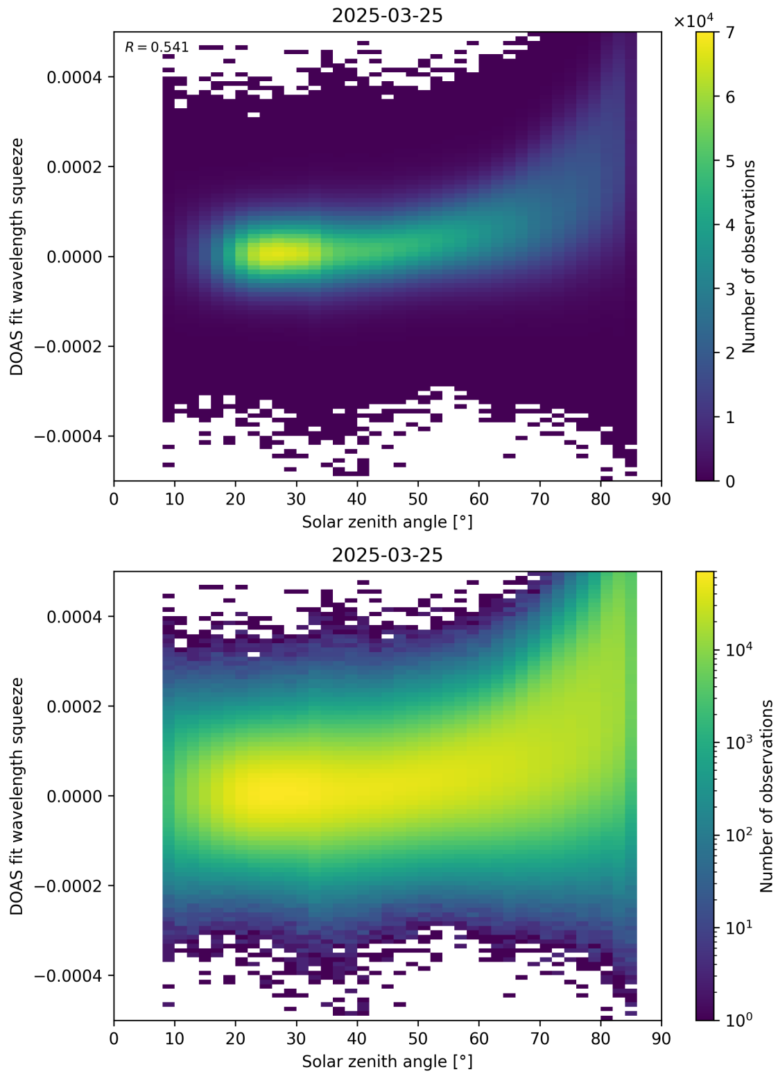
Figure 169: Scatter density plot of “Solar zenith angle” against “DOAS fit wavelength squeeze” for 2025-03-24 to 2025-03-26.
