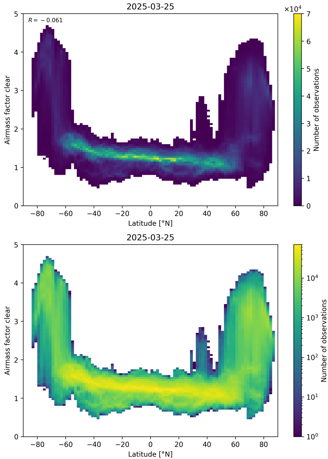
Figure 156: Scatter density plot of “Latitude” against “Airmass factor clear” for 2025-03-24 to 2025-03-26.
