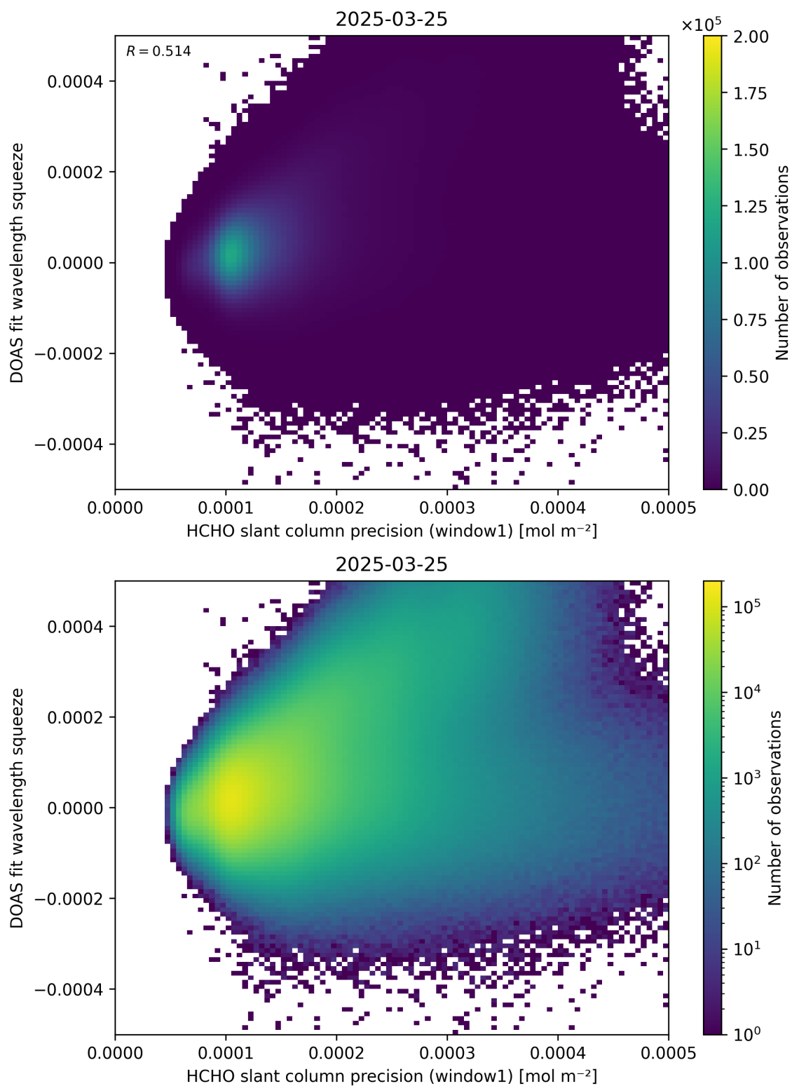
Figure 90: Scatter density plot of “HCHO slant column precision (window1)” against “DOAS fit wavelength squeeze” for 2025-03-24 to 2025-03-26.
