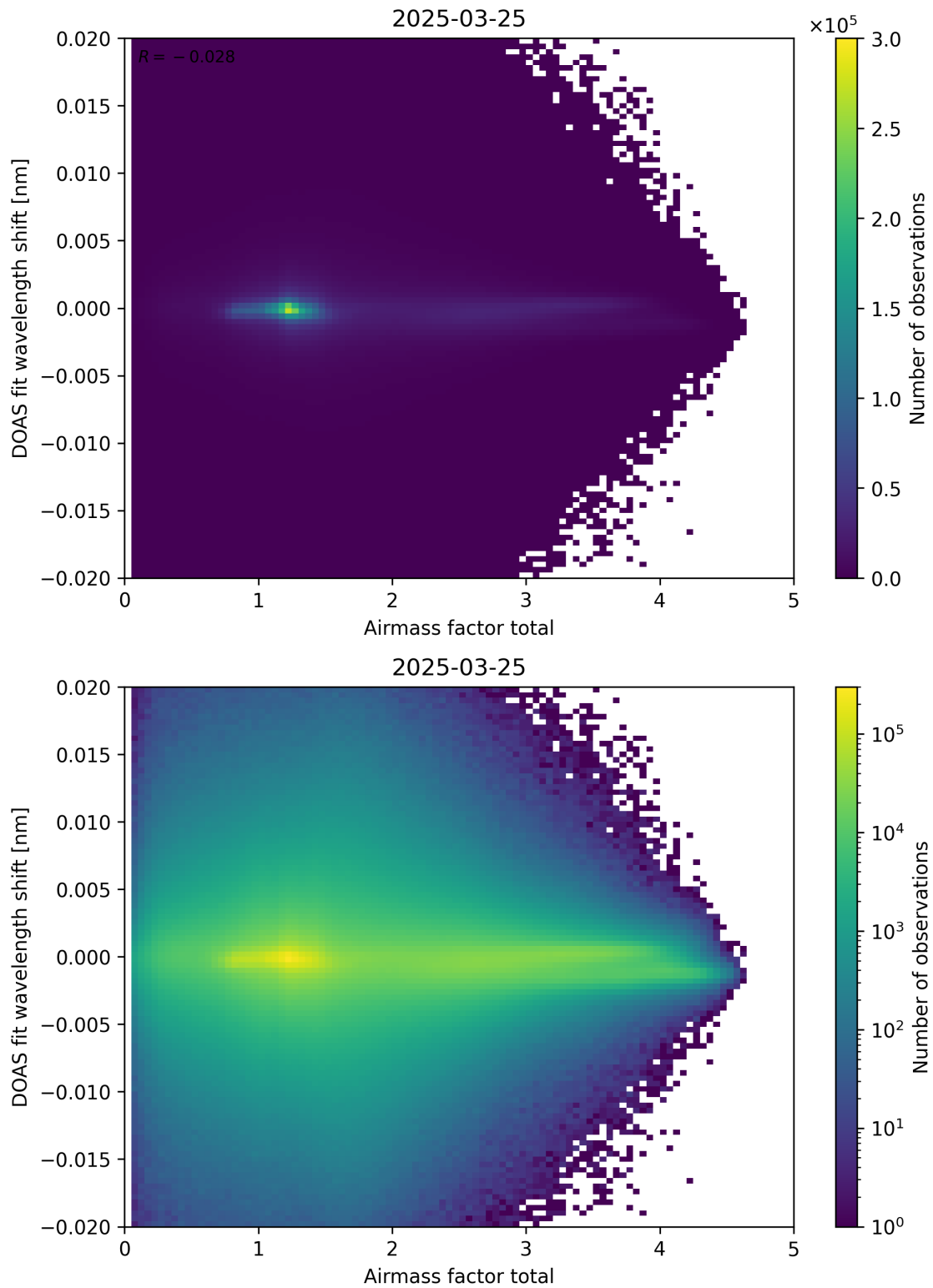
Figure 98: Scatter density plot of “Airmass factor total” against “DOAS fit wavelength shift” for 2025-03-24 to 2025-03-26.
