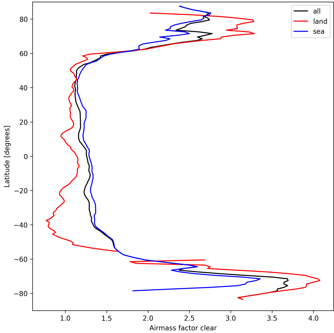
Figure 28: Zonal average of “Airmass factor clear” for 2025-03-24 to 2025-03-26.
