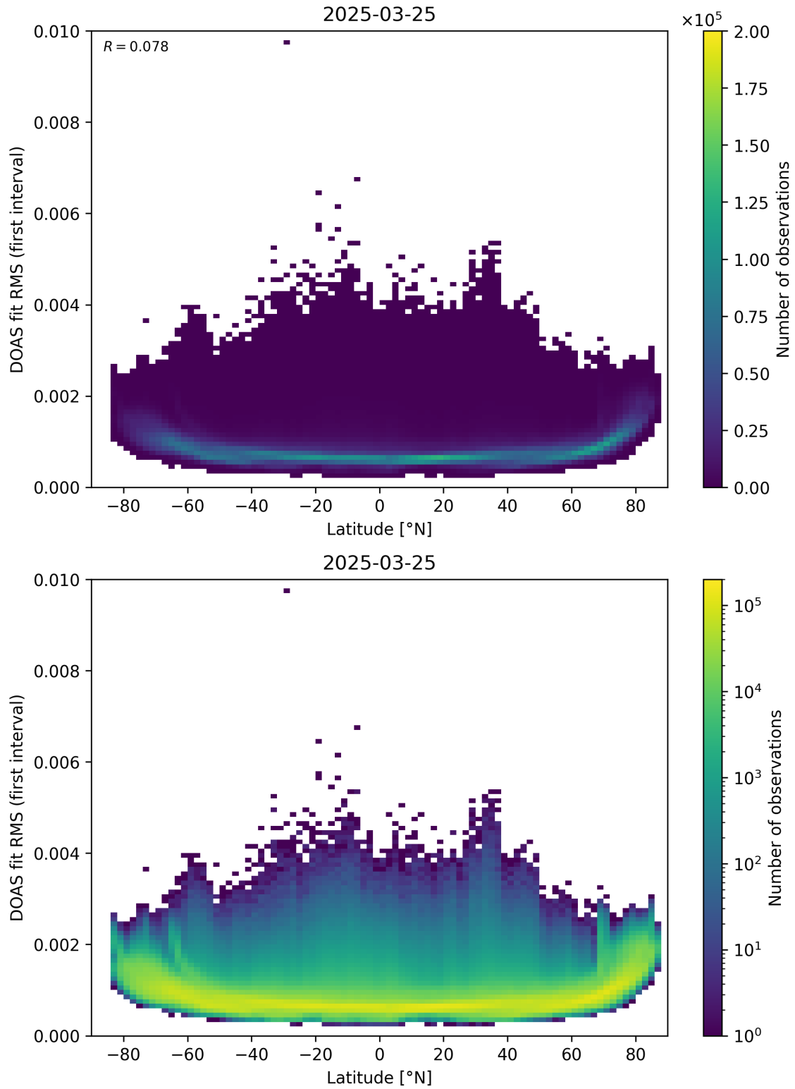
Figure 153: Scatter density plot of “Latitude” against “DOAS fit RMS (first interval)” for 2025-03-24 to 2025-03-26.
