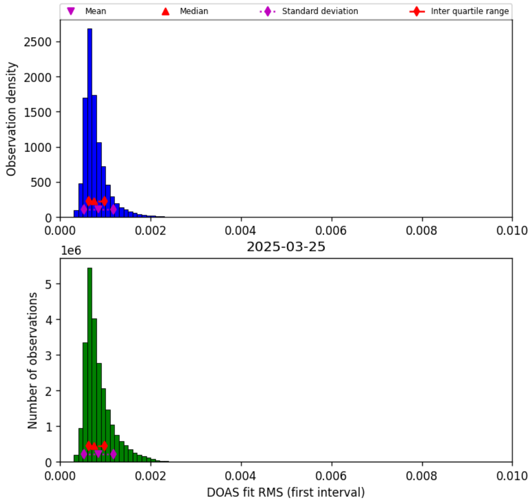
Figure 46: Histogram of “DOAS fit RMS (first interval)” for 2025-03-24 to 2025-03-26
