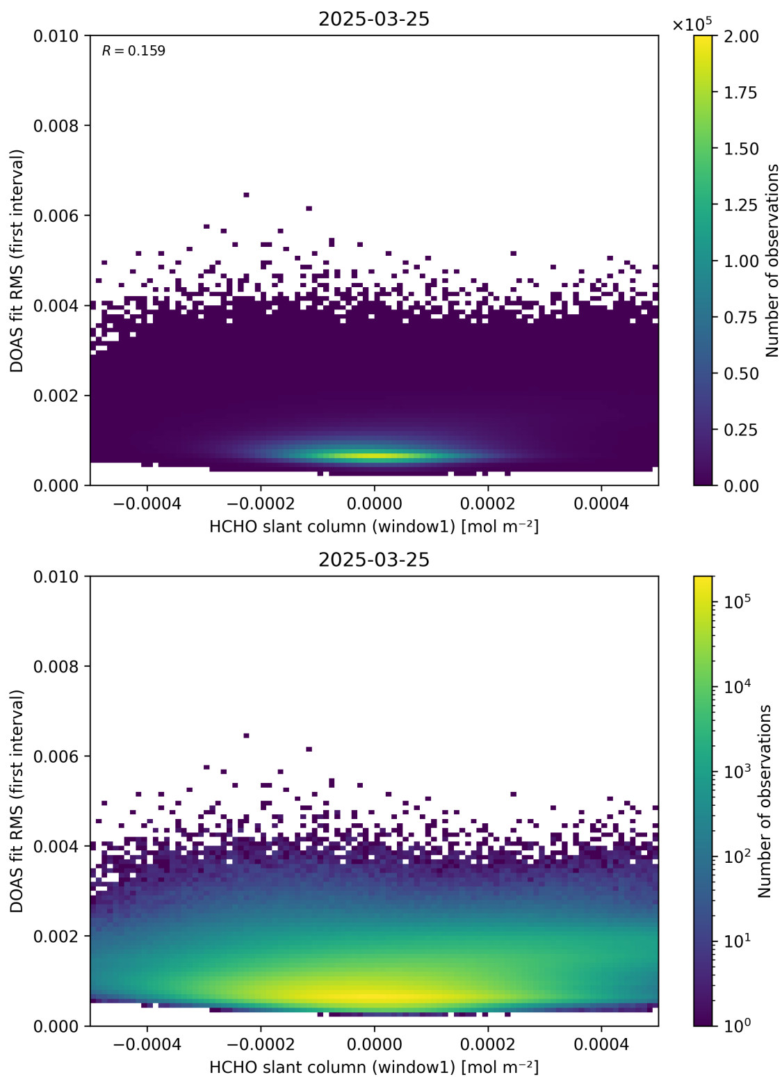
Figure 78: Scatter density plot of “HCHO slant column (window1)” against “DOAS fit RMS (first interval)” for 2025-03-24 to 2025-03-26.
