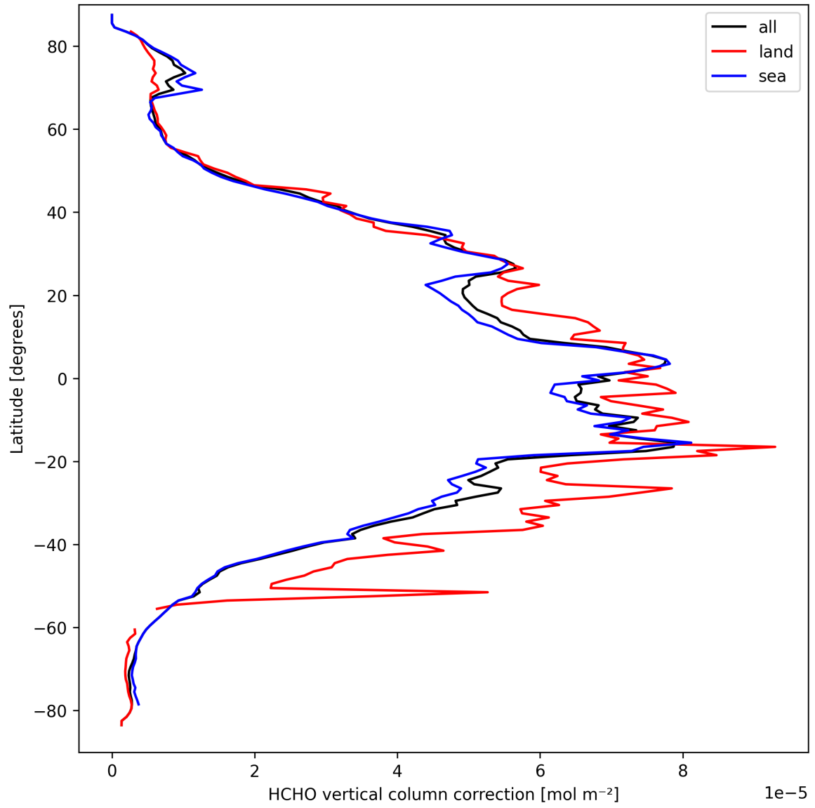
Figure 23: Zonal average of “HCHO vertical column correction” for 2025-03-24 to 2025-03-26.
