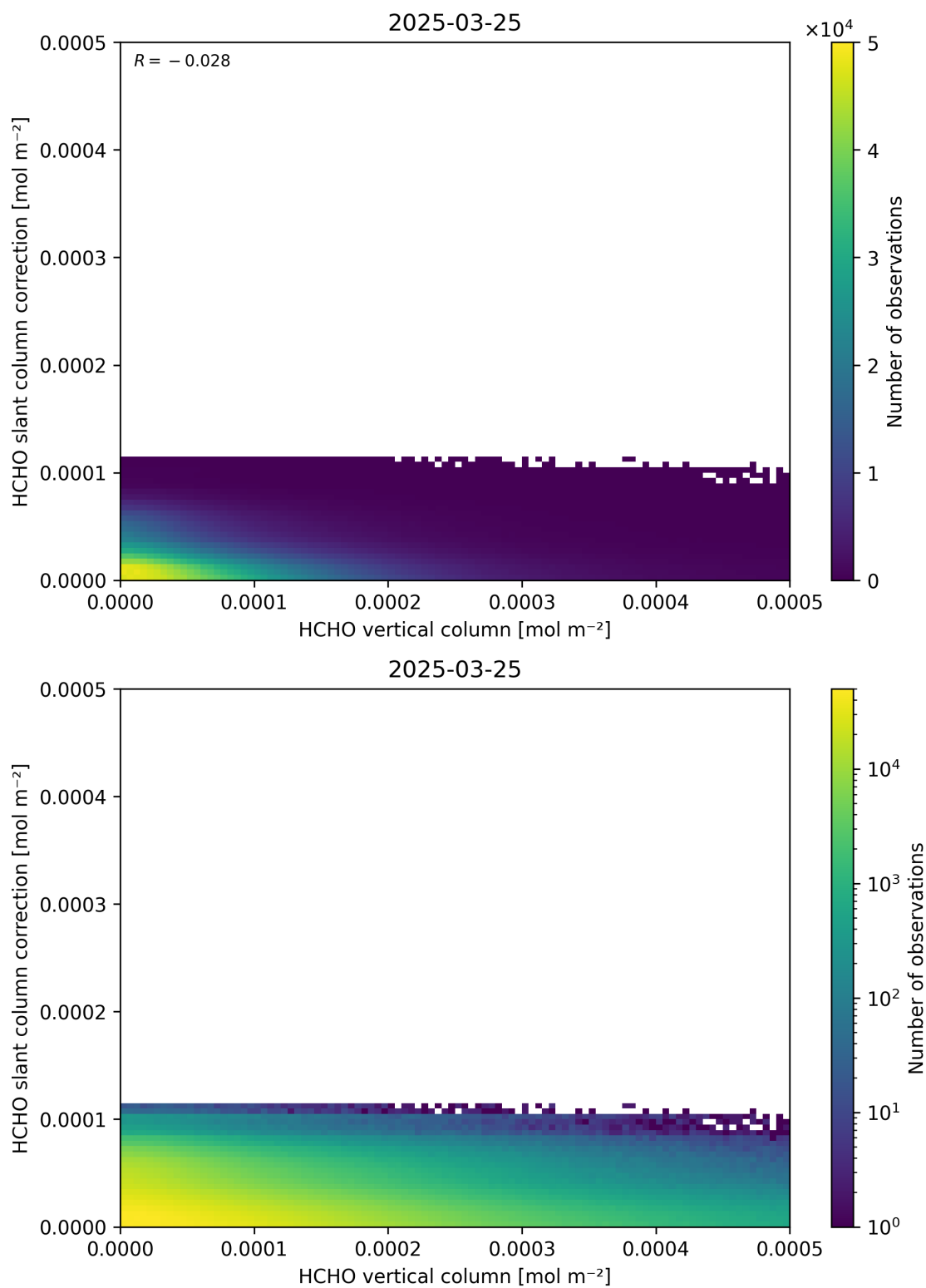
Figure 128: Scatter density plot of “HCHO vertical column” against “HCHO slant column correction” for 2025-03-24 to 2025-03-26.
