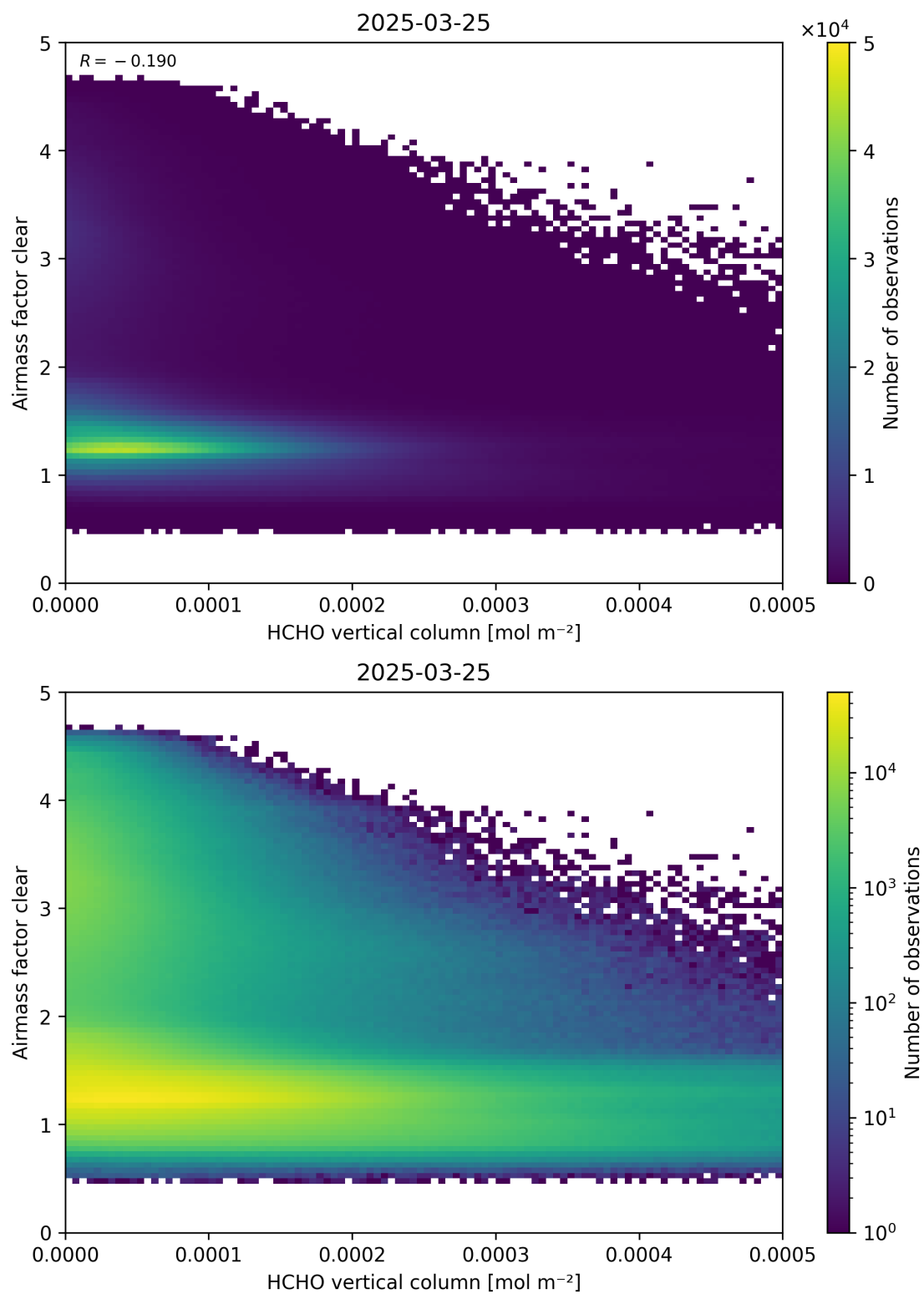
Figure 126: Scatter density plot of “HCHO vertical column” against “Airmass factor clear” for 2025-03-24 to 2025-03-26.
