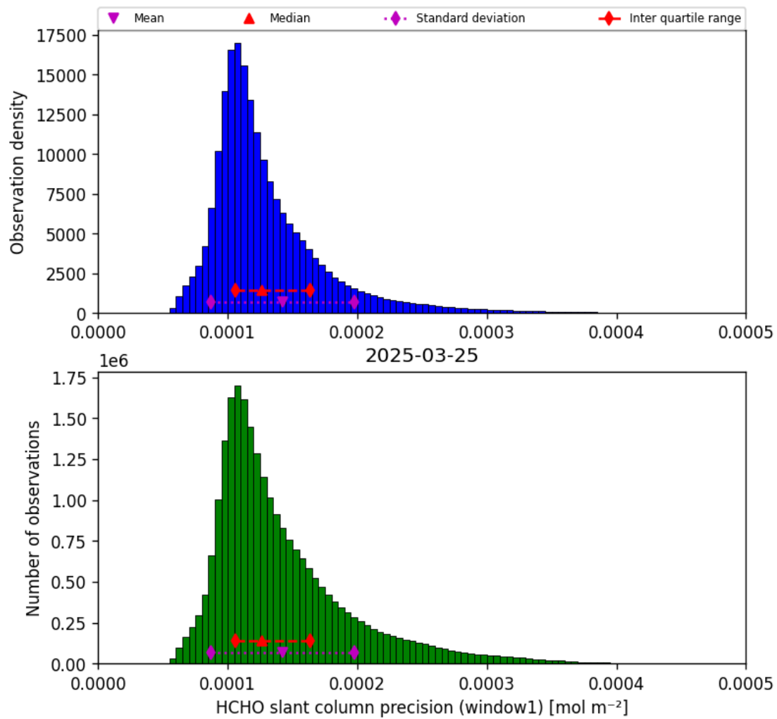
Figure 39: Histogram of “HCHO slant column precision (window1)” for 2025-03-24 to 2025-03-26
