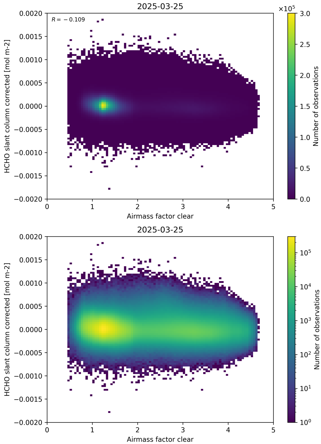
Figure 74: Scatter density plot of “Airmass factor clear” against “HCHO slant column corrected” for 2025-03-24 to 2025-03-26.
