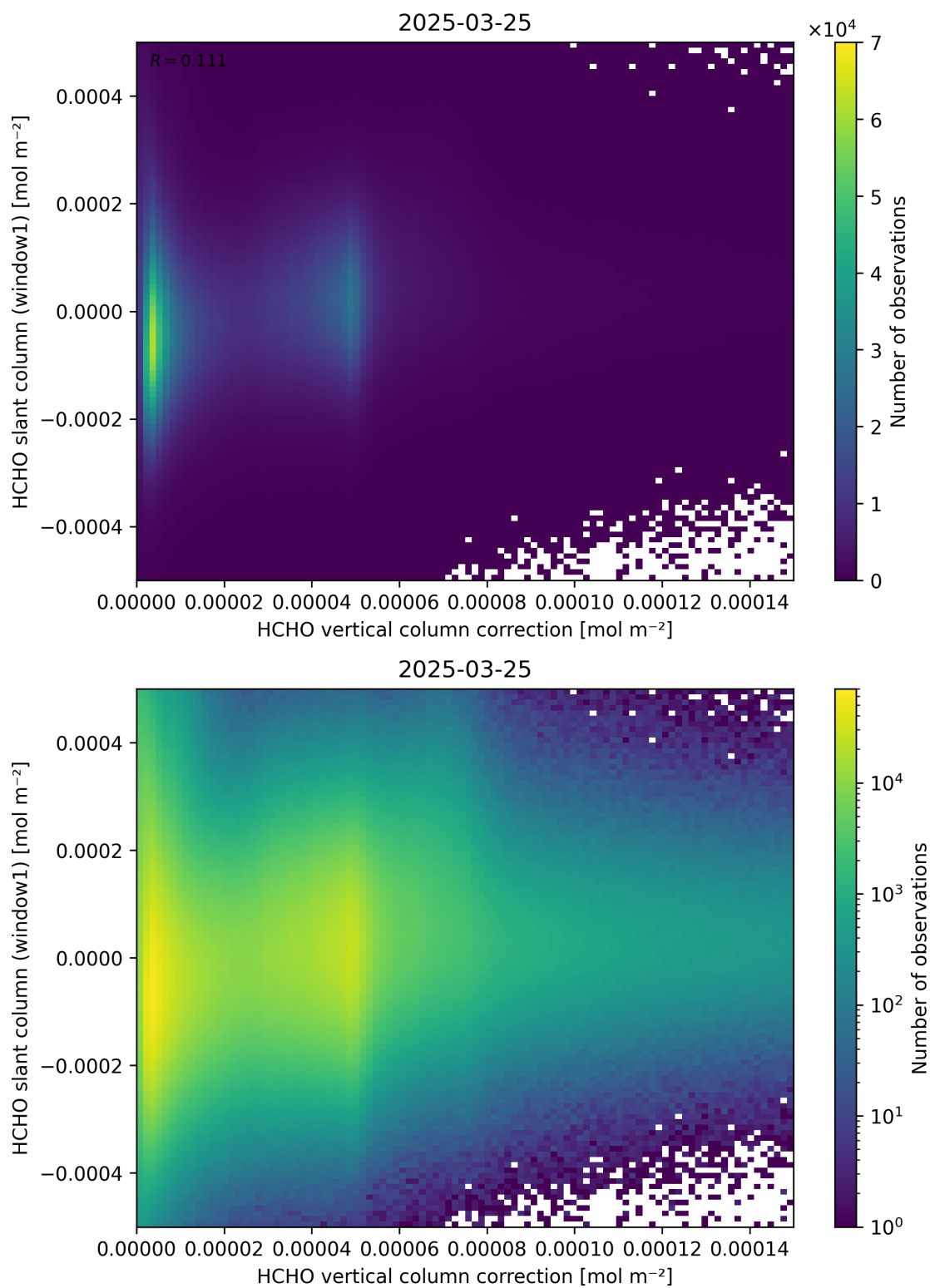
Figure 118: Scatter density plot of “HCHO vertical column correction” against “HCHO slant column (window1)” for 2025-03-24 to 2025-03-26.
