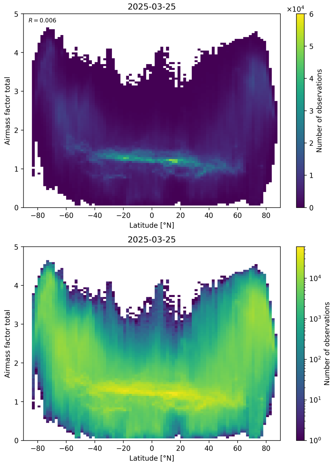
Figure 161: Scatter density plot of “Latitude” against “Airmass factor total” for 2025-03-24 to 2025-03-26.
