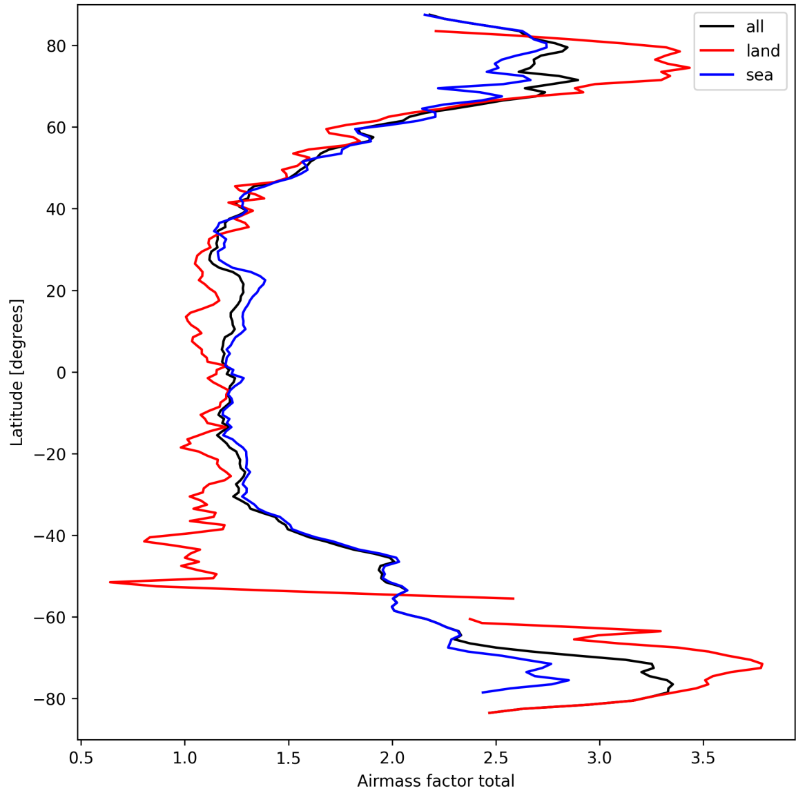
Figure 26: Zonal average of “Airmass factor total” for 2025-03-24 to 2025-03-26.
