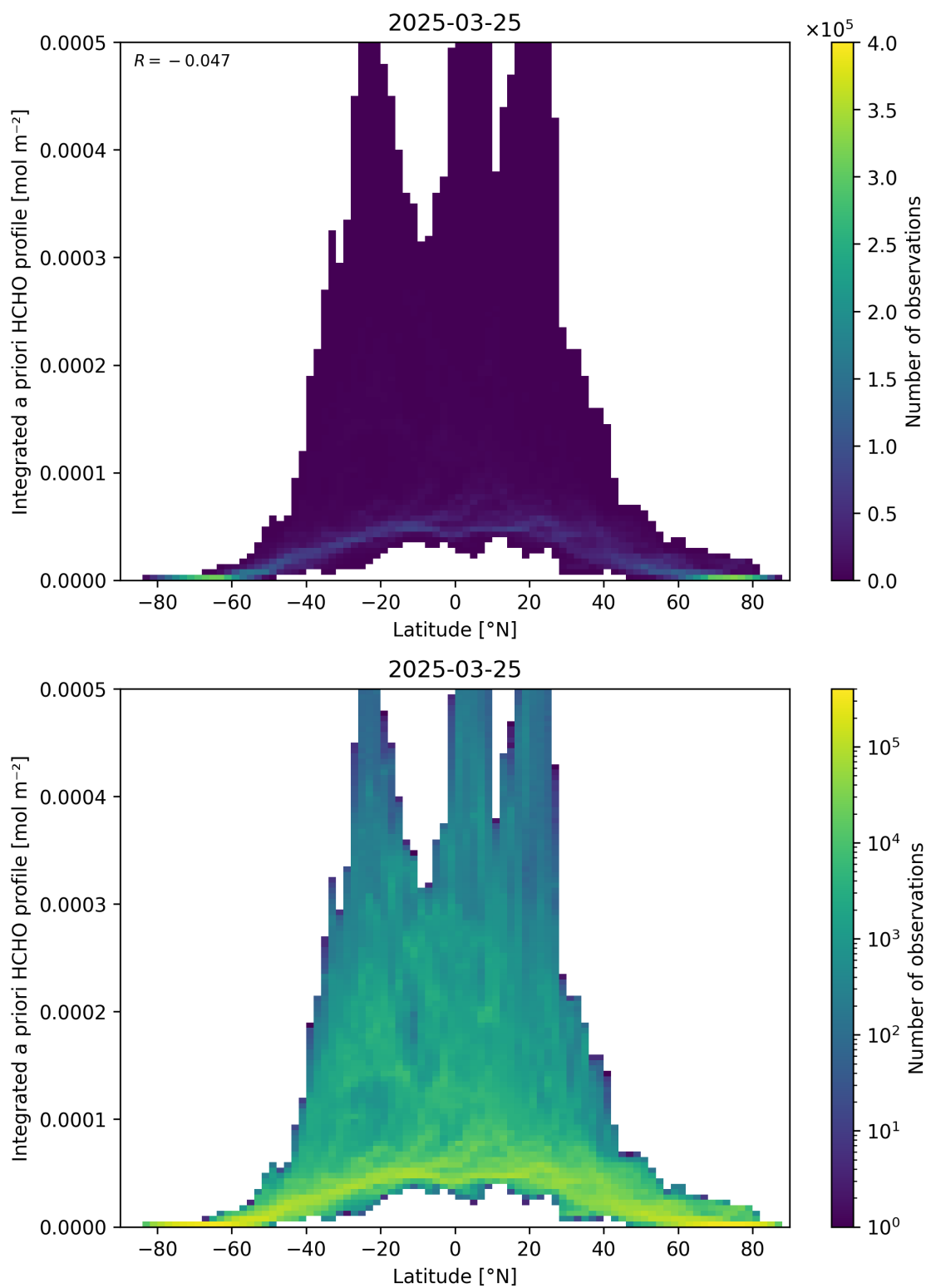
Figure 166: Scatter density plot of “Latitude” against “Integrated a priori HCHO profile” for 2025-03-24 to 2025-03-26.
