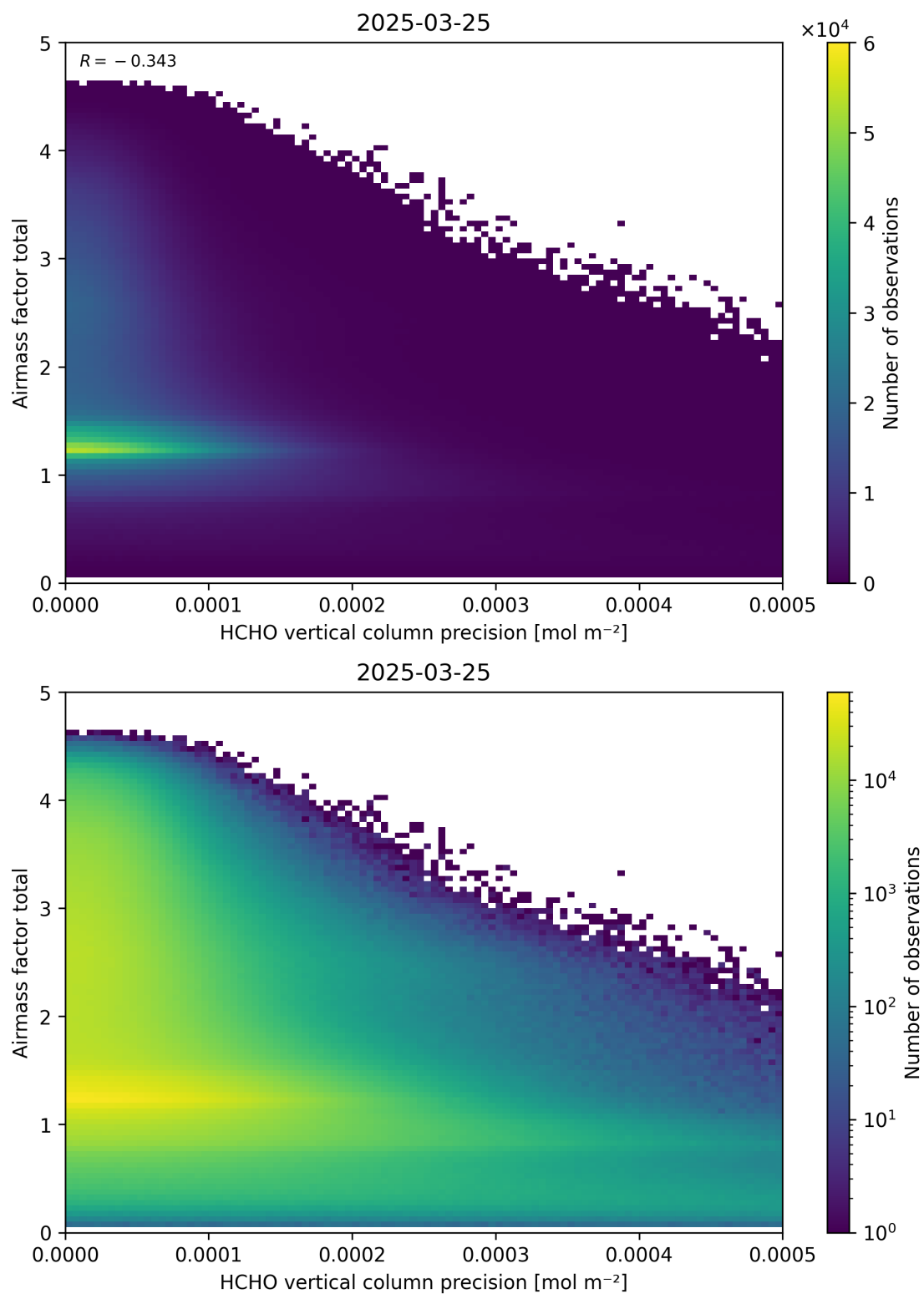
Figure 144: Scatter density plot of “HCHO vertical column precision” against “Airmass factor total” for 2025-03-24 to 2025-03-26.
