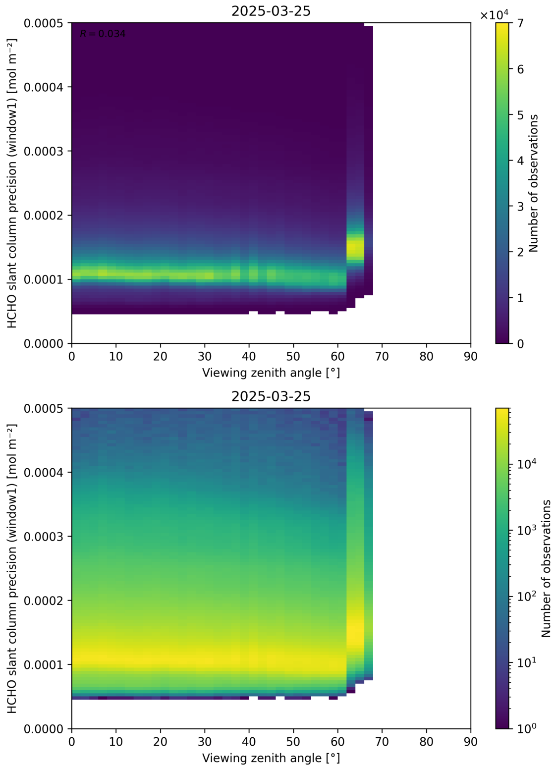
Figure 189: Scatter density plot of “Viewing zenith angle” against “HCHO slant column precision (window1)” for 2025-03-24 to 2025-03-26.
