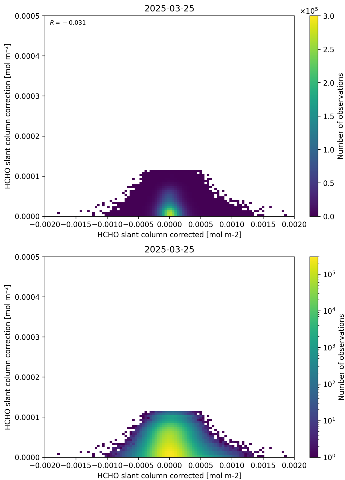
Figure 77: Scatter density plot of “HCHO slant column corrected” against “HCHO slant column correction” for 2025-03-24 to 2025-03-26.
