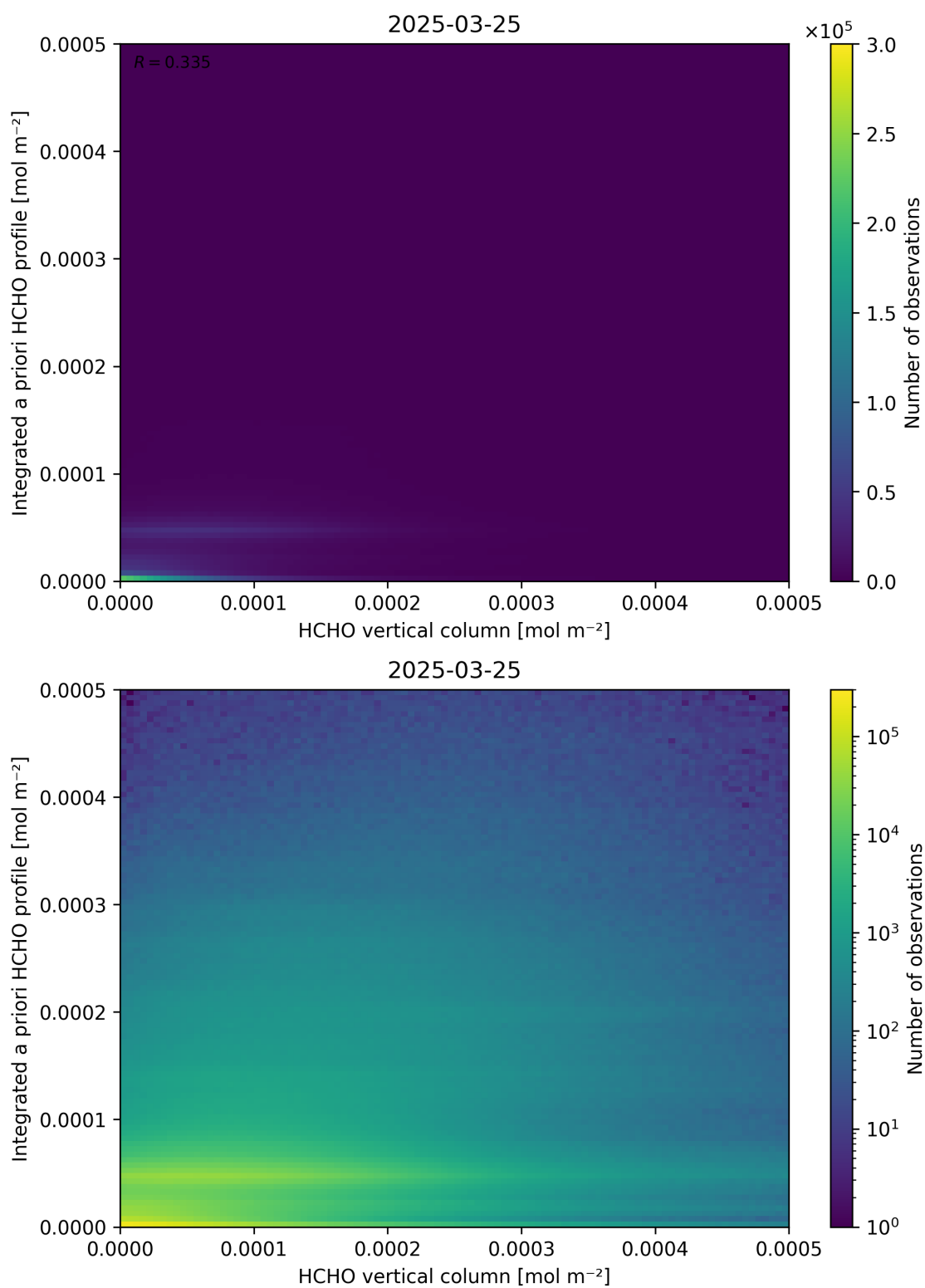
Figure 135: Scatter density plot of “HCHO vertical column” against “Integrated a priori HCHO profile” for 2025-03-24 to 2025-03-26.
