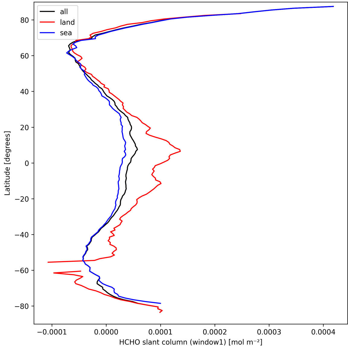
Figure 24: Zonal average of “HCHO slant column (window1)” for 2025-03-24 to 2025-03-26.
