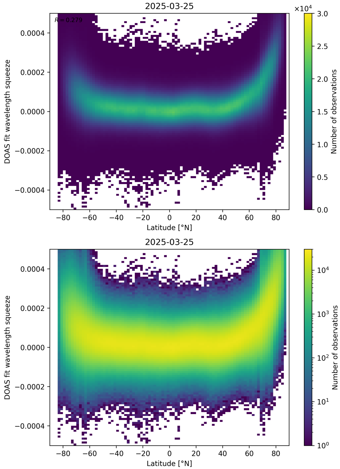
Figure 155: Scatter density plot of “Latitude” against “DOAS fit wavelength squeeze” for 2025-03-24 to 2025-03-26.
