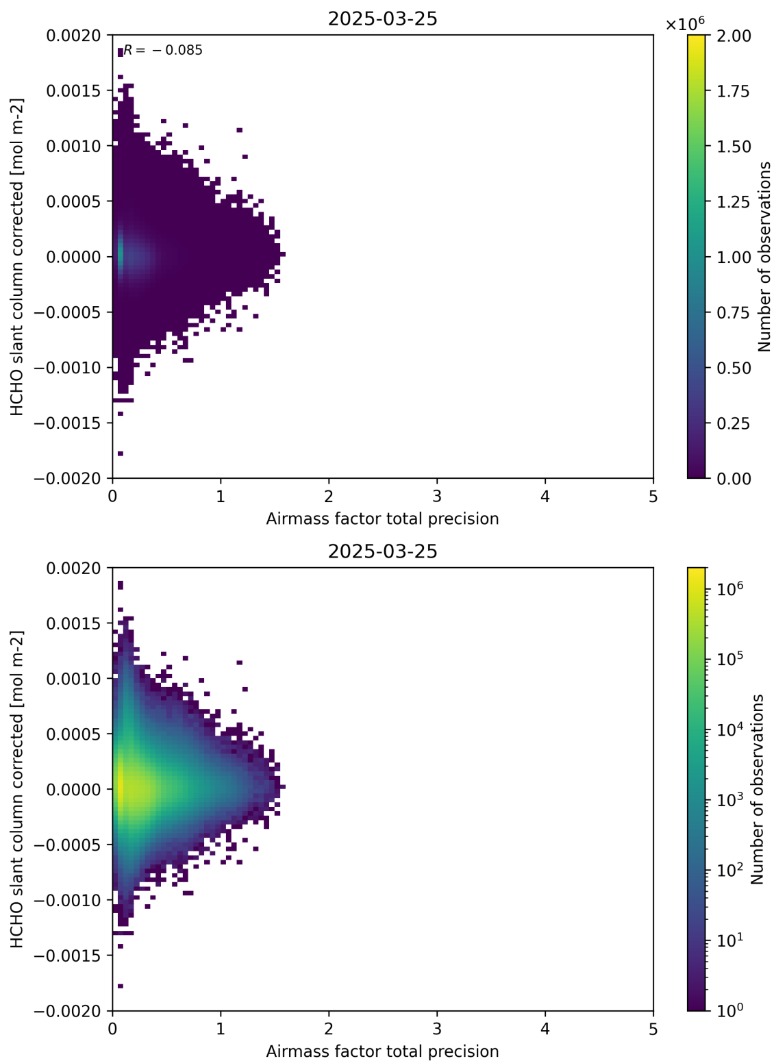
Figure 109: Scatter density plot of “Airmass factor total precision” against “HCHO slant column corrected” for 2025-03-24 to 2025-03-26.
