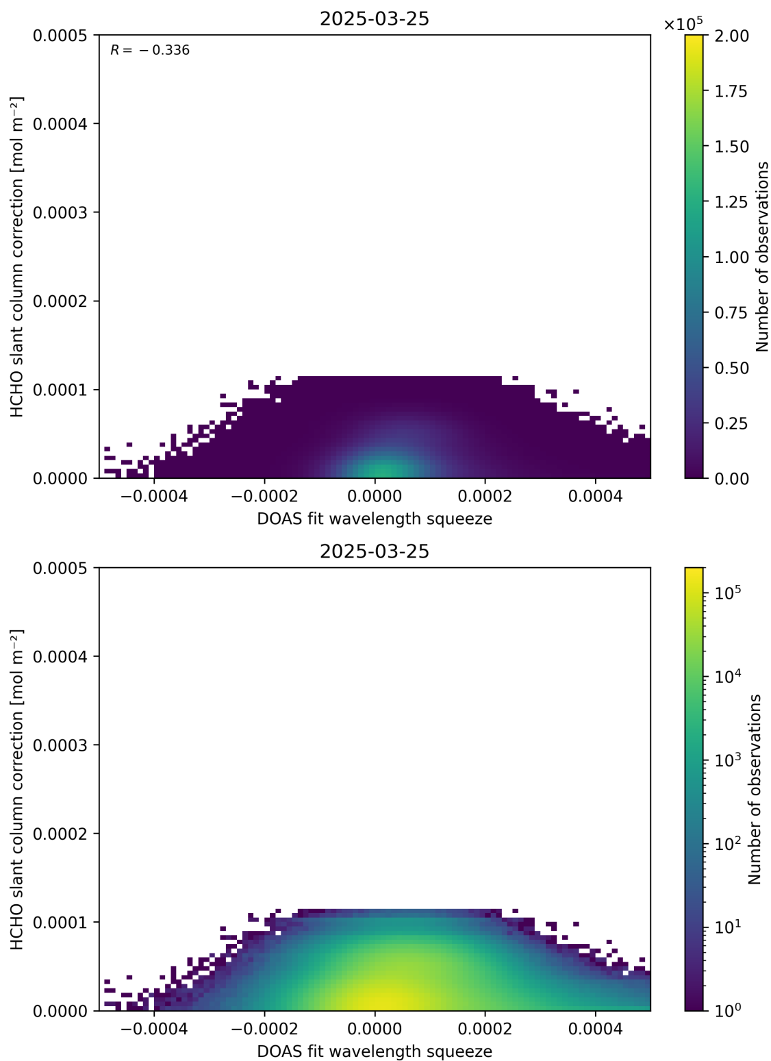
Figure 70: Scatter density plot of “DOAS fit wavelength squeeze” against “HCHO slant column correction” for 2025-03-24 to 2025-03-26.
