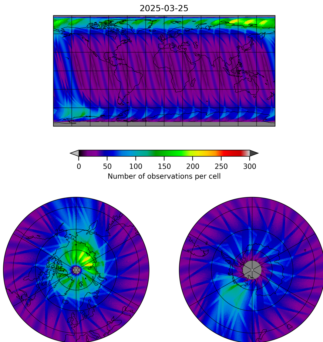
Figure 19: Map of the number of observations for 2025-03-24 to 2025-03-26
