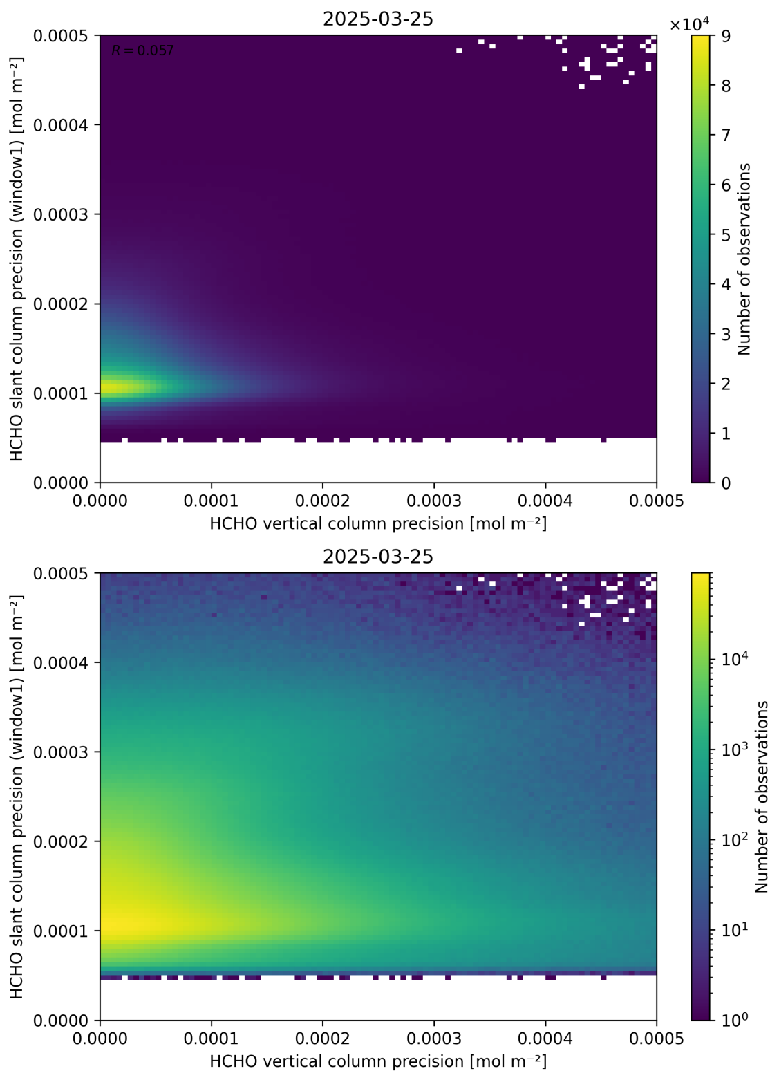
Figure 143: Scatter density plot of “HCHO vertical column precision” against “HCHO slant column precision (window1)” for 2025-03-24 to 2025-03-26.
