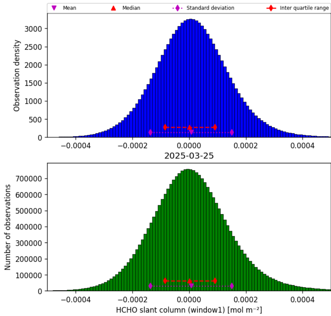
Figure 38: Histogram of “HCHO slant column (window1)” for 2025-03-24 to 2025-03-26
