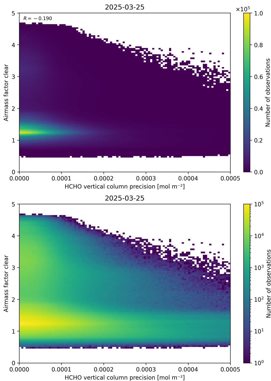
Figure 139: Scatter density plot of “HCHO vertical column precision” against “Airmass factor clear” for 2025-03-24 to 2025-03-26.
