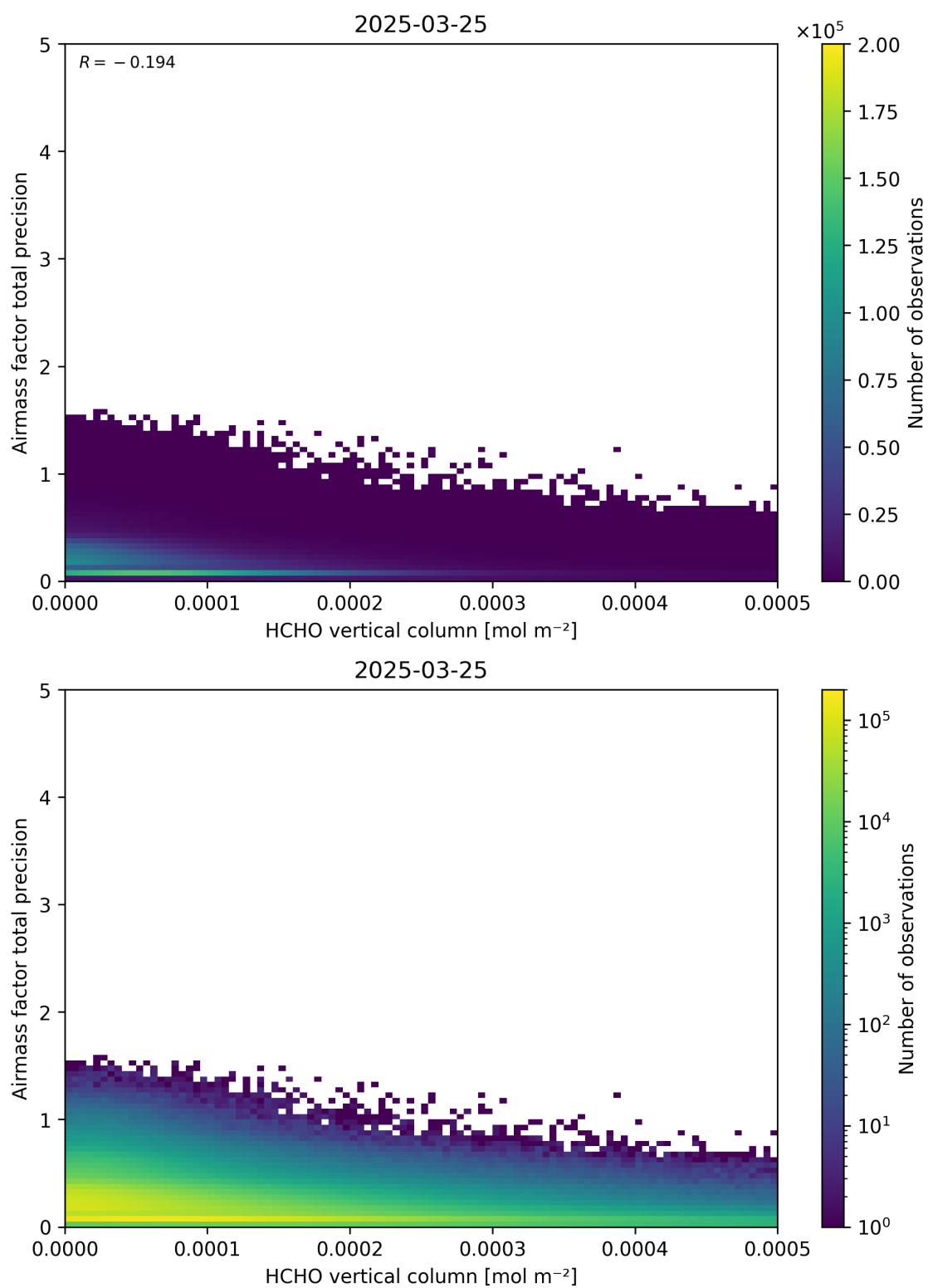
Figure 132: Scatter density plot of “HCHO vertical column” against “Airmass factor total precision” for 2025-03-24 to 2025-03-26.
