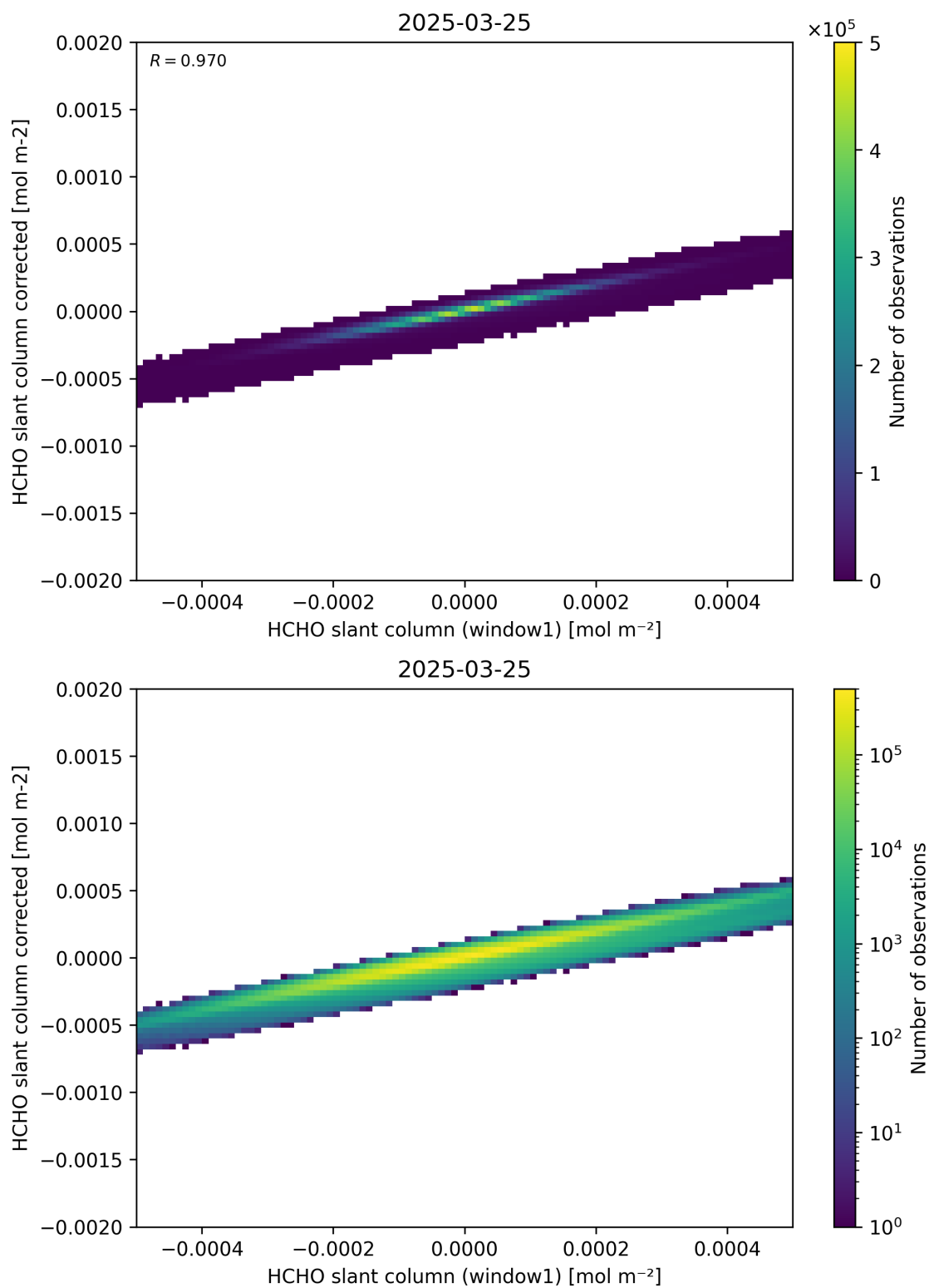
Figure 82: Scatter density plot of “HCHO slant column (window1)” against “HCHO slant column corrected” for 2025-03-24 to 2025-03-26.
