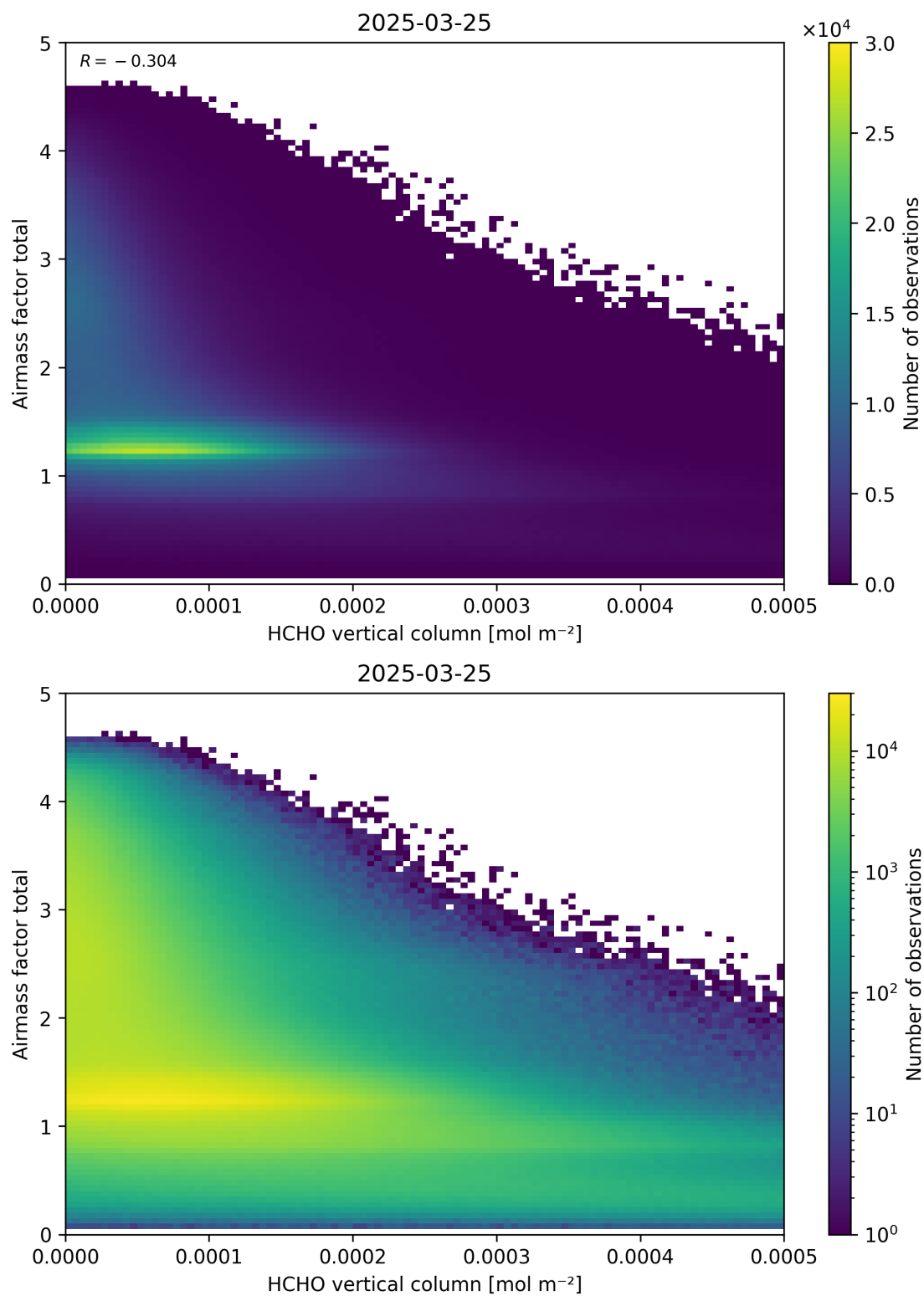
Figure 131: Scatter density plot of “HCHO vertical column” against “Airmass factor total” for 2025-03-24 to 2025-03-26.
