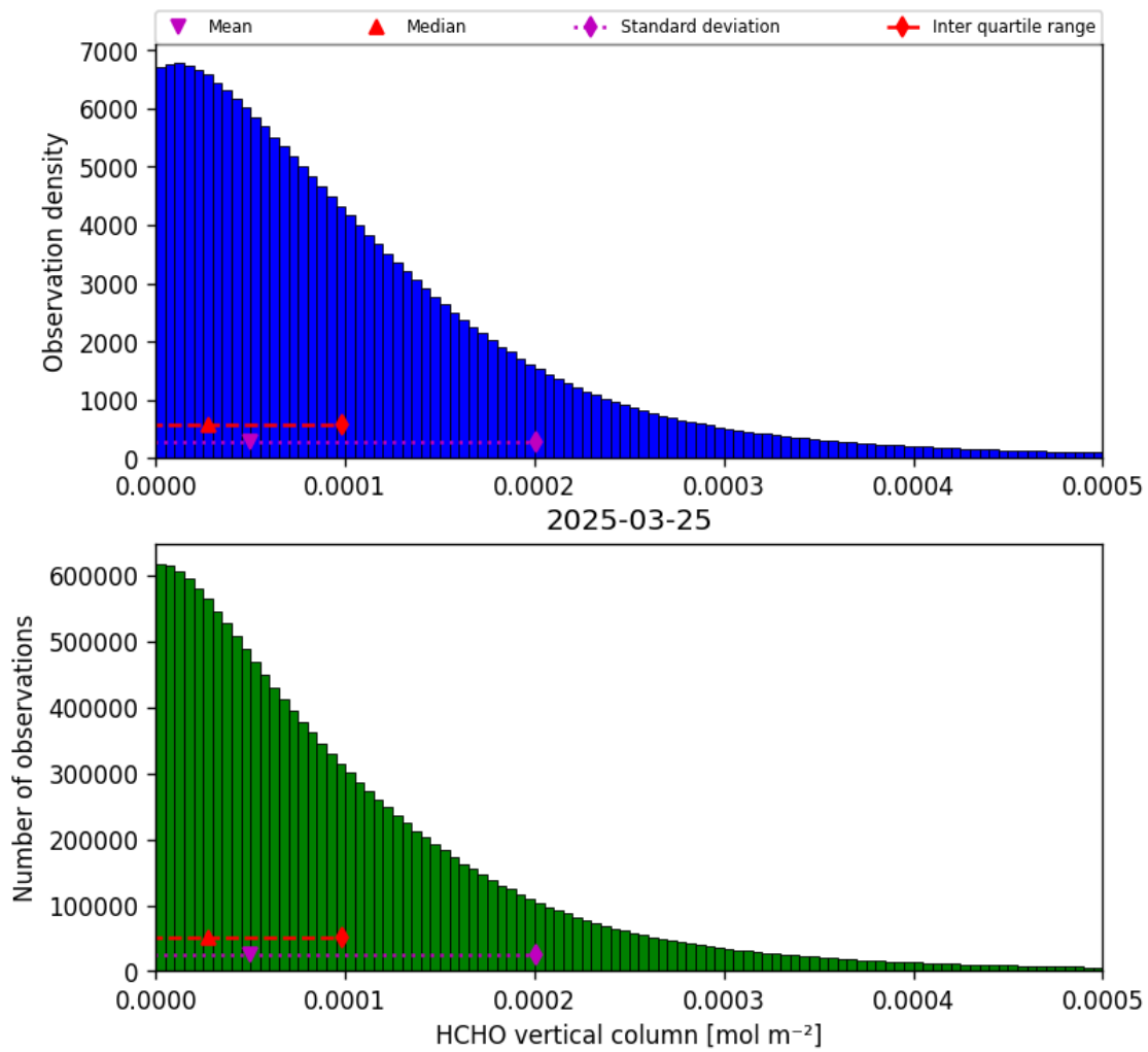
Figure 35: Histogram of “HCHO vertical column” for 2025-03-24 to 2025-03-26
