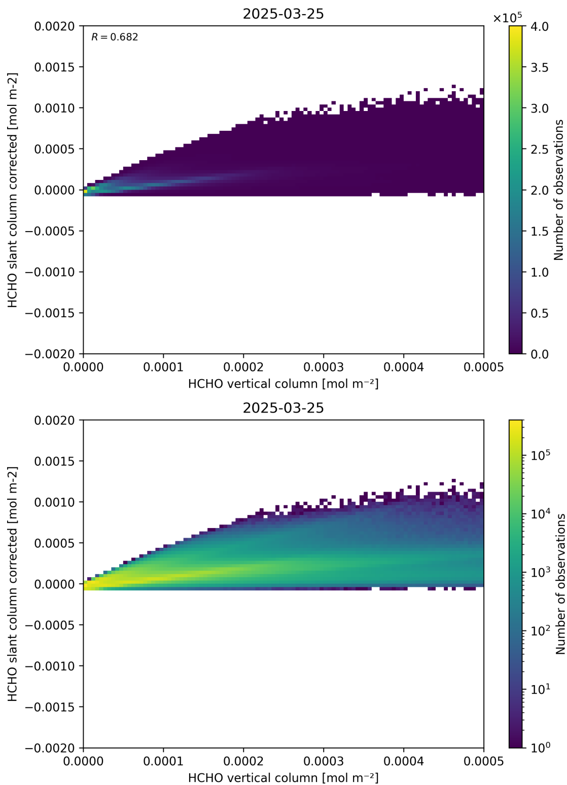
Figure 127: Scatter density plot of “HCHO vertical column” against “HCHO slant column corrected” for 2025-03-24 to 2025-03-26.
