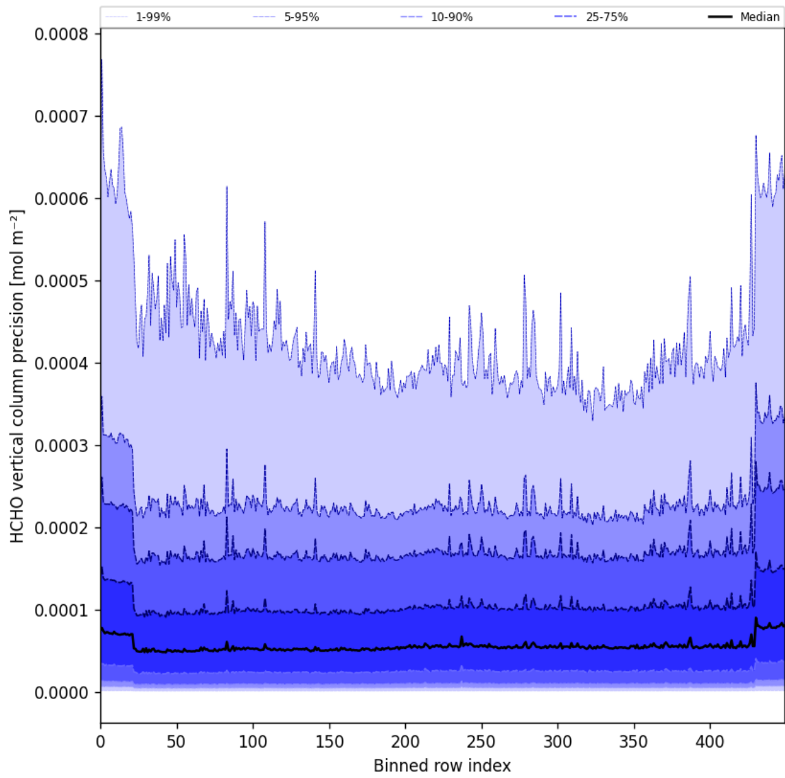
Figure 50: Along track statistics of “HCHO vertical column precision” for 2025-03-24 to 2025-03-26
