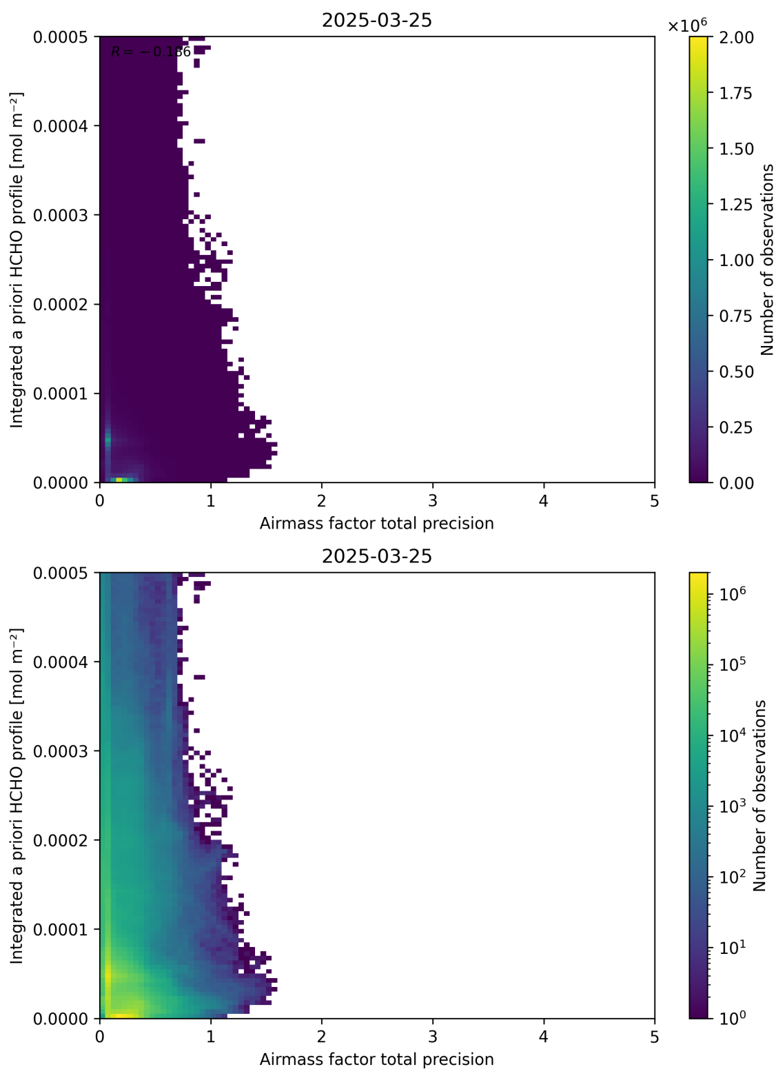
Figure 111: Scatter density plot of “Airmass factor total precision” against “Integrated a priori HCHO profile” for 2025-03-24 to 2025-03-26.
