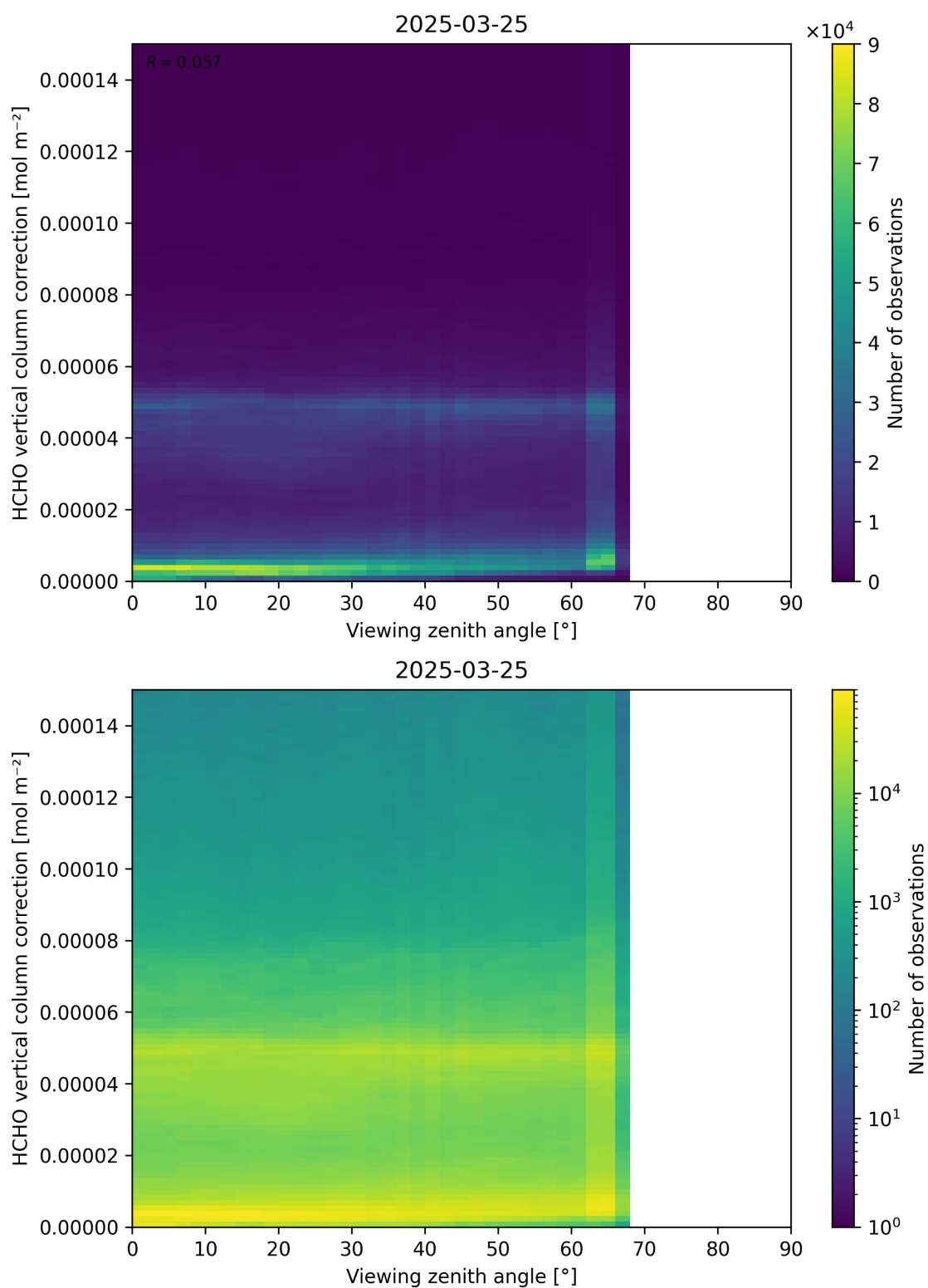
Figure 193: Scatter density plot of “Viewing zenith angle” against “HCHO vertical column correction” for 2025-03-24 to 2025-03-26.
