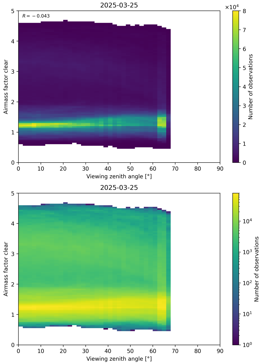
Figure 185: Scatter density plot of “Viewing zenith angle” against “Airmass factor clear” for 2025-03-24 to 2025-03-26.
