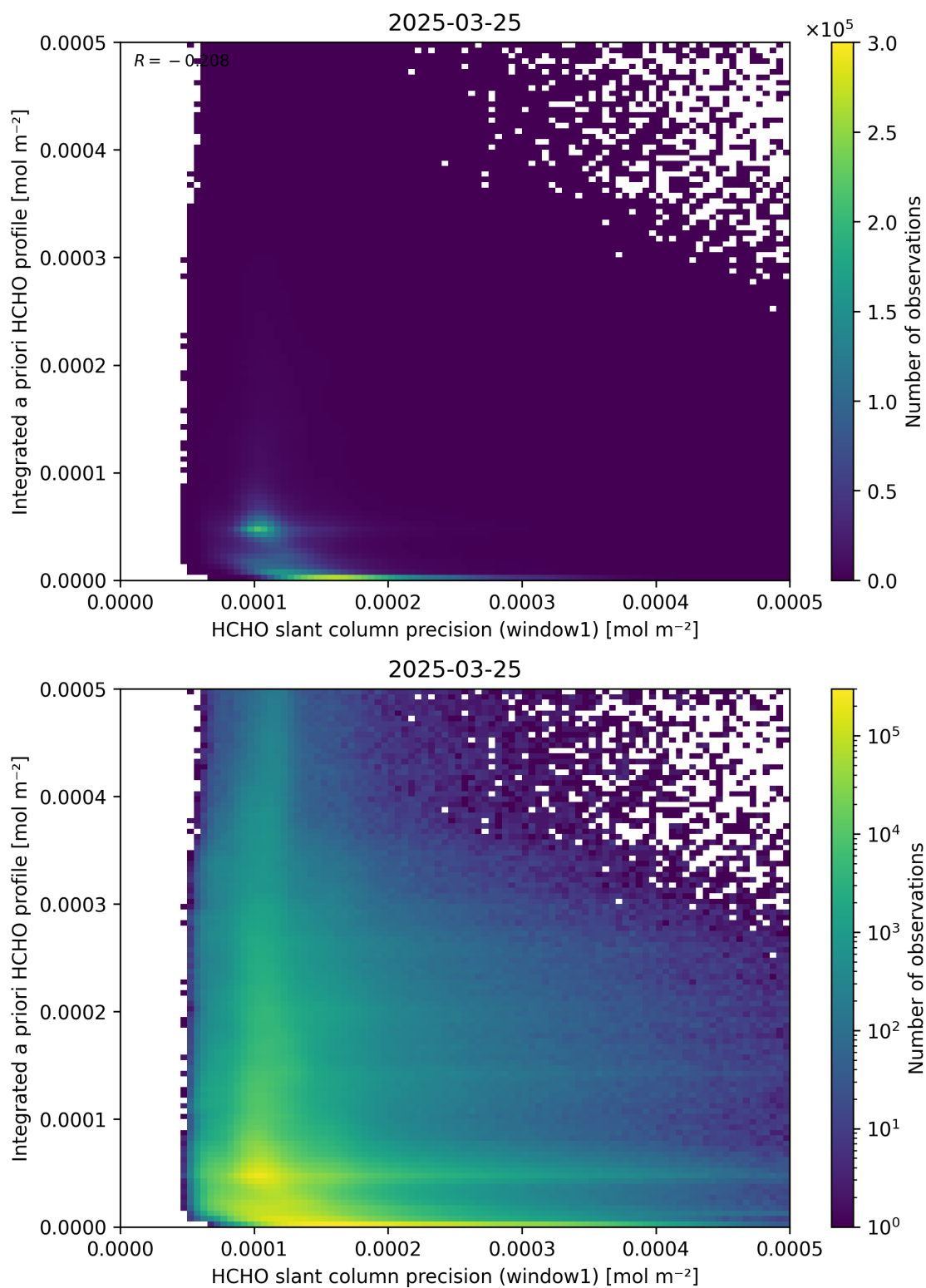
Figure 96: Scatter density plot of “HCHO slant column precision (window1)” against “Integrated a priori HCHO profile” for 2025-03-24 to 2025-03-26.
