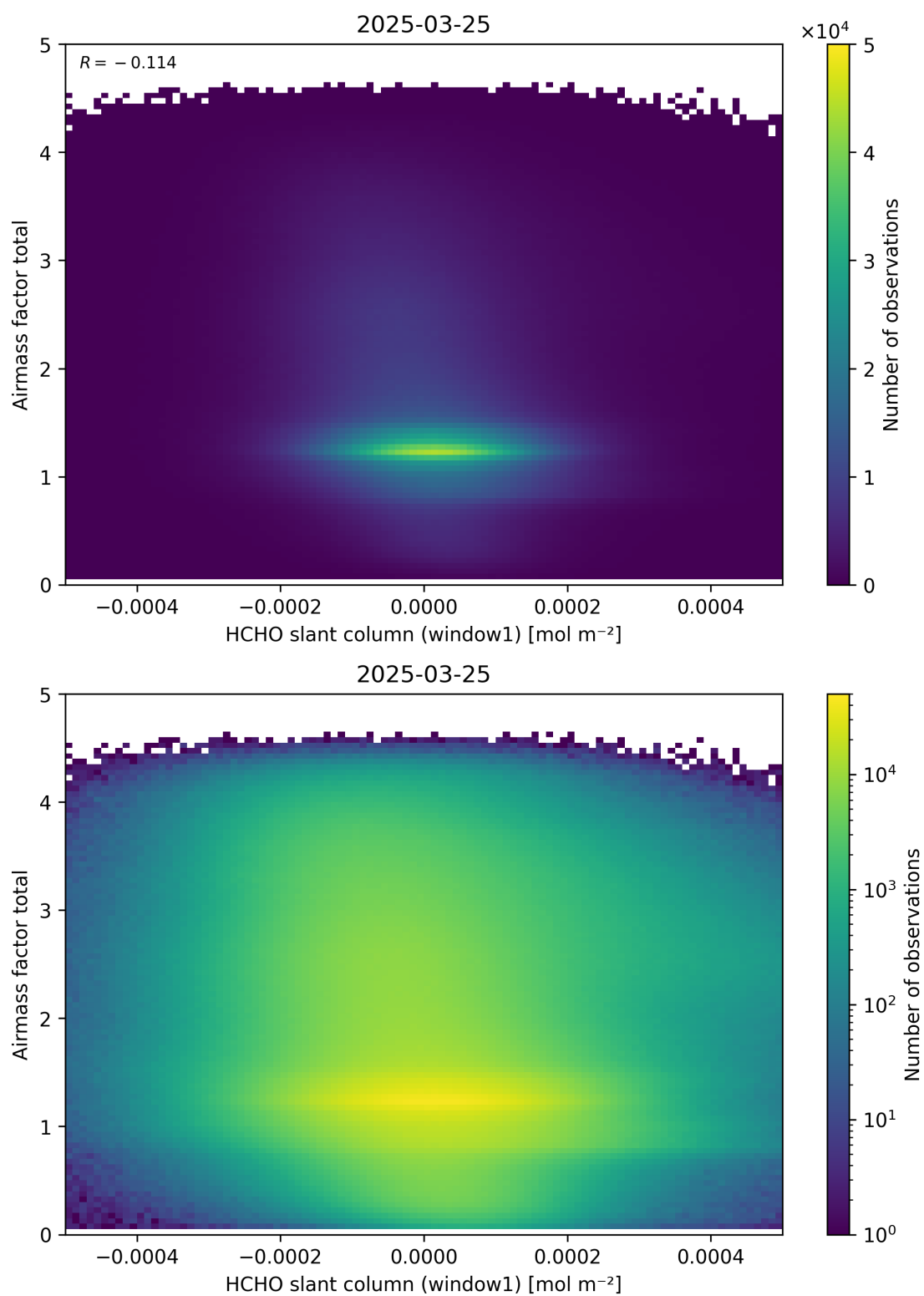
Figure 85: Scatter density plot of “HCHO slant column (window1)” against “Airmass factor total” for 2025-03-24 to 2025-03-26.
