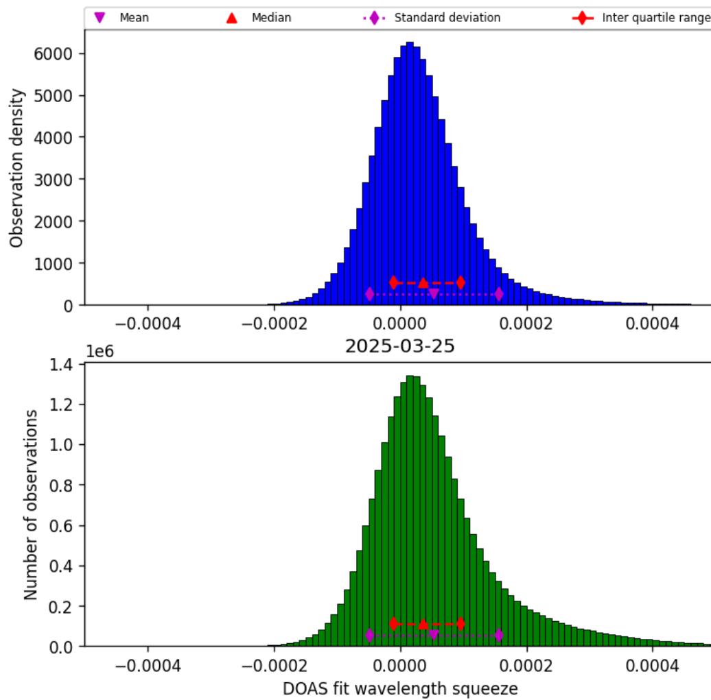
Figure 45: Histogram of “DOAS fit wavelength squeeze” for 2025-03-24 to 2025-03-26
