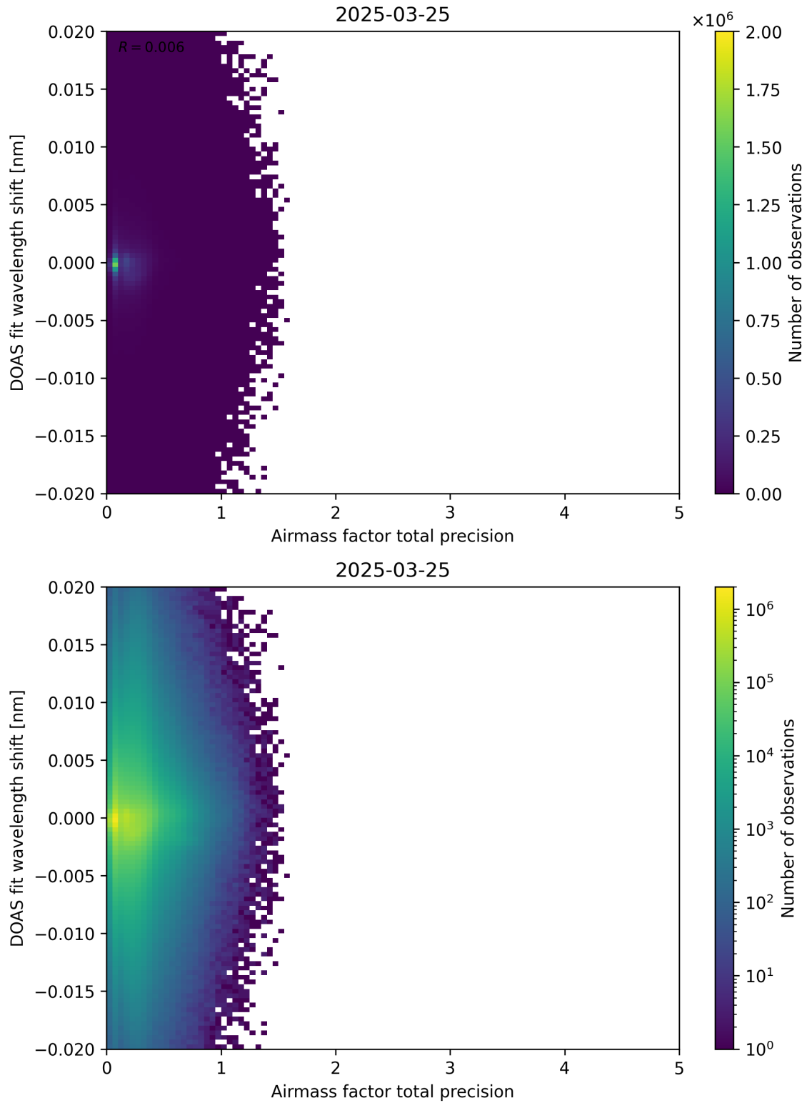
Figure 106: Scatter density plot of “Airmass factor total precision” against “DOAS fit wavelength shift” for 2025-03-24 to 2025-03-26.
