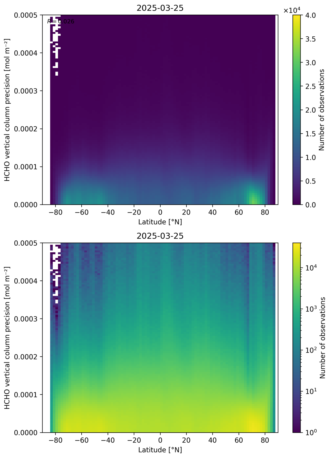
Figure 165: Scatter density plot of “Latitude” against “HCHO vertical column precision” for 2025-03-24 to 2025-03-26.
