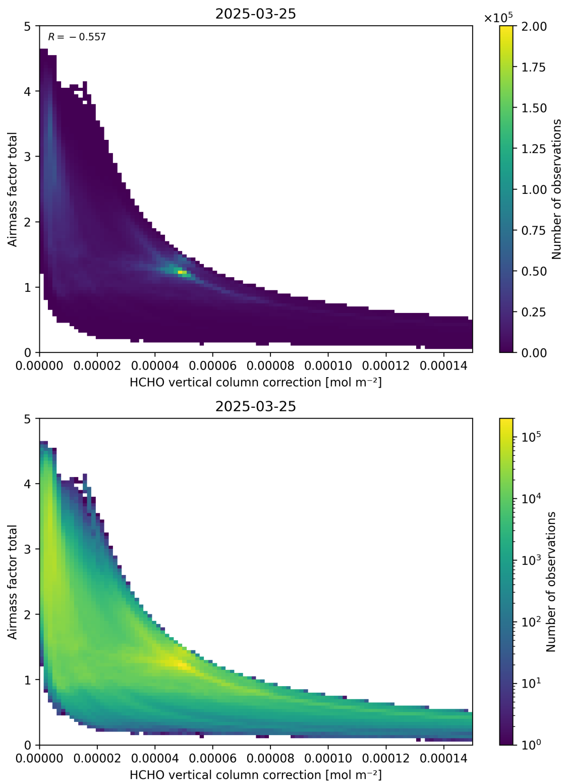
Figure 120: Scatter density plot of “HCHO vertical column correction” against “Airmass factor total” for 2025-03-24 to 2025-03-26.
