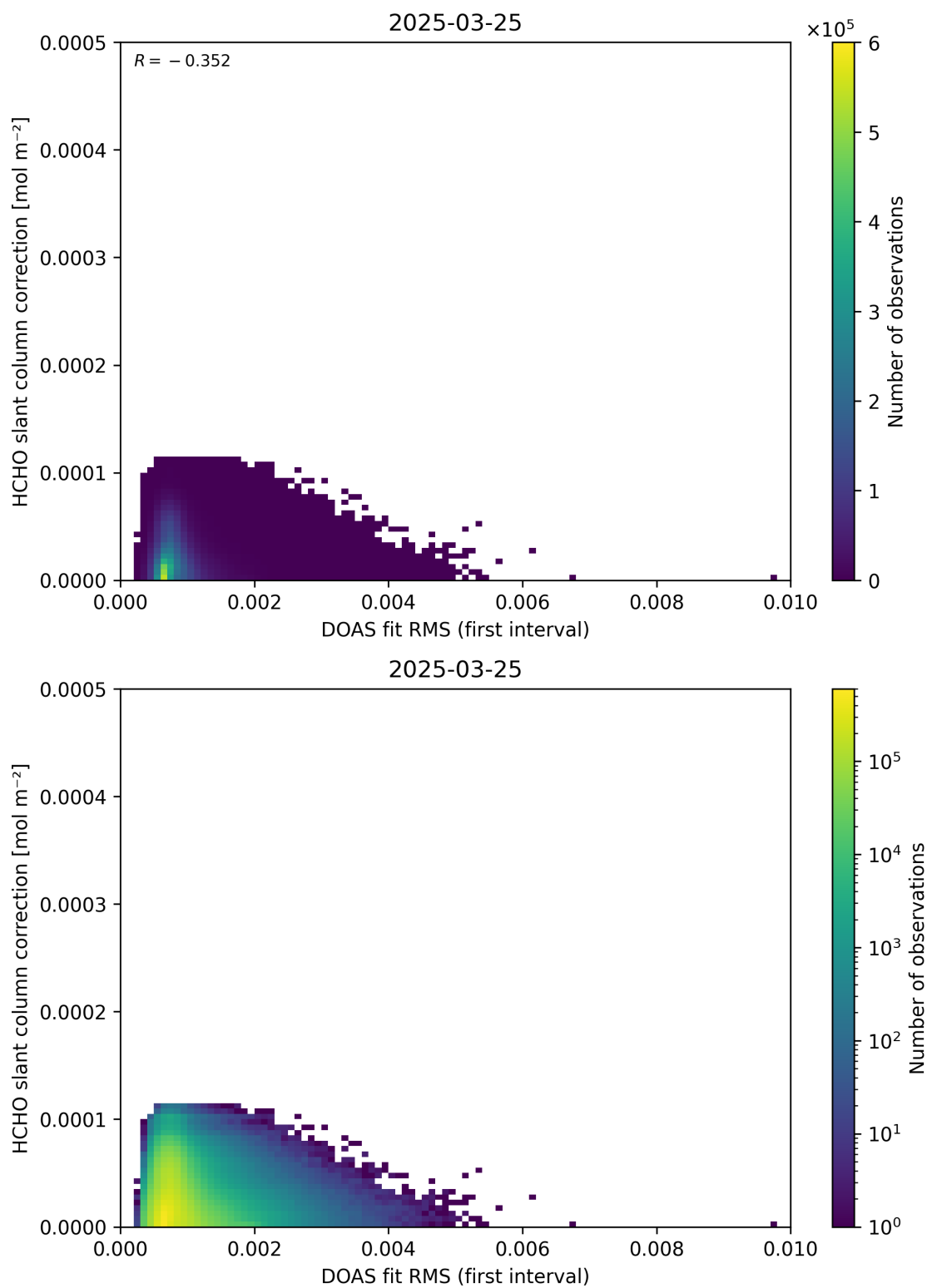
Figure 63: Scatter density plot of “DOAS fit RMS (first interval)” against “HCHO slant column correction” for 2025-03-24 to 2025-03-26.
