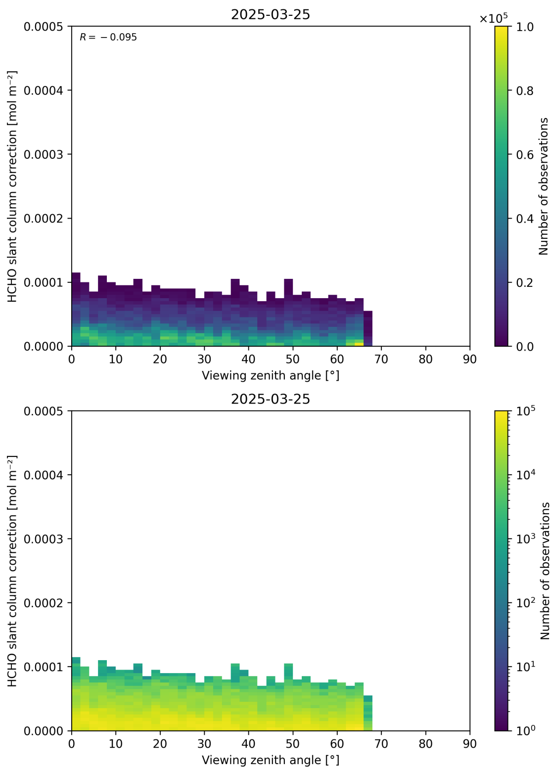
Figure 187: Scatter density plot of “Viewing zenith angle” against “HCHO slant column correction” for 2025-03-24 to 2025-03-26.
