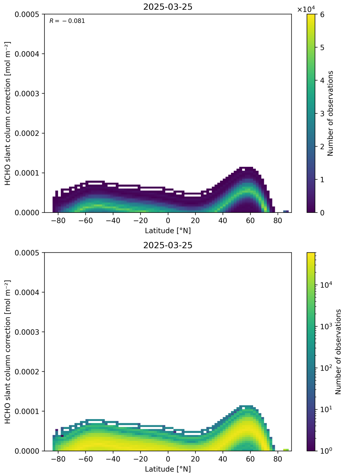
Figure 158: Scatter density plot of “Latitude” against “HCHO slant column correction” for 2025-03-24 to 2025-03-26.
