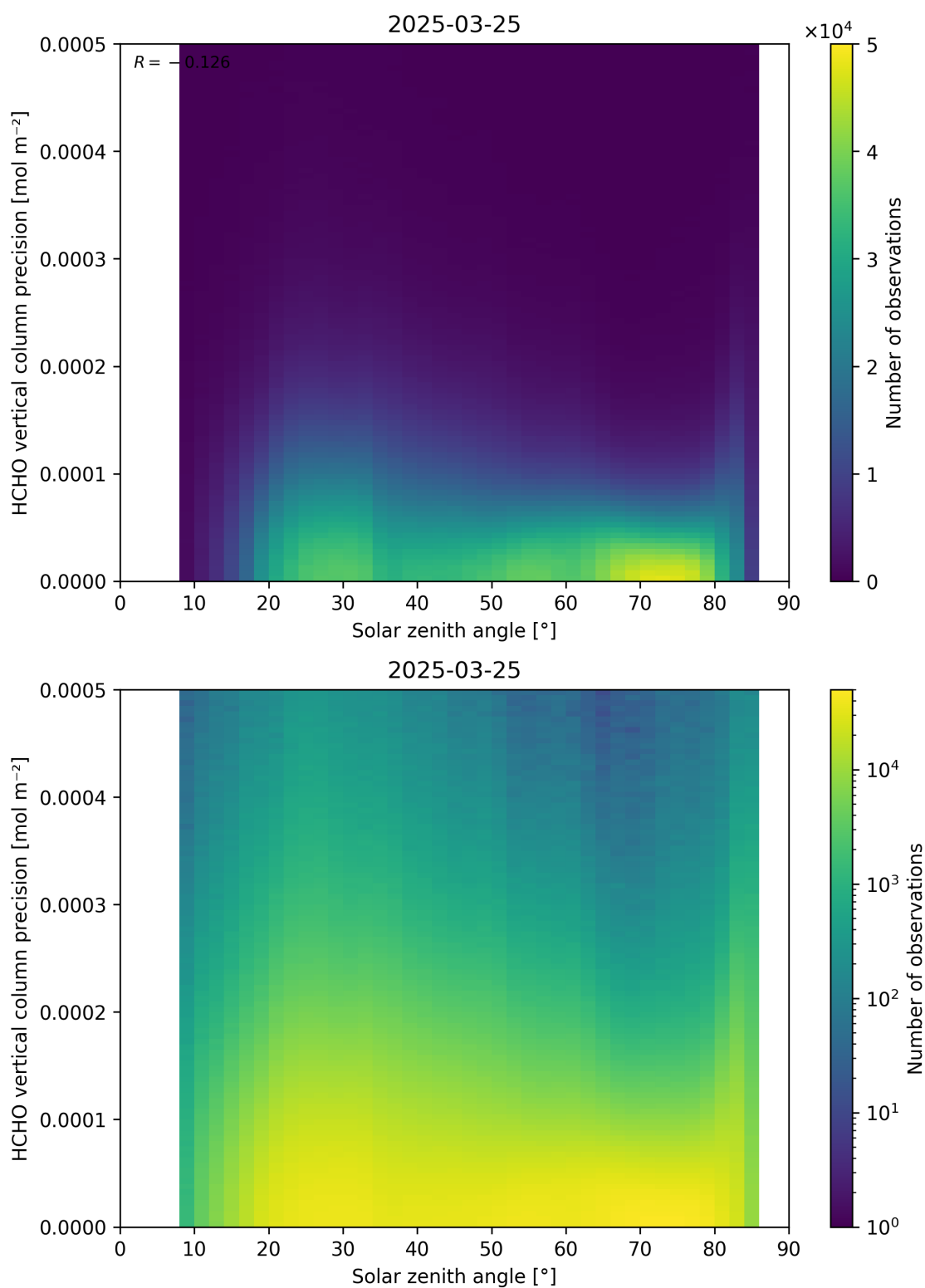
Figure 179: Scatter density plot of “Solar zenith angle” against “HCHO vertical column precision” for 2025-03-24 to 2025-03-26.
