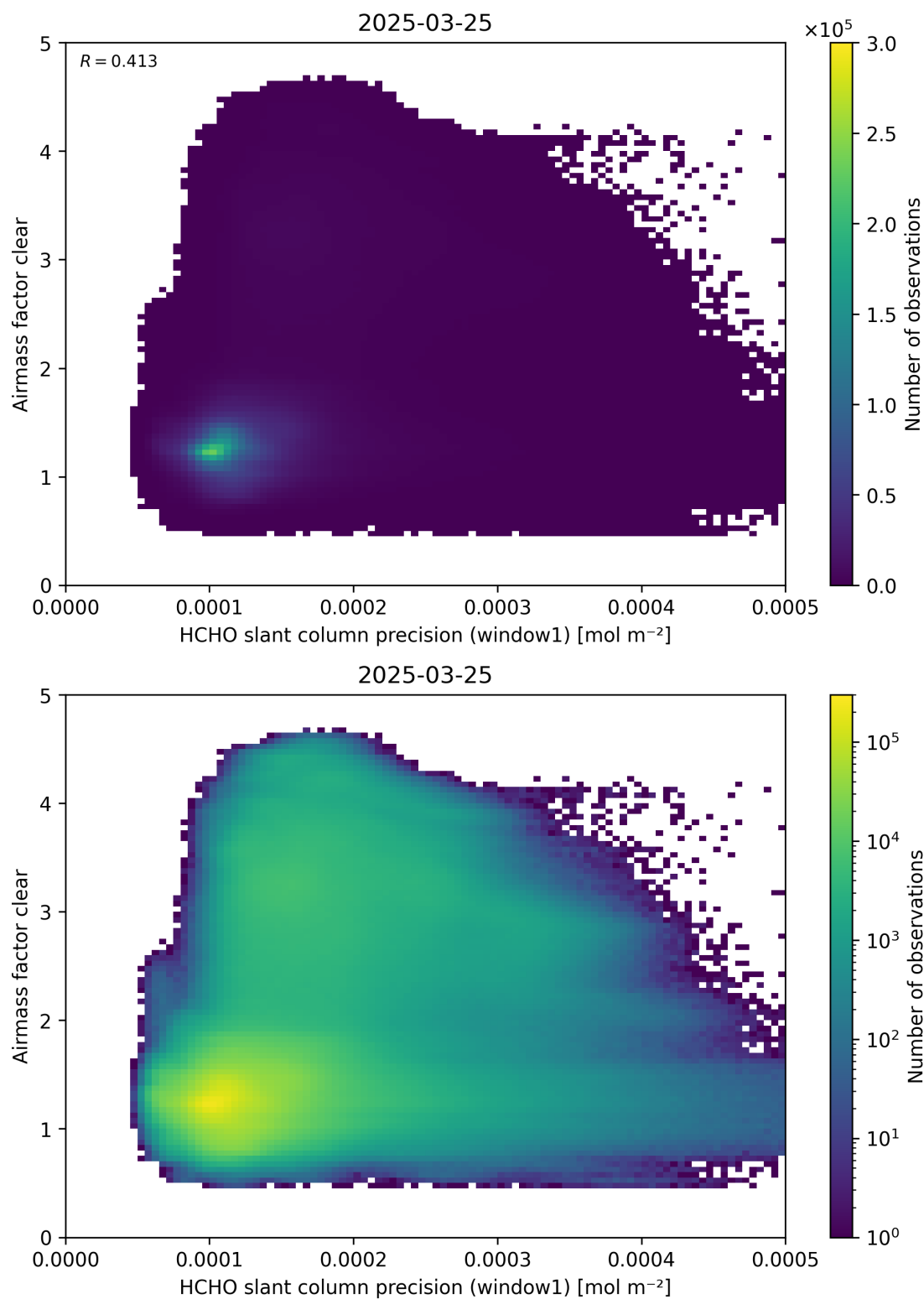
Figure 91: Scatter density plot of “HCHO slant column precision (window1)” against “Airmass factor clear” for 2025-03-24 to 2025-03-26.
