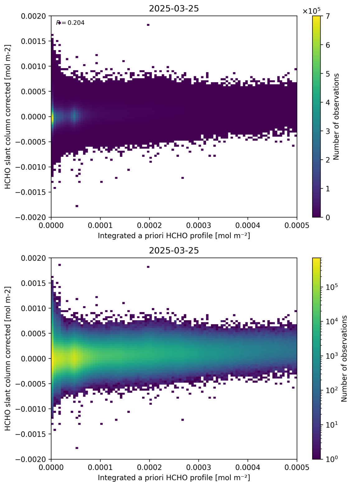
Figure 151: Scatter density plot of “Integrated a priori HCHO profile” against “HCHO slant column corrected” for 2025-03-24 to 2025-03-26.
