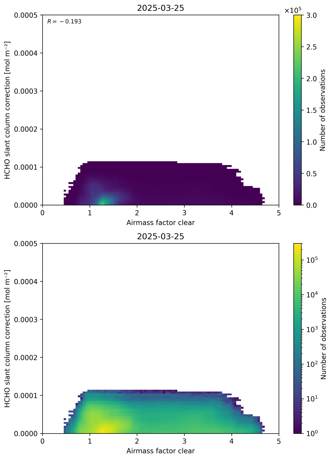
Figure 75: Scatter density plot of “Airmass factor clear” against “HCHO slant column correction” for 2025-03-24 to 2025-03-26.
