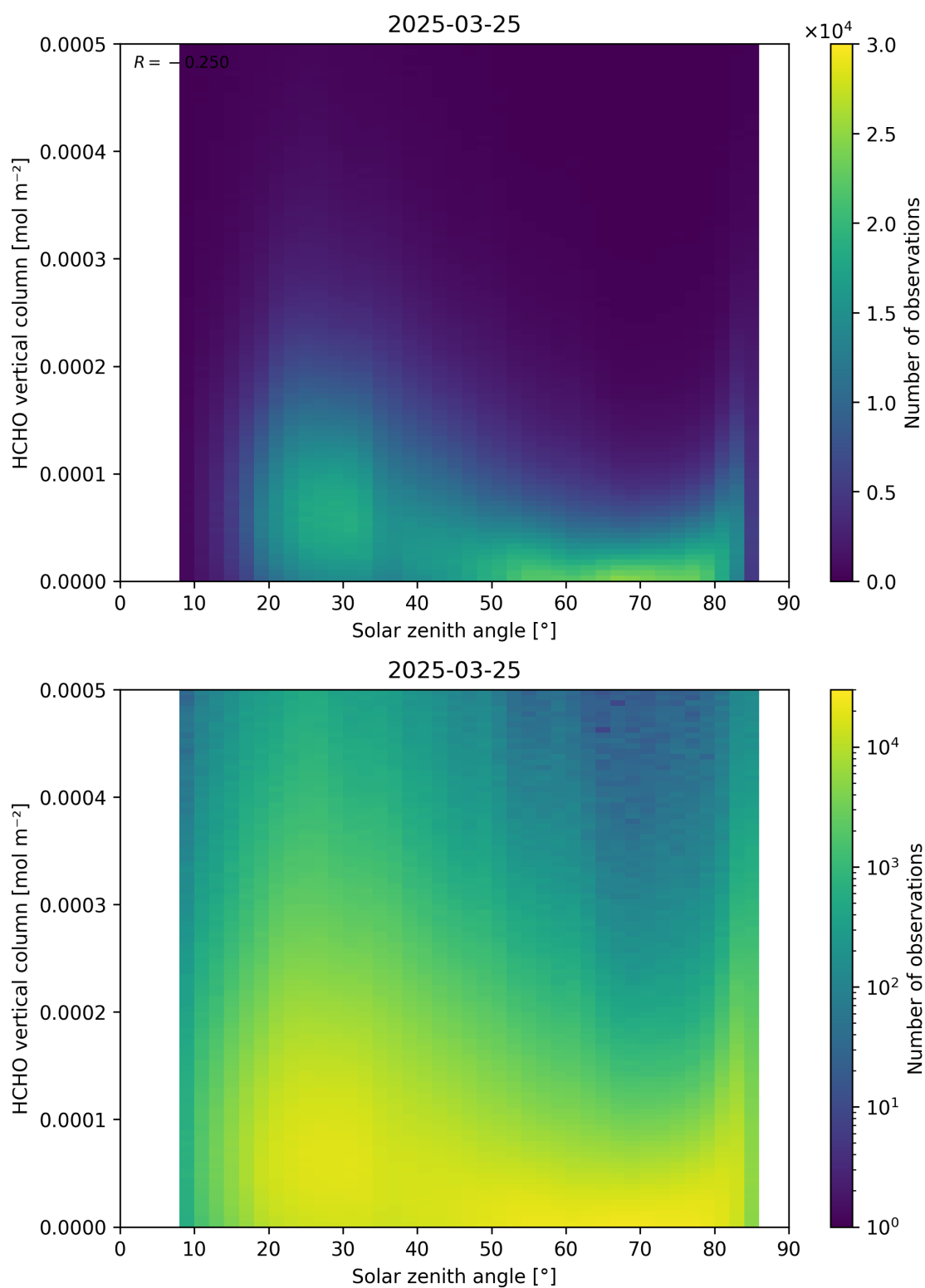
Figure 177: Scatter density plot of “Solar zenith angle” against “HCHO vertical column” for 2025-03-24 to 2025-03-26.
