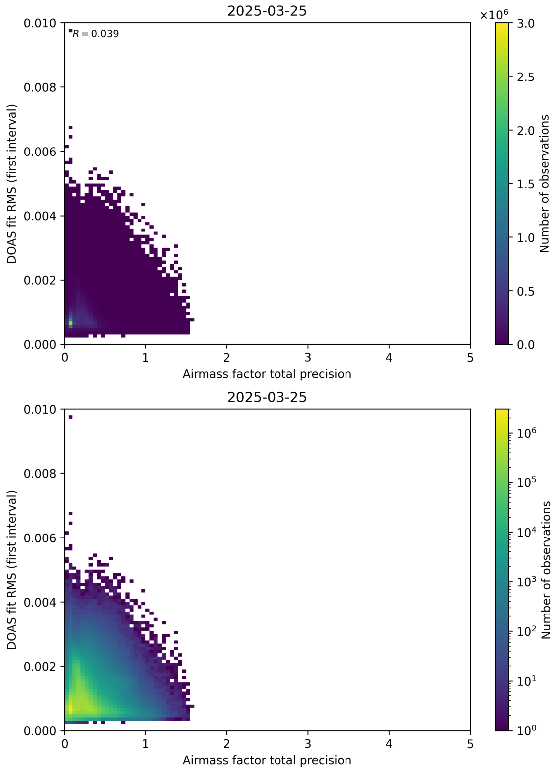
Figure 105: Scatter density plot of “Airmass factor total precision” against “DOAS fit RMS (first interval)” for 2025-03-24 to 2025-03-26.
