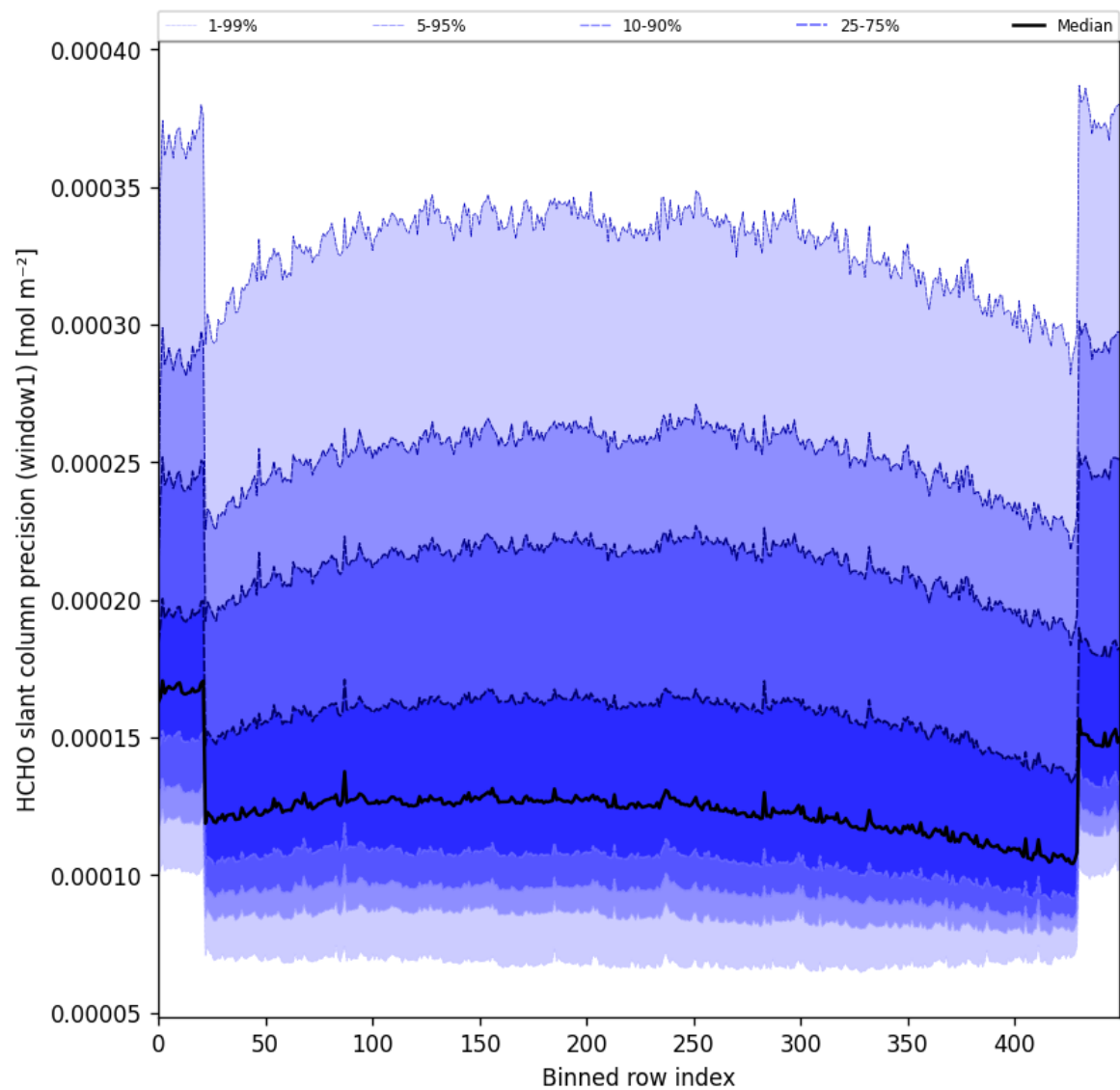
Figure 53: Along track statistics of “HCHO slant column precision (window1)” for 2025-03-24 to 2025-03-26
