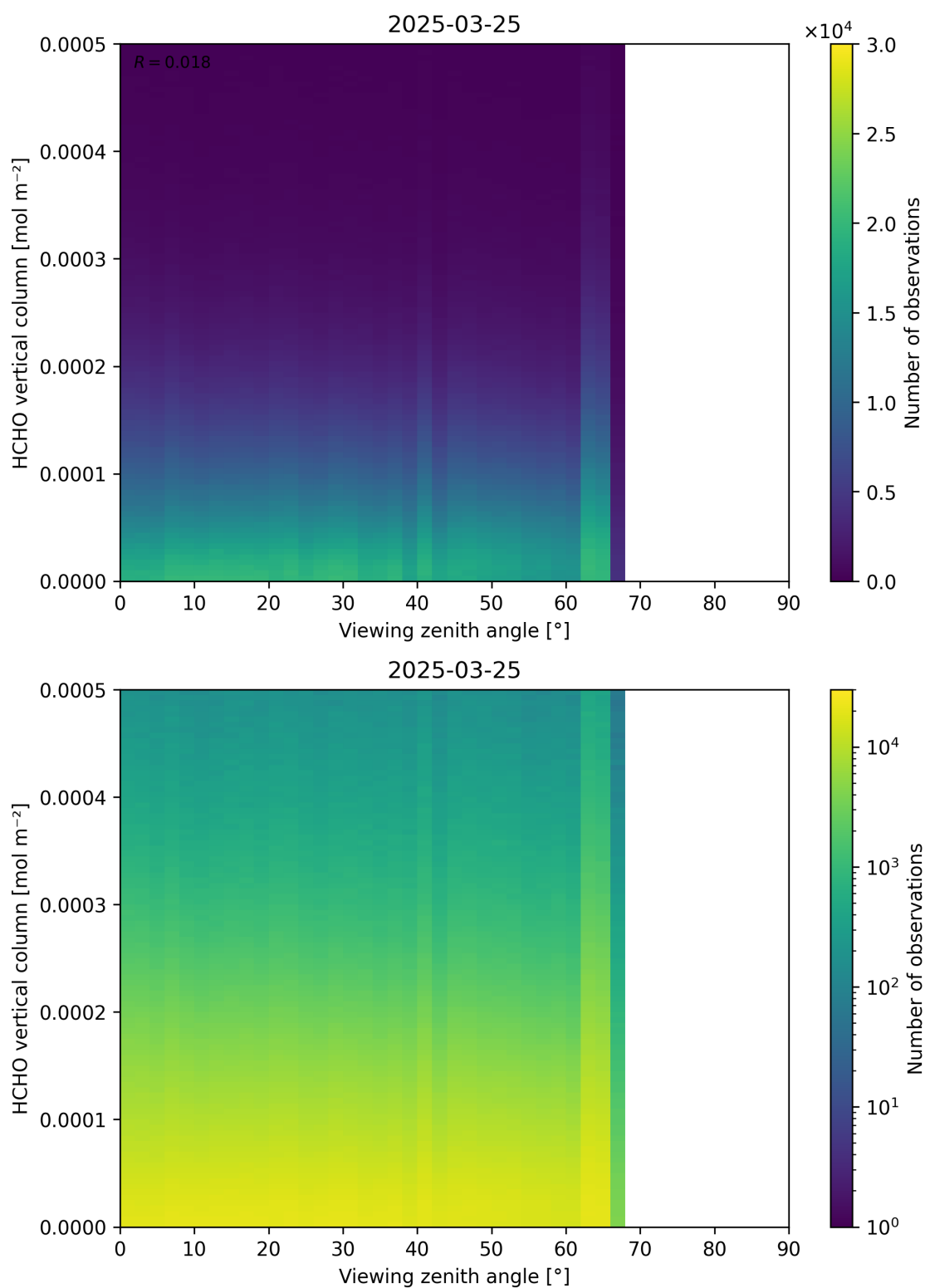
Figure 192: Scatter density plot of “Viewing zenith angle” against “HCHO vertical column” for 2025-03-24 to 2025-03-26.
