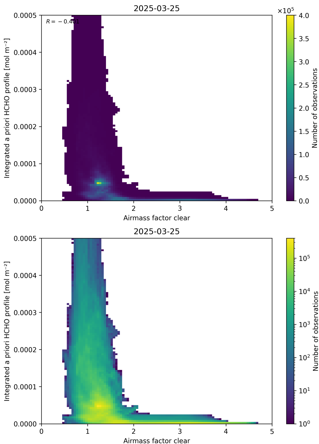
Figure 76: Scatter density plot of “Airmass factor clear” against “Integrated a priori HCHO profile” for 2025-03-24 to 2025-03-26.
