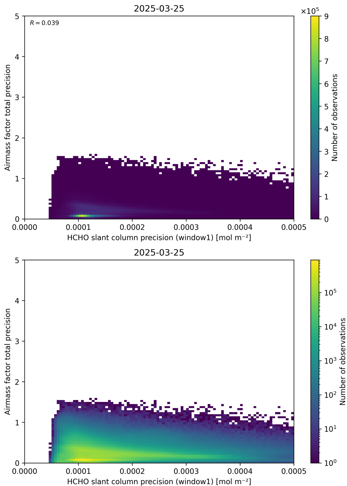
Figure 95: Scatter density plot of “HCHO slant column precision (window1)” against “Airmass factor total precision” for 2025-03-24 to 2025-03-26.
