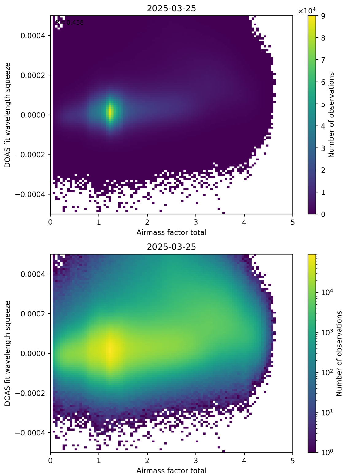
Figure 99: Scatter density plot of “Airmass factor total” against “DOAS fit wavelength squeeze” for 2025-03-24 to 2025-03-26.
