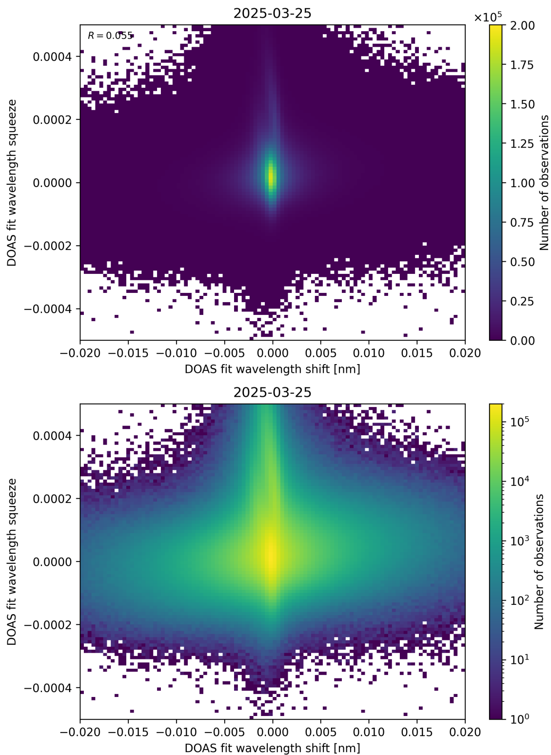
Figure 65: Scatter density plot of “DOAS fit wavelength shift” against “DOAS fit wavelength squeeze” for 2025-03-24 to 2025-03-26.
