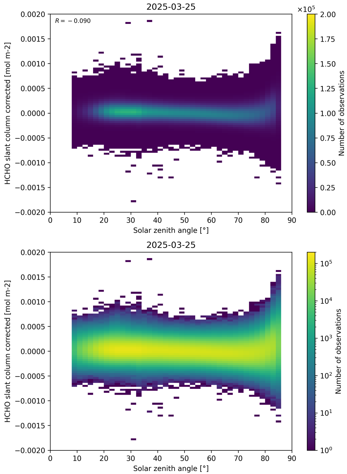
Figure 171: Scatter density plot of “Solar zenith angle” against “HCHO slant column corrected” for 2025-03-24 to 2025-03-26.
