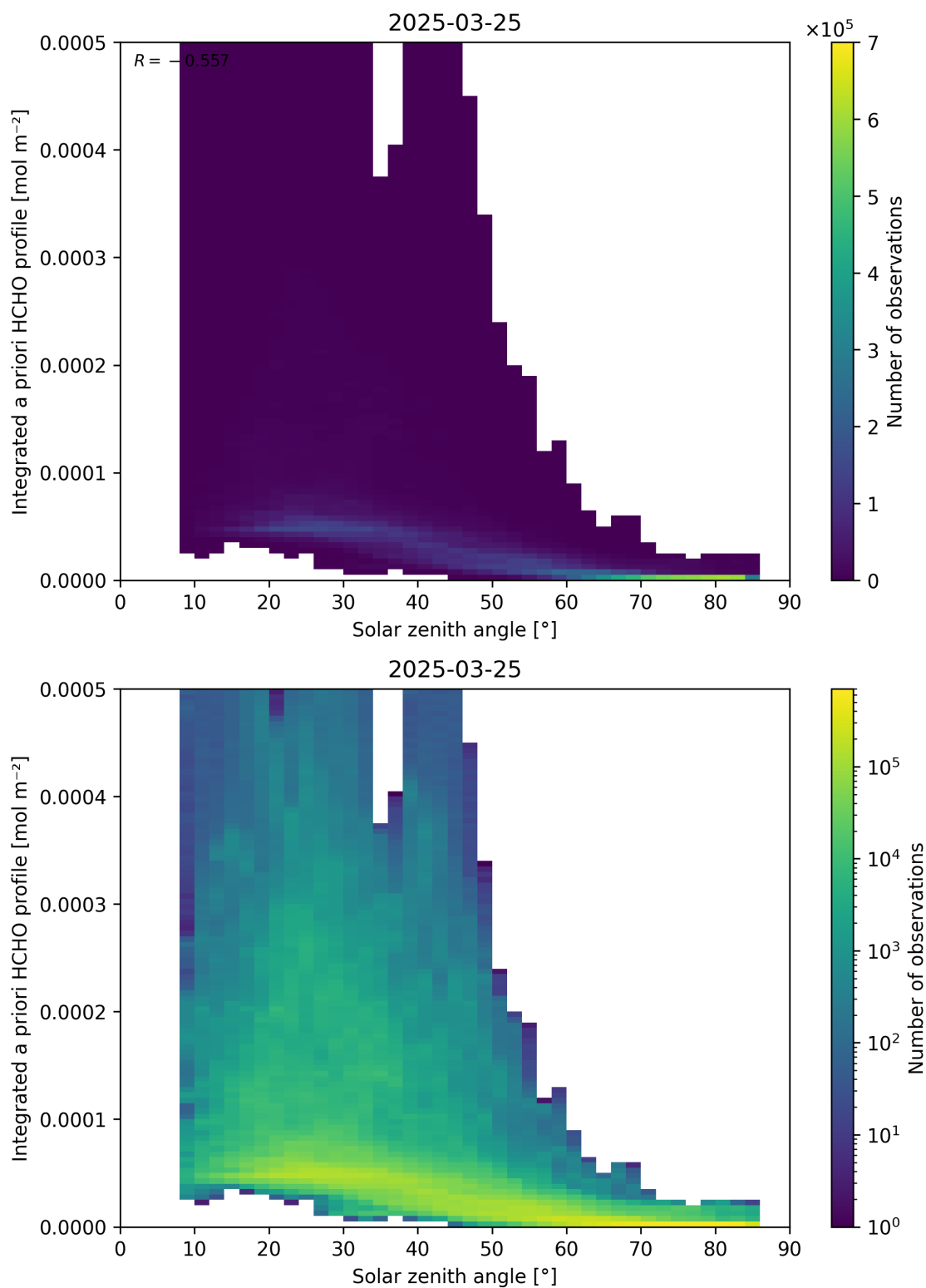
Figure 180: Scatter density plot of “Solar zenith angle” against “Integrated a priori HCHO profile” for 2025-03-24 to 2025-03-26.
