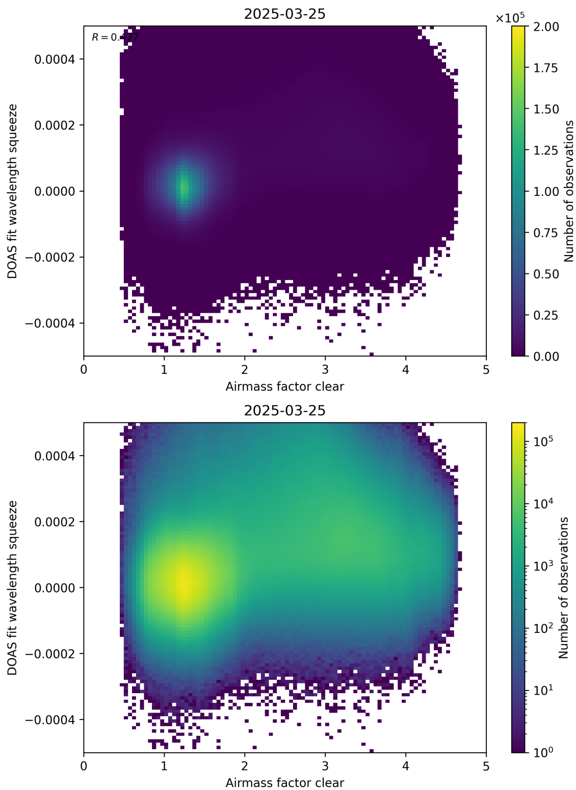
Figure 73: Scatter density plot of “Airmass factor clear” against “DOAS fit wavelength squeeze” for 2025-03-24 to 2025-03-26.
