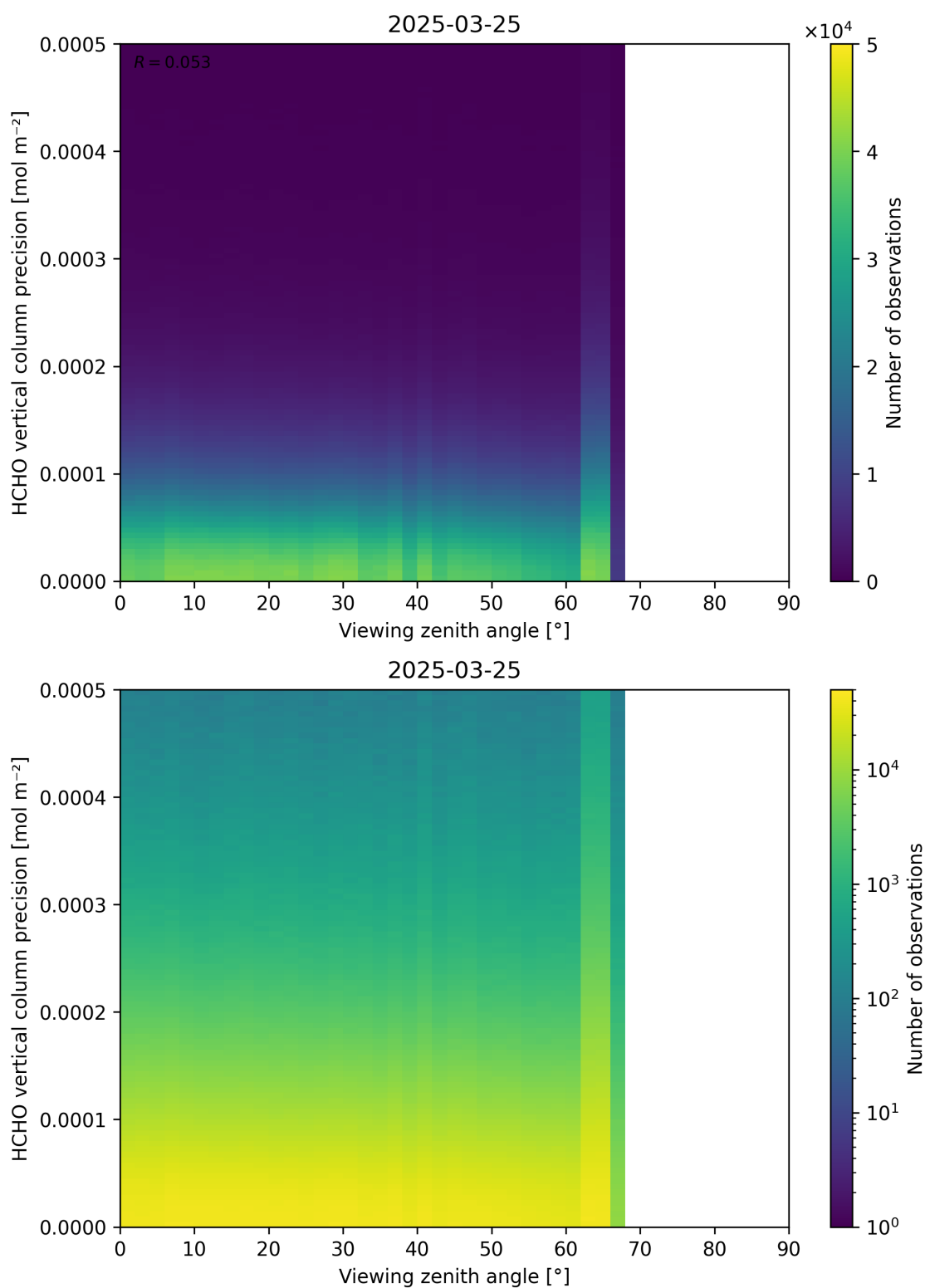
Figure 194: Scatter density plot of “Viewing zenith angle” against “HCHO vertical column precision” for 2025-03-24 to 2025-03-26.
