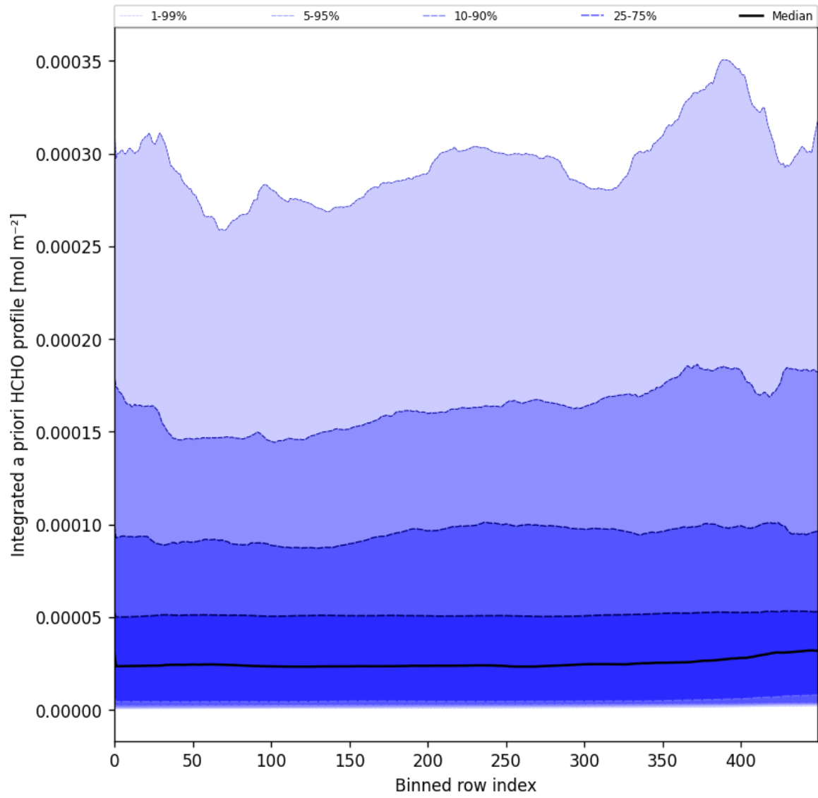
Figure 57: Along track statistics of “Integrated a priori HCHO profile” for 2025-03-24 to 2025-03-26
