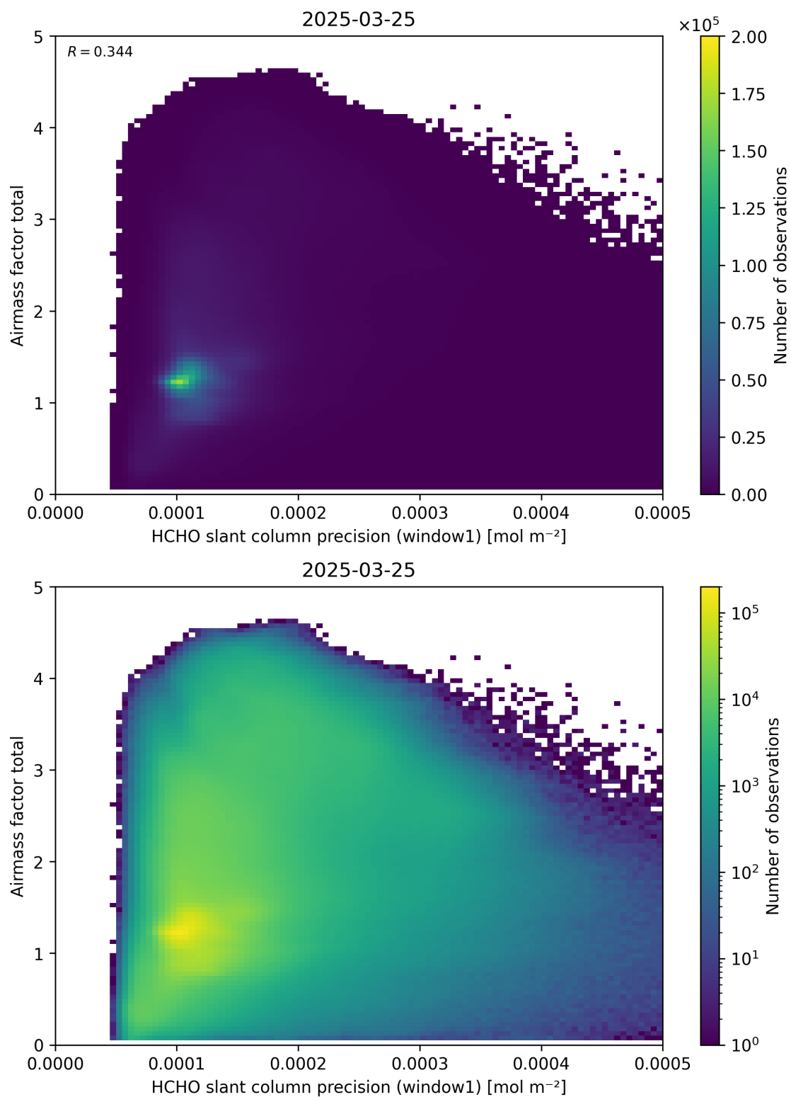
Figure 94: Scatter density plot of “HCHO slant column precision (window1)” against “Airmass factor total” for 2025-03-24 to 2025-03-26.
