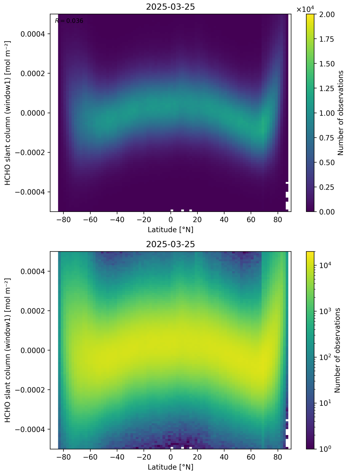
Figure 159: Scatter density plot of “Latitude” against “HCHO slant column (window1)” for 2025-03-24 to 2025-03-26.
