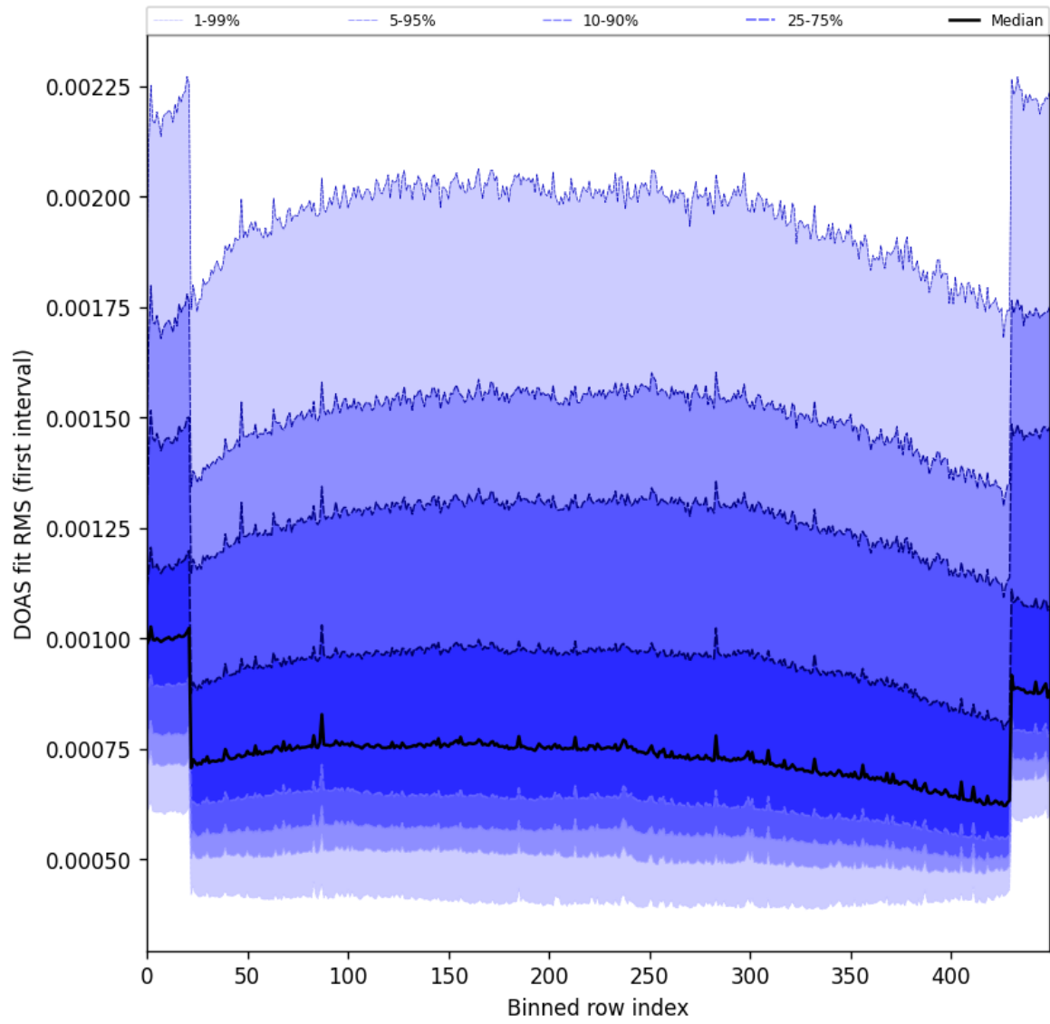
Figure 60: Along track statistics of “DOAS fit RMS (first interval)” for 2025-03-24 to 2025-03-26
