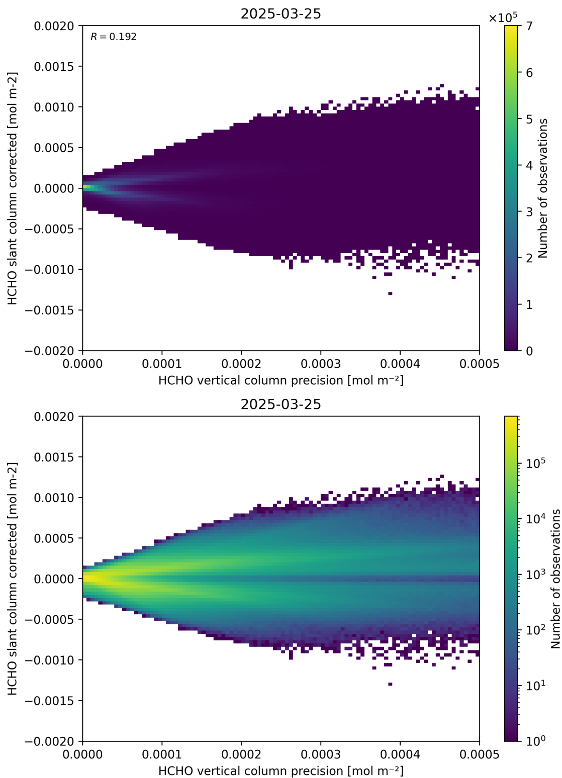
Figure 140: Scatter density plot of “HCHO vertical column precision” against “HCHO slant column corrected” for 2025-03-24 to 2025-03-26.
