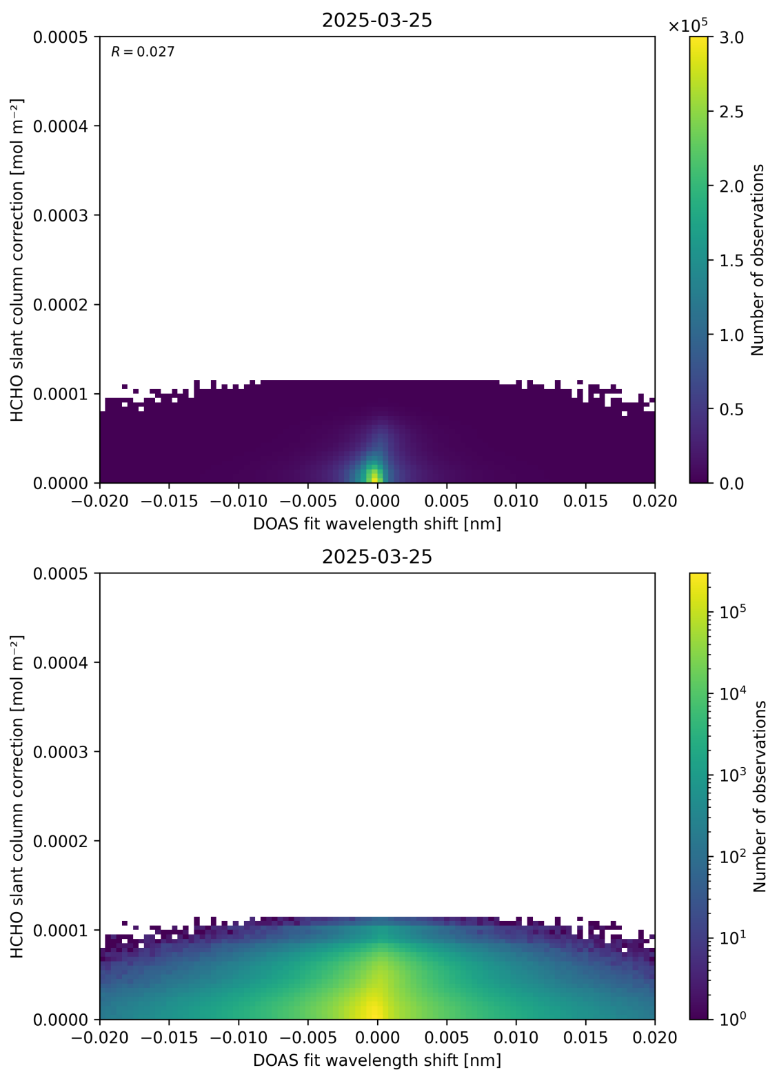
Figure 67: Scatter density plot of “DOAS fit wavelength shift” against “HCHO slant column correction” for 2025-03-24 to 2025-03-26.
