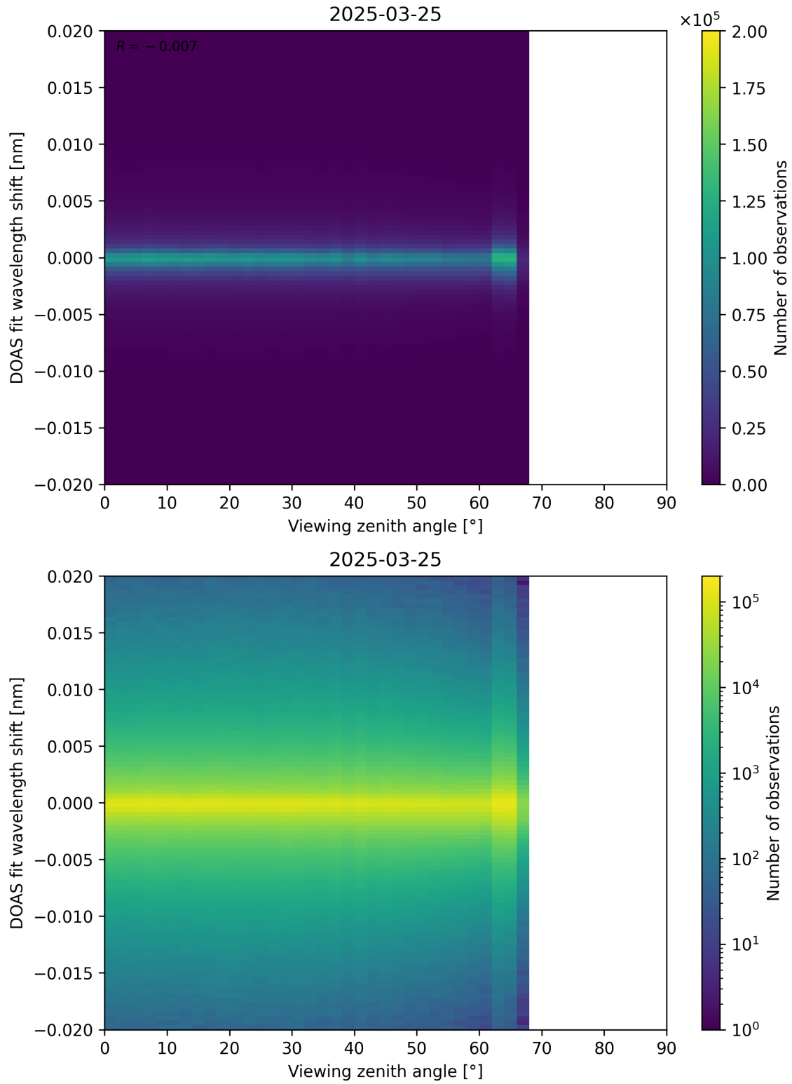
Figure 183: Scatter density plot of “Viewing zenith angle” against “DOAS fit wavelength shift” for 2025-03-24 to 2025-03-26.
