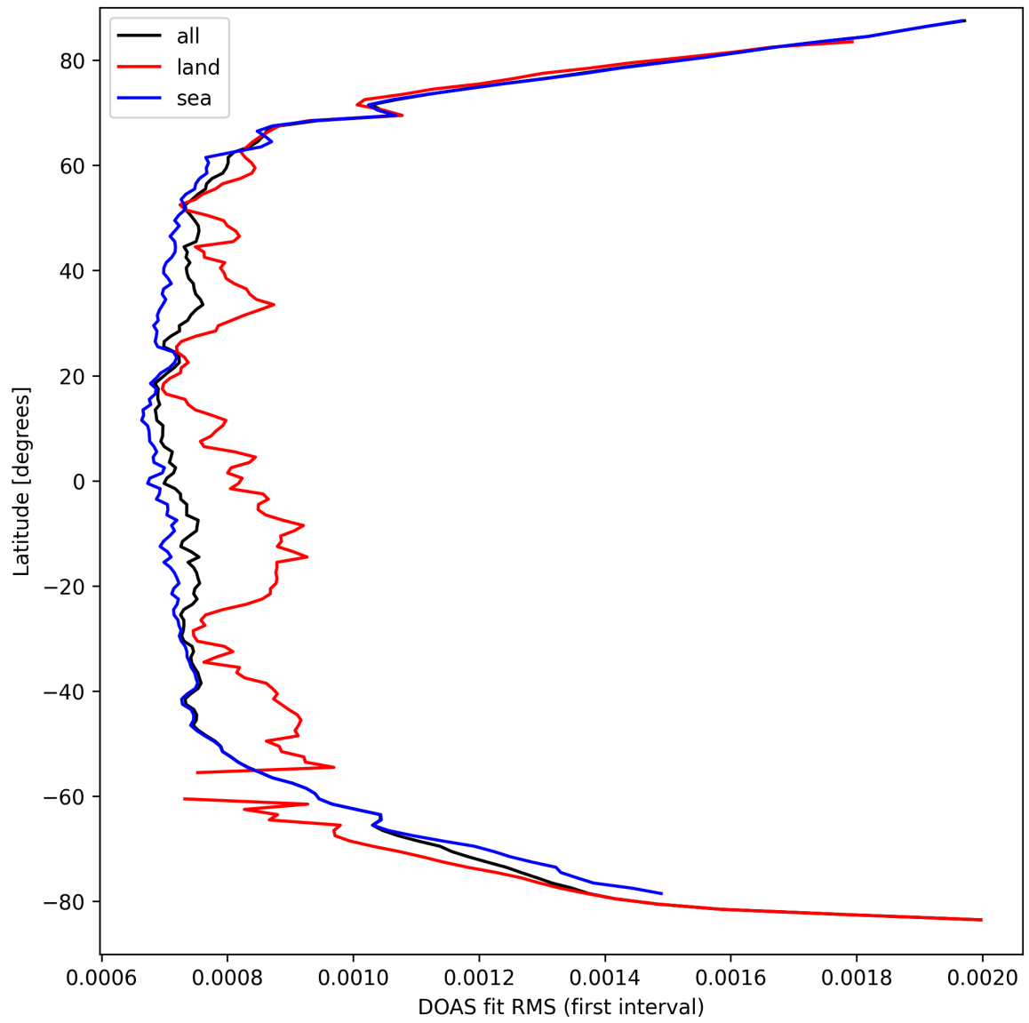
Figure 32: Zonal average of “DOAS fit RMS (first interval)” for 2025-03-24 to 2025-03-26.
