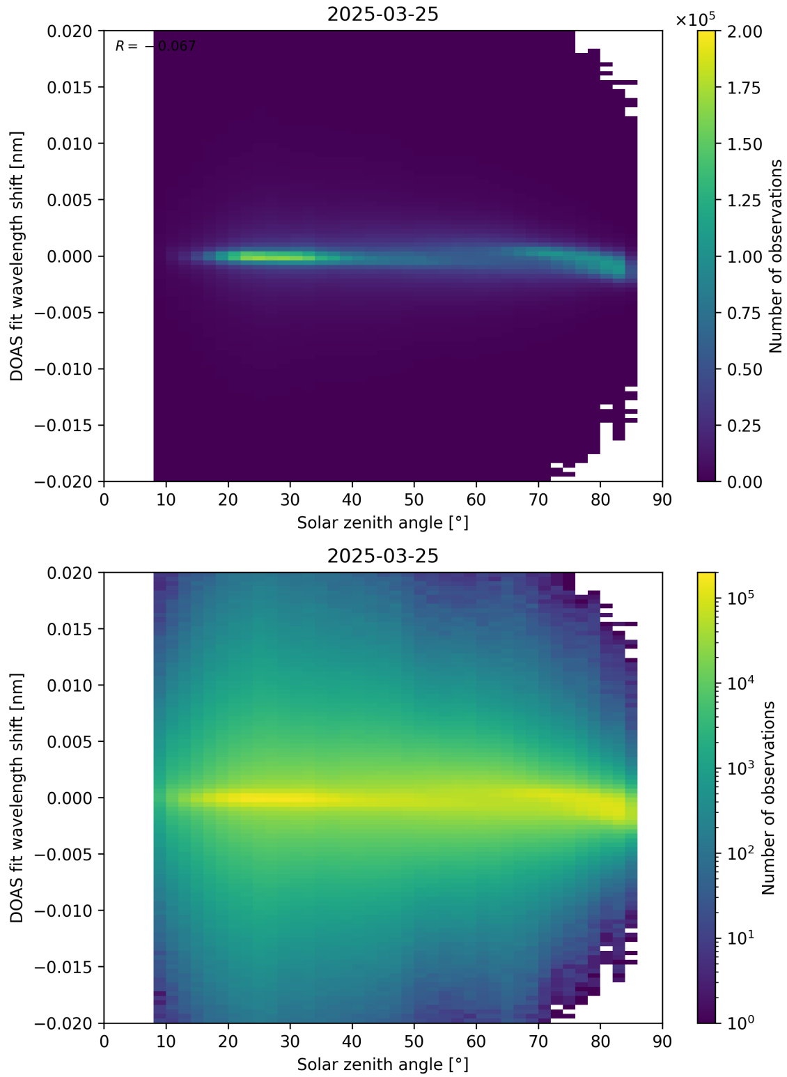
Figure 168: Scatter density plot of “Solar zenith angle” against “DOAS fit wavelength shift” for 2025-03-24 to 2025-03-26.
