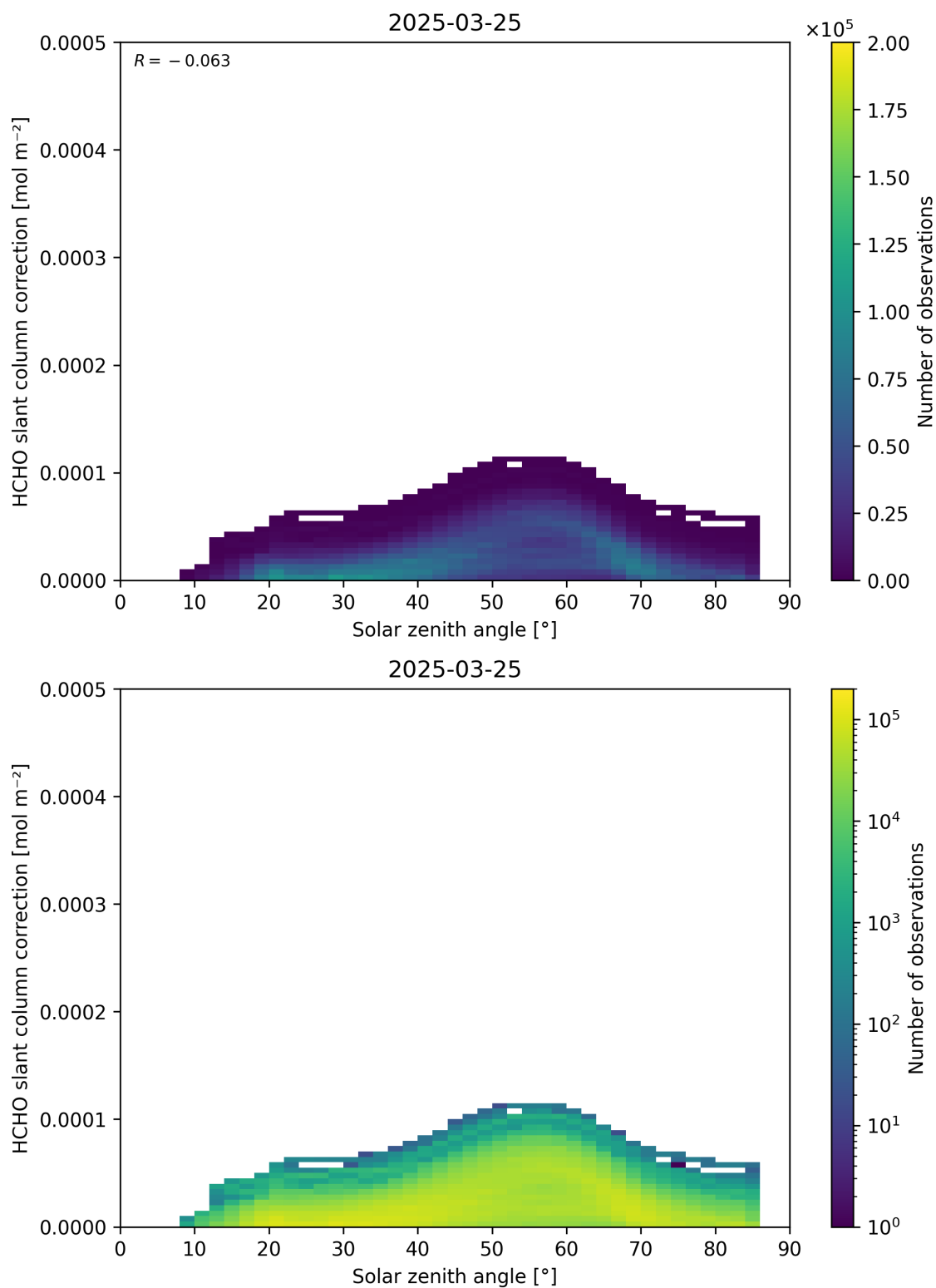
Figure 172: Scatter density plot of “Solar zenith angle” against “HCHO slant column correction” for 2025-03-24 to 2025-03-26.
