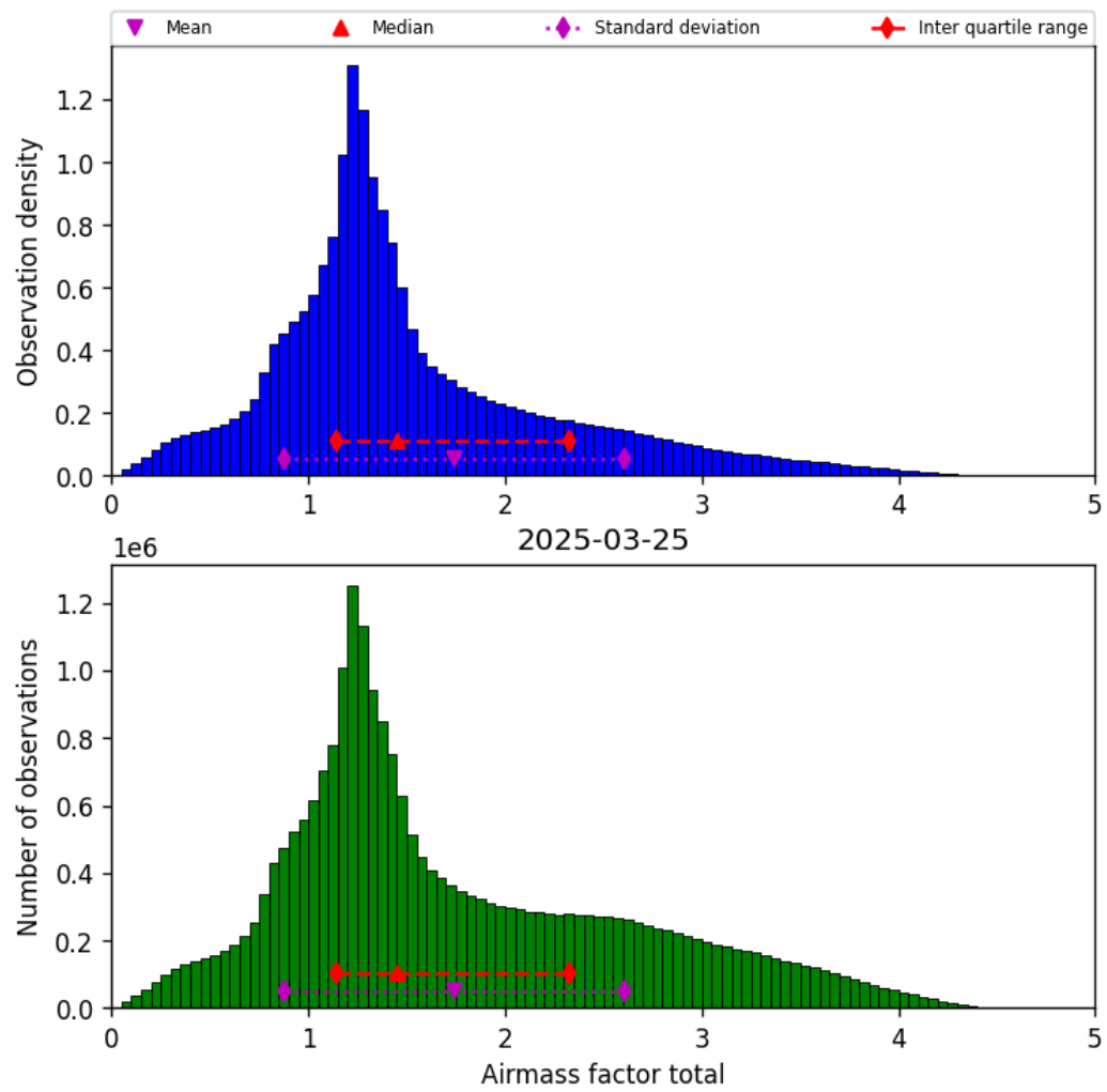
Figure 40: Histogram of “Airmass factor total” for 2025-03-24 to 2025-03-26
