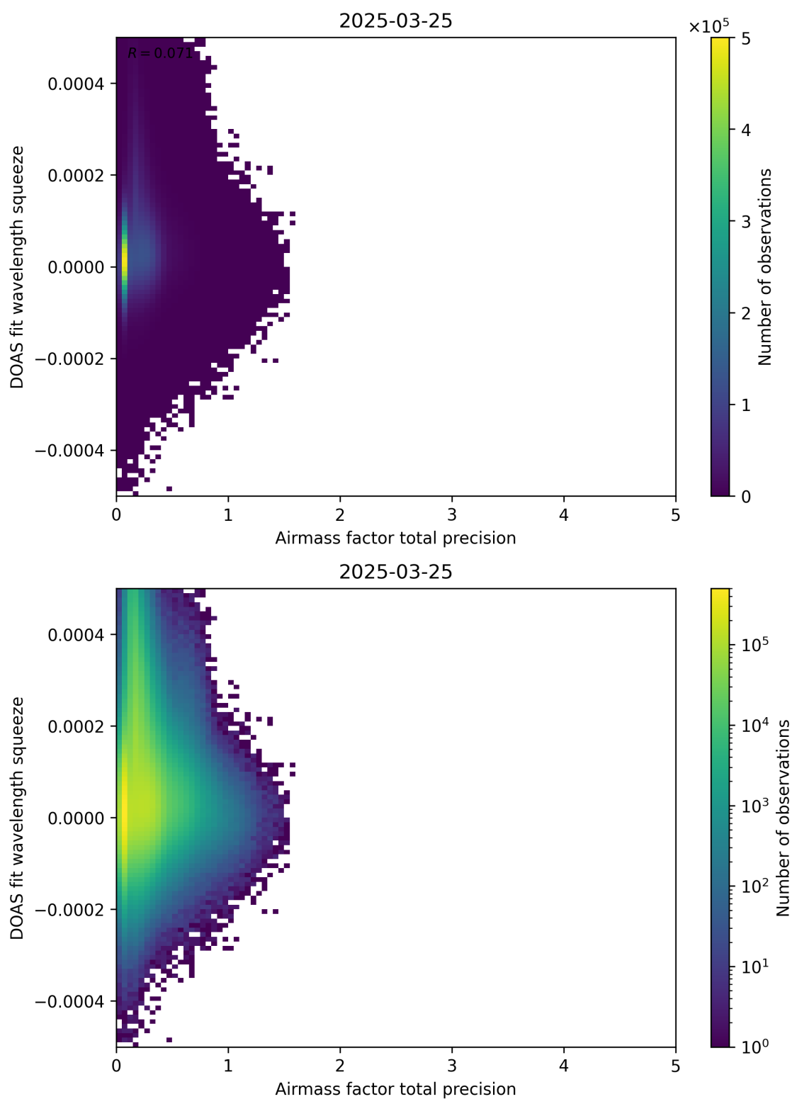
Figure 107: Scatter density plot of “Airmass factor total precision” against “DOAS fit wavelength squeeze” for 2025-03-24 to 2025-03-26.
