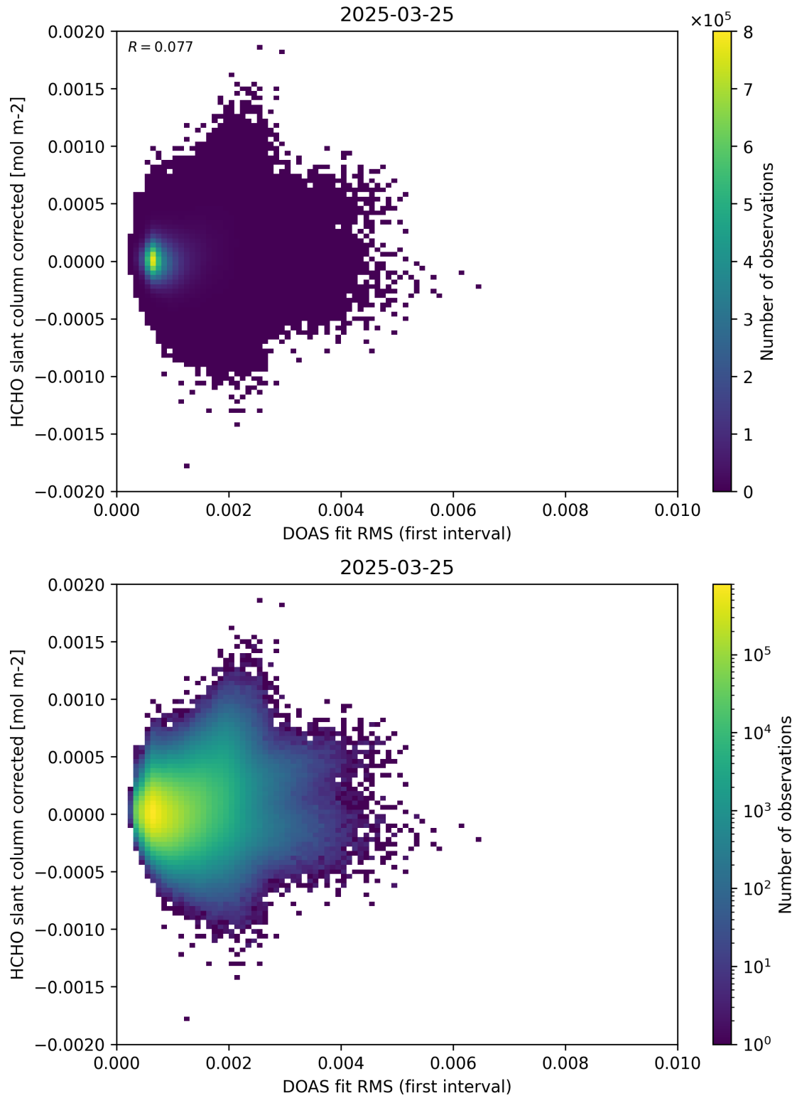
Figure 62: Scatter density plot of “DOAS fit RMS (first interval)” against “HCHO slant column corrected” for 2025-03-24 to 2025-03-26.
