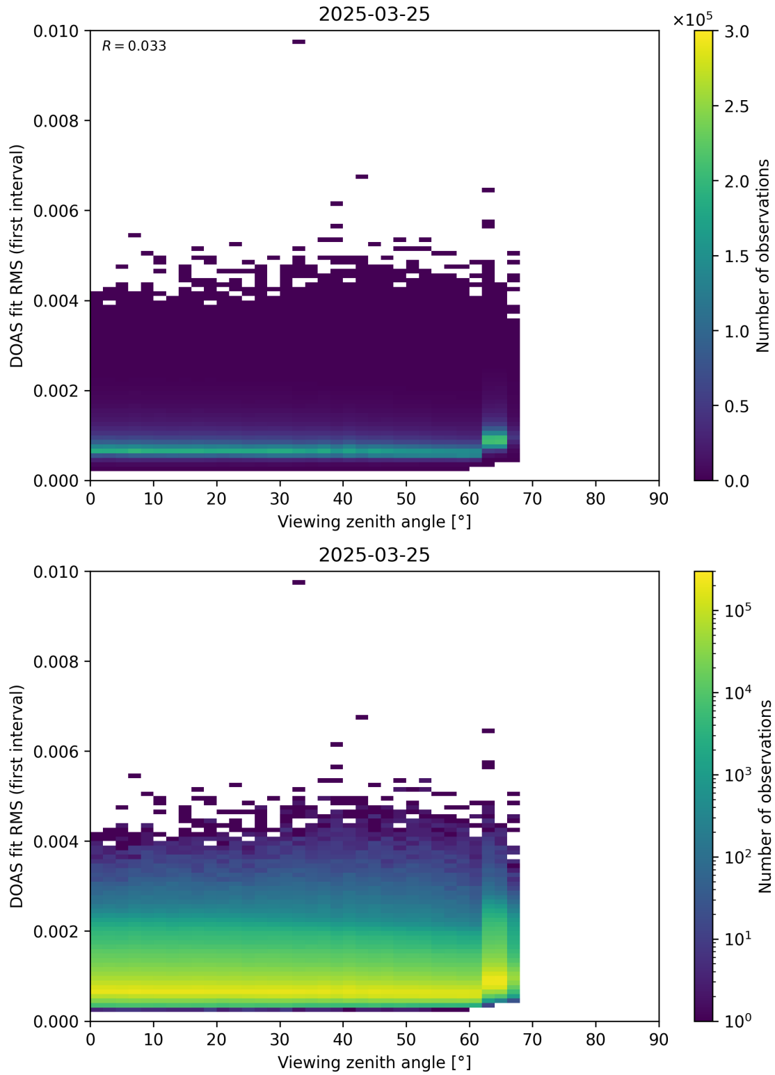
Figure 182: Scatter density plot of “Viewing zenith angle” against “DOAS fit RMS (first interval)” for 2025-03-24 to 2025-03-26.
