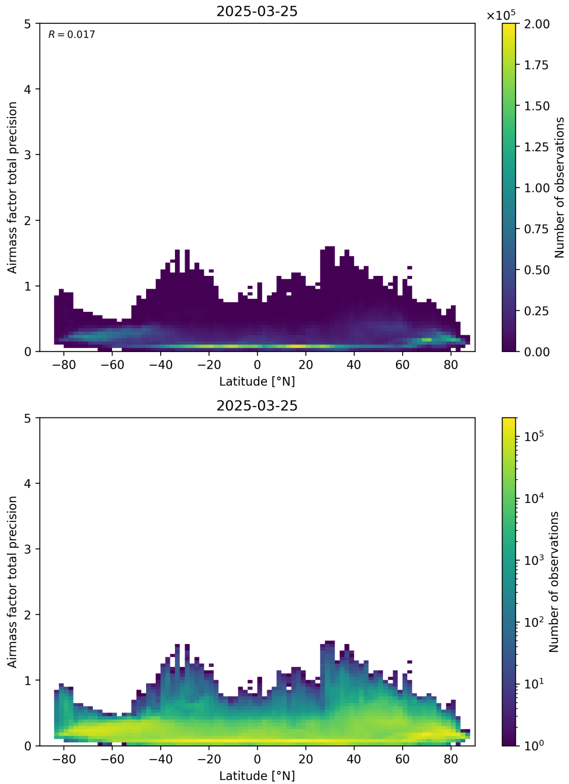
Figure 162: Scatter density plot of “Latitude” against “Airmass factor total precision” for 2025-03-24 to 2025-03-26.
