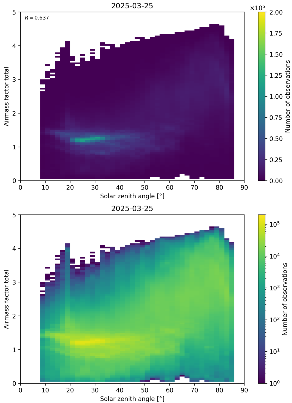
Figure 175: Scatter density plot of “Solar zenith angle” against “Airmass factor total” for 2025-03-24 to 2025-03-26.
