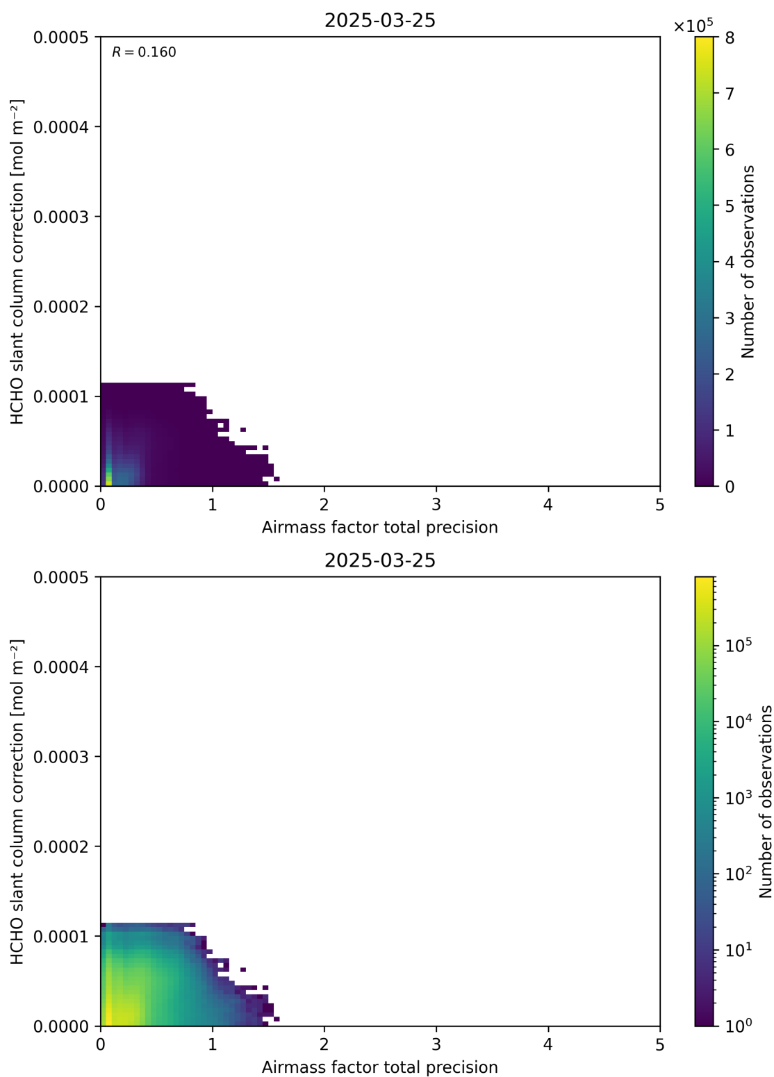
Figure 110: Scatter density plot of “Airmass factor total precision” against “HCHO slant column correction” for 2025-03-24 to 2025-03-26.
