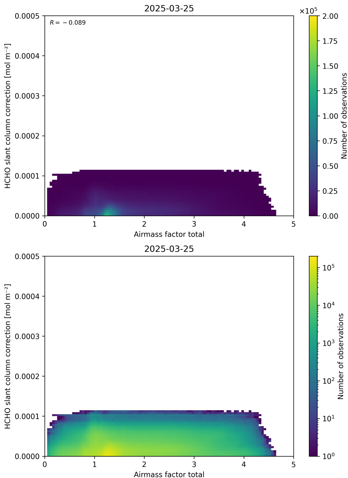
Figure 102: Scatter density plot of “Airmass factor total” against “HCHO slant column correction” for 2025-03-24 to 2025-03-26.
