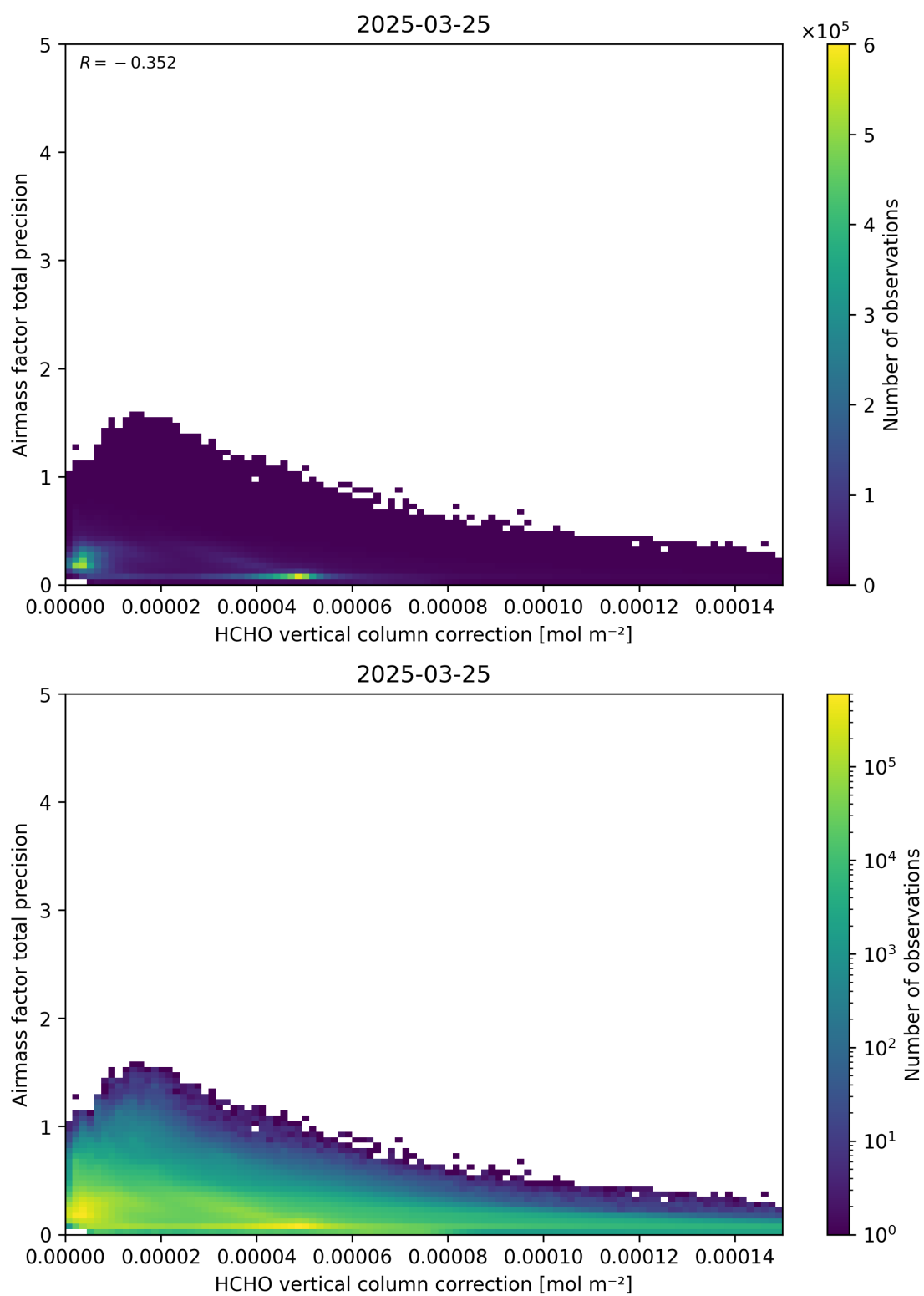
Figure 121: Scatter density plot of “HCHO vertical column correction” against “Airmass factor total precision” for 2025-03-24 to 2025-03-26.
