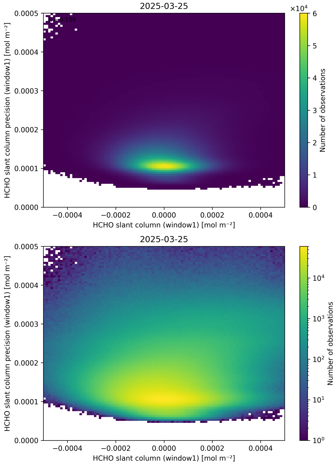
Figure 84: Scatter density plot of “HCHO slant column (window1)” against “HCHO slant column precision (window1)” for 2025-03-24 to 2025-03-26.
