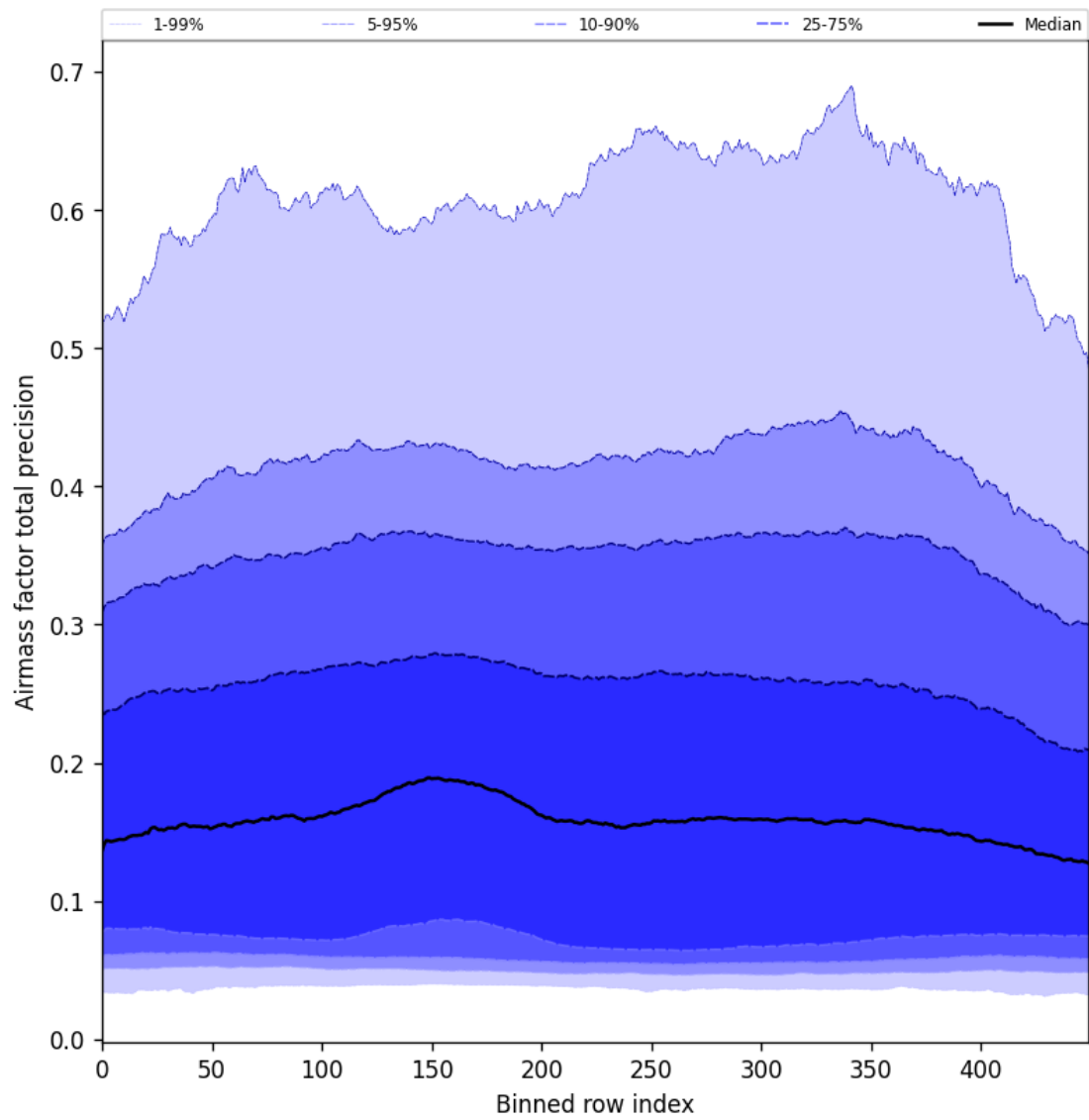
Figure 55: Along track statistics of “Airmass factor total precision” for 2025-03-24 to 2025-03-26
