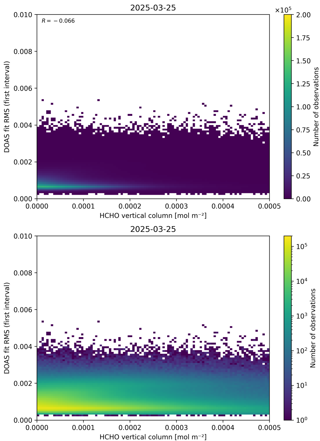
Figure 123: Scatter density plot of “HCHO vertical column” against “DOAS fit RMS (first interval)” for 2025-03-24 to 2025-03-26.
