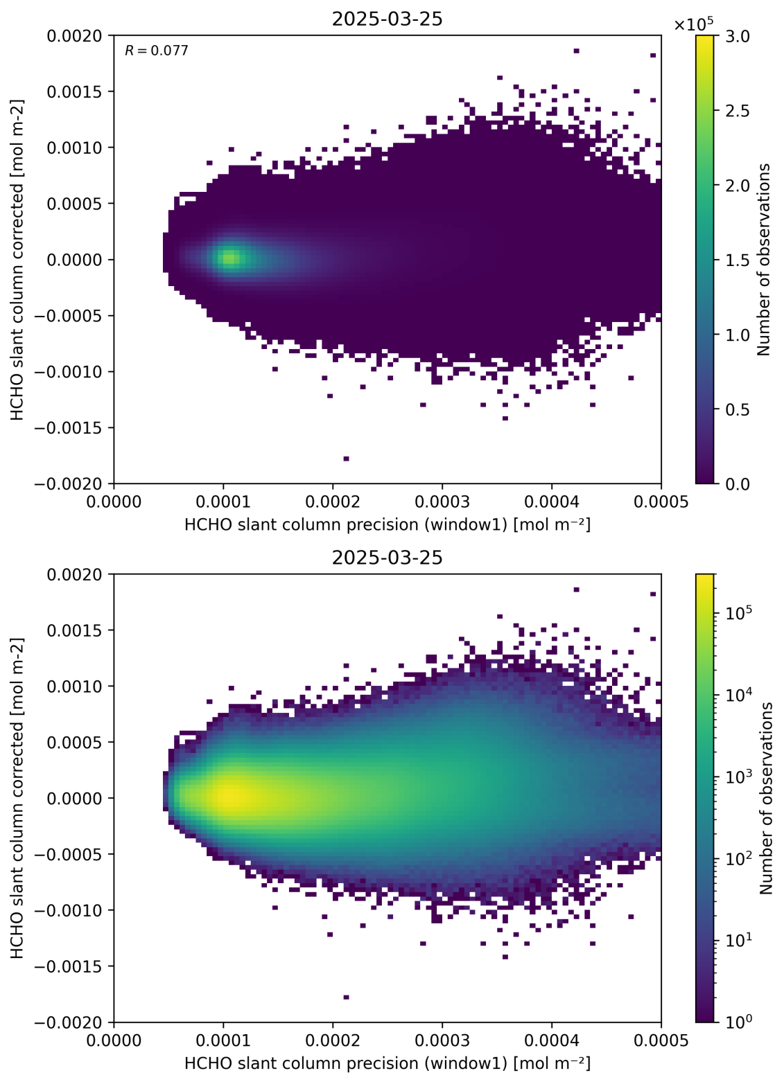
Figure 92: Scatter density plot of “HCHO slant column precision (window1)” against “HCHO slant column corrected” for 2025-03-24 to 2025-03-26.
