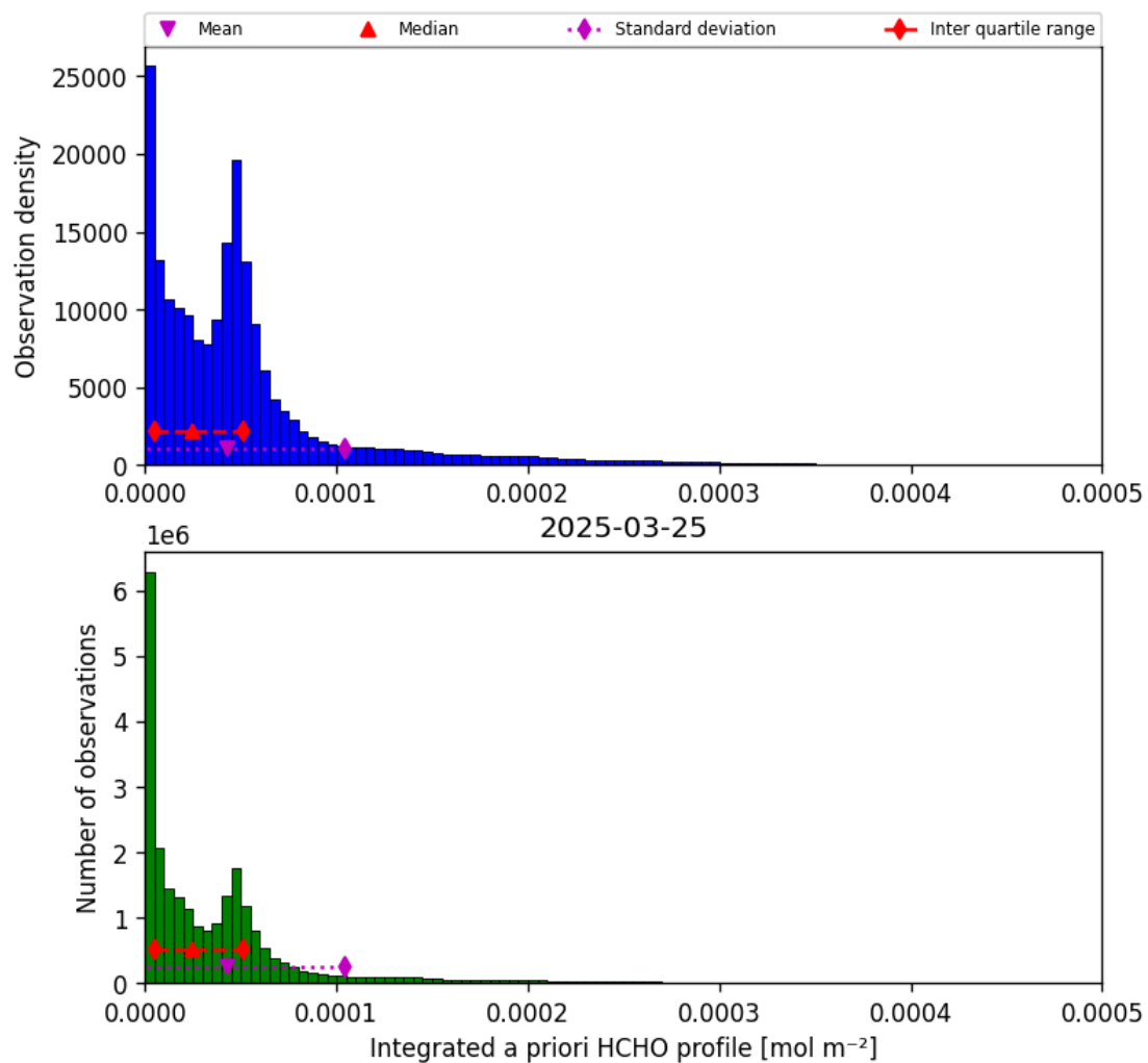
Figure 43: Histogram of “Integrated a priori HCHO profile” for 2025-03-24 to 2025-03-26
