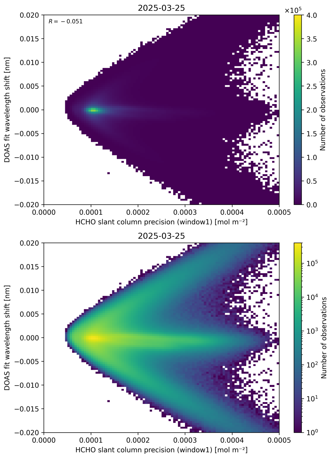
Figure 89: Scatter density plot of “HCHO slant column precision (window1)” against “DOAS fit wavelength shift” for 2025-03-24 to 2025-03-26.
