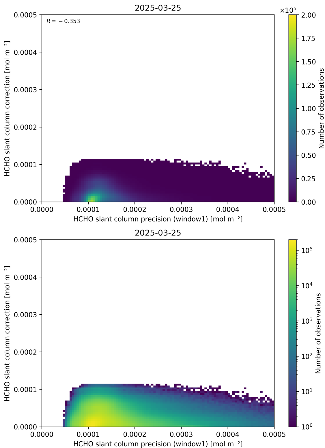
Figure 93: Scatter density plot of “HCHO slant column precision (window1)” against “HCHO slant column correction” for 2025-03-24 to 2025-03-26.
