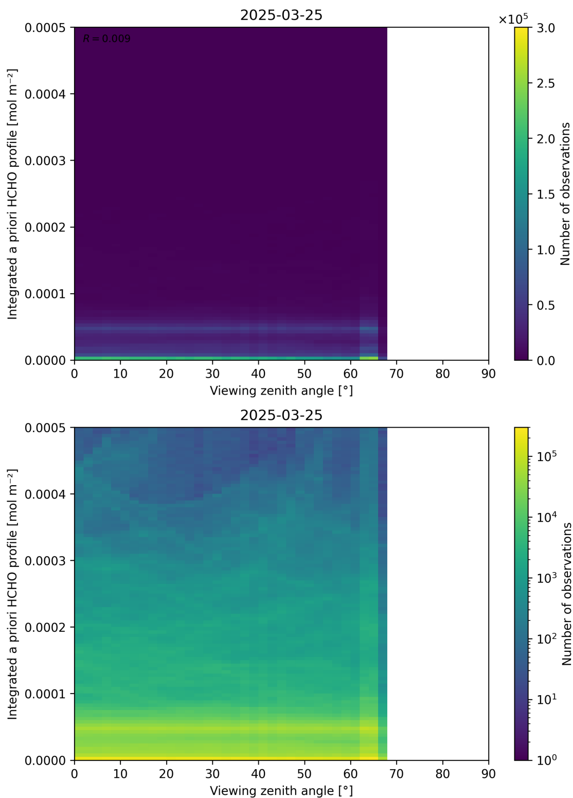
Figure 195: Scatter density plot of “Viewing zenith angle” against “Integrated a priori HCHO profile” for 2025-03-24 to 2025-03-26.
