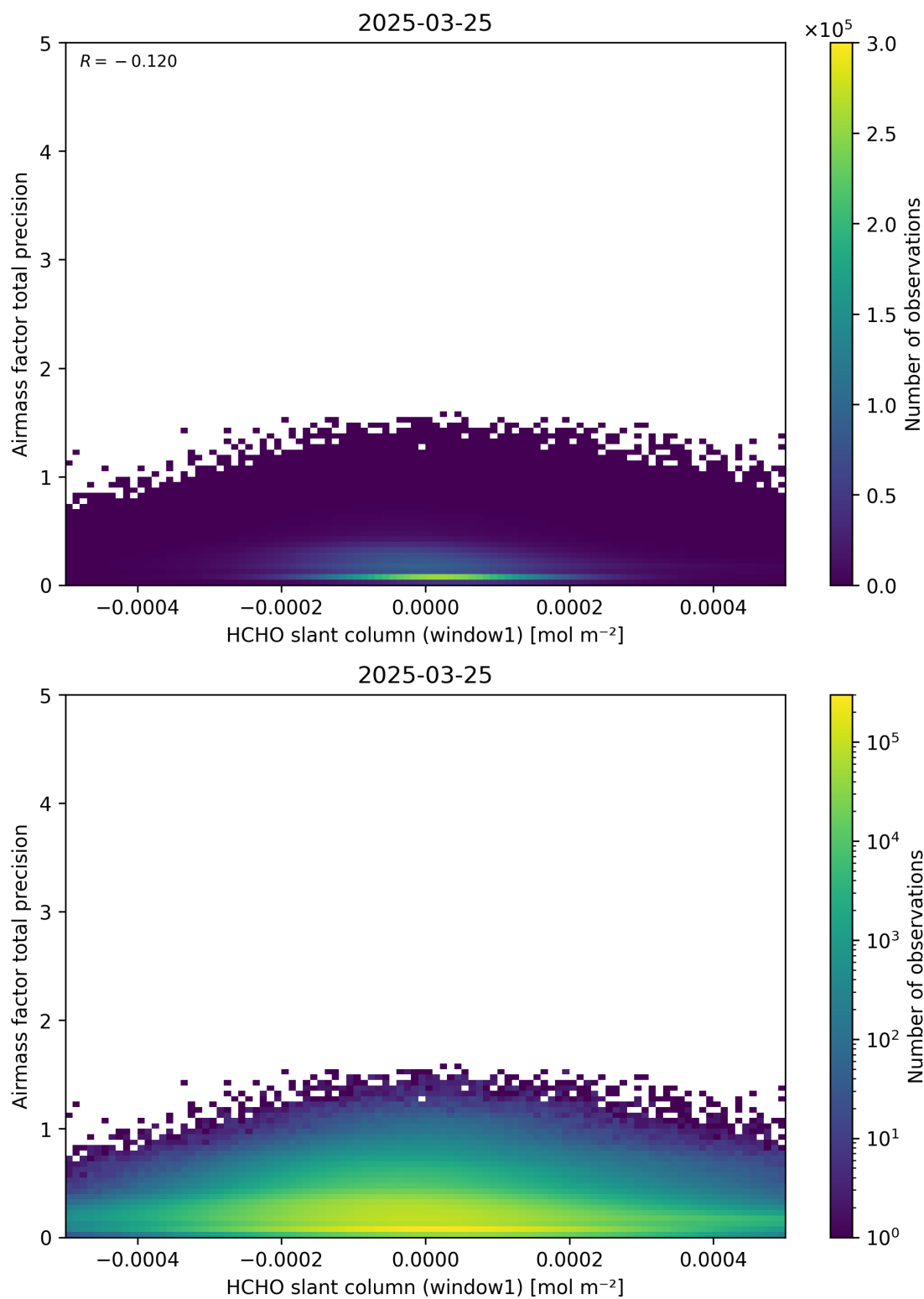
Figure 86: Scatter density plot of “HCHO slant column (window1)” against “Airmass factor total precision” for 2025-03-24 to 2025-03-26.
