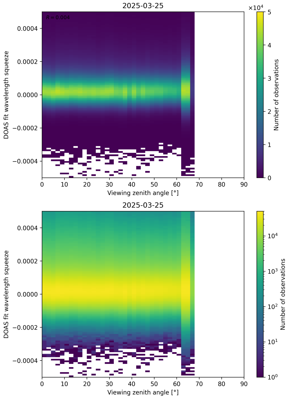
Figure 184: Scatter density plot of “Viewing zenith angle” against “DOAS fit wavelength squeeze” for 2025-03-24 to 2025-03-26.
