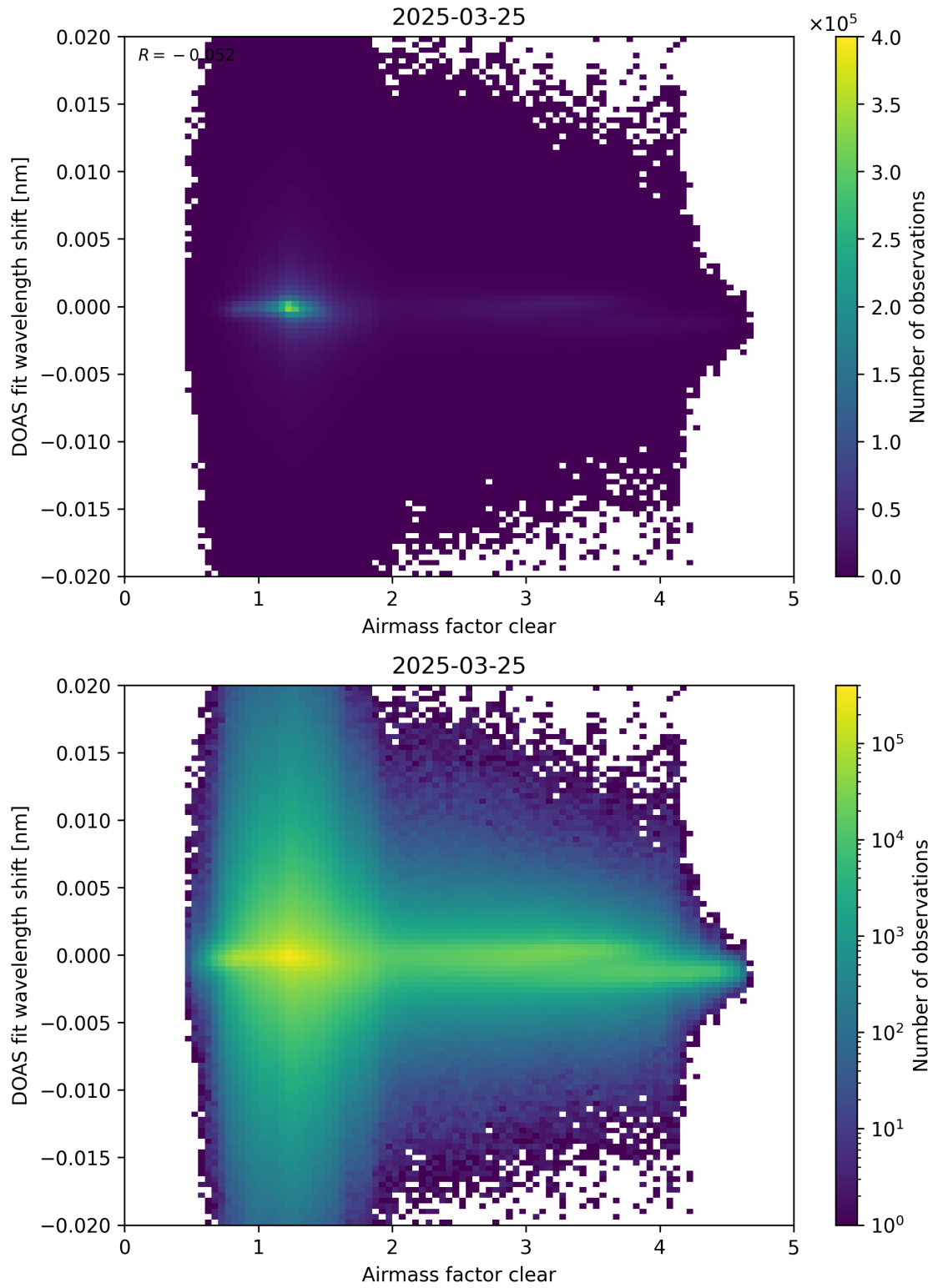
Figure 72: Scatter density plot of “Airmass factor clear” against “DOAS fit wavelength shift” for 2025-03-24 to 2025-03-26.
