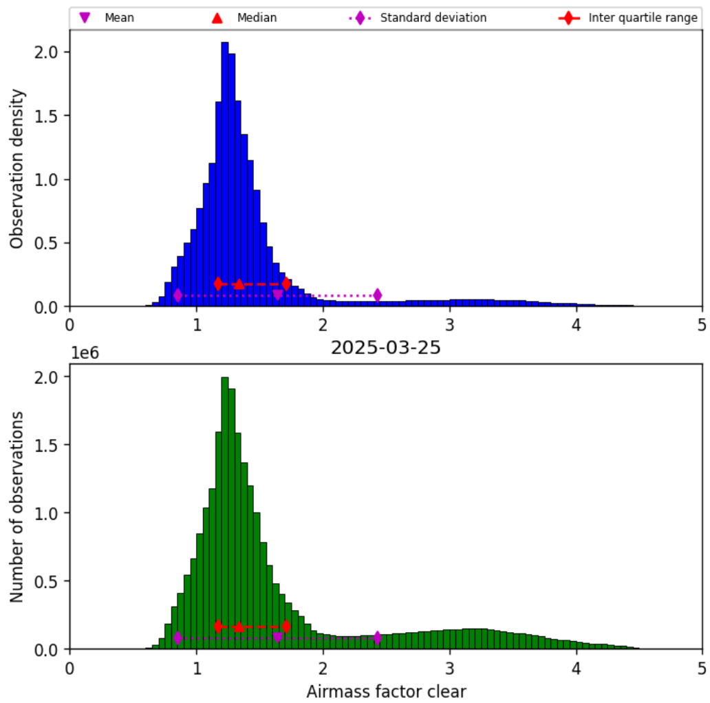
Figure 42: Histogram of “Airmass factor clear” for 2025-03-24 to 2025-03-26
