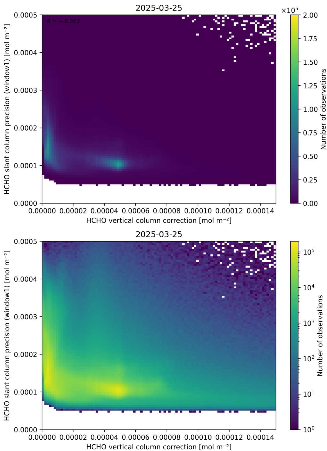
Figure 119: Scatter density plot of “HCHO vertical column correction” against “HCHO slant column precision (window1)” for 2025-03-24 to 2025-03-26.
