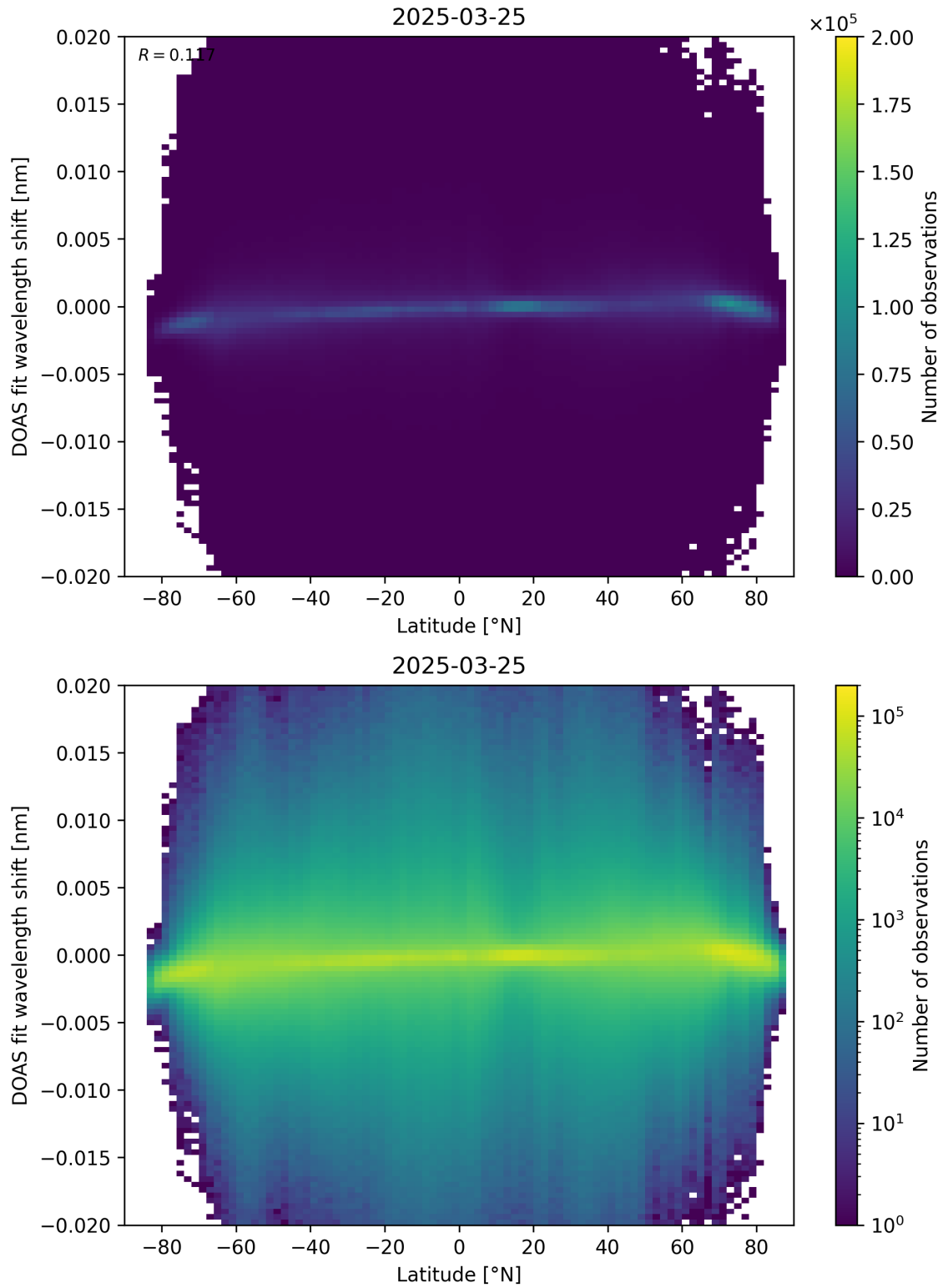
Figure 154: Scatter density plot of “Latitude” against “DOAS fit wavelength shift” for 2025-03-24 to 2025-03-26.
