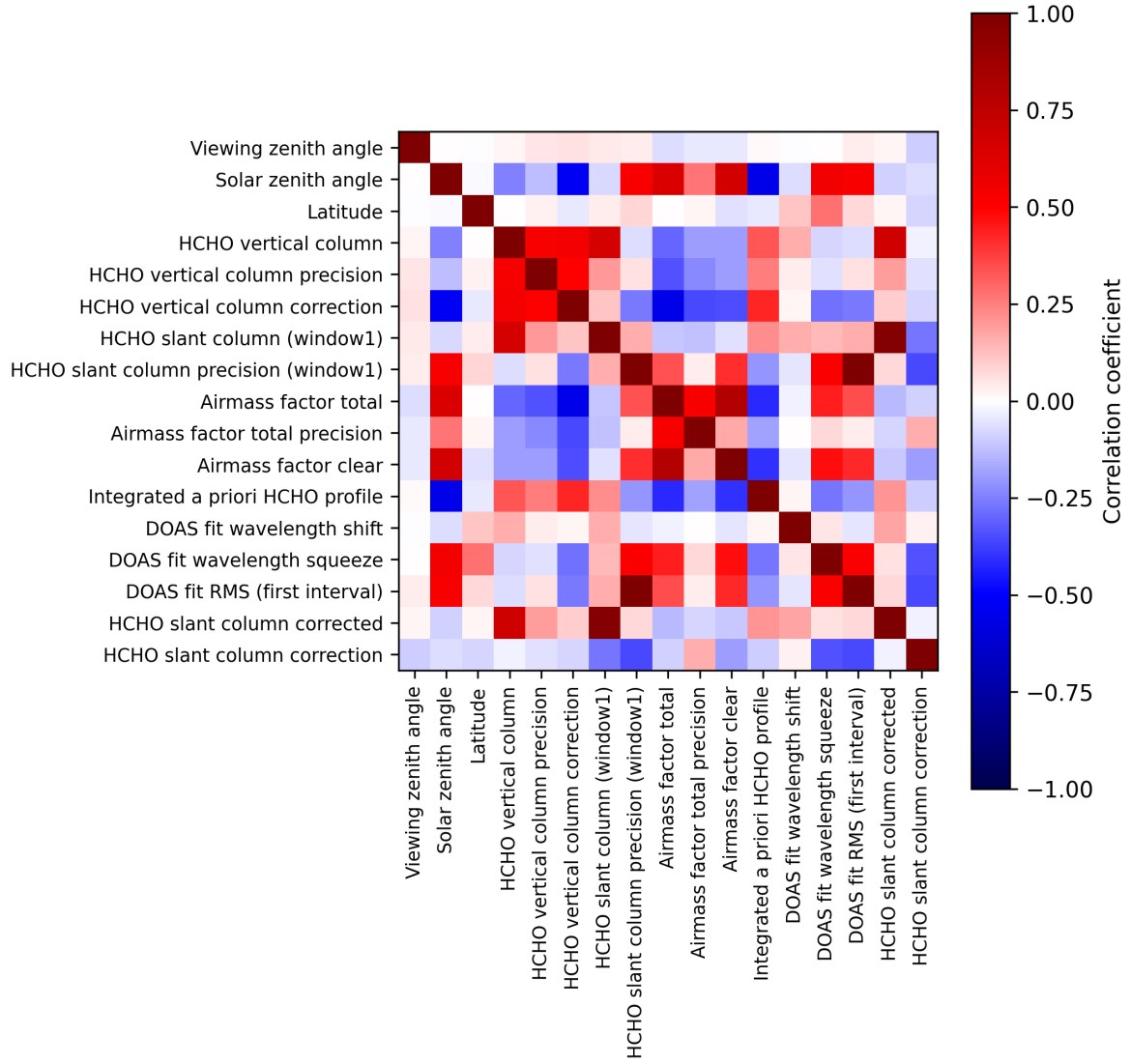
Figure 2: Map of correlation matrix for 2025-03-24 to 2025-03-26.
