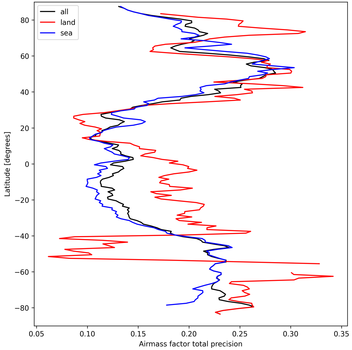
Figure 27: Zonal average of “Airmass factor total precision” for 2025-03-24 to 2025-03-26.
