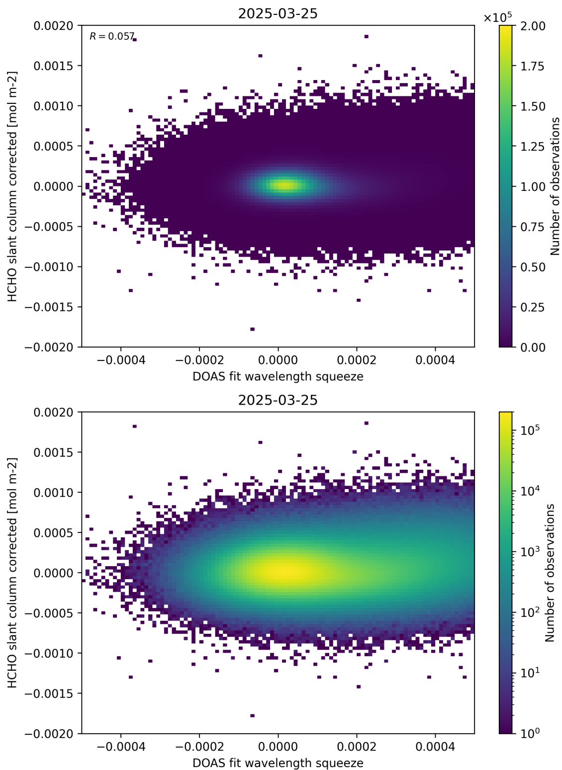
Figure 69: Scatter density plot of “DOAS fit wavelength squeeze” against “HCHO slant column corrected” for 2025-03-24 to 2025-03-26.
