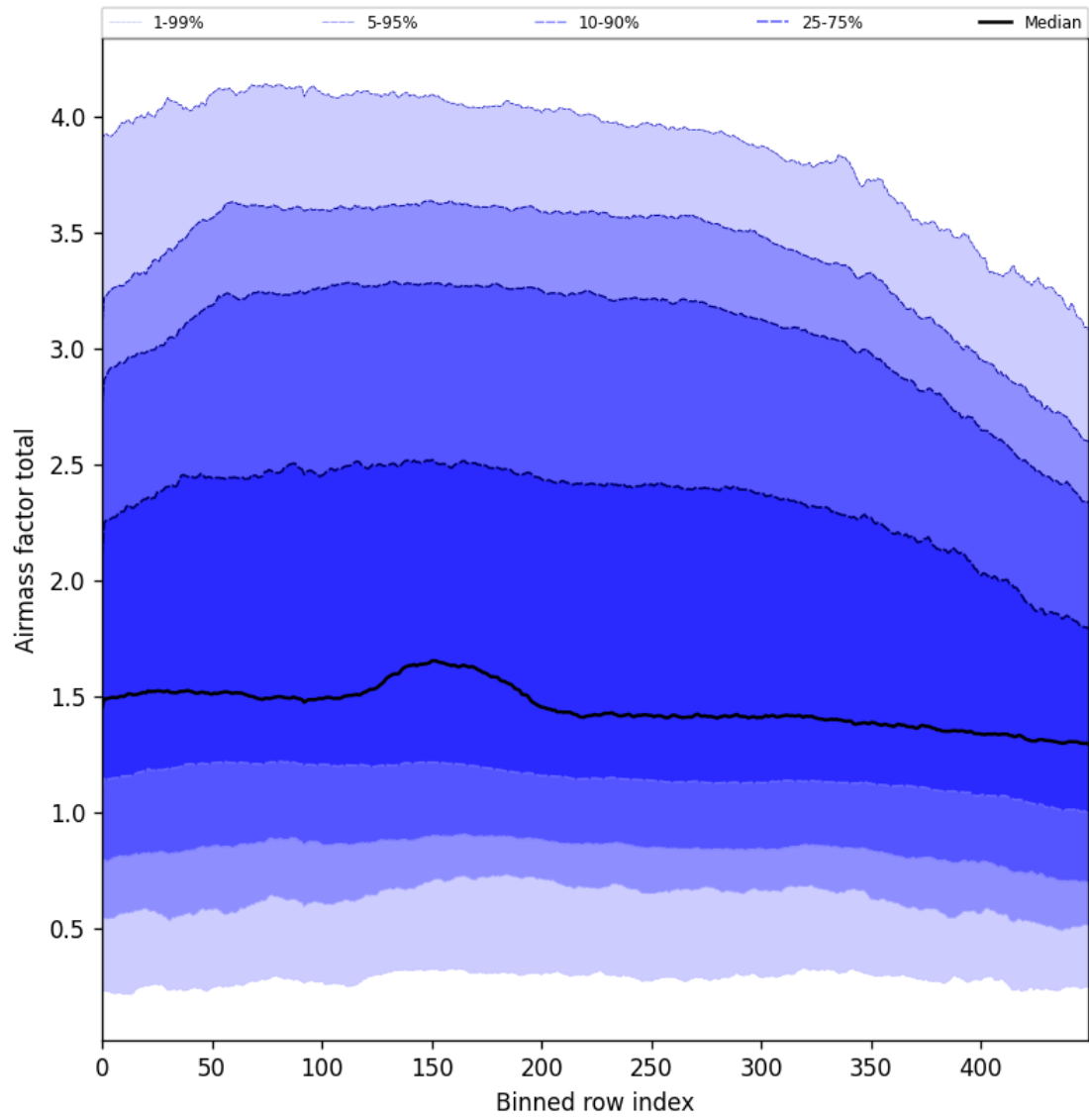
Figure 54: Along track statistics of “Airmass factor total” for 2025-03-24 to 2025-03-26
