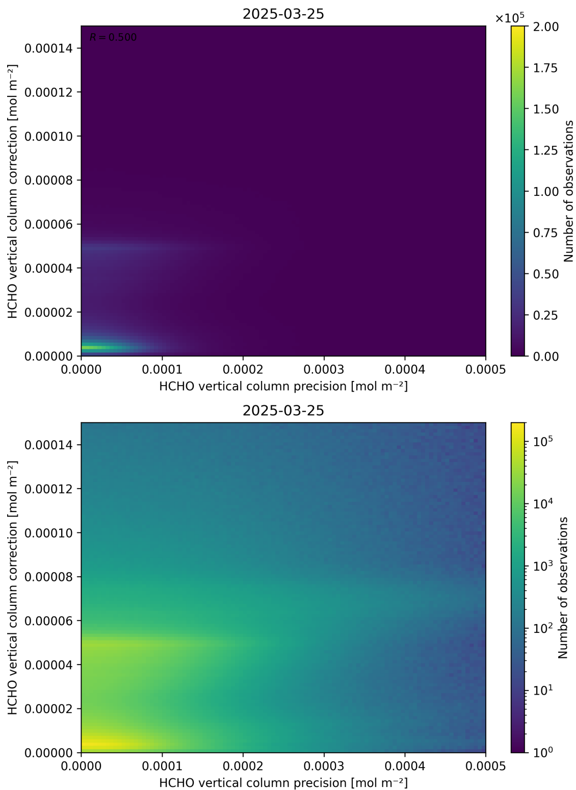
Figure 146: Scatter density plot of “HCHO vertical column precision” against “HCHO vertical column correction” for 2025-03-24 to 2025-03-26.
