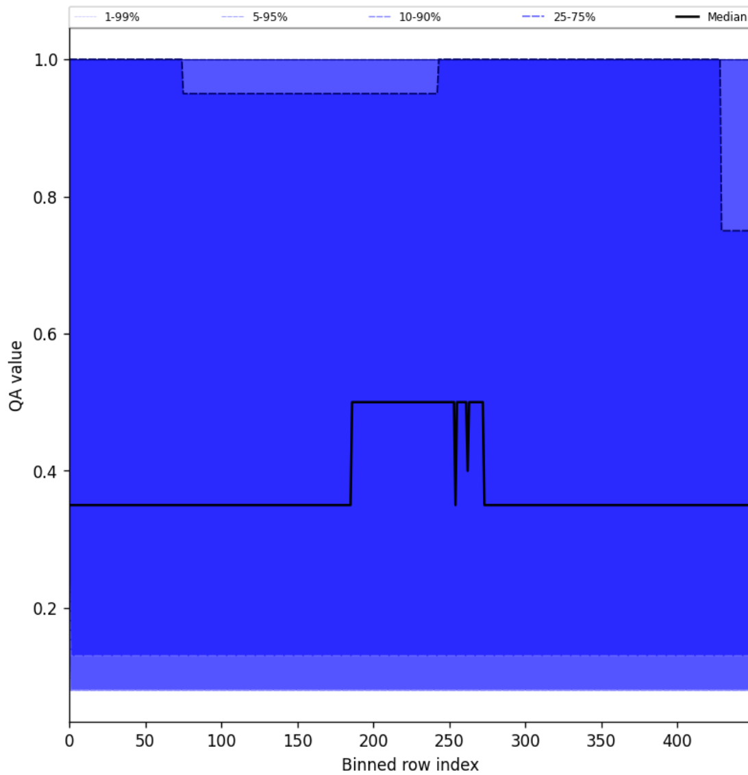
Figure 48: Along track statistics of “QA value” for 2025-03-24 to 2025-03-26
