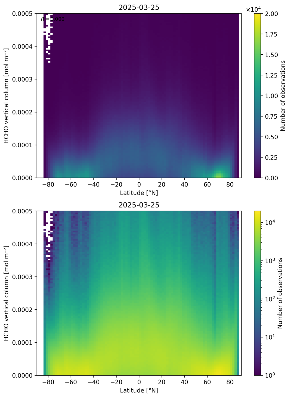
Figure 163: Scatter density plot of “Latitude” against “HCHO vertical column” for 2025-03-24 to 2025-03-26.
