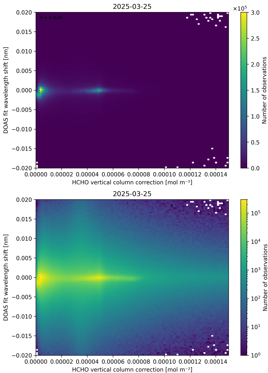
Figure 113: Scatter density plot of “HCHO vertical column correction” against “DOAS fit wavelength shift” for 2025-03-24 to 2025-03-26.
