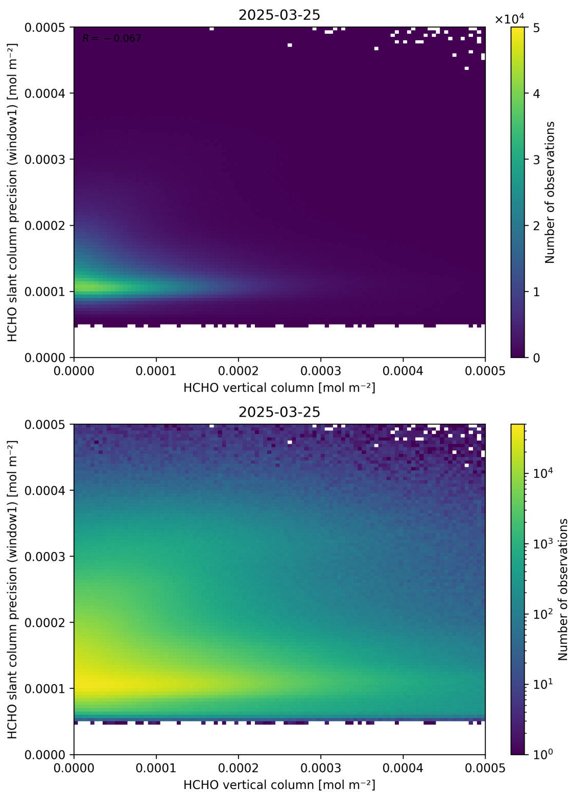
Figure 130: Scatter density plot of “HCHO vertical column” against “HCHO slant column precision (window1)” for 2025-03-24 to 2025-03-26.
