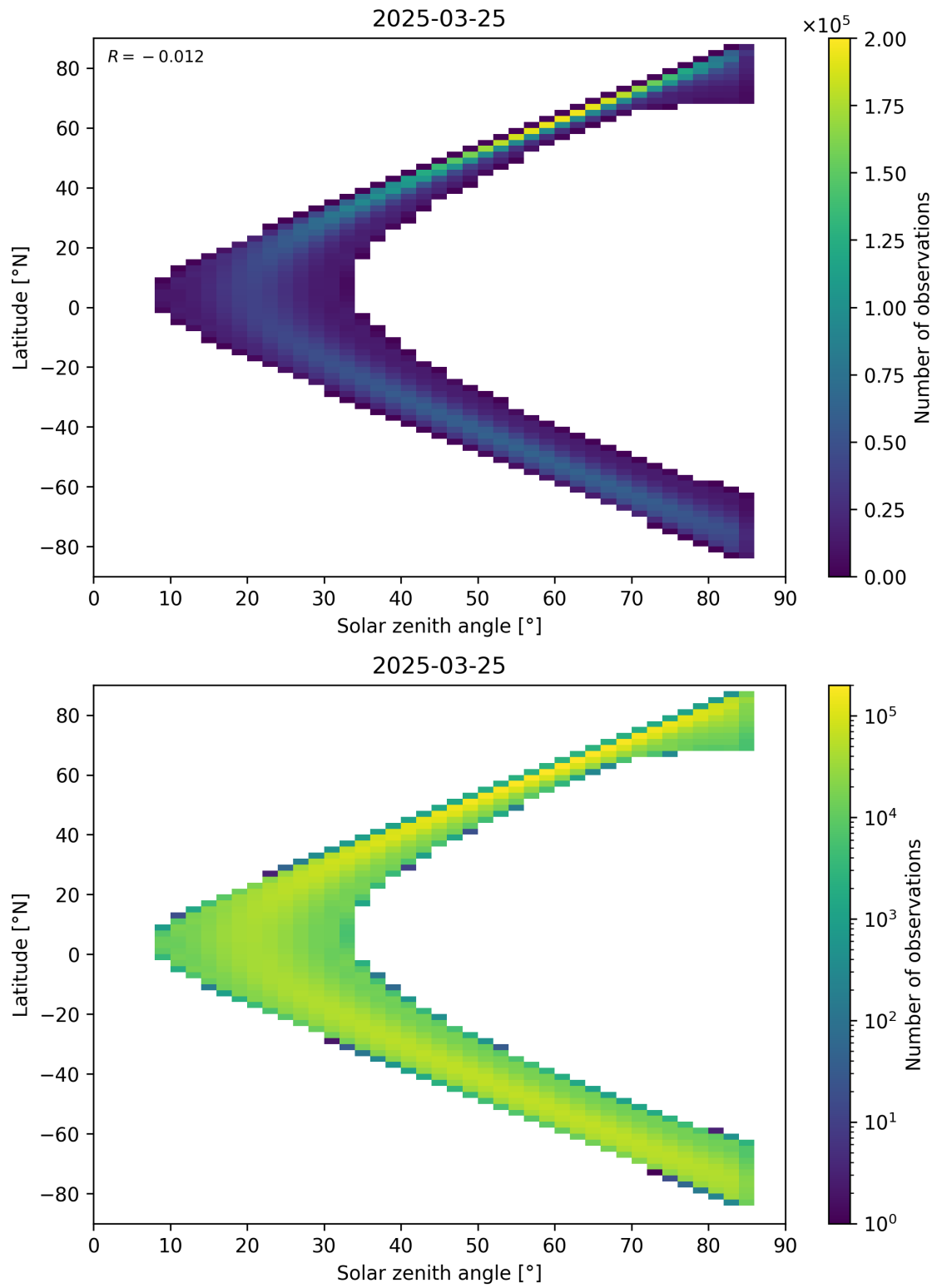
Figure 181: Scatter density plot of “Solar zenith angle” against “Latitude” for 2025-03-24 to 2025-03-26.
