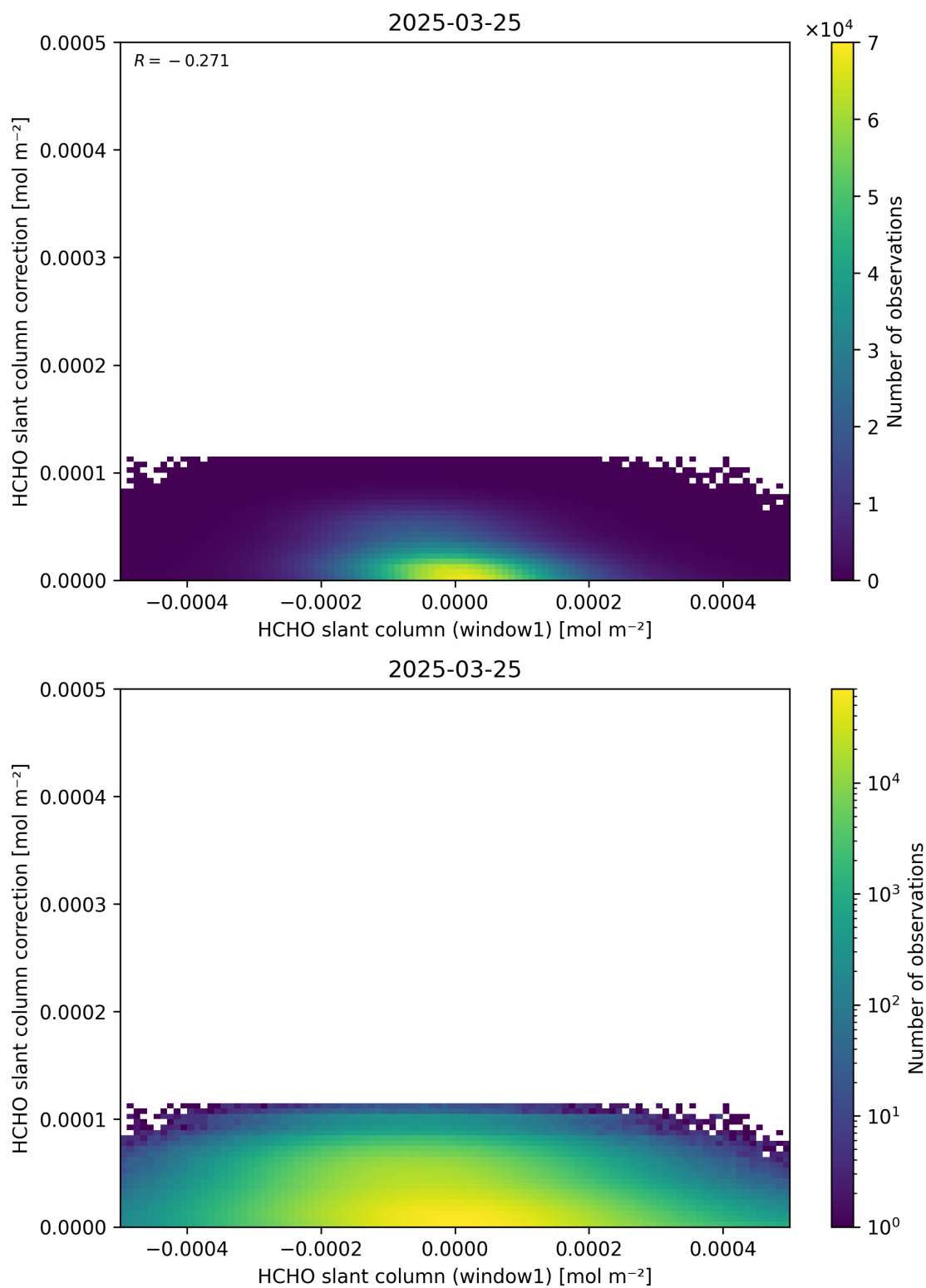
Figure 83: Scatter density plot of “HCHO slant column (window1)” against “HCHO slant column correction” for 2025-03-24 to 2025-03-26.
