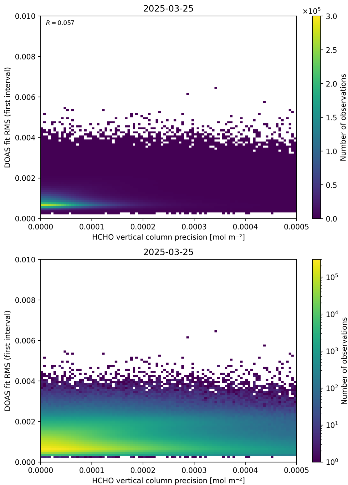
Figure 136: Scatter density plot of “HCHO vertical column precision” against “DOAS fit RMS (first interval)” for 2025-03-24 to 2025-03-26.
