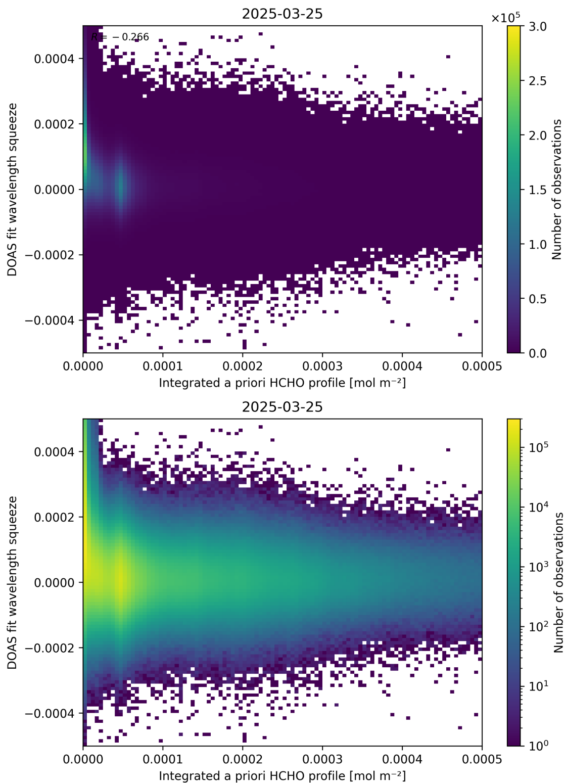
Figure 150: Scatter density plot of “Integrated a priori HCHO profile” against “DOAS fit wavelength squeeze” for 2025-03-24 to 2025-03-26.
