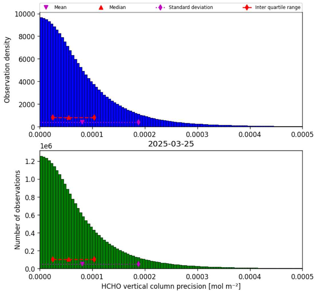
Figure 36: Histogram of “HCHO vertical column precision” for 2025-03-24 to 2025-03-26
