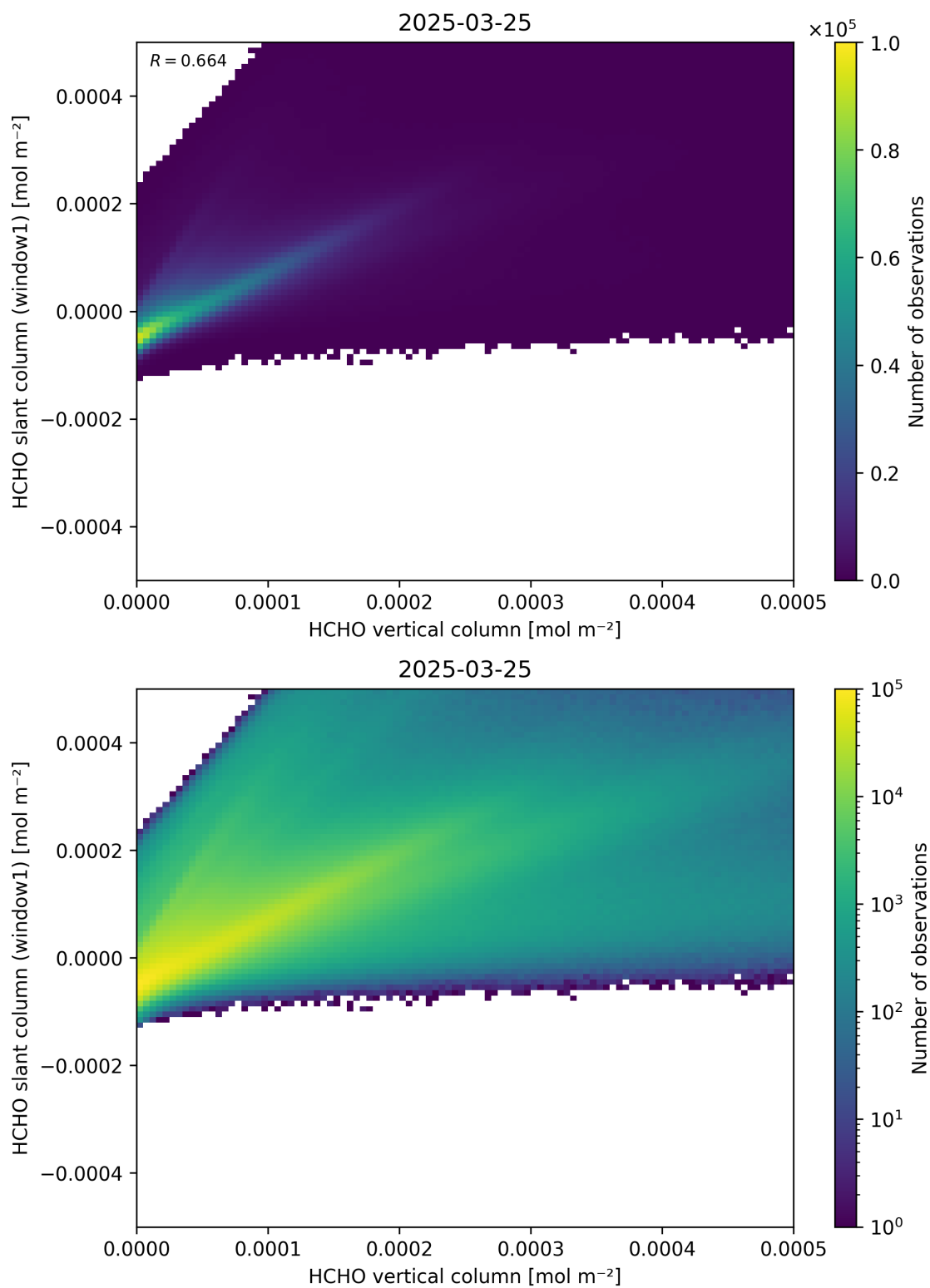
Figure 129: Scatter density plot of “HCHO vertical column” against “HCHO slant column (window1)” for 2025-03-24 to 2025-03-26.
