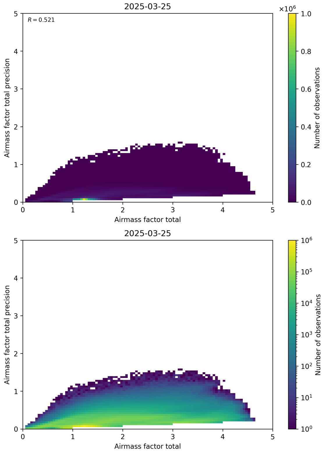
Figure 103: Scatter density plot of “Airmass factor total” against “Airmass factor total precision” for 2025-03-24 to 2025-03-26.
