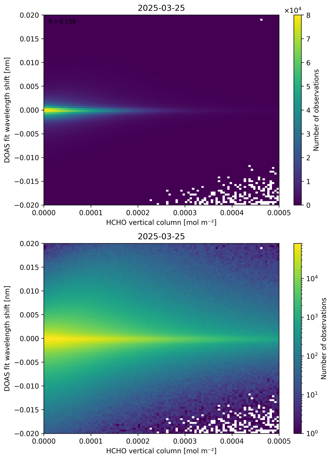
Figure 124: Scatter density plot of “HCHO vertical column” against “DOAS fit wavelength shift” for 2025-03-24 to 2025-03-26.
