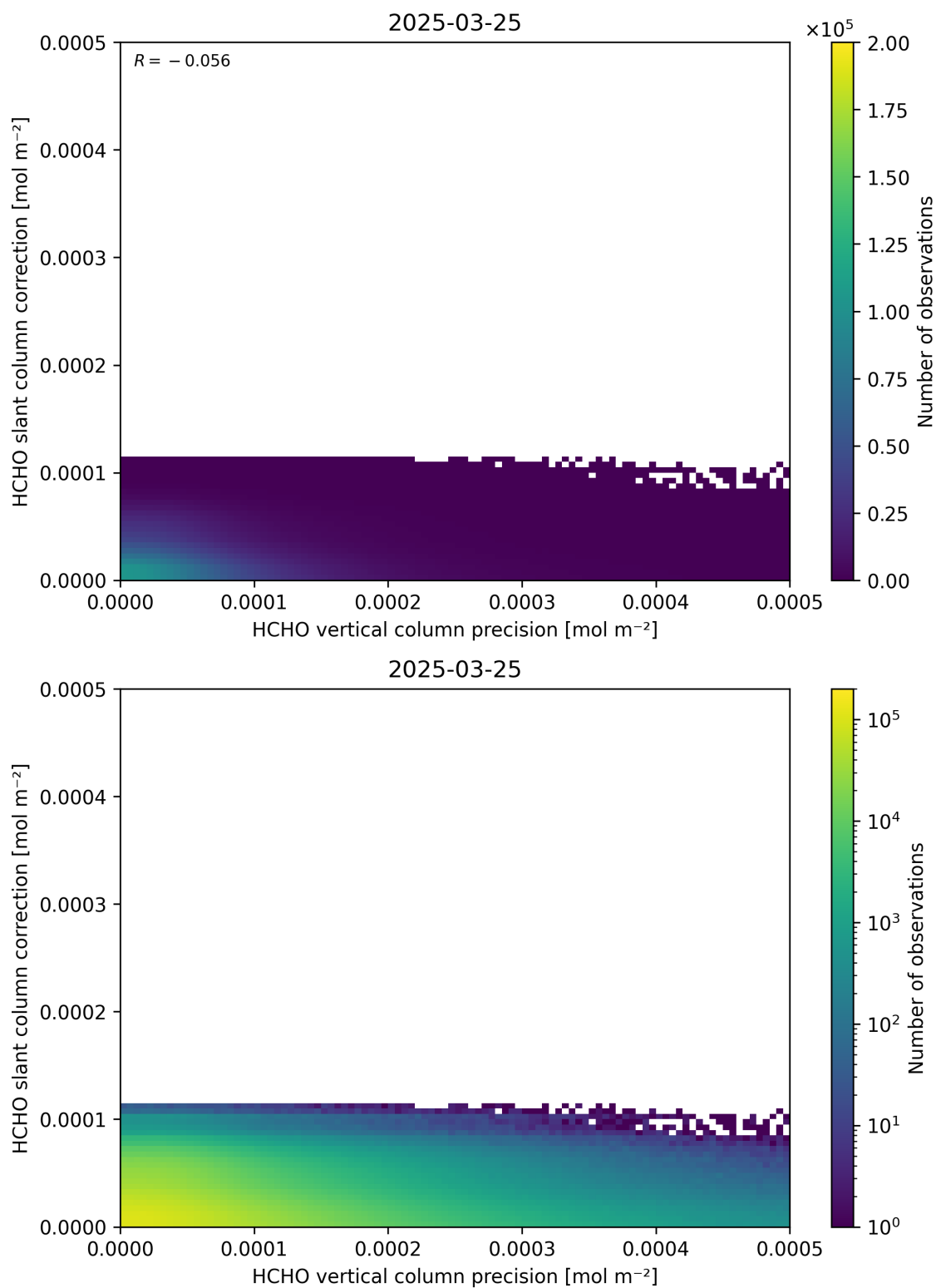
Figure 141: Scatter density plot of “HCHO vertical column precision” against “HCHO slant column correction” for 2025-03-24 to 2025-03-26.
