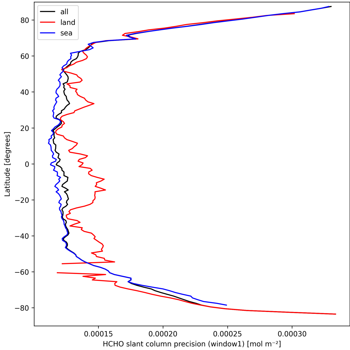
Figure 25: Zonal average of "HCHO slant column precision (window1)" for 2025-03-24 to 2025-03-26.
