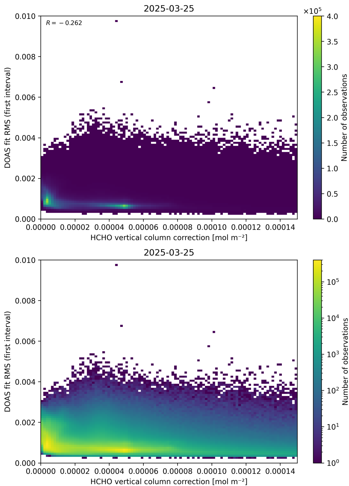
Figure 112: Scatter density plot of “HCHO vertical column correction” against “DOAS fit RMS (first interval)” for 2025-03-24 to 2025-03-26.
