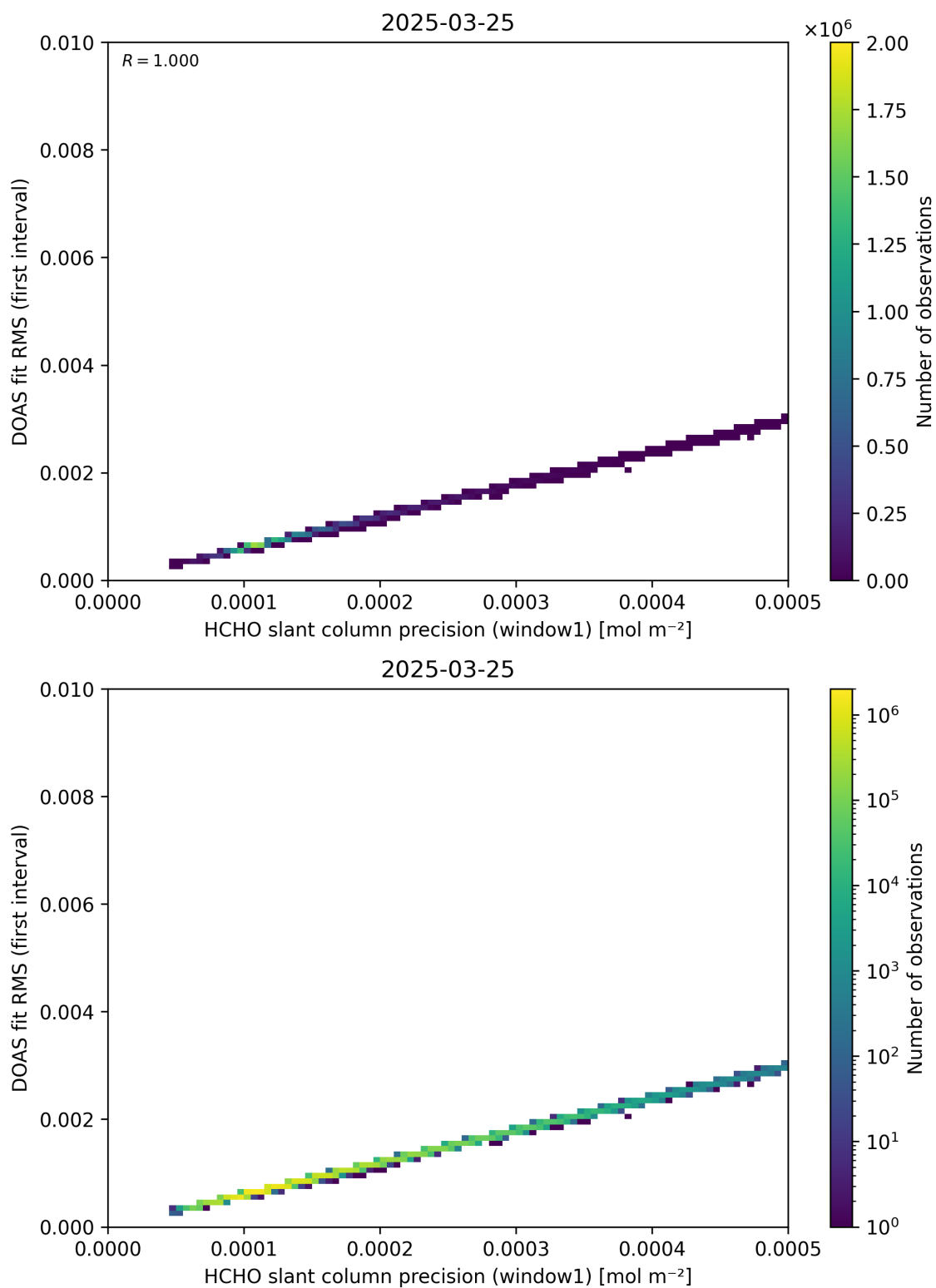
Figure 88: Scatter density plot of “HCHO slant column precision (window1)” against “DOAS fit RMS (first interval)” for 2025-03-24 to 2025-03-26.
