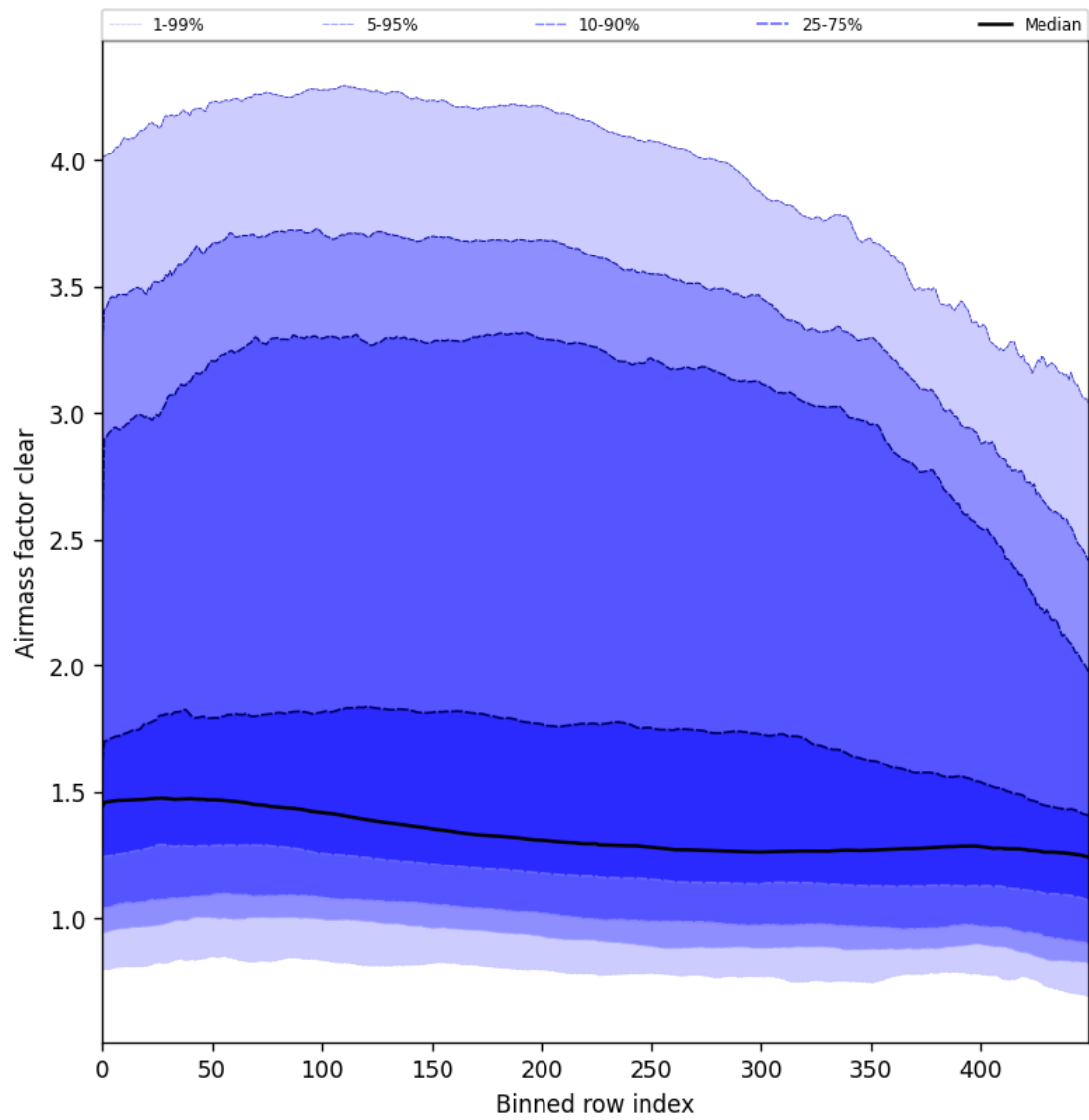
Figure 56: Along track statistics of “Airmass factor clear” for 2025-03-24 to 2025-03-26
