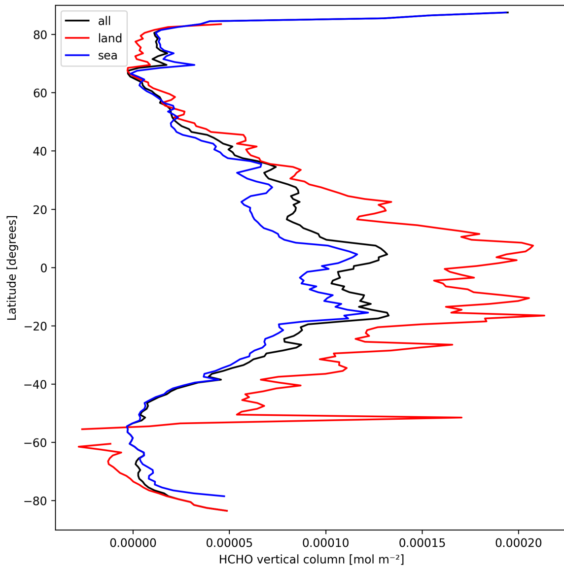
Figure 21: Zonal average of “HCHO vertical column” for 2025-03-24 to 2025-03-26.
