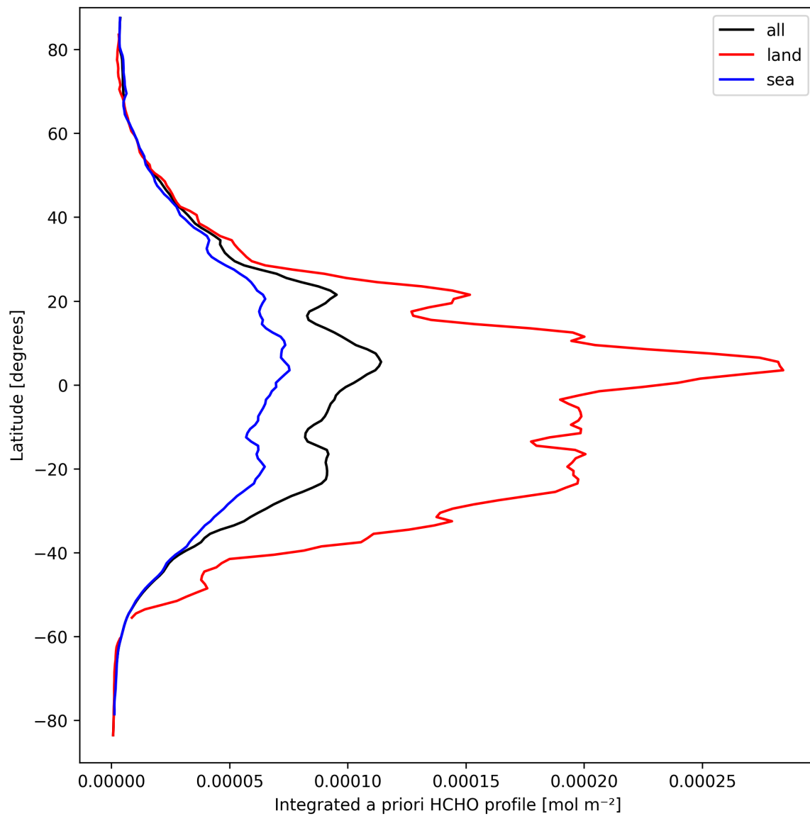
Figure 29: Zonal average of “Integrated a priori HCHO profile” for 2025-03-24 to 2025-03-26.
