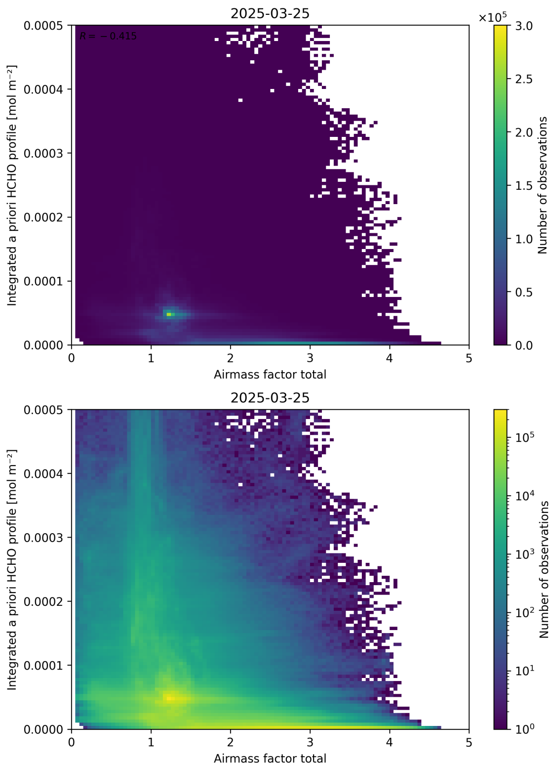
Figure 104: Scatter density plot of “Airmass factor total” against “Integrated a priori HCHO profile” for 2025-03-24 to 2025-03-26.
