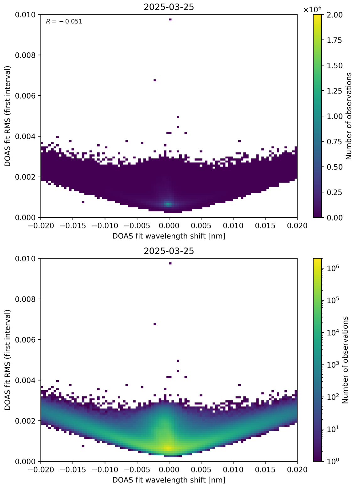
Figure 64: Scatter density plot of “DOAS fit wavelength shift” against “DOAS fit RMS (first interval)” for 2025-03-24 to 2025-03-26.
