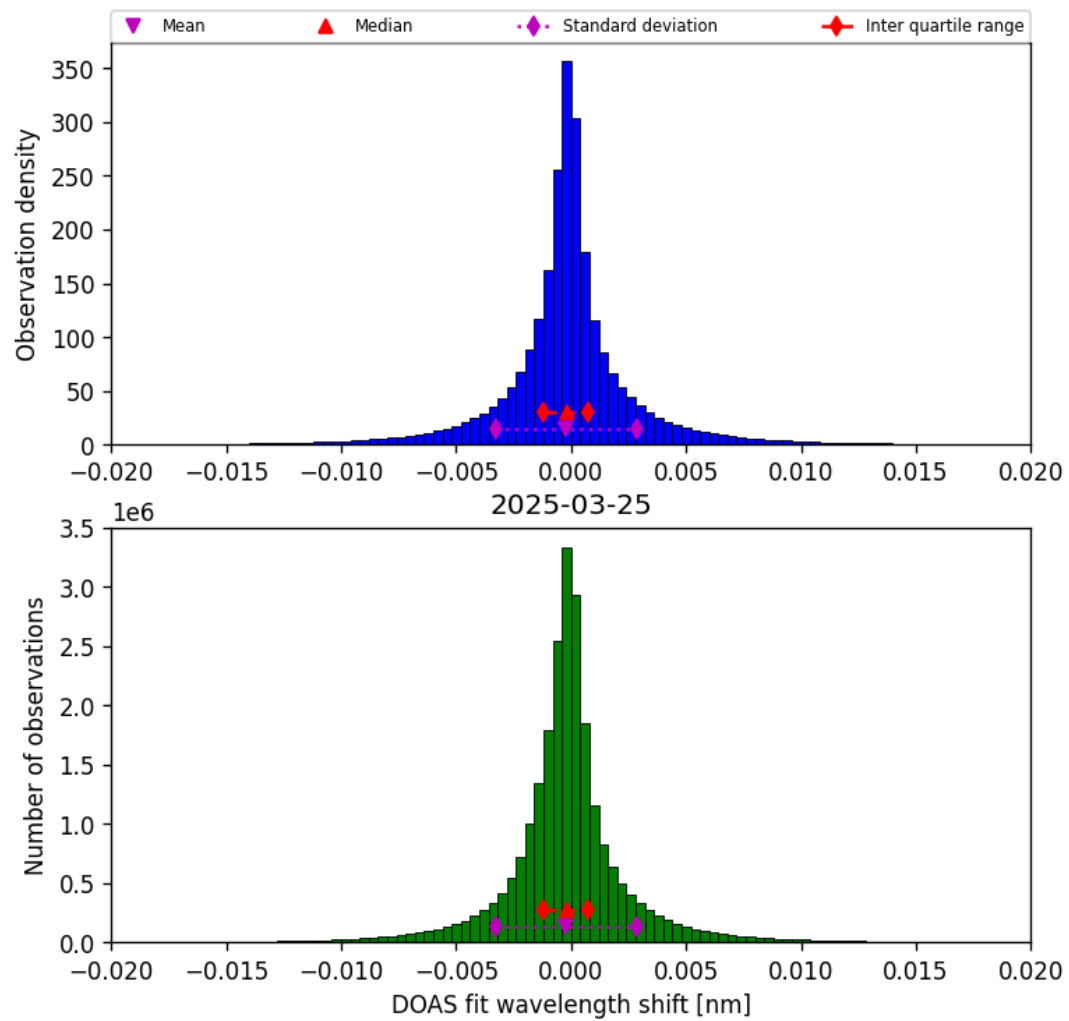
Figure 44: Histogram of “DOAS fit wavelength shift” for 2025-03-24 to 2025-03-26
