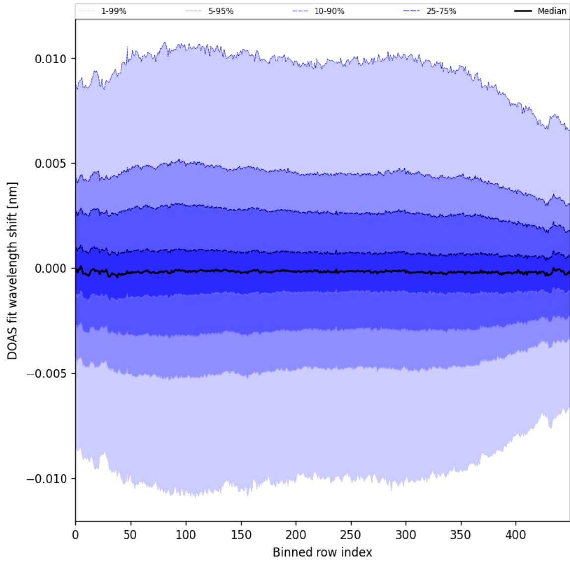
Figure 58: Along track statistics of “DOAS fit wavelength shift” for 2025-03-24 to 2025-03-26
