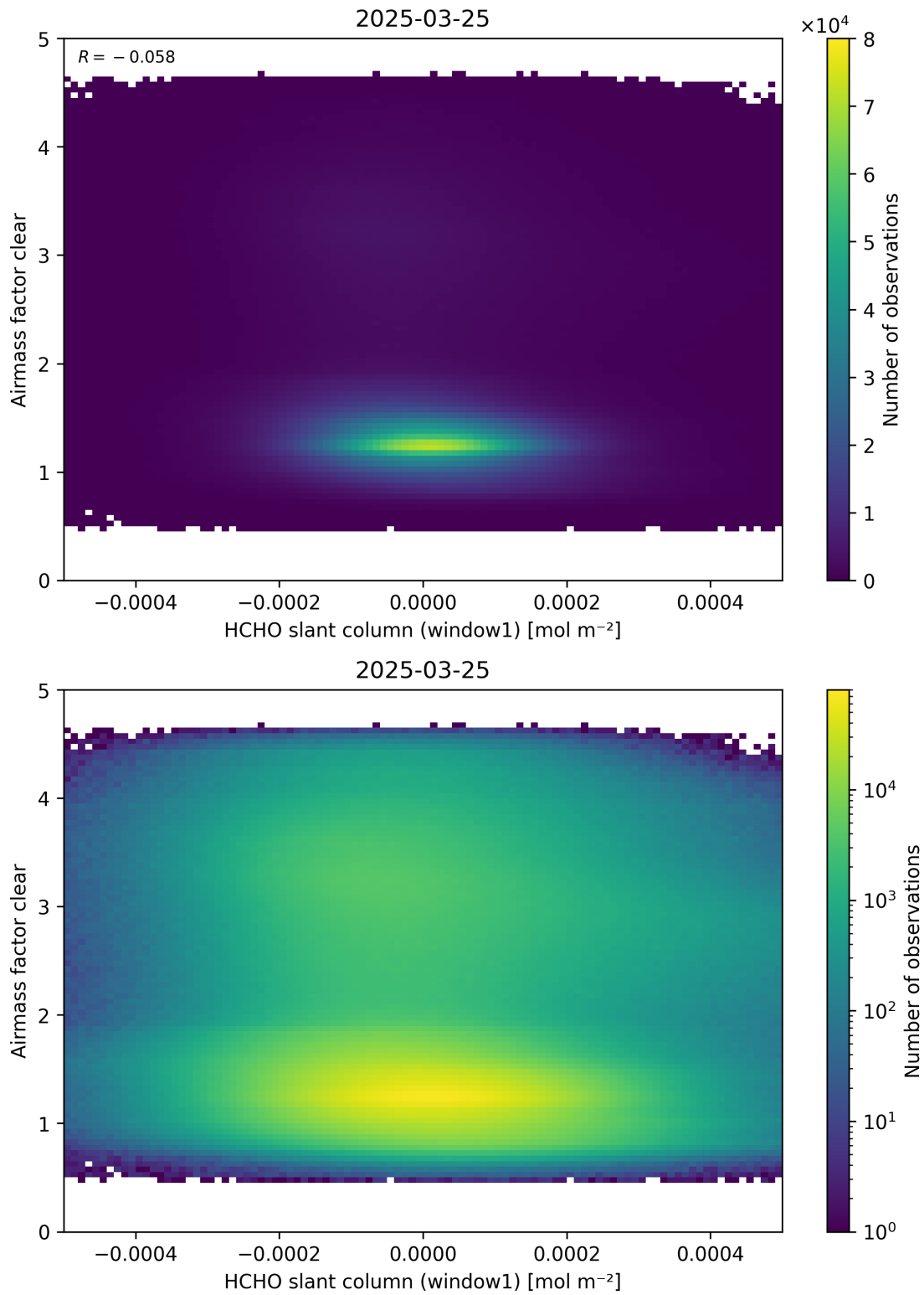
Figure 81: Scatter density plot of “HCHO slant column (window1)” against “Airmass factor clear” for 2025-03-24 to 2025-03-26.
