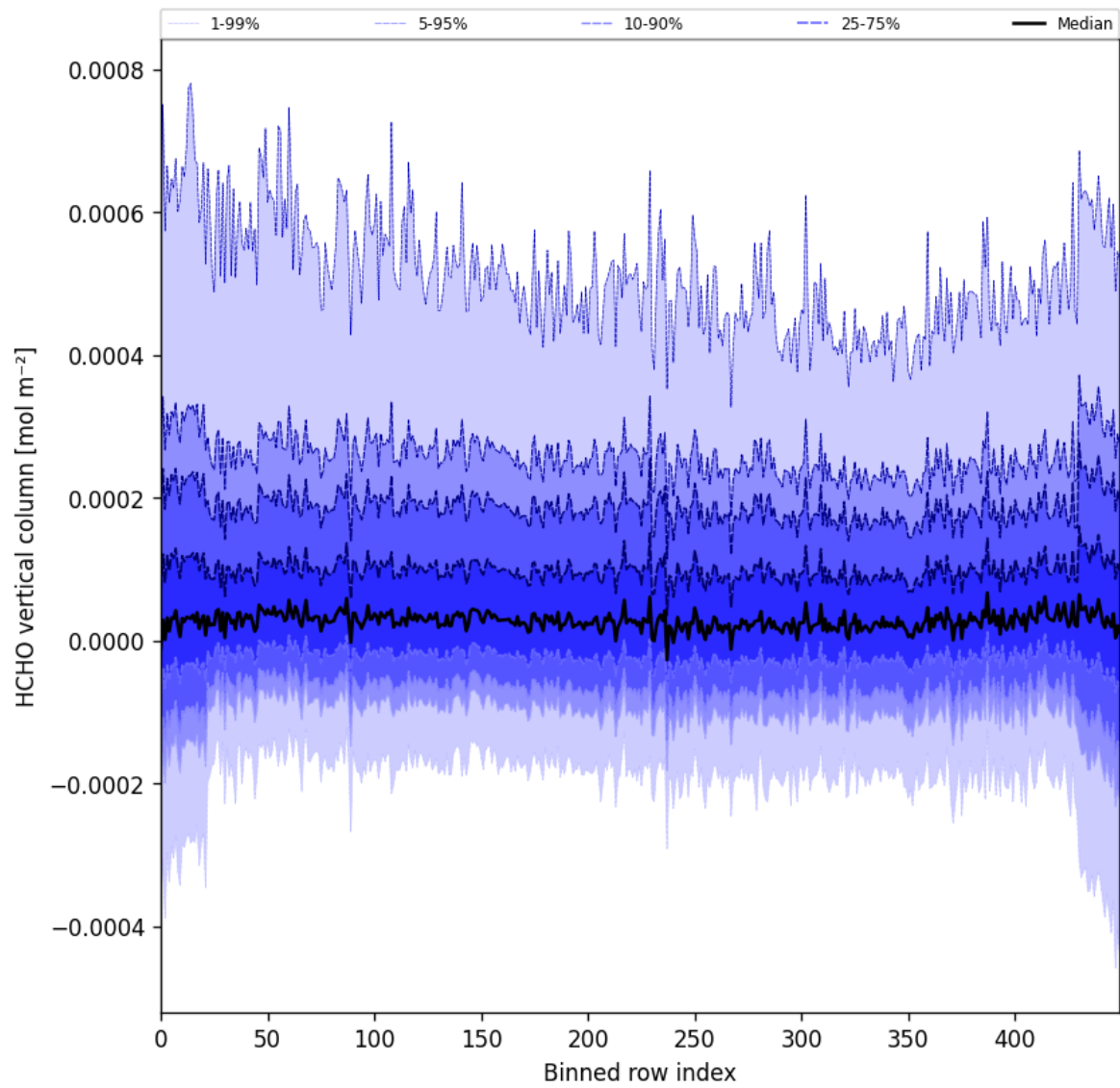
Figure 49: Along track statistics of “HCHO vertical column” for 2025-03-24 to 2025-03-26
