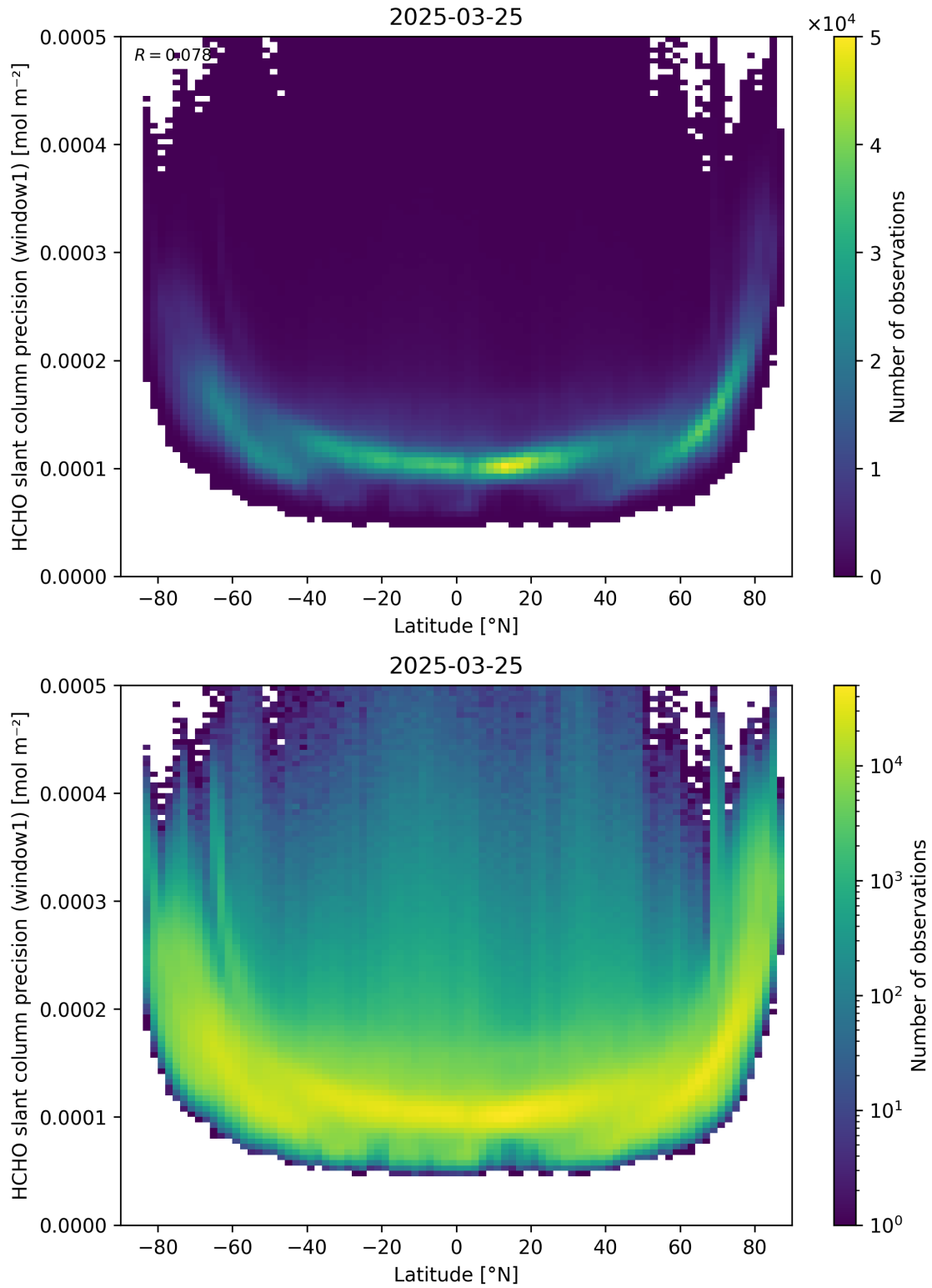
Figure 160: Scatter density plot of “Latitude” against “HCHO slant column precision (window1)” for 2025-03-24 to 2025-03-26.
