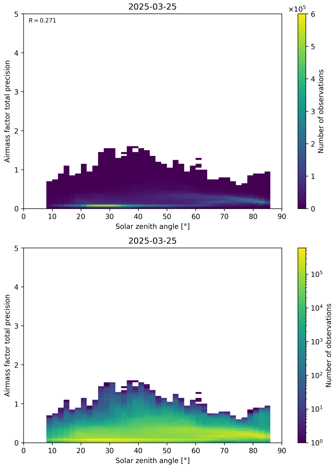
Figure 176: Scatter density plot of “Solar zenith angle” against “Airmass factor total precision” for 2025-03-24 to 2025-03-26.
