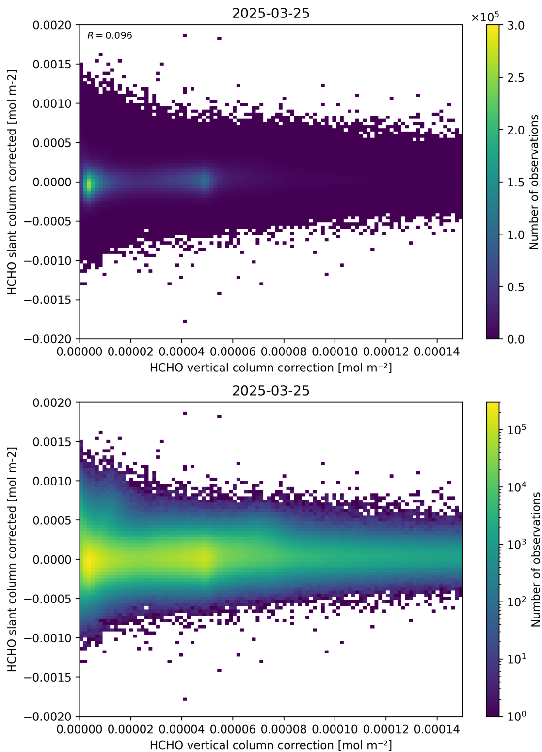
Figure 116: Scatter density plot of “HCHO vertical column correction” against “HCHO slant column corrected” for 2025-03-24 to 2025-03-26.
