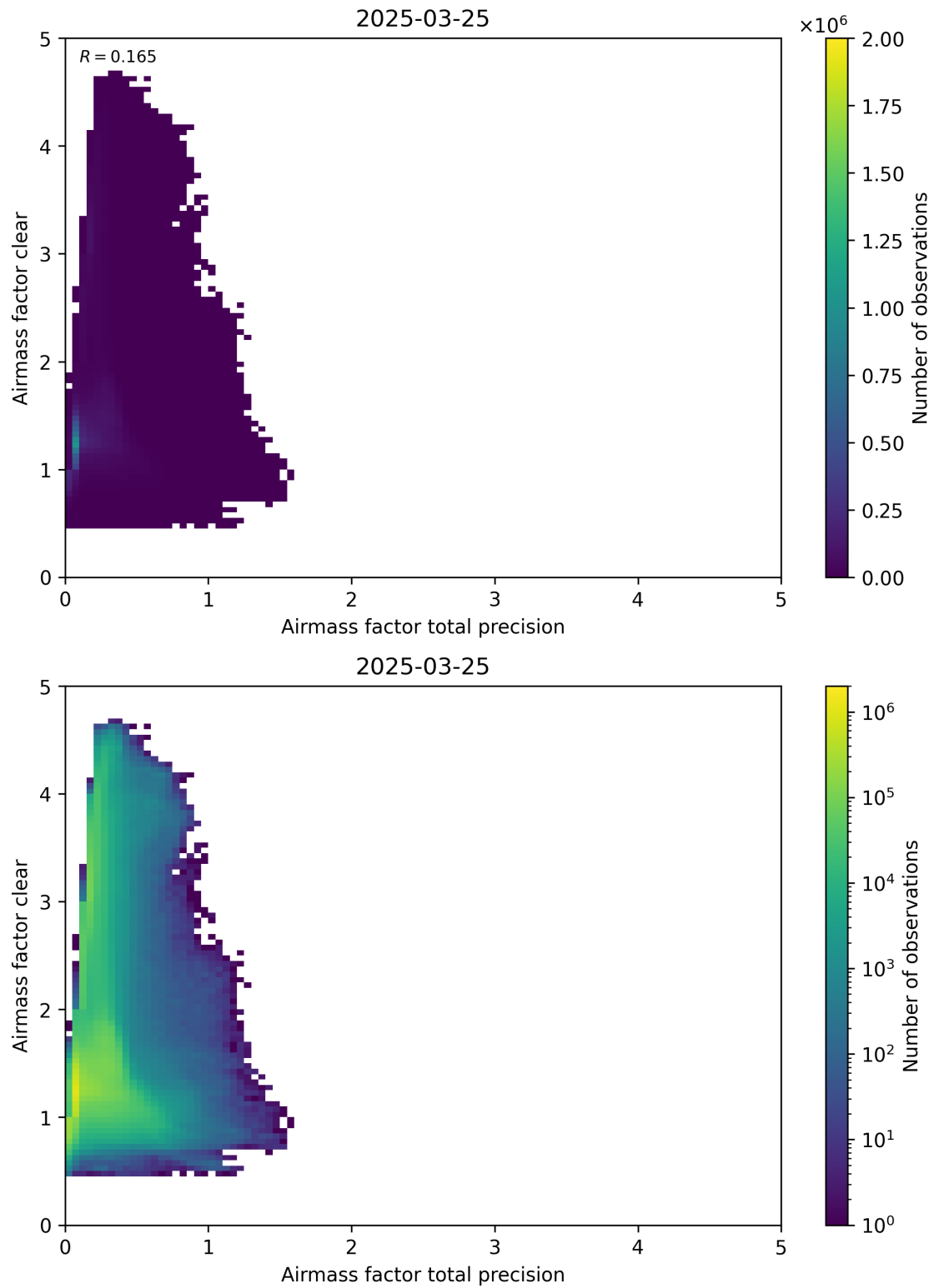
Figure 108: Scatter density plot of “Airmass factor total precision” against “Airmass factor clear” for 2025-03-24 to 2025-03-26.
