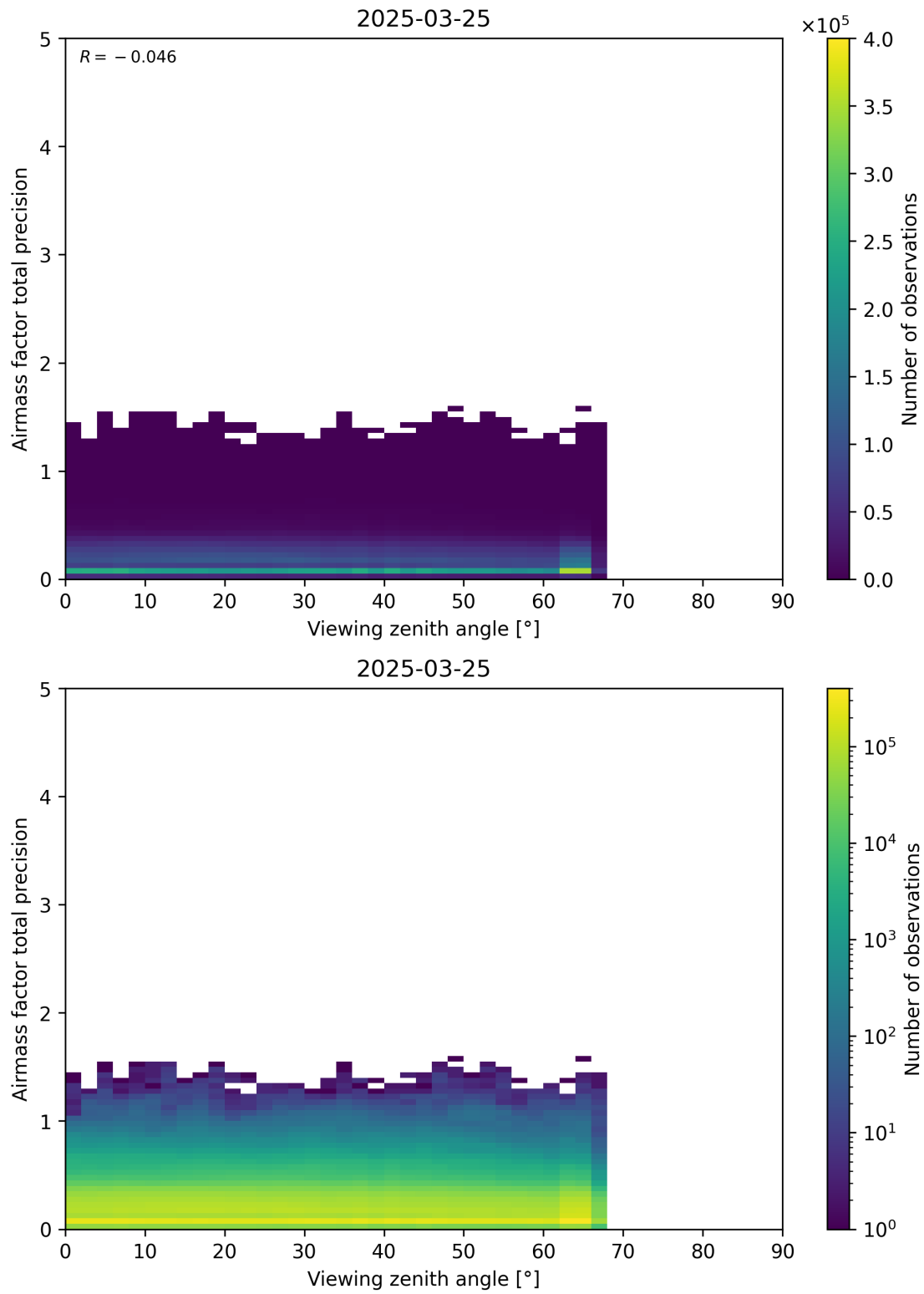
Figure 191: Scatter density plot of “Viewing zenith angle” against “Airmass factor total precision” for 2025-03-24 to 2025-03-26.
