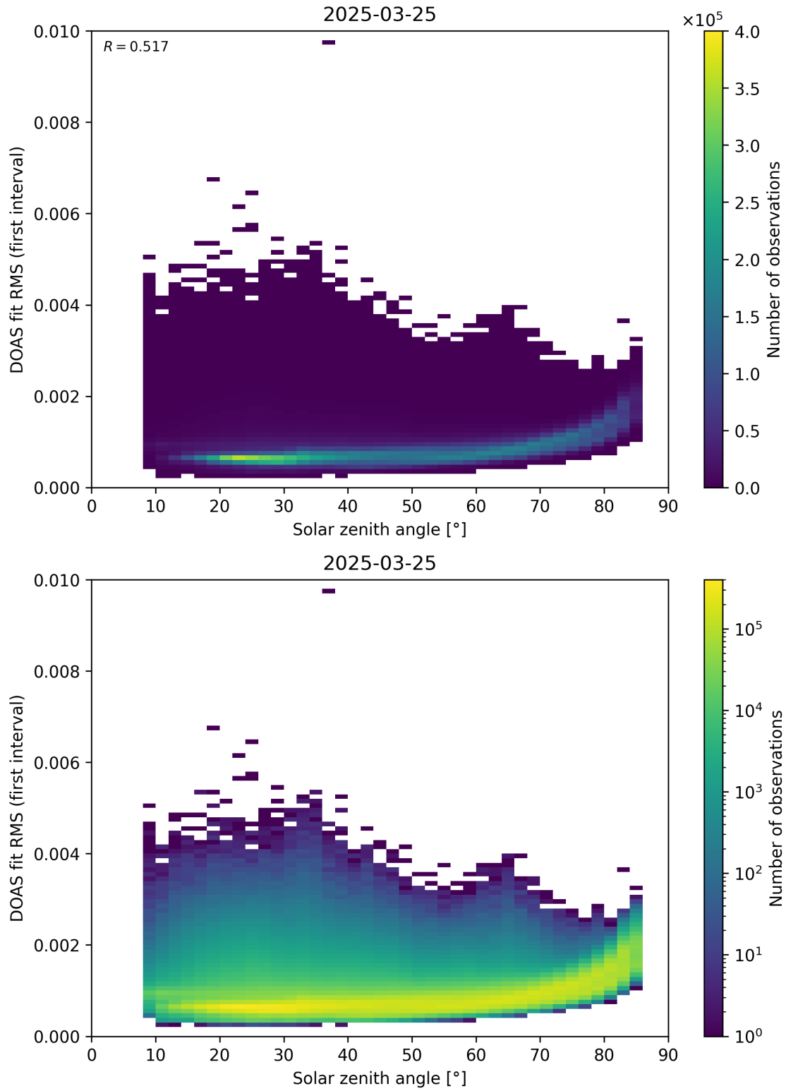
Figure 167: Scatter density plot of “Solar zenith angle” against “DOAS fit RMS (first interval)” for 2025-03-24 to 2025-03-26.
