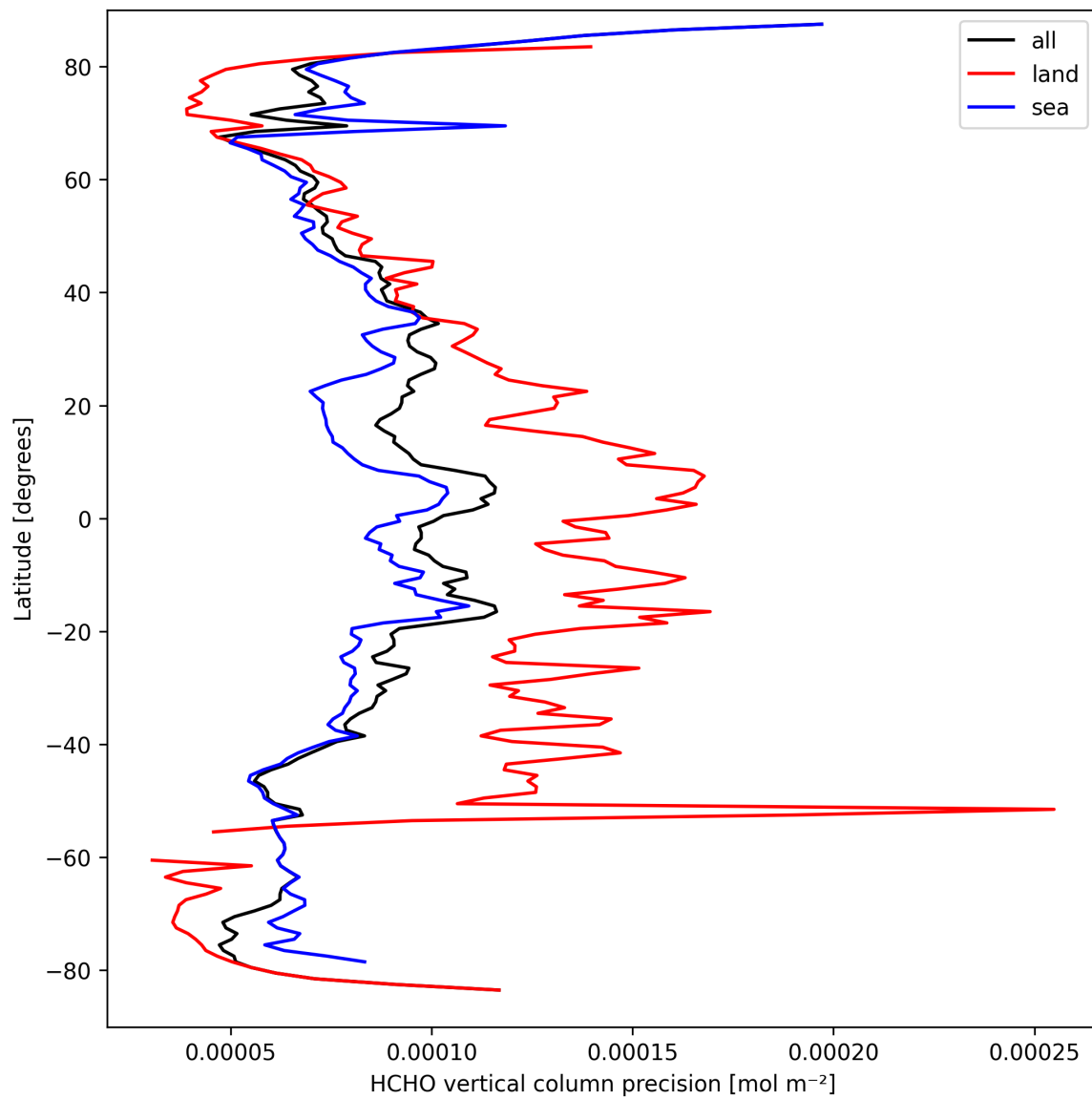
Figure 22: Zonal average of “HCHO vertical column precision” for 2025-03-24 to 2025-03-26.
