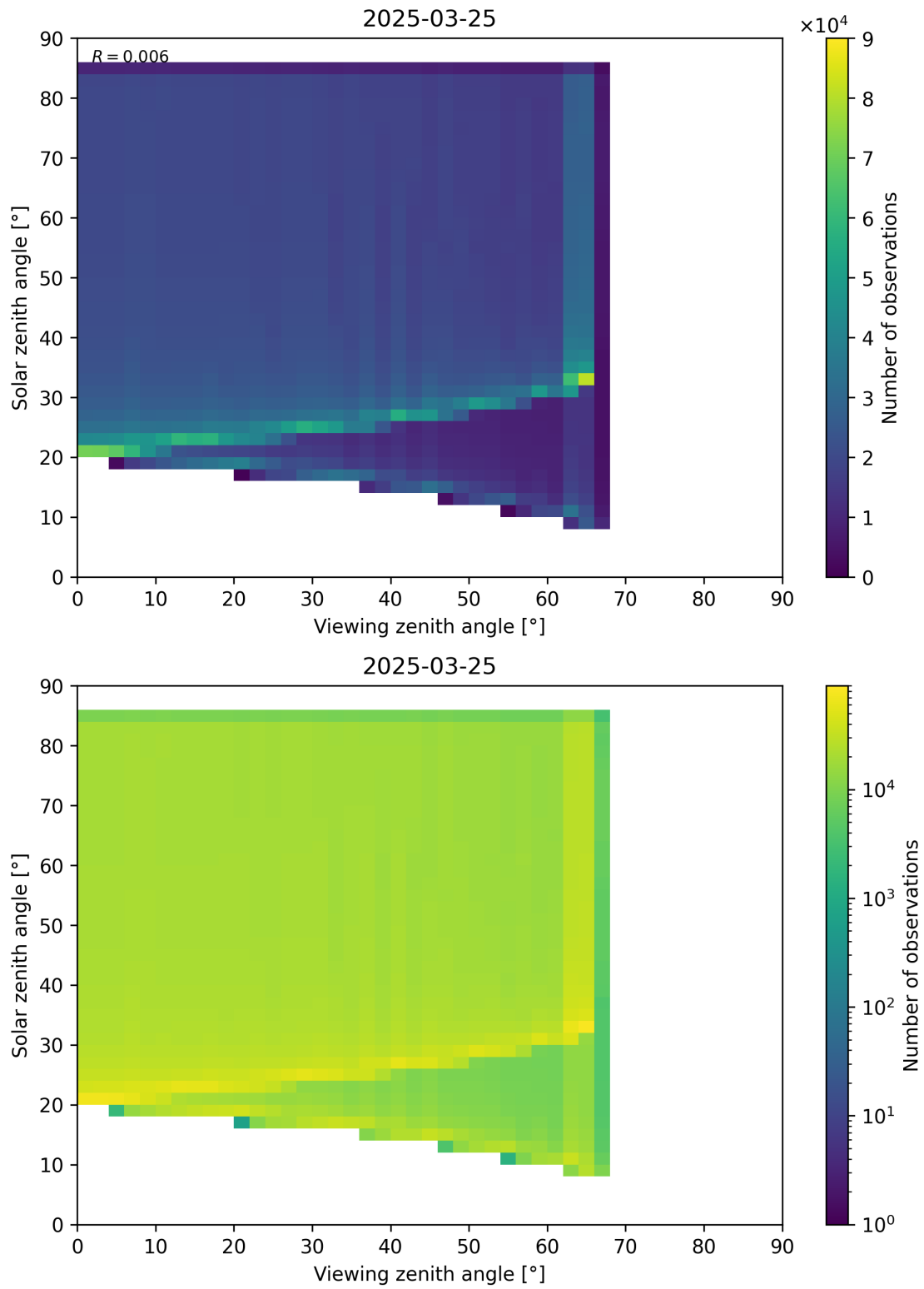
Figure 197: Scatter density plot of “Viewing zenith angle” against “Solar zenith angle” for 2025-03-24 to 2025-03-26.
