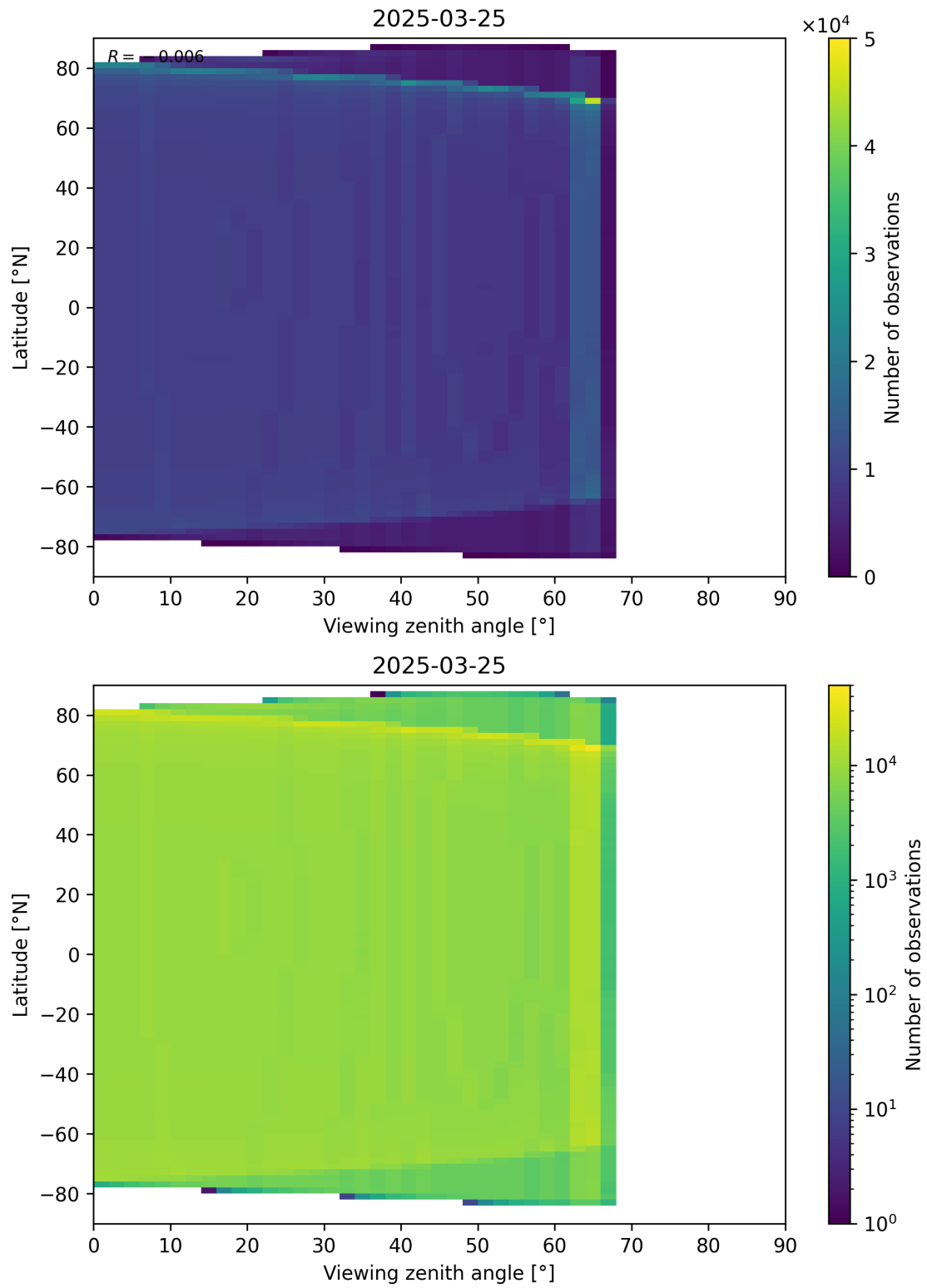
Figure 196: Scatter density plot of “Viewing zenith angle” against “Latitude” for 2025-03-24 to 2025-03-26.
