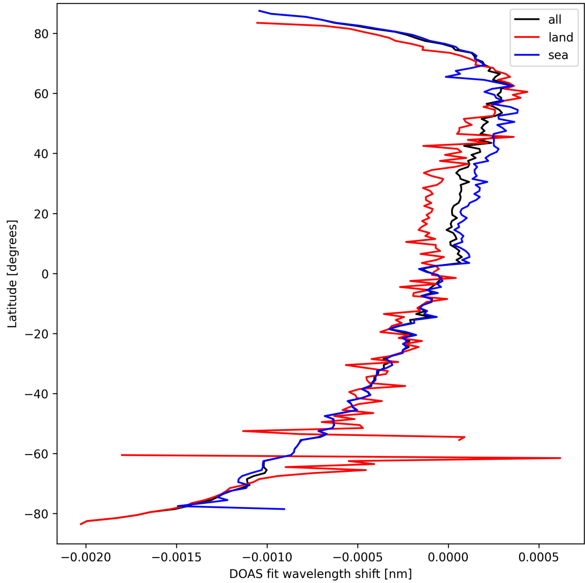
Figure 30: Zonal average of “DOAS fit wavelength shift” for 2025-03-24 to 2025-03-26.
