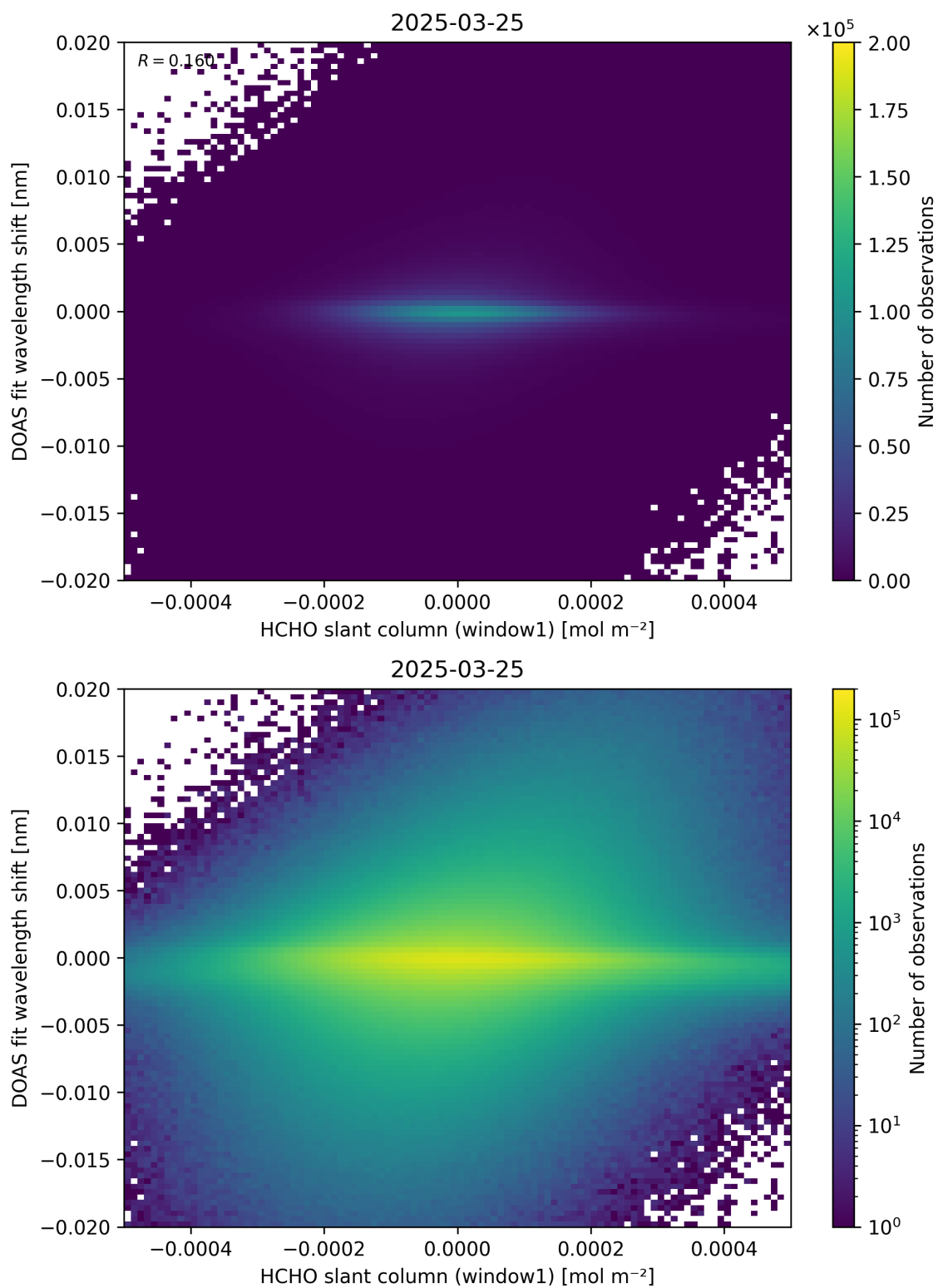
Figure 79: Scatter density plot of “HCHO slant column (window1)” against “DOAS fit wavelength shift” for 2025-03-24 to 2025-03-26.
