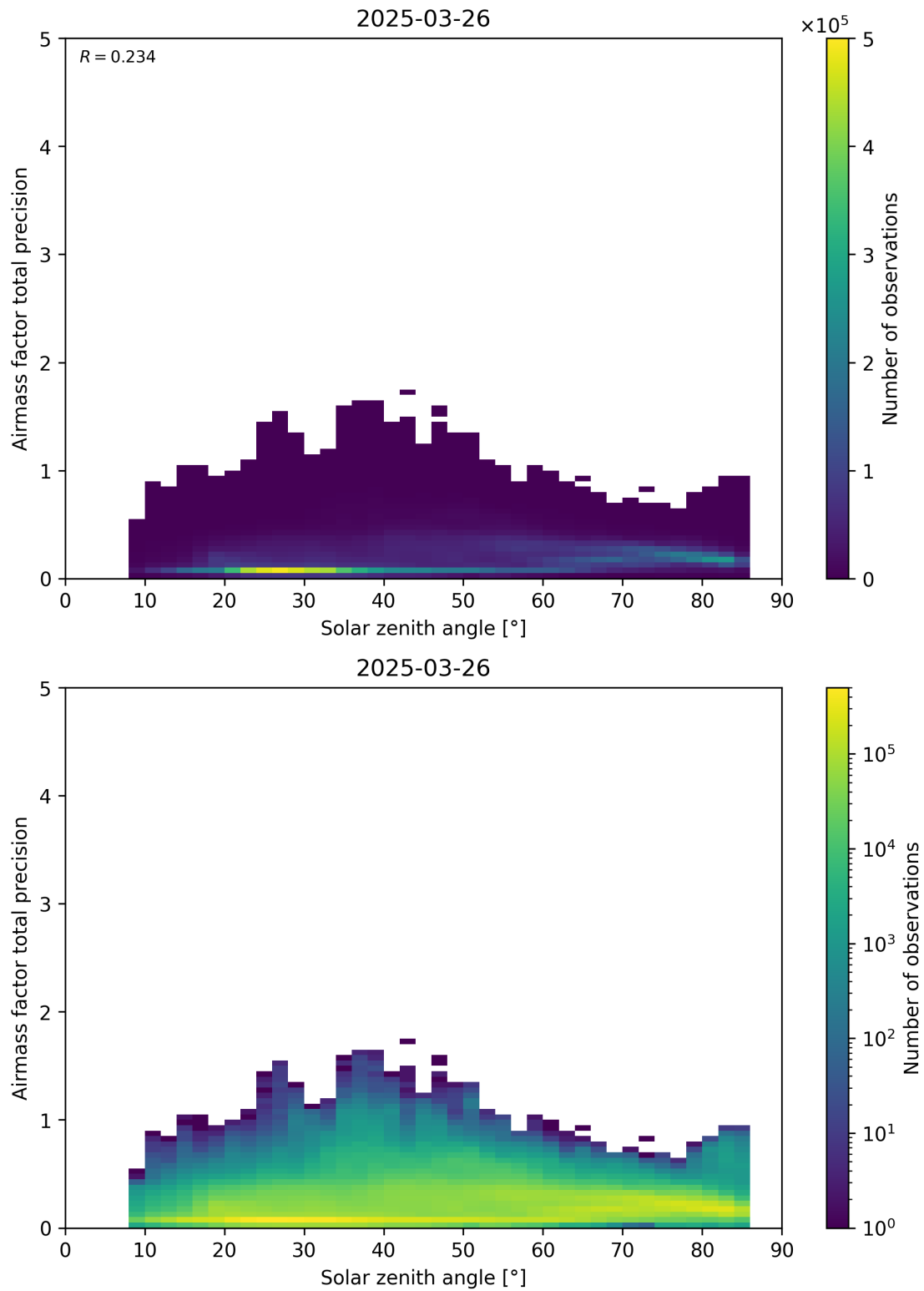
Figure 176: Scatter density plot of “Solar zenith angle” against “Airmass factor total precision” for 2025-03-25 to 2025-03-27.
