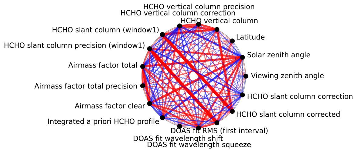
Figure 1: Map of correlation graph for 2025-03-25 to 2025-03-27.
