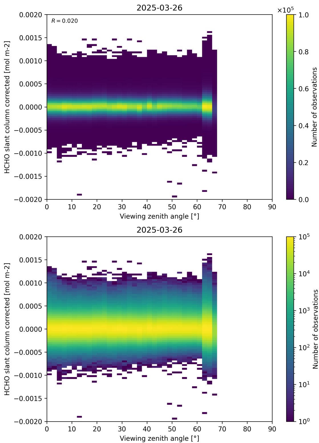
Figure 186: Scatter density plot of “Viewing zenith angle” against “HCHO slant column corrected” for 2025-03-25 to 2025-03-27.
