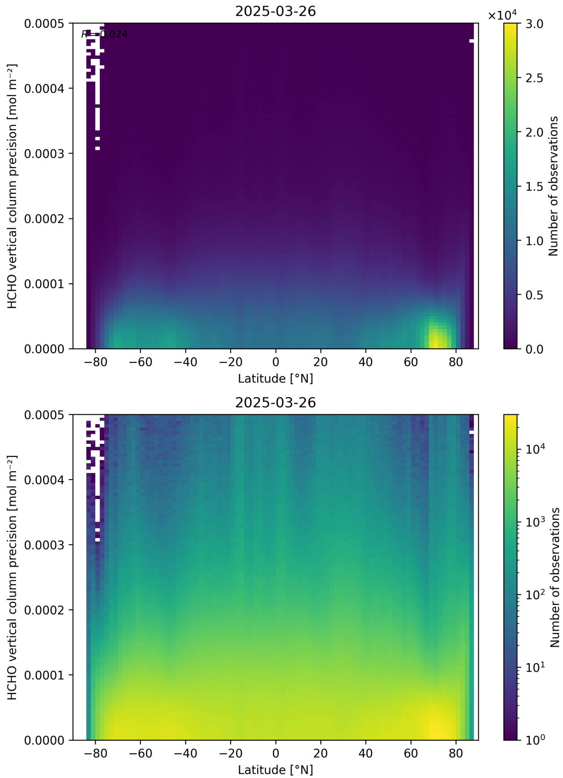
Figure 165: Scatter density plot of “Latitude” against “HCHO vertical column precision” for 2025-03-25 to 2025-03-27.
