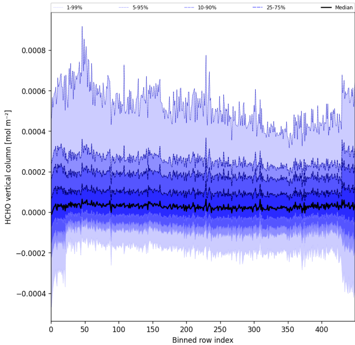
Figure 49: Along track statistics of “HCHO vertical column” for 2025-03-25 to 2025-03-27
