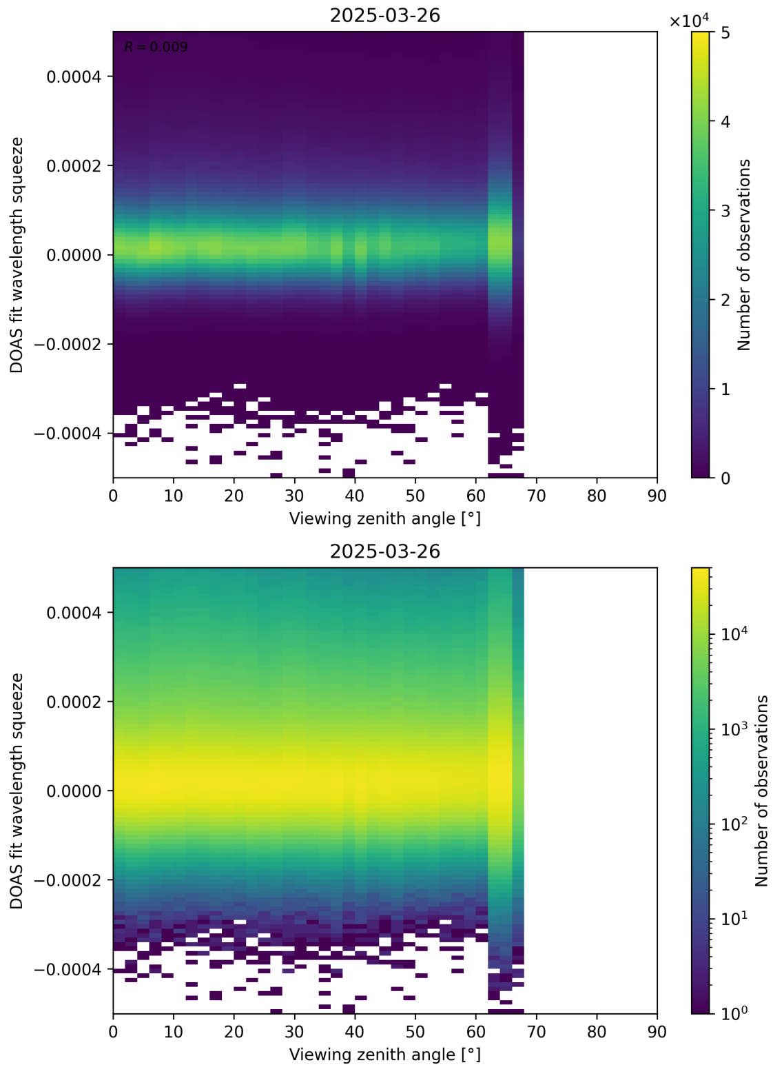
Figure 184: Scatter density plot of “Viewing zenith angle” against “DOAS fit wavelength squeeze” for 2025-03-25 to 2025-03-27.
