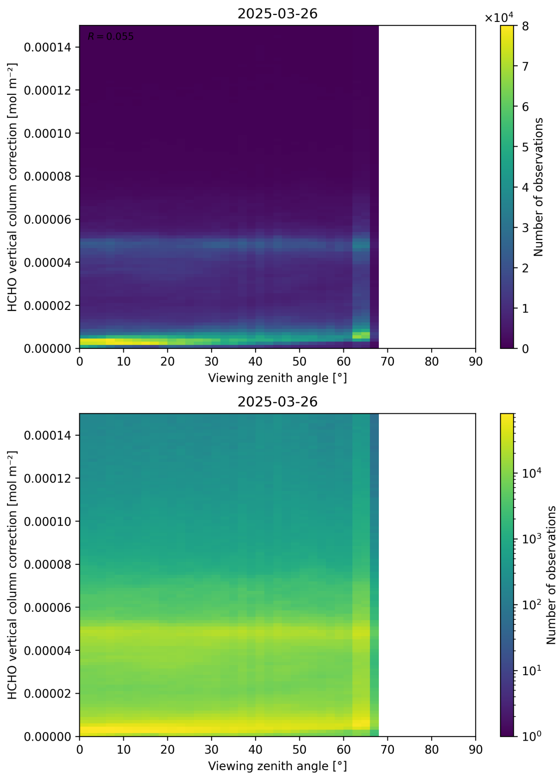
Figure 193: Scatter density plot of “Viewing zenith angle” against “HCHO vertical column correction” for 2025-03-25 to 2025-03-27.
