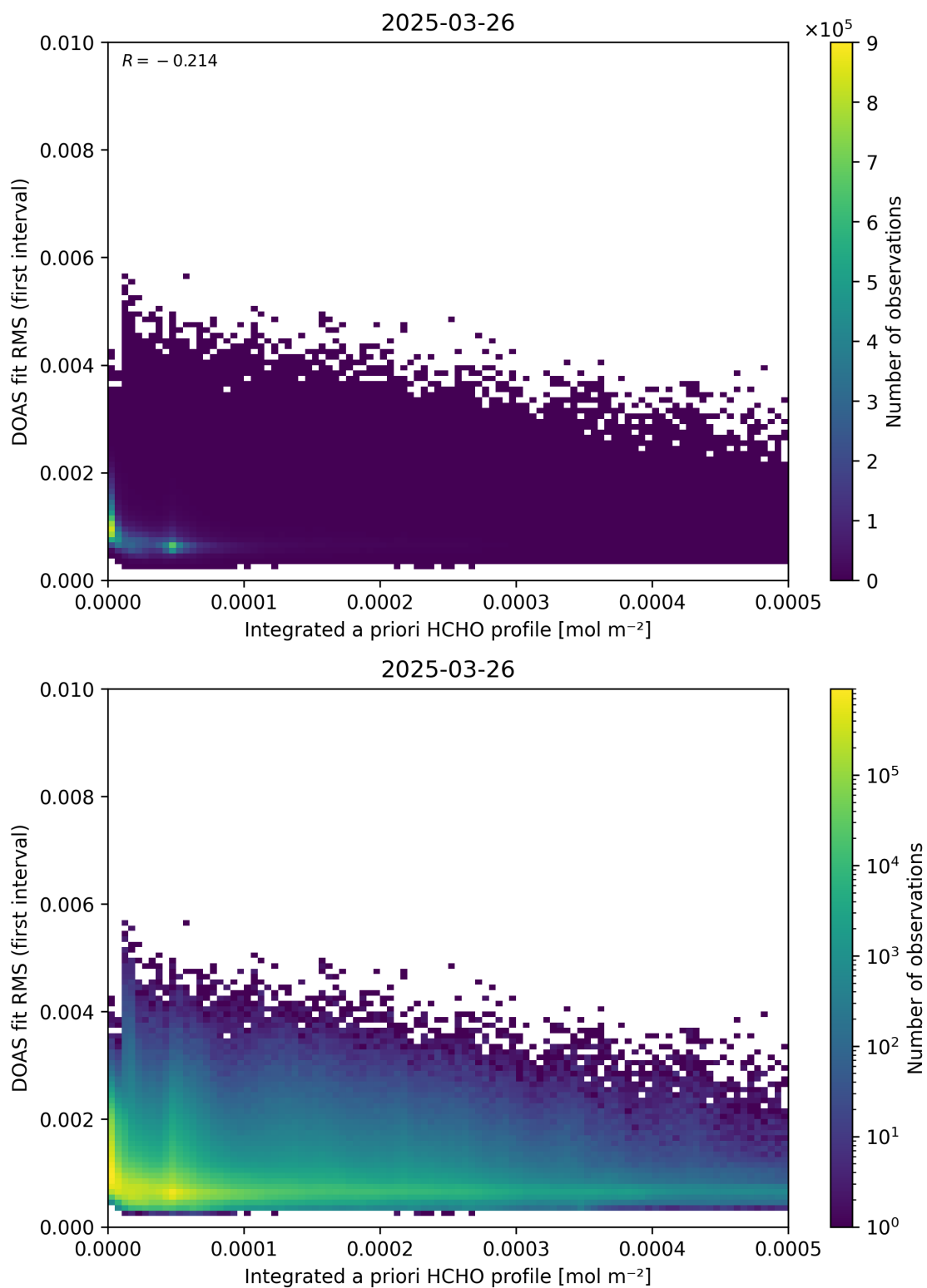
Figure 148: Scatter density plot of “Integrated a priori HCHO profile” against “DOAS fit RMS (first interval)” for 2025-03-25 to 2025-03-27.
