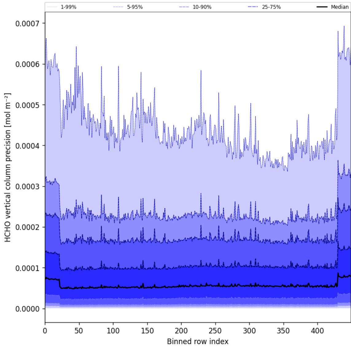
Figure 50: Along track statistics of “HCHO vertical column precision” for 2025-03-25 to 2025-03-27
