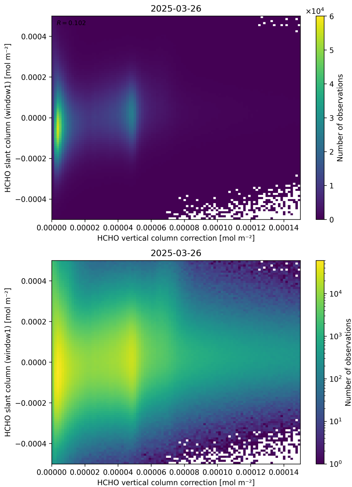
Figure 118: Scatter density plot of “HCHO vertical column correction” against “HCHO slant column (window1)” for 2025-03-25 to 2025-03-27.
