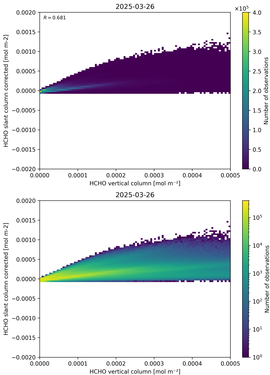
Figure 127: Scatter density plot of “HCHO vertical column” against “HCHO slant column corrected” for 2025-03-25 to 2025-03-27.
