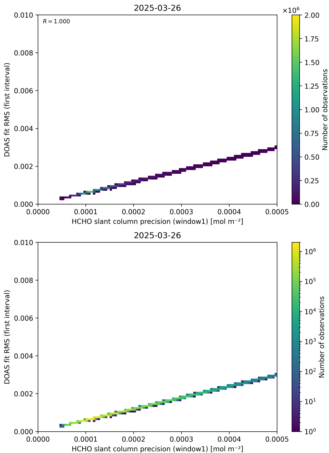
Figure 88: Scatter density plot of “HCHO slant column precision (window1)” against “DOAS fit RMS (first interval)” for 2025-03-25 to 2025-03-27.
