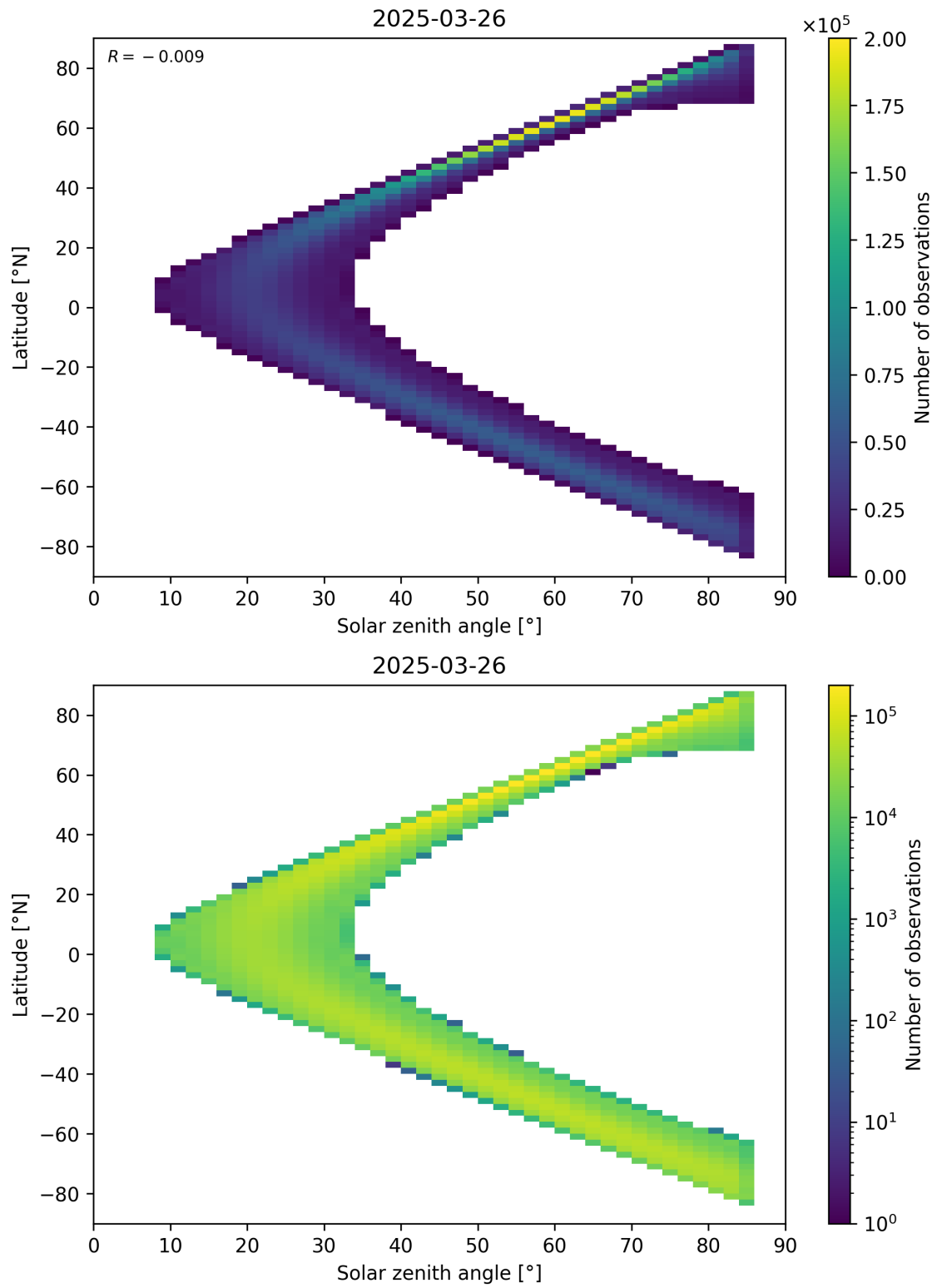
Figure 181: Scatter density plot of “Solar zenith angle” against “Latitude” for 2025-03-25 to 2025-03-27.
