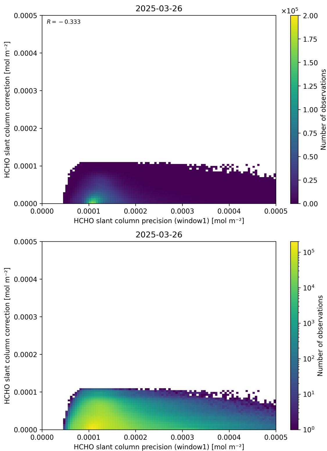
Figure 93: Scatter density plot of “HCHO slant column precision (window1)” against “HCHO slant column correction” for 2025-03-25 to 2025-03-27.
