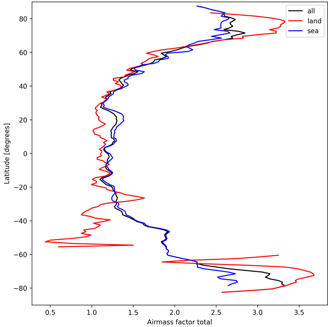
Figure 26: Zonal average of “Airmass factor total” for 2025-03-25 to 2025-03-27.
