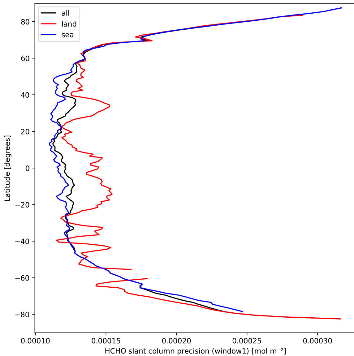
Figure 25: Zonal average of “HCHO slant column precision (window1)” for 2025-03-25 to 2025-03-27.
