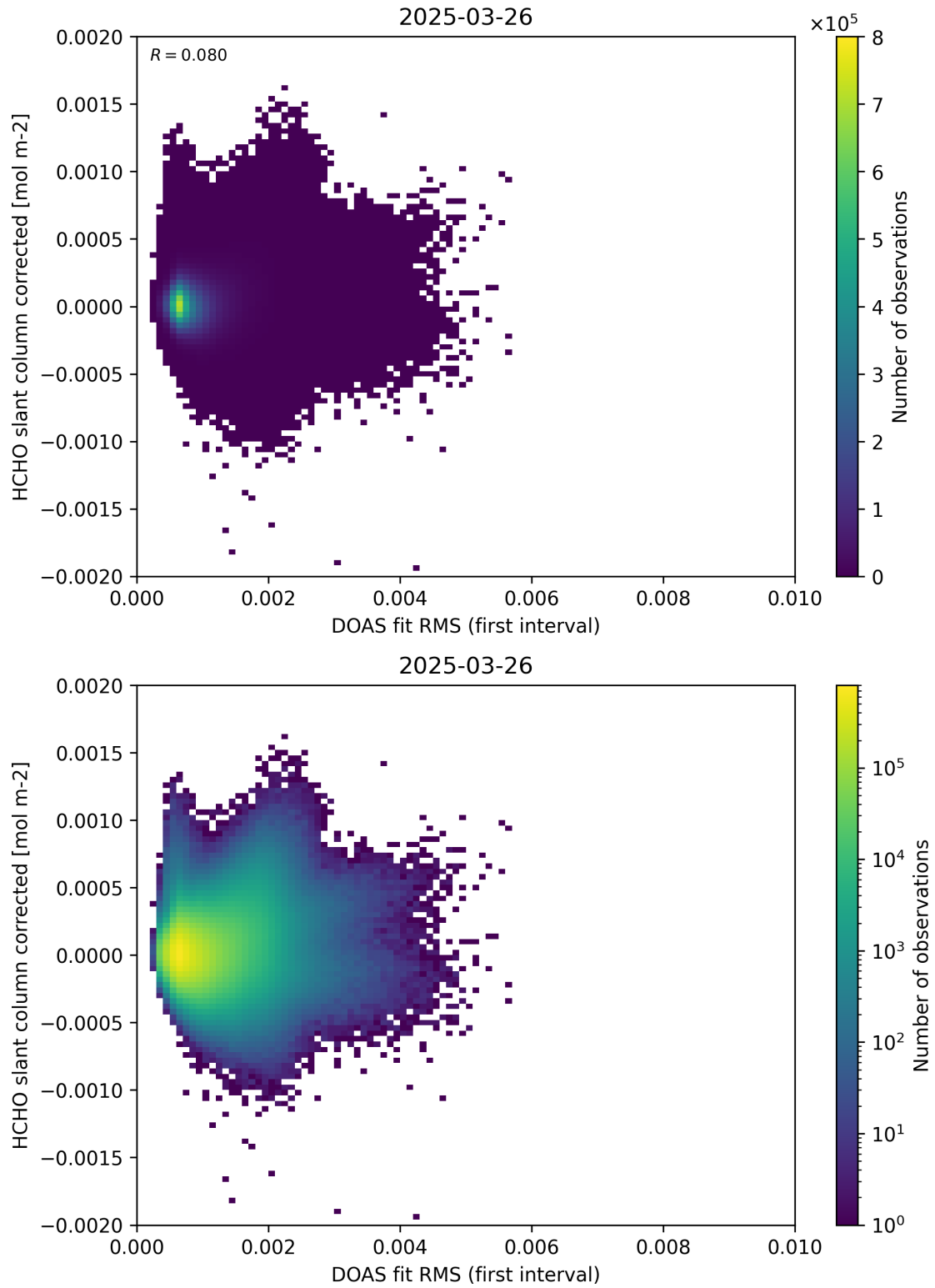
Figure 62: Scatter density plot of “DOAS fit RMS (first interval)” against “HCHO slant column corrected” for 2025-03-25 to 2025-03-27.
