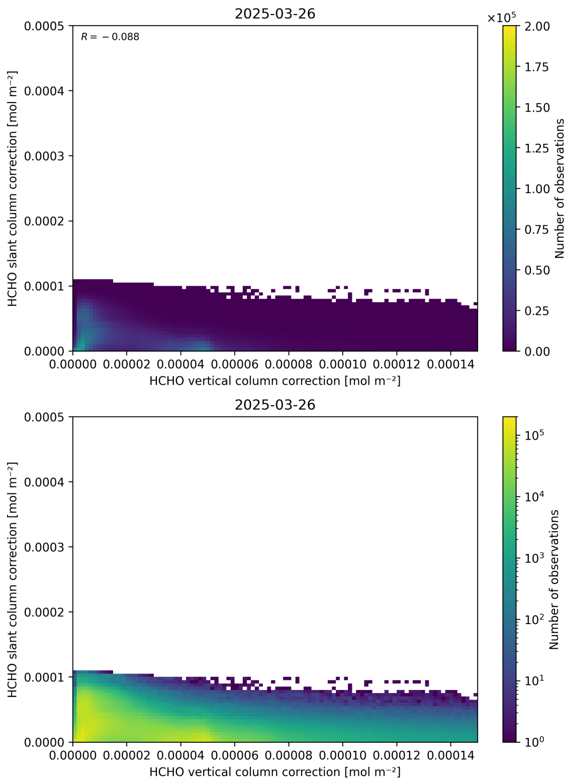
Figure 117: Scatter density plot of “HCHO vertical column correction” against “HCHO slant column correction” for 2025-03-25 to 2025-03-27.
