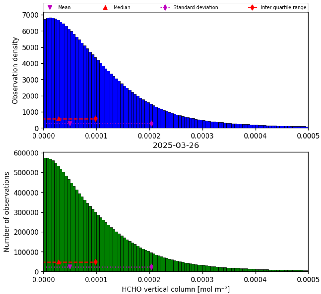
Figure 35: Histogram of “HCHO vertical column” for 2025-03-25 to 2025-03-27
