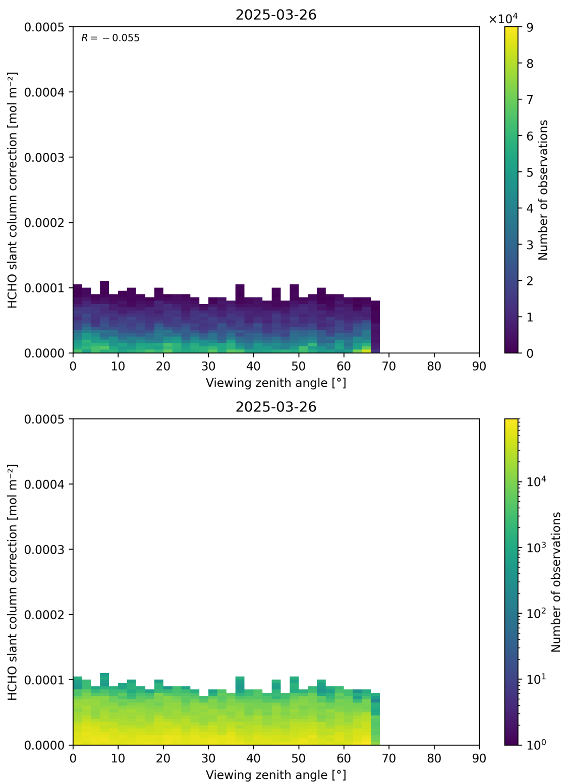
Figure 187: Scatter density plot of “Viewing zenith angle” against “HCHO slant column correction” for 2025-03-25 to 2025-03-27.
