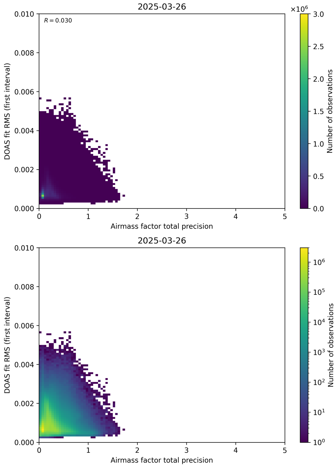
Figure 105: Scatter density plot of “Airmass factor total precision” against “DOAS fit RMS (first interval)” for 2025-03-25 to 2025-03-27.
