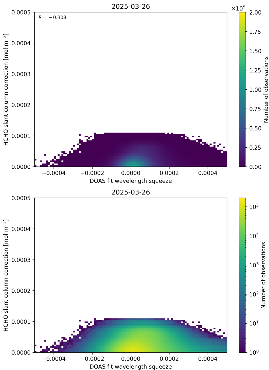
Figure 70: Scatter density plot of “DOAS fit wavelength squeeze” against “HCHO slant column correction” for 2025-03-25 to 2025-03-27.
