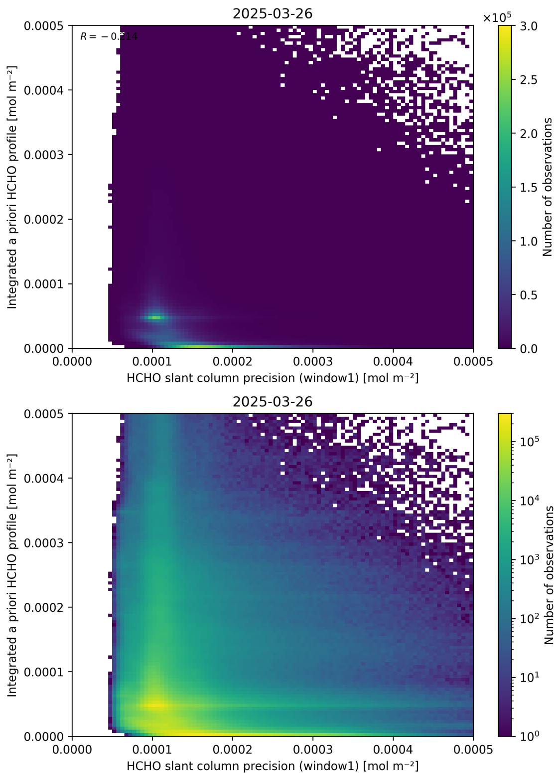
Figure 96: Scatter density plot of “HCHO slant column precision (window1)” against “Integrated a priori HCHO profile” for 2025-03-25 to 2025-03-27.
