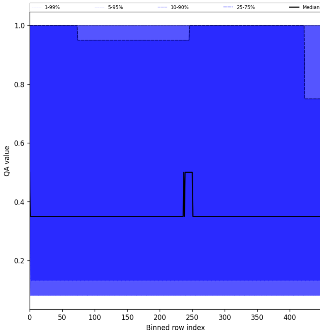
Figure 48: Along track statistics of “QA value” for 2025-03-25 to 2025-03-27
