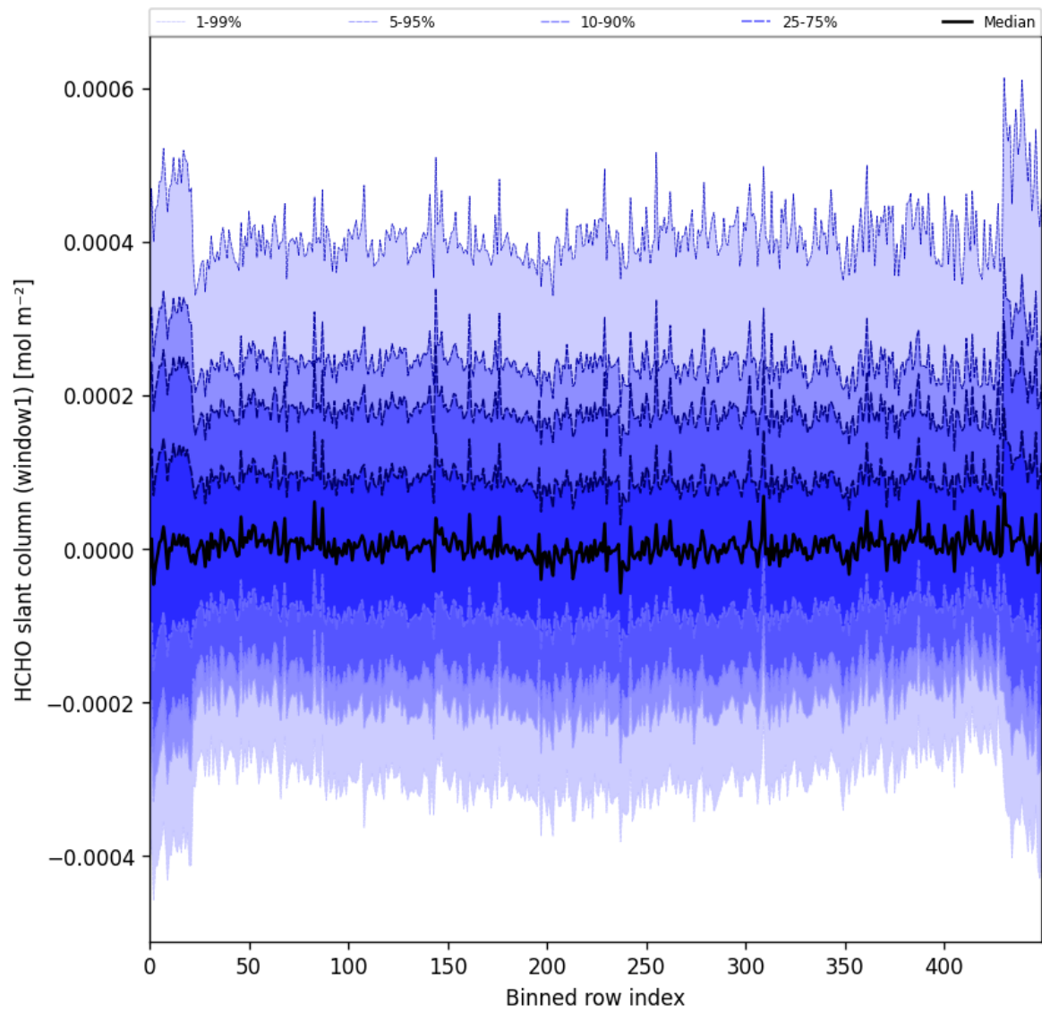
Figure 52: Along track statistics of “HCHO slant column (window1)” for 2025-03-25 to 2025-03-27
