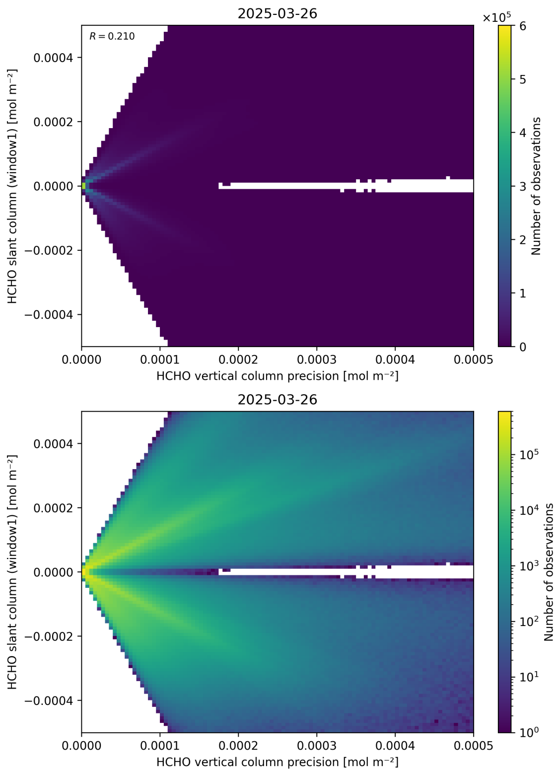
Figure 142: Scatter density plot of “HCHO vertical column precision” against “HCHO slant column (window1)” for 2025-03-25 to 2025-03-27.
