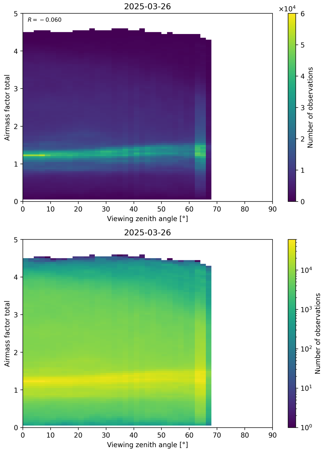
Figure 190: Scatter density plot of “Viewing zenith angle” against “Airmass factor total” for 2025-03-25 to 2025-03-27.
