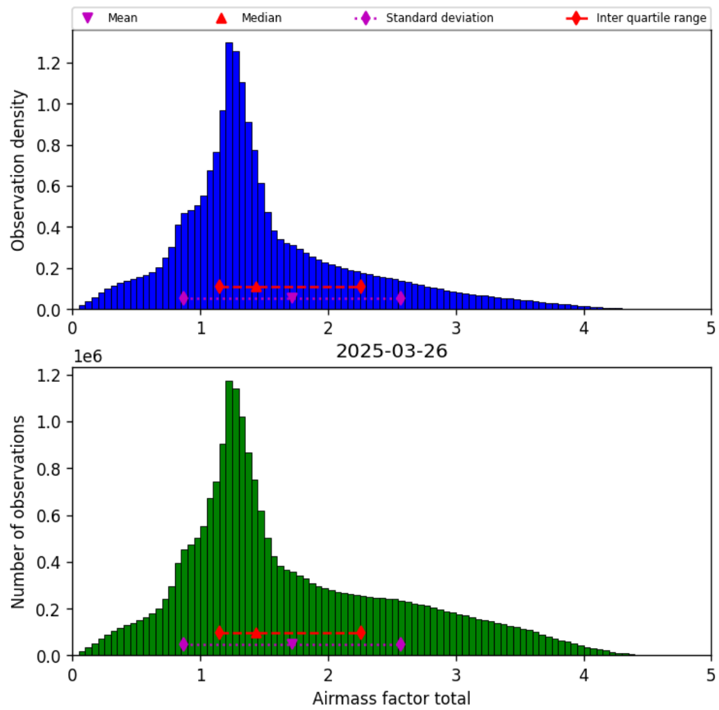
Figure 40: Histogram of “Airmass factor total” for 2025-03-25 to 2025-03-27
