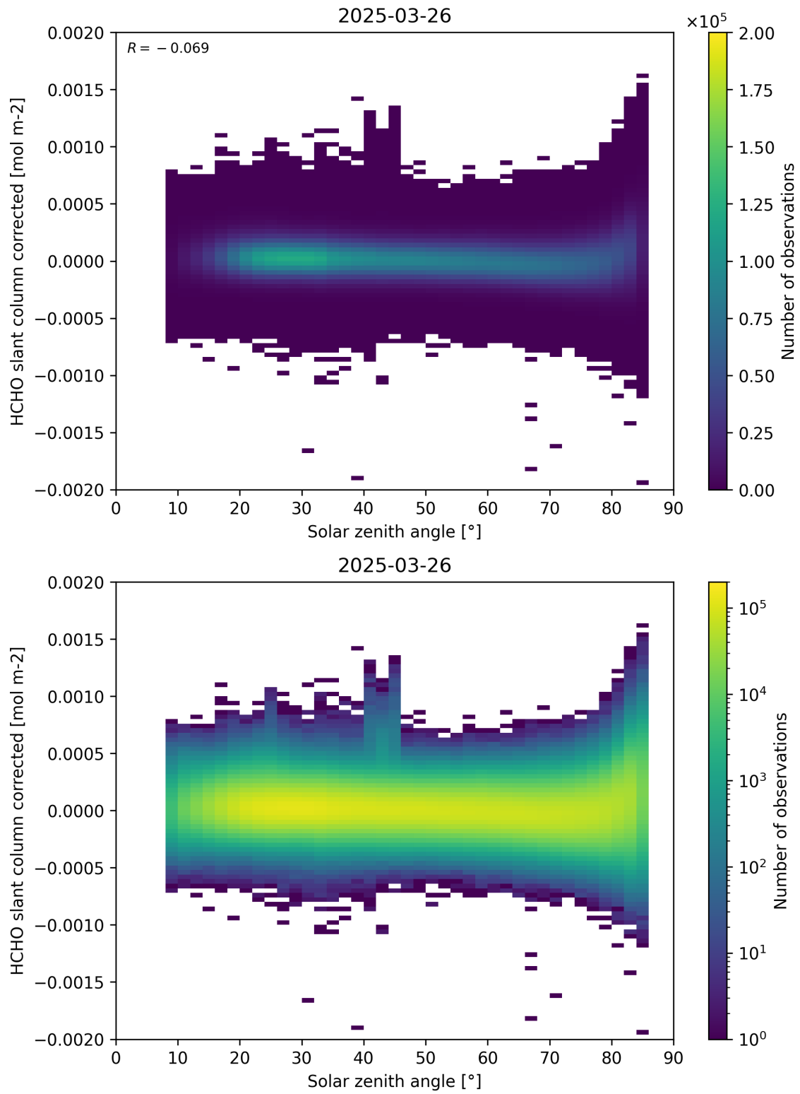
Figure 171: Scatter density plot of “Solar zenith angle” against “HCHO slant column corrected” for 2025-03-25 to 2025-03-27.
