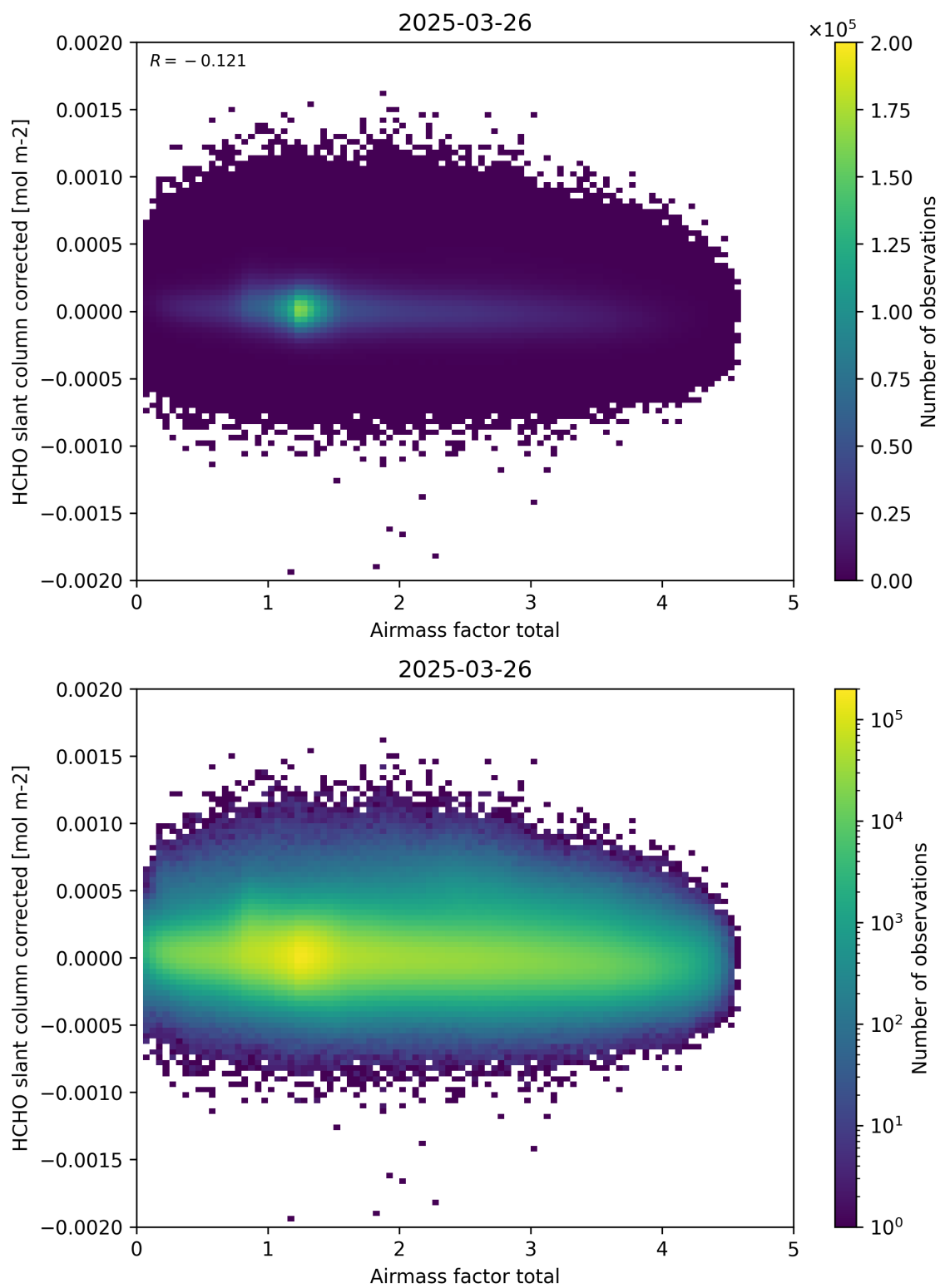
Figure 101: Scatter density plot of “Airmass factor total” against “HCHO slant column corrected” for 2025-03-25 to 2025-03-27.
