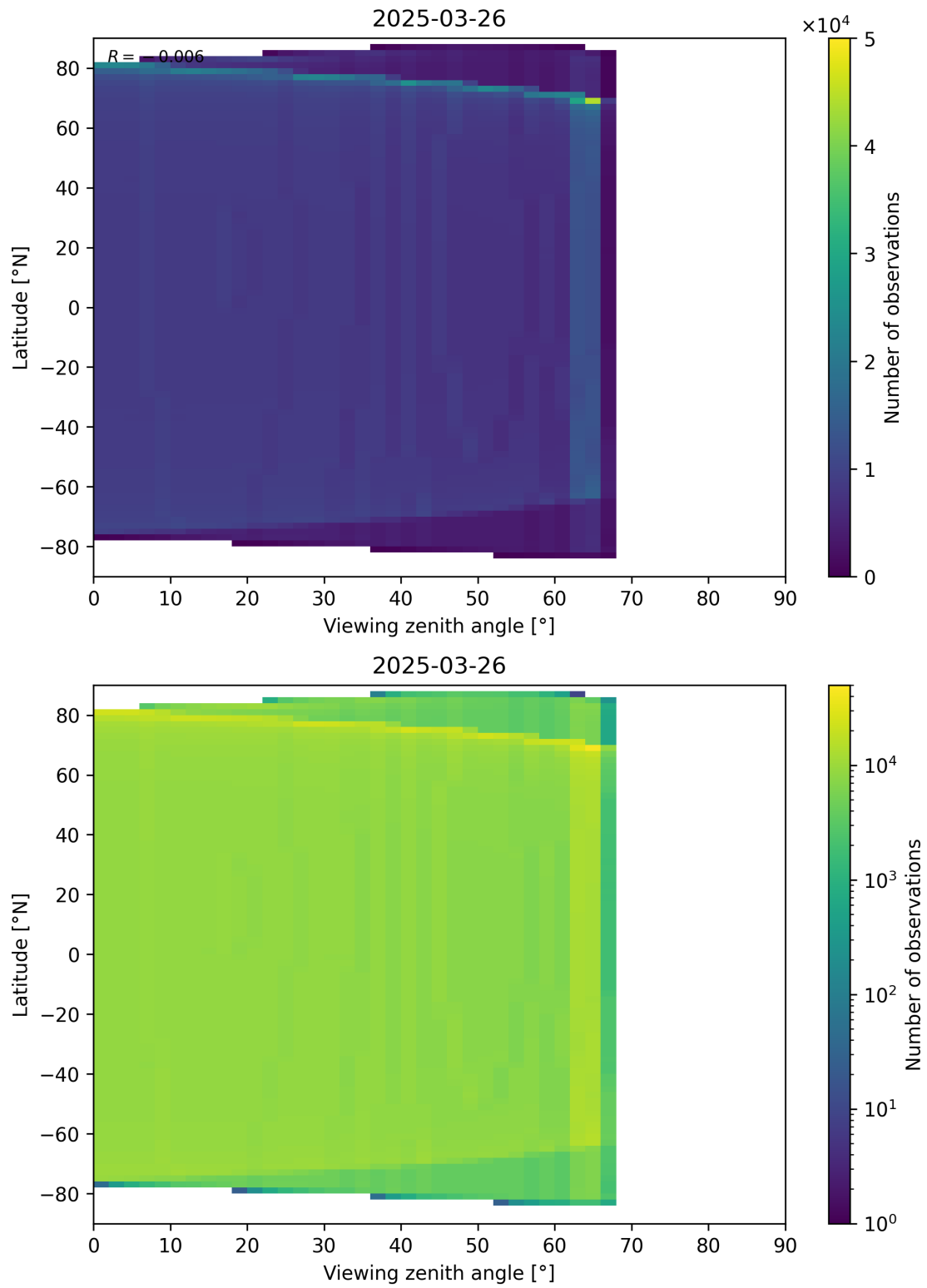
Figure 196: Scatter density plot of “Viewing zenith angle” against “Latitude” for 2025-03-25 to 2025-03-27.
