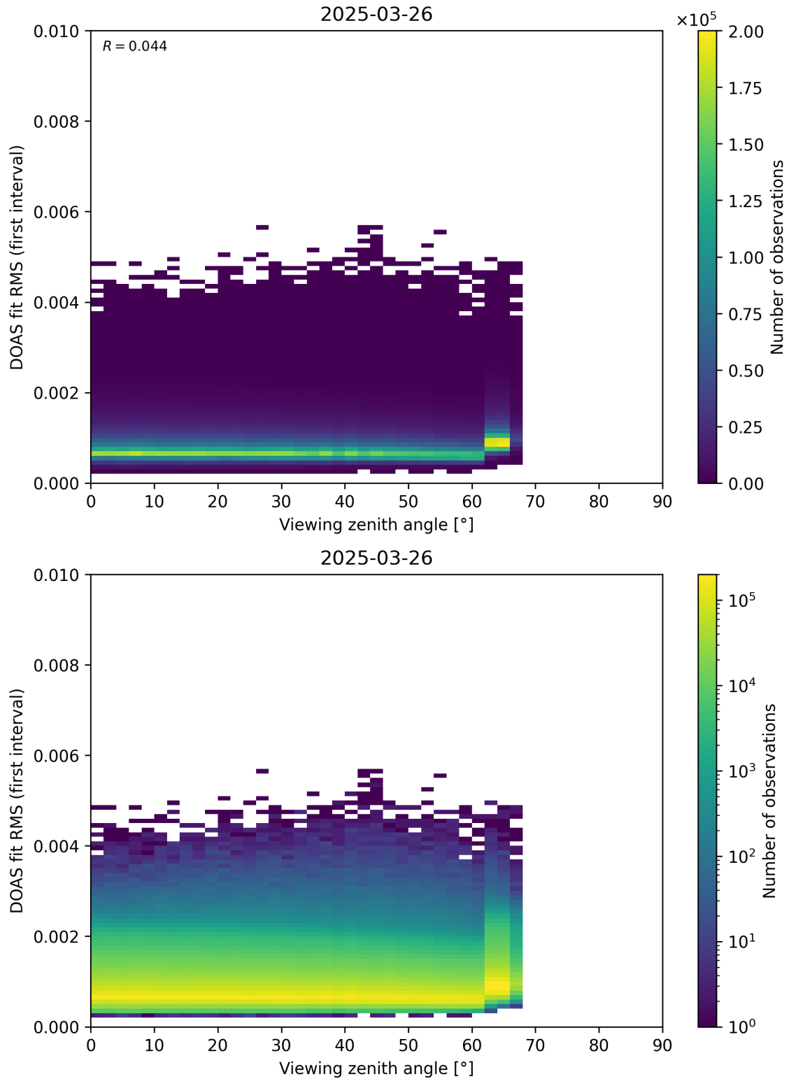
Figure 182: Scatter density plot of “Viewing zenith angle” against “DOAS fit RMS (first interval)” for 2025-03-25 to 2025-03-27.
