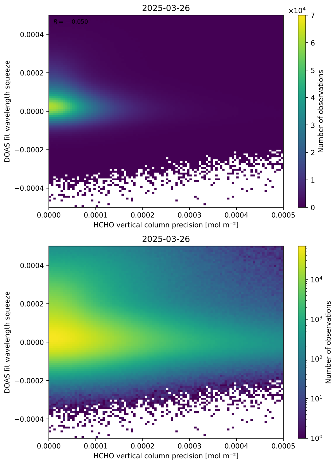
Figure 138: Scatter density plot of “HCHO vertical column precision” against “DOAS fit wavelength squeeze” for 2025-03-25 to 2025-03-27.
