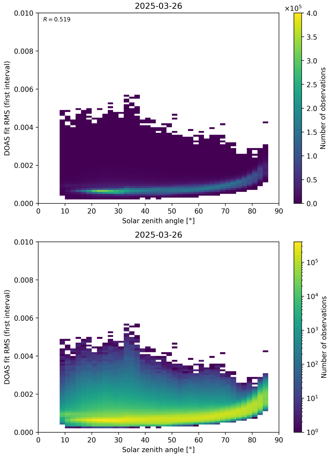
Figure 167: Scatter density plot of “Solar zenith angle” against “DOAS fit RMS (first interval)” for 2025-03-25 to 2025-03-27.
