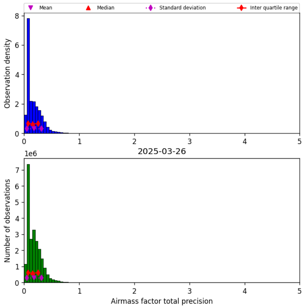
Figure 41: Histogram of “Airmass factor total precision” for 2025-03-25 to 2025-03-27
