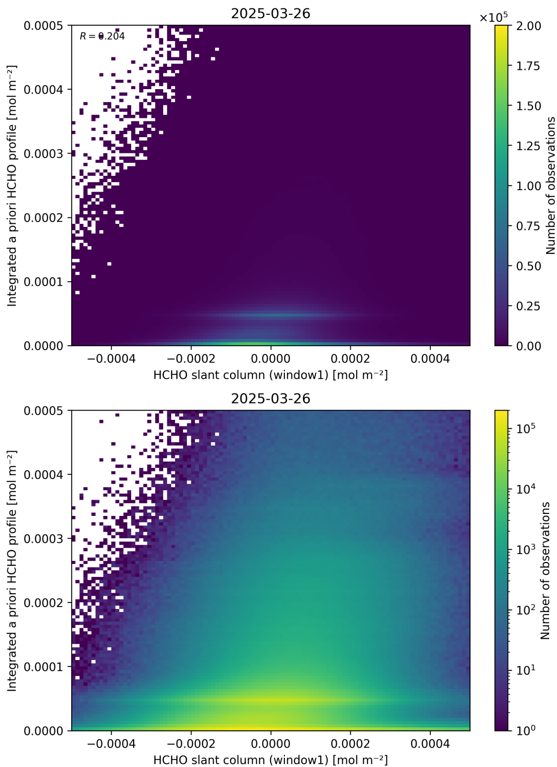
Figure 87: Scatter density plot of “HCHO slant column (window1)” against “Integrated a priori HCHO profile” for 2025-03-25 to 2025-03-27.
