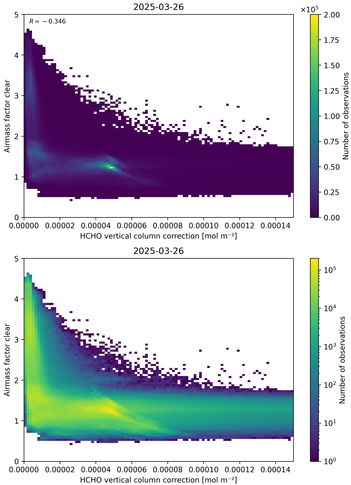
Figure 115: Scatter density plot of “HCHO vertical column correction” against “Airmass factor clear” for 2025-03-25 to 2025-03-27.
