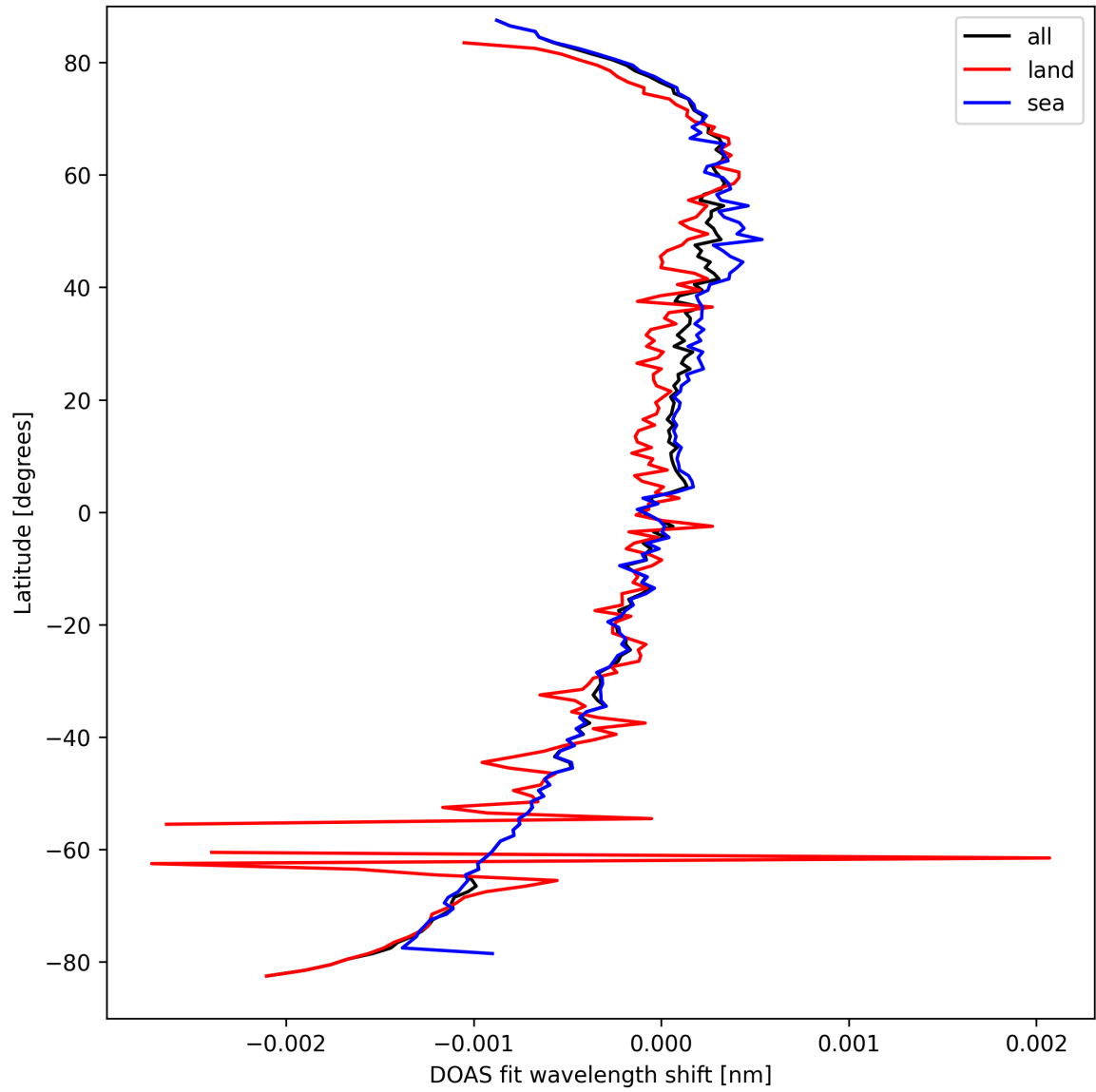
Figure 30: Zonal average of “DOAS fit wavelength shift” for 2025-03-25 to 2025-03-27.
