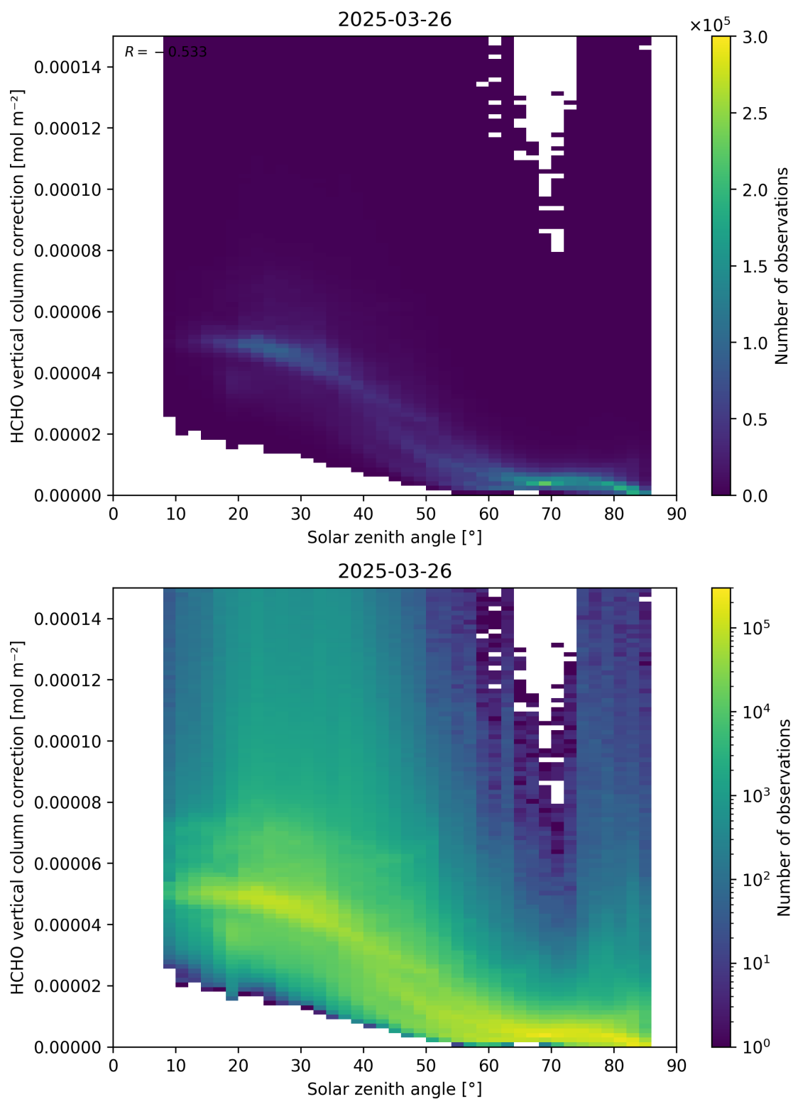
Figure 178: Scatter density plot of “Solar zenith angle” against “HCHO vertical column correction” for 2025-03-25 to 2025-03-27.
