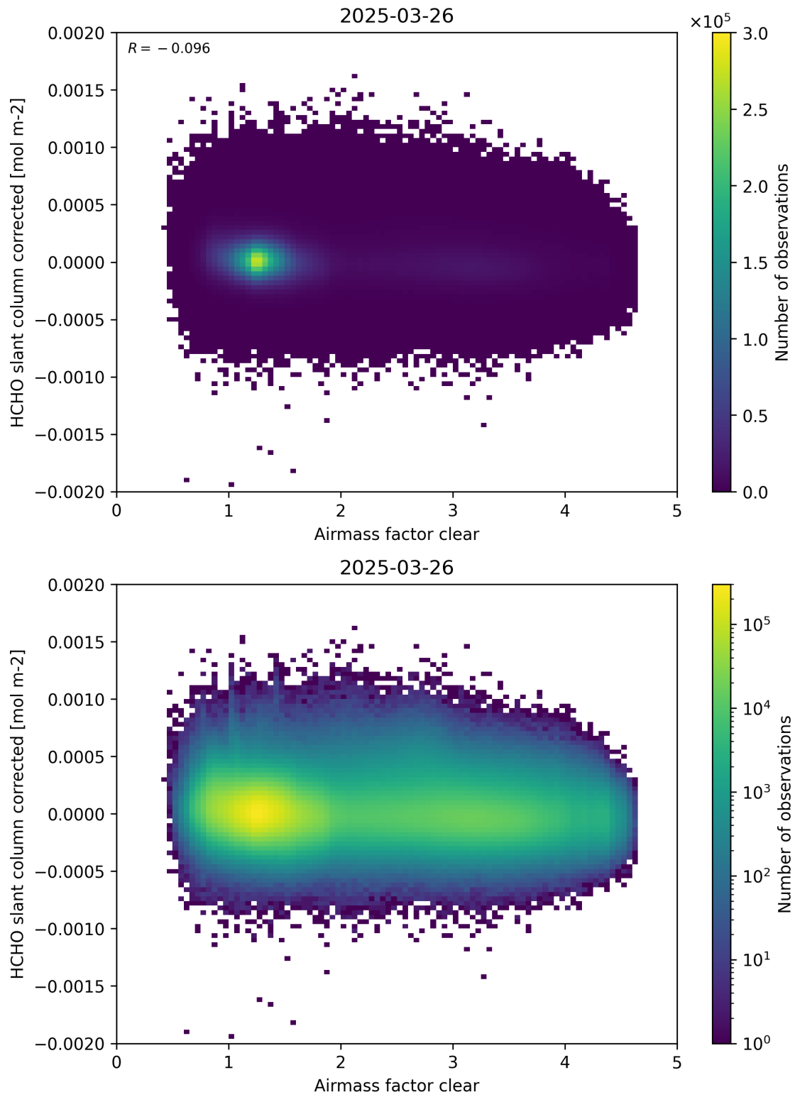
Figure 74: Scatter density plot of “Airmass factor clear” against “HCHO slant column corrected” for 2025-03-25 to 2025-03-27.
