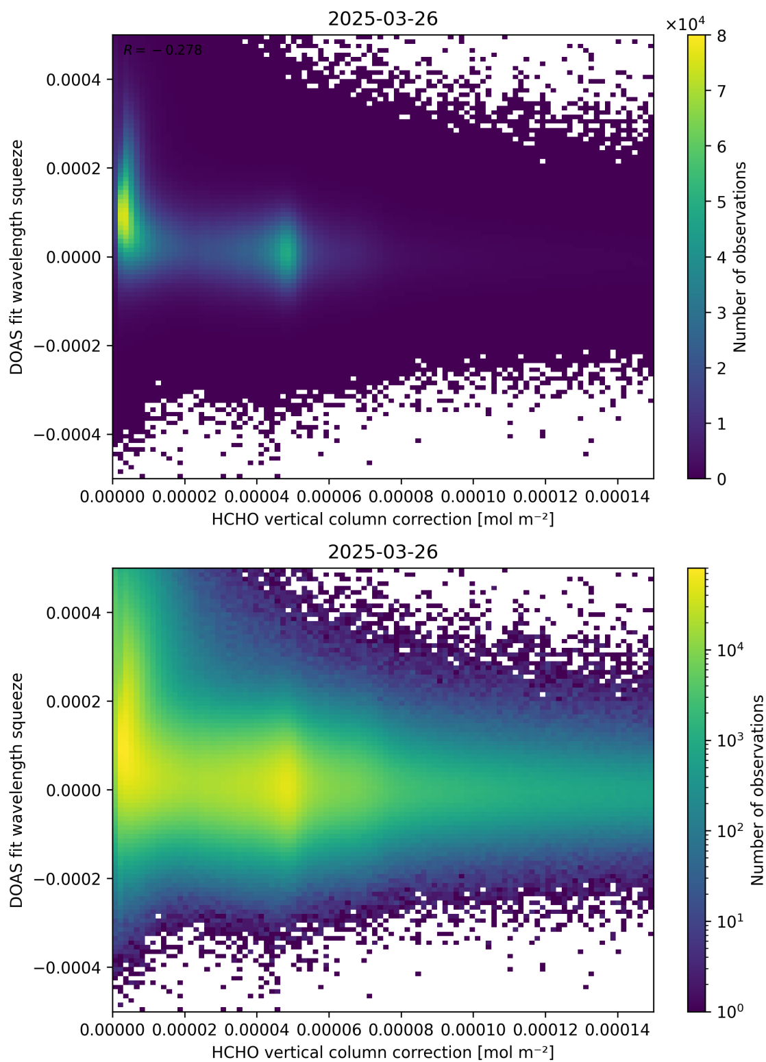
Figure 114: Scatter density plot of “HCHO vertical column correction” against “DOAS fit wavelength squeeze” for 2025-03-25 to 2025-03-27.
