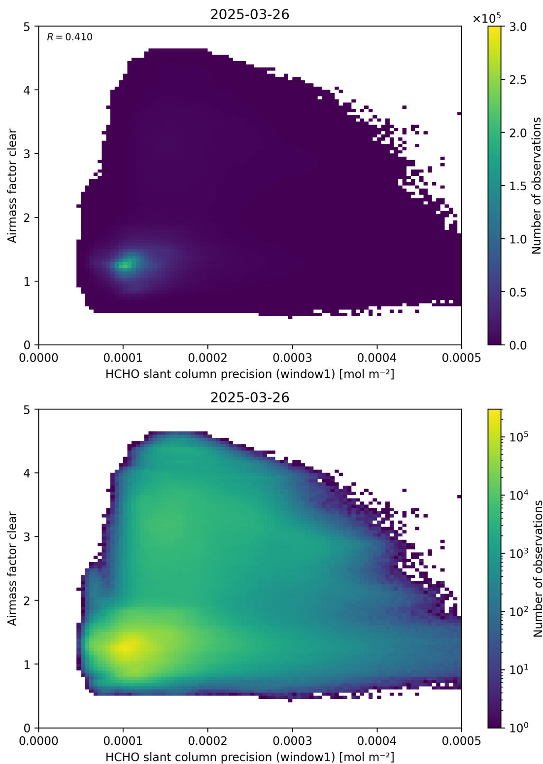
Figure 91: Scatter density plot of “HCHO slant column precision (window1)” against “Airmass factor clear” for 2025-03-25 to 2025-03-27.
