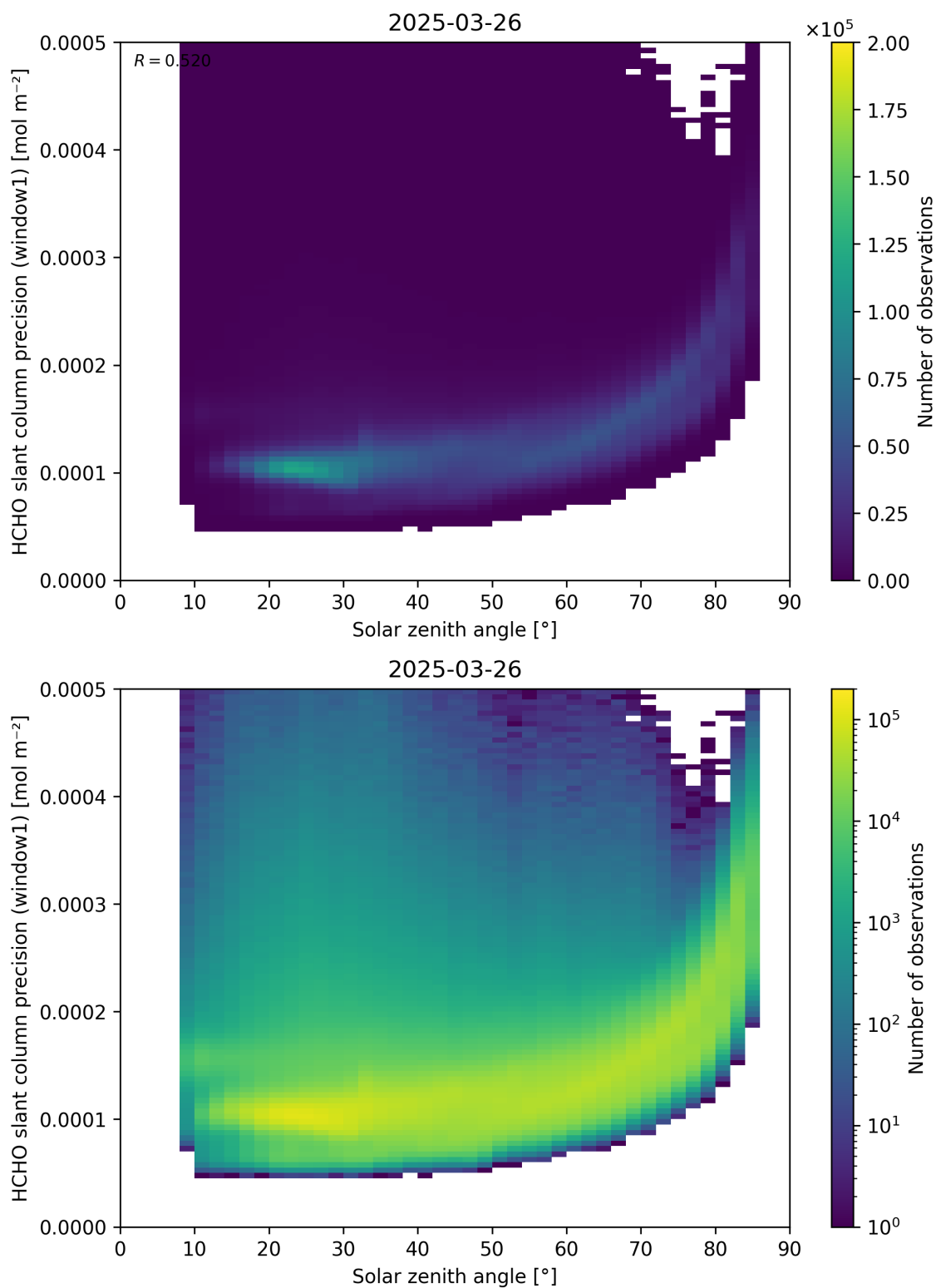
Figure 174: Scatter density plot of “Solar zenith angle” against “HCHO slant column precision (window1)” for 2025-03-25 to 2025-03-27.
