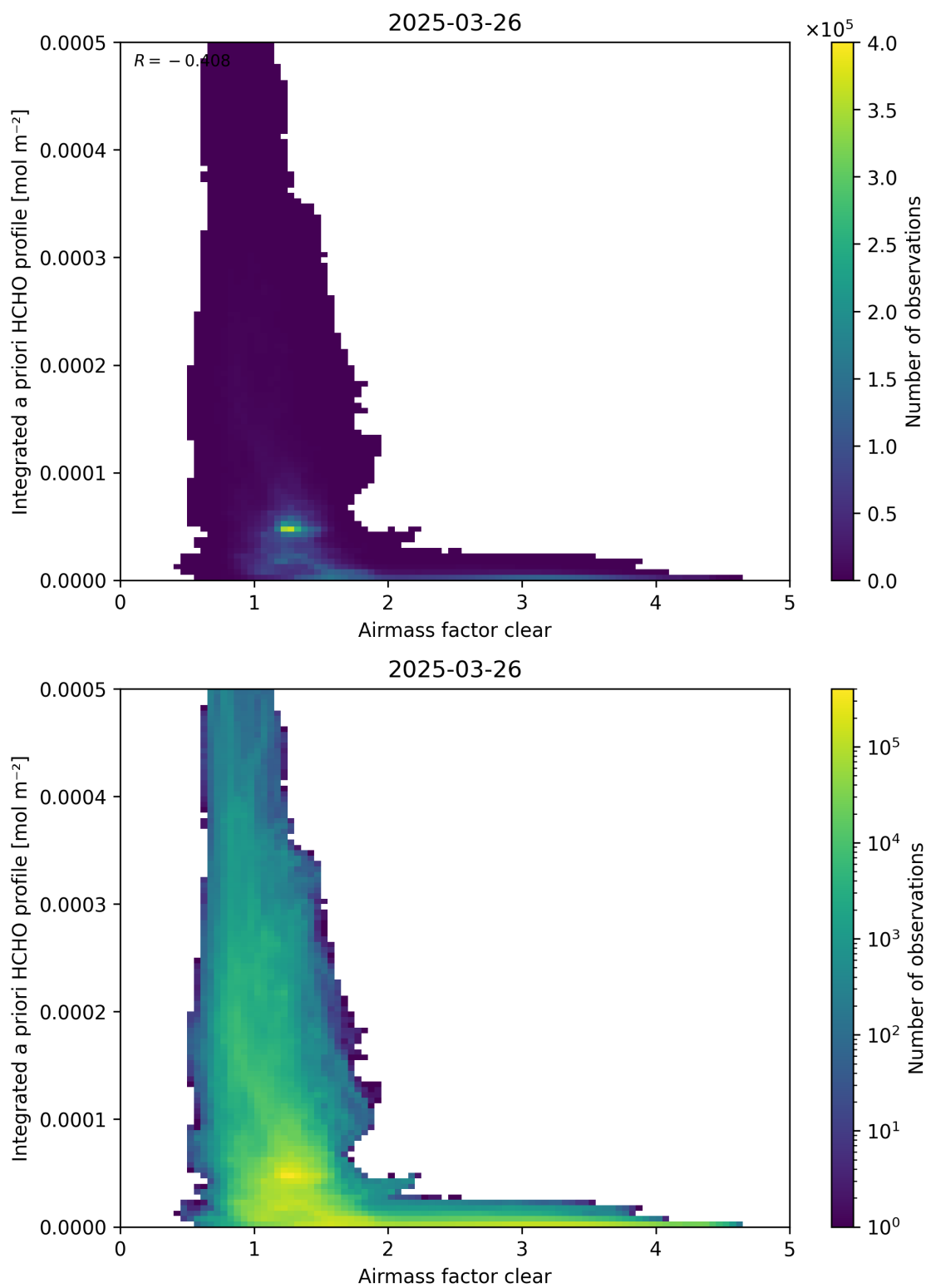
Figure 76: Scatter density plot of “Airmass factor clear” against “Integrated a priori HCHO profile” for 2025-03-25 to 2025-03-27.
