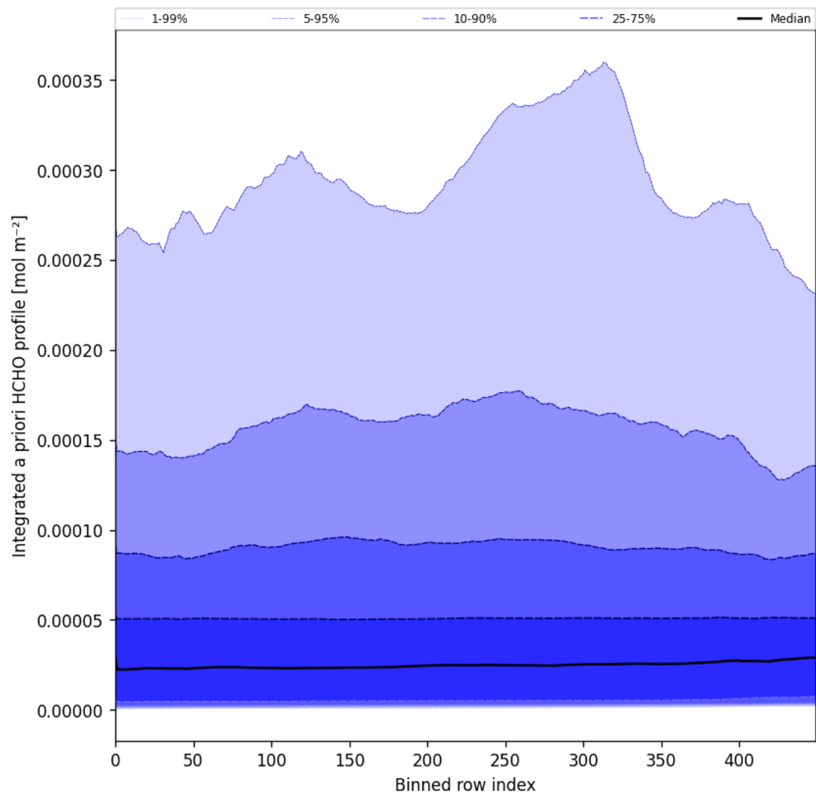
Figure 57: Along track statistics of “Integrated a priori HCHO profile” for 2025-03-25 to 2025-03-27
