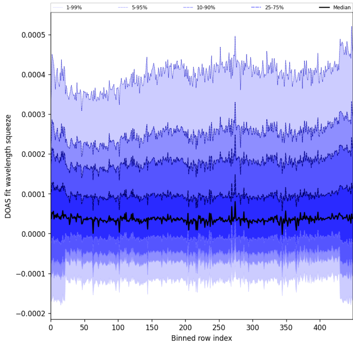
Figure 59: Along track statistics of “DOAS fit wavelength squeeze” for 2025-03-25 to 2025-03-27
