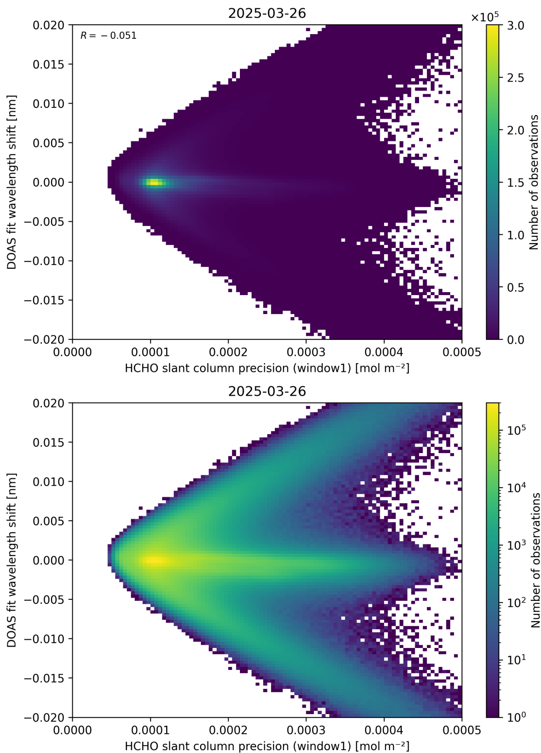
Figure 89: Scatter density plot of “HCHO slant column precision (window1)” against “DOAS fit wavelength shift” for 2025-03-25 to 2025-03-27.
