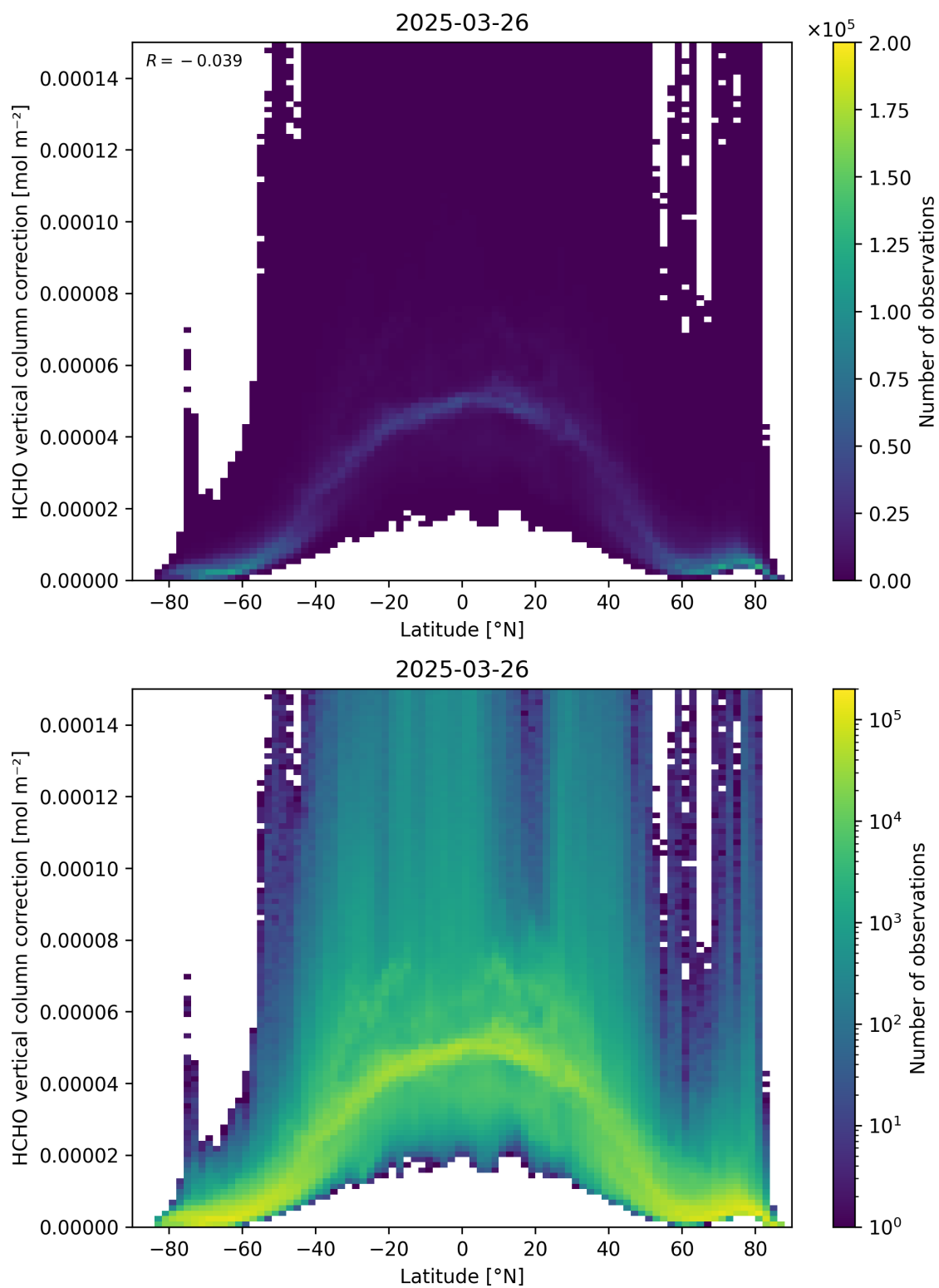
Figure 164: Scatter density plot of “Latitude” against “HCHO vertical column correction” for 2025-03-25 to 2025-03-27.
