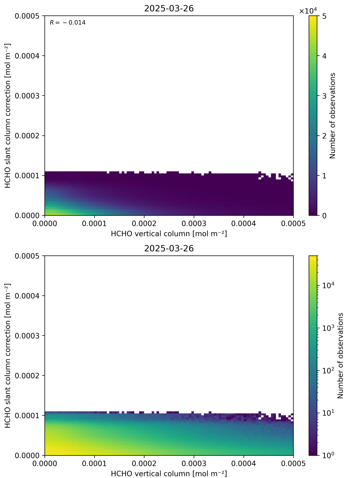
Figure 128: Scatter density plot of “HCHO vertical column” against “HCHO slant column correction” for 2025-03-25 to 2025-03-27.
