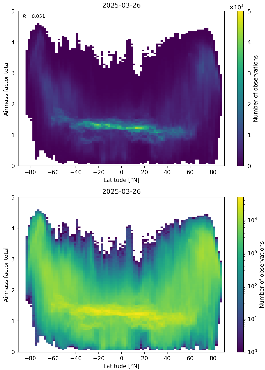
Figure 161: Scatter density plot of “Latitude” against “Airmass factor total” for 2025-03-25 to 2025-03-27.
