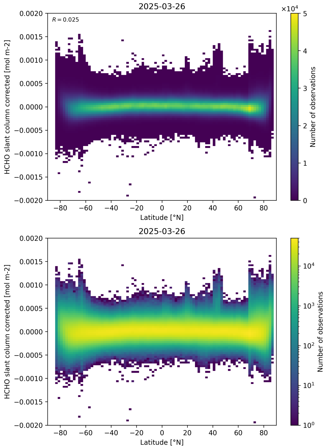
Figure 157: Scatter density plot of “Latitude” against “HCHO slant column corrected” for 2025-03-25 to 2025-03-27.
