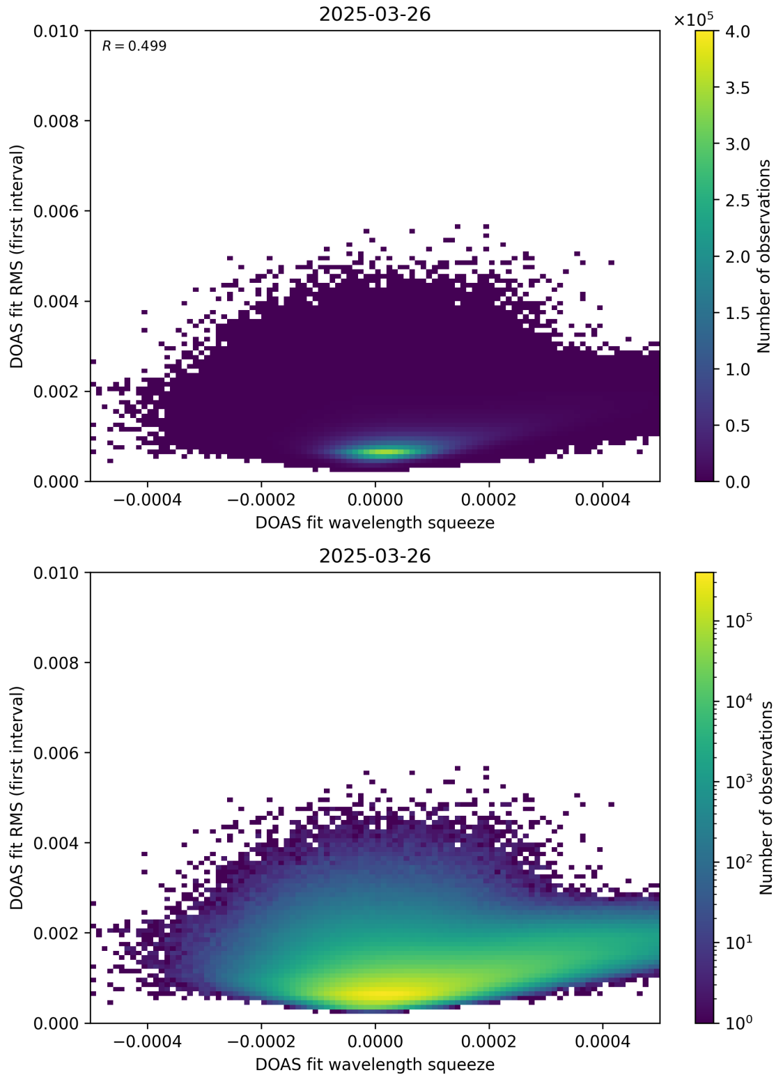
Figure 68: Scatter density plot of “DOAS fit wavelength squeeze” against “DOAS fit RMS (first interval)” for 2025-03-25 to 2025-03-27.
