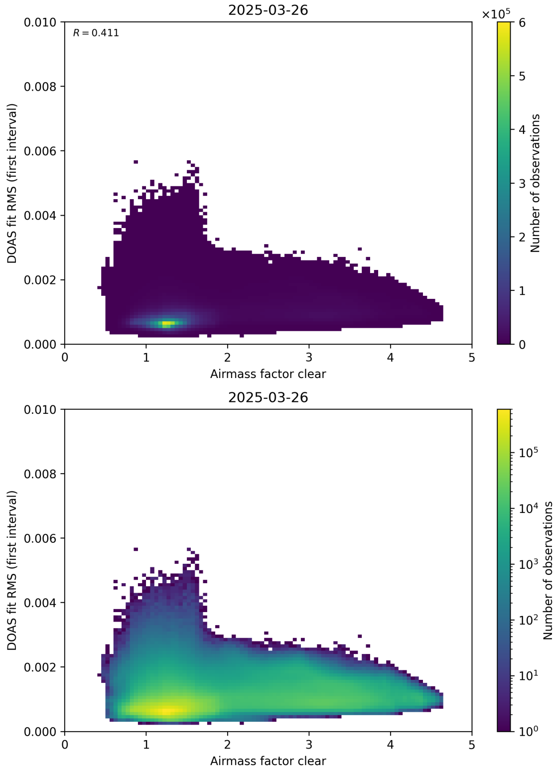
Figure 71: Scatter density plot of “Airmass factor clear” against “DOAS fit RMS (first interval)” for 2025-03-25 to 2025-03-27.
