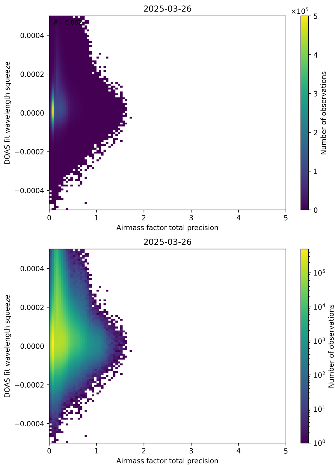
Figure 107: Scatter density plot of “Airmass factor total precision” against “DOAS fit wavelength squeeze” for 2025-03-25 to 2025-03-27.
