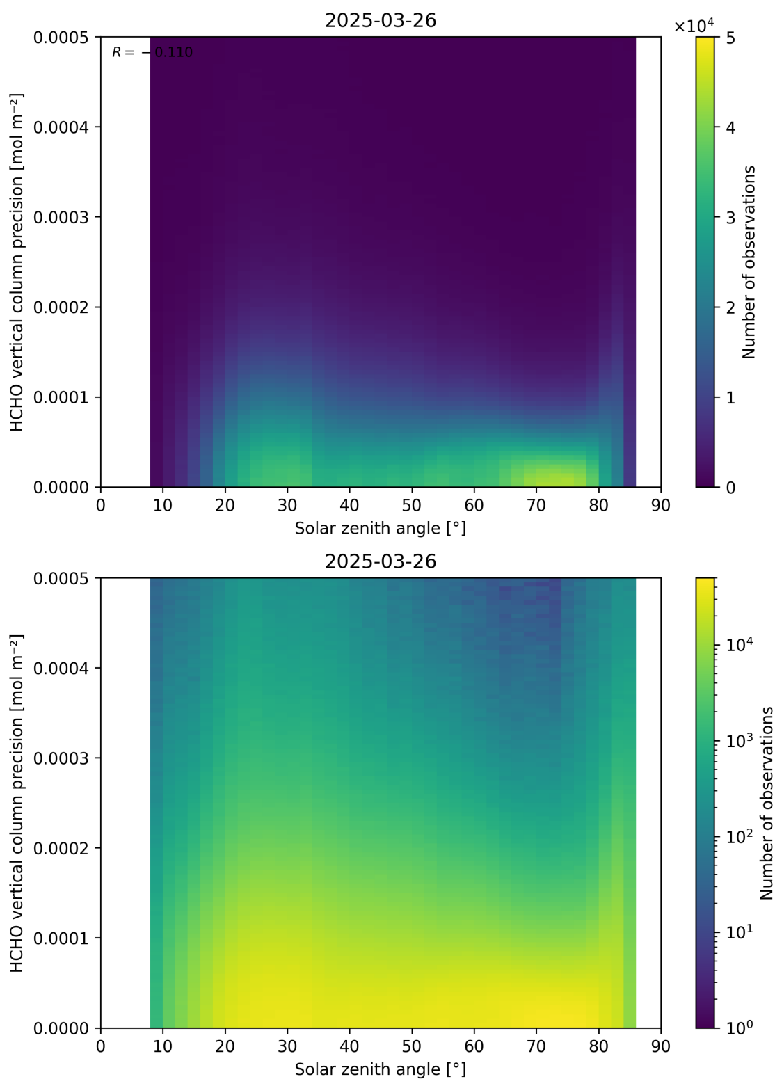
Figure 179: Scatter density plot of “Solar zenith angle” against “HCHO vertical column precision” for 2025-03-25 to 2025-03-27.
