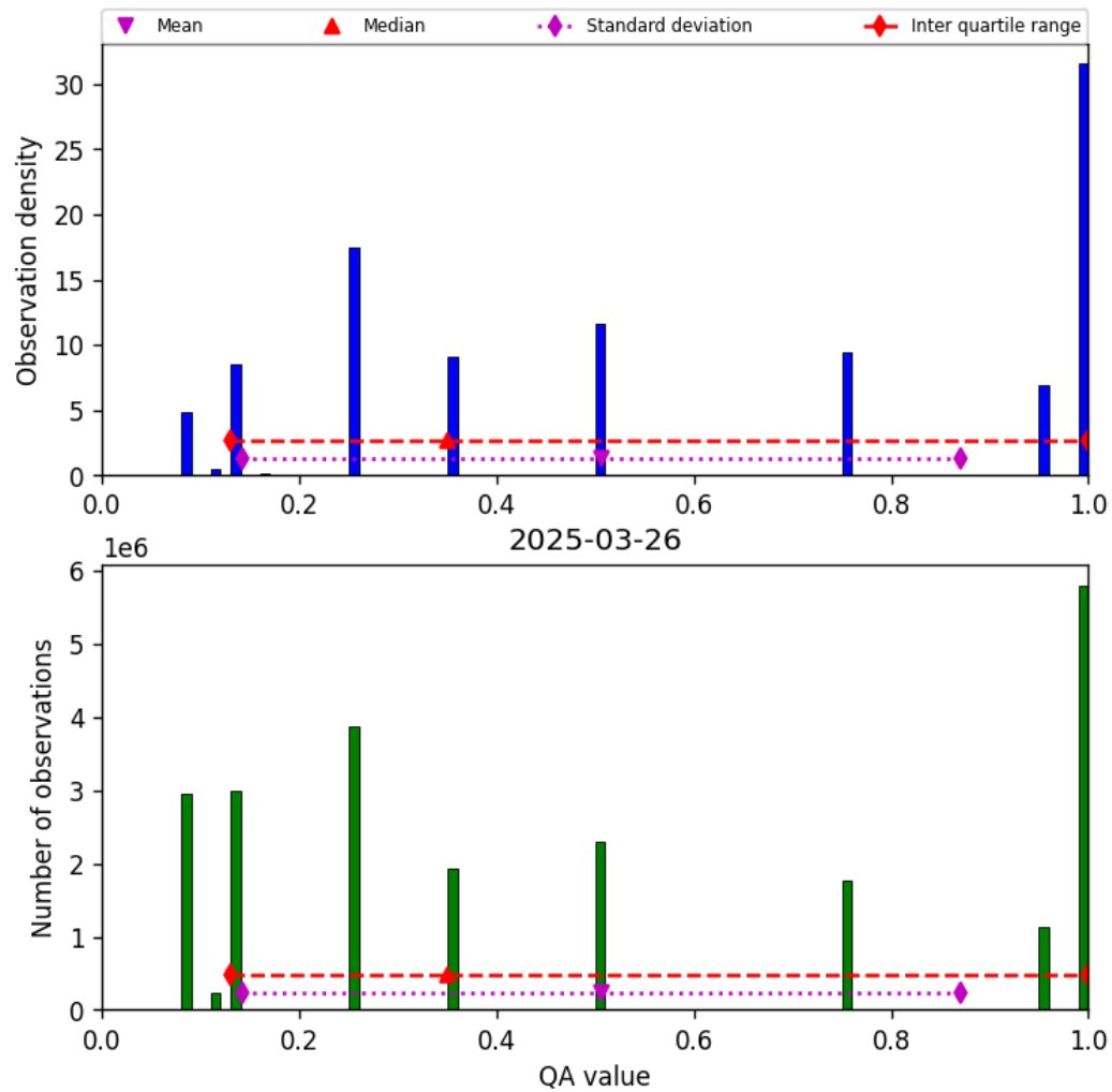
Figure 34: Histogram of “QA value” for 2025-03-25 to 2025-03-27
