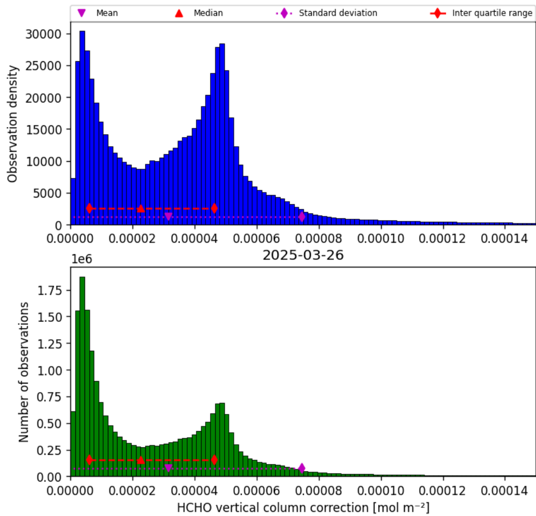
Figure 37: Histogram of “HCHO vertical column correction” for 2025-03-25 to 2025-03-27
