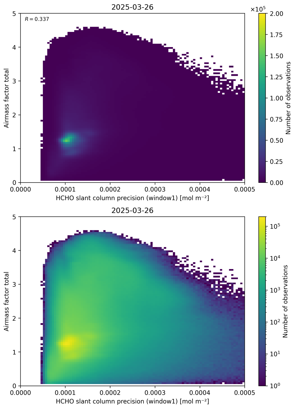
Figure 94: Scatter density plot of “HCHO slant column precision (window1)” against “Airmass factor total” for 2025-03-25 to 2025-03-27.
