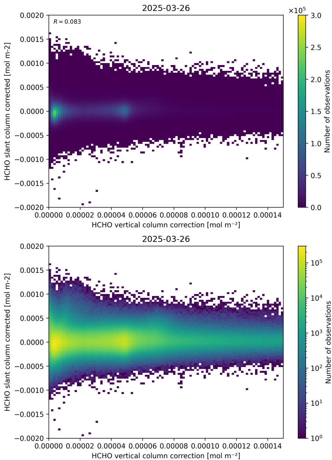
Figure 116: Scatter density plot of “HCHO vertical column correction” against “HCHO slant column corrected” for 2025-03-25 to 2025-03-27.
