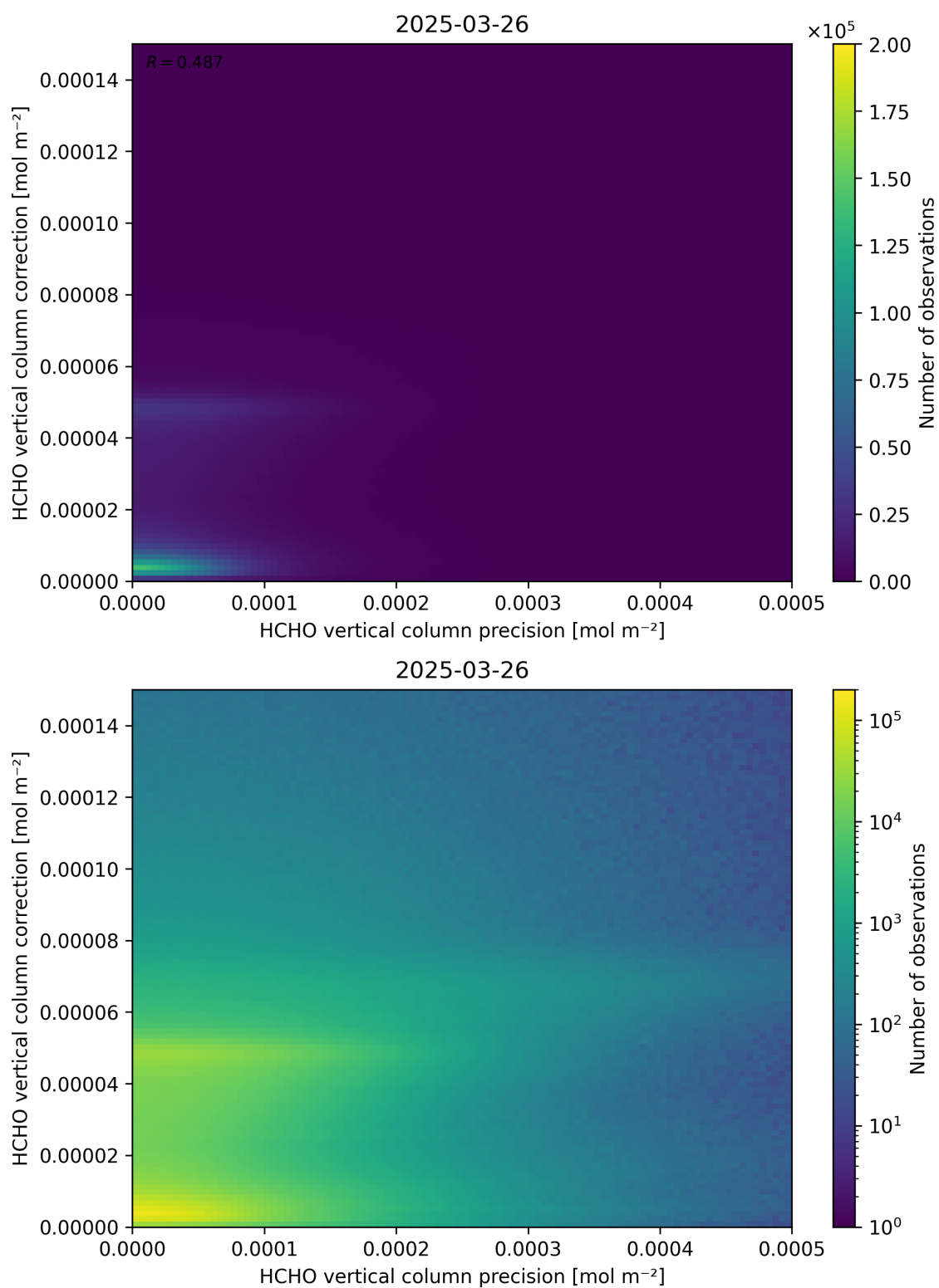
Figure 146: Scatter density plot of “HCHO vertical column precision” against “HCHO vertical column correction” for 2025-03-25 to 2025-03-27.
