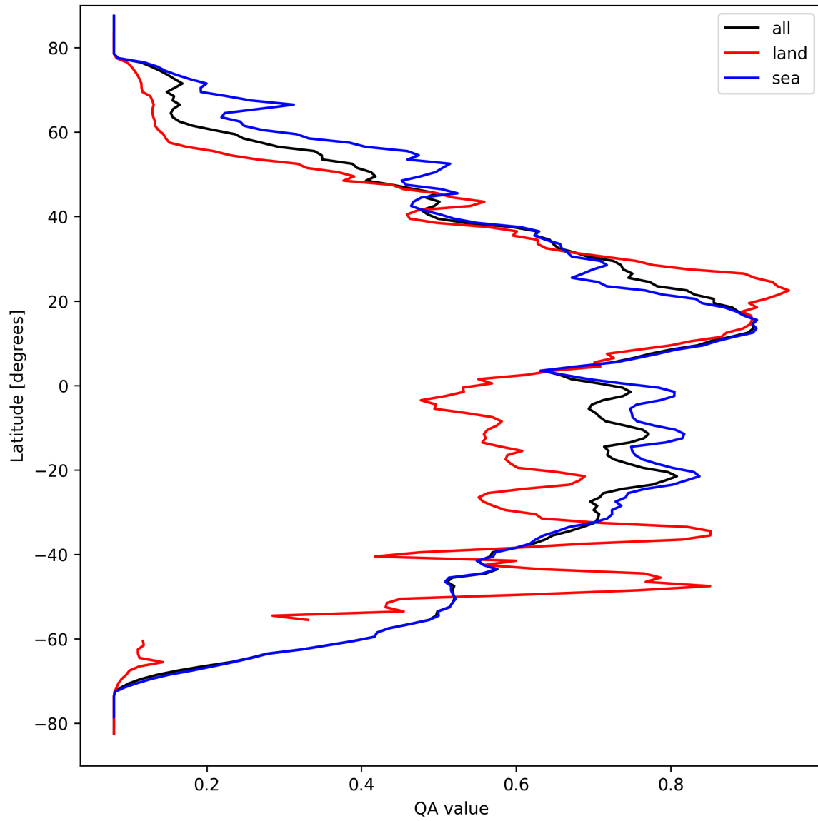
Figure 20: Zonal average of “QA value” for 2025-03-25 to 2025-03-27.
