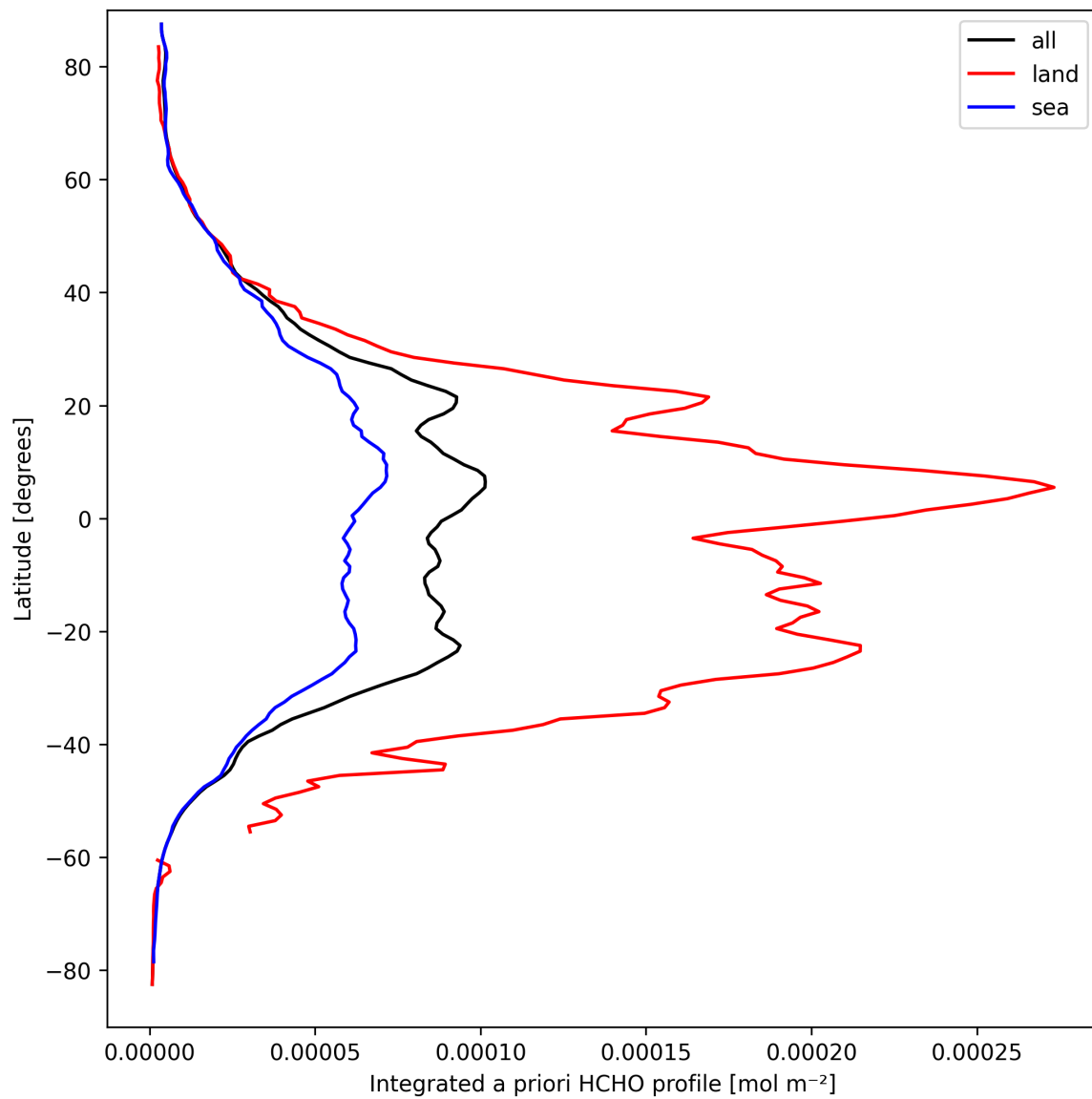
Figure 29: Zonal average of “Integrated a priori HCHO profile” for 2025-03-25 to 2025-03-27.
