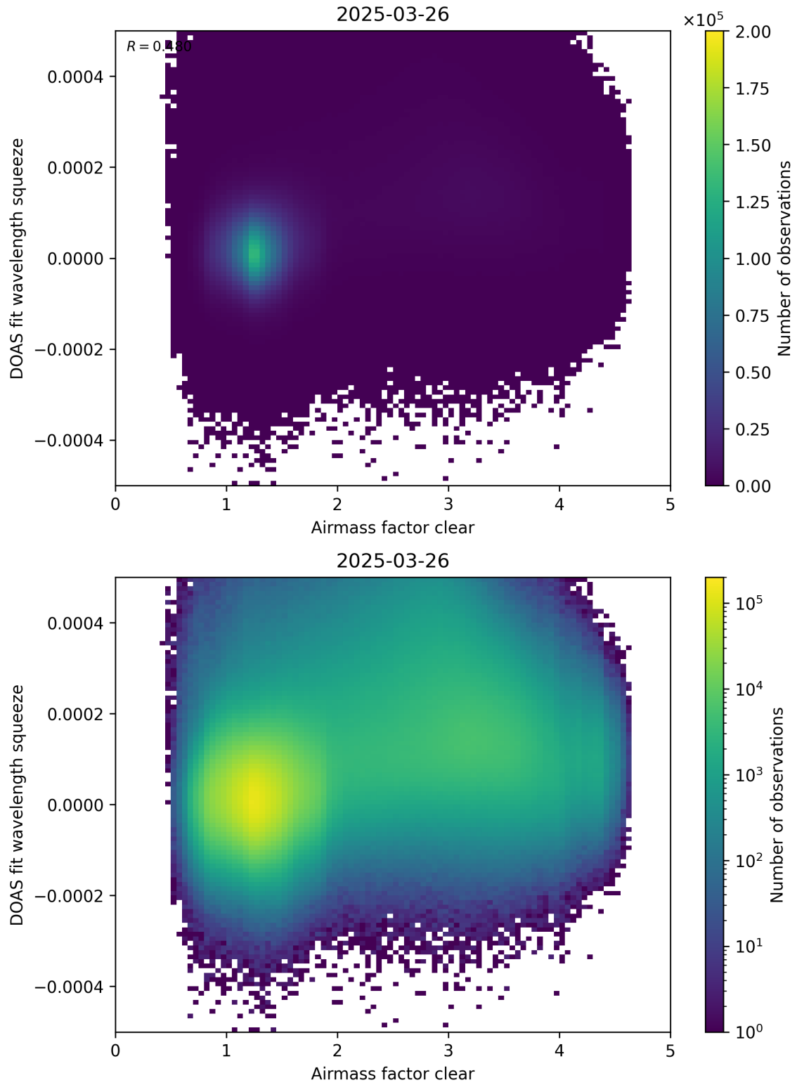
Figure 73: Scatter density plot of “Airmass factor clear” against “DOAS fit wavelength squeeze” for 2025-03-25 to 2025-03-27.
