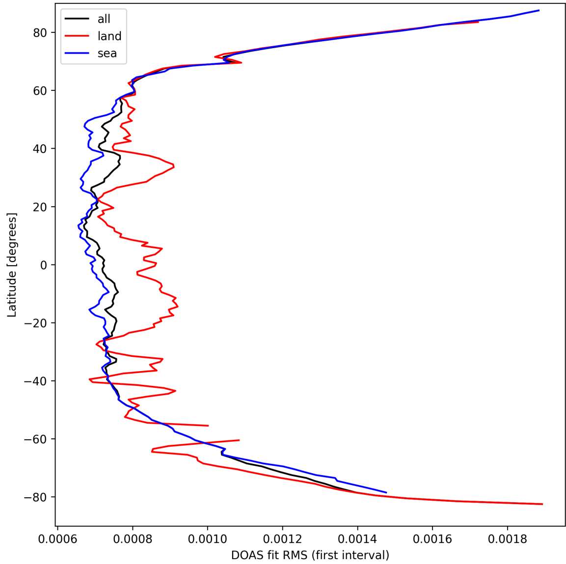
Figure 32: Zonal average of “DOAS fit RMS (first interval)” for 2025-03-25 to 2025-03-27.
