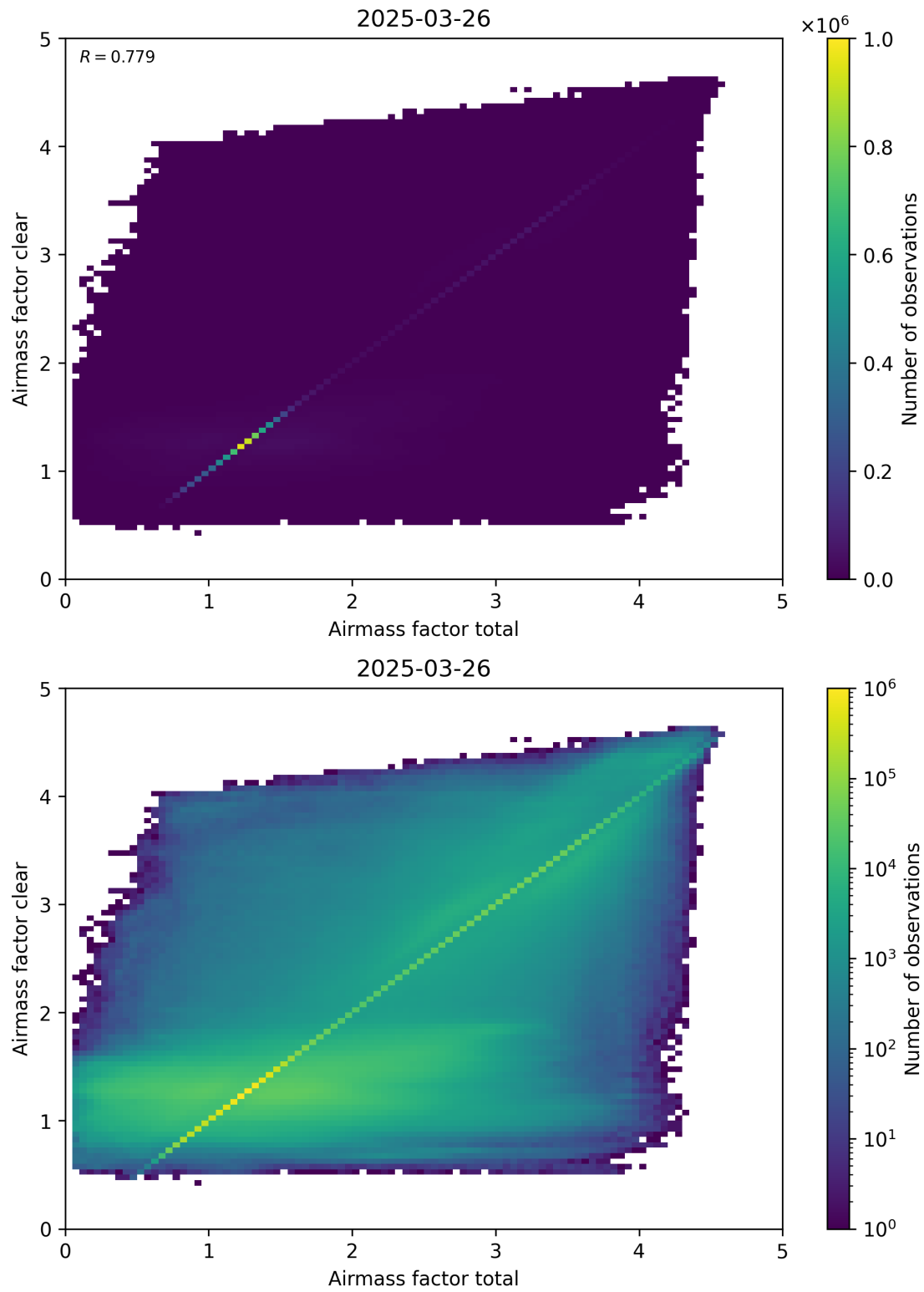
Figure 100: Scatter density plot of “Airmass factor total” against “Airmass factor clear” for 2025-03-25 to 2025-03-27.
