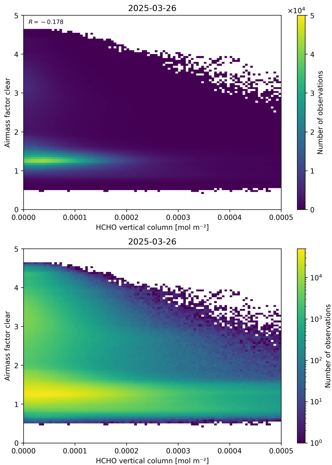
Figure 126: Scatter density plot of “HCHO vertical column” against “Airmass factor clear” for 2025-03-25 to 2025-03-27.
