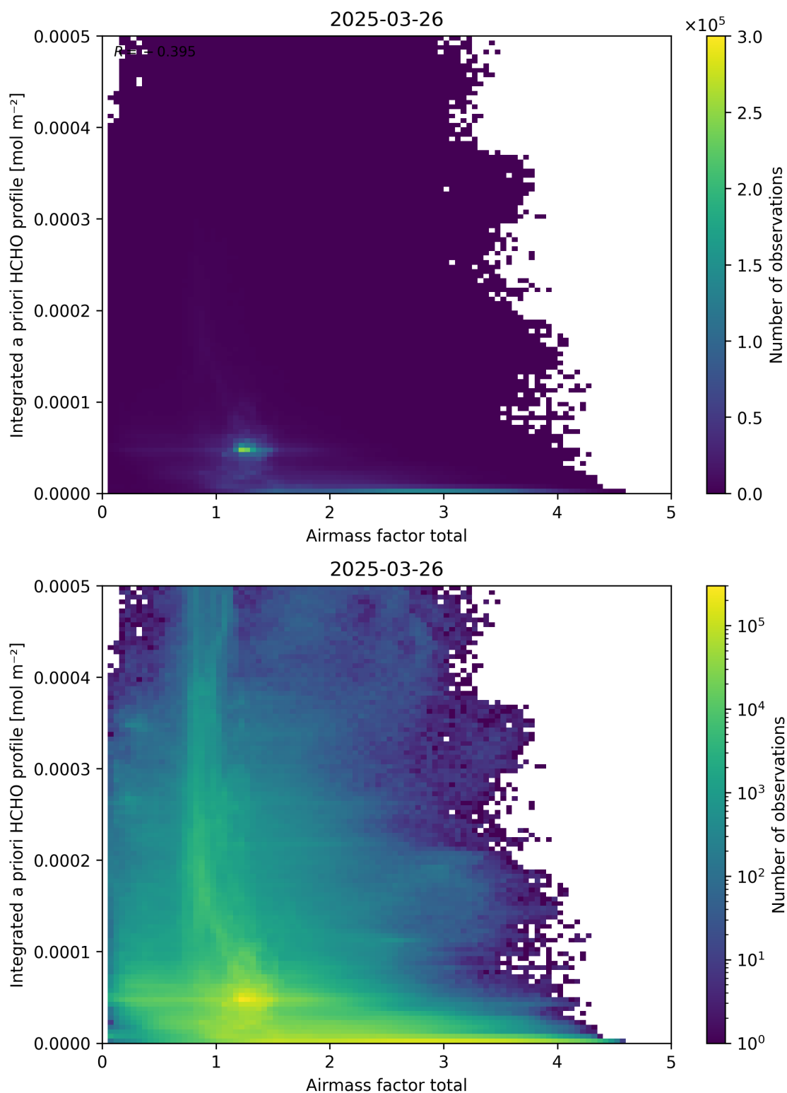
Figure 104: Scatter density plot of “Airmass factor total” against “Integrated a priori HCHO profile” for 2025-03-25 to 2025-03-27.
