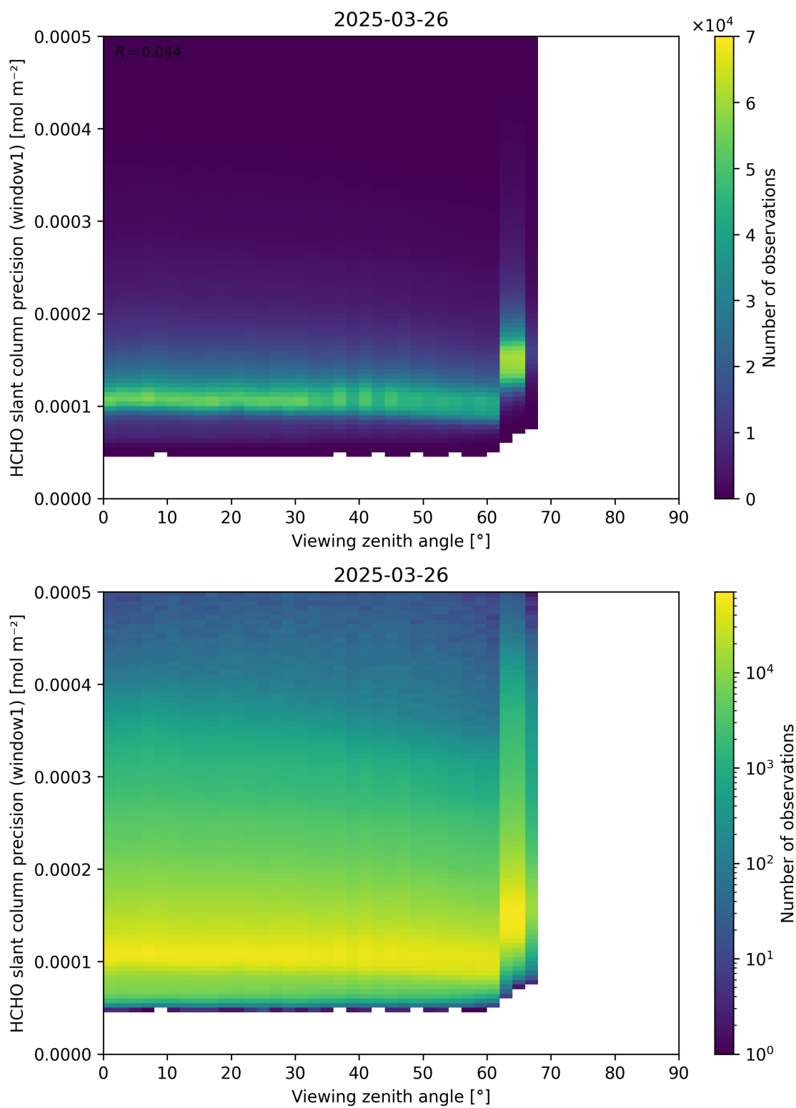
Figure 189: Scatter density plot of “Viewing zenith angle” against “HCHO slant column precision (window1)” for 2025-03-25 to 2025-03-27.
