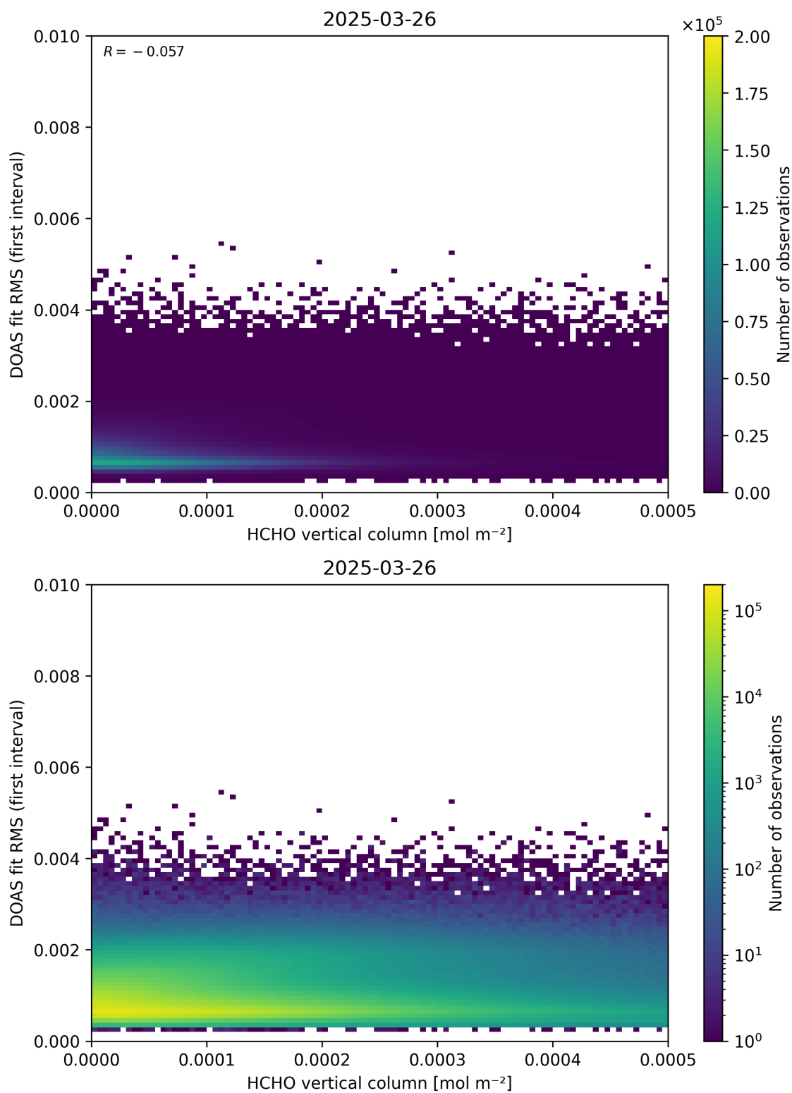
Figure 123: Scatter density plot of “HCHO vertical column” against “DOAS fit RMS (first interval)” for 2025-03-25 to 2025-03-27.
