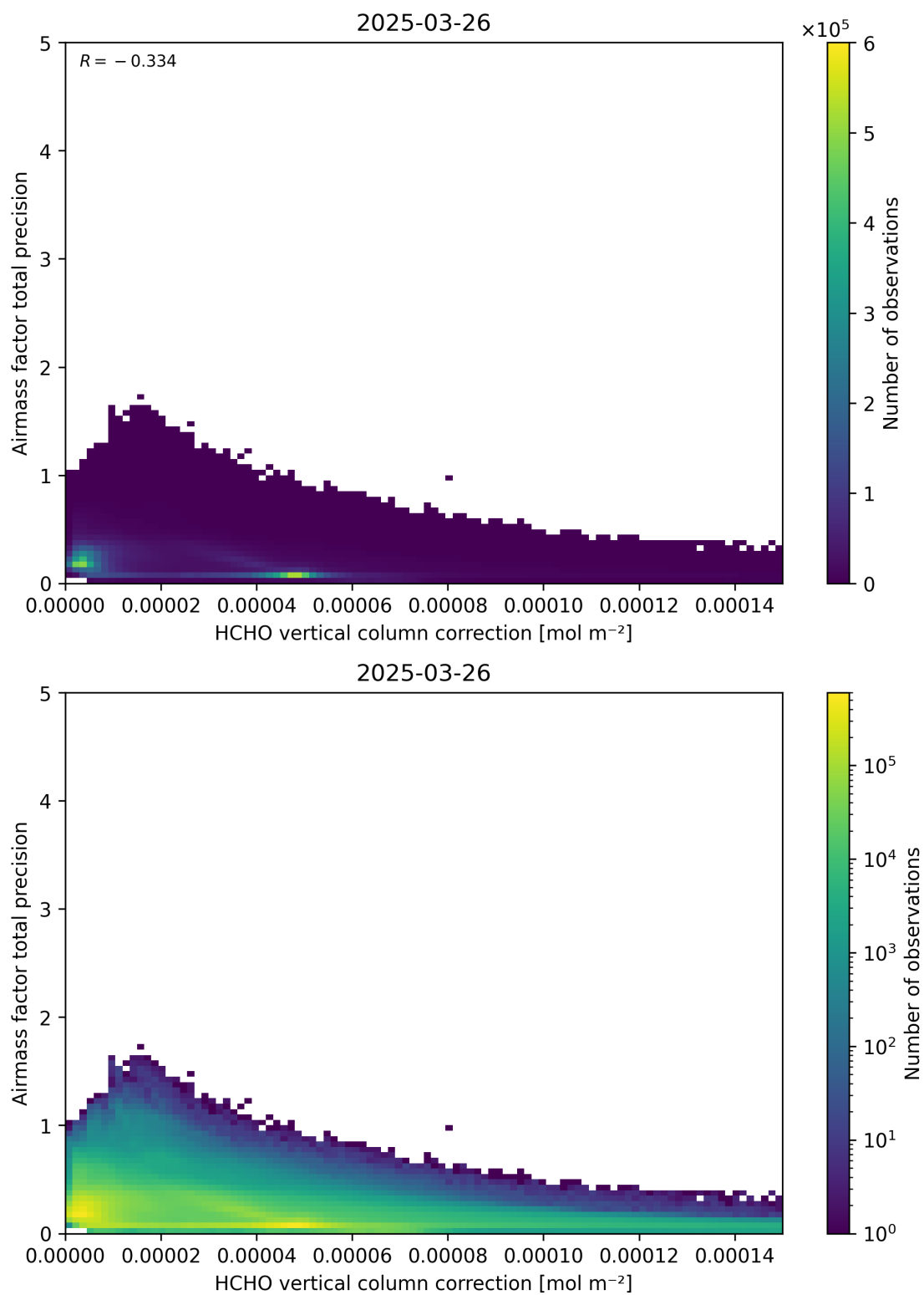
Figure 121: Scatter density plot of “HCHO vertical column correction” against “Airmass factor total precision” for 2025-03-25 to 2025-03-27.
