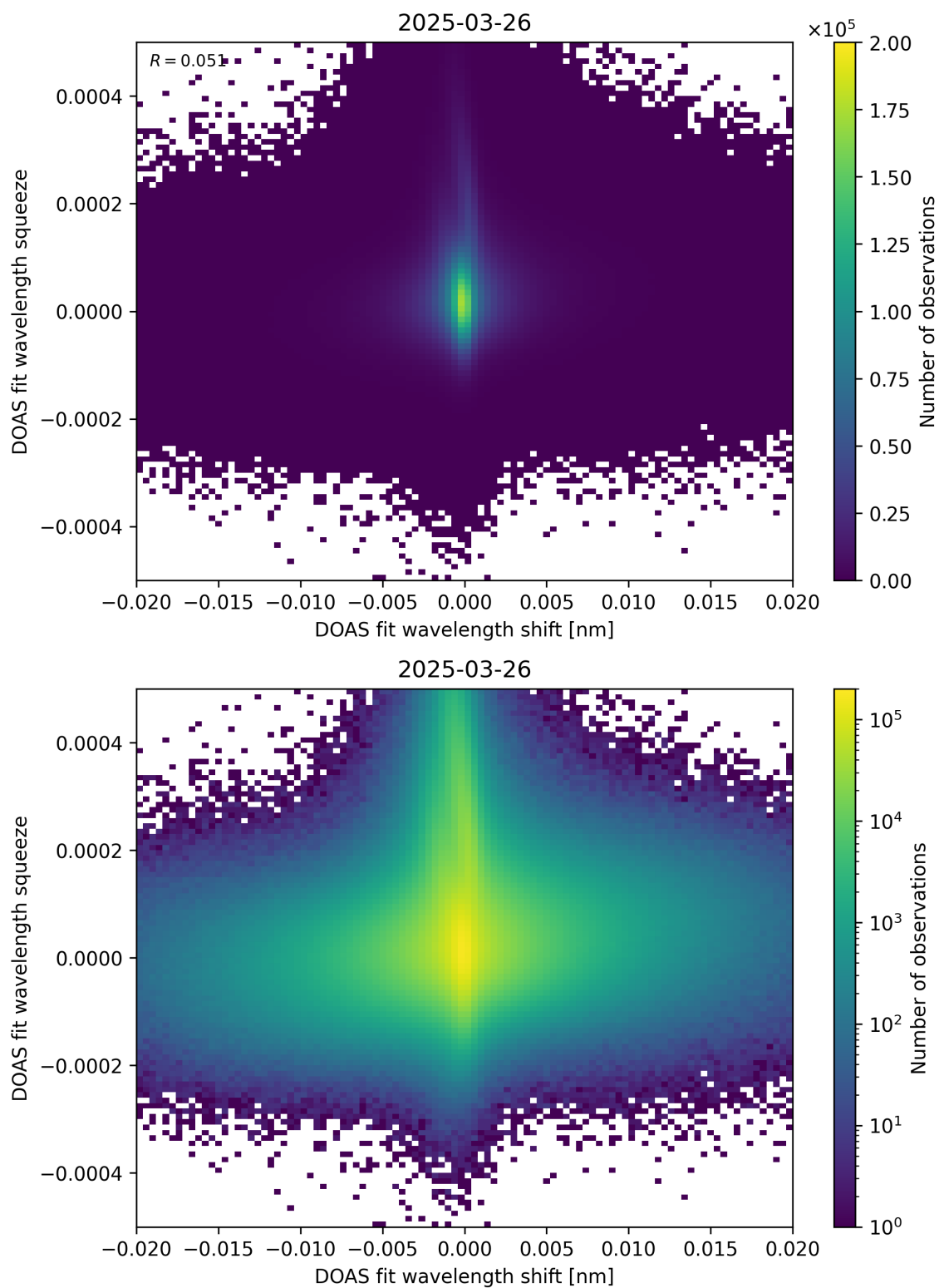
Figure 65: Scatter density plot of “DOAS fit wavelength shift” against “DOAS fit wavelength squeeze” for 2025-03-25 to 2025-03-27.
