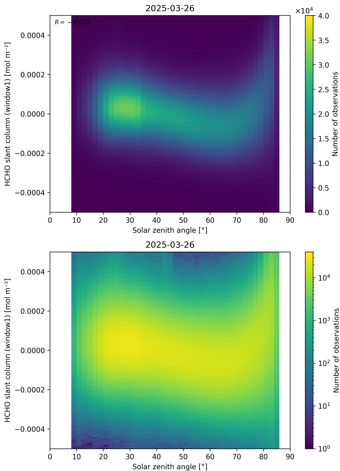
Figure 173: Scatter density plot of “Solar zenith angle” against “HCHO slant column (window1)” for 2025-03-25 to 2025-03-27.
