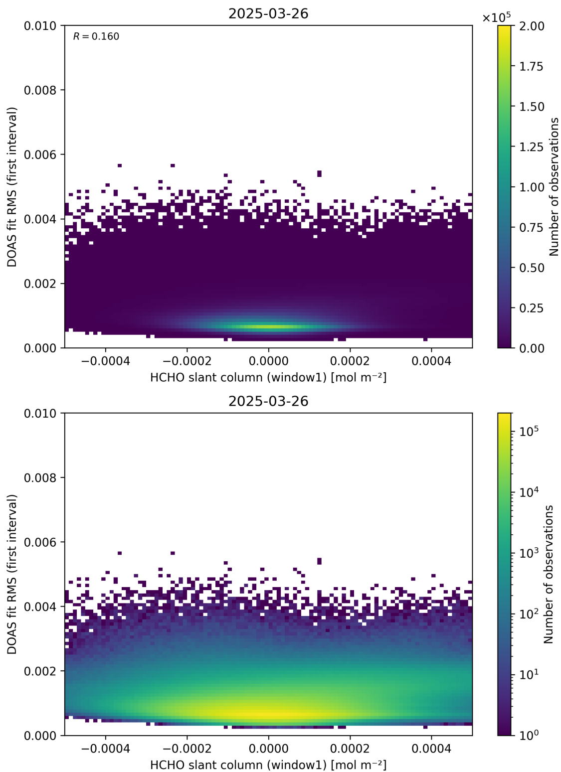
Figure 78: Scatter density plot of “HCHO slant column (window1)” against “DOAS fit RMS (first interval)” for 2025-03-25 to 2025-03-27.
