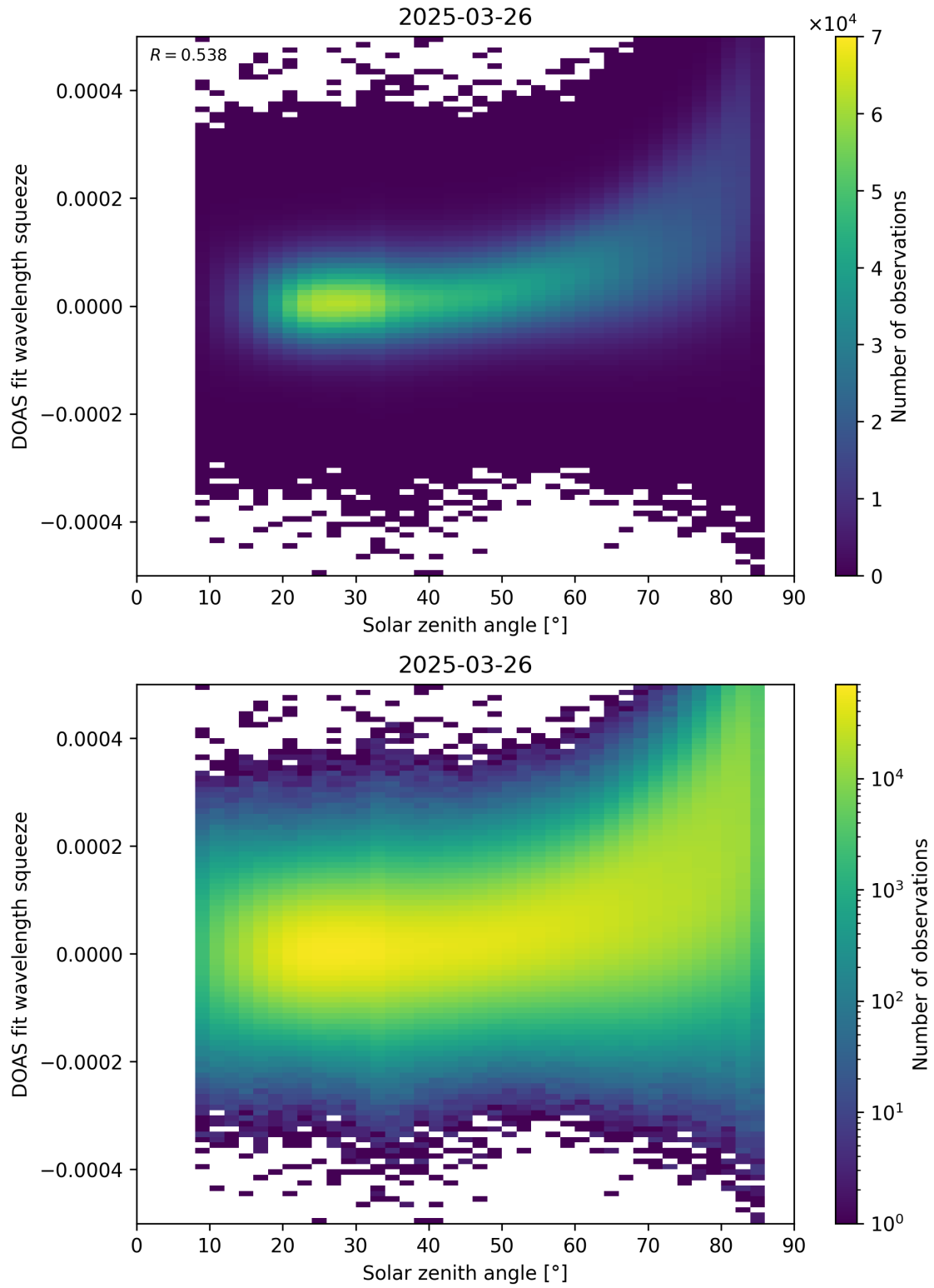
Figure 169: Scatter density plot of “Solar zenith angle” against “DOAS fit wavelength squeeze” for 2025-03-25 to 2025-03-27.
