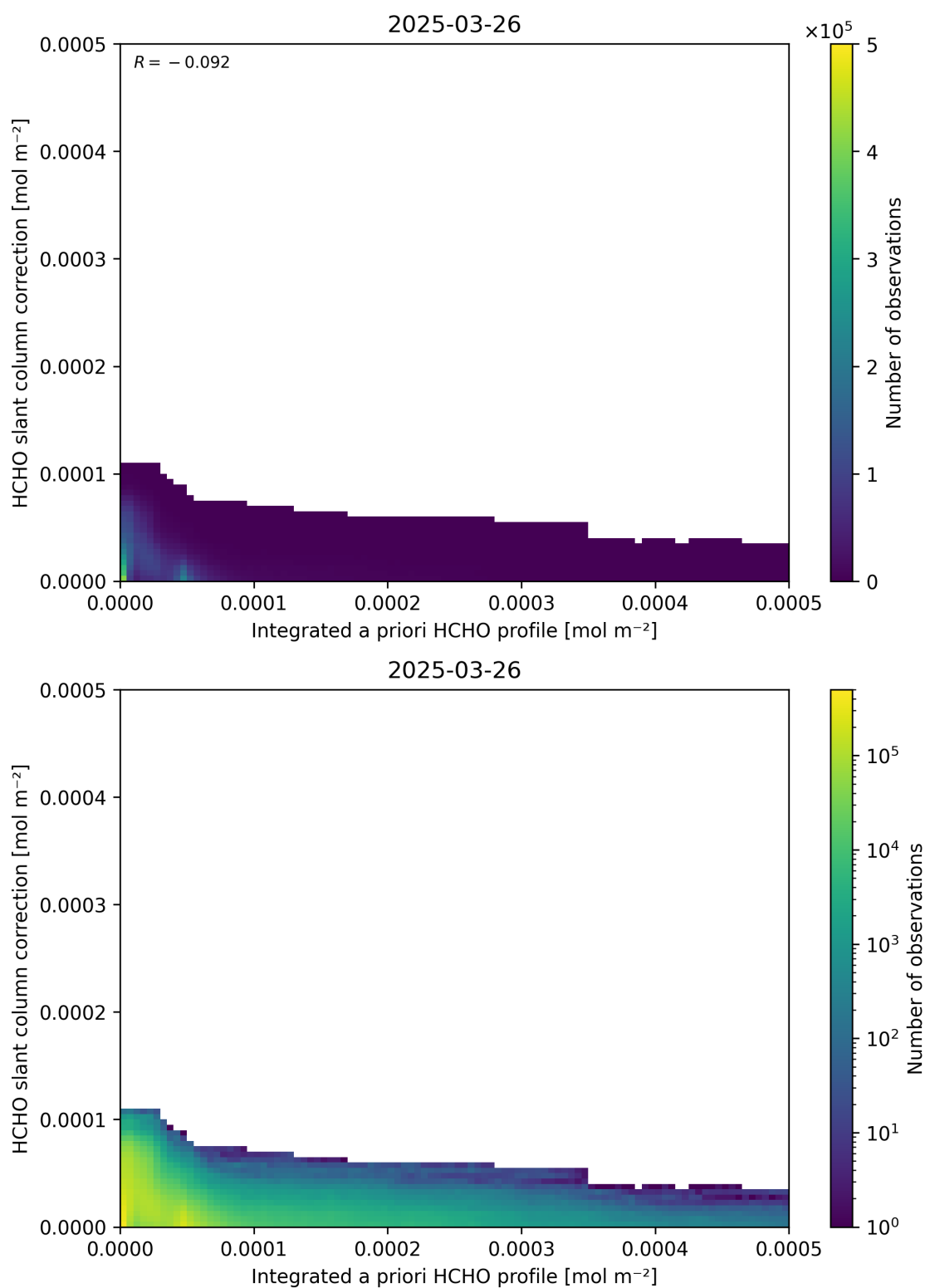
Figure 152: Scatter density plot of “Integrated a priori HCHO profile” against “HCHO slant column correction” for 2025-03-25 to 2025-03-27.
