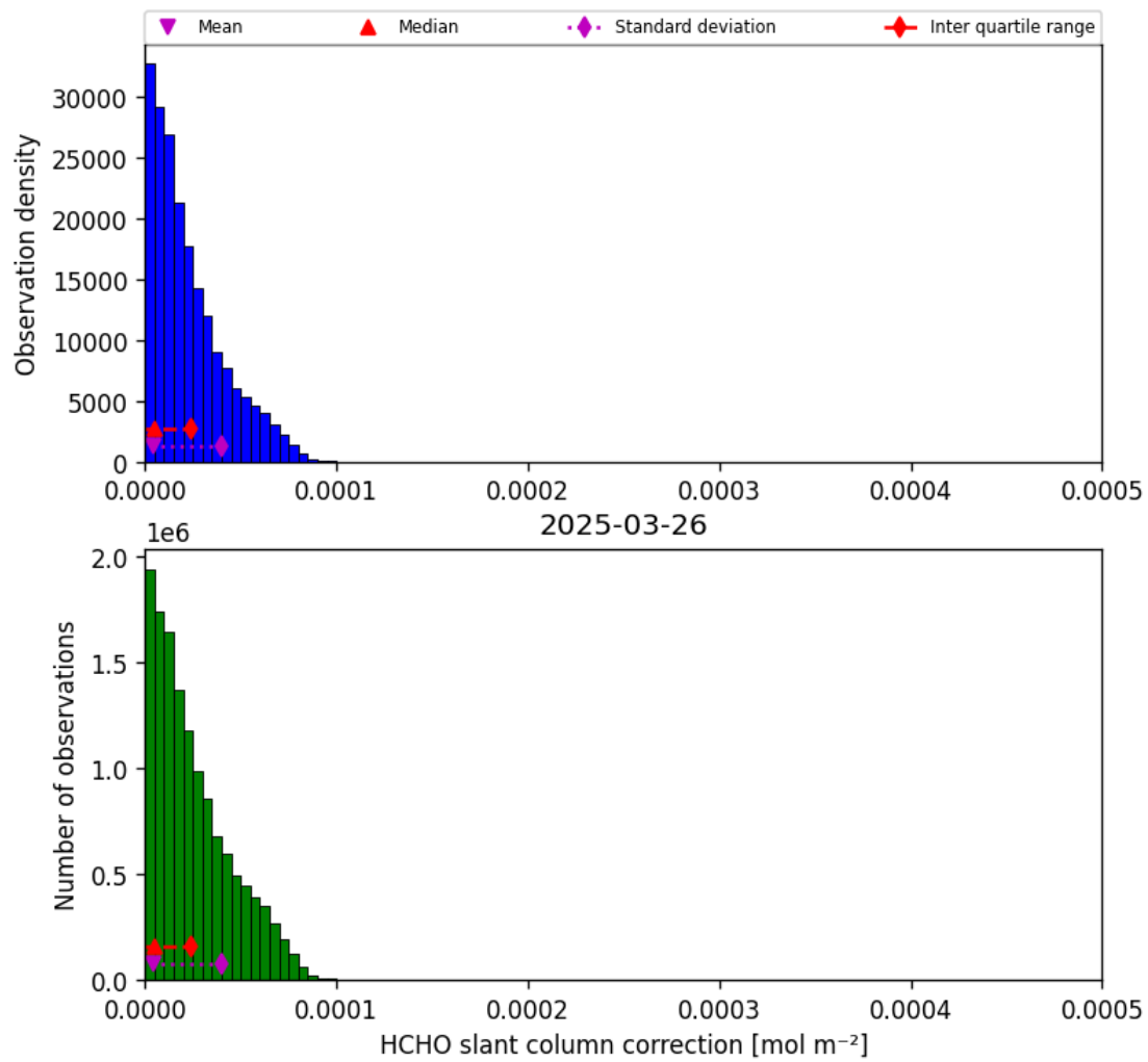
Figure 47: Histogram of “HCHO slant column correction” for 2025-03-25 to 2025-03-27
