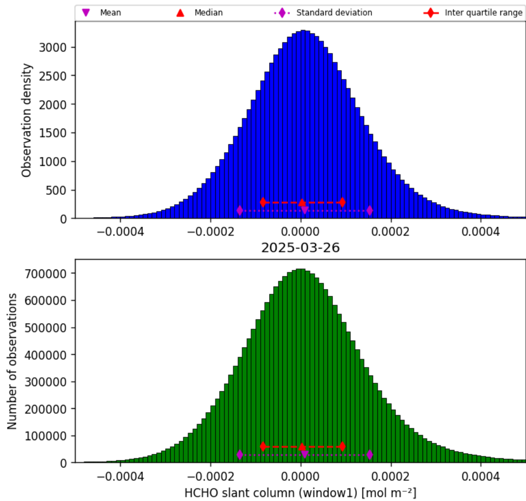
Figure 38: Histogram of “HCHO slant column (window1)” for 2025-03-25 to 2025-03-27
