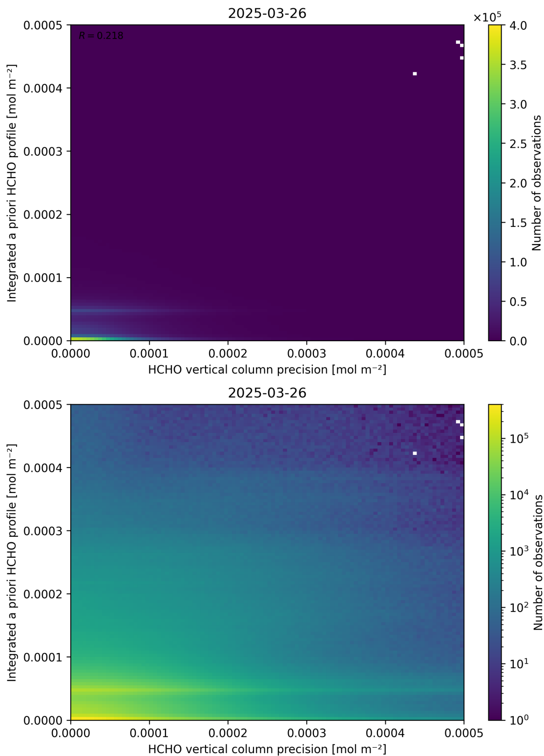
Figure 147: Scatter density plot of “HCHO vertical column precision” against “Integrated a priori HCHO profile” for 2025-03-25 to 2025-03-27.
