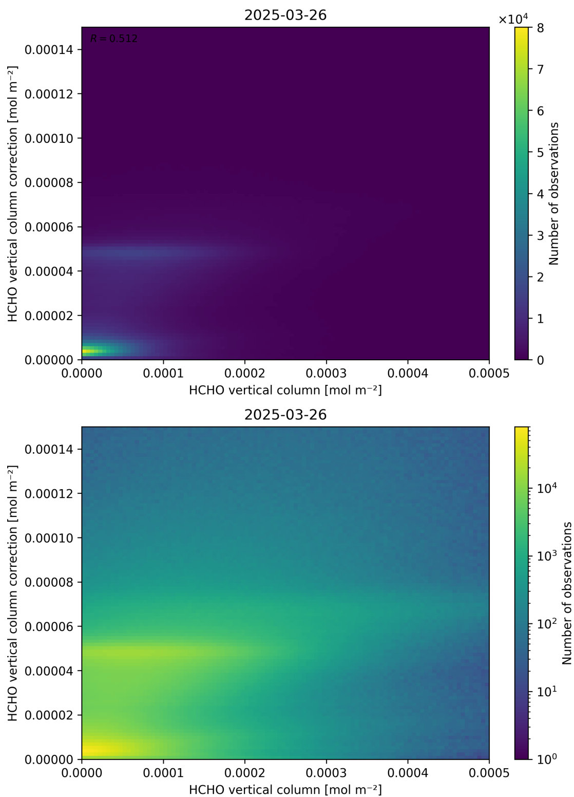
Figure 133: Scatter density plot of “HCHO vertical column” against “HCHO vertical column correction” for 2025-03-25 to 2025-03-27.
