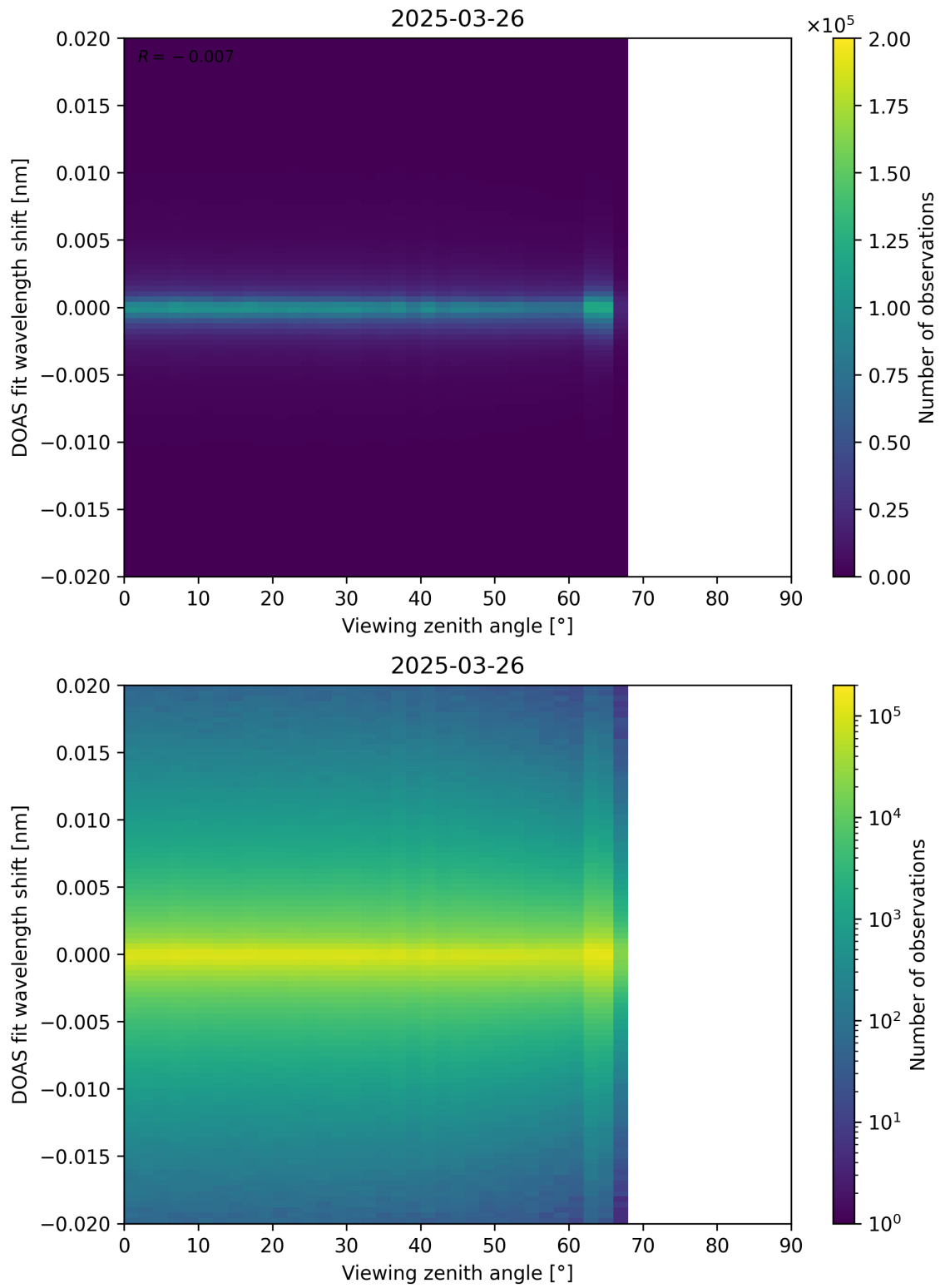
Figure 183: Scatter density plot of “Viewing zenith angle” against “DOAS fit wavelength shift” for 2025-03-25 to 2025-03-27.
