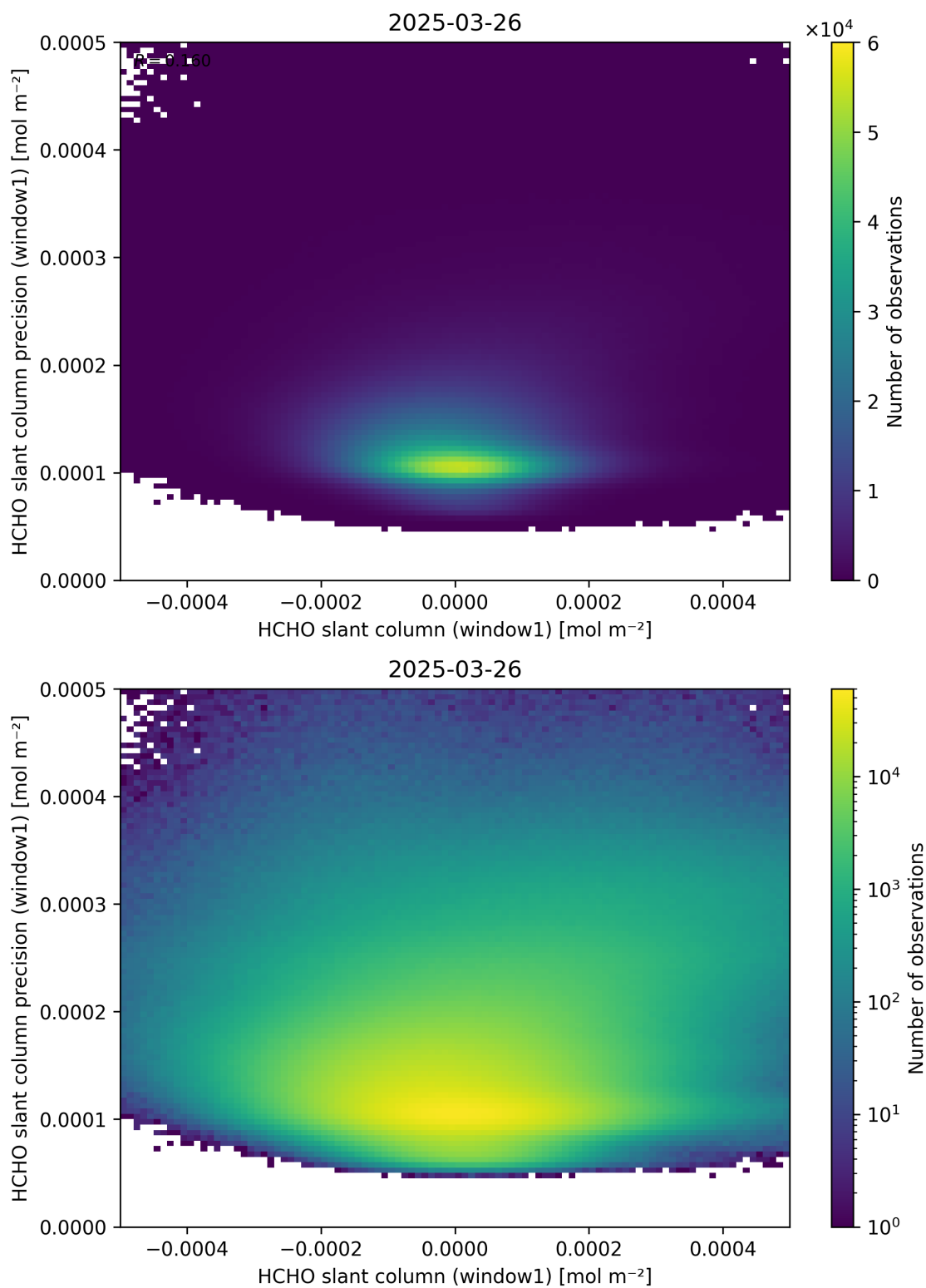
Figure 84: Scatter density plot of “HCHO slant column (window1)” against “HCHO slant column precision (window1)” for 2025-03-25 to 2025-03-27.
