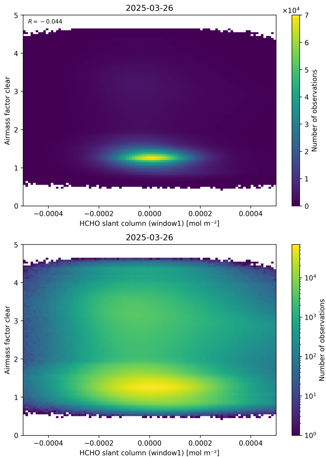
Figure 81: Scatter density plot of “HCHO slant column (window1)” against “Airmass factor clear” for 2025-03-25 to 2025-03-27.
