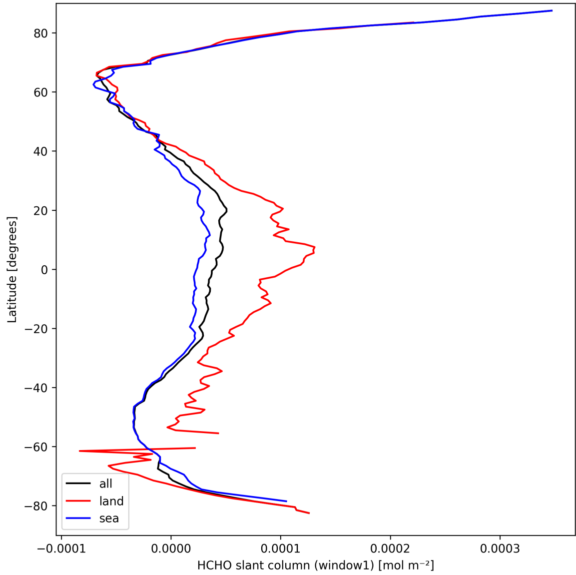
Figure 24: Zonal average of “HCHO slant column (window1)” for 2025-03-25 to 2025-03-27.
