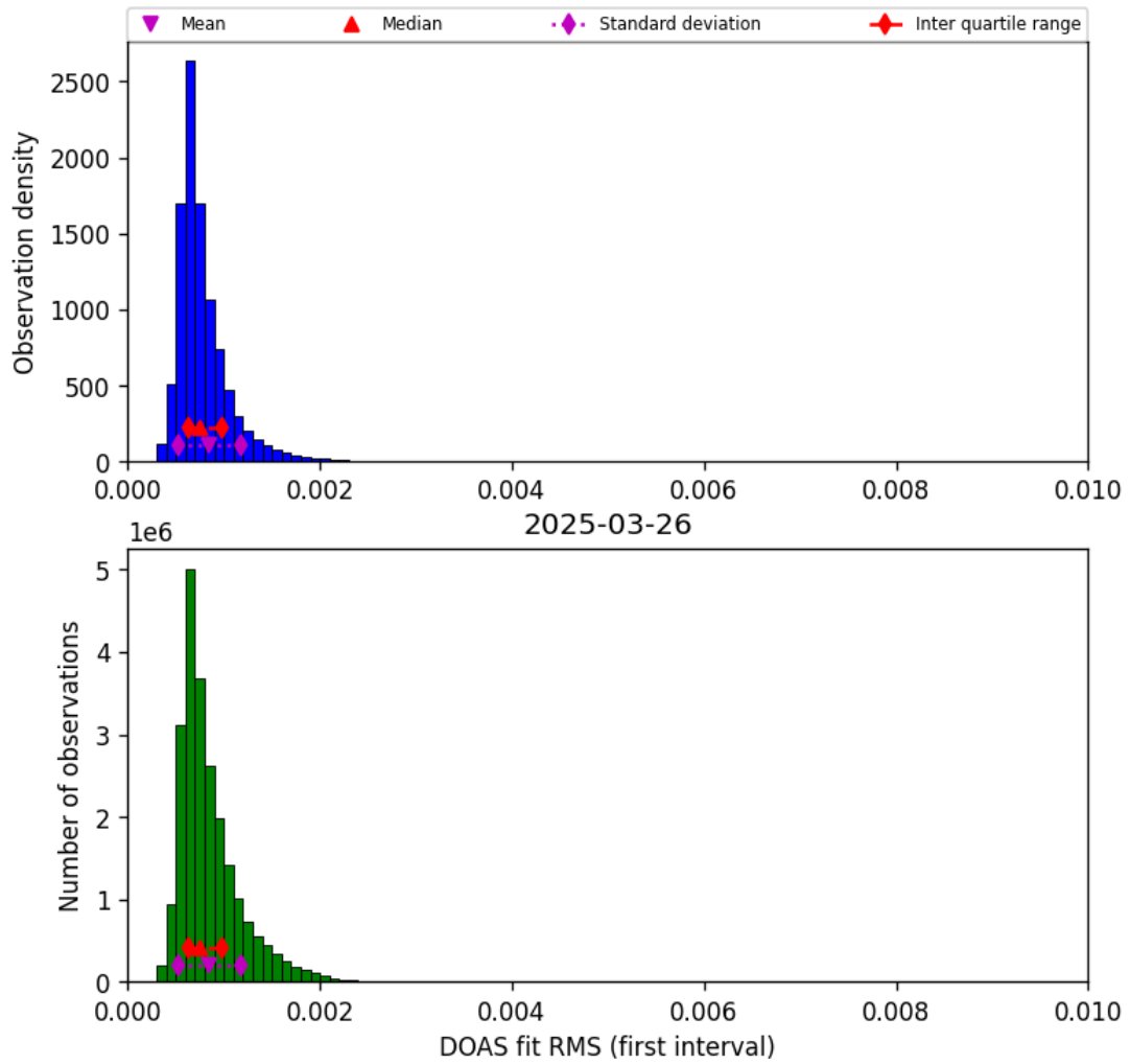
Figure 46: Histogram of “DOAS fit RMS (first interval)” for 2025-03-25 to 2025-03-27
