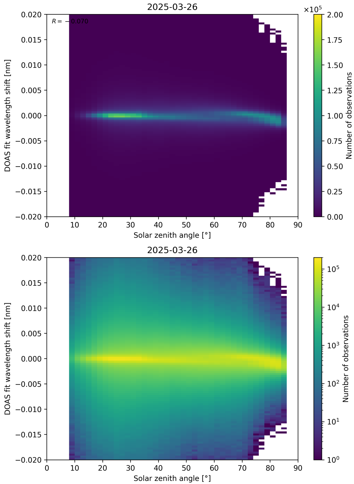
Figure 168: Scatter density plot of “Solar zenith angle” against “DOAS fit wavelength shift” for 2025-03-25 to 2025-03-27.
