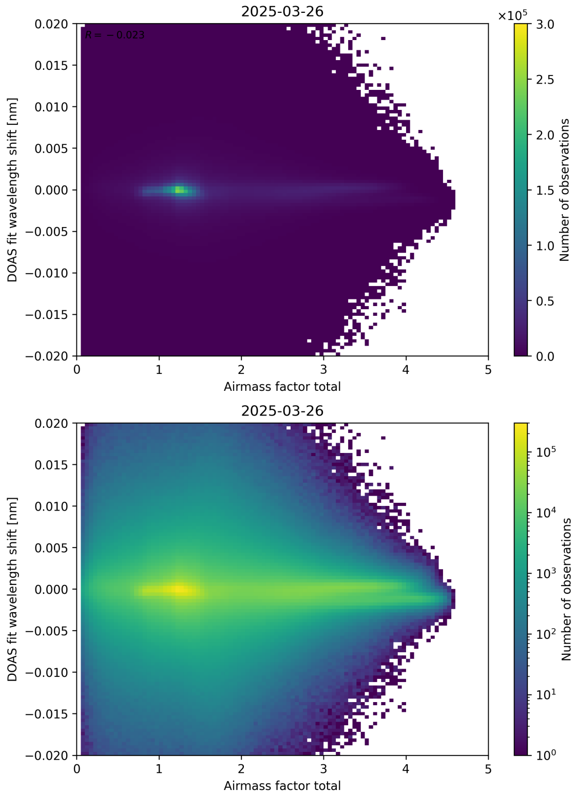
Figure 98: Scatter density plot of “Airmass factor total” against “DOAS fit wavelength shift” for 2025-03-25 to 2025-03-27.
