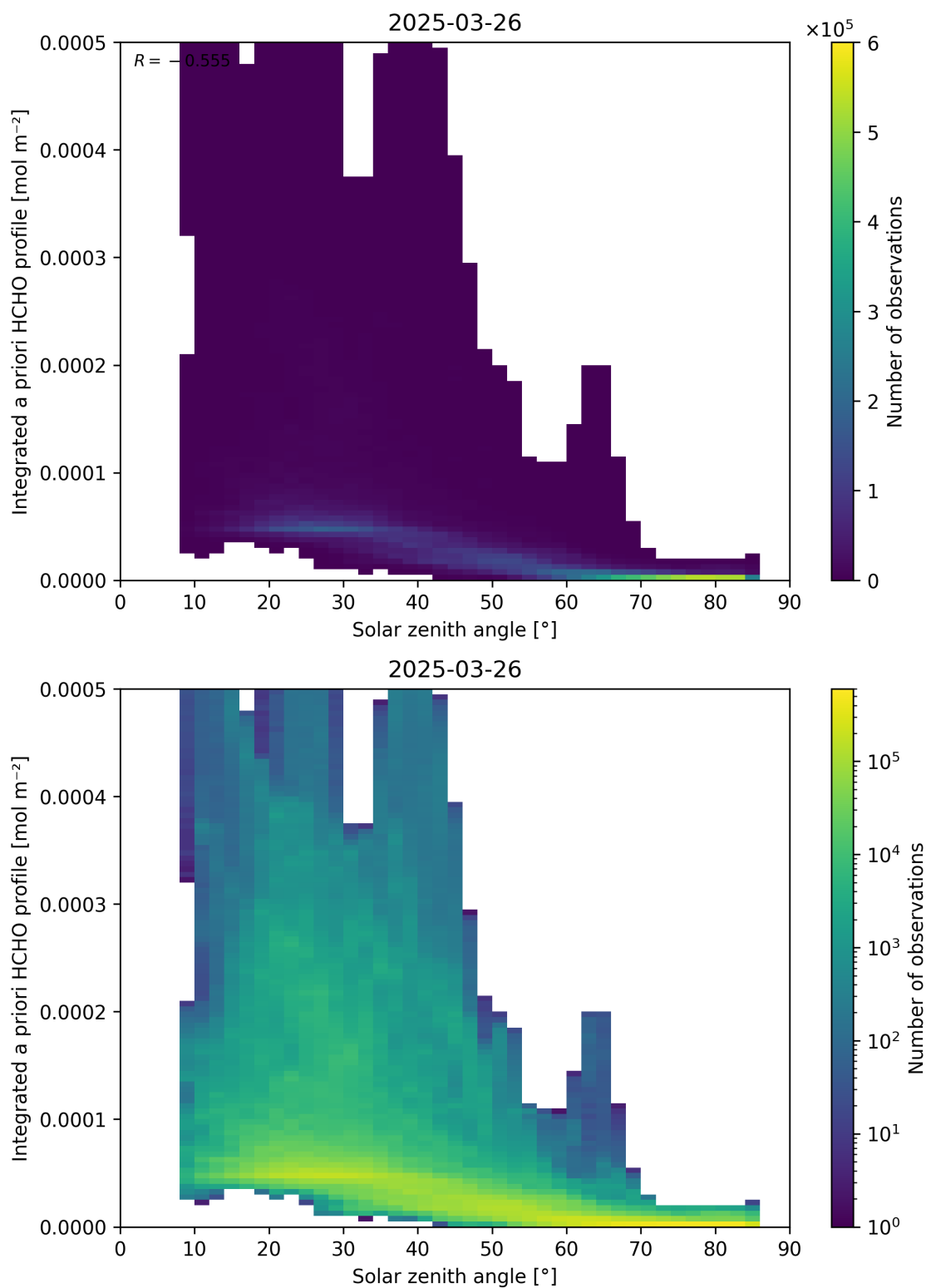
Figure 180: Scatter density plot of “Solar zenith angle” against “Integrated a priori HCHO profile” for 2025-03-25 to 2025-03-27.
