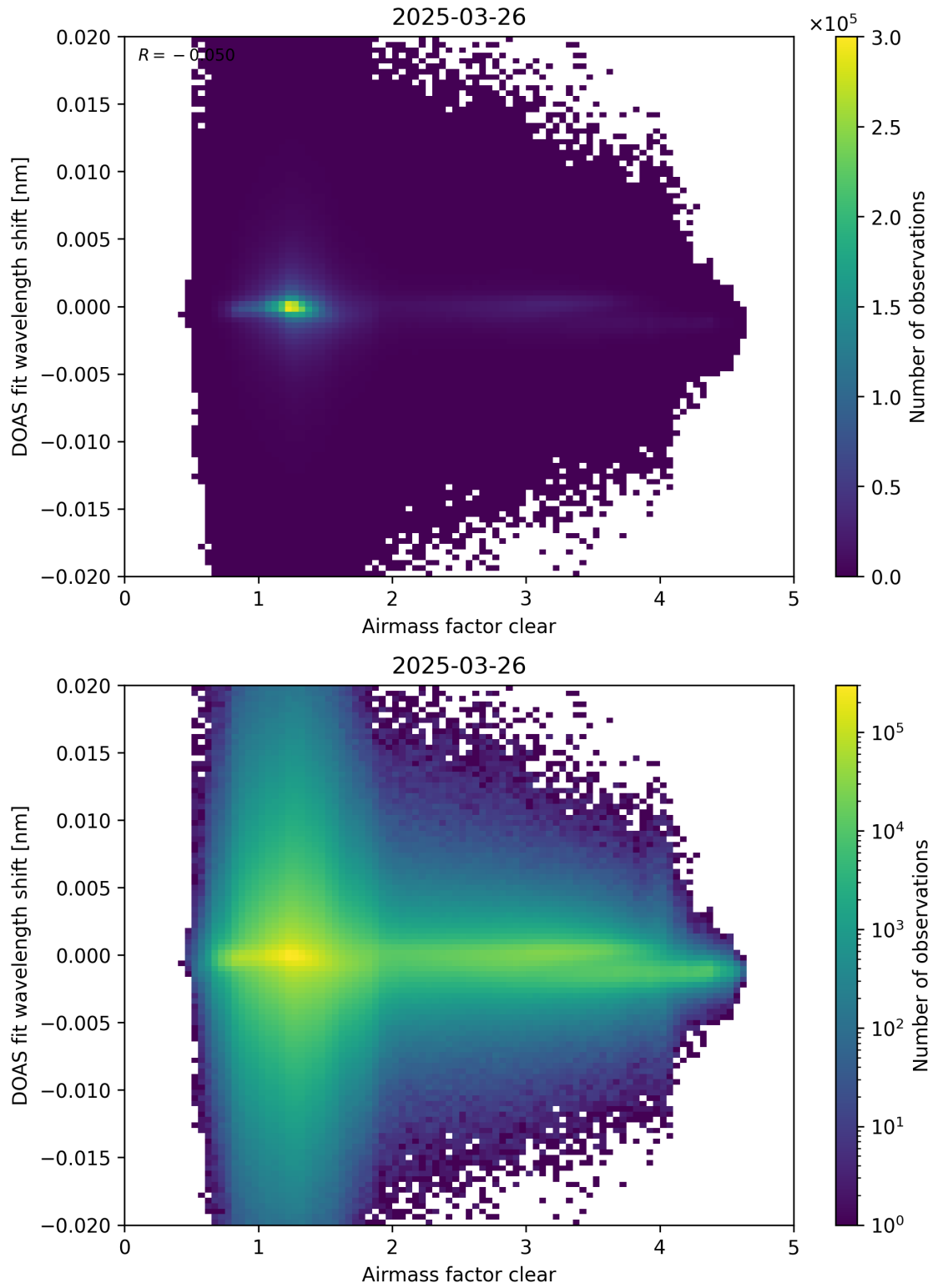
Figure 72: Scatter density plot of “Airmass factor clear” against “DOAS fit wavelength shift” for 2025-03-25 to 2025-03-27.
