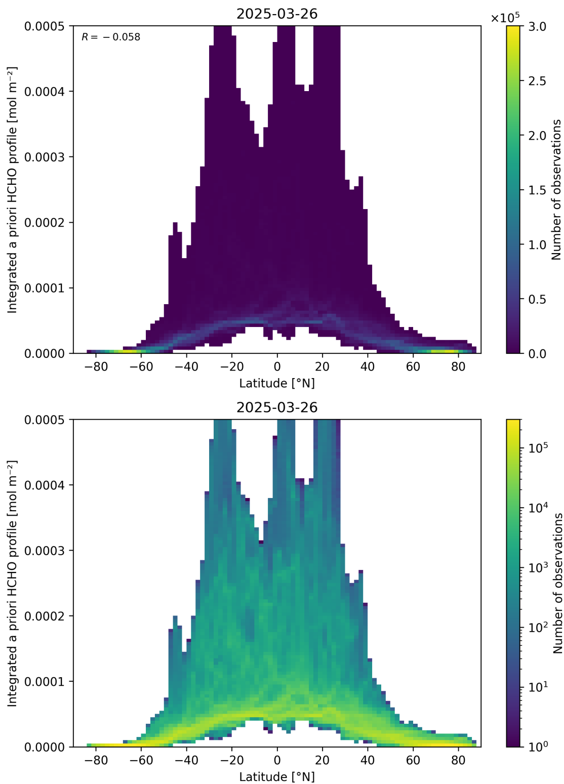
Figure 166: Scatter density plot of “Latitude” against “Integrated a priori HCHO profile” for 2025-03-25 to 2025-03-27.
