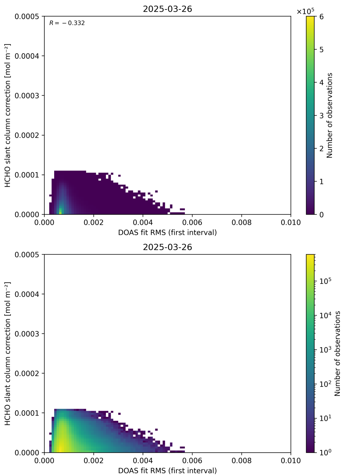
Figure 63: Scatter density plot of “DOAS fit RMS (first interval)” against “HCHO slant column correction” for 2025-03-25 to 2025-03-27.
