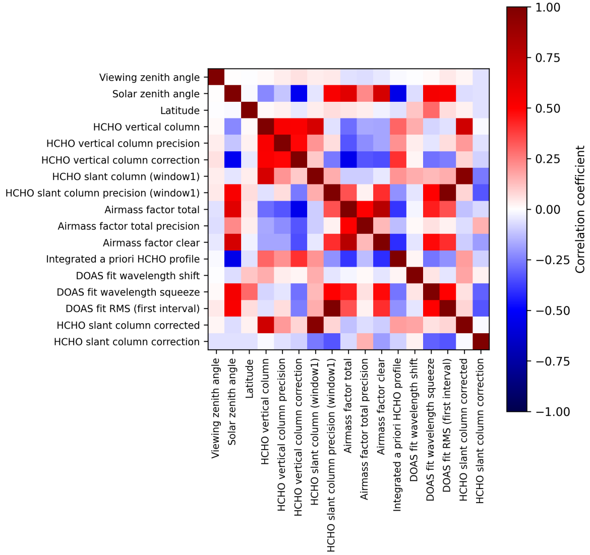
Figure 2: Map of correlation matrix for 2025-03-25 to 2025-03-27.
