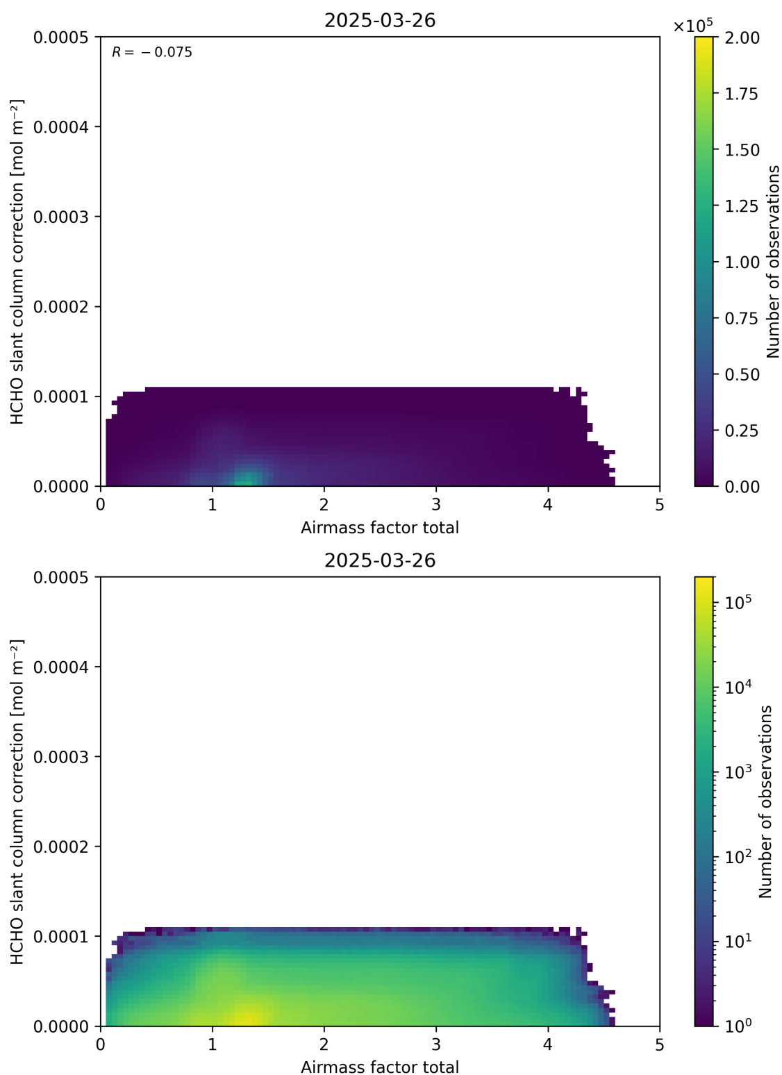
Figure 102: Scatter density plot of “Airmass factor total” against “HCHO slant column correction” for 2025-03-25 to 2025-03-27.
