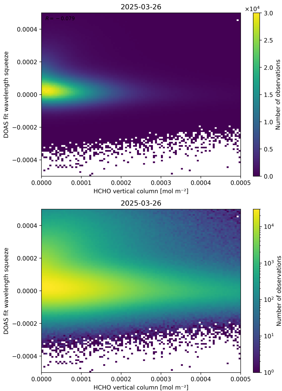
Figure 125: Scatter density plot of “HCHO vertical column” against “DOAS fit wavelength squeeze” for 2025-03-25 to 2025-03-27.
