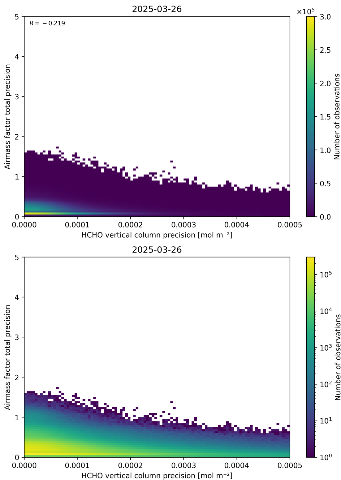
Figure 145: Scatter density plot of “HCHO vertical column precision” against “Airmass factor total precision” for 2025-03-25 to 2025-03-27.
