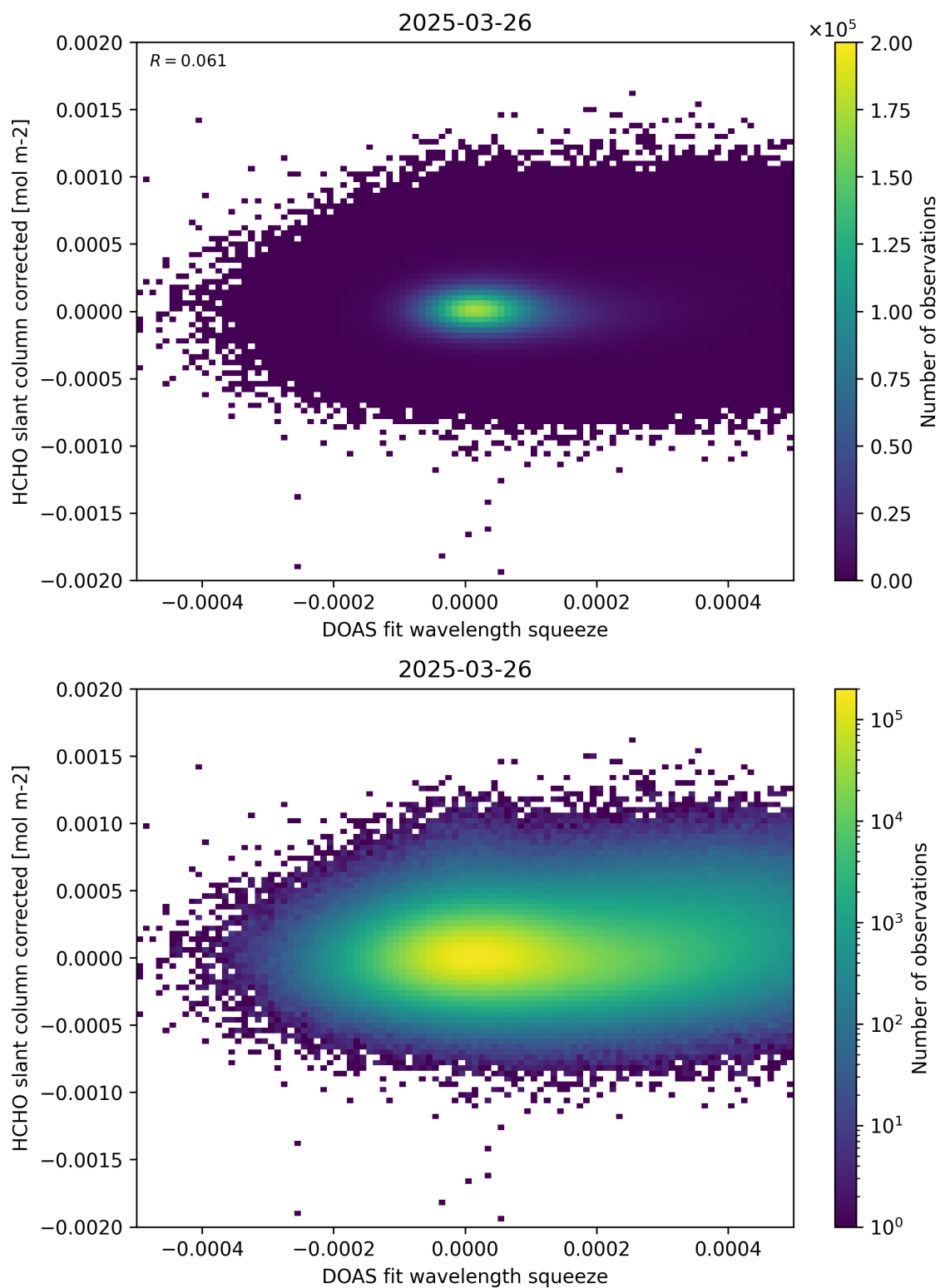
Figure 69: Scatter density plot of “DOAS fit wavelength squeeze” against “HCHO slant column corrected” for 2025-03-25 to 2025-03-27.
