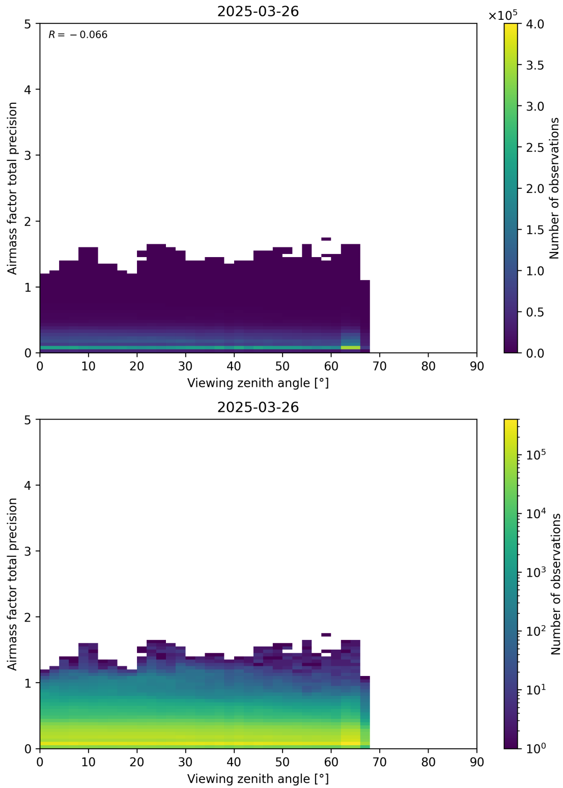
Figure 191: Scatter density plot of “Viewing zenith angle” against “Airmass factor total precision” for 2025-03-25 to 2025-03-27.
