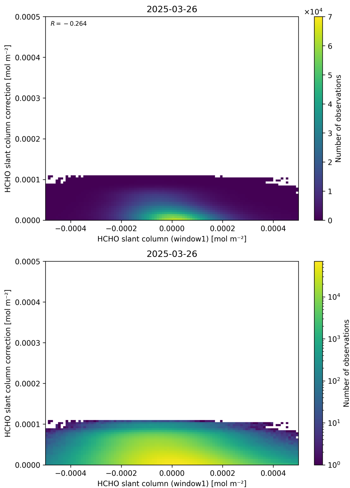
Figure 83: Scatter density plot of “HCHO slant column (window1)” against “HCHO slant column correction” for 2025-03-25 to 2025-03-27.
