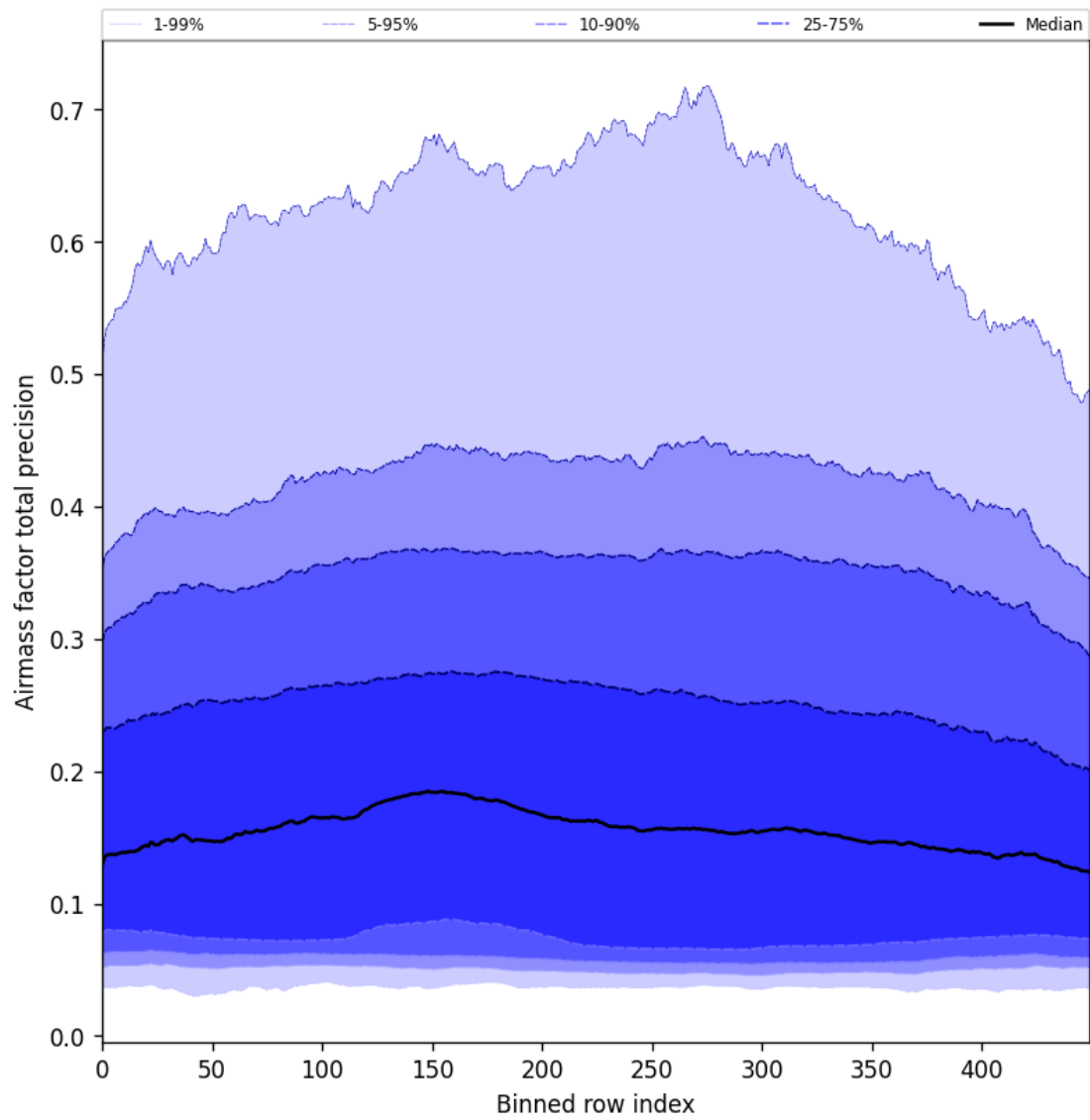
Figure 55: Along track statistics of “Airmass factor total precision” for 2025-03-25 to 2025-03-27
