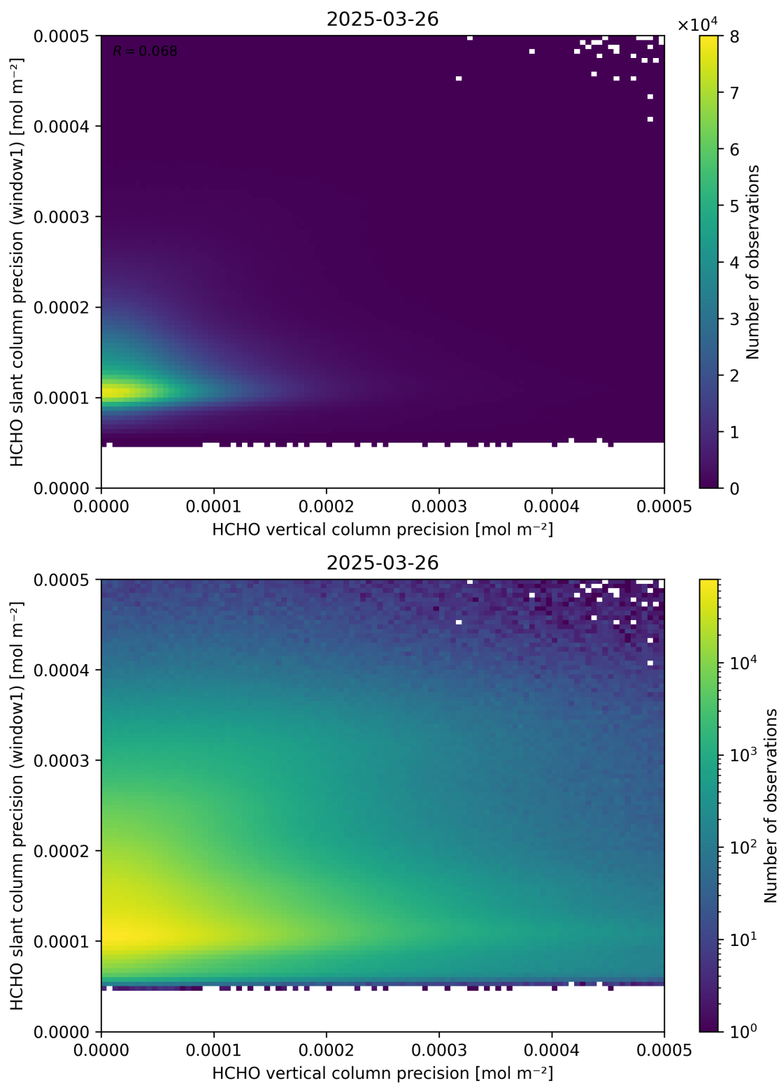
Figure 143: Scatter density plot of “HCHO vertical column precision” against “HCHO slant column precision (window1)” for 2025-03-25 to 2025-03-27.
