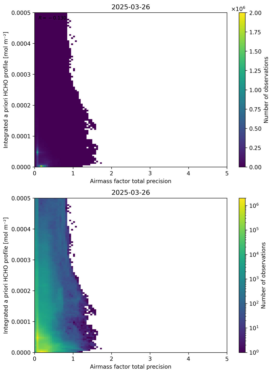
Figure 111: Scatter density plot of “Airmass factor total precision” against “Integrated a priori HCHO profile” for 2025-03-25 to 2025-03-27.
