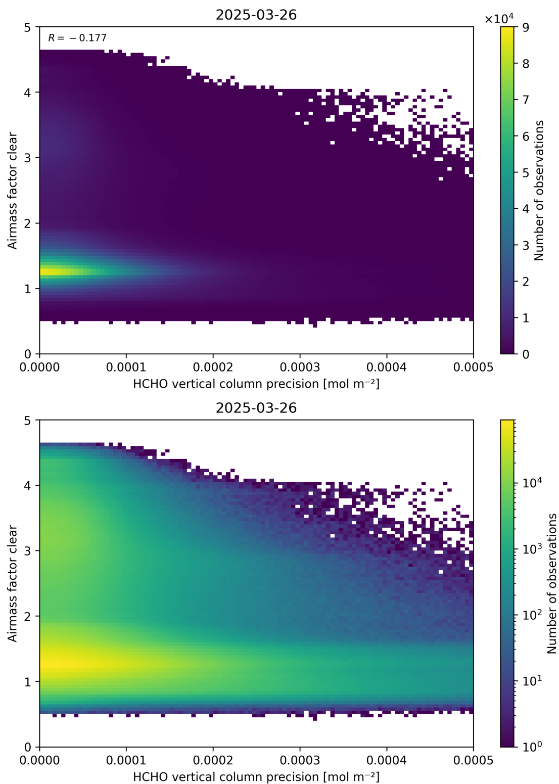
Figure 139: Scatter density plot of “HCHO vertical column precision” against “Airmass factor clear” for 2025-03-25 to 2025-03-27.
