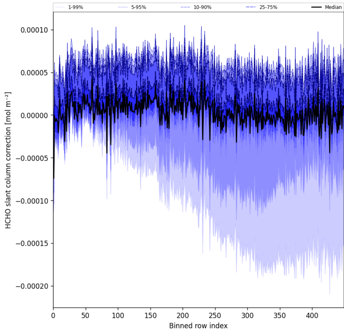
Figure 61: Along track statistics of “HCHO slant column correction” for 2025-03-25 to 2025-03-27
