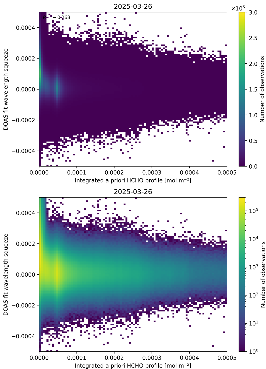
Figure 150: Scatter density plot of “Integrated a priori HCHO profile” against “DOAS fit wavelength squeeze” for 2025-03-25 to 2025-03-27.
