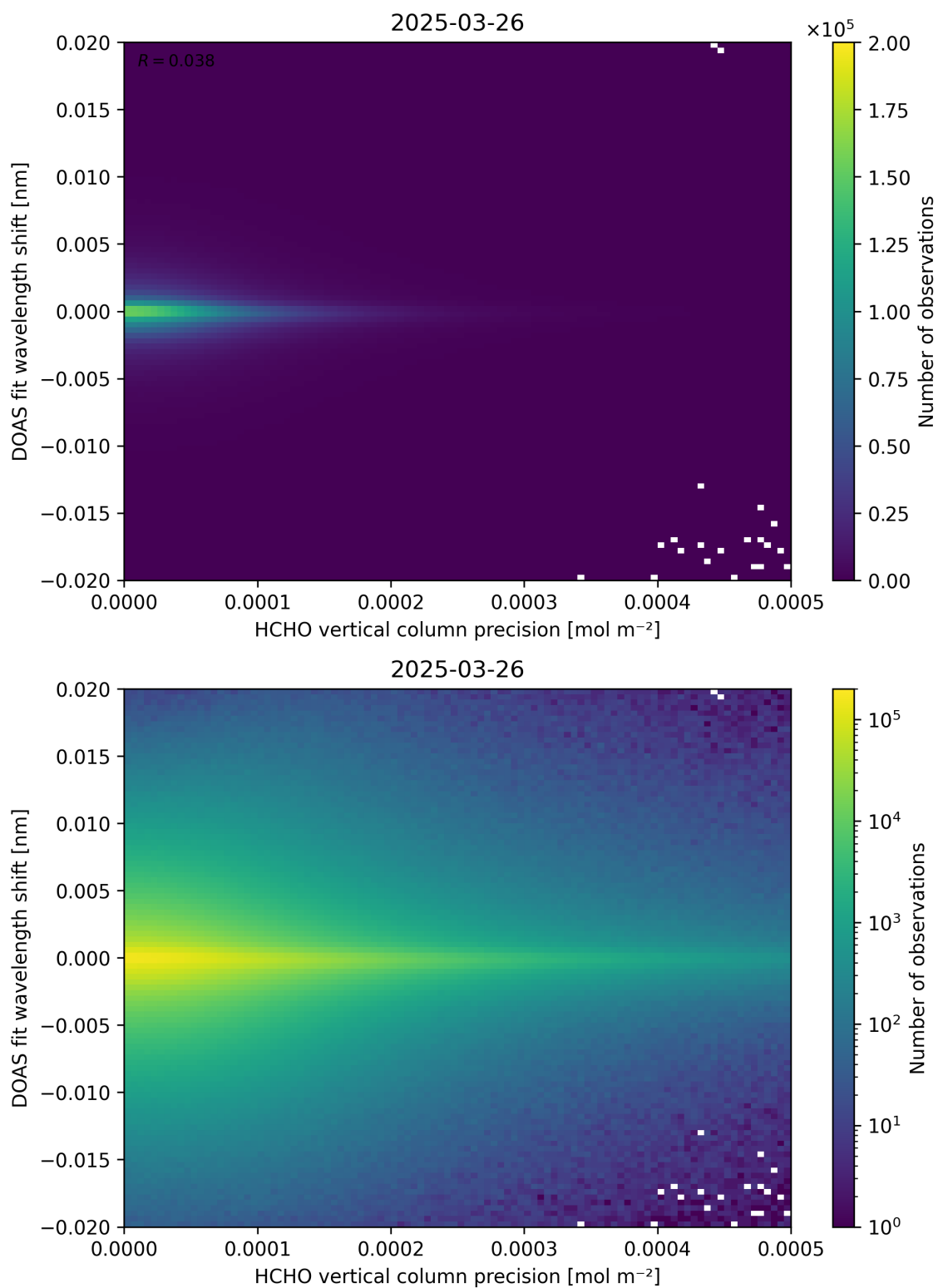
Figure 137: Scatter density plot of “HCHO vertical column precision” against “DOAS fit wavelength shift” for 2025-03-25 to 2025-03-27.
