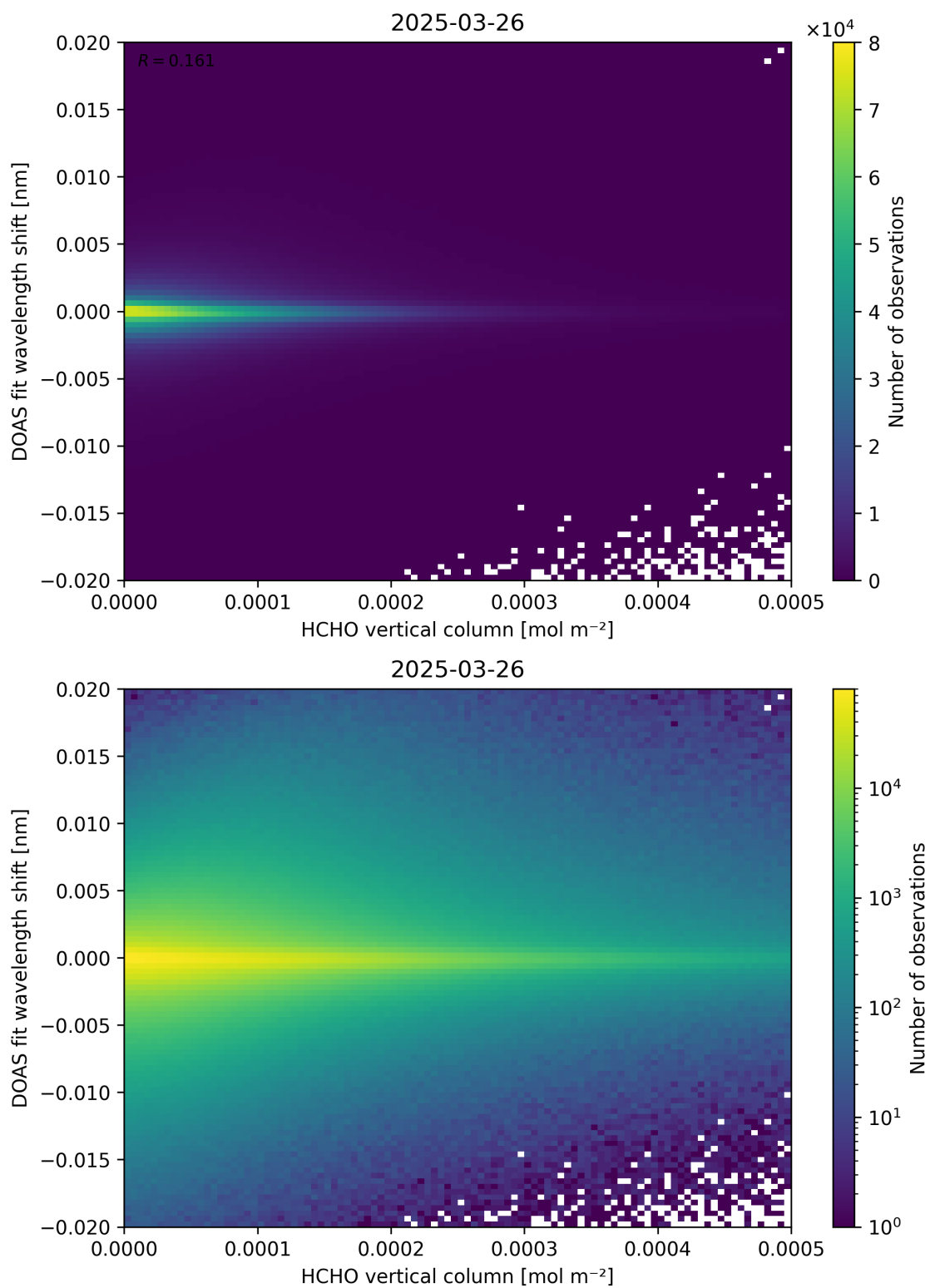
Figure 124: Scatter density plot of “HCHO vertical column” against “DOAS fit wavelength shift” for 2025-03-25 to 2025-03-27.
