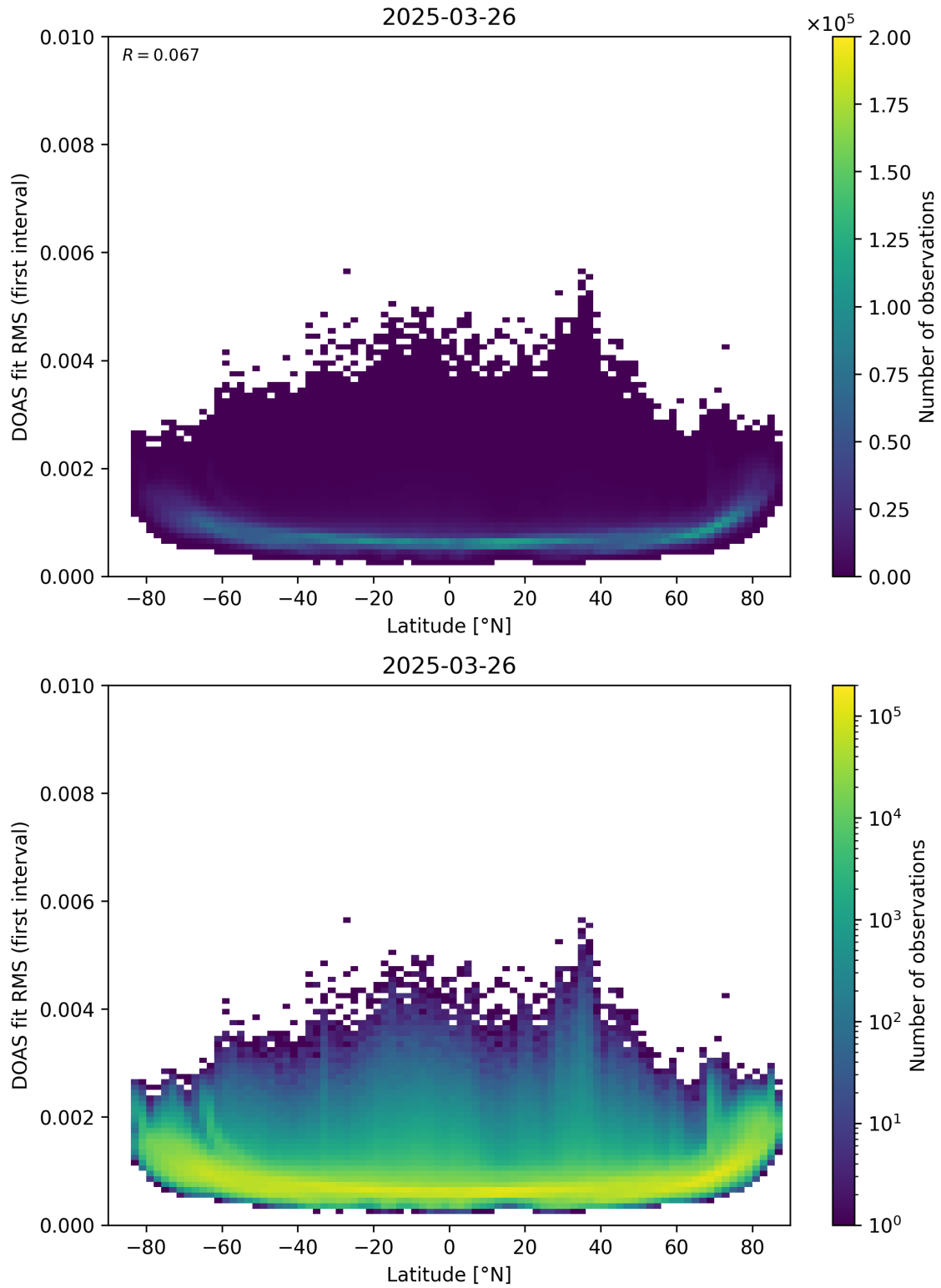
Figure 153: Scatter density plot of “Latitude” against “DOAS fit RMS (first interval)” for 2025-03-25 to 2025-03-27.
