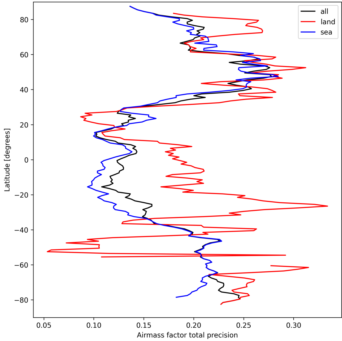
Figure 27: Zonal average of “Airmass factor total precision” for 2025-03-25 to 2025-03-27.
