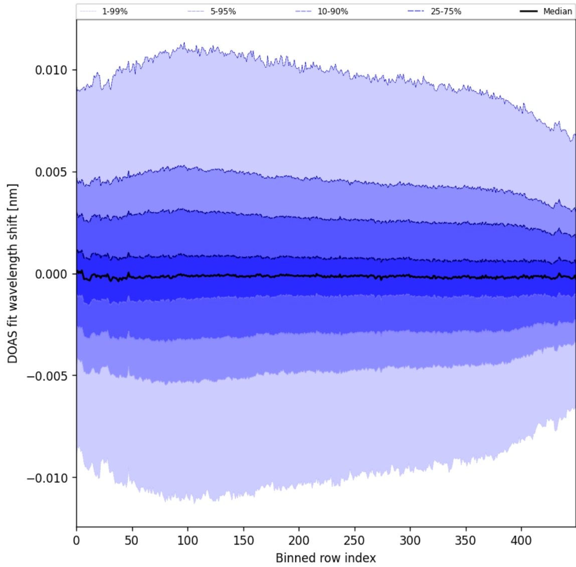
Figure 58: Along track statistics of “DOAS fit wavelength shift” for 2025-03-25 to 2025-03-27
