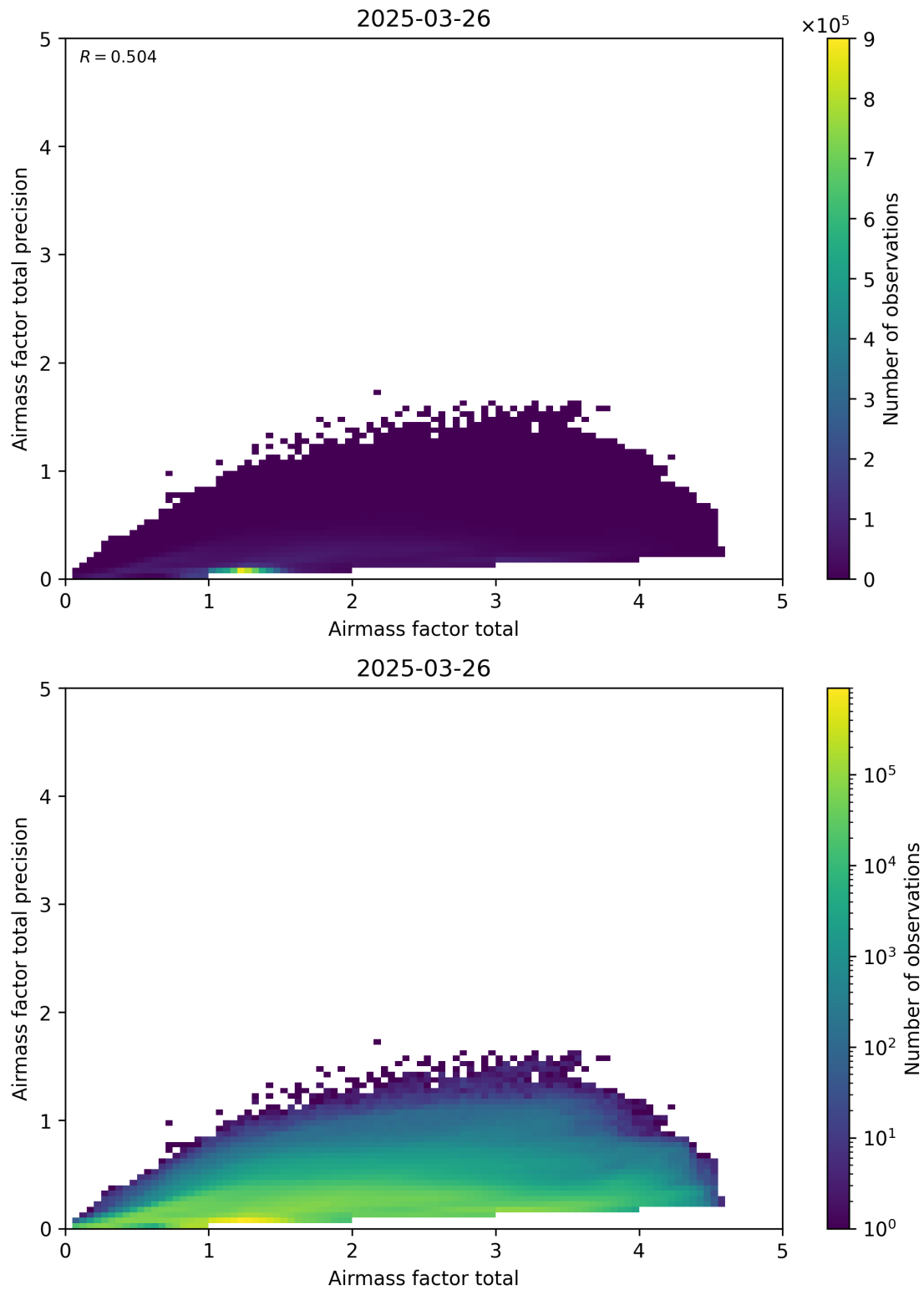
Figure 103: Scatter density plot of “Airmass factor total” against “Airmass factor total precision” for 2025-03-25 to 2025-03-27.
