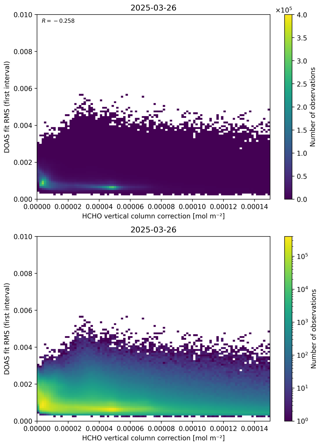
Figure 112: Scatter density plot of “HCHO vertical column correction” against “DOAS fit RMS (first interval)” for 2025-03-25 to 2025-03-27.
