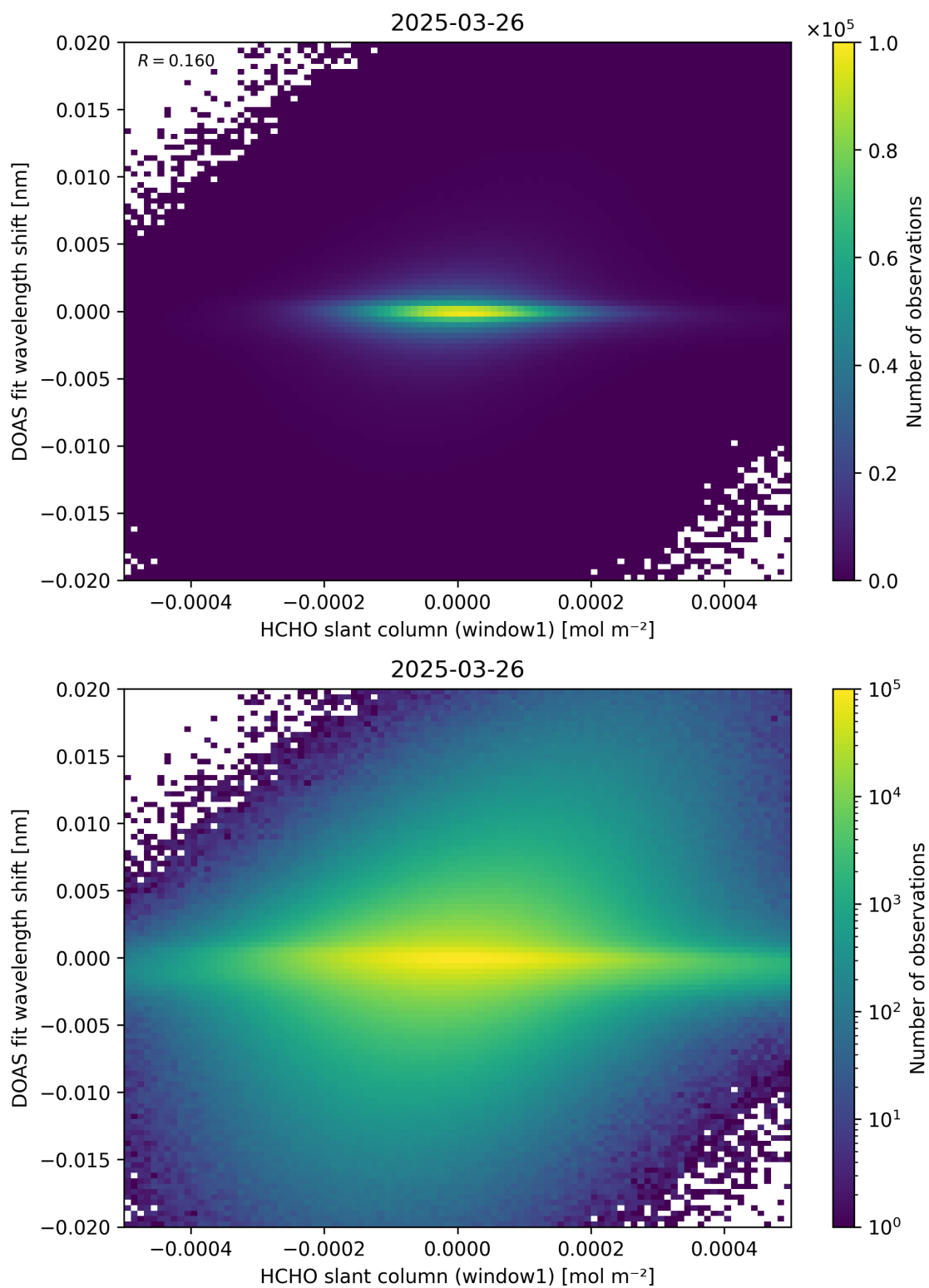
Figure 79: Scatter density plot of “HCHO slant column (window1)” against “DOAS fit wavelength shift” for 2025-03-25 to 2025-03-27.
