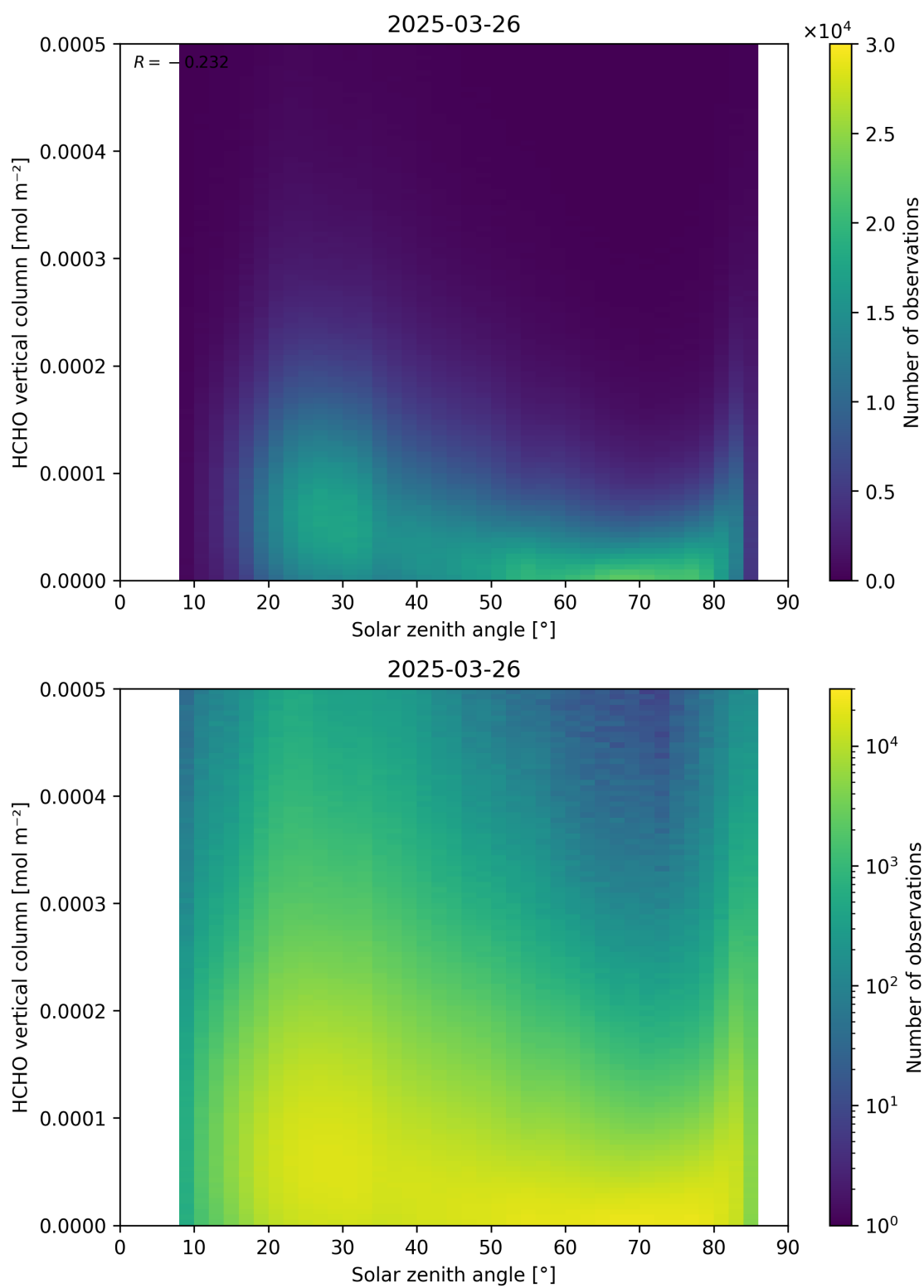
Figure 177: Scatter density plot of “Solar zenith angle” against “HCHO vertical column” for 2025-03-25 to 2025-03-27.
