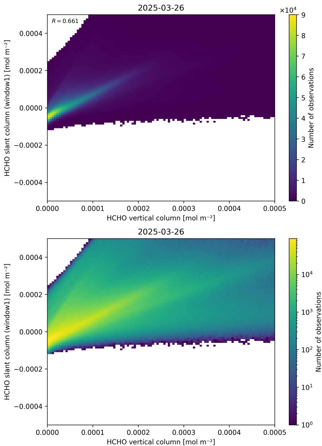
Figure 129: Scatter density plot of “HCHO vertical column” against “HCHO slant column (window1)” for 2025-03-25 to 2025-03-27.
