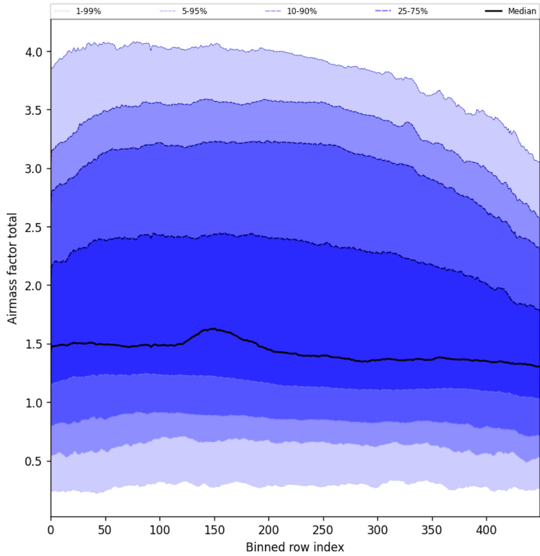
Figure 54: Along track statistics of “Airmass factor total” for 2025-03-25 to 2025-03-27
