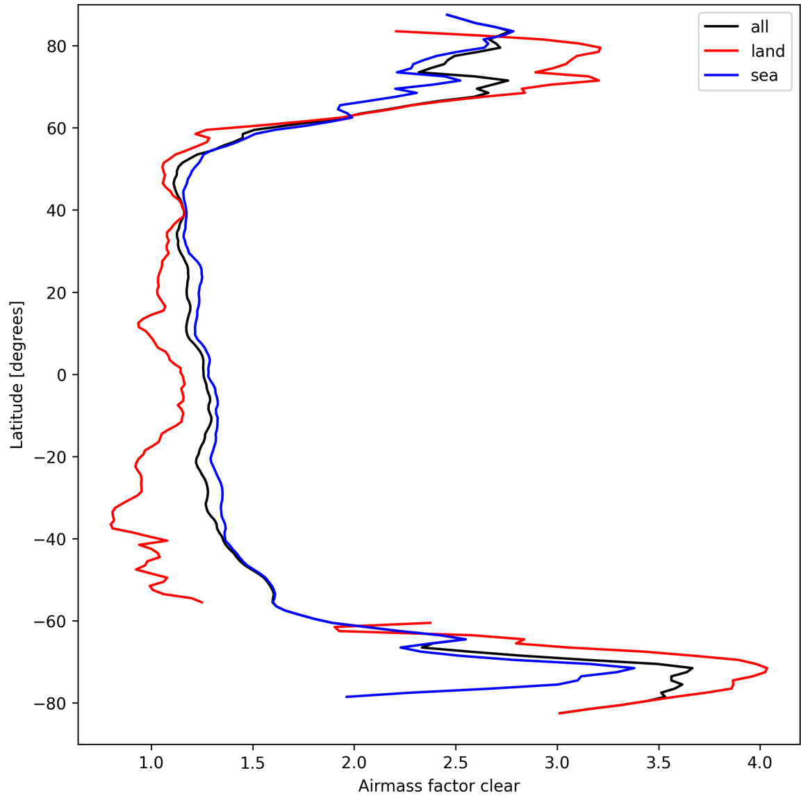
Figure 28: Zonal average of “Airmass factor clear” for 2025-03-25 to 2025-03-27.
