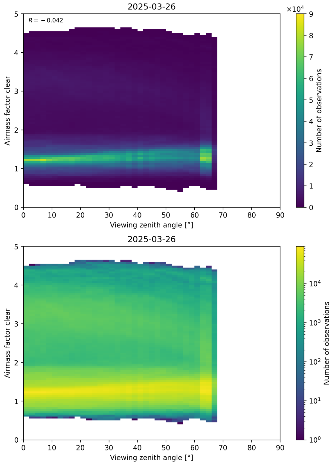
Figure 185: Scatter density plot of “Viewing zenith angle” against “Airmass factor clear” for 2025-03-25 to 2025-03-27.
