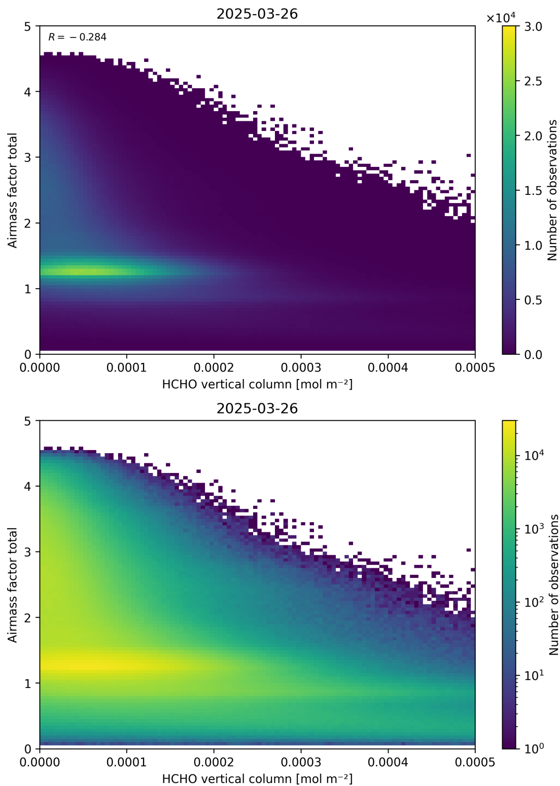
Figure 131: Scatter density plot of “HCHO vertical column” against “Airmass factor total” for 2025-03-25 to 2025-03-27.
