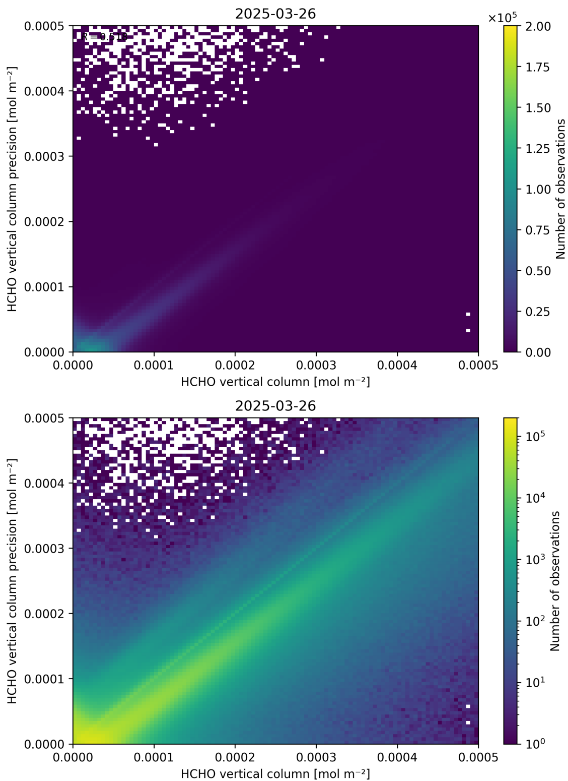
Figure 134: Scatter density plot of “HCHO vertical column” against “HCHO vertical column precision” for 2025-03-25 to 2025-03-27.
