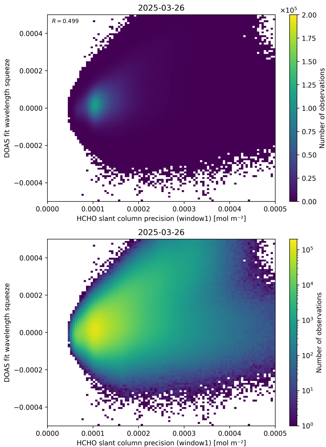
Figure 90: Scatter density plot of “HCHO slant column precision (window1)” against “DOAS fit wavelength squeeze” for 2025-03-25 to 2025-03-27.
