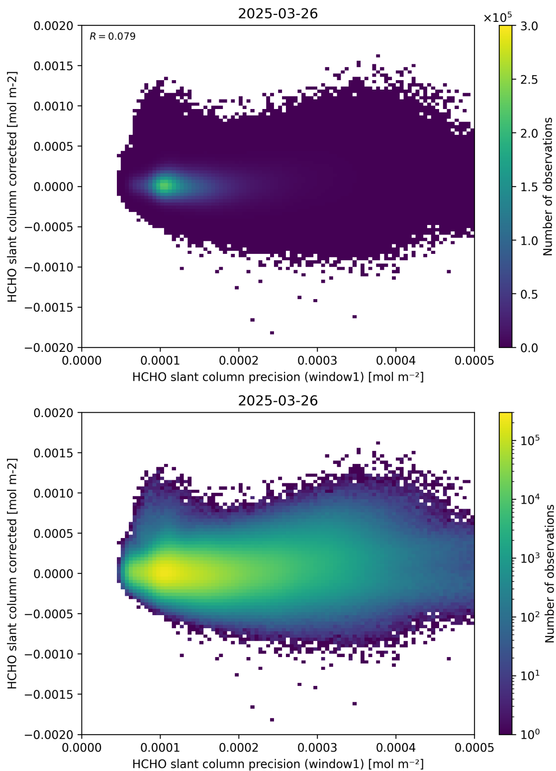
Figure 92: Scatter density plot of “HCHO slant column precision (window1)” against “HCHO slant column corrected” for 2025-03-25 to 2025-03-27.
