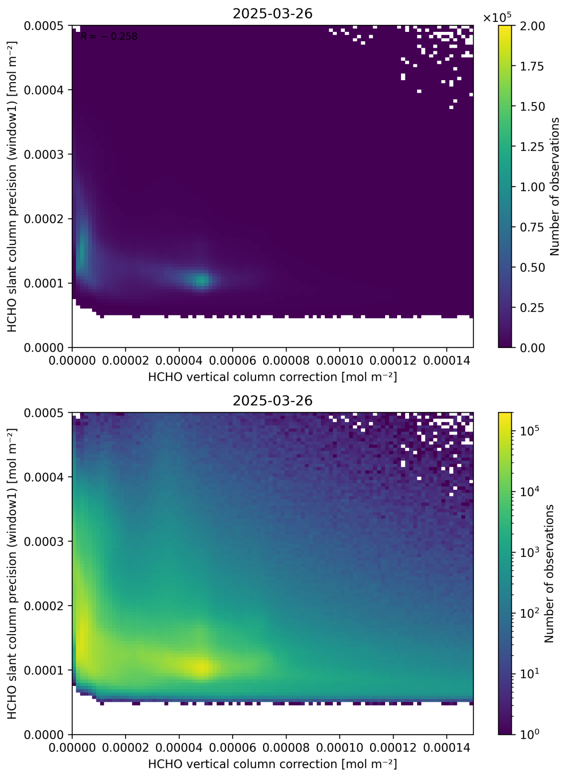
Figure 119: Scatter density plot of “HCHO vertical column correction” against “HCHO slant column precision (window1)” for 2025-03-25 to 2025-03-27.
