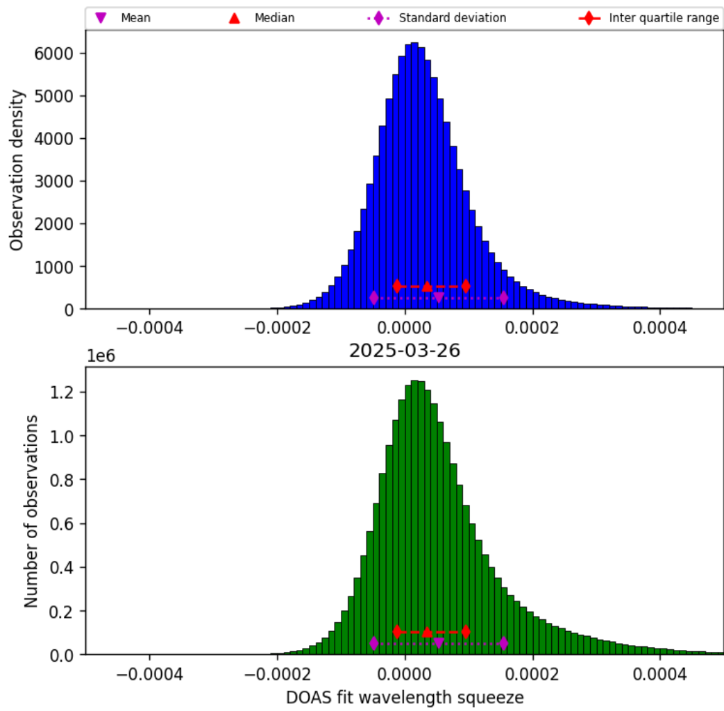
Figure 45: Histogram of “DOAS fit wavelength squeeze” for 2025-03-25 to 2025-03-27
