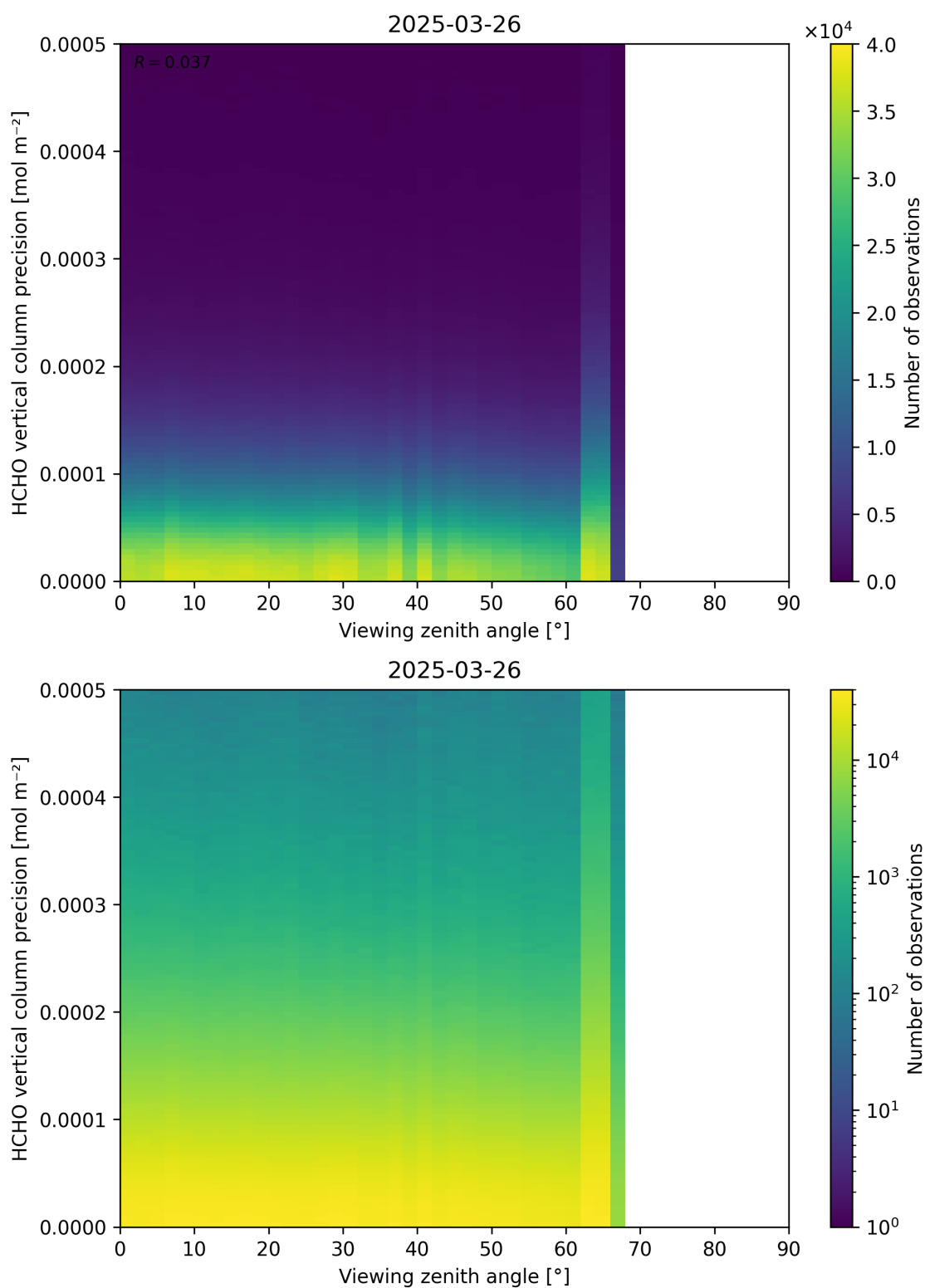
Figure 194: Scatter density plot of “Viewing zenith angle” against “HCHO vertical column precision” for 2025-03-25 to 2025-03-27.
