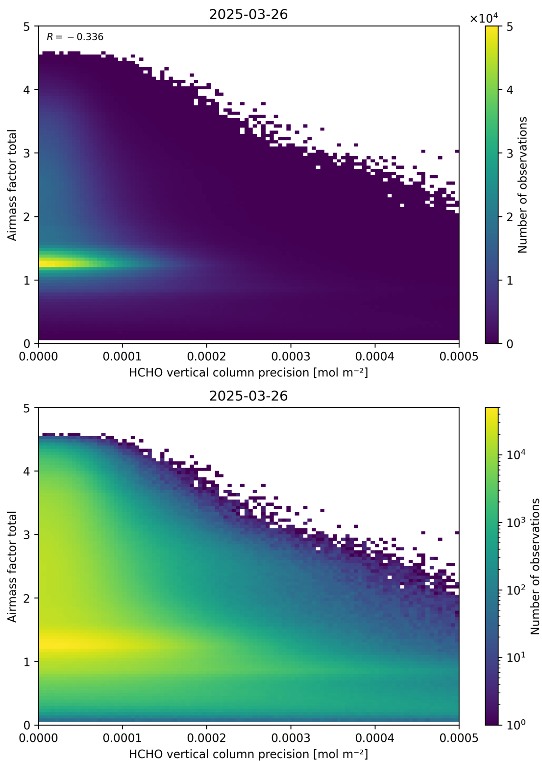
Figure 144: Scatter density plot of “HCHO vertical column precision” against “Airmass factor total” for 2025-03-25 to 2025-03-27.
