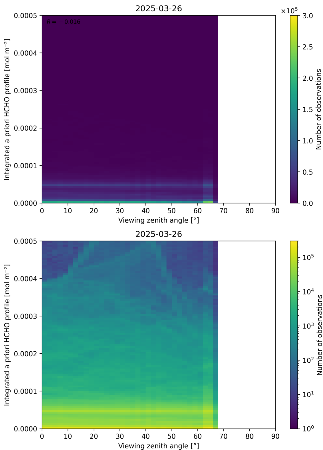
Figure 195: Scatter density plot of “Viewing zenith angle” against “Integrated a priori HCHO profile” for 2025-03-25 to 2025-03-27.
