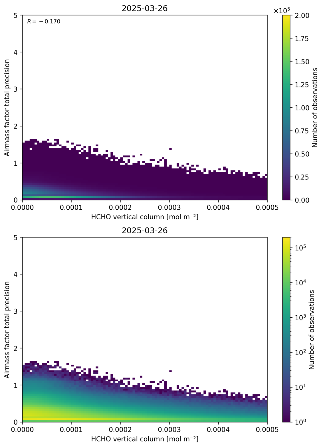
Figure 132: Scatter density plot of “HCHO vertical column” against “Airmass factor total precision” for 2025-03-25 to 2025-03-27.
