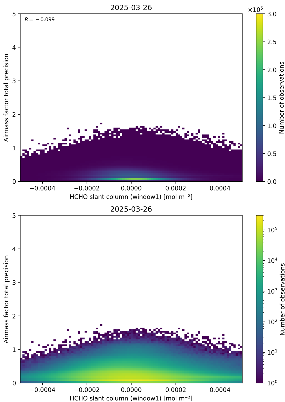
Figure 86: Scatter density plot of “HCHO slant column (window1)” against “Airmass factor total precision” for 2025-03-25 to 2025-03-27.
