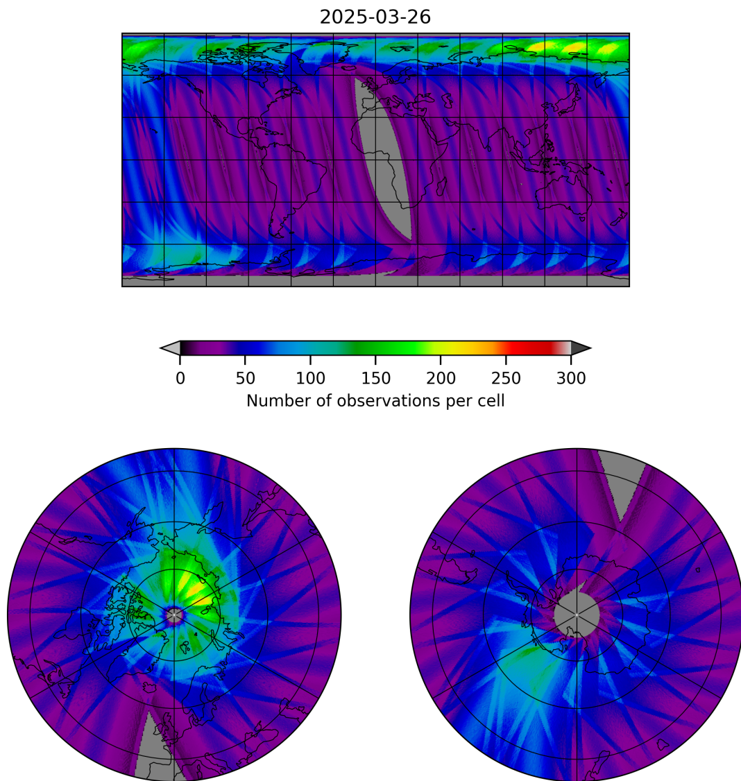
Figure 19: Map of the number of observations for 2025-03-25 to 2025-03-27
