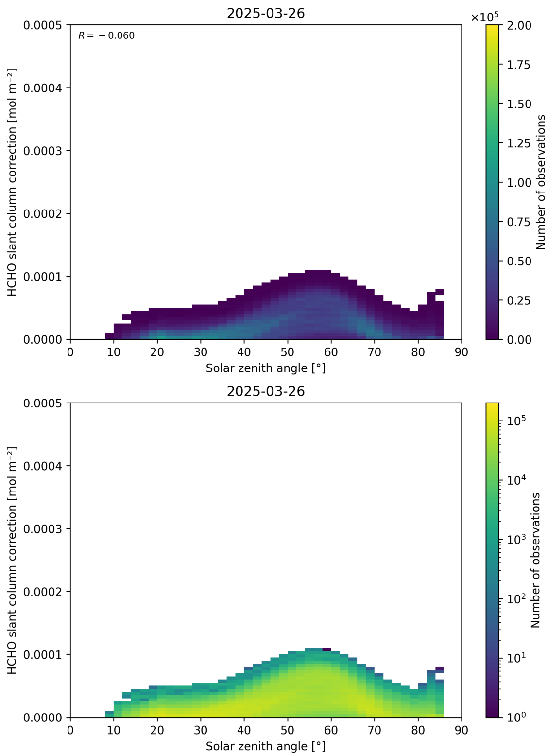
Figure 172: Scatter density plot of “Solar zenith angle” against “HCHO slant column correction” for 2025-03-25 to 2025-03-27.
