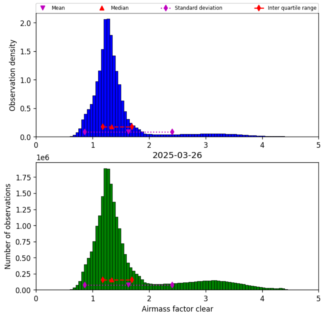
Figure 42: Histogram of “Airmass factor clear” for 2025-03-25 to 2025-03-27
