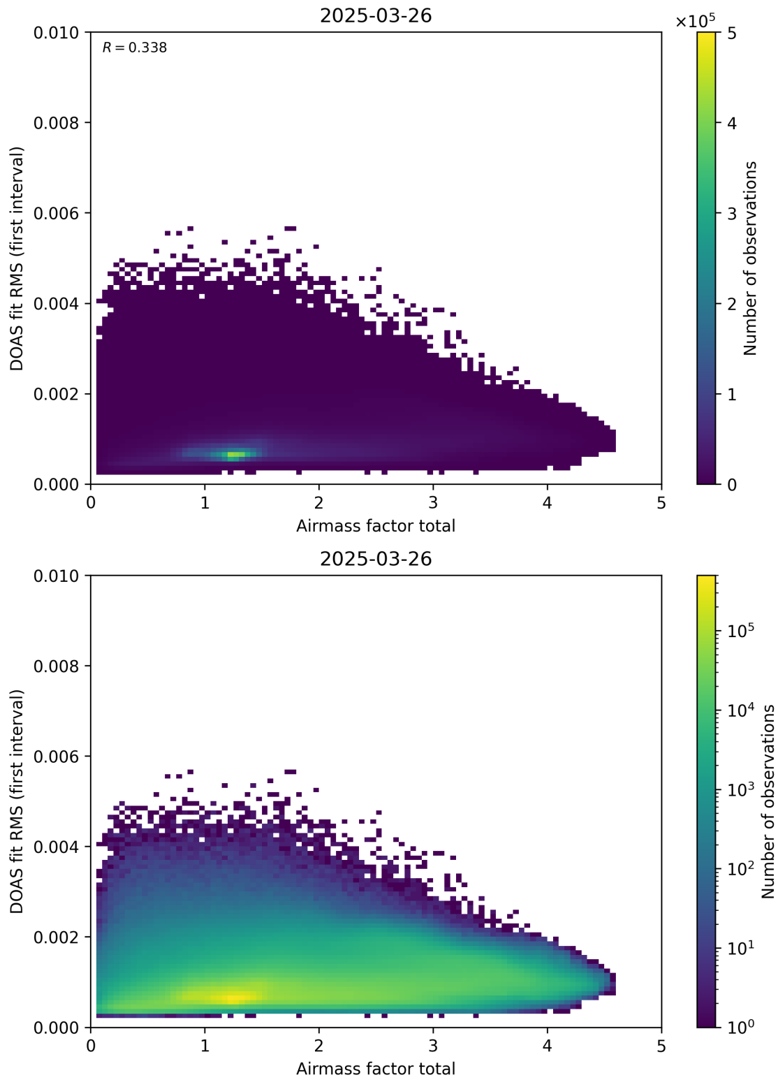
Figure 97: Scatter density plot of “Airmass factor total” against “DOAS fit RMS (first interval)” for 2025-03-25 to 2025-03-27.
