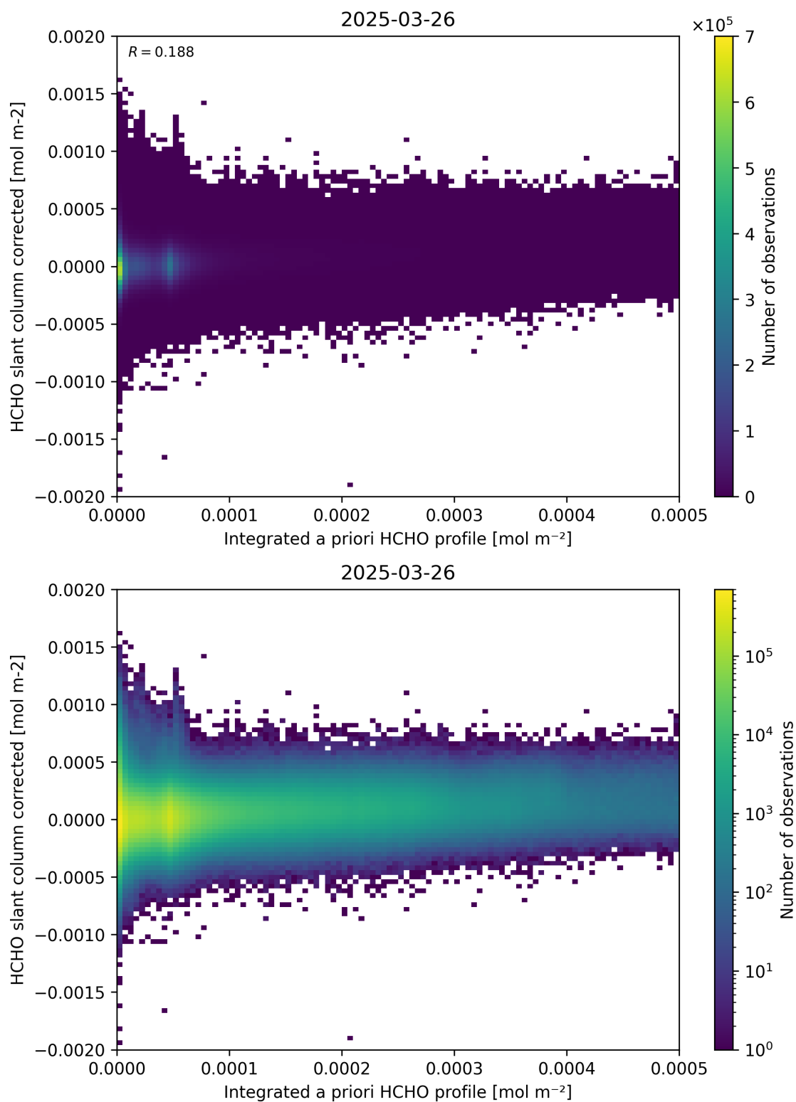
Figure 151: Scatter density plot of “Integrated a priori HCHO profile” against “HCHO slant column corrected” for 2025-03-25 to 2025-03-27.
