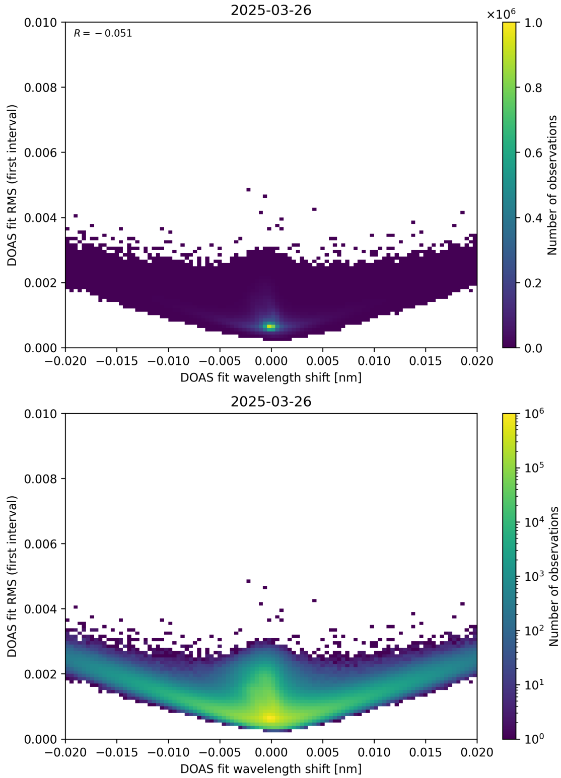
Figure 64: Scatter density plot of “DOAS fit wavelength shift” against “DOAS fit RMS (first interval)” for 2025-03-25 to 2025-03-27.
