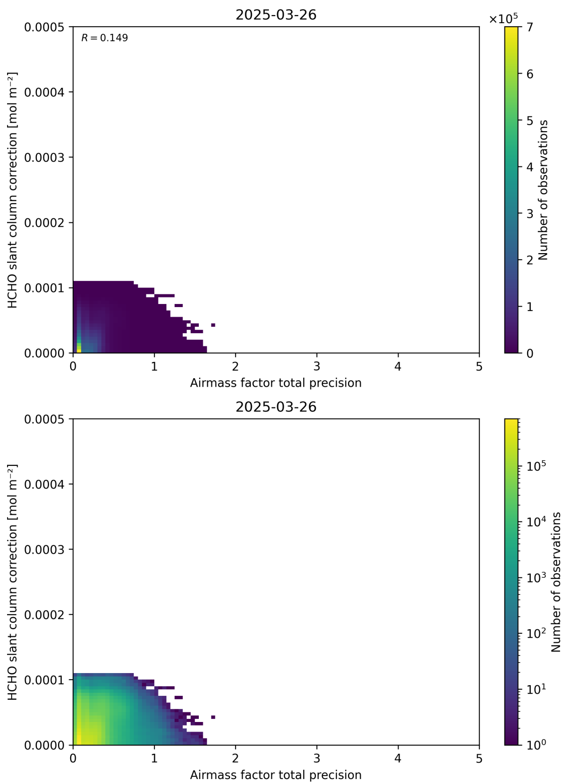
Figure 110: Scatter density plot of “Airmass factor total precision” against “HCHO slant column correction” for 2025-03-25 to 2025-03-27.
