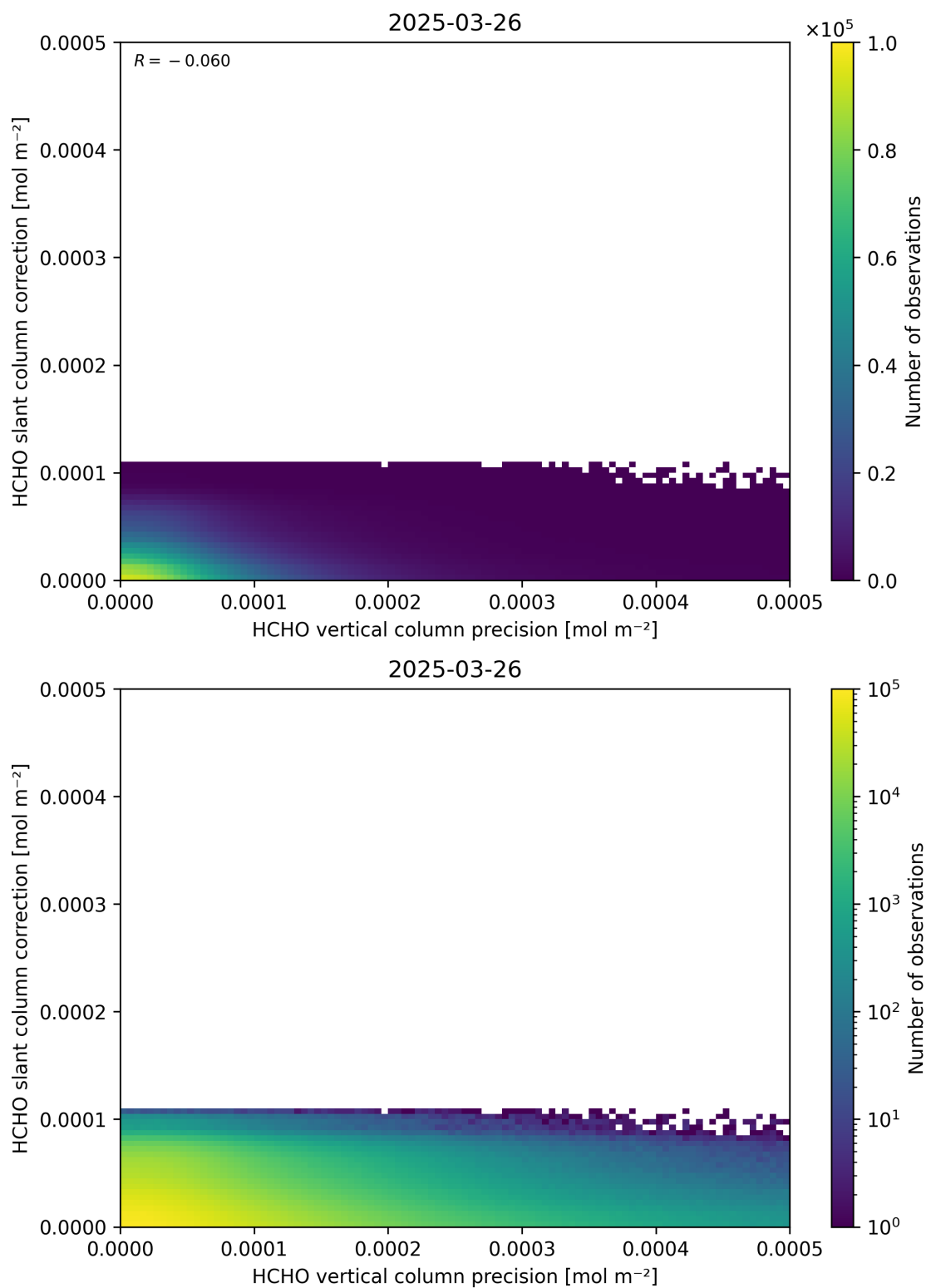
Figure 141: Scatter density plot of “HCHO vertical column precision” against “HCHO slant column correction” for 2025-03-25 to 2025-03-27.
