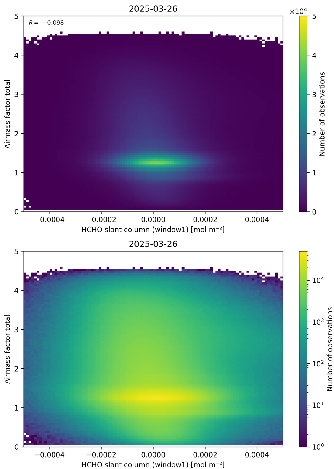
Figure 85: Scatter density plot of “HCHO slant column (window1)” against “Airmass factor total” for 2025-03-25 to 2025-03-27.
