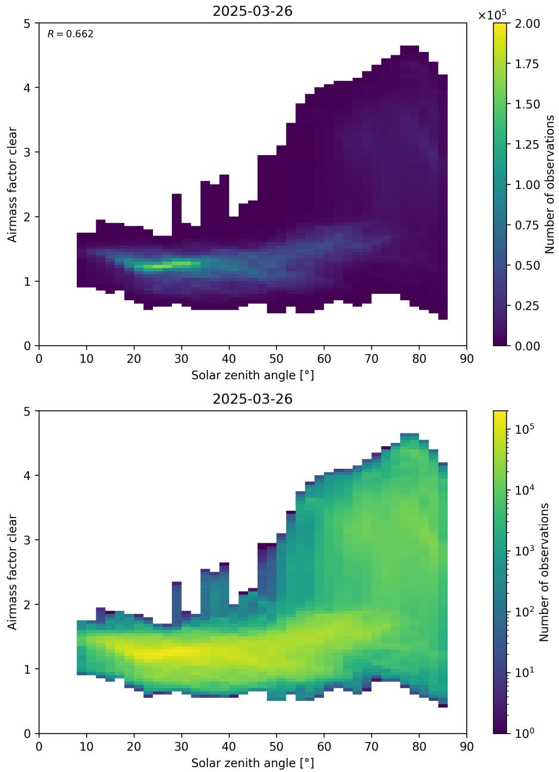
Figure 170: Scatter density plot of “Solar zenith angle” against “Airmass factor clear” for 2025-03-25 to 2025-03-27.
