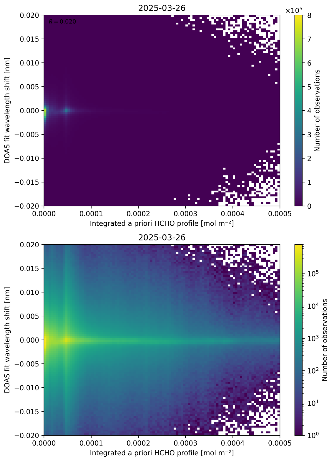
Figure 149: Scatter density plot of “Integrated a priori HCHO profile” against “DOAS fit wavelength shift” for 2025-03-25 to 2025-03-27.
