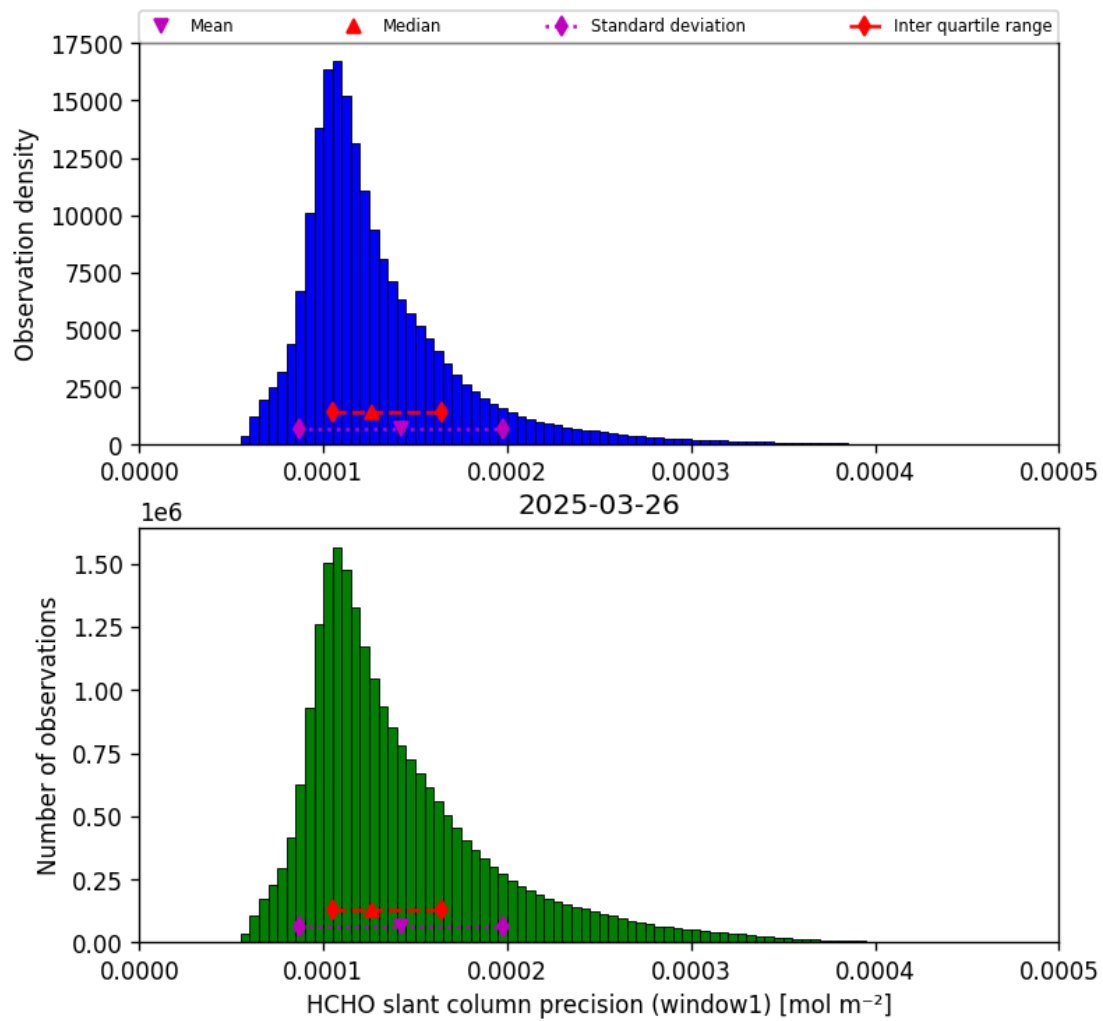
Figure 39: Histogram of “HCHO slant column precision (window1)” for 2025-03-25 to 2025-03-27
