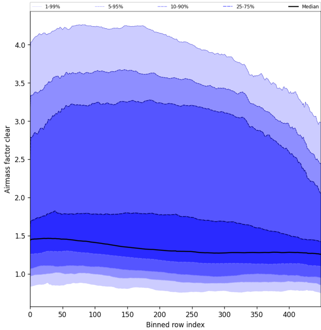
Figure 56: Along track statistics of “Air mass factor clear” for 2025-03-25 to 2025-03-27
