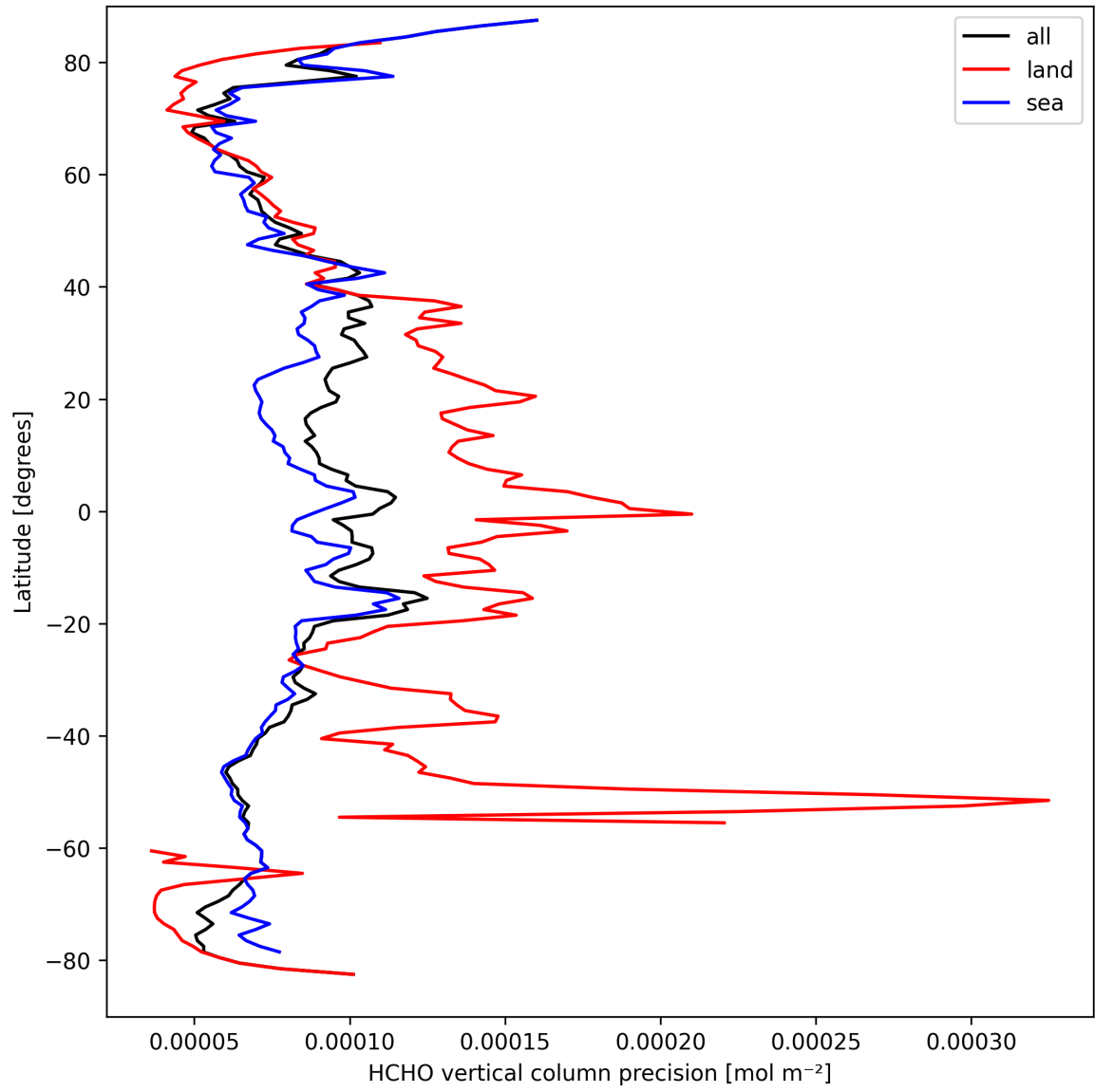
Figure 22: Zonal average of “HCHO vertical column precision” for 2025-03-25 to 2025-03-27.
