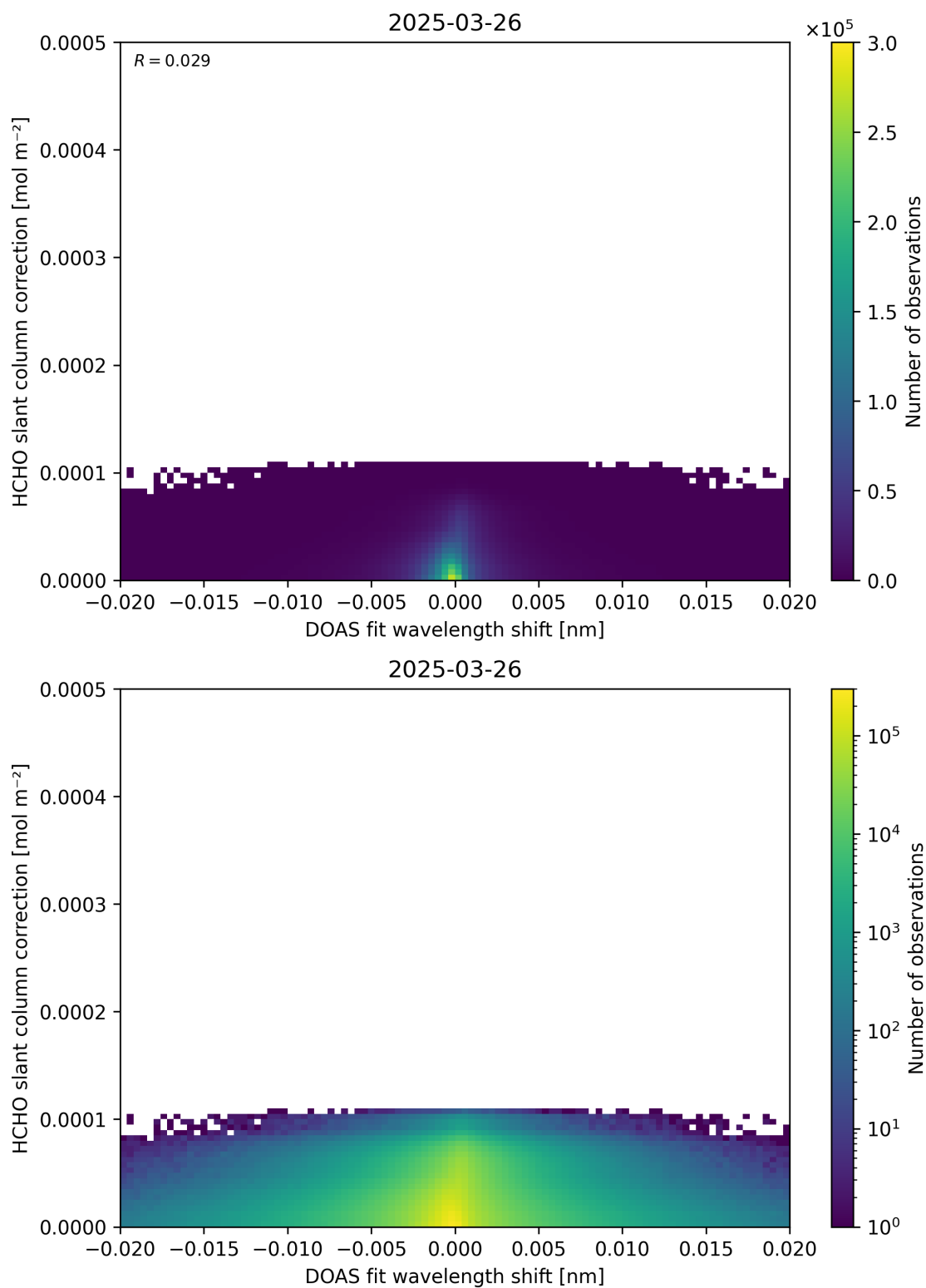
Figure 67: Scatter density plot of “DOAS fit wavelength shift” against “HCHO slant column correction” for 2025-03-25 to 2025-03-27.
