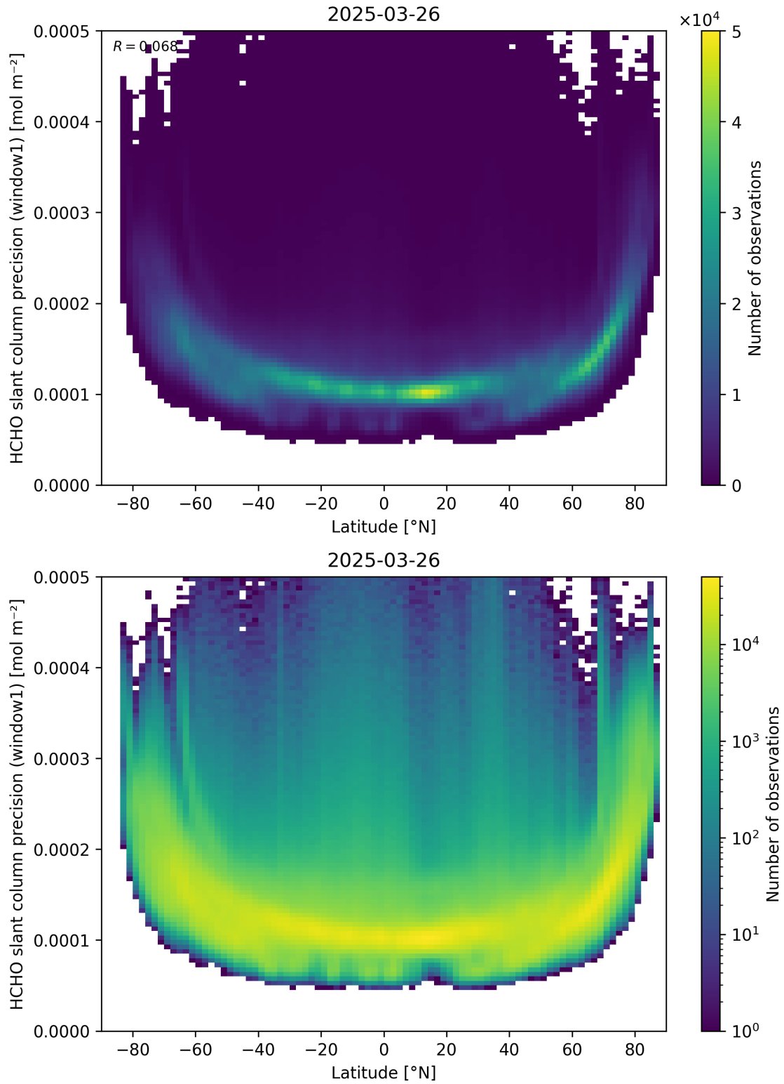
Figure 160: Scatter density plot of “Latitude” against “HCHO slant column precision (window1)” for 2025-03-25 to 2025-03-27.
