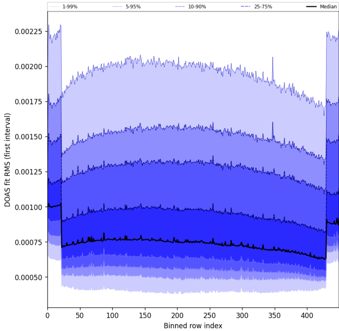
Figure 60: Along track statistics of “DOAS fit RMS (first interval)” for 2025-03-25 to 2025-03-27
