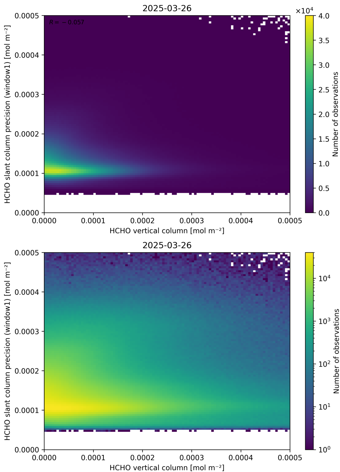
Figure 130: Scatter density plot of “HCHO vertical column” against “HCHO slant column precision (window1)” for 2025-03-25 to 2025-03-27.
