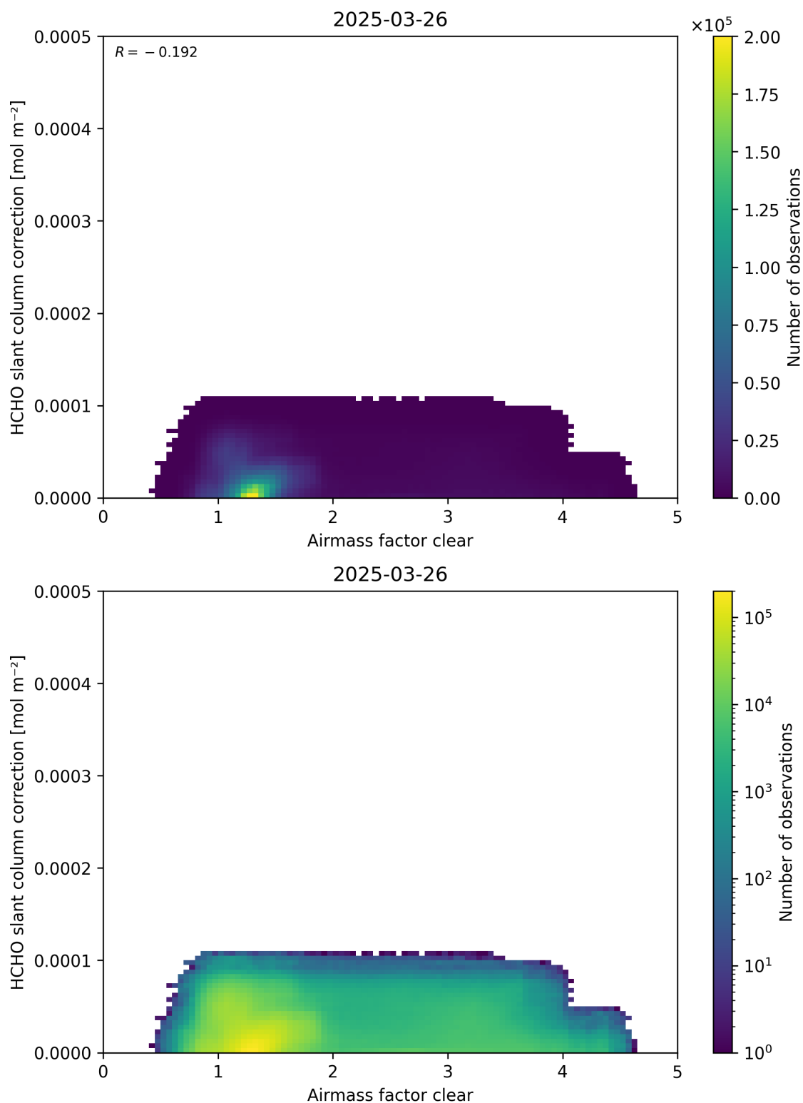
Figure 75: Scatter density plot of “Airmass factor clear” against “HCHO slant column correction” for 2025-03-25 to 2025-03-27.
