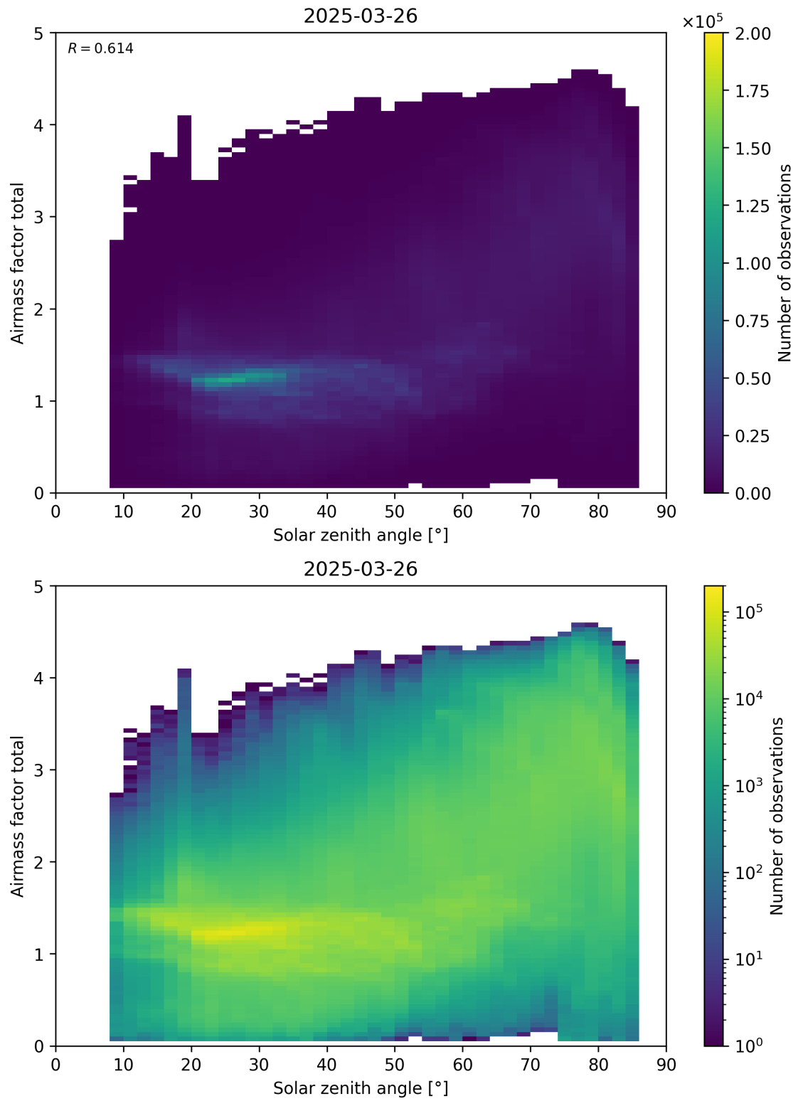
Figure 175: Scatter density plot of “Solar zenith angle” against “Airmass factor total” for 2025-03-25 to 2025-03-27.
