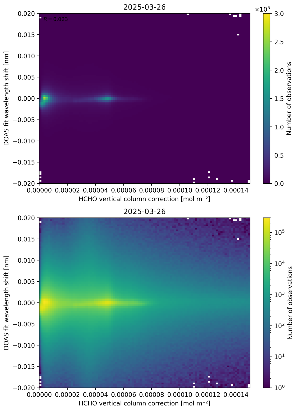
Figure 113: Scatter density plot of “HCHO vertical column correction” against “DOAS fit wavelength shift” for 2025-03-25 to 2025-03-27.
