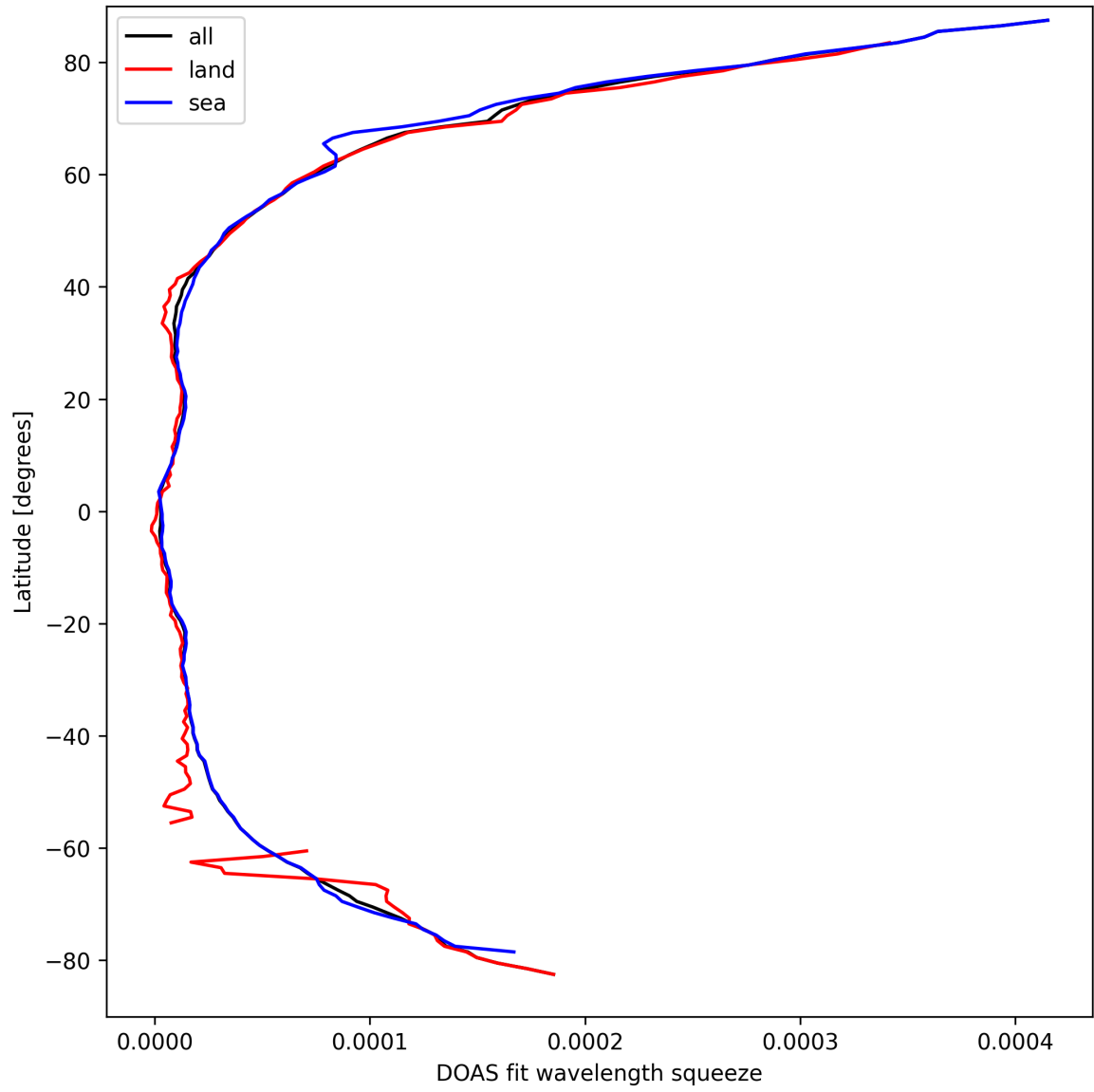
Figure 31: Zonal average of “DOAS fit wavelength squeeze” for 2025-03-25 to 2025-03-27.
