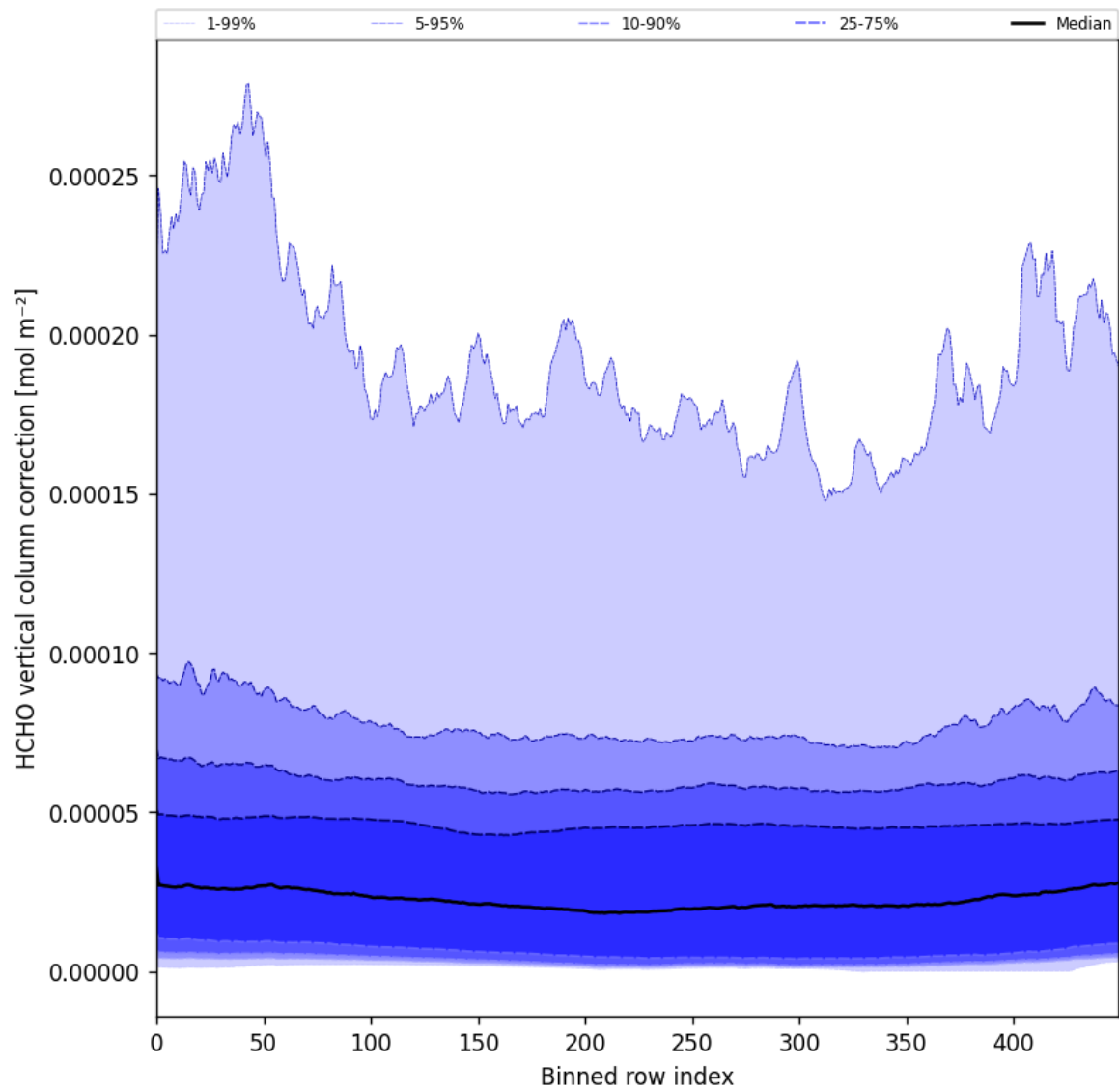
Figure 51: Along track statistics of “HCHO vertical column correction” for 2025-03-25 to 2025-03-27
