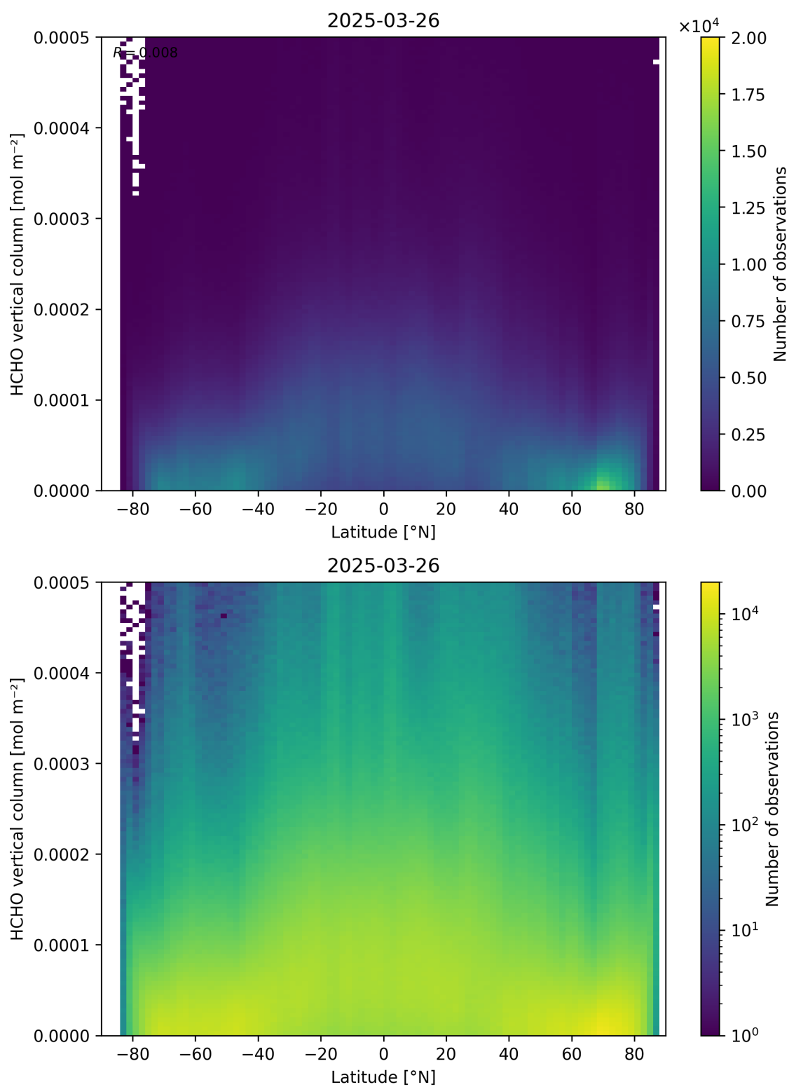
Figure 163: Scatter density plot of “Latitude” against “HCHO vertical column” for 2025-03-25 to 2025-03-27.
