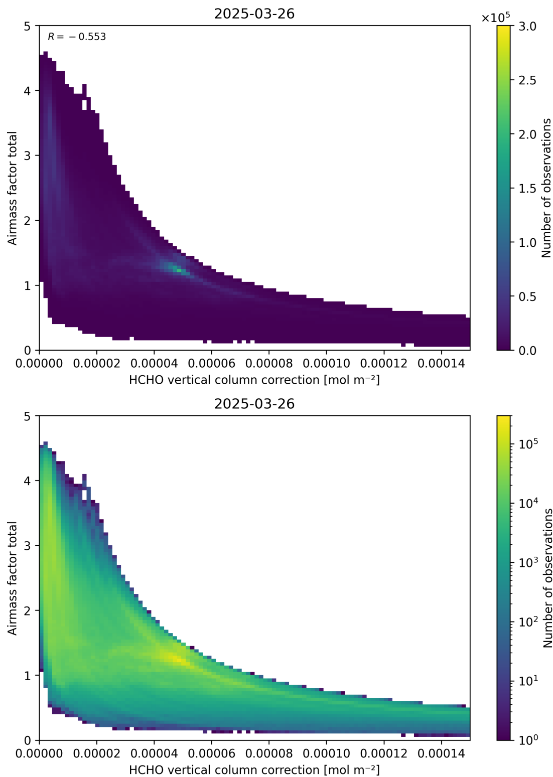
Figure 120: Scatter density plot of “HCHO vertical column correction” against “Airmass factor total” for 2025-03-25 to 2025-03-27.
