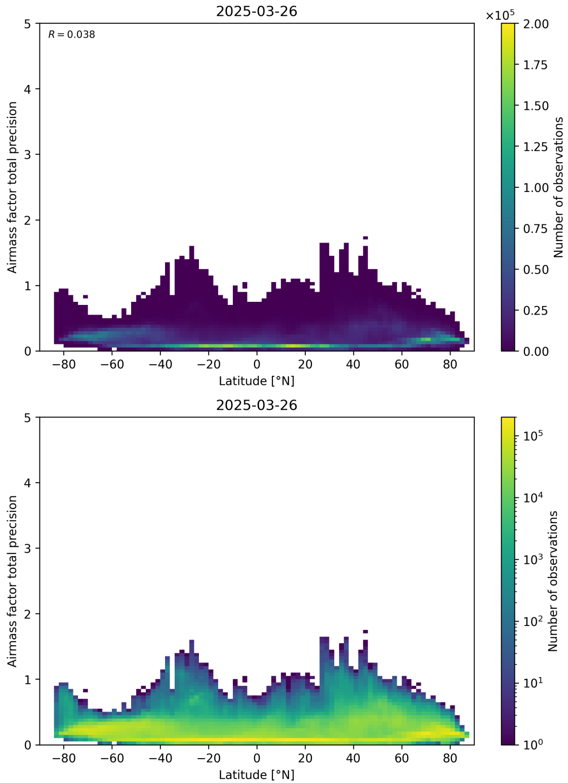
Figure 162: Scatter density plot of “Latitude” against “Airmass factor total precision” for 2025-03-25 to 2025-03-27.
