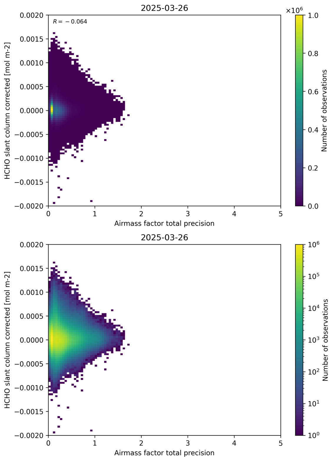
Figure 109: Scatter density plot of “Airmass factor total precision” against “HCHO slant column corrected” for 2025-03-25 to 2025-03-27.
