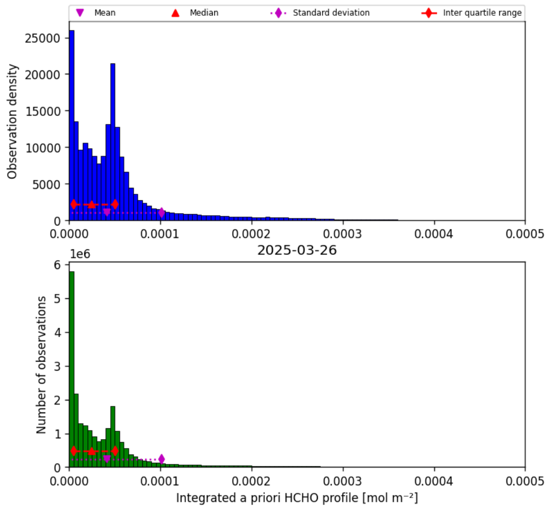
Figure 43: Histogram of “Integrated a priori HCHO profile” for 2025-03-25 to 2025-03-27
