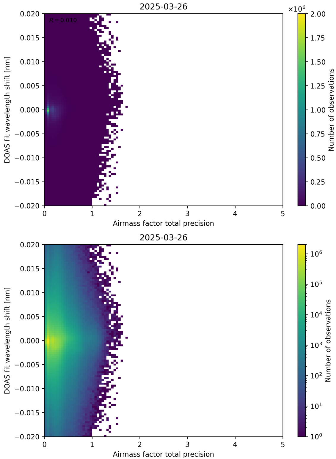
Figure 106: Scatter density plot of “Airmass factor total precision” against “DOAS fit wavelength shift” for 2025-03-25 to 2025-03-27.
