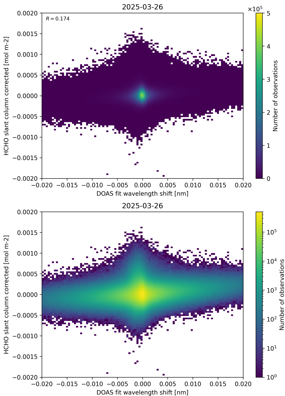
Figure 66: Scatter density plot of “DOAS fit wavelength shift” against “HCHO slant column corrected” for 2025-03-25 to 2025-03-27.
