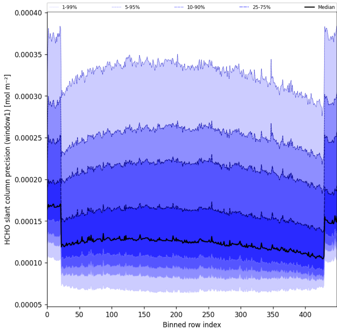
Figure 53: Along track statistics of “HCHO slant column precision (window1)” for 2025-03-25 to 2025-03-27
