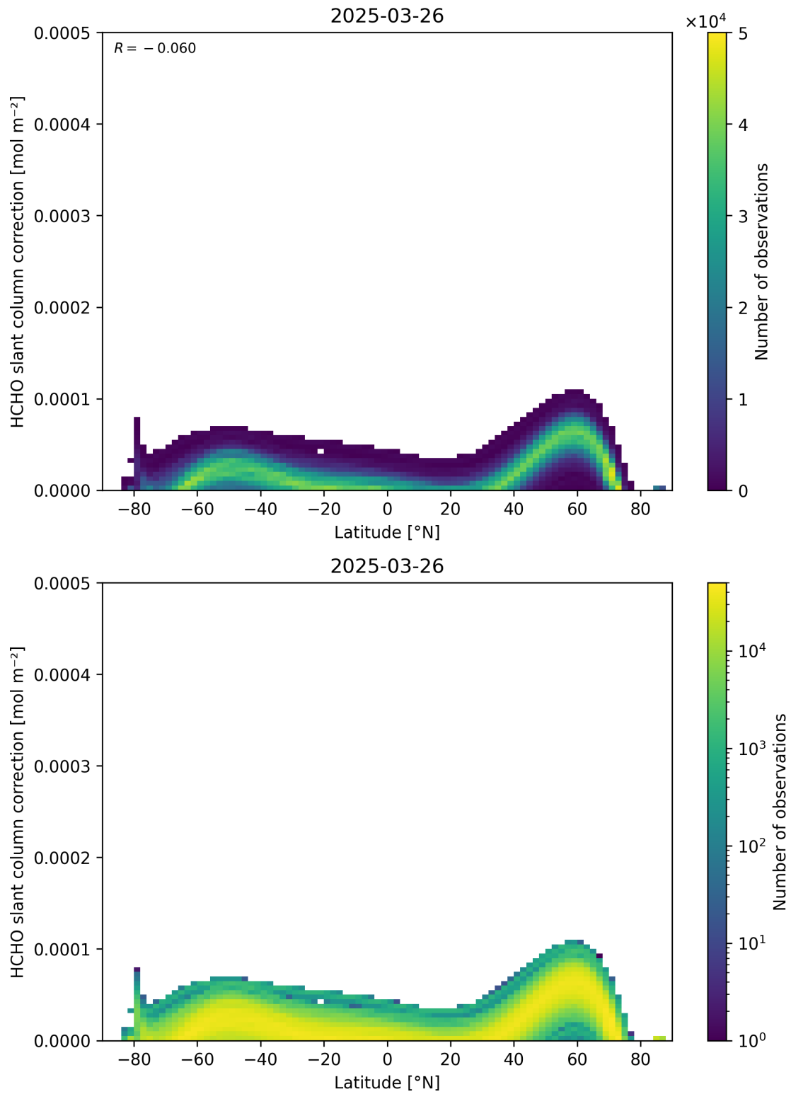
Figure 158: Scatter density plot of “Latitude” against “HCHO slant column correction” for 2025-03-25 to 2025-03-27.
