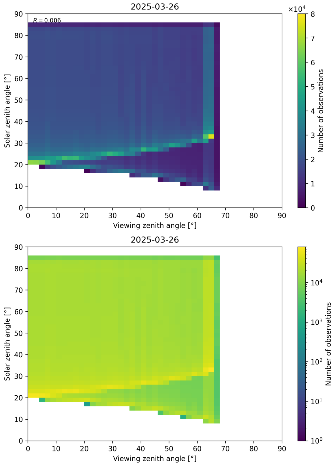
Figure 197: Scatter density plot of “Viewing zenith angle” against “Solar zenith angle” for 2025-03-25 to 2025-03-27.
