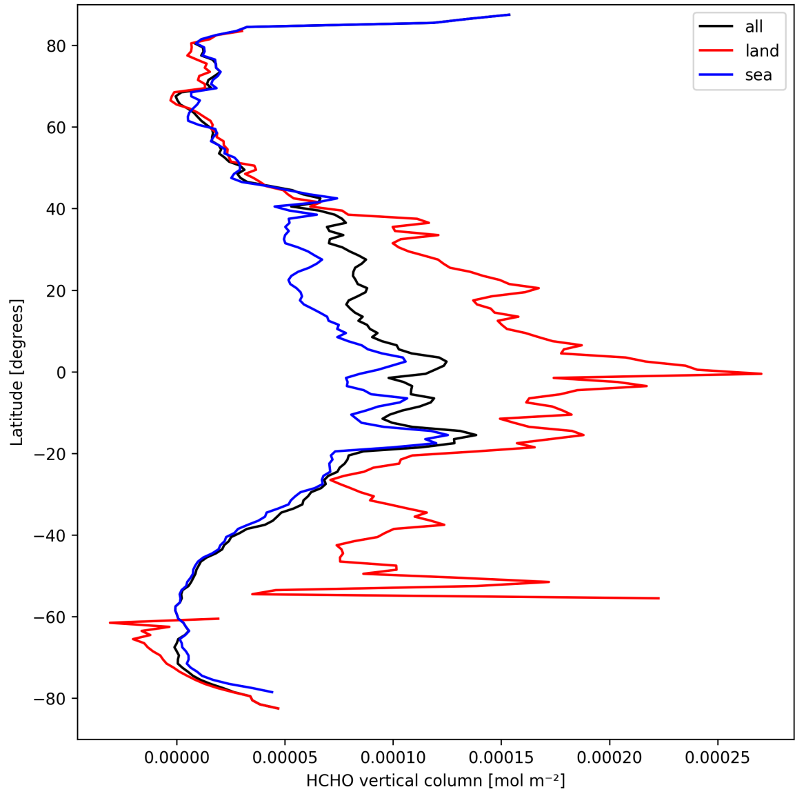
Figure 21: Zonal average of “HCHO vertical column” for 2025-03-25 to 2025-03-27.
