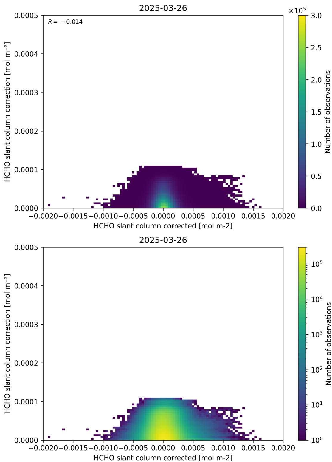
Figure 77: Scatter density plot of “HCHO slant column corrected” against “HCHO slant column correction” for 2025-03-25 to 2025-03-27.
