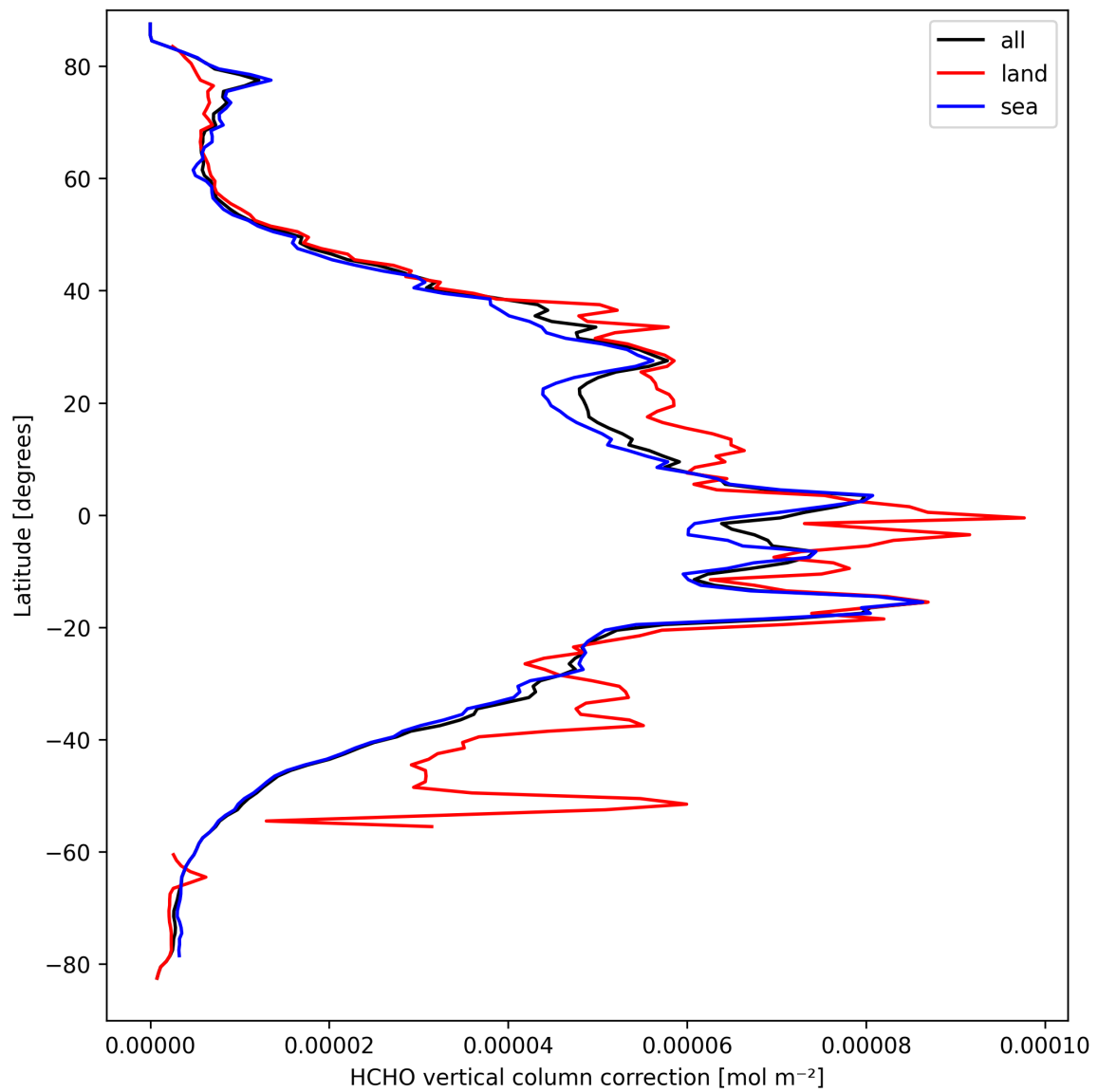
Figure 23: Zonal average of “HCHO vertical column correction” for 2025-03-25 to 2025-03-27.
