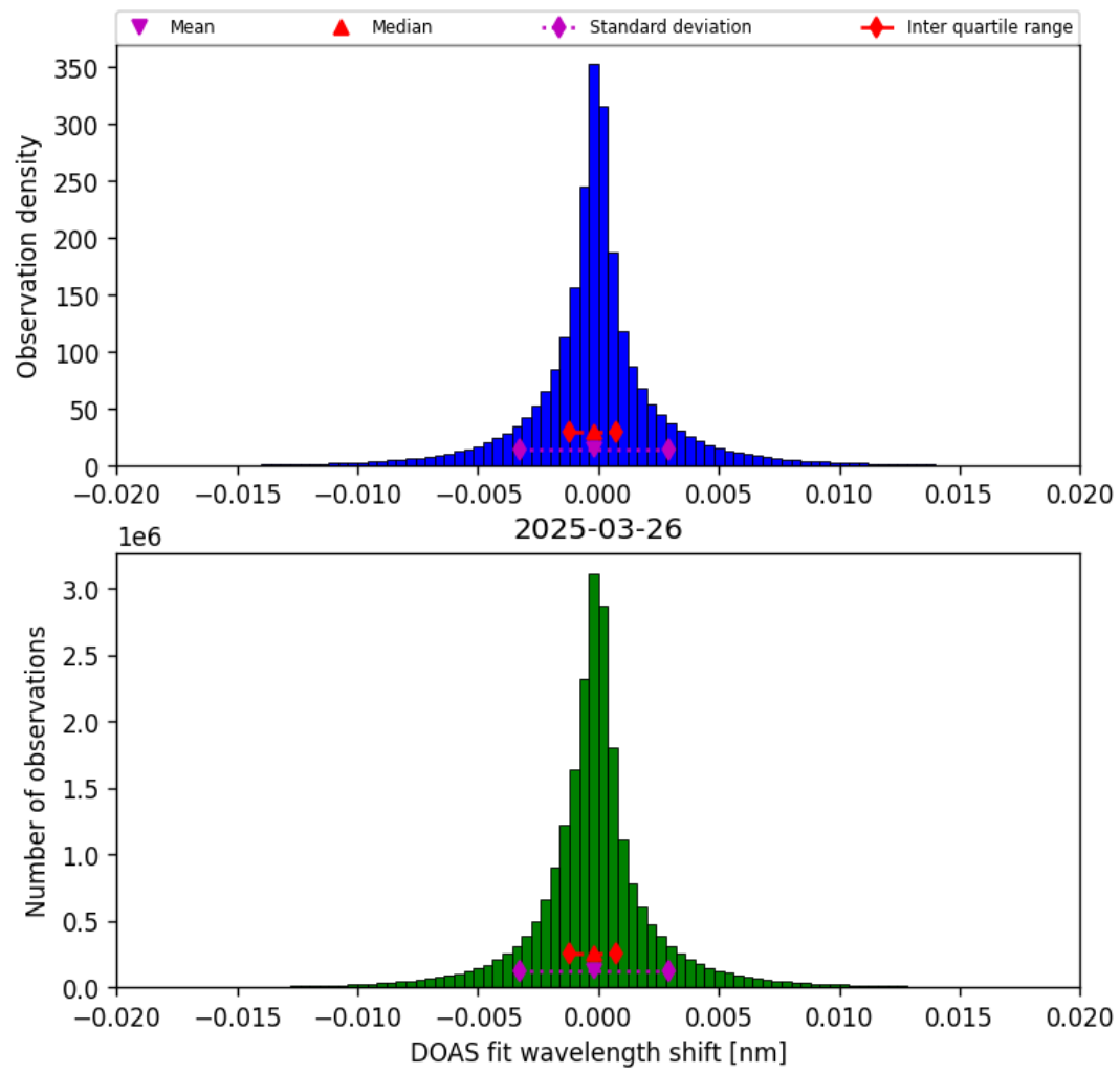
Figure 44: Histogram of “DOAS fit wavelength shift” for 2025-03-25 to 2025-03-27
