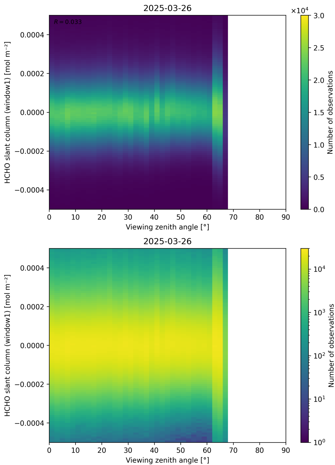
Figure 188: Scatter density plot of “Viewing zenith angle” against “HCHO slant column (window1)” for 2025-03-25 to 2025-03-27.
