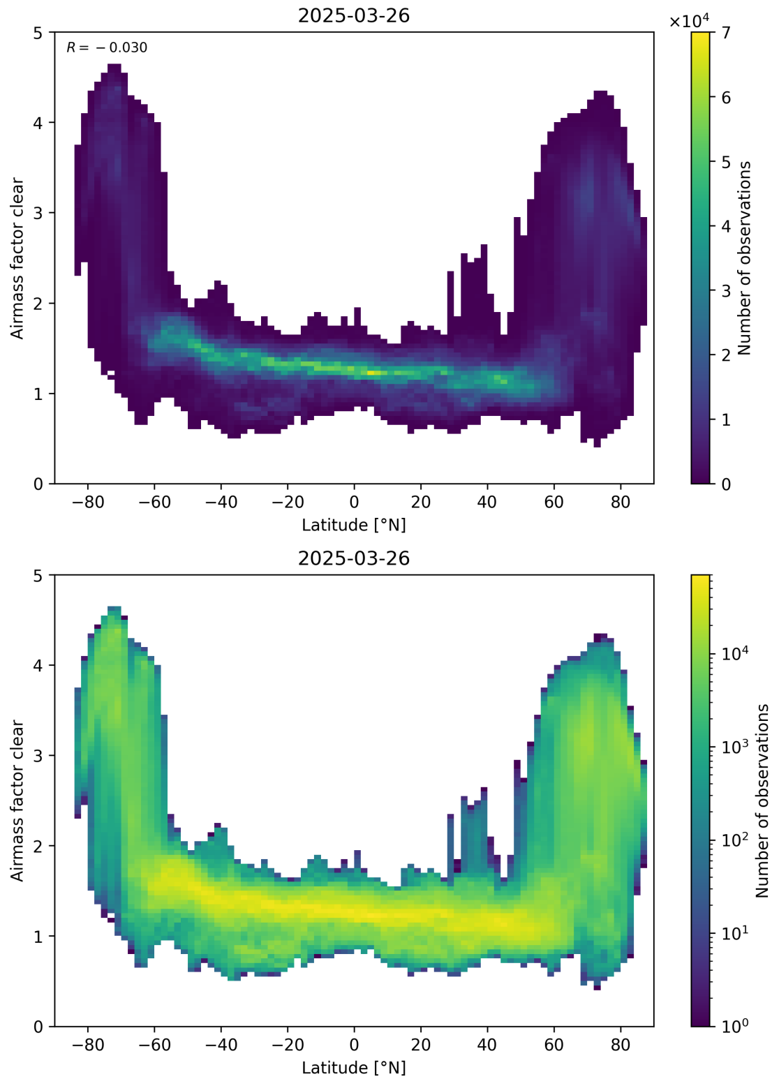
Figure 156: Scatter density plot of “Latitude” against “Airmass factor clear” for 2025-03-25 to 2025-03-27.
