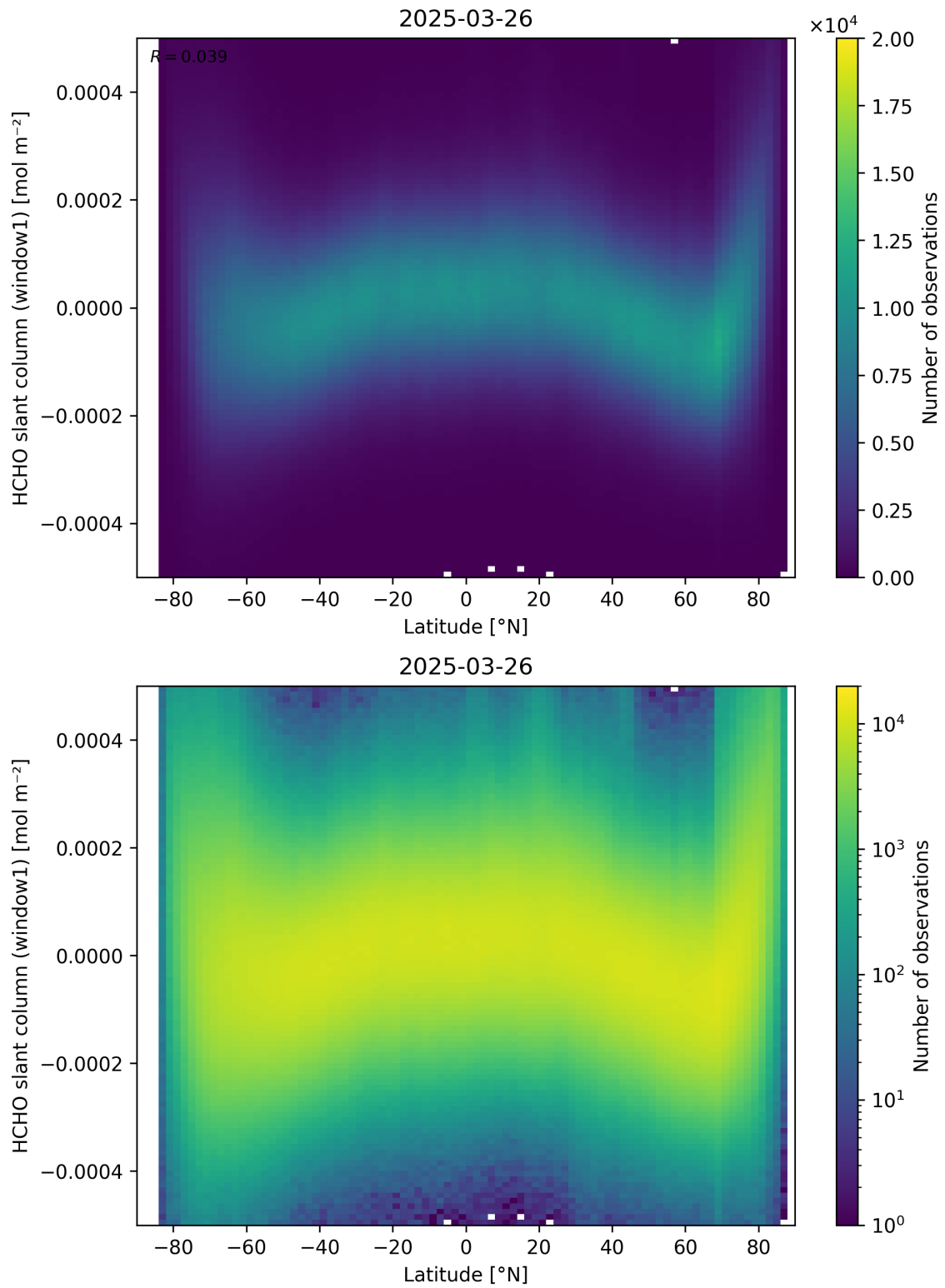
Figure 159: Scatter density plot of “Latitude” against “HCHO slant column (window1)” for 2025-03-25 to 2025-03-27.
