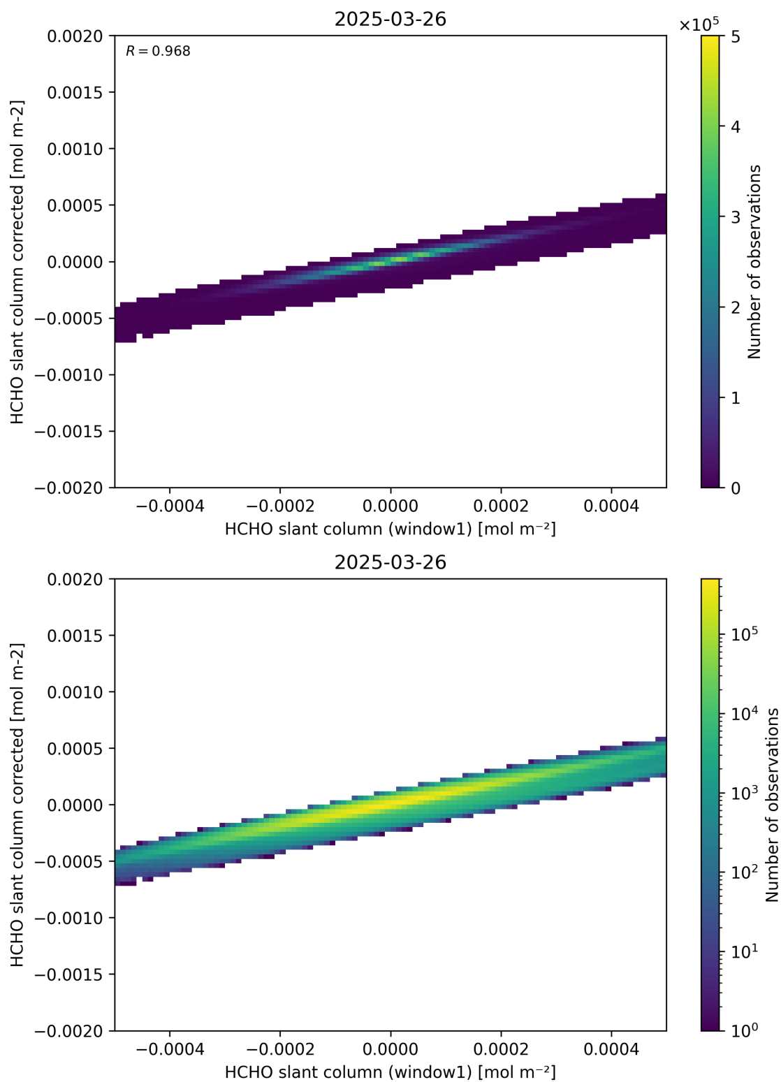
Figure 82: Scatter density plot of “HCHO slant column (window1)” against “HCHO slant column corrected” for 2025-03-25 to 2025-03-27.
