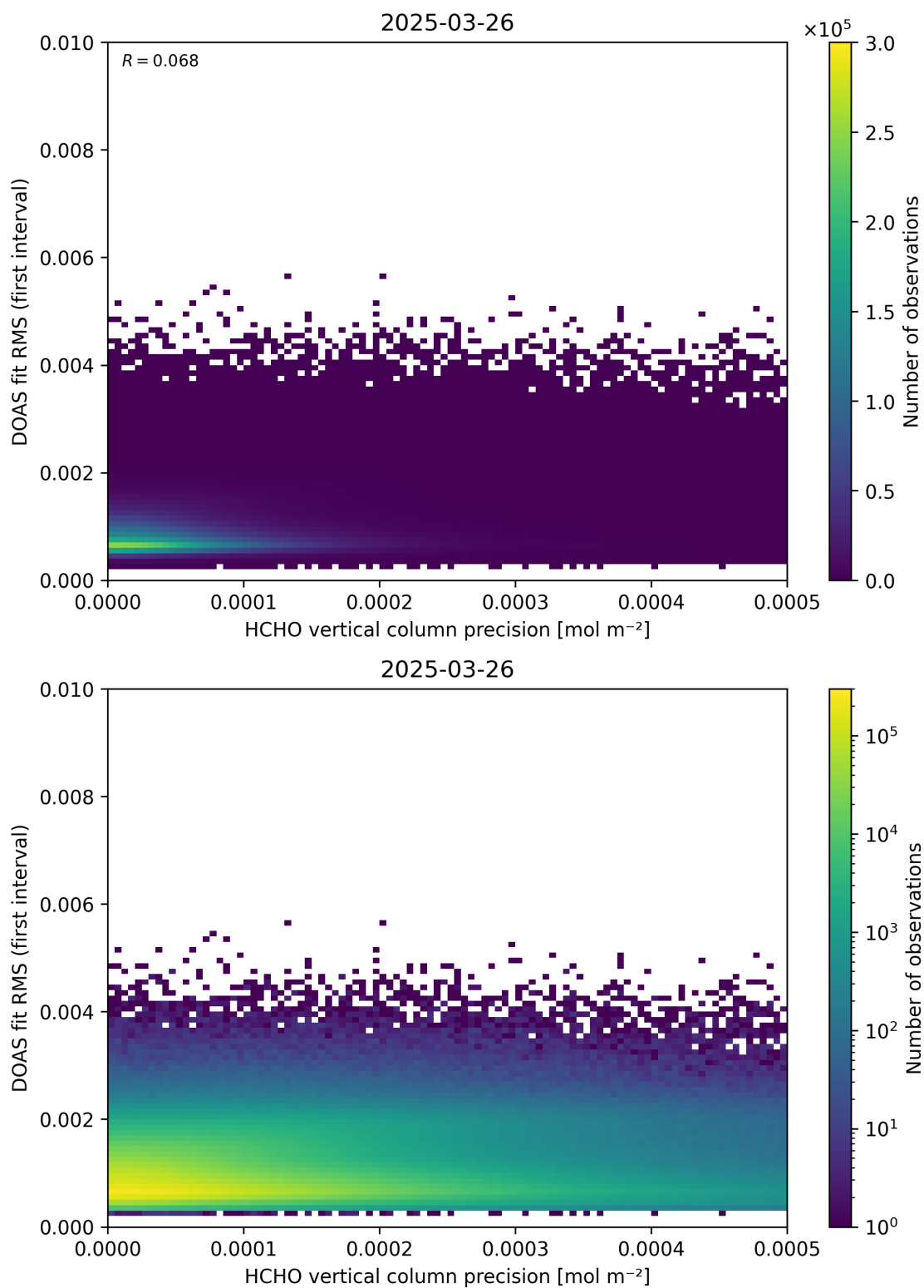
Figure 136: Scatter density plot of “HCHO vertical column precision” against “DOAS fit RMS (first interval)” for 2025-03-25 to 2025-03-27.
