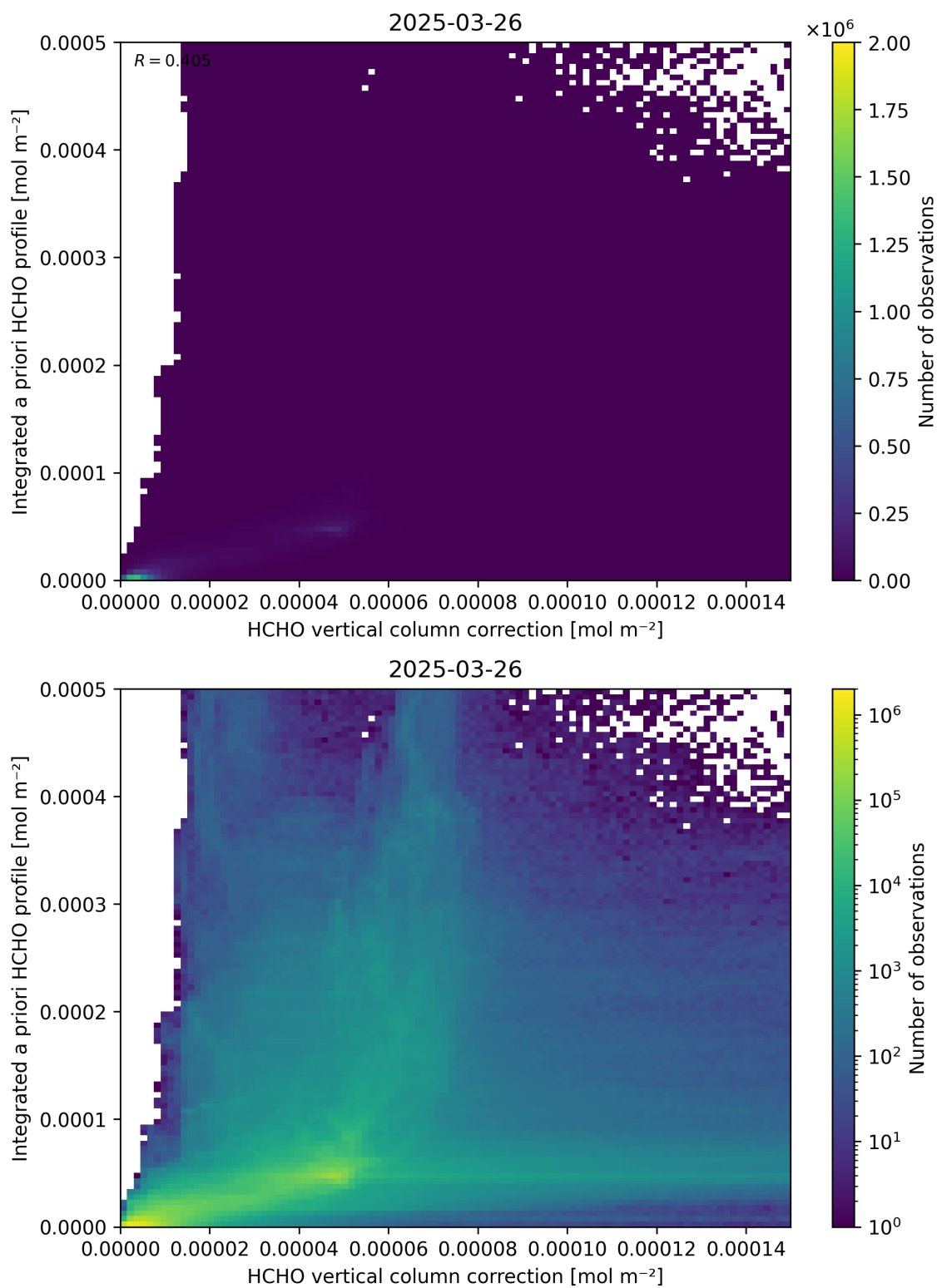
Figure 122: Scatter density plot of “HCHO vertical column correction” against “Integrated a priori HCHO profile” for 2025-03-25 to 2025-03-27.
