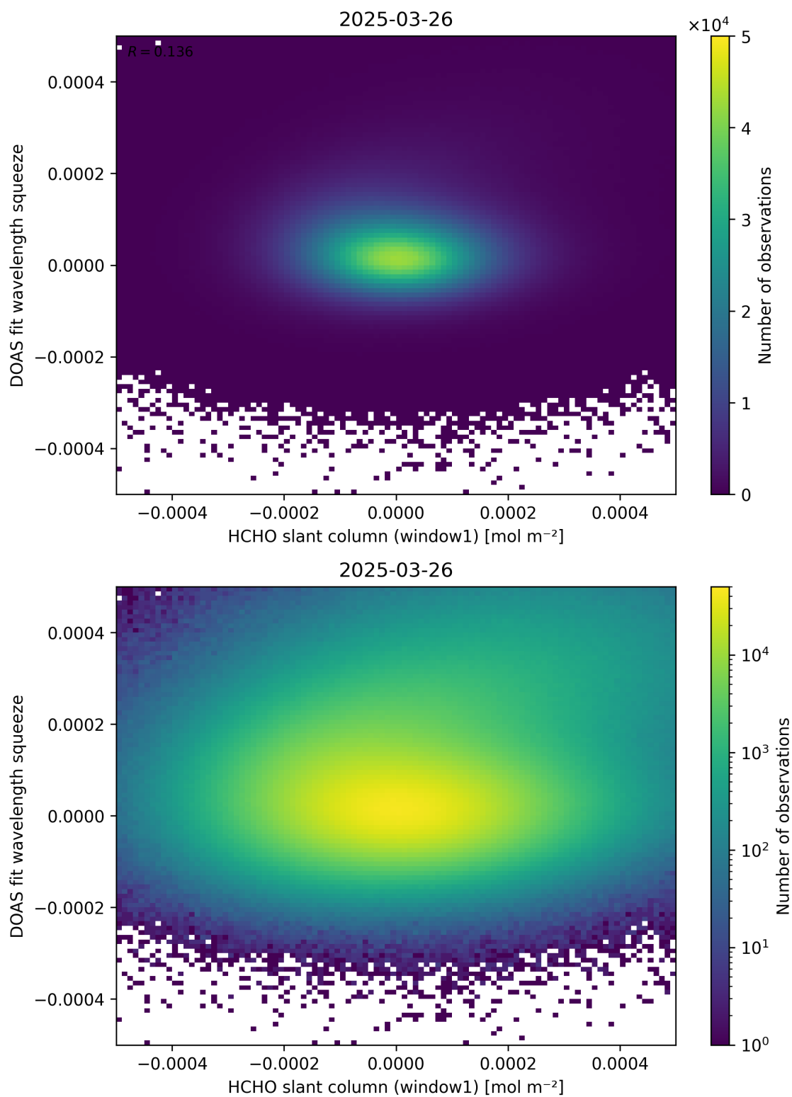
Figure 80: Scatter density plot of “HCHO slant column (window1)” against “DOAS fit wavelength squeeze” for 2025-03-25 to 2025-03-27.
