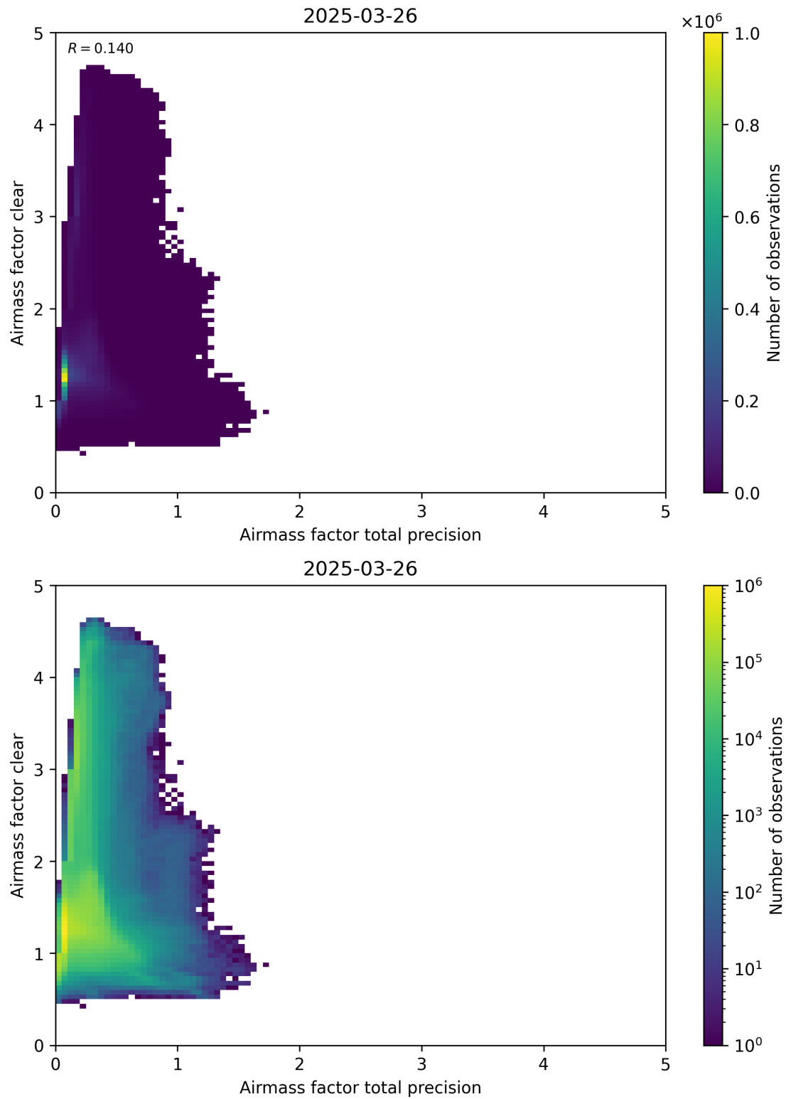
Figure 108: Scatter density plot of “Airmass factor total precision” against “Airmass factor clear” for 2025-03-25 to 2025-03-27.
