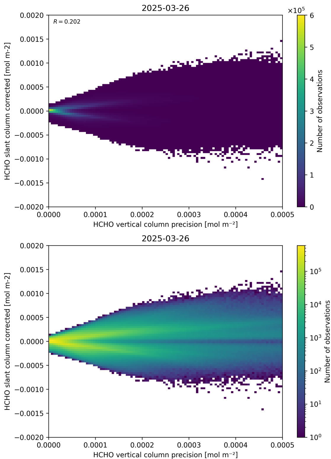
Figure 140: Scatter density plot of “HCHO vertical column precision” against “HCHO slant column corrected” for 2025-03-25 to 2025-03-27.
