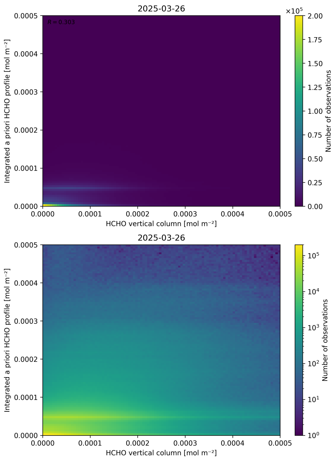
Figure 135: Scatter density plot of “HCHO vertical column” against “Integrated a priori HCHO profile” for 2025-03-25 to 2025-03-27.
