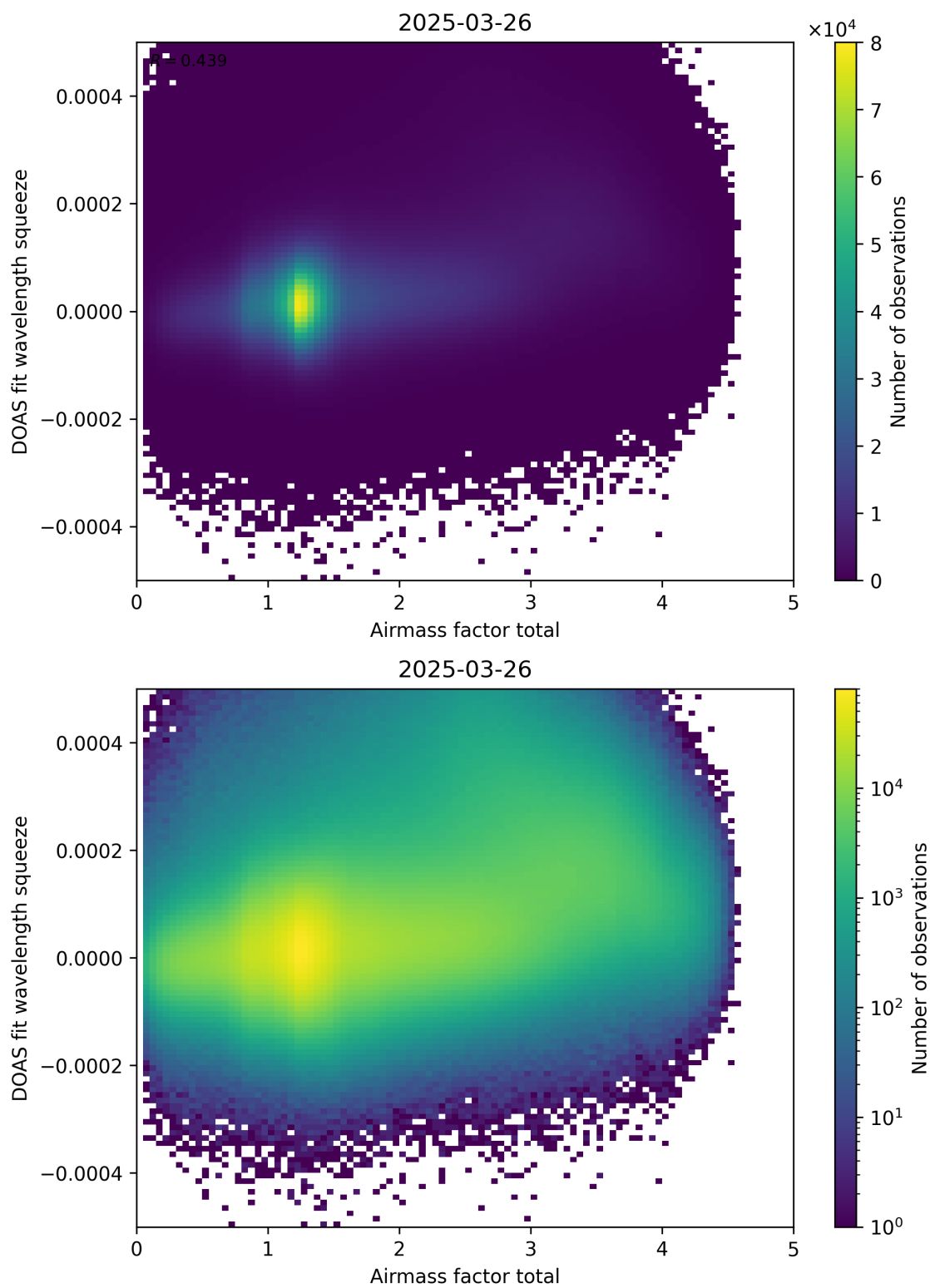
Figure 99: Scatter density plot of “Airmass factor total” against “DOAS fit wavelength squeeze” for 2025-03-25 to 2025-03-27.
