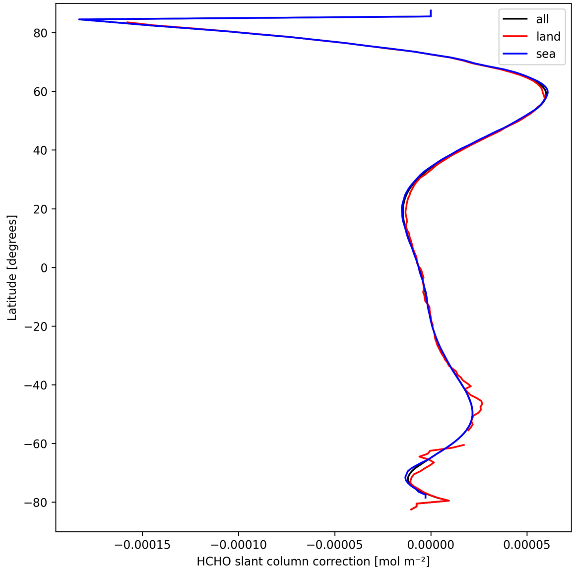
Figure 33: Zonal average of “HCHO slant column correction” for 2025-03-25 to 2025-03-27.
