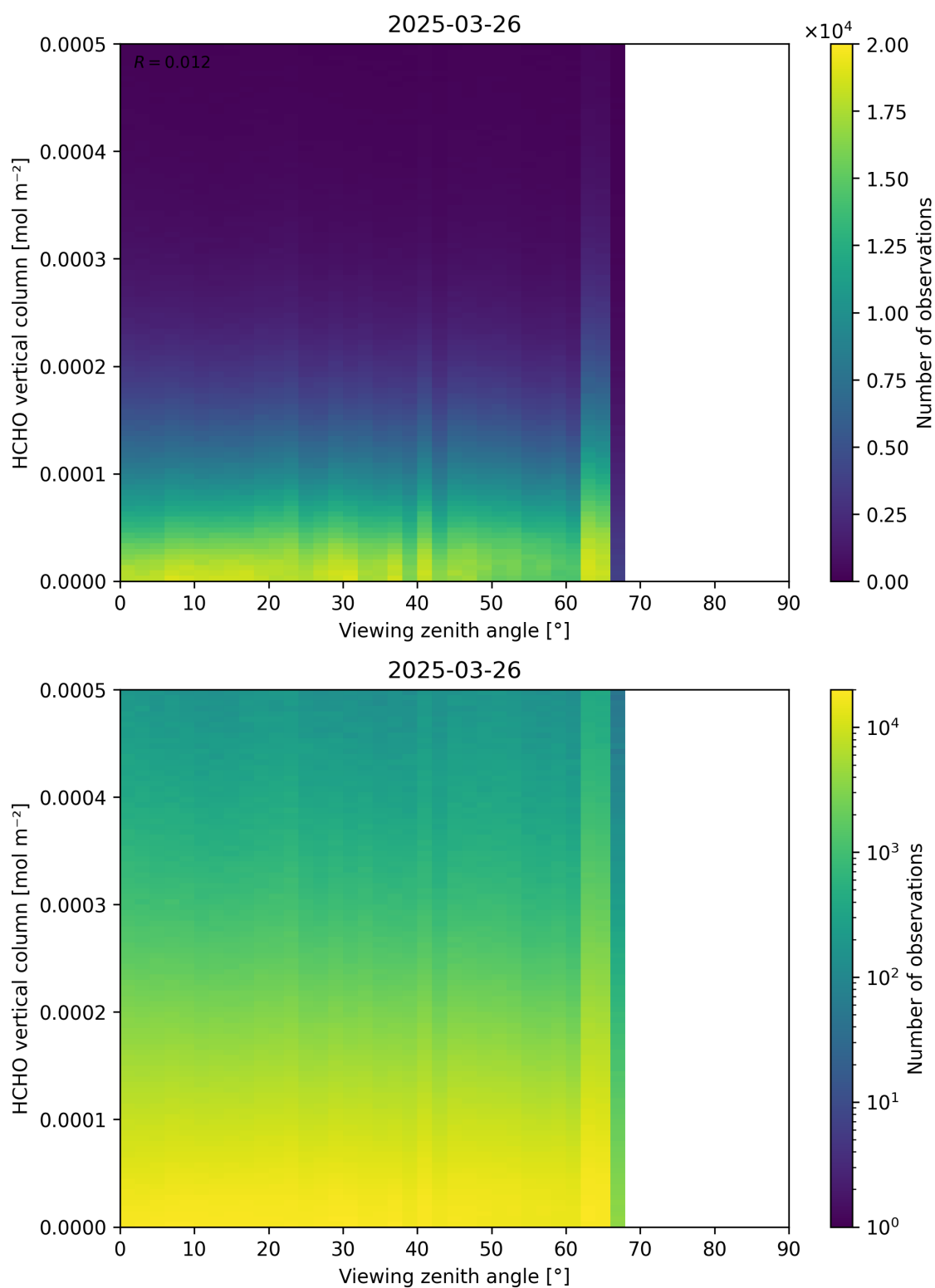
Figure 192: Scatter density plot of “Viewing zenith angle” against “HCHO vertical column” for 2025-03-25 to 2025-03-27.
