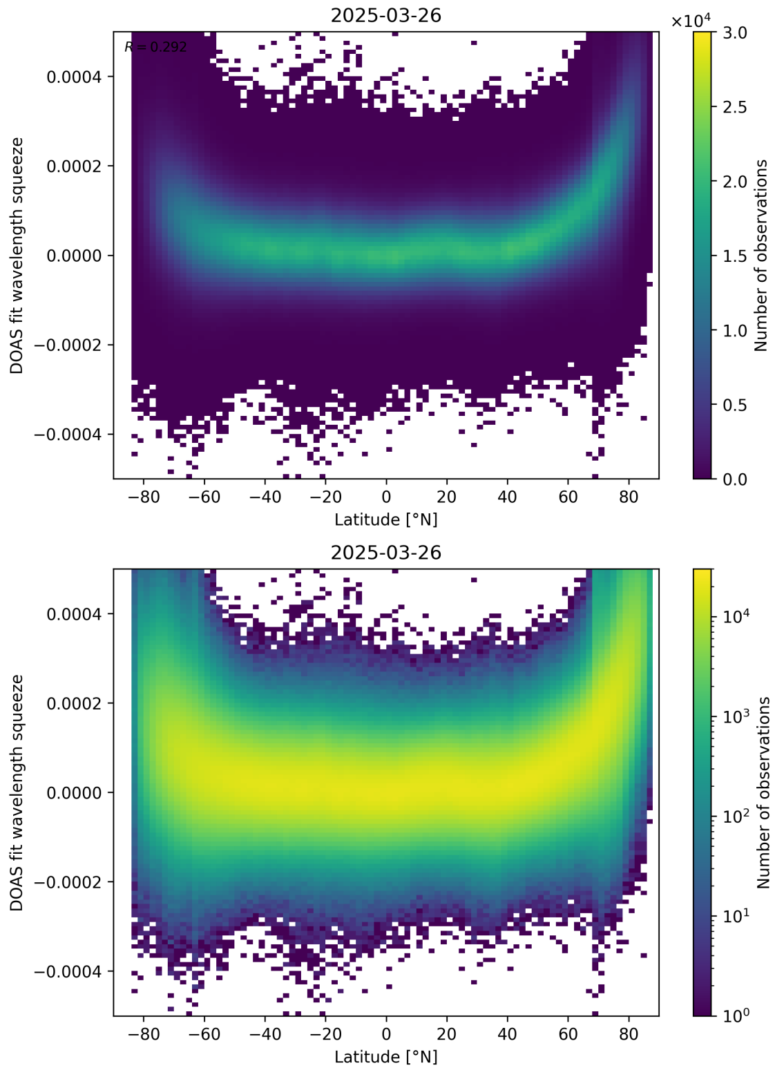
Figure 155: Scatter density plot of “Latitude” against “DOAS fit wavelength squeeze” for 2025-03-25 to 2025-03-27.
