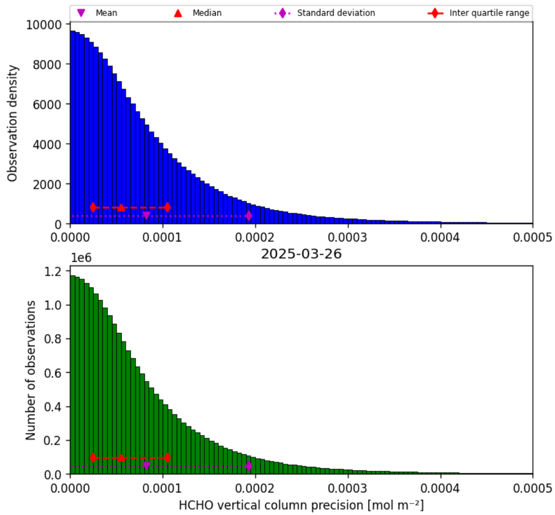
Figure 36: Histogram of “HCHO vertical column precision” for 2025-03-25 to 2025-03-27
