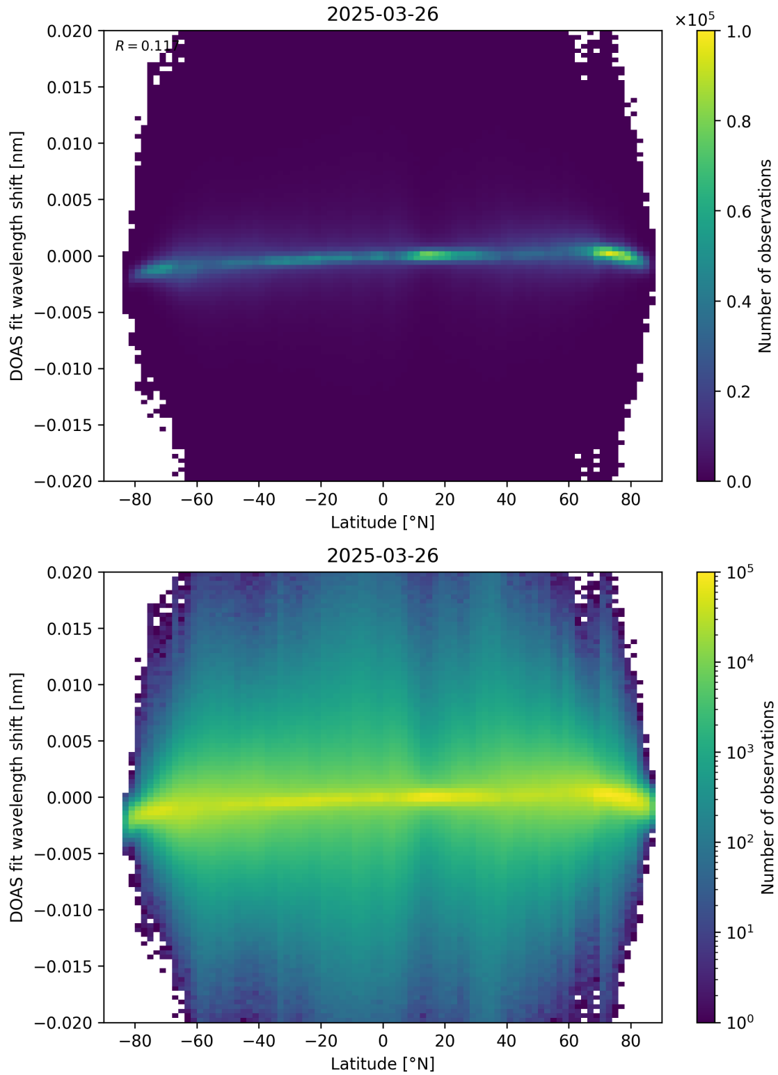
Figure 154: Scatter density plot of “Latitude” against “DOAS fit wavelength shift” for 2025-03-25 to 2025-03-27.
