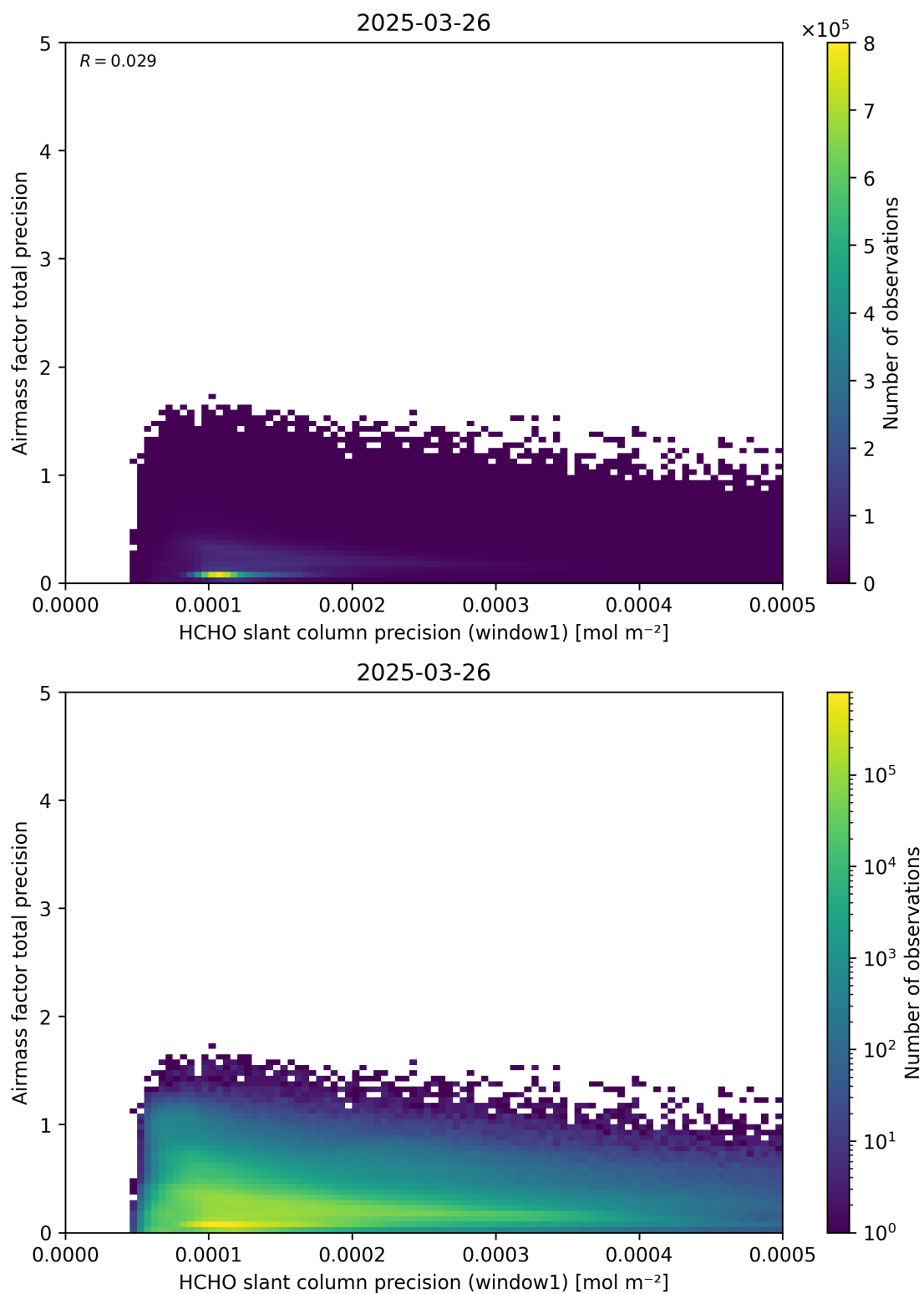
Figure 95: Scatter density plot of “HCHO slant column precision (window1)” against “Airmass factor total precision” for 2025-03-25 to 2025-03-27.
