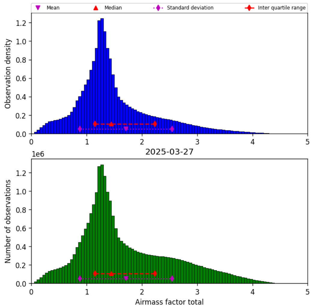
Figure 40: Histogram of “Airmass factor total” for 2025-03-26 to 2025-03-28
