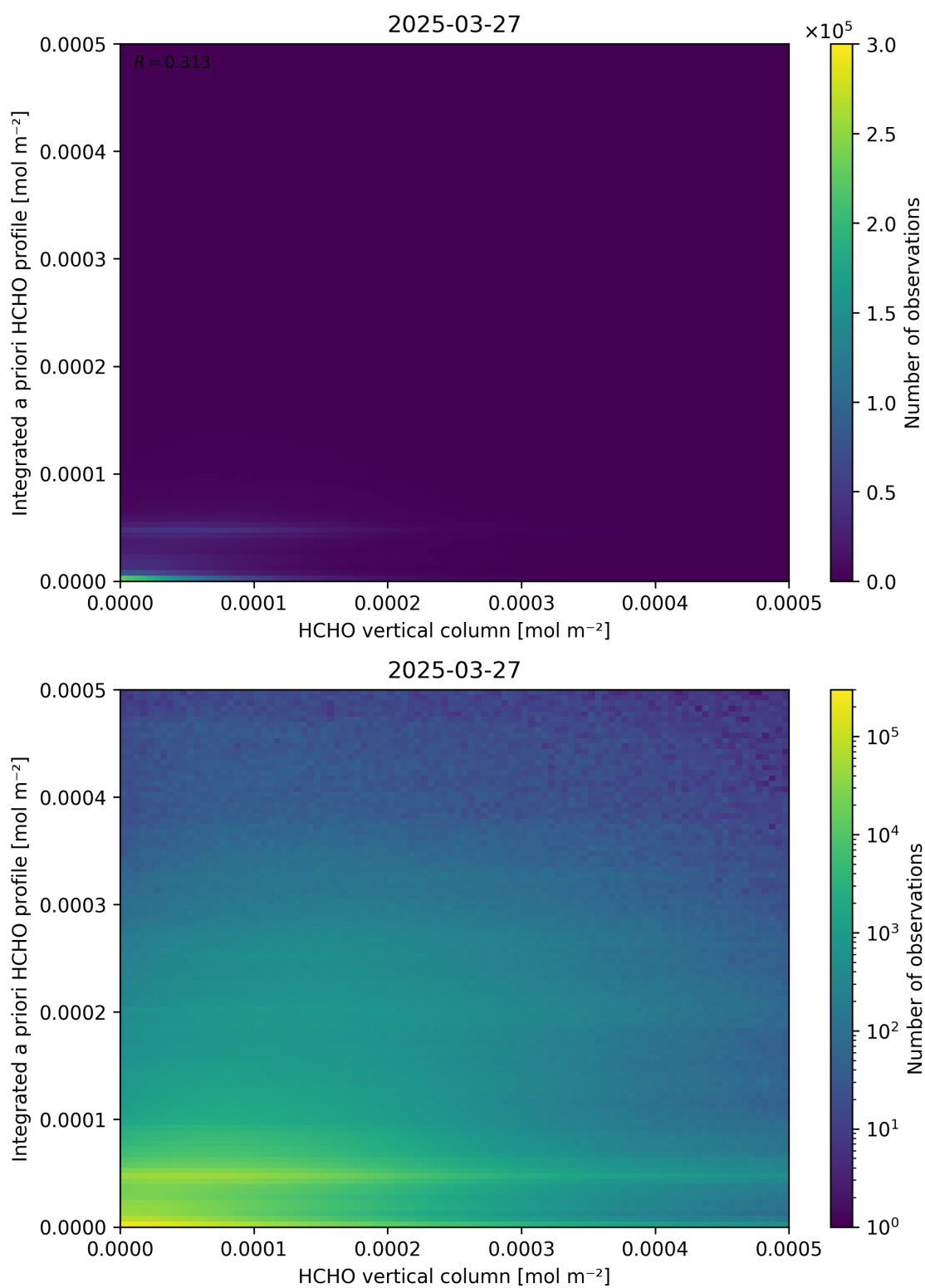
Figure 135: Scatter density plot of “HCHO vertical column” against “Integrated a priori HCHO profile” for 2025-03-26 to 2025-03-28.
