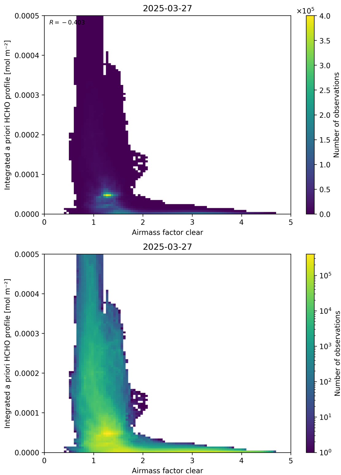
Figure 76: Scatter density plot of “Airmass factor clear” against “Integrated a priori HCHO profile” for 2025-03-26 to 2025-03-28.
