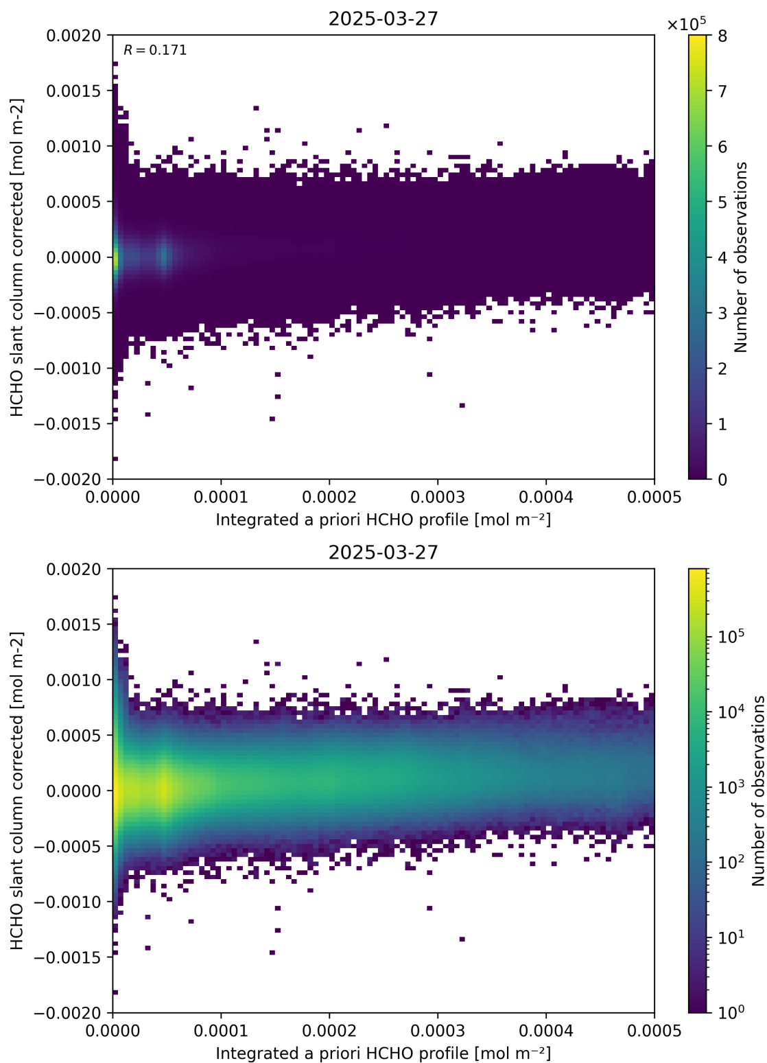
Figure 151: Scatter density plot of “Integrated a priori HCHO profile” against “HCHO slant column corrected” for 2025-03-26 to 2025-03-28.
