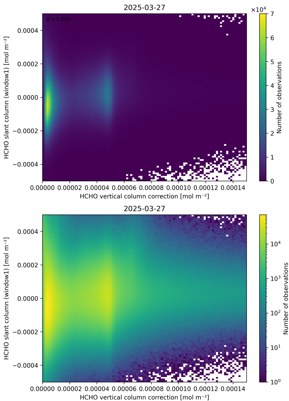
Figure 118: Scatter density plot of “HCHO vertical column correction” against “HCHO slant column (window1)” for 2025-03-26 to 2025-03-28.
