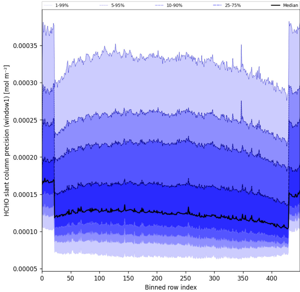
Figure 53: Along track statistics of “HCHO slant column precision (window1)” for 2025-03-26 to 2025-03-28
