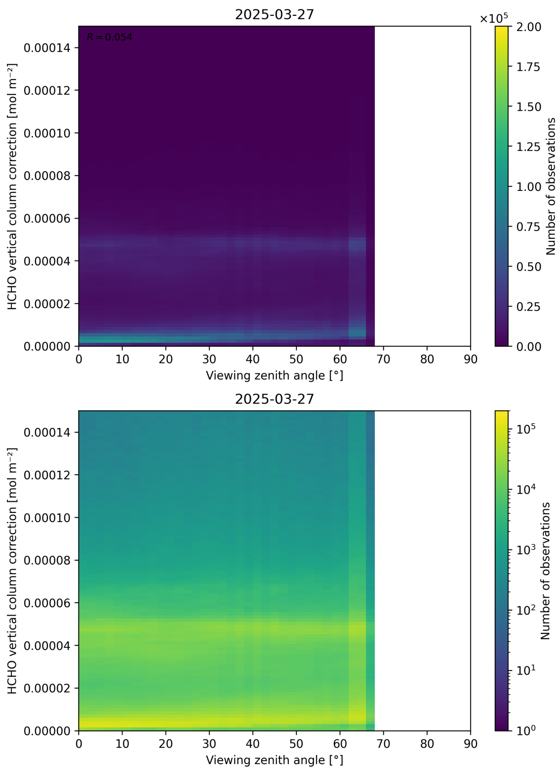
Figure 193: Scatter density plot of “Viewing zenith angle” against “HCHO vertical column correction” for 2025-03-26 to 2025-03-28.
