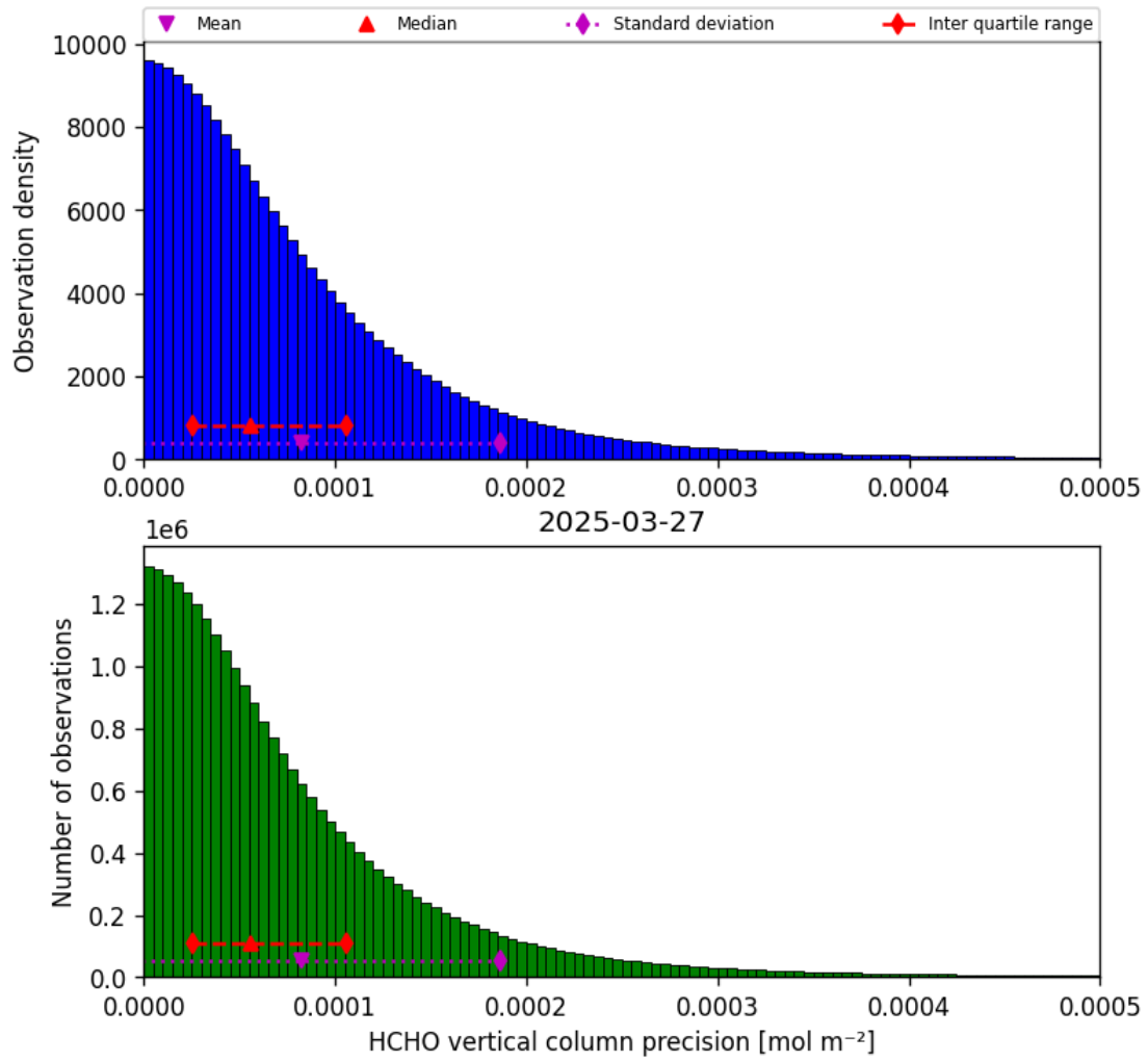
Figure 36: Histogram of “HCHO vertical column precision” for 2025-03-26 to 2025-03-28
