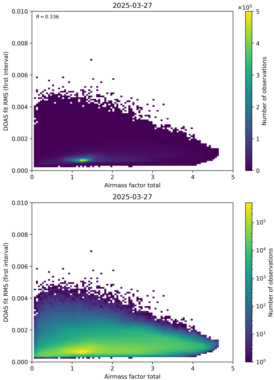
Figure 97: Scatter density plot of “Airmass factor total” against “DOAS fit RMS (first interval)” for 2025-03-26 to 2025-03-28.
