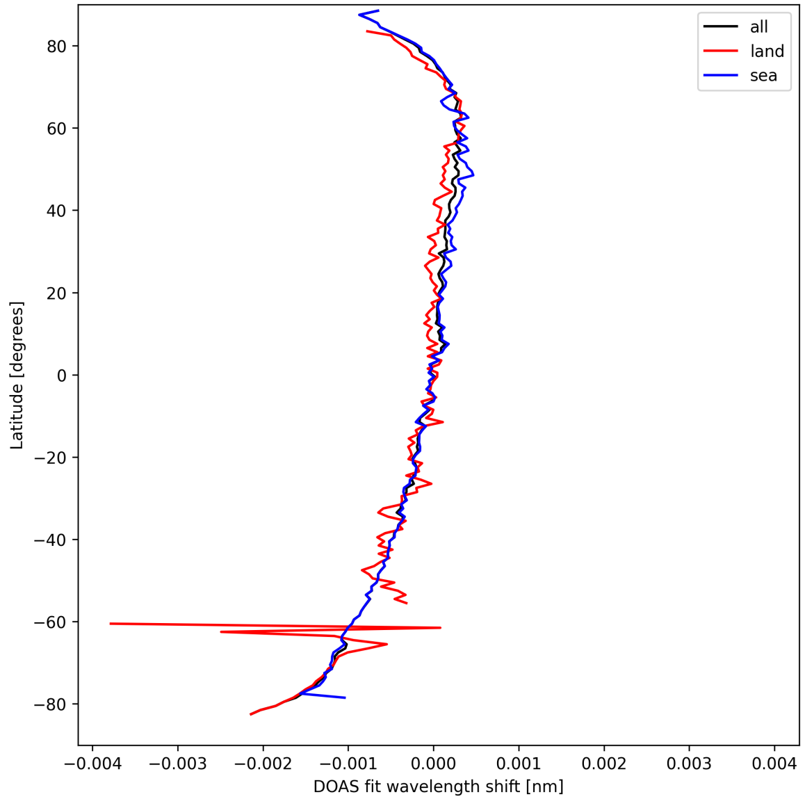
Figure 30: Zonal average of “DOAS fit wavelength shift” for 2025-03-26 to 2025-03-28.
