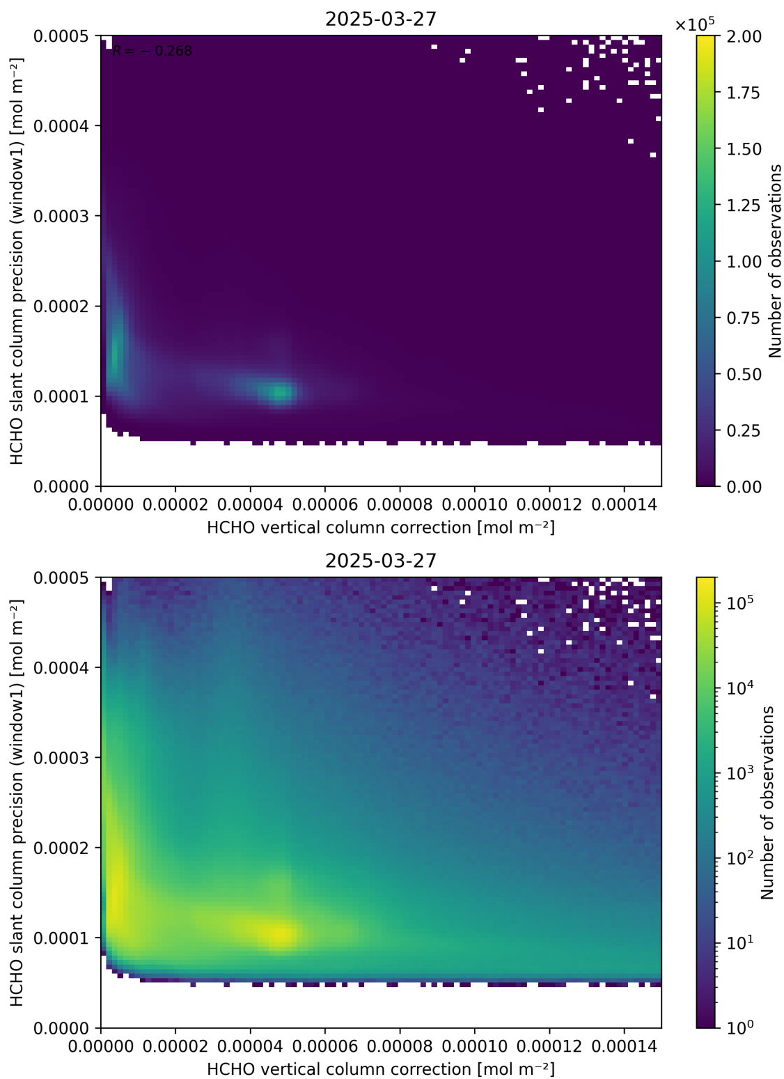
Figure 119: Scatter density plot of “HCHO vertical column correction” against “HCHO slant column precision (window1)” for 2025-03-26 to 2025-03-28.
