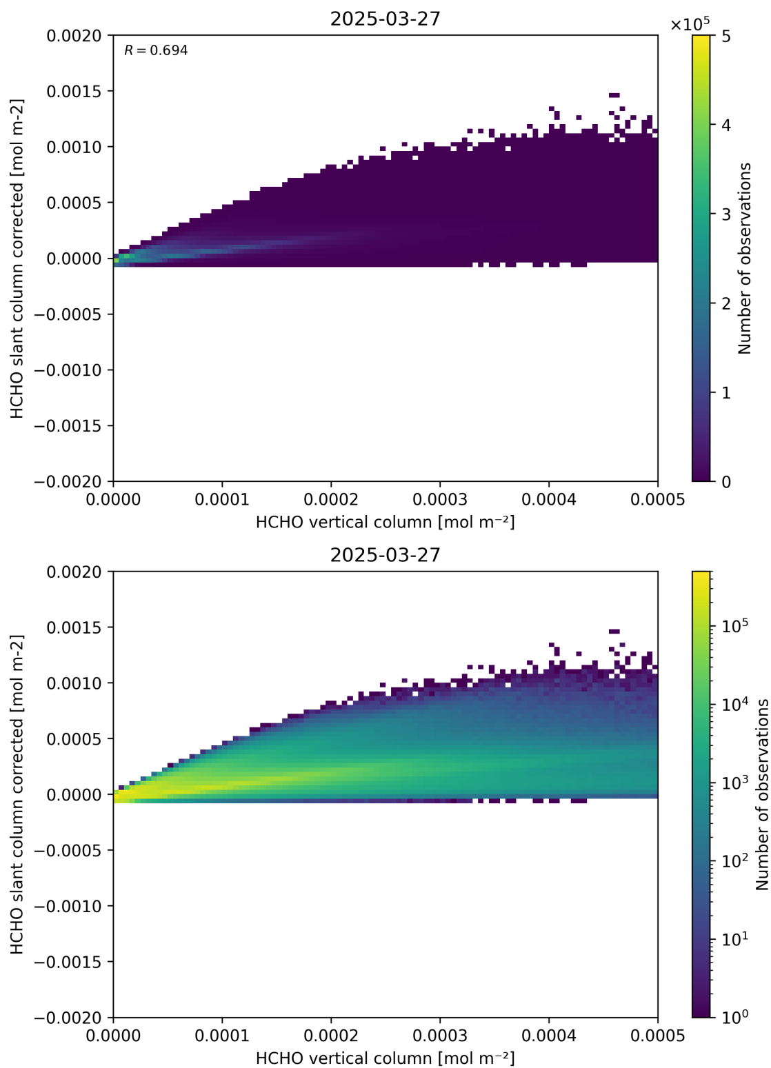
Figure 127: Scatter density plot of “HCHO vertical column” against “HCHO slant column corrected” for 2025-03-26 to 2025-03-28.
