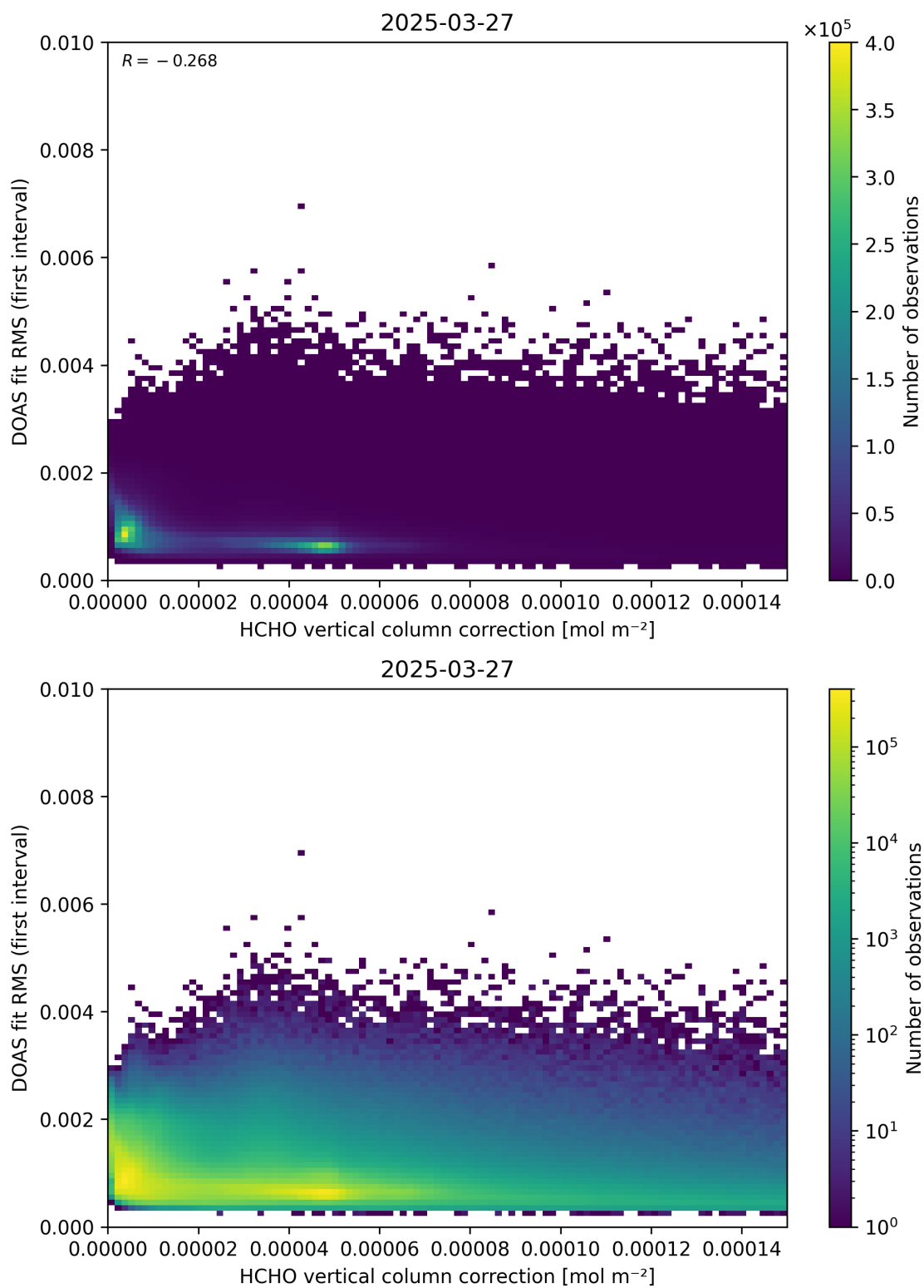
Figure 112: Scatter density plot of “HCHO vertical column correction” against “DOAS fit RMS (first interval)” for 2025-03-26 to 2025-03-28.
