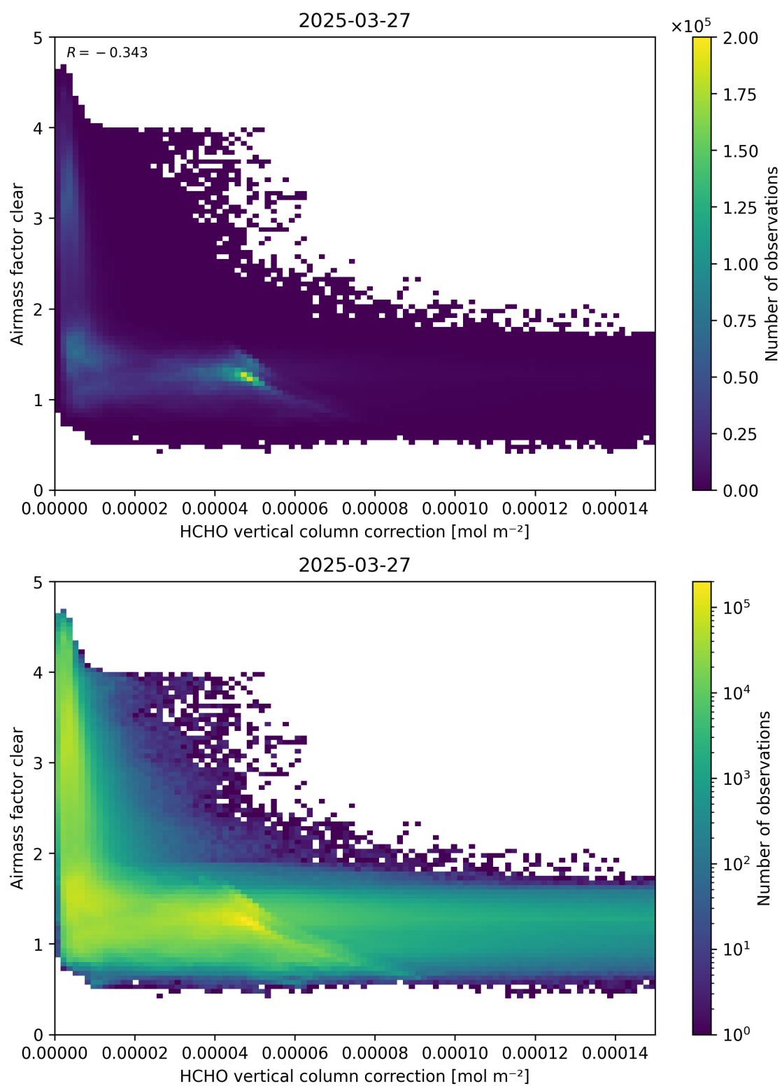
Figure 115: Scatter density plot of “HCHO vertical column correction” against “Airmass factor clear” for 2025-03-26 to 2025-03-28.
