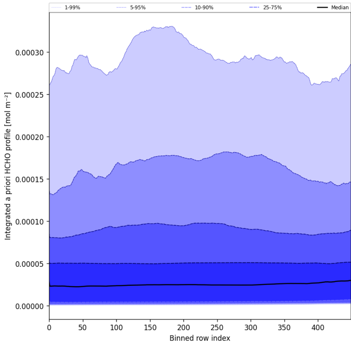
Figure 57: Along track statistics of "Integrated a priori HCHO profile" for 2025-03-26 to 2025-03-28
