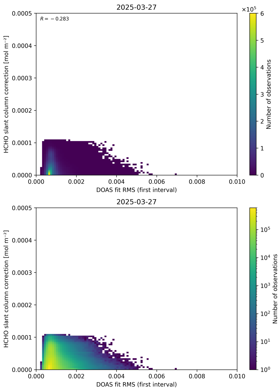
Figure 63: Scatter density plot of “DOAS fit RMS (first interval)” against “HCHO slant column correction” for 2025-03-26 to 2025-03-28.
