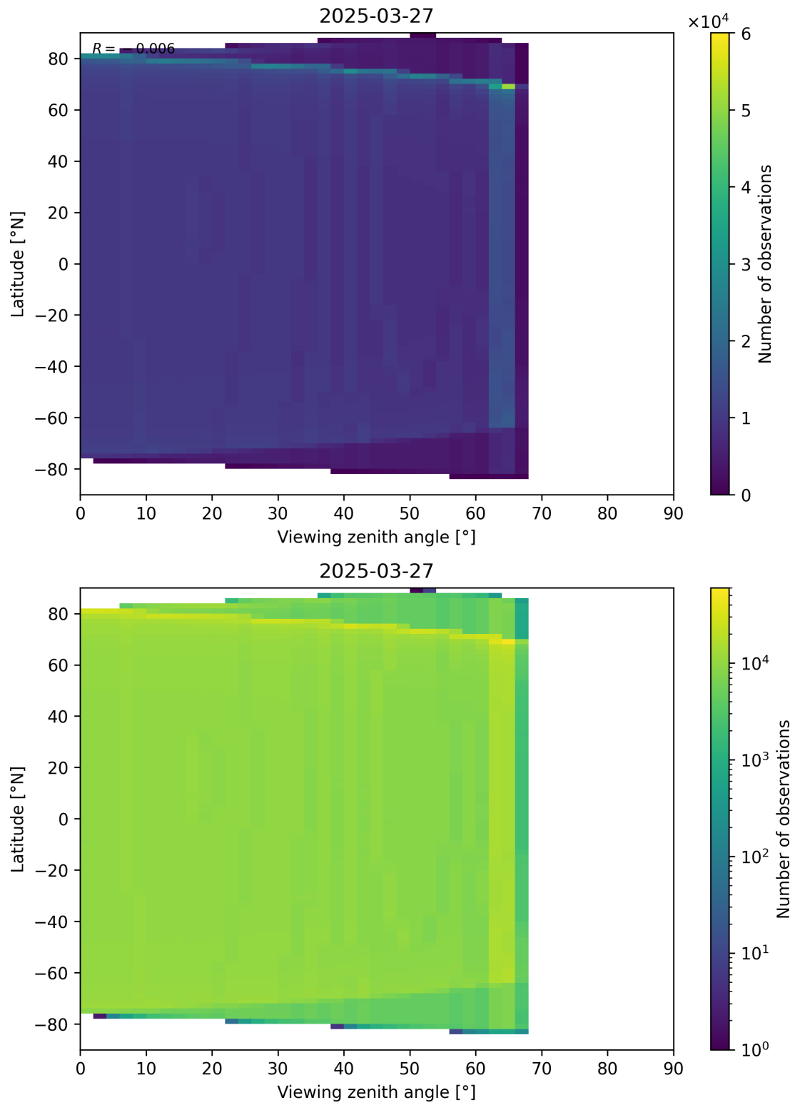
Figure 196: Scatter density plot of “Viewing zenith angle” against “Latitude” for 2025-03-26 to 2025-03-28.
