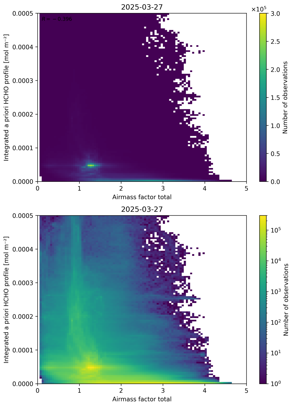
Figure 104: Scatter density plot of “Airmass factor total” against “Integrated a priori HCHO profile” for 2025-03-26 to 2025-03-28.
