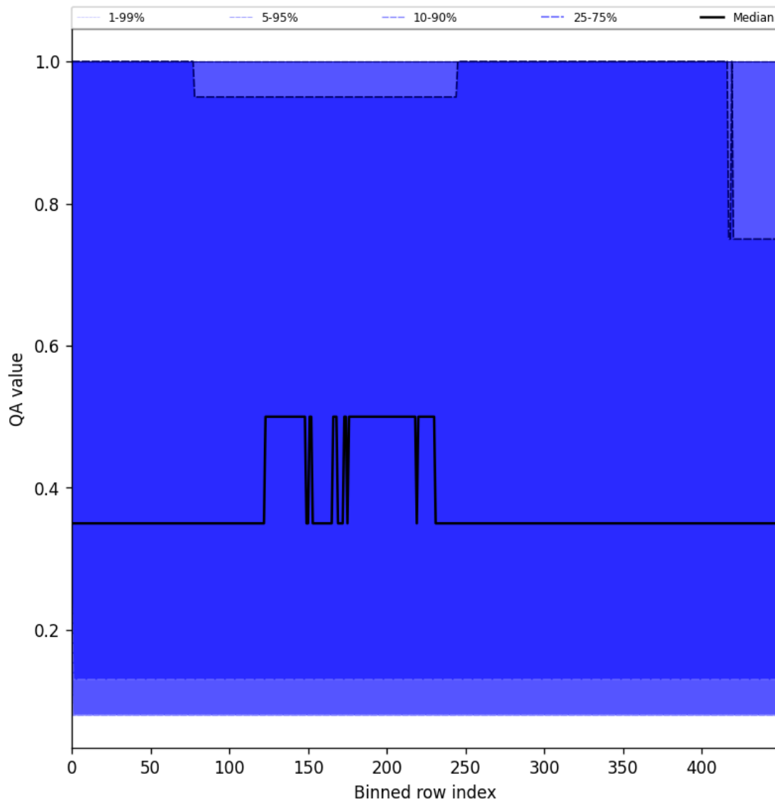
Figure 48: Along track statistics of “QA value” for 2025-03-26 to 2025-03-28
