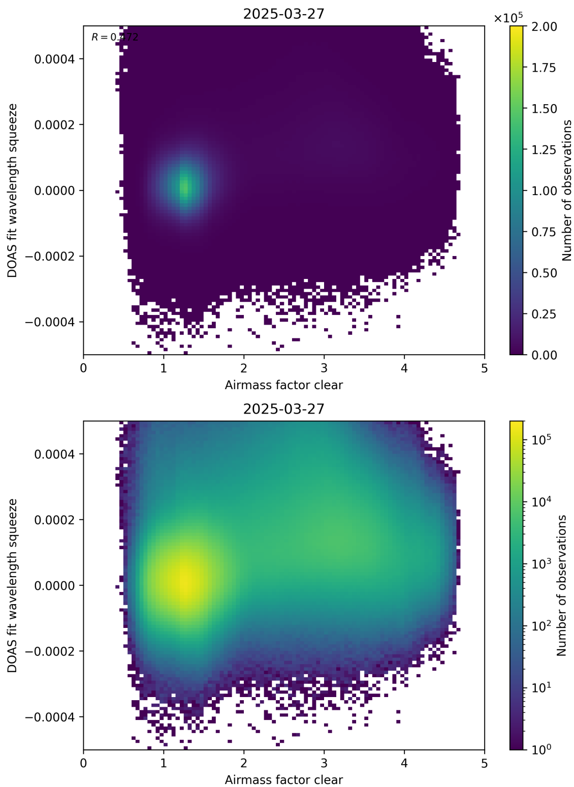
Figure 73: Scatter density plot of “Airmass factor clear” against “DOAS fit wavelength squeeze” for 2025-03-26 to 2025-03-28.
