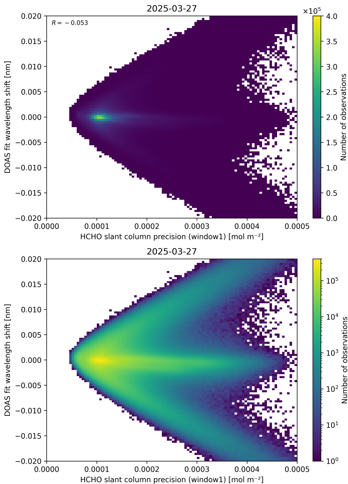
Figure 89: Scatter density plot of “HCHO slant column precision (window1)” against “DOAS fit wavelength shift” for 2025-03-26 to 2025-03-28.
