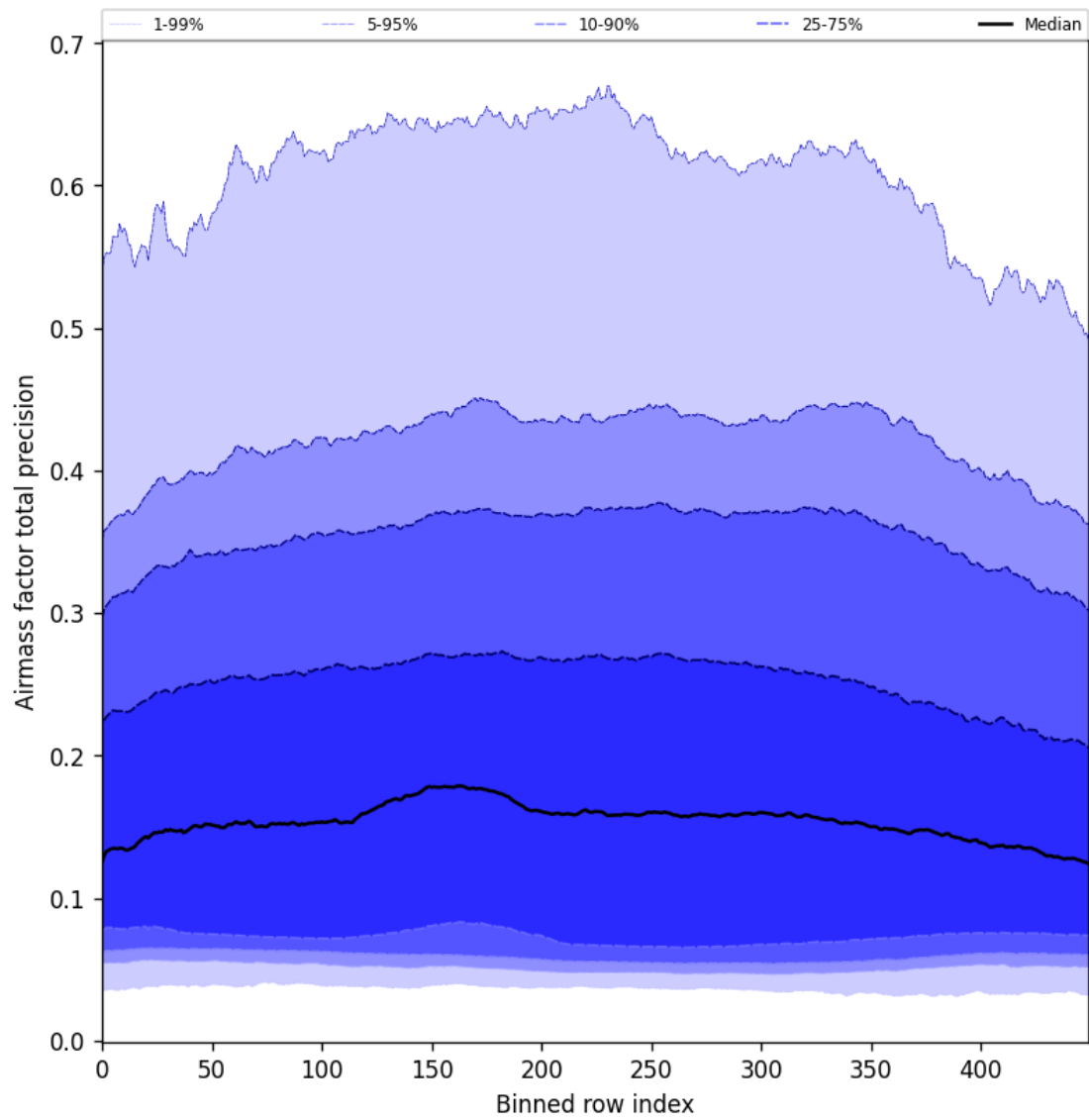
Figure 55: Along track statistics of “Airmass factor total precision” for 2025-03-26 to 2025-03-28
