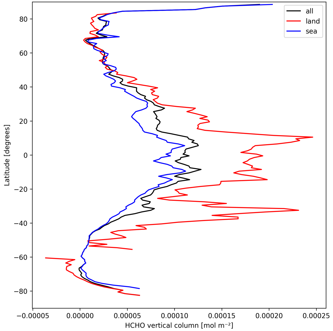
Figure 21: Zonal average of “HCHO vertical column” for 2025-03-26 to 2025-03-28.
