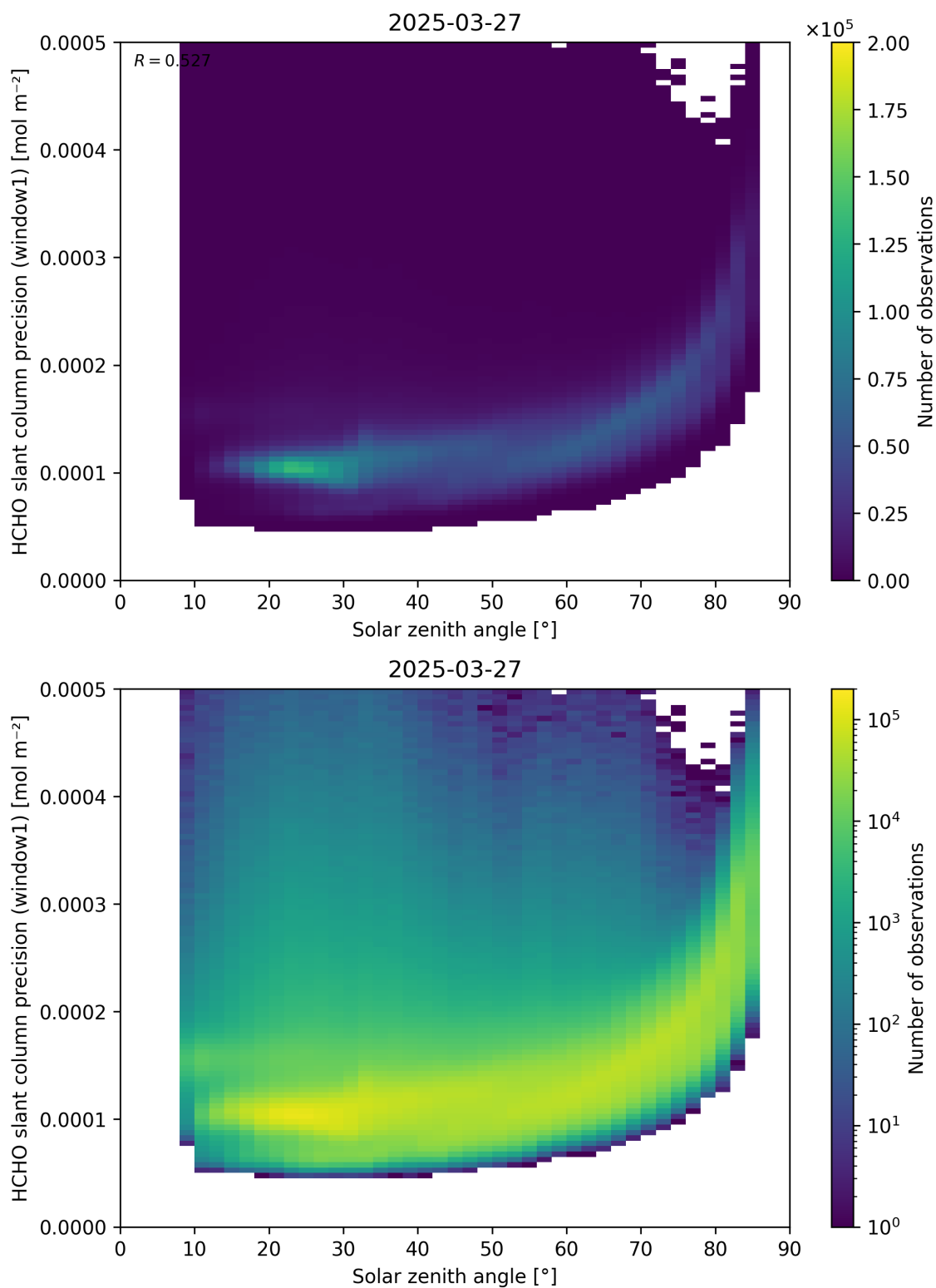
Figure 174: Scatter density plot of “Solar zenith angle” against “HCHO slant column precision (window1)” for 2025-03-26 to 2025-03-28.
