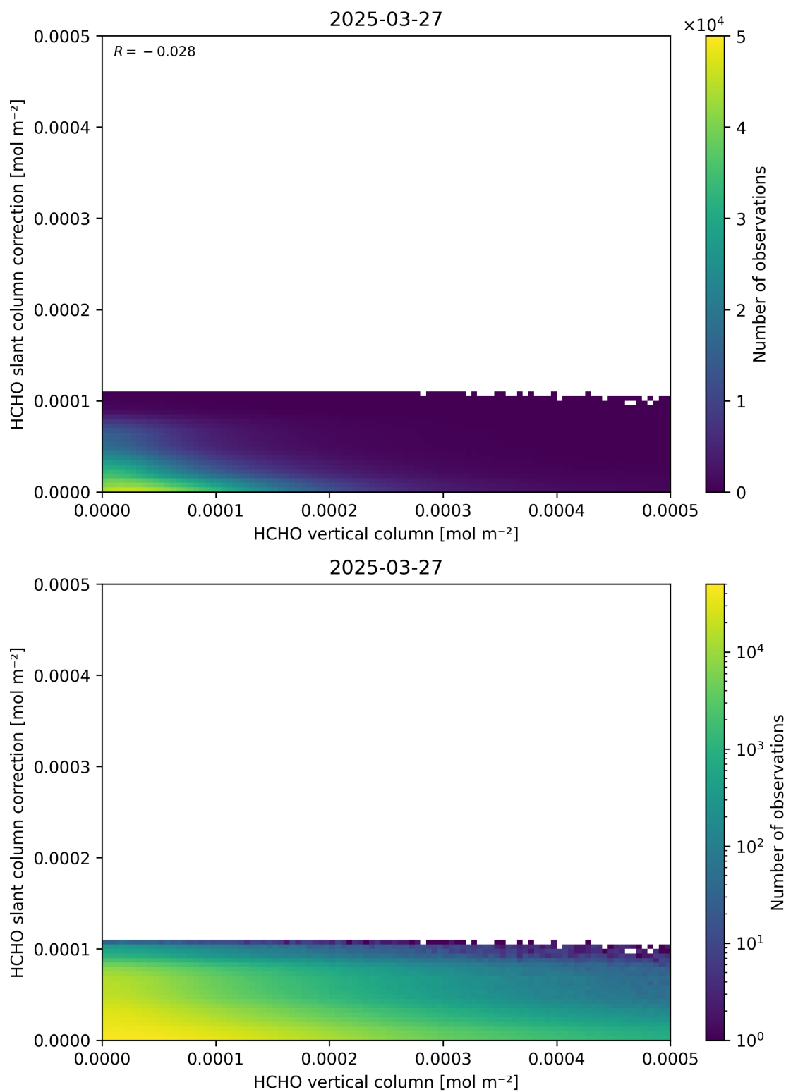
Figure 128: Scatter density plot of “HCHO vertical column” against “HCHO slant column correction” for 2025-03-26 to 2025-03-28.
