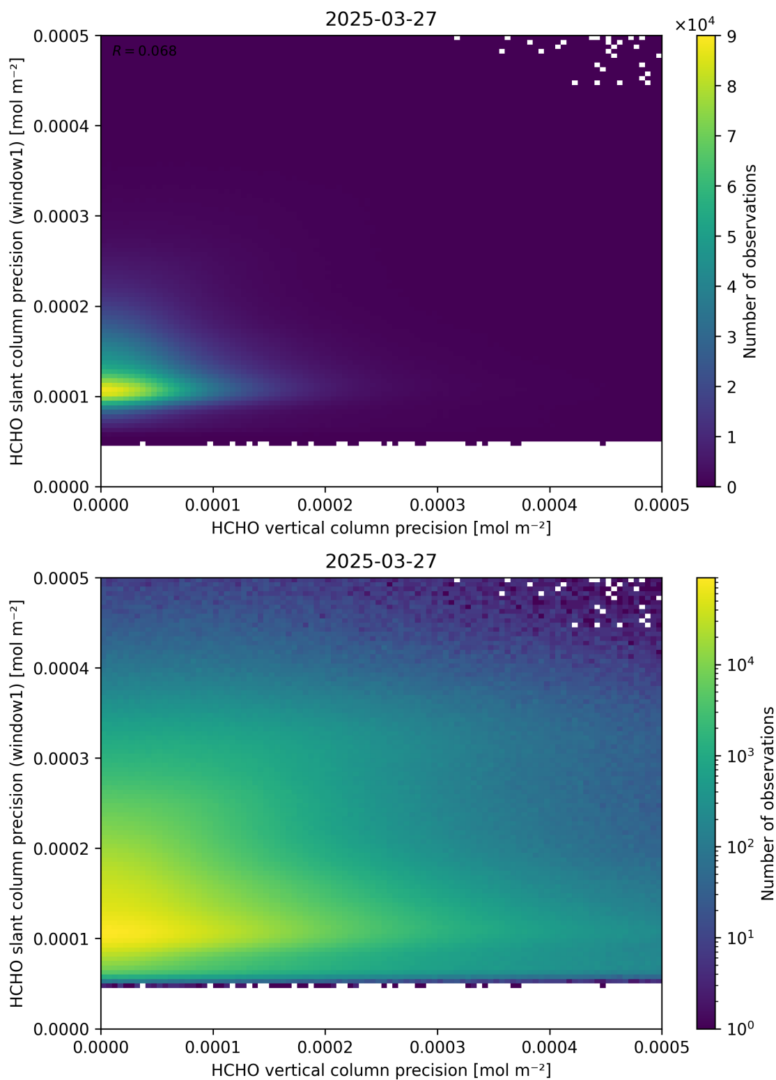
Figure 143: Scatter density plot of “HCHO vertical column precision” against “HCHO slant column precision (window1)” for 2025-03-26 to 2025-03-28.
