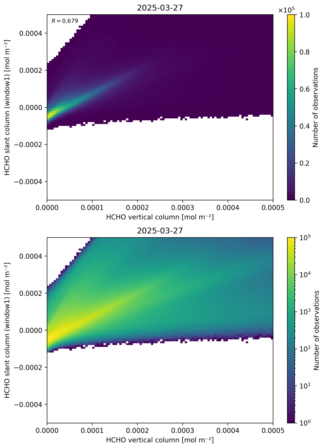
Figure 129: Scatter density plot of “HCHO vertical column” against “HCHO slant column (window1)” for 2025-03-26 to 2025-03-28.
