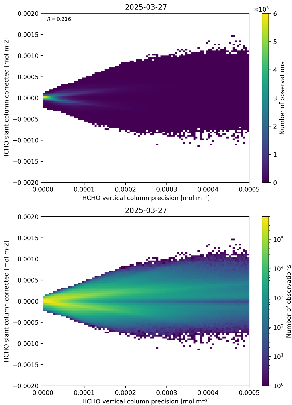
Figure 140: Scatter density plot of “HCHO vertical column precision” against “HCHO slant column corrected” for 2025-03-26 to 2025-03-28.
