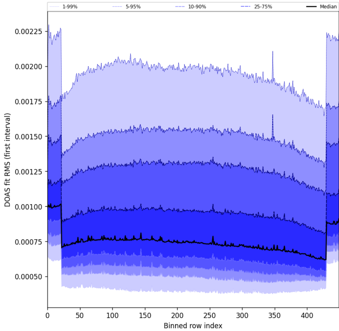
Figure 60: Along track statistics of “DOAS fit RMS (first interval)” for 2025-03-26 to 2025-03-28
