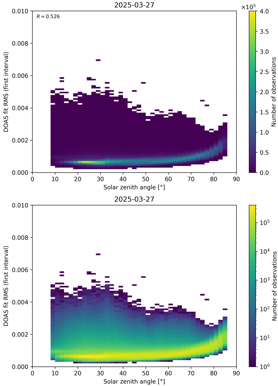
Figure 167: Scatter density plot of “Solar zenith angle” against “DOAS fit RMS (first interval)” for 2025-03-26 to 2025-03-28.
