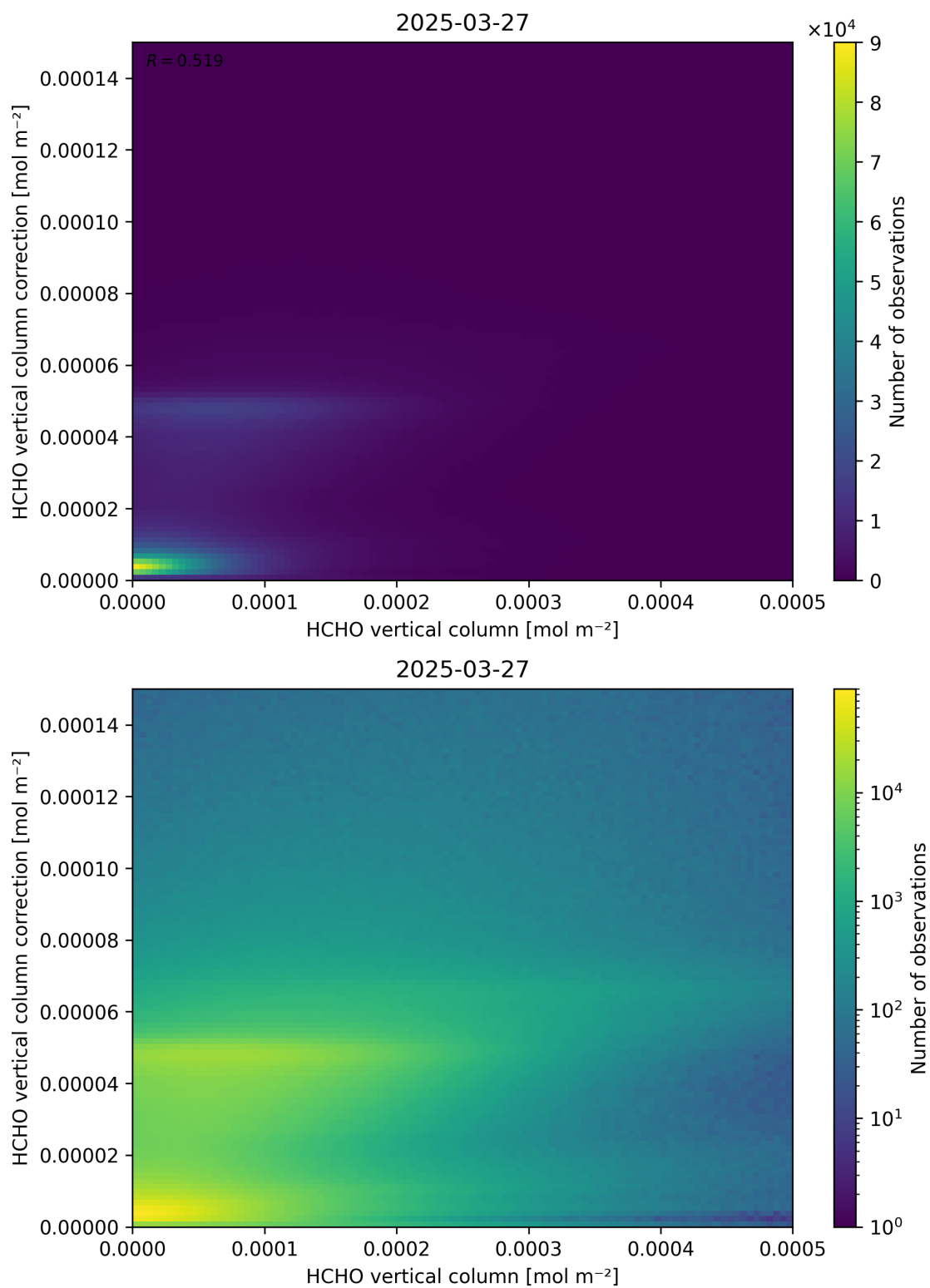
Figure 133: Scatter density plot of “HCHO vertical column” against “HCHO vertical column correction” for 2025-03-26 to 2025-03-28.
