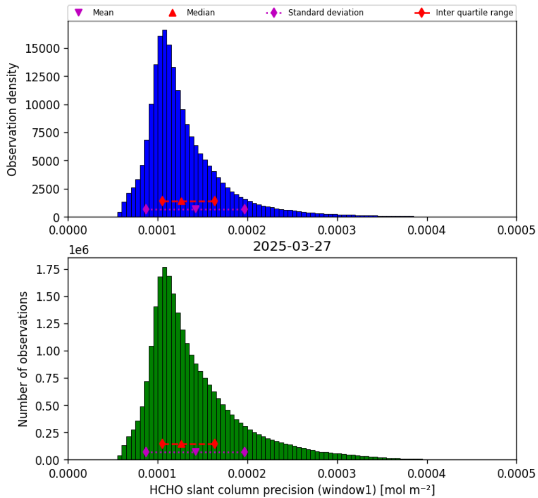
Figure 39: Histogram of “HCHO slant column precision (window1)” for 2025-03-26 to 2025-03-28
