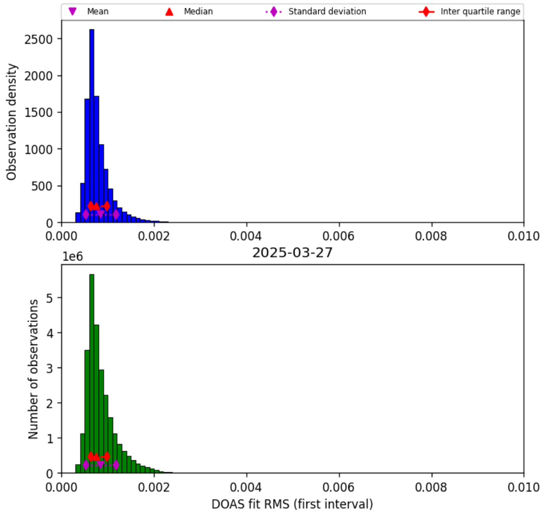
Figure 46: Histogram of “DOAS fit RMS (first interval)” for 2025-03-26 to 2025-03-28
