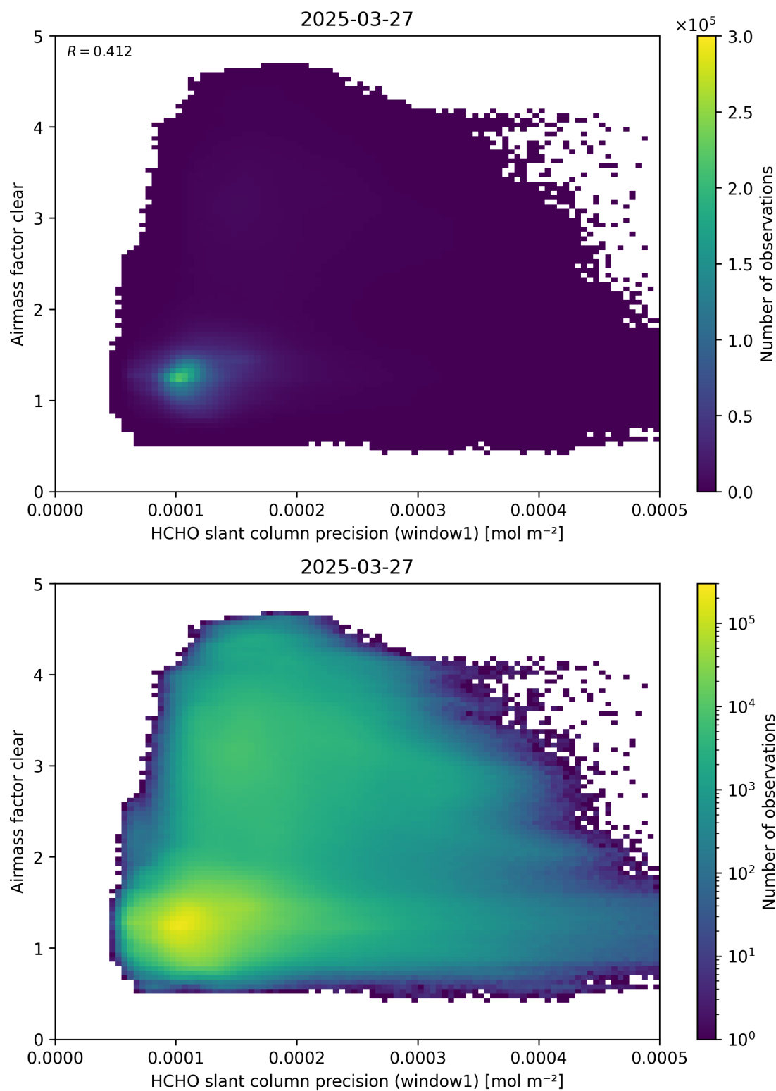
Figure 91: Scatter density plot of “HCHO slant column precision (window1)” against “Airmass factor clear” for 2025-03-26 to 2025-03-28.
