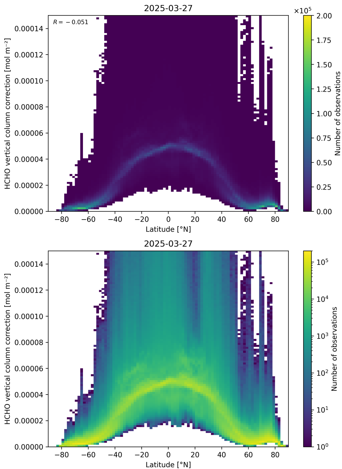
Figure 164: Scatter density plot of “Latitude” against “HCHO vertical column correction” for 2025-03-26 to 2025-03-28.
