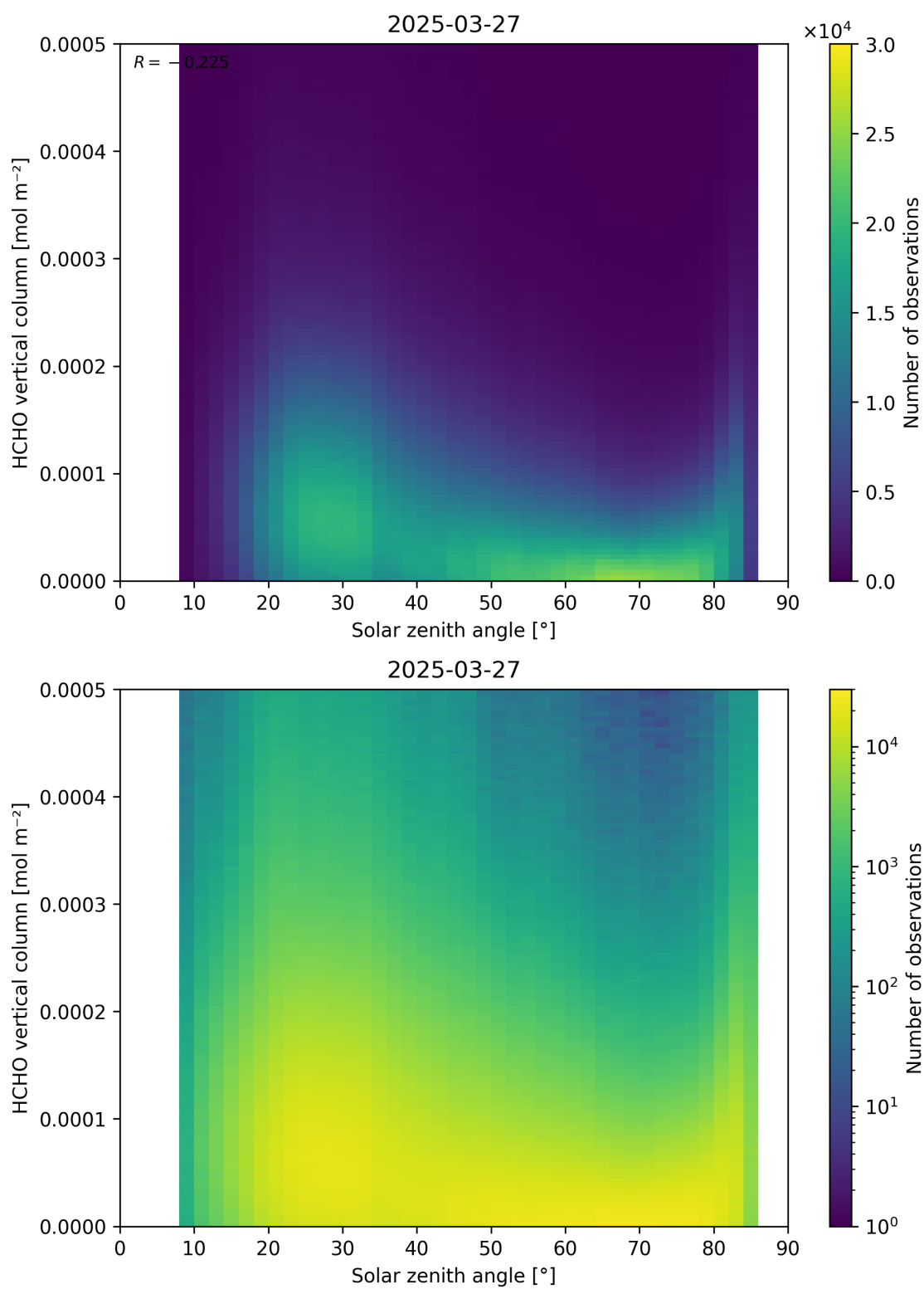
Figure 177: Scatter density plot of “Solar zenith angle” against “HCHO vertical column” for 2025-03-26 to 2025-03-28.
