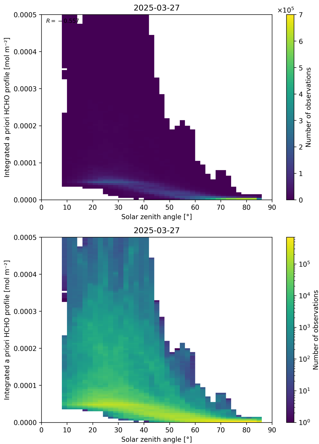
Figure 180: Scatter density plot of “Solar zenith angle” against “Integrated a priori HCHO profile” for 2025-03-26 to 2025-03-28.
