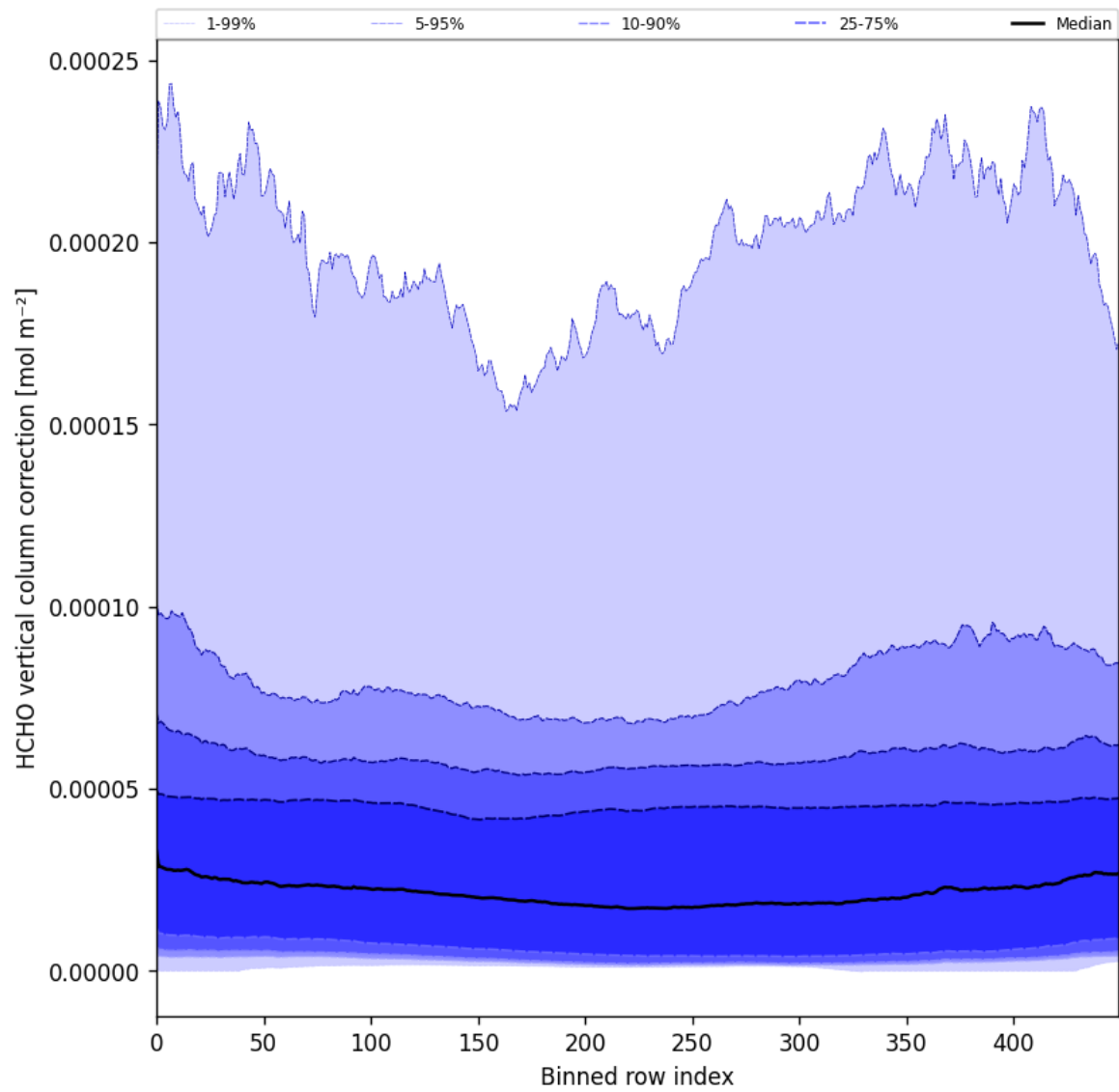
Figure 51: Along track statistics of “HCHO vertical column correction” for 2025-03-26 to 2025-03-28
