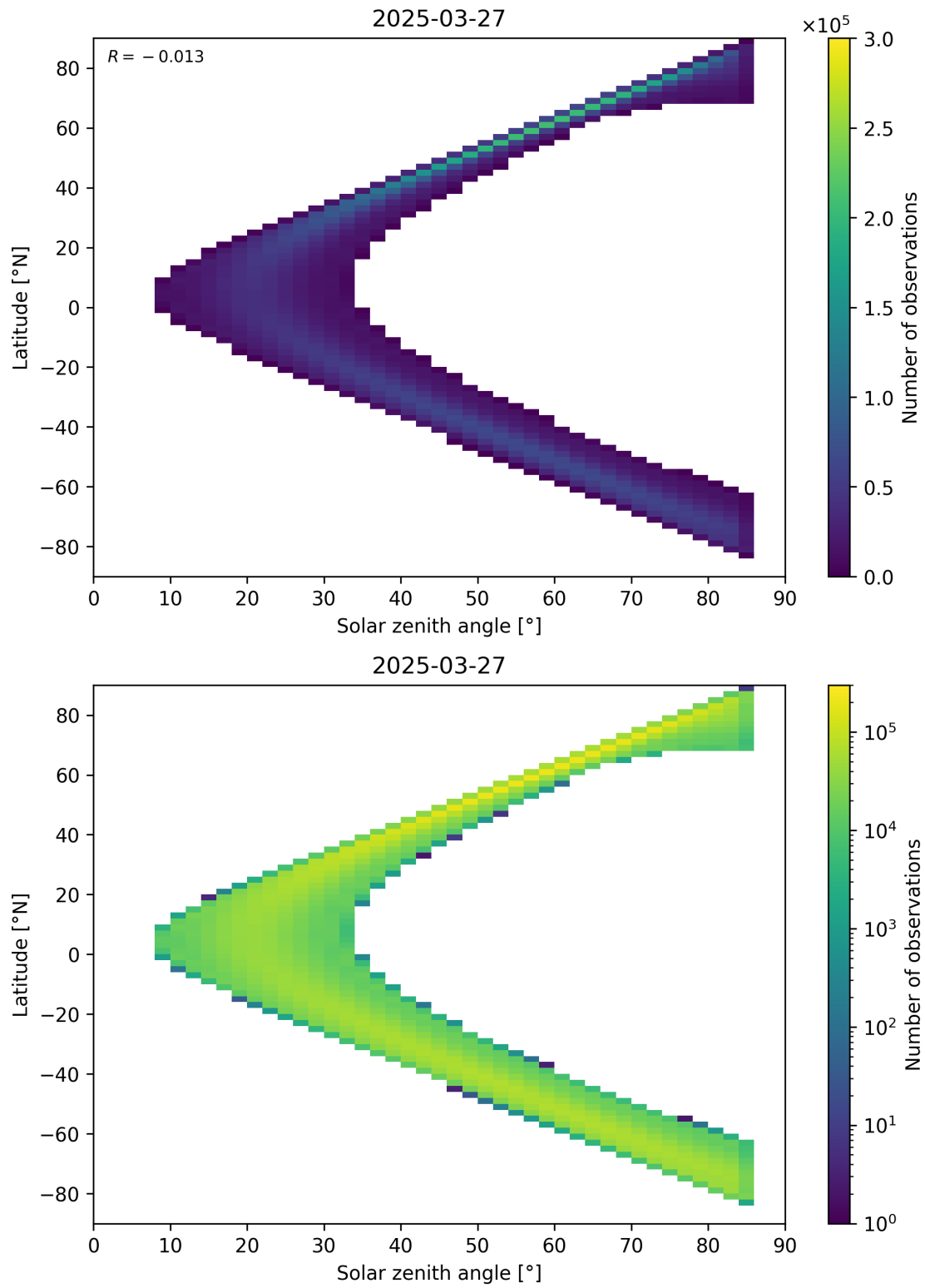
Figure 181: Scatter density plot of “Solar zenith angle” against “Latitude” for 2025-03-26 to 2025-03-28.
