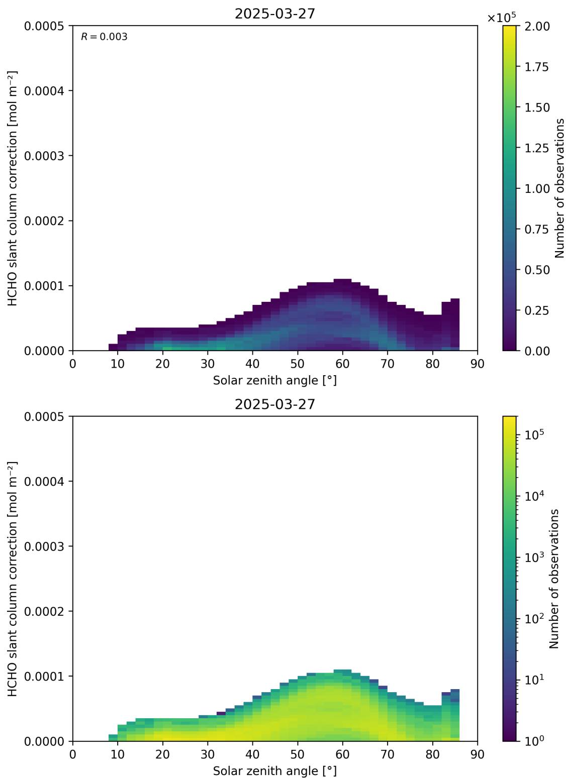
Figure 172: Scatter density plot of “Solar zenith angle” against “HCHO slant column correction” for 2025-03-26 to 2025-03-28.
