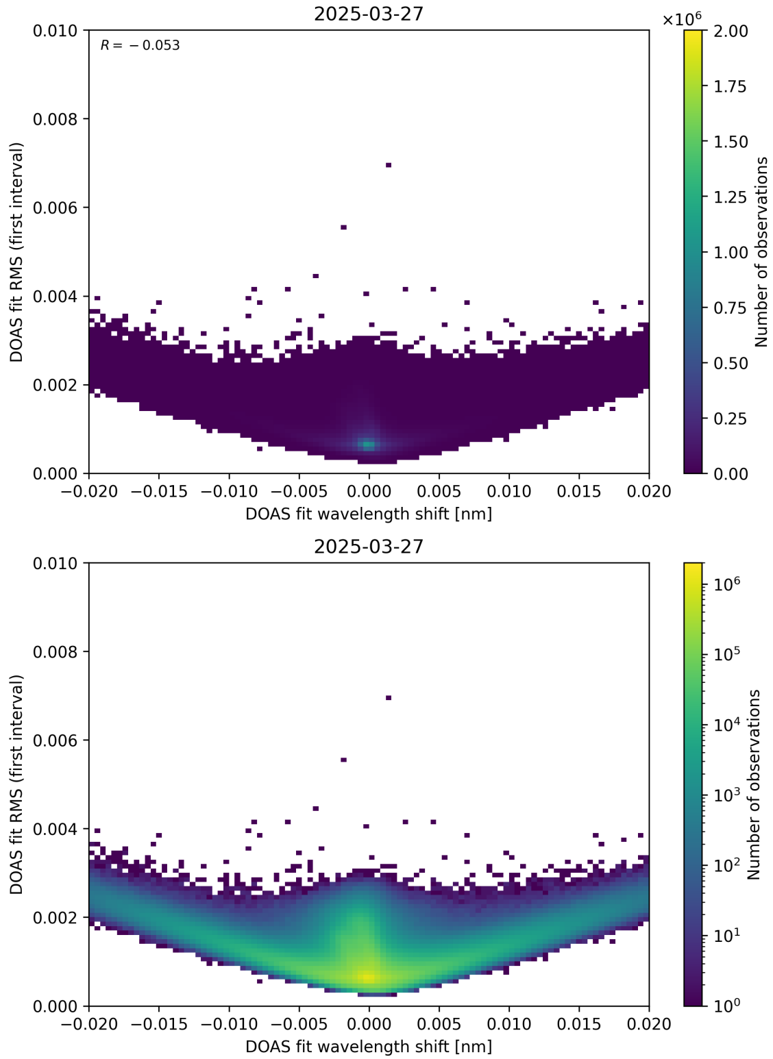
Figure 64: Scatter density plot of “DOAS fit wavelength shift” against “DOAS fit RMS (first interval)” for 2025-03-26 to 2025-03-28.
