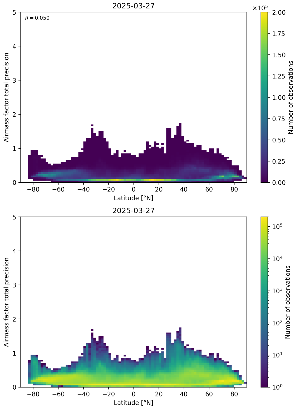
Figure 162: Scatter density plot of “Latitude” against “Airmass factor total precision” for 2025-03-26 to 2025-03-28.
