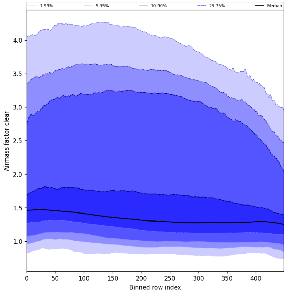
Figure 56: Along track statistics of “Air mass factor clear” for 2025-03-26 to 2025-03-28
