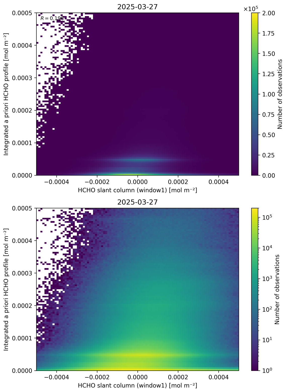
Figure 87: Scatter density plot of “HCHO slant column (window1)” against “Integrated a priori HCHO profile” for 2025-03-26 to 2025-03-28.
