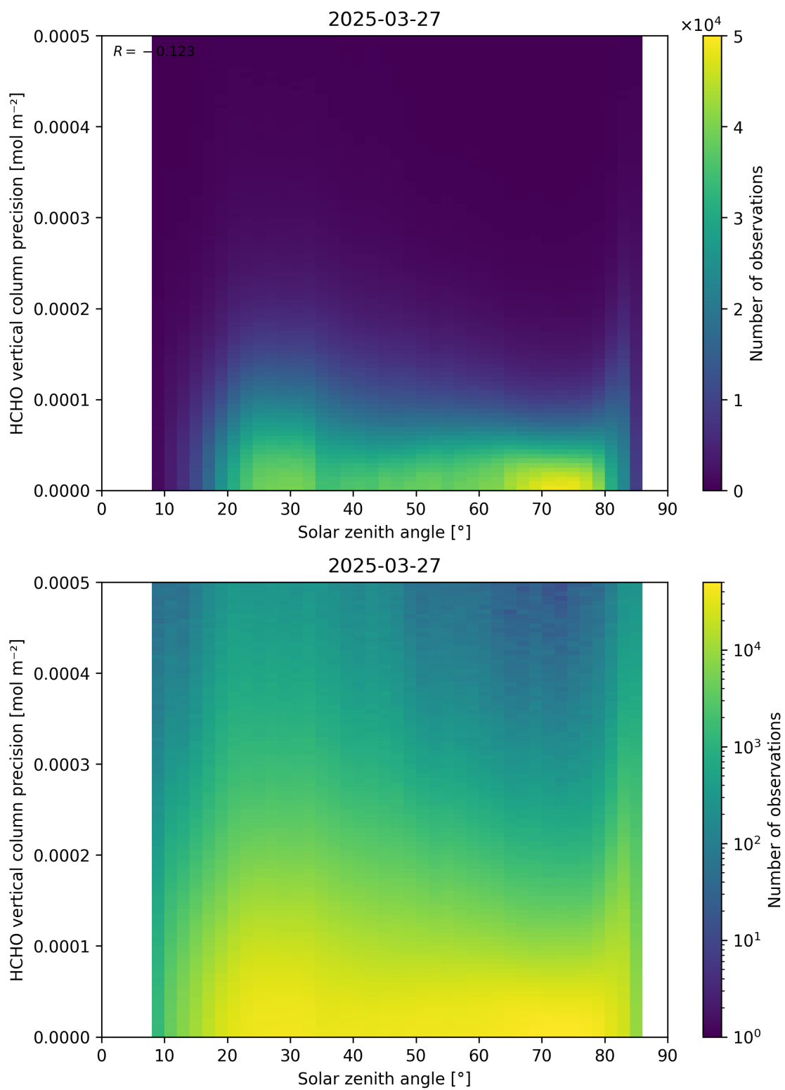
Figure 179: Scatter density plot of “Solar zenith angle” against “HCHO vertical column precision” for 2025-03-26 to 2025-03-28.
