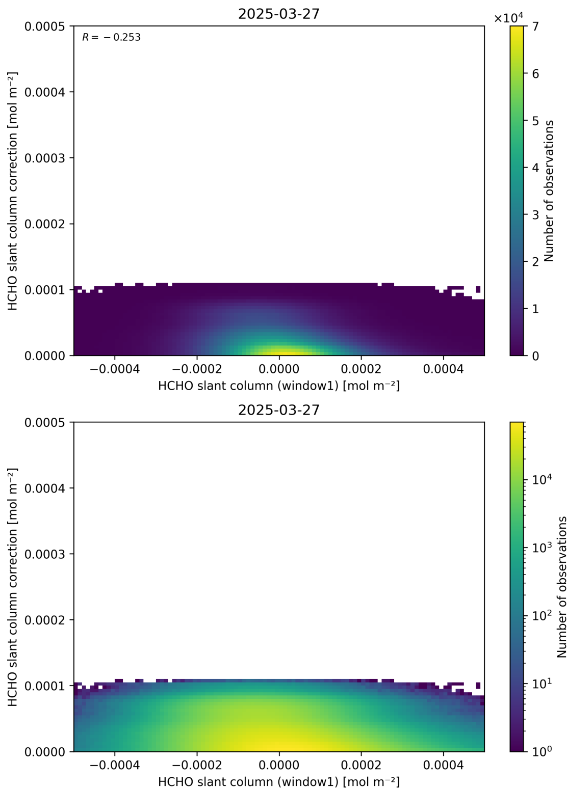
Figure 83: Scatter density plot of “HCHO slant column (window1)” against “HCHO slant column correction” for 2025-03-26 to 2025-03-28.
