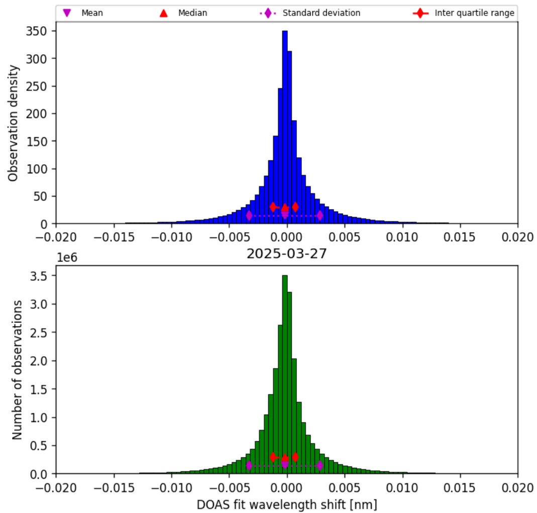
Figure 44: Histogram of “DOAS fit wavelength shift” for 2025-03-26 to 2025-03-28
