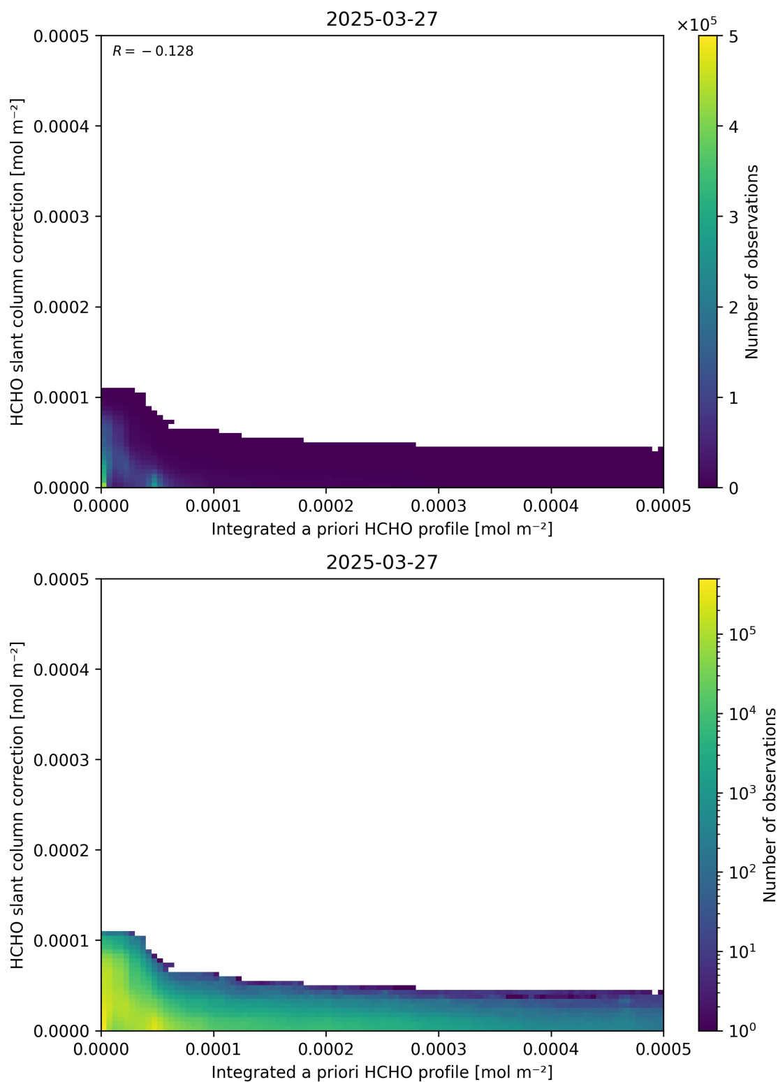
Figure 152: Scatter density plot of “Integrated a priori HCHO profile” against “HCHO slant column correction” for 2025-03-26 to 2025-03-28.
