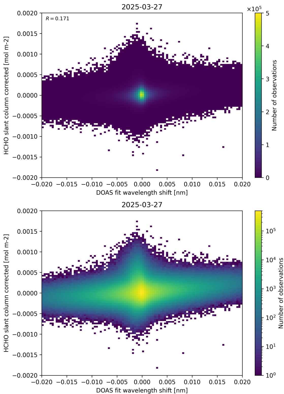
Figure 66: Scatter density plot of “DOAS fit wavelength shift” against “HCHO slant column corrected” for 2025-03-26 to 2025-03-28.
