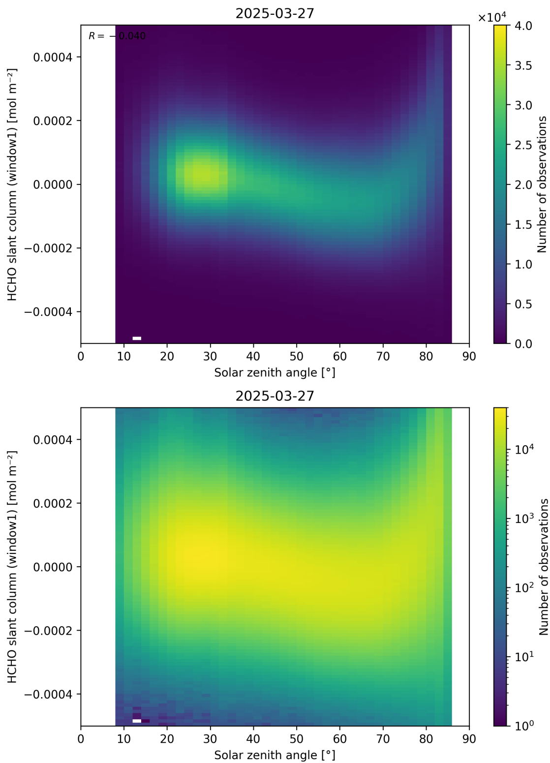
Figure 173: Scatter density plot of “Solar zenith angle” against “HCHO slant column (window1)” for 2025-03-26 to 2025-03-28.
