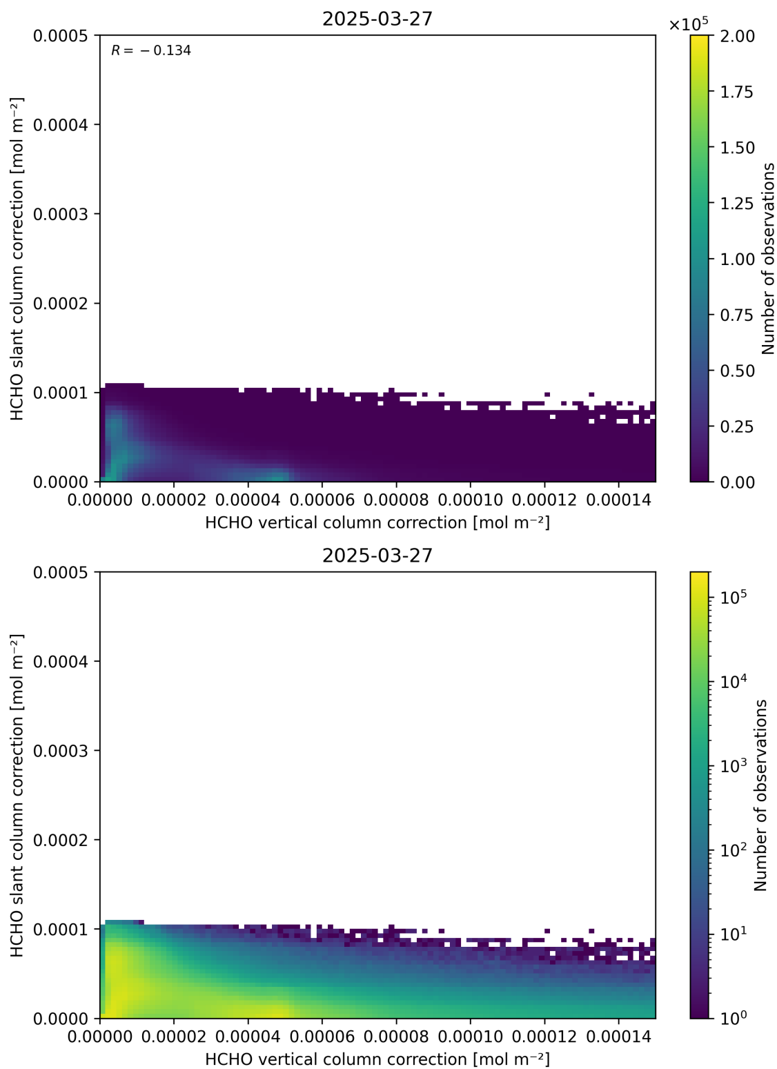
Figure 117: Scatter density plot of “HCHO vertical column correction” against “HCHO slant column correction” for 2025-03-26 to 2025-03-28.
