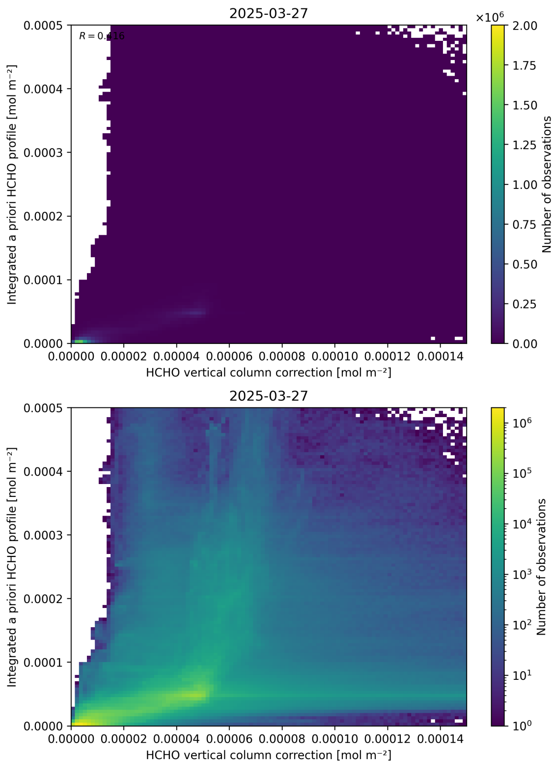
Figure 122: Scatter density plot of “HCHO vertical column correction” against “Integrated a priori HCHO profile” for 2025-03-26 to 2025-03-28.
