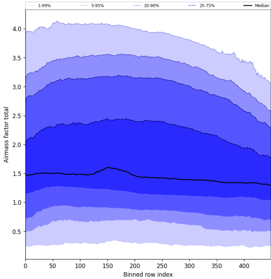
Figure 54: Along track statistics of “Airmass factor total” for 2025-03-26 to 2025-03-28
