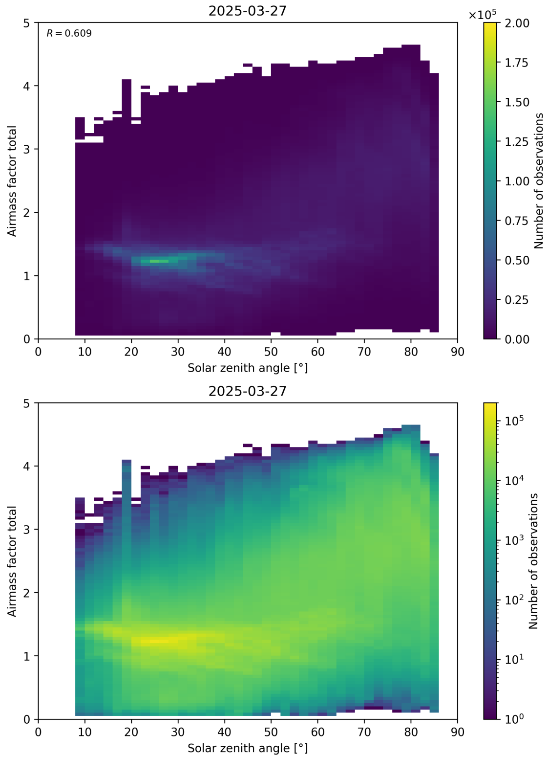
Figure 175: Scatter density plot of “Solar zenith angle” against “Airmass factor total” for 2025-03-26 to 2025-03-28.
