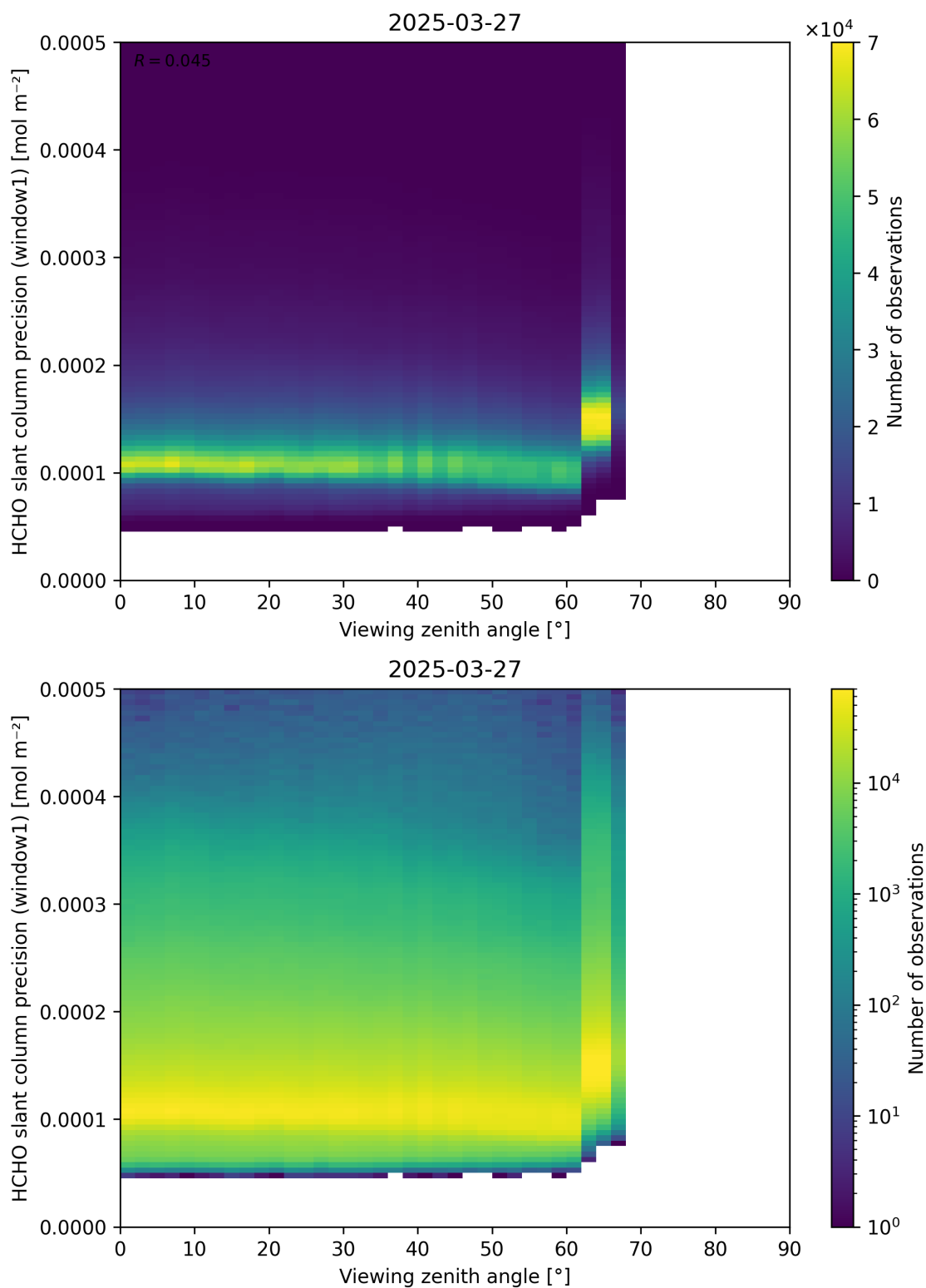
Figure 189: Scatter density plot of “Viewing zenith angle” against “HCHO slant column precision (window1)” for 2025-03-26 to 2025-03-28.
