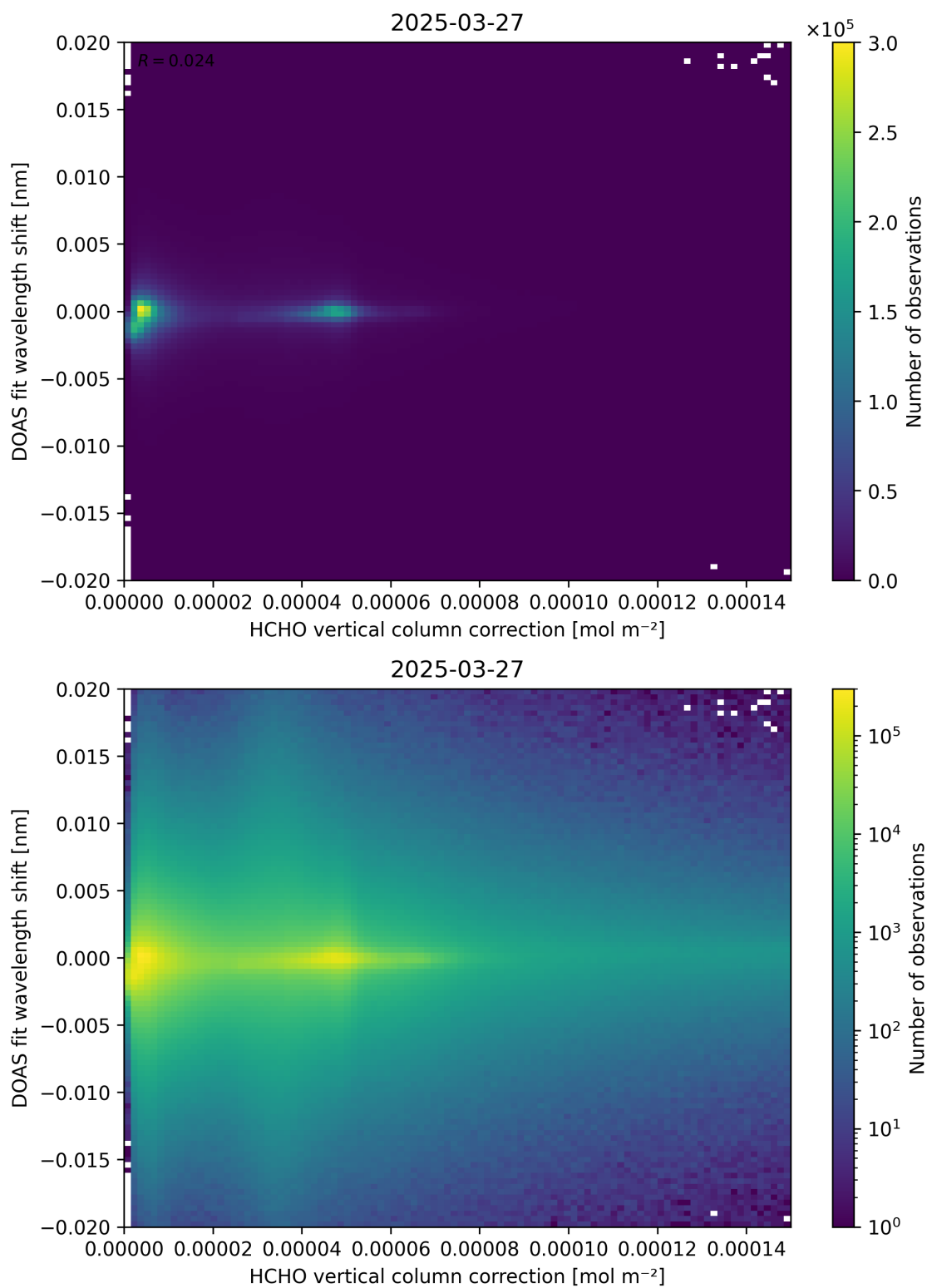
Figure 113: Scatter density plot of “HCHO vertical column correction” against “DOAS fit wavelength shift” for 2025-03-26 to 2025-03-28.
