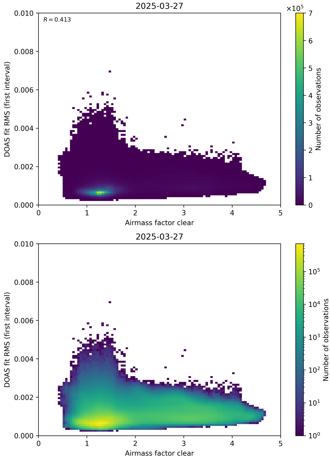
Figure 71: Scatter density plot of “Airmass factor clear” against “DOAS fit RMS (first interval)” for 2025-03-26 to 2025-03-28.
