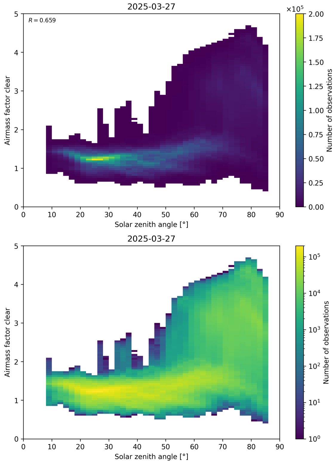
Figure 170: Scatter density plot of “Solar zenith angle” against “Airmass factor clear” for 2025-03-26 to 2025-03-28.
