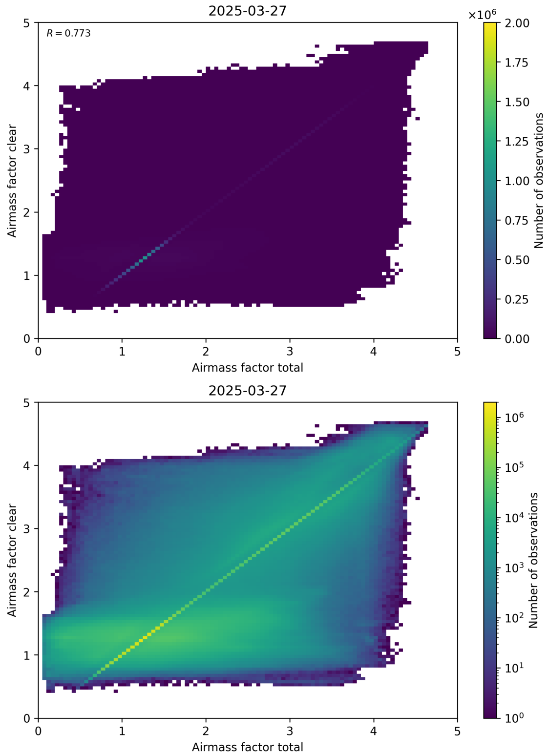
Figure 100: Scatter density plot of “Airmass factor total” against “Airmass factor clear” for 2025-03-26 to 2025-03-28.
