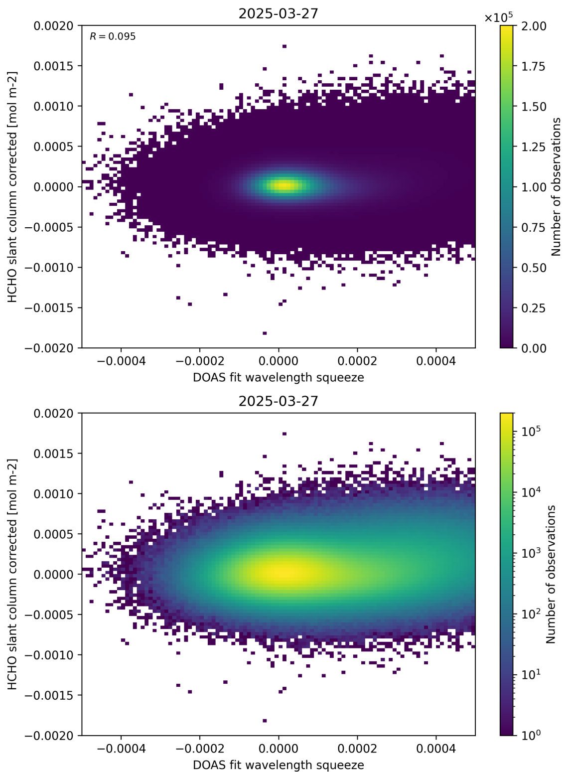
Figure 69: Scatter density plot of “DOAS fit wavelength squeeze” against “HCHO slant column corrected” for 2025-03-26 to 2025-03-28.
