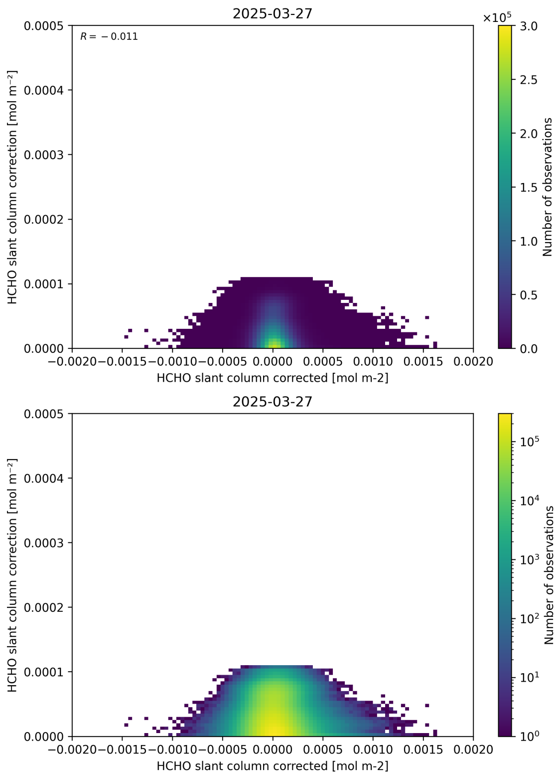
Figure 77: Scatter density plot of “HCHO slant column corrected” against “HCHO slant column correction” for 2025-03-26 to 2025-03-28.
