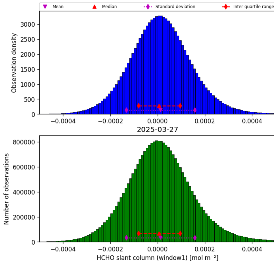
Figure 38: Histogram of “HCHO slant column (window1)” for 2025-03-26 to 2025-03-28
