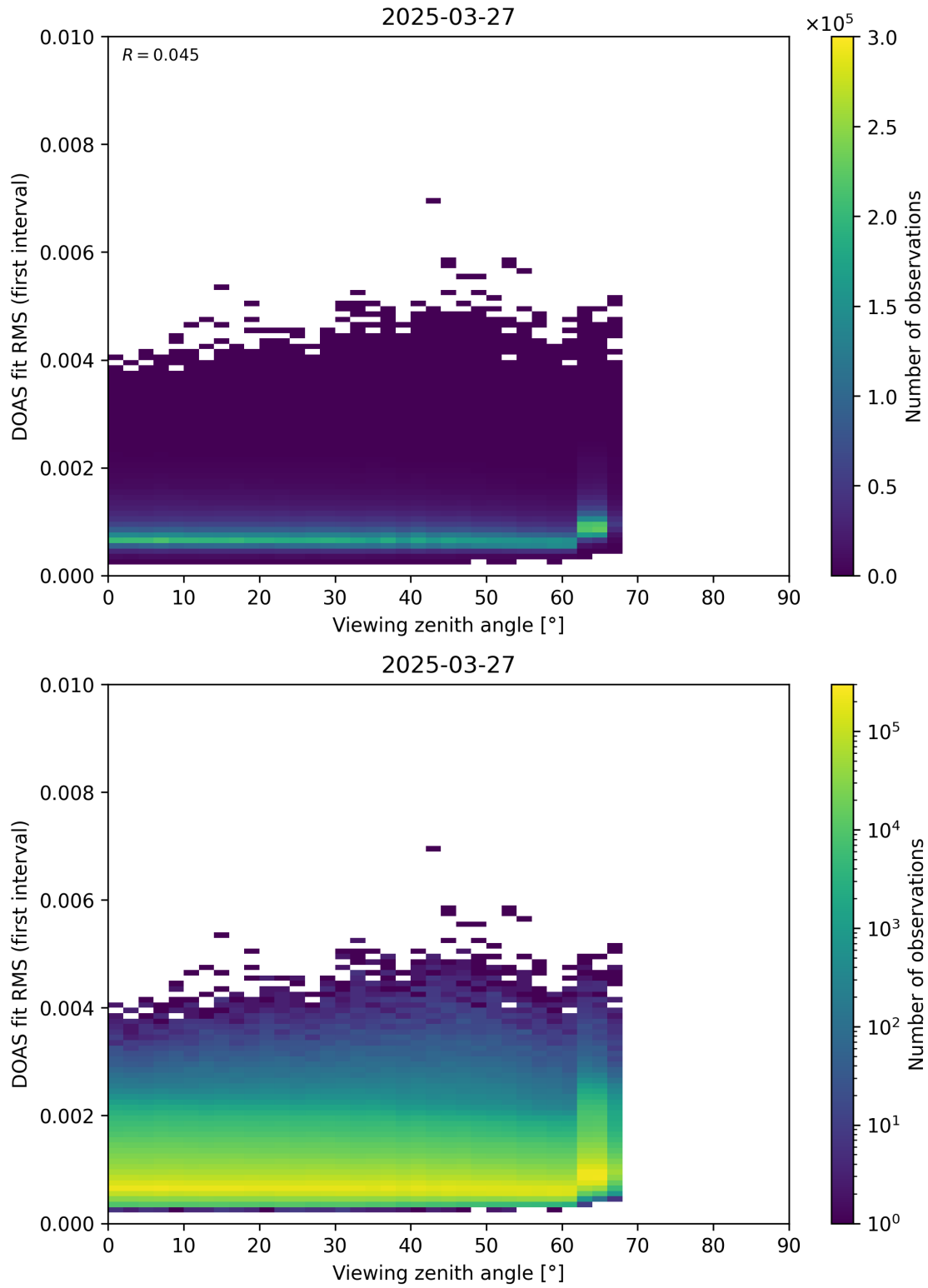
Figure 182: Scatter density plot of “Viewing zenith angle” against “DOAS fit RMS (first interval)” for 2025-03-26 to 2025-03-28.
