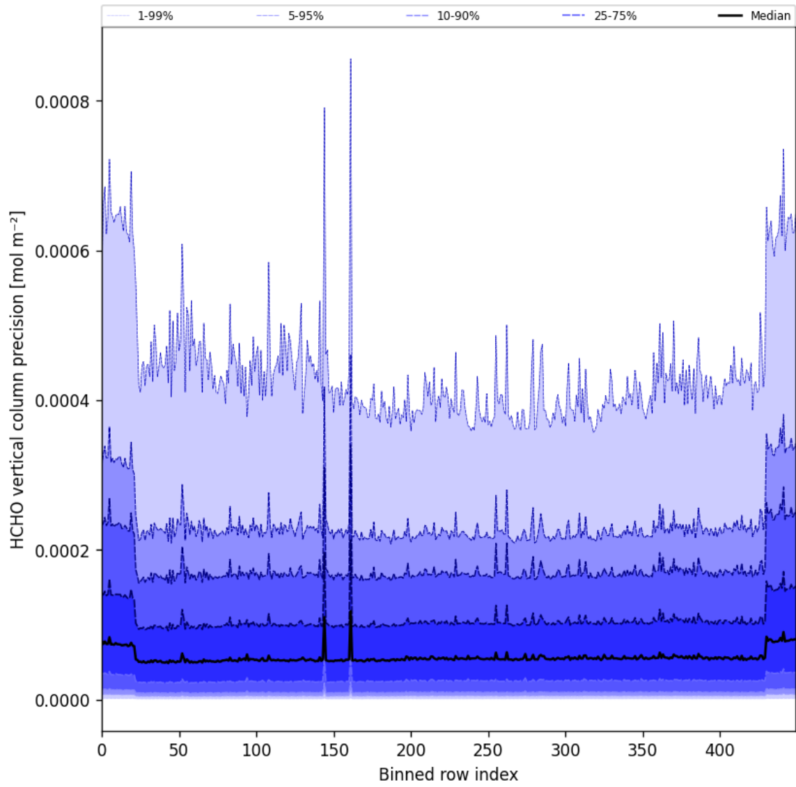
Figure 50: Along track statistics of “HCHO vertical column precision” for 2025-03-26 to 2025-03-28
