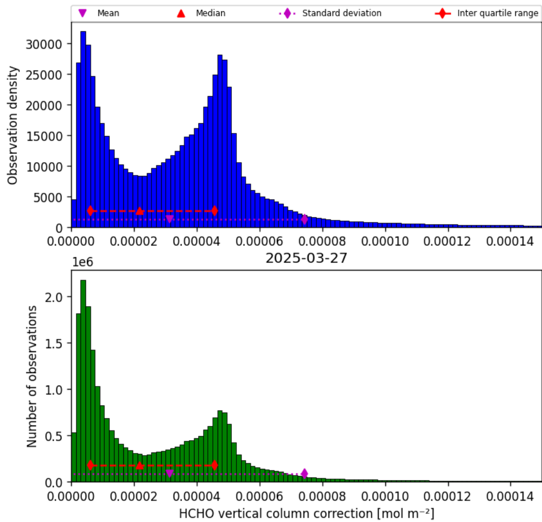
Figure 37: Histogram of “HCHO vertical column correction” for 2025-03-26 to 2025-03-28
