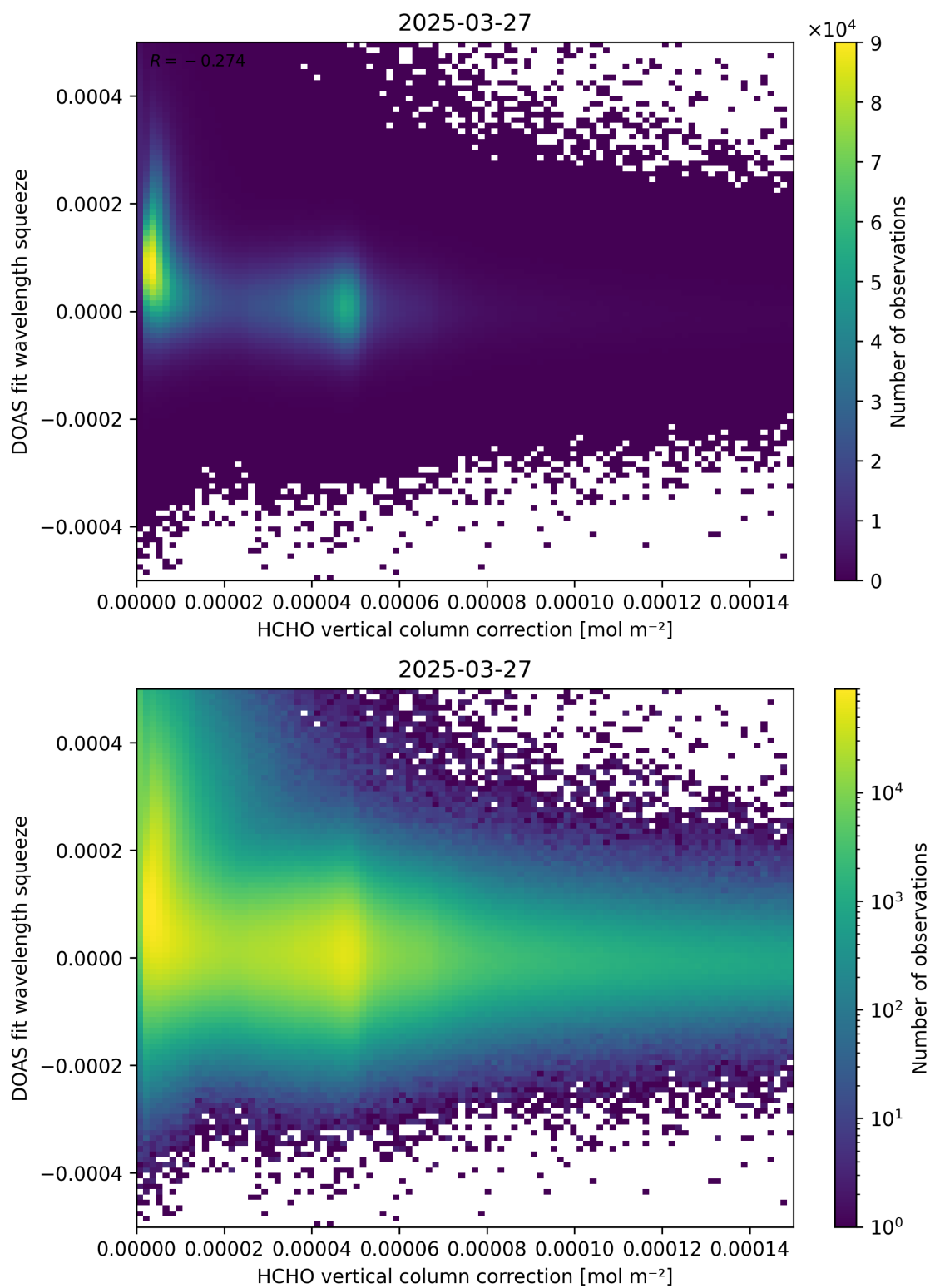
Figure 114: Scatter density plot of “HCHO vertical column correction” against “DOAS fit wavelength squeeze” for 2025-03-26 to 2025-03-28.
