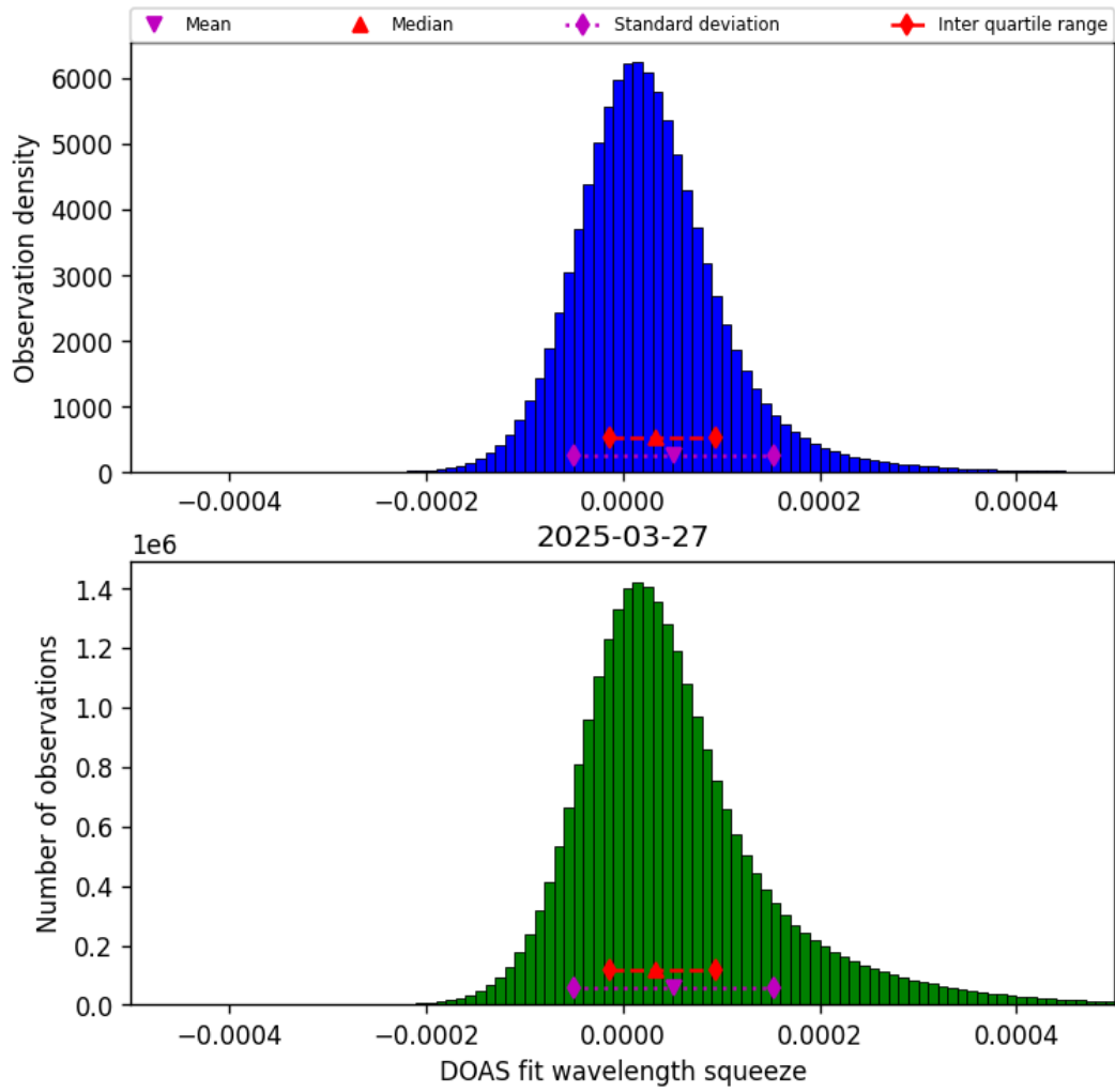
Figure 45: Histogram of “DOAS fit wavelength squeeze” for 2025-03-26 to 2025-03-28
