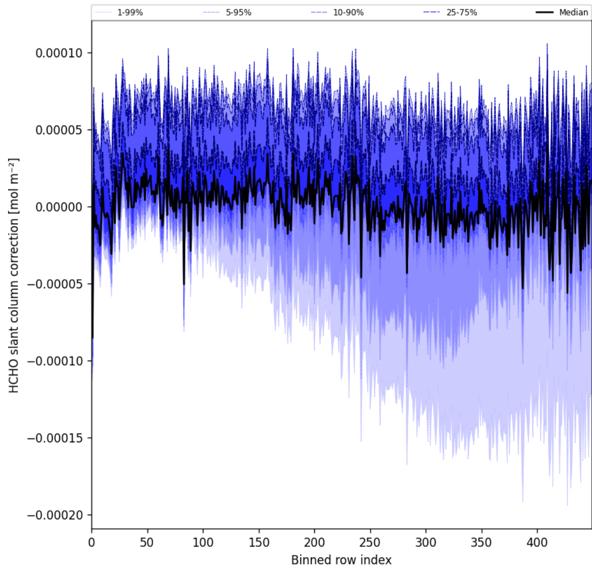
Figure 61: Along track statistics of “HCHO slant column correction” for 2025-03-26 to 2025-03-28
