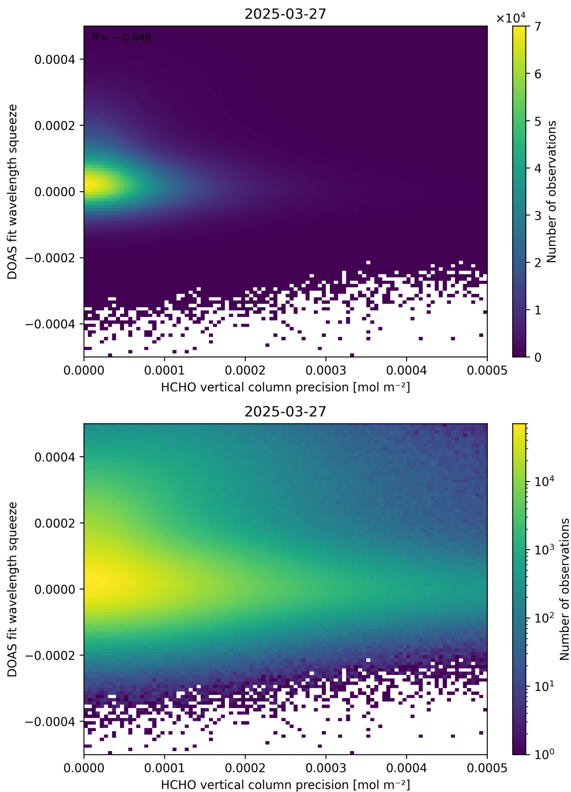
Figure 138: Scatter density plot of “HCHO vertical column precision” against “DOAS fit wavelength squeeze” for 2025-03-26 to 2025-03-28.
