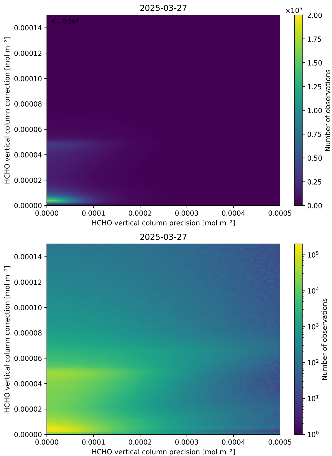
Figure 146: Scatter density plot of “HCHO vertical column precision” against “HCHO vertical column correction” for 2025-03-26 to 2025-03-28.
