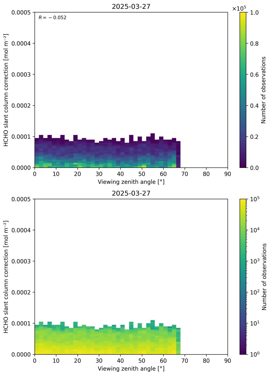
Figure 187: Scatter density plot of “Viewing zenith angle” against “HCHO slant column correction” for 2025-03-26 to 2025-03-28.
