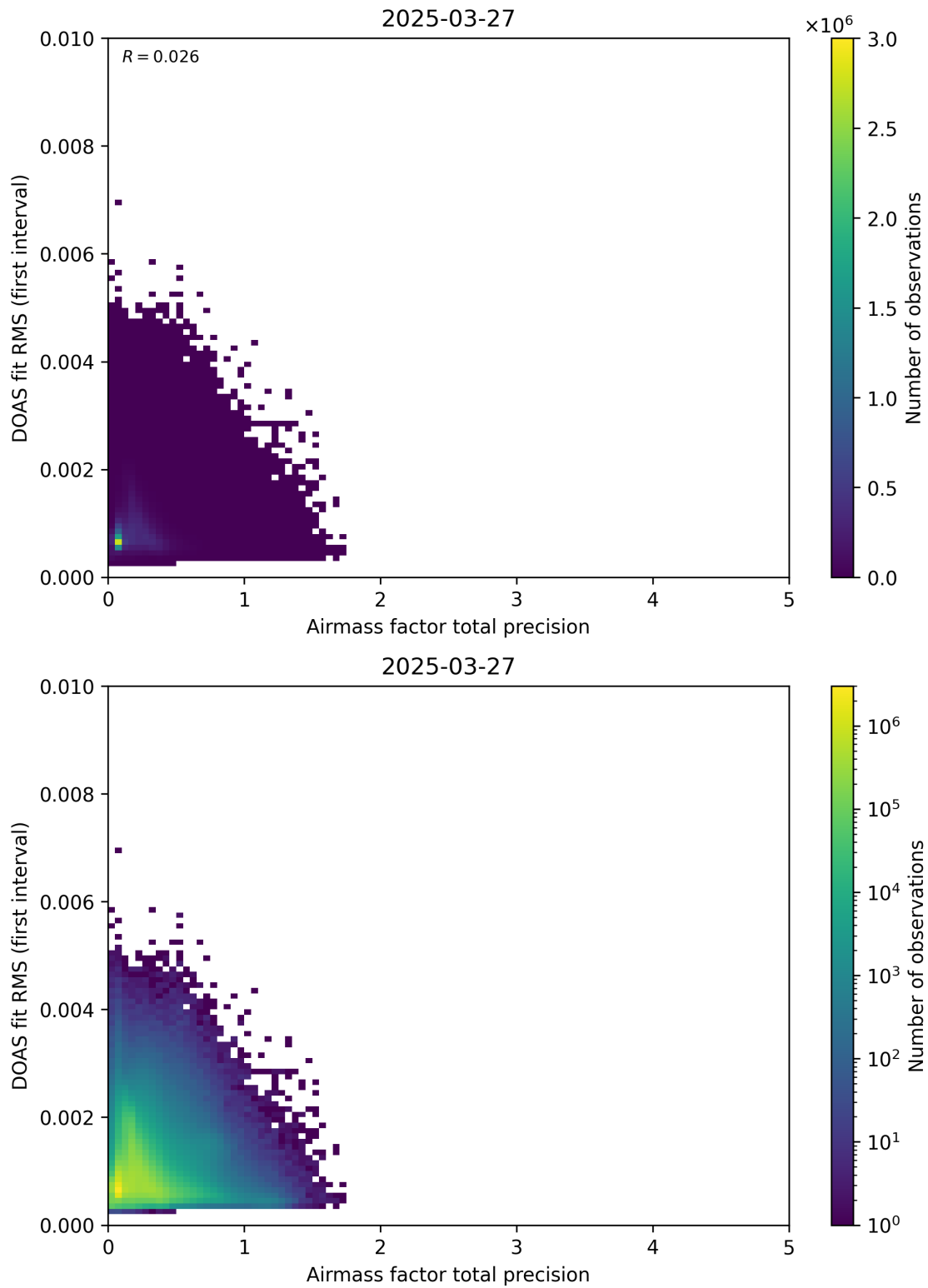
Figure 105: Scatter density plot of “Airmass factor total precision” against “DOAS fit RMS (first interval)” for 2025-03-26 to 2025-03-28.
