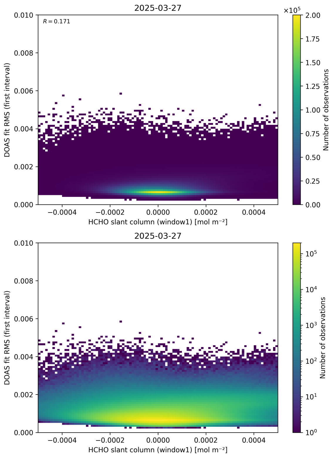
Figure 78: Scatter density plot of “HCHO slant column (window1)” against “DOAS fit RMS (first interval)” for 2025-03-26 to 2025-03-28.
