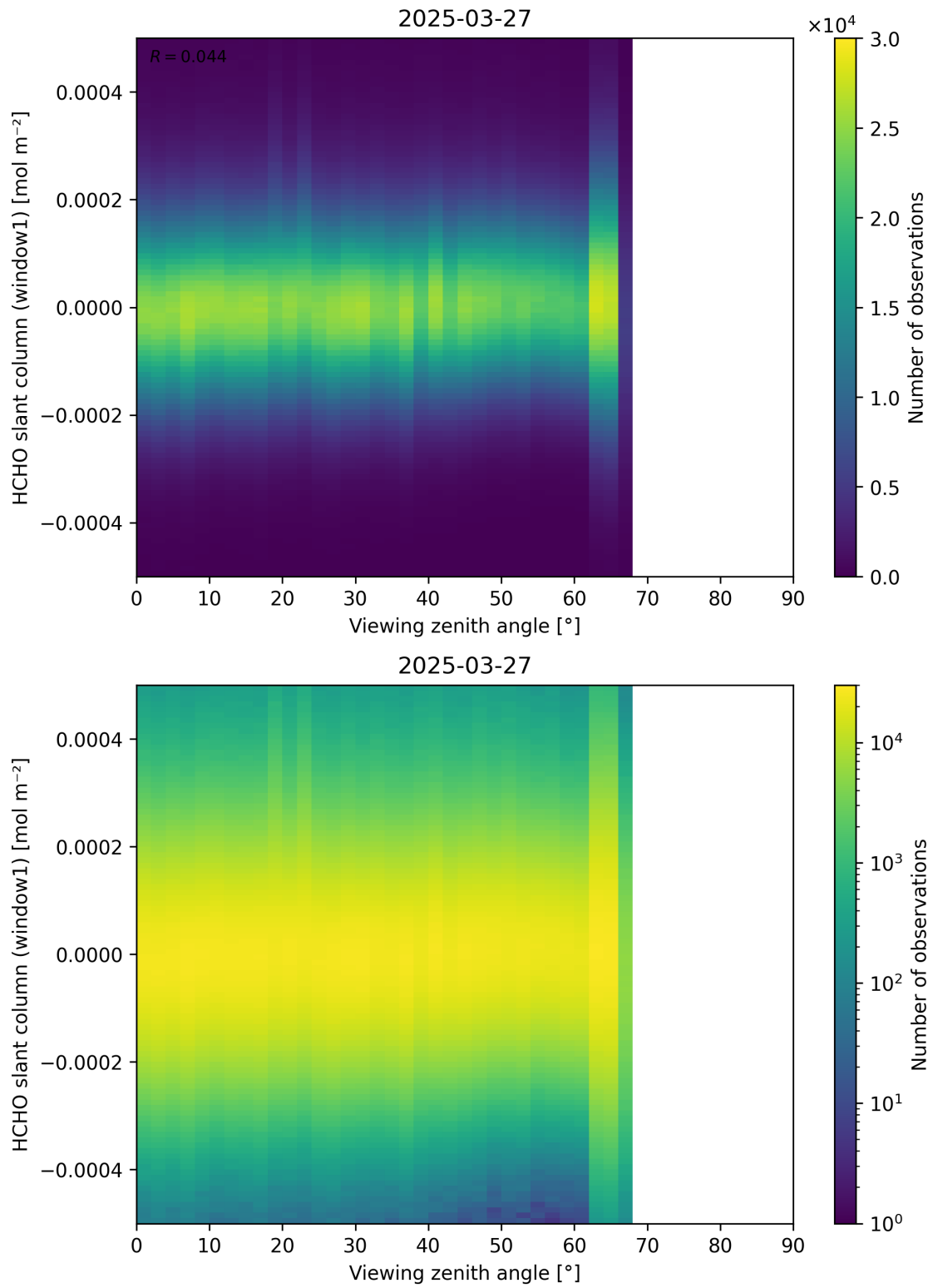
Figure 188: Scatter density plot of “Viewing zenith angle” against “HCHO slant column (window1)” for 2025-03-26 to 2025-03-28.
