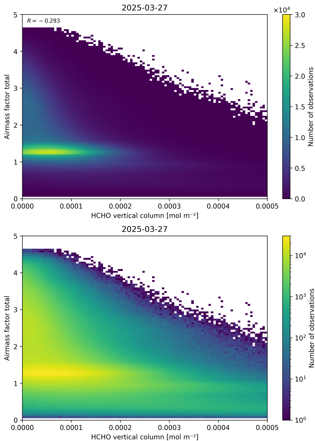
Figure 131: Scatter density plot of “HCHO vertical column” against “Airmass factor total” for 2025-03-26 to 2025-03-28.
