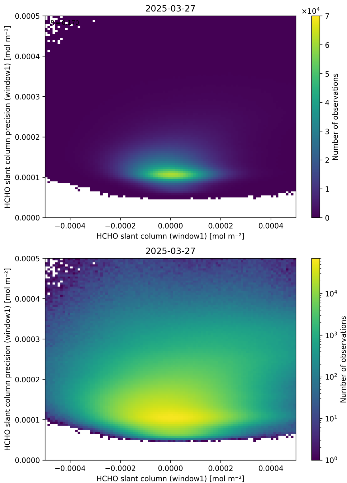
Figure 84: Scatter density plot of “HCHO slant column (window1)” against “HCHO slant column precision (window1)” for 2025-03-26 to 2025-03-28.
