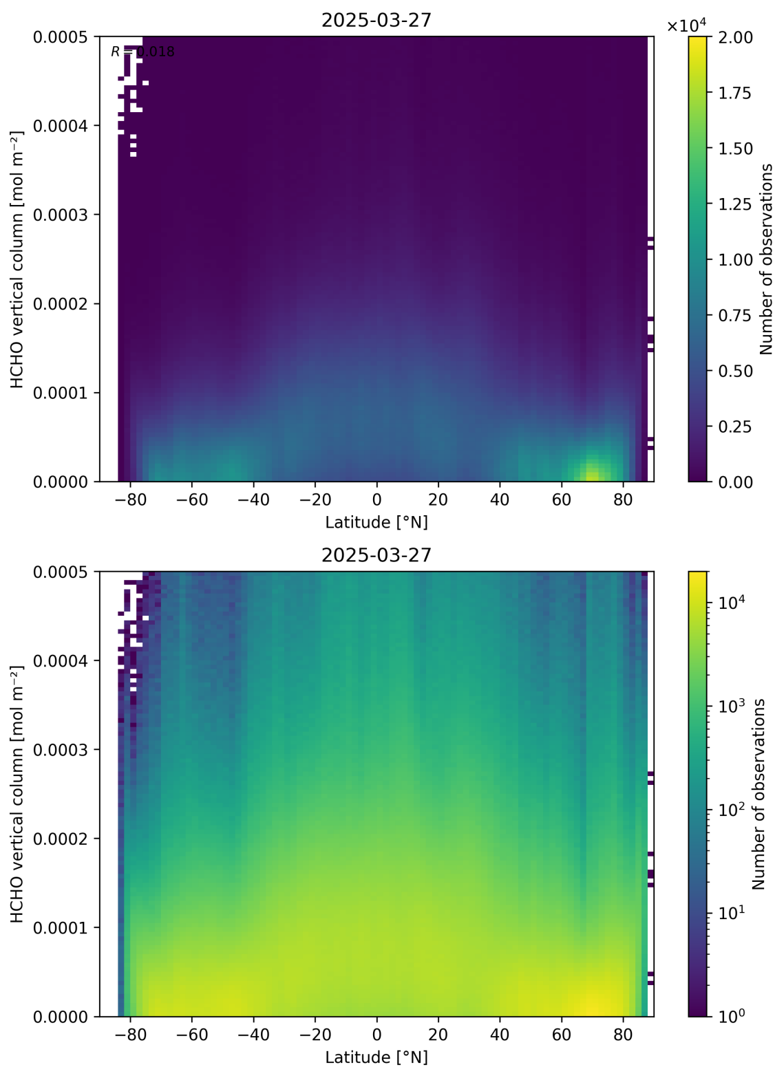
Figure 163: Scatter density plot of “Latitude” against “HCHO vertical column” for 2025-03-26 to 2025-03-28.
