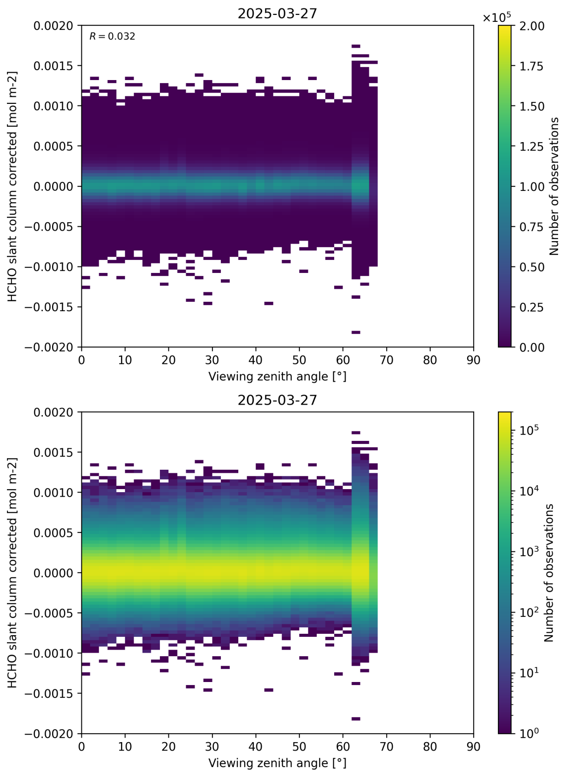
Figure 186: Scatter density plot of “Viewing zenith angle” against “HCHO slant column corrected” for 2025-03-26 to 2025-03-28.
