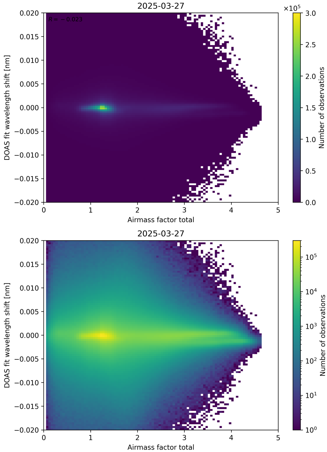
Figure 98: Scatter density plot of “Airmass factor total” against “DOAS fit wavelength shift” for 2025-03-26 to 2025-03-28.
