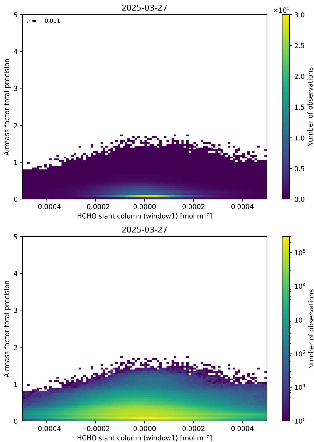
Figure 86: Scatter density plot of “HCHO slant column (window1)” against “Airmass factor total precision” for 2025-03-26 to 2025-03-28.
