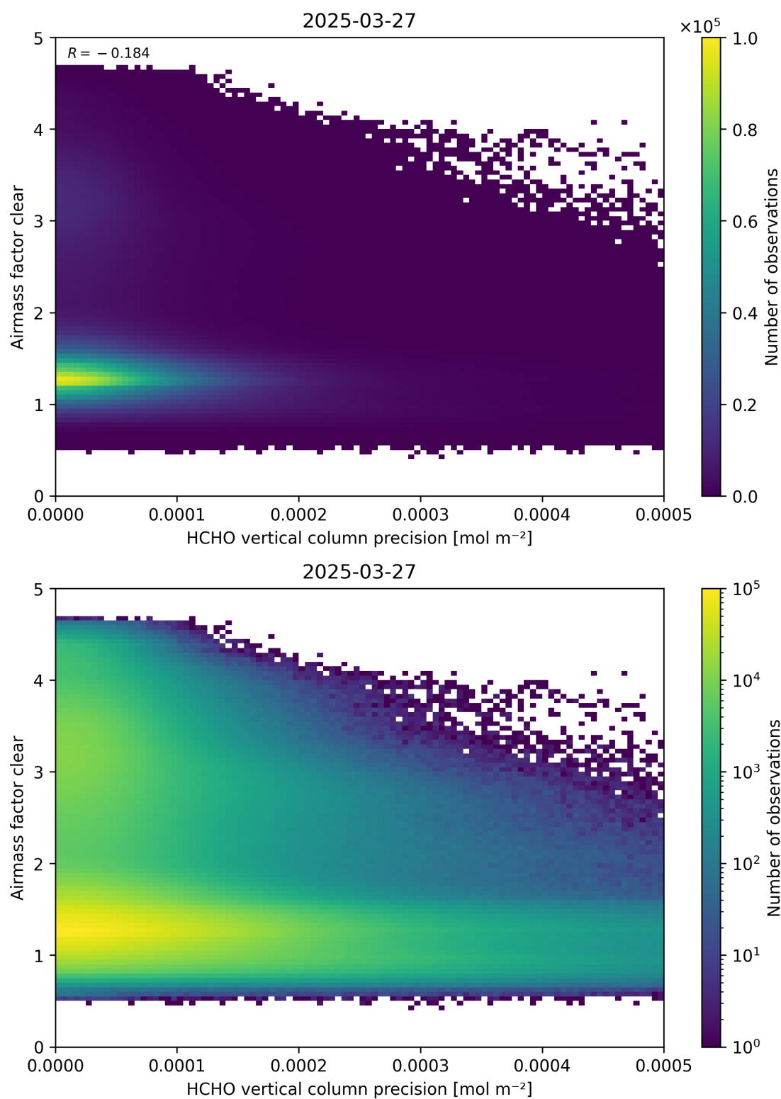
Figure 139: Scatter density plot of “HCHO vertical column precision” against “Airmass factor clear” for 2025-03-26 to 2025-03-28.
