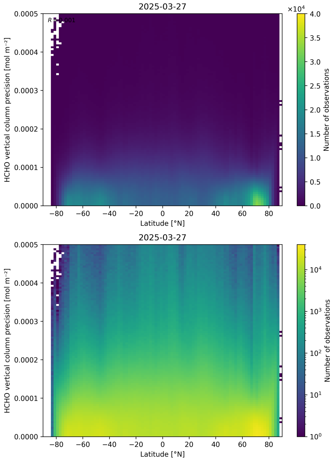
Figure 165: Scatter density plot of “Latitude” against “HCHO vertical column precision” for 2025-03-26 to 2025-03-28.
