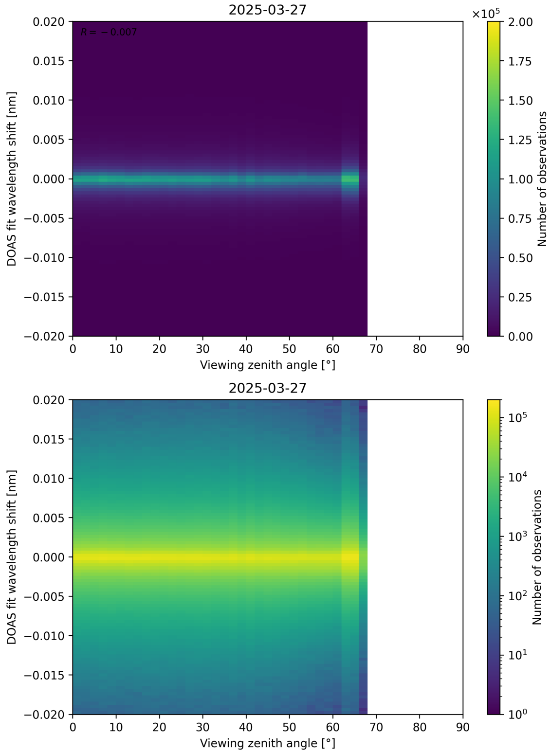
Figure 183: Scatter density plot of “Viewing zenith angle” against “DOAS fit wavelength shift” for 2025-03-26 to 2025-03-28.
