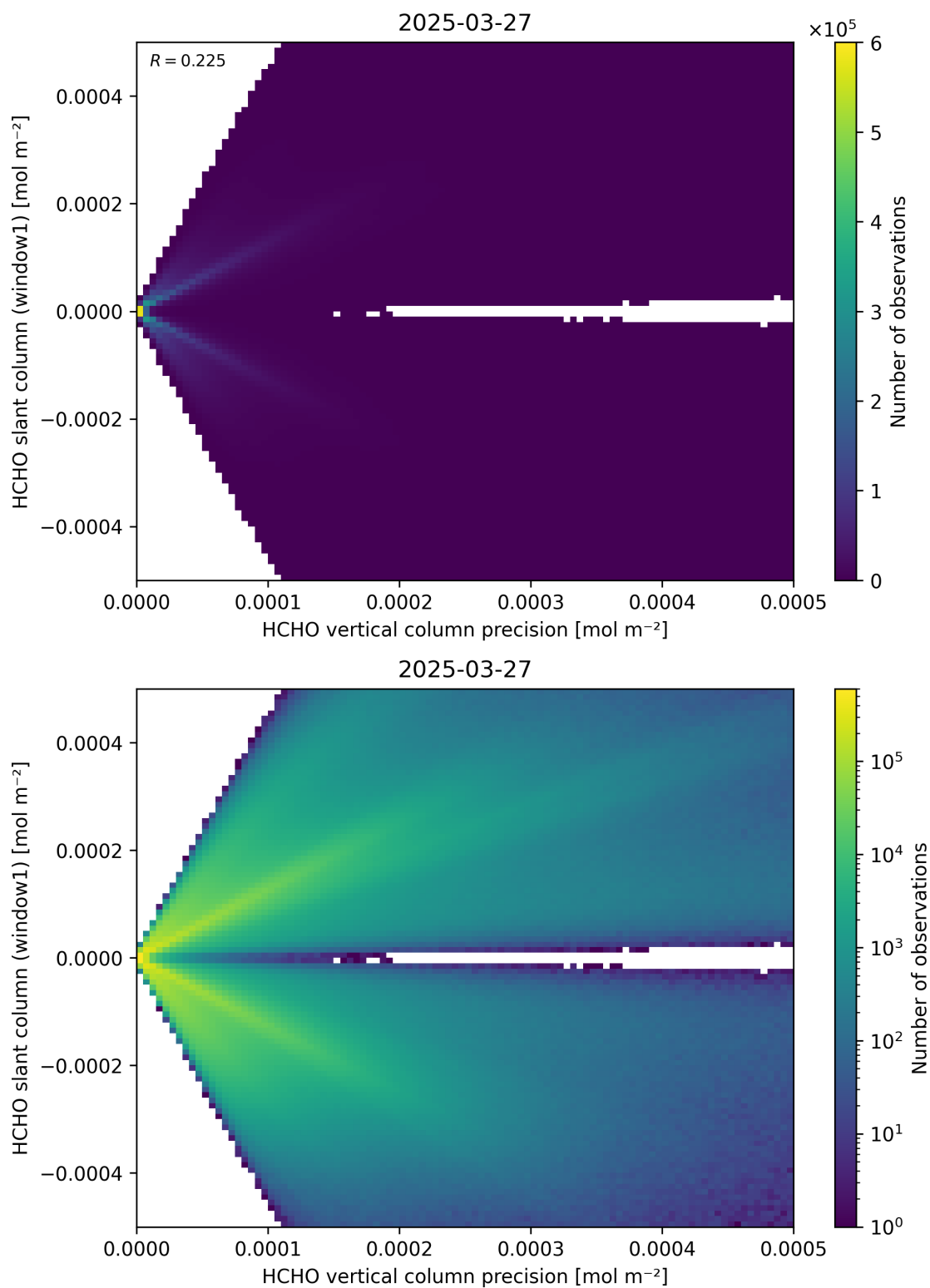
Figure 142: Scatter density plot of “HCHO vertical column precision” against “HCHO slant column (window1)” for 2025-03-26 to 2025-03-28.
