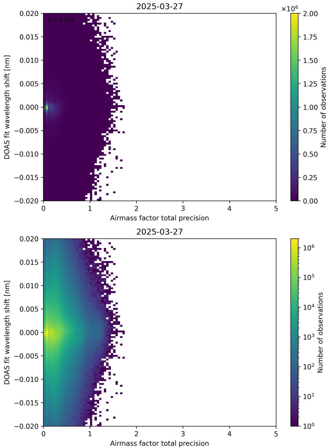
Figure 106: Scatter density plot of “Airmass factor total precision” against “DOAS fit wavelength shift” for 2025-03-26 to 2025-03-28.
