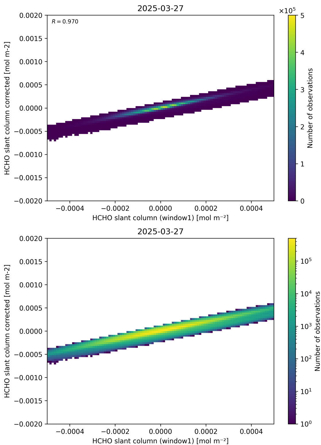
Figure 82: Scatter density plot of “HCHO slant column (window1)” against “HCHO slant column corrected” for 2025-03-26 to 2025-03-28.
