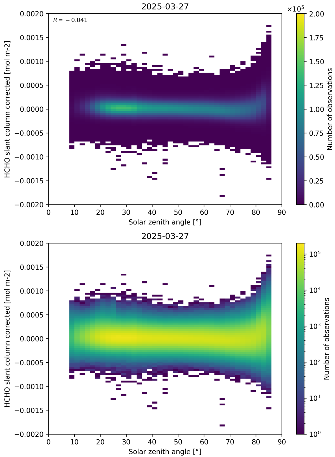
Figure 171: Scatter density plot of “Solar zenith angle” against “HCHO slant column corrected” for 2025-03-26 to 2025-03-28.
