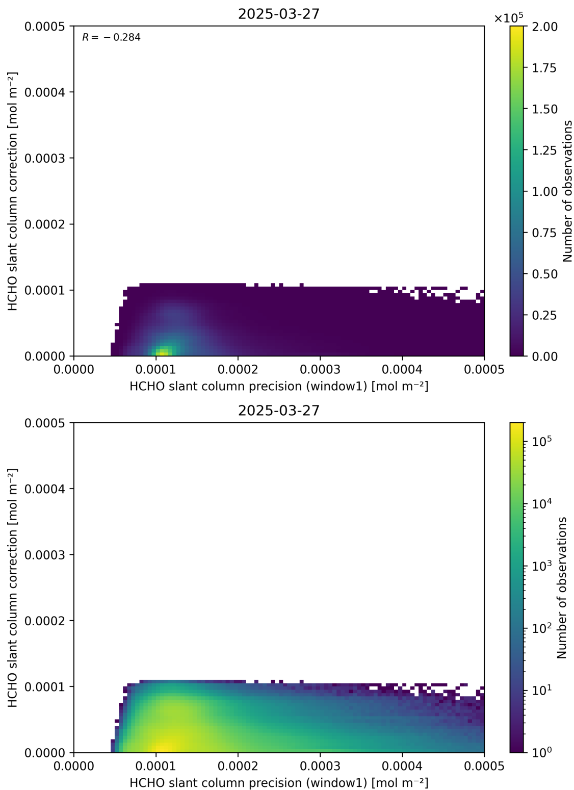
Figure 93: Scatter density plot of “HCHO slant column precision (window1)” against “HCHO slant column correction” for 2025-03-26 to 2025-03-28.
