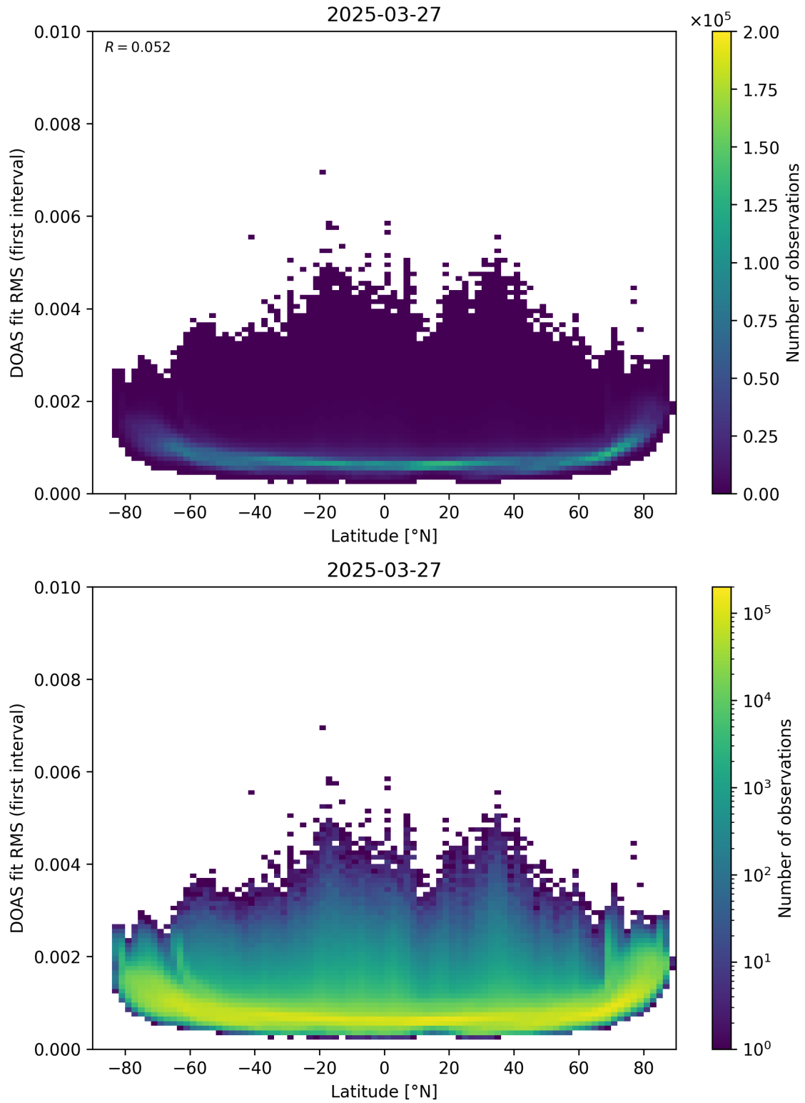
Figure 153: Scatter density plot of “Latitude” against “DOAS fit RMS (first interval)” for 2025-03-26 to 2025-03-28.
