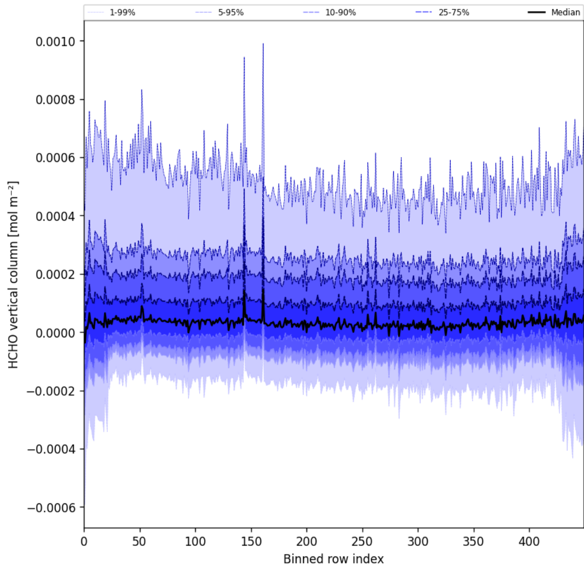
Figure 49: Along track statistics of “HCHO vertical column” for 2025-03-26 to 2025-03-28
