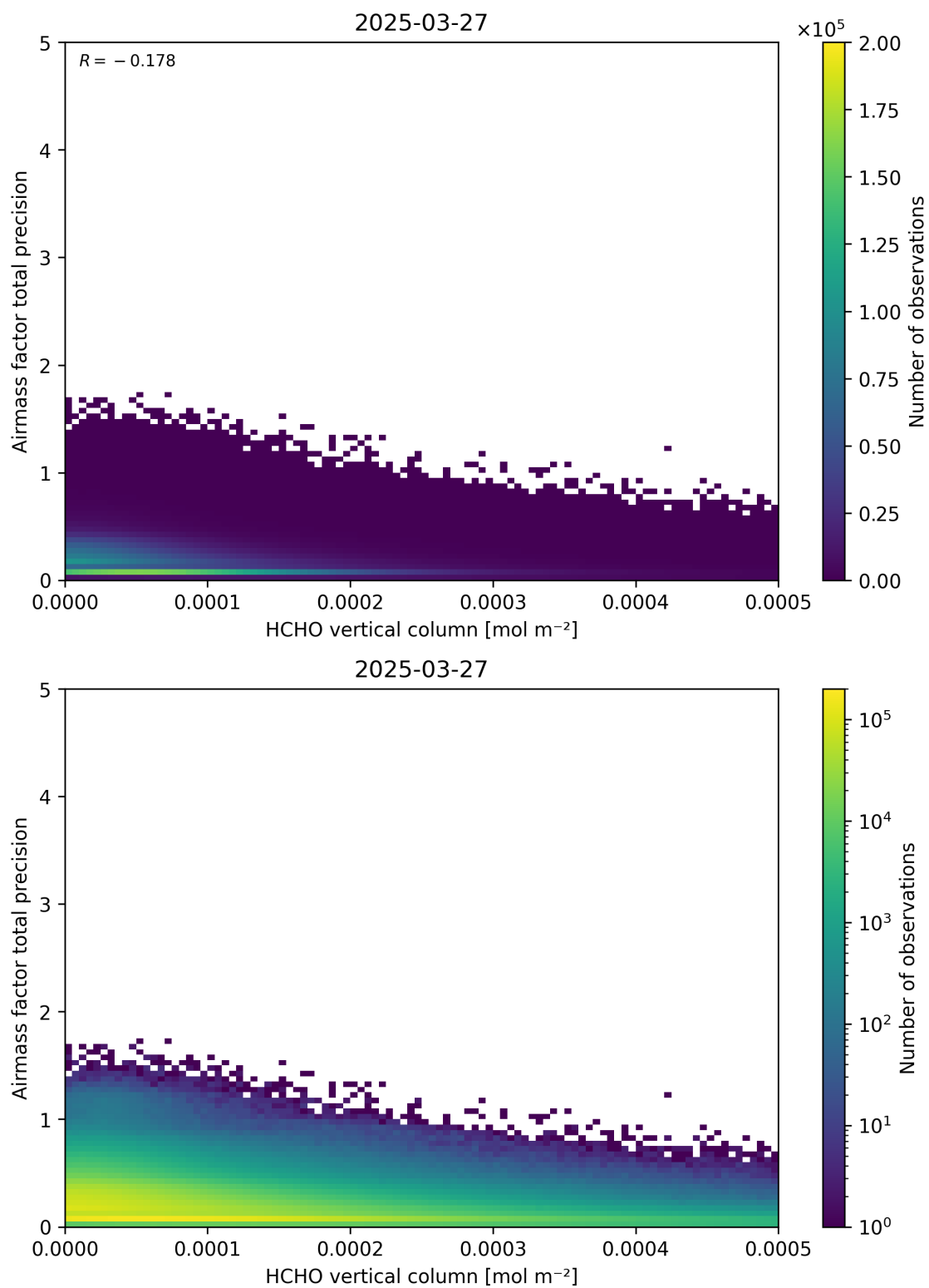
Figure 132: Scatter density plot of “HCHO vertical column” against “Airmass factor total precision” for 2025-03-26 to 2025-03-28.
