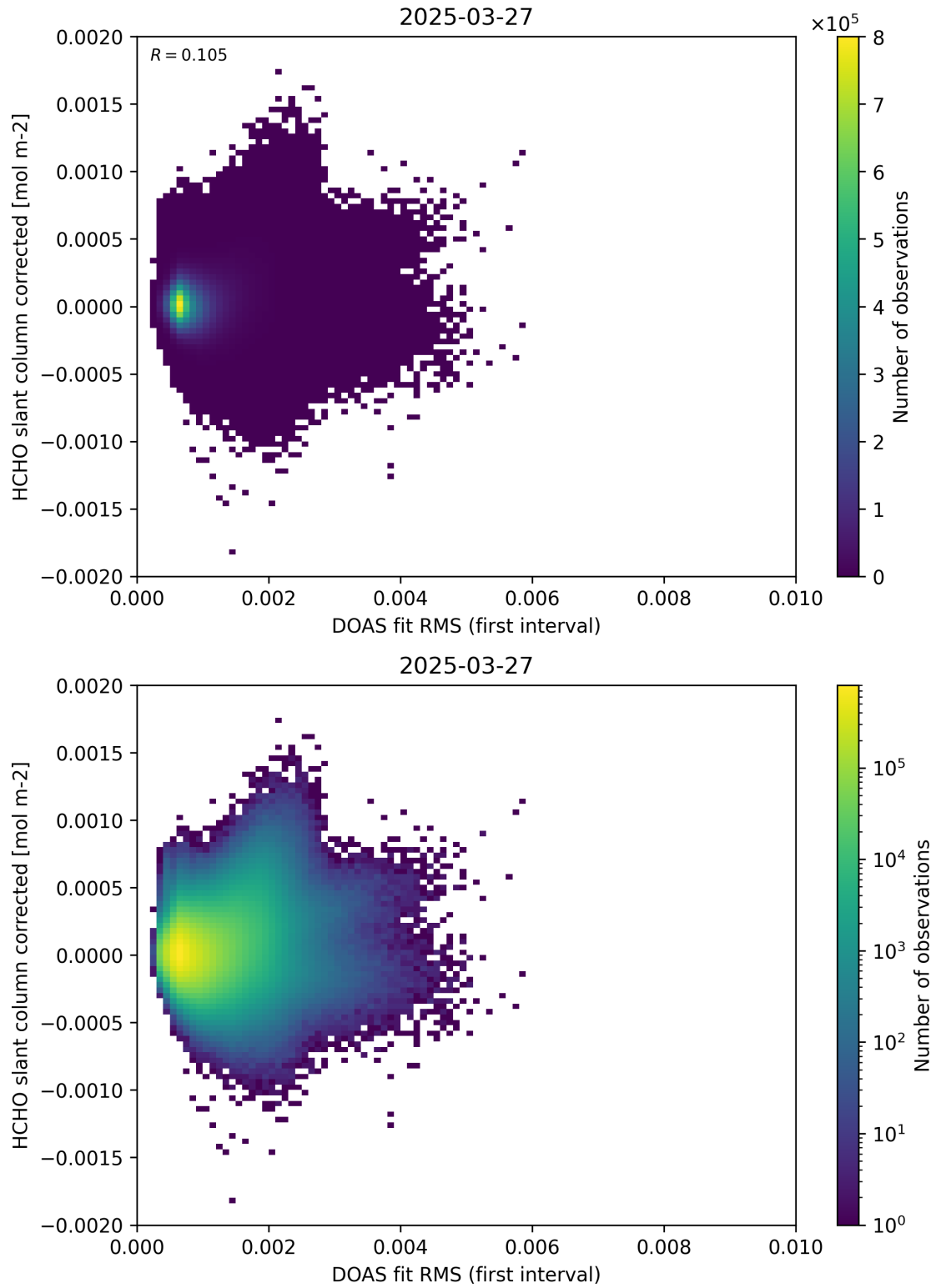
Figure 62: Scatter density plot of “DOAS fit RMS (first interval)” against “HCHO slant column corrected” for 2025-03-26 to 2025-03-28.
