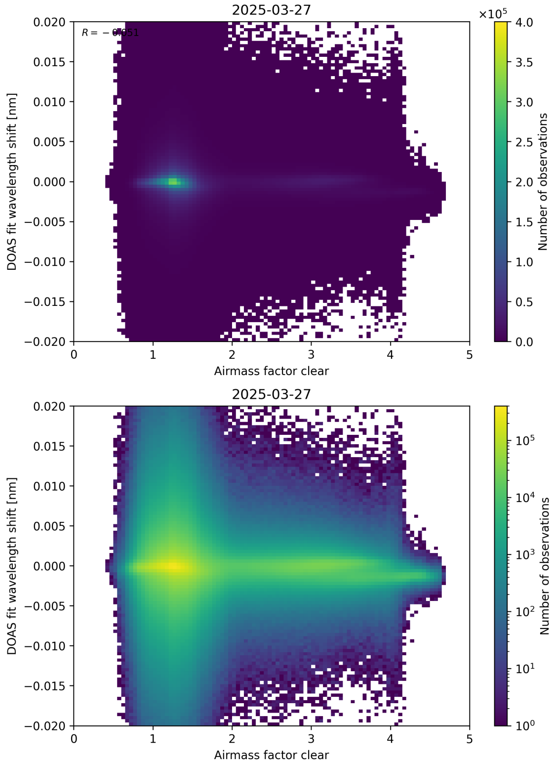
Figure 72: Scatter density plot of “Airmass factor clear” against “DOAS fit wavelength shift” for 2025-03-26 to 2025-03-28.
