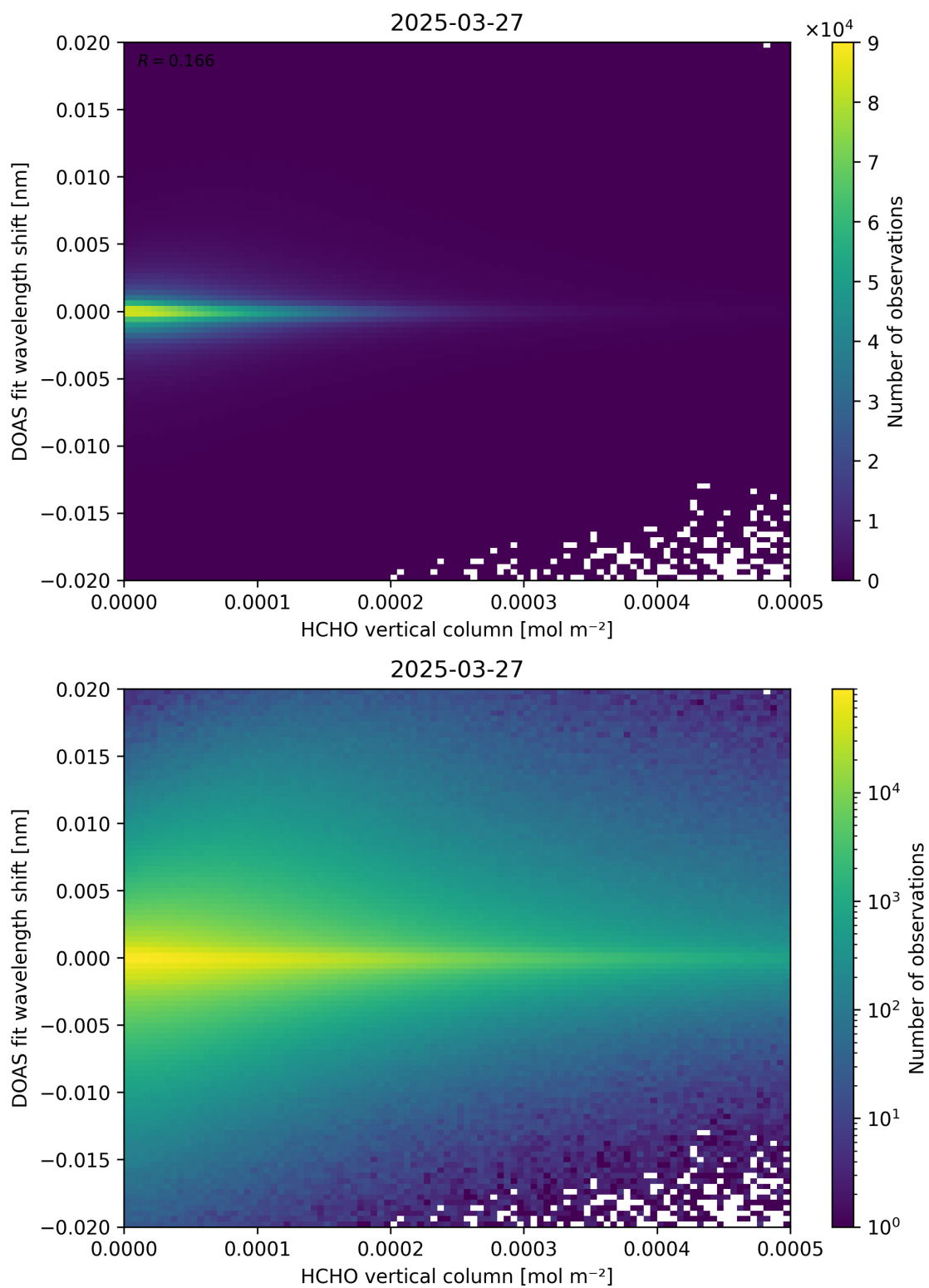
Figure 124: Scatter density plot of “HCHO vertical column” against “DOAS fit wavelength shift” for 2025-03-26 to 2025-03-28.
