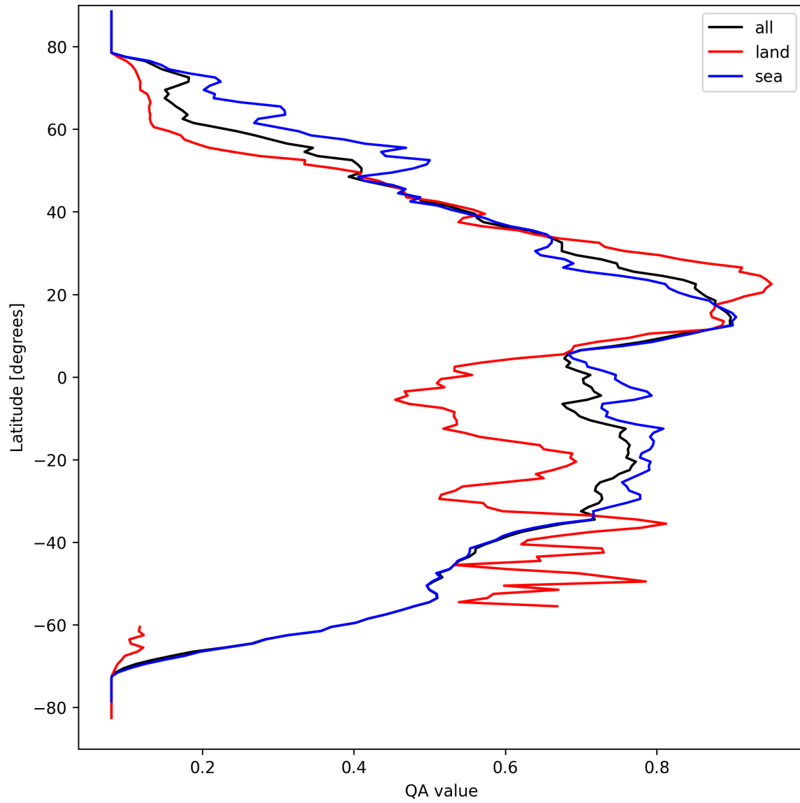
Figure 20: Zonal average of “QA value” for 2025-03-26 to 2025-03-28.
