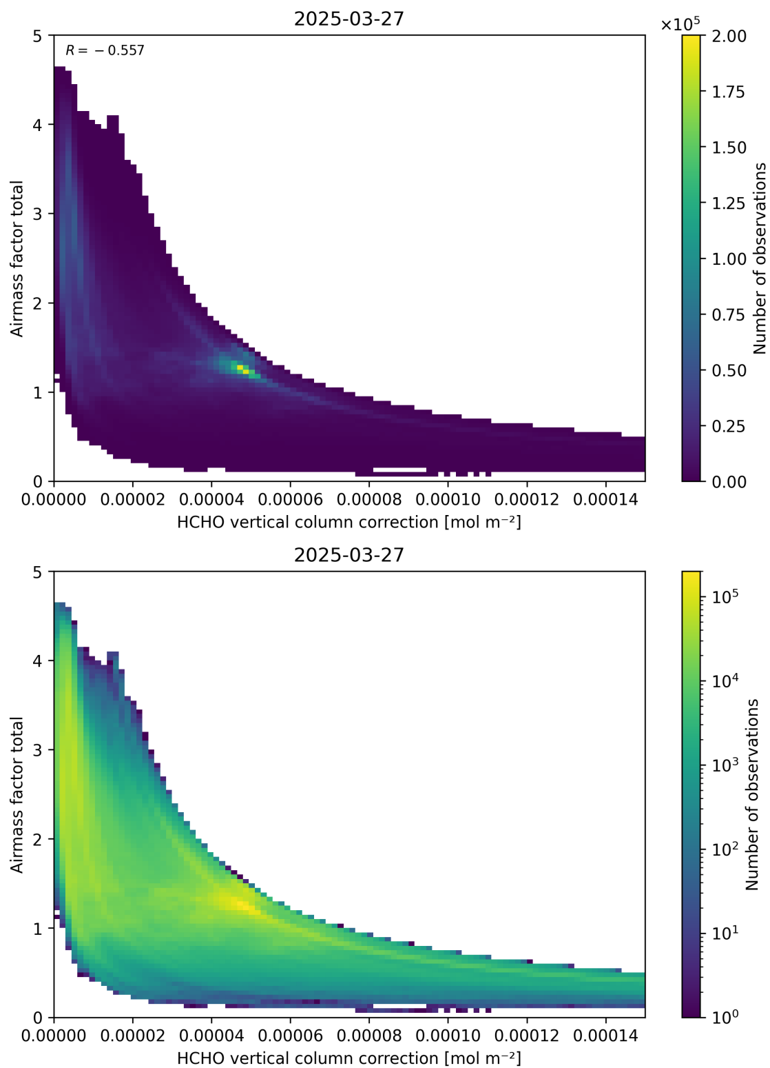
Figure 120: Scatter density plot of “HCHO vertical column correction” against “Airmass factor total” for 2025-03-26 to 2025-03-28.
