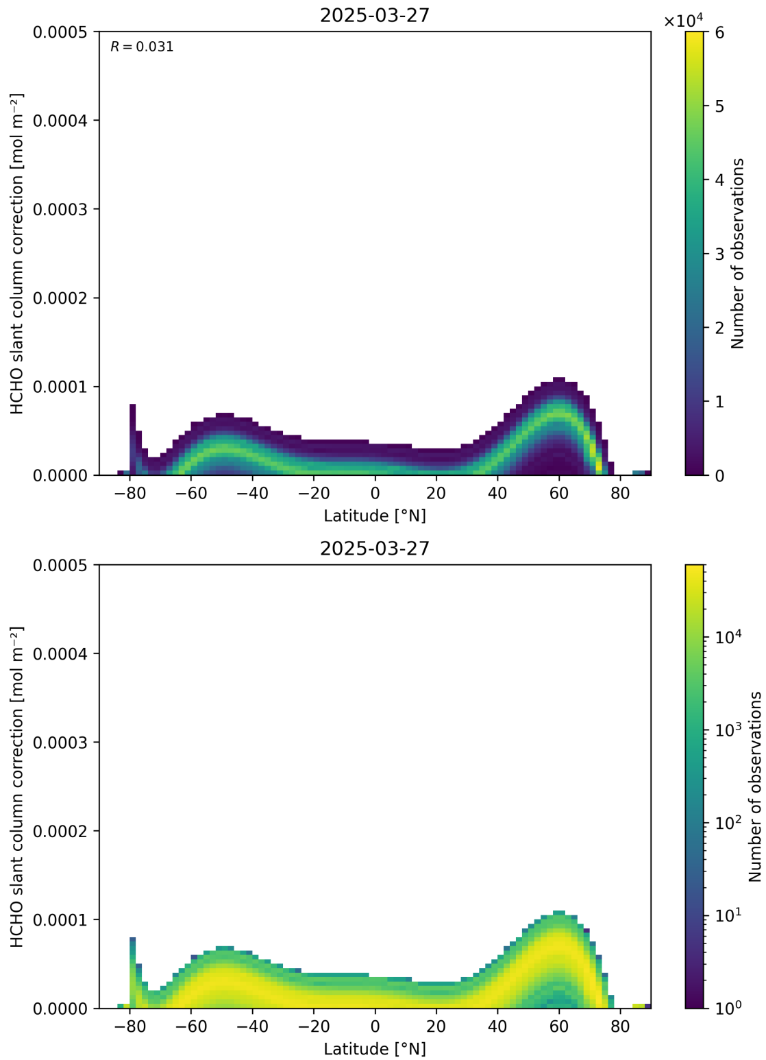
Figure 158: Scatter density plot of “Latitude” against “HCHO slant column correction” for 2025-03-26 to 2025-03-28.
