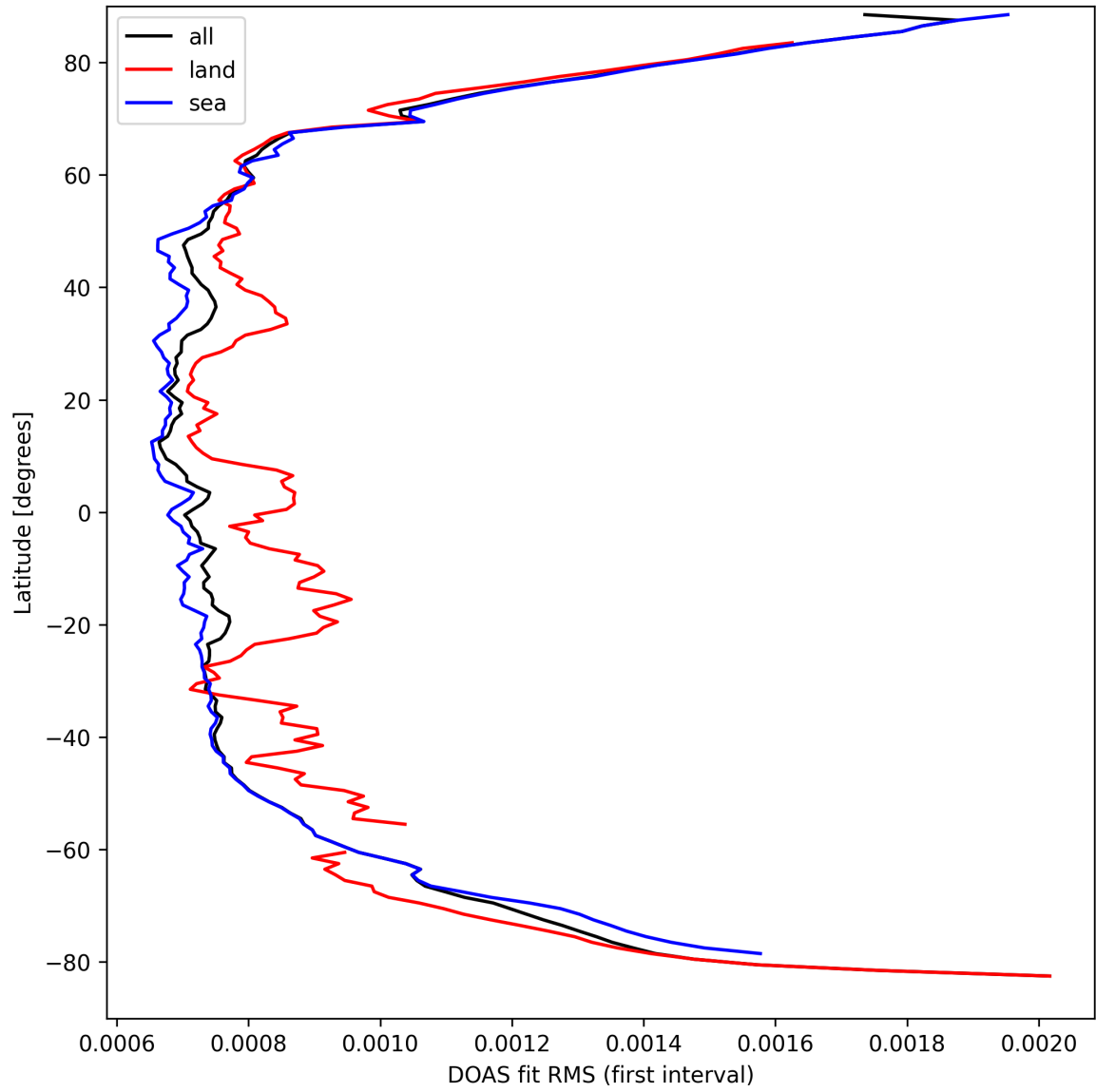
Figure 32: Zonal average of “DOAS fit RMS (first interval)” for 2025-03-26 to 2025-03-28.
