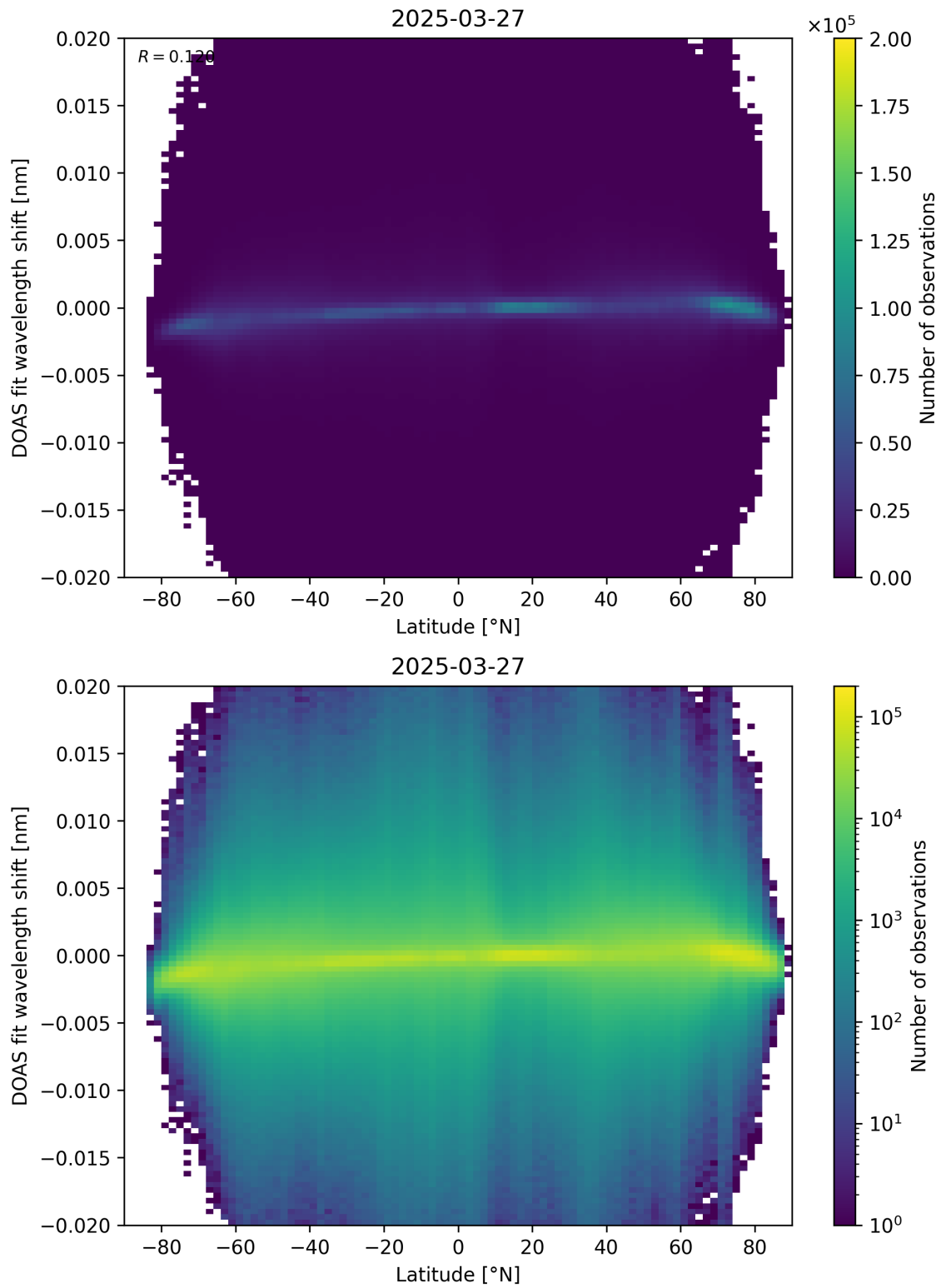
Figure 154: Scatter density plot of “Latitude” against “DOAS fit wavelength shift” for 2025-03-26 to 2025-03-28.
