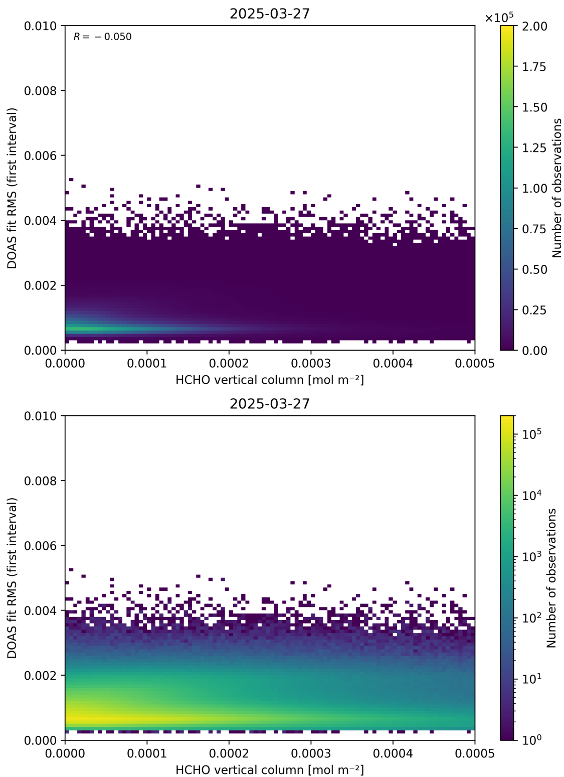
Figure 123: Scatter density plot of “HCHO vertical column” against “DOAS fit RMS (first interval)” for 2025-03-26 to 2025-03-28.
