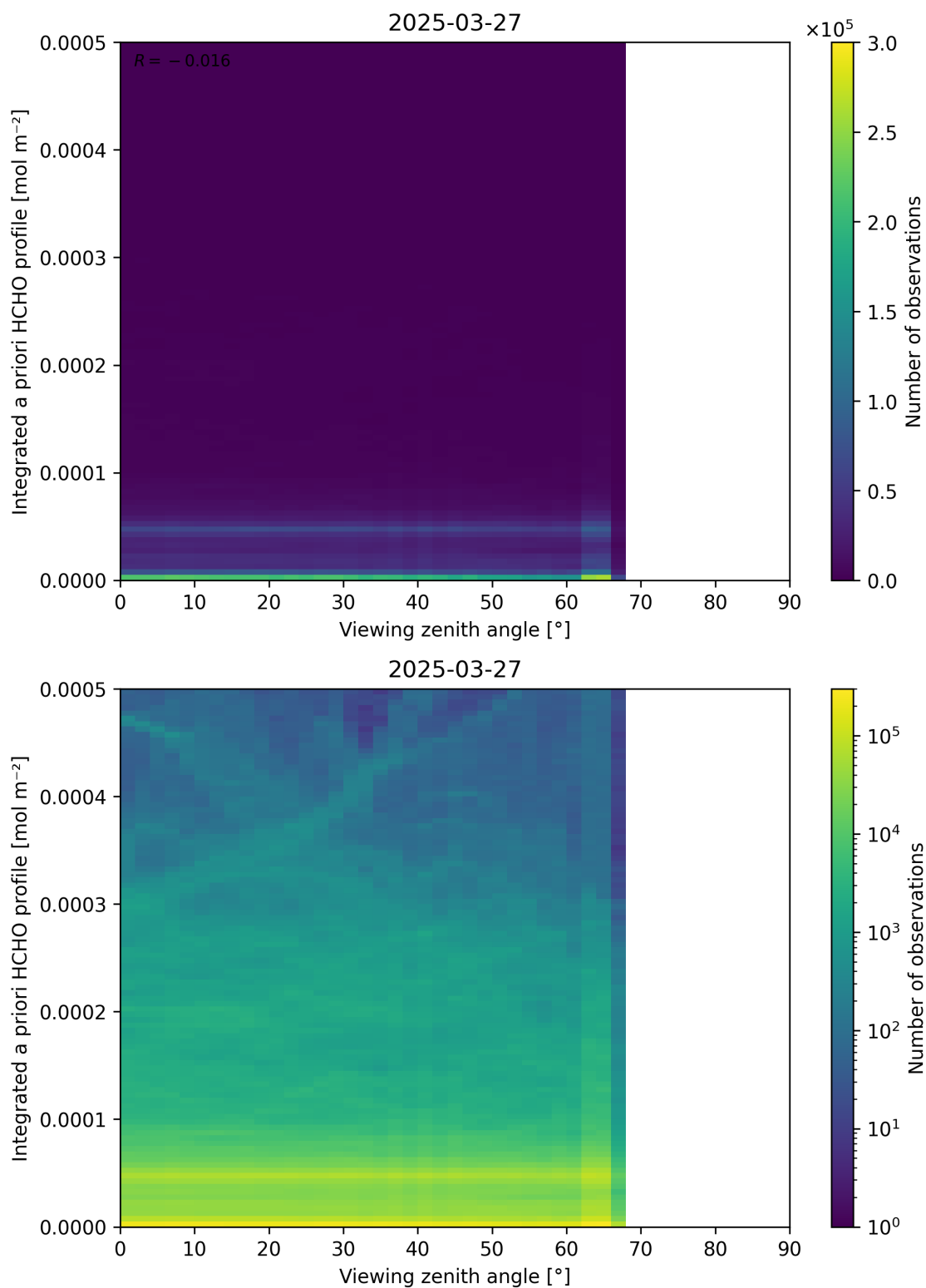
Figure 195: Scatter density plot of “Viewing zenith angle” against “Integrated a priori HCHO profile” for 2025-03-26 to 2025-03-28.
