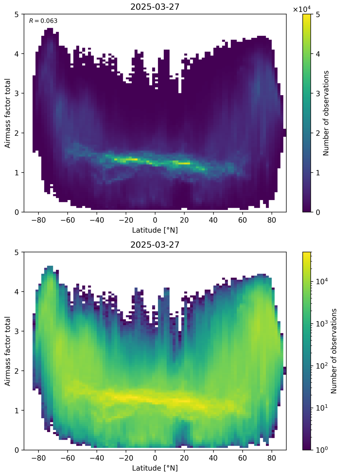
Figure 161: Scatter density plot of “Latitude” against “Airmass factor total” for 2025-03-26 to 2025-03-28.
