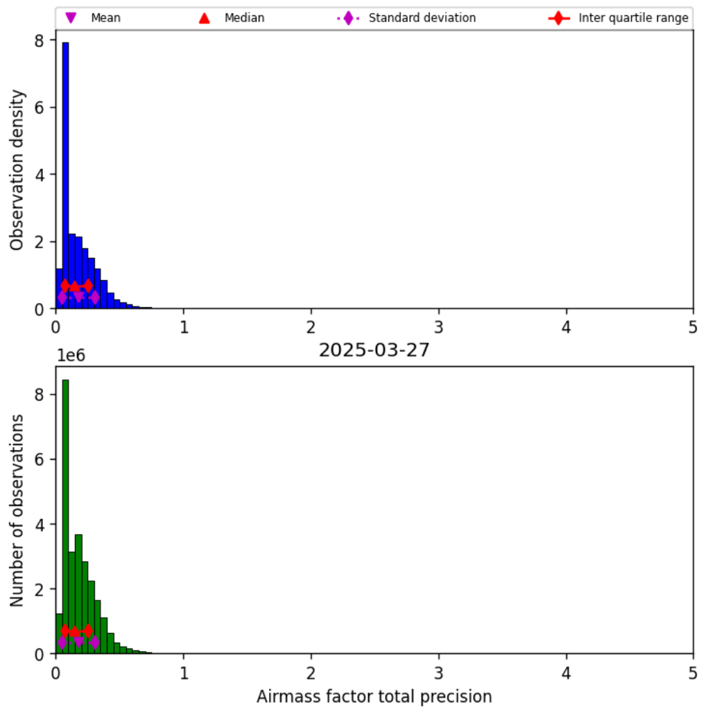
Figure 41: Histogram of “Airmass factor total precision” for 2025-03-26 to 2025-03-28
