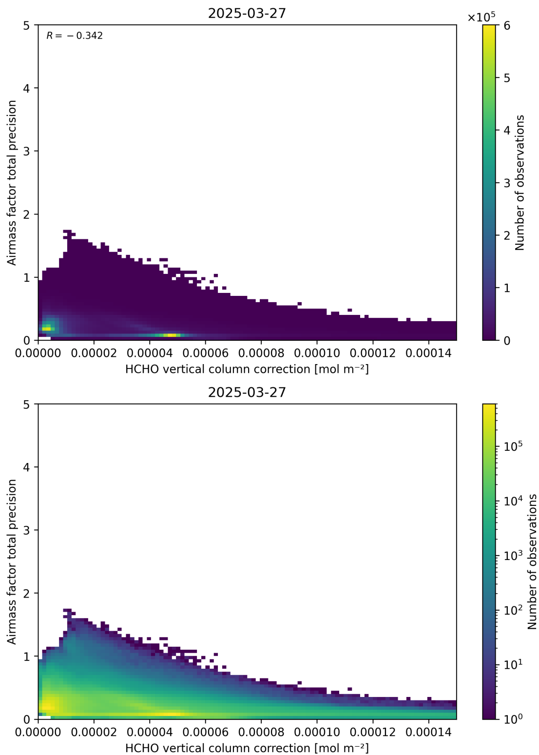
Figure 121: Scatter density plot of “HCHO vertical column correction” against “Airmass factor total precision” for 2025-03-26 to 2025-03-28.
