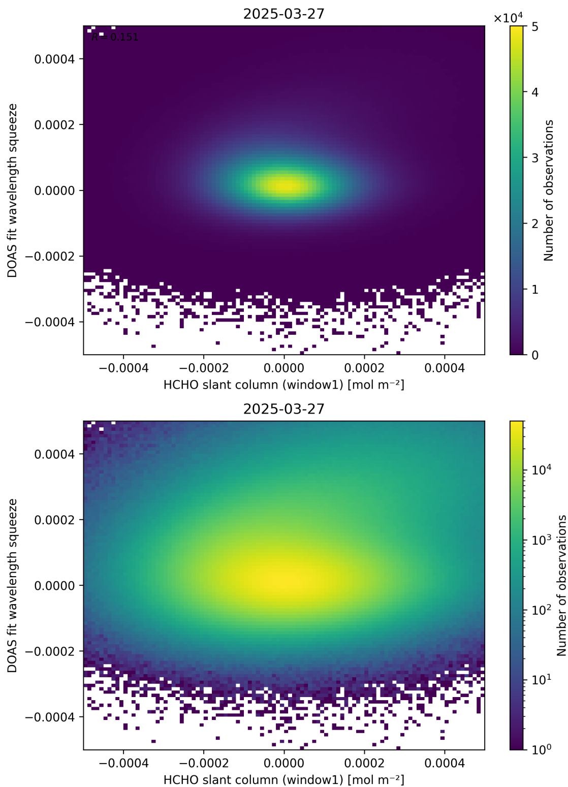
Figure 80: Scatter density plot of “HCHO slant column (window1)” against “DOAS fit wavelength squeeze” for 2025-03-26 to 2025-03-28.
