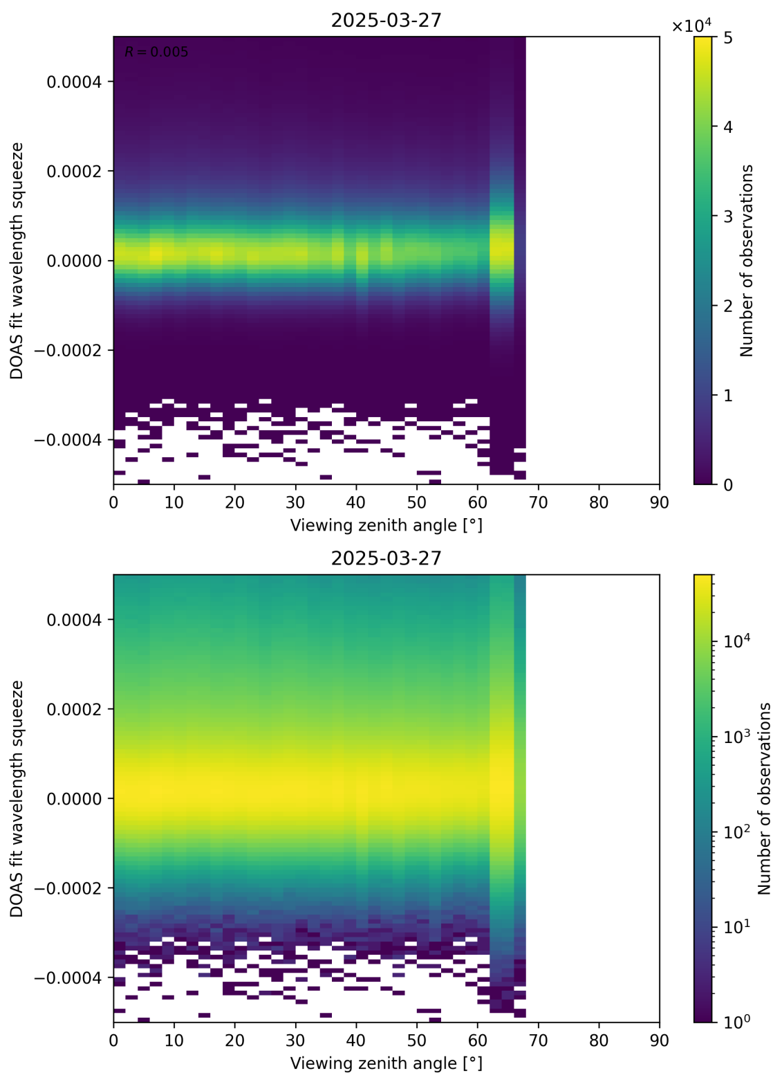
Figure 184: Scatter density plot of “Viewing zenith angle” against “DOAS fit wavelength squeeze” for 2025-03-26 to 2025-03-28.
