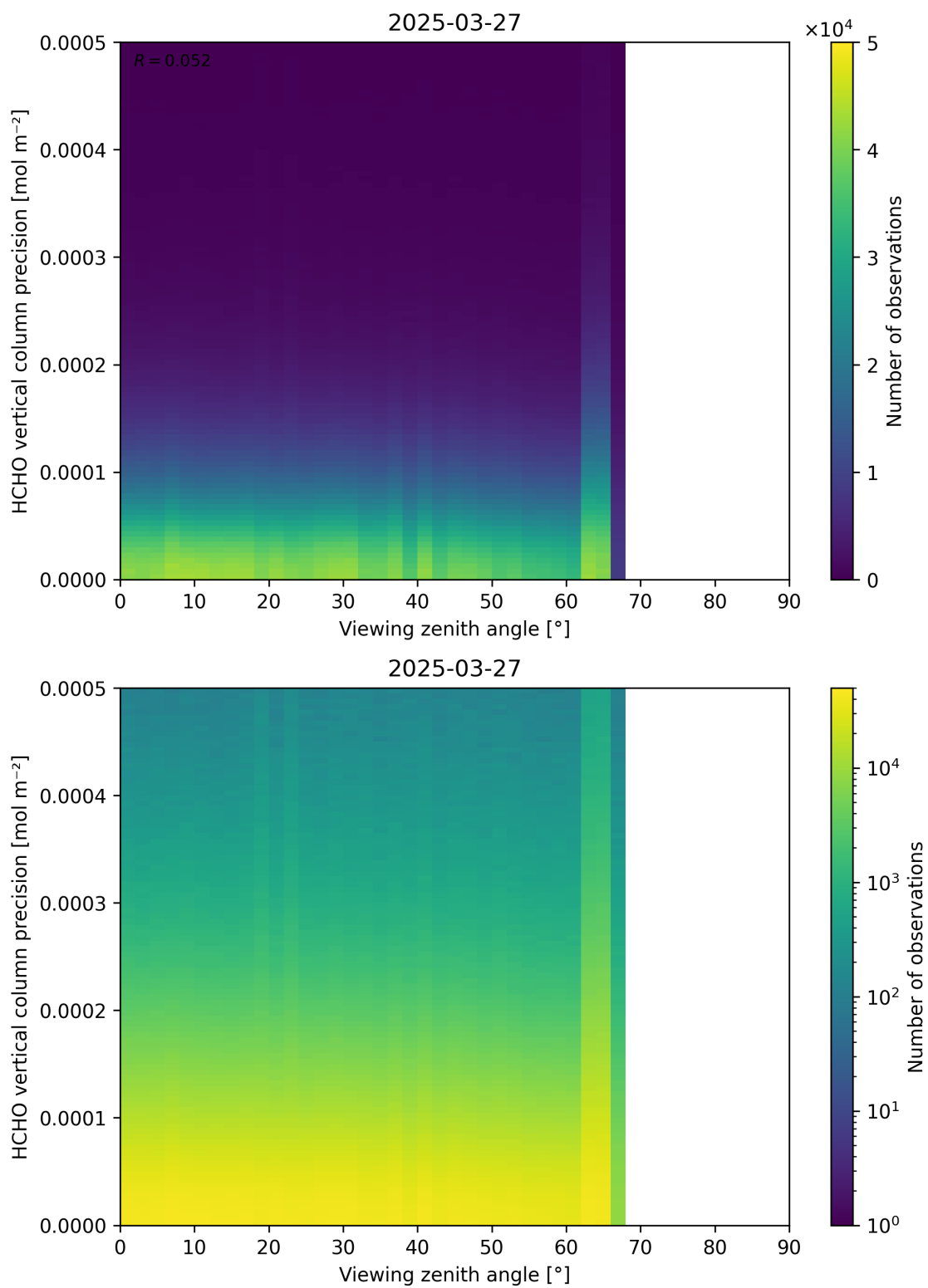
Figure 194: Scatter density plot of “Viewing zenith angle” against “HCHO vertical column precision” for 2025-03-26 to 2025-03-28.
