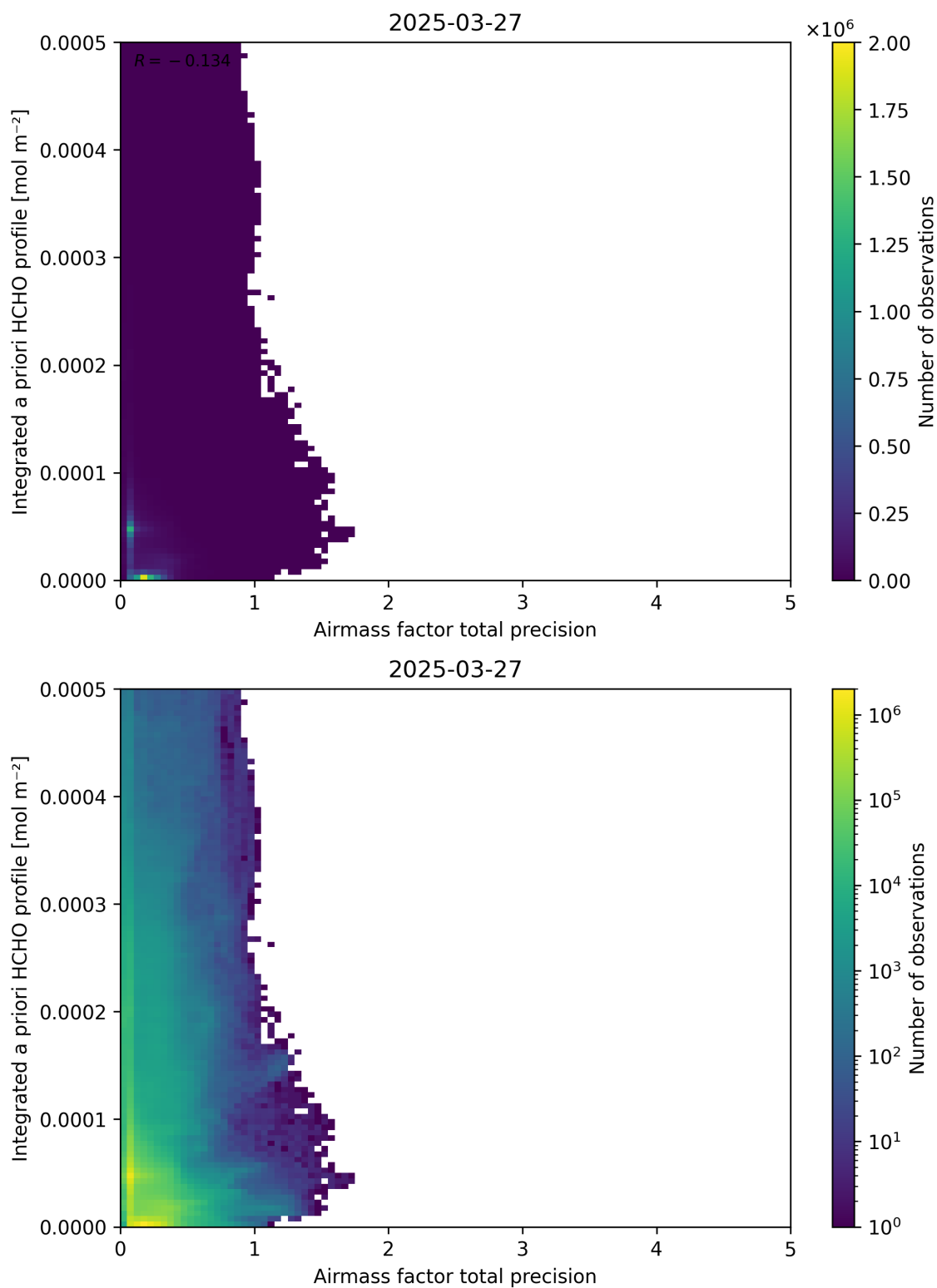
Figure 111: Scatter density plot of “Airmass factor total precision” against “Integrated a priori HCHO profile” for 2025-03-26 to 2025-03-28.
