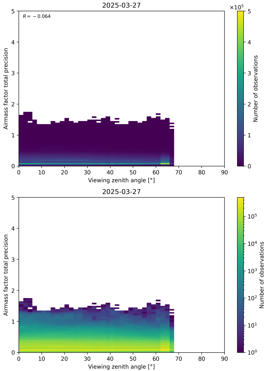
Figure 191: Scatter density plot of “Viewing zenith angle” against “Airmass factor total precision” for 2025-03-26 to 2025-03-28.
