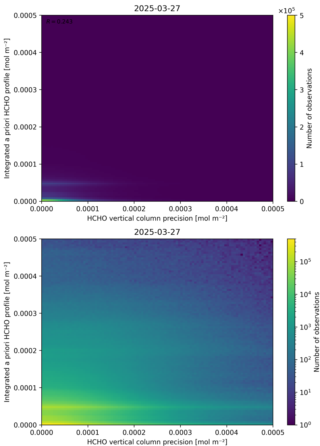
Figure 147: Scatter density plot of “HCHO vertical column precision” against “Integrated a priori HCHO profile” for 2025-03-26 to 2025-03-28.
