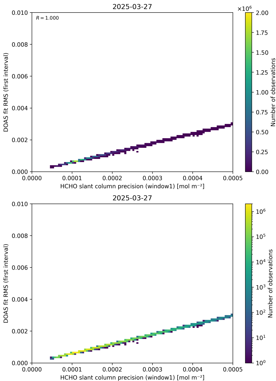
Figure 88: Scatter density plot of “HCHO slant column precision (window1)” against “DOAS fit RMS (first interval)” for 2025-03-26 to 2025-03-28.
