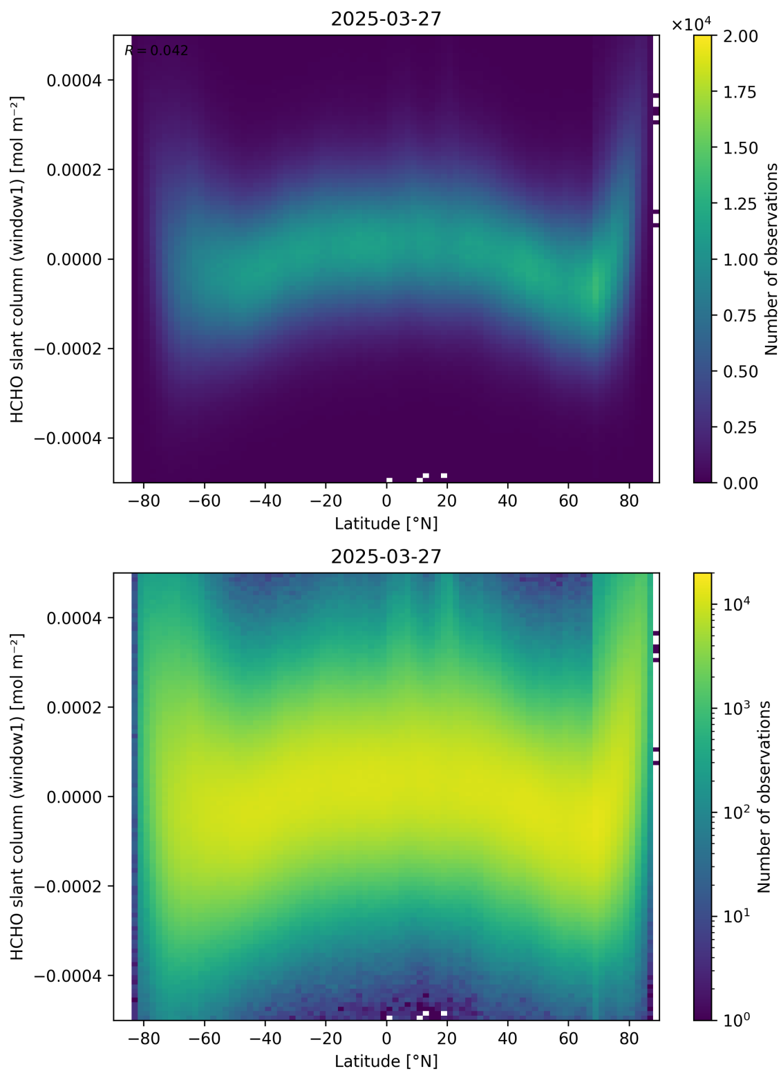
Figure 159: Scatter density plot of “Latitude” against “HCHO slant column (window1)” for 2025-03-26 to 2025-03-28.
