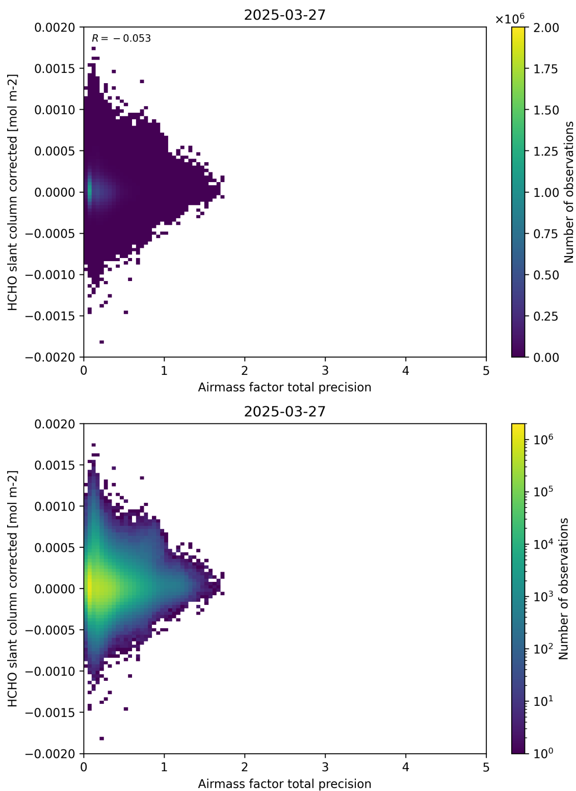
Figure 109: Scatter density plot of “Airmass factor total precision” against “HCHO slant column corrected” for 2025-03-26 to 2025-03-28.
