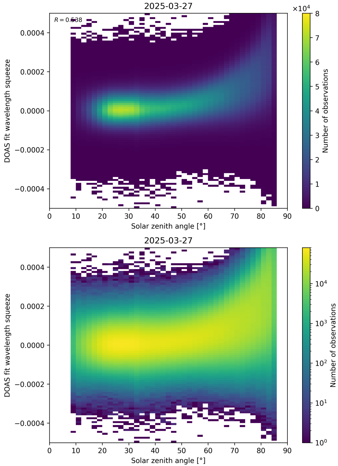
Figure 169: Scatter density plot of “Solar zenith angle” against “DOAS fit wavelength squeeze” for 2025-03-26 to 2025-03-28.
