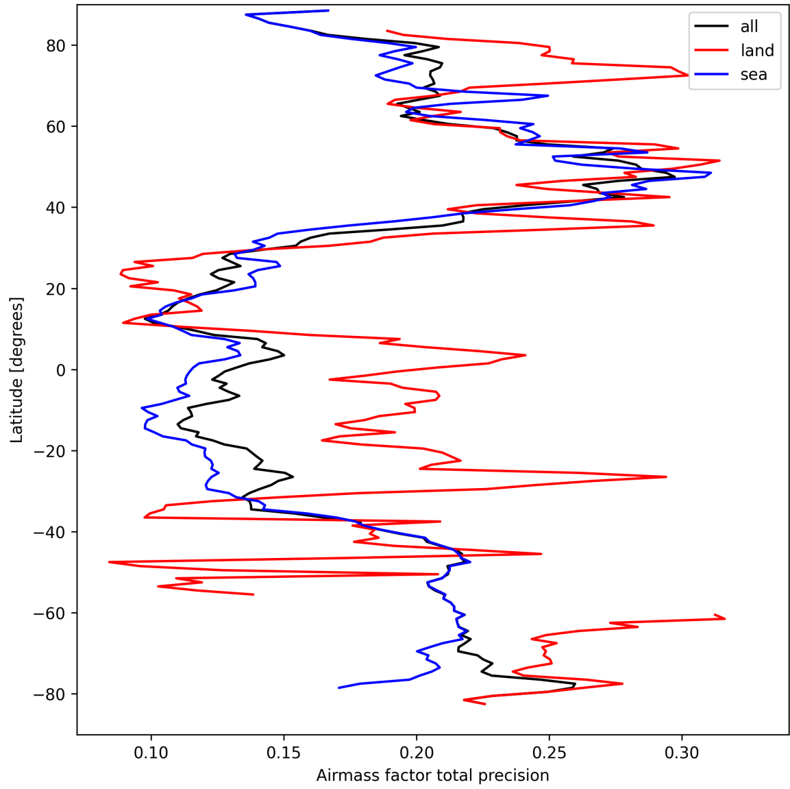
Figure 27: Zonal average of “Airmass factor total precision” for 2025-03-26 to 2025-03-28.
