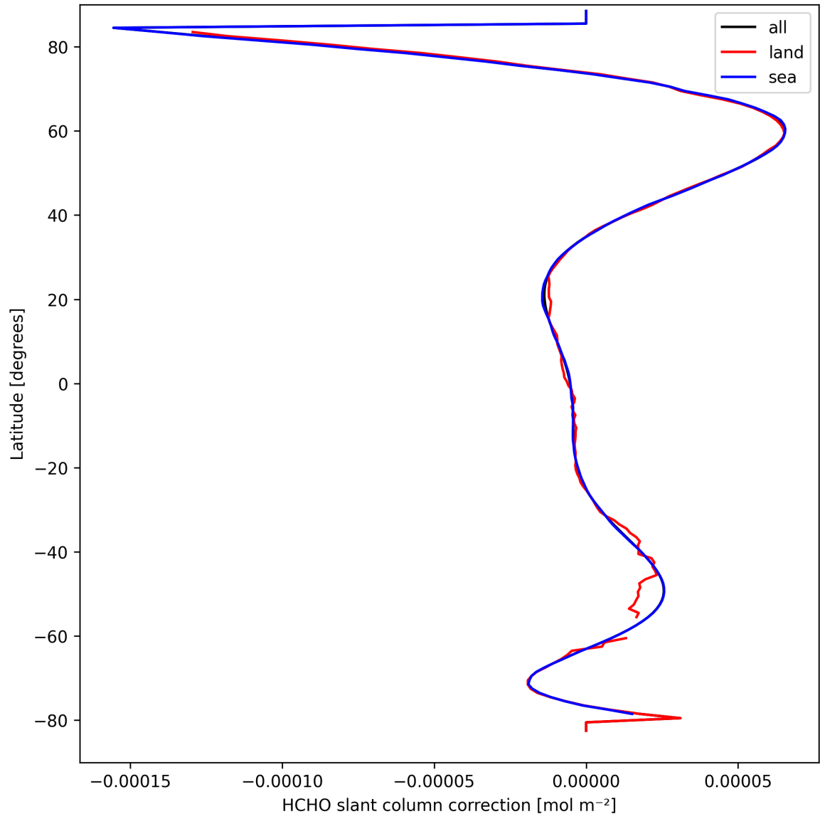
Figure 33: Zonal average of “HCHO slant column correction” for 2025-03-26 to 2025-03-28.
