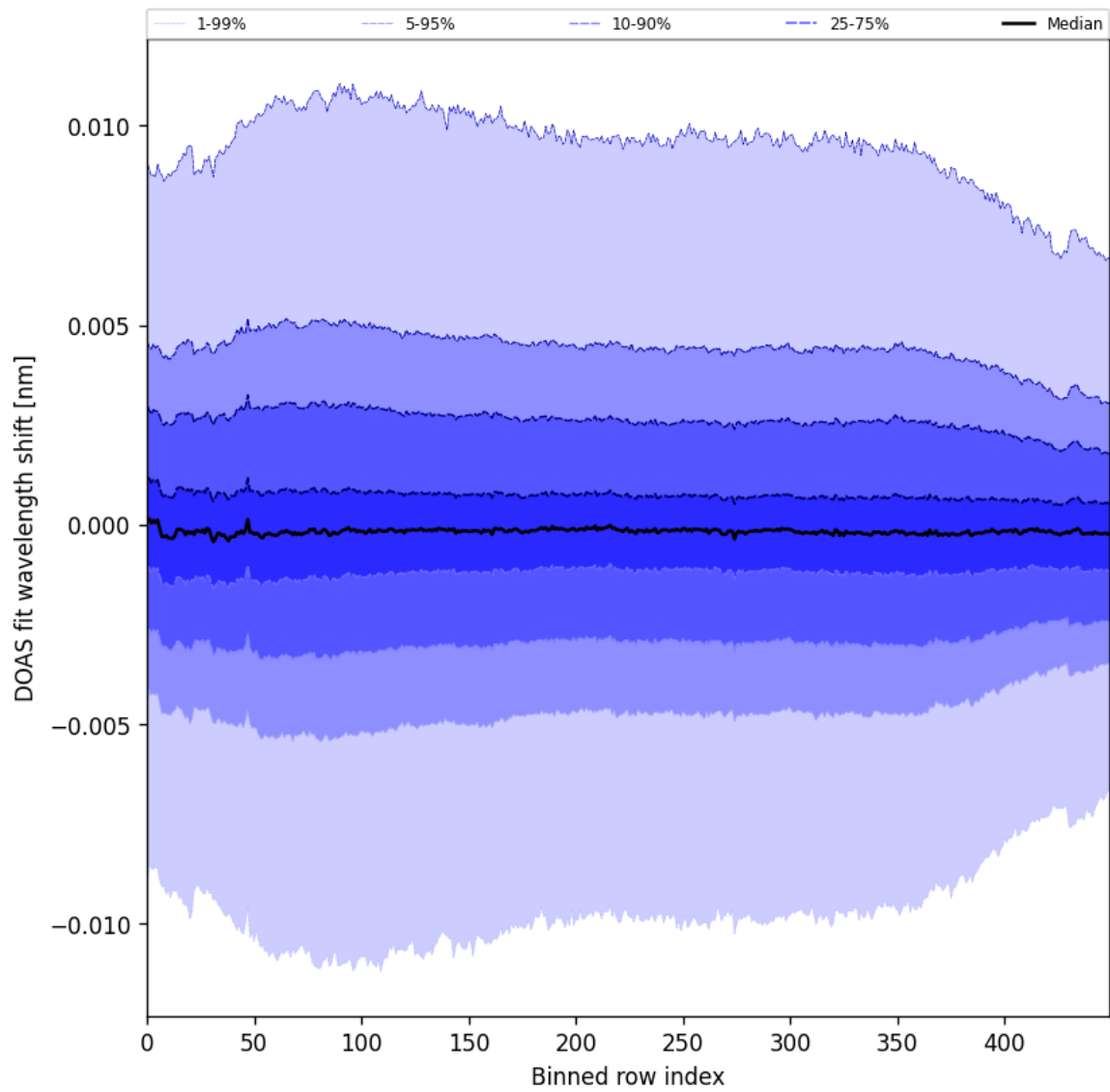
Figure 58: Along track statistics of “DOAS fit wavelength shift” for 2025-03-26 to 2025-03-28
