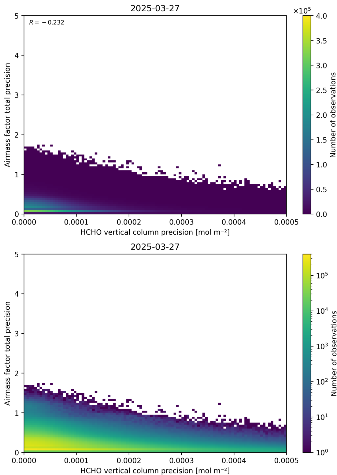
Figure 145: Scatter density plot of “HCHO vertical column precision” against “Airmass factor total precision” for 2025-03-26 to 2025-03-28.
