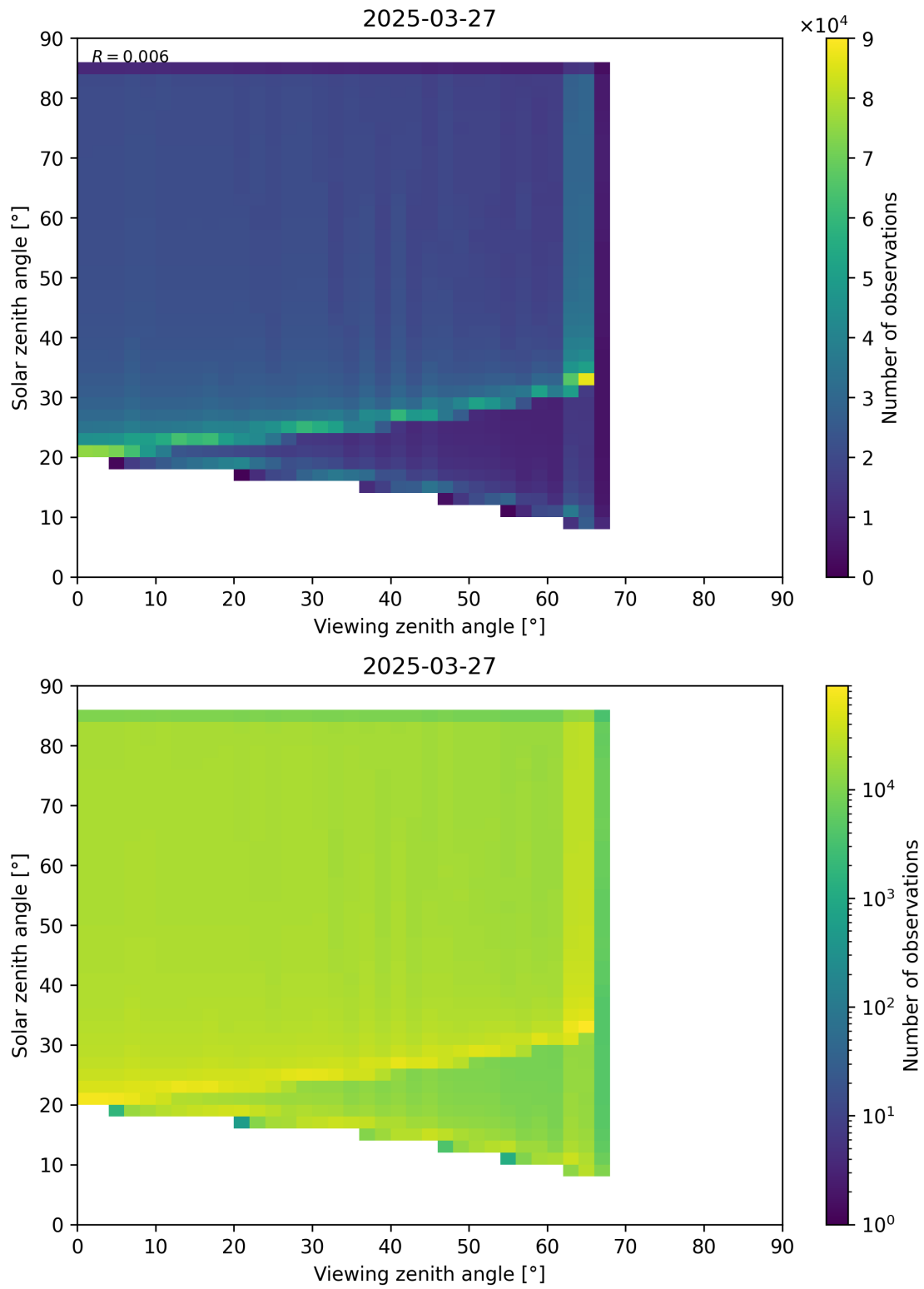
Figure 197: Scatter density plot of “Viewing zenith angle” against “Solar zenith angle” for 2025-03-26 to 2025-03-28.
