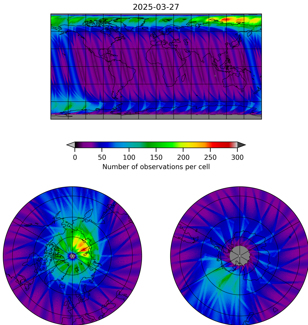
Figure 19: Map of the number of observations for 2025-03-26 to 2025-03-28
