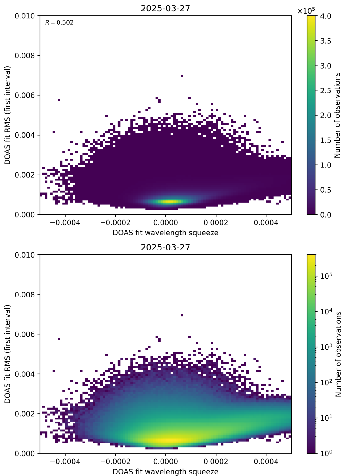
Figure 68: Scatter density plot of “DOAS fit wavelength squeeze” against “DOAS fit RMS (first interval)” for 2025-03-26 to 2025-03-28.
