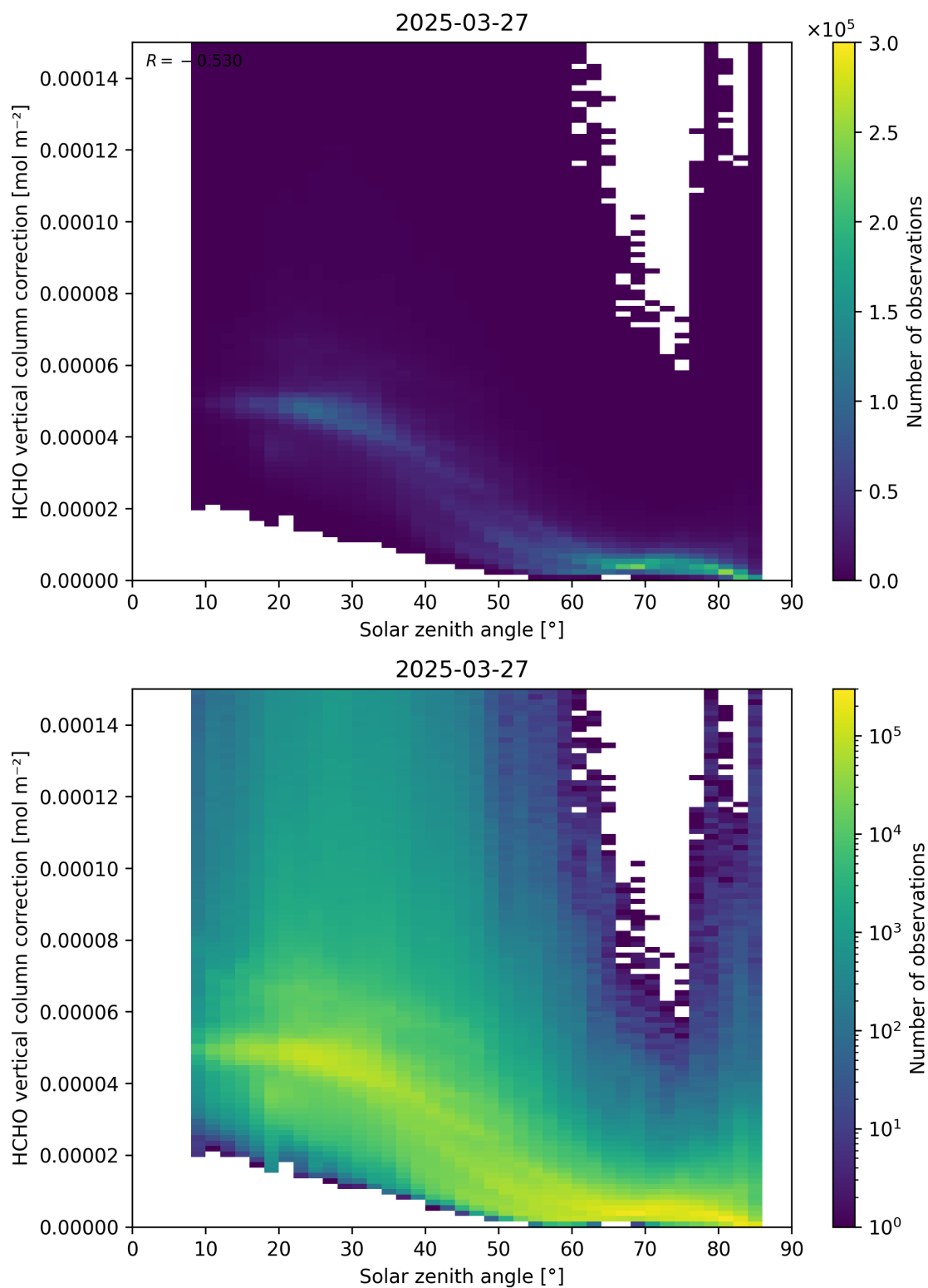
Figure 178: Scatter density plot of “Solar zenith angle” against “HCHO vertical column correction” for 2025-03-26 to 2025-03-28.
