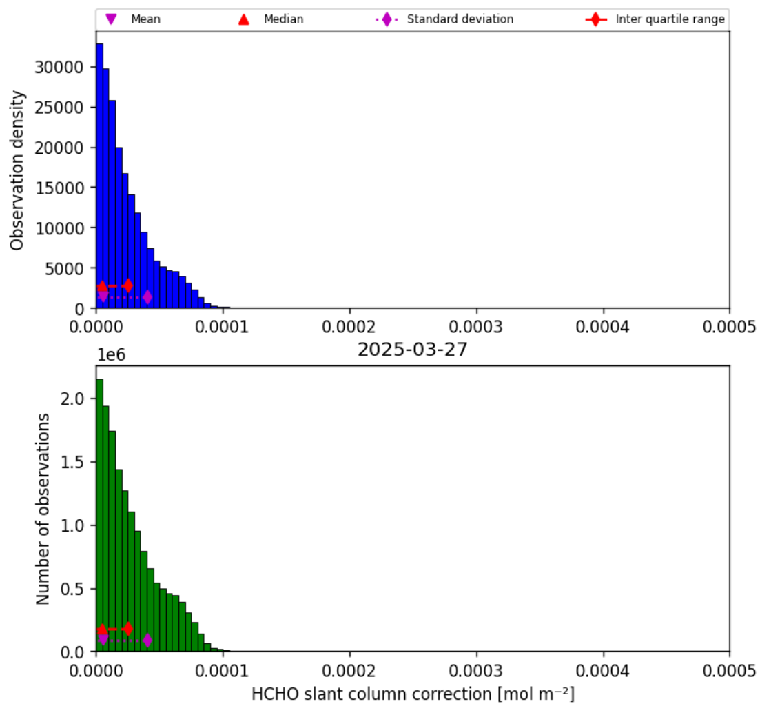
Figure 47: Histogram of “HCHO slant column correction” for 2025-03-26 to 2025-03-28
