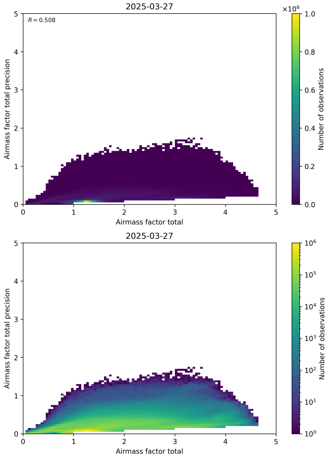
Figure 103: Scatter density plot of “Airmass factor total” against “Airmass factor total precision” for 2025-03-26 to 2025-03-28.
