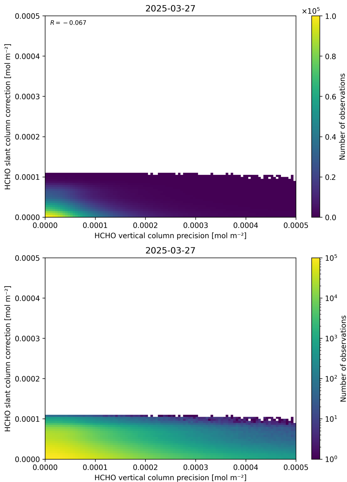
Figure 141: Scatter density plot of “HCHO vertical column precision” against “HCHO slant column correction” for 2025-03-26 to 2025-03-28.
