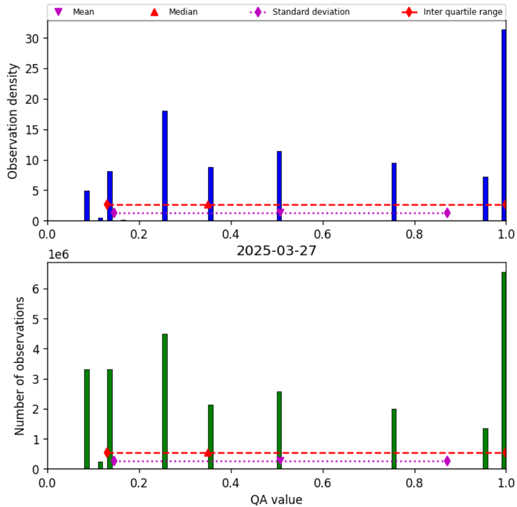
Figure 34: Histogram of “QA value” for 2025-03-26 to 2025-03-28
