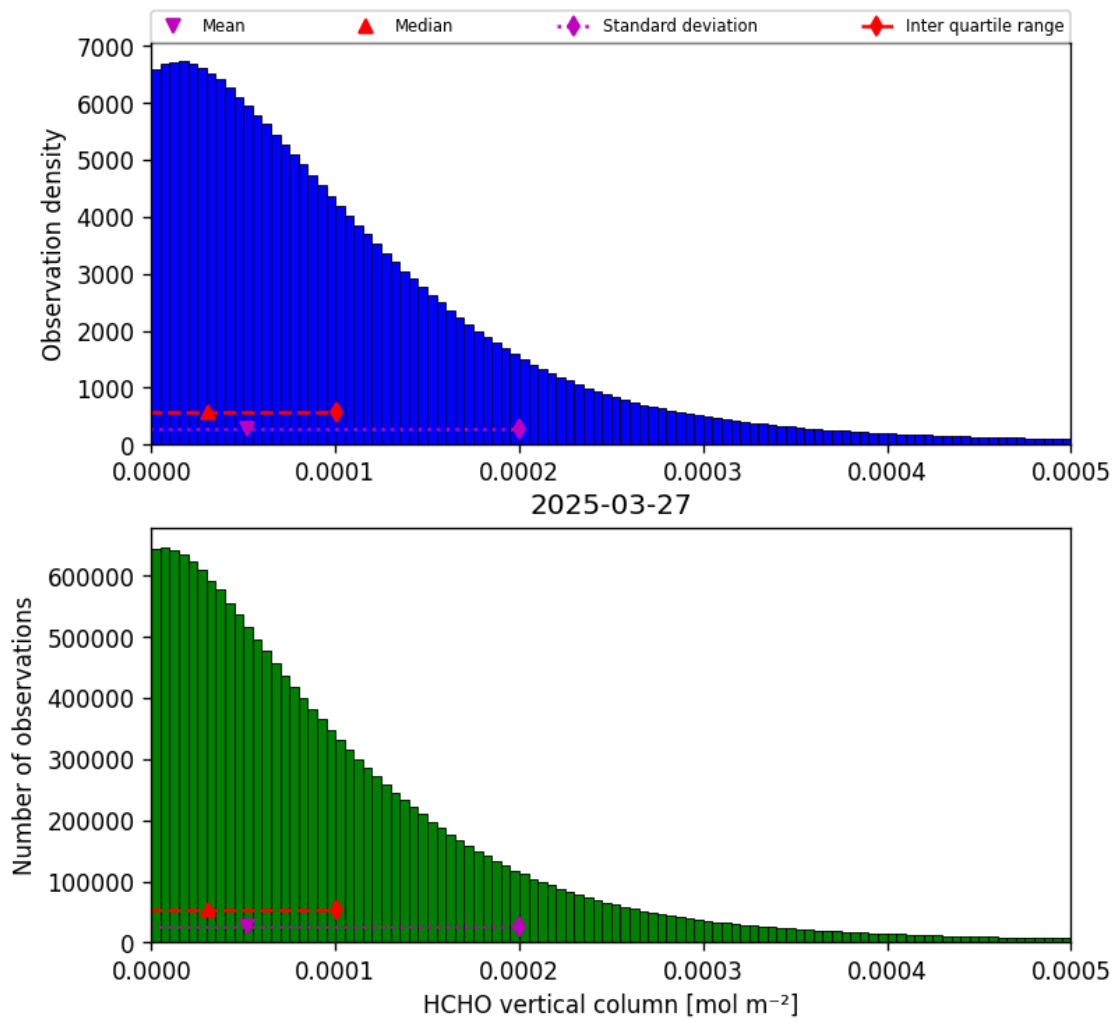
Figure 35: Histogram of “HCHO vertical column” for 2025-03-26 to 2025-03-28
