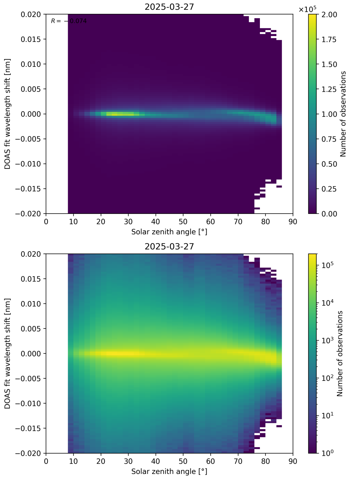
Figure 168: Scatter density plot of “Solar zenith angle” against “DOAS fit wavelength shift” for 2025-03-26 to 2025-03-28.
