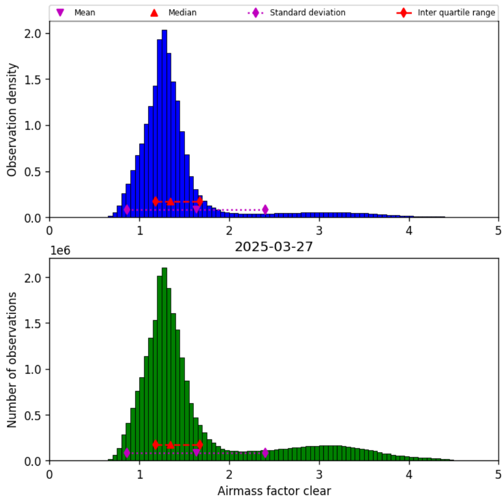
Figure 42: Histogram of “Airmass factor clear” for 2025-03-26 to 2025-03-28
