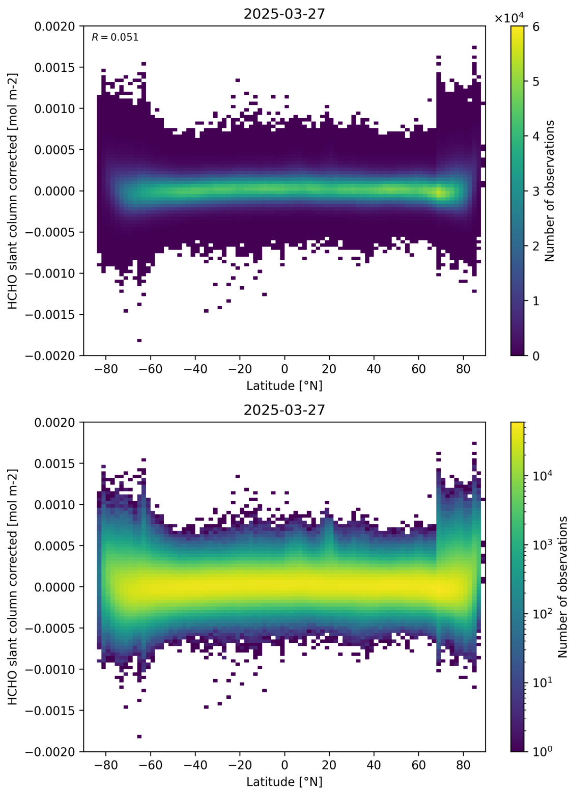
Figure 157: Scatter density plot of “Latitude” against “HCHO slant column corrected” for 2025-03-26 to 2025-03-28.
