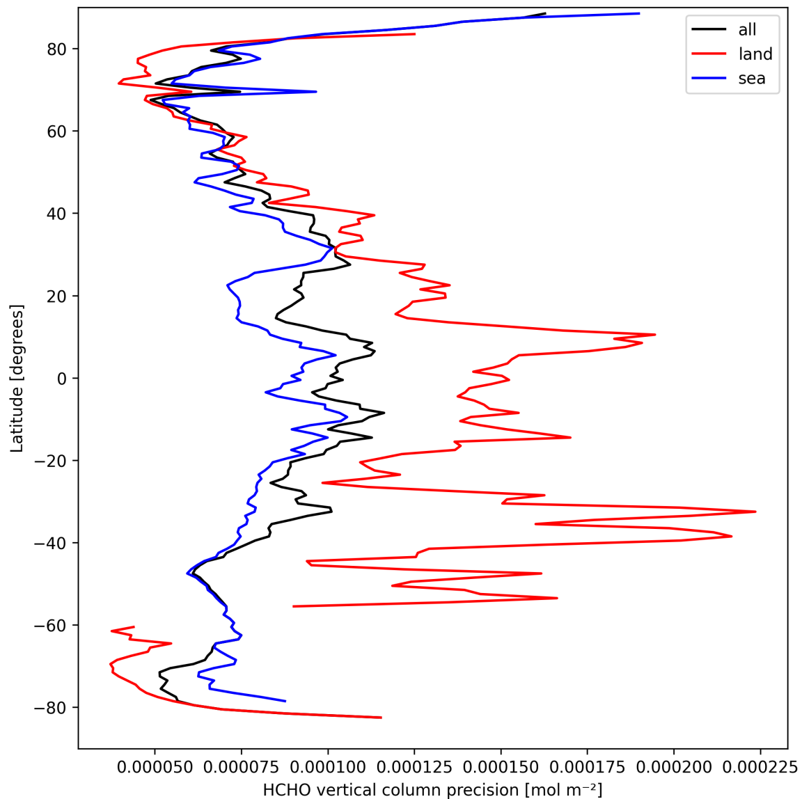
Figure 22: Zonal average of “HCHO vertical column precision” for 2025-03-26 to 2025-03-28.
