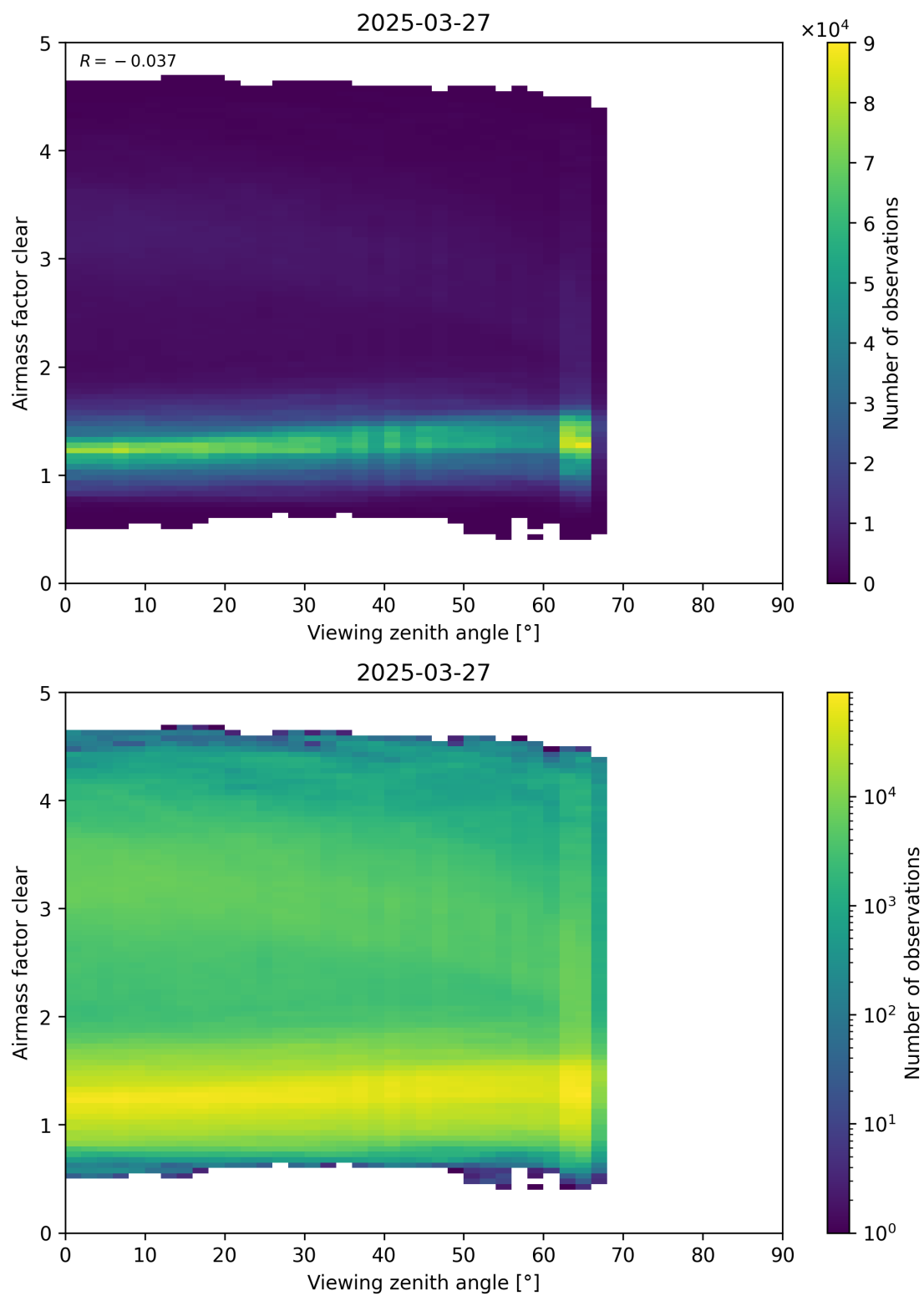
Figure 185: Scatter density plot of “Viewing zenith angle” against “Airmass factor clear” for 2025-03-26 to 2025-03-28.
