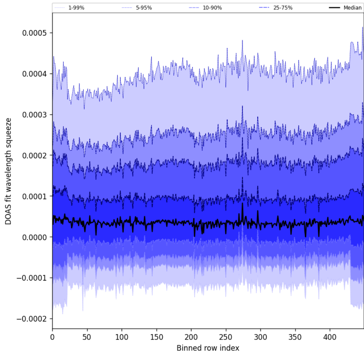
Figure 59: Along track statistics of “DOAS fit wavelength squeeze” for 2025-03-26 to 2025-03-28
