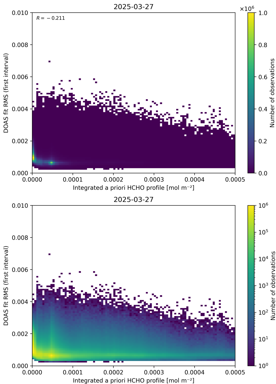
Figure 148: Scatter density plot of “Integrated a priori HCHO profile” against “DOAS fit RMS (first interval)” for 2025-03-26 to 2025-03-28.
