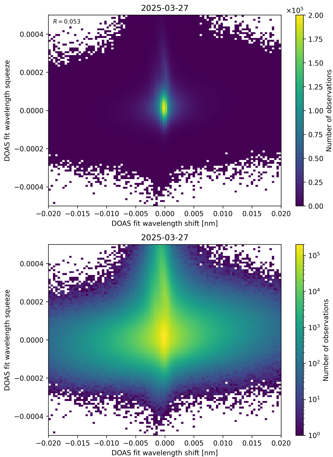
Figure 65: Scatter density plot of “DOAS fit wavelength shift” against “DOAS fit wavelength squeeze” for 2025-03-26 to 2025-03-28.
