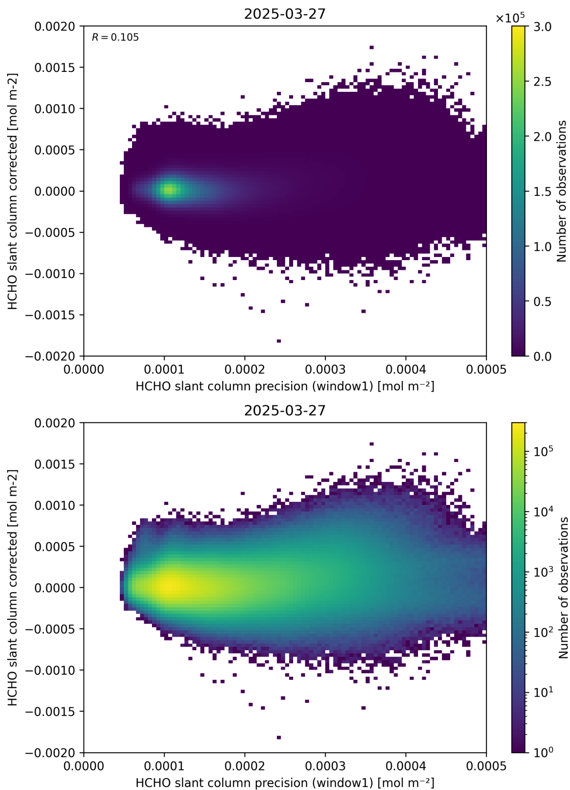
Figure 92: Scatter density plot of “HCHO slant column precision (window1)” against “HCHO slant column corrected” for 2025-03-26 to 2025-03-28.
