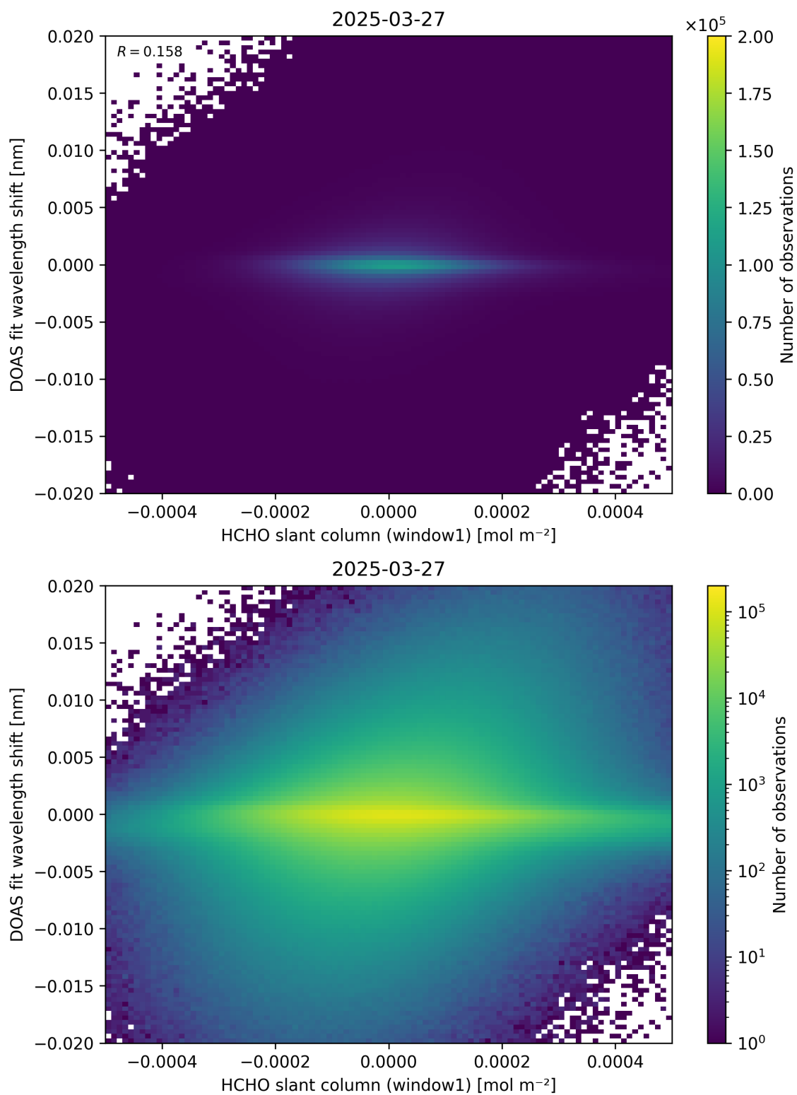
Figure 79: Scatter density plot of “HCHO slant column (window1)” against “DOAS fit wavelength shift” for 2025-03-26 to 2025-03-28.
