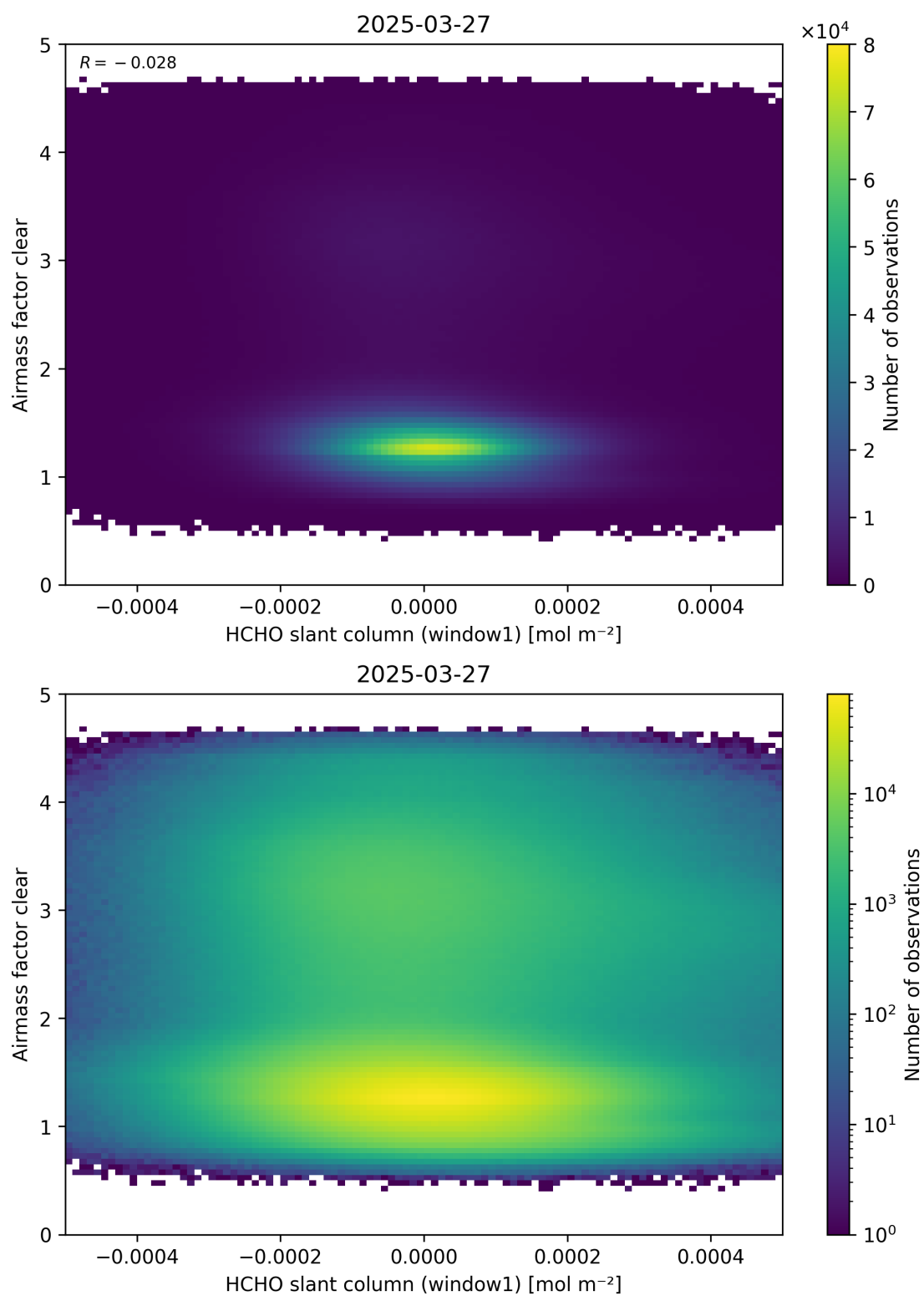
Figure 81: Scatter density plot of “HCHO slant column (window1)” against “Airmass factor clear” for 2025-03-26 to 2025-03-28.
