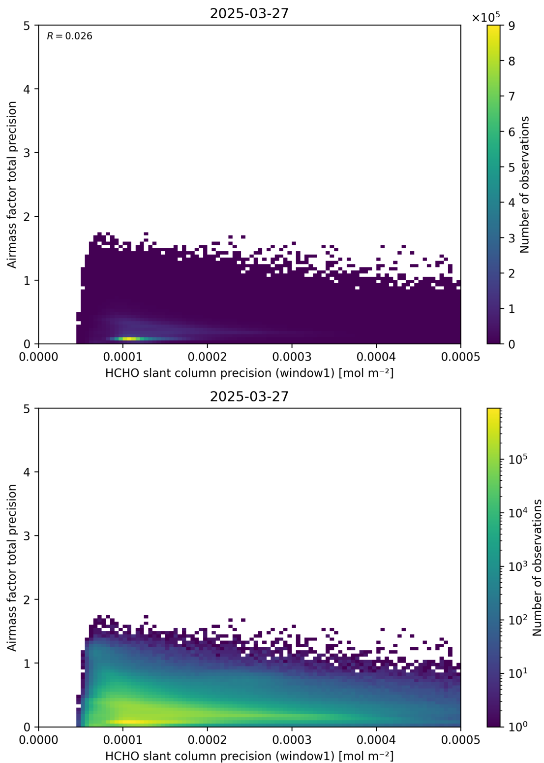
Figure 95: Scatter density plot of “HCHO slant column precision (window1)” against “Airmass factor total precision” for 2025-03-26 to 2025-03-28.
