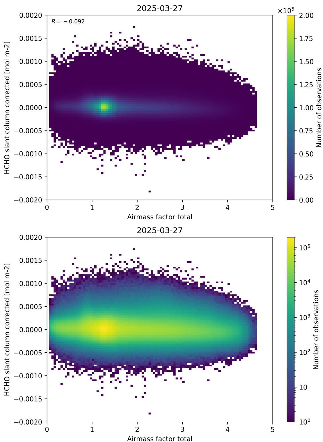
Figure 101: Scatter density plot of “Airmass factor total” against “HCHO slant column corrected” for 2025-03-26 to 2025-03-28.
