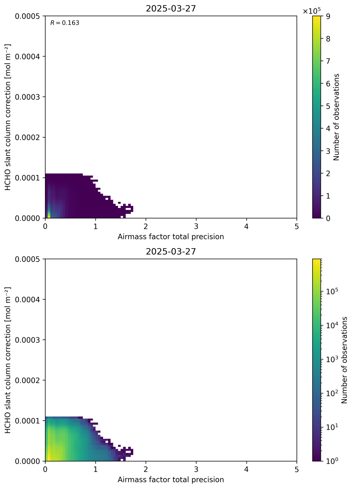
Figure 110: Scatter density plot of “Airmass factor total precision” against “HCHO slant column correction” for 2025-03-26 to 2025-03-28.
