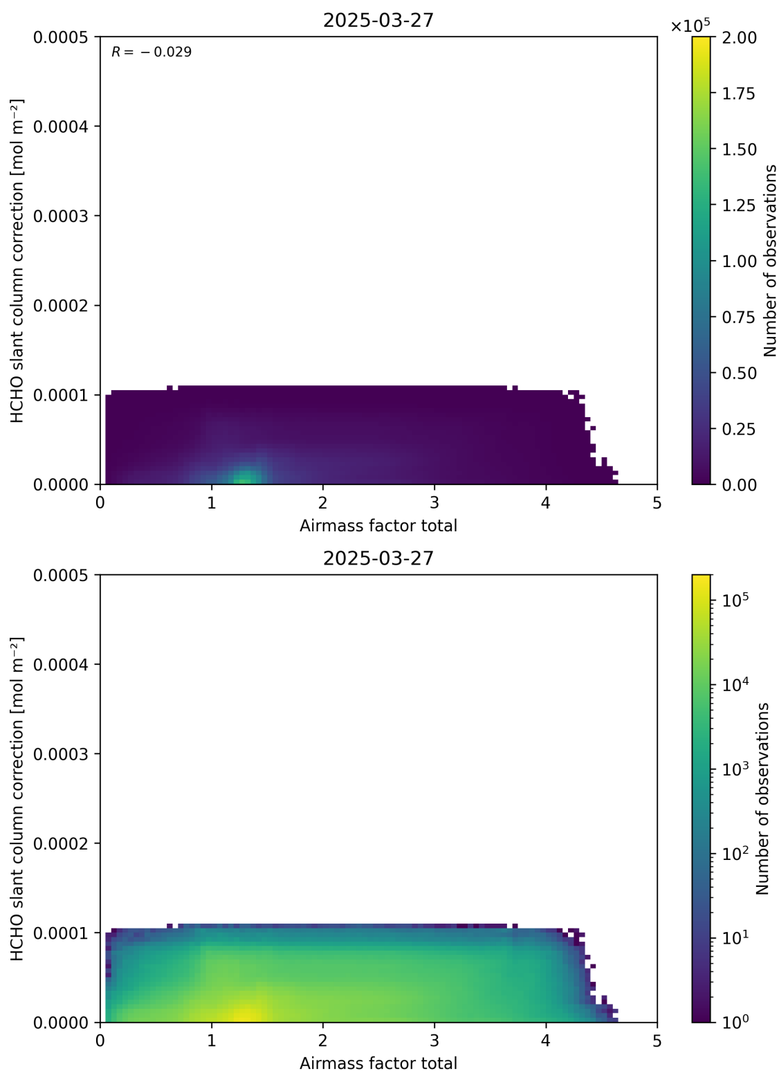
Figure 102: Scatter density plot of “Airmass factor total” against “HCHO slant column correction” for 2025-03-26 to 2025-03-28.
