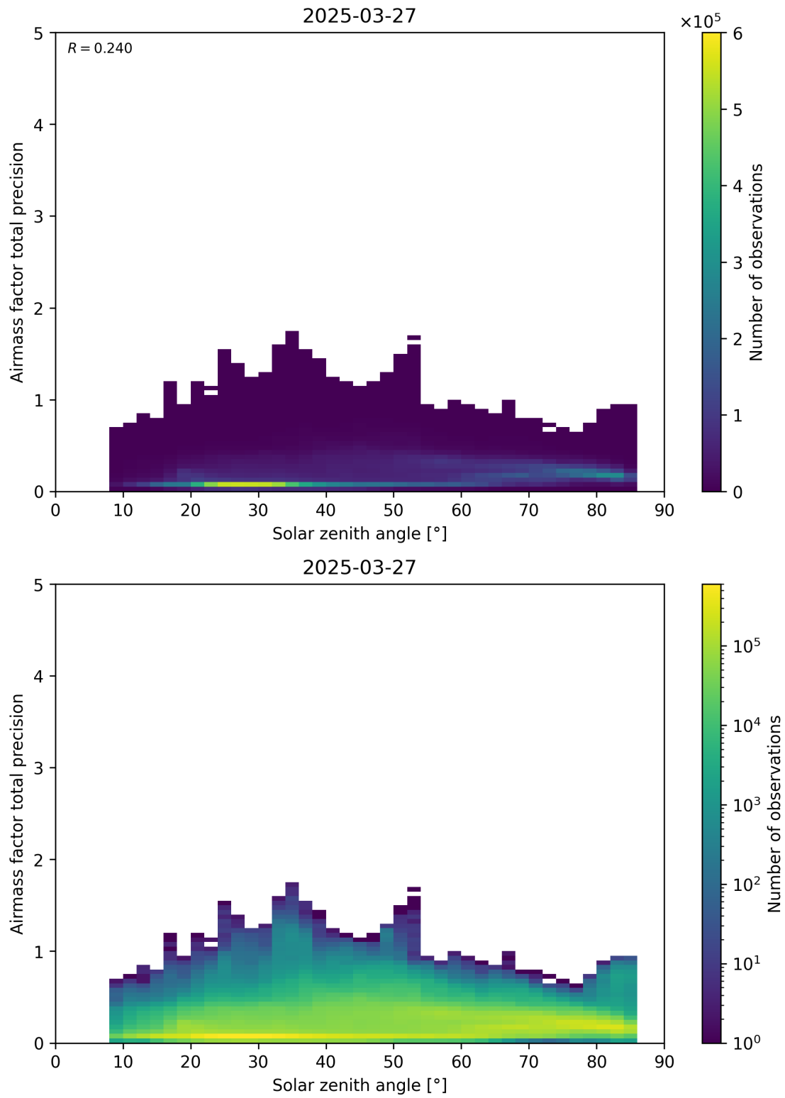
Figure 176: Scatter density plot of “Solar zenith angle” against “Airmass factor total precision” for 2025-03-26 to 2025-03-28.
