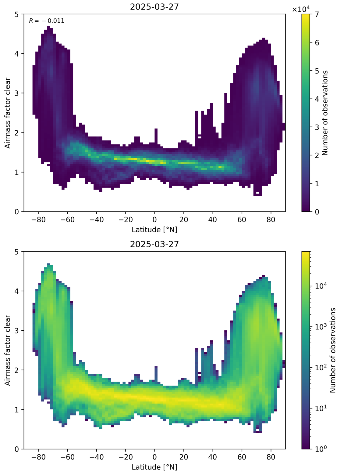
Figure 156: Scatter density plot of “Latitude” against “Airmass factor clear” for 2025-03-26 to 2025-03-28.
