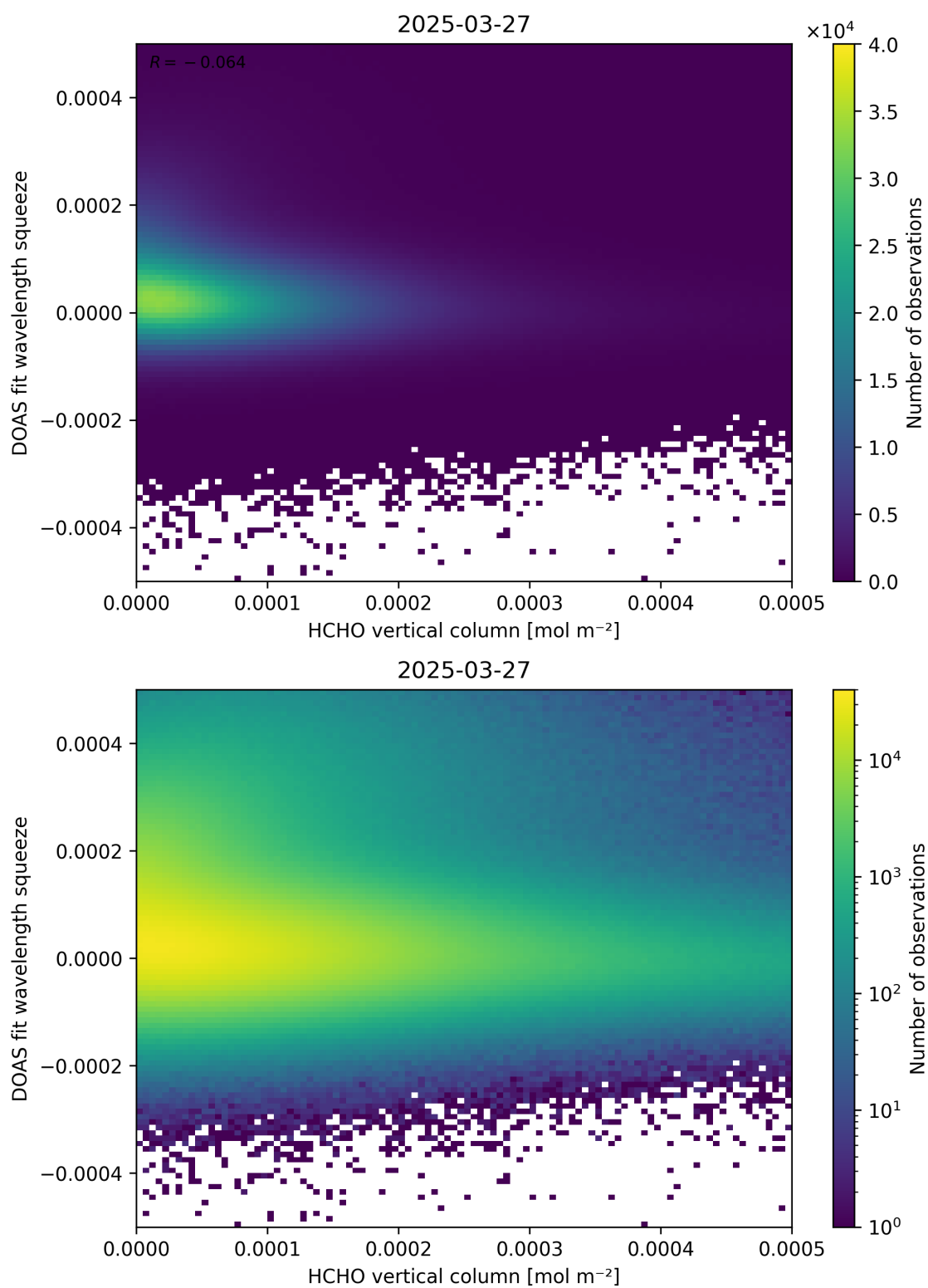
Figure 125: Scatter density plot of “HCHO vertical column” against “DOAS fit wavelength squeeze” for 2025-03-26 to 2025-03-28.
