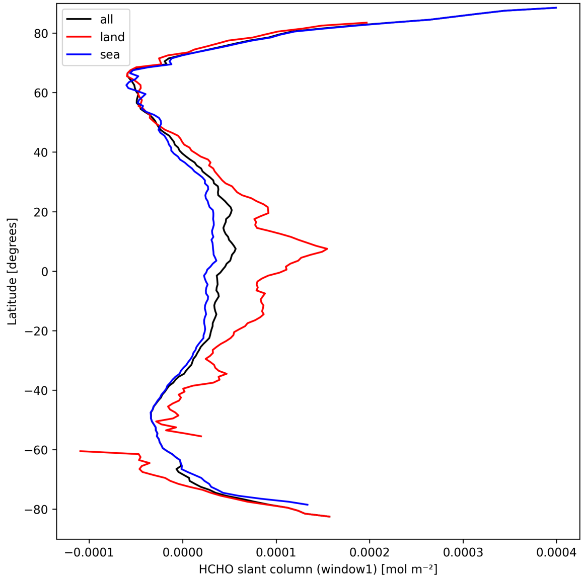
Figure 24: Zonal average of “HCHO slant column (window1)” for 2025-03-26 to 2025-03-28.
