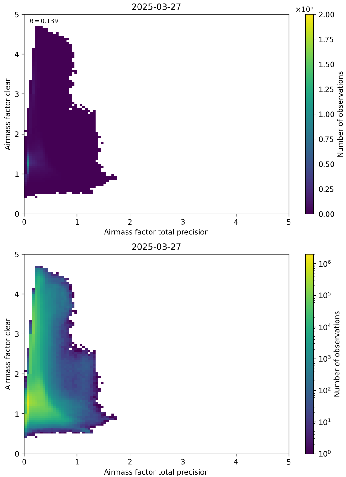
Figure 108: Scatter density plot of “Airmass factor total precision” against “Airmass factor clear” for 2025-03-26 to 2025-03-28.
