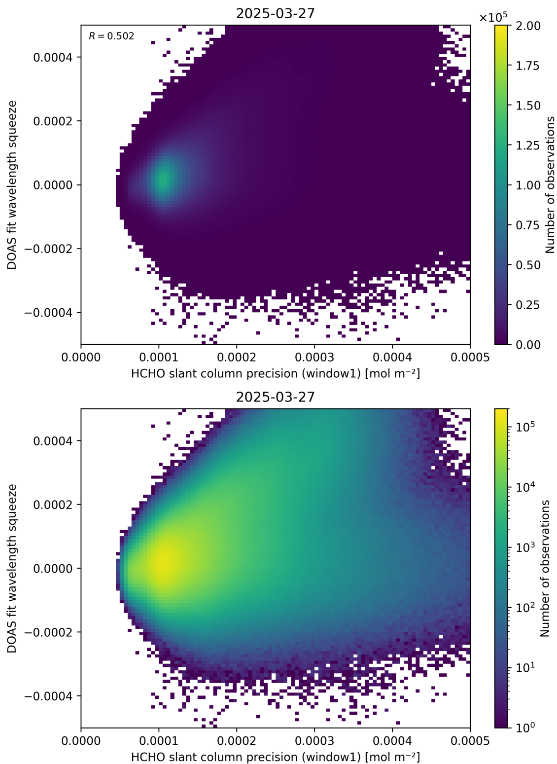
Figure 90: Scatter density plot of “HCHO slant column precision (window1)” against “DOAS fit wavelength squeeze” for 2025-03-26 to 2025-03-28.
