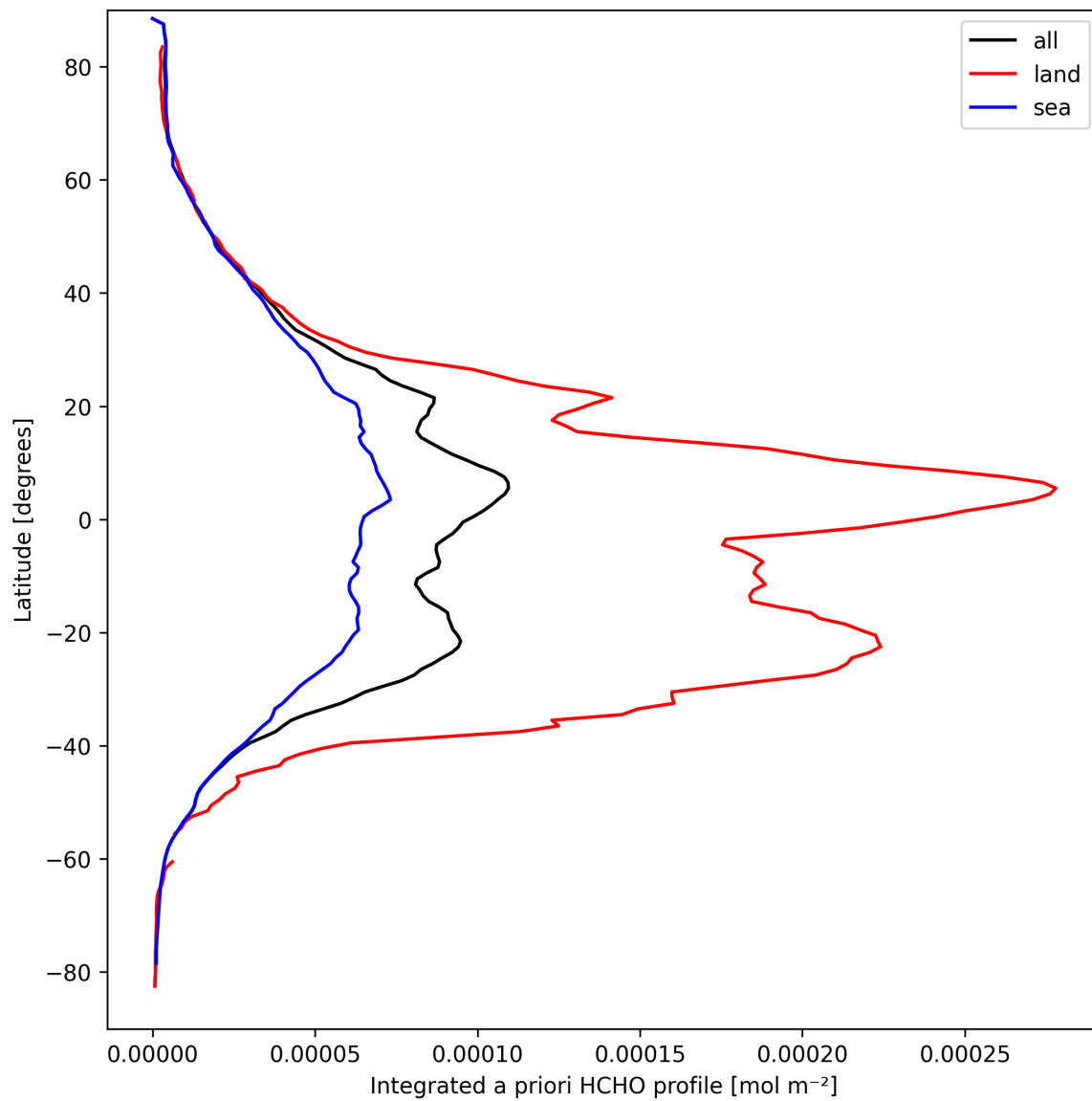
Figure 29: Zonal average of “Integrated a priori HCHO profile” for 2025-03-26 to 2025-03-28.
