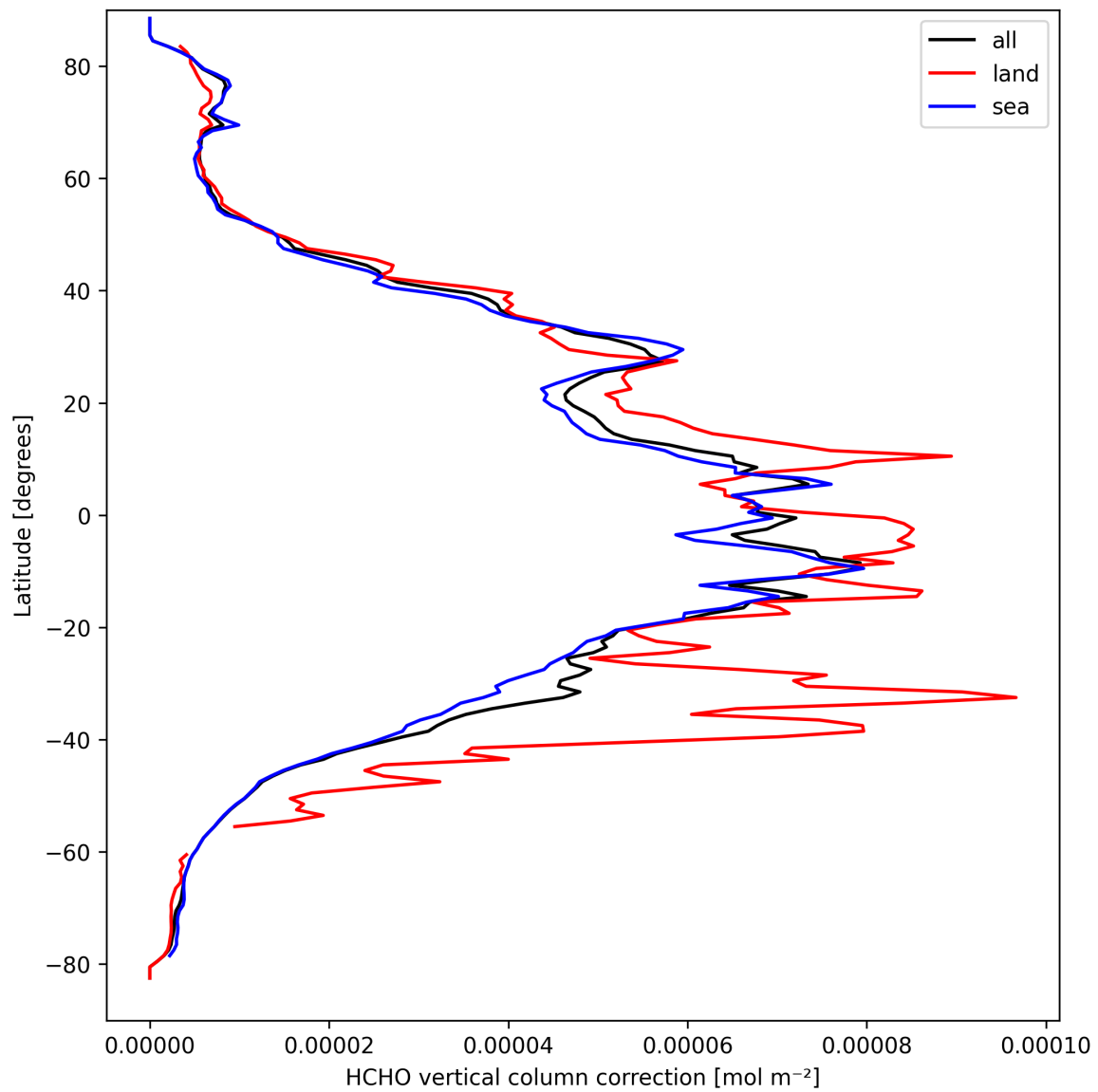
Figure 23: Zonal average of “HCHO vertical column correction” for 2025-03-26 to 2025-03-28.
