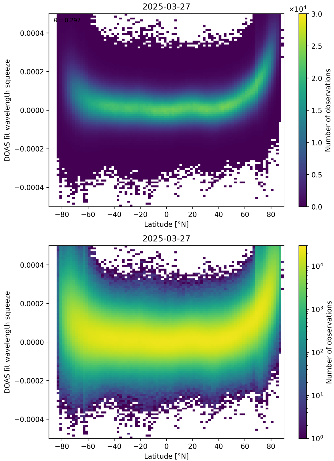
Figure 155: Scatter density plot of “Latitude” against “DOAS fit wavelength squeeze” for 2025-03-26 to 2025-03-28.
