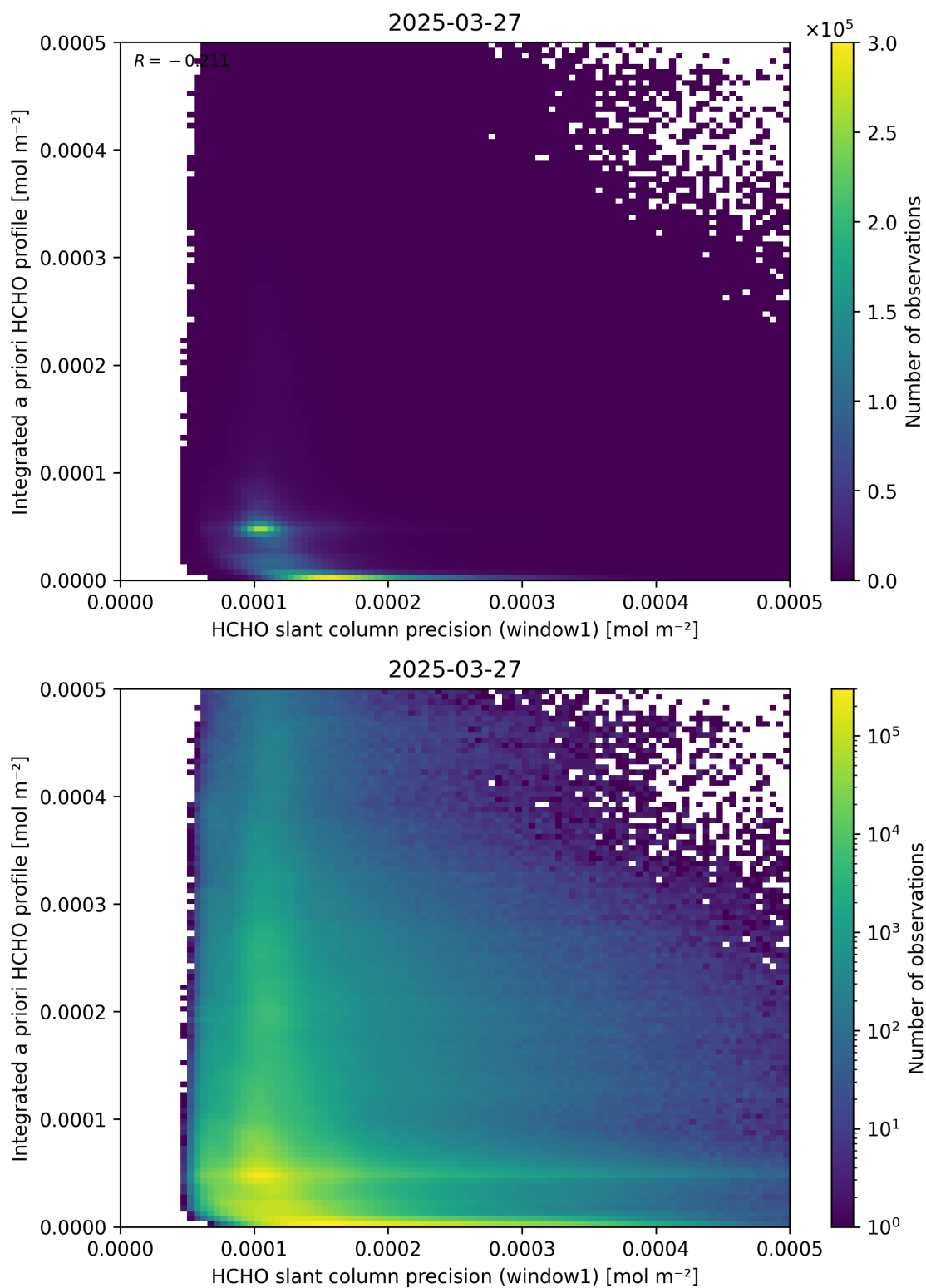
Figure 96: Scatter density plot of “HCHO slant column precision (window1)” against “Integrated a priori HCHO profile” for 2025-03-26 to 2025-03-28.
