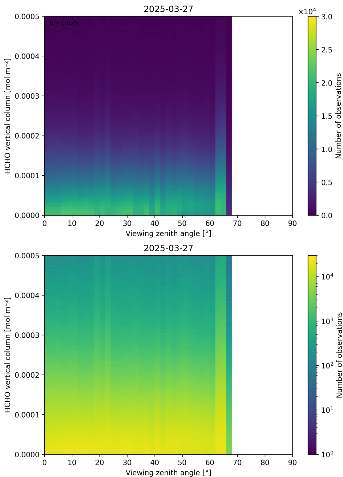
Figure 192: Scatter density plot of “Viewing zenith angle” against “HCHO vertical column” for 2025-03-26 to 2025-03-28.
