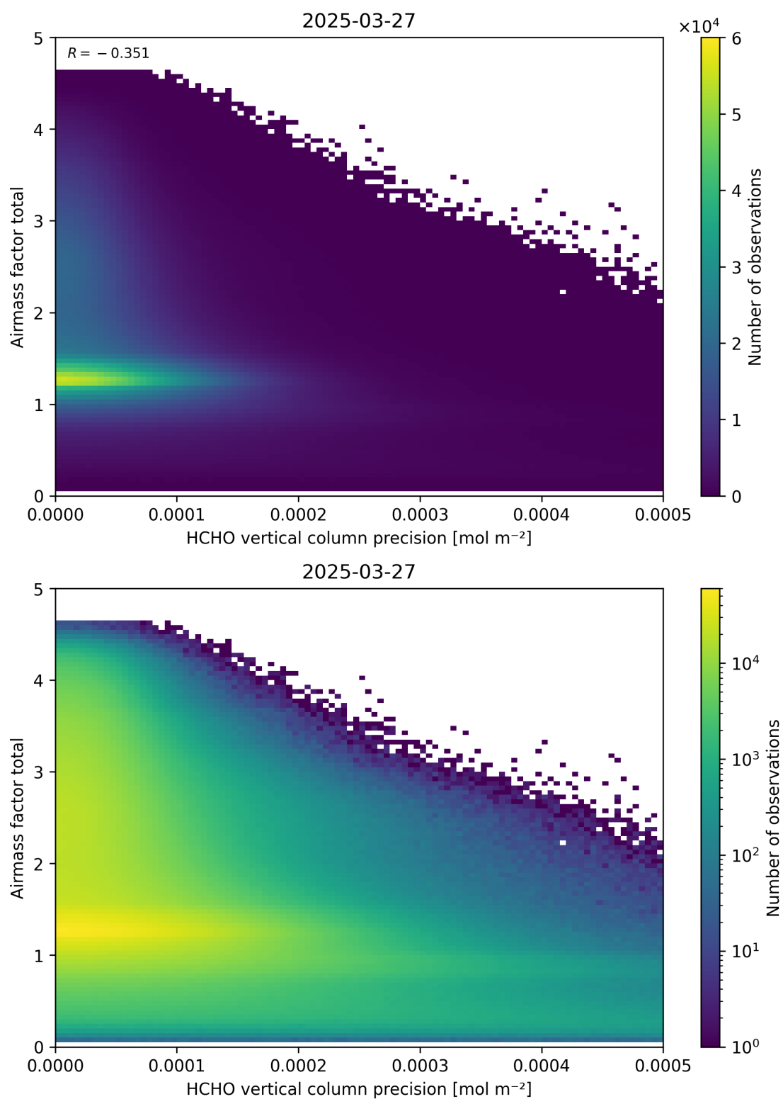
Figure 144: Scatter density plot of “HCHO vertical column precision” against “Airmass factor total” for 2025-03-26 to 2025-03-28.
