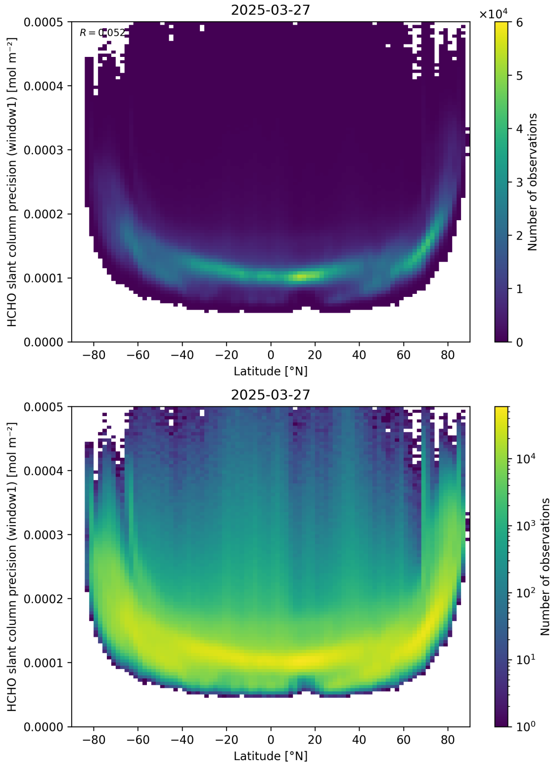
Figure 160: Scatter density plot of “Latitude” against “HCHO slant column precision (window1)” for 2025-03-26 to 2025-03-28.
