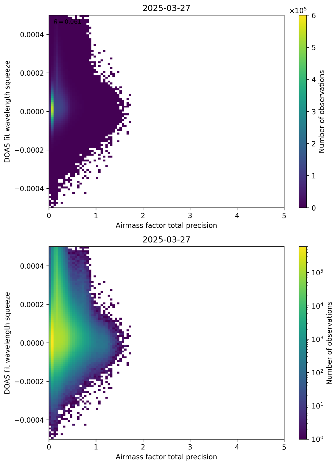
Figure 107: Scatter density plot of “Airmass factor total precision” against “DOAS fit wavelength squeeze” for 2025-03-26 to 2025-03-28.
