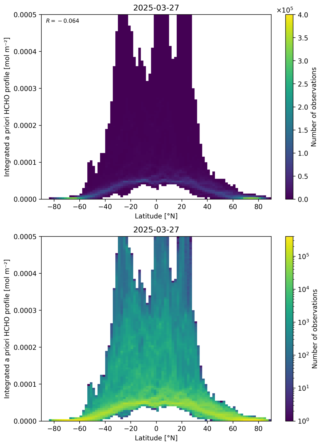
Figure 166: Scatter density plot of “Latitude” against “Integrated a priori HCHO profile” for 2025-03-26 to 2025-03-28.
