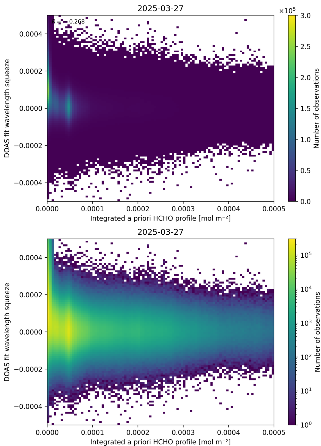
Figure 150: Scatter density plot of “Integrated a priori HCHO profile” against “DOAS fit wavelength squeeze” for 2025-03-26 to 2025-03-28.
