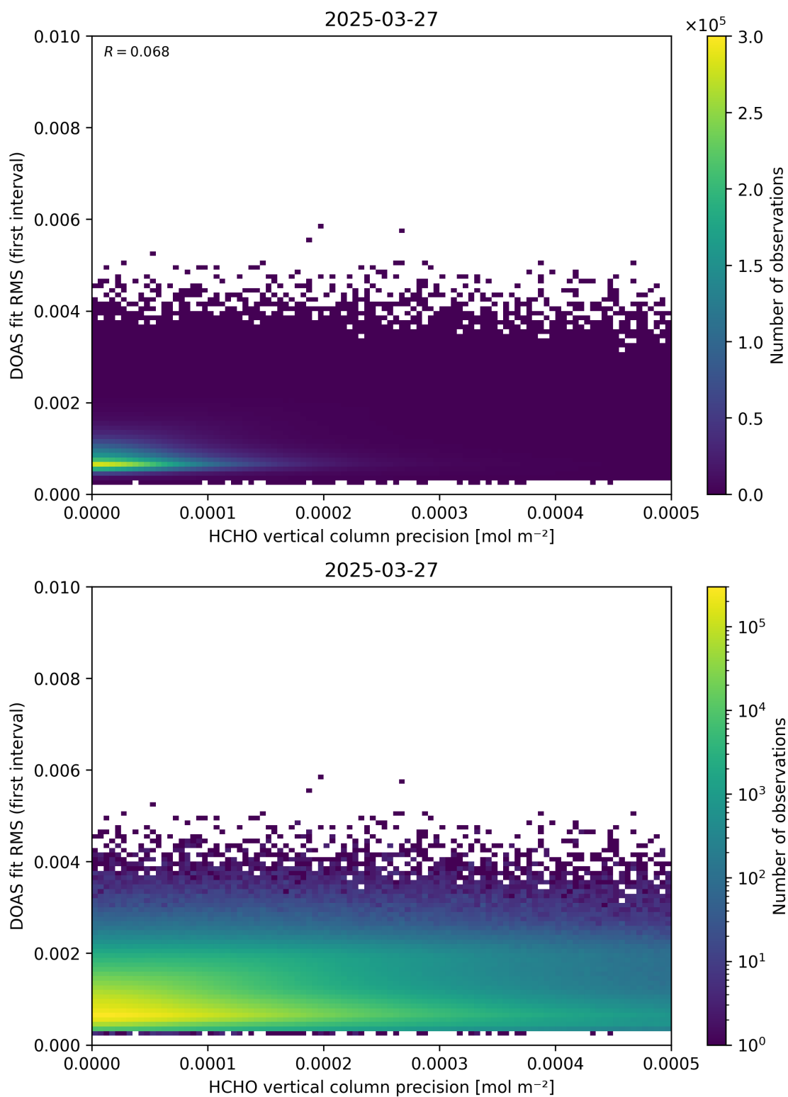
Figure 136: Scatter density plot of “HCHO vertical column precision” against “DOAS fit RMS (first interval)” for 2025-03-26 to 2025-03-28.
