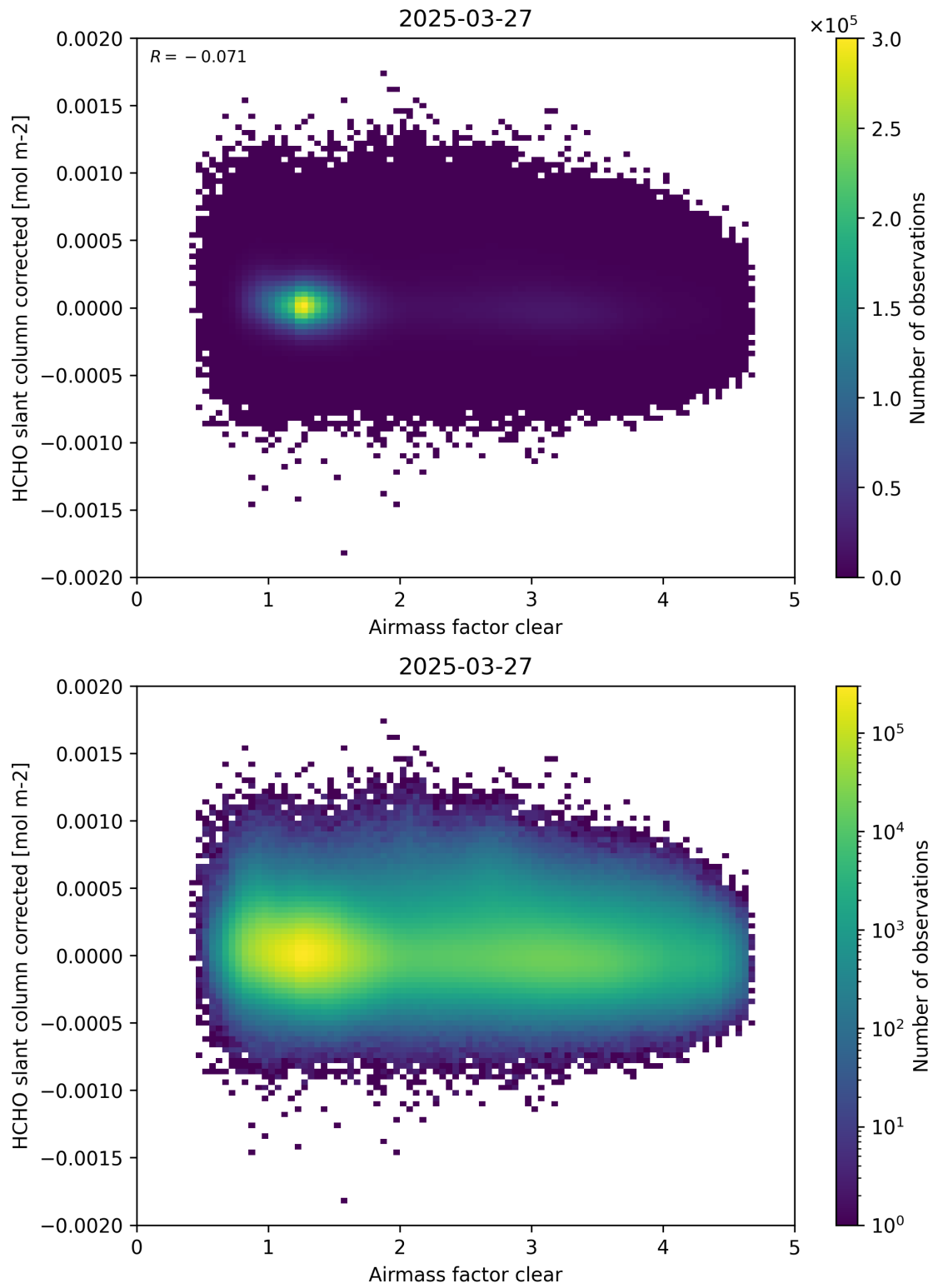
Figure 74: Scatter density plot of “Airmass factor clear” against “HCHO slant column corrected” for 2025-03-26 to 2025-03-28.
