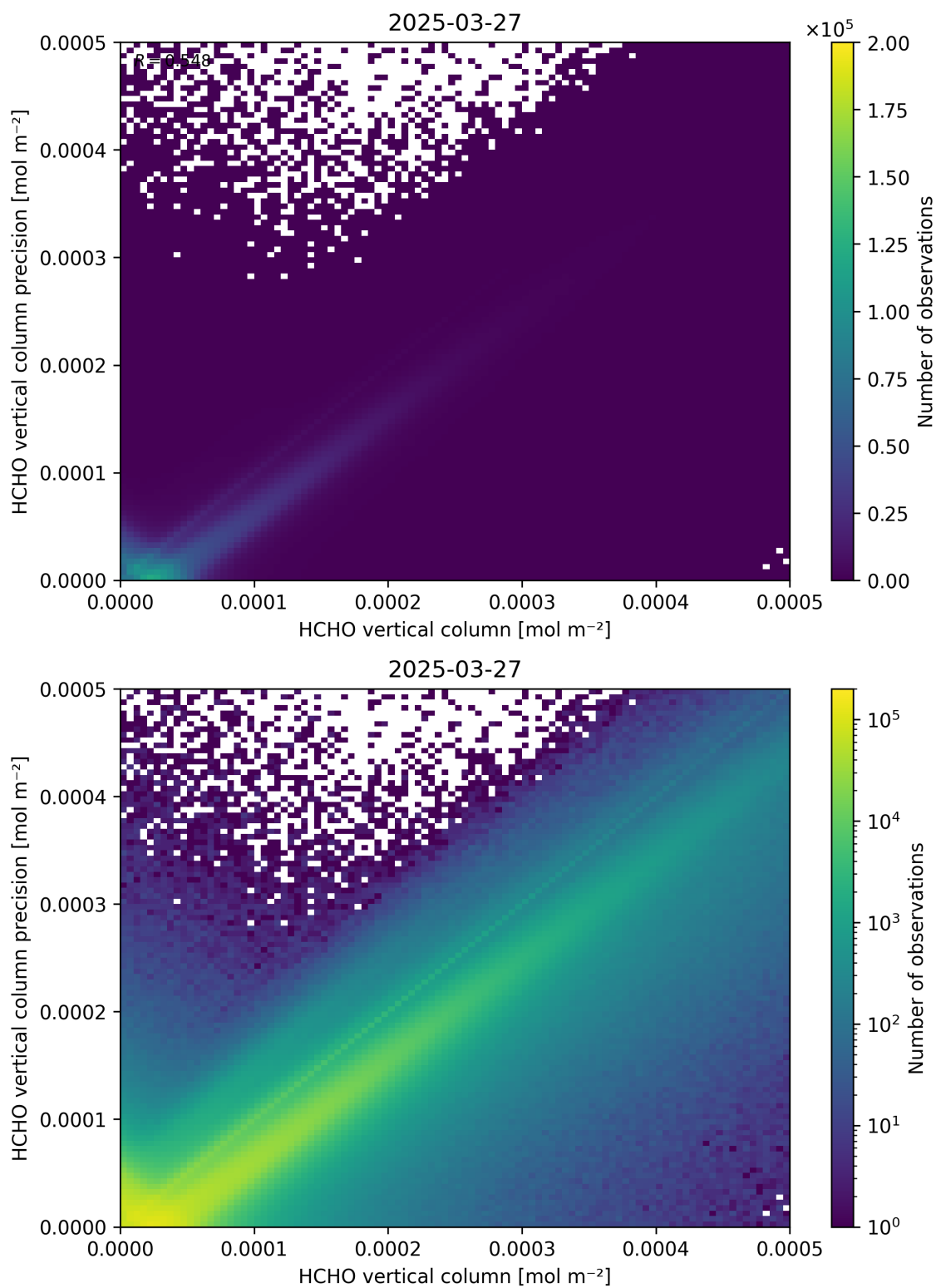
Figure 134: Scatter density plot of “HCHO vertical column” against “HCHO vertical column precision” for 2025-03-26 to 2025-03-28.
