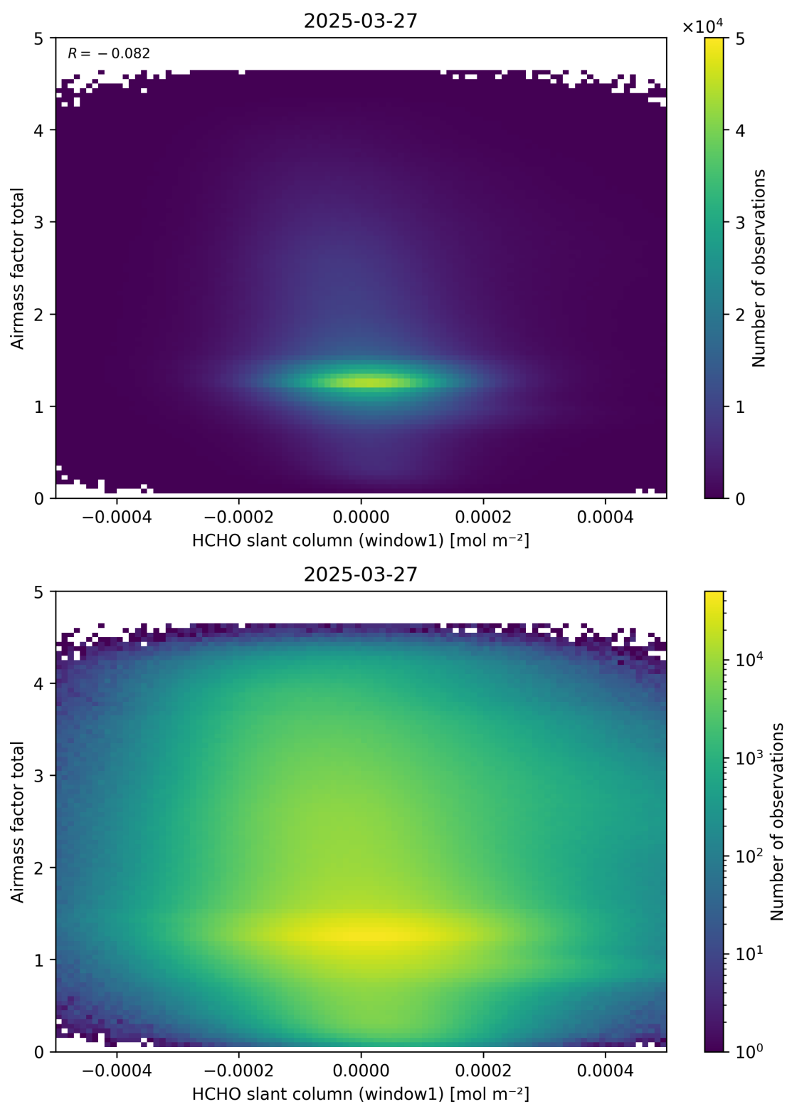
Figure 85: Scatter density plot of “HCHO slant column (window1)” against “Airmass factor total” for 2025-03-26 to 2025-03-28.
