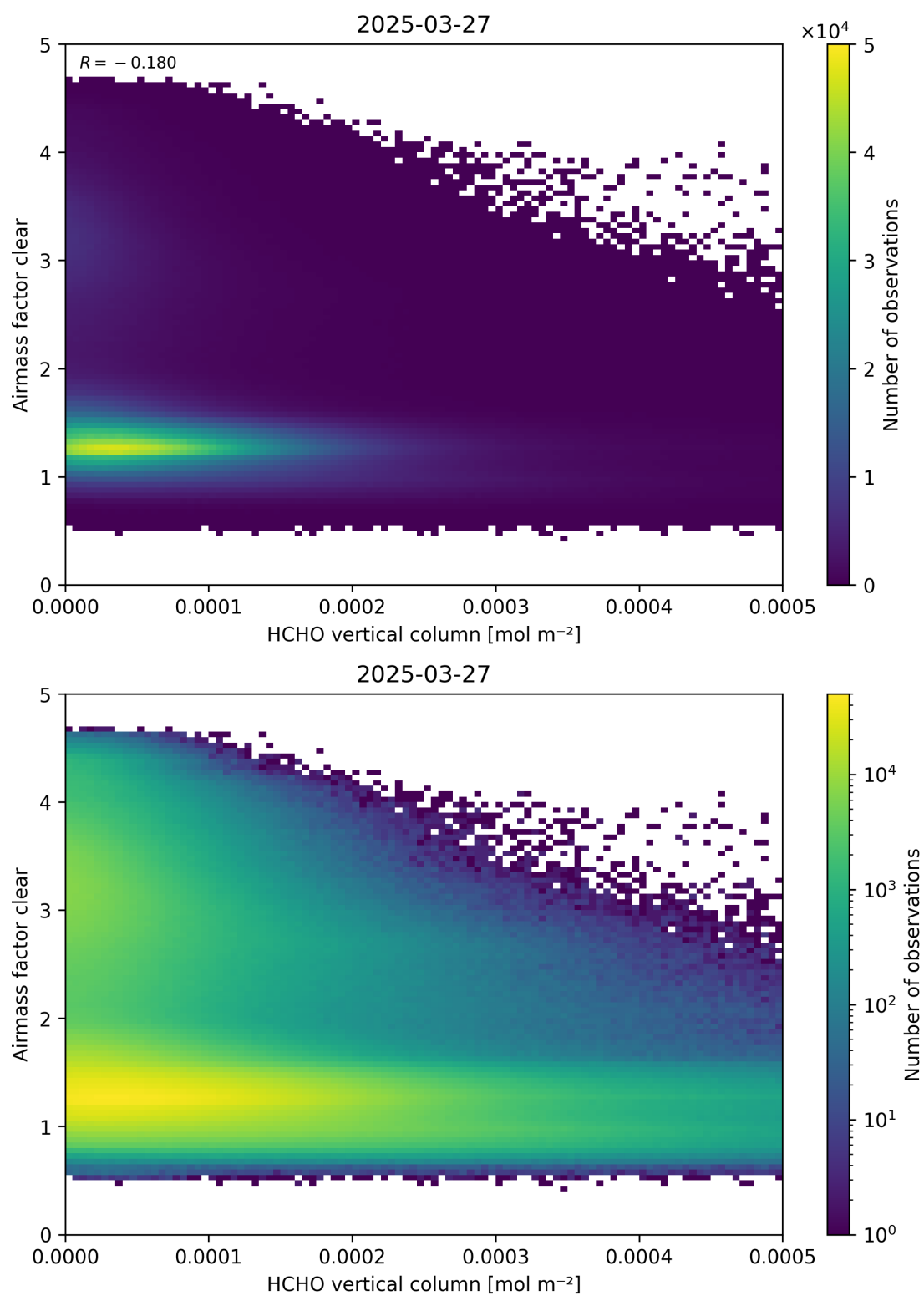
Figure 126: Scatter density plot of “HCHO vertical column” against “Airmass factor clear” for 2025-03-26 to 2025-03-28.
