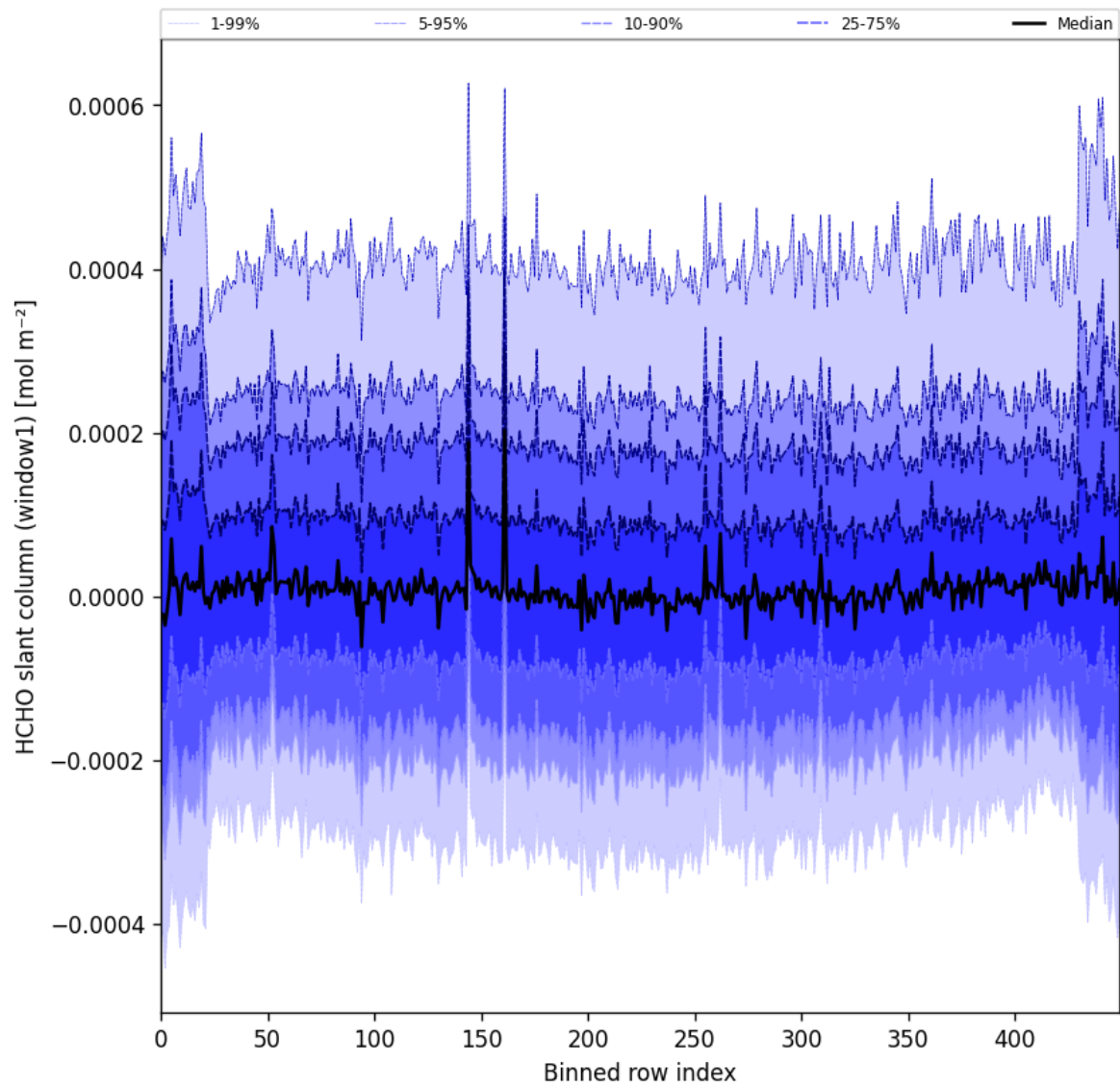
Figure 52: Along track statistics of “HCHO slant column (window1)” for 2025-03-26 to 2025-03-28
