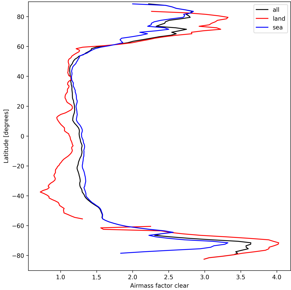
Figure 28: Zonal average of “Airmass factor clear” for 2025-03-26 to 2025-03-28.
