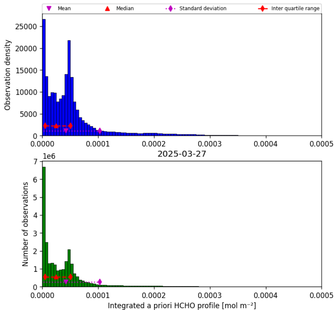
Figure 43: Histogram of “Integrated a priori HCHO profile” for 2025-03-26 to 2025-03-28
