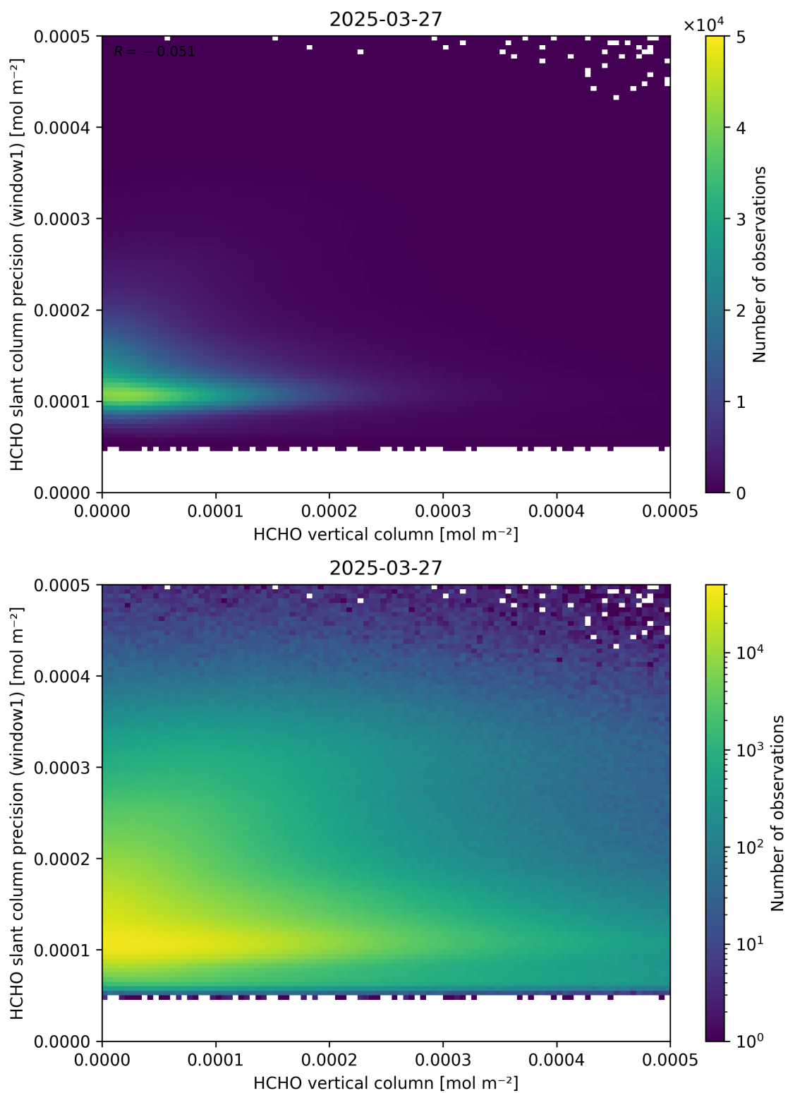
Figure 130: Scatter density plot of “HCHO vertical column” against “HCHO slant column precision (window1)” for 2025-03-26 to 2025-03-28.
