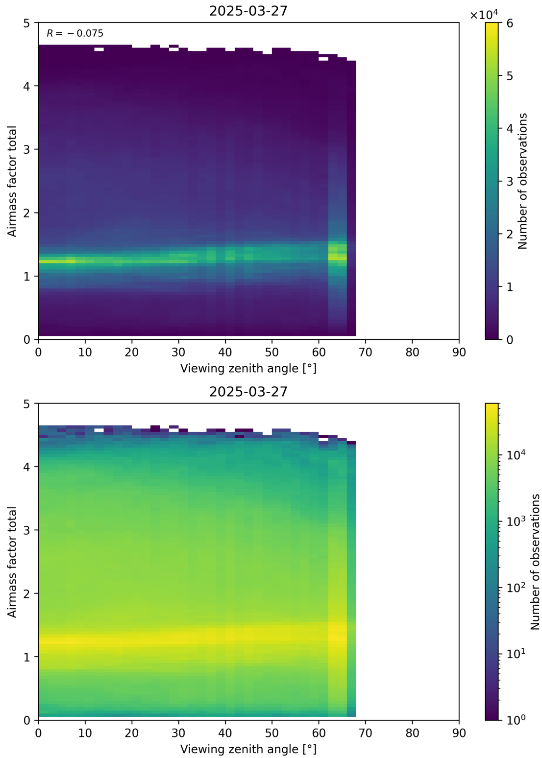
Figure 190: Scatter density plot of “Viewing zenith angle” against “Airmass factor total” for 2025-03-26 to 2025-03-28.
