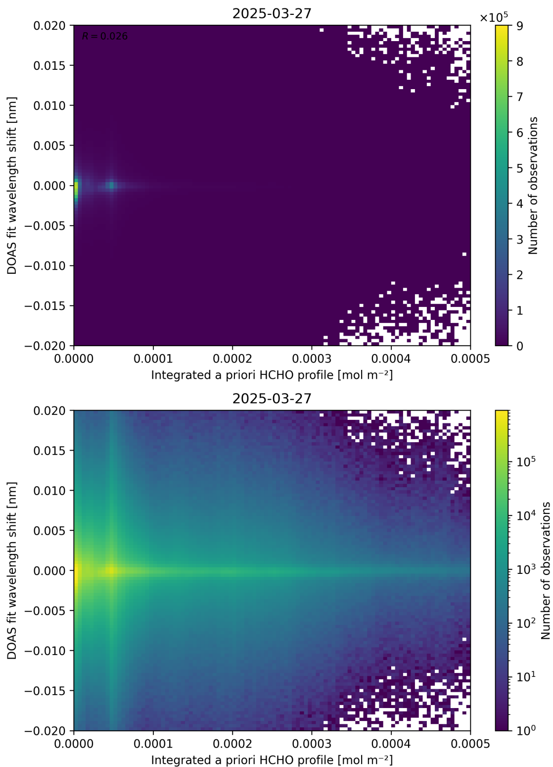
Figure 149: Scatter density plot of “Integrated a priori HCHO profile” against “DOAS fit wavelength shift” for 2025-03-26 to 2025-03-28.
