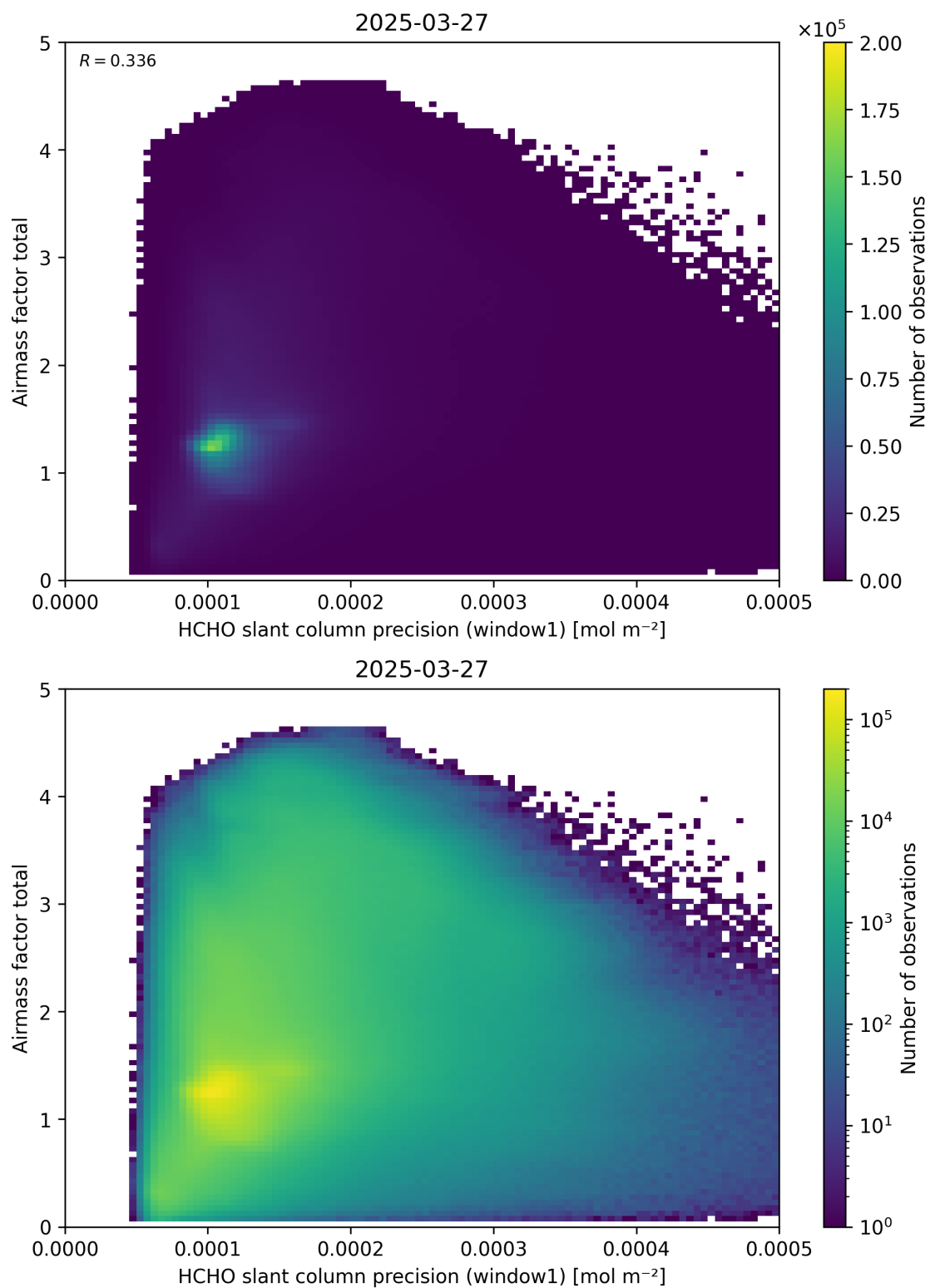
Figure 94: Scatter density plot of “HCHO slant column precision (window1)” against “Airmass factor total” for 2025-03-26 to 2025-03-28.
