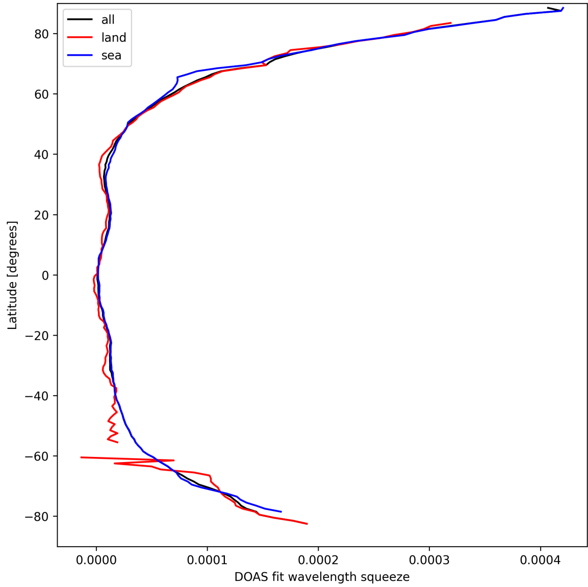
Figure 31: Zonal average of “DOAS fit wavelength squeeze” for 2025-03-26 to 2025-03-28.
