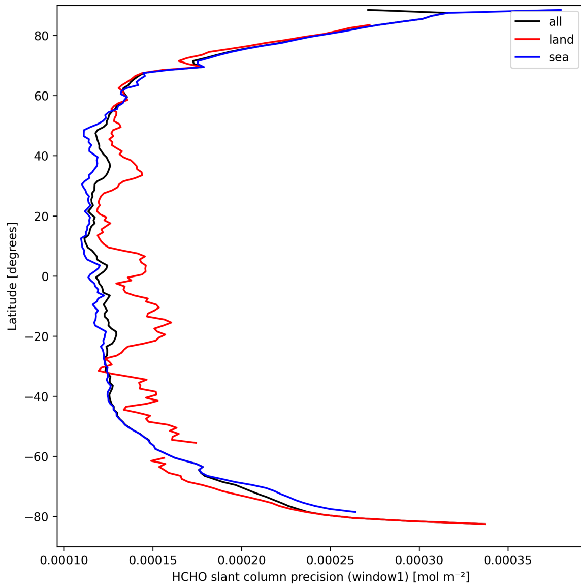
Figure 25: Zonal average of “HCHO slant column precision (window1)” for 2025-03-26 to 2025-03-28.
