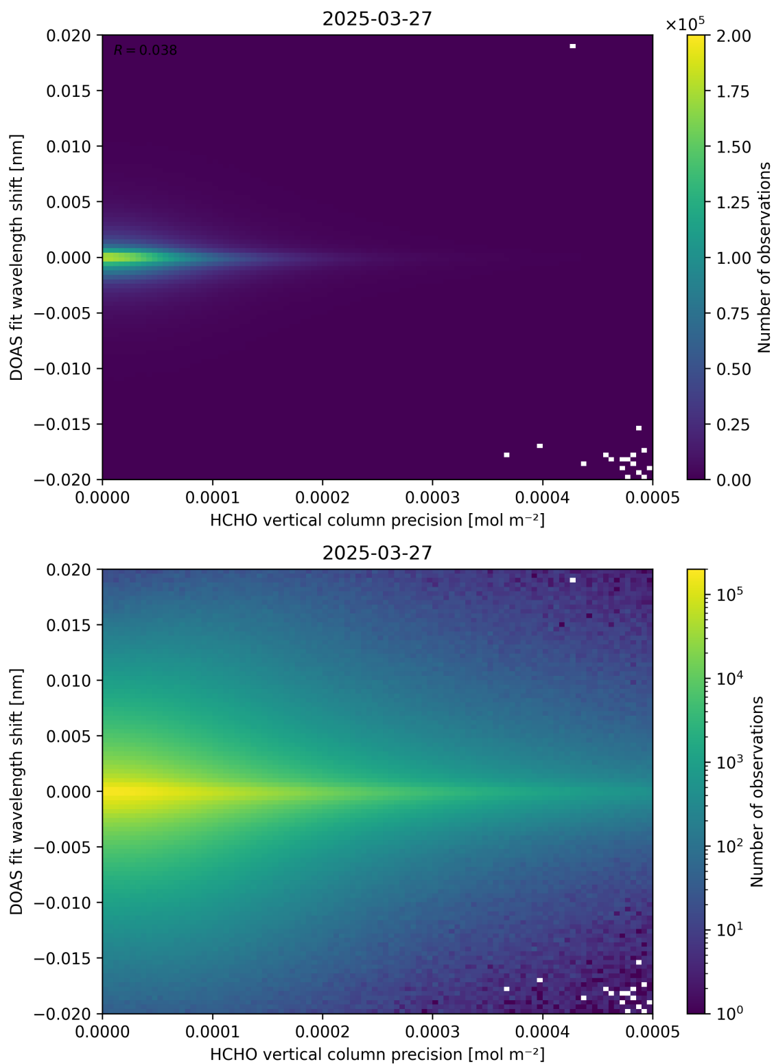
Figure 137: Scatter density plot of “HCHO vertical column precision” against “DOAS fit wavelength shift” for 2025-03-26 to 2025-03-28.
