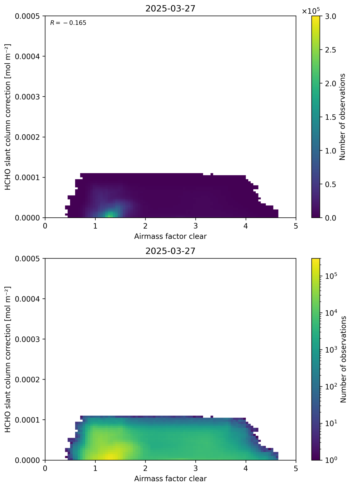
Figure 75: Scatter density plot of “Airmass factor clear” against “HCHO slant column correction” for 2025-03-26 to 2025-03-28.
