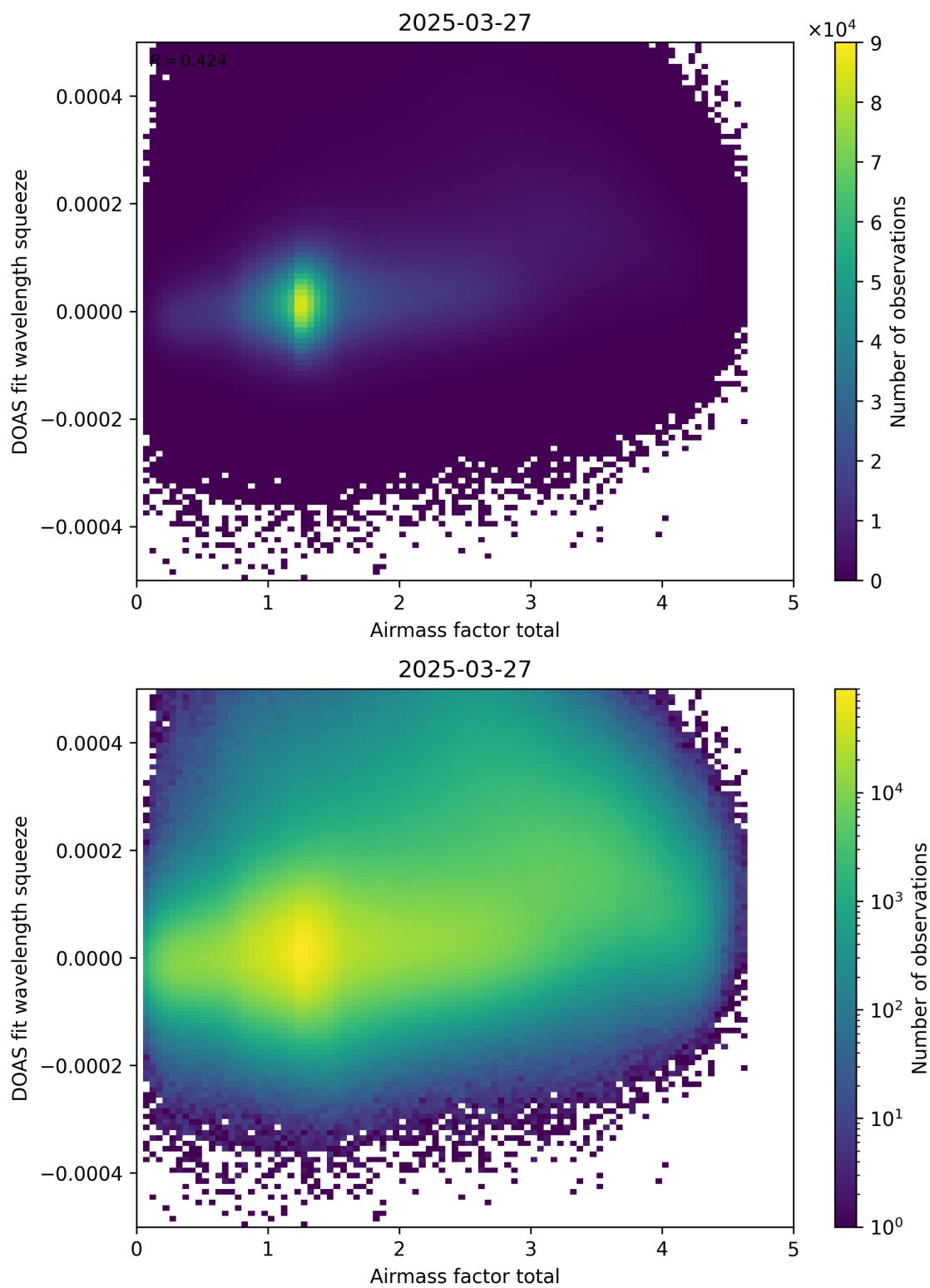
Figure 99: Scatter density plot of “Airmass factor total” against “DOAS fit wavelength squeeze” for 2025-03-26 to 2025-03-28.
