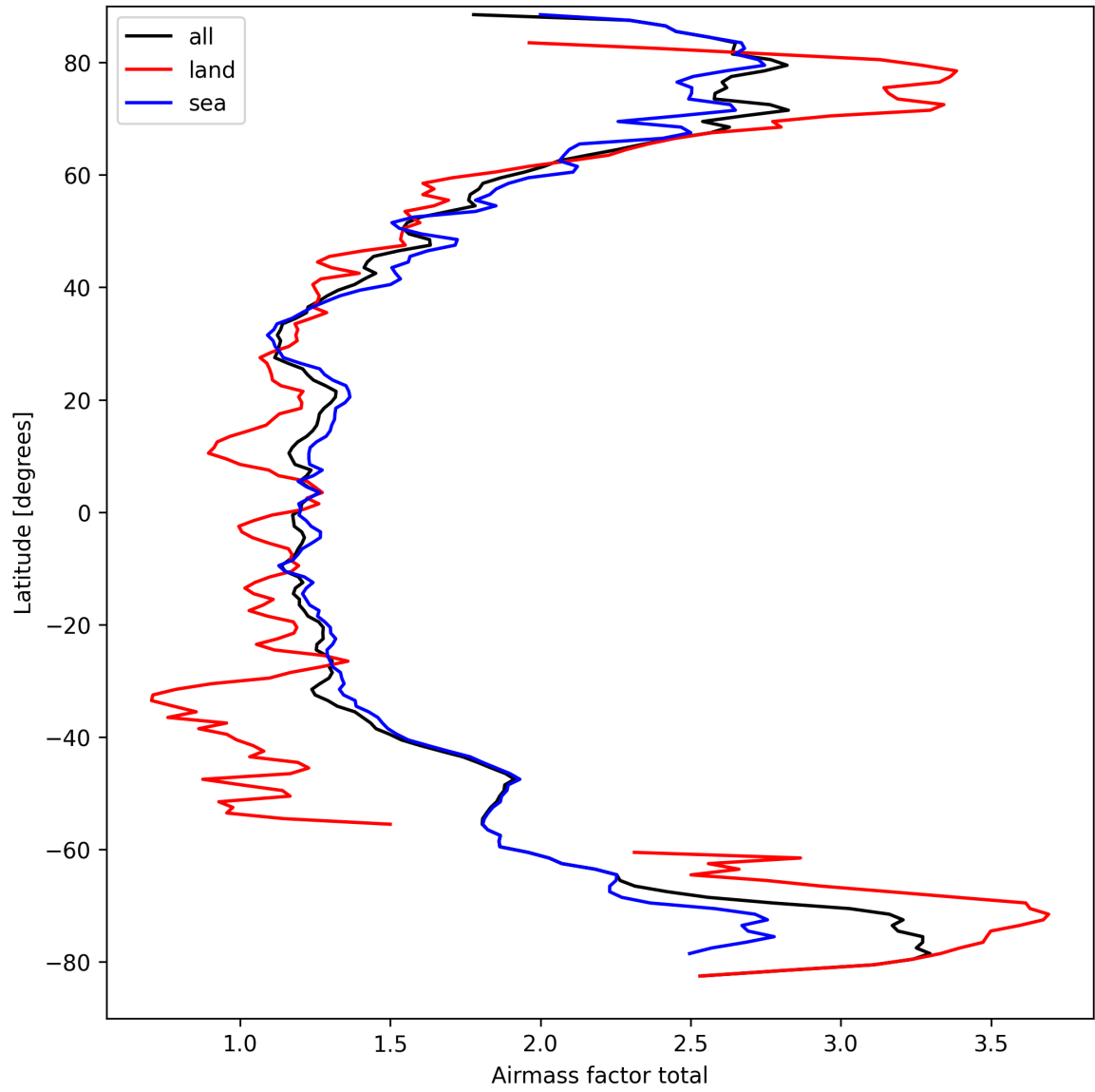
Figure 26: Zonal average of “Airmass factor total” for 2025-03-26 to 2025-03-28.
