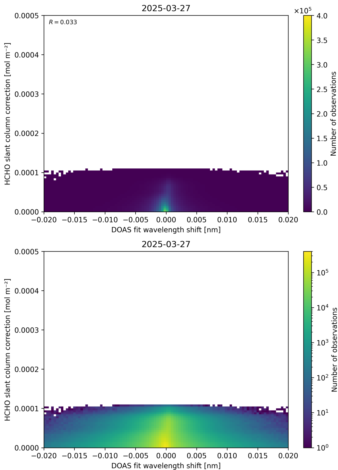
Figure 67: Scatter density plot of “DOAS fit wavelength shift” against “HCHO slant column correction” for 2025-03-26 to 2025-03-28.
