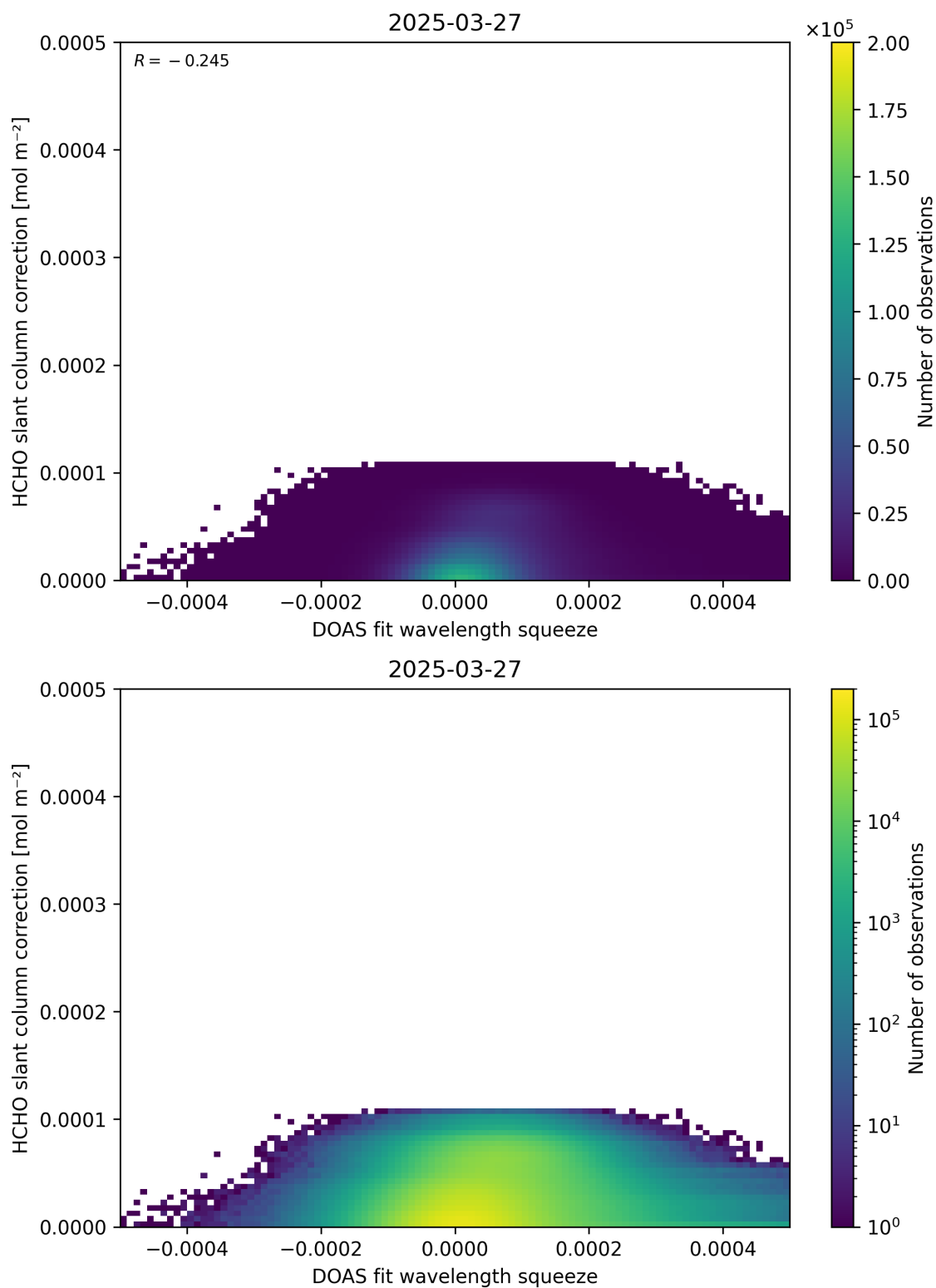
Figure 70: Scatter density plot of “DOAS fit wavelength squeeze” against “HCHO slant column correction” for 2025-03-26 to 2025-03-28.
