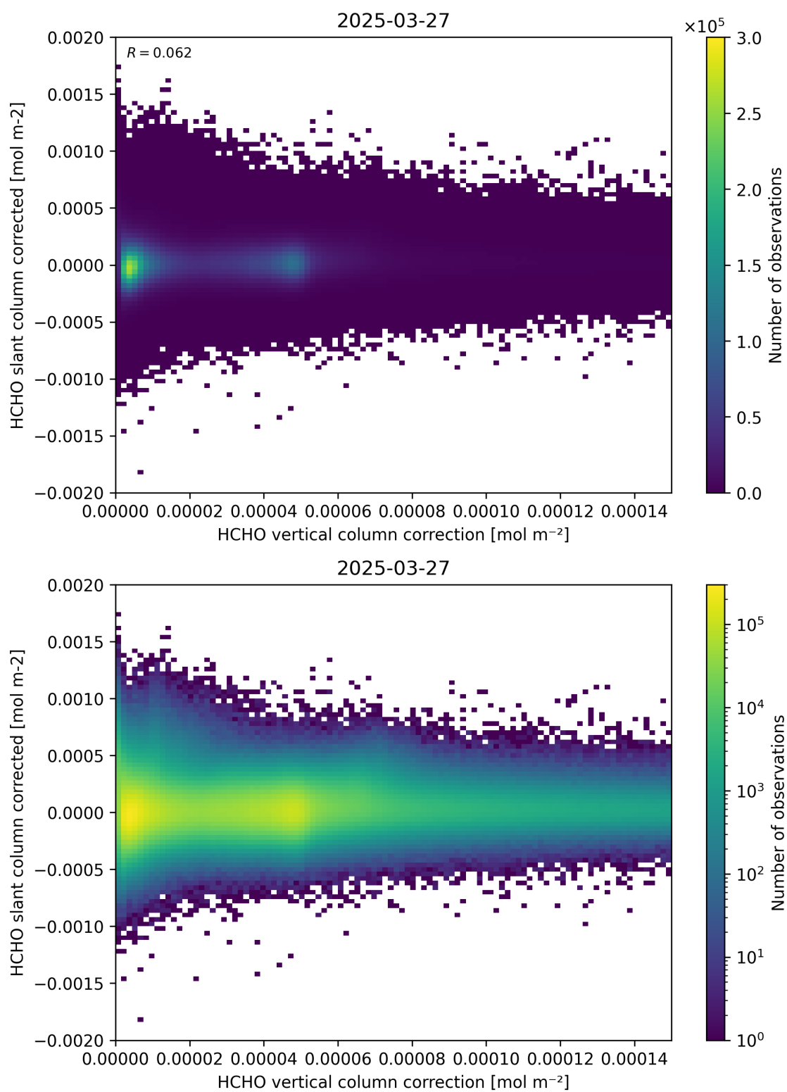
Figure 116: Scatter density plot of “HCHO vertical column correction” against “HCHO slant column corrected” for 2025-03-26 to 2025-03-28.
