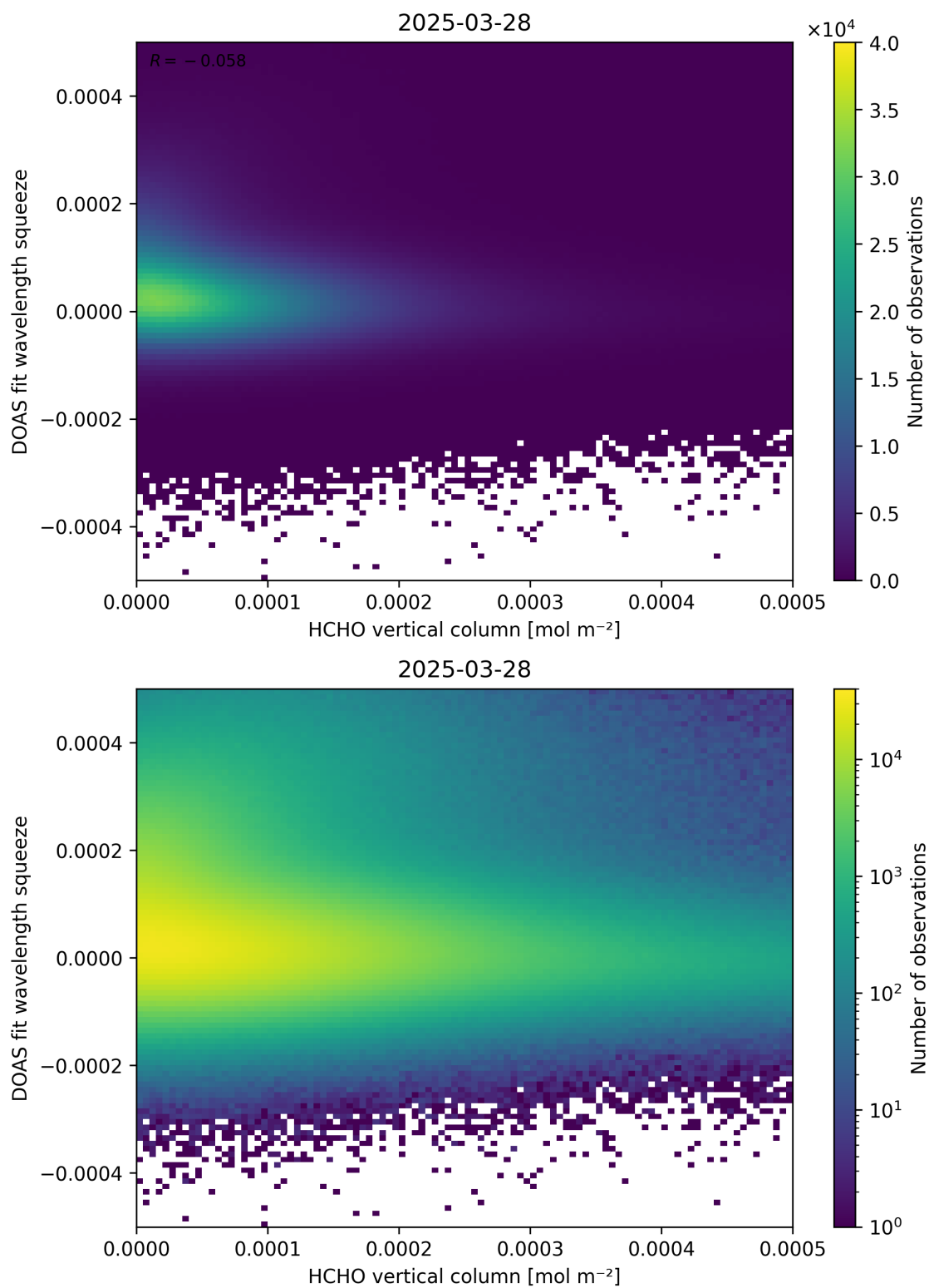
Figure 125: Scatter density plot of “HCHO vertical column” against “DOAS fit wavelength squeeze” for 2025-03-28 to 2025-03-29.
