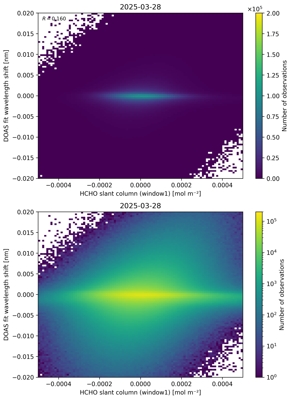
Figure 79: Scatter density plot of “HCHO slant column (window1)” against “DOAS fit wavelength shift” for 2025-03-28 to 2025-03-29.
