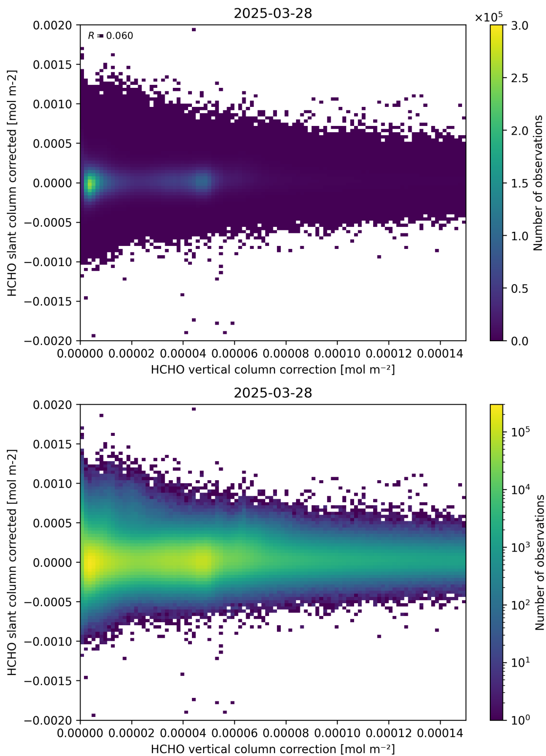
Figure 116: Scatter density plot of “HCHO vertical column correction” against “HCHO slant column corrected” for 2025-03-28 to 2025-03-29.
