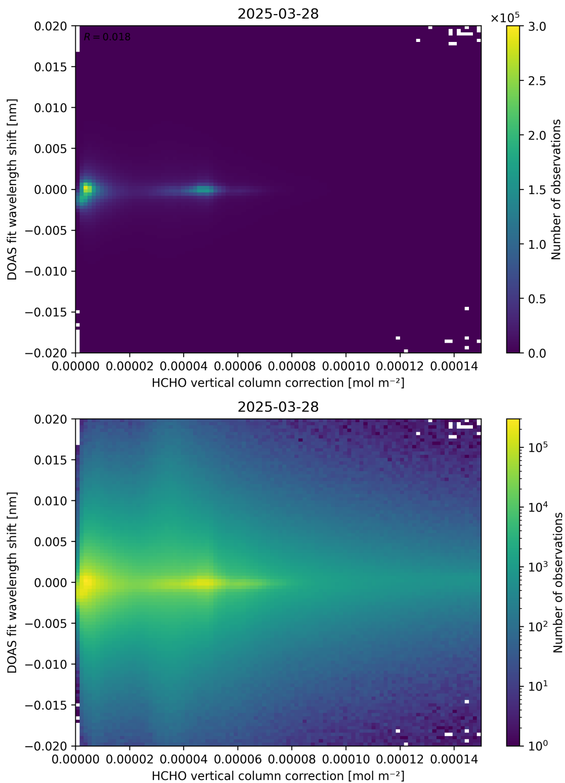
Figure 113: Scatter density plot of “HCHO vertical column correction” against “DOAS fit wavelength shift” for 2025-03-28 to 2025-03-29.
