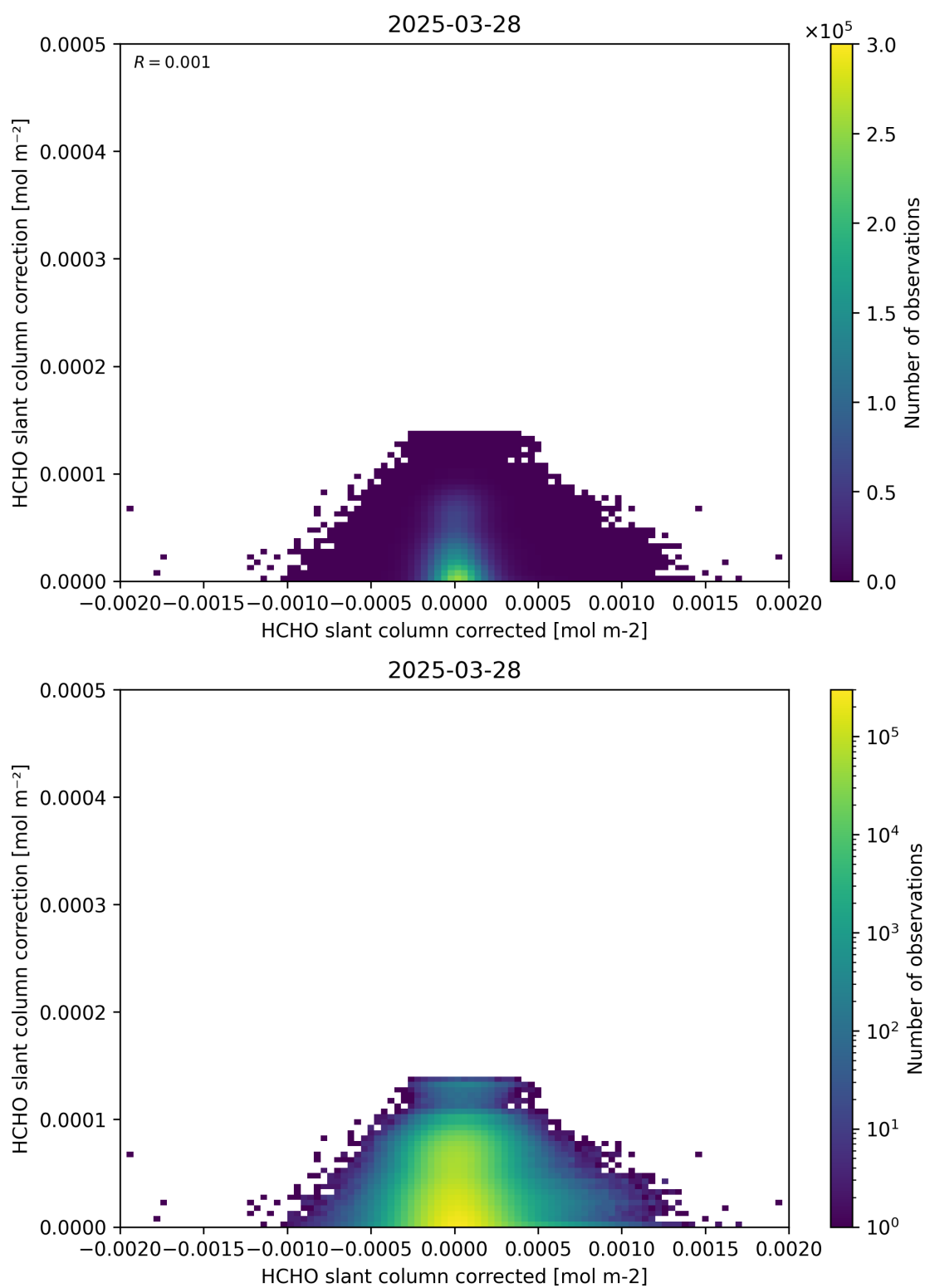
Figure 77: Scatter density plot of “HCHO slant column corrected” against “HCHO slant column correction” for 2025-03-28 to 2025-03-29.
