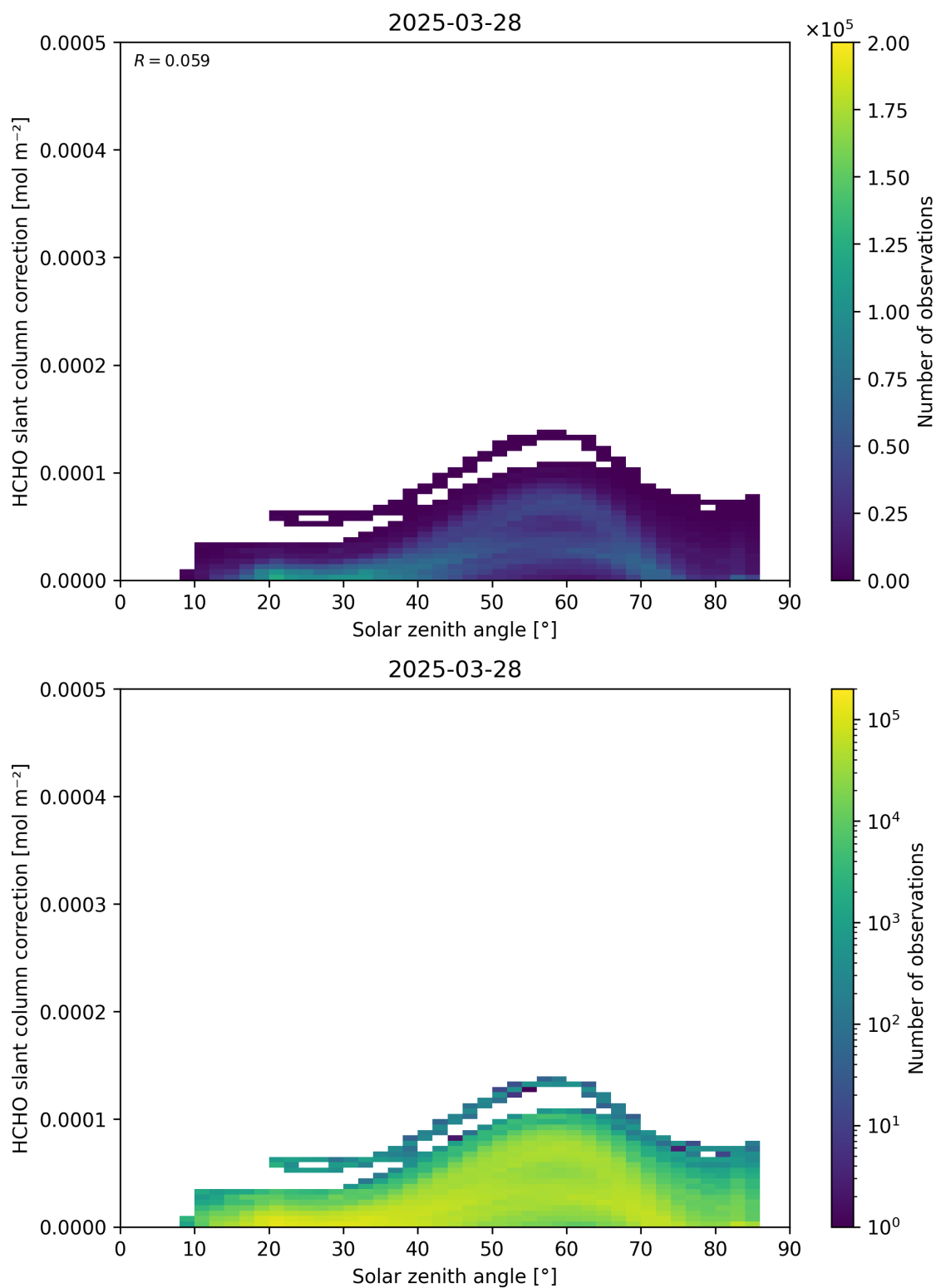
Figure 172: Scatter density plot of “Solar zenith angle” against “HCHO slant column correction” for 2025-03-28 to 2025-03-29.
