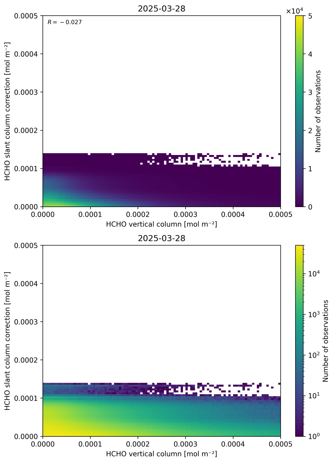
Figure 128: Scatter density plot of “HCHO vertical column” against “HCHO slant column correction” for 2025-03-28 to 2025-03-29.
