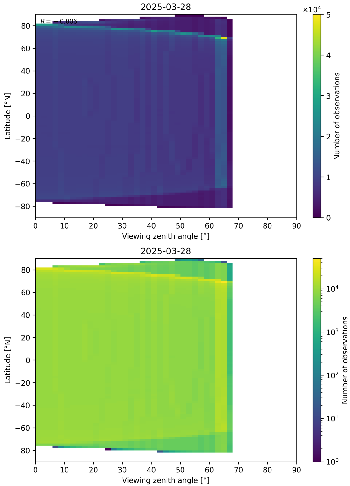
Figure 196: Scatter density plot of “Viewing zenith angle” against “Latitude” for 2025-03-28 to 2025-03-29.
