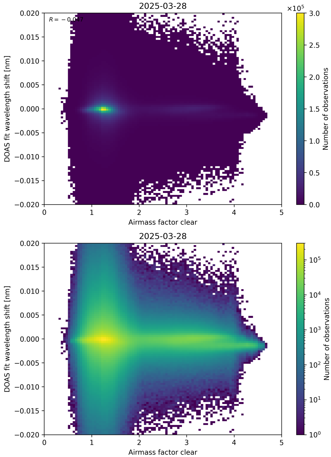
Figure 72: Scatter density plot of “Airmass factor clear” against “DOAS fit wavelength shift” for 2025-03-28 to 2025-03-29.
