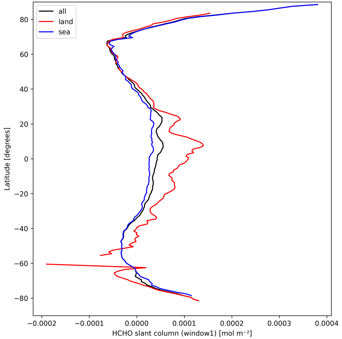
Figure 24: Zonal average of “HCHO slant column (window1)” for 2025-03-28 to 2025-03-29.
