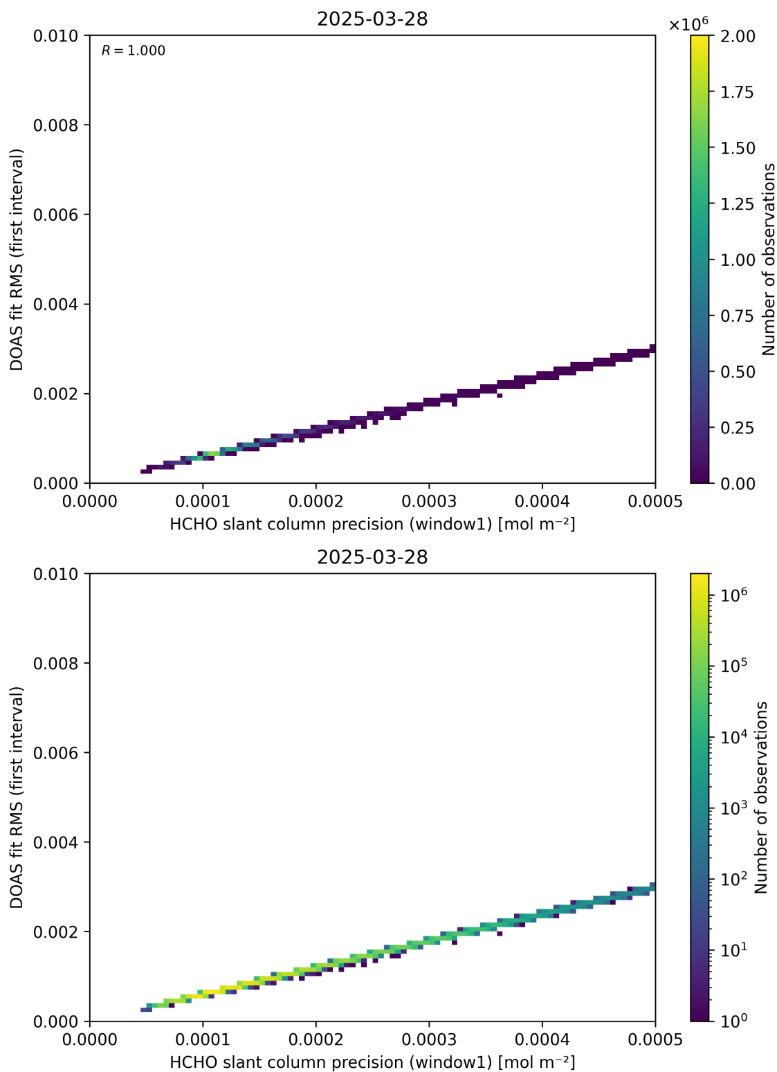
Figure 88: Scatter density plot of “HCHO slant column precision (window1)” against “DOAS fit RMS (first interval)” for 2025-03-28 to 2025-03-29.
