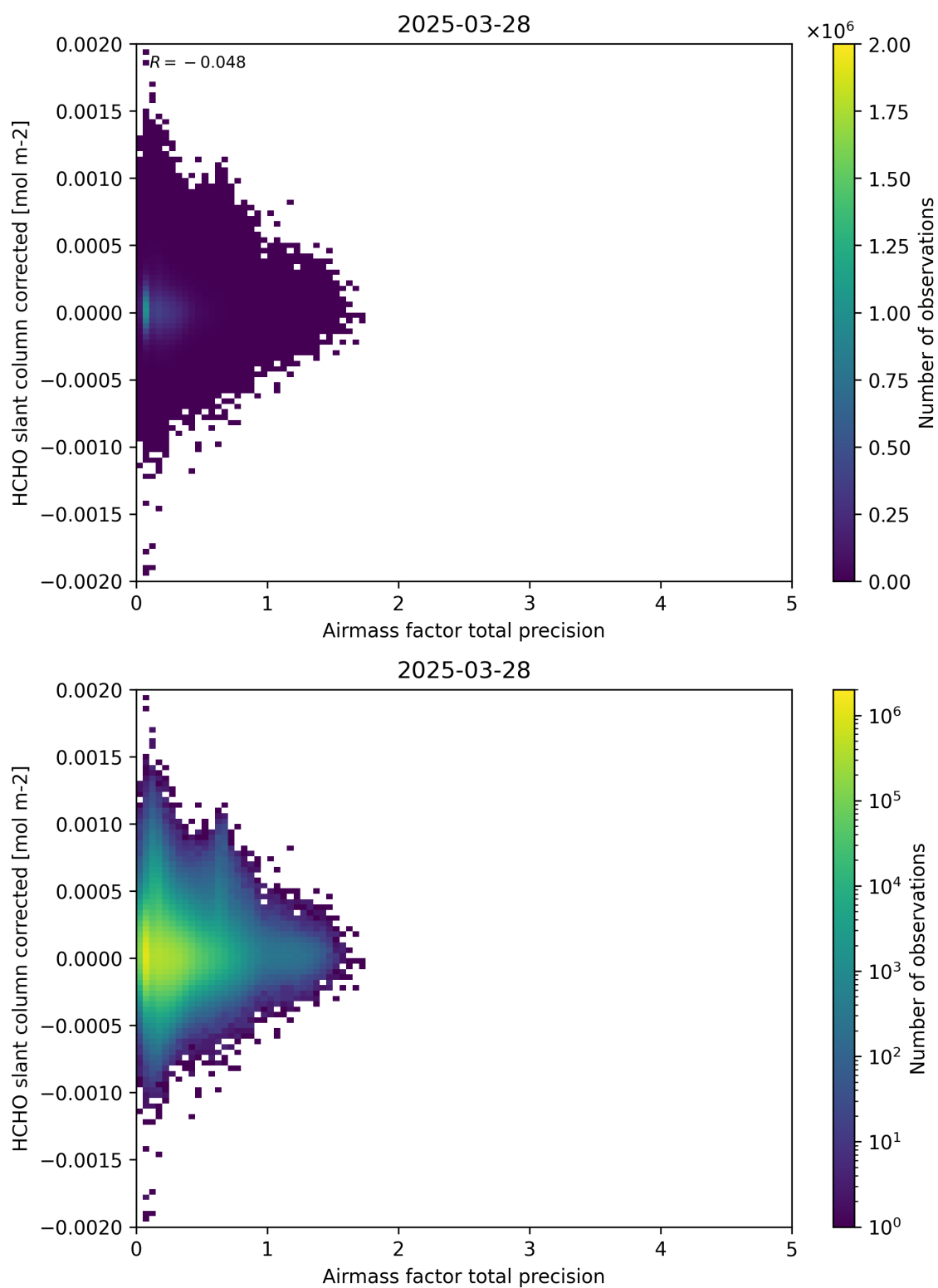
Figure 109: Scatter density plot of “Airmass factor total precision” against “HCHO slant column corrected” for 2025-03-28 to 2025-03-29.
