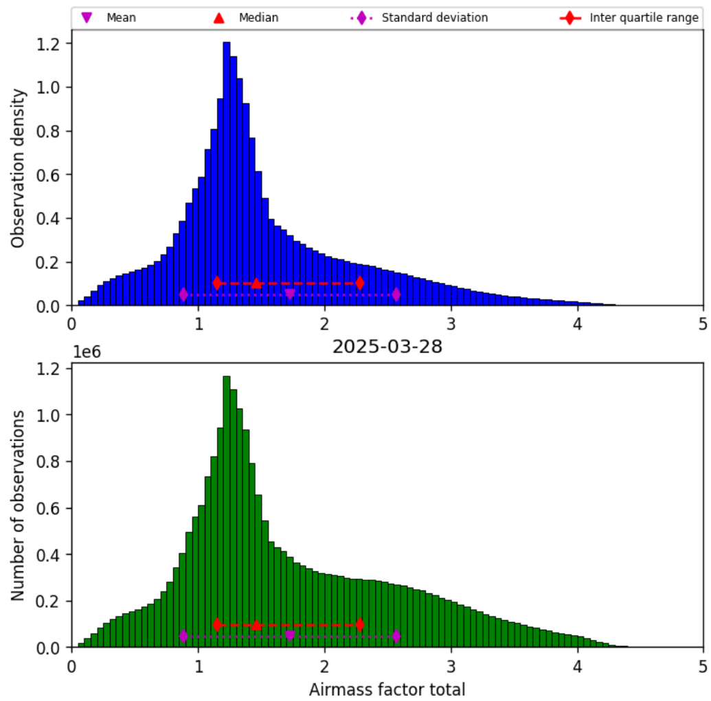
Figure 40: Histogram of “Airmass factor total” for 2025-03-28 to 2025-03-29
