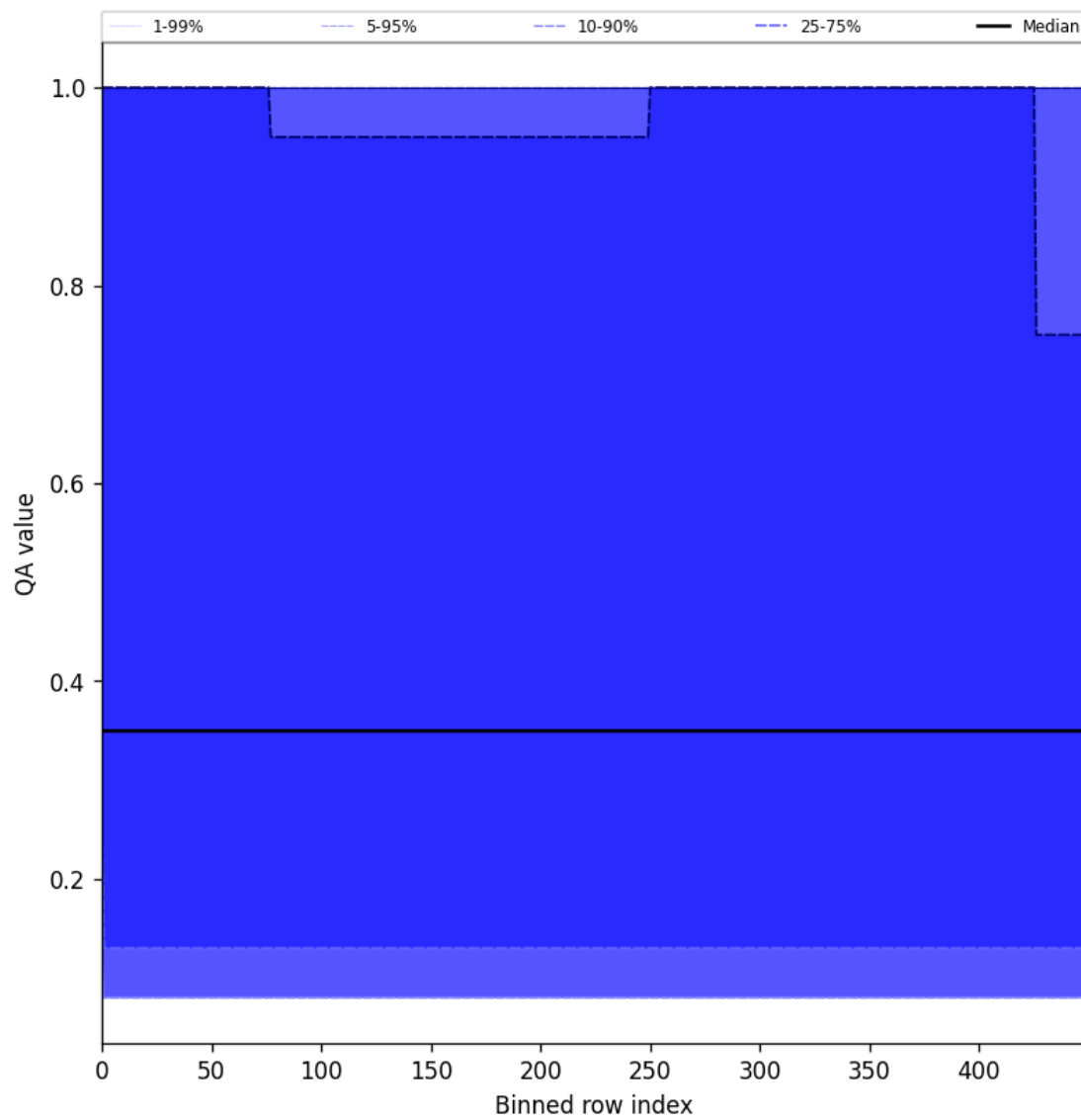
Figure 48: Along track statistics of “QA value” for 2025-03-28 to 2025-03-29
