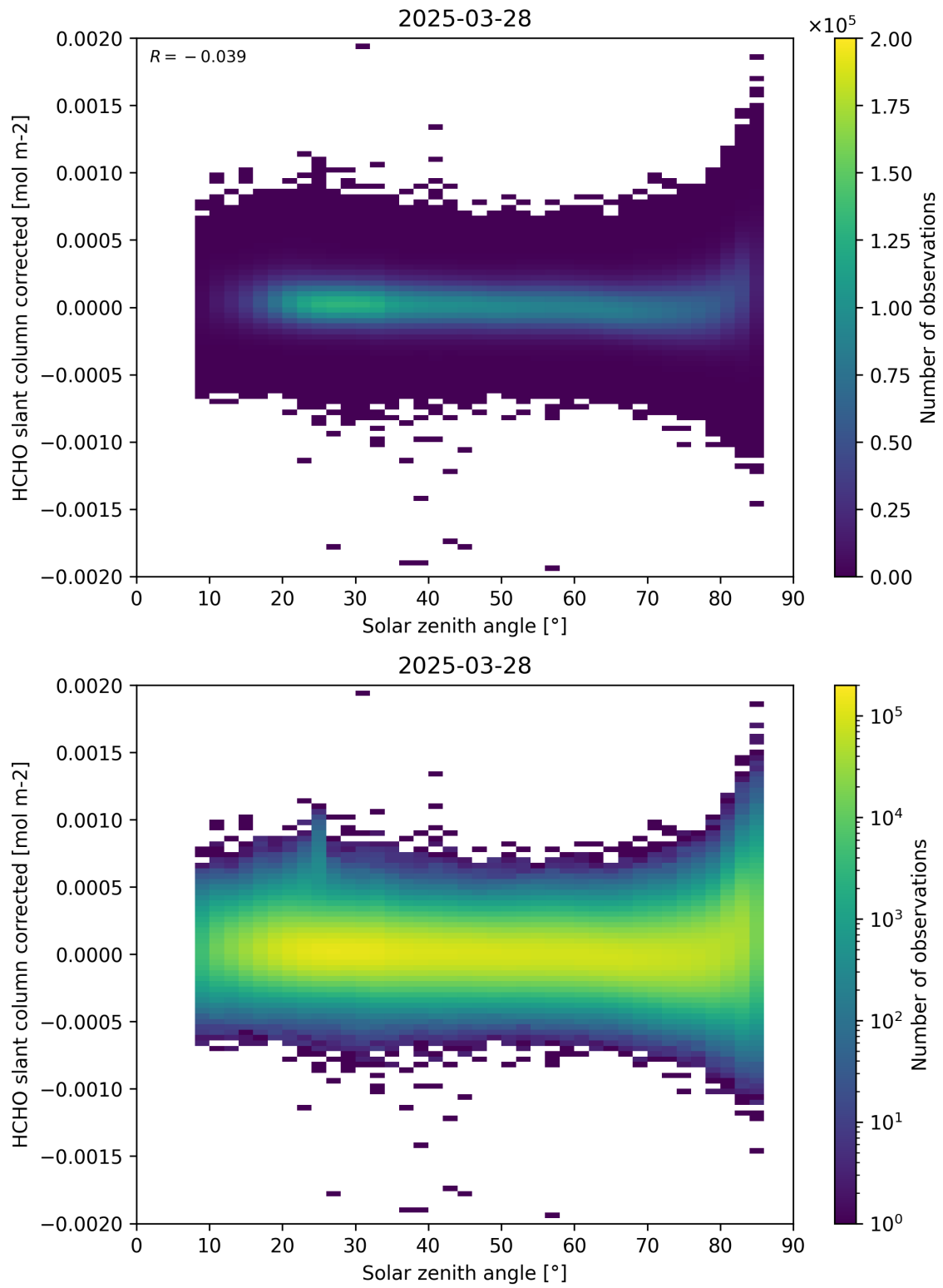
Figure 171: Scatter density plot of “Solar zenith angle” against “HCHO slant column corrected” for 2025-03-28 to 2025-03-29.
