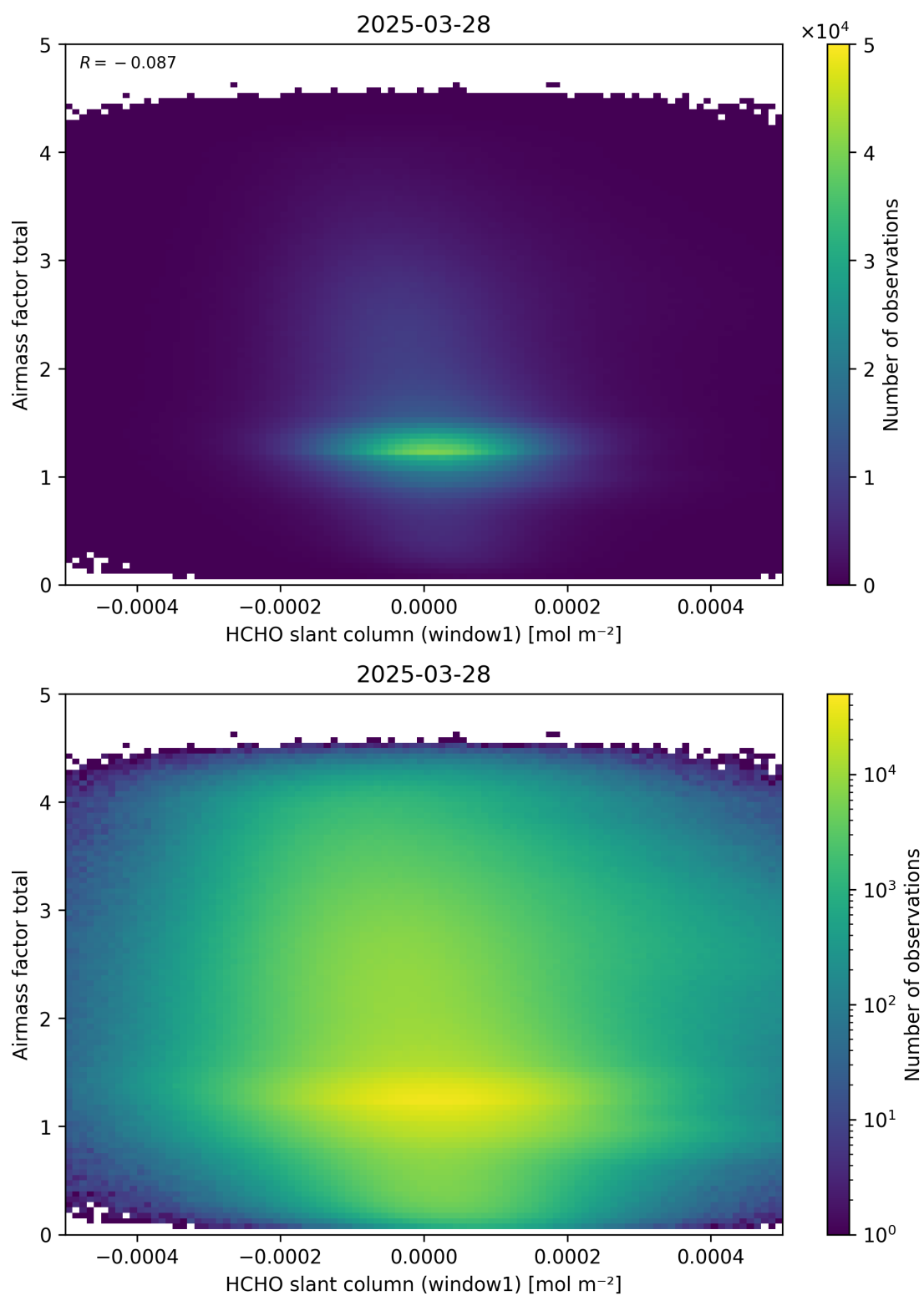
Figure 85: Scatter density plot of “HCHO slant column (window1)” against “Airmass factor total” for 2025-03-28 to 2025-03-29.
