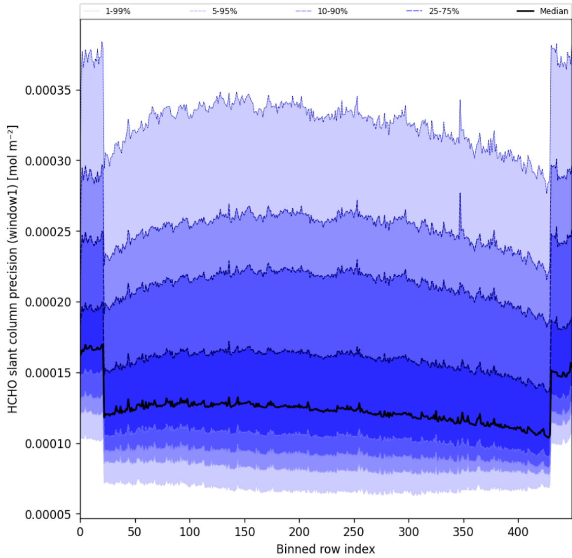
Figure 53: Along track statistics of “HCHO slant column precision (window1)” for 2025-03-28 to 2025-03-29
