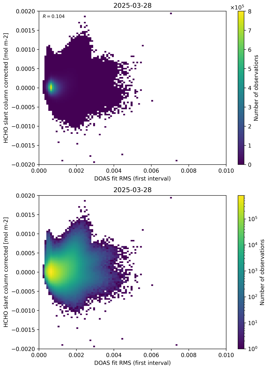
Figure 62: Scatter density plot of “DOAS fit RMS (first interval)” against “HCHO slant column corrected” for 2025-03-28 to 2025-03-29.
