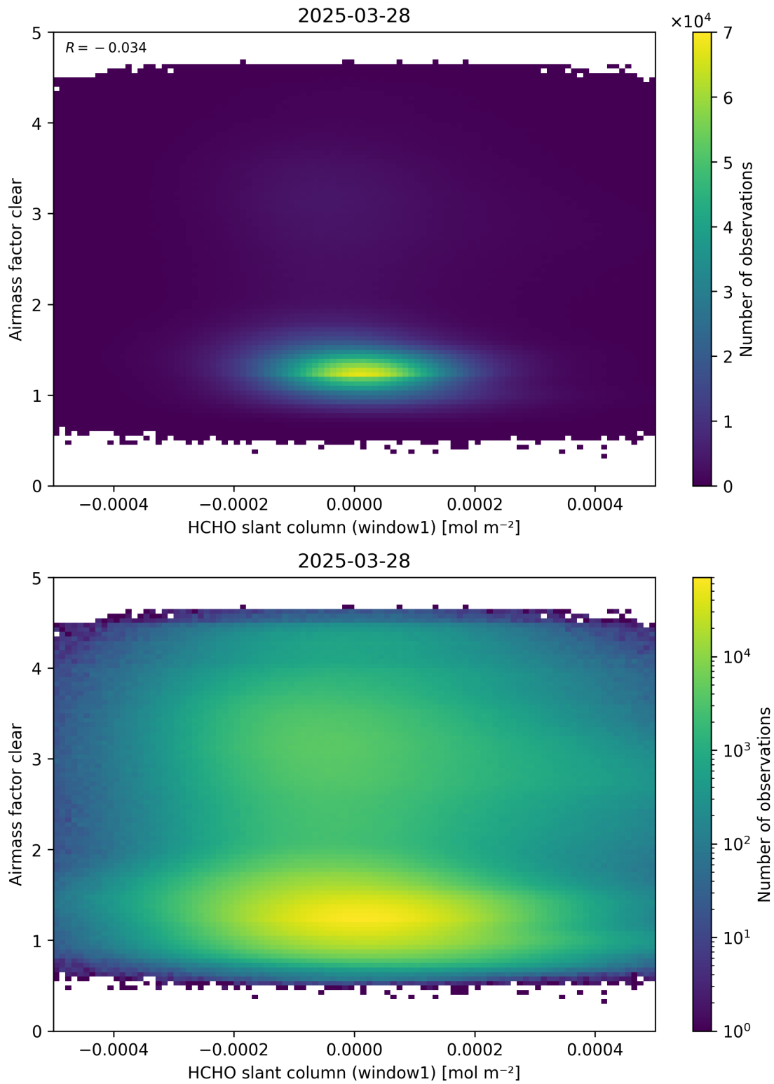
Figure 81: Scatter density plot of “HCHO slant column (window1)” against “Airmass factor clear” for 2025-03-28 to 2025-03-29.
