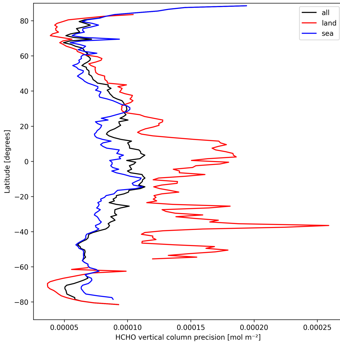
Figure 22: Zonal average of “HCHO vertical column precision” for 2025-03-28 to 2025-03-29.
