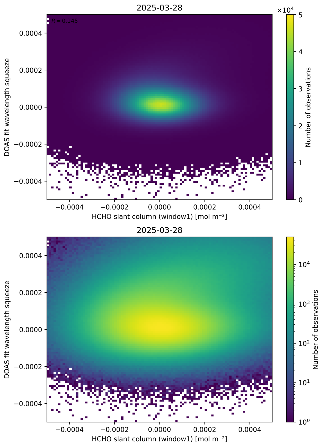
Figure 80: Scatter density plot of “HCHO slant column (window1)” against “DOAS fit wavelength squeeze” for 2025-03-28 to 2025-03-29.
