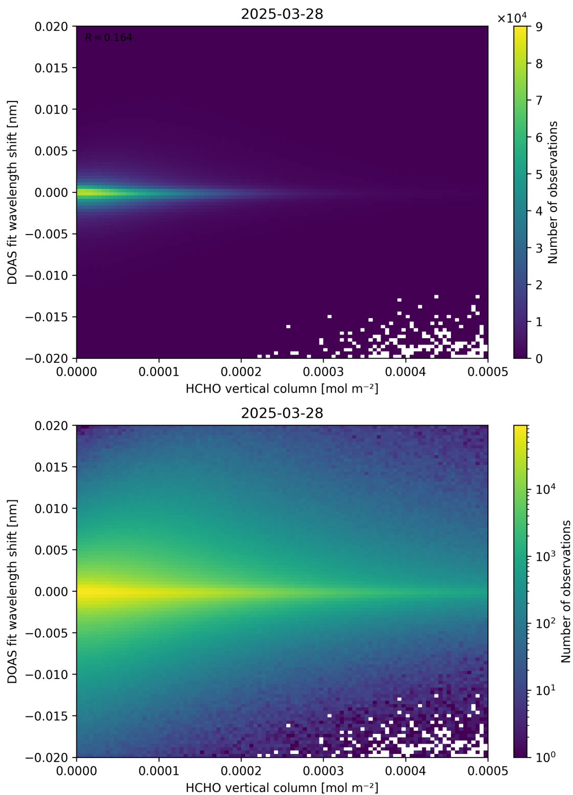
Figure 124: Scatter density plot of “HCHO vertical column” against “DOAS fit wavelength shift” for 2025-03-28 to 2025-03-29.
