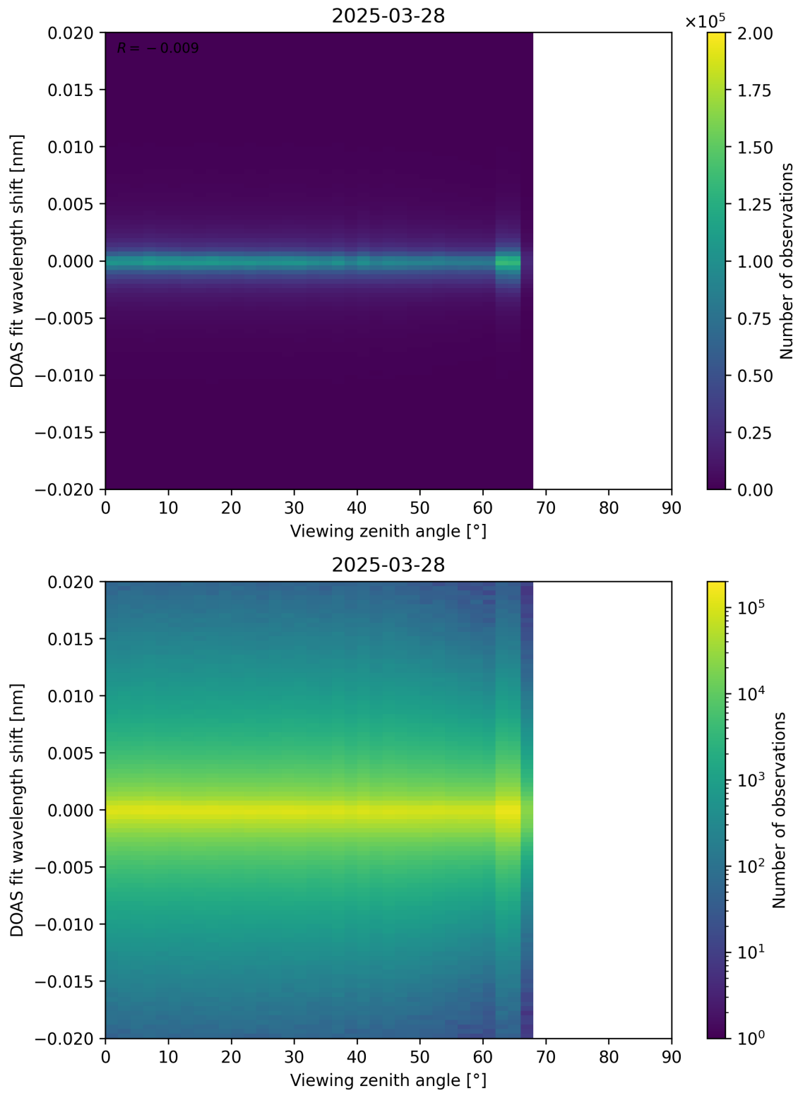
Figure 183: Scatter density plot of “Viewing zenith angle” against “DOAS fit wavelength shift” for 2025-03-28 to 2025-03-29.
