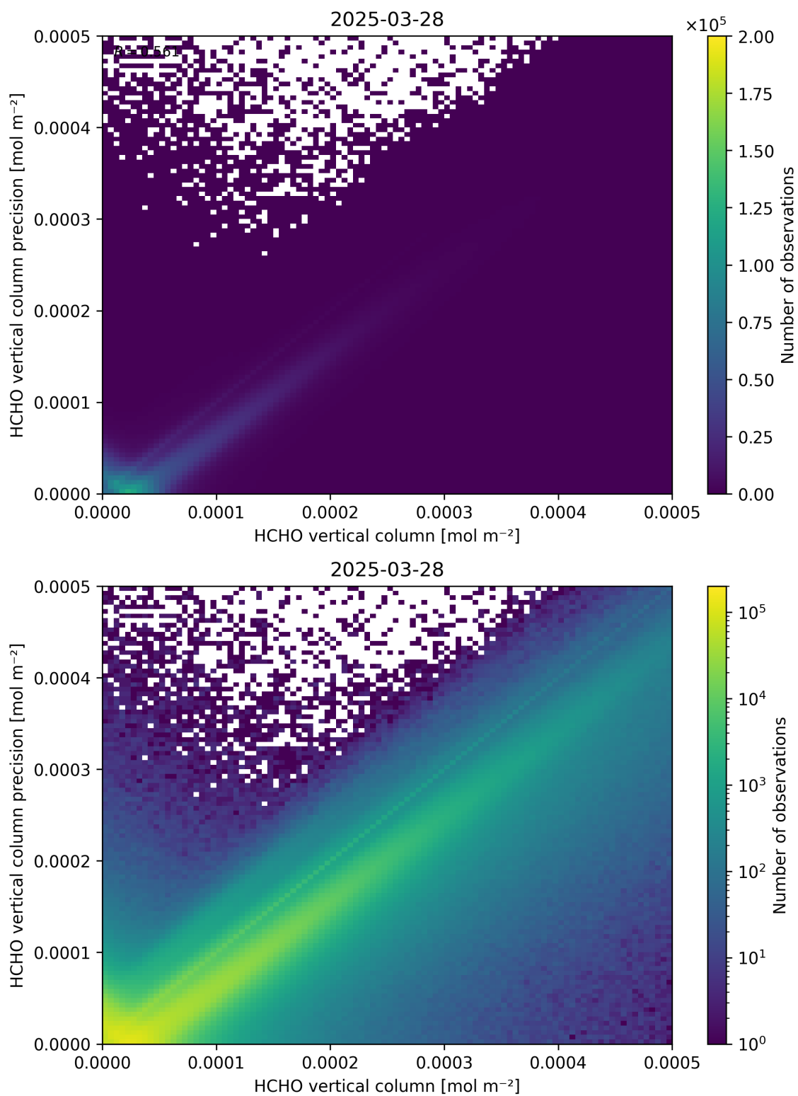
Figure 134: Scatter density plot of “HCHO vertical column” against “HCHO vertical column precision” for 2025-03-28 to 2025-03-29.
