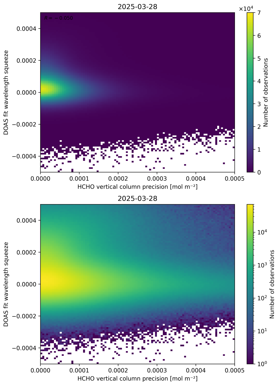
Figure 138: Scatter density plot of “HCHO vertical column precision” against “DOAS fit wavelength squeeze” for 2025-03-28 to 2025-03-29.
