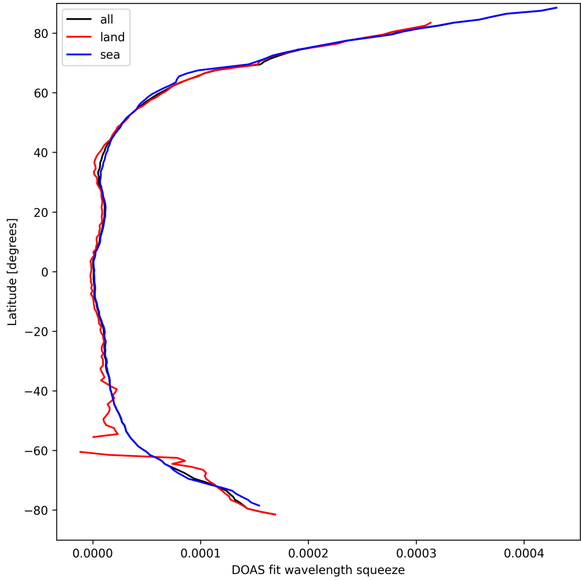
Figure 31: Zonal average of “DOAS fit wavelength squeeze” for 2025-03-28 to 2025-03-29.
