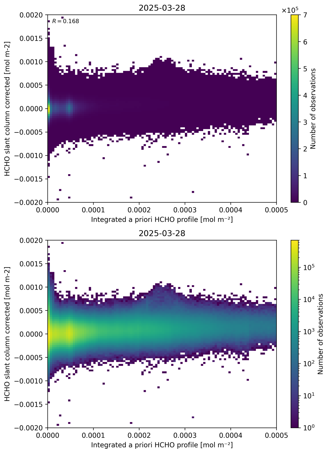
Figure 151: Scatter density plot of “Integrated a priori HCHO profile” against “HCHO slant column corrected” for 2025-03-28 to 2025-03-29.
