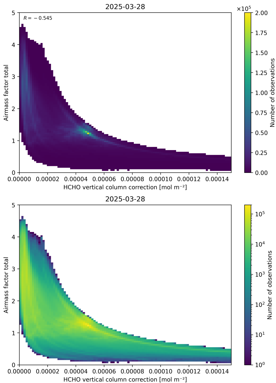
Figure 120: Scatter density plot of “HCHO vertical column correction” against “Airmass factor total” for 2025-03-28 to 2025-03-29.
