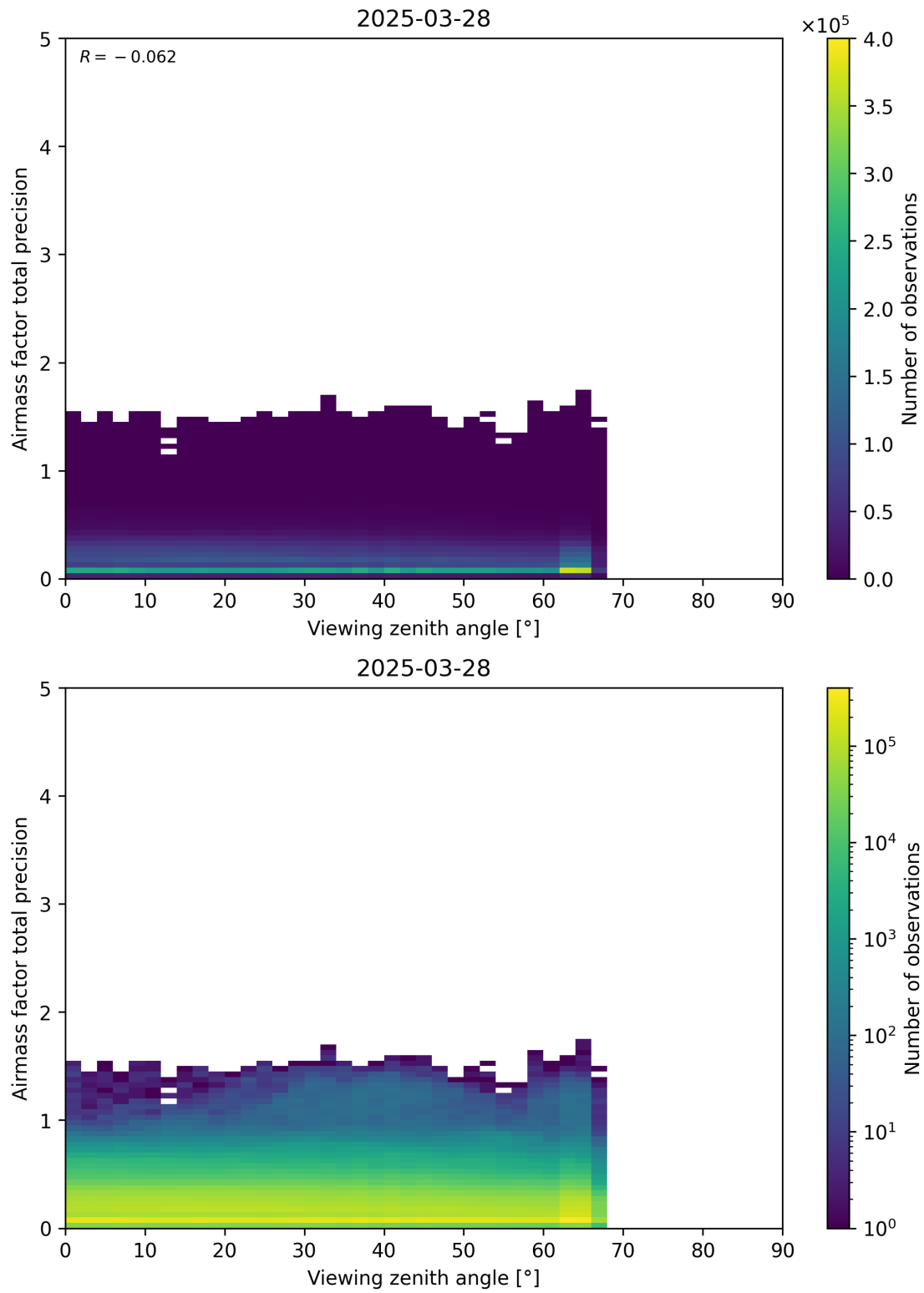
Figure 191: Scatter density plot of “Viewing zenith angle” against “Airmass factor total precision” for 2025-03-28 to 2025-03-29.
