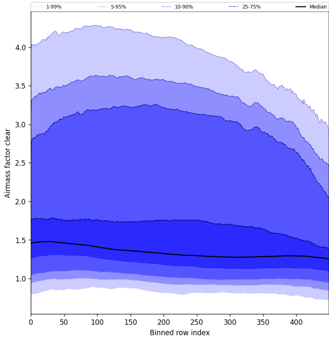
Figure 56: Along track statistics of “Airmass factor clear” for 2025-03-28 to 2025-03-29
