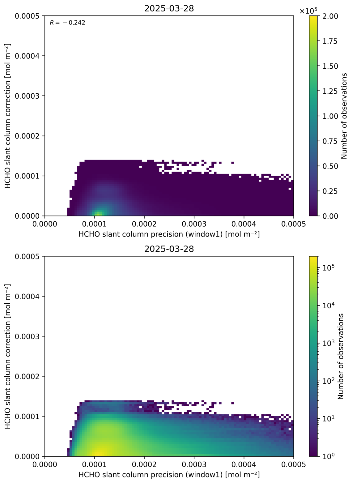
Figure 93: Scatter density plot of “HCHO slant column precision (window1)” against “HCHO slant column correction” for 2025-03-28 to 2025-03-29.
