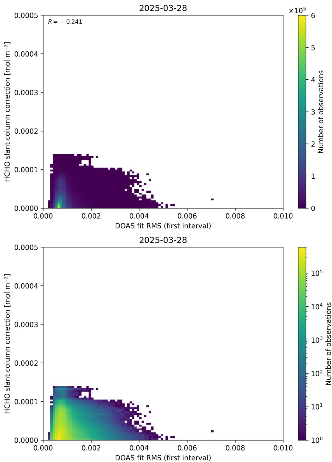
Figure 63: Scatter density plot of “DOAS fit RMS (first interval)” against “HCHO slant column correction” for 2025-03-28 to 2025-03-29.
