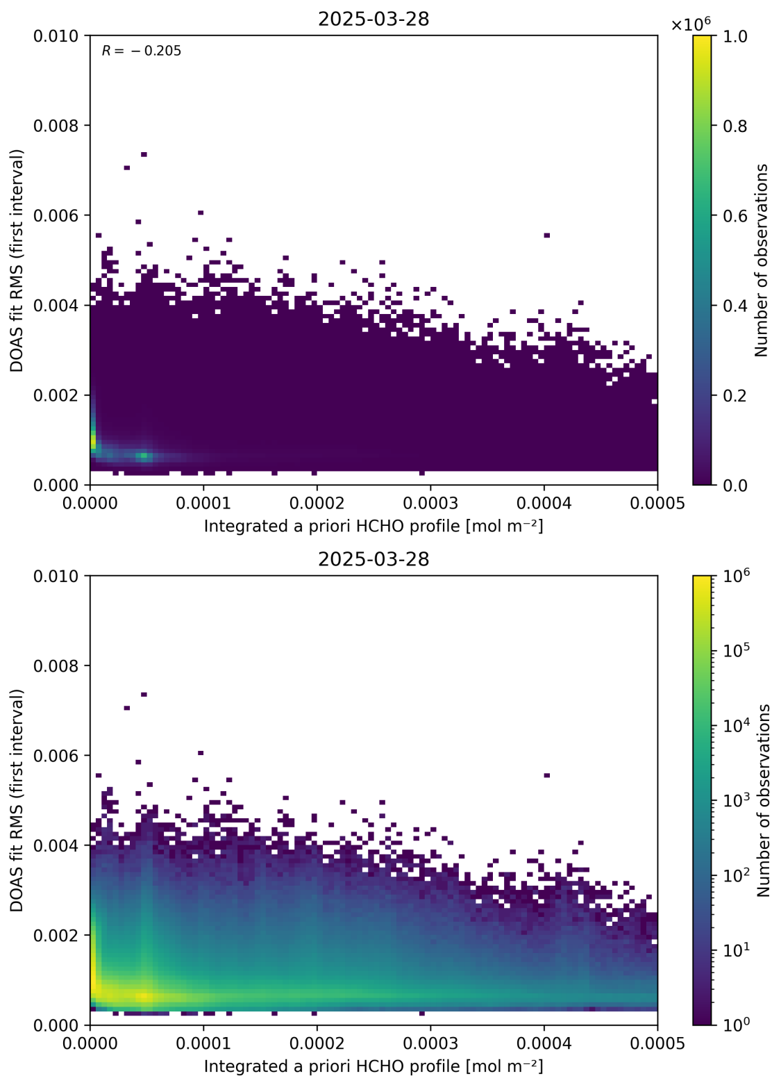
Figure 148: Scatter density plot of “Integrated a priori HCHO profile” against “DOAS fit RMS (first interval)” for 2025-03-28 to 2025-03-29.
