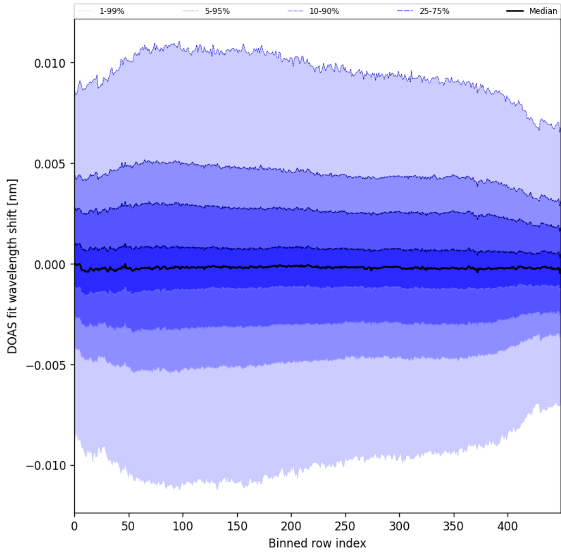
Figure 58: Along track statistics of “DOAS fit wavelength shift” for 2025-03-28 to 2025-03-29
