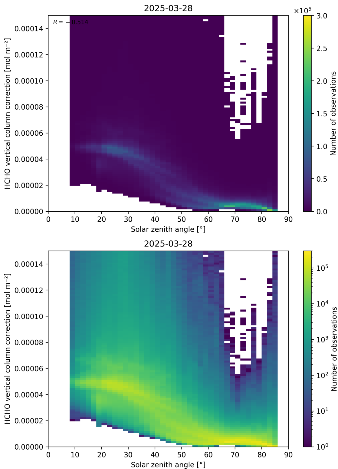
Figure 178: Scatter density plot of “Solar zenith angle” against “HCHO vertical column correction” for 2025-03-28 to 2025-03-29.
