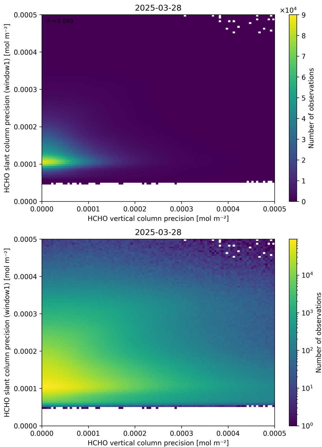
Figure 143: Scatter density plot of “HCHO vertical column precision” against “HCHO slant column precision (window1)” for 2025-03-28 to 2025-03-29.
