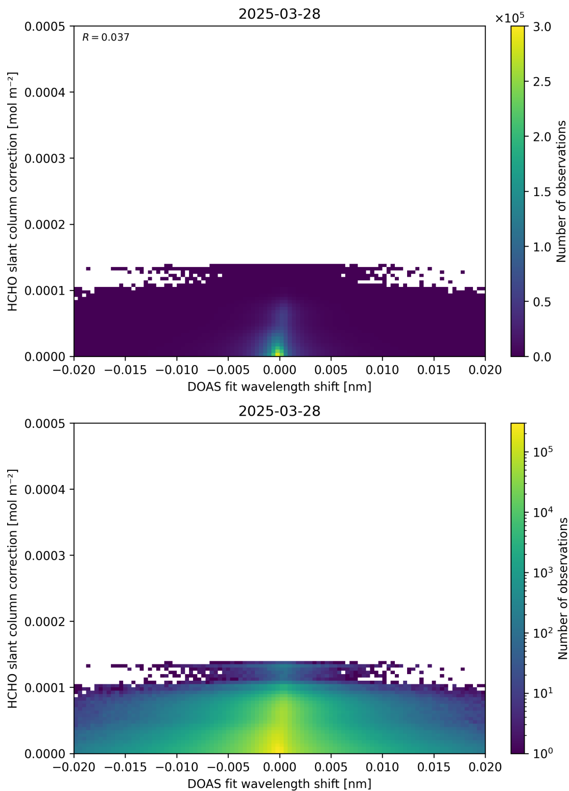
Figure 67: Scatter density plot of “DOAS fit wavelength shift” against “HCHO slant column correction” for 2025-03-28 to 2025-03-29.
