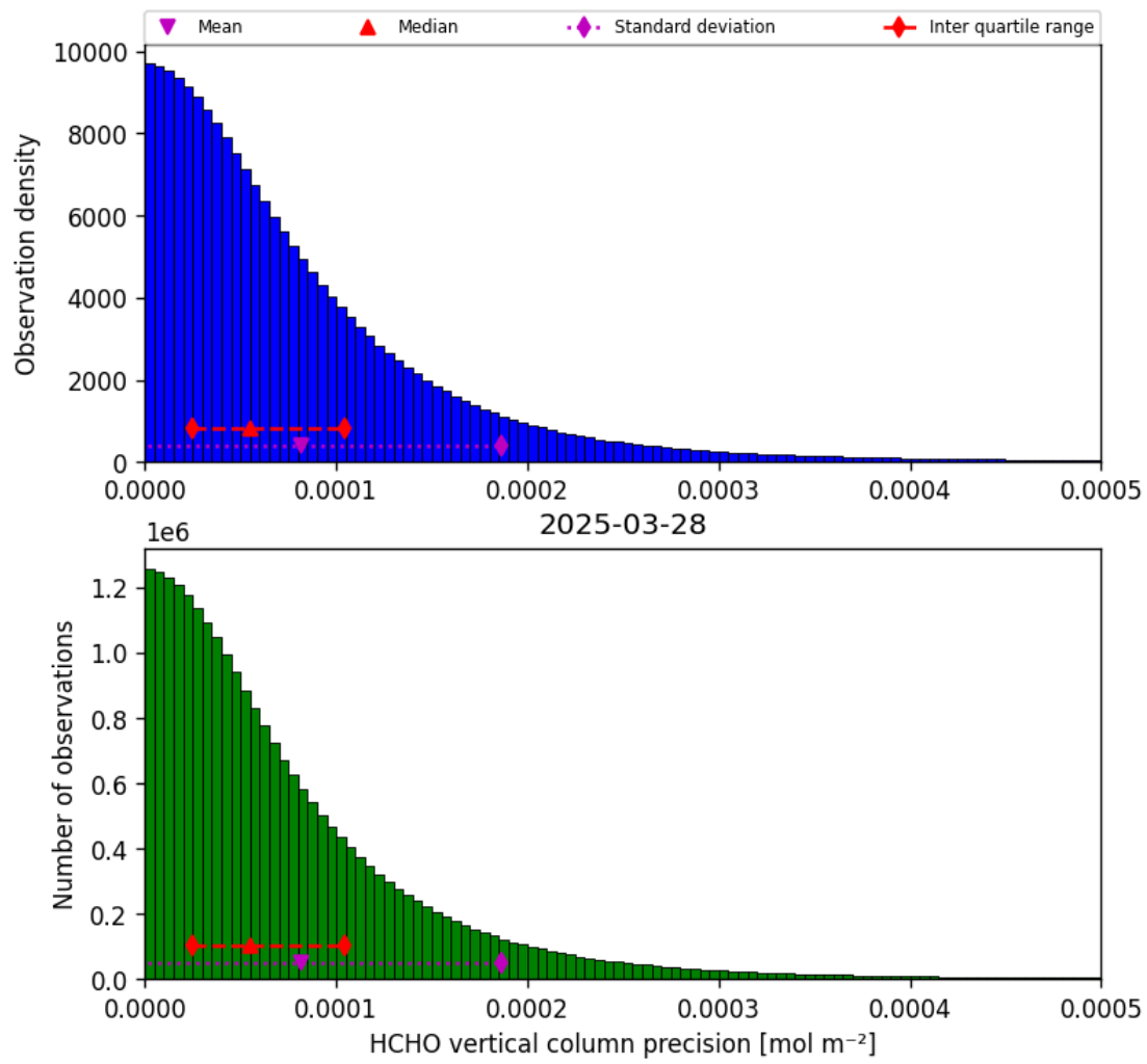
Figure 36: Histogram of “HCHO vertical column precision” for 2025-03-28 to 2025-03-29
