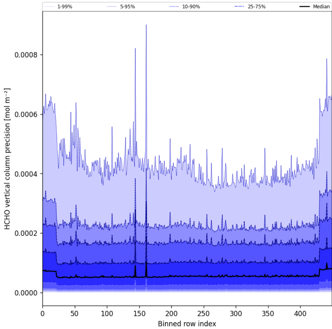
Figure 50: Along track statistics of “HCHO vertical column precision” for 2025-03-28 to 2025-03-29
