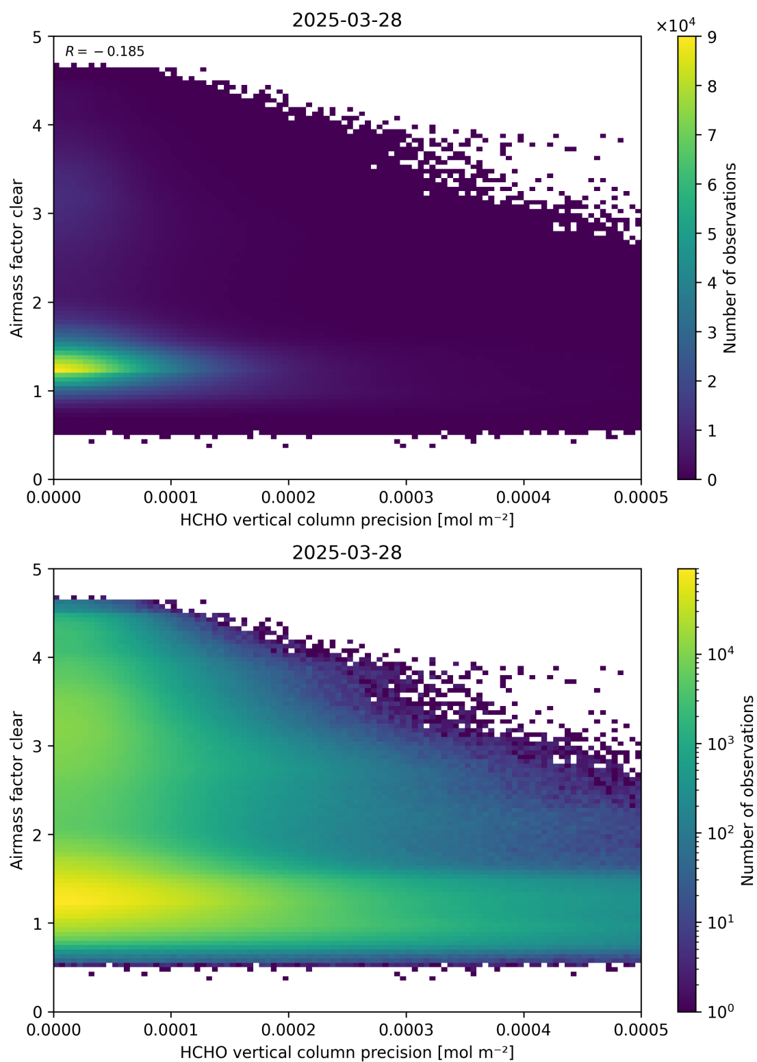
Figure 139: Scatter density plot of “HCHO vertical column precision” against “Airmass factor clear” for 2025-03-28 to 2025-03-29.
