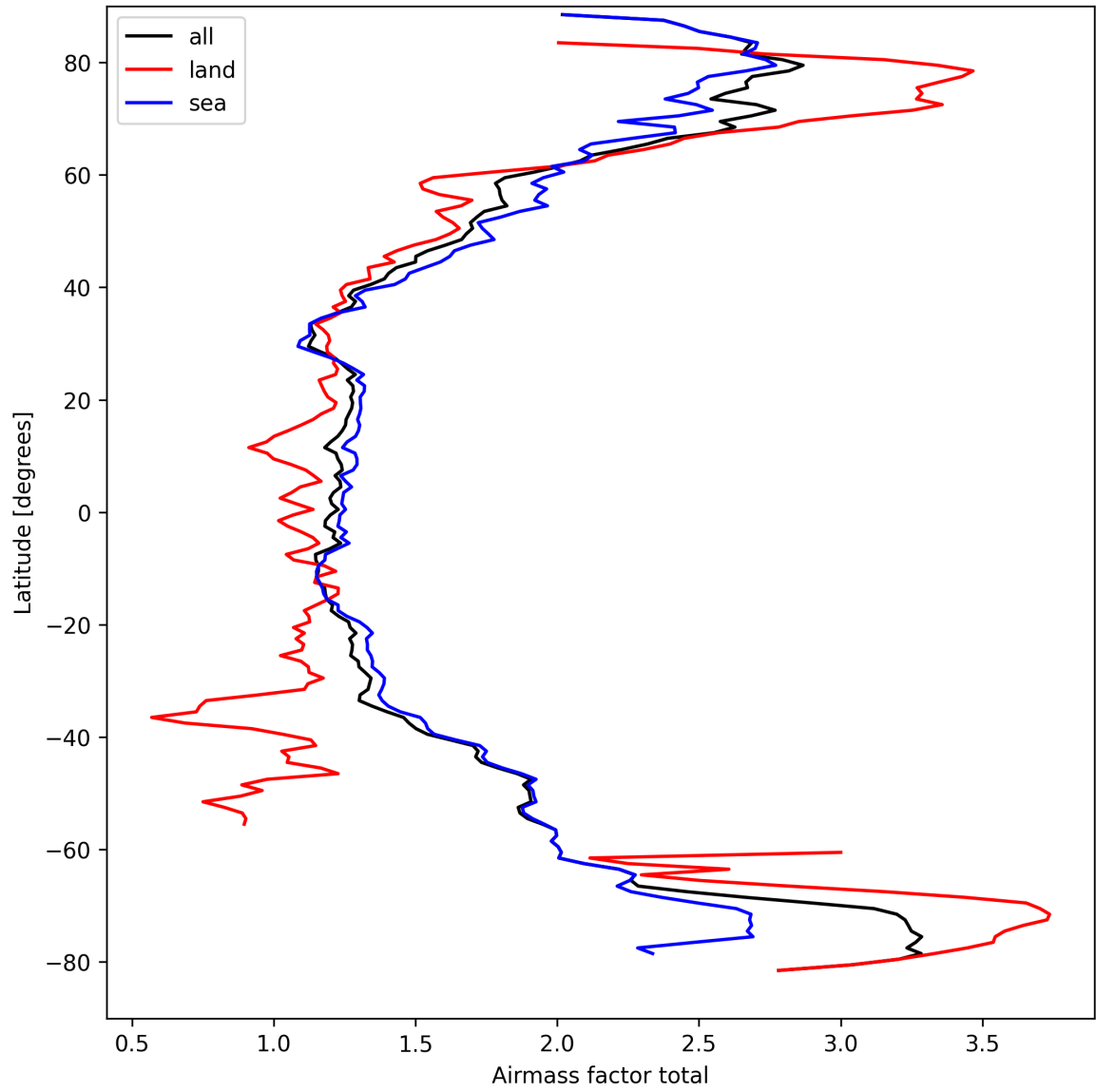
Figure 26: Zonal average of “Airmass factor total” for 2025-03-28 to 2025-03-29.
