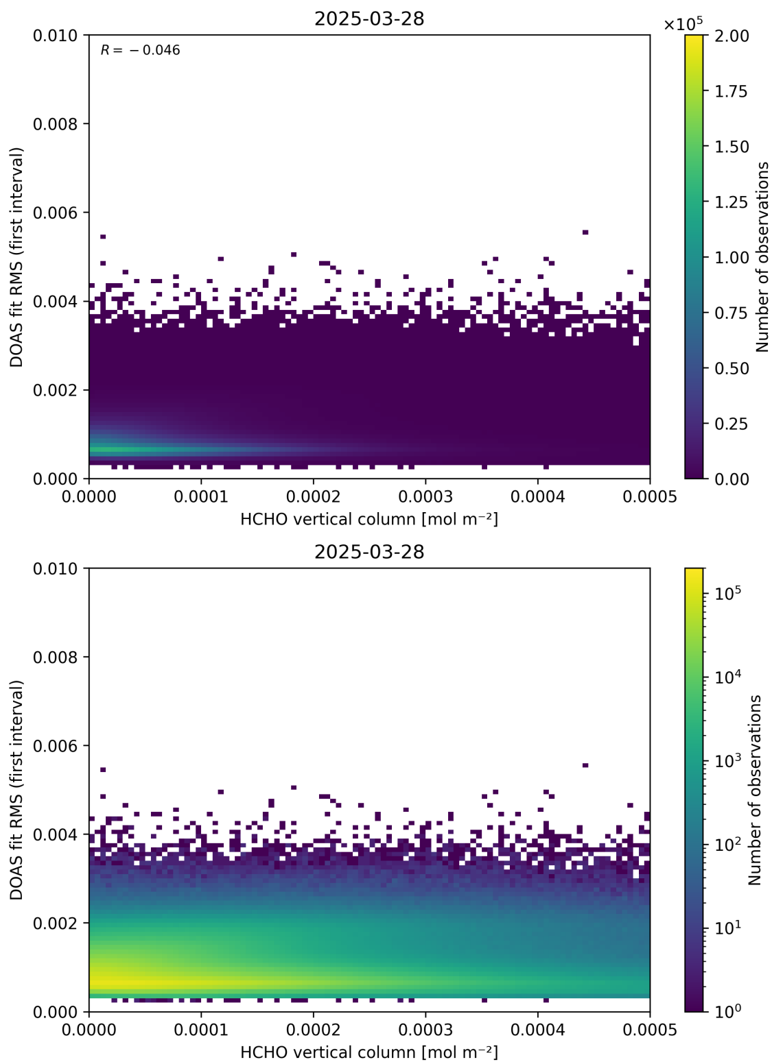
Figure 123: Scatter density plot of “HCHO vertical column” against “DOAS fit RMS (first interval)” for 2025-03-28 to 2025-03-29.
