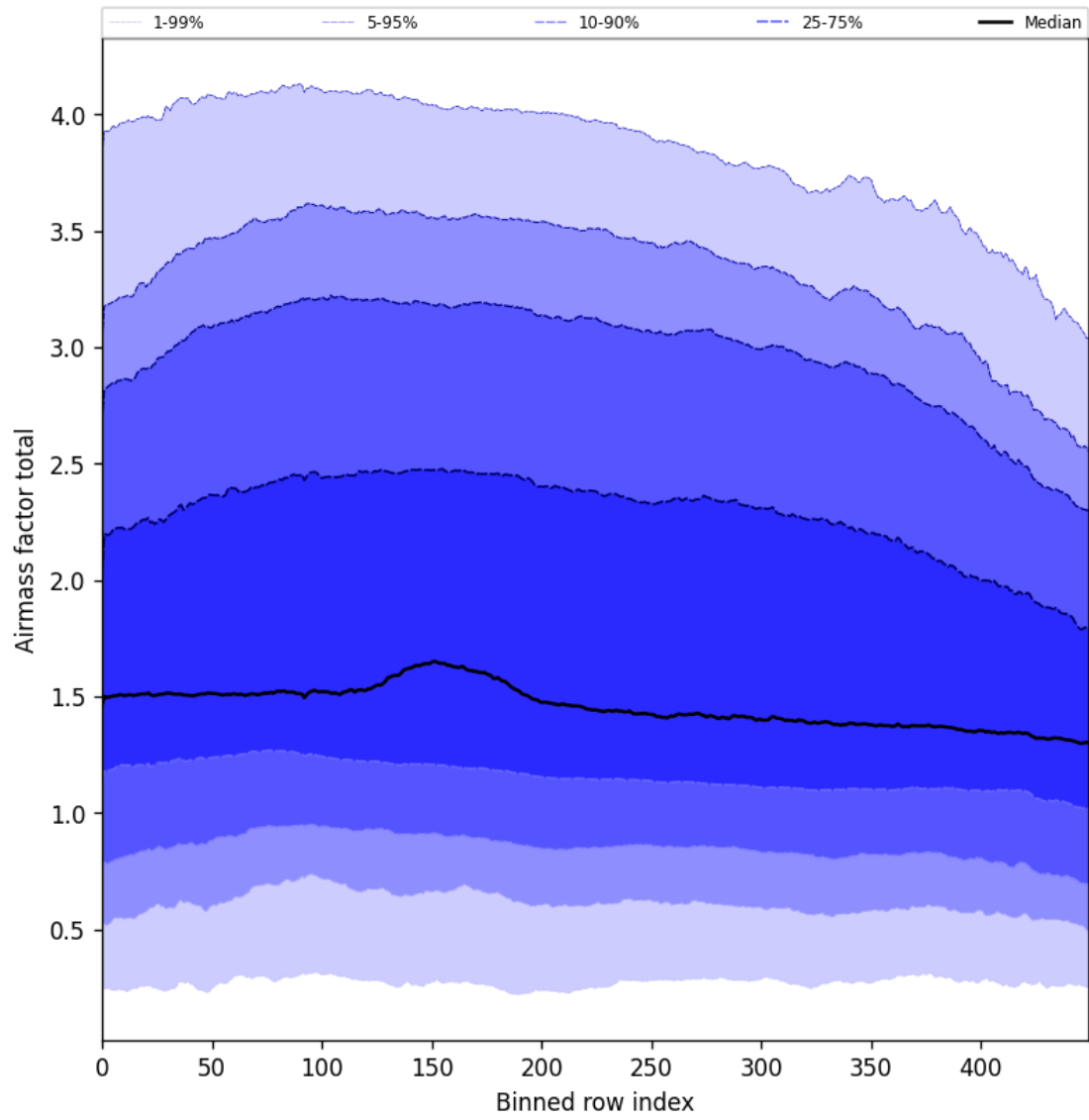
Figure 54: Along track statistics of “Airmass factor total” for 2025-03-28 to 2025-03-29
