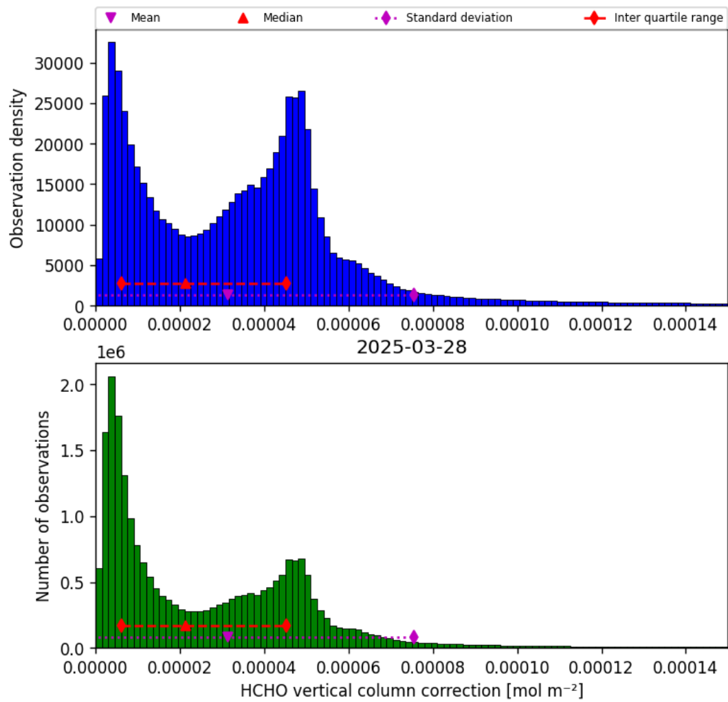
Figure 37: Histogram of “HCHO vertical column correction” for 2025-03-28 to 2025-03-29
