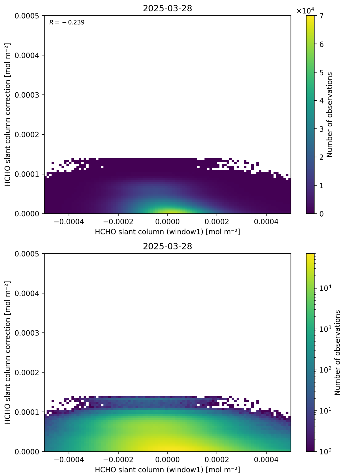
Figure 83: Scatter density plot of “HCHO slant column (window1)” against “HCHO slant column correction” for 2025-03-28 to 2025-03-29.
