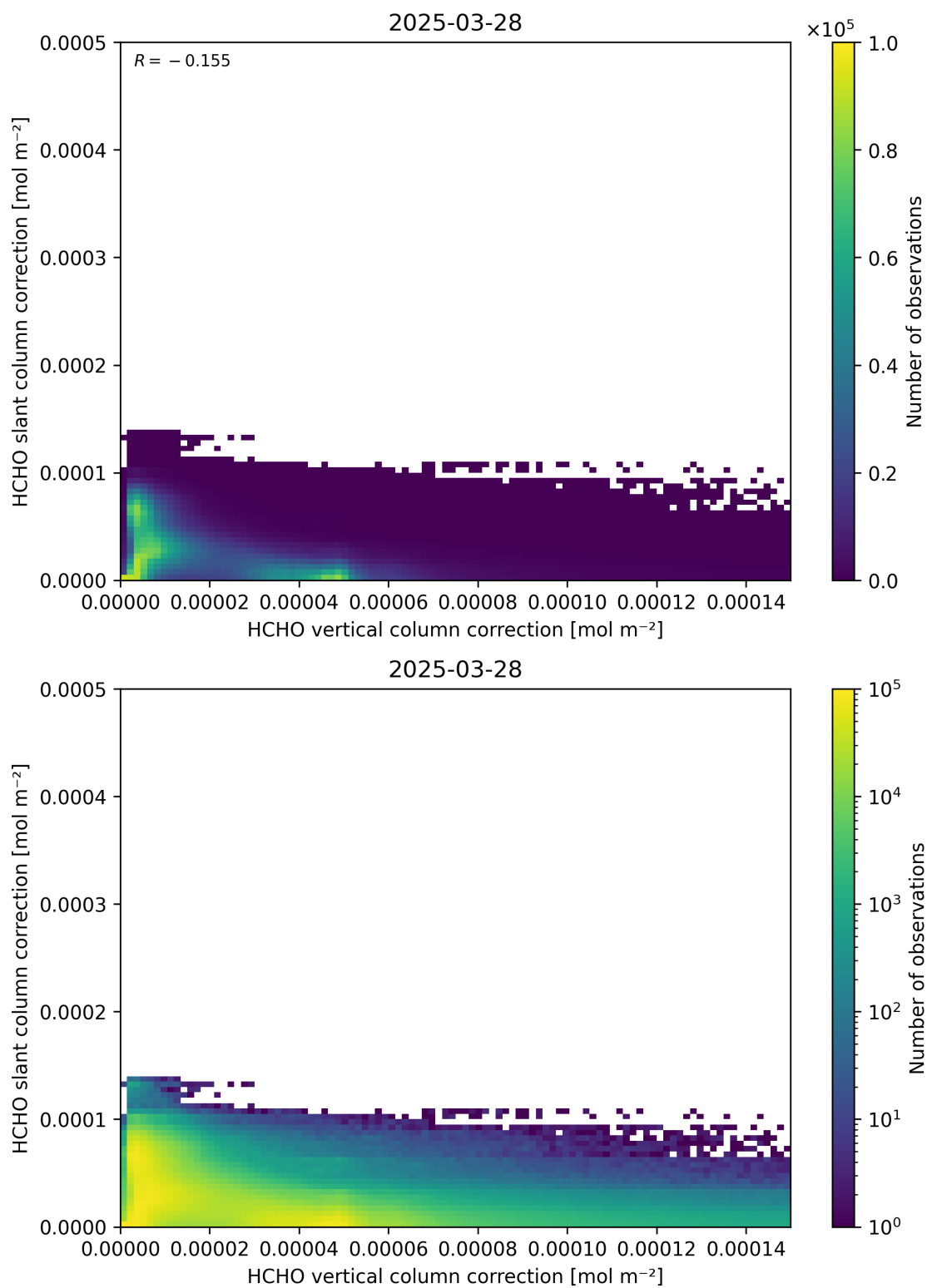
Figure 117: Scatter density plot of “HCHO vertical column correction” against “HCHO slant column correction” for 2025-03-28 to 2025-03-29.
