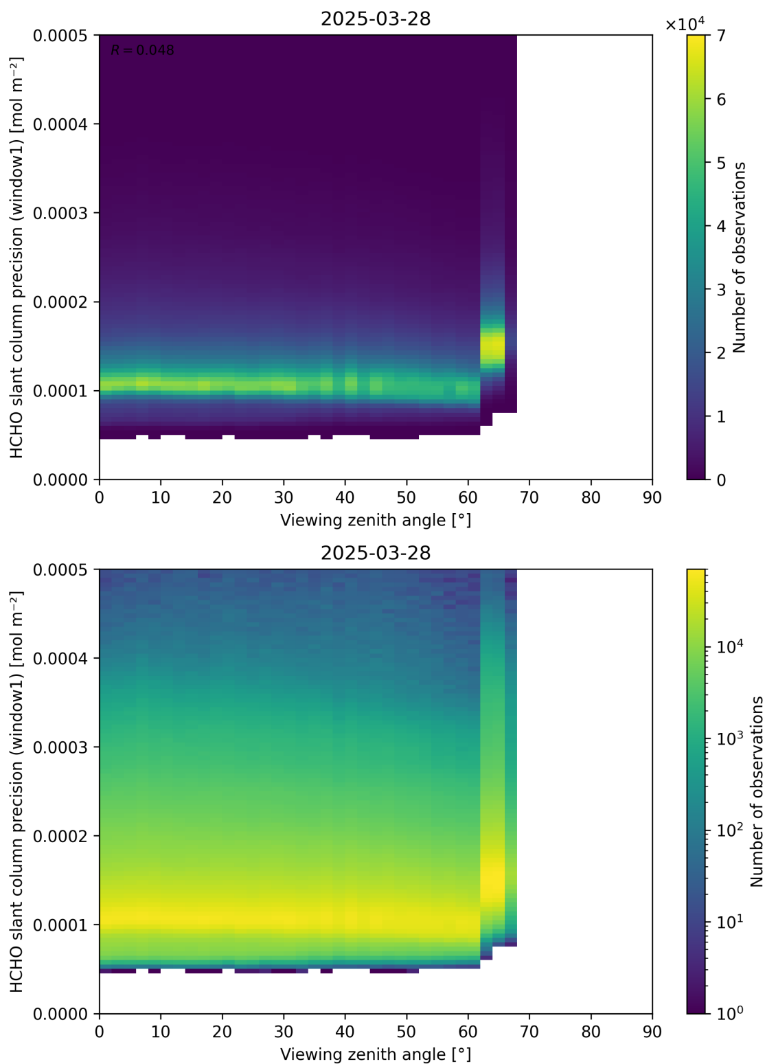
Figure 189: Scatter density plot of “Viewing zenith angle” against “HCHO slant column precision (window1)” for 2025-03-28 to 2025-03-29.
