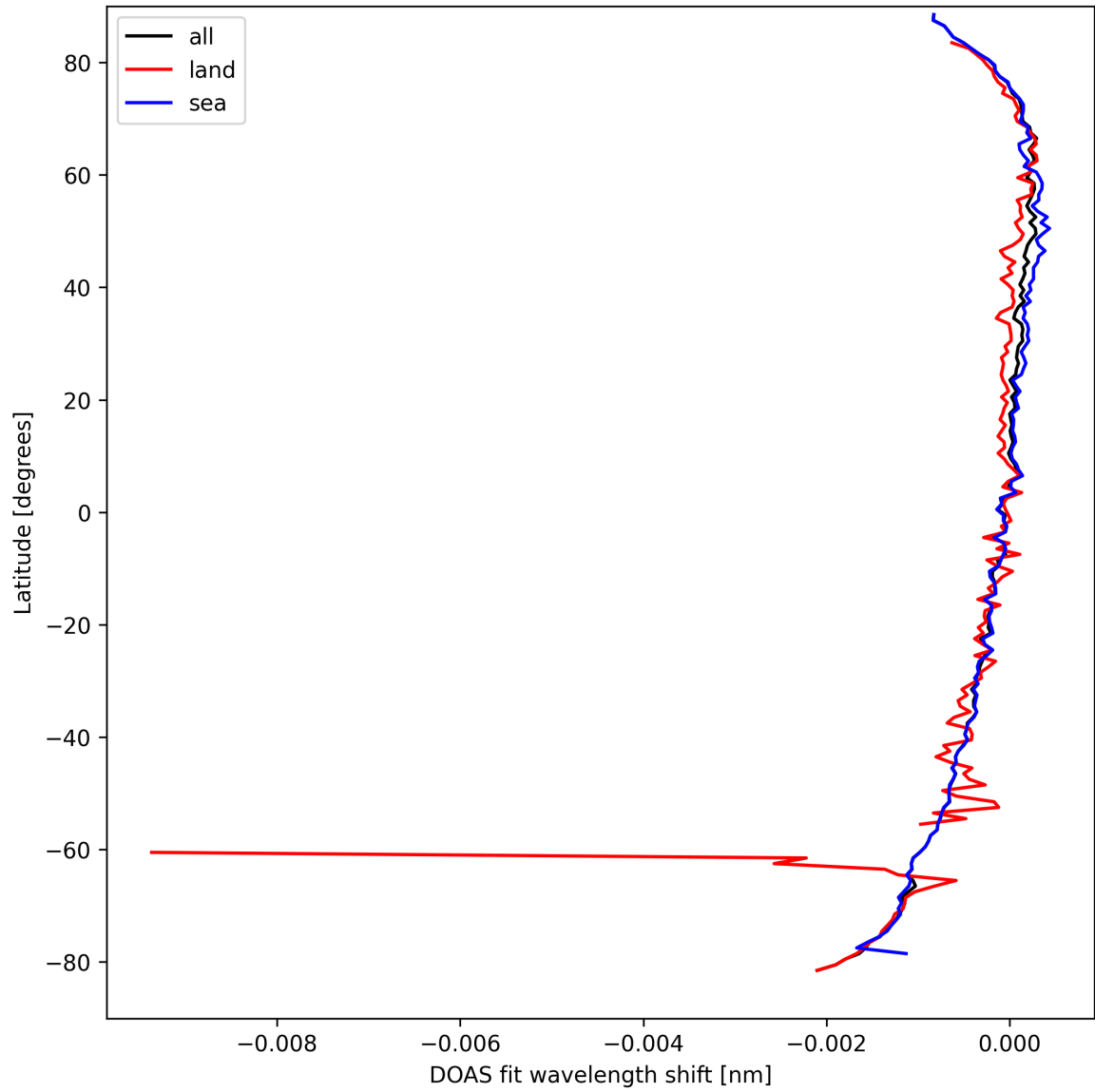
Figure 30: Zonal average of “DOAS fit wavelength shift” for 2025-03-28 to 2025-03-29.
