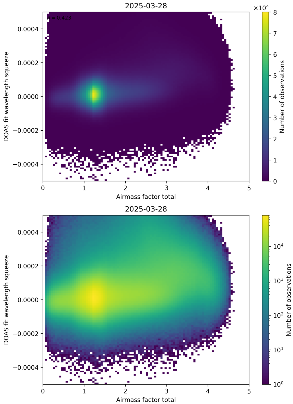
Figure 99: Scatter density plot of “Airmass factor total” against “DOAS fit wavelength squeeze” for 2025-03-28 to 2025-03-29.
