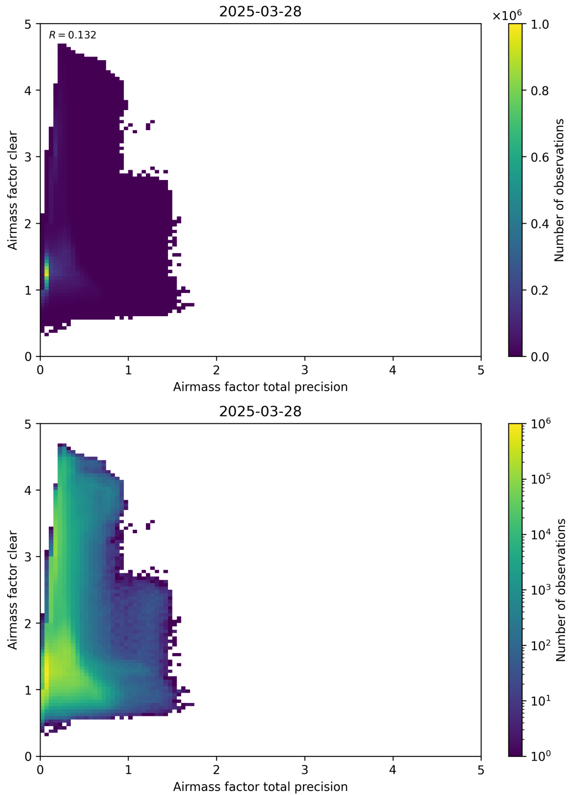
Figure 108: Scatter density plot of “Airmass factor total precision” against “Airmass factor clear” for 2025-03-28 to 2025-03-29.
