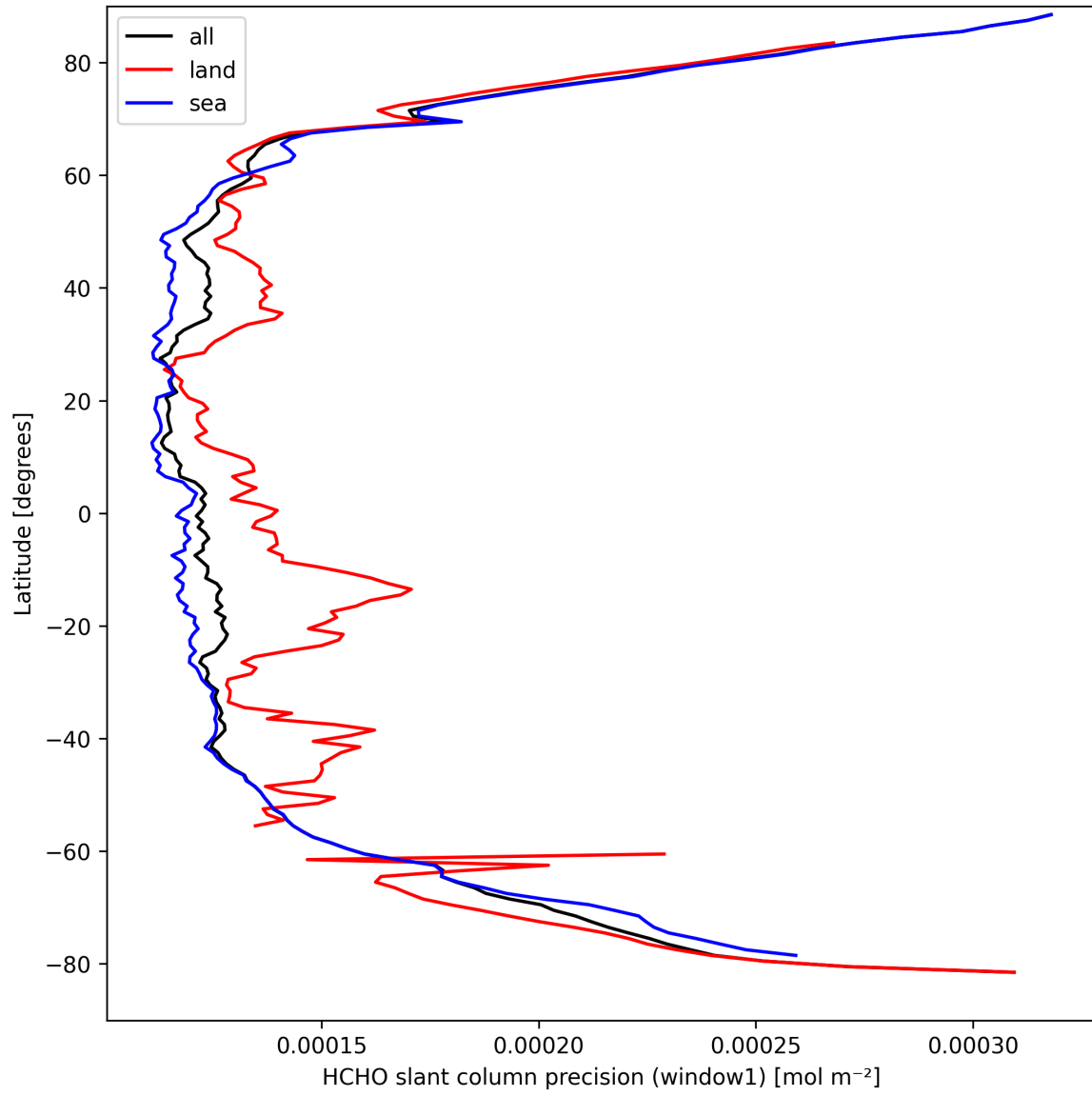
Figure 25: Zonal average of "HCHO slant column precision (window1)" for 2025-03-28 to 2025-03-29.
