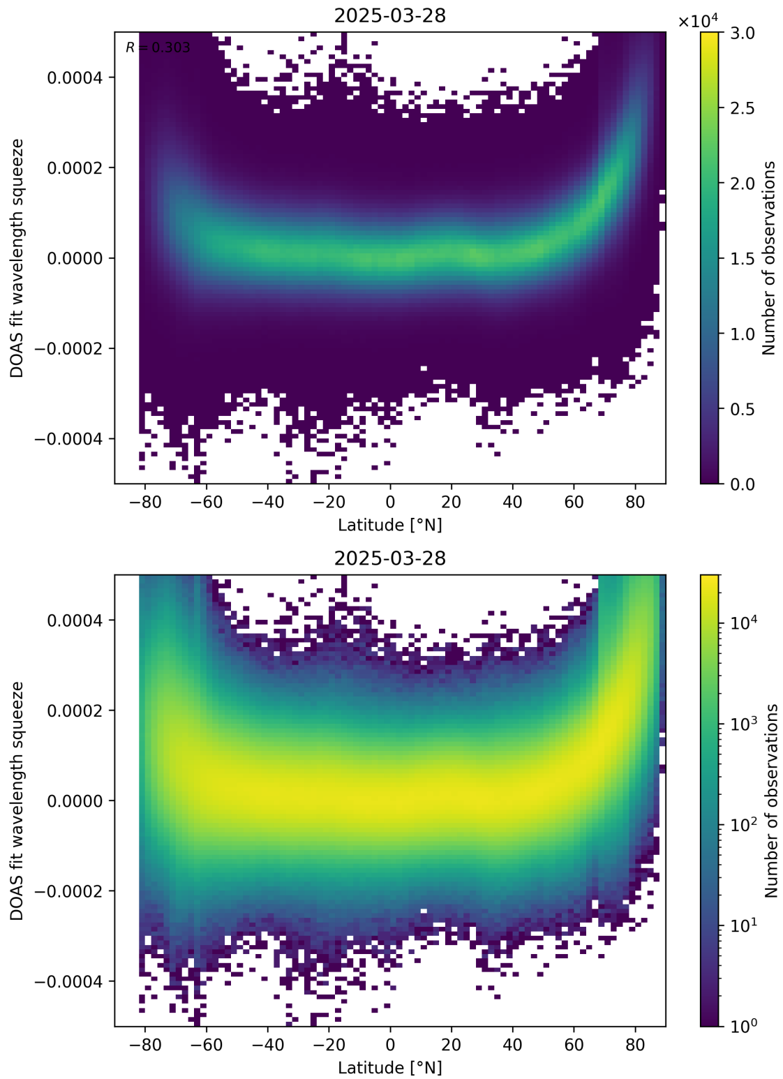
Figure 155: Scatter density plot of “Latitude” against “DOAS fit wavelength squeeze” for 2025-03-28 to 2025-03-29.
