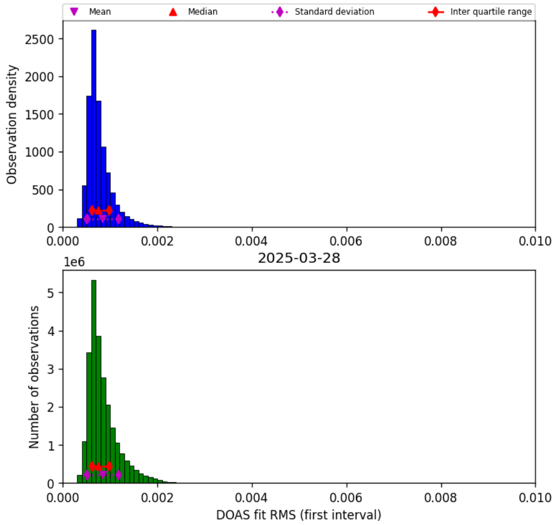
Figure 46: Histogram of “DOAS fit RMS (first interval)” for 2025-03-28 to 2025-03-29
