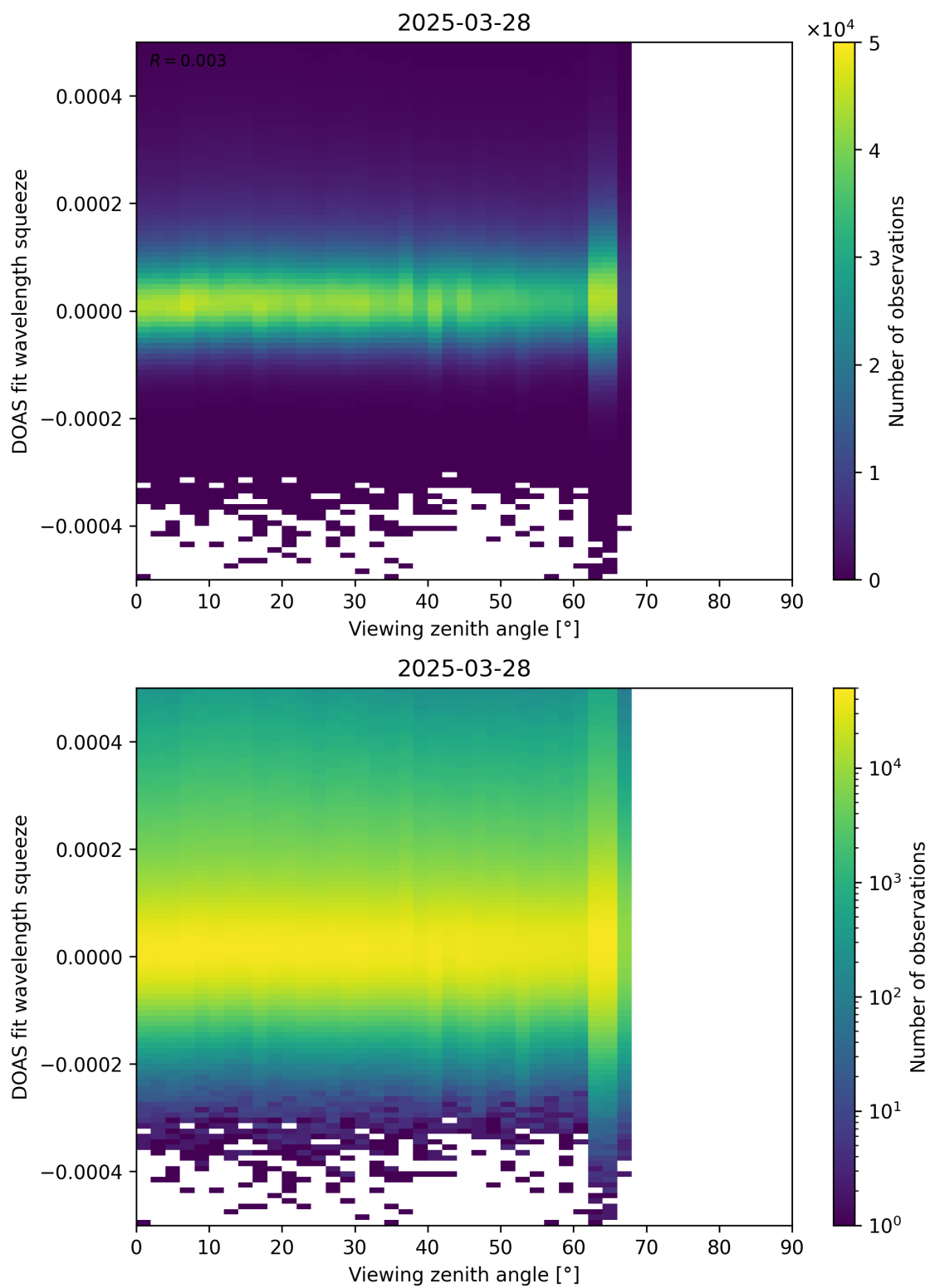
Figure 184: Scatter density plot of “Viewing zenith angle” against “DOAS fit wavelength squeeze” for 2025-03-28 to 2025-03-29.
