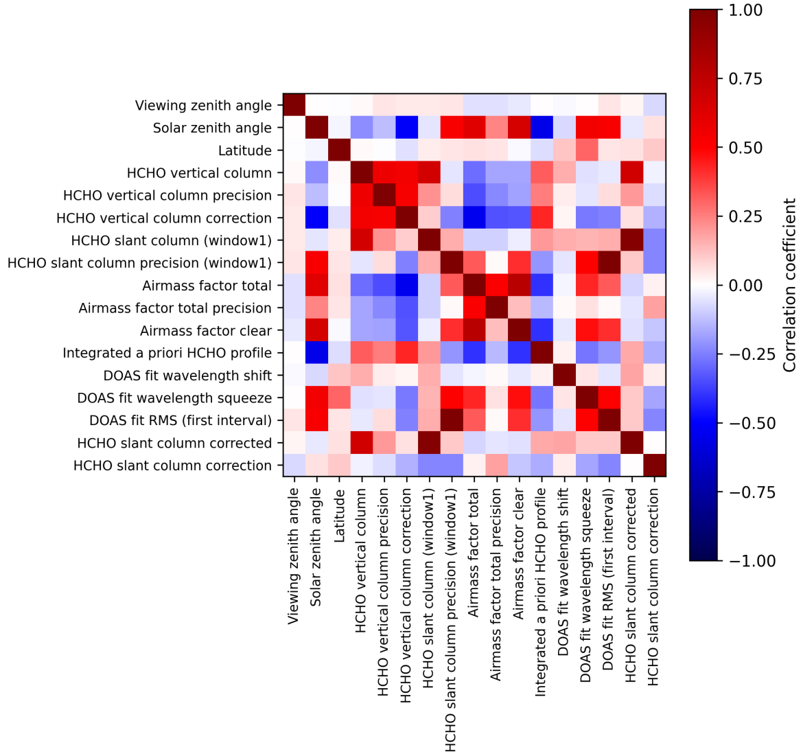
Figure 2: Map of correlation matrix for 2025-03-28 to 2025-03-29.
