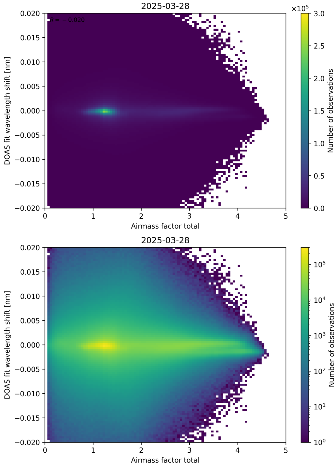
Figure 98: Scatter density plot of “Airmass factor total” against “DOAS fit wavelength shift” for 2025-03-28 to 2025-03-29.
