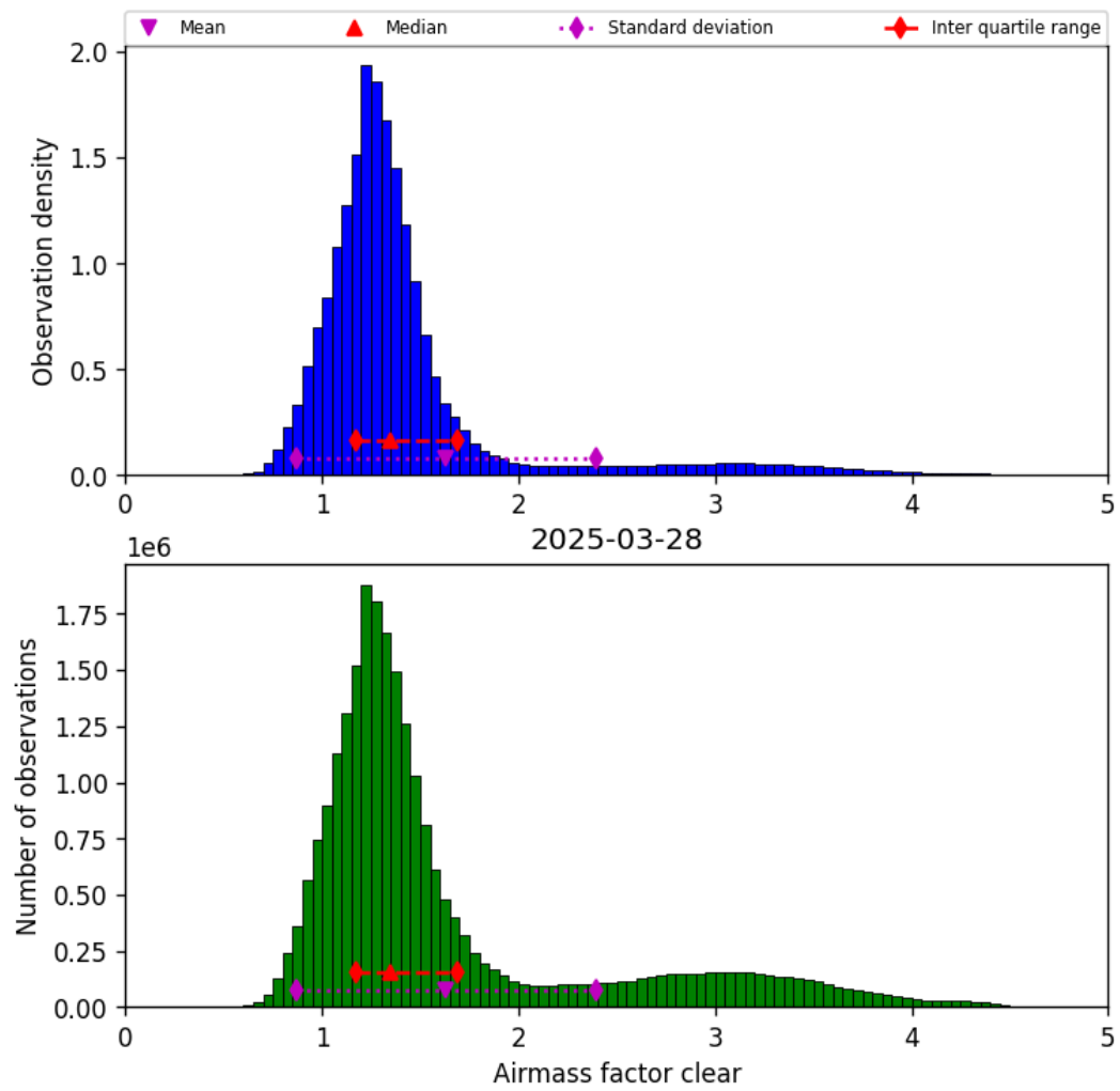
Figure 42: Histogram of “Airmass factor clear” for 2025-03-28 to 2025-03-29
