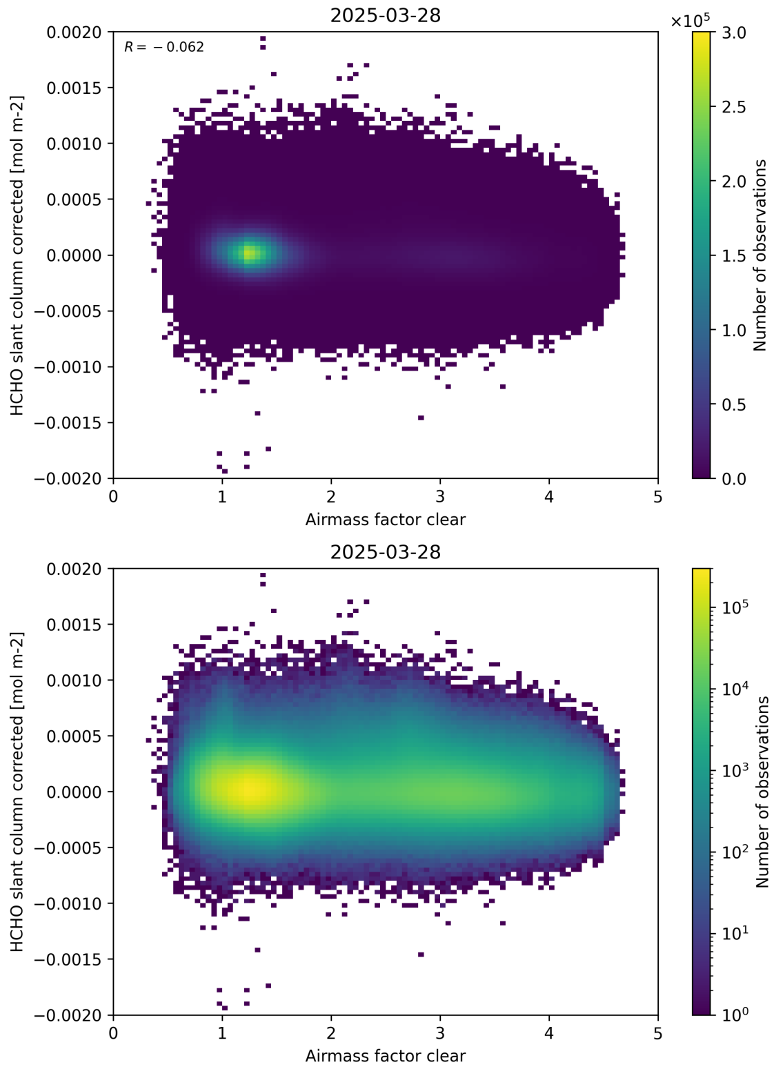
Figure 74: Scatter density plot of “Airmass factor clear” against “HCHO slant column corrected” for 2025-03-28 to 2025-03-29.
