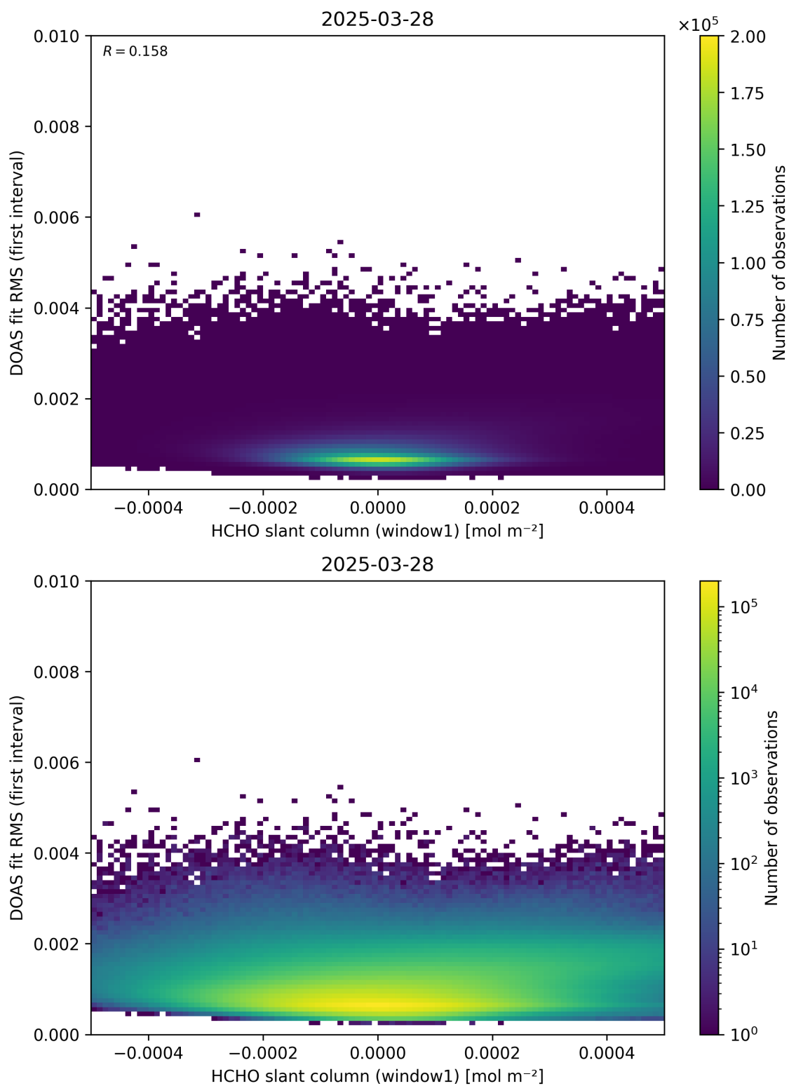
Figure 78: Scatter density plot of “HCHO slant column (window1)” against “DOAS fit RMS (first interval)” for 2025-03-28 to 2025-03-29.
