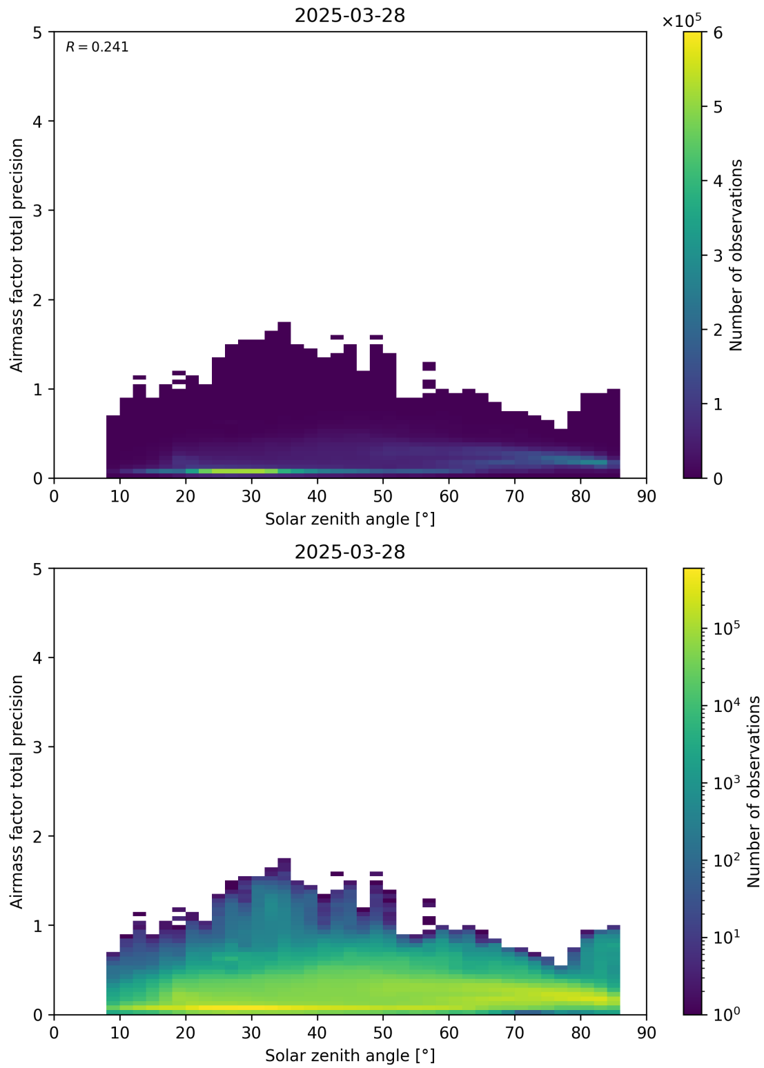
Figure 176: Scatter density plot of “Solar zenith angle” against “Airmass factor total precision” for 2025-03-28 to 2025-03-29.
