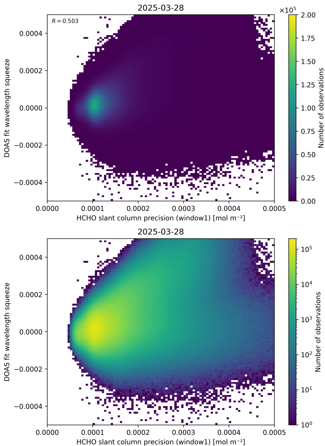
Figure 90: Scatter density plot of “HCHO slant column precision (window1)” against “DOAS fit wavelength squeeze” for 2025-03-28 to 2025-03-29.
