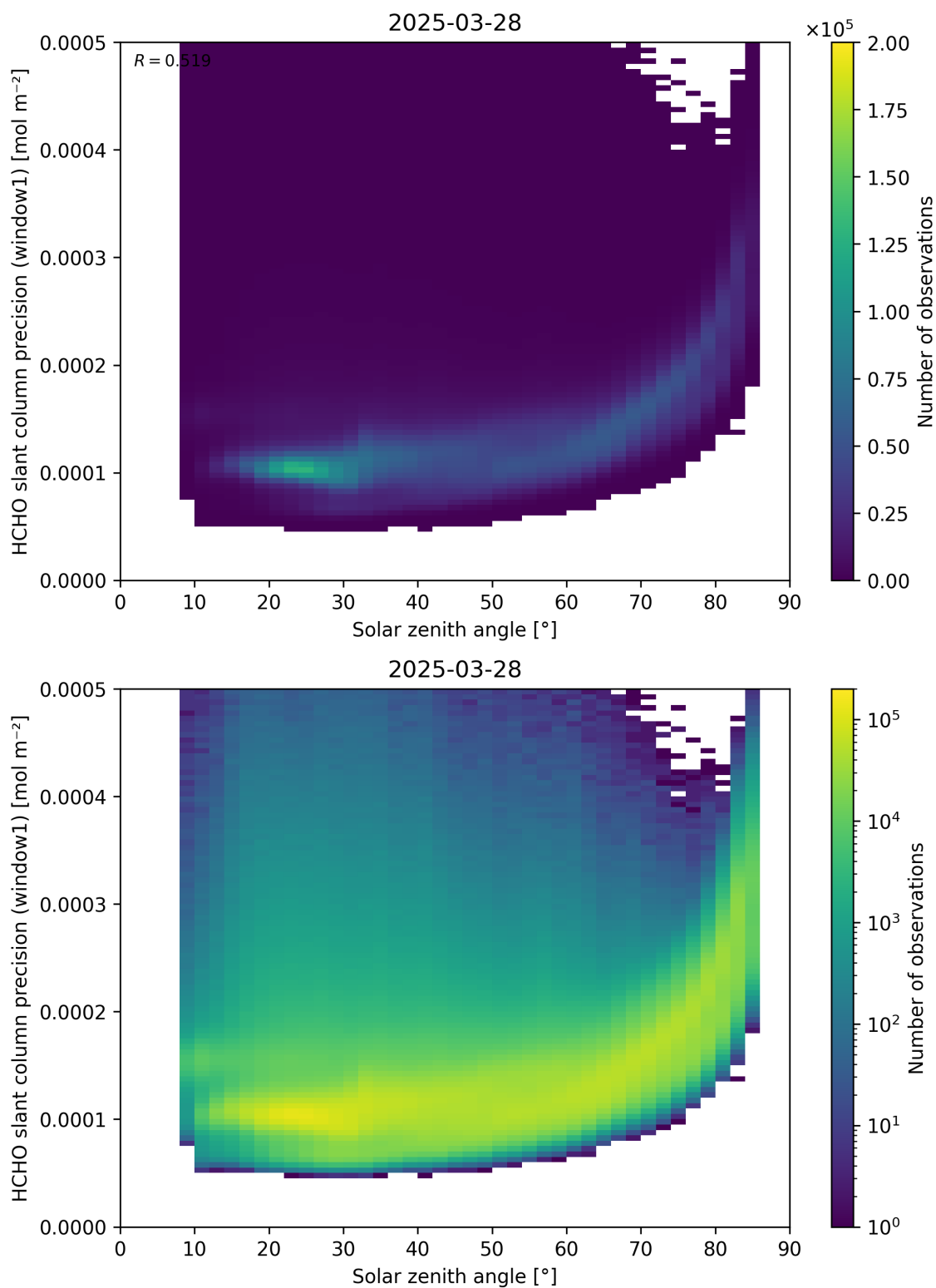
Figure 174: Scatter density plot of “Solar zenith angle” against “HCHO slant column precision (window1)” for 2025-03-28 to 2025-03-29.
