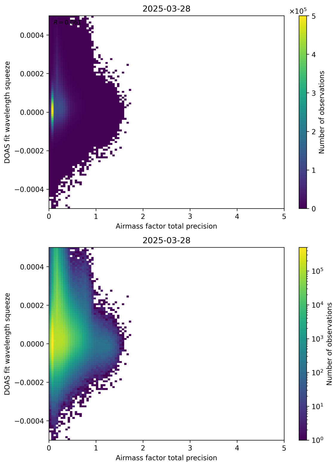
Figure 107: Scatter density plot of “Airmass factor total precision” against “DOAS fit wavelength squeeze” for 2025-03-28 to 2025-03-29.
