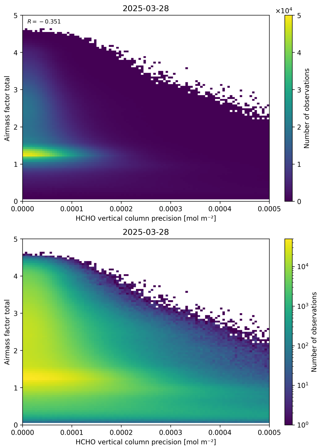
Figure 144: Scatter density plot of “HCHO vertical column precision” against “Airmass factor total” for 2025-03-28 to 2025-03-29.
