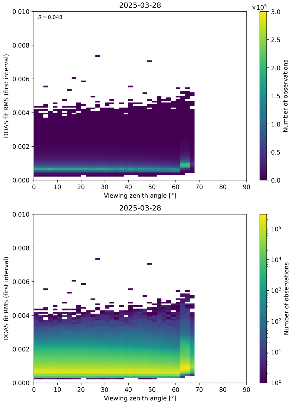
Figure 182: Scatter density plot of “Viewing zenith angle” against “DOAS fit RMS (first interval)” for 2025-03-28 to 2025-03-29.
