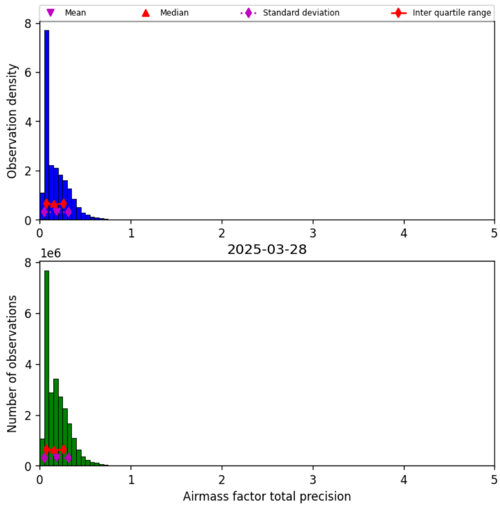
Figure 41: Histogram of “Airmass factor total precision” for 2025-03-28 to 2025-03-29
