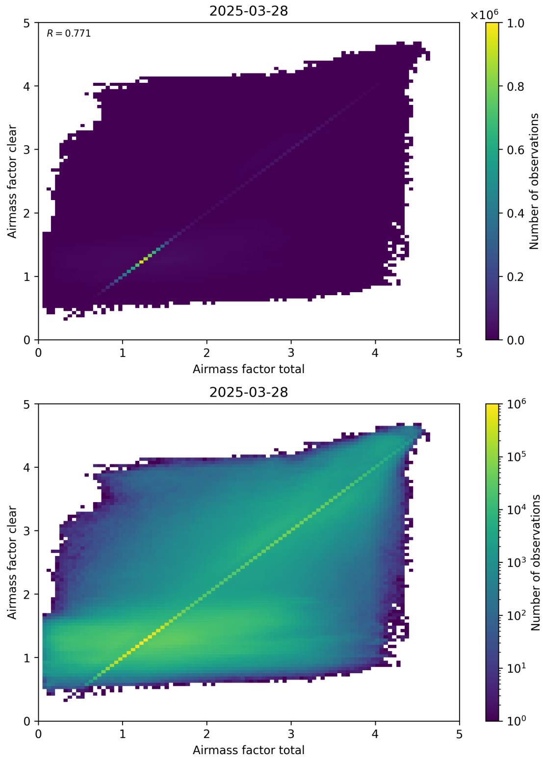
Figure 100: Scatter density plot of “Airmass factor total” against “Airmass factor clear” for 2025-03-28 to 2025-03-29.
