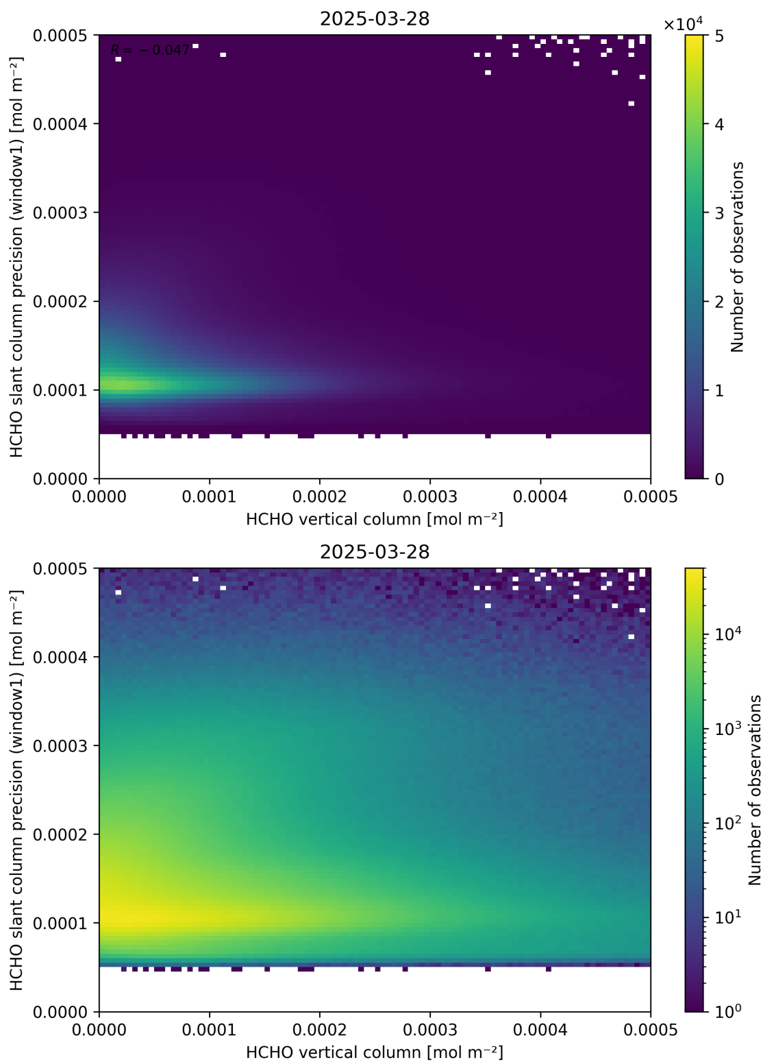
Figure 130: Scatter density plot of “HCHO vertical column” against “HCHO slant column precision (window1)” for 2025-03-28 to 2025-03-29.
