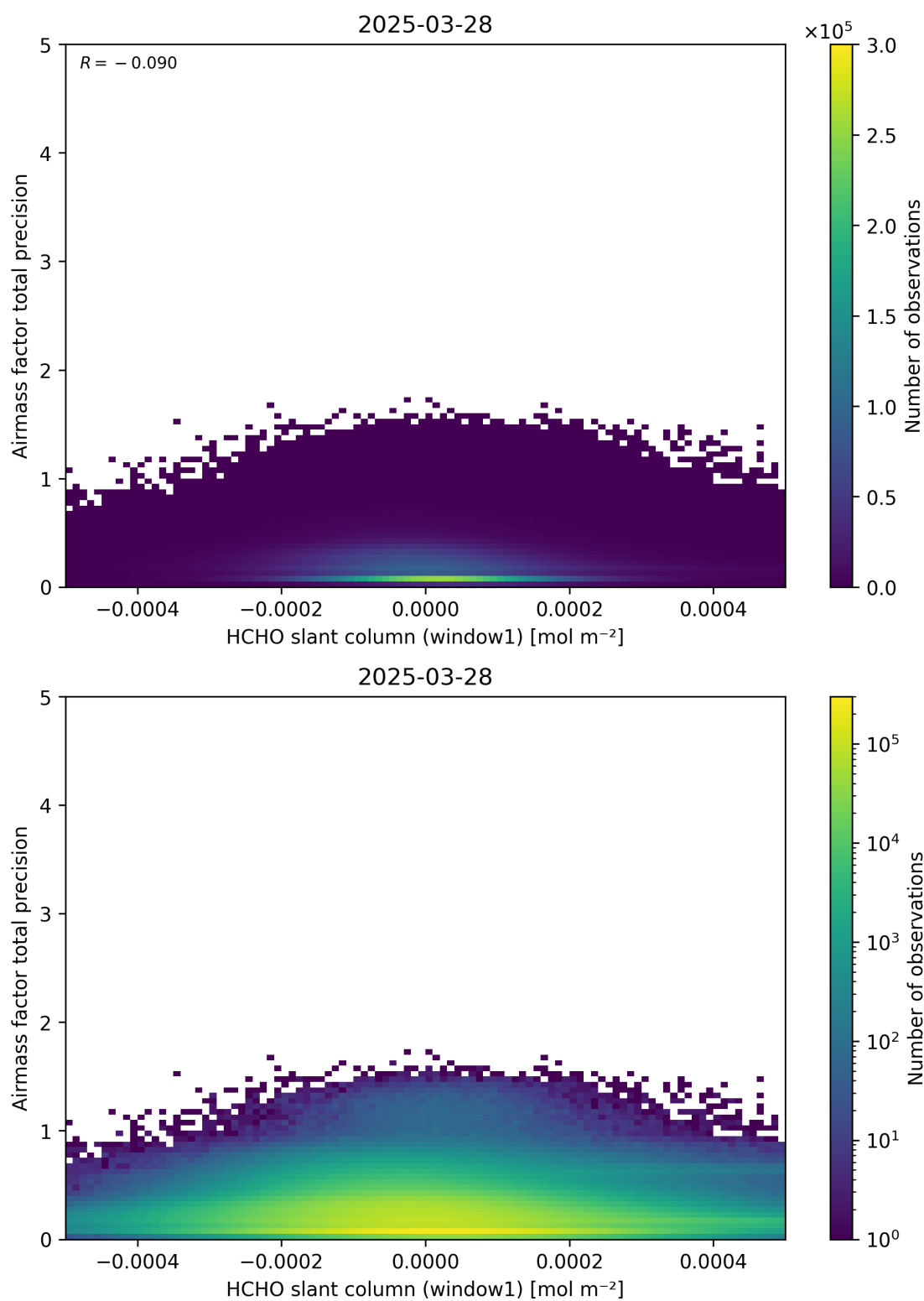
Figure 86: Scatter density plot of “HCHO slant column (window1)” against “Airmass factor total precision” for 2025-03-28 to 2025-03-29.
