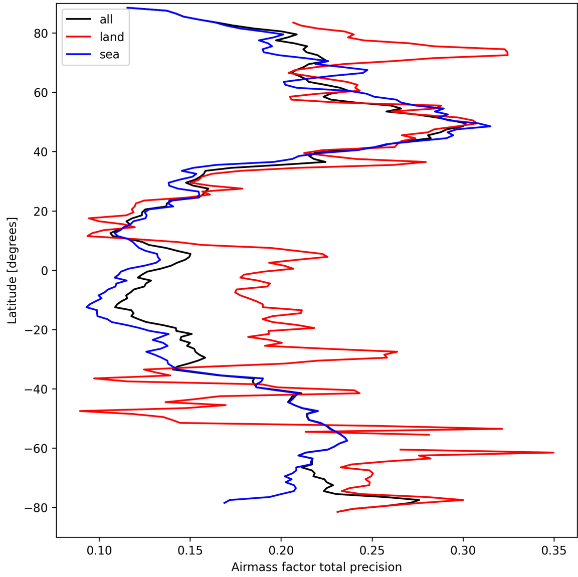
Figure 27: Zonal average of “Airmass factor total precision” for 2025-03-28 to 2025-03-29.
