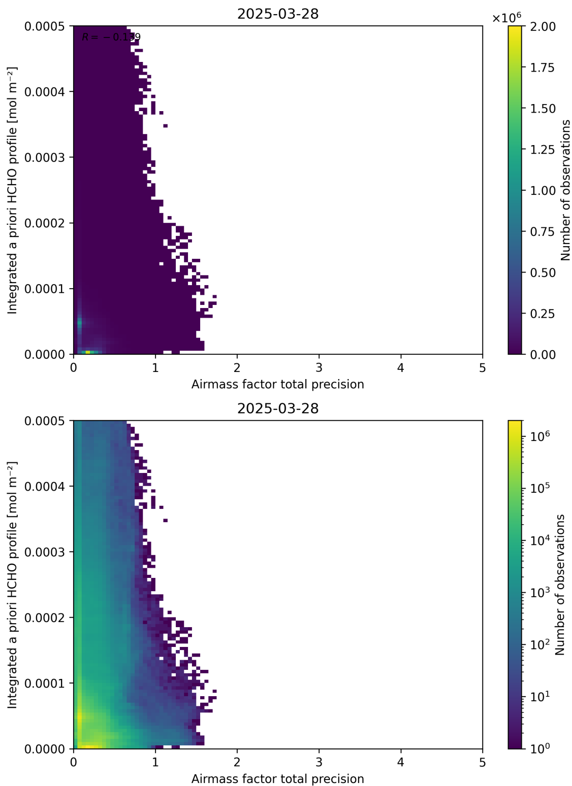
Figure 111: Scatter density plot of “Airmass factor total precision” against “Integrated a priori HCHO profile” for 2025-03-28 to 2025-03-29.
