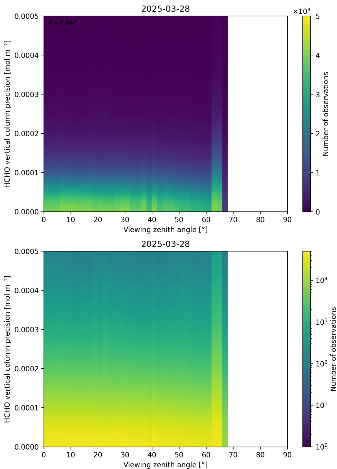
Figure 194: Scatter density plot of “Viewing zenith angle” against “HCHO vertical column precision” for 2025-03-28 to 2025-03-29.
