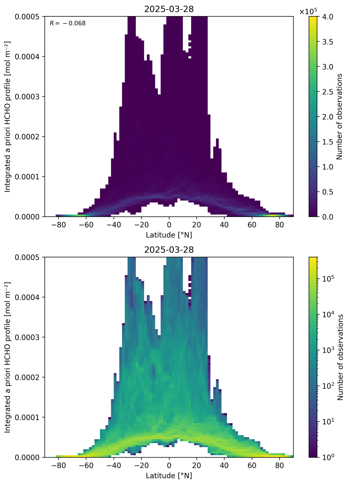
Figure 166: Scatter density plot of “Latitude” against “Integrated a priori HCHO profile” for 2025-03-28 to 2025-03-29.
