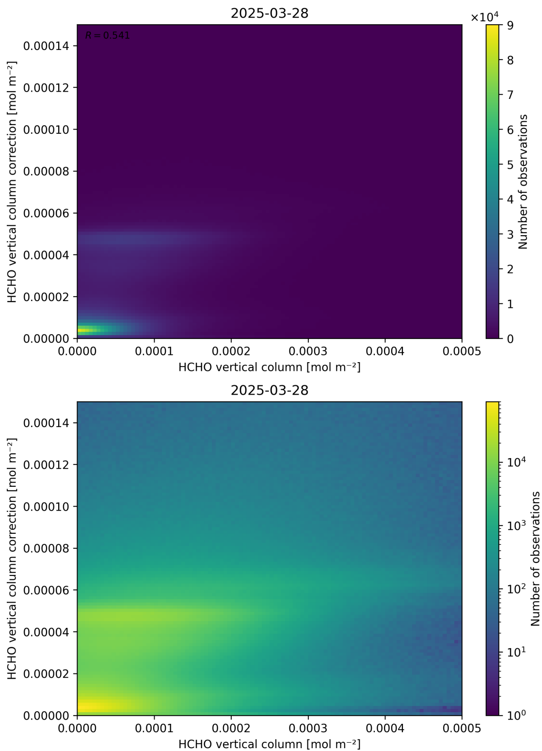
Figure 133: Scatter density plot of “HCHO vertical column” against “HCHO vertical column correction” for 2025-03-28 to 2025-03-29.
