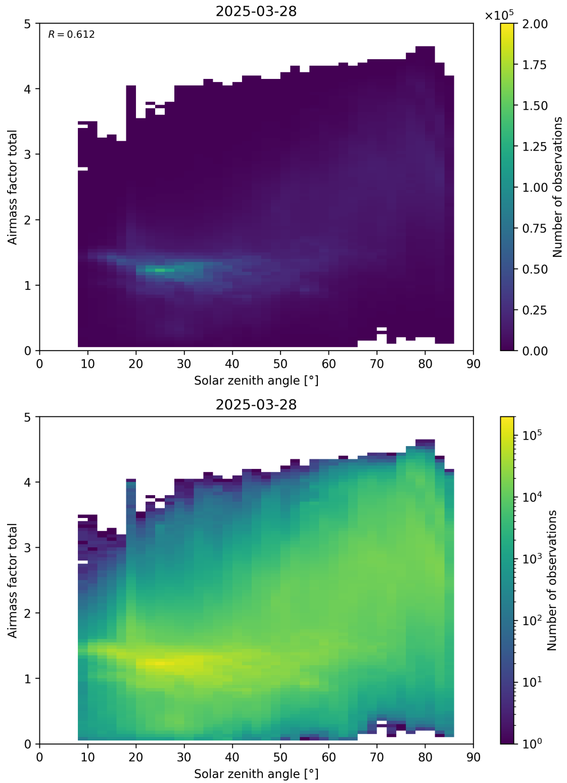
Figure 175: Scatter density plot of “Solar zenith angle” against “Airmass factor total” for 2025-03-28 to 2025-03-29.
