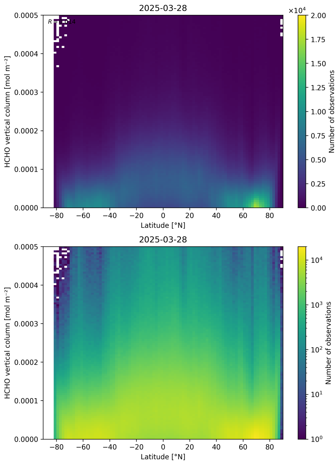
Figure 163: Scatter density plot of “Latitude” against “HCHO vertical column” for 2025-03-28 to 2025-03-29.
