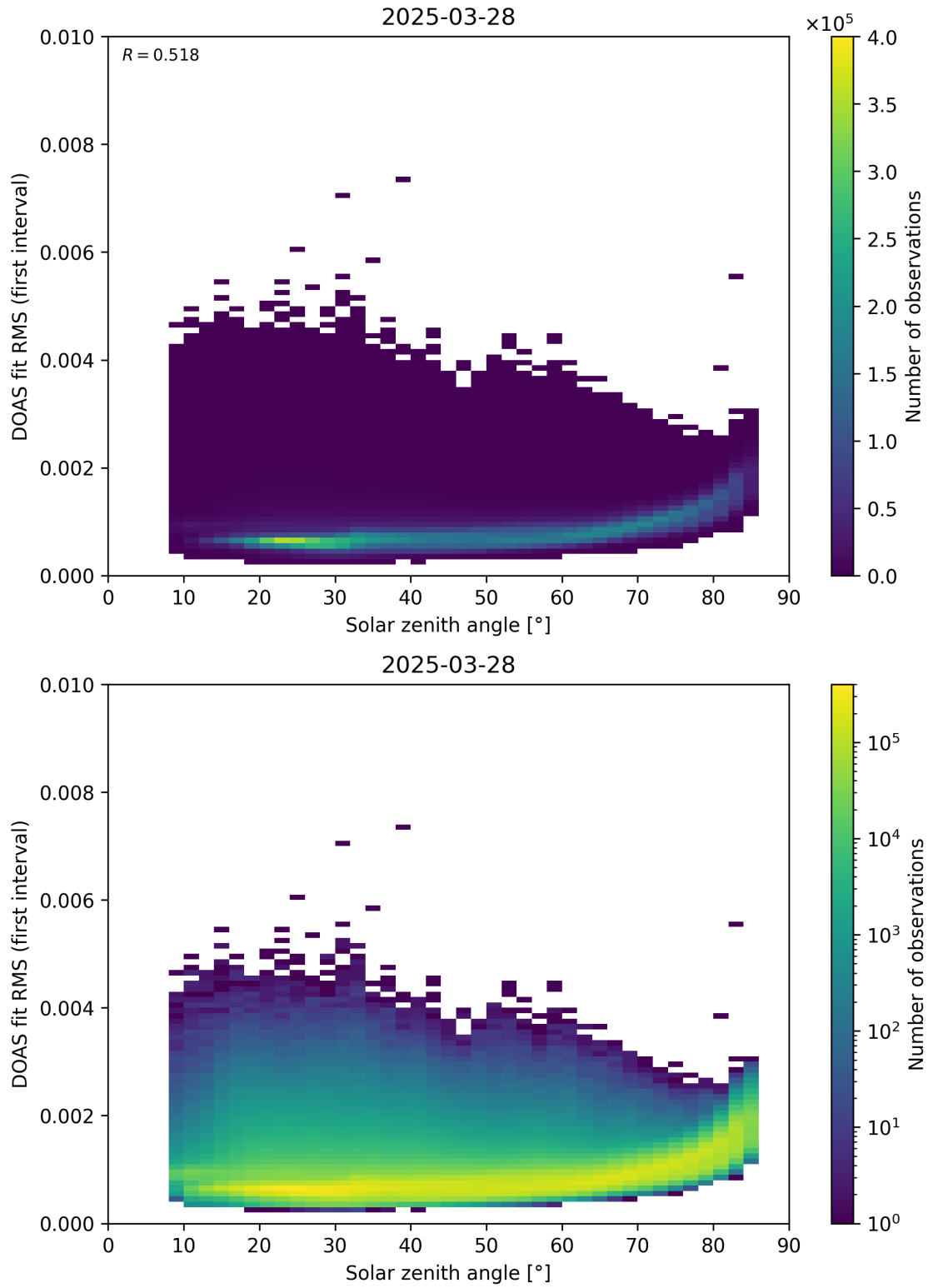
Figure 167: Scatter density plot of “Solar zenith angle” against “DOAS fit RMS (first interval)” for 2025-03-28 to 2025-03-29.
