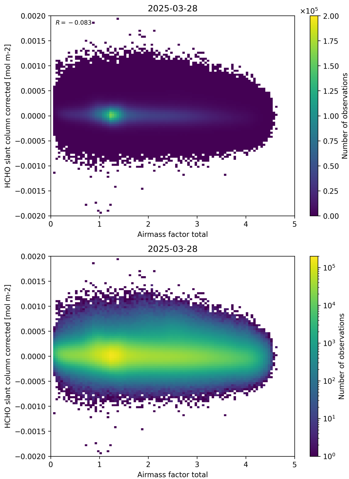
Figure 101: Scatter density plot of “Airmass factor total” against “HCHO slant column corrected” for 2025-03-28 to 2025-03-29.
