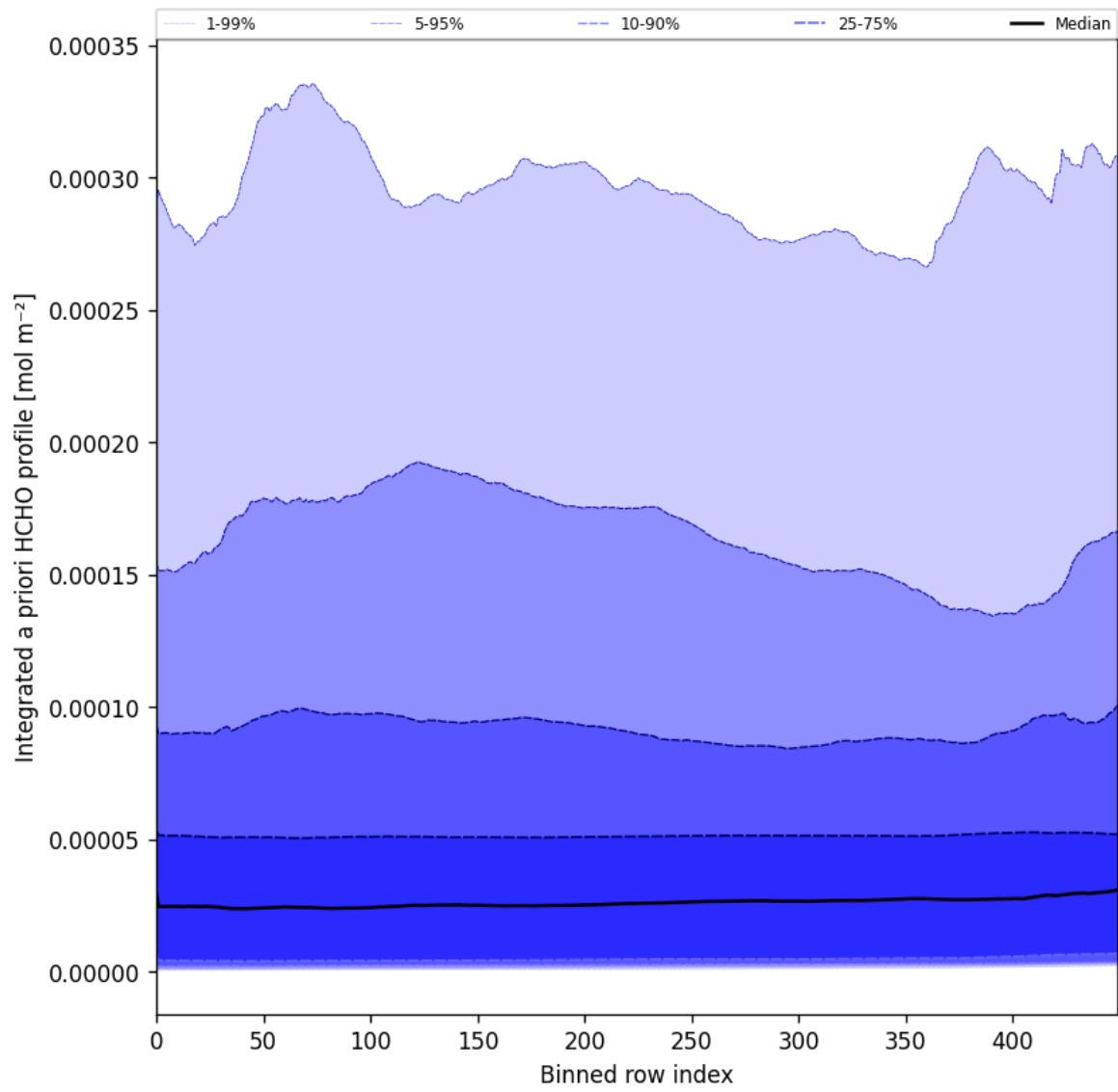
Figure 57: Along track statistics of “Integrated a priori HCHO profile” for 2025-03-28 to 2025-03-29
