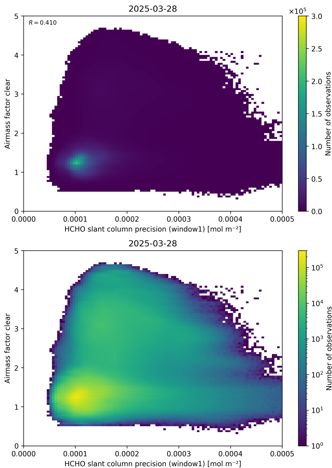
Figure 91: Scatter density plot of “HCHO slant column precision (window1)” against “Airmass factor clear” for 2025-03-28 to 2025-03-29.
