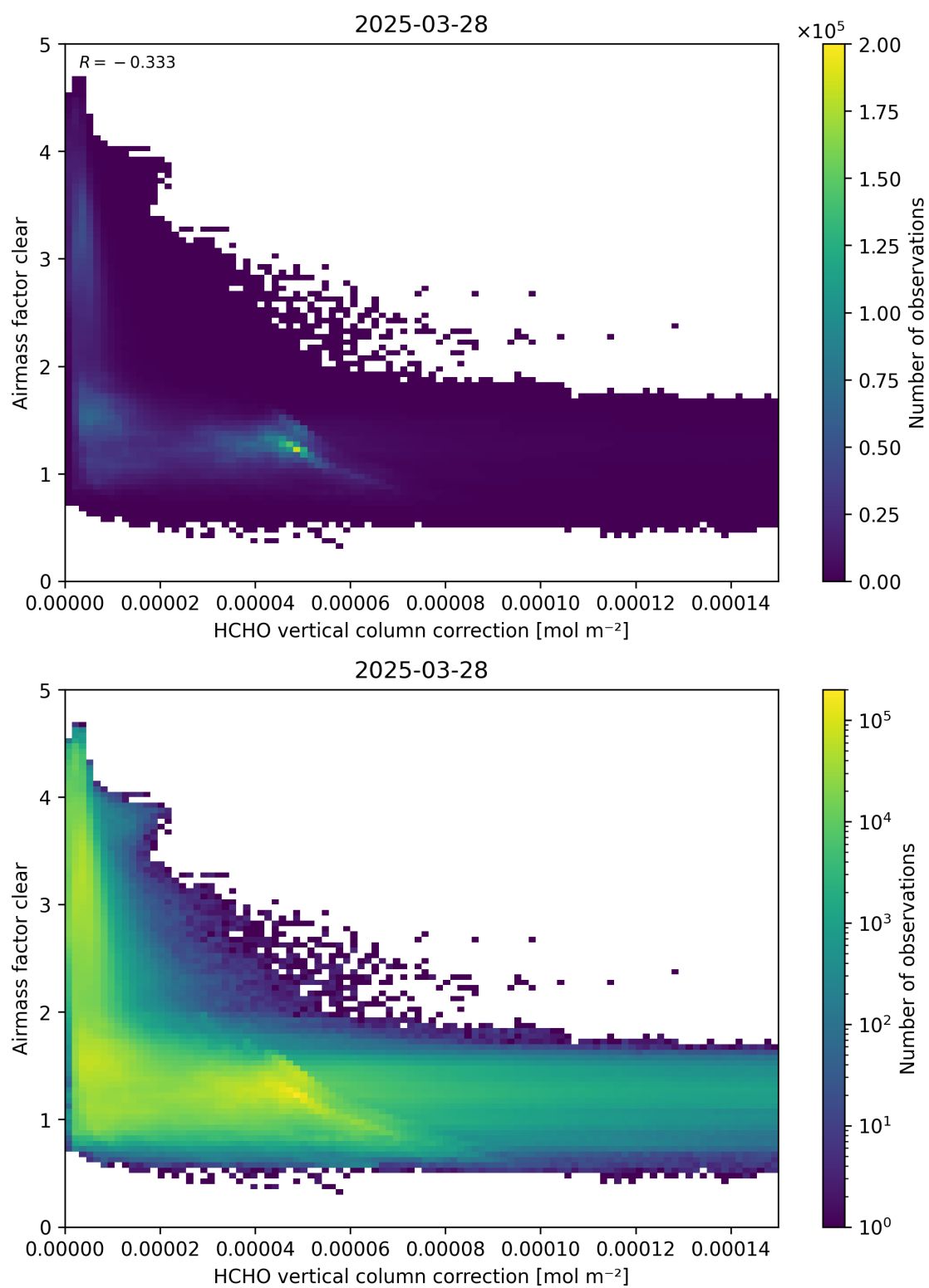
Figure 115: Scatter density plot of “HCHO vertical column correction” against “Airmass factor clear” for 2025-03-28 to 2025-03-29.
