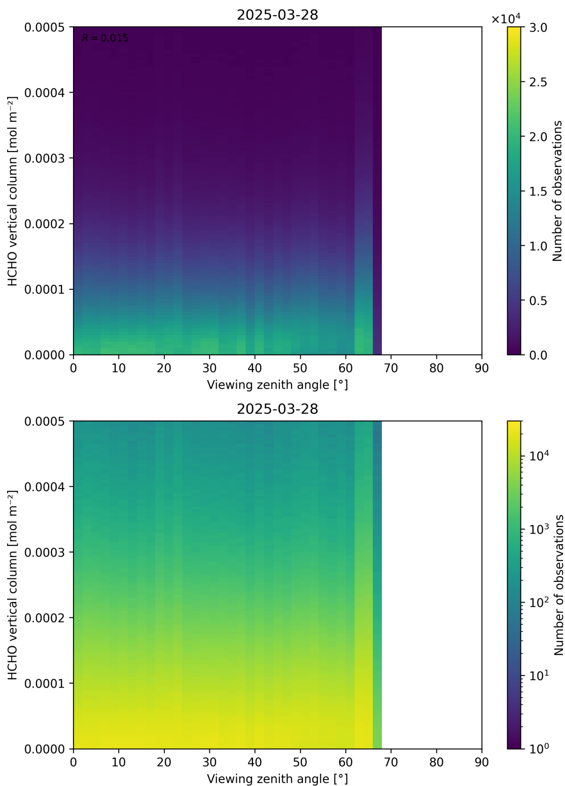
Figure 192: Scatter density plot of “Viewing zenith angle” against “HCHO vertical column” for 2025-03-28 to 2025-03-29.
