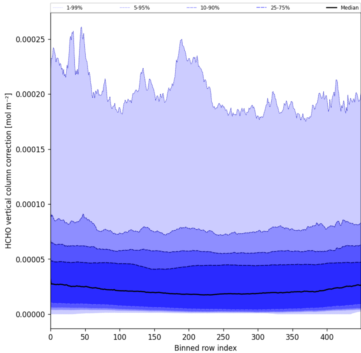
Figure 51: Along track statistics of “HCHO vertical column correction” for 2025-03-28 to 2025-03-29
