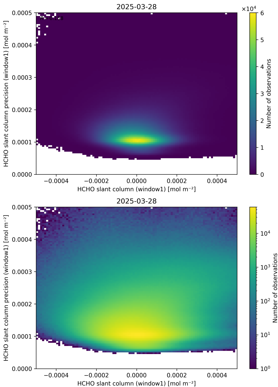
Figure 84: Scatter density plot of “HCHO slant column (window1)” against “HCHO slant column precision (window1)” for 2025-03-28 to 2025-03-29.
