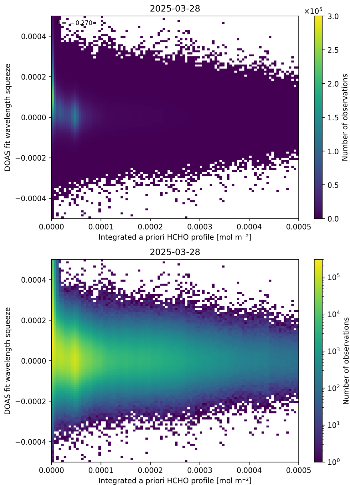
Figure 150: Scatter density plot of “Integrated a priori HCHO profile” against “DOAS fit wavelength squeeze” for 2025-03-28 to 2025-03-29.
