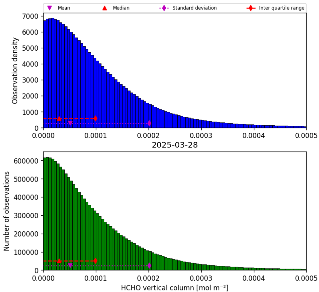
Figure 35: Histogram of “HCHO vertical column” for 2025-03-28 to 2025-03-29
