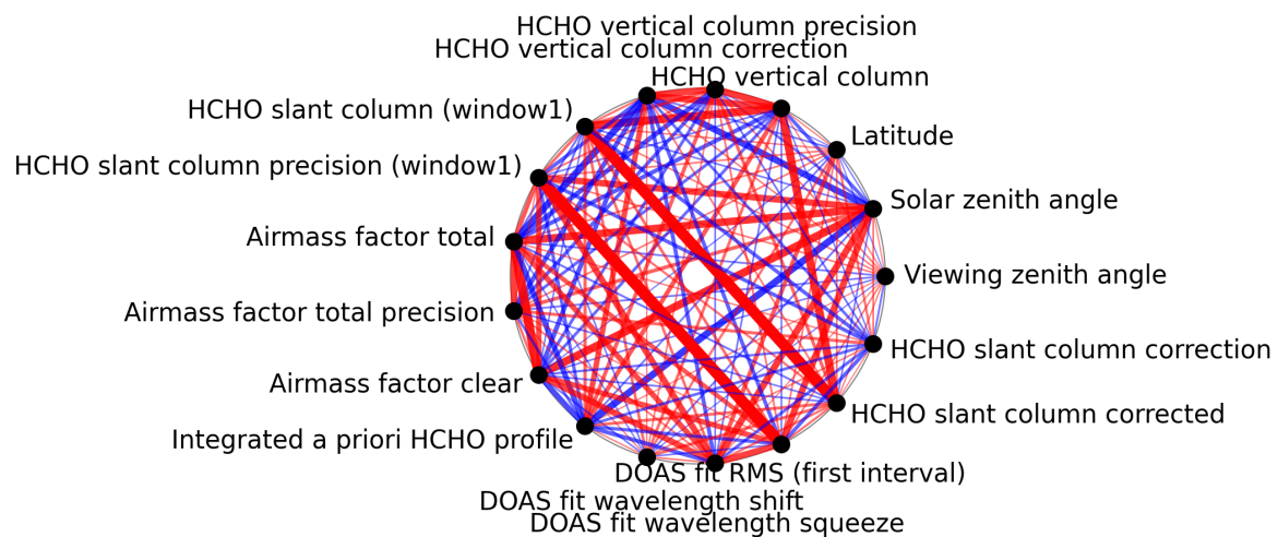
Figure 1: Map of correlation graph for 2025-03-28 to 2025-03-29.
