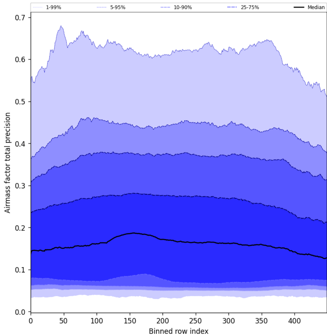
Figure 55: Along track statistics of “Airmass factor total precision” for 2025-03-28 to 2025-03-29
