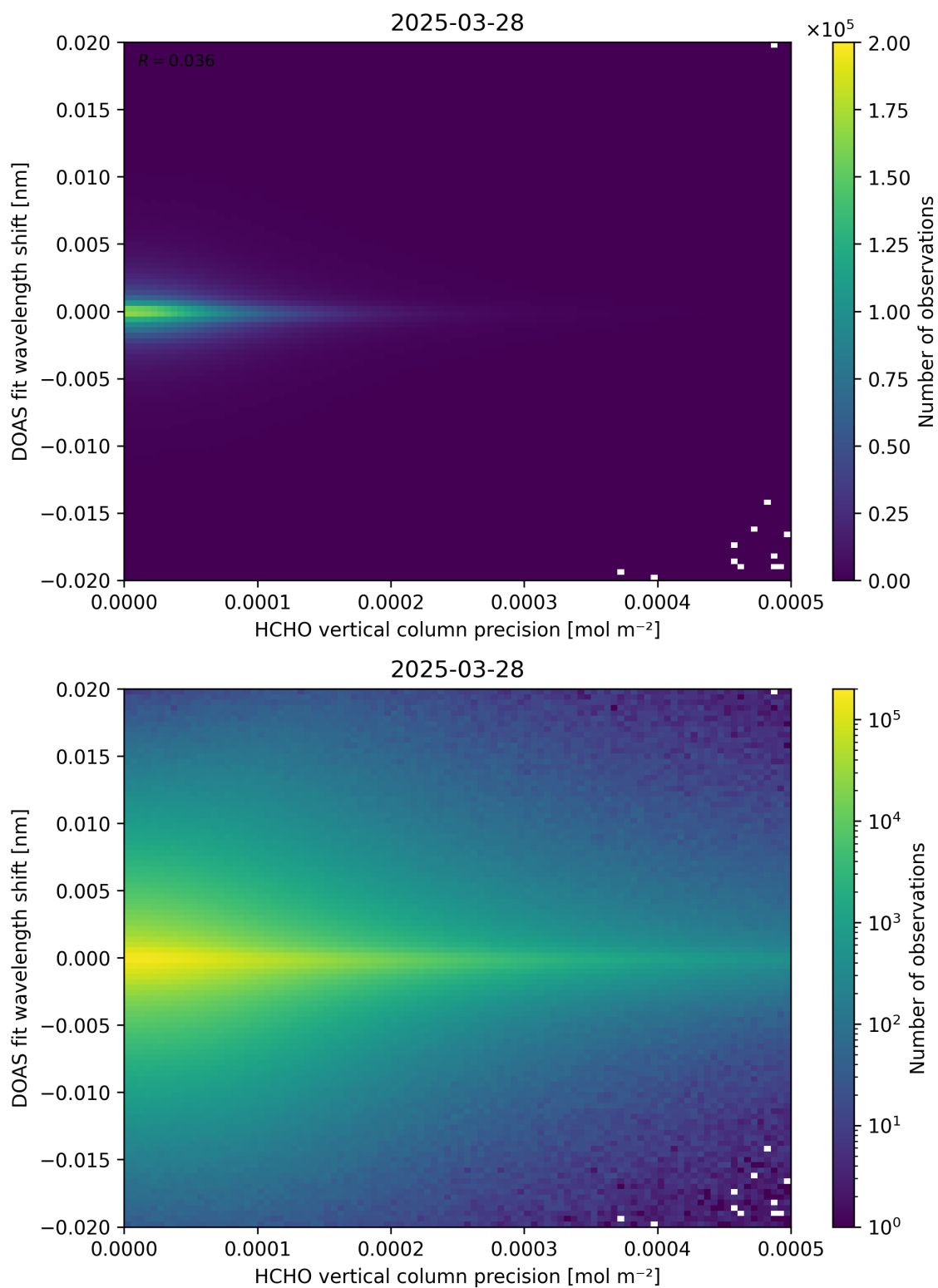
Figure 137: Scatter density plot of “HCHO vertical column precision” against “DOAS fit wavelength shift” for 2025-03-28 to 2025-03-29.
