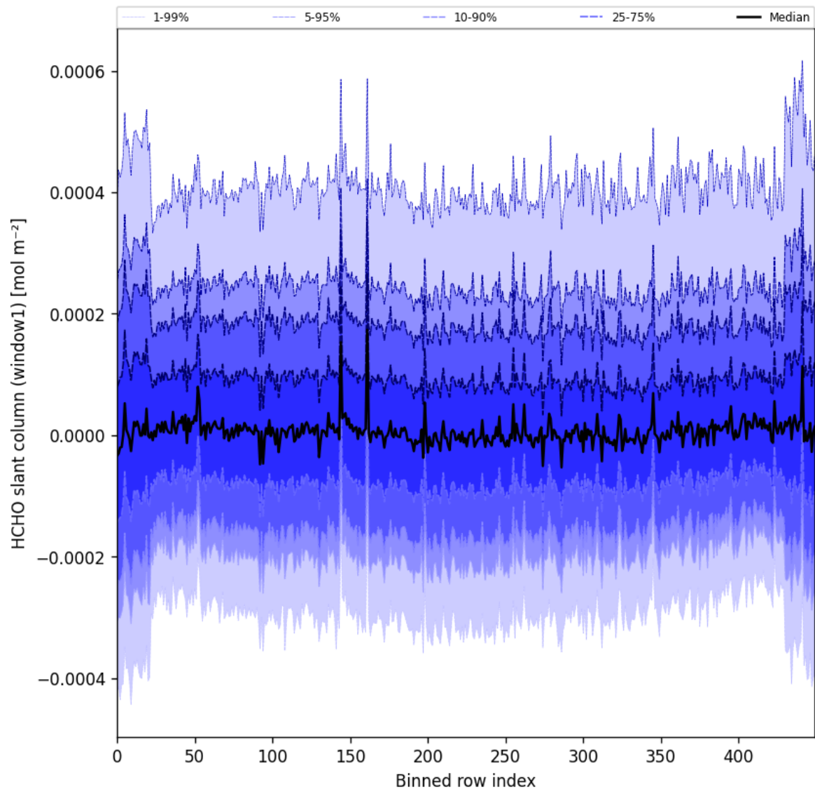
Figure 52: Along track statistics of “HCHO slant column (window1)” for 2025-03-28 to 2025-03-29
