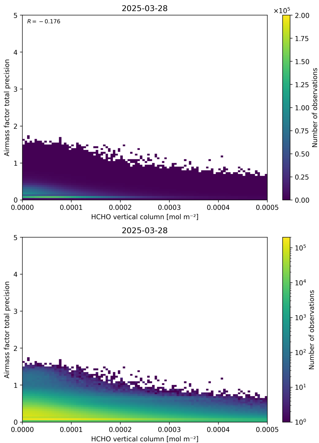
Figure 132: Scatter density plot of “HCHO vertical column” against “Airmass factor total precision” for 2025-03-28 to 2025-03-29.
