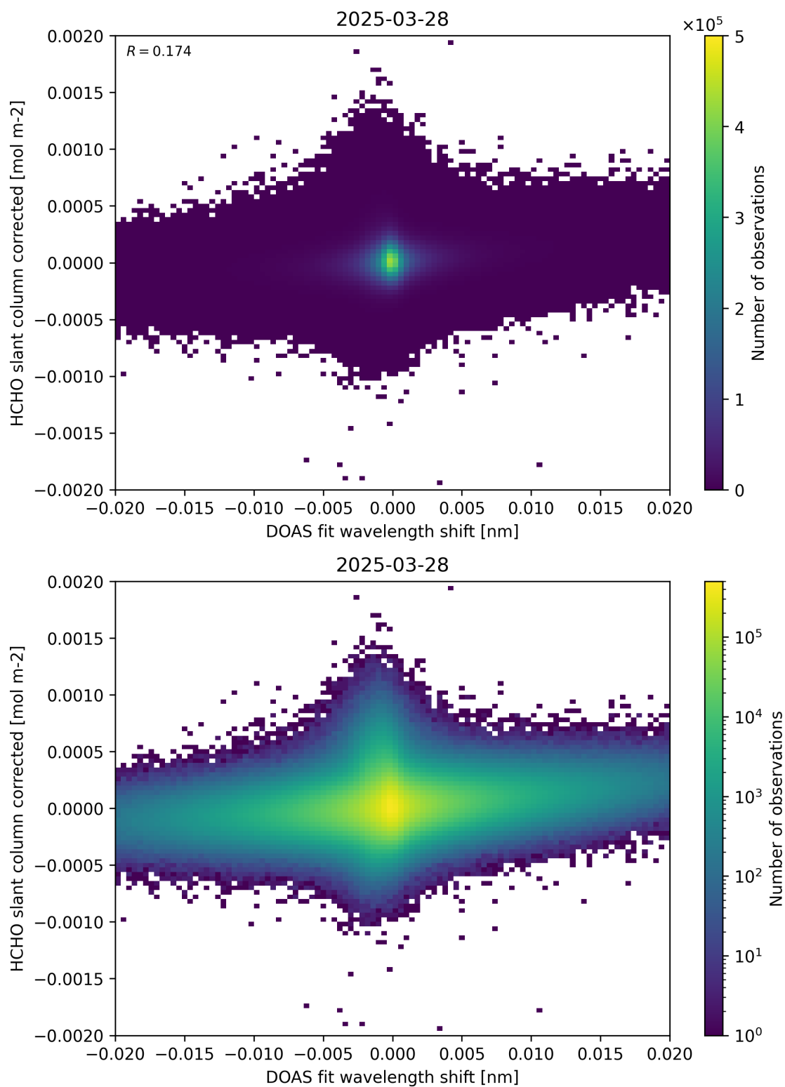
Figure 66: Scatter density plot of “DOAS fit wavelength shift” against “HCHO slant column corrected” for 2025-03-28 to 2025-03-29.
