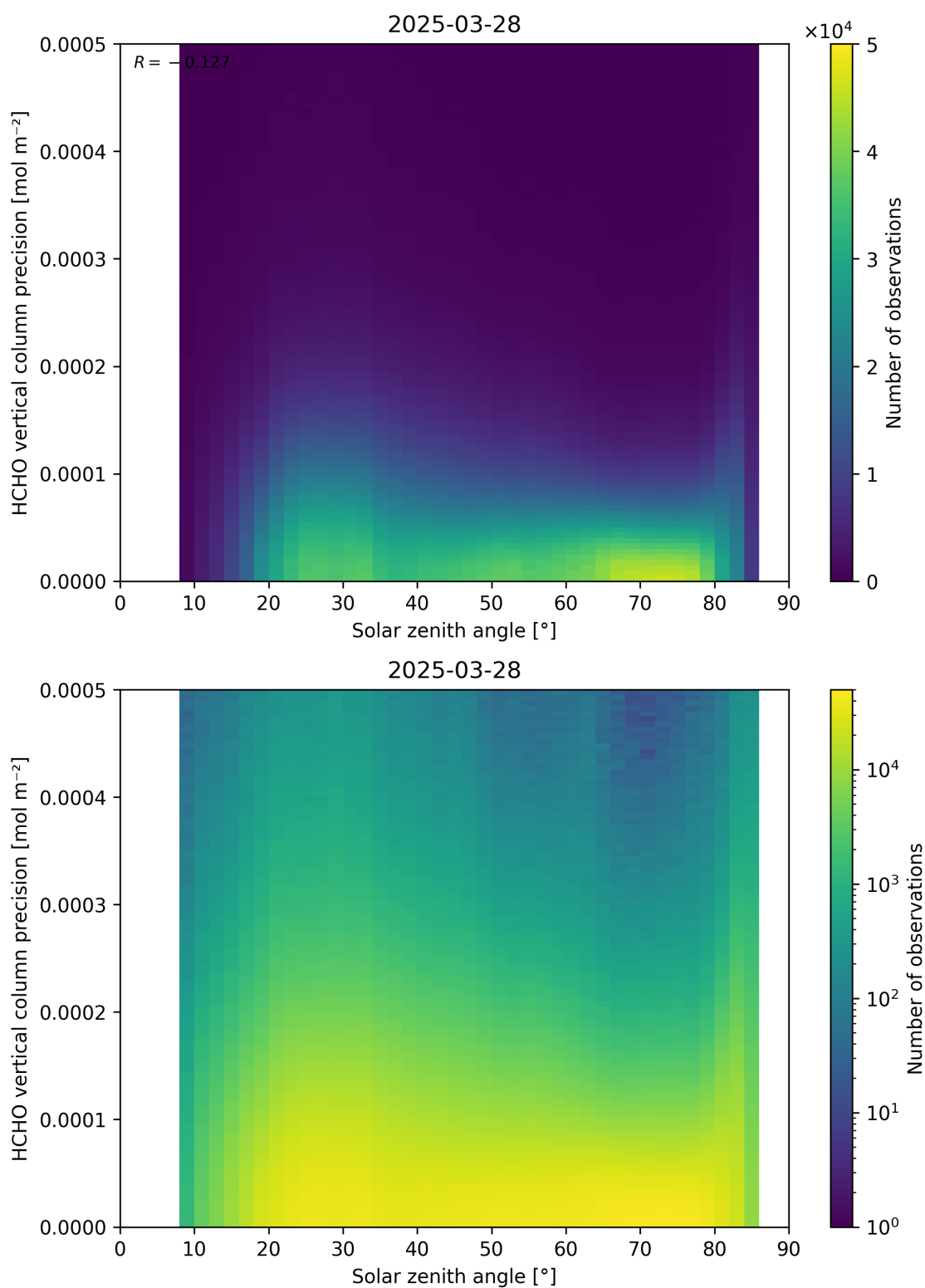
Figure 179: Scatter density plot of “Solar zenith angle” against “HCHO vertical column precision” for 2025-03-28 to 2025-03-29.
