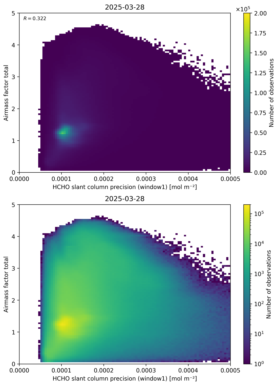
Figure 94: Scatter density plot of “HCHO slant column precision (window1)” against “Airmass factor total” for 2025-03-28 to 2025-03-29.
