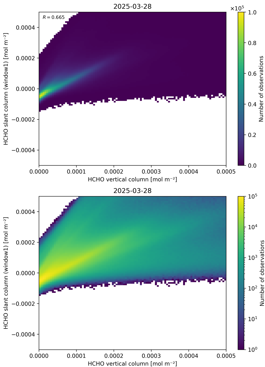
Figure 129: Scatter density plot of “HCHO vertical column” against “HCHO slant column (window1)” for 2025-03-28 to 2025-03-29.
