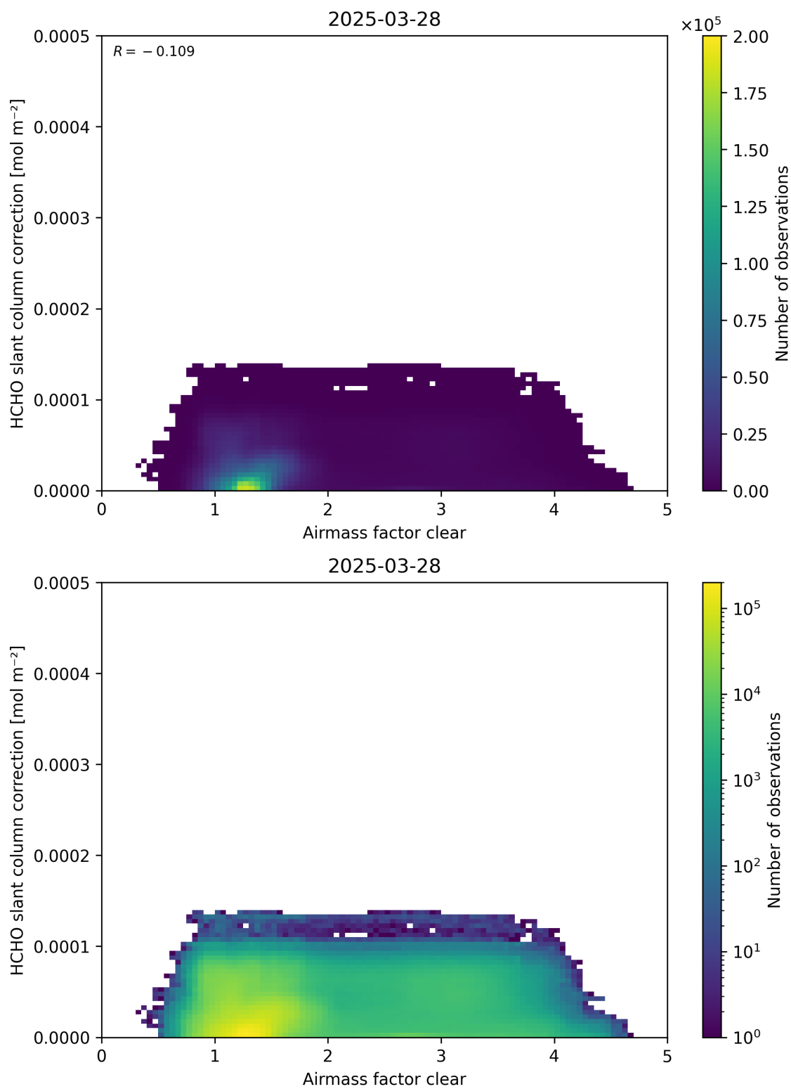
Figure 75: Scatter density plot of “Airmass factor clear” against “HCHO slant column correction” for 2025-03-28 to 2025-03-29.
