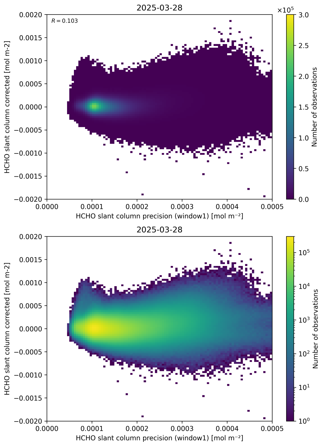
Figure 92: Scatter density plot of “HCHO slant column precision (window1)” against “HCHO slant column corrected” for 2025-03-28 to 2025-03-29.
