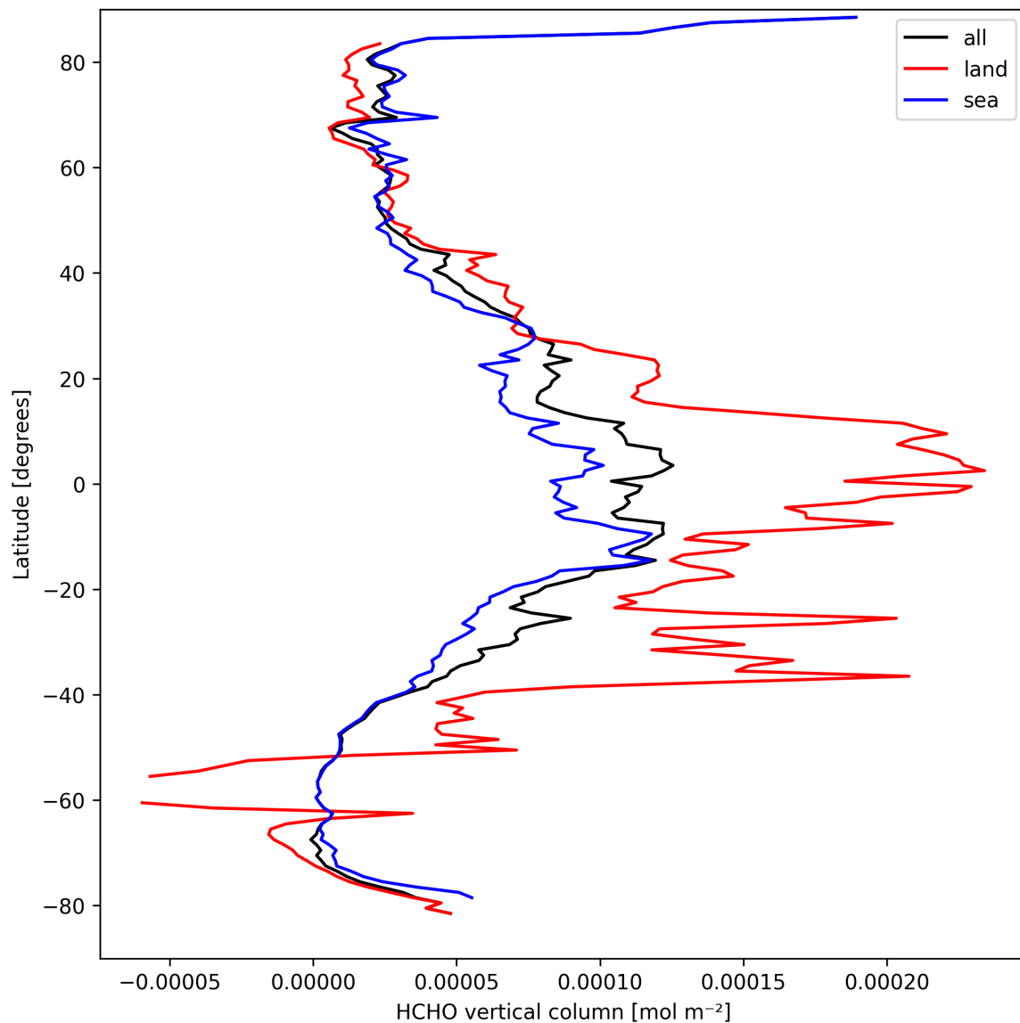
Figure 21: Zonal average of “HCHO vertical column” for 2025-03-28 to 2025-03-29.
