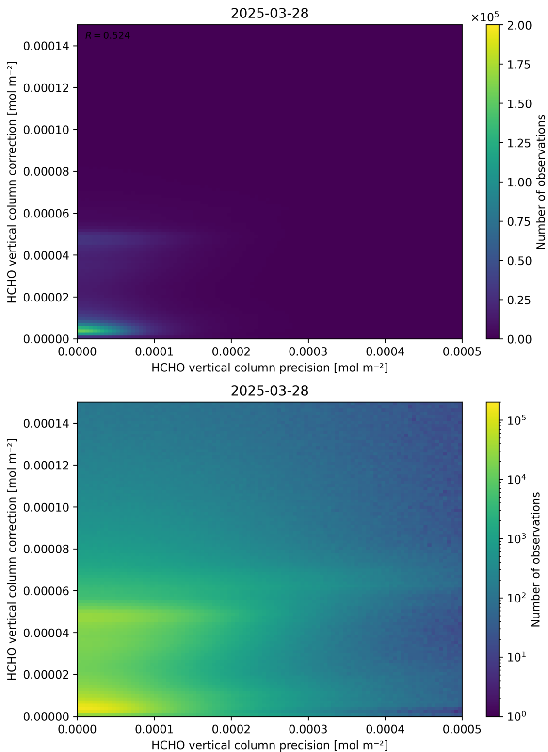
Figure 146: Scatter density plot of “HCHO vertical column precision” against “HCHO vertical column correction” for 2025-03-28 to 2025-03-29.
