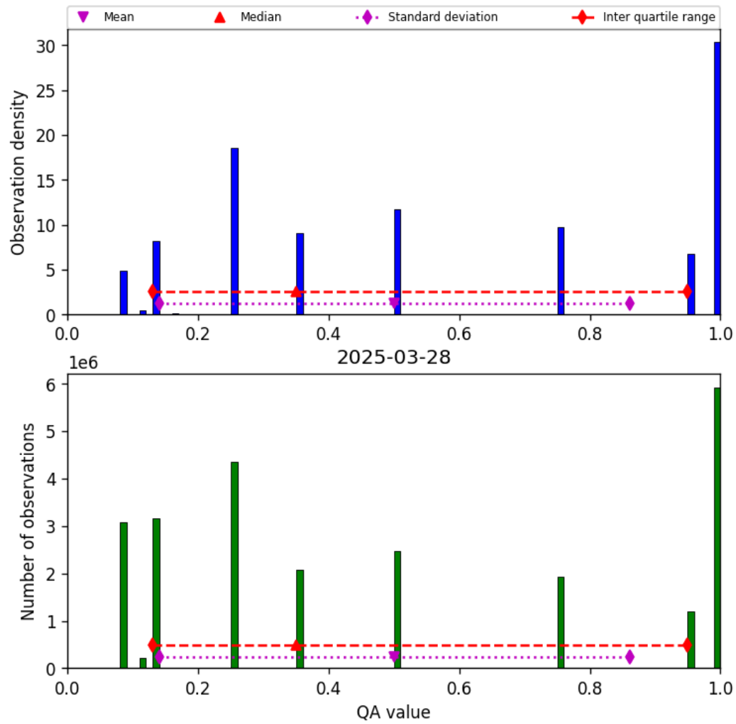
Figure 34: Histogram of “QA value” for 2025-03-28 to 2025-03-29
