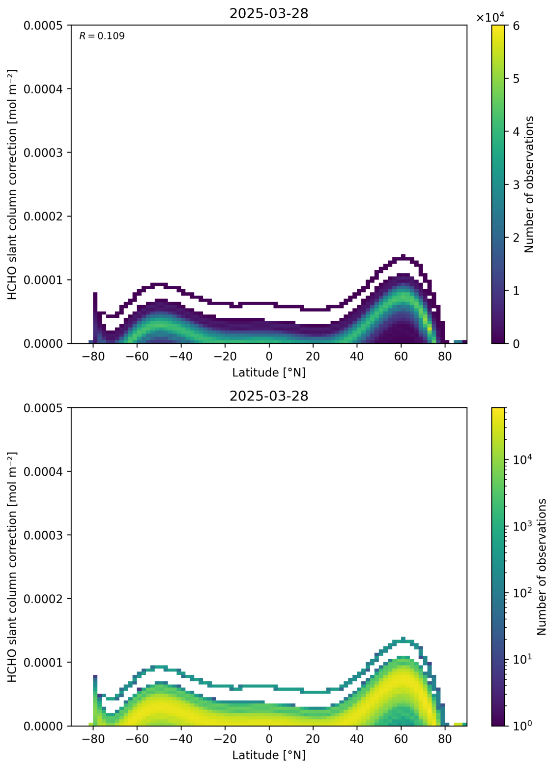
Figure 158: Scatter density plot of “Latitude” against “HCHO slant column correction” for 2025-03-28 to 2025-03-29.
