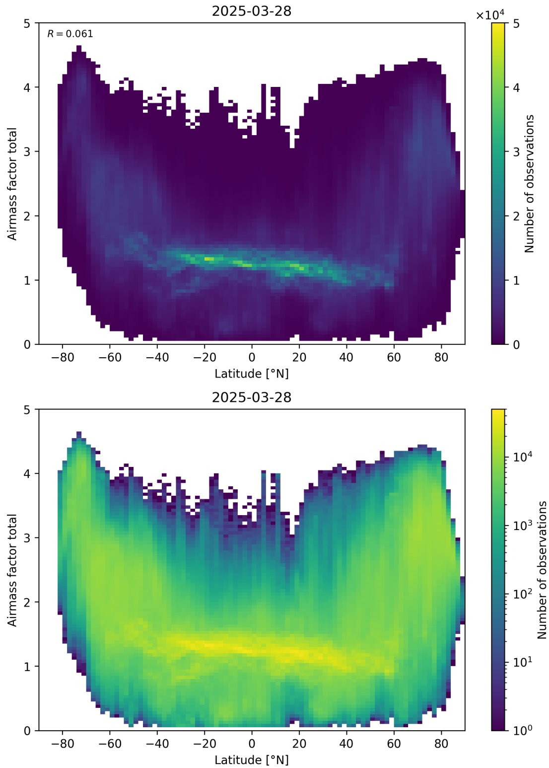
Figure 161: Scatter density plot of “Latitude” against “Airmass factor total” for 2025-03-28 to 2025-03-29.
