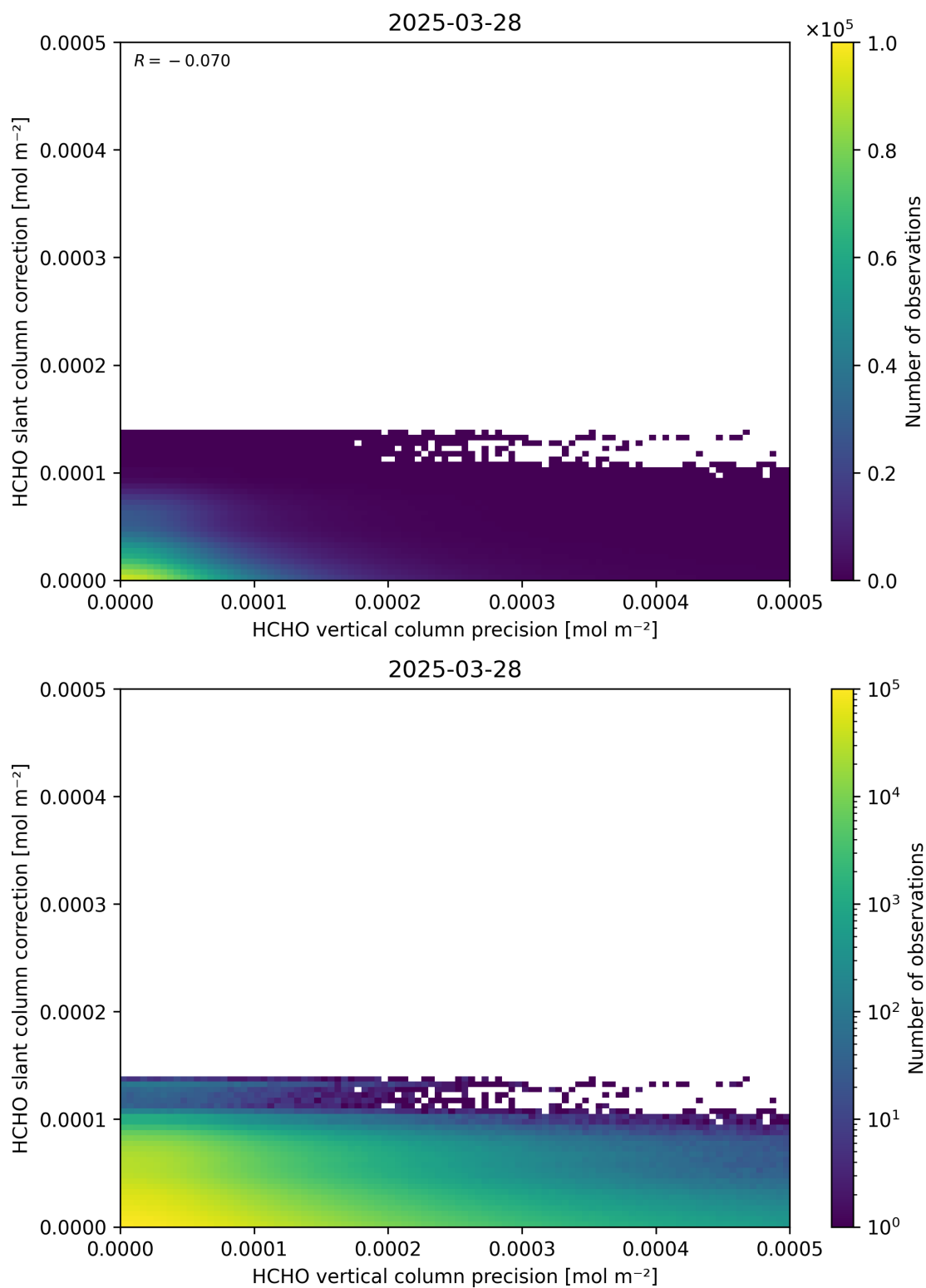
Figure 141: Scatter density plot of “HCHO vertical column precision” against “HCHO slant column correction” for 2025-03-28 to 2025-03-29.
