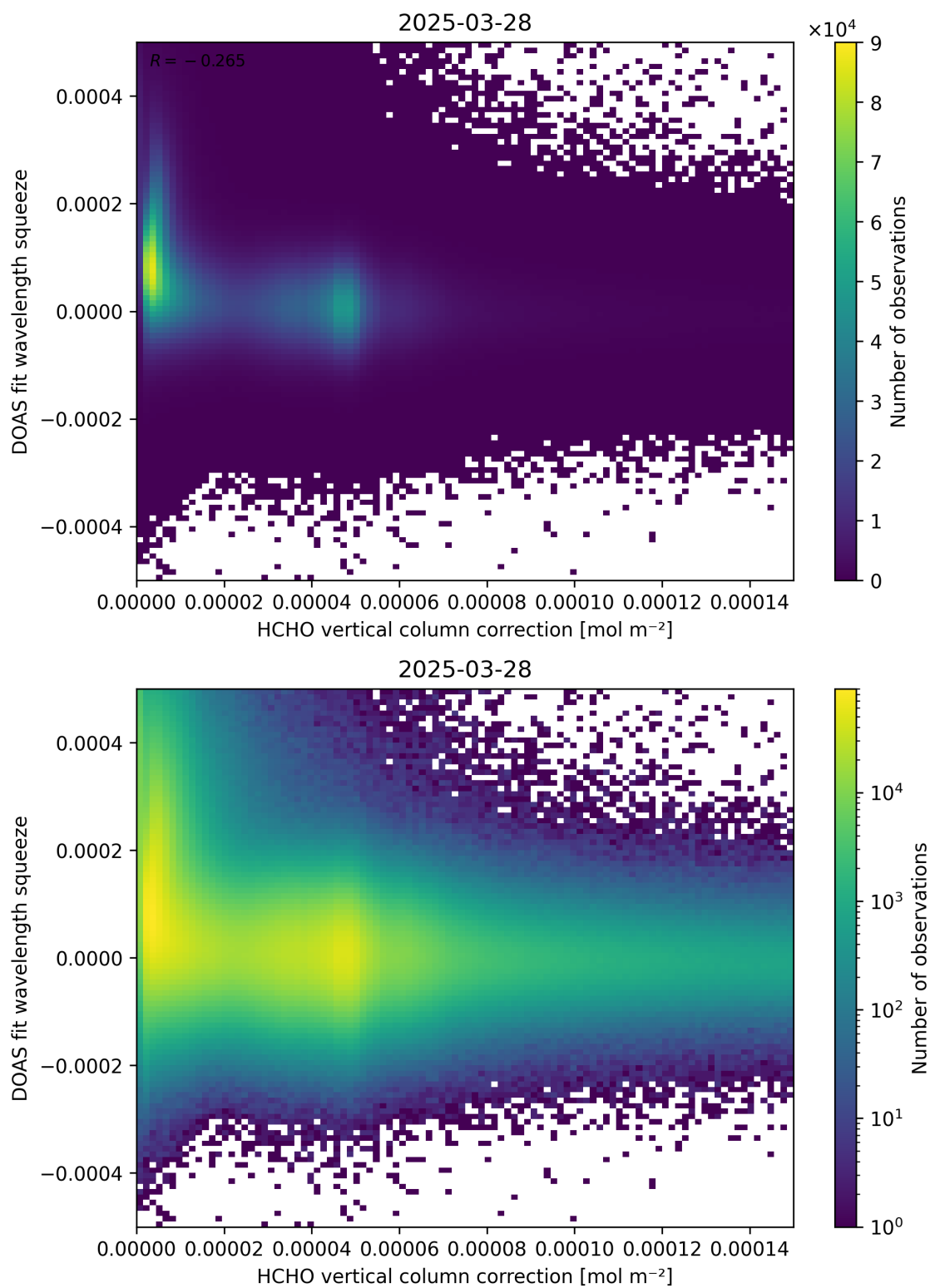
Figure 114: Scatter density plot of “HCHO vertical column correction” against “DOAS fit wavelength squeeze” for 2025-03-28 to 2025-03-29.
