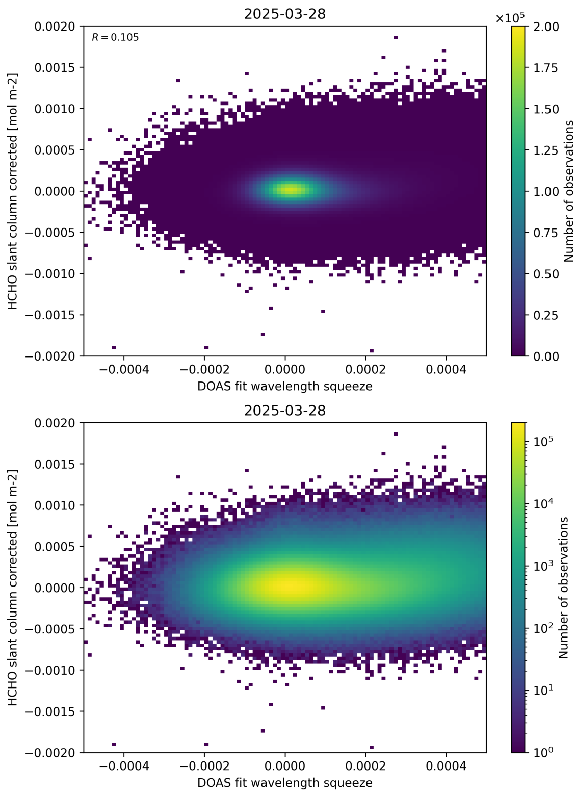
Figure 69: Scatter density plot of “DOAS fit wavelength squeeze” against “HCHO slant column corrected” for 2025-03-28 to 2025-03-29.
