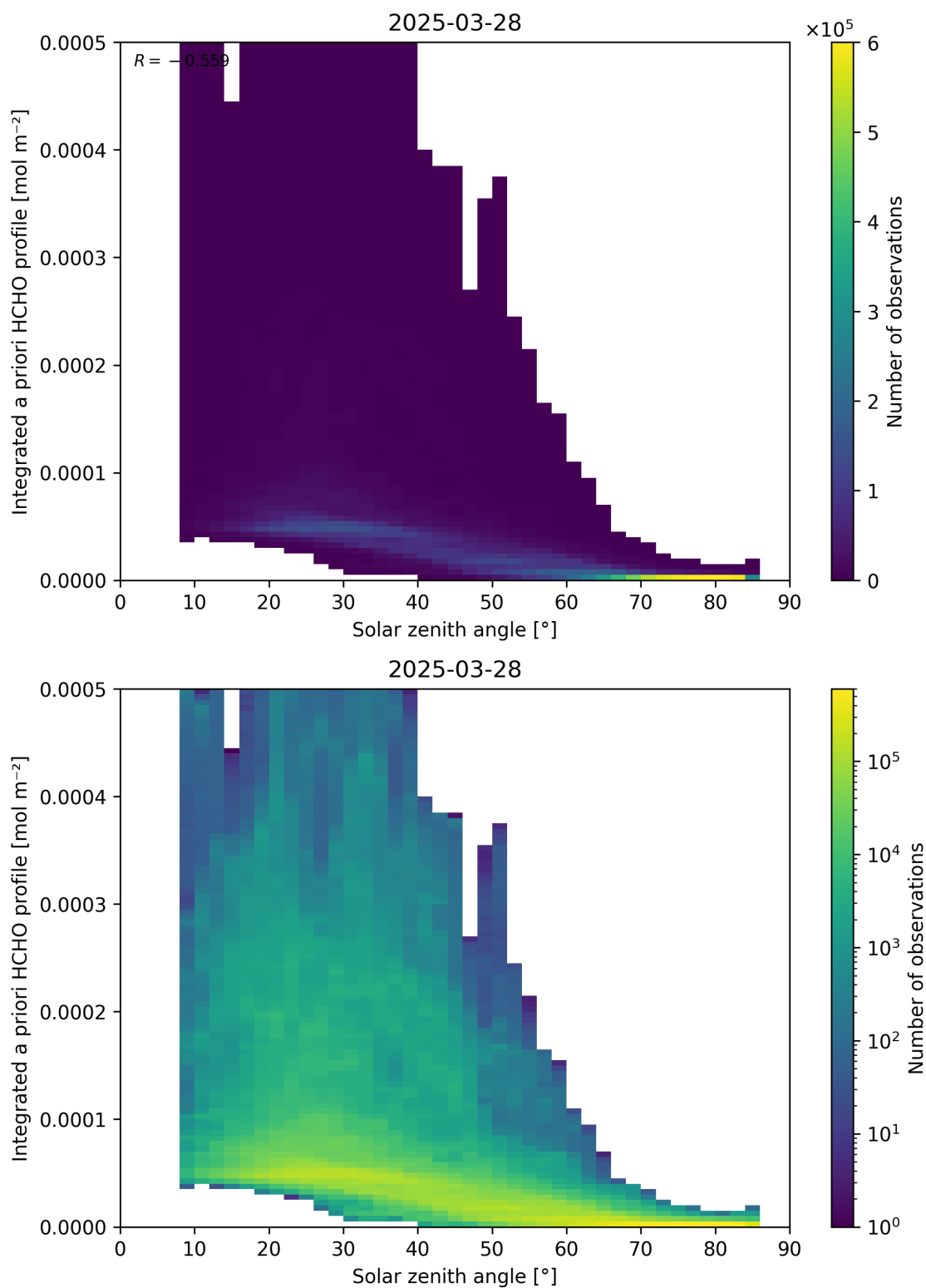
Figure 180: Scatter density plot of “Solar zenith angle” against “Integrated a priori HCHO profile” for 2025-03-28 to 2025-03-29.
