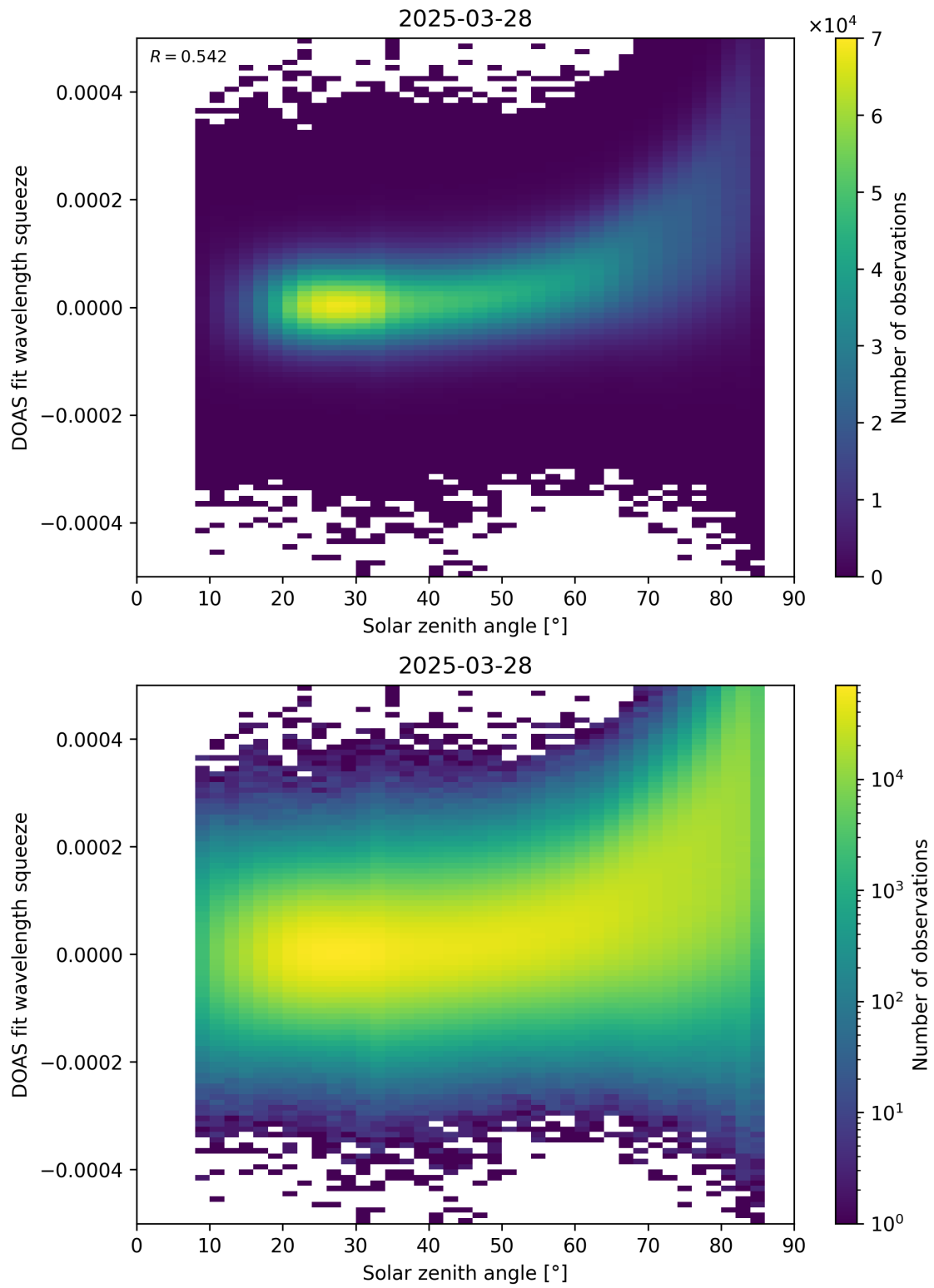
Figure 169: Scatter density plot of “Solar zenith angle” against “DOAS fit wavelength squeeze” for 2025-03-28 to 2025-03-29.
