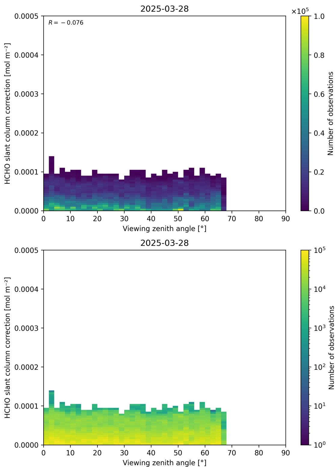
Figure 187: Scatter density plot of “Viewing zenith angle” against “HCHO slant column correction” for 2025-03-28 to 2025-03-29.
