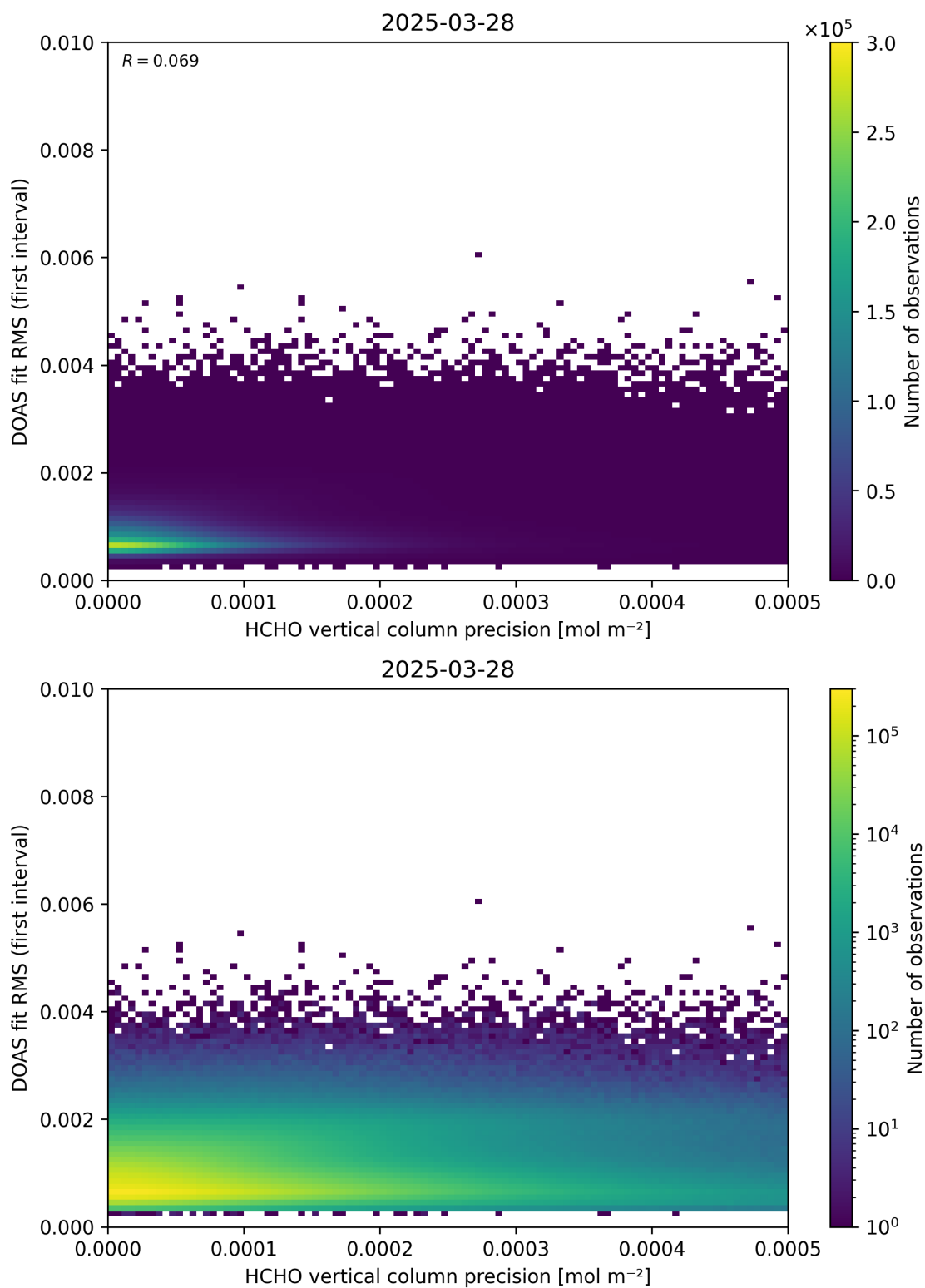
Figure 136: Scatter density plot of “HCHO vertical column precision” against “DOAS fit RMS (first interval)” for 2025-03-28 to 2025-03-29.
