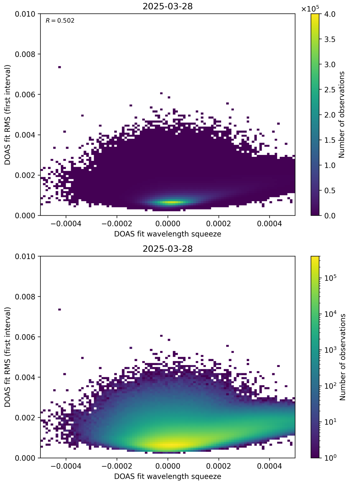
Figure 68: Scatter density plot of “DOAS fit wavelength squeeze” against “DOAS fit RMS (first interval)” for 2025-03-28 to 2025-03-29.
