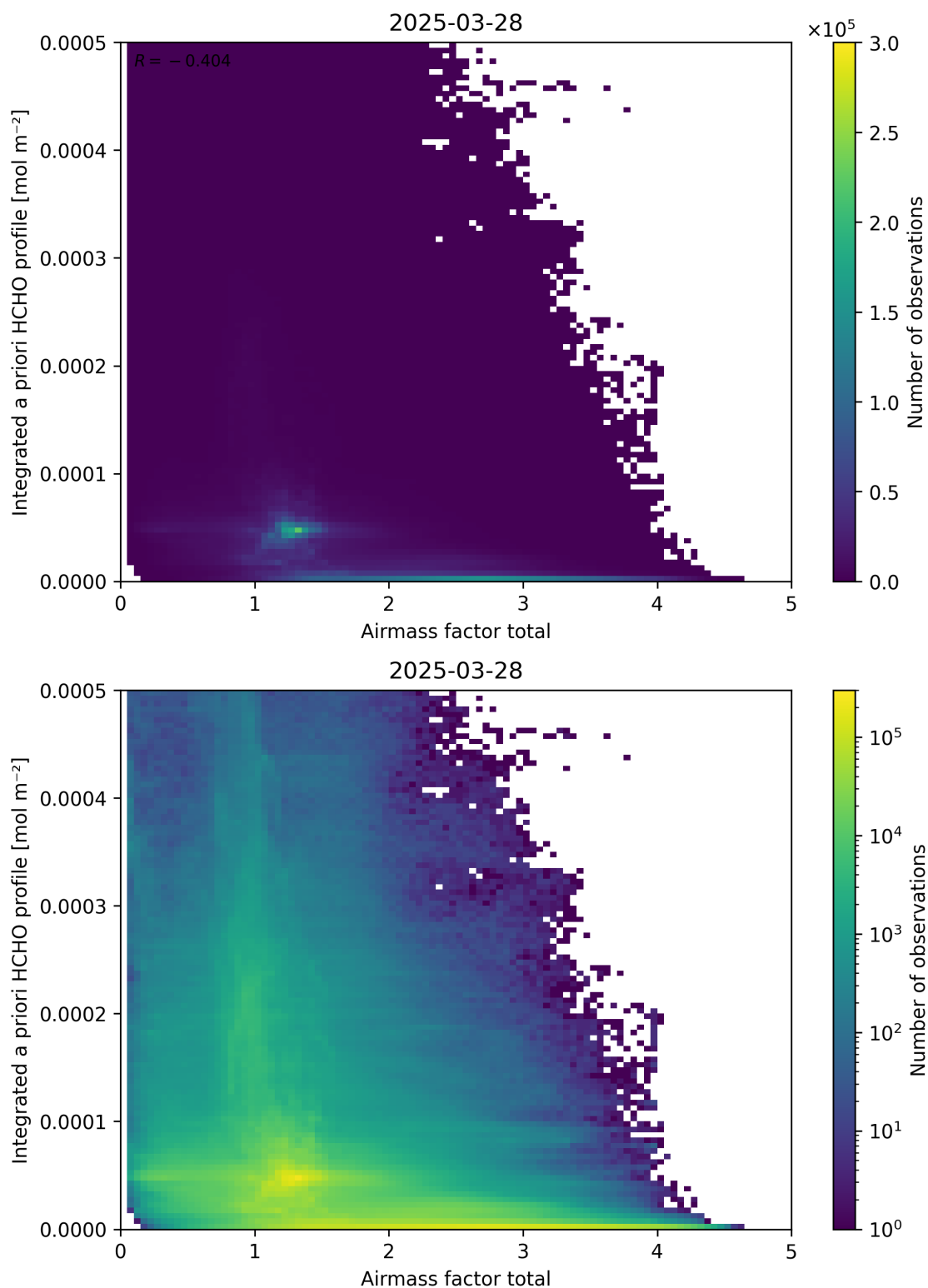
Figure 104: Scatter density plot of “Airmass factor total” against “Integrated a priori HCHO profile” for 2025-03-28 to 2025-03-29.
