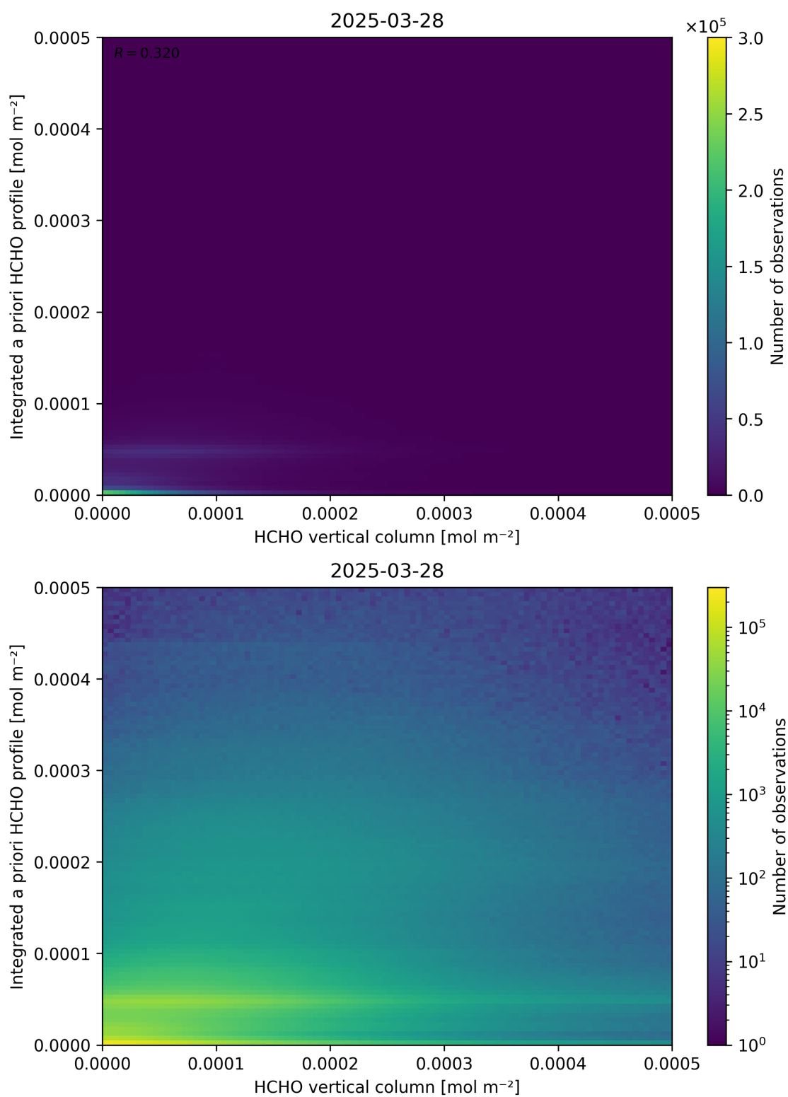
Figure 135: Scatter density plot of “HCHO vertical column” against “Integrated a priori HCHO profile” for 2025-03-28 to 2025-03-29.
