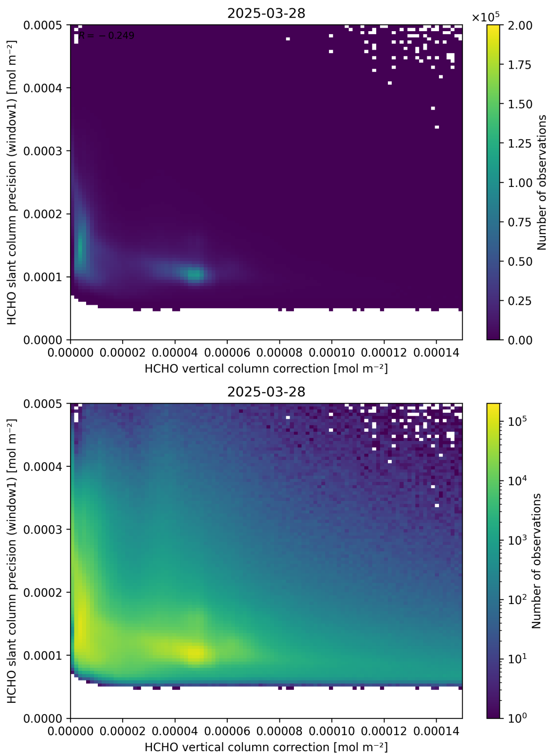
Figure 119: Scatter density plot of “HCHO vertical column correction” against “HCHO slant column precision (window1)” for 2025-03-28 to 2025-03-29.
