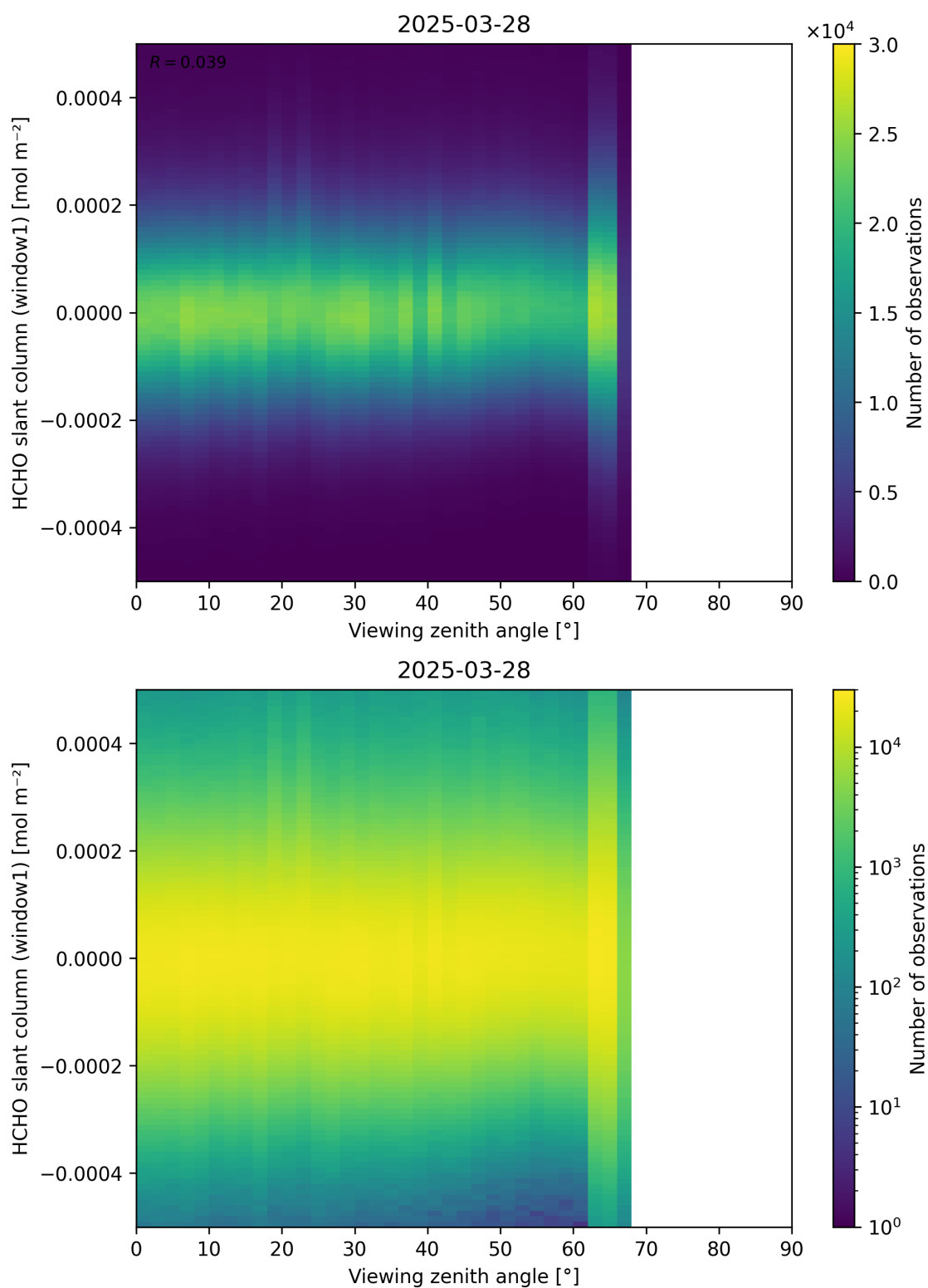
Figure 188: Scatter density plot of “Viewing zenith angle” against “HCHO slant column (window1)” for 2025-03-28 to 2025-03-29.
