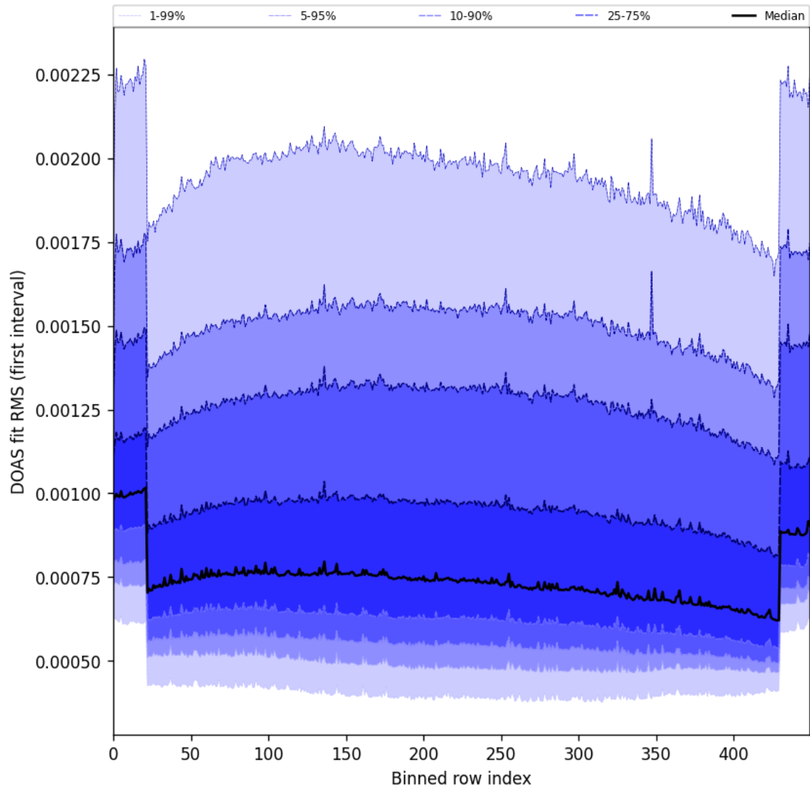
Figure 60: Along track statistics of “DOAS fit RMS (first interval)” for 2025-03-28 to 2025-03-29
