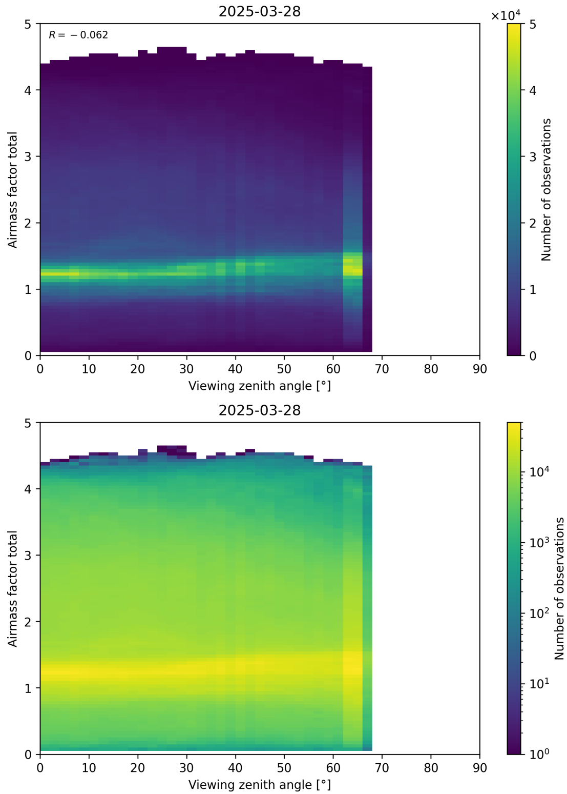
Figure 190: Scatter density plot of “Viewing zenith angle” against “Airmass factor total” for 2025-03-28 to 2025-03-29.
