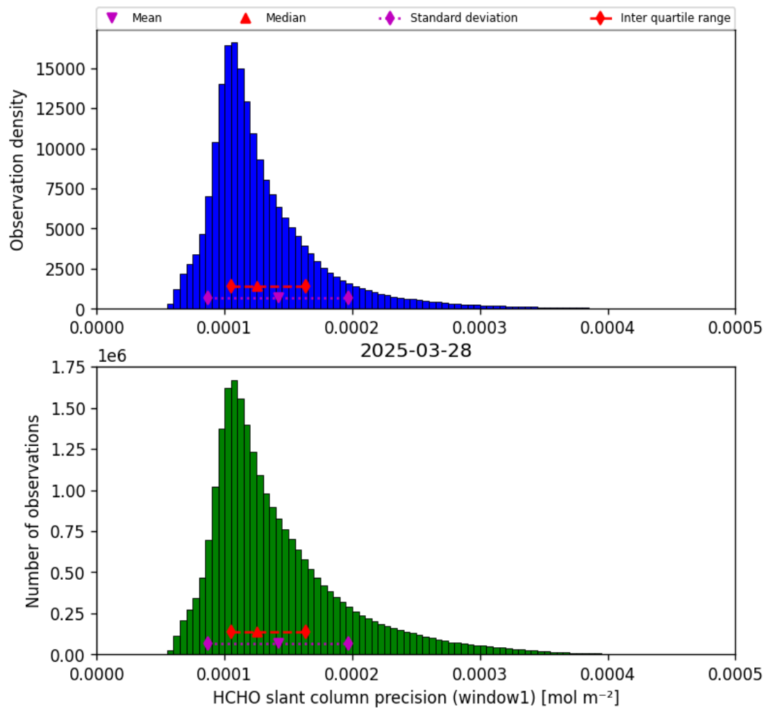
Figure 39: Histogram of “HCHO slant column precision (window1)” for 2025-03-28 to 2025-03-29
