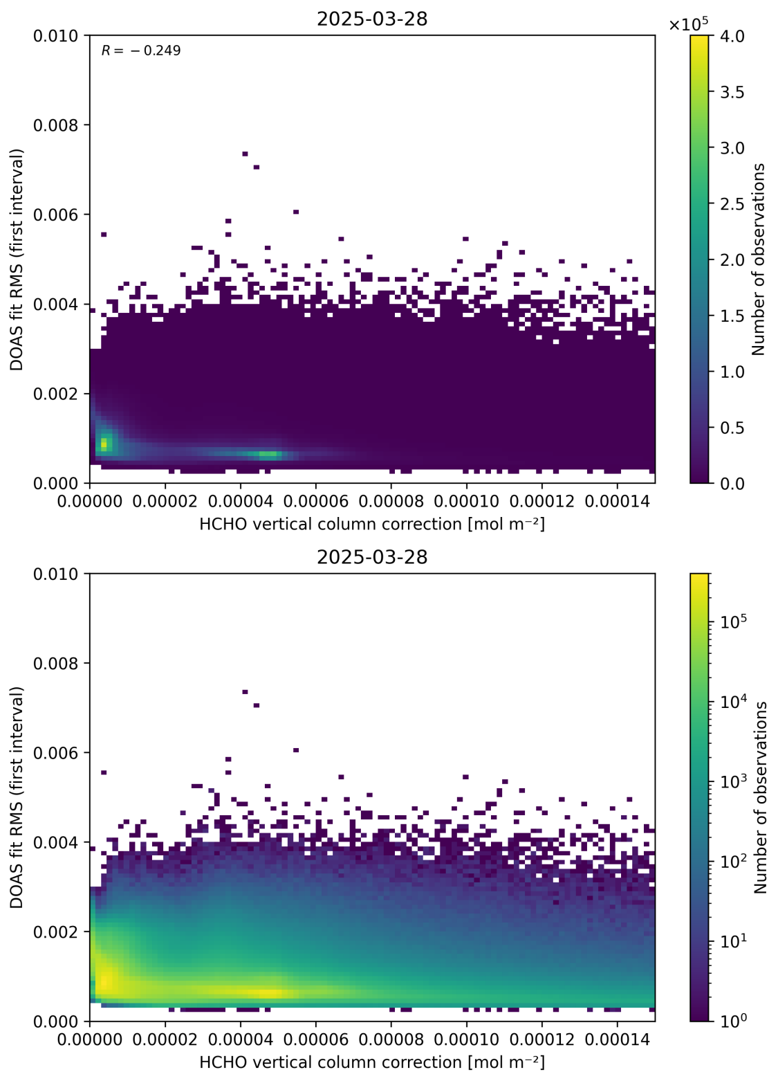
Figure 112: Scatter density plot of “HCHO vertical column correction” against “DOAS fit RMS (first interval)” for 2025-03-28 to 2025-03-29.
