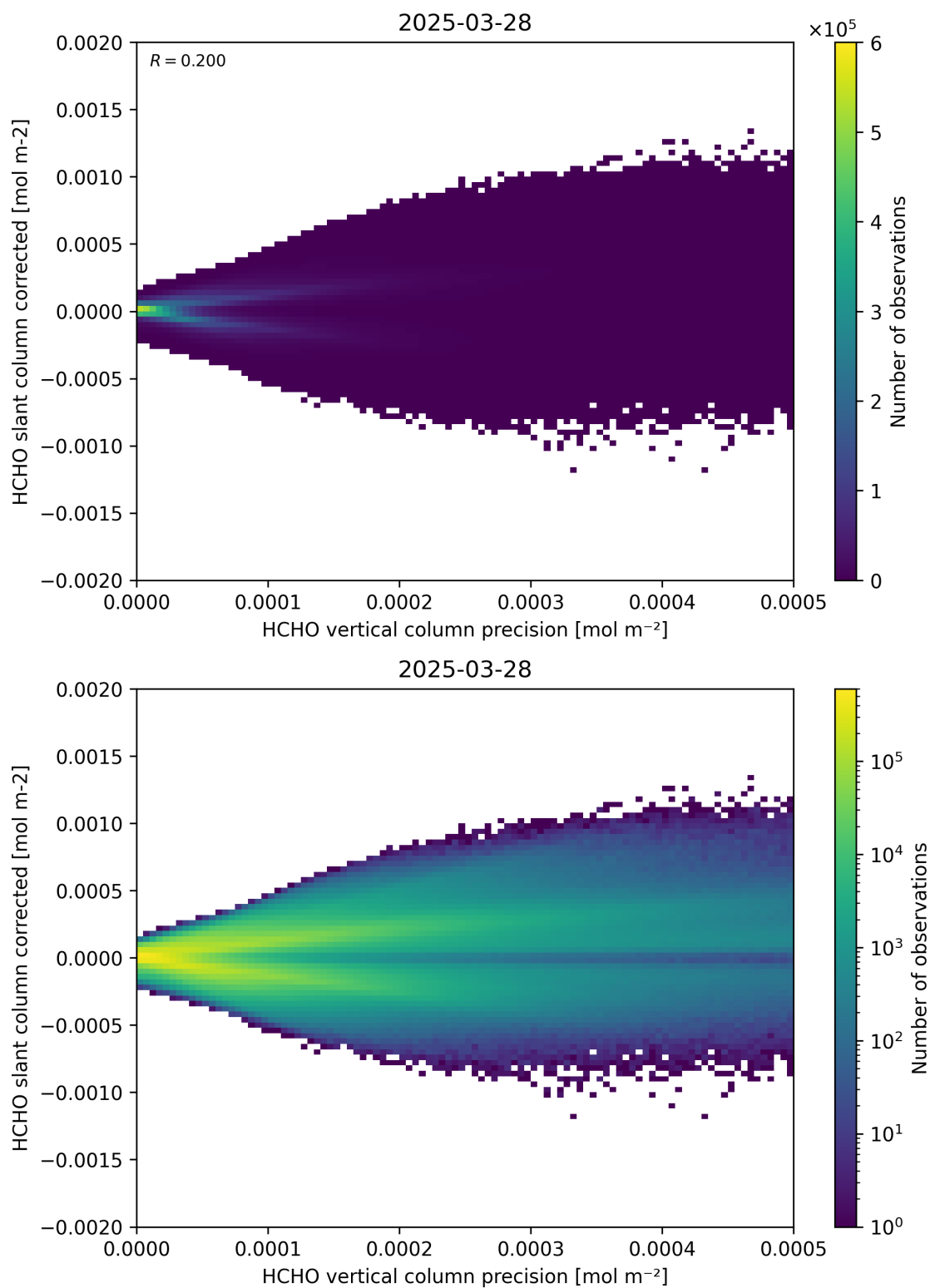
Figure 140: Scatter density plot of “HCHO vertical column precision” against “HCHO slant column corrected” for 2025-03-28 to 2025-03-29.
