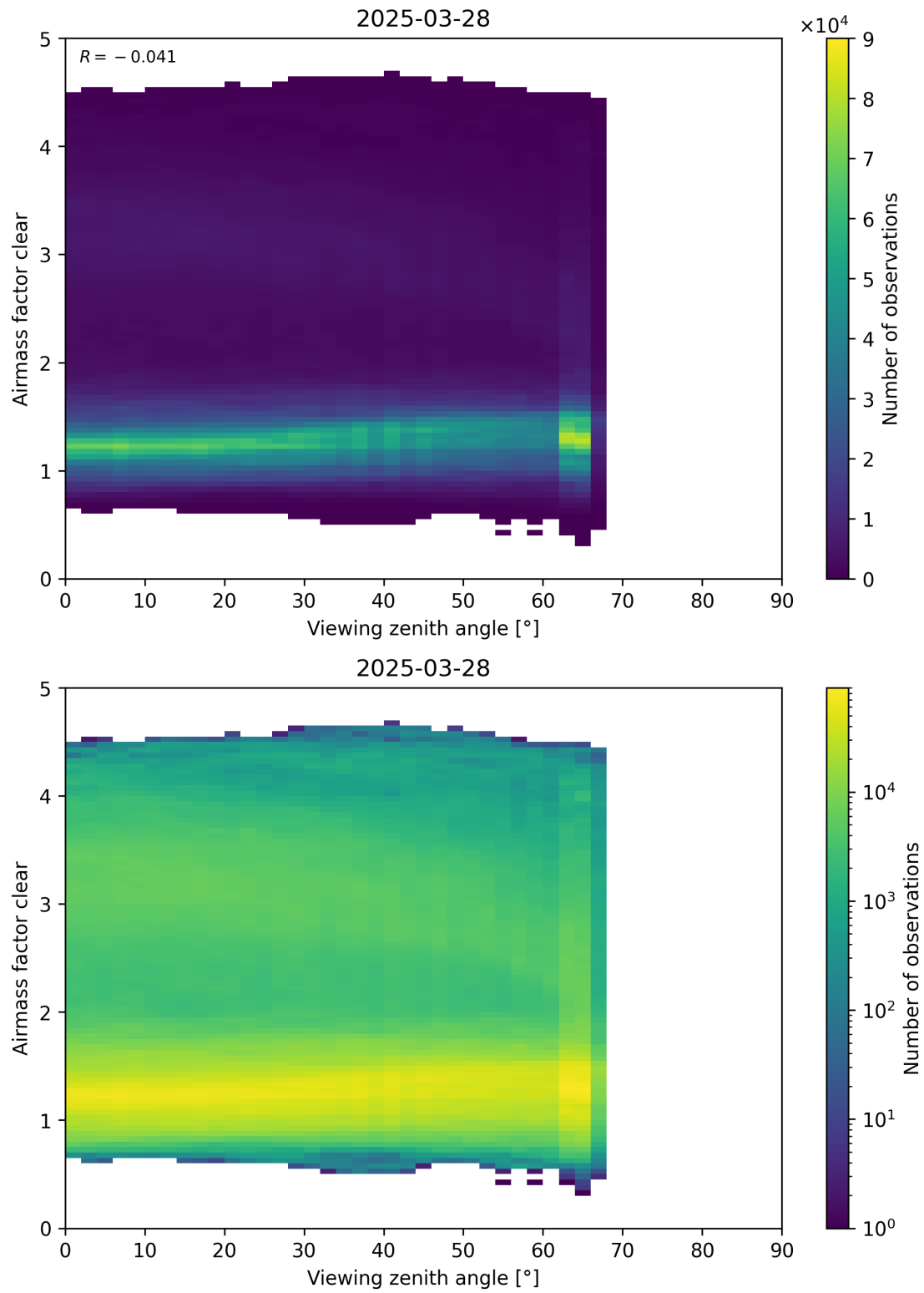
Figure 185: Scatter density plot of “Viewing zenith angle” against “Airmass factor clear” for 2025-03-28 to 2025-03-29.
