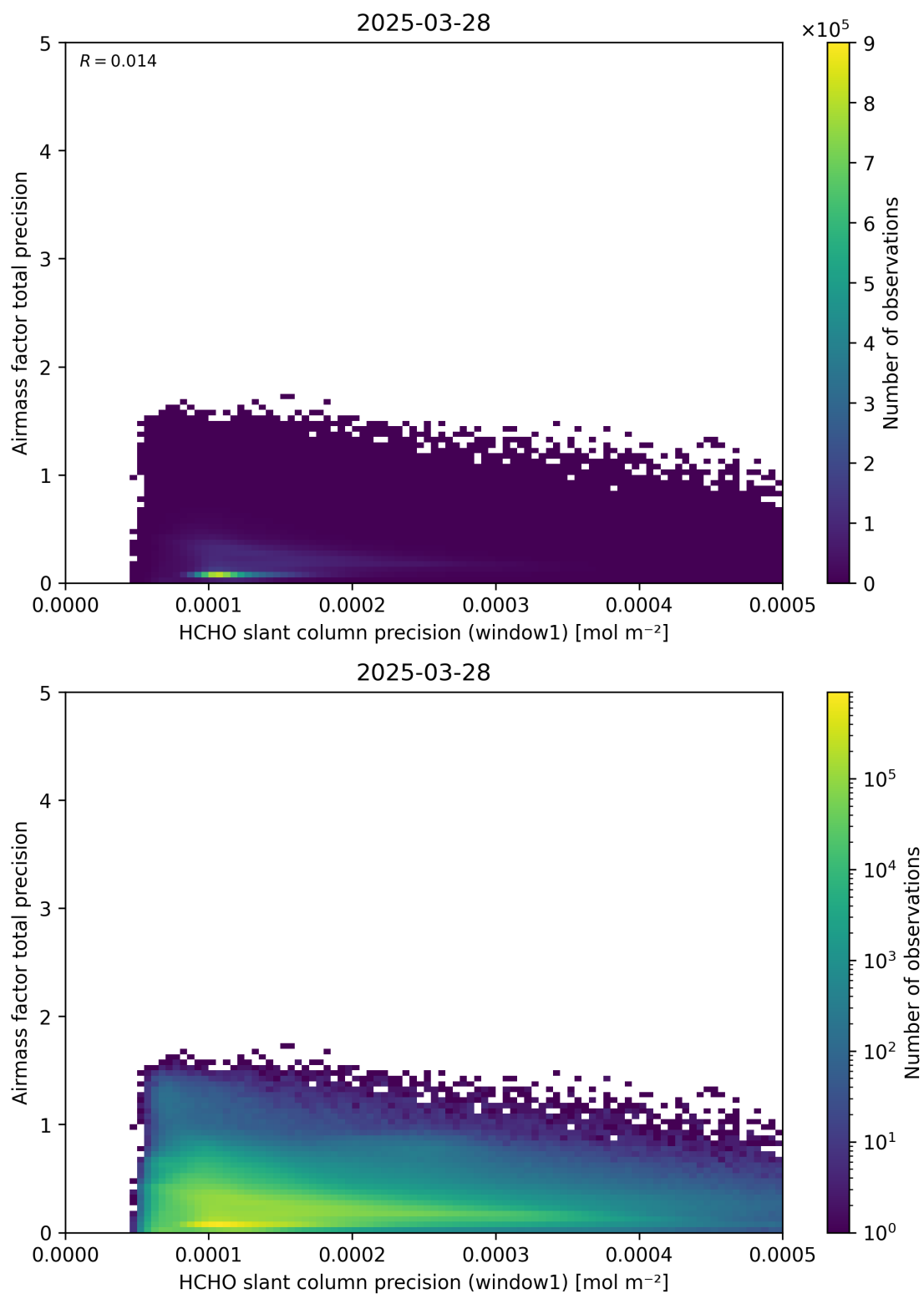
Figure 95: Scatter density plot of “HCHO slant column precision (window1)” against “Airmass factor total precision” for 2025-03-28 to 2025-03-29.
