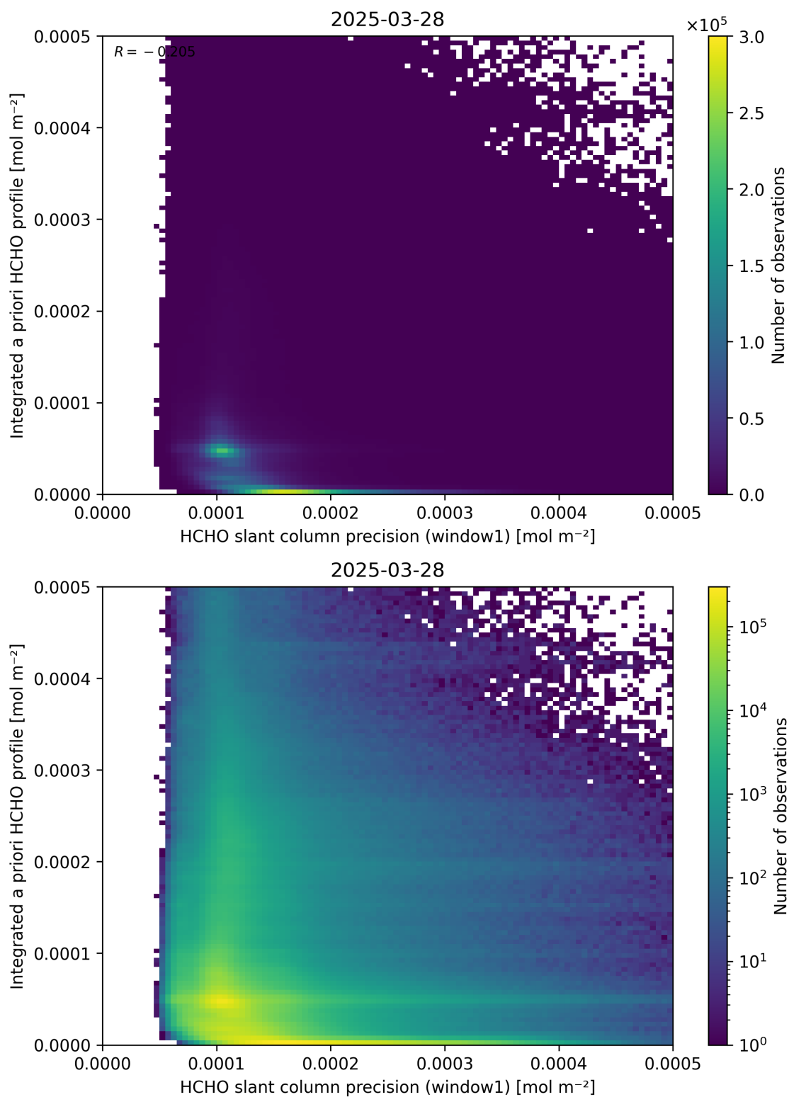
Figure 96: Scatter density plot of “HCHO slant column precision (window1)” against “Integrated a priori HCHO profile” for 2025-03-28 to 2025-03-29.
