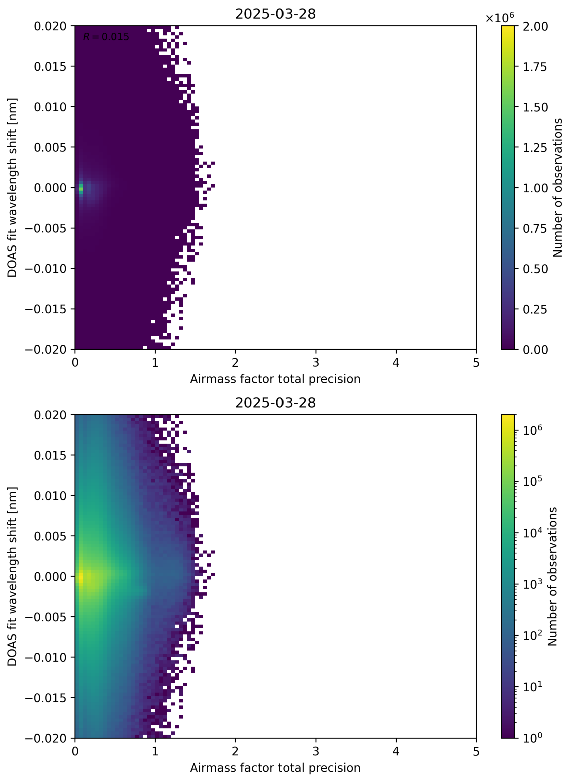
Figure 106: Scatter density plot of “Airmass factor total precision” against “DOAS fit wavelength shift” for 2025-03-28 to 2025-03-29.
