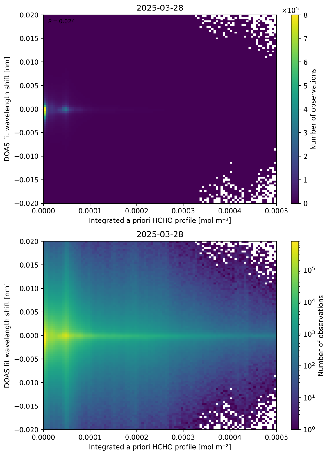
Figure 149: Scatter density plot of “Integrated a priori HCHO profile” against “DOAS fit wavelength shift” for 2025-03-28 to 2025-03-29.
