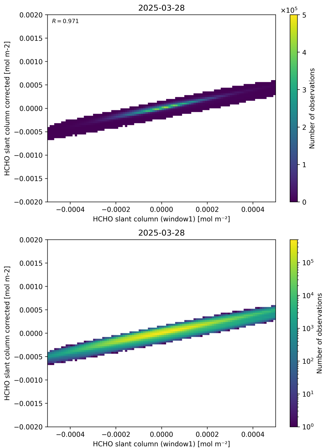
Figure 82: Scatter density plot of “HCHO slant column (window1)” against “HCHO slant column corrected” for 2025-03-28 to 2025-03-29.
