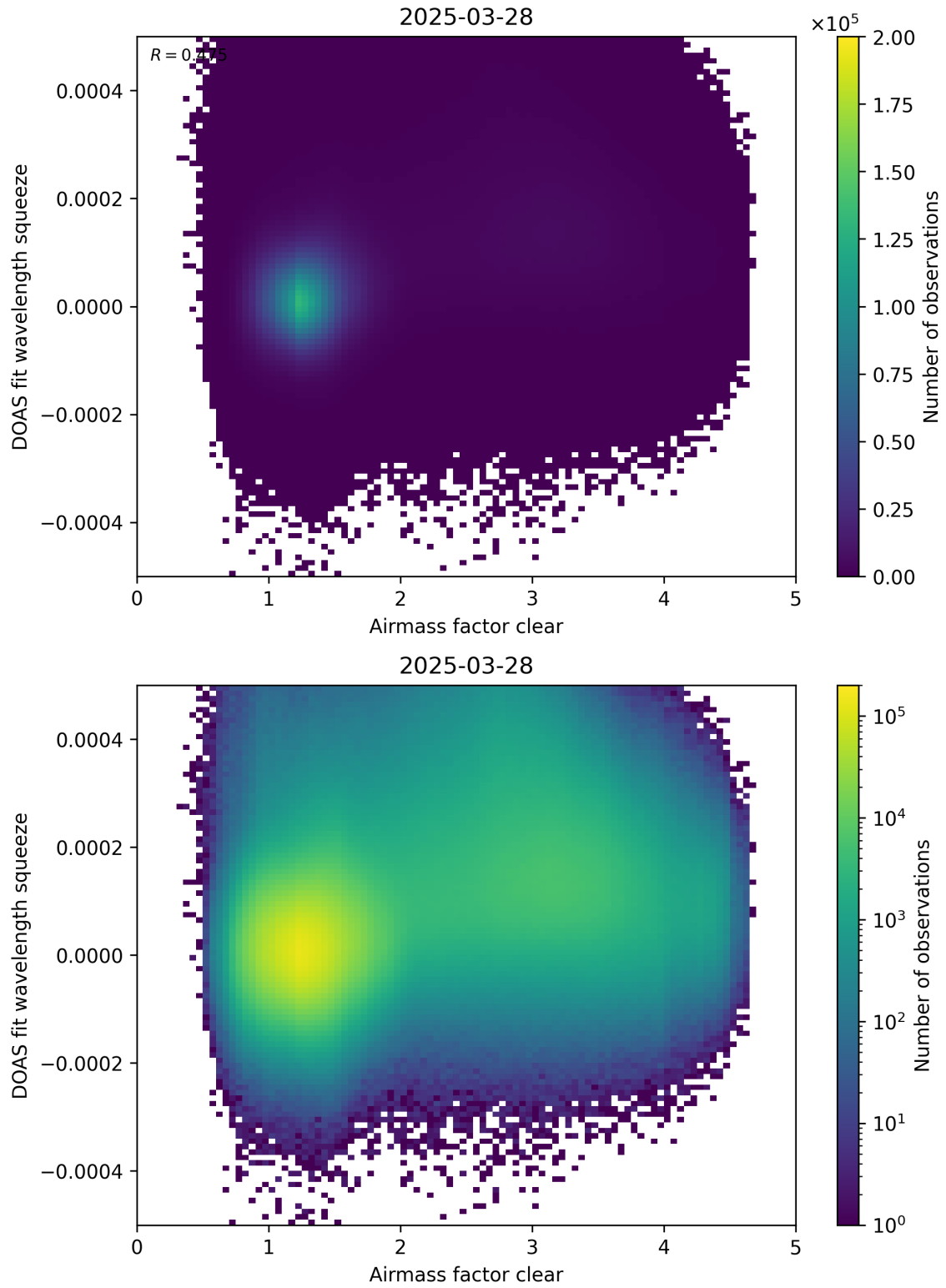
Figure 73: Scatter density plot of “Airmass factor clear” against “DOAS fit wavelength squeeze” for 2025-03-28 to 2025-03-29.
