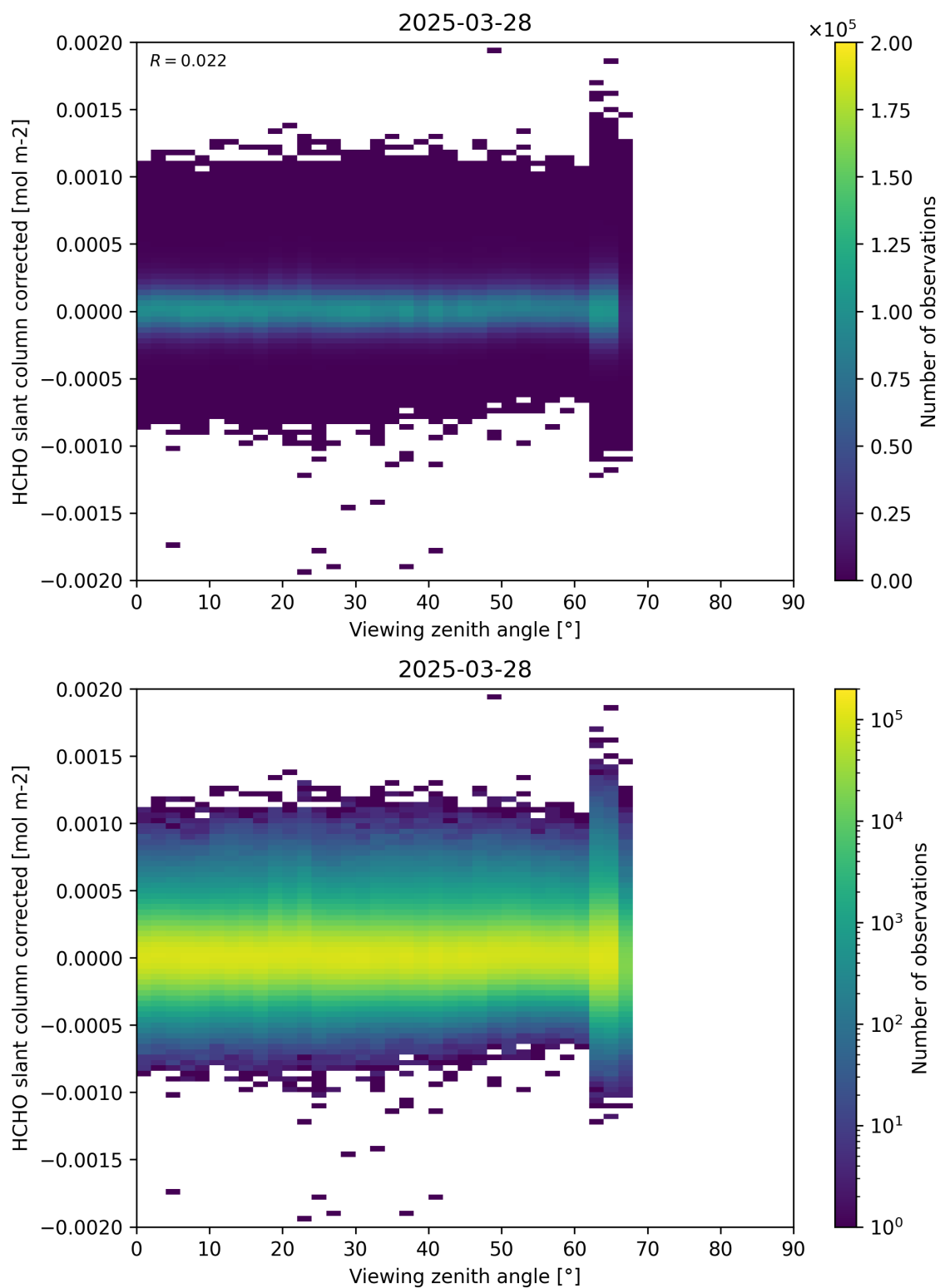
Figure 186: Scatter density plot of “Viewing zenith angle” against “HCHO slant column corrected” for 2025-03-28 to 2025-03-29.
