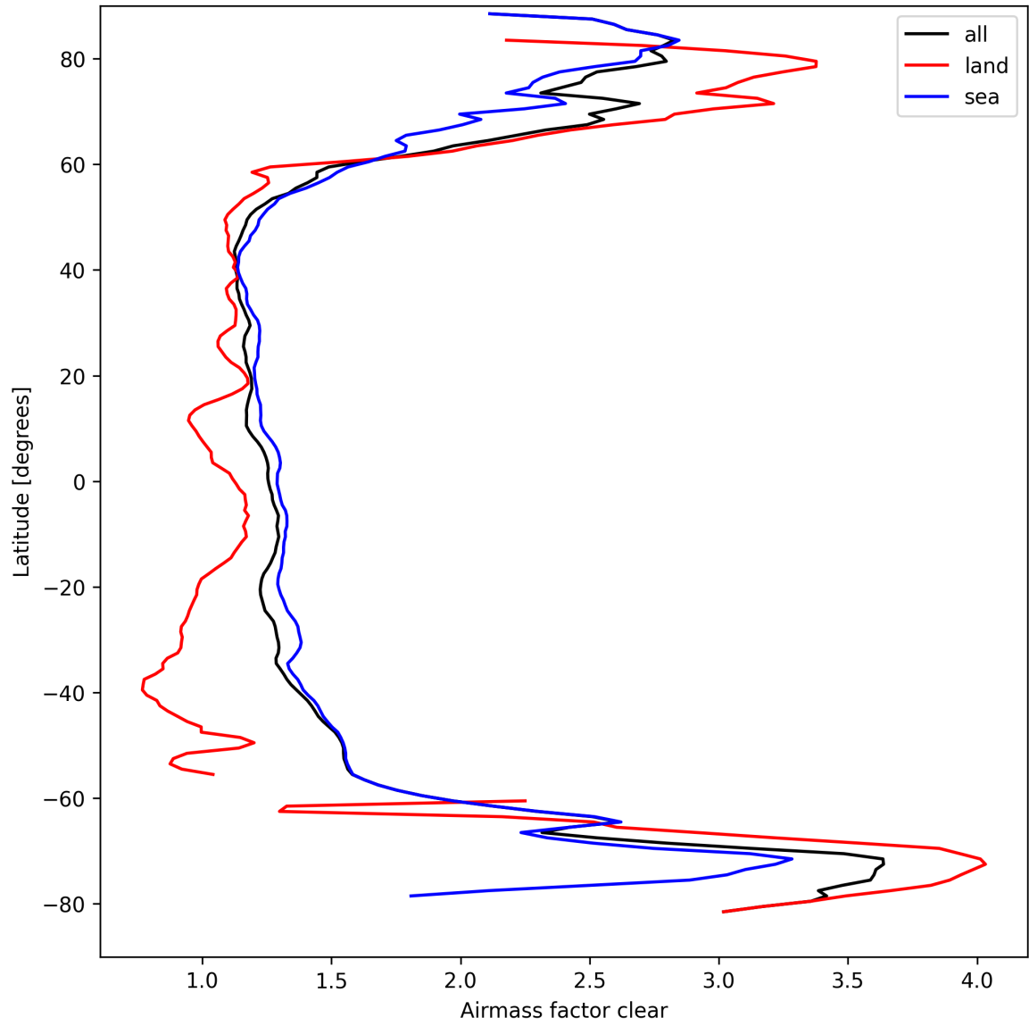
Figure 28: Zonal average of “Airmass factor clear” for 2025-03-28 to 2025-03-29.
