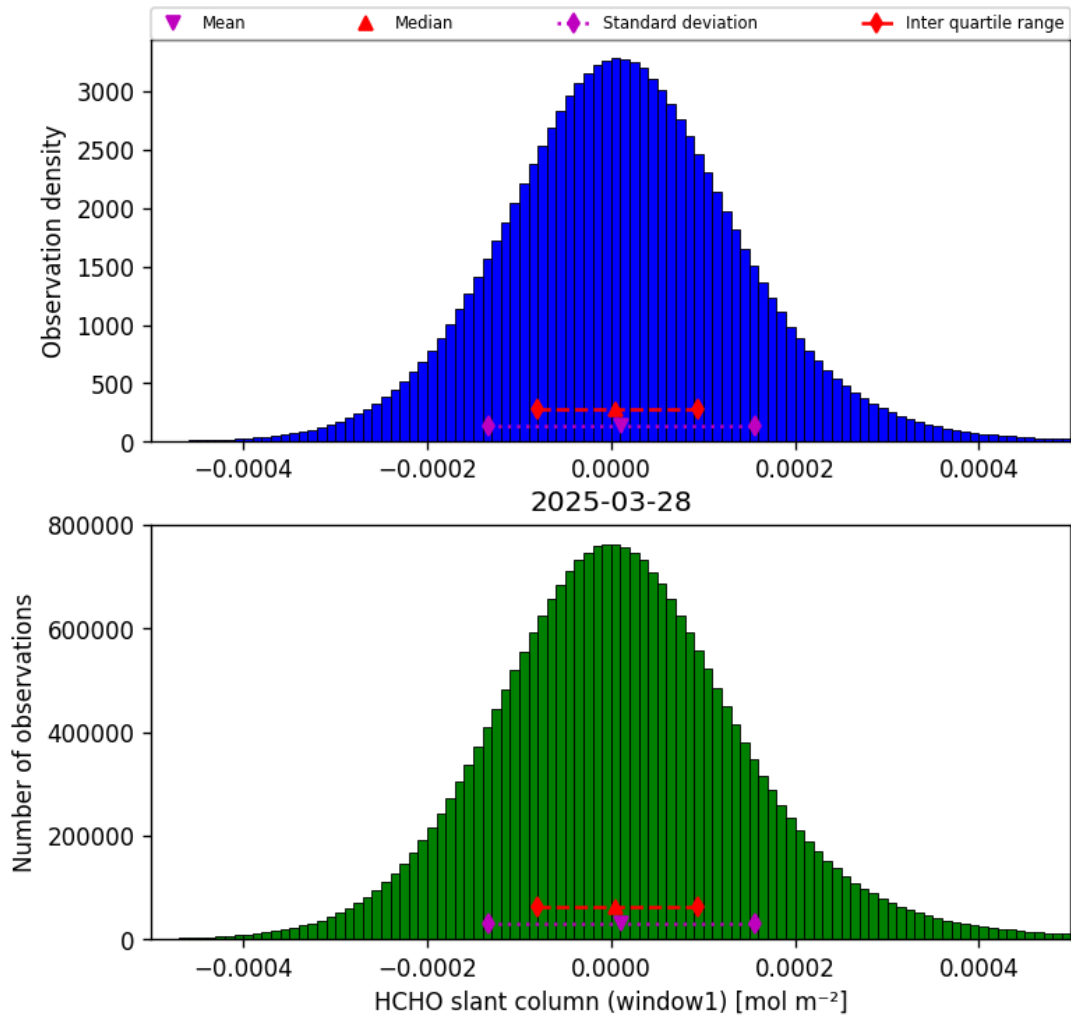
Figure 38: Histogram of “HCHO slant column (window1)” for 2025-03-28 to 2025-03-29
