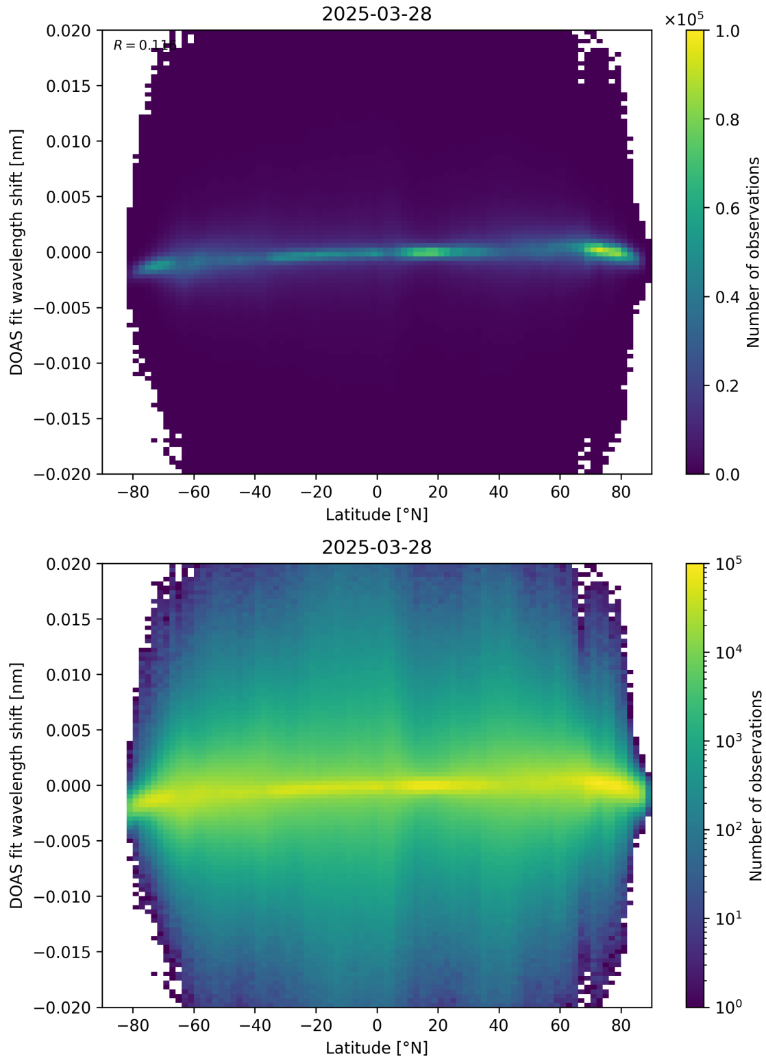
Figure 154: Scatter density plot of “Latitude” against “DOAS fit wavelength shift” for 2025-03-28 to 2025-03-29.
