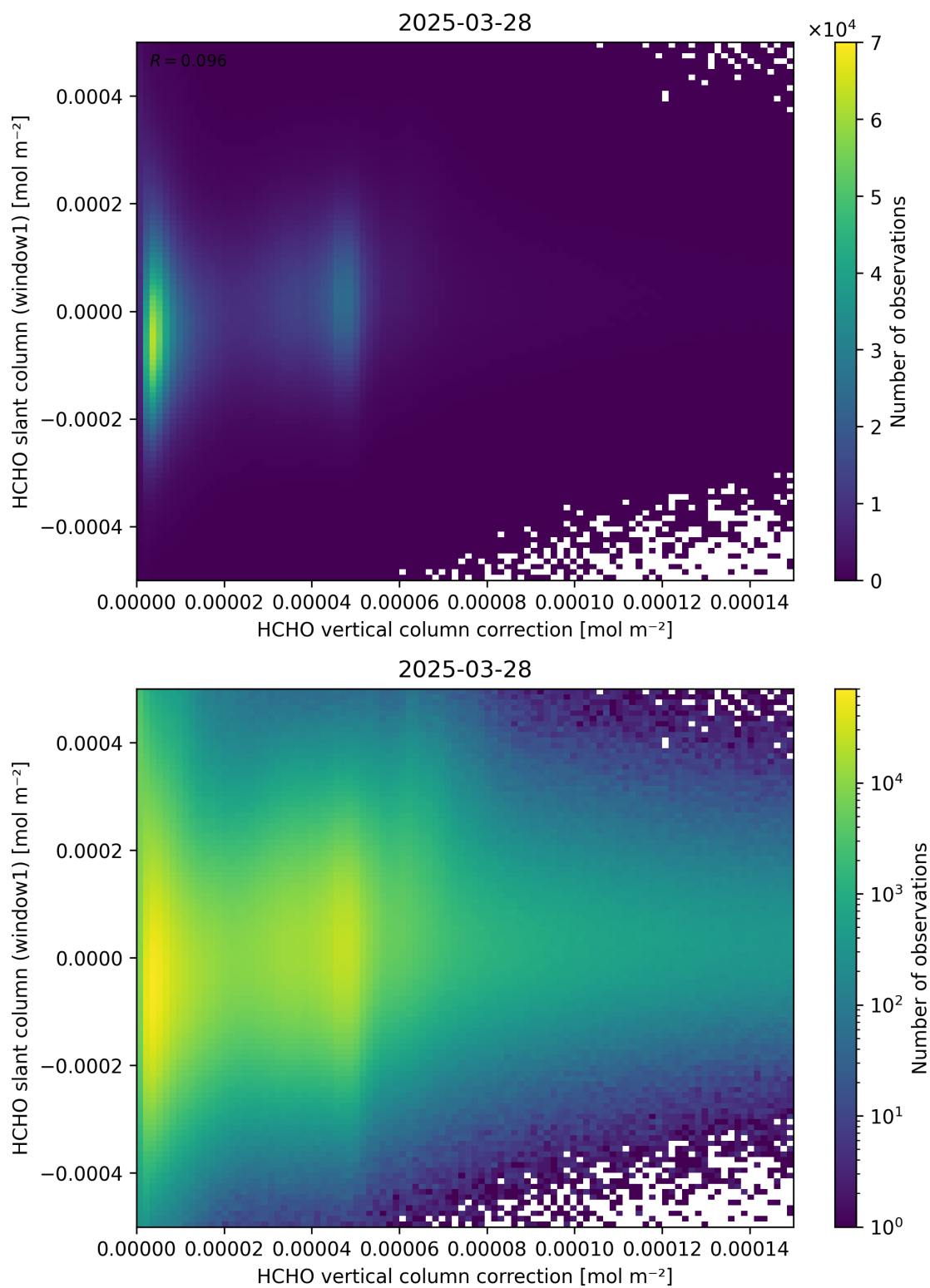
Figure 118: Scatter density plot of “HCHO vertical column correction” against “HCHO slant column (window1)” for 2025-03-28 to 2025-03-29.
