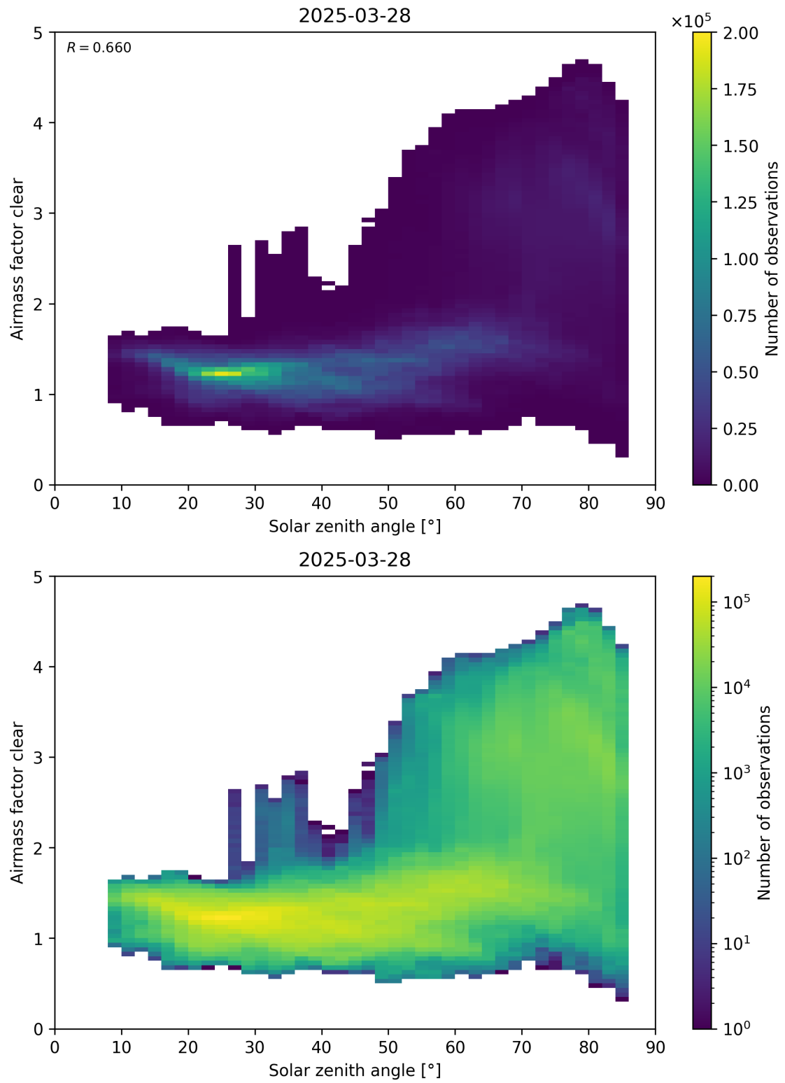
Figure 170: Scatter density plot of “Solar zenith angle” against “Airmass factor clear” for 2025-03-28 to 2025-03-29.
