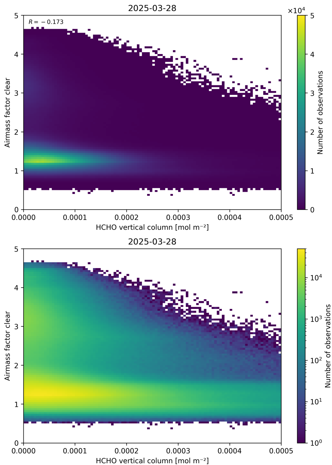
Figure 126: Scatter density plot of “HCHO vertical column” against “Airmass factor clear” for 2025-03-28 to 2025-03-29.
