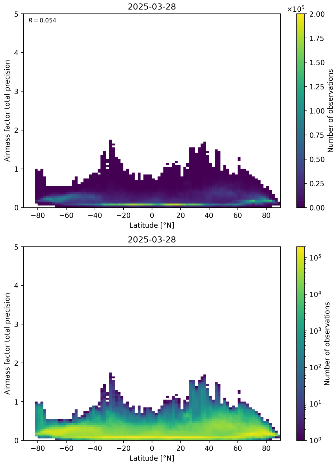
Figure 162: Scatter density plot of “Latitude” against “Airmass factor total precision” for 2025-03-28 to 2025-03-29.
