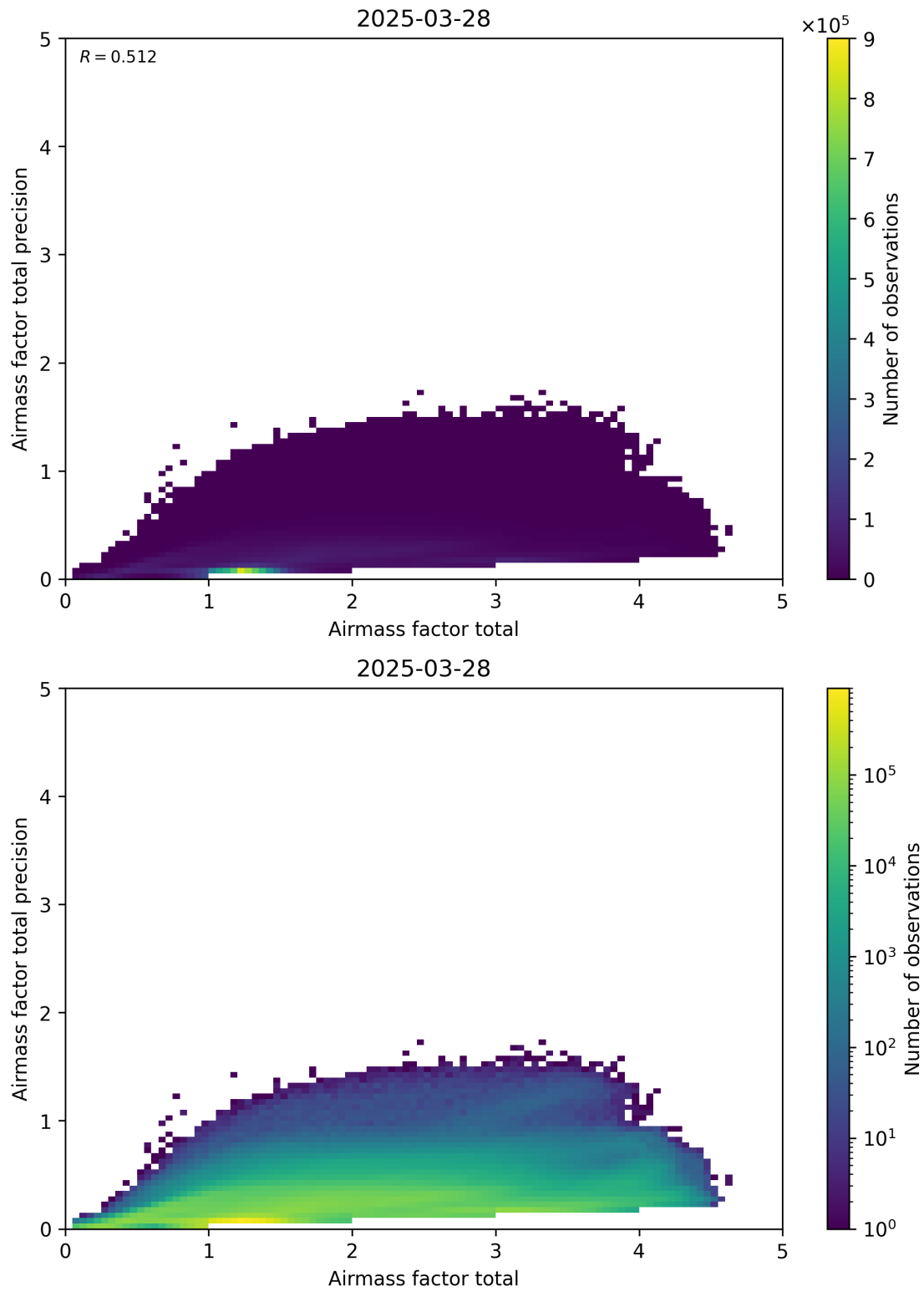
Figure 103: Scatter density plot of “Airmass factor total” against “Airmass factor total precision” for 2025-03-28 to 2025-03-29.
