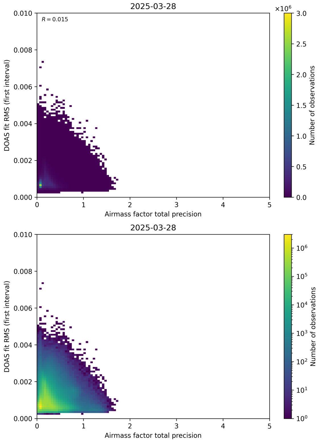
Figure 105: Scatter density plot of “Airmass factor total precision” against “DOAS fit RMS (first interval)” for 2025-03-28 to 2025-03-29.
