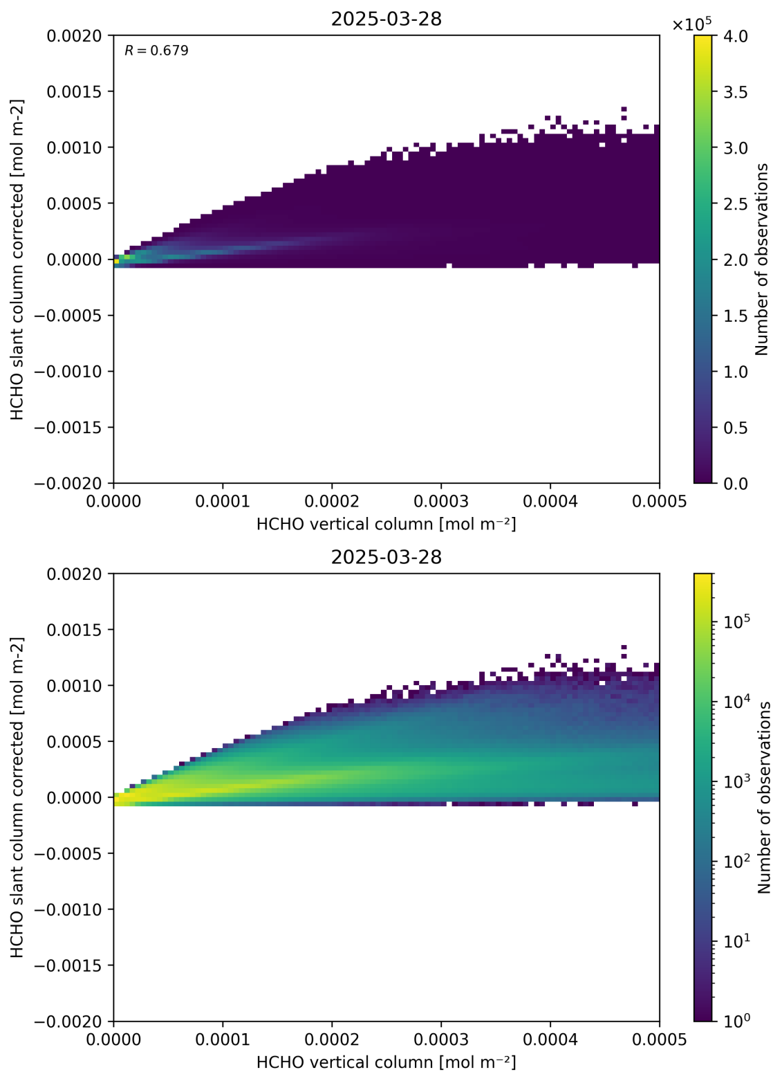
Figure 127: Scatter density plot of “HCHO vertical column” against “HCHO slant column corrected” for 2025-03-28 to 2025-03-29.
