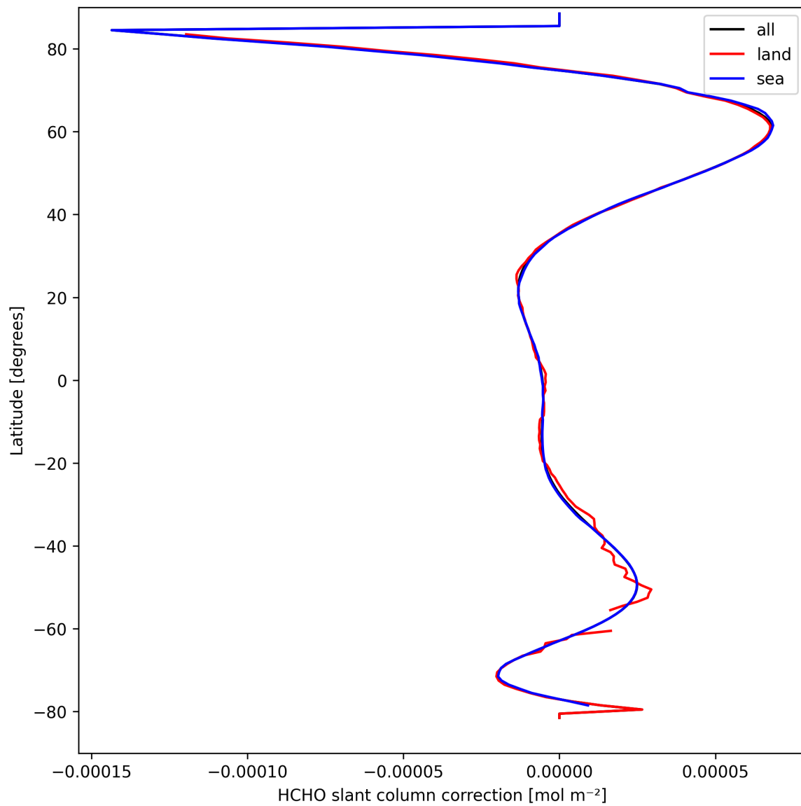
Figure 33: Zonal average of “HCHO slant column correction” for 2025-03-28 to 2025-03-29.
