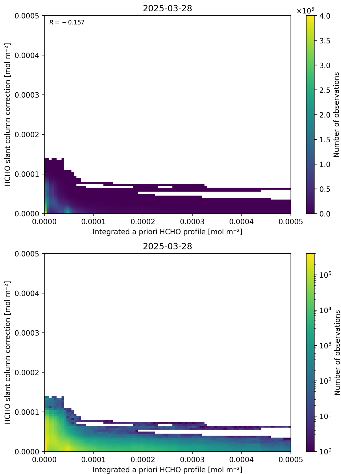
Figure 152: Scatter density plot of “Integrated a priori HCHO profile” against “HCHO slant column correction” for 2025-03-28 to 2025-03-29.
