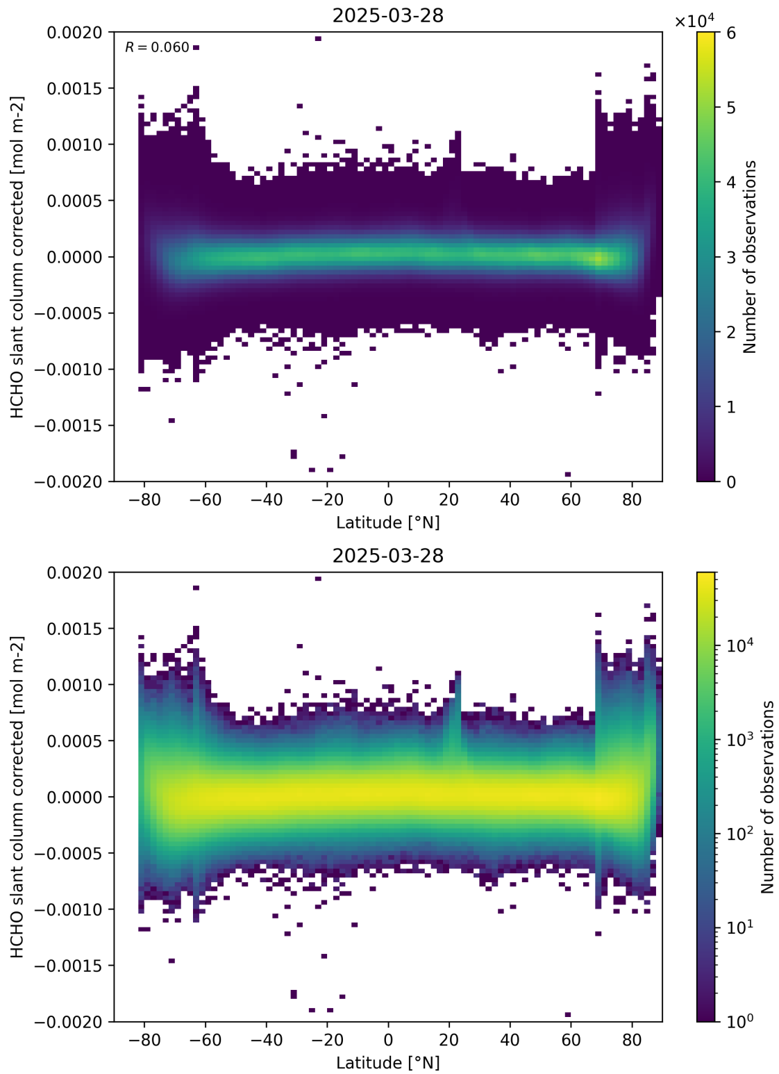
Figure 157: Scatter density plot of “Latitude” against “HCHO slant column corrected” for 2025-03-28 to 2025-03-29.
