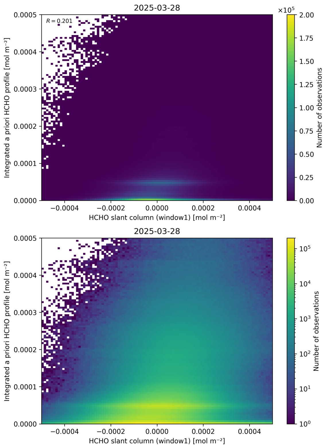
Figure 87: Scatter density plot of “HCHO slant column (window1)” against “Integrated a priori HCHO profile” for 2025-03-28 to 2025-03-29.
