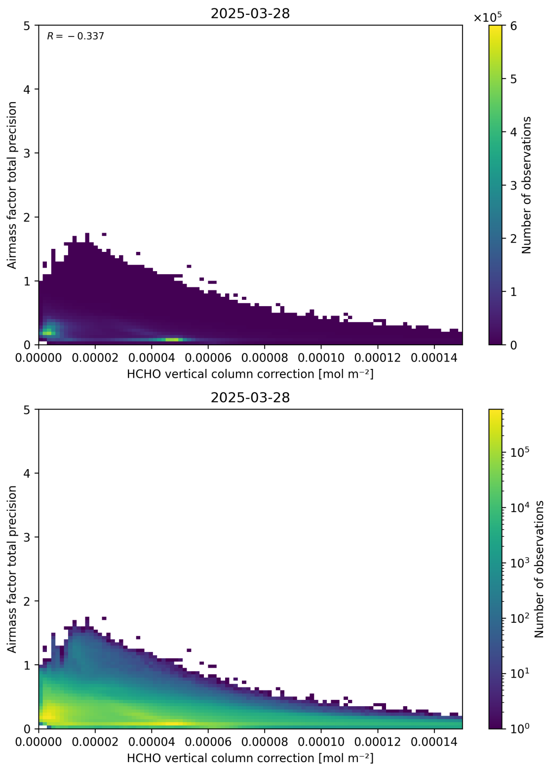
Figure 121: Scatter density plot of “HCHO vertical column correction” against “Airmass factor total precision” for 2025-03-28 to 2025-03-29.
