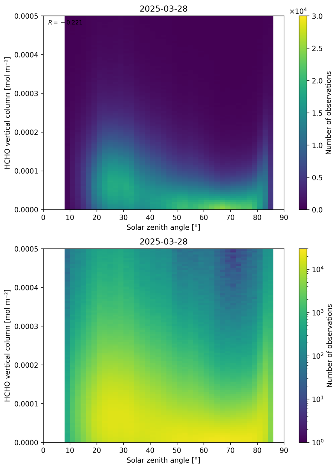
Figure 177: Scatter density plot of “Solar zenith angle” against “HCHO vertical column” for 2025-03-28 to 2025-03-29.
