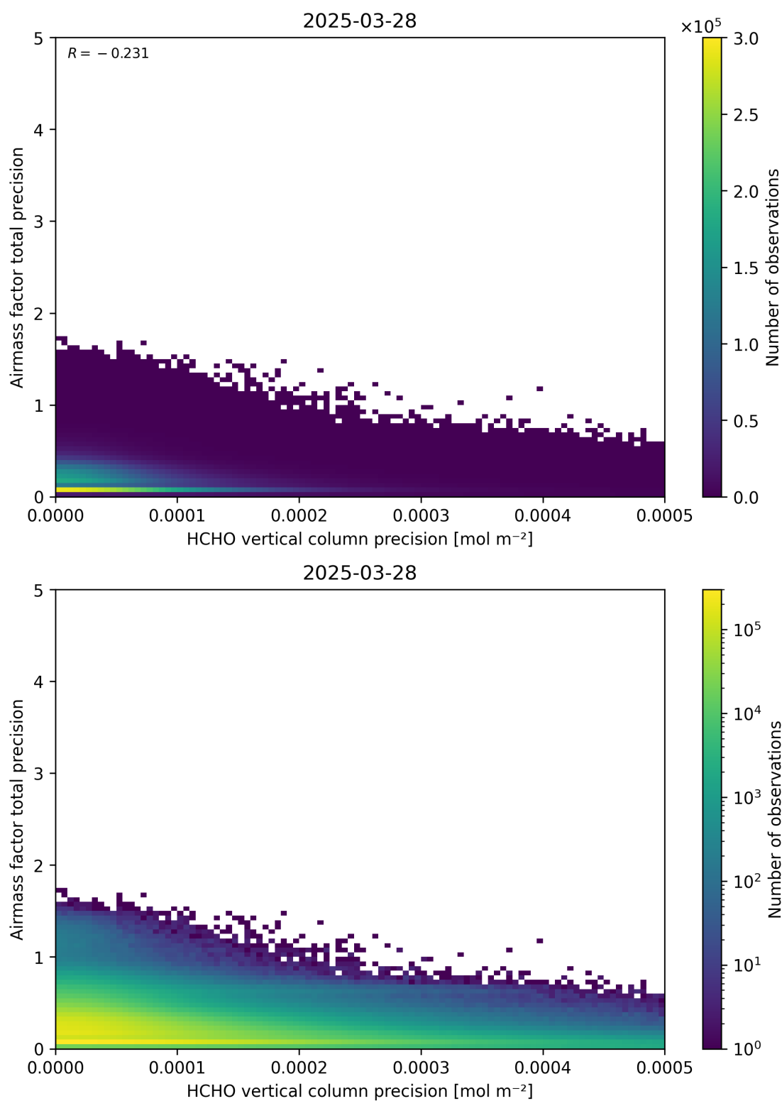
Figure 145: Scatter density plot of “HCHO vertical column precision” against “Airmass factor total precision” for 2025-03-28 to 2025-03-29.
