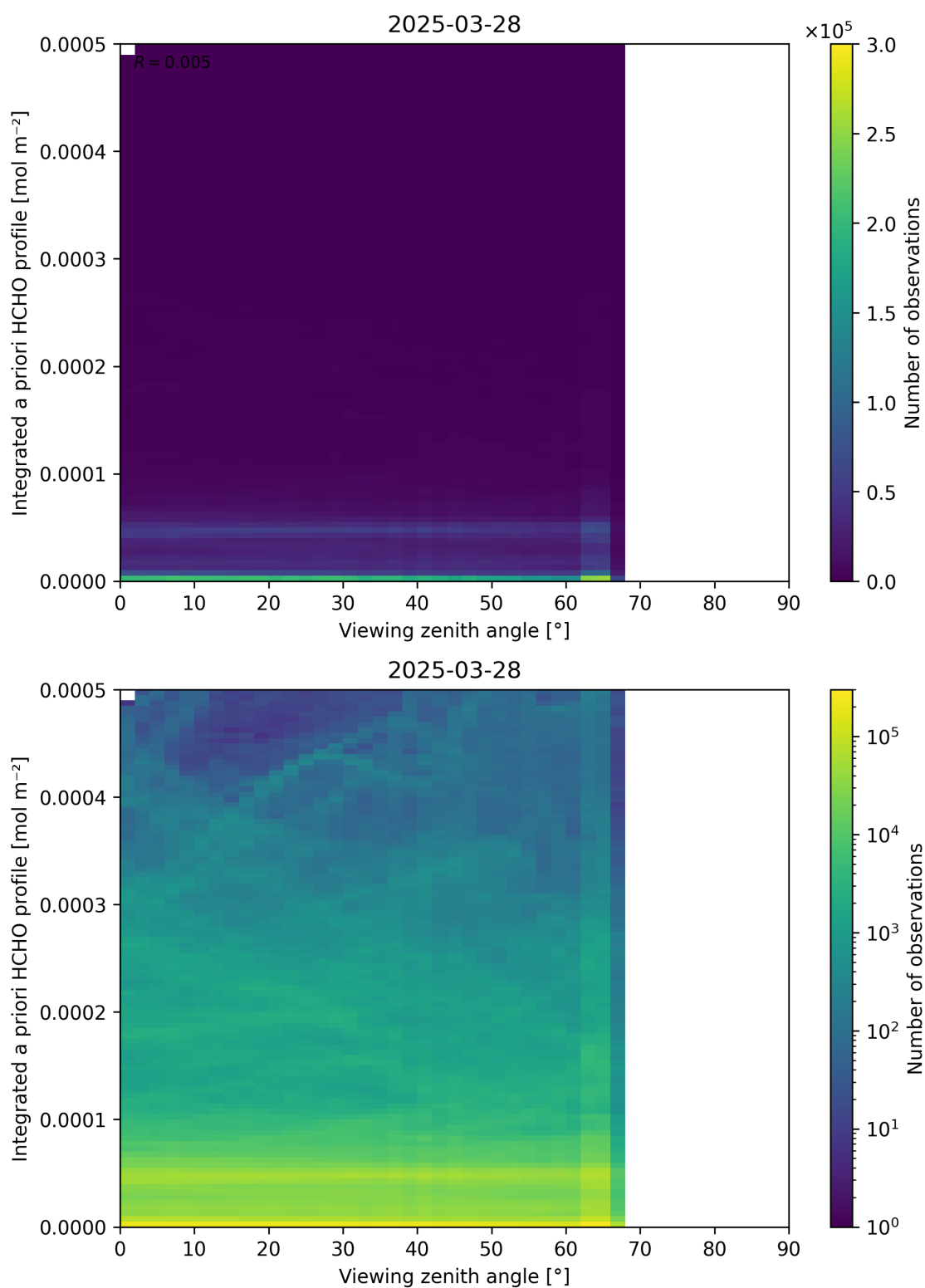
Figure 195: Scatter density plot of “Viewing zenith angle” against “Integrated a priori HCHO profile” for 2025-03-28 to 2025-03-29.
