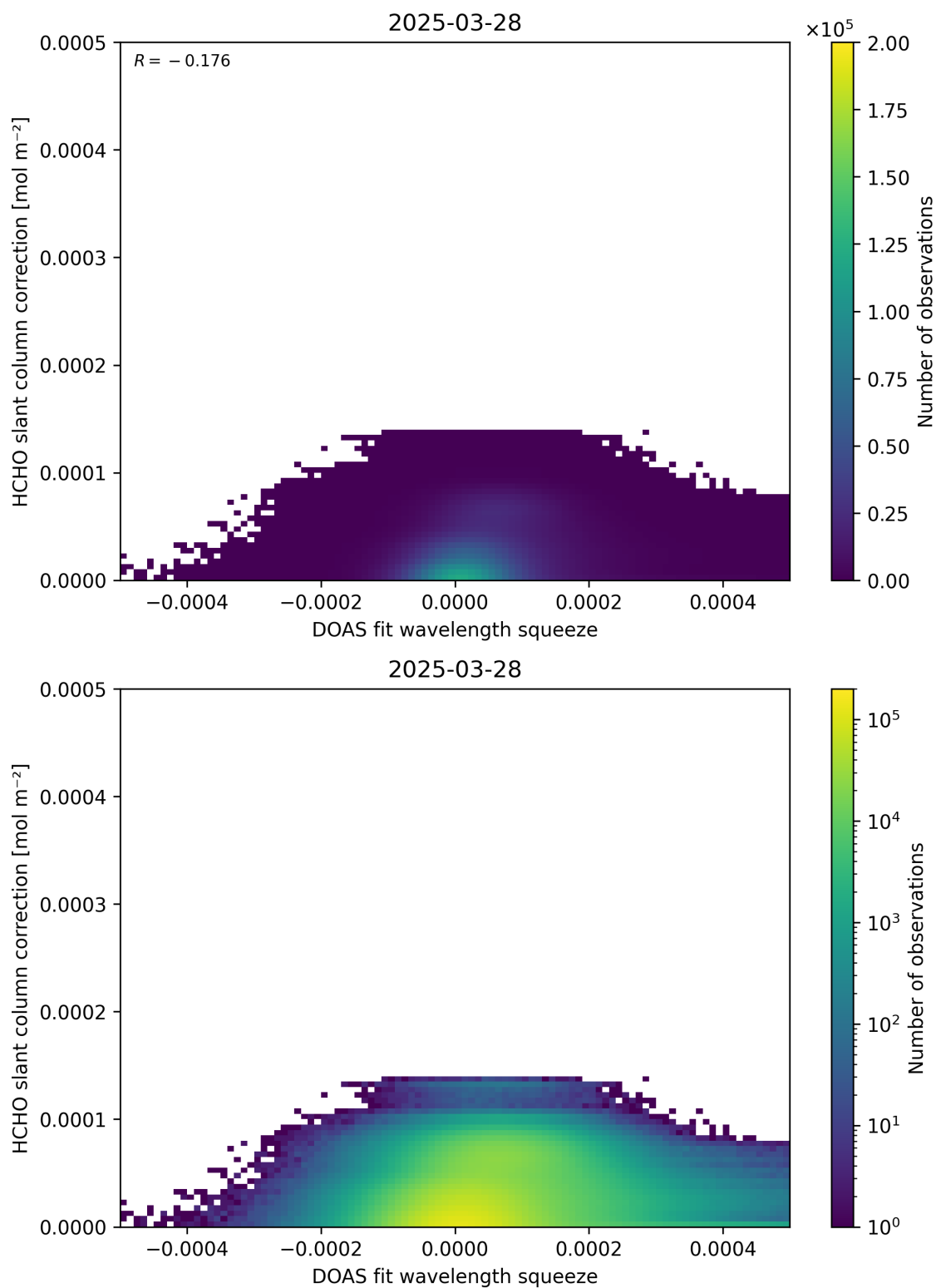
Figure 70: Scatter density plot of “DOAS fit wavelength squeeze” against “HCHO slant column correction” for 2025-03-28 to 2025-03-29.
