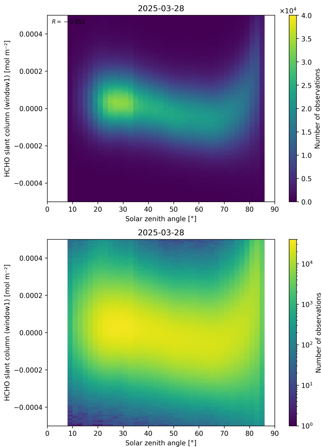
Figure 173: Scatter density plot of “Solar zenith angle” against “HCHO slant column (window1)” for 2025-03-28 to 2025-03-29.
