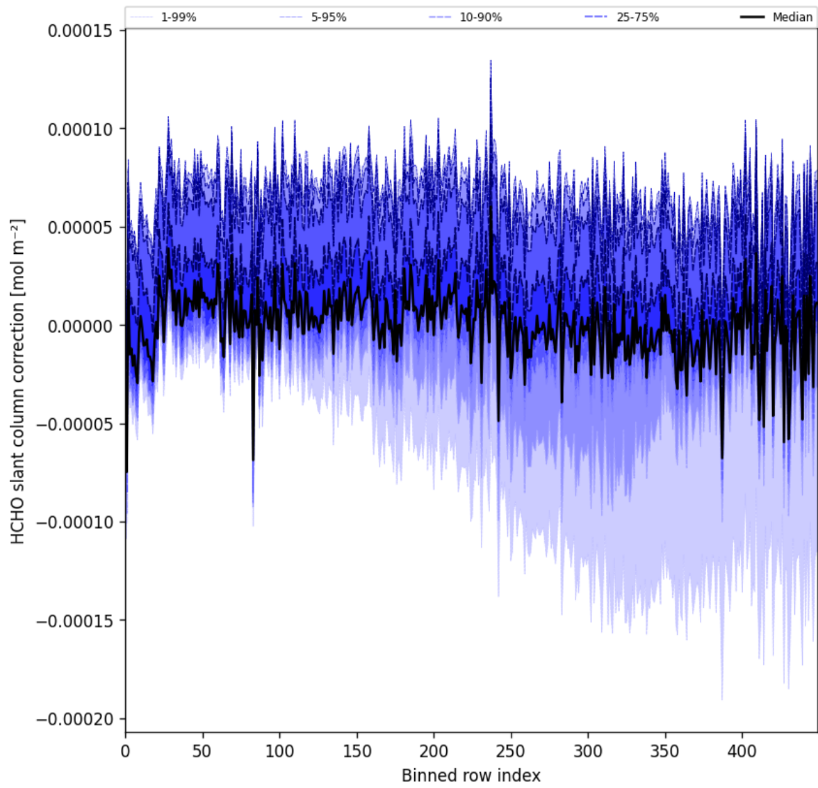
Figure 61: Along track statistics of “HCHO slant column correction” for 2025-03-28 to 2025-03-29
