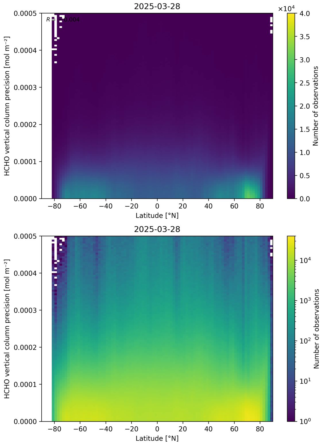
Figure 165: Scatter density plot of “Latitude” against “HCHO vertical column precision” for 2025-03-28 to 2025-03-29.
