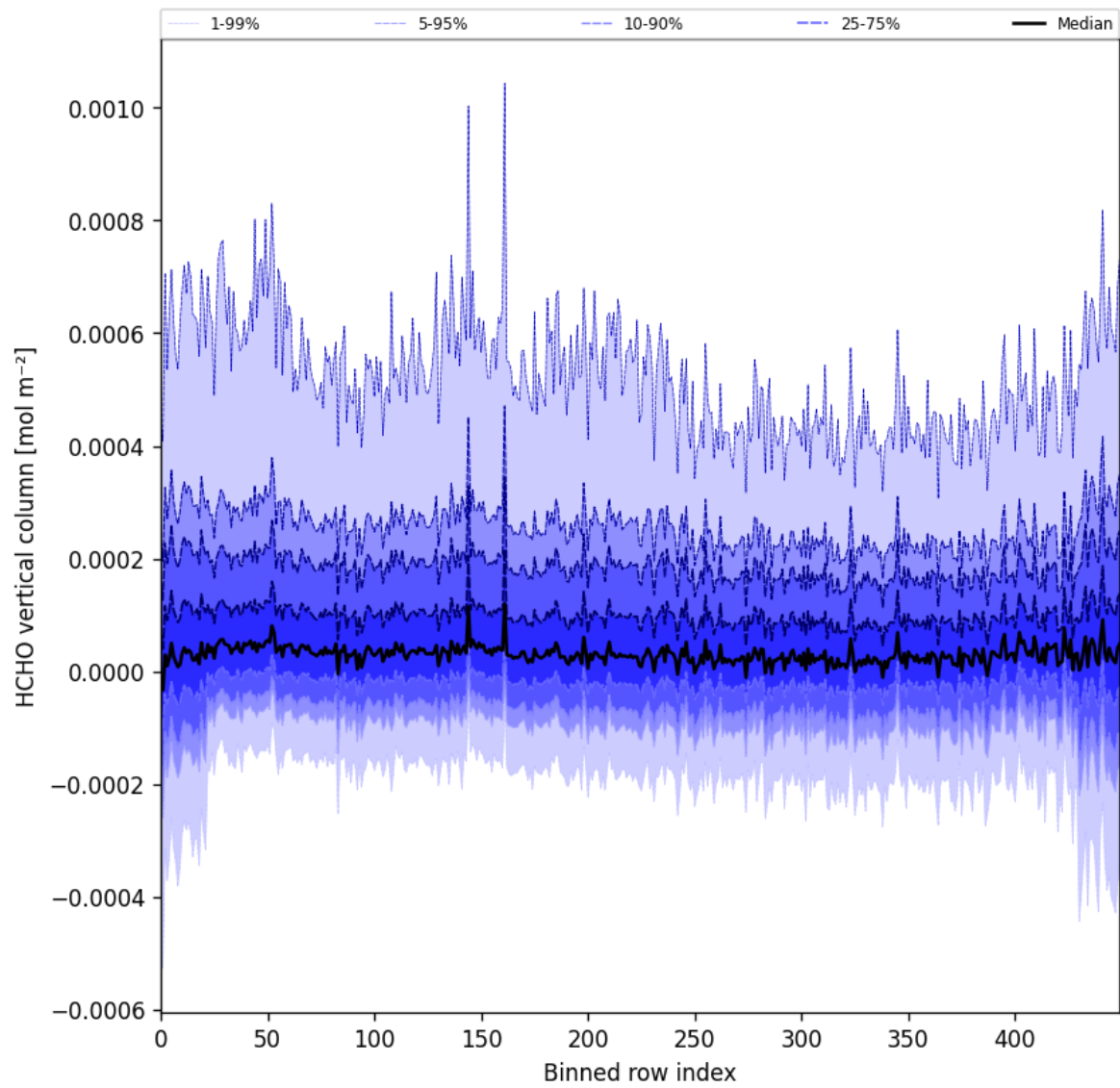
Figure 49: Along track statistics of “HCHO vertical column” for 2025-03-28 to 2025-03-29
