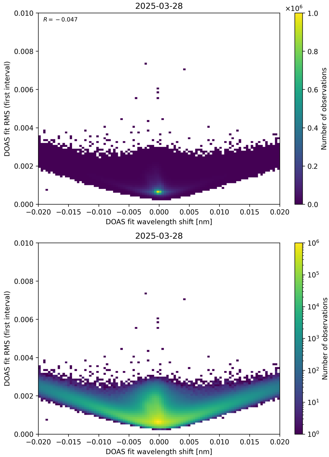
Figure 64: Scatter density plot of “DOAS fit wavelength shift” against “DOAS fit RMS (first interval)” for 2025-03-28 to 2025-03-29.
