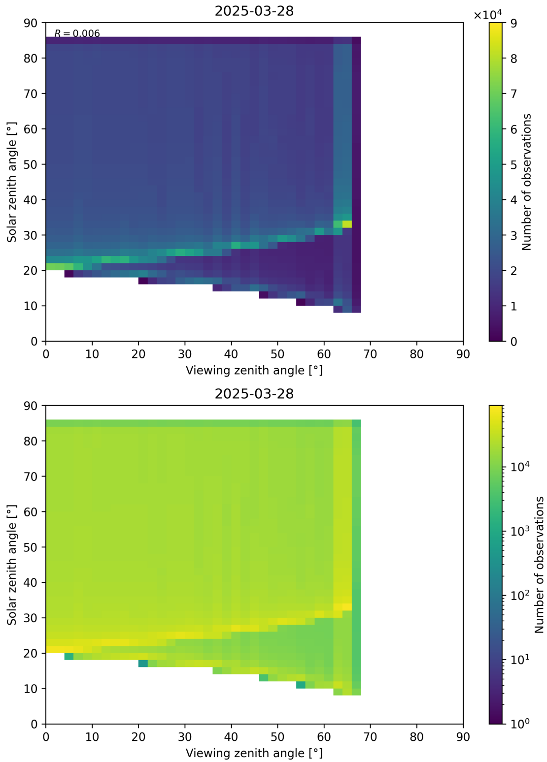
Figure 197: Scatter density plot of “Viewing zenith angle” against “Solar zenith angle” for 2025-03-28 to 2025-03-29.
