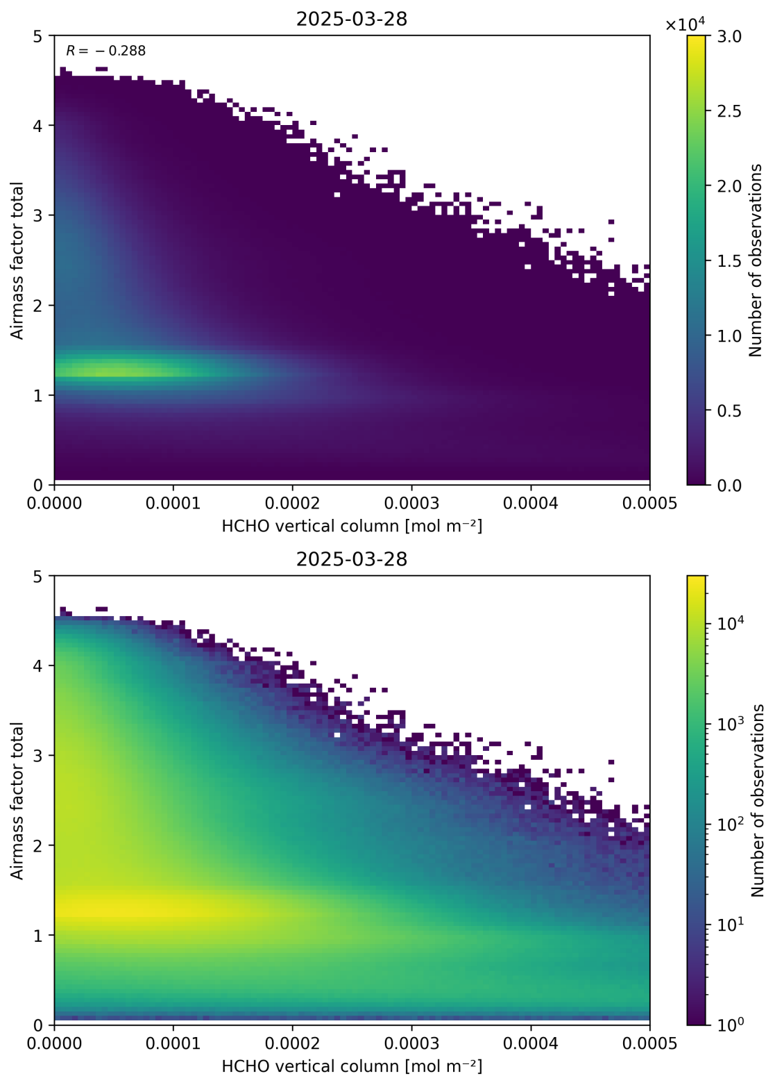
Figure 131: Scatter density plot of “HCHO vertical column” against “Airmass factor total” for 2025-03-28 to 2025-03-29.
