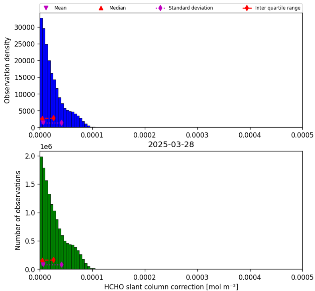
Figure 47: Histogram of “HCHO slant column correction” for 2025-03-28 to 2025-03-29
