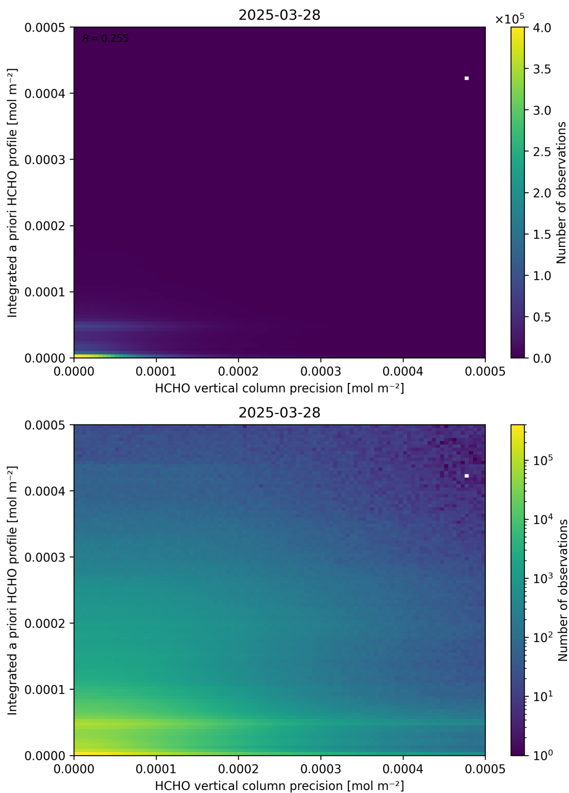
Figure 147: Scatter density plot of “HCHO vertical column precision” against “Integrated a priori HCHO profile” for 2025-03-28 to 2025-03-29.
