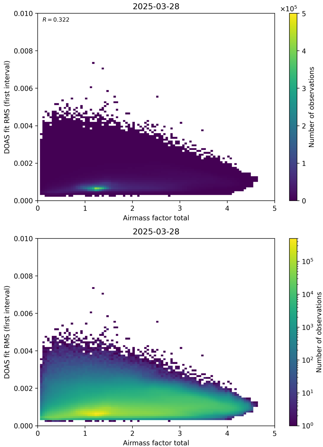
Figure 97: Scatter density plot of “Airmass factor total” against “DOAS fit RMS (first interval)” for 2025-03-28 to 2025-03-29.
