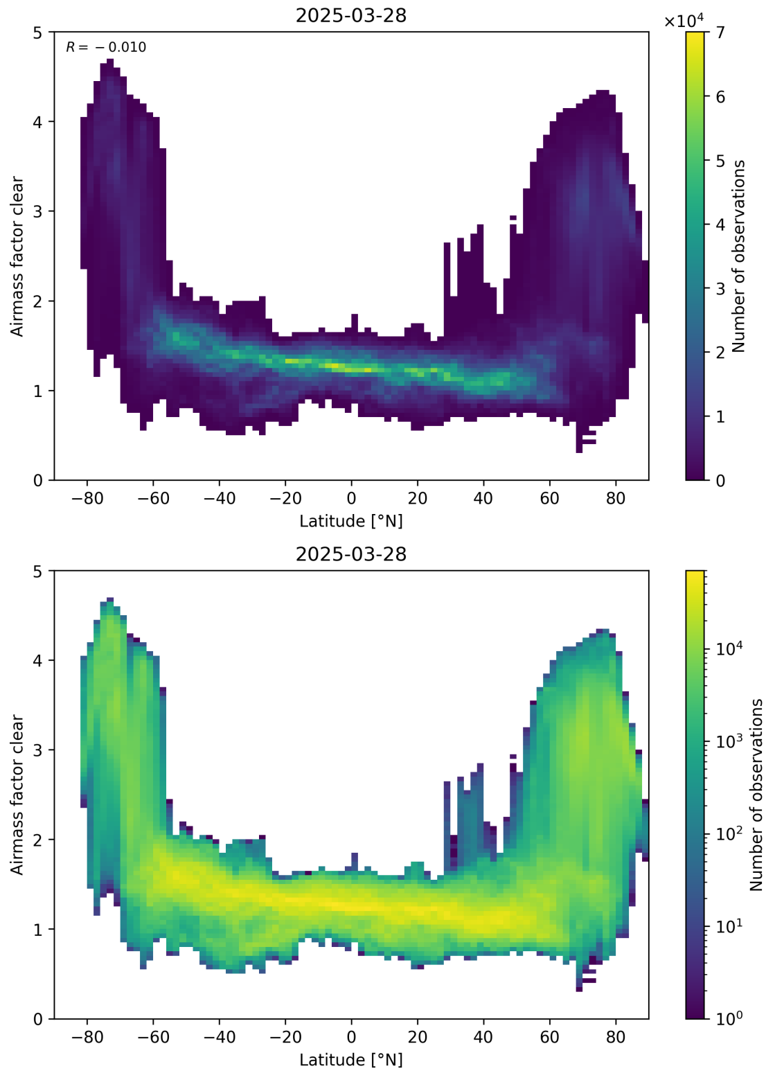
Figure 156: Scatter density plot of “Latitude” against “Airmass factor clear” for 2025-03-28 to 2025-03-29.
