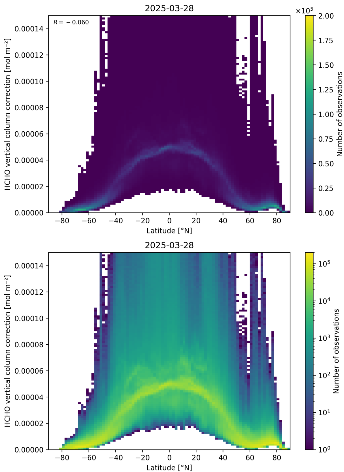
Figure 164: Scatter density plot of “Latitude” against “HCHO vertical column correction” for 2025-03-28 to 2025-03-29.
