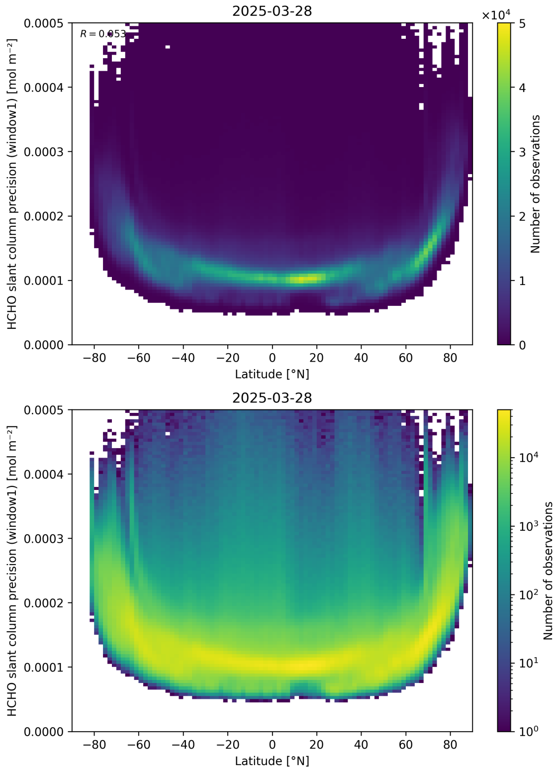
Figure 160: Scatter density plot of “Latitude” against “HCHO slant column precision (window1)” for 2025-03-28 to 2025-03-29.
