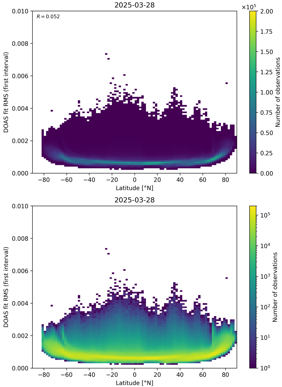
Figure 153: Scatter density plot of “Latitude” against “DOAS fit RMS (first interval)” for 2025-03-28 to 2025-03-29.
