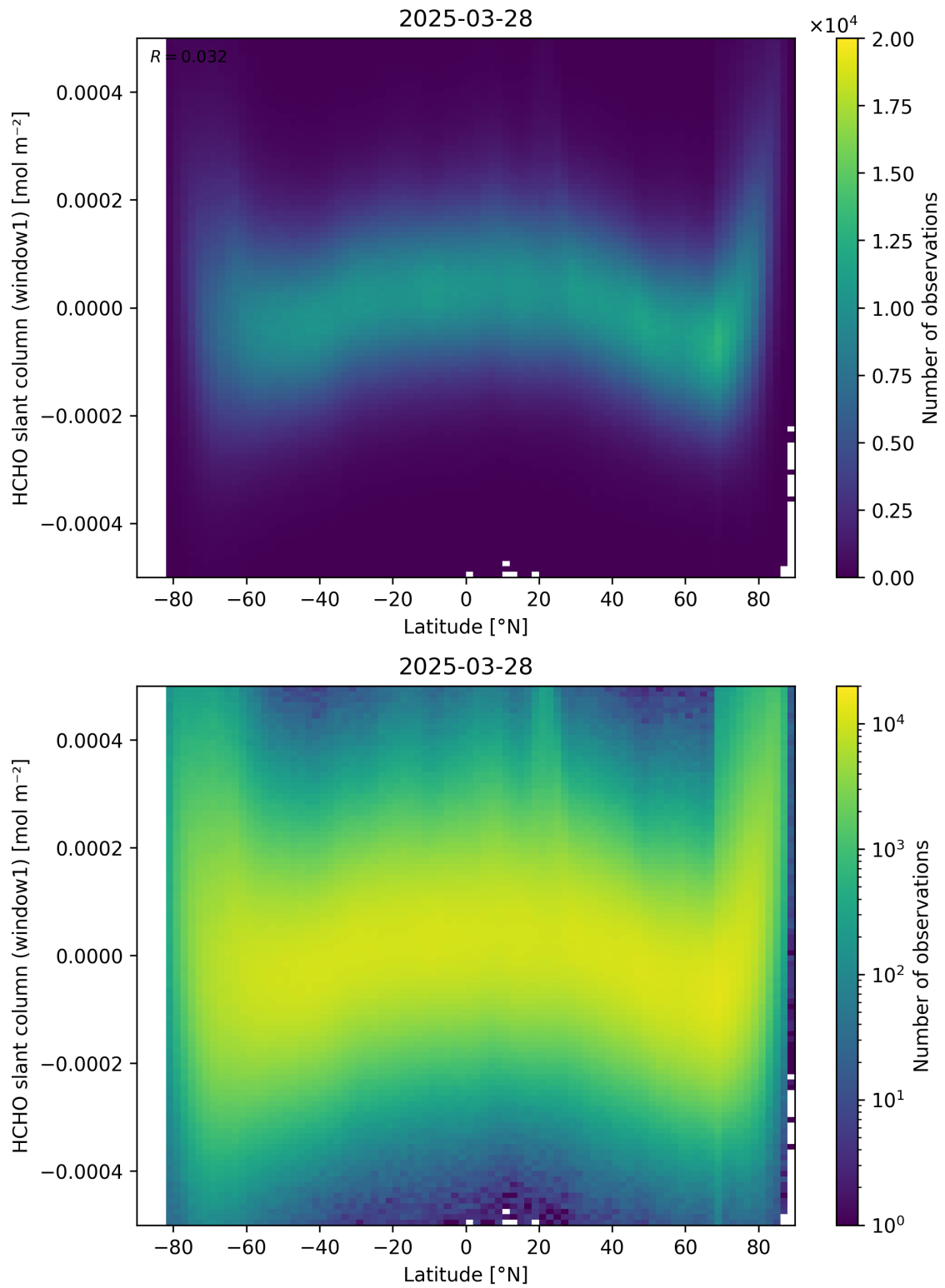
Figure 159: Scatter density plot of “Latitude” against “HCHO slant column (window1)” for 2025-03-28 to 2025-03-29.
