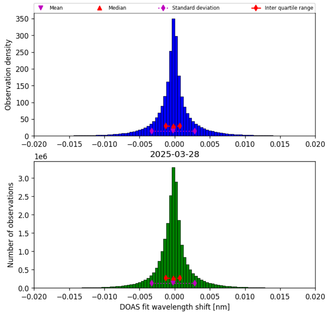
Figure 44: Histogram of “DOAS fit wavelength shift” for 2025-03-28 to 2025-03-29
