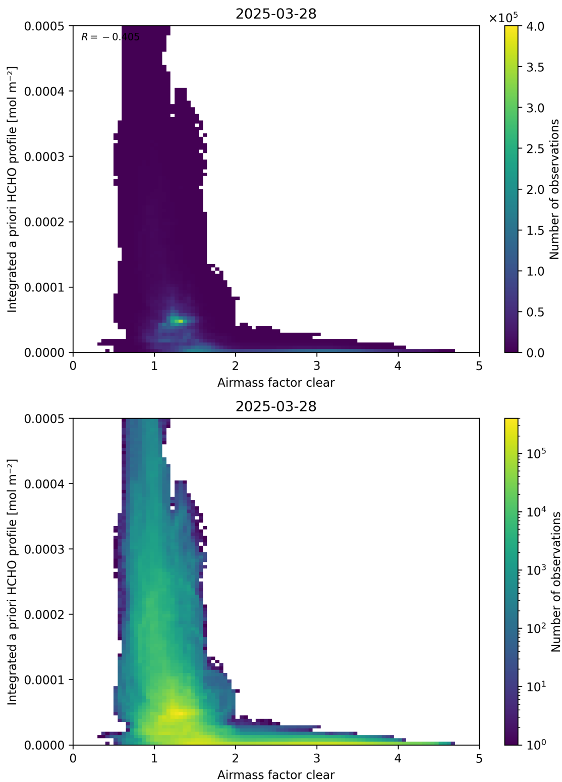
Figure 76: Scatter density plot of “Airmass factor clear” against “Integrated a priori HCHO profile” for 2025-03-28 to 2025-03-29.
