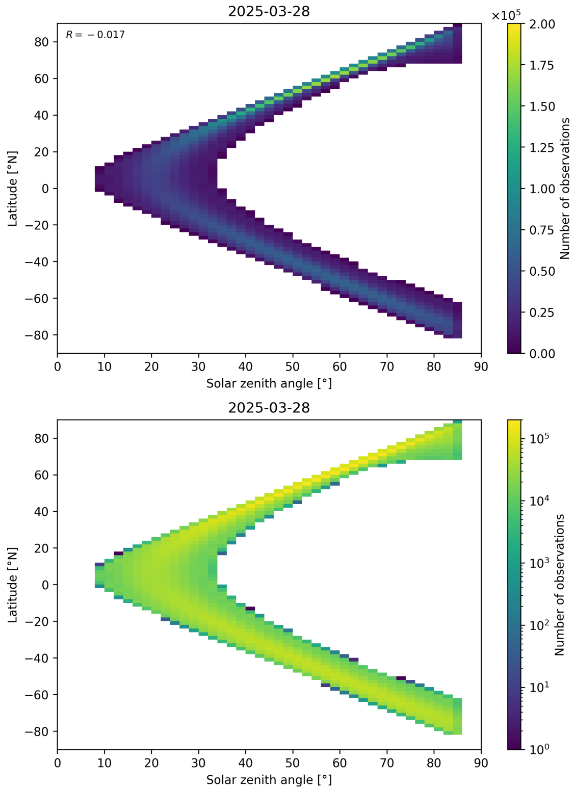
Figure 181: Scatter density plot of “Solar zenith angle” against “Latitude” for 2025-03-28 to 2025-03-29.
