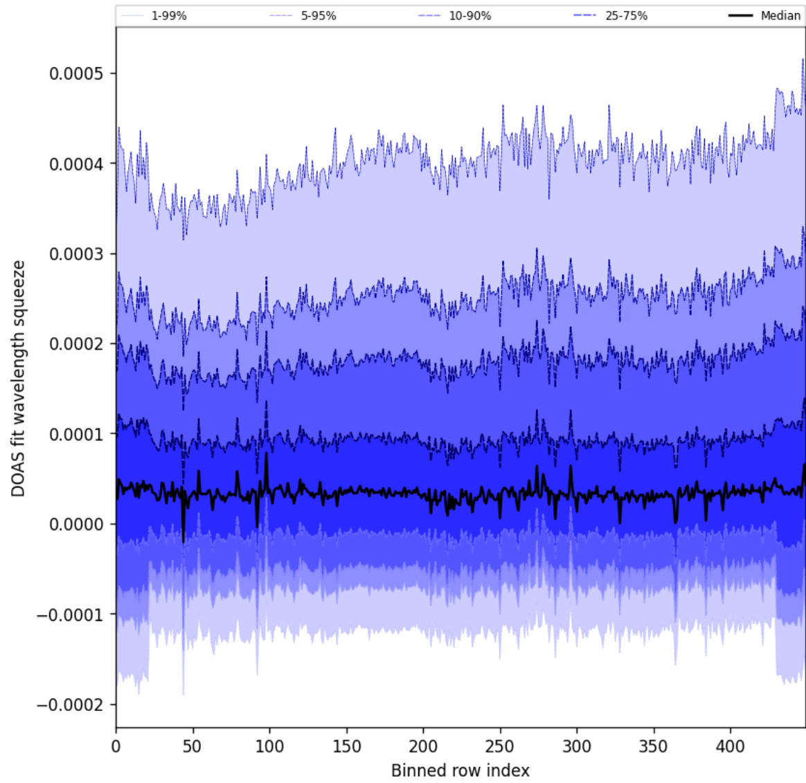
Figure 59: Along track statistics of “DOAS fit wavelength squeeze” for 2025-03-28 to 2025-03-29
