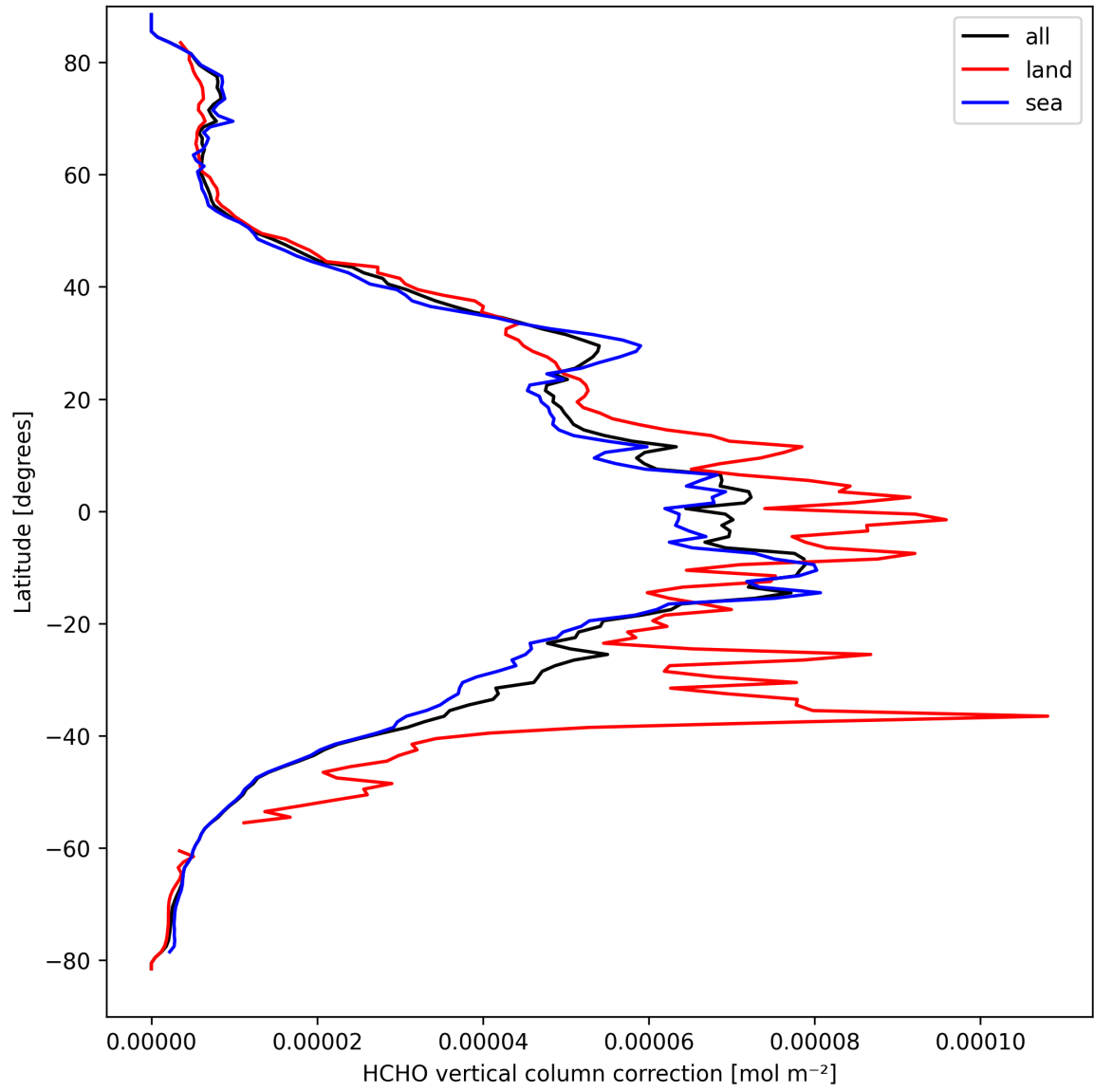
Figure 23: Zonal average of “HCHO vertical column correction” for 2025-03-28 to 2025-03-29.
