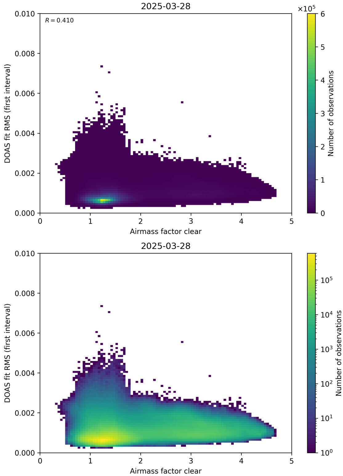
Figure 71: Scatter density plot of “Airmass factor clear” against “DOAS fit RMS (first interval)” for 2025-03-28 to 2025-03-29.
