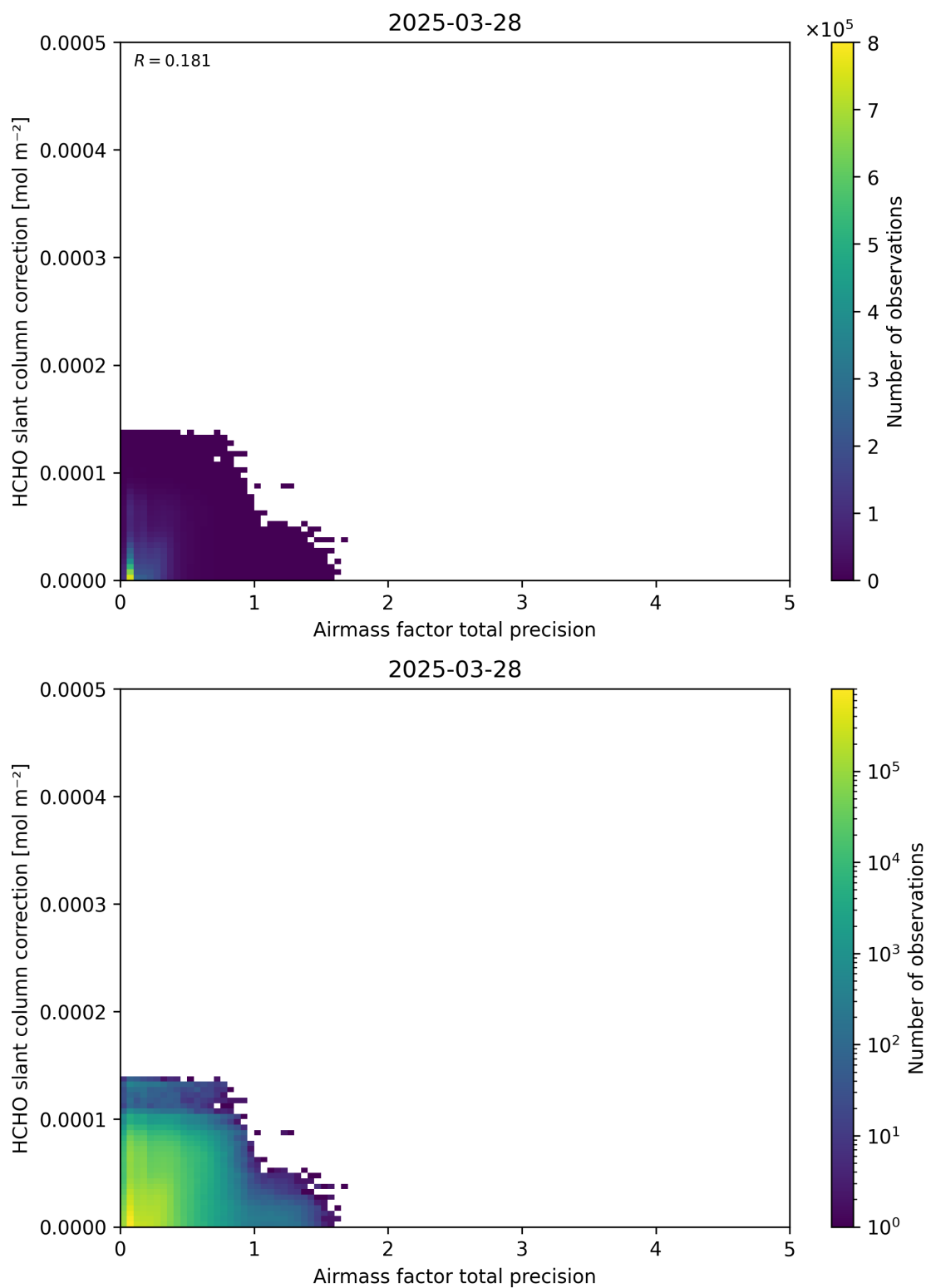
Figure 110: Scatter density plot of “Airmass factor total precision” against “HCHO slant column correction” for 2025-03-28 to 2025-03-29.
