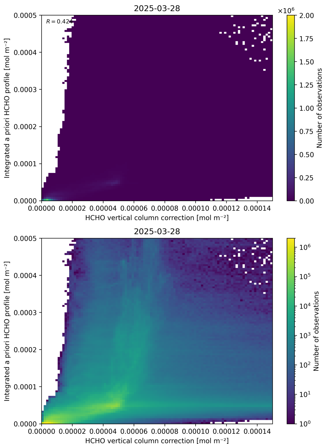
Figure 122: Scatter density plot of “HCHO vertical column correction” against “Integrated a priori HCHO profile” for 2025-03-28 to 2025-03-29.
