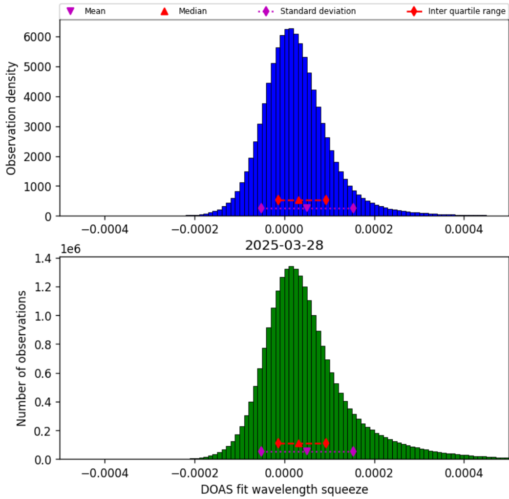
Figure 45: Histogram of “DOAS fit wavelength squeeze” for 2025-03-28 to 2025-03-29
