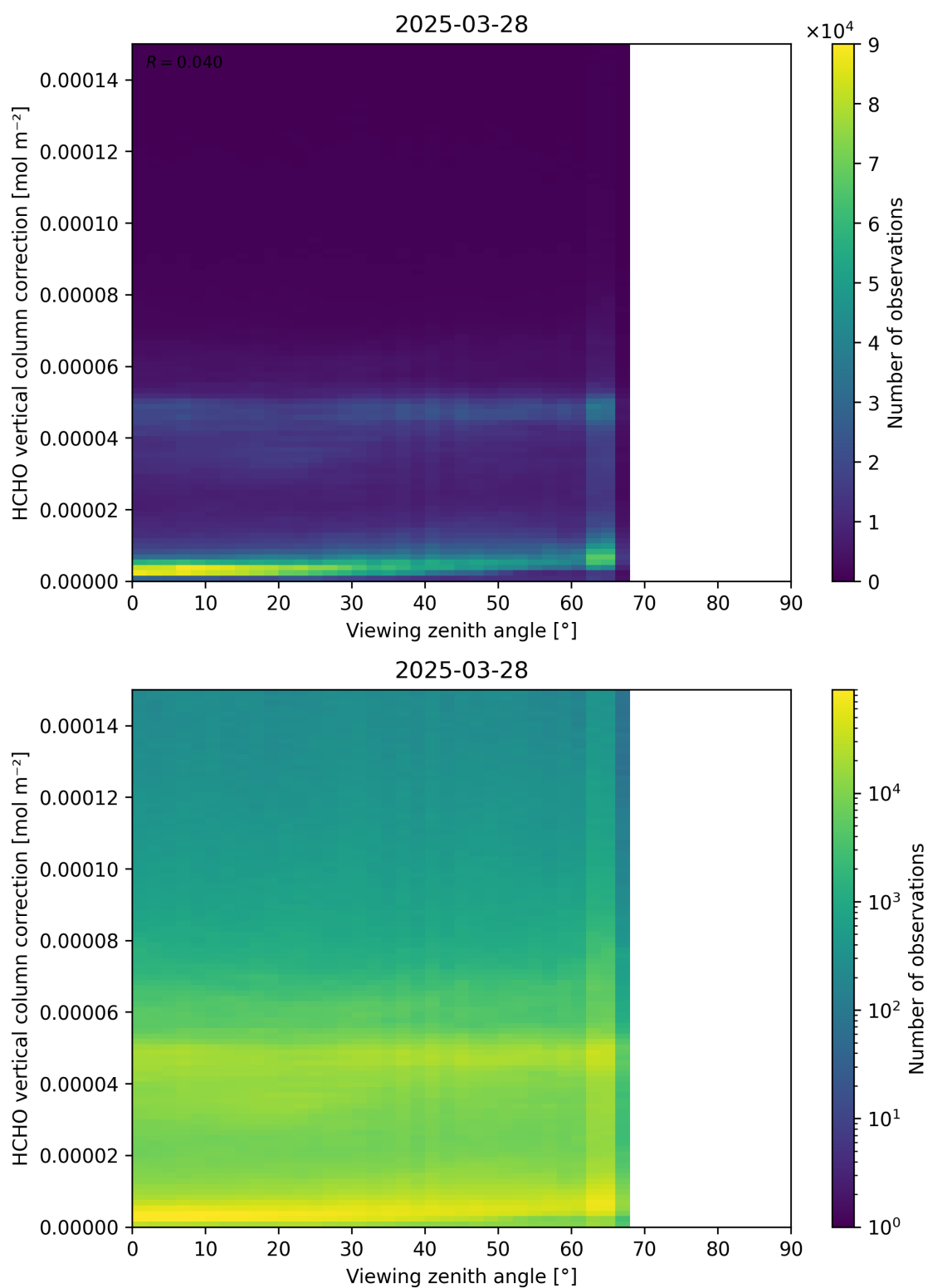
Figure 193: Scatter density plot of “Viewing zenith angle” against “HCHO vertical column correction” for 2025-03-28 to 2025-03-29.
