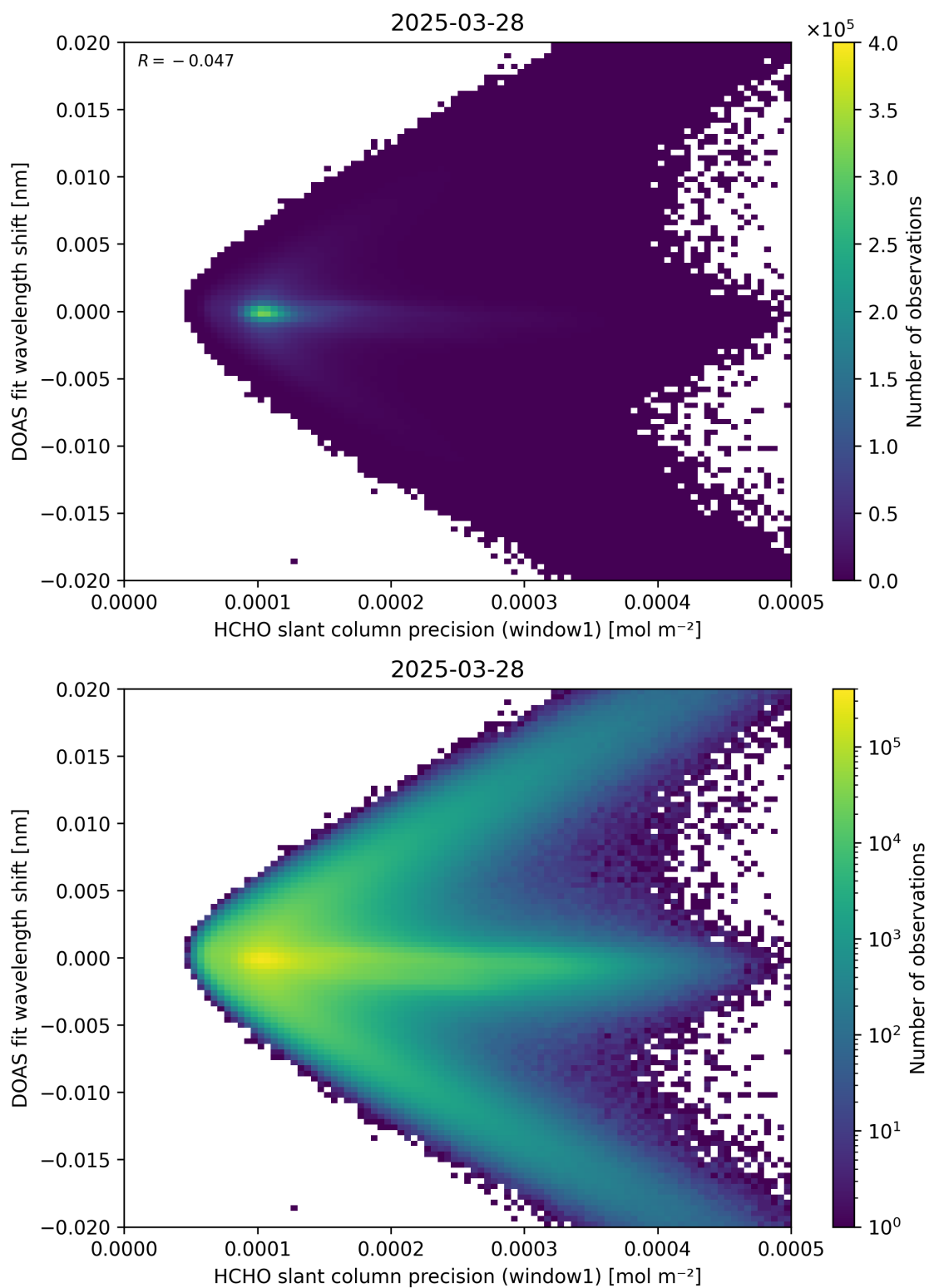
Figure 89: Scatter density plot of “HCHO slant column precision (window1)” against “DOAS fit wavelength shift” for 2025-03-28 to 2025-03-29.
