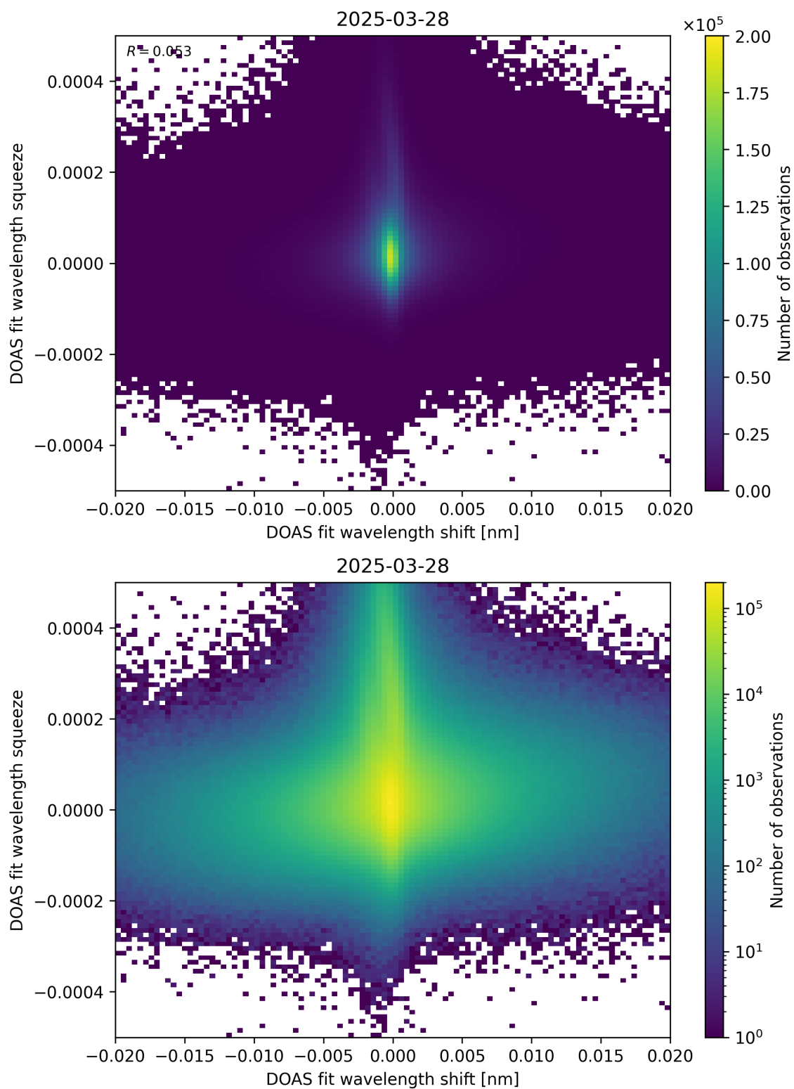
Figure 65: Scatter density plot of “DOAS fit wavelength shift” against “DOAS fit wavelength squeeze” for 2025-03-28 to 2025-03-29.
