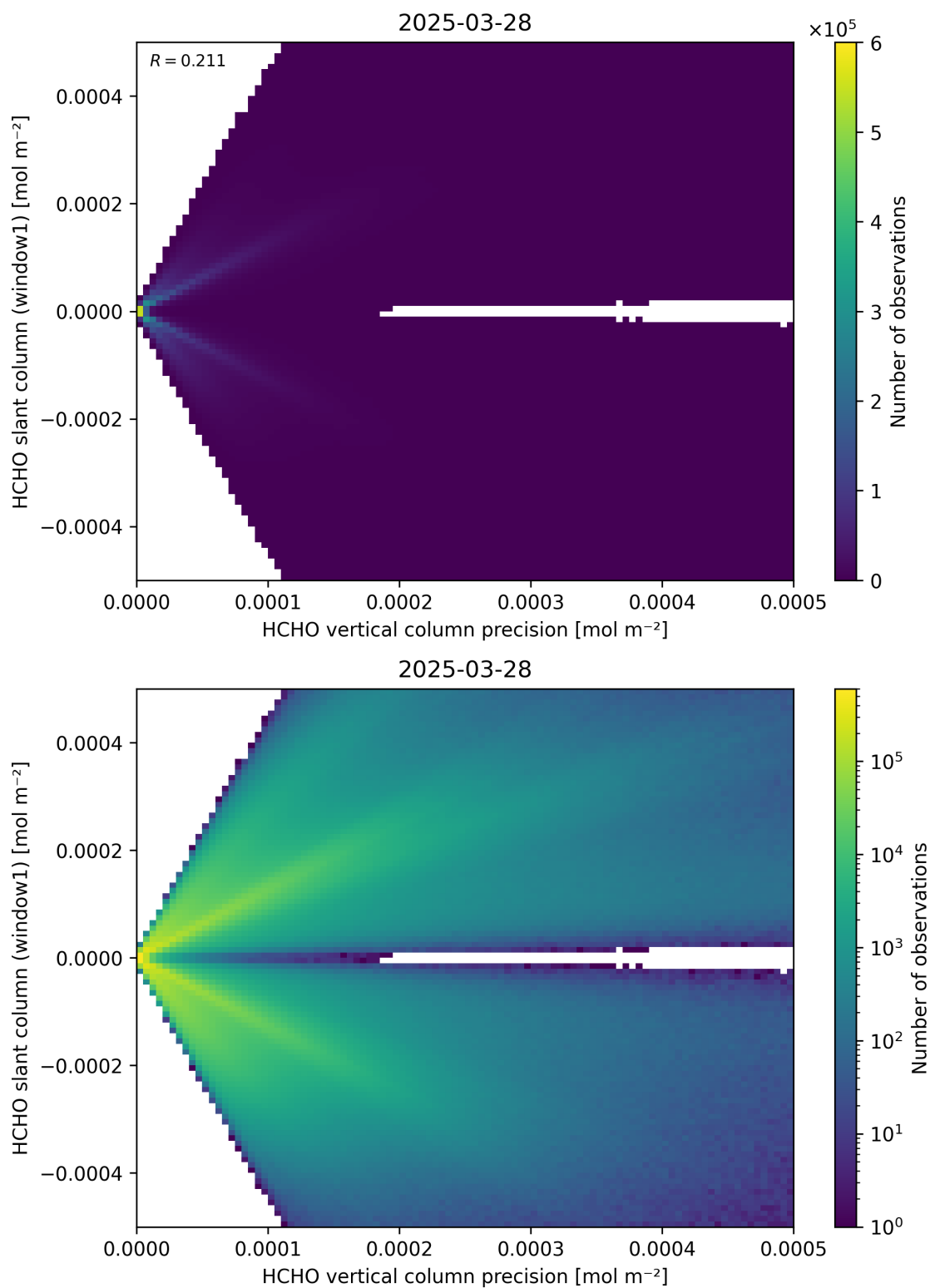
Figure 142: Scatter density plot of “HCHO vertical column precision” against “HCHO slant column (window1)” for 2025-03-28 to 2025-03-29.
