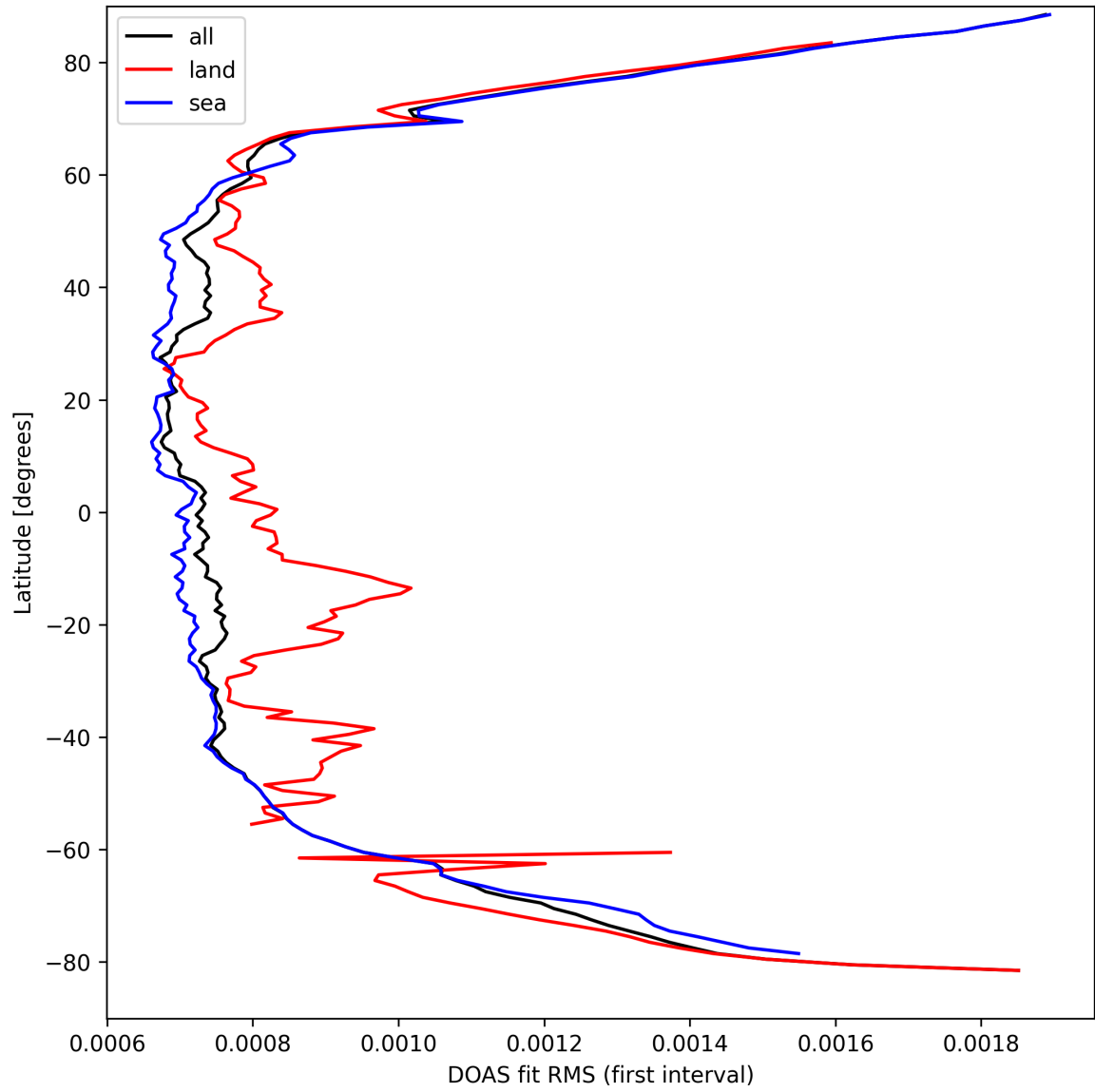
Figure 32: Zonal average of "DOAS fit RMS (first interval)" for 2025-03-28 to 2025-03-29.
