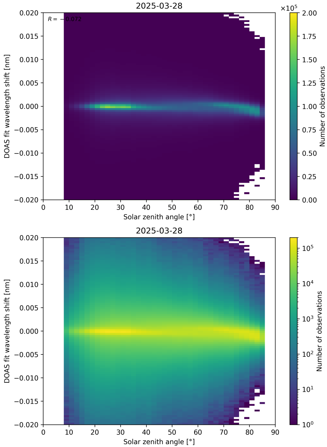
Figure 168: Scatter density plot of “Solar zenith angle” against “DOAS fit wavelength shift” for 2025-03-28 to 2025-03-29.
