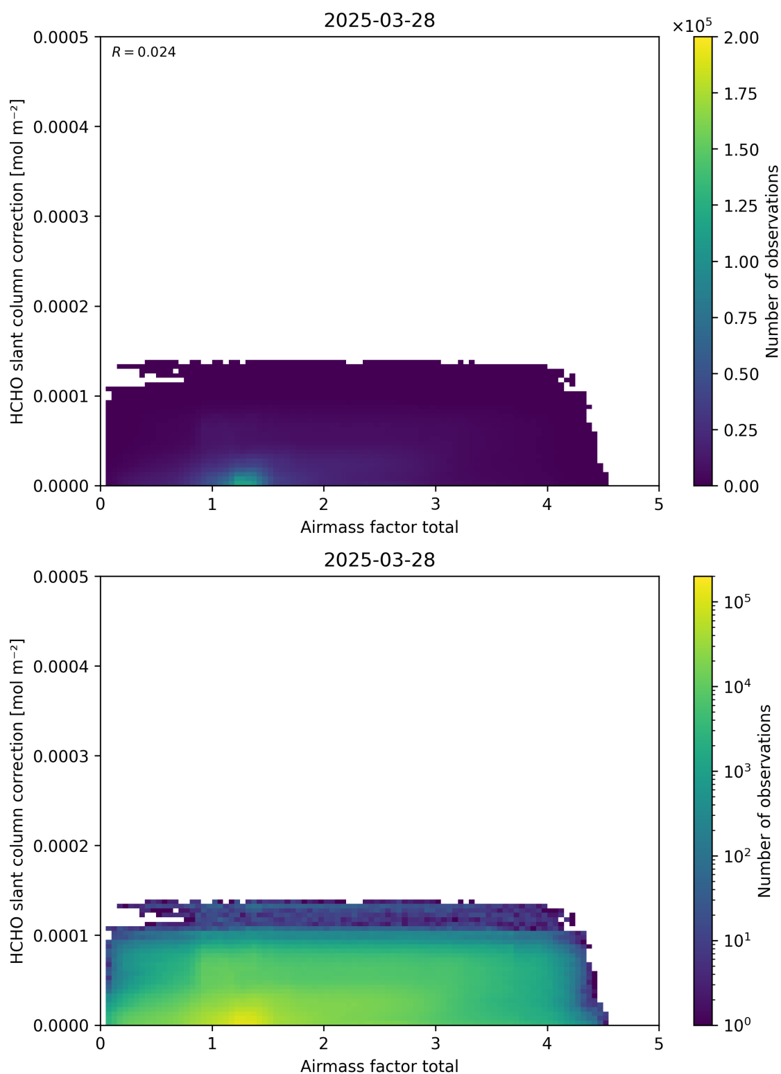
Figure 102: Scatter density plot of “Airmass factor total” against “HCHO slant column correction” for 2025-03-28 to 2025-03-29.
