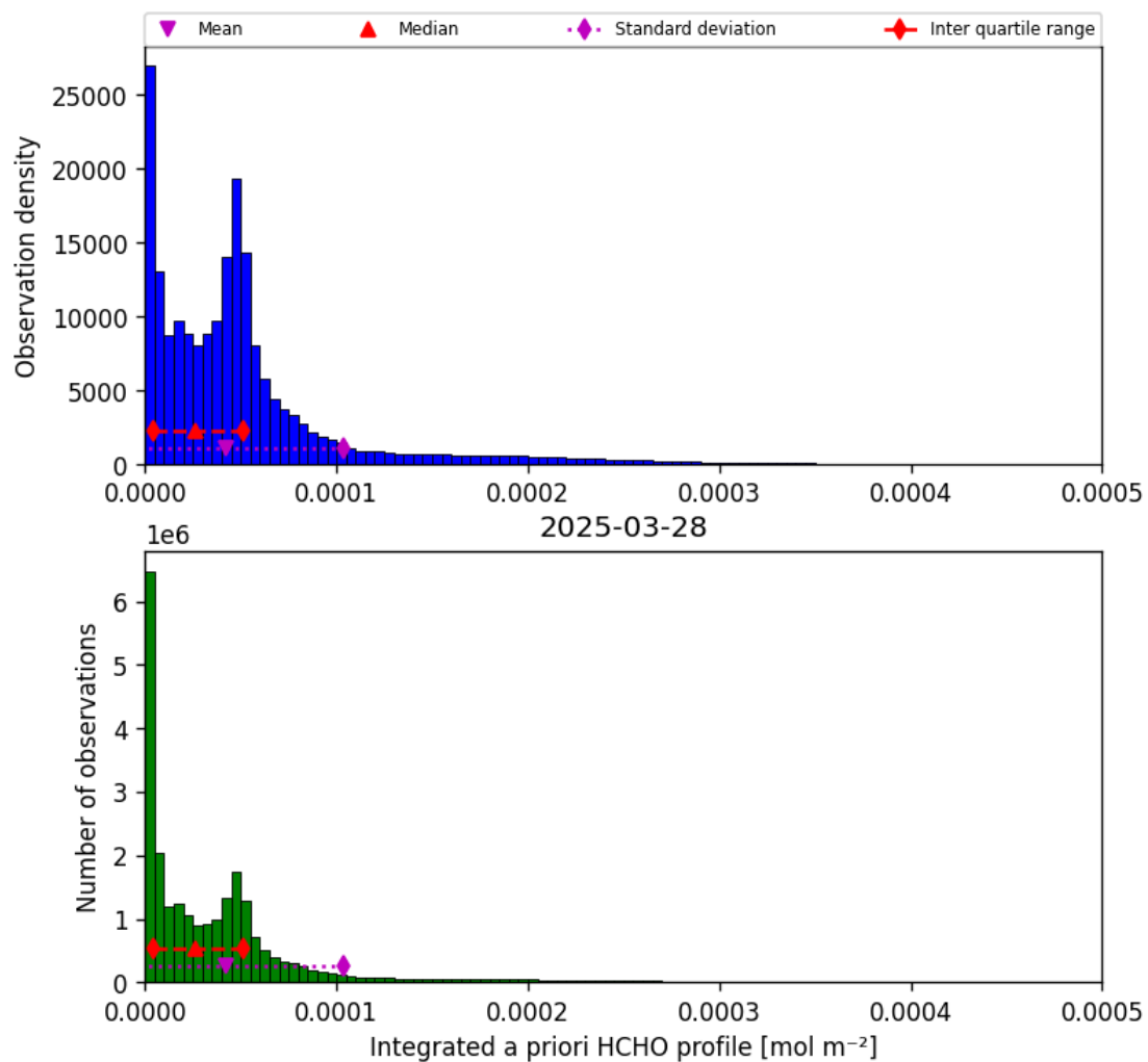
Figure 43: Histogram of “Integrated a priori HCHO profile” for 2025-03-28 to 2025-03-29
