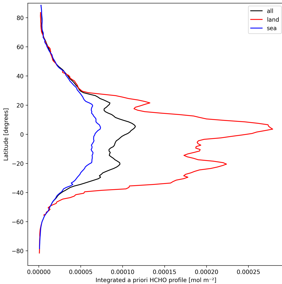
Figure 29: Zonal average of “Integrated a priori HCHO profile” for 2025-03-28 to 2025-03-29.
