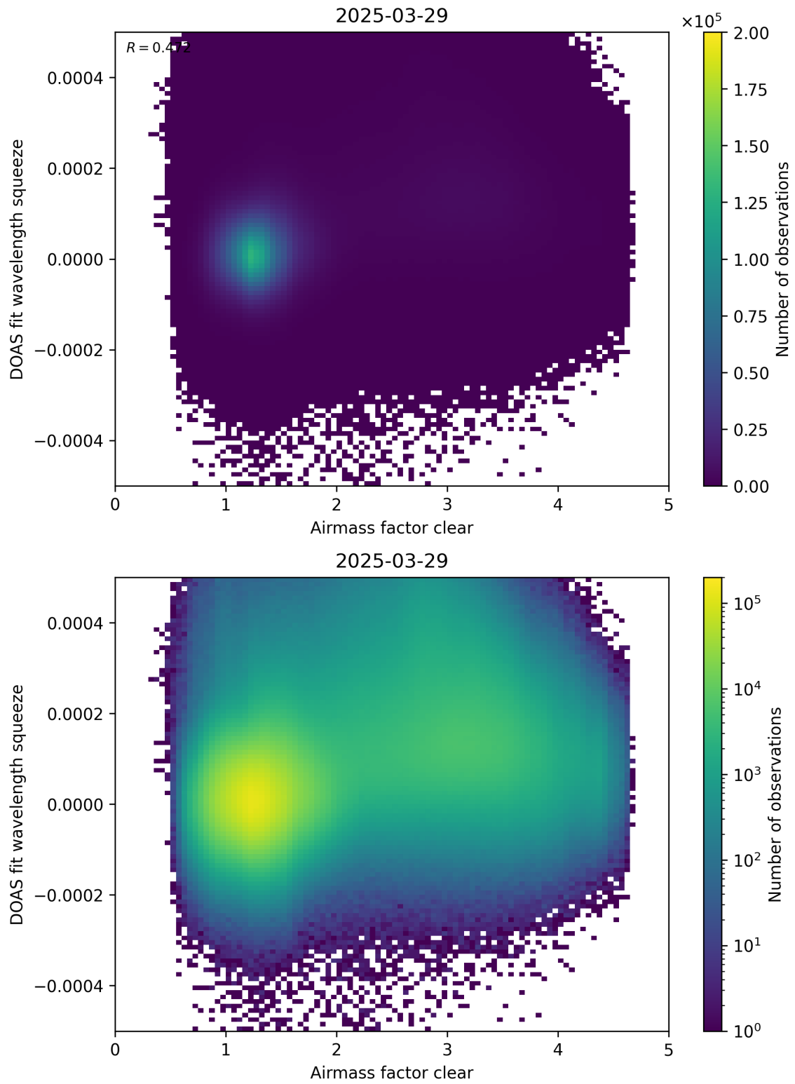
Figure 73: Scatter density plot of “Airmass factor clear” against “DOAS fit wavelength squeeze” for 2025-03-28 to 2025-03-30.
