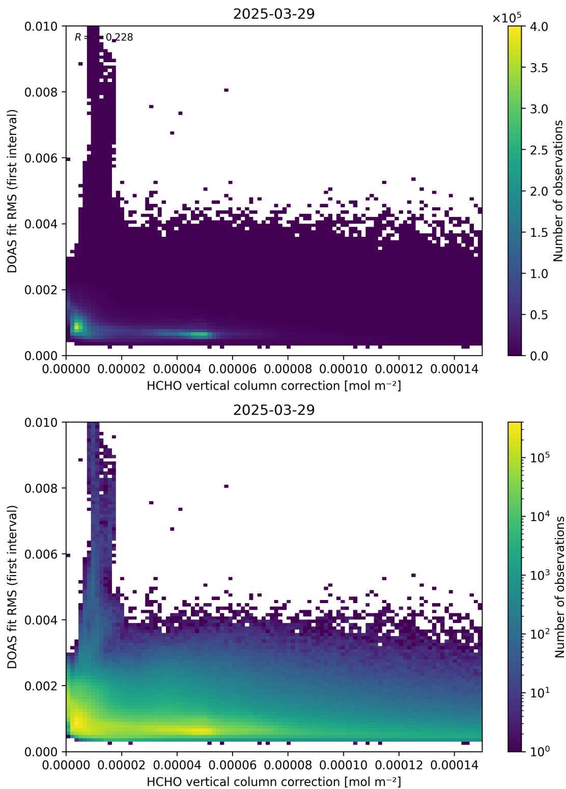
Figure 112: Scatter density plot of “HCHO vertical column correction” against “DOAS fit RMS (first interval)” for 2025-03-28 to 2025-03-30.
