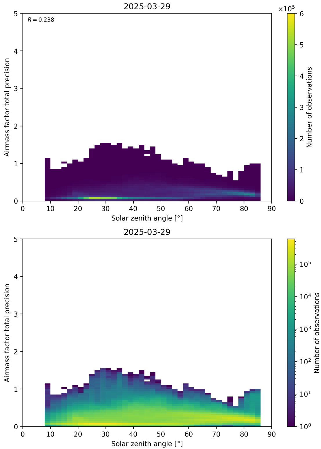
Figure 176: Scatter density plot of “Solar zenith angle” against “Airmass factor total precision” for 2025-03-28 to 2025-03-30.
