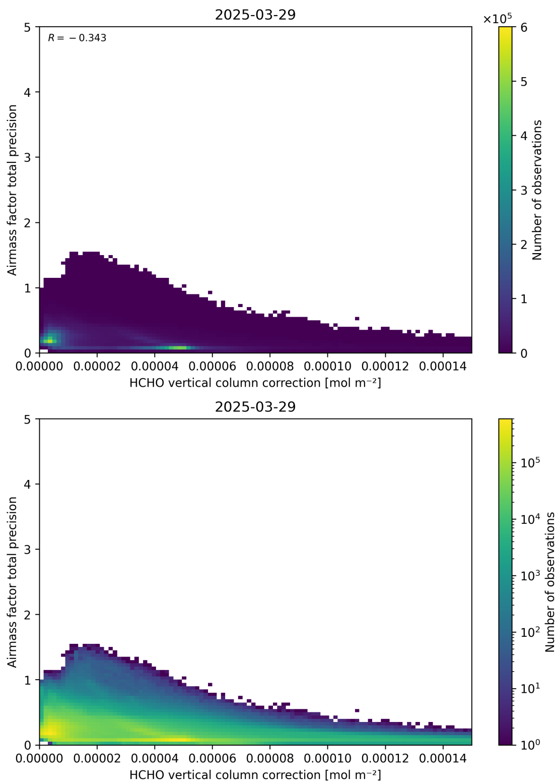
Figure 121: Scatter density plot of “HCHO vertical column correction” against “Airmass factor total precision” for 2025-03-28 to 2025-03-30.
