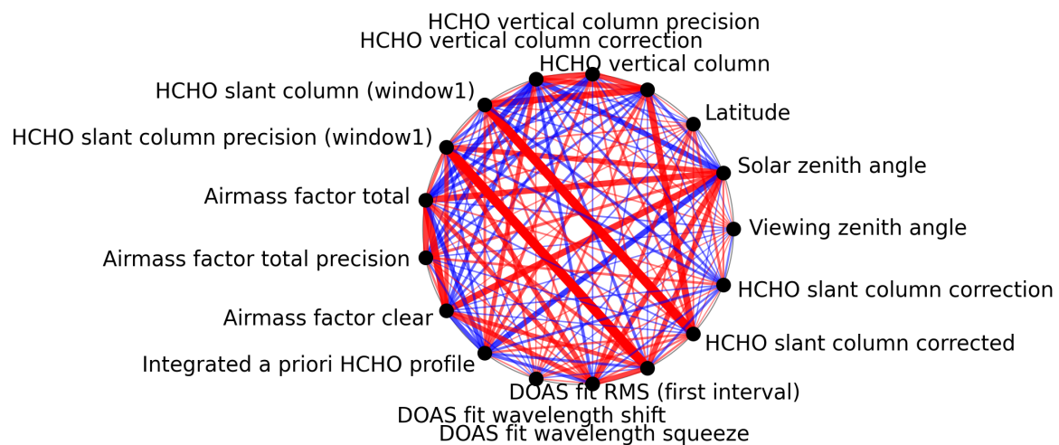
Figure 1: Map of correlation graph for 2025-03-28 to 2025-03-30.
