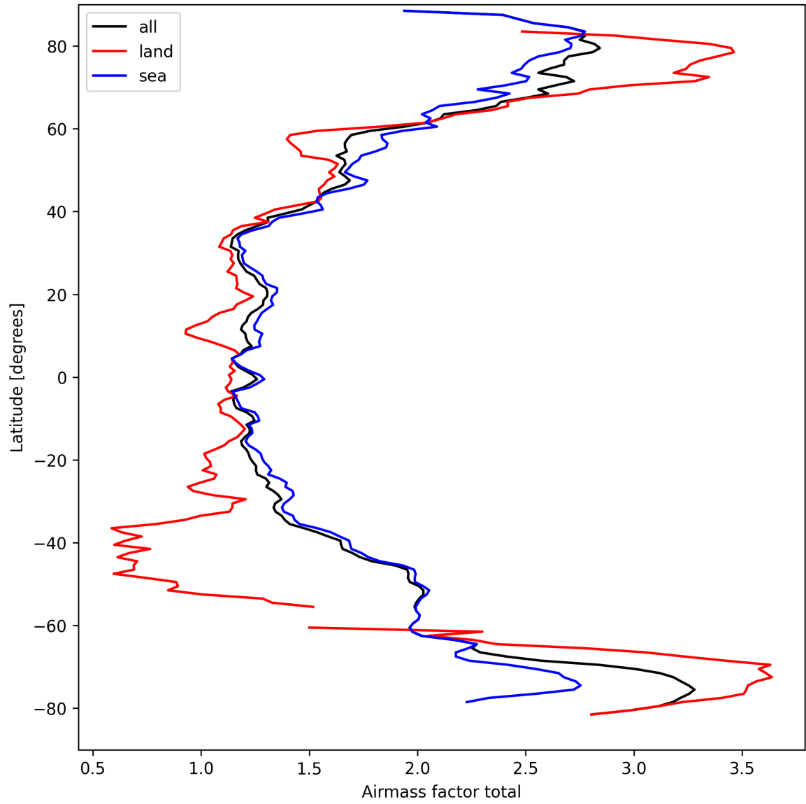
Figure 26: Zonal average of “Airmass factor total” for 2025-03-28 to 2025-03-30.
