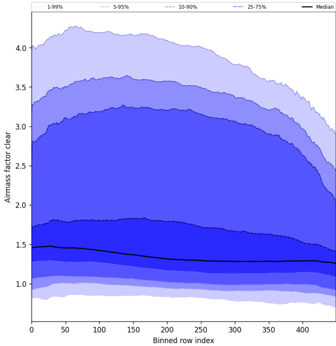
Figure 56: Along track statistics of “Air mass factor clear” for 2025-03-28 to 2025-03-30
