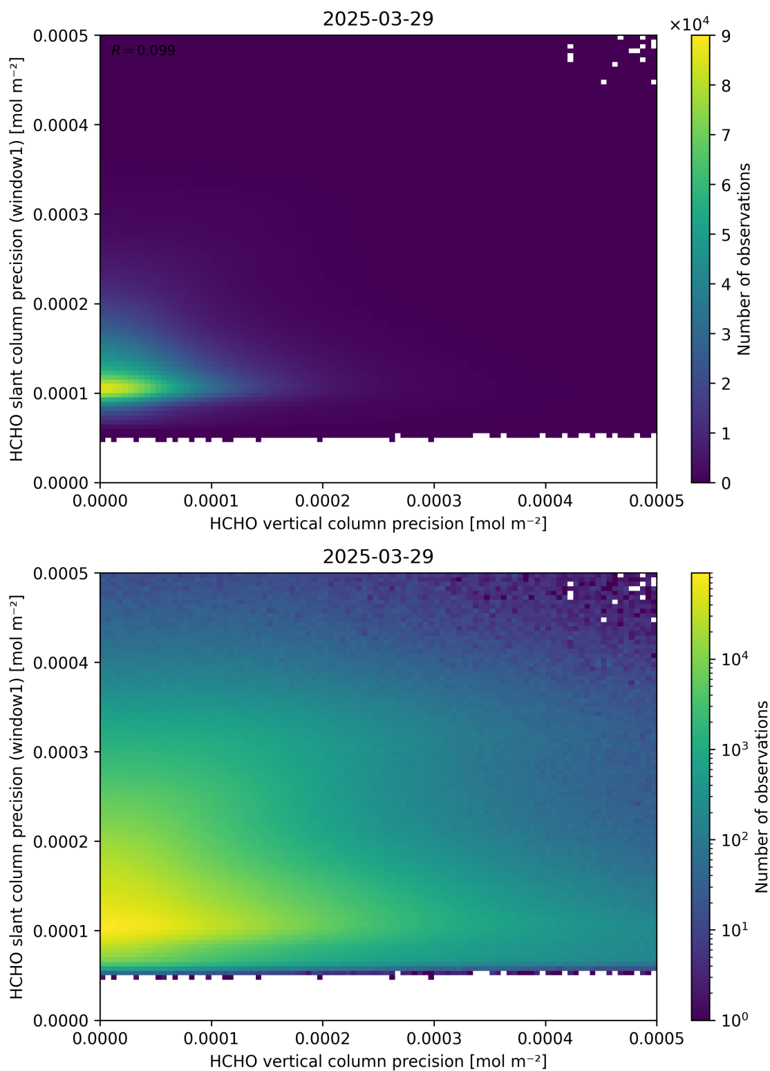
Figure 143: Scatter density plot of “HCHO vertical column precision” against “HCHO slant column precision (window1)” for 2025-03-28 to 2025-03-30.
