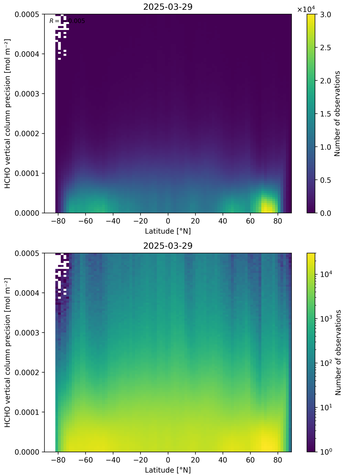
Figure 165: Scatter density plot of “Latitude” against “HCHO vertical column precision” for 2025-03-28 to 2025-03-30.
