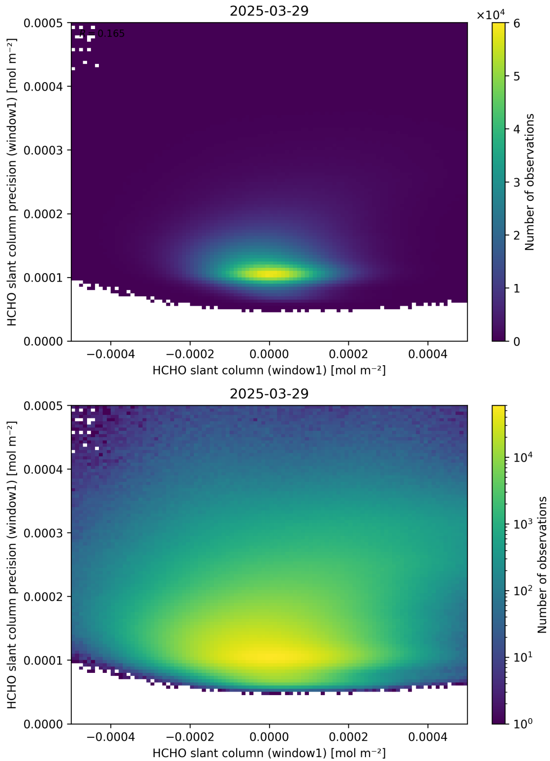
Figure 84: Scatter density plot of “HCHO slant column (window1)” against “HCHO slant column precision (window1)” for 2025-03-28 to 2025-03-30.
