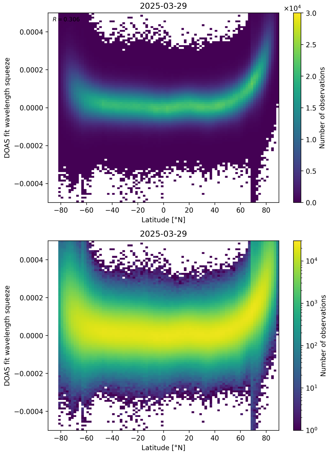
Figure 155: Scatter density plot of “Latitude” against “DOAS fit wavelength squeeze” for 2025-03-28 to 2025-03-30.
