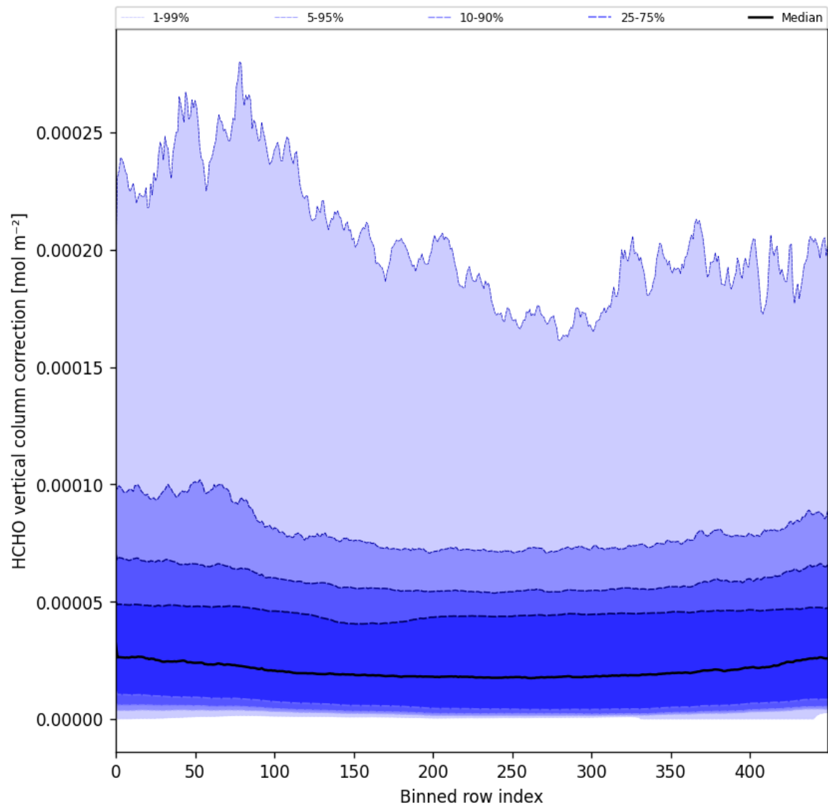
Figure 51: Along track statistics of “HCHO vertical column correction” for 2025-03-28 to 2025-03-30
