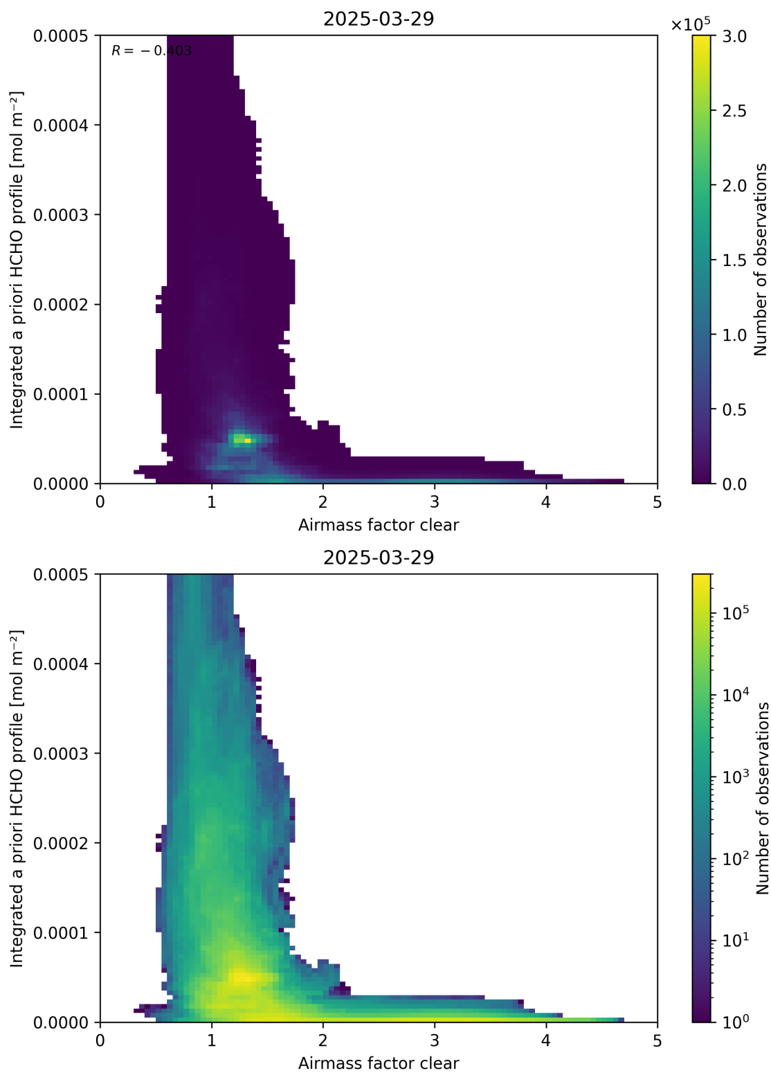
Figure 76: Scatter density plot of “Airmass factor clear” against “Integrated a priori HCHO profile” for 2025-03-28 to 2025-03-30.
