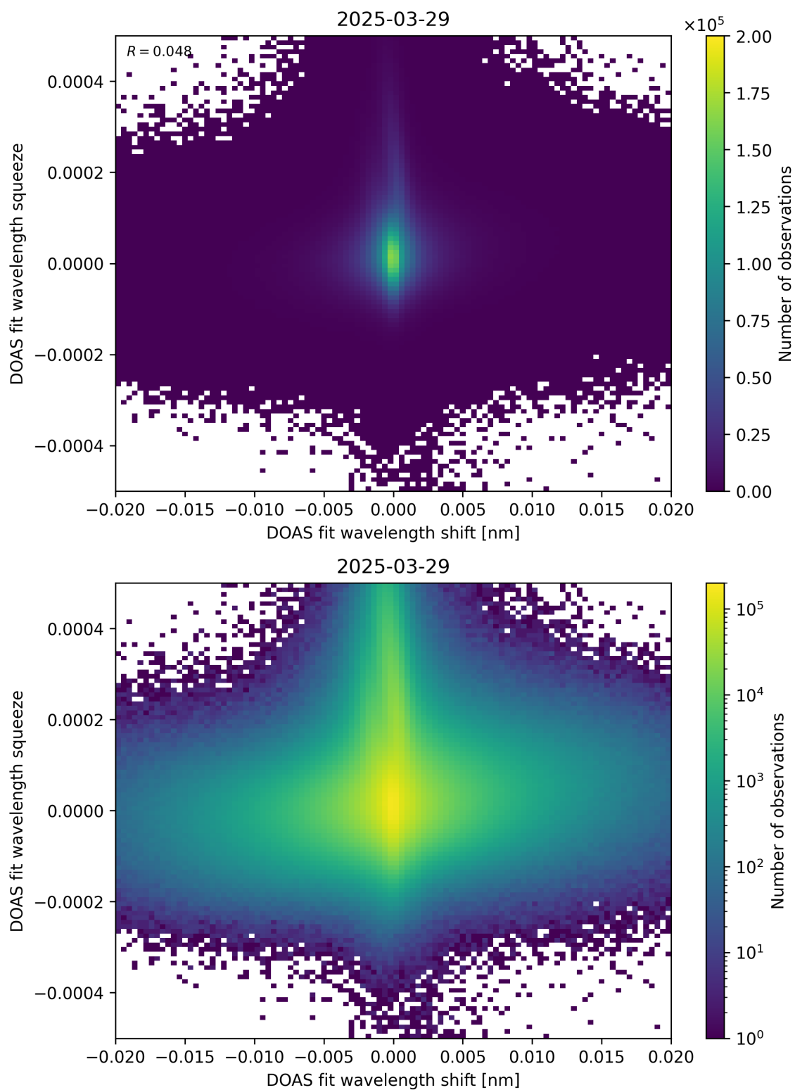
Figure 65: Scatter density plot of “DOAS fit wavelength shift” against “DOAS fit wavelength squeeze” for 2025-03-28 to 2025-03-30.
