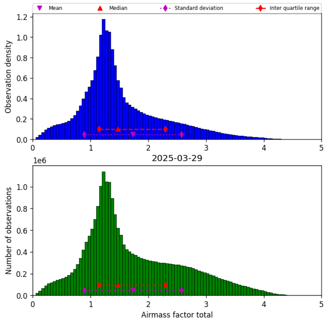
Figure 40: Histogram of “Airmass factor total” for 2025-03-28 to 2025-03-30
