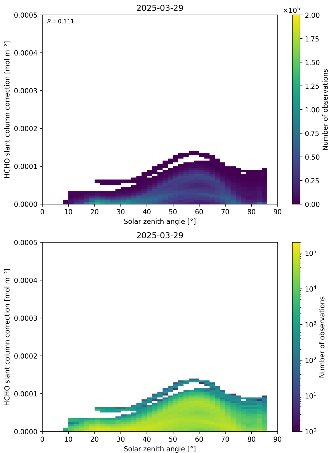
Figure 172: Scatter density plot of “Solar zenith angle” against “HCHO slant column correction” for 2025-03-28 to 2025-03-30.
