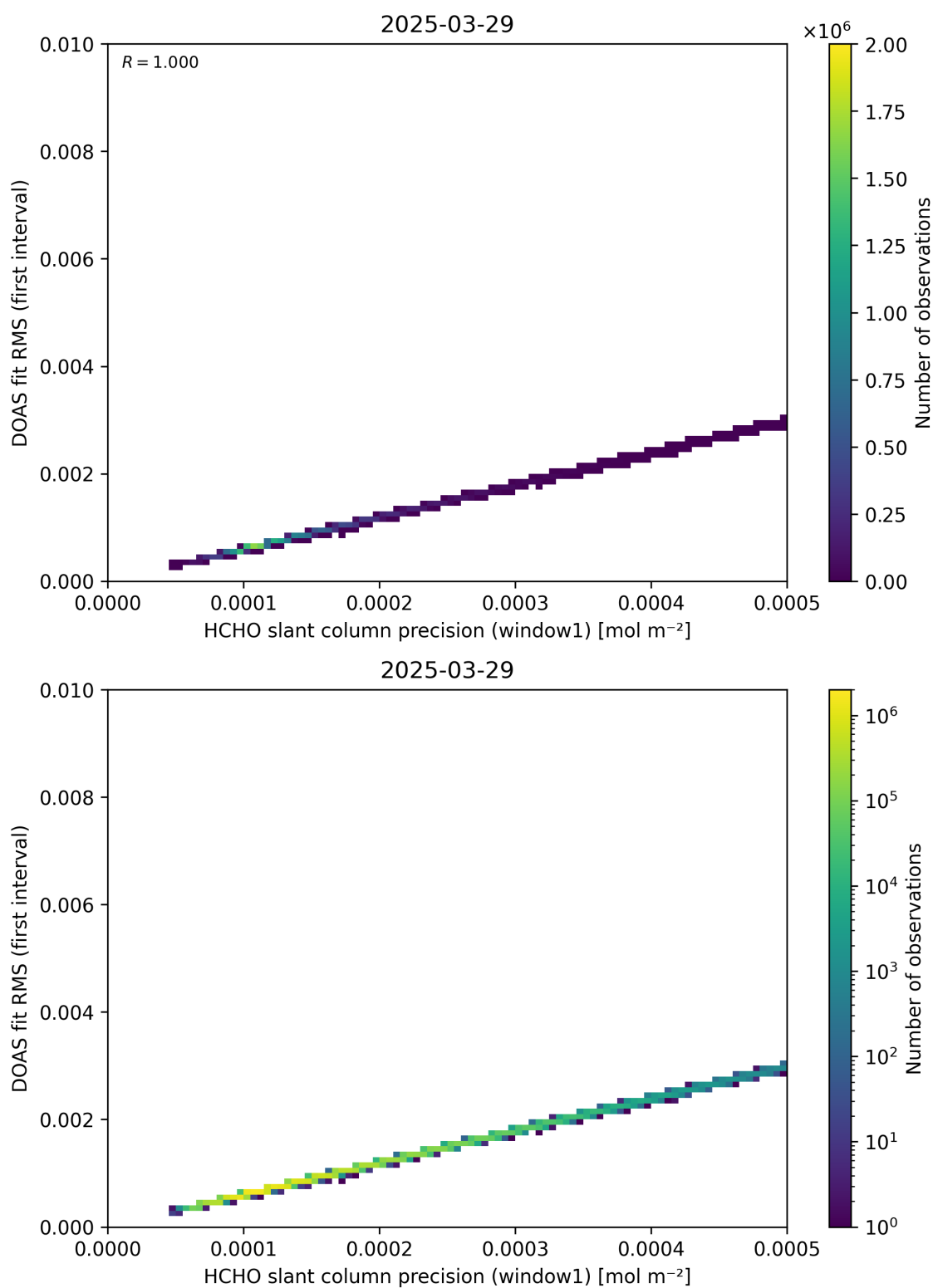
Figure 88: Scatter density plot of “HCHO slant column precision (window1)” against “DOAS fit RMS (first interval)” for 2025-03-28 to 2025-03-30.
