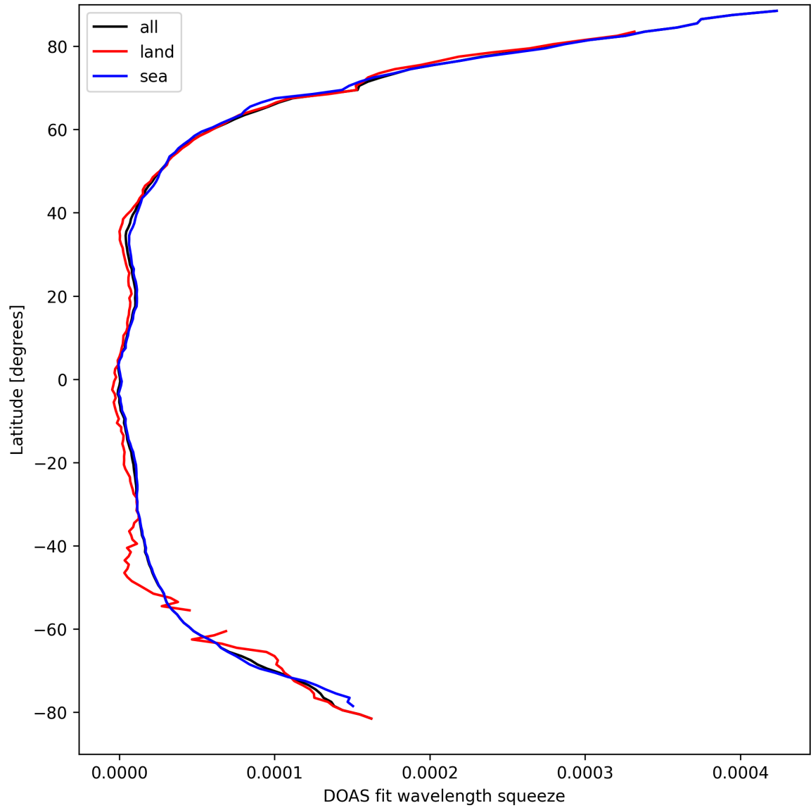
Figure 31: Zonal average of “DOAS fit wavelength squeeze” for 2025-03-28 to 2025-03-30.
