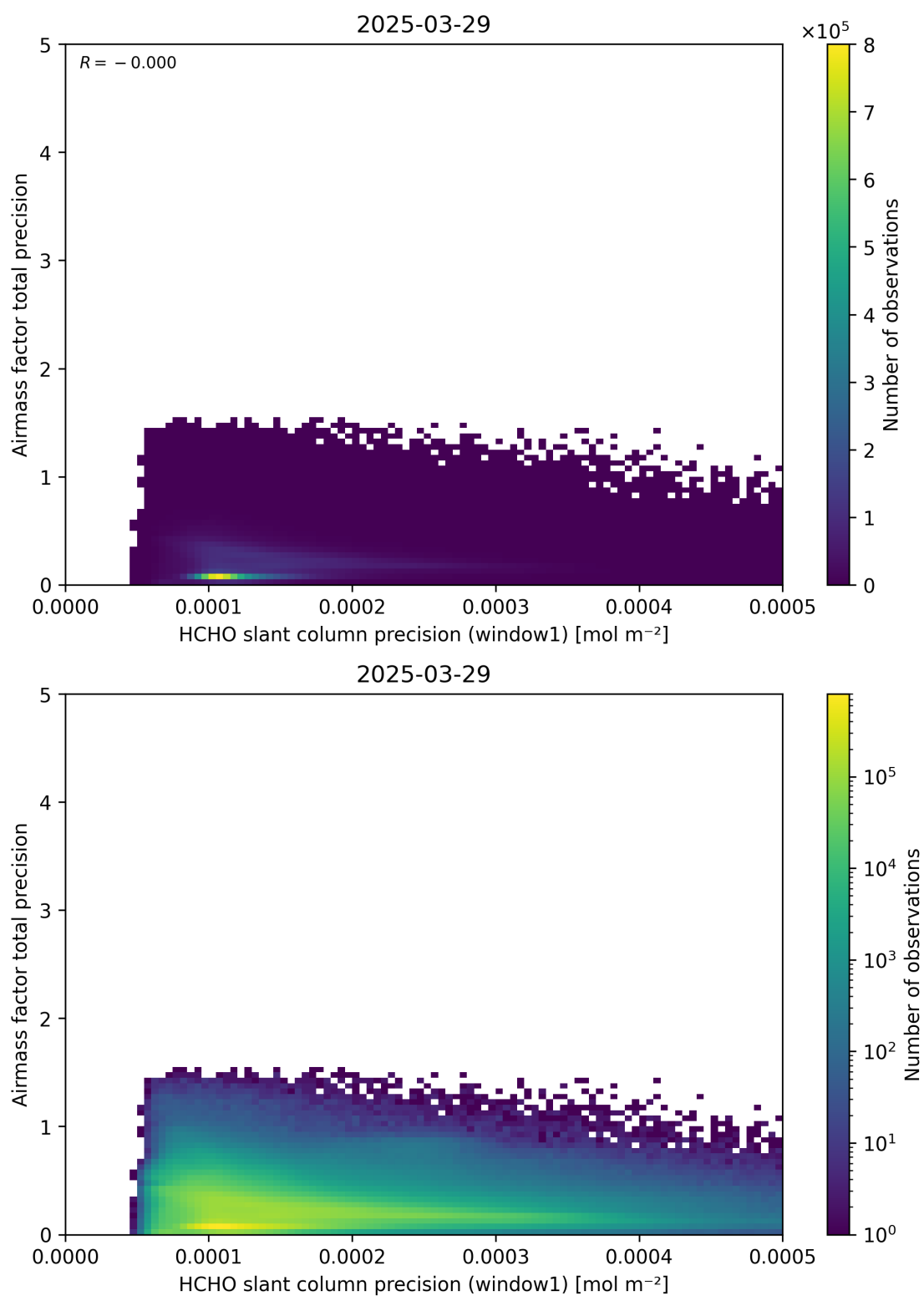
Figure 95: Scatter density plot of “HCHO slant column precision (window1)” against “Airmass factor total precision” for 2025-03-28 to 2025-03-30.
