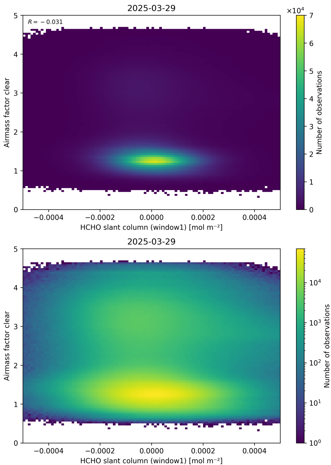
Figure 81: Scatter density plot of “HCHO slant column (window1)” against “Airmass factor clear” for 2025-03-28 to 2025-03-30.
