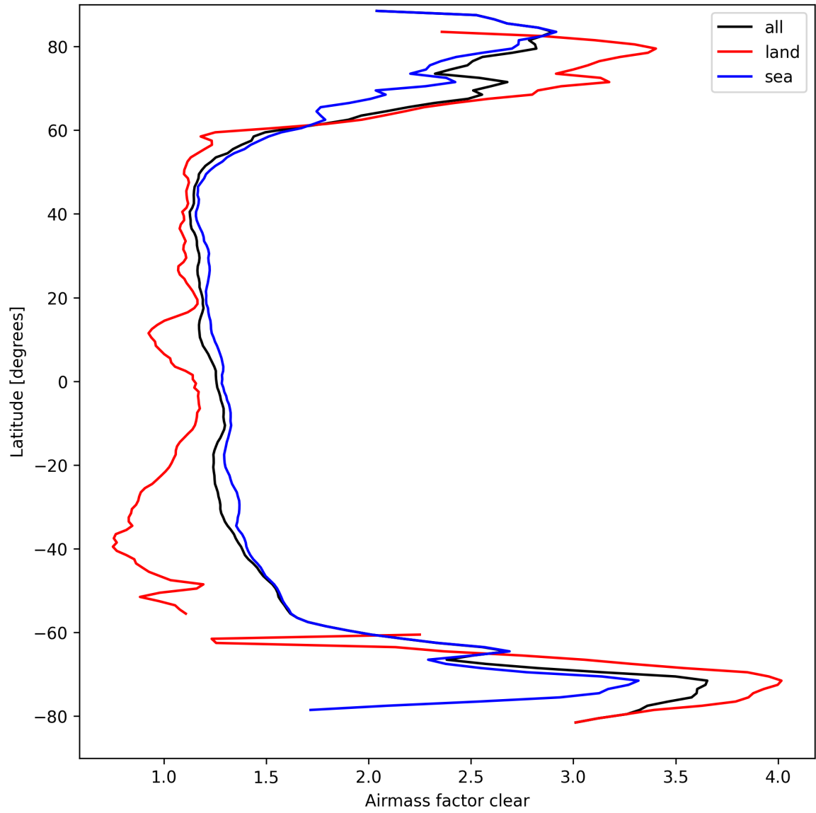
Figure 28: Zonal average of “Airmass factor clear” for 2025-03-28 to 2025-03-30.
