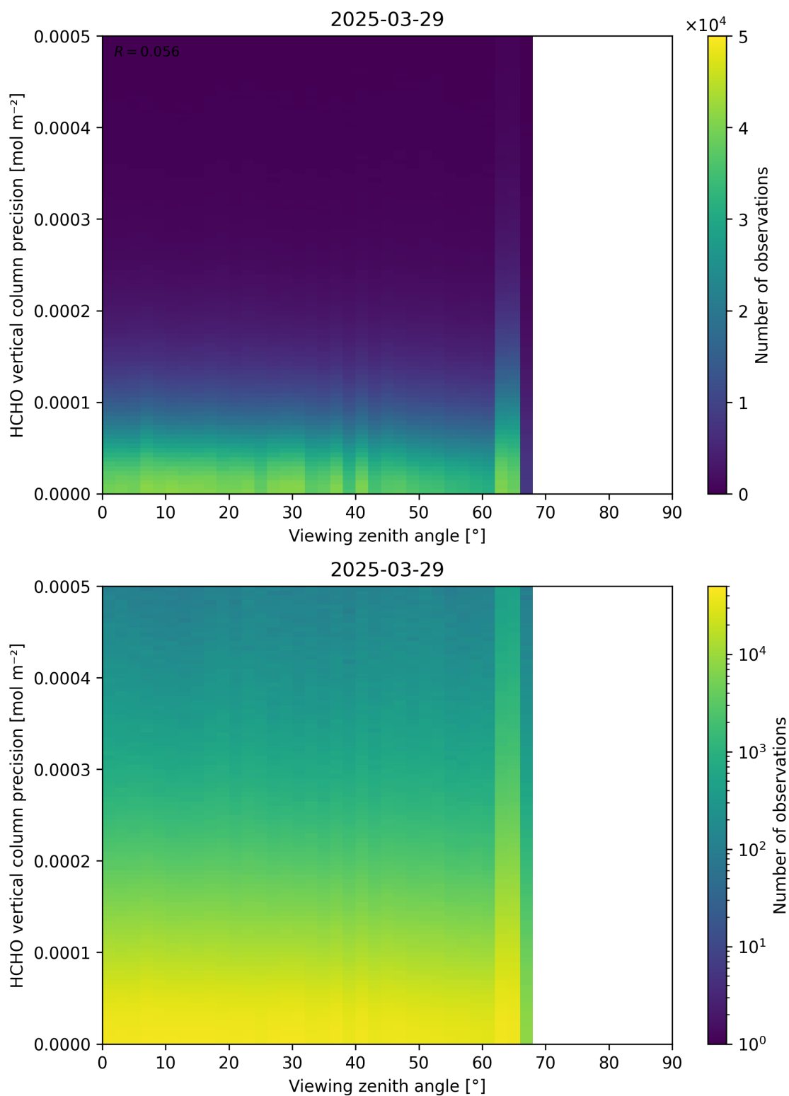
Figure 194: Scatter density plot of “Viewing zenith angle” against “HCHO vertical column precision” for 2025-03-28 to 2025-03-30.
