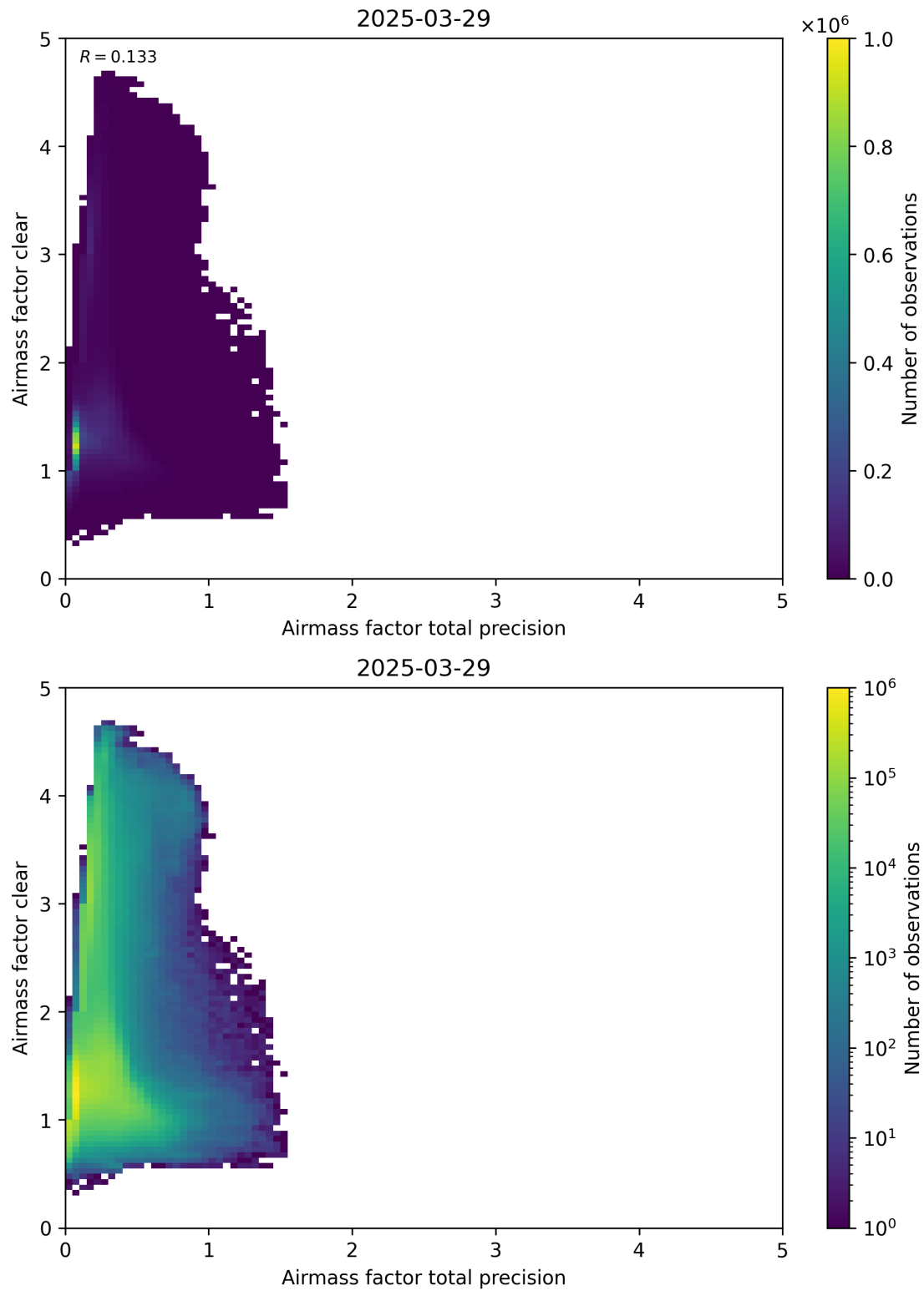
Figure 108: Scatter density plot of “Airmass factor total precision” against “Airmass factor clear” for 2025-03-28 to 2025-03-30.
