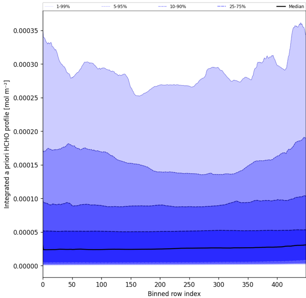
Figure 57: Along track statistics of "Integrated a priori HCHO profile" for 2025-03-28 to 2025-03-30
