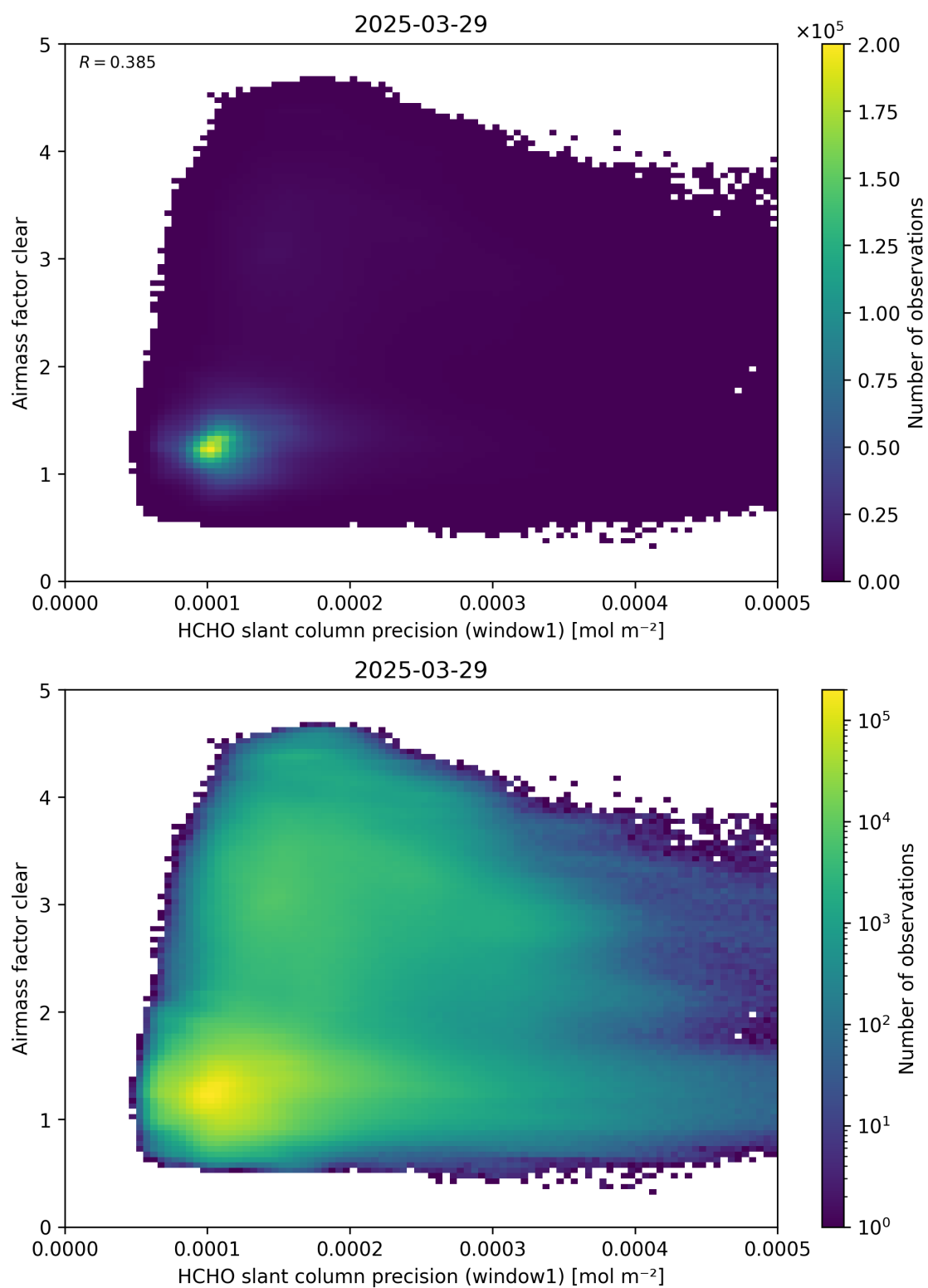
Figure 91: Scatter density plot of “HCHO slant column precision (window1)” against “Airmass factor clear” for 2025-03-28 to 2025-03-30.
