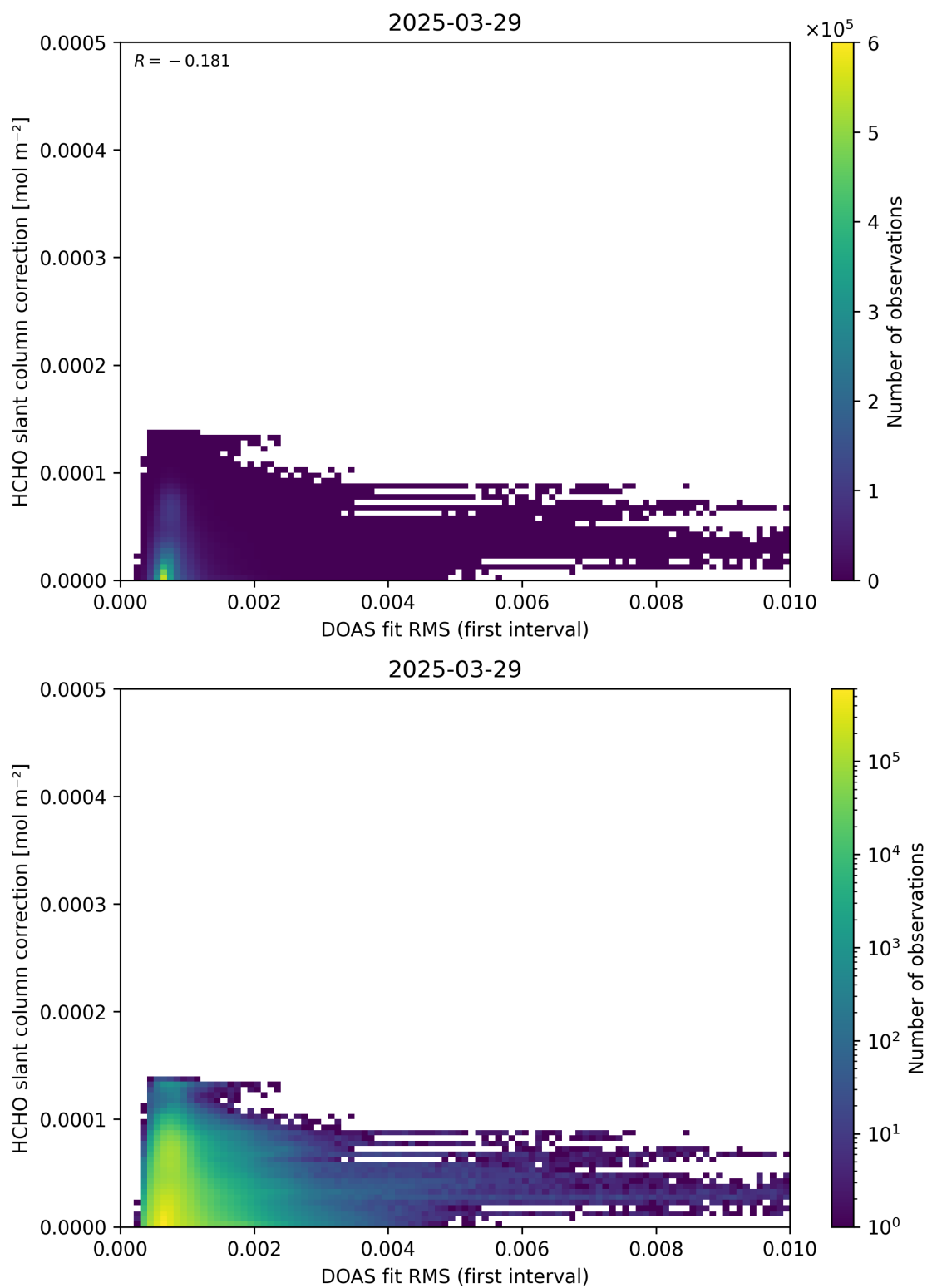
Figure 63: Scatter density plot of “DOAS fit RMS (first interval)” against “HCHO slant column correction” for 2025-03-28 to 2025-03-30.
