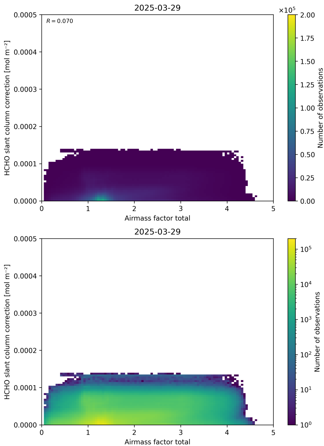
Figure 102: Scatter density plot of “Airmass factor total” against “HCHO slant column correction” for 2025-03-28 to 2025-03-30.
