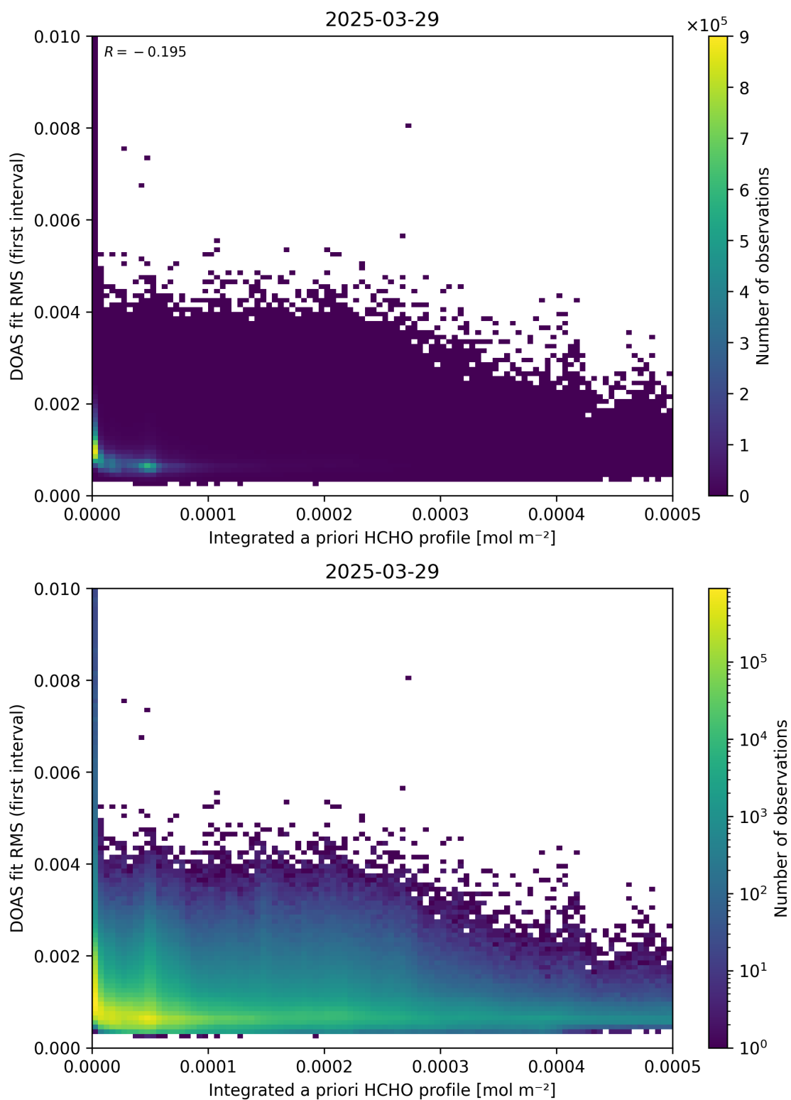
Figure 148: Scatter density plot of “Integrated a priori HCHO profile” against “DOAS fit RMS (first interval)” for 2025-03-28 to 2025-03-30.
