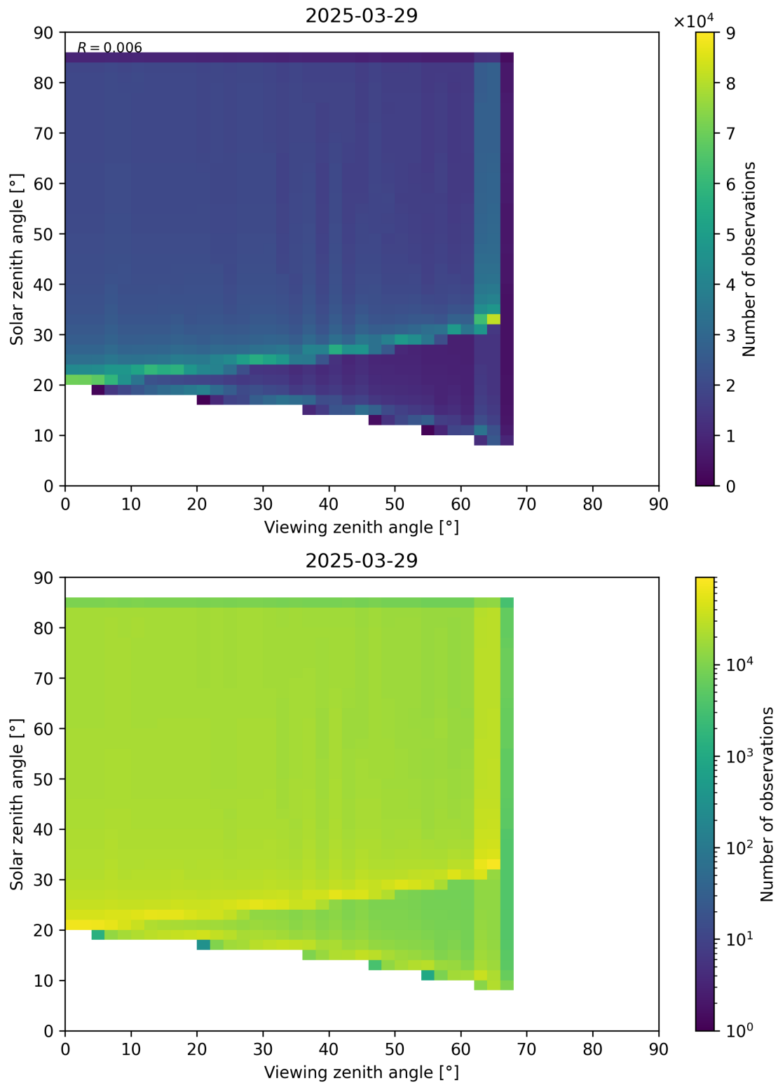
Figure 197: Scatter density plot of “Viewing zenith angle” against “Solar zenith angle” for 2025-03-28 to 2025-03-30.
