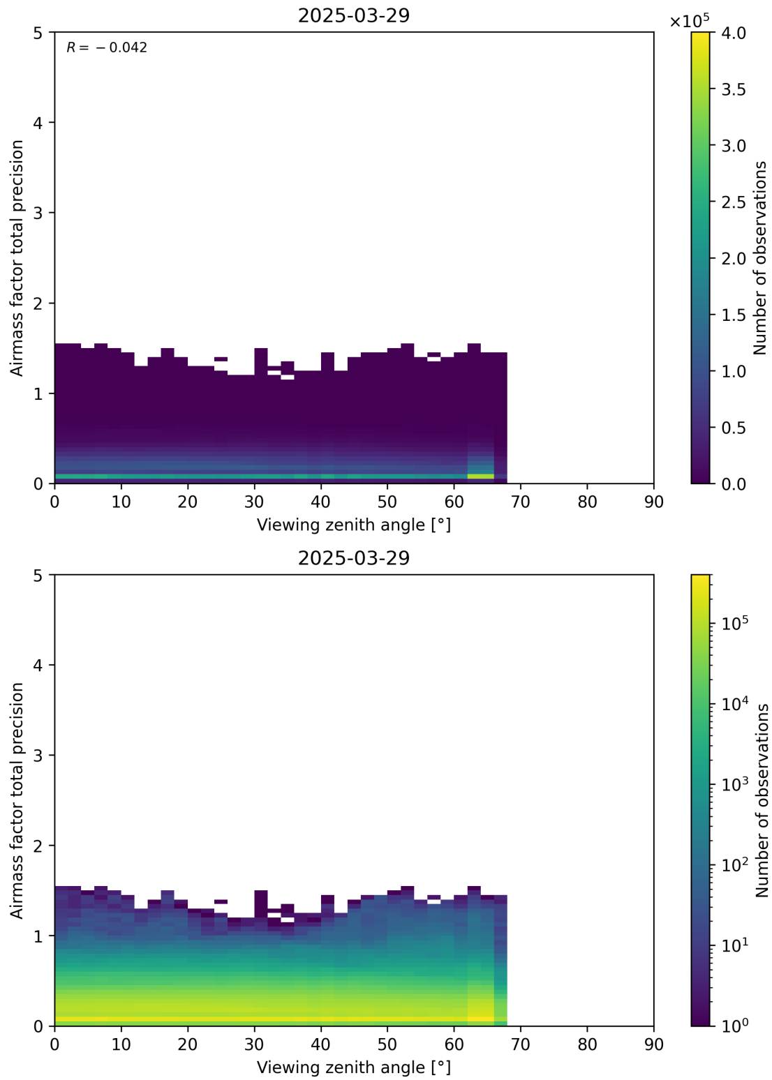
Figure 191: Scatter density plot of “Viewing zenith angle” against “Airmass factor total precision” for 2025-03-28 to 2025-03-30.
