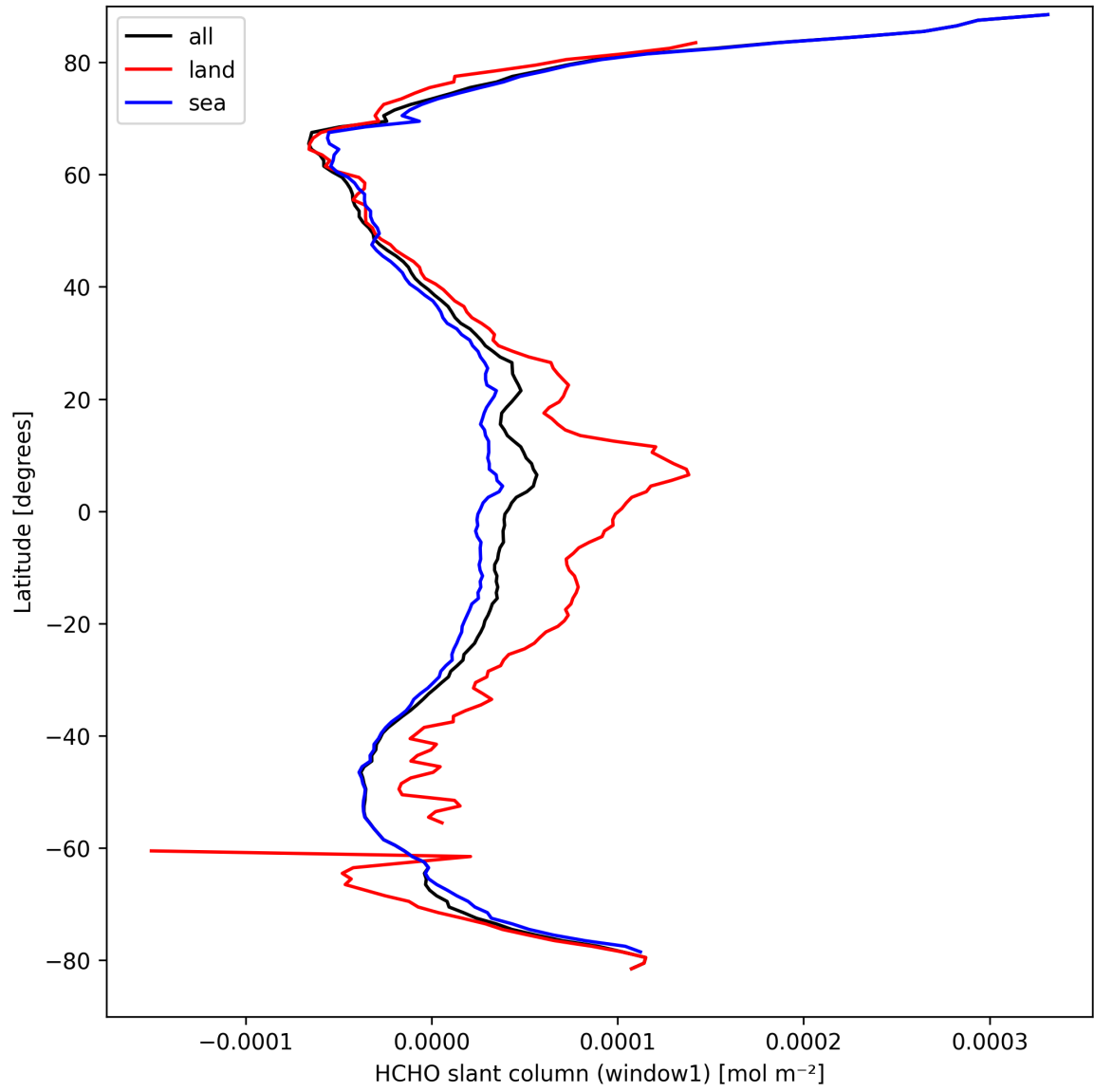
Figure 24: Zonal average of “HCHO slant column (window1)” for 2025-03-28 to 2025-03-30.
