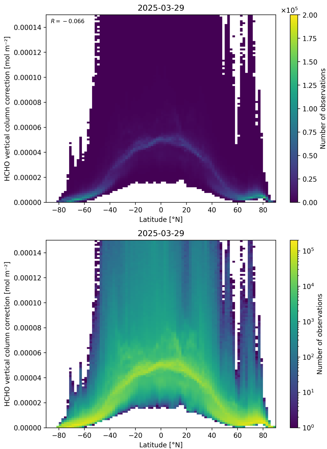
Figure 164: Scatter density plot of “Latitude” against “HCHO vertical column correction” for 2025-03-28 to 2025-03-30.
