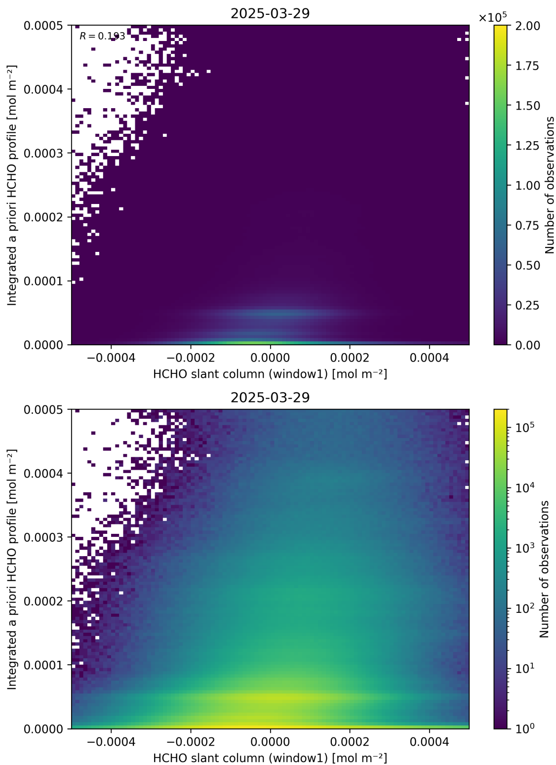
Figure 87: Scatter density plot of “HCHO slant column (window1)” against “Integrated a priori HCHO profile” for 2025-03-28 to 2025-03-30.
