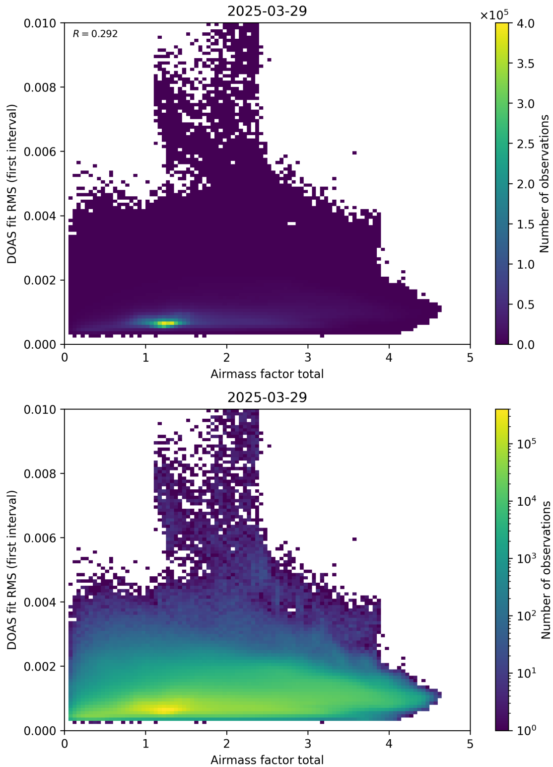
Figure 97: Scatter density plot of “Airmass factor total” against “DOAS fit RMS (first interval)” for 2025-03-28 to 2025-03-30.
