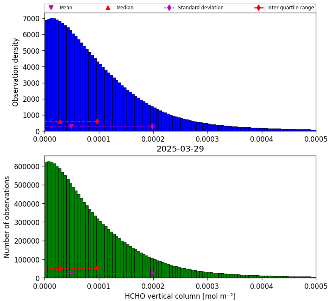
Figure 35: Histogram of “HCHO vertical column” for 2025-03-28 to 2025-03-30
