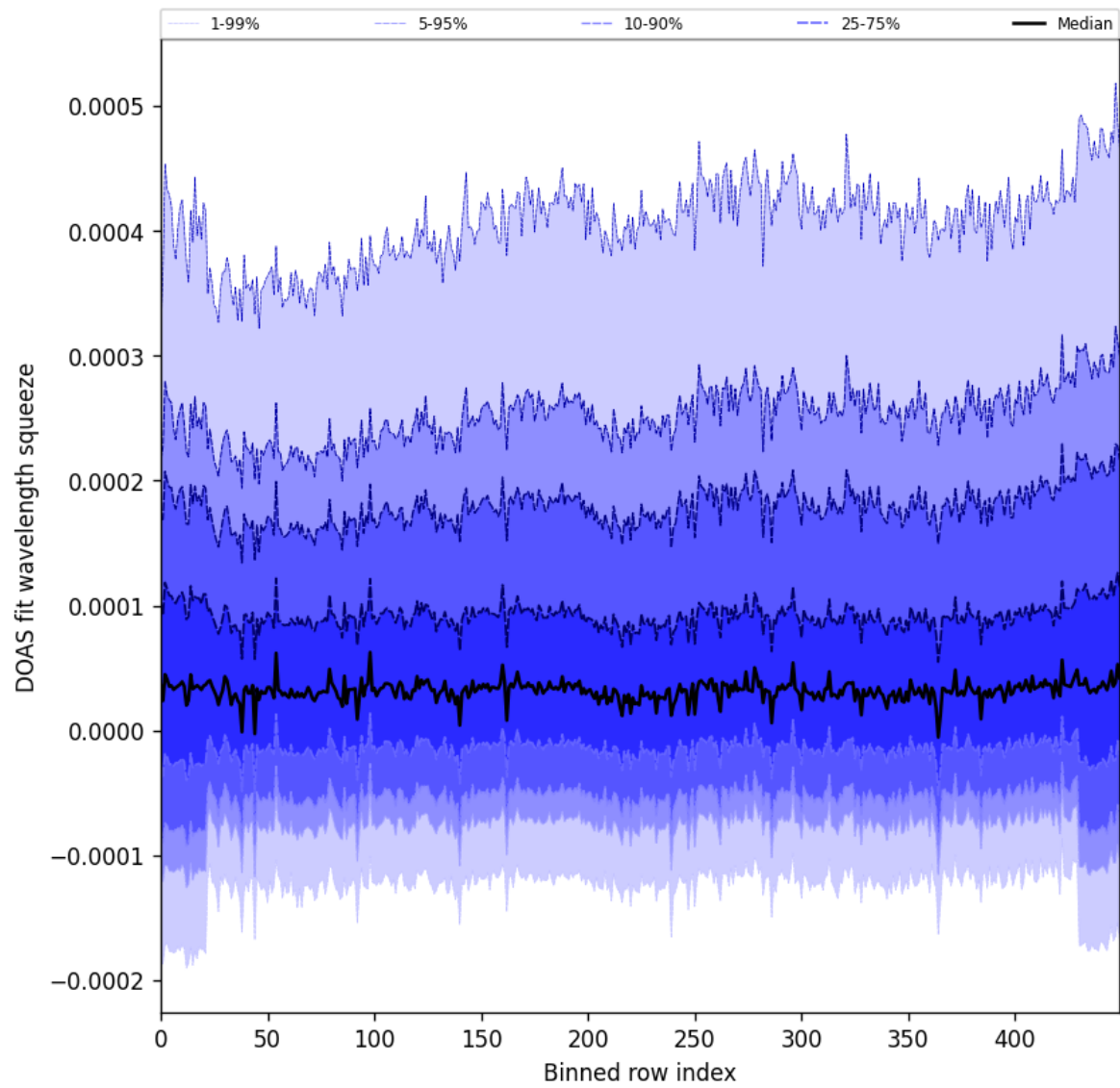
Figure 59: Along track statistics of “DOAS fit wavelength squeeze” for 2025-03-28 to 2025-03-30
