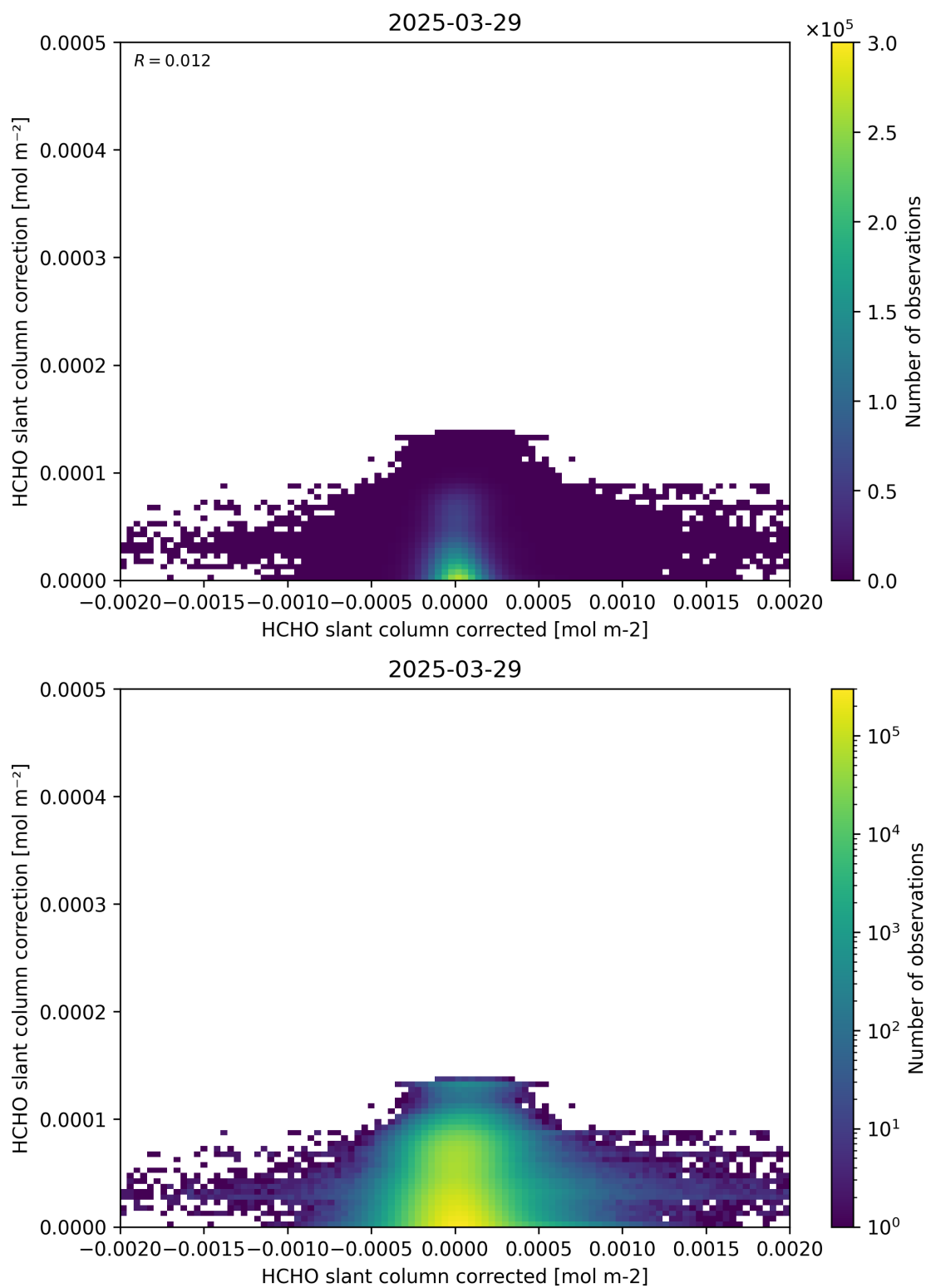
Figure 77: Scatter density plot of “HCHO slant column corrected” against “HCHO slant column correction” for 2025-03-28 to 2025-03-30.
