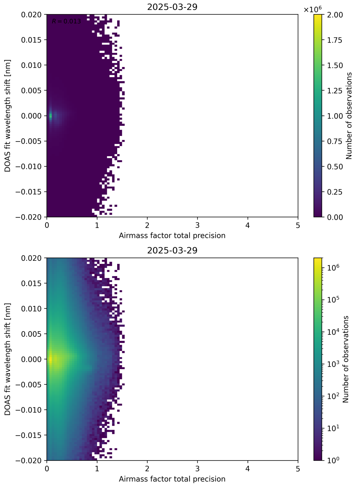
Figure 106: Scatter density plot of “Airmass factor total precision” against “DOAS fit wavelength shift” for 2025-03-28 to 2025-03-30.
