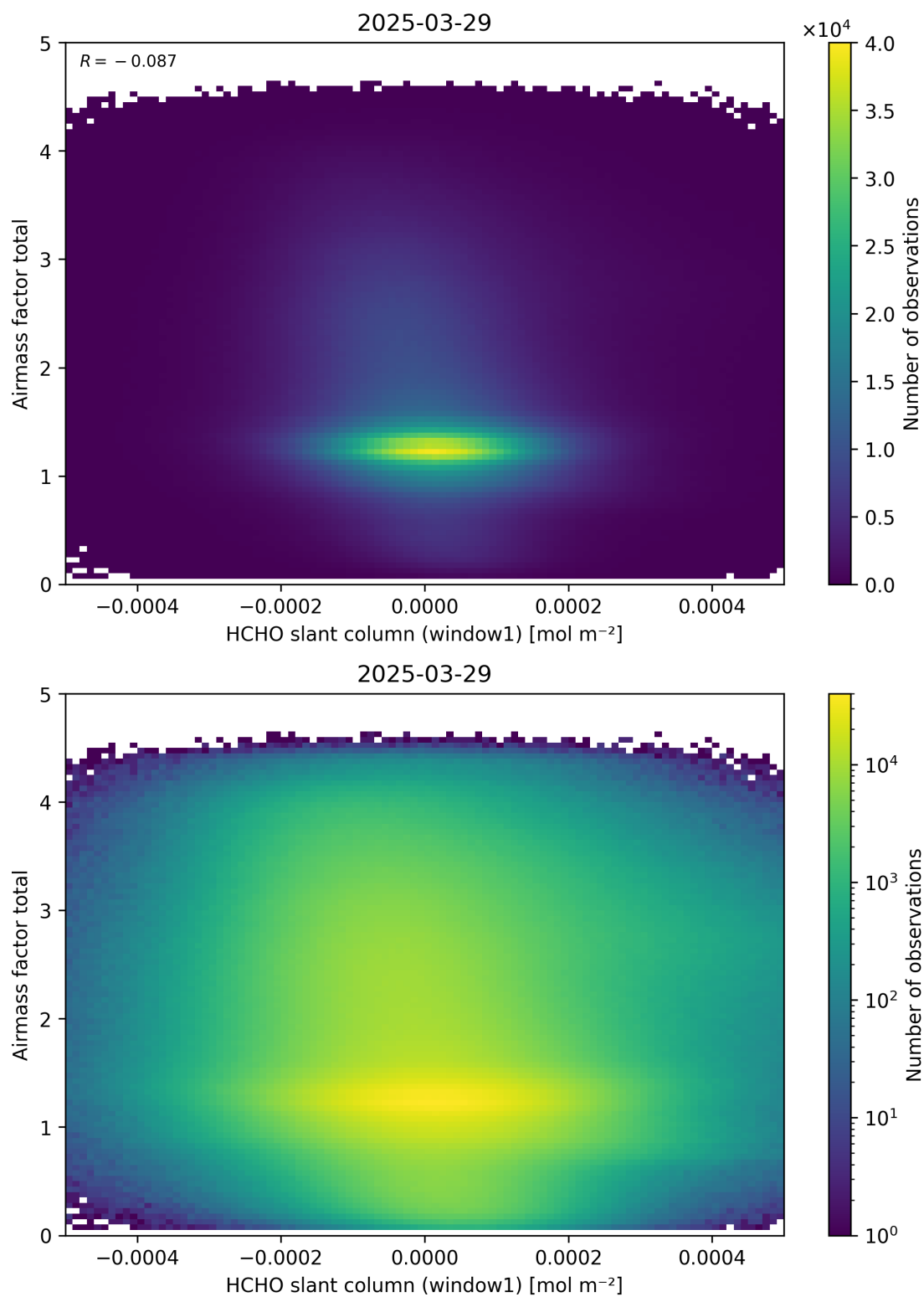
Figure 85: Scatter density plot of “HCHO slant column (window1)” against “Airmass factor total” for 2025-03-28 to 2025-03-30.
