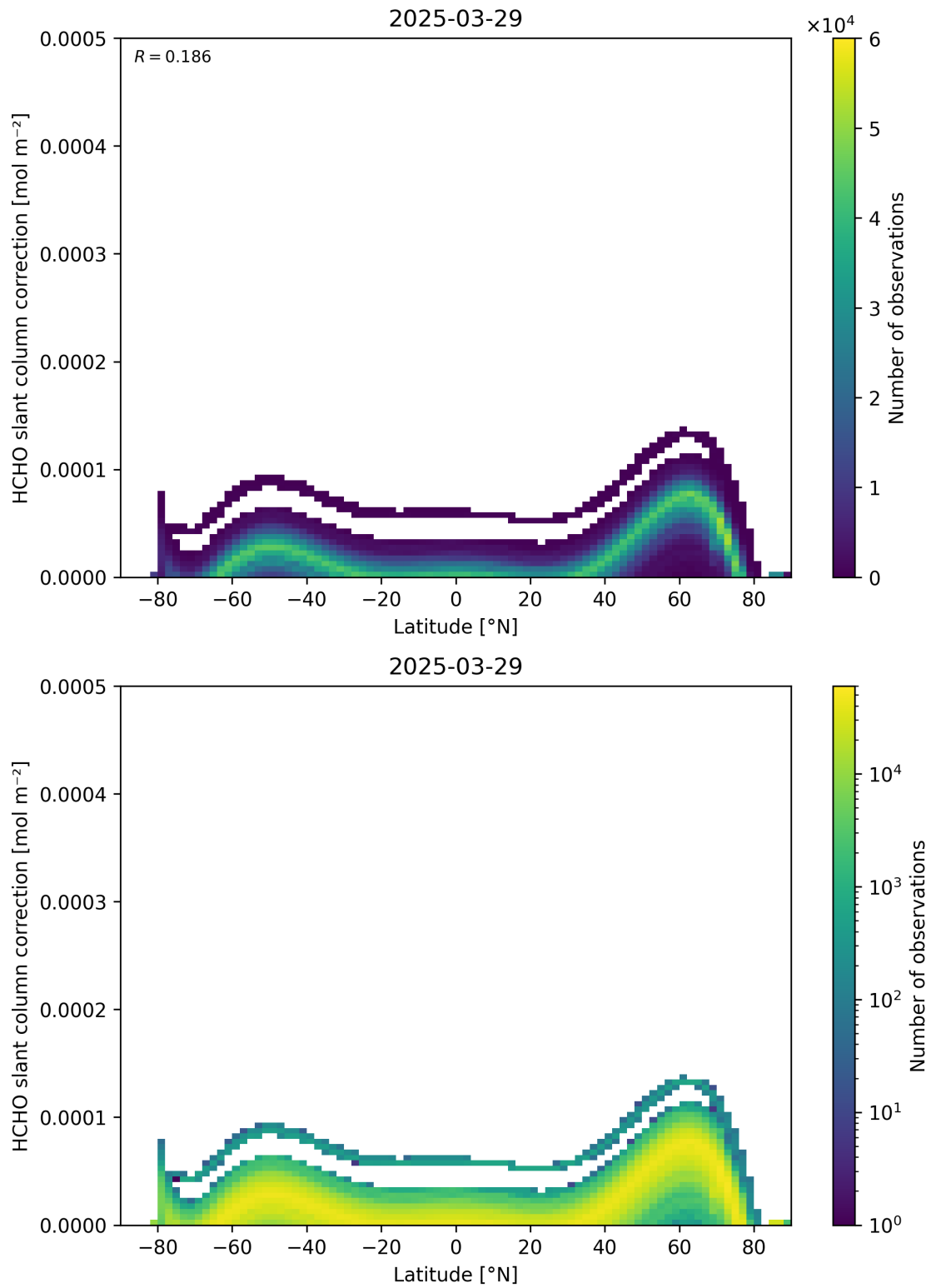
Figure 158: Scatter density plot of “Latitude” against “HCHO slant column correction” for 2025-03-28 to 2025-03-30.
