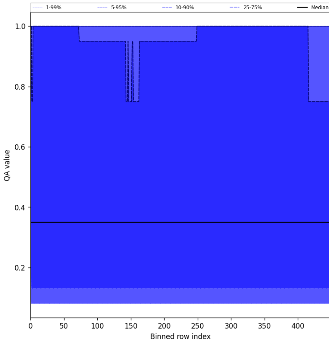
Figure 48: Along track statistics of “QA value” for 2025-03-28 to 2025-03-30
