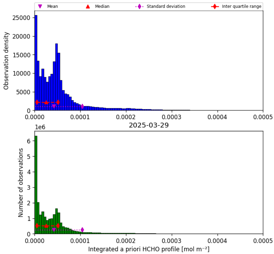
Figure 43: Histogram of “Integrated a priori HCHO profile” for 2025-03-28 to 2025-03-30
