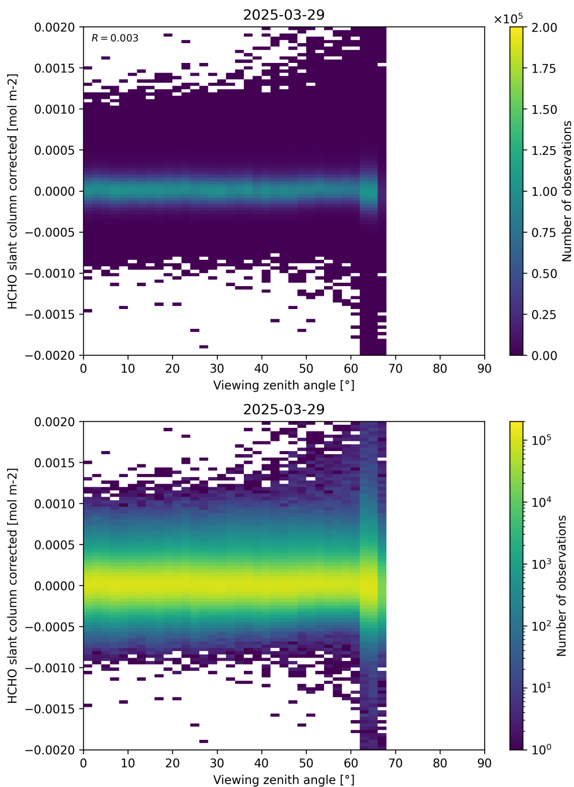
Figure 186: Scatter density plot of “Viewing zenith angle” against “HCHO slant column corrected” for 2025-03-28 to 2025-03-30.
