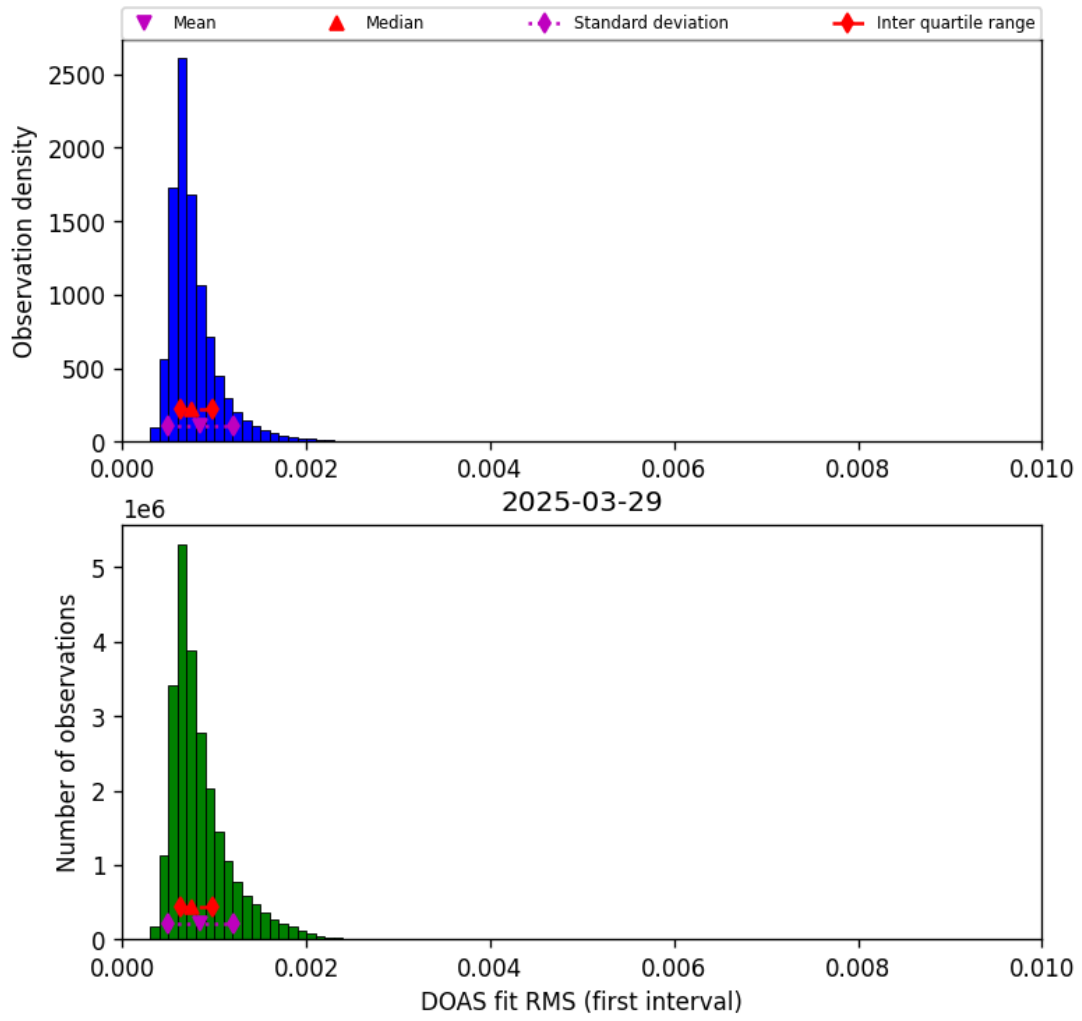
Figure 46: Histogram of “DOAS fit RMS (first interval)” for 2025-03-28 to 2025-03-30
