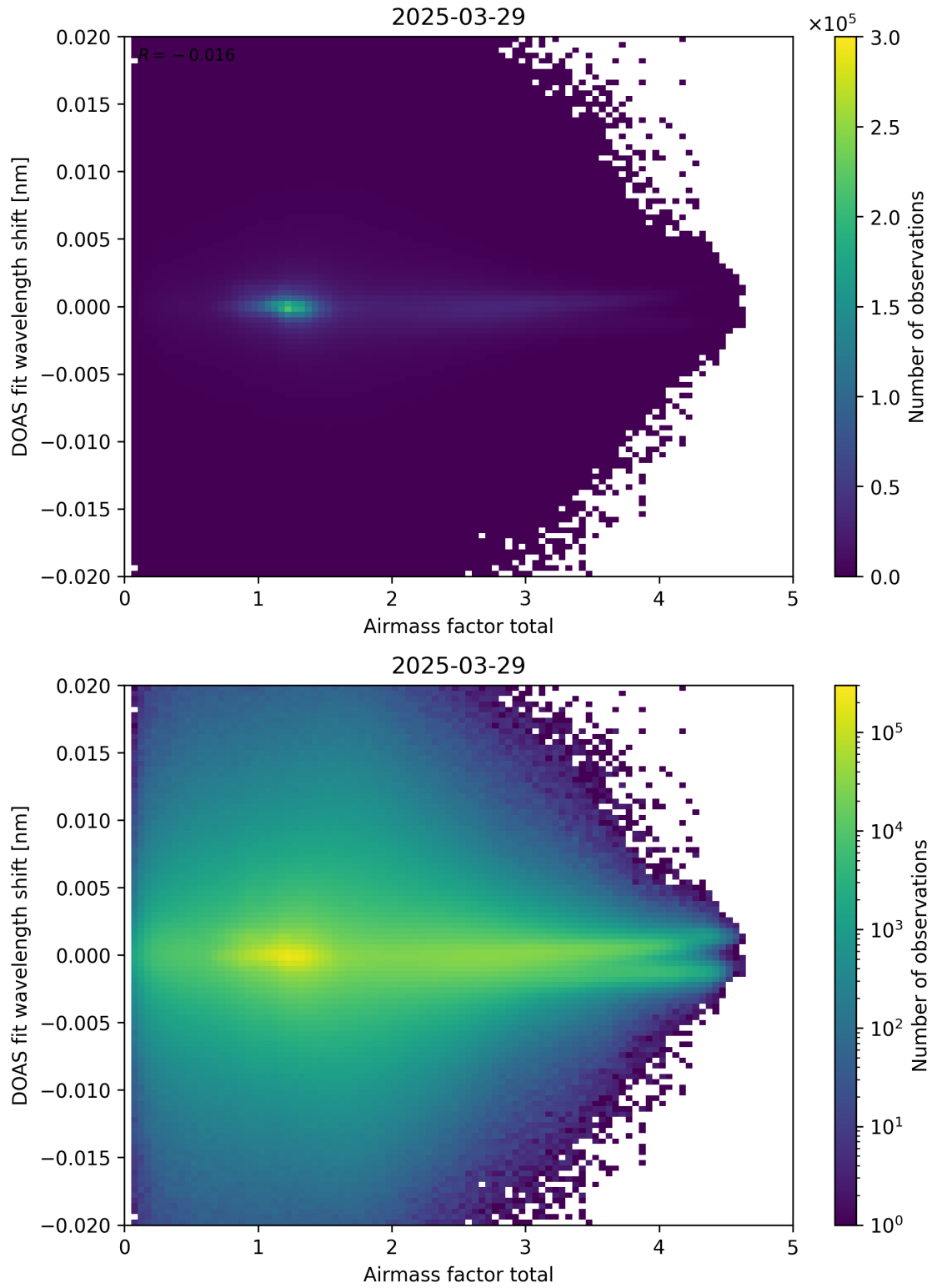
Figure 98: Scatter density plot of “Airmass factor total” against “DOAS fit wavelength shift” for 2025-03-28 to 2025-03-30.
