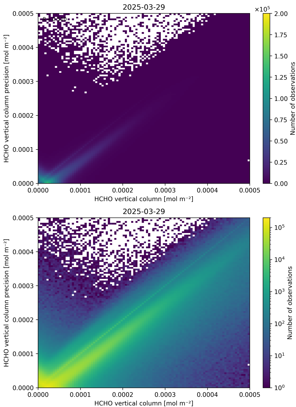
Figure 134: Scatter density plot of “HCHO vertical column” against “HCHO vertical column precision” for 2025-03-28 to 2025-03-30.
