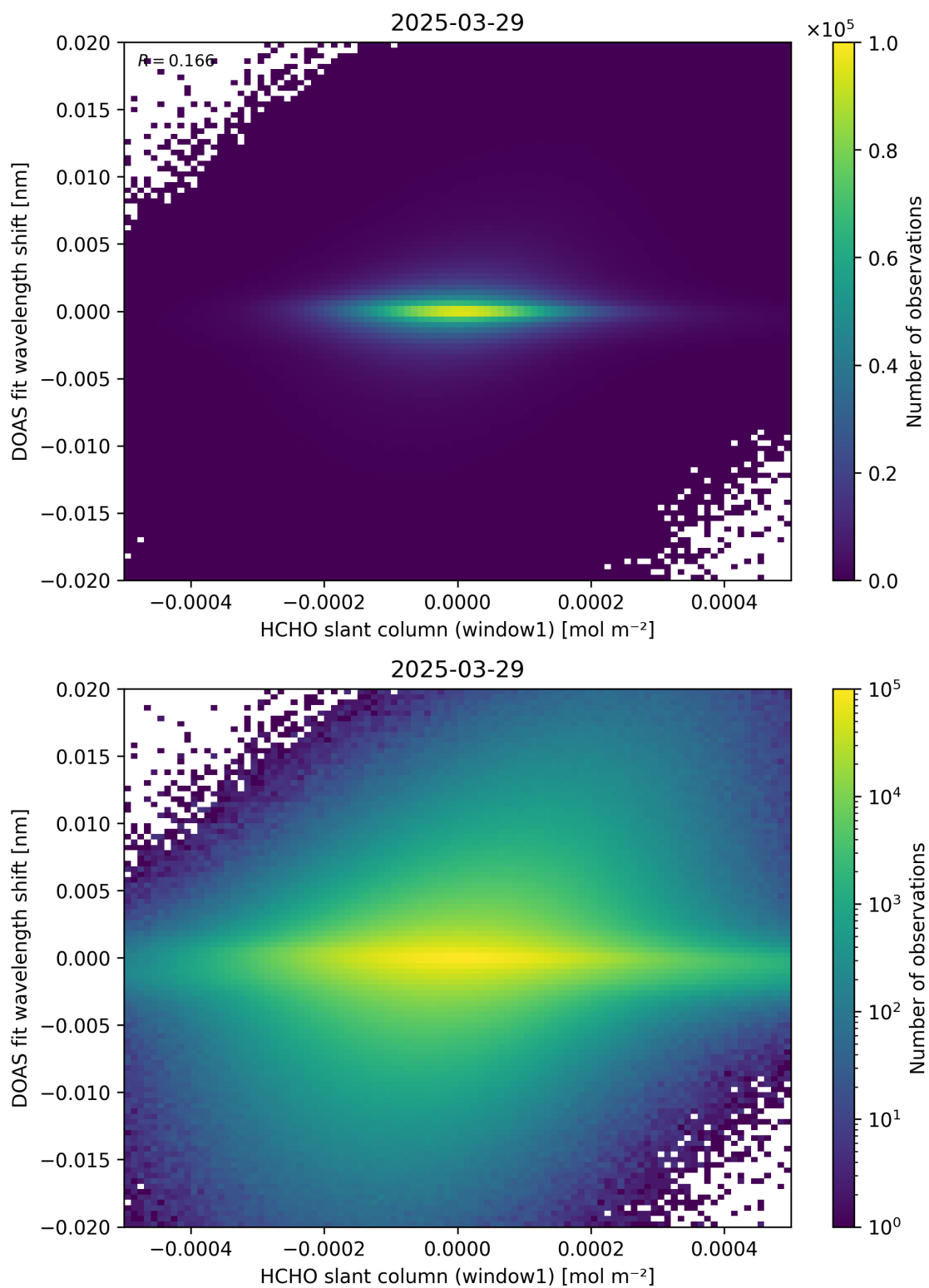
Figure 79: Scatter density plot of “HCHO slant column (window1)” against “DOAS fit wavelength shift” for 2025-03-28 to 2025-03-30.
