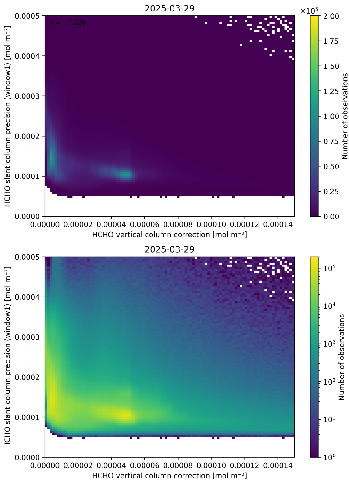
Figure 119: Scatter density plot of “HCHO vertical column correction” against “HCHO slant column precision (window1)” for 2025-03-28 to 2025-03-30.
