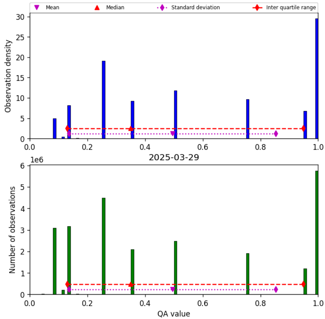
Figure 34: Histogram of “QA value” for 2025-03-28 to 2025-03-30
