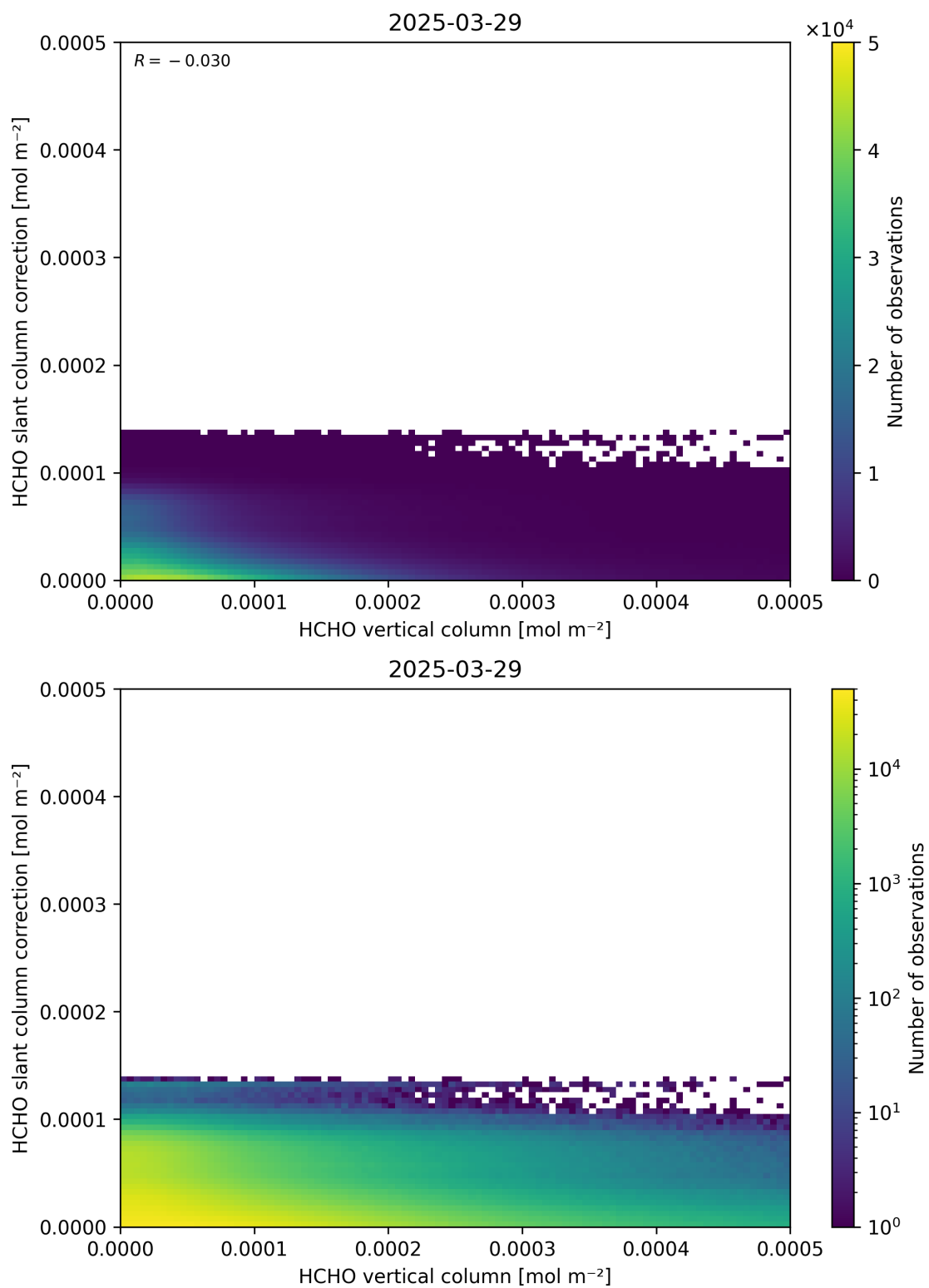
Figure 128: Scatter density plot of “HCHO vertical column” against “HCHO slant column correction” for 2025-03-28 to 2025-03-30.
