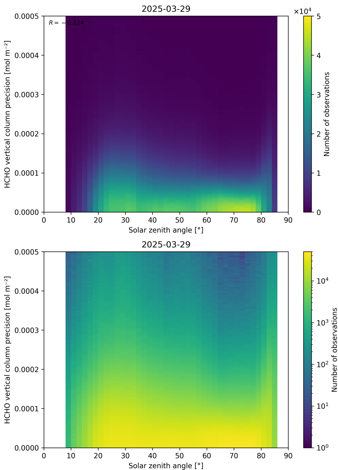
Figure 179: Scatter density plot of “Solar zenith angle” against “HCHO vertical column precision” for 2025-03-28 to 2025-03-30.
