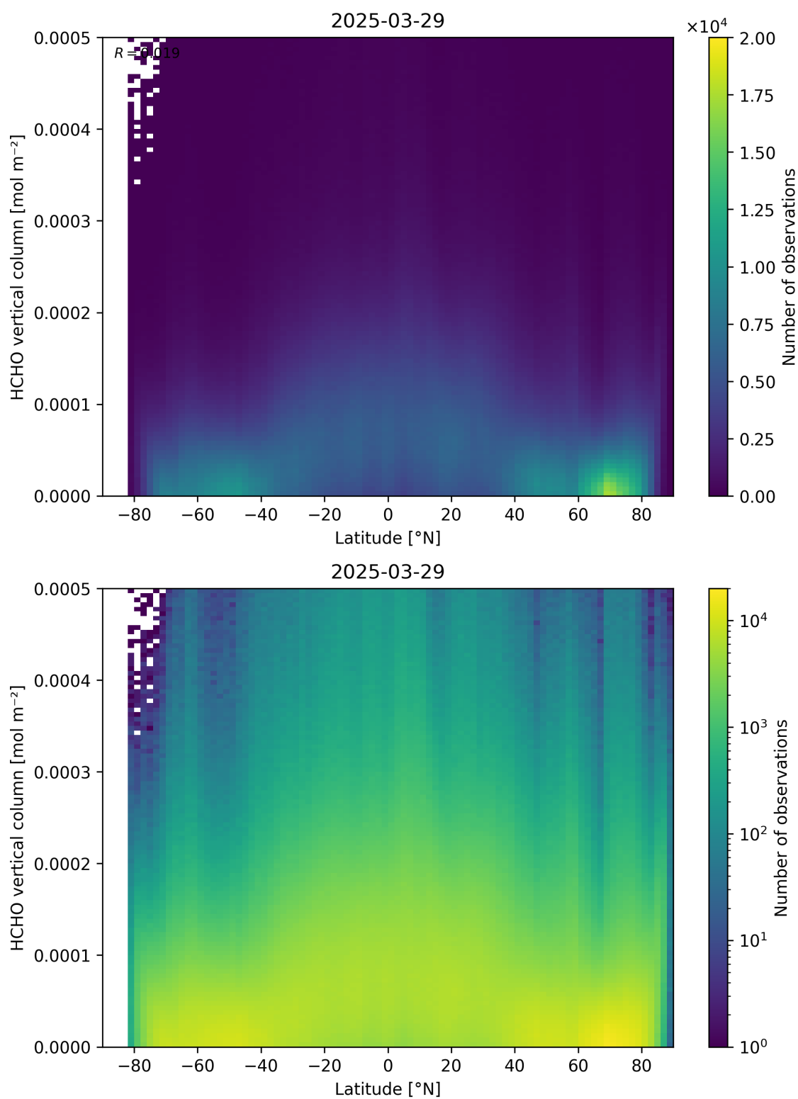
Figure 163: Scatter density plot of “Latitude” against “HCHO vertical column” for 2025-03-28 to 2025-03-30.
