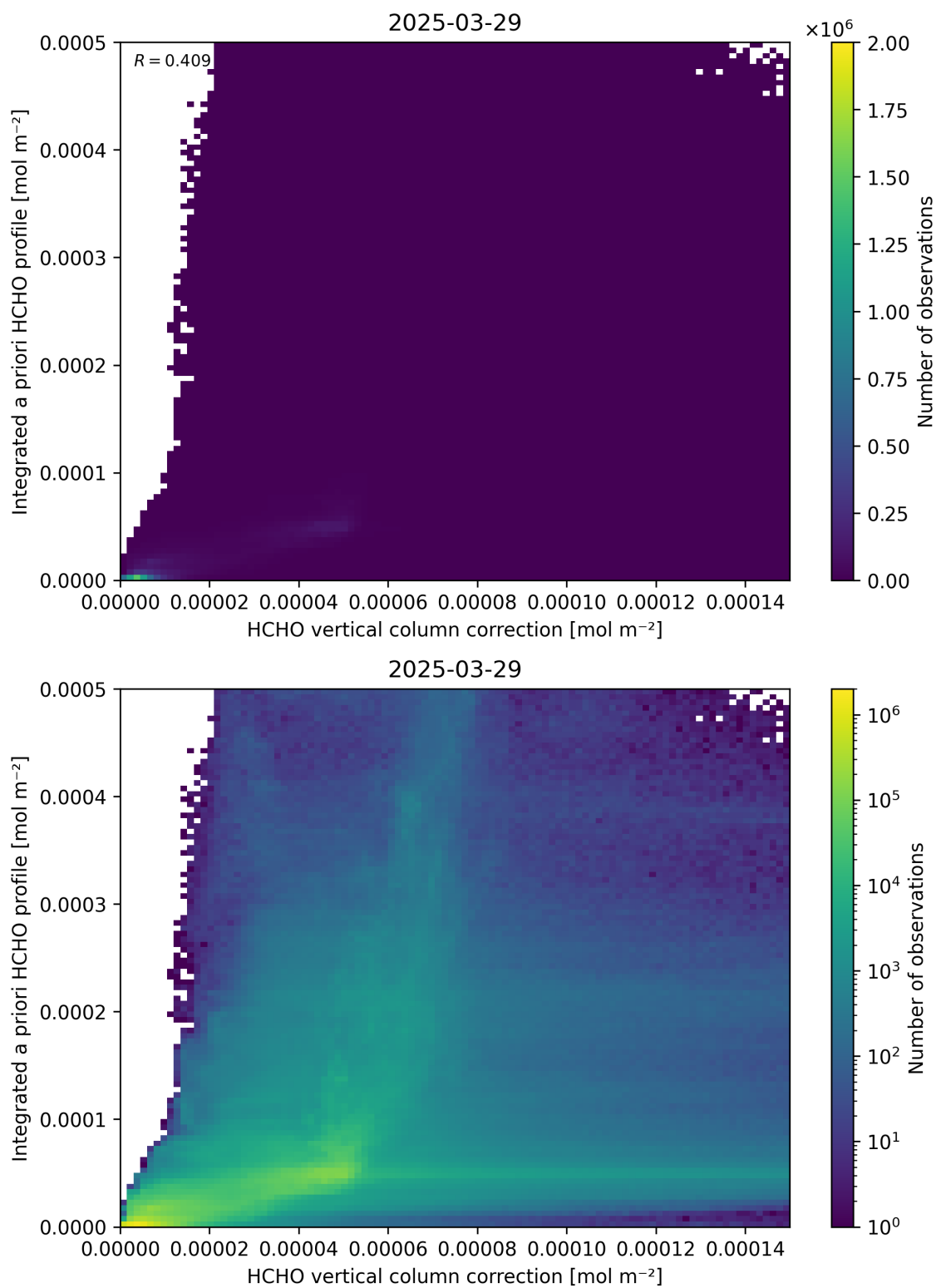
Figure 122: Scatter density plot of “HCHO vertical column correction” against “Integrated a priori HCHO profile” for 2025-03-28 to 2025-03-30.
