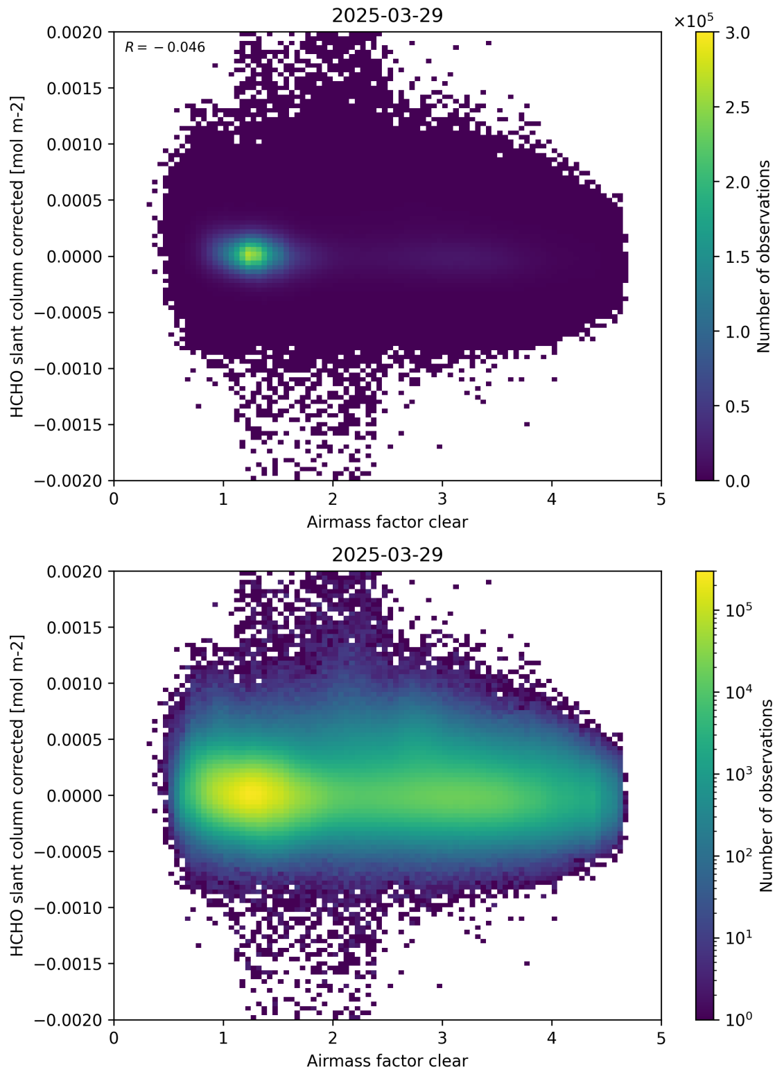
Figure 74: Scatter density plot of “Airmass factor clear” against “HCHO slant column corrected” for 2025-03-28 to 2025-03-30.
