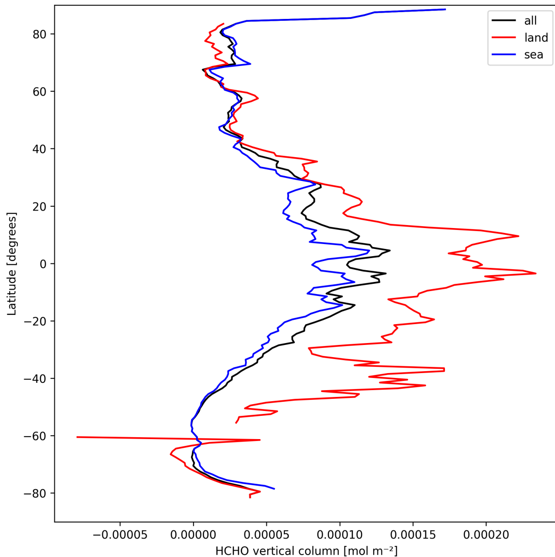
Figure 21: Zonal average of “HCHO vertical column” for 2025-03-28 to 2025-03-30.
