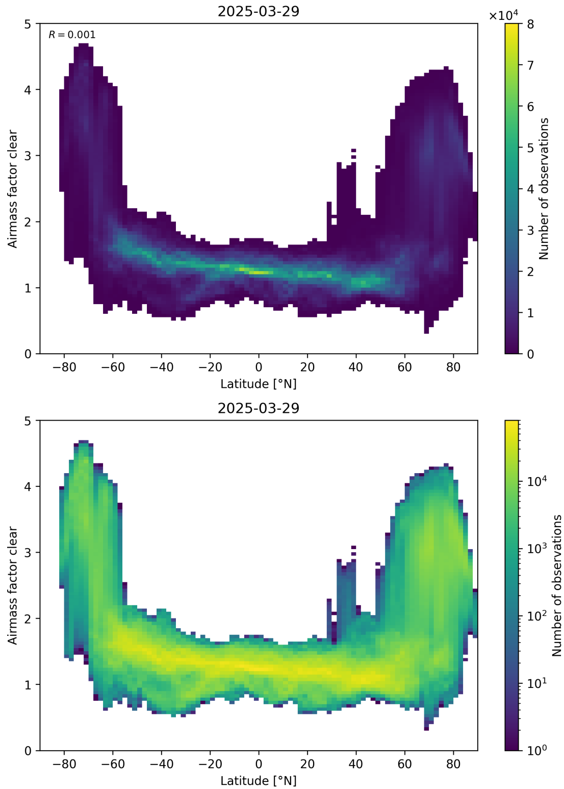
Figure 156: Scatter density plot of “Latitude” against “Airmass factor clear” for 2025-03-28 to 2025-03-30.
