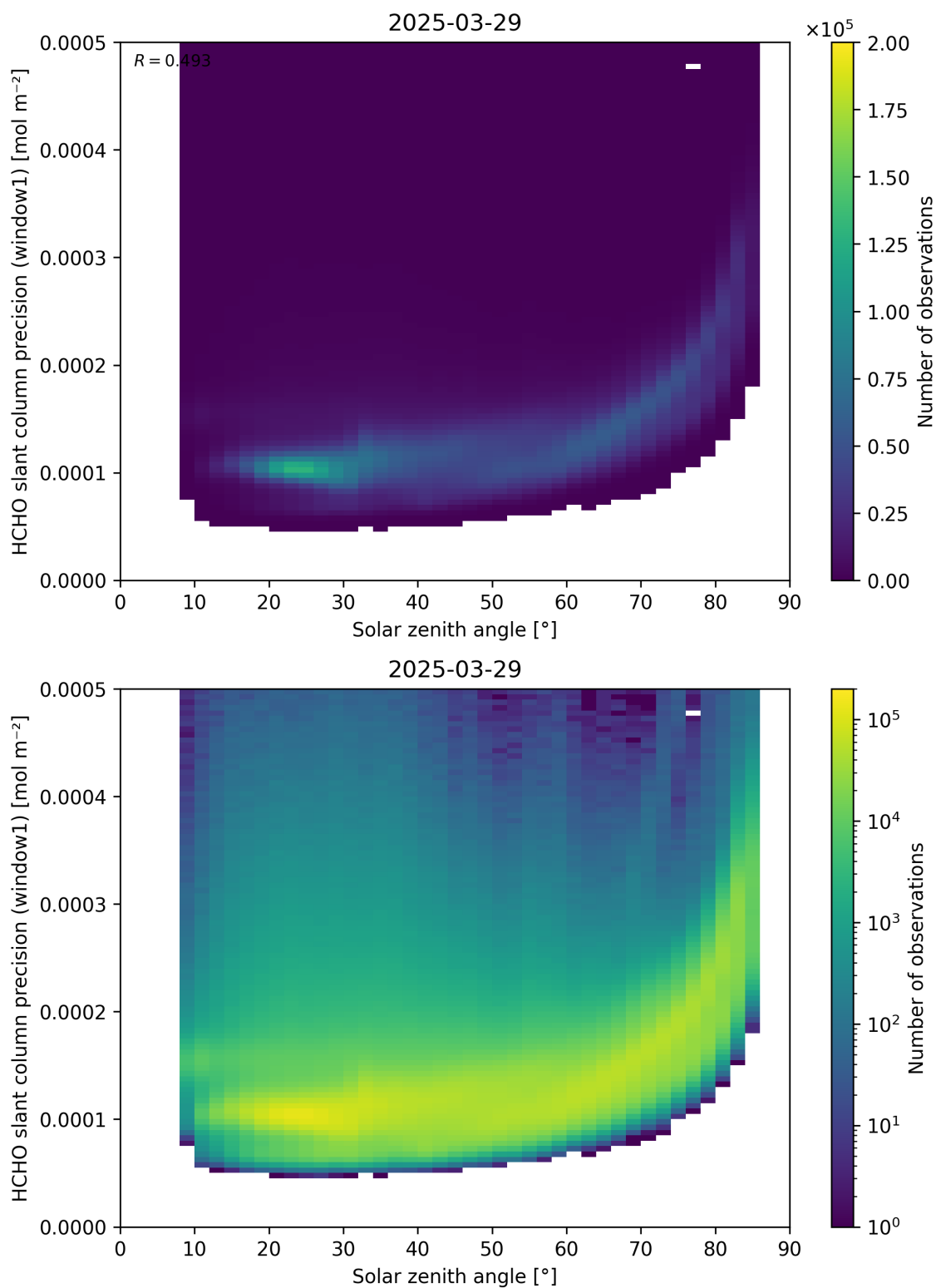
Figure 174: Scatter density plot of “Solar zenith angle” against “HCHO slant column precision (window1)” for 2025-03-28 to 2025-03-30.
