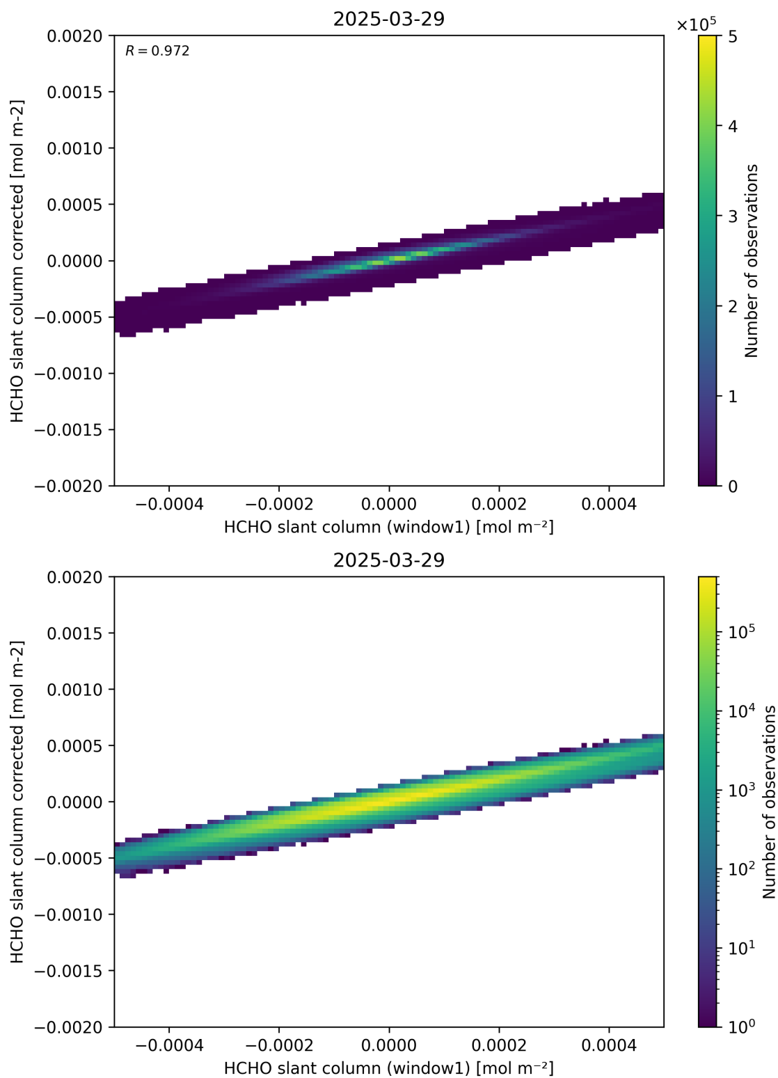
Figure 82: Scatter density plot of “HCHO slant column (window1)” against “HCHO slant column corrected” for 2025-03-28 to 2025-03-30.
