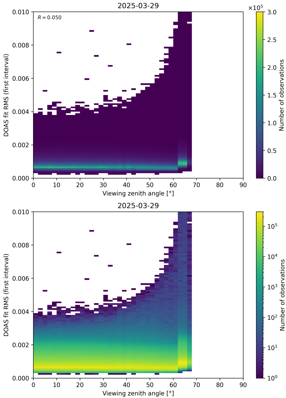
Figure 182: Scatter density plot of “Viewing zenith angle” against “DOAS fit RMS (first interval)” for 2025-03-28 to 2025-03-30.
