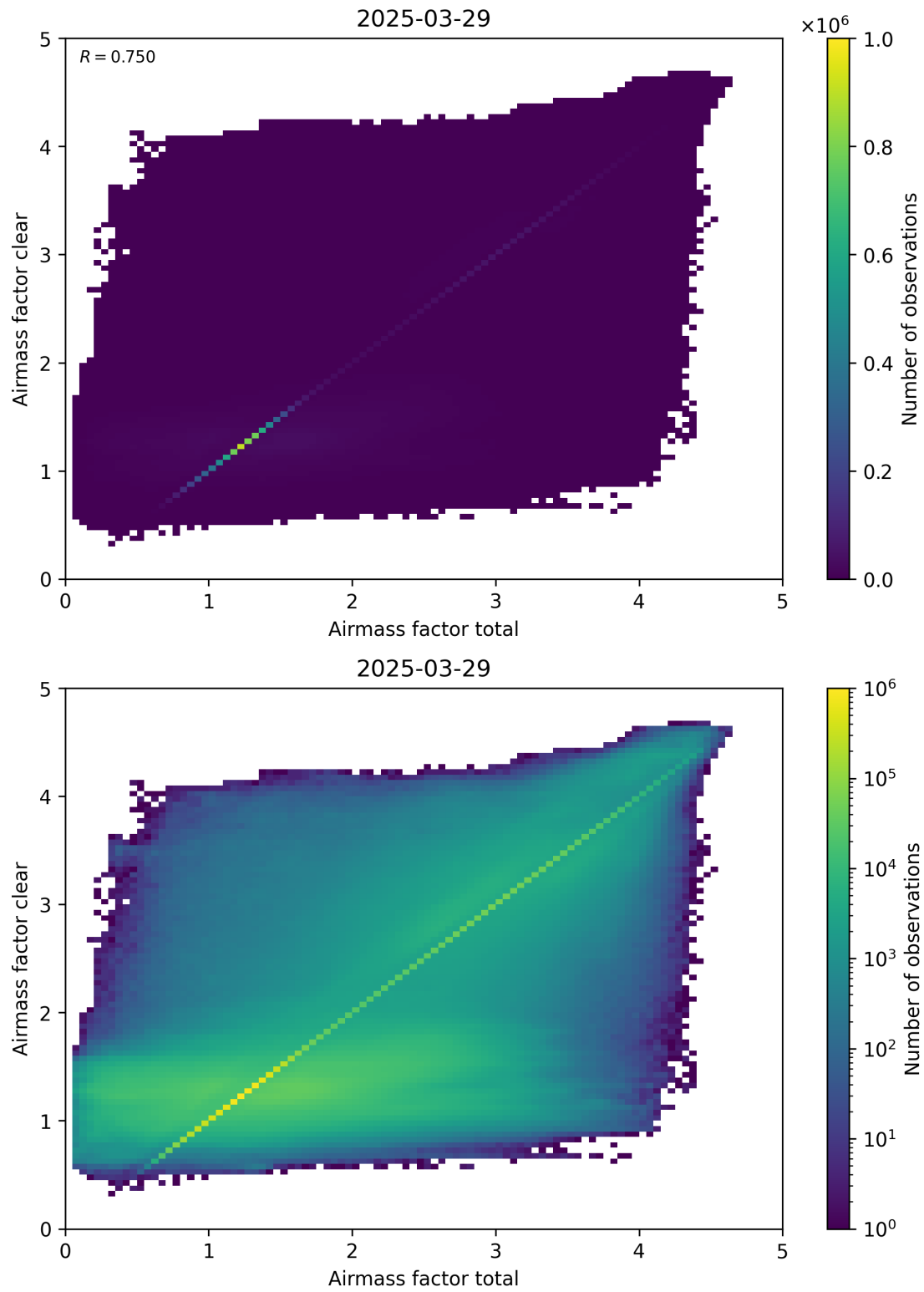
Figure 100: Scatter density plot of “Airmass factor total” against “Airmass factor clear” for 2025-03-28 to 2025-03-30.
