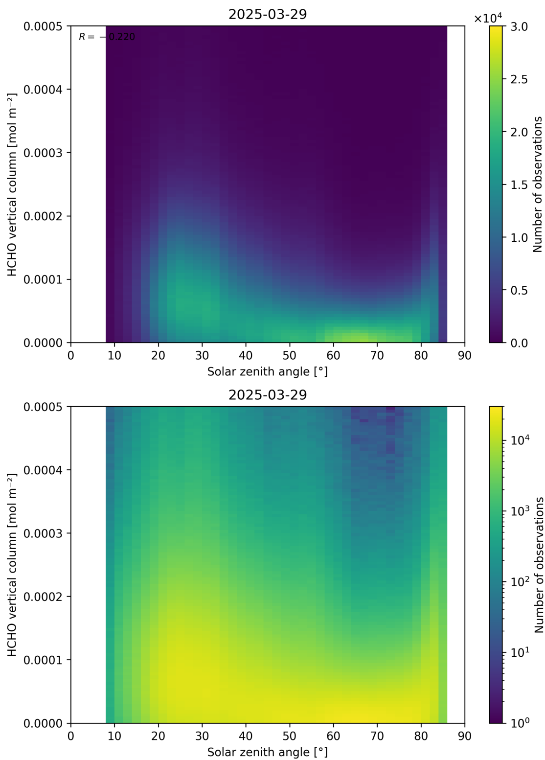
Figure 177: Scatter density plot of “Solar zenith angle” against “HCHO vertical column” for 2025-03-28 to 2025-03-30.
