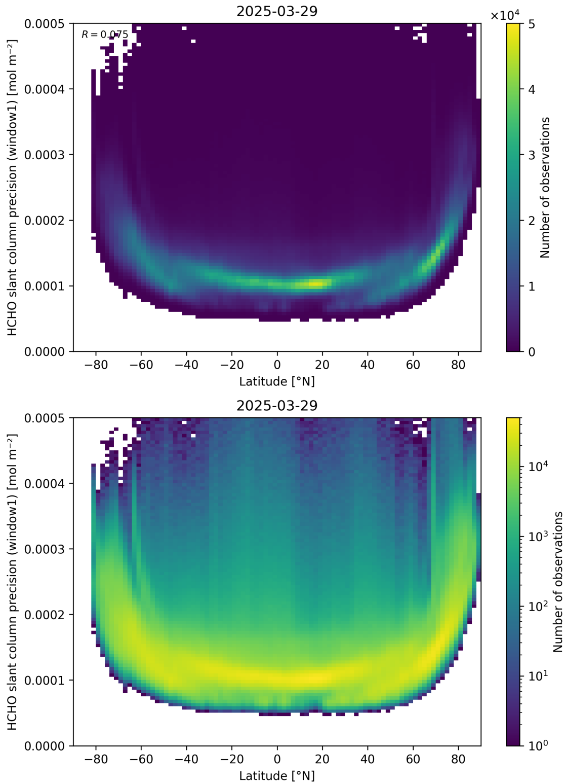
Figure 160: Scatter density plot of “Latitude” against “HCHO slant column precision (window1)” for 2025-03-28 to 2025-03-30.
