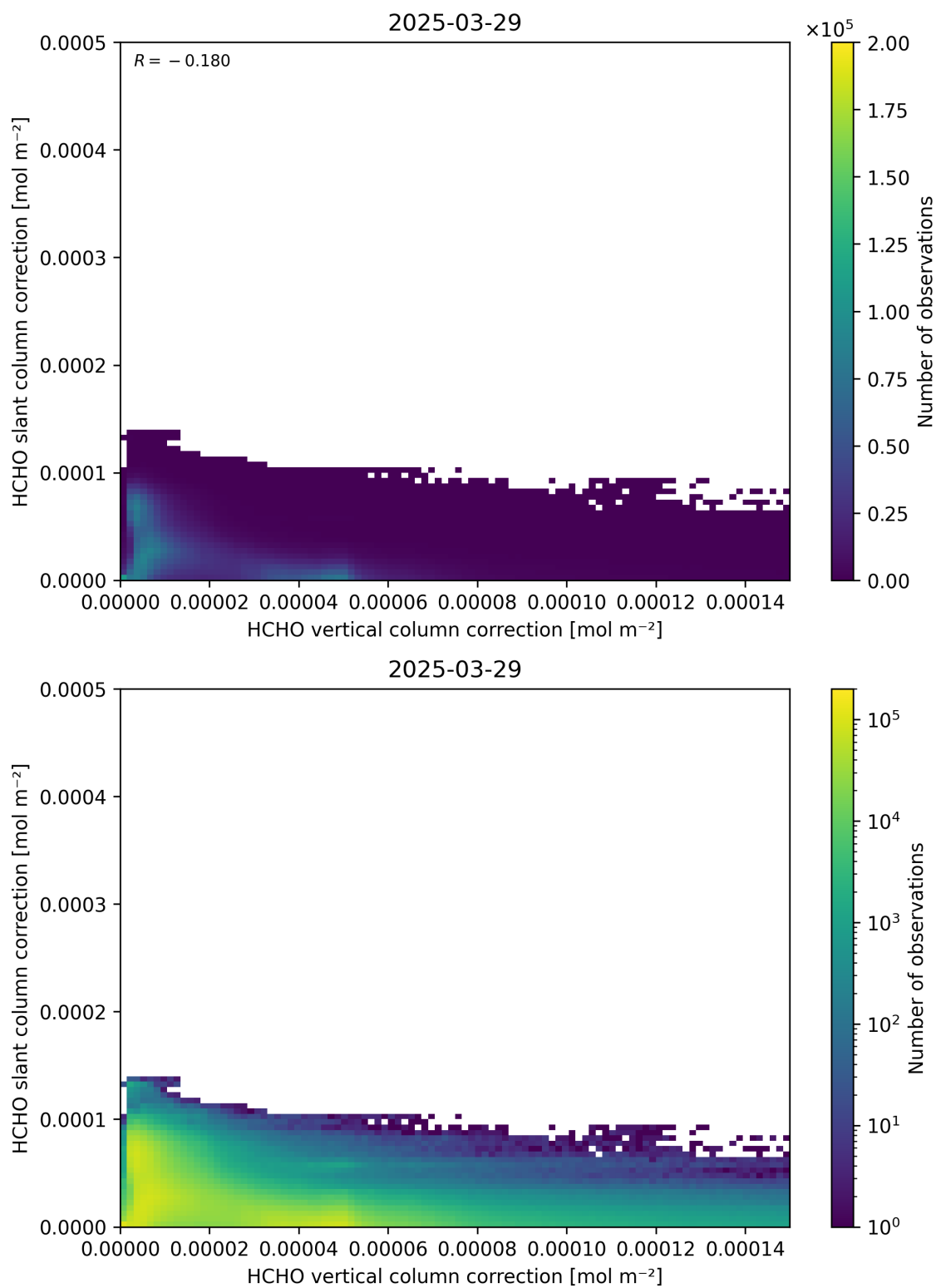
Figure 117: Scatter density plot of “HCHO vertical column correction” against “HCHO slant column correction” for 2025-03-28 to 2025-03-30.
