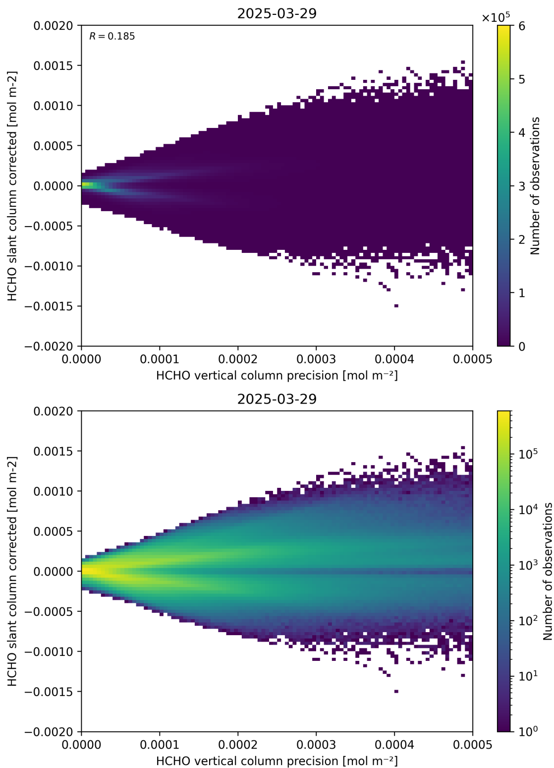
Figure 140: Scatter density plot of “HCHO vertical column precision” against “HCHO slant column corrected” for 2025-03-28 to 2025-03-30.
