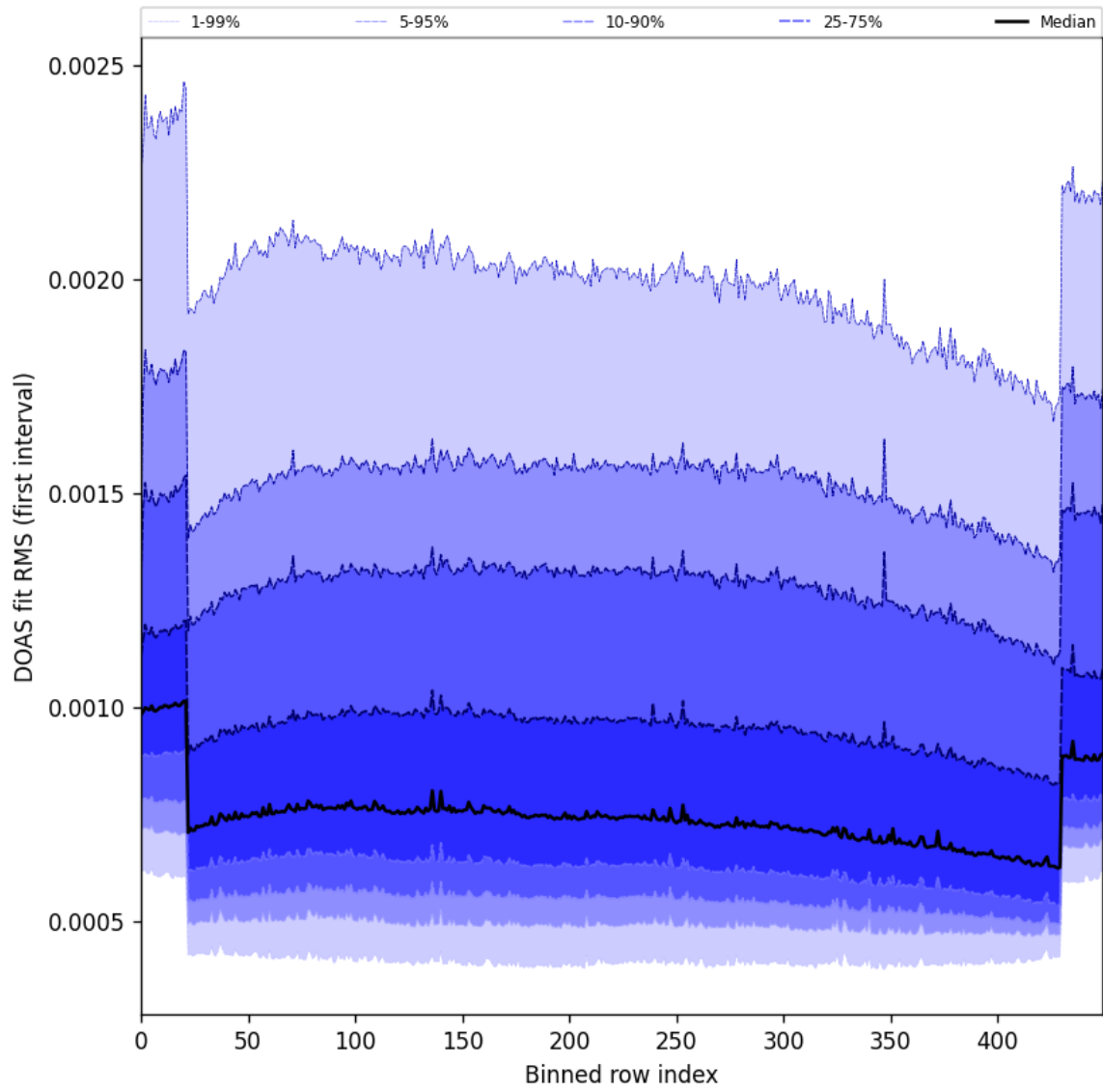
Figure 60: Along track statistics of “DOAS fit RMS (first interval)” for 2025-03-28 to 2025-03-30
