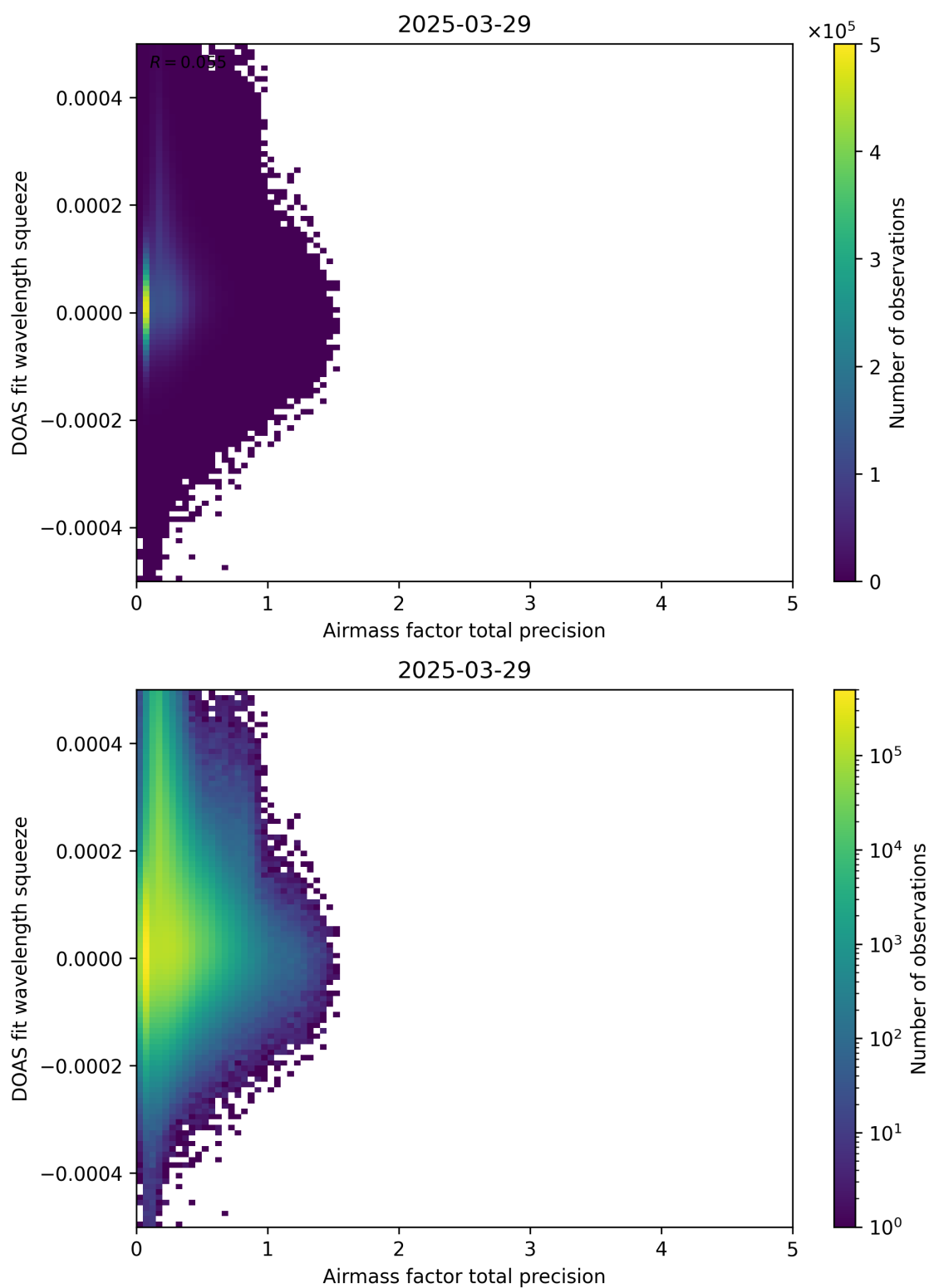
Figure 107: Scatter density plot of “Airmass factor total precision” against “DOAS fit wavelength squeeze” for 2025-03-28 to 2025-03-30.
