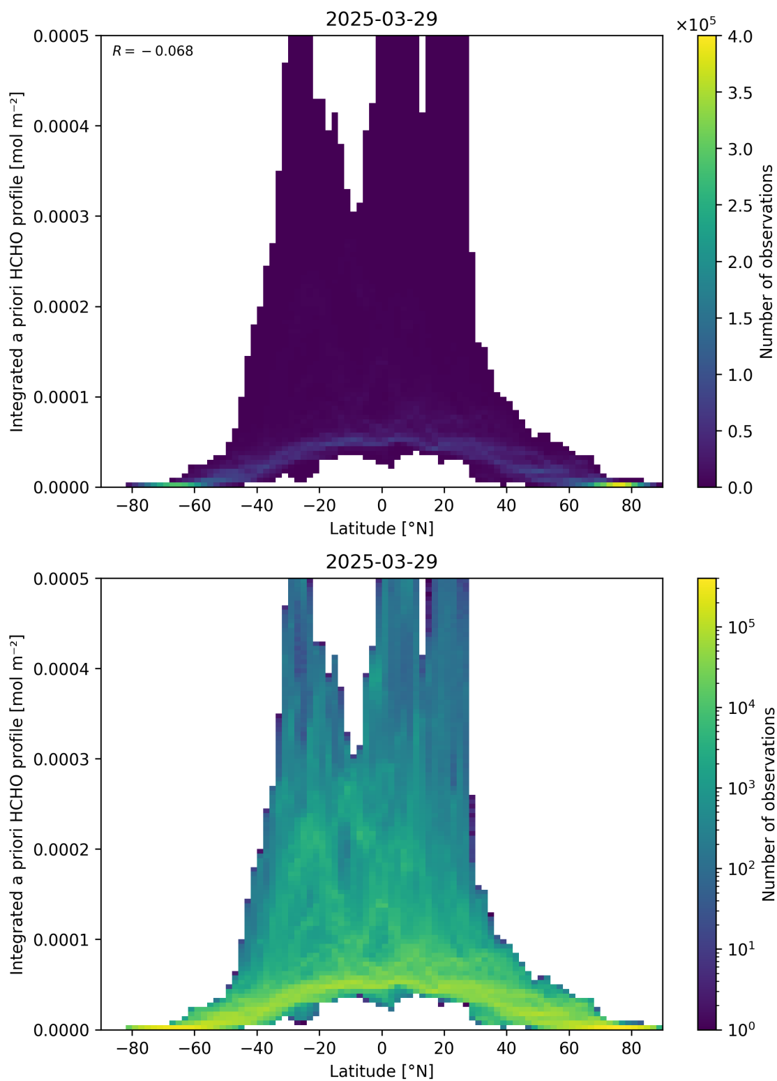
Figure 166: Scatter density plot of “Latitude” against “Integrated a priori HCHO profile” for 2025-03-28 to 2025-03-30.
