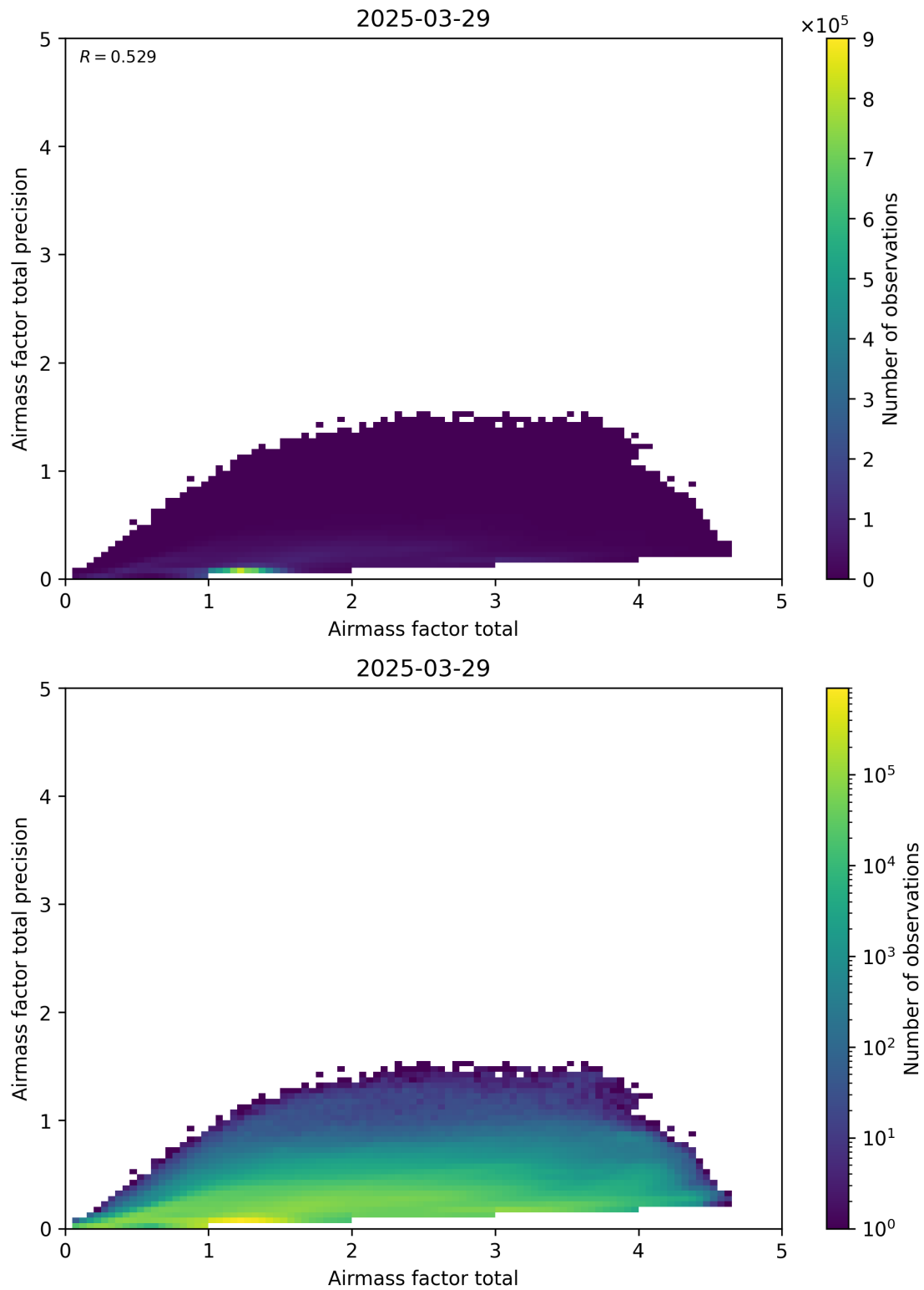
Figure 103: Scatter density plot of “Airmass factor total” against “Airmass factor total precision” for 2025-03-28 to 2025-03-30.
