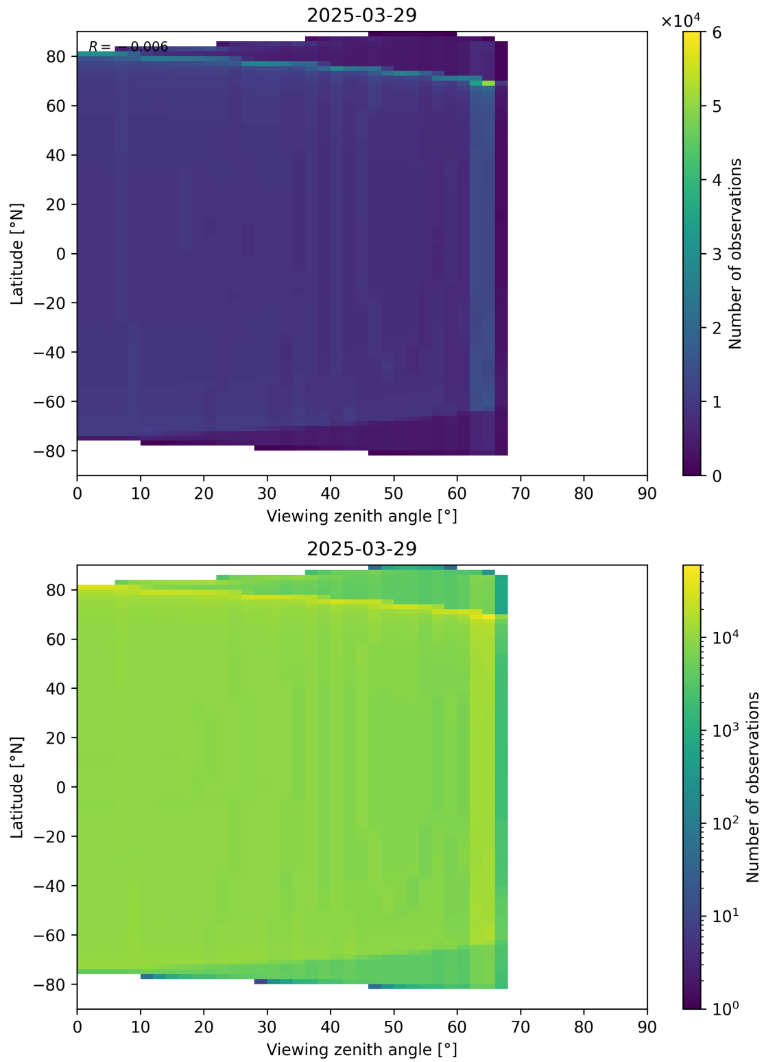
Figure 196: Scatter density plot of “Viewing zenith angle” against “Latitude” for 2025-03-28 to 2025-03-30.
