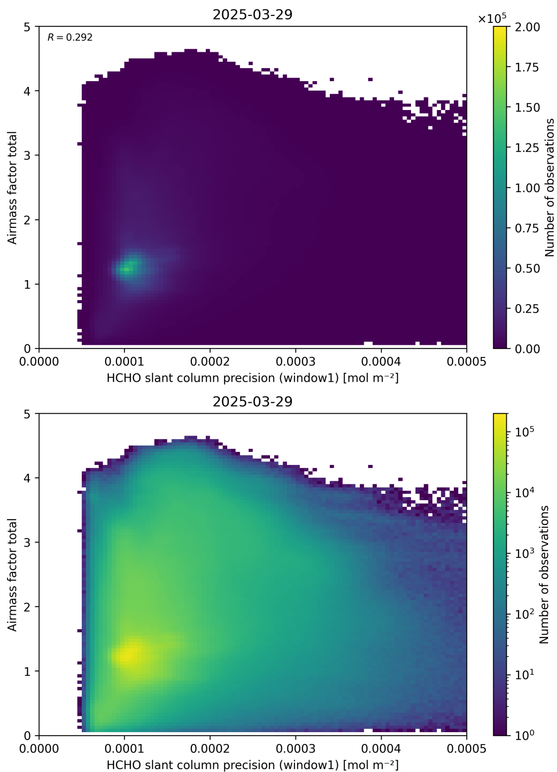
Figure 94: Scatter density plot of “HCHO slant column precision (window1)” against “Airmass factor total” for 2025-03-28 to 2025-03-30.
