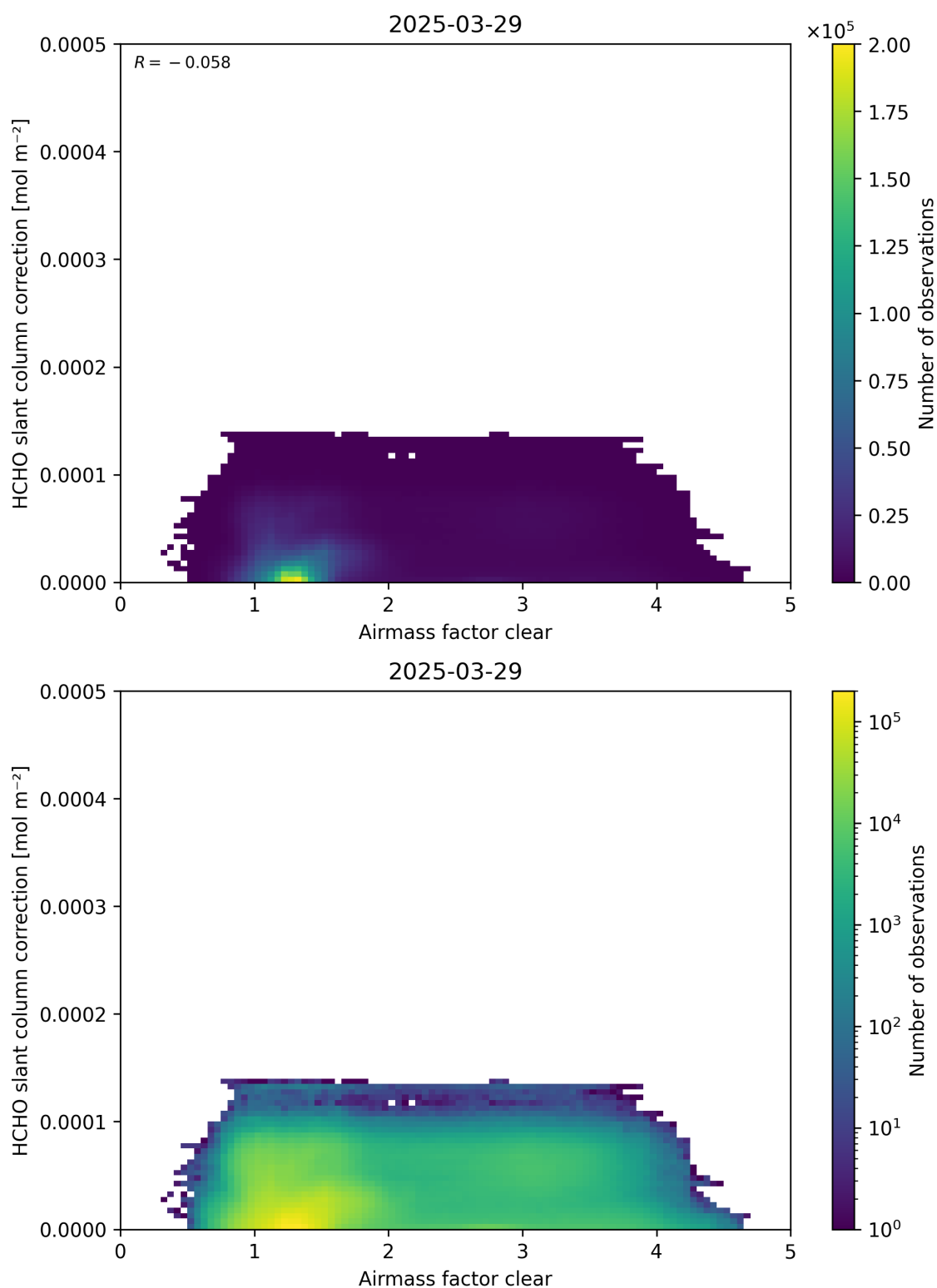
Figure 75: Scatter density plot of “Airmass factor clear” against “HCHO slant column correction” for 2025-03-28 to 2025-03-30.
