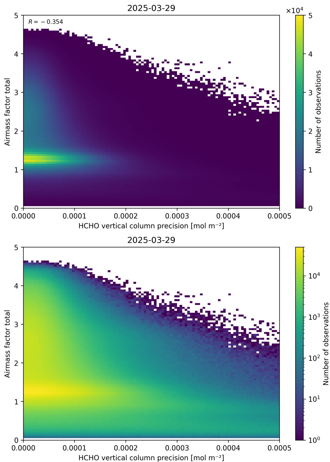
Figure 144: Scatter density plot of “HCHO vertical column precision” against “Airmass factor total” for 2025-03-28 to 2025-03-30.
