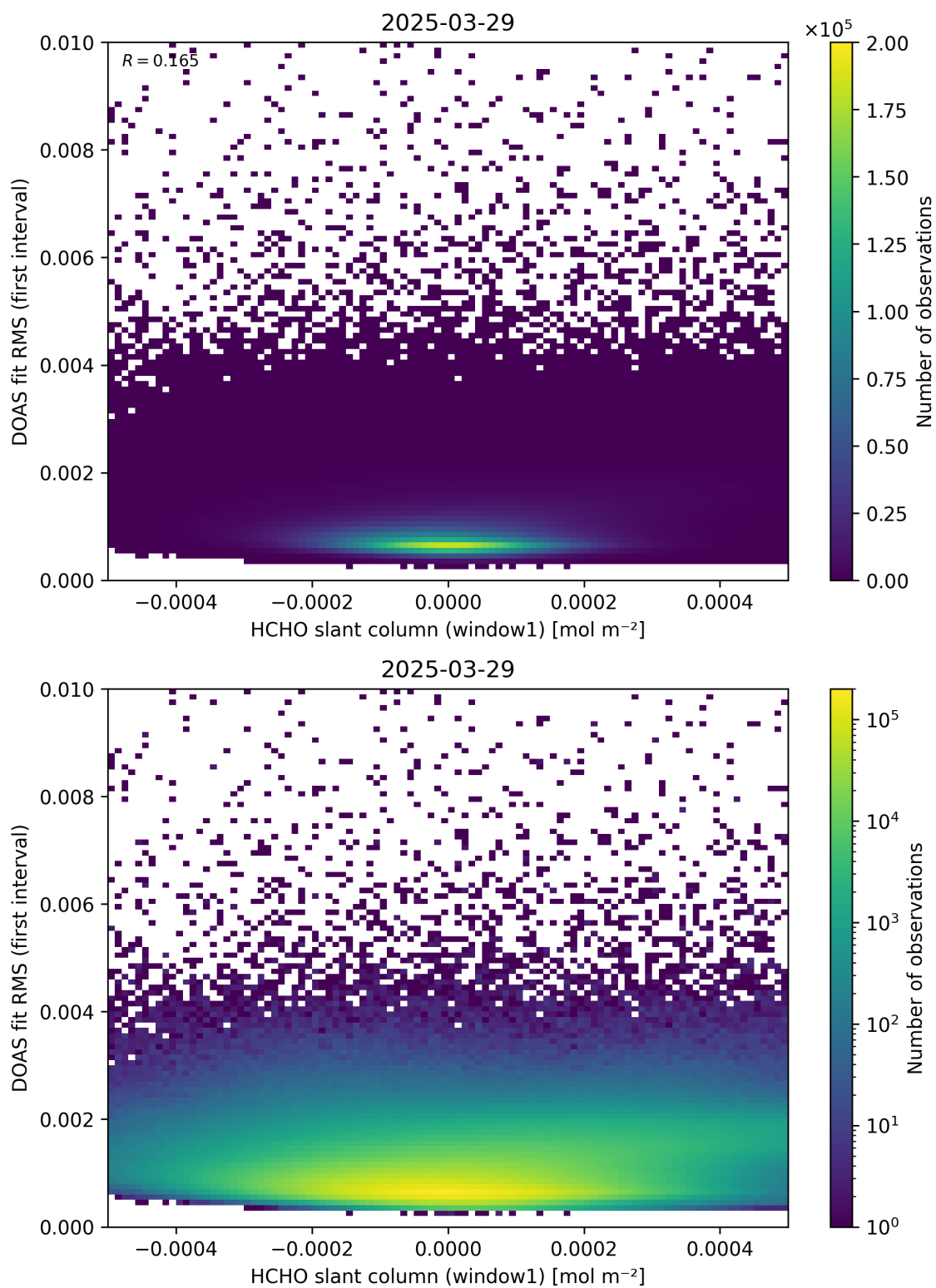
Figure 78: Scatter density plot of “HCHO slant column (window1)” against “DOAS fit RMS (first interval)” for 2025-03-28 to 2025-03-30.
