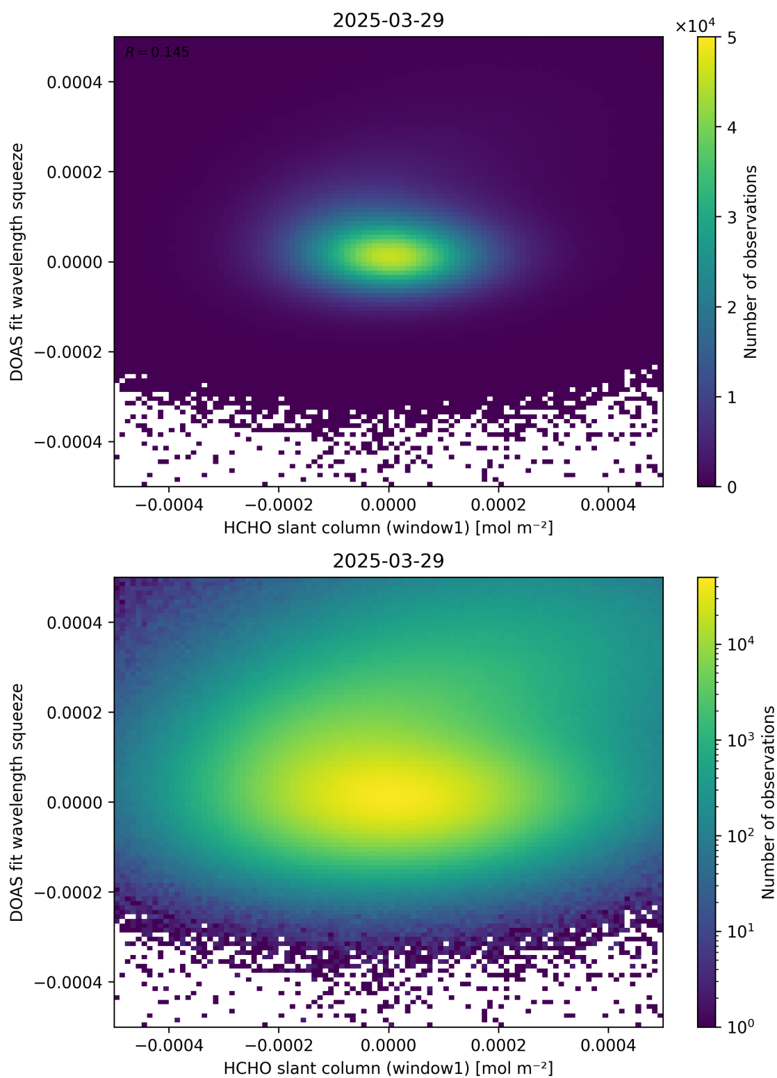
Figure 80: Scatter density plot of “HCHO slant column (window1)” against “DOAS fit wavelength squeeze” for 2025-03-28 to 2025-03-30.
