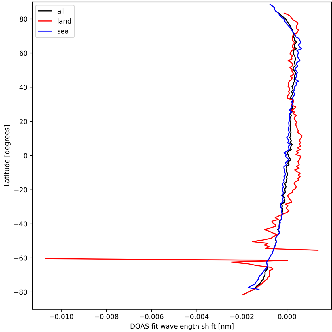
Figure 30: Zonal average of "DOAS fit wavelength shift" for 2025-03-28 to 2025-03-30.
