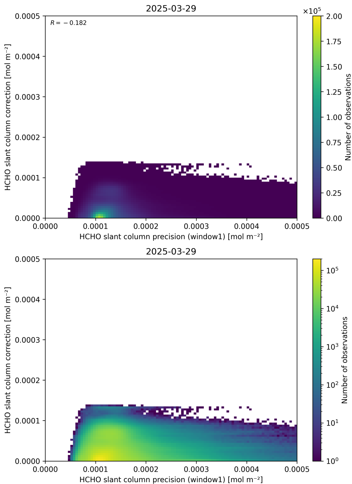
Figure 93: Scatter density plot of “HCHO slant column precision (window1)” against “HCHO slant column correction” for 2025-03-28 to 2025-03-30.
