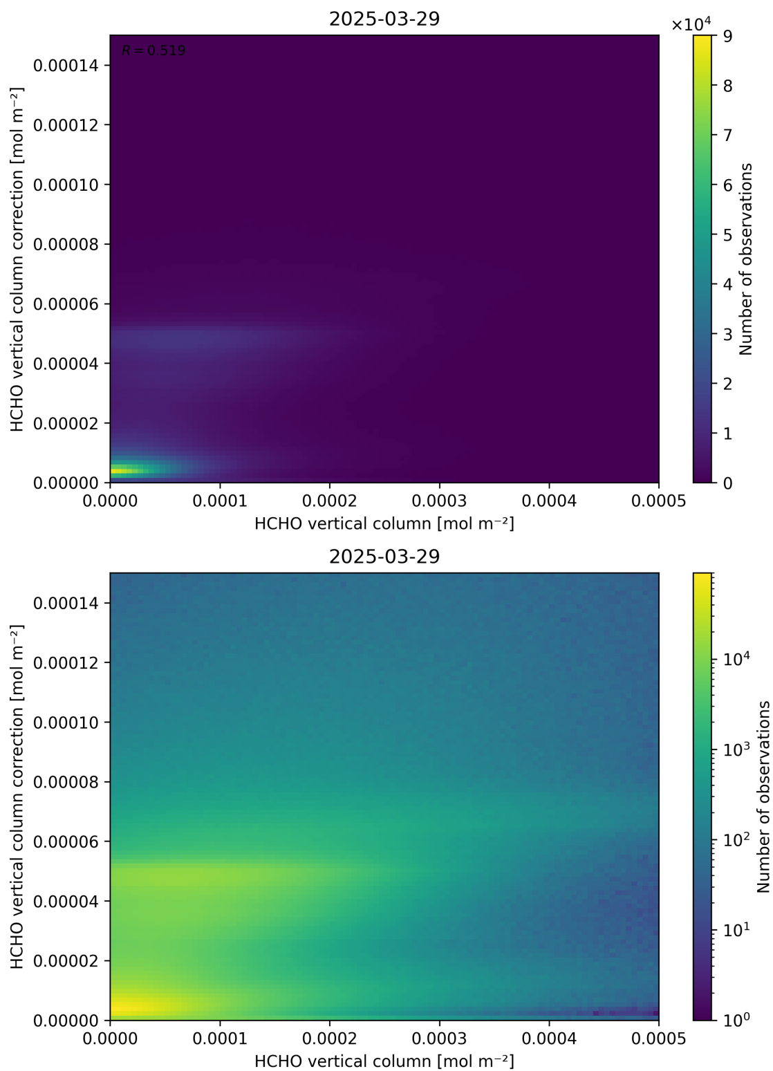
Figure 133: Scatter density plot of “HCHO vertical column” against “HCHO vertical column correction” for 2025-03-28 to 2025-03-30.
