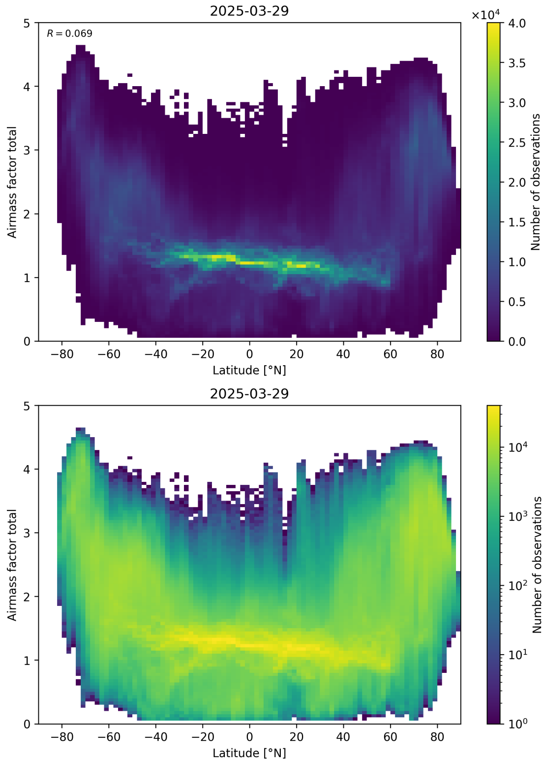
Figure 161: Scatter density plot of “Latitude” against “Airmass factor total” for 2025-03-28 to 2025-03-30.
