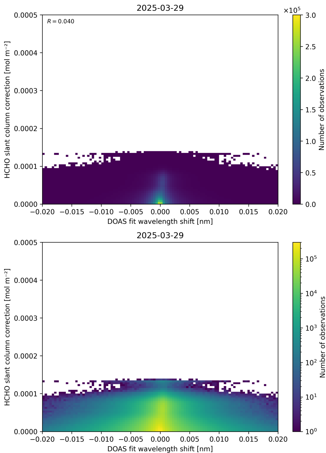
Figure 67: Scatter density plot of “DOAS fit wavelength shift” against “HCHO slant column correction” for 2025-03-28 to 2025-03-30.
