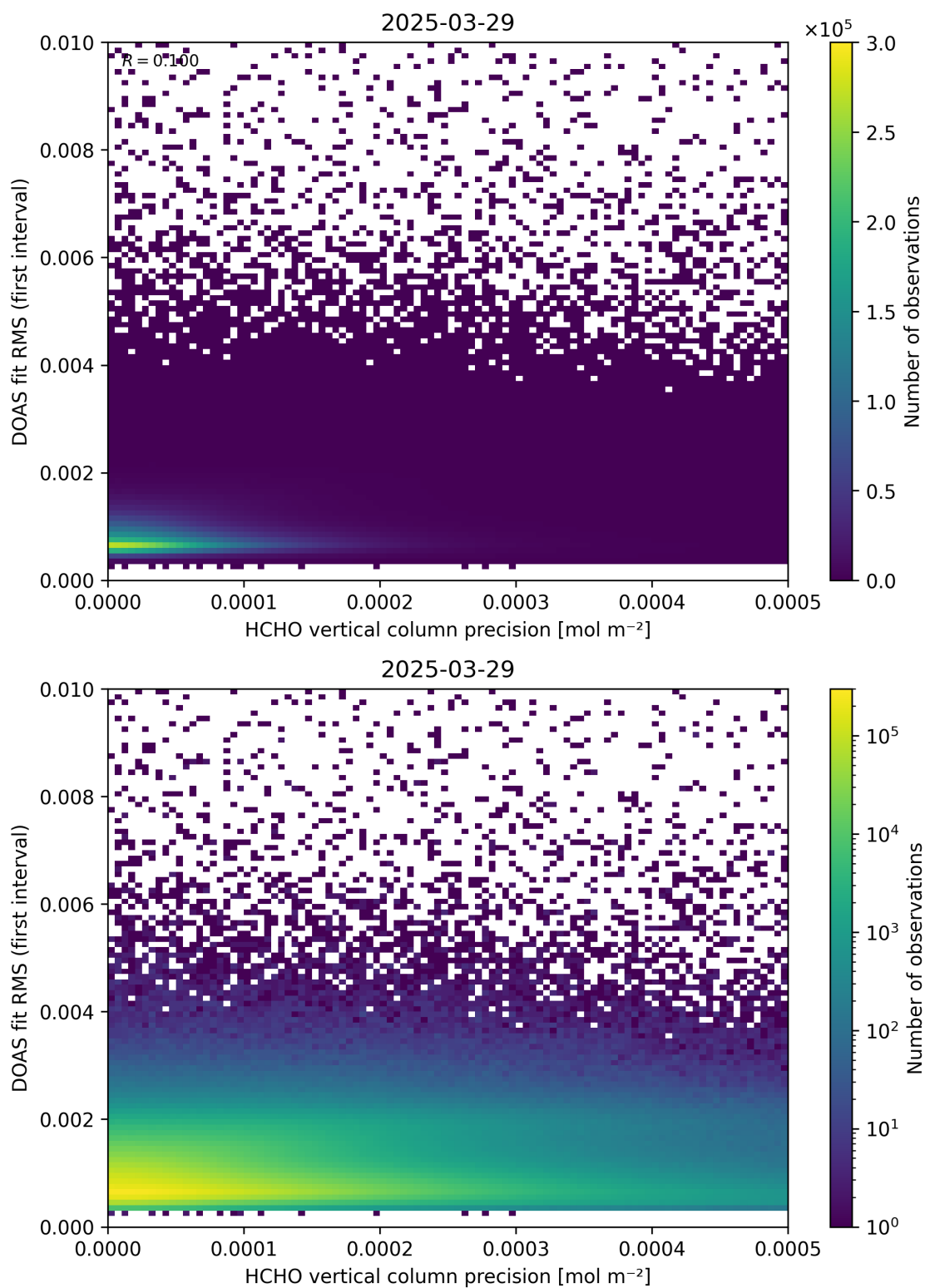
Figure 136: Scatter density plot of “HCHO vertical column precision” against “DOAS fit RMS (first interval)” for 2025-03-28 to 2025-03-30.
