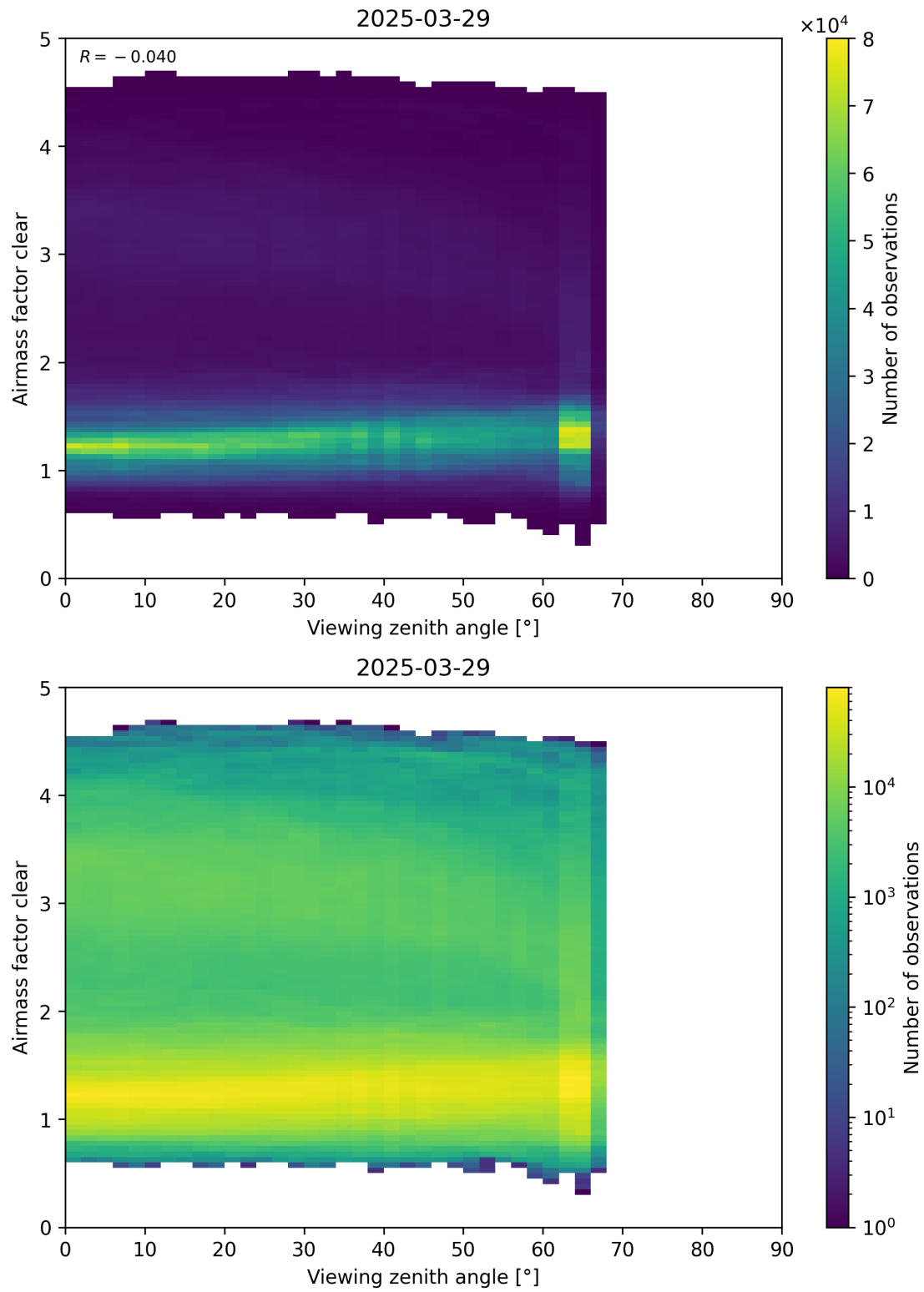
Figure 185: Scatter density plot of “Viewing zenith angle” against “Airmass factor clear” for 2025-03-28 to 2025-03-30.
