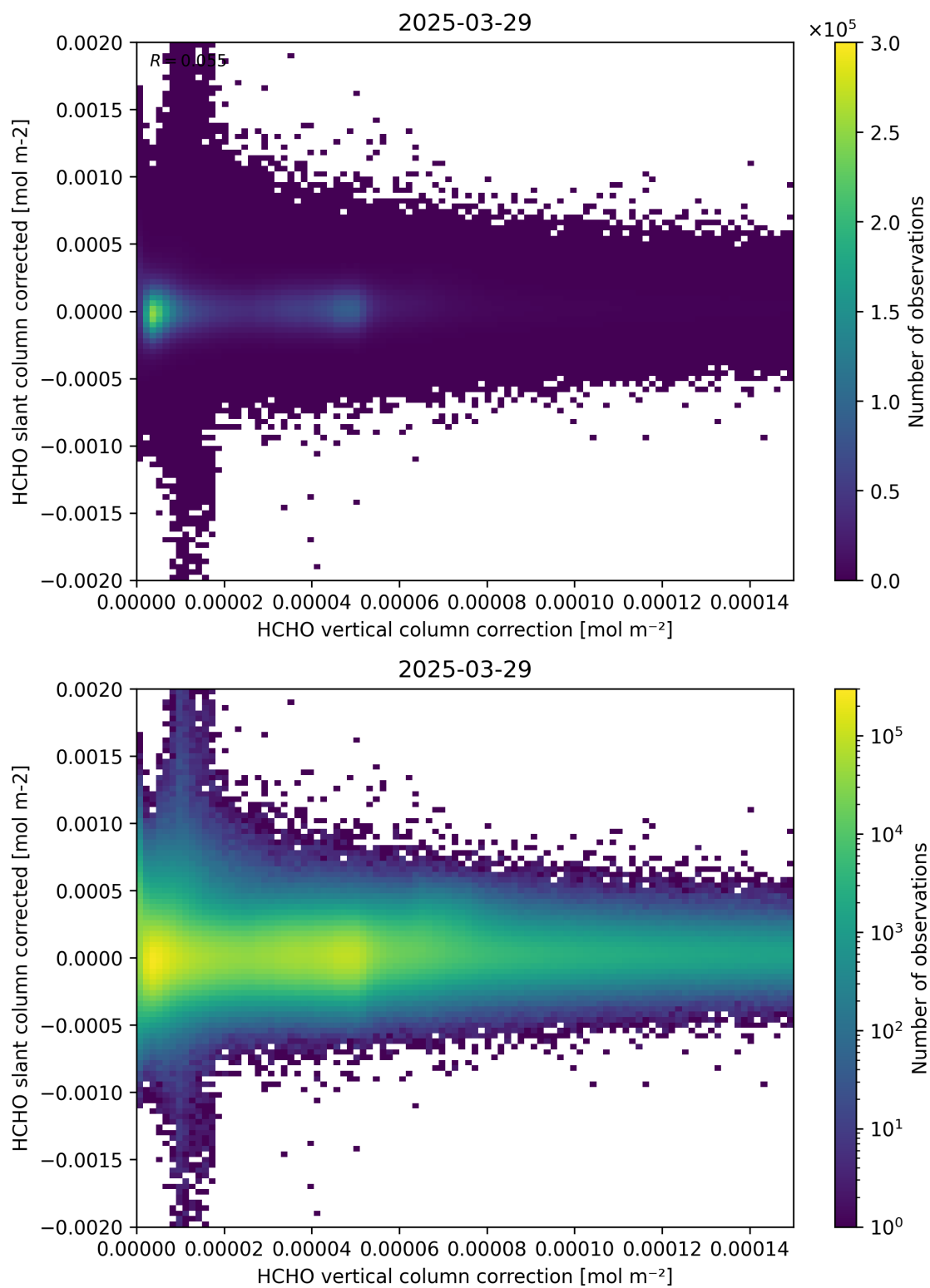
Figure 116: Scatter density plot of “HCHO vertical column correction” against “HCHO slant column corrected” for 2025-03-28 to 2025-03-30.
