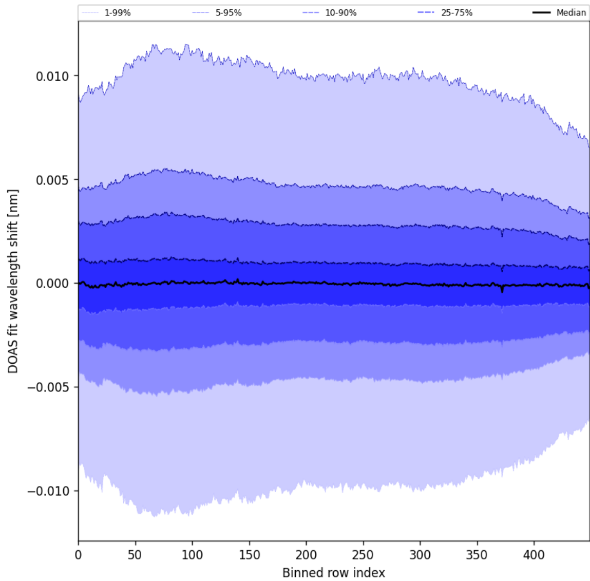
Figure 58: Along track statistics of “DOAS fit wavelength shift” for 2025-03-28 to 2025-03-30
