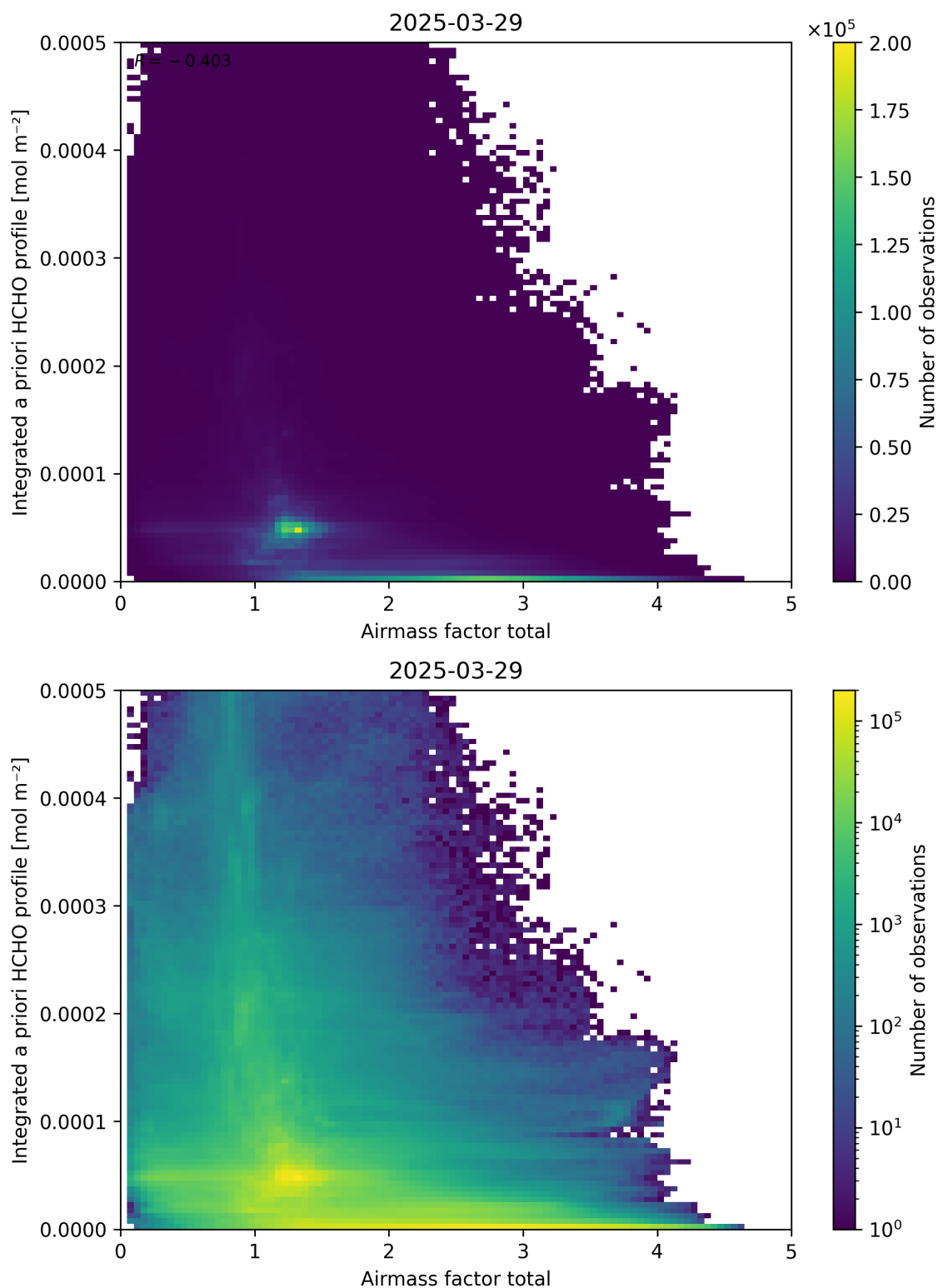
Figure 104: Scatter density plot of “Airmass factor total” against “Integrated a priori HCHO profile” for 2025-03-28 to 2025-03-30.
