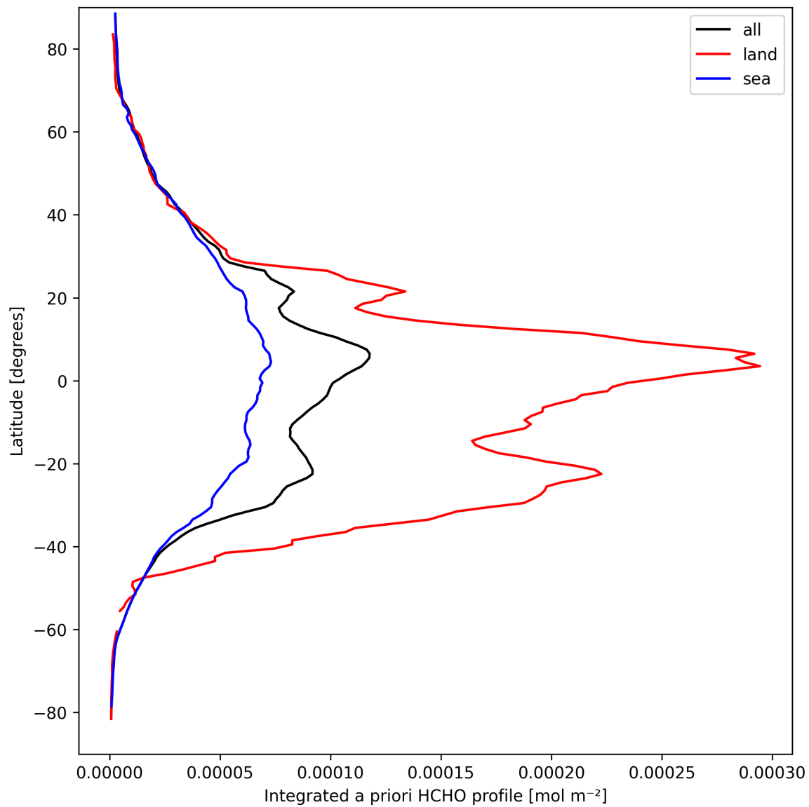
Figure 29: Zonal average of “Integrated a priori HCHO profile” for 2025-03-28 to 2025-03-30.
