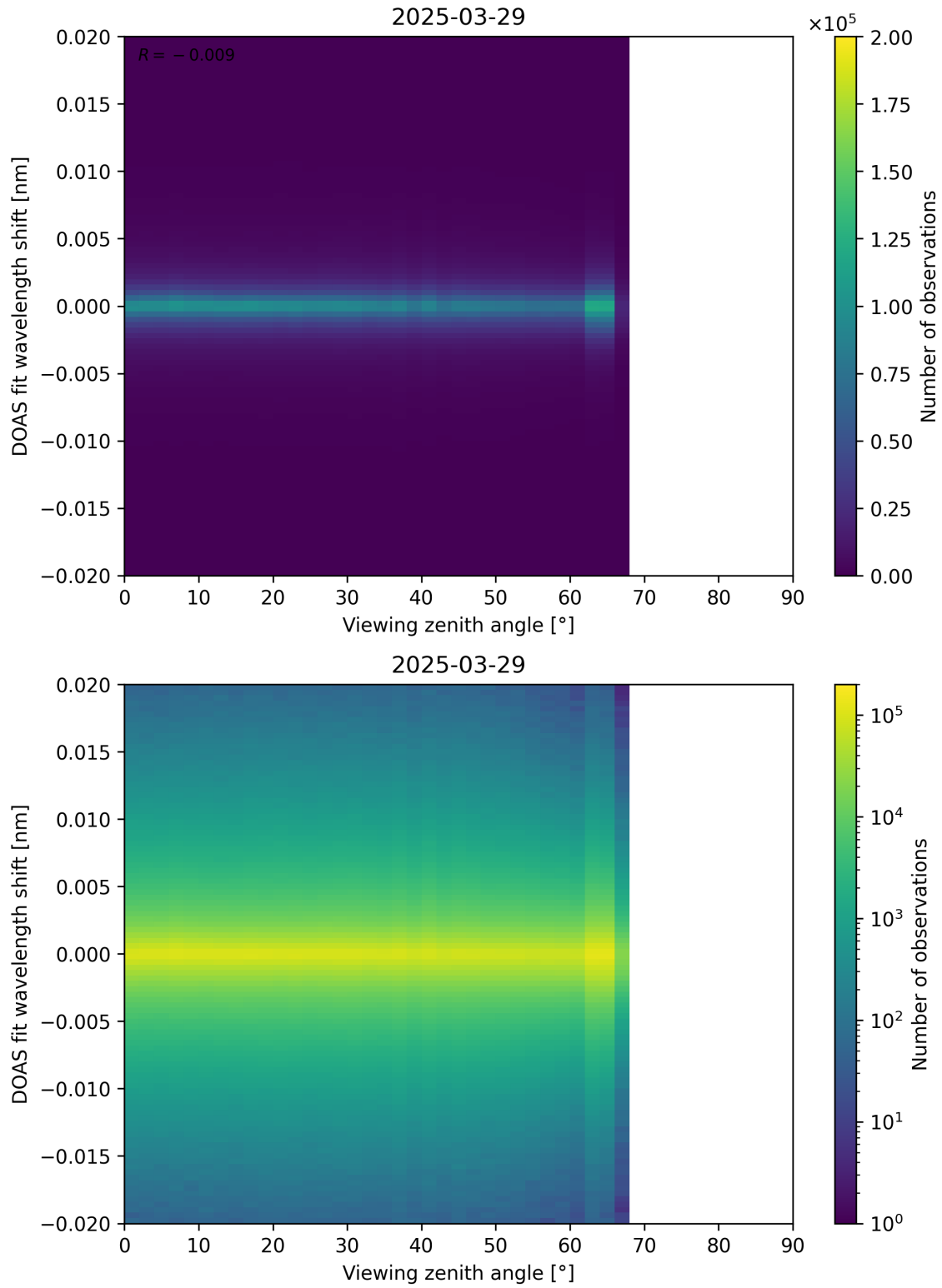
Figure 183: Scatter density plot of “Viewing zenith angle” against “DOAS fit wavelength shift” for 2025-03-28 to 2025-03-30.
