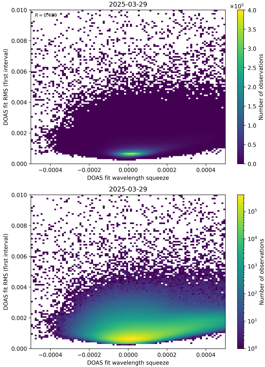
Figure 68: Scatter density plot of “DOAS fit wavelength squeeze” against “DOAS fit RMS (first interval)” for 2025-03-28 to 2025-03-30.
