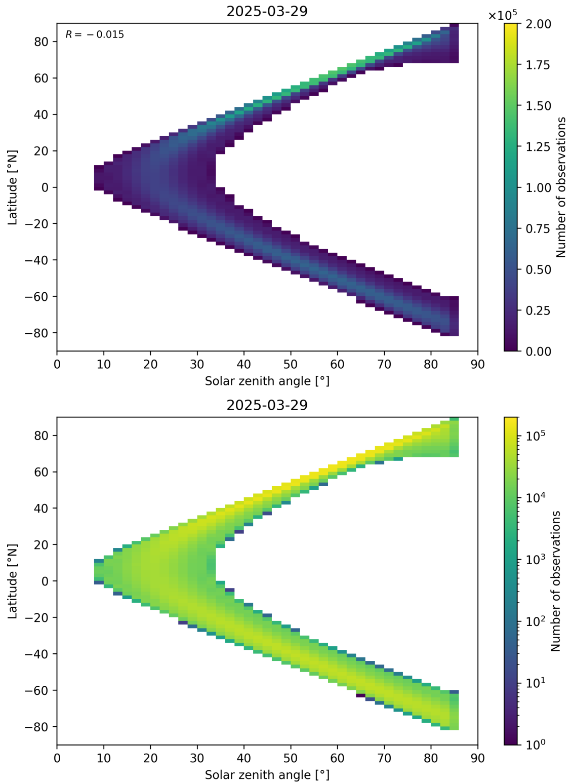
Figure 181: Scatter density plot of “Solar zenith angle” against “Latitude” for 2025-03-28 to 2025-03-30.
