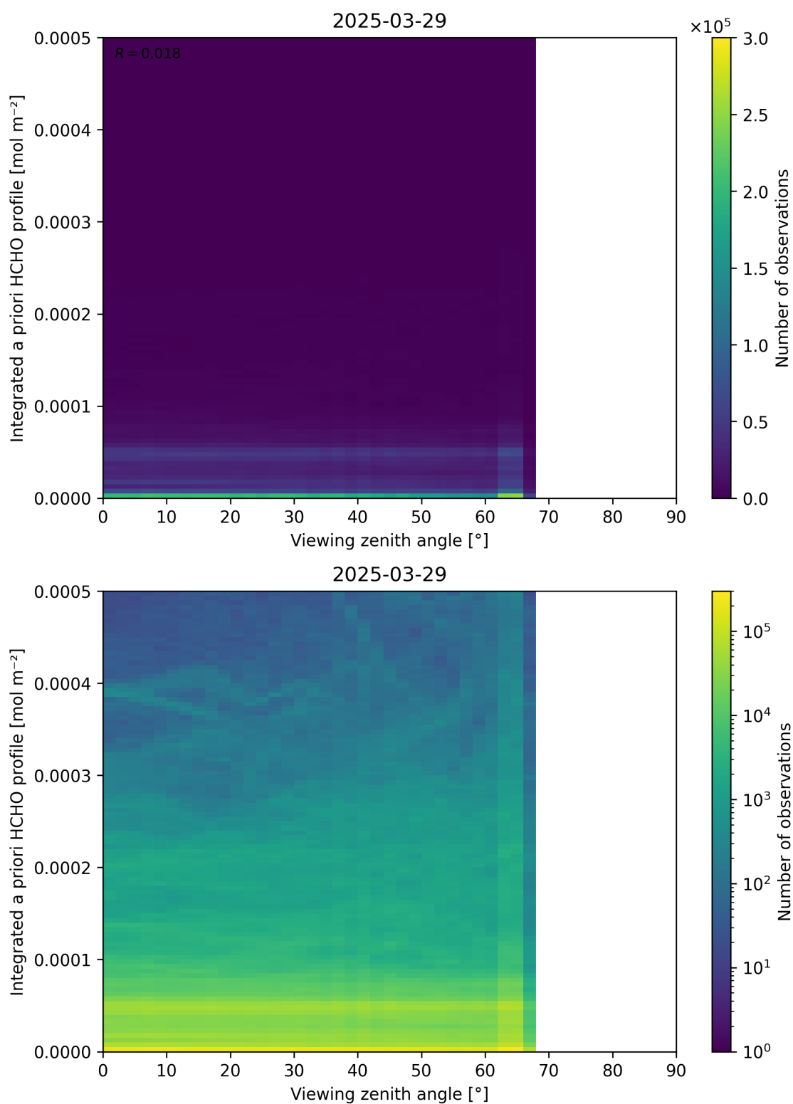
Figure 195: Scatter density plot of “Viewing zenith angle” against “Integrated a priori HCHO profile” for 2025-03-28 to 2025-03-30.
