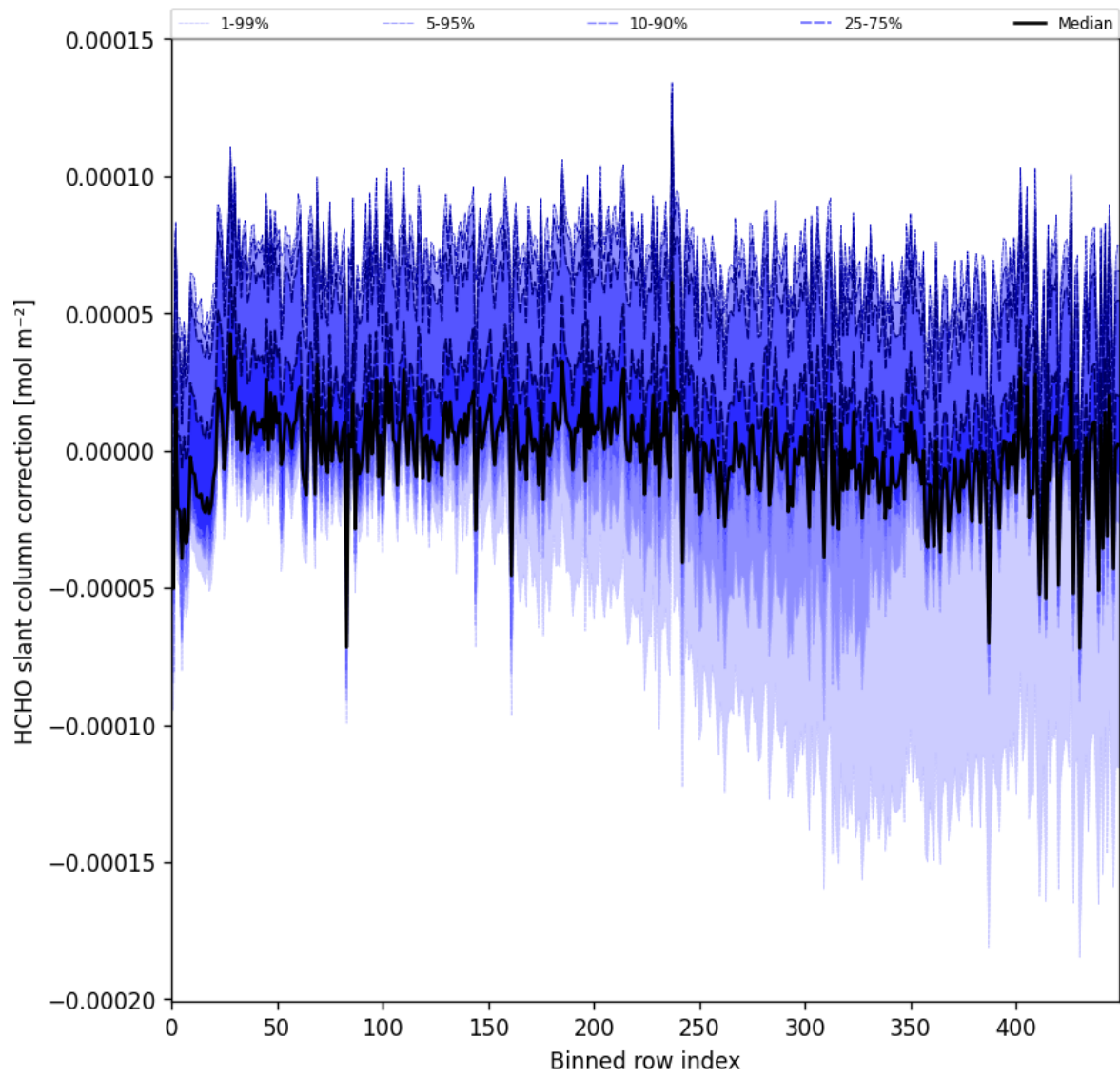
Figure 61: Along track statistics of “HCHO slant column correction” for 2025-03-28 to 2025-03-30
