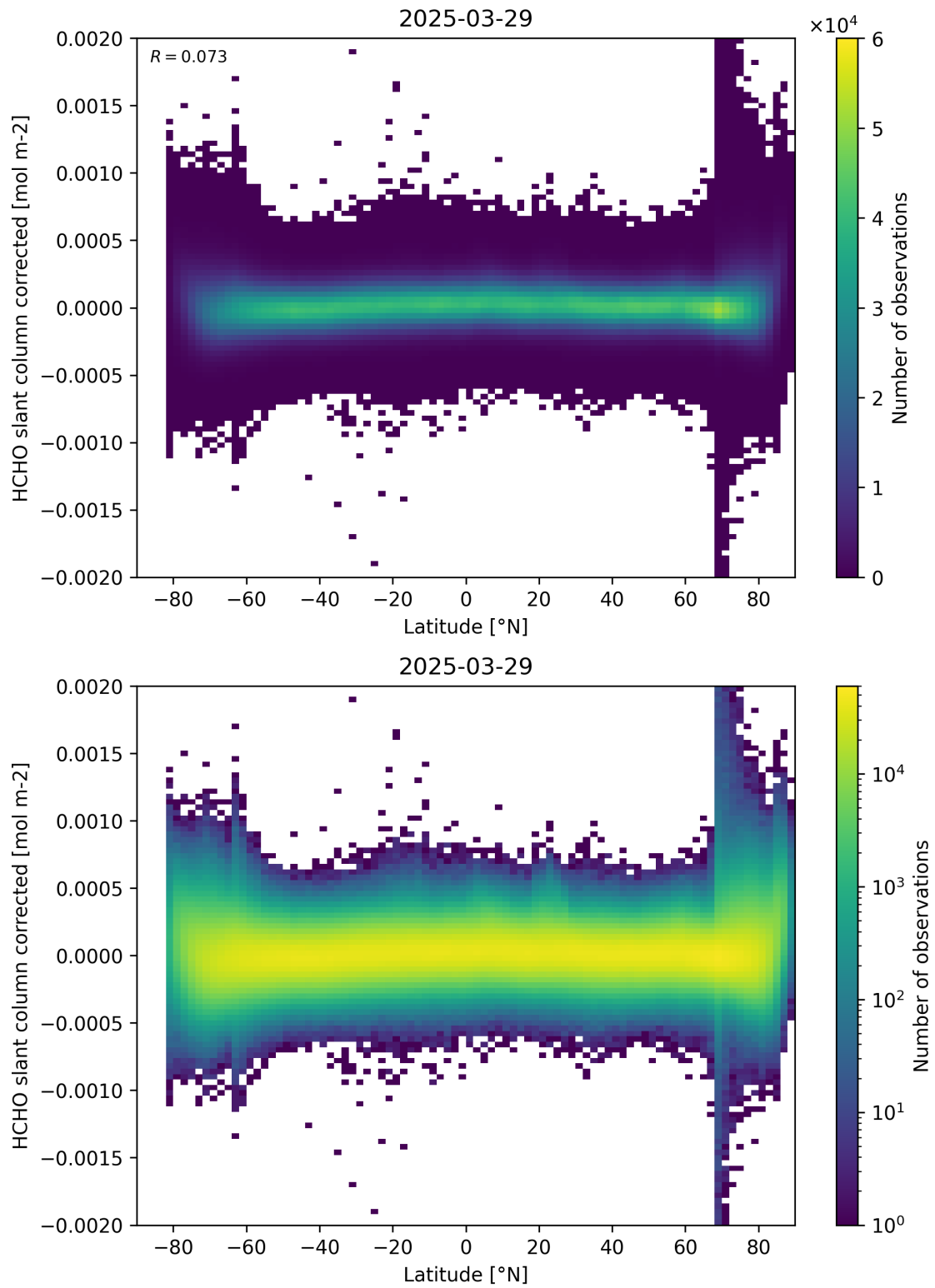
Figure 157: Scatter density plot of “Latitude” against “HCHO slant column corrected” for 2025-03-28 to 2025-03-30.
