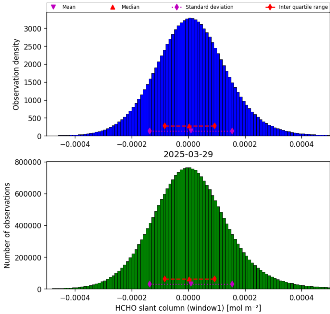
Figure 38: Histogram of “HCHO slant column (window1)” for 2025-03-28 to 2025-03-30
