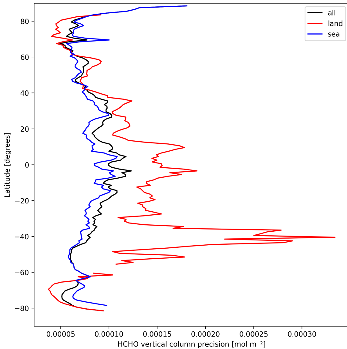
Figure 22: Zonal average of “HCHO vertical column precision” for 2025-03-28 to 2025-03-30.
