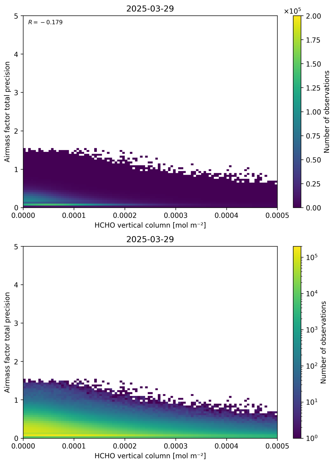
Figure 132: Scatter density plot of “HCHO vertical column” against “Airmass factor total precision” for 2025-03-28 to 2025-03-30.
