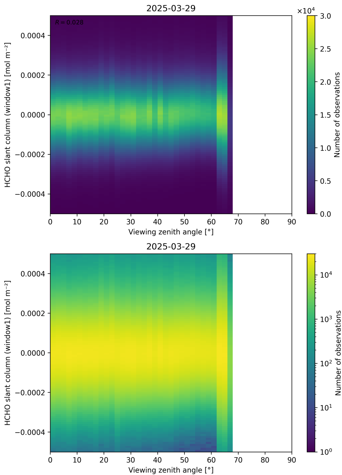
Figure 188: Scatter density plot of “Viewing zenith angle” against “HCHO slant column (window1)” for 2025-03-28 to 2025-03-30.
