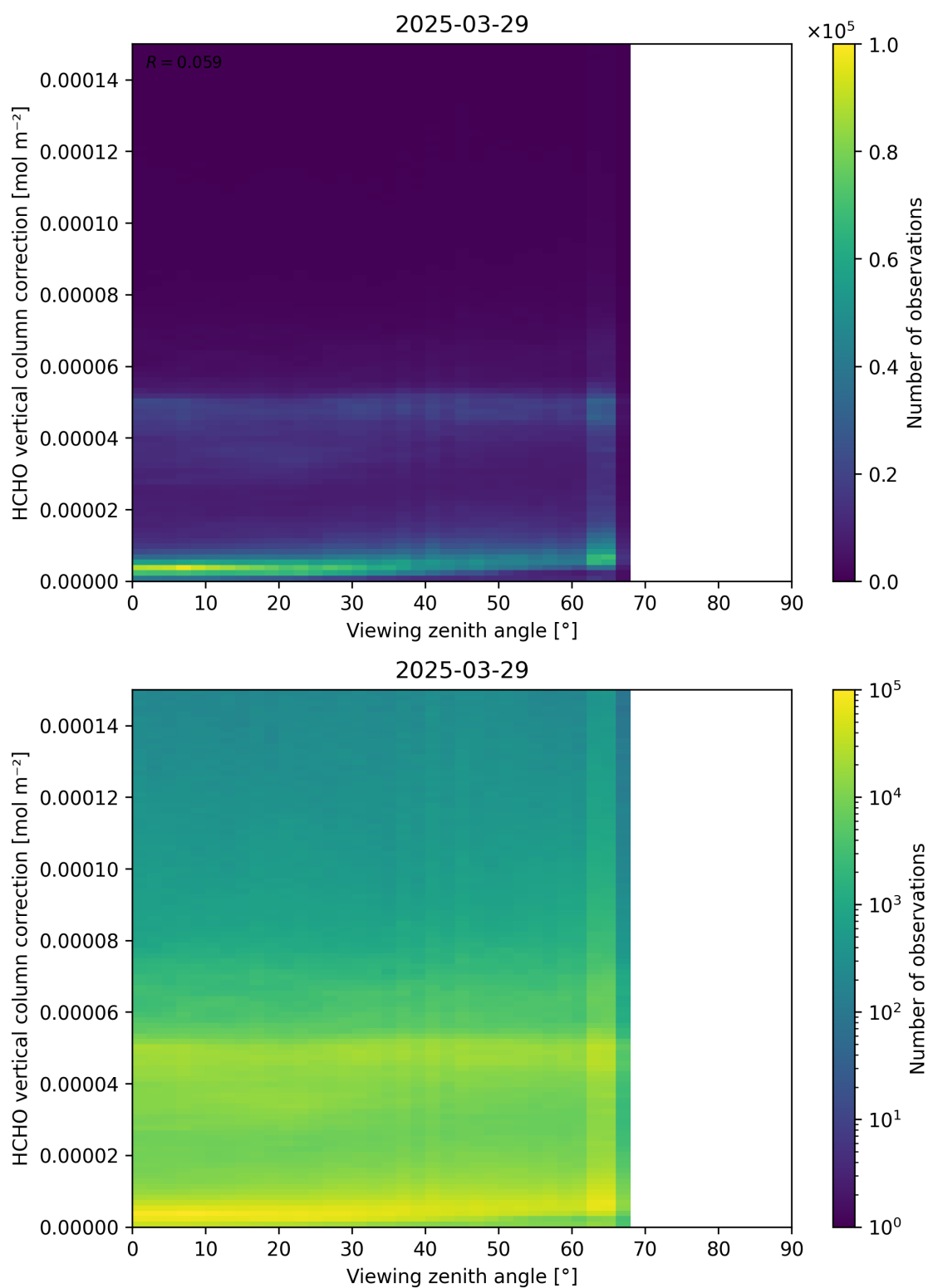
Figure 193: Scatter density plot of “Viewing zenith angle” against “HCHO vertical column correction” for 2025-03-28 to 2025-03-30.
