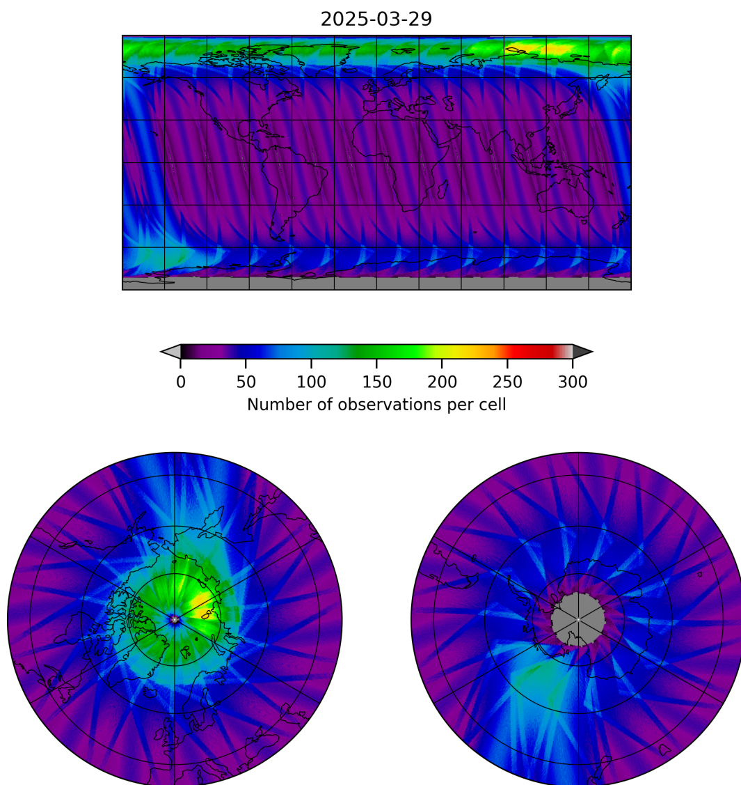
Figure 19: Map of the number of observations for 2025-03-28 to 2025-03-30
