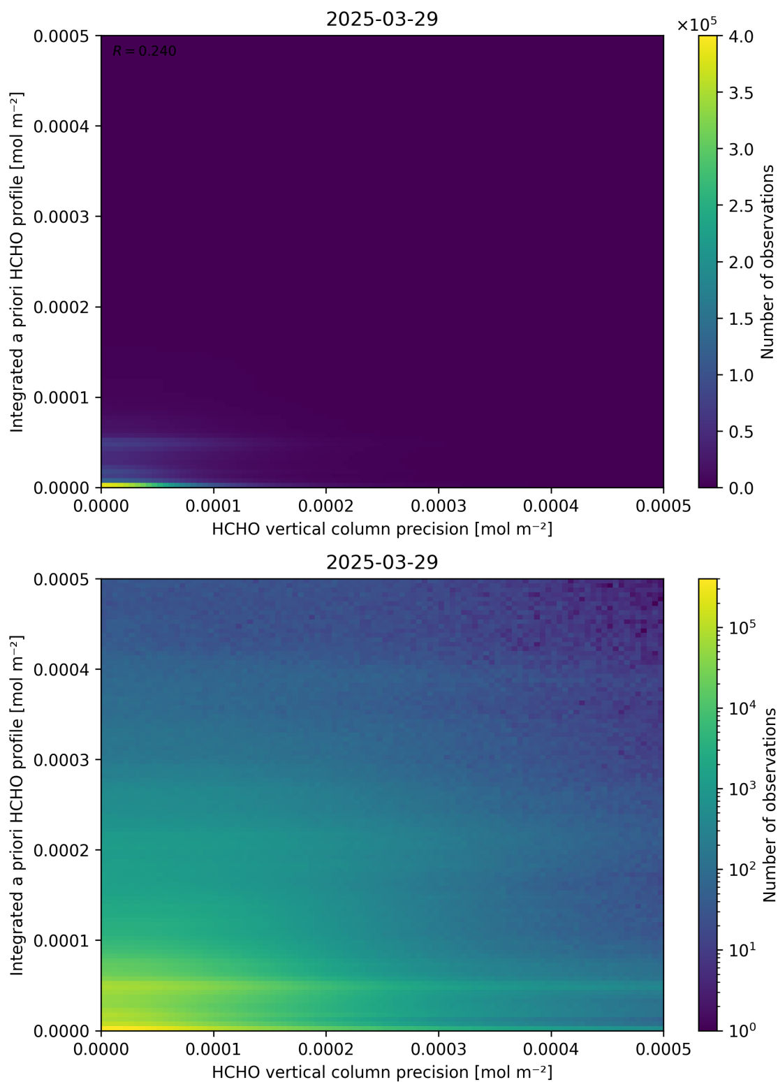
Figure 147: Scatter density plot of “HCHO vertical column precision” against “Integrated a priori HCHO profile” for 2025-03-28 to 2025-03-30.
