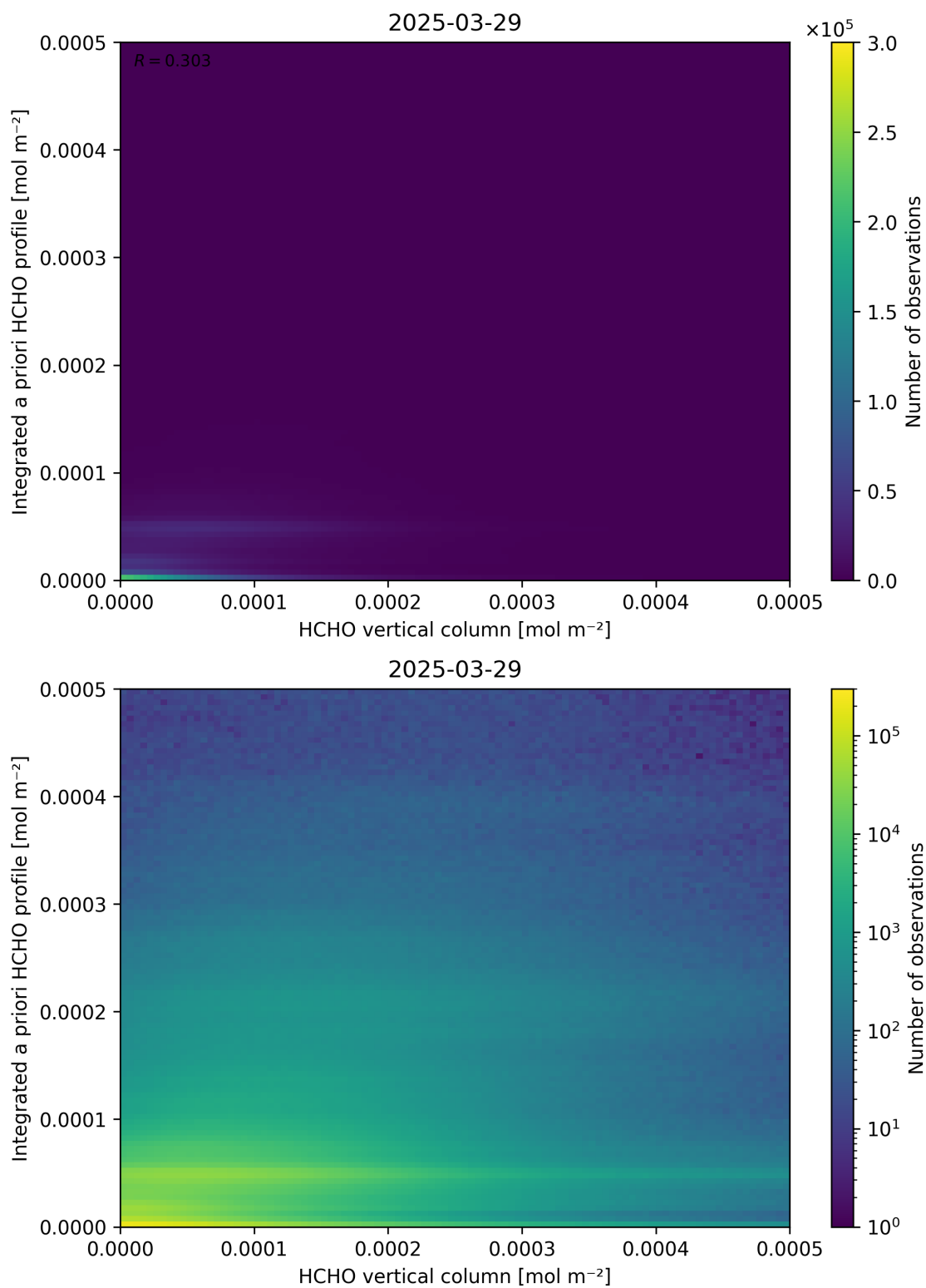
Figure 135: Scatter density plot of “HCHO vertical column” against “Integrated a priori HCHO profile” for 2025-03-28 to 2025-03-30.
