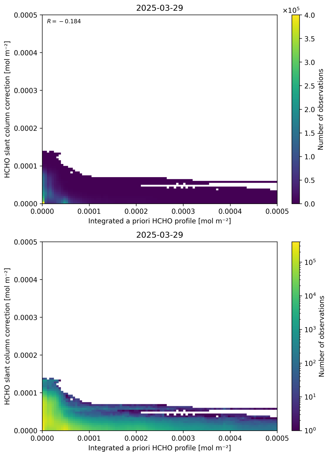
Figure 152: Scatter density plot of “Integrated a priori HCHO profile” against “HCHO slant column correction” for 2025-03-28 to 2025-03-30.
