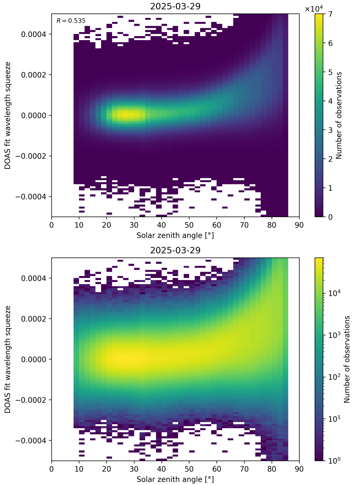
Figure 169: Scatter density plot of “Solar zenith angle” against “DOAS fit wavelength squeeze” for 2025-03-28 to 2025-03-30.
