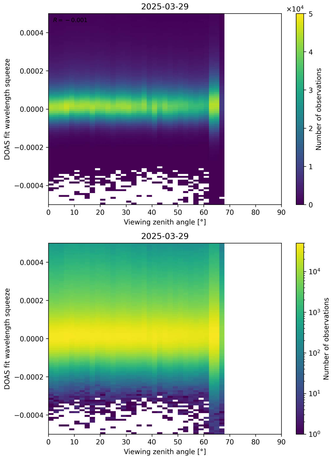
Figure 184: Scatter density plot of “Viewing zenith angle” against “DOAS fit wavelength squeeze” for 2025-03-28 to 2025-03-30.
