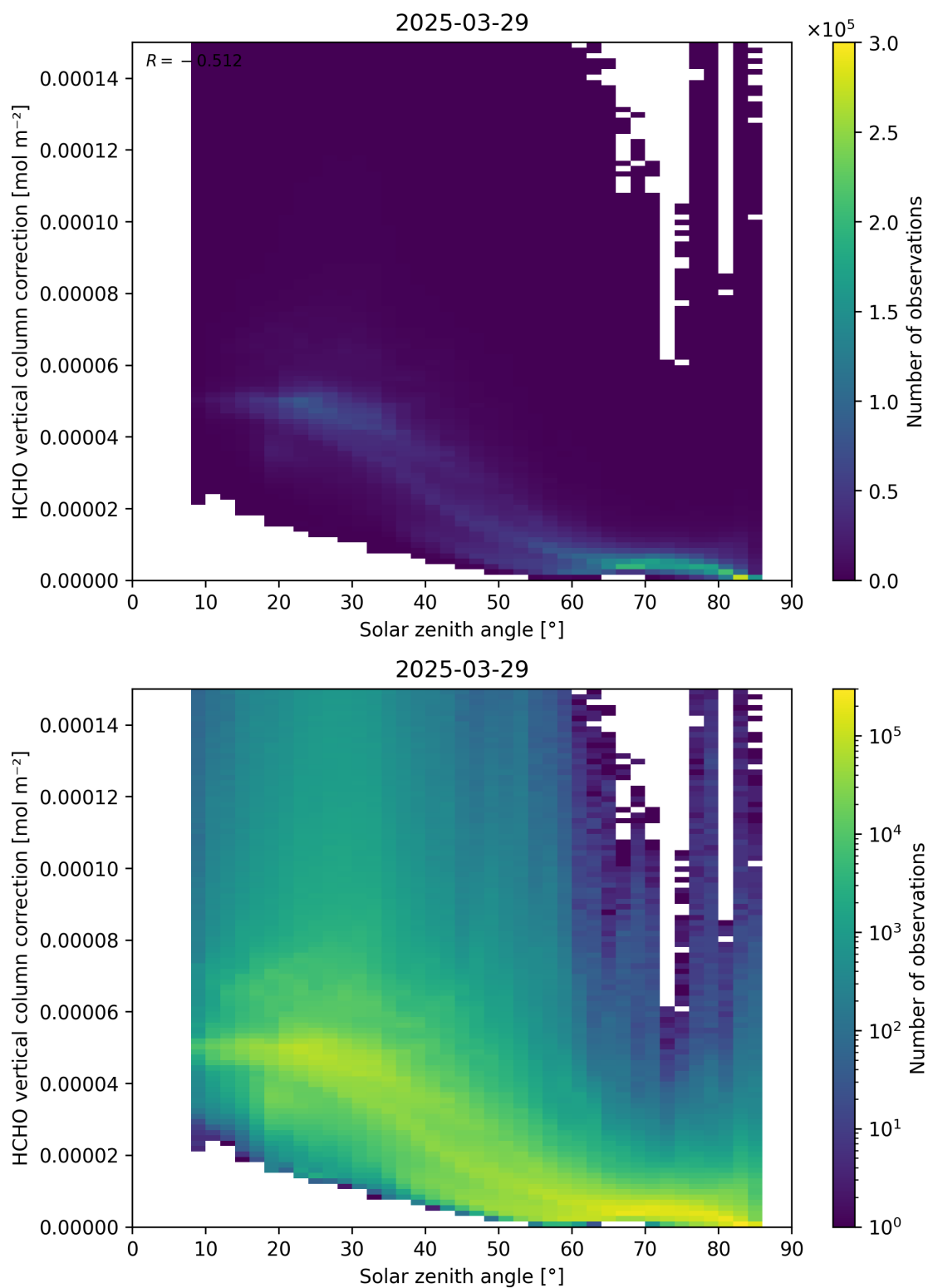
Figure 178: Scatter density plot of “Solar zenith angle” against “HCHO vertical column correction” for 2025-03-28 to 2025-03-30.
