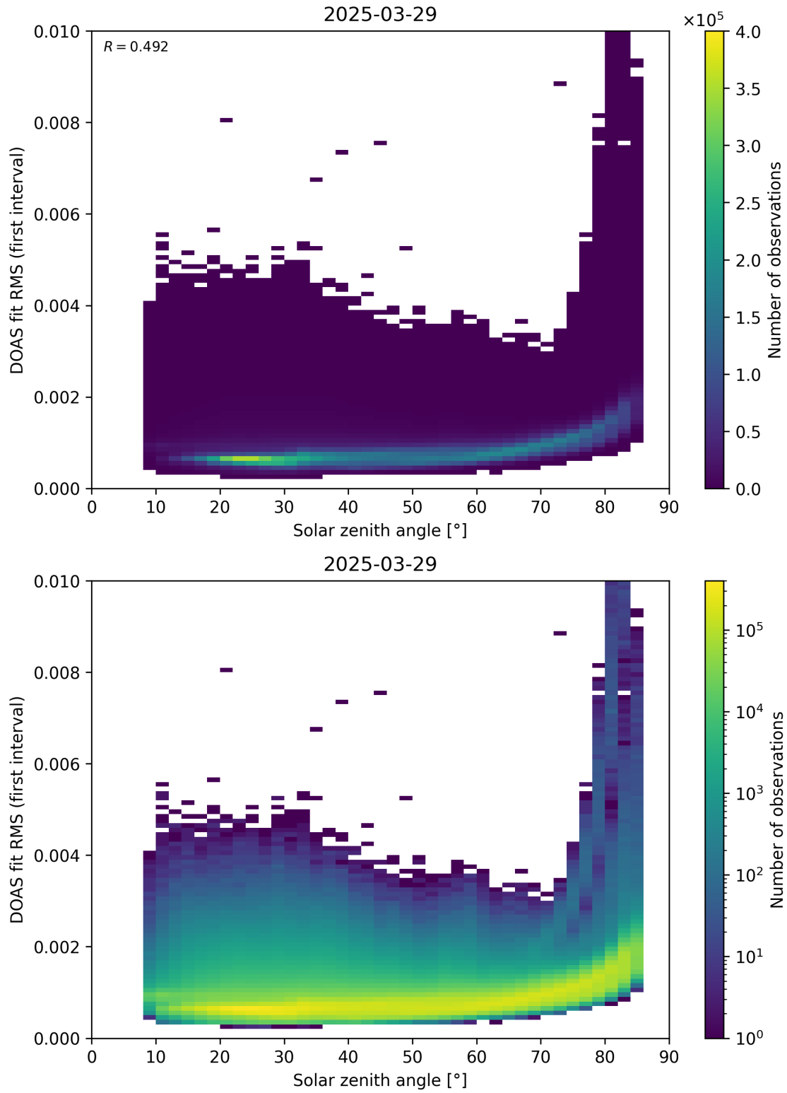
Figure 167: Scatter density plot of “Solar zenith angle” against “DOAS fit RMS (first interval)” for 2025-03-28 to 2025-03-30.
