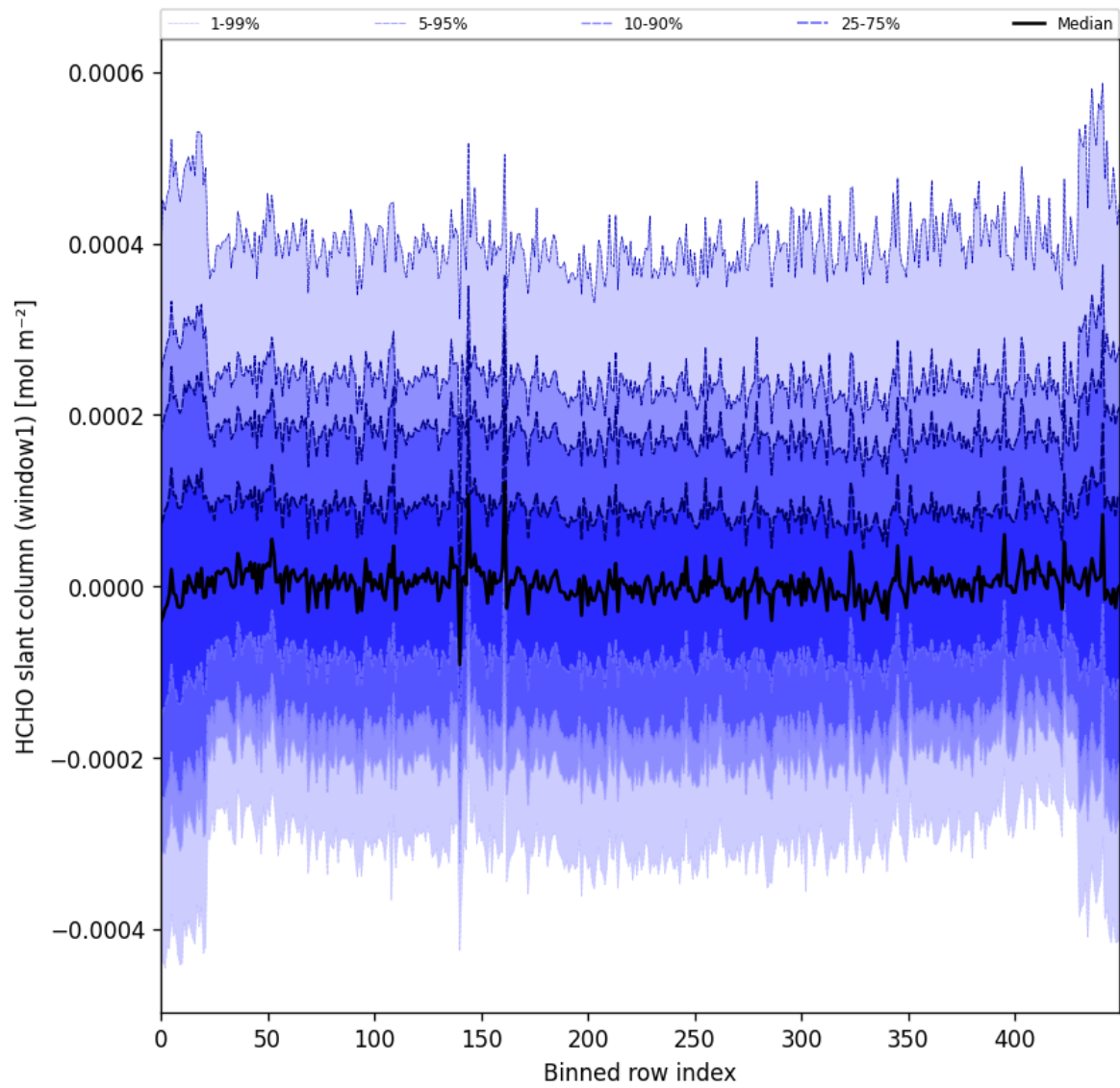
Figure 52: Along track statistics of “HCHO slant column (window1)” for 2025-03-28 to 2025-03-30
