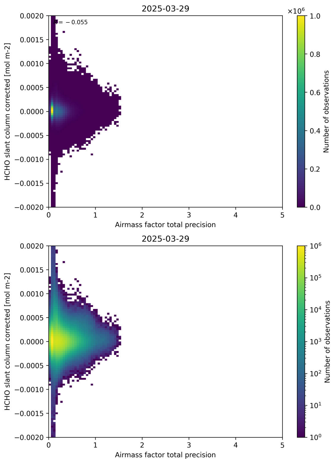
Figure 109: Scatter density plot of “Airmass factor total precision” against “HCHO slant column corrected” for 2025-03-28 to 2025-03-30.
