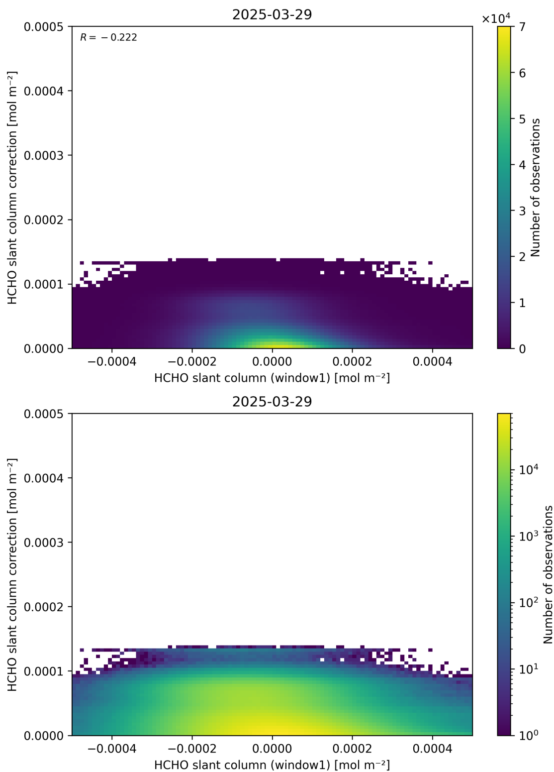
Figure 83: Scatter density plot of “HCHO slant column (window1)” against “HCHO slant column correction” for 2025-03-28 to 2025-03-30.
