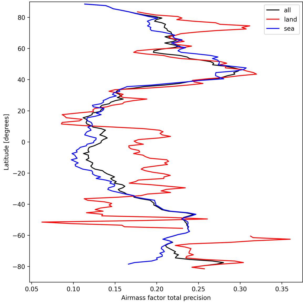
Figure 27: Zonal average of “Airmass factor total precision” for 2025-03-28 to 2025-03-30.
