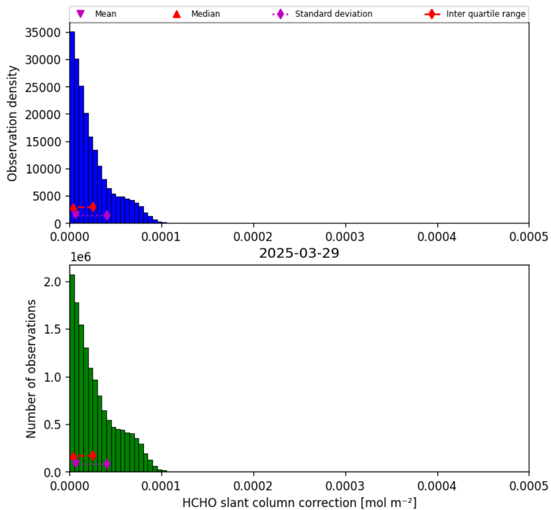
Figure 47: Histogram of “HCHO slant column correction” for 2025-03-28 to 2025-03-30
