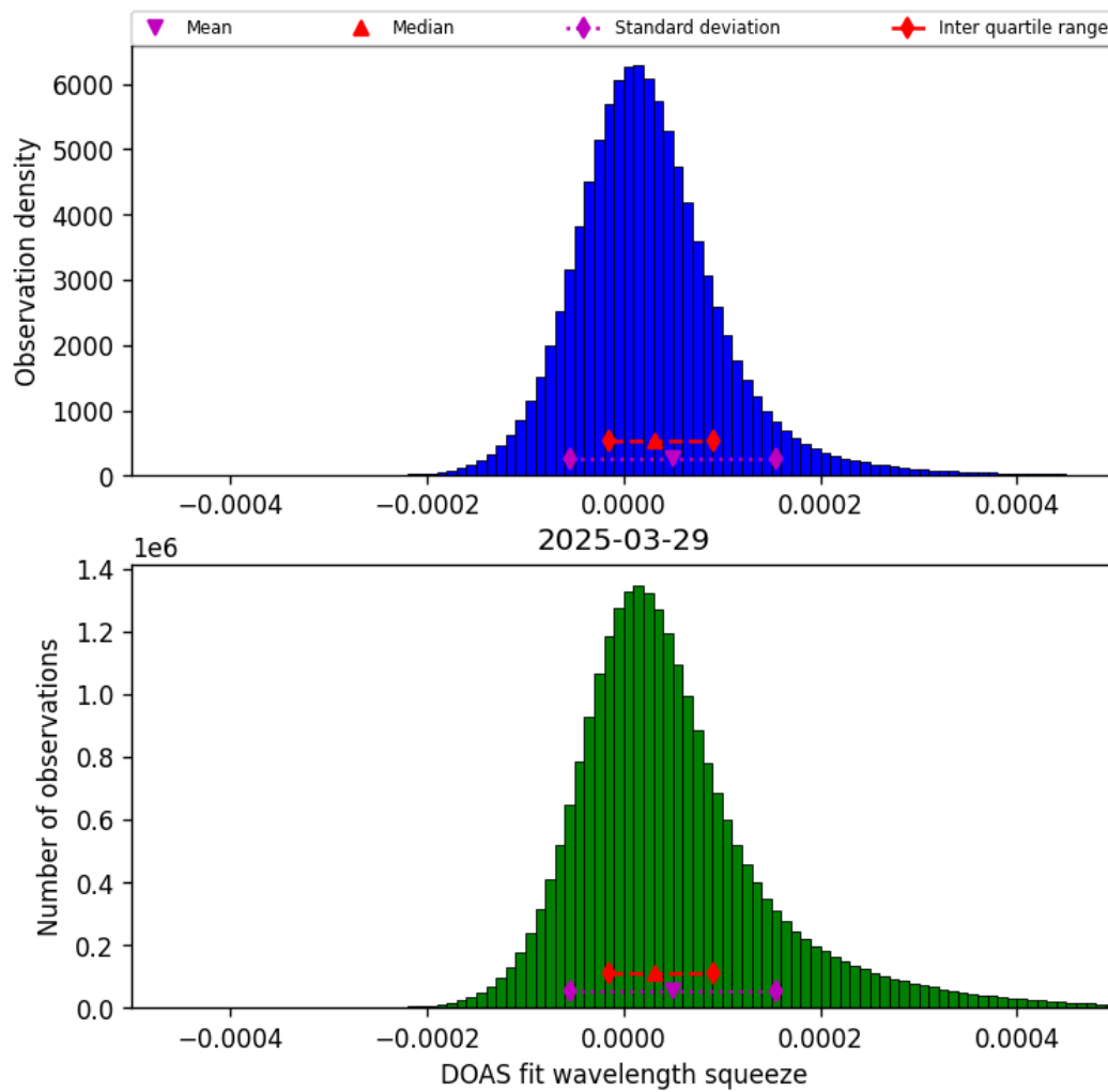
Figure 45: Histogram of “DOAS fit wavelength squeeze” for 2025-03-28 to 2025-03-30
