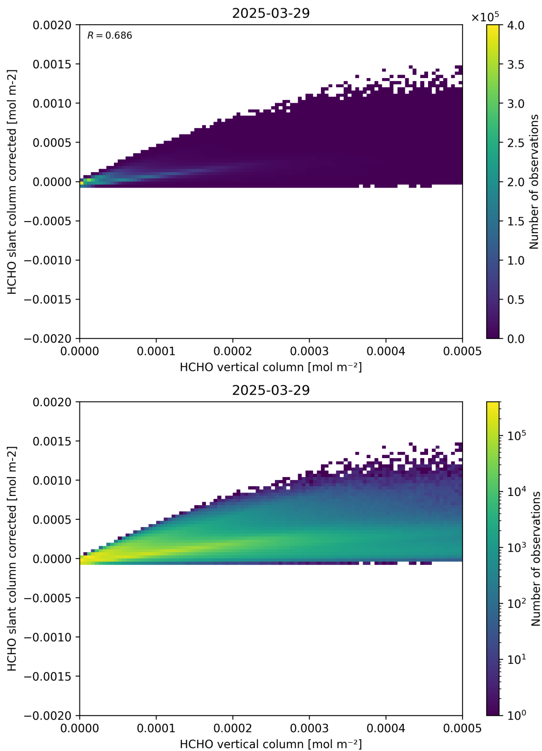
Figure 127: Scatter density plot of “HCHO vertical column” against “HCHO slant column corrected” for 2025-03-28 to 2025-03-30.
