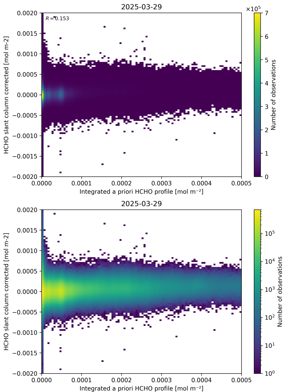
Figure 151: Scatter density plot of “Integrated a priori HCHO profile” against “HCHO slant column corrected” for 2025-03-28 to 2025-03-30.
