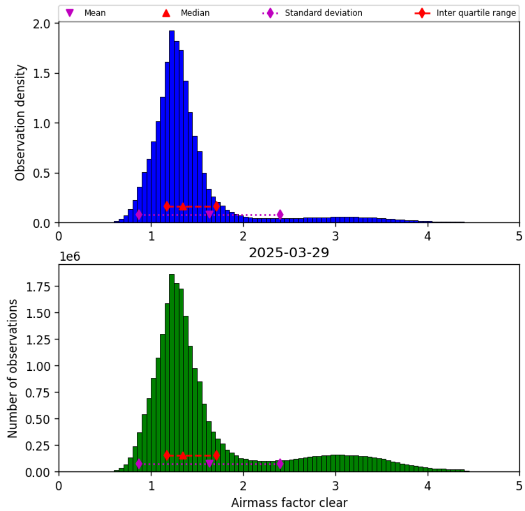
Figure 42: Histogram of “Airmass factor clear” for 2025-03-28 to 2025-03-30
