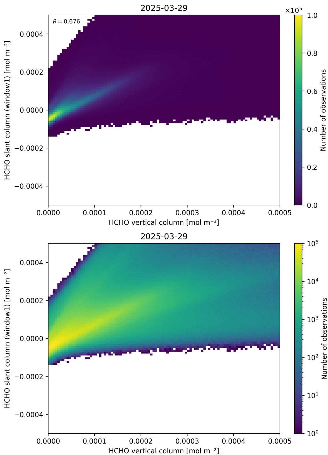
Figure 129: Scatter density plot of “HCHO vertical column” against “HCHO slant column (window1)” for 2025-03-28 to 2025-03-30.
