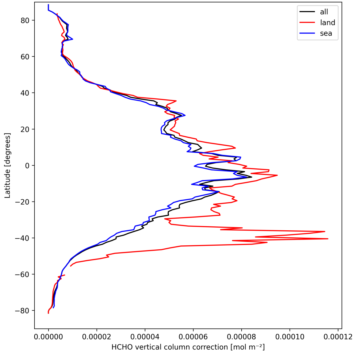
Figure 23: Zonal average of “HCHO vertical column correction” for 2025-03-28 to 2025-03-30.
