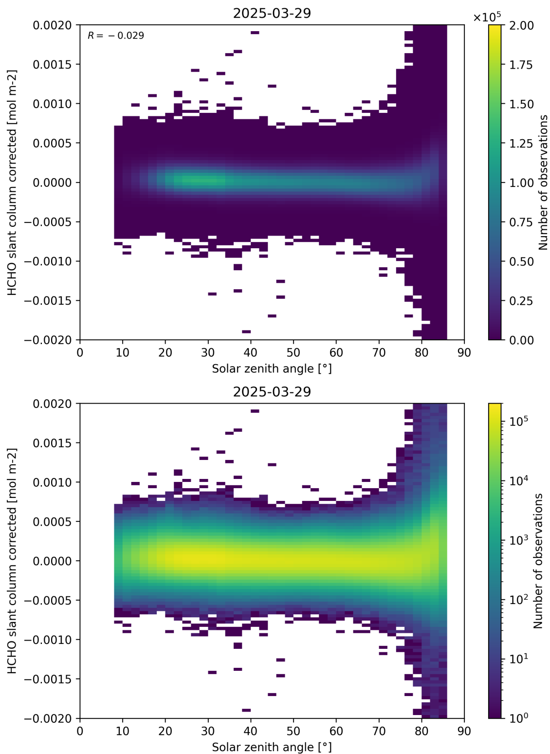
Figure 171: Scatter density plot of “Solar zenith angle” against “HCHO slant column corrected” for 2025-03-28 to 2025-03-30.
