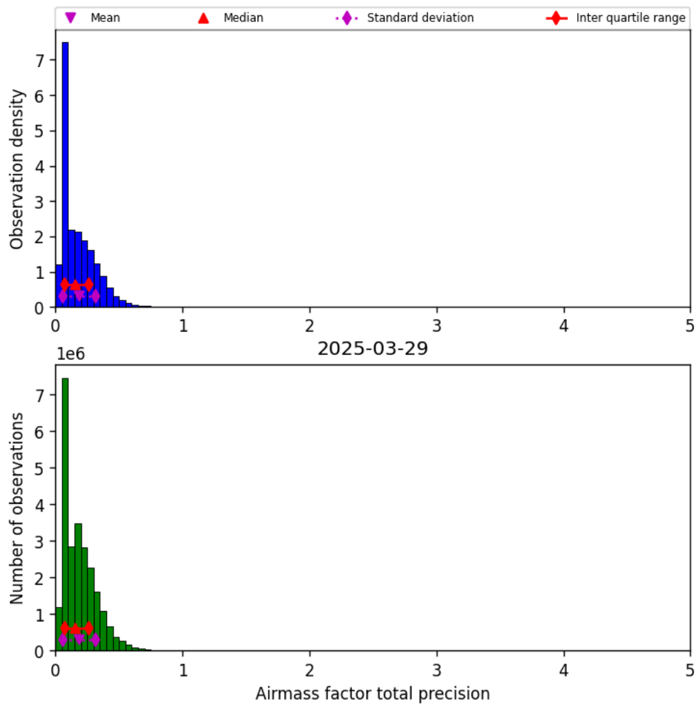
Figure 41: Histogram of “Airmass factor total precision” for 2025-03-28 to 2025-03-30
