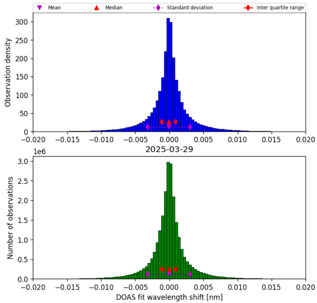
Figure 44: Histogram of “DOAS fit wavelength shift” for 2025-03-28 to 2025-03-30
