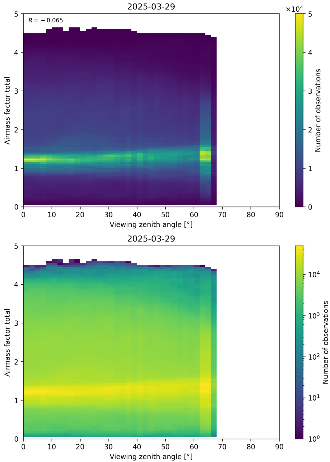
Figure 190: Scatter density plot of “Viewing zenith angle” against “Airmass factor total” for 2025-03-28 to 2025-03-30.
