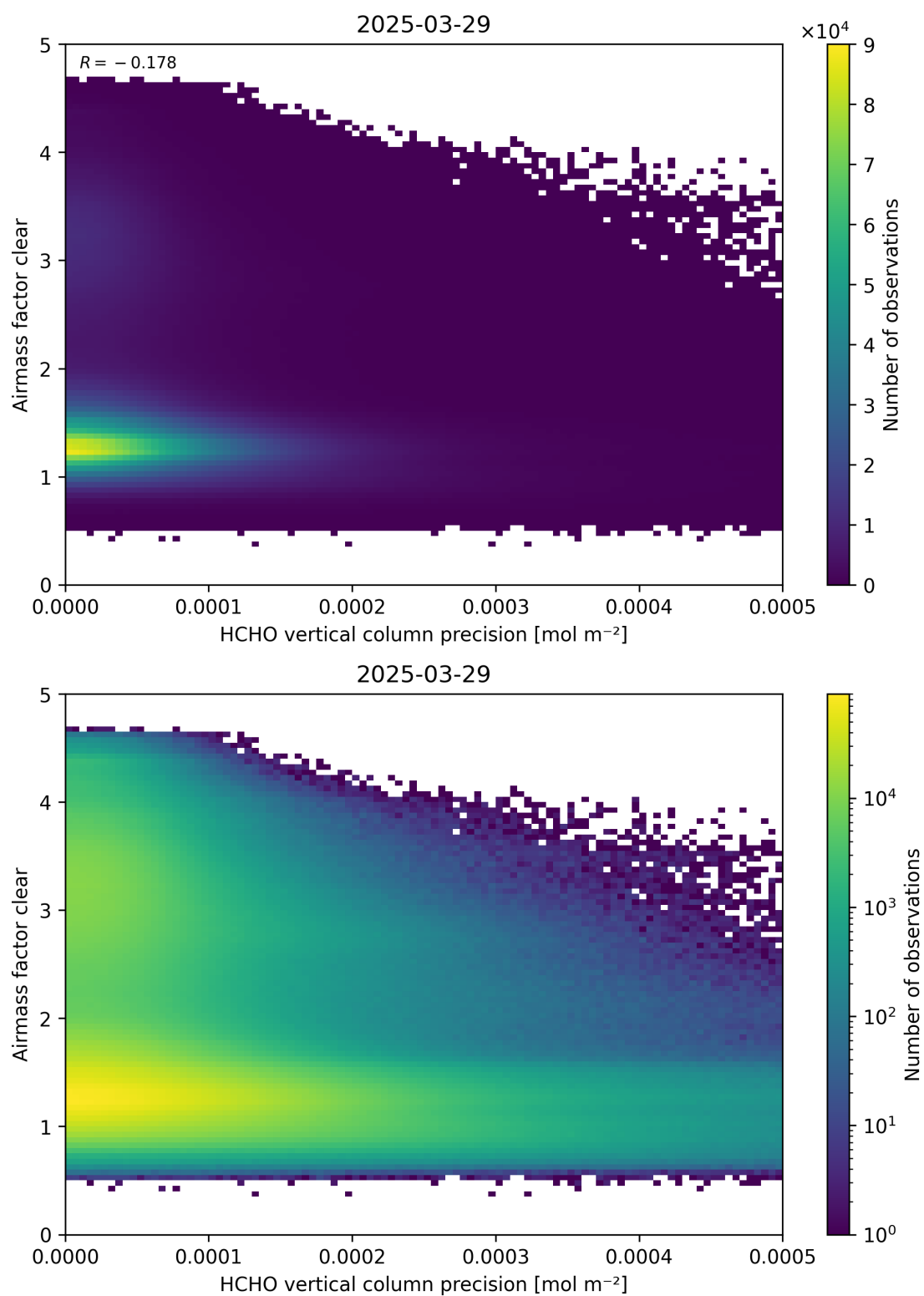
Figure 139: Scatter density plot of “HCHO vertical column precision” against “Airmass factor clear” for 2025-03-28 to 2025-03-30.
