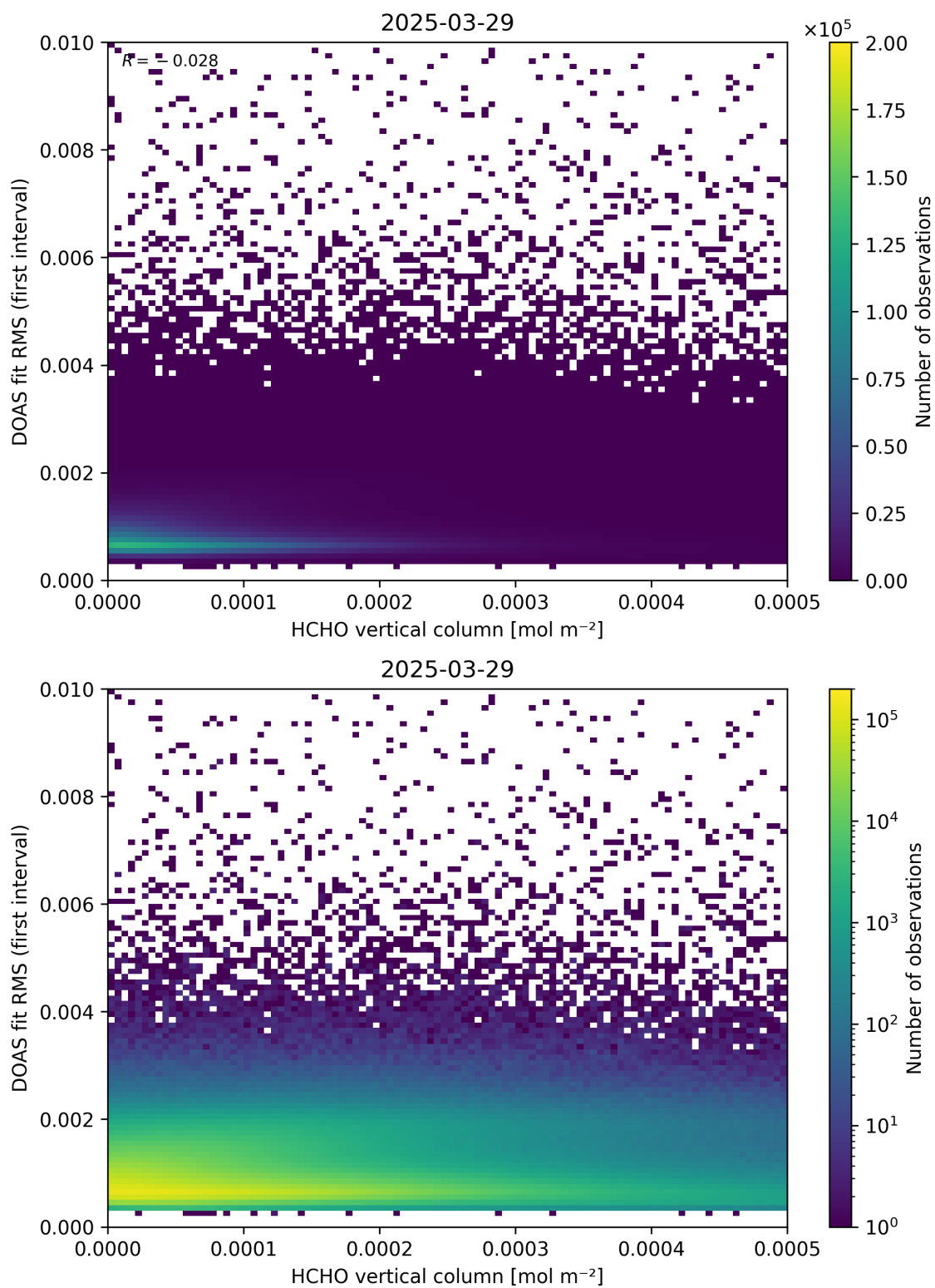
Figure 123: Scatter density plot of “HCHO vertical column” against “DOAS fit RMS (first interval)” for 2025-03-28 to 2025-03-30.
