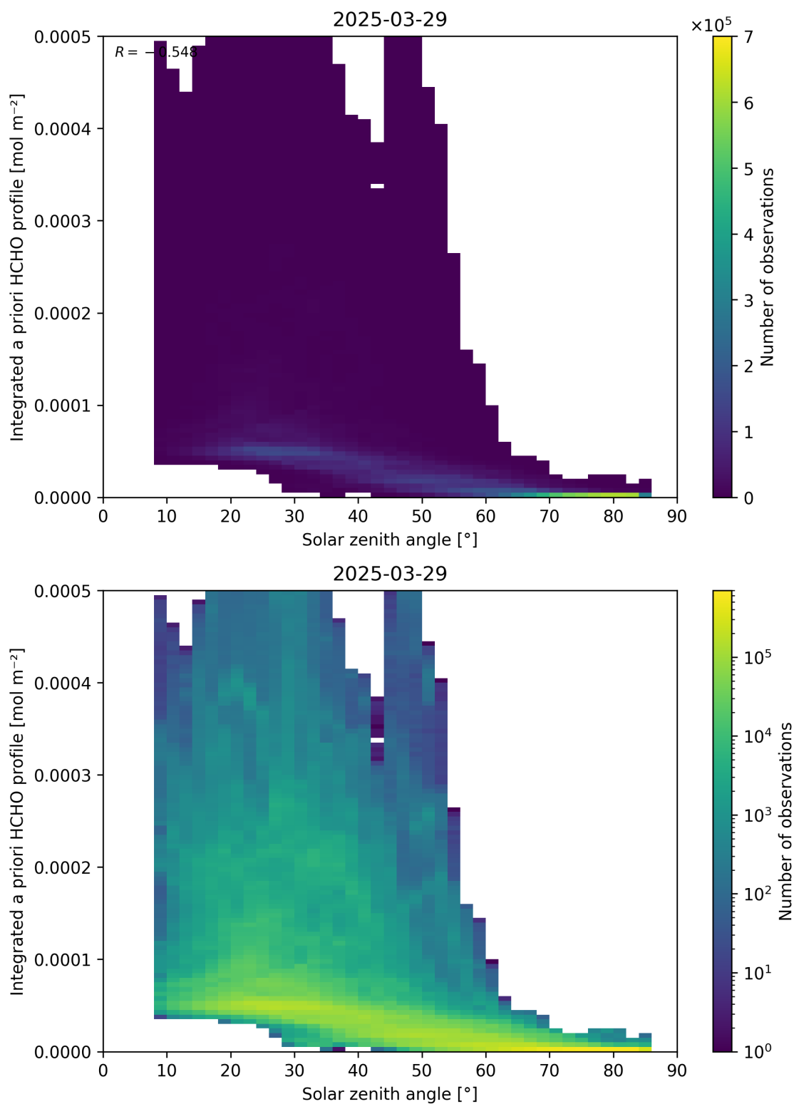
Figure 180: Scatter density plot of “Solar zenith angle” against “Integrated a priori HCHO profile” for 2025-03-28 to 2025-03-30.
