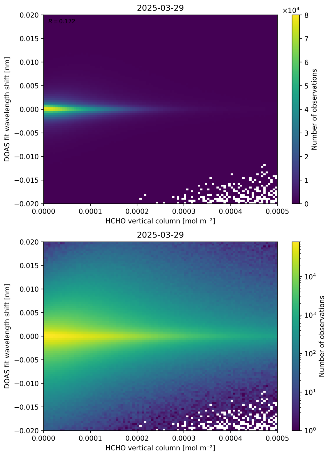
Figure 124: Scatter density plot of “HCHO vertical column” against “DOAS fit wavelength shift” for 2025-03-28 to 2025-03-30.
