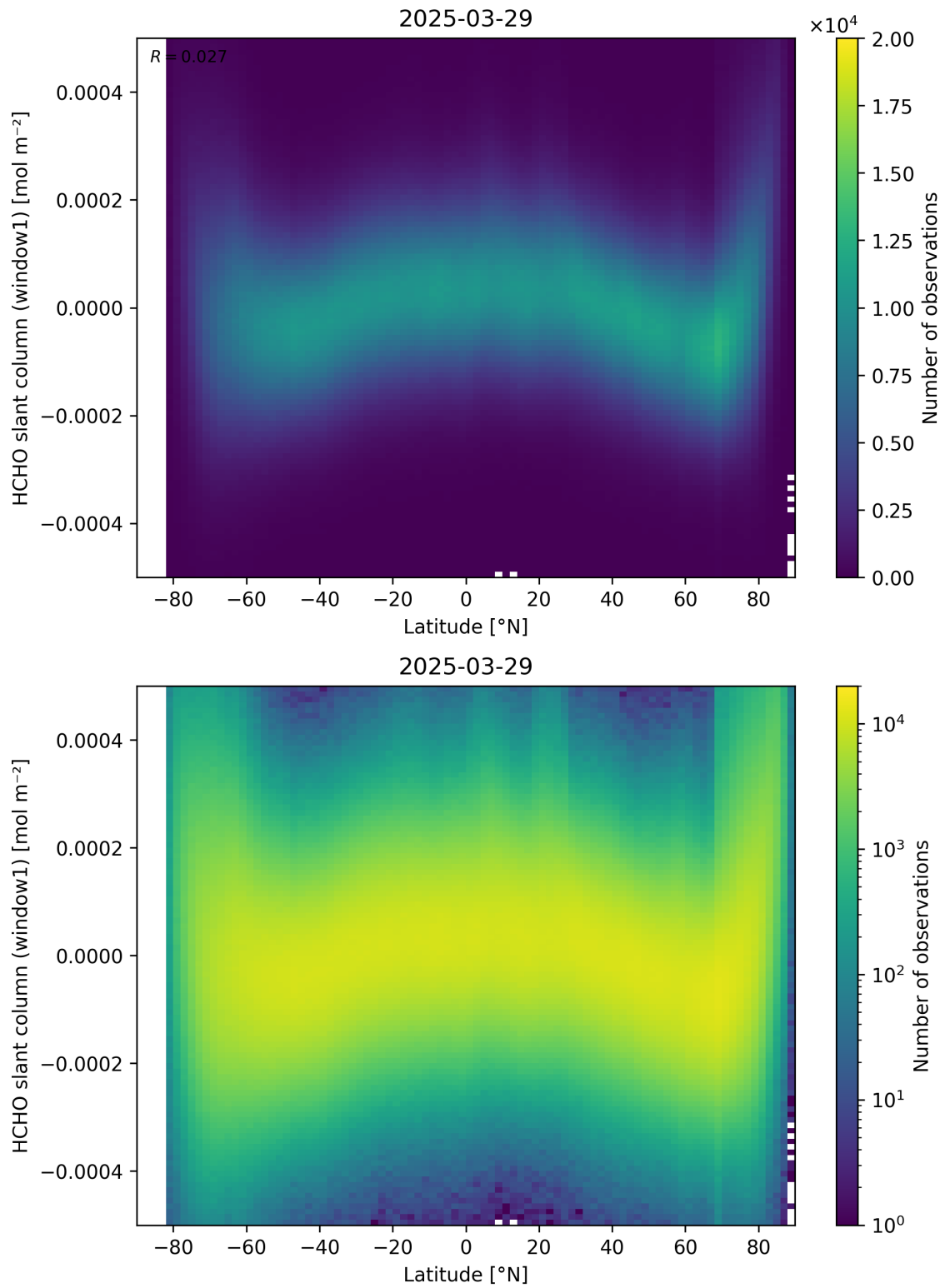
Figure 159: Scatter density plot of “Latitude” against “HCHO slant column (window1)” for 2025-03-28 to 2025-03-30.
