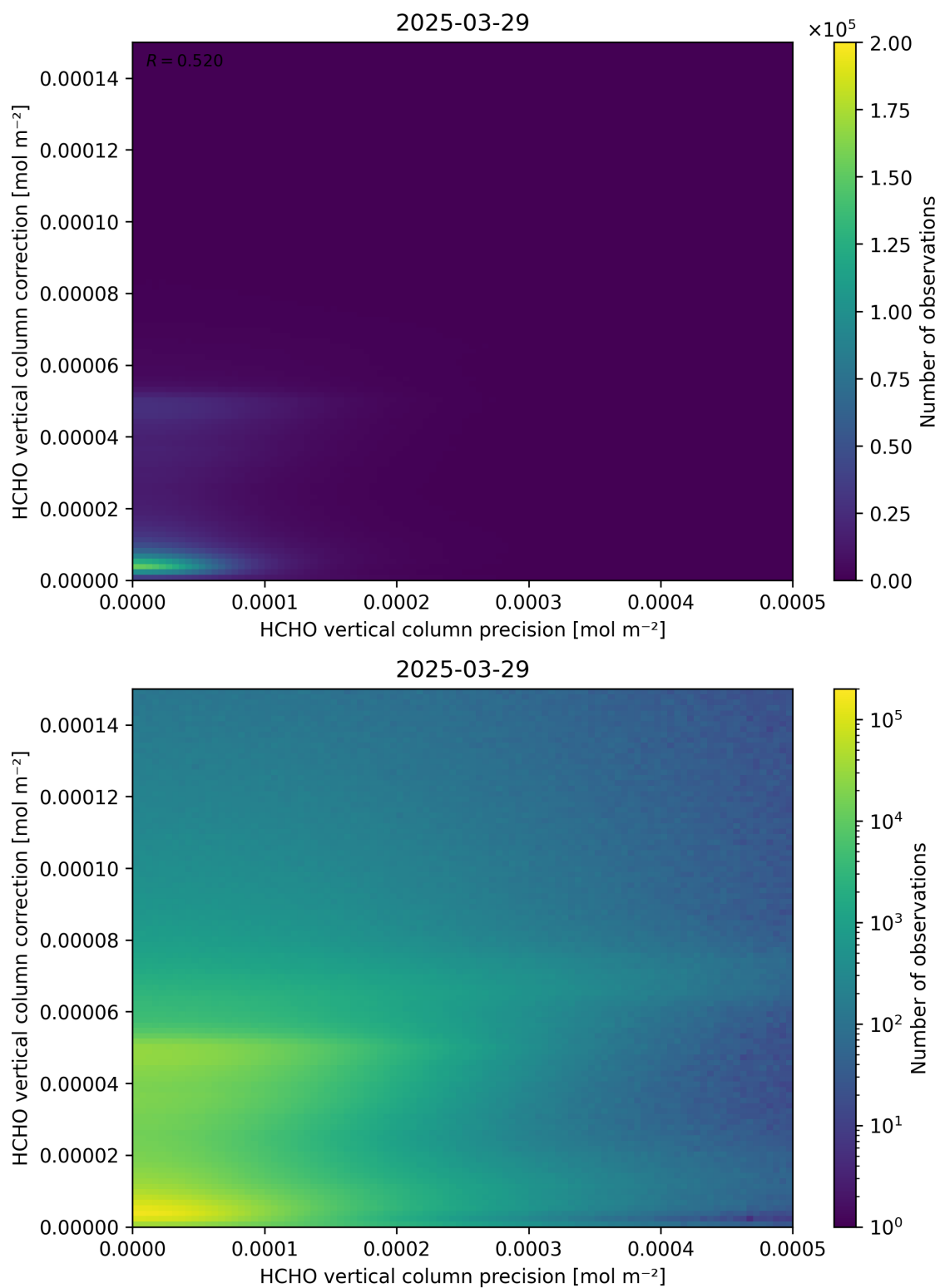
Figure 146: Scatter density plot of “HCHO vertical column precision” against “HCHO vertical column correction” for 2025-03-28 to 2025-03-30.
