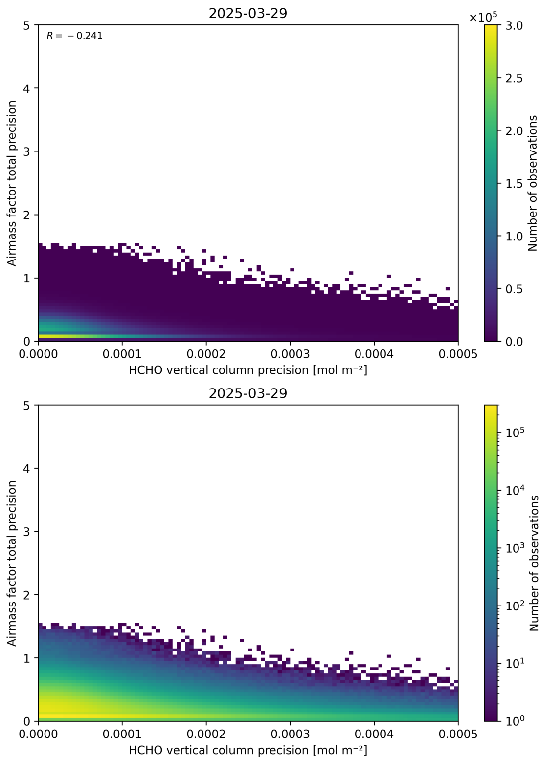
Figure 145: Scatter density plot of “HCHO vertical column precision” against “Airmass factor total precision” for 2025-03-28 to 2025-03-30.
