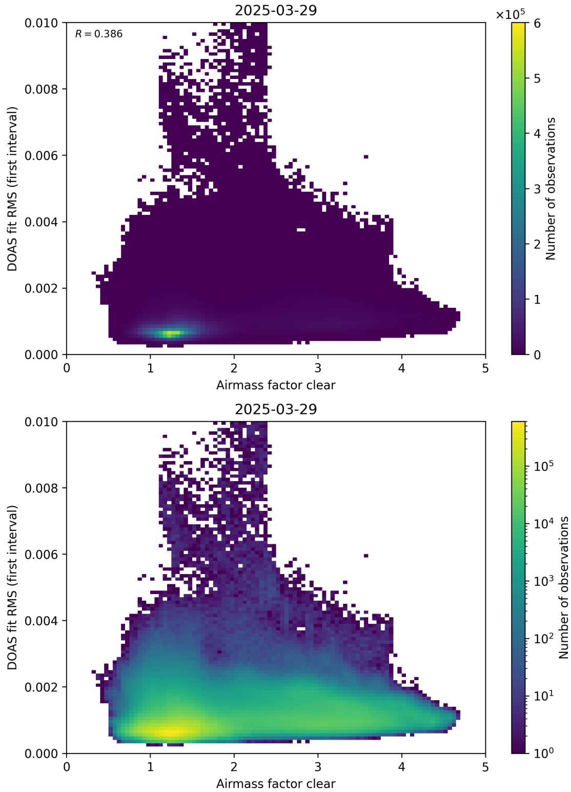
Figure 71: Scatter density plot of “Airmass factor clear” against “DOAS fit RMS (first interval)” for 2025-03-28 to 2025-03-30.
