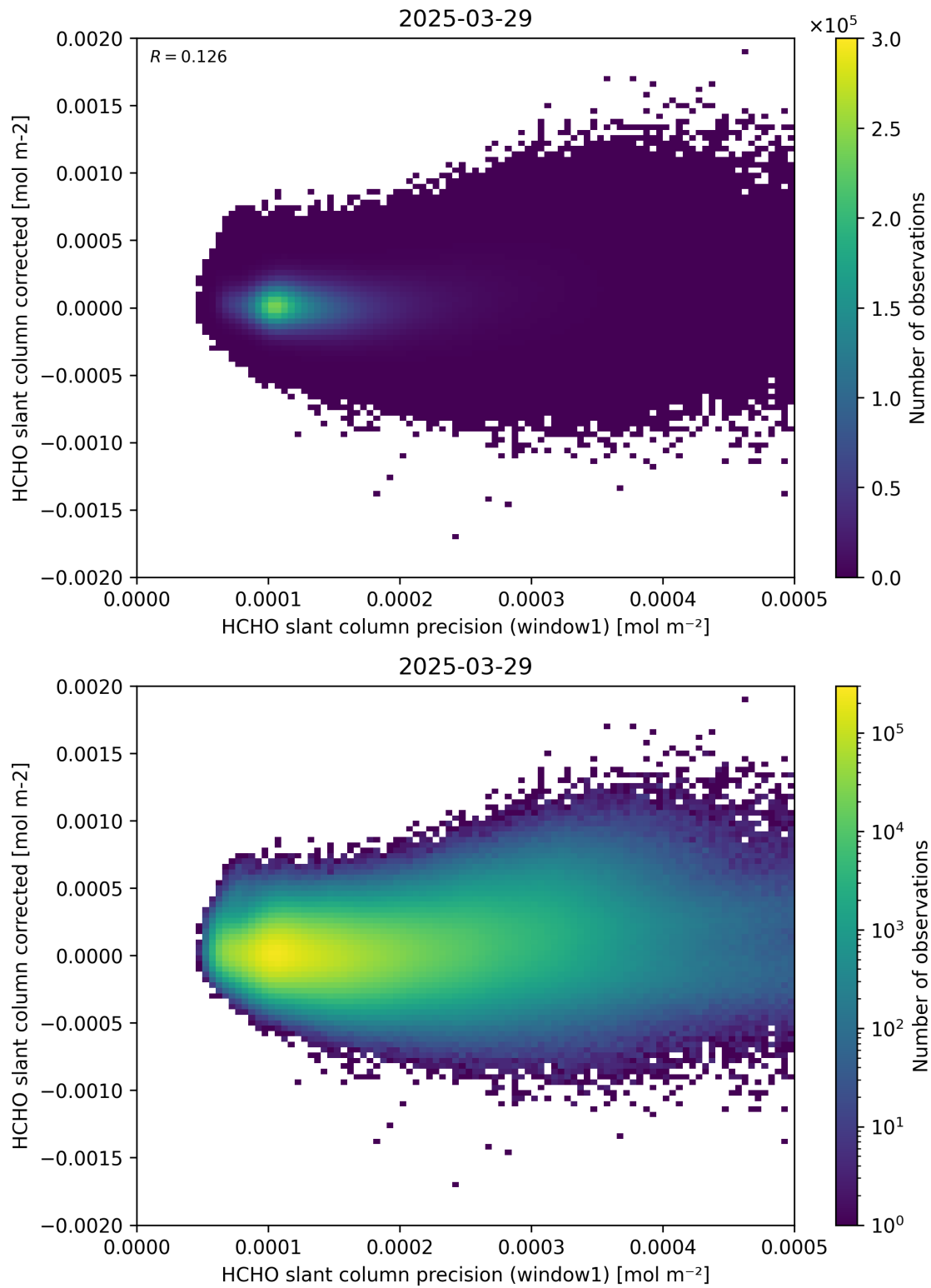
Figure 92: Scatter density plot of “HCHO slant column precision (window1)” against “HCHO slant column corrected” for 2025-03-28 to 2025-03-30.
