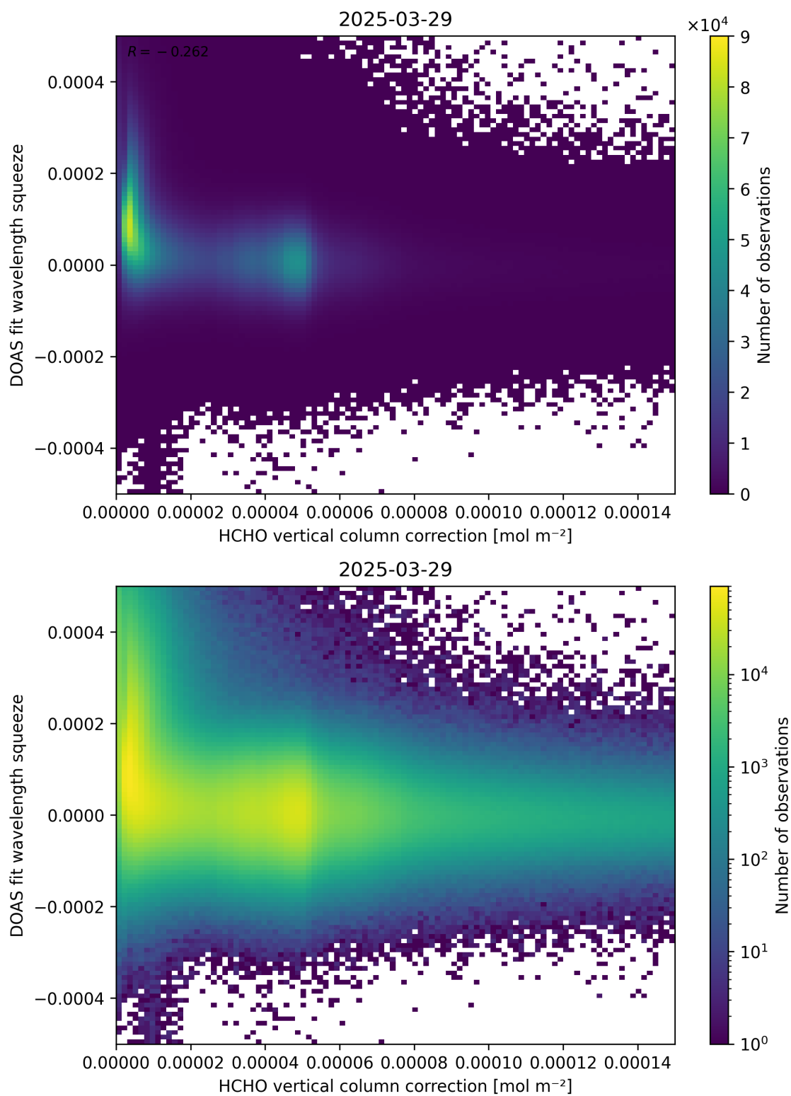
Figure 114: Scatter density plot of “HCHO vertical column correction” against “DOAS fit wavelength squeeze” for 2025-03-28 to 2025-03-30.
