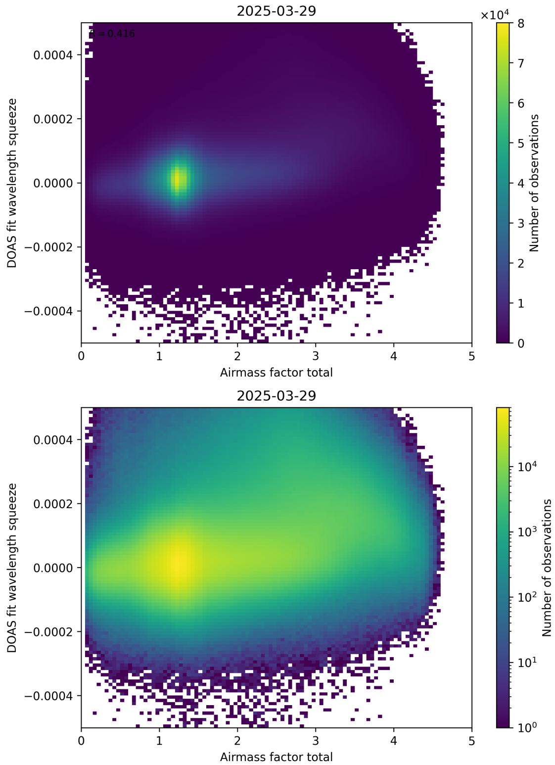
Figure 99: Scatter density plot of “Airmass factor total” against “DOAS fit wavelength squeeze” for 2025-03-28 to 2025-03-30.
