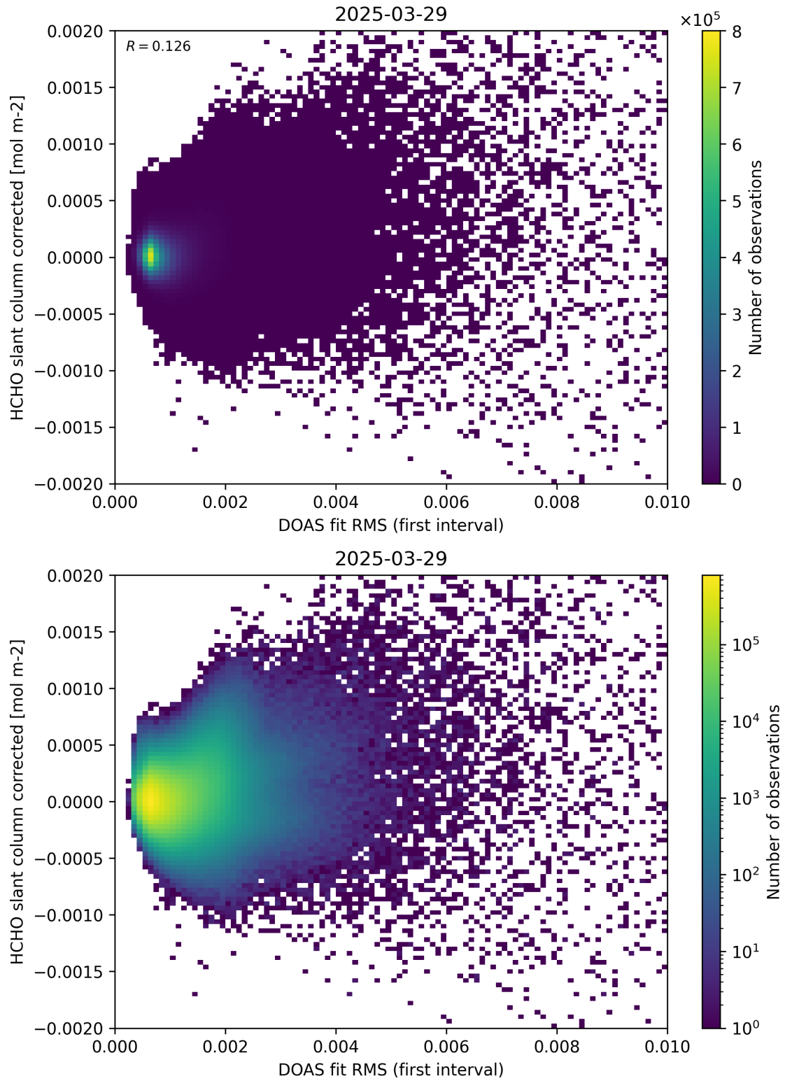
Figure 62: Scatter density plot of “DOAS fit RMS (first interval)” against “HCHO slant column corrected” for 2025-03-28 to 2025-03-30.
