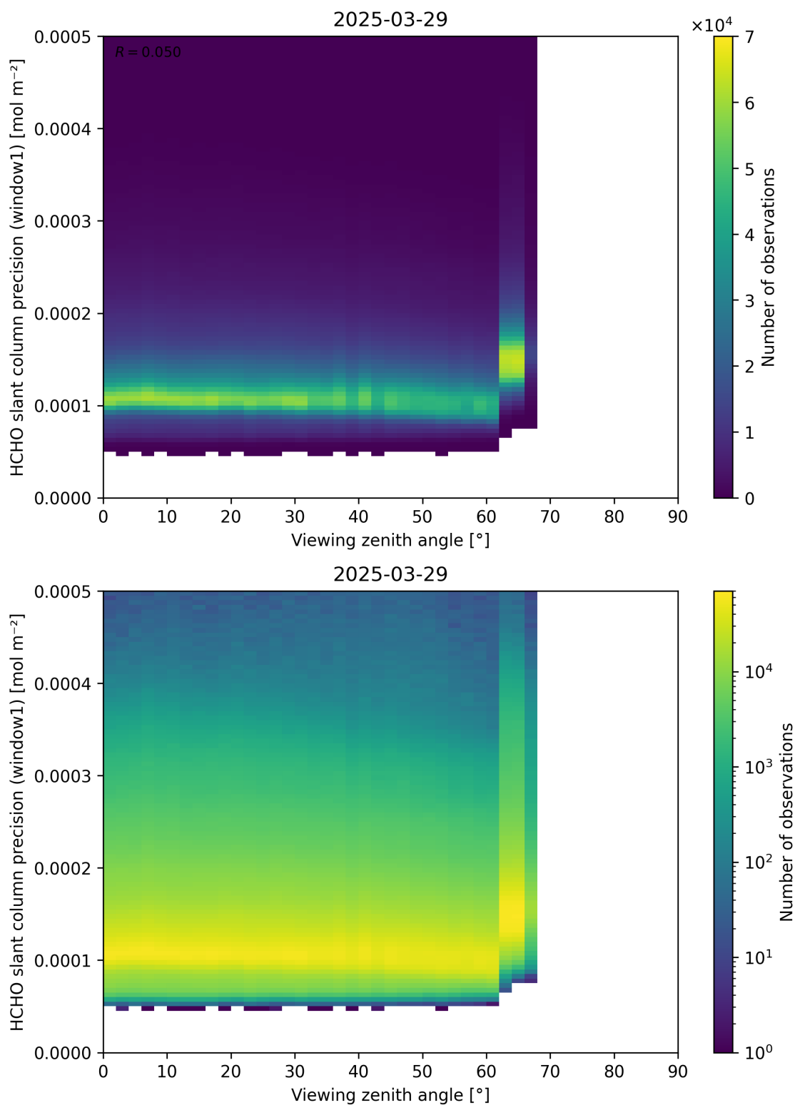
Figure 189: Scatter density plot of “Viewing zenith angle” against “HCHO slant column precision (window1)” for 2025-03-28 to 2025-03-30.
