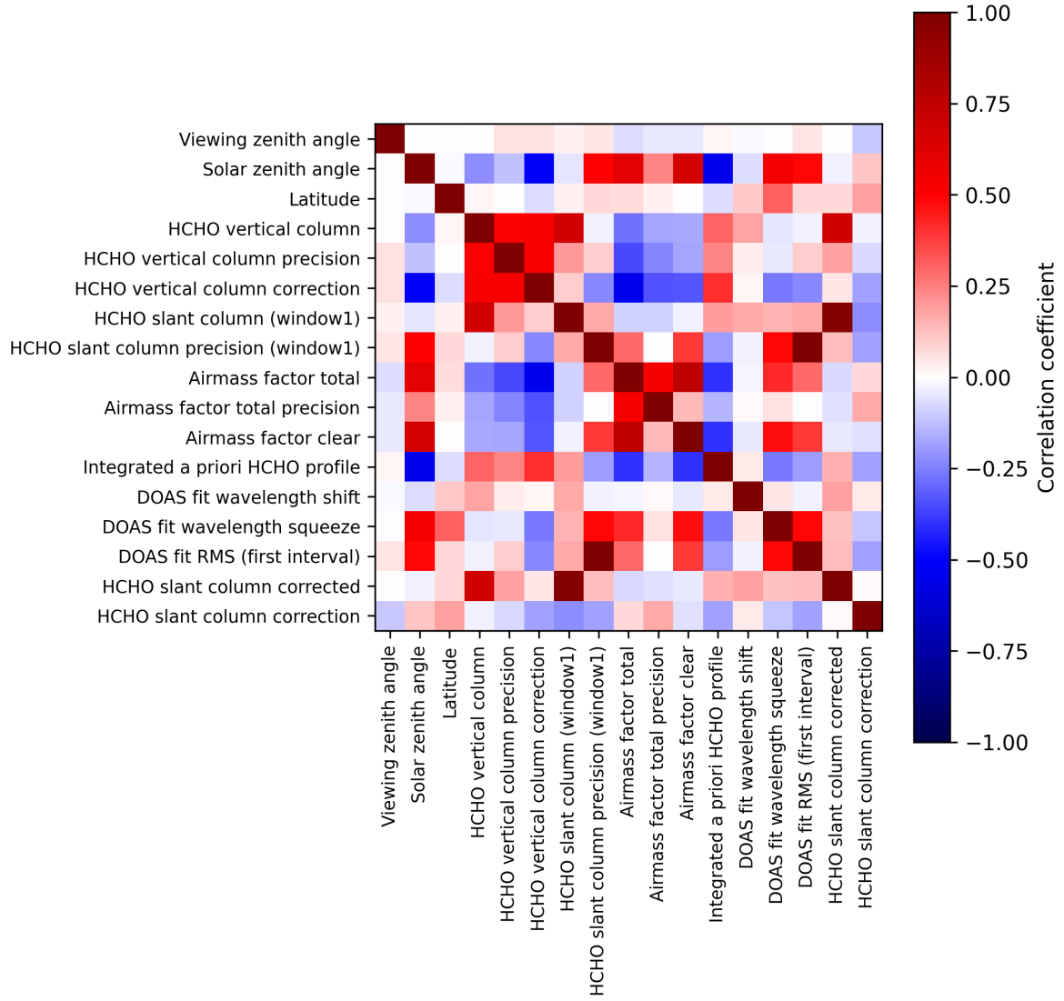
Figure 2: Map of correlation matrix for 2025-03-28 to 2025-03-30.
