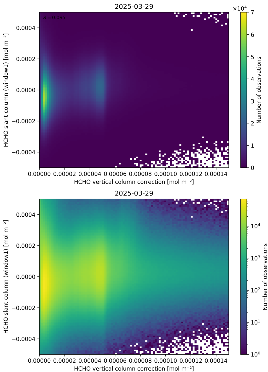
Figure 118: Scatter density plot of “HCHO vertical column correction” against “HCHO slant column (window1)” for 2025-03-28 to 2025-03-30.
