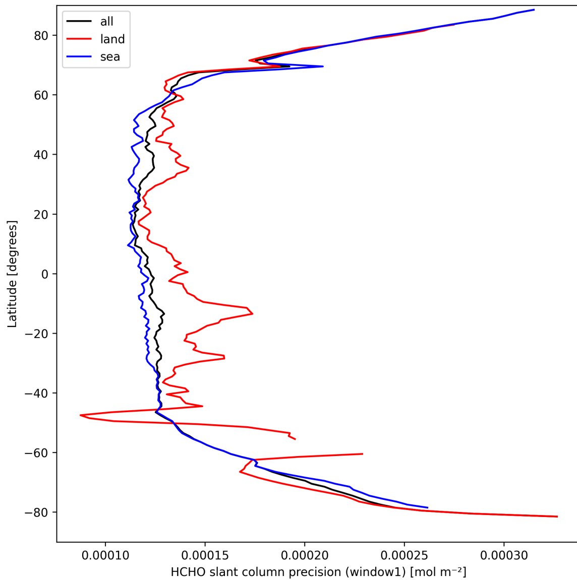
Figure 25: Zonal average of “HCHO slant column precision (window1)” for 2025-03-28 to 2025-03-30.
