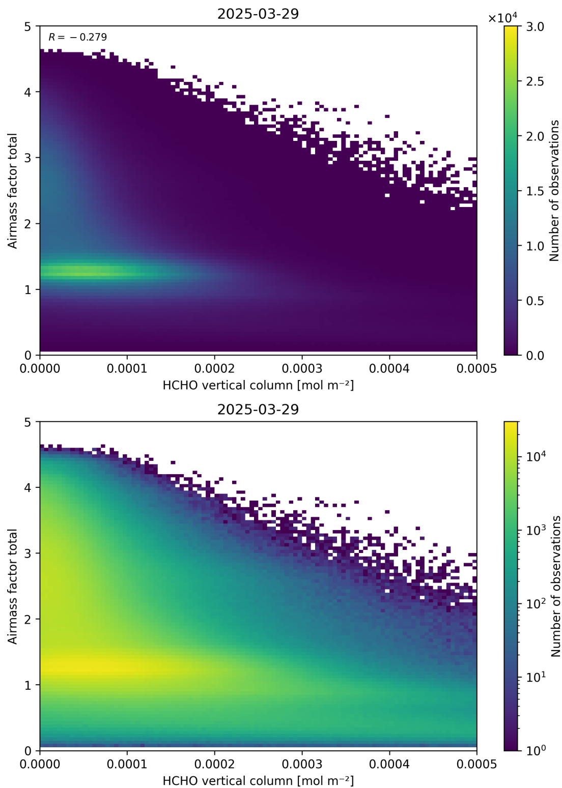
Figure 131: Scatter density plot of “HCHO vertical column” against “Airmass factor total” for 2025-03-28 to 2025-03-30.
