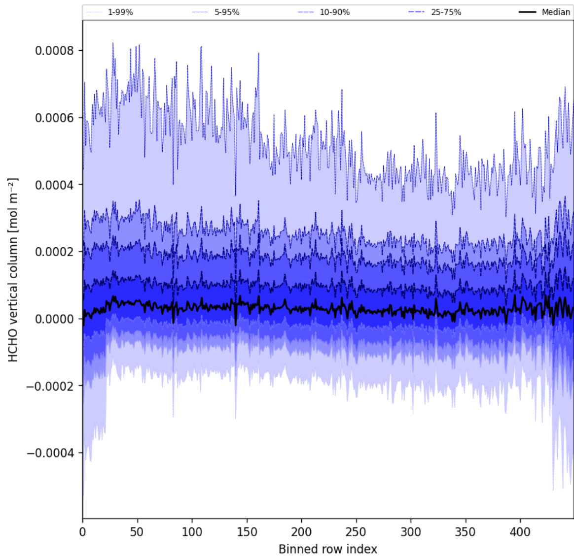
Figure 49: Along track statistics of “HCHO vertical column” for 2025-03-28 to 2025-03-30
