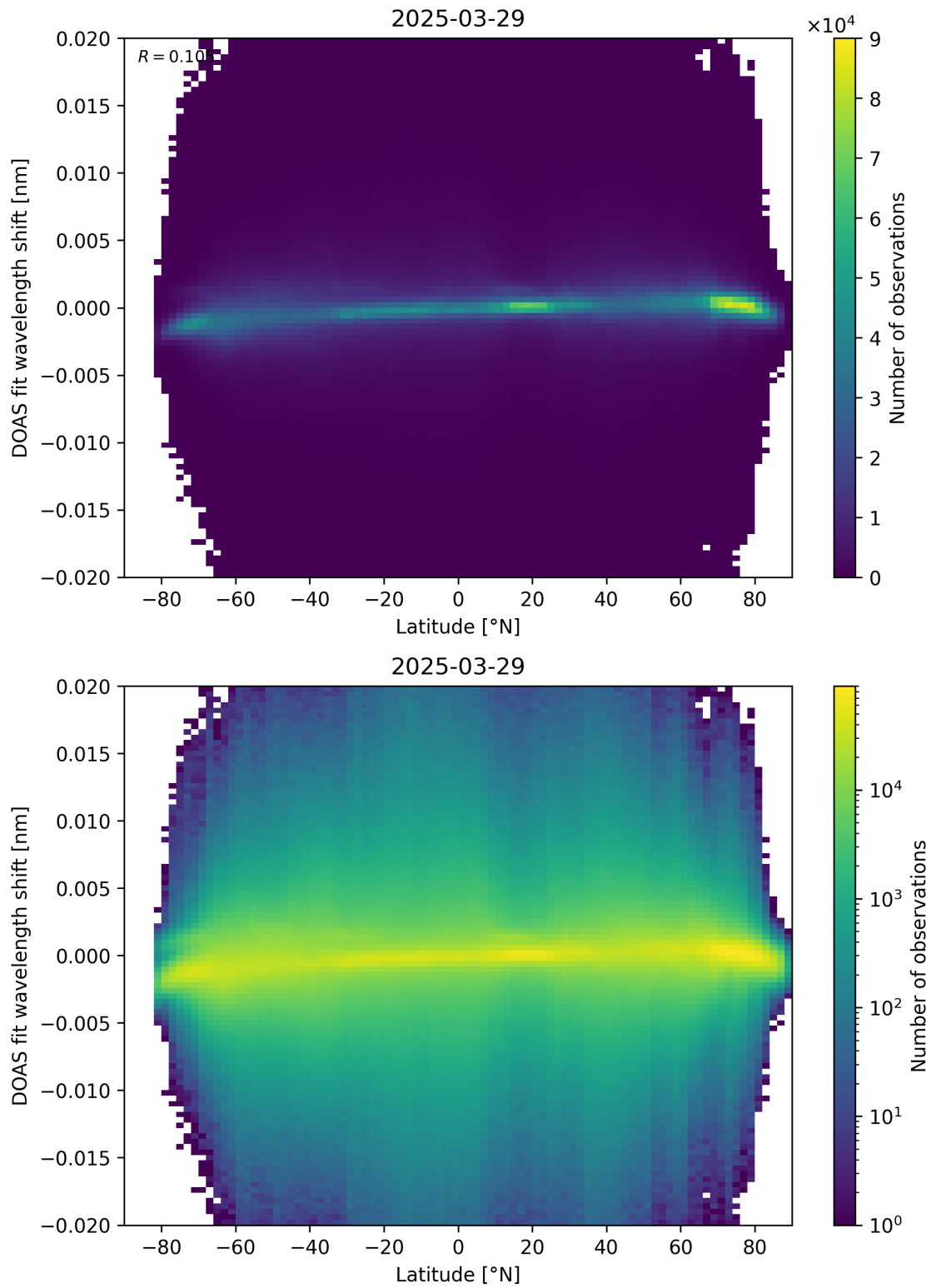
Figure 154: Scatter density plot of “Latitude” against “DOAS fit wavelength shift” for 2025-03-28 to 2025-03-30.
