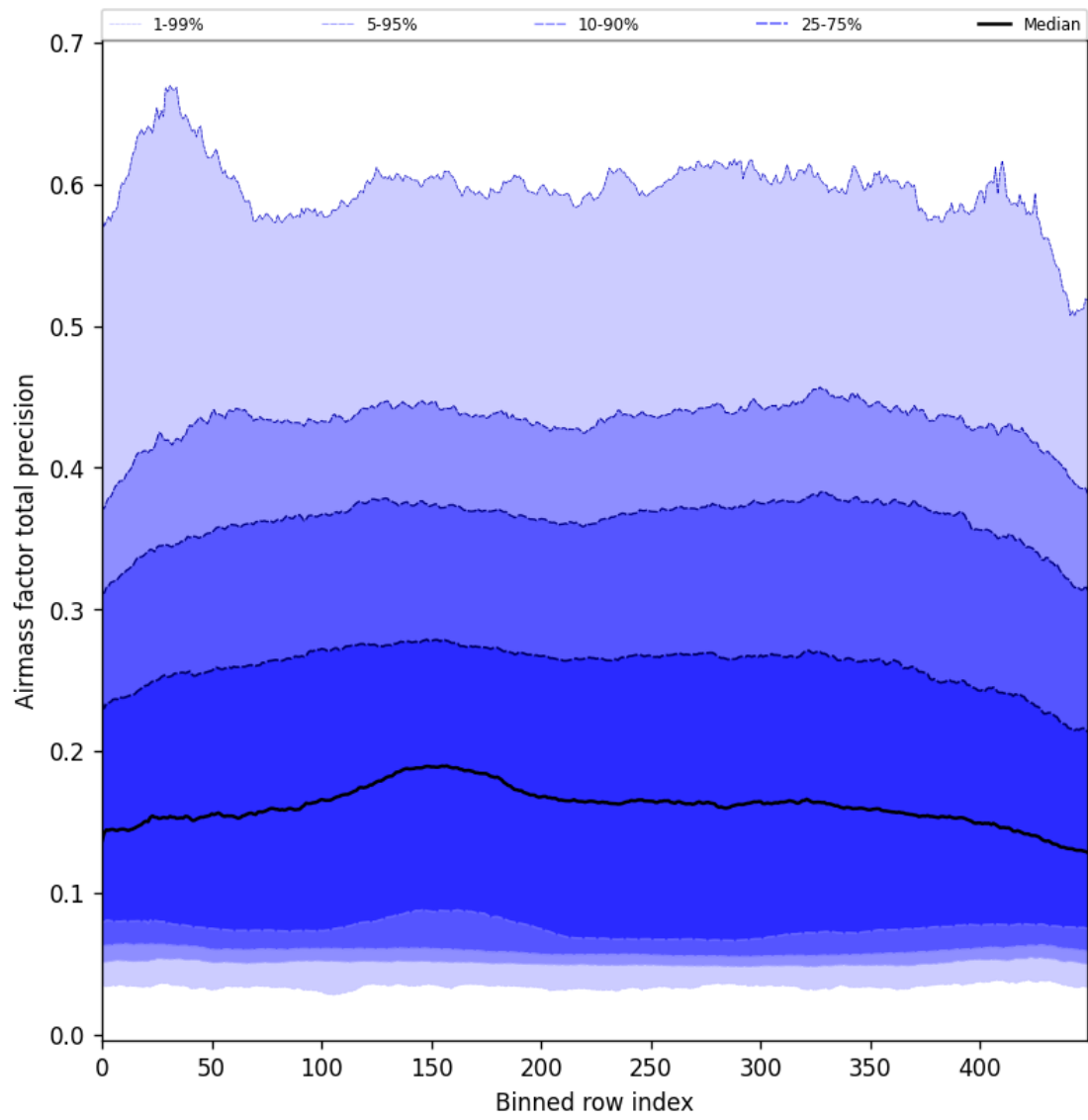
Figure 55: Along track statistics of “Airmass factor total precision” for 2025-03-28 to 2025-03-30
