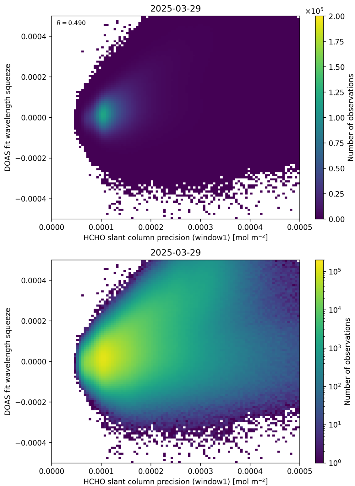
Figure 90: Scatter density plot of “HCHO slant column precision (window1)” against “DOAS fit wavelength squeeze” for 2025-03-28 to 2025-03-30.
