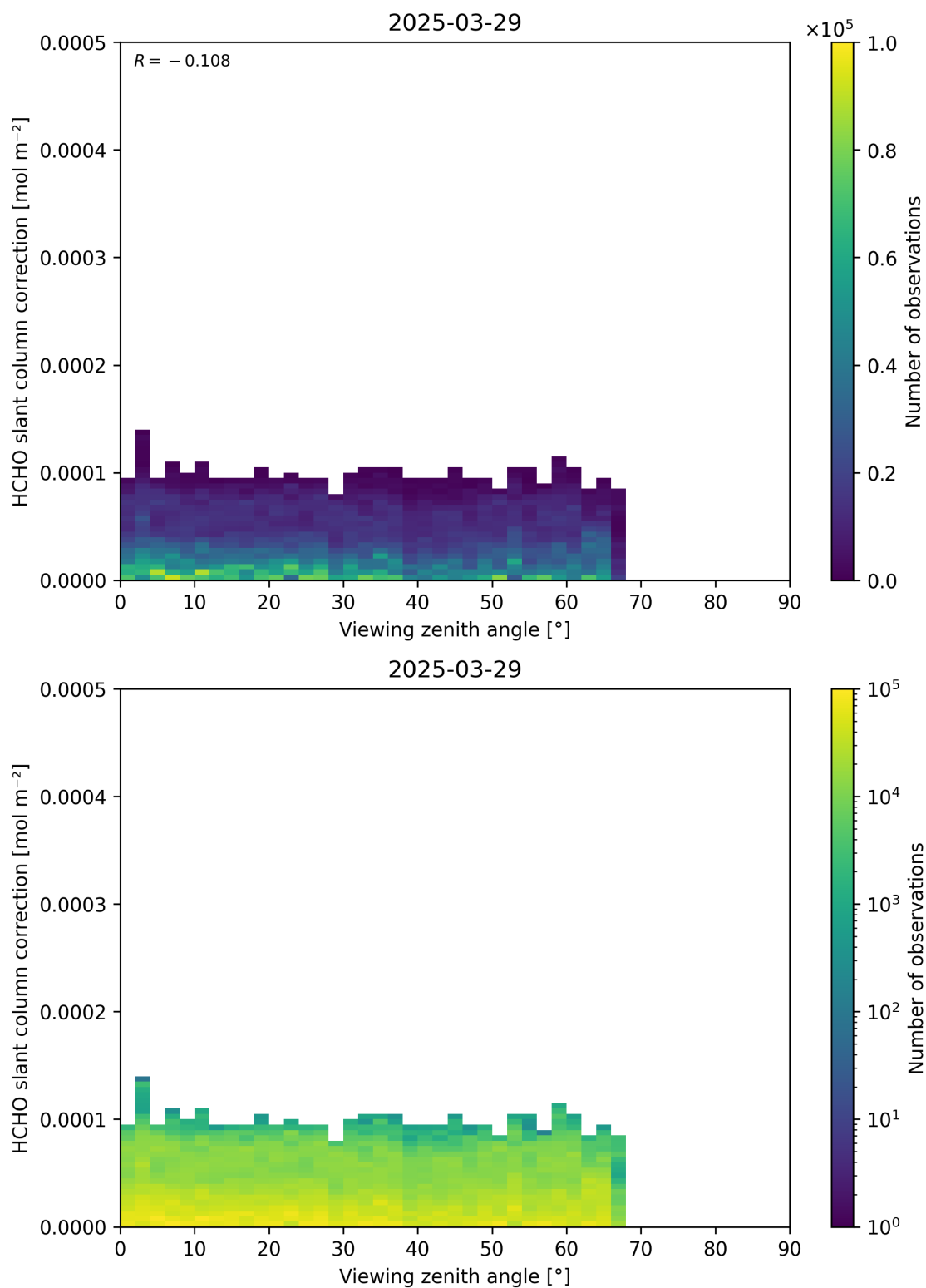
Figure 187: Scatter density plot of “Viewing zenith angle” against “HCHO slant column correction” for 2025-03-28 to 2025-03-30.
