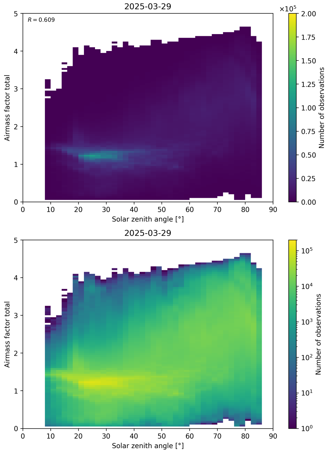
Figure 175: Scatter density plot of “Solar zenith angle” against “Airmass factor total” for 2025-03-28 to 2025-03-30.
