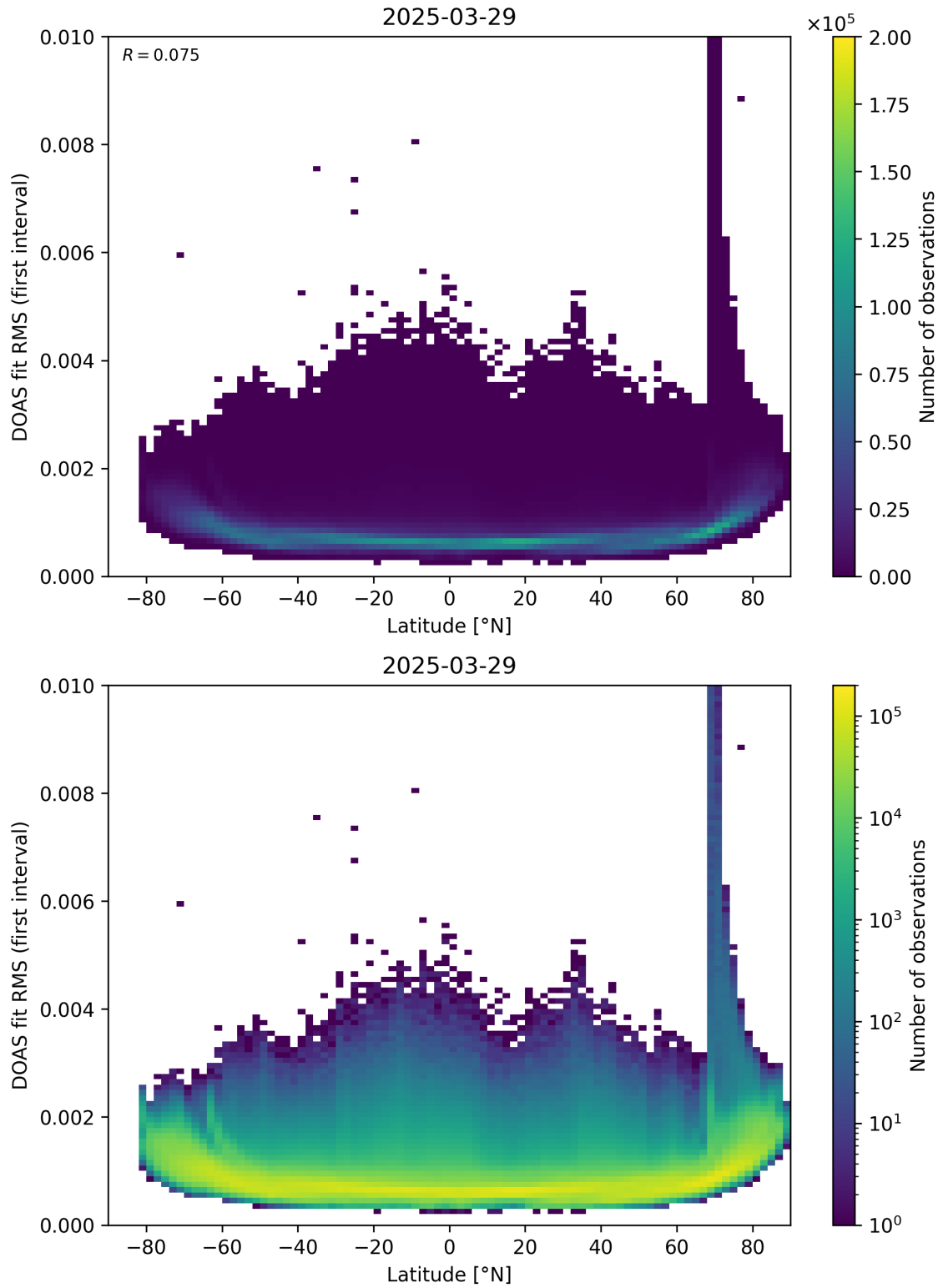
Figure 153: Scatter density plot of “Latitude” against “DOAS fit RMS (first interval)” for 2025-03-28 to 2025-03-30.
