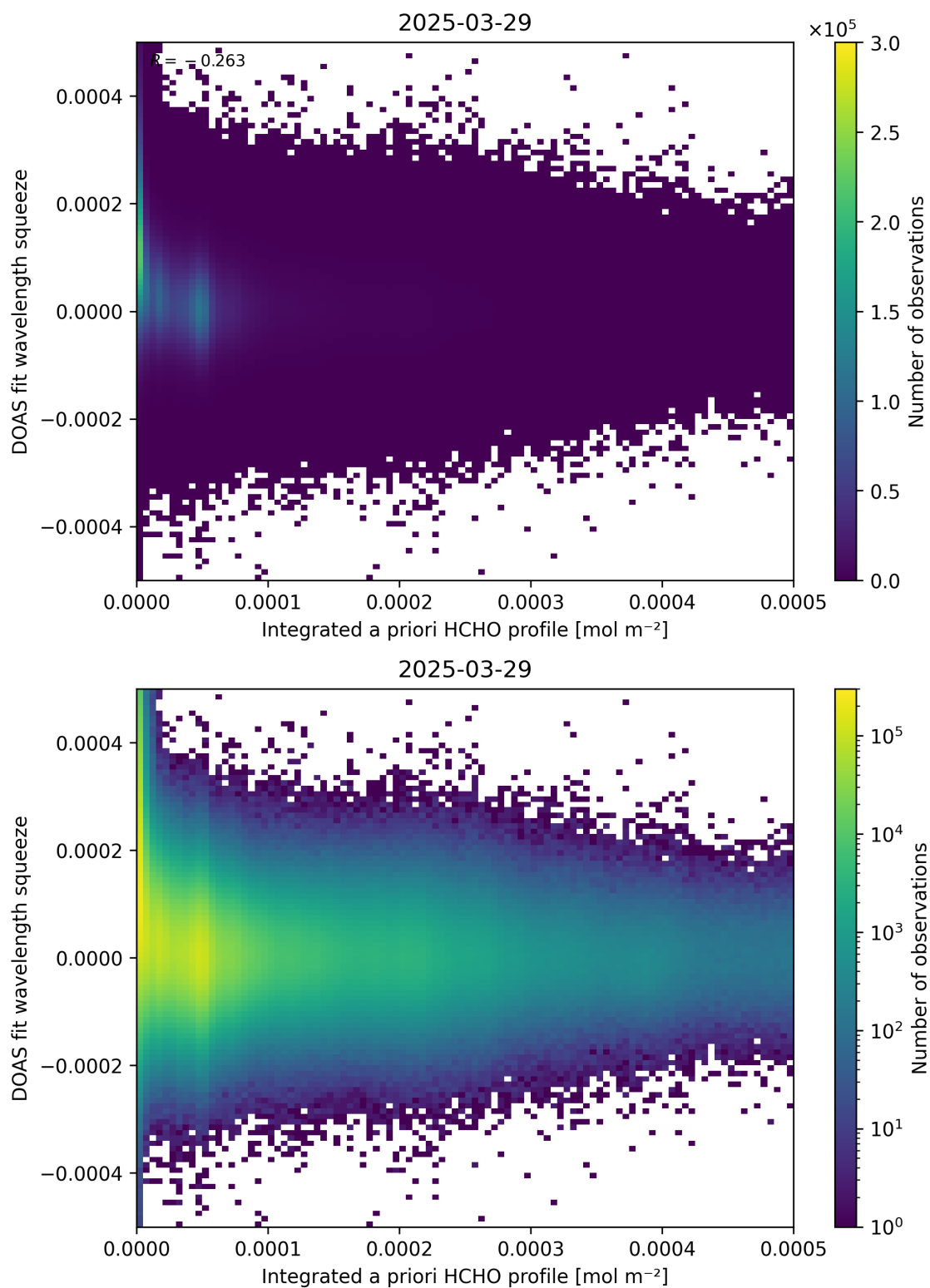
Figure 150: Scatter density plot of “Integrated a priori HCHO profile” against “DOAS fit wavelength squeeze” for 2025-03-28 to 2025-03-30.
