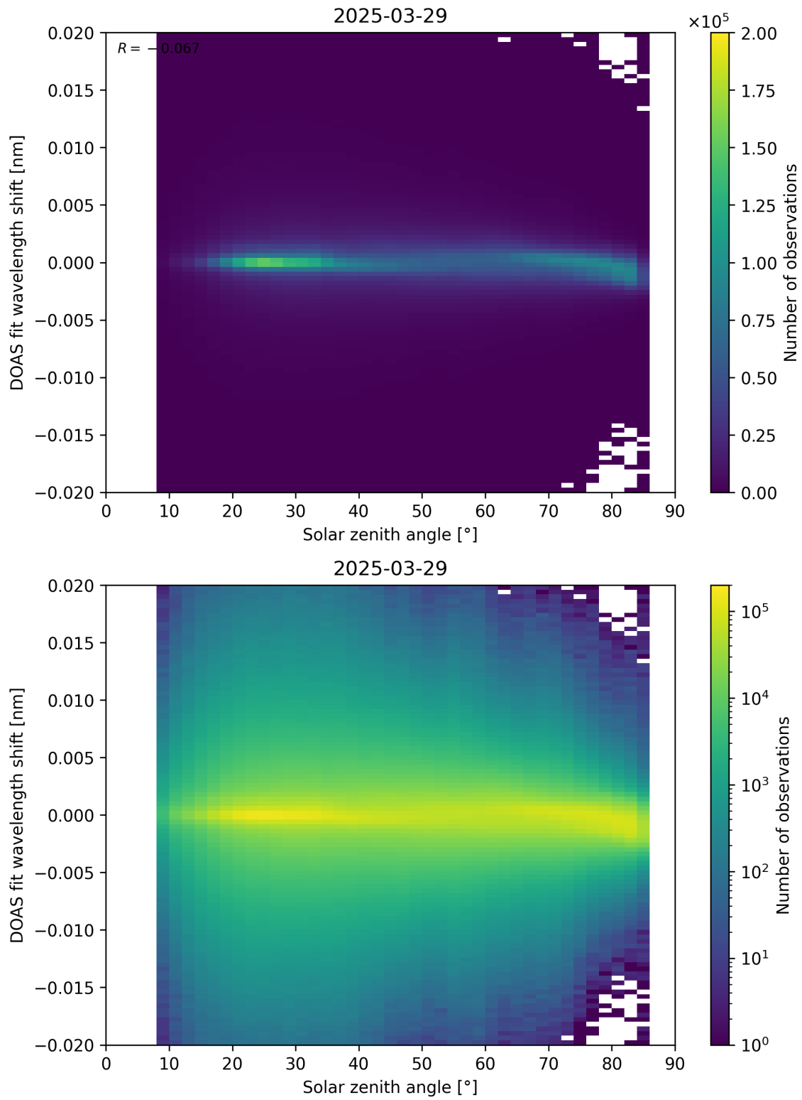
Figure 168: Scatter density plot of “Solar zenith angle” against “DOAS fit wavelength shift” for 2025-03-28 to 2025-03-30.
