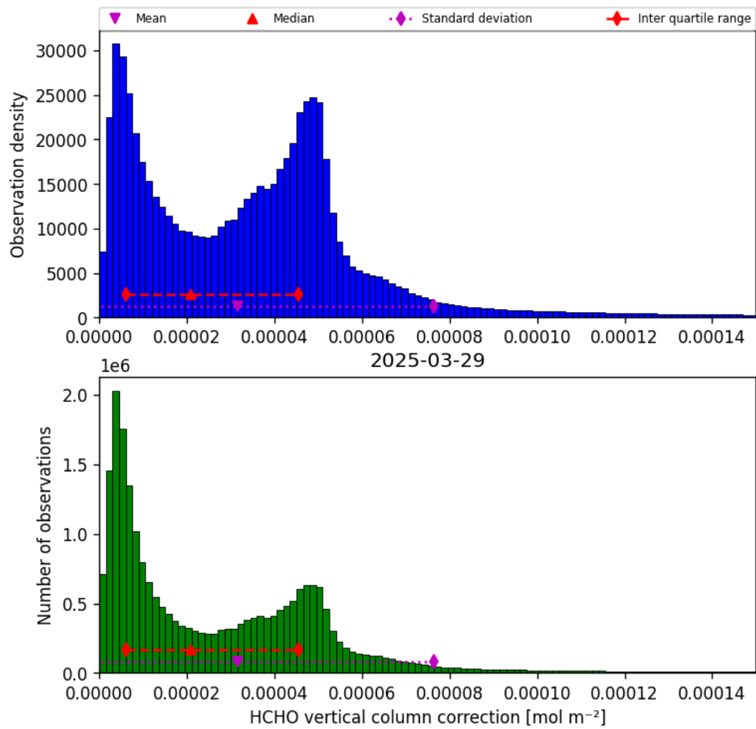
Figure 37: Histogram of “HCHO vertical column correction” for 2025-03-28 to 2025-03-30
