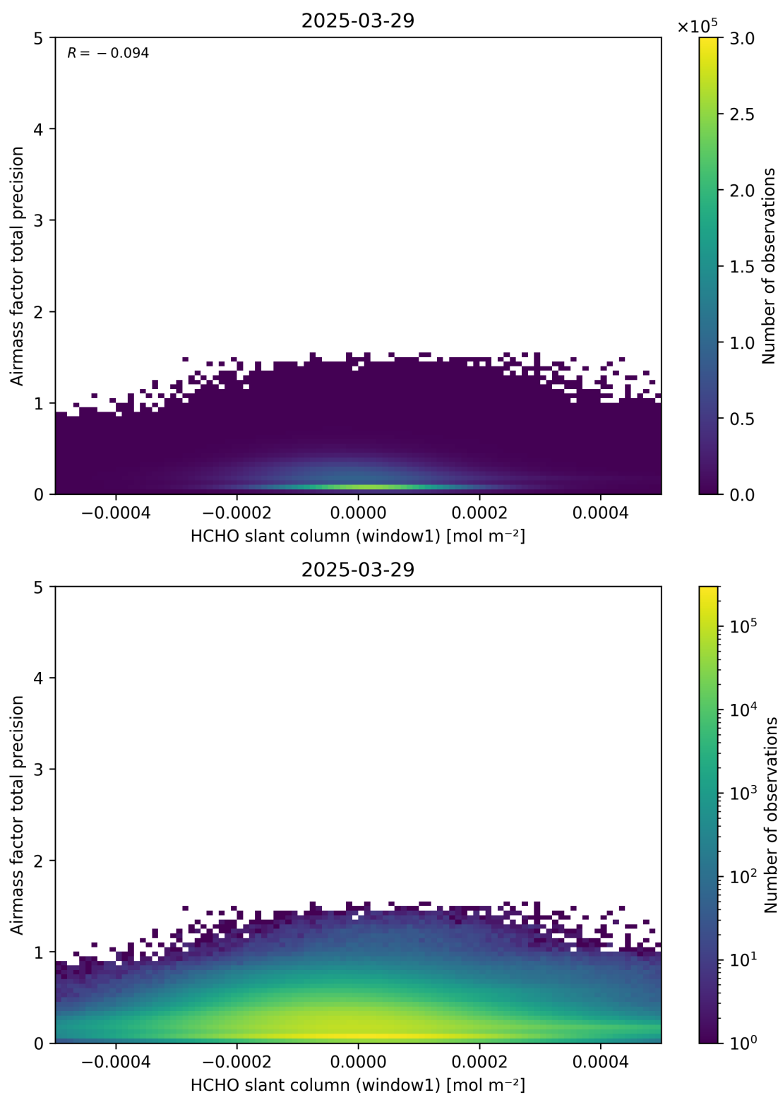
Figure 86: Scatter density plot of “HCHO slant column (window1)” against “Airmass factor total precision” for 2025-03-28 to 2025-03-30.
