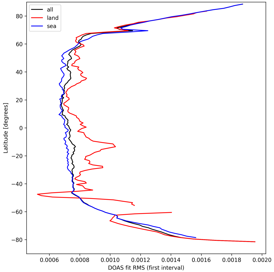
Figure 32: Zonal average of "DOAS fit RMS (first interval)" for 2025-03-28 to 2025-03-30.
