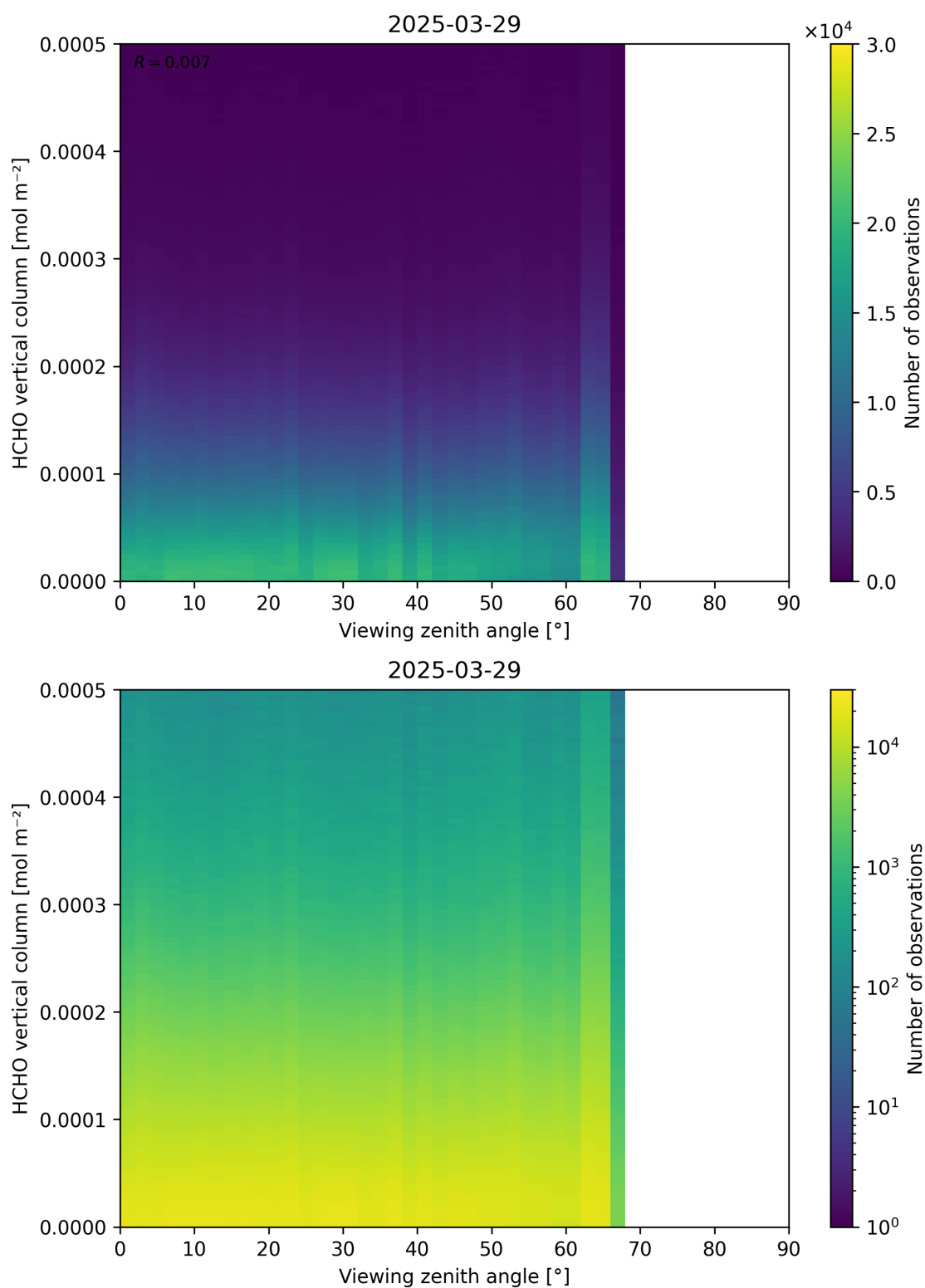
Figure 192: Scatter density plot of “Viewing zenith angle” against “HCHO vertical column” for 2025-03-28 to 2025-03-30.
