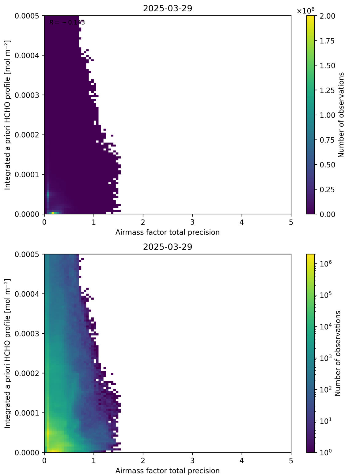
Figure 111: Scatter density plot of “Airmass factor total precision” against “Integrated a priori HCHO profile” for 2025-03-28 to 2025-03-30.
