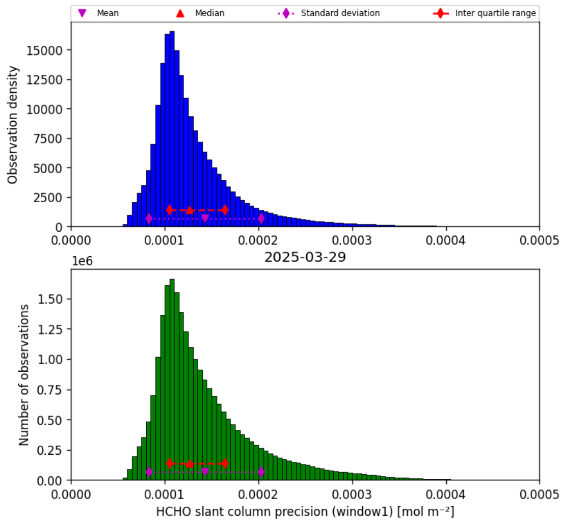
Figure 39: Histogram of “HCHO slant column precision (window1)” for 2025-03-28 to 2025-03-30
