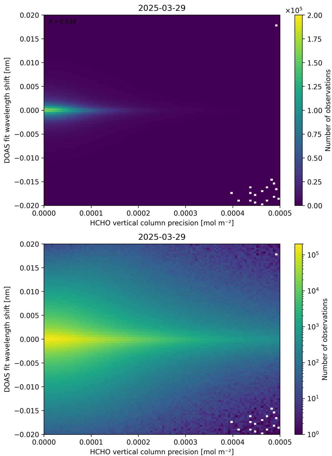
Figure 137: Scatter density plot of “HCHO vertical column precision” against “DOAS fit wavelength shift” for 2025-03-28 to 2025-03-30.
