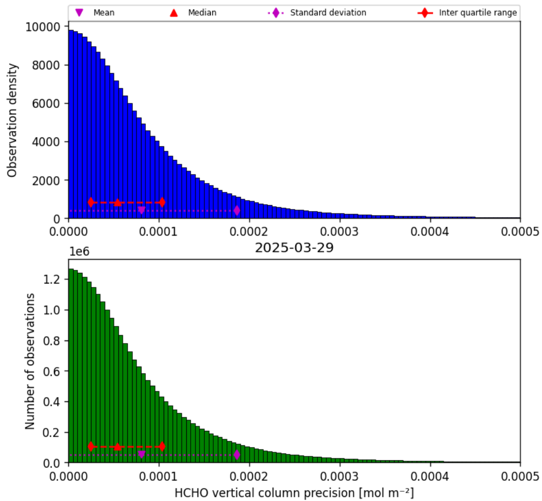
Figure 36: Histogram of “HCHO vertical column precision” for 2025-03-28 to 2025-03-30
