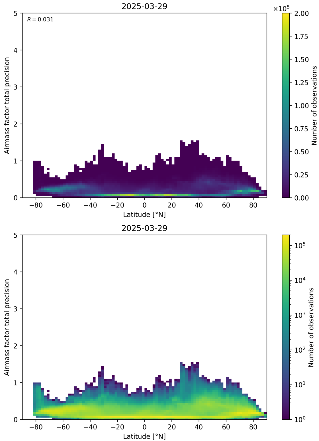
Figure 162: Scatter density plot of “Latitude” against “Airmass factor total precision” for 2025-03-28 to 2025-03-30.
