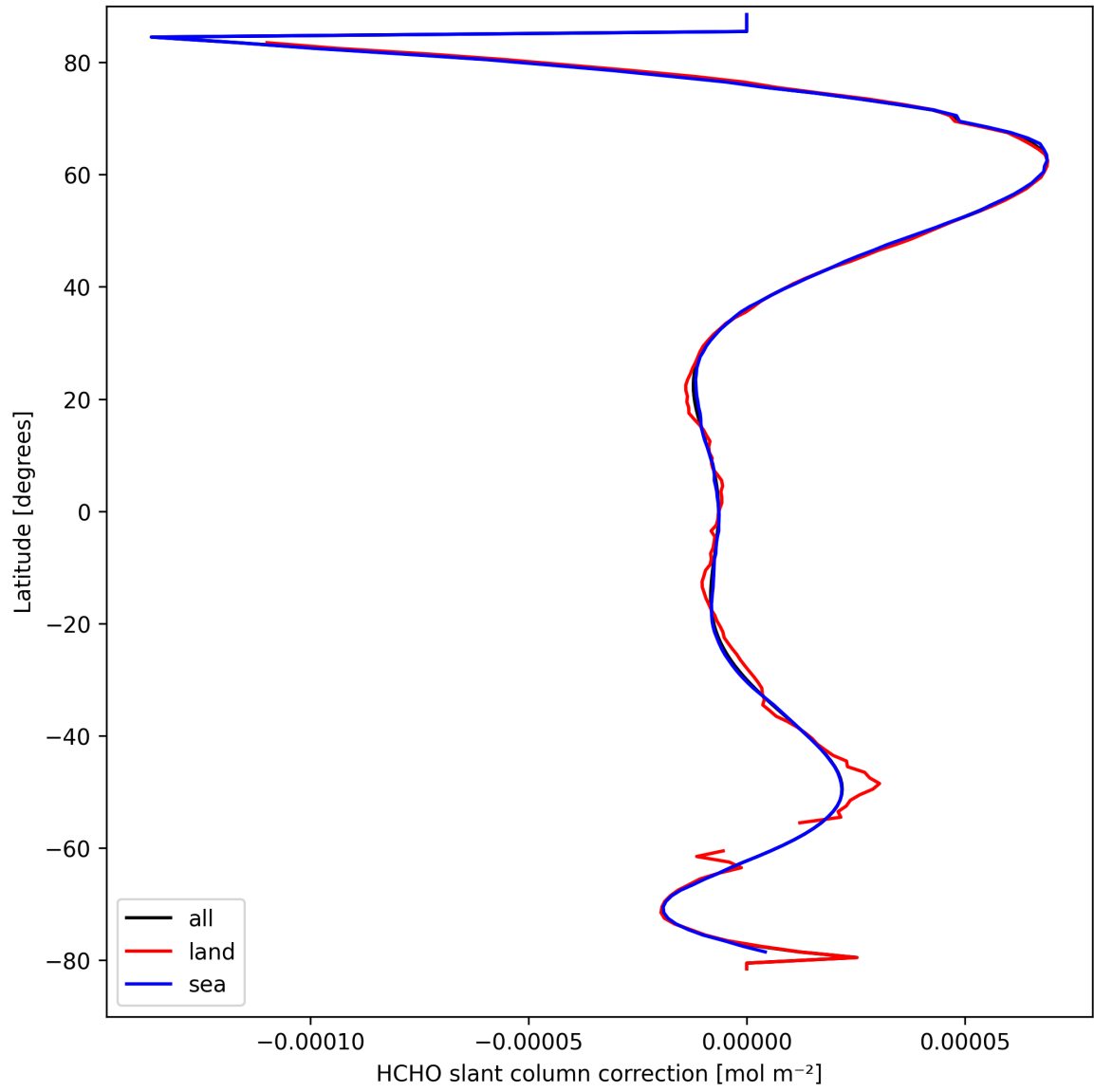
Figure 33: Zonal average of "HCHO slant column correction" for 2025-03-28 to 2025-03-30.
