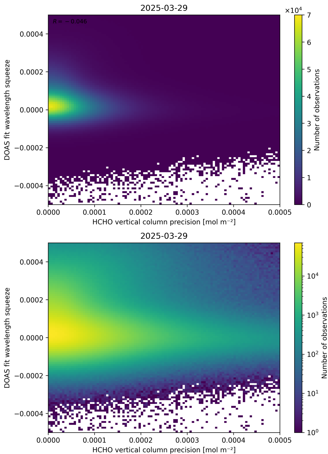
Figure 138: Scatter density plot of “HCHO vertical column precision” against “DOAS fit wavelength squeeze” for 2025-03-28 to 2025-03-30.
