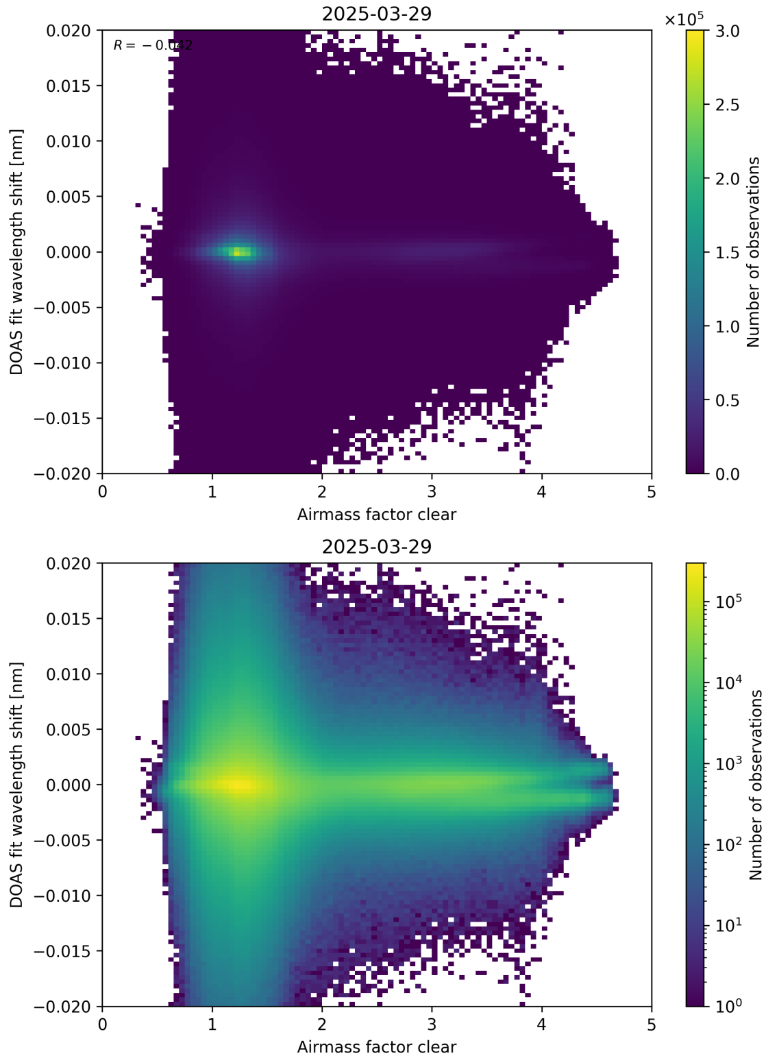
Figure 72: Scatter density plot of “Airmass factor clear” against “DOAS fit wavelength shift” for 2025-03-28 to 2025-03-30.
