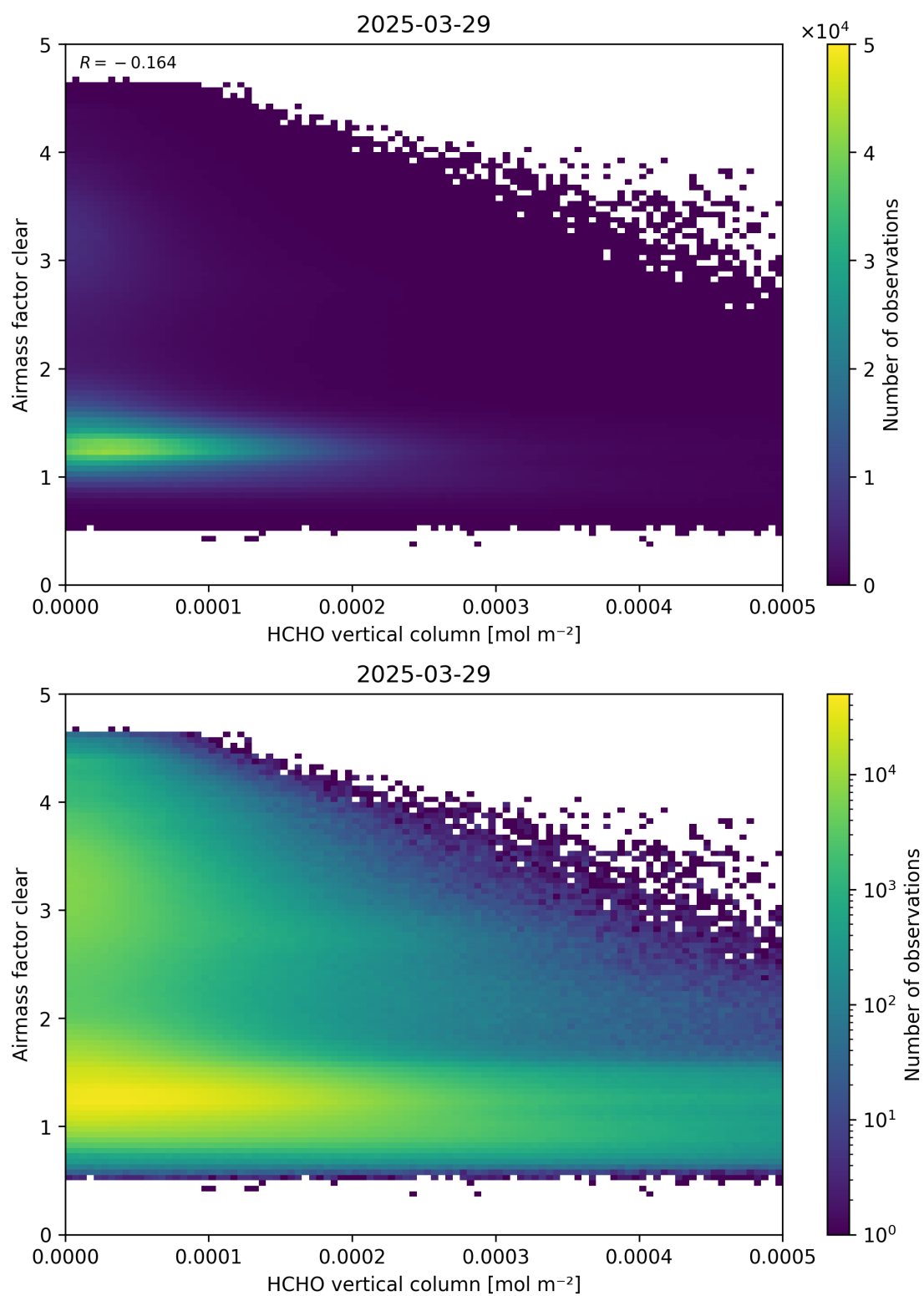
Figure 126: Scatter density plot of “HCHO vertical column” against “Airmass factor clear” for 2025-03-28 to 2025-03-30.
