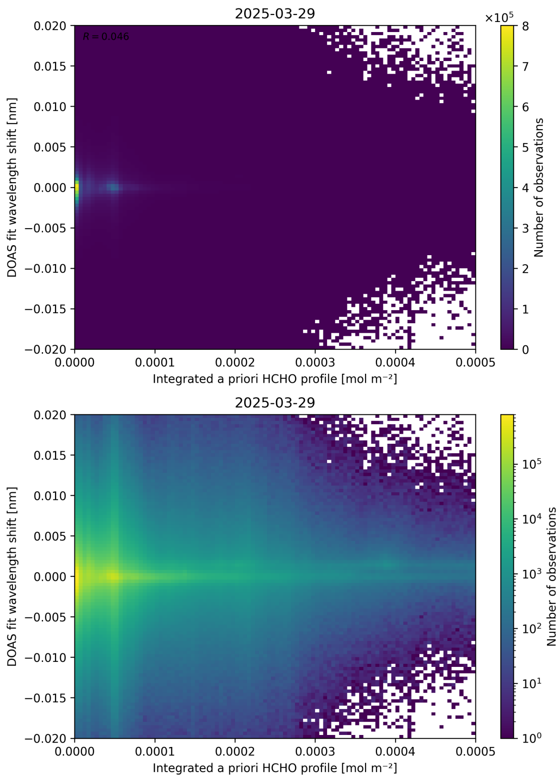
Figure 149: Scatter density plot of “Integrated a priori HCHO profile” against “DOAS fit wavelength shift” for 2025-03-28 to 2025-03-30.
