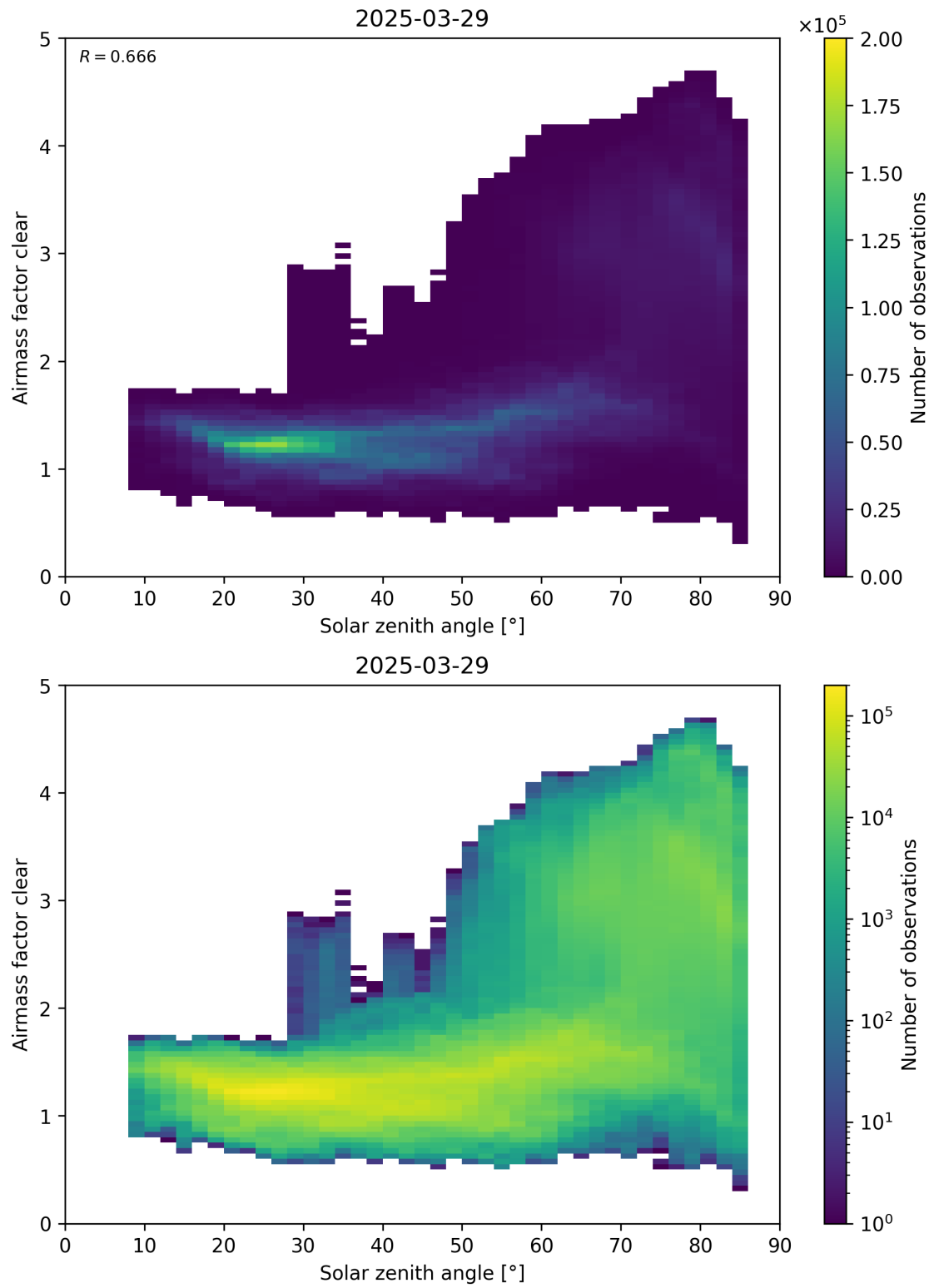
Figure 170: Scatter density plot of “Solar zenith angle” against “Airmass factor clear” for 2025-03-28 to 2025-03-30.
