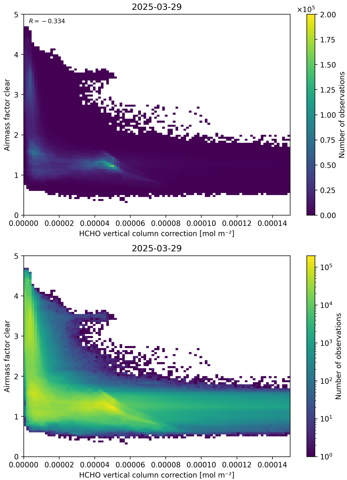
Figure 115: Scatter density plot of “HCHO vertical column correction” against “Airmass factor clear” for 2025-03-28 to 2025-03-30.
