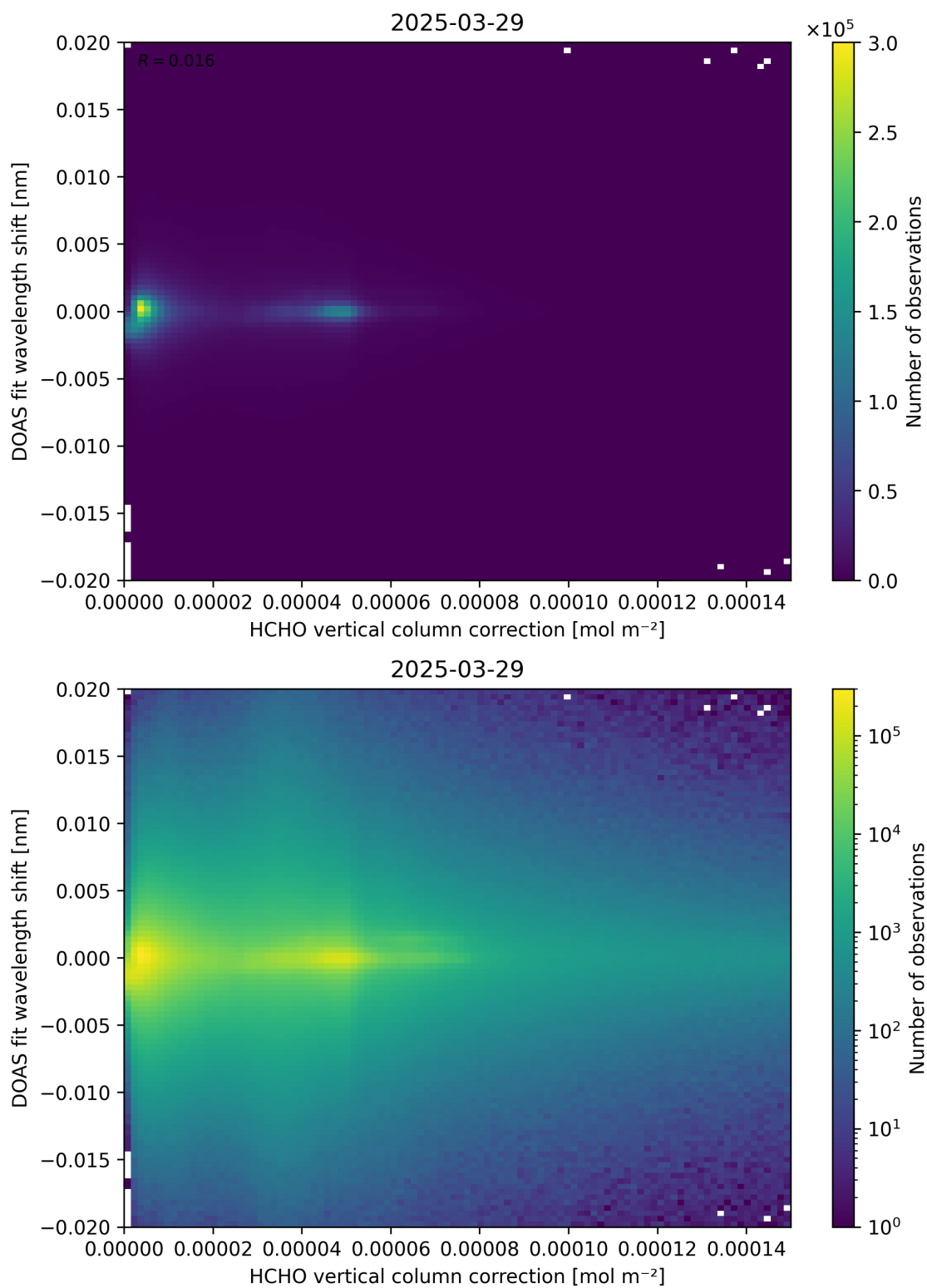
Figure 113: Scatter density plot of “HCHO vertical column correction” against “DOAS fit wavelength shift” for 2025-03-28 to 2025-03-30.
