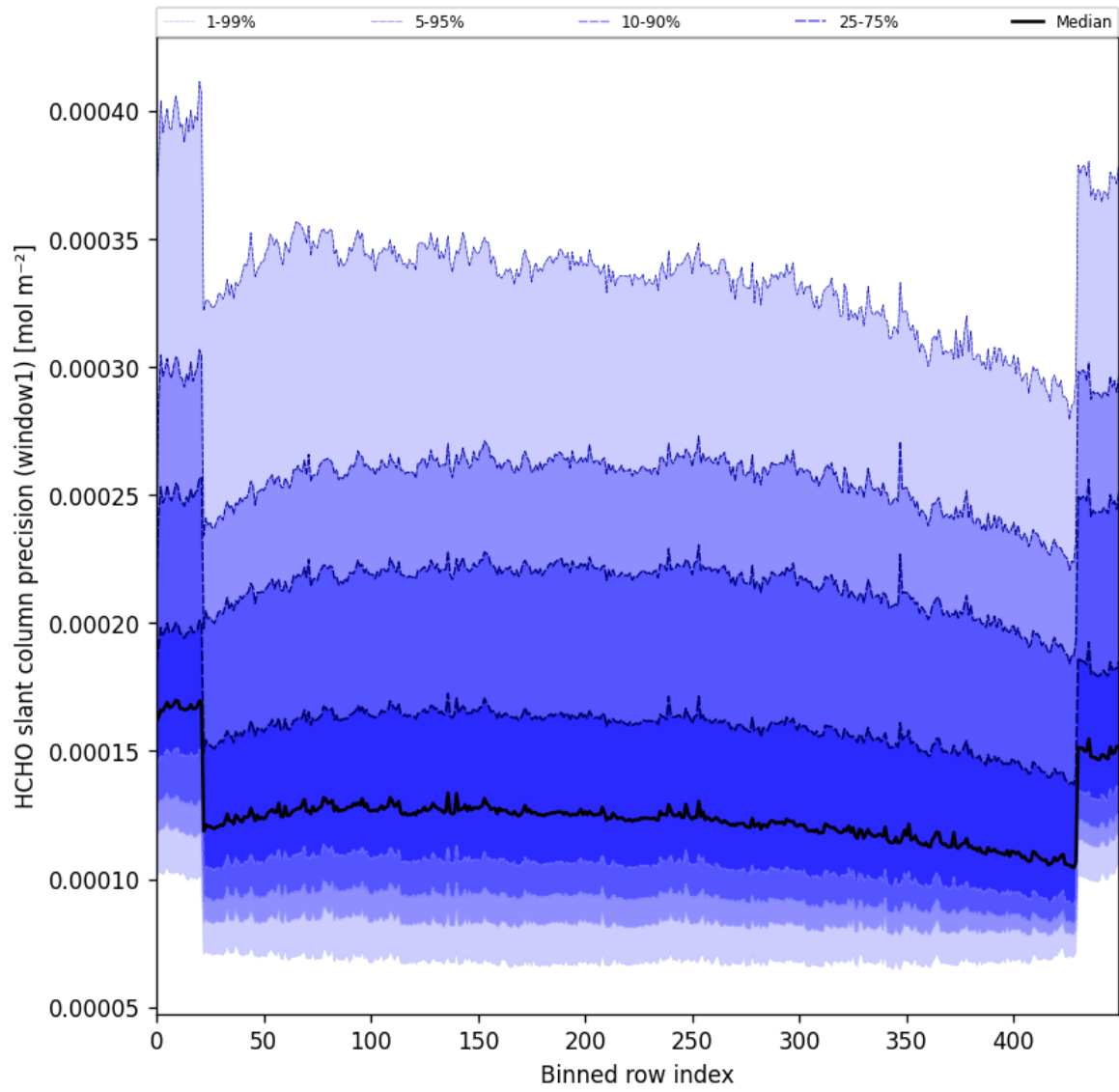
Figure 53: Along track statistics of “HCHO slant column precision (window1)” for 2025-03-28 to 2025-03-30
