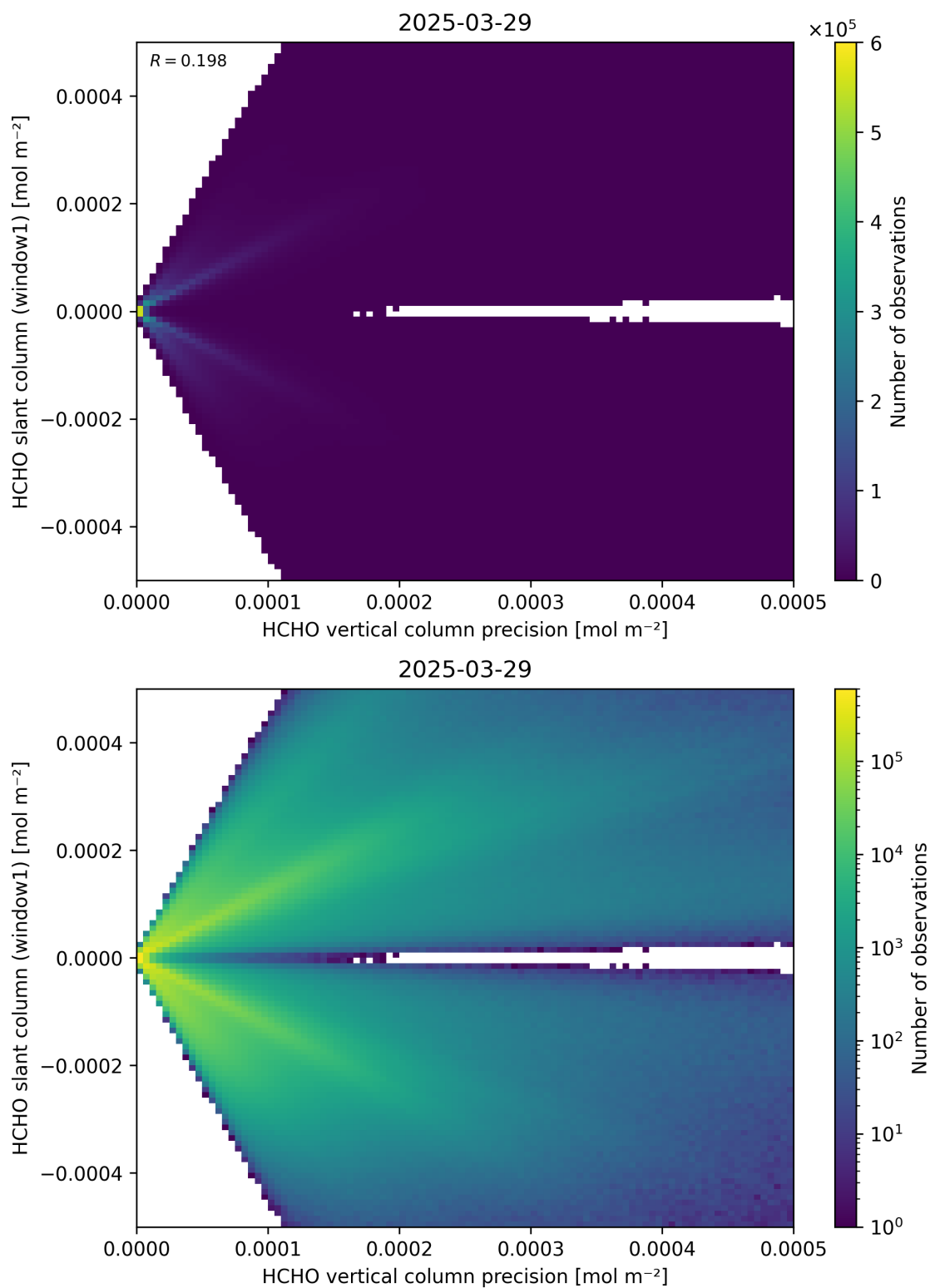
Figure 142: Scatter density plot of “HCHO vertical column precision” against “HCHO slant column (window1)” for 2025-03-28 to 2025-03-30.
