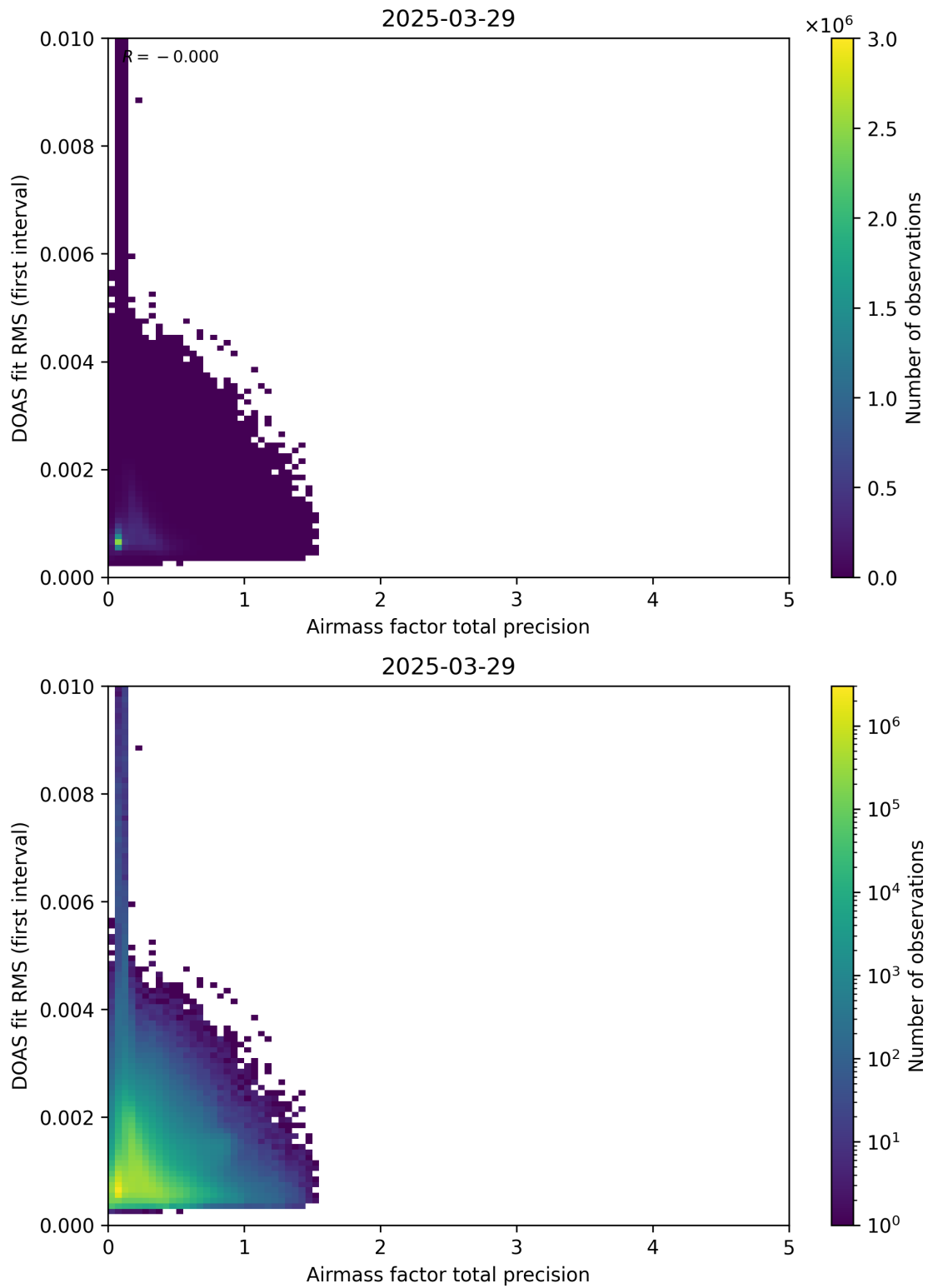
Figure 105: Scatter density plot of “Airmass factor total precision” against “DOAS fit RMS (first interval)” for 2025-03-28 to 2025-03-30.
