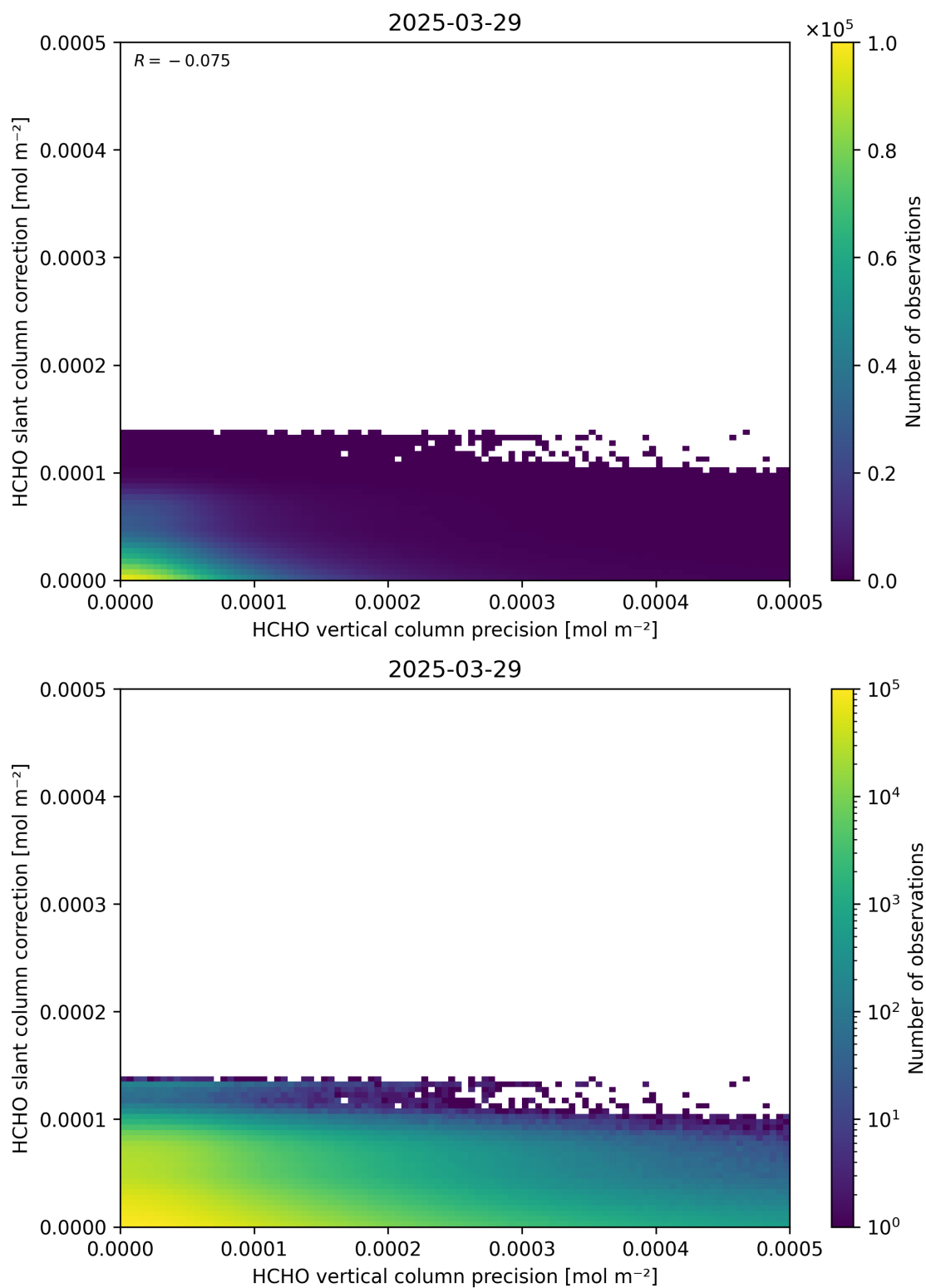
Figure 141: Scatter density plot of “HCHO vertical column precision” against “HCHO slant column correction” for 2025-03-28 to 2025-03-30.
