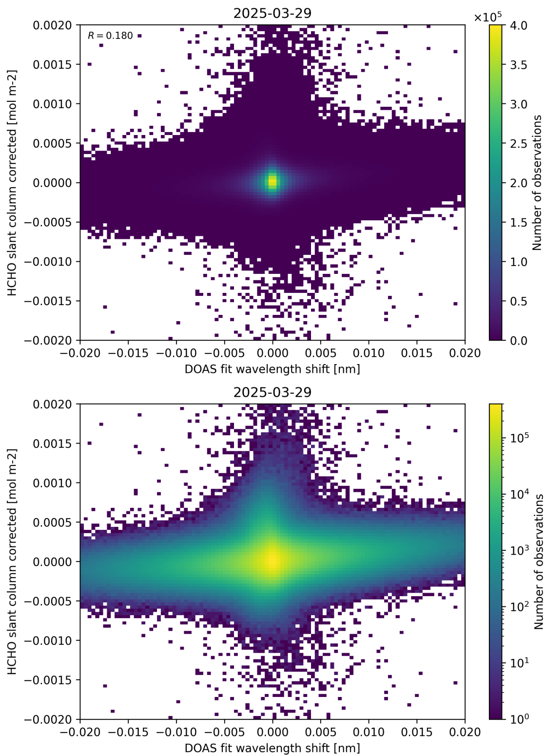
Figure 66: Scatter density plot of “DOAS fit wavelength shift” against “HCHO slant column corrected” for 2025-03-28 to 2025-03-30.
