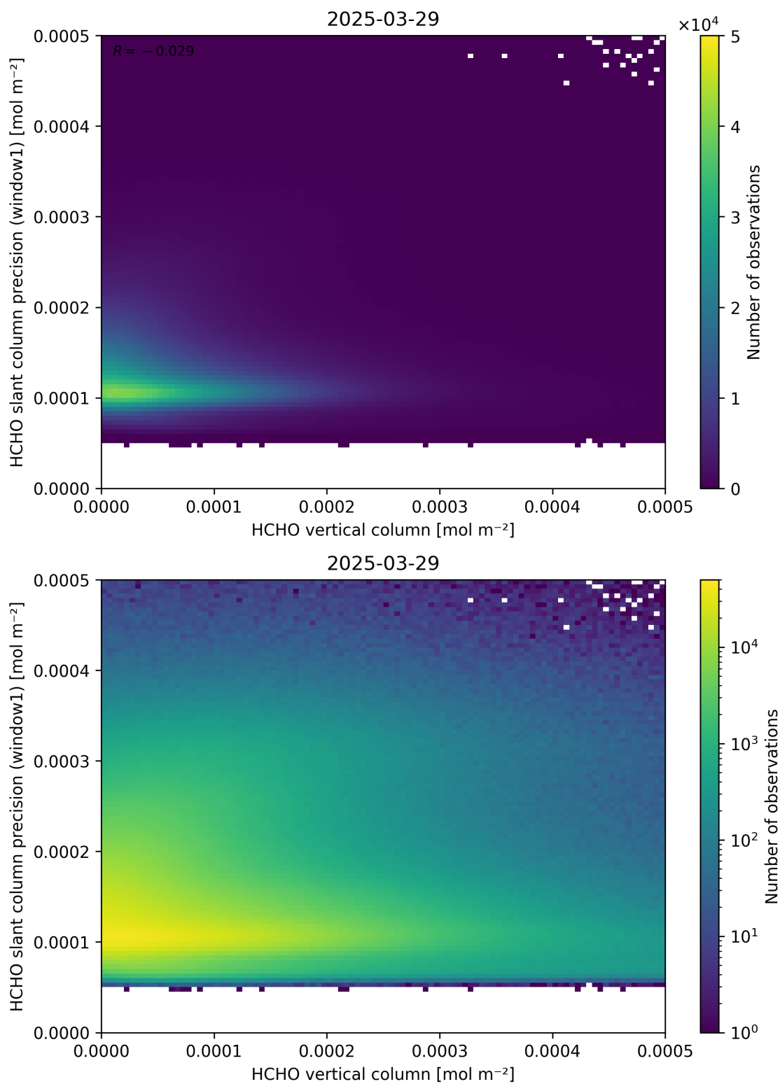
Figure 130: Scatter density plot of “HCHO vertical column” against “HCHO slant column precision (window1)” for 2025-03-28 to 2025-03-30.
