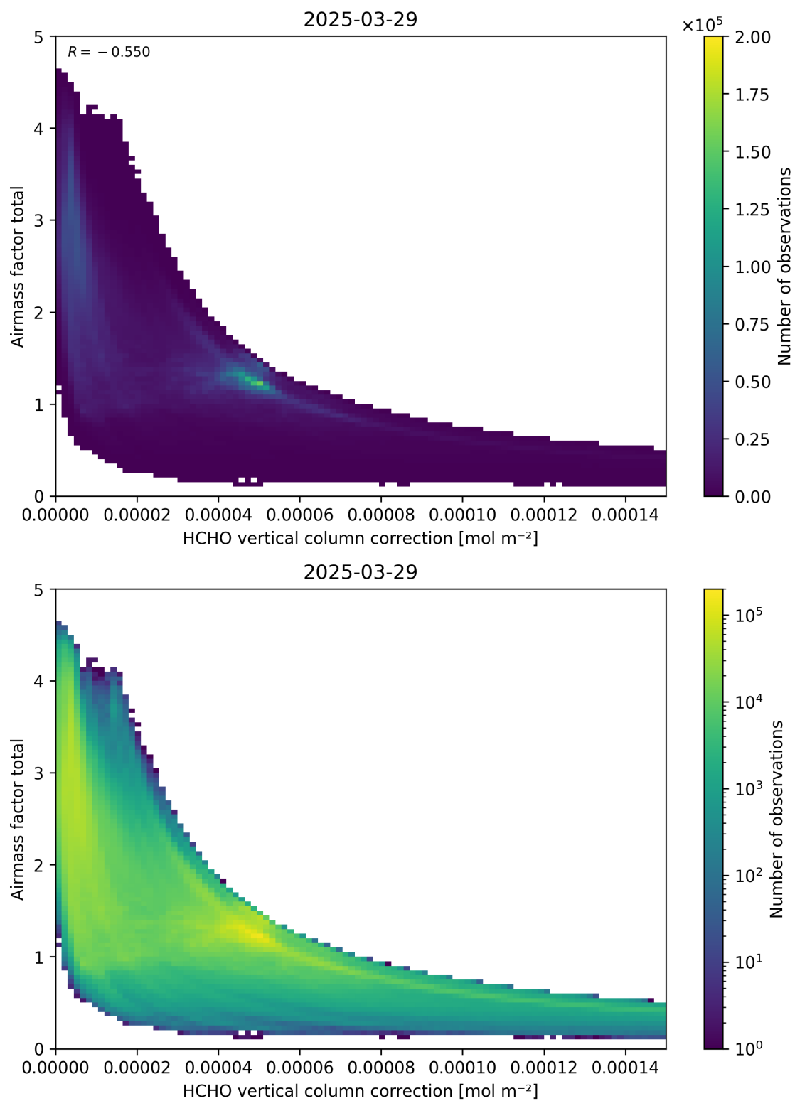
Figure 120: Scatter density plot of “HCHO vertical column correction” against “Airmass factor total” for 2025-03-28 to 2025-03-30.
