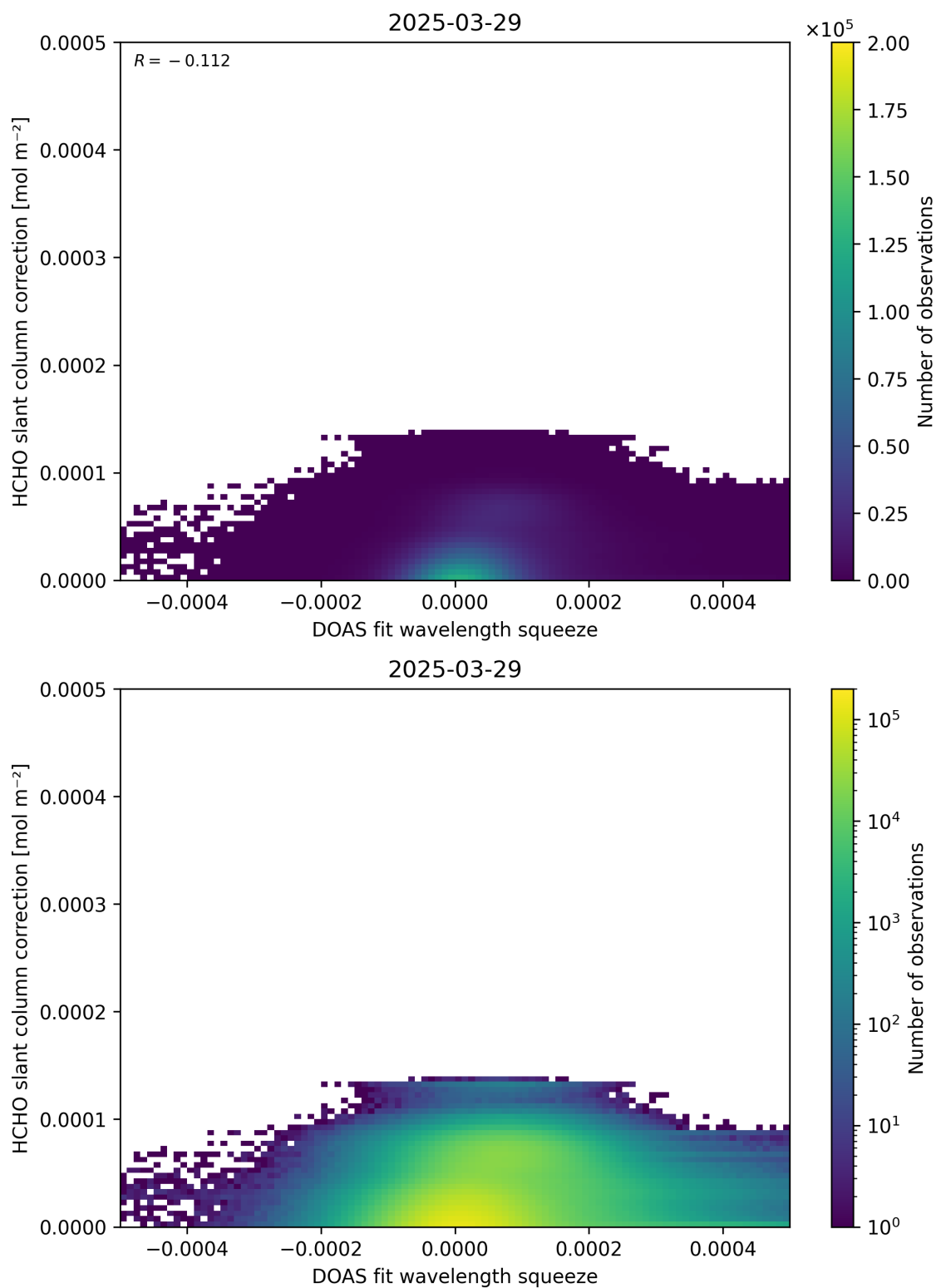
Figure 70: Scatter density plot of “DOAS fit wavelength squeeze” against “HCHO slant column correction” for 2025-03-28 to 2025-03-30.
