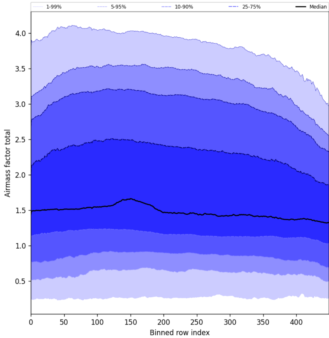
Figure 54: Along track statistics of “Airmass factor total” for 2025-03-28 to 2025-03-30
