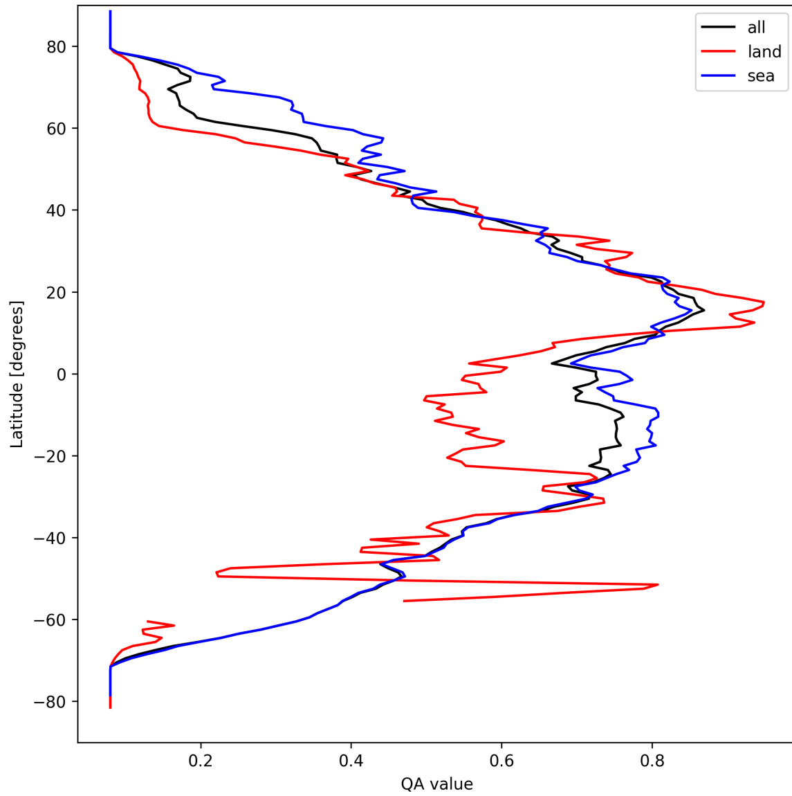
Figure 20: Zonal average of “QA value” for 2025-03-28 to 2025-03-30.
