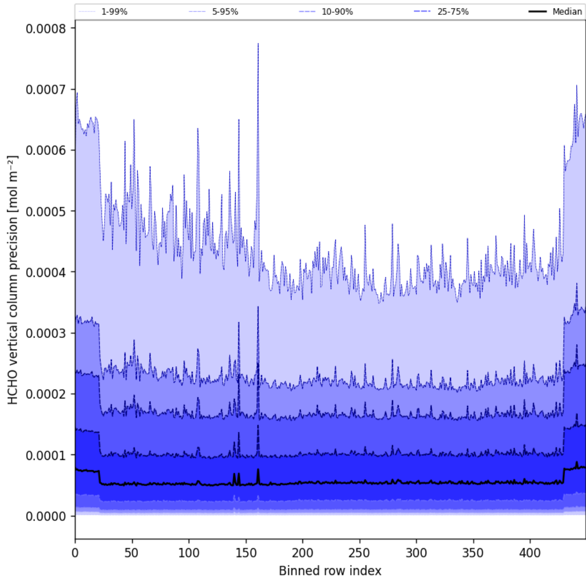
Figure 50: Along track statistics of "HCHO vertical column precision" for 2025-03-28 to 2025-03-30
