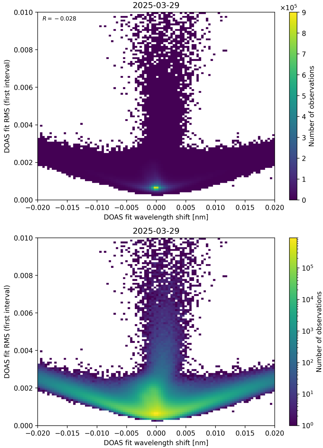
Figure 64: Scatter density plot of “DOAS fit wavelength shift” against “DOAS fit RMS (first interval)” for 2025-03-28 to 2025-03-30.
