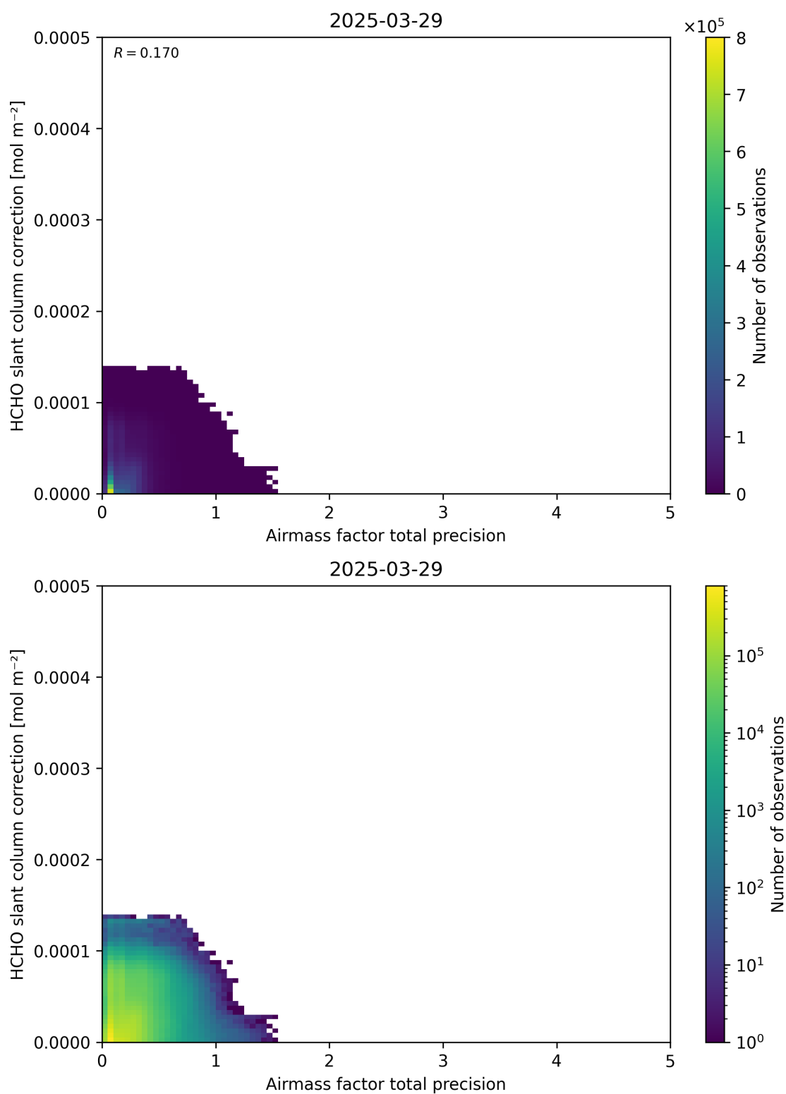
Figure 110: Scatter density plot of “Airmass factor total precision” against “HCHO slant column correction” for 2025-03-28 to 2025-03-30.
