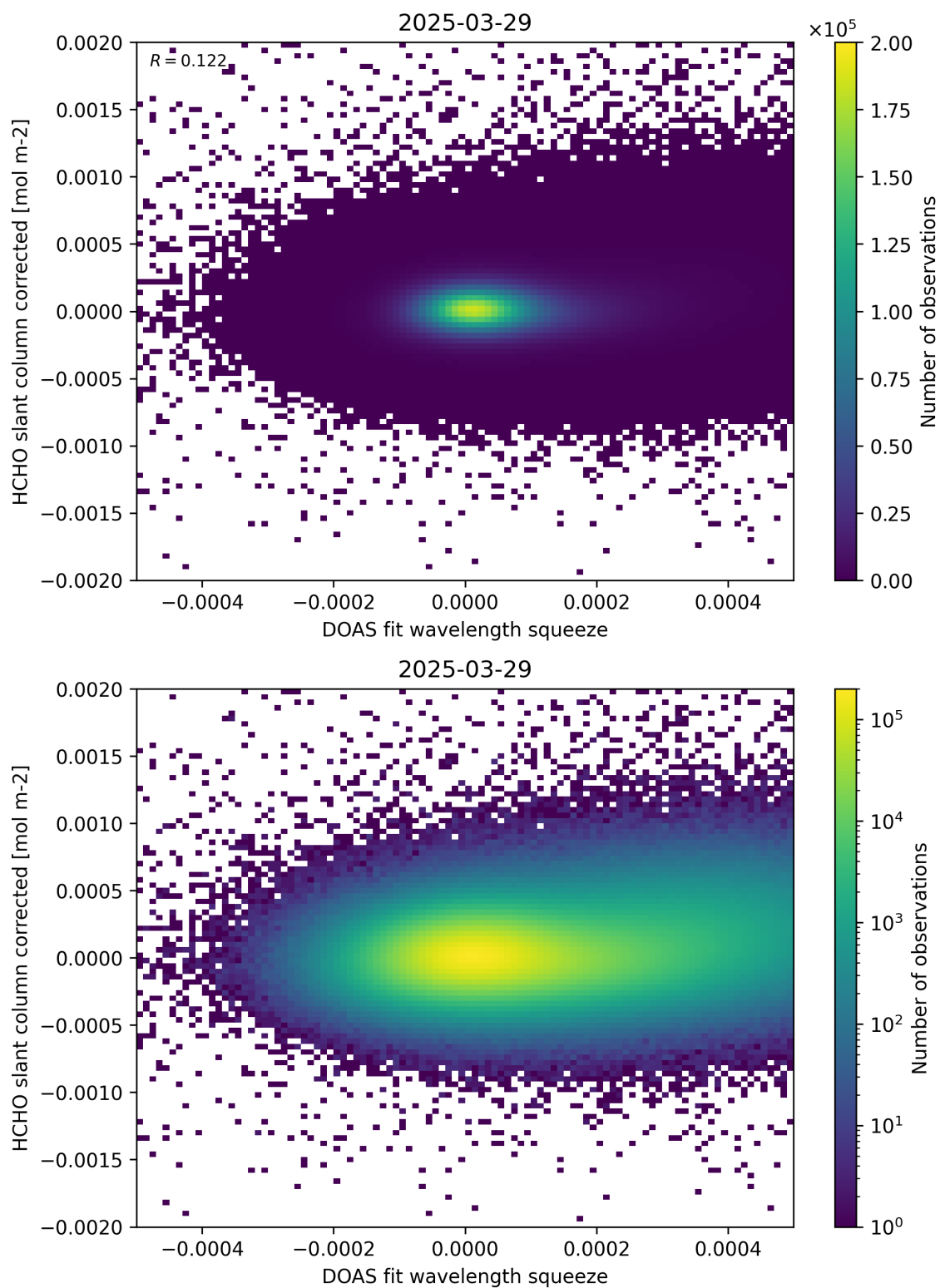
Figure 69: Scatter density plot of “DOAS fit wavelength squeeze” against “HCHO slant column corrected” for 2025-03-28 to 2025-03-30.
