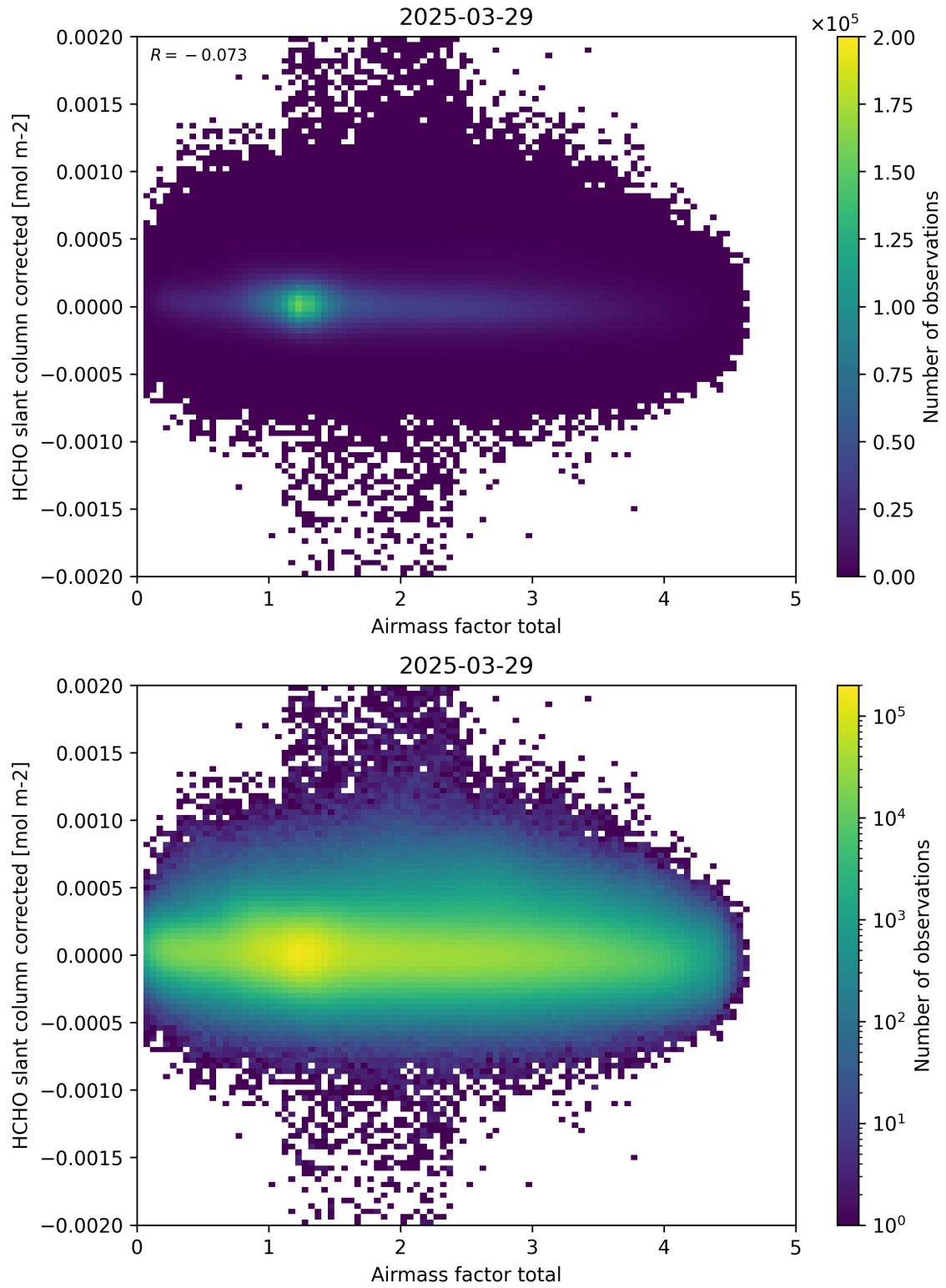
Figure 101: Scatter density plot of “Airmass factor total” against “HCHO slant column corrected” for 2025-03-28 to 2025-03-30.
