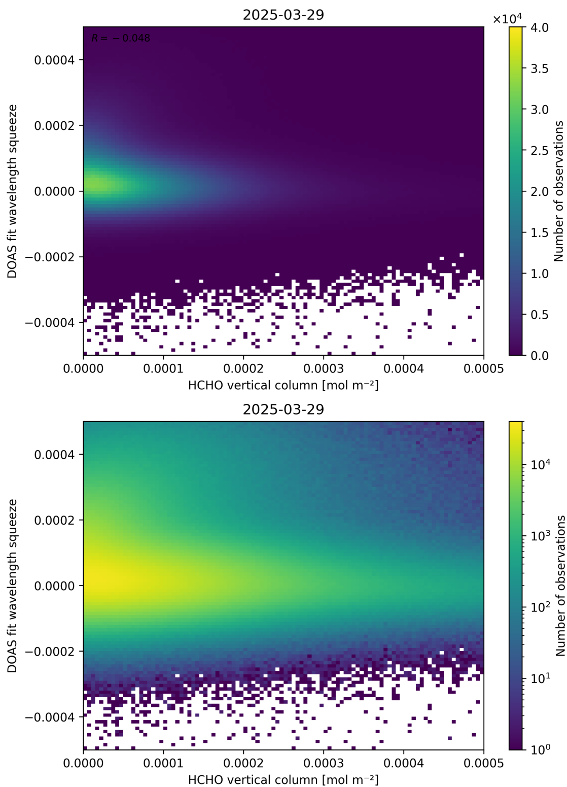
Figure 125: Scatter density plot of “HCHO vertical column” against “DOAS fit wavelength squeeze” for 2025-03-28 to 2025-03-30.
