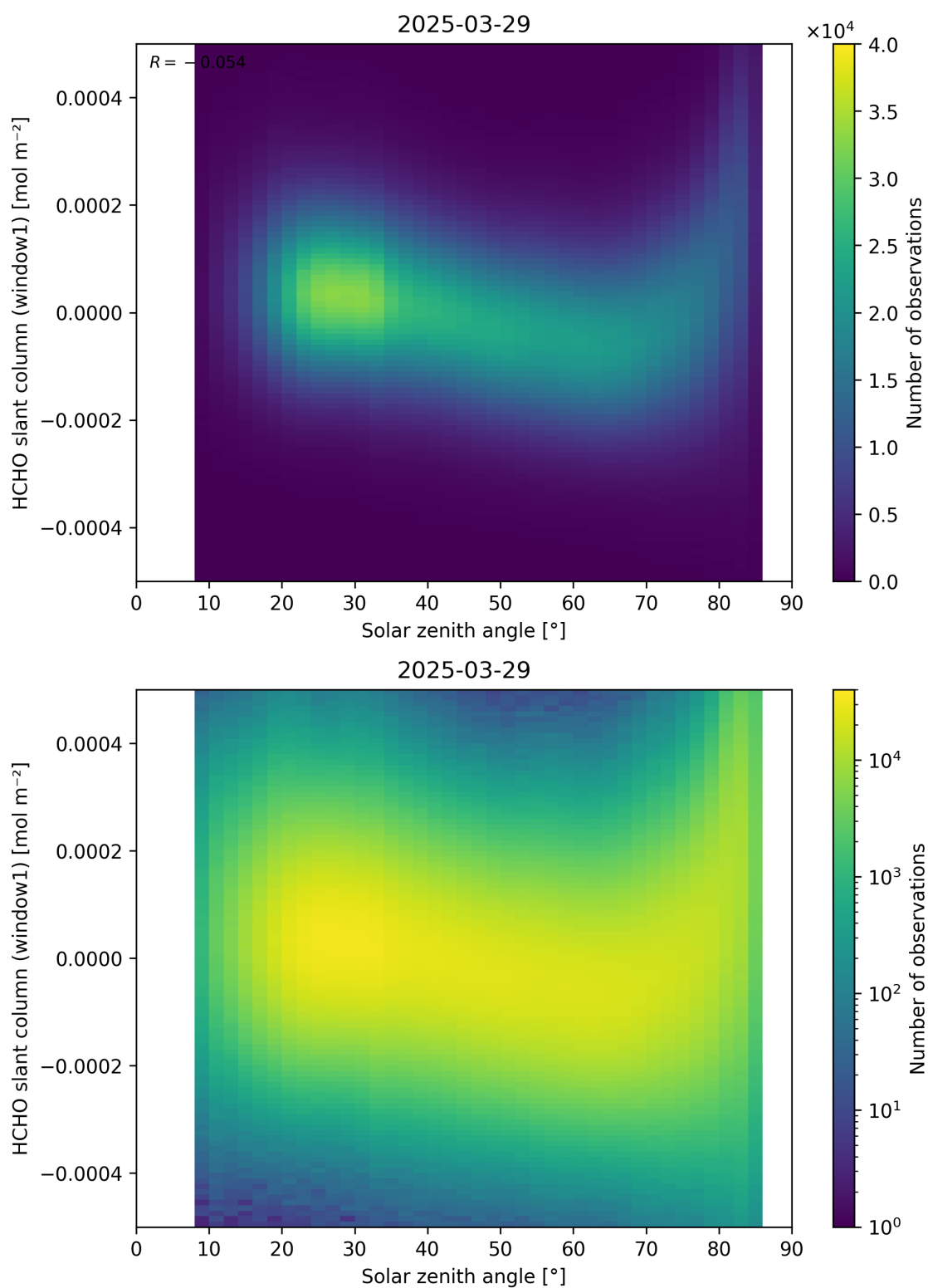
Figure 173: Scatter density plot of “Solar zenith angle” against “HCHO slant column (window1)” for 2025-03-28 to 2025-03-30.
