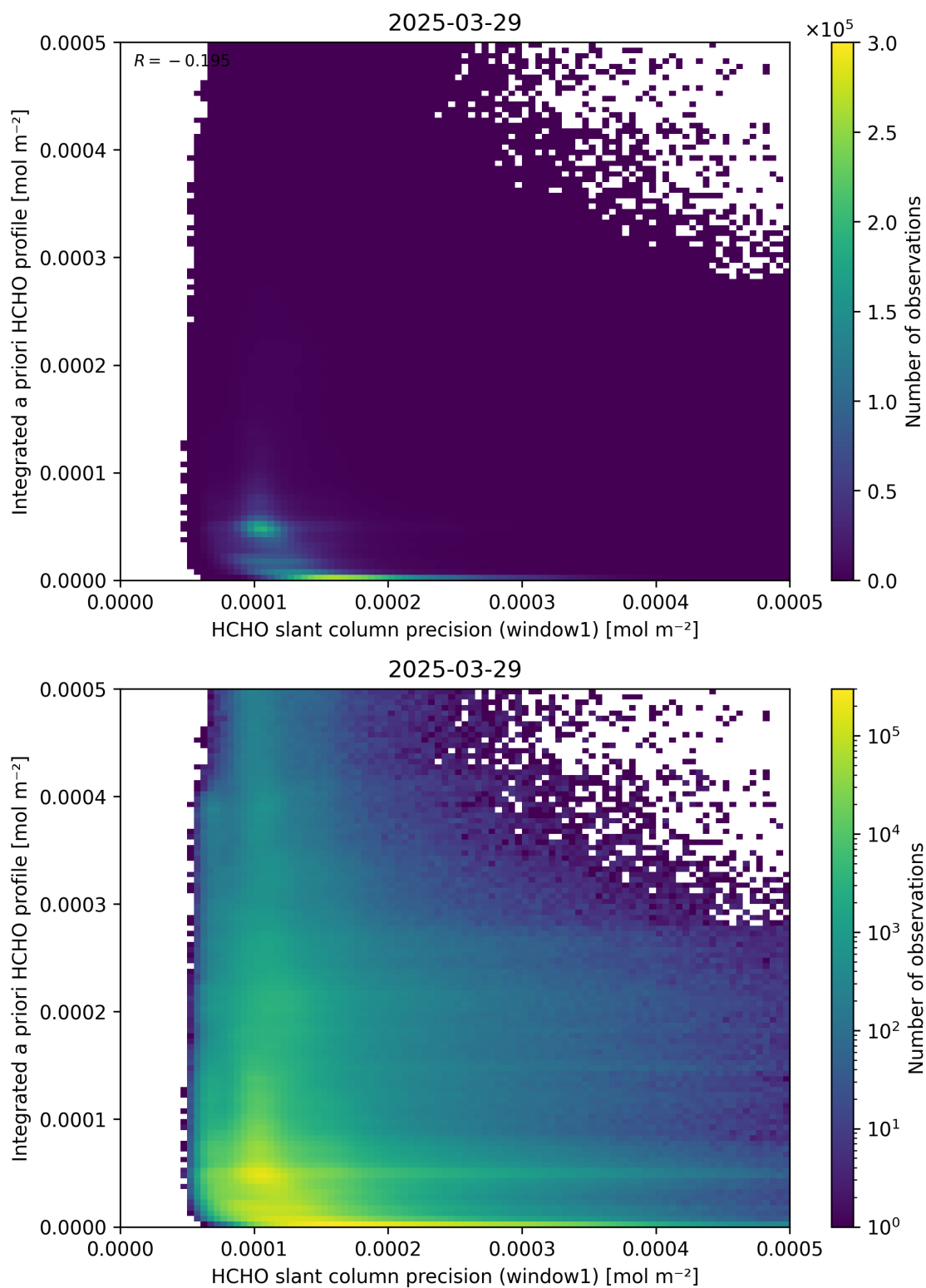
Figure 96: Scatter density plot of “HCHO slant column precision (window1)” against “Integrated a priori HCHO profile” for 2025-03-28 to 2025-03-30.
