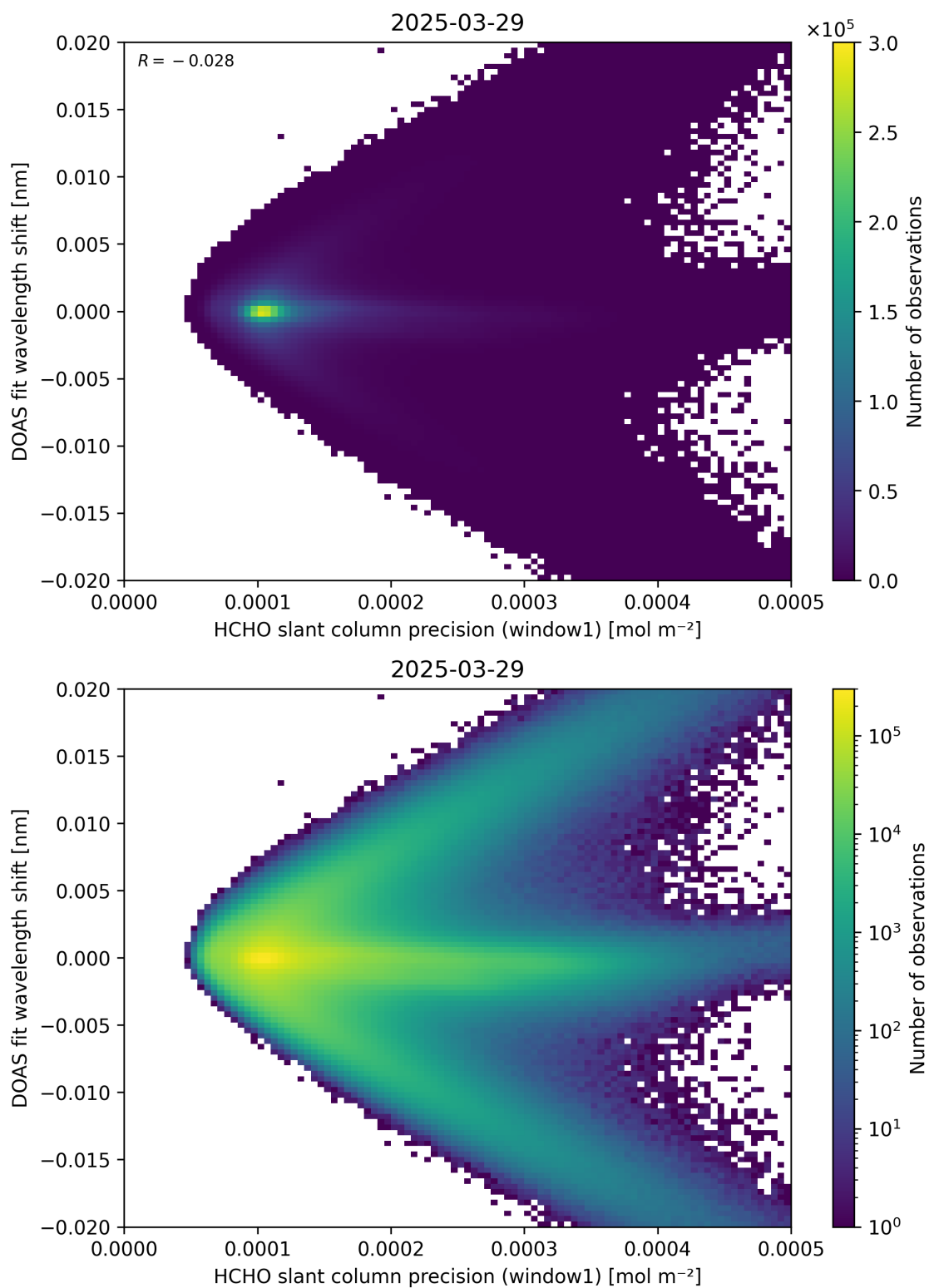
Figure 89: Scatter density plot of “HCHO slant column precision (window1)” against “DOAS fit wavelength shift” for 2025-03-28 to 2025-03-30.
