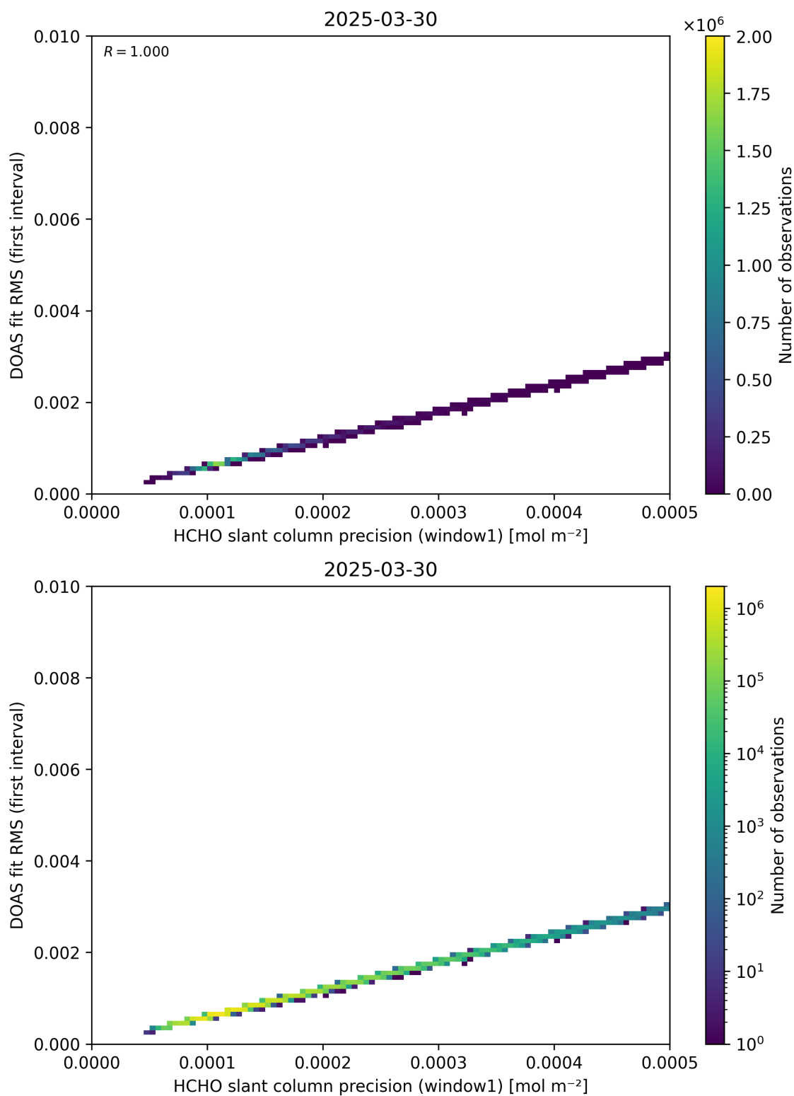
Figure 88: Scatter density plot of “HCHO slant column precision (window1)” against “DOAS fit RMS (first interval)” for 2025-03-29 to 2025-03-31.
