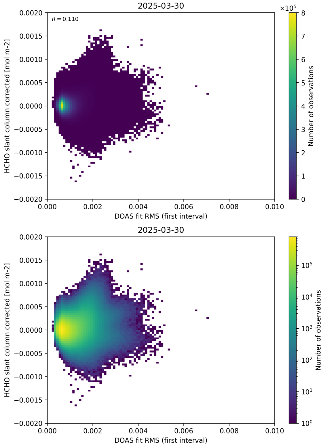
Figure 62: Scatter density plot of “DOAS fit RMS (first interval)” against “HCHO slant column corrected” for 2025-03-29 to 2025-03-31.
