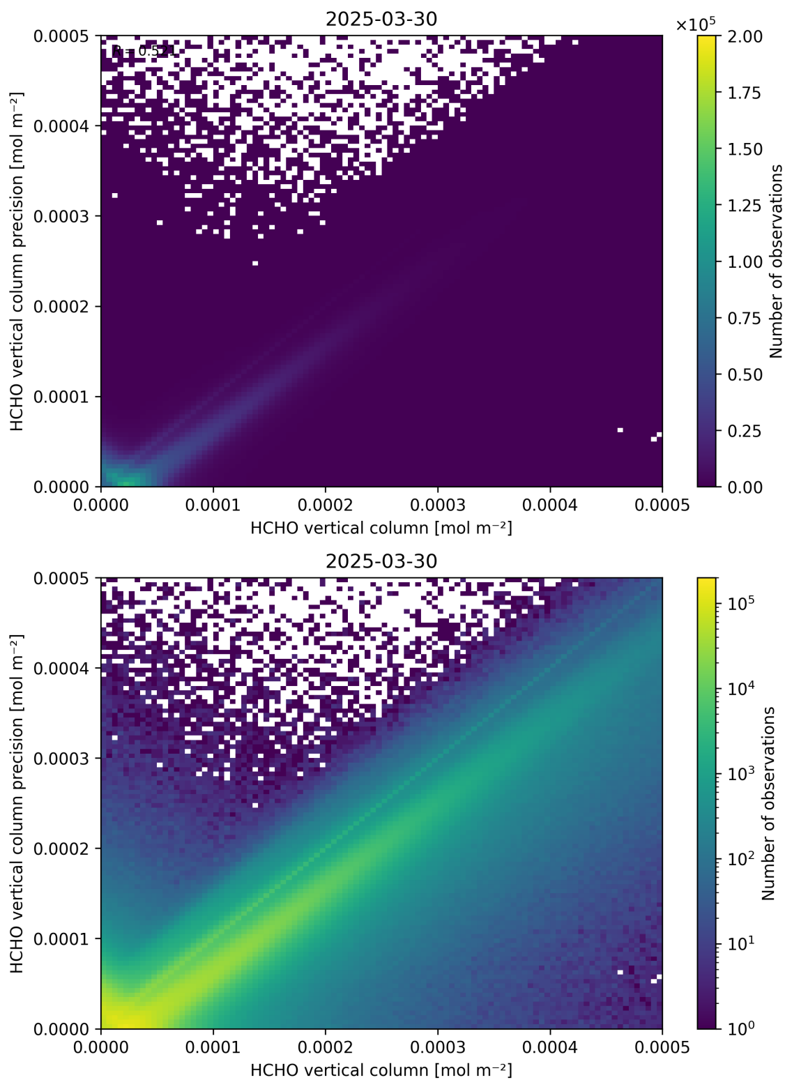
Figure 134: Scatter density plot of “HCHO vertical column” against “HCHO vertical column precision” for 2025-03-29 to 2025-03-31.
