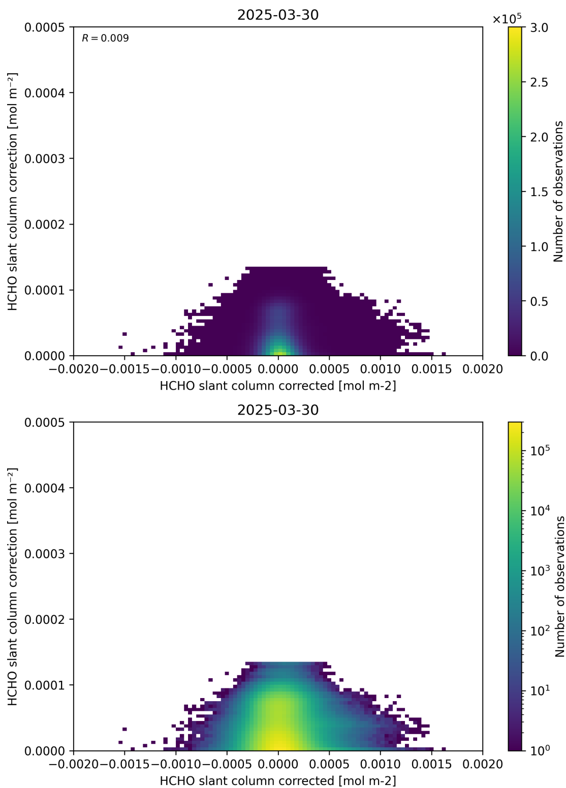
Figure 77: Scatter density plot of “HCHO slant column corrected” against “HCHO slant column correction” for 2025-03-29 to 2025-03-31.
