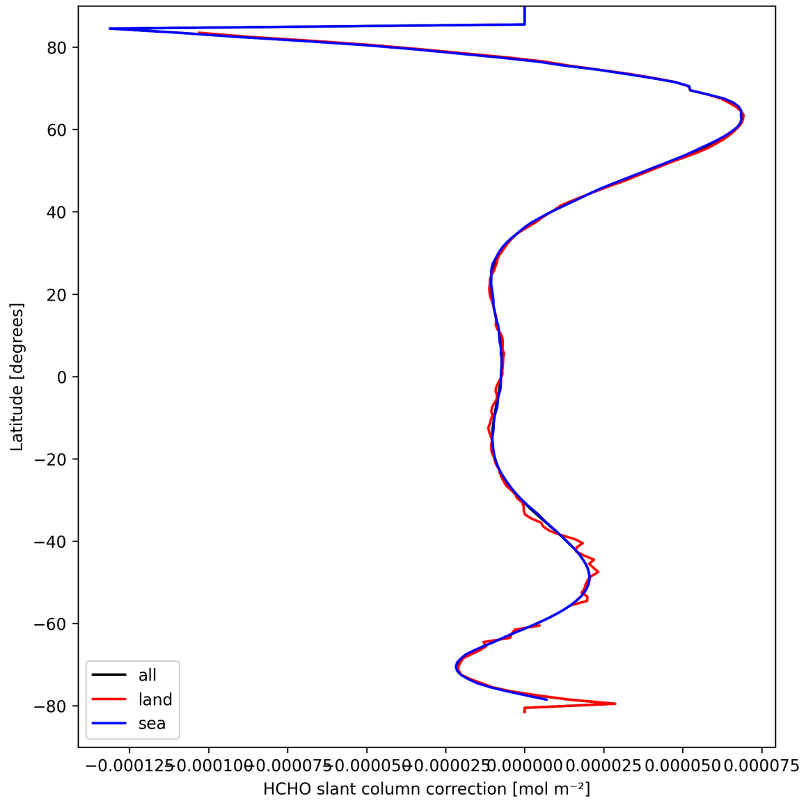
Figure 33: Zonal average of “HCHO slant column correction” for 2025-03-29 to 2025-03-31.
