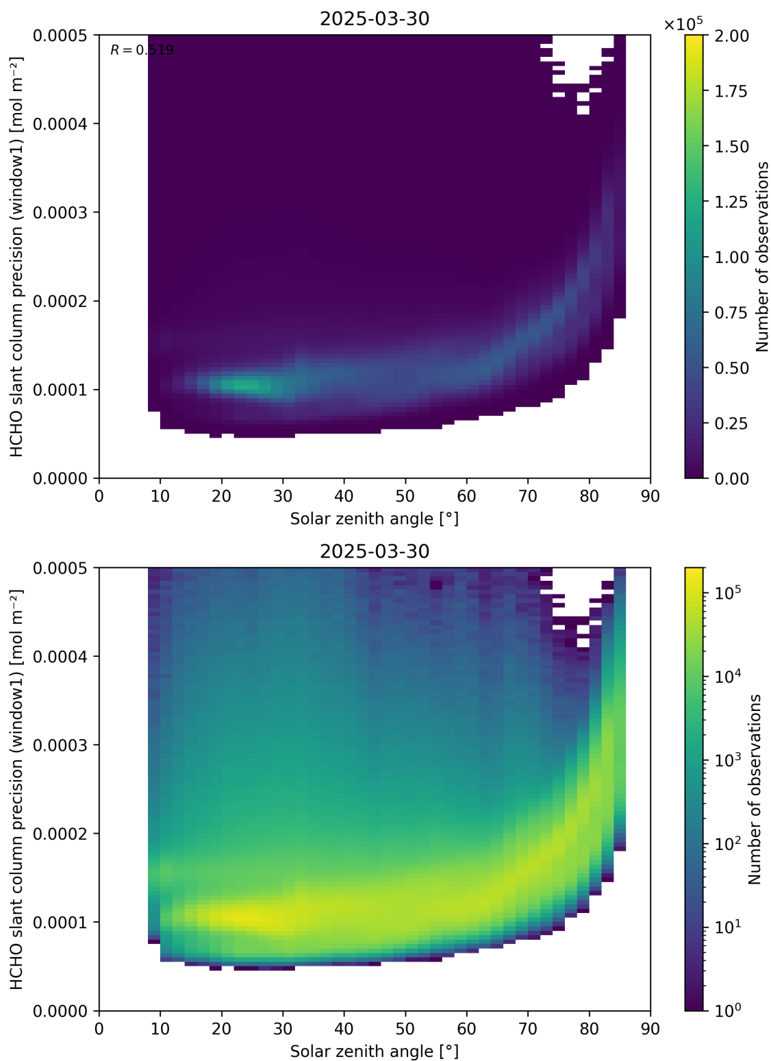
Figure 174: Scatter density plot of “Solar zenith angle” against “HCHO slant column precision (window1)” for 2025-03-29 to 2025-03-31.
