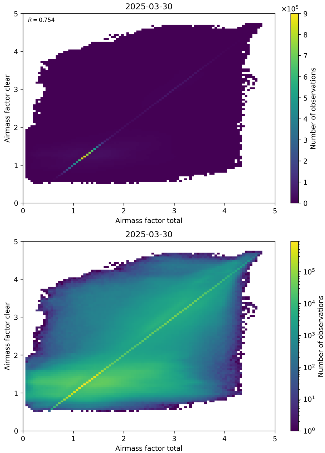
Figure 100: Scatter density plot of “Airmass factor total” against “Airmass factor clear” for 2025-03-29 to 2025-03-31.
