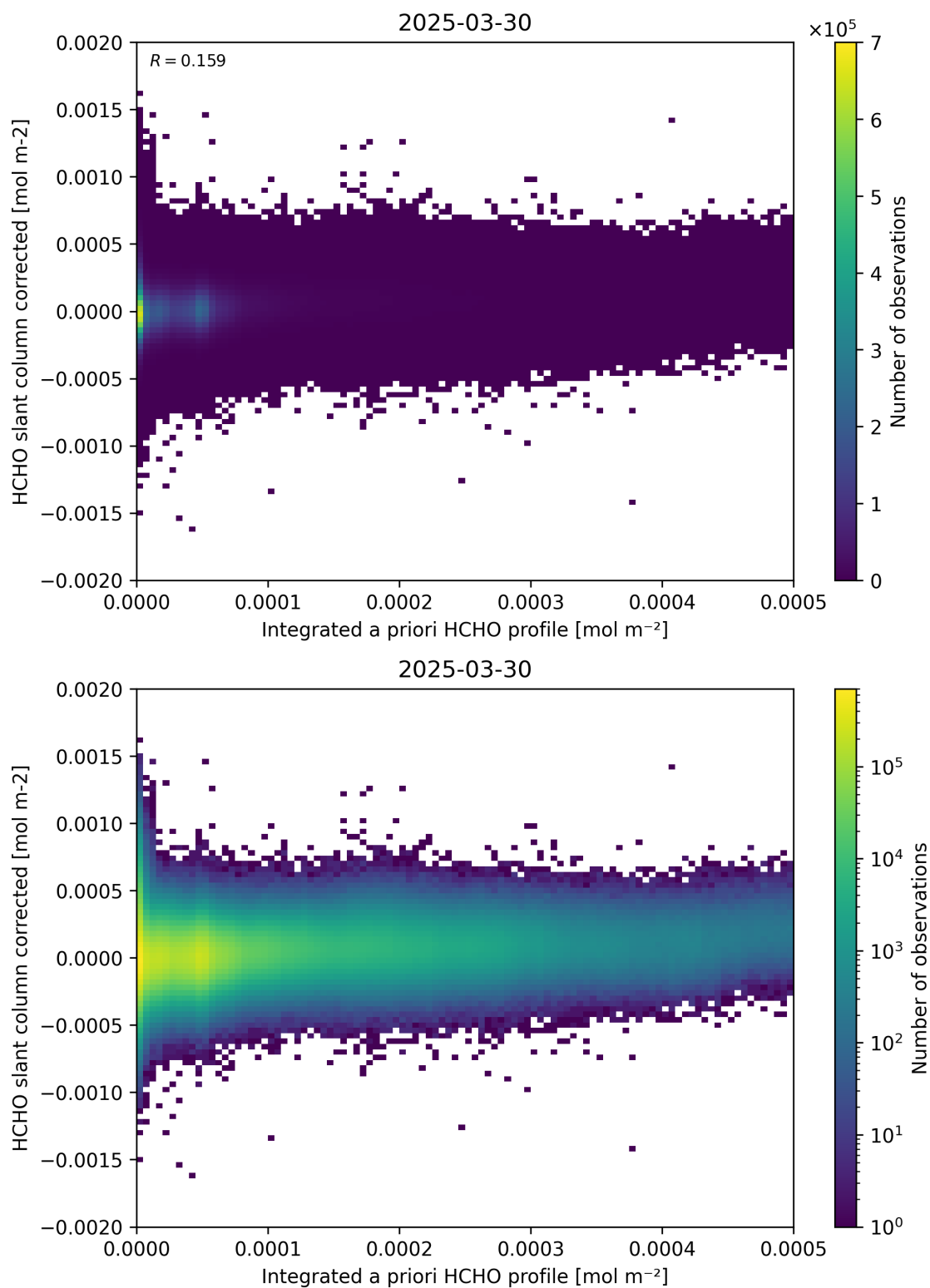
Figure 151: Scatter density plot of “Integrated a priori HCHO profile” against “HCHO slant column corrected” for 2025-03-29 to 2025-03-31.
