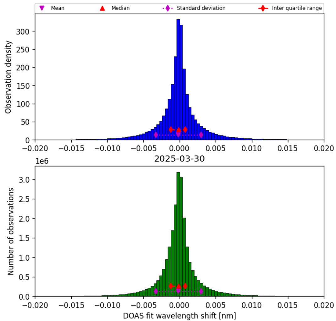
Figure 44: Histogram of “DOAS fit wavelength shift” for 2025-03-29 to 2025-03-31
