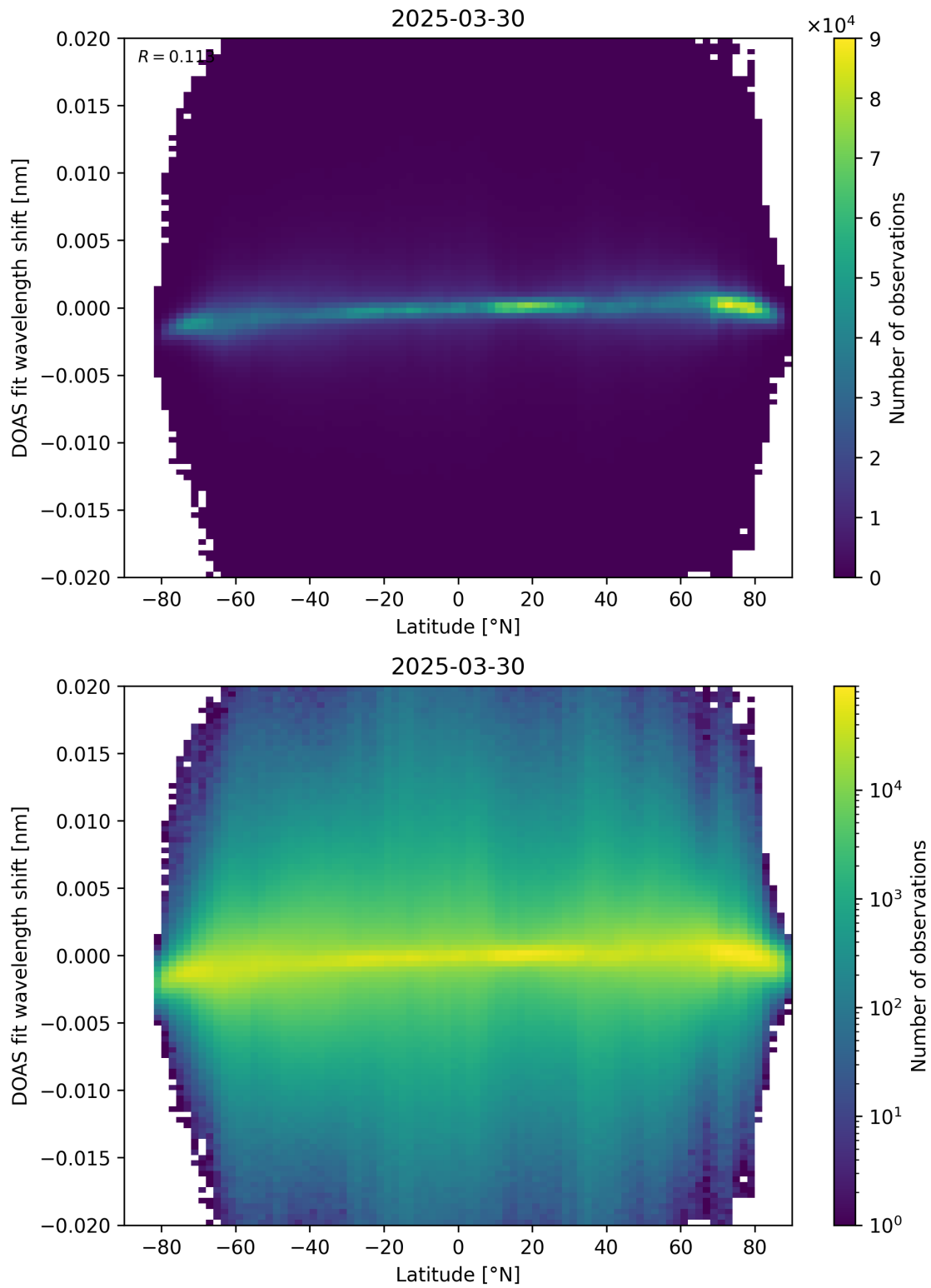
Figure 154: Scatter density plot of “Latitude” against “DOAS fit wavelength shift” for 2025-03-29 to 2025-03-31.
