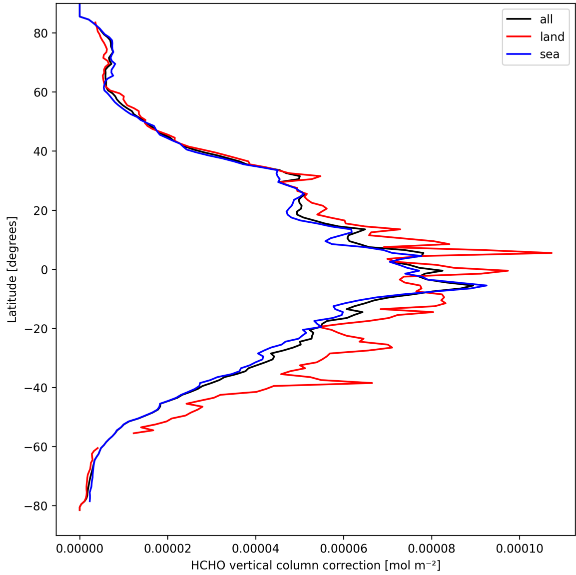
Figure 23: Zonal average of “HCHO vertical column correction” for 2025-03-29 to 2025-03-31.
