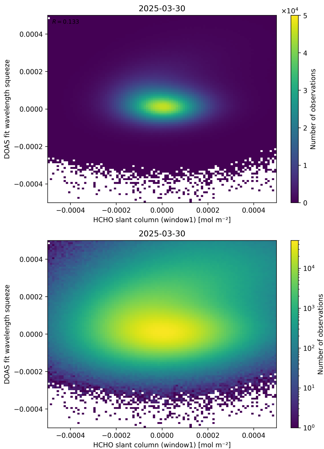
Figure 80: Scatter density plot of “HCHO slant column (window1)” against “DOAS fit wavelength squeeze” for 2025-03-29 to 2025-03-31.
