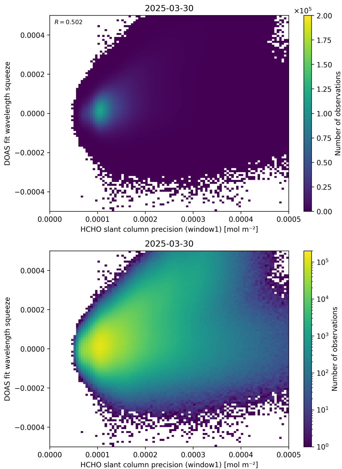
Figure 90: Scatter density plot of “HCHO slant column precision (window1)” against “DOAS fit wavelength squeeze” for 2025-03-29 to 2025-03-31.
