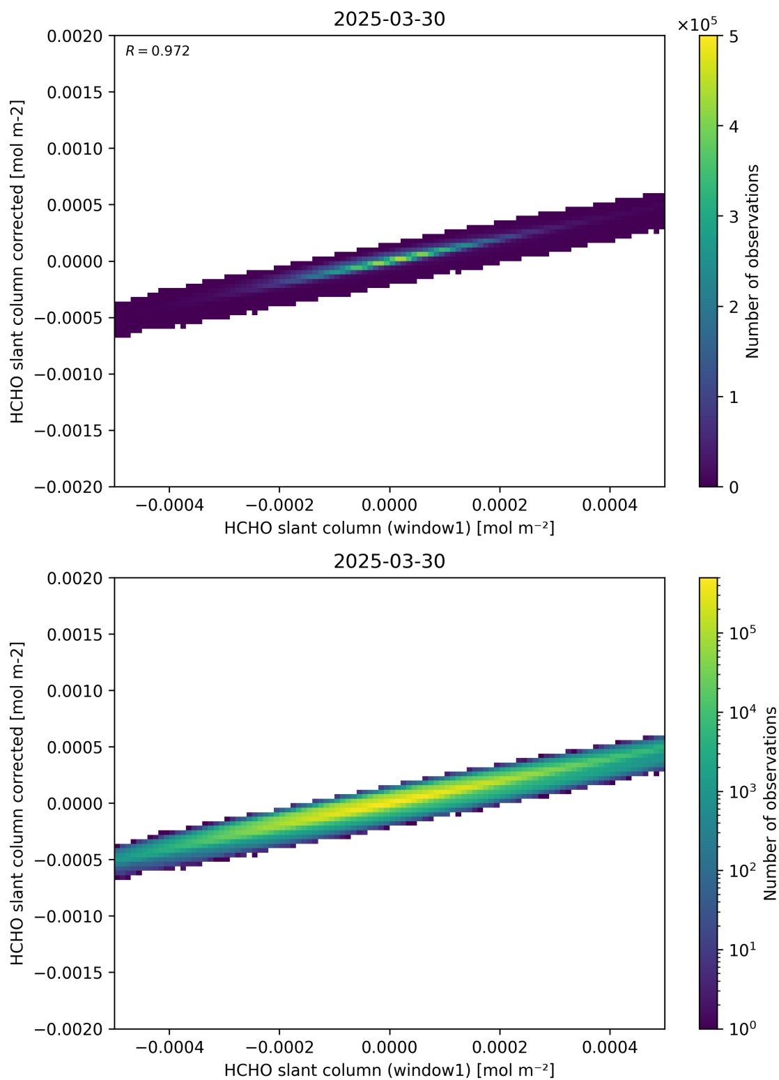
Figure 82: Scatter density plot of “HCHO slant column (window1)” against “HCHO slant column corrected” for 2025-03-29 to 2025-03-31.
