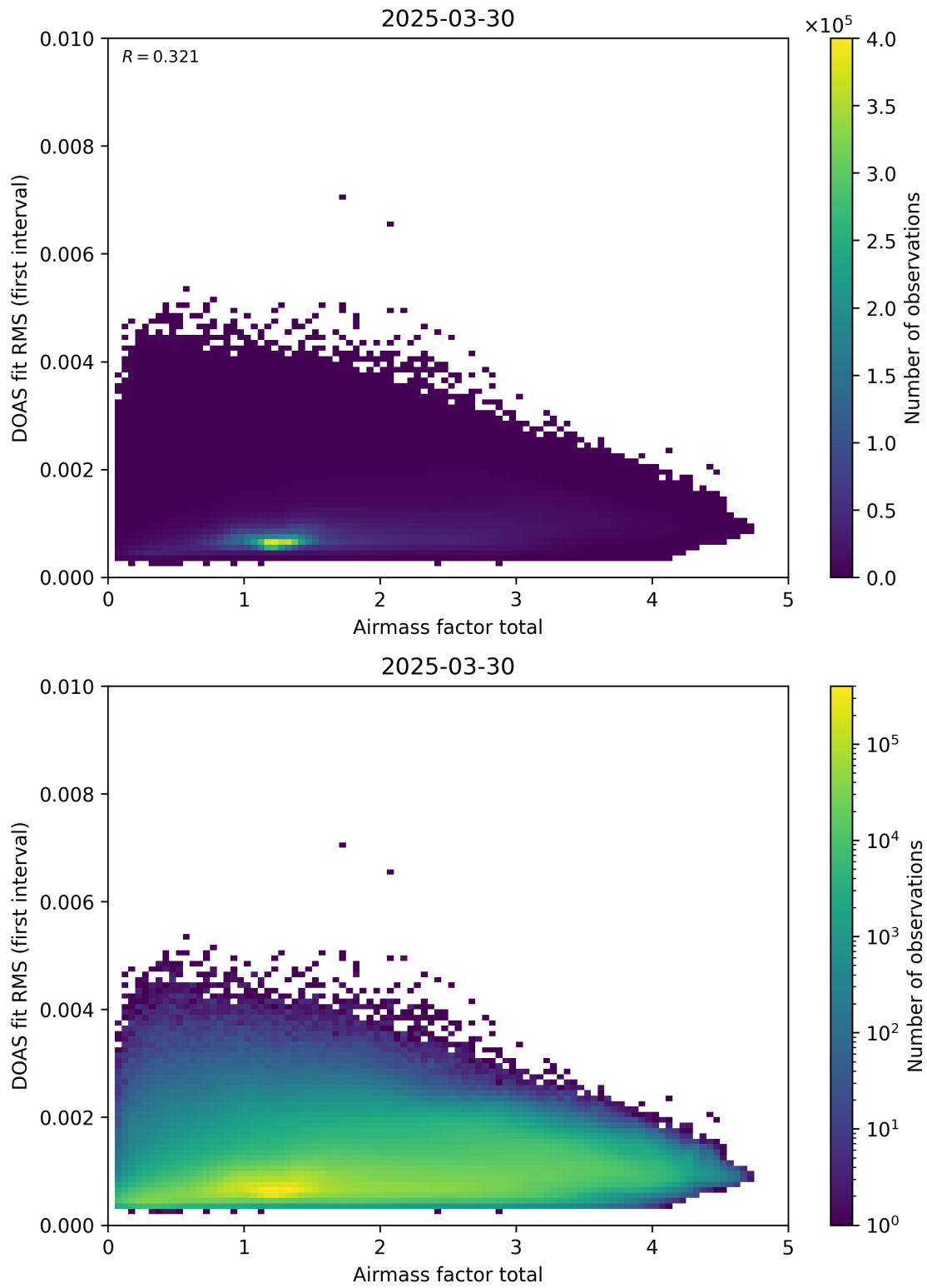
Figure 97: Scatter density plot of “Airmass factor total” against “DOAS fit RMS (first interval)” for 2025-03-29 to 2025-03-31.
