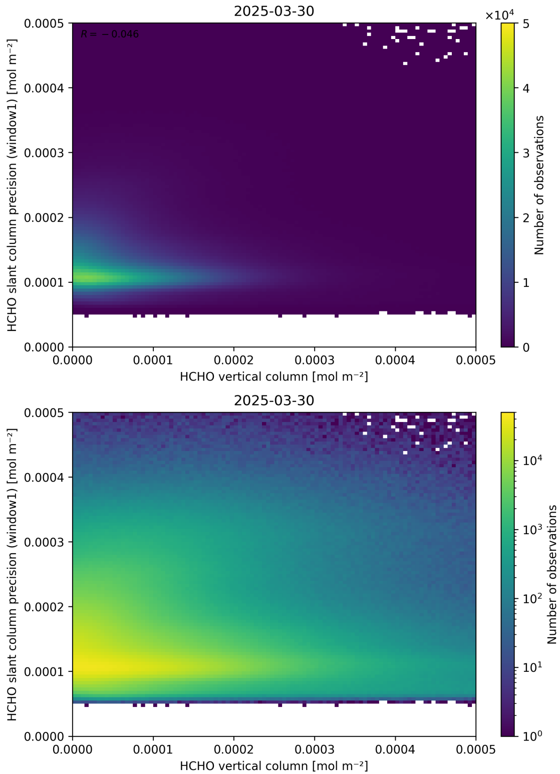
Figure 130: Scatter density plot of “HCHO vertical column” against “HCHO slant column precision (window1)” for 2025-03-29 to 2025-03-31.
