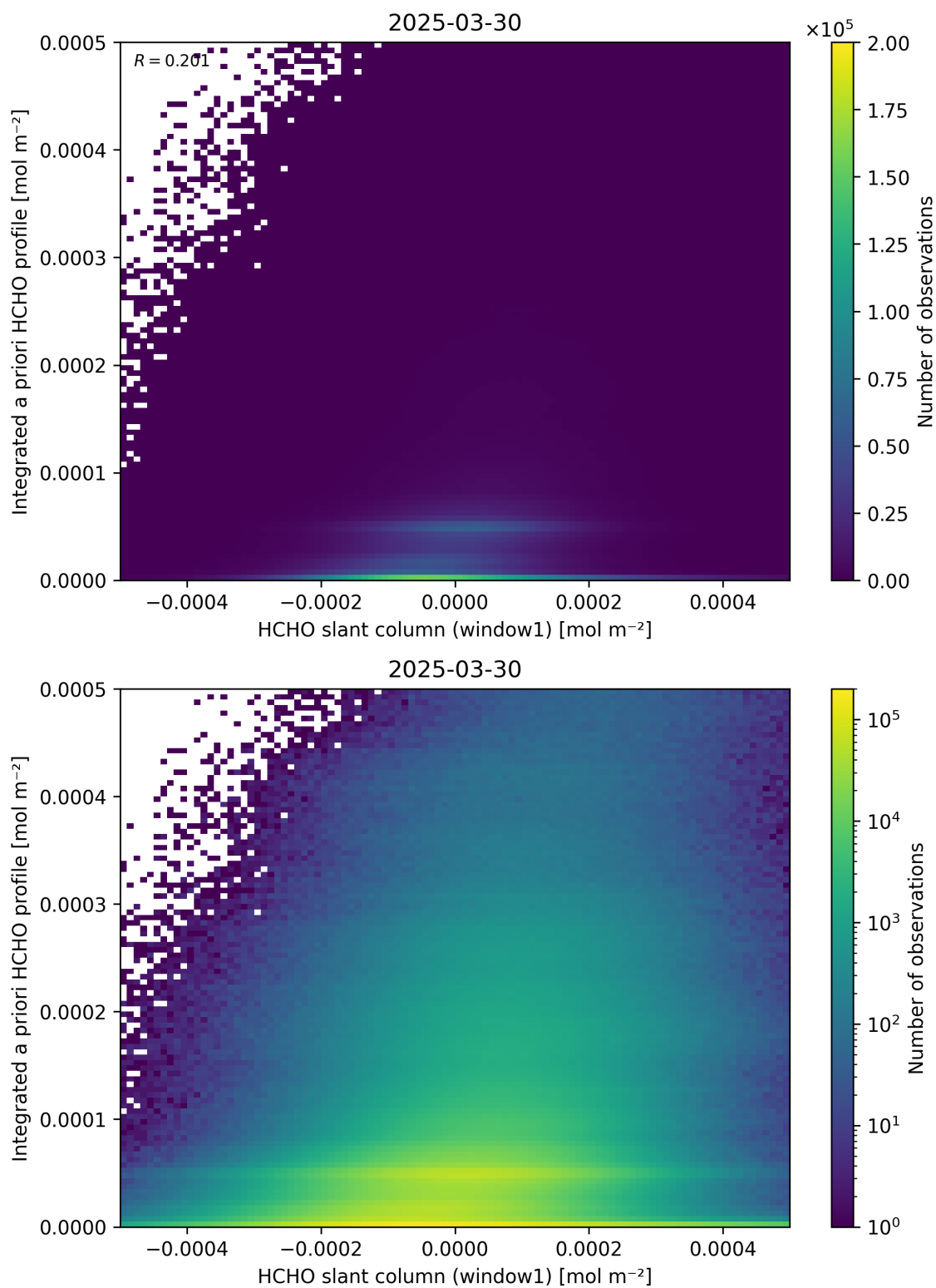
Figure 87: Scatter density plot of “HCHO slant column (window1)” against “Integrated a priori HCHO profile” for 2025-03-29 to 2025-03-31.
