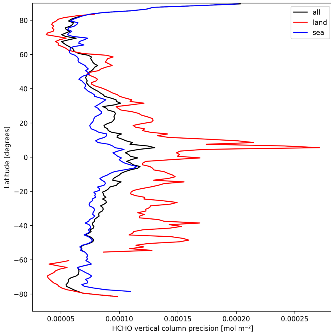
Figure 22: Zonal average of “HCHO vertical column precision” for 2025-03-29 to 2025-03-31.
