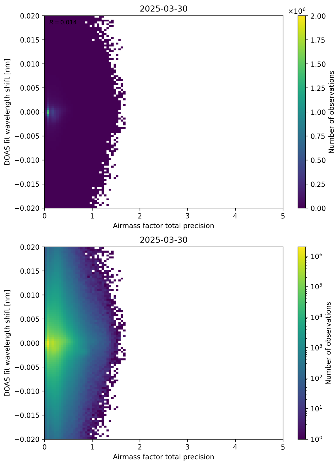
Figure 106: Scatter density plot of “Airmass factor total precision” against “DOAS fit wavelength shift” for 2025-03-29 to 2025-03-31.
