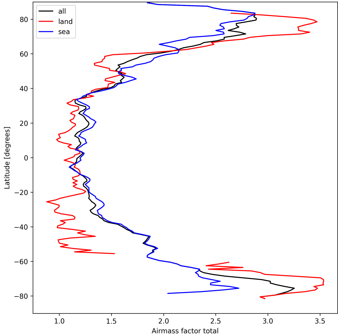
Figure 26: Zonal average of “Airmass factor total” for 2025-03-29 to 2025-03-31.
