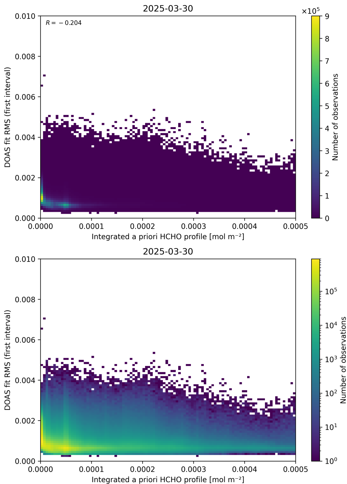
Figure 148: Scatter density plot of “Integrated a priori HCHO profile” against “DOAS fit RMS (first interval)” for 2025-03-29 to 2025-03-31.
