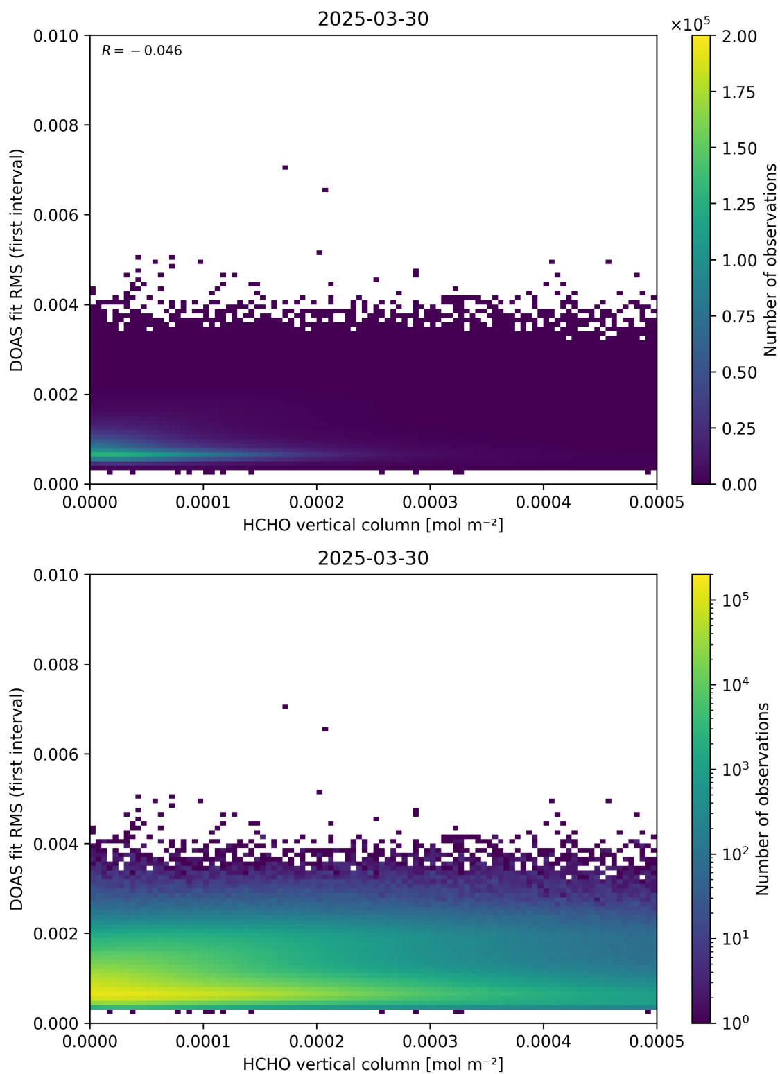
Figure 123: Scatter density plot of “HCHO vertical column” against “DOAS fit RMS (first interval)” for 2025-03-29 to 2025-03-31.
