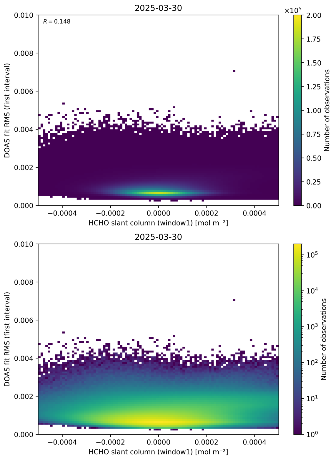
Figure 78: Scatter density plot of “HCHO slant column (window1)” against “DOAS fit RMS (first interval)” for 2025-03-29 to 2025-03-31.
