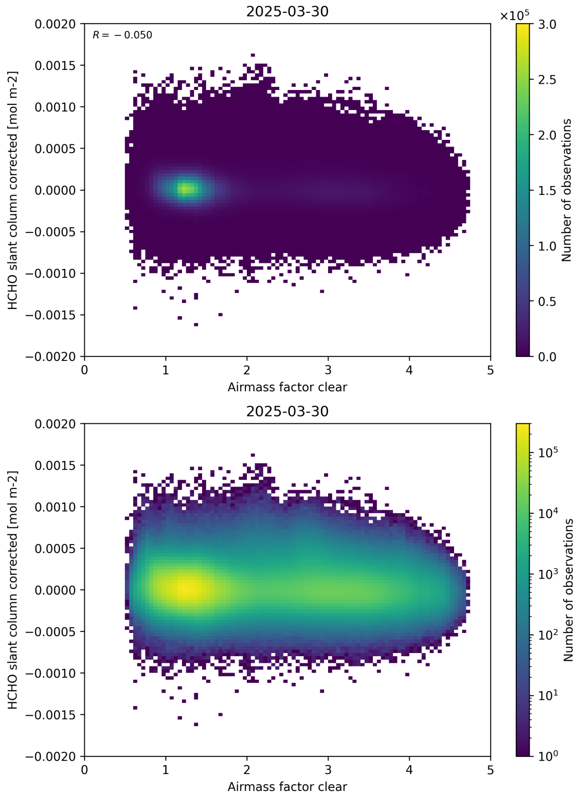
Figure 74: Scatter density plot of “Airmass factor clear” against “HCHO slant column corrected” for 2025-03-29 to 2025-03-31.
