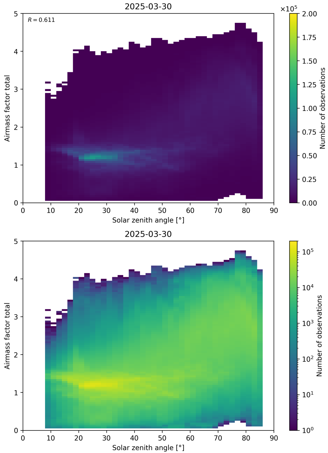
Figure 175: Scatter density plot of “Solar zenith angle” against “Airmass factor total” for 2025-03-29 to 2025-03-31.
