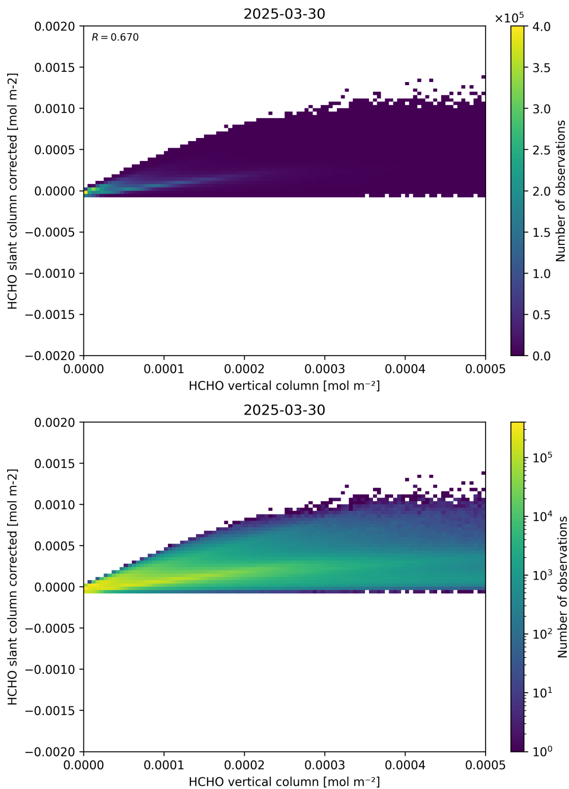
Figure 127: Scatter density plot of “HCHO vertical column” against “HCHO slant column corrected” for 2025-03-29 to 2025-03-31.
