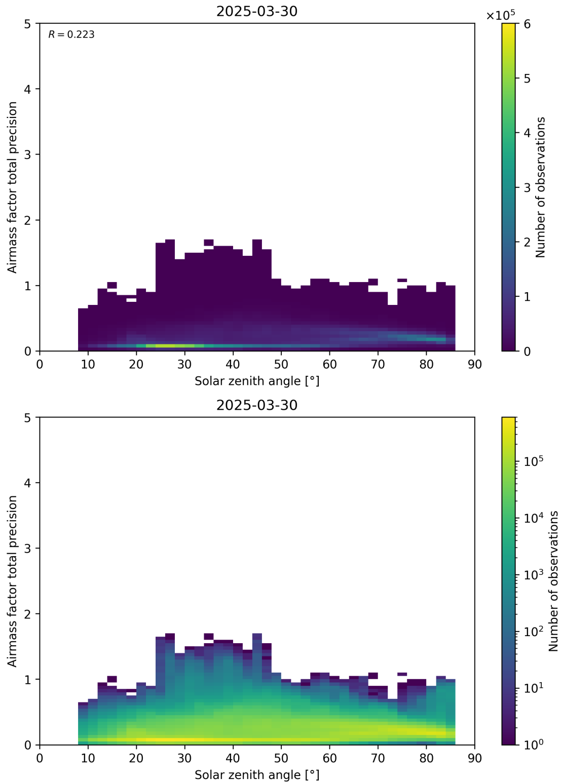
Figure 176: Scatter density plot of “Solar zenith angle” against “Airmass factor total precision” for 2025-03-29 to 2025-03-31.
