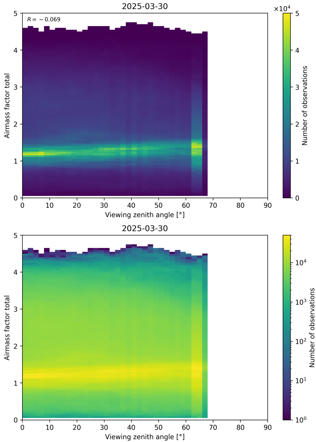
Figure 190: Scatter density plot of “Viewing zenith angle” against “Airmass factor total” for 2025-03-29 to 2025-03-31.
