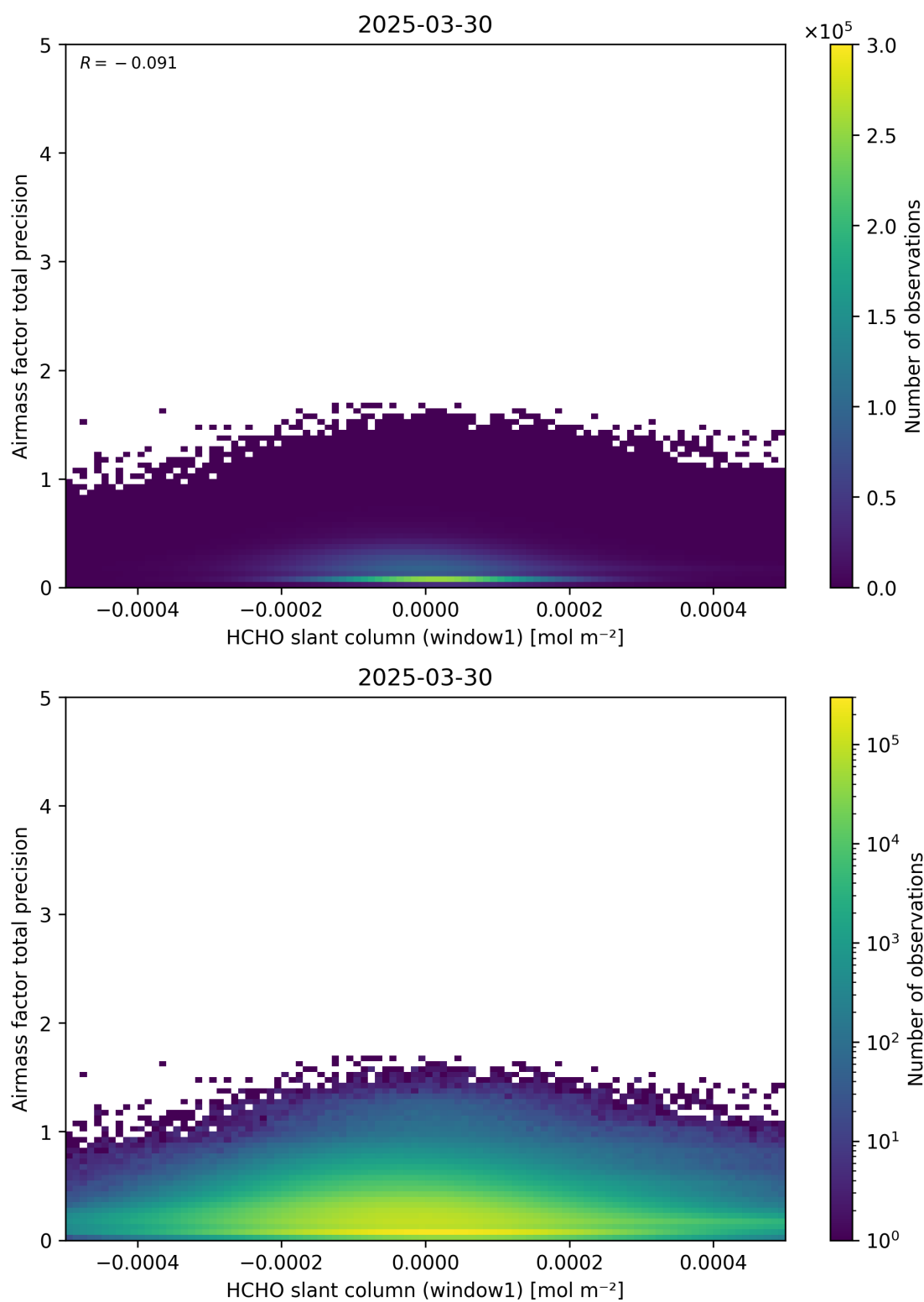
Figure 86: Scatter density plot of “HCHO slant column (window1)” against “Airmass factor total precision” for 2025-03-29 to 2025-03-31.
