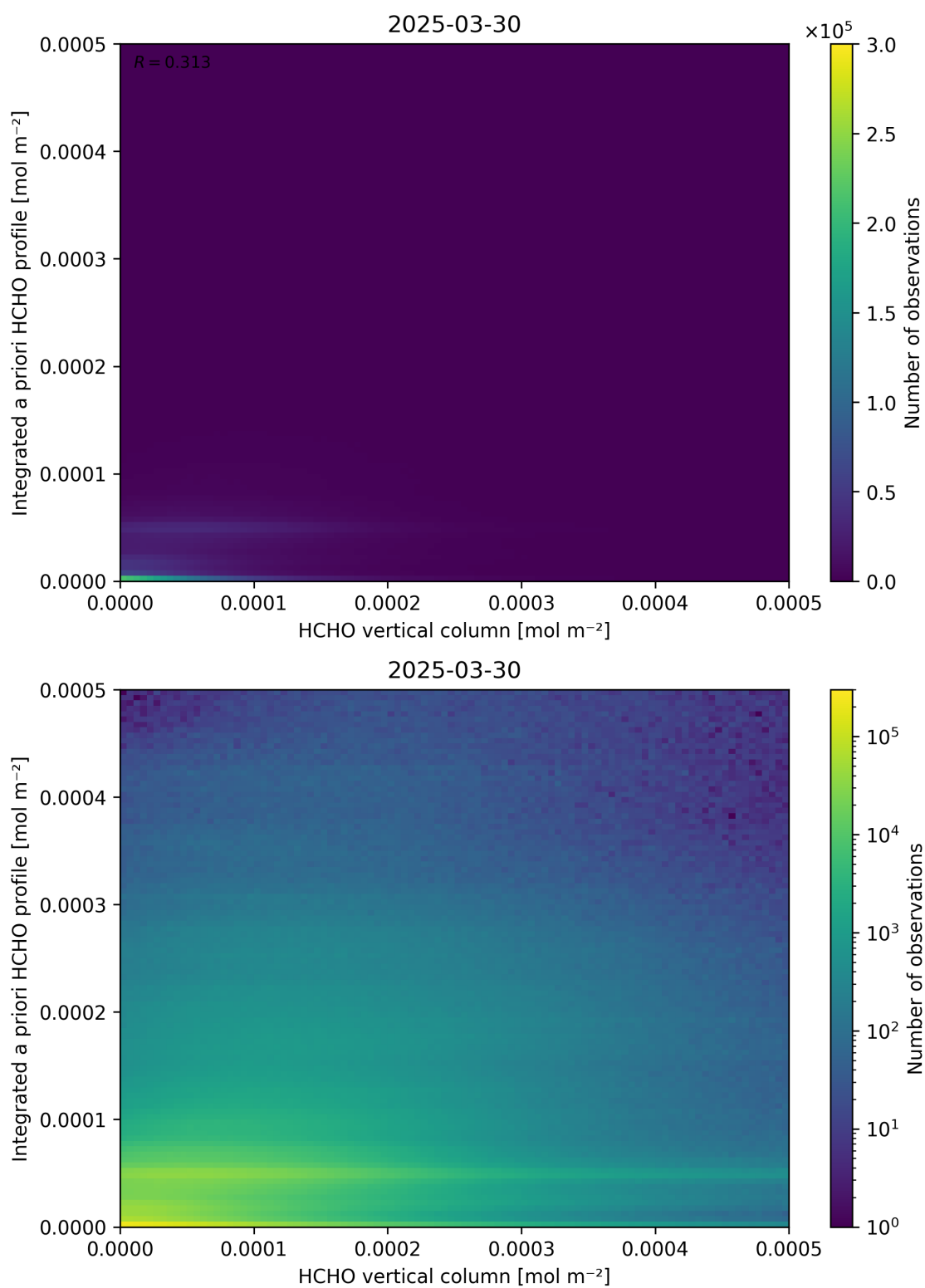
Figure 135: Scatter density plot of “HCHO vertical column” against “Integrated a priori HCHO profile” for 2025-03-29 to 2025-03-31.
