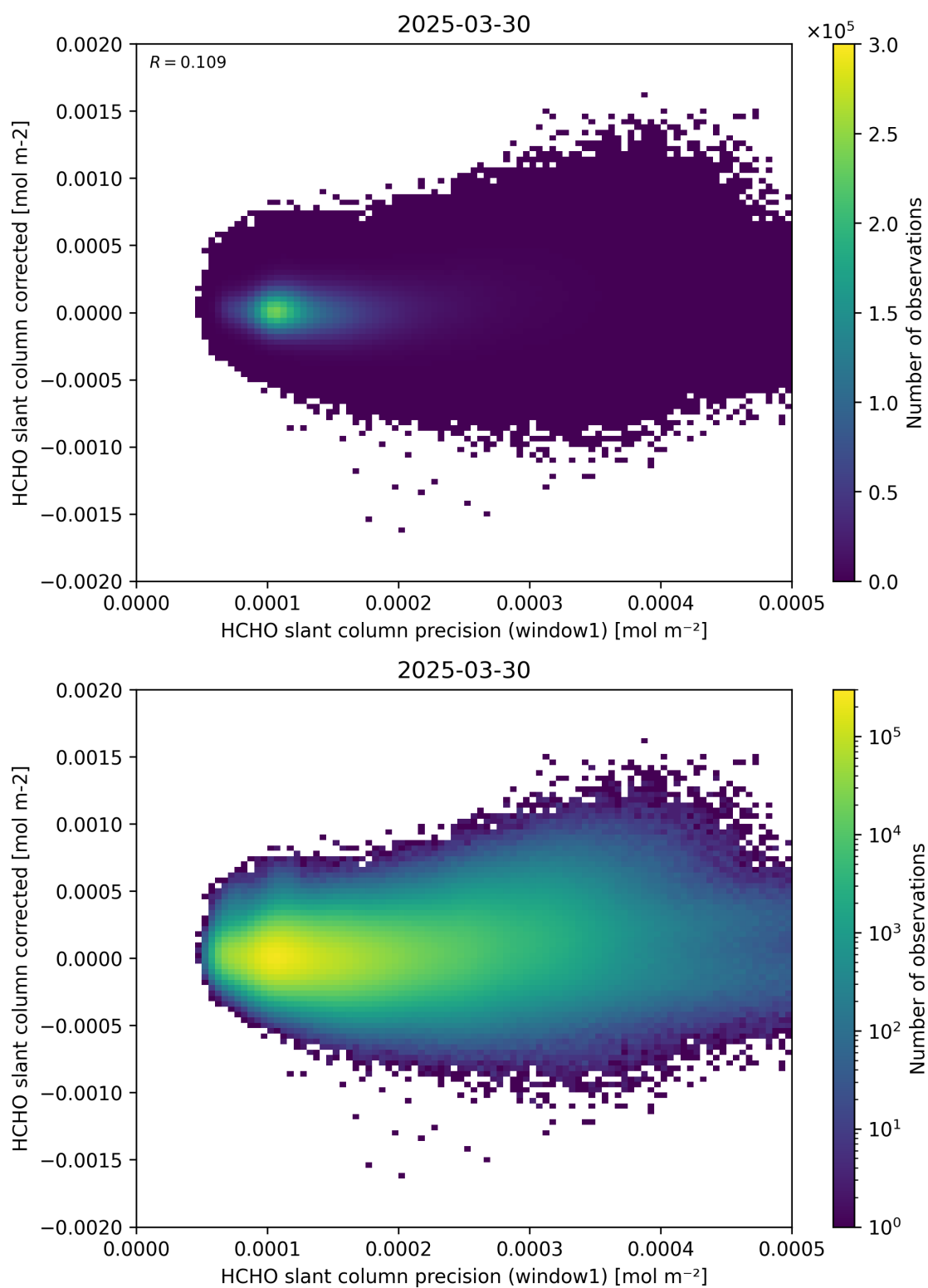
Figure 92: Scatter density plot of “HCHO slant column precision (window1)” against “HCHO slant column corrected” for 2025-03-29 to 2025-03-31.
