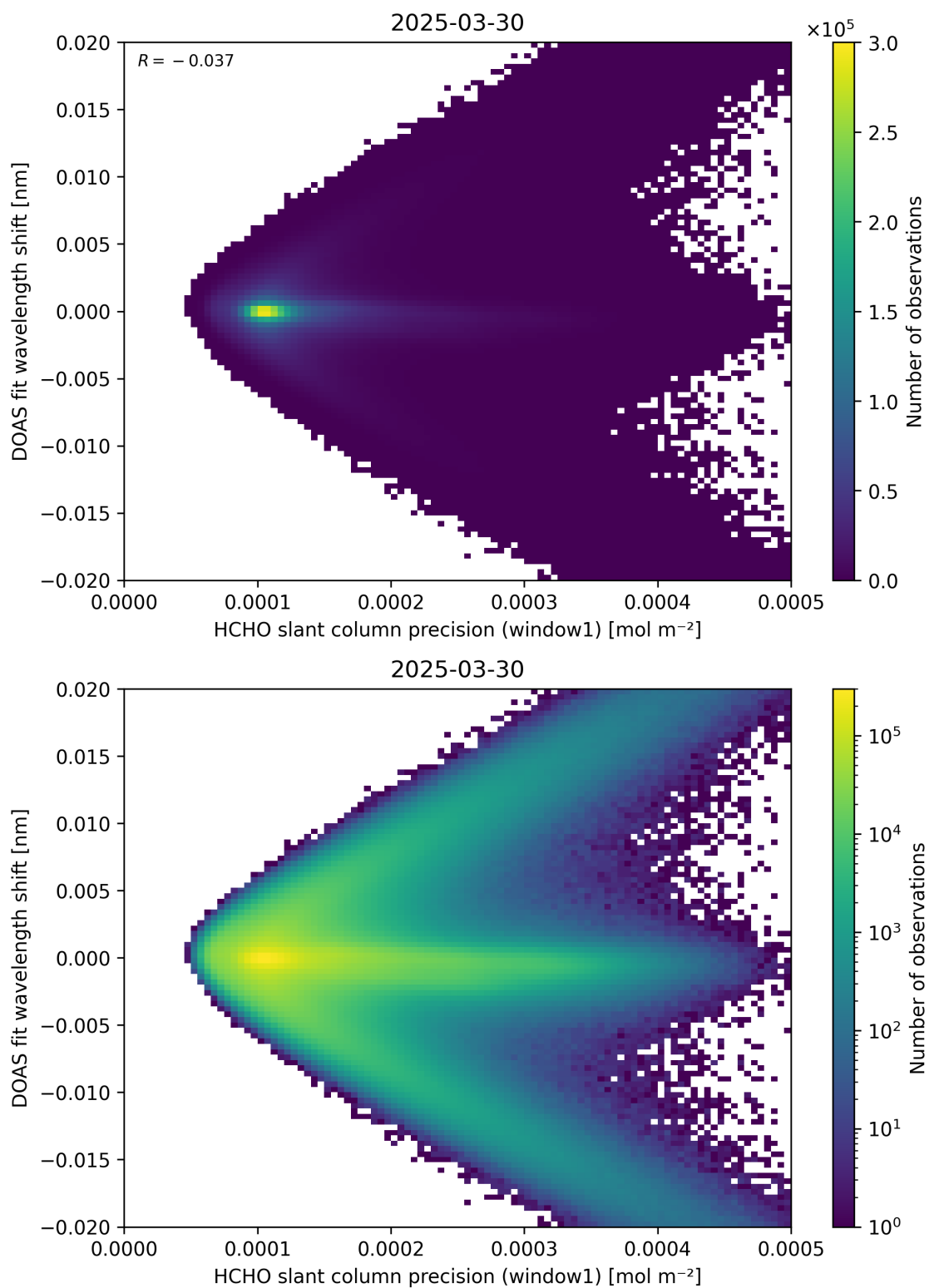
Figure 89: Scatter density plot of “HCHO slant column precision (window1)” against “DOAS fit wavelength shift” for 2025-03-29 to 2025-03-31.
