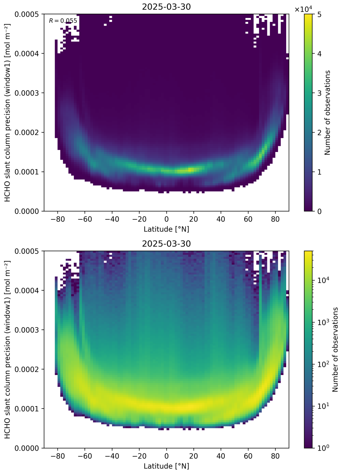
Figure 160: Scatter density plot of “Latitude” against “HCHO slant column precision (window1)” for 2025-03-29 to 2025-03-31.
