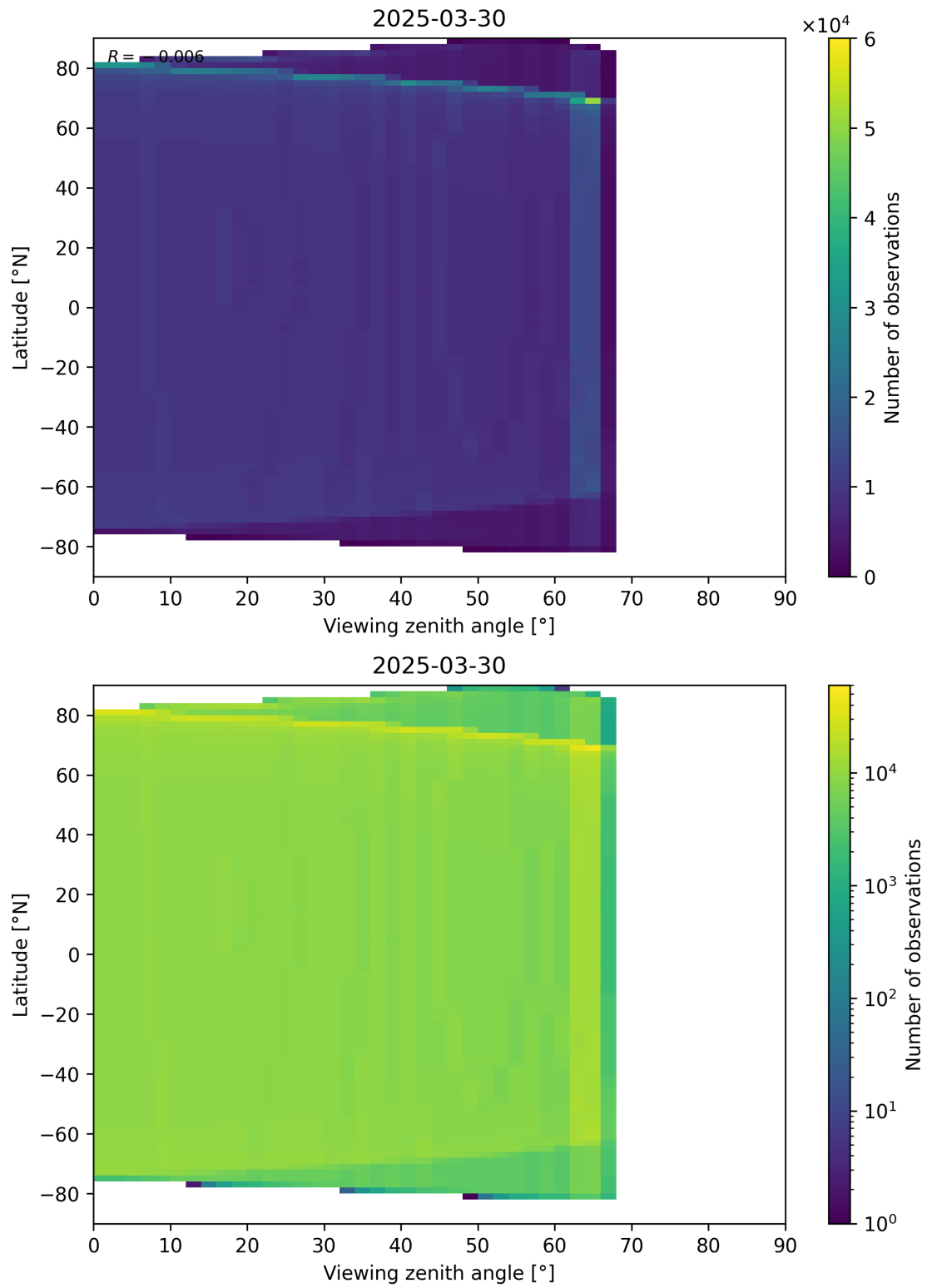
Figure 196: Scatter density plot of “Viewing zenith angle” against “Latitude” for 2025-03-29 to 2025-03-31.
