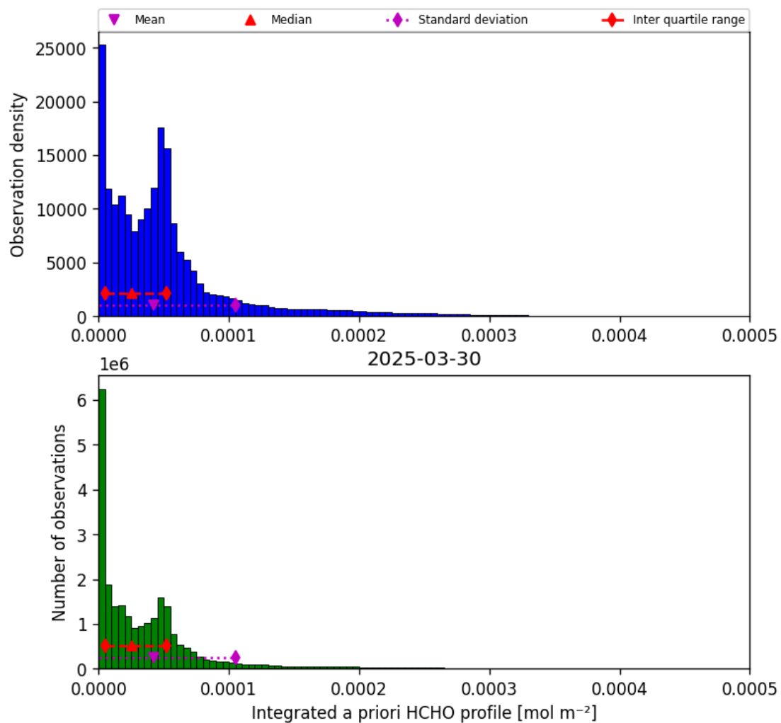
Figure 43: Histogram of “Integrated a priori HCHO profile” for 2025-03-29 to 2025-03-31
