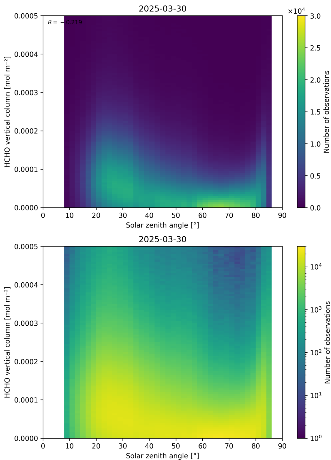
Figure 177: Scatter density plot of “Solar zenith angle” against “HCHO vertical column” for 2025-03-29 to 2025-03-31.
