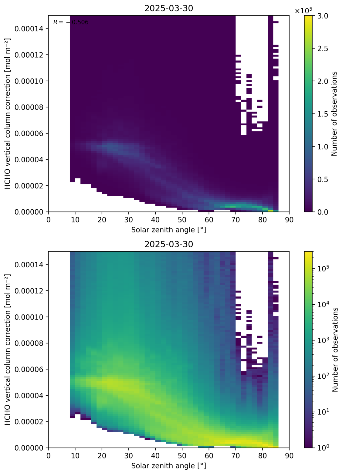
Figure 178: Scatter density plot of “Solar zenith angle” against “HCHO vertical column correction” for 2025-03-29 to 2025-03-31.
