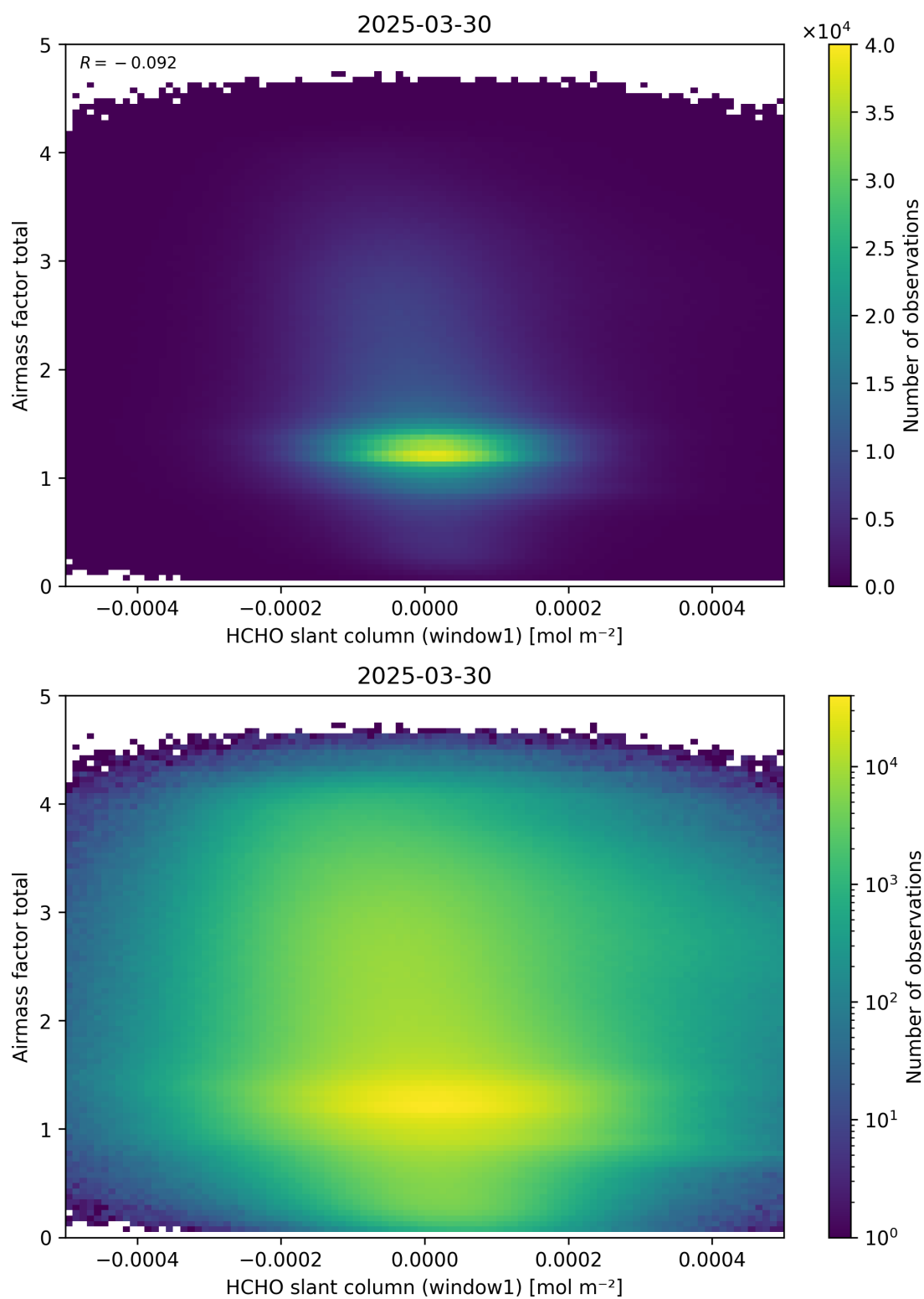
Figure 85: Scatter density plot of “HCHO slant column (window1)” against “Airmass factor total” for 2025-03-29 to 2025-03-31.
