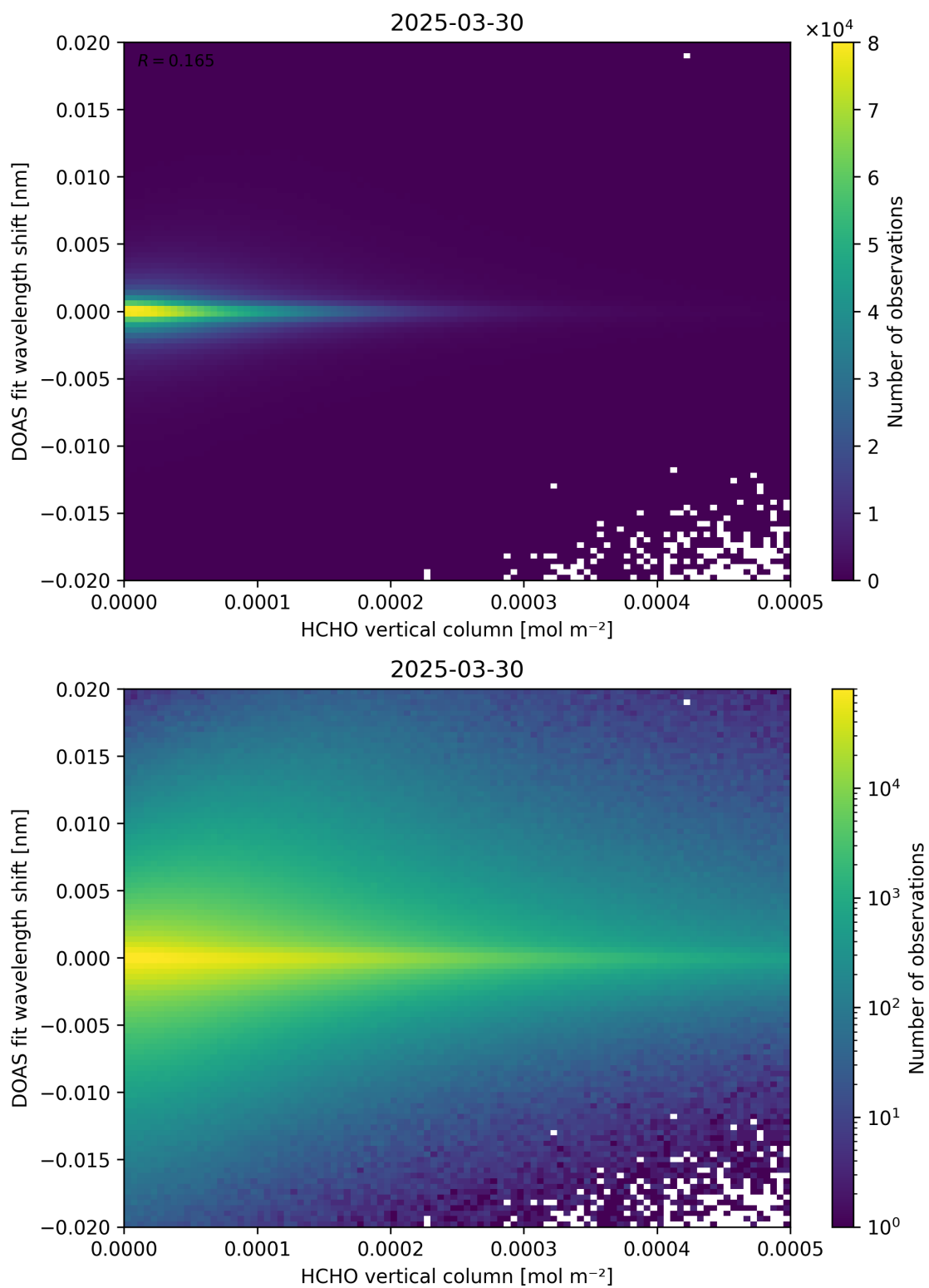
Figure 124: Scatter density plot of “HCHO vertical column” against “DOAS fit wavelength shift” for 2025-03-29 to 2025-03-31.
