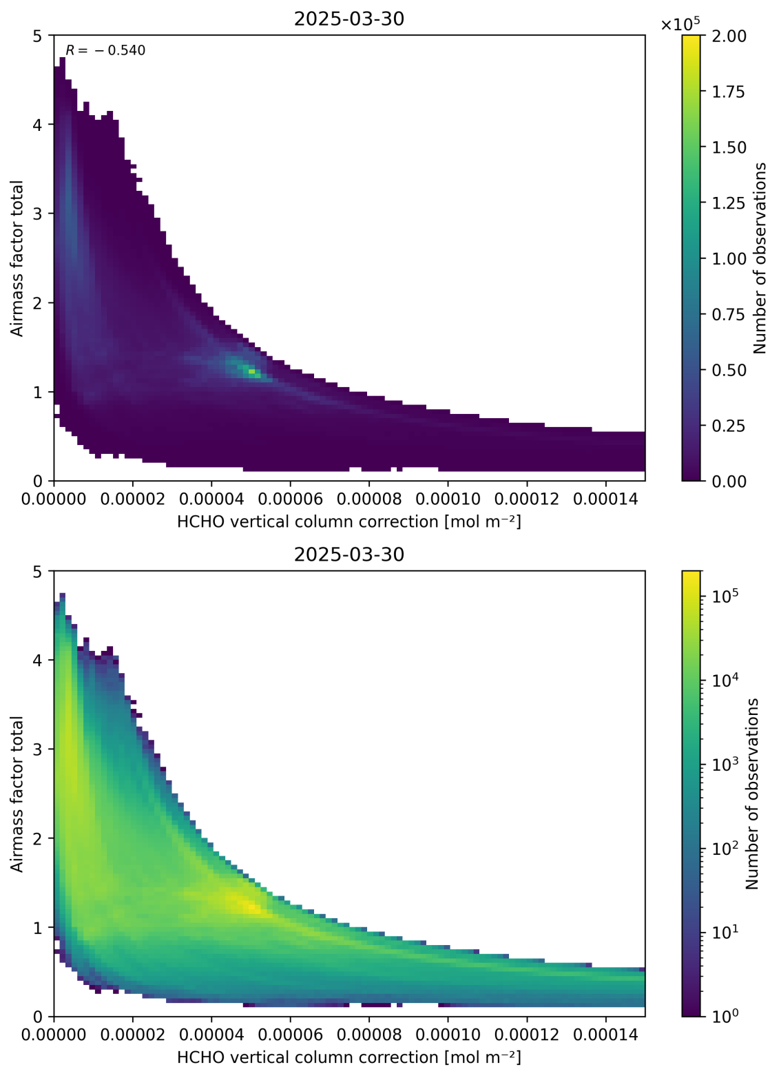
Figure 120: Scatter density plot of “HCHO vertical column correction” against “Airmass factor total” for 2025-03-29 to 2025-03-31.
