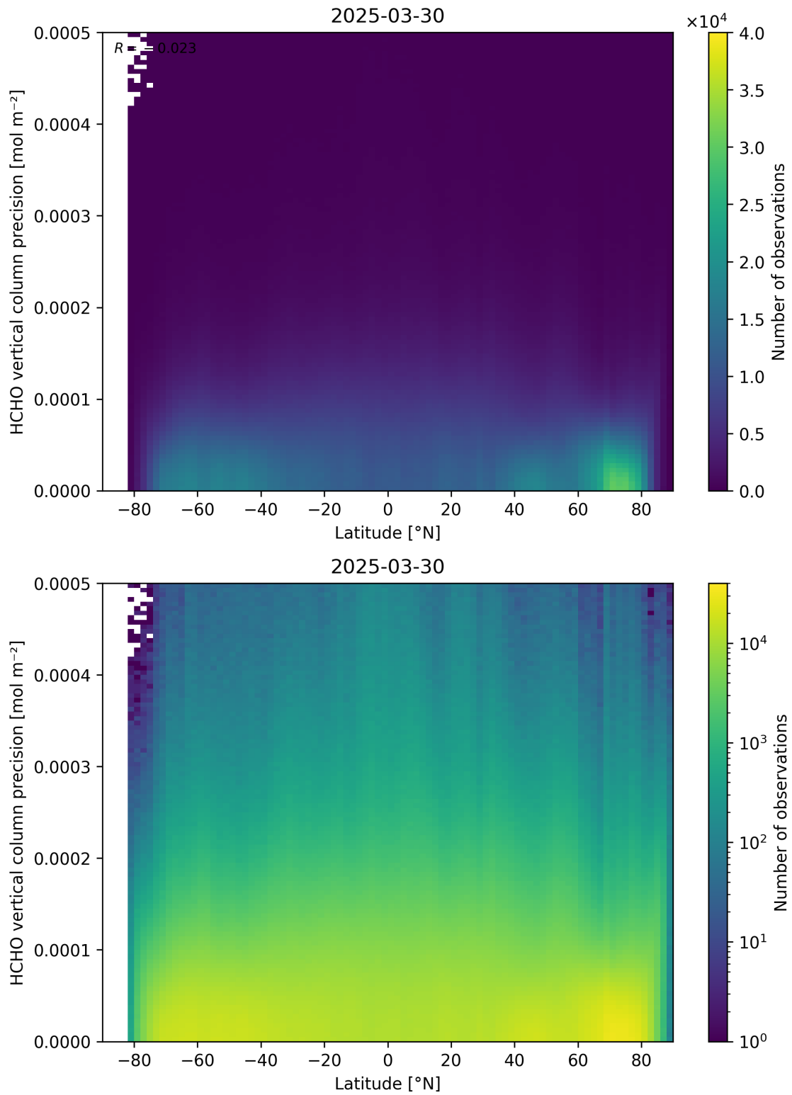
Figure 165: Scatter density plot of “Latitude” against “HCHO vertical column precision” for 2025-03-29 to 2025-03-31.
