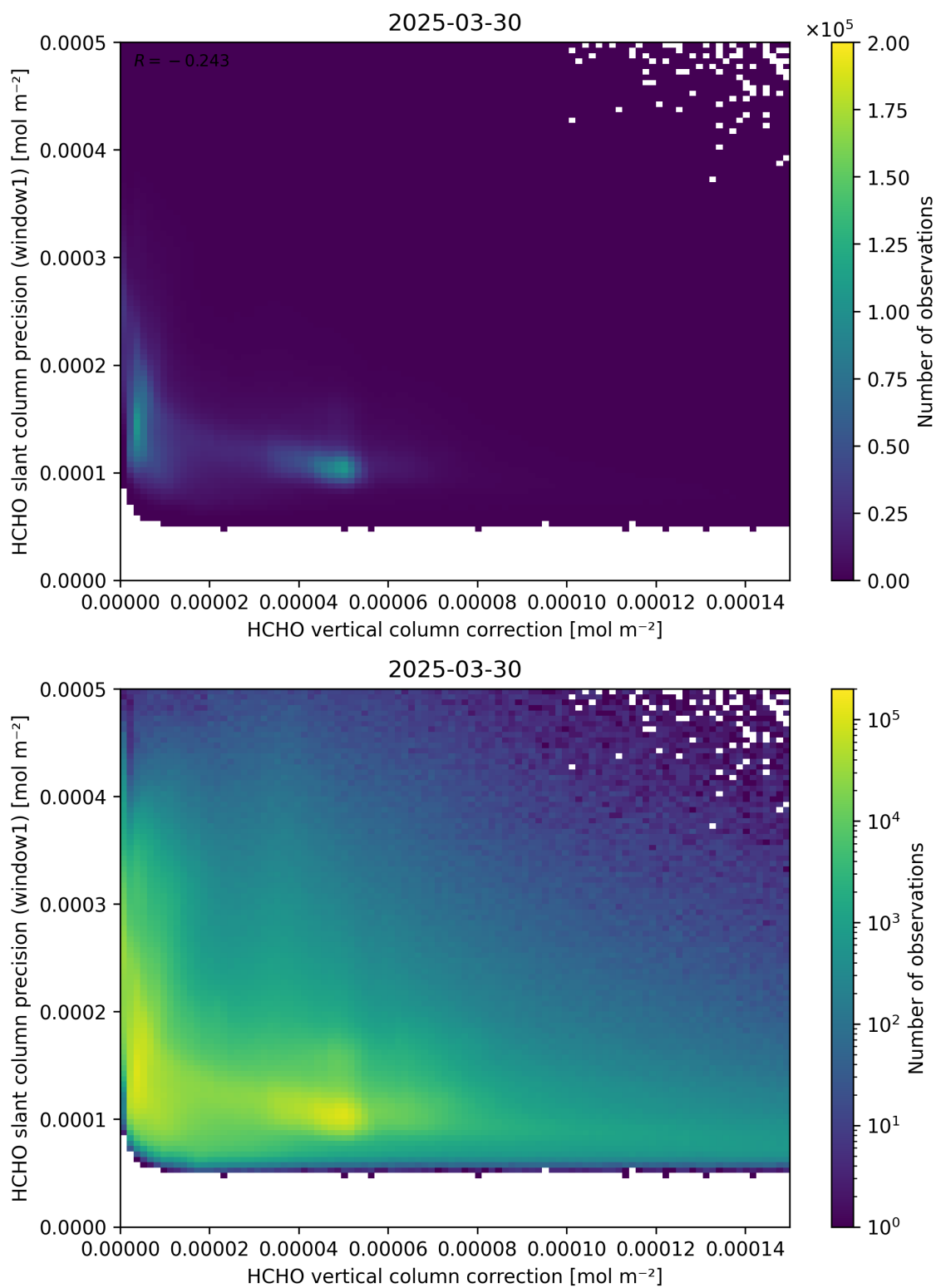
Figure 119: Scatter density plot of “HCHO vertical column correction” against “HCHO slant column precision (window1)” for 2025-03-29 to 2025-03-31.
