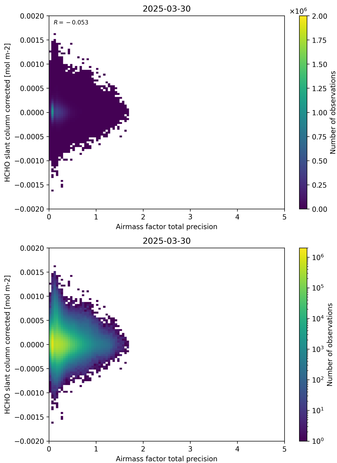
Figure 109: Scatter density plot of “Airmass factor total precision” against “HCHO slant column corrected” for 2025-03-29 to 2025-03-31.
