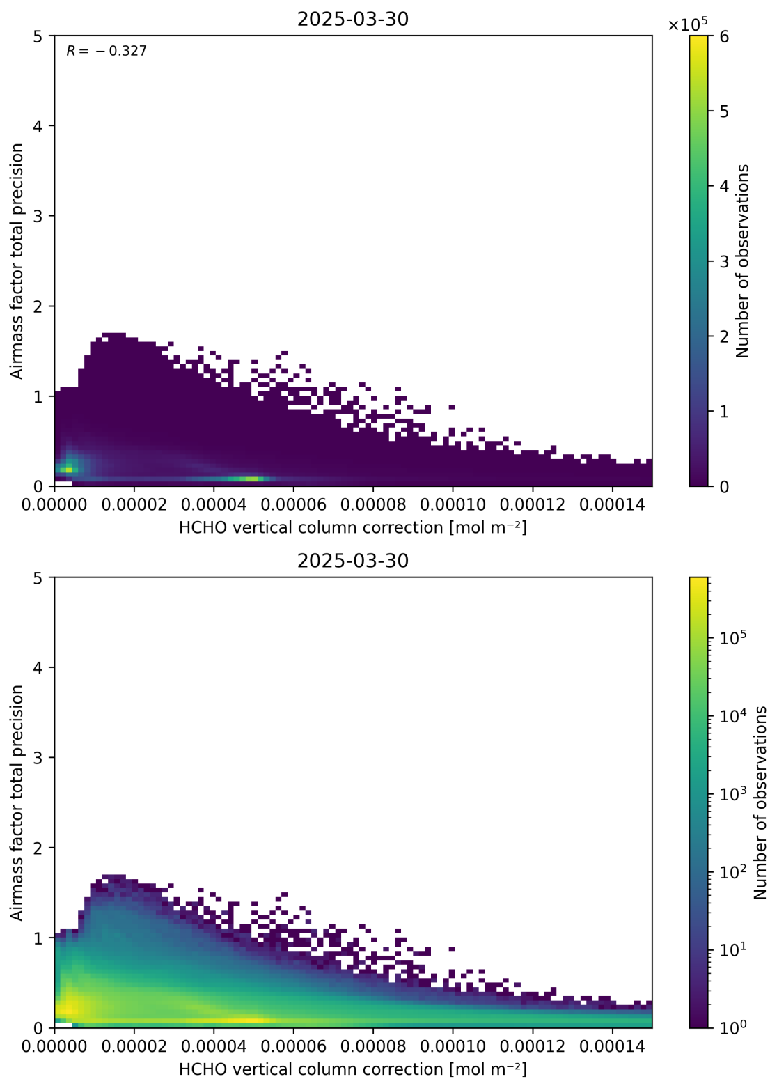
Figure 121: Scatter density plot of “HCHO vertical column correction” against “Airmass factor total precision” for 2025-03-29 to 2025-03-31.
