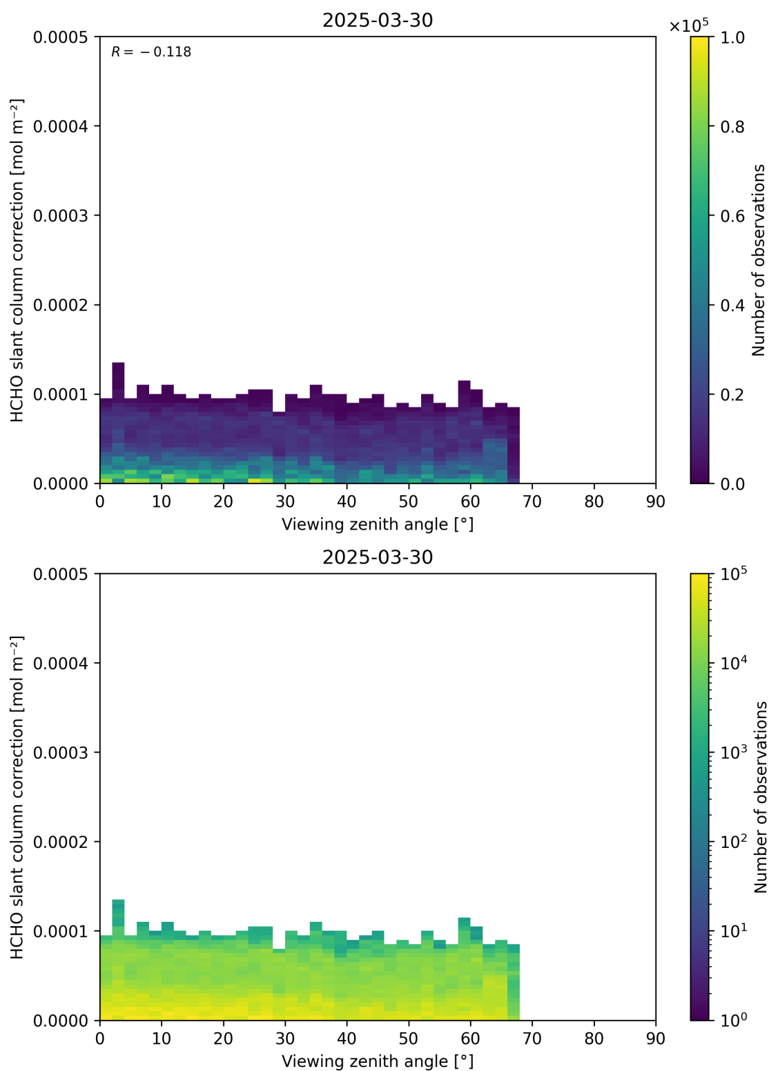
Figure 187: Scatter density plot of “Viewing zenith angle” against “HCHO slant column correction” for 2025-03-29 to 2025-03-31.
