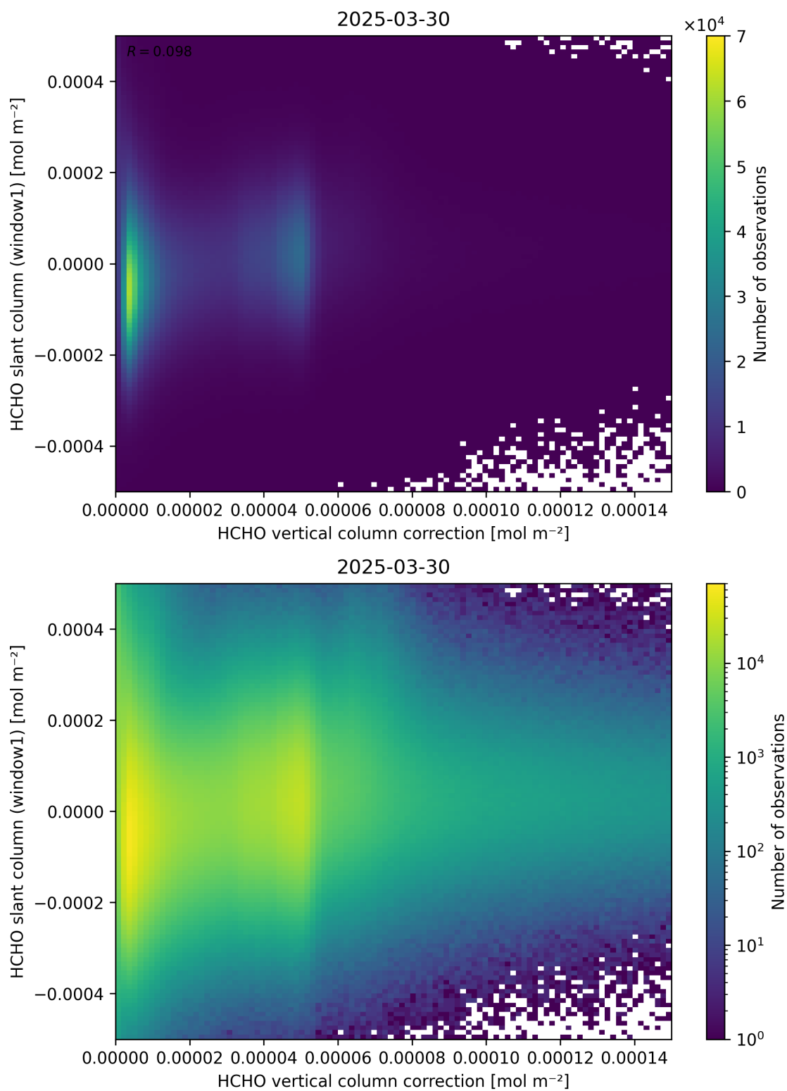
Figure 118: Scatter density plot of “HCHO vertical column correction” against “HCHO slant column (window1)” for 2025-03-29 to 2025-03-31.
