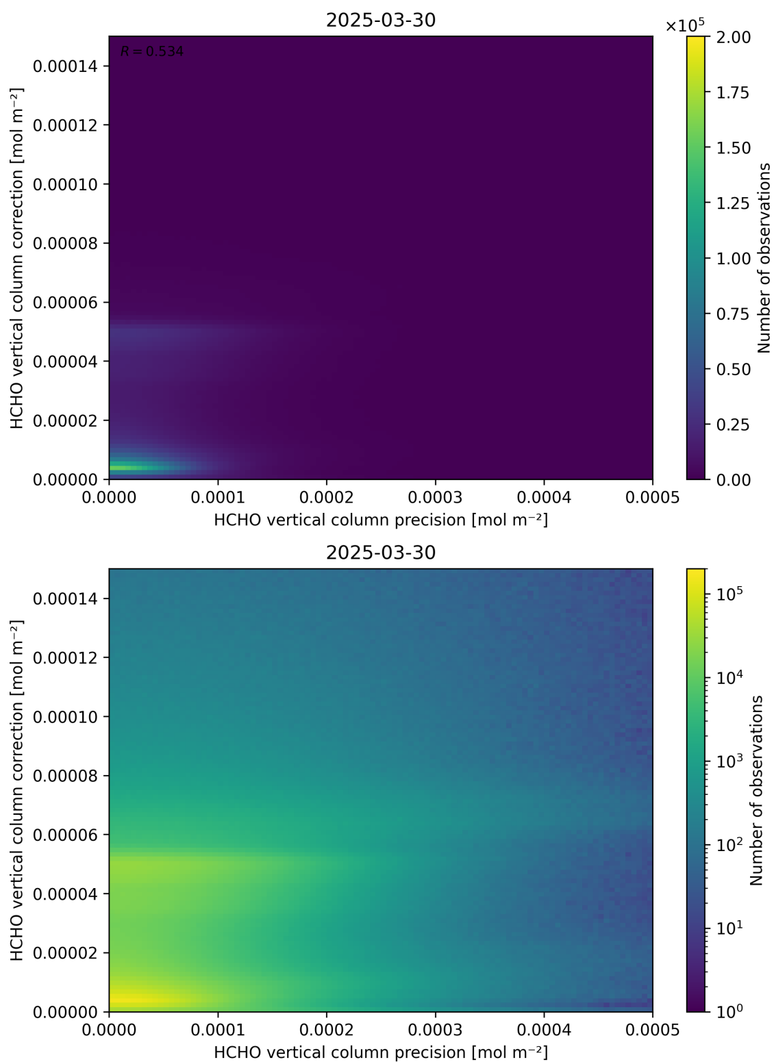
Figure 146: Scatter density plot of “HCHO vertical column precision” against “HCHO vertical column correction” for 2025-03-29 to 2025-03-31.
