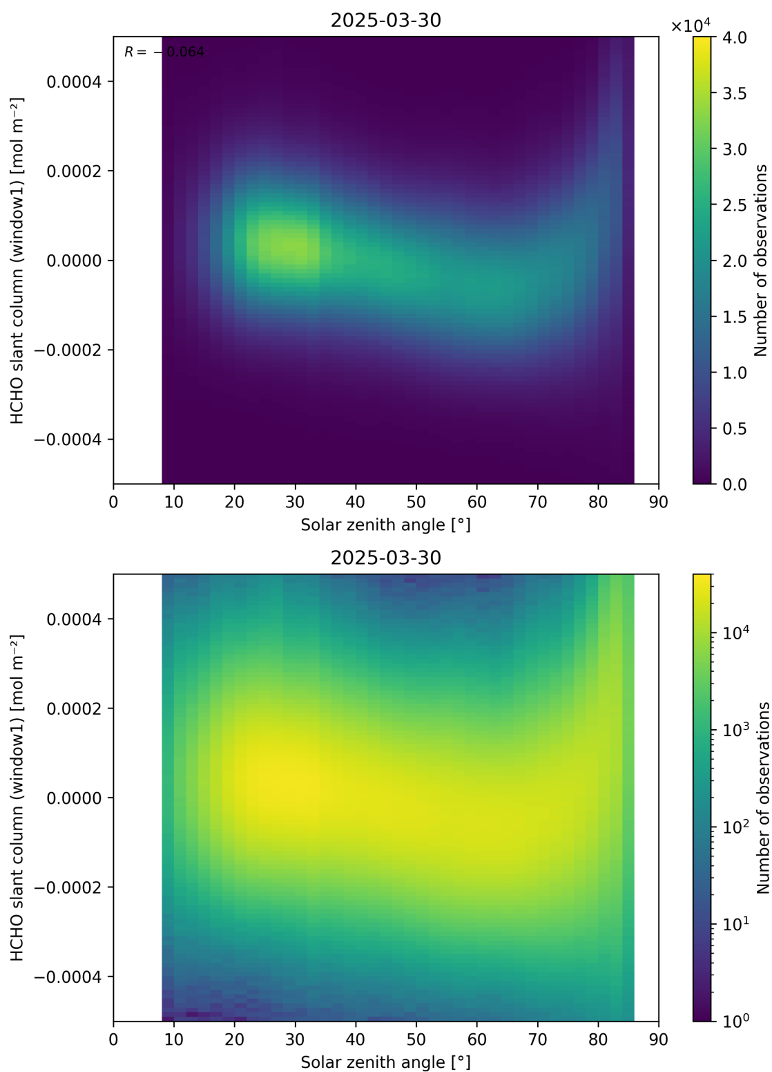
Figure 173: Scatter density plot of “Solar zenith angle” against “HCHO slant column (window1)” for 2025-03-29 to 2025-03-31.
