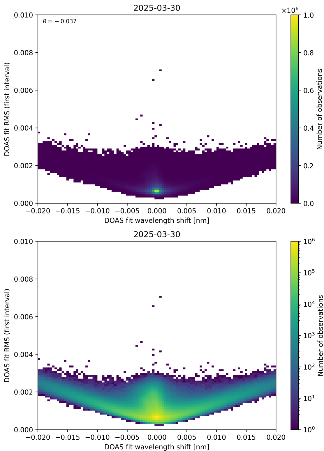
Figure 64: Scatter density plot of “DOAS fit wavelength shift” against “DOAS fit RMS (first interval)” for 2025-03-29 to 2025-03-31.
