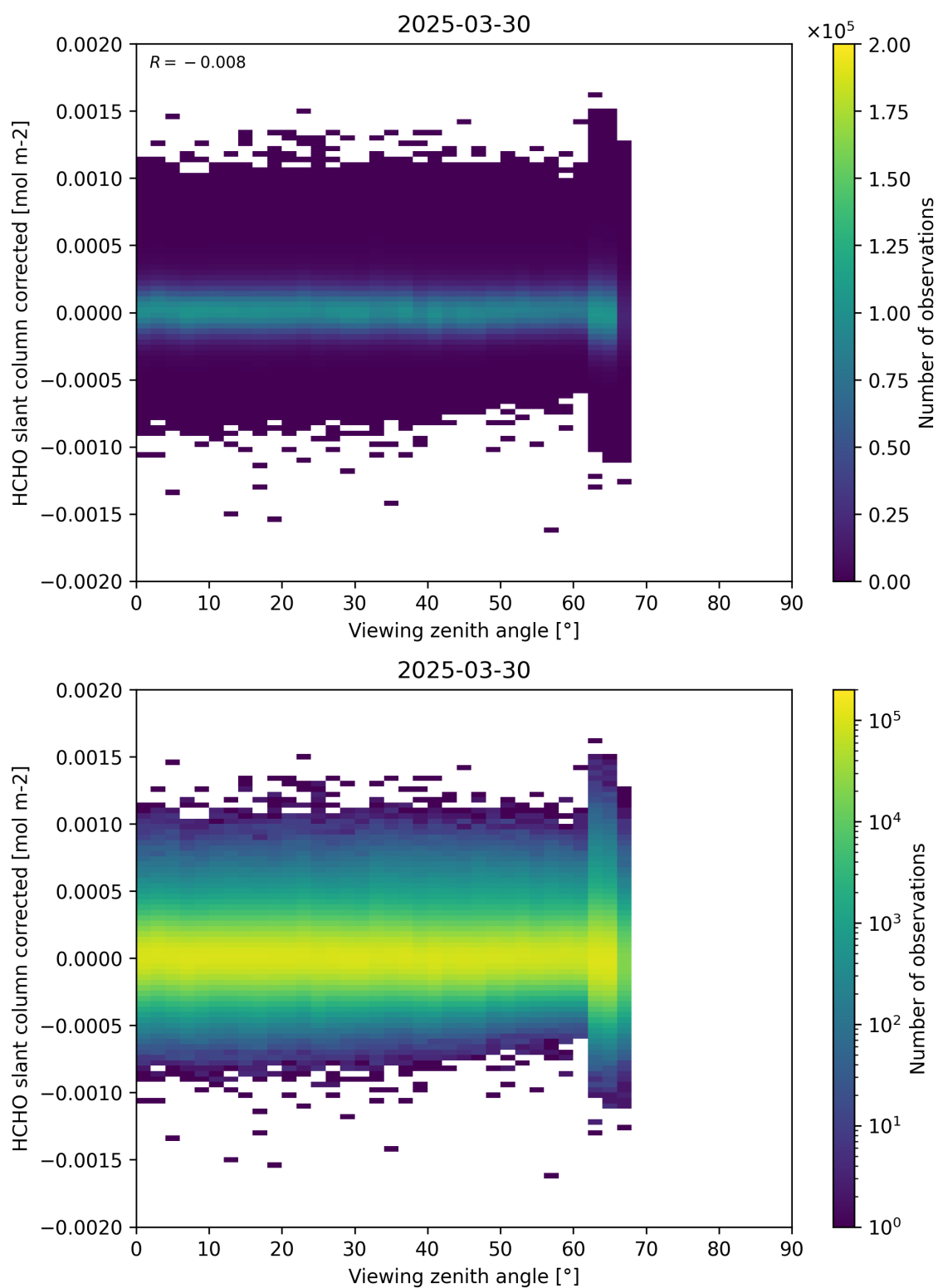
Figure 186: Scatter density plot of “Viewing zenith angle” against “HCHO slant column corrected” for 2025-03-29 to 2025-03-31.
