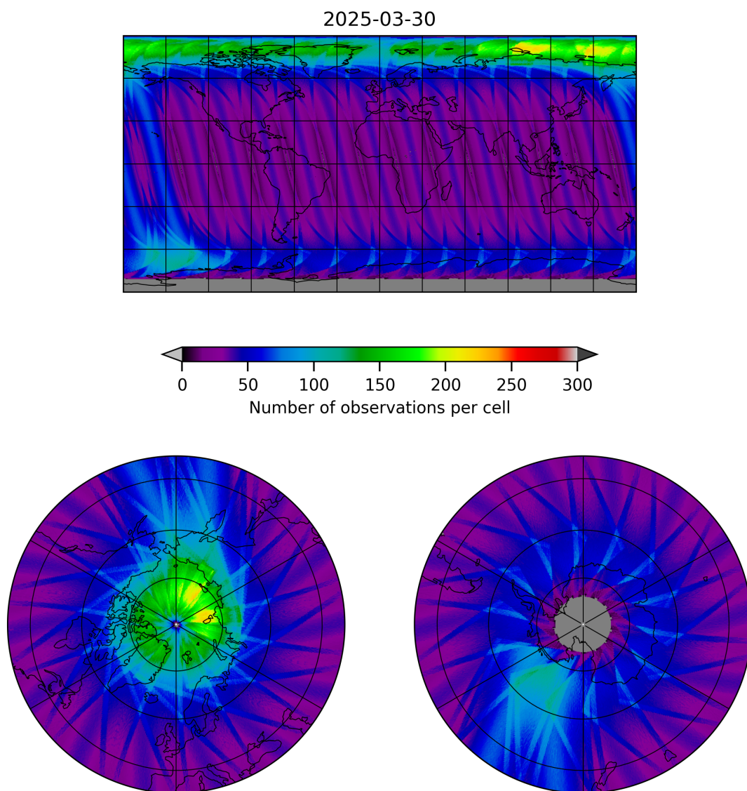
Figure 19: Map of the number of observations for 2025-03-29 to 2025-03-31
