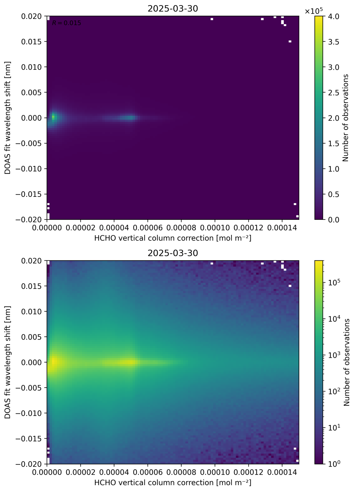
Figure 113: Scatter density plot of “HCHO vertical column correction” against “DOAS fit wavelength shift” for 2025-03-29 to 2025-03-31.
