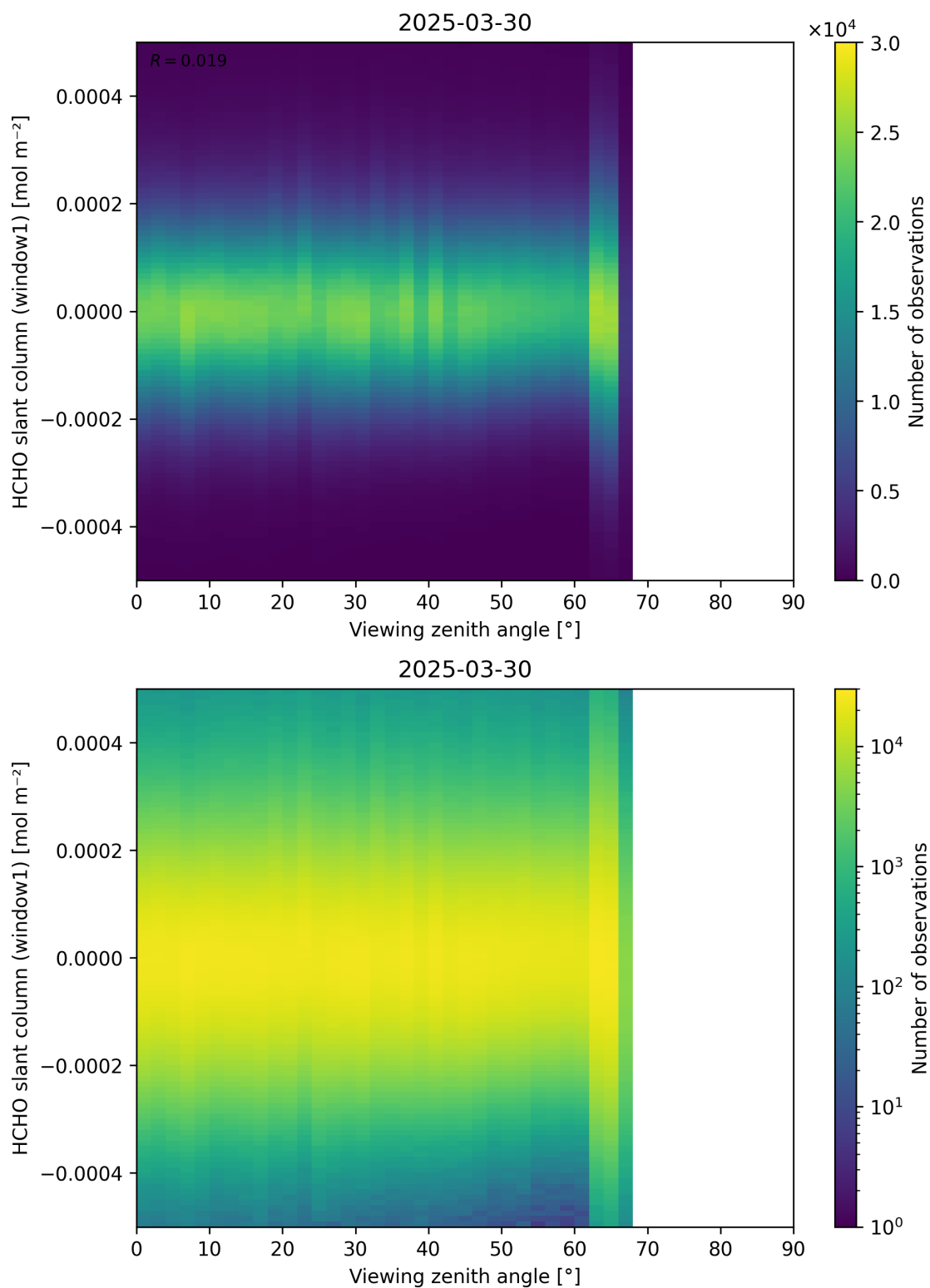
Figure 188: Scatter density plot of “Viewing zenith angle” against “HCHO slant column (window1)” for 2025-03-29 to 2025-03-31.
