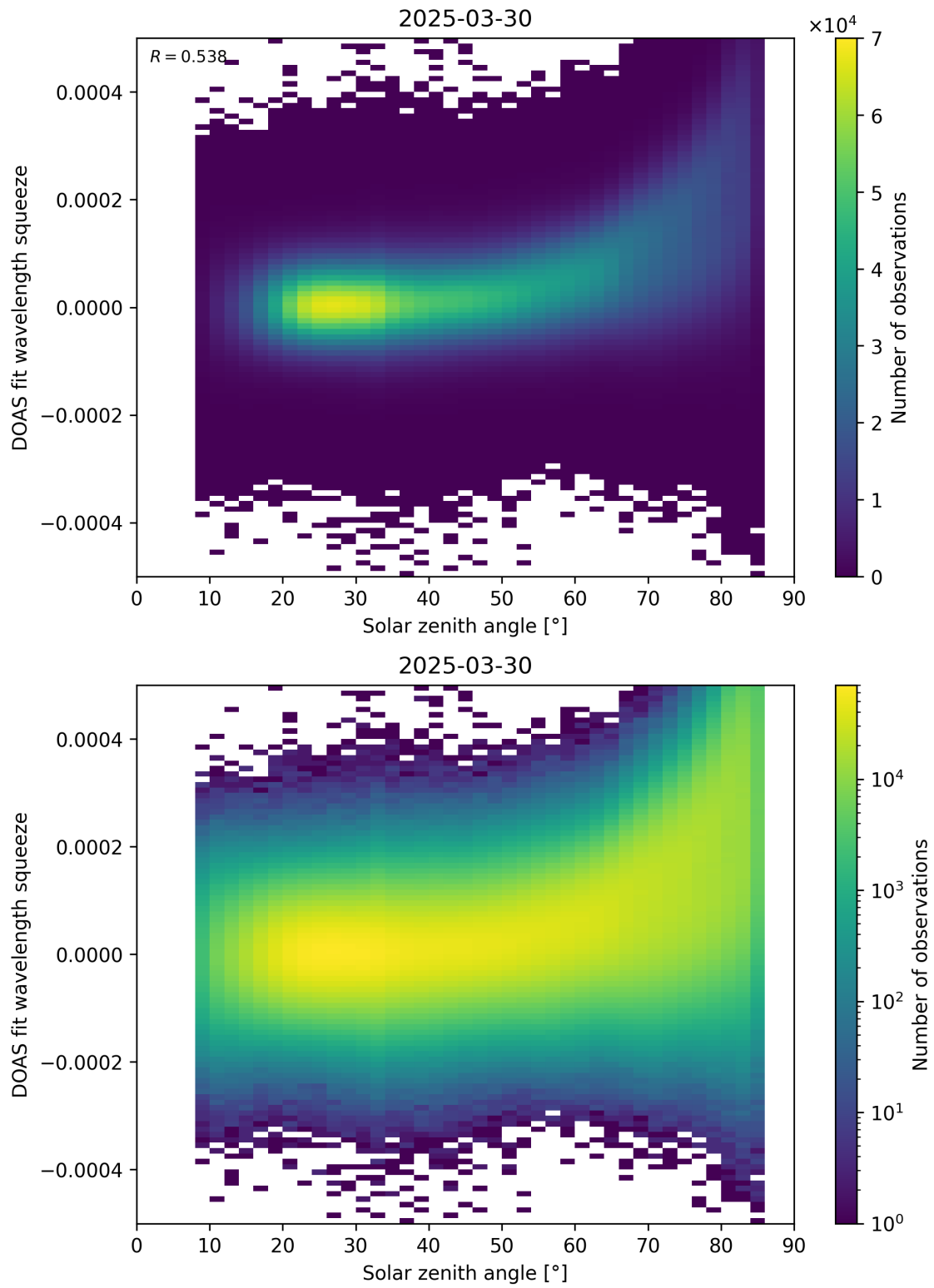
Figure 169: Scatter density plot of “Solar zenith angle” against “DOAS fit wavelength squeeze” for 2025-03-29 to 2025-03-31.
