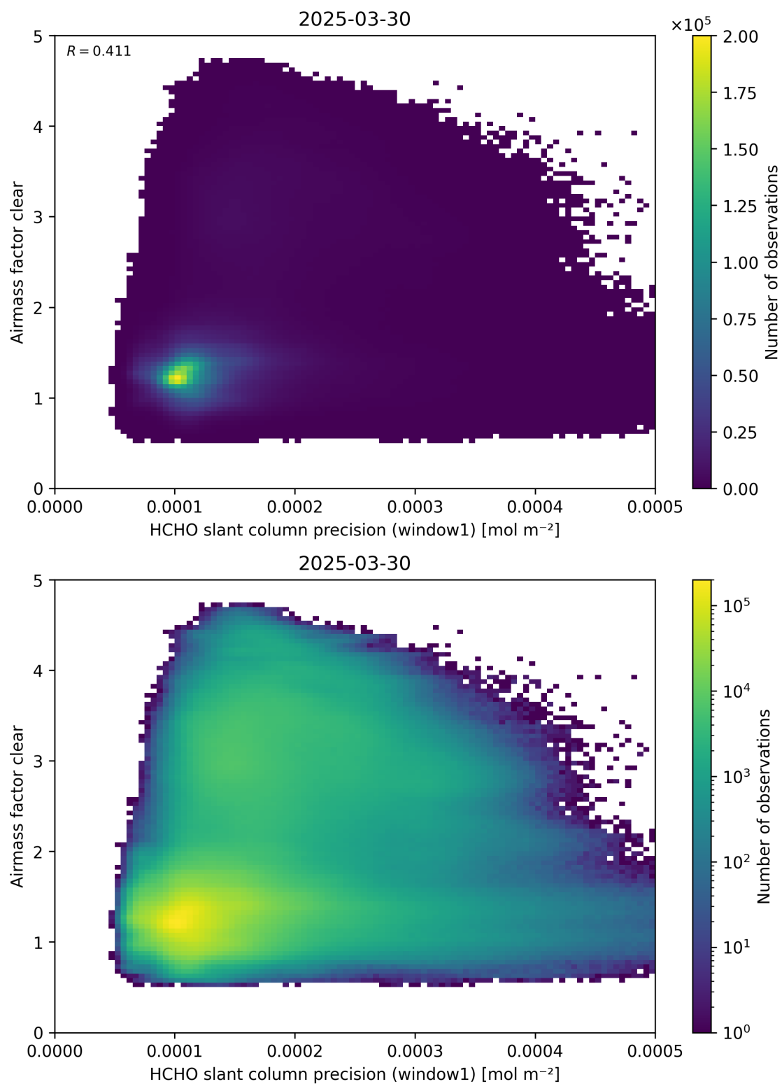
Figure 91: Scatter density plot of “HCHO slant column precision (window1)” against “Airmass factor clear” for 2025-03-29 to 2025-03-31.
