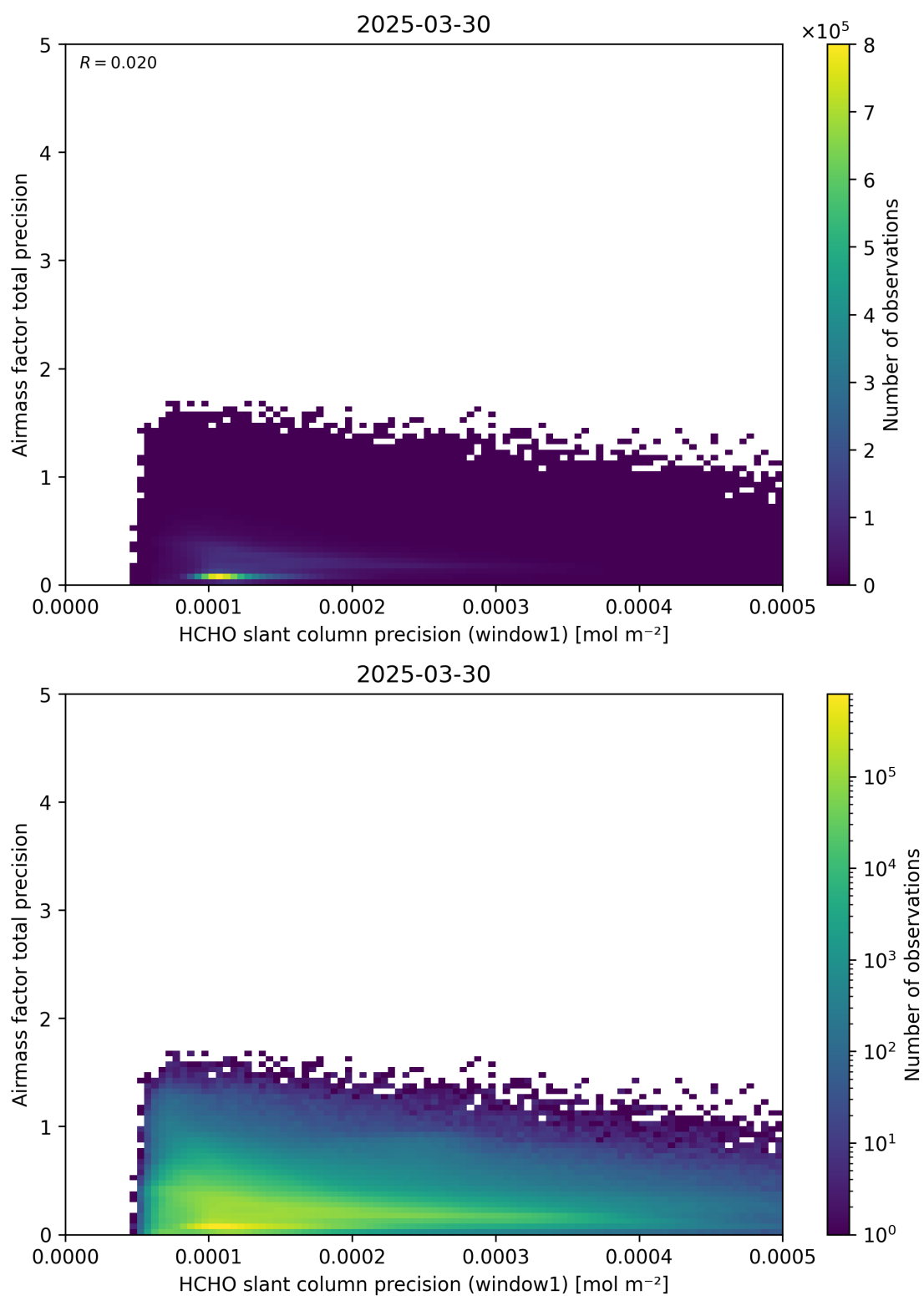
Figure 95: Scatter density plot of “HCHO slant column precision (window1)” against “Airmass factor total precision” for 2025-03-29 to 2025-03-31.
