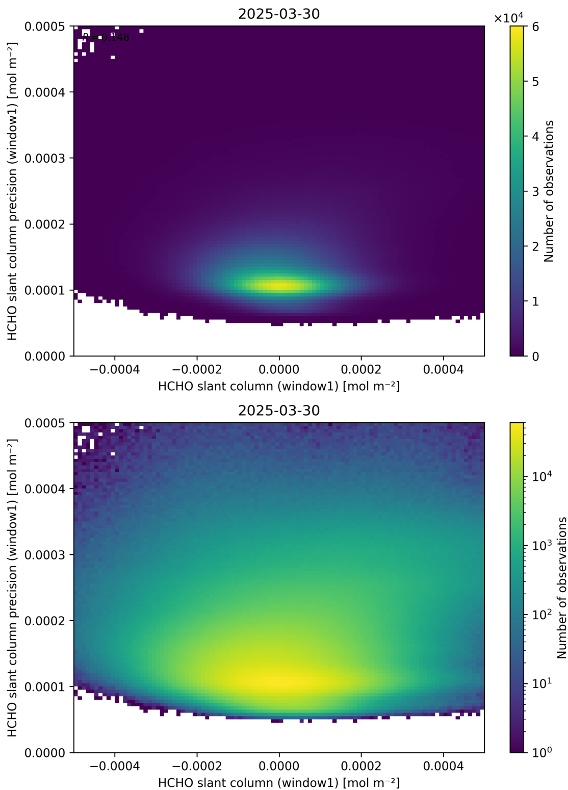
Figure 84: Scatter density plot of “HCHO slant column (window1)” against “HCHO slant column precision (window1)” for 2025-03-29 to 2025-03-31.
