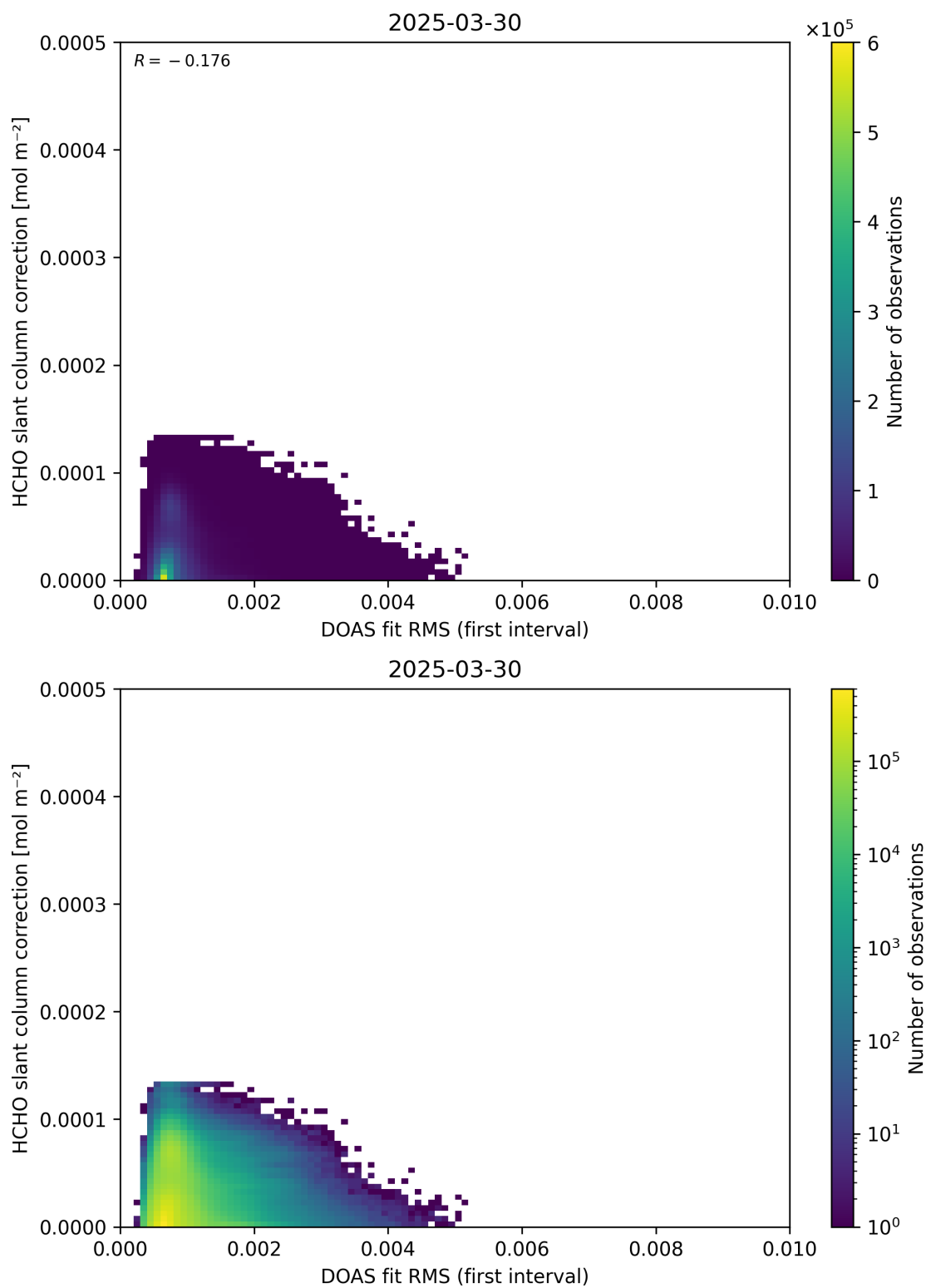
Figure 63: Scatter density plot of “DOAS fit RMS (first interval)” against “HCHO slant column correction” for 2025-03-29 to 2025-03-31.
