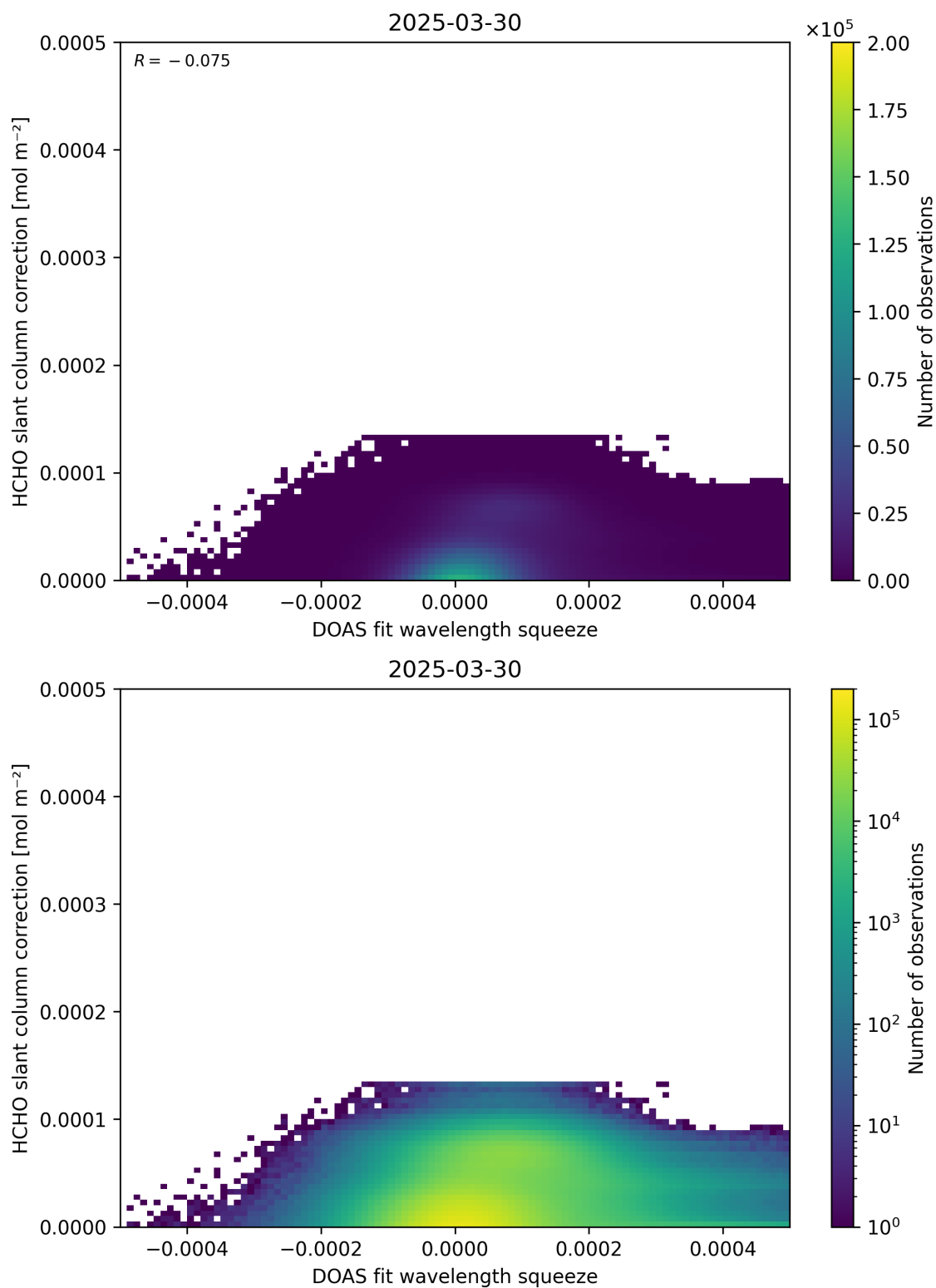
Figure 70: Scatter density plot of “DOAS fit wavelength squeeze” against “HCHO slant column correction” for 2025-03-29 to 2025-03-31.
