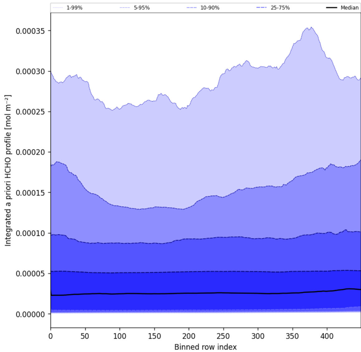
Figure 57: Along track statistics of “Integrated a priori HCHO profile” for 2025-03-29 to 2025-03-31
