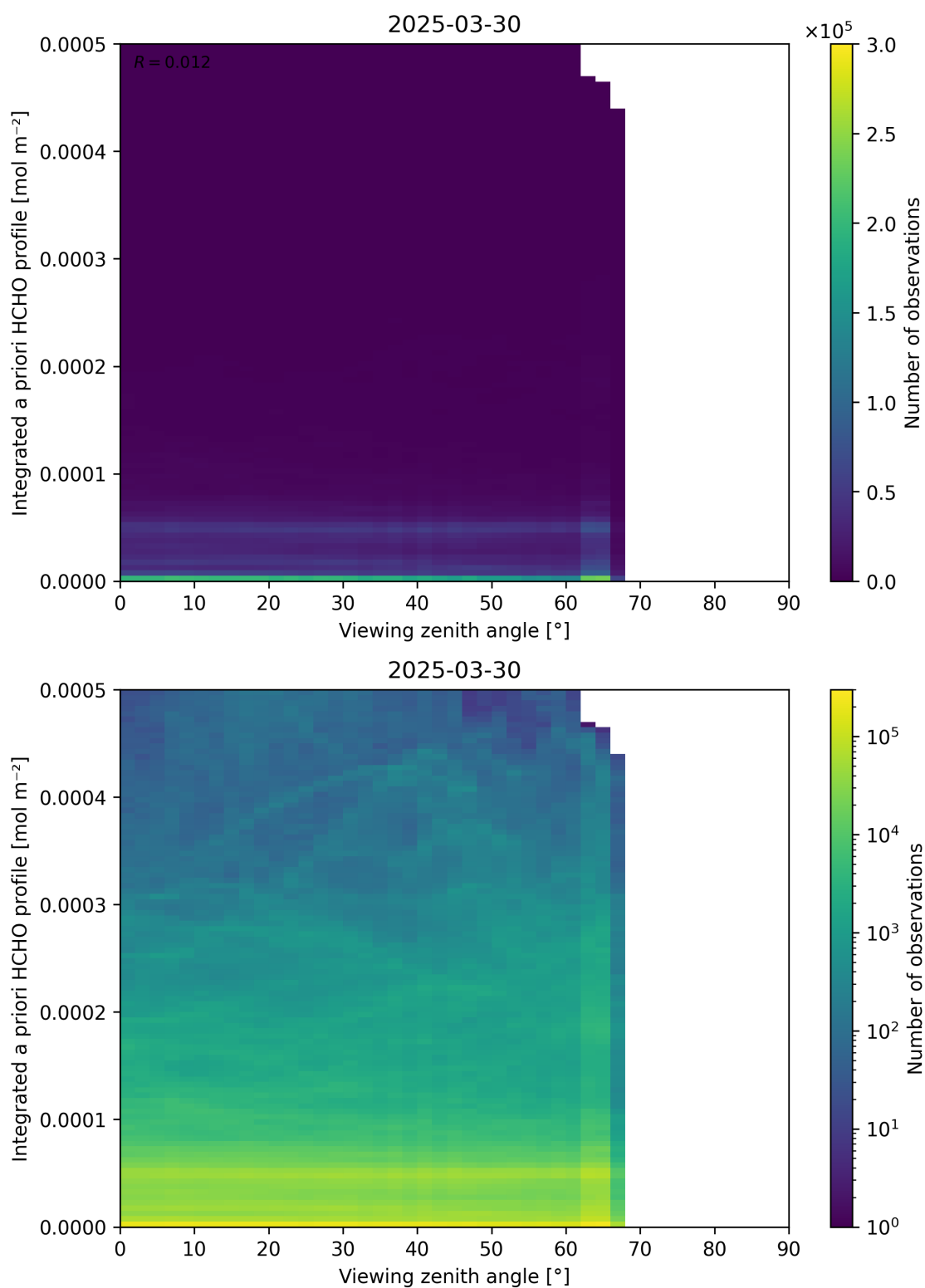
Figure 195: Scatter density plot of “Viewing zenith angle” against “Integrated a priori HCHO profile” for 2025-03-29 to 2025-03-31.
