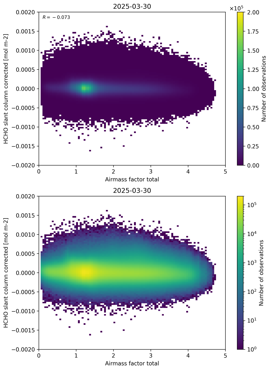
Figure 101: Scatter density plot of “Airmass factor total” against “HCHO slant column corrected” for 2025-03-29 to 2025-03-31.
