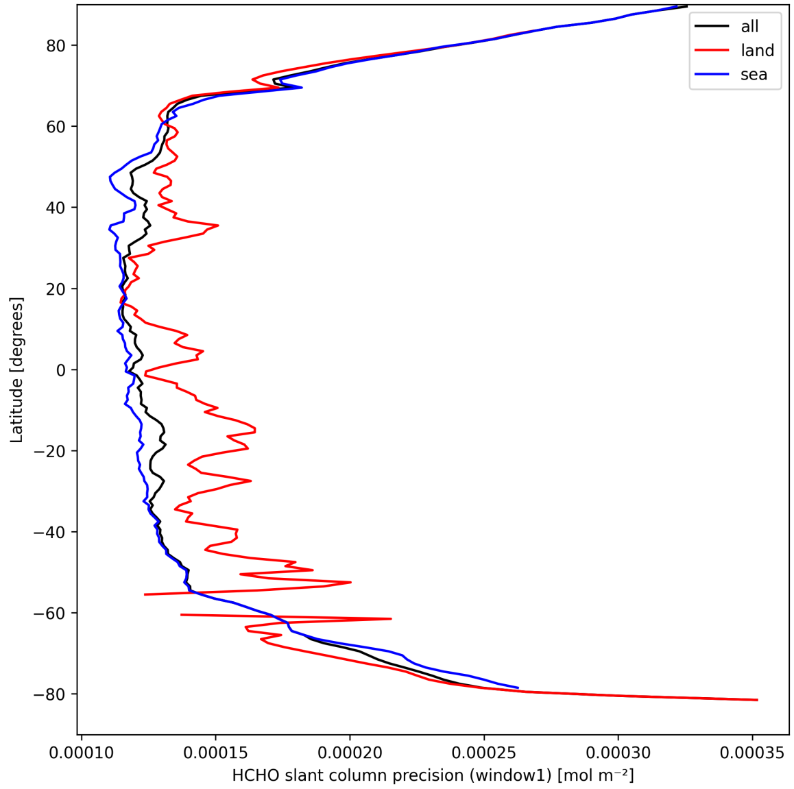
Figure 25: Zonal average of “HCHO slant column precision (window1)” for 2025-03-29 to 2025-03-31.
