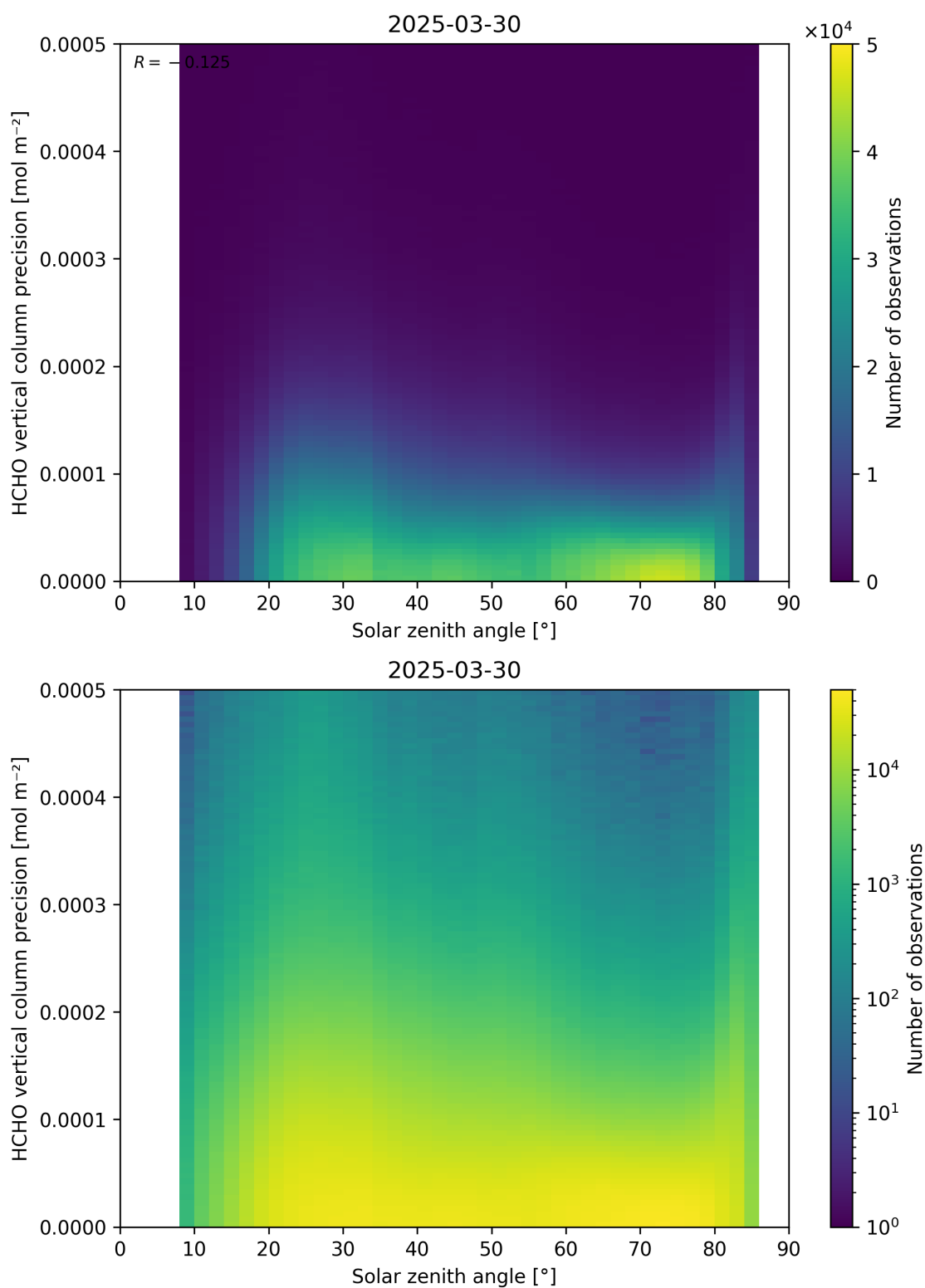
Figure 179: Scatter density plot of “Solar zenith angle” against “HCHO vertical column precision” for 2025-03-29 to 2025-03-31.
