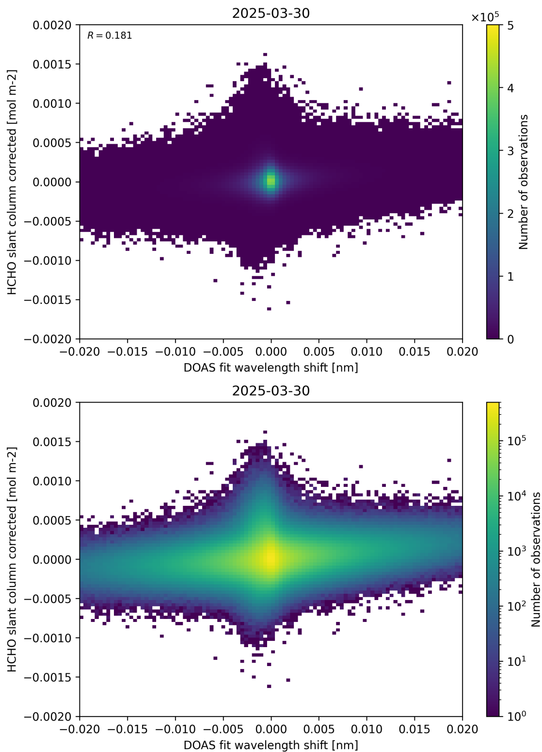
Figure 66: Scatter density plot of “DOAS fit wavelength shift” against “HCHO slant column corrected” for 2025-03-29 to 2025-03-31.
