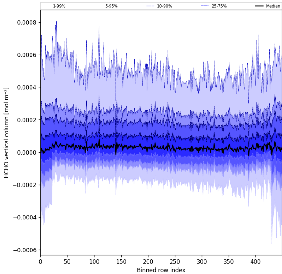
Figure 49: Along track statistics of “HCHO vertical column” for 2025-03-29 to 2025-03-31
