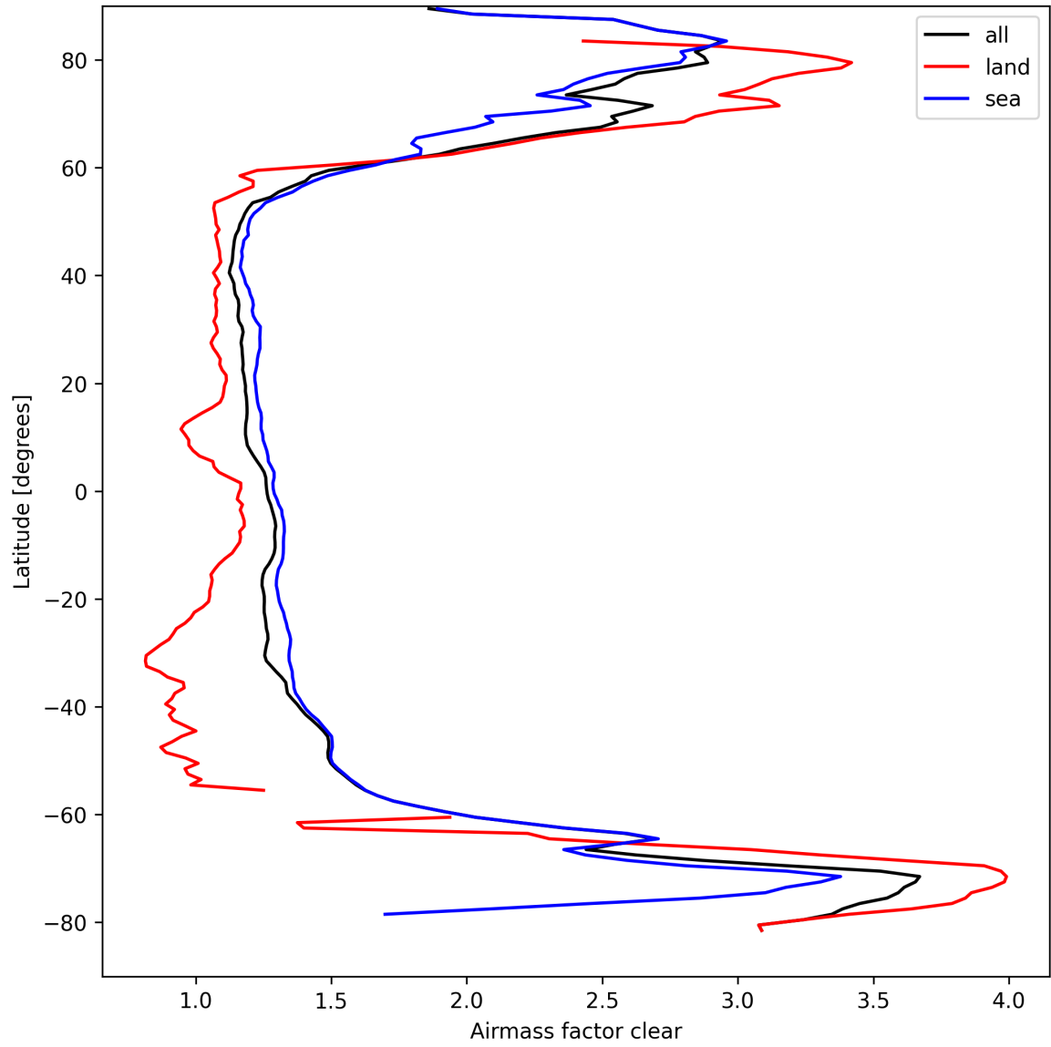
Figure 28: Zonal average of “Airmass factor clear” for 2025-03-29 to 2025-03-31.
