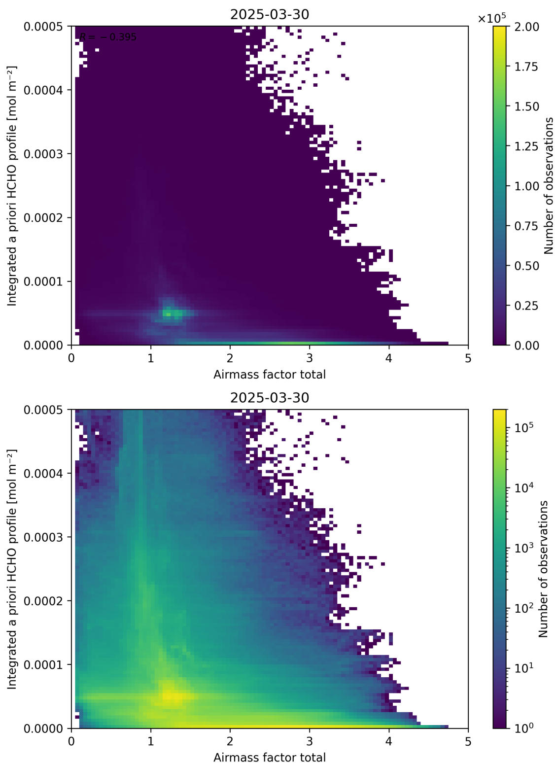
Figure 104: Scatter density plot of “Airmass factor total” against “Integrated a priori HCHO profile” for 2025-03-29 to 2025-03-31.
