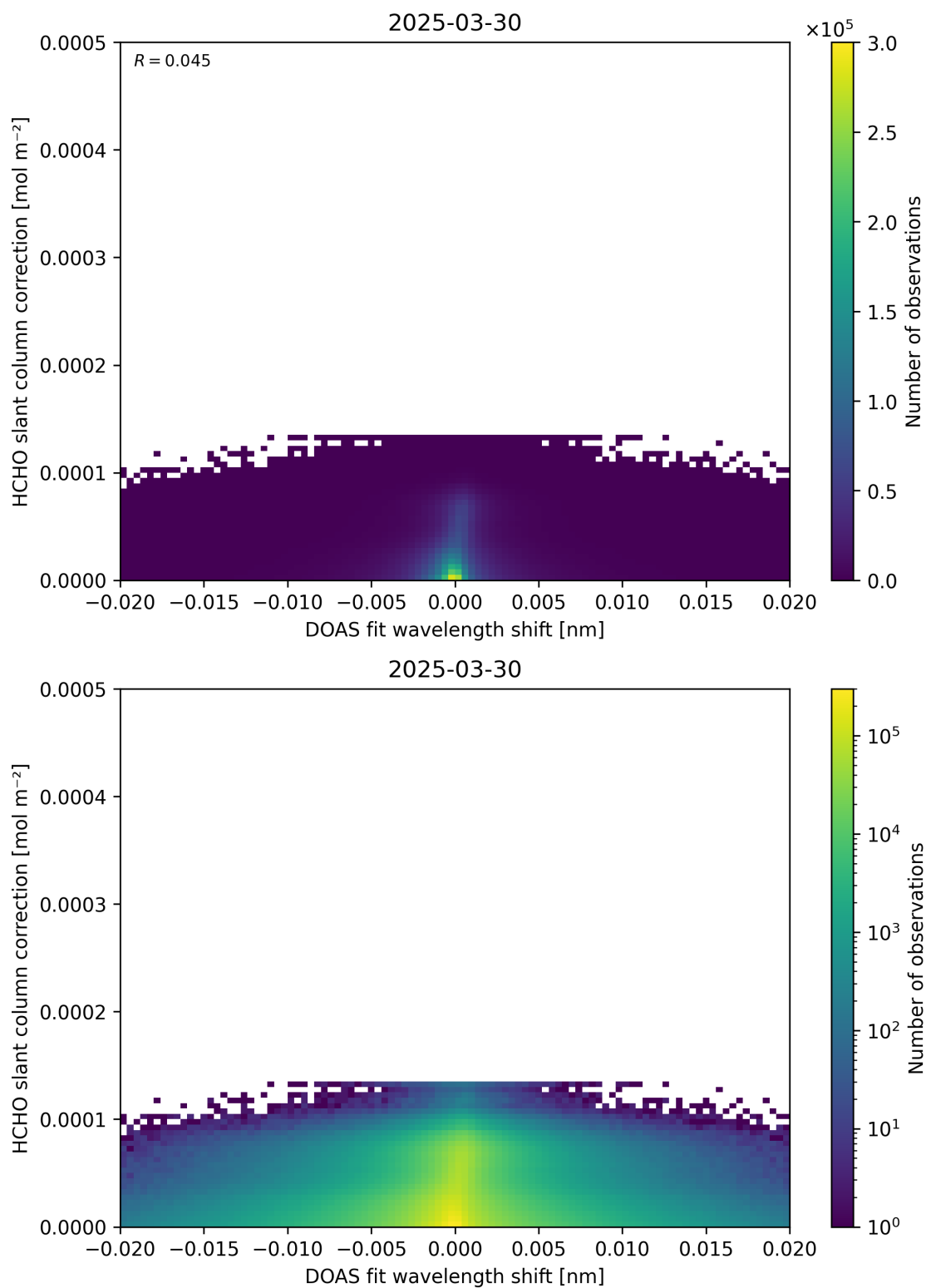
Figure 67: Scatter density plot of “DOAS fit wavelength shift” against “HCHO slant column correction” for 2025-03-29 to 2025-03-31.
