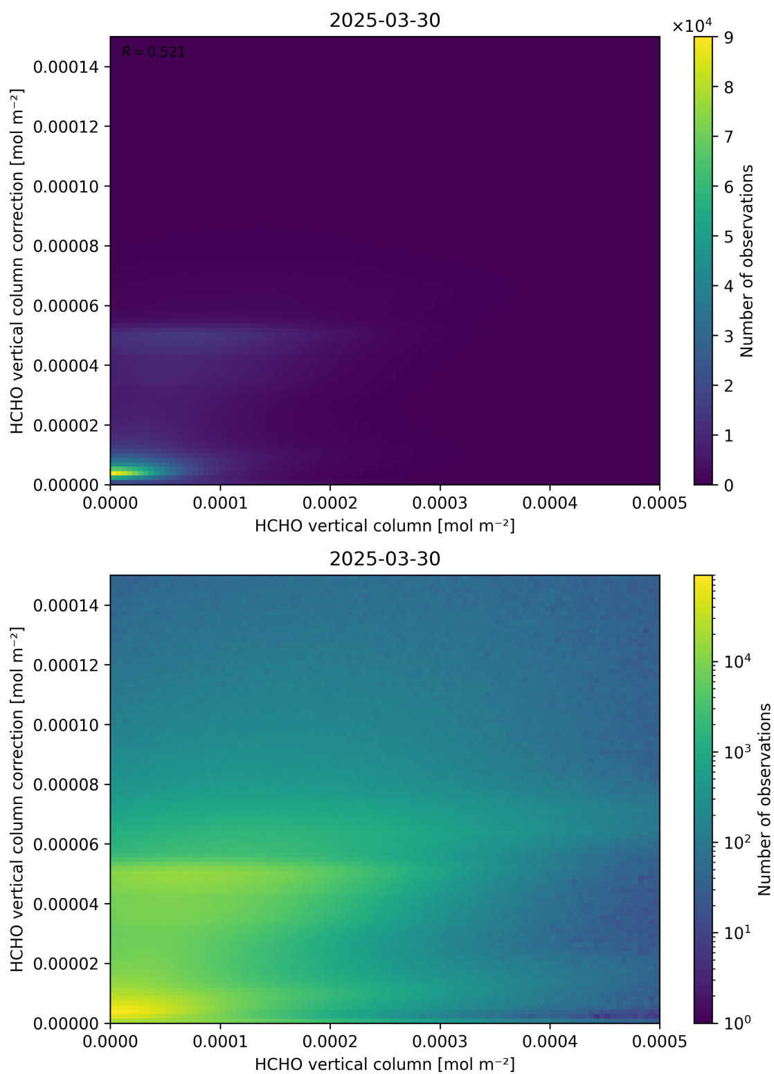
Figure 133: Scatter density plot of “HCHO vertical column” against “HCHO vertical column correction” for 2025-03-29 to 2025-03-31.
