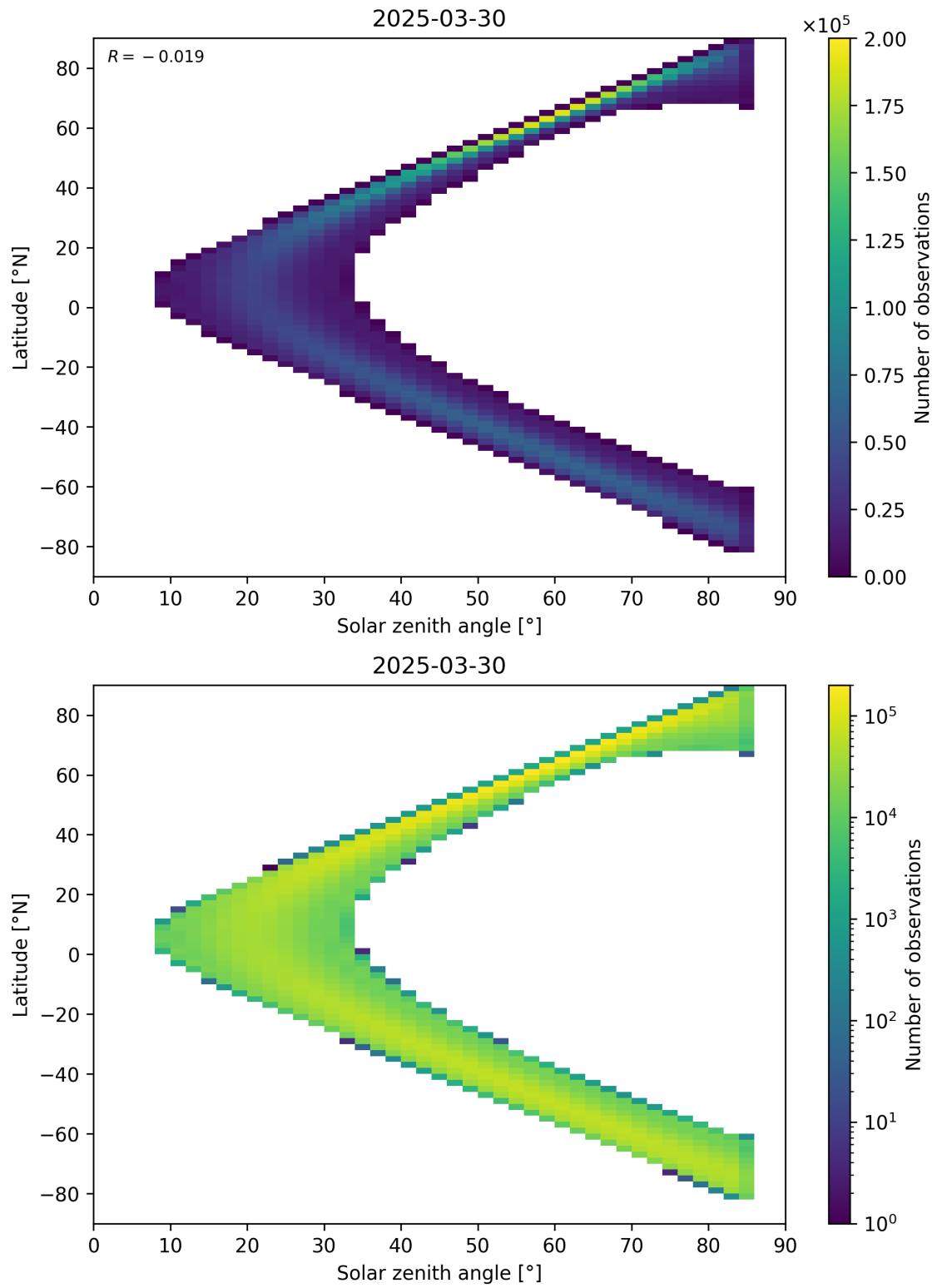
Figure 181: Scatter density plot of “Solar zenith angle” against “Latitude” for 2025-03-29 to 2025-03-31.
