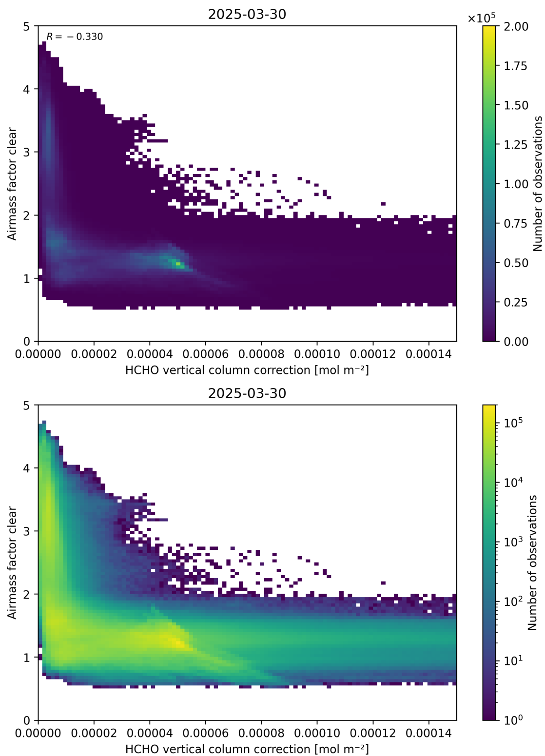
Figure 115: Scatter density plot of “HCHO vertical column correction” against “Airmass factor clear” for 2025-03-29 to 2025-03-31.
