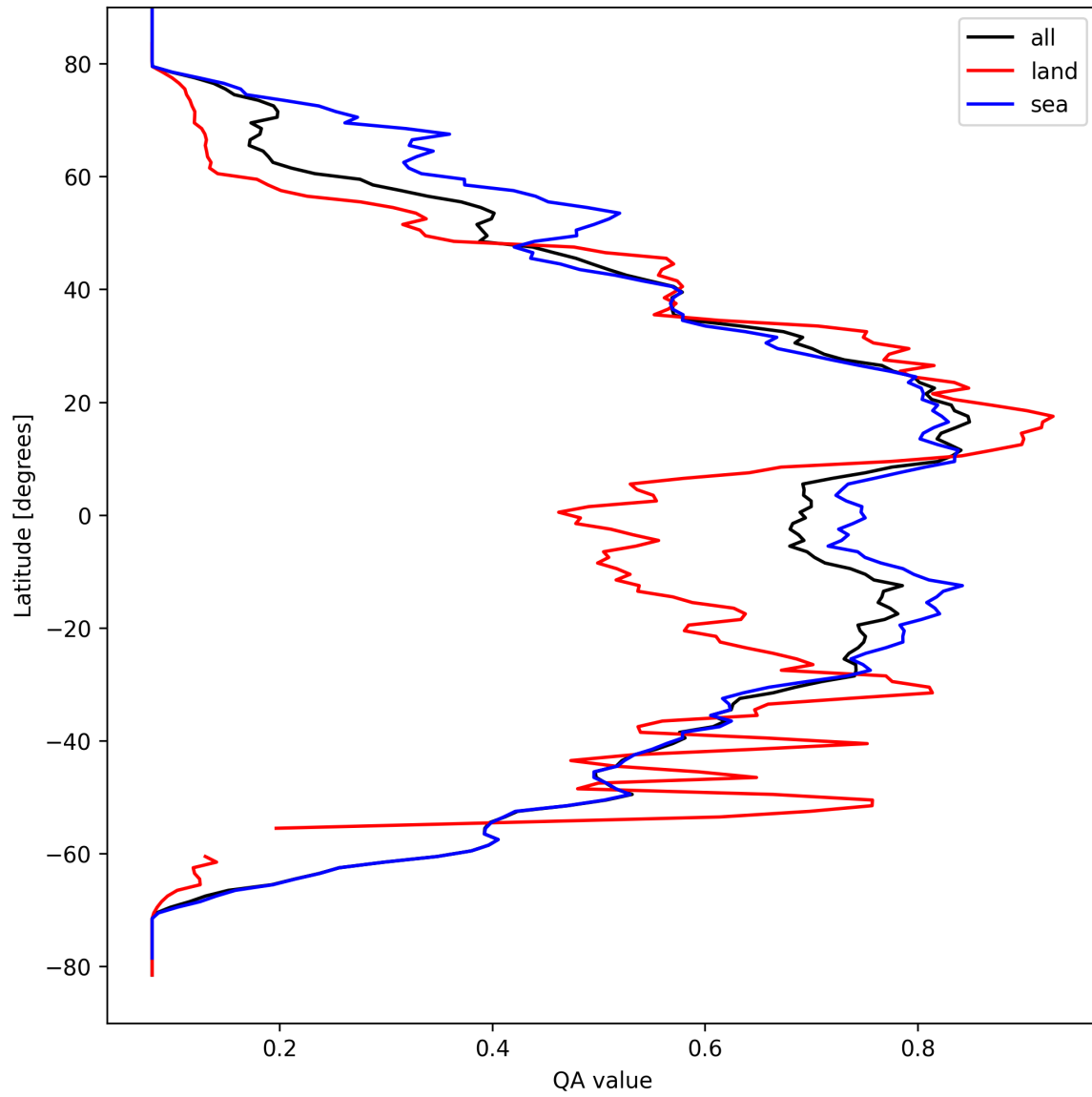
Figure 20: Zonal average of “QA value” for 2025-03-29 to 2025-03-31.
