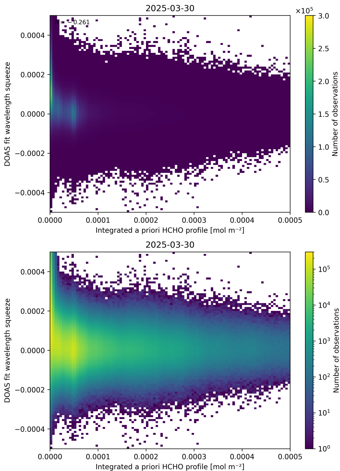
Figure 150: Scatter density plot of “Integrated a priori HCHO profile” against “DOAS fit wavelength squeeze” for 2025-03-29 to 2025-03-31.
