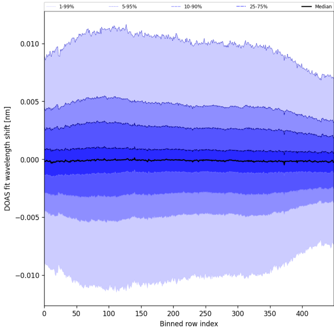
Figure 58: Along track statistics of “DOAS fit wavelength shift” for 2025-03-29 to 2025-03-31
