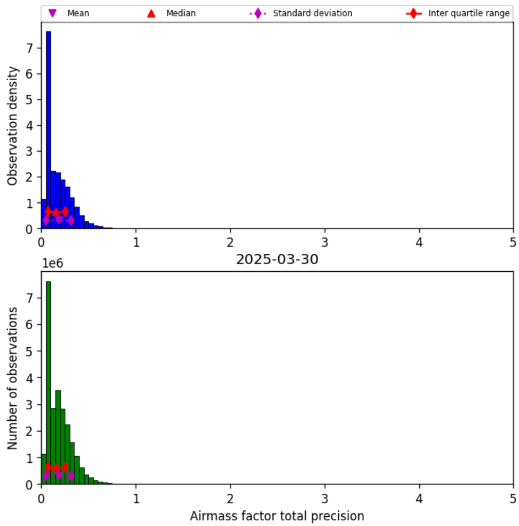
Figure 41: Histogram of “Airmass factor total precision” for 2025-03-29 to 2025-03-31
