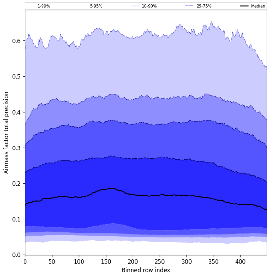
Figure 55: Along track statistics of “Airmass factor total precision” for 2025-03-29 to 2025-03-31
