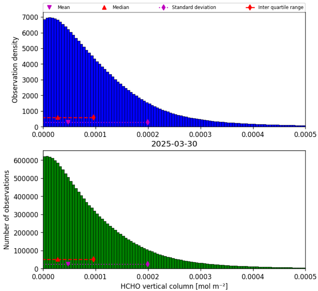
Figure 35: Histogram of “HCHO vertical column” for 2025-03-29 to 2025-03-31
