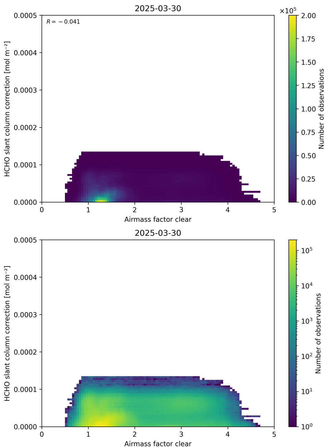
Figure 75: Scatter density plot of “Airmass factor clear” against “HCHO slant column correction” for 2025-03-29 to 2025-03-31.
