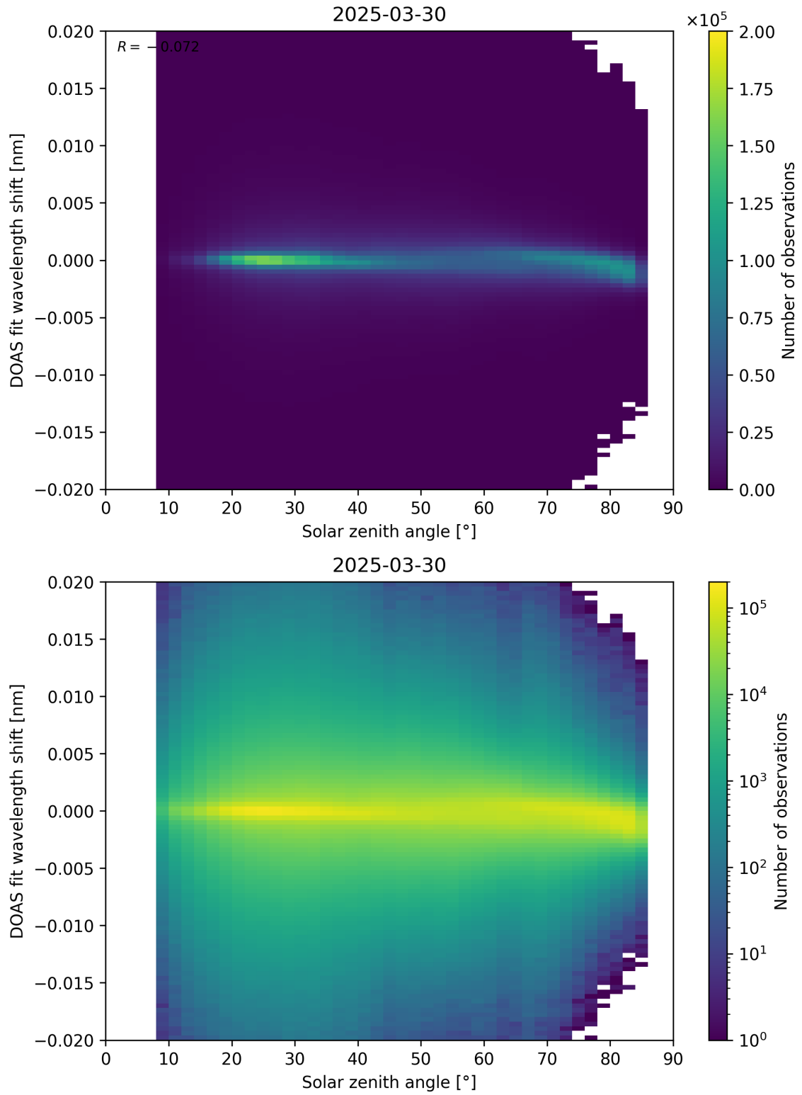
Figure 168: Scatter density plot of “Solar zenith angle” against “DOAS fit wavelength shift” for 2025-03-29 to 2025-03-31.
