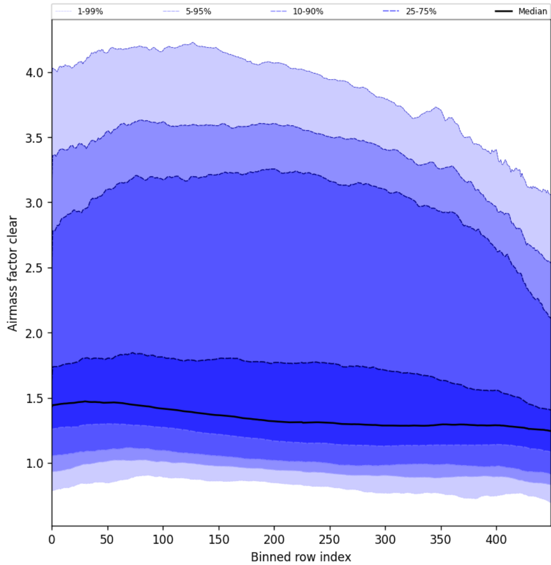
Figure 56: Along track statistics of “Air mass factor clear” for 2025-03-29 to 2025-03-31
