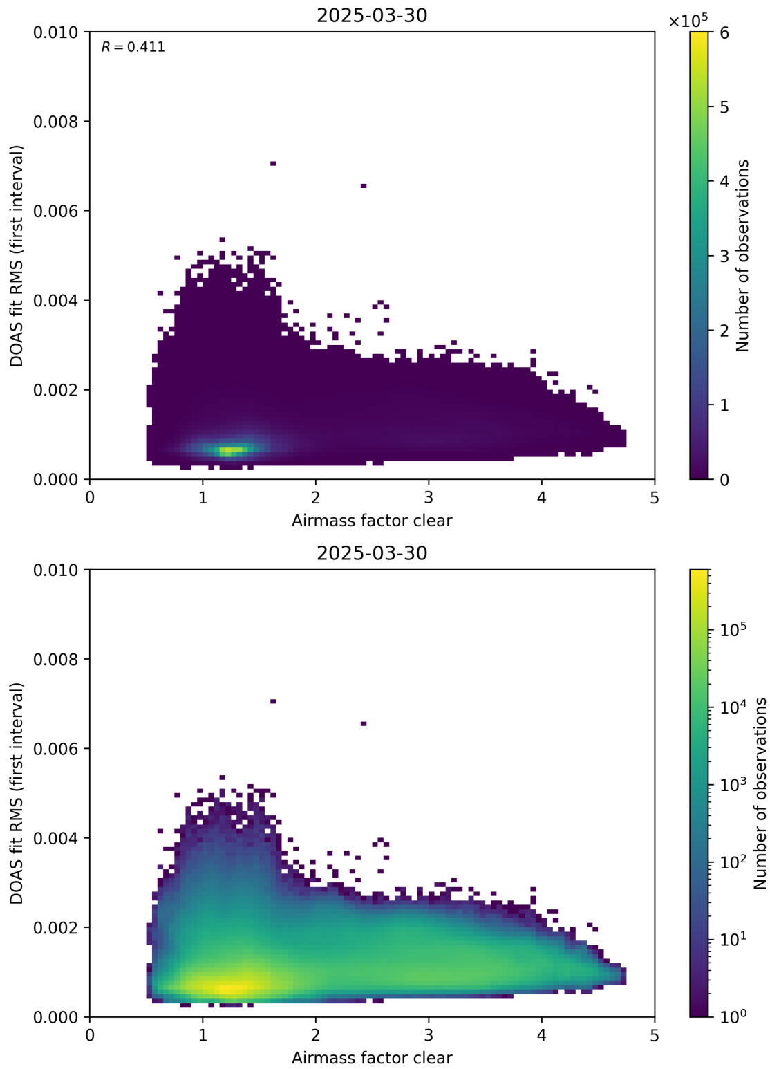
Figure 71: Scatter density plot of “Airmass factor clear” against “DOAS fit RMS (first interval)” for 2025-03-29 to 2025-03-31.
