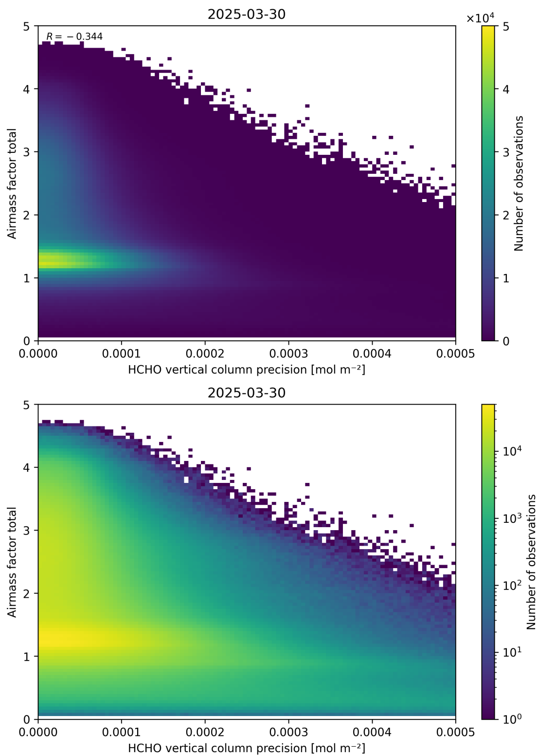
Figure 144: Scatter density plot of “HCHO vertical column precision” against “Airmass factor total” for 2025-03-29 to 2025-03-31.
