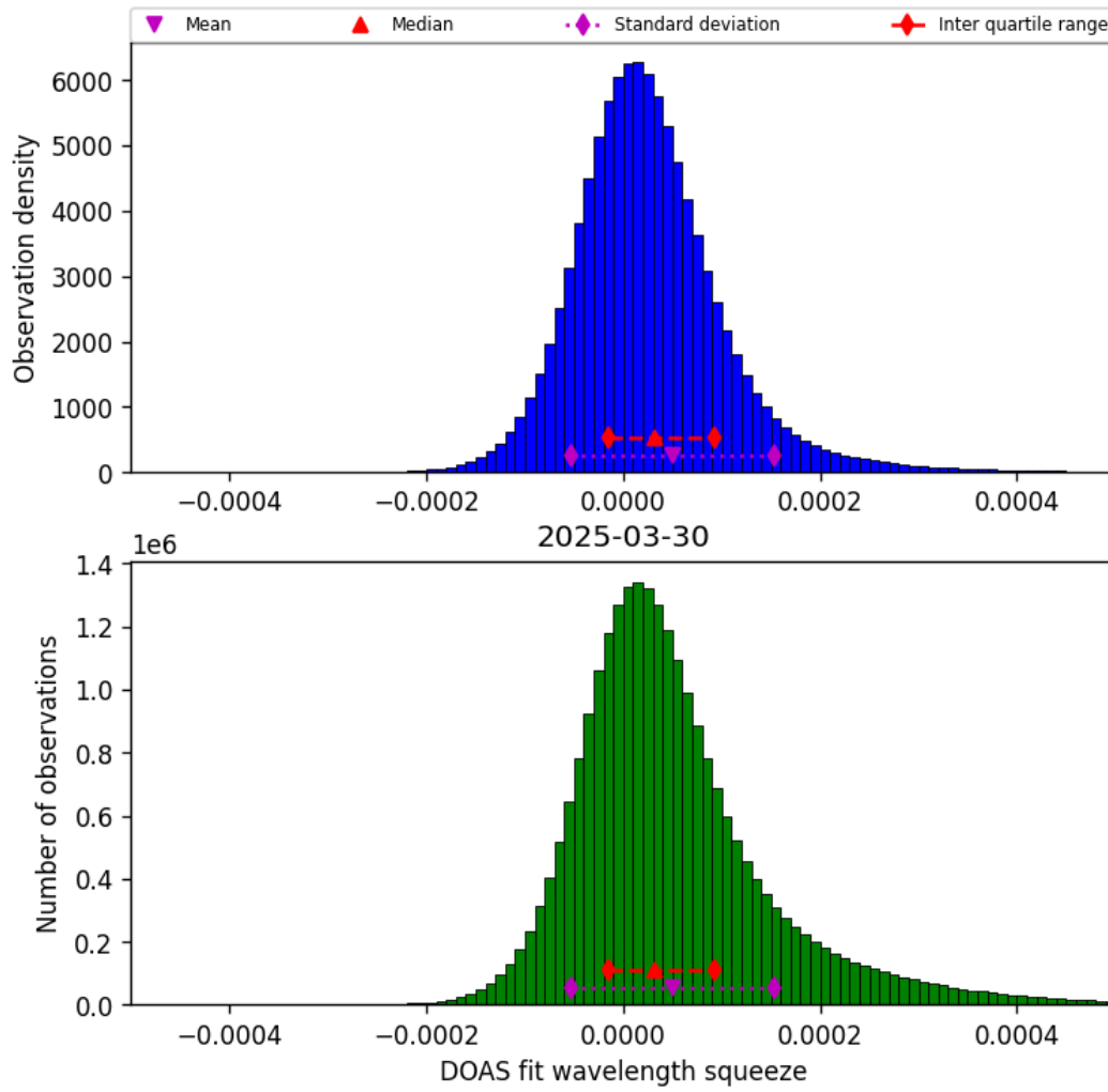
Figure 45: Histogram of “DOAS fit wavelength squeeze” for 2025-03-29 to 2025-03-31
