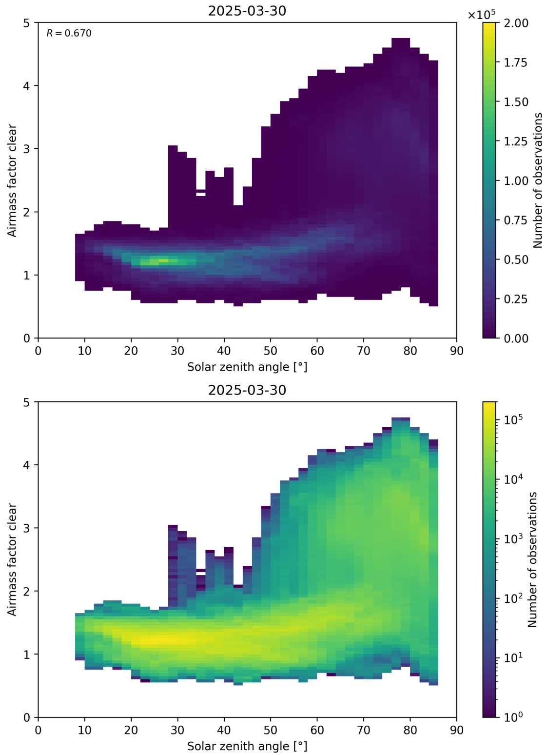
Figure 170: Scatter density plot of “Solar zenith angle” against “Airmass factor clear” for 2025-03-29 to 2025-03-31.
