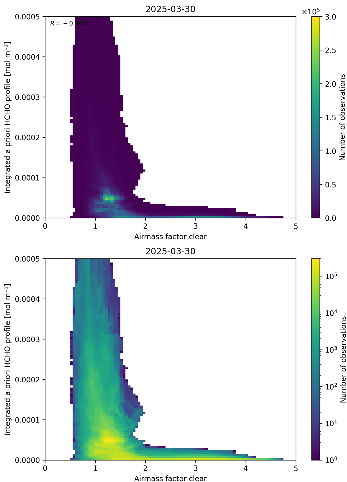
Figure 76: Scatter density plot of “Airmass factor clear” against “Integrated a priori HCHO profile” for 2025-03-29 to 2025-03-31.
