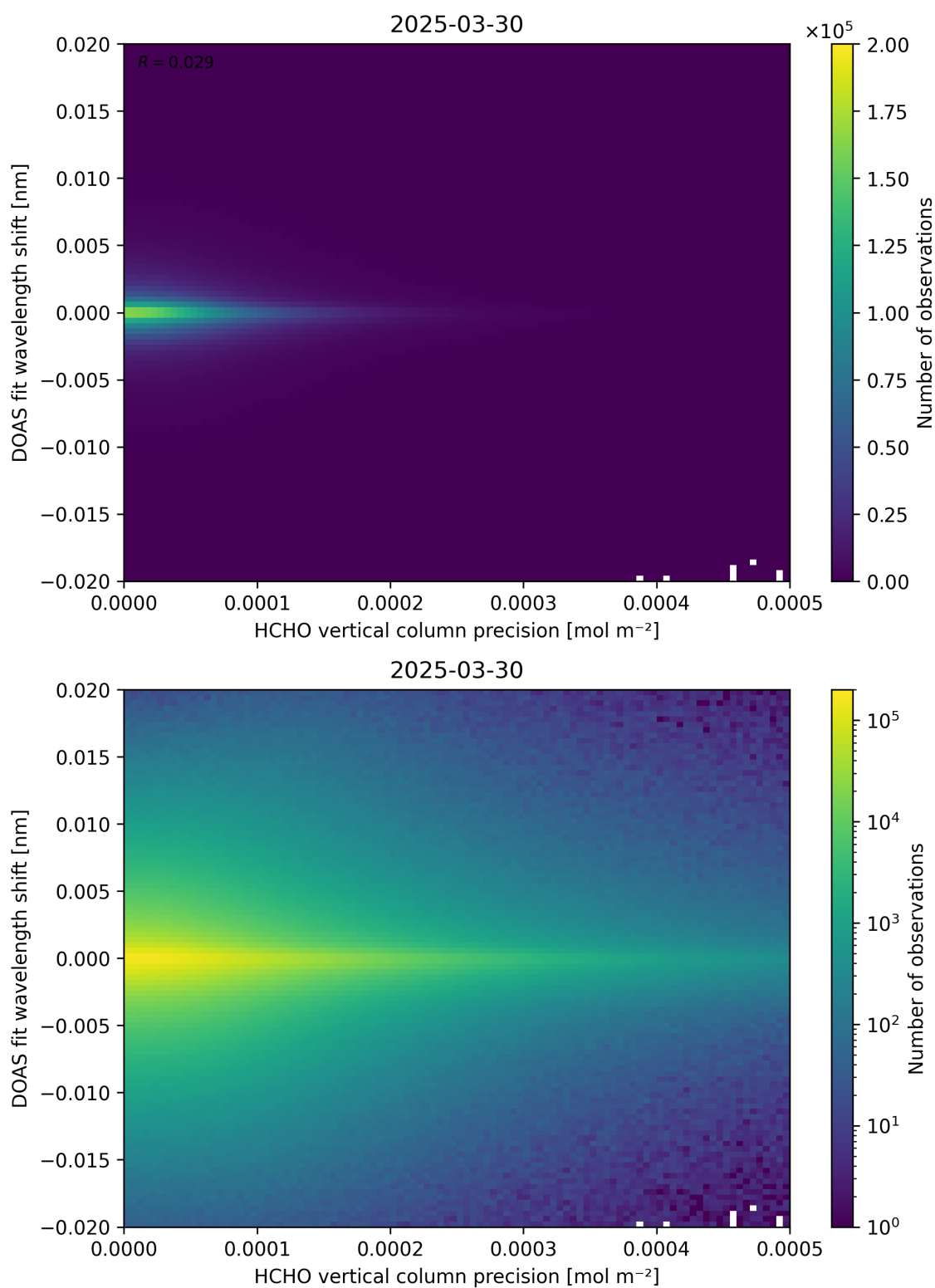
Figure 137: Scatter density plot of “HCHO vertical column precision” against “DOAS fit wavelength shift” for 2025-03-29 to 2025-03-31.
