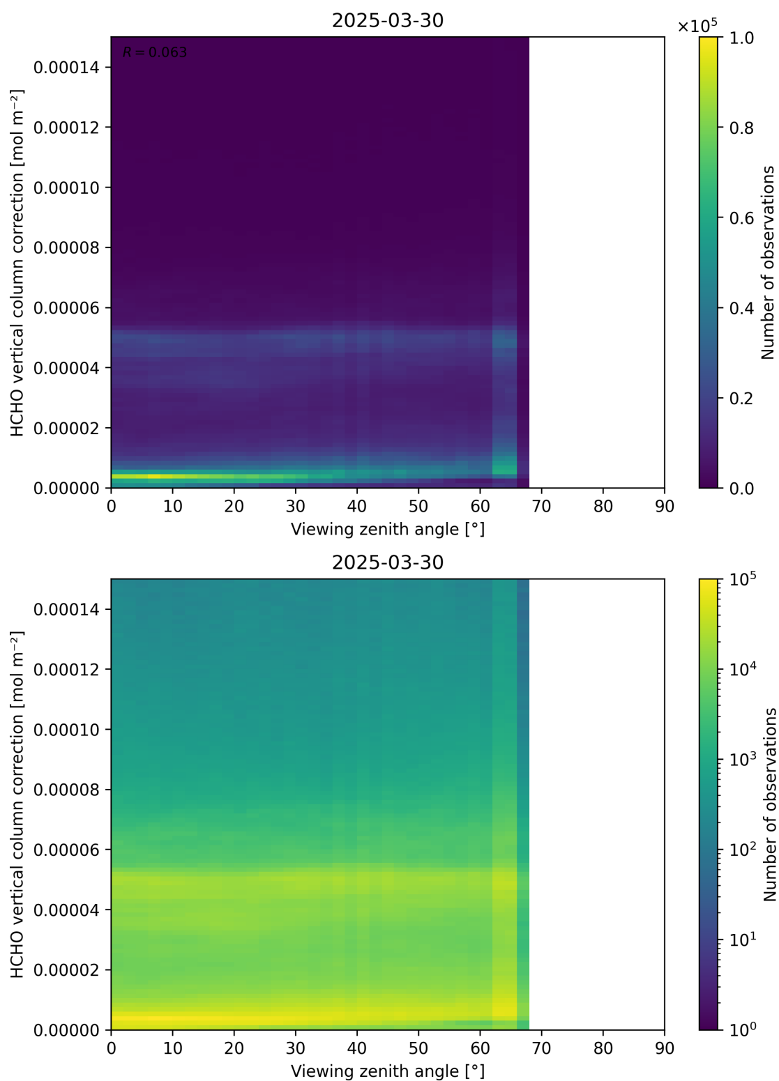
Figure 193: Scatter density plot of “Viewing zenith angle” against “HCHO vertical column correction” for 2025-03-29 to 2025-03-31.
