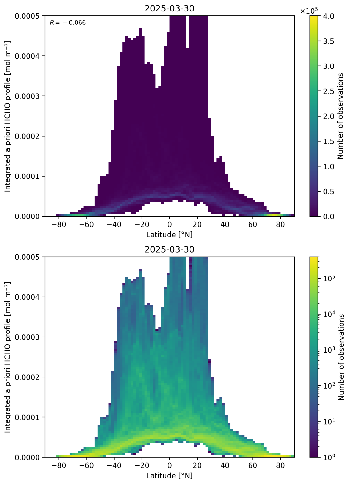
Figure 166: Scatter density plot of “Latitude” against “Integrated a priori HCHO profile” for 2025-03-29 to 2025-03-31.
