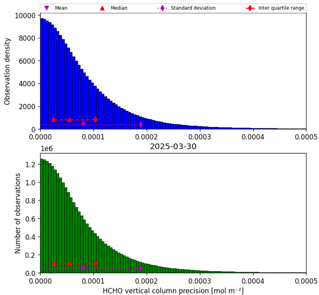
Figure 36: Histogram of “HCHO vertical column precision” for 2025-03-29 to 2025-03-31
