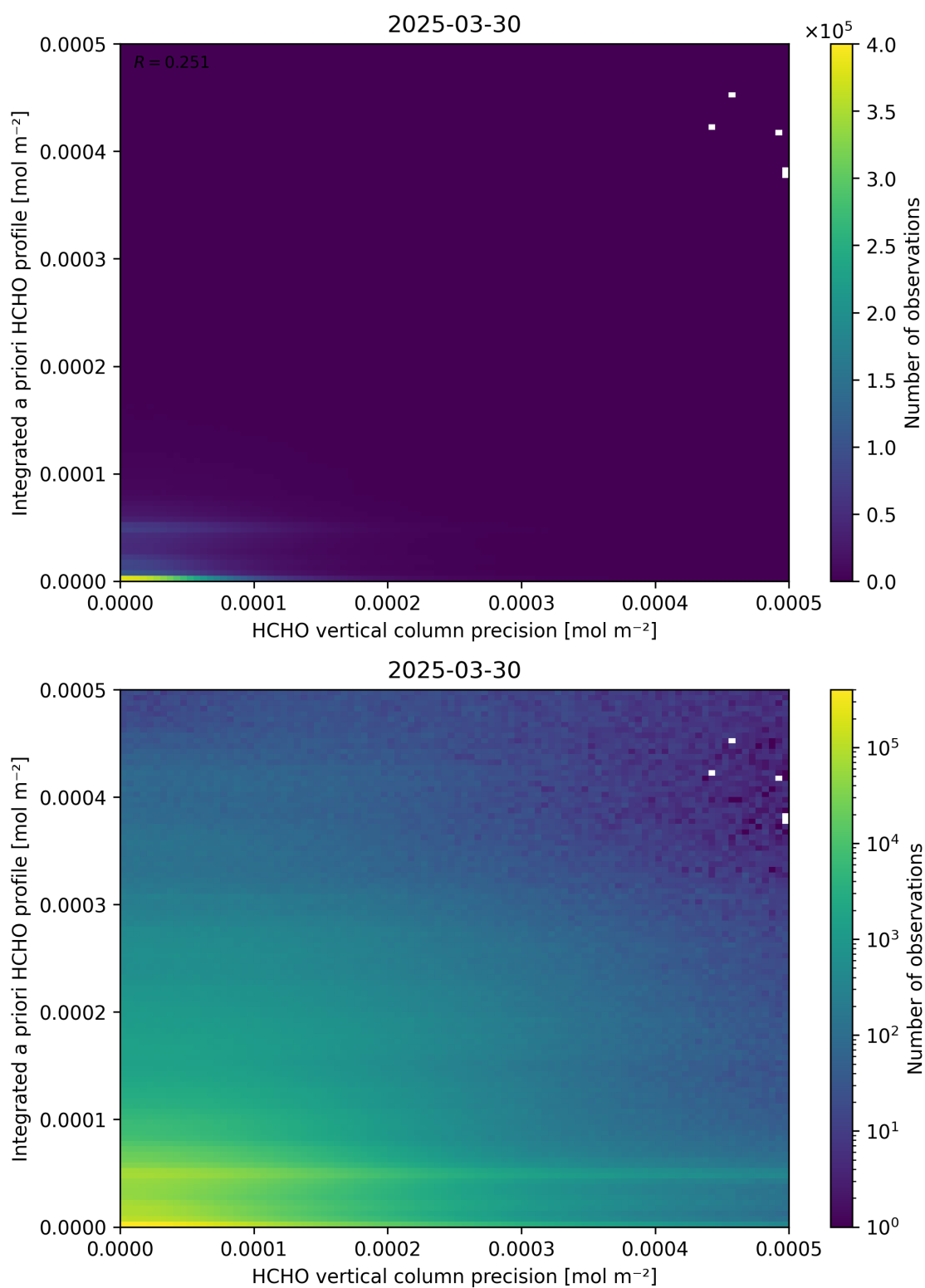
Figure 147: Scatter density plot of “HCHO vertical column precision” against “Integrated a priori HCHO profile” for 2025-03-29 to 2025-03-31.
