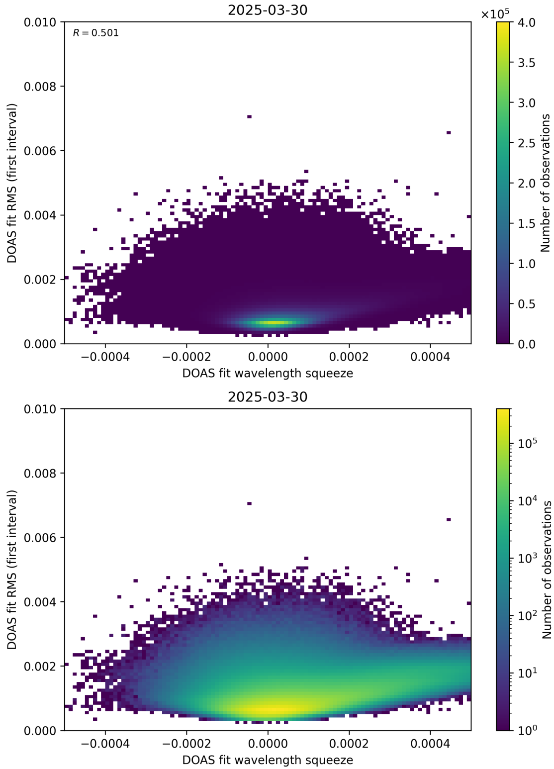
Figure 68: Scatter density plot of “DOAS fit wavelength squeeze” against “DOAS fit RMS (first interval)” for 2025-03-29 to 2025-03-31.
