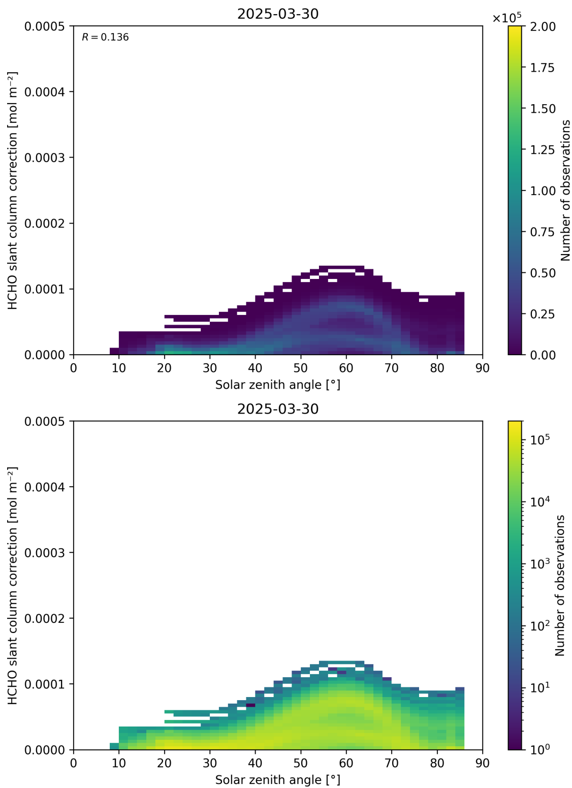
Figure 172: Scatter density plot of “Solar zenith angle” against “HCHO slant column correction” for 2025-03-29 to 2025-03-31.
