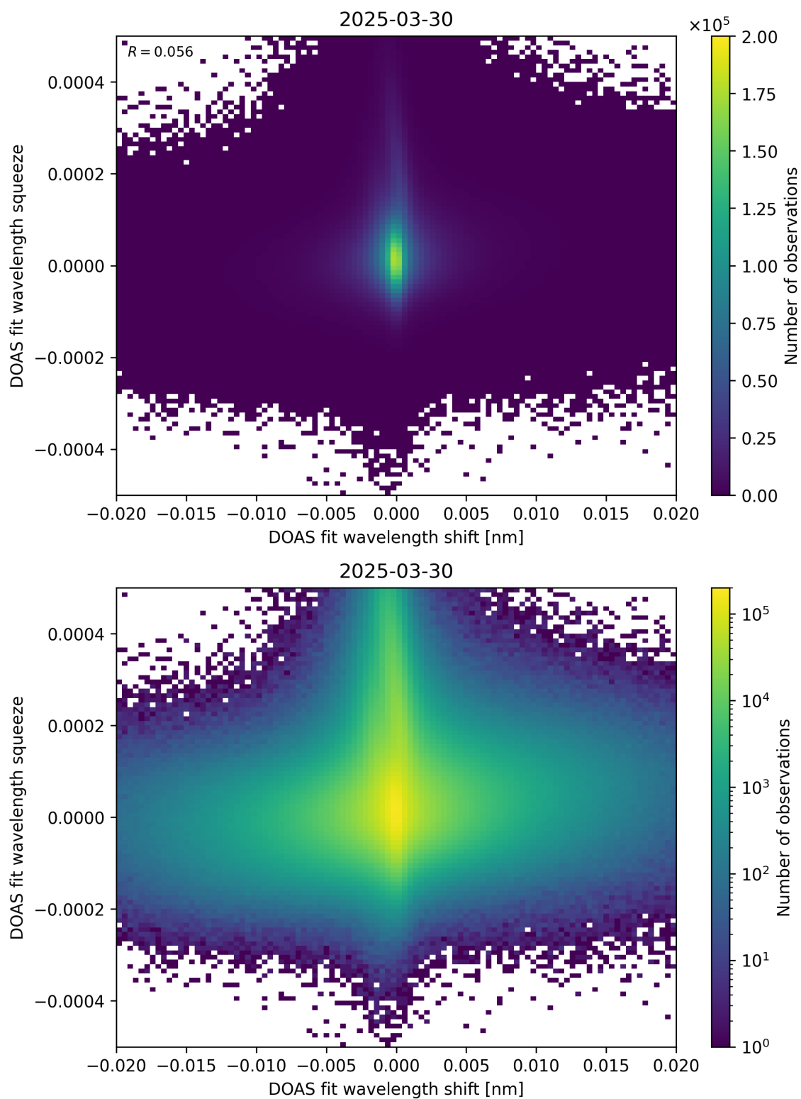
Figure 65: Scatter density plot of “DOAS fit wavelength shift” against “DOAS fit wavelength squeeze” for 2025-03-29 to 2025-03-31.
