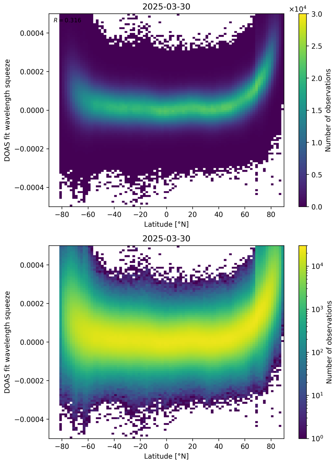
Figure 155: Scatter density plot of “Latitude” against “DOAS fit wavelength squeeze” for 2025-03-29 to 2025-03-31.
