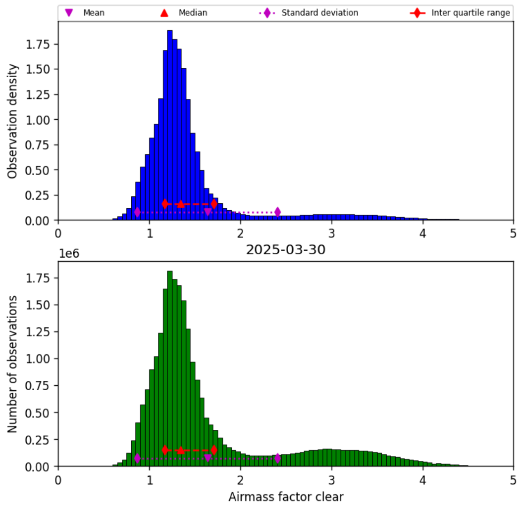
Figure 42: Histogram of “Airmass factor clear” for 2025-03-29 to 2025-03-31
