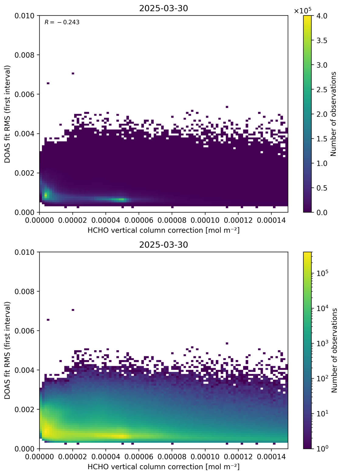
Figure 112: Scatter density plot of “HCHO vertical column correction” against “DOAS fit RMS (first interval)” for 2025-03-29 to 2025-03-31.
