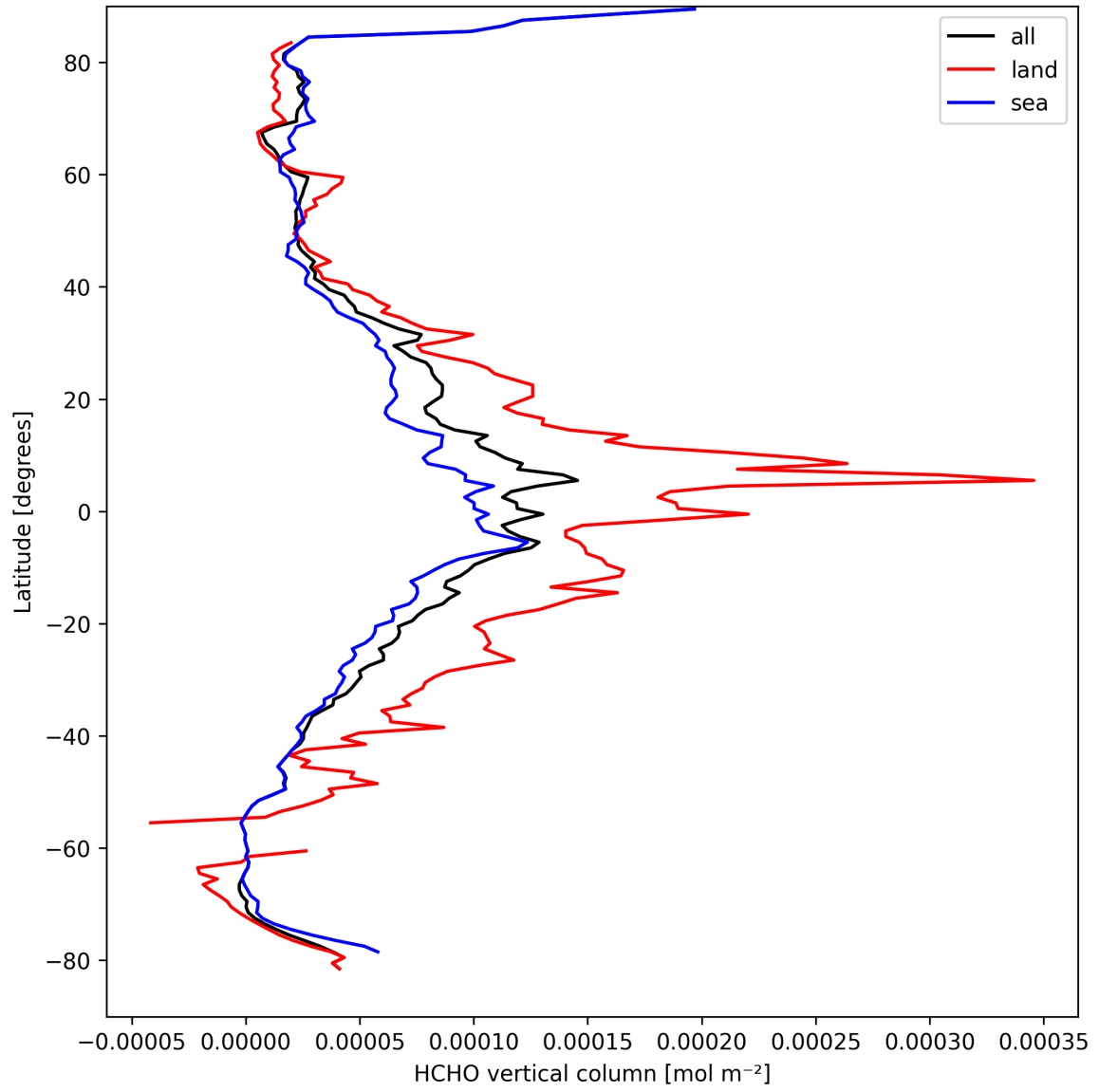
Figure 21: Zonal average of “HCHO vertical column” for 2025-03-29 to 2025-03-31.
