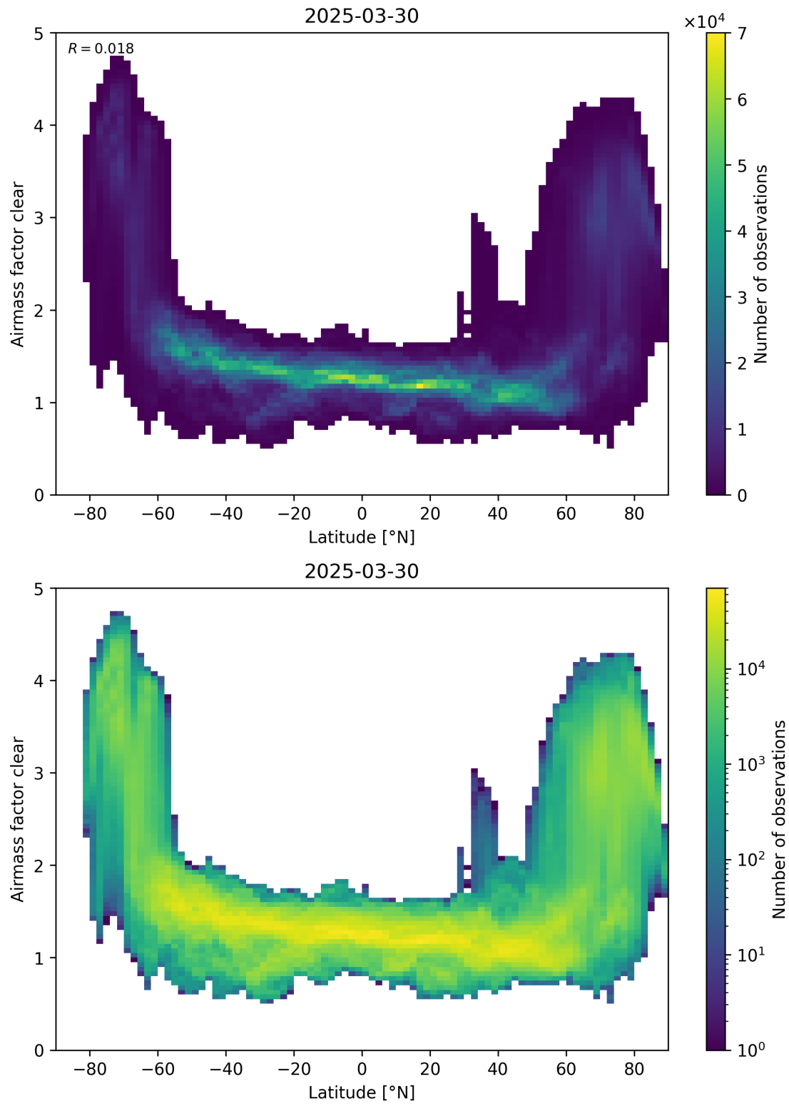
Figure 156: Scatter density plot of “Latitude” against “Airmass factor clear” for 2025-03-29 to 2025-03-31.
