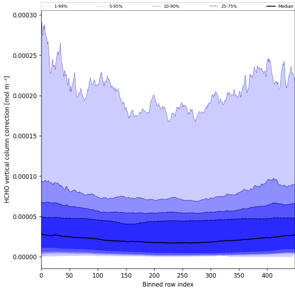
Figure 51: Along track statistics of “HCHO vertical column correction” for 2025-03-29 to 2025-03-31
