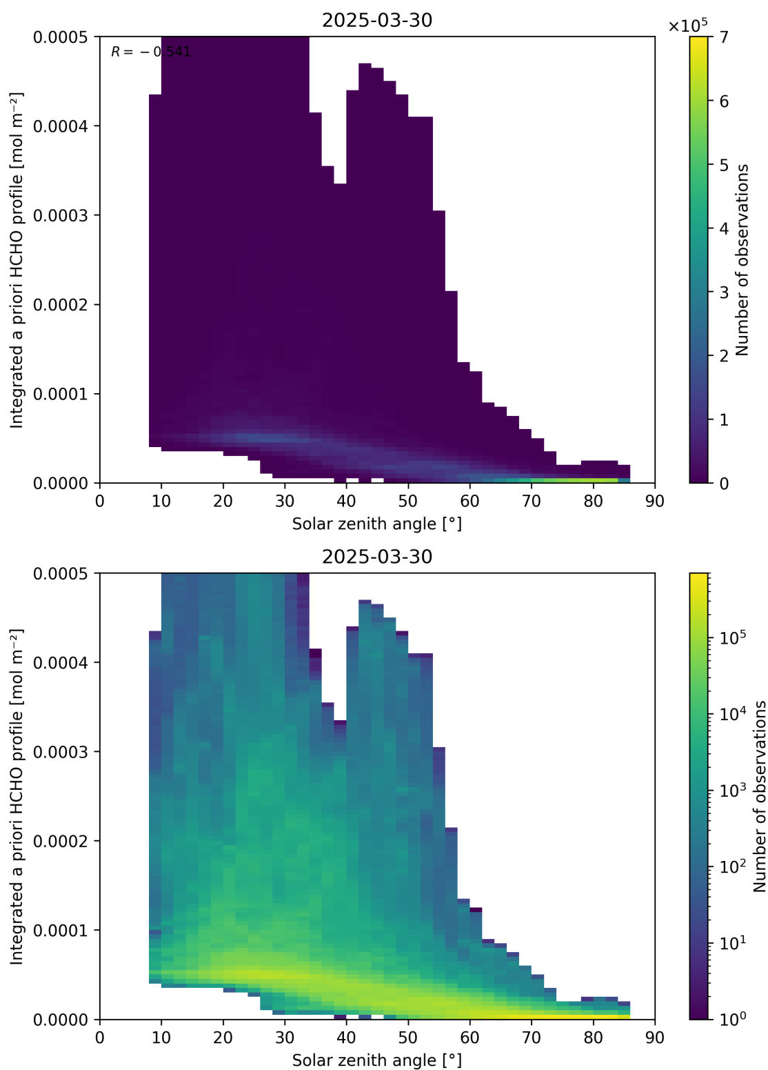
Figure 180: Scatter density plot of “Solar zenith angle” against “Integrated a priori HCHO profile” for 2025-03-29 to 2025-03-31.
