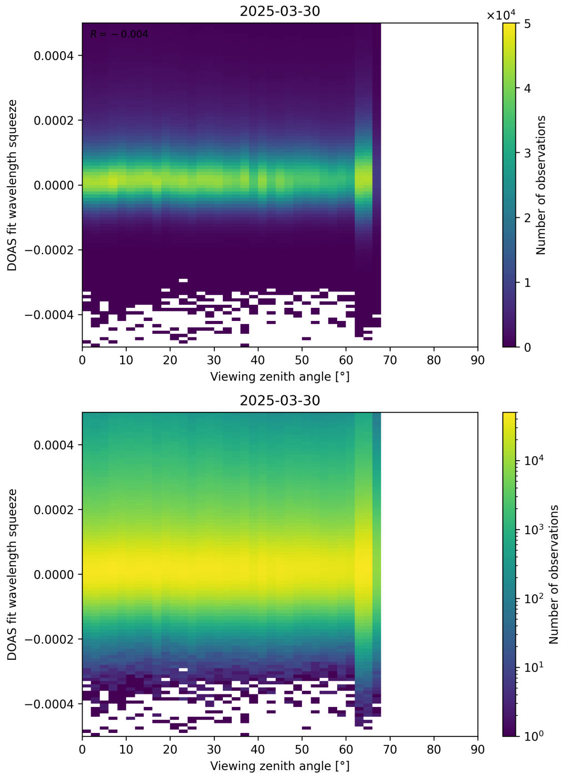
Figure 184: Scatter density plot of “Viewing zenith angle” against “DOAS fit wavelength squeeze” for 2025-03-29 to 2025-03-31.
