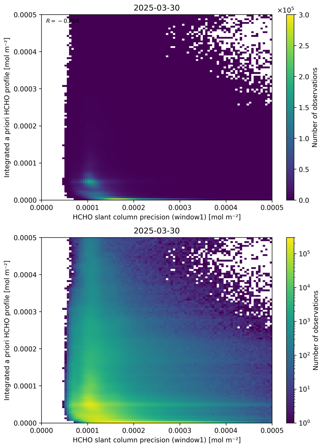
Figure 96: Scatter density plot of “HCHO slant column precision (window1)” against “Integrated a priori HCHO profile” for 2025-03-29 to 2025-03-31.
