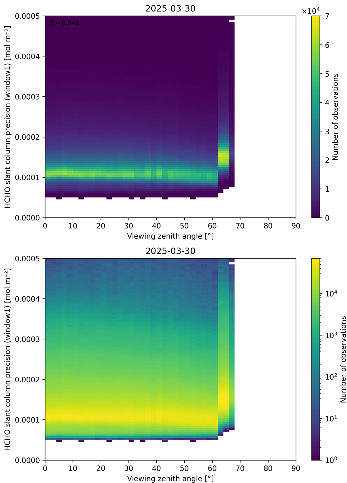
Figure 189: Scatter density plot of “Viewing zenith angle” against “HCHO slant column precision (window1)” for 2025-03-29 to 2025-03-31.
