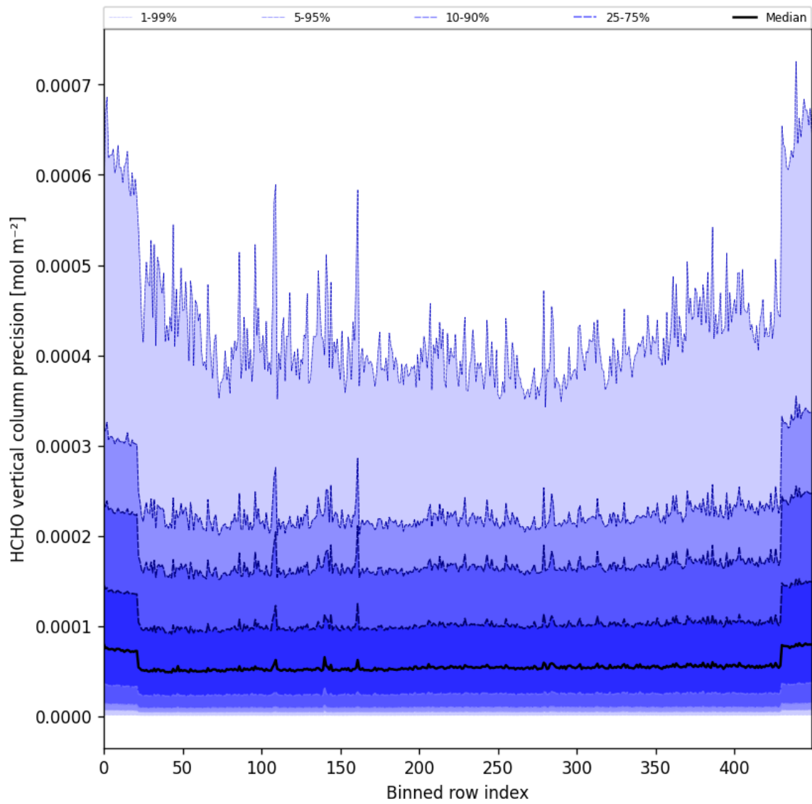
Figure 50: Along track statistics of “HCHO vertical column precision” for 2025-03-29 to 2025-03-31
