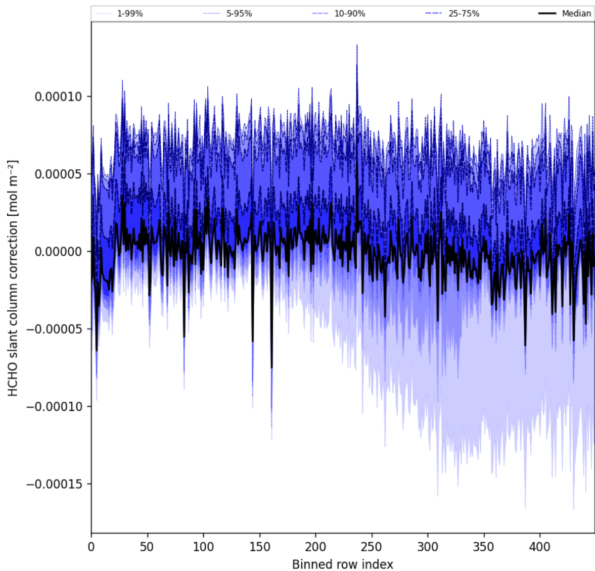
Figure 61: Along track statistics of “HCHO slant column correction” for 2025-03-29 to 2025-03-31
