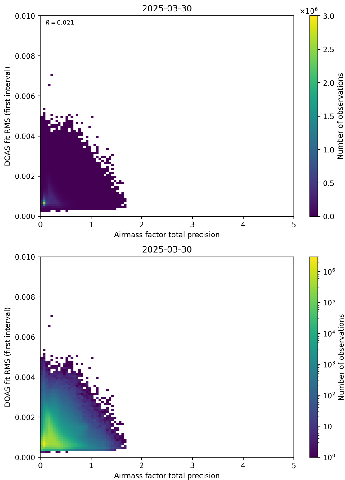
Figure 105: Scatter density plot of “Airmass factor total precision” against “DOAS fit RMS (first interval)” for 2025-03-29 to 2025-03-31.
