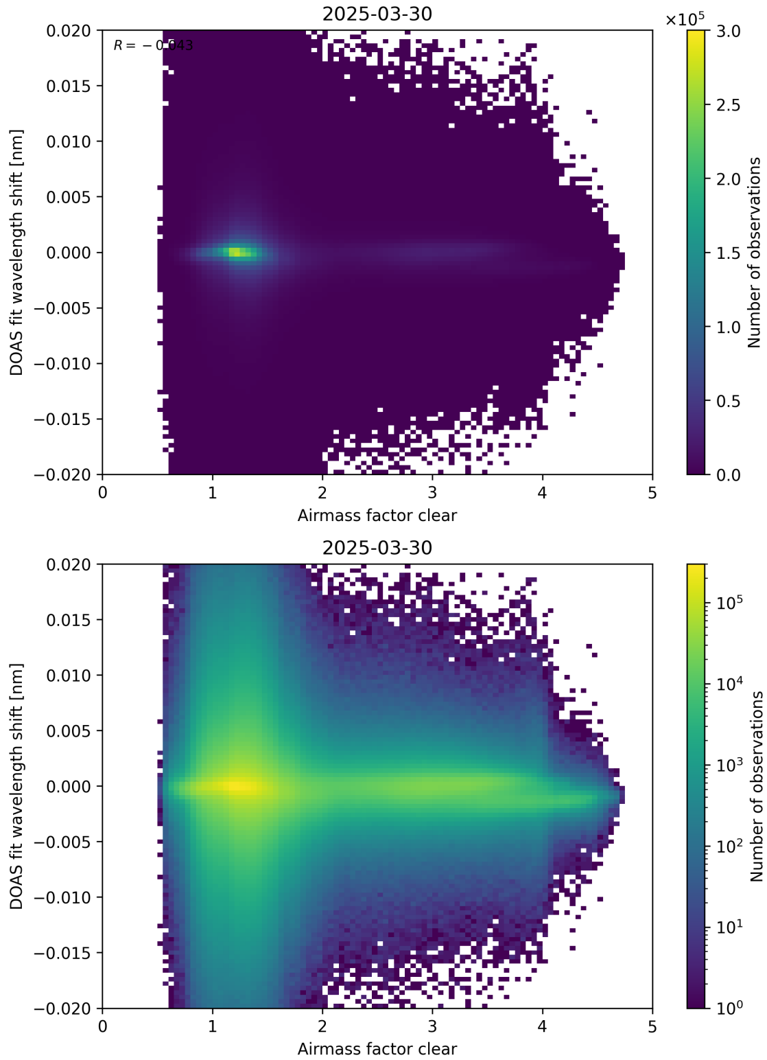
Figure 72: Scatter density plot of “Airmass factor clear” against “DOAS fit wavelength shift” for 2025-03-29 to 2025-03-31.
