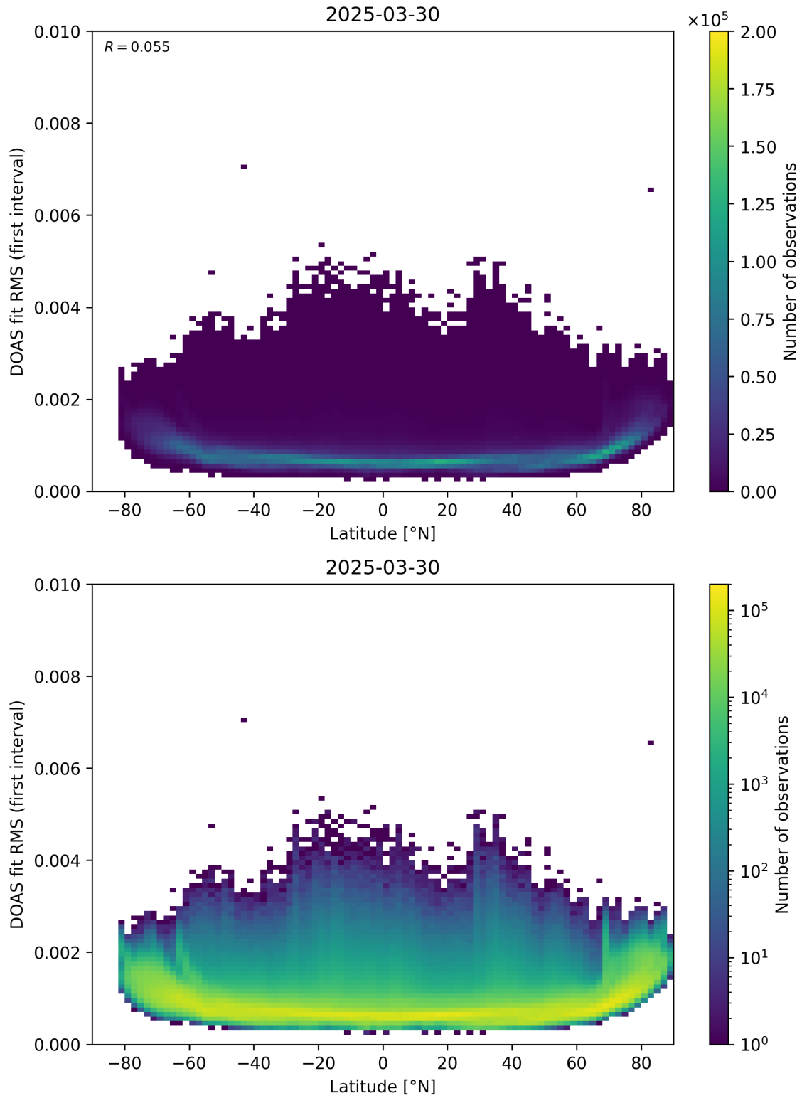
Figure 153: Scatter density plot of “Latitude” against “DOAS fit RMS (first interval)” for 2025-03-29 to 2025-03-31.
