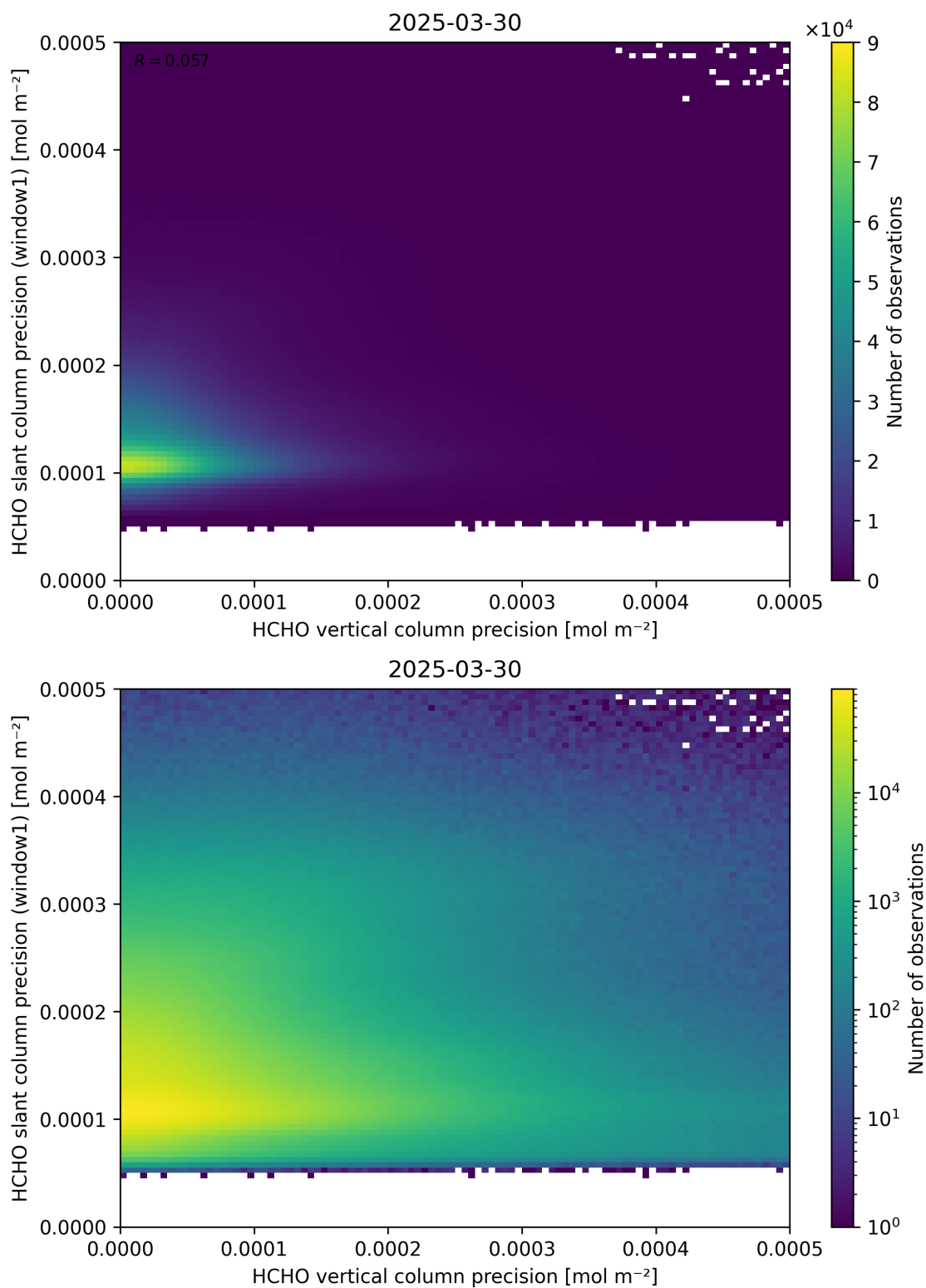
Figure 143: Scatter density plot of “HCHO vertical column precision” against “HCHO slant column precision (window1)” for 2025-03-29 to 2025-03-31.
