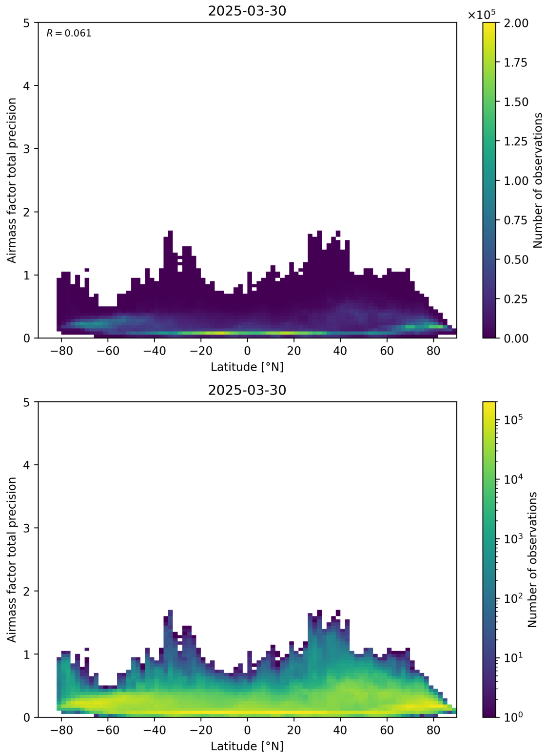
Figure 162: Scatter density plot of “Latitude” against “Airmass factor total precision” for 2025-03-29 to 2025-03-31.
