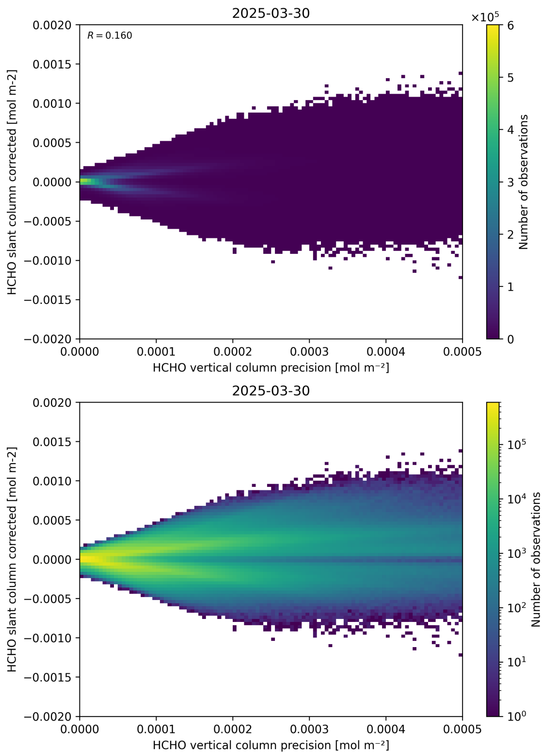
Figure 140: Scatter density plot of “HCHO vertical column precision” against “HCHO slant column corrected” for 2025-03-29 to 2025-03-31.
