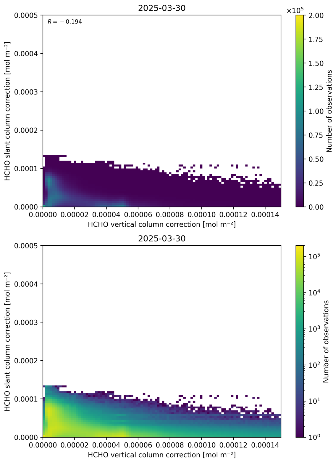
Figure 117: Scatter density plot of “HCHO vertical column correction” against “HCHO slant column correction” for 2025-03-29 to 2025-03-31.
