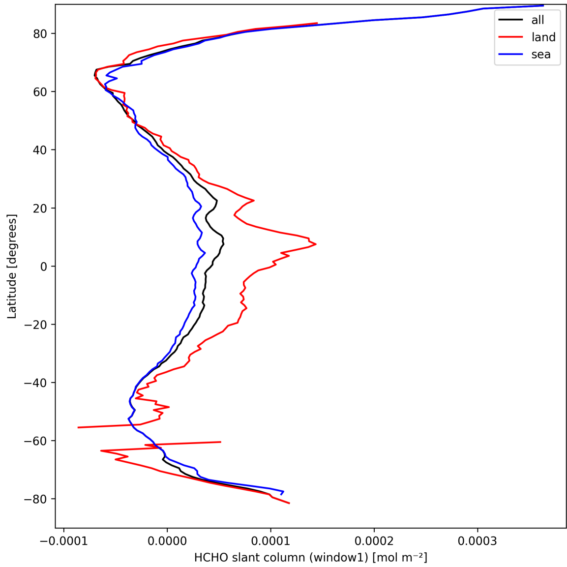
Figure 24: Zonal average of “HCHO slant column (window1)” for 2025-03-29 to 2025-03-31.
