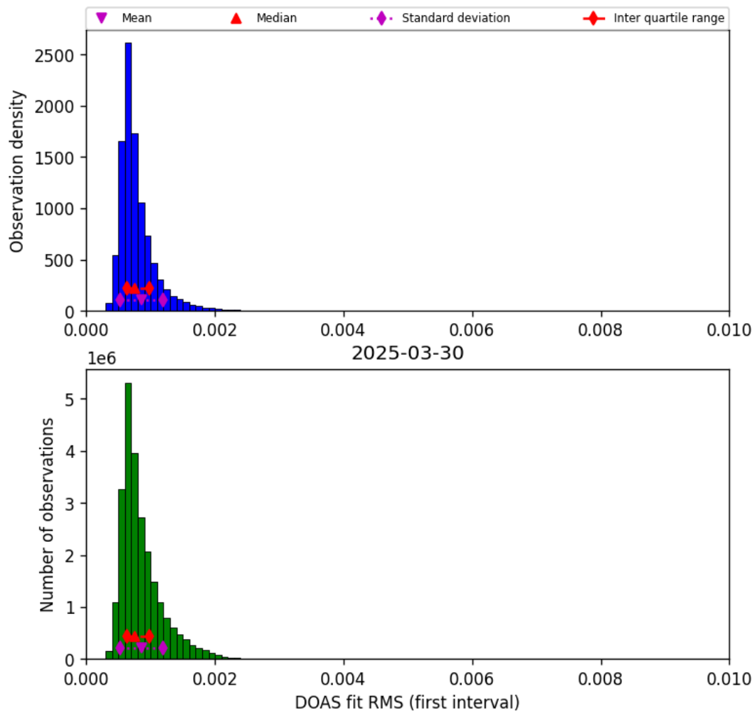
Figure 46: Histogram of “DOAS fit RMS (first interval)” for 2025-03-29 to 2025-03-31
