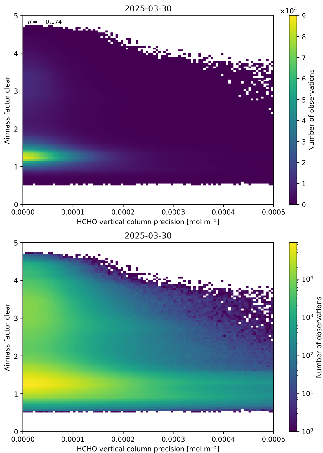
Figure 139: Scatter density plot of “HCHO vertical column precision” against “Airmass factor clear” for 2025-03-29 to 2025-03-31.
