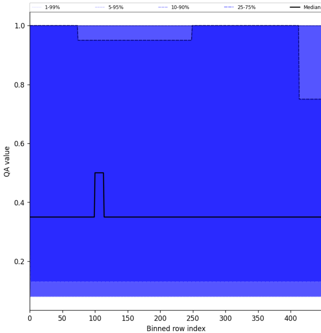
Figure 48: Along track statistics of “QA value” for 2025-03-29 to 2025-03-31
