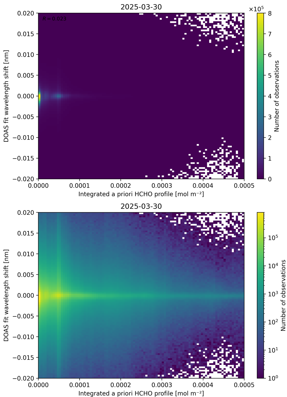
Figure 149: Scatter density plot of “Integrated a priori HCHO profile” against “DOAS fit wavelength shift” for 2025-03-29 to 2025-03-31.
