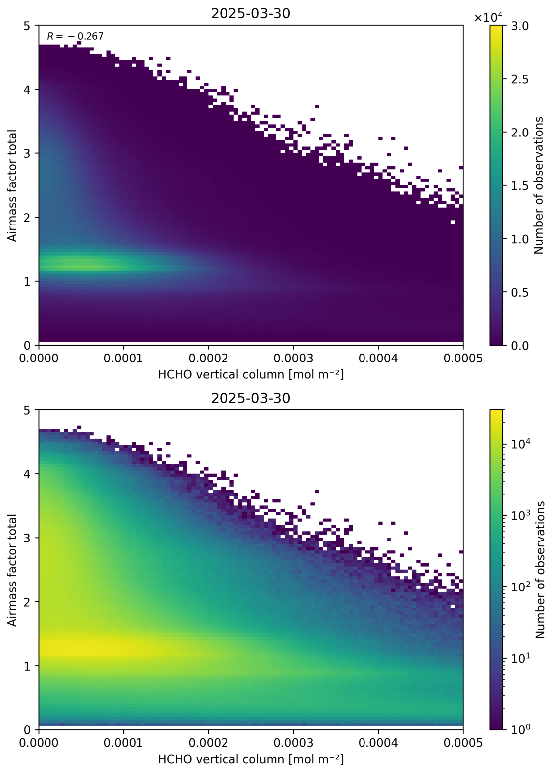
Figure 131: Scatter density plot of “HCHO vertical column” against “Airmass factor total” for 2025-03-29 to 2025-03-31.
