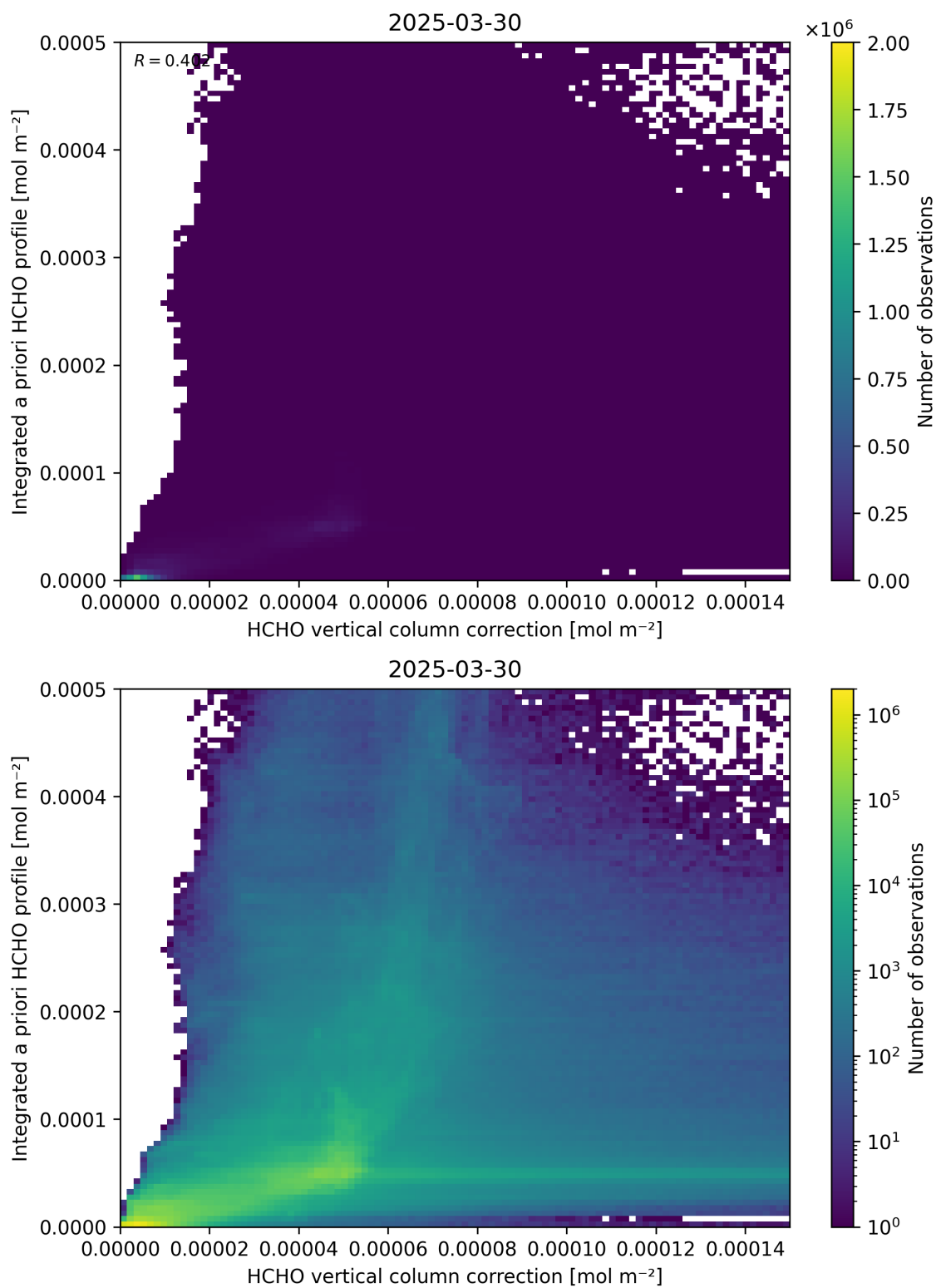
Figure 122: Scatter density plot of “HCHO vertical column correction” against “Integrated a priori HCHO profile” for 2025-03-29 to 2025-03-31.
