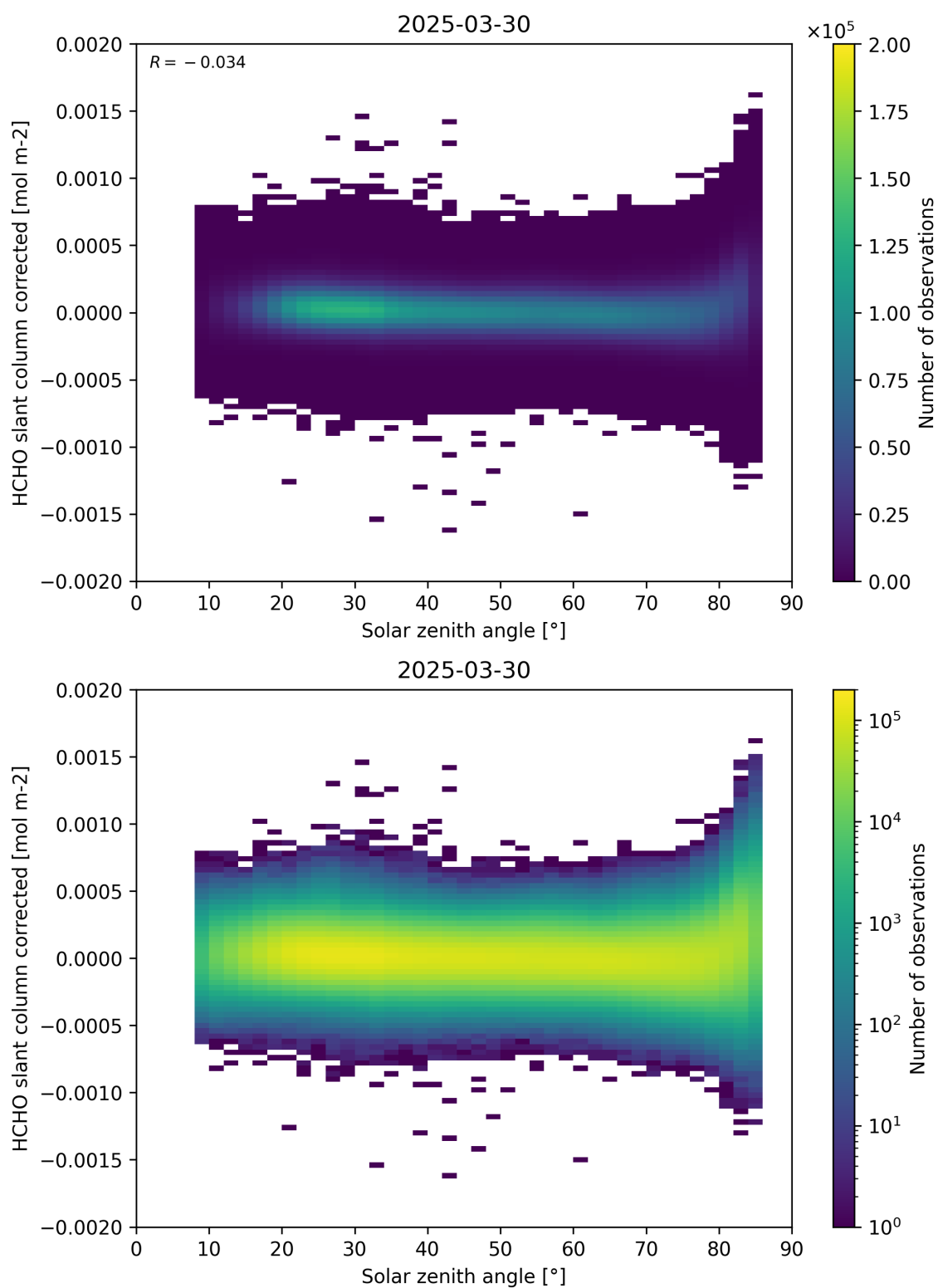
Figure 171: Scatter density plot of “Solar zenith angle” against “HCHO slant column corrected” for 2025-03-29 to 2025-03-31.
