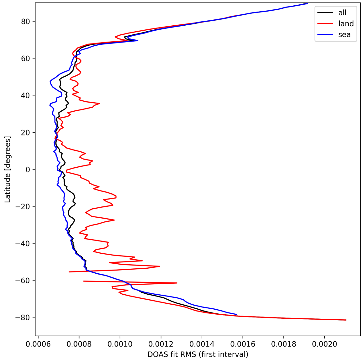
Figure 32: Zonal average of “DOAS fit RMS (first interval)” for 2025-03-29 to 2025-03-31.
