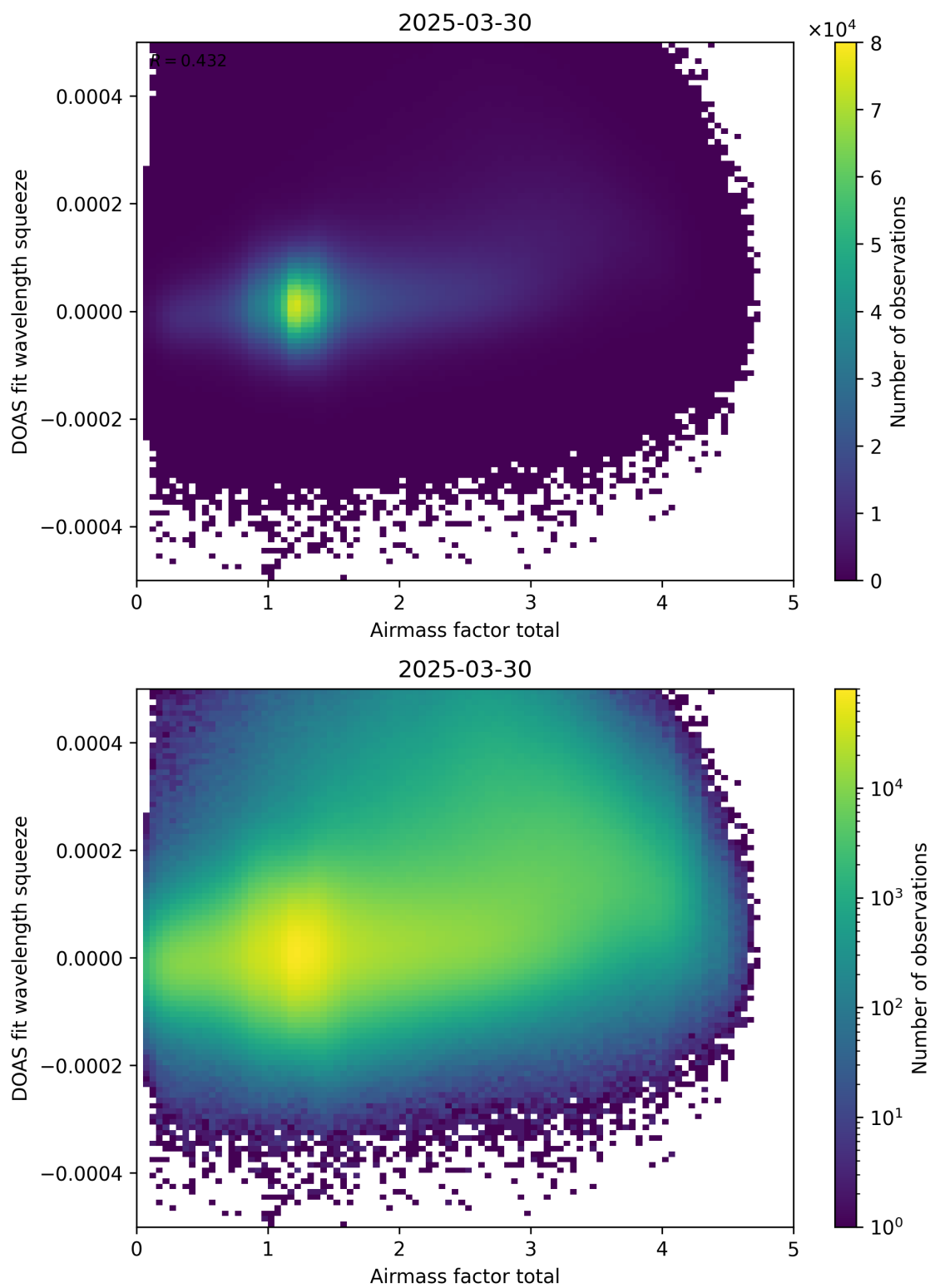
Figure 99: Scatter density plot of “Airmass factor total” against “DOAS fit wavelength squeeze” for 2025-03-29 to 2025-03-31.
