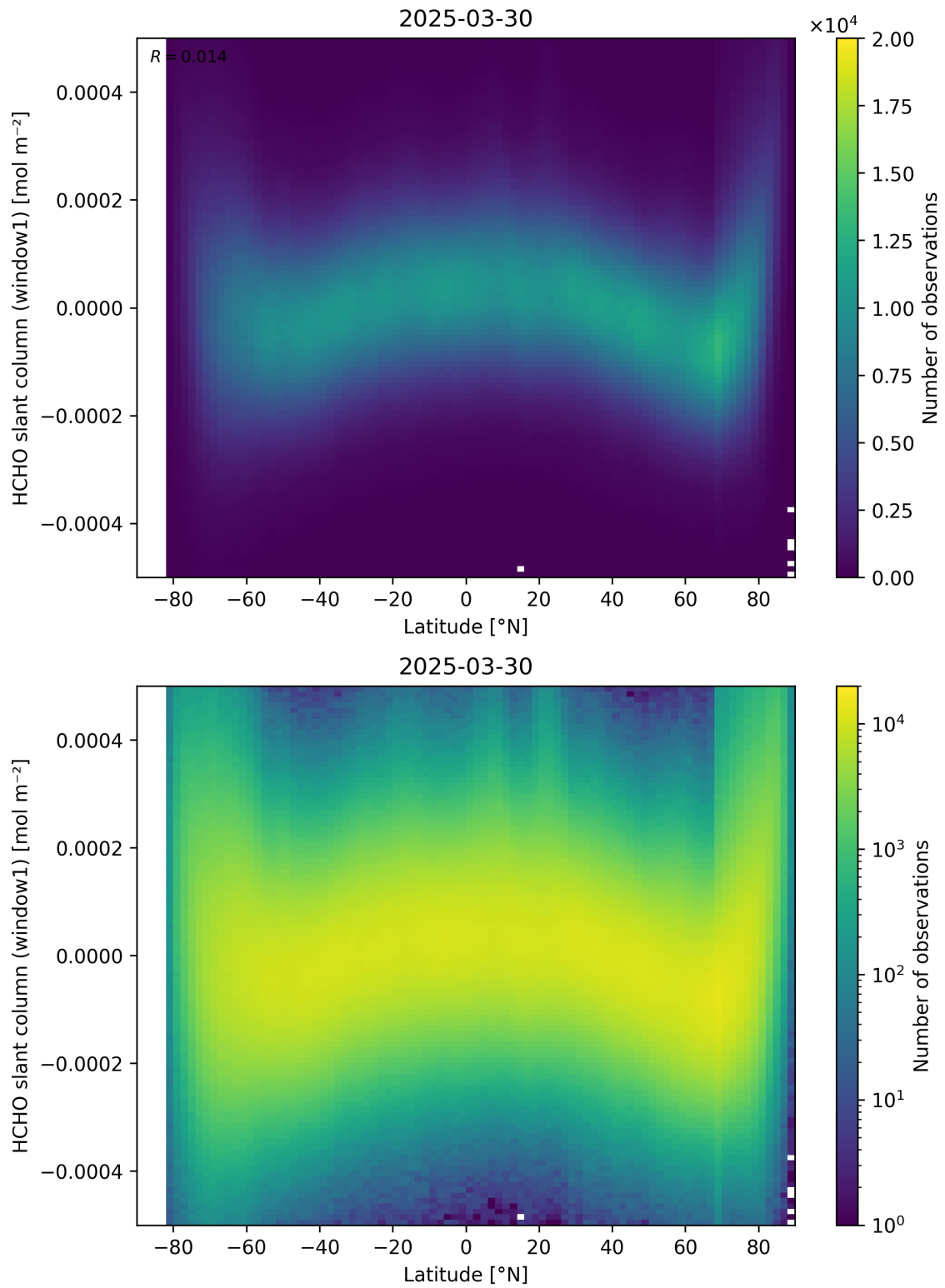
Figure 159: Scatter density plot of “Latitude” against “HCHO slant column (window1)” for 2025-03-29 to 2025-03-31.
