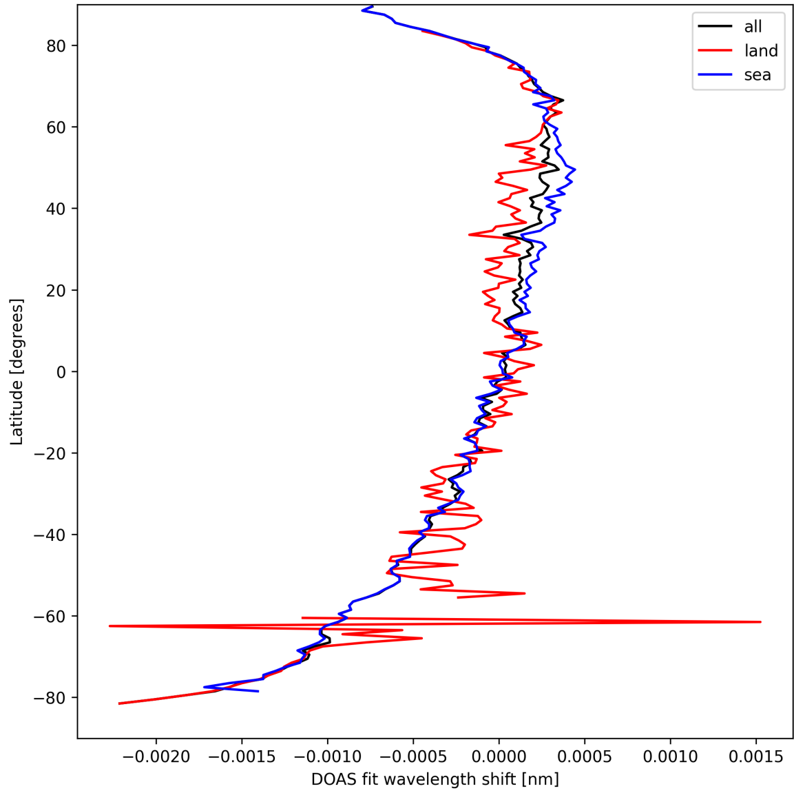
Figure 30: Zonal average of "DOAS fit wavelength shift" for 2025-03-29 to 2025-03-31.
