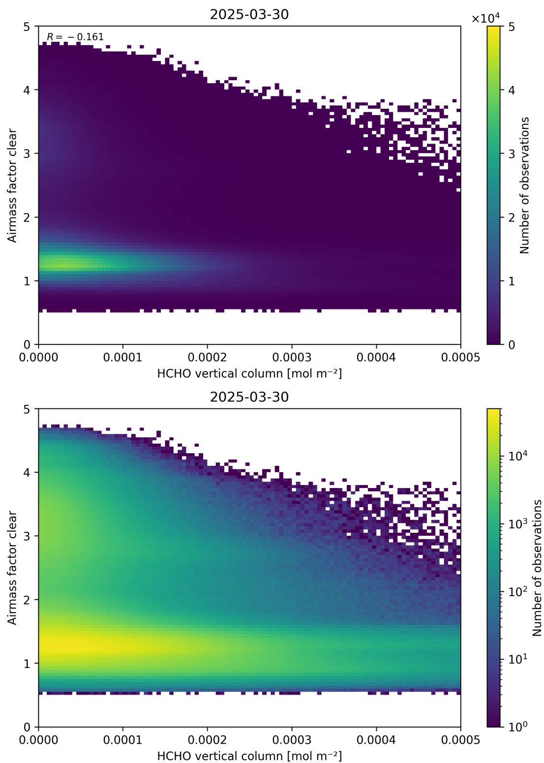
Figure 126: Scatter density plot of “HCHO vertical column” against “Airmass factor clear” for 2025-03-29 to 2025-03-31.
