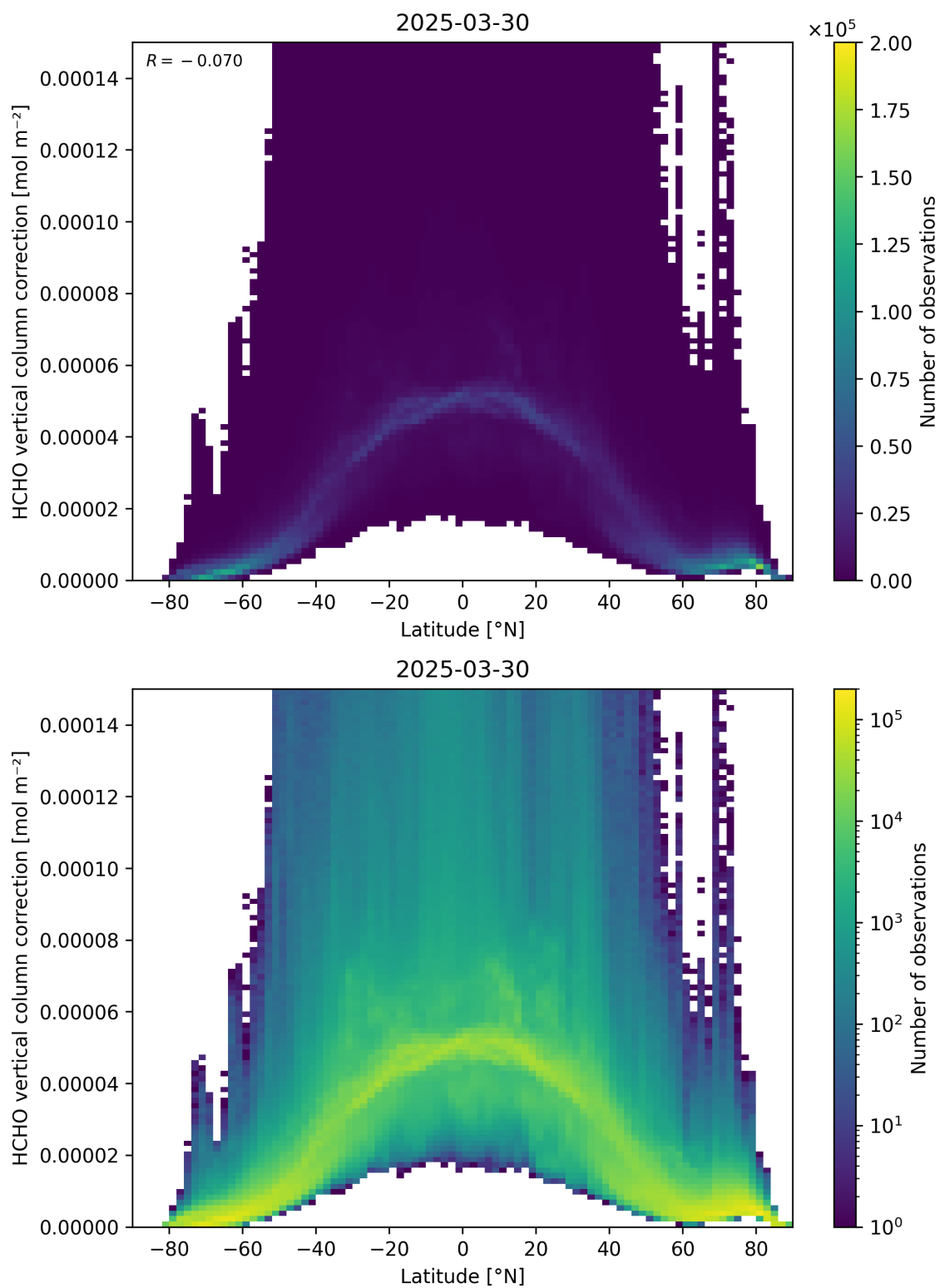
Figure 164: Scatter density plot of “Latitude” against “HCHO vertical column correction” for 2025-03-29 to 2025-03-31.
