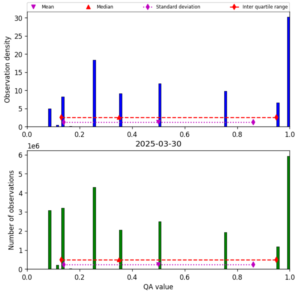
Figure 34: Histogram of “QA value” for 2025-03-29 to 2025-03-31
