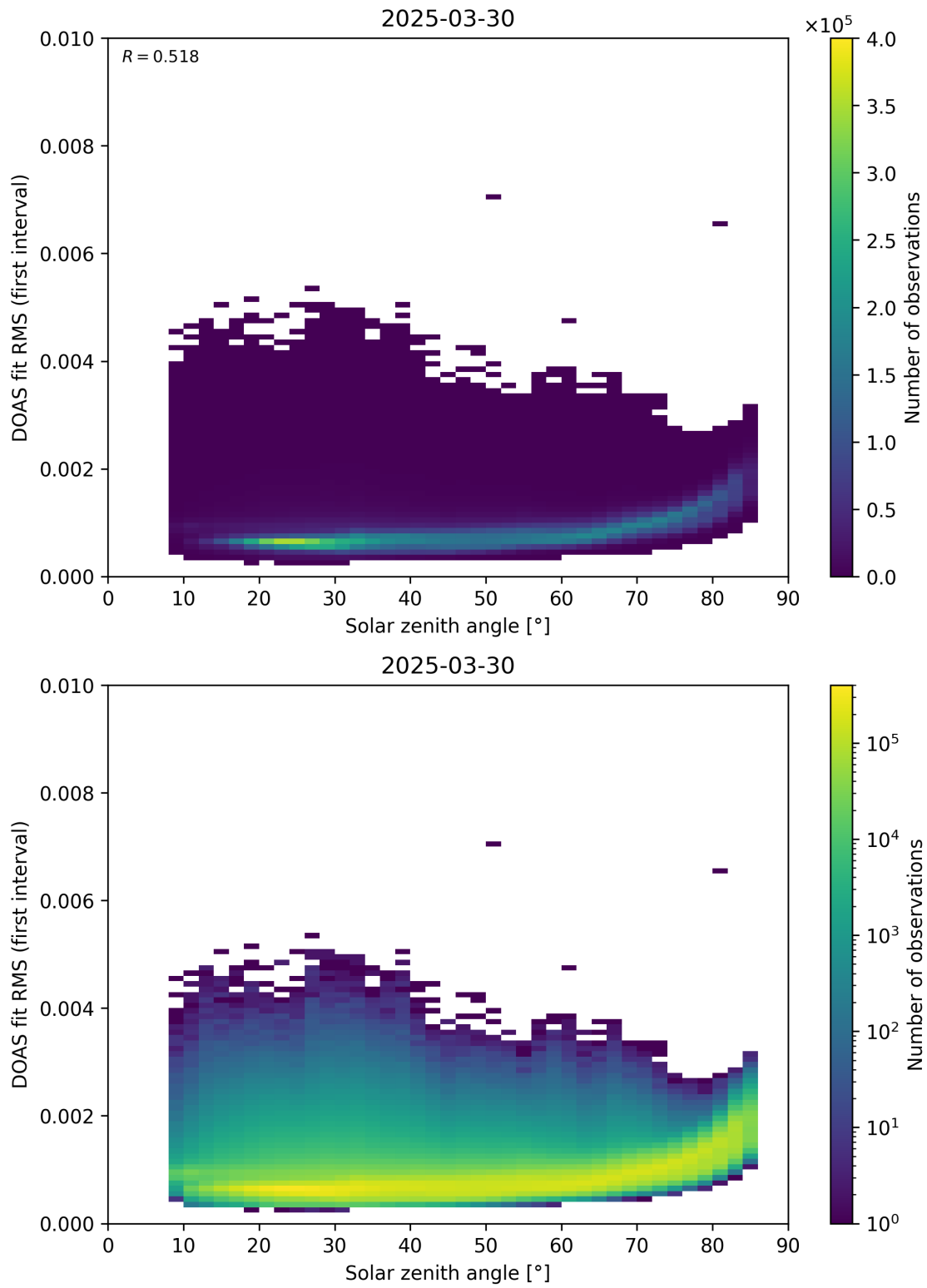
Figure 167: Scatter density plot of “Solar zenith angle” against “DOAS fit RMS (first interval)” for 2025-03-29 to 2025-03-31.
