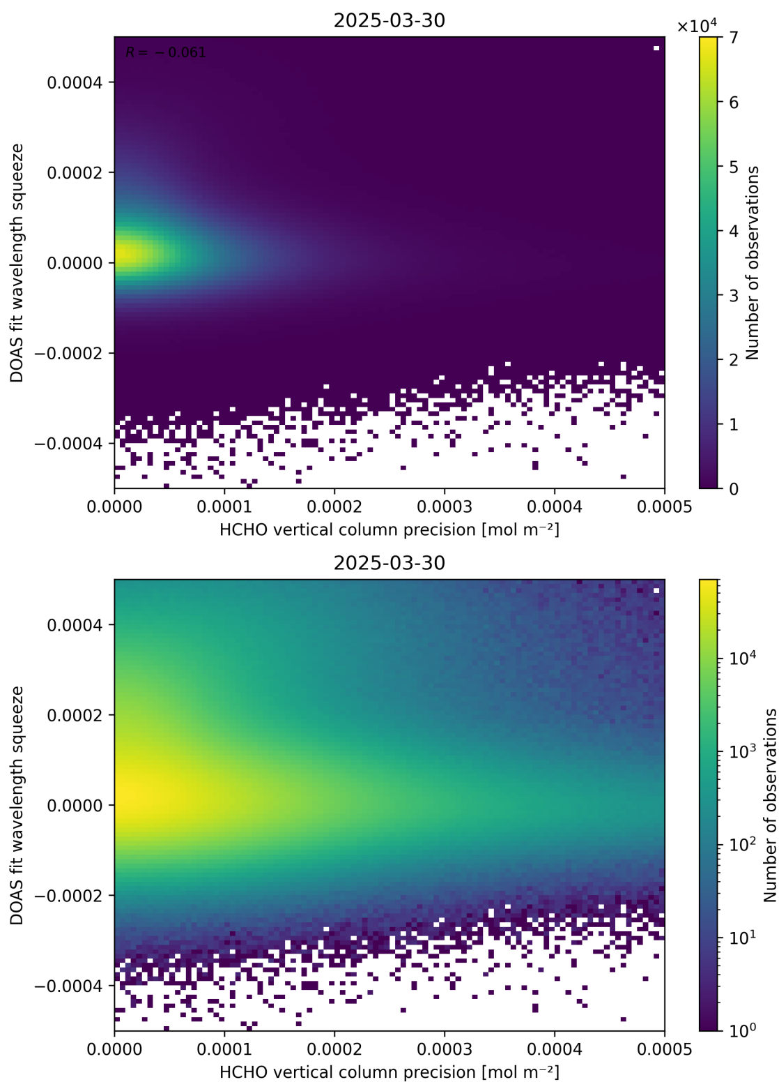
Figure 138: Scatter density plot of “HCHO vertical column precision” against “DOAS fit wavelength squeeze” for 2025-03-29 to 2025-03-31.
