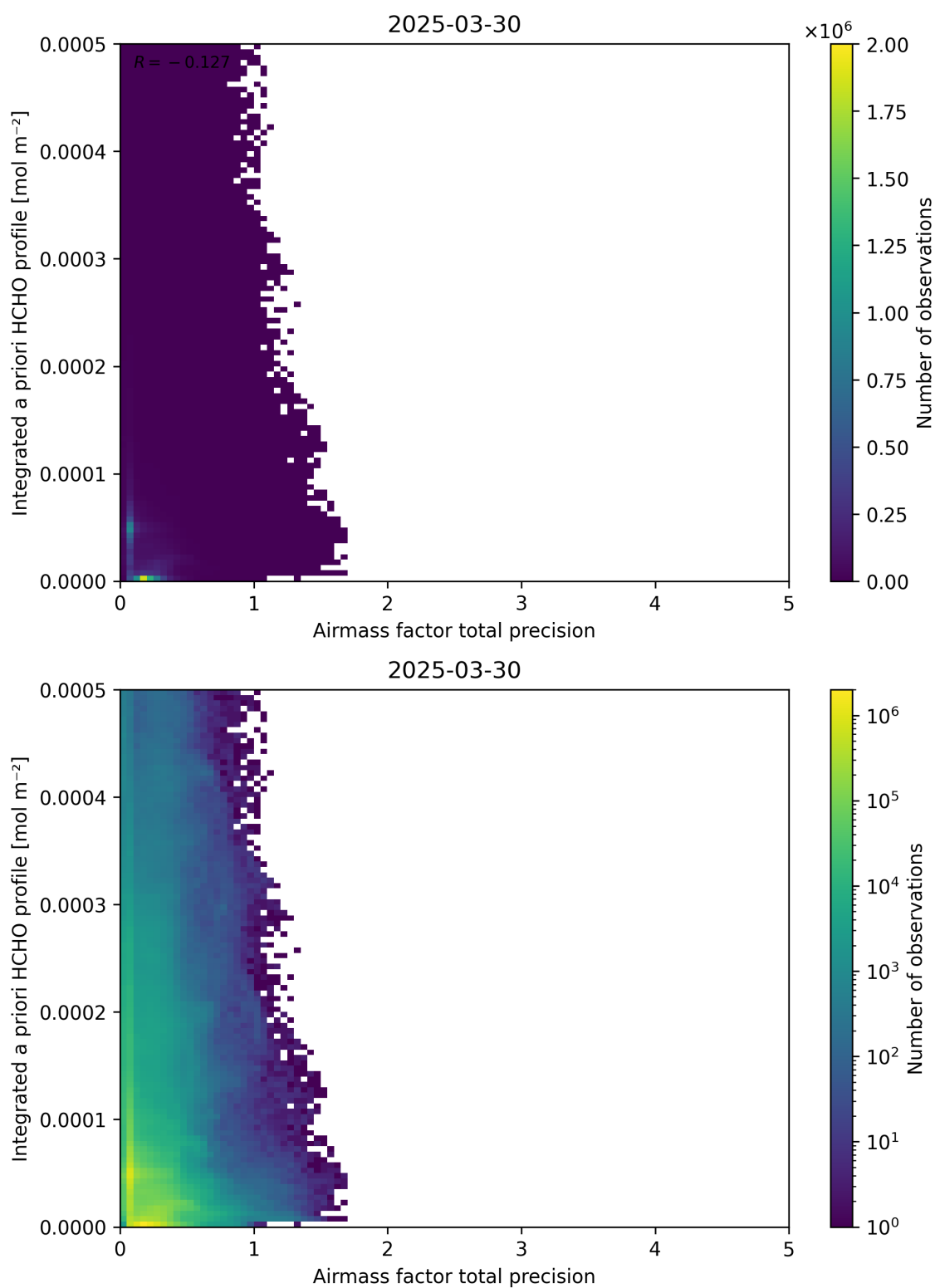
Figure 111: Scatter density plot of “Airmass factor total precision” against “Integrated a priori HCHO profile” for 2025-03-29 to 2025-03-31.
