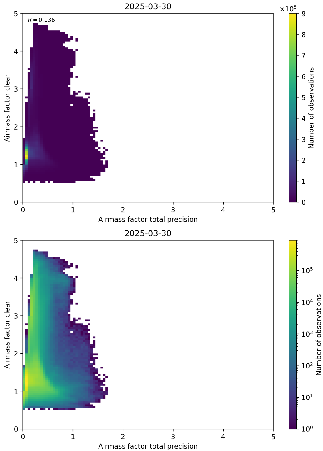
Figure 108: Scatter density plot of “Airmass factor total precision” against “Airmass factor clear” for 2025-03-29 to 2025-03-31.
