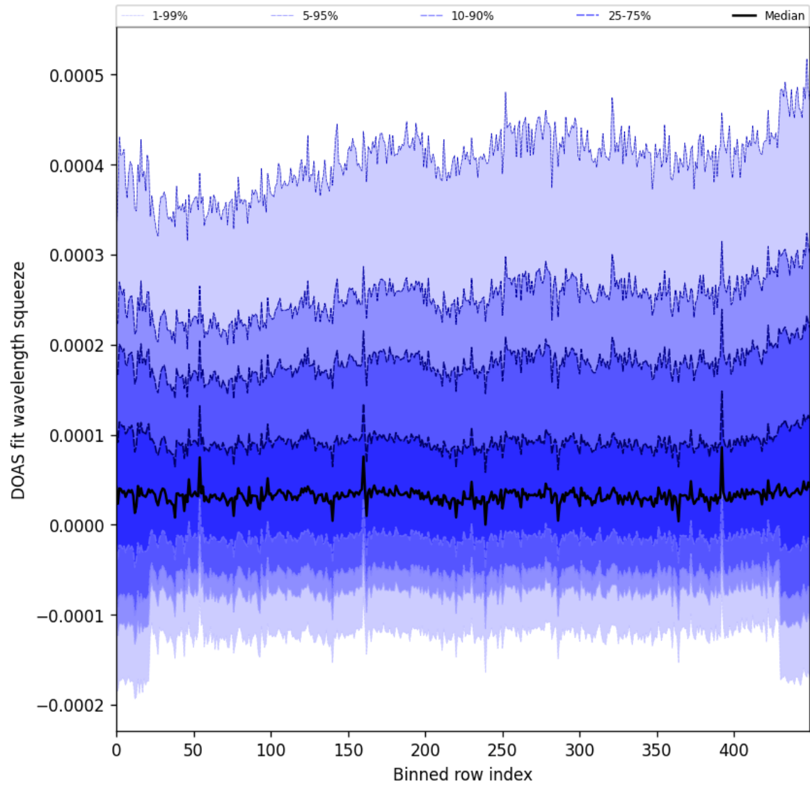
Figure 59: Along track statistics of “DOAS fit wavelength squeeze” for 2025-03-29 to 2025-03-31
