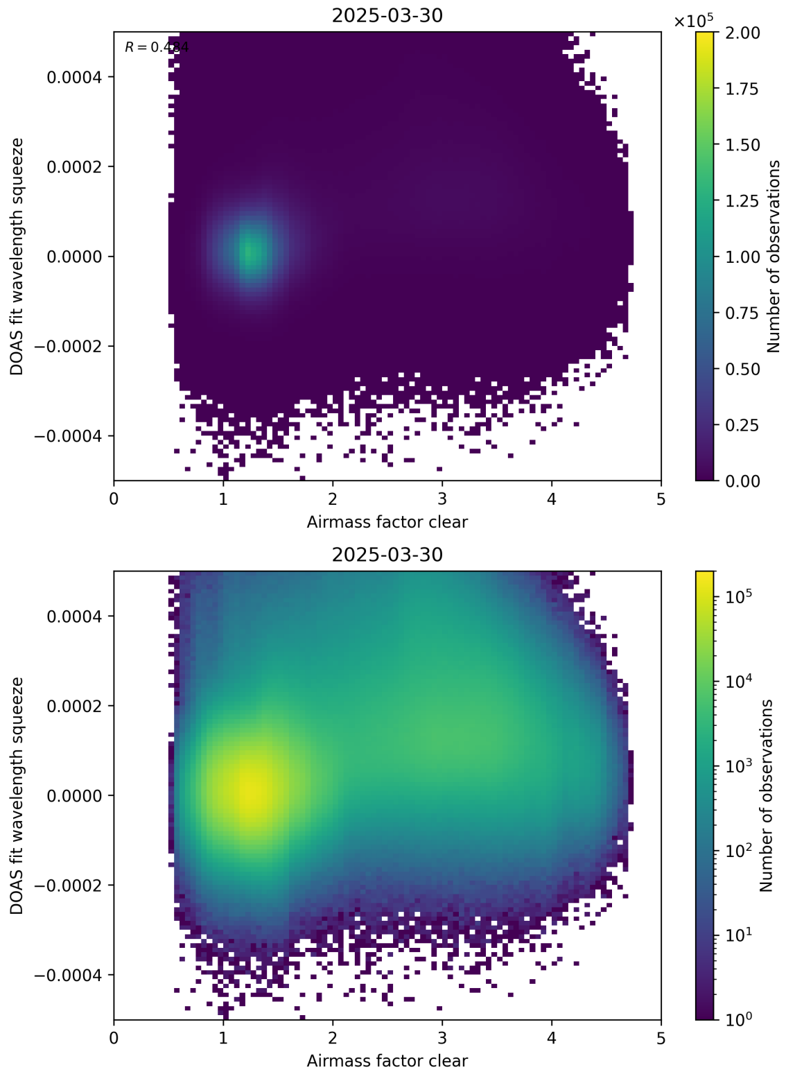
Figure 73: Scatter density plot of “Airmass factor clear” against “DOAS fit wavelength squeeze” for 2025-03-29 to 2025-03-31.
