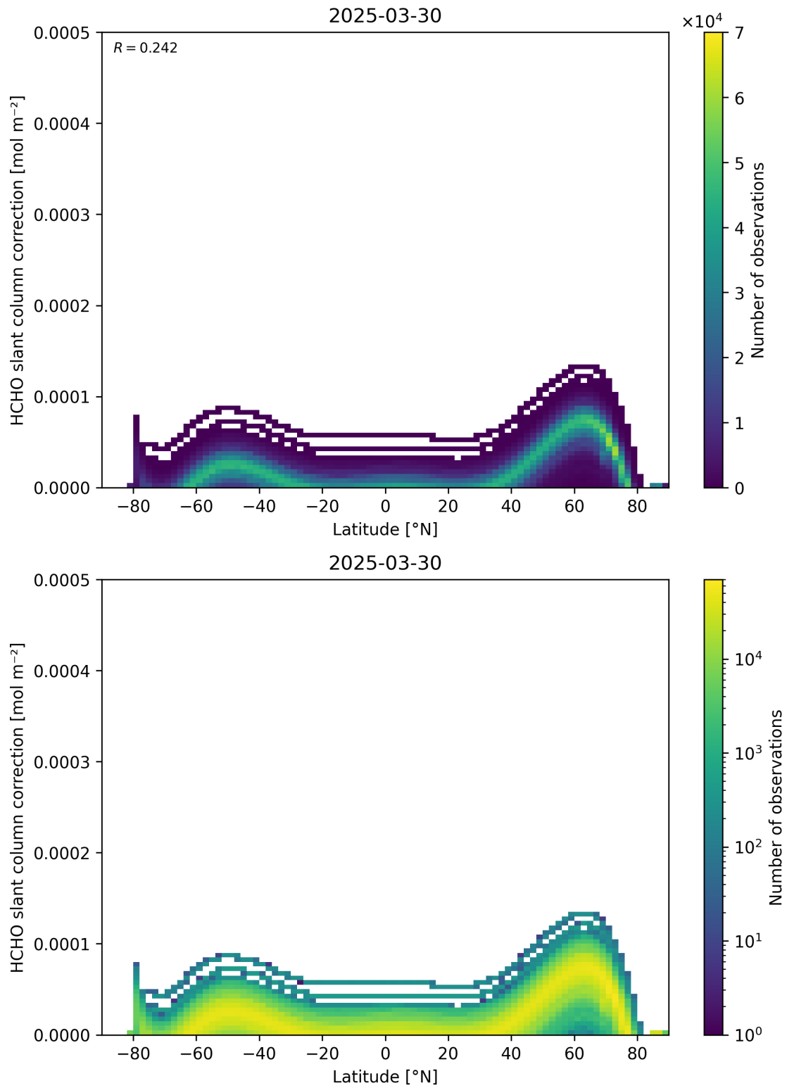
Figure 158: Scatter density plot of “Latitude” against “HCHO slant column correction” for 2025-03-29 to 2025-03-31.
