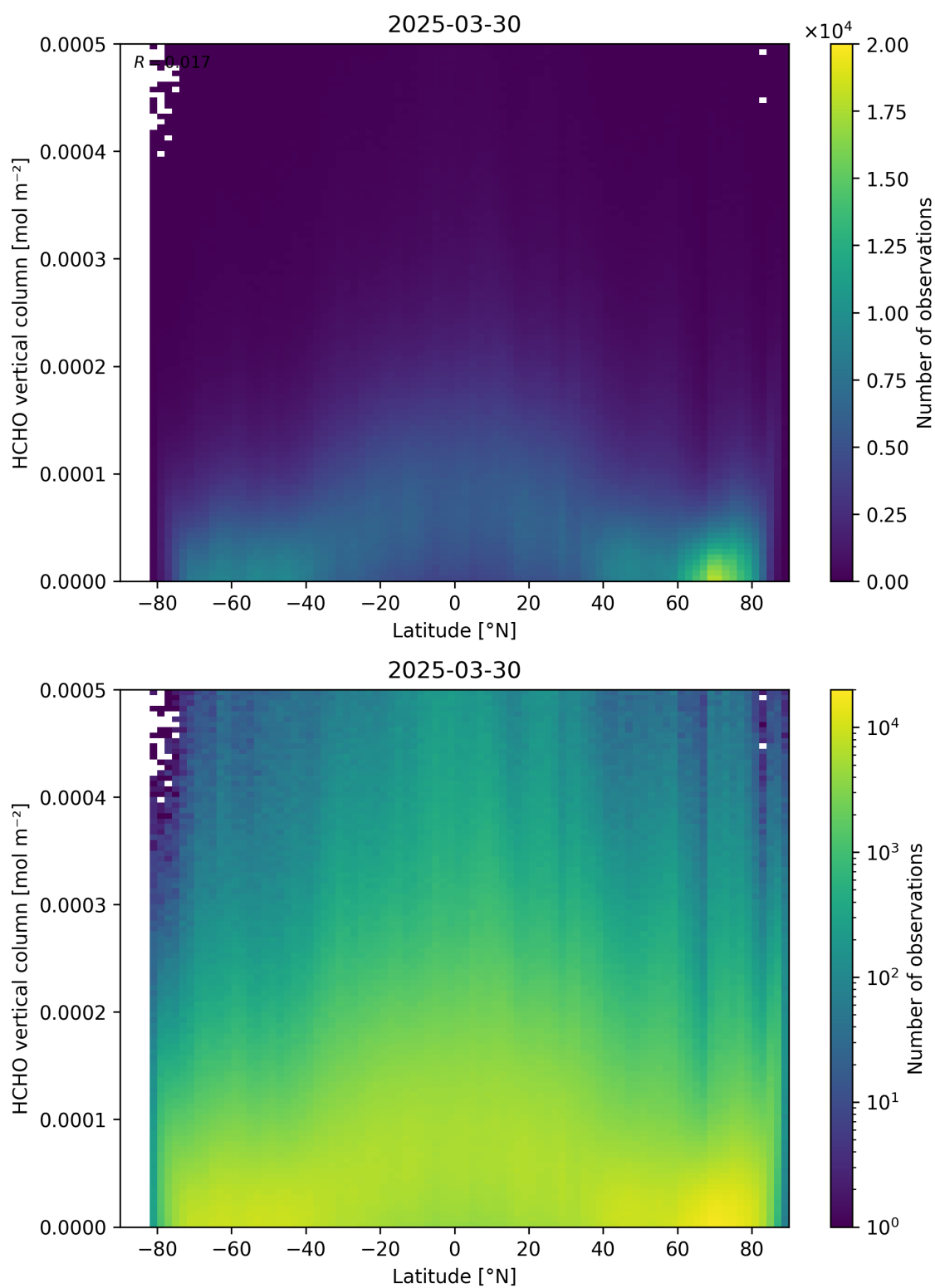
Figure 163: Scatter density plot of “Latitude” against “HCHO vertical column” for 2025-03-29 to 2025-03-31.
