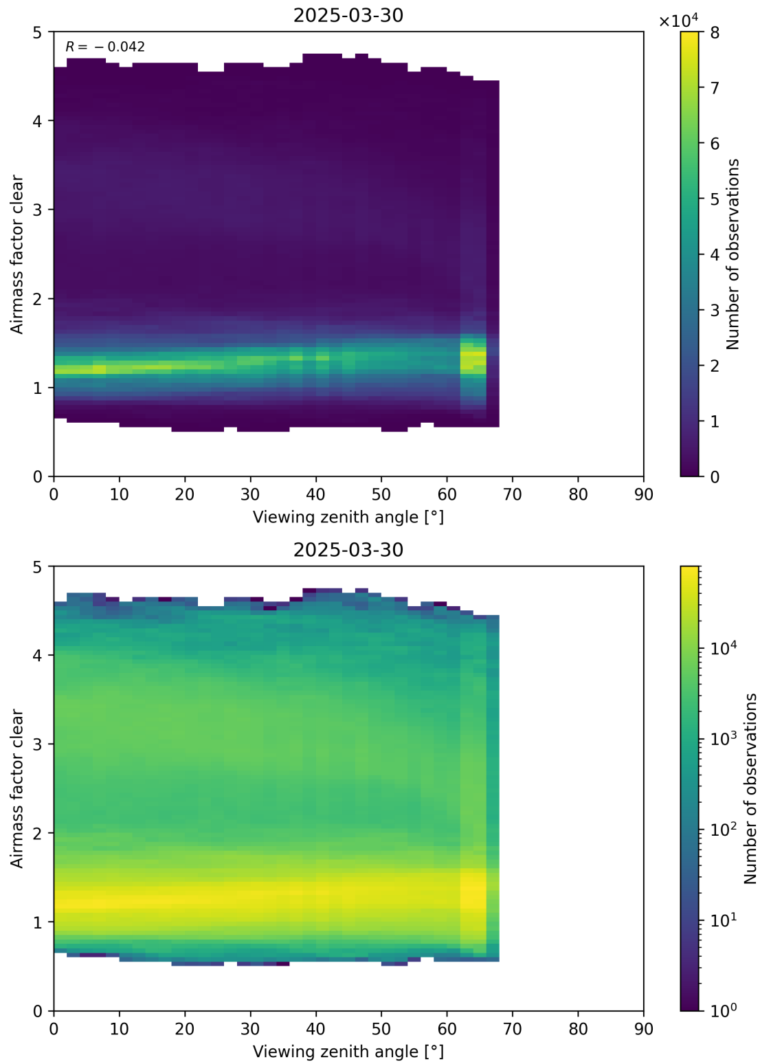
Figure 185: Scatter density plot of “Viewing zenith angle” against “Airmass factor clear” for 2025-03-29 to 2025-03-31.
