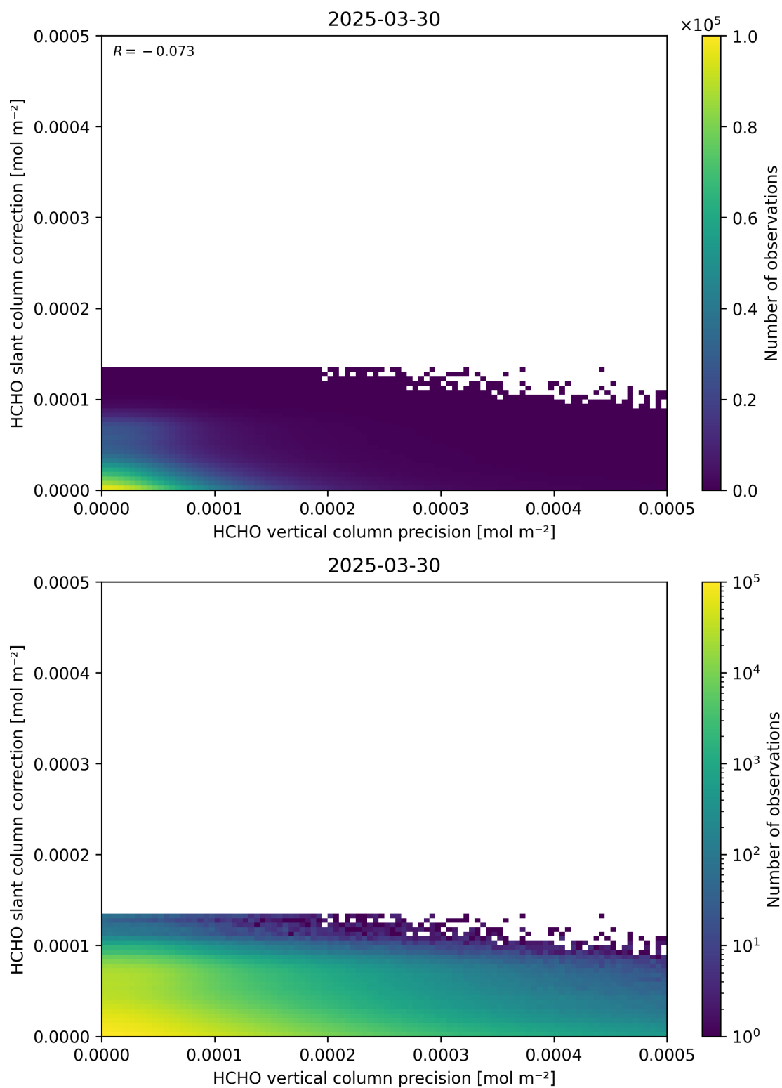
Figure 141: Scatter density plot of “HCHO vertical column precision” against “HCHO slant column correction” for 2025-03-29 to 2025-03-31.
