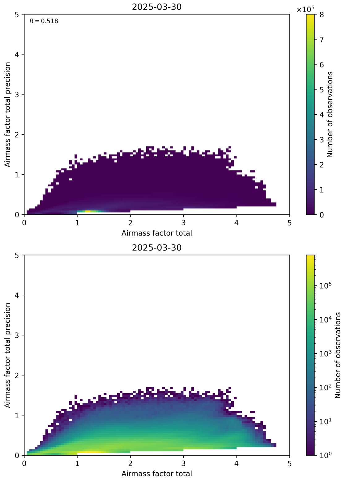
Figure 103: Scatter density plot of “Airmass factor total” against “Airmass factor total precision” for 2025-03-29 to 2025-03-31.
