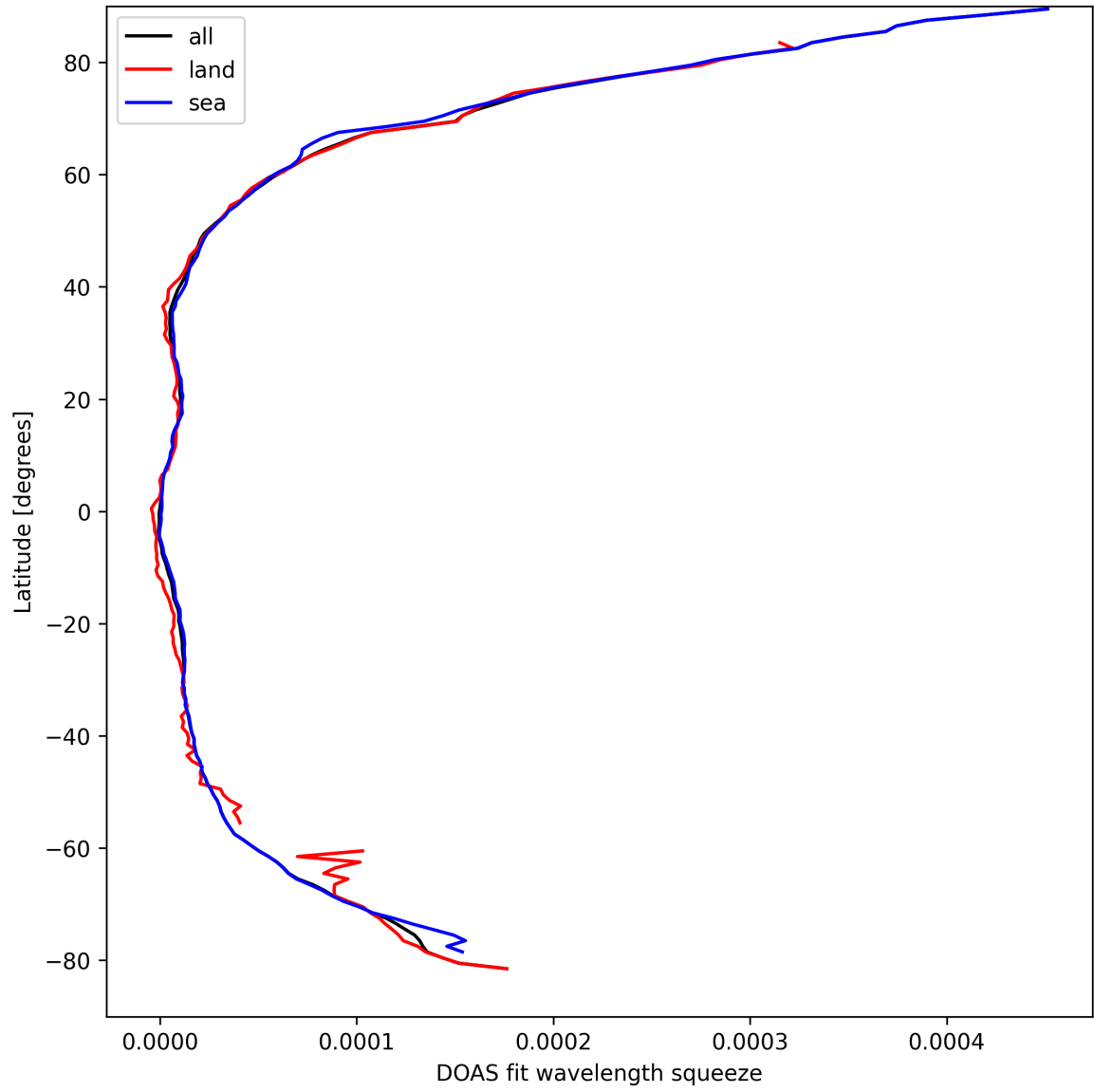
Figure 31: Zonal average of “DOAS fit wavelength squeeze” for 2025-03-29 to 2025-03-31.
