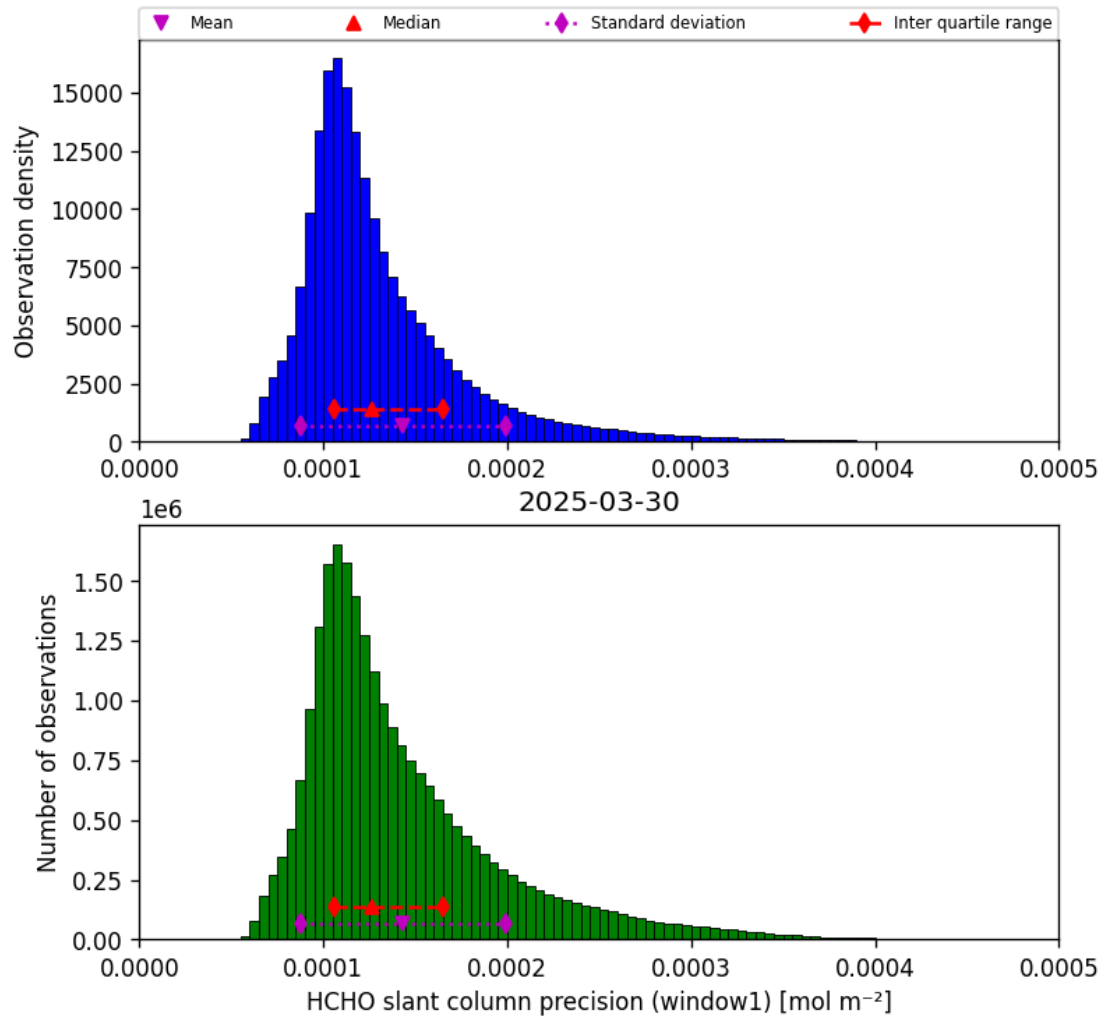
Figure 39: Histogram of “HCHO slant column precision (window1)” for 2025-03-29 to 2025-03-31
