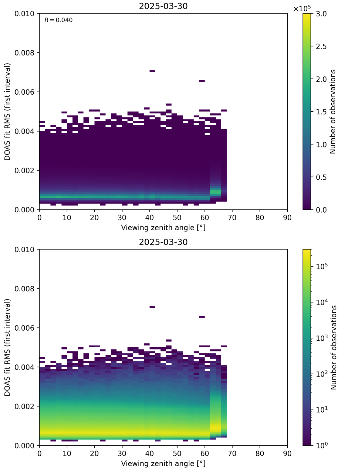
Figure 182: Scatter density plot of “Viewing zenith angle” against “DOAS fit RMS (first interval)” for 2025-03-29 to 2025-03-31.
