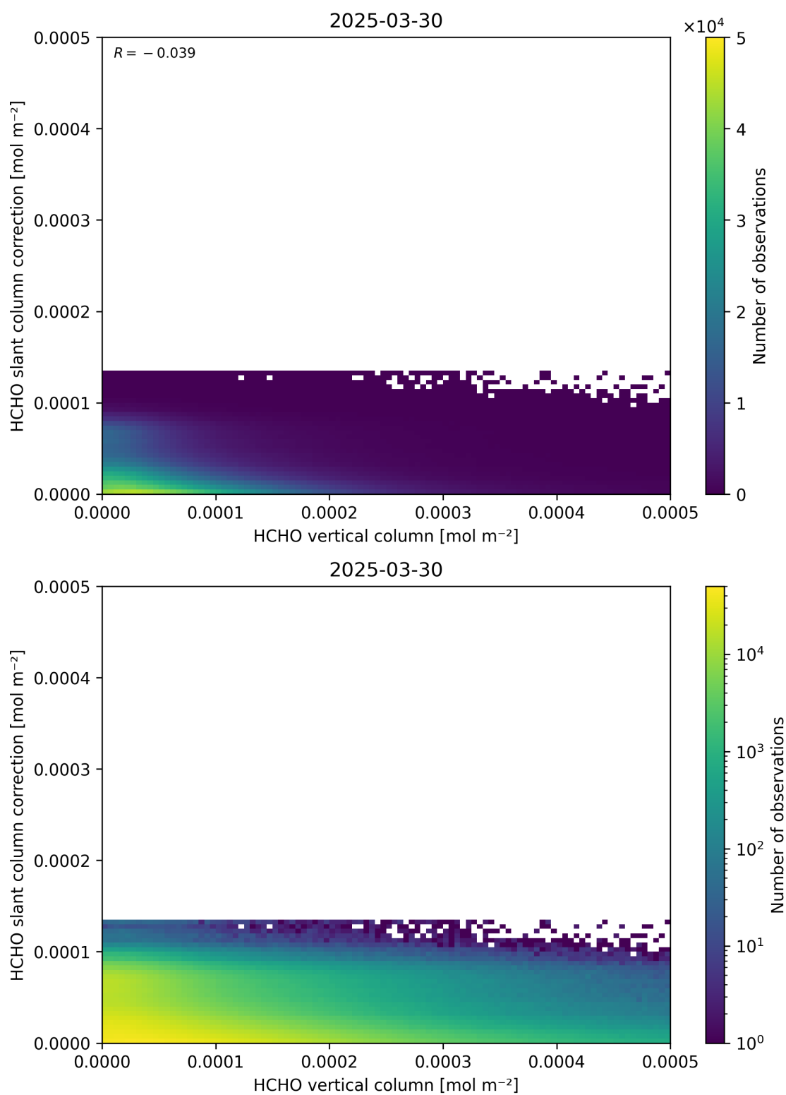
Figure 128: Scatter density plot of “HCHO vertical column” against “HCHO slant column correction” for 2025-03-29 to 2025-03-31.
