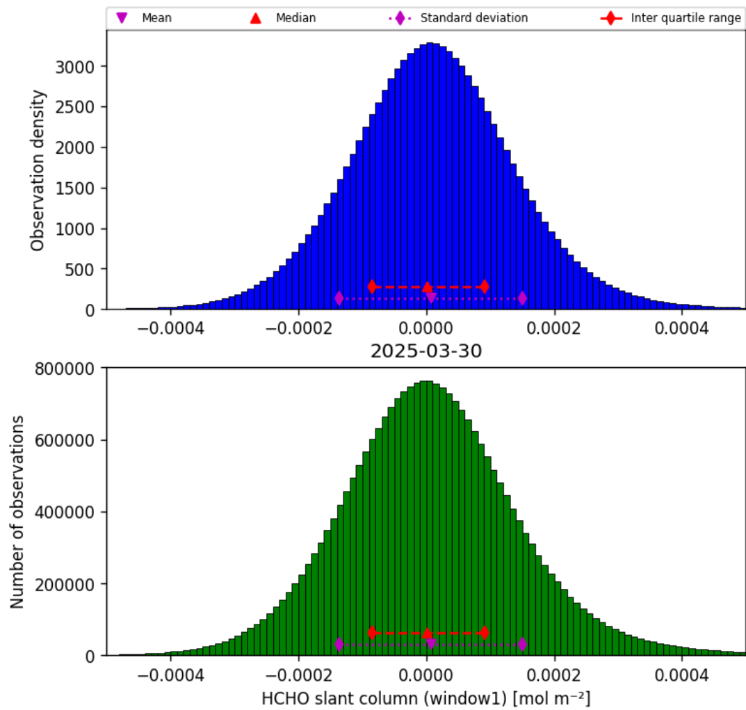
Figure 38: Histogram of “HCHO slant column (window1)” for 2025-03-29 to 2025-03-31
