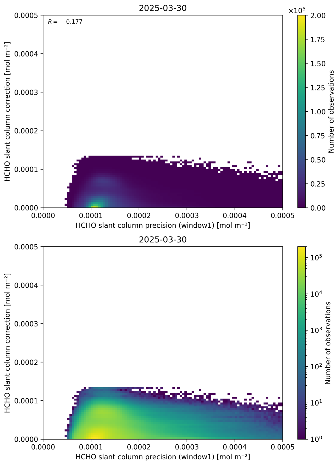
Figure 93: Scatter density plot of “HCHO slant column precision (window1)” against “HCHO slant column correction” for 2025-03-29 to 2025-03-31.
