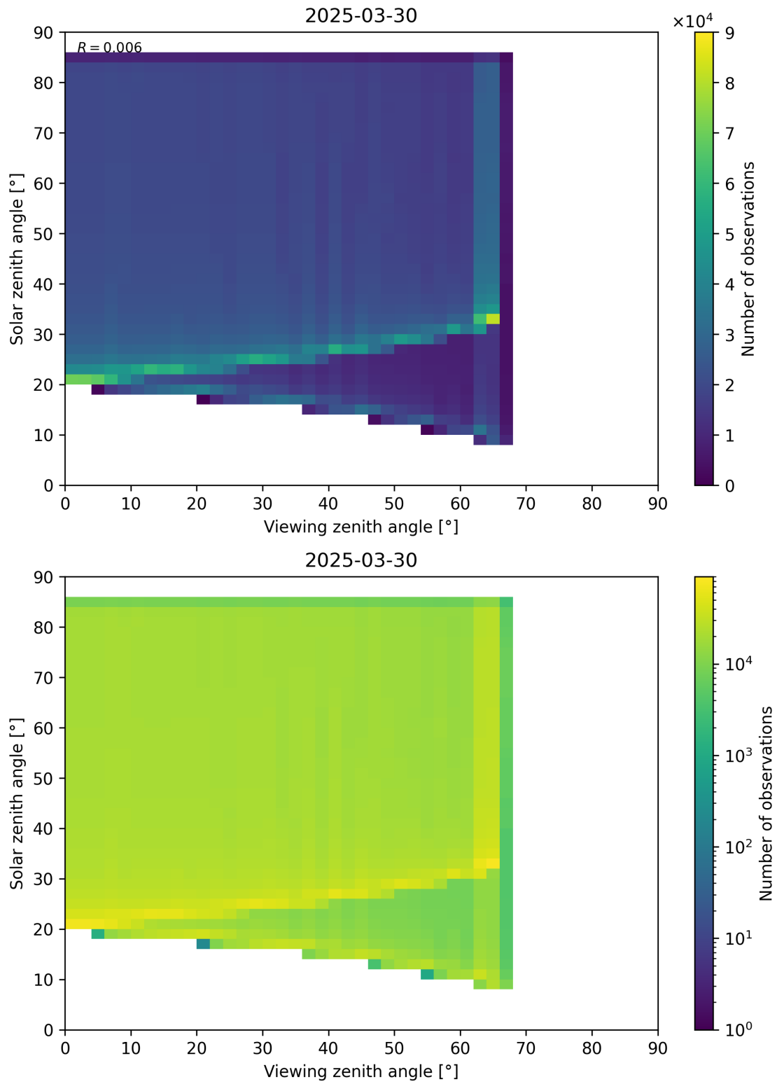
Figure 197: Scatter density plot of “Viewing zenith angle” against “Solar zenith angle” for 2025-03-29 to 2025-03-31.
