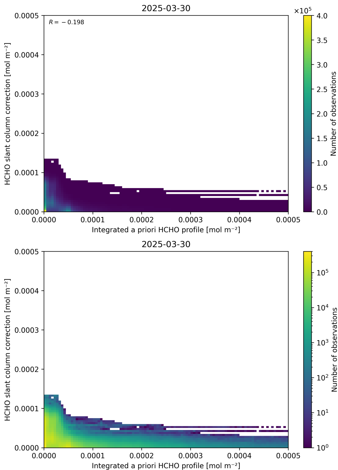
Figure 152: Scatter density plot of “Integrated a priori HCHO profile” against “HCHO slant column correction” for 2025-03-29 to 2025-03-31.
