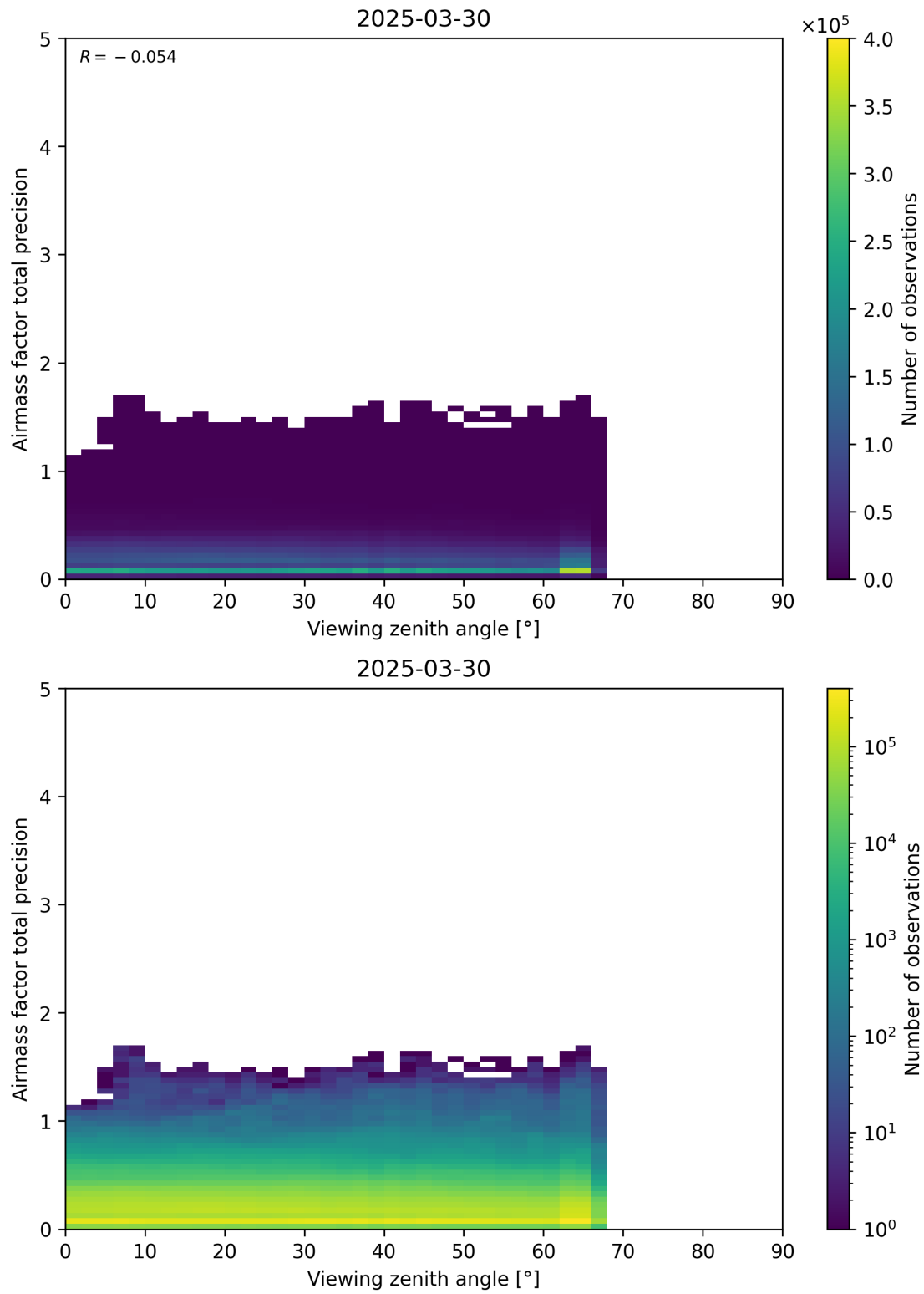
Figure 191: Scatter density plot of “Viewing zenith angle” against “Airmass factor total precision” for 2025-03-29 to 2025-03-31.
