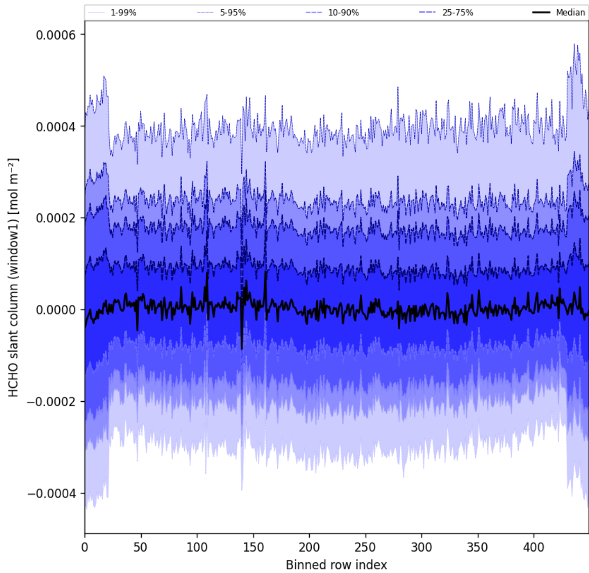
Figure 52: Along track statistics of “HCHO slant column (window1)” for 2025-03-29 to 2025-03-31
