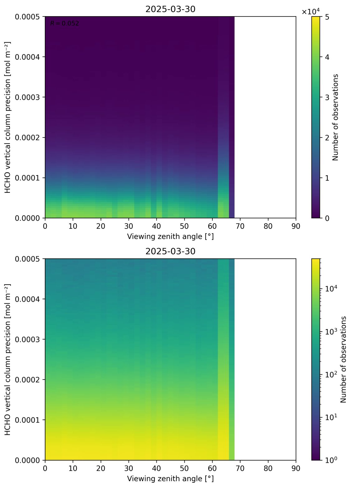
Figure 194: Scatter density plot of “Viewing zenith angle” against “HCHO vertical column precision” for 2025-03-29 to 2025-03-31.
