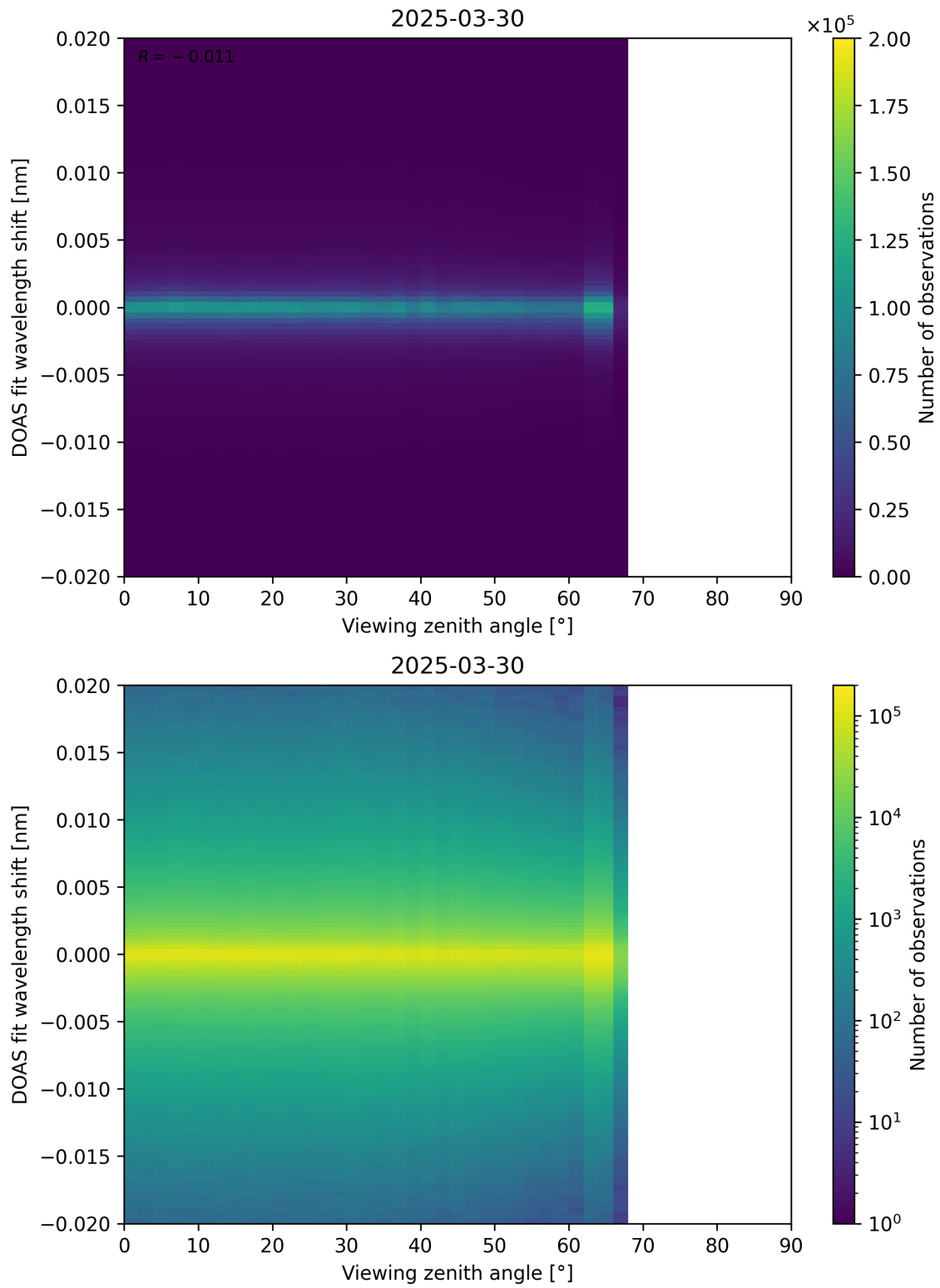
Figure 183: Scatter density plot of “Viewing zenith angle” against “DOAS fit wavelength shift” for 2025-03-29 to 2025-03-31.
