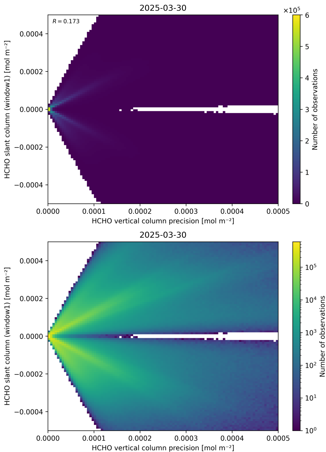
Figure 142: Scatter density plot of “HCHO vertical column precision” against “HCHO slant column (window1)” for 2025-03-29 to 2025-03-31.
