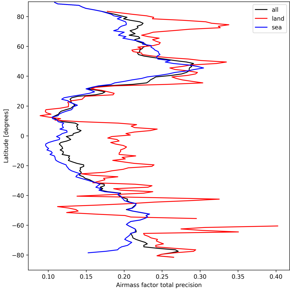
Figure 27: Zonal average of “Airmass factor total precision” for 2025-03-29 to 2025-03-31.
