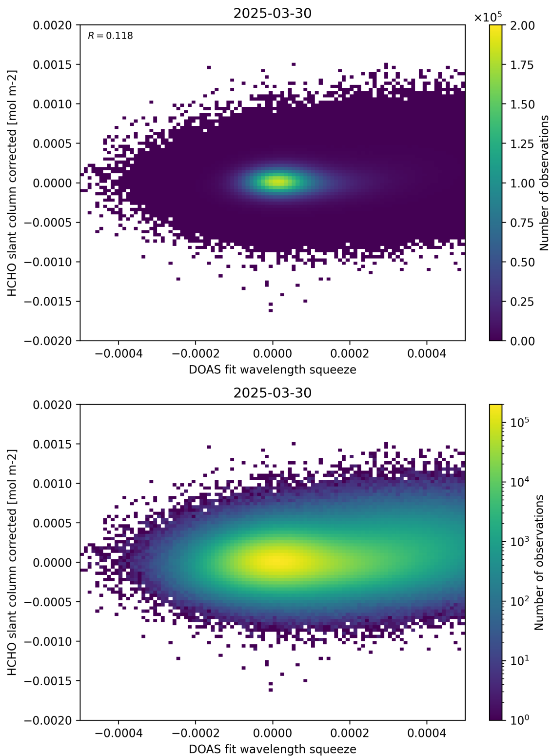
Figure 69: Scatter density plot of “DOAS fit wavelength squeeze” against “HCHO slant column corrected” for 2025-03-29 to 2025-03-31.
