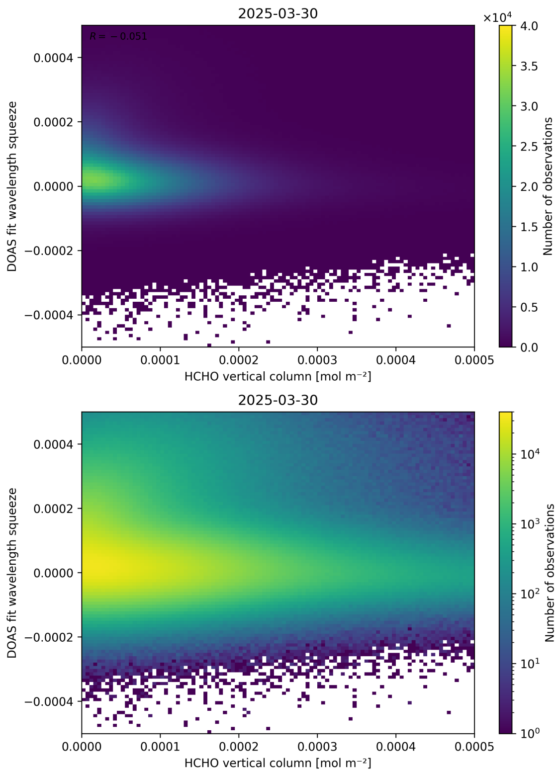
Figure 125: Scatter density plot of “HCHO vertical column” against “DOAS fit wavelength squeeze” for 2025-03-29 to 2025-03-31.
