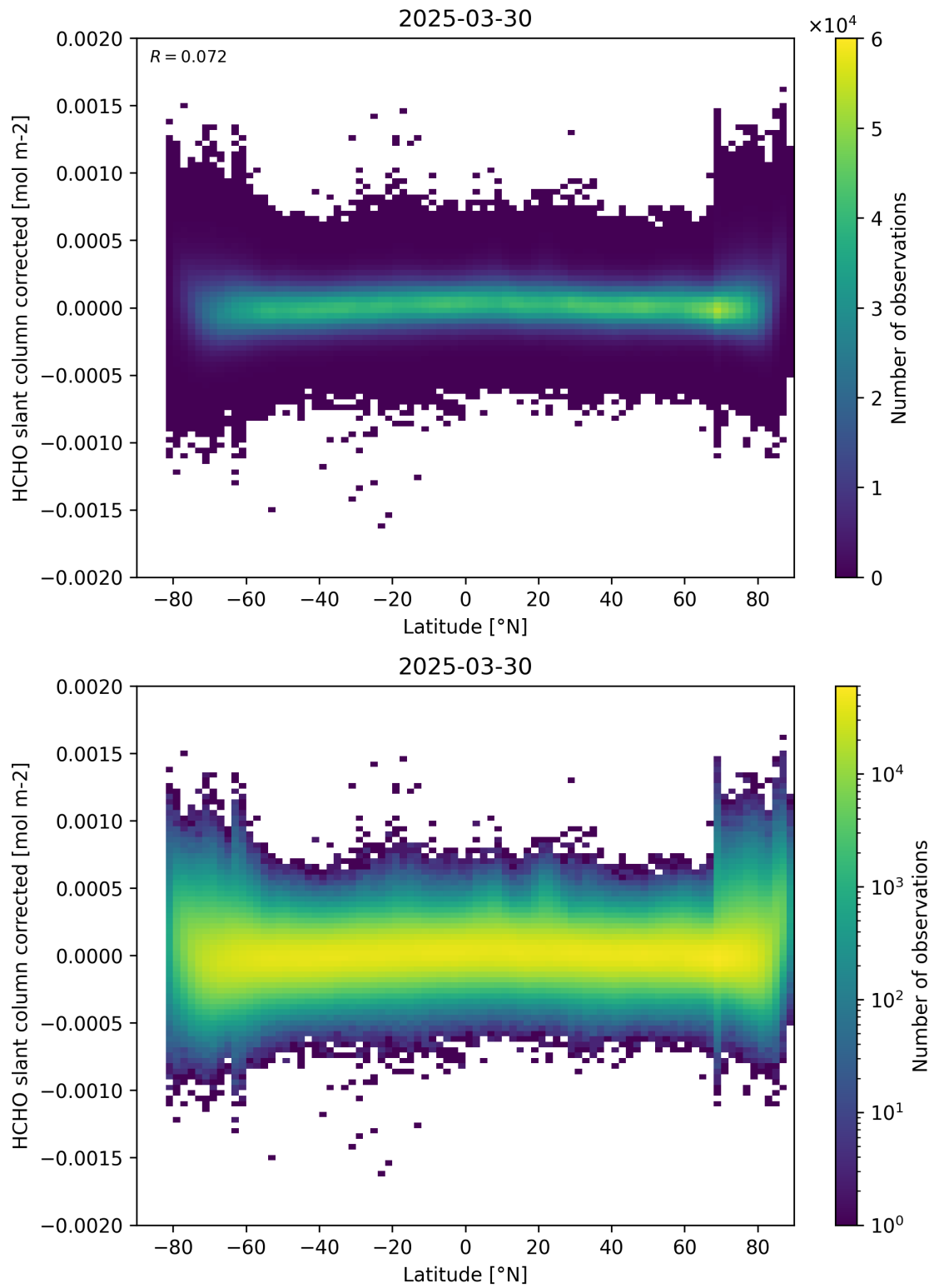
Figure 157: Scatter density plot of “Latitude” against “HCHO slant column corrected” for 2025-03-29 to 2025-03-31.
