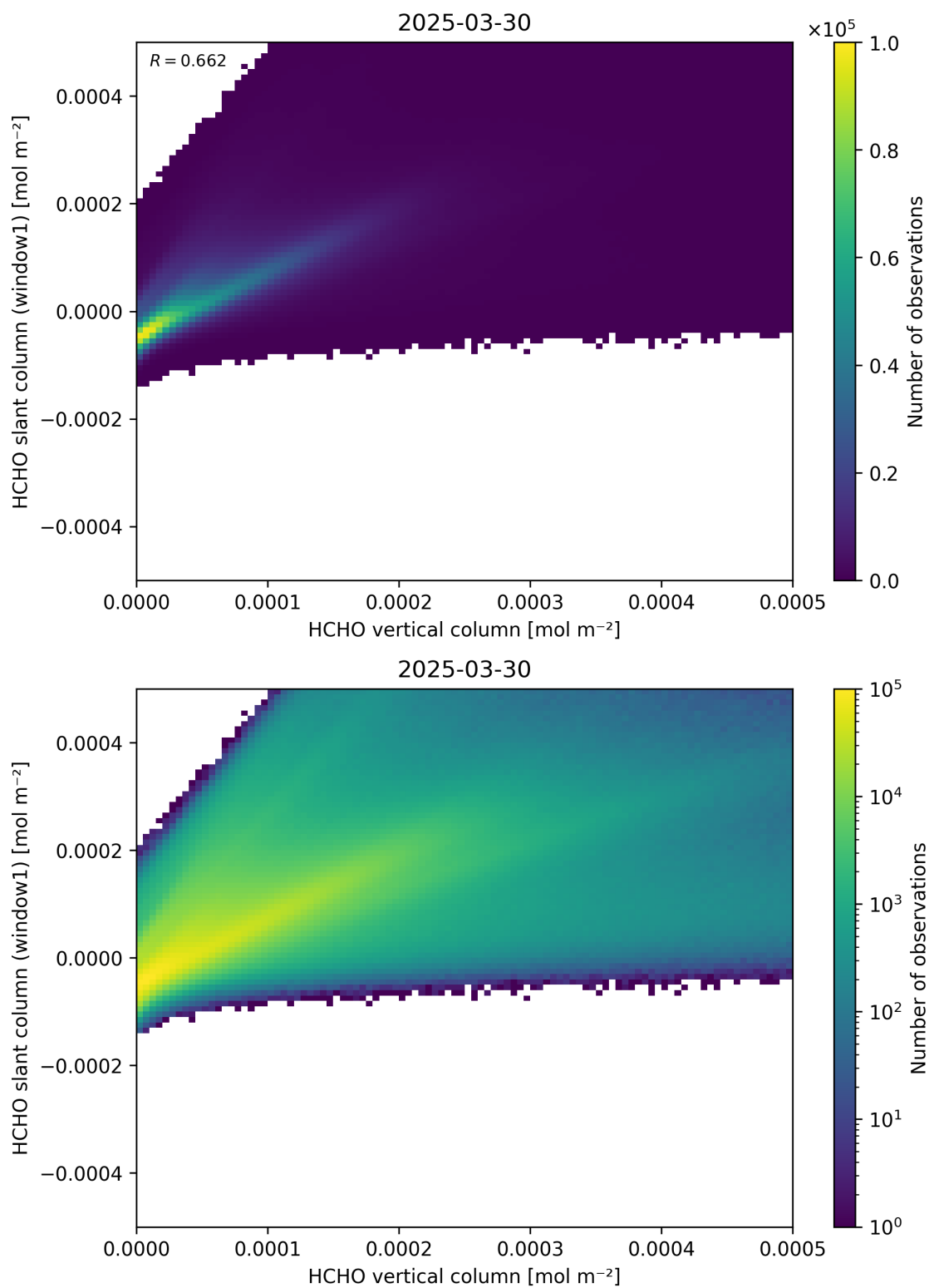
Figure 129: Scatter density plot of “HCHO vertical column” against “HCHO slant column (window1)” for 2025-03-29 to 2025-03-31.
