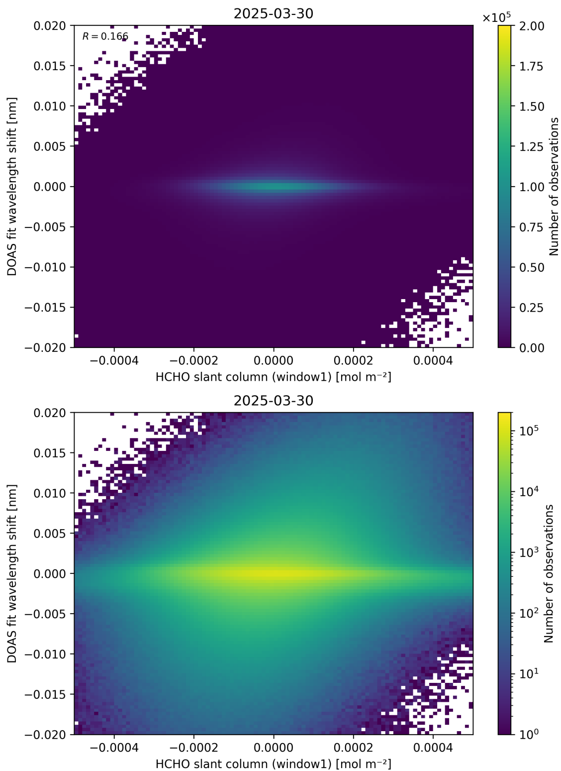
Figure 79: Scatter density plot of “HCHO slant column (window1)” against “DOAS fit wavelength shift” for 2025-03-29 to 2025-03-31.
