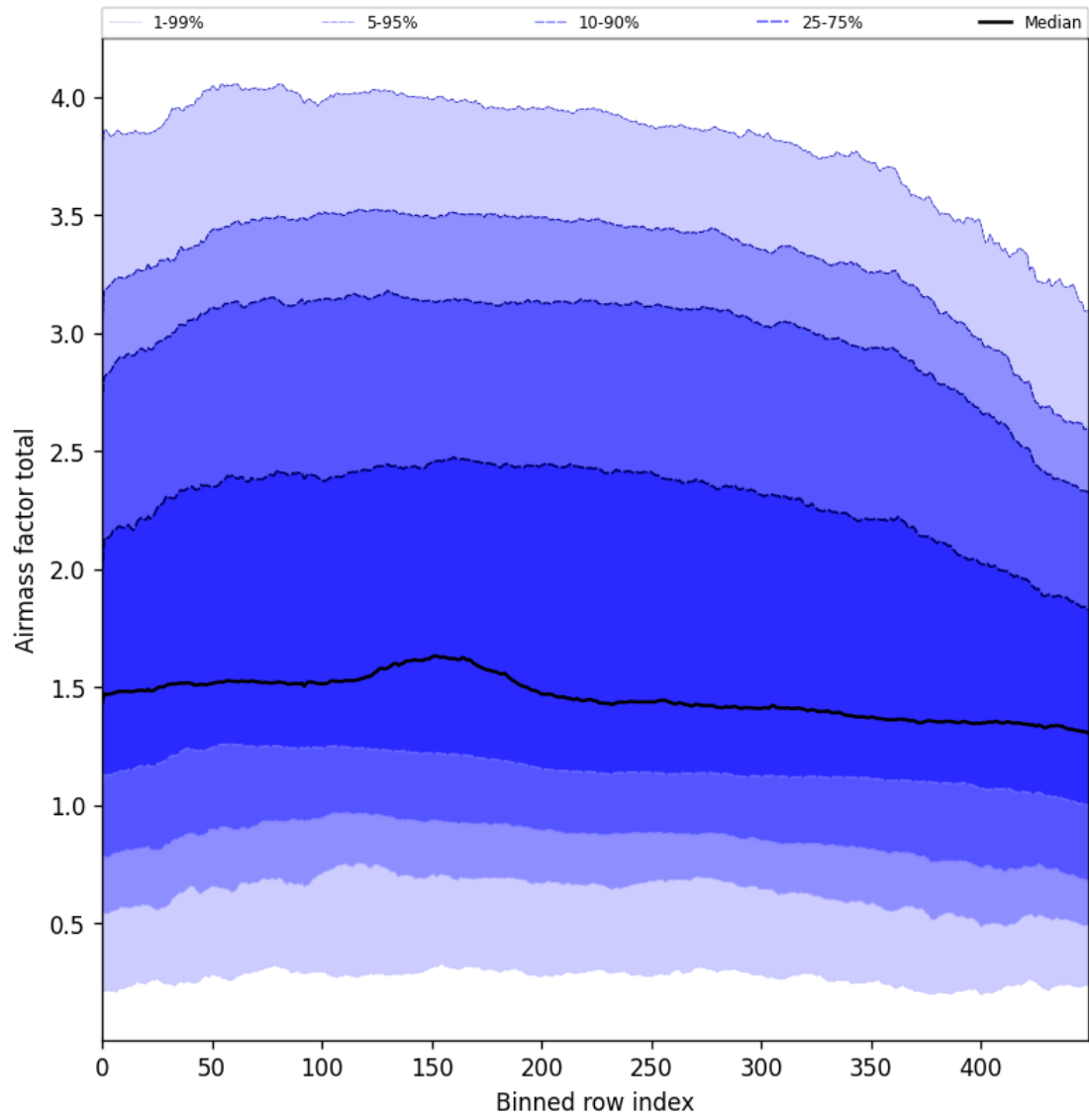
Figure 54: Along track statistics of “Airmass factor total” for 2025-03-29 to 2025-03-31
