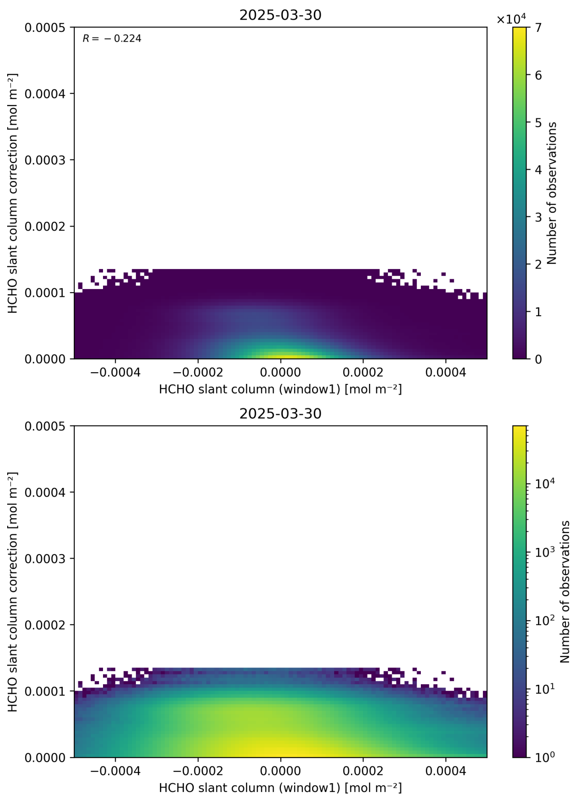
Figure 83: Scatter density plot of “HCHO slant column (window1)” against “HCHO slant column correction” for 2025-03-29 to 2025-03-31.
