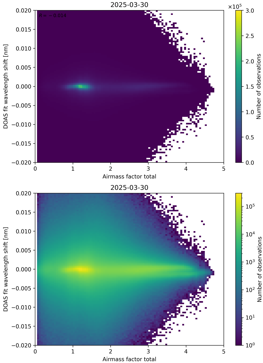
Figure 98: Scatter density plot of “Airmass factor total” against “DOAS fit wavelength shift” for 2025-03-29 to 2025-03-31.
