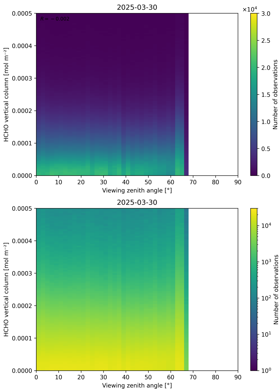
Figure 192: Scatter density plot of “Viewing zenith angle” against “HCHO vertical column” for 2025-03-29 to 2025-03-31.
