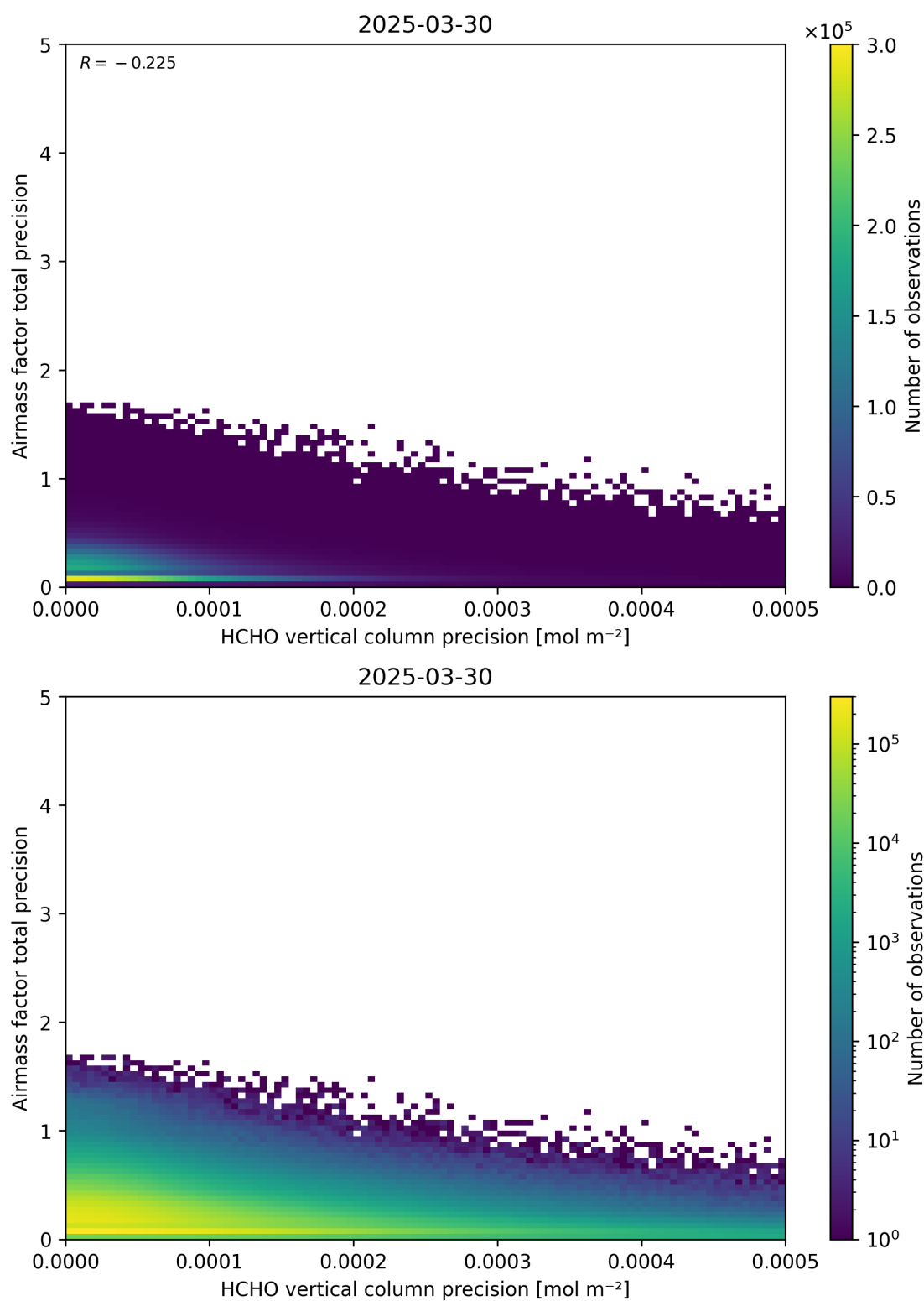
Figure 145: Scatter density plot of “HCHO vertical column precision” against “Airmass factor total precision” for 2025-03-29 to 2025-03-31.
