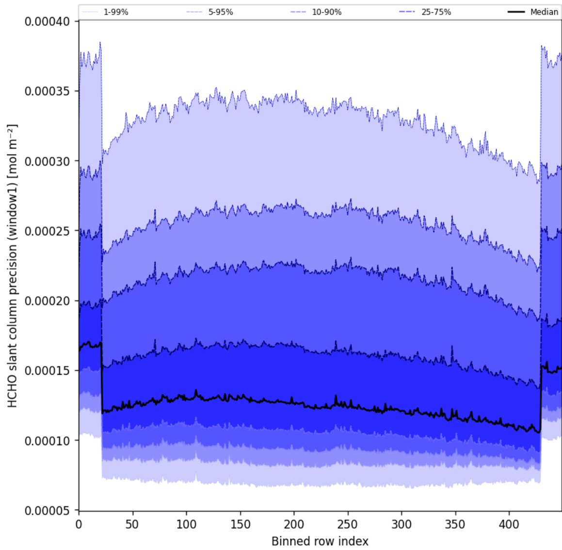
Figure 53: Along track statistics of “HCHO slant column precision (window1)” for 2025-03-29 to 2025-03-31
