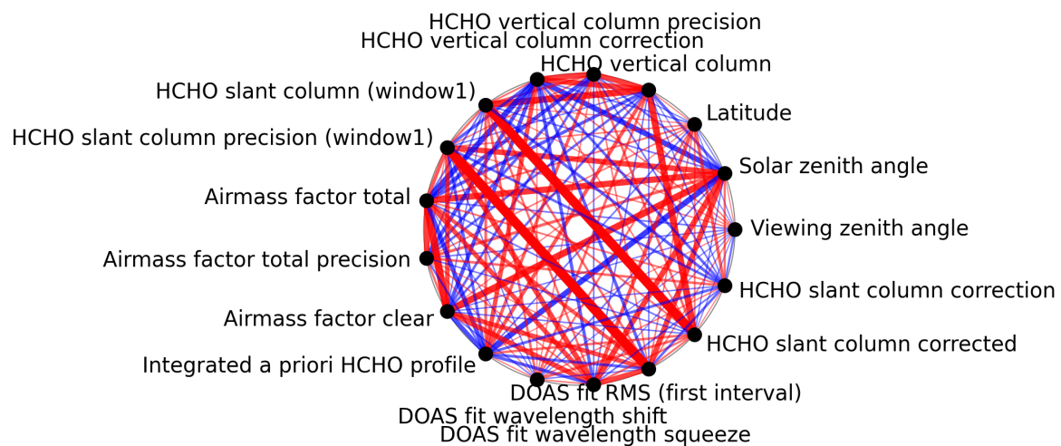
Figure 1: Map of correlation graph for 2025-03-29 to 2025-03-31.
