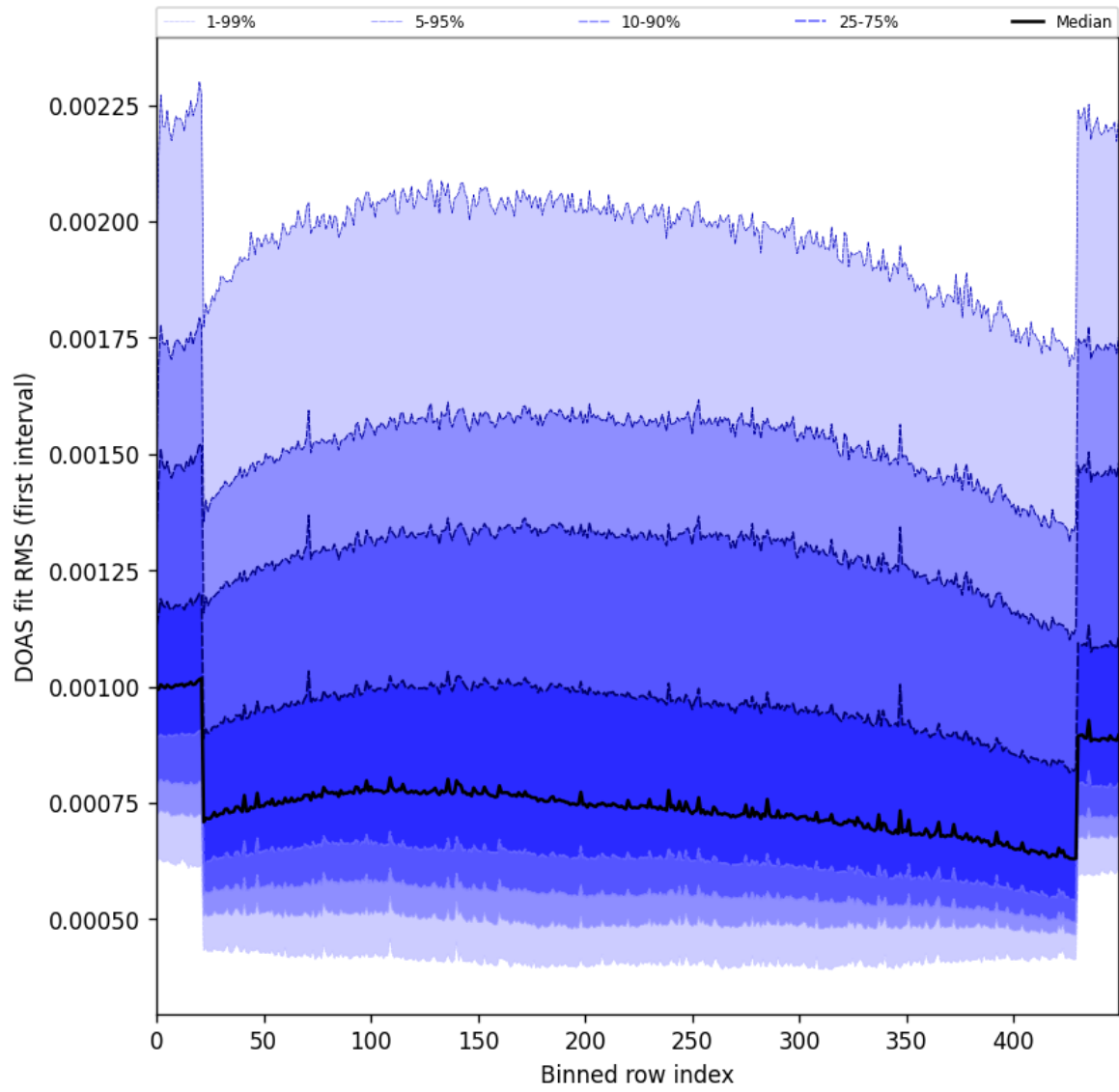
Figure 60: Along track statistics of “DOAS fit RMS (first interval)” for 2025-03-29 to 2025-03-31
