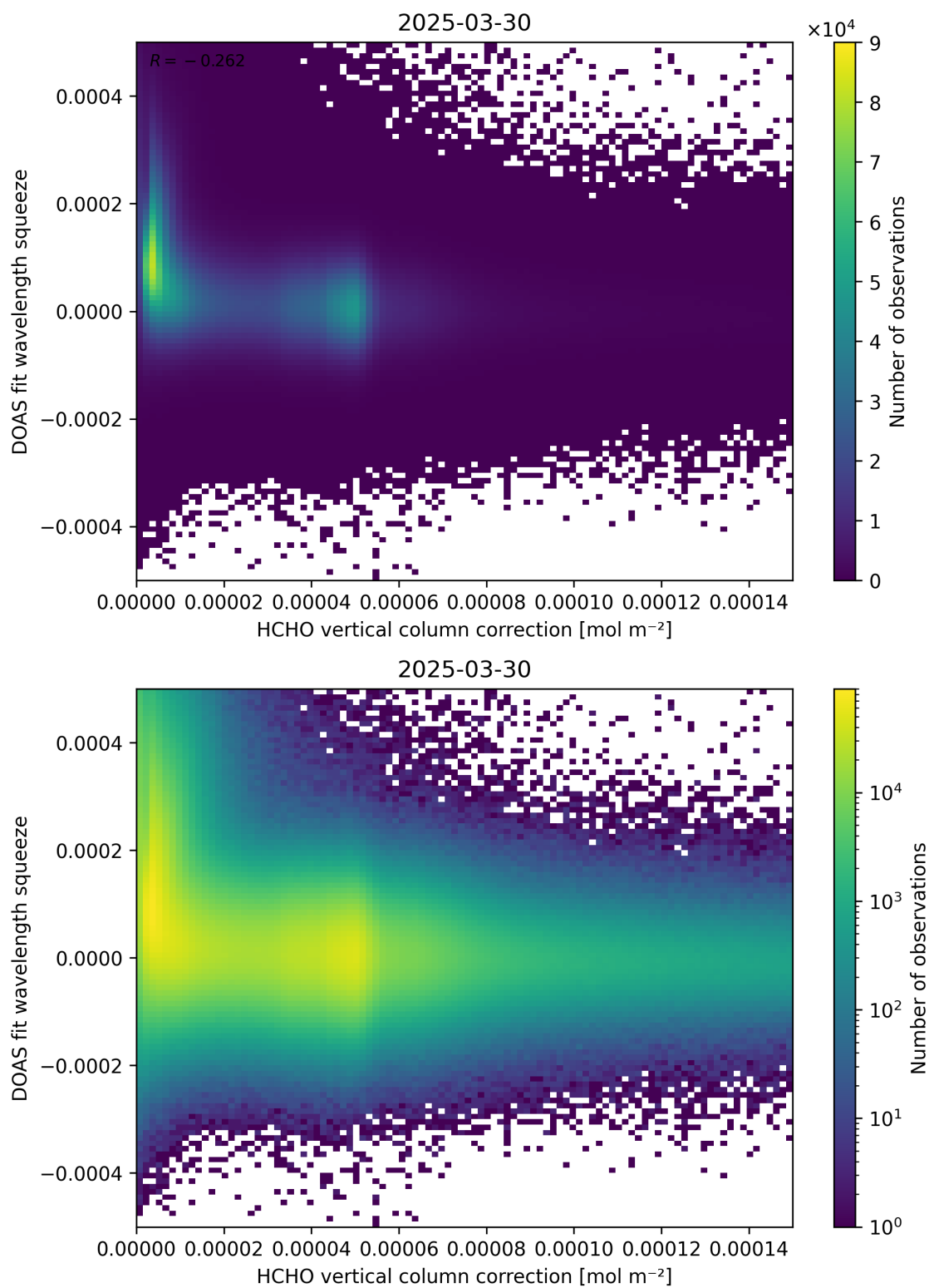
Figure 114: Scatter density plot of “HCHO vertical column correction” against “DOAS fit wavelength squeeze” for 2025-03-29 to 2025-03-31.
