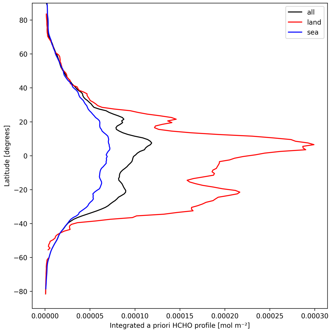
Figure 29: Zonal average of “Integrated a priori HCHO profile” for 2025-03-29 to 2025-03-31.
