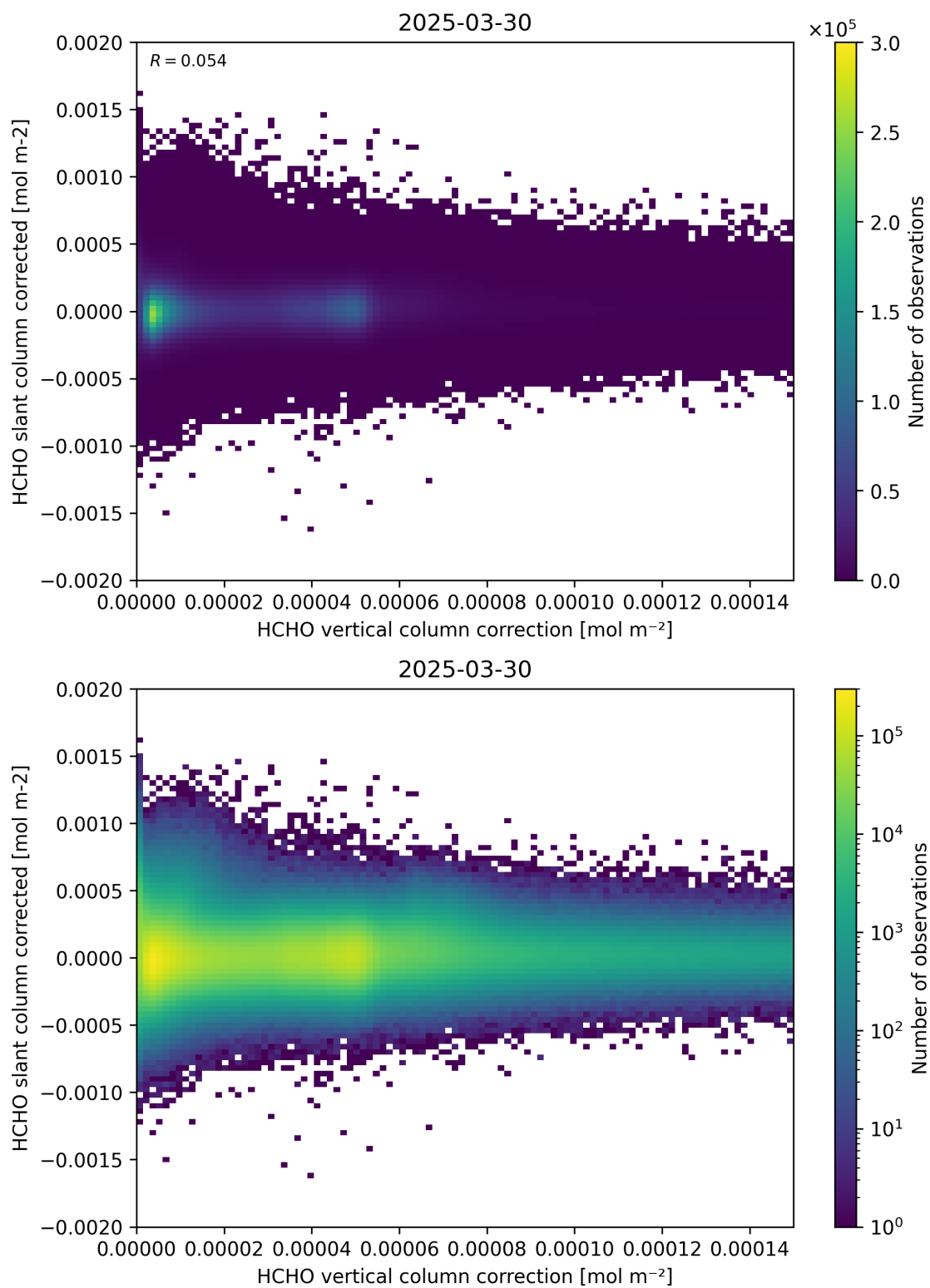
Figure 116: Scatter density plot of “HCHO vertical column correction” against “HCHO slant column corrected” for 2025-03-29 to 2025-03-31.
