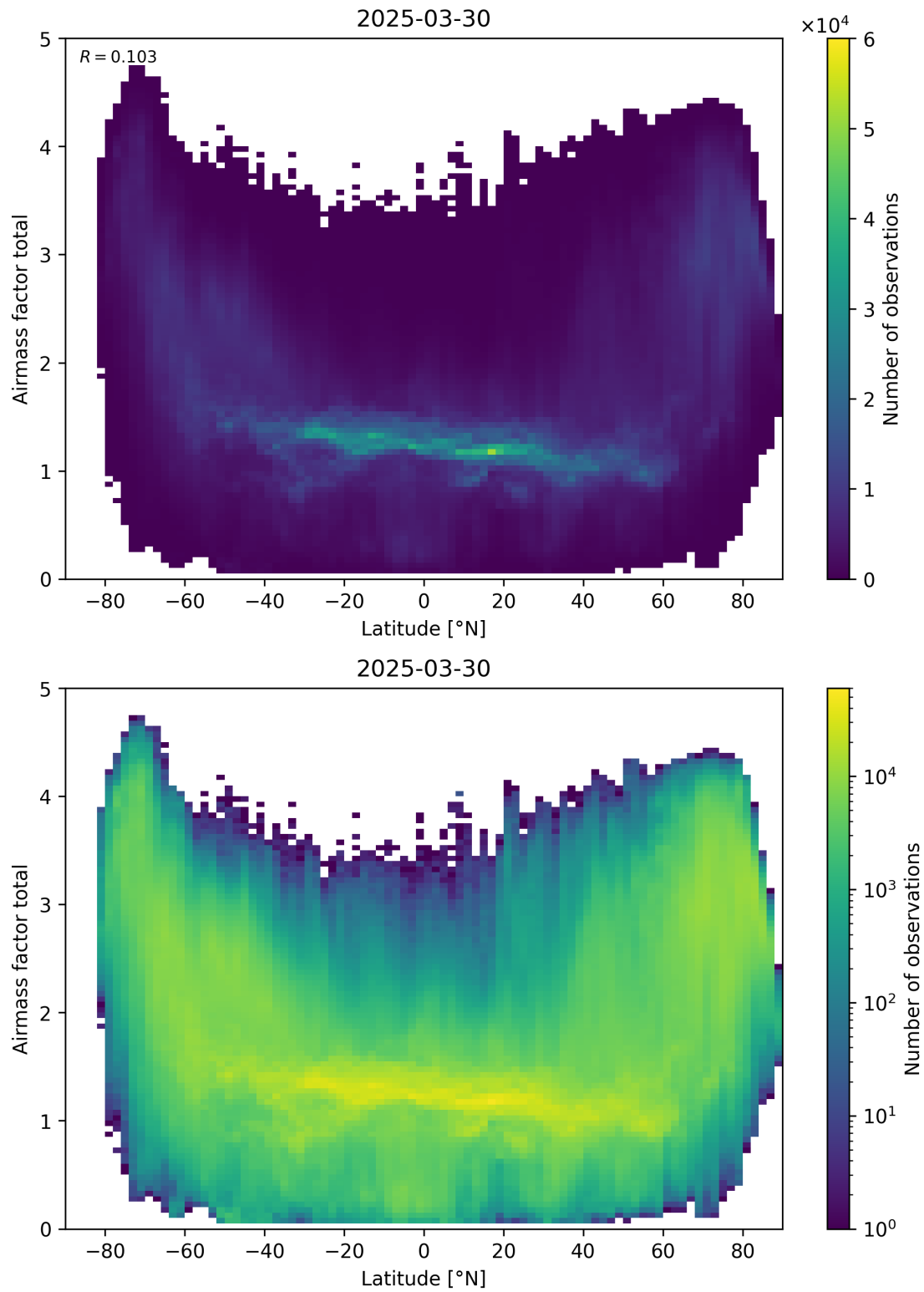
Figure 161: Scatter density plot of “Latitude” against “Airmass factor total” for 2025-03-29 to 2025-03-31.
