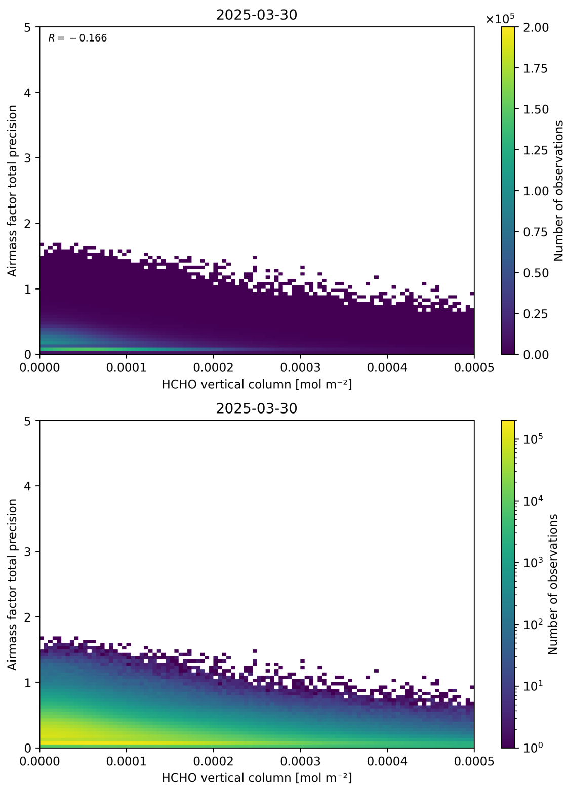
Figure 132: Scatter density plot of “HCHO vertical column” against “Airmass factor total precision” for 2025-03-29 to 2025-03-31.
