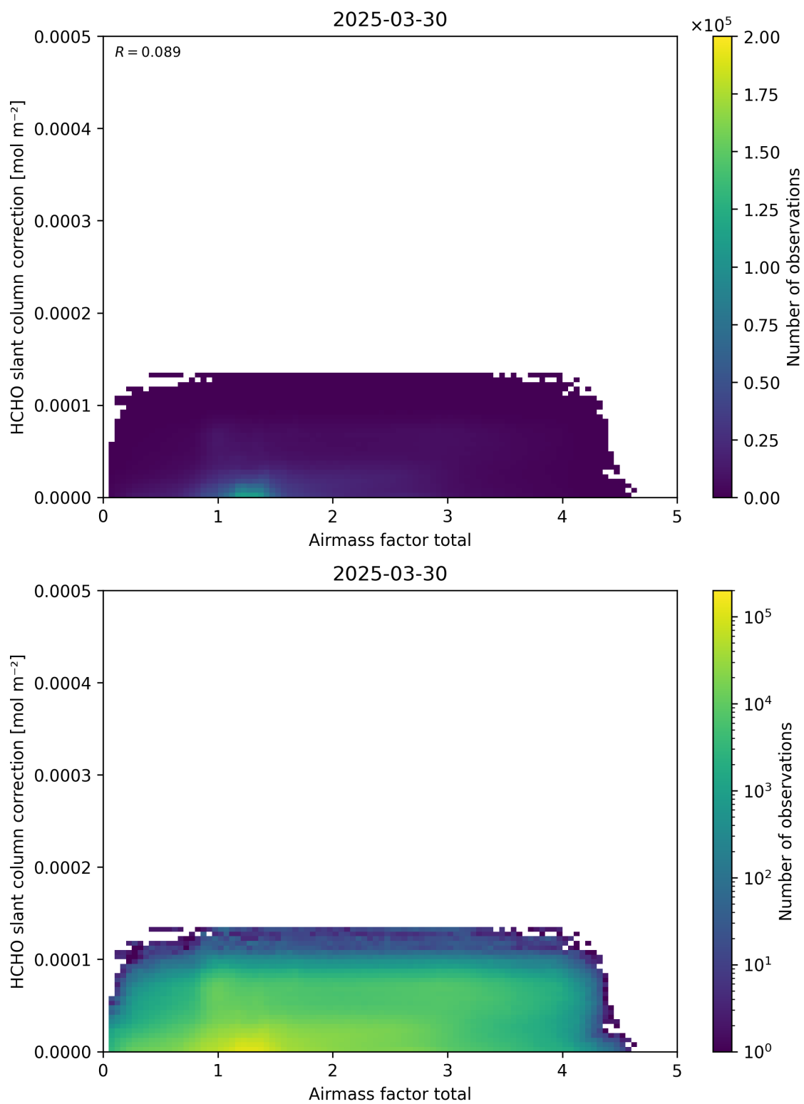
Figure 102: Scatter density plot of “Airmass factor total” against “HCHO slant column correction” for 2025-03-29 to 2025-03-31.
