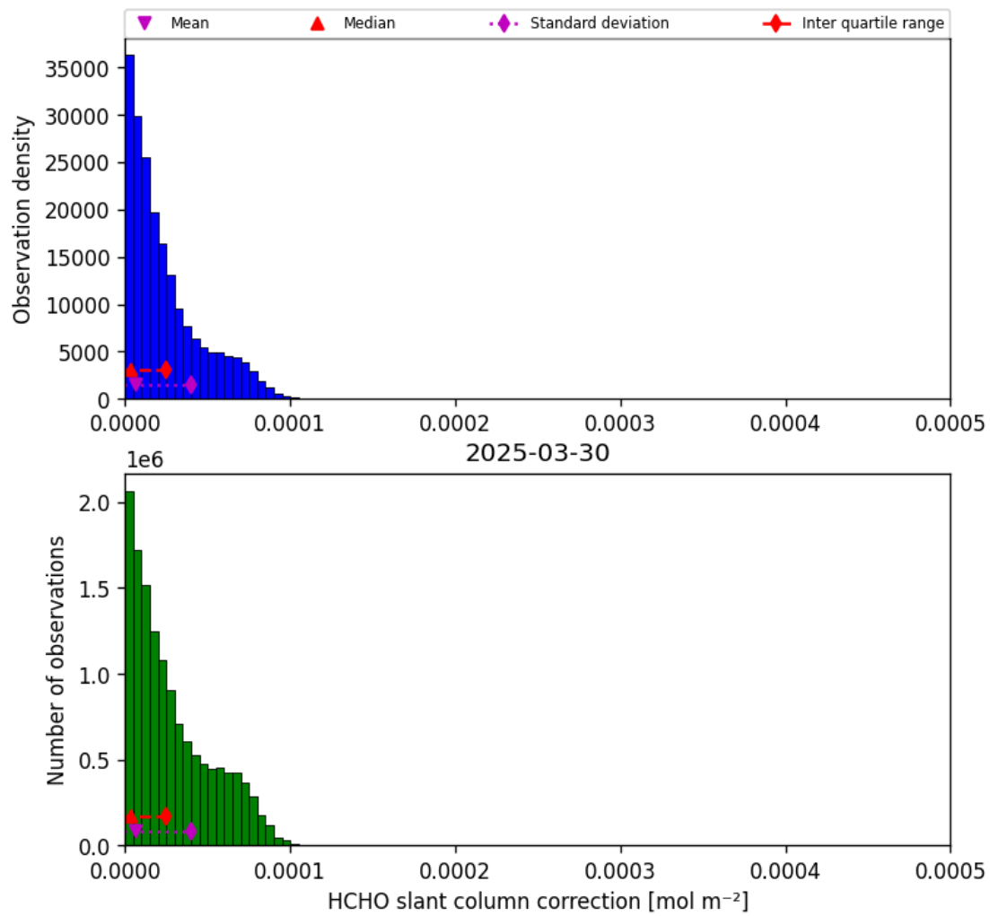
Figure 47: Histogram of “HCHO slant column correction” for 2025-03-29 to 2025-03-31
