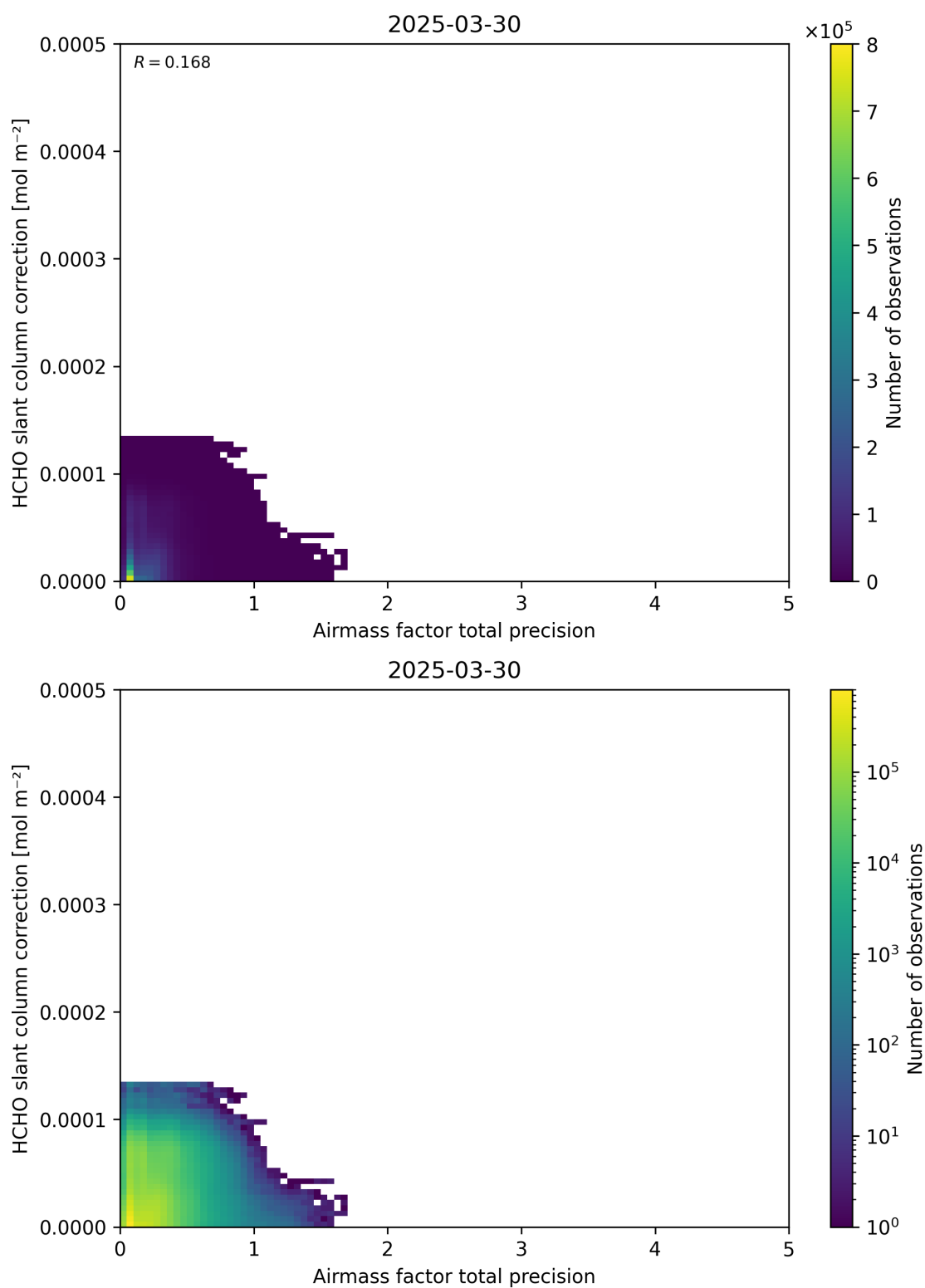
Figure 110: Scatter density plot of “Airmass factor total precision” against “HCHO slant column correction” for 2025-03-29 to 2025-03-31.
