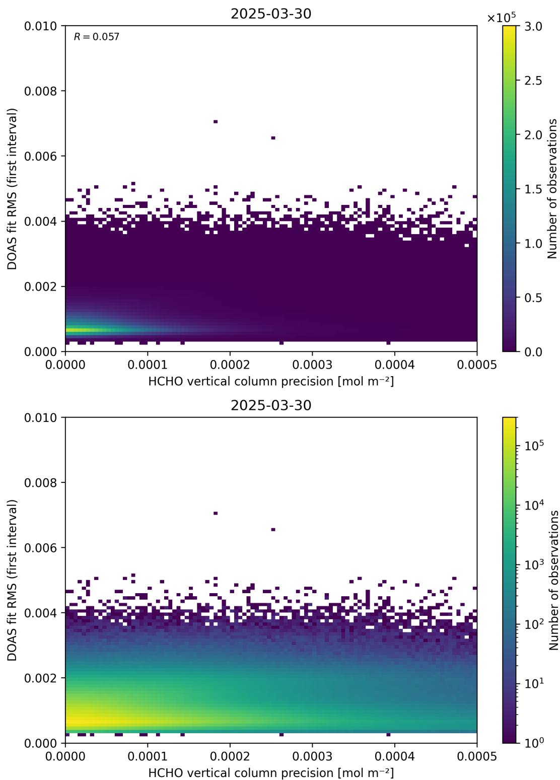
Figure 136: Scatter density plot of “HCHO vertical column precision” against “DOAS fit RMS (first interval)” for 2025-03-29 to 2025-03-31.
