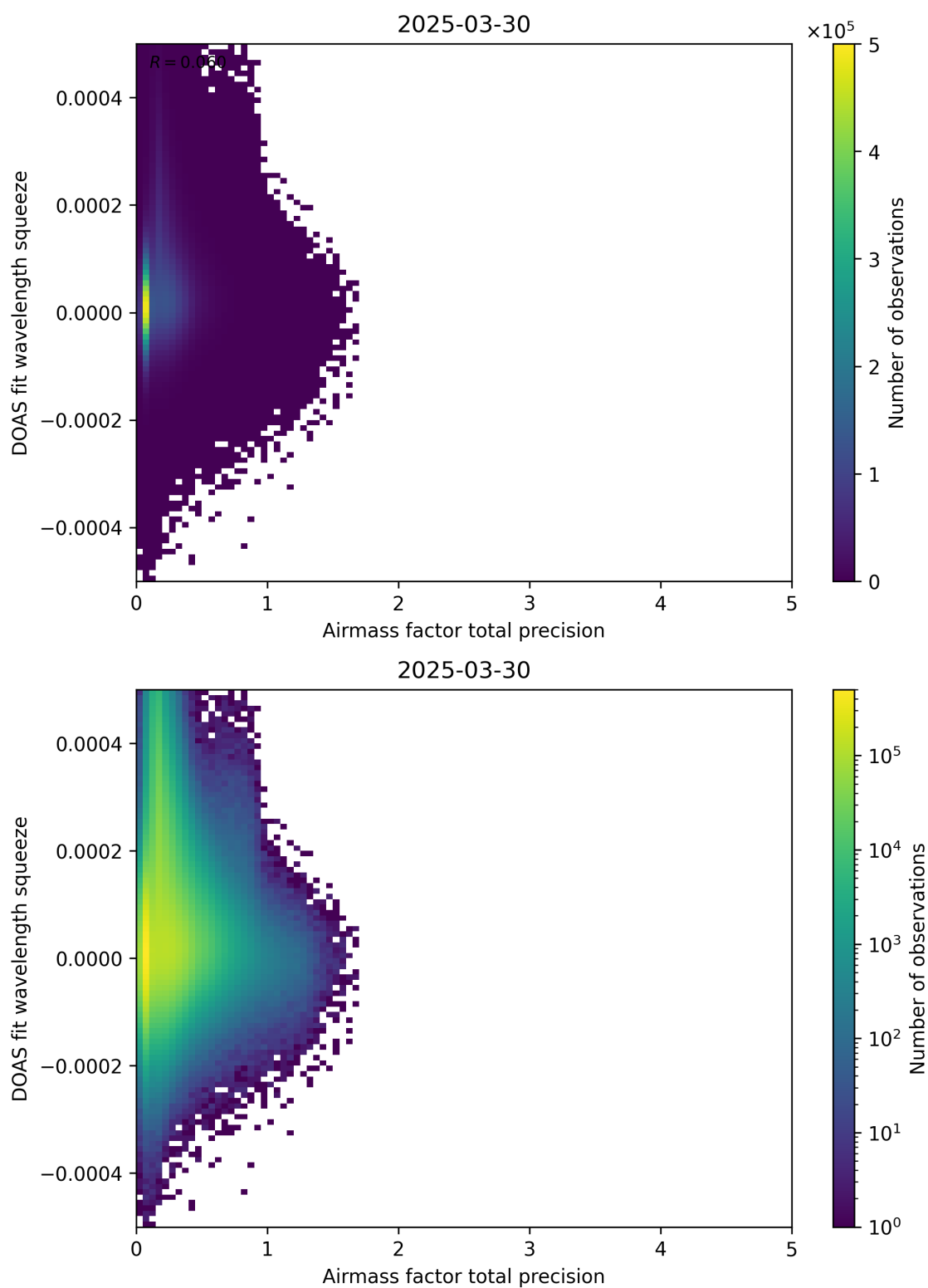
Figure 107: Scatter density plot of “Airmass factor total precision” against “DOAS fit wavelength squeeze” for 2025-03-29 to 2025-03-31.
