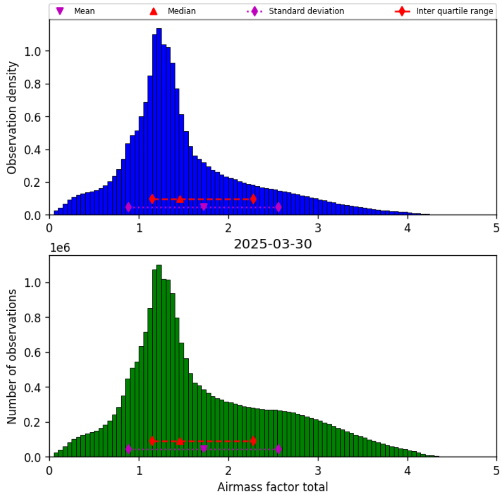
Figure 40: Histogram of “Airmass factor total” for 2025-03-29 to 2025-03-31
