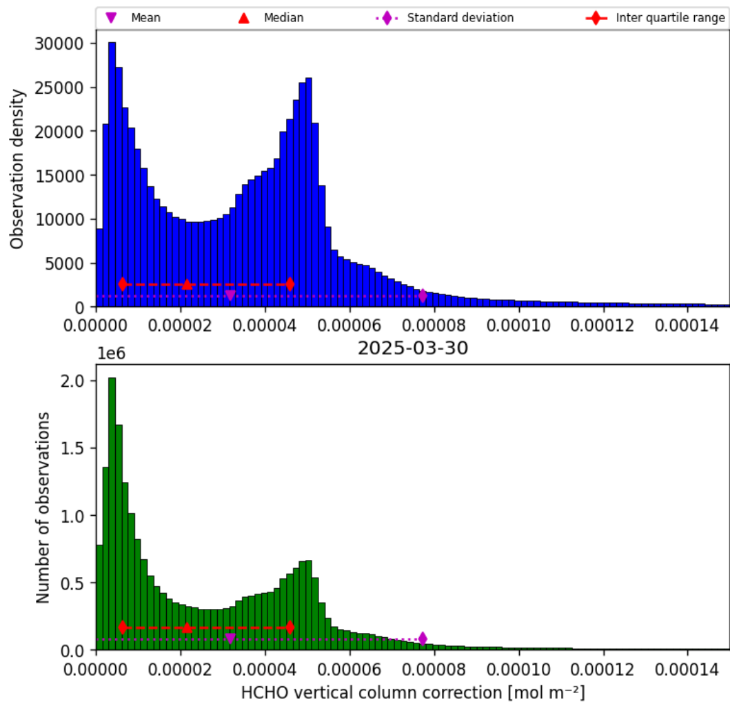
Figure 37: Histogram of “HCHO vertical column correction” for 2025-03-29 to 2025-03-31
