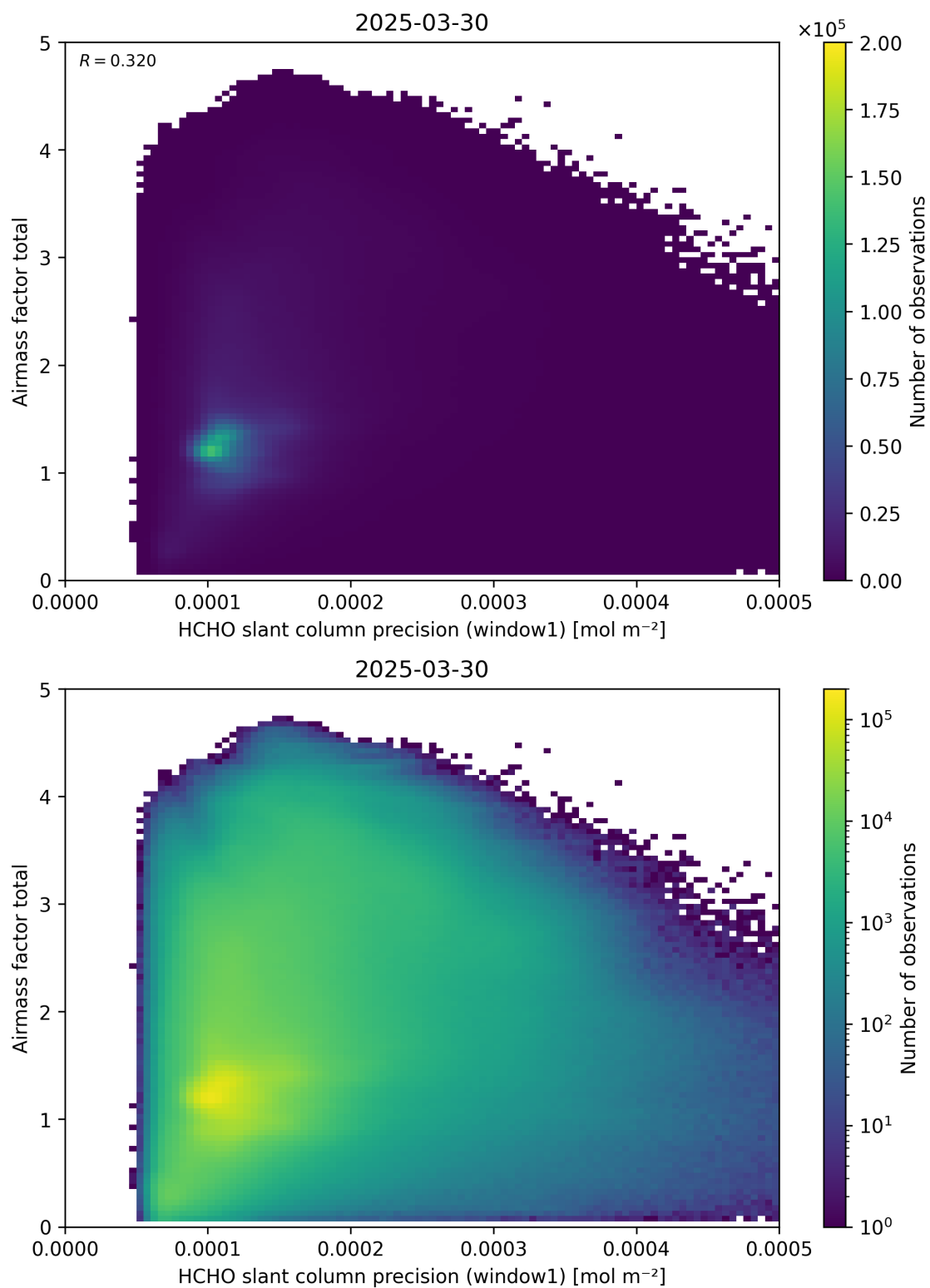
Figure 94: Scatter density plot of “HCHO slant column precision (window1)” against “Airmass factor total” for 2025-03-29 to 2025-03-31.
