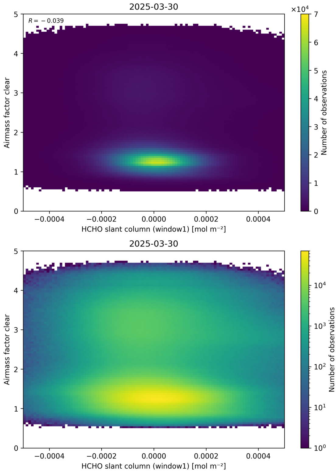
Figure 81: Scatter density plot of “HCHO slant column (window1)” against “Airmass factor clear” for 2025-03-29 to 2025-03-31.
