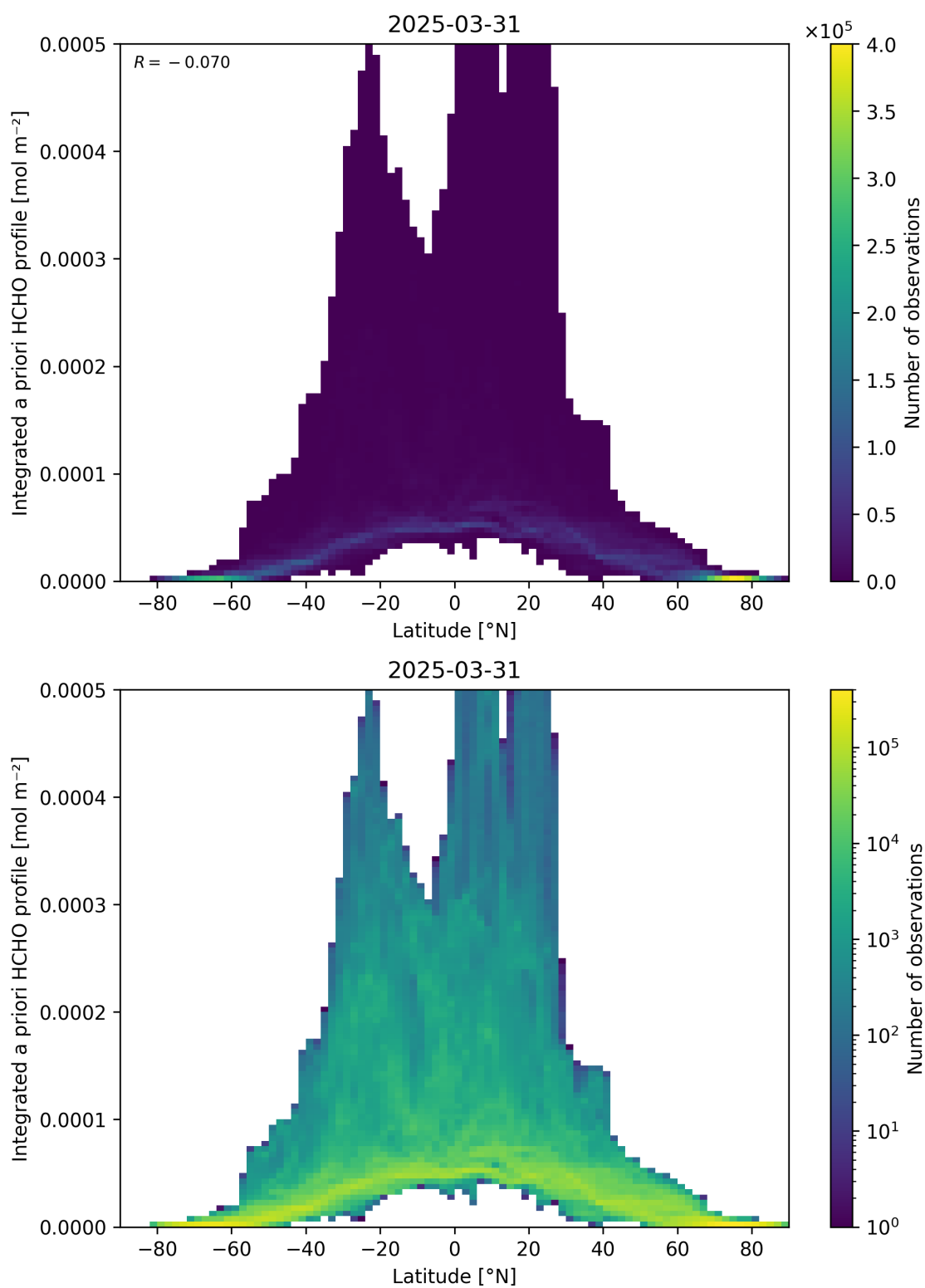
Figure 166: Scatter density plot of “Latitude” against “Integrated a priori HCHO profile” for 2025-03-30 to 2025-04-01.
