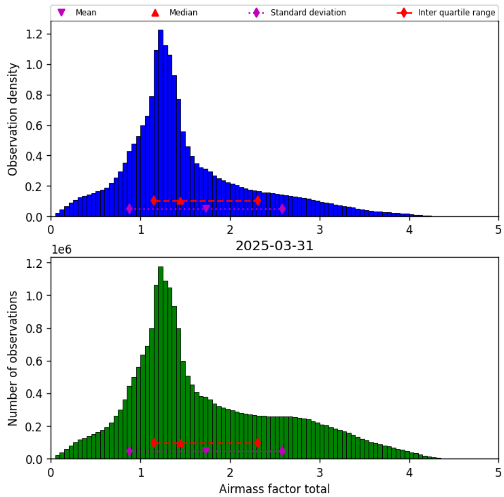
Figure 40: Histogram of “Airmass factor total” for 2025-03-30 to 2025-04-01
