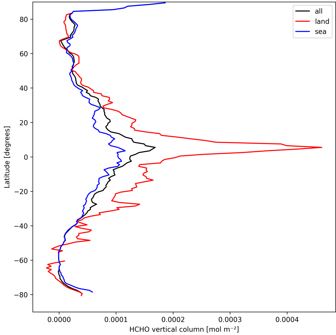
Figure 21: Zonal average of “HCHO vertical column” for 2025-03-30 to 2025-04-01.
