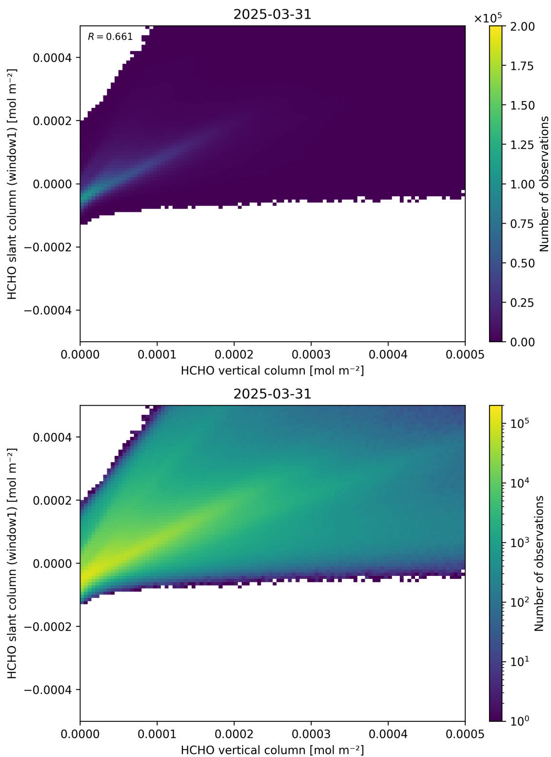
Figure 129: Scatter density plot of “HCHO vertical column” against “HCHO slant column (window1)” for 2025-03-30 to 2025-04-01.
