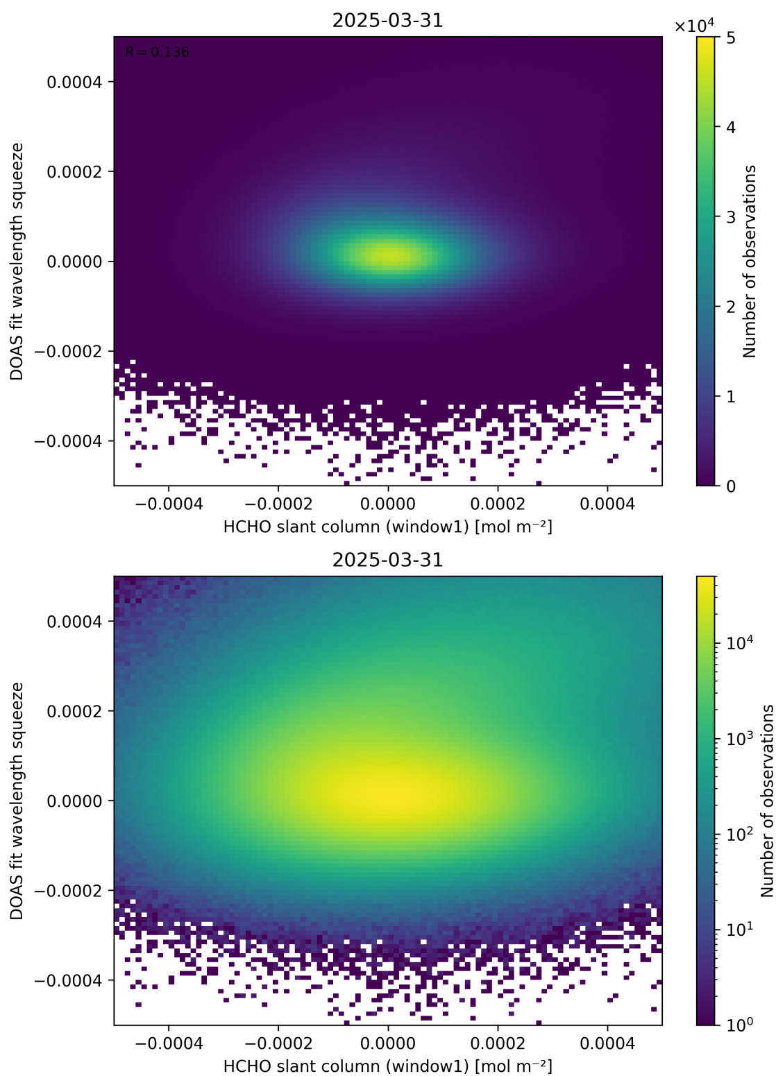
Figure 80: Scatter density plot of “HCHO slant column (window1)” against “DOAS fit wavelength squeeze” for 2025-03-30 to 2025-04-01.
