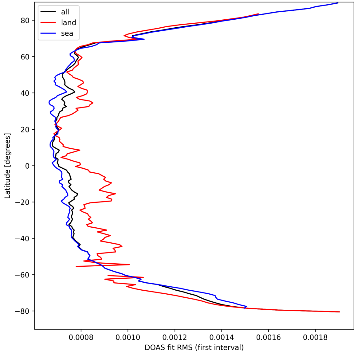
Figure 32: Zonal average of "DOAS fit RMS (first interval)" for 2025-03-30 to 2025-04-01.
