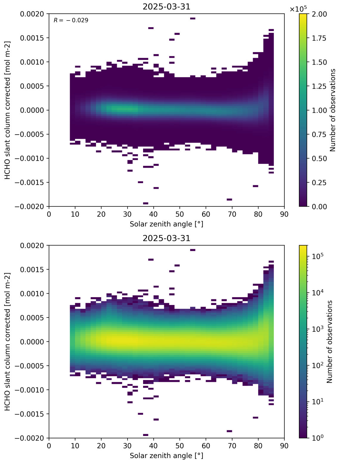
Figure 171: Scatter density plot of “Solar zenith angle” against “HCHO slant column corrected” for 2025-03-30 to 2025-04-01.
