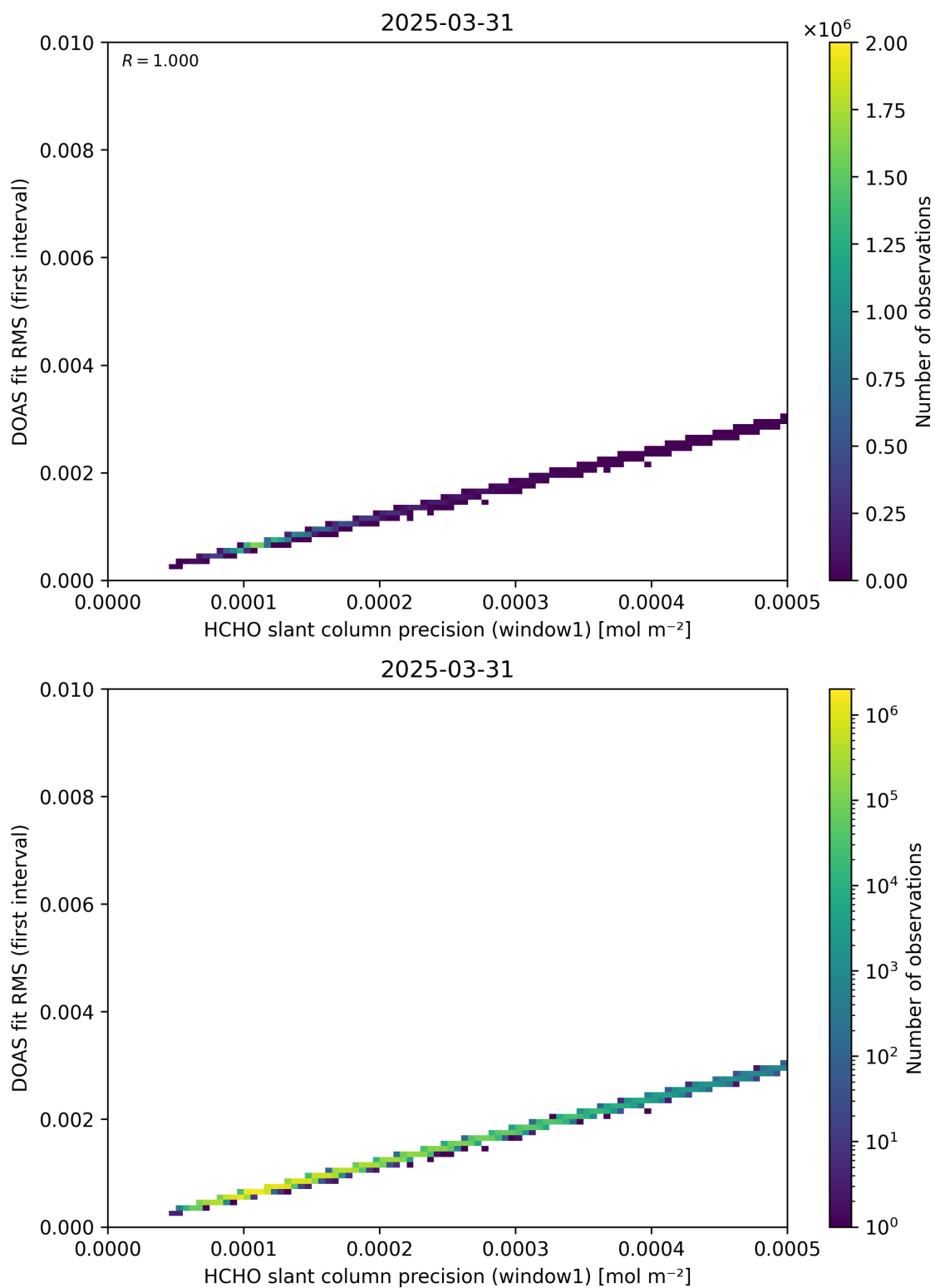
Figure 88: Scatter density plot of “HCHO slant column precision (window1)” against “DOAS fit RMS (first interval)” for 2025-03-30 to 2025-04-01.
