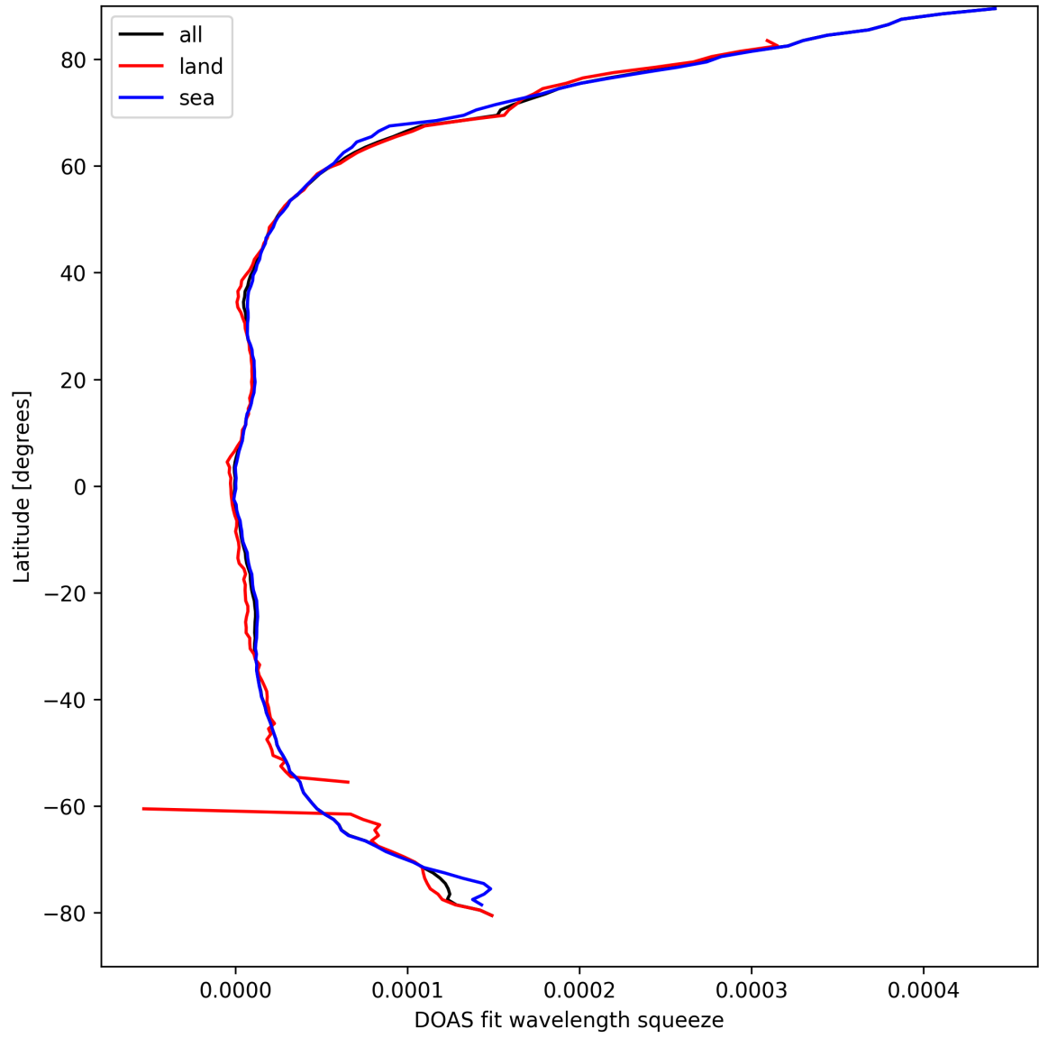
Figure 31: Zonal average of “DOAS fit wavelength squeeze” for 2025-03-30 to 2025-04-01.
