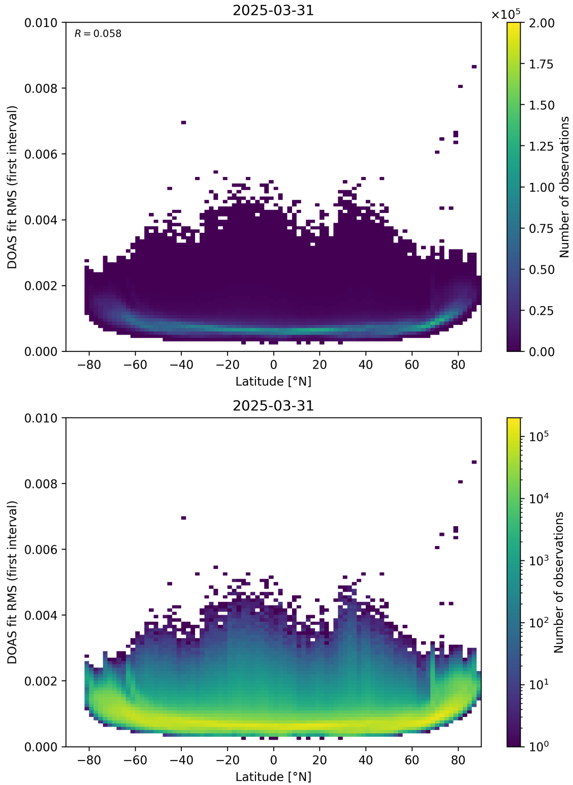
Figure 153: Scatter density plot of “Latitude” against “DOAS fit RMS (first interval)” for 2025-03-30 to 2025-04-01.
