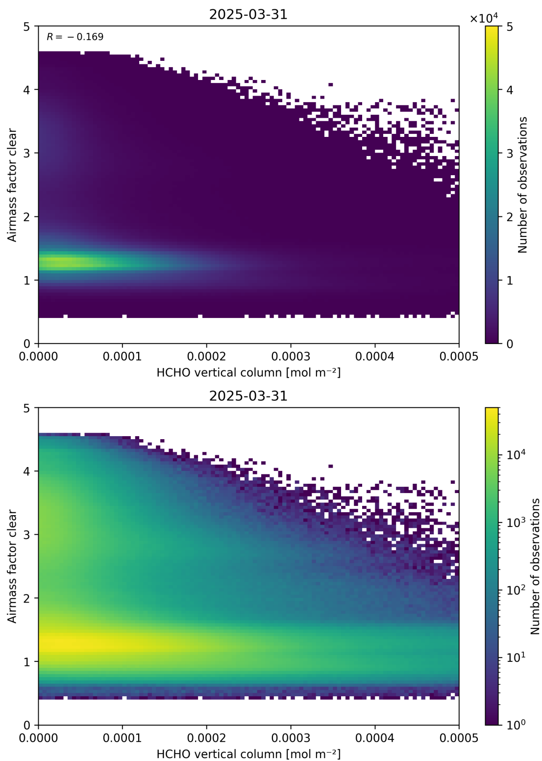
Figure 126: Scatter density plot of “HCHO vertical column” against “Airmass factor clear” for 2025-03-30 to 2025-04-01.
