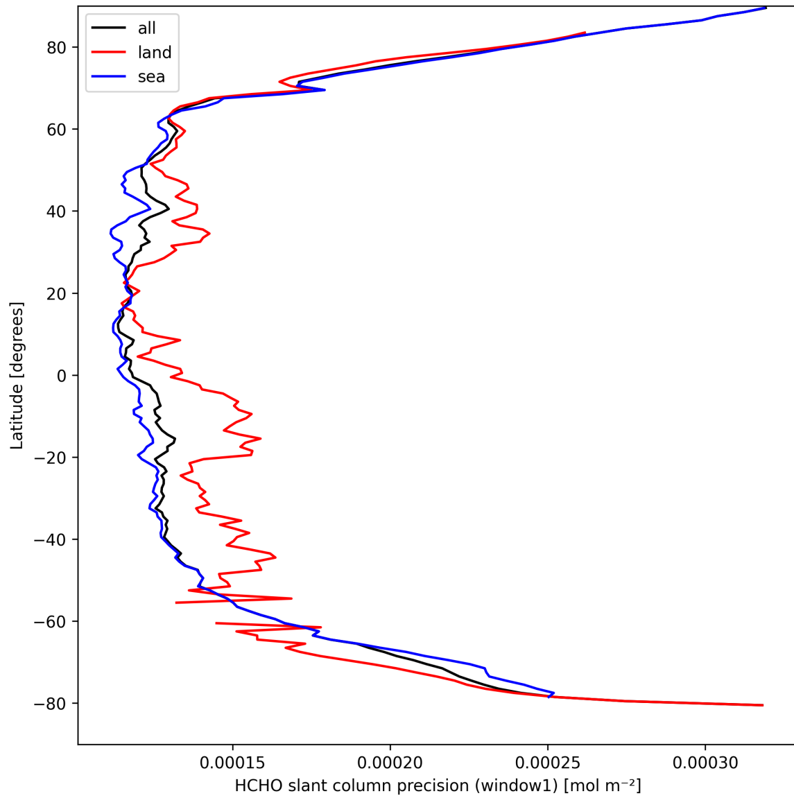
Figure 25: Zonal average of “HCHO slant column precision (window1)” for 2025-03-30 to 2025-04-01.
