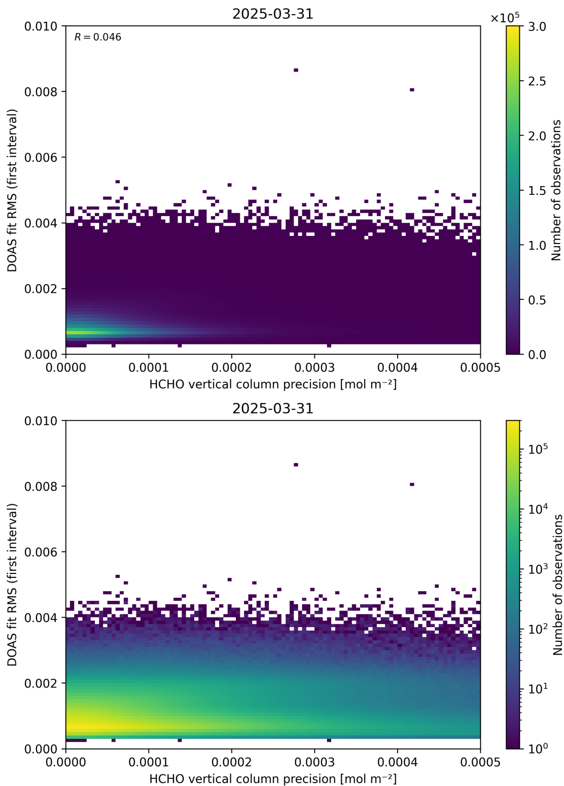
Figure 136: Scatter density plot of “HCHO vertical column precision” against “DOAS fit RMS (first interval)” for 2025-03-30 to 2025-04-01.
