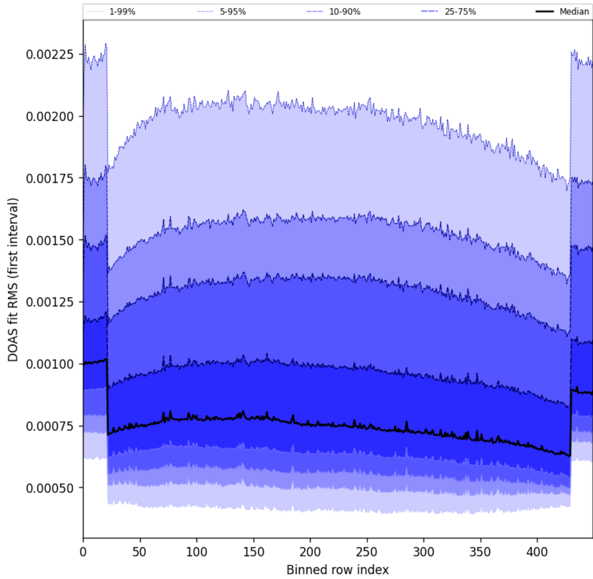
Figure 60: Along track statistics of “DOAS fit RMS (first interval)” for 2025-03-30 to 2025-04-01
