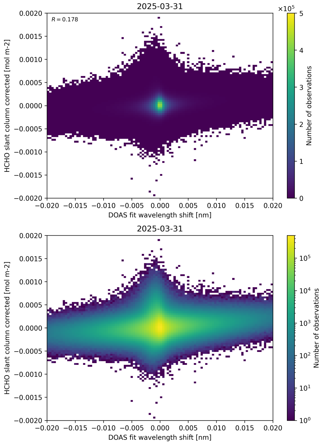
Figure 66: Scatter density plot of “DOAS fit wavelength shift” against “HCHO slant column corrected” for 2025-03-30 to 2025-04-01.
