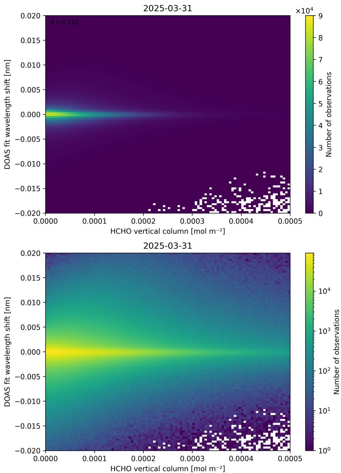
Figure 124: Scatter density plot of “HCHO vertical column” against “DOAS fit wavelength shift” for 2025-03-30 to 2025-04-01.
