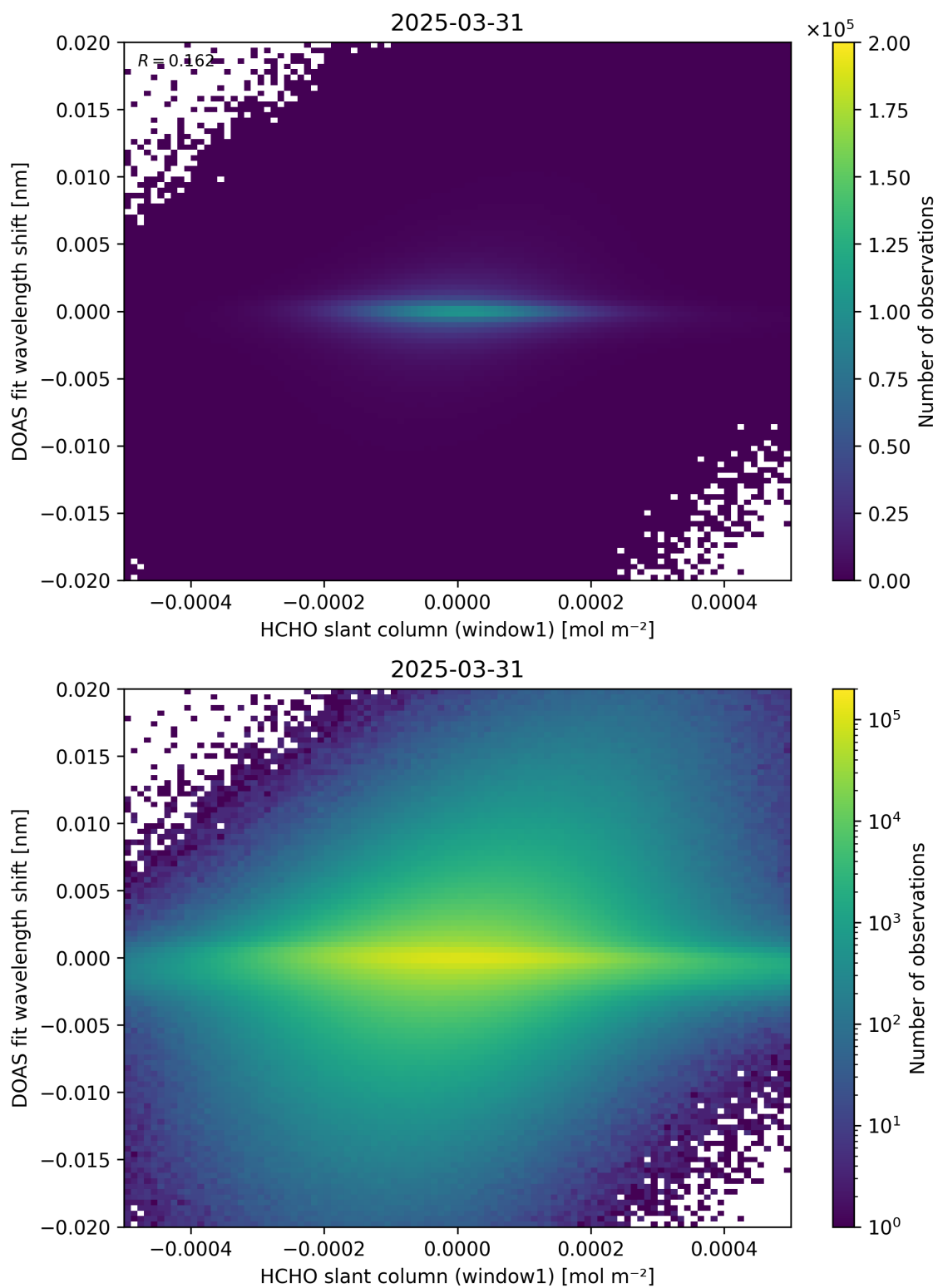
Figure 79: Scatter density plot of “HCHO slant column (window1)” against “DOAS fit wavelength shift” for 2025-03-30 to 2025-04-01.
