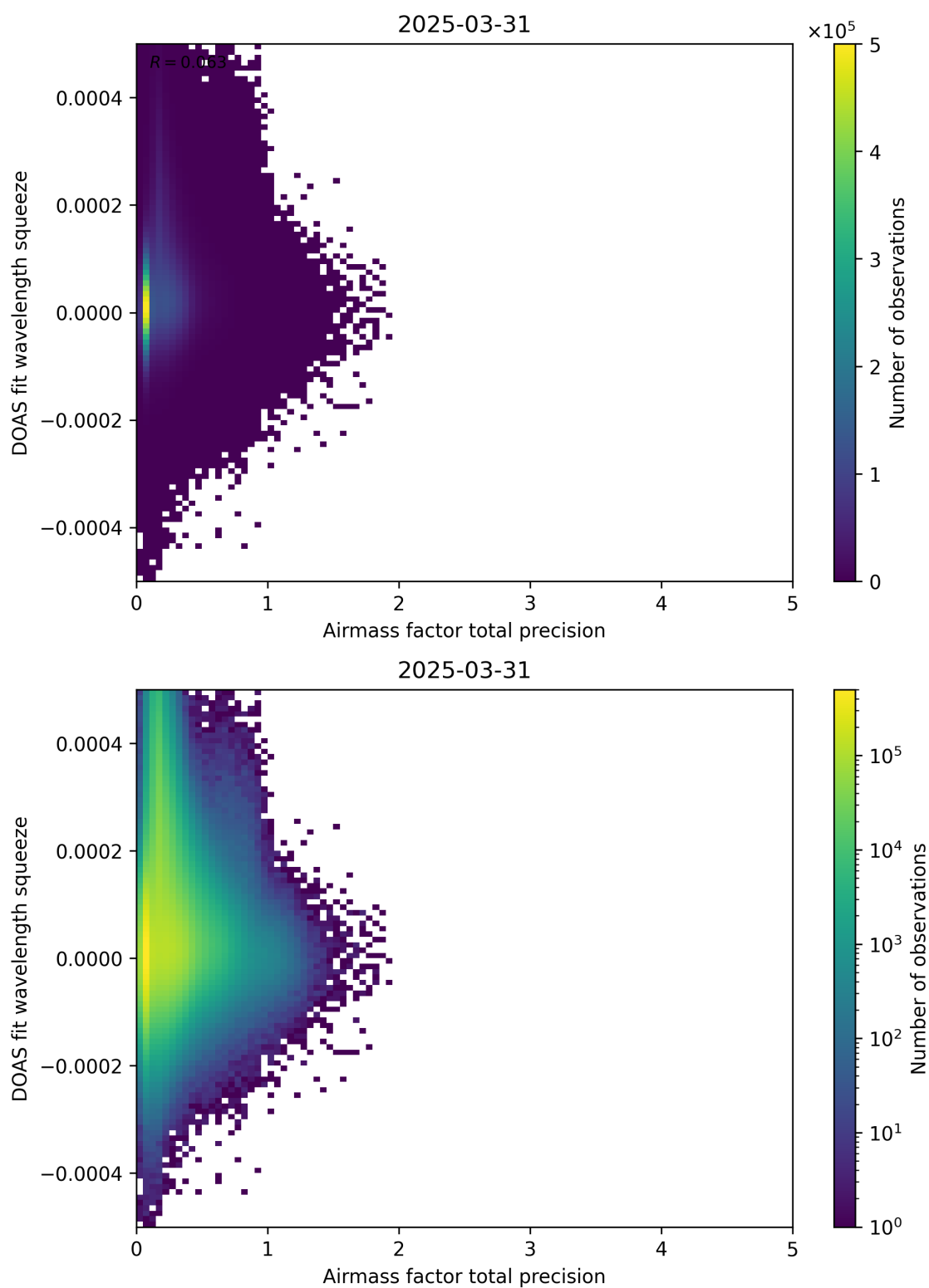
Figure 107: Scatter density plot of “Airmass factor total precision” against “DOAS fit wavelength squeeze” for 2025-03-30 to 2025-04-01.
