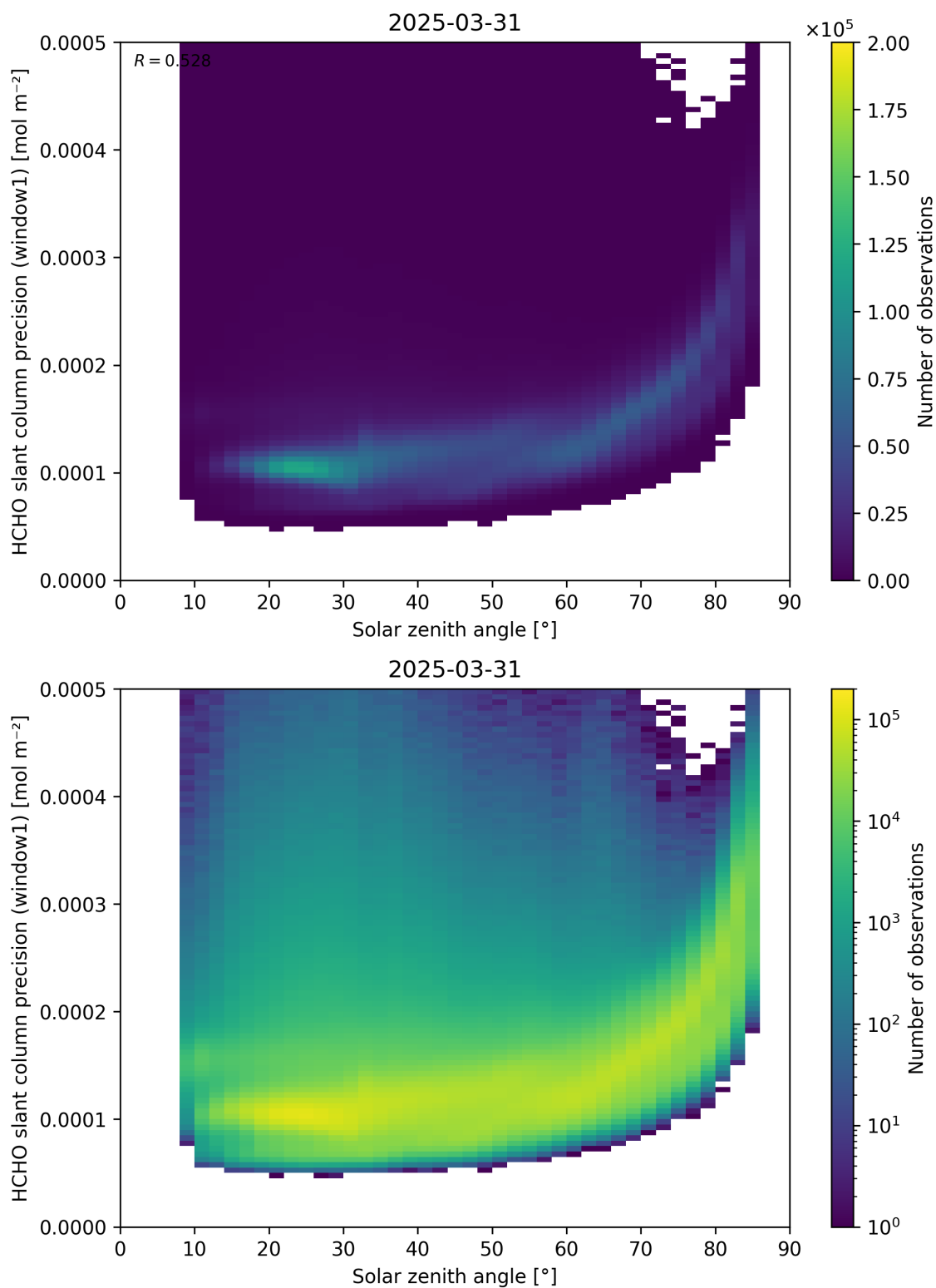
Figure 174: Scatter density plot of “Solar zenith angle” against “HCHO slant column precision (window1)” for 2025-03-30 to 2025-04-01.
