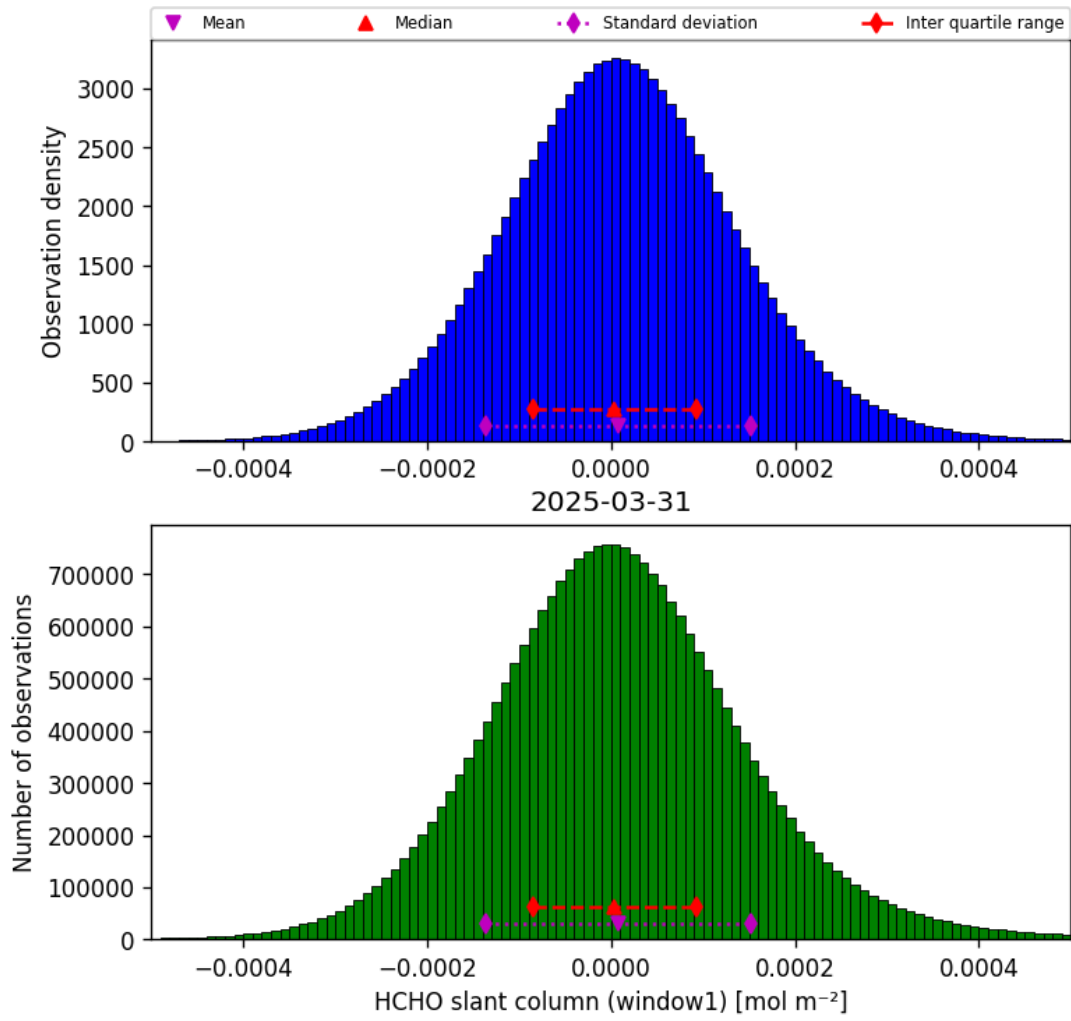
Figure 38: Histogram of “HCHO slant column (window1)” for 2025-03-30 to 2025-04-01
