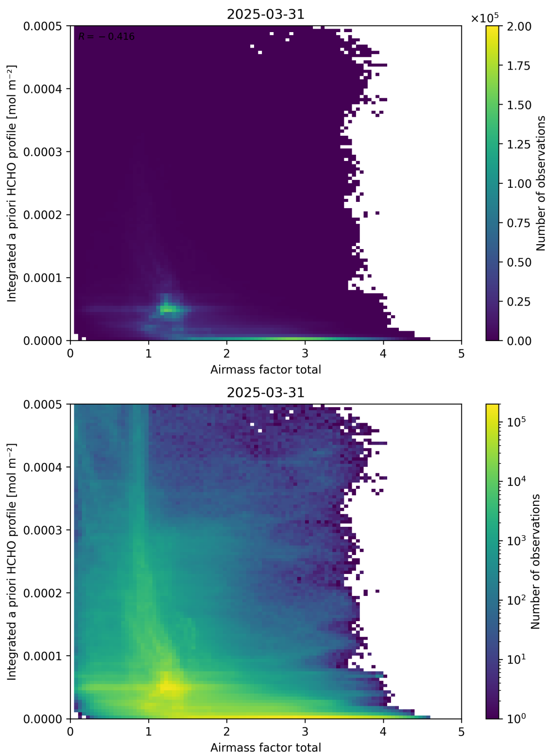
Figure 104: Scatter density plot of “Airmass factor total” against “Integrated a priori HCHO profile” for 2025-03-30 to 2025-04-01.
