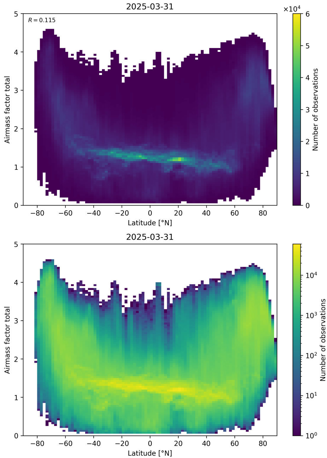
Figure 161: Scatter density plot of “Latitude” against “Airmass factor total” for 2025-03-30 to 2025-04-01.
