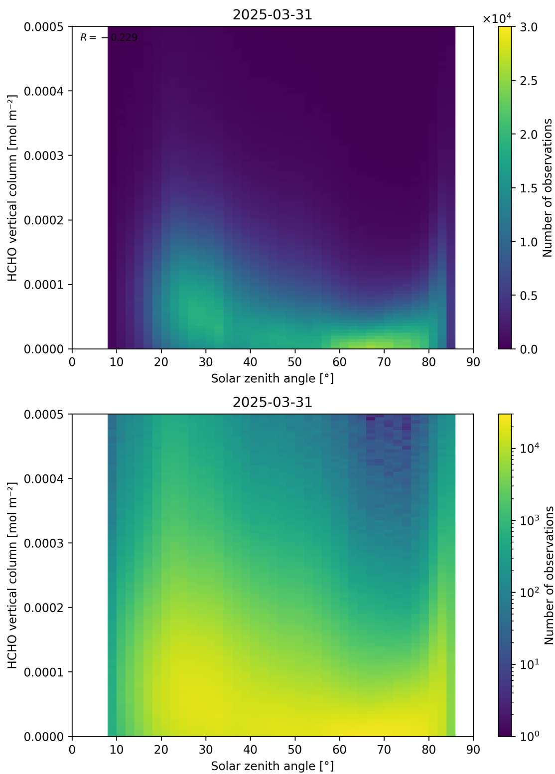
Figure 177: Scatter density plot of “Solar zenith angle” against “HCHO vertical column” for 2025-03-30 to 2025-04-01.
