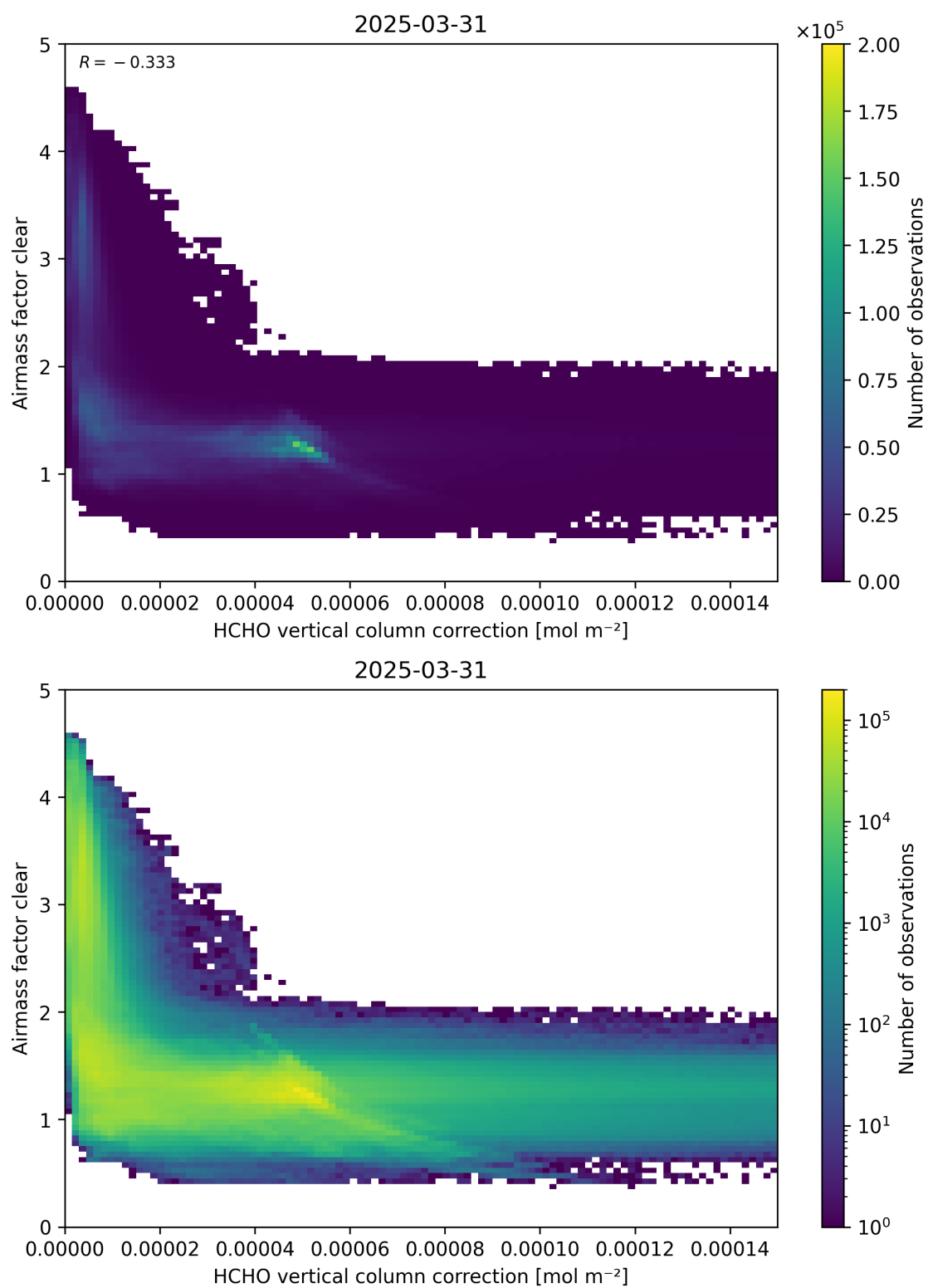
Figure 115: Scatter density plot of “HCHO vertical column correction” against “Airmass factor clear” for 2025-03-30 to 2025-04-01.
