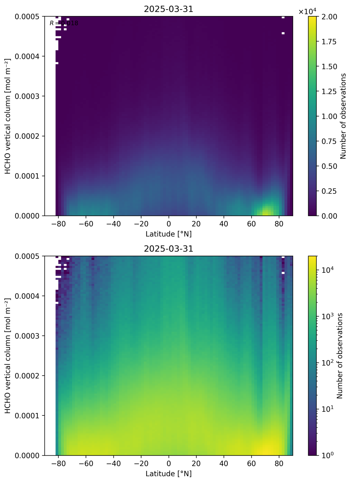
Figure 163: Scatter density plot of “Latitude” against “HCHO vertical column” for 2025-03-30 to 2025-04-01.
