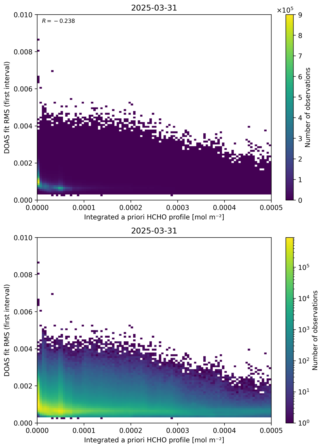
Figure 148: Scatter density plot of “Integrated a priori HCHO profile” against “DOAS fit RMS (first interval)” for 2025-03-30 to 2025-04-01.
