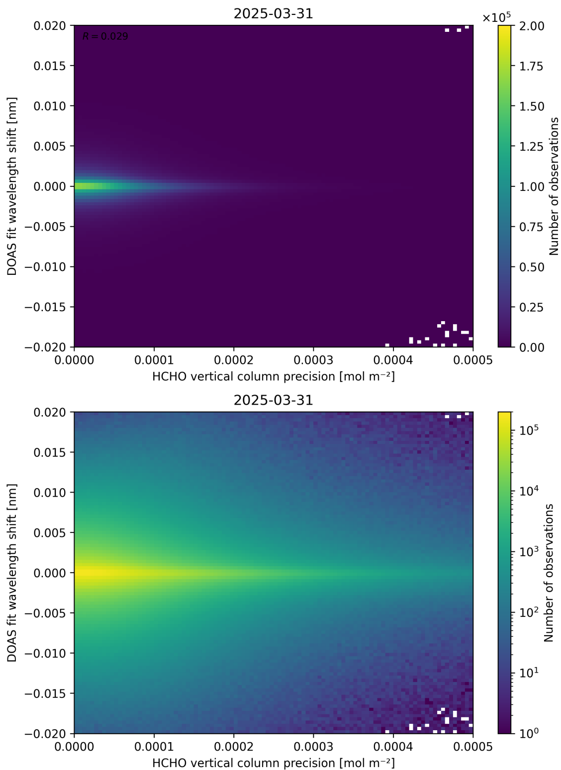
Figure 137: Scatter density plot of “HCHO vertical column precision” against “DOAS fit wavelength shift” for 2025-03-30 to 2025-04-01.
