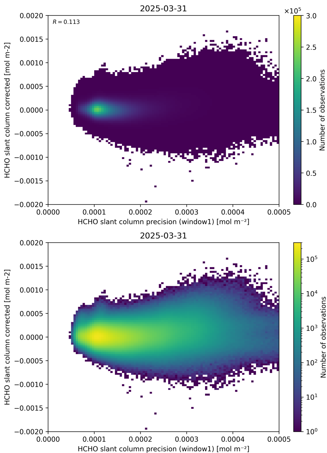
Figure 92: Scatter density plot of “HCHO slant column precision (window1)” against “HCHO slant column corrected” for 2025-03-30 to 2025-04-01.
