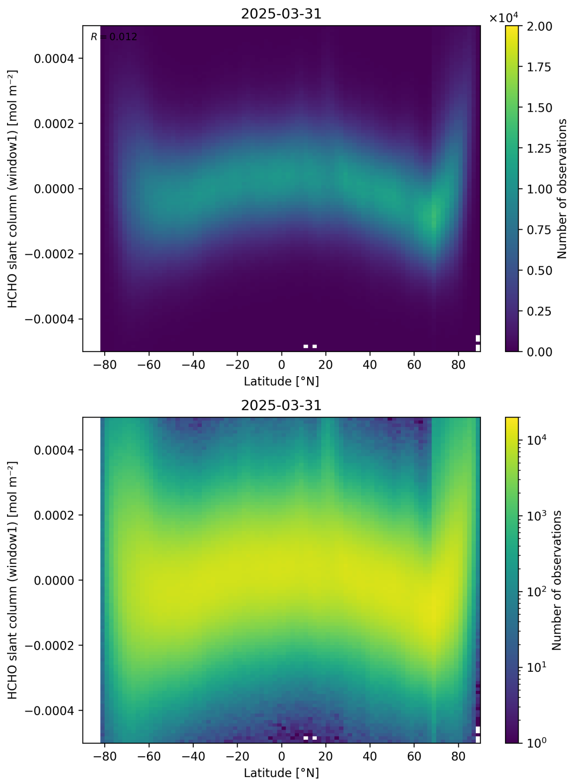
Figure 159: Scatter density plot of “Latitude” against “HCHO slant column (window1)” for 2025-03-30 to 2025-04-01.
