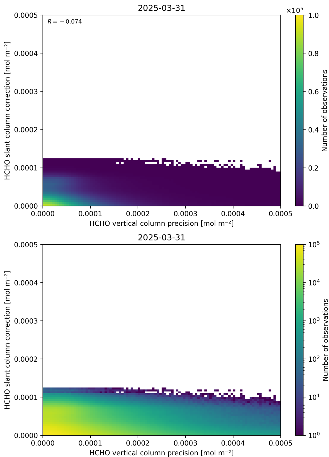
Figure 141: Scatter density plot of “HCHO vertical column precision” against “HCHO slant column correction” for 2025-03-30 to 2025-04-01.
