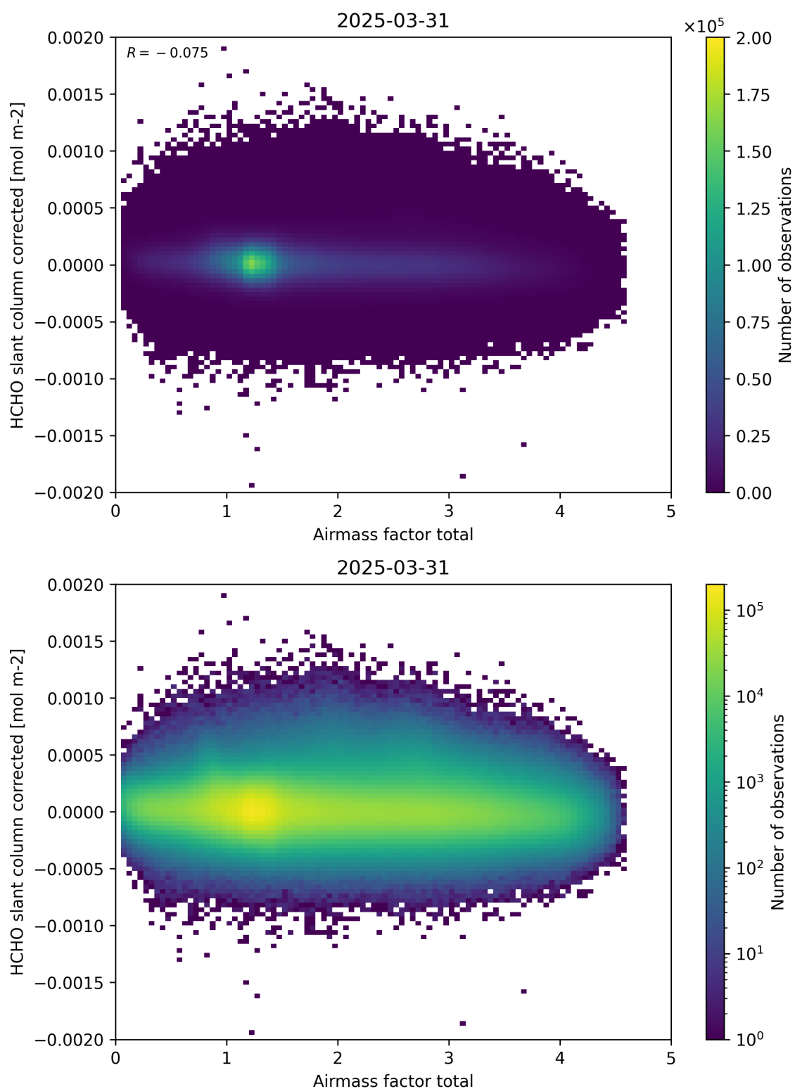
Figure 101: Scatter density plot of “Airmass factor total” against “HCHO slant column corrected” for 2025-03-30 to 2025-04-01.
