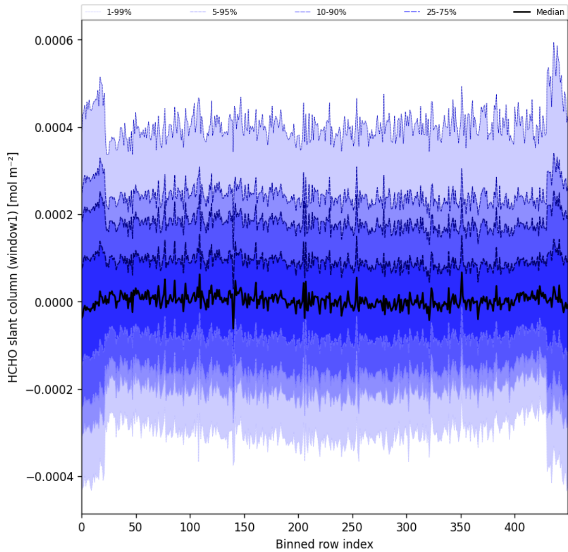
Figure 52: Along track statistics of “HCHO slant column (window1)” for 2025-03-30 to 2025-04-01
