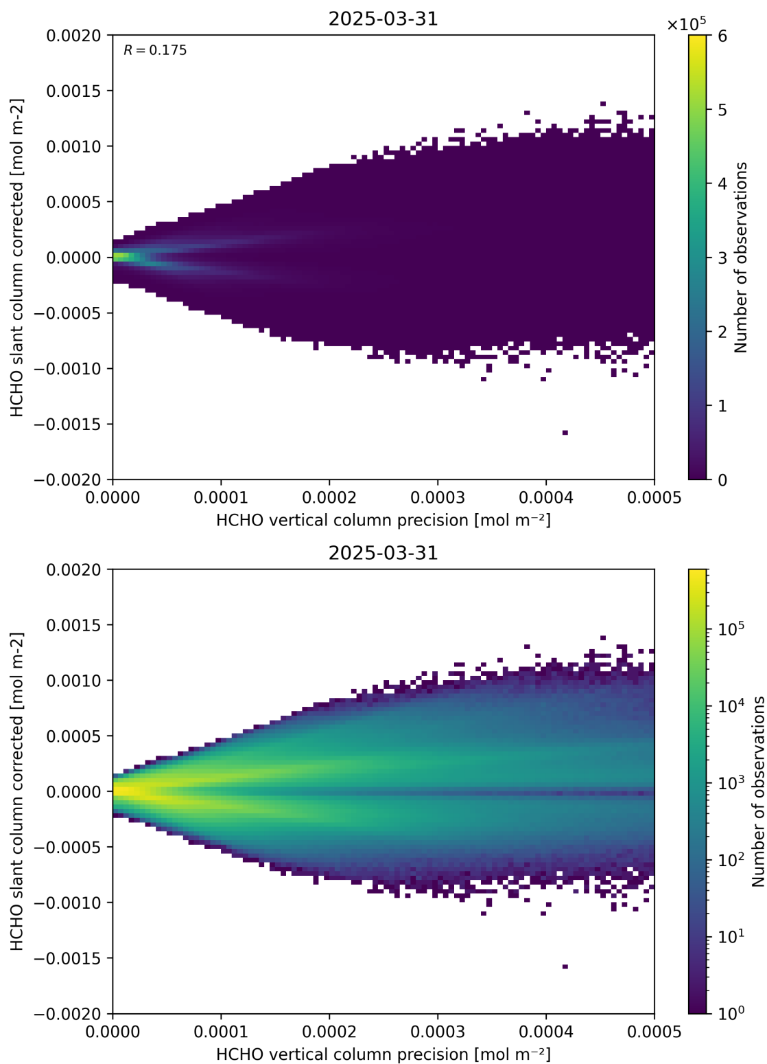
Figure 140: Scatter density plot of “HCHO vertical column precision” against “HCHO slant column corrected” for 2025-03-30 to 2025-04-01.
