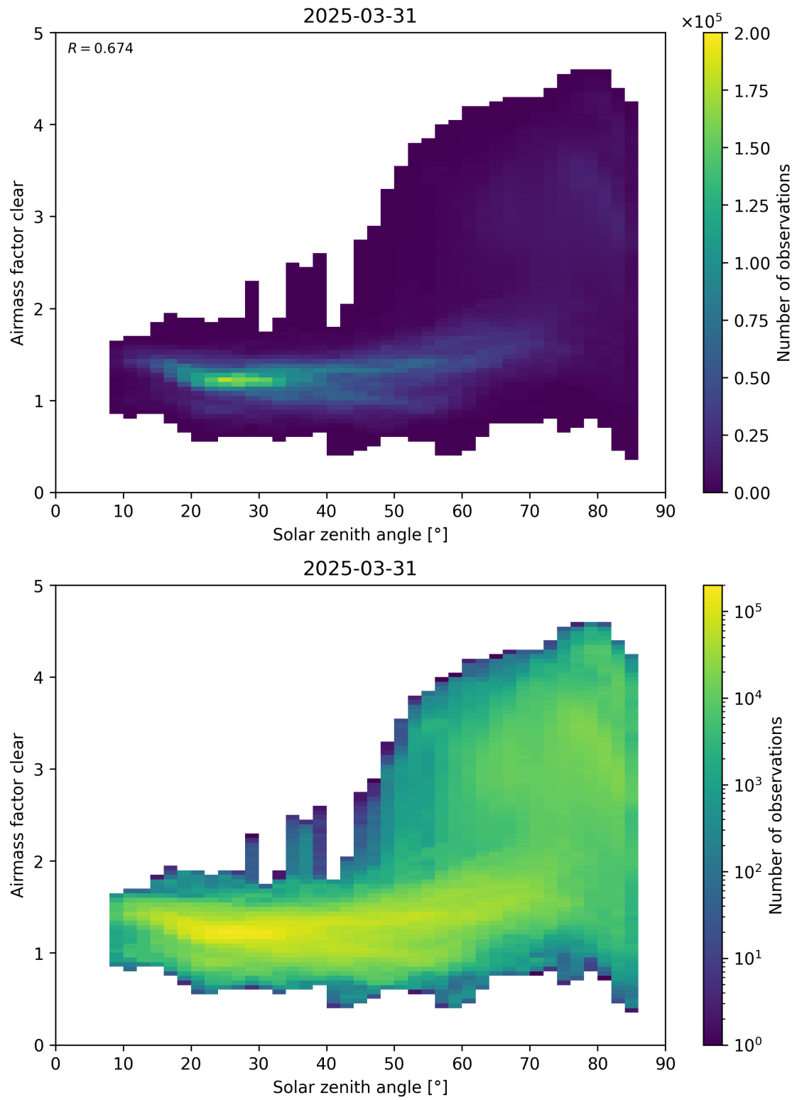
Figure 170: Scatter density plot of “Solar zenith angle” against “Airmass factor clear” for 2025-03-30 to 2025-04-01.
