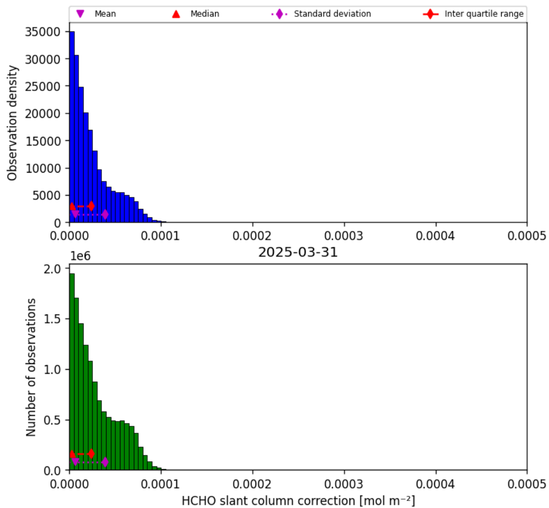
Figure 47: Histogram of "HCHO slant column correction" for 2025-03-30 to 2025-04-01
