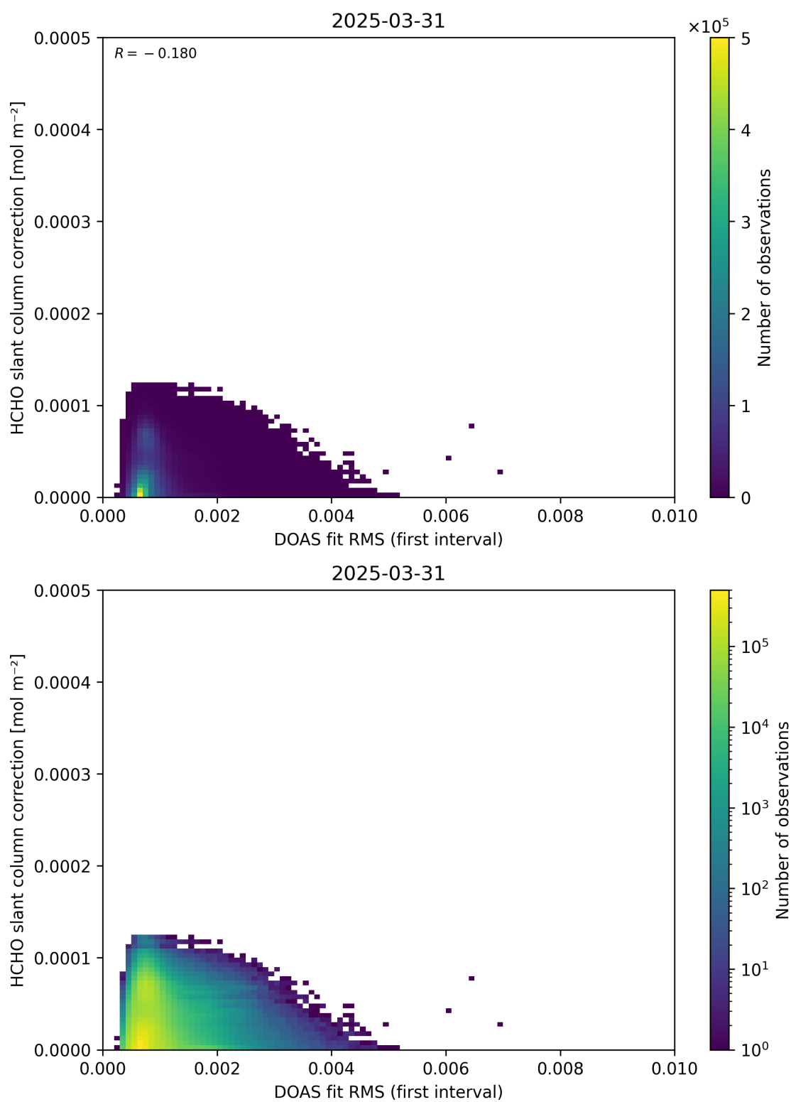
Figure 63: Scatter density plot of “DOAS fit RMS (first interval)” against “HCHO slant column correction” for 2025-03-30 to 2025-04-01.
