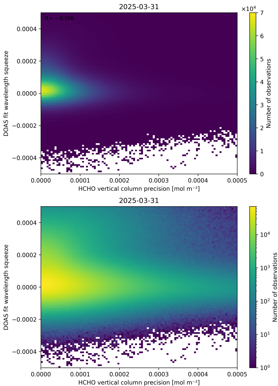
Figure 138: Scatter density plot of “HCHO vertical column precision” against “DOAS fit wavelength squeeze” for 2025-03-30 to 2025-04-01.
