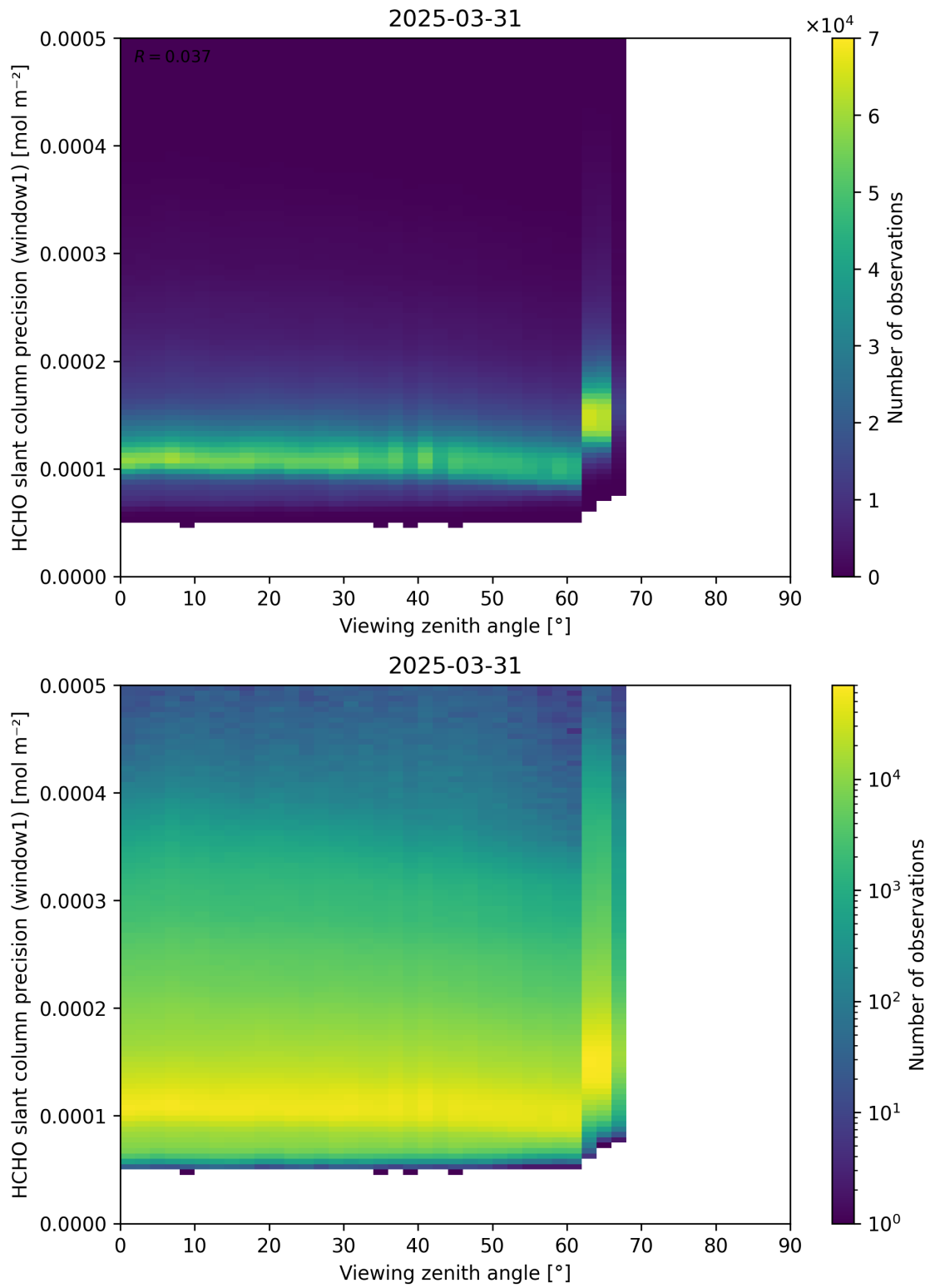
Figure 189: Scatter density plot of “Viewing zenith angle” against “HCHO slant column precision (window1)” for 2025-03-30 to 2025-04-01.
