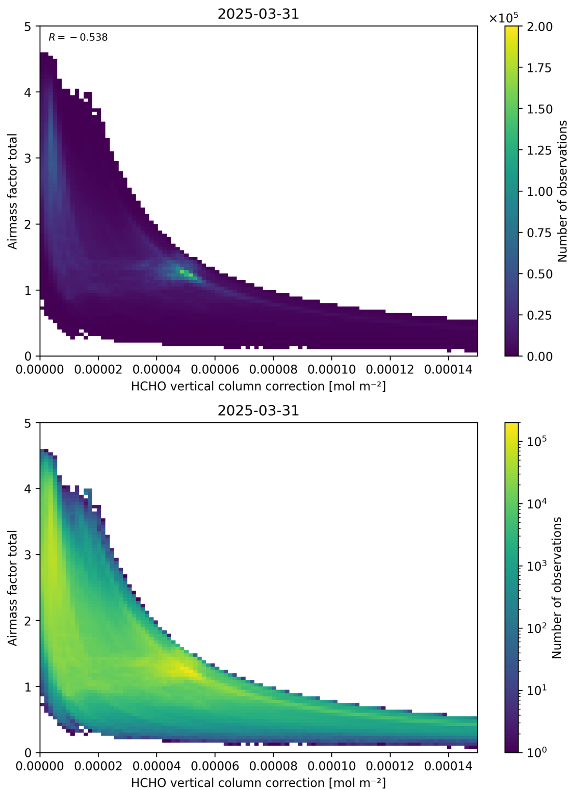
Figure 120: Scatter density plot of “HCHO vertical column correction” against “Airmass factor total” for 2025-03-30 to 2025-04-01.
