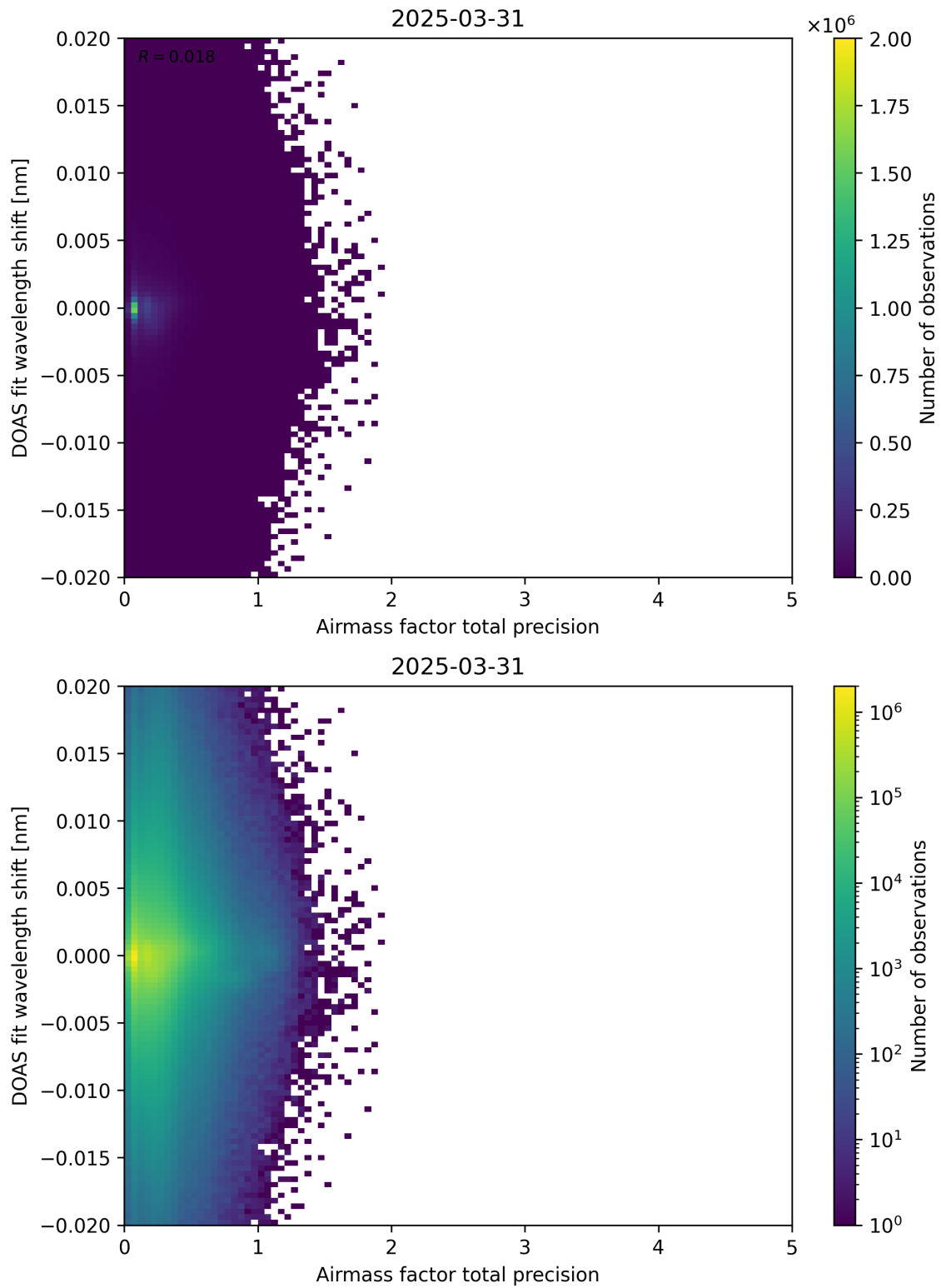
Figure 106: Scatter density plot of “Airmass factor total precision” against “DOAS fit wavelength shift” for 2025-03-30 to 2025-04-01.
