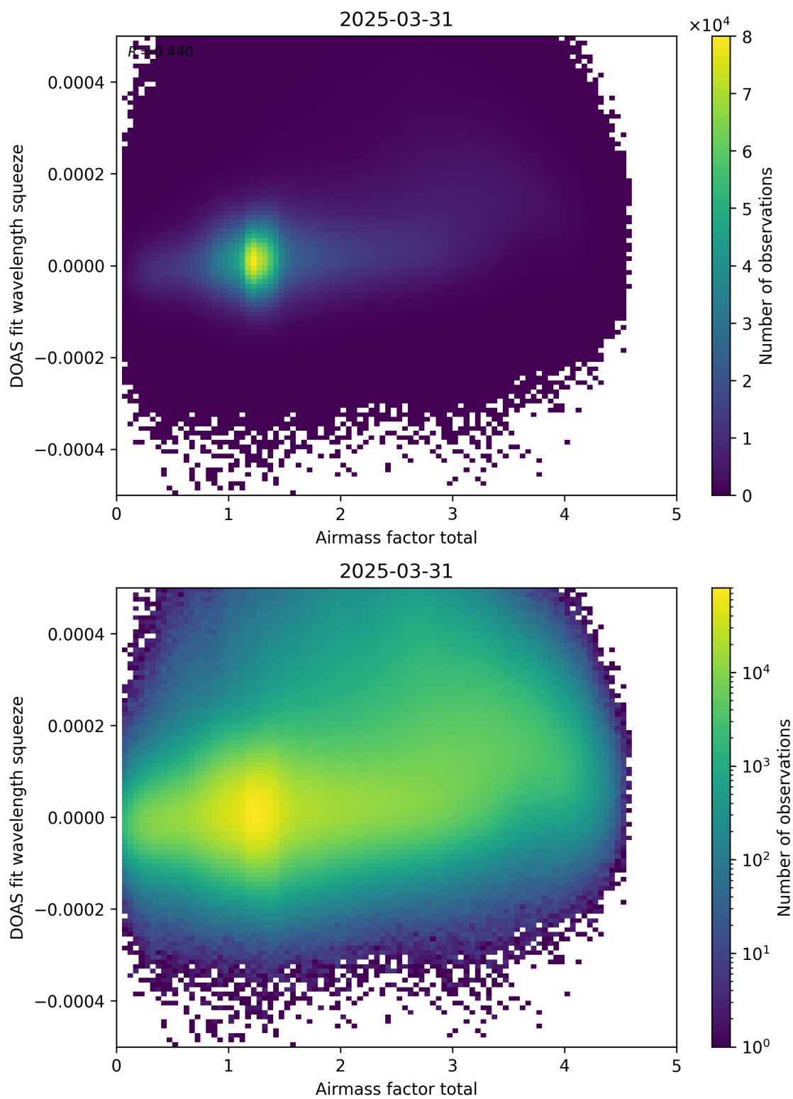
Figure 99: Scatter density plot of “Airmass factor total” against “DOAS fit wavelength squeeze” for 2025-03-30 to 2025-04-01.
