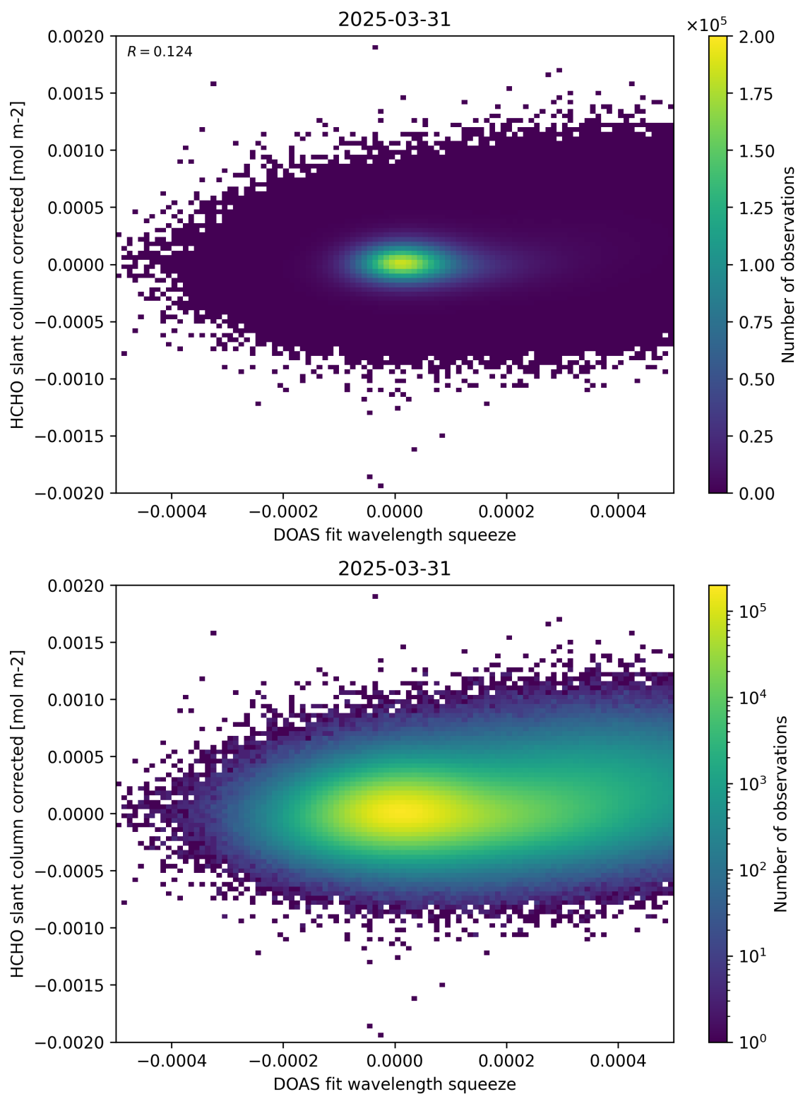
Figure 69: Scatter density plot of “DOAS fit wavelength squeeze” against “HCHO slant column corrected” for 2025-03-30 to 2025-04-01.
