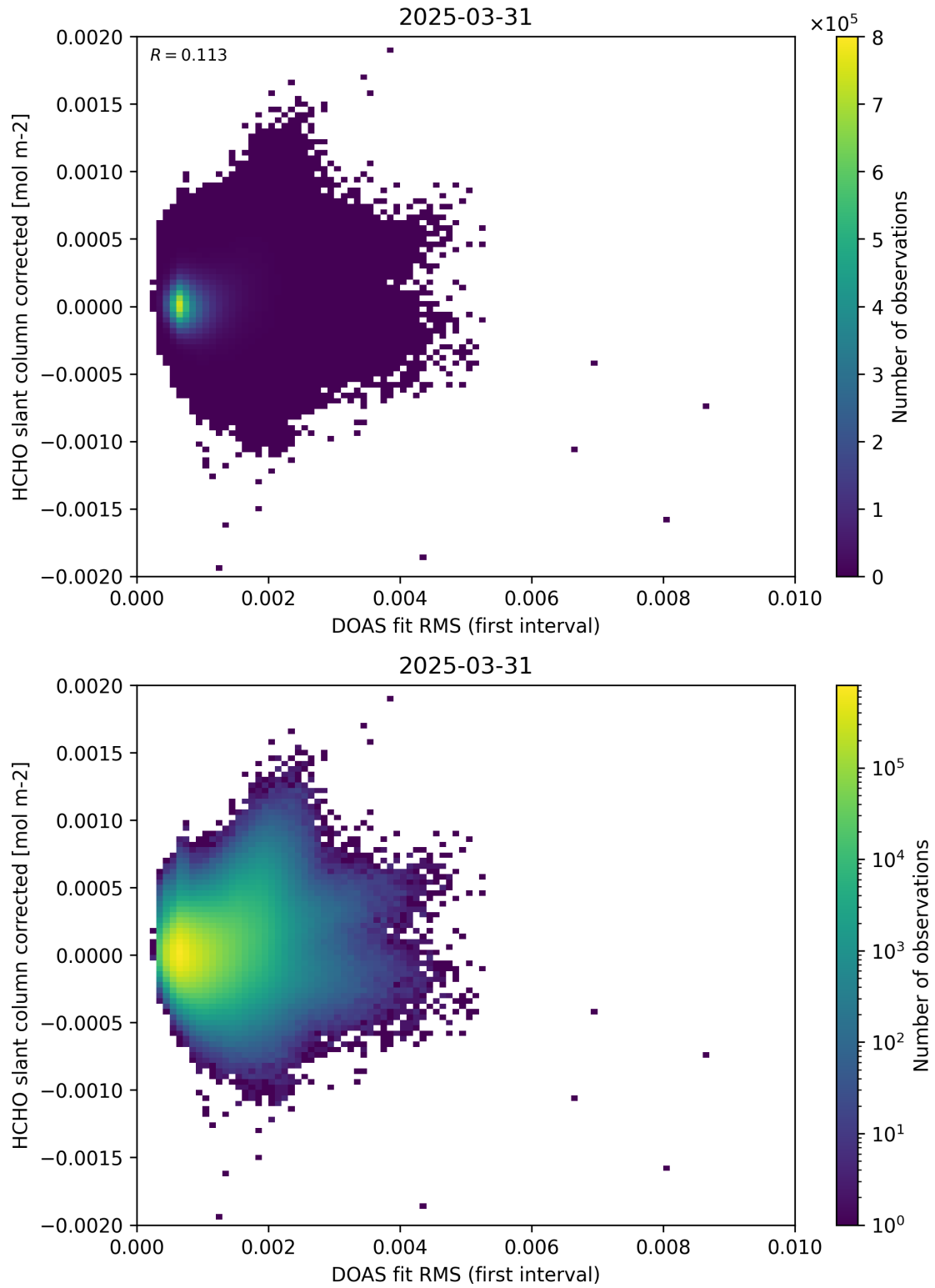
Figure 62: Scatter density plot of “DOAS fit RMS (first interval)” against “HCHO slant column corrected” for 2025-03-30 to 2025-04-01.
