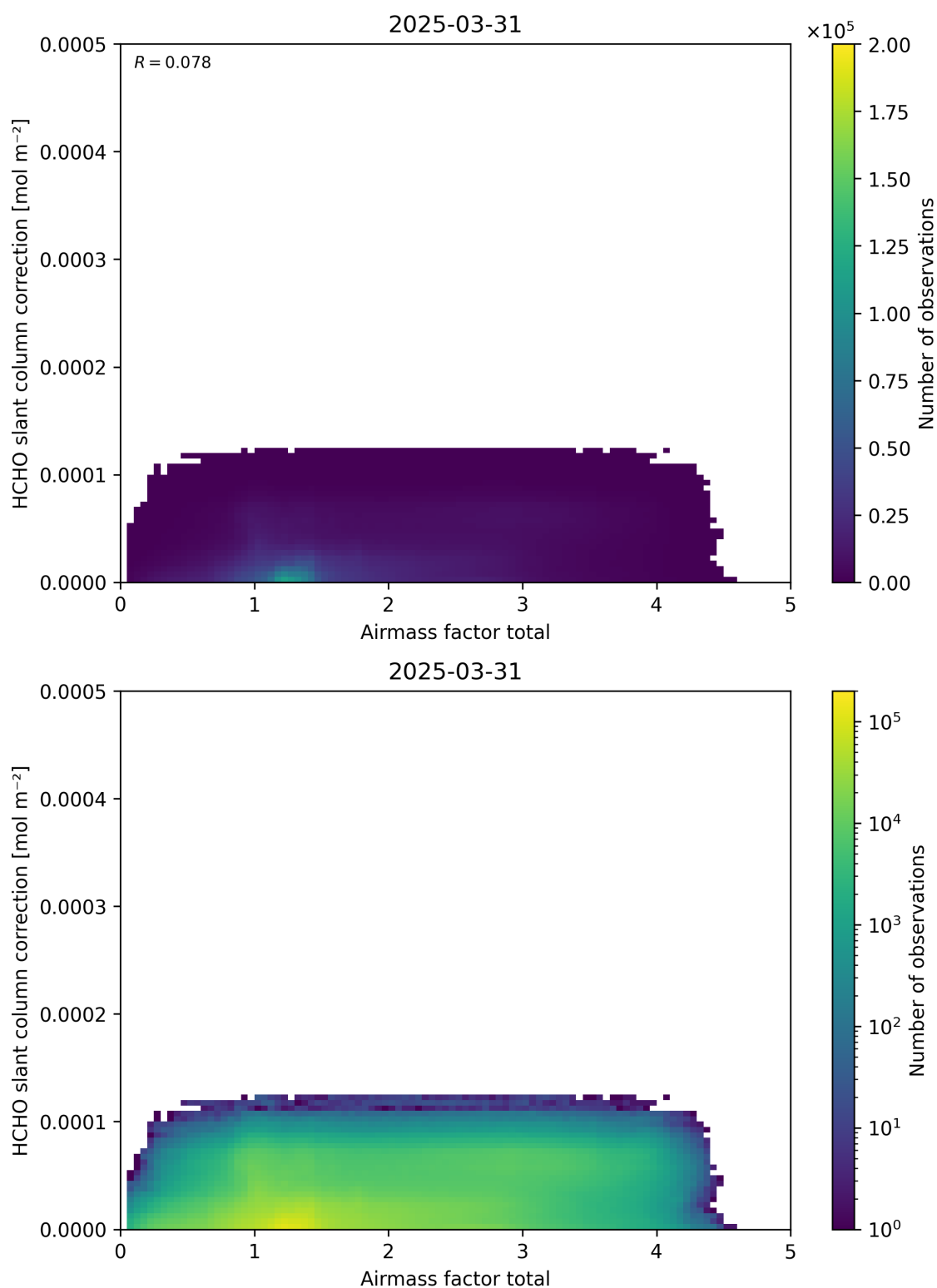
Figure 102: Scatter density plot of “Airmass factor total” against “HCHO slant column correction” for 2025-03-30 to 2025-04-01.
