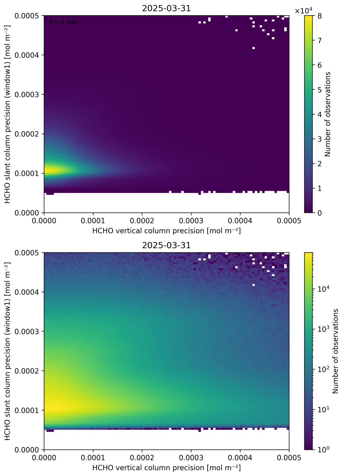
Figure 143: Scatter density plot of “HCHO vertical column precision” against “HCHO slant column precision (window1)” for 2025-03-30 to 2025-04-01.
