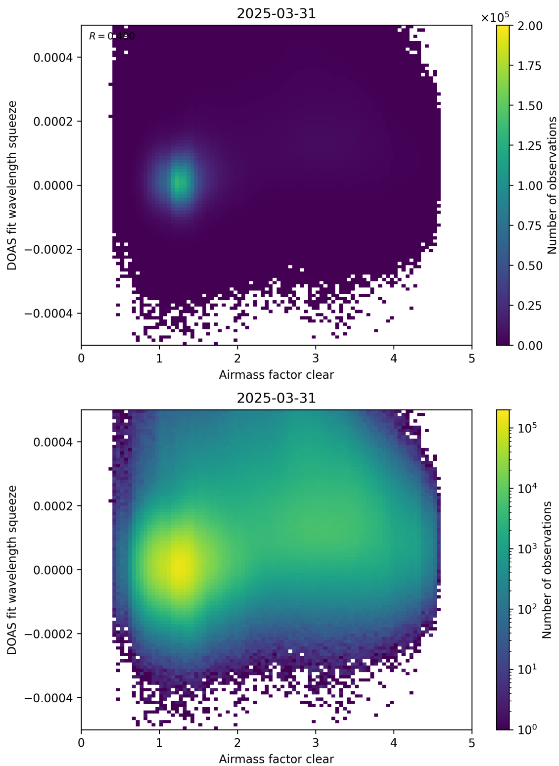
Figure 73: Scatter density plot of “Airmass factor clear” against “DOAS fit wavelength squeeze” for 2025-03-30 to 2025-04-01.
