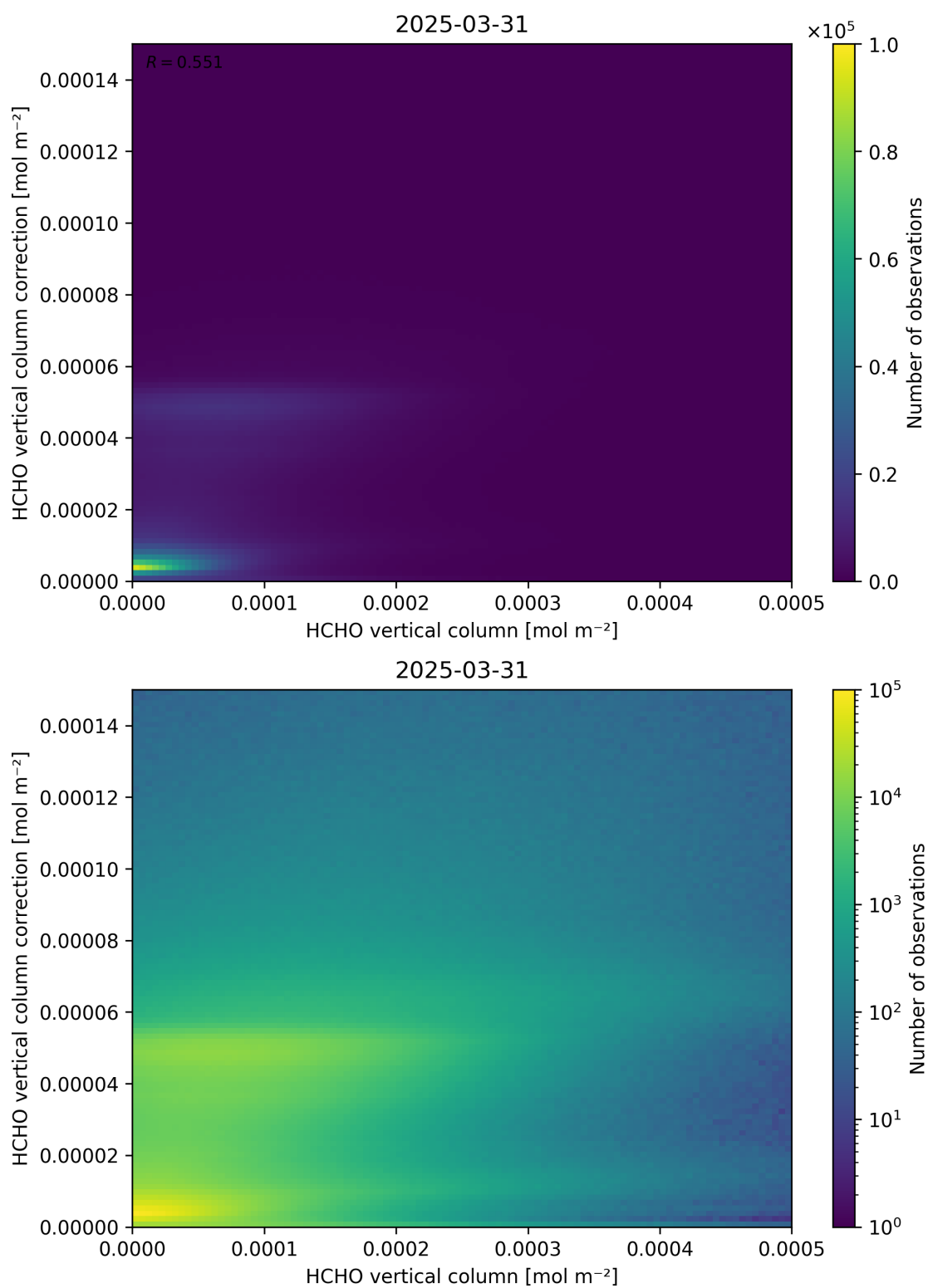
Figure 133: Scatter density plot of “HCHO vertical column” against “HCHO vertical column correction” for 2025-03-30 to 2025-04-01.
