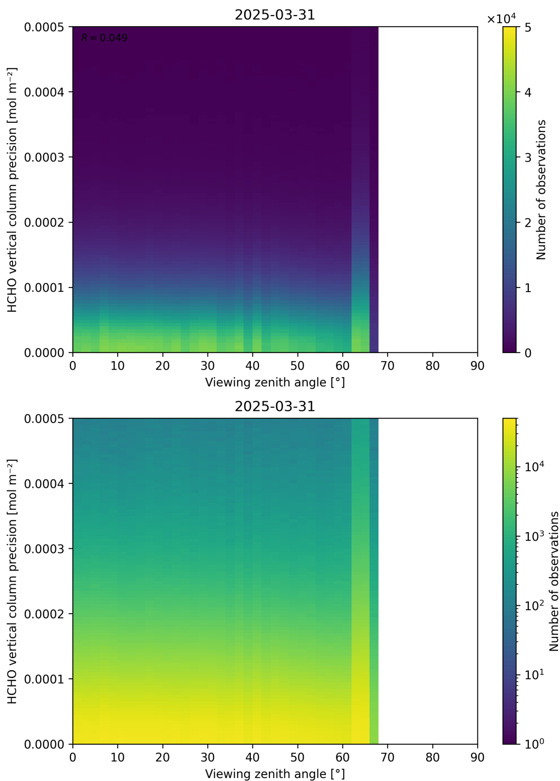
Figure 194: Scatter density plot of “Viewing zenith angle” against “HCHO vertical column precision” for 2025-03-30 to 2025-04-01.
