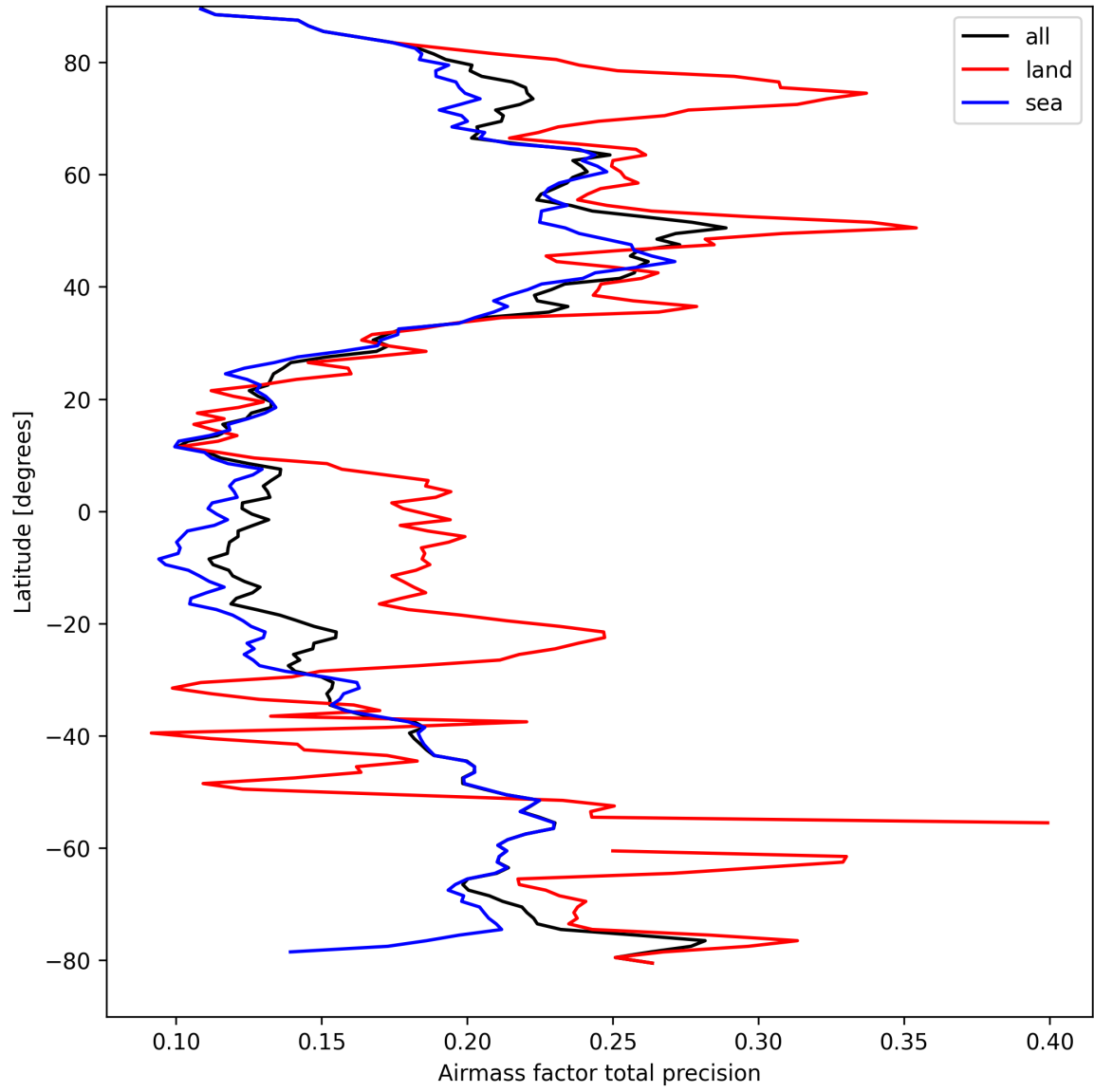
Figure 27: Zonal average of “Airmass factor total precision” for 2025-03-30 to 2025-04-01.
