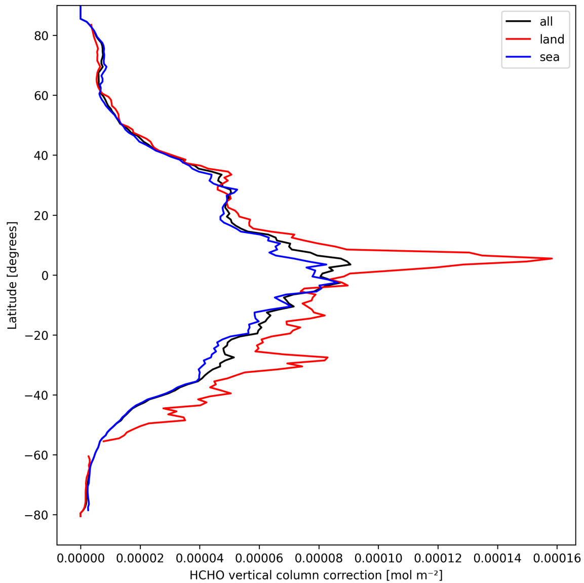
Figure 23: Zonal average of “HCHO vertical column correction” for 2025-03-30 to 2025-04-01.
