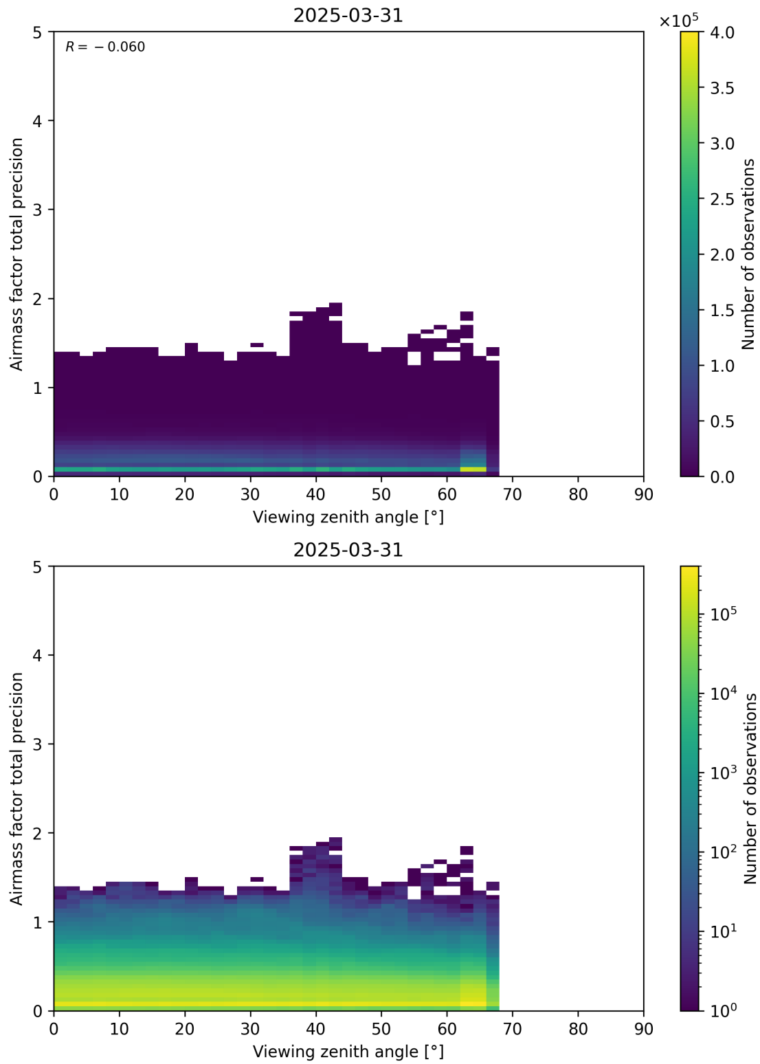
Figure 191: Scatter density plot of “Viewing zenith angle” against “Airmass factor total precision” for 2025-03-30 to 2025-04-01.
