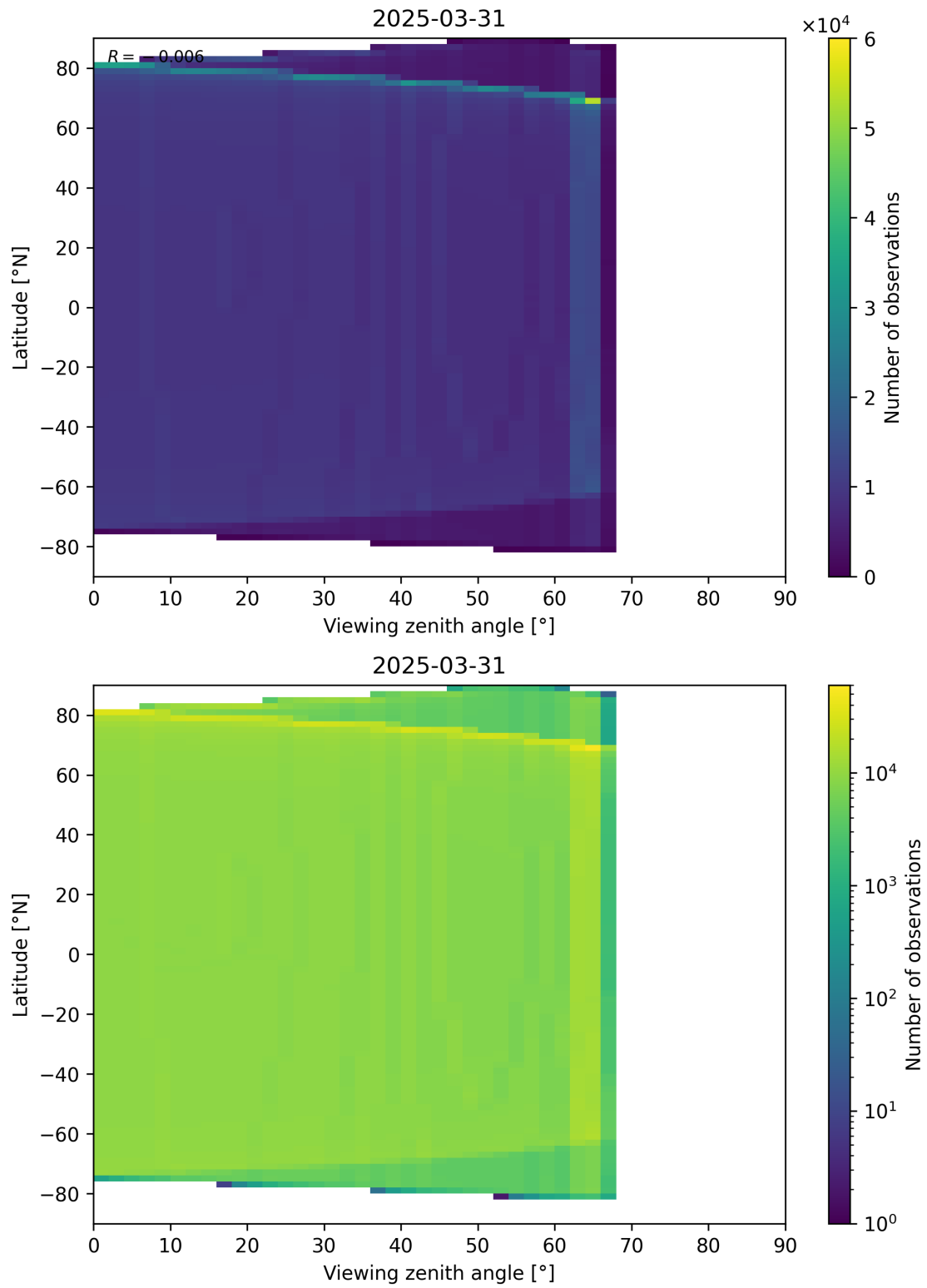
Figure 196: Scatter density plot of “Viewing zenith angle” against “Latitude” for 2025-03-30 to 2025-04-01.
