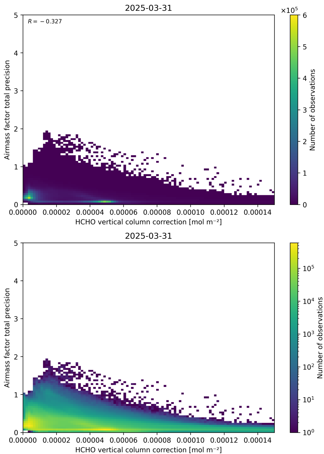
Figure 121: Scatter density plot of “HCHO vertical column correction” against “Airmass factor total precision” for 2025-03-30 to 2025-04-01.
