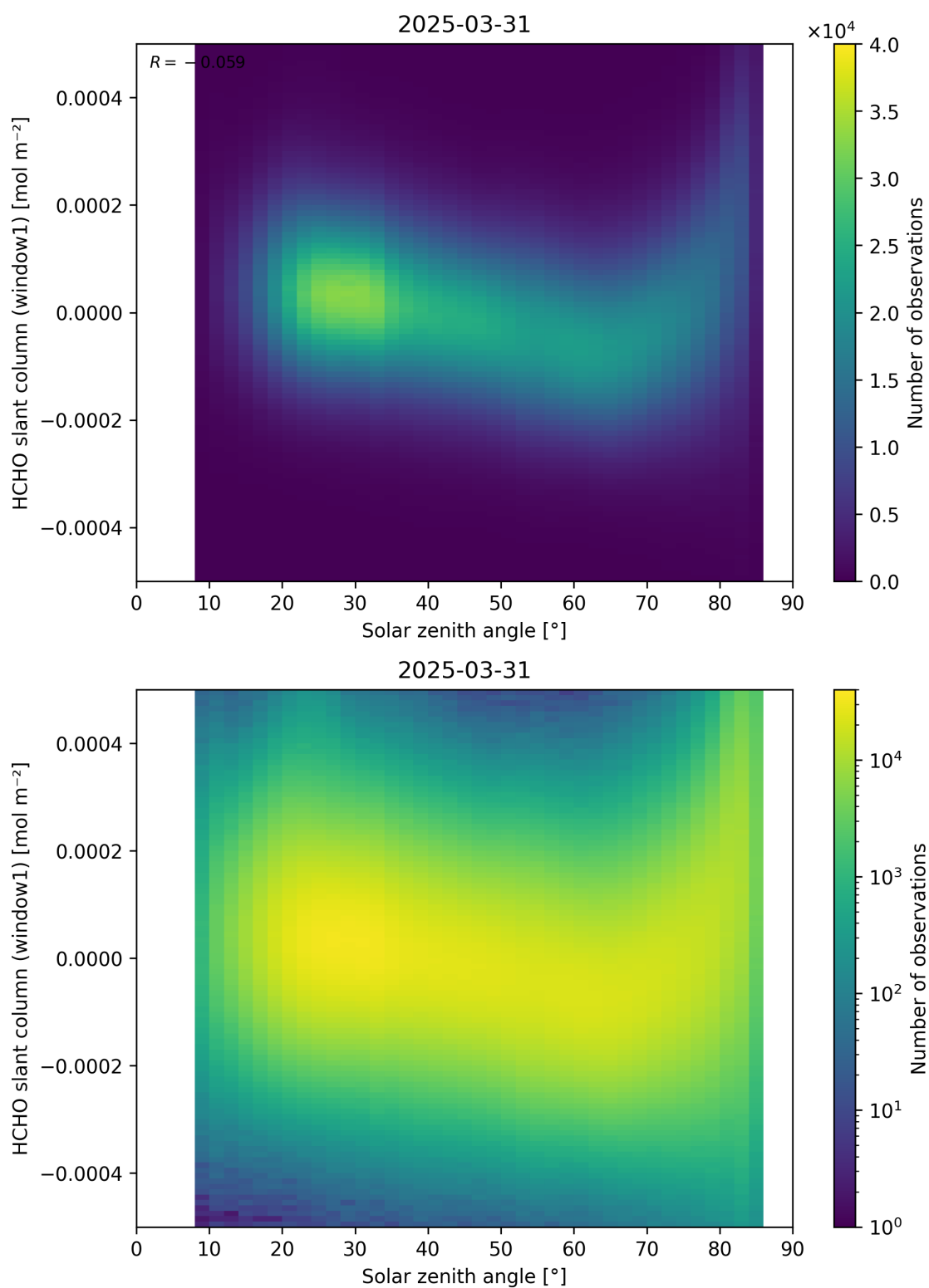
Figure 173: Scatter density plot of “Solar zenith angle” against “HCHO slant column (window1)” for 2025-03-30 to 2025-04-01.
