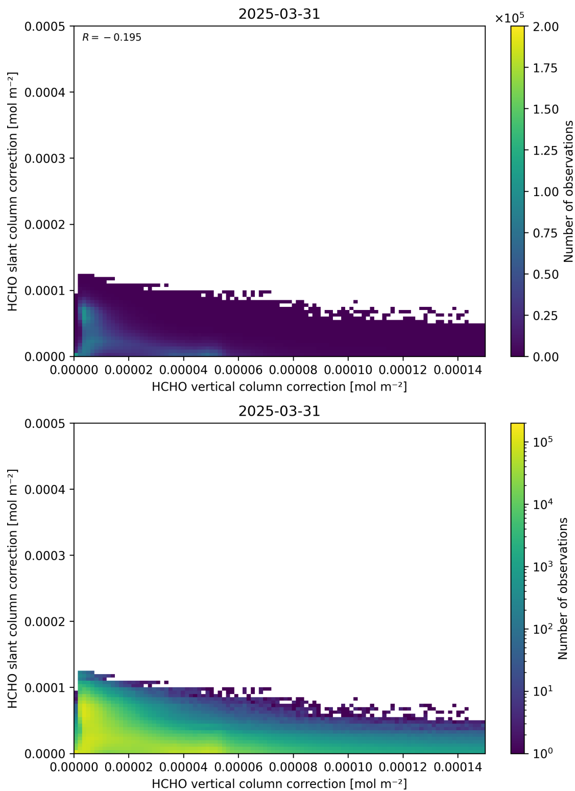
Figure 117: Scatter density plot of “HCHO vertical column correction” against “HCHO slant column correction” for 2025-03-30 to 2025-04-01.
