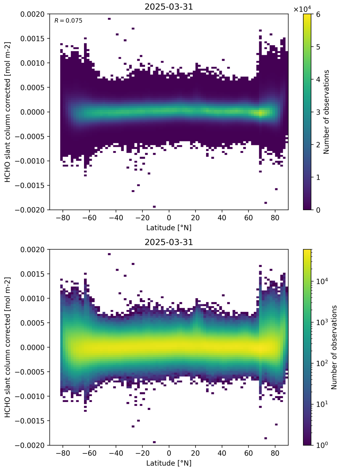
Figure 157: Scatter density plot of “Latitude” against “HCHO slant column corrected” for 2025-03-30 to 2025-04-01.
