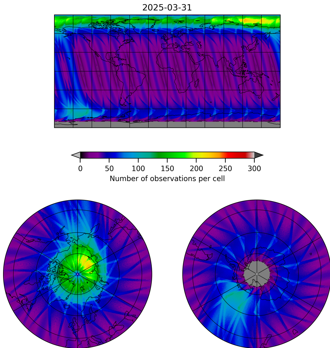
Figure 19: Map of the number of observations for 2025-03-30 to 2025-04-01
