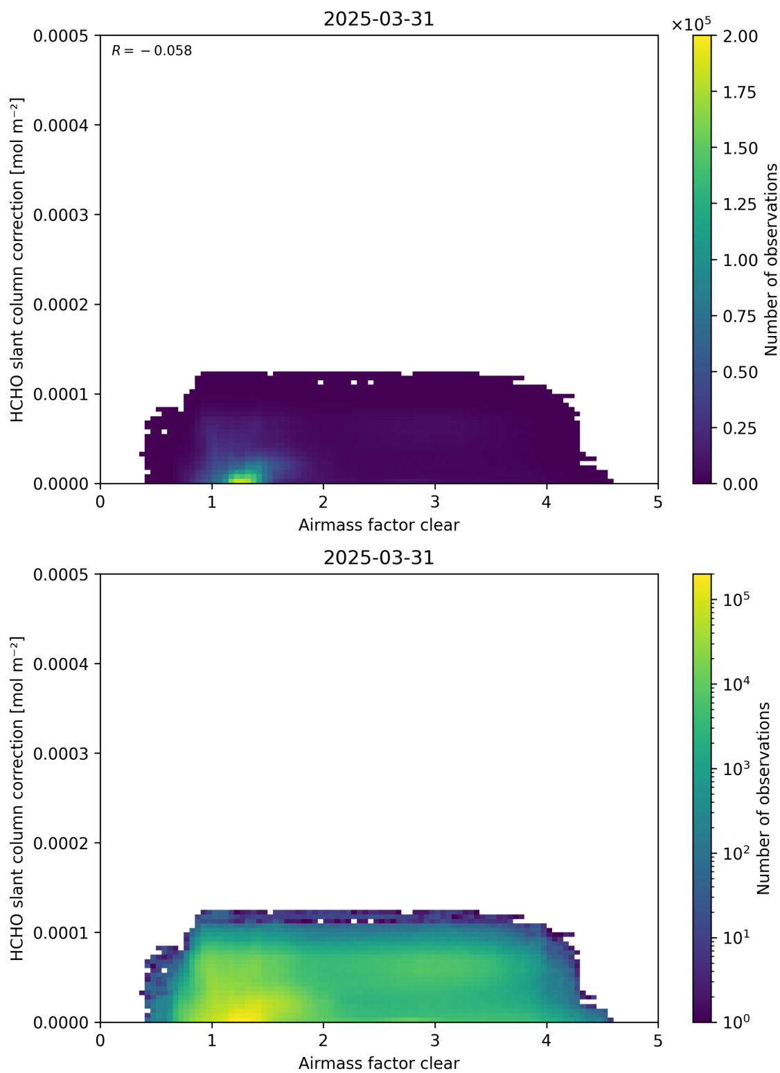
Figure 75: Scatter density plot of “Airmass factor clear” against “HCHO slant column correction” for 2025-03-30 to 2025-04-01.
