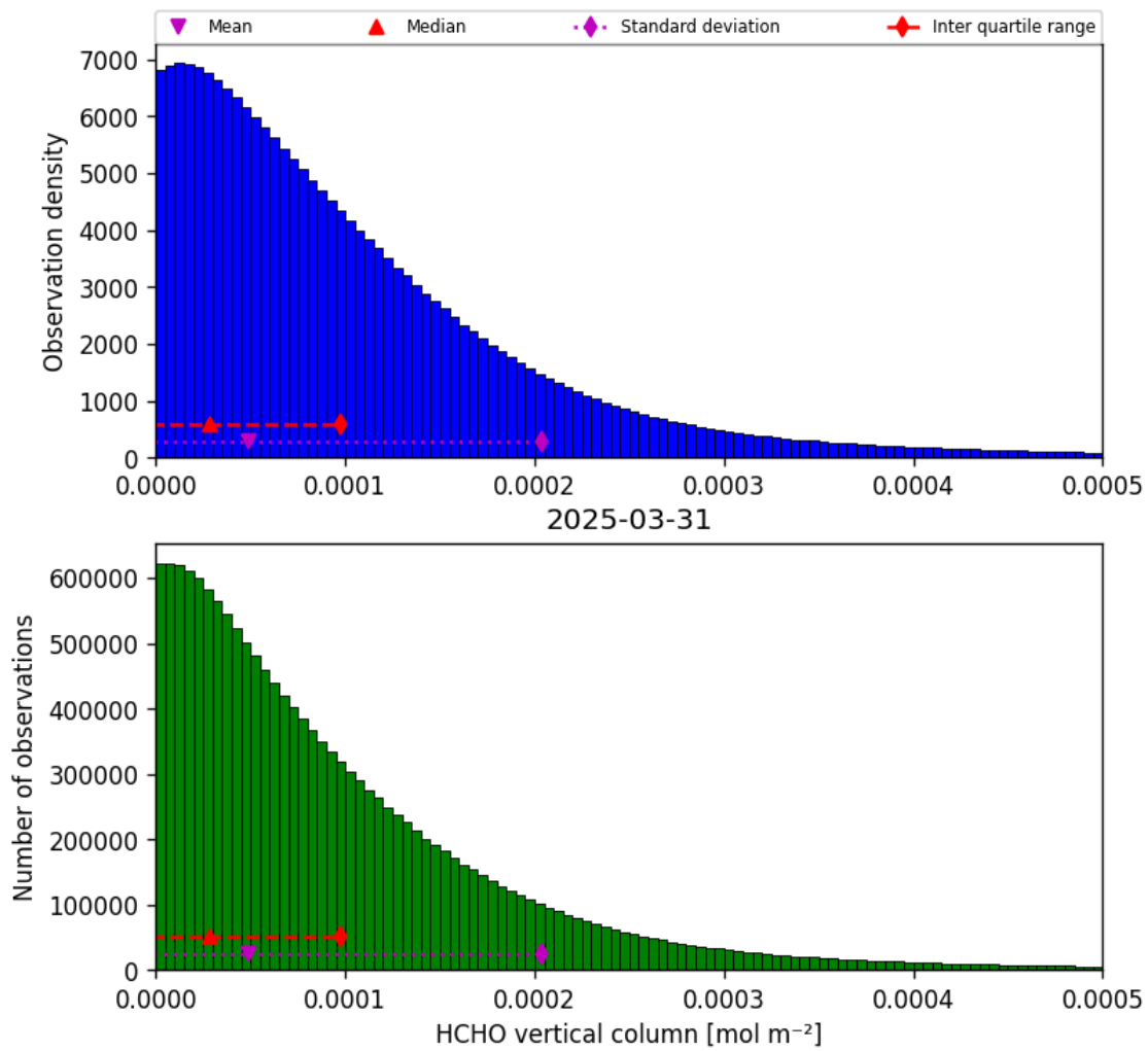
Figure 35: Histogram of “HCHO vertical column” for 2025-03-30 to 2025-04-01
