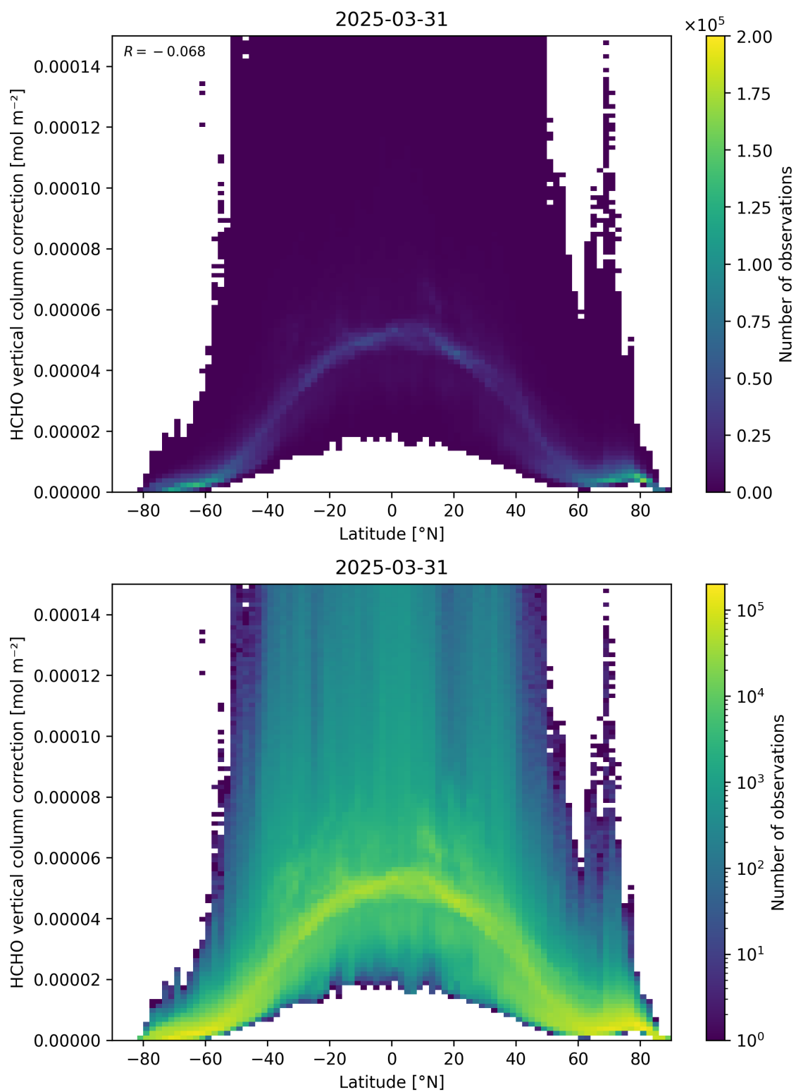
Figure 164: Scatter density plot of “Latitude” against “HCHO vertical column correction” for 2025-03-30 to 2025-04-01.
