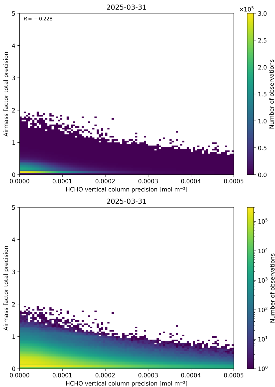
Figure 145: Scatter density plot of “HCHO vertical column precision” against “Airmass factor total precision” for 2025-03-30 to 2025-04-01.
