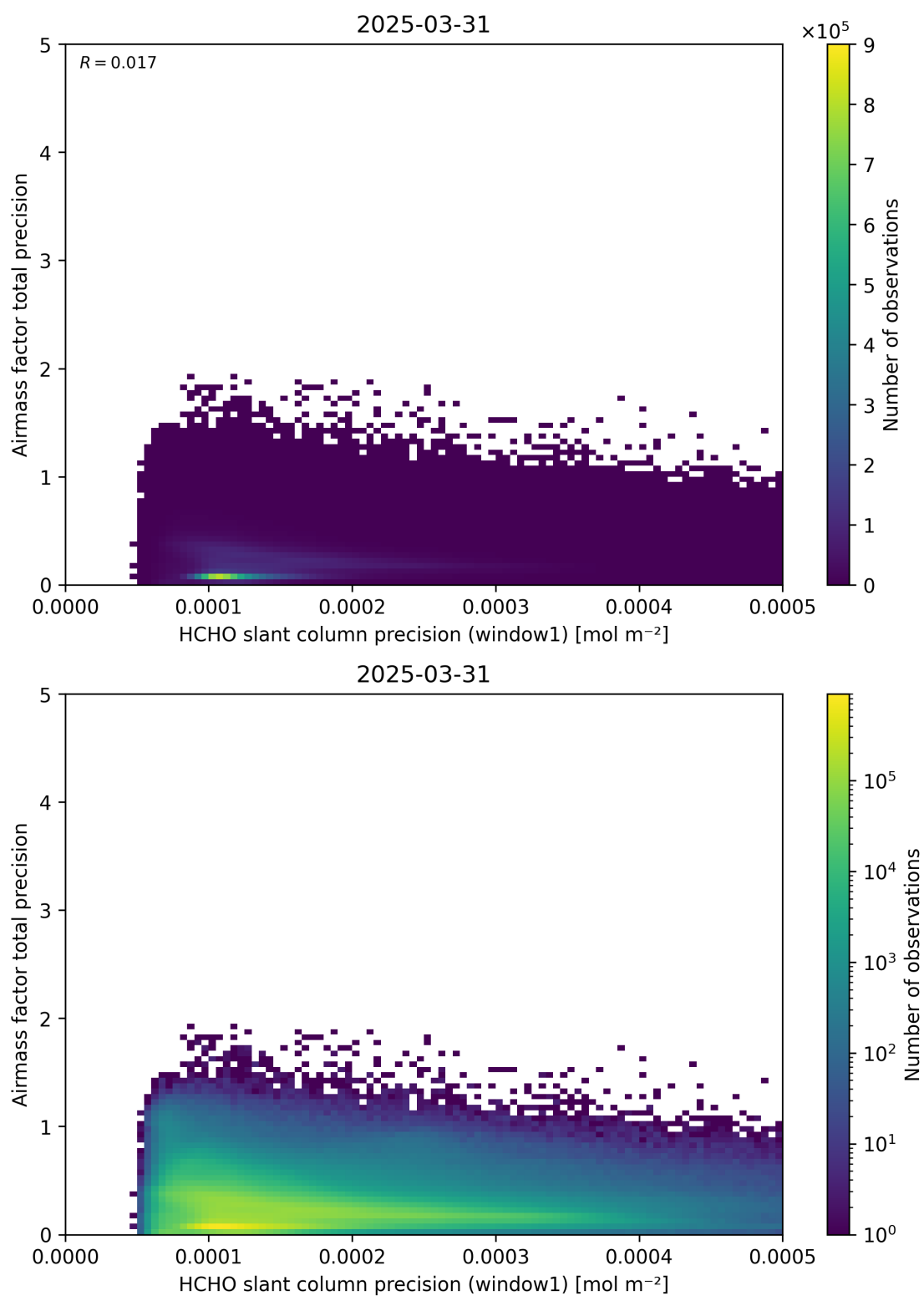
Figure 95: Scatter density plot of “HCHO slant column precision (window1)” against “Airmass factor total precision” for 2025-03-30 to 2025-04-01.
