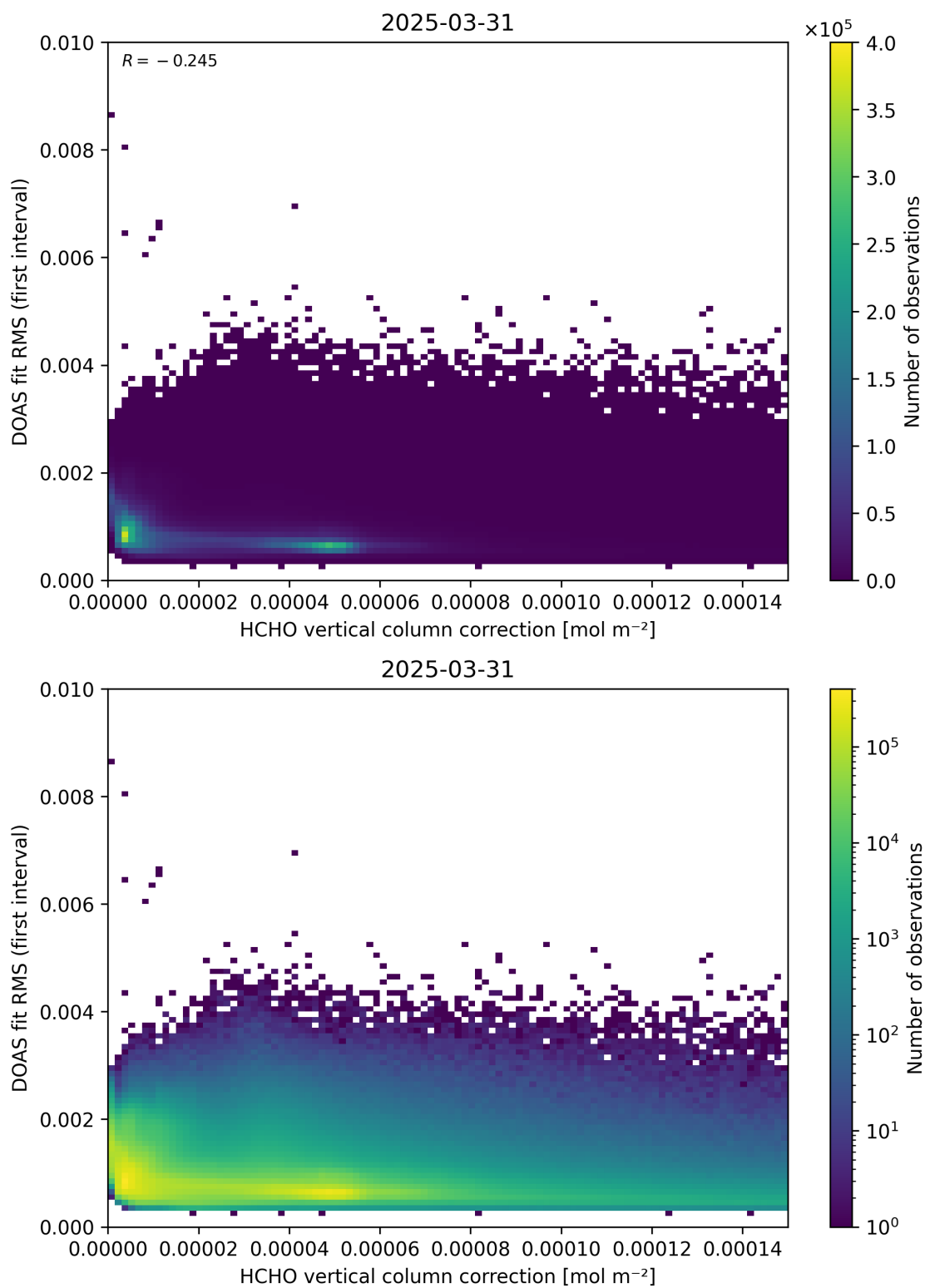
Figure 112: Scatter density plot of “HCHO vertical column correction” against “DOAS fit RMS (first interval)” for 2025-03-30 to 2025-04-01.
