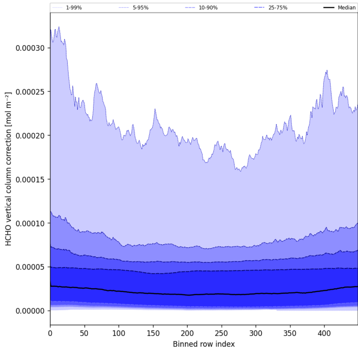
Figure 51: Along track statistics of "HCHO vertical column correction" for 2025-03-30 to 2025-04-01
