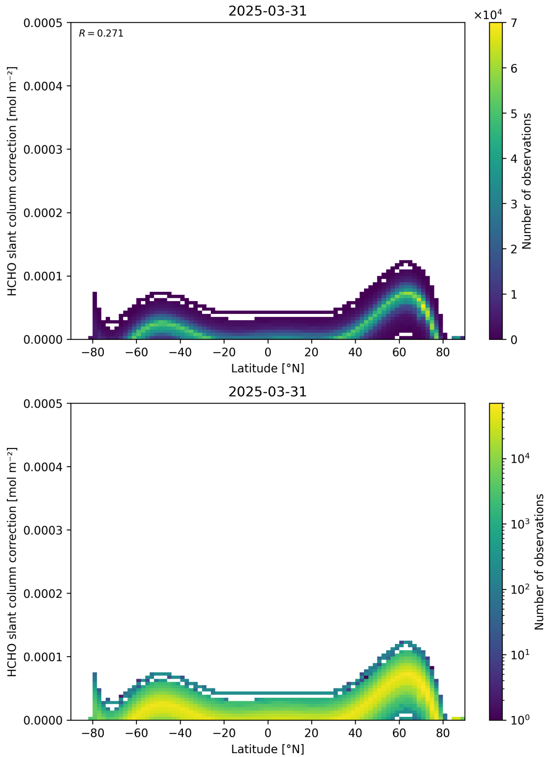
Figure 158: Scatter density plot of “Latitude” against “HCHO slant column correction” for 2025-03-30 to 2025-04-01.
