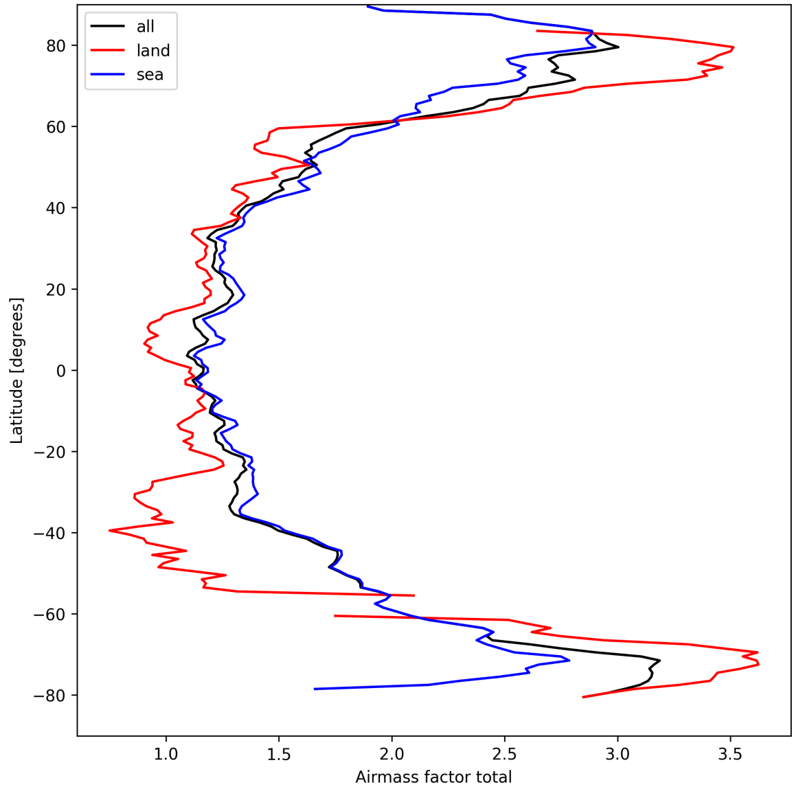
Figure 26: Zonal average of “Airmass factor total” for 2025-03-30 to 2025-04-01.
