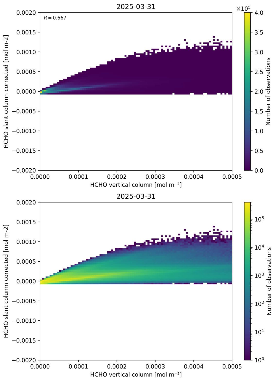
Figure 127: Scatter density plot of “HCHO vertical column” against “HCHO slant column corrected” for 2025-03-30 to 2025-04-01.
