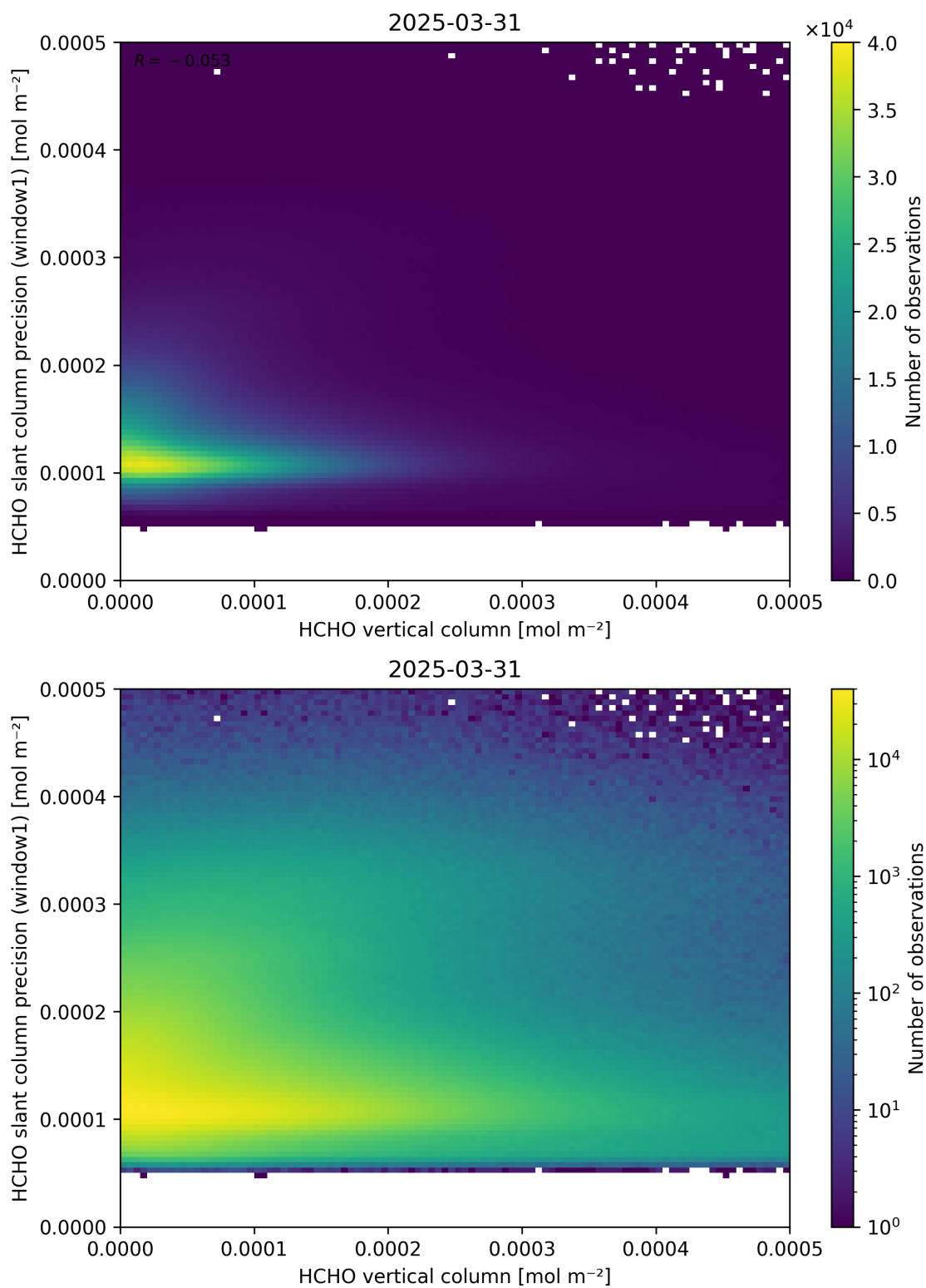
Figure 130: Scatter density plot of “HCHO vertical column” against “HCHO slant column precision (window1)” for 2025-03-30 to 2025-04-01.
