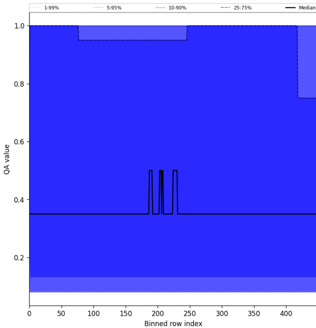
Figure 48: Along track statistics of “QA value” for 2025-03-30 to 2025-04-01
