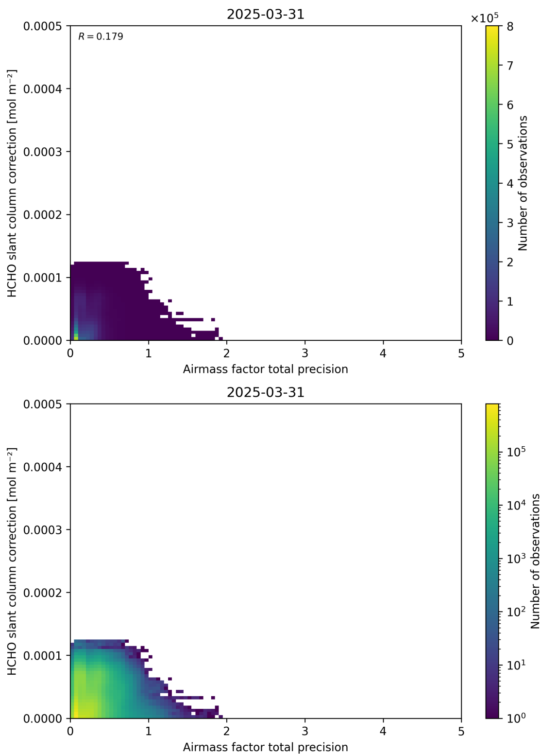
Figure 110: Scatter density plot of “Airmass factor total precision” against “HCHO slant column correction” for 2025-03-30 to 2025-04-01.
