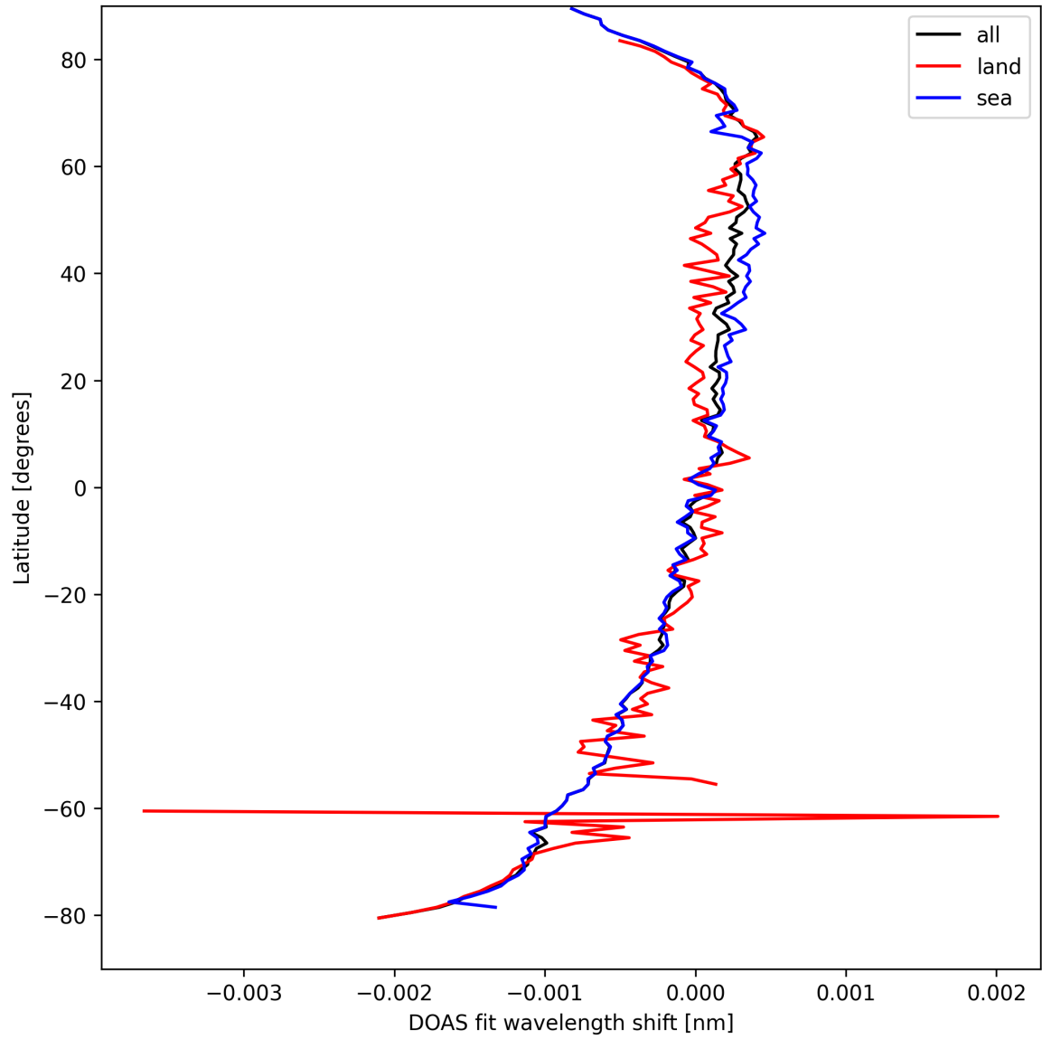
Figure 30: Zonal average of "DOAS fit wavelength shift" for 2025-03-30 to 2025-04-01.
