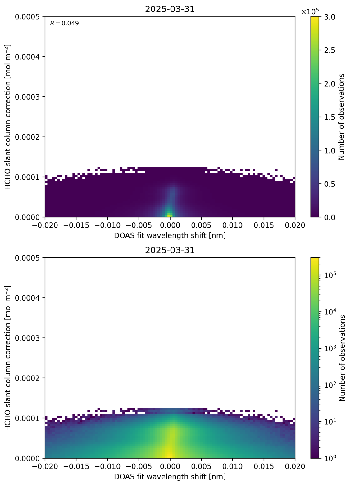
Figure 67: Scatter density plot of “DOAS fit wavelength shift” against “HCHO slant column correction” for 2025-03-30 to 2025-04-01.
