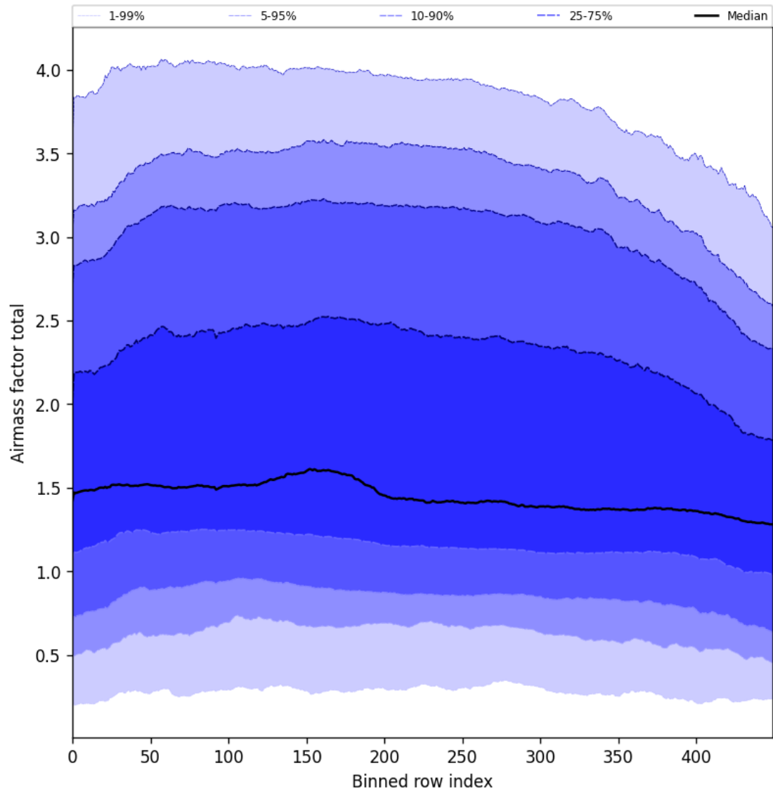
Figure 54: Along track statistics of “Airmass factor total” for 2025-03-30 to 2025-04-01
