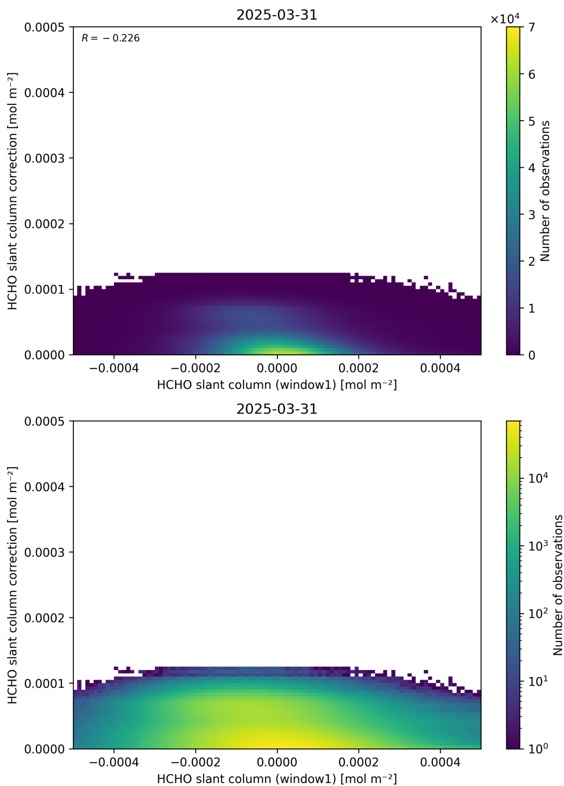
Figure 83: Scatter density plot of “HCHO slant column (window1)” against “HCHO slant column correction” for 2025-03-30 to 2025-04-01.
