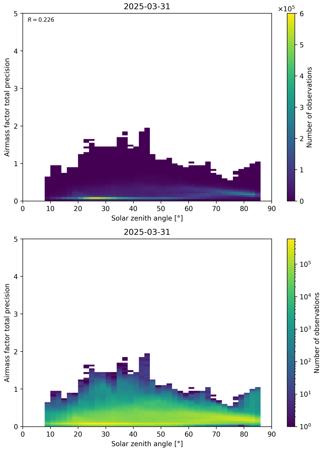
Figure 176: Scatter density plot of “Solar zenith angle” against “Airmass factor total precision” for 2025-03-30 to 2025-04-01.
