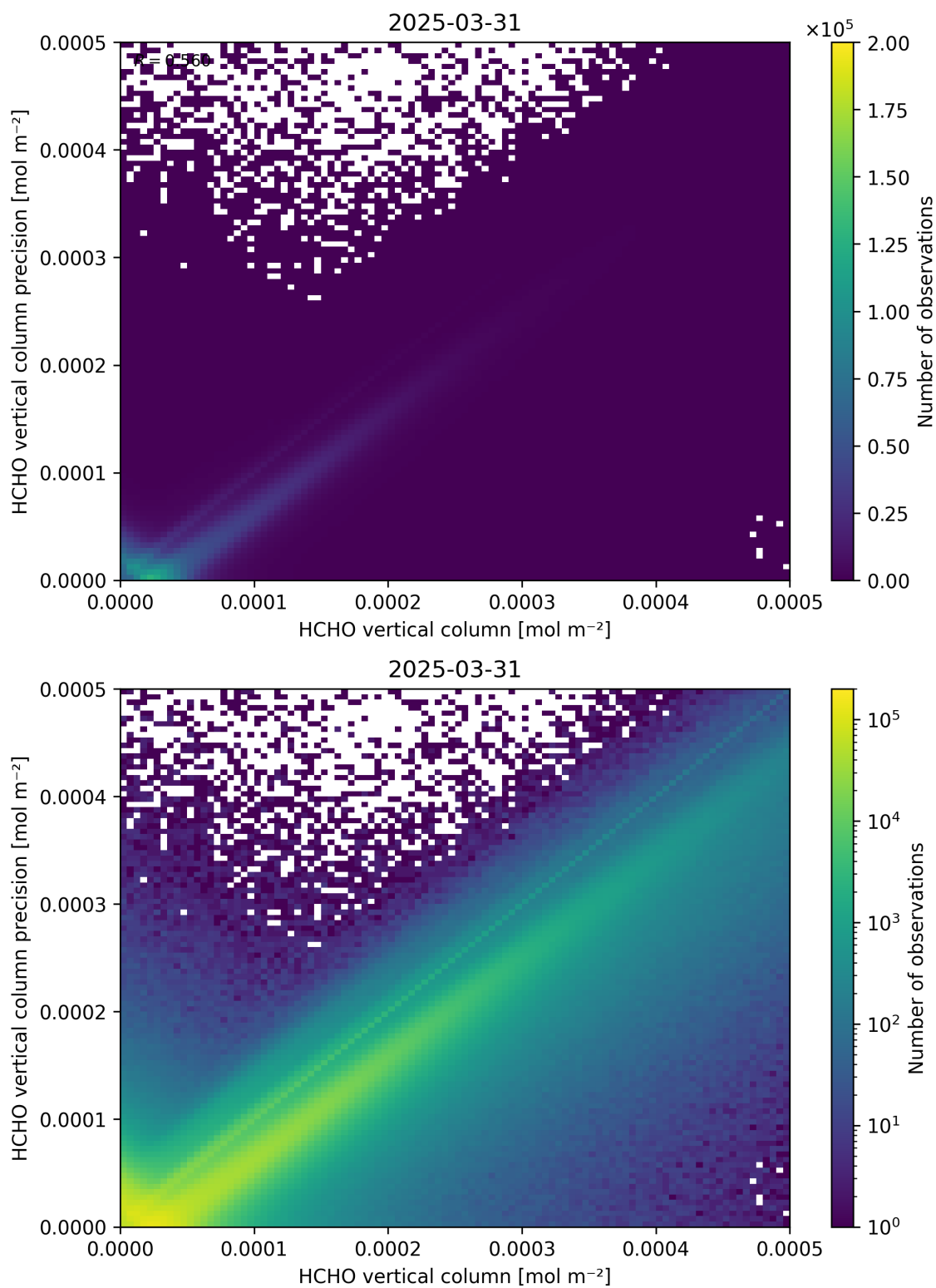
Figure 134: Scatter density plot of “HCHO vertical column” against “HCHO vertical column precision” for 2025-03-30 to 2025-04-01.
