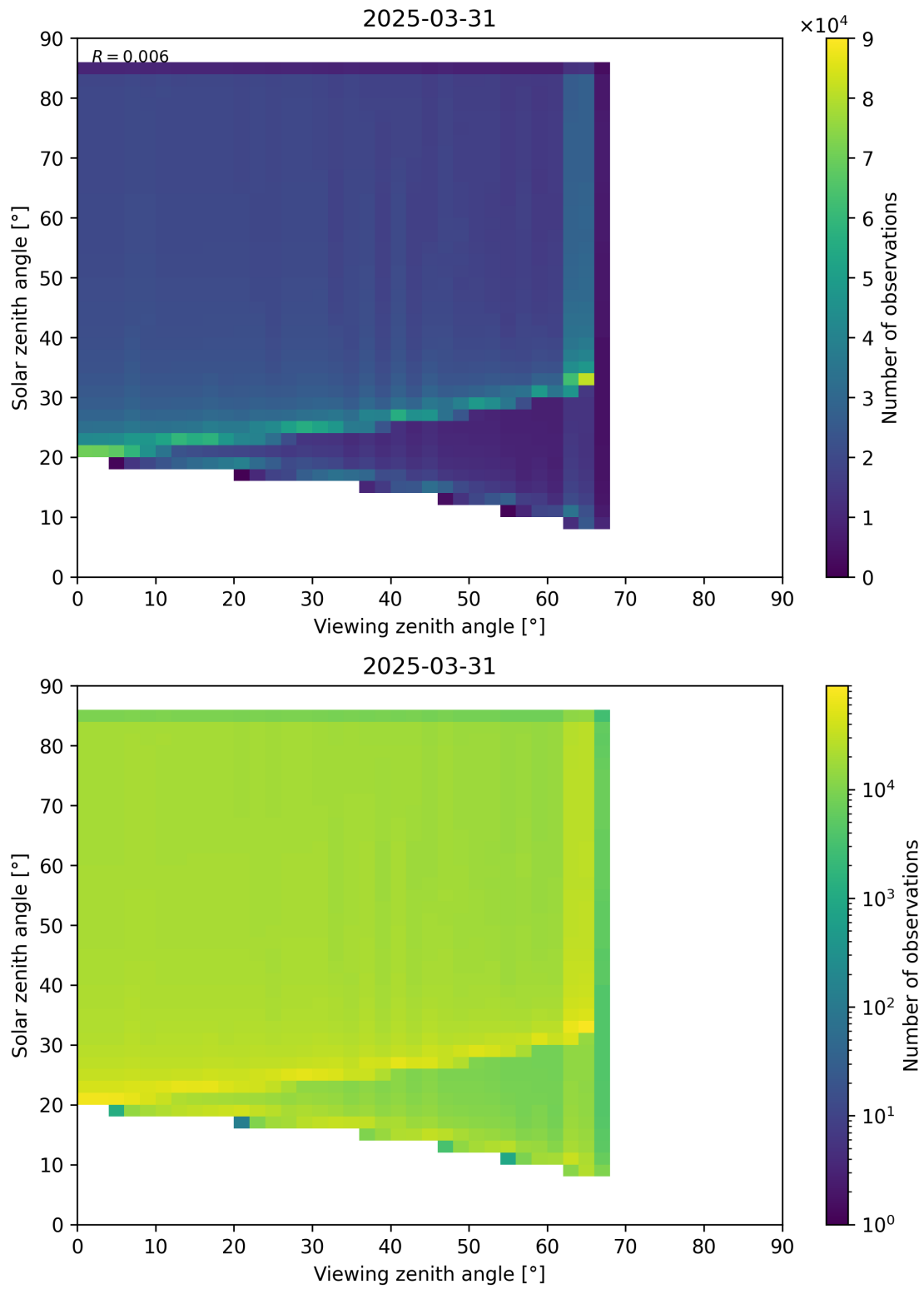
Figure 197: Scatter density plot of “Viewing zenith angle” against “Solar zenith angle” for 2025-03-30 to 2025-04-01.
