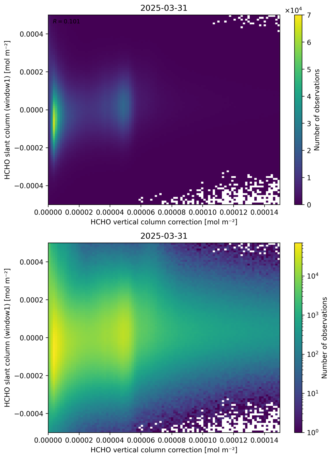
Figure 118: Scatter density plot of “HCHO vertical column correction” against “HCHO slant column (window1)” for 2025-03-30 to 2025-04-01.
