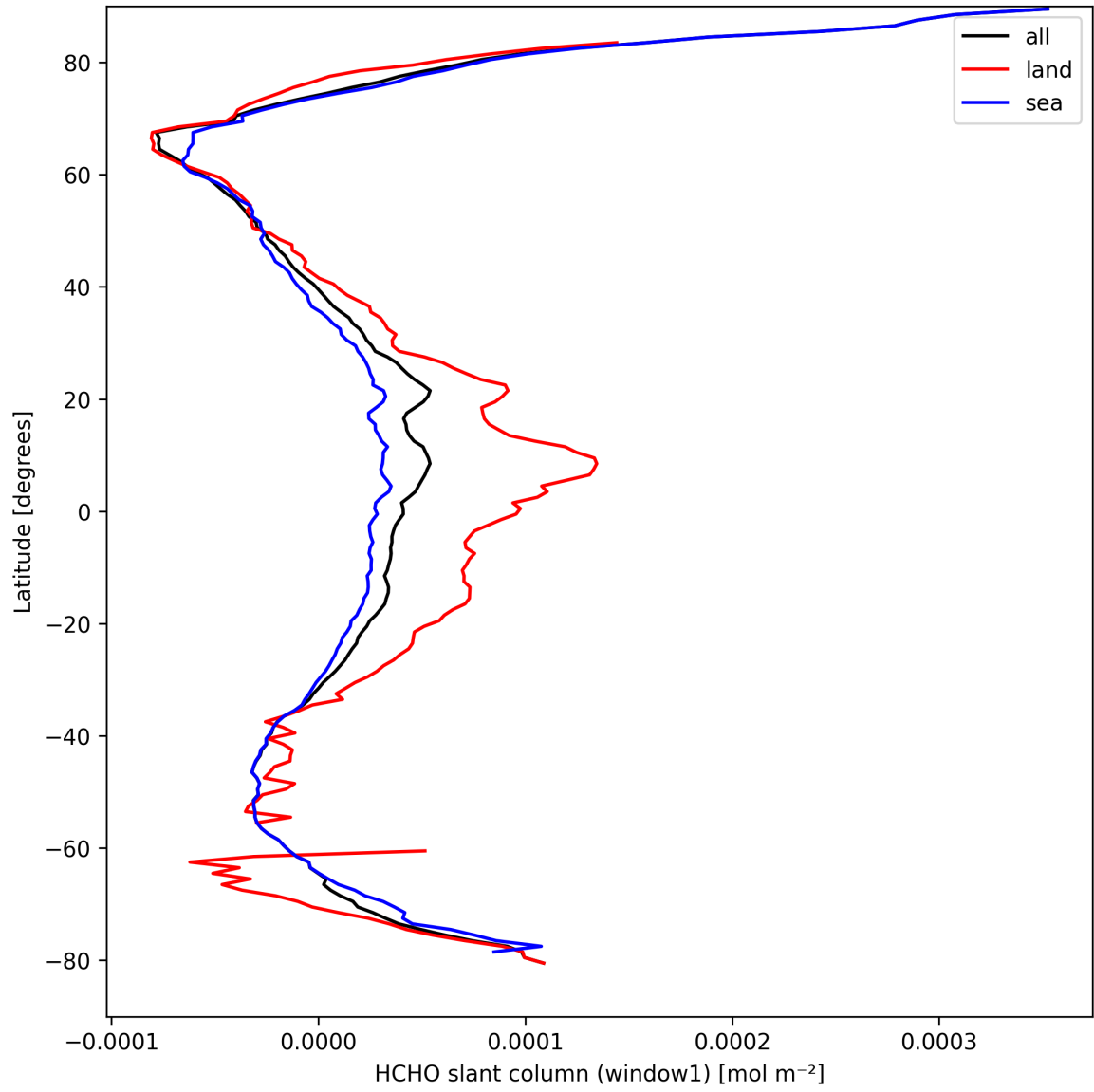
Figure 24: Zonal average of “HCHO slant column (window1)” for 2025-03-30 to 2025-04-01.
