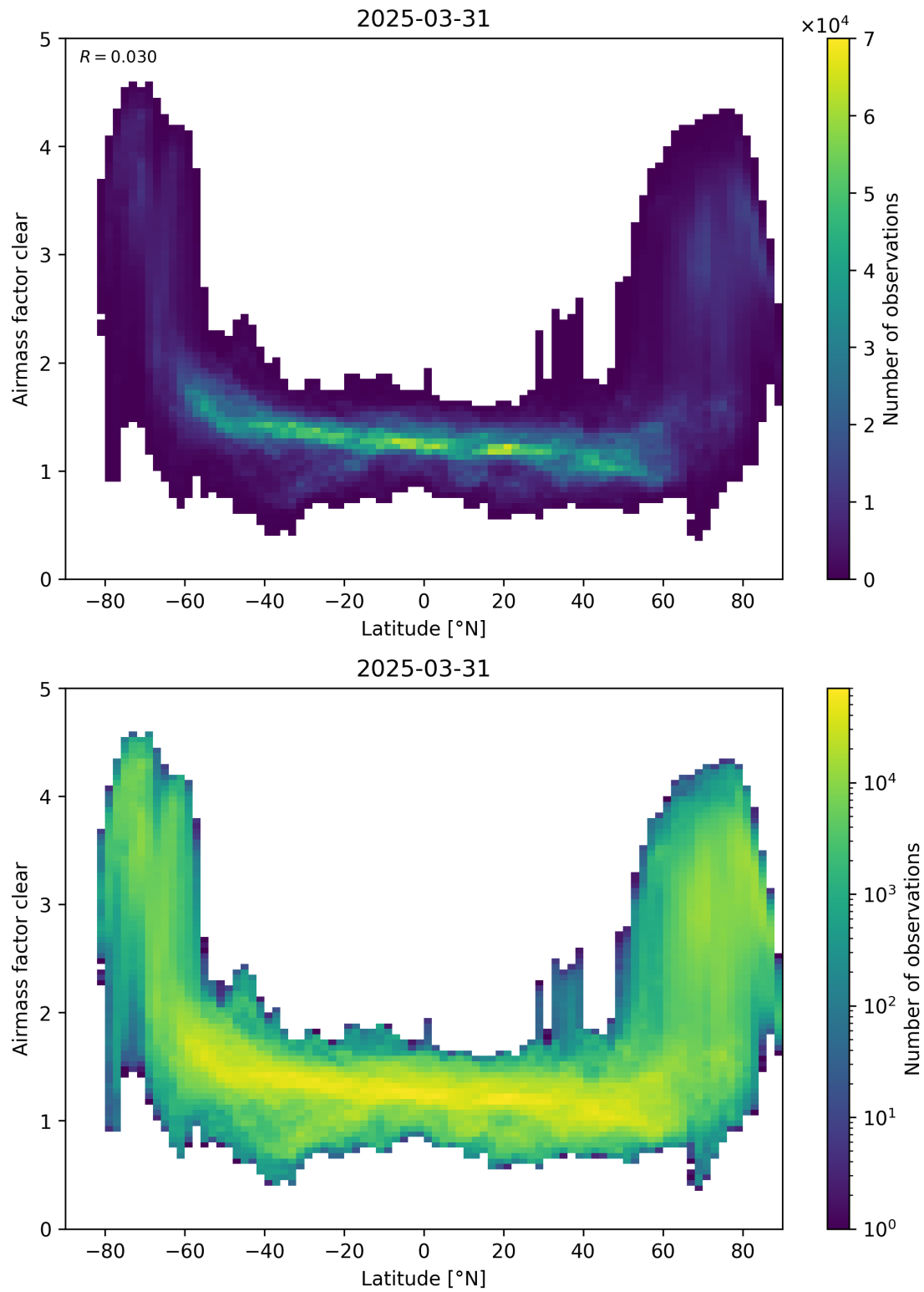
Figure 156: Scatter density plot of “Latitude” against “Airmass factor clear” for 2025-03-30 to 2025-04-01.
