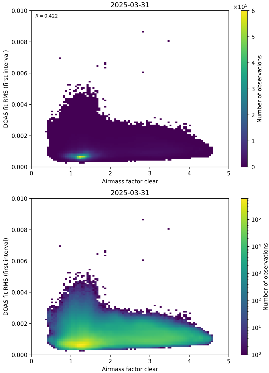
Figure 71: Scatter density plot of “Airmass factor clear” against “DOAS fit RMS (first interval)” for 2025-03-30 to 2025-04-01.
