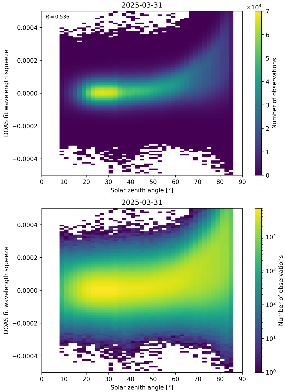
Figure 169: Scatter density plot of “Solar zenith angle” against “DOAS fit wavelength squeeze” for 2025-03-30 to 2025-04-01.
