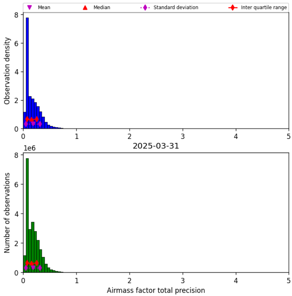
Figure 41: Histogram of “Airmass factor total precision” for 2025-03-30 to 2025-04-01
