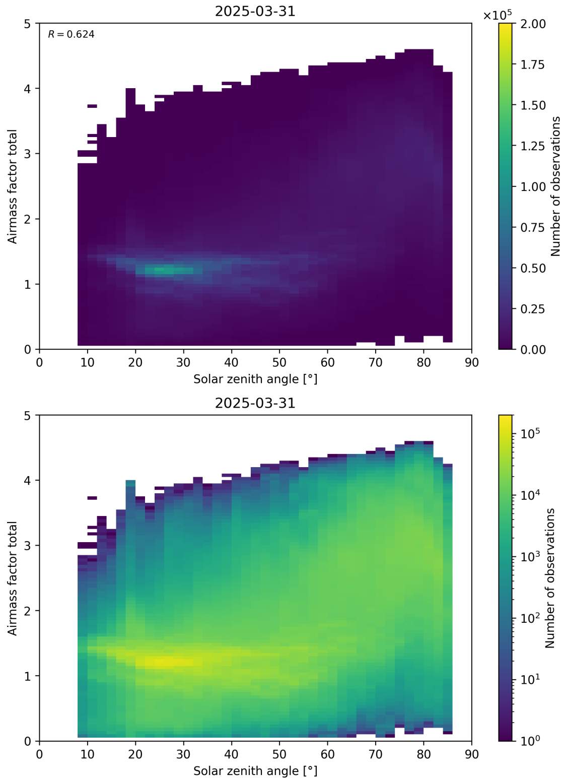
Figure 175: Scatter density plot of “Solar zenith angle” against “Airmass factor total” for 2025-03-30 to 2025-04-01.
