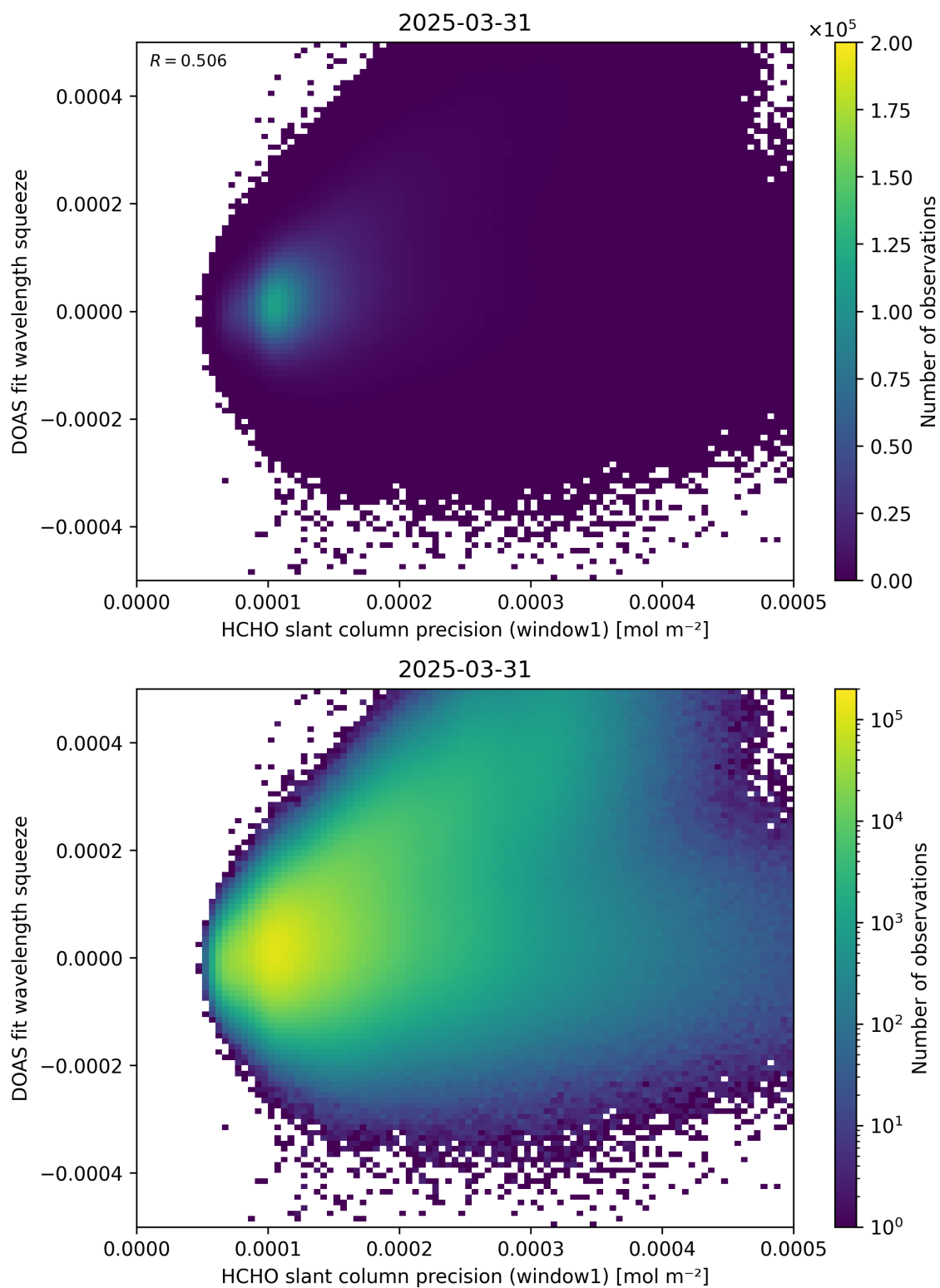
Figure 90: Scatter density plot of “HCHO slant column precision (window1)” against “DOAS fit wavelength squeeze” for 2025-03-30 to 2025-04-01.
