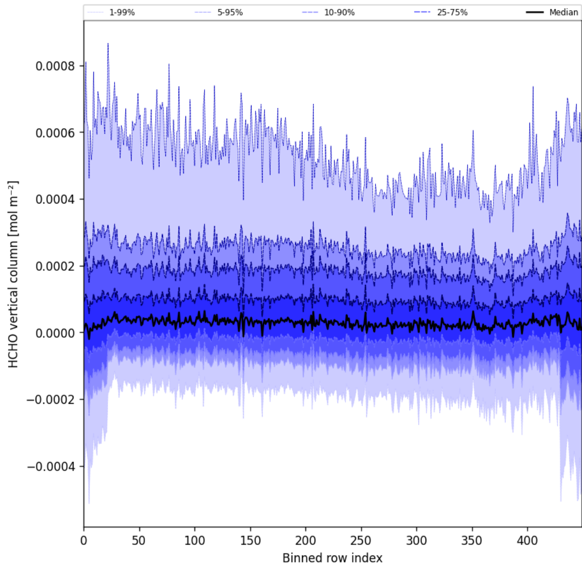
Figure 49: Along track statistics of “HCHO vertical column” for 2025-03-30 to 2025-04-01
