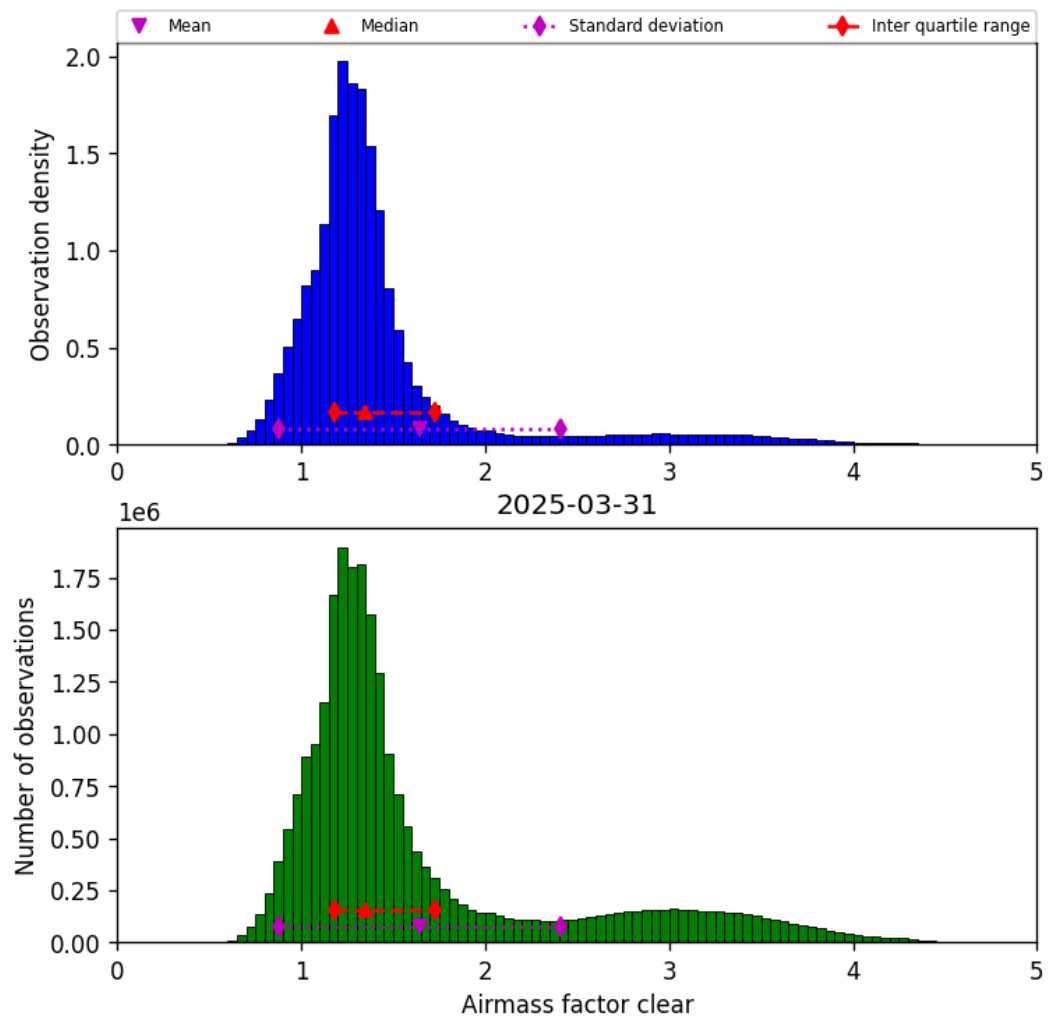
Figure 42: Histogram of “Airmass factor clear” for 2025-03-30 to 2025-04-01
