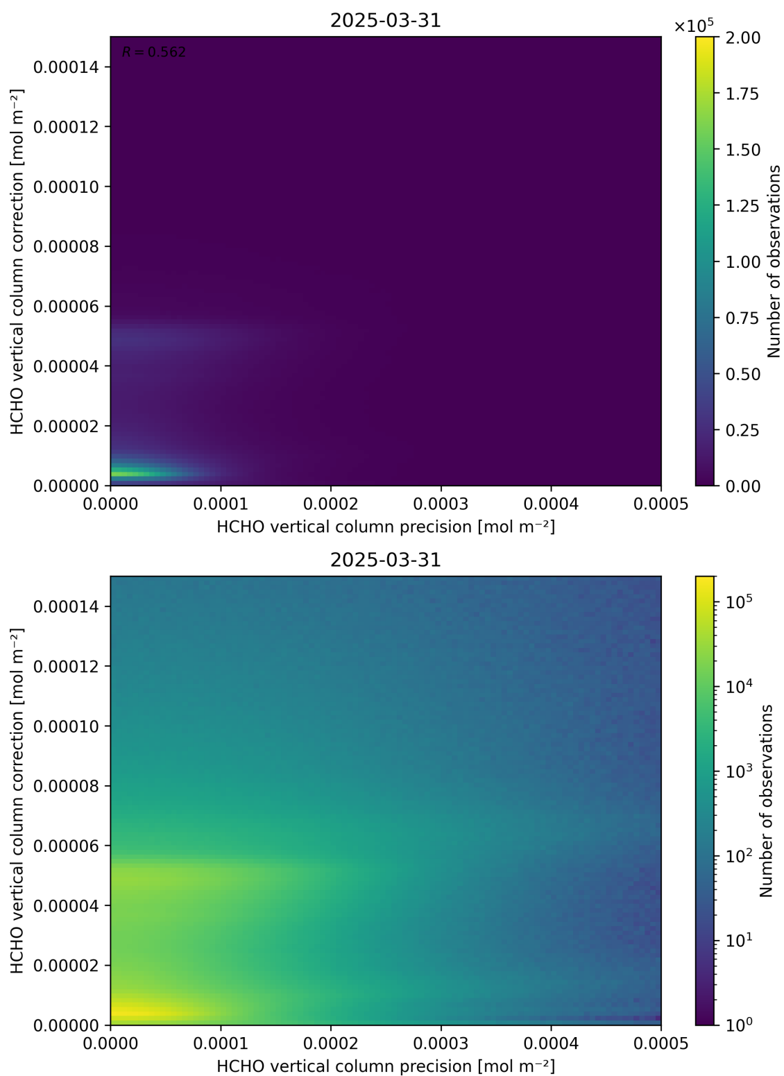
Figure 146: Scatter density plot of “HCHO vertical column precision” against “HCHO vertical column correction” for 2025-03-30 to 2025-04-01.
