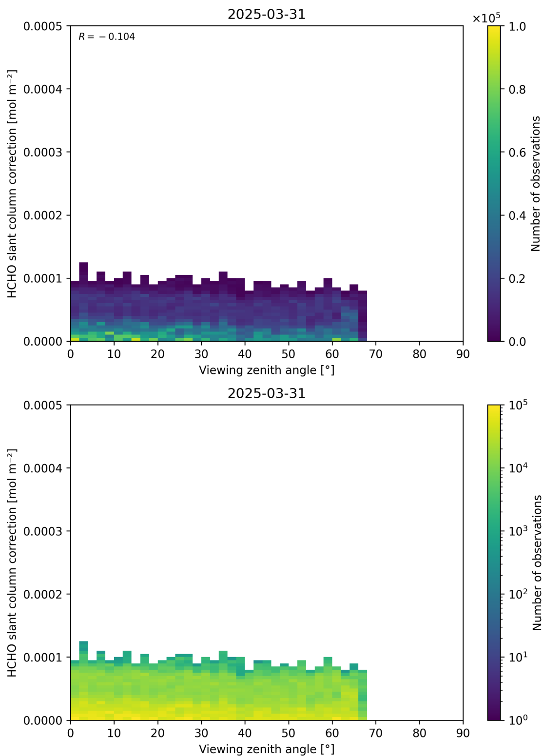
Figure 187: Scatter density plot of “Viewing zenith angle” against “HCHO slant column correction” for 2025-03-30 to 2025-04-01.
