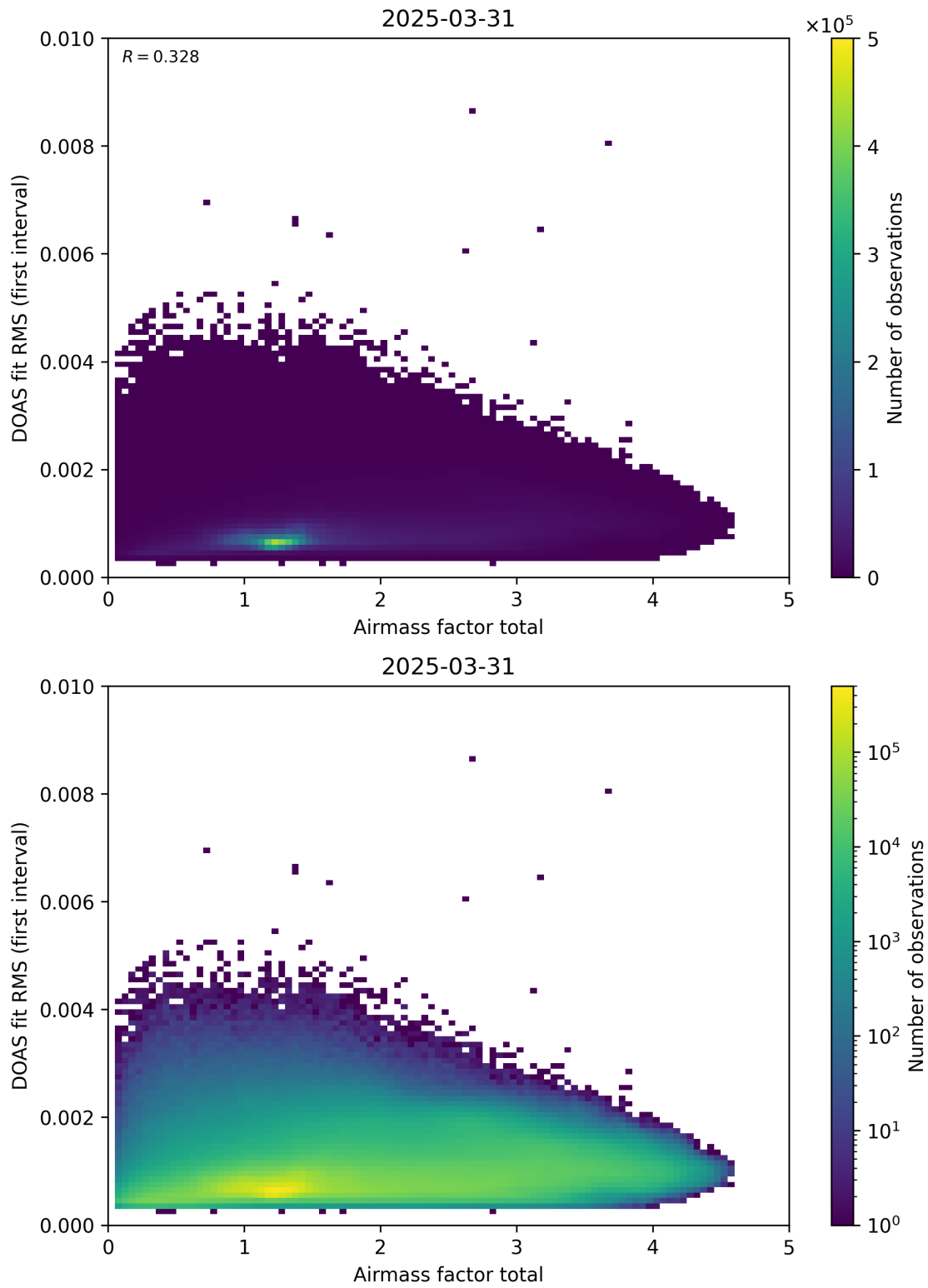
Figure 97: Scatter density plot of “Airmass factor total” against “DOAS fit RMS (first interval)” for 2025-03-30 to 2025-04-01.
