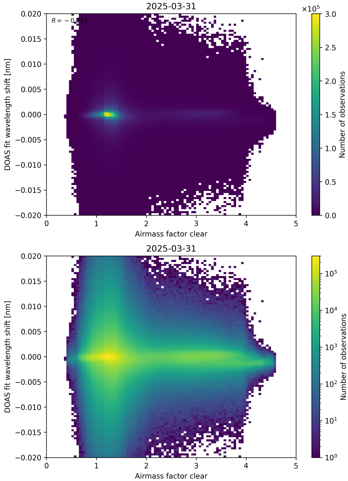
Figure 72: Scatter density plot of “Airmass factor clear” against “DOAS fit wavelength shift” for 2025-03-30 to 2025-04-01.
