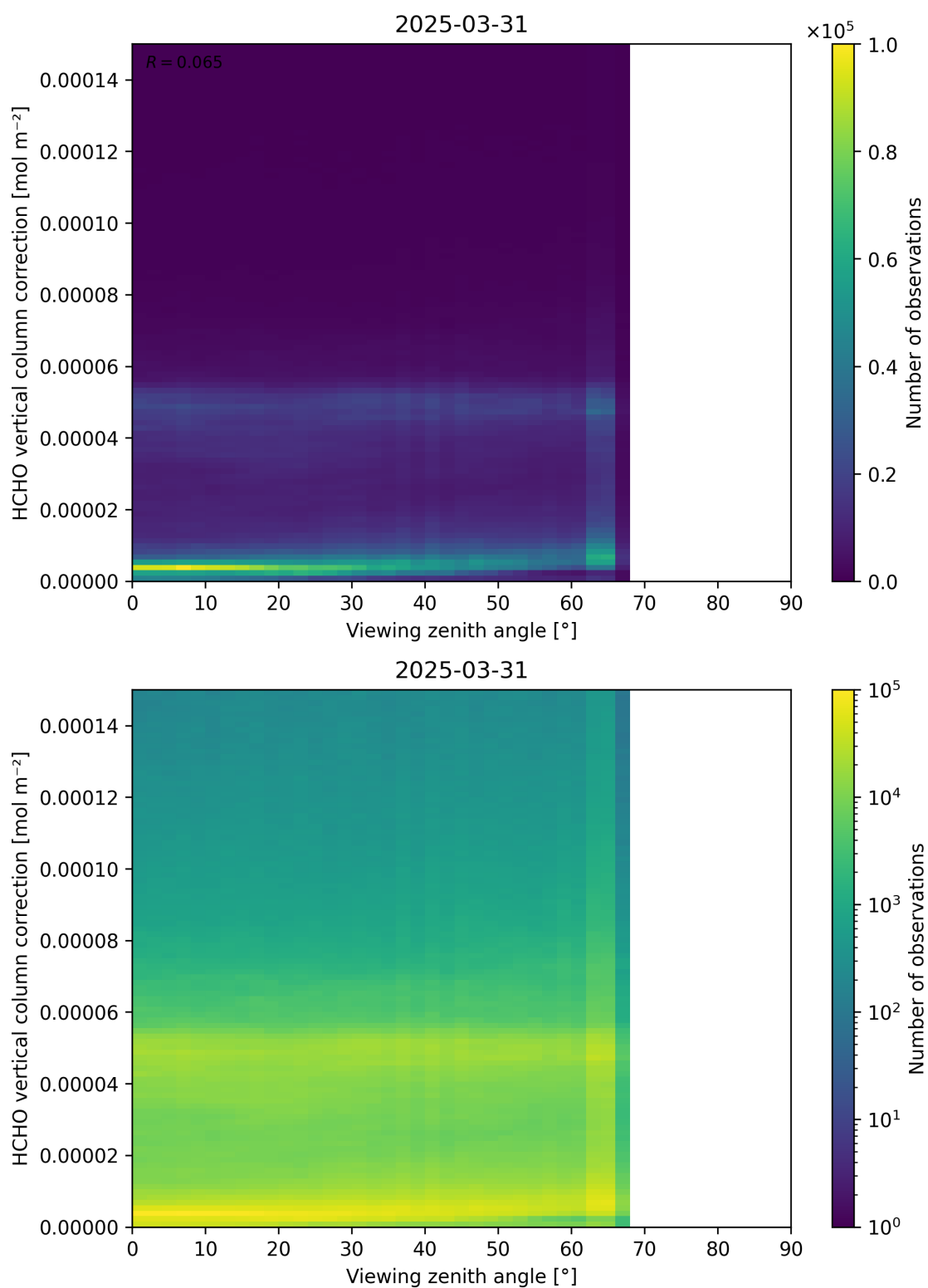
Figure 193: Scatter density plot of “Viewing zenith angle” against “HCHO vertical column correction” for 2025-03-30 to 2025-04-01.
