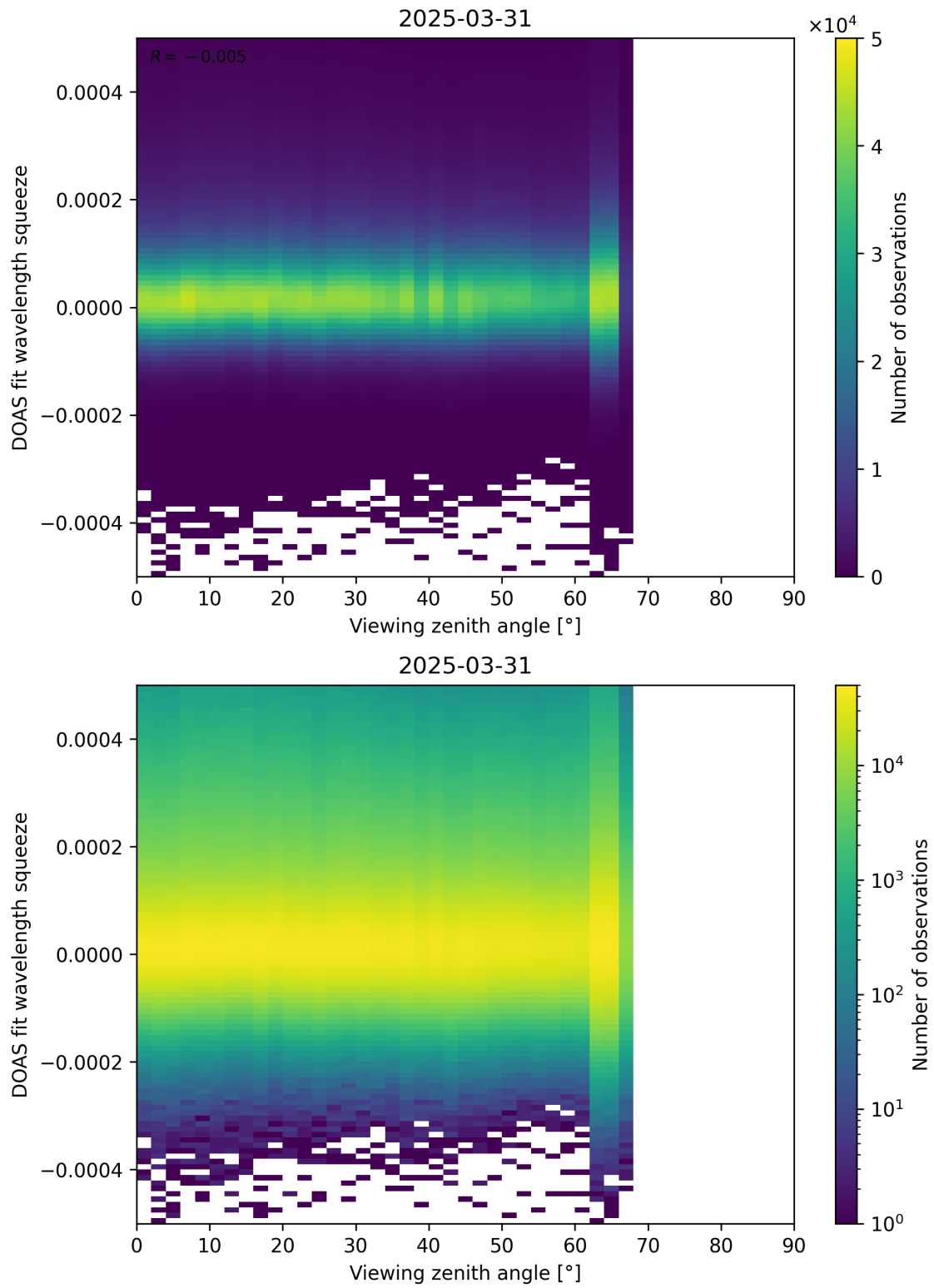
Figure 184: Scatter density plot of “Viewing zenith angle” against “DOAS fit wavelength squeeze” for 2025-03-30 to 2025-04-01.
