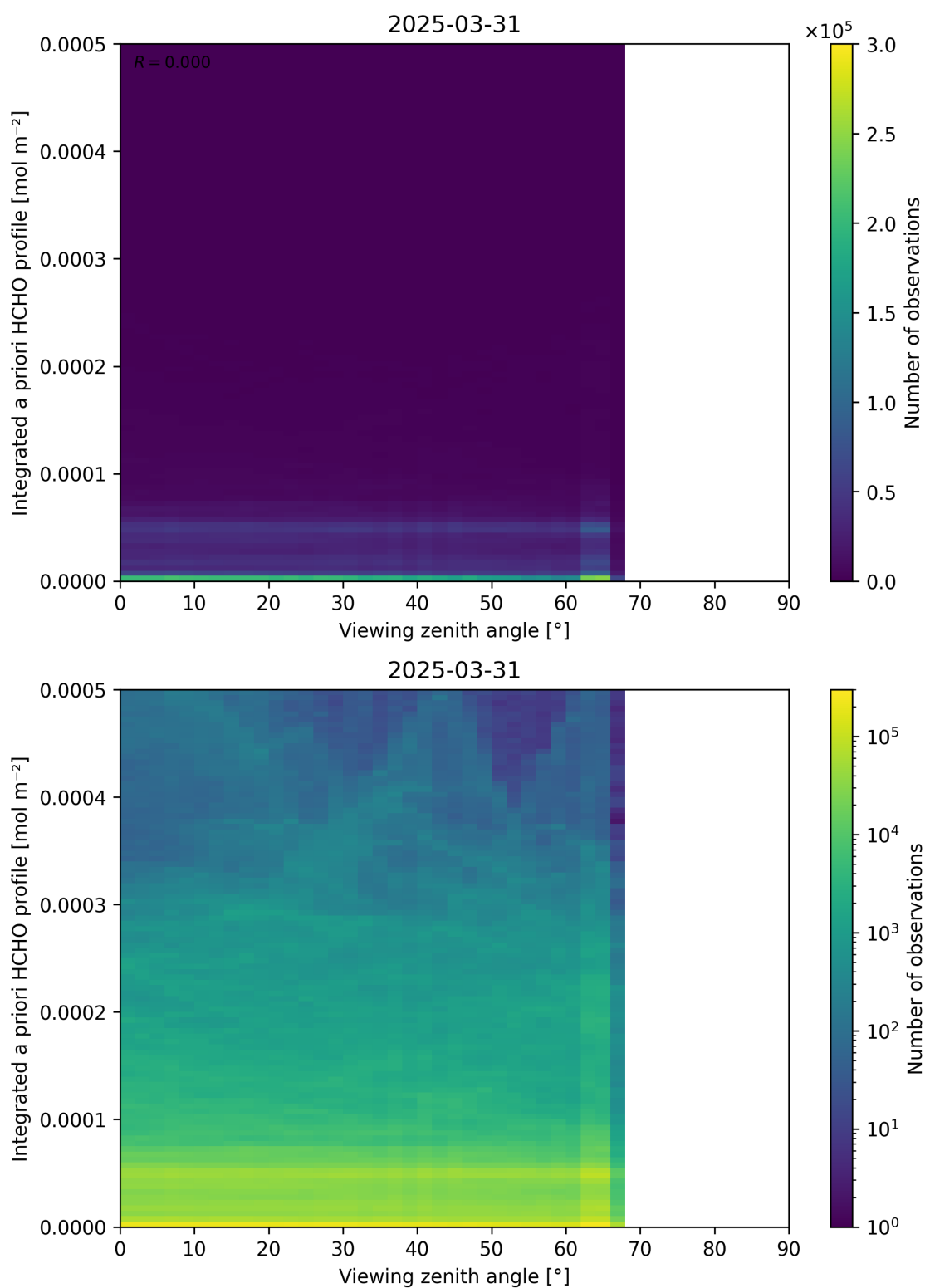
Figure 195: Scatter density plot of “Viewing zenith angle” against “Integrated a priori HCHO profile” for 2025-03-30 to 2025-04-01.
