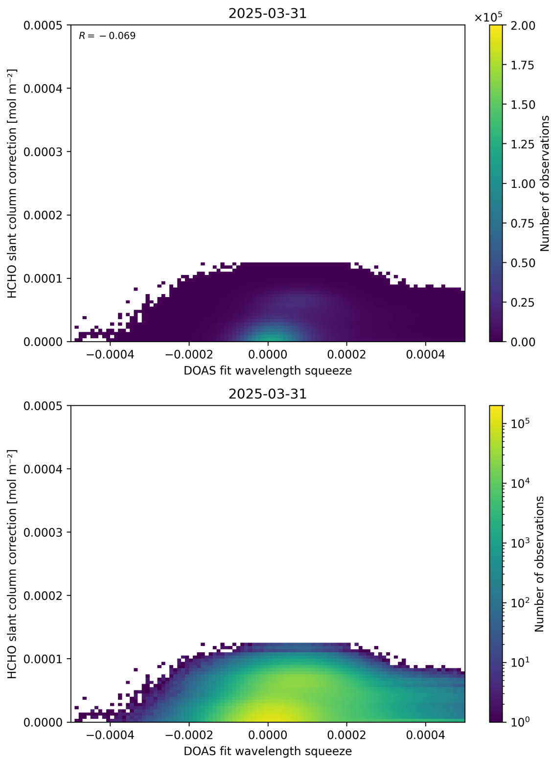
Figure 70: Scatter density plot of “DOAS fit wavelength squeeze” against “HCHO slant column correction” for 2025-03-30 to 2025-04-01.
