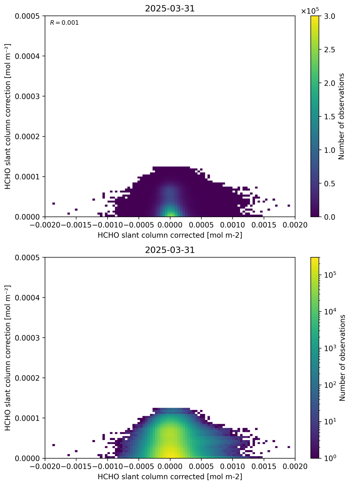
Figure 77: Scatter density plot of “HCHO slant column corrected” against “HCHO slant column correction” for 2025-03-30 to 2025-04-01.
