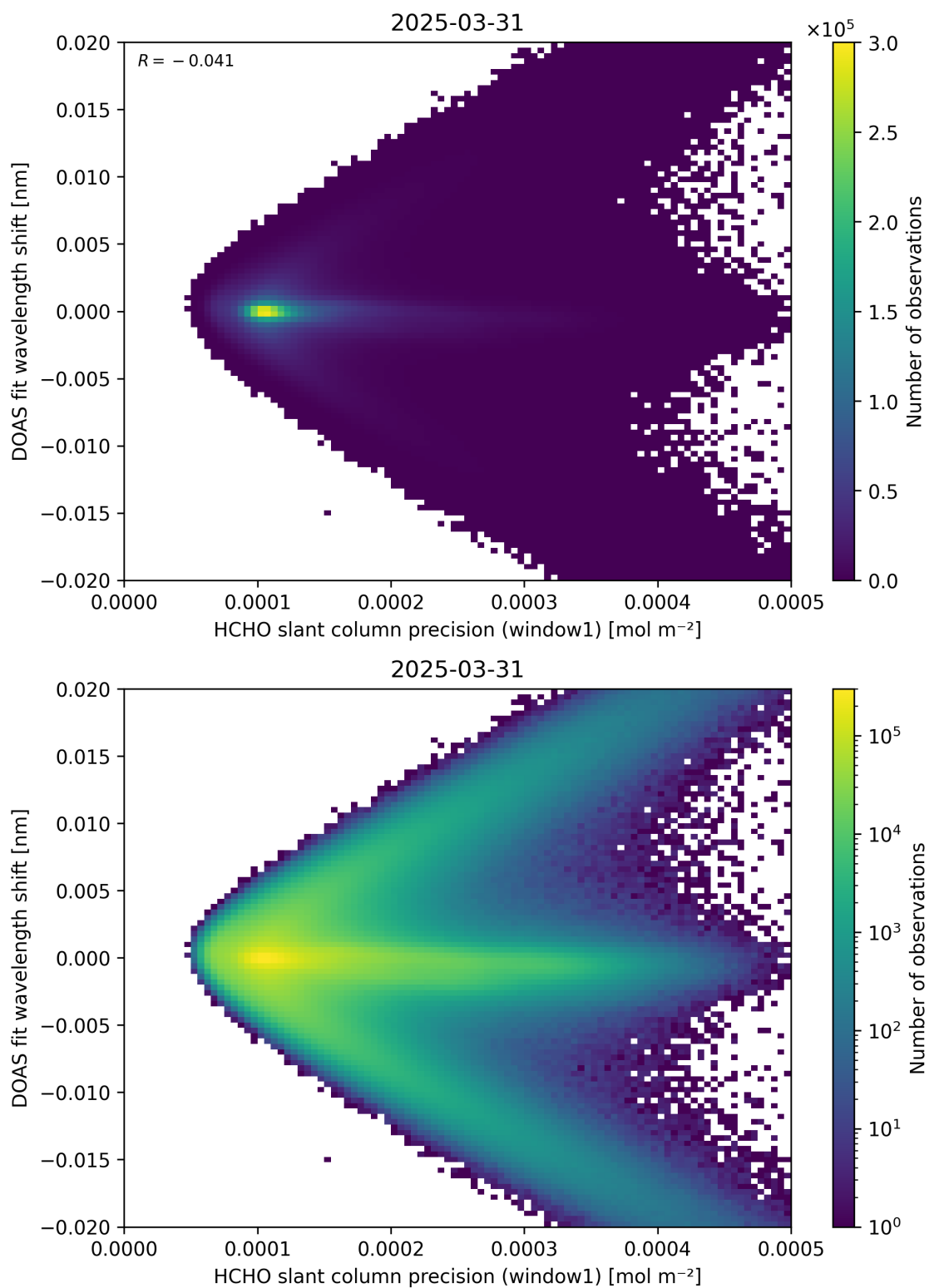
Figure 89: Scatter density plot of “HCHO slant column precision (window1)” against “DOAS fit wavelength shift” for 2025-03-30 to 2025-04-01.
