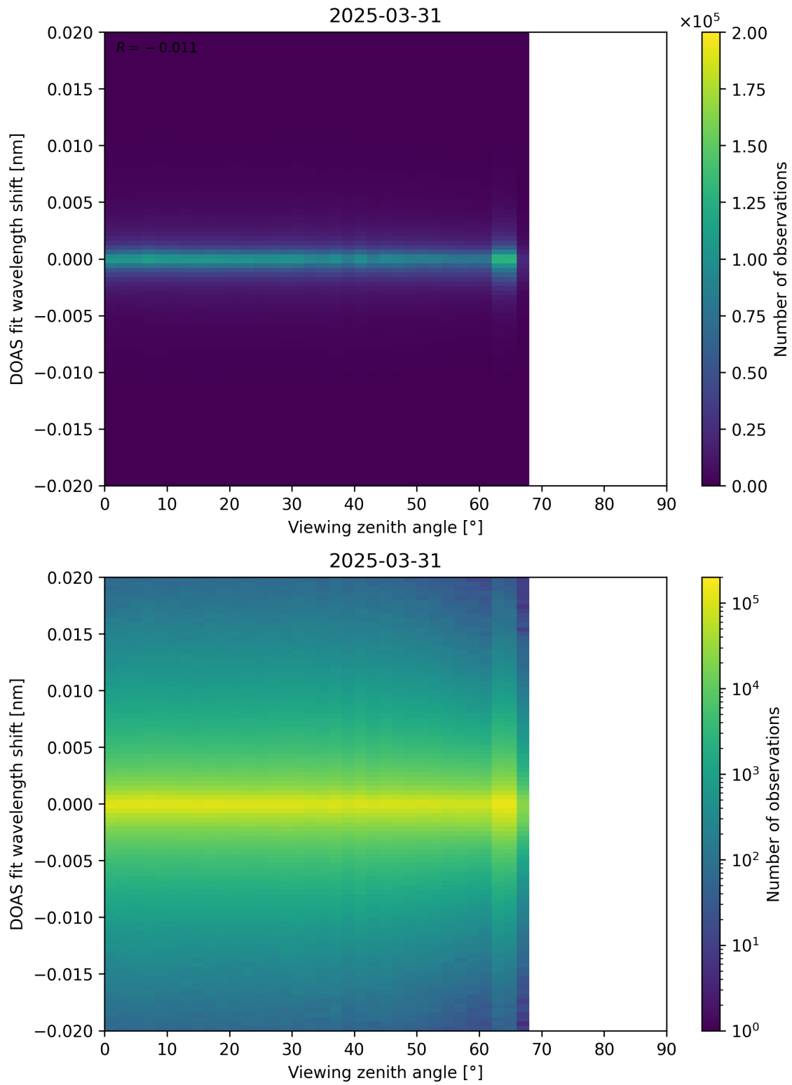
Figure 183: Scatter density plot of “Viewing zenith angle” against “DOAS fit wavelength shift” for 2025-03-30 to 2025-04-01.
