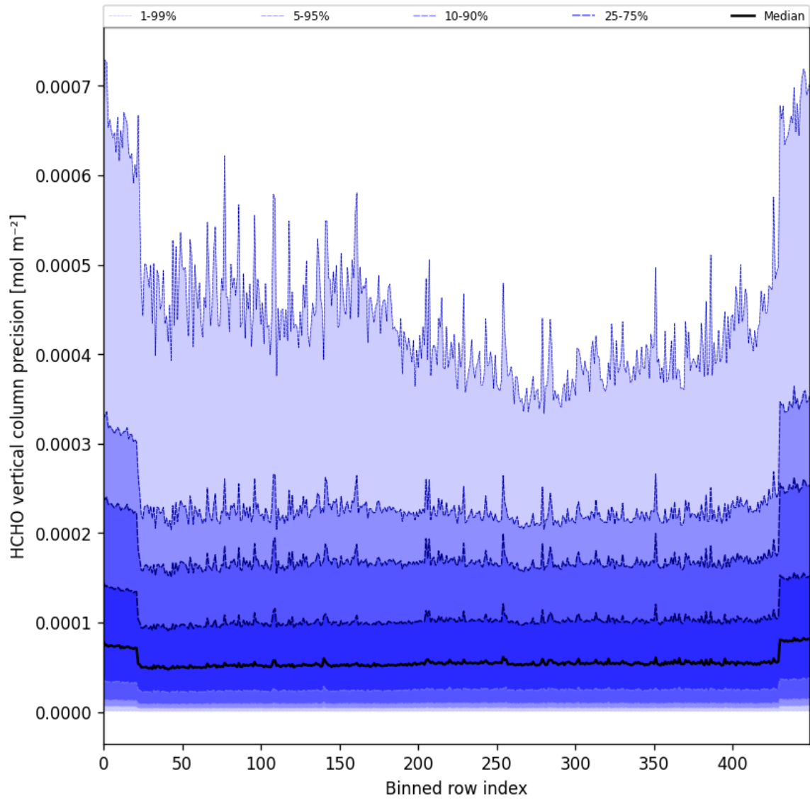
Figure 50: Along track statistics of “HCHO vertical column precision” for 2025-03-30 to 2025-04-01
