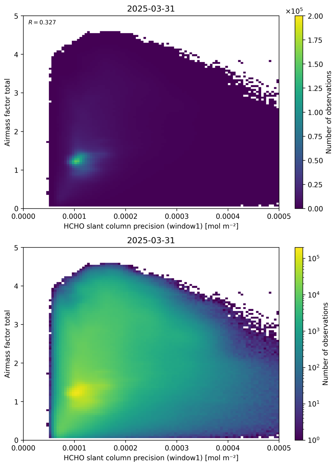
Figure 94: Scatter density plot of “HCHO slant column precision (window1)” against “Airmass factor total” for 2025-03-30 to 2025-04-01.
