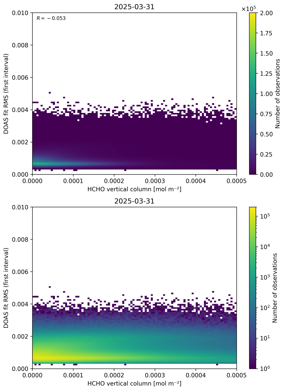
Figure 123: Scatter density plot of “HCHO vertical column” against “DOAS fit RMS (first interval)” for 2025-03-30 to 2025-04-01.
