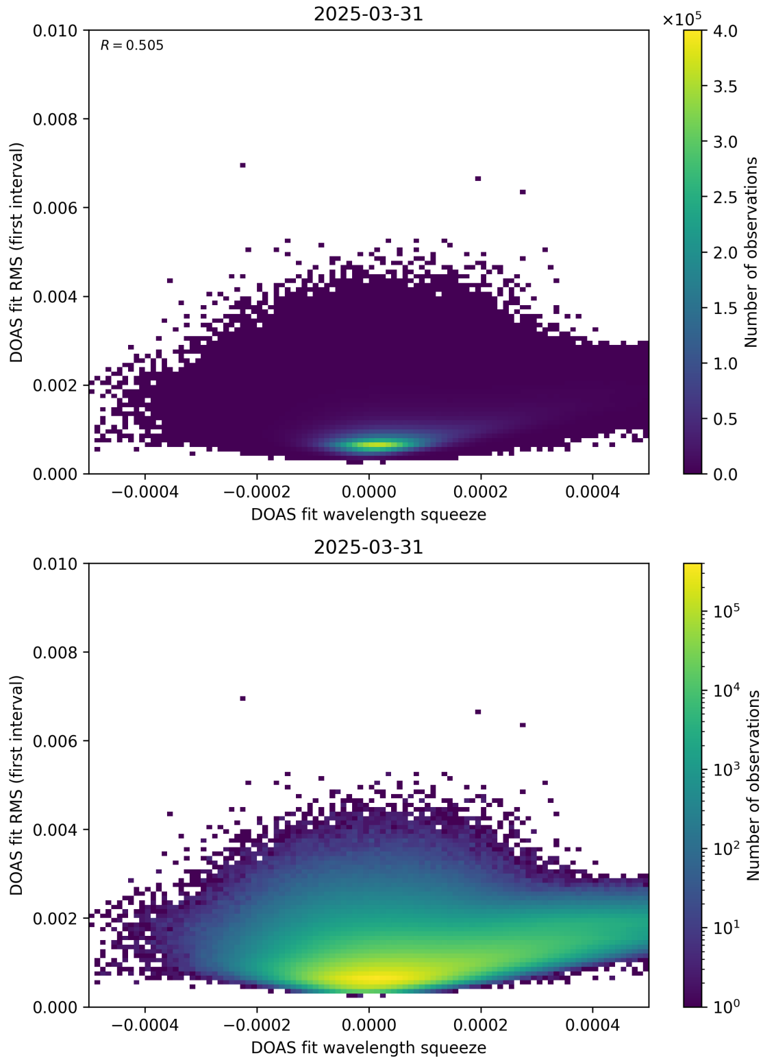
Figure 68: Scatter density plot of “DOAS fit wavelength squeeze” against “DOAS fit RMS (first interval)” for 2025-03-30 to 2025-04-01.
