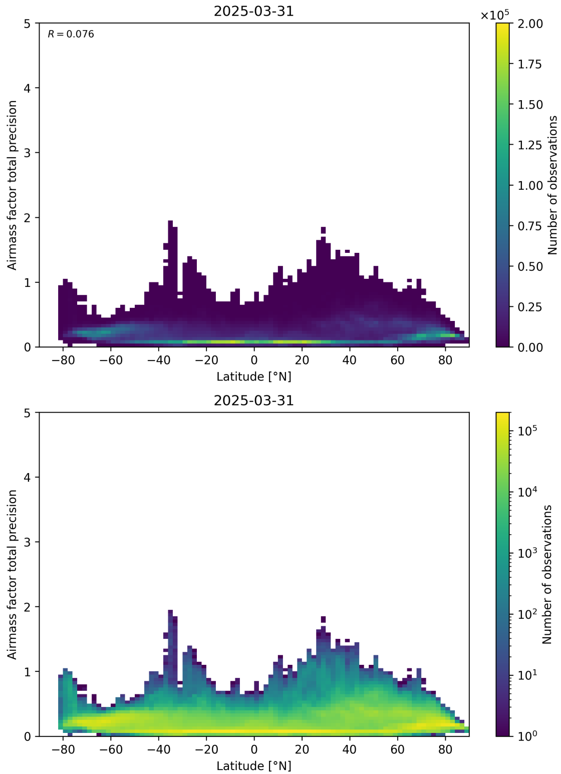
Figure 162: Scatter density plot of “Latitude” against “Airmass factor total precision” for 2025-03-30 to 2025-04-01.
