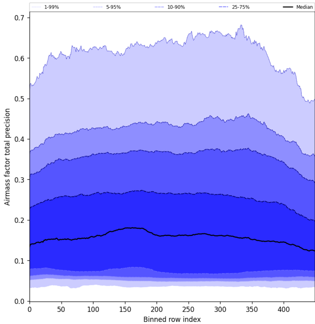
Figure 55: Along track statistics of “Airmass factor total precision” for 2025-03-30 to 2025-04-01
