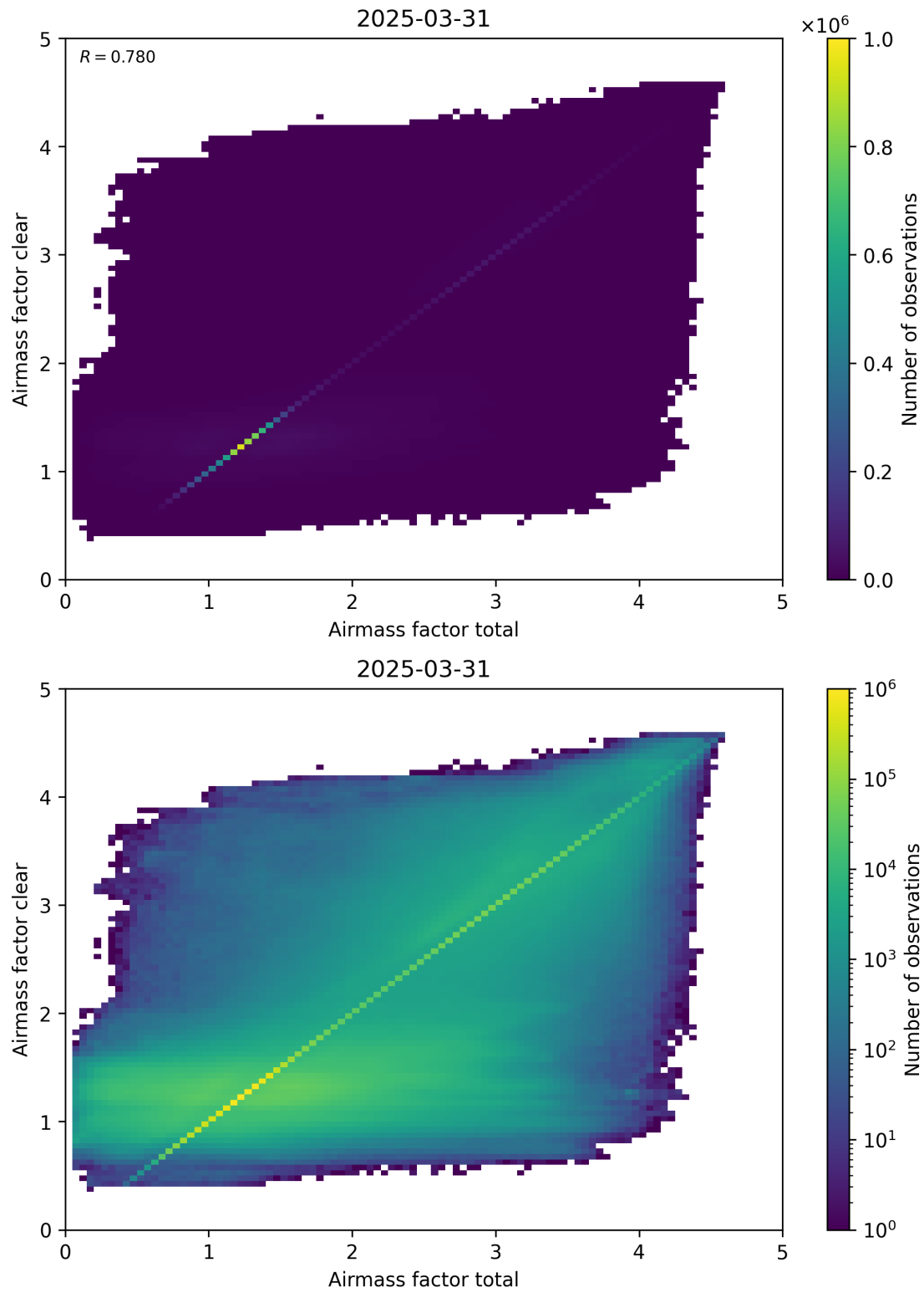
Figure 100: Scatter density plot of “Airmass factor total” against “Airmass factor clear” for 2025-03-30 to 2025-04-01.
