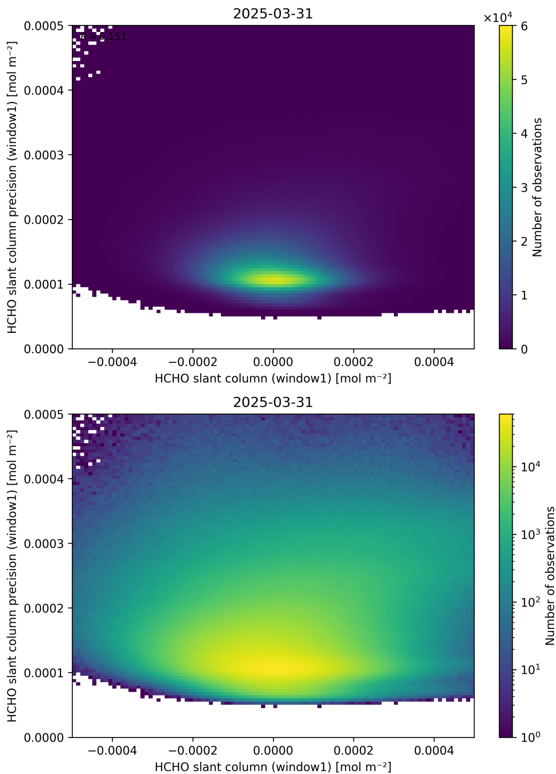
Figure 84: Scatter density plot of “HCHO slant column (window1)” against “HCHO slant column precision (window1)” for 2025-03-30 to 2025-04-01.
