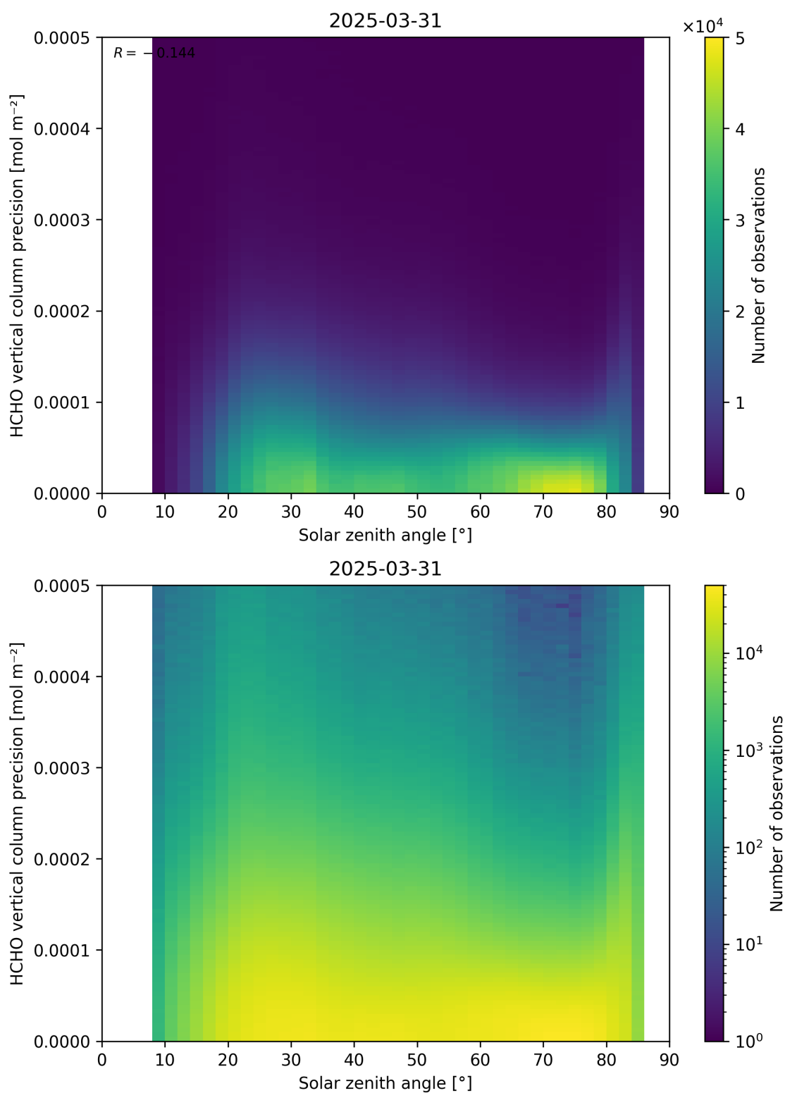
Figure 179: Scatter density plot of “Solar zenith angle” against “HCHO vertical column precision” for 2025-03-30 to 2025-04-01.
