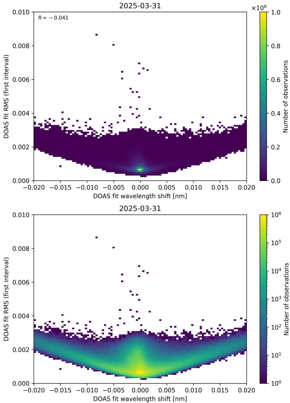
Figure 64: Scatter density plot of “DOAS fit wavelength shift” against “DOAS fit RMS (first interval)” for 2025-03-30 to 2025-04-01.
