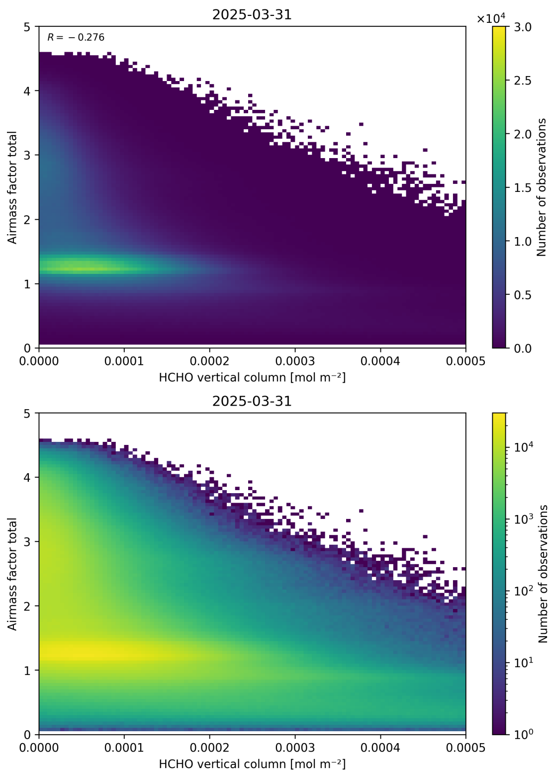
Figure 131: Scatter density plot of “HCHO vertical column” against “Airmass factor total” for 2025-03-30 to 2025-04-01.
