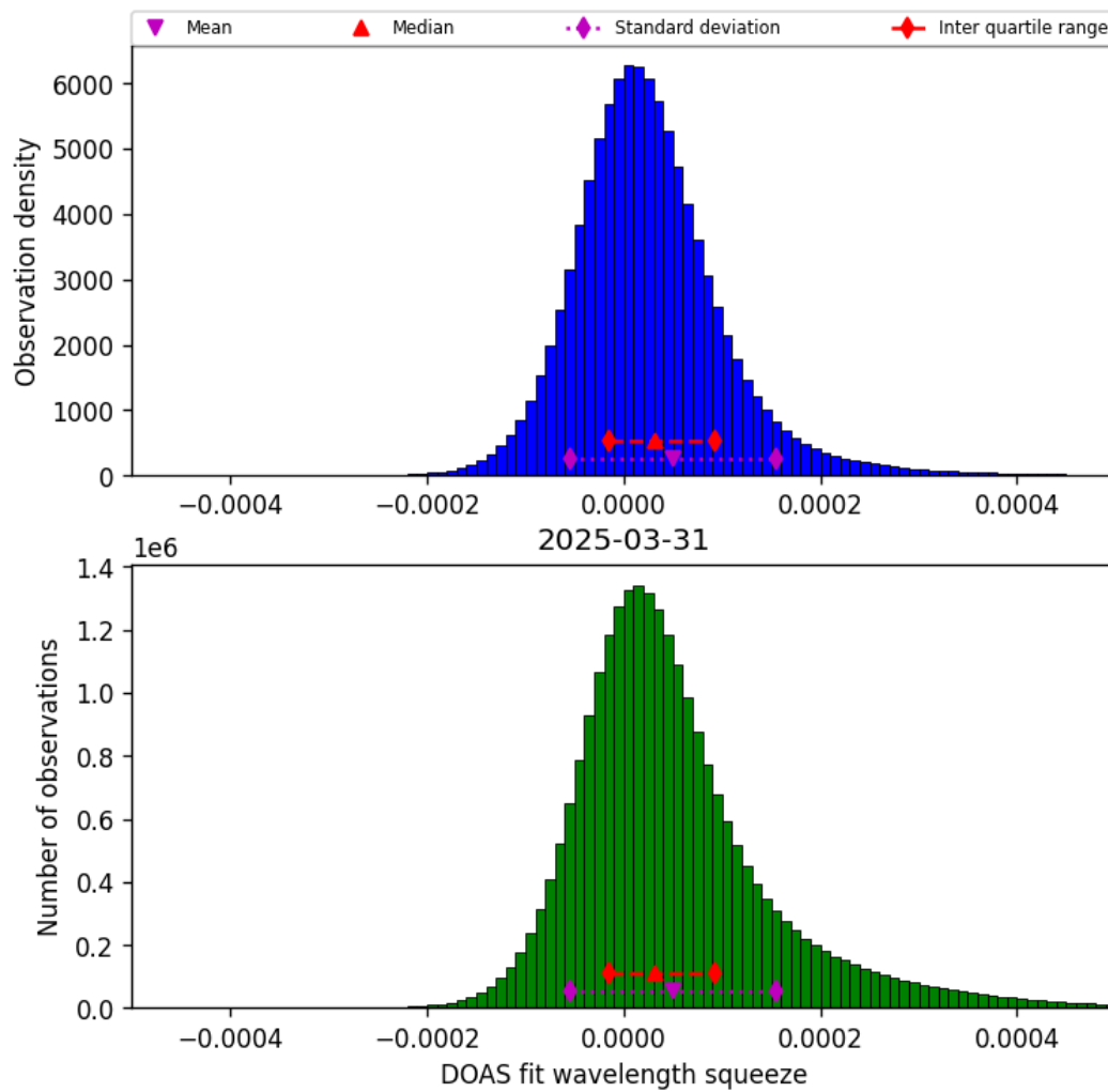
Figure 45: Histogram of “DOAS fit wavelength squeeze” for 2025-03-30 to 2025-04-01
