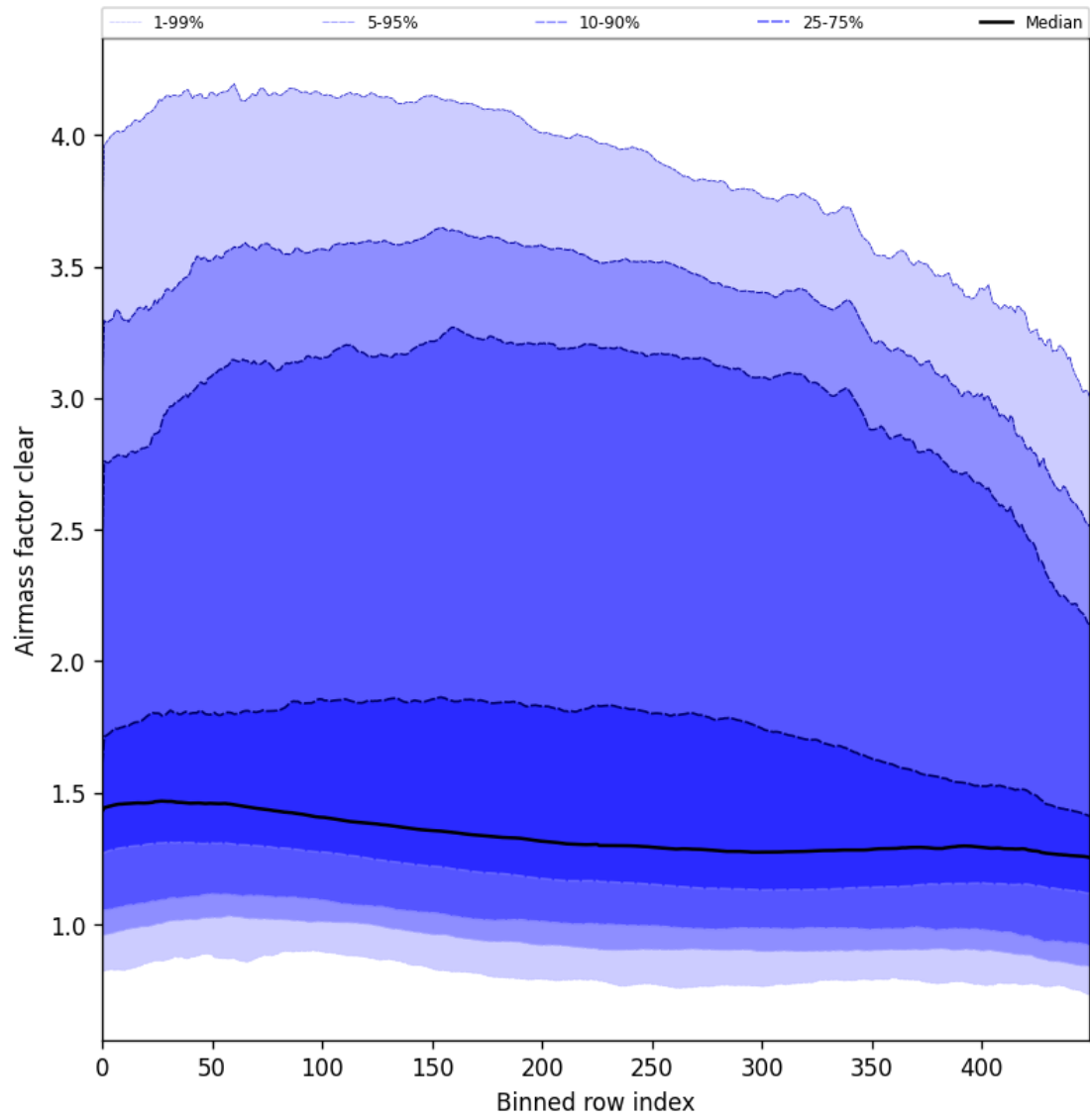
Figure 56: Along track statistics of “Airmass factor clear” for 2025-03-30 to 2025-04-01
