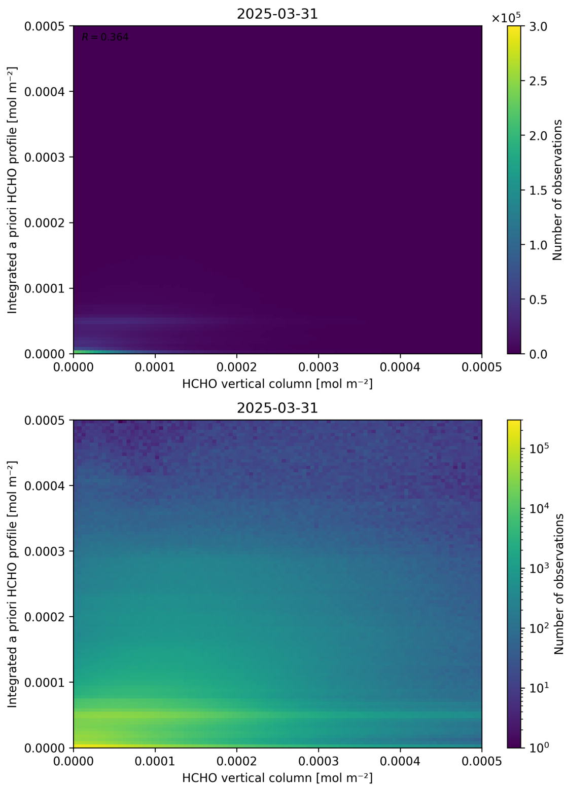
Figure 135: Scatter density plot of “HCHO vertical column” against “Integrated a priori HCHO profile” for 2025-03-30 to 2025-04-01.
