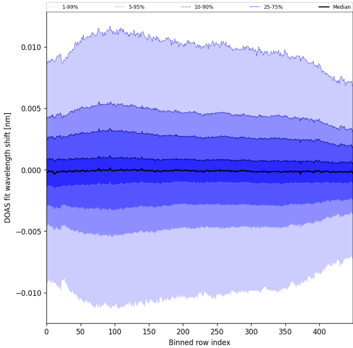
Figure 58: Along track statistics of “DOAS fit wavelength shift” for 2025-03-30 to 2025-04-01
