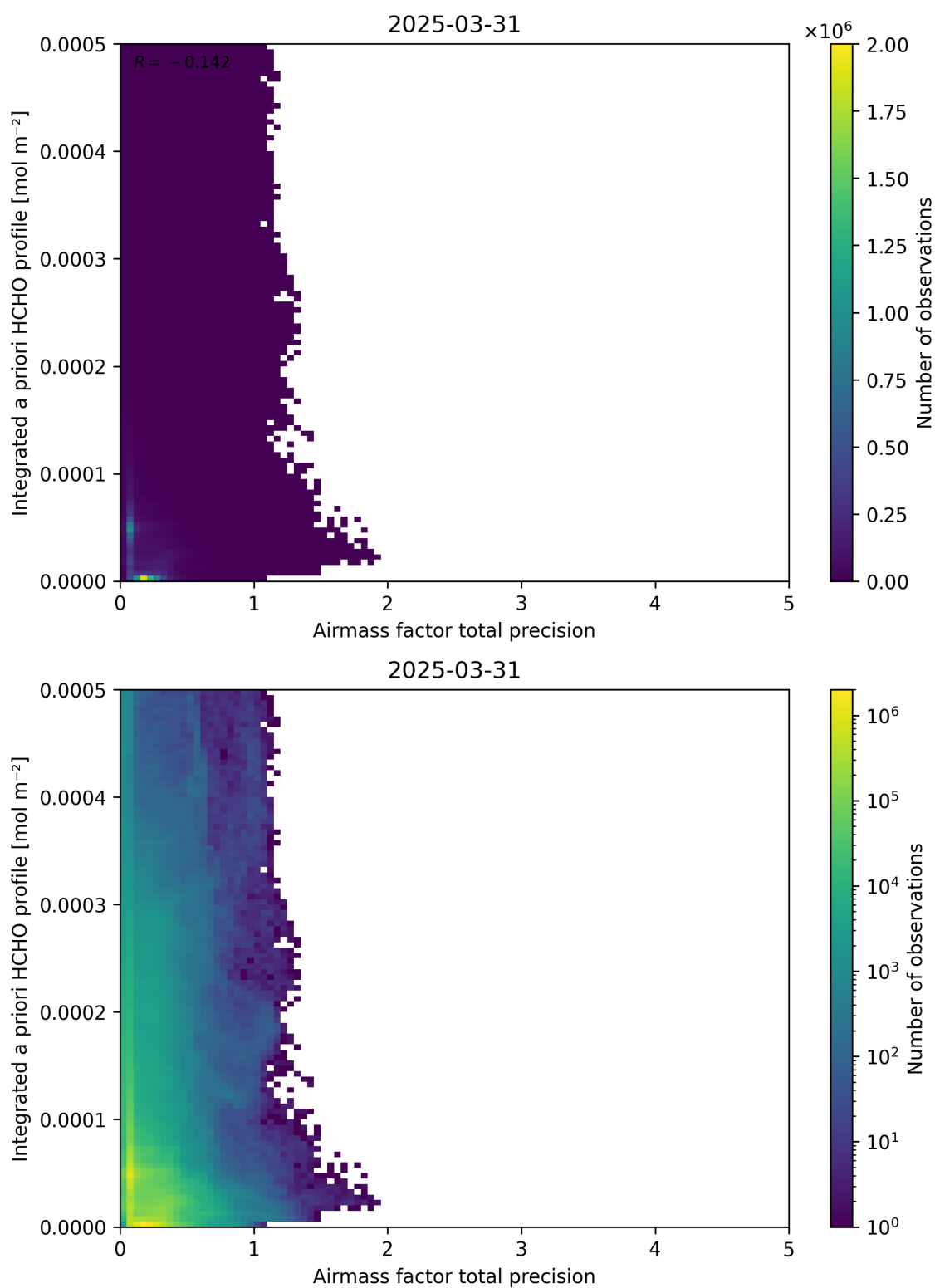
Figure 111: Scatter density plot of “Airmass factor total precision” against “Integrated a priori HCHO profile” for 2025-03-30 to 2025-04-01.
