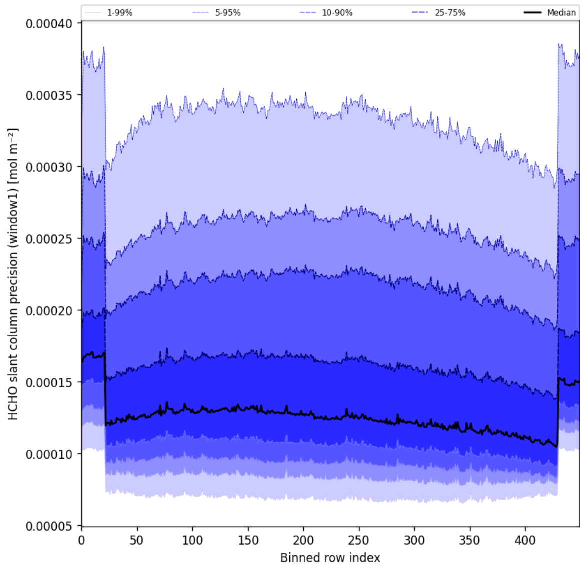
Figure 53: Along track statistics of “HCHO slant column precision (window1)” for 2025-03-30 to 2025-04-01
