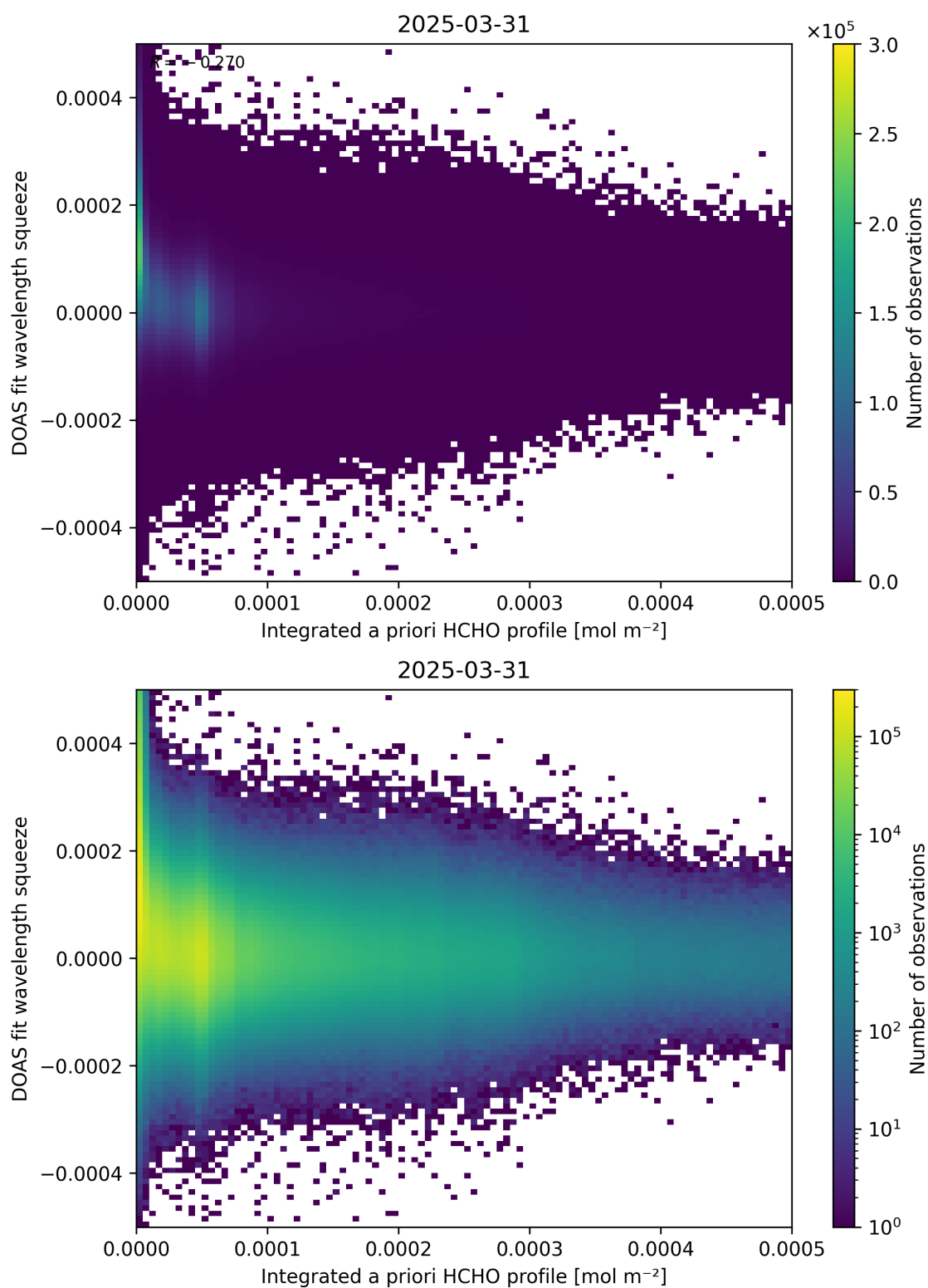
Figure 150: Scatter density plot of “Integrated a priori HCHO profile” against “DOAS fit wavelength squeeze” for 2025-03-30 to 2025-04-01.
