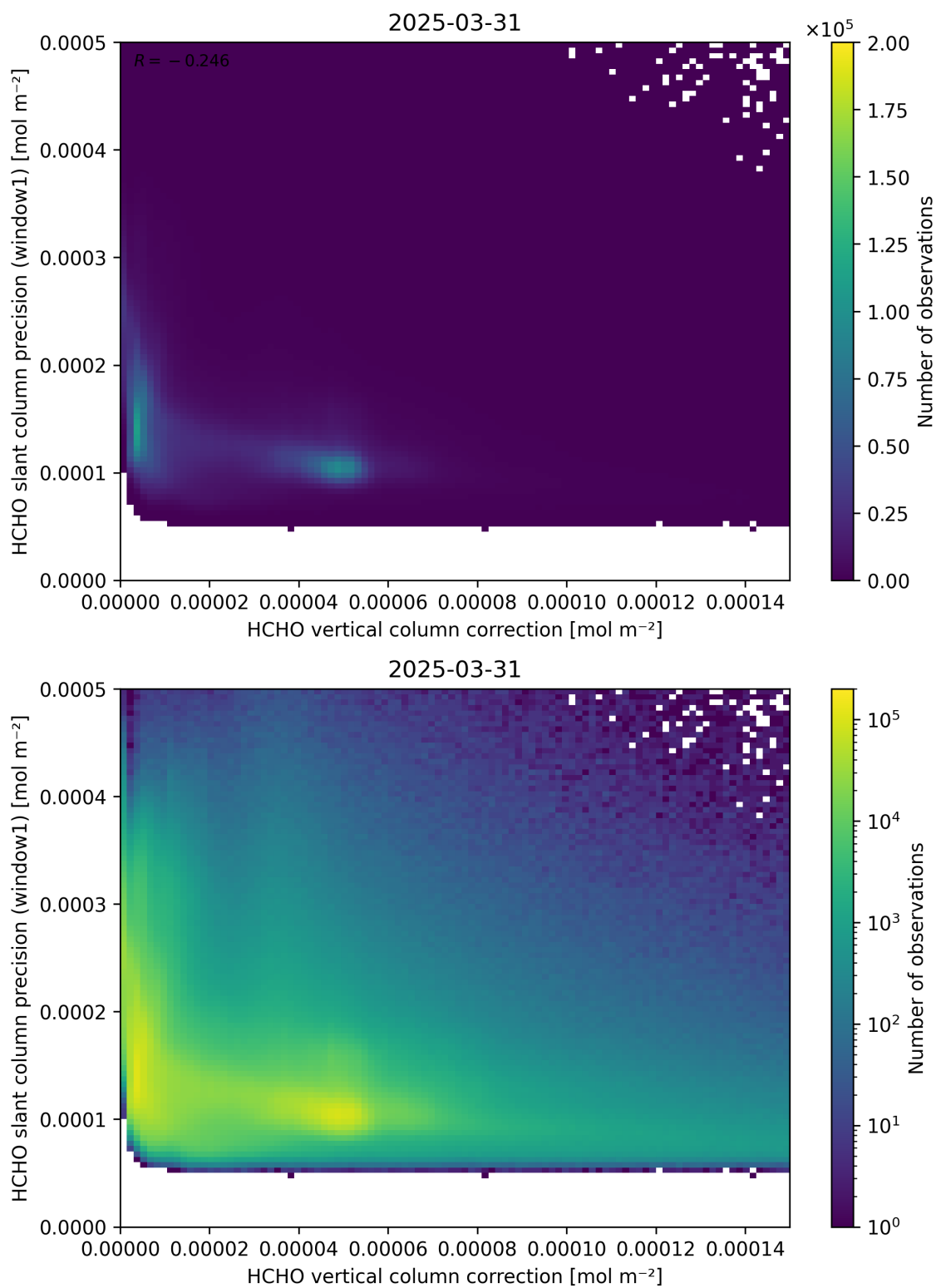
Figure 119: Scatter density plot of “HCHO vertical column correction” against “HCHO slant column precision (window1)” for 2025-03-30 to 2025-04-01.
