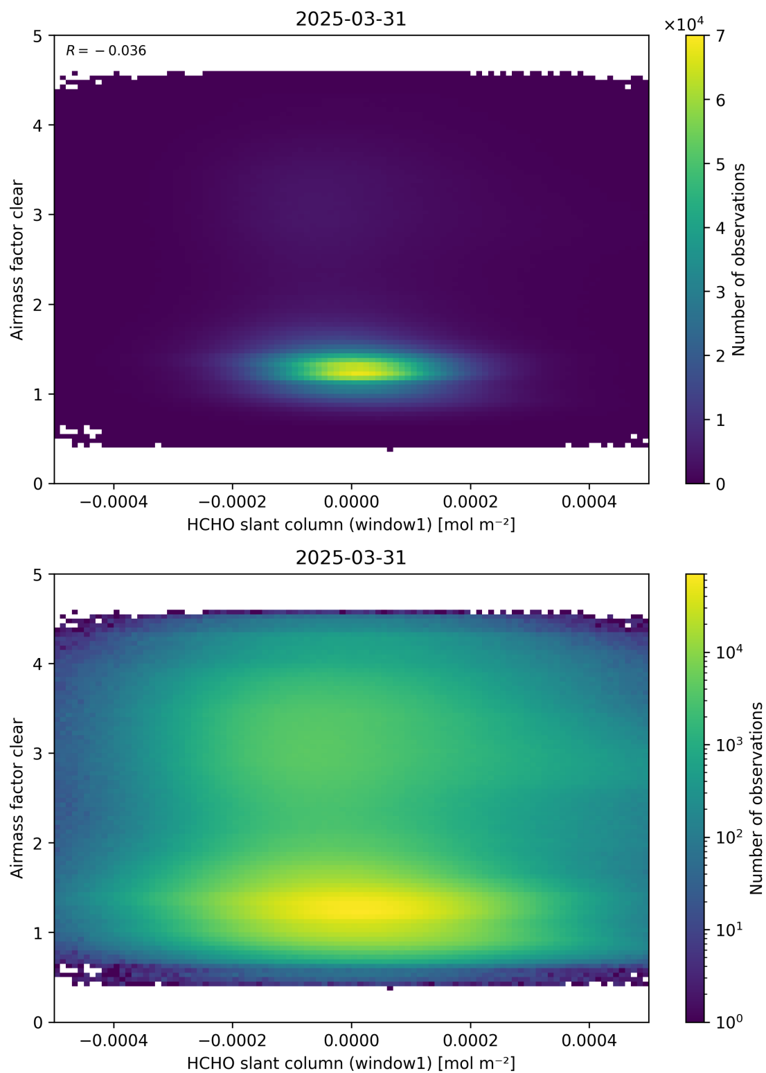
Figure 81: Scatter density plot of “HCHO slant column (window1)” against “Airmass factor clear” for 2025-03-30 to 2025-04-01.
