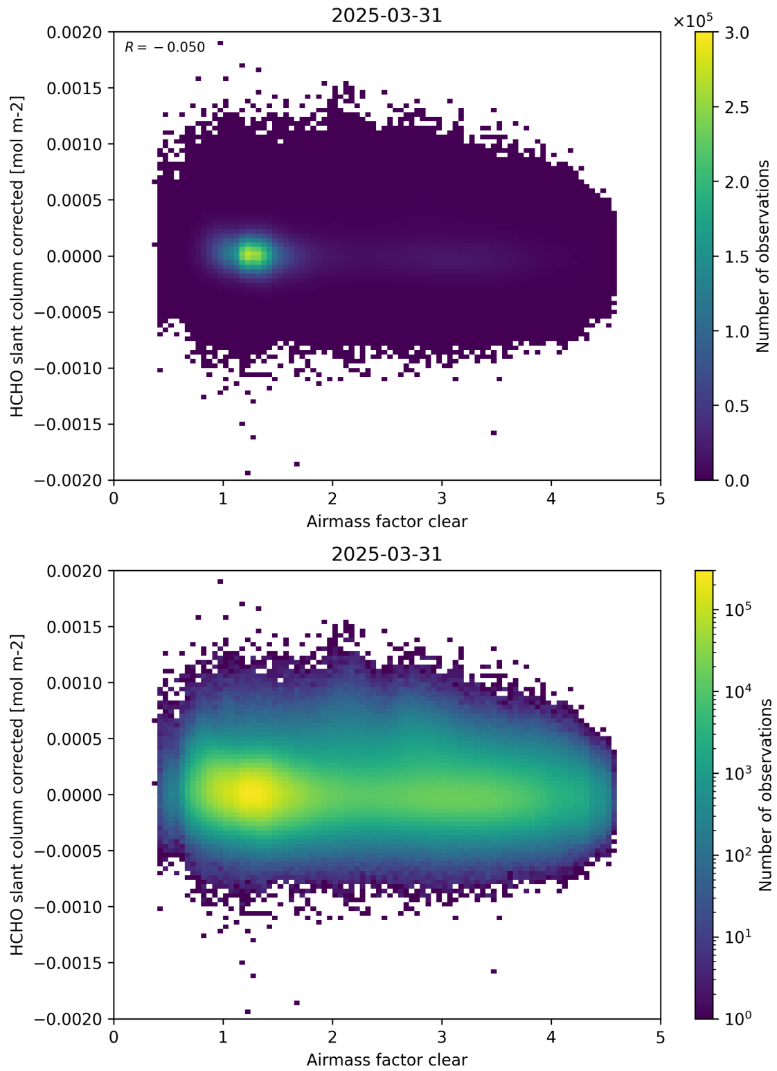
Figure 74: Scatter density plot of “Airmass factor clear” against “HCHO slant column corrected” for 2025-03-30 to 2025-04-01.
