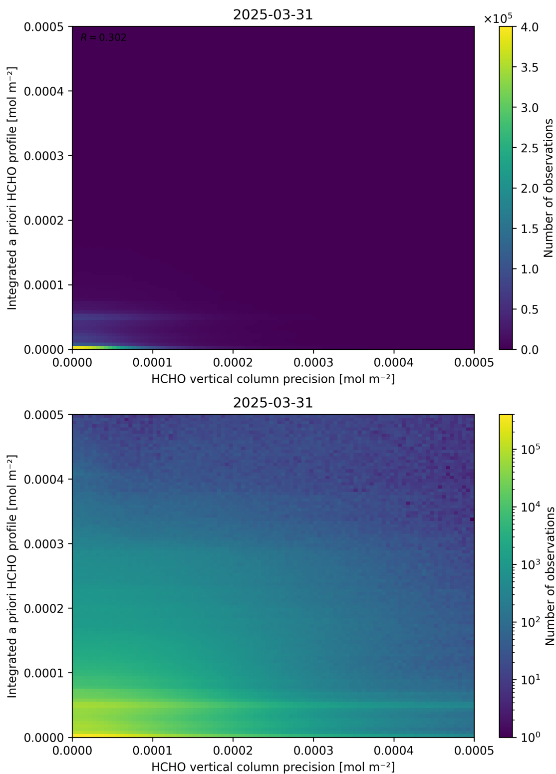
Figure 147: Scatter density plot of “HCHO vertical column precision” against “Integrated a priori HCHO profile” for 2025-03-30 to 2025-04-01.
