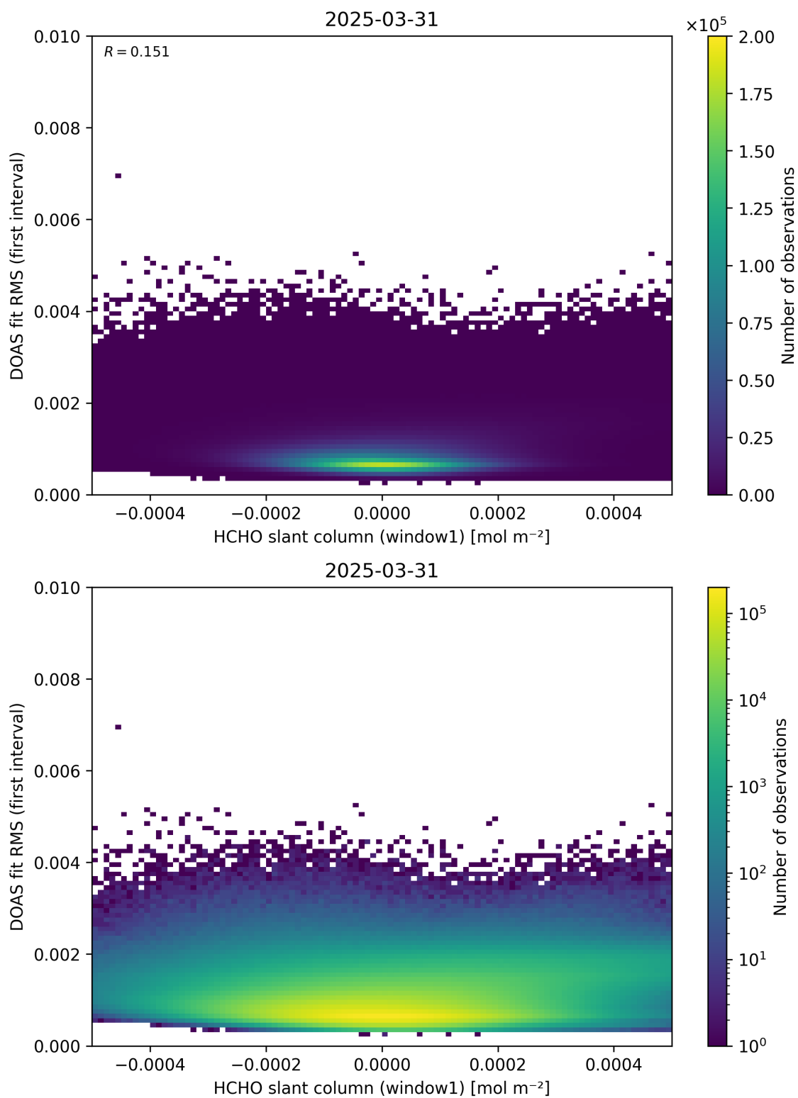
Figure 78: Scatter density plot of “HCHO slant column (window1)” against “DOAS fit RMS (first interval)” for 2025-03-30 to 2025-04-01.
