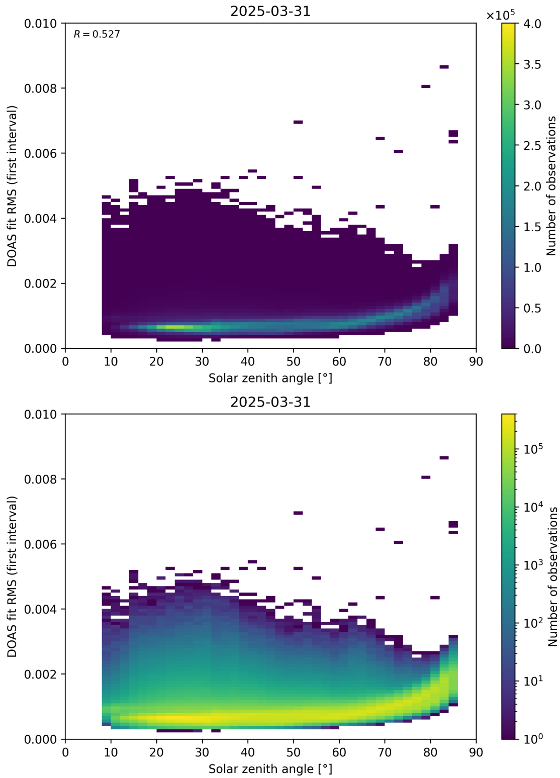
Figure 167: Scatter density plot of “Solar zenith angle” against “DOAS fit RMS (first interval)” for 2025-03-30 to 2025-04-01.
