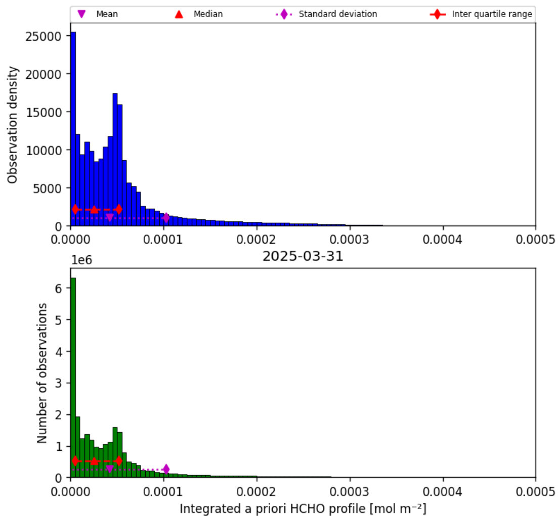
Figure 43: Histogram of “Integrated a priori HCHO profile” for 2025-03-30 to 2025-04-01
