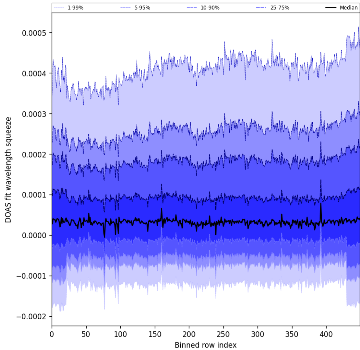
Figure 59: Along track statistics of “DOAS fit wavelength squeeze” for 2025-03-30 to 2025-04-01
