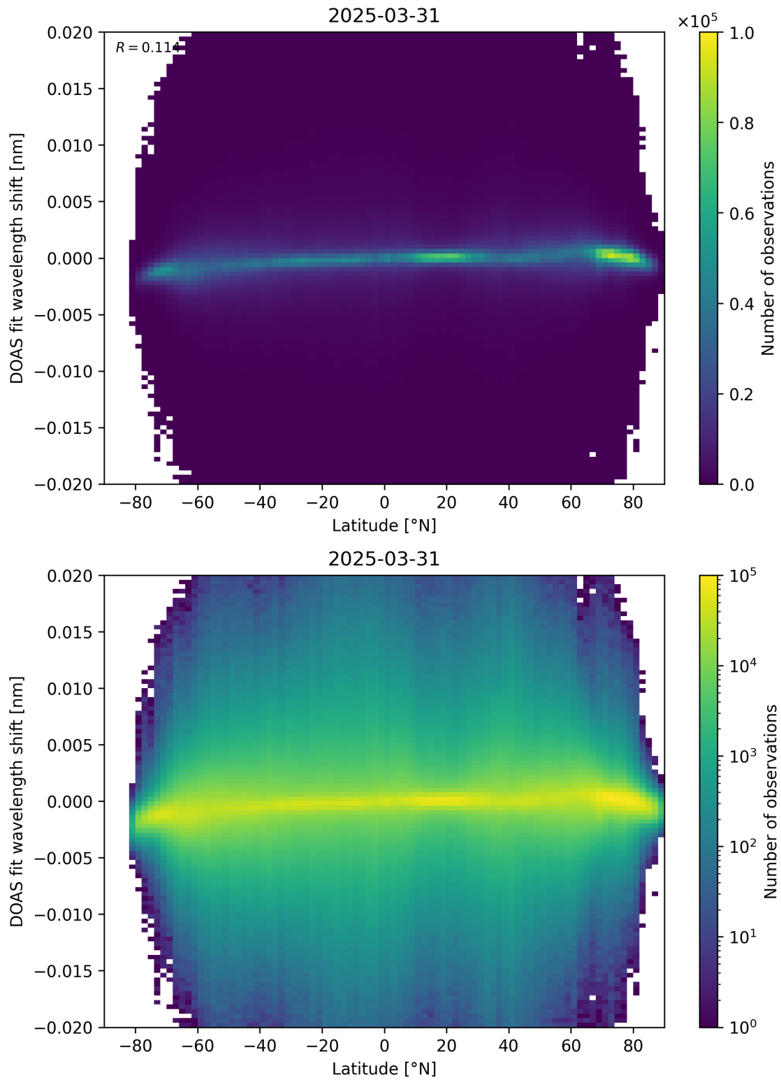
Figure 154: Scatter density plot of “Latitude” against “DOAS fit wavelength shift” for 2025-03-30 to 2025-04-01.
