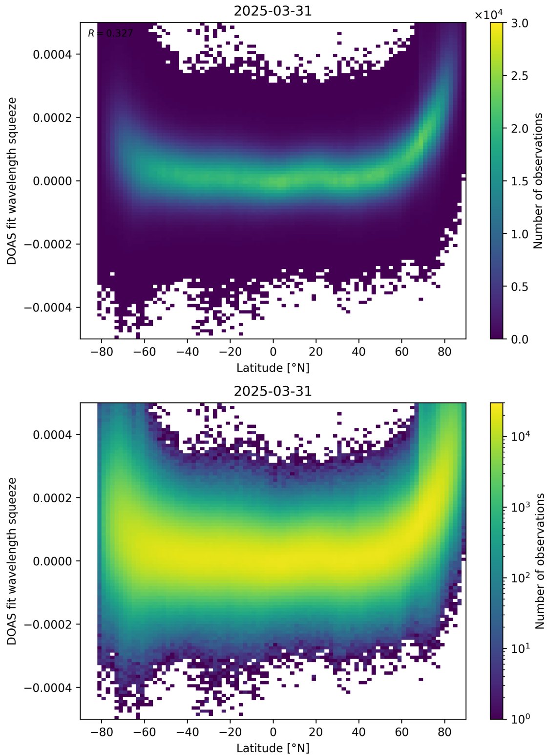
Figure 155: Scatter density plot of “Latitude” against “DOAS fit wavelength squeeze” for 2025-03-30 to 2025-04-01.
