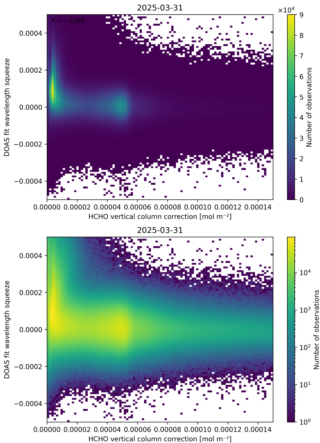
Figure 114: Scatter density plot of “HCHO vertical column correction” against “DOAS fit wavelength squeeze” for 2025-03-30 to 2025-04-01.
