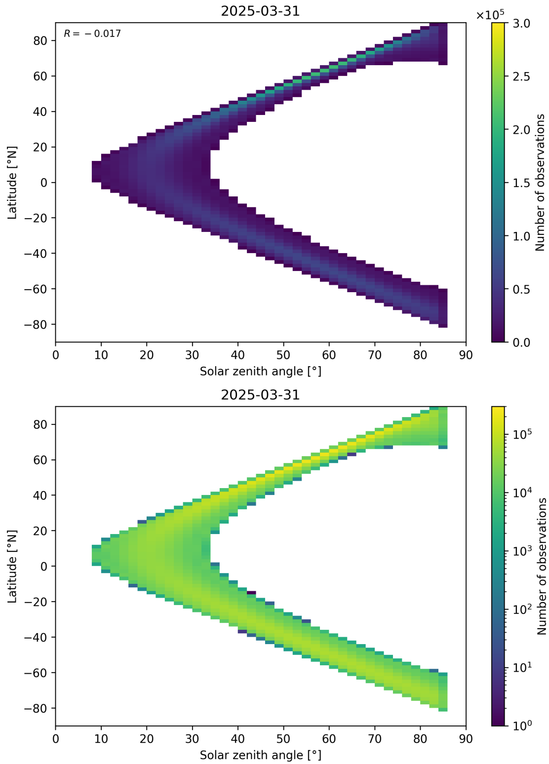
Figure 181: Scatter density plot of “Solar zenith angle” against “Latitude” for 2025-03-30 to 2025-04-01.
