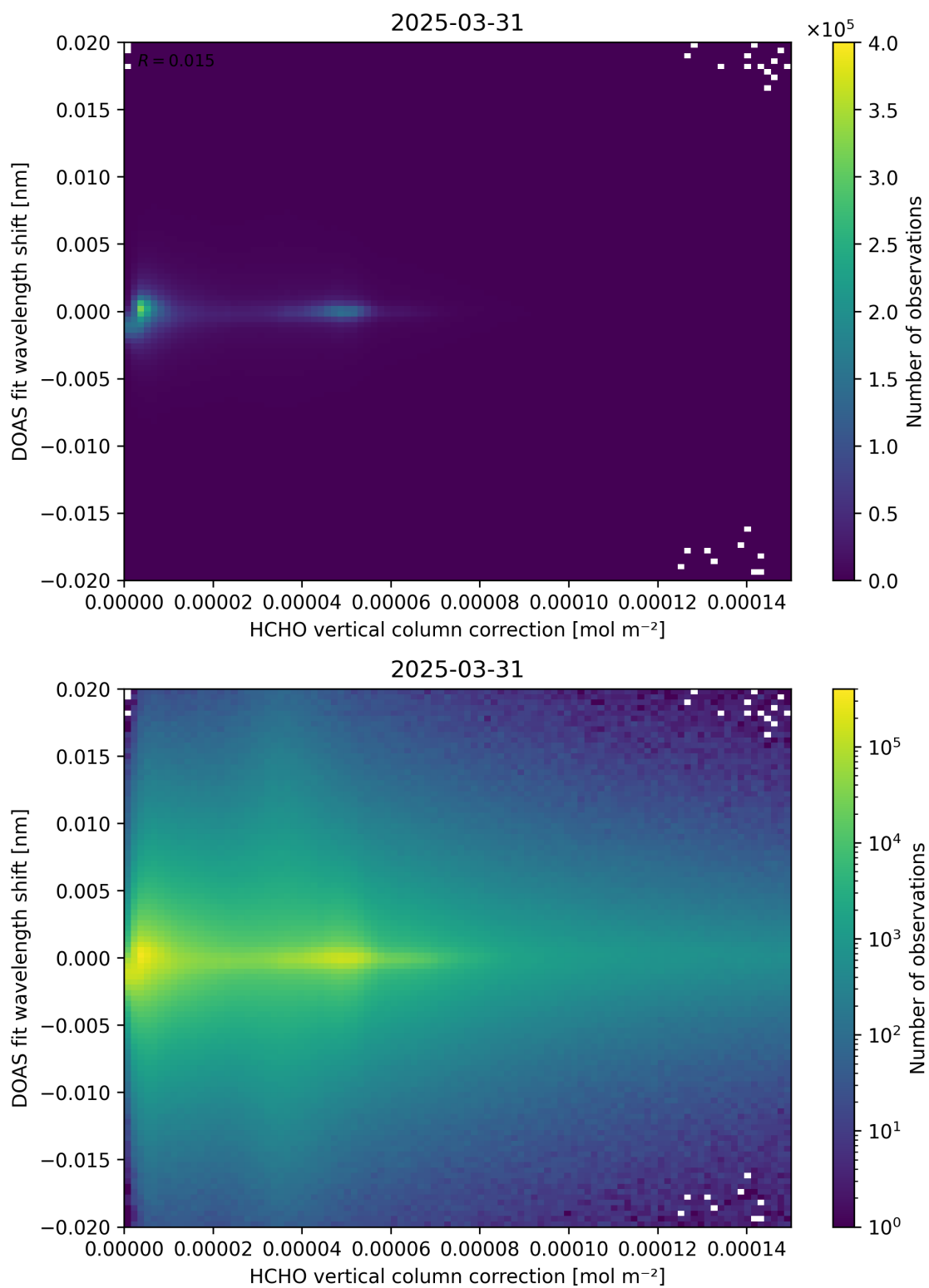
Figure 113: Scatter density plot of “HCHO vertical column correction” against “DOAS fit wavelength shift” for 2025-03-30 to 2025-04-01.
