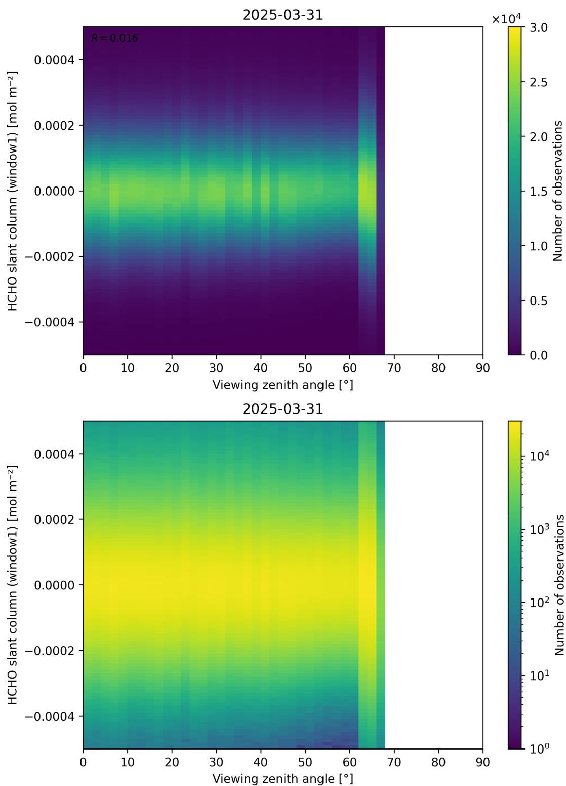
Figure 188: Scatter density plot of “Viewing zenith angle” against “HCHO slant column (window1)” for 2025-03-30 to 2025-04-01.
