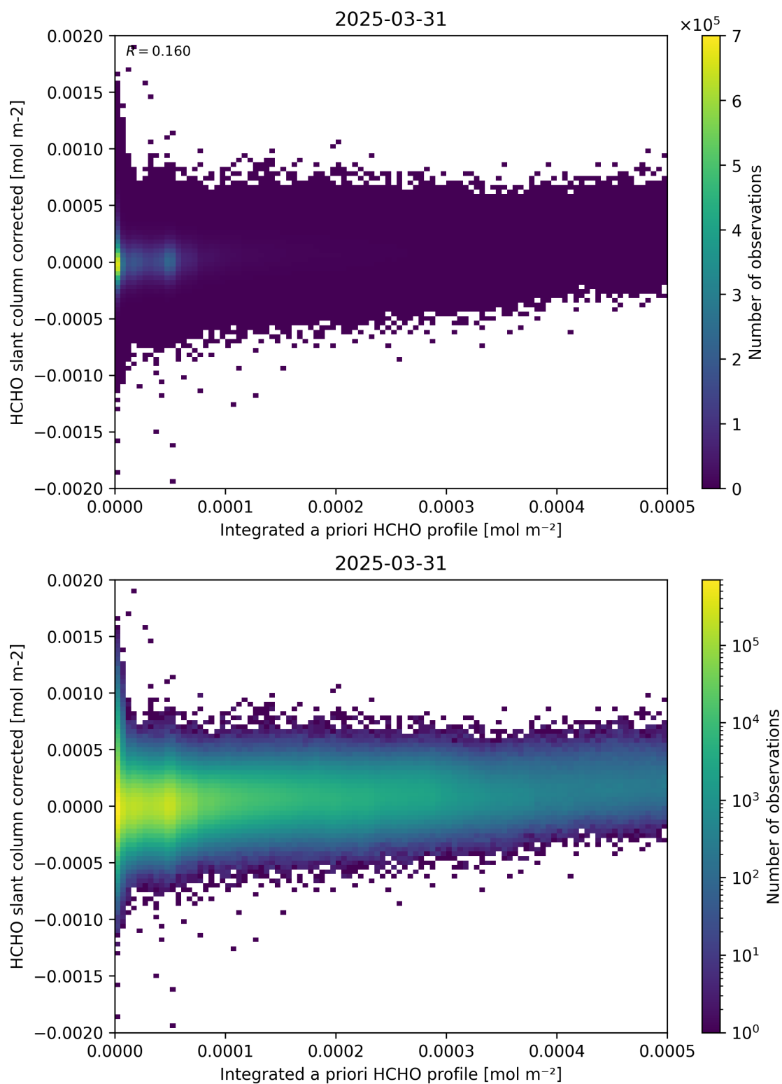
Figure 151: Scatter density plot of “Integrated a priori HCHO profile” against “HCHO slant column corrected” for 2025-03-30 to 2025-04-01.
