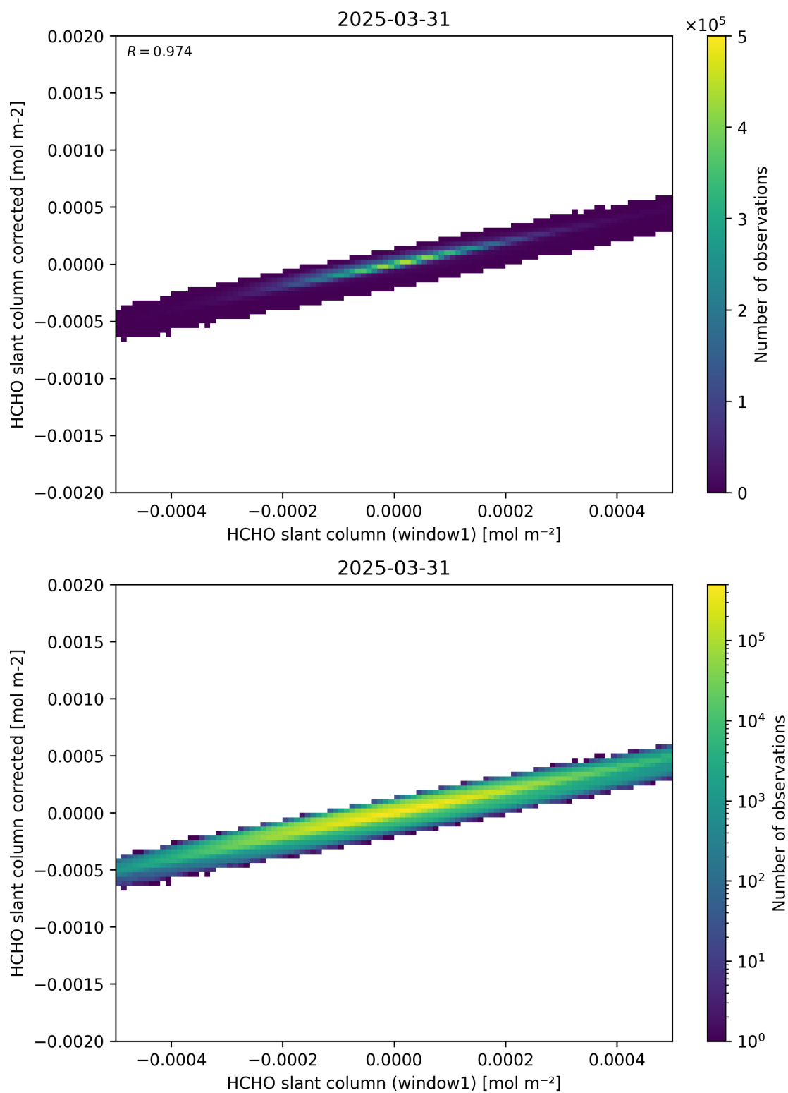
Figure 82: Scatter density plot of “HCHO slant column (window1)” against “HCHO slant column corrected” for 2025-03-30 to 2025-04-01.
