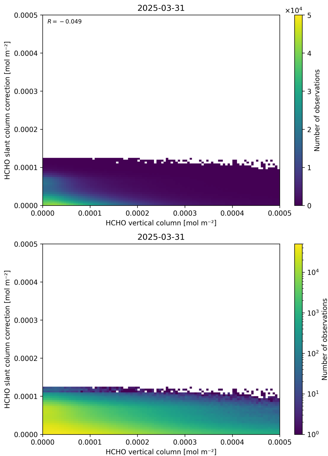
Figure 128: Scatter density plot of “HCHO vertical column” against “HCHO slant column correction” for 2025-03-30 to 2025-04-01.
