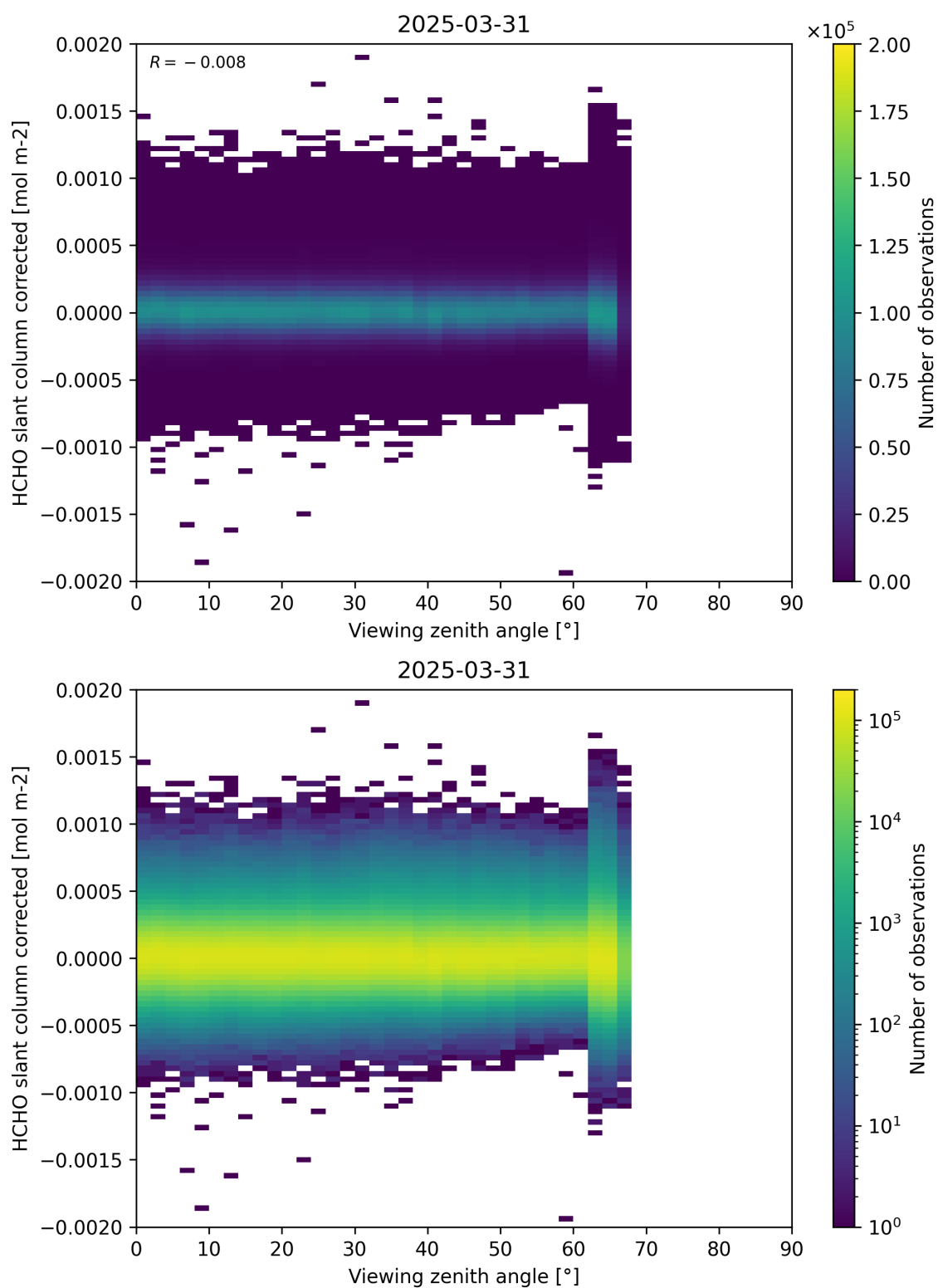
Figure 186: Scatter density plot of “Viewing zenith angle” against “HCHO slant column corrected” for 2025-03-30 to 2025-04-01.
