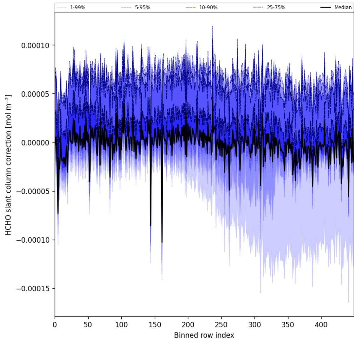
Figure 61: Along track statistics of “HCHO slant column correction” for 2025-03-30 to 2025-04-01
