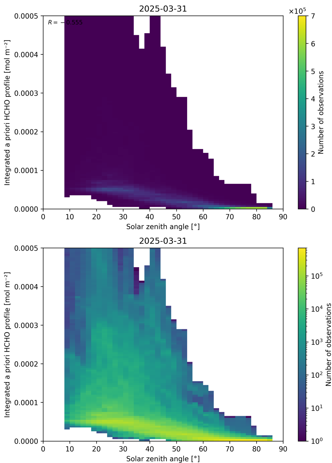
Figure 180: Scatter density plot of “Solar zenith angle” against “Integrated a priori HCHO profile” for 2025-03-30 to 2025-04-01.
