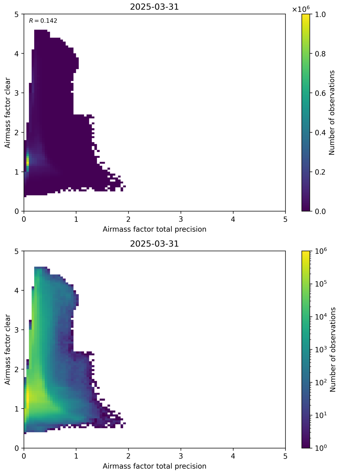
Figure 108: Scatter density plot of “Airmass factor total precision” against “Airmass factor clear” for 2025-03-30 to 2025-04-01.
