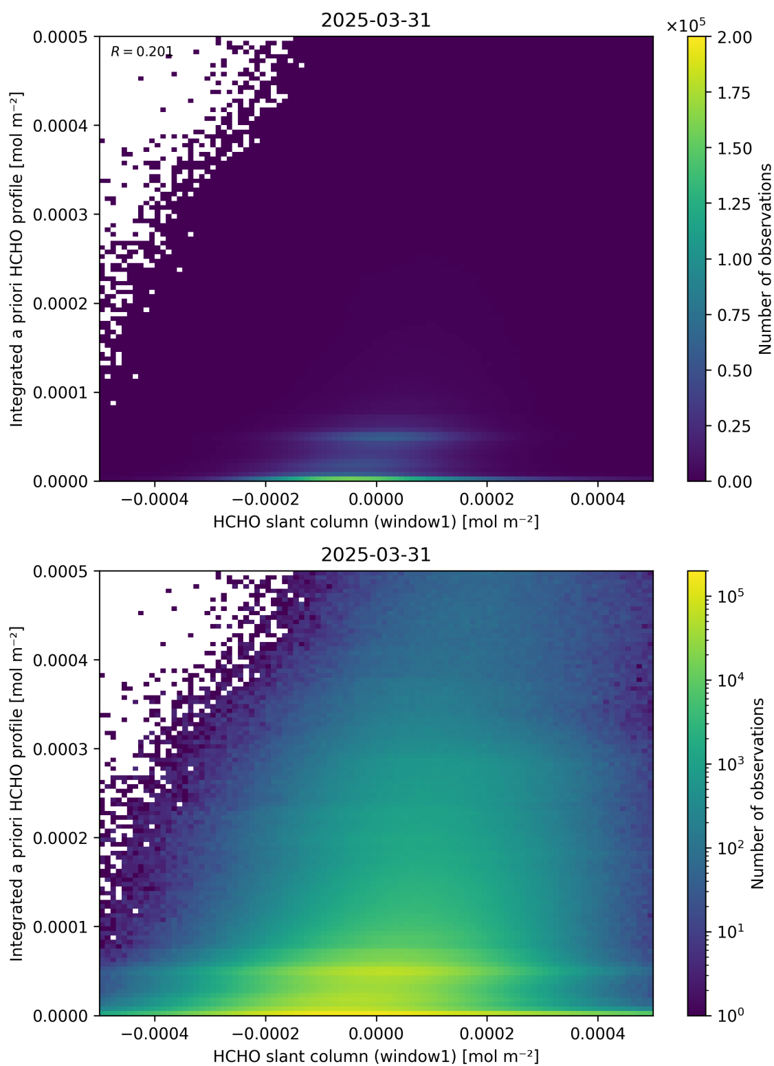
Figure 87: Scatter density plot of “HCHO slant column (window1)” against “Integrated a priori HCHO profile” for 2025-03-30 to 2025-04-01.
