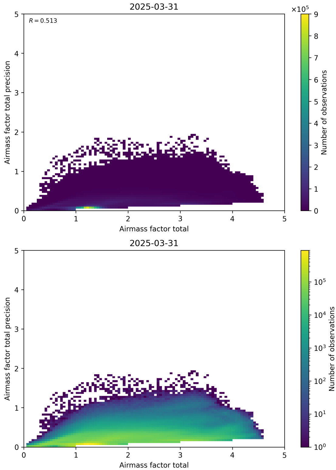
Figure 103: Scatter density plot of “Airmass factor total” against “Airmass factor total precision” for 2025-03-30 to 2025-04-01.
