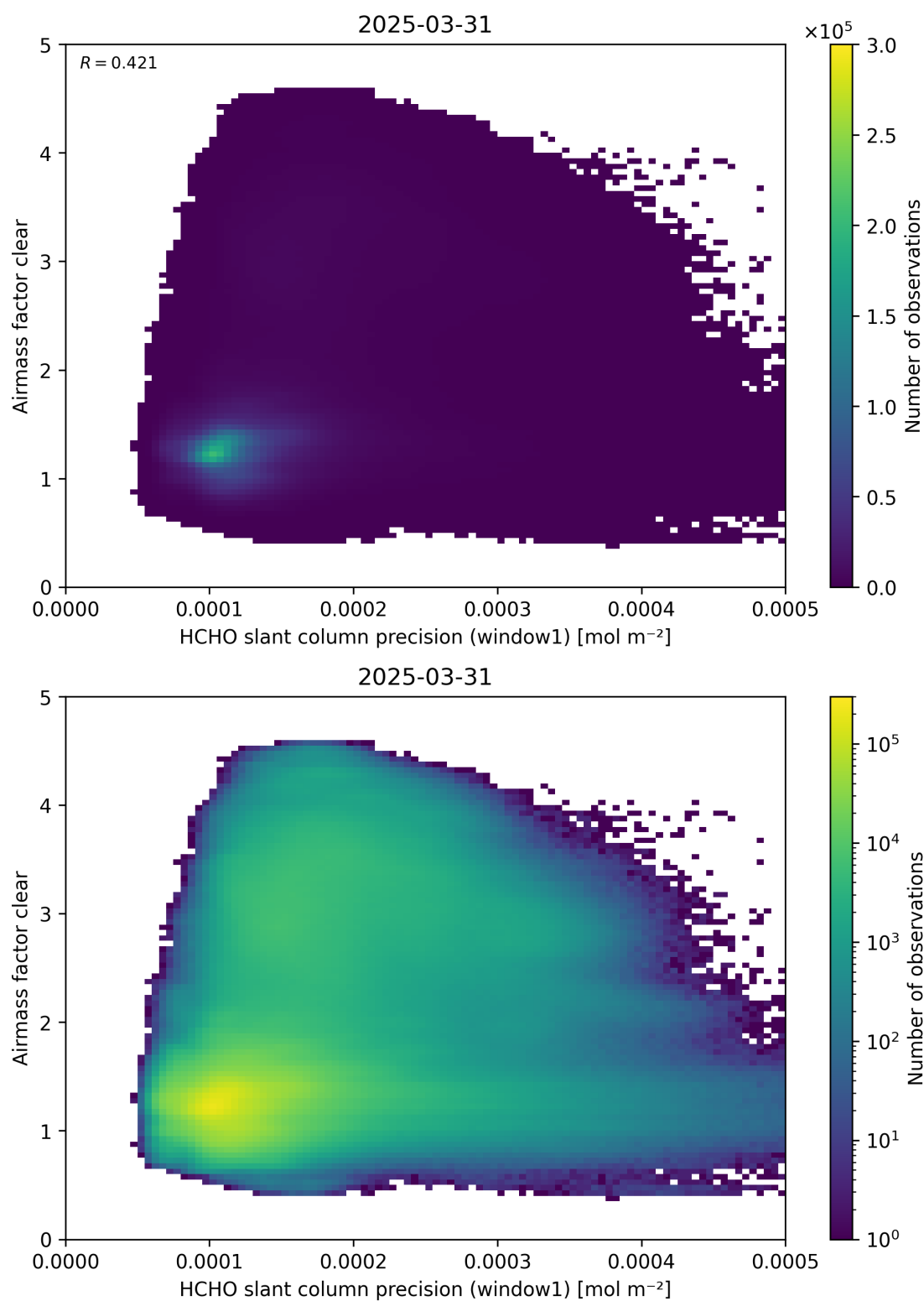
Figure 91: Scatter density plot of “HCHO slant column precision (window1)” against “Airmass factor clear” for 2025-03-30 to 2025-04-01.
