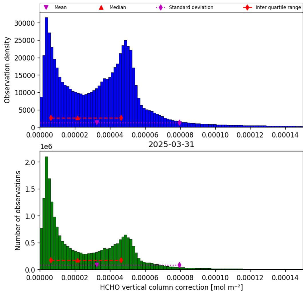
Figure 37: Histogram of “HCHO vertical column correction” for 2025-03-30 to 2025-04-01
