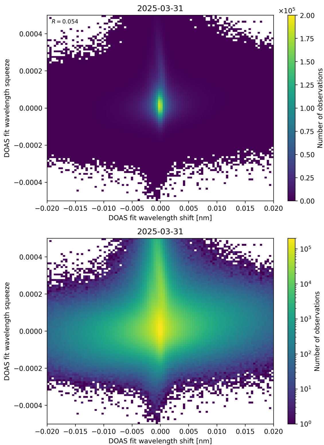
Figure 65: Scatter density plot of “DOAS fit wavelength shift” against “DOAS fit wavelength squeeze” for 2025-03-30 to 2025-04-01.
