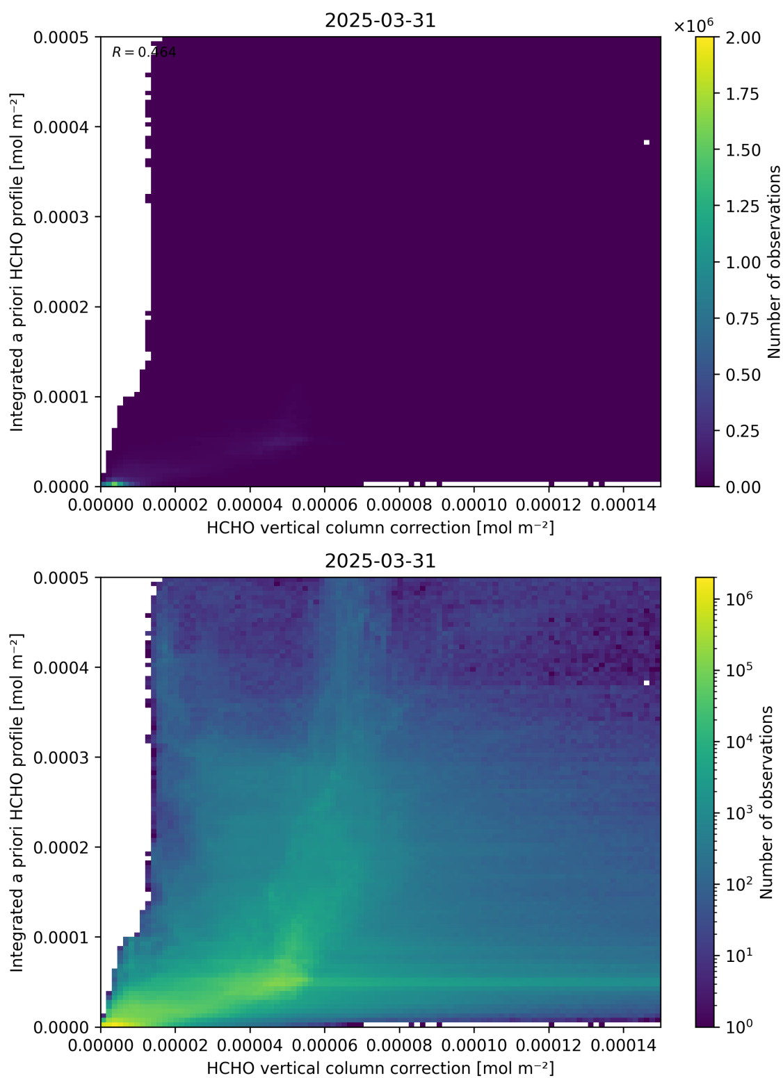
Figure 122: Scatter density plot of “HCHO vertical column correction” against “Integrated a priori HCHO profile” for 2025-03-30 to 2025-04-01.
