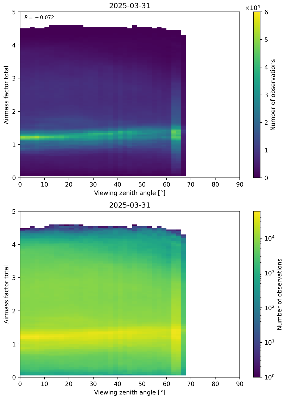
Figure 190: Scatter density plot of “Viewing zenith angle” against “Airmass factor total” for 2025-03-30 to 2025-04-01.
