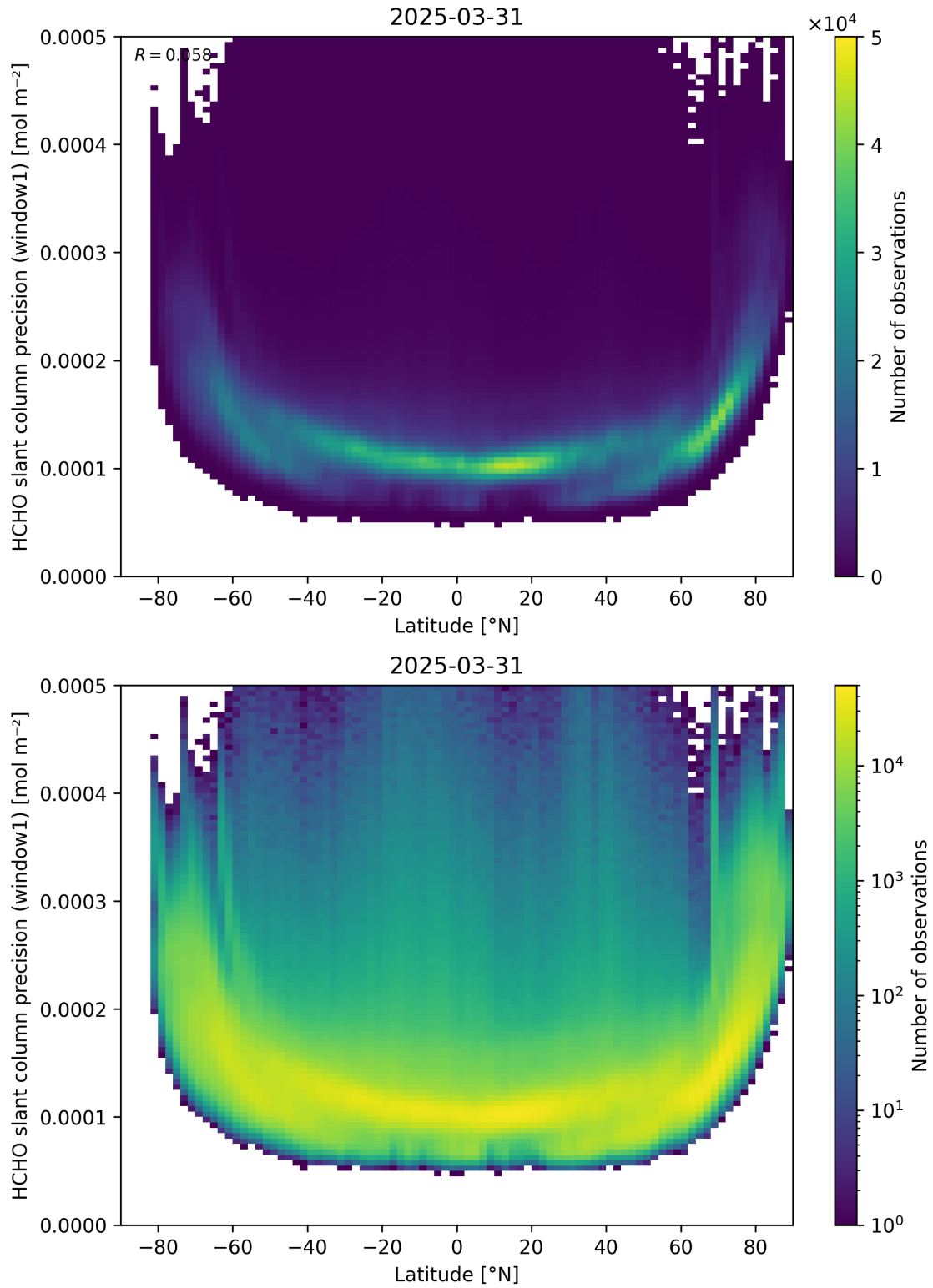
Figure 160: Scatter density plot of “Latitude” against “HCHO slant column precision (window1)” for 2025-03-30 to 2025-04-01.
