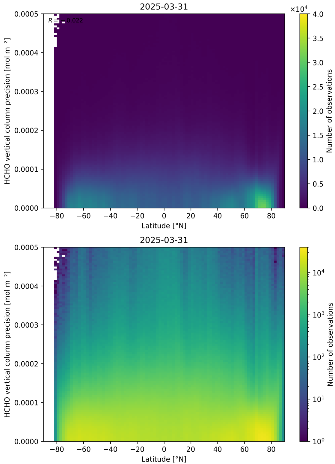
Figure 165: Scatter density plot of “Latitude” against “HCHO vertical column precision” for 2025-03-30 to 2025-04-01.
