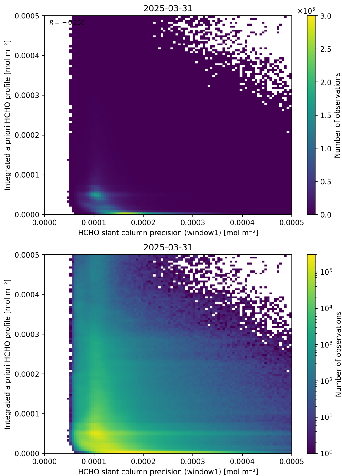
Figure 96: Scatter density plot of “HCHO slant column precision (window1)” against “Integrated a priori HCHO profile” for 2025-03-30 to 2025-04-01.
