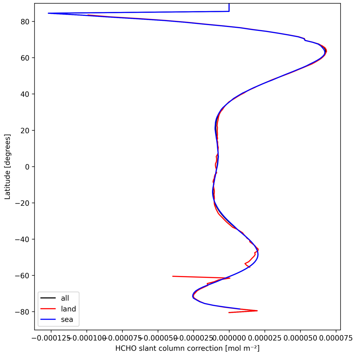
Figure 33: Zonal average of “HCHO slant column correction” for 2025-03-30 to 2025-04-01.
