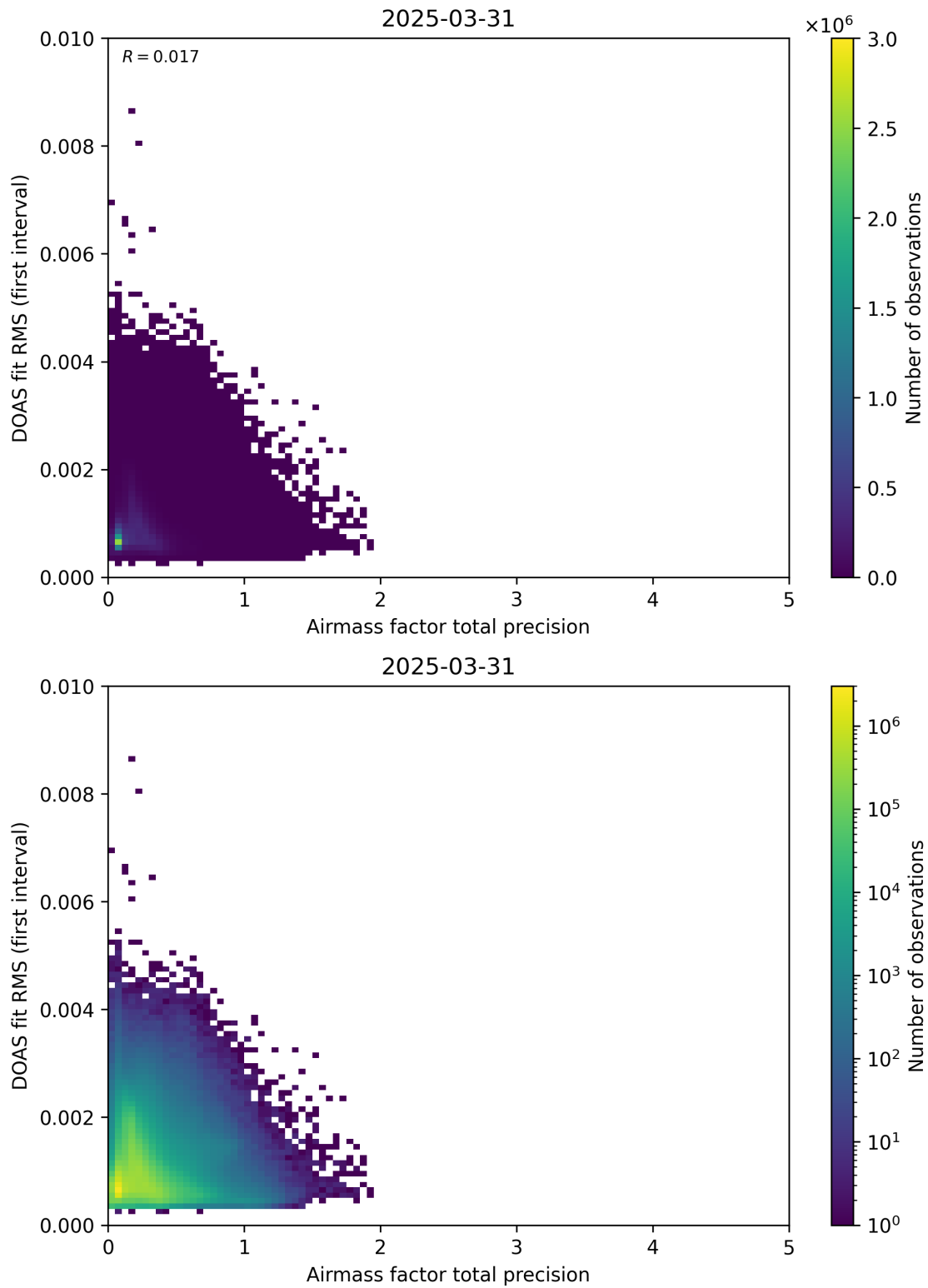
Figure 105: Scatter density plot of “Airmass factor total precision” against “DOAS fit RMS (first interval)” for 2025-03-30 to 2025-04-01.
