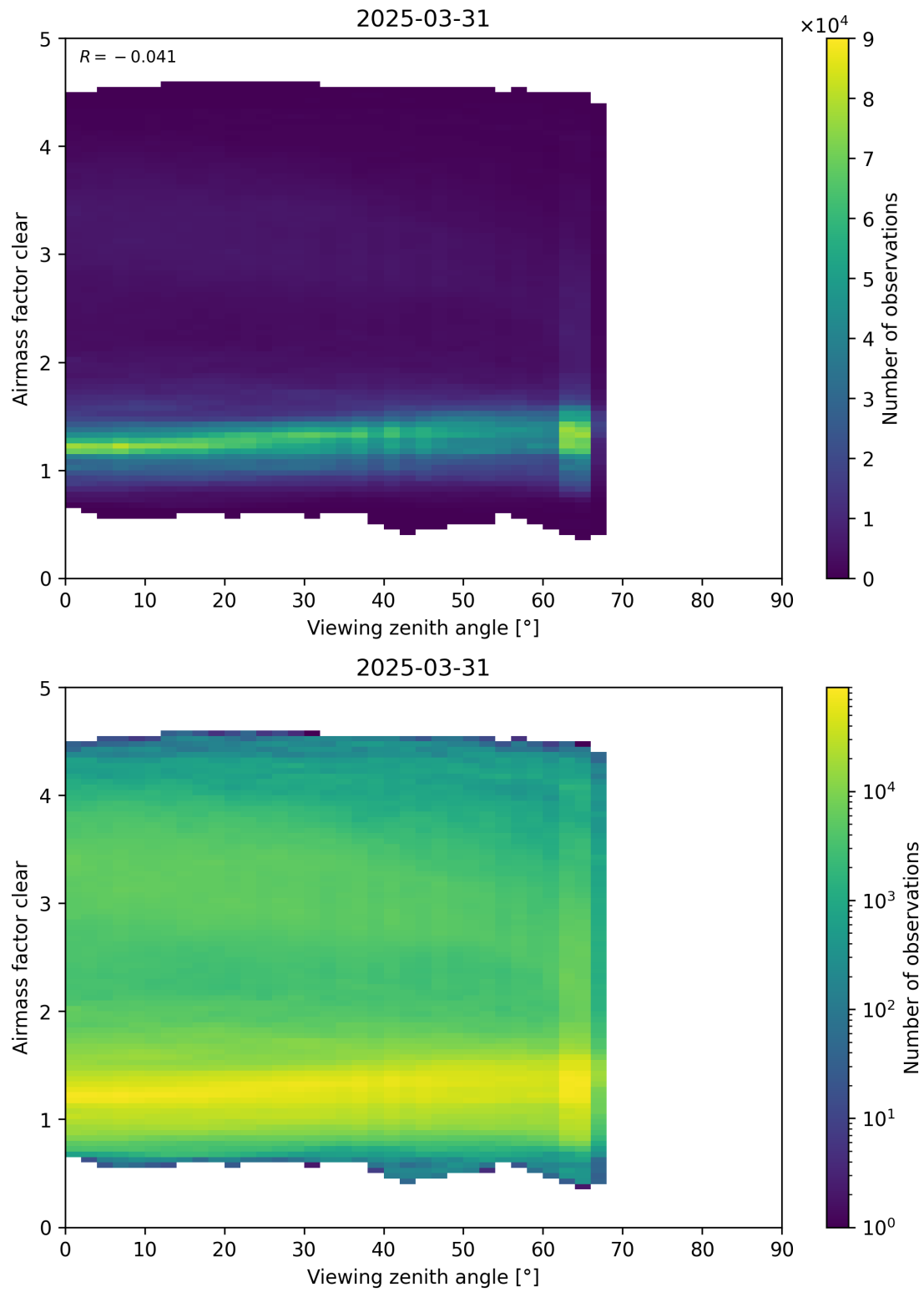
Figure 185: Scatter density plot of “Viewing zenith angle” against “Airmass factor clear” for 2025-03-30 to 2025-04-01.
