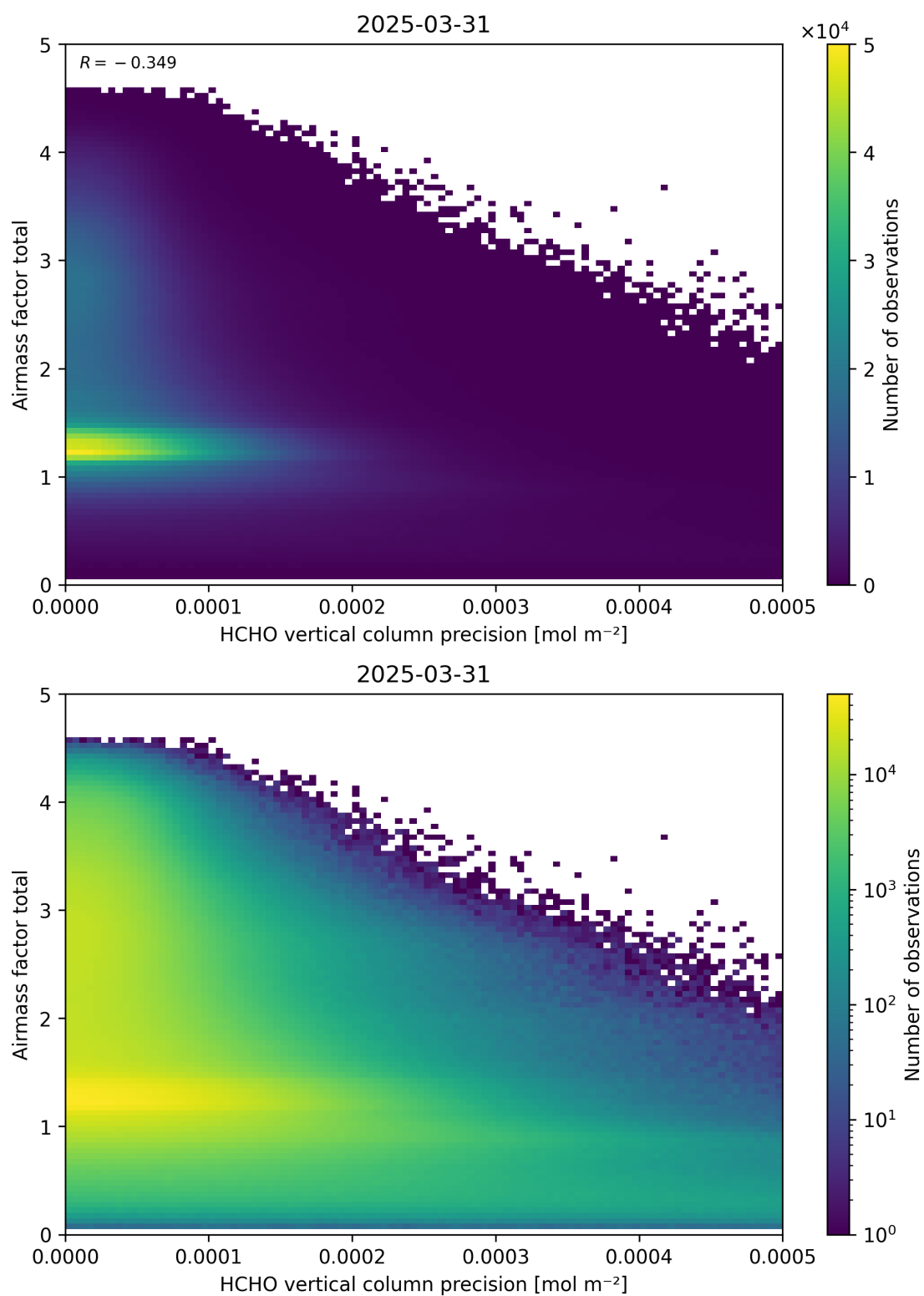
Figure 144: Scatter density plot of “HCHO vertical column precision” against “Airmass factor total” for 2025-03-30 to 2025-04-01.
