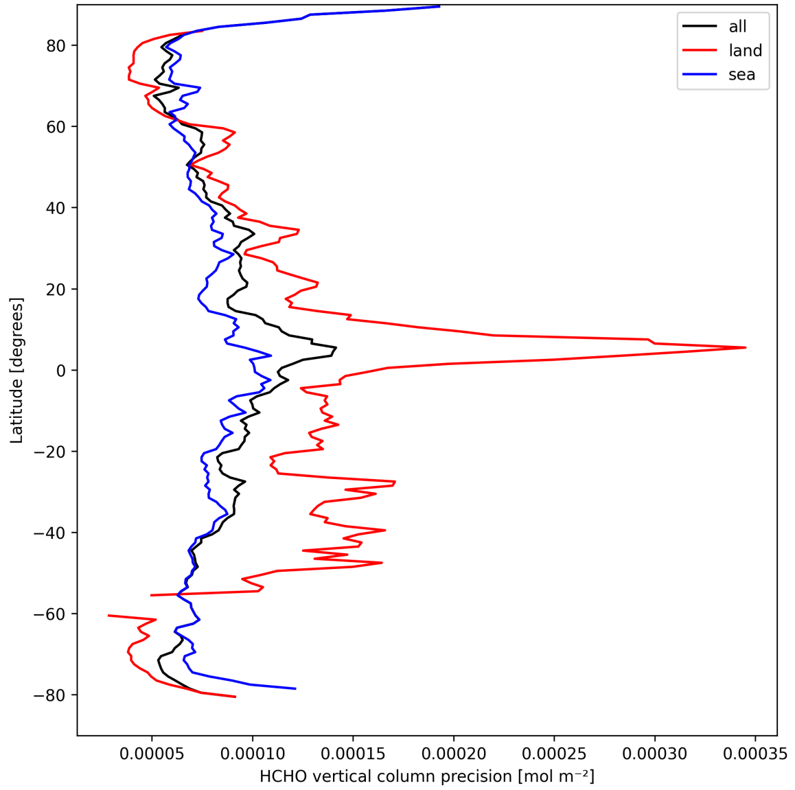
Figure 22: Zonal average of "HCHO vertical column precision" for 2025-03-30 to 2025-04-01.
