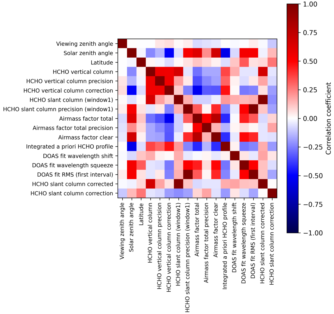
Figure 2: Map of correlation matrix for 2025-03-30 to 2025-04-01.
