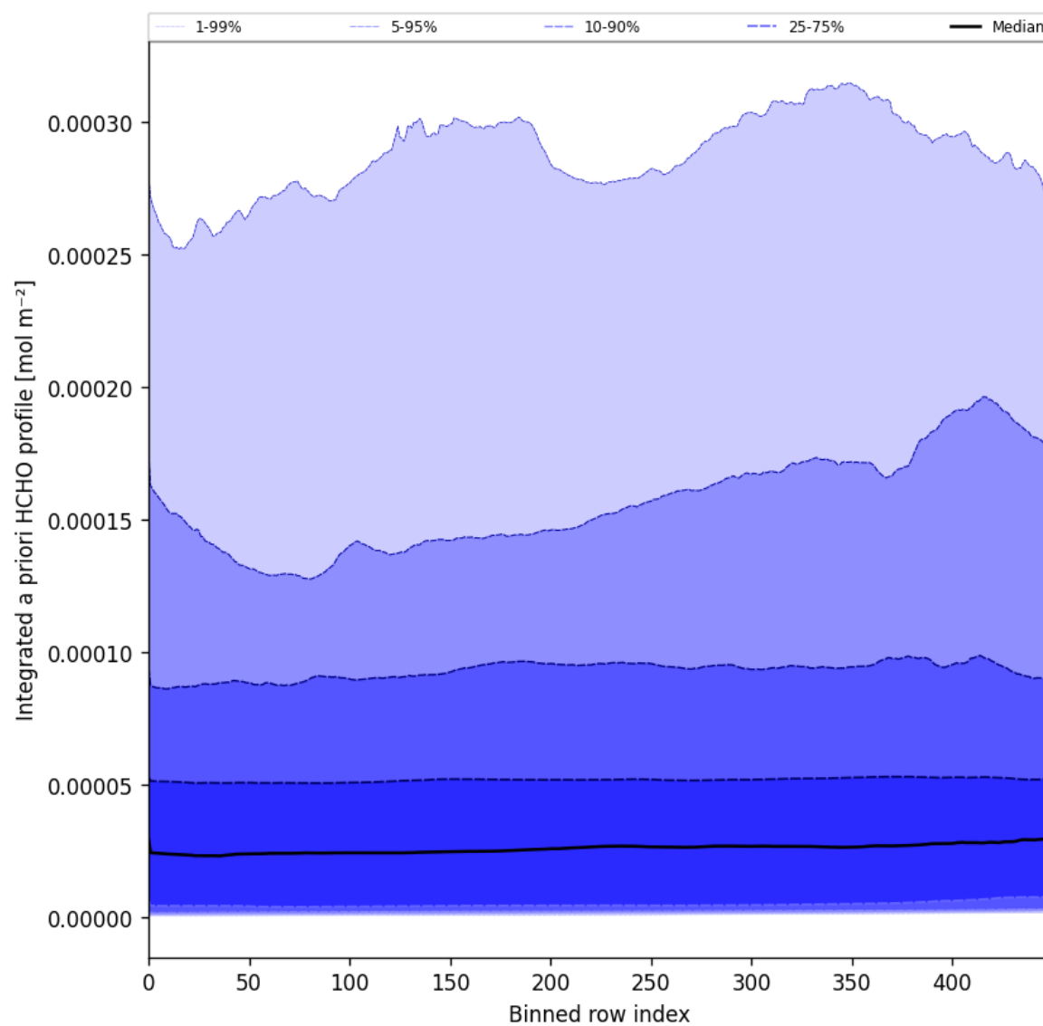
Figure 57: Along track statistics of “Integrated a priori HCHO profile” for 2025-03-30 to 2025-04-01
