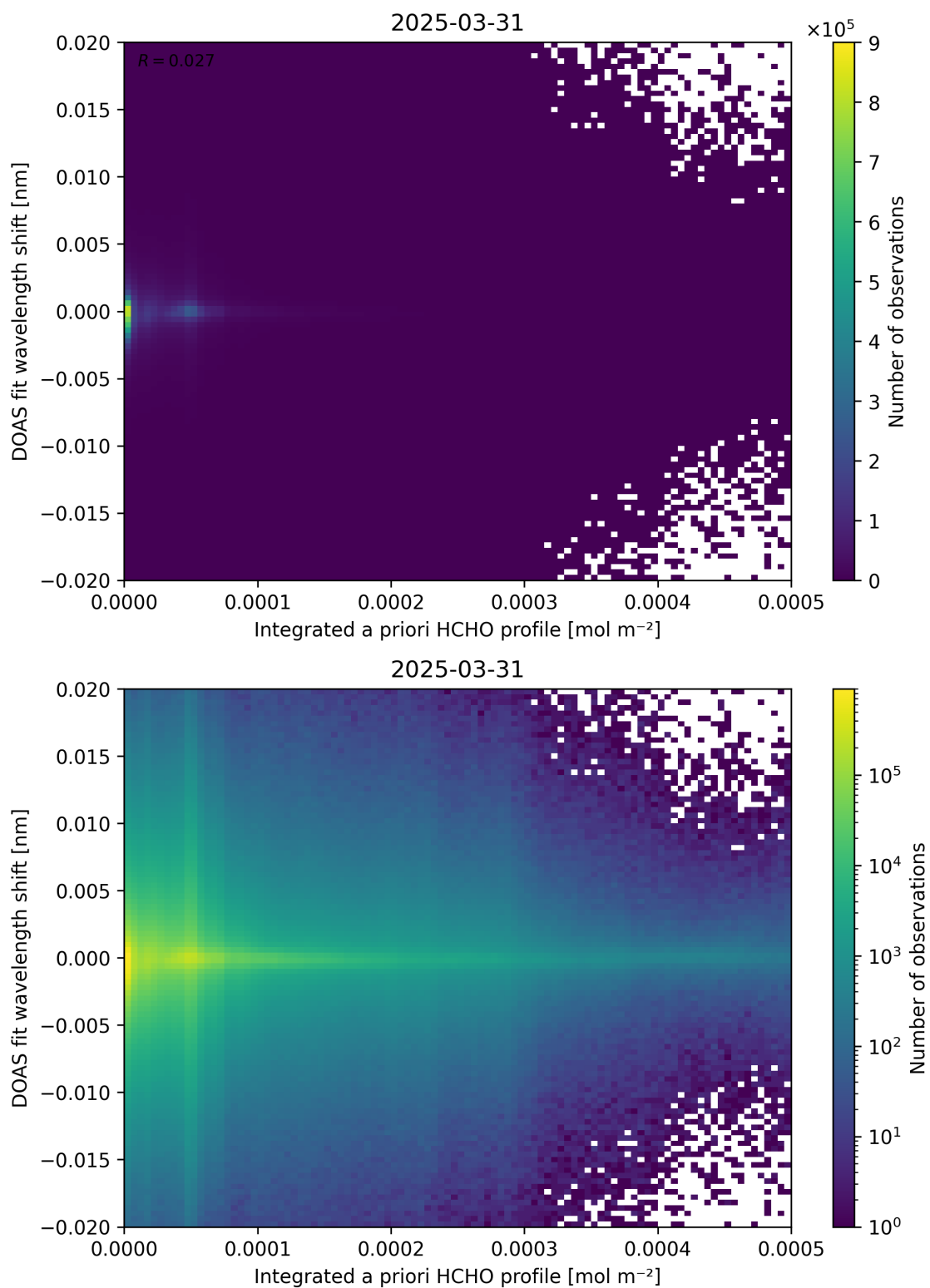
Figure 149: Scatter density plot of “Integrated a priori HCHO profile” against “DOAS fit wavelength shift” for 2025-03-30 to 2025-04-01.
