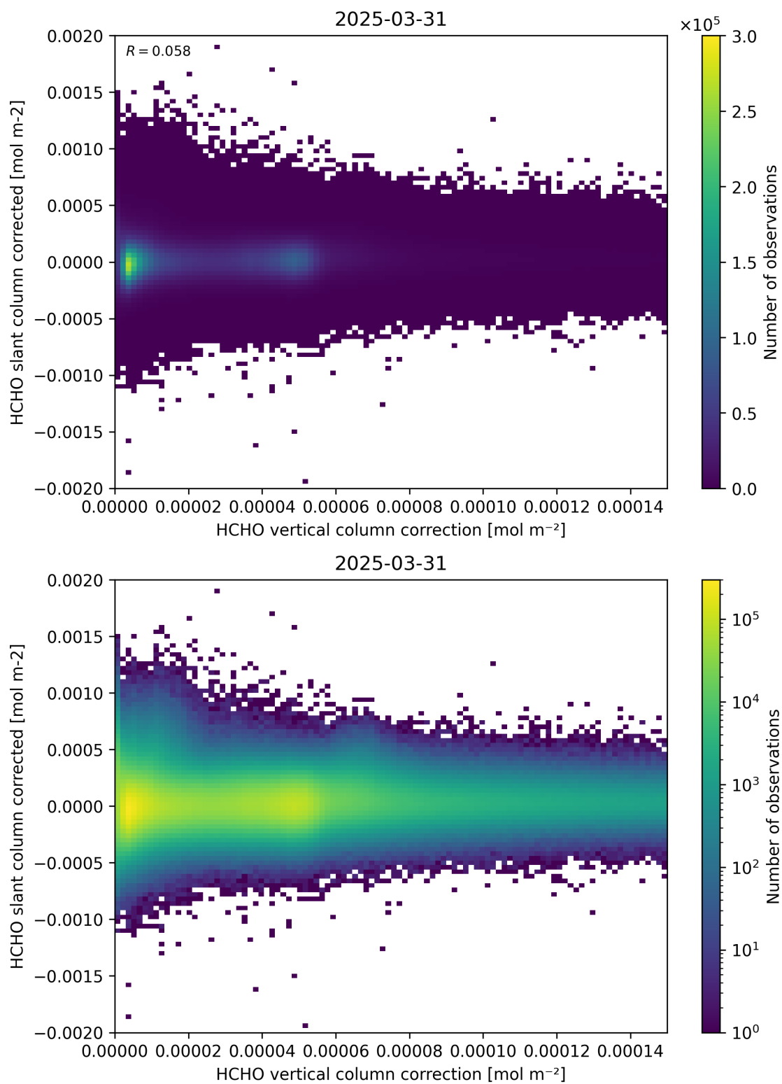
Figure 116: Scatter density plot of “HCHO vertical column correction” against “HCHO slant column corrected” for 2025-03-30 to 2025-04-01.
