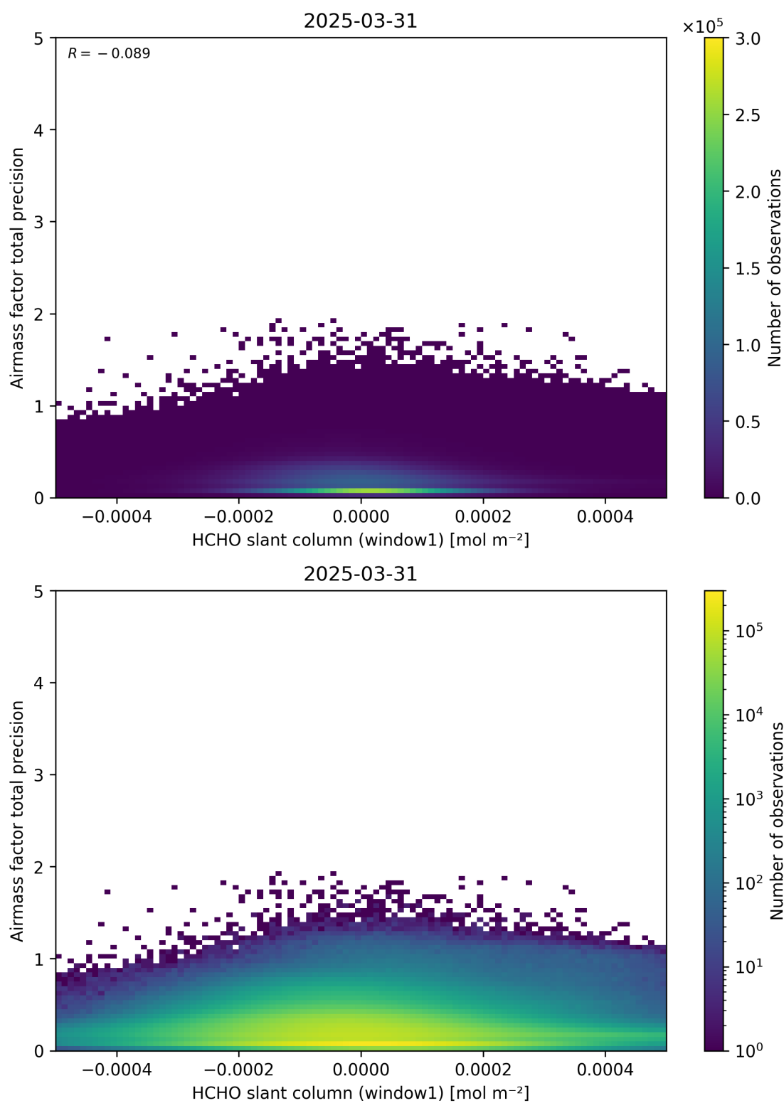
Figure 86: Scatter density plot of “HCHO slant column (window1)” against “Airmass factor total precision” for 2025-03-30 to 2025-04-01.
