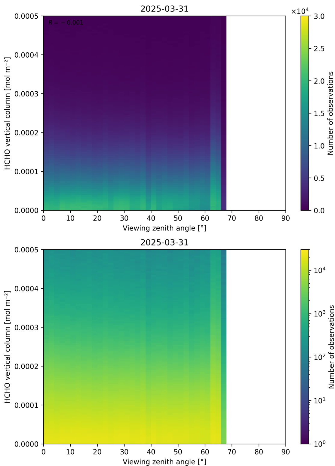
Figure 192: Scatter density plot of “Viewing zenith angle” against “HCHO vertical column” for 2025-03-30 to 2025-04-01.
