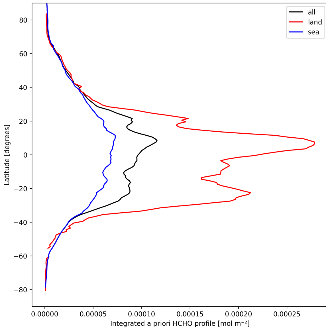
Figure 29: Zonal average of “Integrated a priori HCHO profile” for 2025-03-30 to 2025-04-01.
