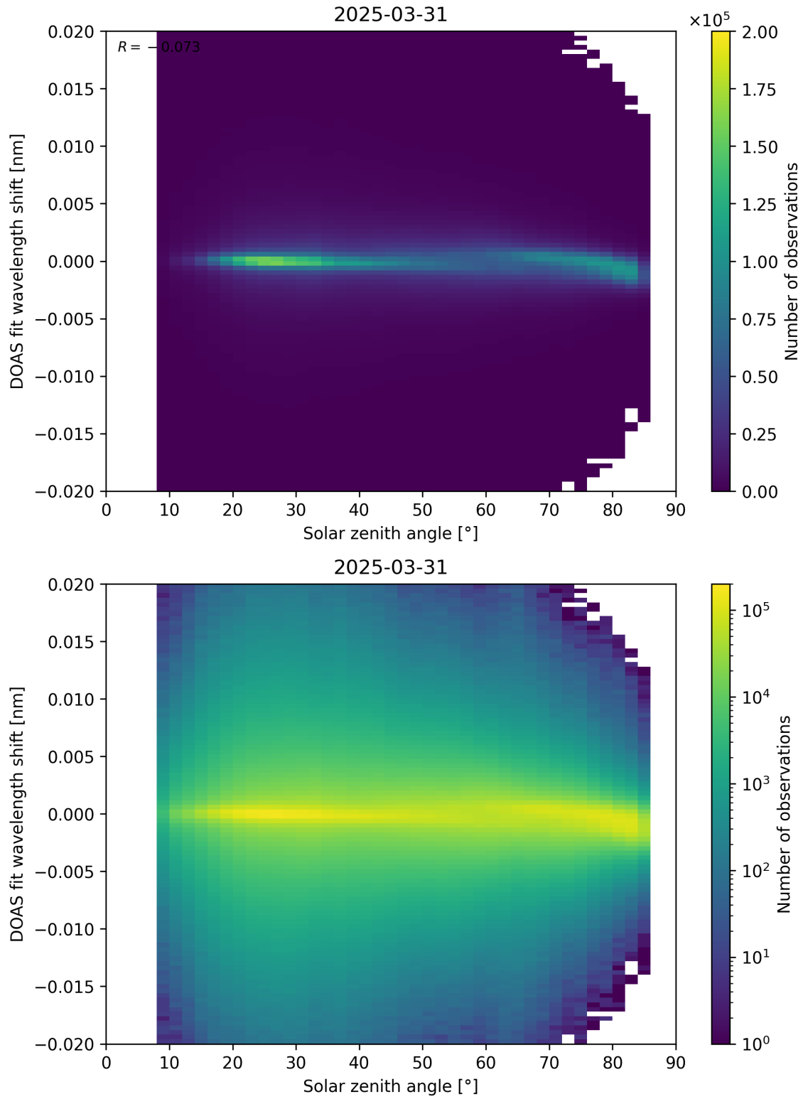
Figure 168: Scatter density plot of “Solar zenith angle” against “DOAS fit wavelength shift” for 2025-03-30 to 2025-04-01.
