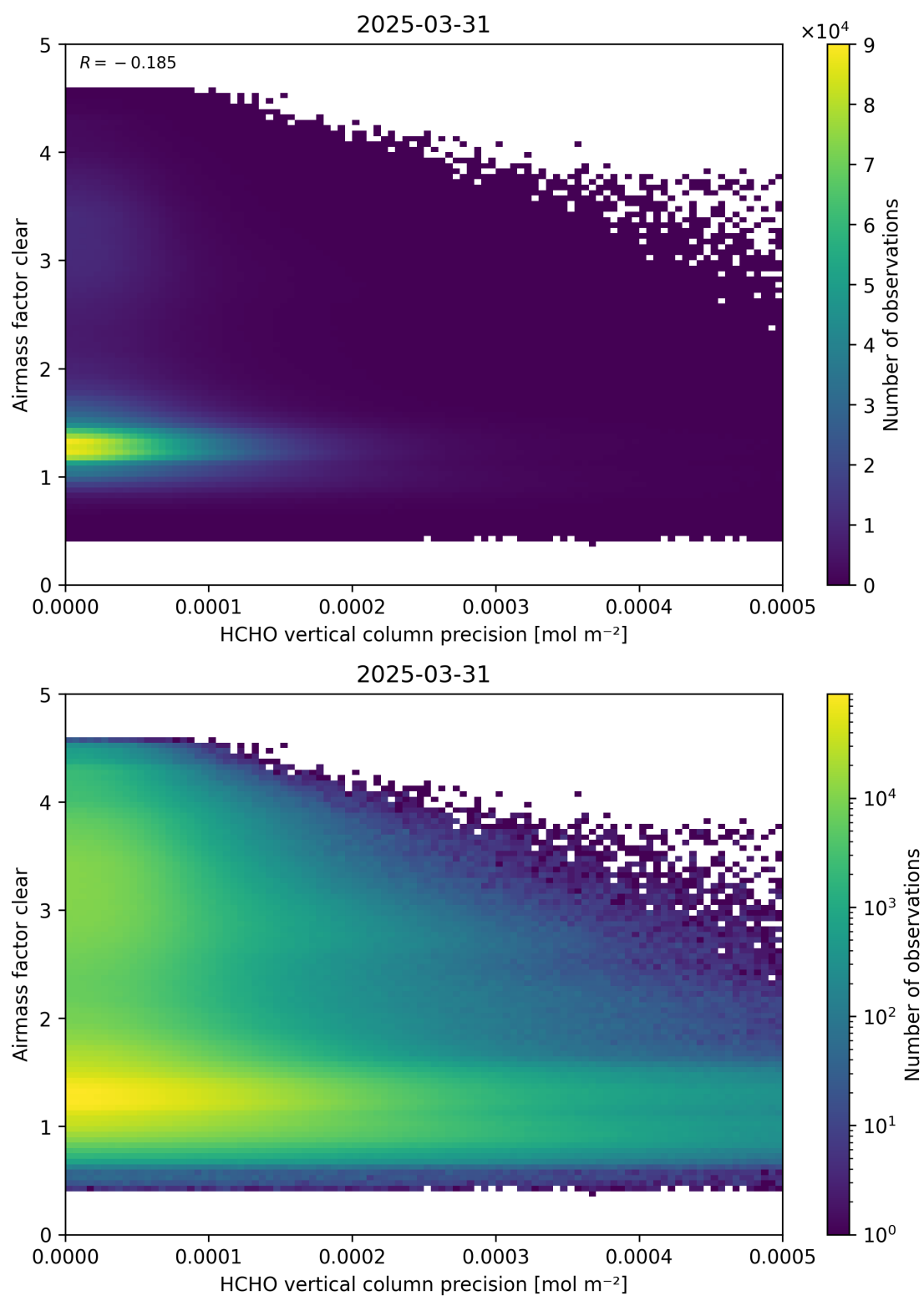
Figure 139: Scatter density plot of “HCHO vertical column precision” against “Airmass factor clear” for 2025-03-30 to 2025-04-01.
