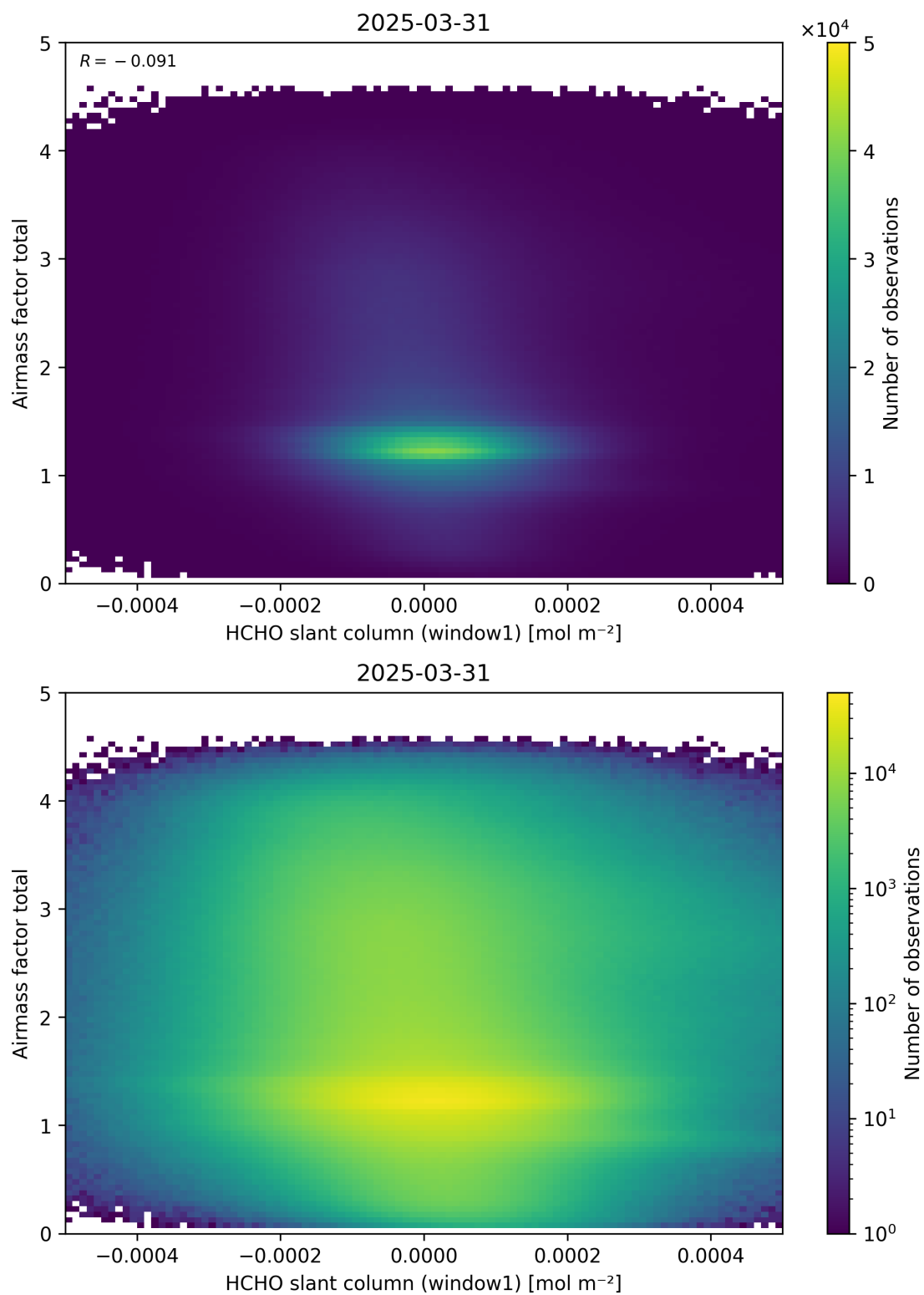
Figure 85: Scatter density plot of “HCHO slant column (window1)” against “Airmass factor total” for 2025-03-30 to 2025-04-01.
