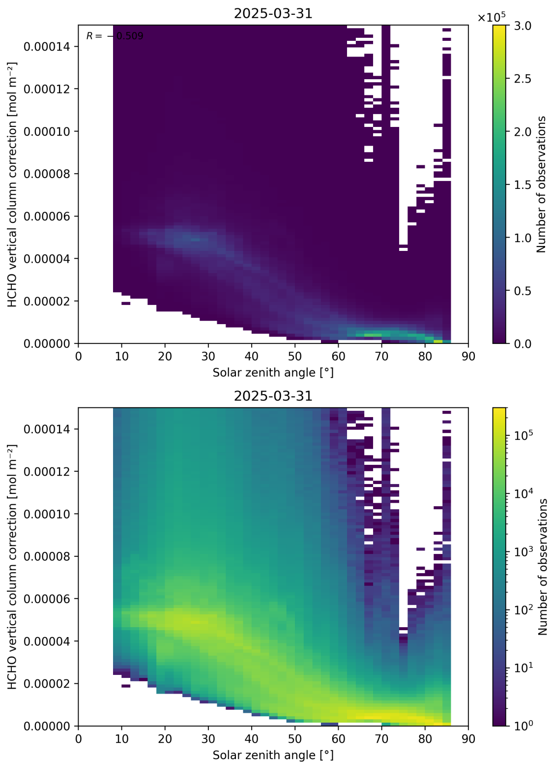
Figure 178: Scatter density plot of “Solar zenith angle” against “HCHO vertical column correction” for 2025-03-30 to 2025-04-01.
