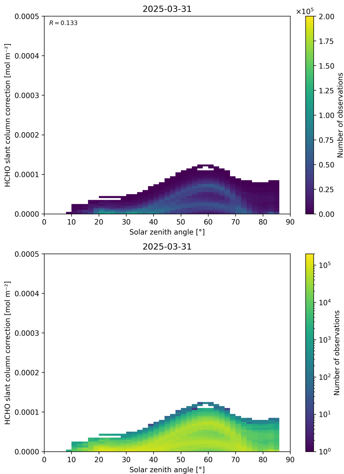
Figure 172: Scatter density plot of “Solar zenith angle” against “HCHO slant column correction” for 2025-03-30 to 2025-04-01.
