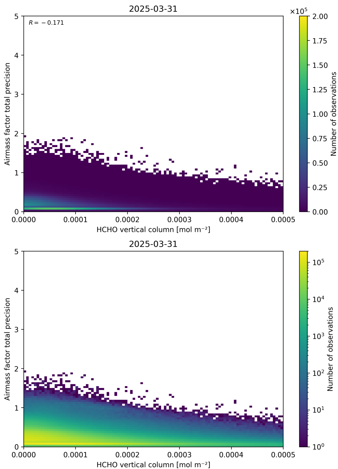
Figure 132: Scatter density plot of “HCHO vertical column” against “Airmass factor total precision” for 2025-03-30 to 2025-04-01.
