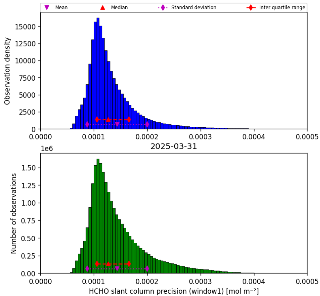
Figure 39: Histogram of “HCHO slant column precision (window1)” for 2025-03-30 to 2025-04-01
