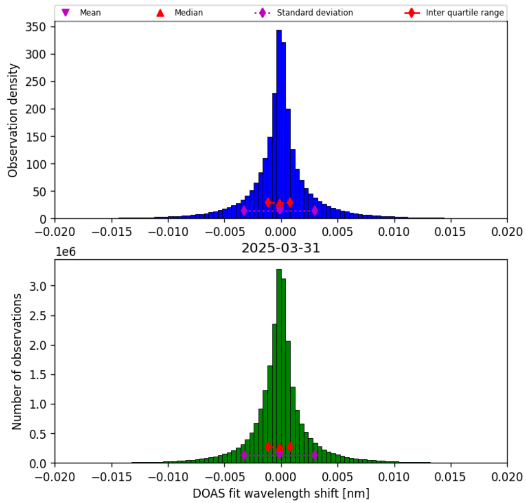
Figure 44: Histogram of “DOAS fit wavelength shift” for 2025-03-30 to 2025-04-01
