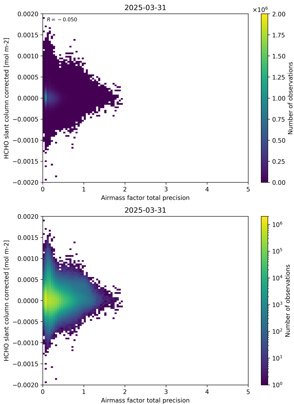
Figure 109: Scatter density plot of “Airmass factor total precision” against “HCHO slant column corrected” for 2025-03-30 to 2025-04-01.
