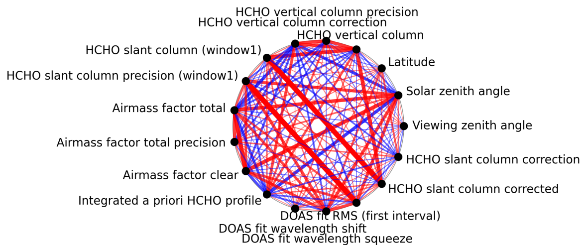
Figure 1: Map of correlation graph for 2025-03-30 to 2025-04-01.
