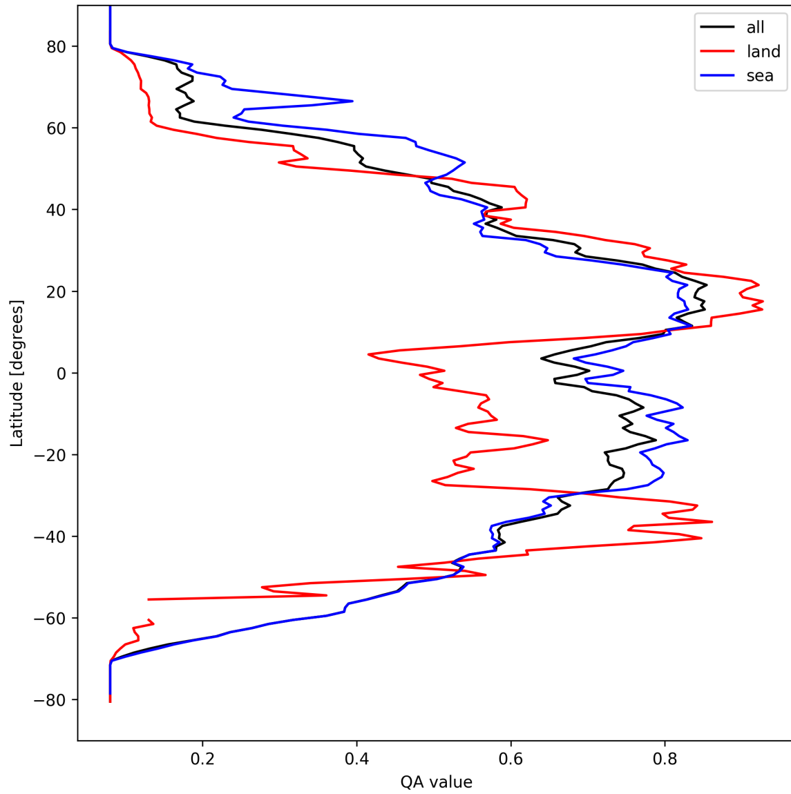
Figure 20: Zonal average of “QA value” for 2025-03-30 to 2025-04-01.
