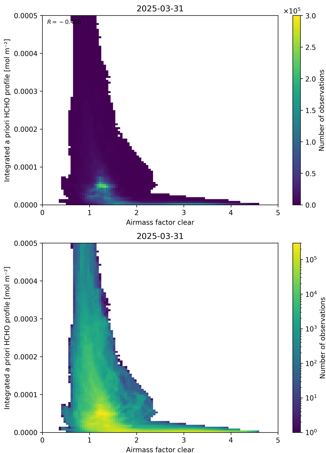
Figure 76: Scatter density plot of “Airmass factor clear” against “Integrated a priori HCHO profile” for 2025-03-30 to 2025-04-01.
