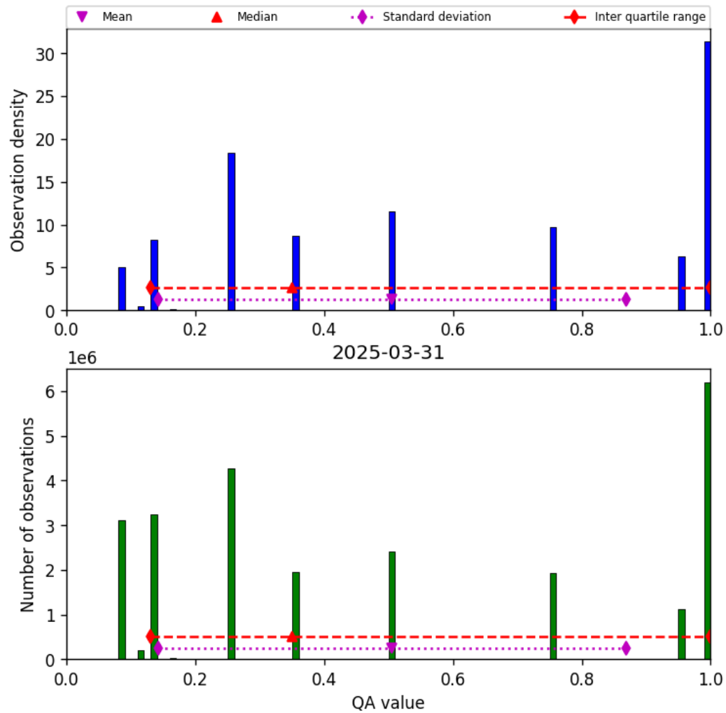
Figure 34: Histogram of “QA value” for 2025-03-30 to 2025-04-01
