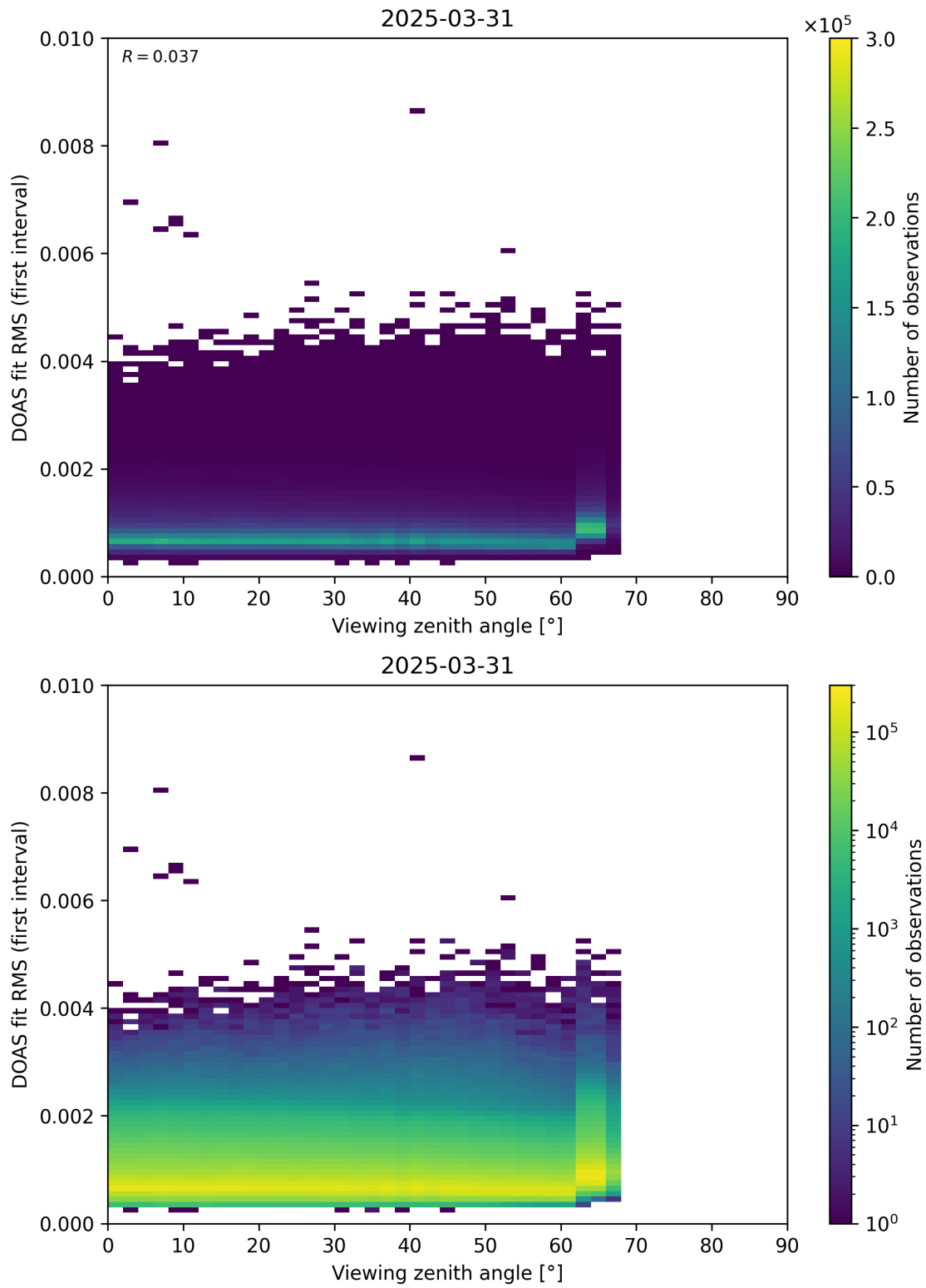
Figure 182: Scatter density plot of “Viewing zenith angle” against “DOAS fit RMS (first interval)” for 2025-03-30 to 2025-04-01.
