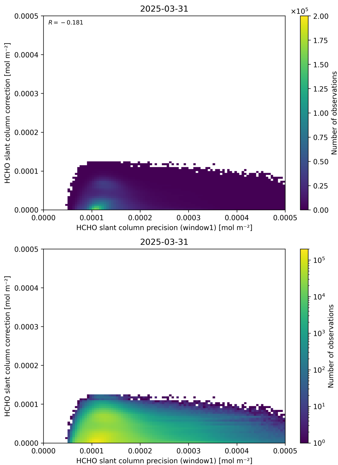
Figure 93: Scatter density plot of “HCHO slant column precision (window1)” against “HCHO slant column correction” for 2025-03-30 to 2025-04-01.
