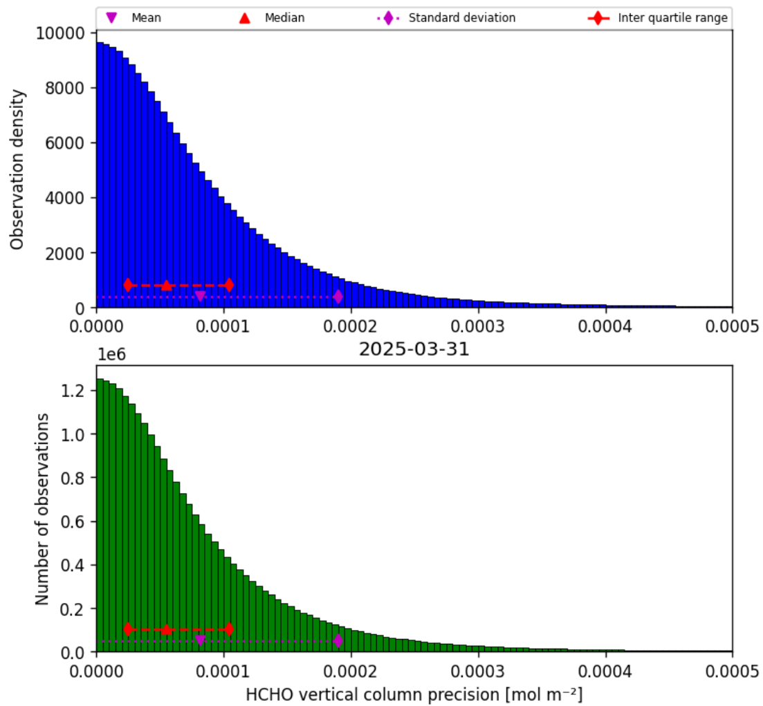
Figure 36: Histogram of “HCHO vertical column precision” for 2025-03-30 to 2025-04-01
