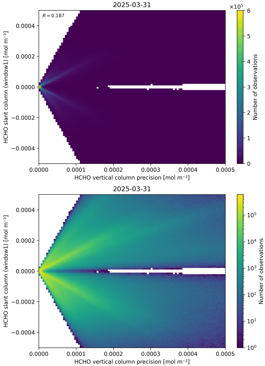
Figure 142: Scatter density plot of “HCHO vertical column precision” against “HCHO slant column (window1)” for 2025-03-30 to 2025-04-01.
