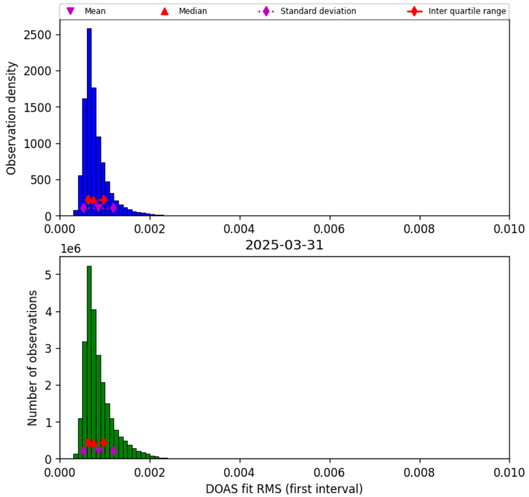
Figure 46: Histogram of “DOAS fit RMS (first interval)” for 2025-03-30 to 2025-04-01
