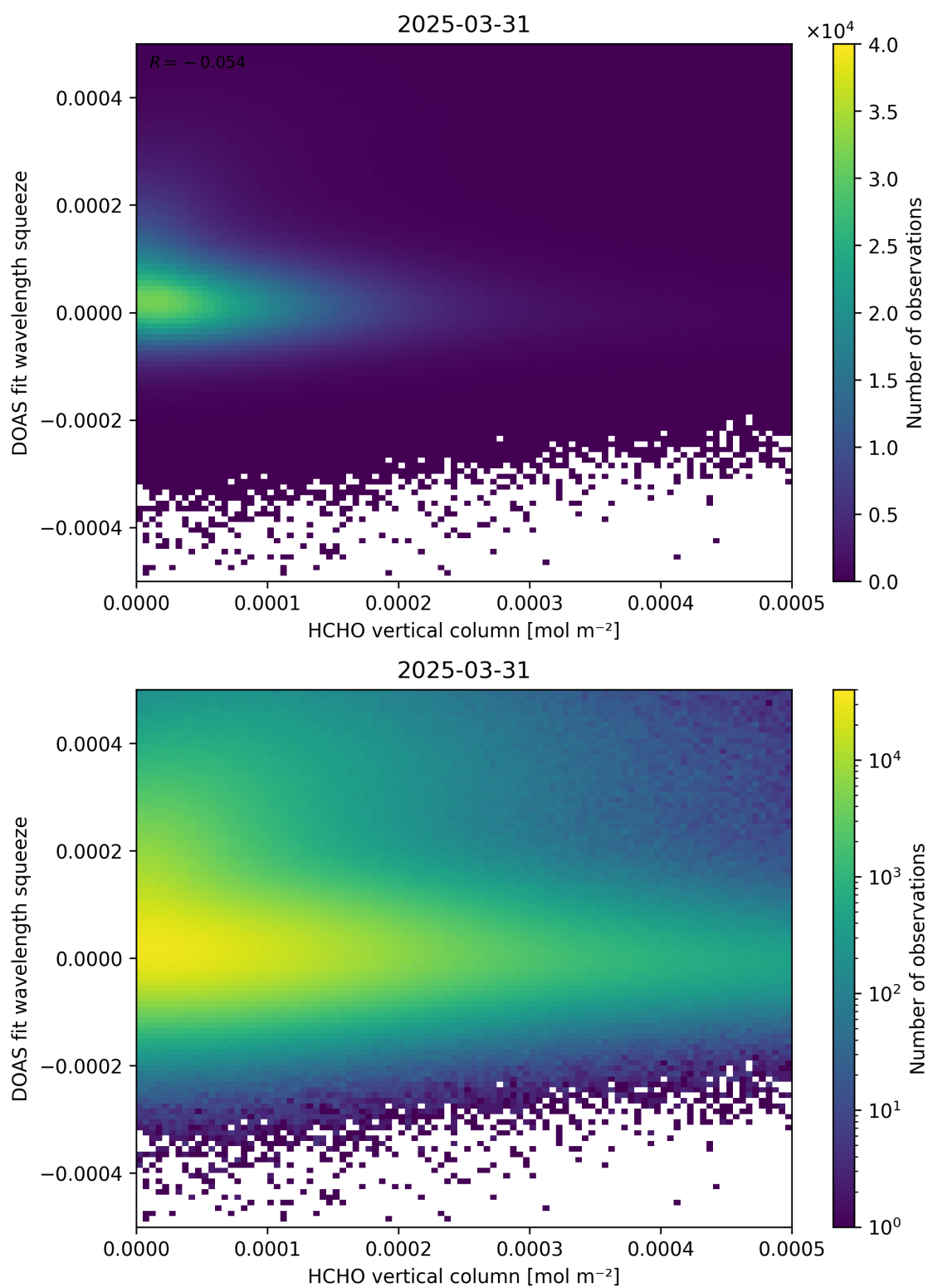
Figure 125: Scatter density plot of “HCHO vertical column” against “DOAS fit wavelength squeeze” for 2025-03-30 to 2025-04-01.
