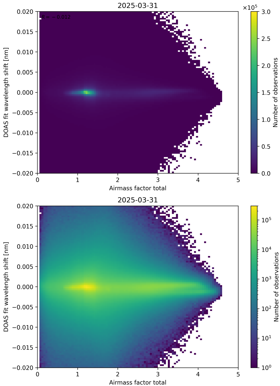
Figure 98: Scatter density plot of “Airmass factor total” against “DOAS fit wavelength shift” for 2025-03-30 to 2025-04-01.
