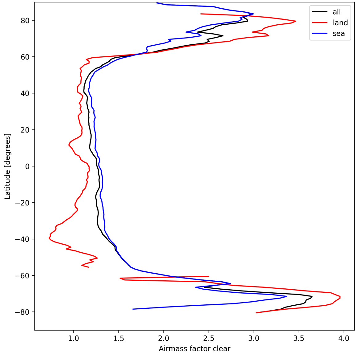
Figure 28: Zonal average of “Airmass factor clear” for 2025-03-30 to 2025-04-01.
