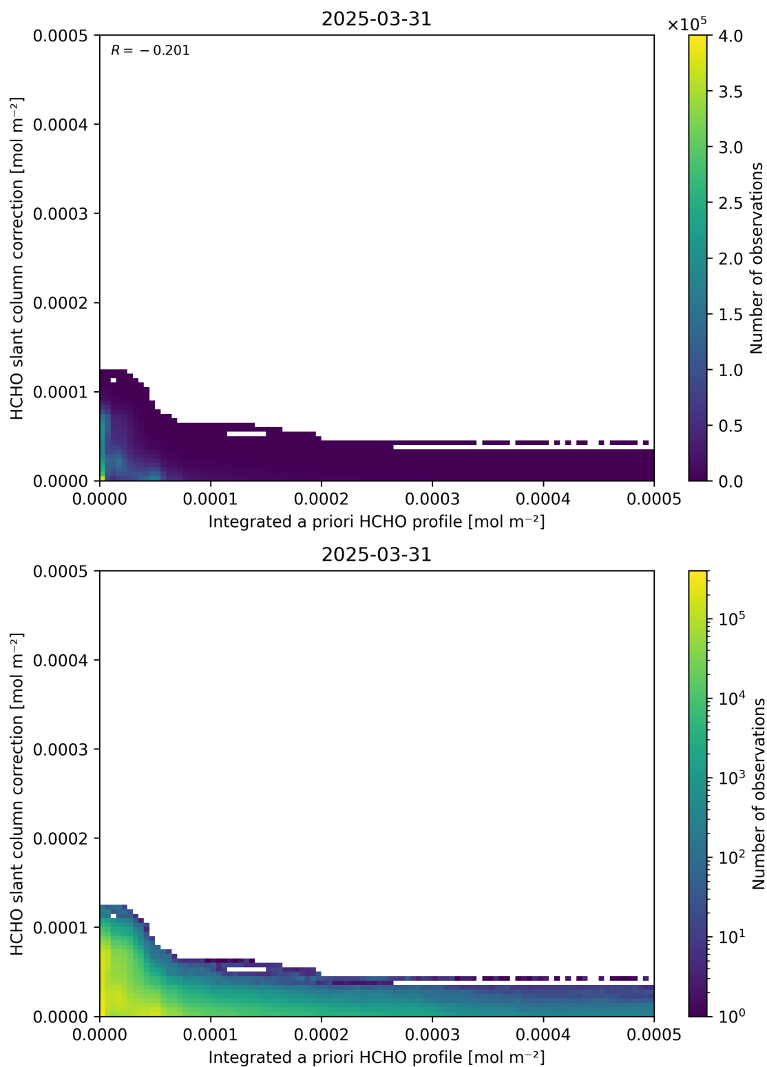
Figure 152: Scatter density plot of “Integrated a priori HCHO profile” against “HCHO slant column correction” for 2025-03-30 to 2025-04-01.
