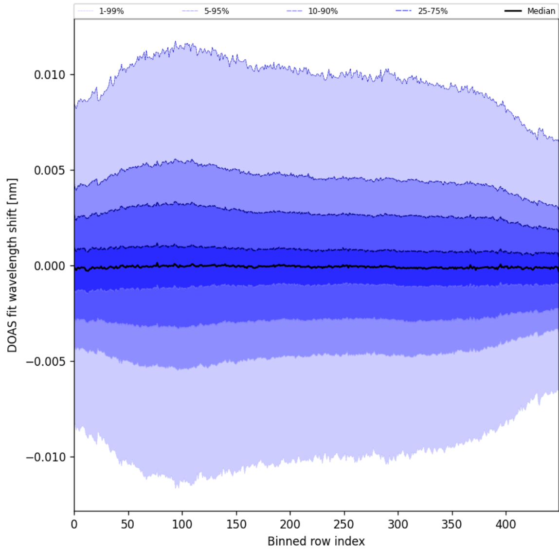
Figure 58: Along track statistics of “DOAS fit wavelength shift” for 2025-03-31 to 2025-04-02
