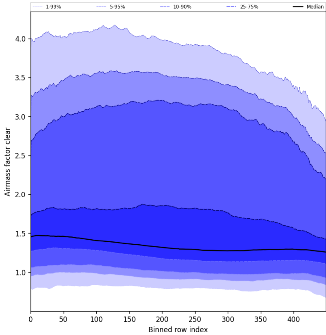
Figure 56: Along track statistics of “Airmass factor clear” for 2025-03-31 to 2025-04-02
