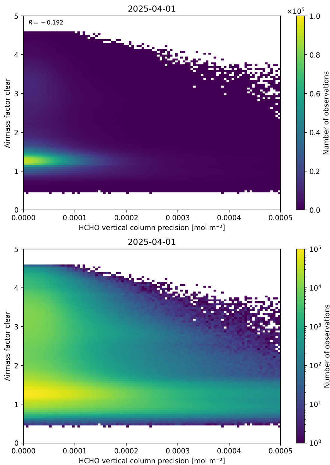
Figure 139: Scatter density plot of “HCHO vertical column precision” against “Airmass factor clear” for 2025-03-31 to 2025-04-02.
