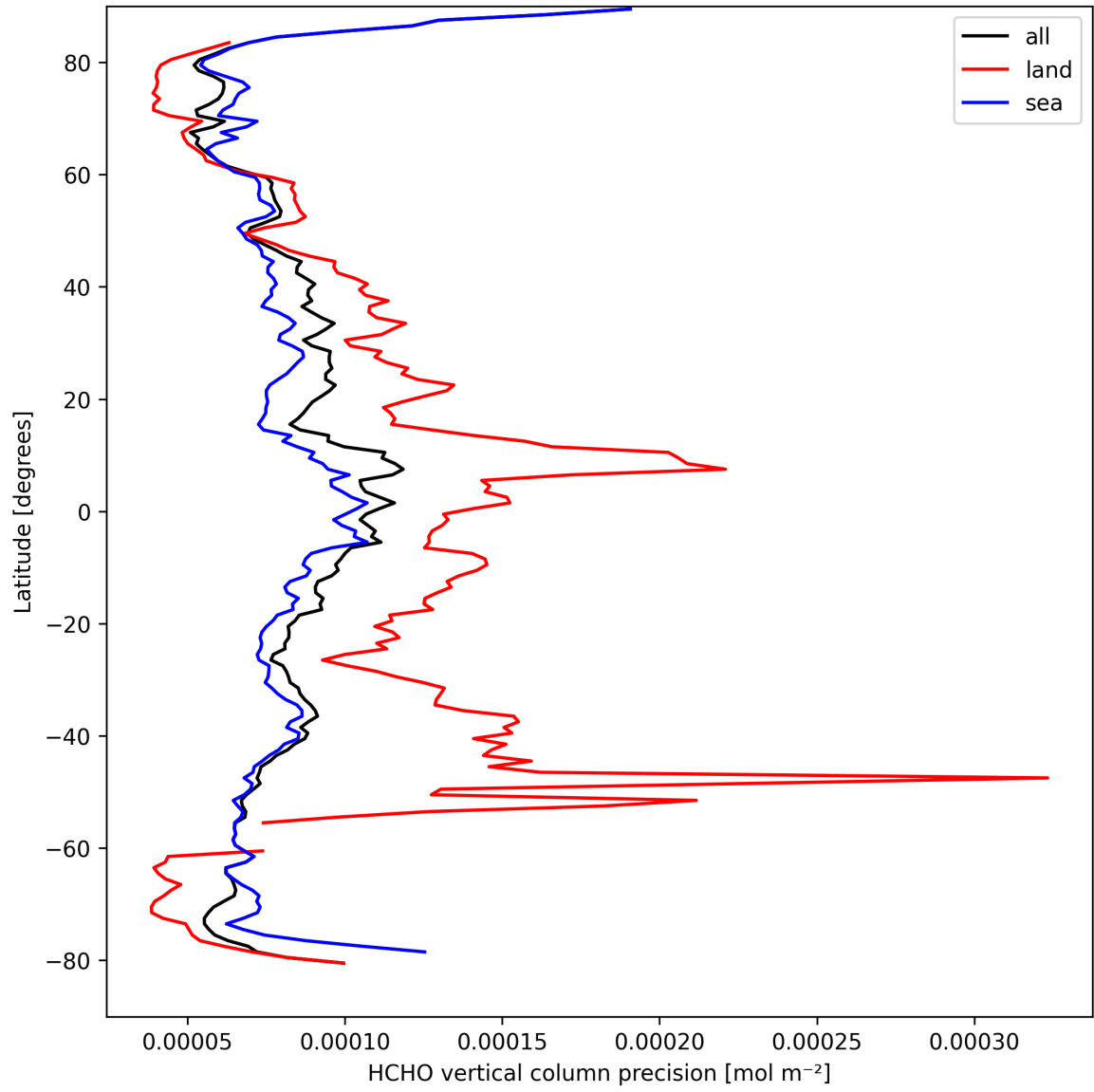
Figure 22: Zonal average of "HCHO vertical column precision" for 2025-03-31 to 2025-04-02.
