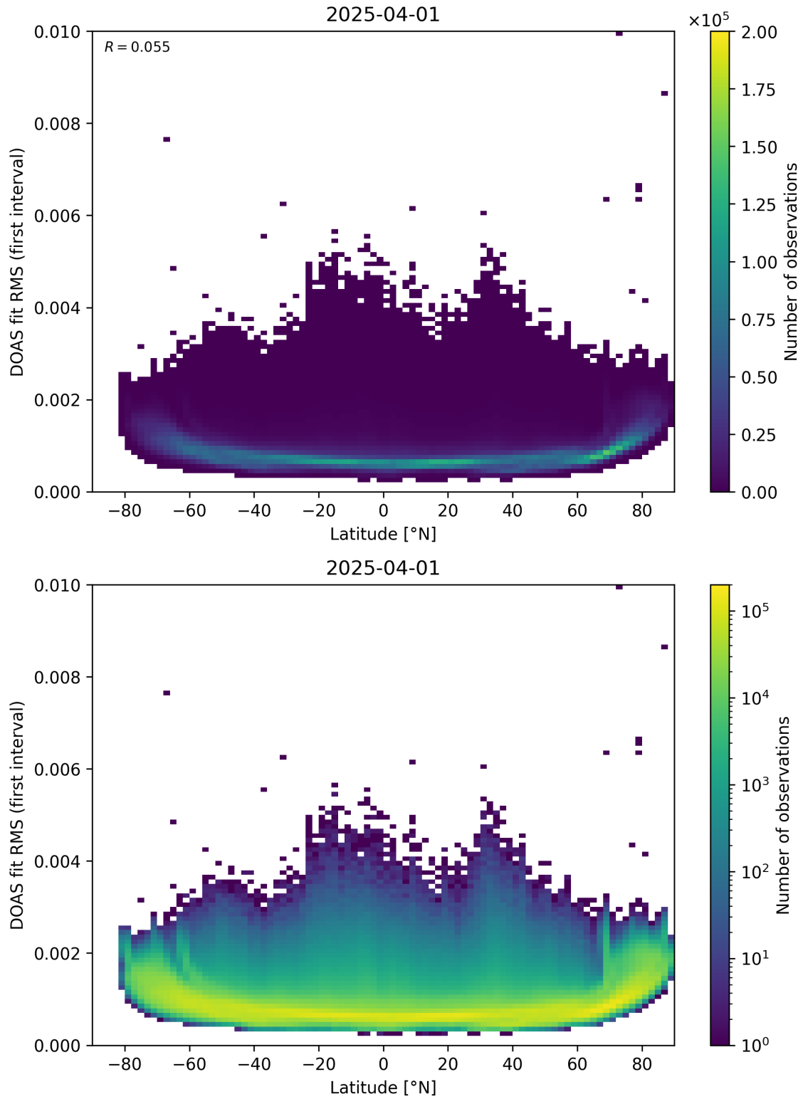
Figure 153: Scatter density plot of “Latitude” against “DOAS fit RMS (first interval)” for 2025-03-31 to 2025-04-02.
