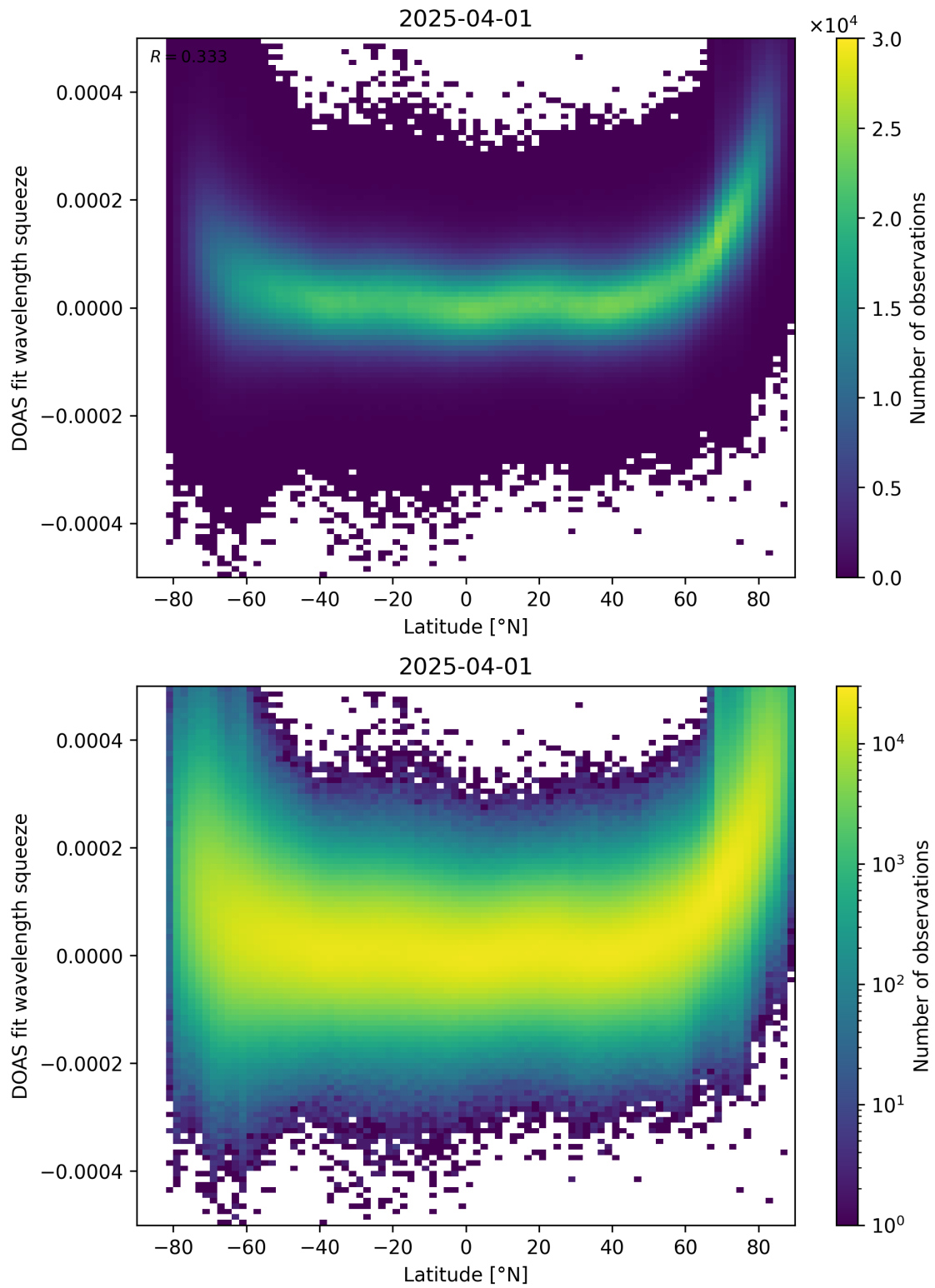
Figure 155: Scatter density plot of “Latitude” against “DOAS fit wavelength squeeze” for 2025-03-31 to 2025-04-02.
