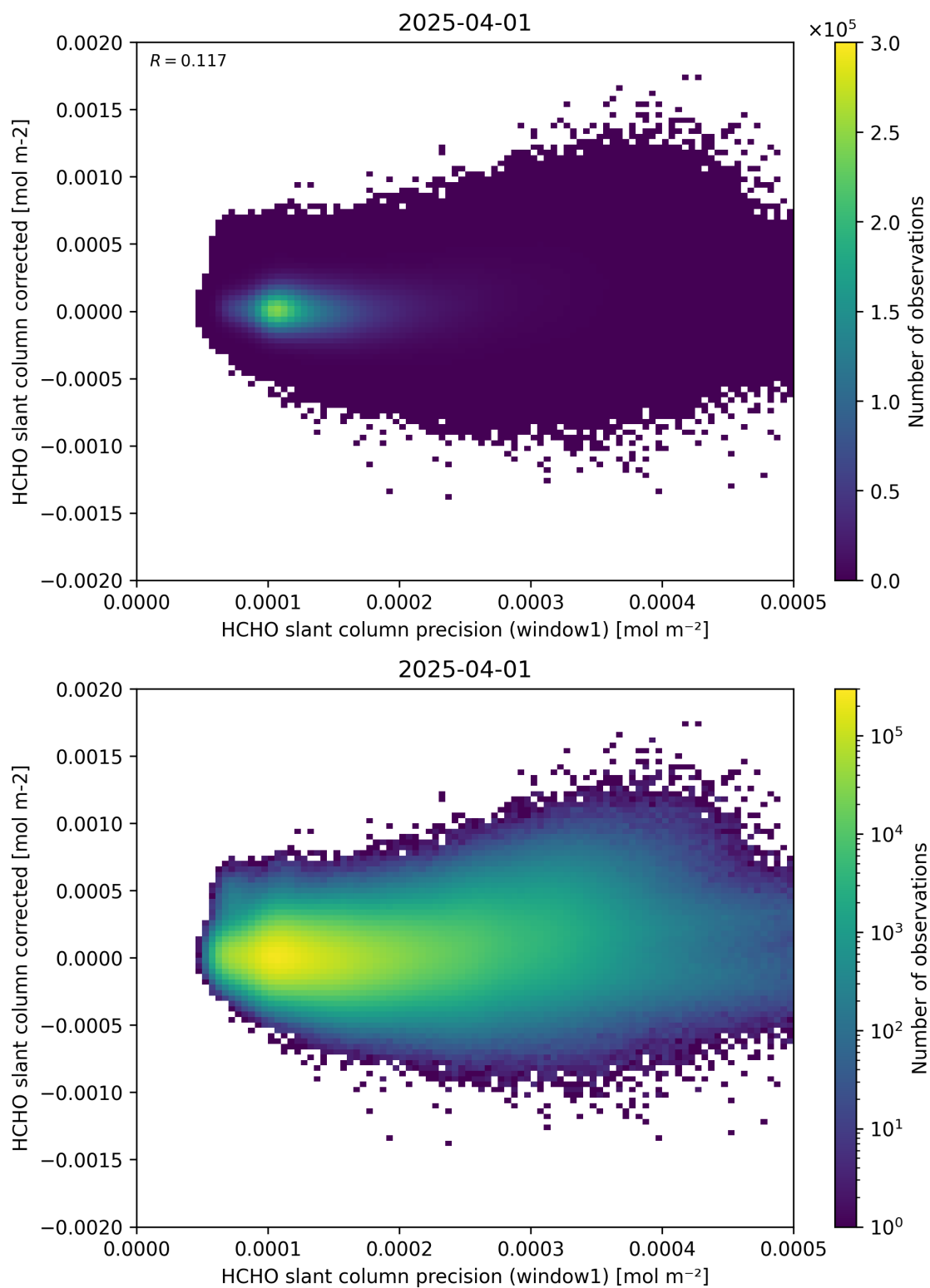
Figure 92: Scatter density plot of “HCHO slant column precision (window1)” against “HCHO slant column corrected” for 2025-03-31 to 2025-04-02.
