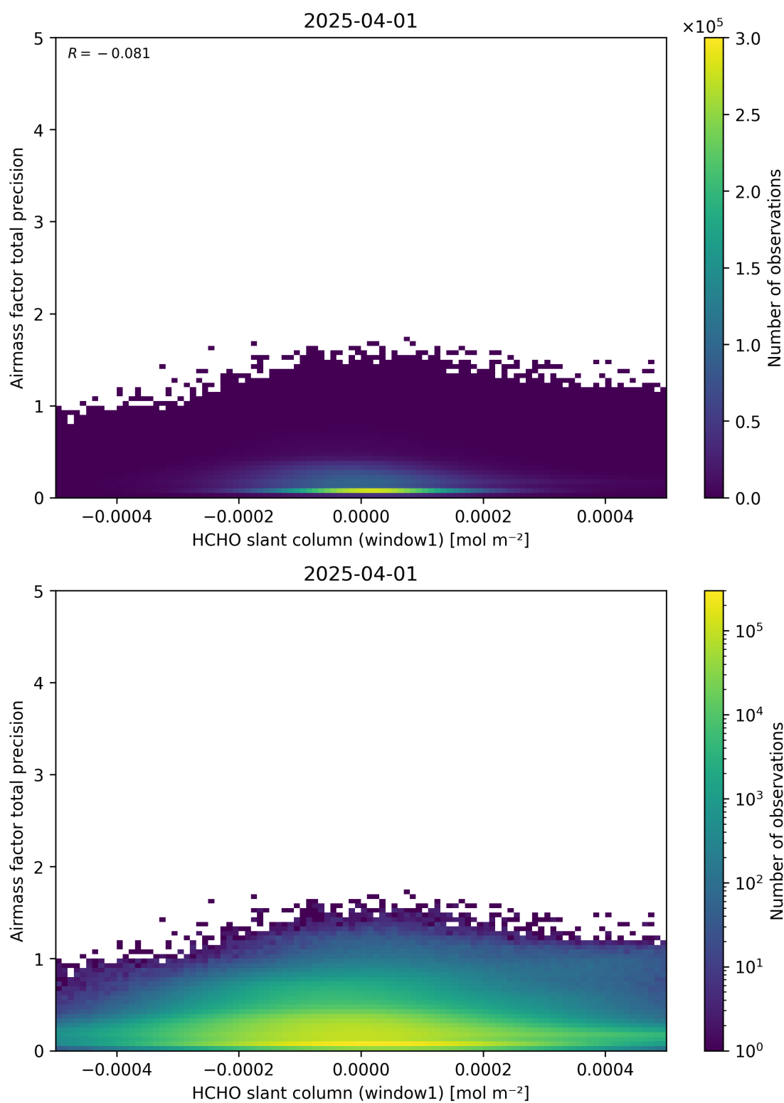
Figure 86: Scatter density plot of “HCHO slant column (window1)” against “Airmass factor total precision” for 2025-03-31 to 2025-04-02.
