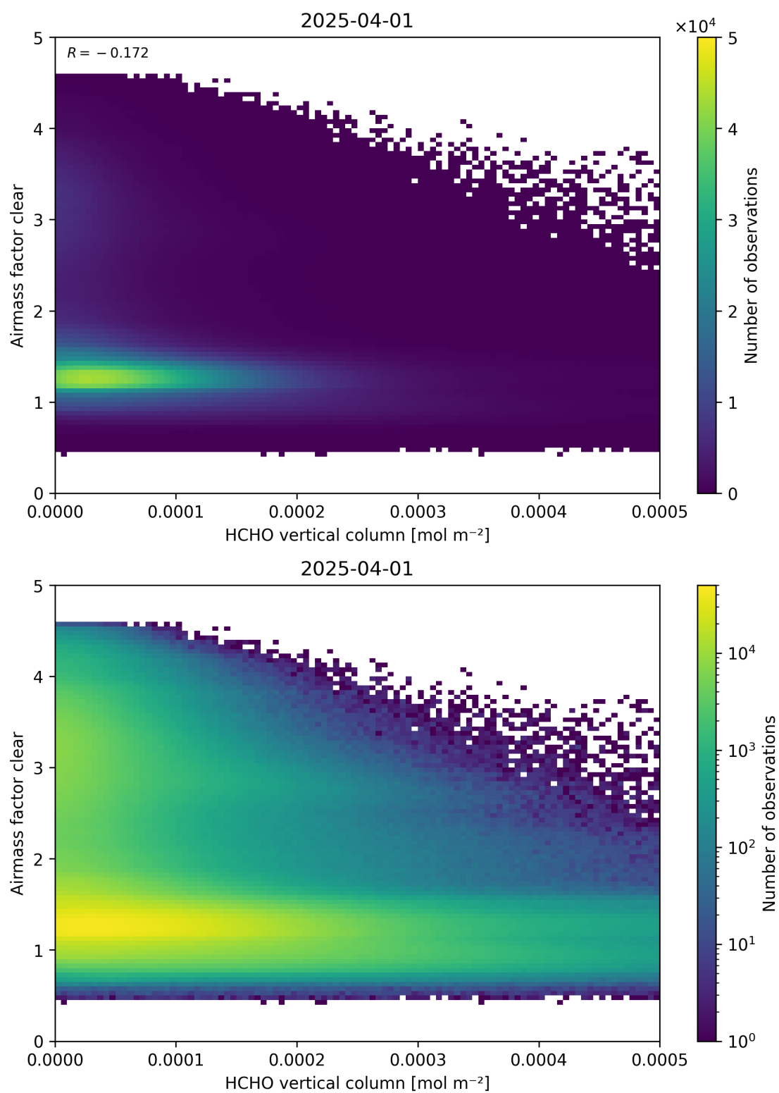
Figure 126: Scatter density plot of “HCHO vertical column” against “Airmass factor clear” for 2025-03-31 to 2025-04-02.
