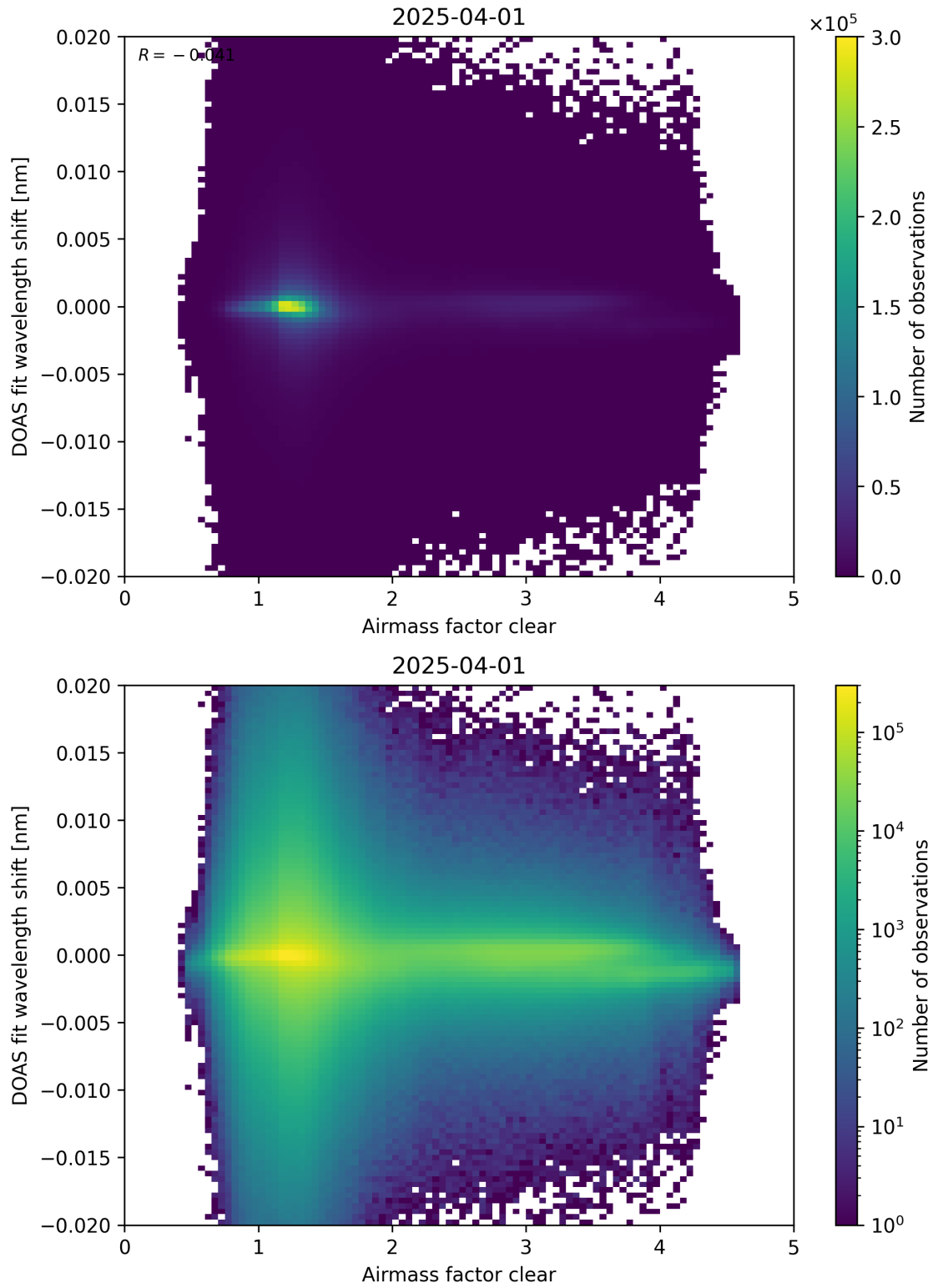
Figure 72: Scatter density plot of “Airmass factor clear” against “DOAS fit wavelength shift” for 2025-03-31 to 2025-04-02.
