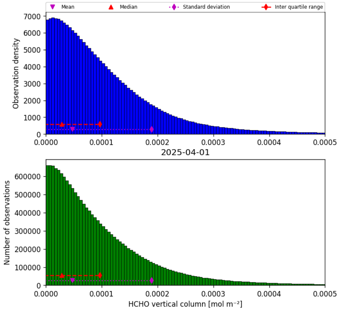
Figure 35: Histogram of “HCHO vertical column” for 2025-03-31 to 2025-04-02
