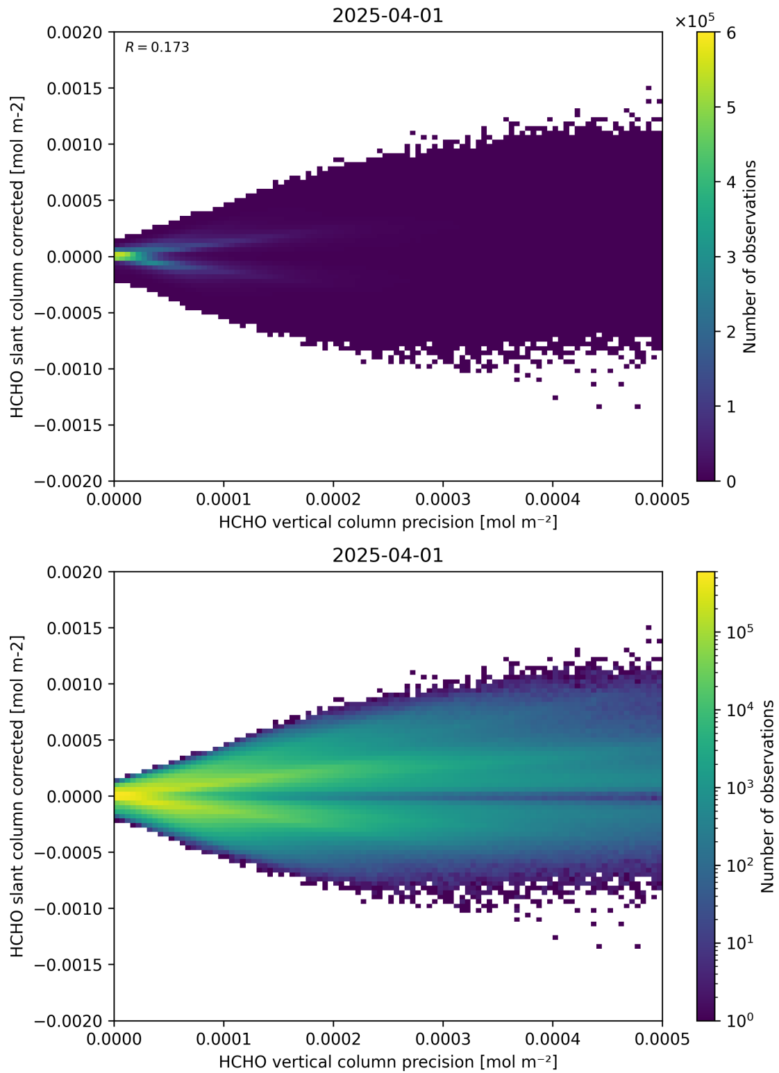
Figure 140: Scatter density plot of “HCHO vertical column precision” against “HCHO slant column corrected” for 2025-03-31 to 2025-04-02.
