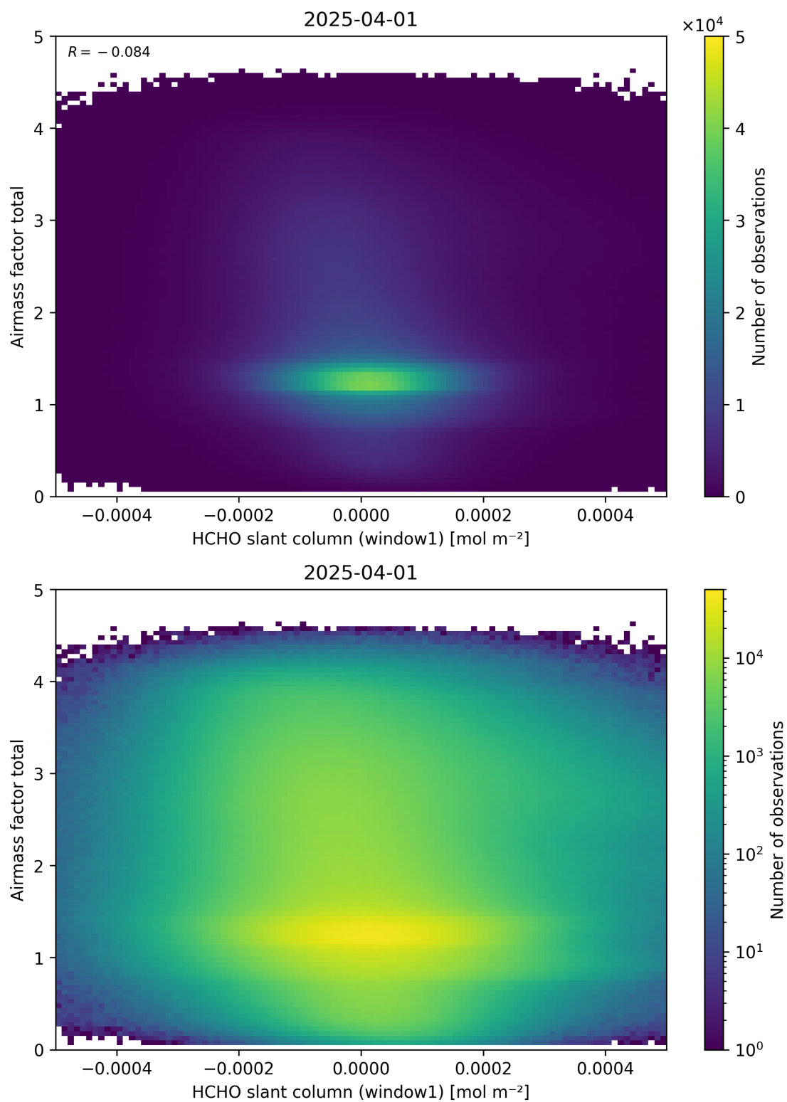
Figure 85: Scatter density plot of “HCHO slant column (window1)” against “Airmass factor total” for 2025-03-31 to 2025-04-02.
