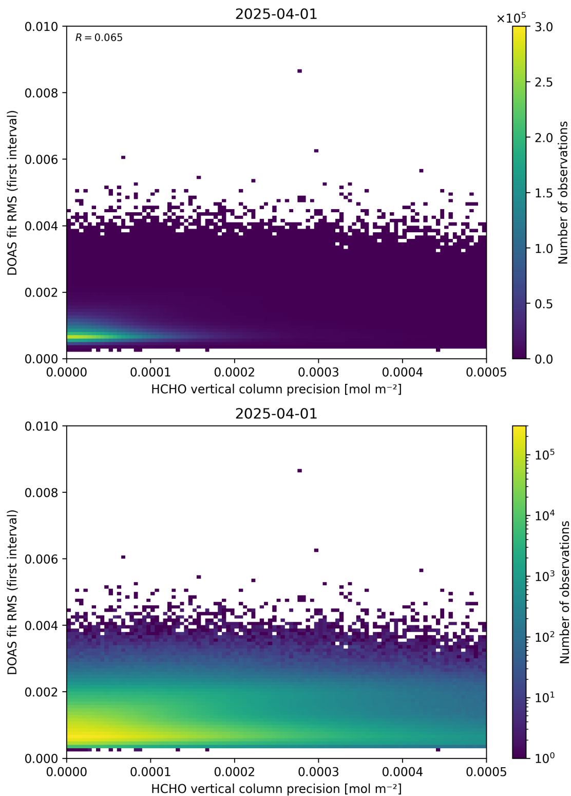
Figure 136: Scatter density plot of “HCHO vertical column precision” against “DOAS fit RMS (first interval)” for 2025-03-31 to 2025-04-02.
