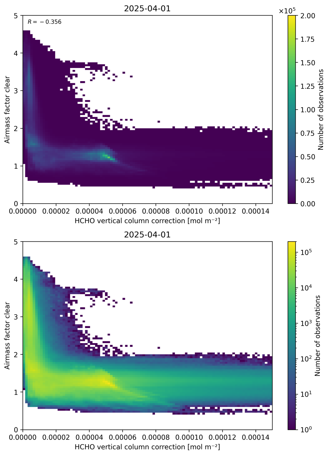
Figure 115: Scatter density plot of “HCHO vertical column correction” against “Airmass factor clear” for 2025-03-31 to 2025-04-02.
