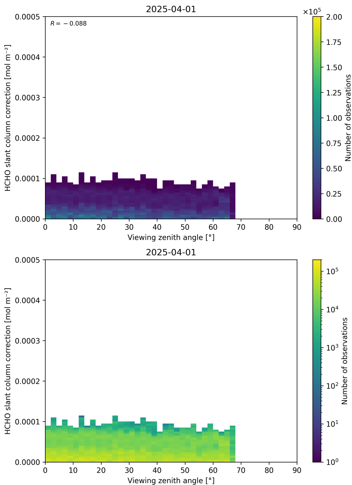
Figure 187: Scatter density plot of “Viewing zenith angle” against “HCHO slant column correction” for 2025-03-31 to 2025-04-02.
