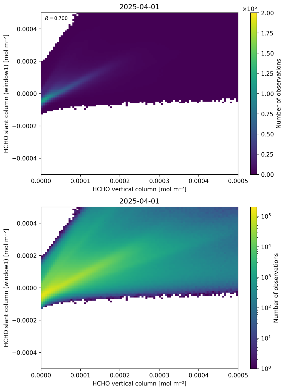
Figure 129: Scatter density plot of “HCHO vertical column” against “HCHO slant column (window1)” for 2025-03-31 to 2025-04-02.
