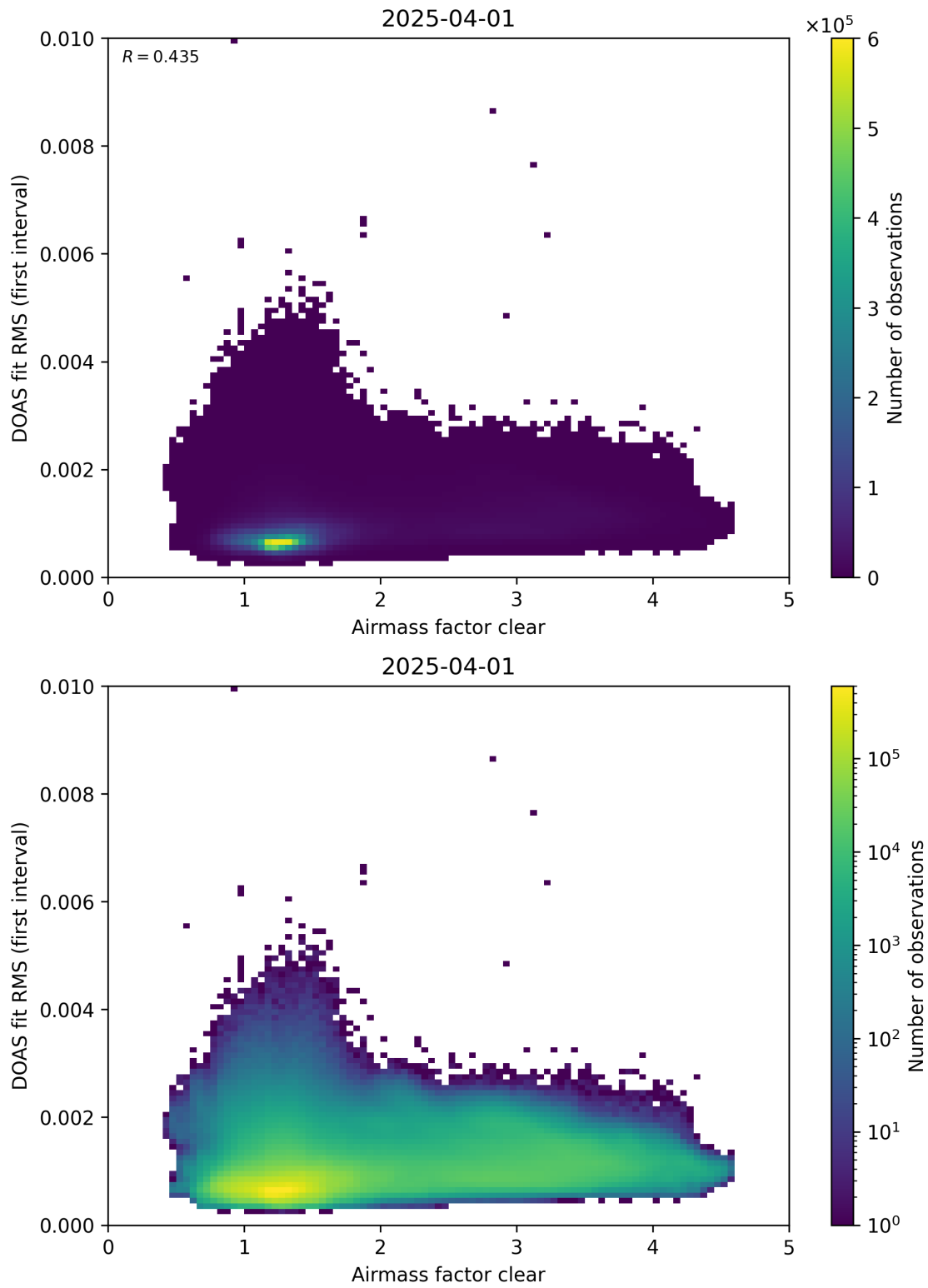
Figure 71: Scatter density plot of “Airmass factor clear” against “DOAS fit RMS (first interval)” for 2025-03-31 to 2025-04-02.
