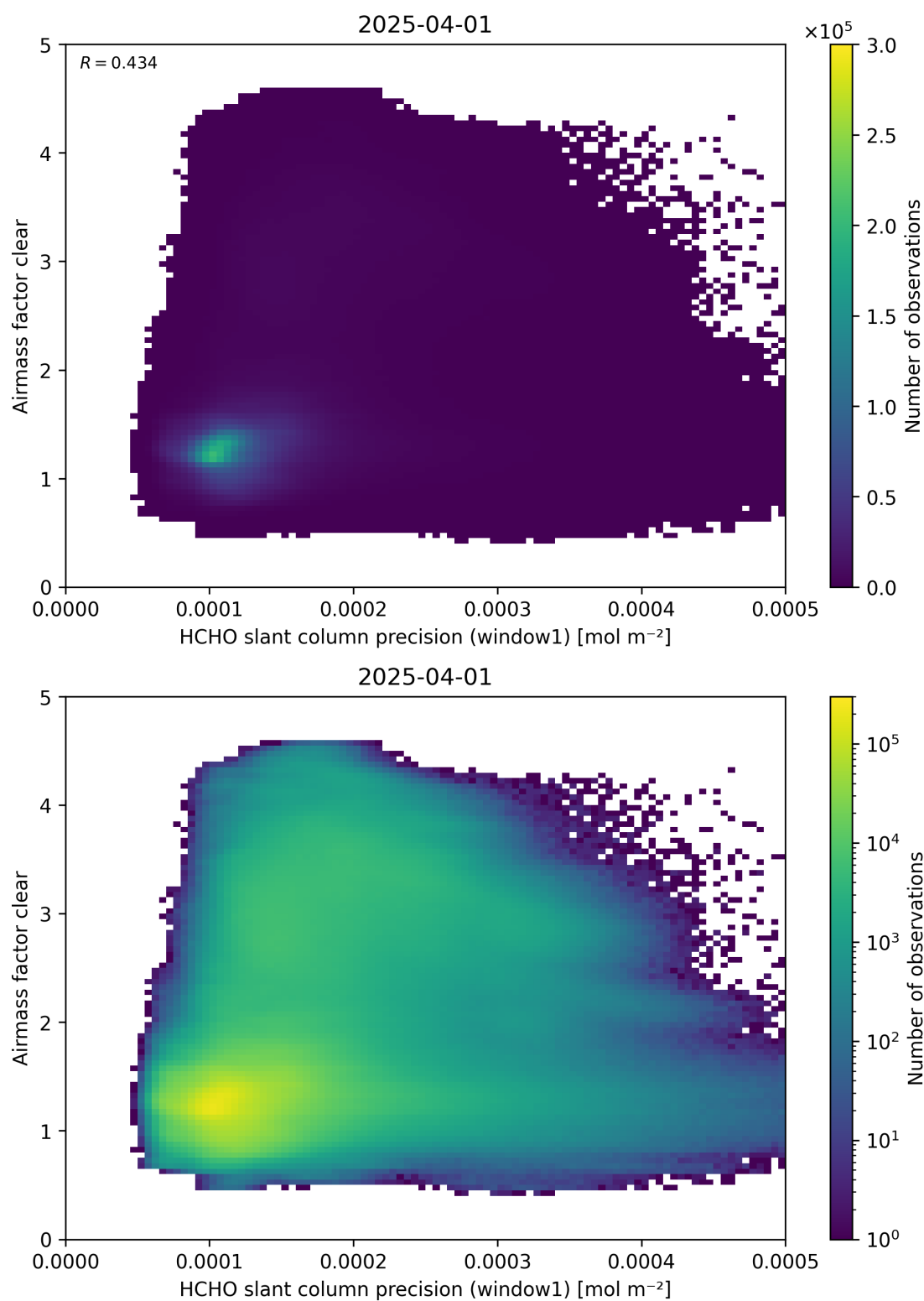
Figure 91: Scatter density plot of “HCHO slant column precision (window1)” against “Airmass factor clear” for 2025-03-31 to 2025-04-02.
