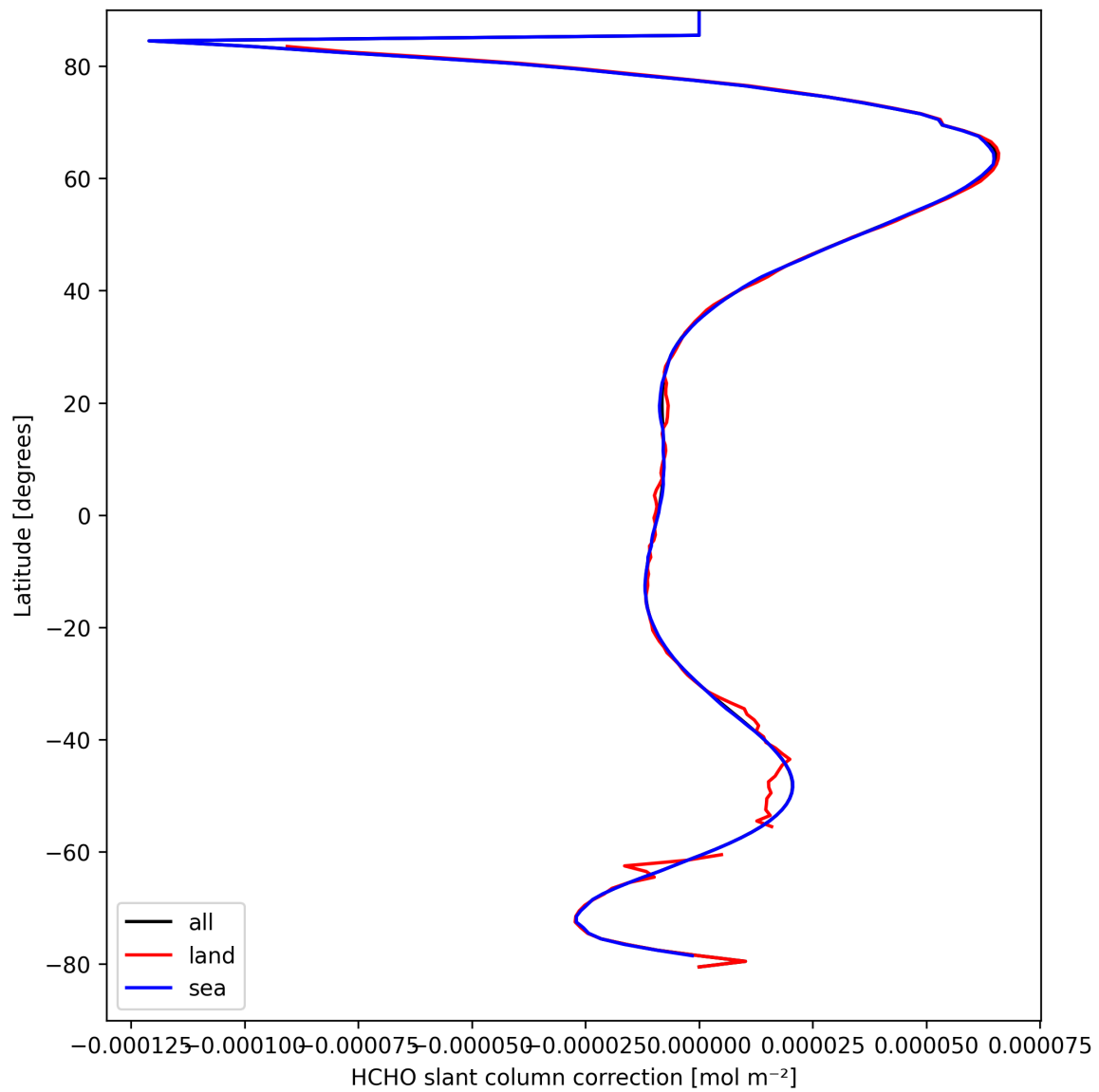
Figure 33: Zonal average of "HCHO slant column correction" for 2025-03-31 to 2025-04-02.
