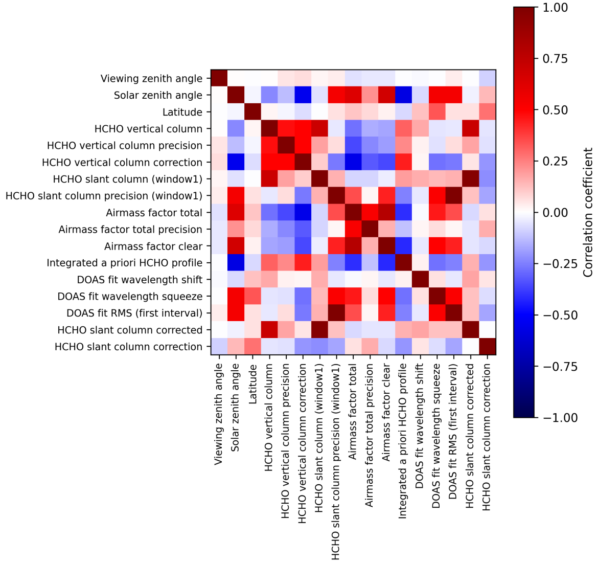
Figure 2: Map of correlation matrix for 2025-03-31 to 2025-04-02.
