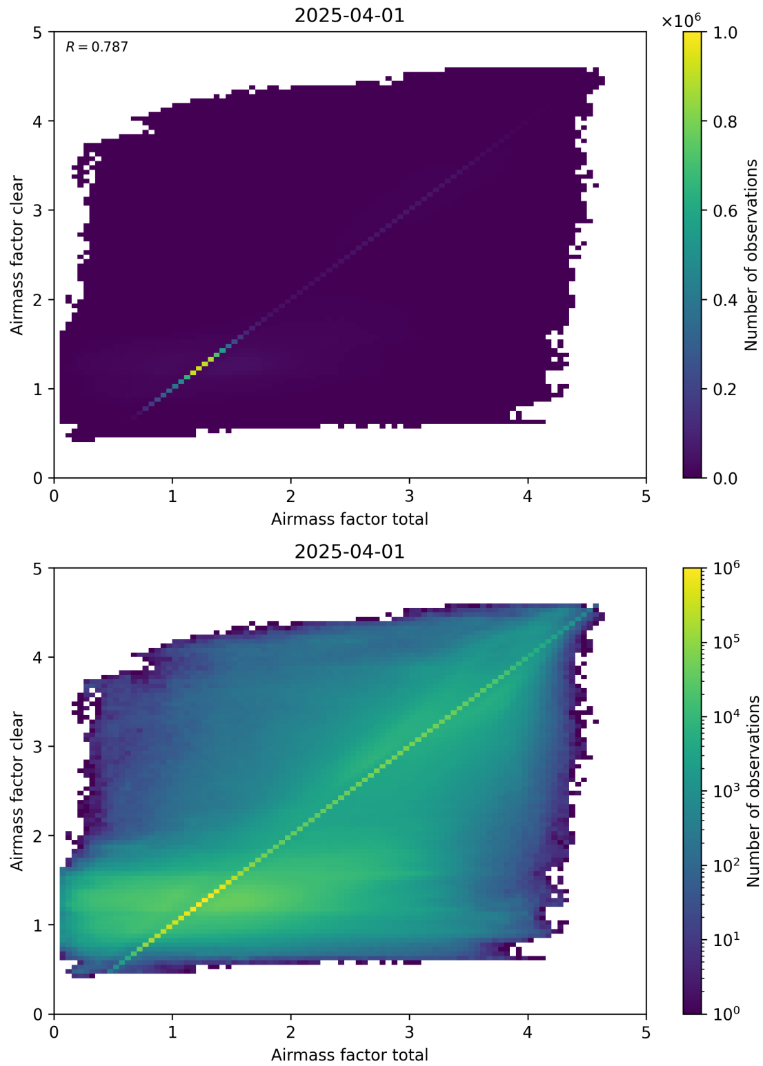
Figure 100: Scatter density plot of “Airmass factor total” against “Airmass factor clear” for 2025-03-31 to 2025-04-02.
