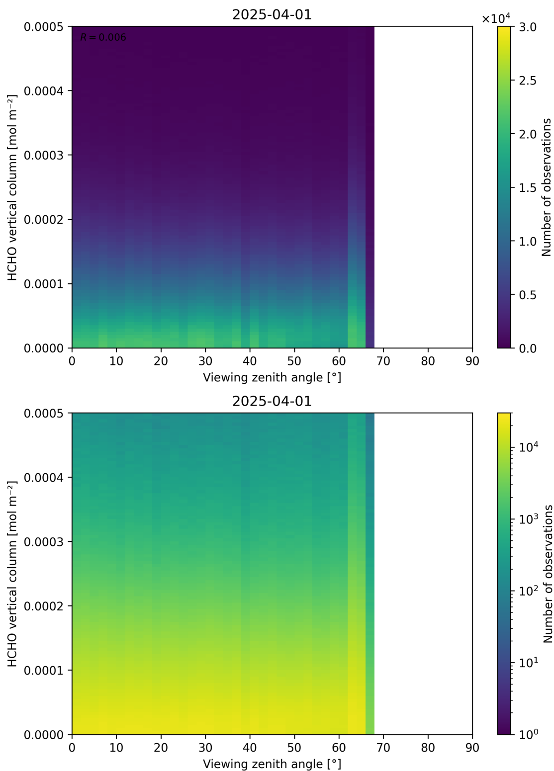
Figure 192: Scatter density plot of “Viewing zenith angle” against “HCHO vertical column” for 2025-03-31 to 2025-04-02.
