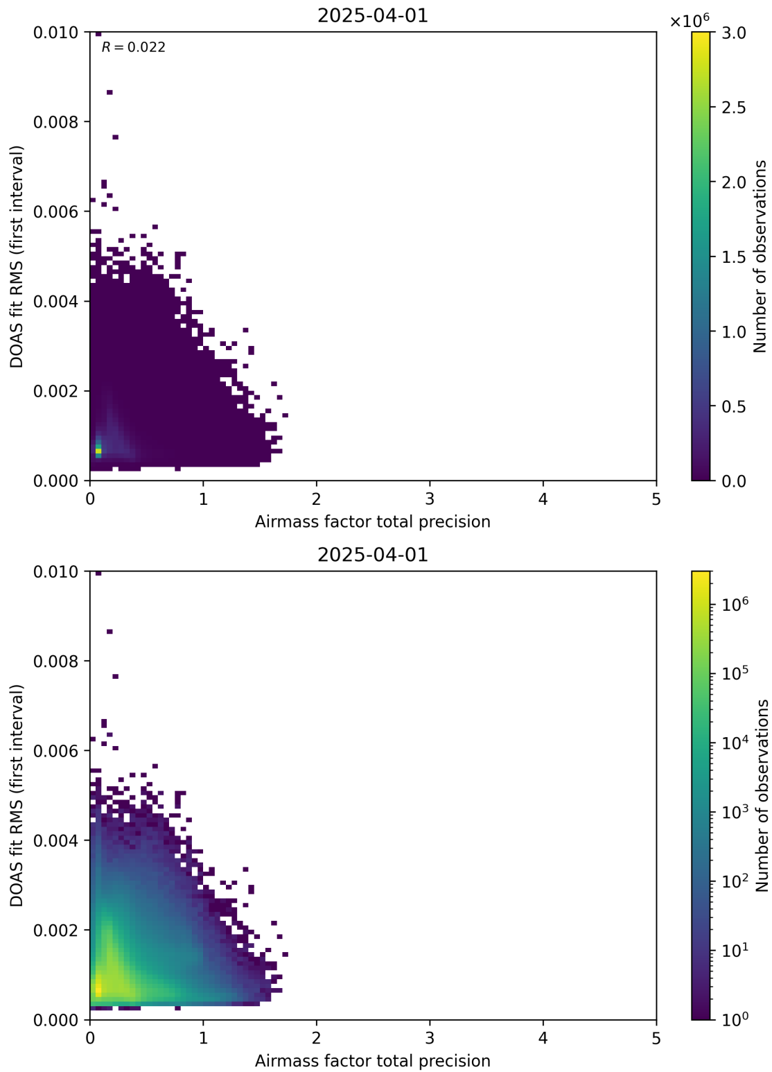
Figure 105: Scatter density plot of “Airmass factor total precision” against “DOAS fit RMS (first interval)” for 2025-03-31 to 2025-04-02.
