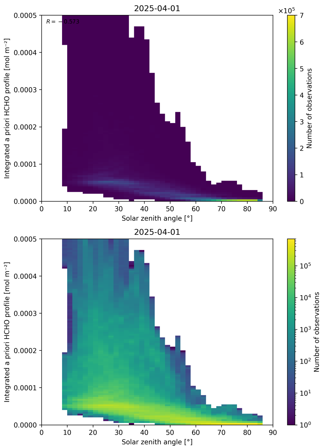
Figure 180: Scatter density plot of “Solar zenith angle” against “Integrated a priori HCHO profile” for 2025-03-31 to 2025-04-02.
