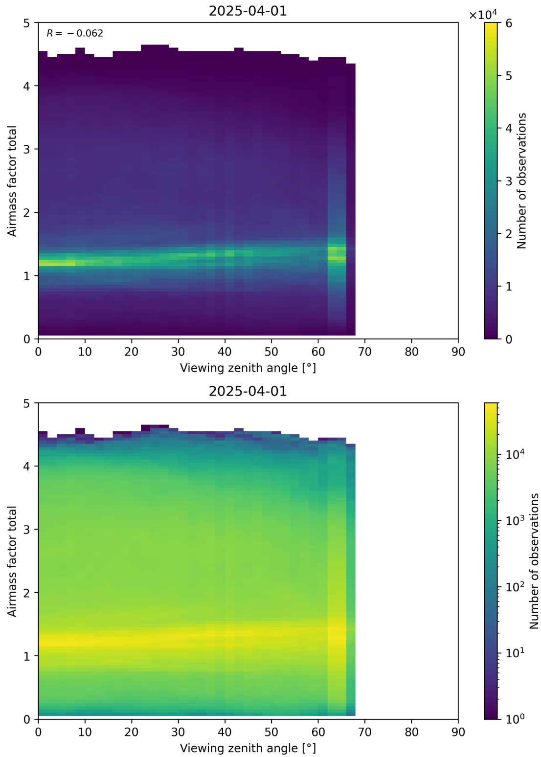
Figure 190: Scatter density plot of “Viewing zenith angle” against “Airmass factor total” for 2025-03-31 to 2025-04-02.
