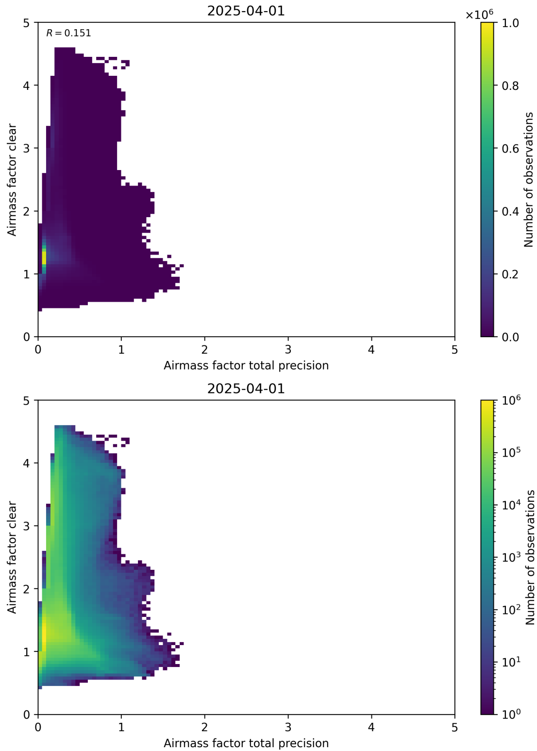
Figure 108: Scatter density plot of “Airmass factor total precision” against “Airmass factor clear” for 2025-03-31 to 2025-04-02.
