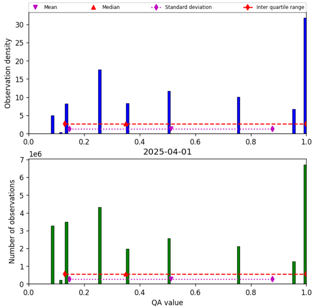
Figure 34: Histogram of “QA value” for 2025-03-31 to 2025-04-02
