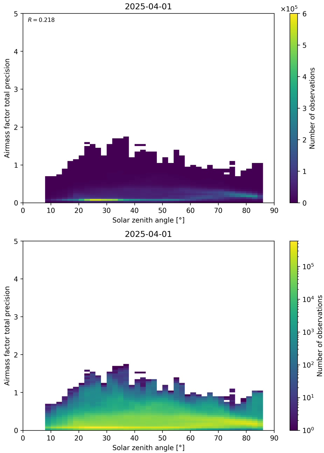
Figure 176: Scatter density plot of “Solar zenith angle” against “Airmass factor total precision” for 2025-03-31 to 2025-04-02.
