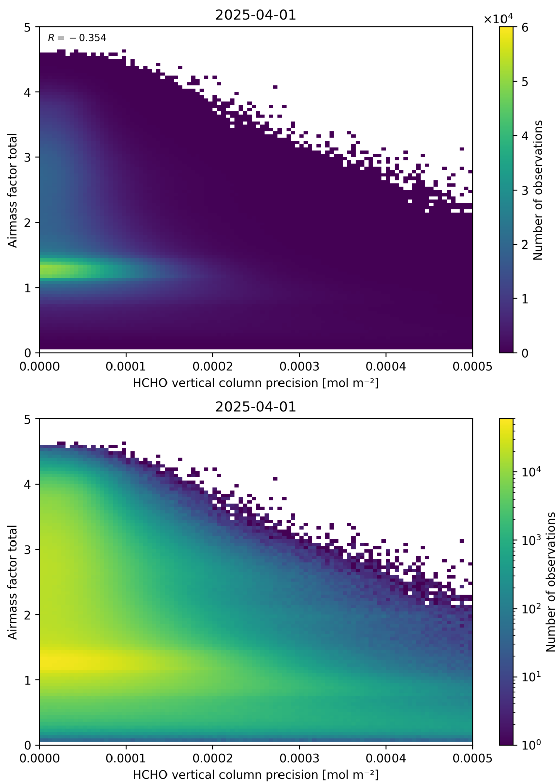
Figure 144: Scatter density plot of “HCHO vertical column precision” against “Airmass factor total” for 2025-03-31 to 2025-04-02.
