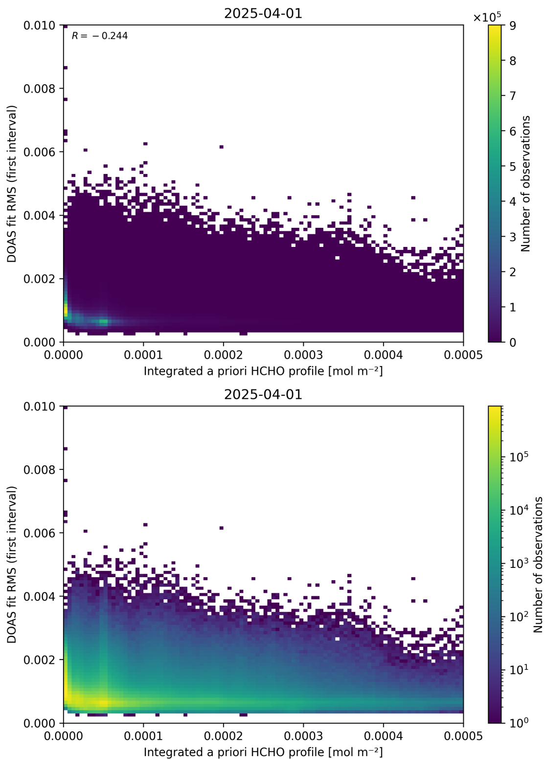
Figure 148: Scatter density plot of “Integrated a priori HCHO profile” against “DOAS fit RMS (first interval)” for 2025-03-31 to 2025-04-02.
