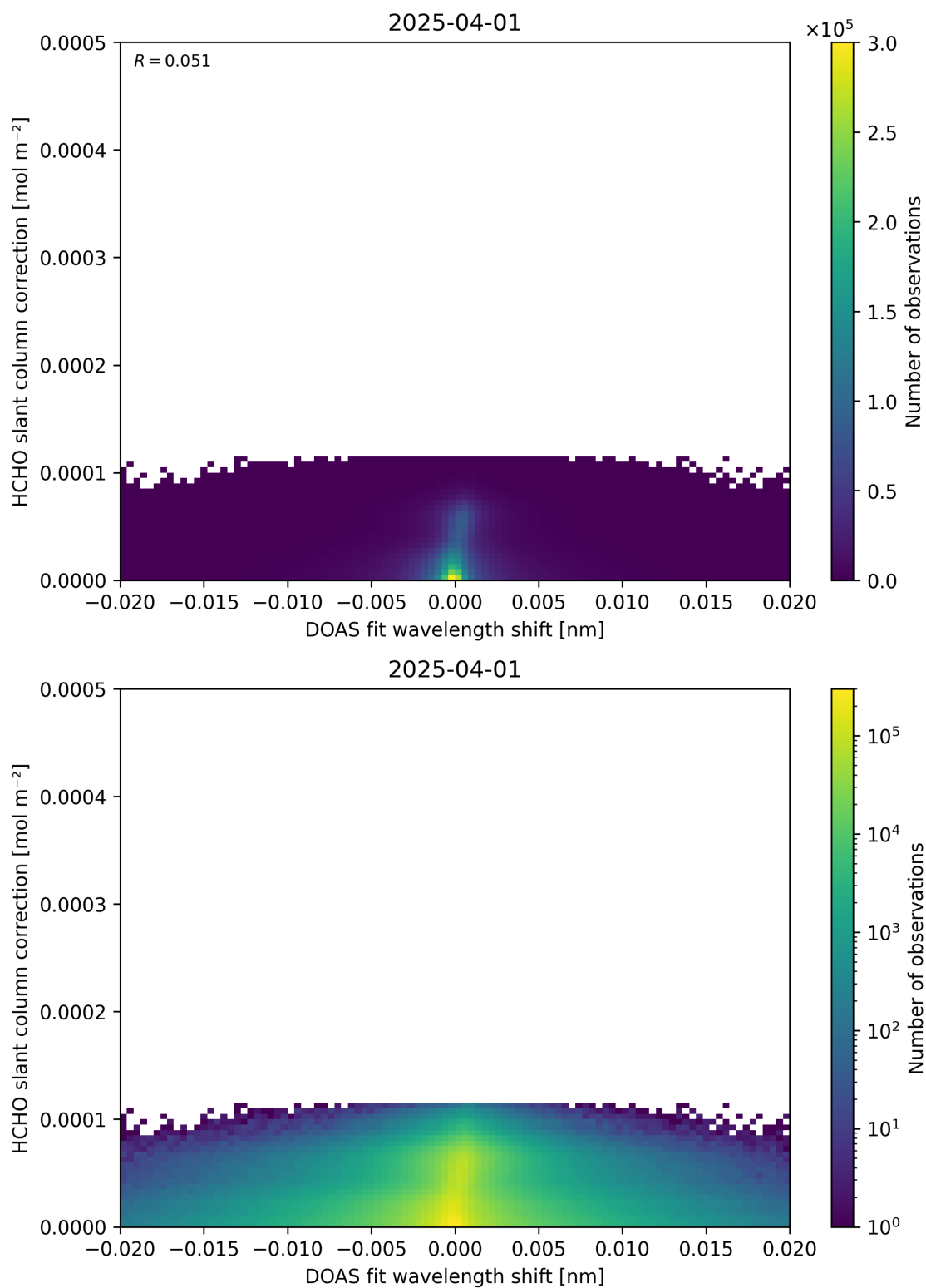
Figure 67: Scatter density plot of “DOAS fit wavelength shift” against “HCHO slant column correction” for 2025-03-31 to 2025-04-02.
