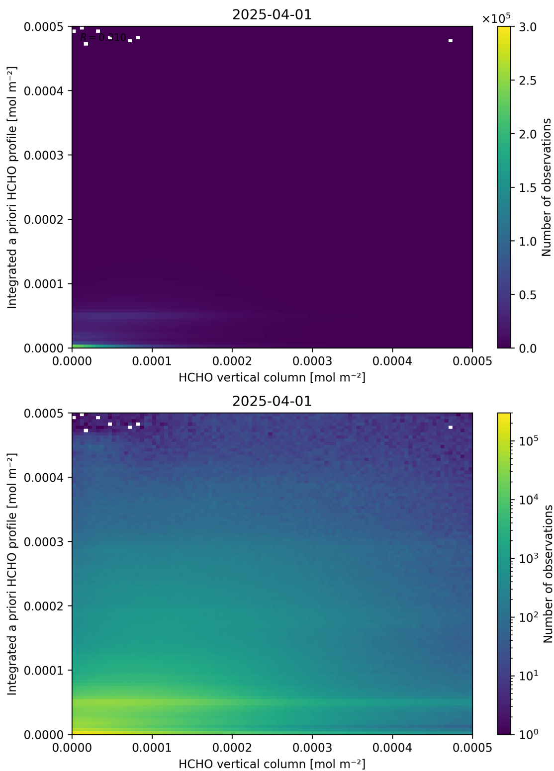
Figure 135: Scatter density plot of “HCHO vertical column” against “Integrated a priori HCHO profile” for 2025-03-31 to 2025-04-02.
