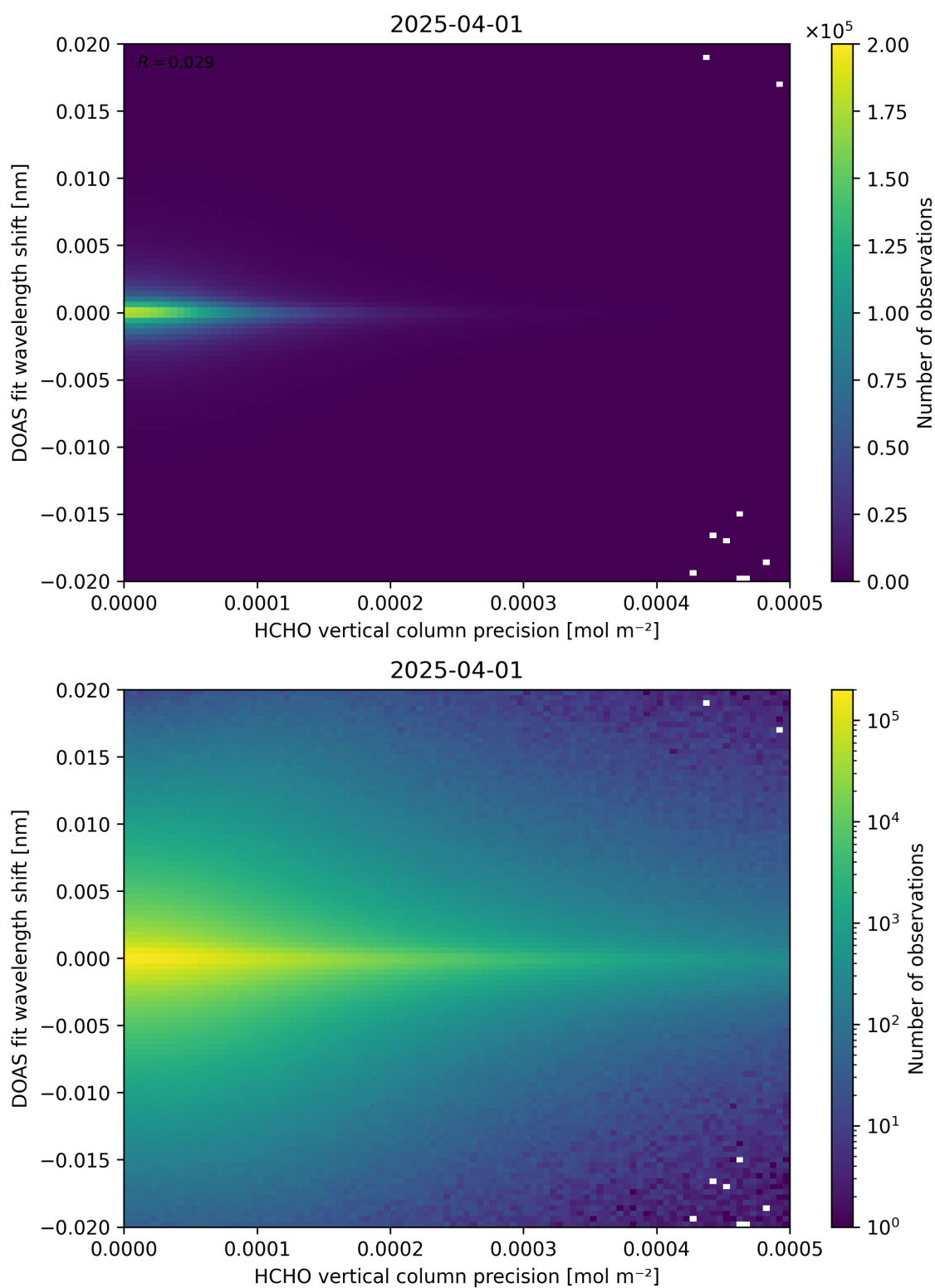
Figure 137: Scatter density plot of “HCHO vertical column precision” against “DOAS fit wavelength shift” for 2025-03-31 to 2025-04-02.
