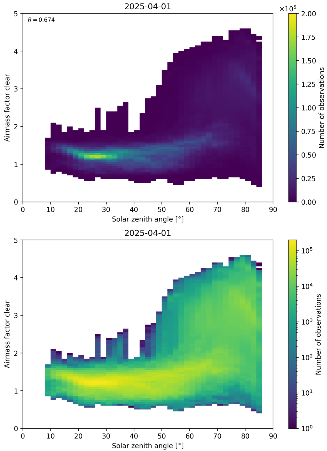
Figure 170: Scatter density plot of “Solar zenith angle” against “Airmass factor clear” for 2025-03-31 to 2025-04-02.
