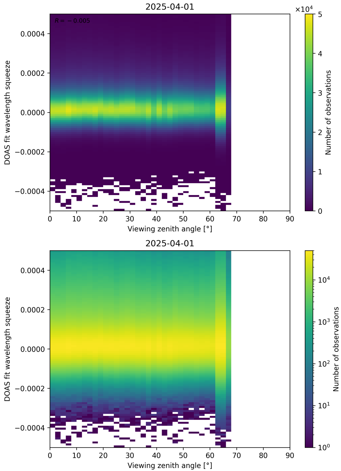
Figure 184: Scatter density plot of “Viewing zenith angle” against “DOAS fit wavelength squeeze” for 2025-03-31 to 2025-04-02.
