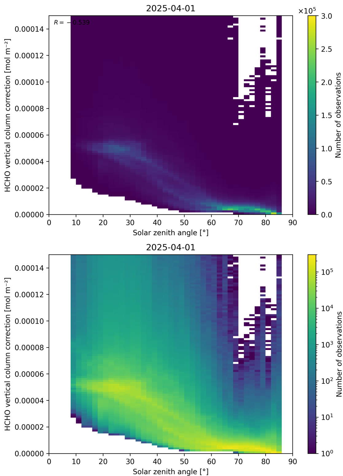
Figure 178: Scatter density plot of “Solar zenith angle” against “HCHO vertical column correction” for 2025-03-31 to 2025-04-02.
