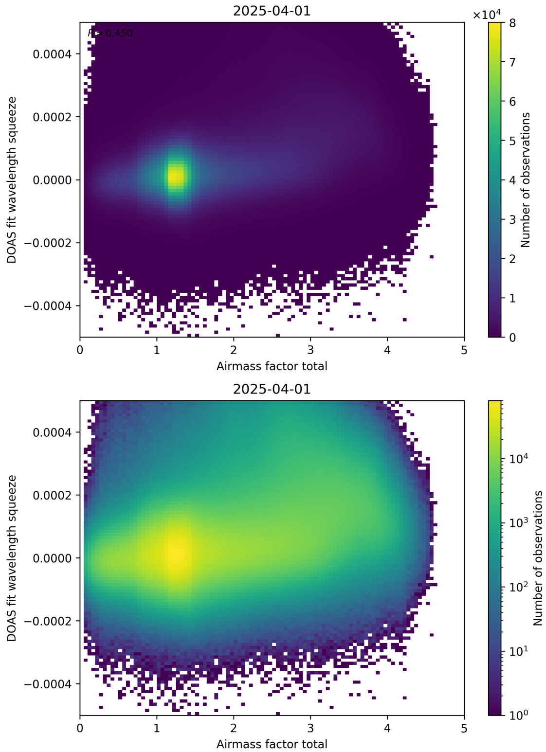
Figure 99: Scatter density plot of “Airmass factor total” against “DOAS fit wavelength squeeze” for 2025-03-31 to 2025-04-02.
