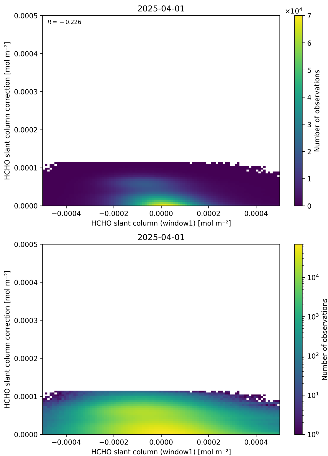
Figure 83: Scatter density plot of “HCHO slant column (window1)” against “HCHO slant column correction” for 2025-03-31 to 2025-04-02.
