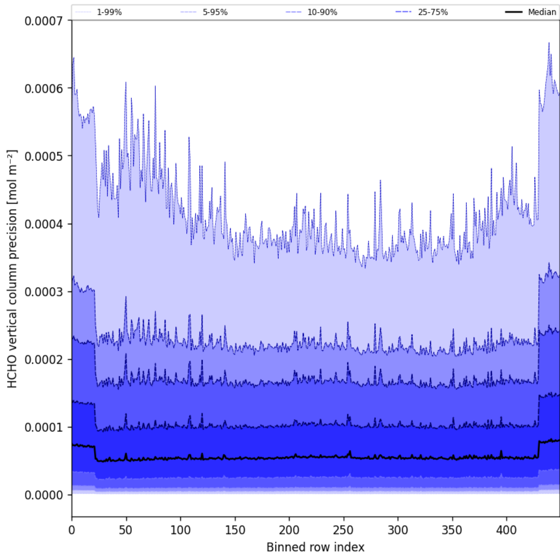
Figure 50: Along track statistics of “HCHO vertical column precision” for 2025-03-31 to 2025-04-02
