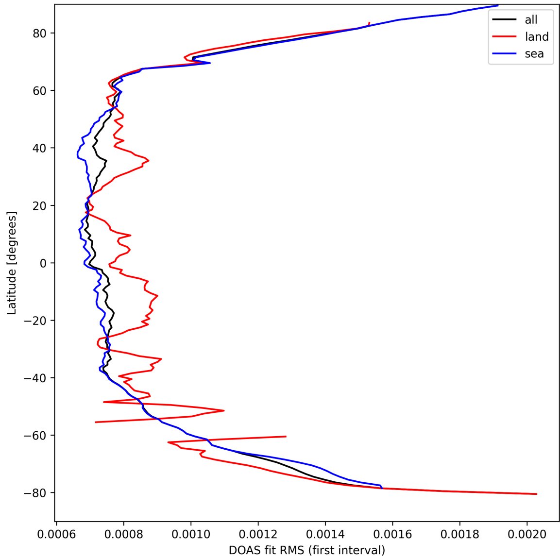
Figure 32: Zonal average of “DOAS fit RMS (first interval)” for 2025-03-31 to 2025-04-02.
