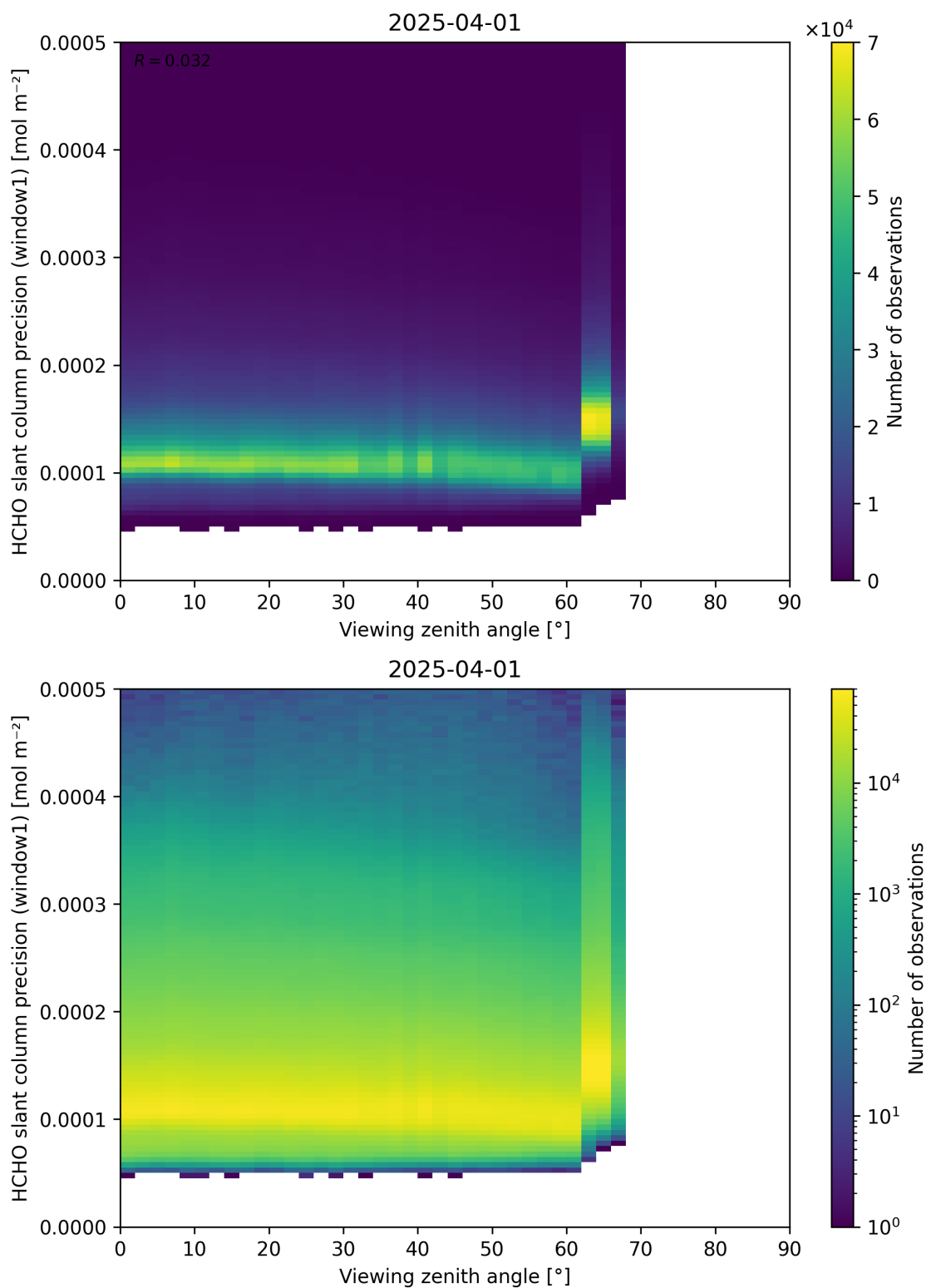
Figure 189: Scatter density plot of “Viewing zenith angle” against “HCHO slant column precision (window1)” for 2025-03-31 to 2025-04-02.
