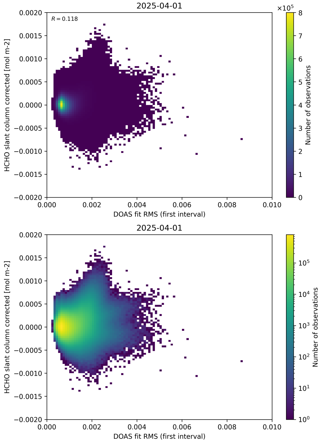
Figure 62: Scatter density plot of “DOAS fit RMS (first interval)” against “HCHO slant column corrected” for 2025-03-31 to 2025-04-02.
