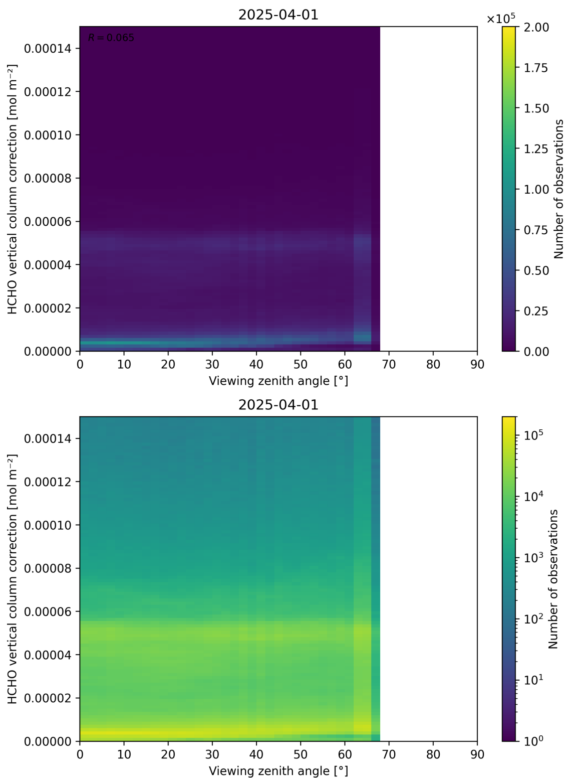
Figure 193: Scatter density plot of “Viewing zenith angle” against “HCHO vertical column correction” for 2025-03-31 to 2025-04-02.
