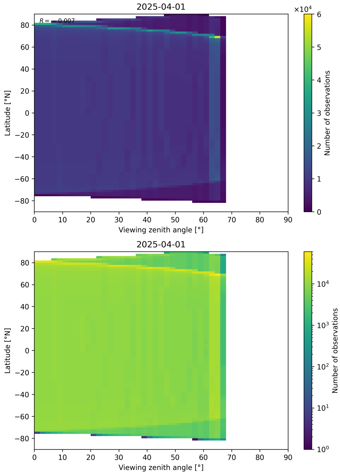
Figure 196: Scatter density plot of “Viewing zenith angle” against “Latitude” for 2025-03-31 to 2025-04-02.
