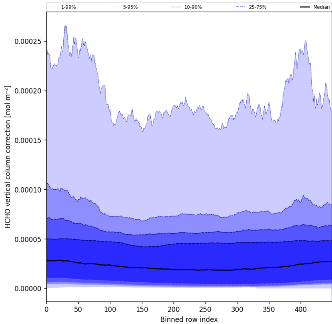
Figure 51: Along track statistics of “HCHO vertical column correction” for 2025-03-31 to 2025-04-02
