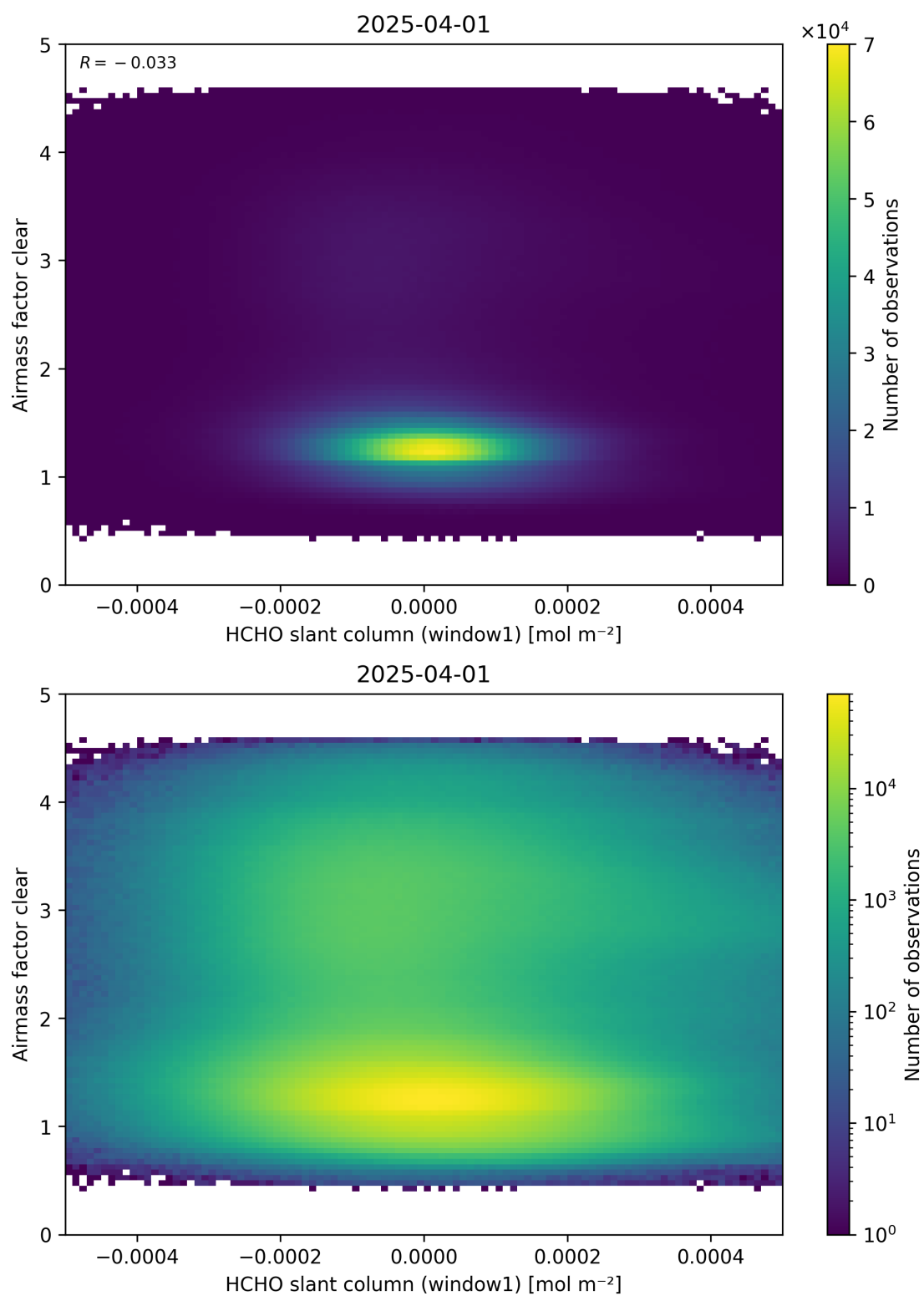
Figure 81: Scatter density plot of “HCHO slant column (window1)” against “Airmass factor clear” for 2025-03-31 to 2025-04-02.
