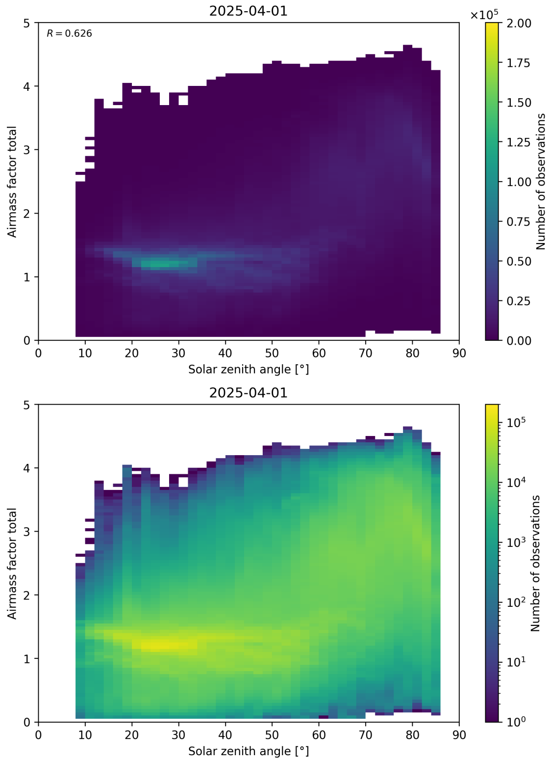
Figure 175: Scatter density plot of “Solar zenith angle” against “Airmass factor total” for 2025-03-31 to 2025-04-02.
