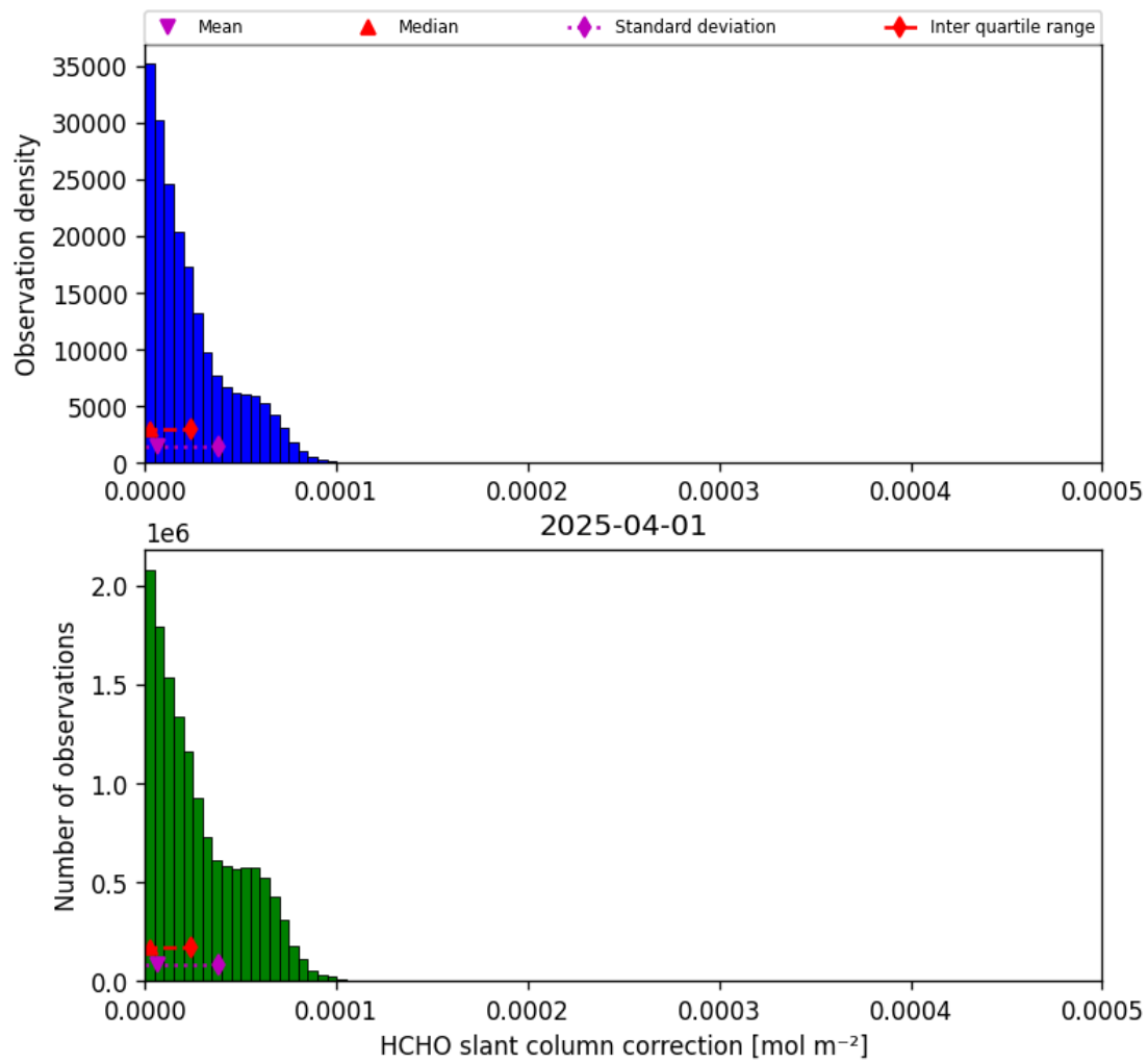
Figure 47: Histogram of “HCHO slant column correction” for 2025-03-31 to 2025-04-02
