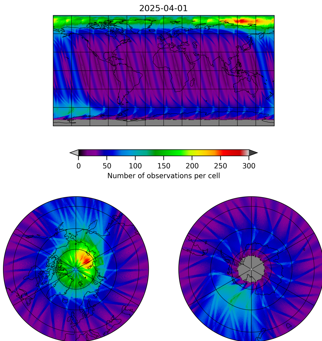
Figure 19: Map of the number of observations for 2025-03-31 to 2025-04-02
