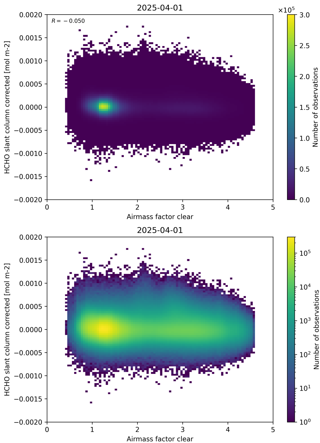
Figure 74: Scatter density plot of “Airmass factor clear” against “HCHO slant column corrected” for 2025-03-31 to 2025-04-02.
