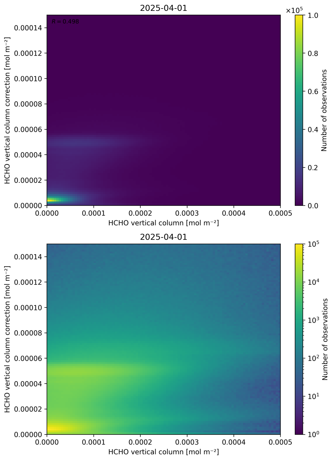
Figure 133: Scatter density plot of “HCHO vertical column” against “HCHO vertical column correction” for 2025-03-31 to 2025-04-02.
