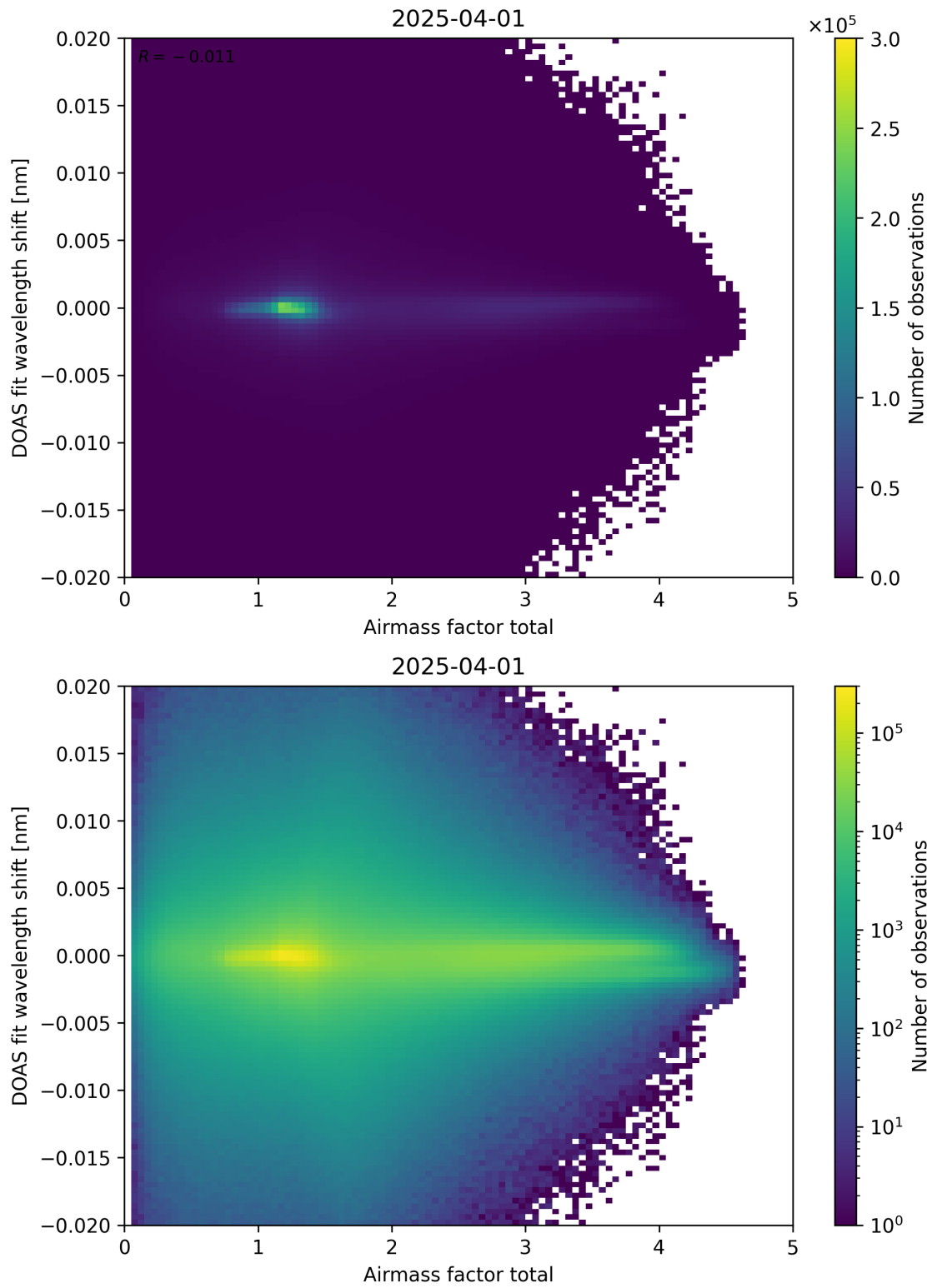
Figure 98: Scatter density plot of “Airmass factor total” against “DOAS fit wavelength shift” for 2025-03-31 to 2025-04-02.
