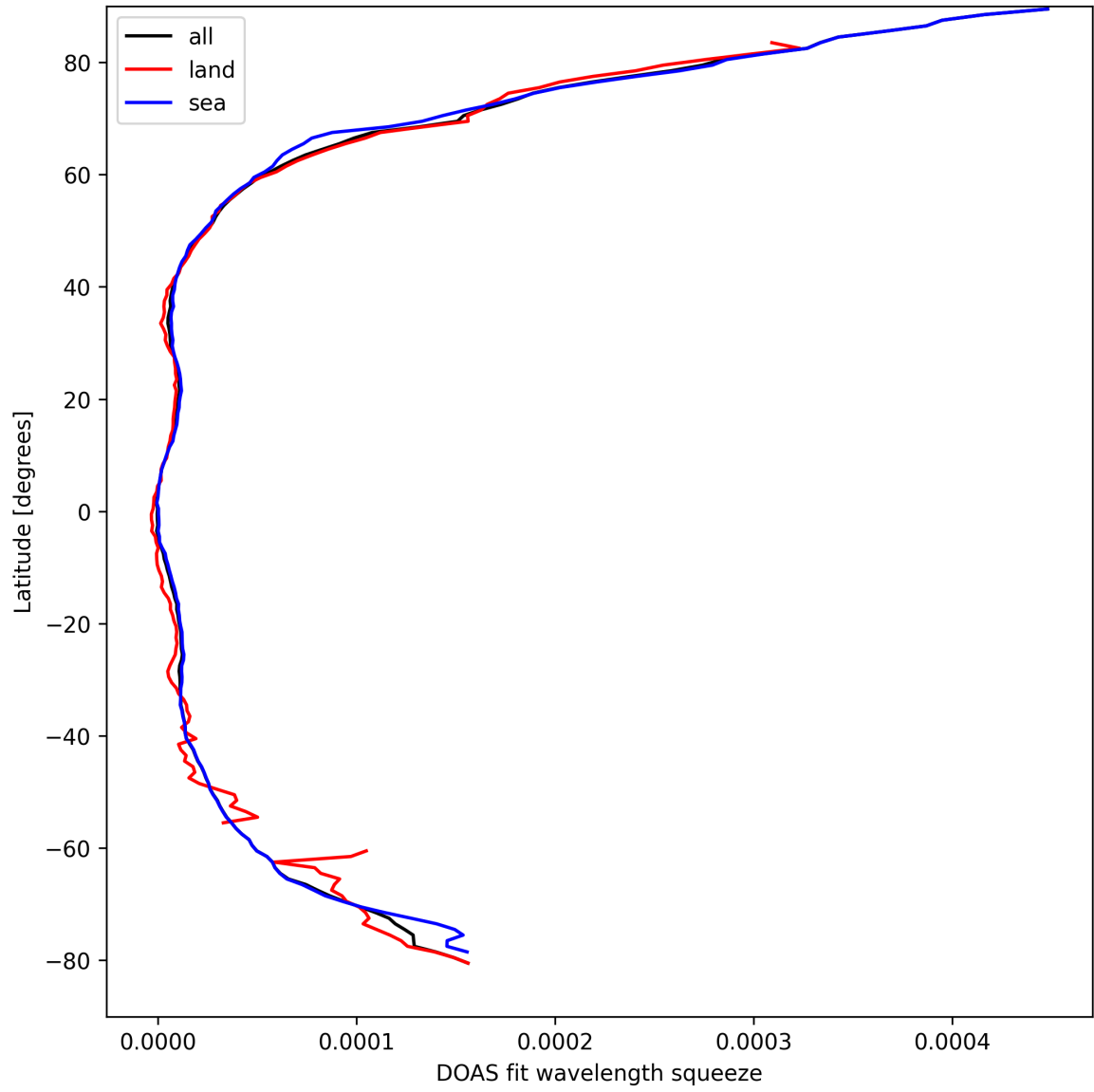
Figure 31: Zonal average of “DOAS fit wavelength squeeze” for 2025-03-31 to 2025-04-02.
