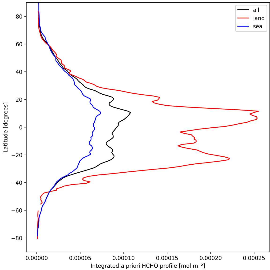
Figure 29: Zonal average of “Integrated a priori HCHO profile” for 2025-03-31 to 2025-04-02.
