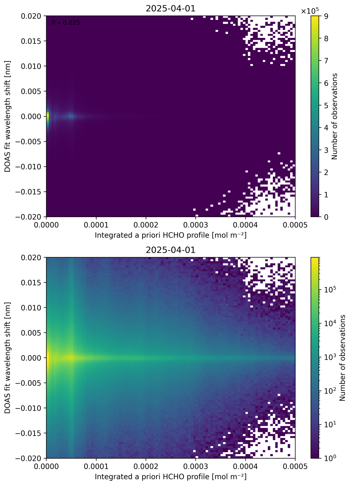
Figure 149: Scatter density plot of “Integrated a priori HCHO profile” against “DOAS fit wavelength shift” for 2025-03-31 to 2025-04-02.
