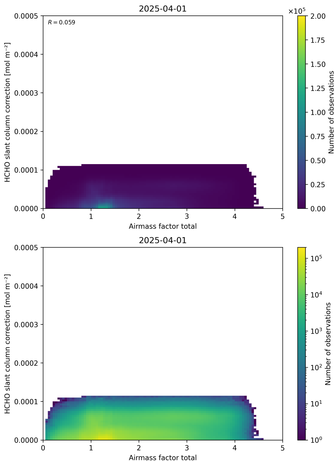
Figure 102: Scatter density plot of “Airmass factor total” against “HCHO slant column correction” for 2025-03-31 to 2025-04-02.
