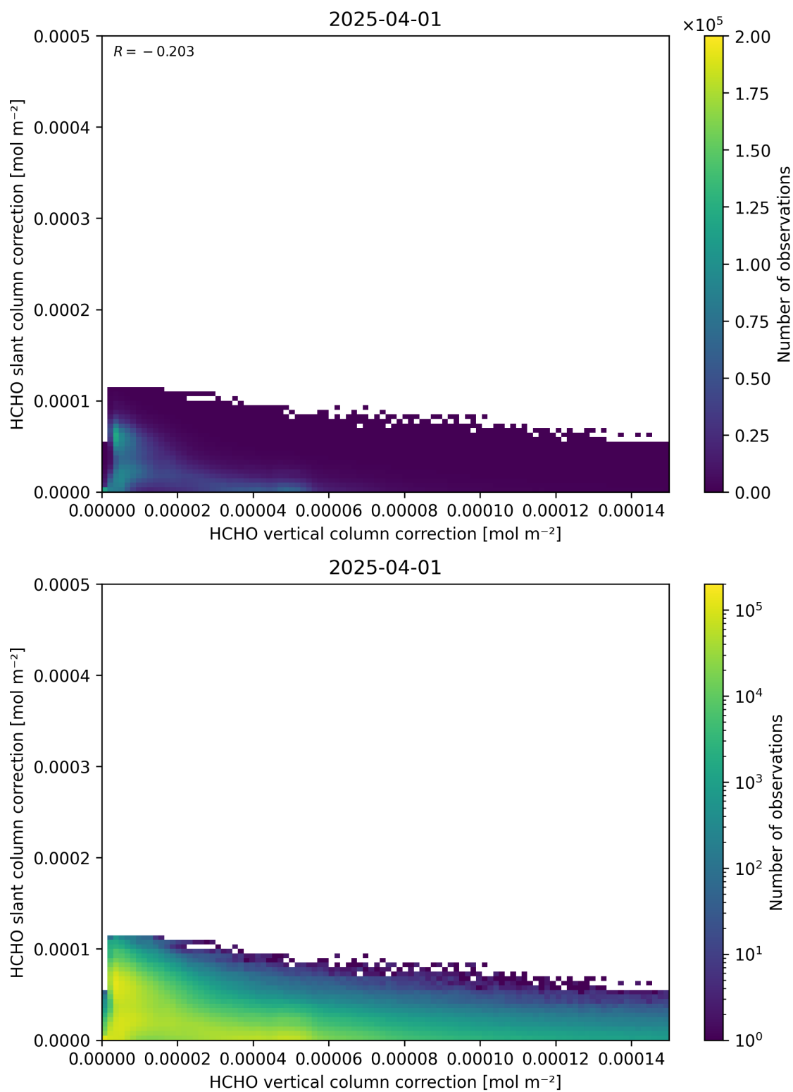
Figure 117: Scatter density plot of “HCHO vertical column correction” against “HCHO slant column correction” for 2025-03-31 to 2025-04-02.
