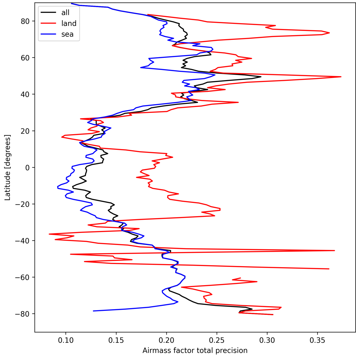
Figure 27: Zonal average of “Airmass factor total precision” for 2025-03-31 to 2025-04-02.
