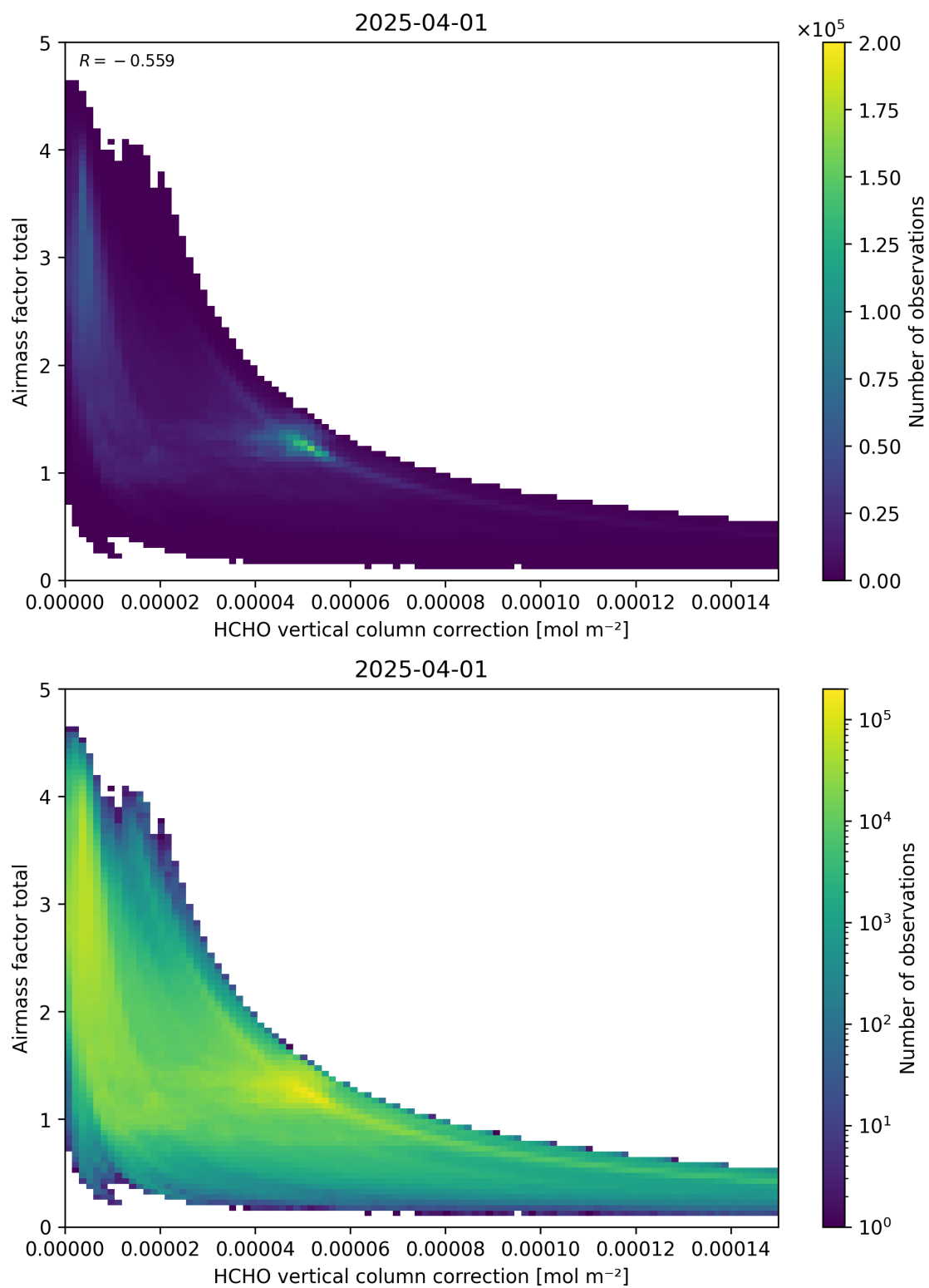
Figure 120: Scatter density plot of “HCHO vertical column correction” against “Airmass factor total” for 2025-03-31 to 2025-04-02.
