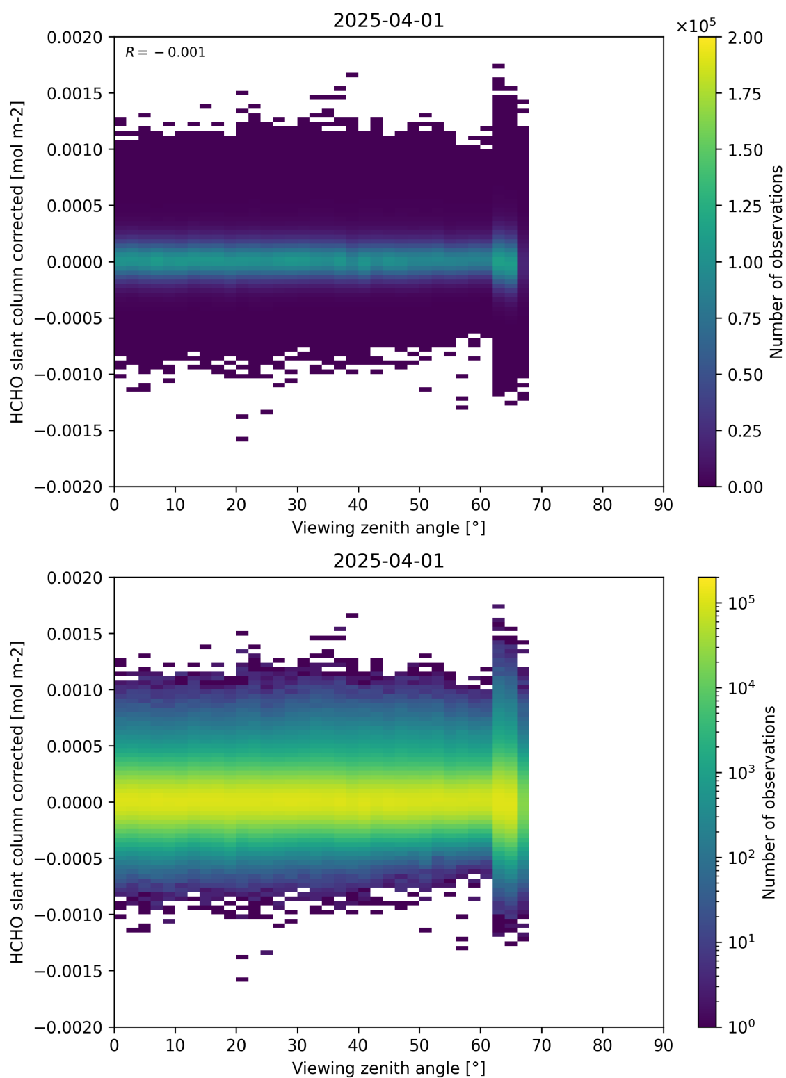
Figure 186: Scatter density plot of “Viewing zenith angle” against “HCHO slant column corrected” for 2025-03-31 to 2025-04-02.
