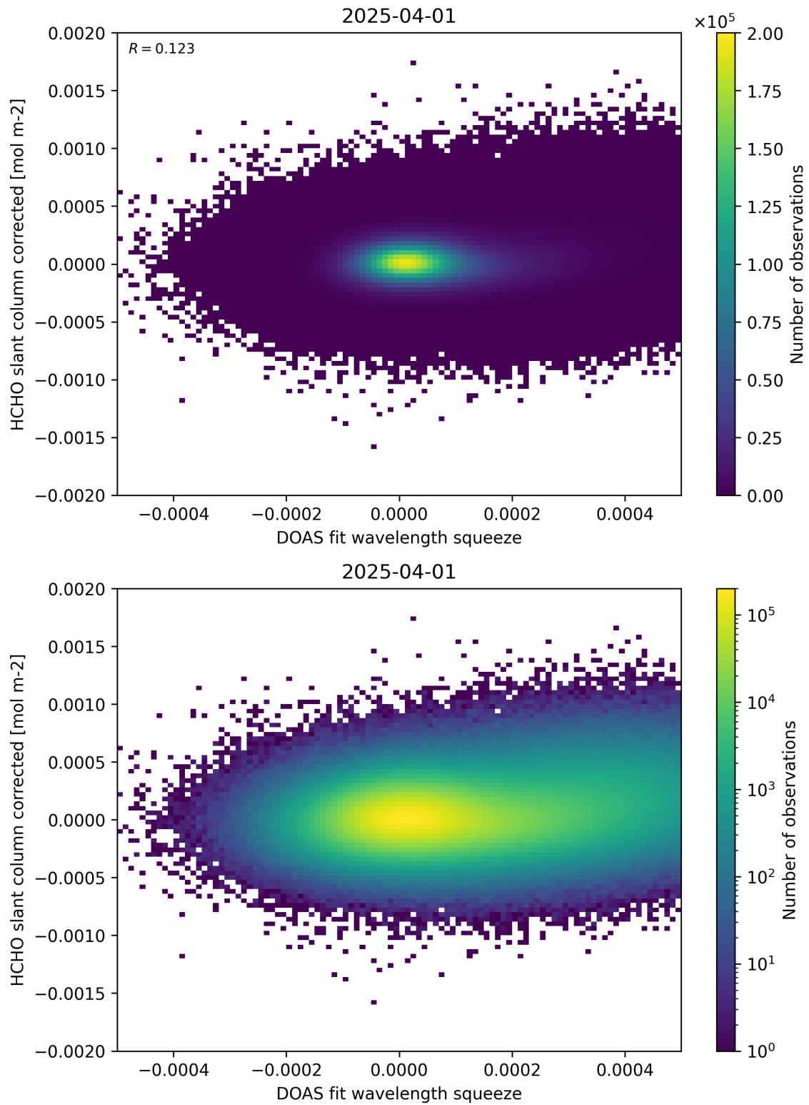
Figure 69: Scatter density plot of “DOAS fit wavelength squeeze” against “HCHO slant column corrected” for 2025-03-31 to 2025-04-02.
