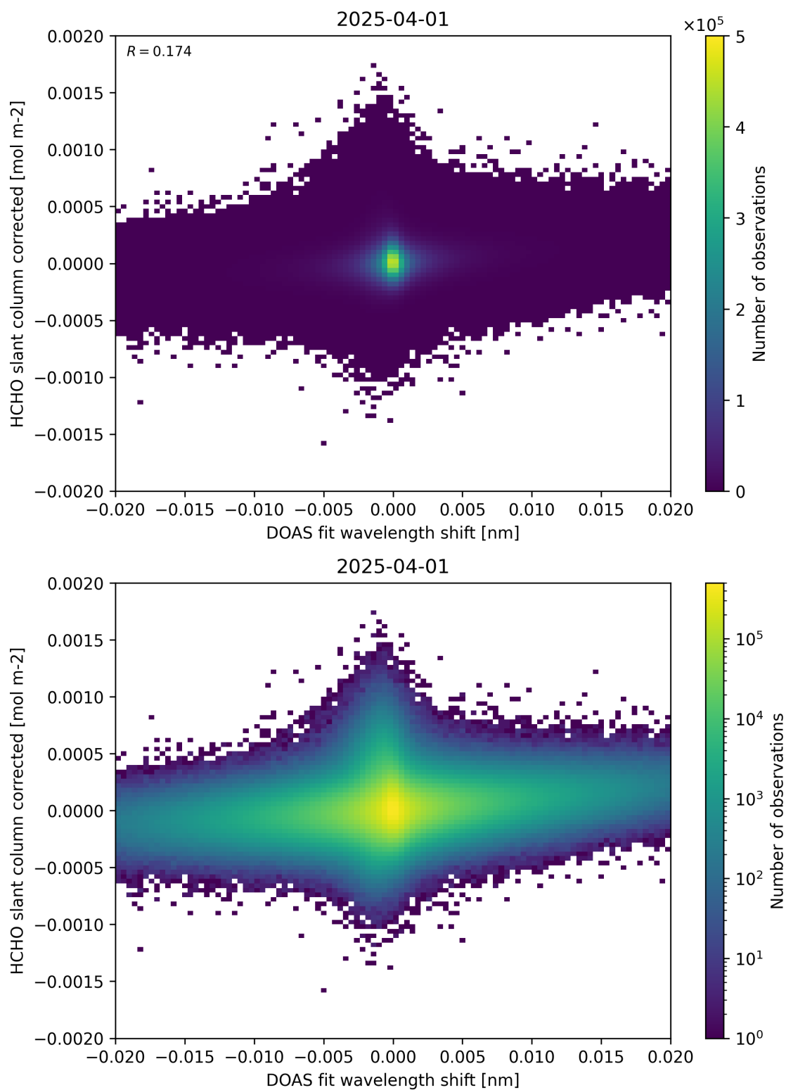
Figure 66: Scatter density plot of “DOAS fit wavelength shift” against “HCHO slant column corrected” for 2025-03-31 to 2025-04-02.
