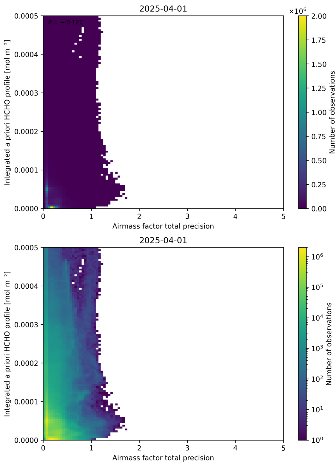
Figure 111: Scatter density plot of “Airmass factor total precision” against “Integrated a priori HCHO profile” for 2025-03-31 to 2025-04-02.
