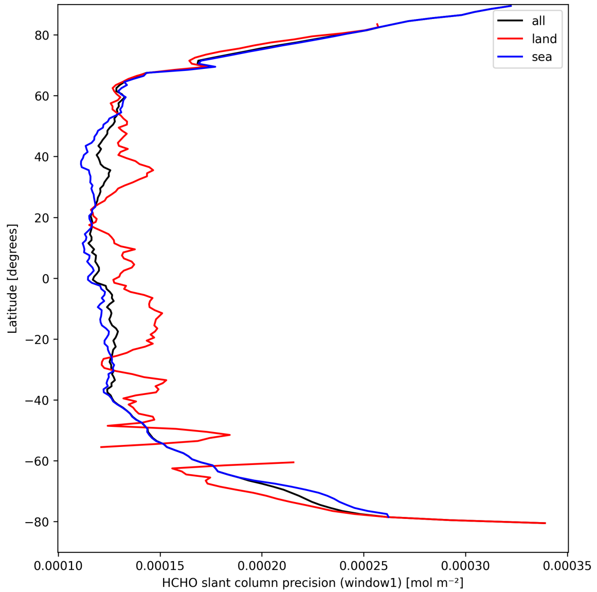
Figure 25: Zonal average of “HCHO slant column precision (window1)” for 2025-03-31 to 2025-04-02.
