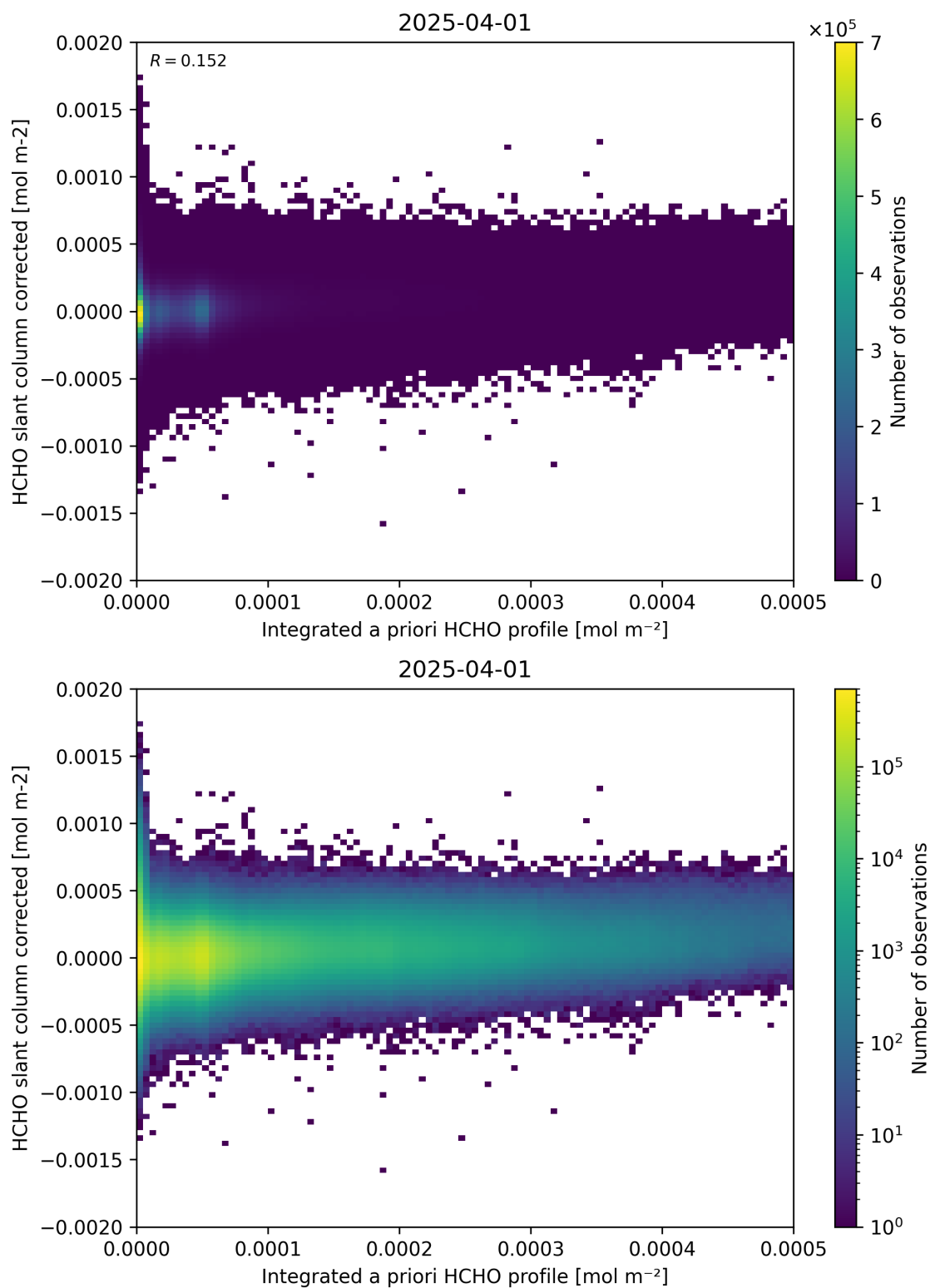
Figure 151: Scatter density plot of “Integrated a priori HCHO profile” against “HCHO slant column corrected” for 2025-03-31 to 2025-04-02.
