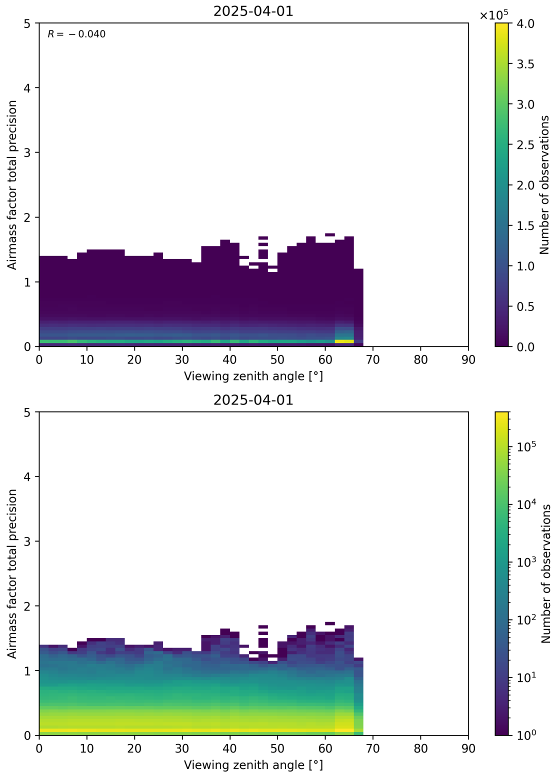
Figure 191: Scatter density plot of “Viewing zenith angle” against “Airmass factor total precision” for 2025-03-31 to 2025-04-02.
