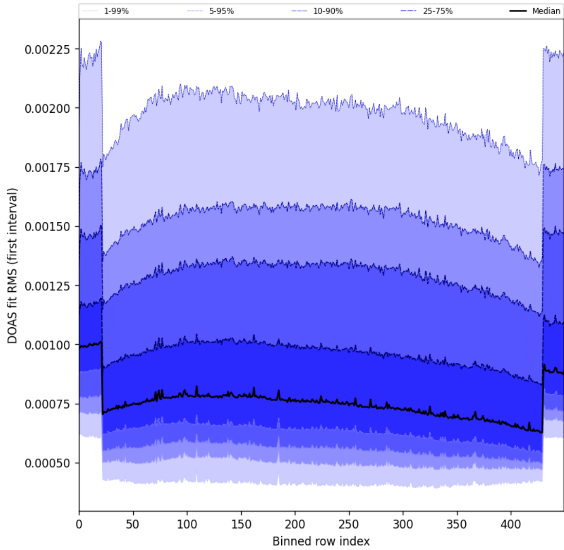
Figure 60: Along track statistics of “DOAS fit RMS (first interval)” for 2025-03-31 to 2025-04-02
