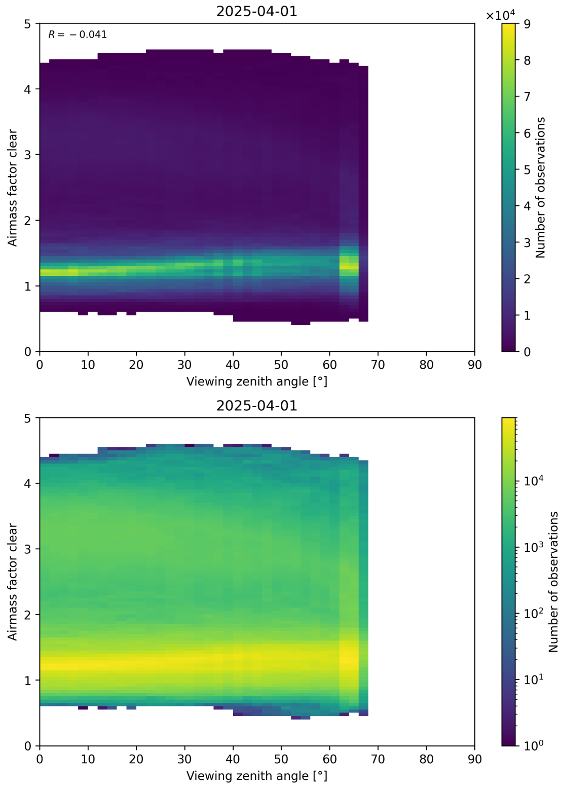
Figure 185: Scatter density plot of “Viewing zenith angle” against “Airmass factor clear” for 2025-03-31 to 2025-04-02.
