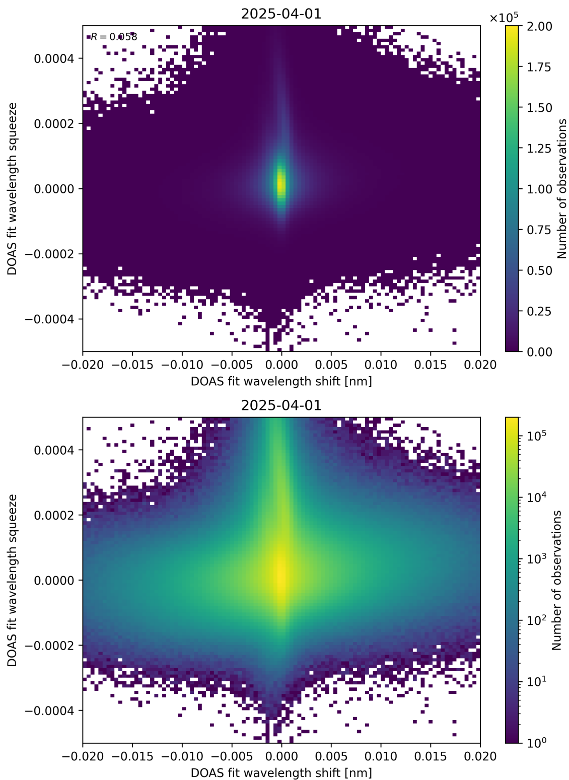
Figure 65: Scatter density plot of “DOAS fit wavelength shift” against “DOAS fit wavelength squeeze” for 2025-03-31 to 2025-04-02.
