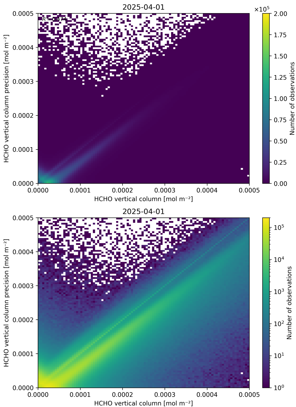
Figure 134: Scatter density plot of “HCHO vertical column” against “HCHO vertical column precision” for 2025-03-31 to 2025-04-02.
