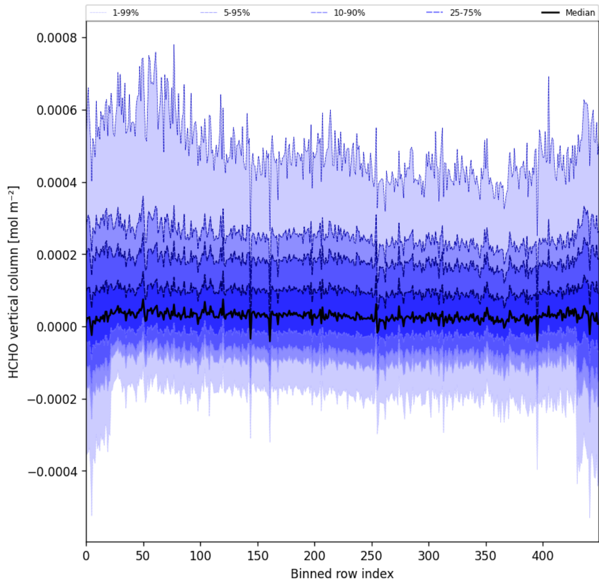
Figure 49: Along track statistics of “HCHO vertical column” for 2025-03-31 to 2025-04-02
