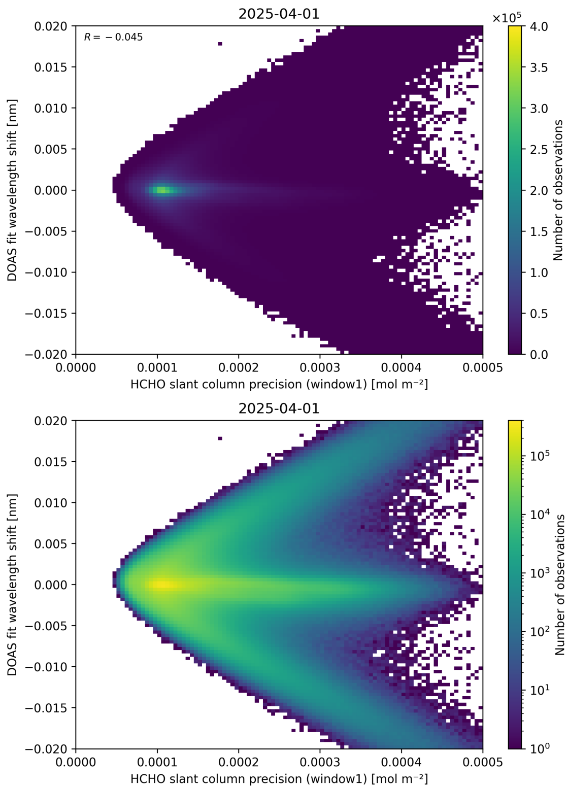
Figure 89: Scatter density plot of “HCHO slant column precision (window1)” against “DOAS fit wavelength shift” for 2025-03-31 to 2025-04-02.
