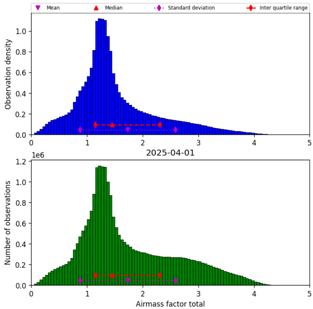
Figure 40: Histogram of “Airmass factor total” for 2025-03-31 to 2025-04-02
