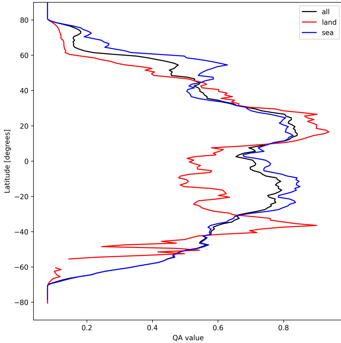
Figure 20: Zonal average of “QA value” for 2025-03-31 to 2025-04-02.
