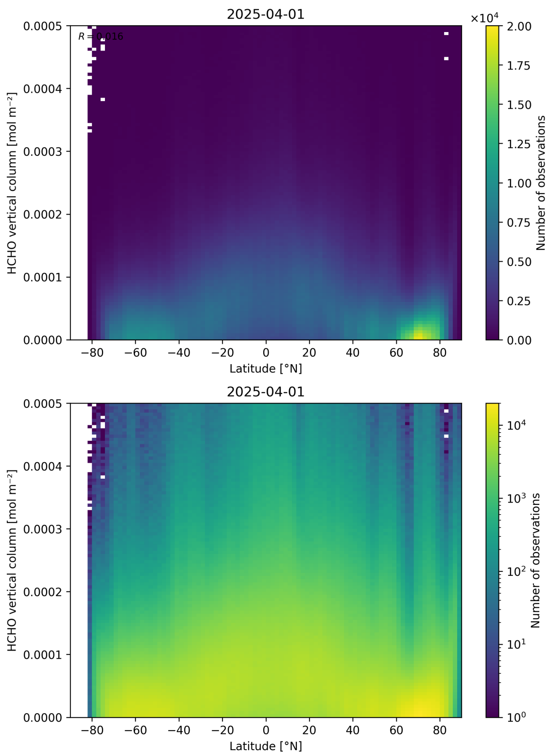
Figure 163: Scatter density plot of “Latitude” against “HCHO vertical column” for 2025-03-31 to 2025-04-02.
