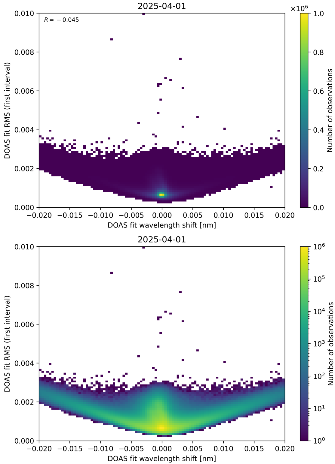
Figure 64: Scatter density plot of “DOAS fit wavelength shift” against “DOAS fit RMS (first interval)” for 2025-03-31 to 2025-04-02.
