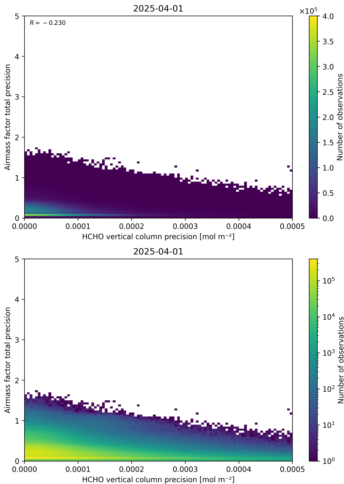
Figure 145: Scatter density plot of “HCHO vertical column precision” against “Airmass factor total precision” for 2025-03-31 to 2025-04-02.
