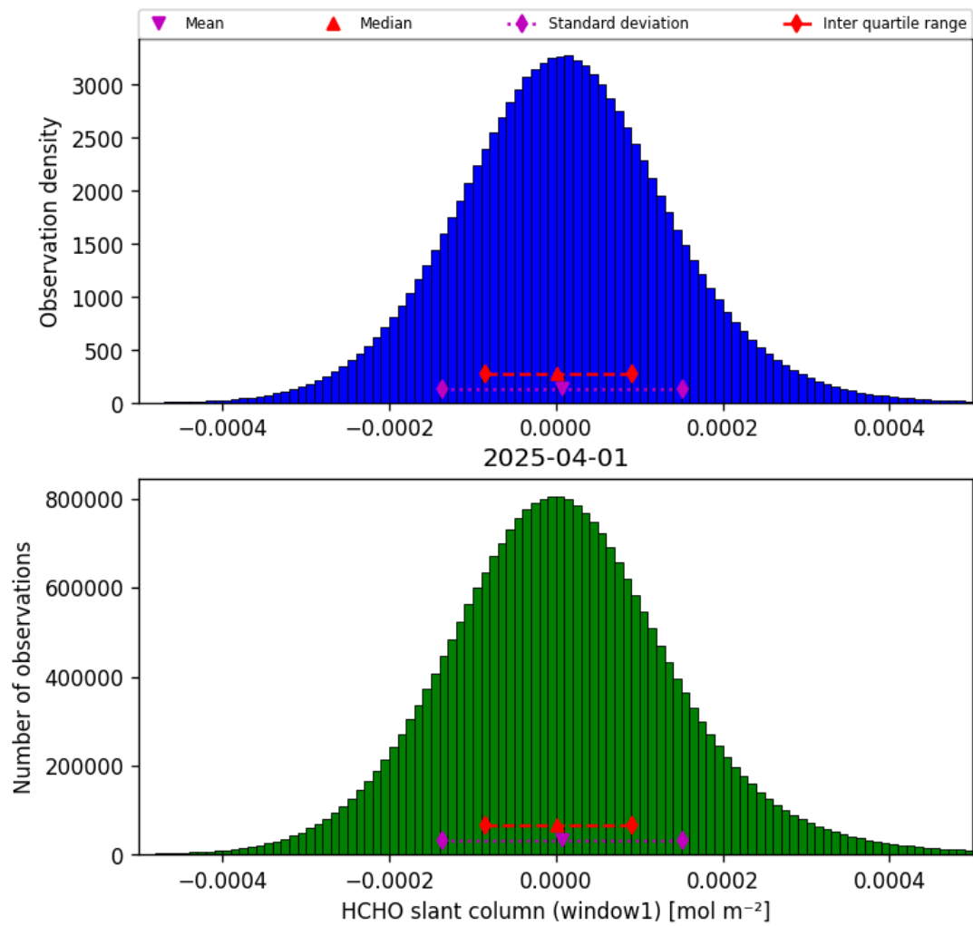
Figure 38: Histogram of “HCHO slant column (window1)” for 2025-03-31 to 2025-04-02
