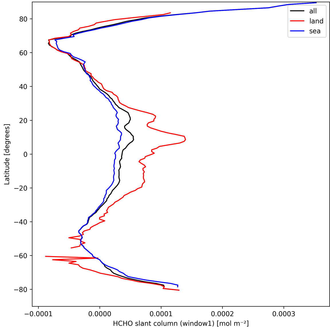
Figure 24: Zonal average of “HCHO slant column (window1)” for 2025-03-31 to 2025-04-02.
