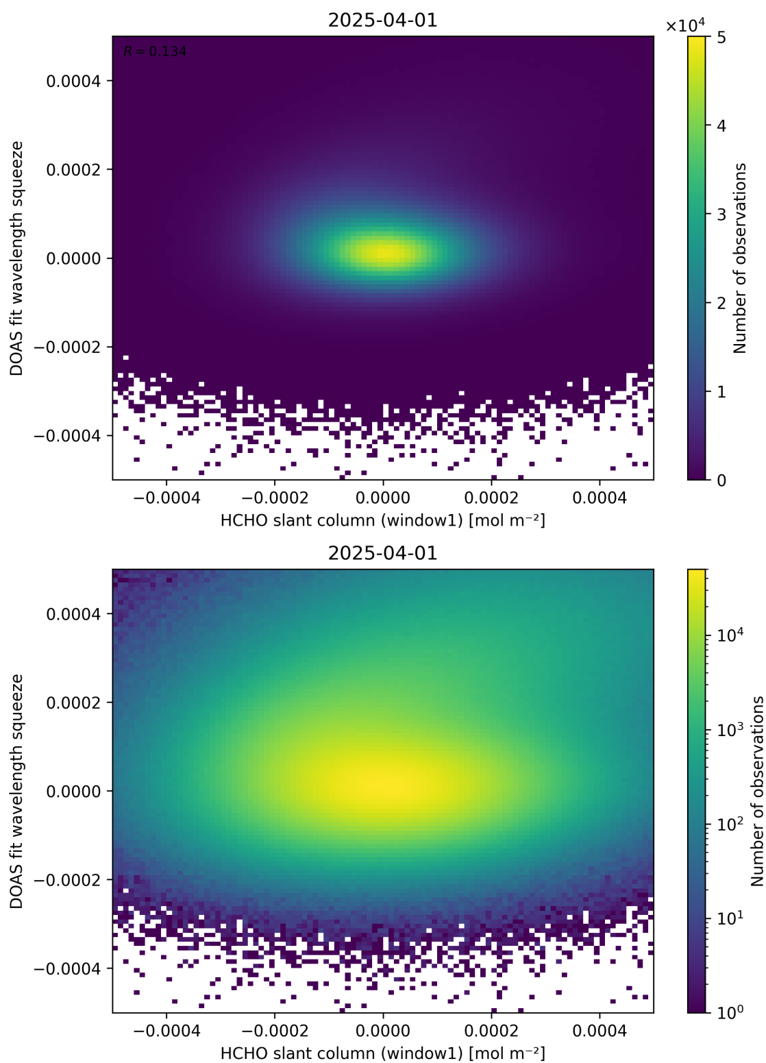
Figure 80: Scatter density plot of “HCHO slant column (window1)” against “DOAS fit wavelength squeeze” for 2025-03-31 to 2025-04-02.
