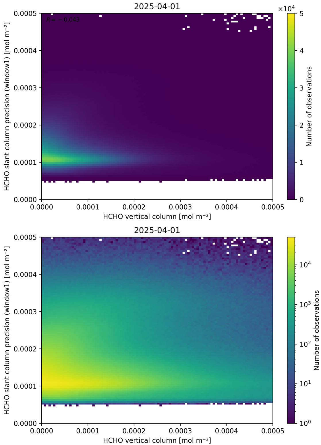
Figure 130: Scatter density plot of “HCHO vertical column” against “HCHO slant column precision (window1)” for 2025-03-31 to 2025-04-02.
