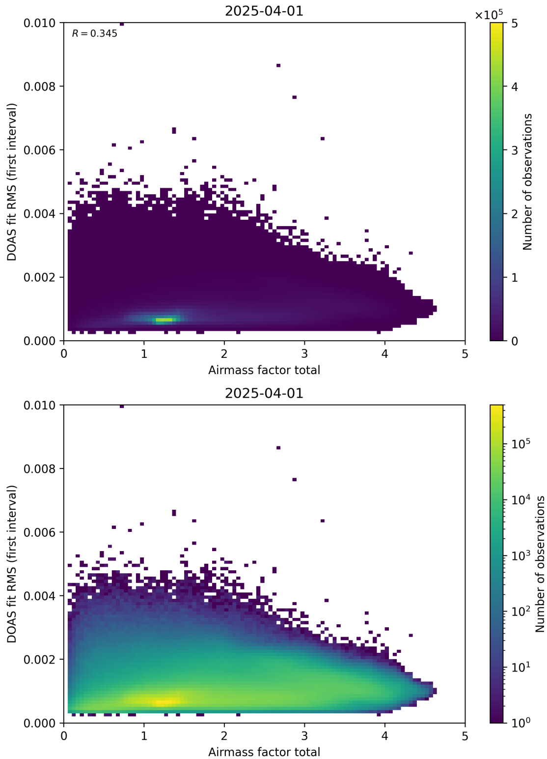
Figure 97: Scatter density plot of “Airmass factor total” against “DOAS fit RMS (first interval)” for 2025-03-31 to 2025-04-02.
