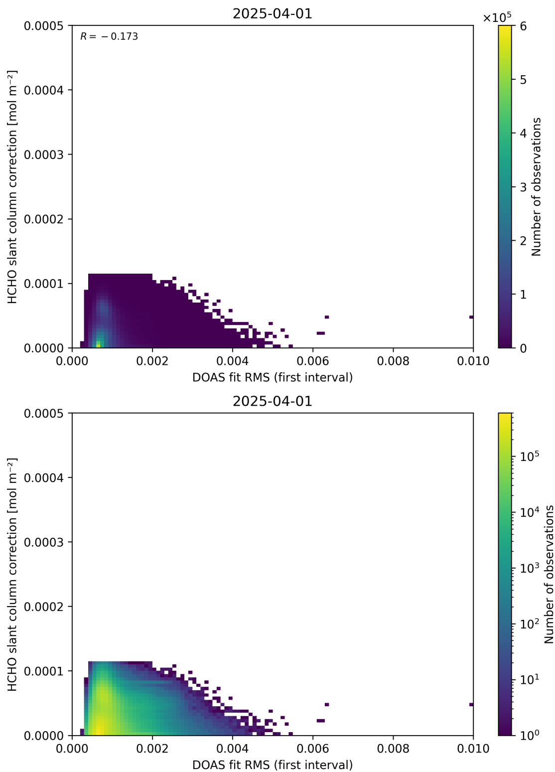
Figure 63: Scatter density plot of “DOAS fit RMS (first interval)” against “HCHO slant column correction” for 2025-03-31 to 2025-04-02.
