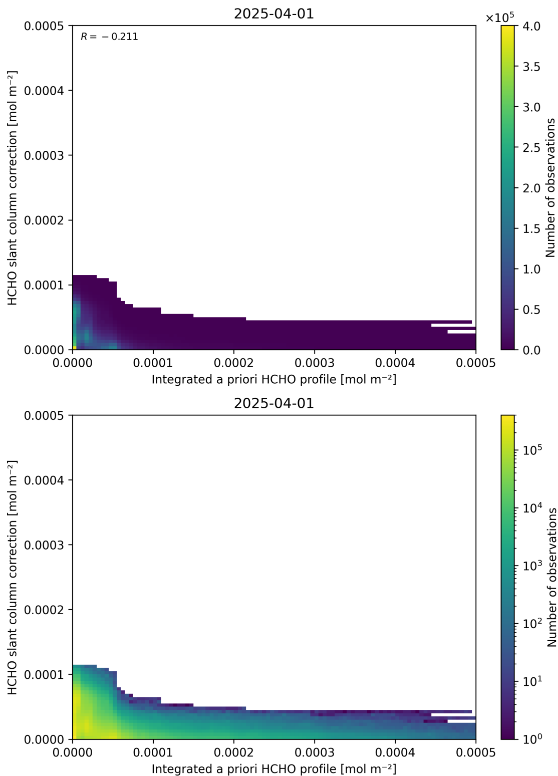
Figure 152: Scatter density plot of “Integrated a priori HCHO profile” against “HCHO slant column correction” for 2025-03-31 to 2025-04-02.
