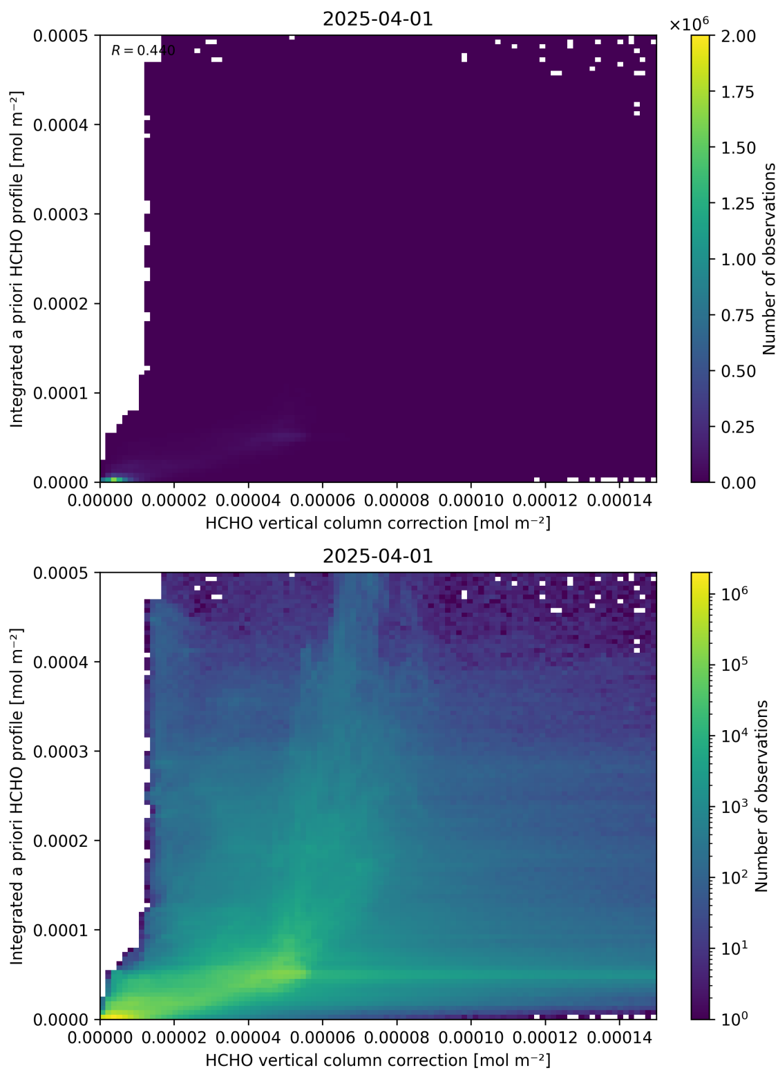
Figure 122: Scatter density plot of “HCHO vertical column correction” against “Integrated a priori HCHO profile” for 2025-03-31 to 2025-04-02.
