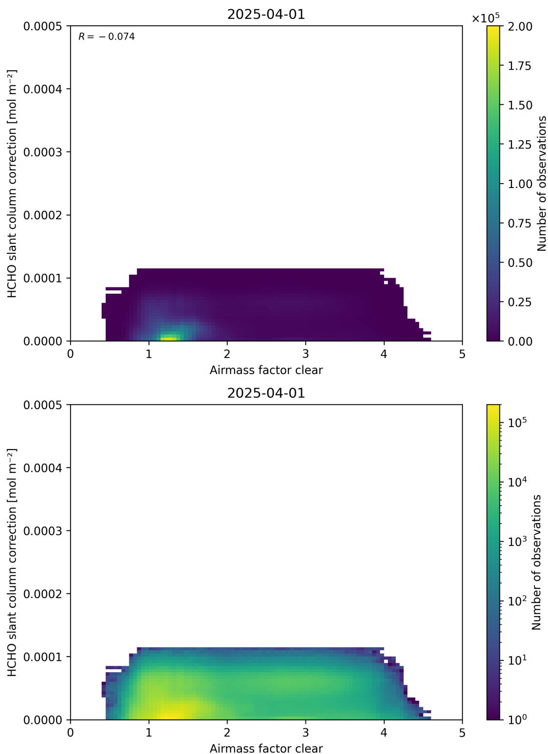
Figure 75: Scatter density plot of “Airmass factor clear” against “HCHO slant column correction” for 2025-03-31 to 2025-04-02.
