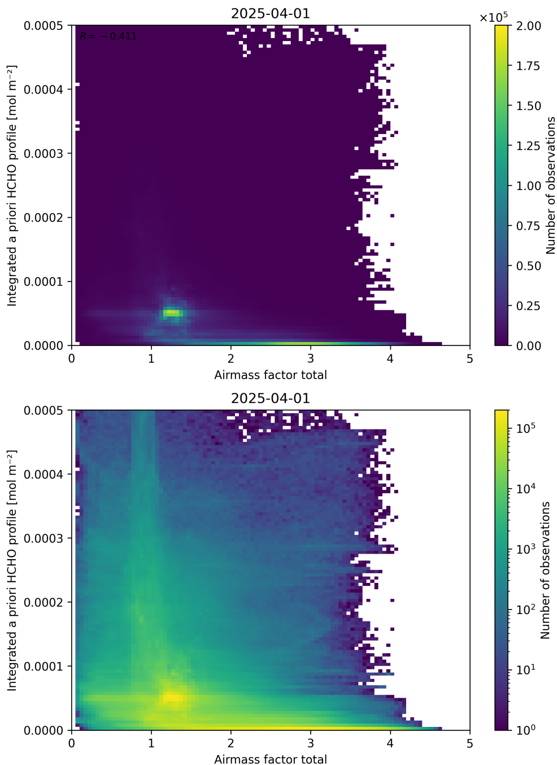
Figure 104: Scatter density plot of “Airmass factor total” against “Integrated a priori HCHO profile” for 2025-03-31 to 2025-04-02.
