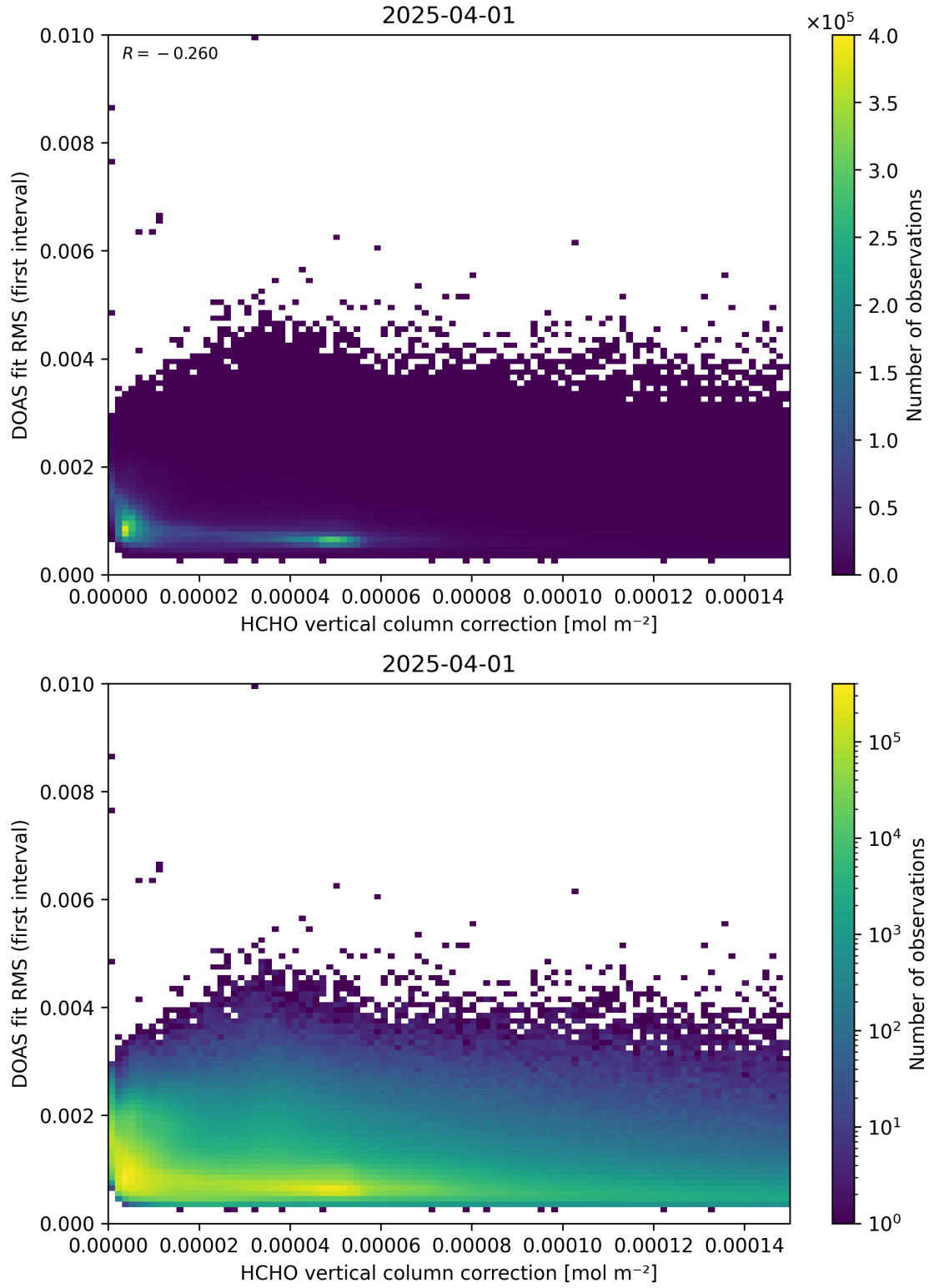
Figure 112: Scatter density plot of “HCHO vertical column correction” against “DOAS fit RMS (first interval)” for 2025-03-31 to 2025-04-02.
