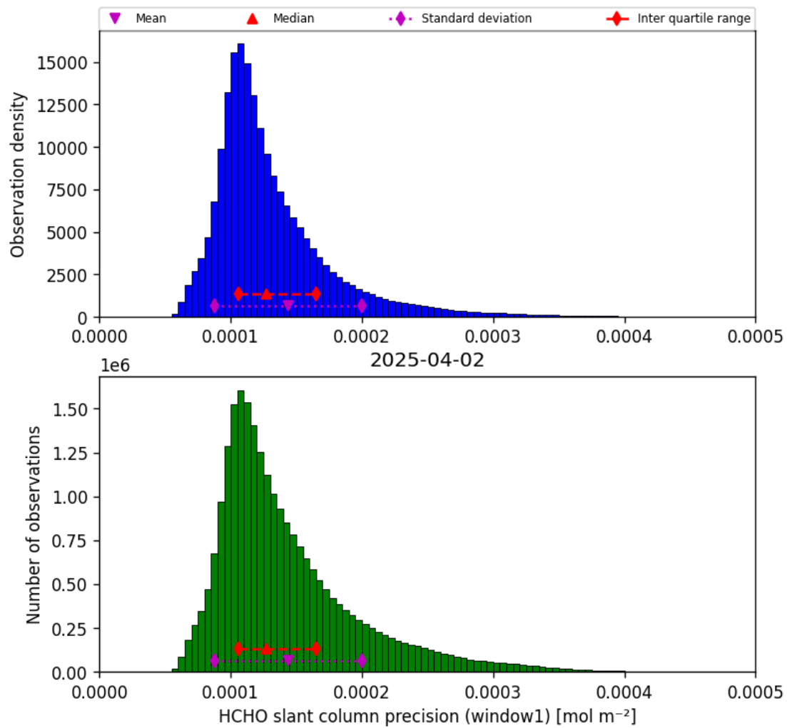
Figure 39: Histogram of “HCHO slant column precision (window1)” for 2025-04-02 to 2025-04-03
