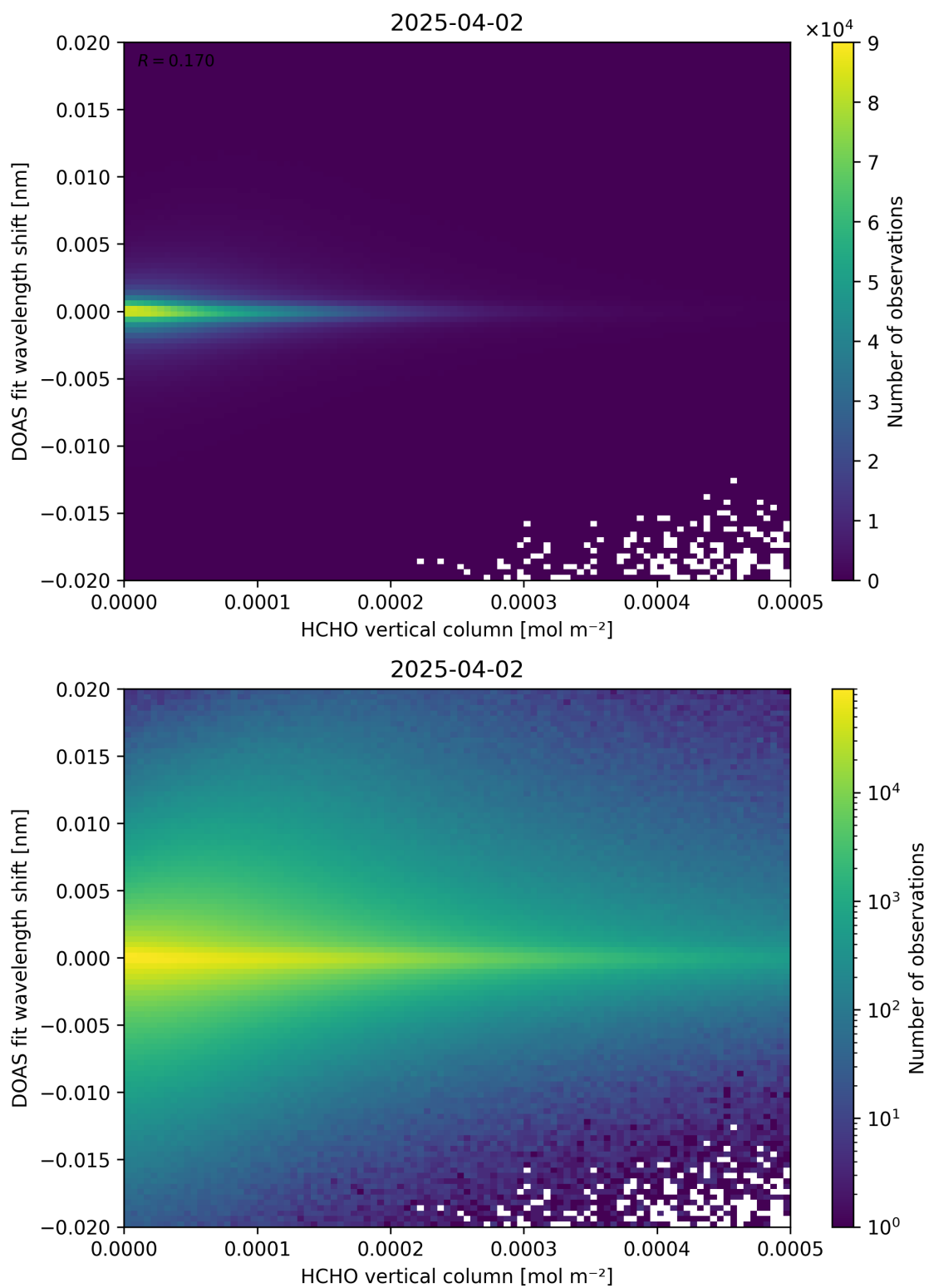
Figure 124: Scatter density plot of “HCHO vertical column” against “DOAS fit wavelength shift” for 2025-04-02 to 2025-04-03.
