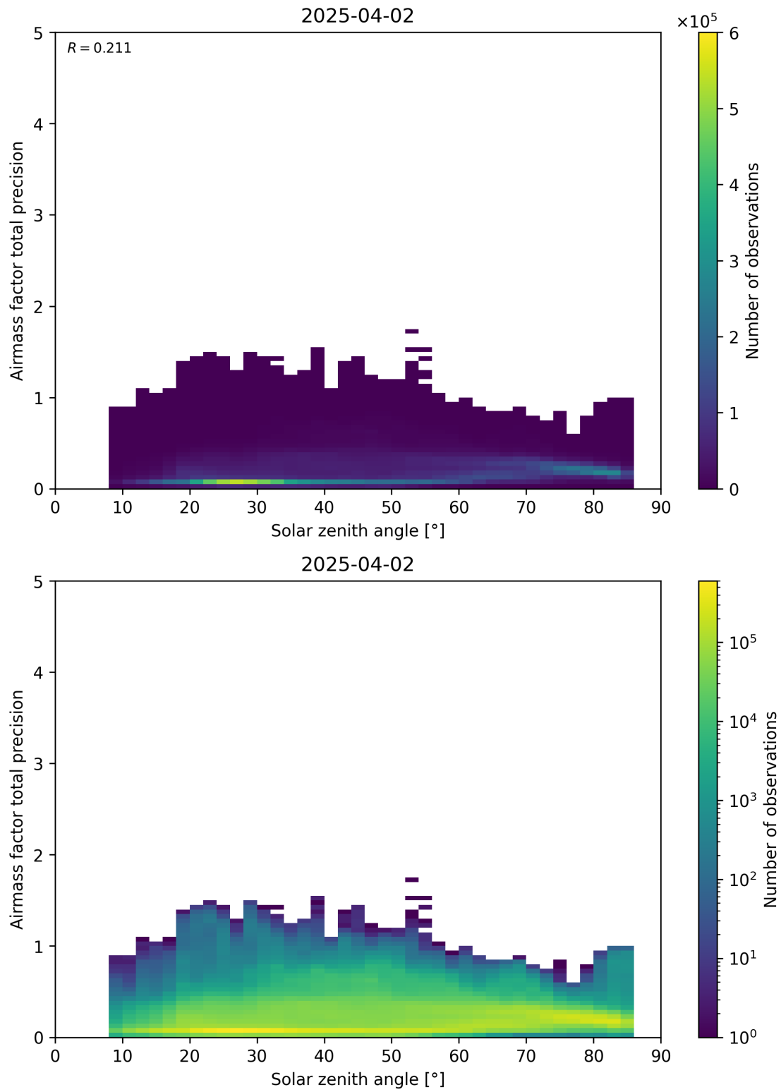
Figure 176: Scatter density plot of “Solar zenith angle” against “Airmass factor total precision” for 2025-04-02 to 2025-04-03.
