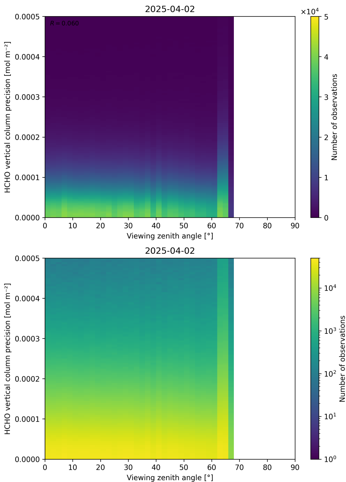
Figure 194: Scatter density plot of “Viewing zenith angle” against “HCHO vertical column precision” for 2025-04-02 to 2025-04-03.
