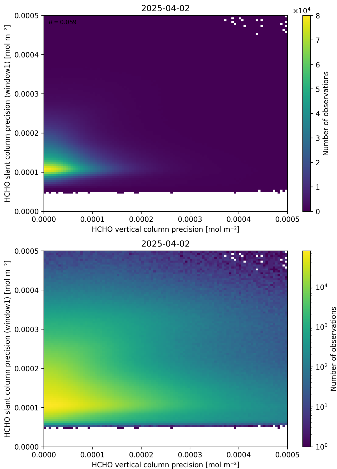
Figure 143: Scatter density plot of “HCHO vertical column precision” against “HCHO slant column precision (window1)” for 2025-04-02 to 2025-04-03.
