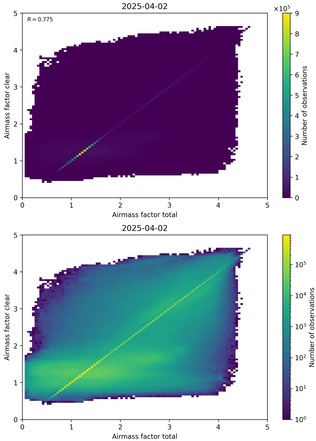
Figure 100: Scatter density plot of “Airmass factor total” against “Airmass factor clear” for 2025-04-02 to 2025-04-03.
