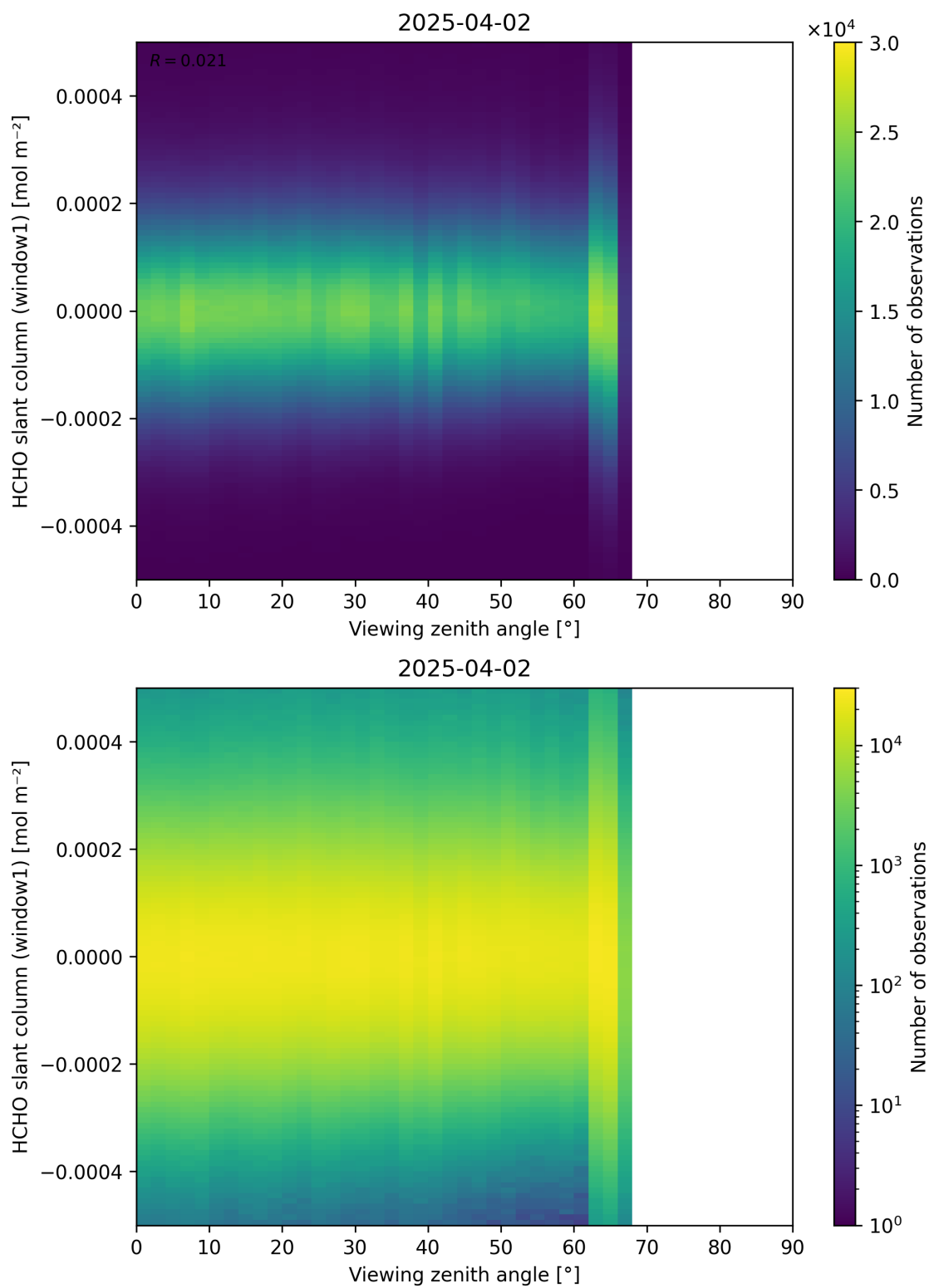
Figure 188: Scatter density plot of “Viewing zenith angle” against “HCHO slant column (window1)” for 2025-04-02 to 2025-04-03.
