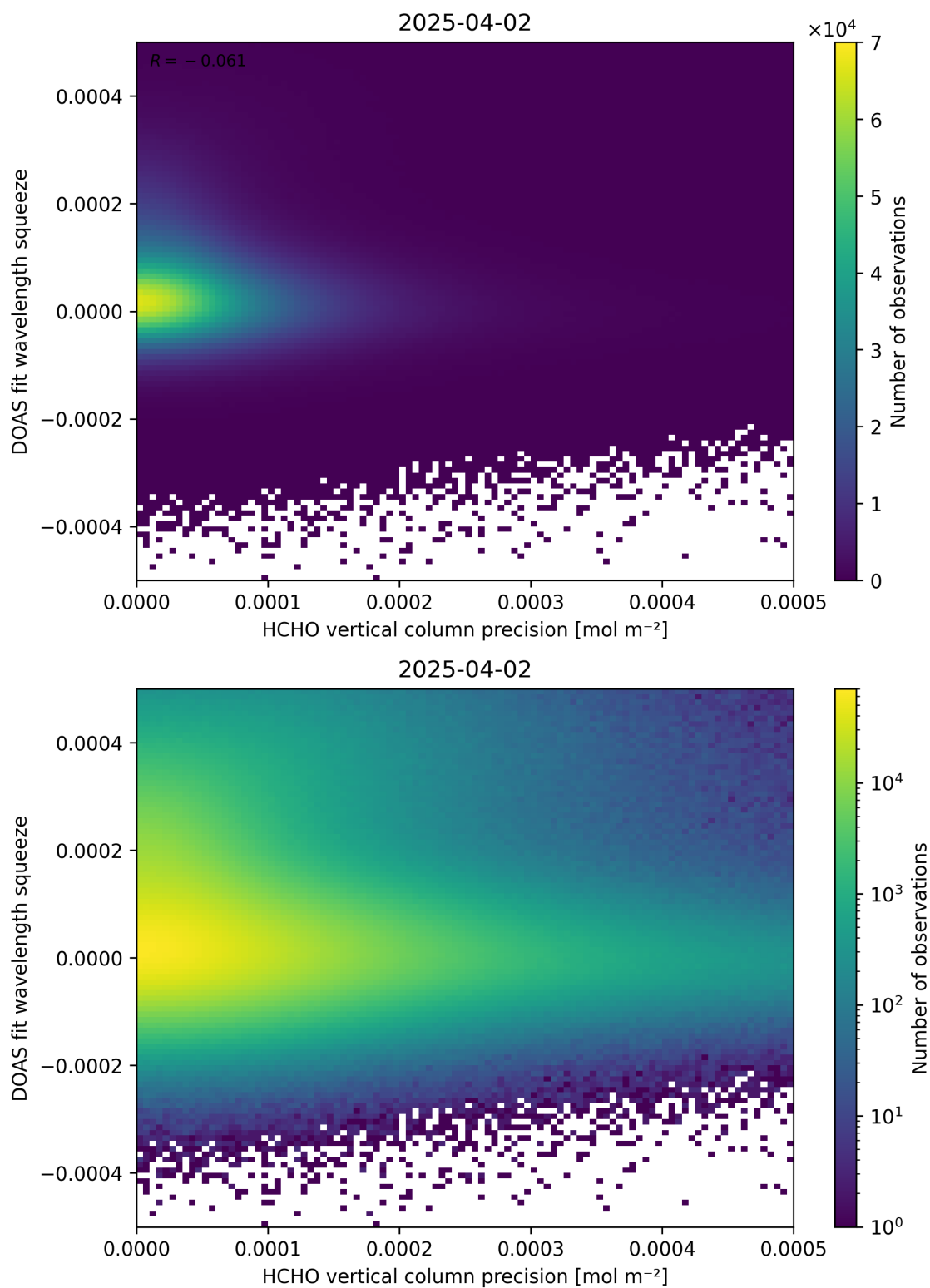
Figure 138: Scatter density plot of “HCHO vertical column precision” against “DOAS fit wavelength squeeze” for 2025-04-02 to 2025-04-03.
