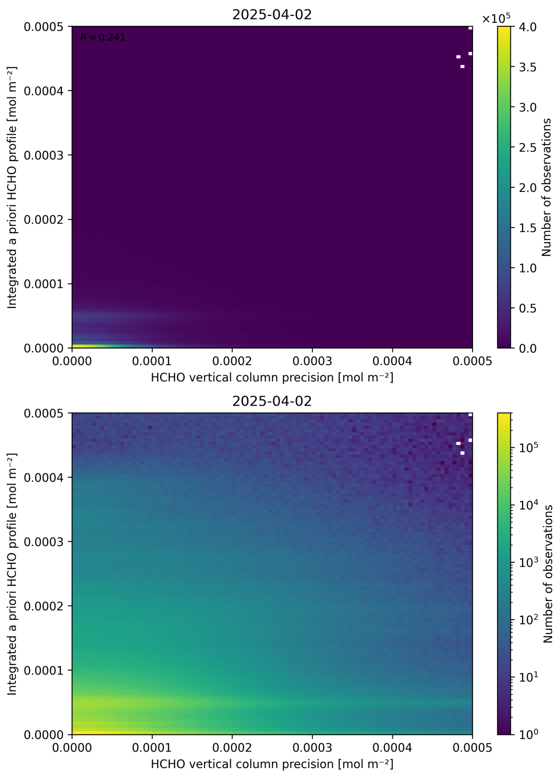
Figure 147: Scatter density plot of “HCHO vertical column precision” against “Integrated a priori HCHO profile” for 2025-04-02 to 2025-04-03.
