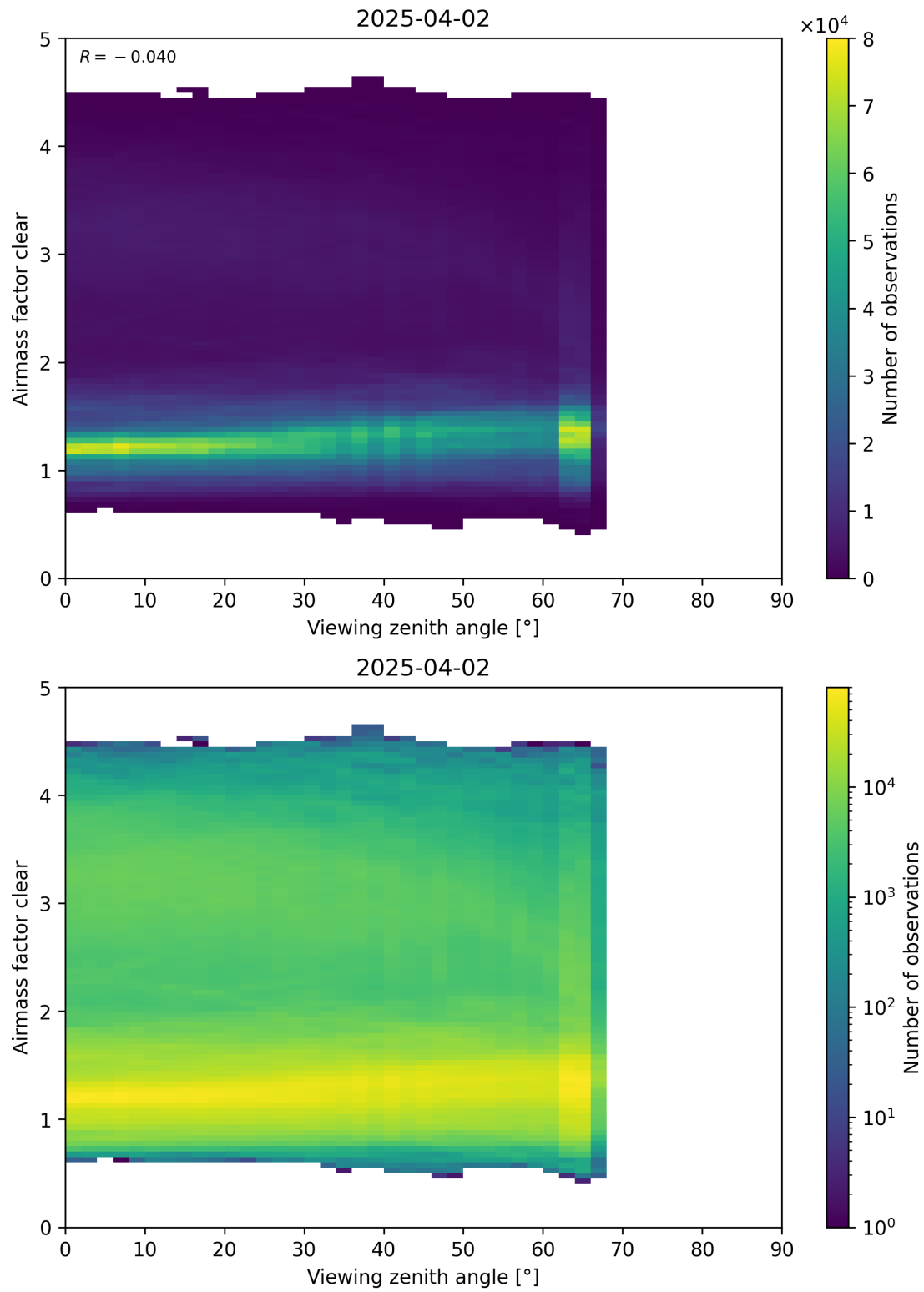
Figure 185: Scatter density plot of “Viewing zenith angle” against “Airmass factor clear” for 2025-04-02 to 2025-04-03.
