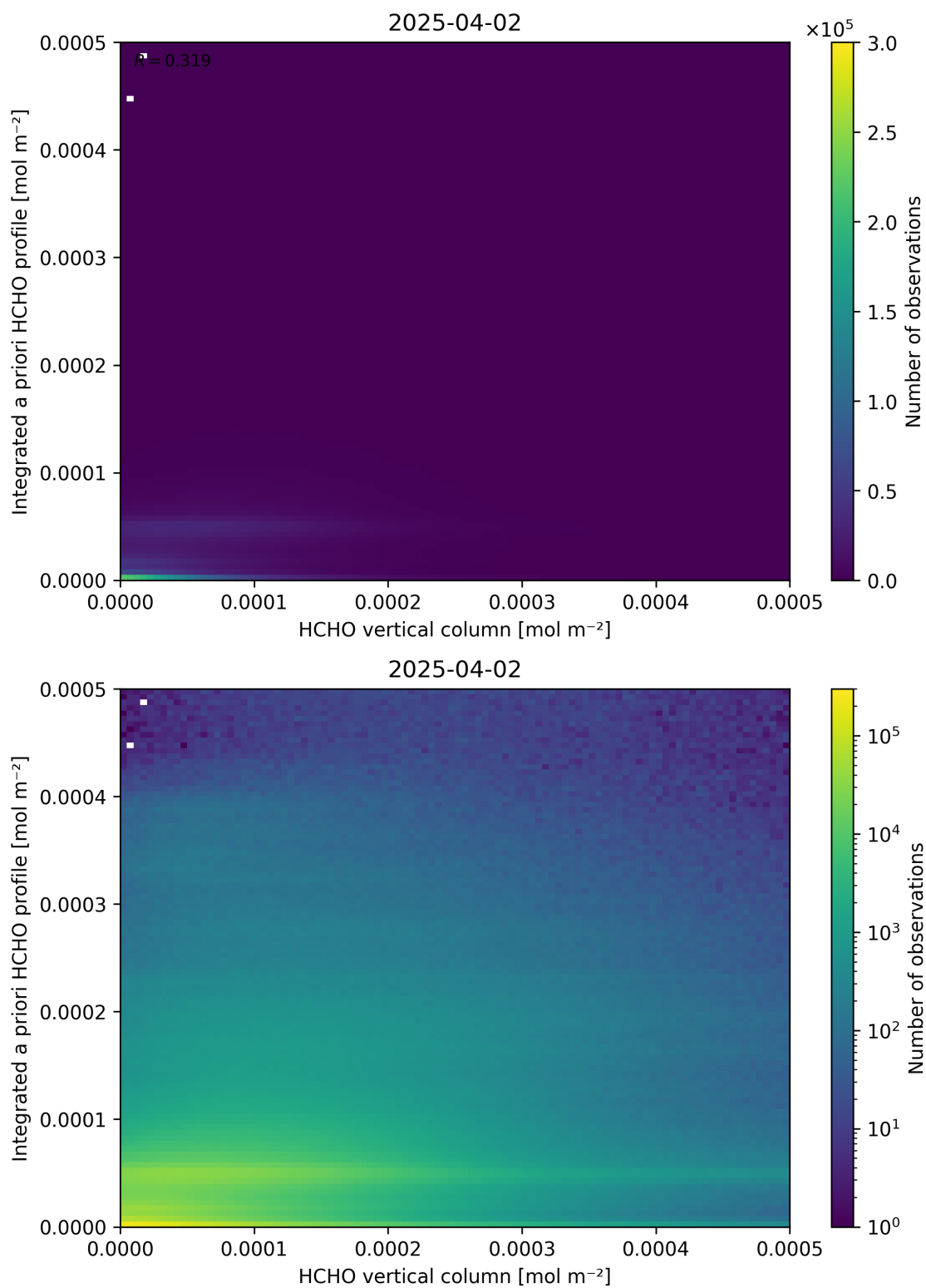
Figure 135: Scatter density plot of “HCHO vertical column” against “Integrated a priori HCHO profile” for 2025-04-02 to 2025-04-03.
