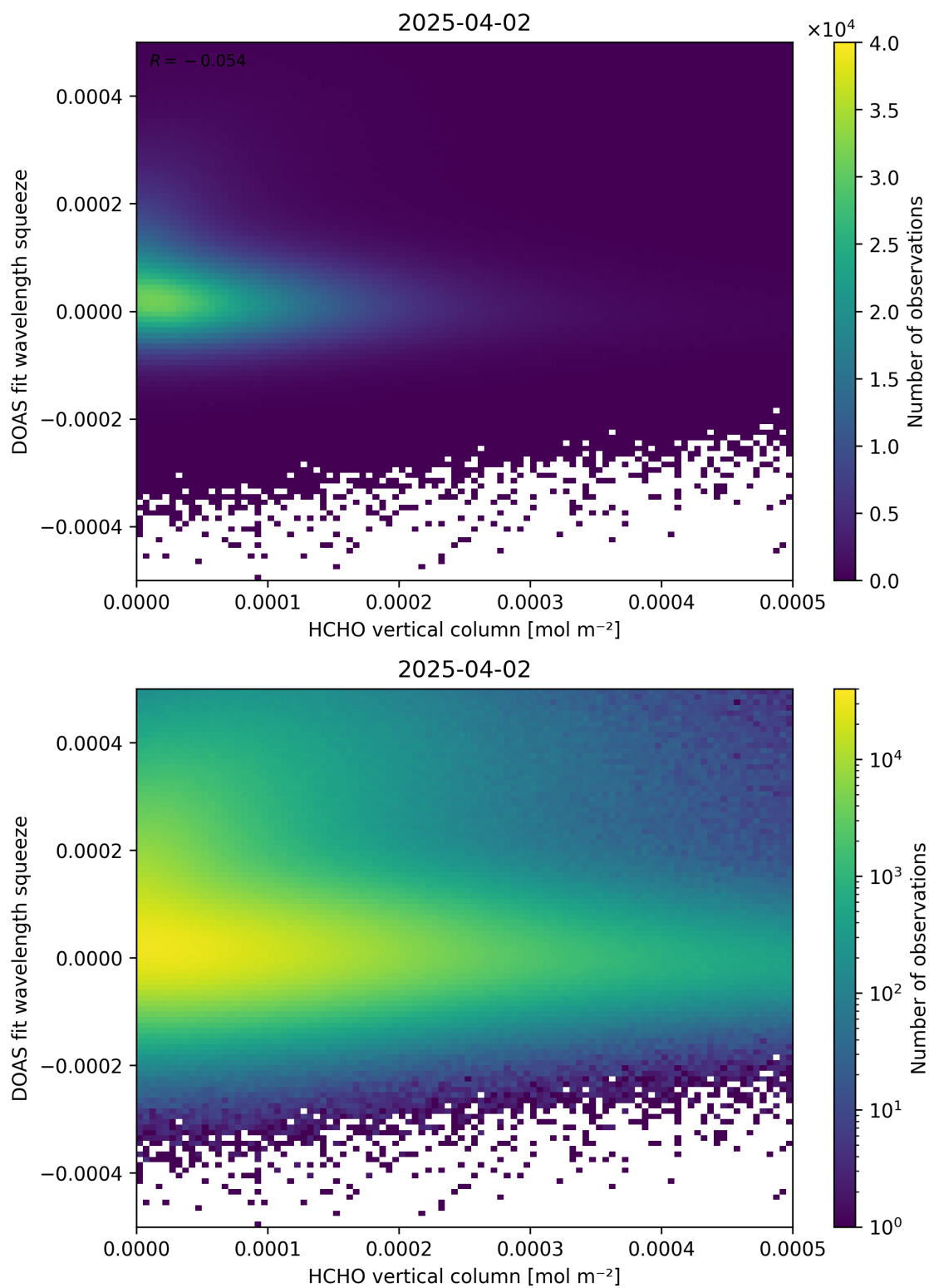
Figure 125: Scatter density plot of “HCHO vertical column” against “DOAS fit wavelength squeeze” for 2025-04-02 to 2025-04-03.
