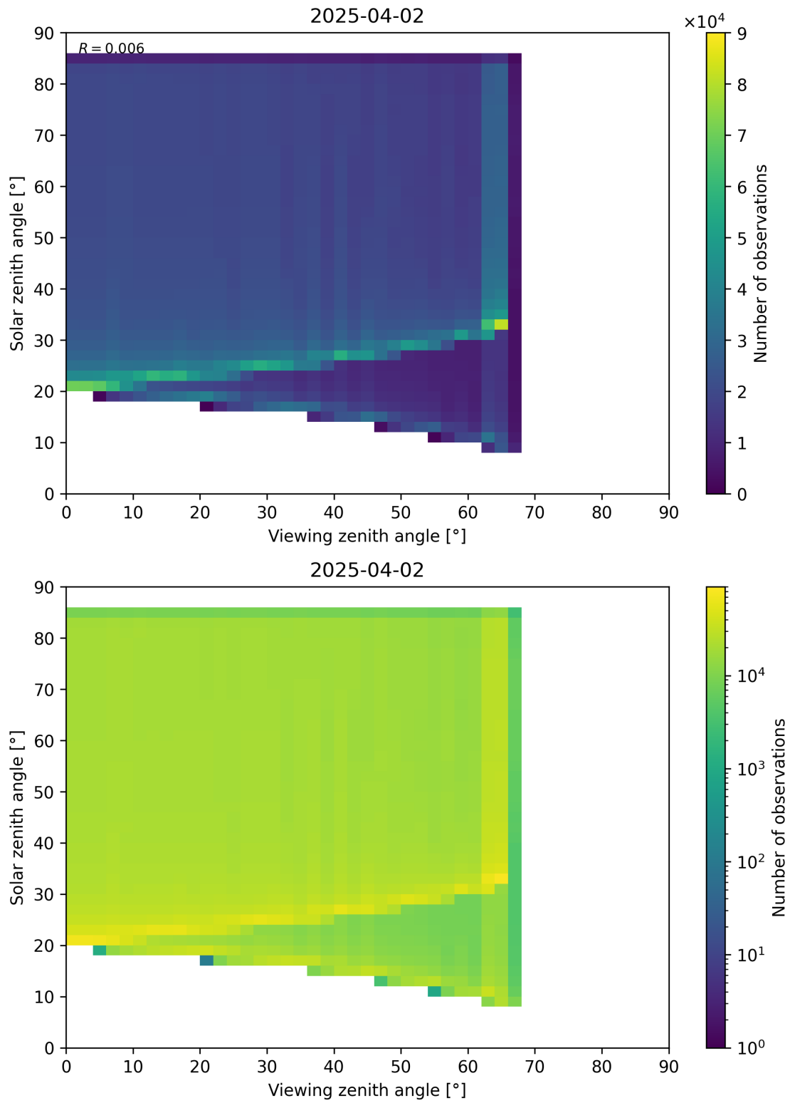
Figure 197: Scatter density plot of “Viewing zenith angle” against “Solar zenith angle” for 2025-04-02 to 2025-04-03.
