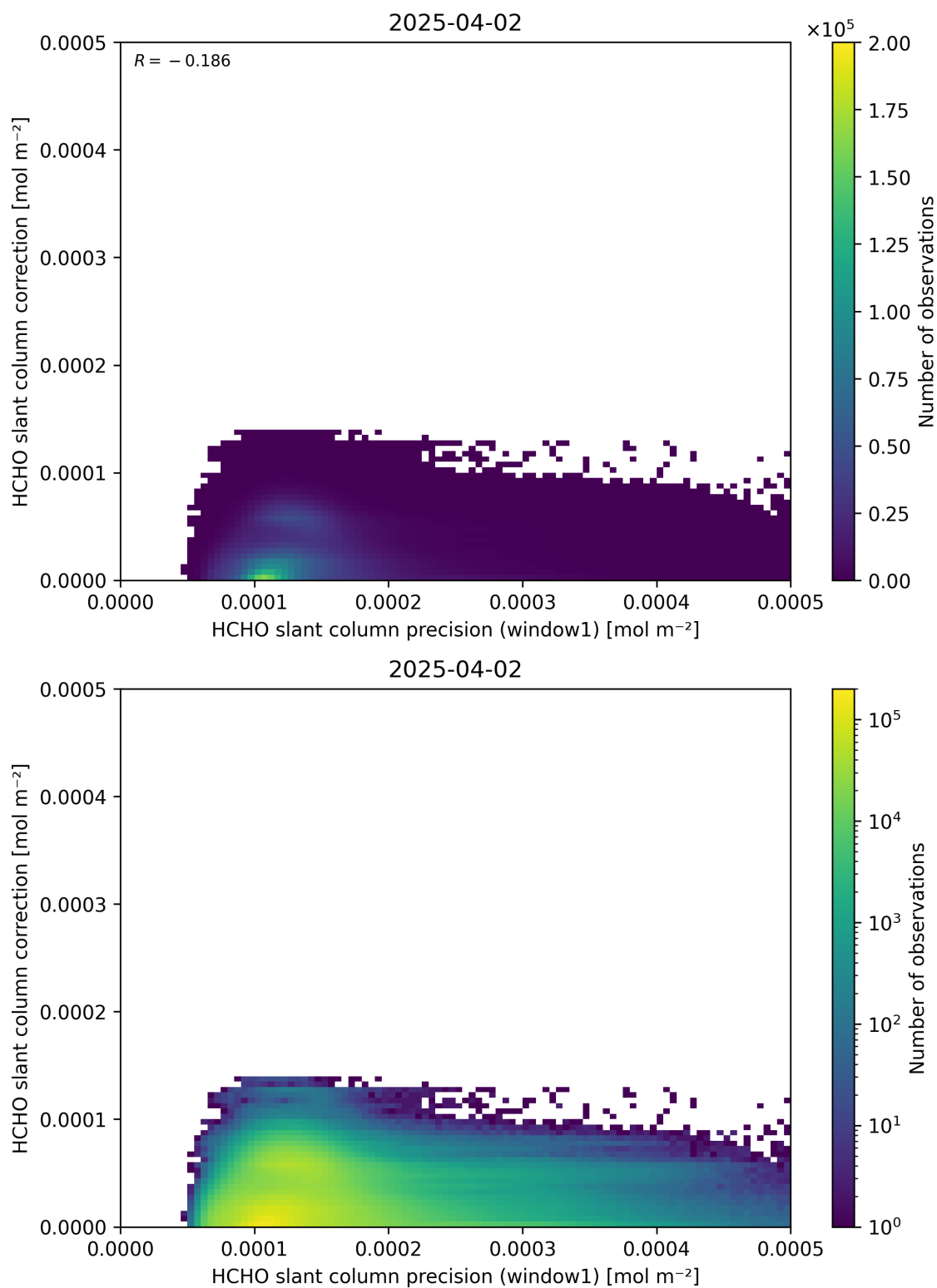
Figure 93: Scatter density plot of “HCHO slant column precision (window1)” against “HCHO slant column correction” for 2025-04-02 to 2025-04-03.
