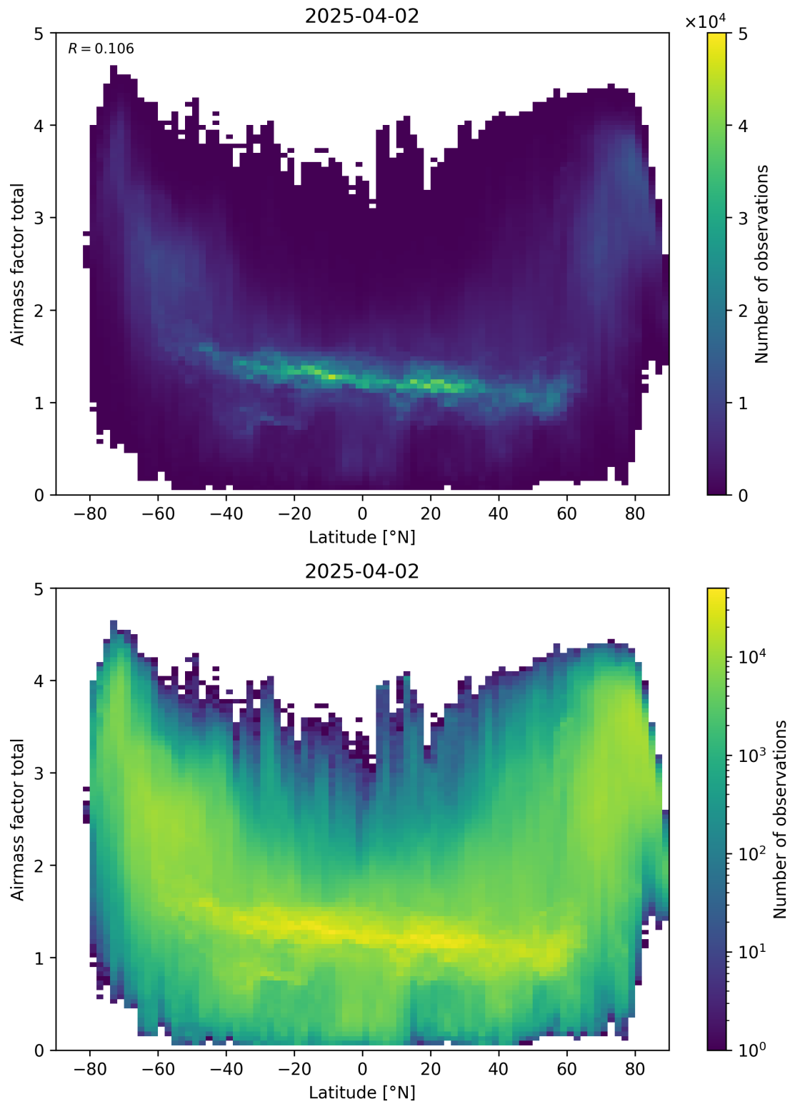
Figure 161: Scatter density plot of “Latitude” against “Airmass factor total” for 2025-04-02 to 2025-04-03.
