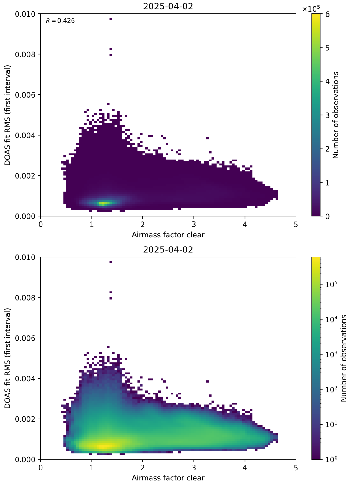
Figure 71: Scatter density plot of “Airmass factor clear” against “DOAS fit RMS (first interval)” for 2025-04-02 to 2025-04-03.
