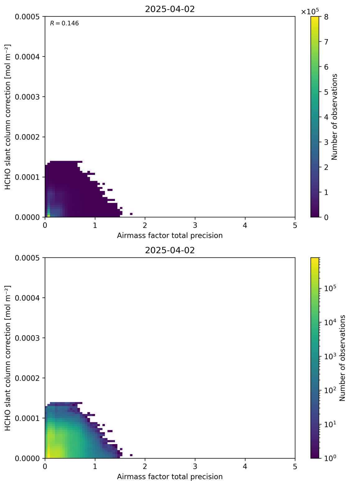
Figure 110: Scatter density plot of “Airmass factor total precision” against “HCHO slant column correction” for 2025-04-02 to 2025-04-03.
