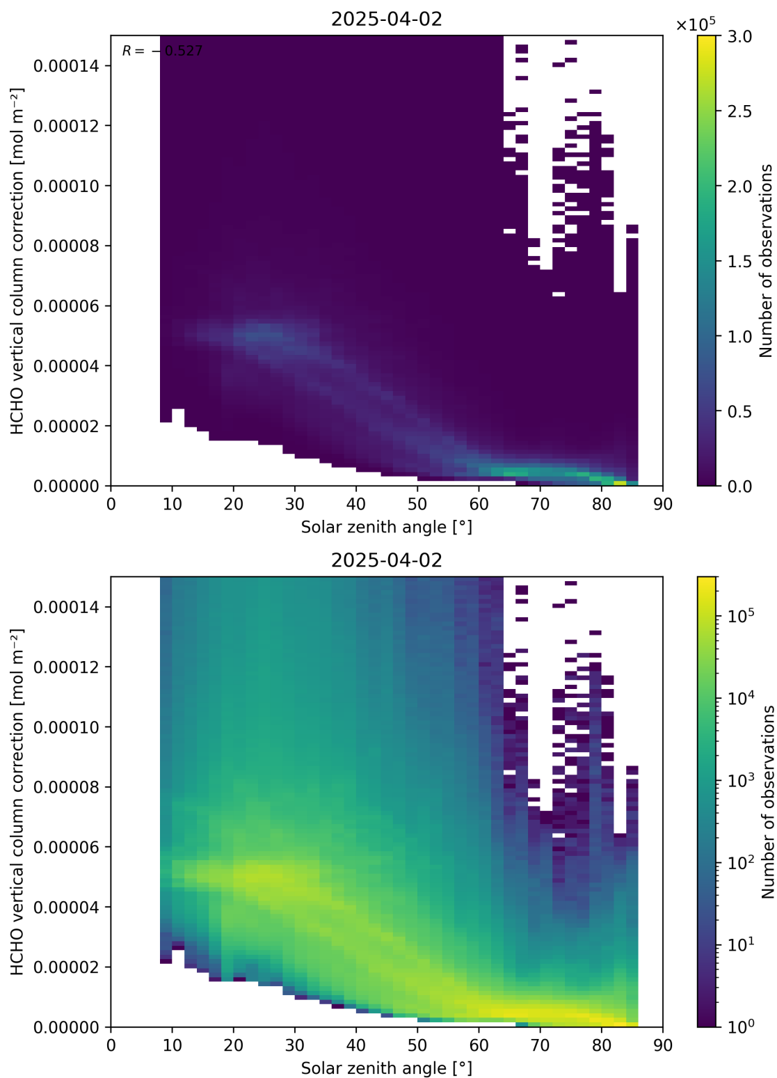
Figure 178: Scatter density plot of “Solar zenith angle” against “HCHO vertical column correction” for 2025-04-02 to 2025-04-03.
