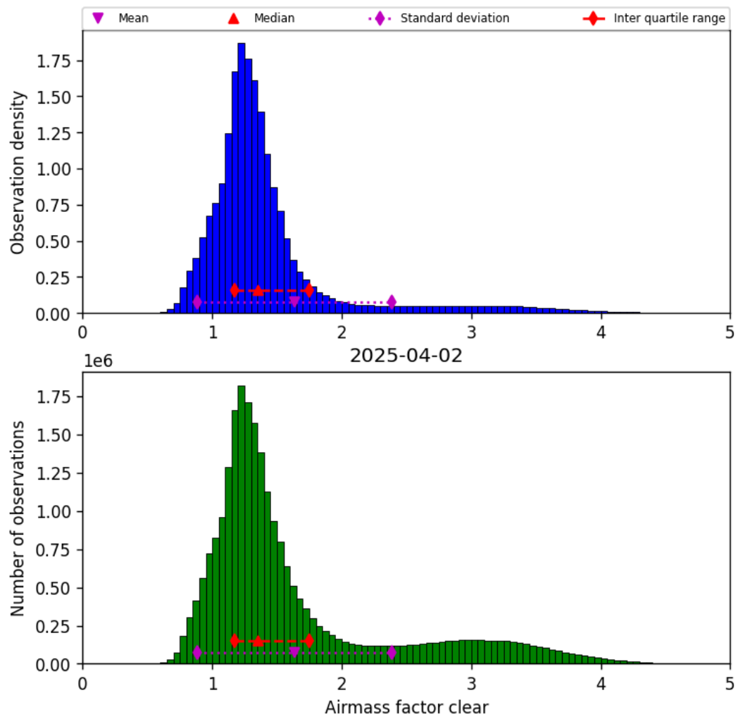
Figure 42: Histogram of “Airmass factor clear” for 2025-04-02 to 2025-04-03
