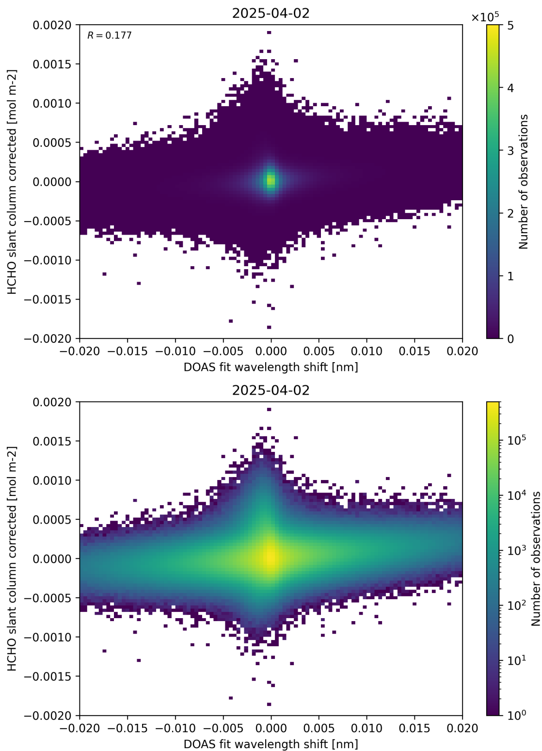
Figure 66: Scatter density plot of “DOAS fit wavelength shift” against “HCHO slant column corrected” for 2025-04-02 to 2025-04-03.
