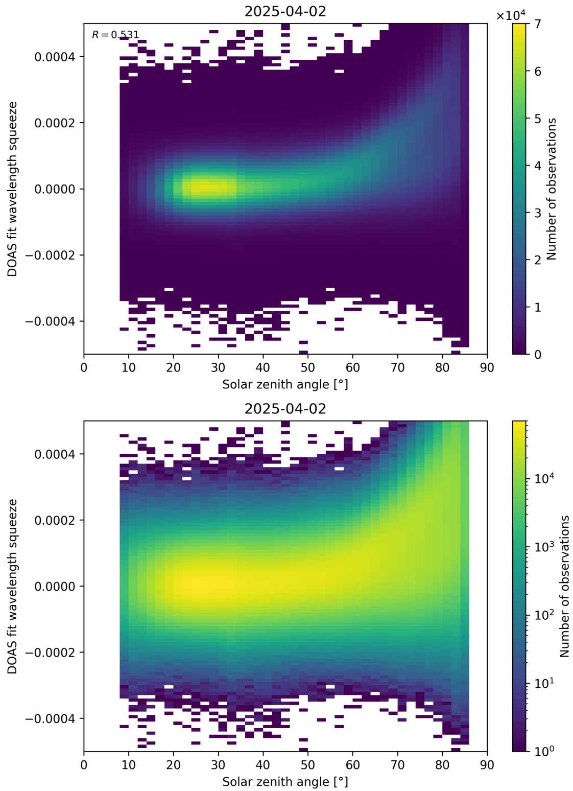
Figure 169: Scatter density plot of “Solar zenith angle” against “DOAS fit wavelength squeeze” for 2025-04-02 to 2025-04-03.
