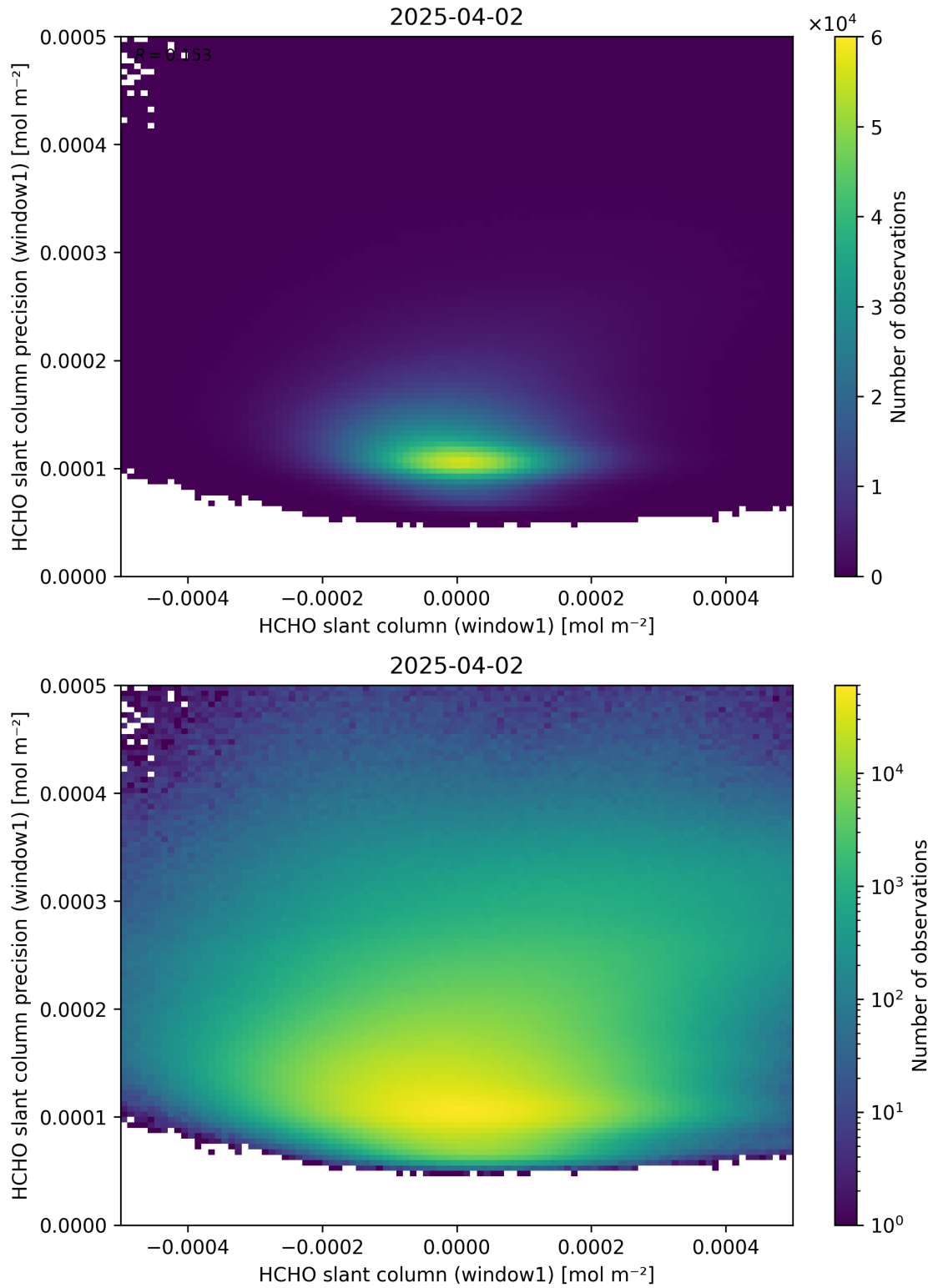
Figure 84: Scatter density plot of “HCHO slant column (window1)” against “HCHO slant column precision (window1)” for 2025-04-02 to 2025-04-03.
