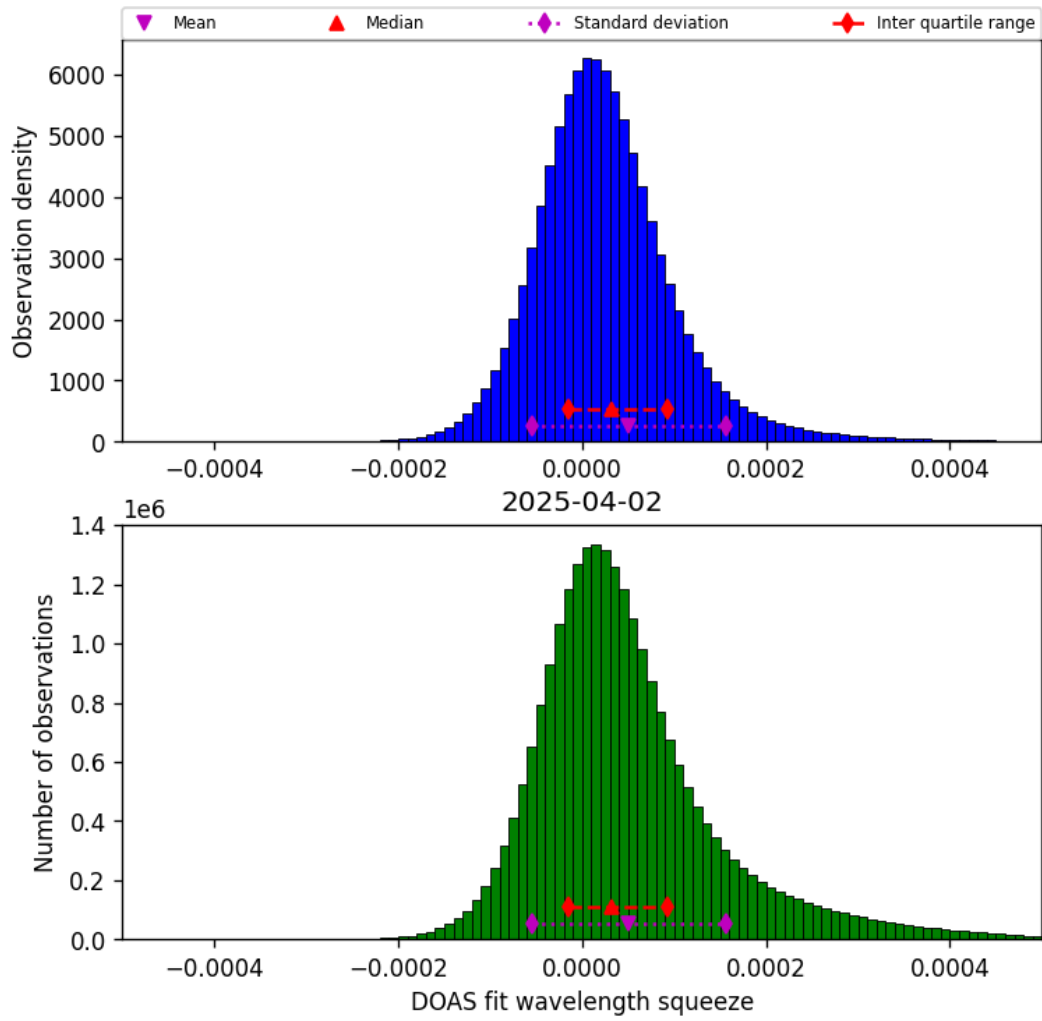
Figure 45: Histogram of “DOAS fit wavelength squeeze” for 2025-04-02 to 2025-04-03
