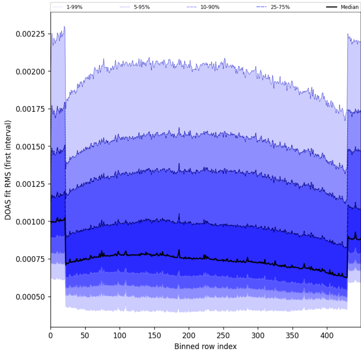
Figure 60: Along track statistics of “DOAS fit RMS (first interval)” for 2025-04-02 to 2025-04-03
