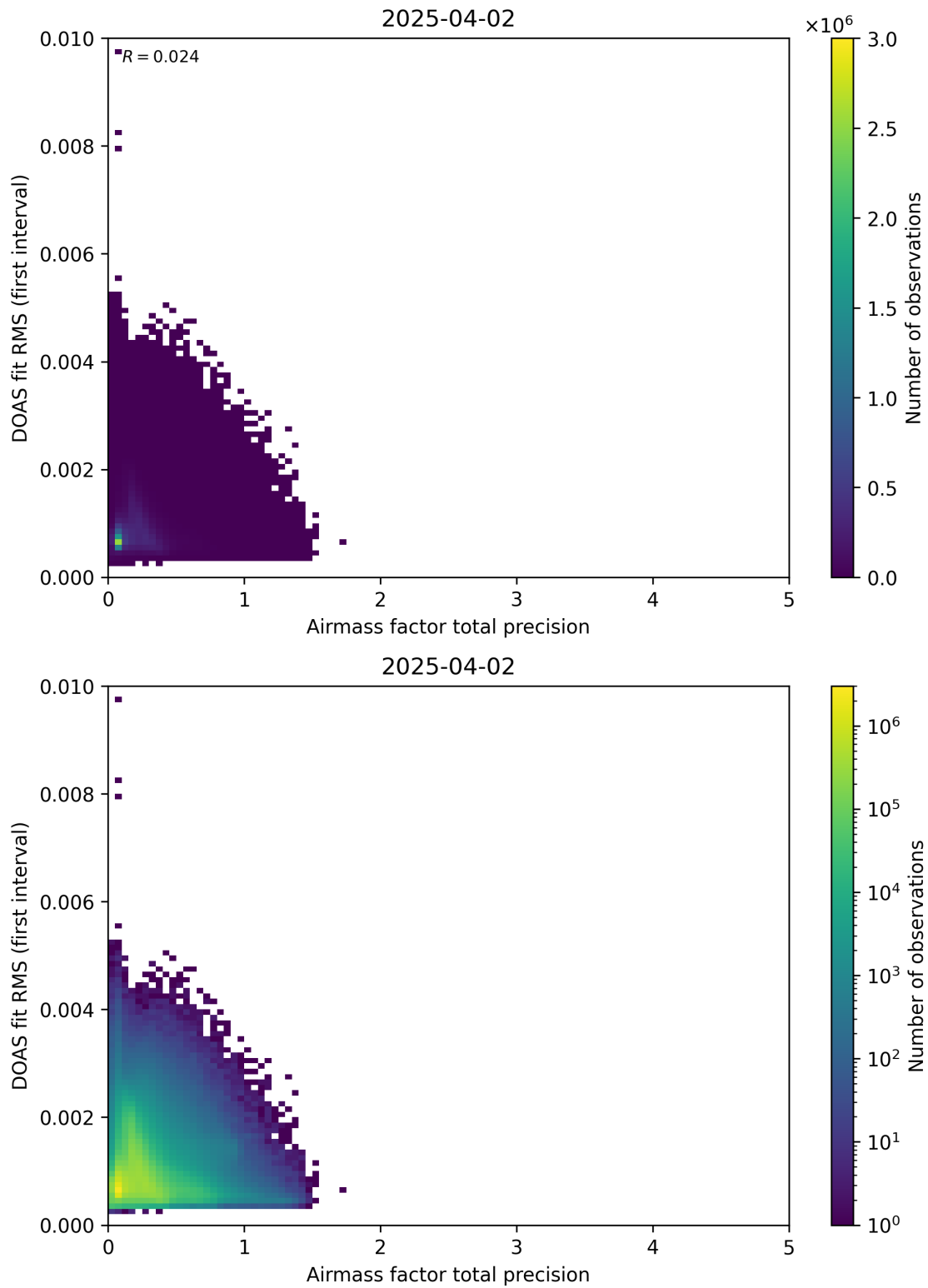
Figure 105: Scatter density plot of “Airmass factor total precision” against “DOAS fit RMS (first interval)” for 2025-04-02 to 2025-04-03.
