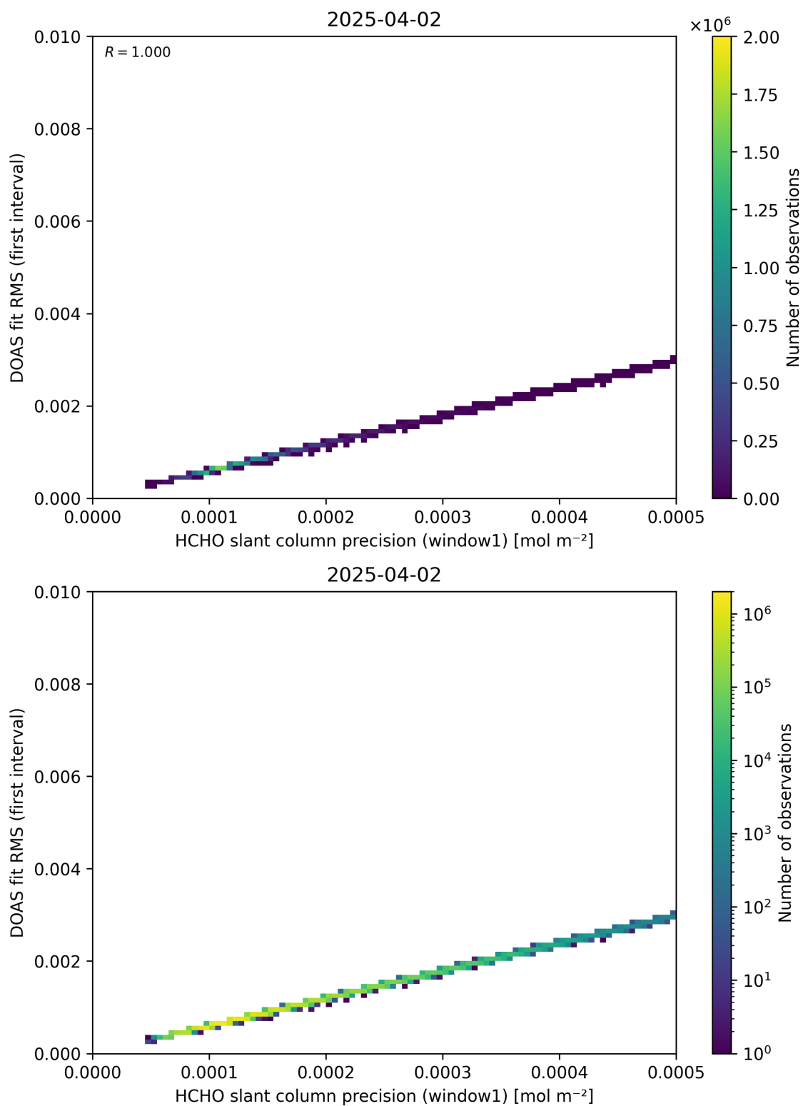
Figure 88: Scatter density plot of “HCHO slant column precision (window1)” against “DOAS fit RMS (first interval)” for 2025-04-02 to 2025-04-03.
