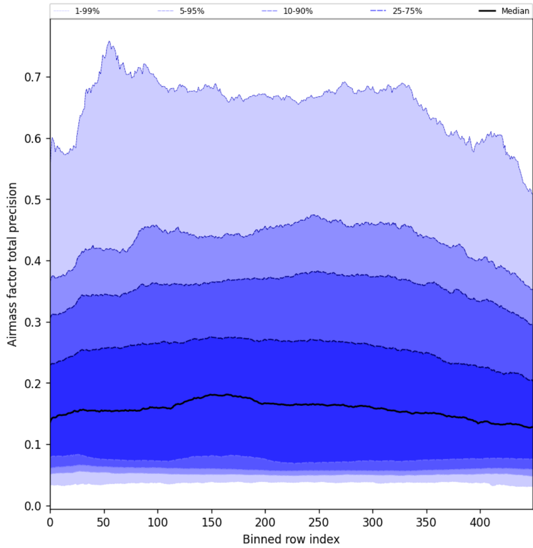
Figure 55: Along track statistics of “Airmass factor total precision” for 2025-04-02 to 2025-04-03
