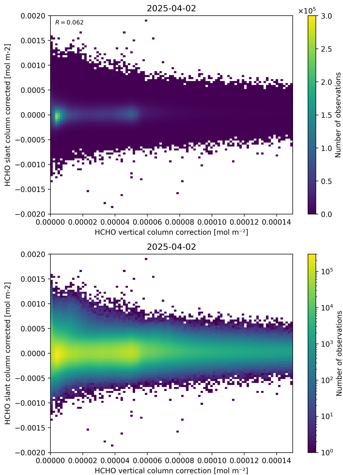
Figure 116: Scatter density plot of “HCHO vertical column correction” against “HCHO slant column corrected” for 2025-04-02 to 2025-04-03.
