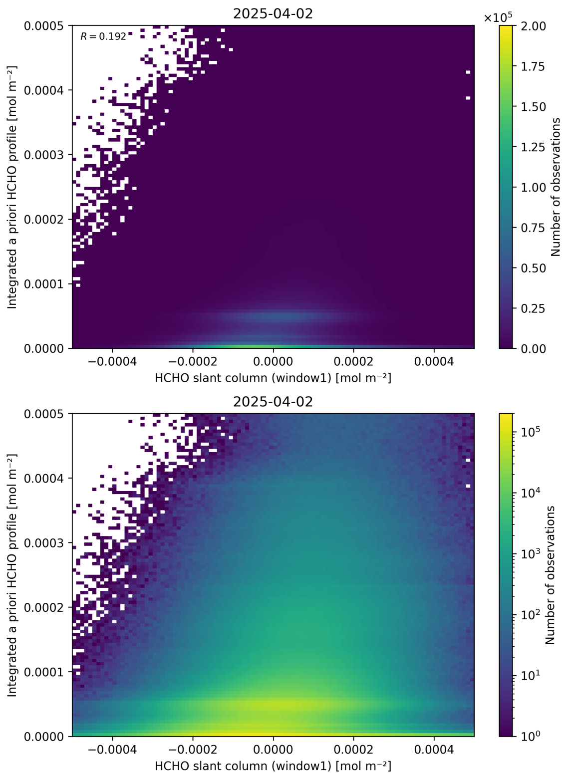
Figure 87: Scatter density plot of “HCHO slant column (window1)” against “Integrated a priori HCHO profile” for 2025-04-02 to 2025-04-03.
