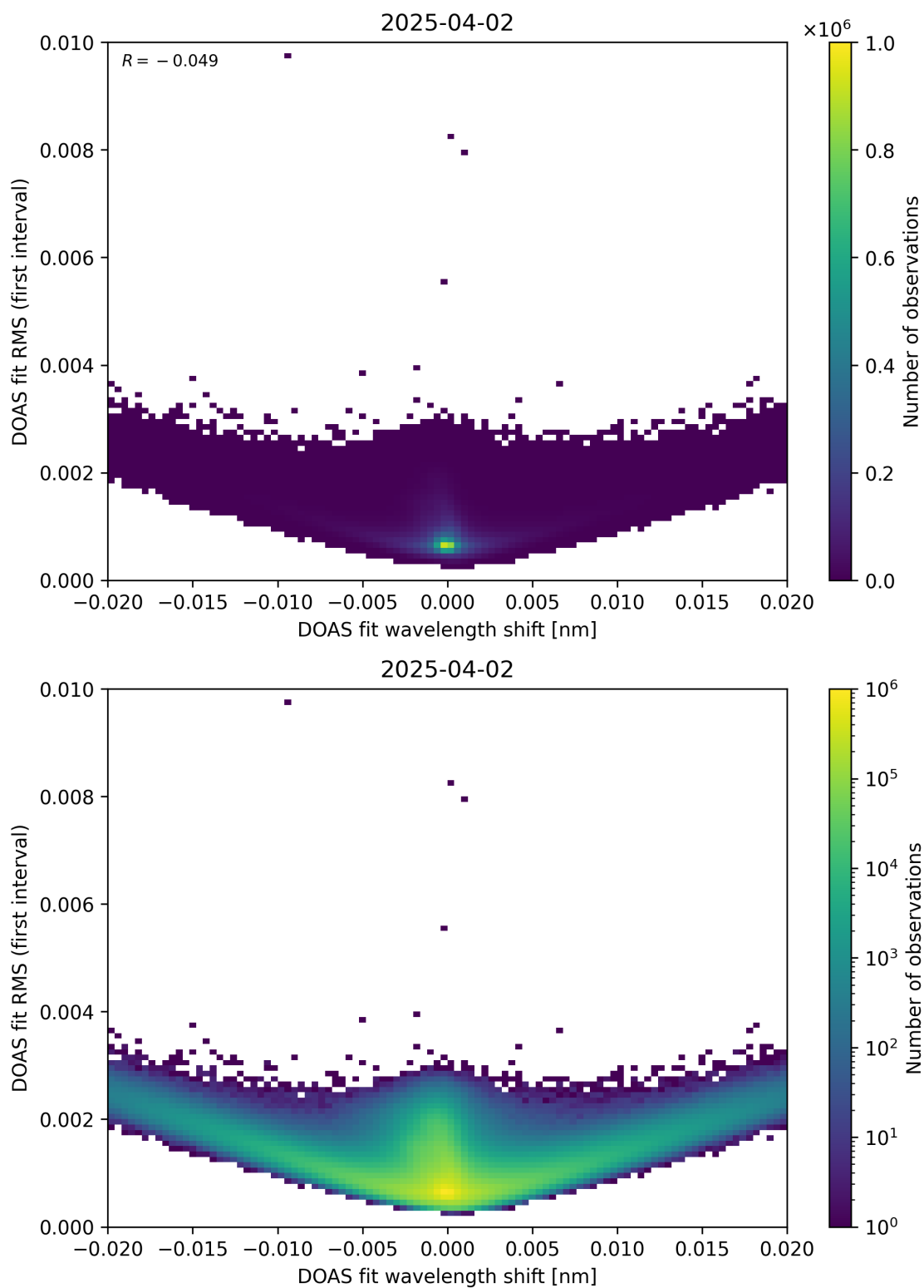
Figure 64: Scatter density plot of “DOAS fit wavelength shift” against “DOAS fit RMS (first interval)” for 2025-04-02 to 2025-04-03.
