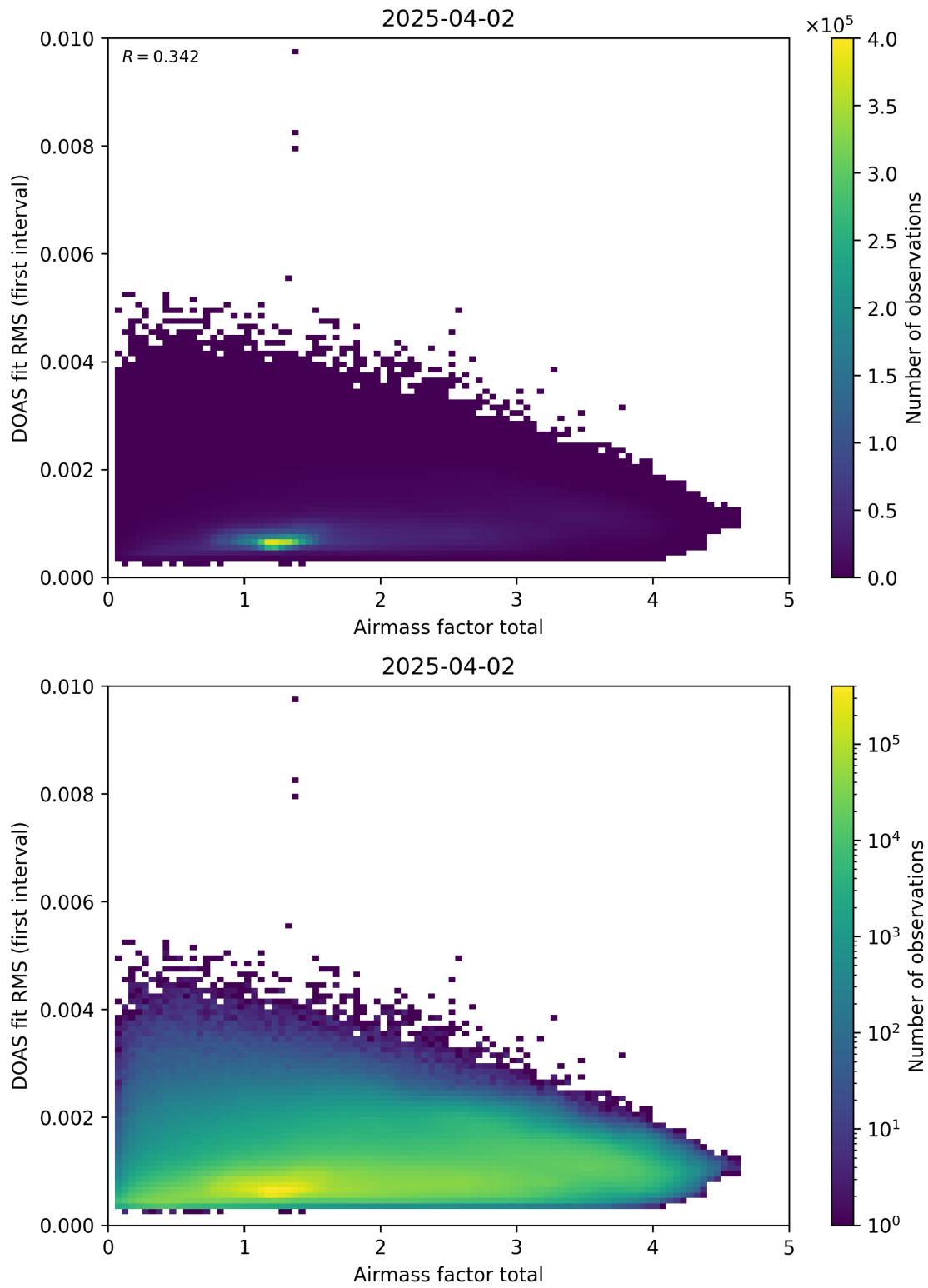
Figure 97: Scatter density plot of “Airmass factor total” against “DOAS fit RMS (first interval)” for 2025-04-02 to 2025-04-03.
