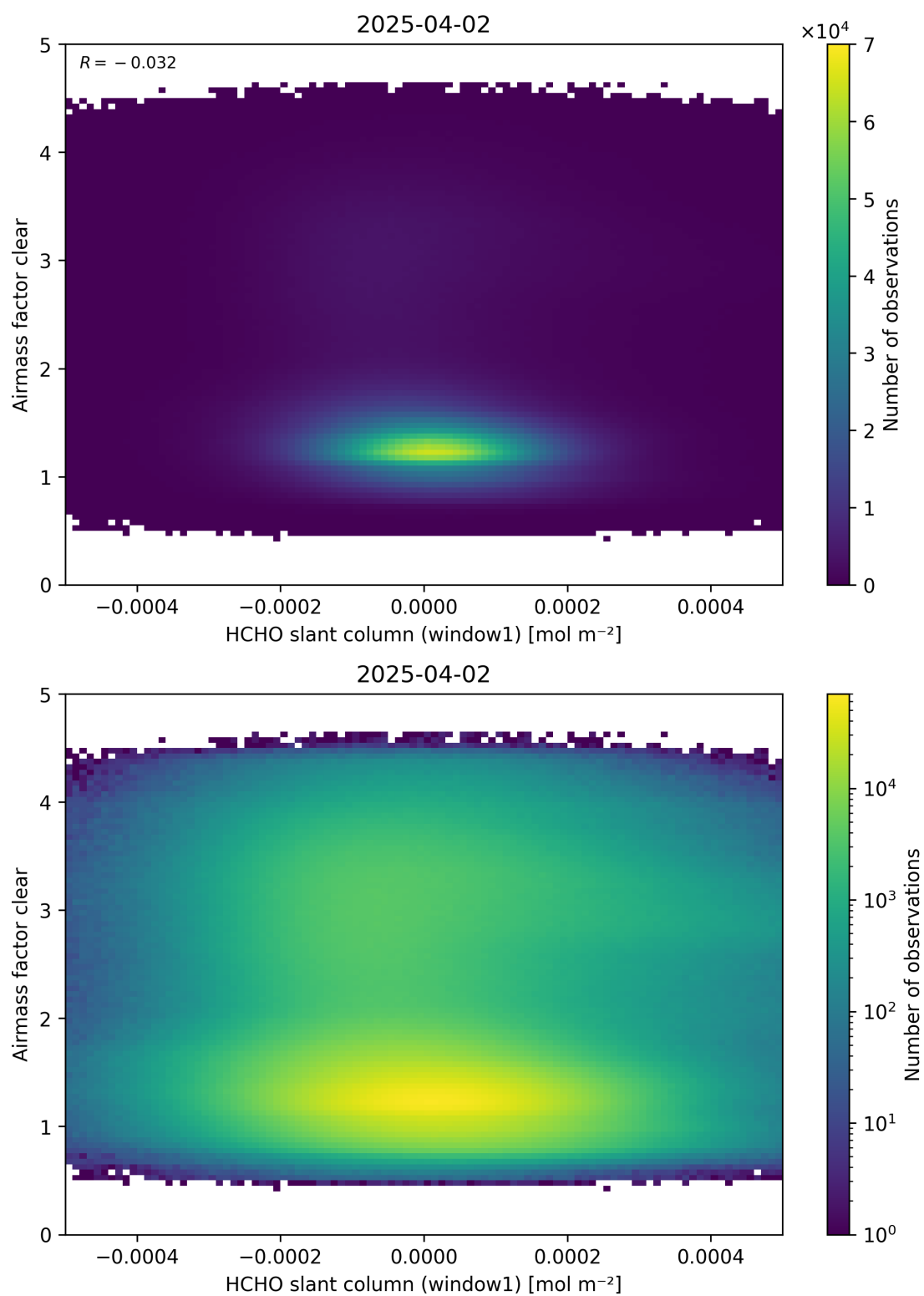
Figure 81: Scatter density plot of “HCHO slant column (window1)” against “Airmass factor clear” for 2025-04-02 to 2025-04-03.
