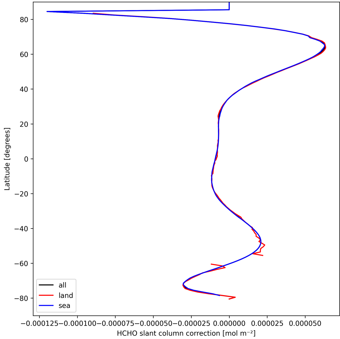
Figure 33: Zonal average of “HCHO slant column correction” for 2025-04-02 to 2025-04-03.
