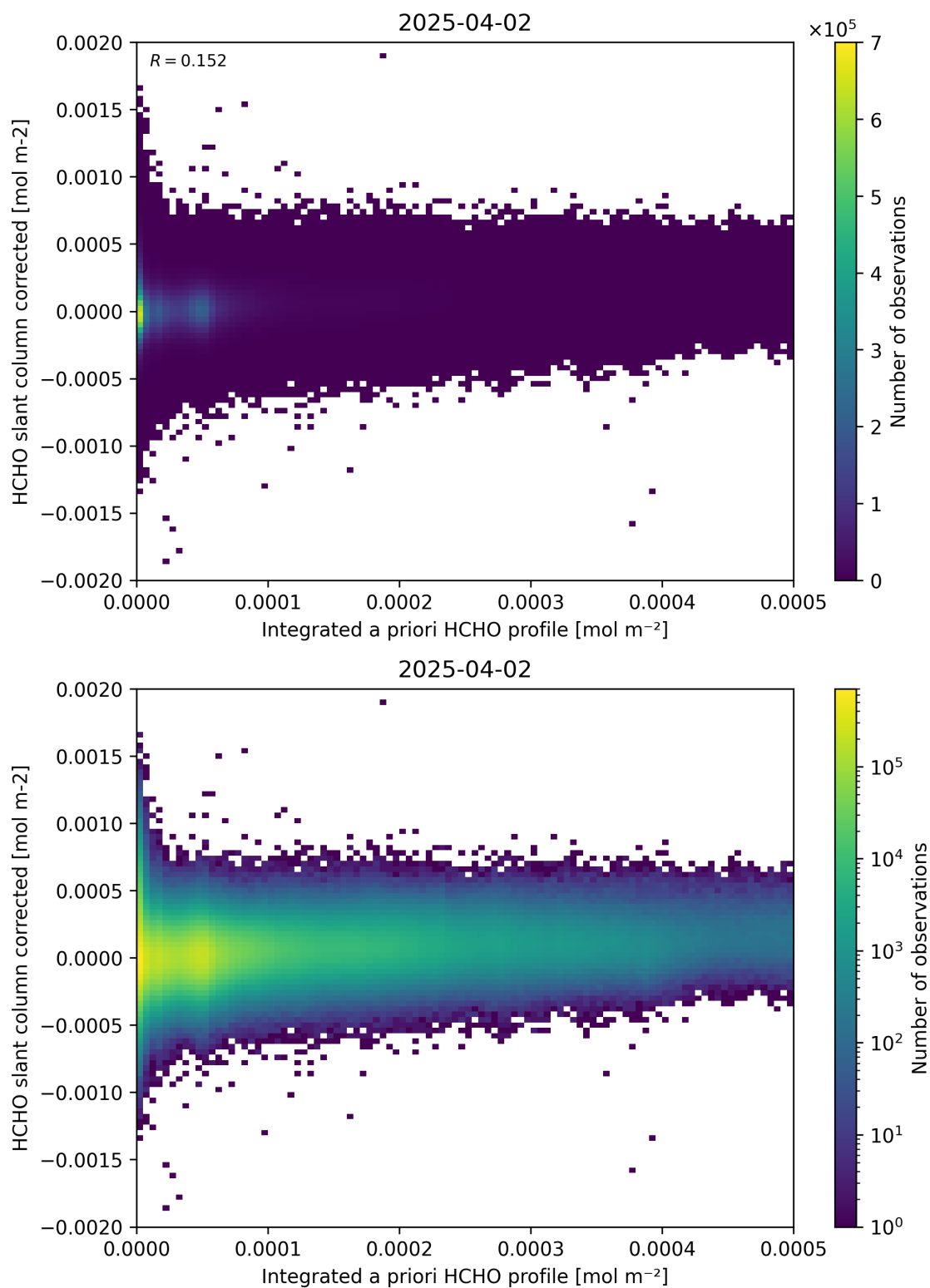
Figure 151: Scatter density plot of “Integrated a priori HCHO profile” against “HCHO slant column corrected” for 2025-04-02 to 2025-04-03.
