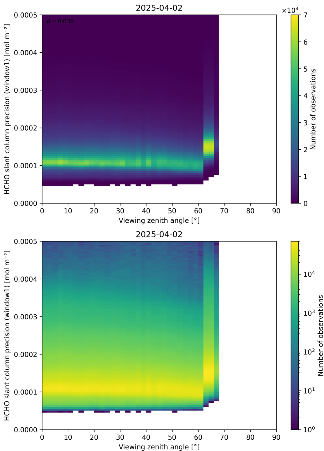
Figure 189: Scatter density plot of “Viewing zenith angle” against “HCHO slant column precision (window1)” for 2025-04-02 to 2025-04-03.
