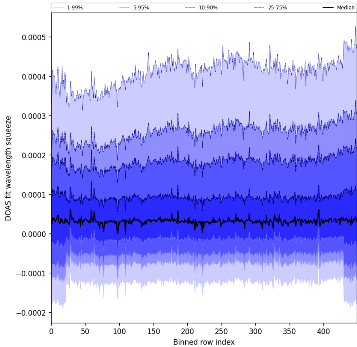
Figure 59: Along track statistics of “DOAS fit wavelength squeeze” for 2025-04-02 to 2025-04-03
