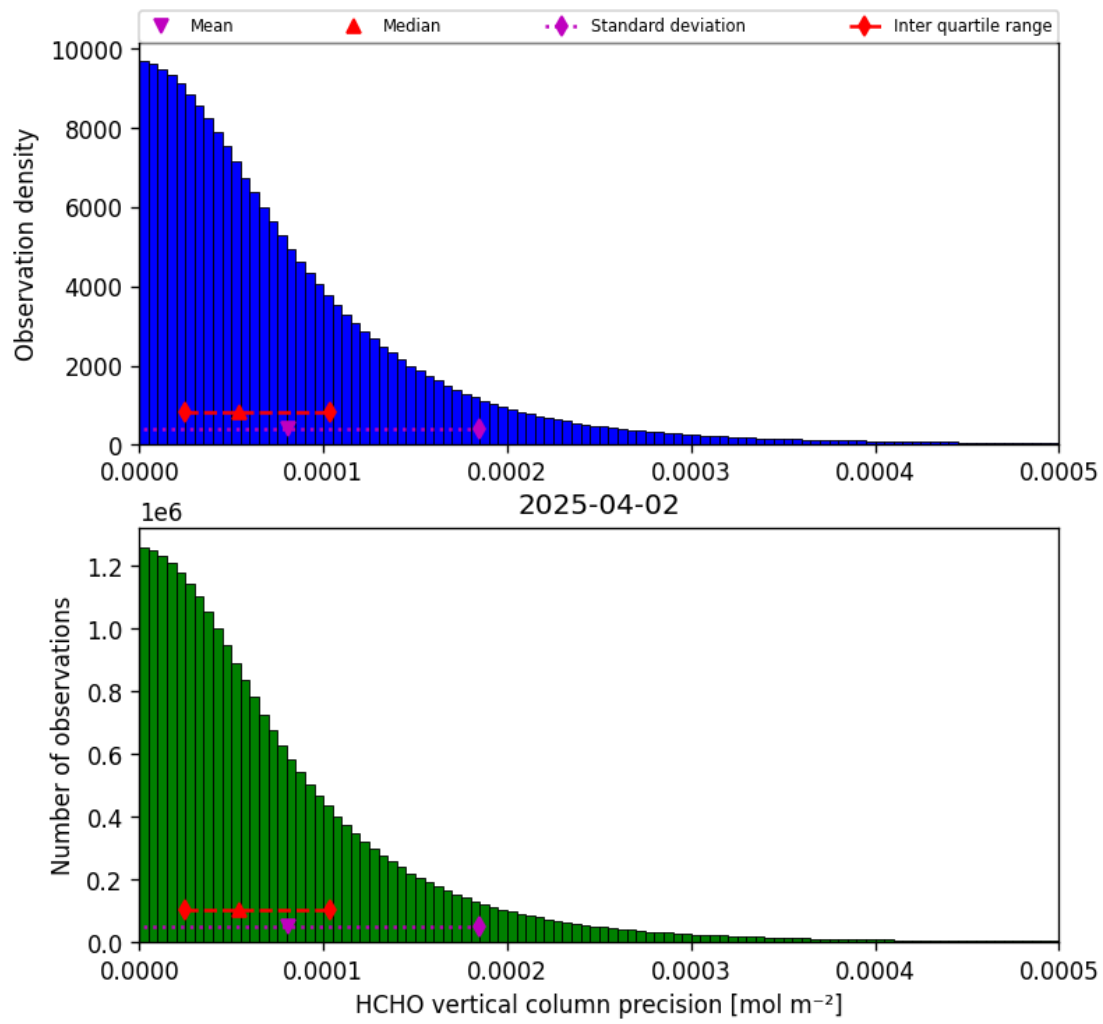
Figure 36: Histogram of “HCHO vertical column precision” for 2025-04-02 to 2025-04-03
