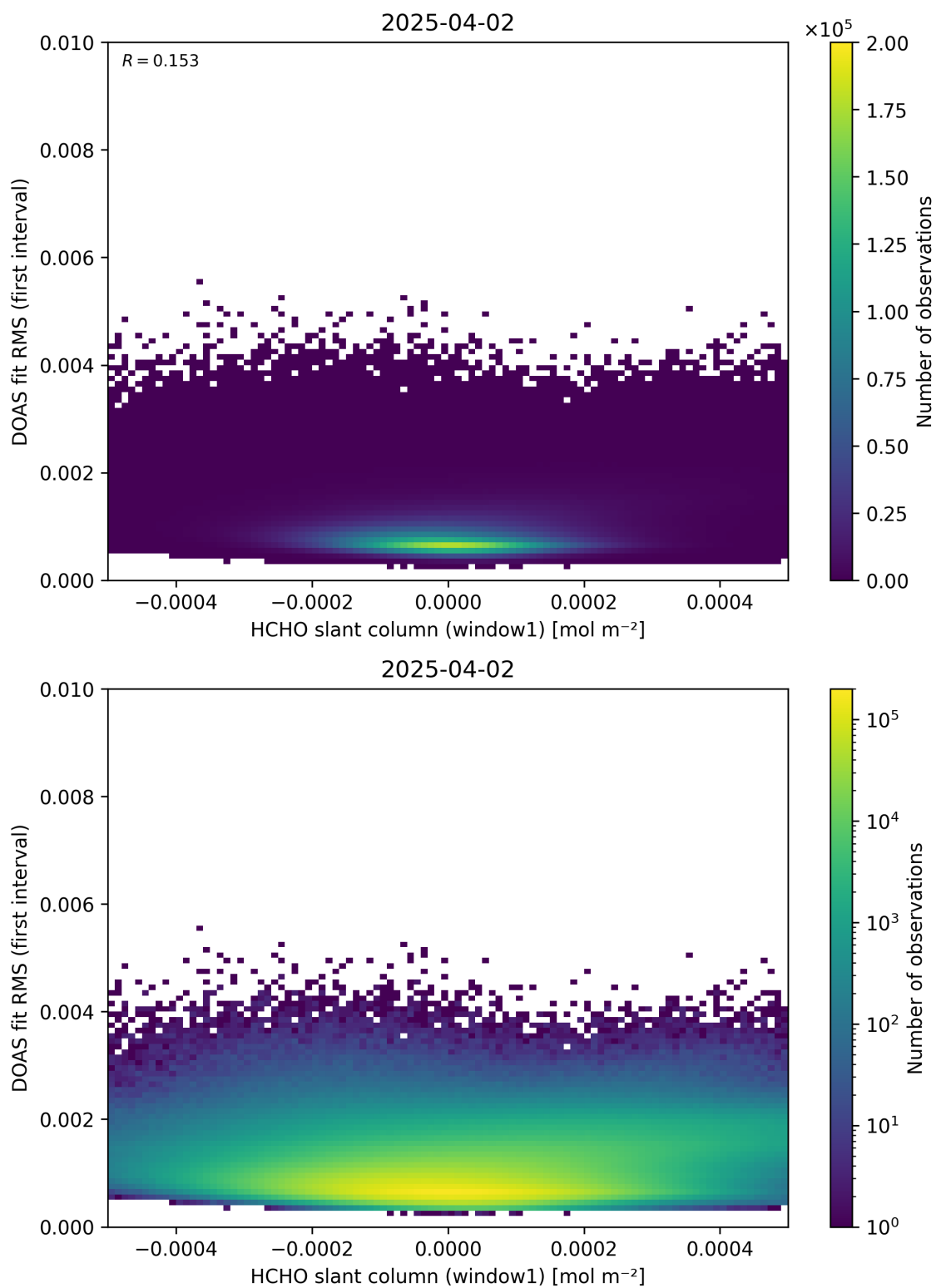
Figure 78: Scatter density plot of “HCHO slant column (window1)” against “DOAS fit RMS (first interval)” for 2025-04-02 to 2025-04-03.
