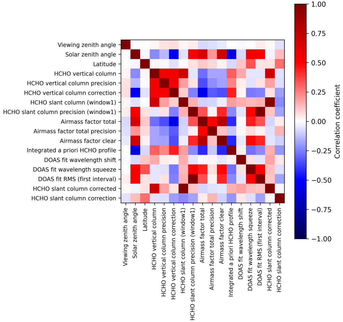
Figure 2: Map of correlation matrix for 2025-04-02 to 2025-04-03.
