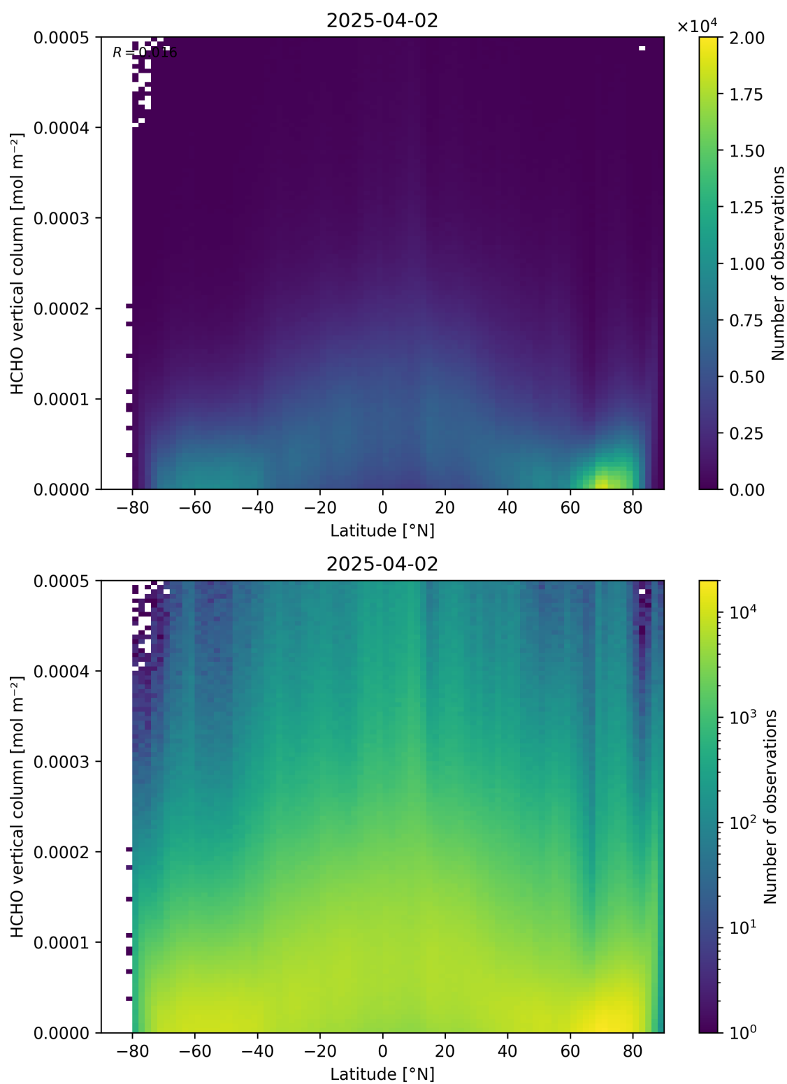
Figure 163: Scatter density plot of “Latitude” against “HCHO vertical column” for 2025-04-02 to 2025-04-03.
