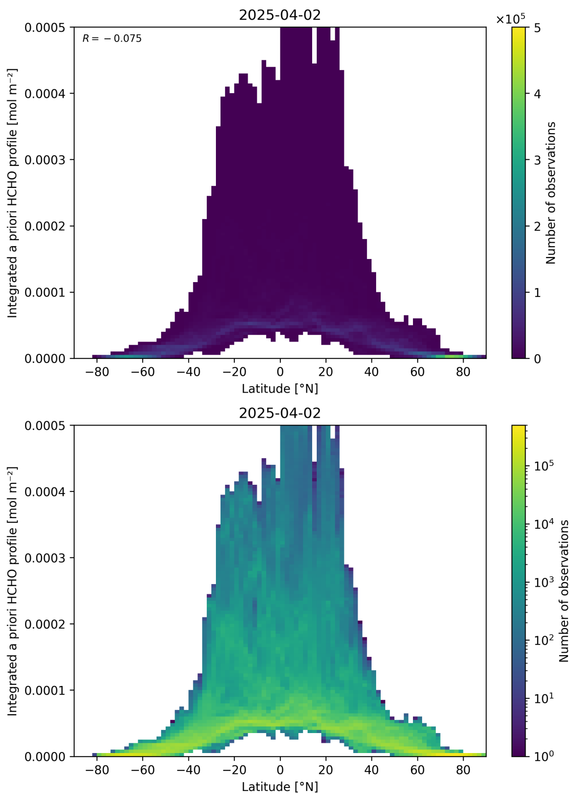
Figure 166: Scatter density plot of “Latitude” against “Integrated a priori HCHO profile” for 2025-04-02 to 2025-04-03.
