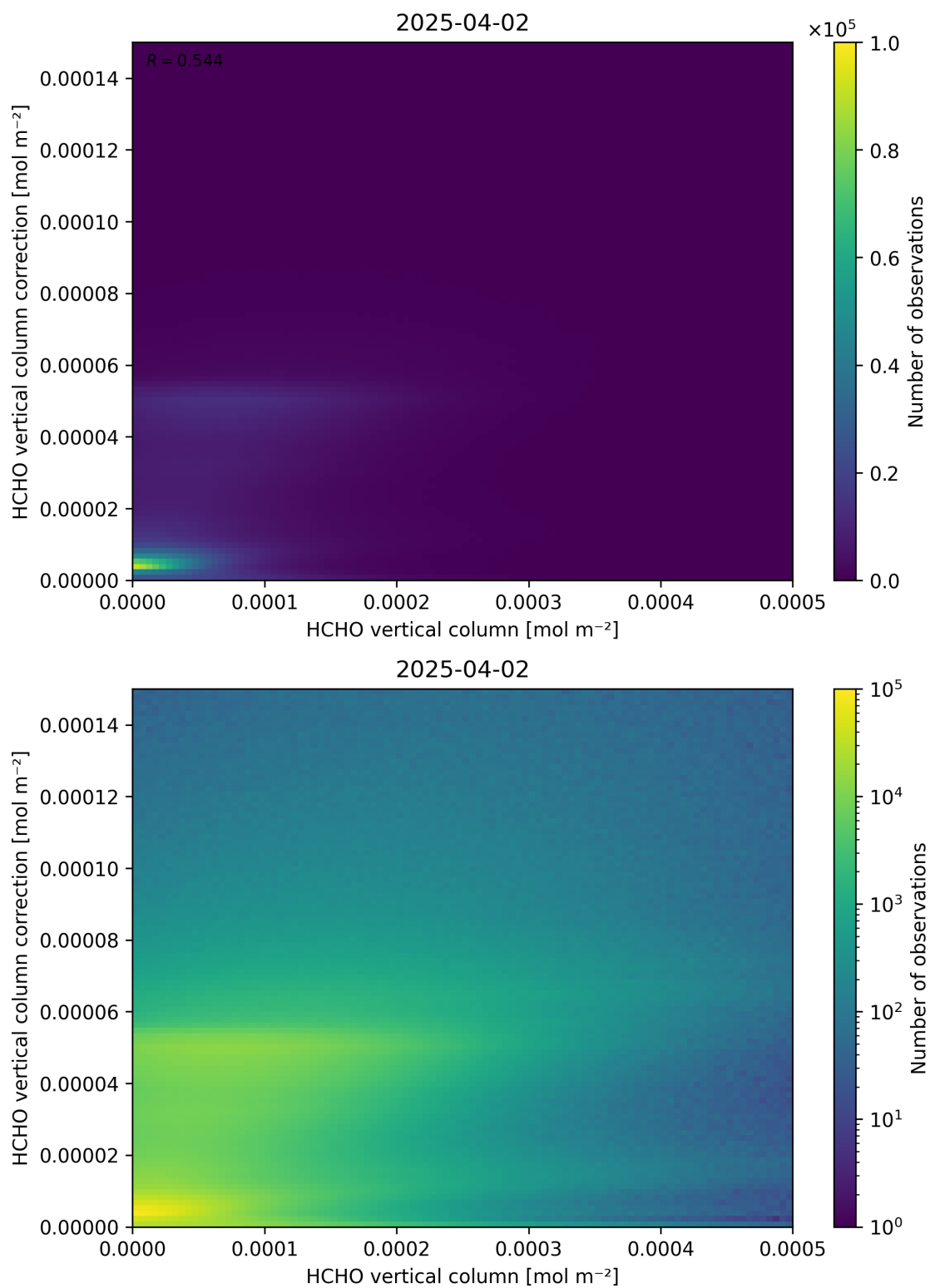
Figure 133: Scatter density plot of “HCHO vertical column” against “HCHO vertical column correction” for 2025-04-02 to 2025-04-03.
