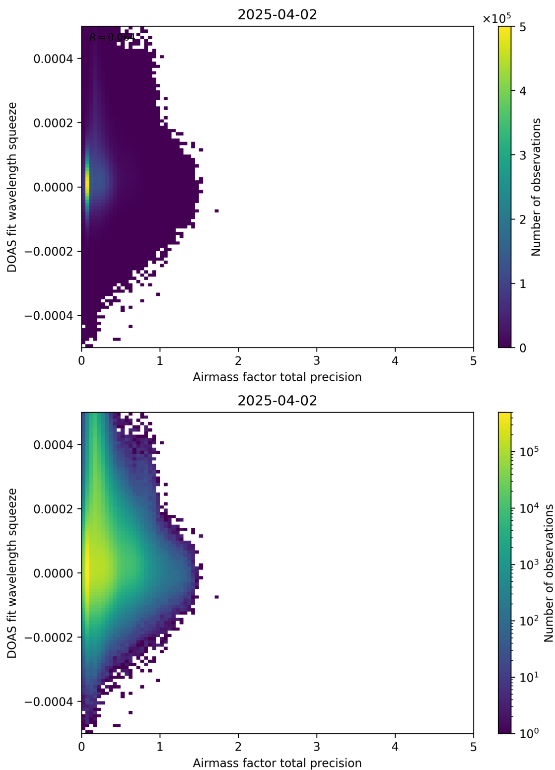
Figure 107: Scatter density plot of “Airmass factor total precision” against “DOAS fit wavelength squeeze” for 2025-04-02 to 2025-04-03.
