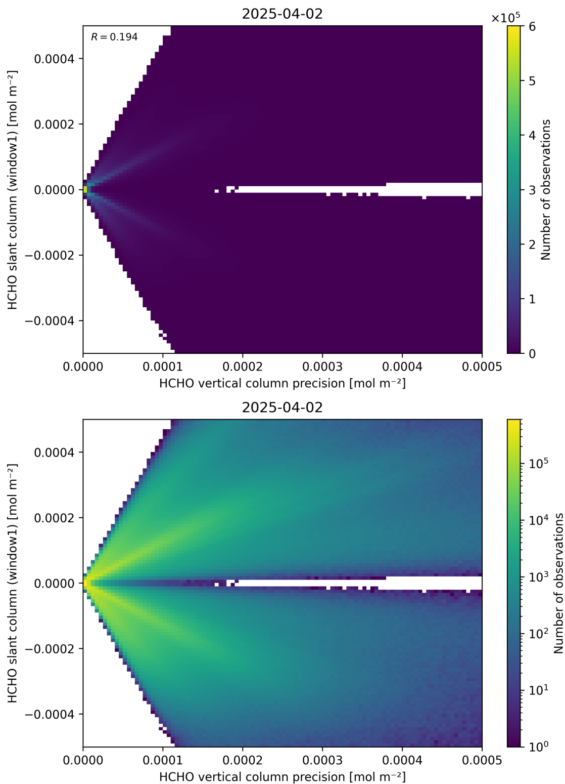
Figure 142: Scatter density plot of “HCHO vertical column precision” against “HCHO slant column (window1)” for 2025-04-02 to 2025-04-03.
