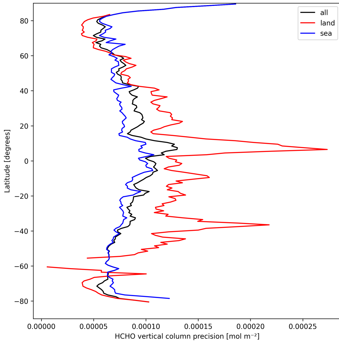
Figure 22: Zonal average of “HCHO vertical column precision” for 2025-04-02 to 2025-04-03.
