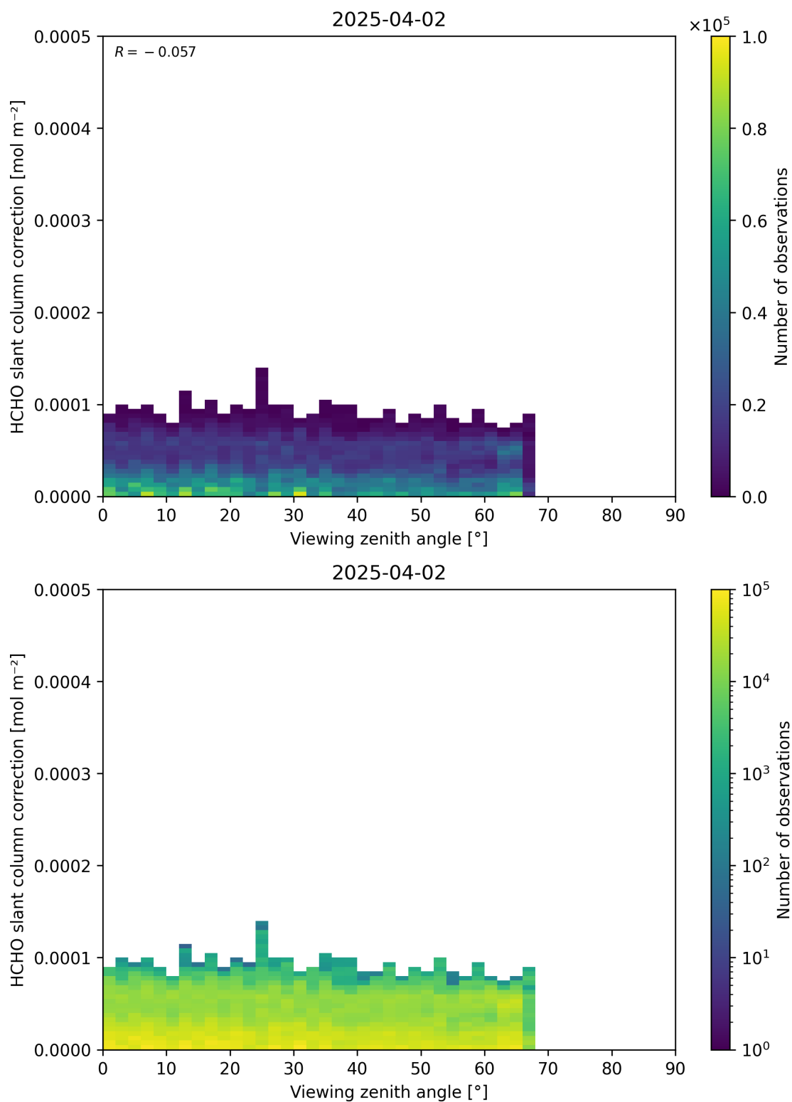
Figure 187: Scatter density plot of “Viewing zenith angle” against “HCHO slant column correction” for 2025-04-02 to 2025-04-03.
