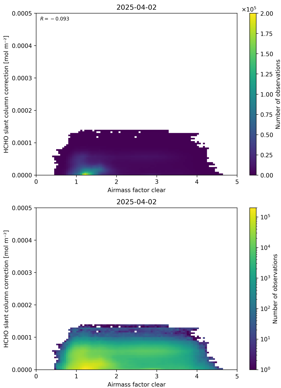
Figure 75: Scatter density plot of “Airmass factor clear” against “HCHO slant column correction” for 2025-04-02 to 2025-04-03.
