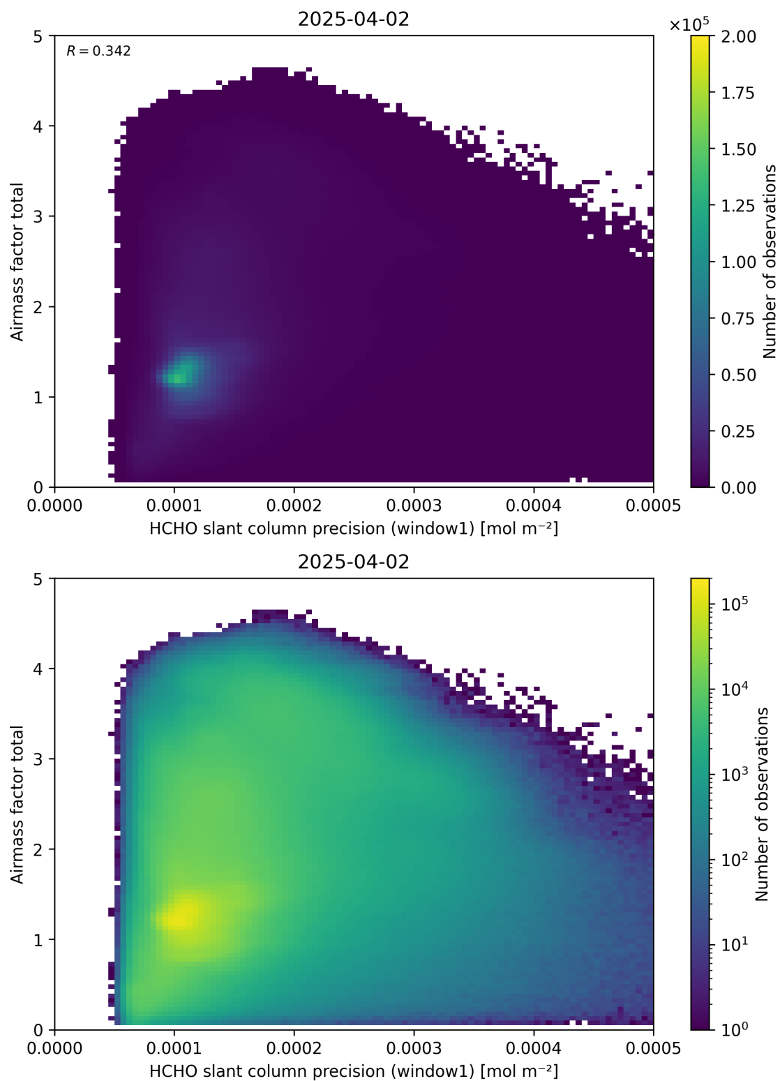
Figure 94: Scatter density plot of “HCHO slant column precision (window1)” against “Airmass factor total” for 2025-04-02 to 2025-04-03.
