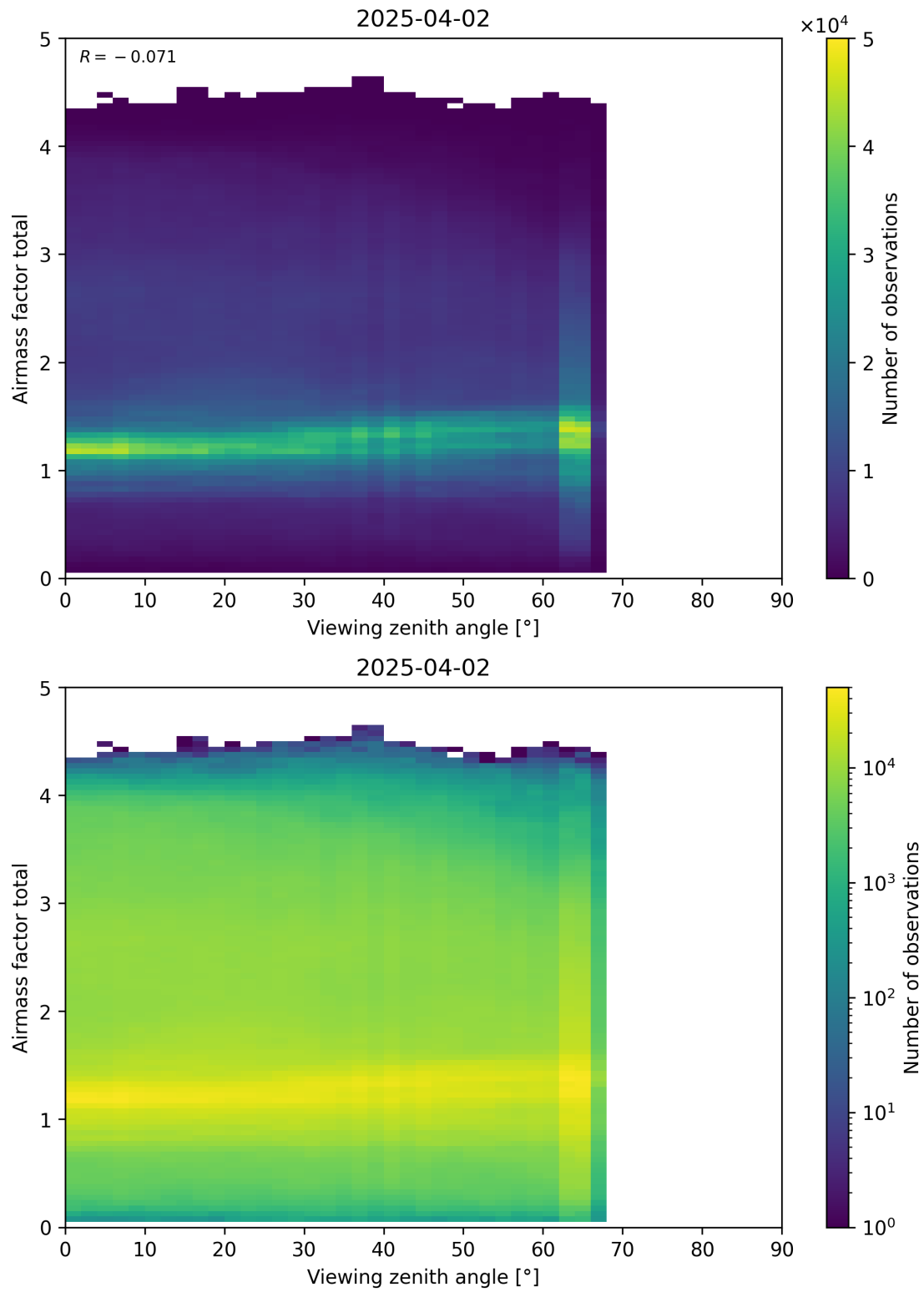
Figure 190: Scatter density plot of “Viewing zenith angle” against “Airmass factor total” for 2025-04-02 to 2025-04-03.
