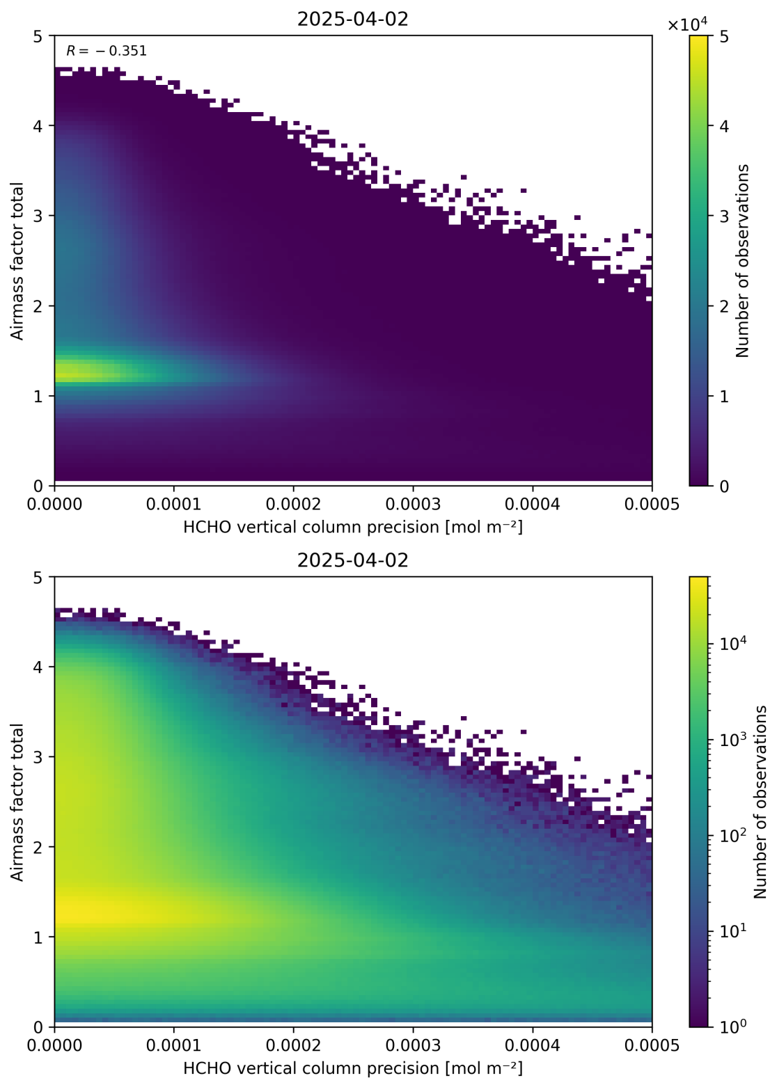
Figure 144: Scatter density plot of “HCHO vertical column precision” against “Airmass factor total” for 2025-04-02 to 2025-04-03.
