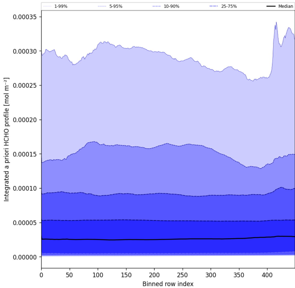
Figure 57: Along track statistics of "Integrated a priori HCHO profile" for 2025-04-02 to 2025-04-03
