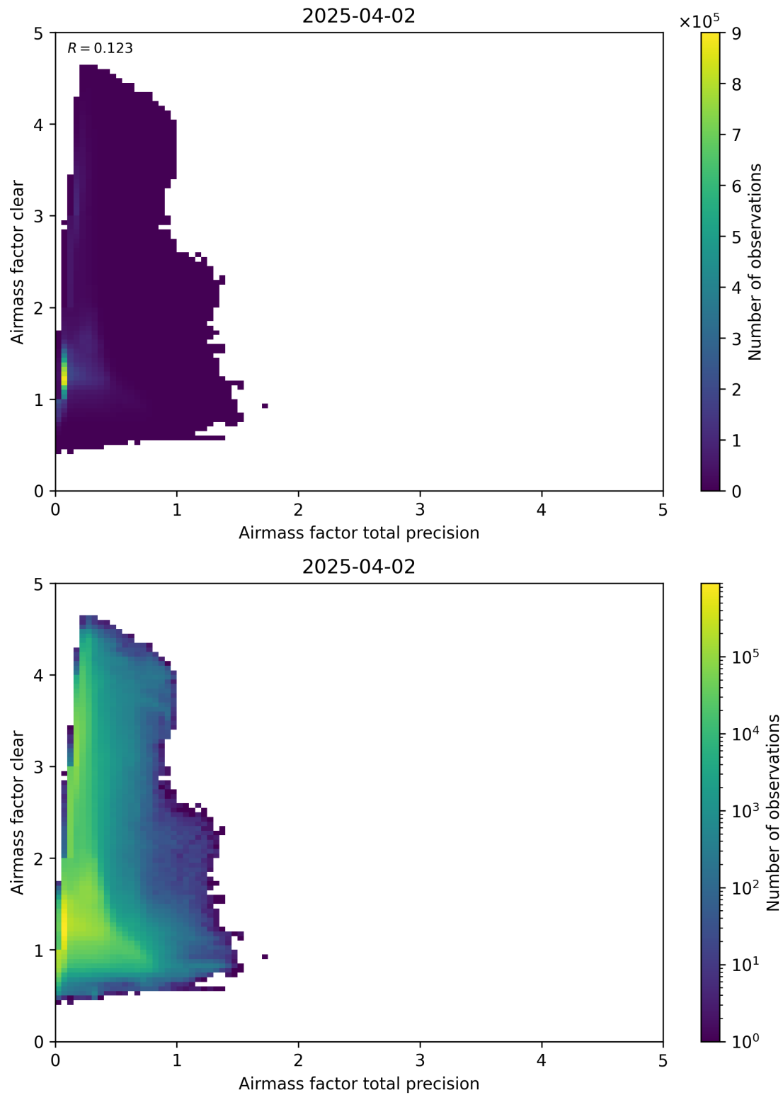
Figure 108: Scatter density plot of “Airmass factor total precision” against “Airmass factor clear” for 2025-04-02 to 2025-04-03.
