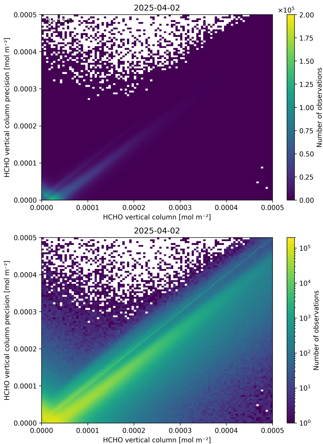
Figure 134: Scatter density plot of “HCHO vertical column” against “HCHO vertical column precision” for 2025-04-02 to 2025-04-03.
