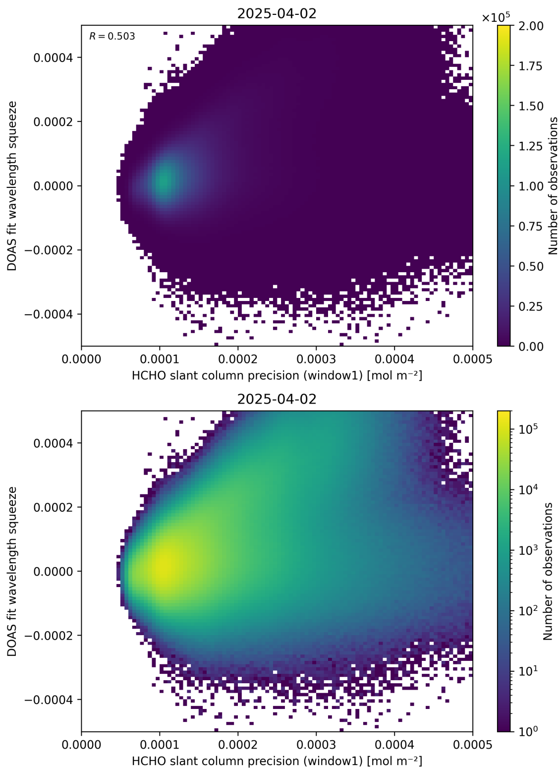
Figure 90: Scatter density plot of “HCHO slant column precision (window1)” against “DOAS fit wavelength squeeze” for 2025-04-02 to 2025-04-03.
