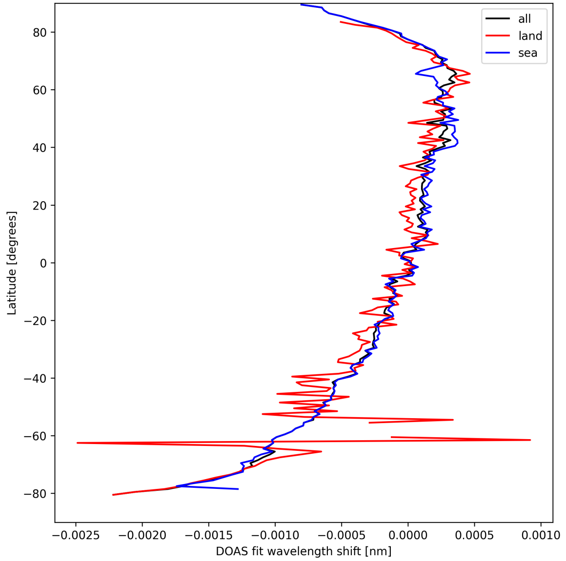
Figure 30: Zonal average of “DOAS fit wavelength shift” for 2025-04-02 to 2025-04-03.
