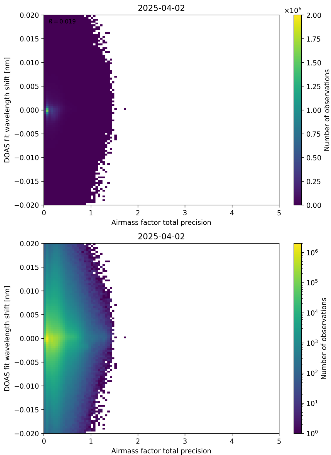
Figure 106: Scatter density plot of “Airmass factor total precision” against “DOAS fit wavelength shift” for 2025-04-02 to 2025-04-03.
