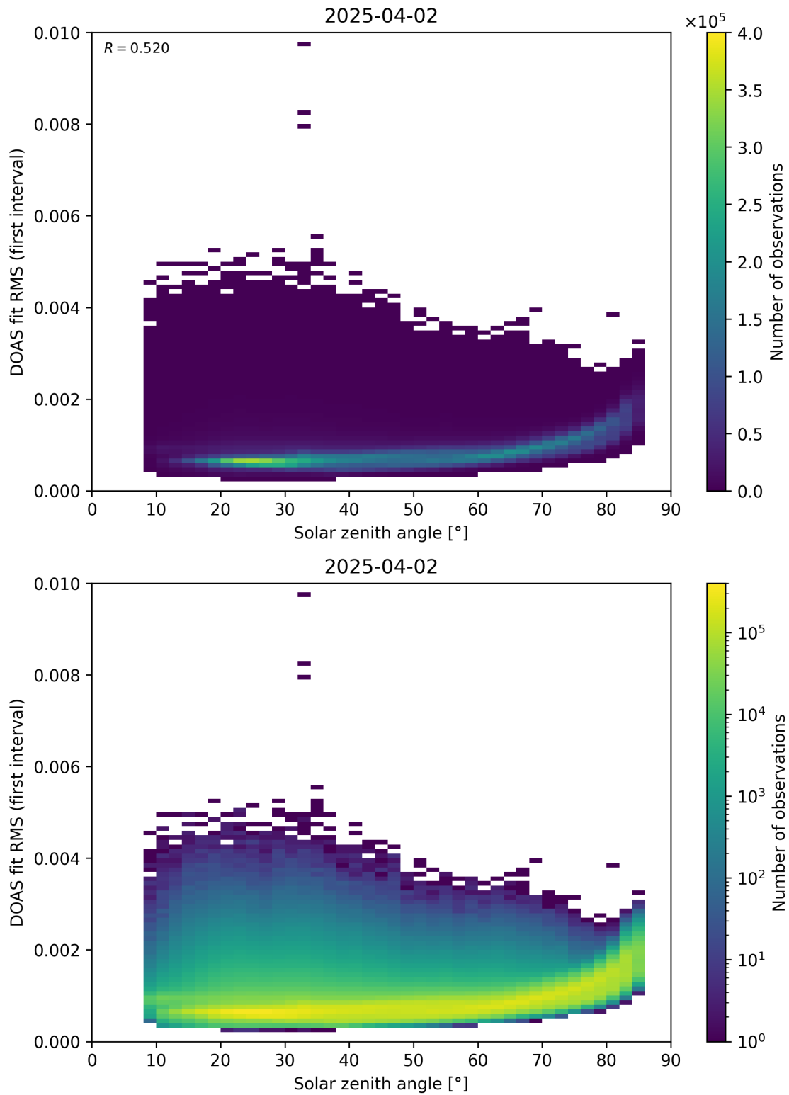
Figure 167: Scatter density plot of “Solar zenith angle” against “DOAS fit RMS (first interval)” for 2025-04-02 to 2025-04-03.
