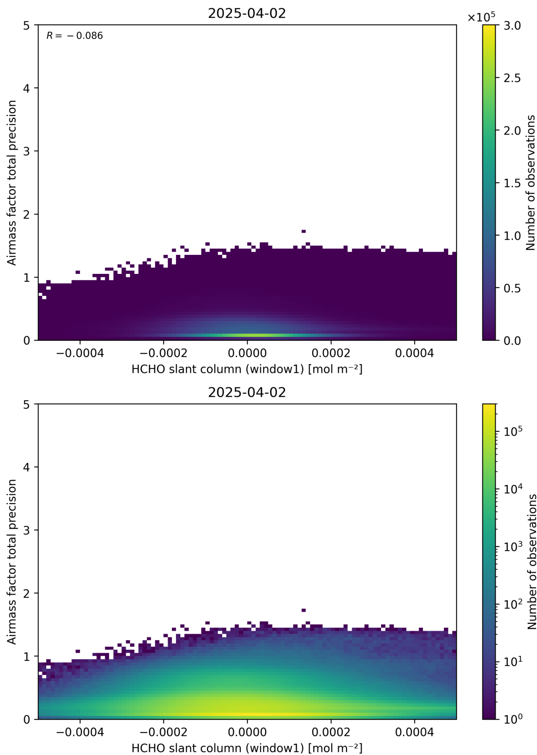
Figure 86: Scatter density plot of “HCHO slant column (window1)” against “Airmass factor total precision” for 2025-04-02 to 2025-04-03.
