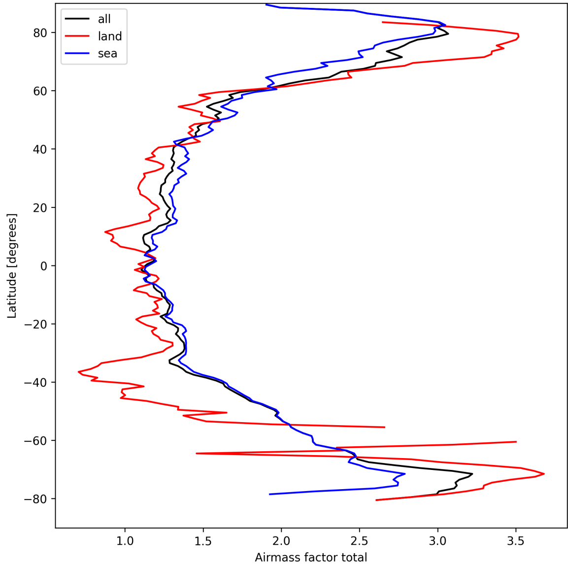
Figure 26: Zonal average of “Airmass factor total” for 2025-04-02 to 2025-04-03.
