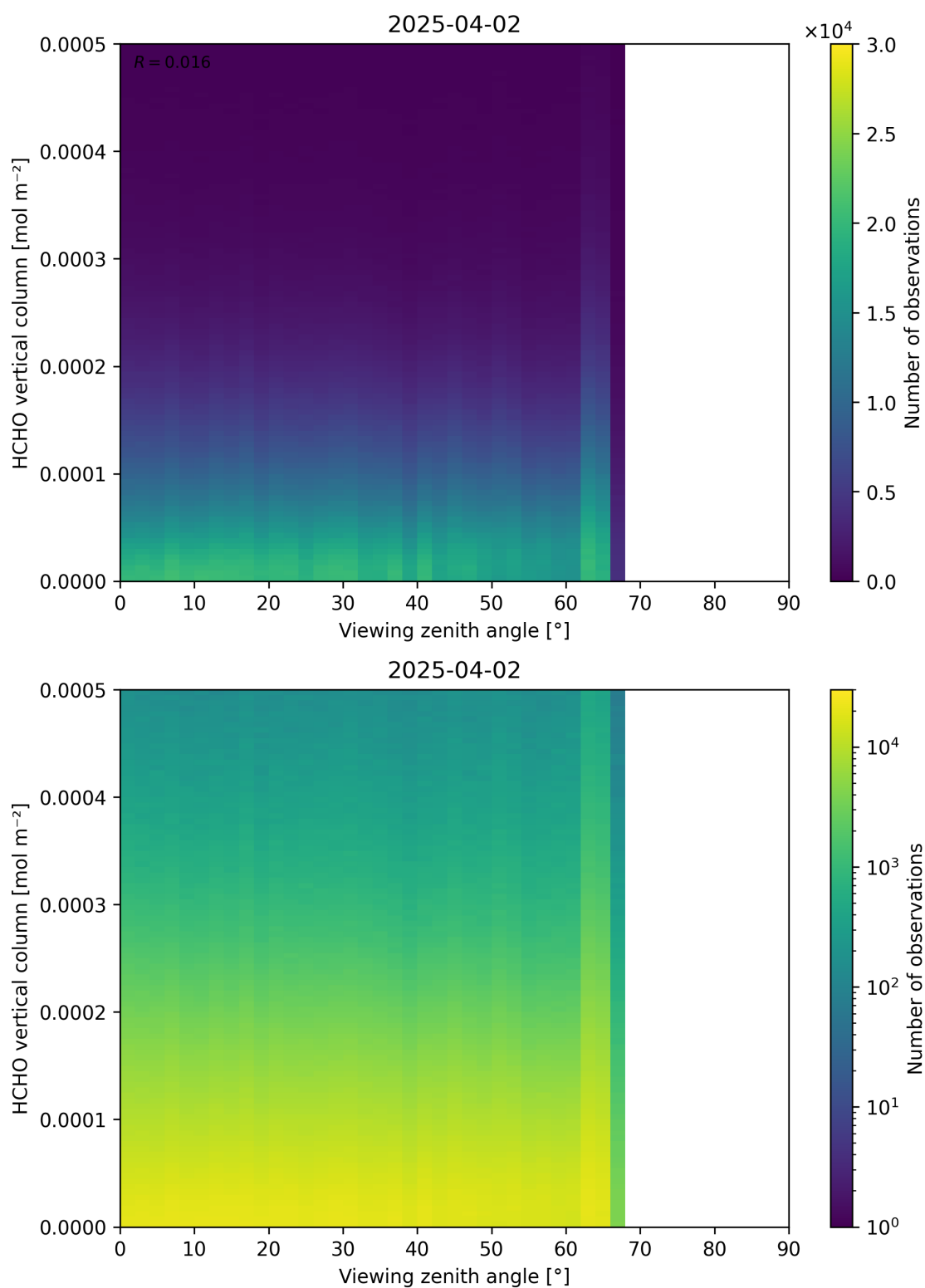
Figure 192: Scatter density plot of “Viewing zenith angle” against “HCHO vertical column” for 2025-04-02 to 2025-04-03.
