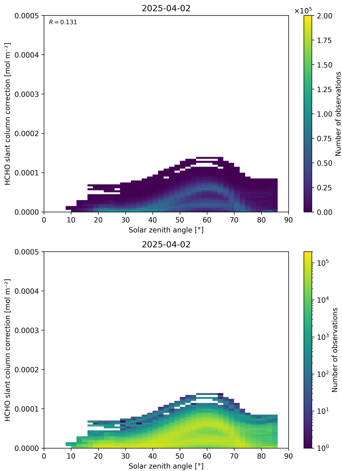
Figure 172: Scatter density plot of “Solar zenith angle” against “HCHO slant column correction” for 2025-04-02 to 2025-04-03.
