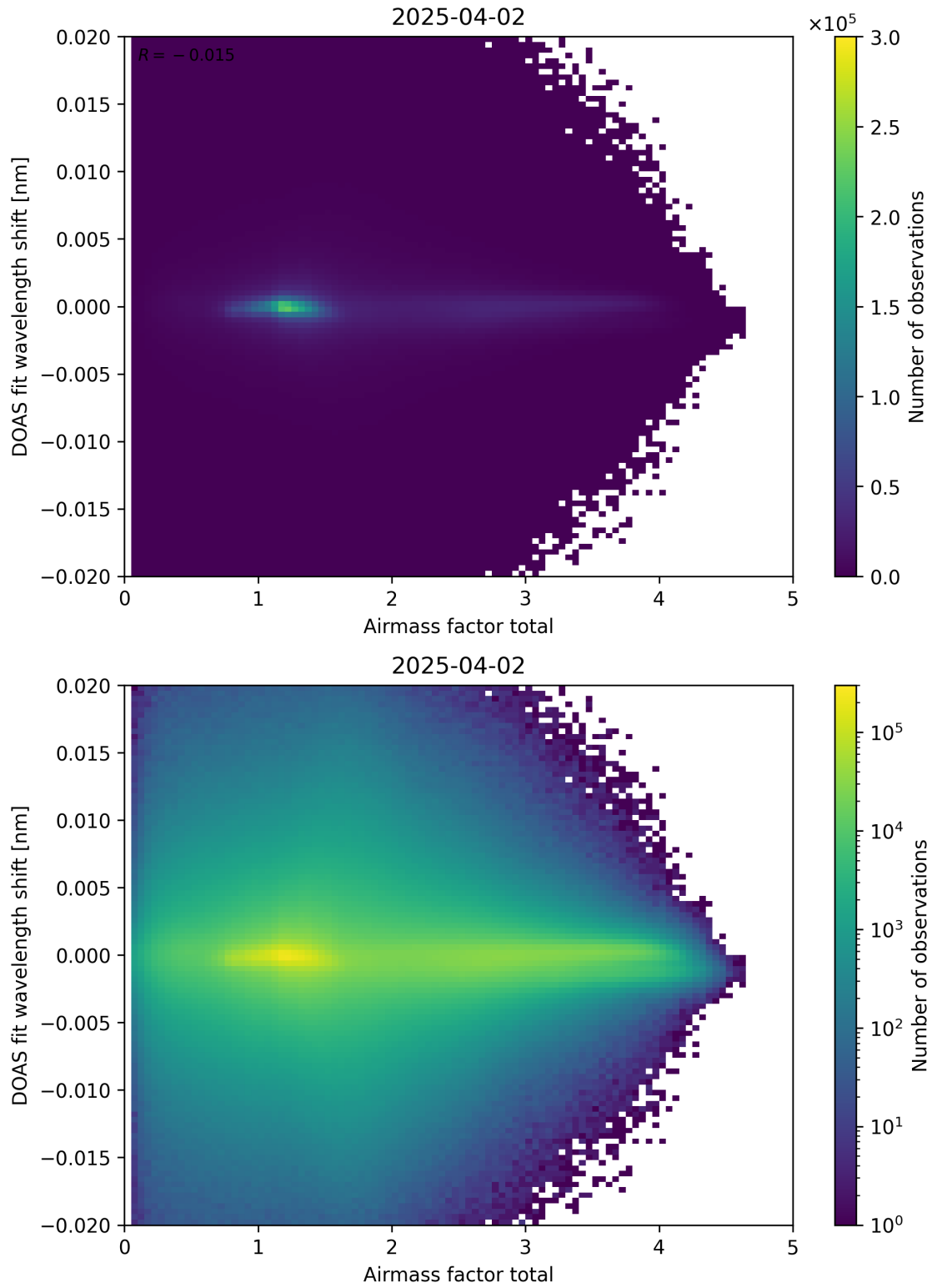
Figure 98: Scatter density plot of “Airmass factor total” against “DOAS fit wavelength shift” for 2025-04-02 to 2025-04-03.
