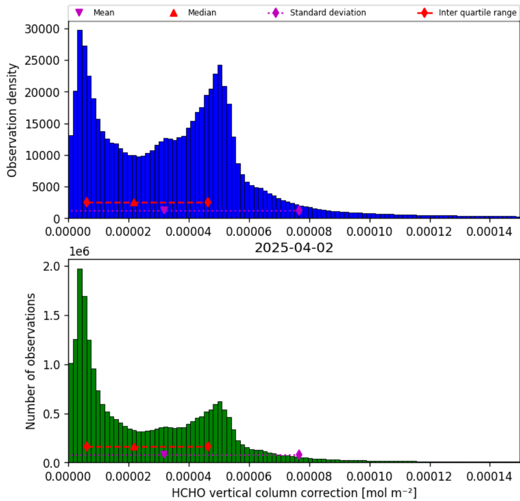
Figure 37: Histogram of “HCHO vertical column correction” for 2025-04-02 to 2025-04-03
