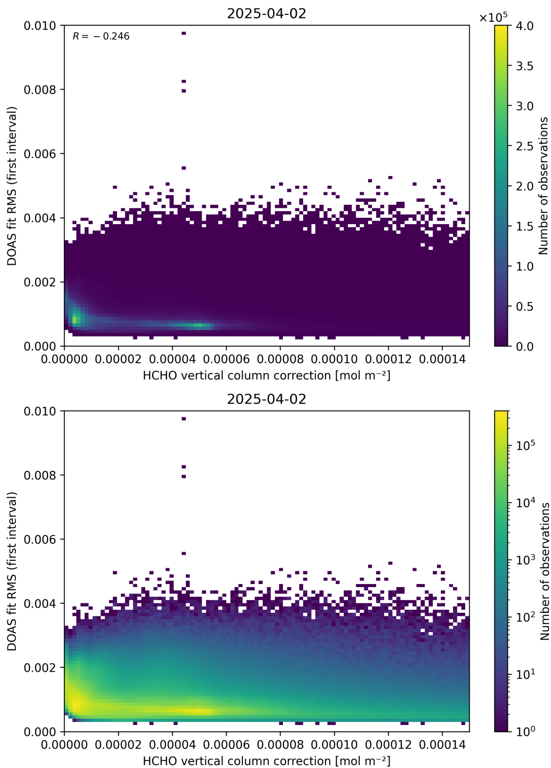
Figure 112: Scatter density plot of “HCHO vertical column correction” against “DOAS fit RMS (first interval)” for 2025-04-02 to 2025-04-03.
