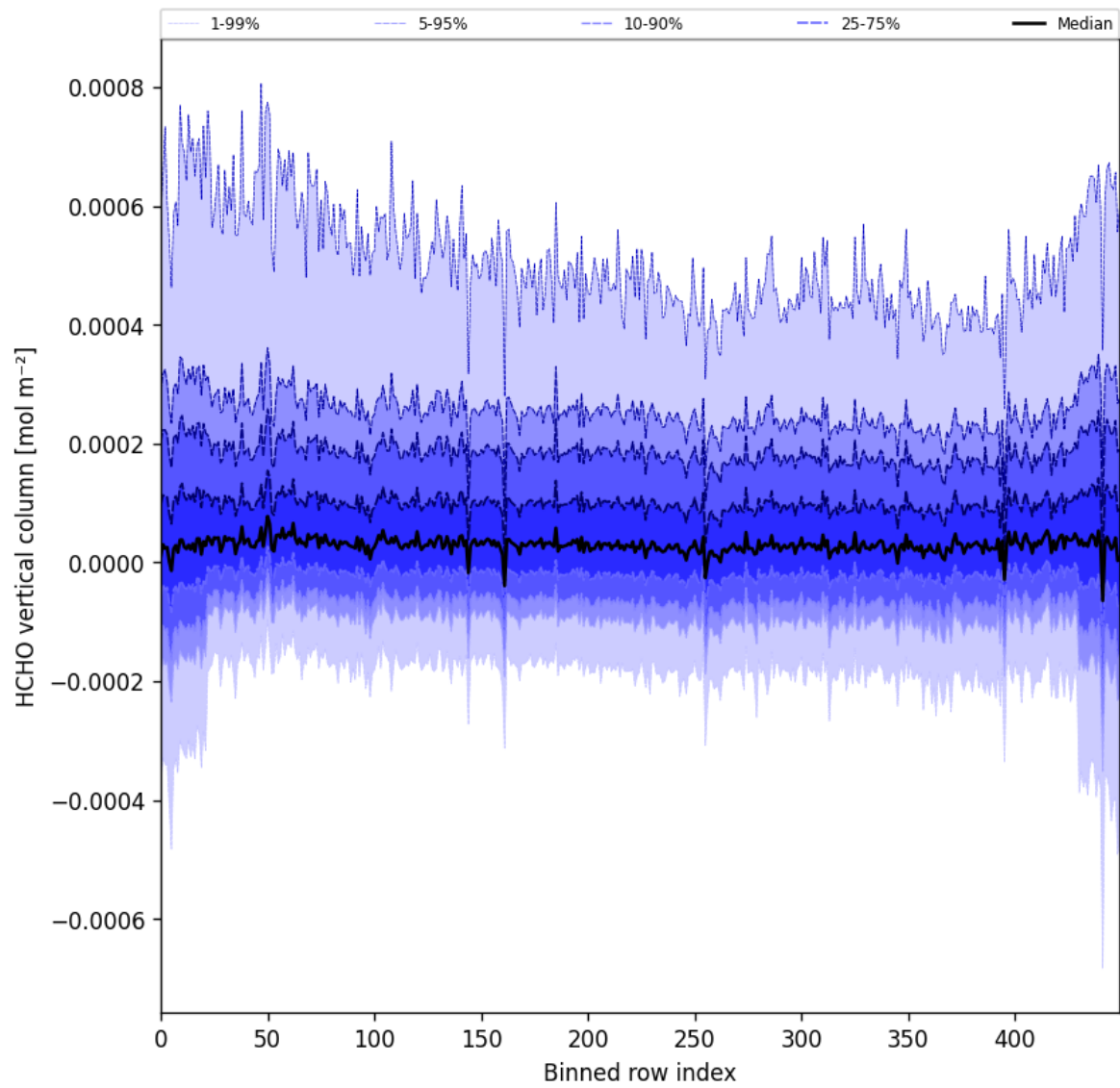
Figure 49: Along track statistics of “HCHO vertical column” for 2025-04-02 to 2025-04-03
