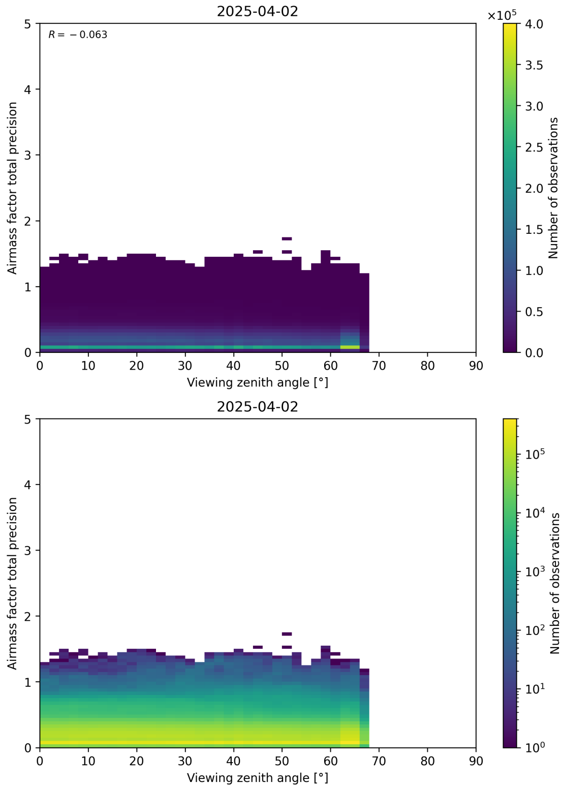
Figure 191: Scatter density plot of “Viewing zenith angle” against “Airmass factor total precision” for 2025-04-02 to 2025-04-03.
