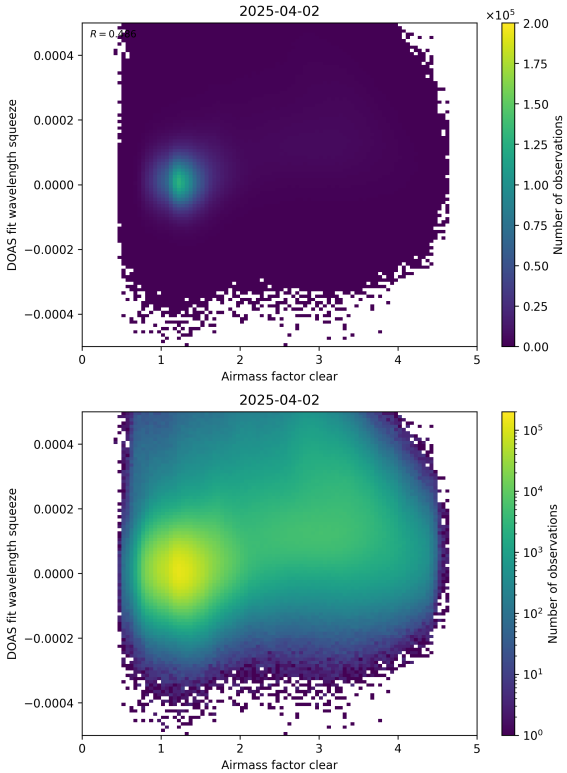
Figure 73: Scatter density plot of “Airmass factor clear” against “DOAS fit wavelength squeeze” for 2025-04-02 to 2025-04-03.
