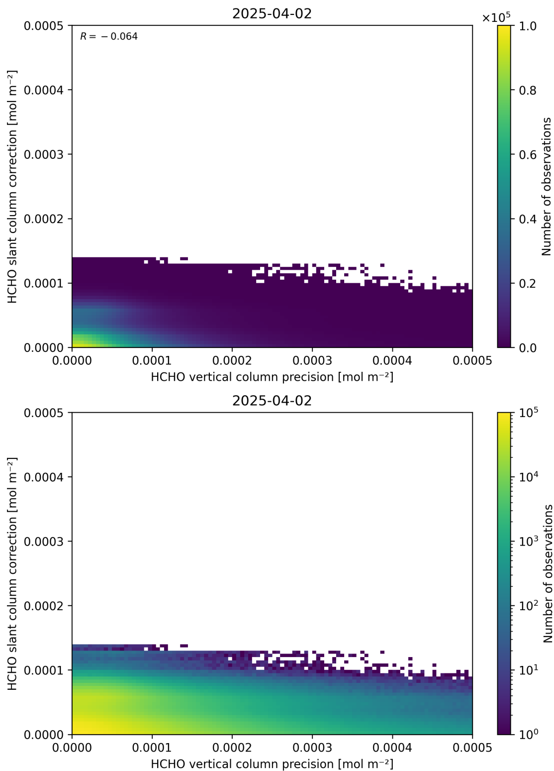
Figure 141: Scatter density plot of “HCHO vertical column precision” against “HCHO slant column correction” for 2025-04-02 to 2025-04-03.
