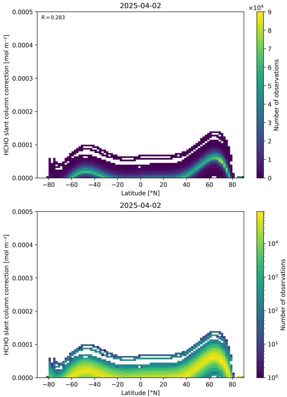
Figure 158: Scatter density plot of “Latitude” against “HCHO slant column correction” for 2025-04-02 to 2025-04-03.
