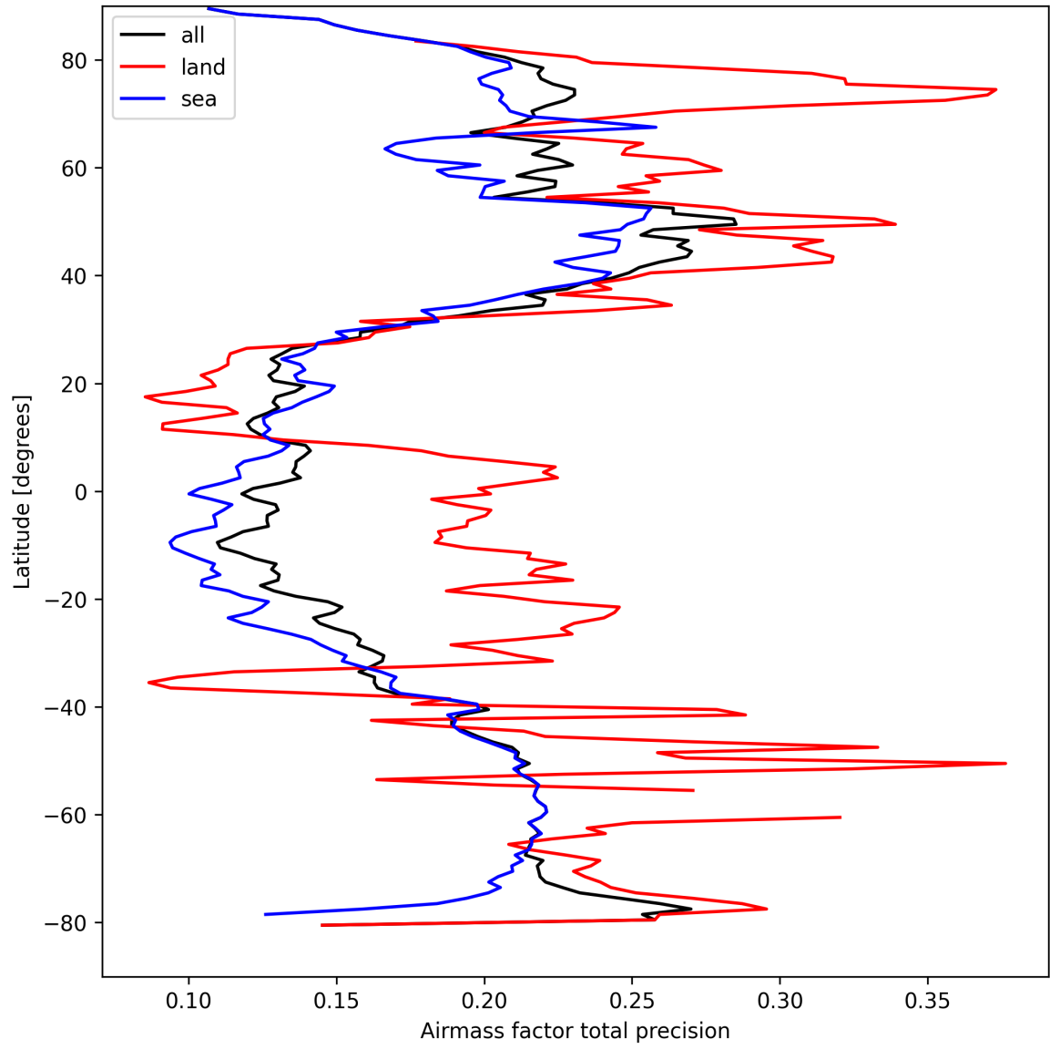
Figure 27: Zonal average of “Airmass factor total precision” for 2025-04-02 to 2025-04-03.
