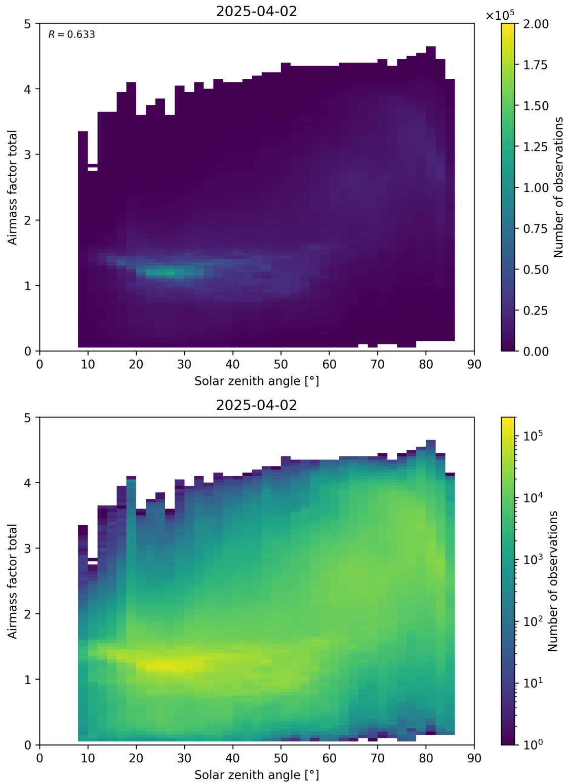
Figure 175: Scatter density plot of “Solar zenith angle” against “Airmass factor total” for 2025-04-02 to 2025-04-03.
