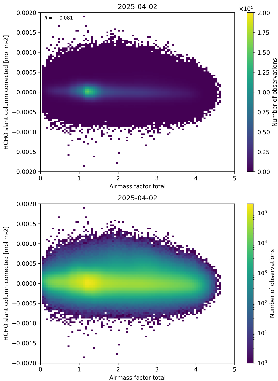
Figure 101: Scatter density plot of “Airmass factor total” against “HCHO slant column corrected” for 2025-04-02 to 2025-04-03.
