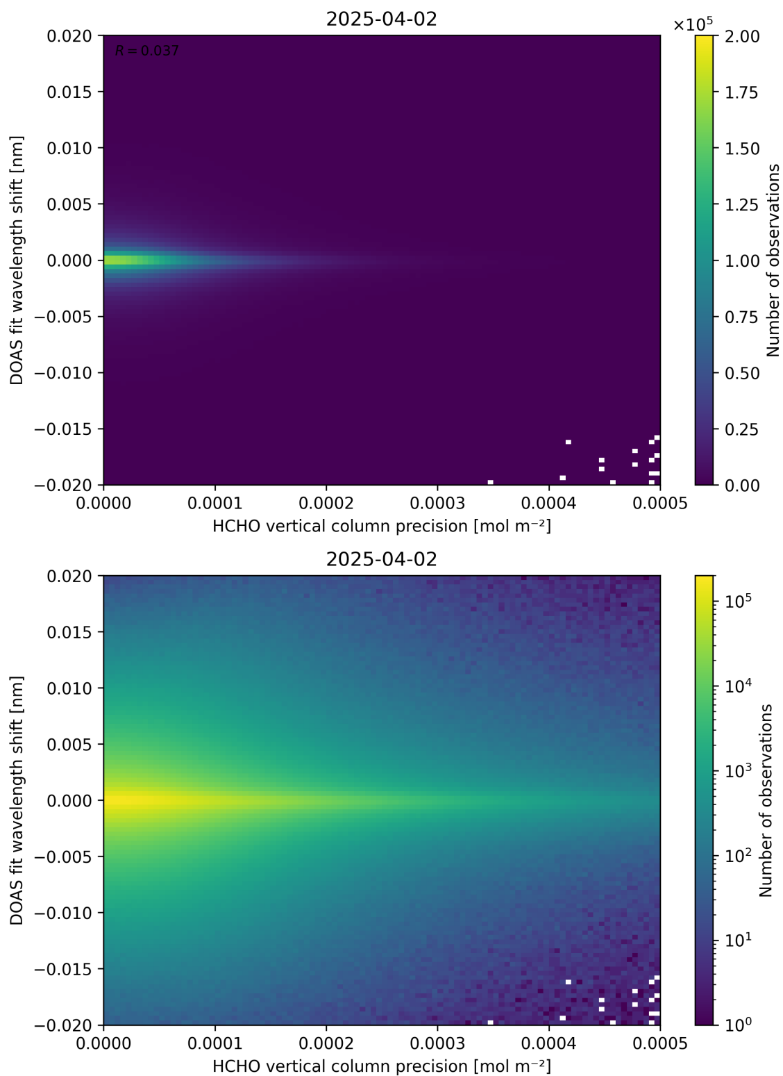
Figure 137: Scatter density plot of “HCHO vertical column precision” against “DOAS fit wavelength shift” for 2025-04-02 to 2025-04-03.
