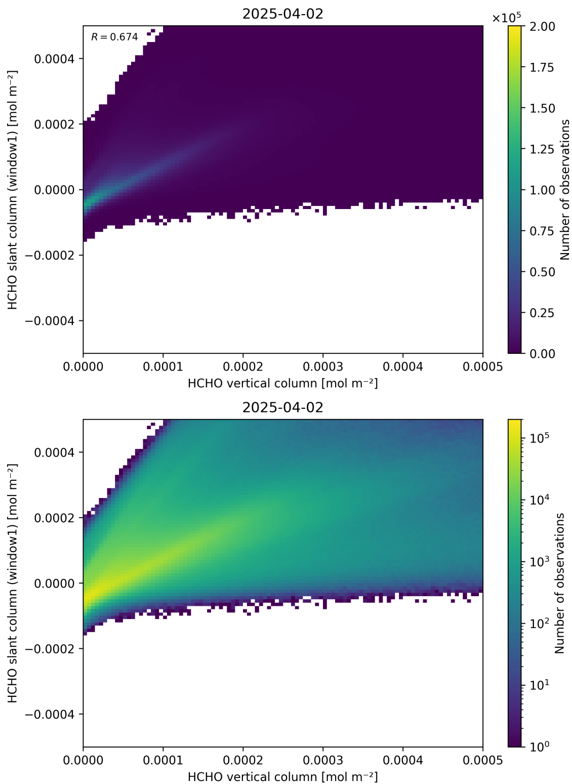
Figure 129: Scatter density plot of “HCHO vertical column” against “HCHO slant column (window1)” for 2025-04-02 to 2025-04-03.
