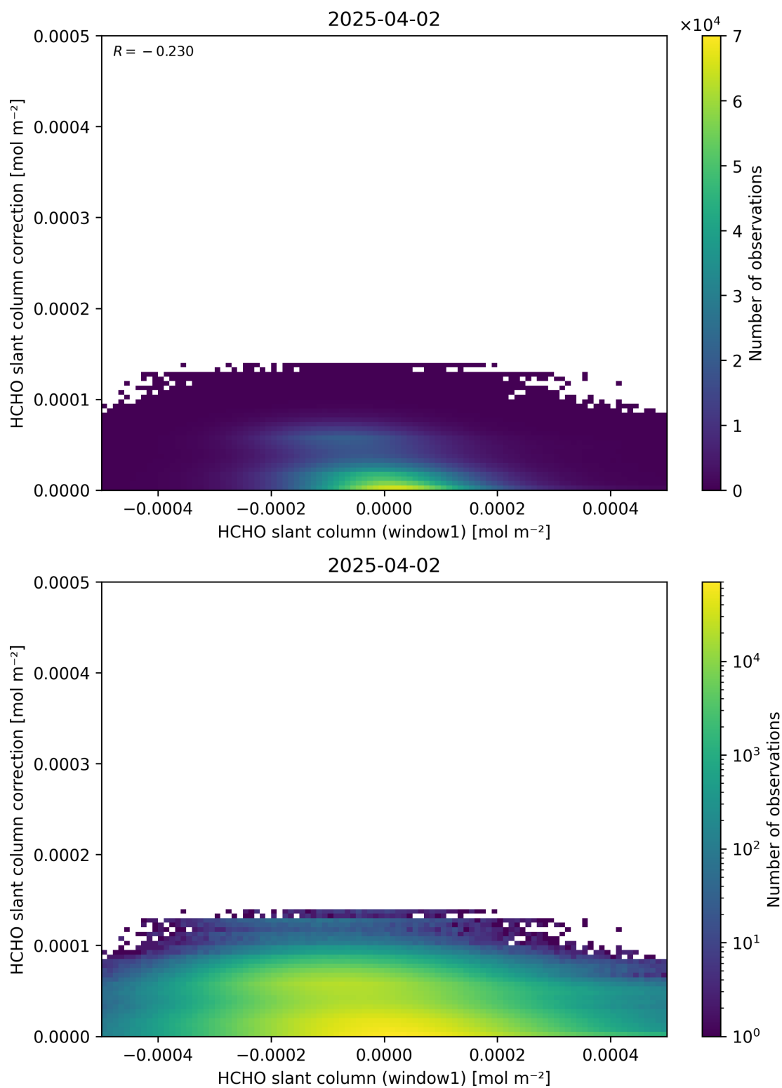
Figure 83: Scatter density plot of “HCHO slant column (window1)” against “HCHO slant column correction” for 2025-04-02 to 2025-04-03.
