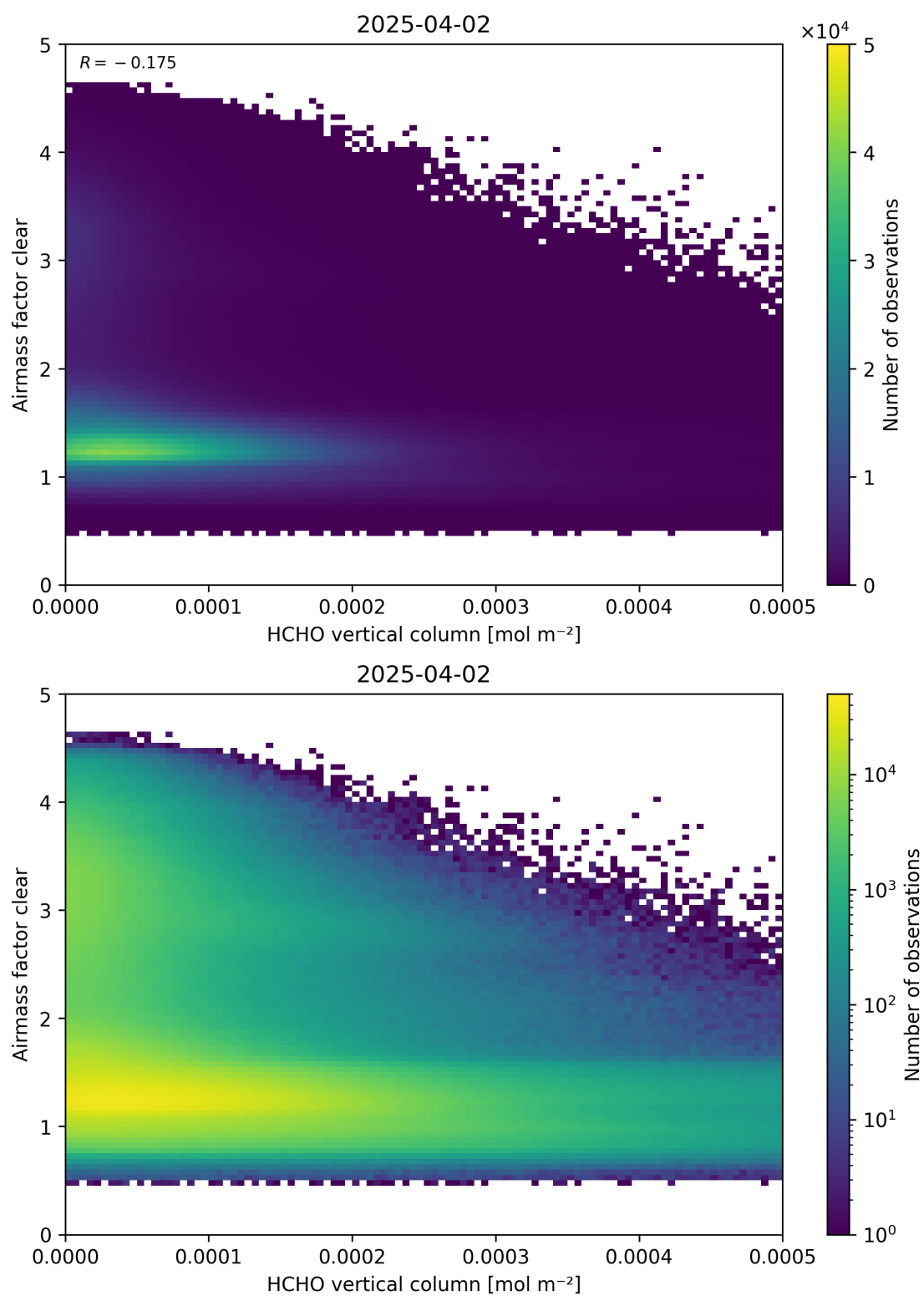
Figure 126: Scatter density plot of “HCHO vertical column” against “Airmass factor clear” for 2025-04-02 to 2025-04-03.
