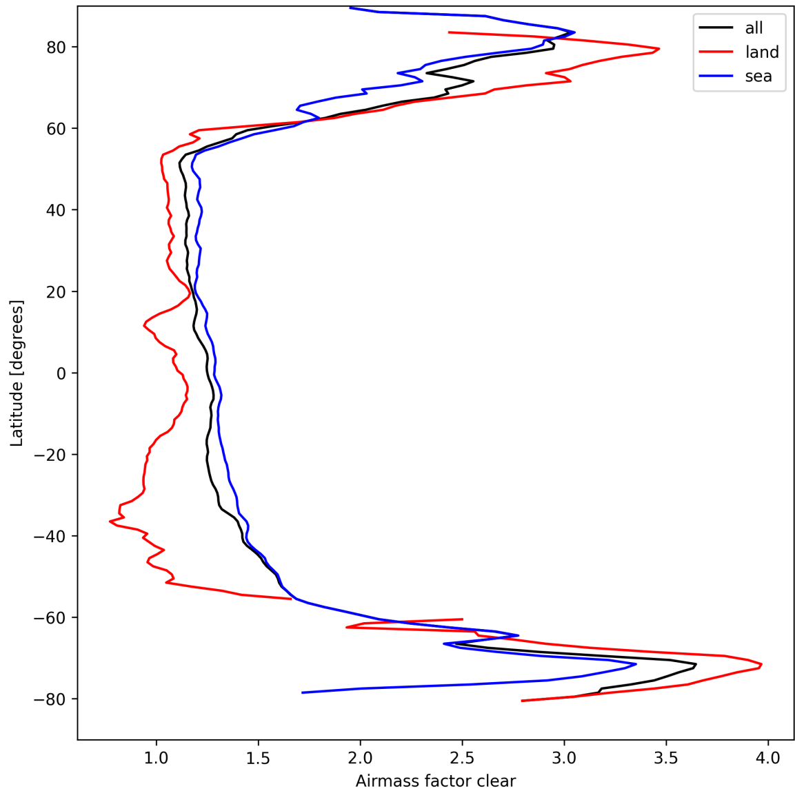
Figure 28: Zonal average of “Airmass factor clear” for 2025-04-02 to 2025-04-03.
