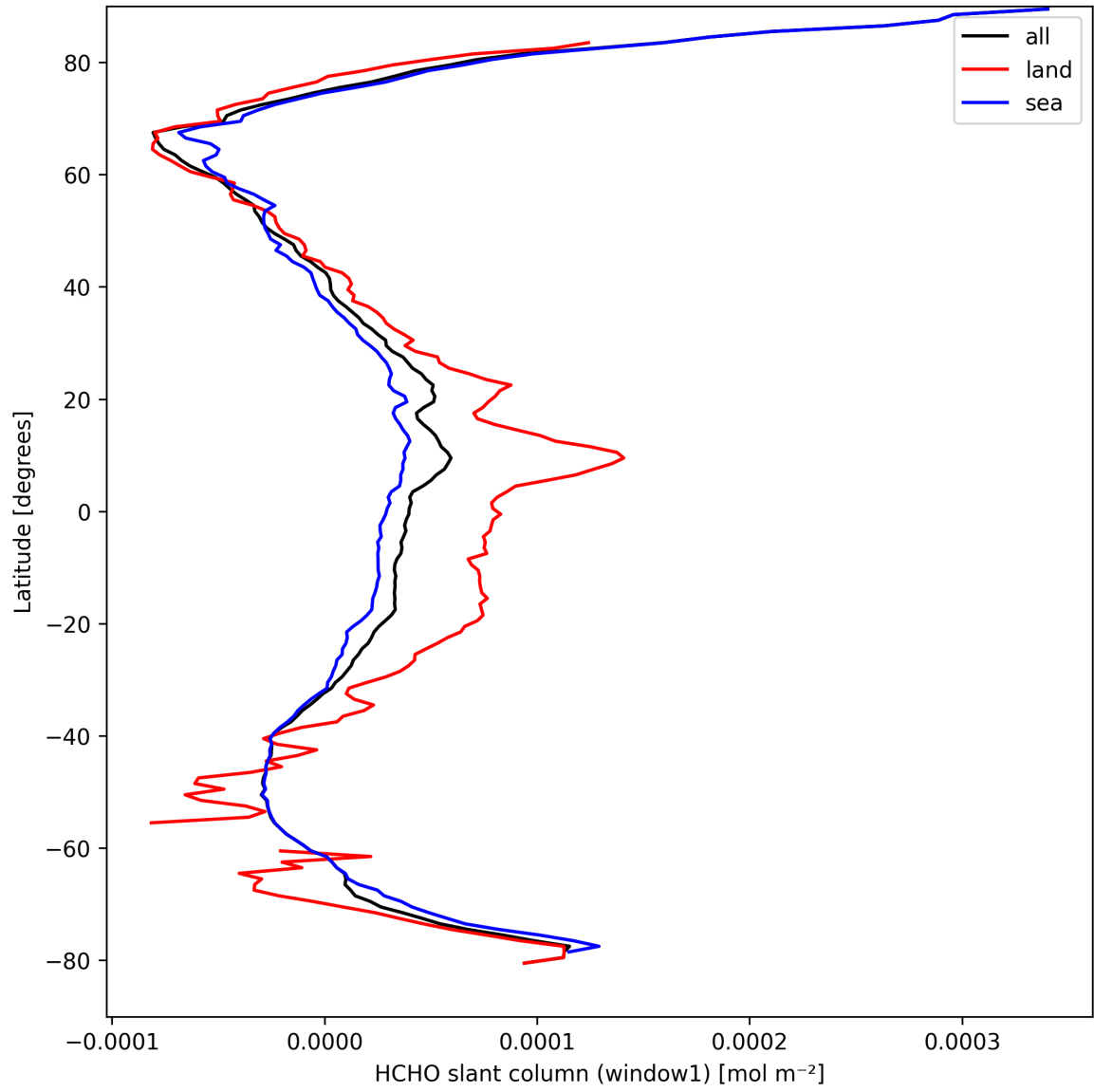
Figure 24: Zonal average of “HCHO slant column (window1)” for 2025-04-02 to 2025-04-03.
