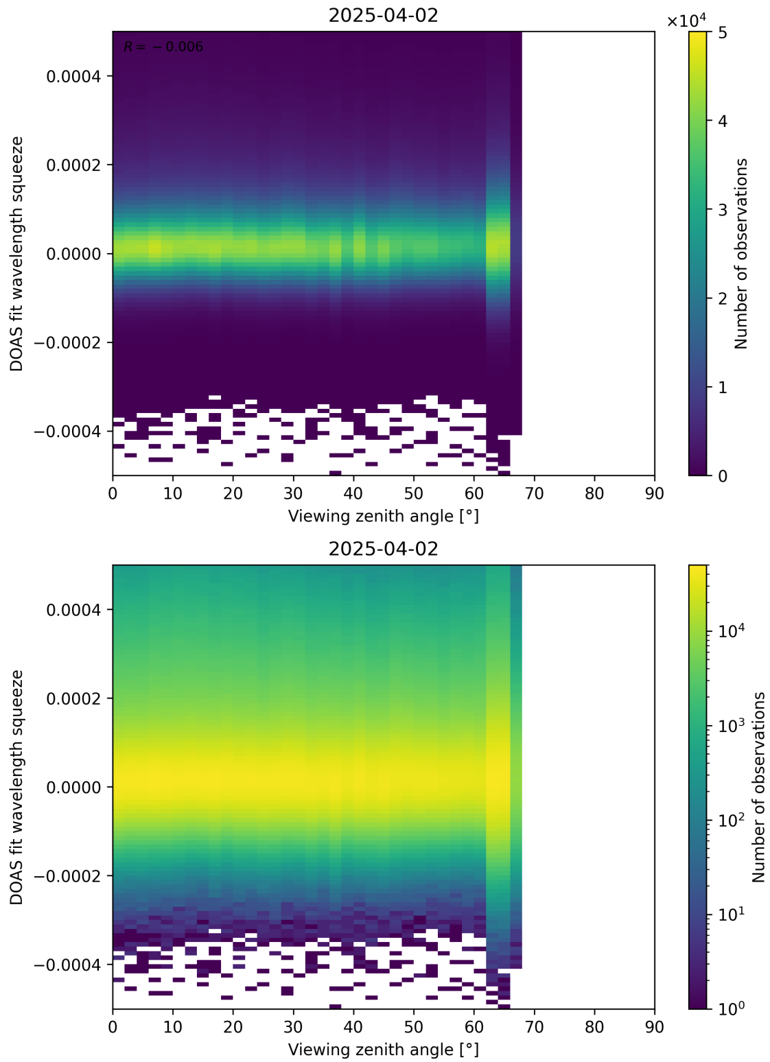
Figure 184: Scatter density plot of “Viewing zenith angle” against “DOAS fit wavelength squeeze” for 2025-04-02 to 2025-04-03.
