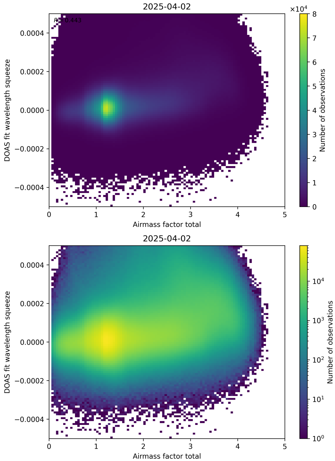
Figure 99: Scatter density plot of “Airmass factor total” against “DOAS fit wavelength squeeze” for 2025-04-02 to 2025-04-03.
