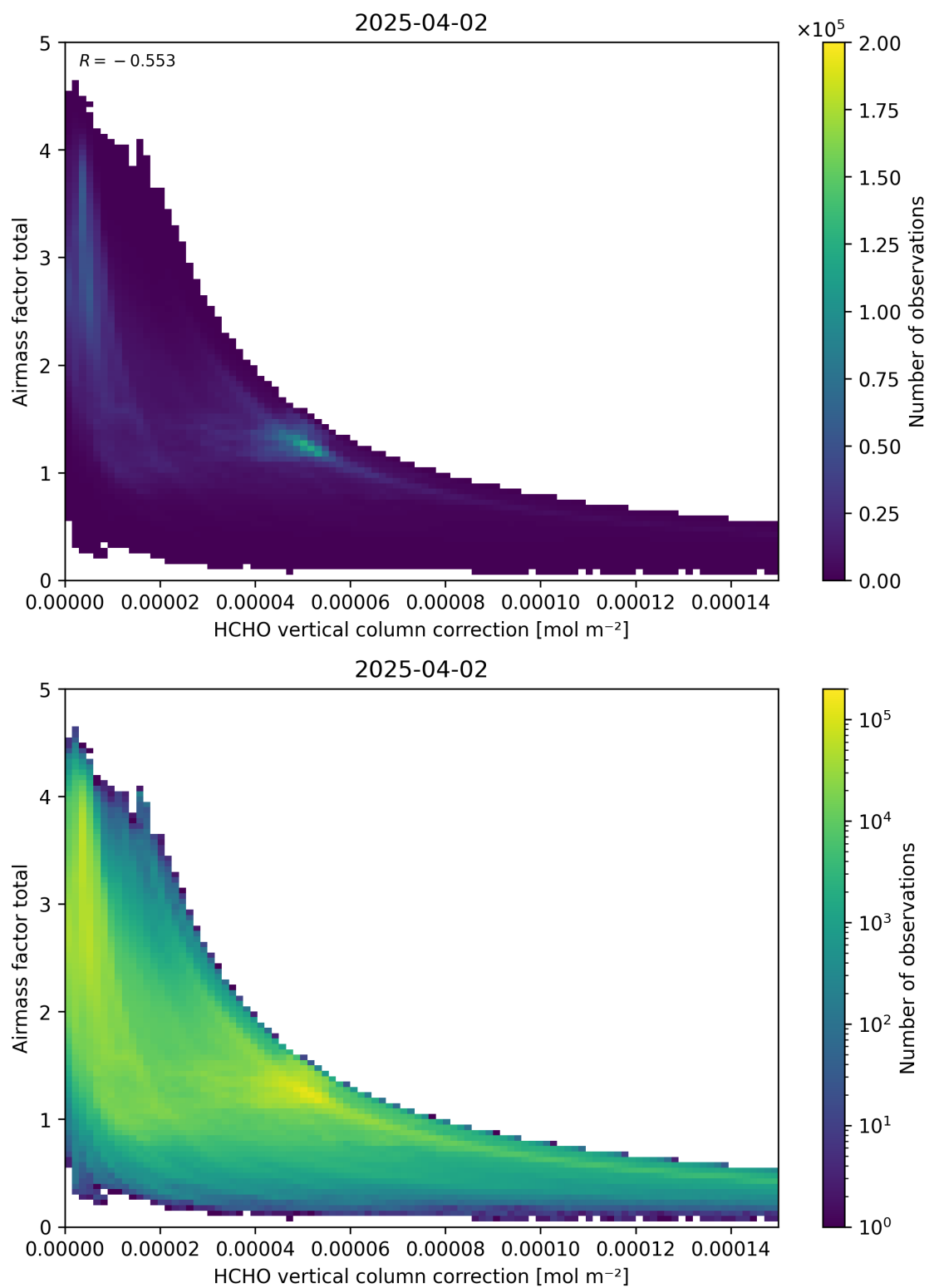
Figure 120: Scatter density plot of “HCHO vertical column correction” against “Airmass factor total” for 2025-04-02 to 2025-04-03.
