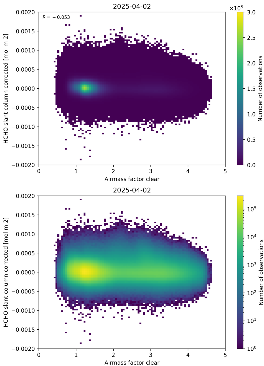
Figure 74: Scatter density plot of “Airmass factor clear” against “HCHO slant column corrected” for 2025-04-02 to 2025-04-03.
