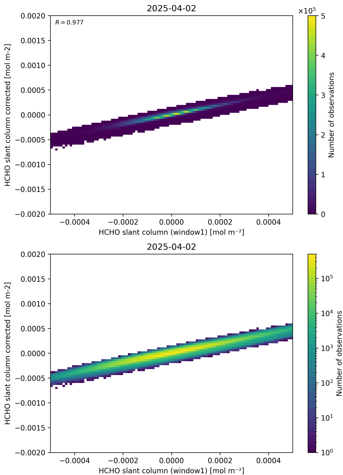
Figure 82: Scatter density plot of “HCHO slant column (window1)” against “HCHO slant column corrected” for 2025-04-02 to 2025-04-03.
