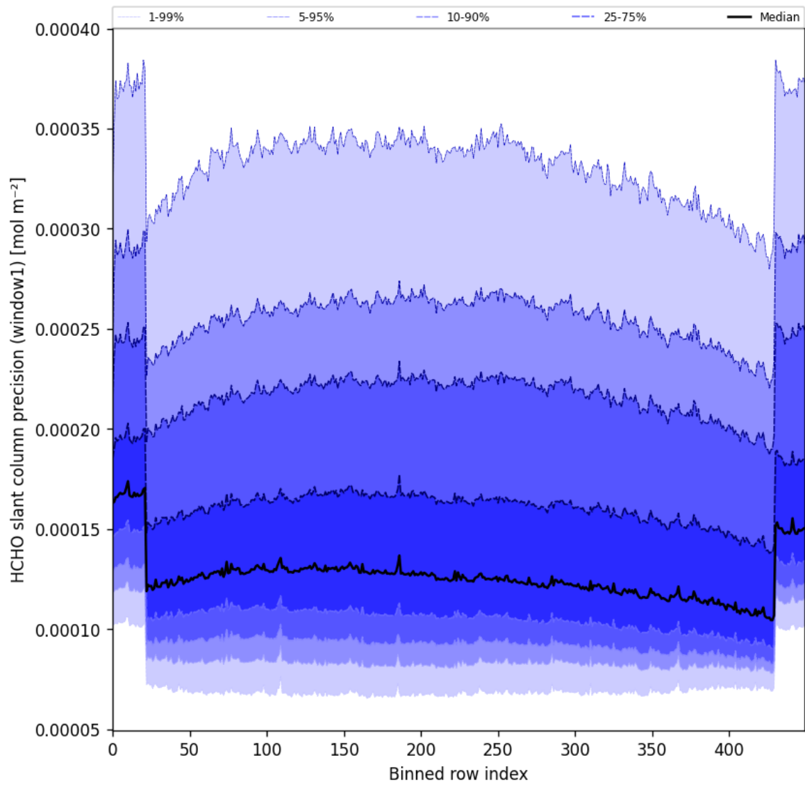
Figure 53: Along track statistics of “HCHO slant column precision (window1)” for 2025-04-02 to 2025-04-03
