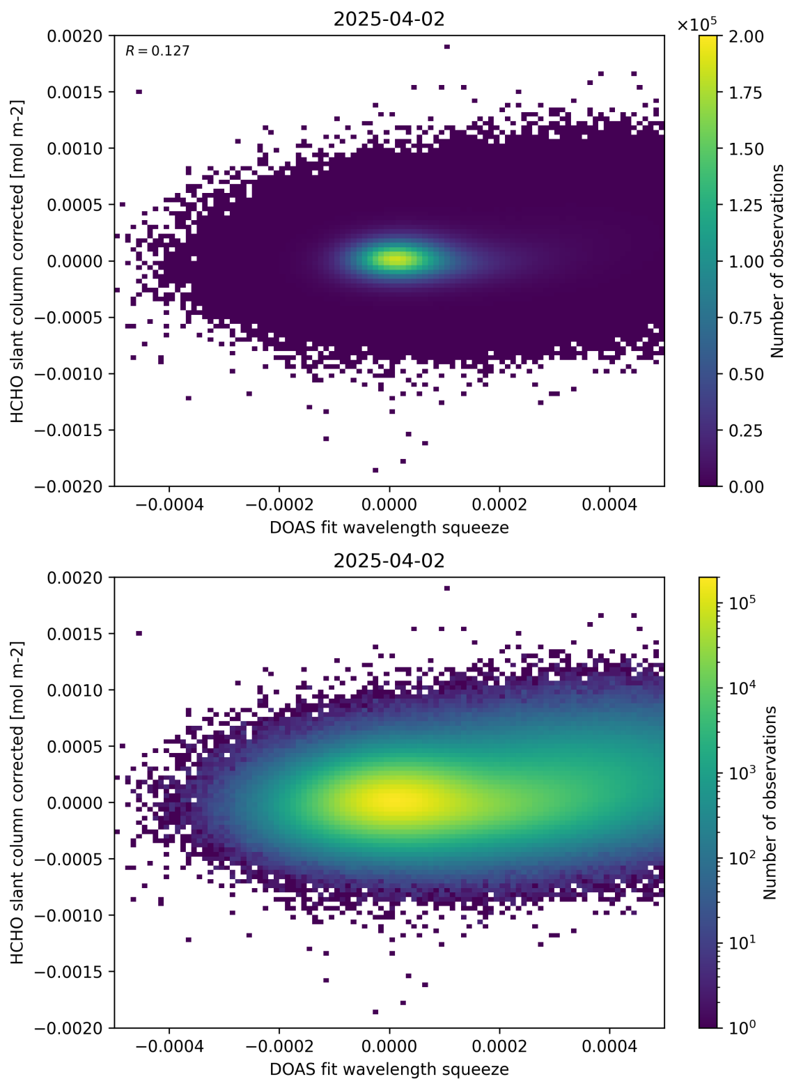
Figure 69: Scatter density plot of “DOAS fit wavelength squeeze” against “HCHO slant column corrected” for 2025-04-02 to 2025-04-03.
