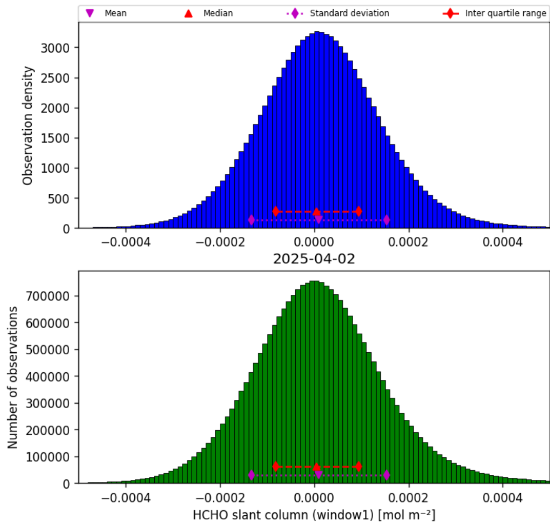
Figure 38: Histogram of “HCHO slant column (window1)” for 2025-04-02 to 2025-04-03
