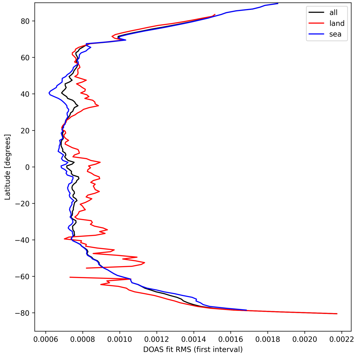
Figure 32: Zonal average of "DOAS fit RMS (first interval)" for 2025-04-02 to 2025-04-03.
