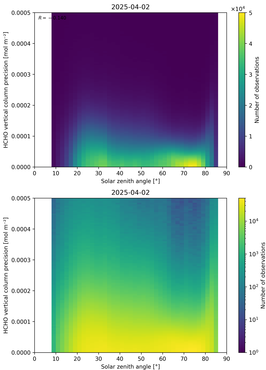
Figure 179: Scatter density plot of “Solar zenith angle” against “HCHO vertical column precision” for 2025-04-02 to 2025-04-03.
