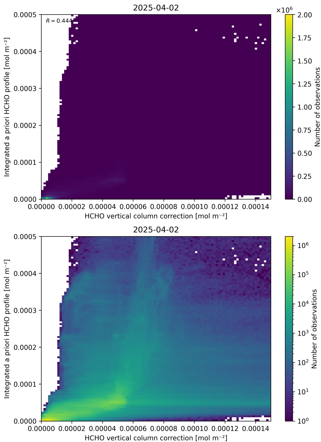
Figure 122: Scatter density plot of “HCHO vertical column correction” against “Integrated a priori HCHO profile” for 2025-04-02 to 2025-04-03.
