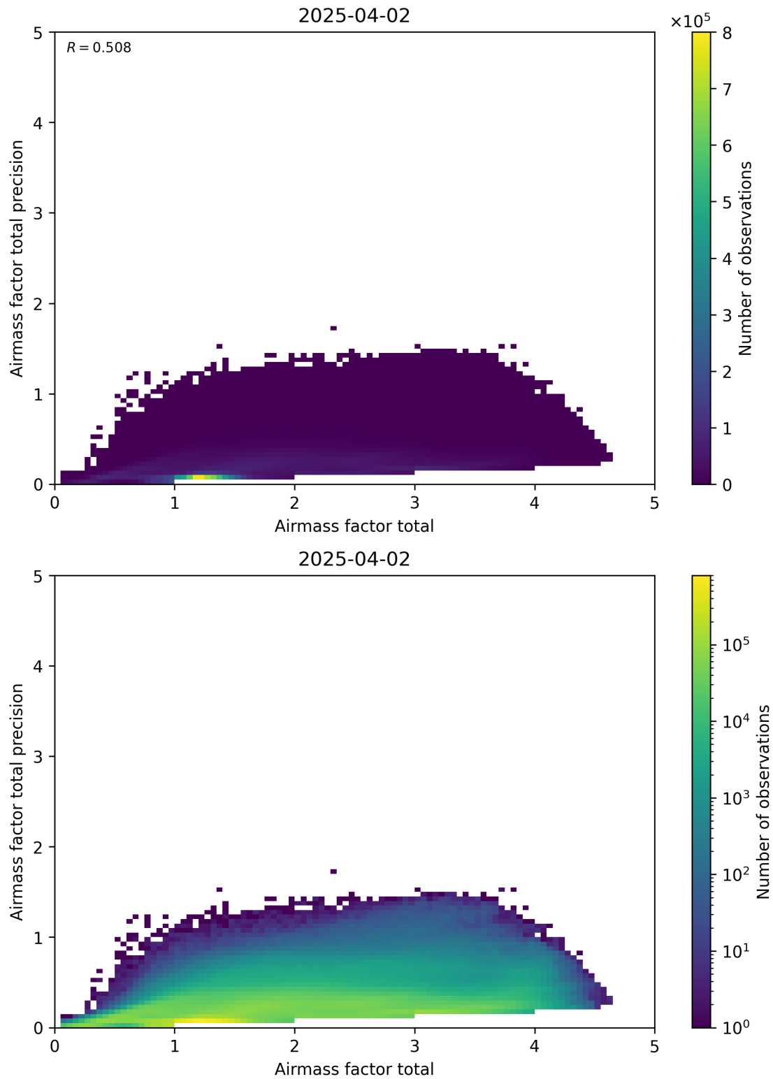
Figure 103: Scatter density plot of “Airmass factor total” against “Airmass factor total precision” for 2025-04-02 to 2025-04-03.
