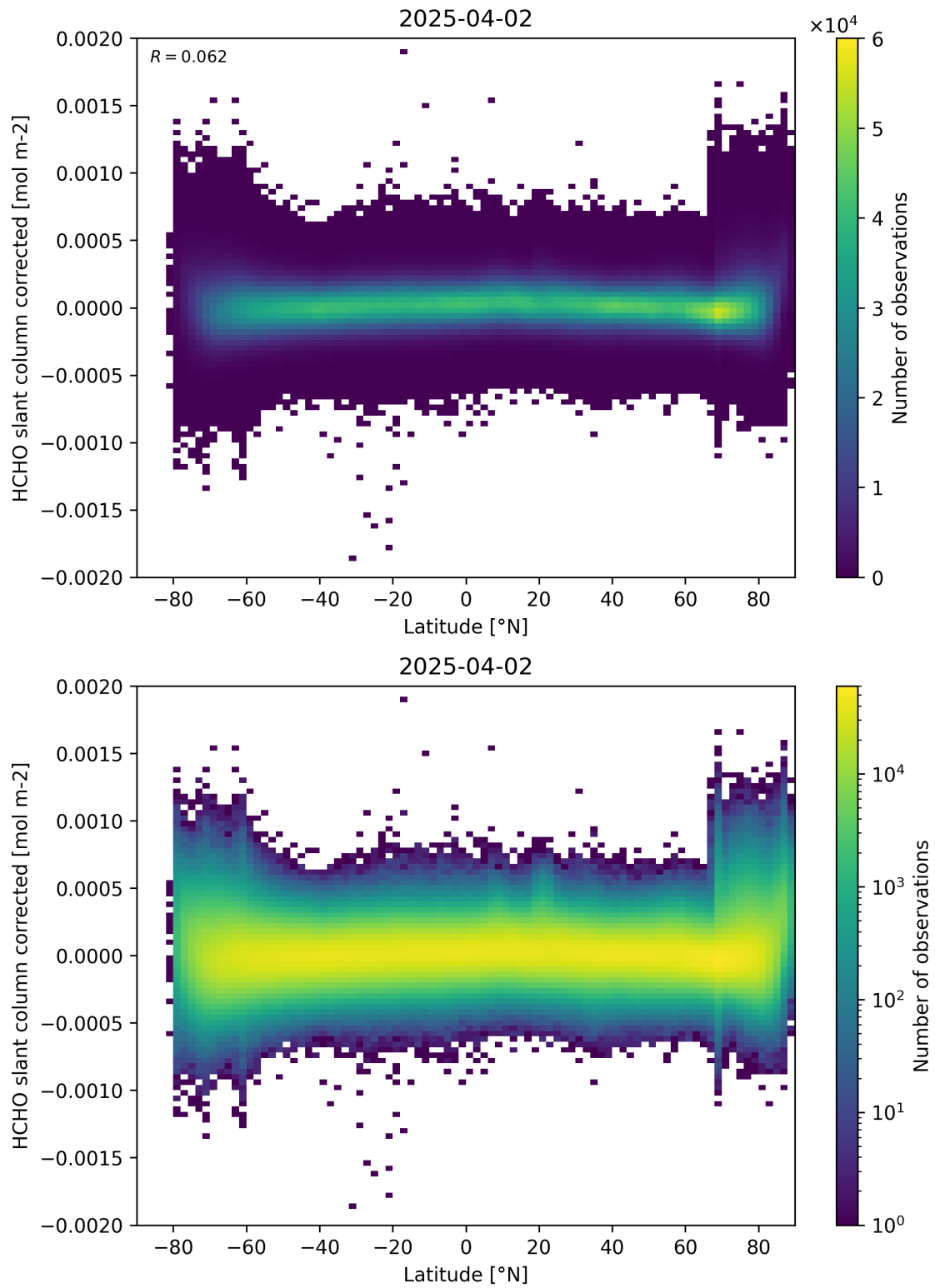
Figure 157: Scatter density plot of “Latitude” against “HCHO slant column corrected” for 2025-04-02 to 2025-04-03.
