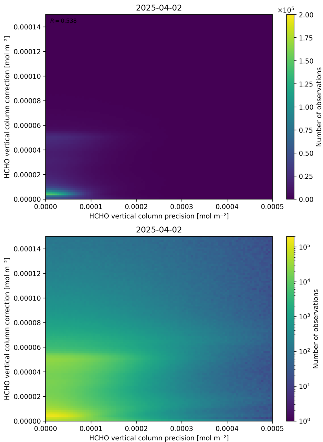
Figure 146: Scatter density plot of “HCHO vertical column precision” against “HCHO vertical column correction” for 2025-04-02 to 2025-04-03.
