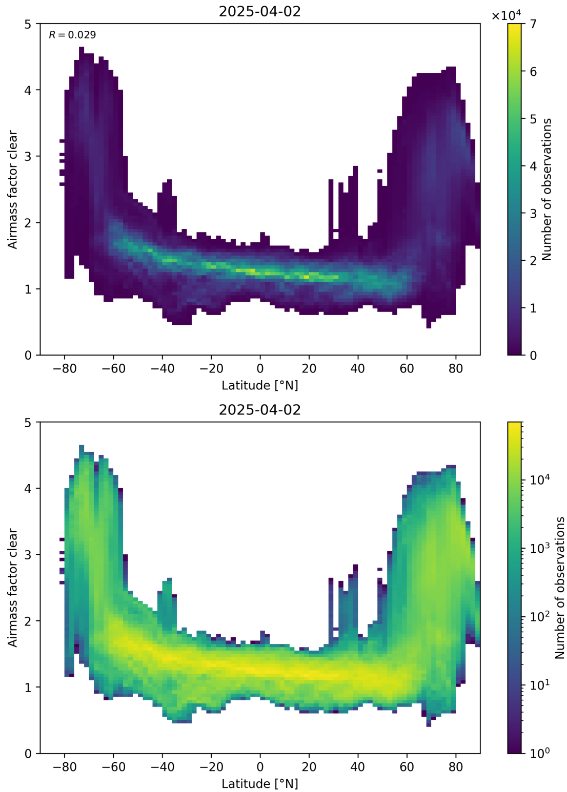
Figure 156: Scatter density plot of “Latitude” against “Airmass factor clear” for 2025-04-02 to 2025-04-03.
