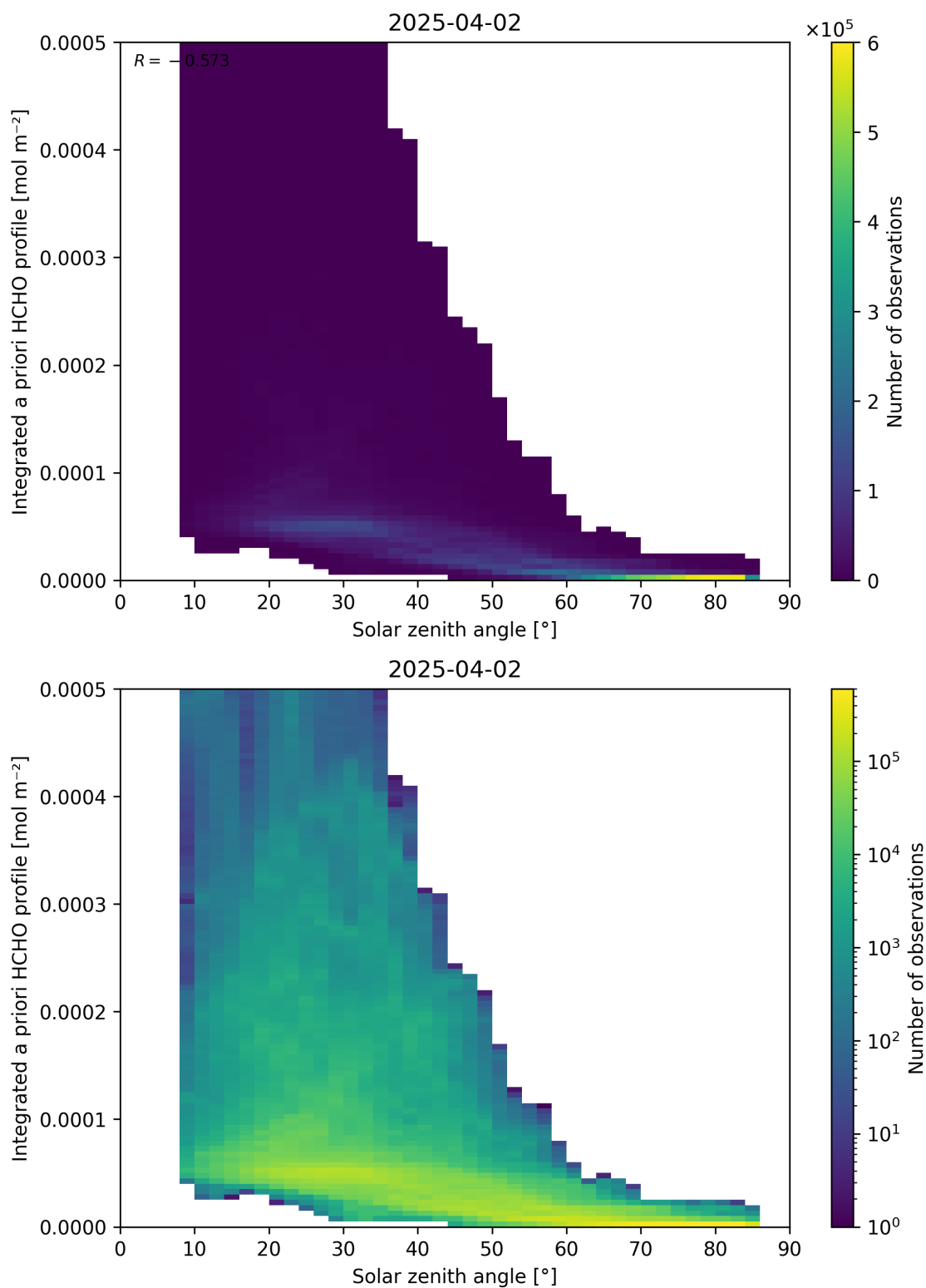
Figure 180: Scatter density plot of “Solar zenith angle” against “Integrated a priori HCHO profile” for 2025-04-02 to 2025-04-03.
