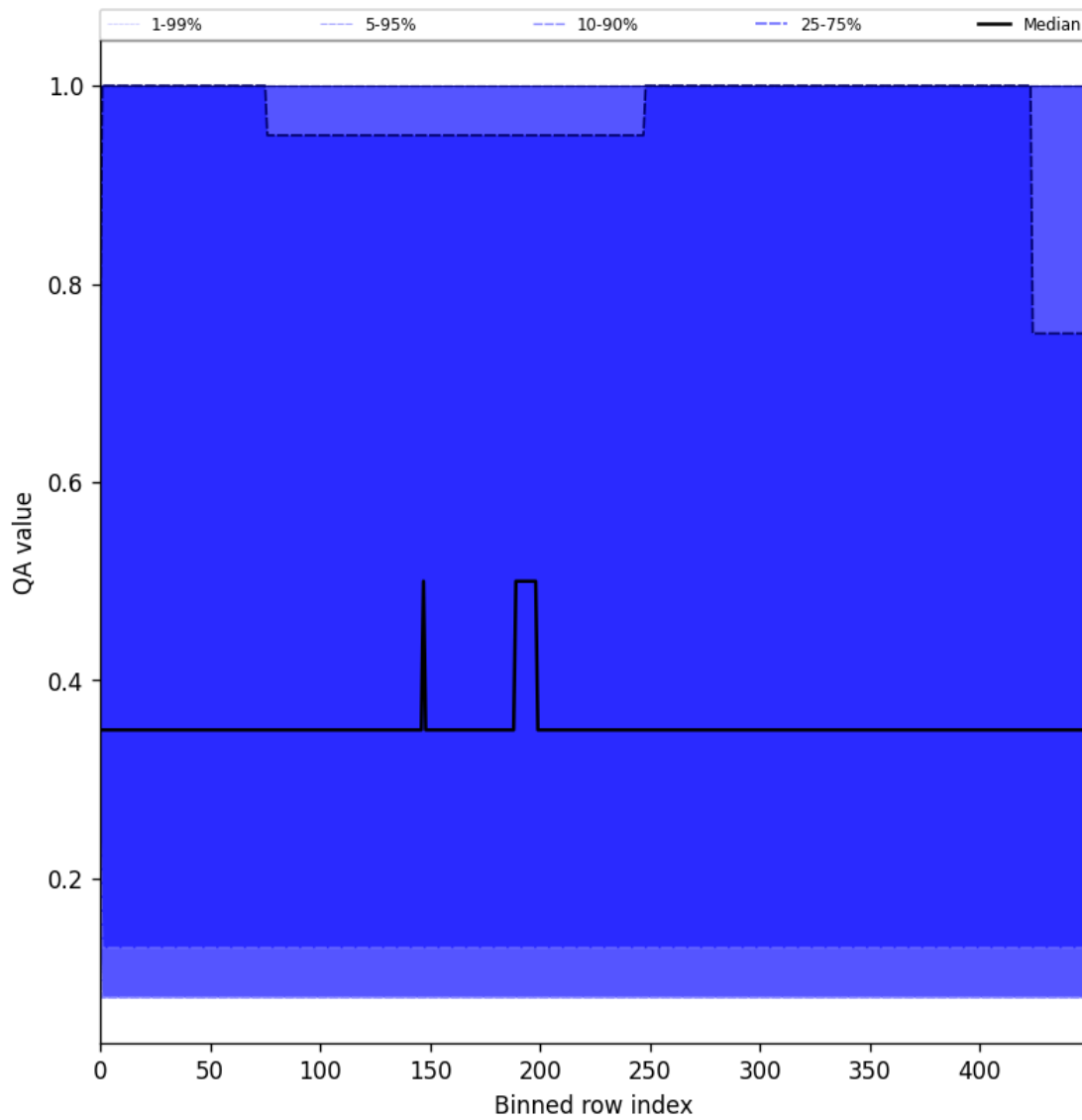
Figure 48: Along track statistics of “QA value” for 2025-04-02 to 2025-04-03
