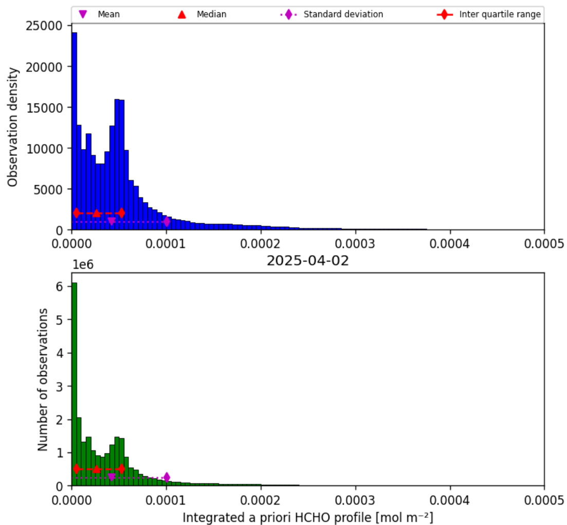
Figure 43: Histogram of “Integrated a priori HCHO profile” for 2025-04-02 to 2025-04-03
