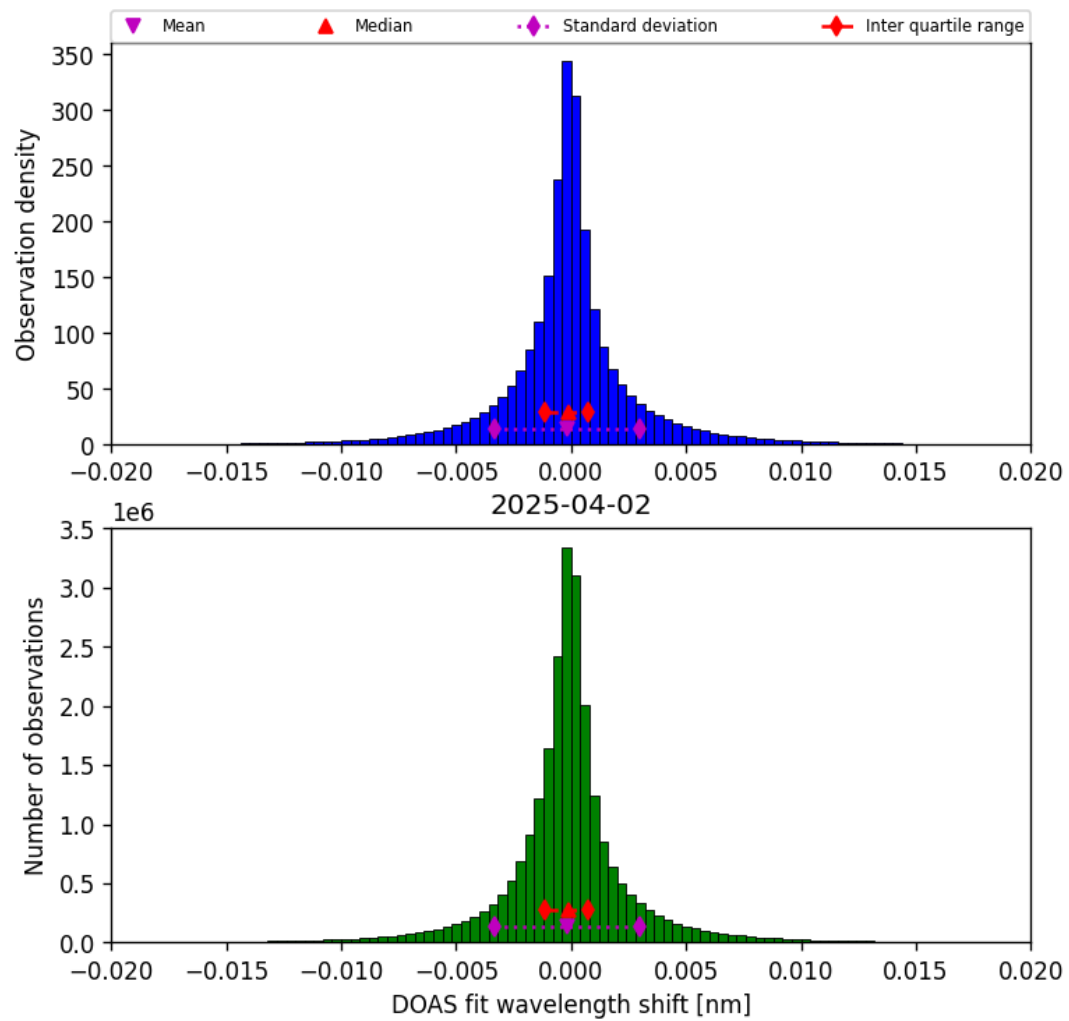
Figure 44: Histogram of “DOAS fit wavelength shift” for 2025-04-02 to 2025-04-03
