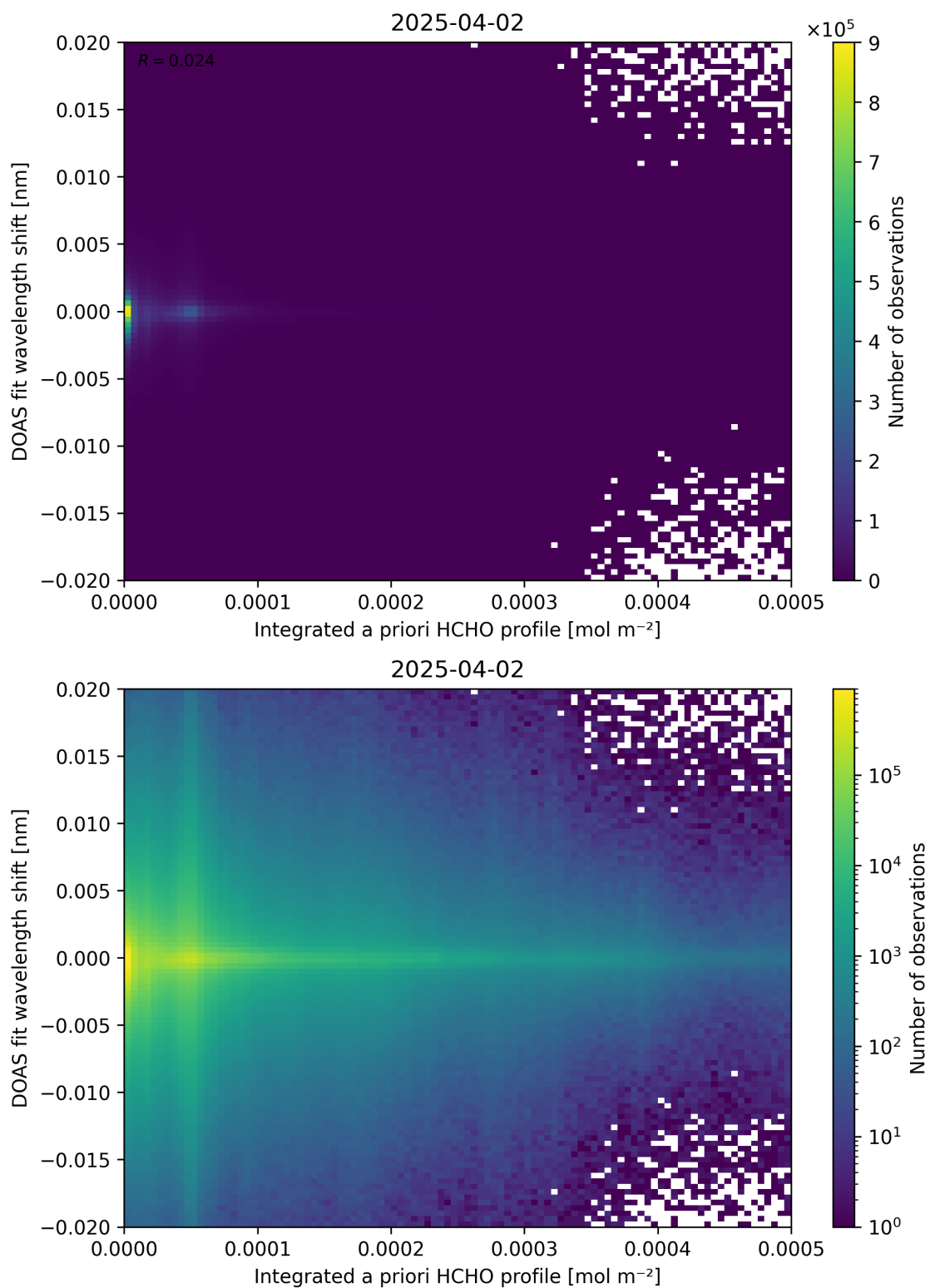
Figure 149: Scatter density plot of “Integrated a priori HCHO profile” against “DOAS fit wavelength shift” for 2025-04-02 to 2025-04-03.
