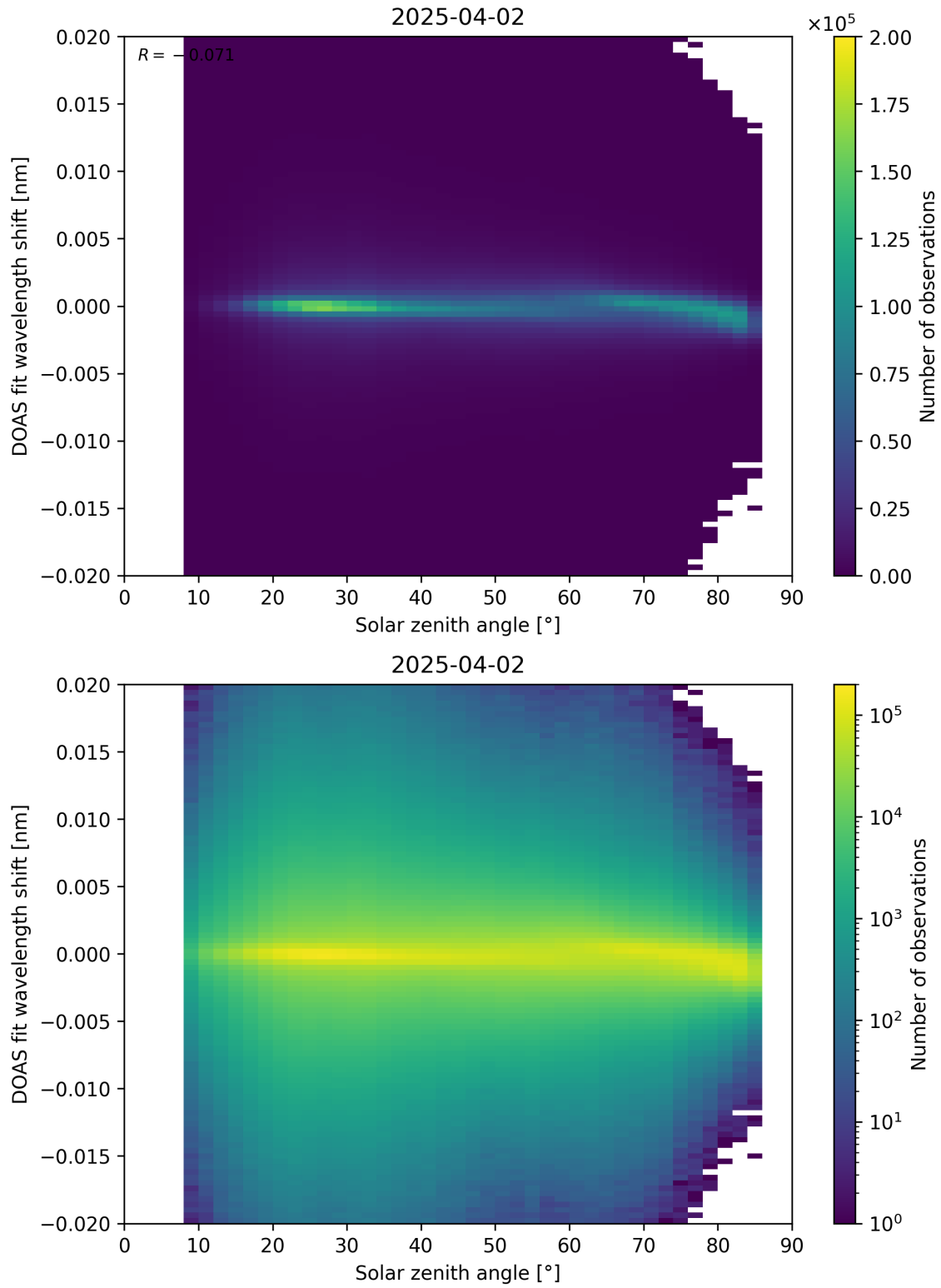
Figure 168: Scatter density plot of “Solar zenith angle” against “DOAS fit wavelength shift” for 2025-04-02 to 2025-04-03.
