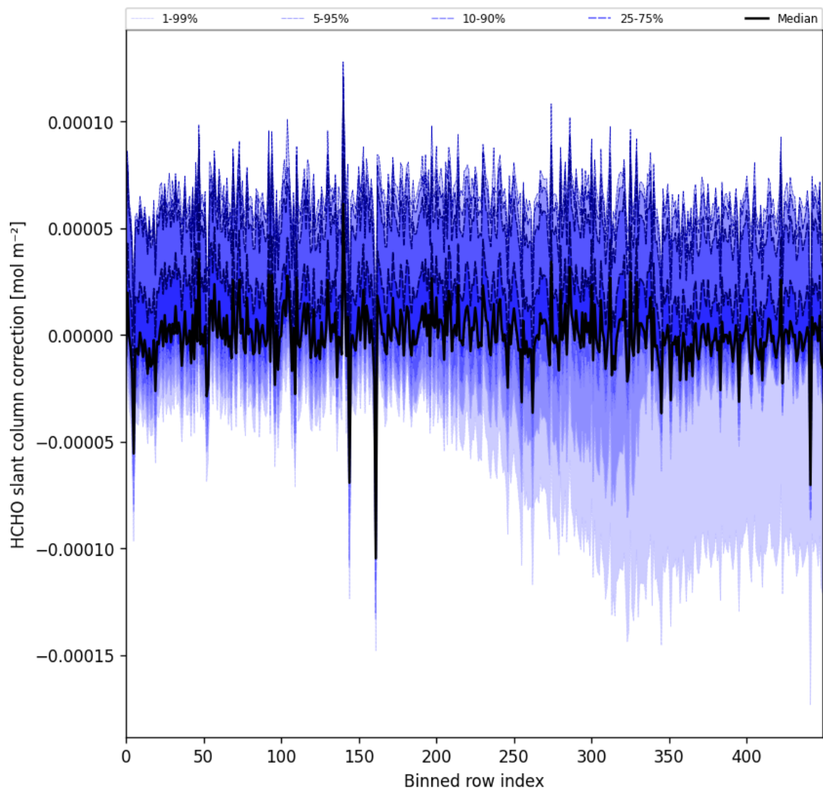
Figure 61: Along track statistics of “HCHO slant column correction” for 2025-04-02 to 2025-04-03
