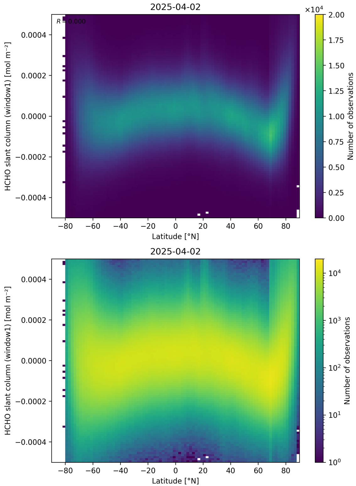
Figure 159: Scatter density plot of “Latitude” against “HCHO slant column (window1)” for 2025-04-02 to 2025-04-03.
