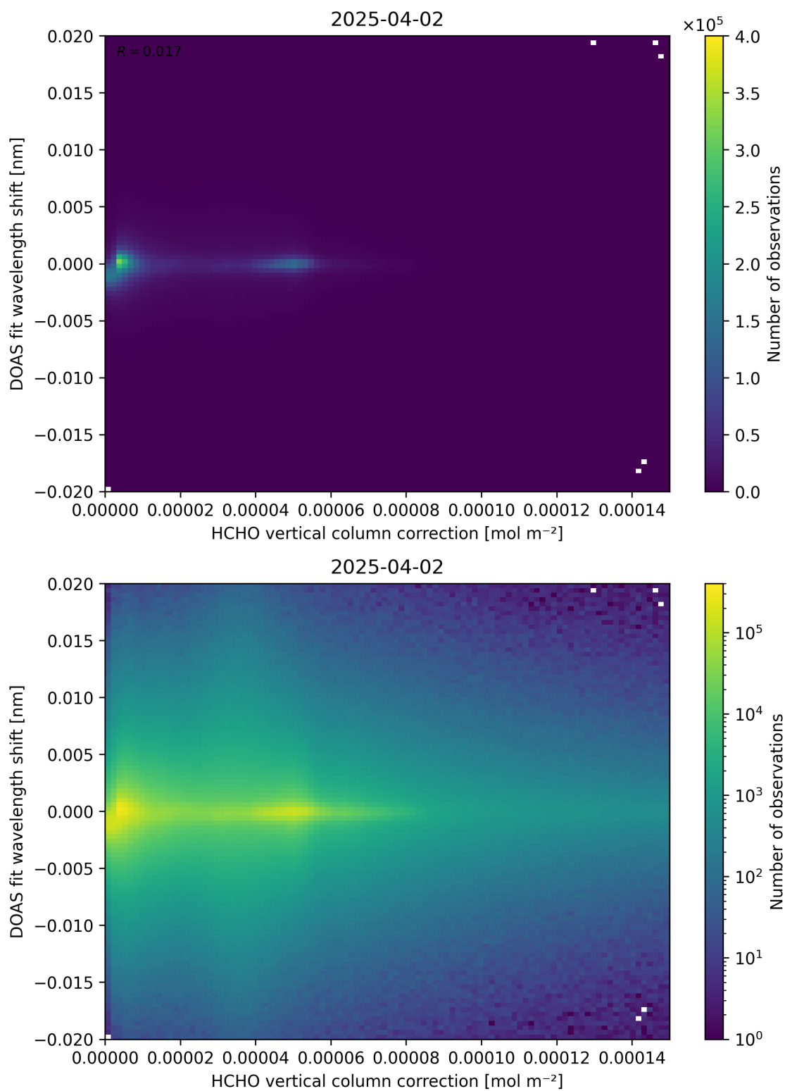
Figure 113: Scatter density plot of “HCHO vertical column correction” against “DOAS fit wavelength shift” for 2025-04-02 to 2025-04-03.
