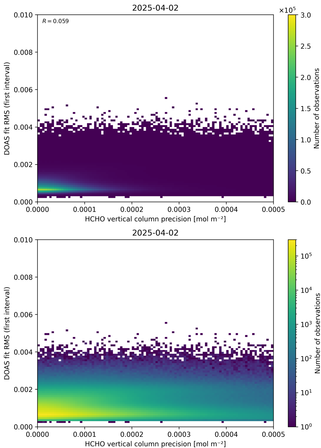
Figure 136: Scatter density plot of “HCHO vertical column precision” against “DOAS fit RMS (first interval)” for 2025-04-02 to 2025-04-03.
