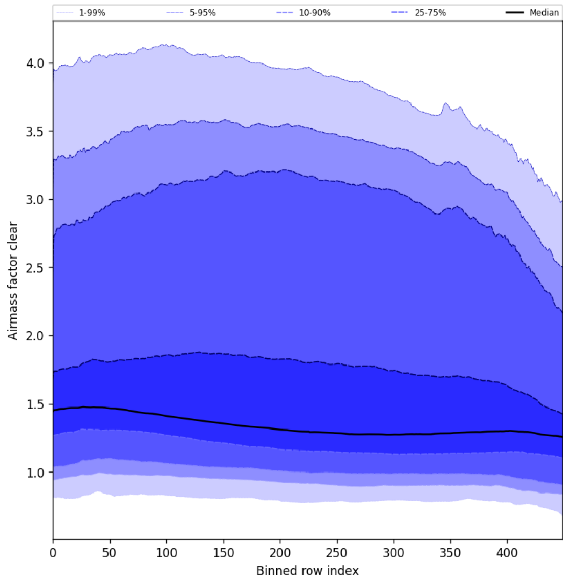
Figure 56: Along track statistics of “Airmass factor clear” for 2025-04-02 to 2025-04-03
