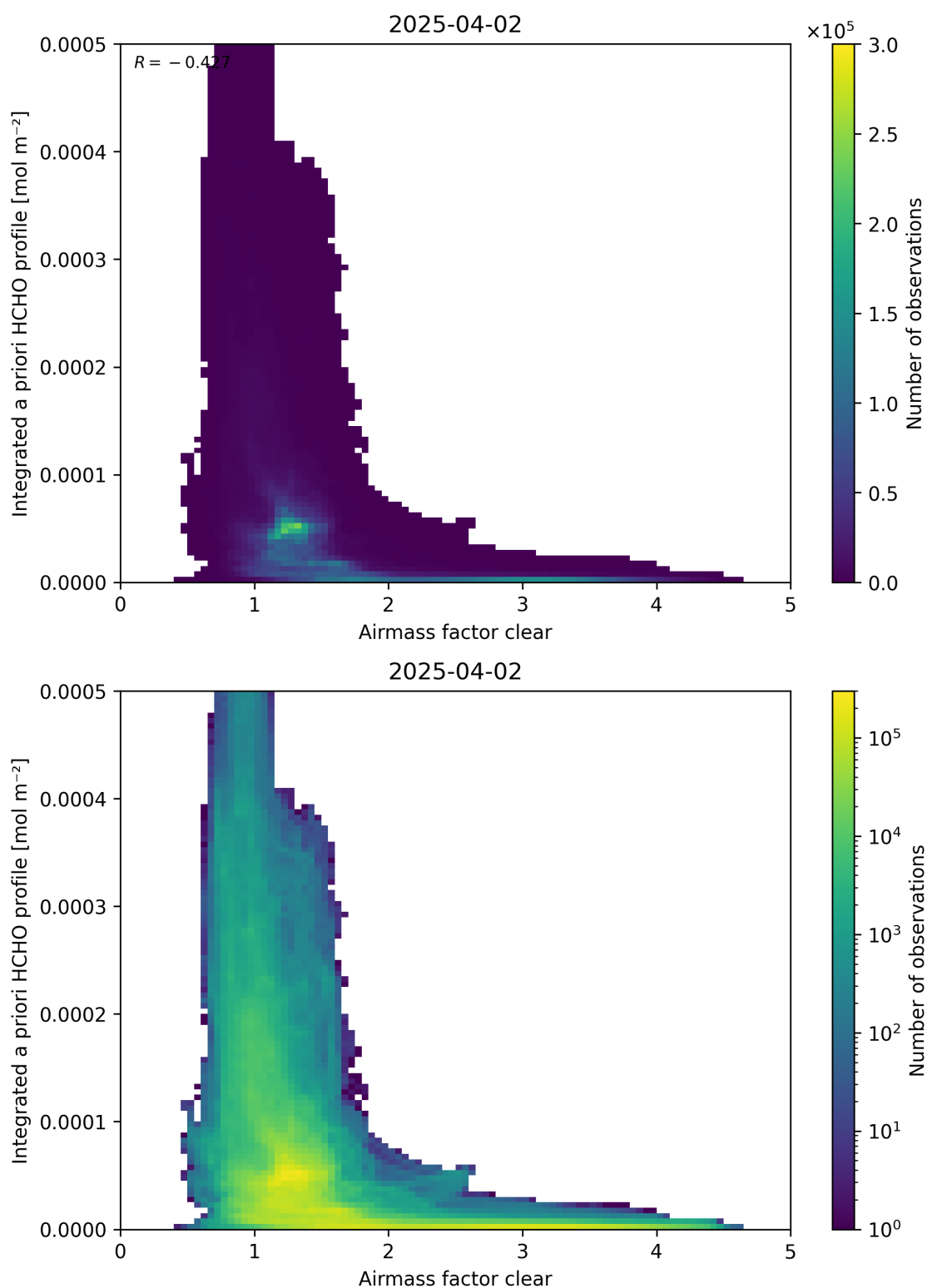
Figure 76: Scatter density plot of “Airmass factor clear” against “Integrated a priori HCHO profile” for 2025-04-02 to 2025-04-03.
