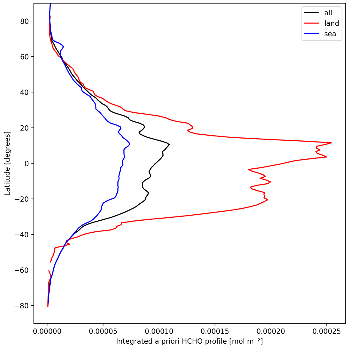
Figure 29: Zonal average of “Integrated a priori HCHO profile” for 2025-04-02 to 2025-04-03.
