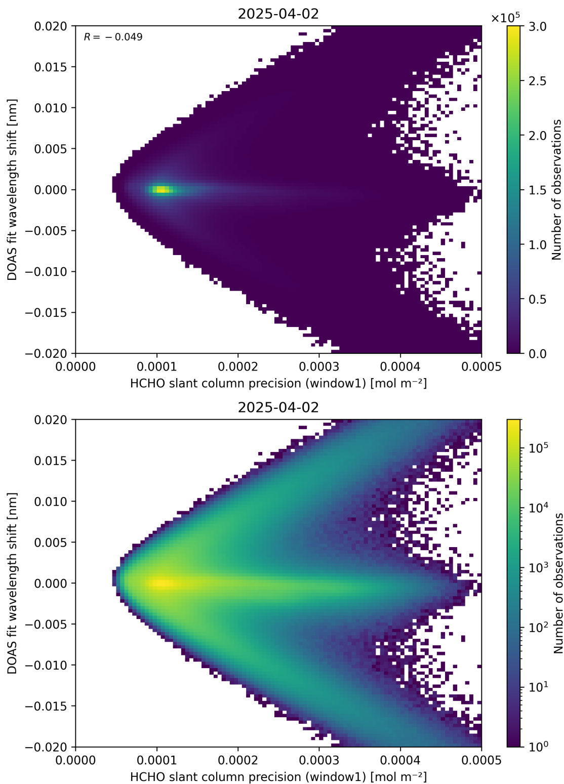
Figure 89: Scatter density plot of “HCHO slant column precision (window1)” against “DOAS fit wavelength shift” for 2025-04-02 to 2025-04-03.
