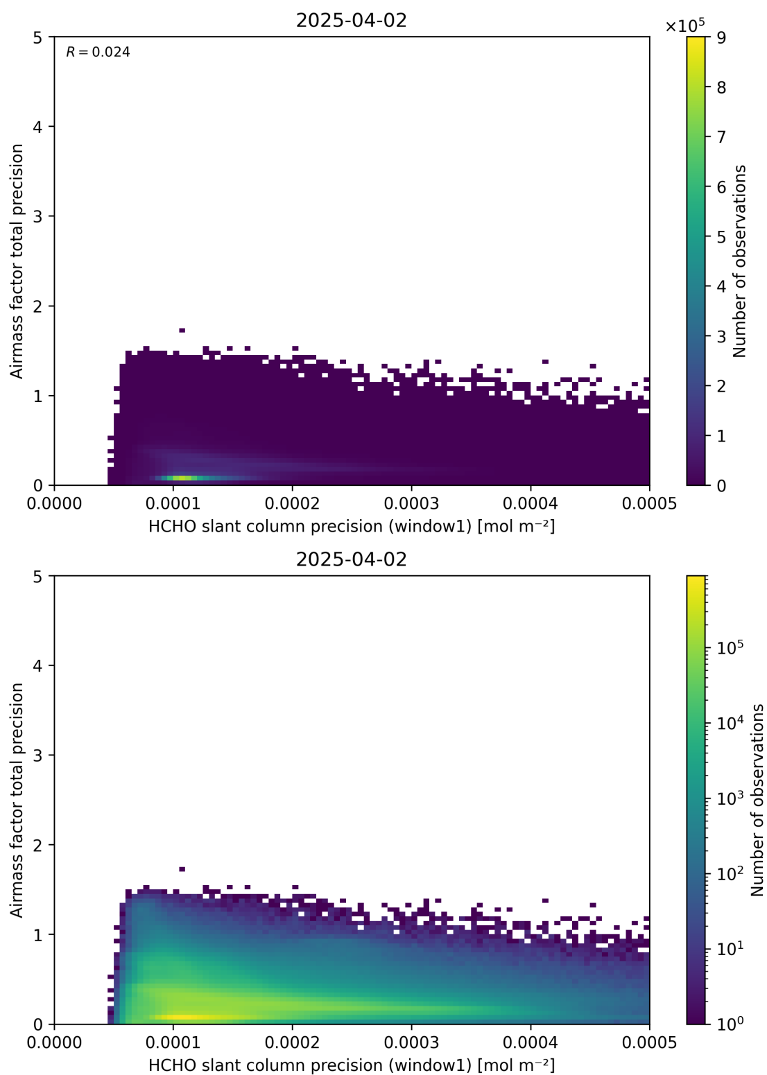
Figure 95: Scatter density plot of “HCHO slant column precision (window1)” against “Airmass factor total precision” for 2025-04-02 to 2025-04-03.
