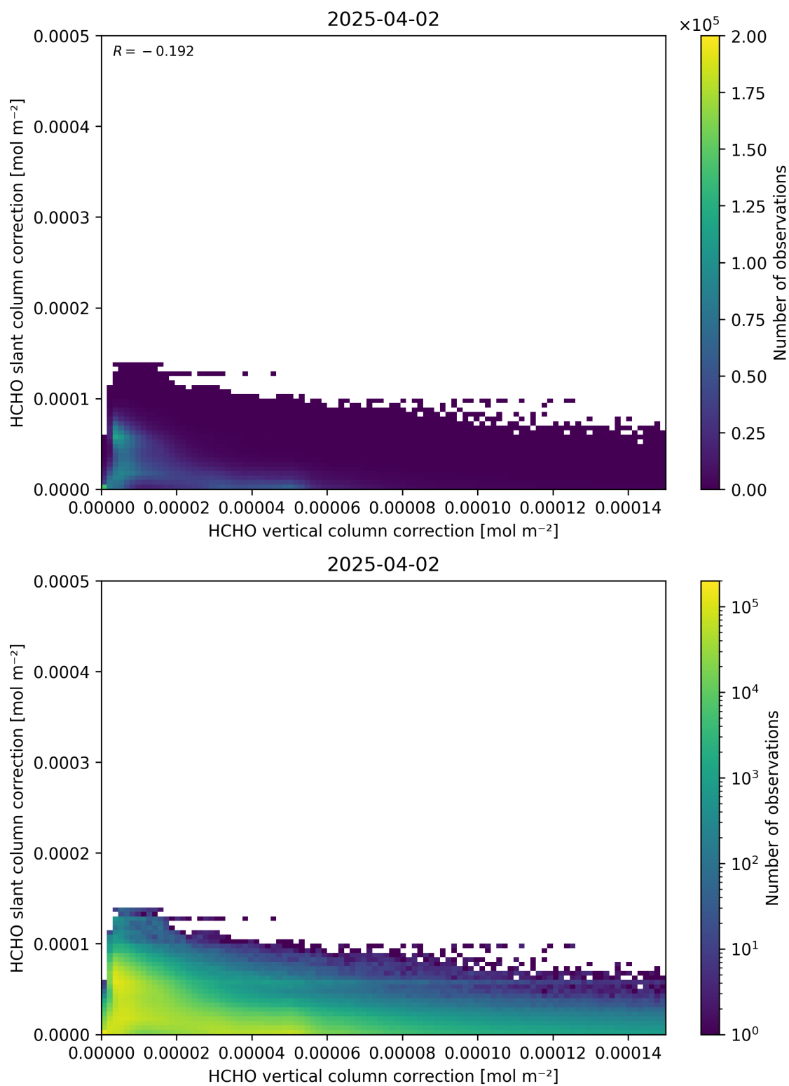
Figure 117: Scatter density plot of “HCHO vertical column correction” against “HCHO slant column correction” for 2025-04-02 to 2025-04-03.
