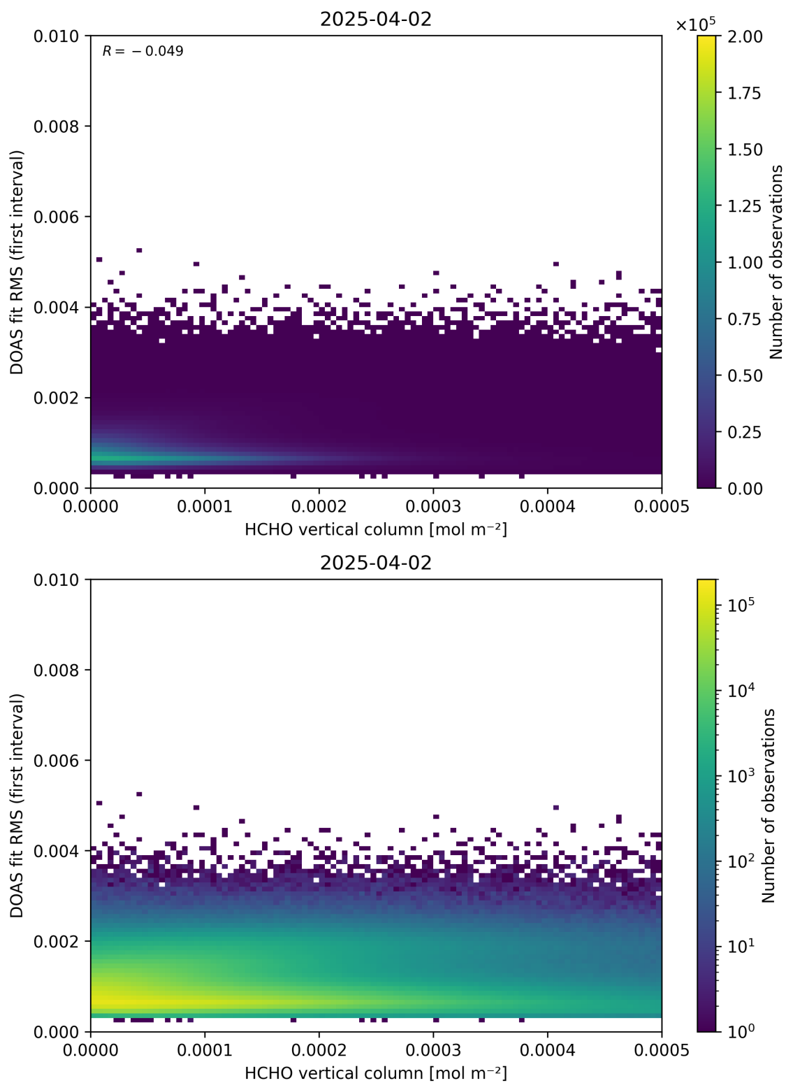
Figure 123: Scatter density plot of “HCHO vertical column” against “DOAS fit RMS (first interval)” for 2025-04-02 to 2025-04-03.
