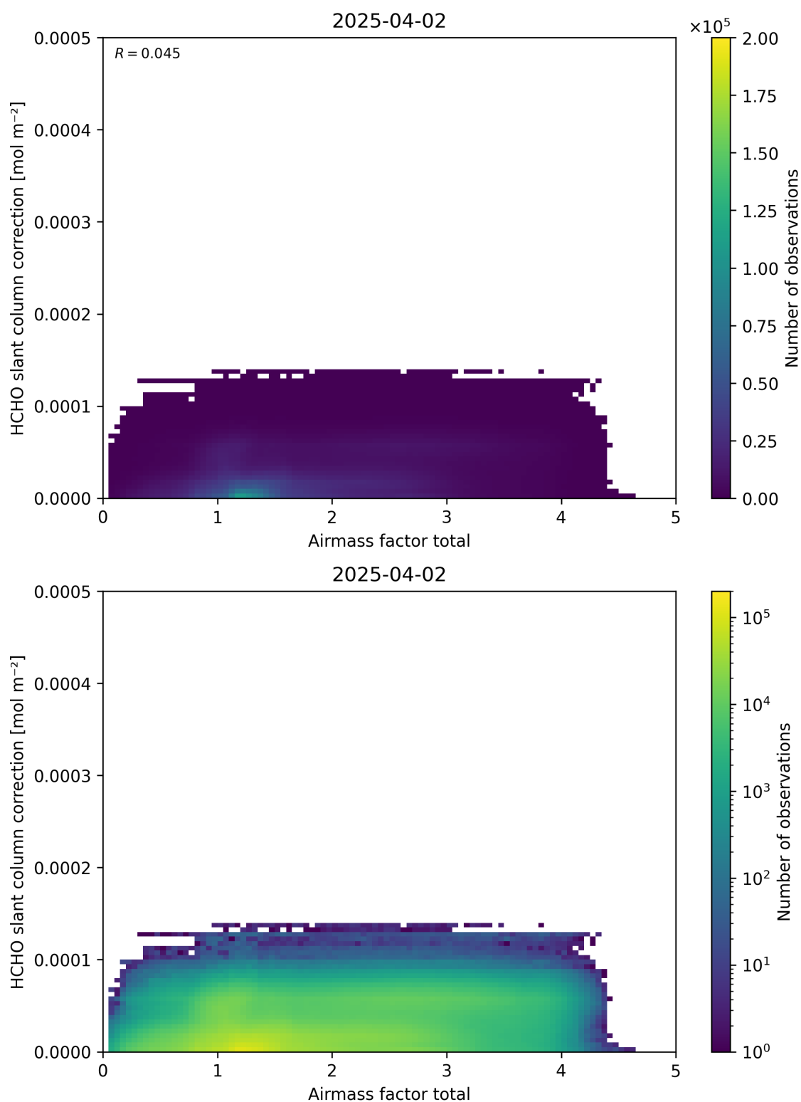
Figure 102: Scatter density plot of “Airmass factor total” against “HCHO slant column correction” for 2025-04-02 to 2025-04-03.
