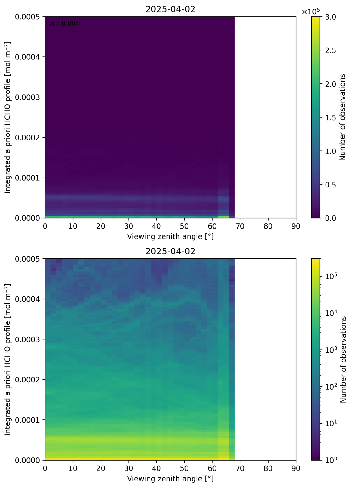
Figure 195: Scatter density plot of “Viewing zenith angle” against “Integrated a priori HCHO profile” for 2025-04-02 to 2025-04-03.
