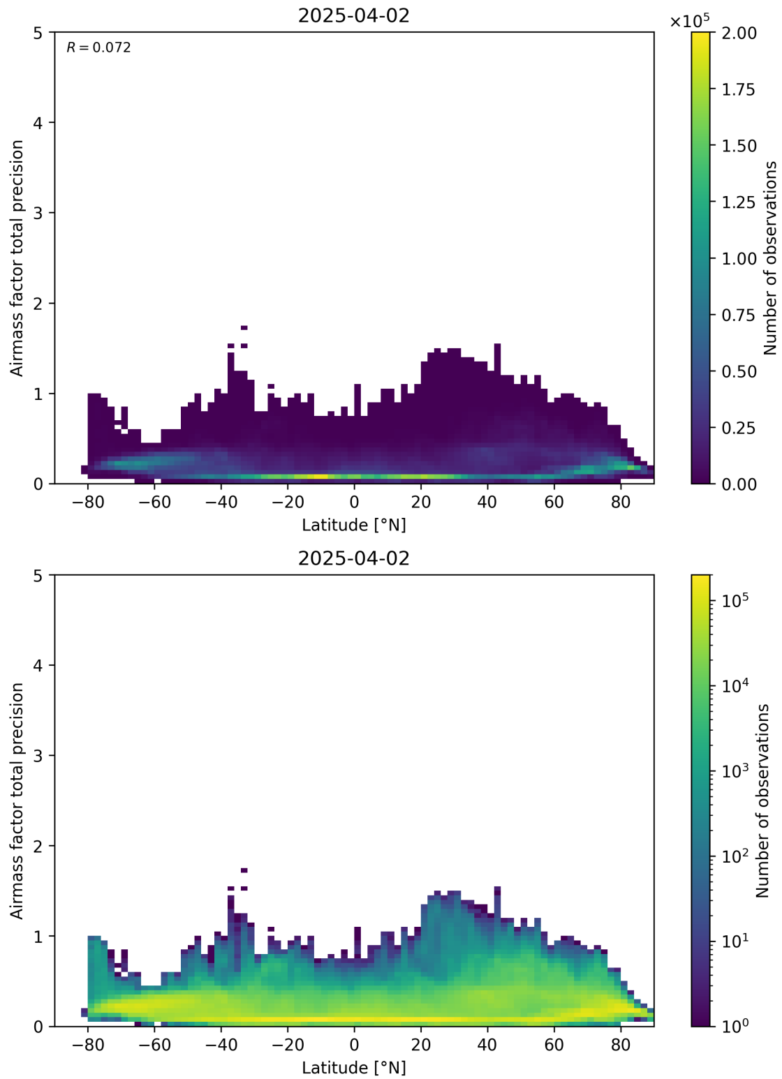
Figure 162: Scatter density plot of “Latitude” against “Airmass factor total precision” for 2025-04-02 to 2025-04-03.
