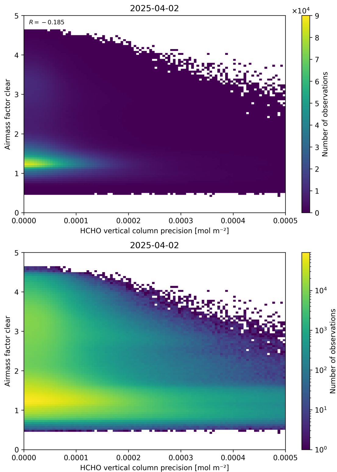
Figure 139: Scatter density plot of “HCHO vertical column precision” against “Airmass factor clear” for 2025-04-02 to 2025-04-03.
