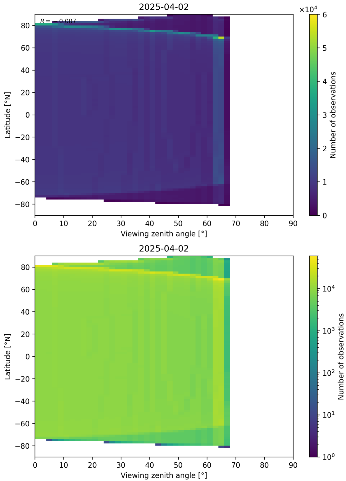
Figure 196: Scatter density plot of “Viewing zenith angle” against “Latitude” for 2025-04-02 to 2025-04-03.
