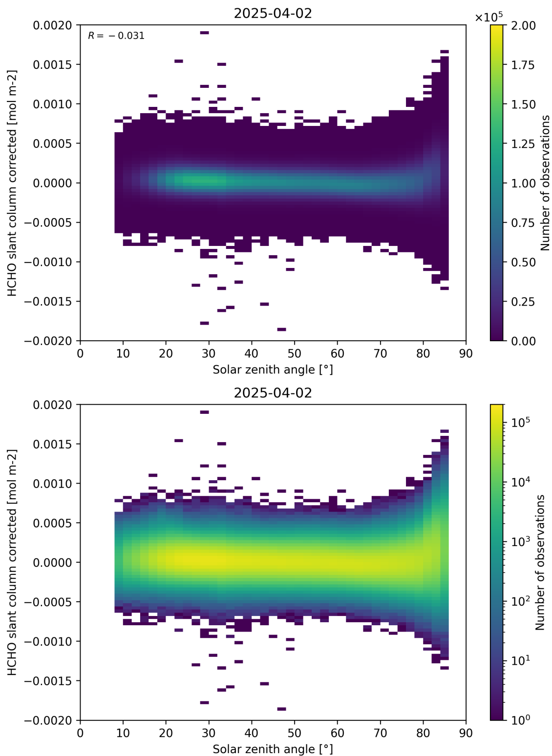
Figure 171: Scatter density plot of “Solar zenith angle” against “HCHO slant column corrected” for 2025-04-02 to 2025-04-03.
