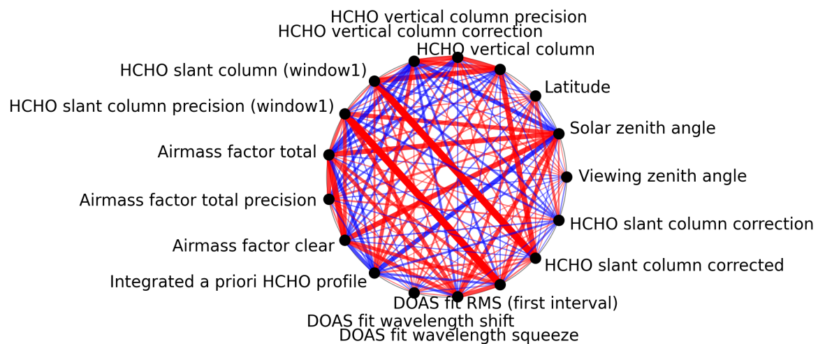
Figure 1: Map of correlation graph for 2025-04-02 to 2025-04-03.
