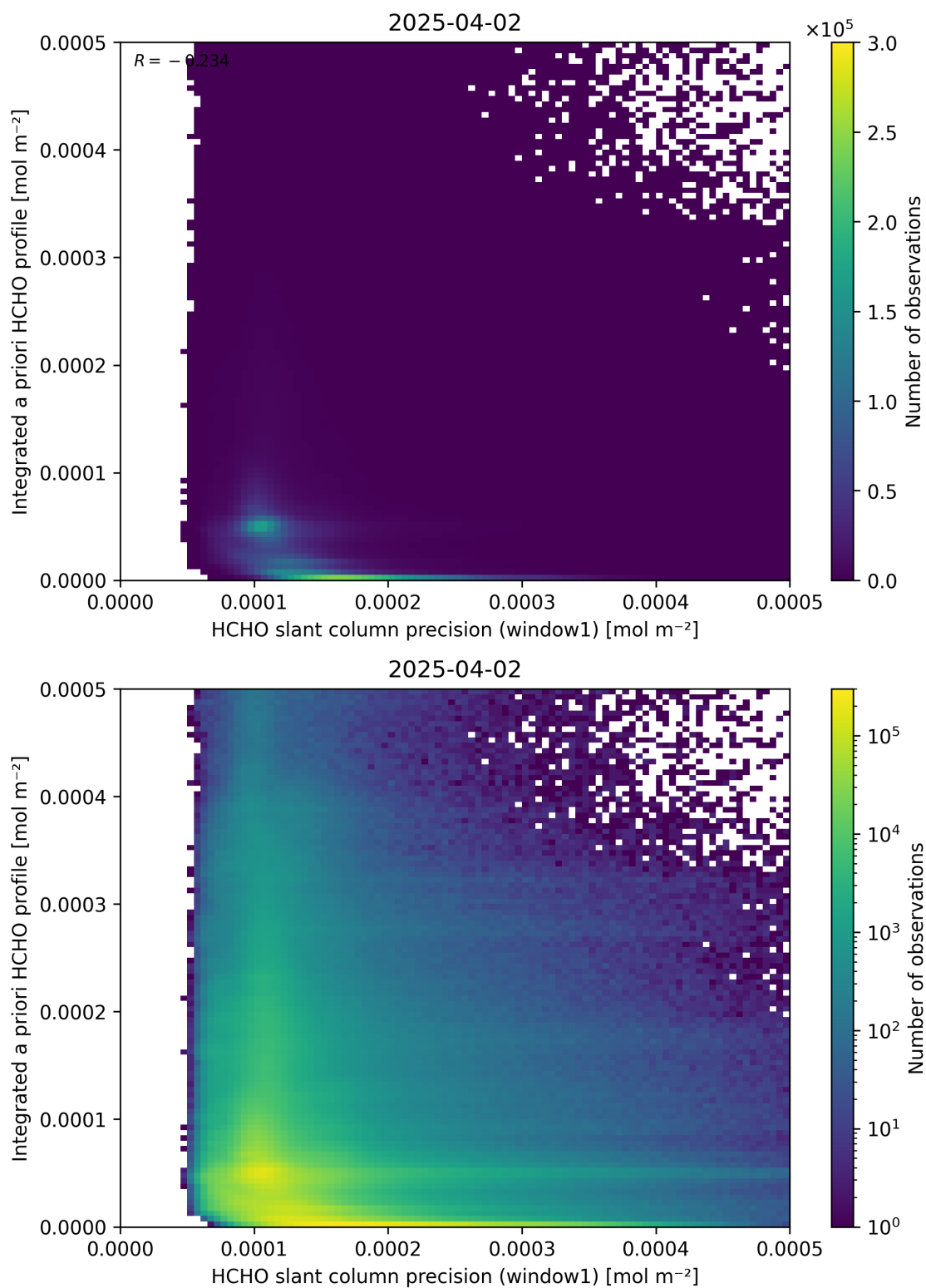
Figure 96: Scatter density plot of “HCHO slant column precision (window1)” against “Integrated a priori HCHO profile” for 2025-04-02 to 2025-04-03.
