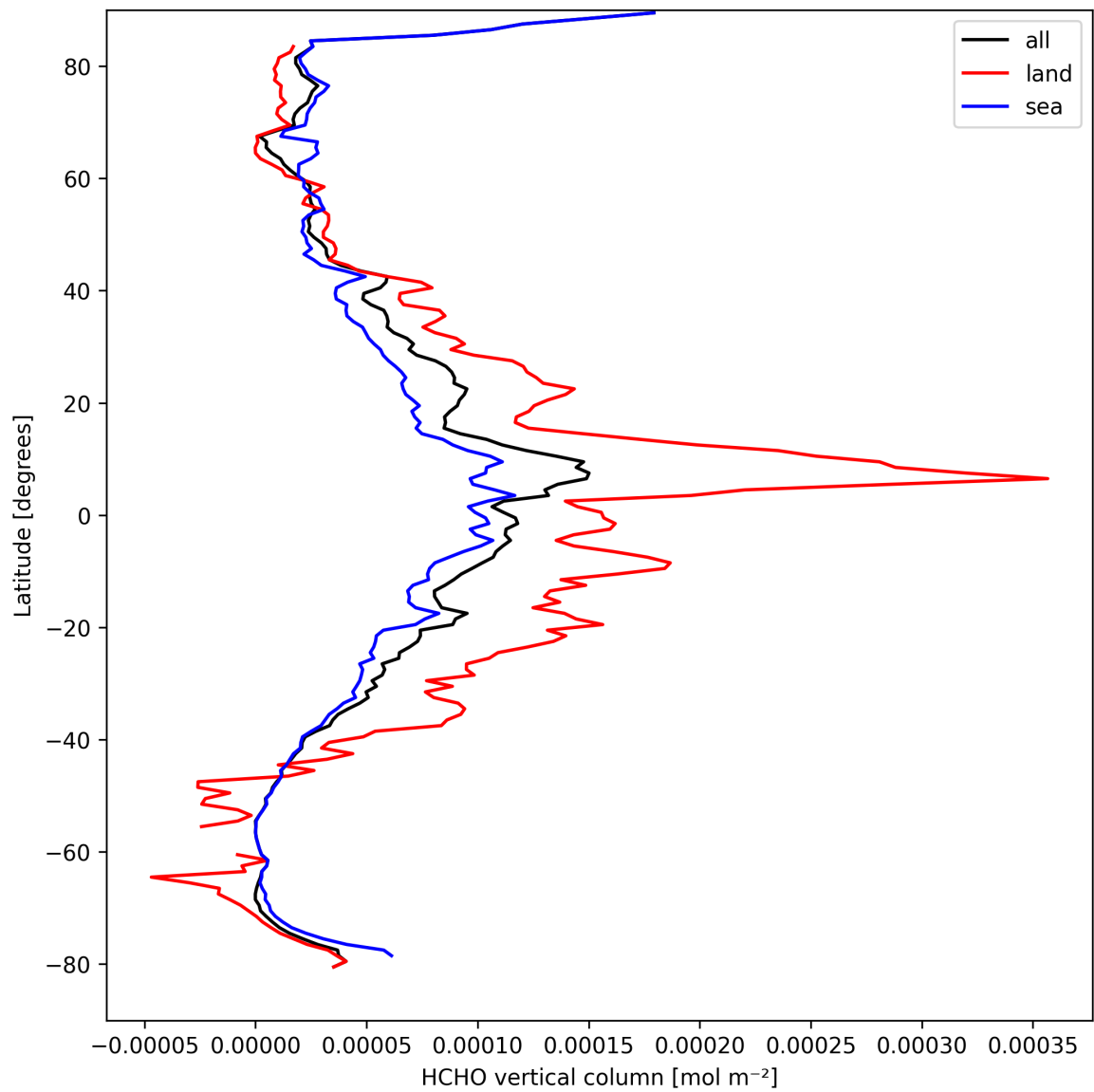
Figure 21: Zonal average of “HCHO vertical column” for 2025-04-02 to 2025-04-03.
