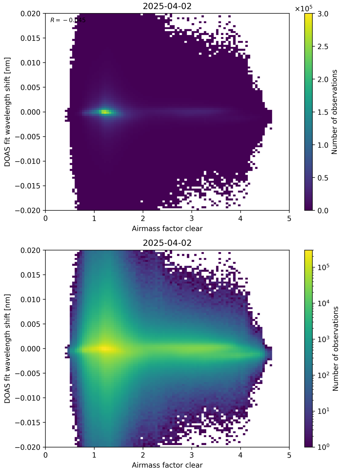
Figure 72: Scatter density plot of “Airmass factor clear” against “DOAS fit wavelength shift” for 2025-04-02 to 2025-04-03.
