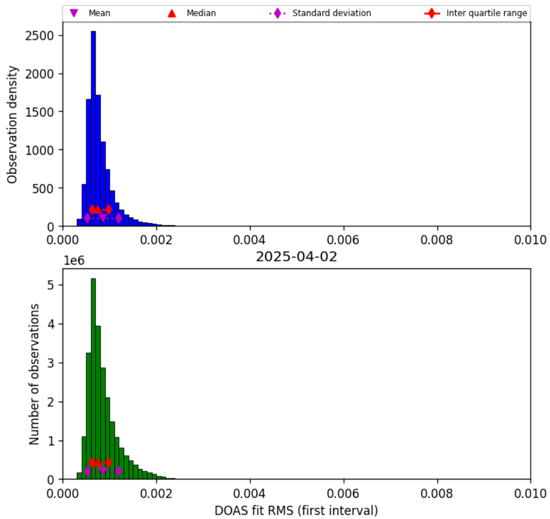
Figure 46: Histogram of “DOAS fit RMS (first interval)” for 2025-04-02 to 2025-04-03
