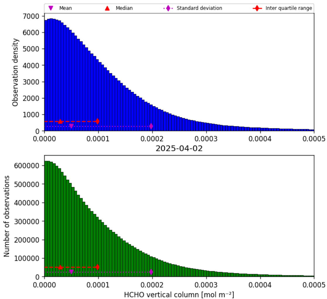
Figure 35: Histogram of “HCHO vertical column” for 2025-04-02 to 2025-04-03
