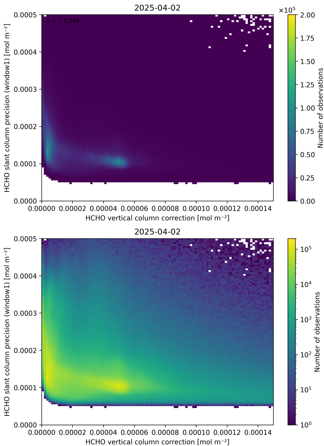
Figure 119: Scatter density plot of “HCHO vertical column correction” against “HCHO slant column precision (window1)” for 2025-04-02 to 2025-04-03.
