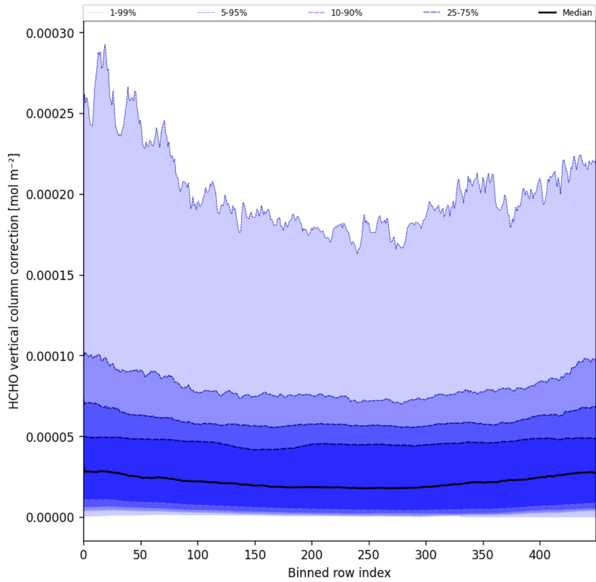
Figure 51: Along track statistics of “HCHO vertical column correction” for 2025-04-02 to 2025-04-03
