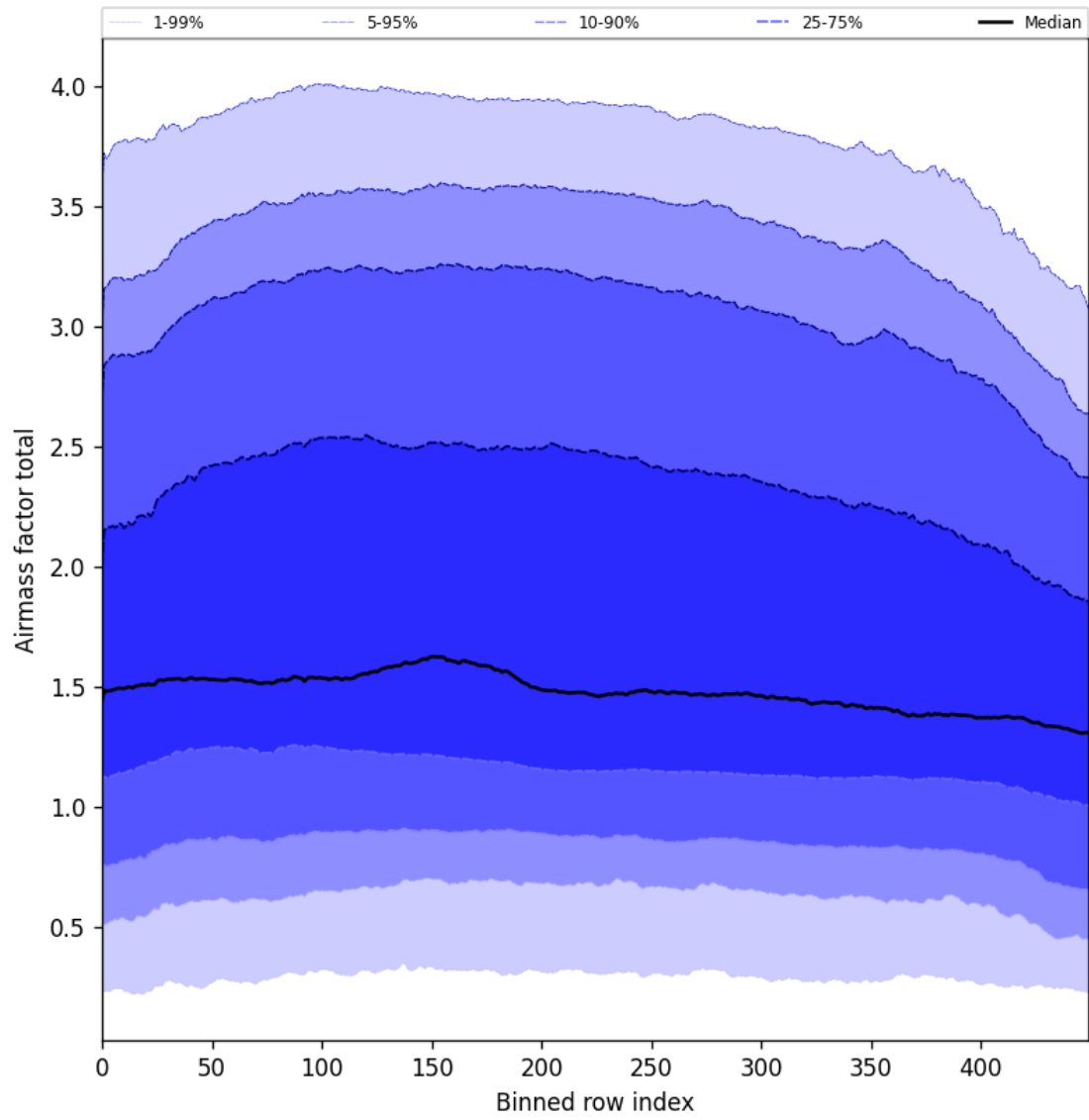
Figure 54: Along track statistics of “Airmass factor total” for 2025-04-02 to 2025-04-03
