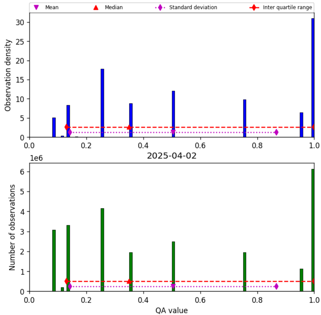
Figure 34: Histogram of “QA value” for 2025-04-02 to 2025-04-03
