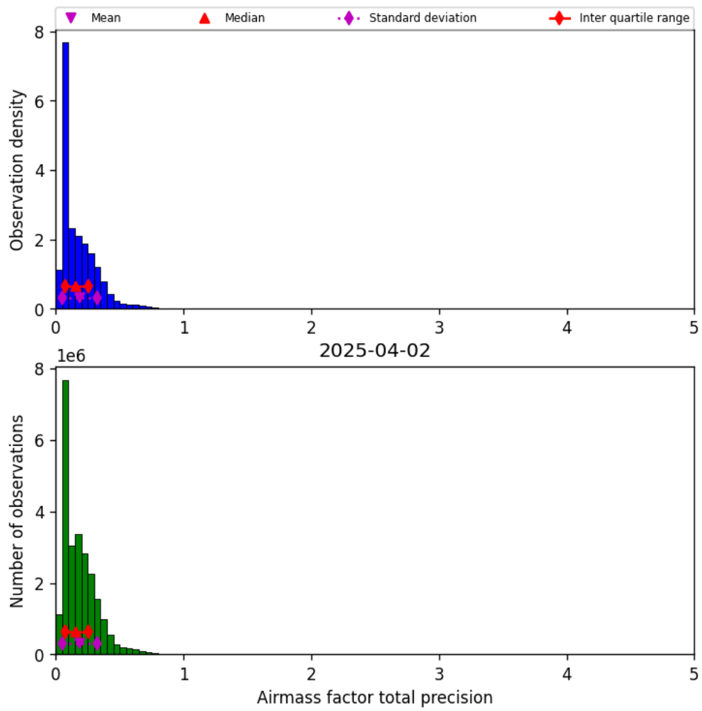
Figure 41: Histogram of “Airmass factor total precision” for 2025-04-02 to 2025-04-03
