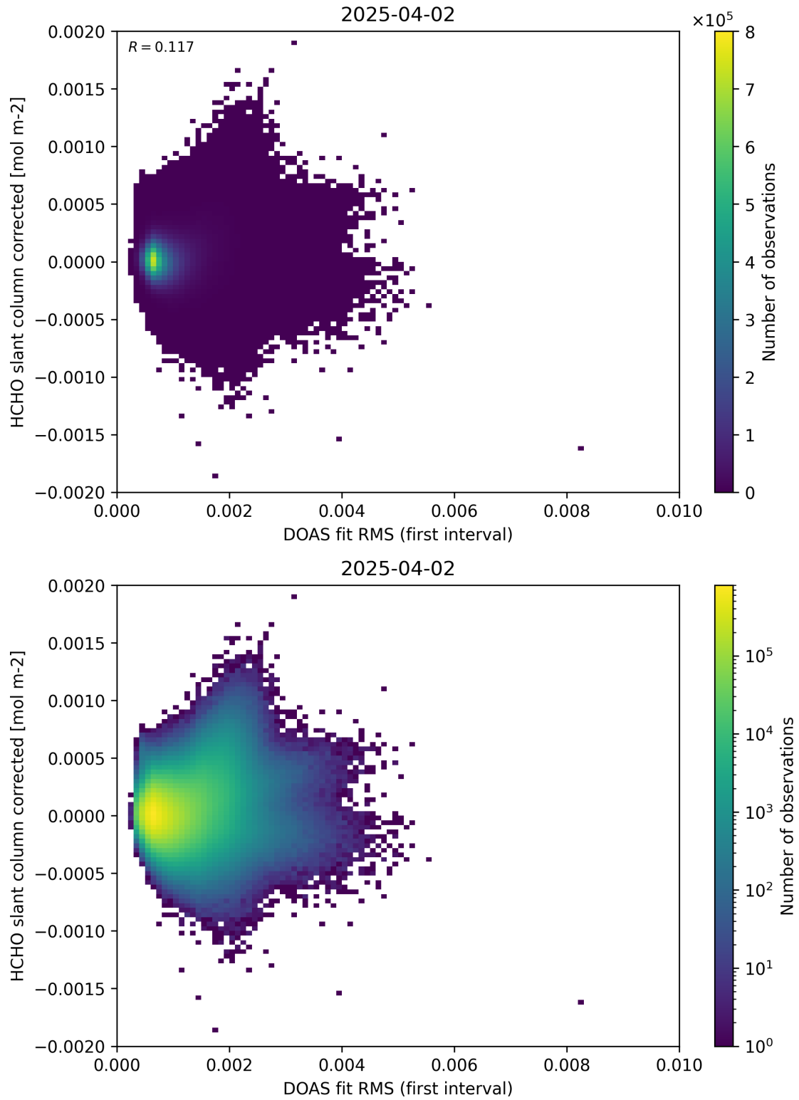
Figure 62: Scatter density plot of “DOAS fit RMS (first interval)” against “HCHO slant column corrected” for 2025-04-02 to 2025-04-03.
