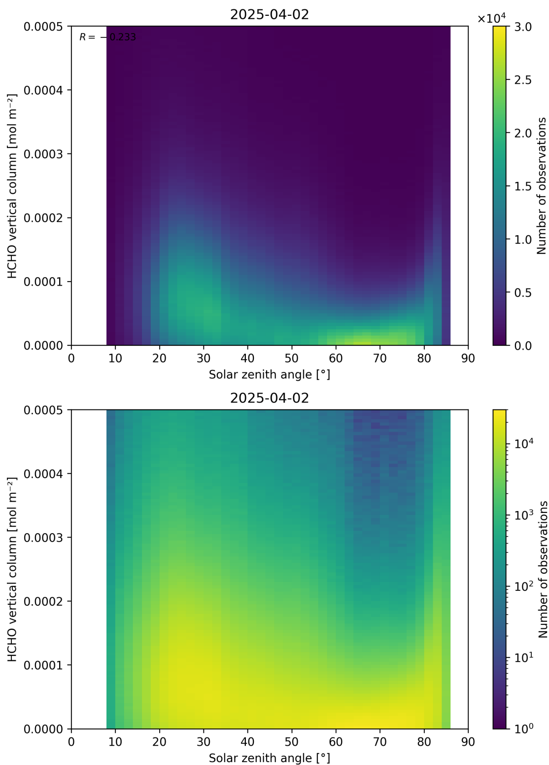
Figure 177: Scatter density plot of “Solar zenith angle” against “HCHO vertical column” for 2025-04-02 to 2025-04-03.
