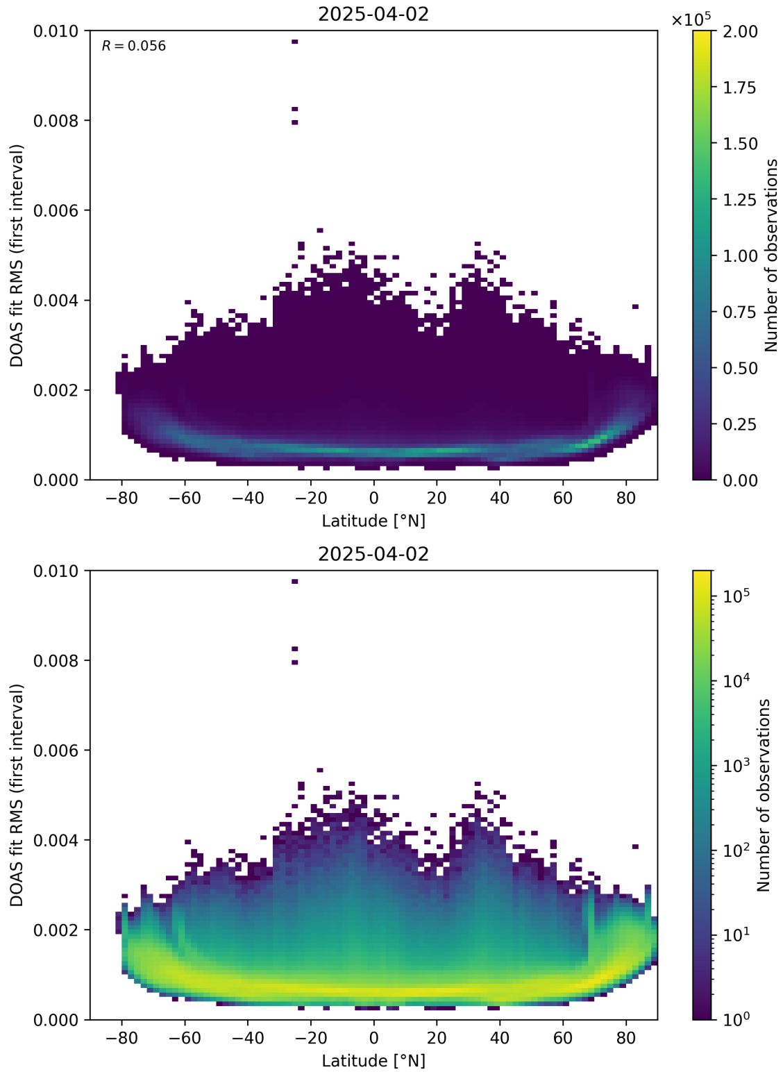
Figure 153: Scatter density plot of “Latitude” against “DOAS fit RMS (first interval)” for 2025-04-02 to 2025-04-03.
