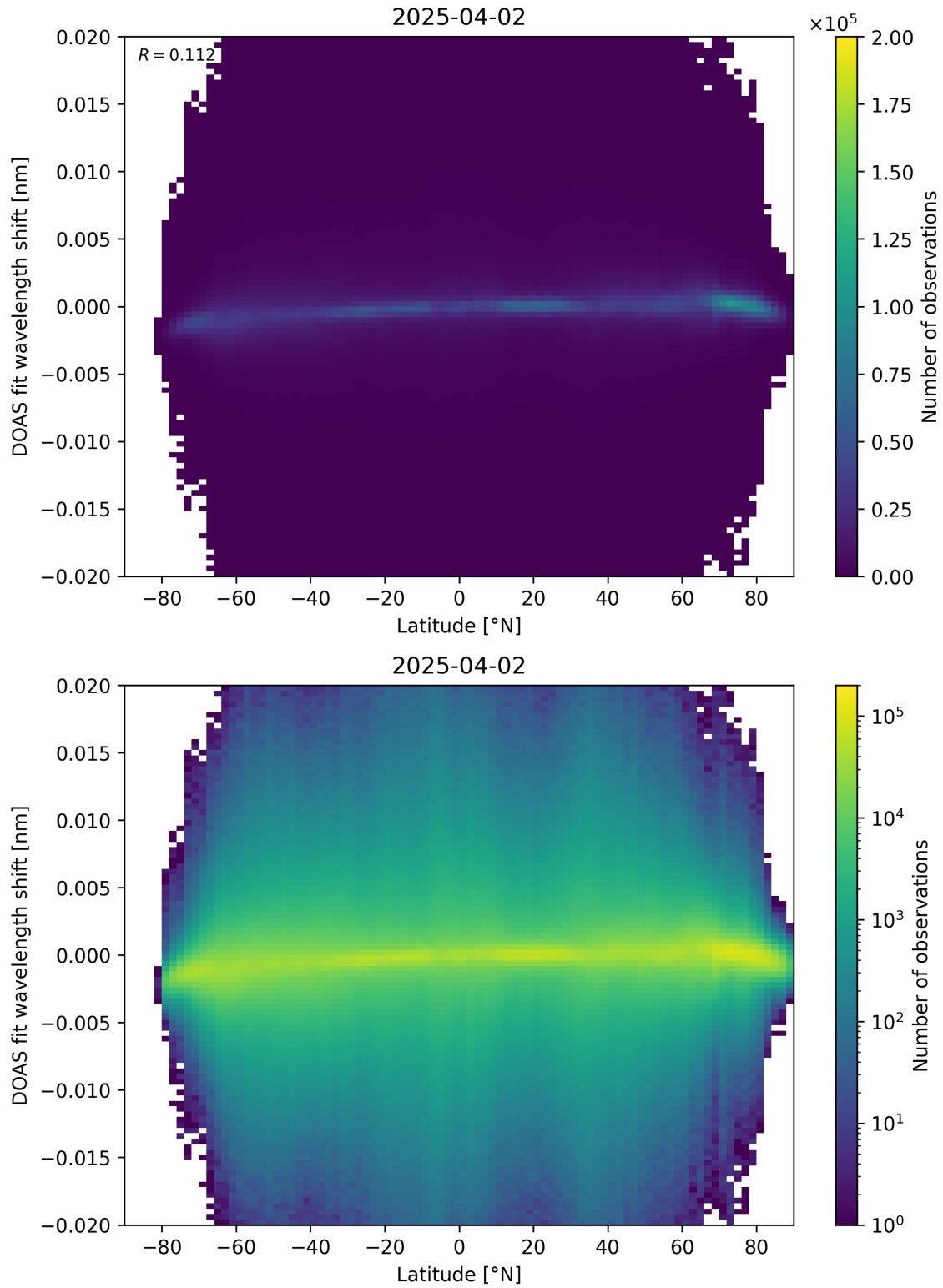
Figure 154: Scatter density plot of “Latitude” against “DOAS fit wavelength shift” for 2025-04-02 to 2025-04-03.
