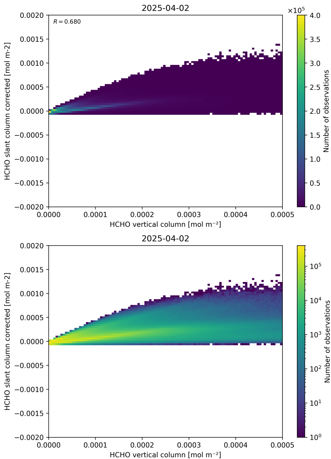
Figure 127: Scatter density plot of “HCHO vertical column” against “HCHO slant column corrected” for 2025-04-02 to 2025-04-03.
