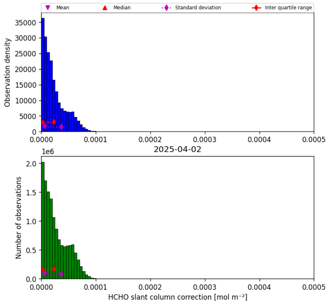
Figure 47: Histogram of “HCHO slant column correction” for 2025-04-02 to 2025-04-03
