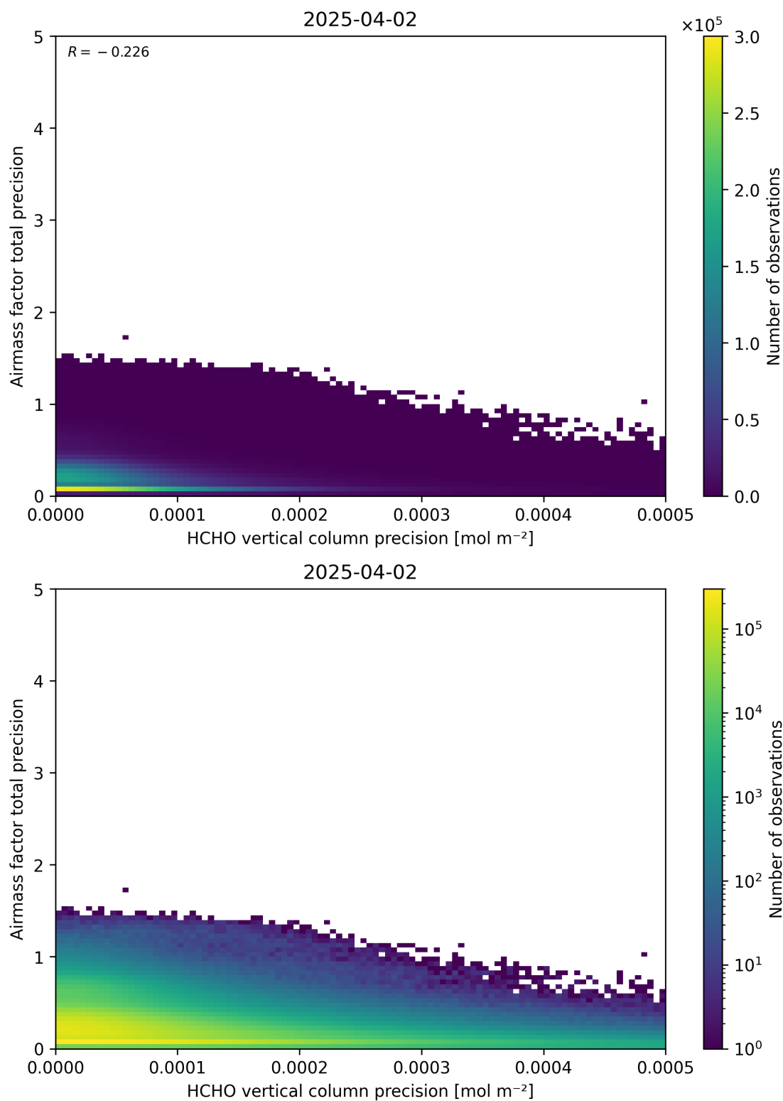
Figure 145: Scatter density plot of “HCHO vertical column precision” against “Airmass factor total precision” for 2025-04-02 to 2025-04-03.
