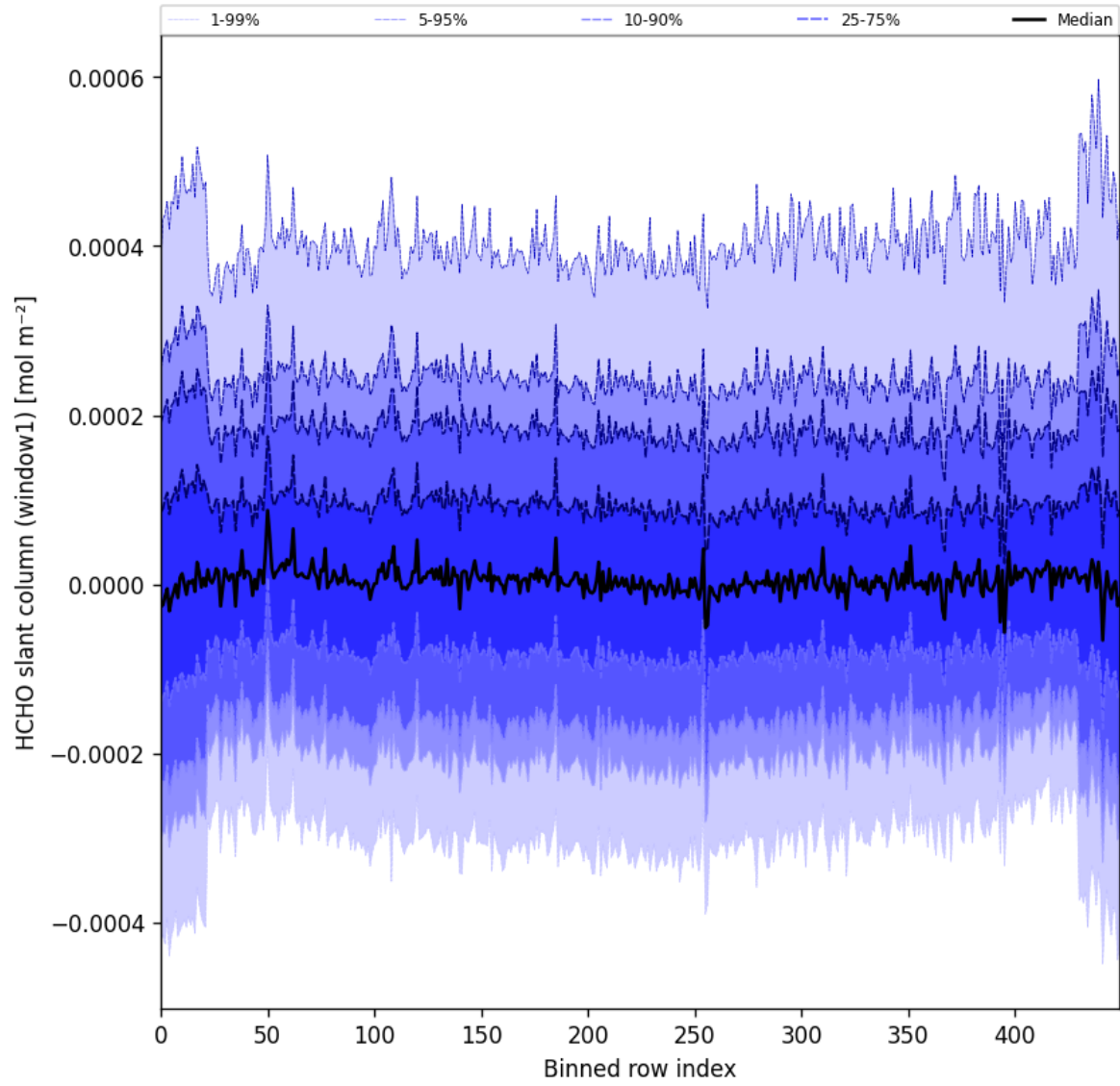
Figure 52: Along track statistics of “HCHO slant column (window1)” for 2025-04-02 to 2025-04-03
