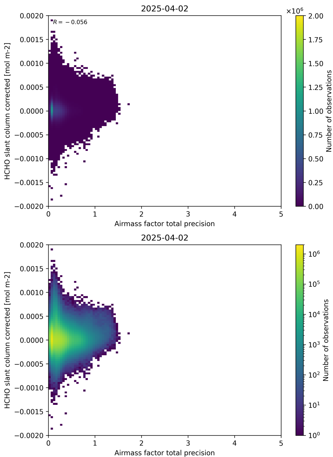
Figure 109: Scatter density plot of “Airmass factor total precision” against “HCHO slant column corrected” for 2025-04-02 to 2025-04-03.
