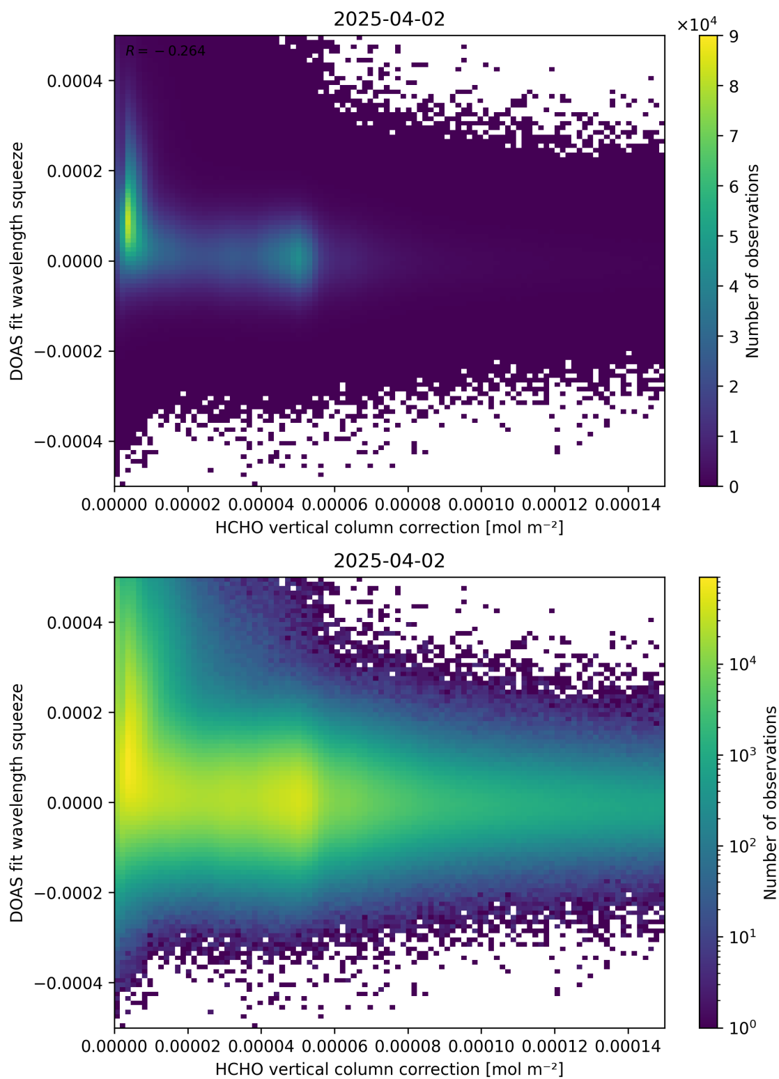
Figure 114: Scatter density plot of “HCHO vertical column correction” against “DOAS fit wavelength squeeze” for 2025-04-02 to 2025-04-03.
