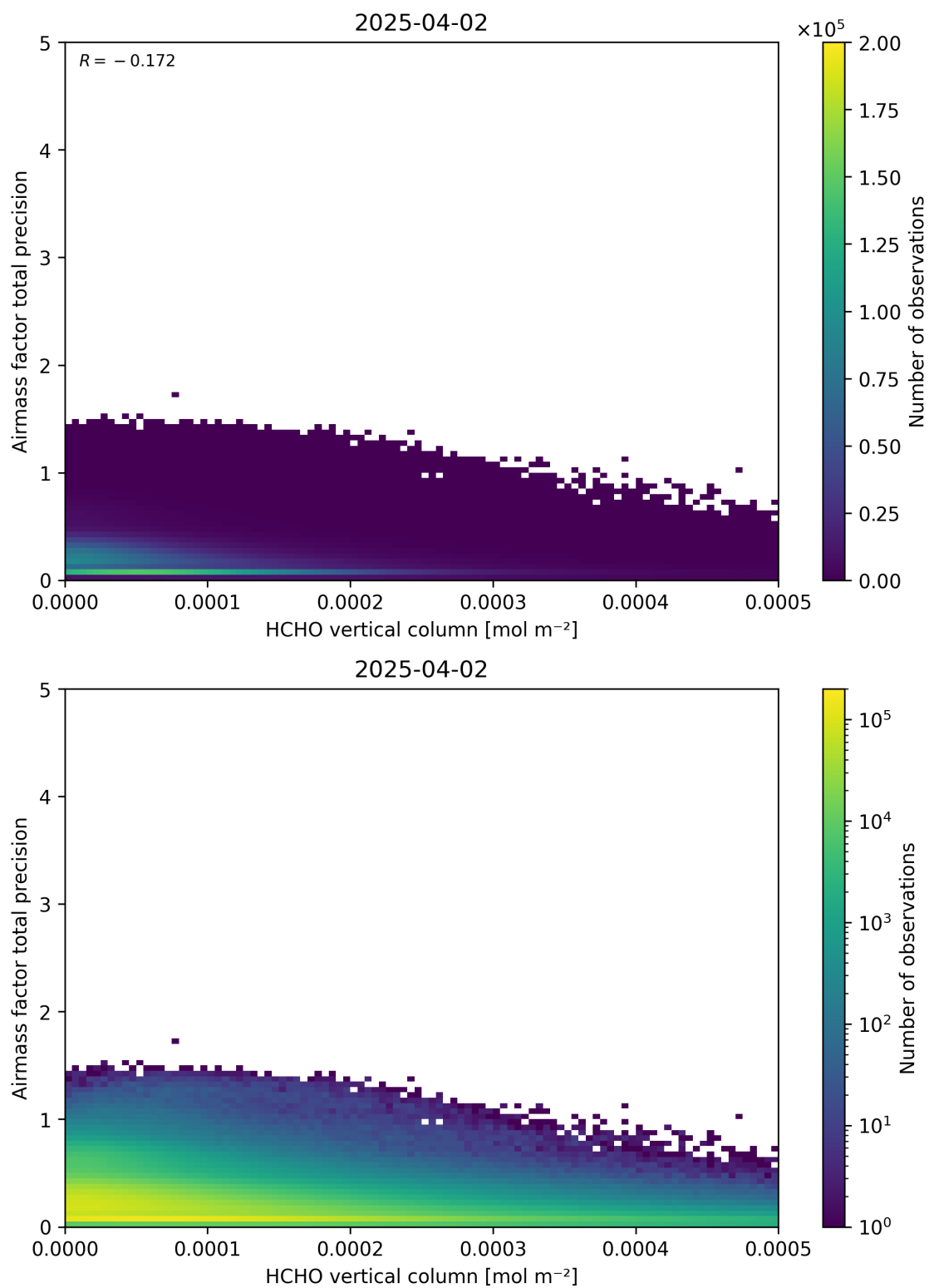
Figure 132: Scatter density plot of “HCHO vertical column” against “Airmass factor total precision” for 2025-04-02 to 2025-04-03.
