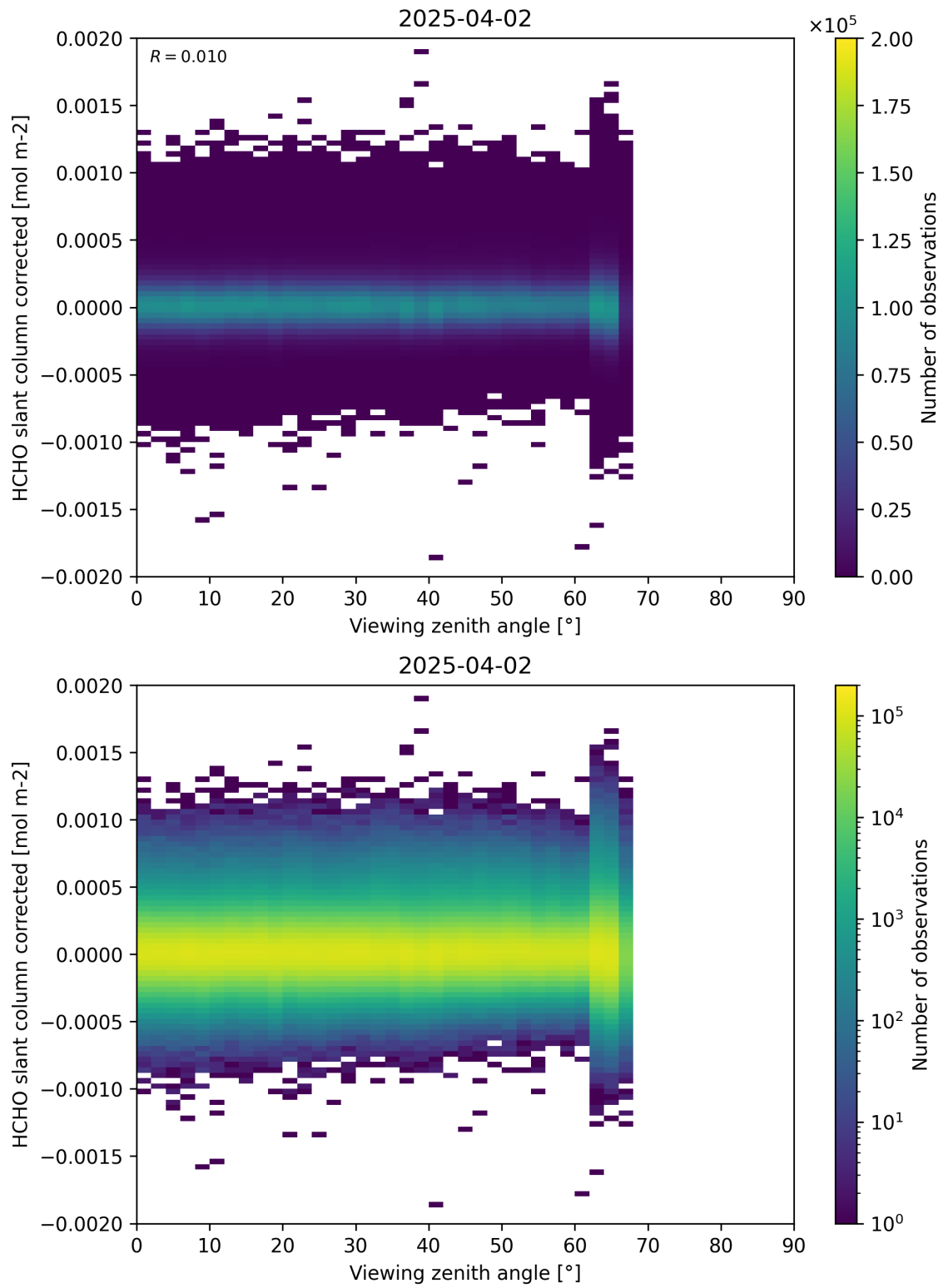
Figure 186: Scatter density plot of “Viewing zenith angle” against “HCHO slant column corrected” for 2025-04-02 to 2025-04-03.
