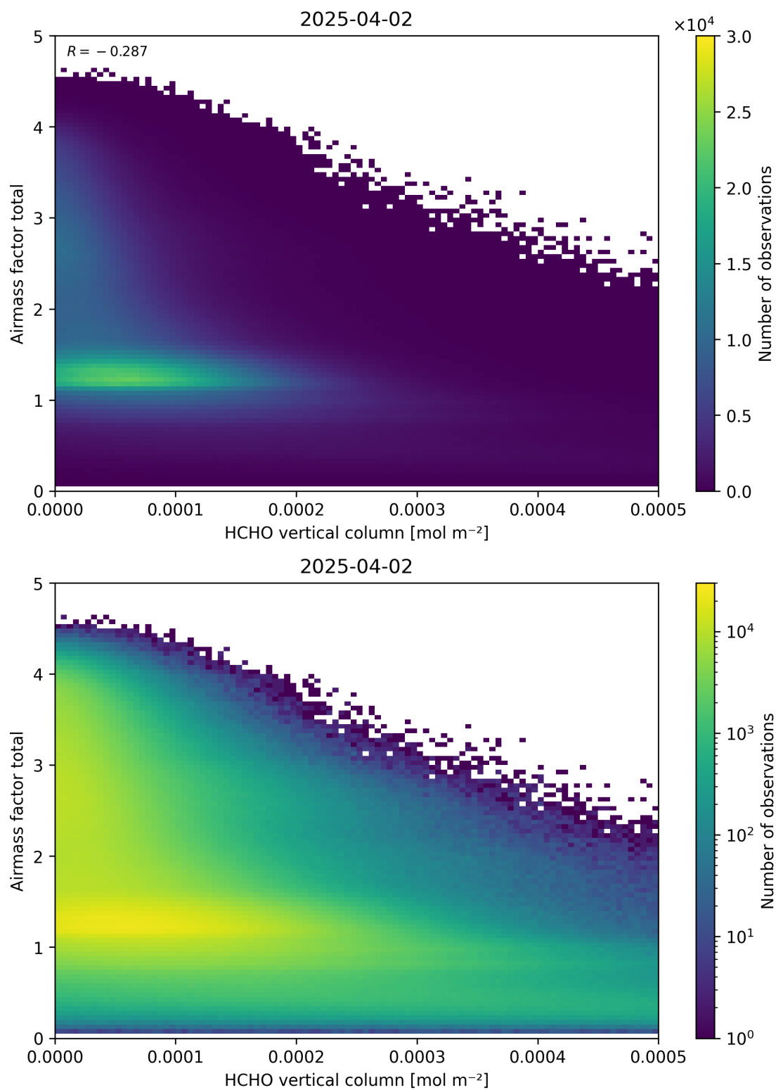
Figure 131: Scatter density plot of “HCHO vertical column” against “Airmass factor total” for 2025-04-02 to 2025-04-03.
