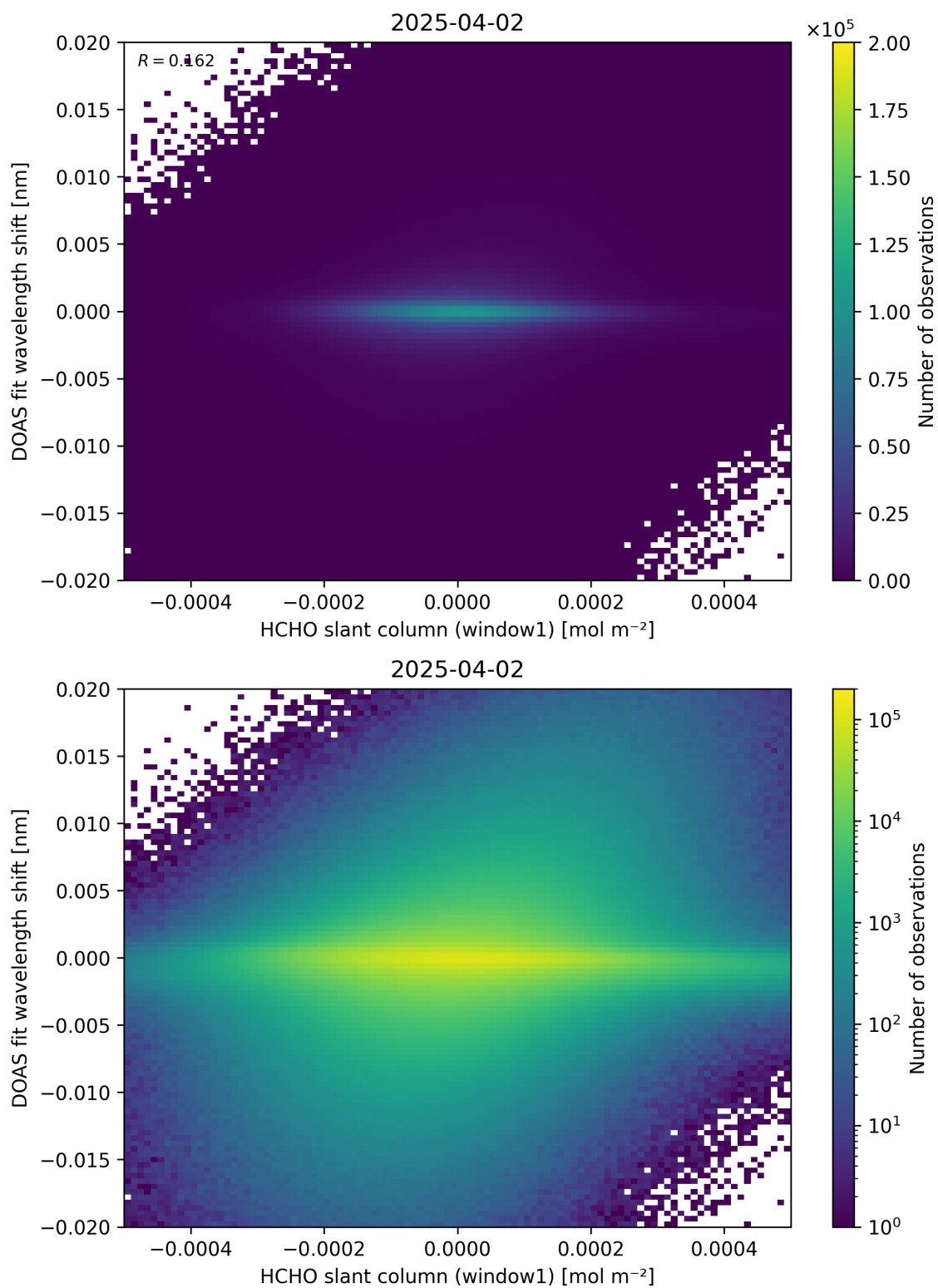
Figure 79: Scatter density plot of “HCHO slant column (window1)” against “DOAS fit wavelength shift” for 2025-04-02 to 2025-04-03.
