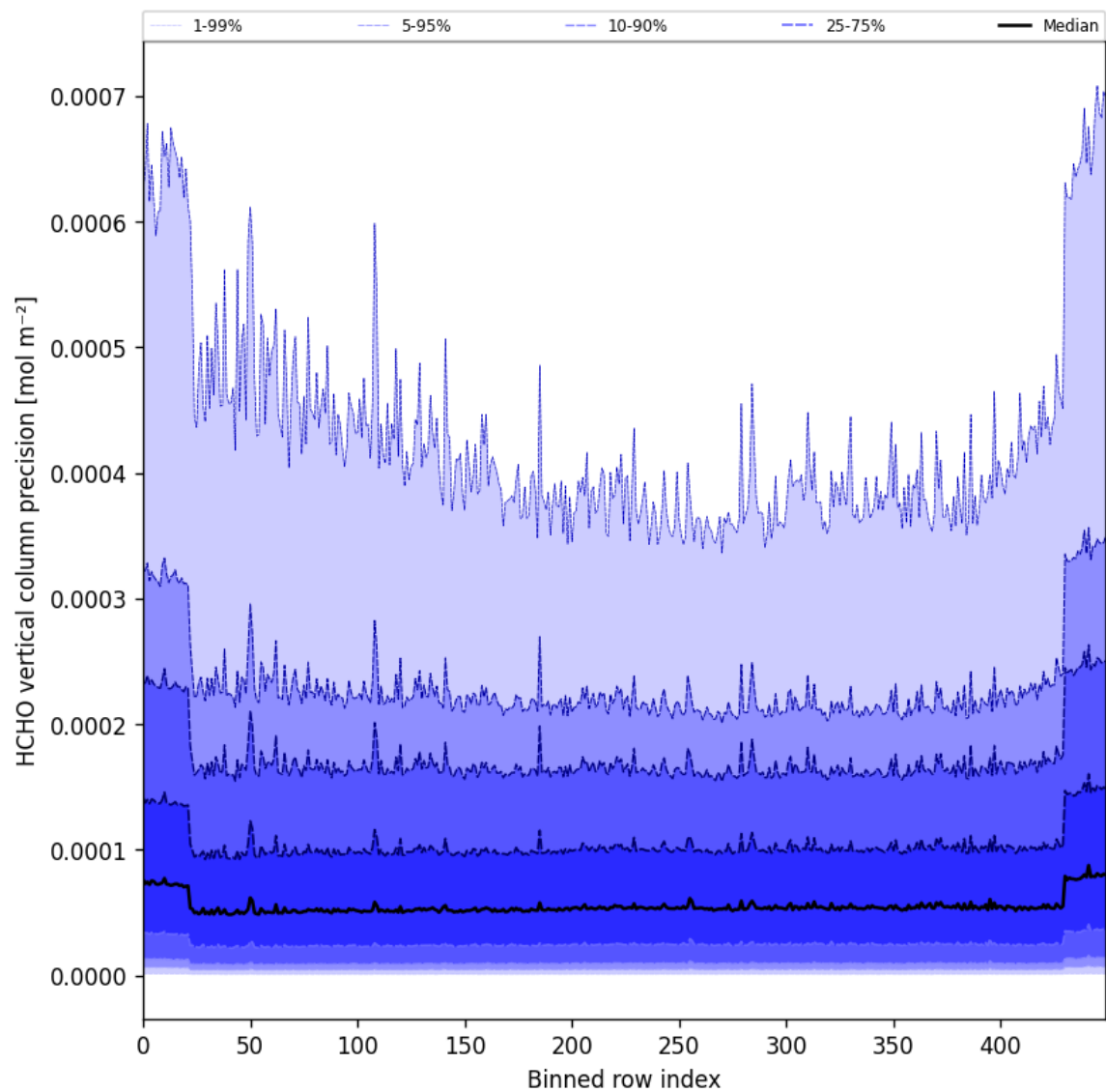
Figure 50: Along track statistics of “HCHO vertical column precision” for 2025-04-02 to 2025-04-03
