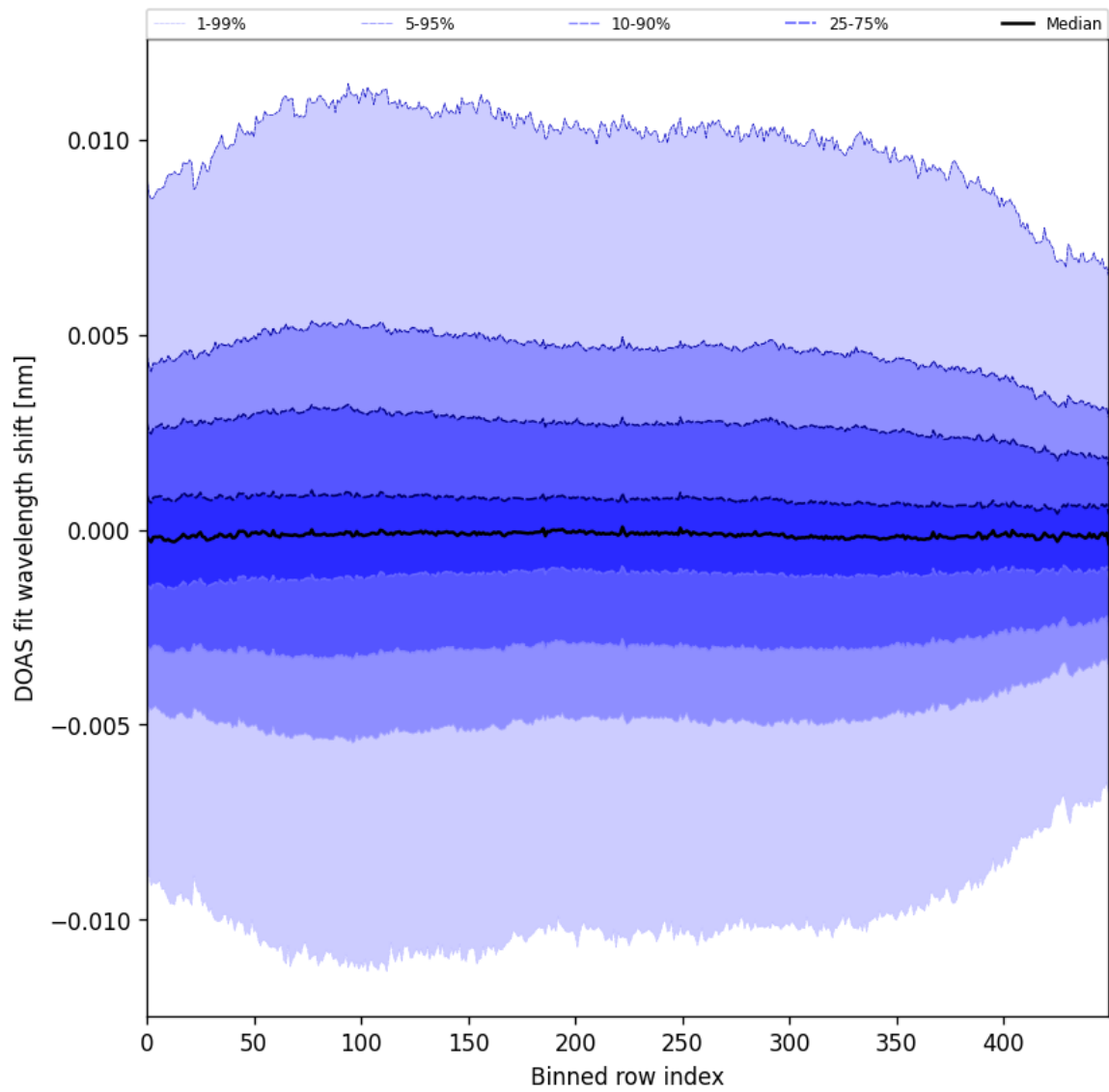
Figure 58: Along track statistics of “DOAS fit wavelength shift” for 2025-04-02 to 2025-04-03
