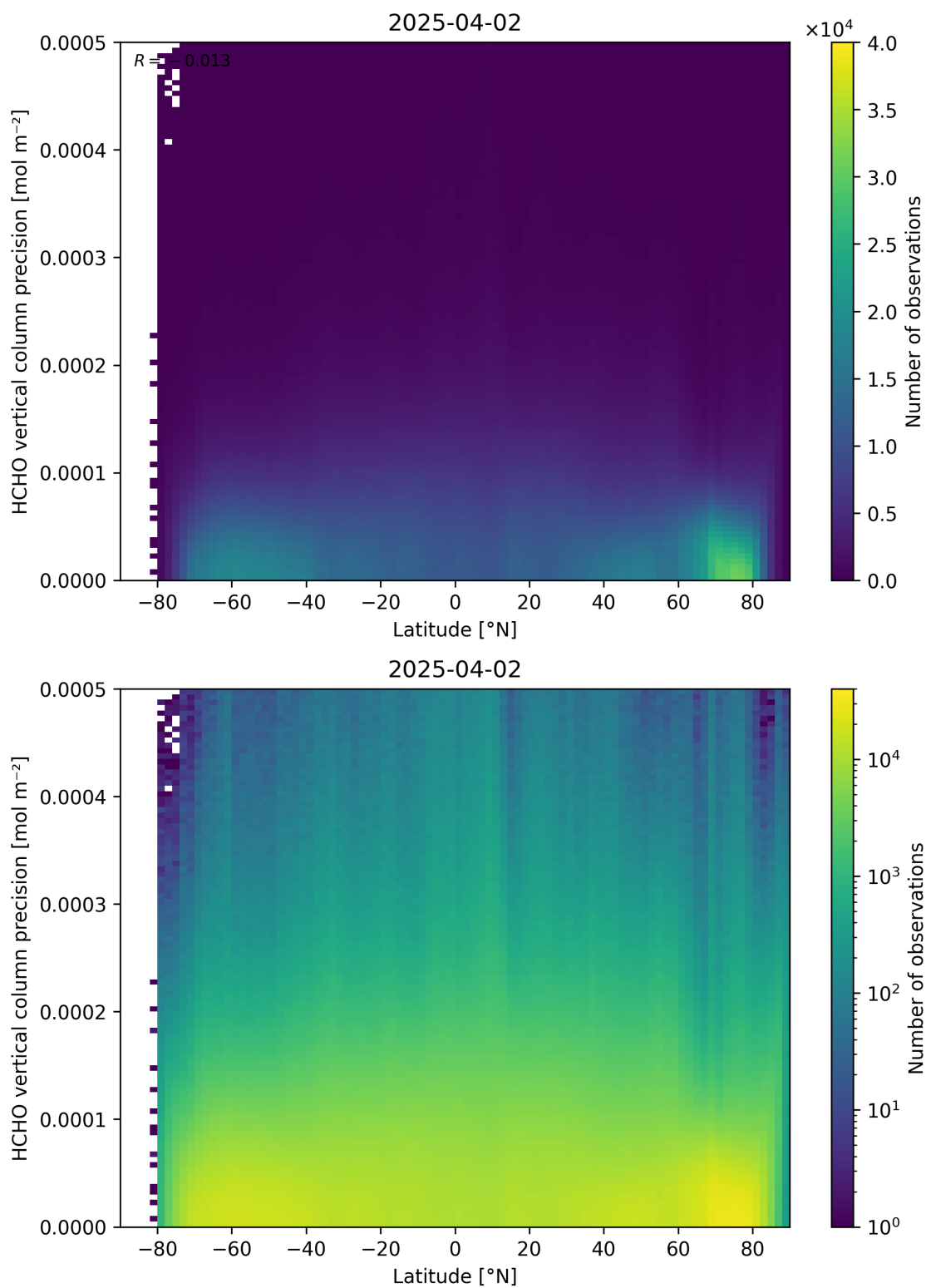
Figure 165: Scatter density plot of “Latitude” against “HCHO vertical column precision” for 2025-04-02 to 2025-04-03.
