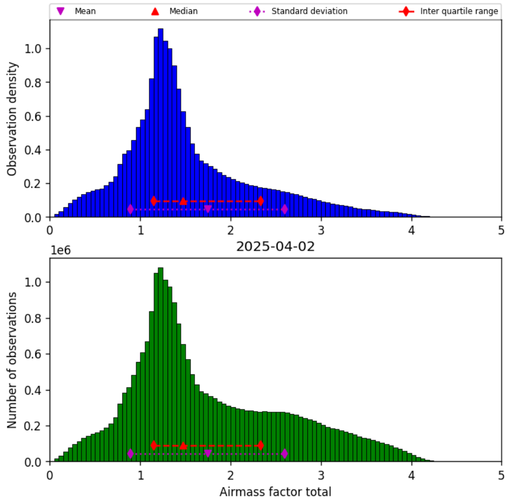
Figure 40: Histogram of “Airmass factor total” for 2025-04-02 to 2025-04-03
