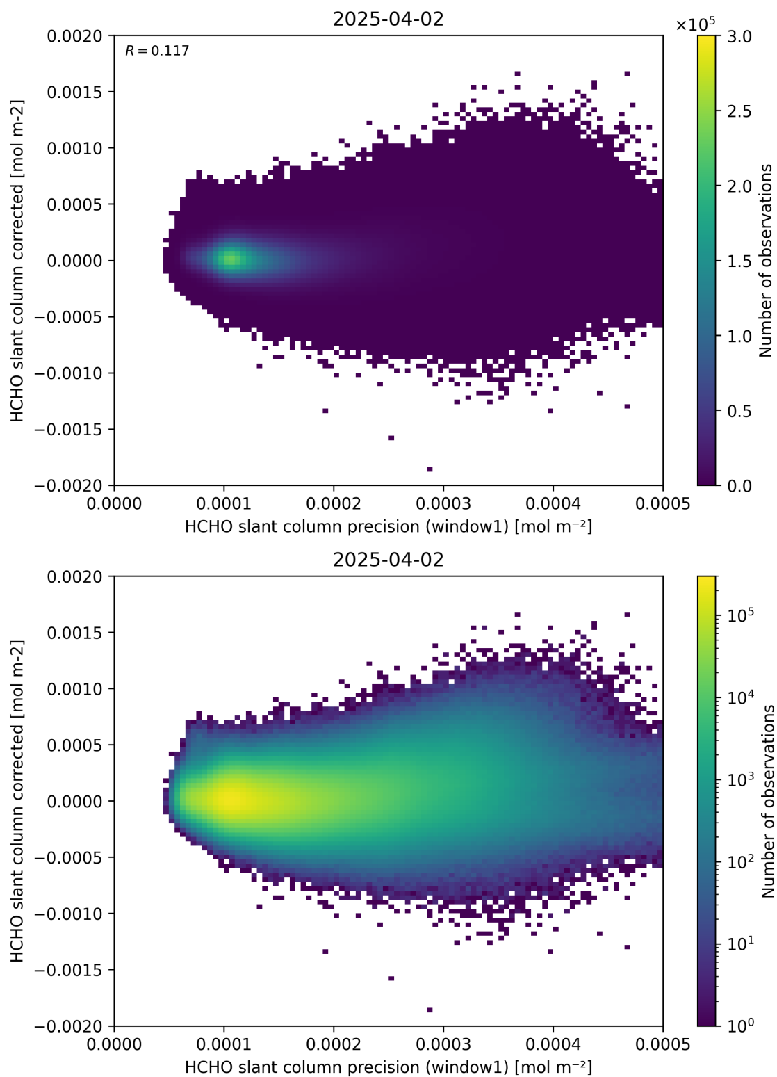
Figure 92: Scatter density plot of “HCHO slant column precision (window1)” against “HCHO slant column corrected” for 2025-04-02 to 2025-04-03.
