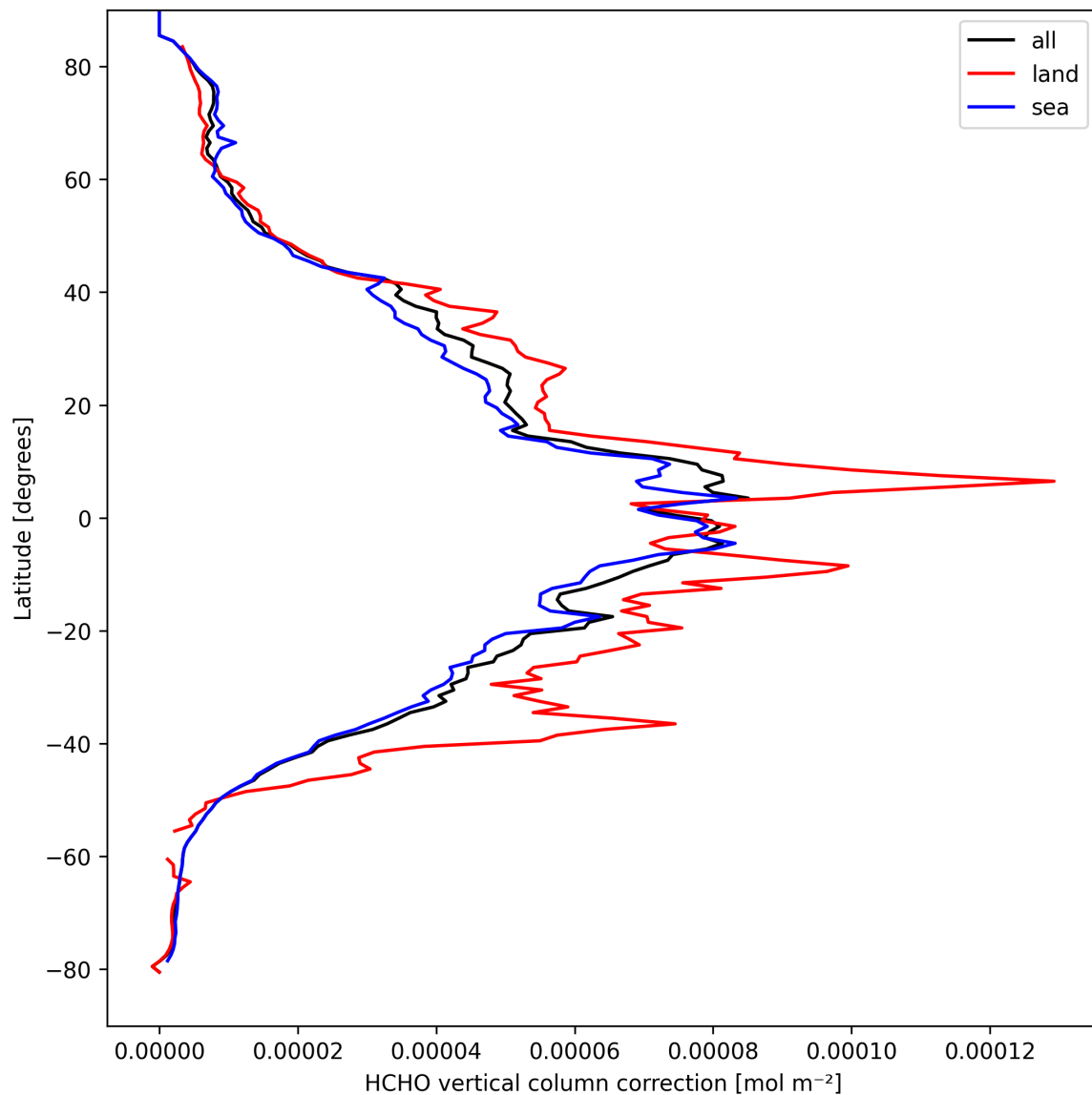
Figure 23: Zonal average of “HCHO vertical column correction” for 2025-04-02 to 2025-04-03.
