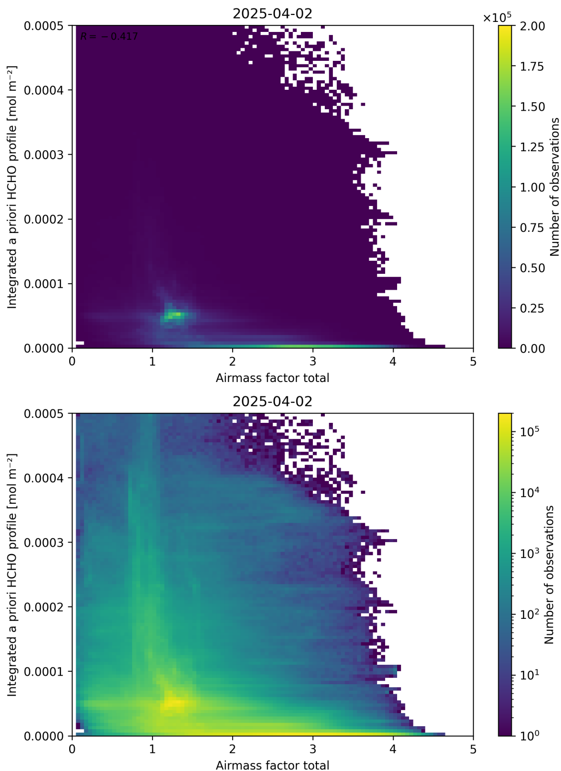
Figure 104: Scatter density plot of “Airmass factor total” against “Integrated a priori HCHO profile” for 2025-04-02 to 2025-04-03.
