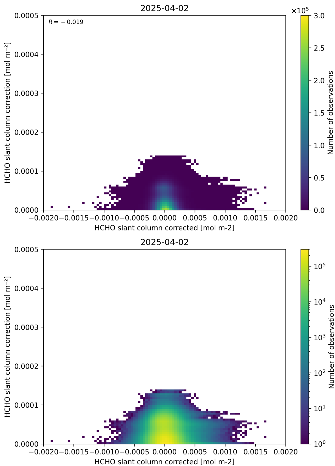
Figure 77: Scatter density plot of “HCHO slant column corrected” against “HCHO slant column correction” for 2025-04-02 to 2025-04-03.
