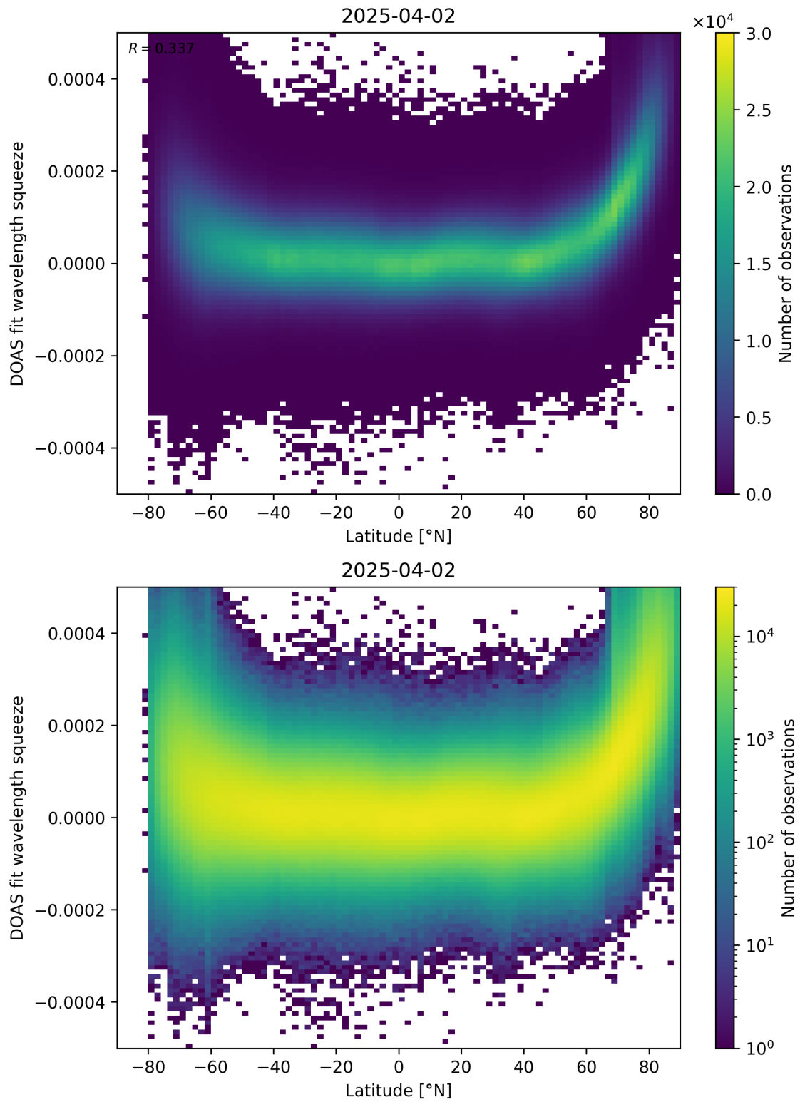
Figure 155: Scatter density plot of “Latitude” against “DOAS fit wavelength squeeze” for 2025-04-02 to 2025-04-03.
