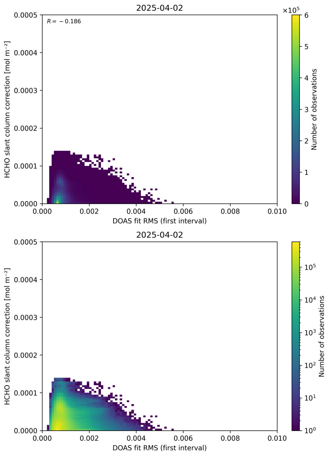
Figure 63: Scatter density plot of “DOAS fit RMS (first interval)” against “HCHO slant column correction” for 2025-04-02 to 2025-04-03.
