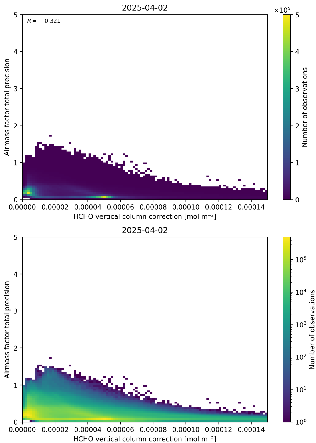
Figure 121: Scatter density plot of “HCHO vertical column correction” against “Airmass factor total precision” for 2025-04-02 to 2025-04-03.
