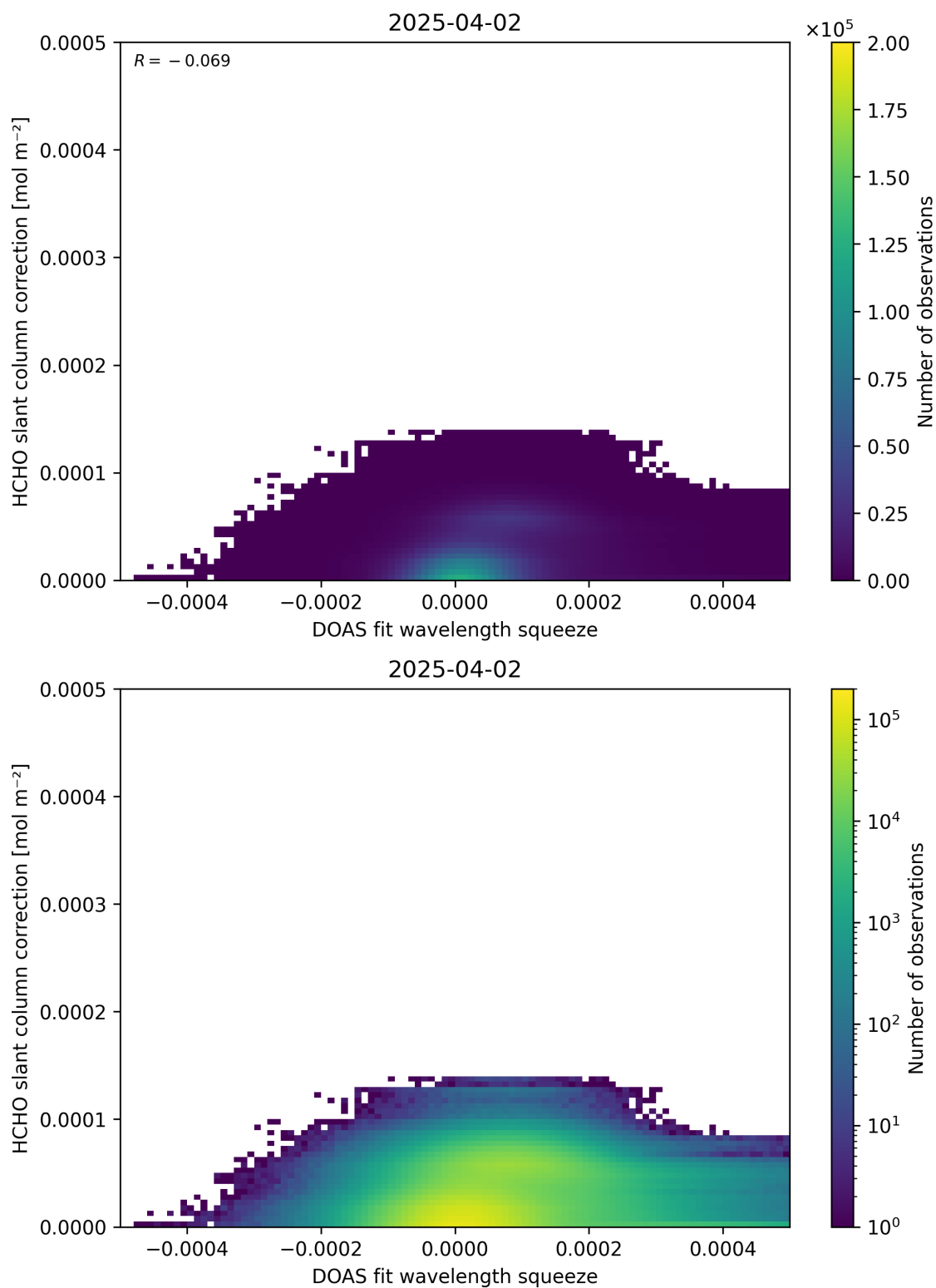
Figure 70: Scatter density plot of “DOAS fit wavelength squeeze” against “HCHO slant column correction” for 2025-04-02 to 2025-04-03.
