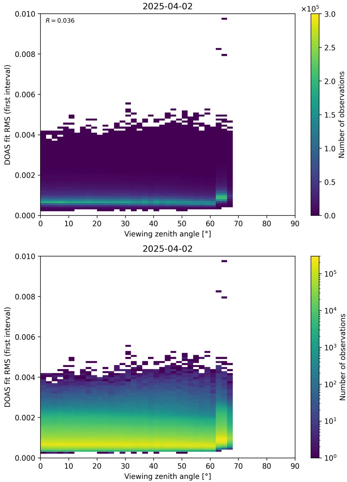
Figure 182: Scatter density plot of “Viewing zenith angle” against “DOAS fit RMS (first interval)” for 2025-04-02 to 2025-04-03.
