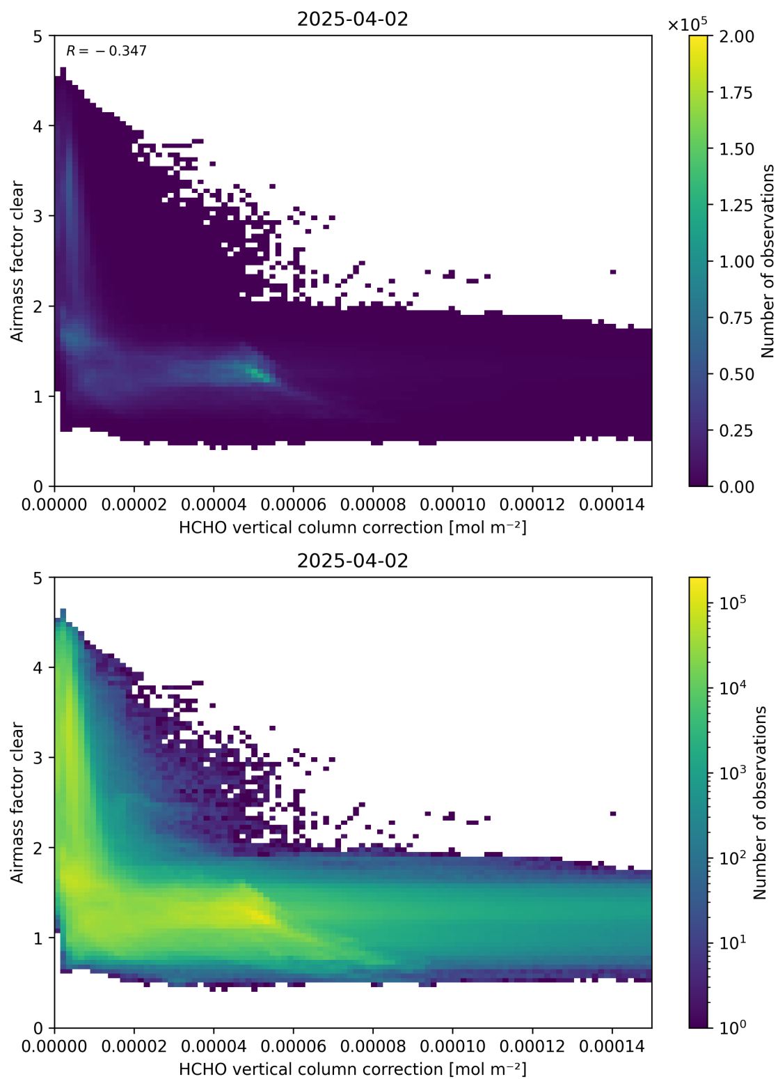
Figure 115: Scatter density plot of “HCHO vertical column correction” against “Airmass factor clear” for 2025-04-02 to 2025-04-03.
