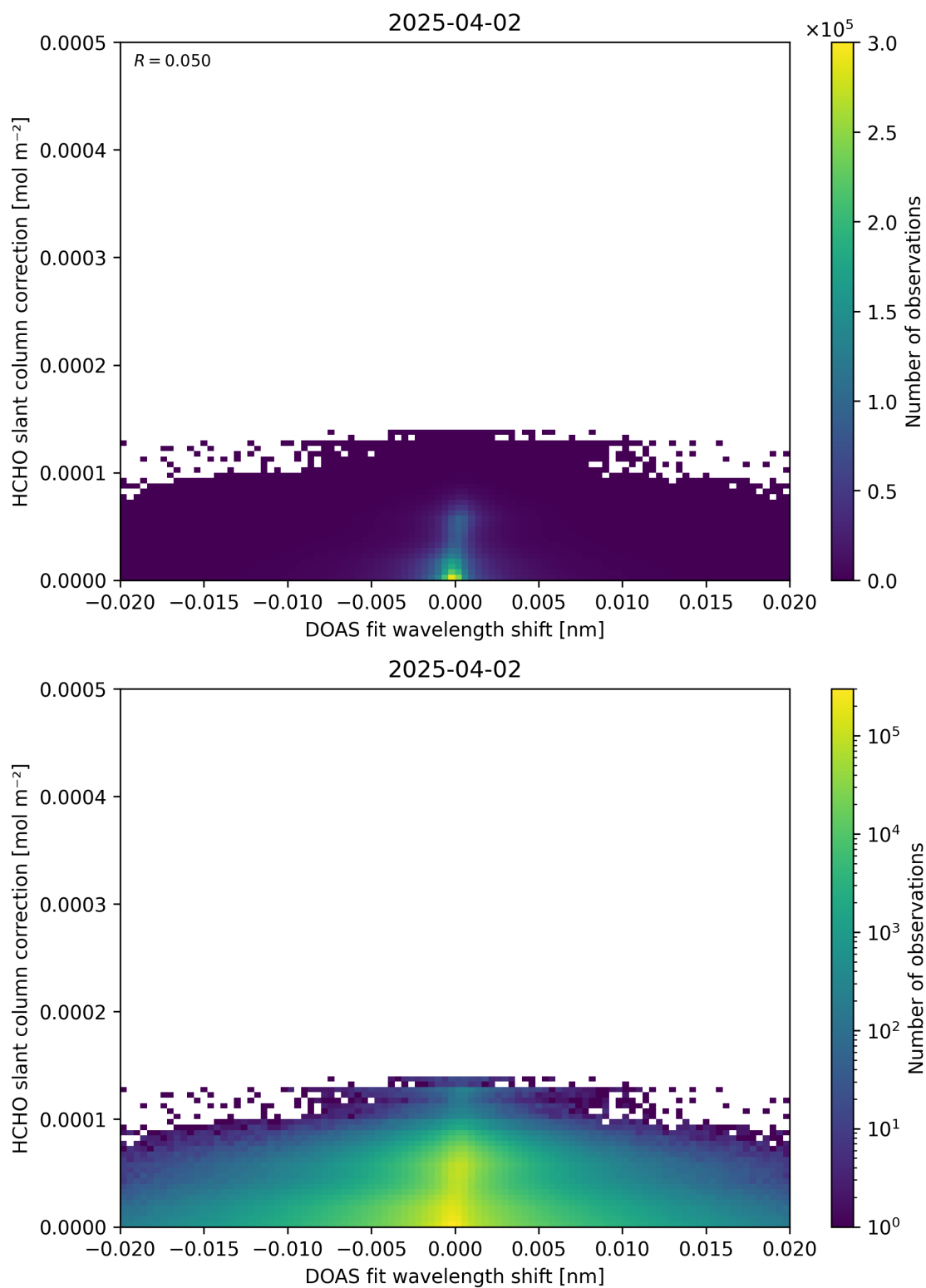
Figure 67: Scatter density plot of “DOAS fit wavelength shift” against “HCHO slant column correction” for 2025-04-02 to 2025-04-03.
