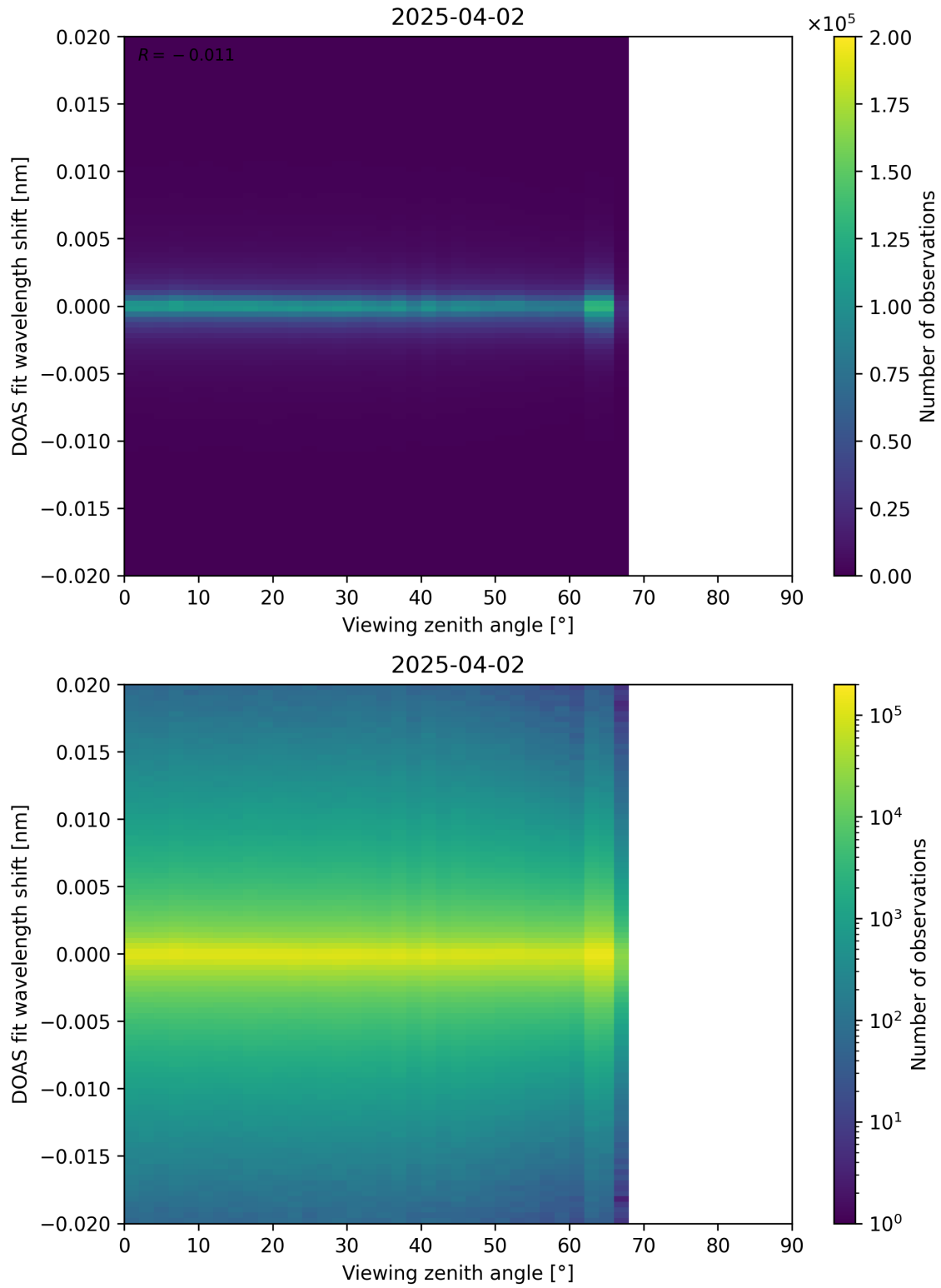
Figure 183: Scatter density plot of “Viewing zenith angle” against “DOAS fit wavelength shift” for 2025-04-02 to 2025-04-03.
