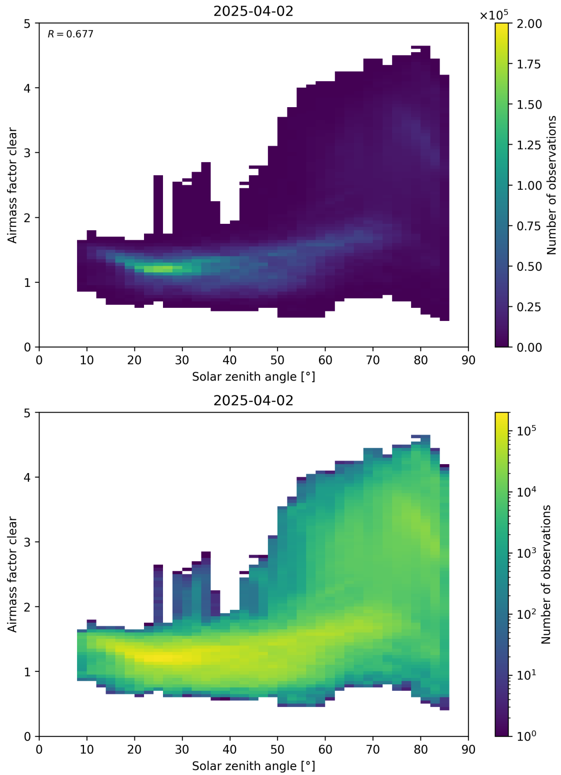
Figure 170: Scatter density plot of “Solar zenith angle” against “Airmass factor clear” for 2025-04-02 to 2025-04-03.
