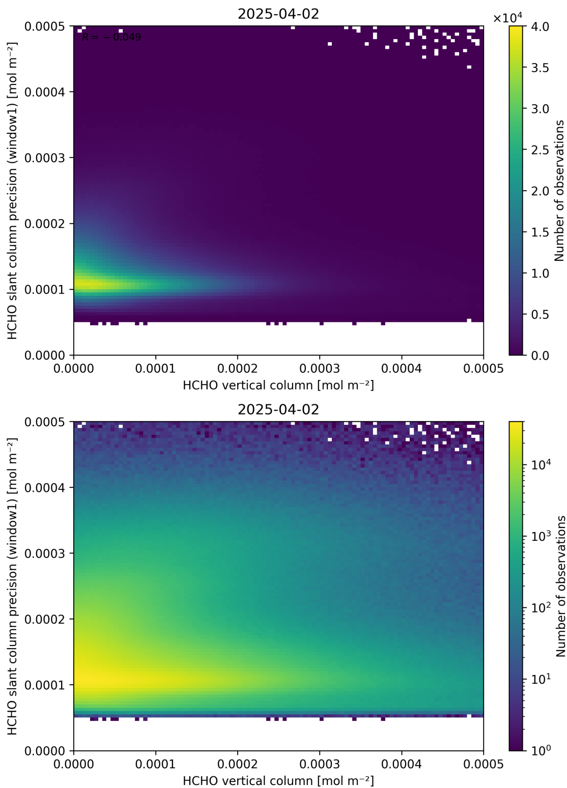
Figure 130: Scatter density plot of “HCHO vertical column” against “HCHO slant column precision (window1)” for 2025-04-02 to 2025-04-03.
