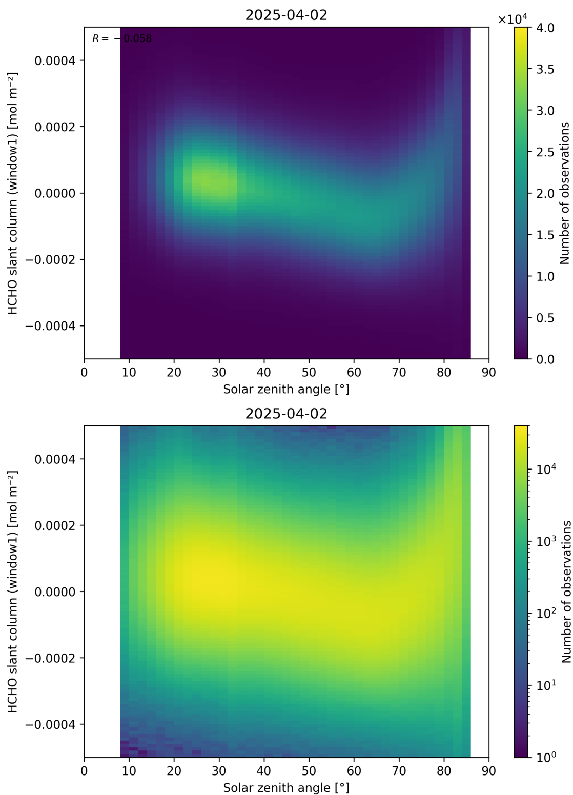
Figure 173: Scatter density plot of “Solar zenith angle” against “HCHO slant column (window1)” for 2025-04-02 to 2025-04-03.
