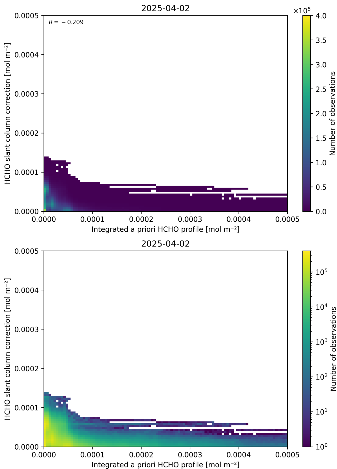
Figure 152: Scatter density plot of “Integrated a priori HCHO profile” against “HCHO slant column correction” for 2025-04-02 to 2025-04-03.
