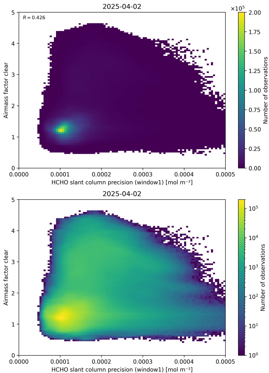
Figure 91: Scatter density plot of “HCHO slant column precision (window1)” against “Airmass factor clear” for 2025-04-02 to 2025-04-03.
