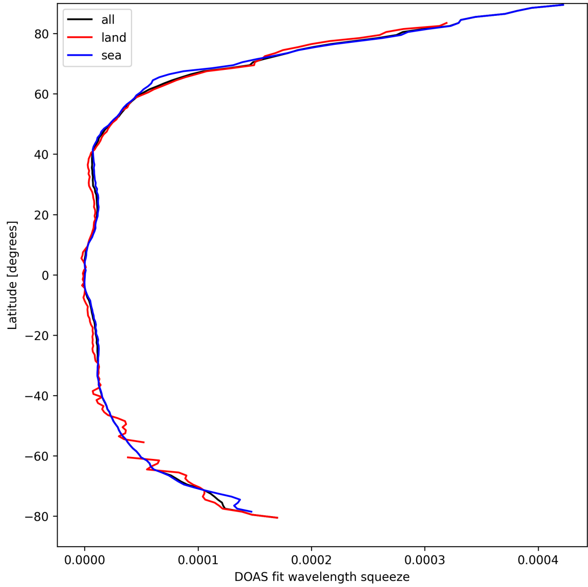
Figure 31: Zonal average of “DOAS fit wavelength squeeze” for 2025-04-02 to 2025-04-03.
