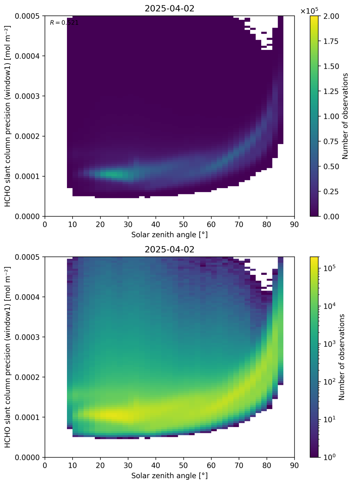
Figure 174: Scatter density plot of “Solar zenith angle” against “HCHO slant column precision (window1)” for 2025-04-02 to 2025-04-03.
