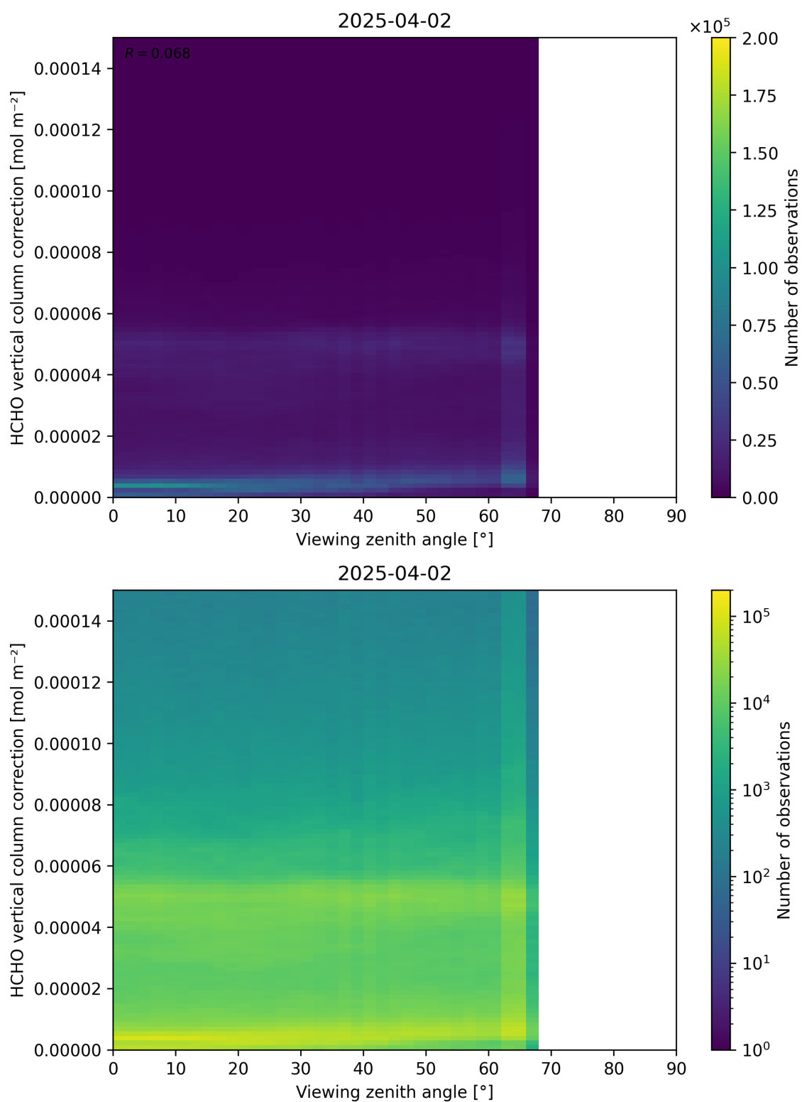
Figure 193: Scatter density plot of “Viewing zenith angle” against “HCHO vertical column correction” for 2025-04-02 to 2025-04-03.
