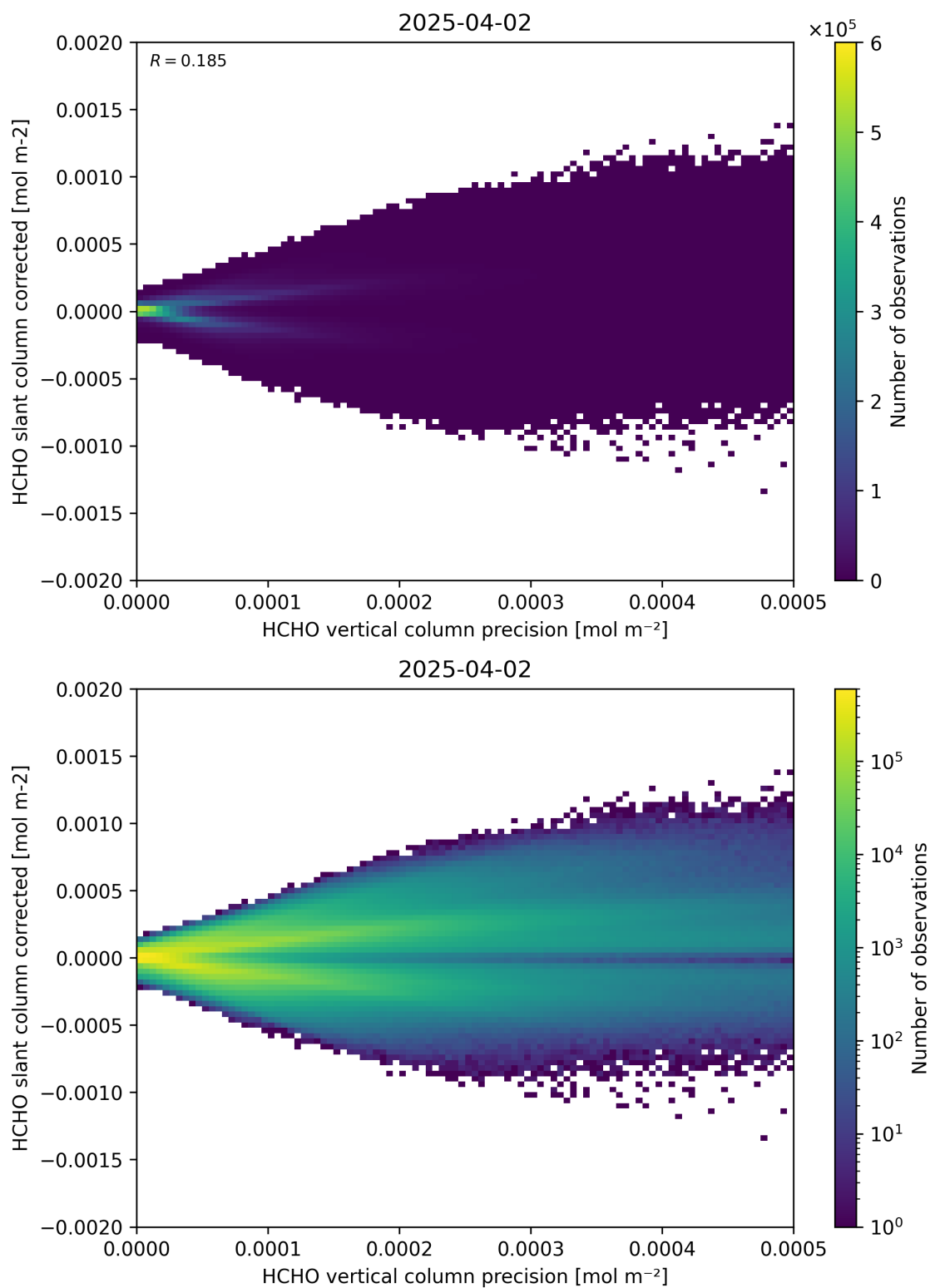
Figure 140: Scatter density plot of “HCHO vertical column precision” against “HCHO slant column corrected” for 2025-04-02 to 2025-04-03.
