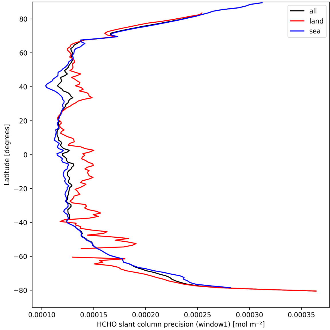
Figure 25: Zonal average of “HCHO slant column precision (window1)” for 2025-04-02 to 2025-04-03.
