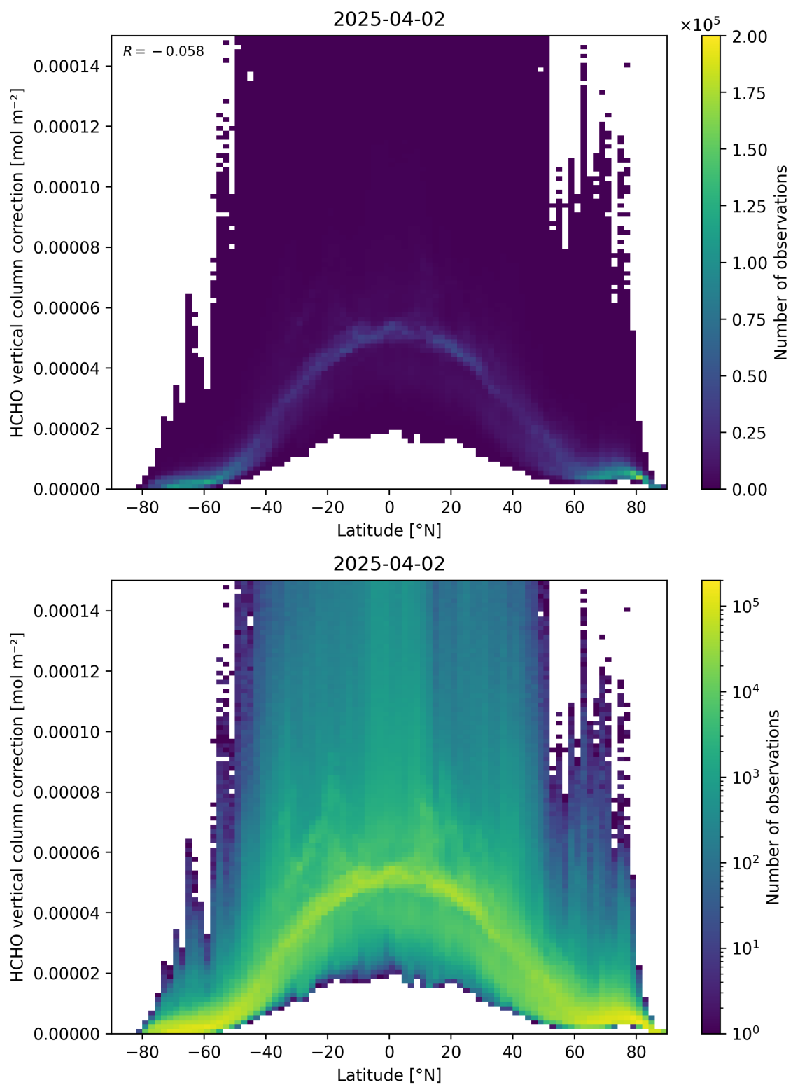
Figure 164: Scatter density plot of “Latitude” against “HCHO vertical column correction” for 2025-04-02 to 2025-04-03.
