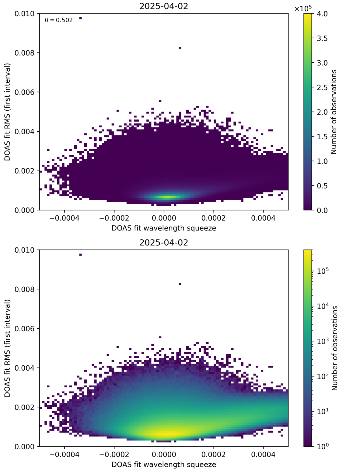
Figure 68: Scatter density plot of “DOAS fit wavelength squeeze” against “DOAS fit RMS (first interval)” for 2025-04-02 to 2025-04-03.
