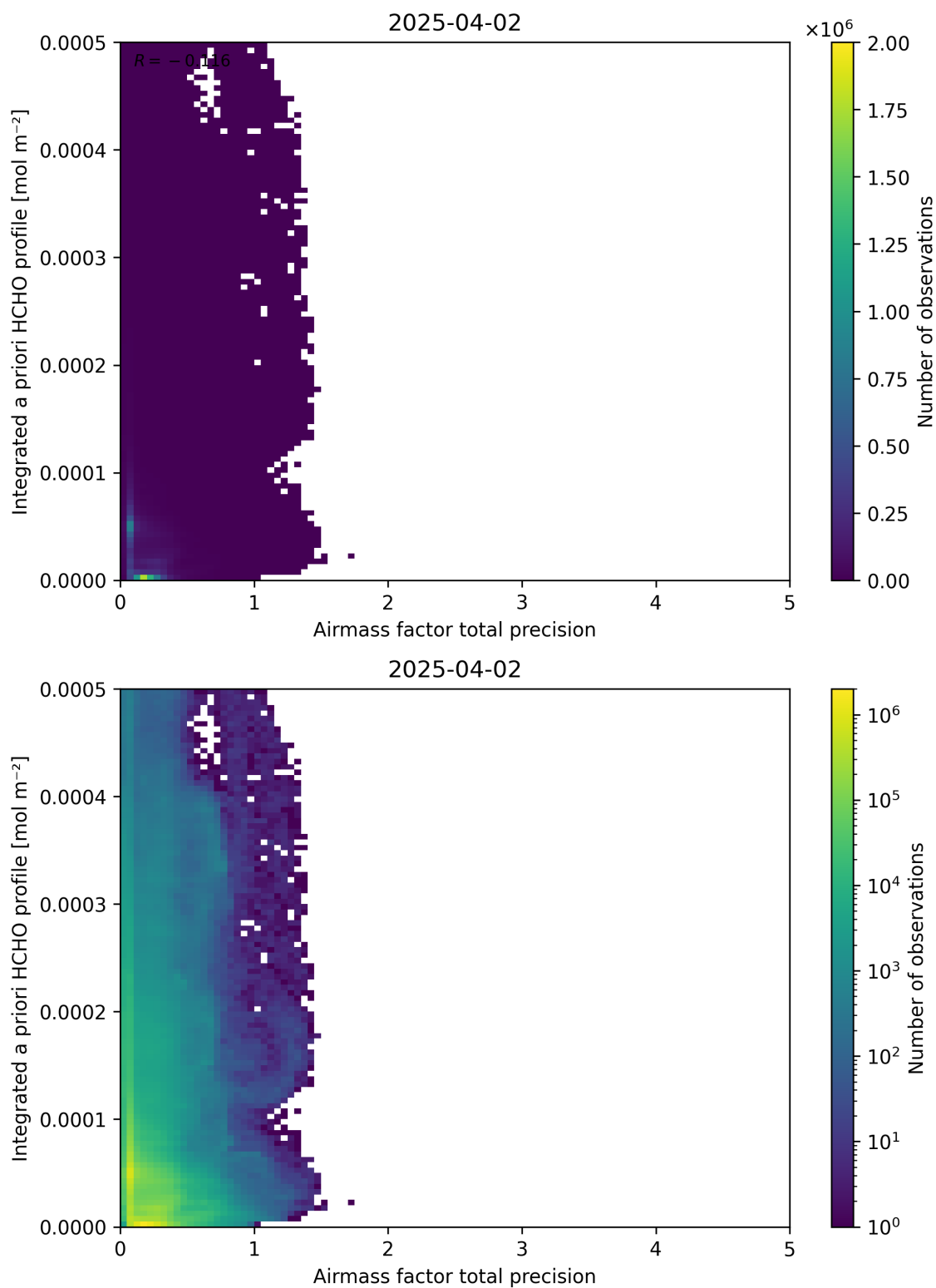
Figure 111: Scatter density plot of “Airmass factor total precision” against “Integrated a priori HCHO profile” for 2025-04-02 to 2025-04-03.
