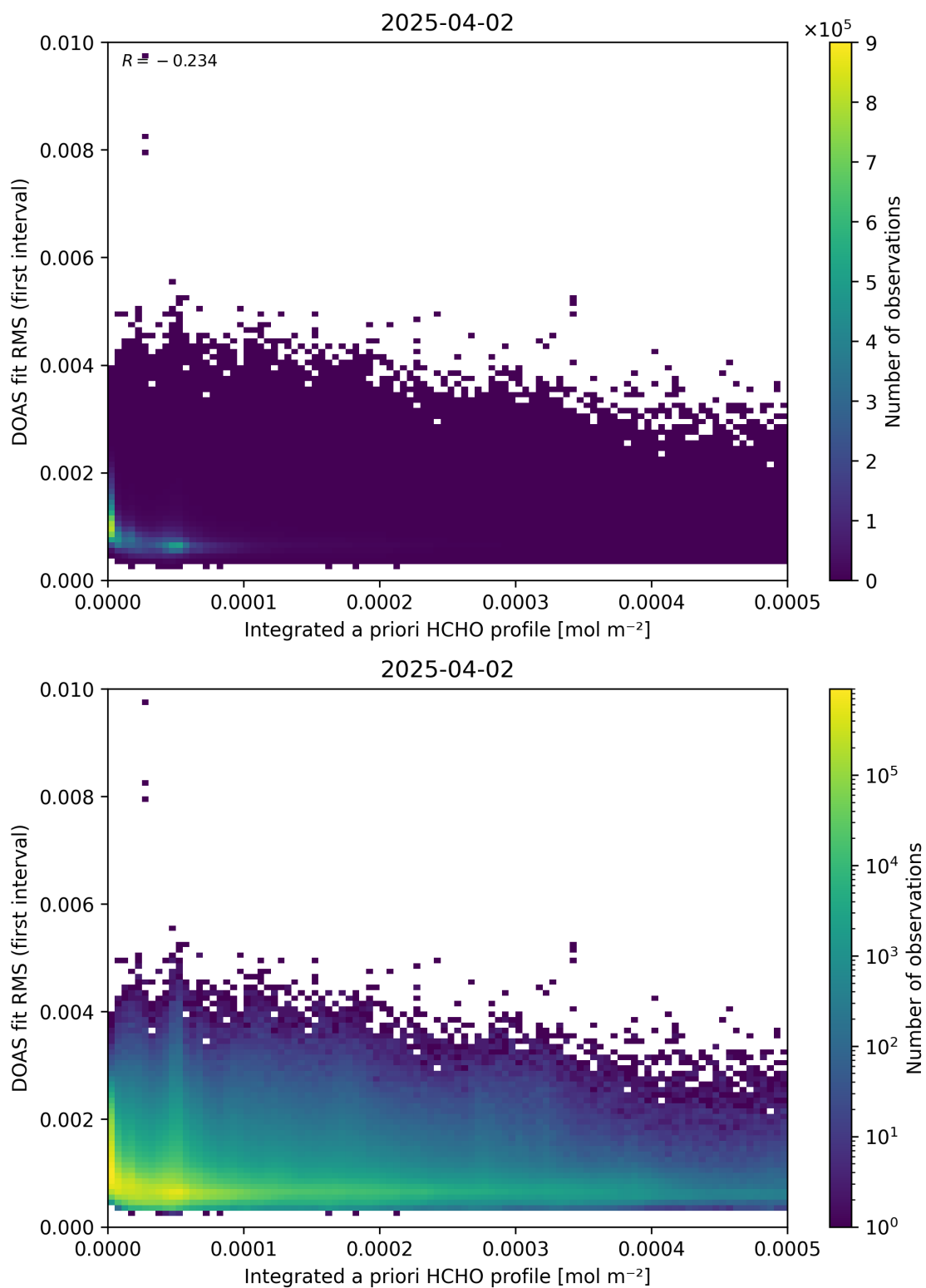
Figure 148: Scatter density plot of “Integrated a priori HCHO profile” against “DOAS fit RMS (first interval)” for 2025-04-02 to 2025-04-03.
