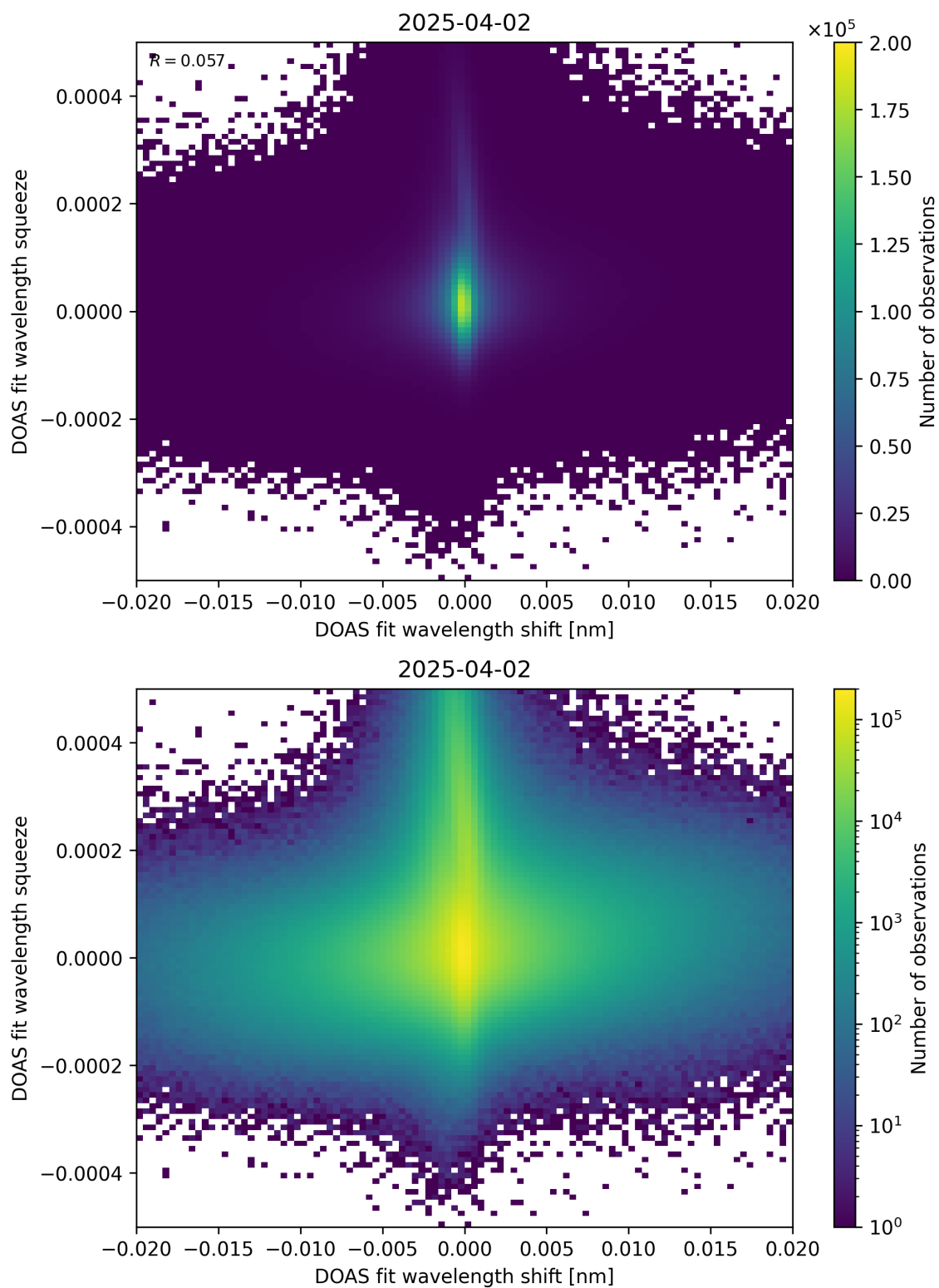
Figure 65: Scatter density plot of “DOAS fit wavelength shift” against “DOAS fit wavelength squeeze” for 2025-04-02 to 2025-04-03.
