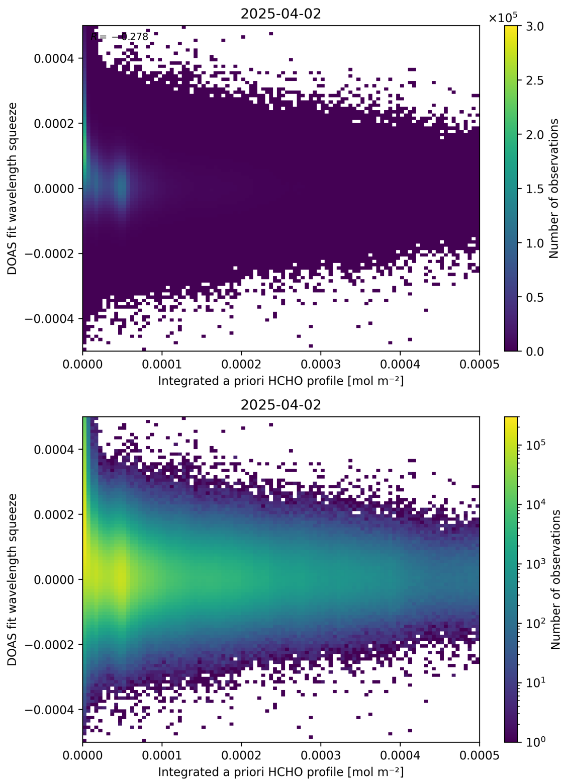
Figure 150: Scatter density plot of “Integrated a priori HCHO profile” against “DOAS fit wavelength squeeze” for 2025-04-02 to 2025-04-03.
