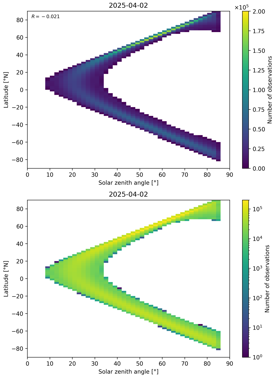
Figure 181: Scatter density plot of “Solar zenith angle” against “Latitude” for 2025-04-02 to 2025-04-03.
