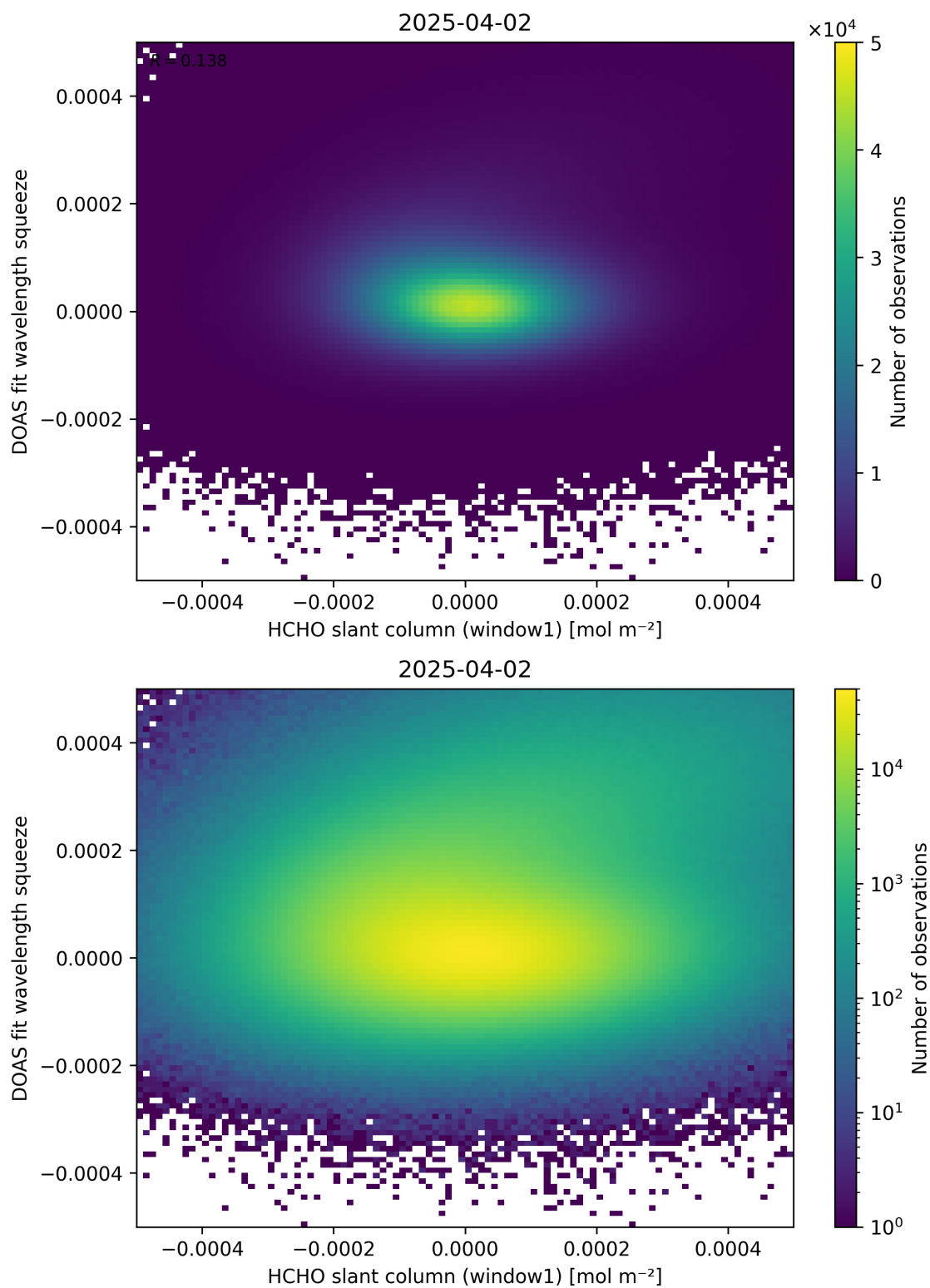
Figure 80: Scatter density plot of “HCHO slant column (window1)” against “DOAS fit wavelength squeeze” for 2025-04-02 to 2025-04-03.
