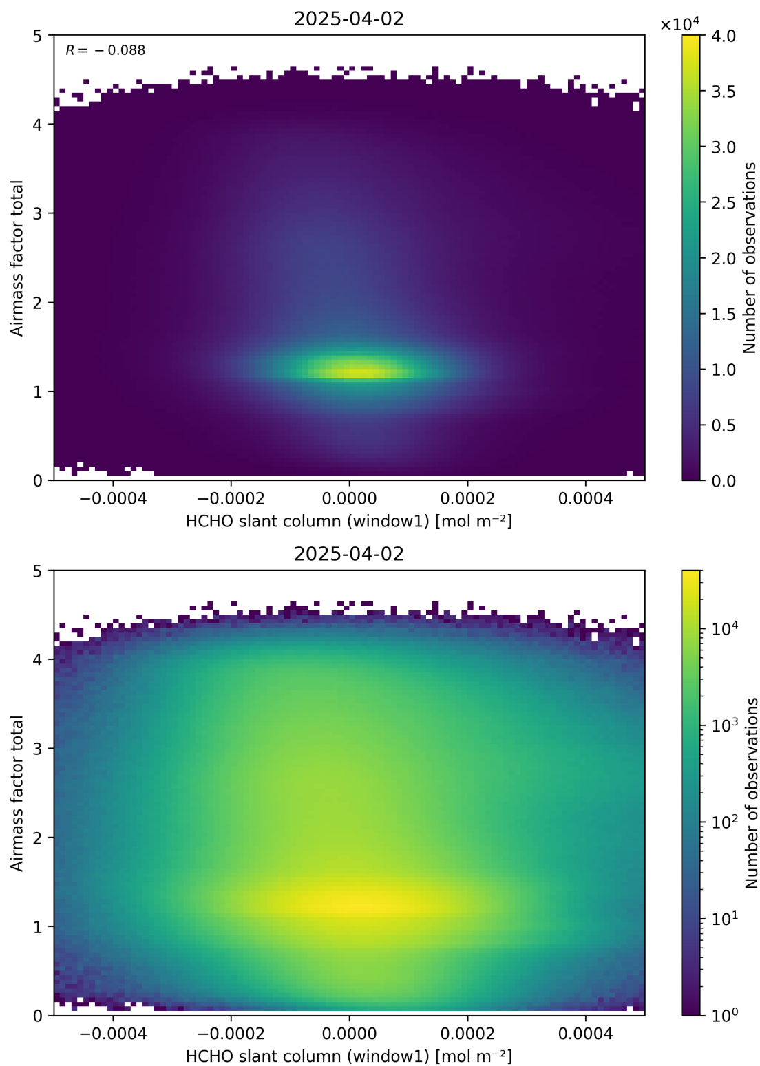
Figure 85: Scatter density plot of “HCHO slant column (window1)” against “Airmass factor total” for 2025-04-02 to 2025-04-03.
