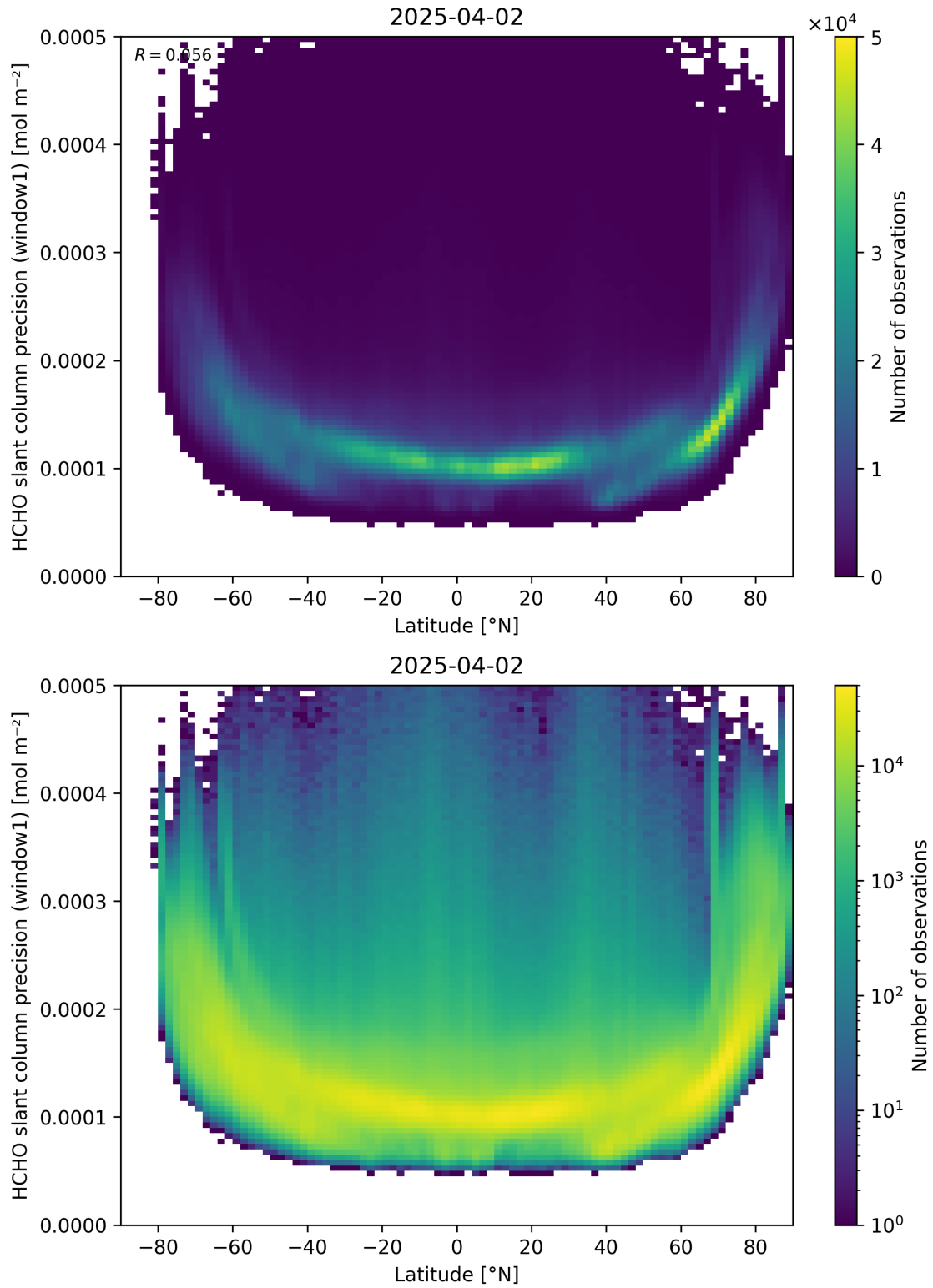
Figure 160: Scatter density plot of “Latitude” against “HCHO slant column precision (window1)” for 2025-04-02 to 2025-04-03.
