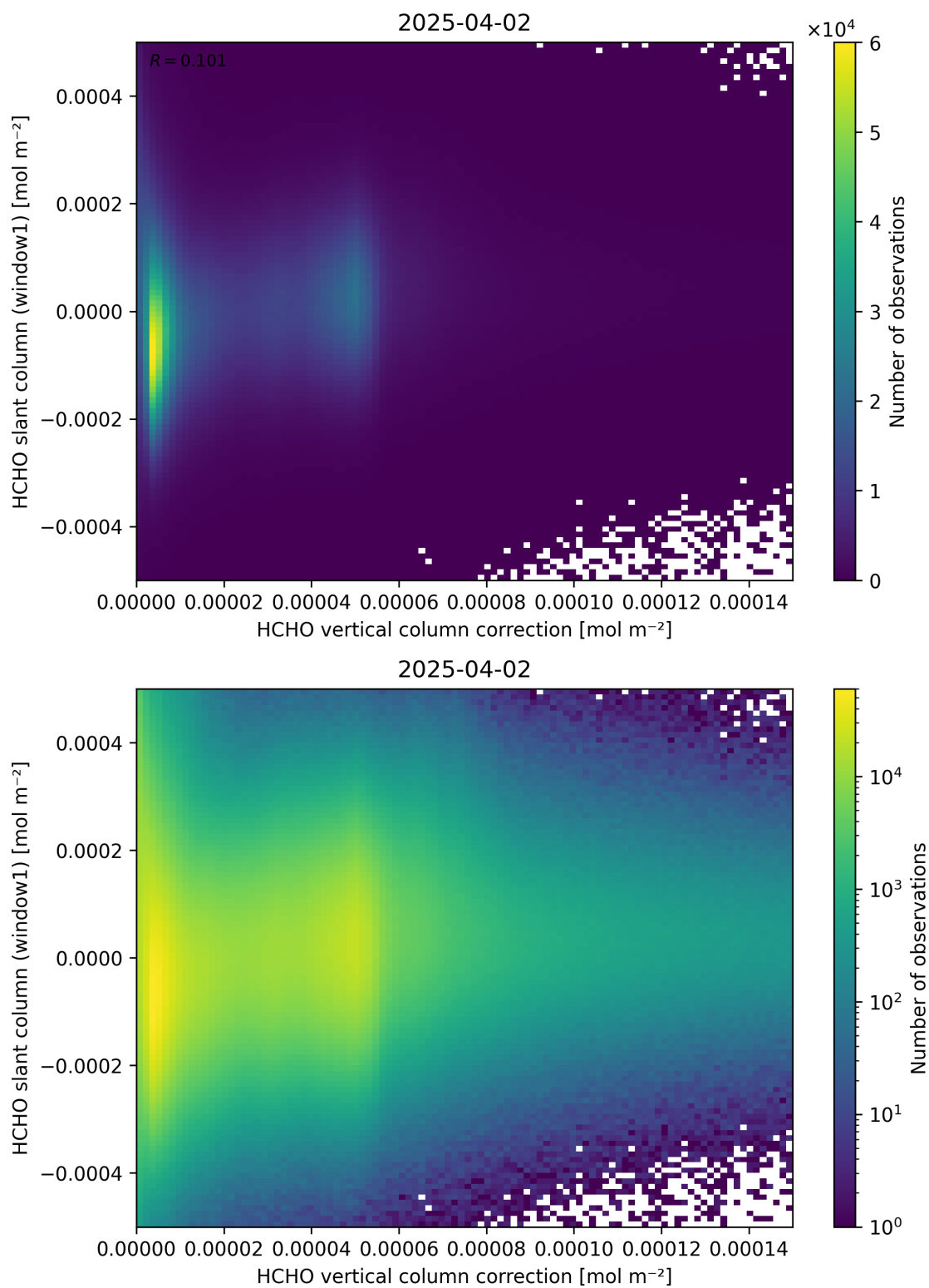
Figure 118: Scatter density plot of “HCHO vertical column correction” against “HCHO slant column (window1)” for 2025-04-02 to 2025-04-03.
