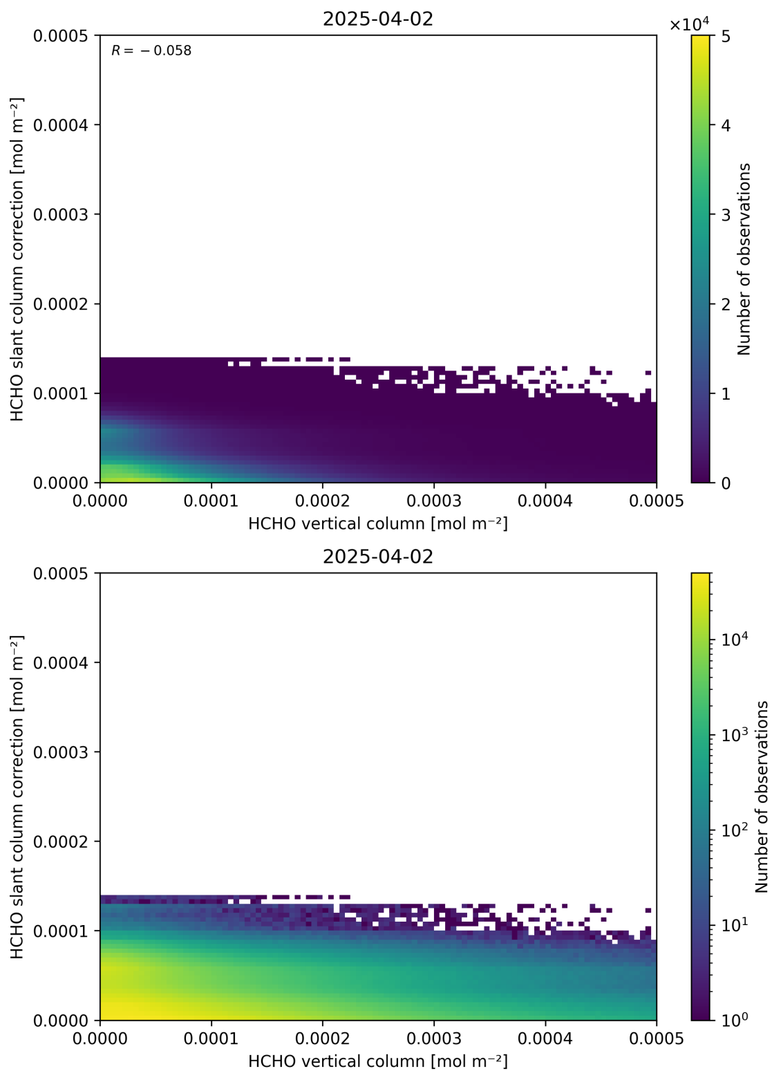
Figure 128: Scatter density plot of “HCHO vertical column” against “HCHO slant column correction” for 2025-04-02 to 2025-04-03.
