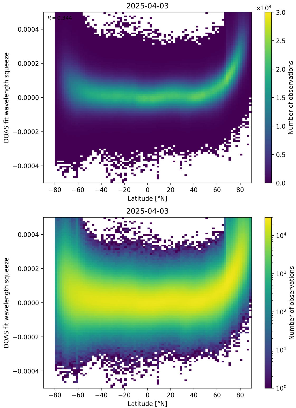
Figure 155: Scatter density plot of “Latitude” against “DOAS fit wavelength squeeze” for 2025-04-03 to 2025-04-04.
