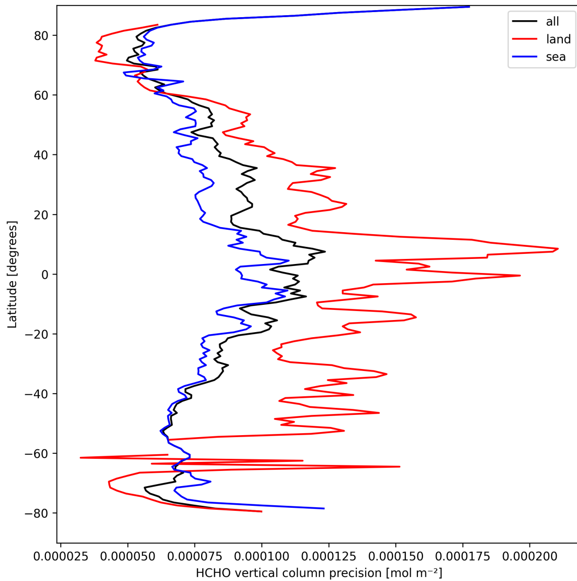
Figure 22: Zonal average of “HCHO vertical column precision” for 2025-04-03 to 2025-04-04.
