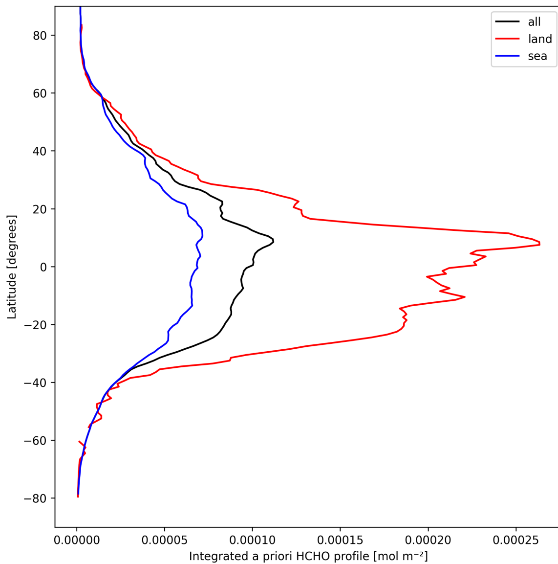
Figure 29: Zonal average of “Integrated a priori HCHO profile” for 2025-04-03 to 2025-04-04.
