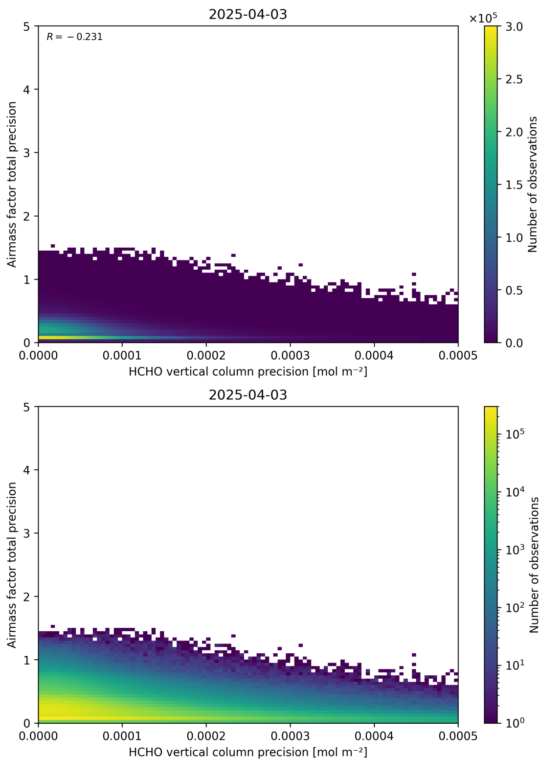
Figure 145: Scatter density plot of “HCHO vertical column precision” against “Airmass factor total precision” for 2025-04-03 to 2025-04-04.
