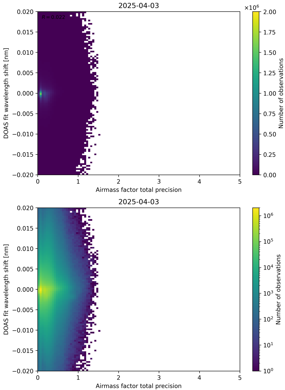
Figure 106: Scatter density plot of “Airmass factor total precision” against “DOAS fit wavelength shift” for 2025-04-03 to 2025-04-04.
