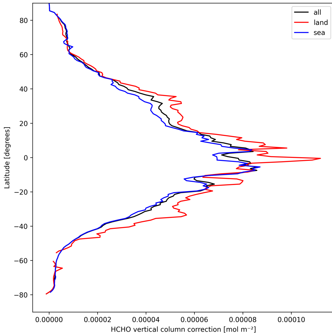
Figure 23: Zonal average of “HCHO vertical column correction” for 2025-04-03 to 2025-04-04.
