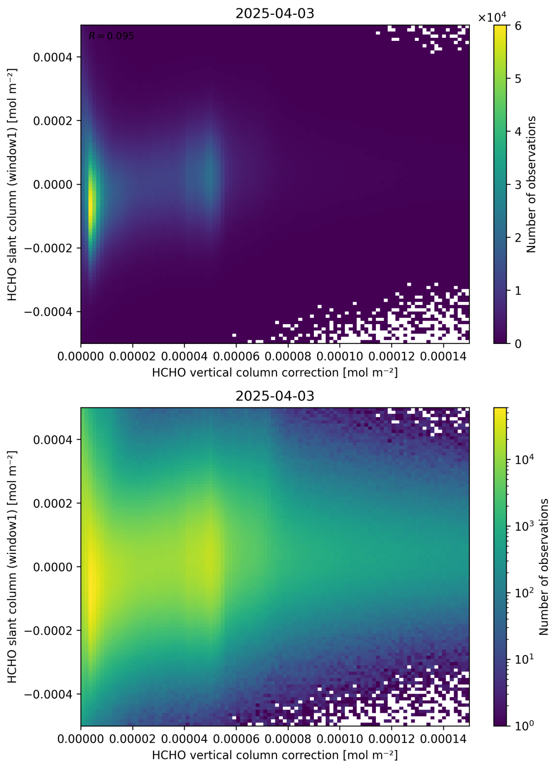
Figure 118: Scatter density plot of “HCHO vertical column correction” against “HCHO slant column (window1)” for 2025-04-03 to 2025-04-04.
