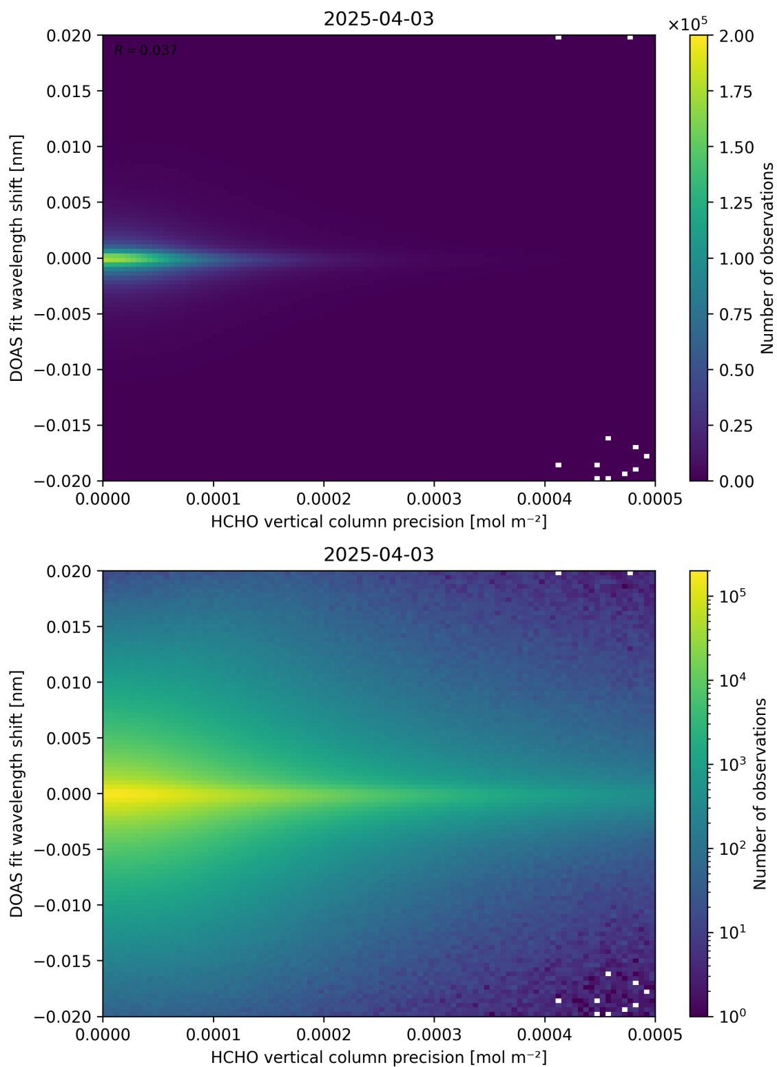
Figure 137: Scatter density plot of “HCHO vertical column precision” against “DOAS fit wavelength shift” for 2025-04-03 to 2025-04-04.
