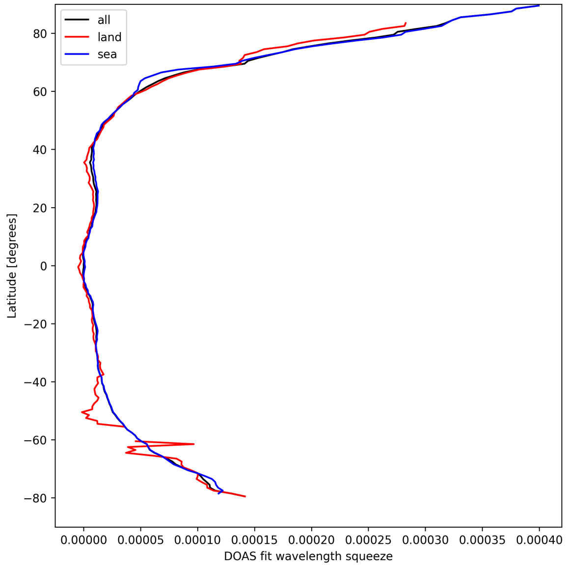
Figure 31: Zonal average of “DOAS fit wavelength squeeze” for 2025-04-03 to 2025-04-04.
