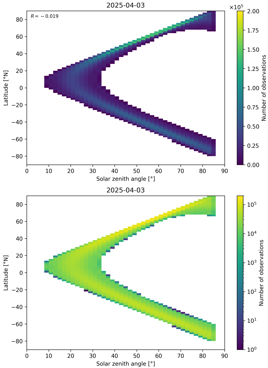
Figure 181: Scatter density plot of “Solar zenith angle” against “Latitude” for 2025-04-03 to 2025-04-04.
