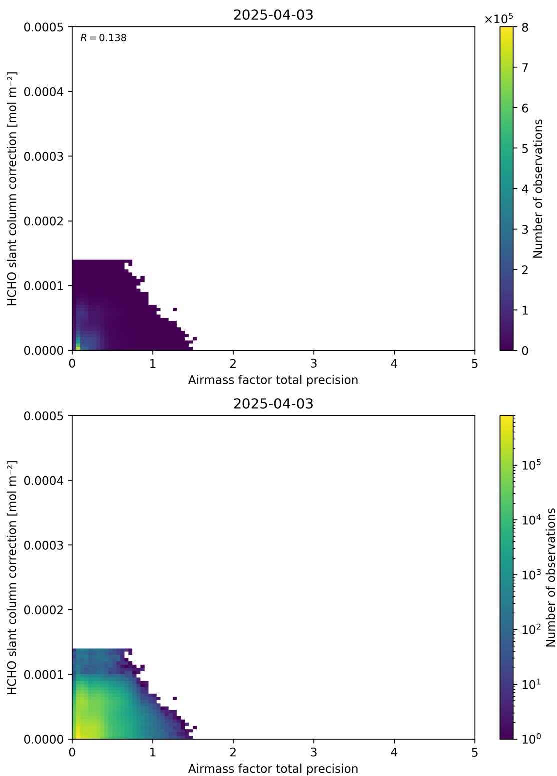
Figure 110: Scatter density plot of “Airmass factor total precision” against “HCHO slant column correction” for 2025-04-03 to 2025-04-04.
