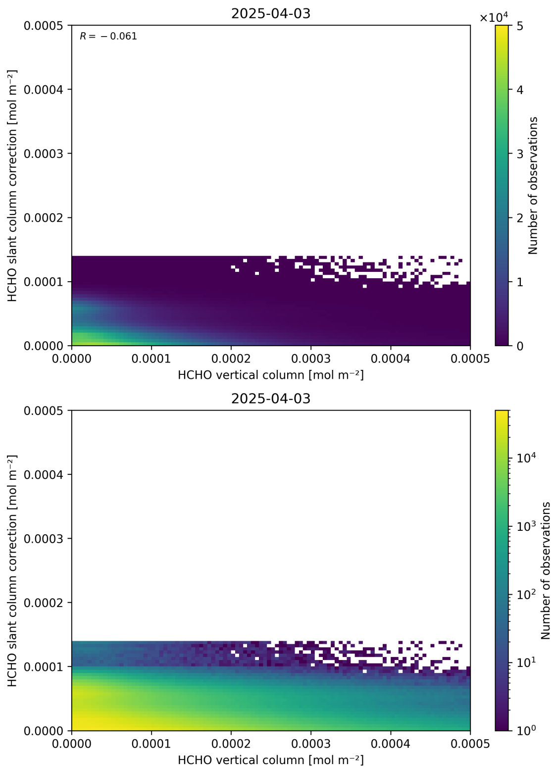
Figure 128: Scatter density plot of “HCHO vertical column” against “HCHO slant column correction” for 2025-04-03 to 2025-04-04.
