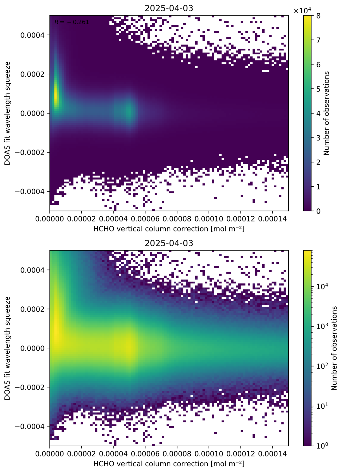
Figure 114: Scatter density plot of “HCHO vertical column correction” against “DOAS fit wavelength squeeze” for 2025-04-03 to 2025-04-04.
