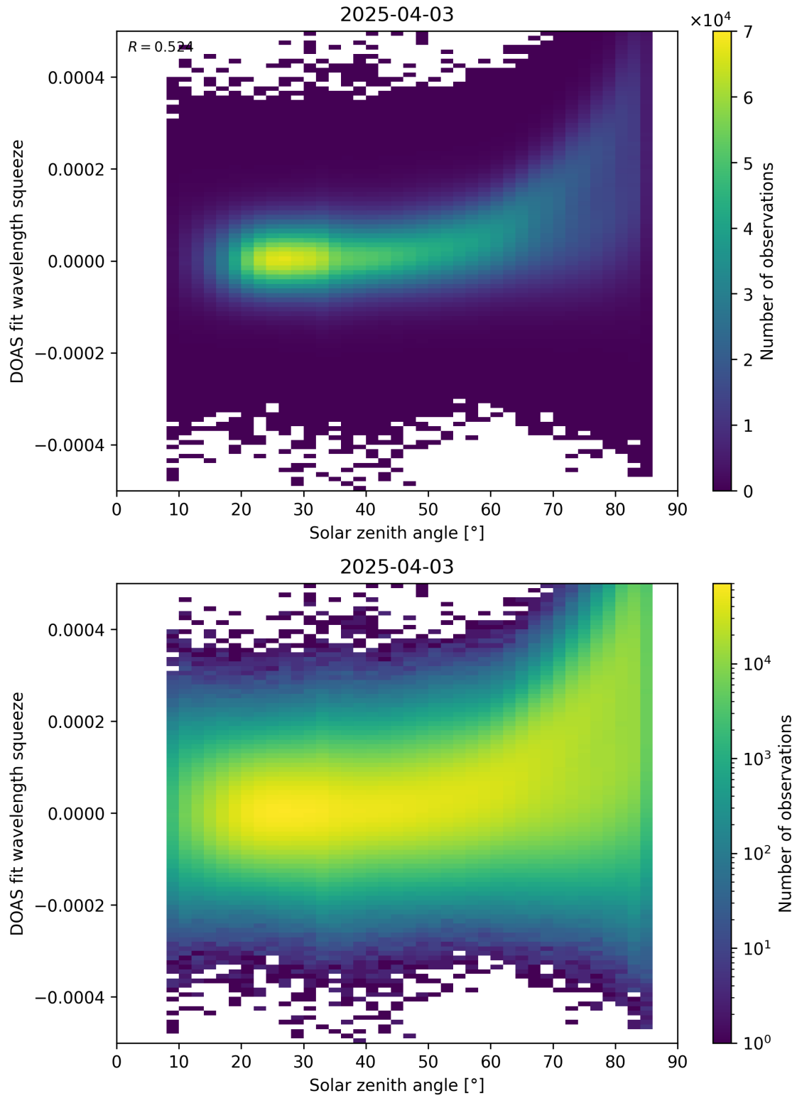
Figure 169: Scatter density plot of “Solar zenith angle” against “DOAS fit wavelength squeeze” for 2025-04-03 to 2025-04-04.
