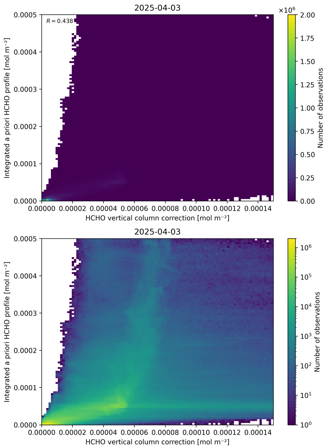
Figure 122: Scatter density plot of “HCHO vertical column correction” against “Integrated a priori HCHO profile” for 2025-04-03 to 2025-04-04.
