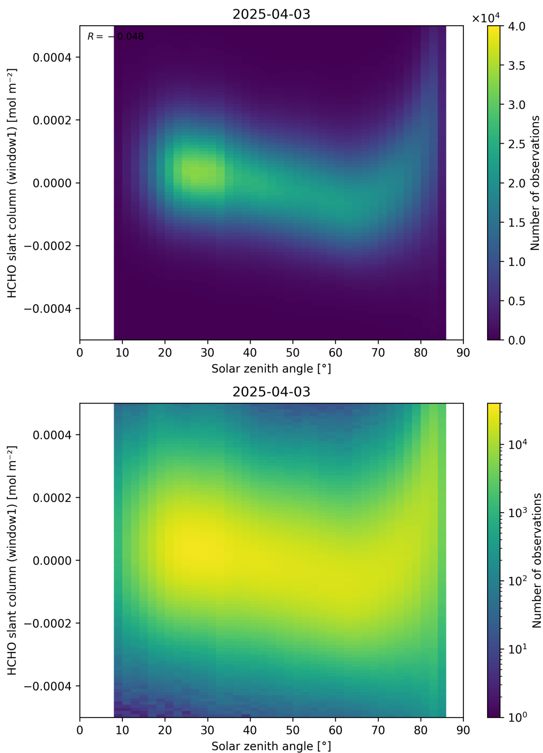
Figure 173: Scatter density plot of “Solar zenith angle” against “HCHO slant column (window1)” for 2025-04-03 to 2025-04-04.
