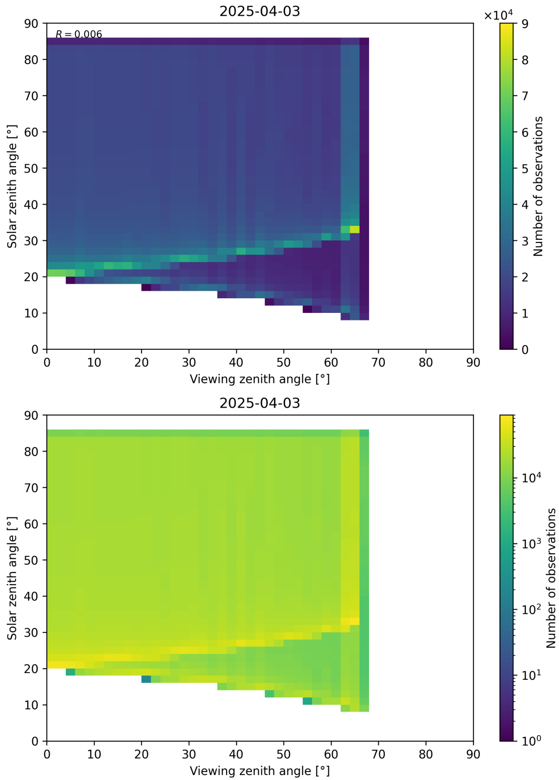
Figure 197: Scatter density plot of “Viewing zenith angle” against “Solar zenith angle” for 2025-04-03 to 2025-04-04.
