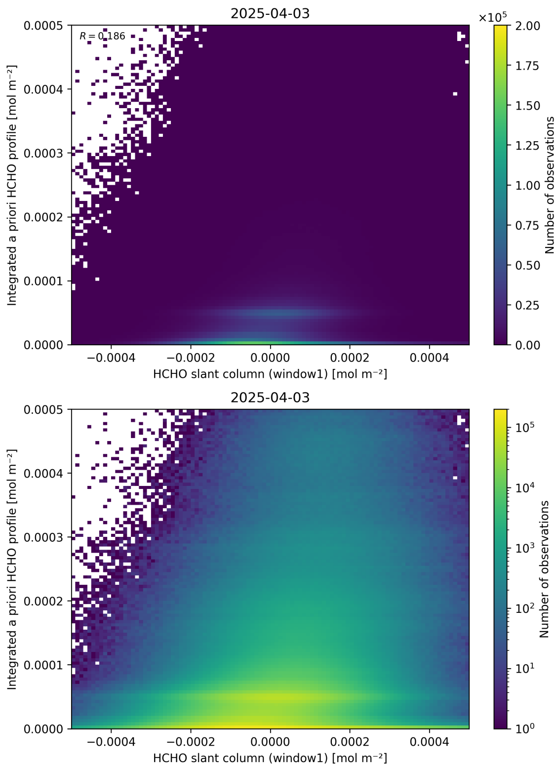
Figure 87: Scatter density plot of “HCHO slant column (window1)” against “Integrated a priori HCHO profile” for 2025-04-03 to 2025-04-04.
