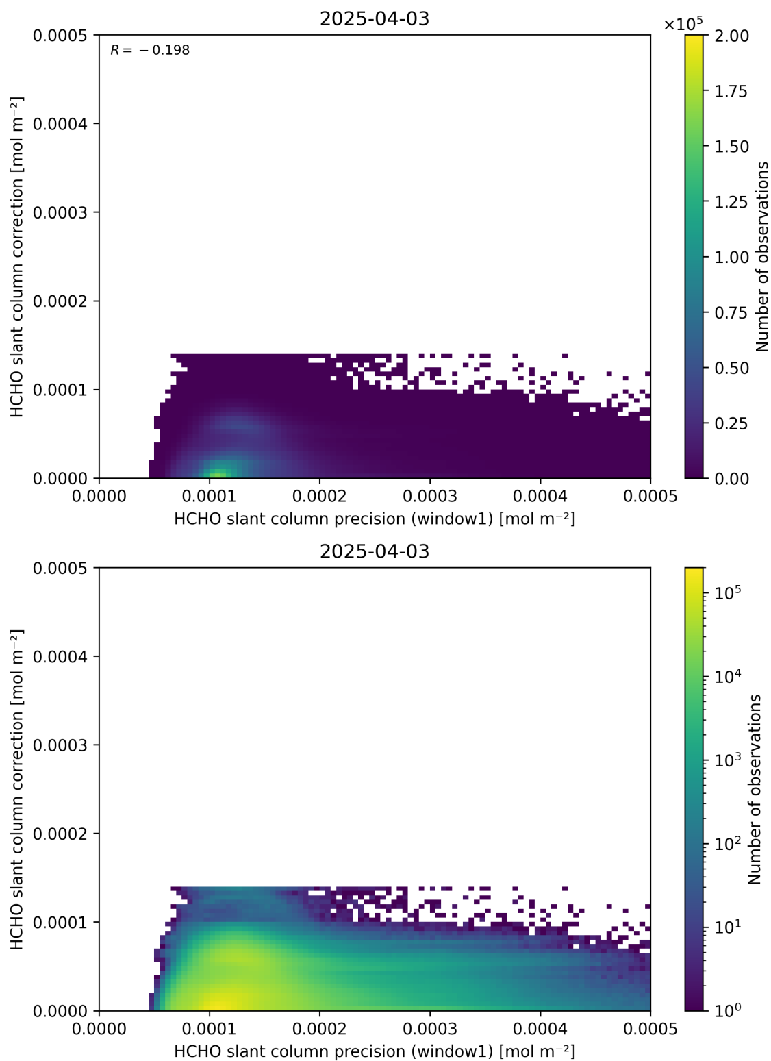
Figure 93: Scatter density plot of “HCHO slant column precision (window1)” against “HCHO slant column correction” for 2025-04-03 to 2025-04-04.
