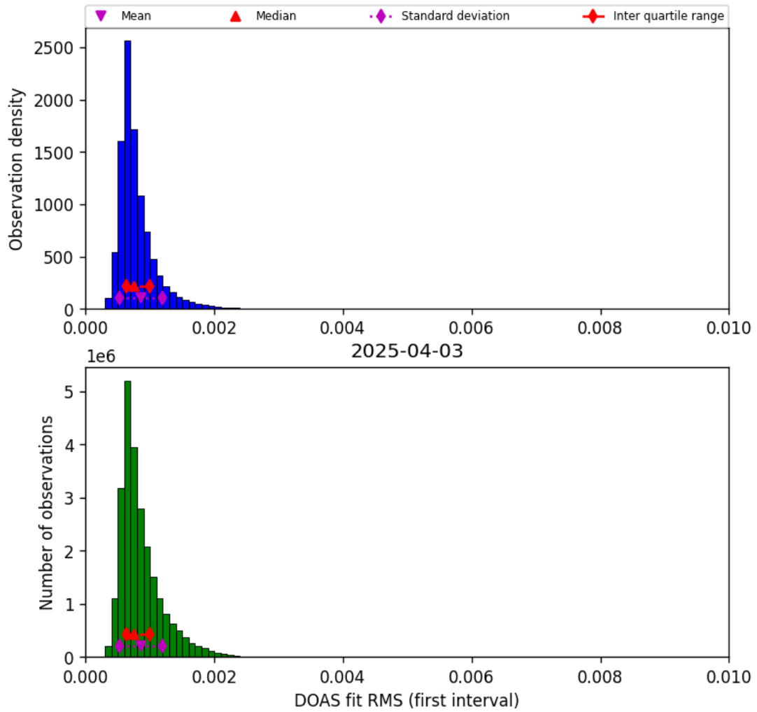
Figure 46: Histogram of “DOAS fit RMS (first interval)” for 2025-04-03 to 2025-04-04
