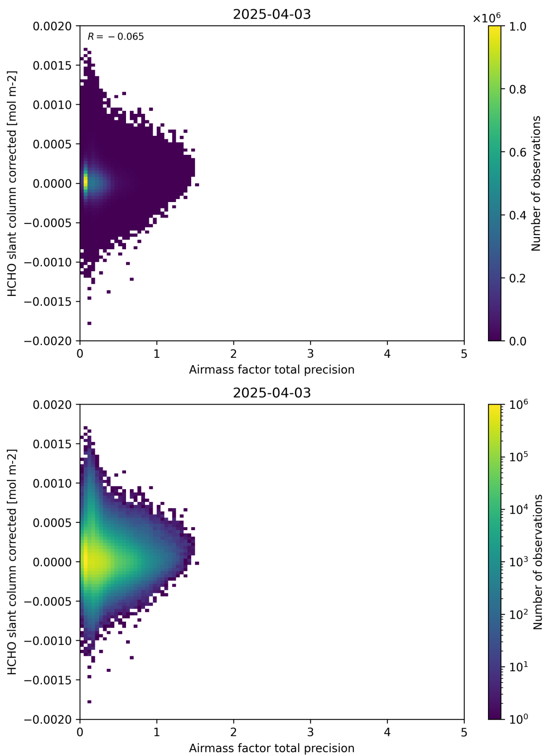
Figure 109: Scatter density plot of “Airmass factor total precision” against “HCHO slant column corrected” for 2025-04-03 to 2025-04-04.
