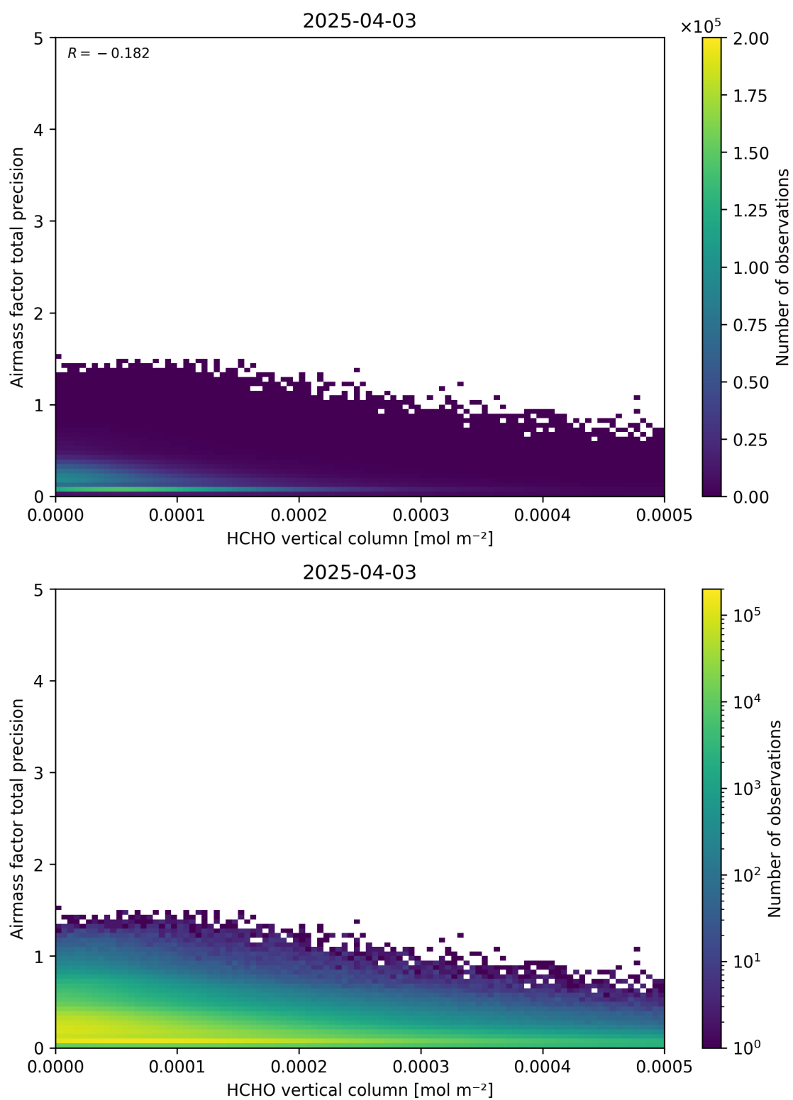
Figure 132: Scatter density plot of “HCHO vertical column” against “Airmass factor total precision” for 2025-04-03 to 2025-04-04.
