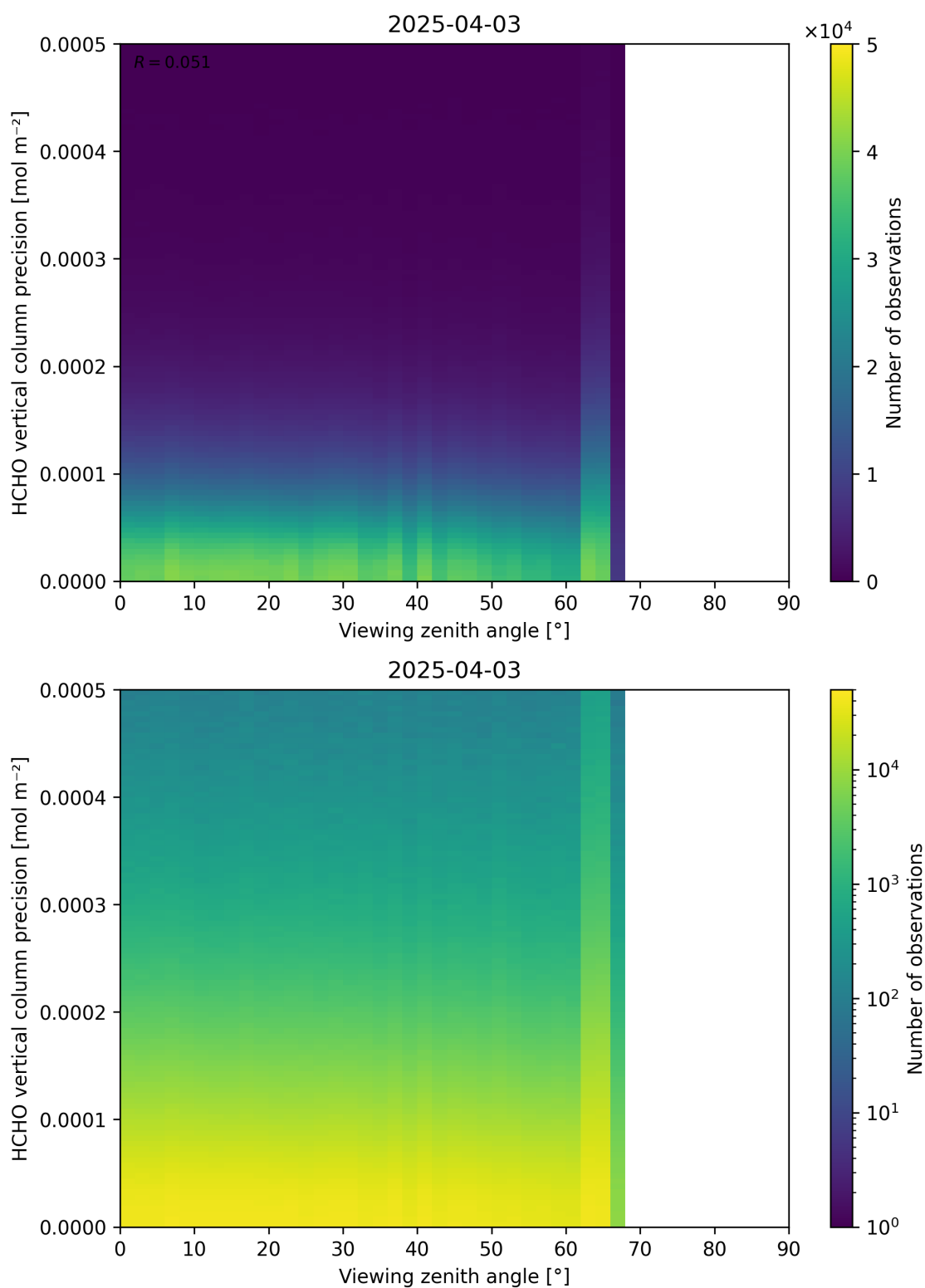
Figure 194: Scatter density plot of “Viewing zenith angle” against “HCHO vertical column precision” for 2025-04-03 to 2025-04-04.
