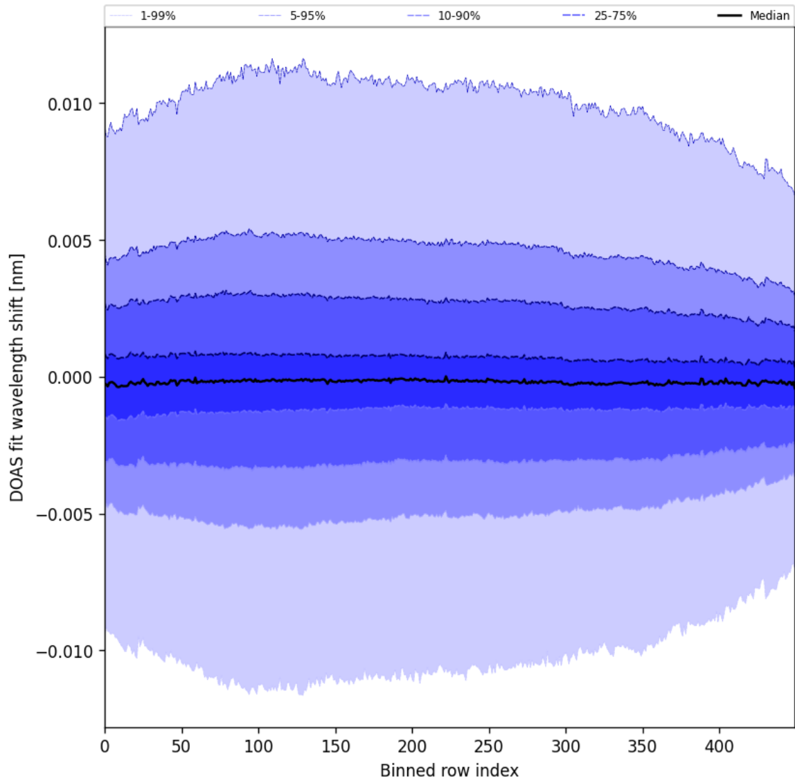
Figure 58: Along track statistics of “DOAS fit wavelength shift” for 2025-04-03 to 2025-04-04
