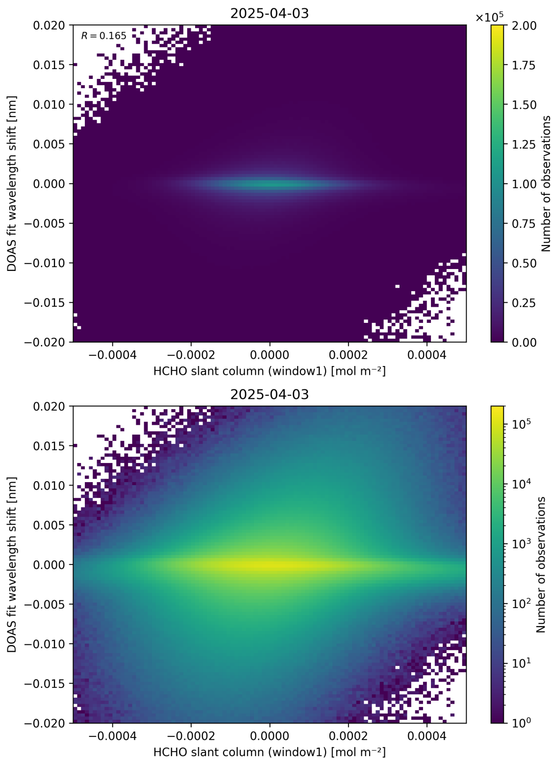
Figure 79: Scatter density plot of “HCHO slant column (window1)” against “DOAS fit wavelength shift” for 2025-04-03 to 2025-04-04.
