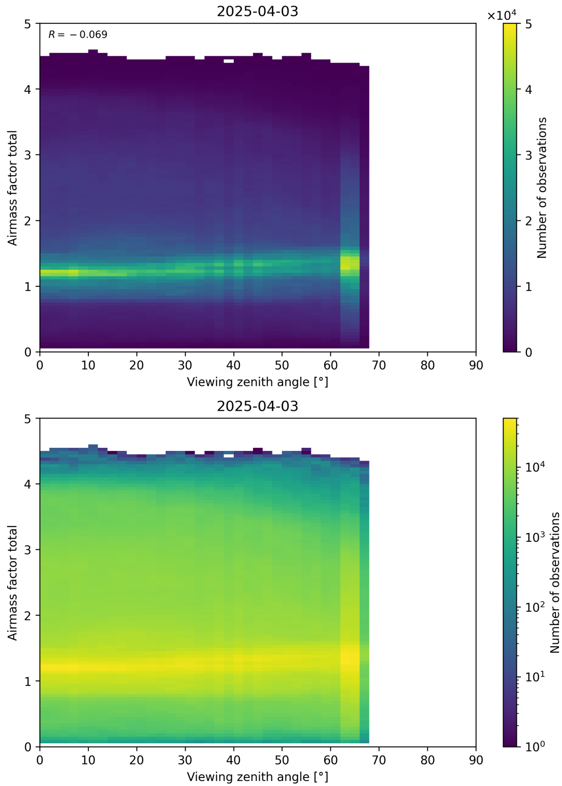
Figure 190: Scatter density plot of “Viewing zenith angle” against “Airmass factor total” for 2025-04-03 to 2025-04-04.
