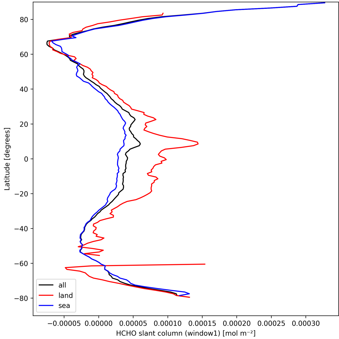
Figure 24: Zonal average of “HCHO slant column (window1)” for 2025-04-03 to 2025-04-04.
