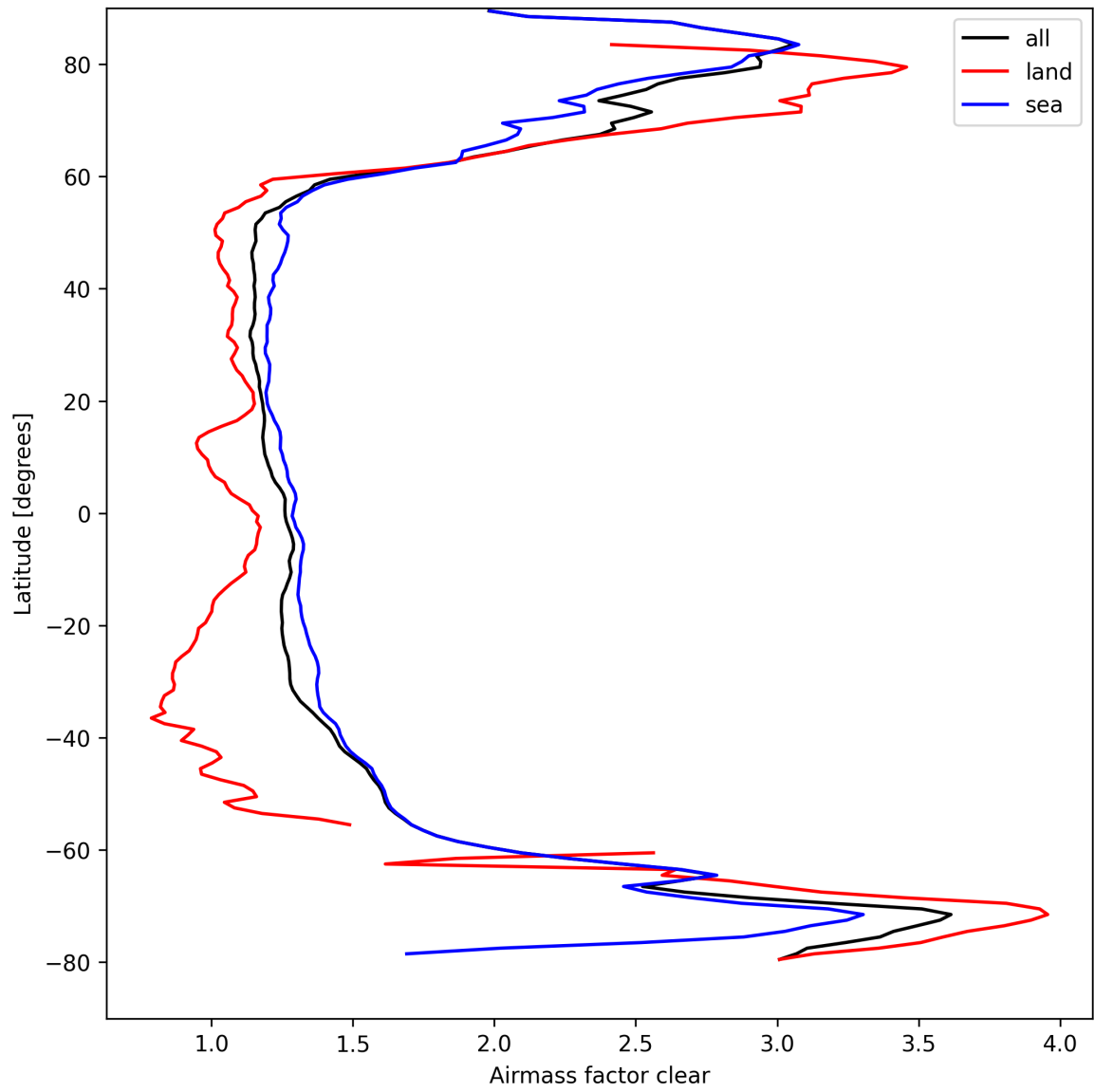
Figure 28: Zonal average of “Airmass factor clear” for 2025-04-03 to 2025-04-04.
