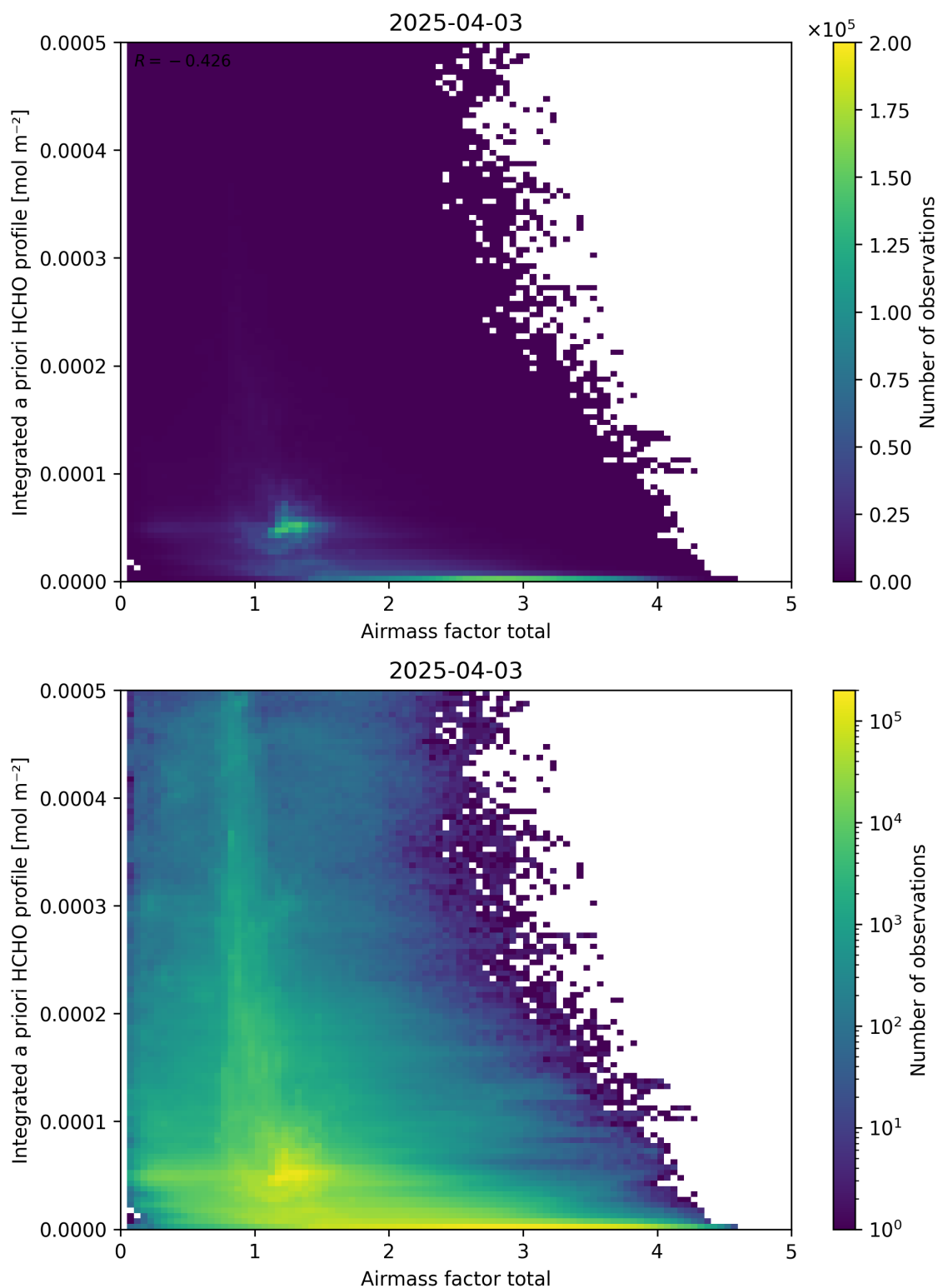
Figure 104: Scatter density plot of “Airmass factor total” against “Integrated a priori HCHO profile” for 2025-04-03 to 2025-04-04.
