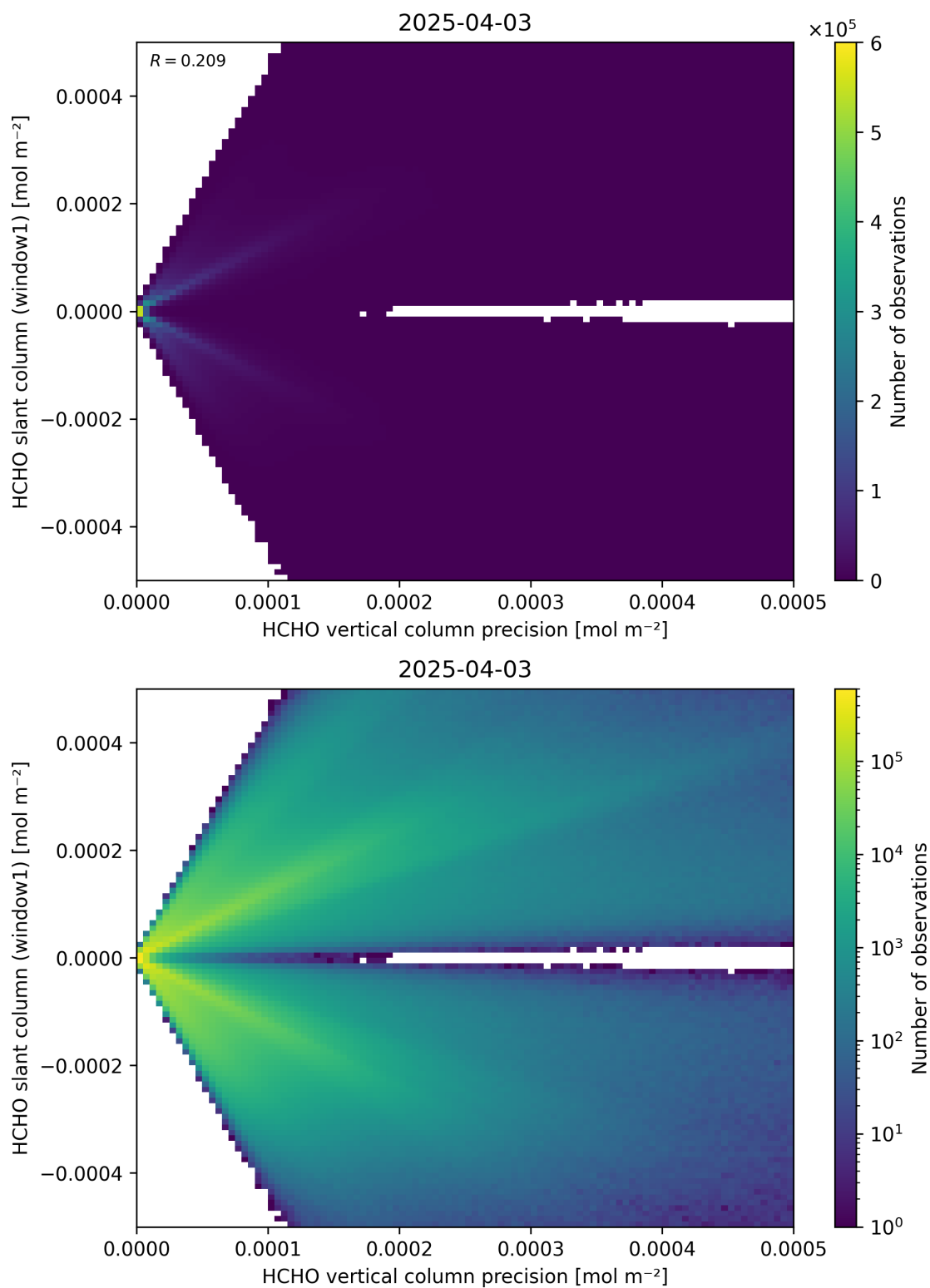
Figure 142: Scatter density plot of “HCHO vertical column precision” against “HCHO slant column (window1)” for 2025-04-03 to 2025-04-04.
