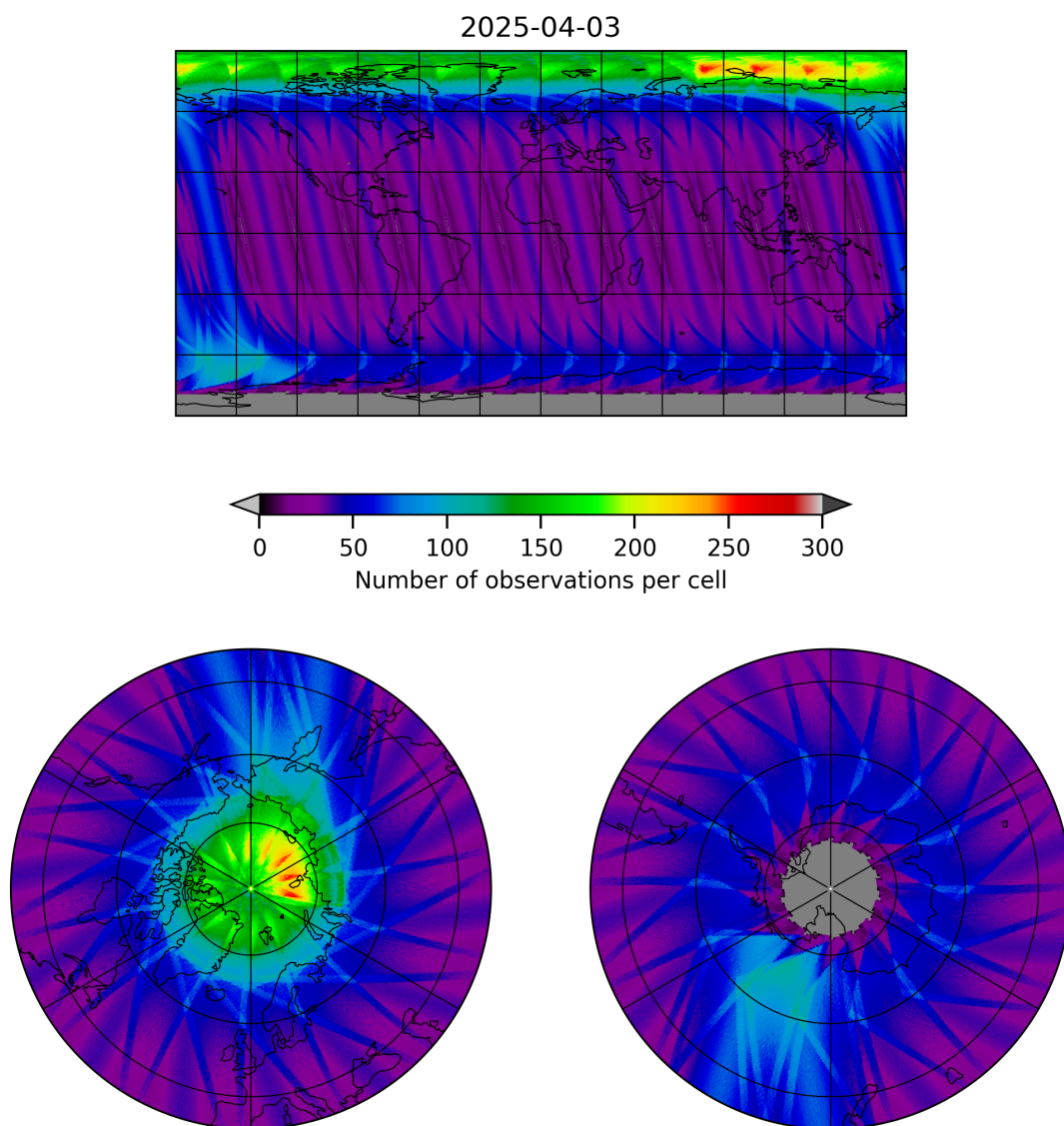
Figure 19: Map of the number of observations for 2025-04-03 to 2025-04-04
