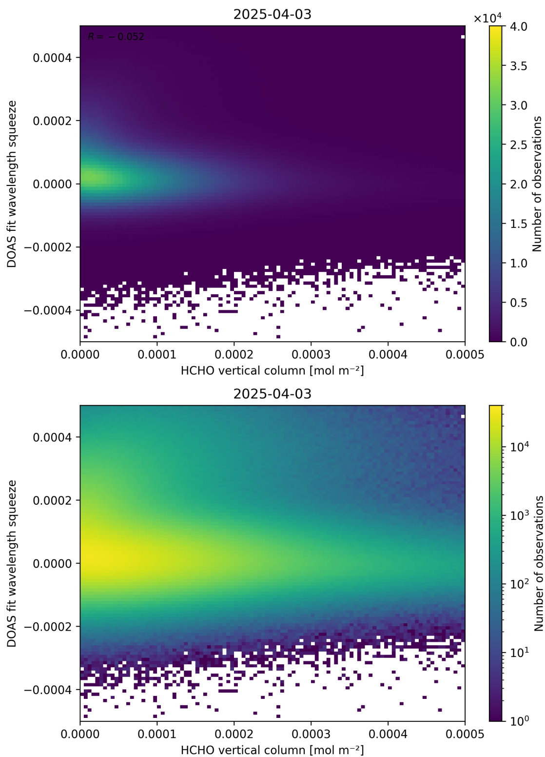
Figure 125: Scatter density plot of “HCHO vertical column” against “DOAS fit wavelength squeeze” for 2025-04-03 to 2025-04-04.
