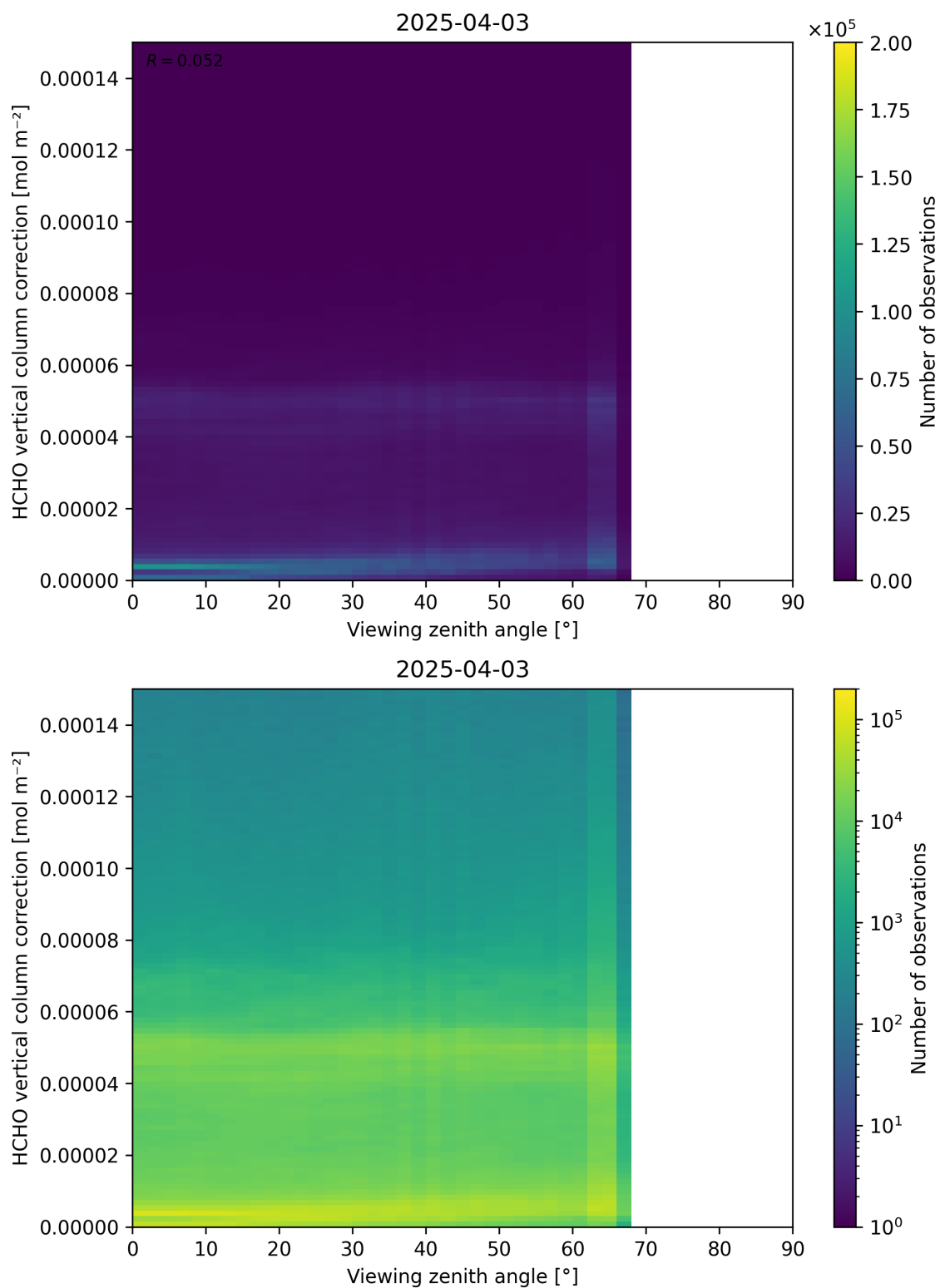
Figure 193: Scatter density plot of “Viewing zenith angle” against “HCHO vertical column correction” for 2025-04-03 to 2025-04-04.
