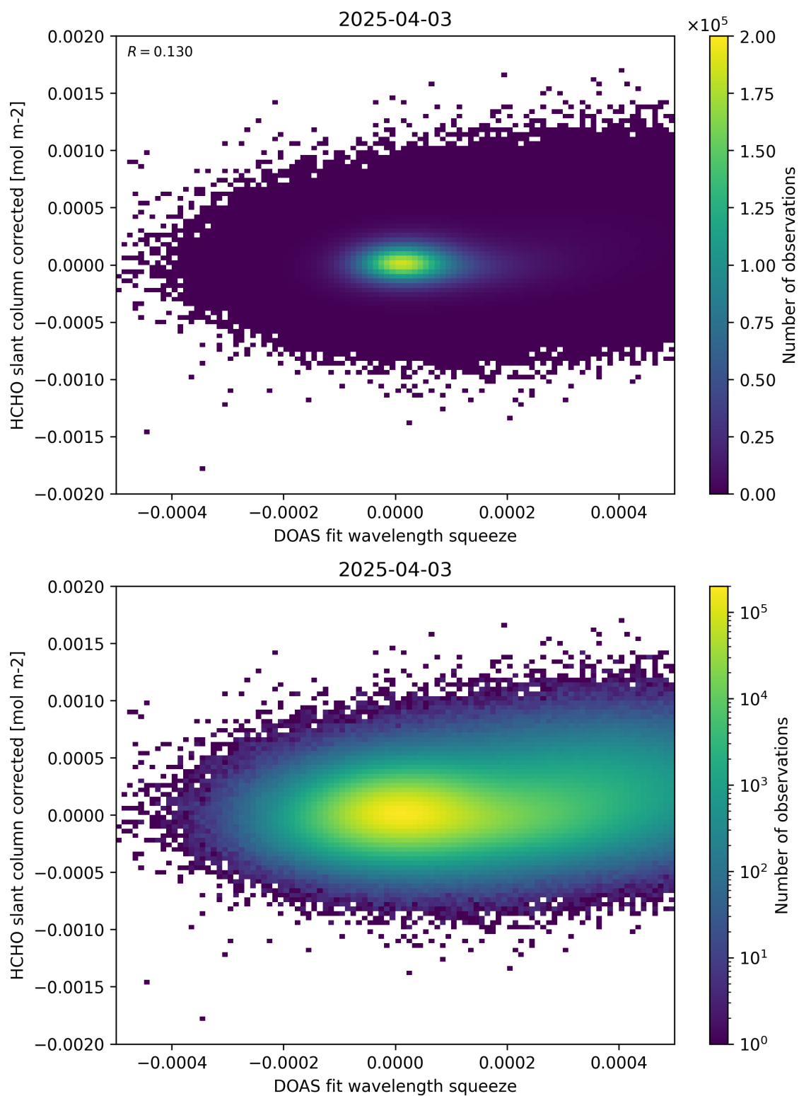
Figure 69: Scatter density plot of “DOAS fit wavelength squeeze” against “HCHO slant column corrected” for 2025-04-03 to 2025-04-04.
