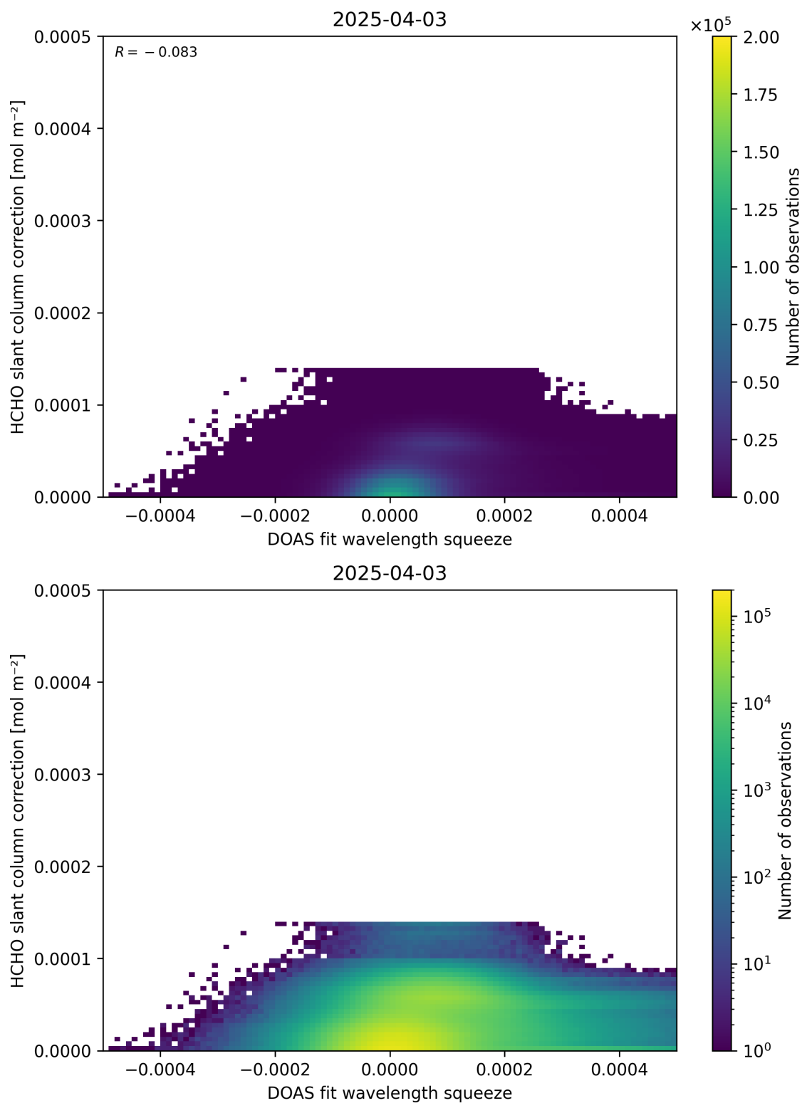
Figure 70: Scatter density plot of “DOAS fit wavelength squeeze” against “HCHO slant column correction” for 2025-04-03 to 2025-04-04.
