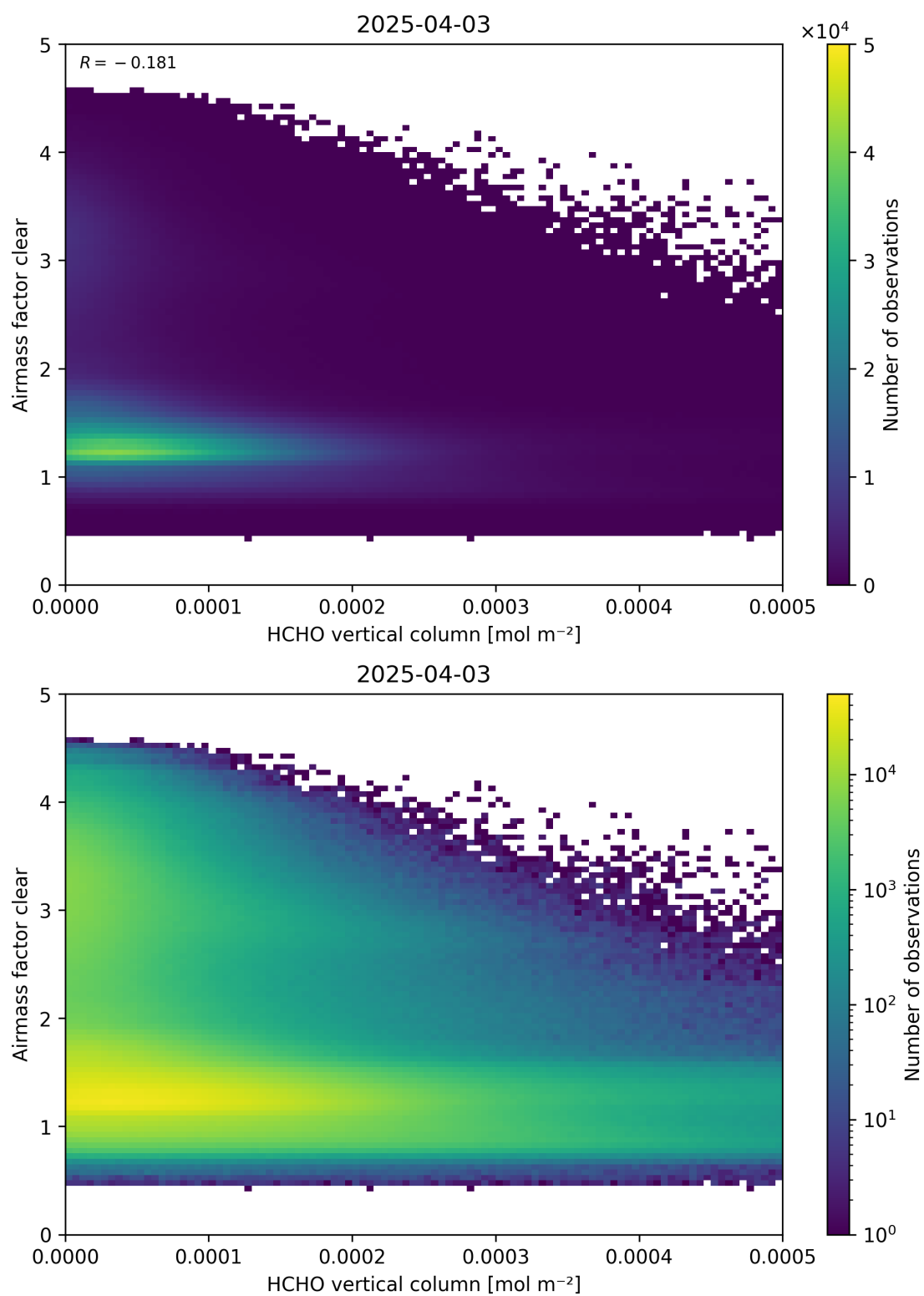
Figure 126: Scatter density plot of “HCHO vertical column” against “Airmass factor clear” for 2025-04-03 to 2025-04-04.
