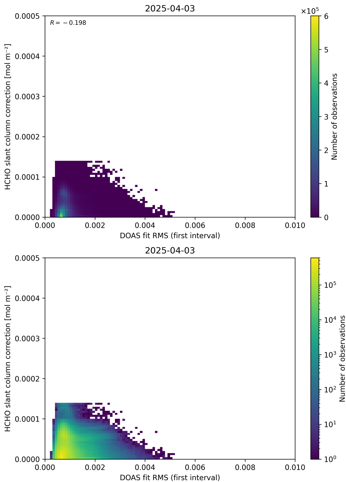
Figure 63: Scatter density plot of “DOAS fit RMS (first interval)” against “HCHO slant column correction” for 2025-04-03 to 2025-04-04.
