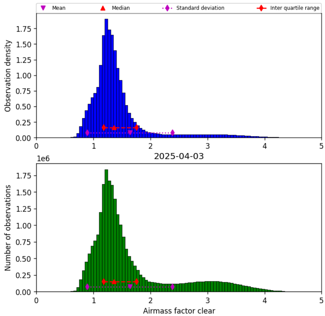
Figure 42: Histogram of “Airmass factor clear” for 2025-04-03 to 2025-04-04
