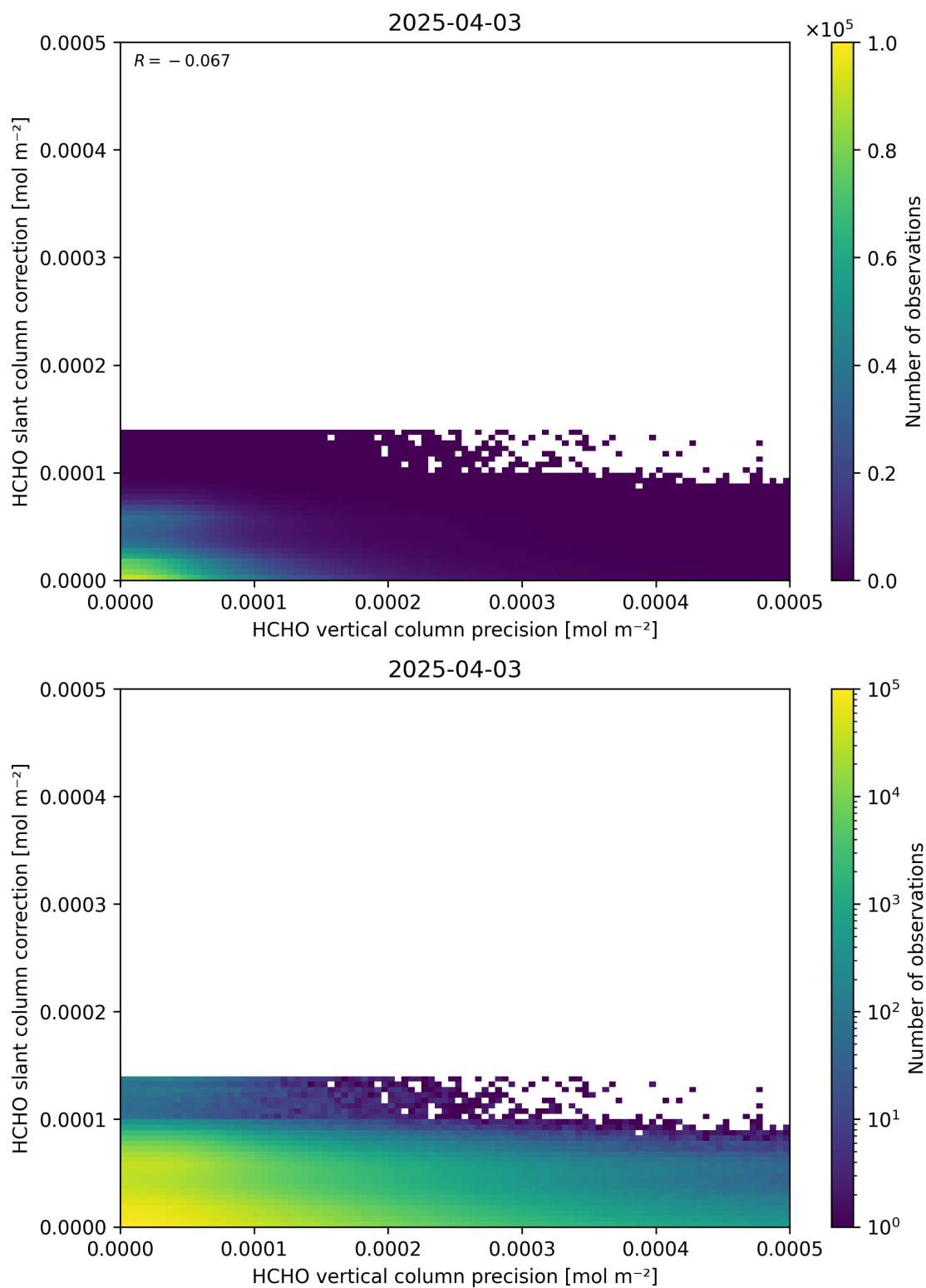
Figure 141: Scatter density plot of “HCHO vertical column precision” against “HCHO slant column correction” for 2025-04-03 to 2025-04-04.
