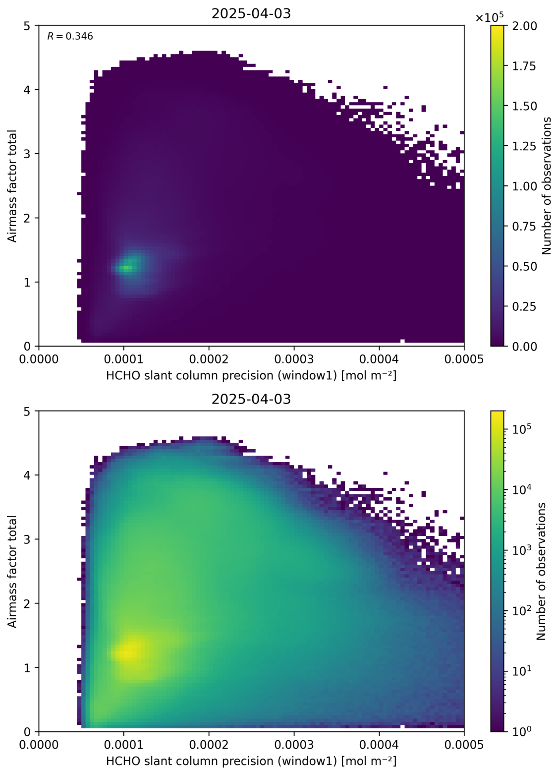
Figure 94: Scatter density plot of “HCHO slant column precision (window1)” against “Airmass factor total” for 2025-04-03 to 2025-04-04.
