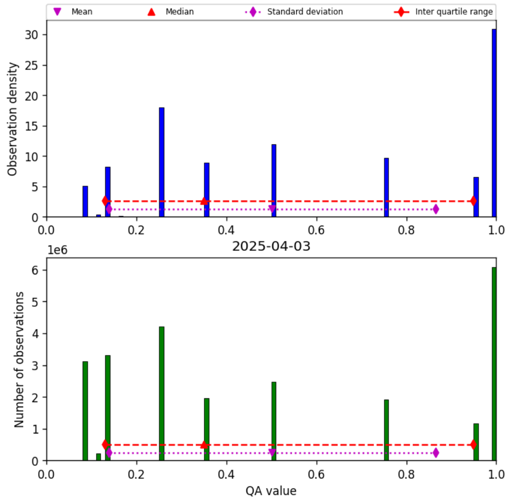
Figure 34: Histogram of “QA value” for 2025-04-03 to 2025-04-04
