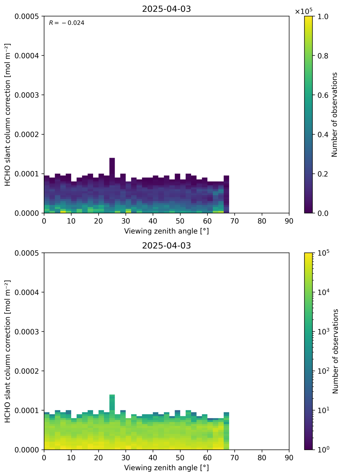
Figure 187: Scatter density plot of “Viewing zenith angle” against “HCHO slant column correction” for 2025-04-03 to 2025-04-04.
