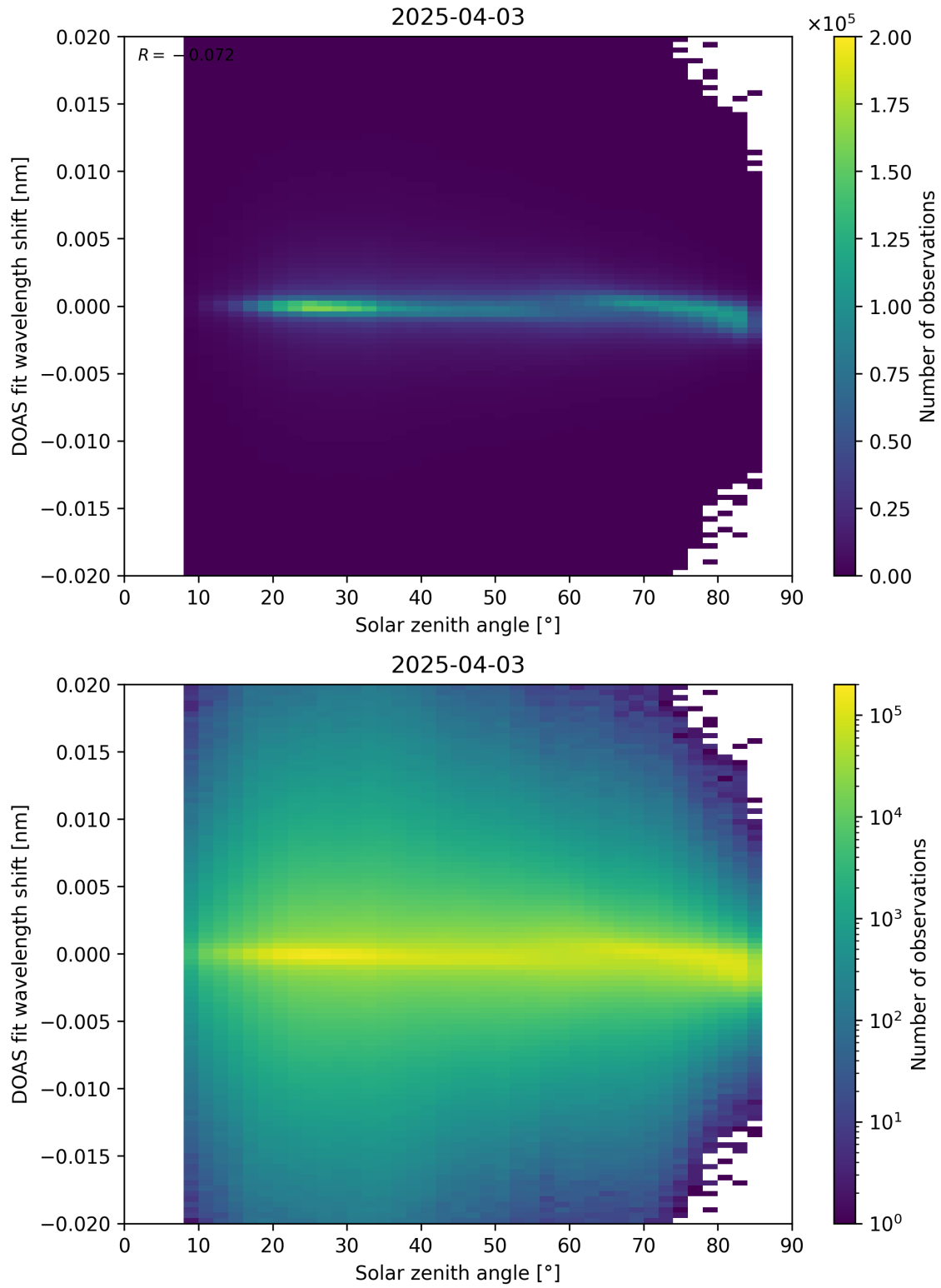
Figure 168: Scatter density plot of “Solar zenith angle” against “DOAS fit wavelength shift” for 2025-04-03 to 2025-04-04.
