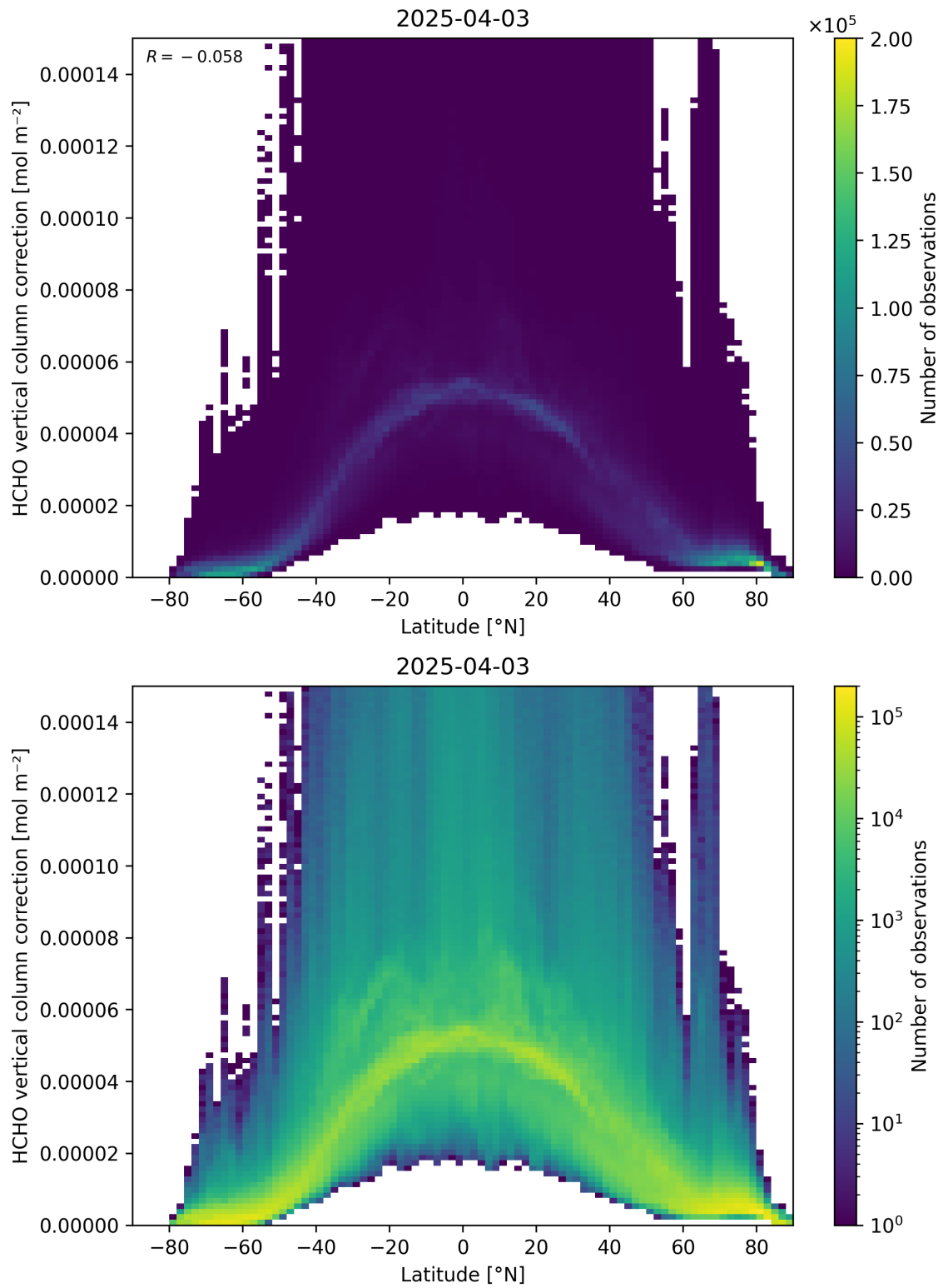
Figure 164: Scatter density plot of “Latitude” against “HCHO vertical column correction” for 2025-04-03 to 2025-04-04.
