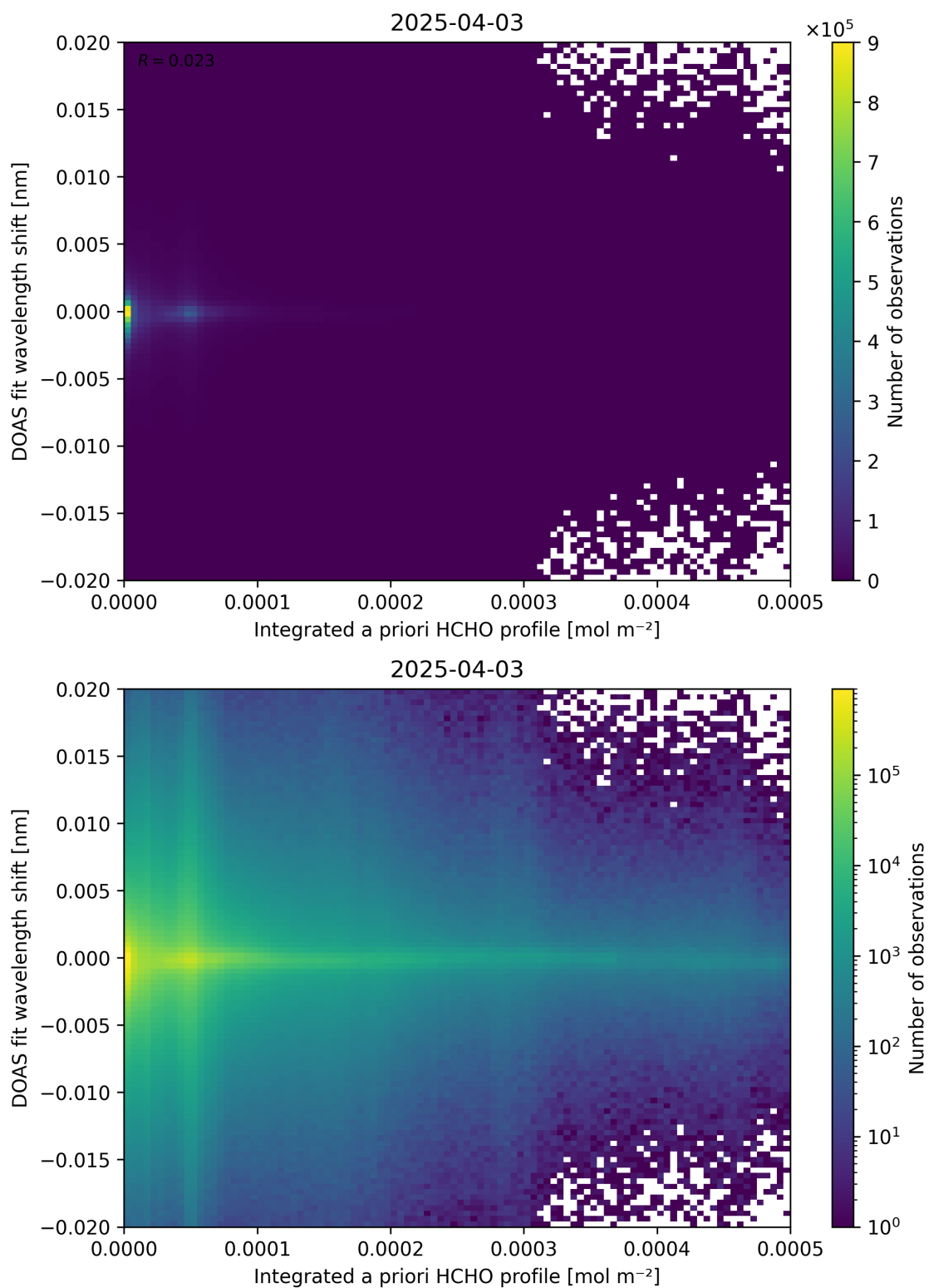
Figure 149: Scatter density plot of “Integrated a priori HCHO profile” against “DOAS fit wavelength shift” for 2025-04-03 to 2025-04-04.
