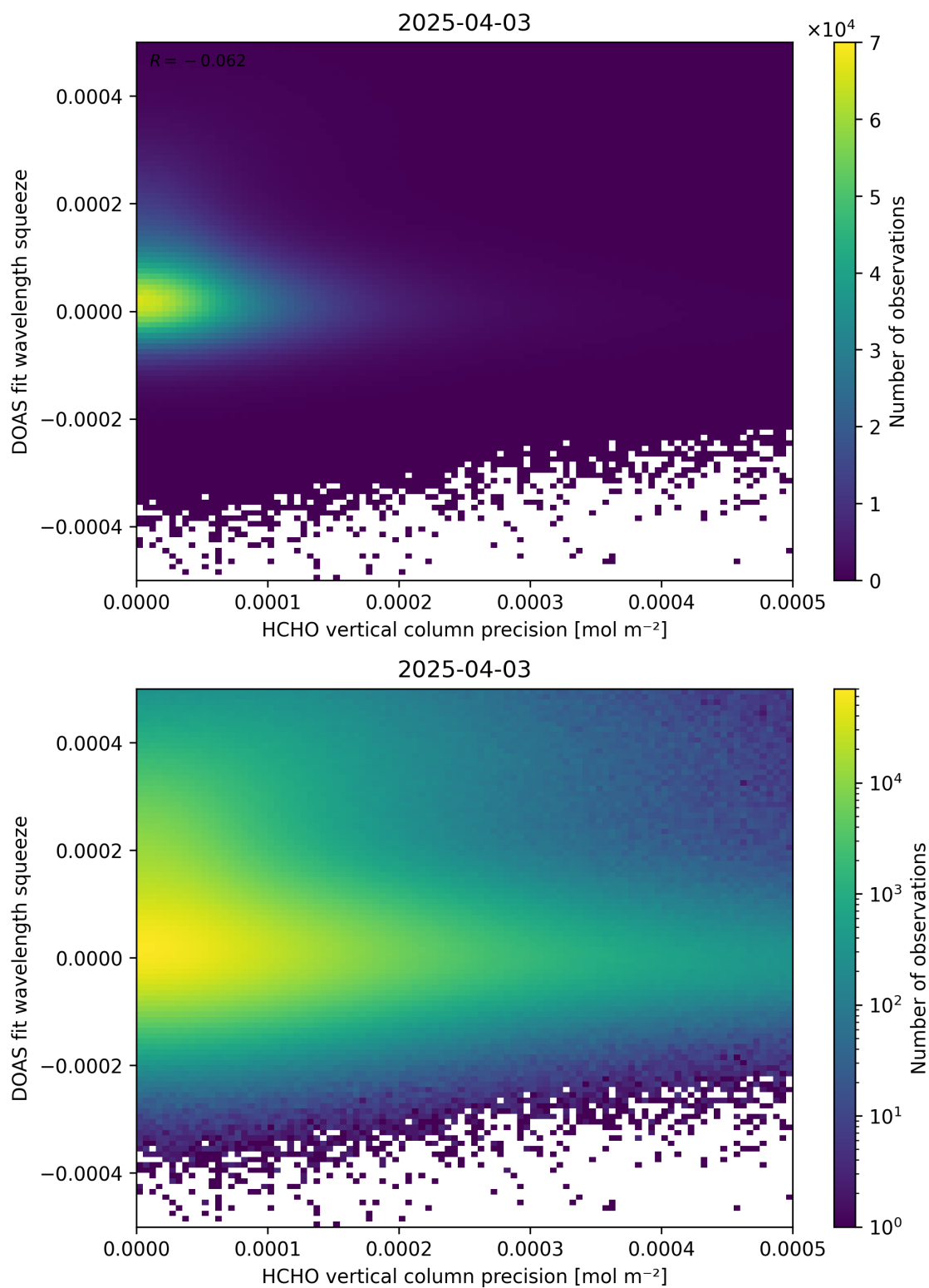
Figure 138: Scatter density plot of “HCHO vertical column precision” against “DOAS fit wavelength squeeze” for 2025-04-03 to 2025-04-04.
