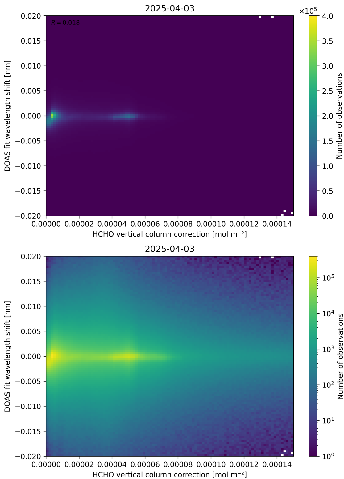
Figure 113: Scatter density plot of “HCHO vertical column correction” against “DOAS fit wavelength shift” for 2025-04-03 to 2025-04-04.
