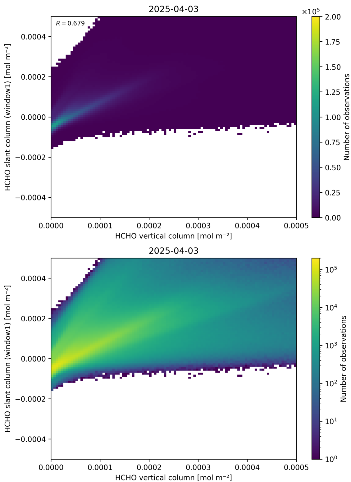
Figure 129: Scatter density plot of “HCHO vertical column” against “HCHO slant column (window1)” for 2025-04-03 to 2025-04-04.
