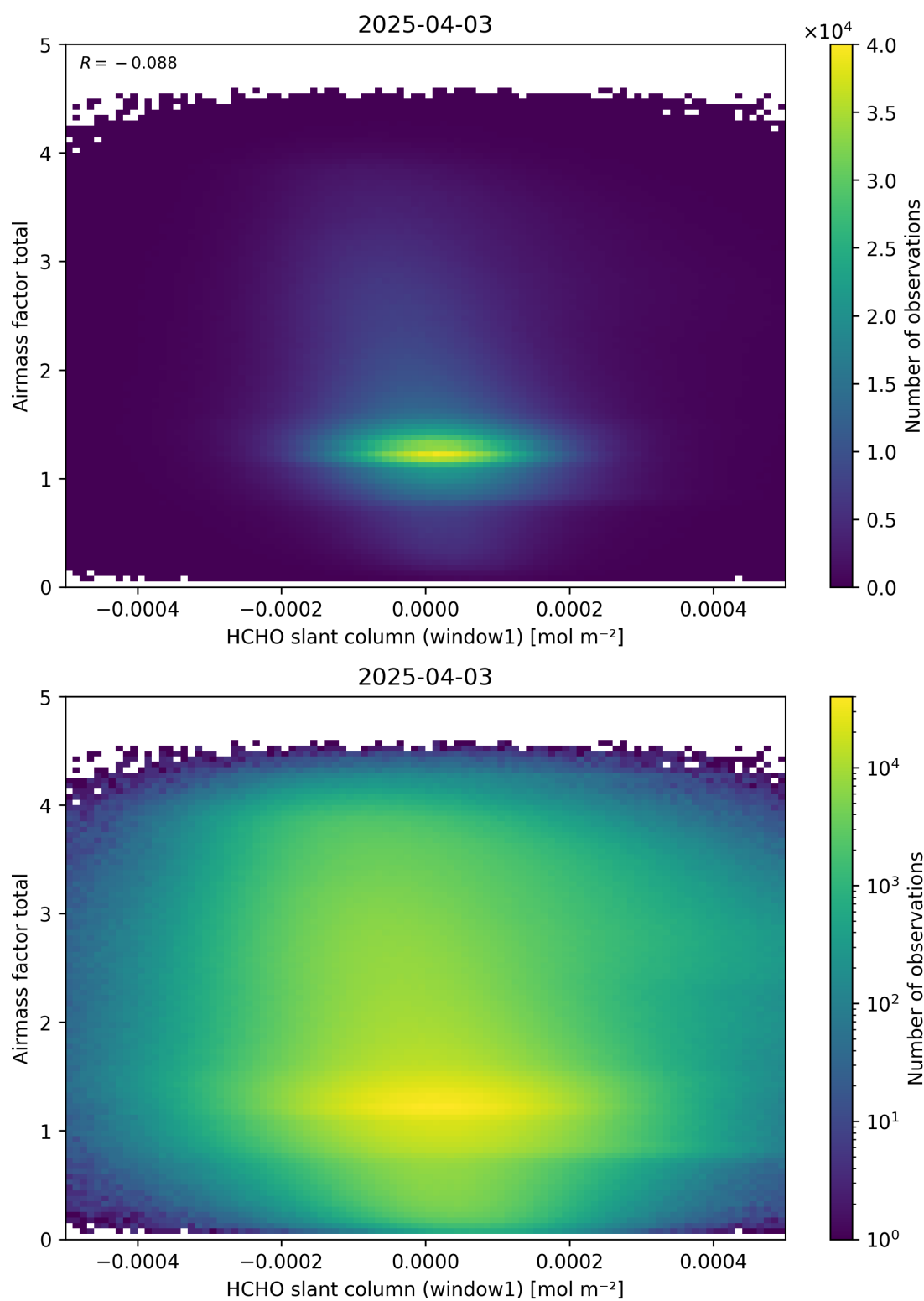
Figure 85: Scatter density plot of “HCHO slant column (window1)” against “Airmass factor total” for 2025-04-03 to 2025-04-04.
