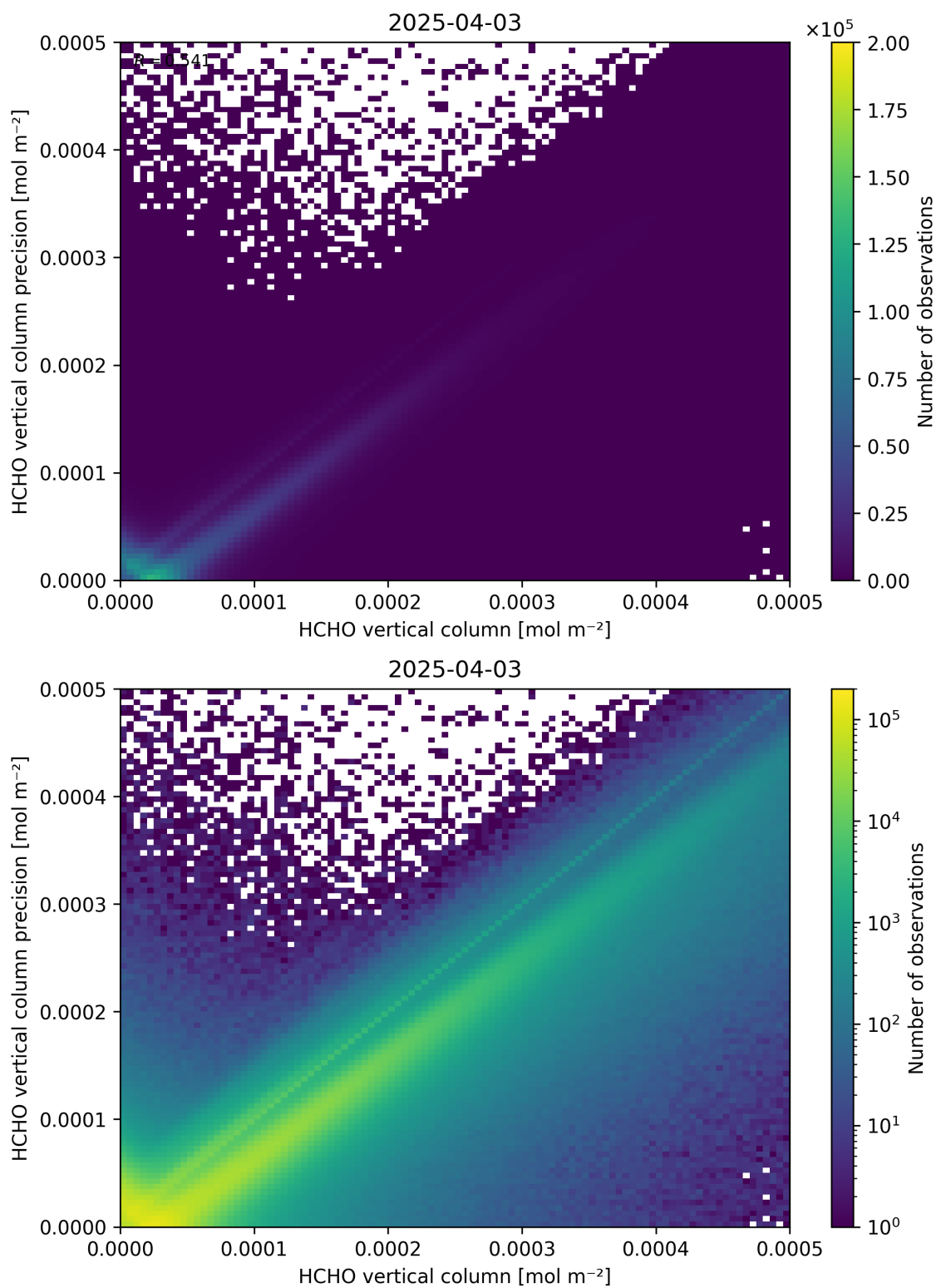
Figure 134: Scatter density plot of “HCHO vertical column” against “HCHO vertical column precision” for 2025-04-03 to 2025-04-04.
