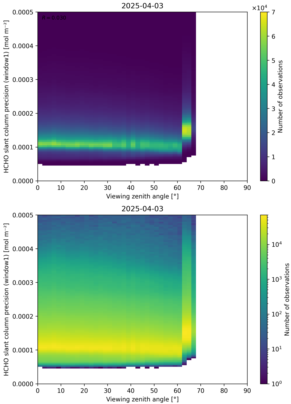
Figure 189: Scatter density plot of “Viewing zenith angle” against “HCHO slant column precision (window1)” for 2025-04-03 to 2025-04-04.
