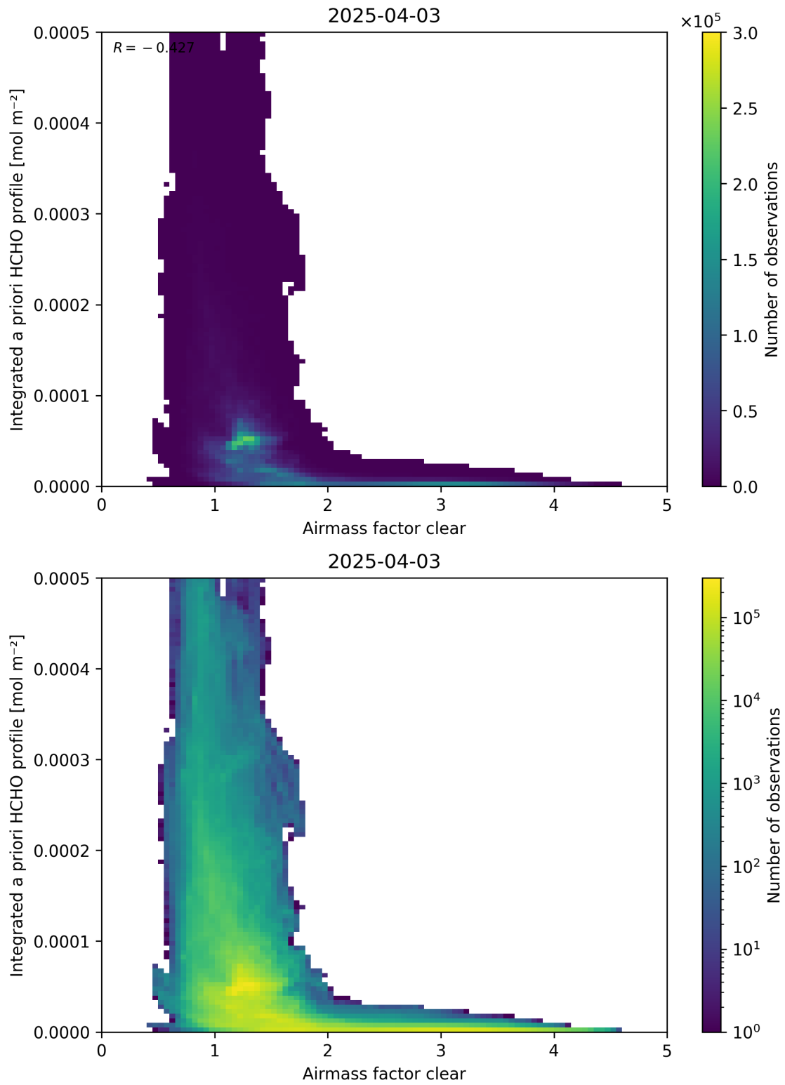
Figure 76: Scatter density plot of “Airmass factor clear” against “Integrated a priori HCHO profile” for 2025-04-03 to 2025-04-04.
