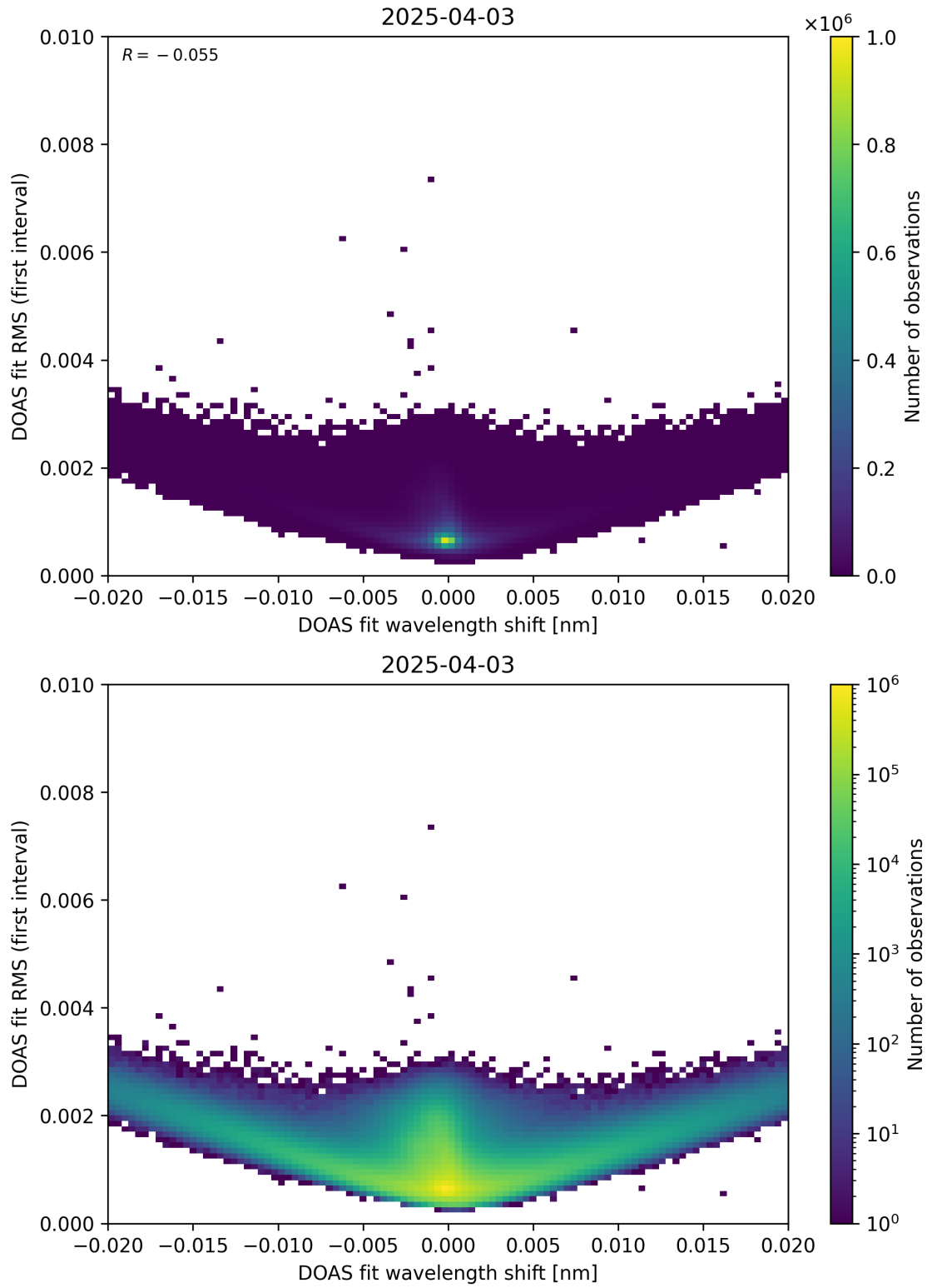
Figure 64: Scatter density plot of “DOAS fit wavelength shift” against “DOAS fit RMS (first interval)” for 2025-04-03 to 2025-04-04.
