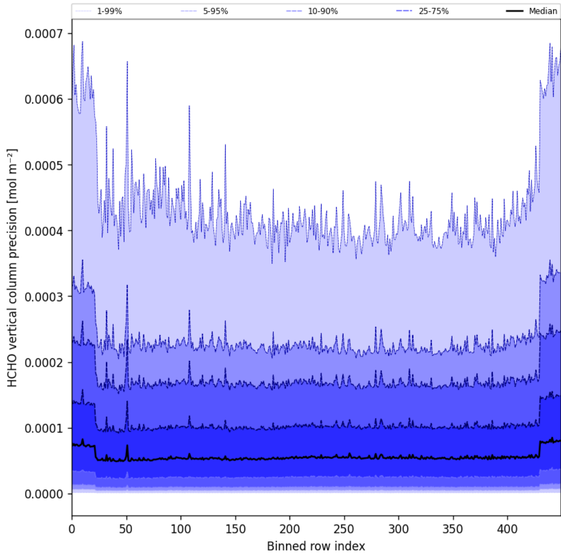
Figure 50: Along track statistics of “HCHO vertical column precision” for 2025-04-03 to 2025-04-04
