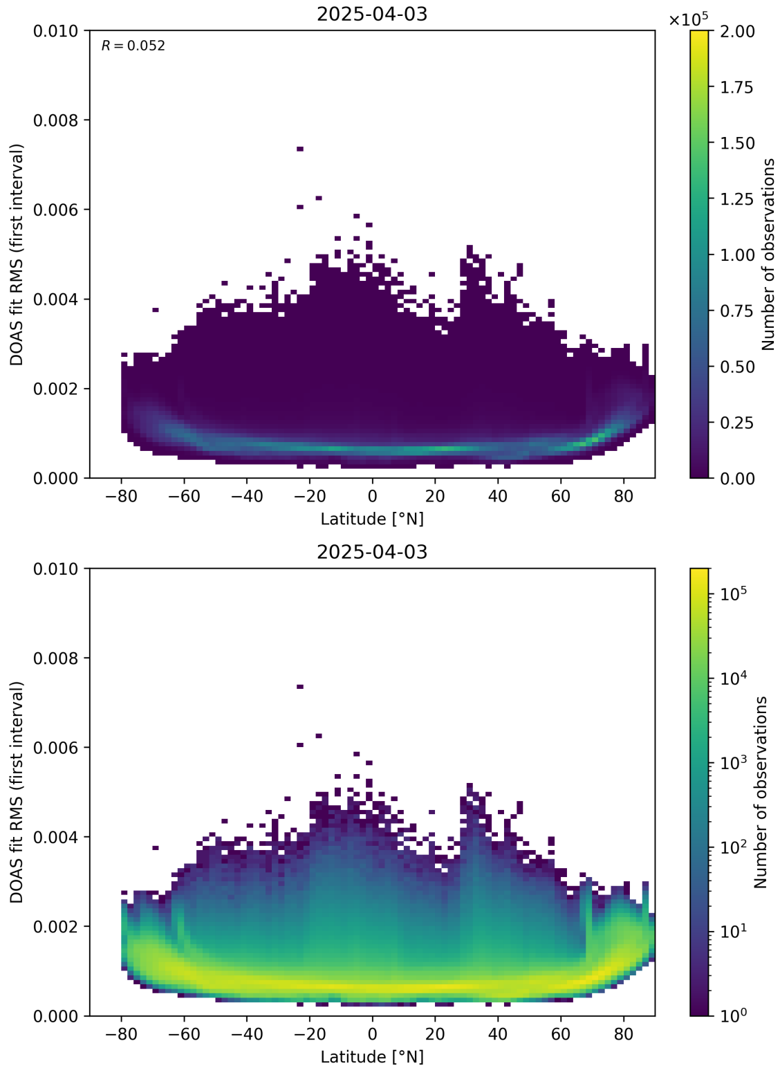
Figure 153: Scatter density plot of “Latitude” against “DOAS fit RMS (first interval)” for 2025-04-03 to 2025-04-04.
