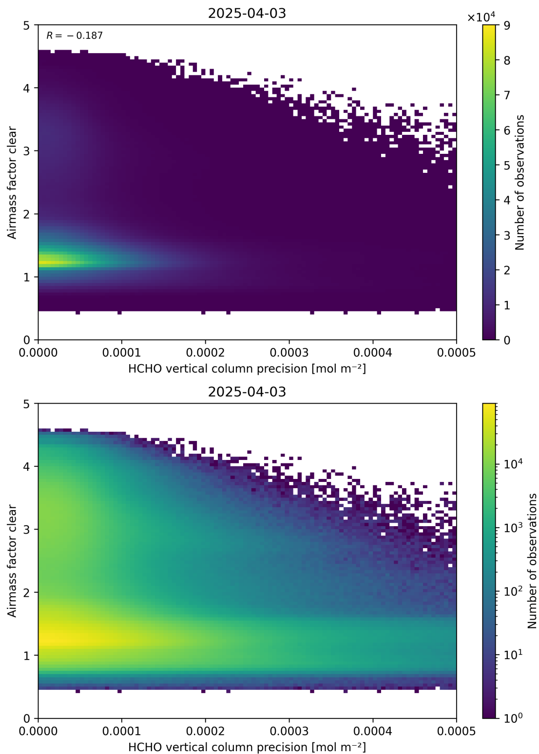
Figure 139: Scatter density plot of “HCHO vertical column precision” against “Airmass factor clear” for 2025-04-03 to 2025-04-04.
