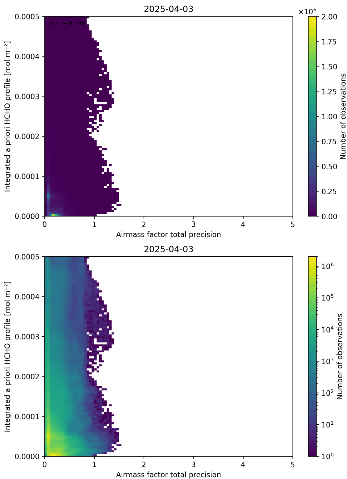
Figure 111: Scatter density plot of “Airmass factor total precision” against “Integrated a priori HCHO profile” for 2025-04-03 to 2025-04-04.
