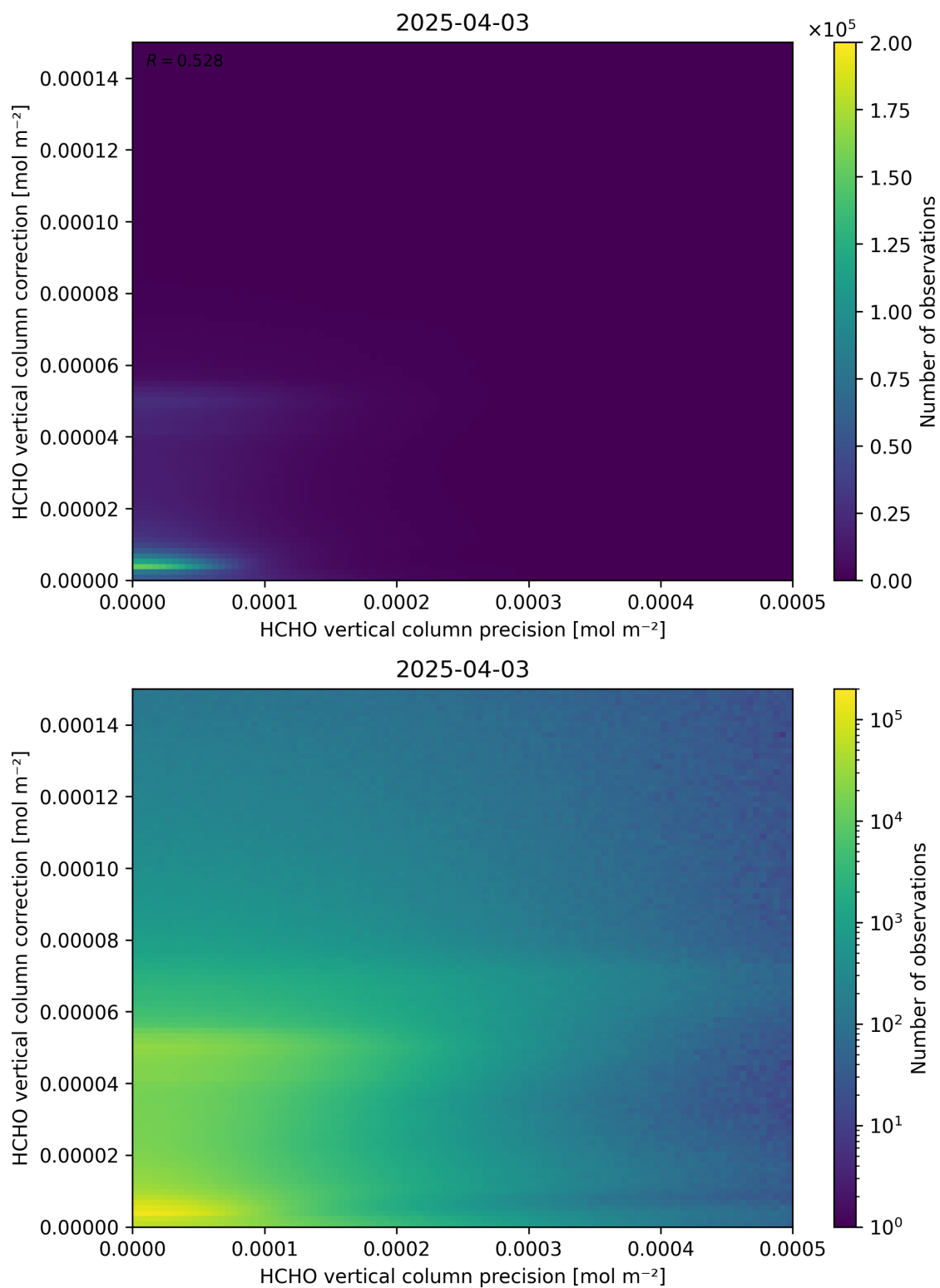
Figure 146: Scatter density plot of “HCHO vertical column precision” against “HCHO vertical column correction” for 2025-04-03 to 2025-04-04.
