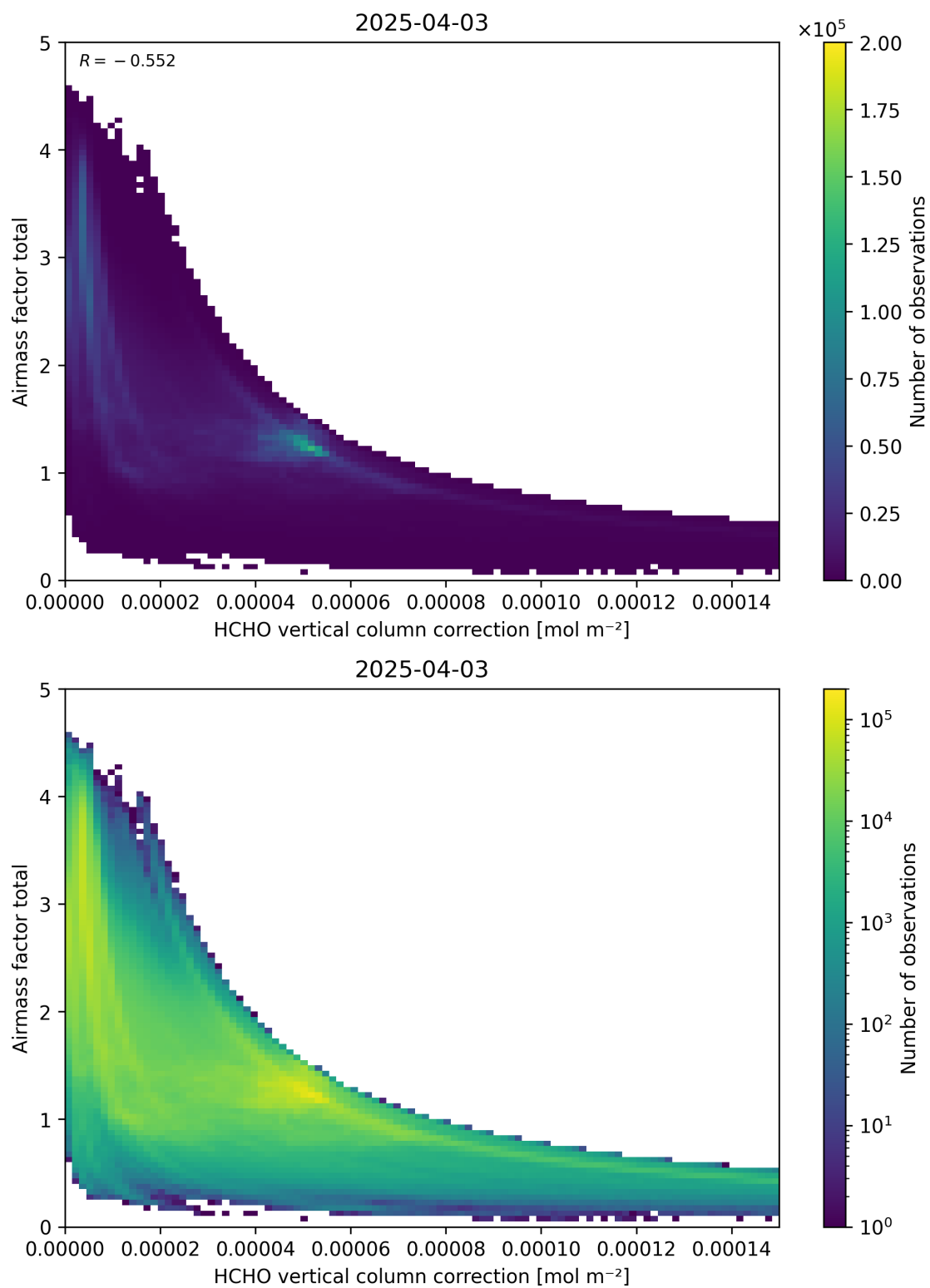
Figure 120: Scatter density plot of “HCHO vertical column correction” against “Airmass factor total” for 2025-04-03 to 2025-04-04.
