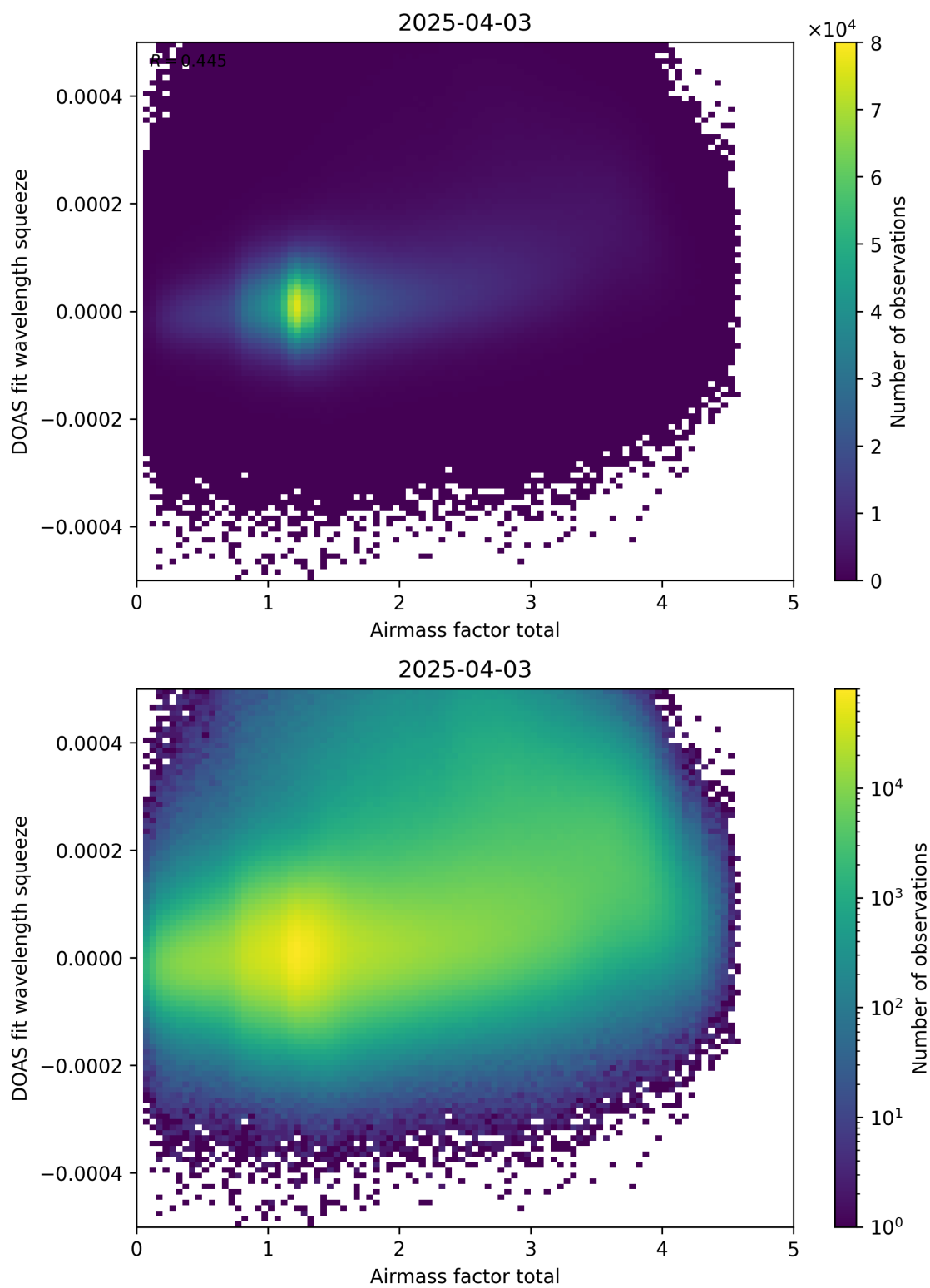
Figure 99: Scatter density plot of “Airmass factor total” against “DOAS fit wavelength squeeze” for 2025-04-03 to 2025-04-04.
