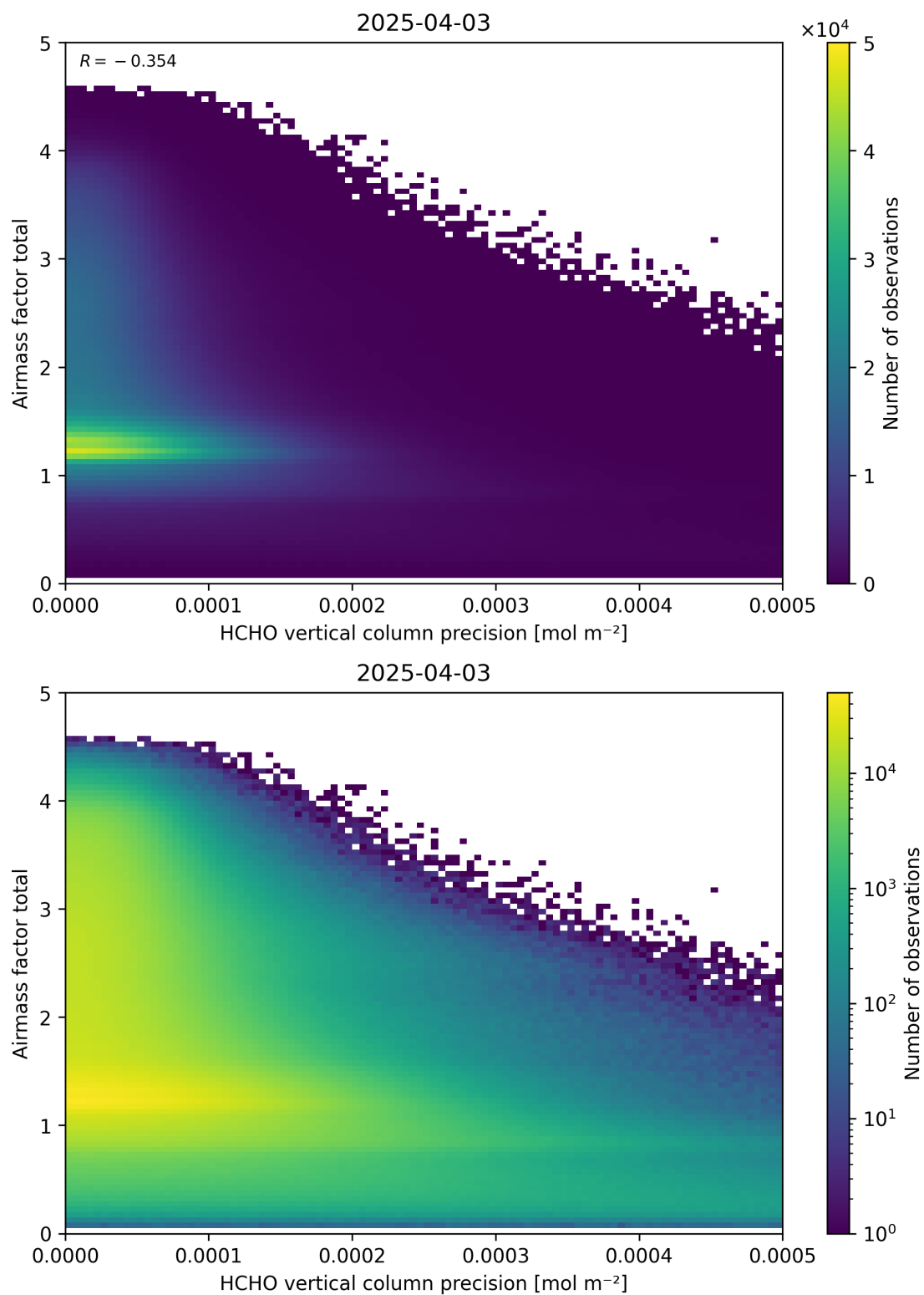
Figure 144: Scatter density plot of “HCHO vertical column precision” against “Airmass factor total” for 2025-04-03 to 2025-04-04.
