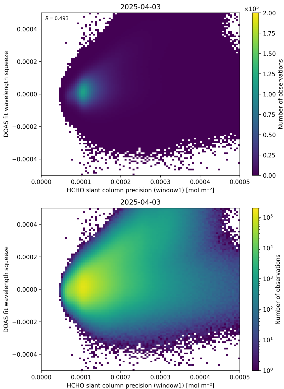
Figure 90: Scatter density plot of “HCHO slant column precision (window1)” against “DOAS fit wavelength squeeze” for 2025-04-03 to 2025-04-04.
