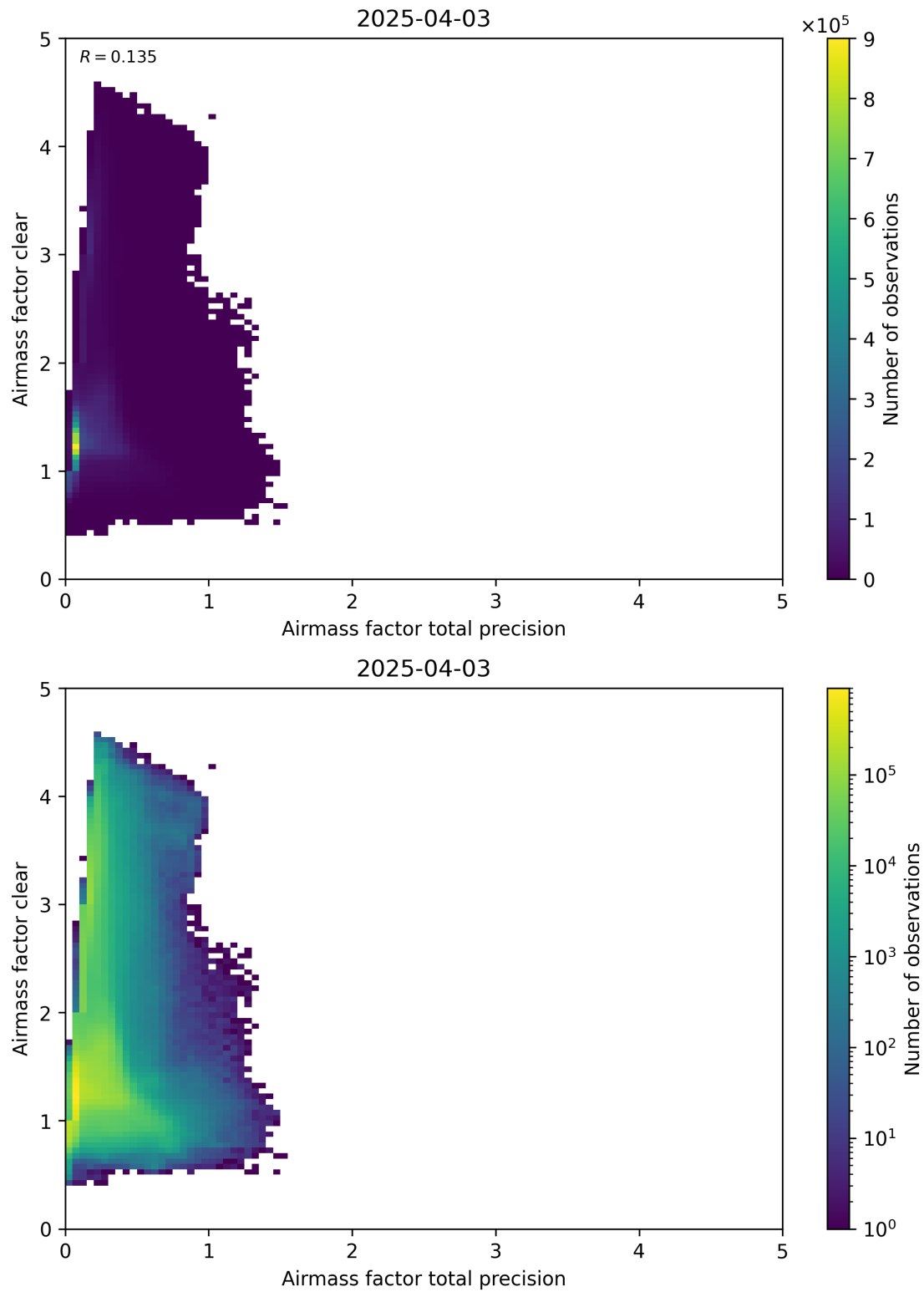
Figure 108: Scatter density plot of “Airmass factor total precision” against “Airmass factor clear” for 2025-04-03 to 2025-04-04.
