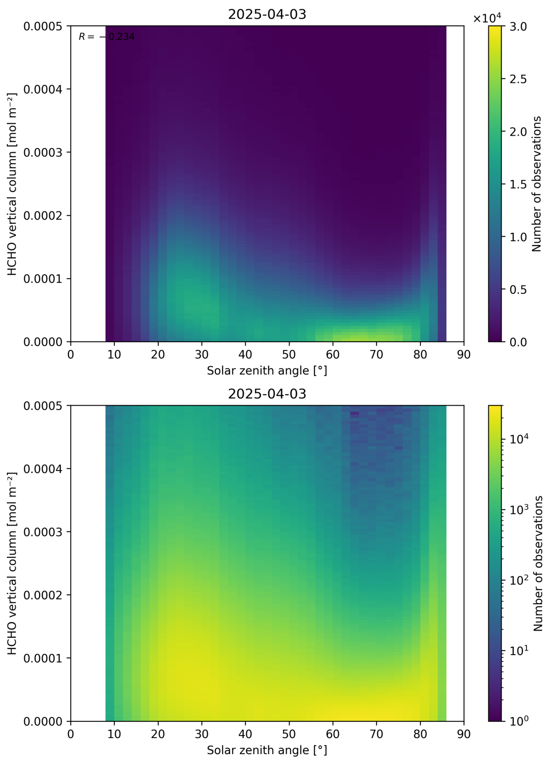
Figure 177: Scatter density plot of “Solar zenith angle” against “HCHO vertical column” for 2025-04-03 to 2025-04-04.
