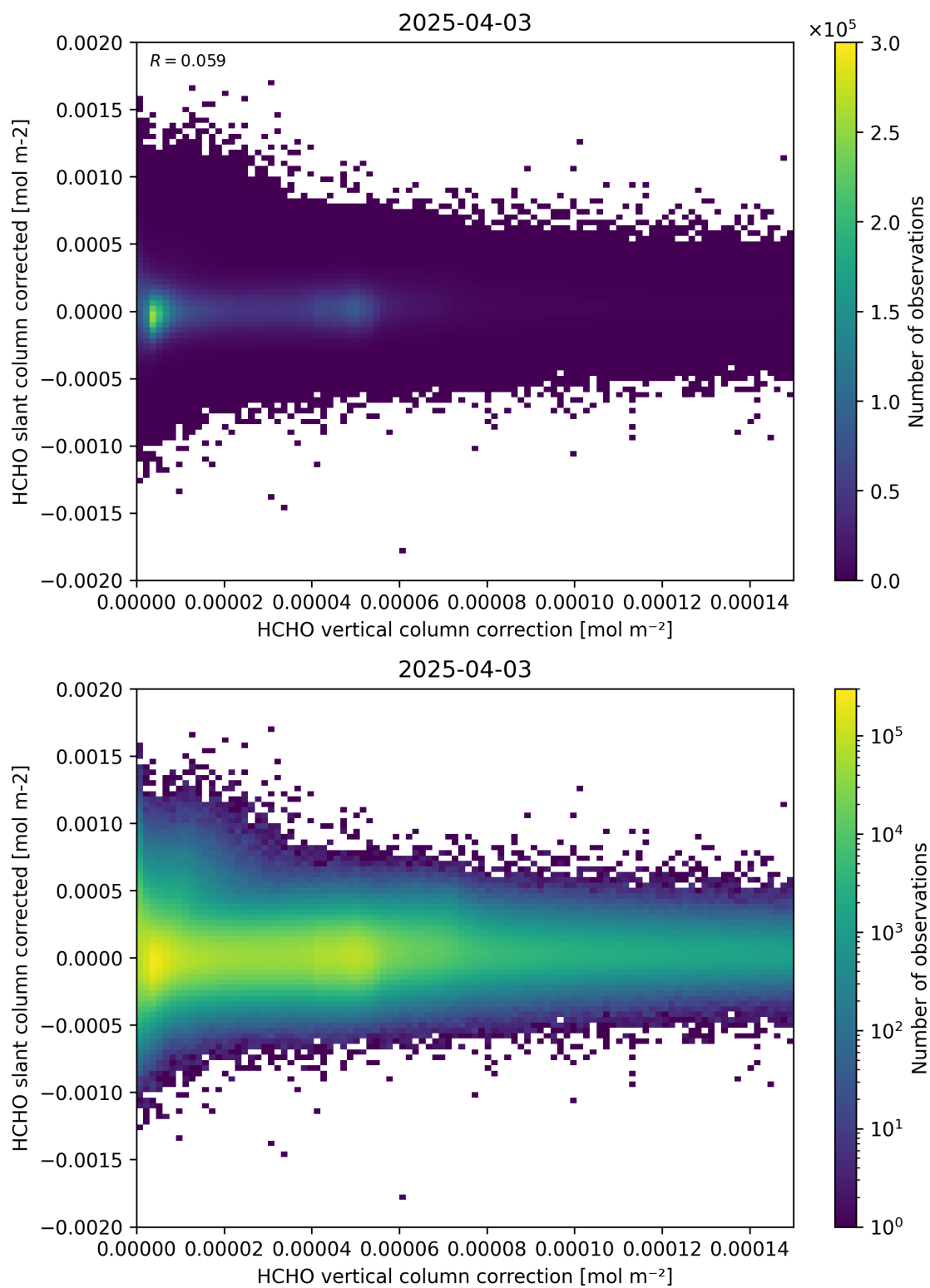
Figure 116: Scatter density plot of “HCHO vertical column correction” against “HCHO slant column corrected” for 2025-04-03 to 2025-04-04.
