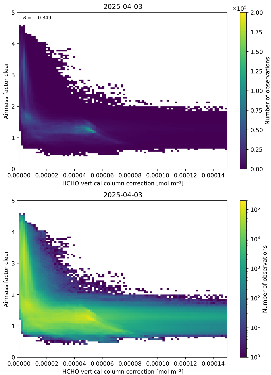
Figure 115: Scatter density plot of “HCHO vertical column correction” against “Airmass factor clear” for 2025-04-03 to 2025-04-04.
