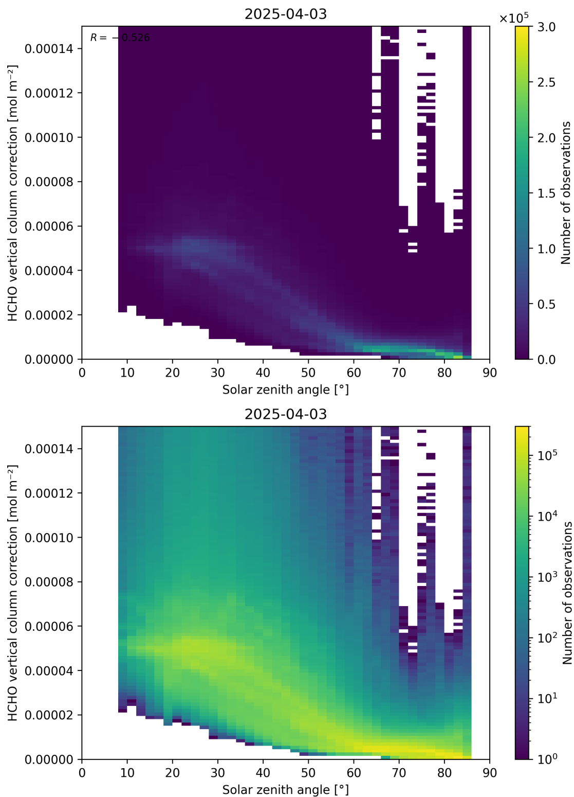
Figure 178: Scatter density plot of “Solar zenith angle” against “HCHO vertical column correction” for 2025-04-03 to 2025-04-04.
