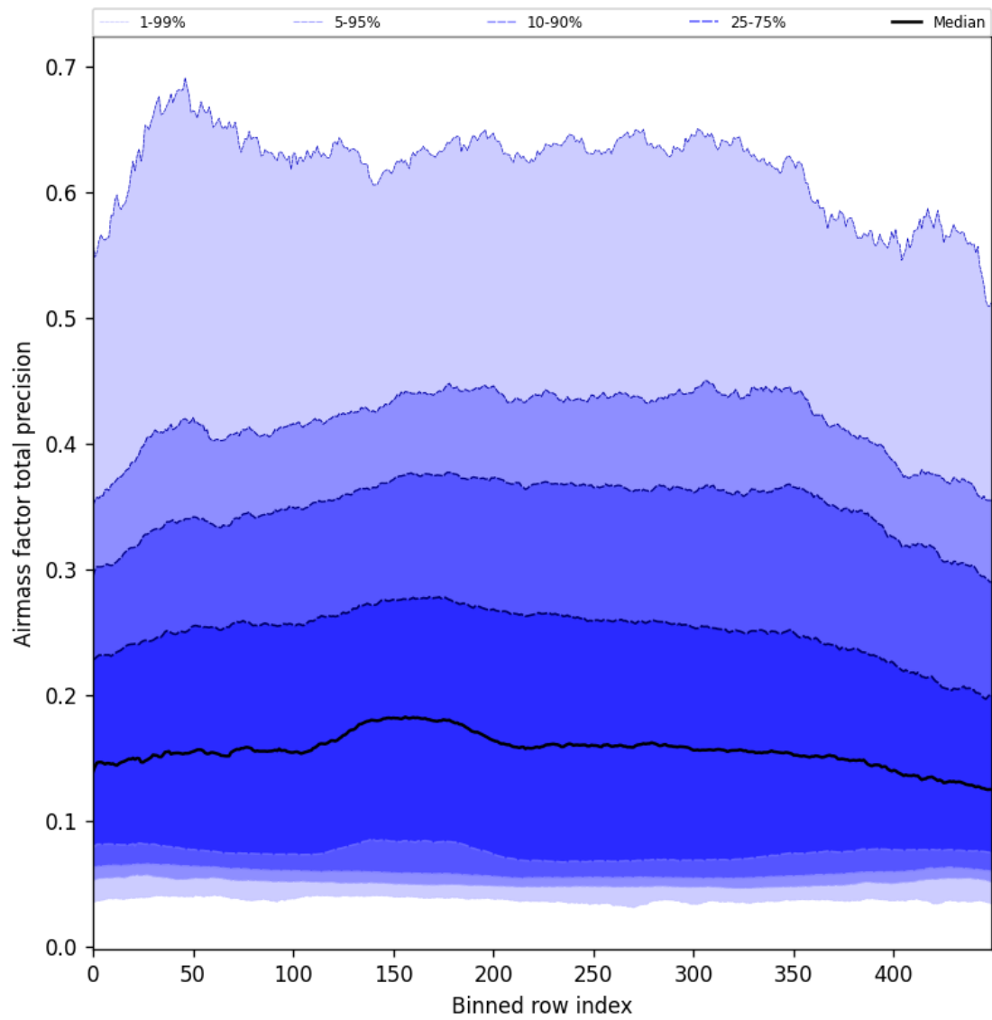
Figure 55: Along track statistics of “Airmass factor total precision” for 2025-04-03 to 2025-04-04
