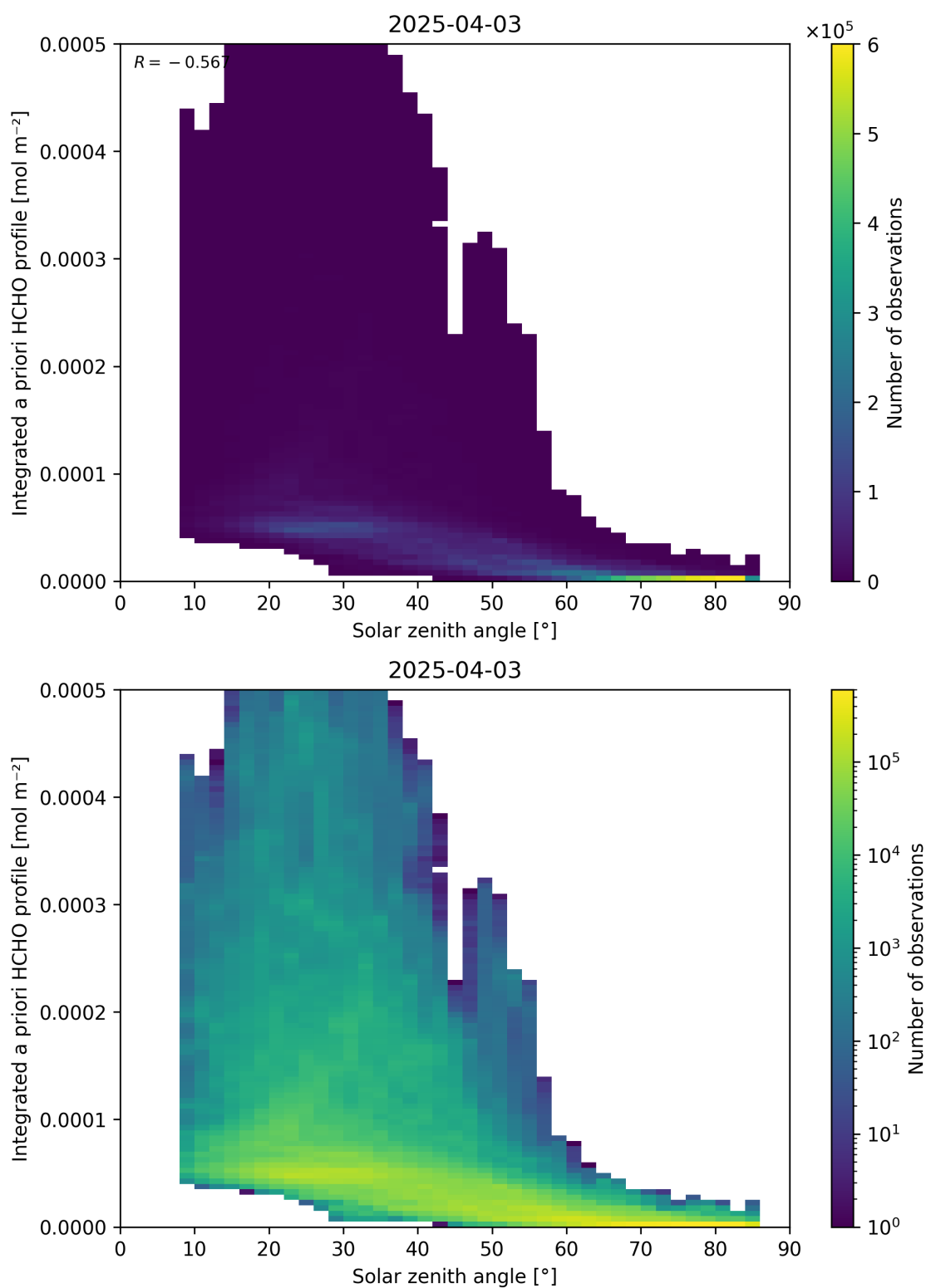
Figure 180: Scatter density plot of “Solar zenith angle” against “Integrated a priori HCHO profile” for 2025-04-03 to 2025-04-04.
