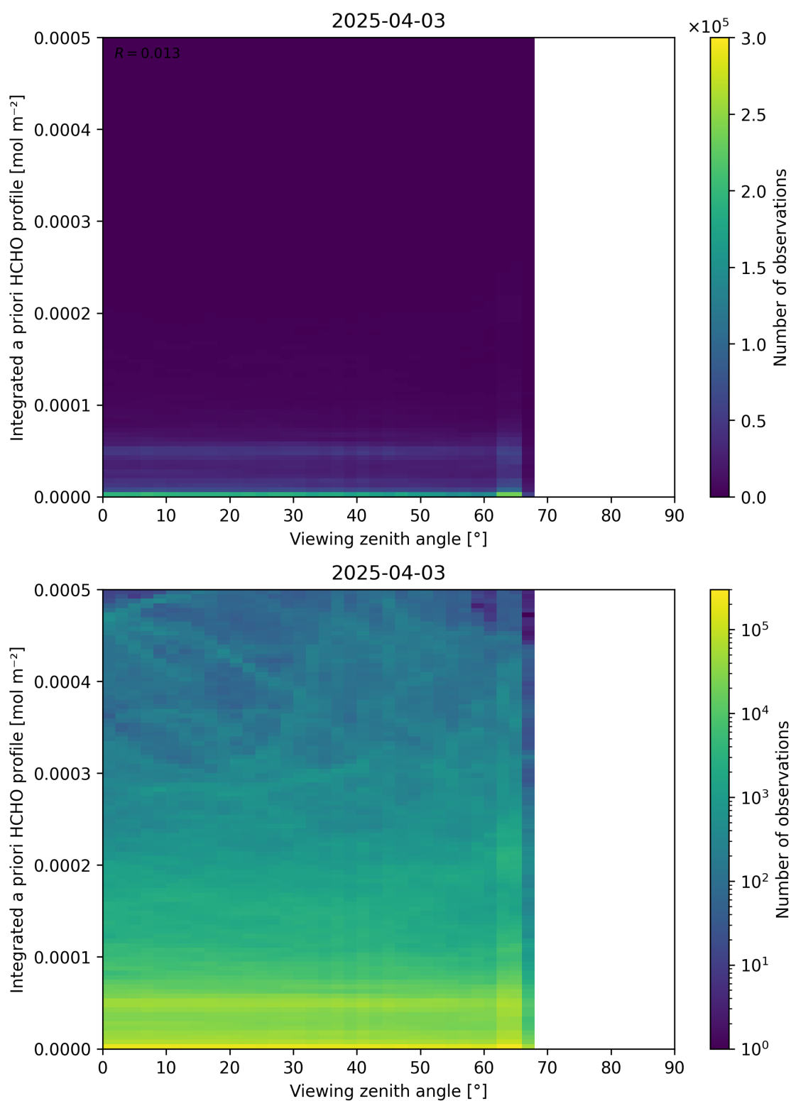
Figure 195: Scatter density plot of “Viewing zenith angle” against “Integrated a priori HCHO profile” for 2025-04-03 to 2025-04-04.
