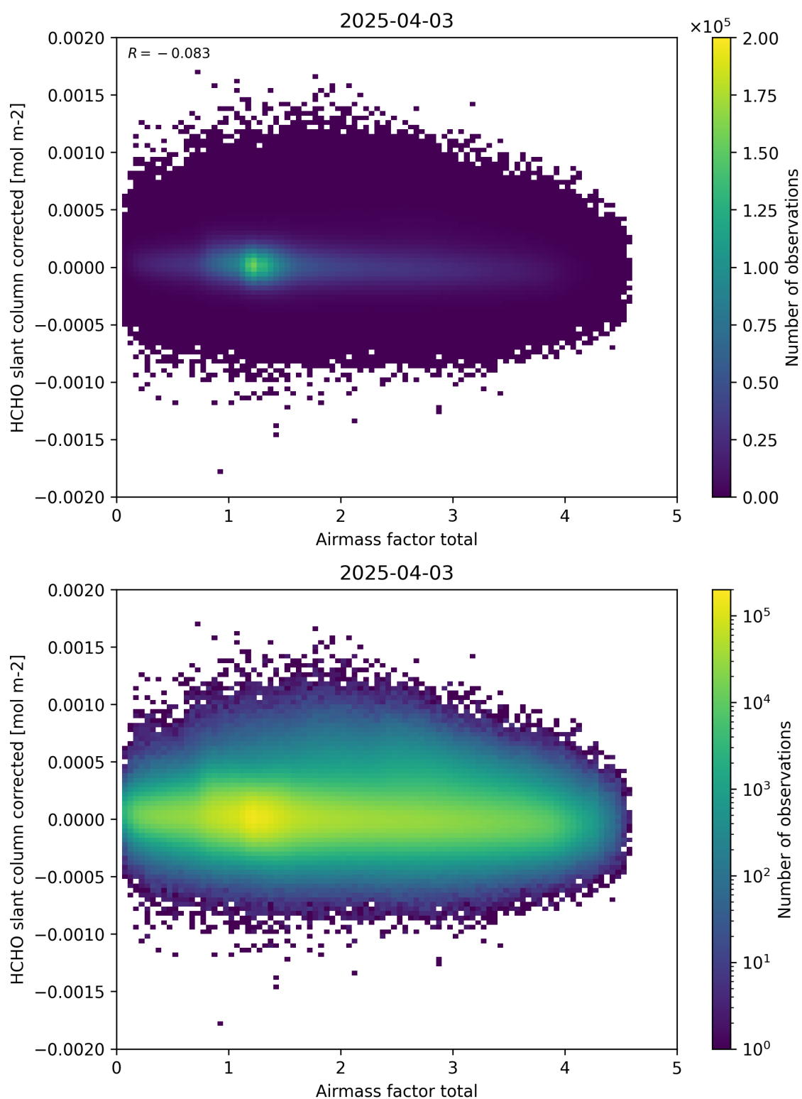
Figure 101: Scatter density plot of “Airmass factor total” against “HCHO slant column corrected” for 2025-04-03 to 2025-04-04.
