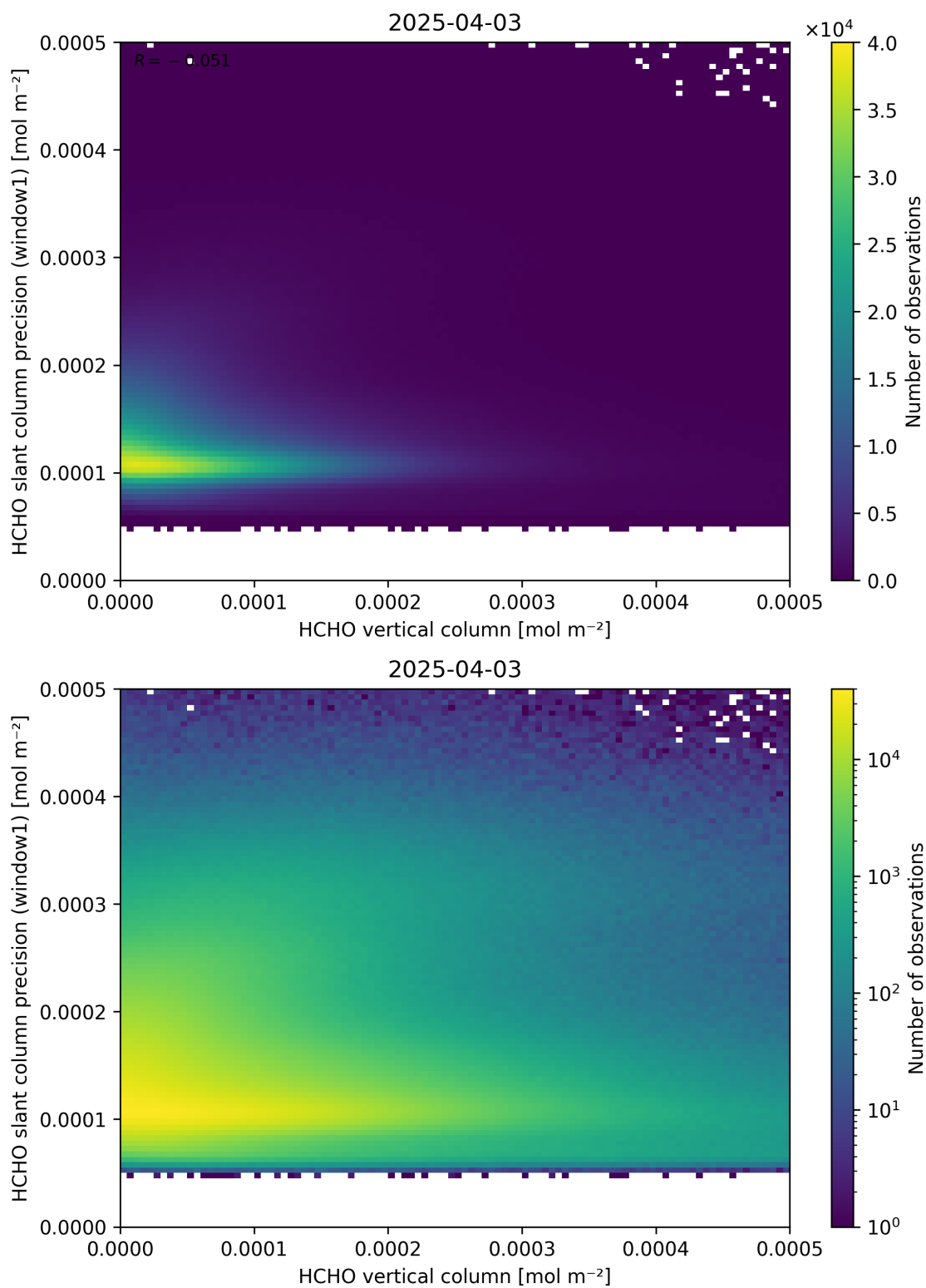
Figure 130: Scatter density plot of “HCHO vertical column” against “HCHO slant column precision (window1)” for 2025-04-03 to 2025-04-04.
