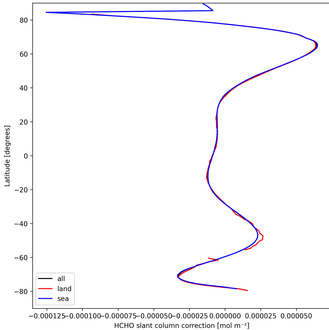
Figure 33: Zonal average of "HCHO slant column correction" for 2025-04-03 to 2025-04-04.
