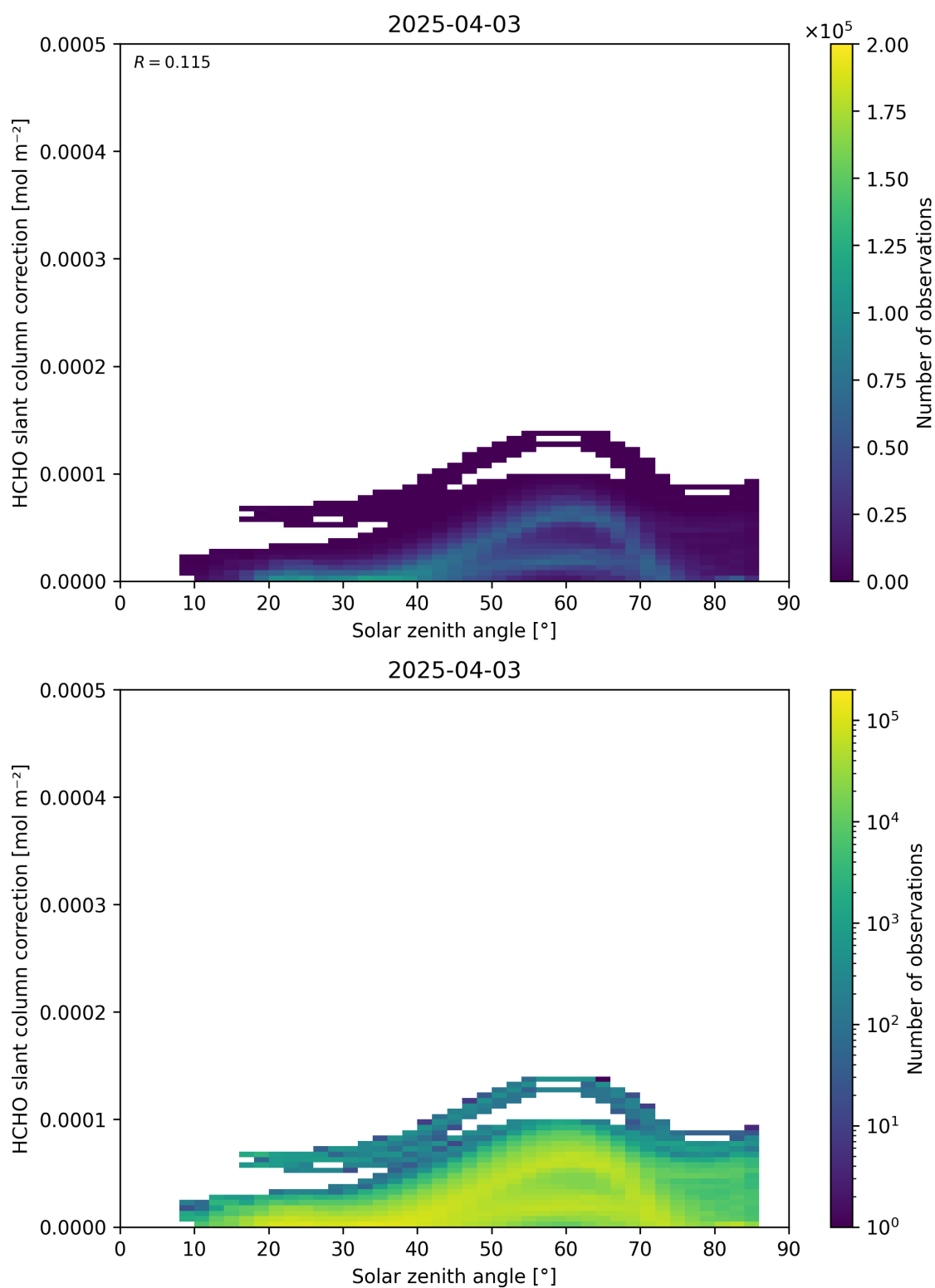
Figure 172: Scatter density plot of “Solar zenith angle” against “HCHO slant column correction” for 2025-04-03 to 2025-04-04.
