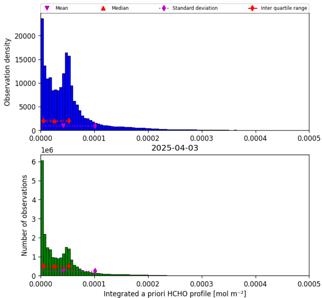
Figure 43: Histogram of “Integrated a priori HCHO profile” for 2025-04-03 to 2025-04-04
