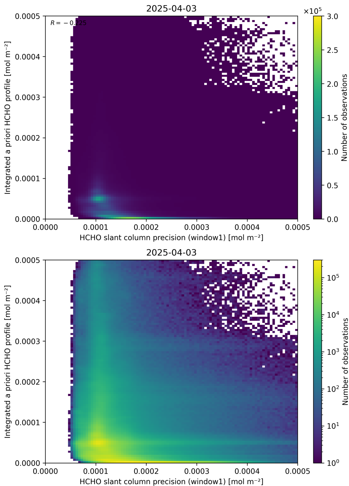
Figure 96: Scatter density plot of “HCHO slant column precision (window1)” against “Integrated a priori HCHO profile” for 2025-04-03 to 2025-04-04.
