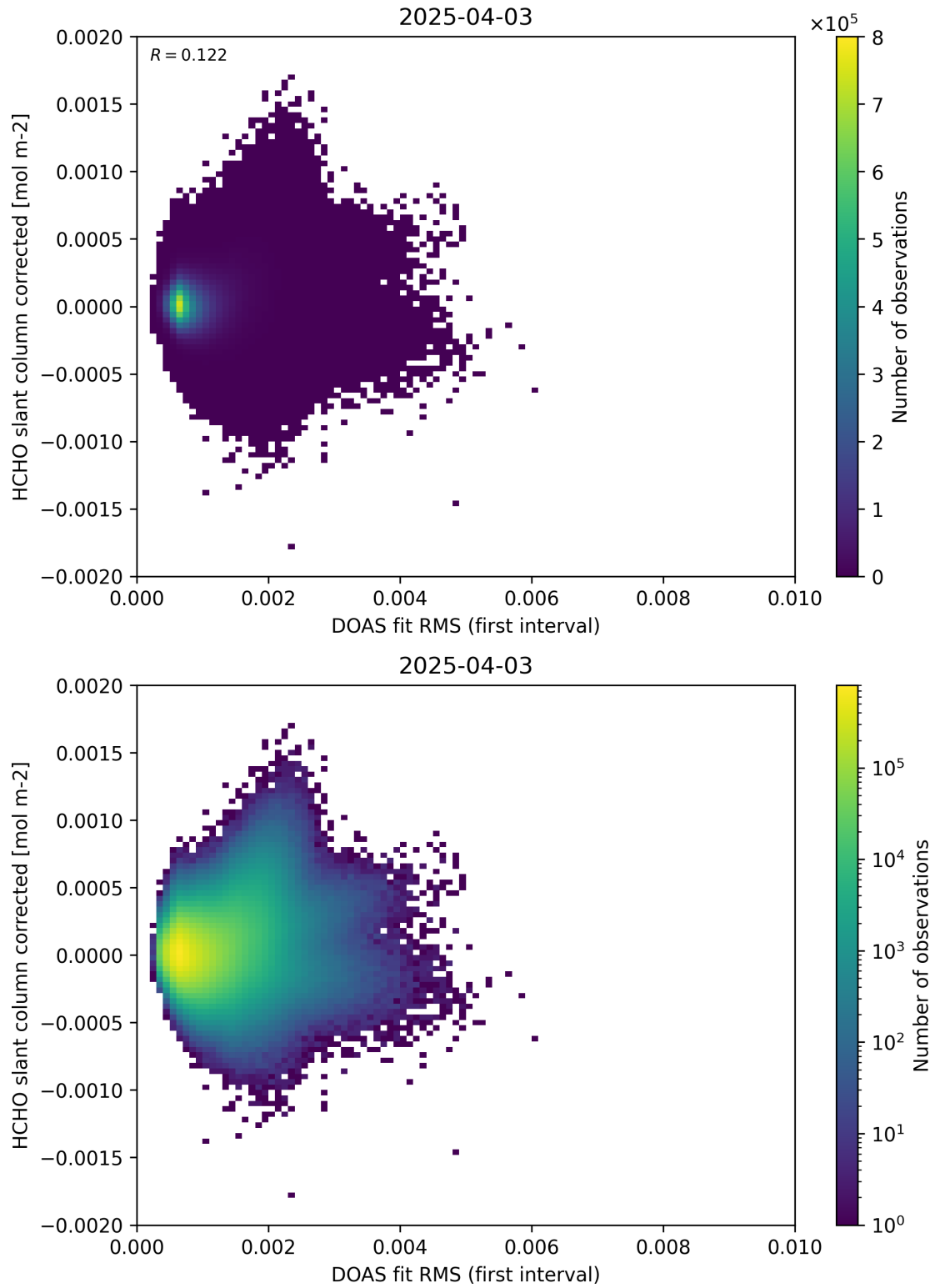
Figure 62: Scatter density plot of “DOAS fit RMS (first interval)” against “HCHO slant column corrected” for 2025-04-03 to 2025-04-04.
