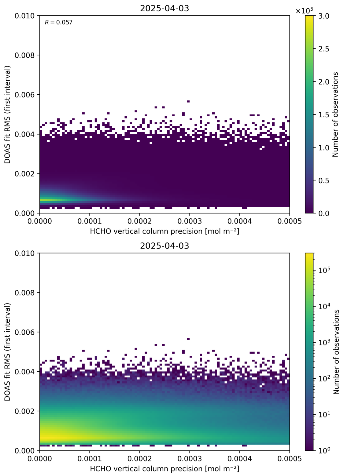
Figure 136: Scatter density plot of “HCHO vertical column precision” against “DOAS fit RMS (first interval)” for 2025-04-03 to 2025-04-04.
