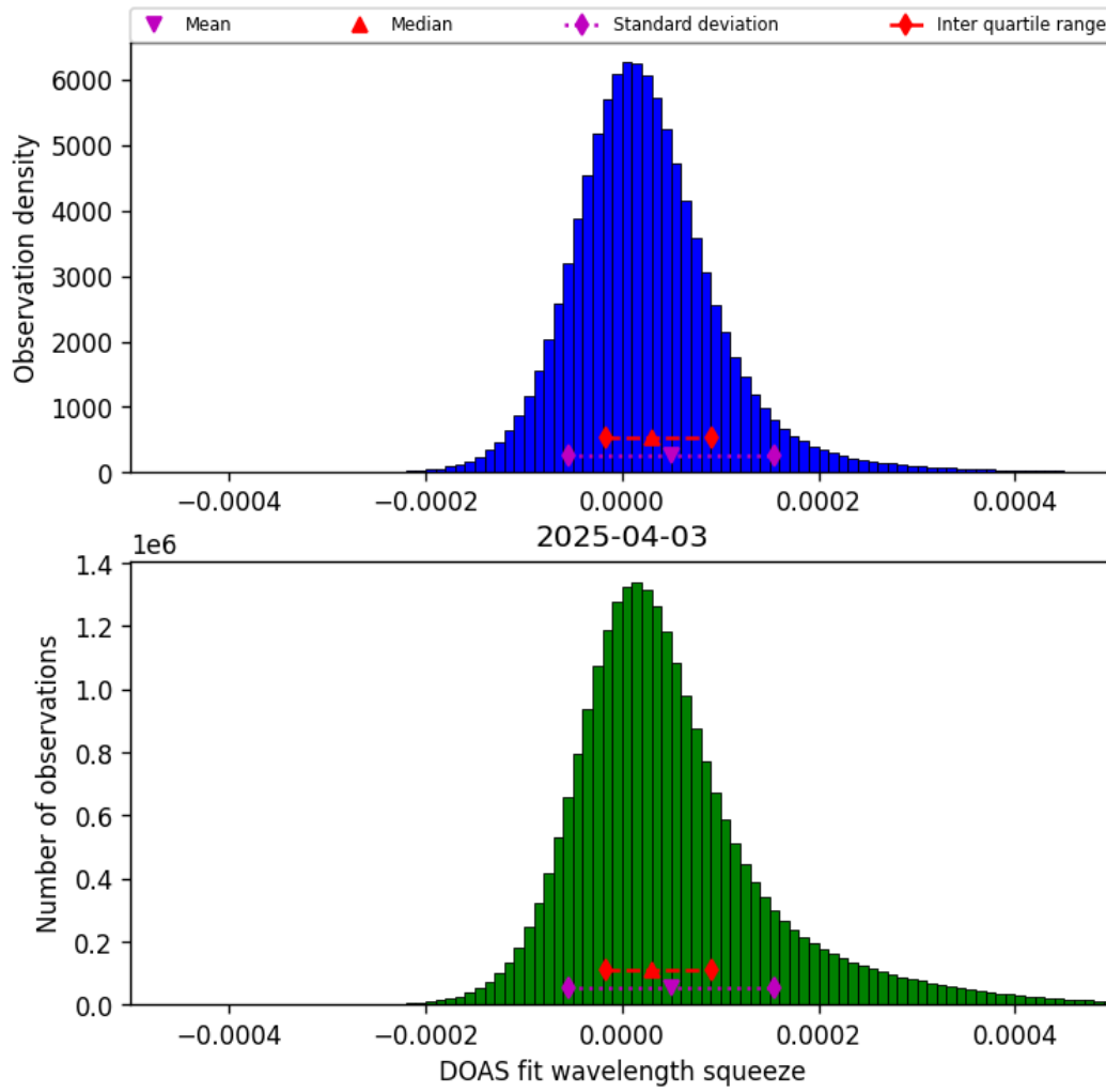
Figure 45: Histogram of “DOAS fit wavelength squeeze” for 2025-04-03 to 2025-04-04
