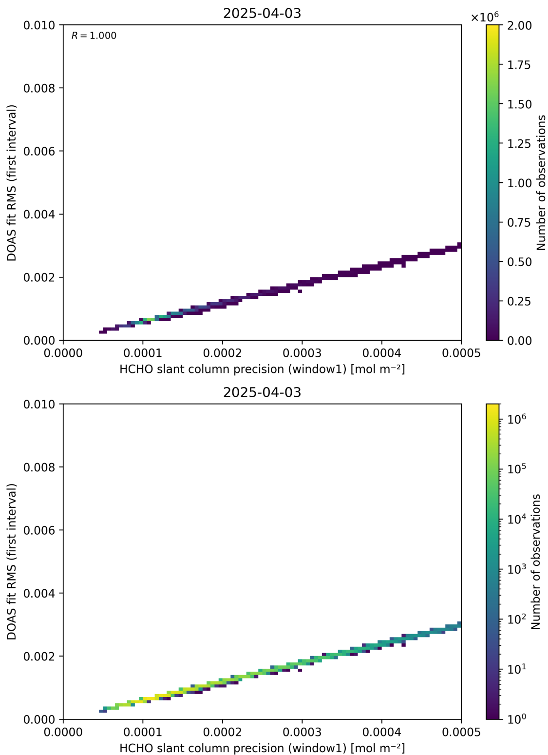
Figure 88: Scatter density plot of “HCHO slant column precision (window1)” against “DOAS fit RMS (first interval)” for 2025-04-03 to 2025-04-04.
