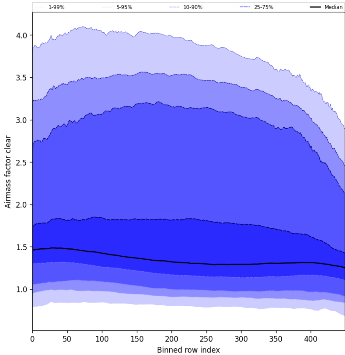
Figure 56: Along track statistics of “Airmass factor clear” for 2025-04-03 to 2025-04-04
