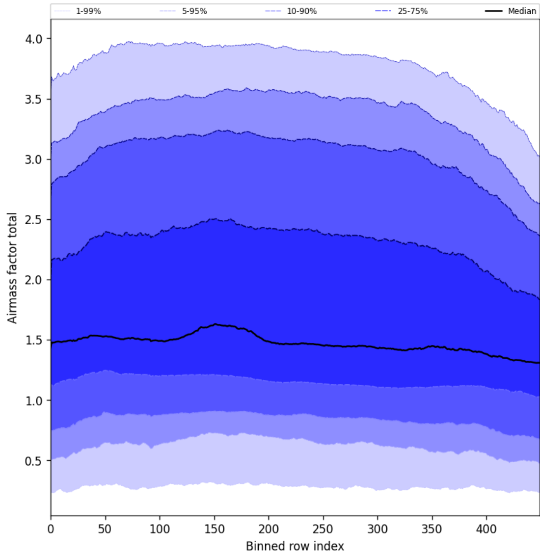
Figure 54: Along track statistics of “Airmass factor total” for 2025-04-03 to 2025-04-04
