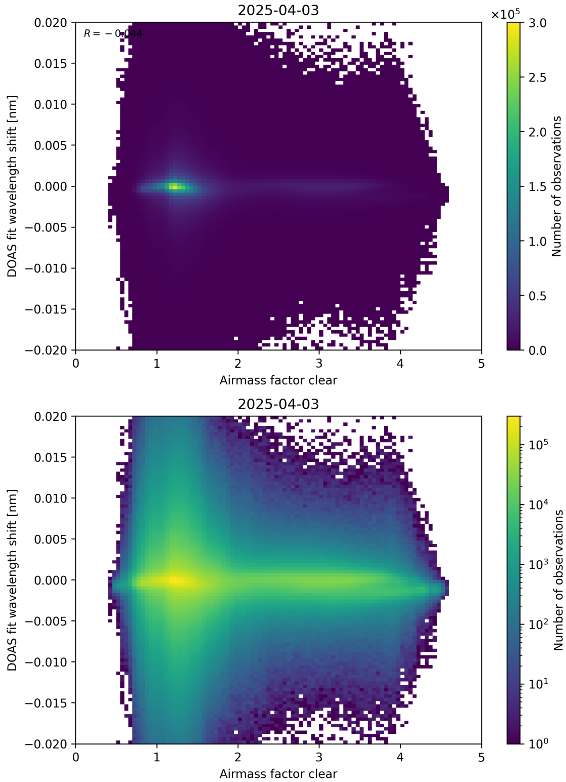
Figure 72: Scatter density plot of “Airmass factor clear” against “DOAS fit wavelength shift” for 2025-04-03 to 2025-04-04.
