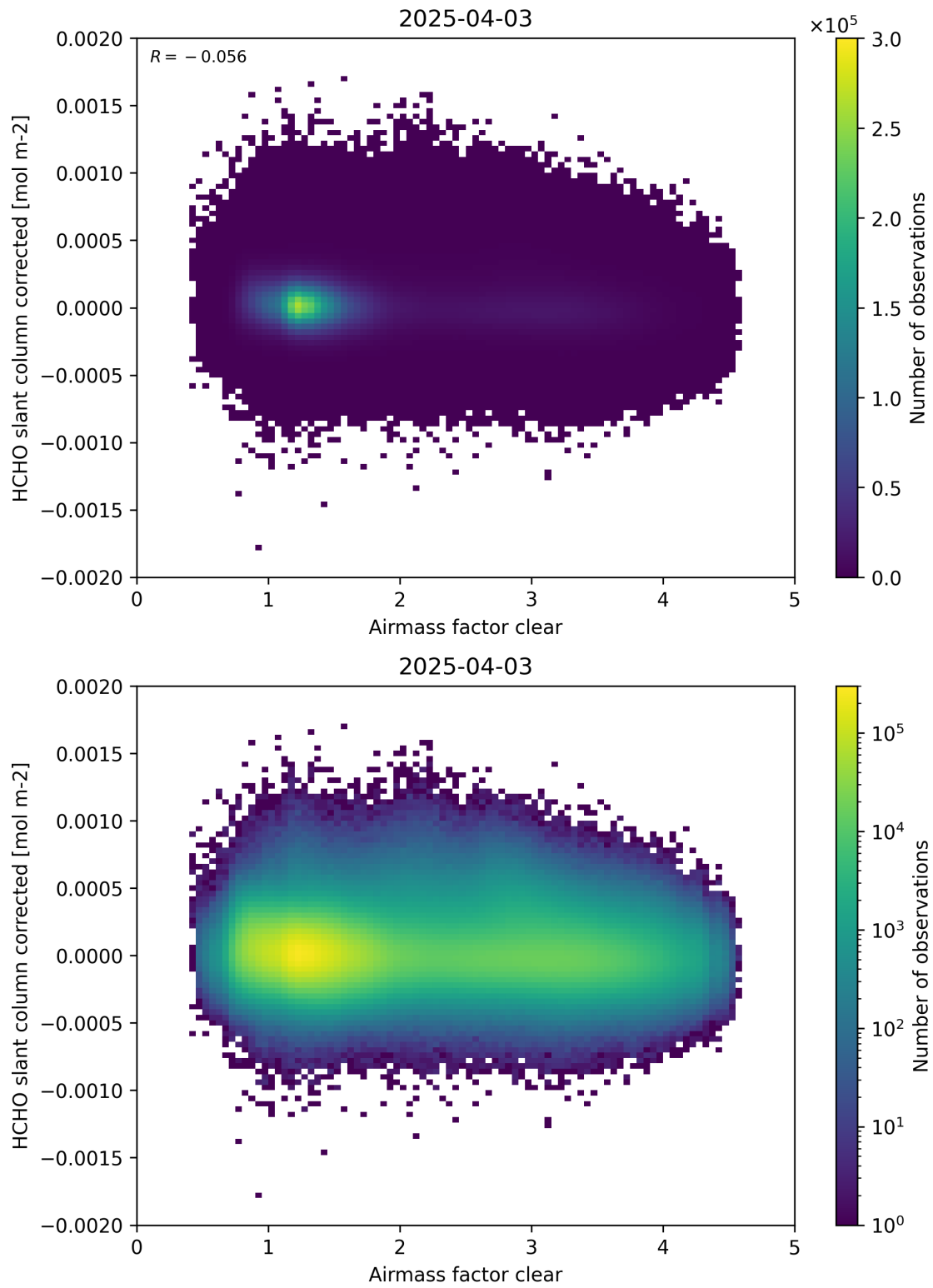
Figure 74: Scatter density plot of “Airmass factor clear” against “HCHO slant column corrected” for 2025-04-03 to 2025-04-04.
