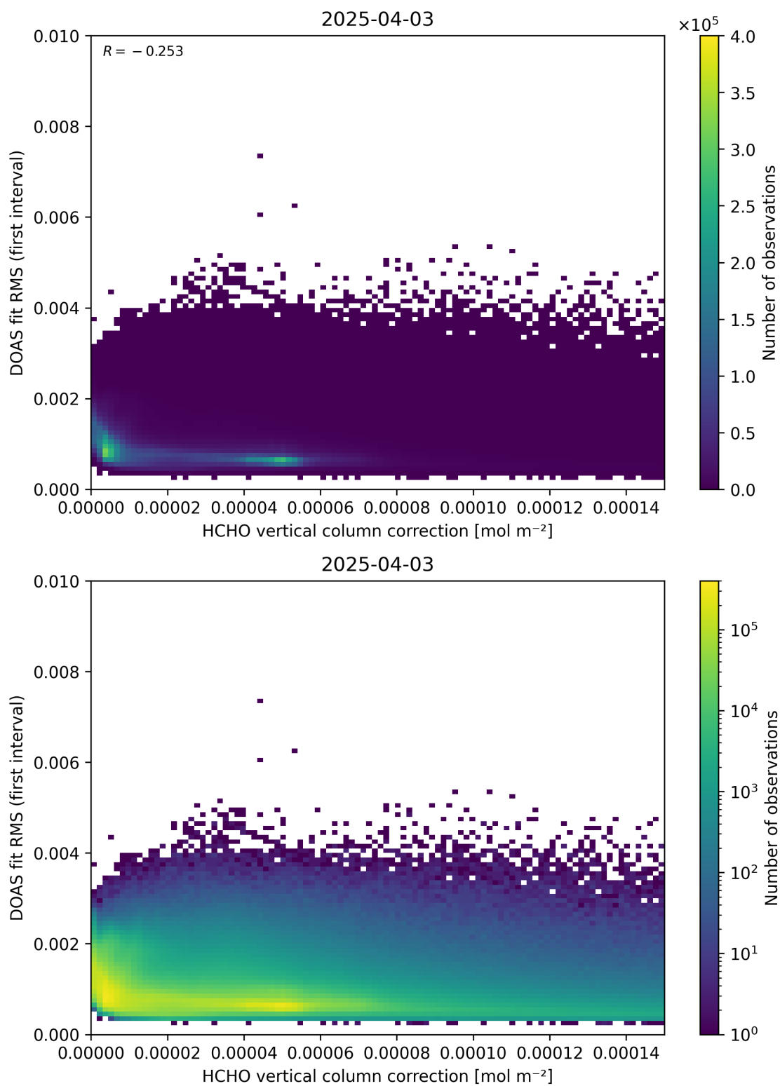
Figure 112: Scatter density plot of “HCHO vertical column correction” against “DOAS fit RMS (first interval)” for 2025-04-03 to 2025-04-04.
