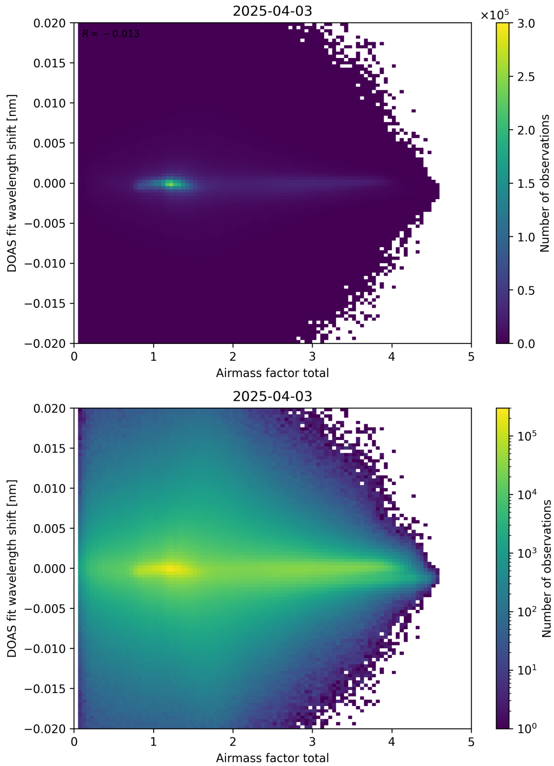
Figure 98: Scatter density plot of “Airmass factor total” against “DOAS fit wavelength shift” for 2025-04-03 to 2025-04-04.
