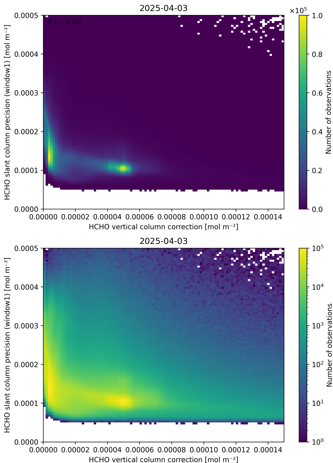
Figure 119: Scatter density plot of “HCHO vertical column correction” against “HCHO slant column precision (window1)” for 2025-04-03 to 2025-04-04.
