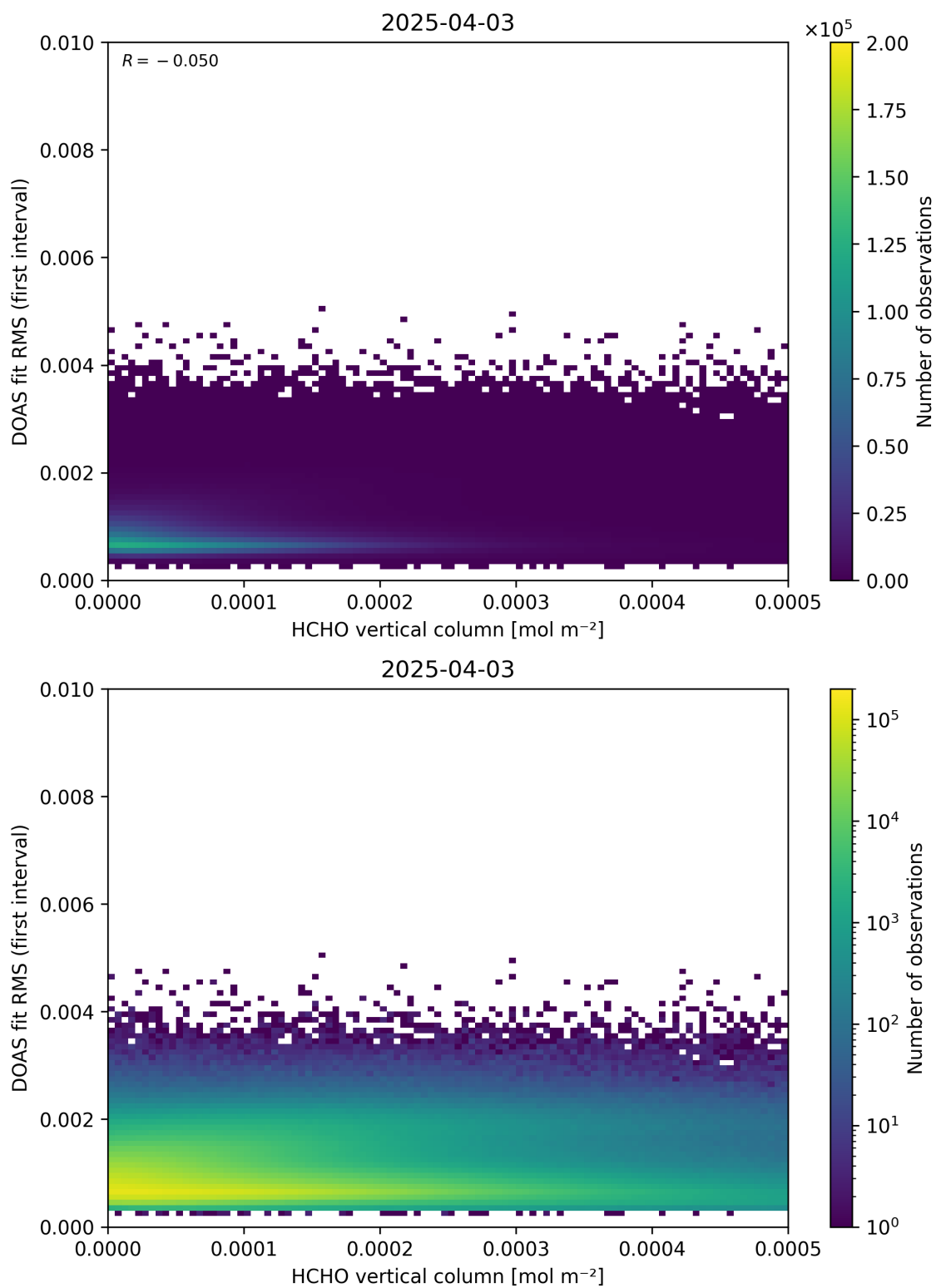
Figure 123: Scatter density plot of “HCHO vertical column” against “DOAS fit RMS (first interval)” for 2025-04-03 to 2025-04-04.
