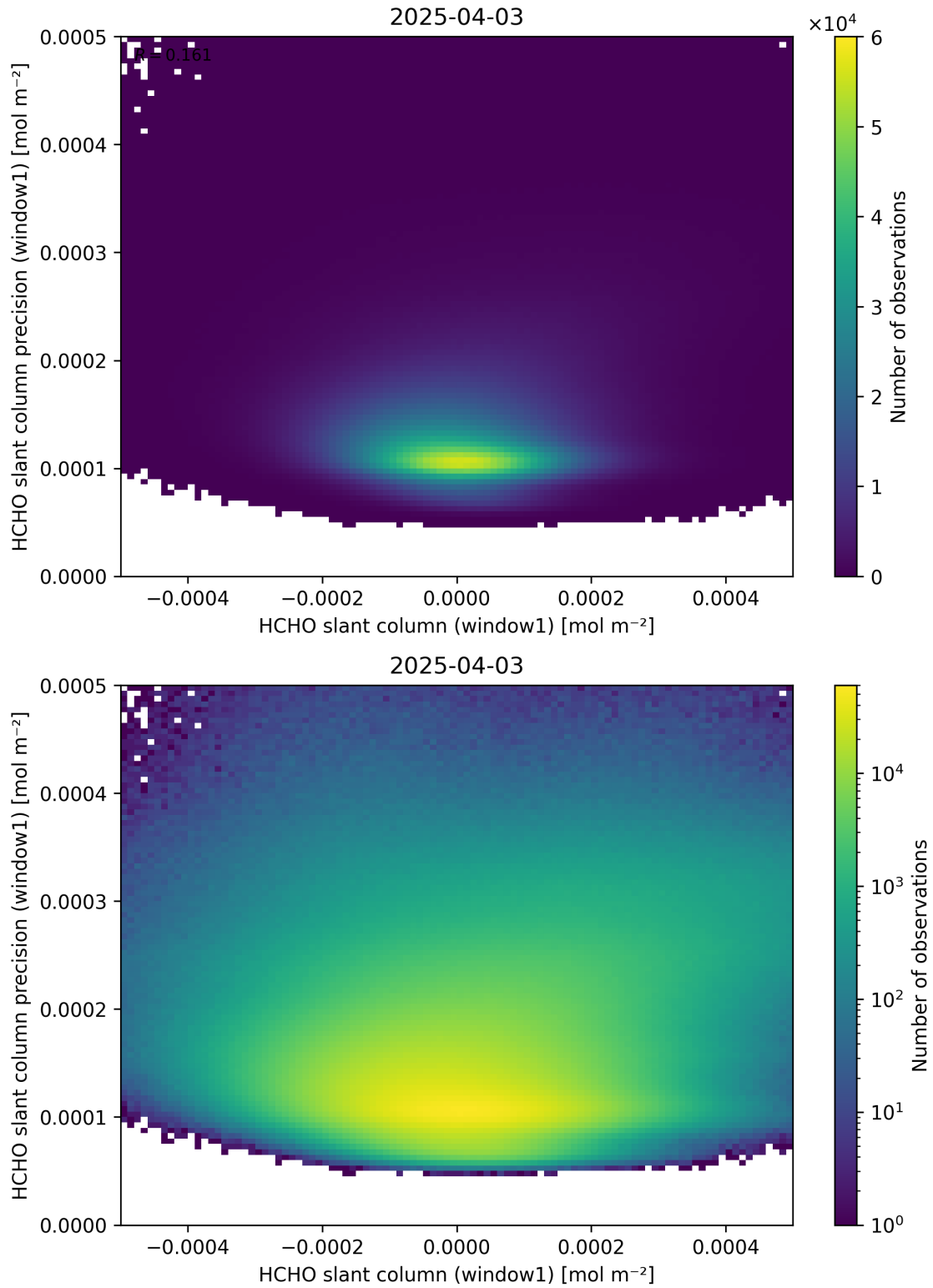
Figure 84: Scatter density plot of “HCHO slant column (window1)” against “HCHO slant column precision (window1)” for 2025-04-03 to 2025-04-04.
