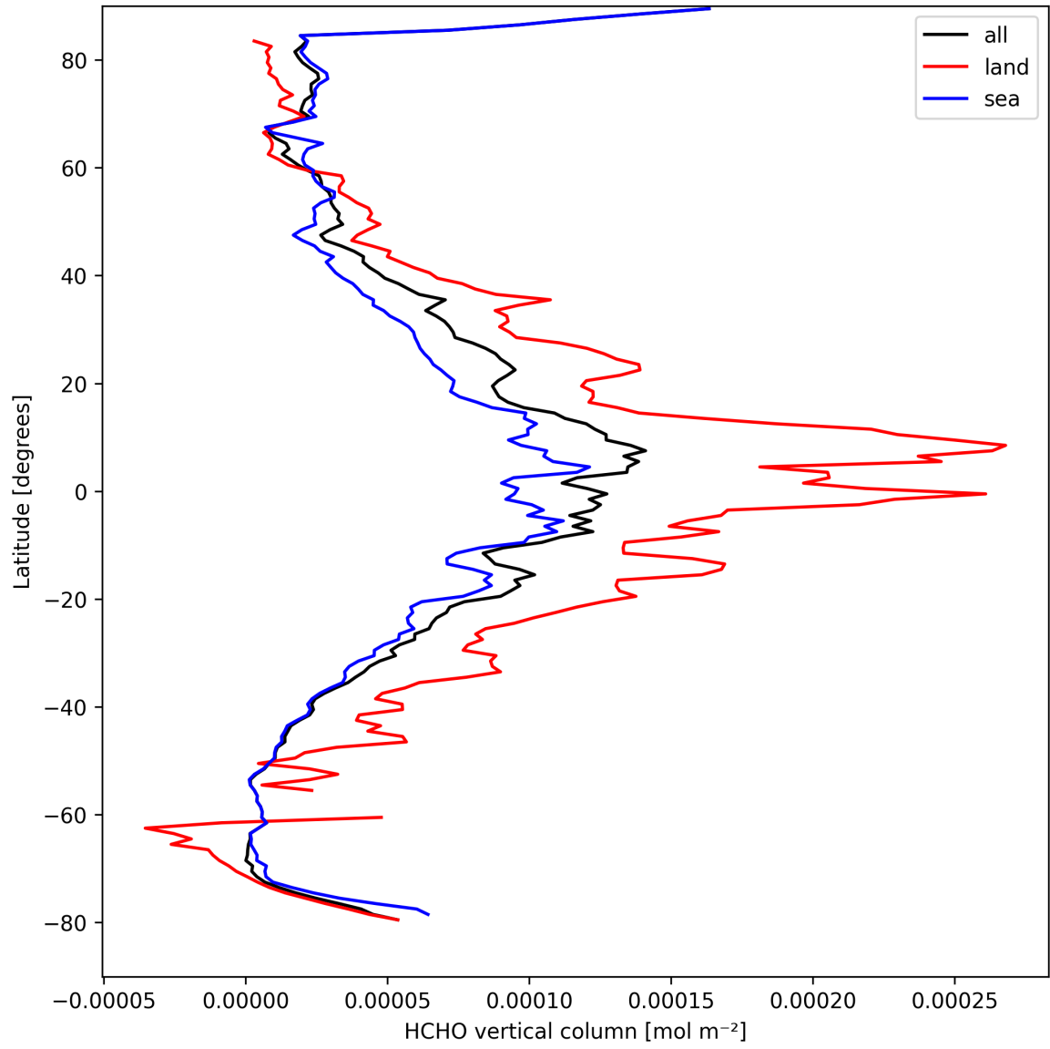
Figure 21: Zonal average of “HCHO vertical column” for 2025-04-03 to 2025-04-04.
