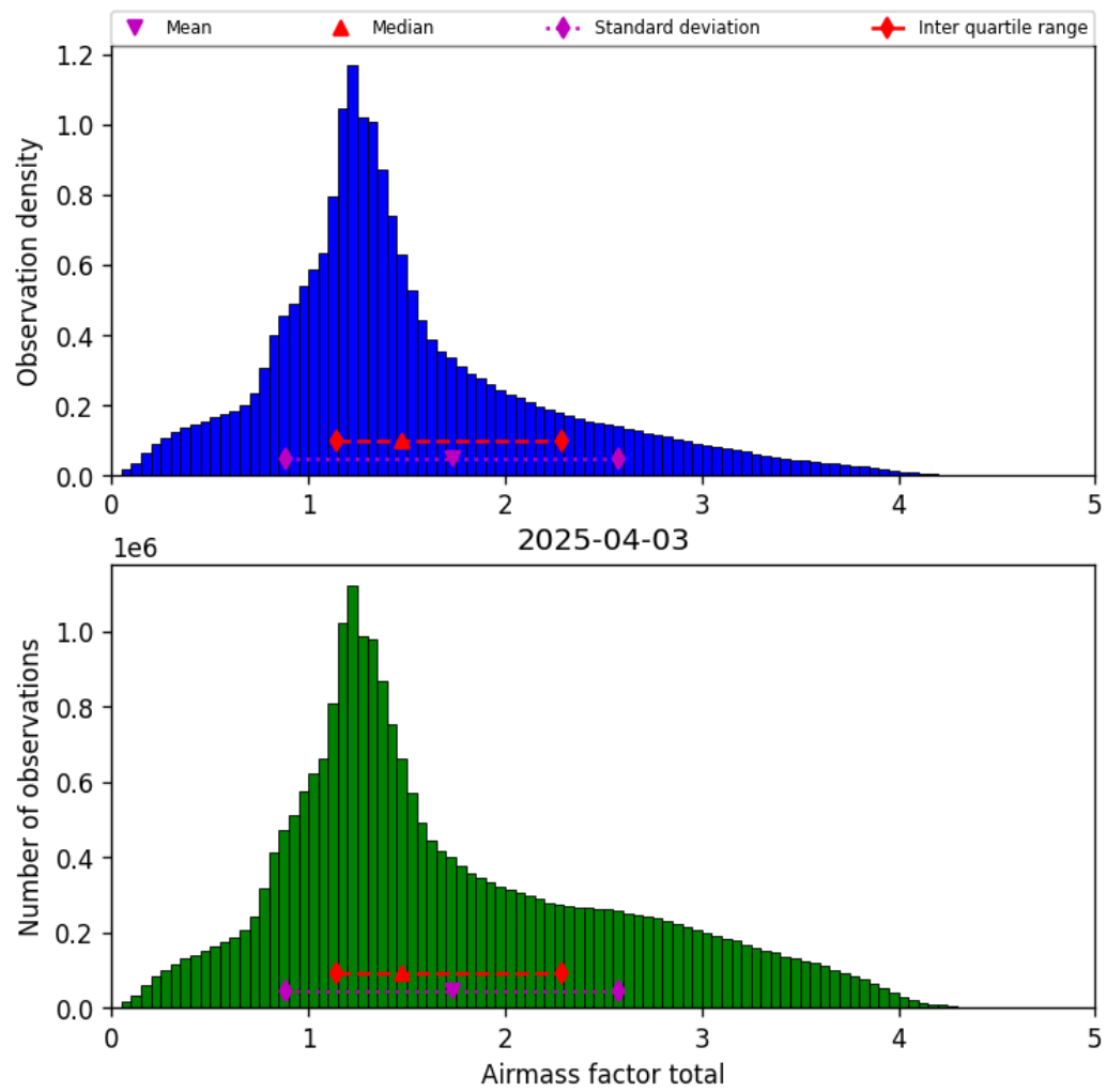
Figure 40: Histogram of “Airmass factor total” for 2025-04-03 to 2025-04-04
