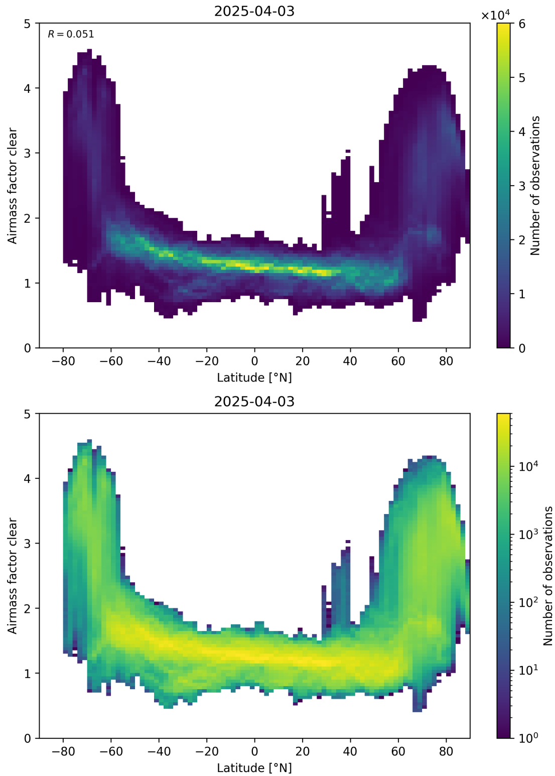
Figure 156: Scatter density plot of “Latitude” against “Airmass factor clear” for 2025-04-03 to 2025-04-04.
