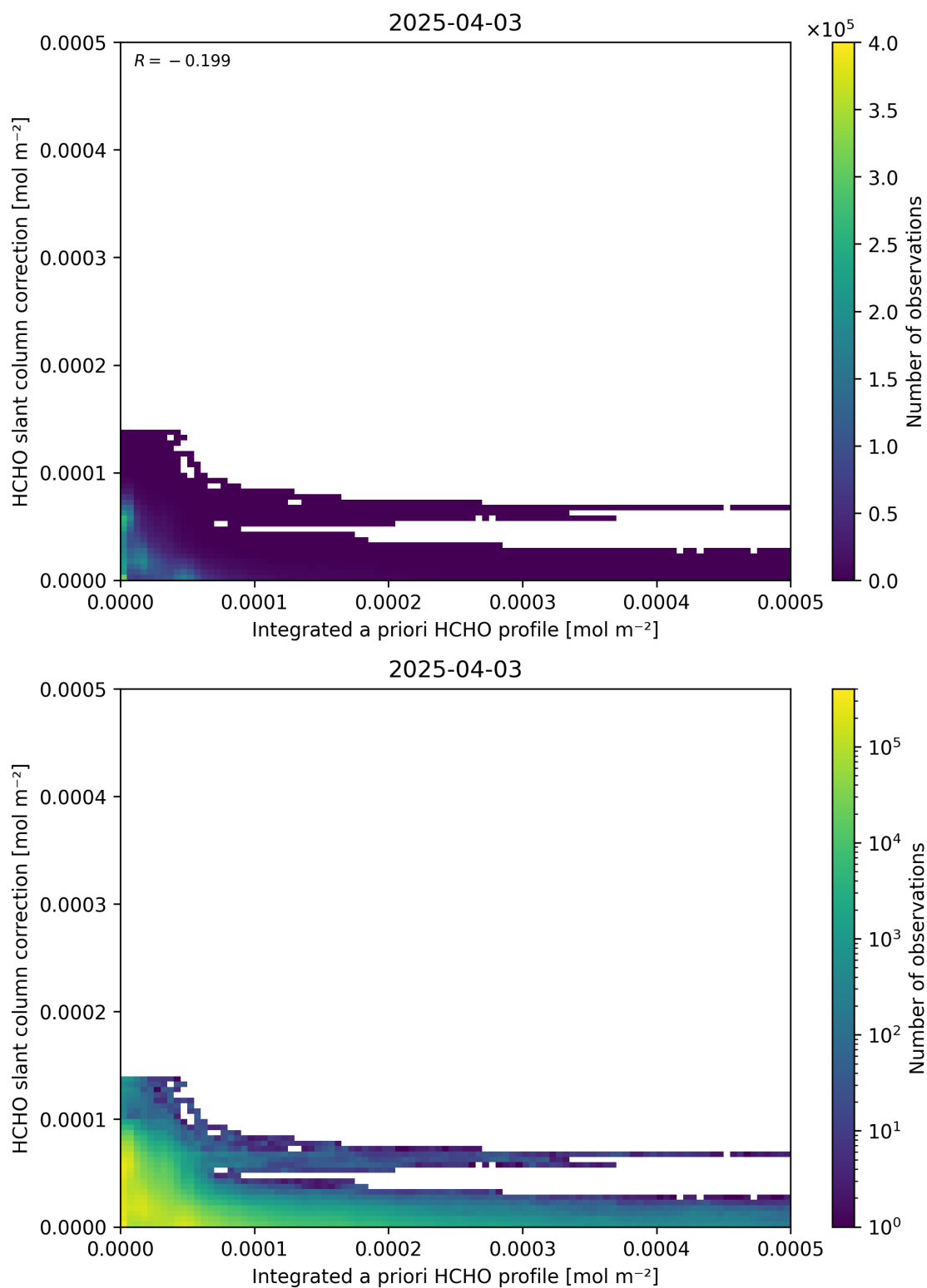
Figure 152: Scatter density plot of “Integrated a priori HCHO profile” against “HCHO slant column correction” for 2025-04-03 to 2025-04-04.
