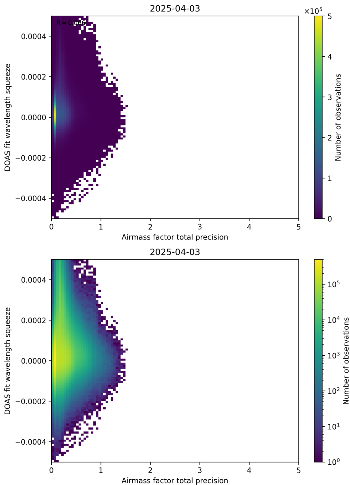
Figure 107: Scatter density plot of “Airmass factor total precision” against “DOAS fit wavelength squeeze” for 2025-04-03 to 2025-04-04.
