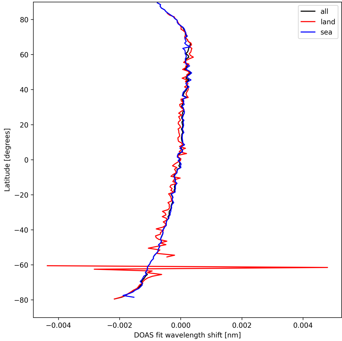
Figure 30: Zonal average of “DOAS fit wavelength shift” for 2025-04-03 to 2025-04-04.
