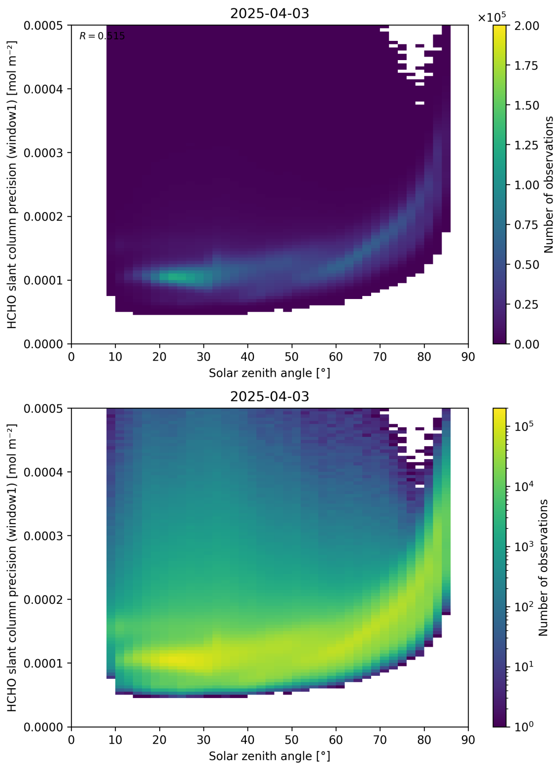
Figure 174: Scatter density plot of “Solar zenith angle” against “HCHO slant column precision (window1)” for 2025-04-03 to 2025-04-04.
