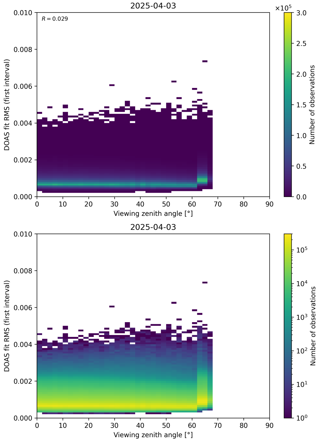
Figure 182: Scatter density plot of “Viewing zenith angle” against “DOAS fit RMS (first interval)” for 2025-04-03 to 2025-04-04.
