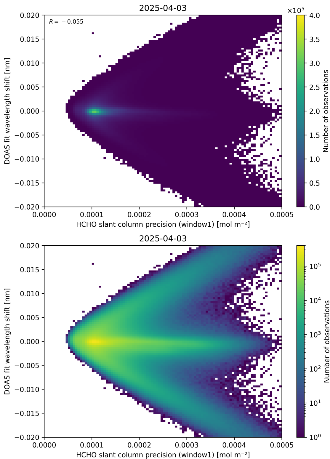
Figure 89: Scatter density plot of “HCHO slant column precision (window1)” against “DOAS fit wavelength shift” for 2025-04-03 to 2025-04-04.
