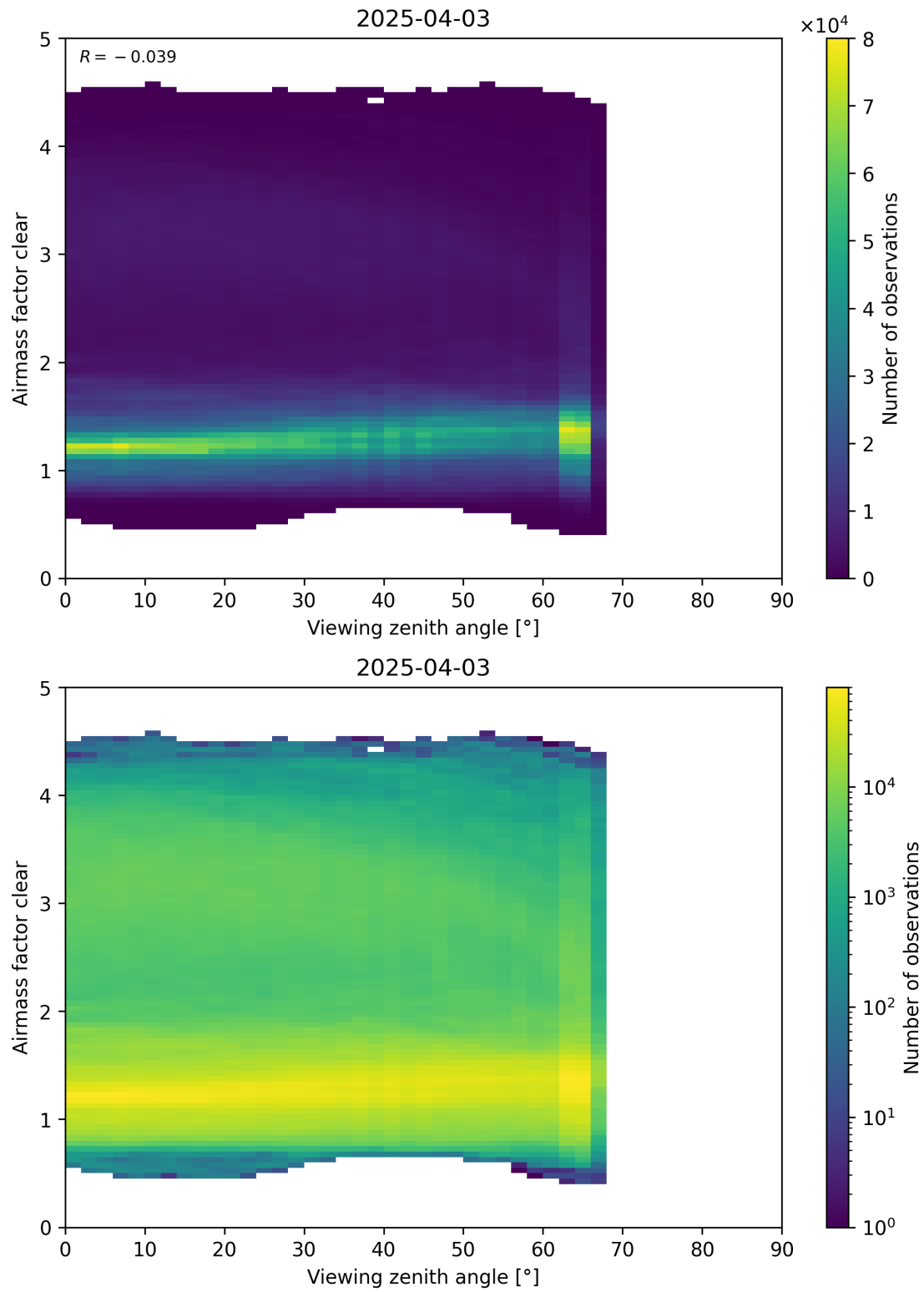
Figure 185: Scatter density plot of “Viewing zenith angle” against “Airmass factor clear” for 2025-04-03 to 2025-04-04.
