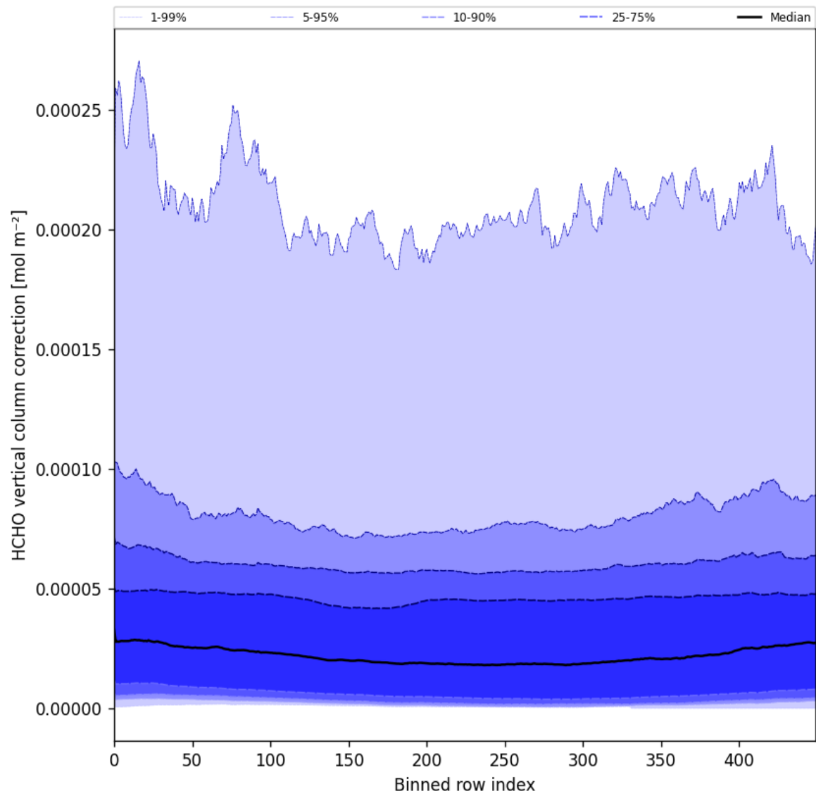
Figure 51: Along track statistics of “HCHO vertical column correction” for 2025-04-03 to 2025-04-04
