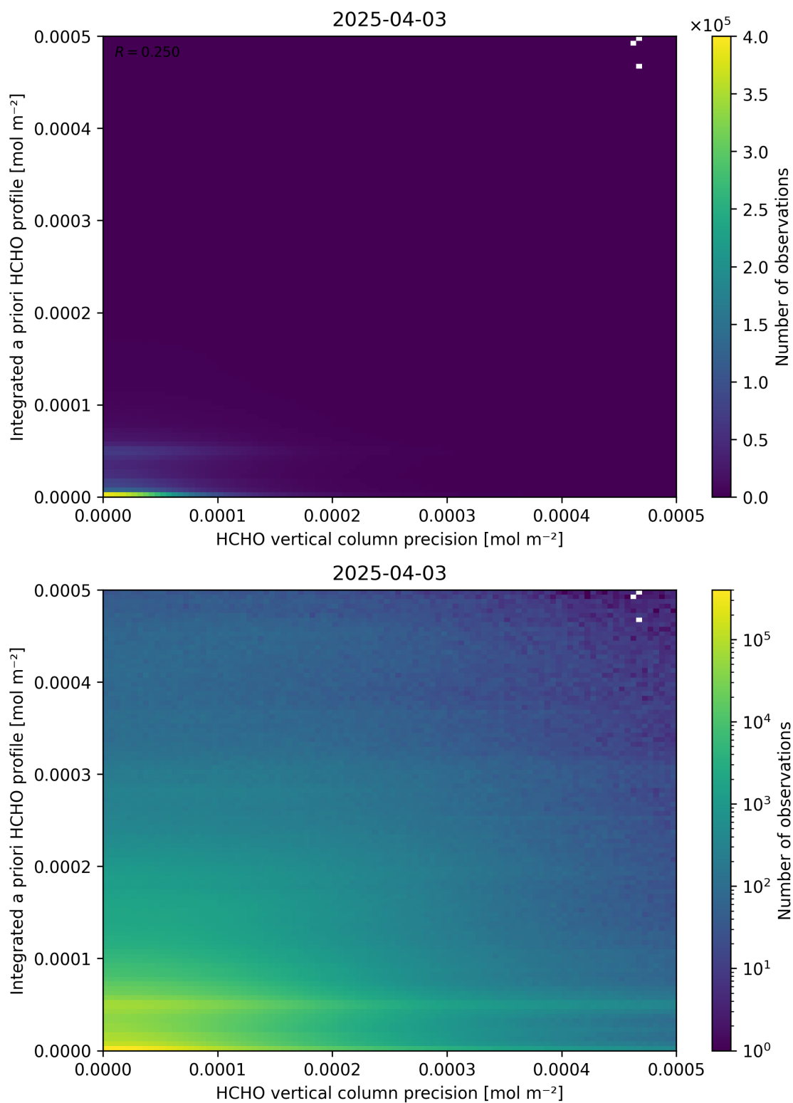
Figure 147: Scatter density plot of “HCHO vertical column precision” against “Integrated a priori HCHO profile” for 2025-04-03 to 2025-04-04.
