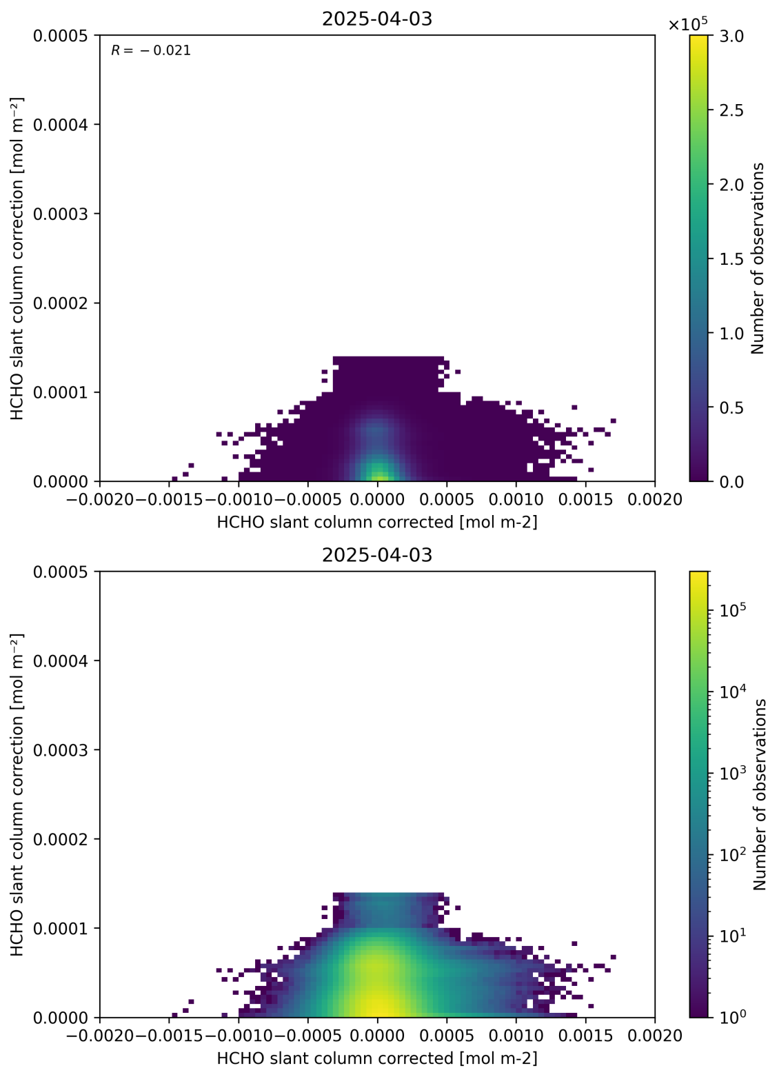
Figure 77: Scatter density plot of “HCHO slant column corrected” against “HCHO slant column correction” for 2025-04-03 to 2025-04-04.
