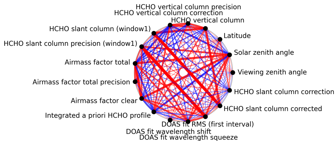
Figure 1: Map of correlation graph for 2025-04-03 to 2025-04-04.
