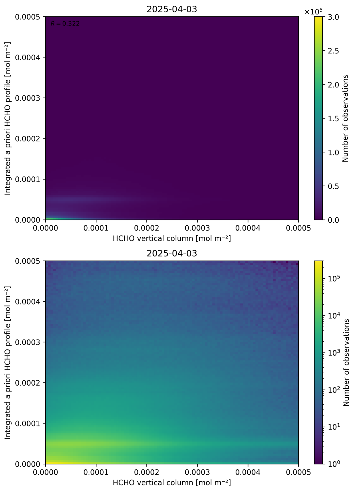
Figure 135: Scatter density plot of “HCHO vertical column” against “Integrated a priori HCHO profile” for 2025-04-03 to 2025-04-04.
