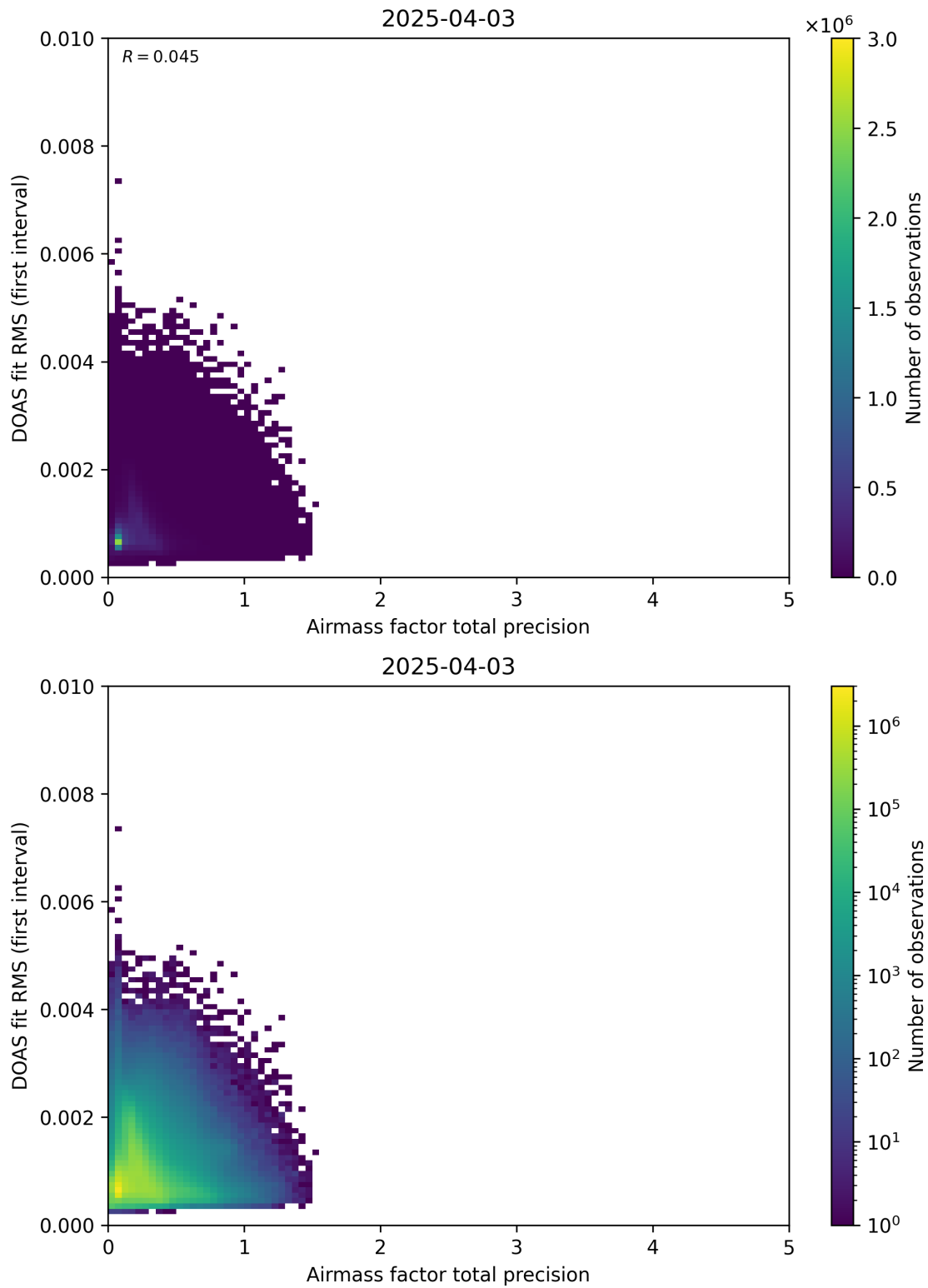
Figure 105: Scatter density plot of “Airmass factor total precision” against “DOAS fit RMS (first interval)” for 2025-04-03 to 2025-04-04.
