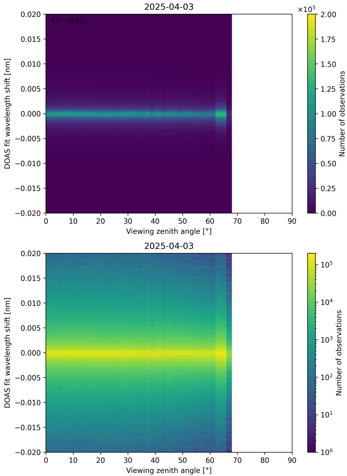
Figure 183: Scatter density plot of “Viewing zenith angle” against “DOAS fit wavelength shift” for 2025-04-03 to 2025-04-04.
