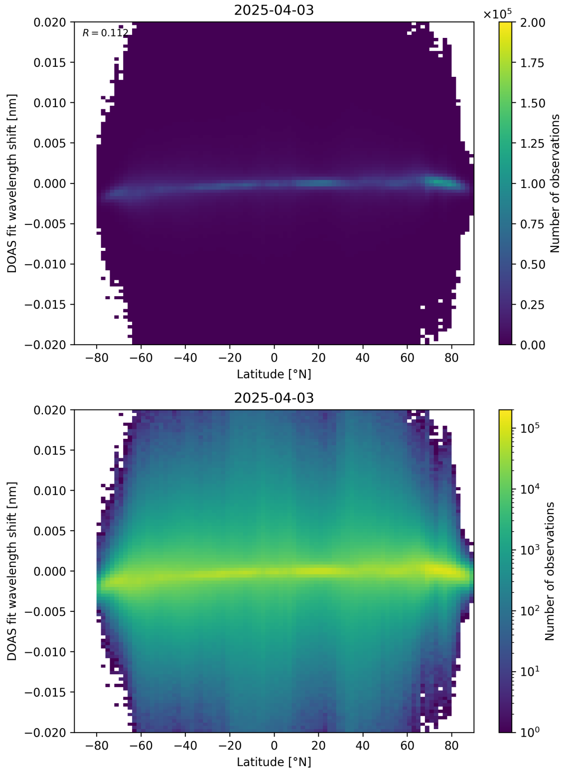
Figure 154: Scatter density plot of “Latitude” against “DOAS fit wavelength shift” for 2025-04-03 to 2025-04-04.
