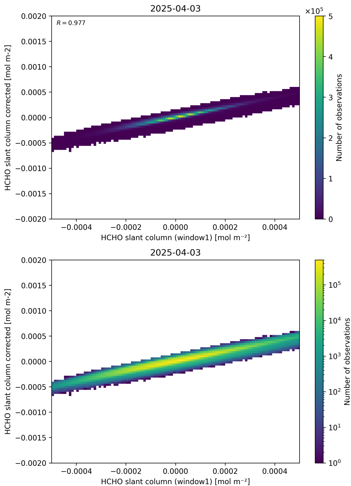
Figure 82: Scatter density plot of “HCHO slant column (window1)” against “HCHO slant column corrected” for 2025-04-03 to 2025-04-04.
