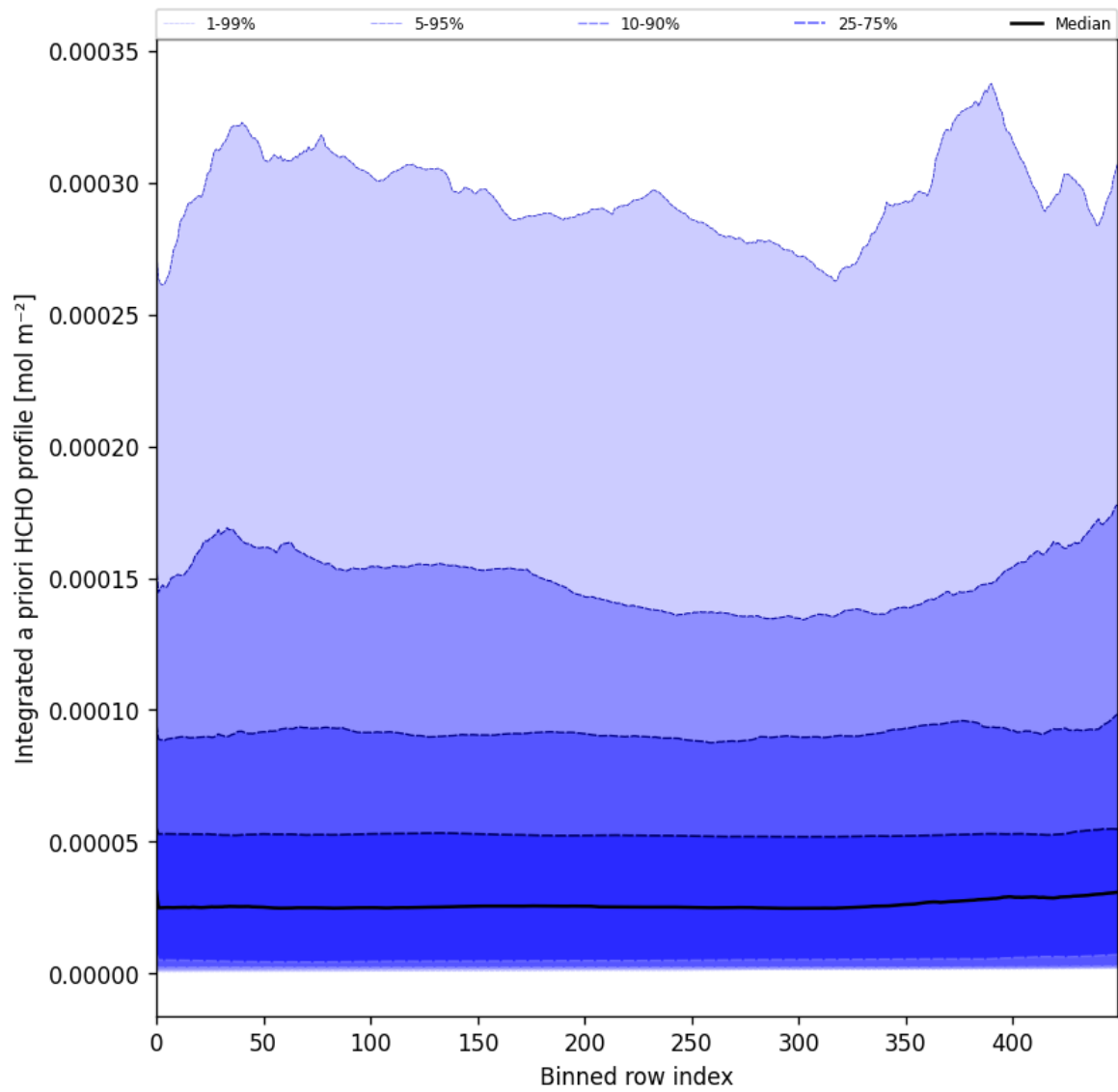
Figure 57: Along track statistics of "Integrated a priori HCHO profile" for 2025-04-03 to 2025-04-04
