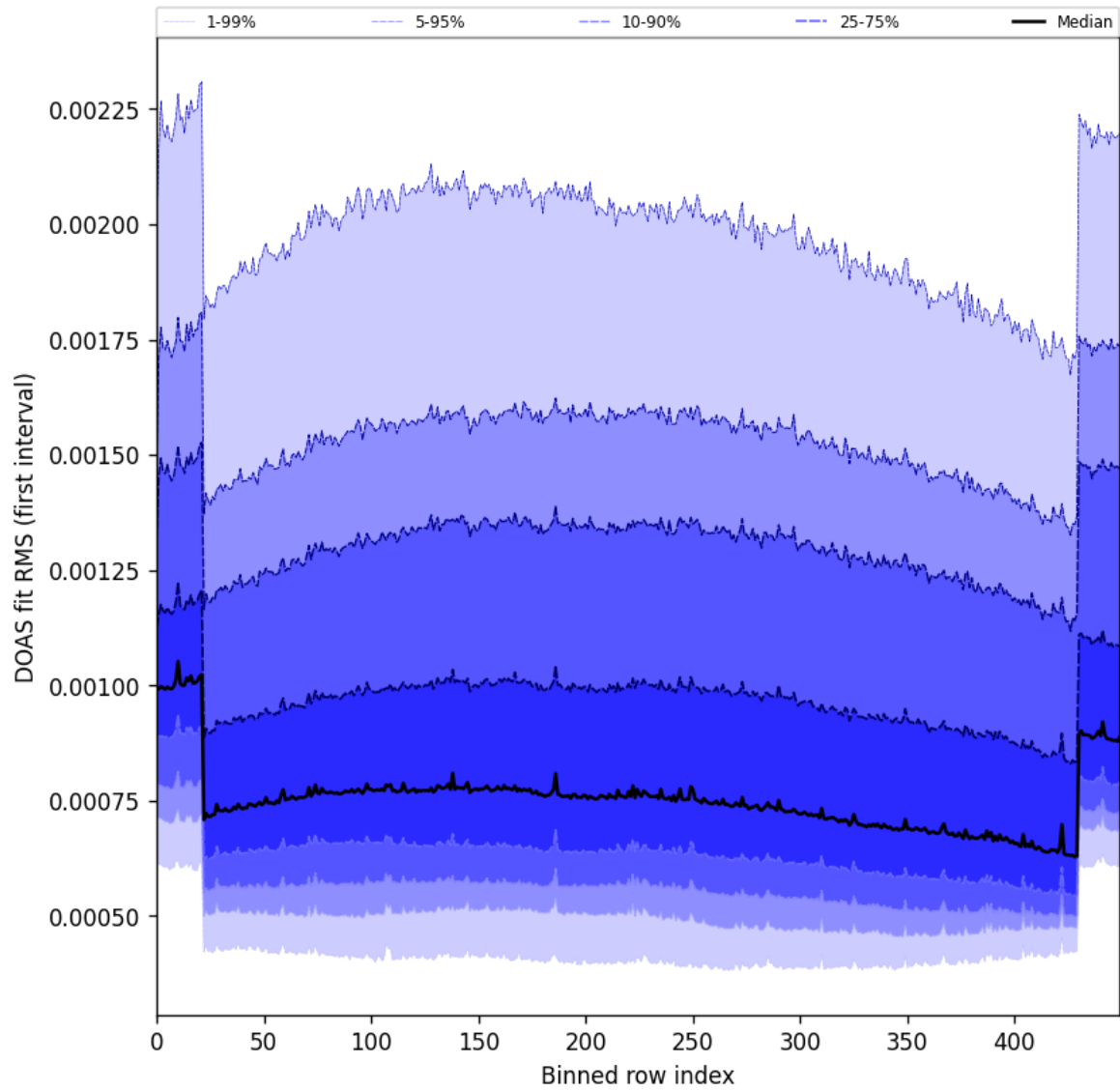
Figure 60: Along track statistics of “DOAS fit RMS (first interval)” for 2025-04-03 to 2025-04-04
