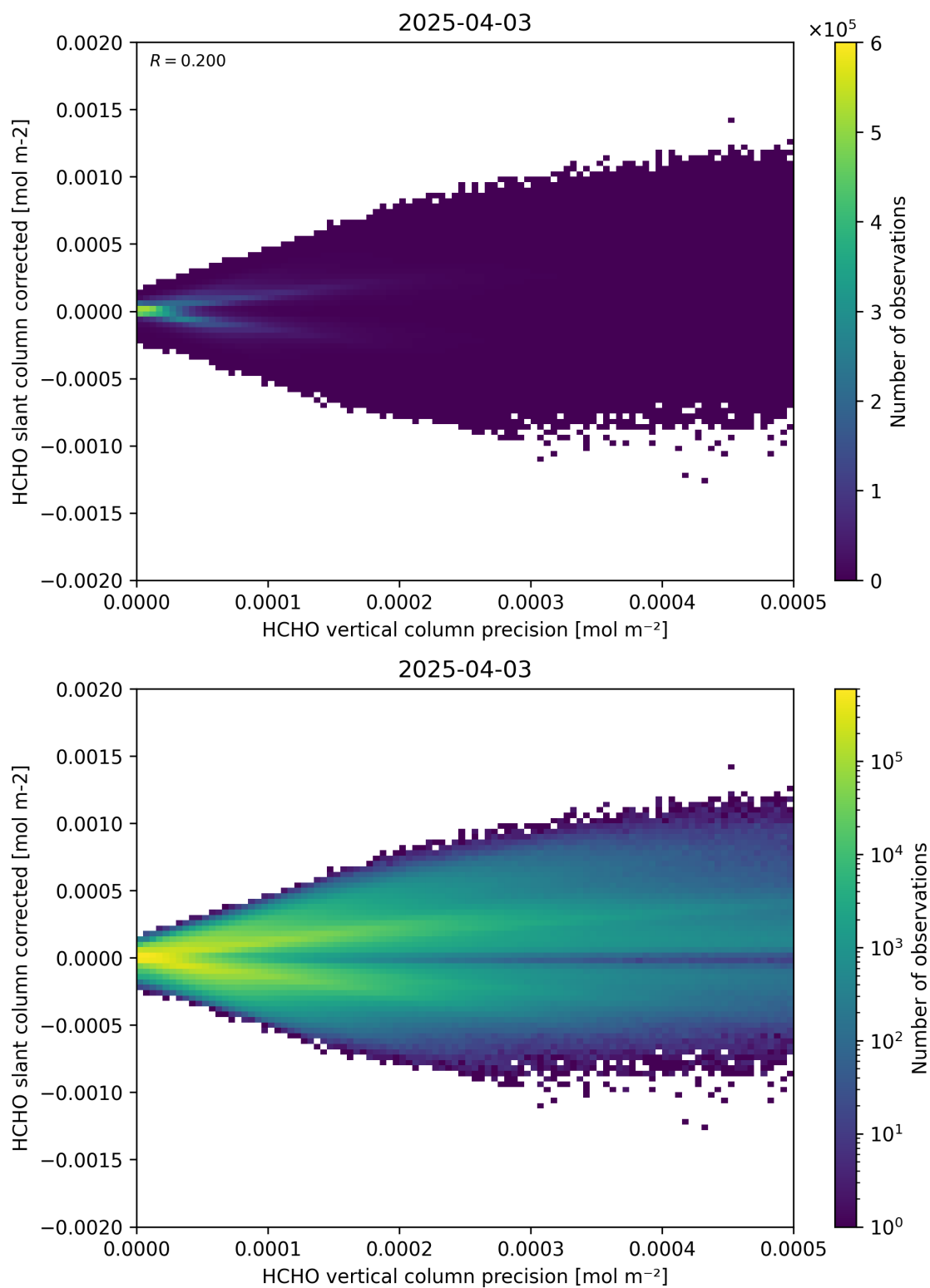
Figure 140: Scatter density plot of “HCHO vertical column precision” against “HCHO slant column corrected” for 2025-04-03 to 2025-04-04.
