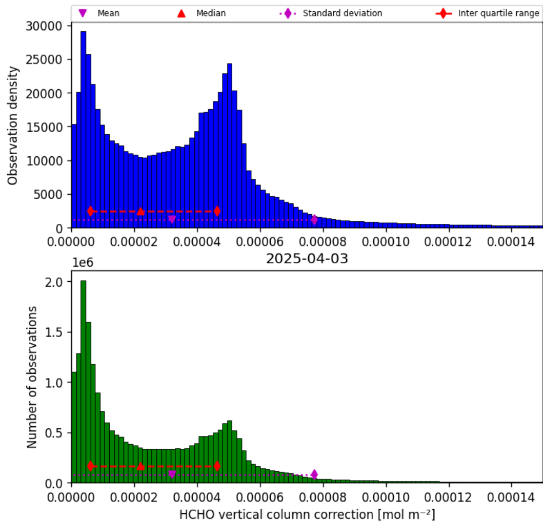
Figure 37: Histogram of “HCHO vertical column correction” for 2025-04-03 to 2025-04-04
