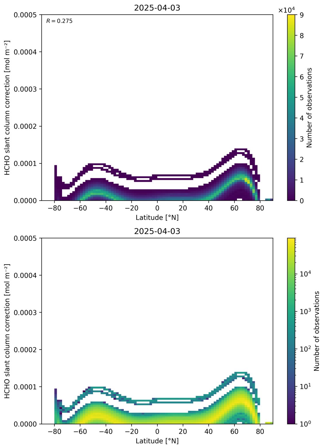
Figure 158: Scatter density plot of “Latitude” against “HCHO slant column correction” for 2025-04-03 to 2025-04-04.
