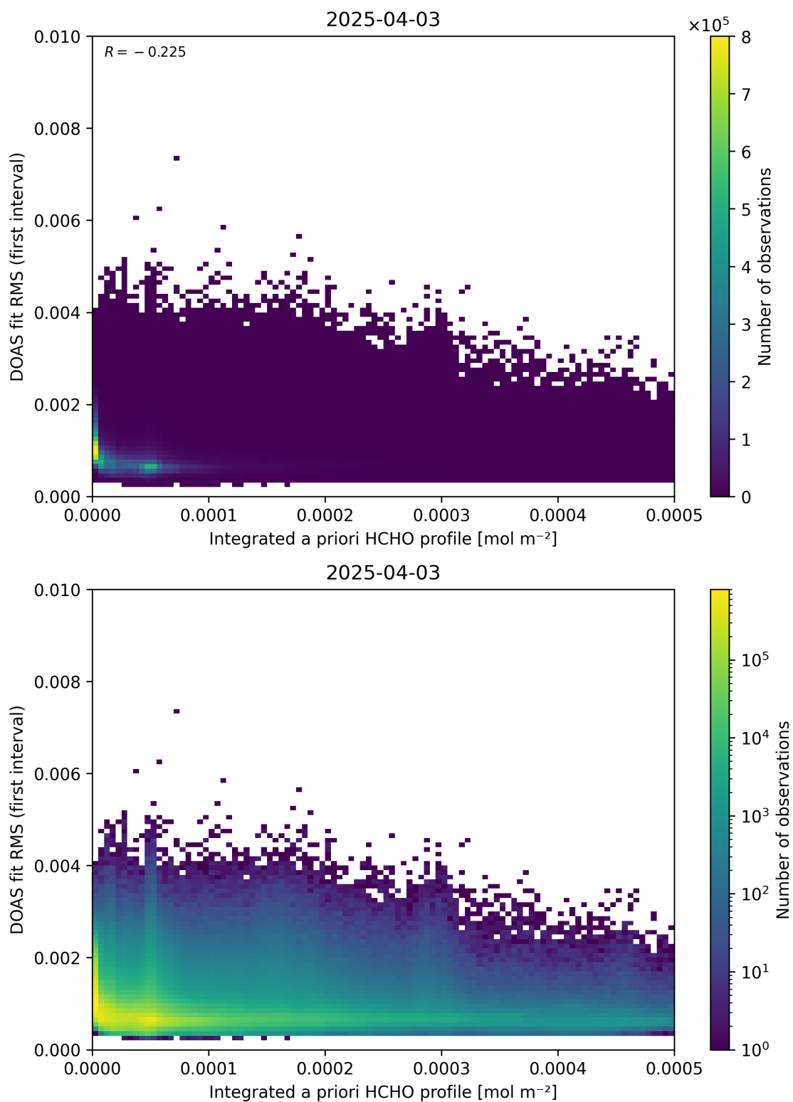
Figure 148: Scatter density plot of “Integrated a priori HCHO profile” against “DOAS fit RMS (first interval)” for 2025-04-03 to 2025-04-04.
