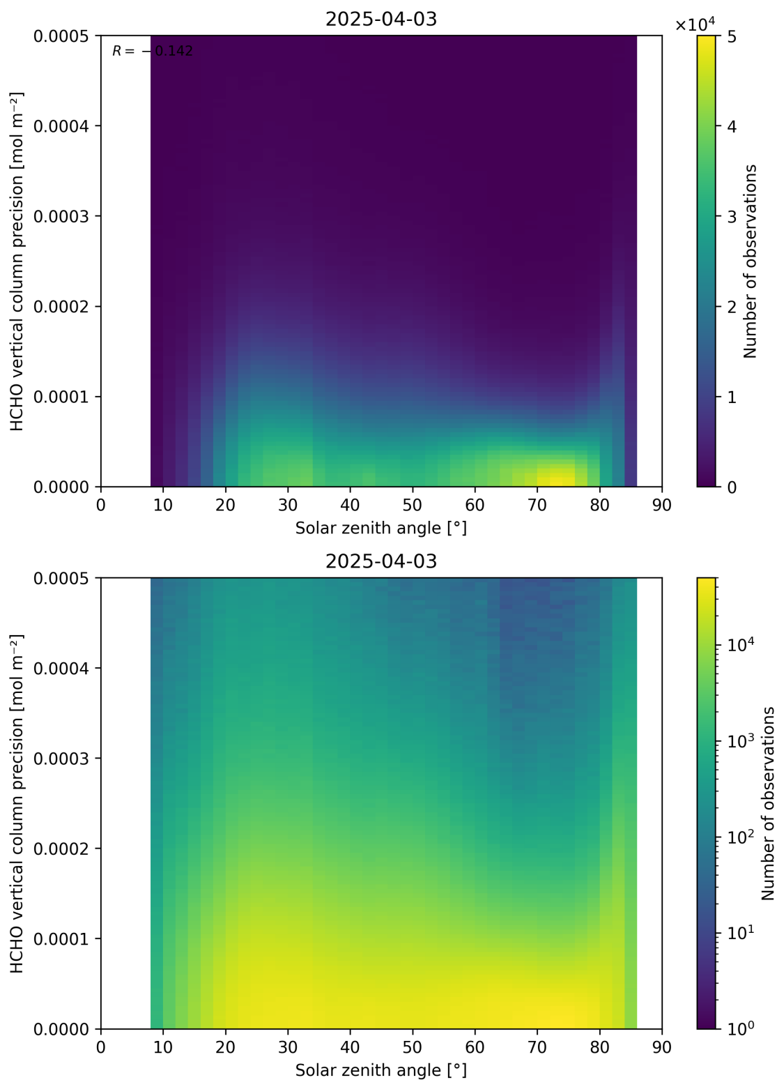
Figure 179: Scatter density plot of “Solar zenith angle” against “HCHO vertical column precision” for 2025-04-03 to 2025-04-04.
