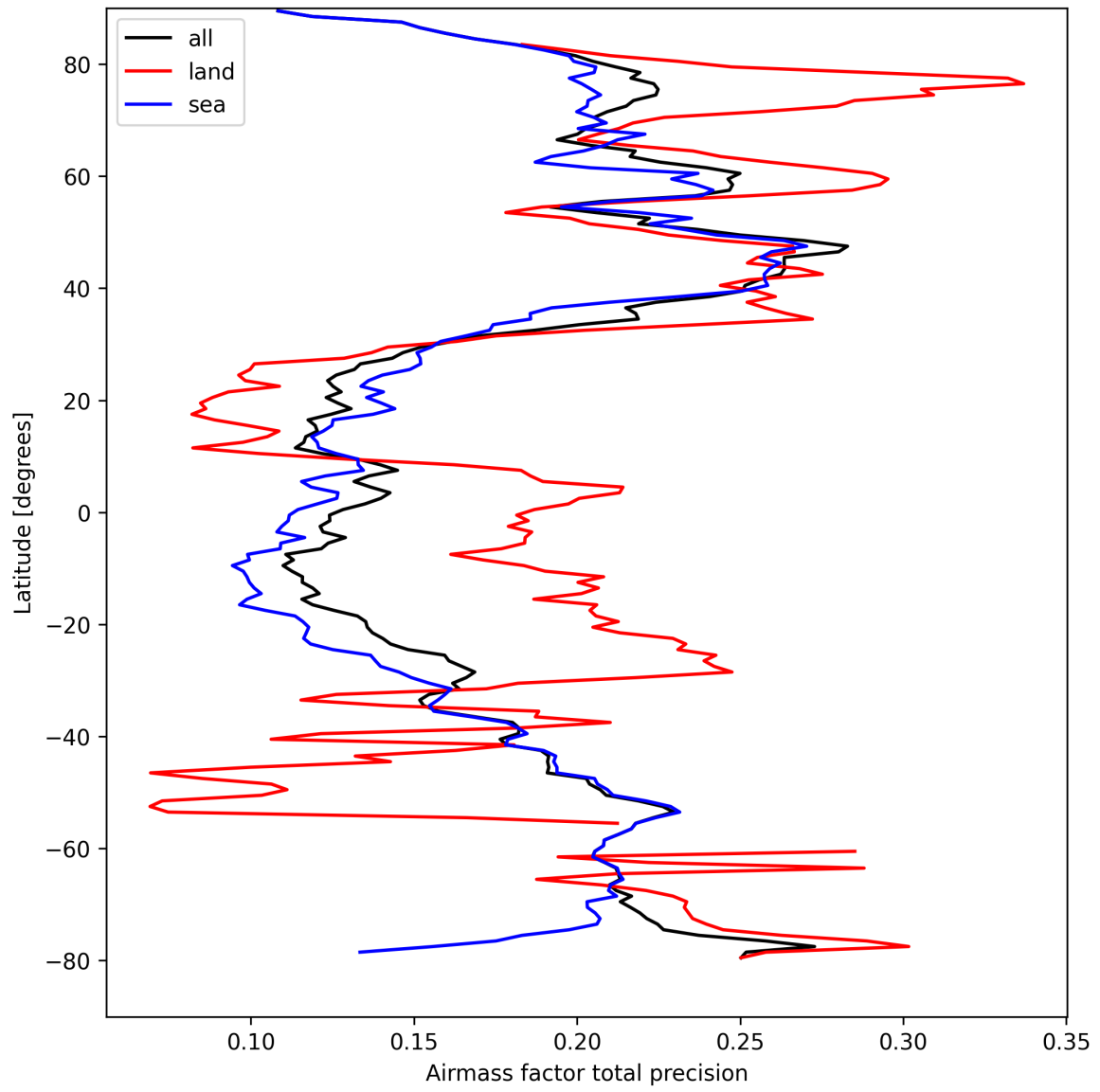
Figure 27: Zonal average of “Airmass factor total precision” for 2025-04-03 to 2025-04-04.
