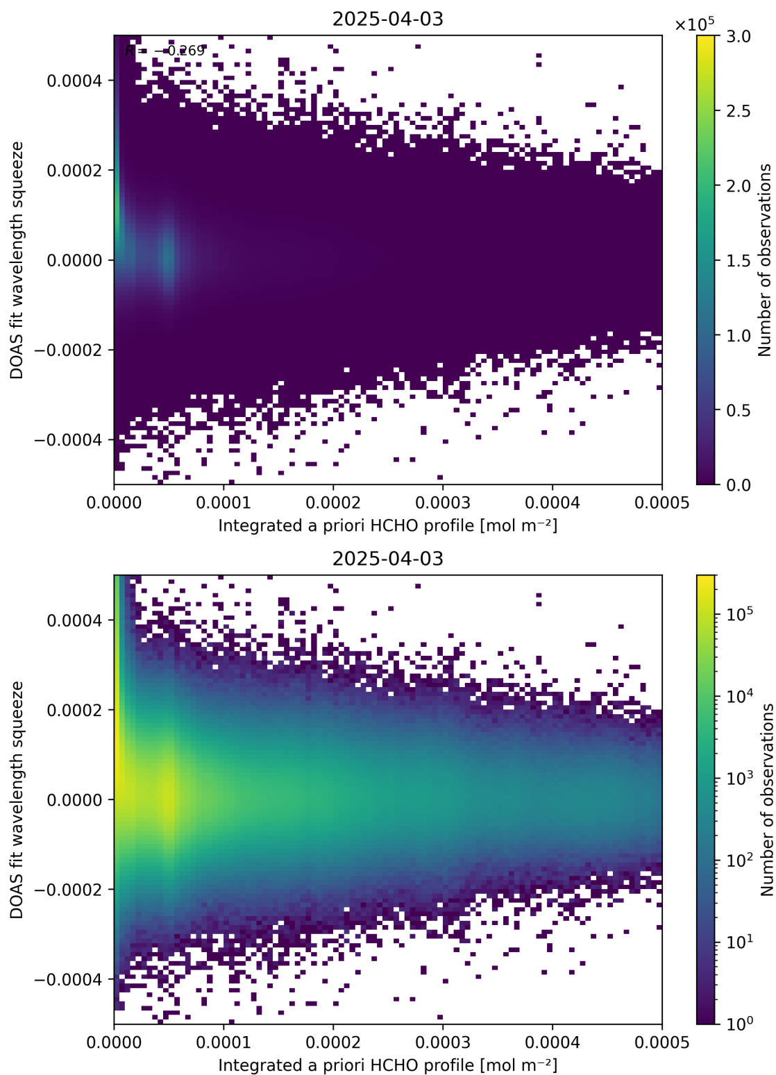
Figure 150: Scatter density plot of “Integrated a priori HCHO profile” against “DOAS fit wavelength squeeze” for 2025-04-03 to 2025-04-04.
