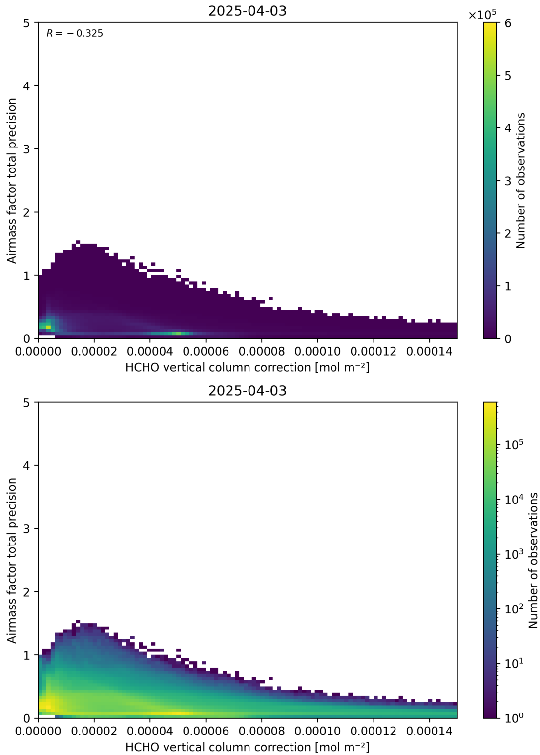
Figure 121: Scatter density plot of “HCHO vertical column correction” against “Airmass factor total precision” for 2025-04-03 to 2025-04-04.
