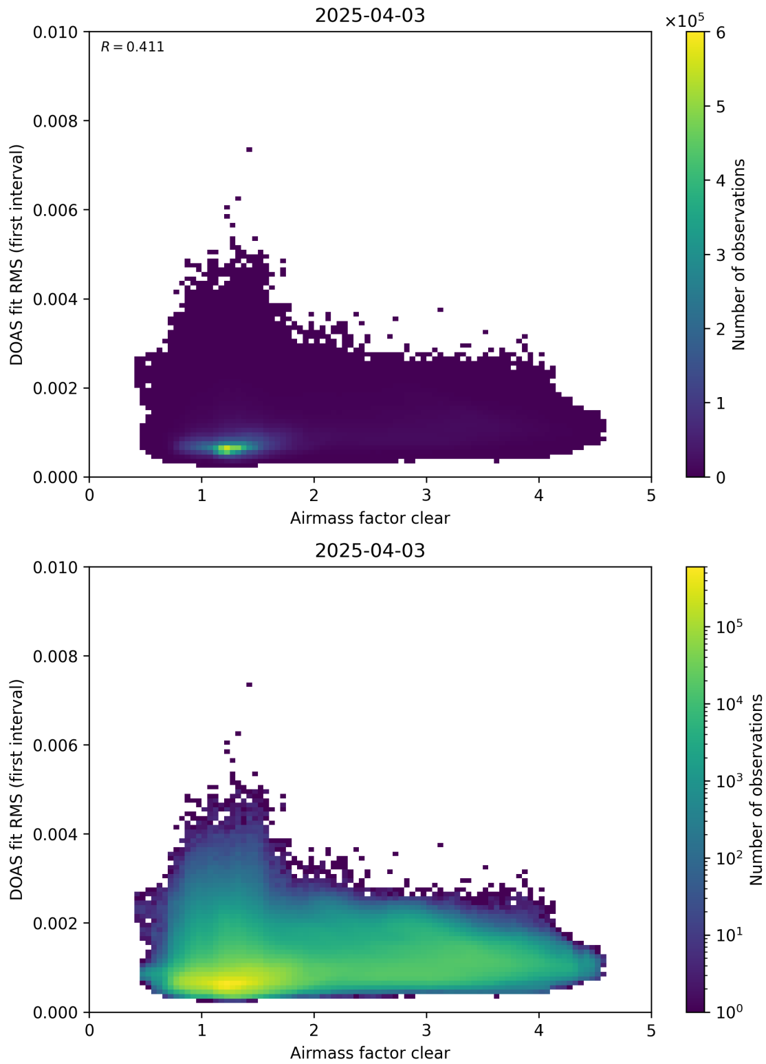
Figure 71: Scatter density plot of “Airmass factor clear” against “DOAS fit RMS (first interval)” for 2025-04-03 to 2025-04-04.
