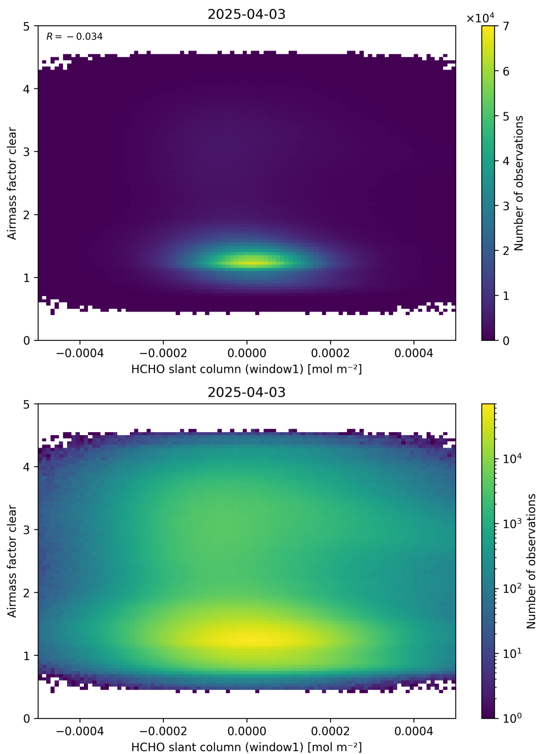
Figure 81: Scatter density plot of “HCHO slant column (window1)” against “Airmass factor clear” for 2025-04-03 to 2025-04-04.
