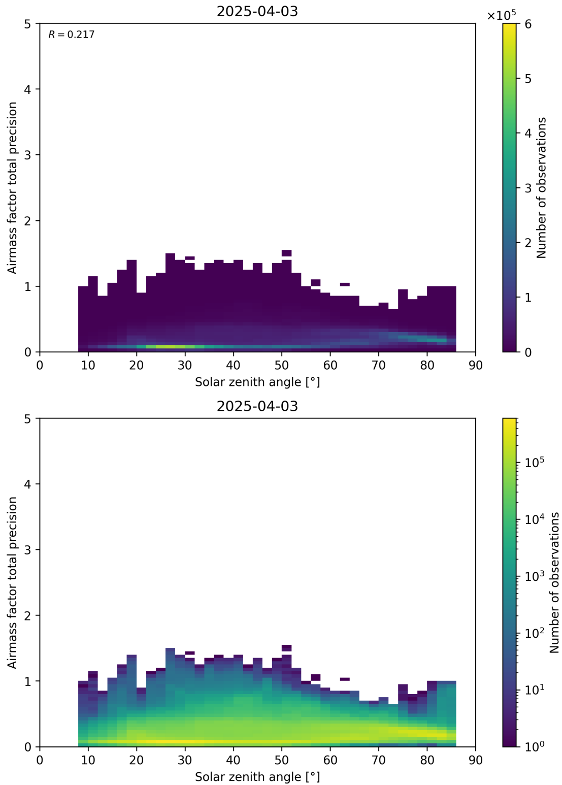
Figure 176: Scatter density plot of “Solar zenith angle” against “Airmass factor total precision” for 2025-04-03 to 2025-04-04.
