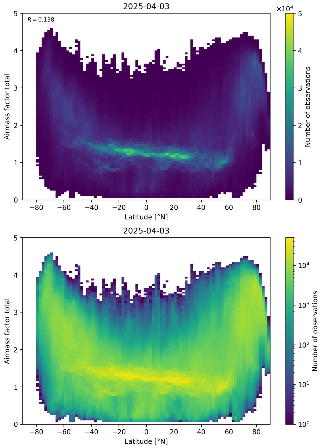
Figure 161: Scatter density plot of “Latitude” against “Airmass factor total” for 2025-04-03 to 2025-04-04.
