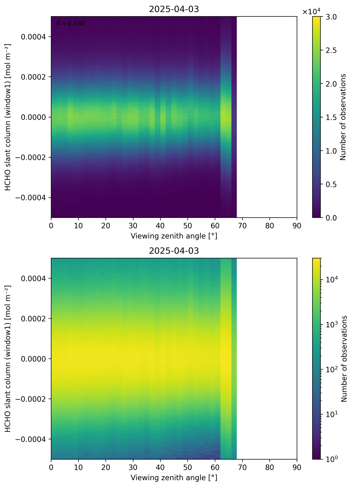
Figure 188: Scatter density plot of “Viewing zenith angle” against “HCHO slant column (window1)” for 2025-04-03 to 2025-04-04.
