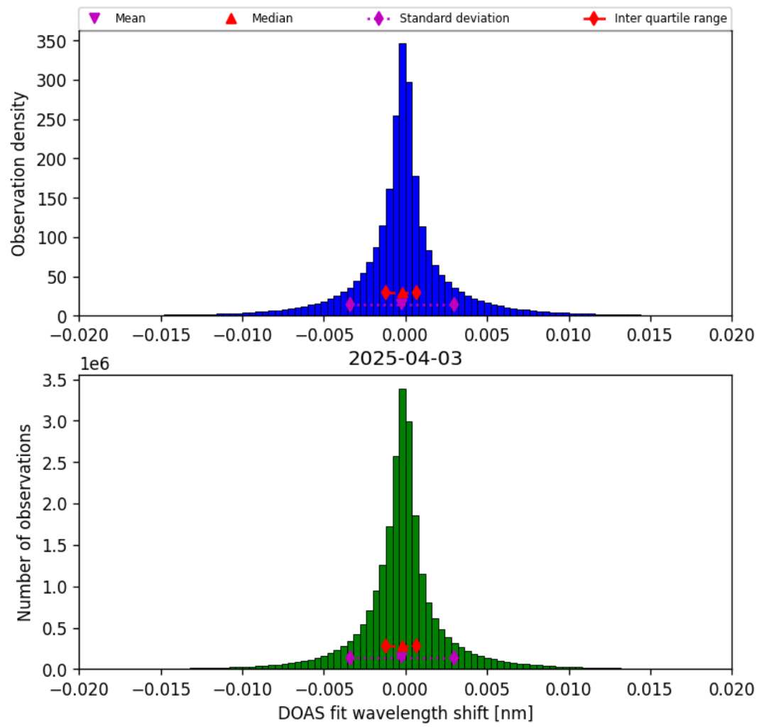
Figure 44: Histogram of “DOAS fit wavelength shift” for 2025-04-03 to 2025-04-04
