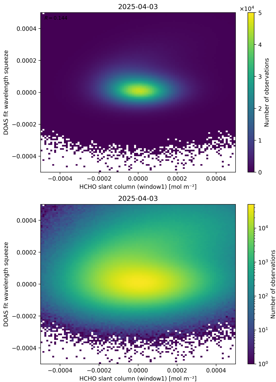
Figure 80: Scatter density plot of “HCHO slant column (window1)” against “DOAS fit wavelength squeeze” for 2025-04-03 to 2025-04-04.
