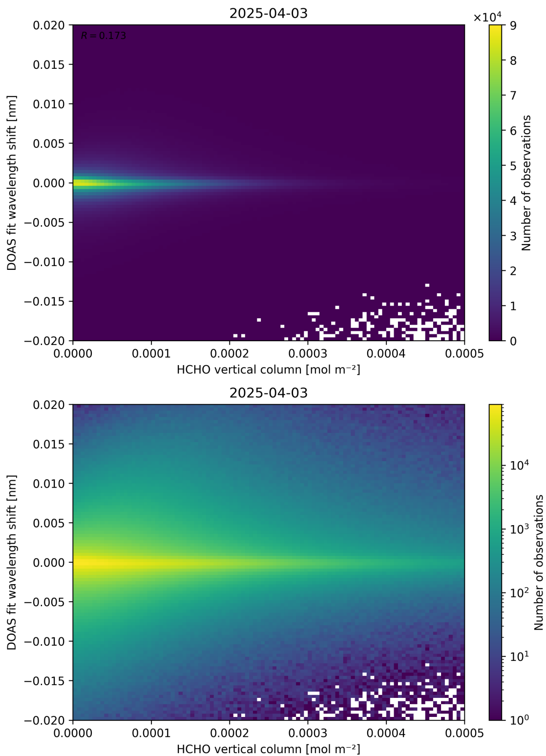
Figure 124: Scatter density plot of “HCHO vertical column” against “DOAS fit wavelength shift” for 2025-04-03 to 2025-04-04.
