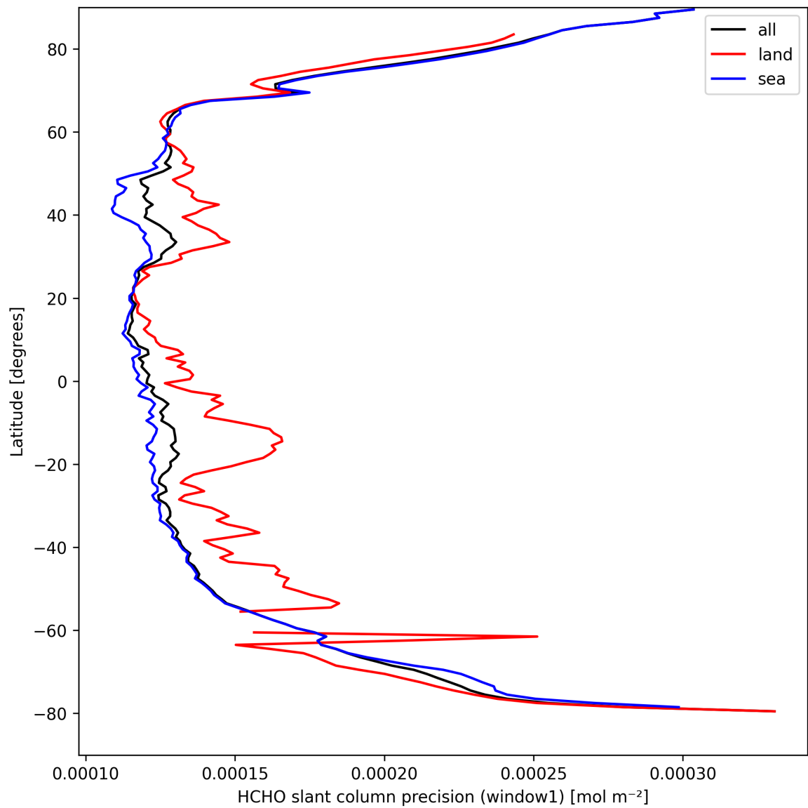
Figure 25: Zonal average of “HCHO slant column precision (window1)” for 2025-04-03 to 2025-04-04.
