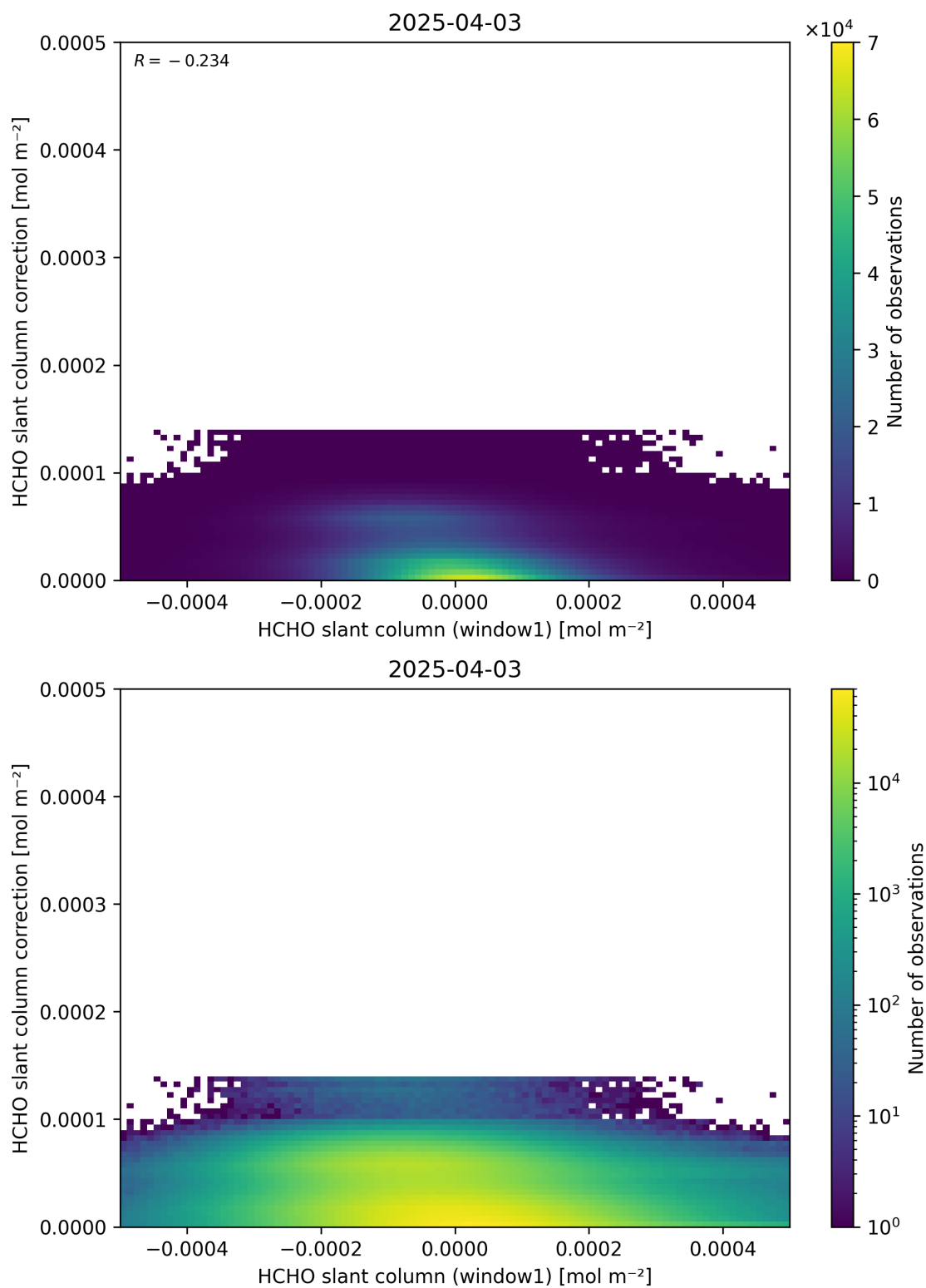
Figure 83: Scatter density plot of “HCHO slant column (window1)” against “HCHO slant column correction” for 2025-04-03 to 2025-04-04.
