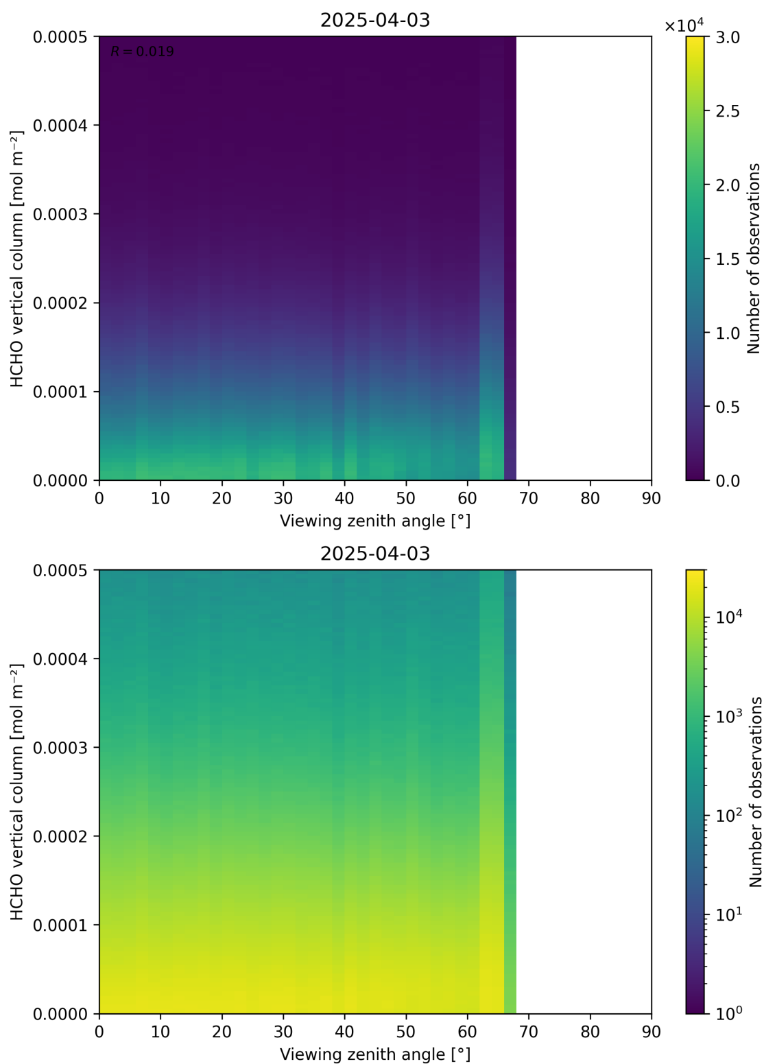
Figure 192: Scatter density plot of “Viewing zenith angle” against “HCHO vertical column” for 2025-04-03 to 2025-04-04.
