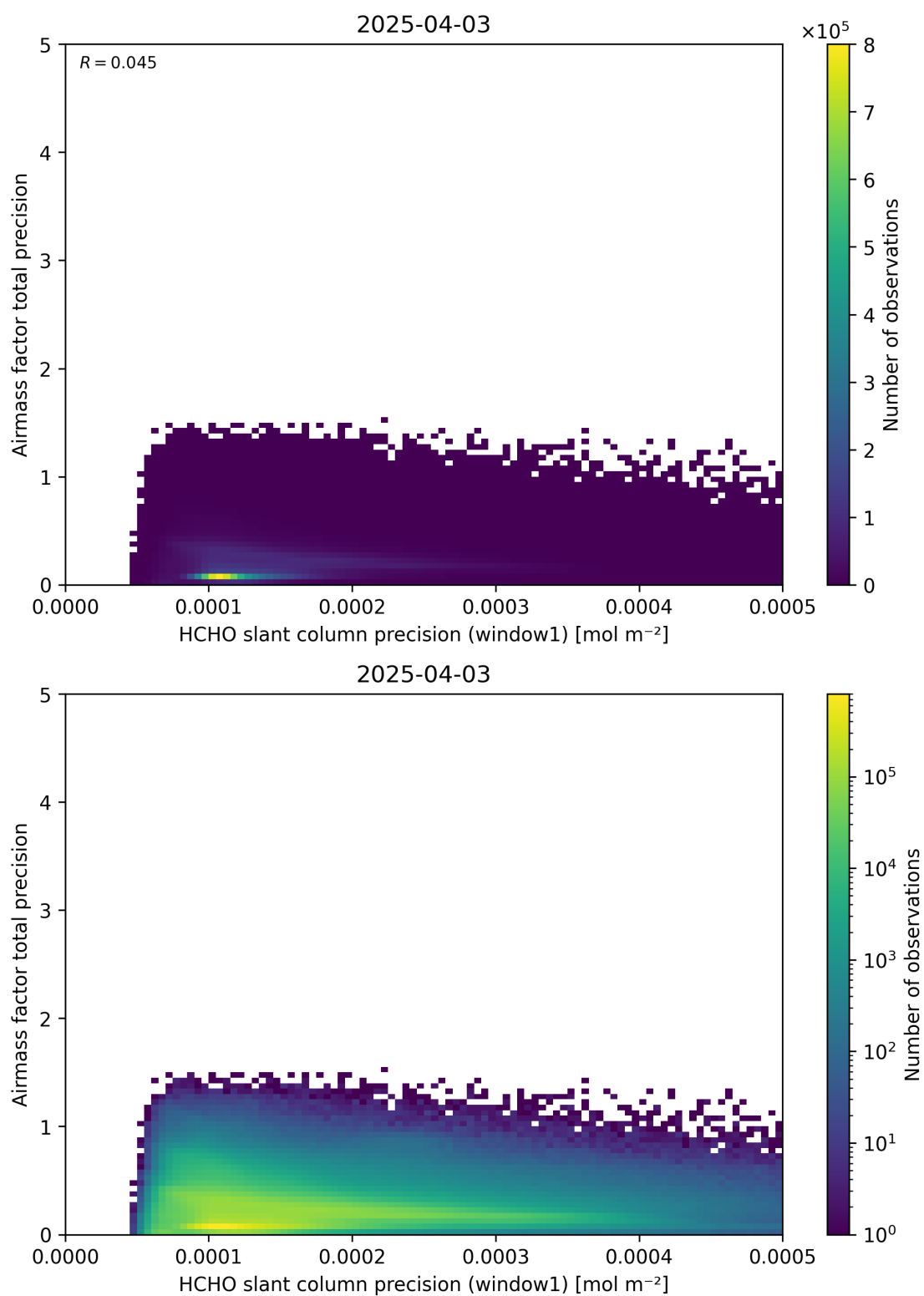
Figure 95: Scatter density plot of “HCHO slant column precision (window1)” against “Airmass factor total precision” for 2025-04-03 to 2025-04-04.
