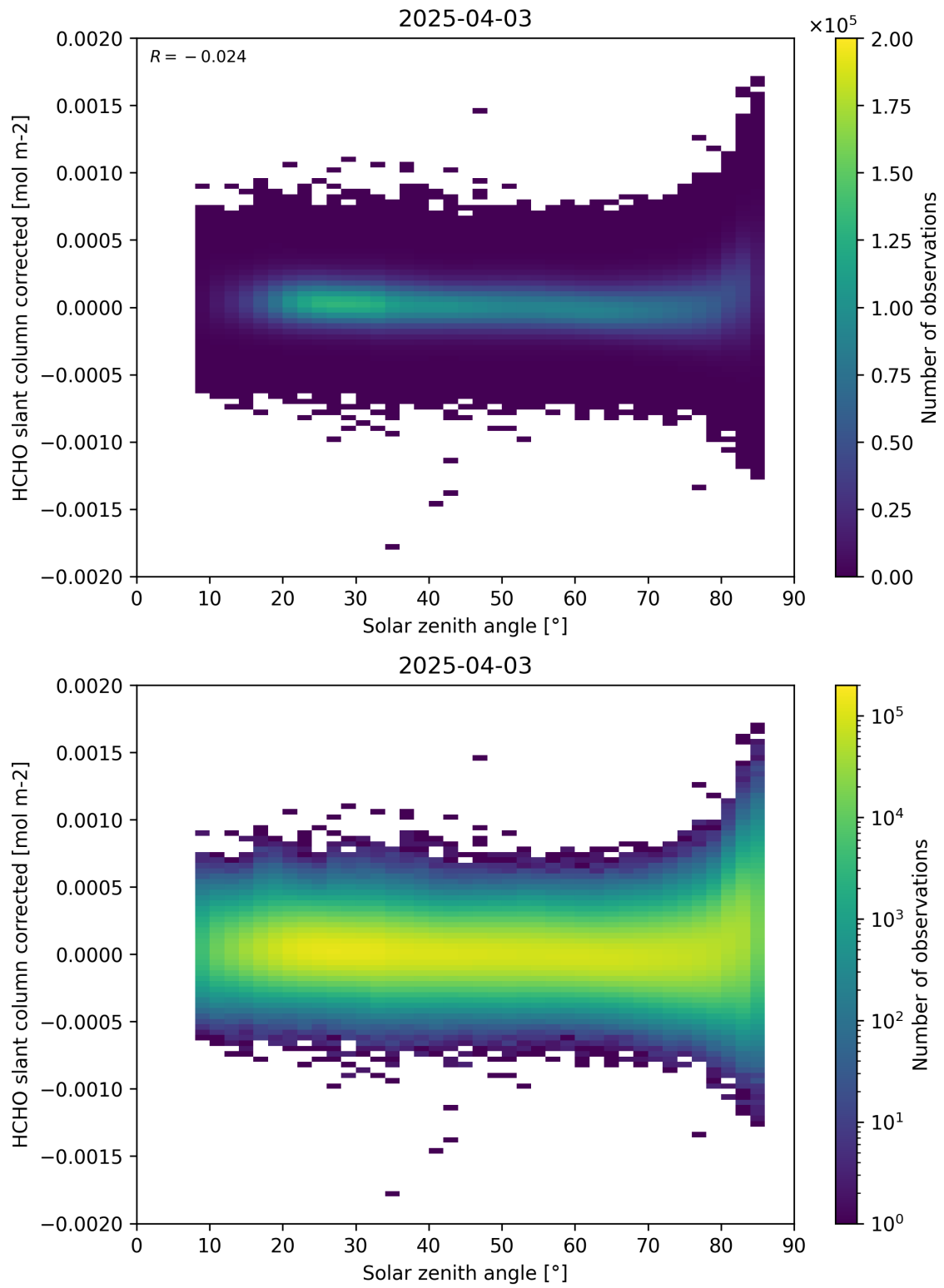
Figure 171: Scatter density plot of “Solar zenith angle” against “HCHO slant column corrected” for 2025-04-03 to 2025-04-04.
