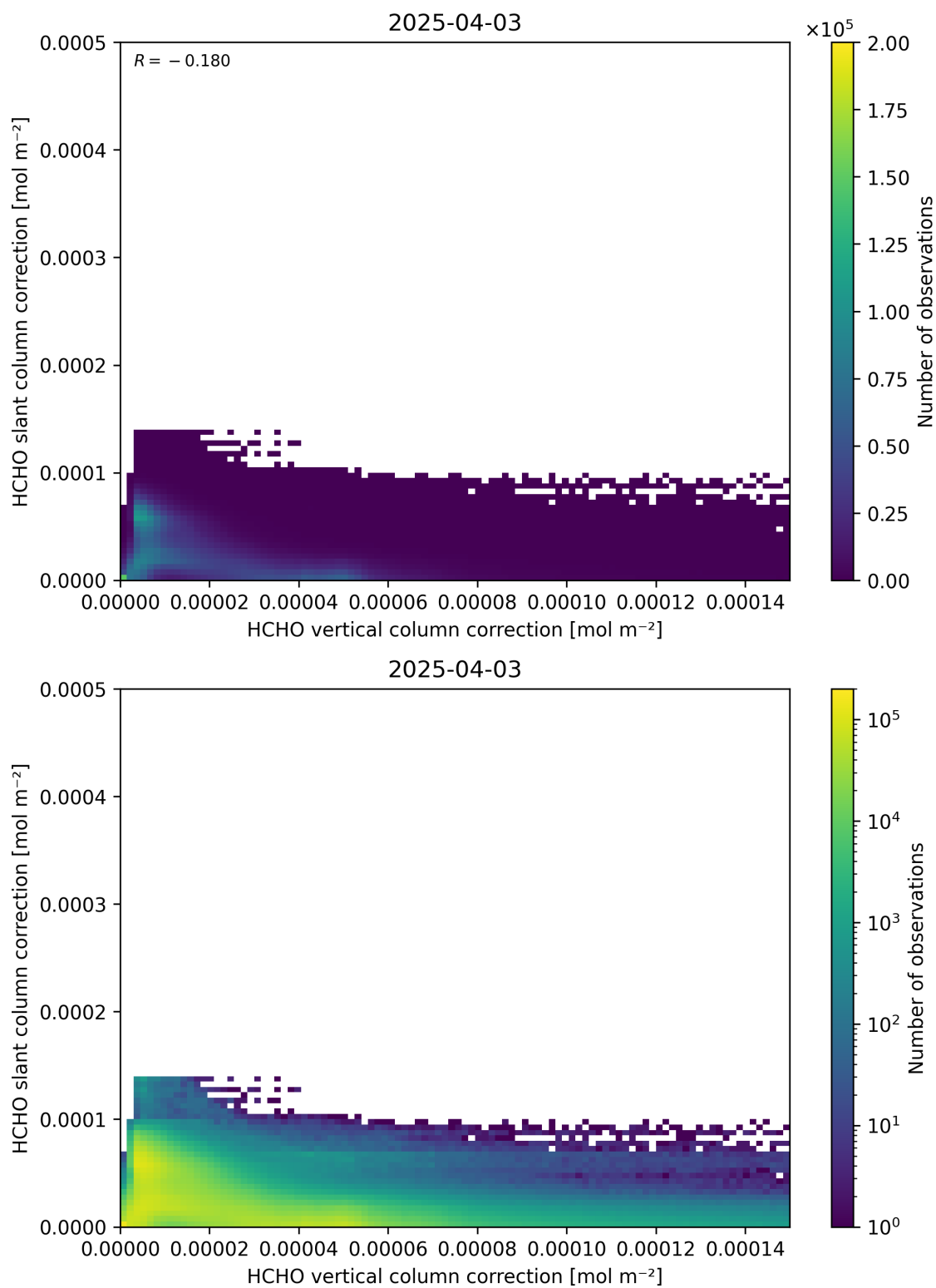
Figure 117: Scatter density plot of “HCHO vertical column correction” against “HCHO slant column correction” for 2025-04-03 to 2025-04-04.
