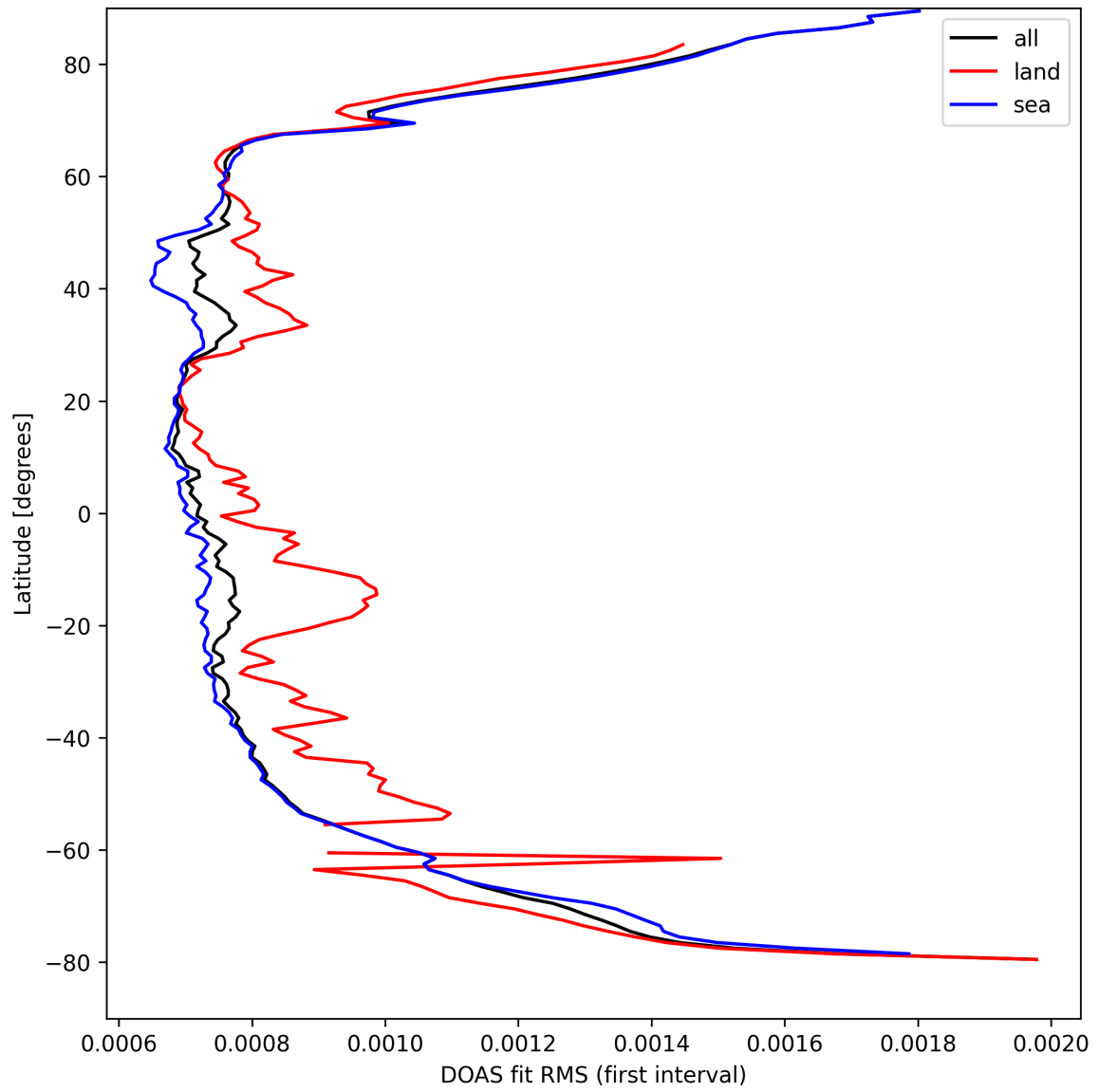
Figure 32: Zonal average of “DOAS fit RMS (first interval)” for 2025-04-03 to 2025-04-04.
