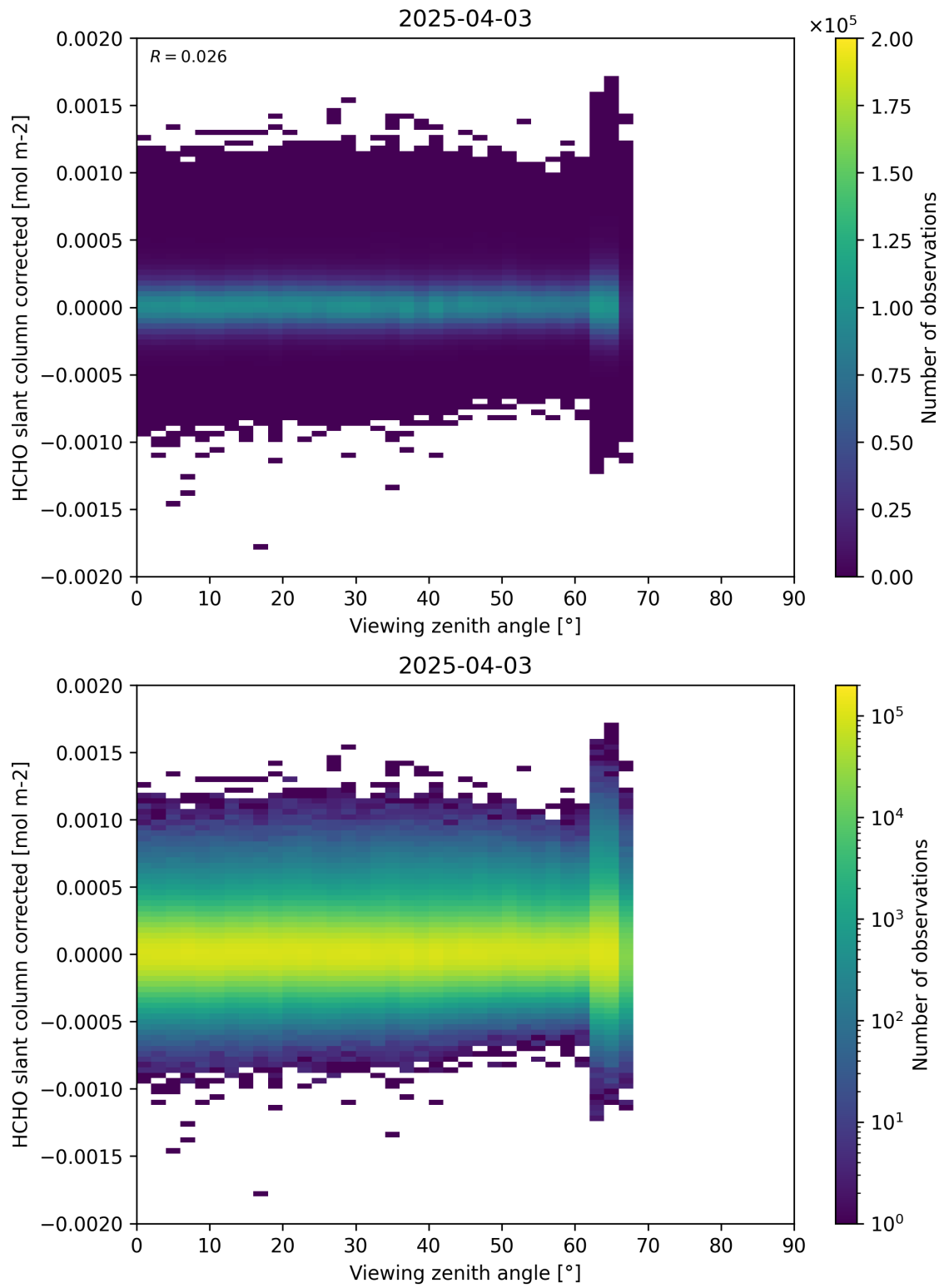
Figure 186: Scatter density plot of “Viewing zenith angle” against “HCHO slant column corrected” for 2025-04-03 to 2025-04-04.
