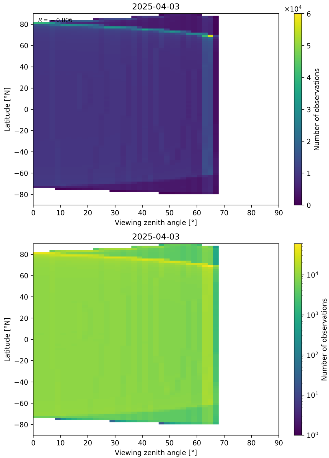
Figure 196: Scatter density plot of “Viewing zenith angle” against “Latitude” for 2025-04-03 to 2025-04-04.
