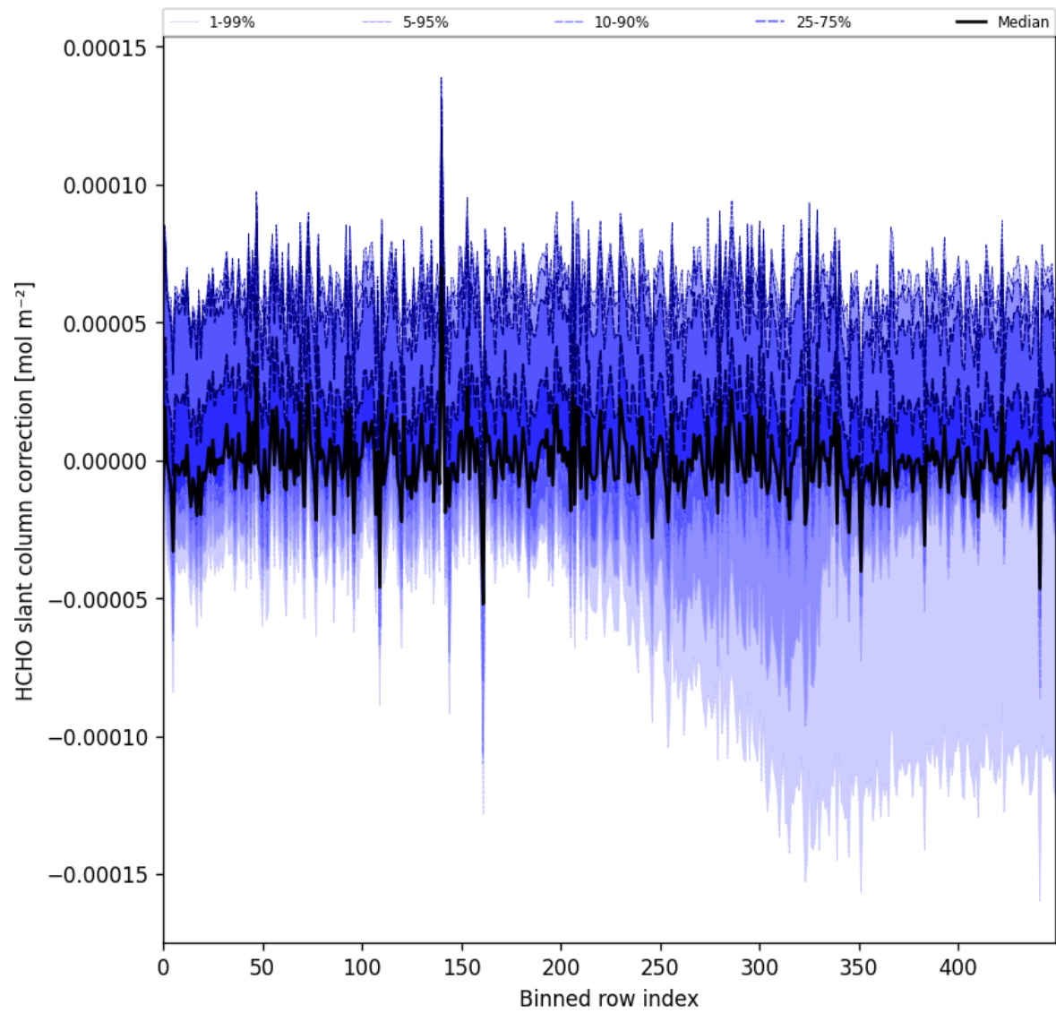
Figure 61: Along track statistics of “HCHO slant column correction” for 2025-04-03 to 2025-04-04
