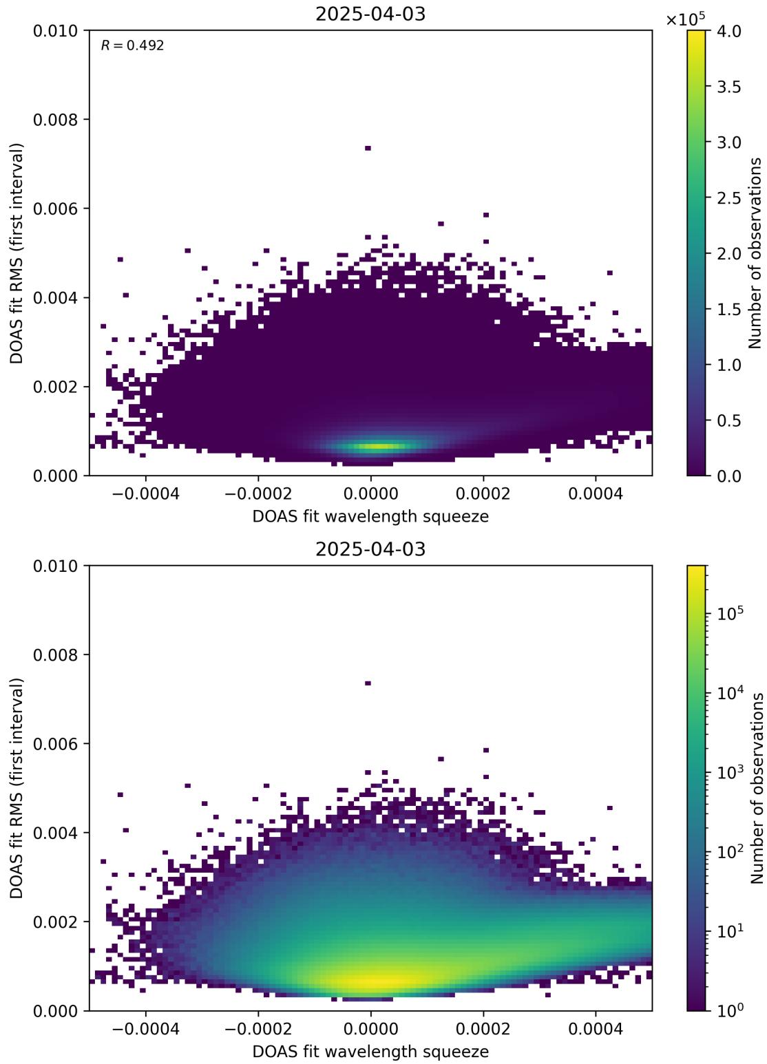
Figure 68: Scatter density plot of “DOAS fit wavelength squeeze” against “DOAS fit RMS (first interval)” for 2025-04-03 to 2025-04-04.
