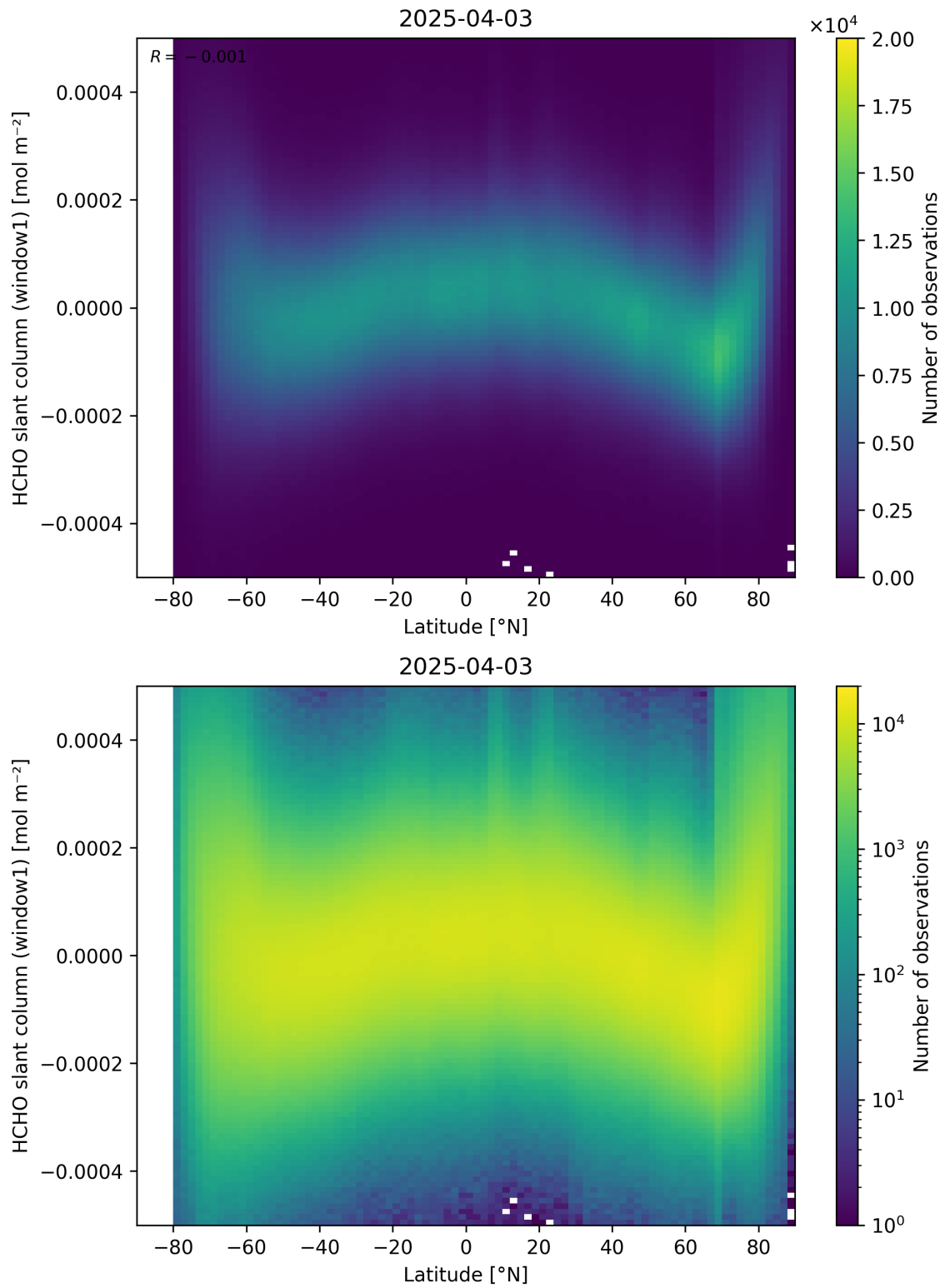
Figure 159: Scatter density plot of “Latitude” against “HCHO slant column (window1)” for 2025-04-03 to 2025-04-04.
