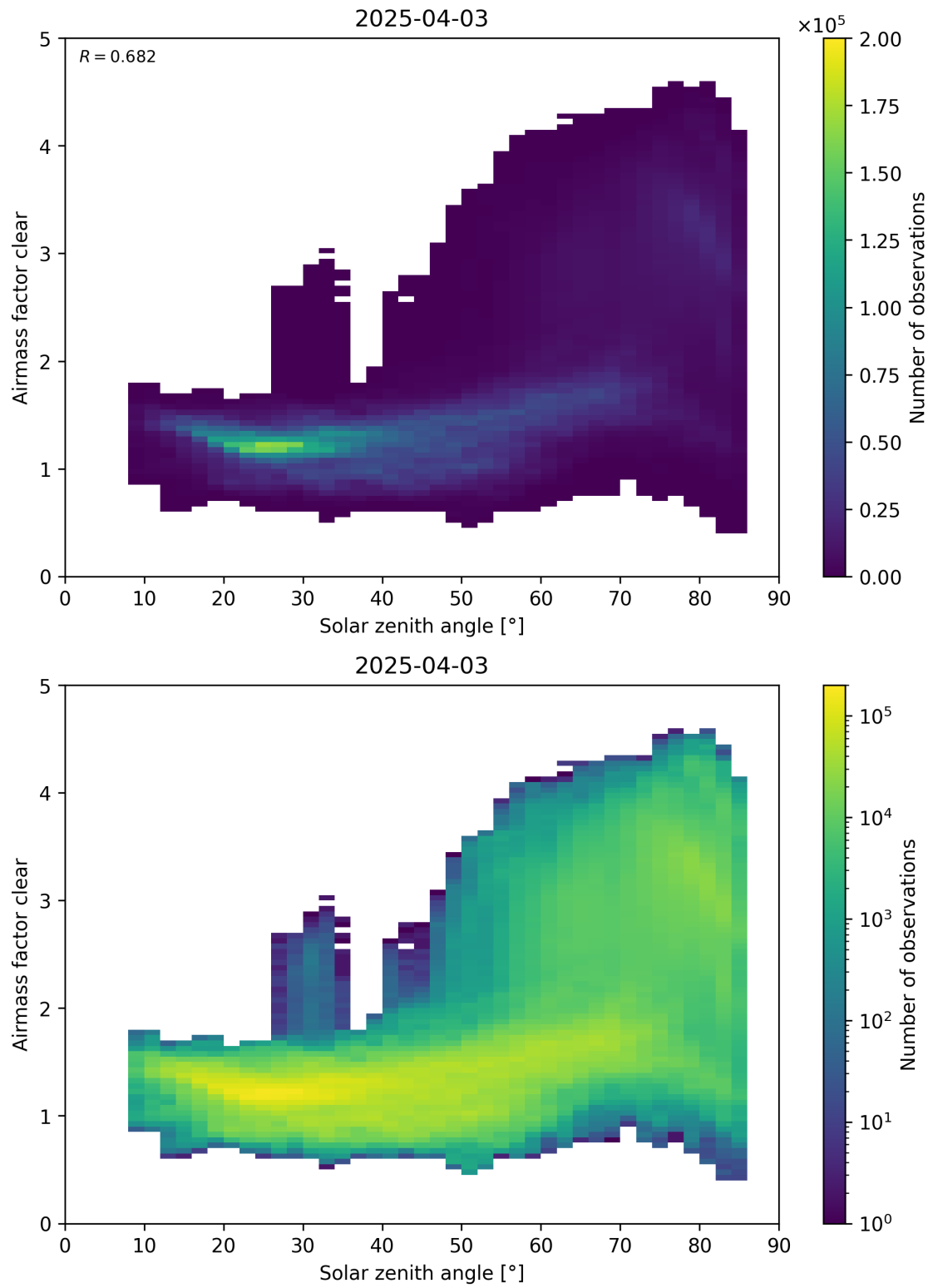
Figure 170: Scatter density plot of “Solar zenith angle” against “Airmass factor clear” for 2025-04-03 to 2025-04-04.
