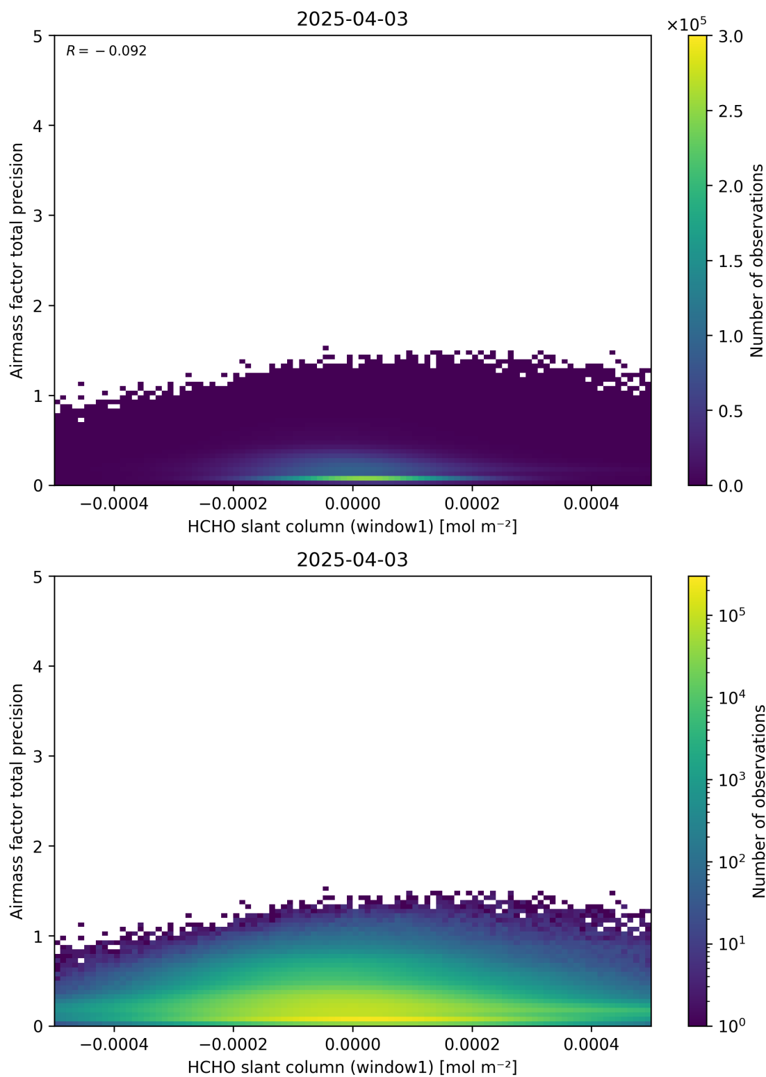
Figure 86: Scatter density plot of “HCHO slant column (window1)” against “Airmass factor total precision” for 2025-04-03 to 2025-04-04.
