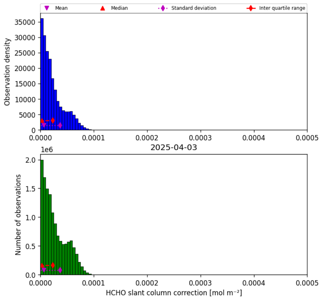
Figure 47: Histogram of “HCHO slant column correction” for 2025-04-03 to 2025-04-04
