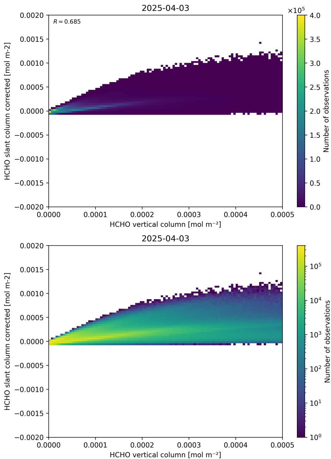
Figure 127: Scatter density plot of “HCHO vertical column” against “HCHO slant column corrected” for 2025-04-03 to 2025-04-04.
