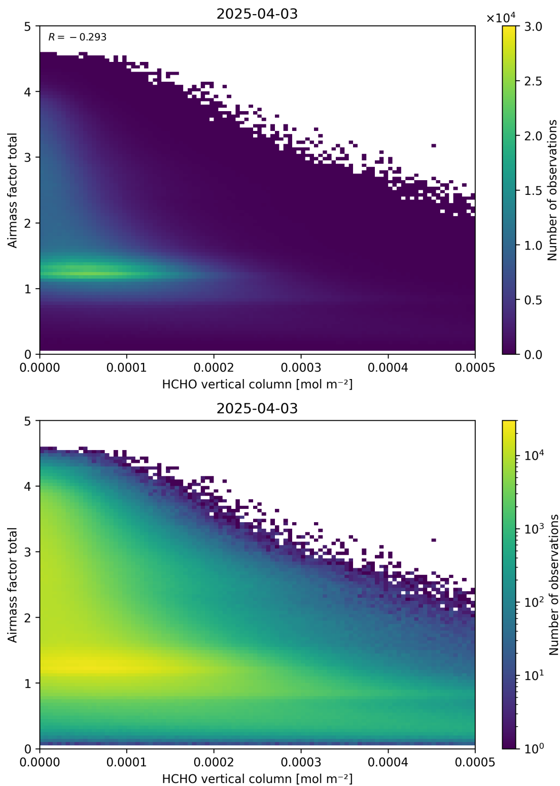
Figure 131: Scatter density plot of “HCHO vertical column” against “Airmass factor total” for 2025-04-03 to 2025-04-04.
