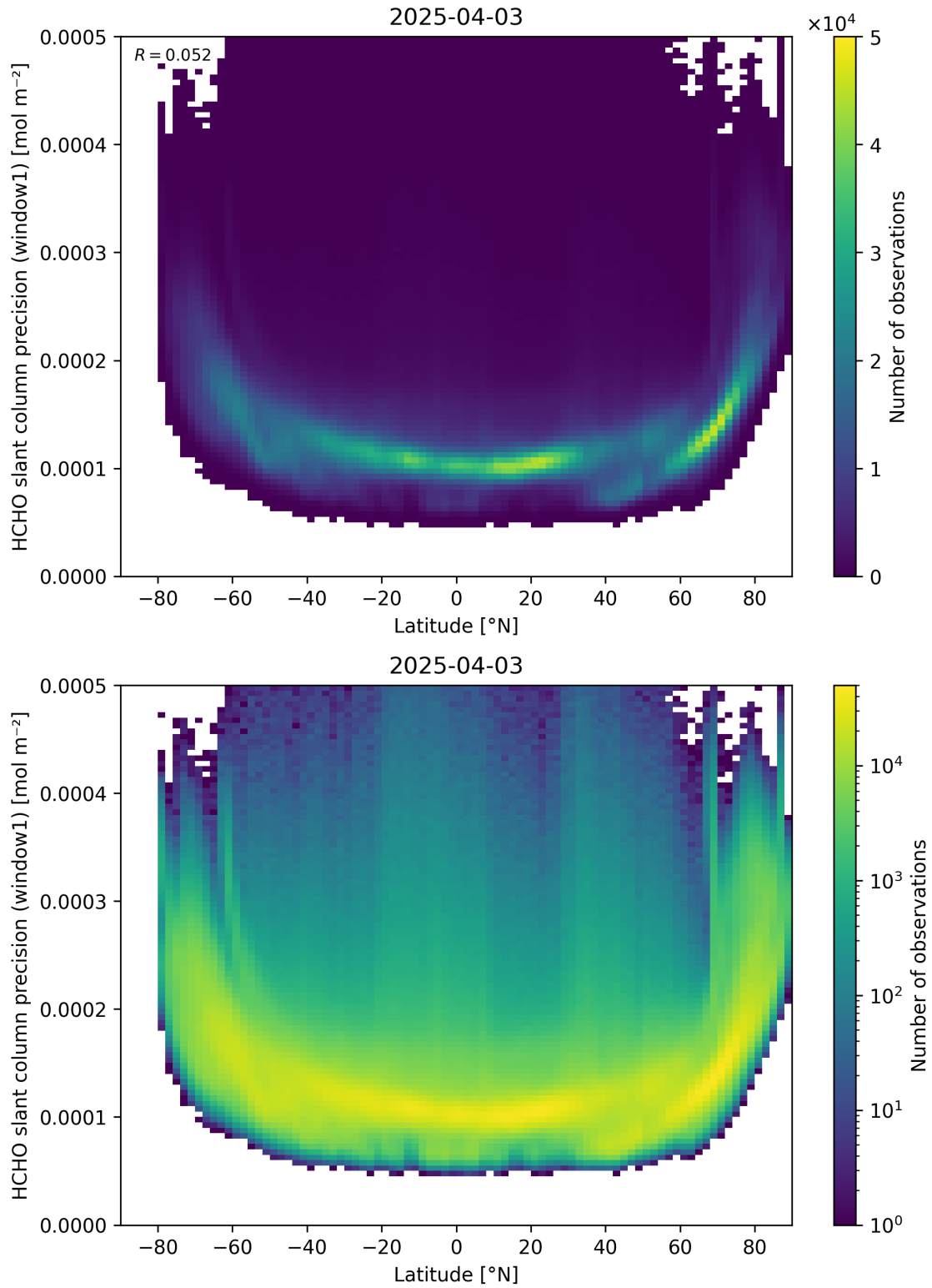
Figure 160: Scatter density plot of “Latitude” against “HCHO slant column precision (window1)” for 2025-04-03 to 2025-04-04.
