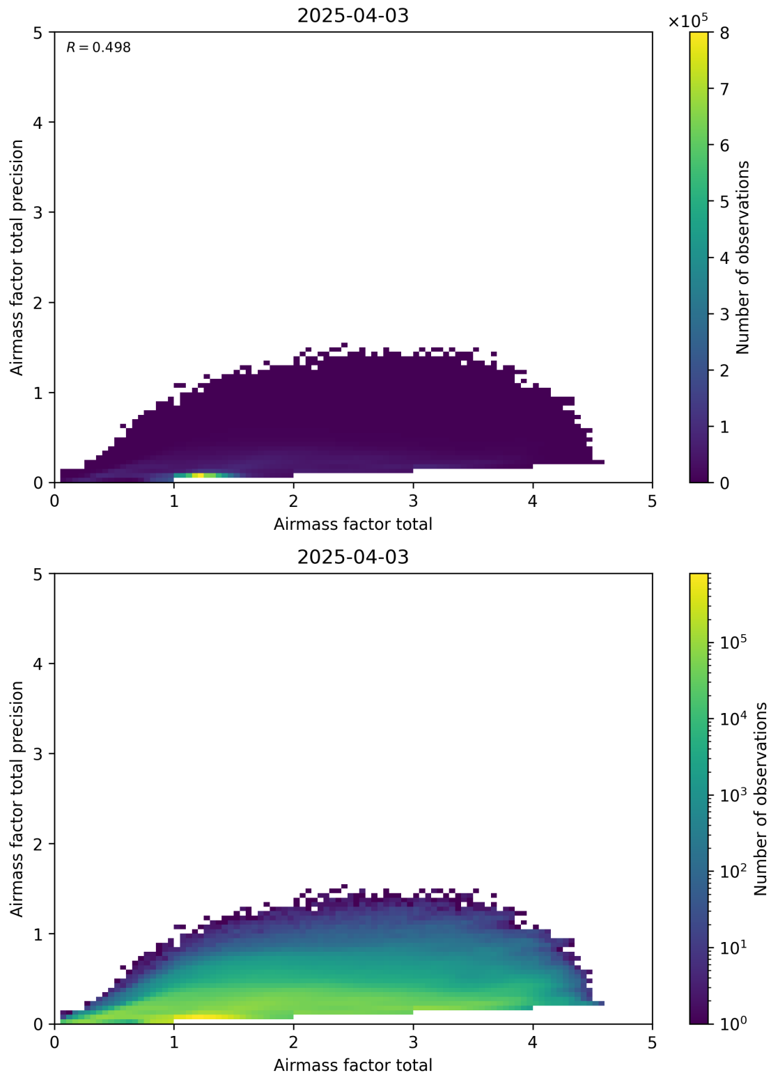
Figure 103: Scatter density plot of “Airmass factor total” against “Airmass factor total precision” for 2025-04-03 to 2025-04-04.
