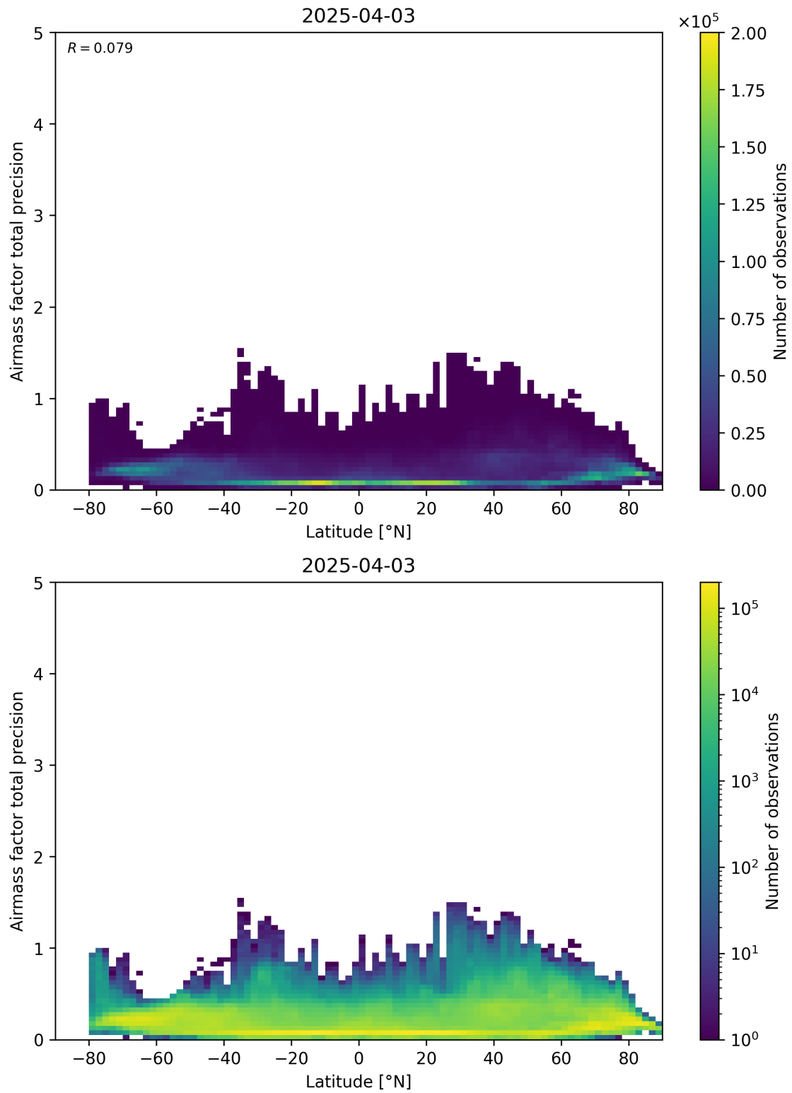
Figure 162: Scatter density plot of “Latitude” against “Airmass factor total precision” for 2025-04-03 to 2025-04-04.
