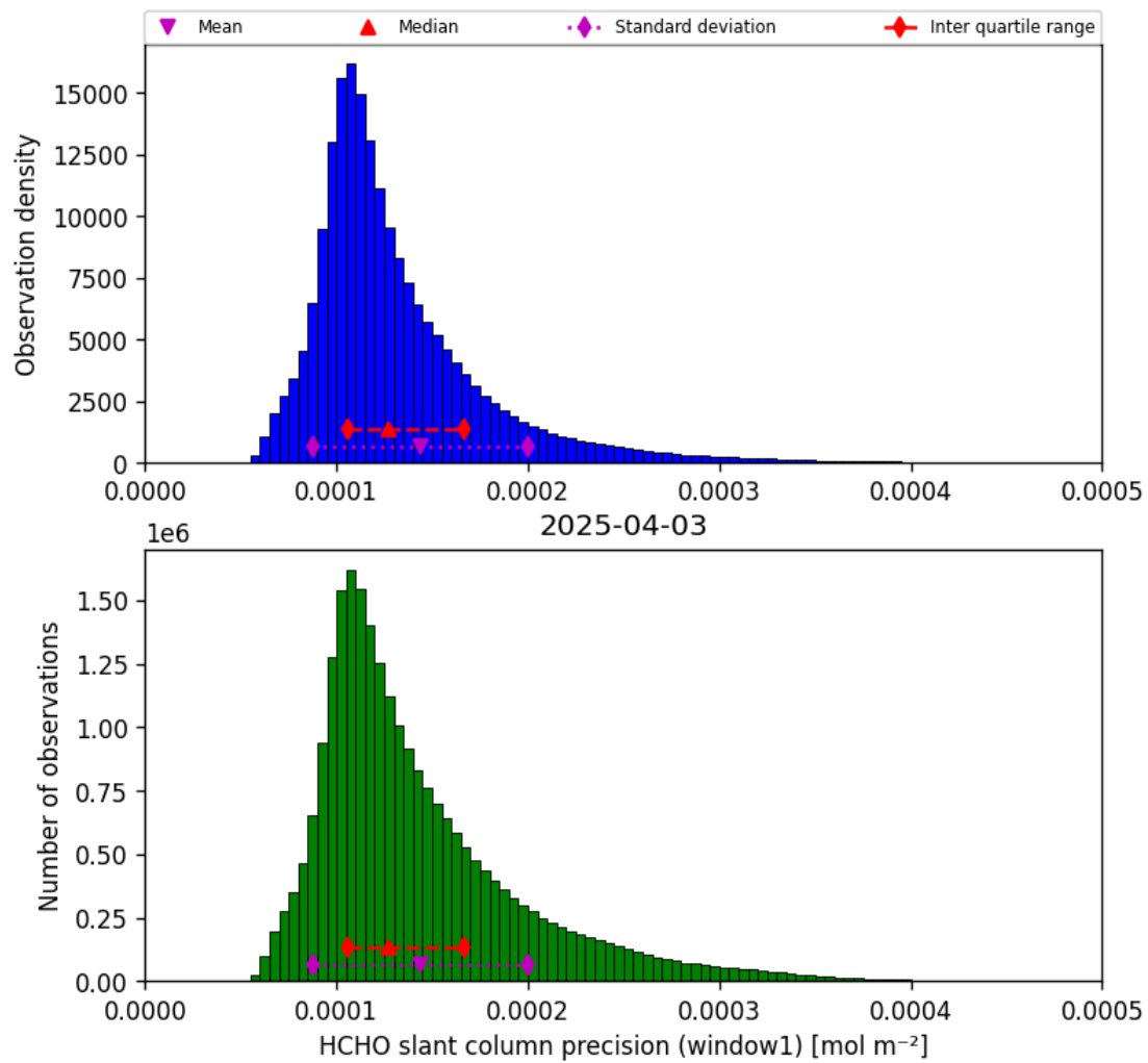
Figure 39: Histogram of “HCHO slant column precision (window1)” for 2025-04-03 to 2025-04-04
