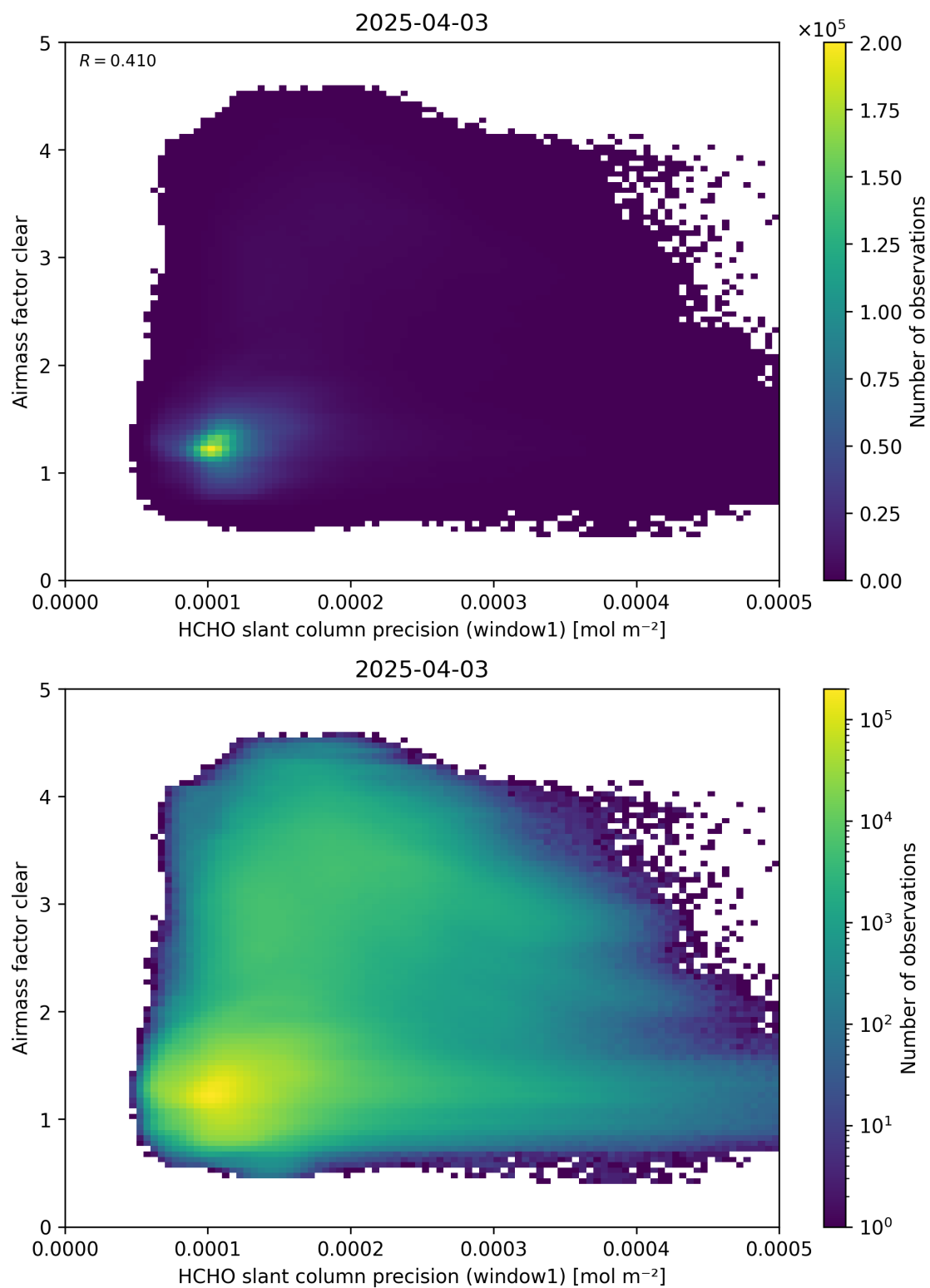
Figure 91: Scatter density plot of “HCHO slant column precision (window1)” against “Airmass factor clear” for 2025-04-03 to 2025-04-04.
