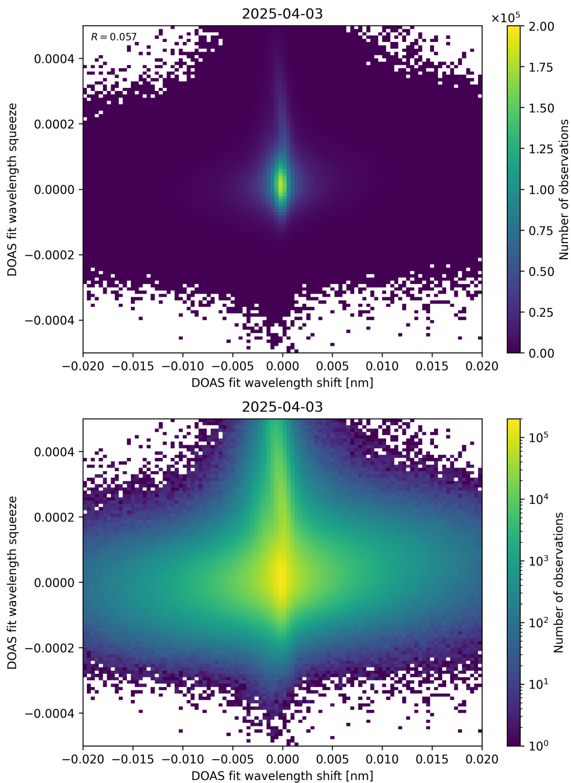
Figure 65: Scatter density plot of “DOAS fit wavelength shift” against “DOAS fit wavelength squeeze” for 2025-04-03 to 2025-04-04.
