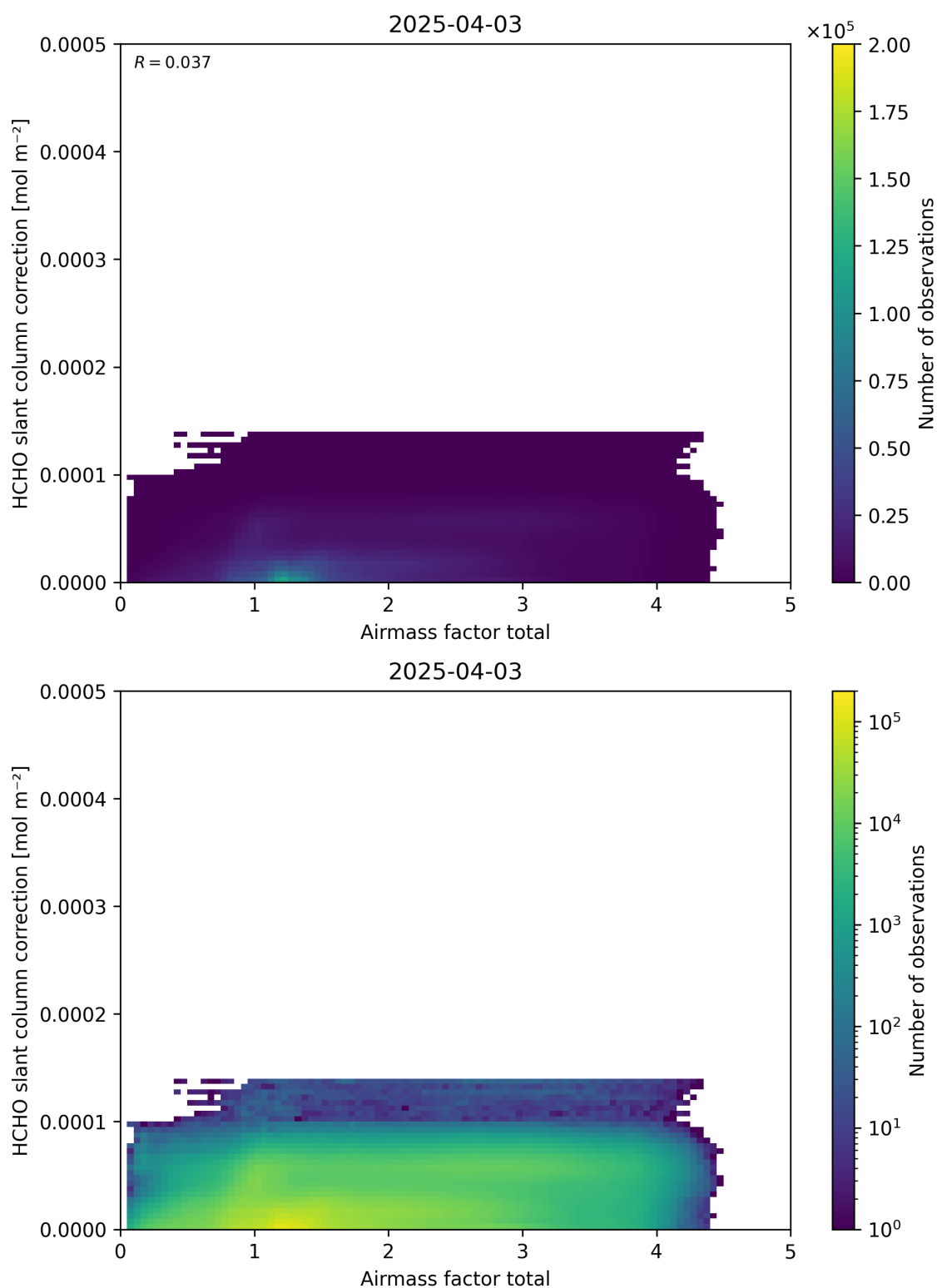
Figure 102: Scatter density plot of “Airmass factor total” against “HCHO slant column correction” for 2025-04-03 to 2025-04-04.
