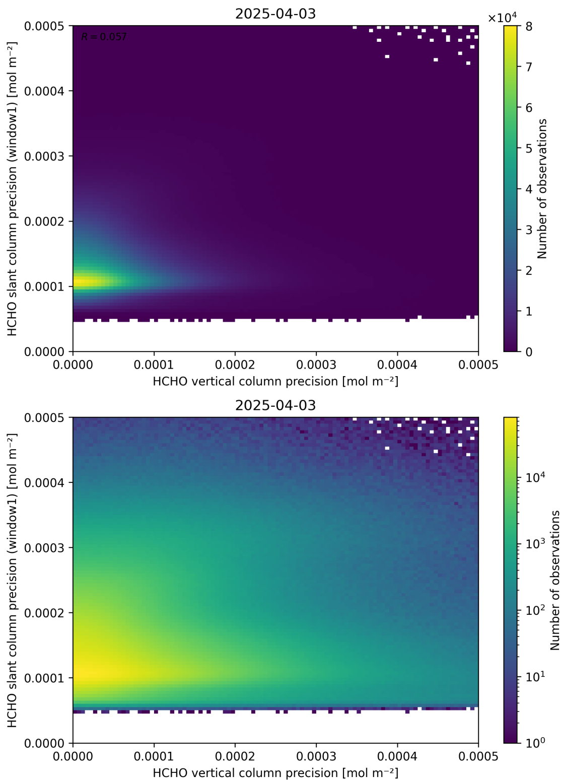
Figure 143: Scatter density plot of “HCHO vertical column precision” against “HCHO slant column precision (window1)” for 2025-04-03 to 2025-04-04.
