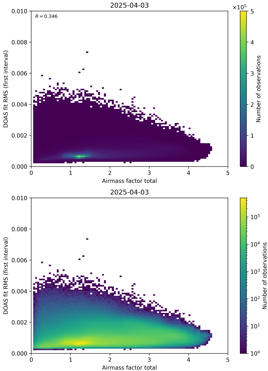
Figure 97: Scatter density plot of “Airmass factor total” against “DOAS fit RMS (first interval)” for 2025-04-03 to 2025-04-04.
