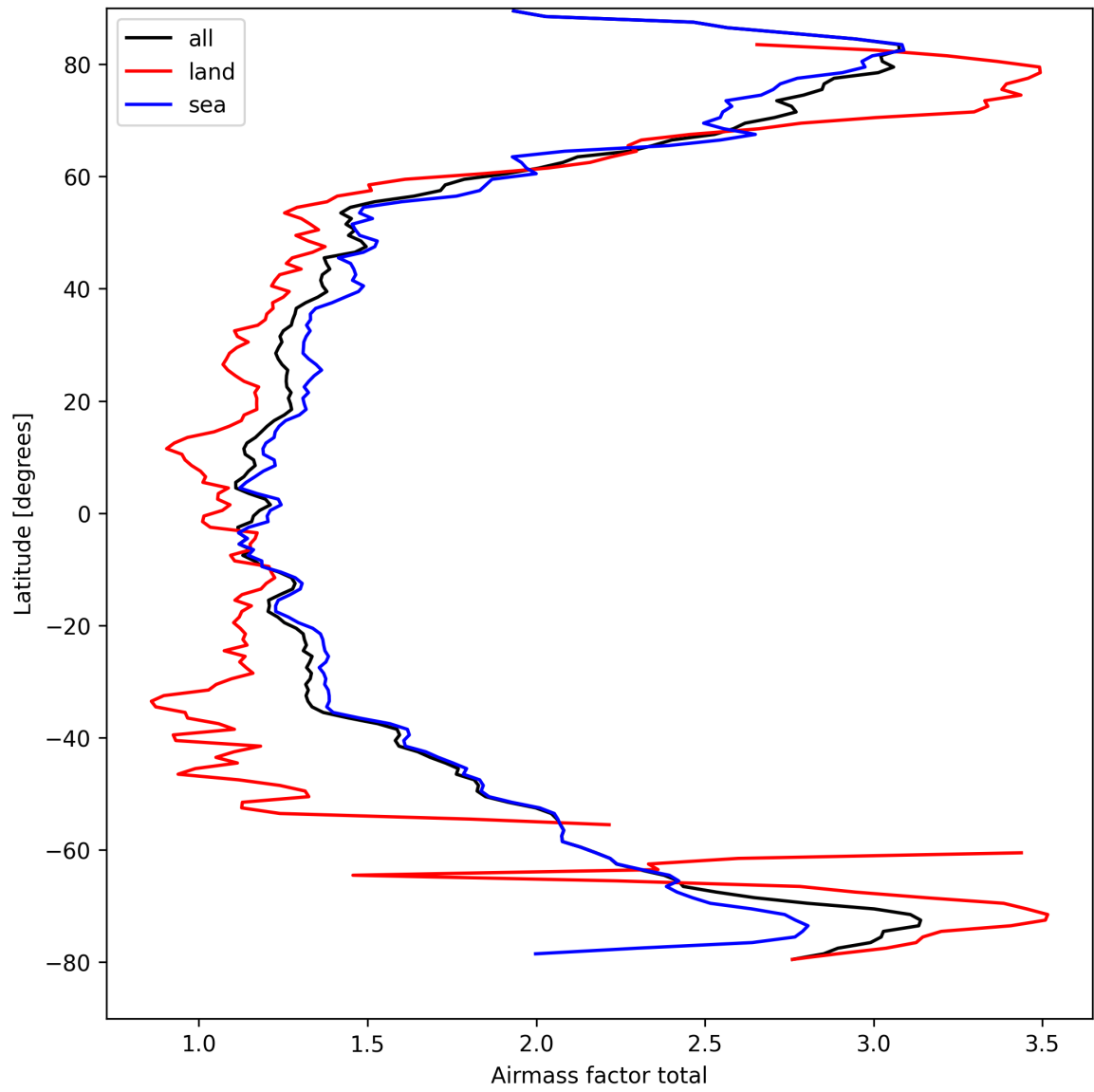
Figure 26: Zonal average of “Airmass factor total” for 2025-04-03 to 2025-04-04.
