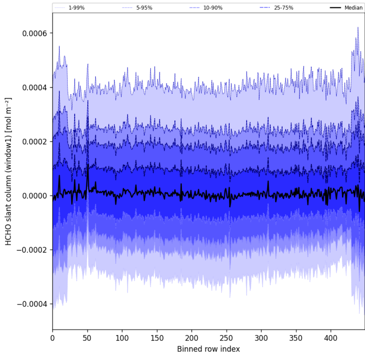
Figure 52: Along track statistics of “HCHO slant column (window1)” for 2025-04-03 to 2025-04-04
