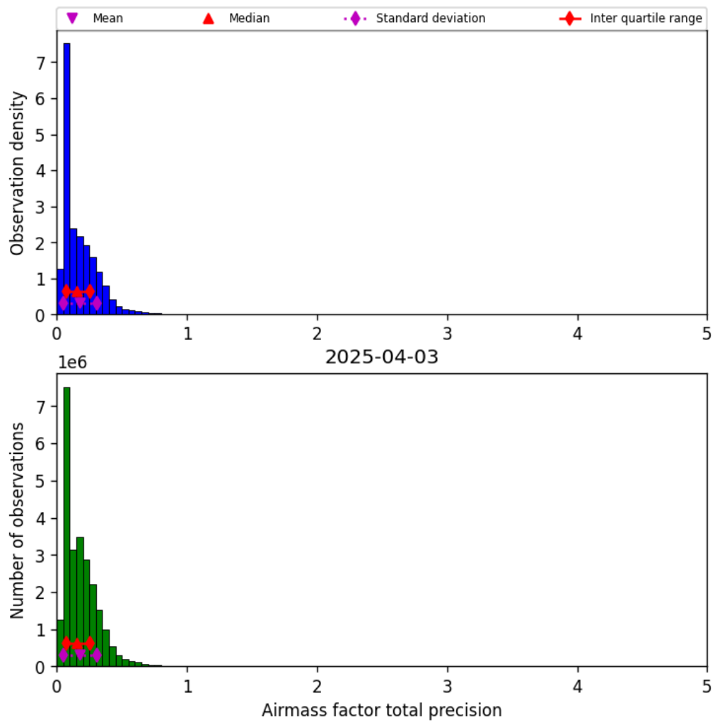
Figure 41: Histogram of “Airmass factor total precision” for 2025-04-03 to 2025-04-04
