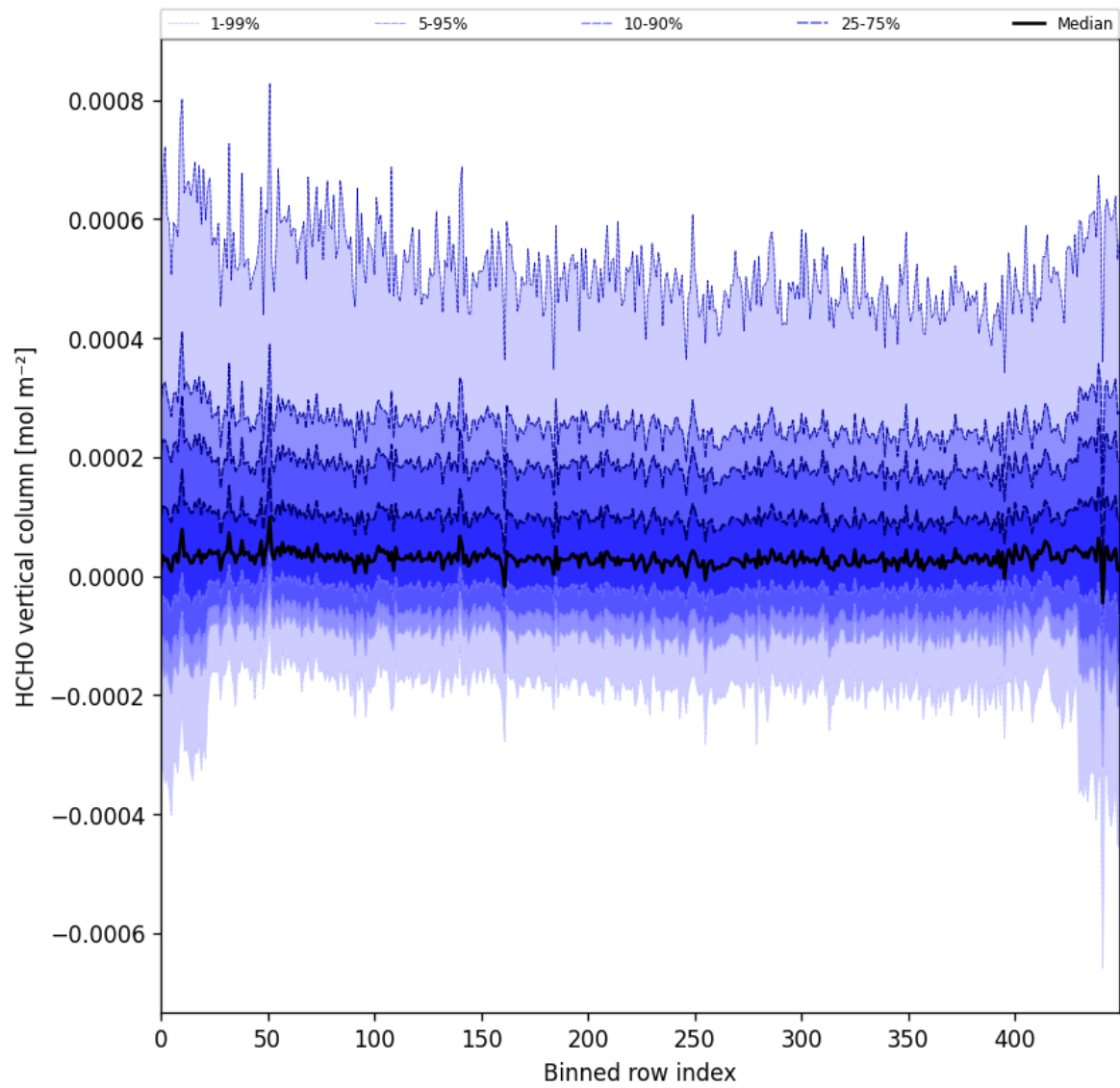
Figure 49: Along track statistics of “HCHO vertical column” for 2025-04-03 to 2025-04-04
