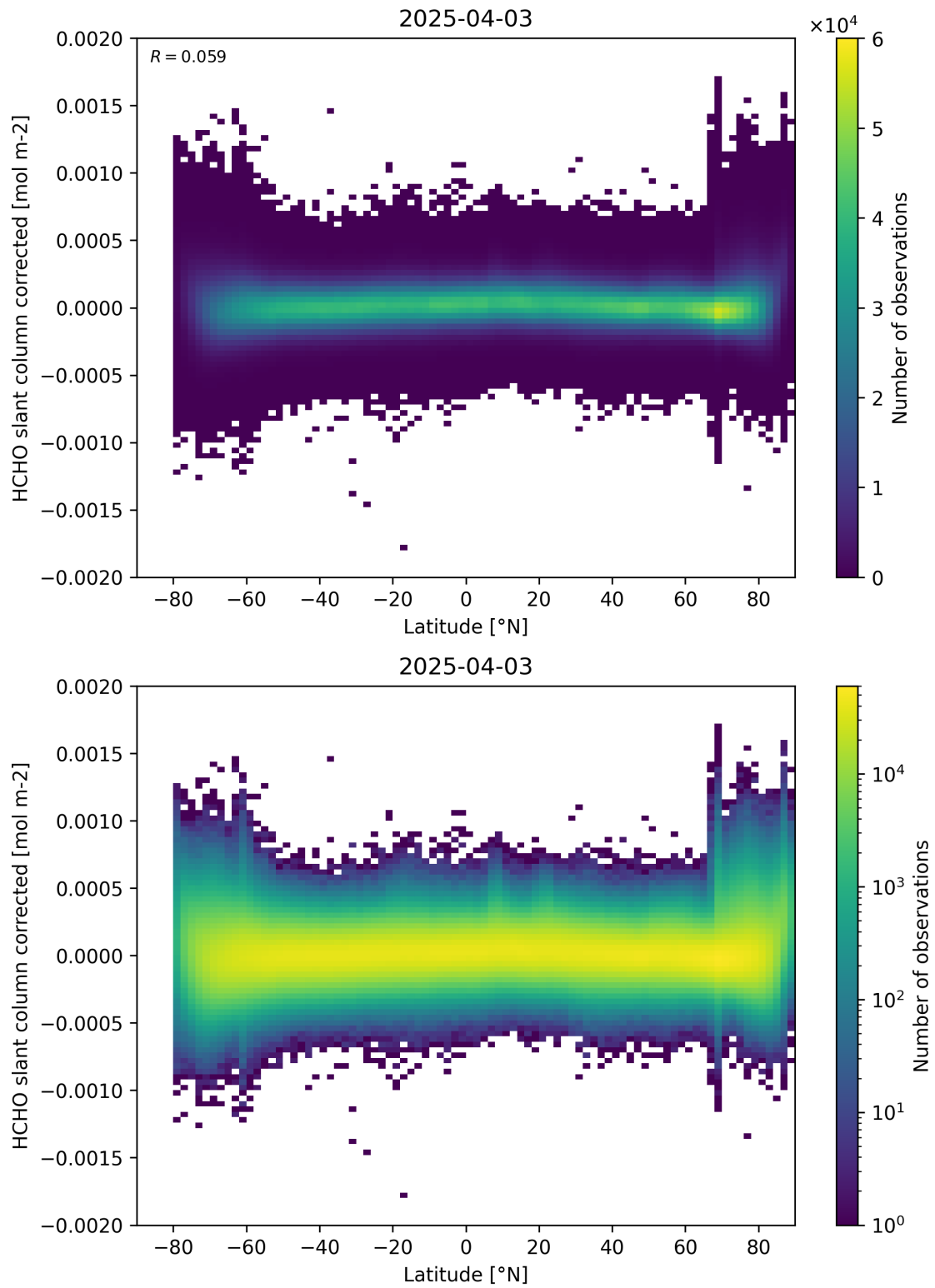
Figure 157: Scatter density plot of “Latitude” against “HCHO slant column corrected” for 2025-04-03 to 2025-04-04.
