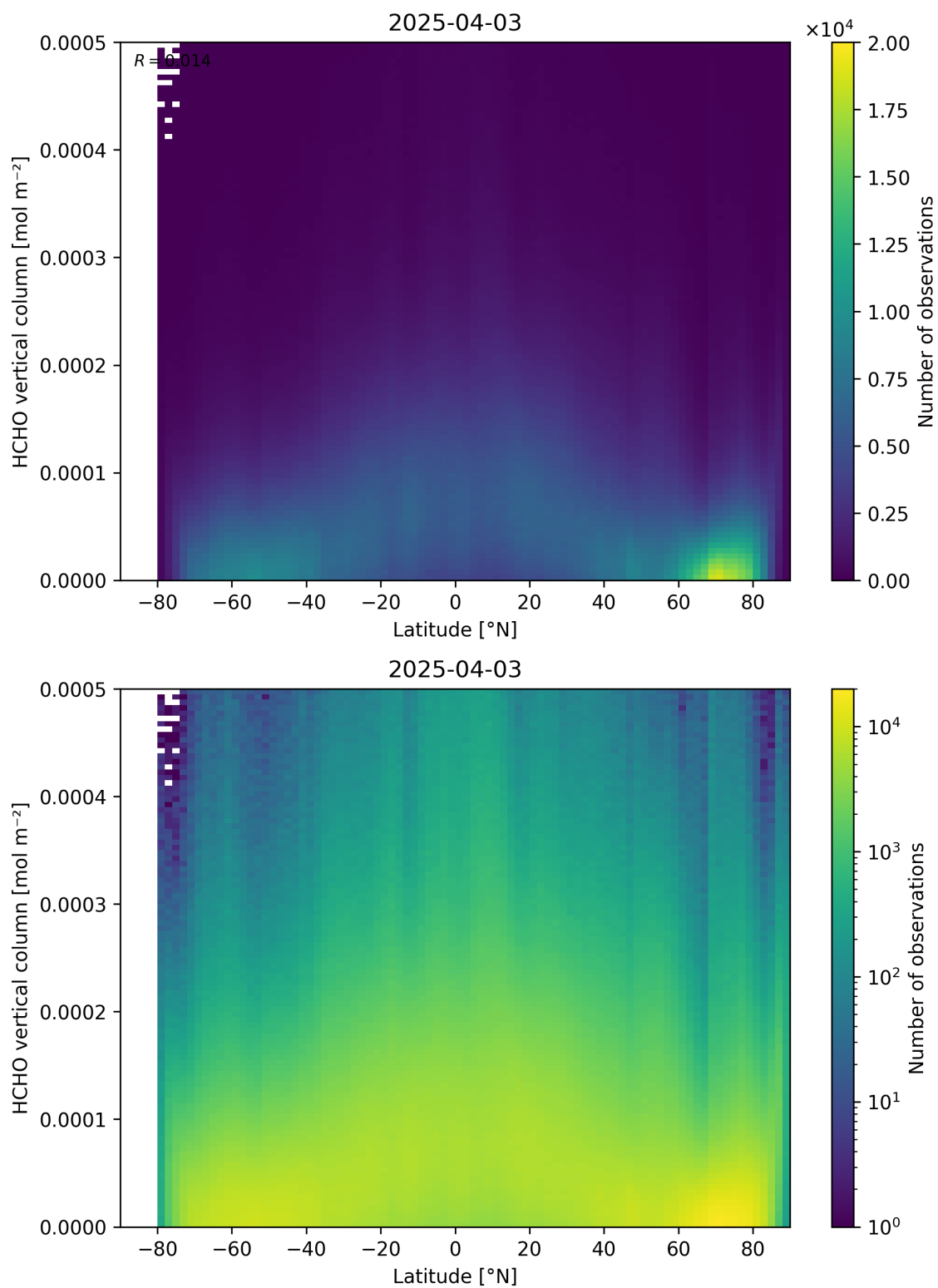
Figure 163: Scatter density plot of “Latitude” against “HCHO vertical column” for 2025-04-03 to 2025-04-04.
