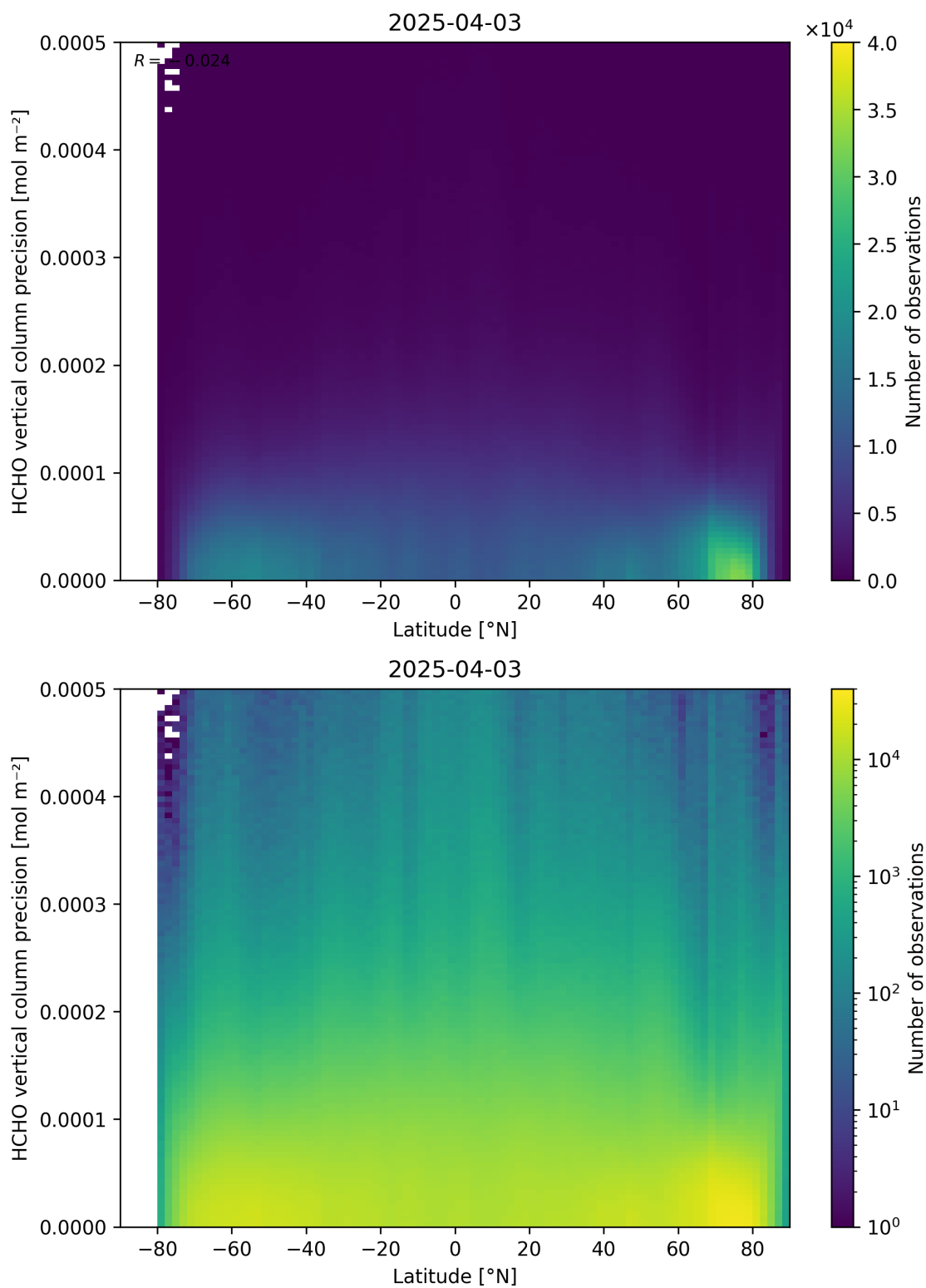
Figure 165: Scatter density plot of “Latitude” against “HCHO vertical column precision” for 2025-04-03 to 2025-04-04.
