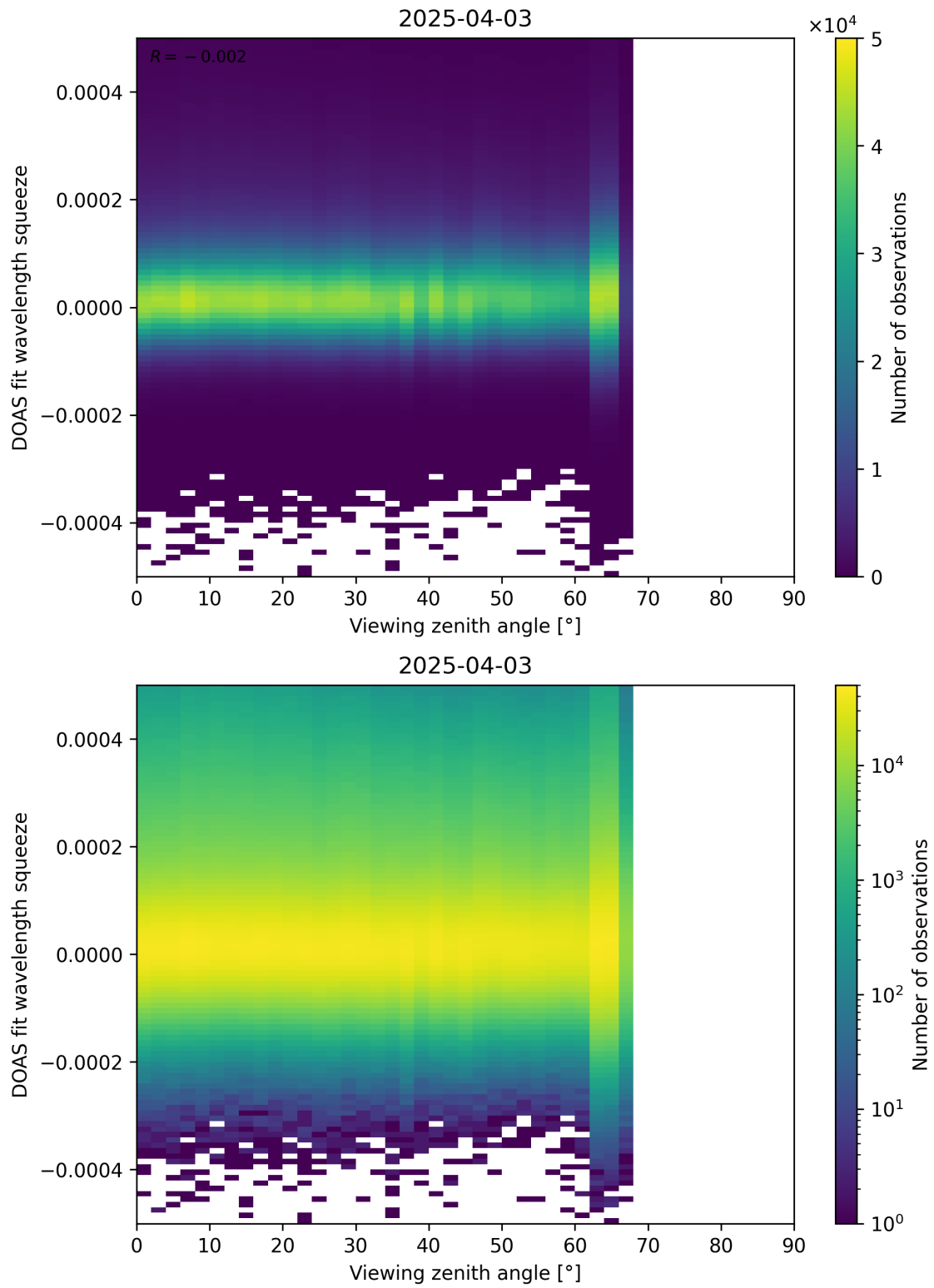
Figure 184: Scatter density plot of “Viewing zenith angle” against “DOAS fit wavelength squeeze” for 2025-04-03 to 2025-04-04.
