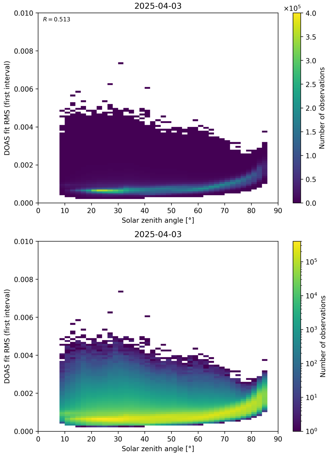
Figure 167: Scatter density plot of “Solar zenith angle” against “DOAS fit RMS (first interval)” for 2025-04-03 to 2025-04-04.
