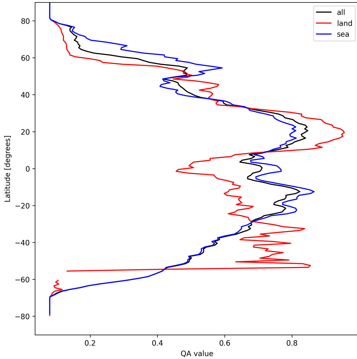
Figure 20: Zonal average of “QA value” for 2025-04-03 to 2025-04-04.
