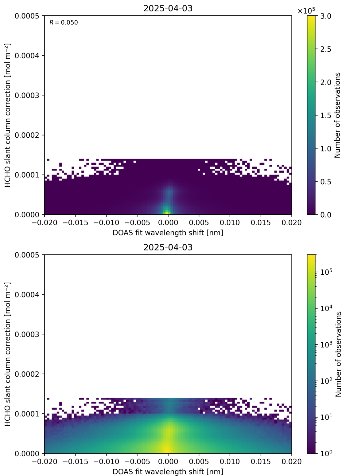
Figure 67: Scatter density plot of “DOAS fit wavelength shift” against “HCHO slant column correction” for 2025-04-03 to 2025-04-04.
