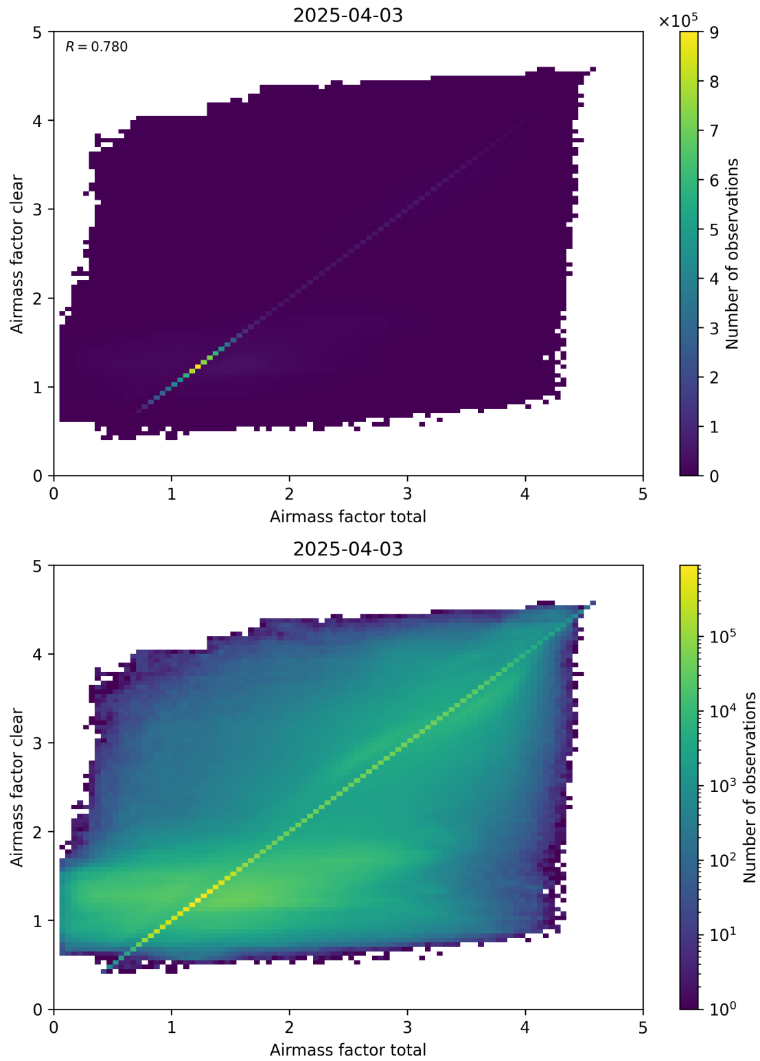
Figure 100: Scatter density plot of “Airmass factor total” against “Airmass factor clear” for 2025-04-03 to 2025-04-04.
