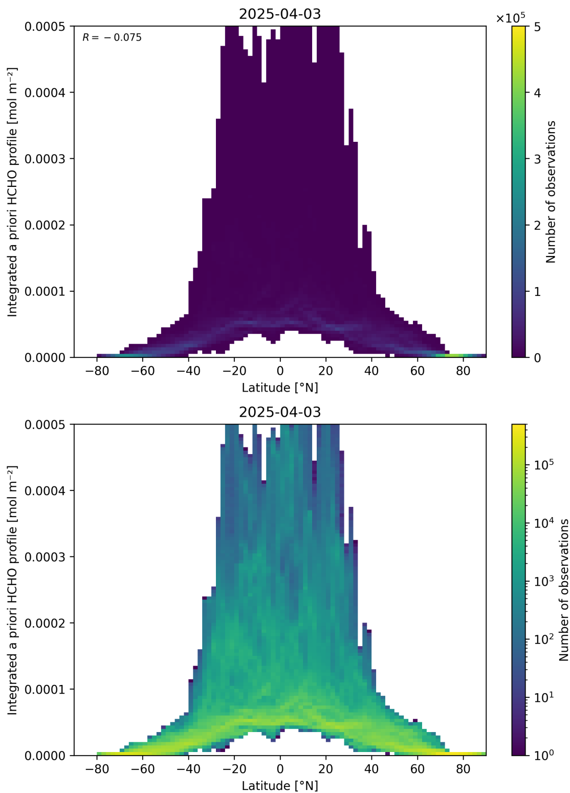
Figure 166: Scatter density plot of “Latitude” against “Integrated a priori HCHO profile” for 2025-04-03 to 2025-04-04.
