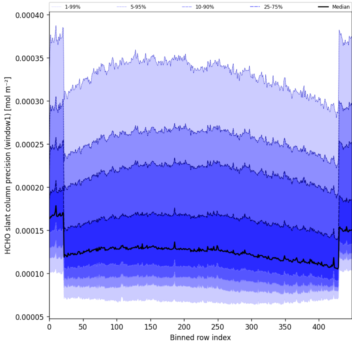
Figure 53: Along track statistics of “HCHO slant column precision (window1)” for 2025-04-03 to 2025-04-04
