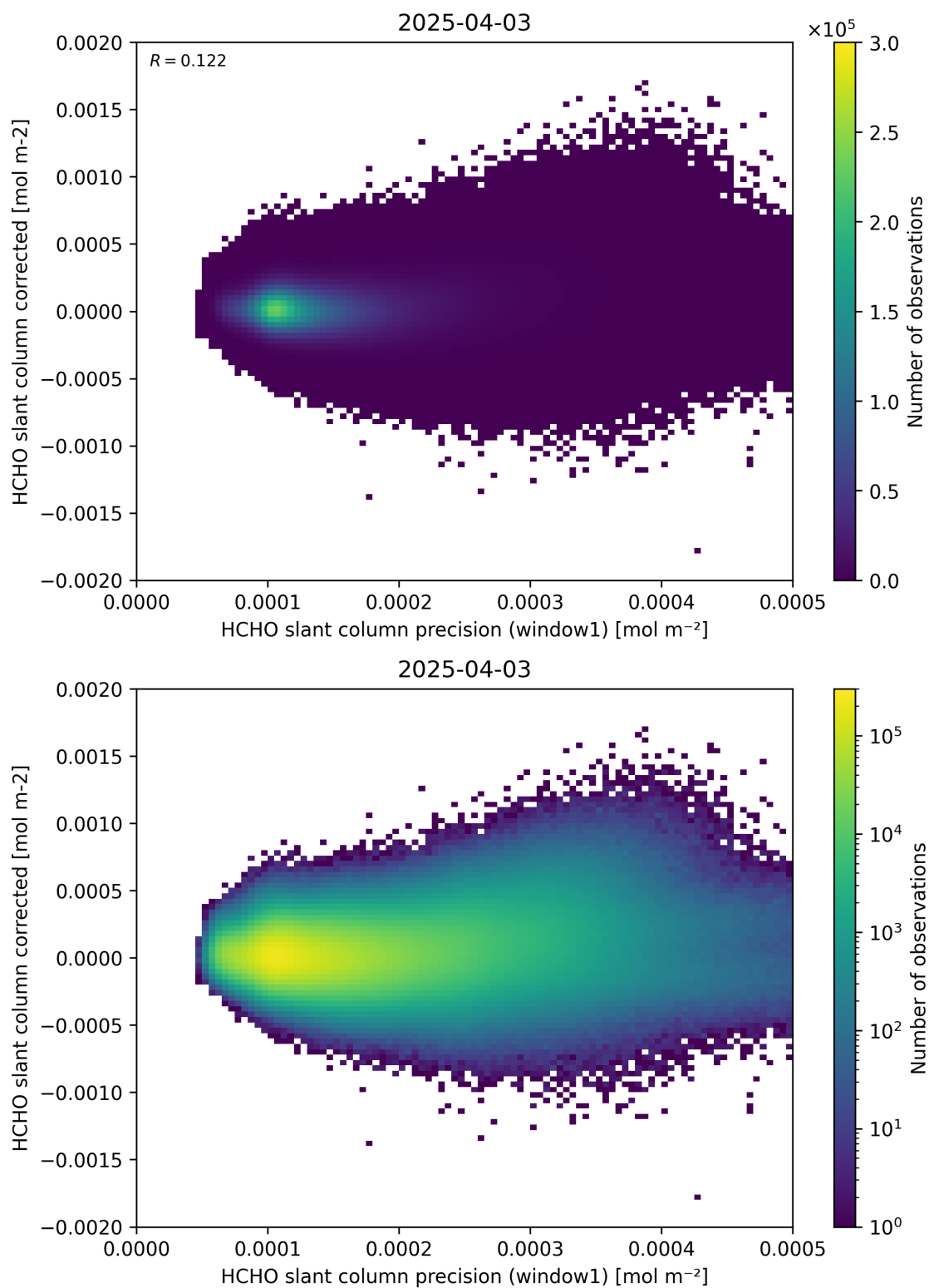
Figure 92: Scatter density plot of “HCHO slant column precision (window1)” against “HCHO slant column corrected” for 2025-04-03 to 2025-04-04.
