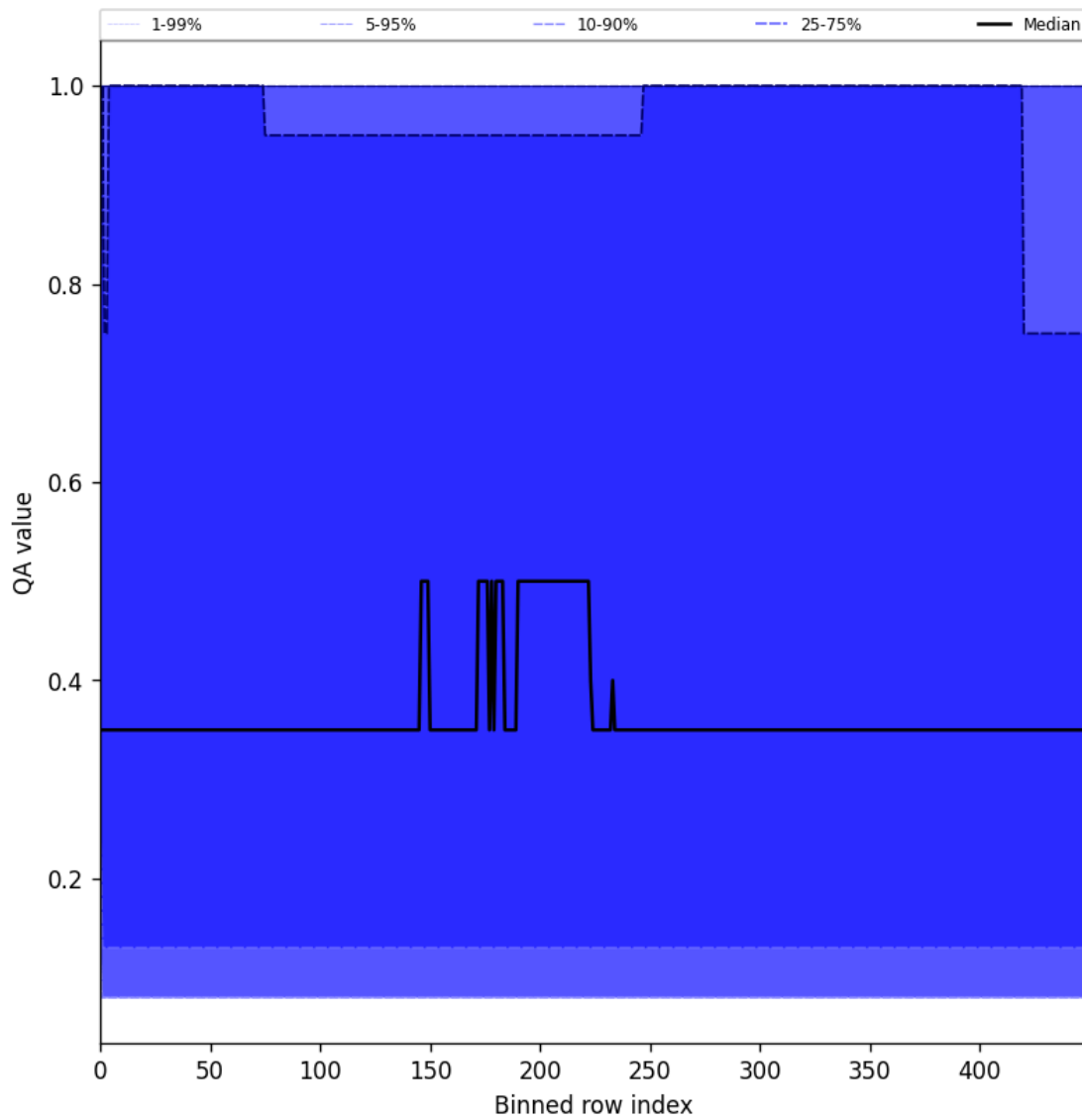
Figure 48: Along track statistics of “QA value” for 2025-04-03 to 2025-04-04
