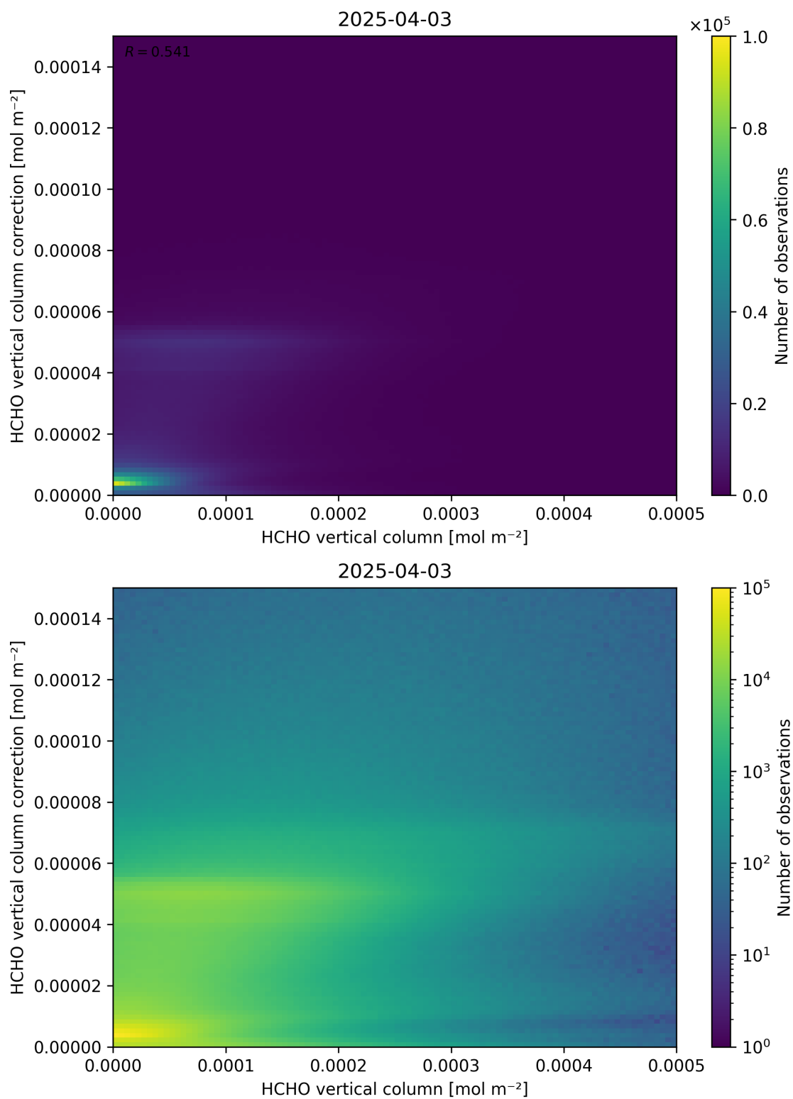
Figure 133: Scatter density plot of “HCHO vertical column” against “HCHO vertical column correction” for 2025-04-03 to 2025-04-04.
