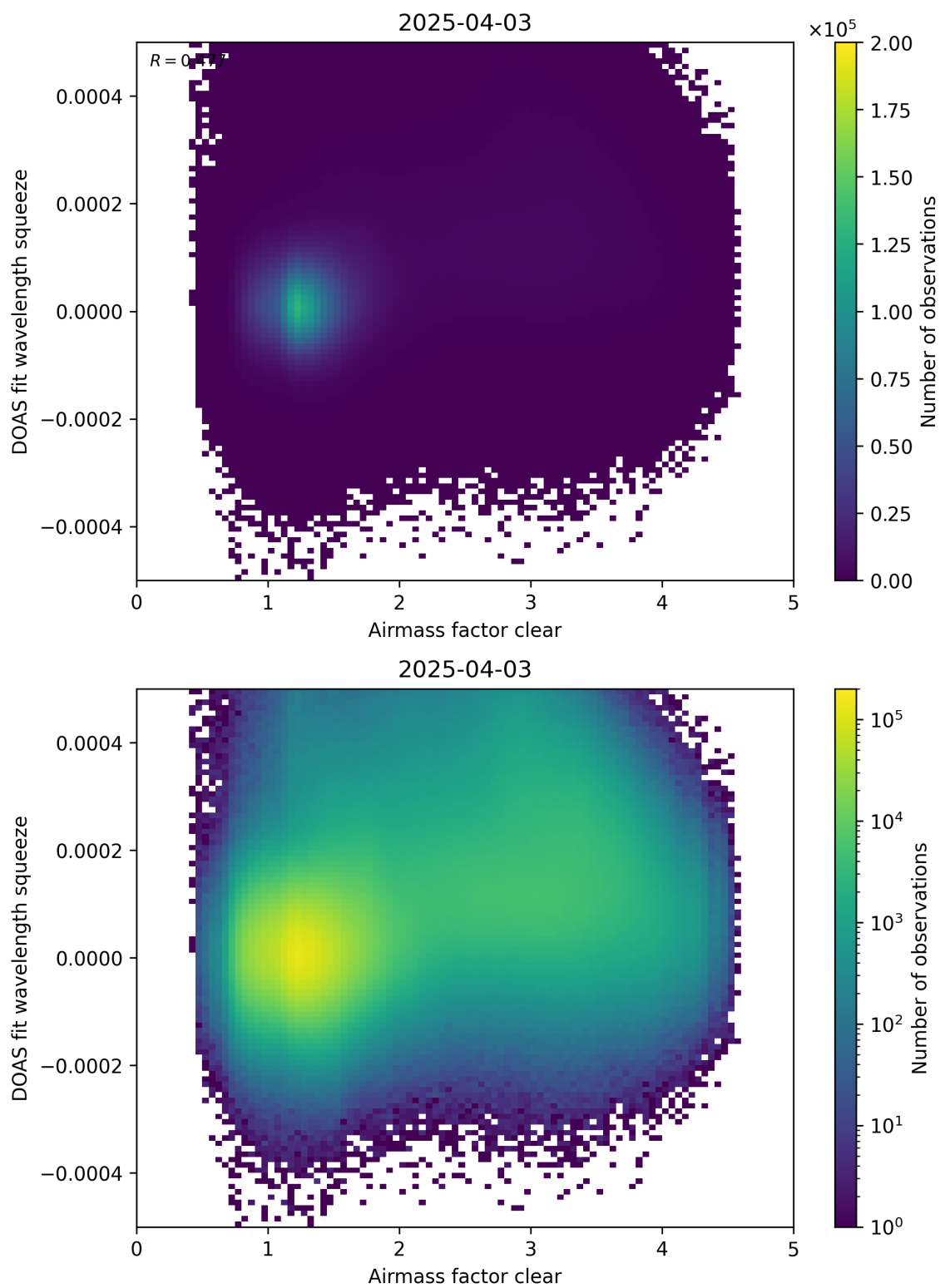
Figure 73: Scatter density plot of “Airmass factor clear” against “DOAS fit wavelength squeeze” for 2025-04-03 to 2025-04-04.
