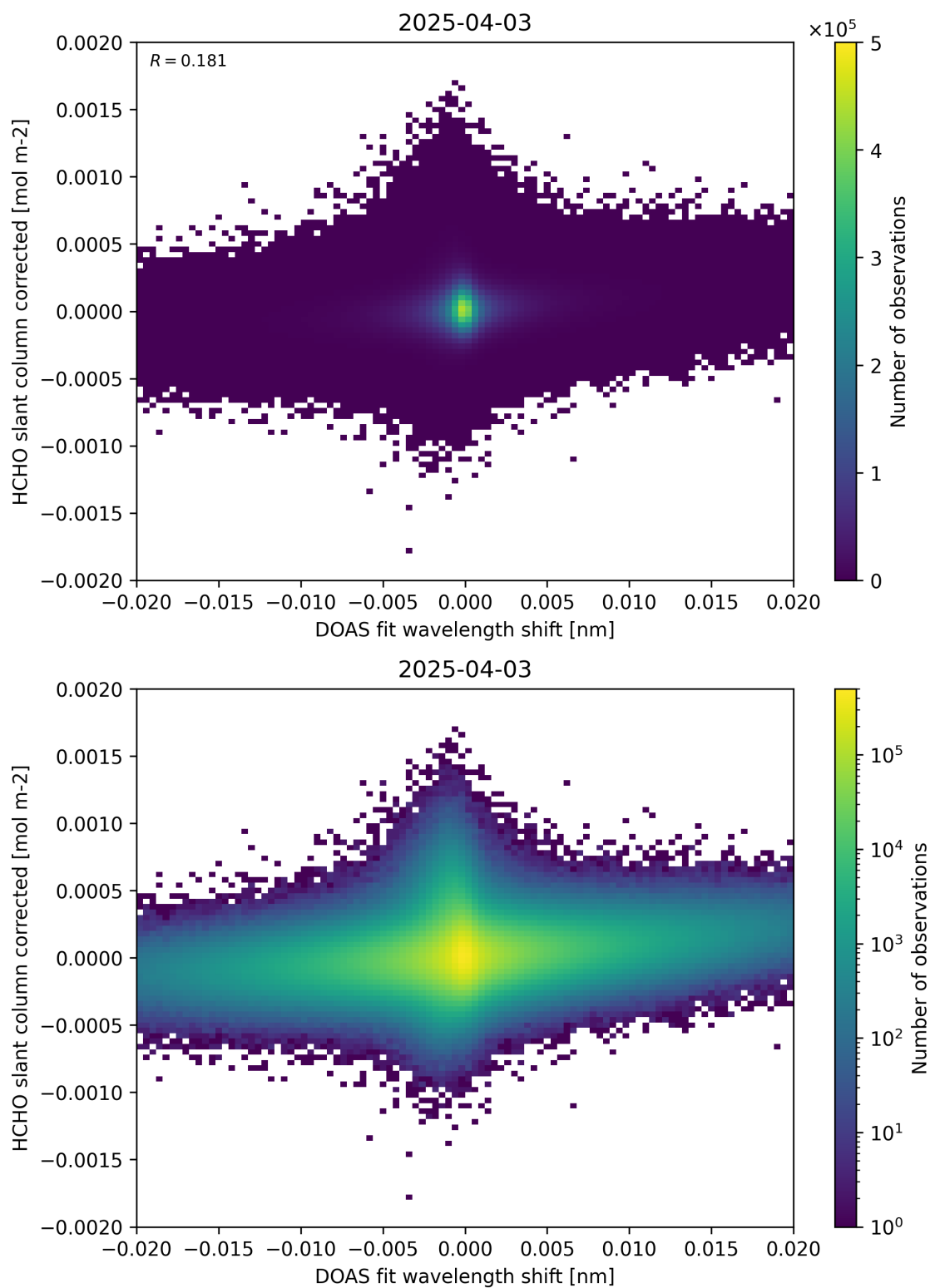
Figure 66: Scatter density plot of “DOAS fit wavelength shift” against “HCHO slant column corrected” for 2025-04-03 to 2025-04-04.
