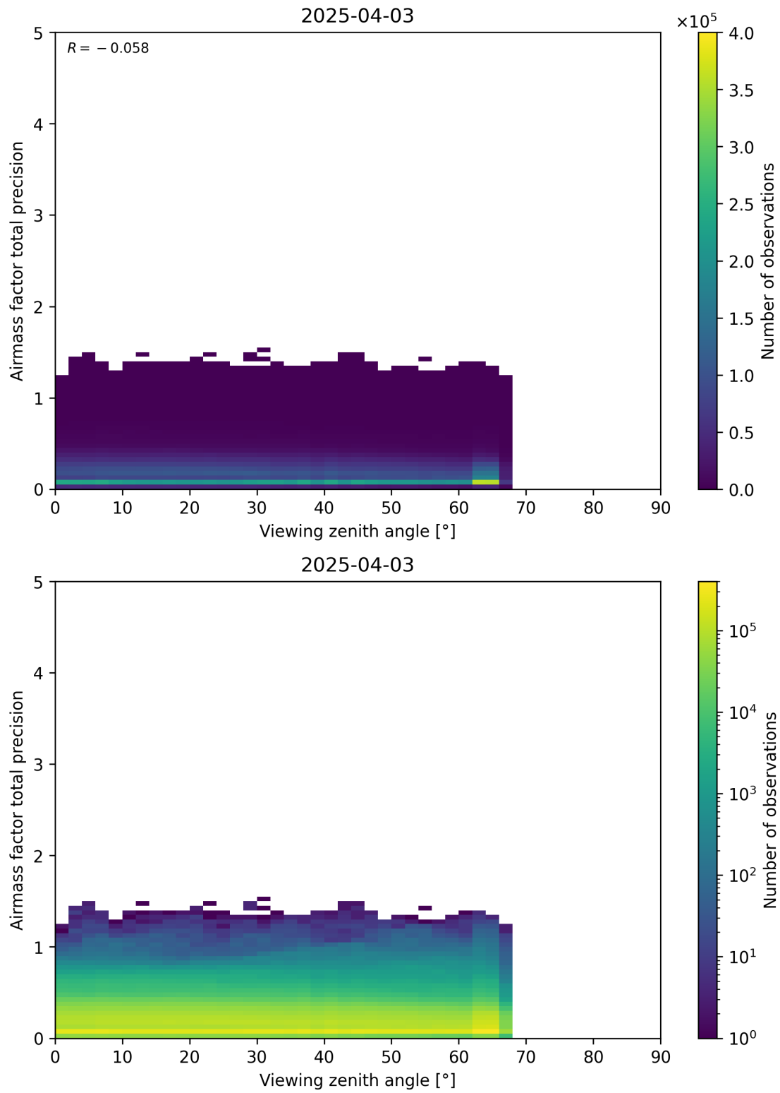
Figure 191: Scatter density plot of “Viewing zenith angle” against “Airmass factor total precision” for 2025-04-03 to 2025-04-04.
