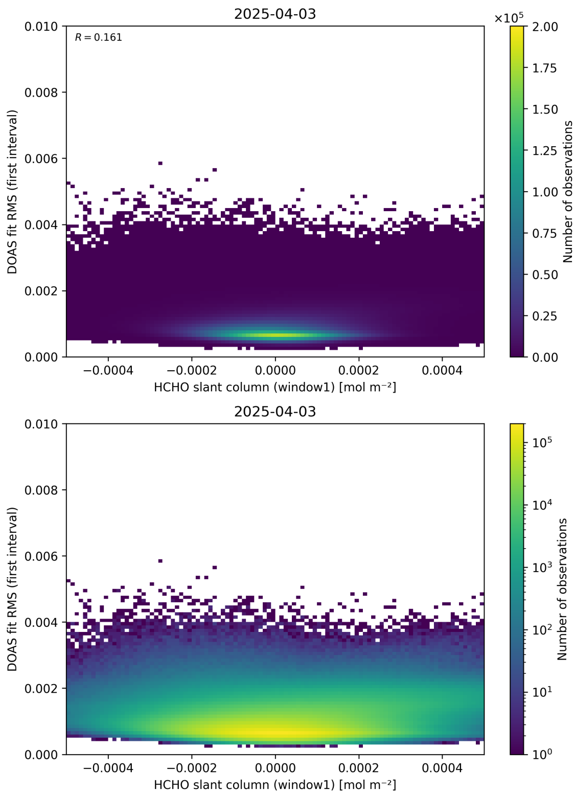
Figure 78: Scatter density plot of “HCHO slant column (window1)” against “DOAS fit RMS (first interval)” for 2025-04-03 to 2025-04-04.
