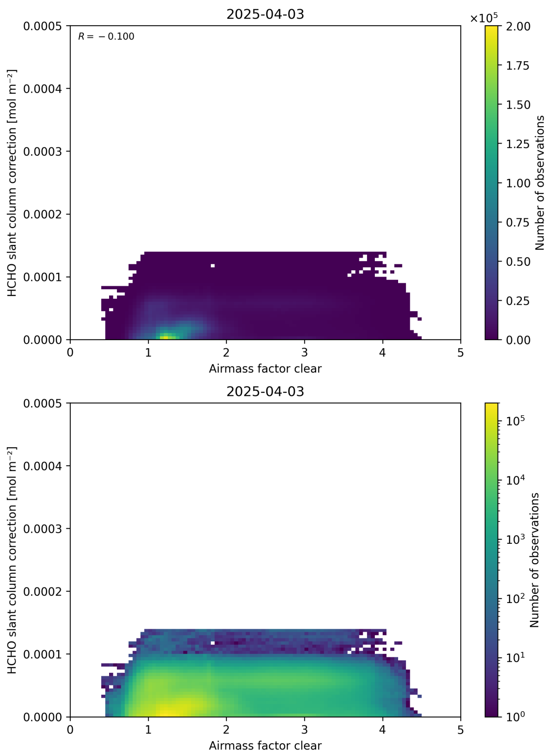
Figure 75: Scatter density plot of “Airmass factor clear” against “HCHO slant column correction” for 2025-04-03 to 2025-04-04.
