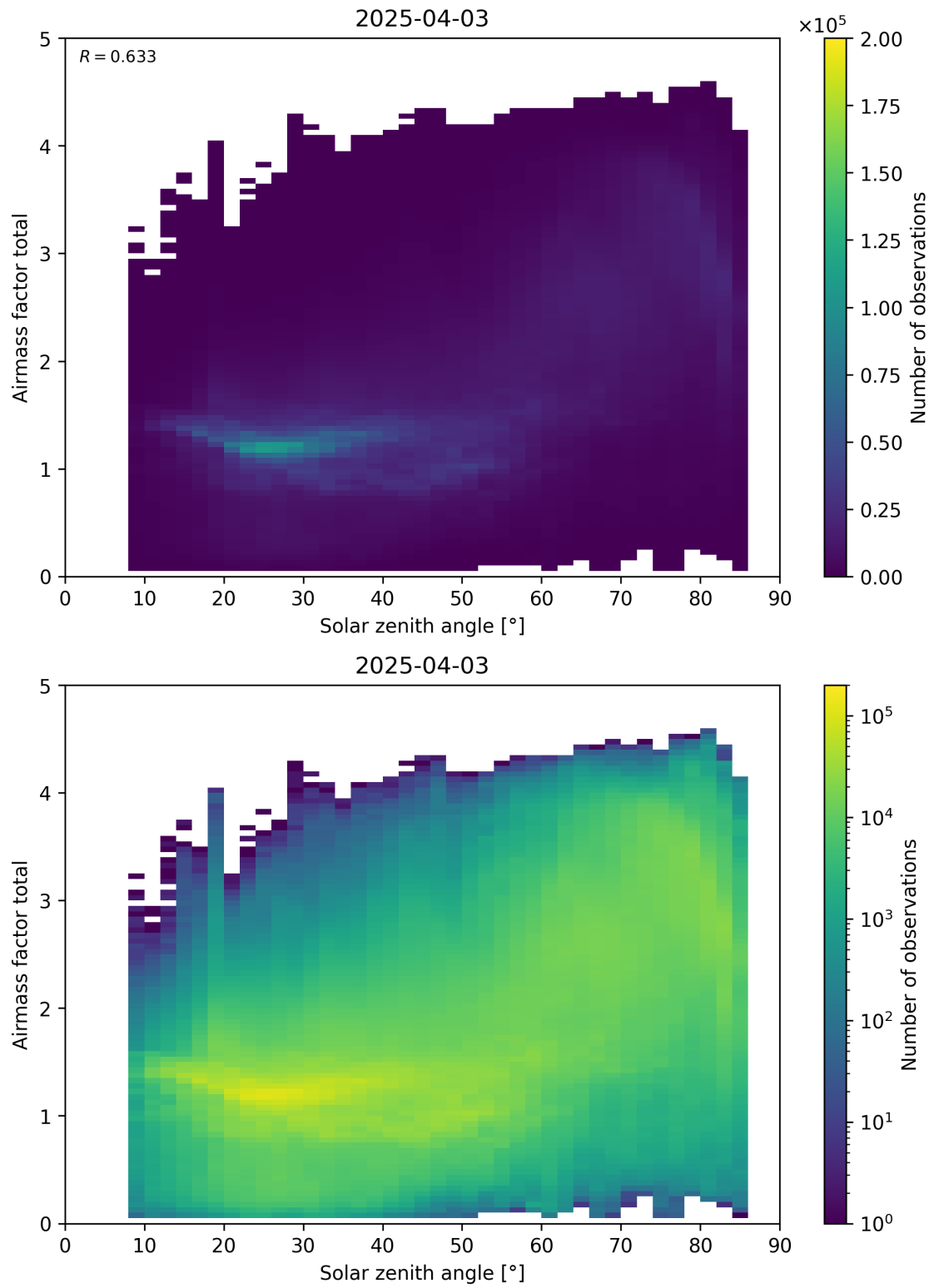
Figure 175: Scatter density plot of “Solar zenith angle” against “Airmass factor total” for 2025-04-03 to 2025-04-04.
