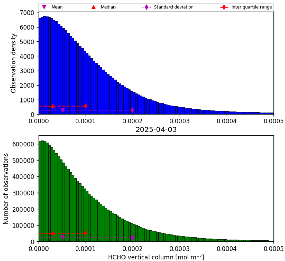
Figure 35: Histogram of “HCHO vertical column” for 2025-04-03 to 2025-04-04
