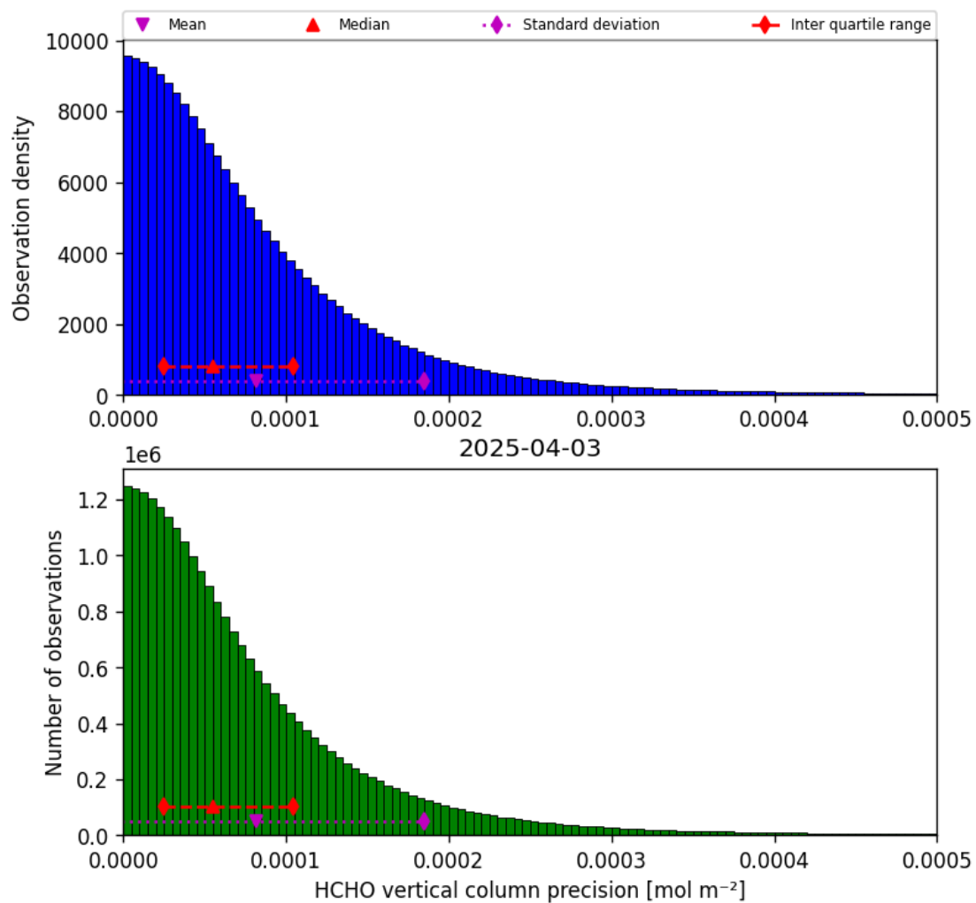
Figure 36: Histogram of “HCHO vertical column precision” for 2025-04-03 to 2025-04-04
