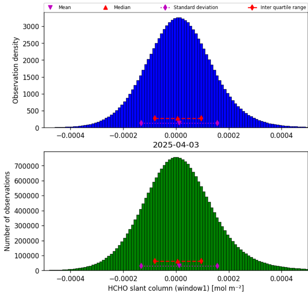
Figure 38: Histogram of “HCHO slant column (window1)” for 2025-04-03 to 2025-04-04
