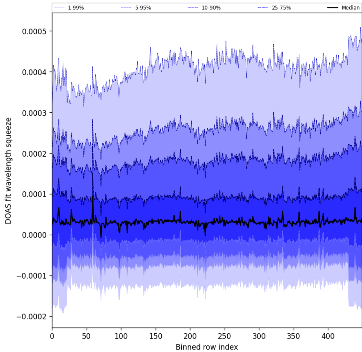
Figure 59: Along track statistics of “DOAS fit wavelength squeeze” for 2025-04-03 to 2025-04-04
