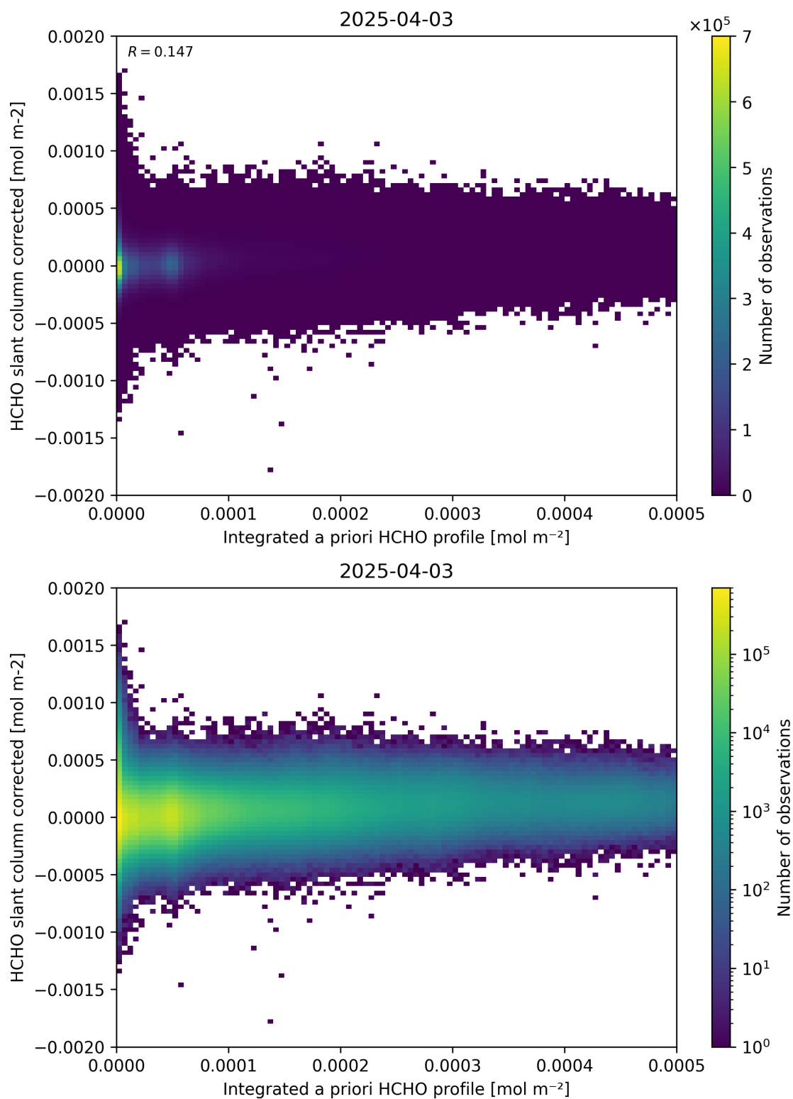
Figure 151: Scatter density plot of “Integrated a priori HCHO profile” against “HCHO slant column corrected” for 2025-04-03 to 2025-04-04.
