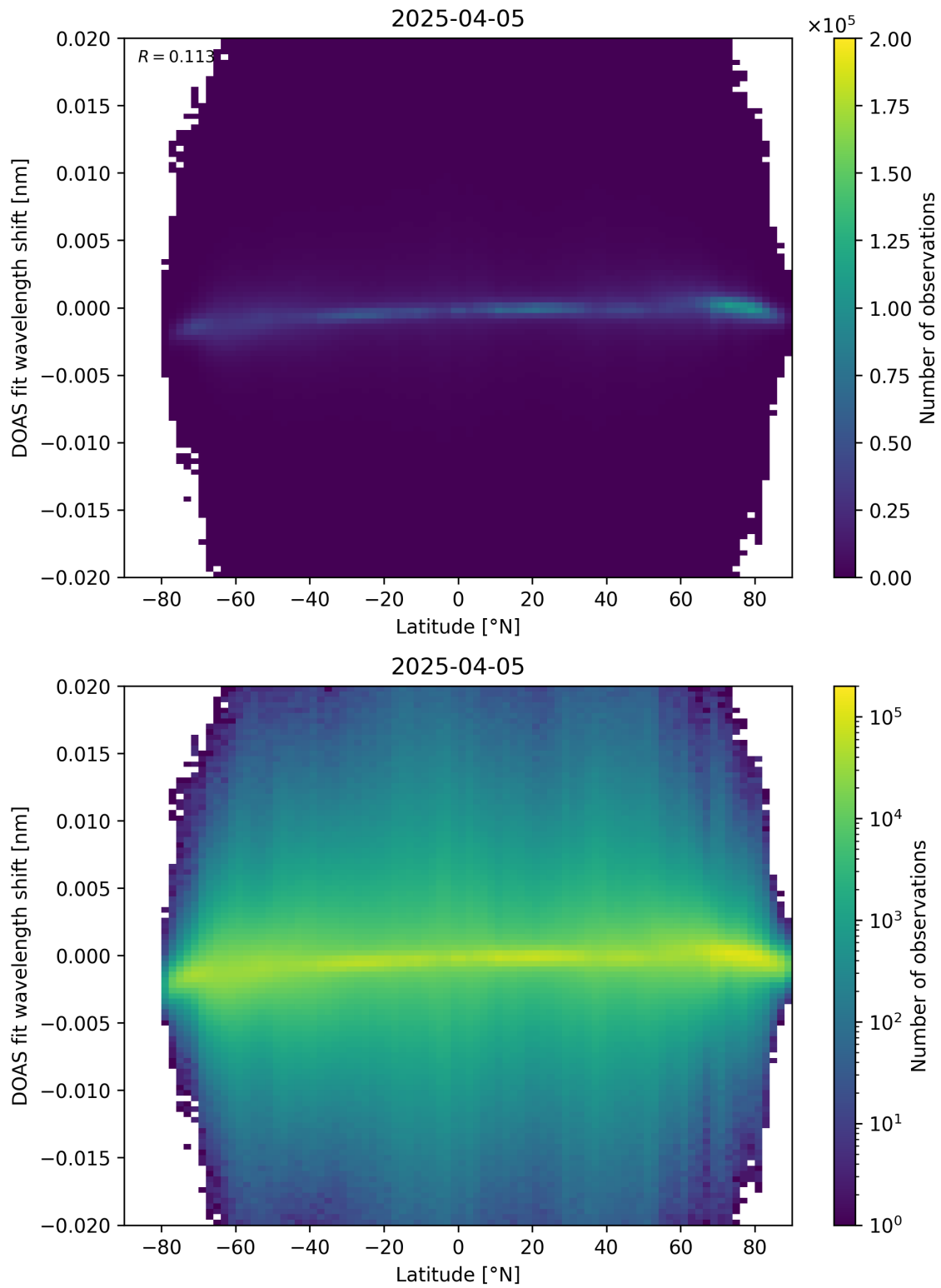
Figure 154: Scatter density plot of “Latitude” against “DOAS fit wavelength shift” for 2025-04-04 to 2025-04-06.
