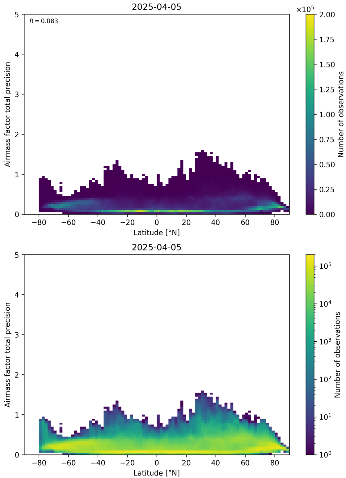
Figure 162: Scatter density plot of “Latitude” against “Airmass factor total precision” for 2025-04-04 to 2025-04-06.
