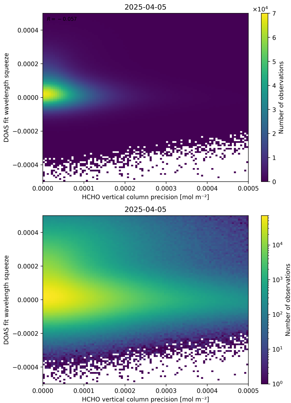
Figure 138: Scatter density plot of “HCHO vertical column precision” against “DOAS fit wavelength squeeze” for 2025-04-04 to 2025-04-06.
