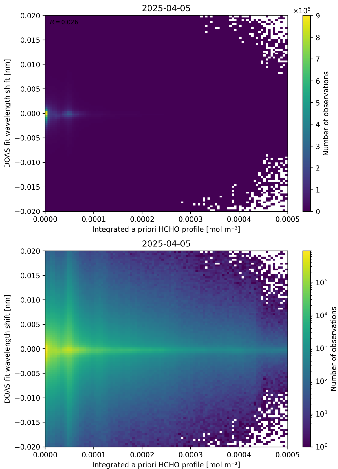
Figure 149: Scatter density plot of “Integrated a priori HCHO profile” against “DOAS fit wavelength shift” for 2025-04-04 to 2025-04-06.
