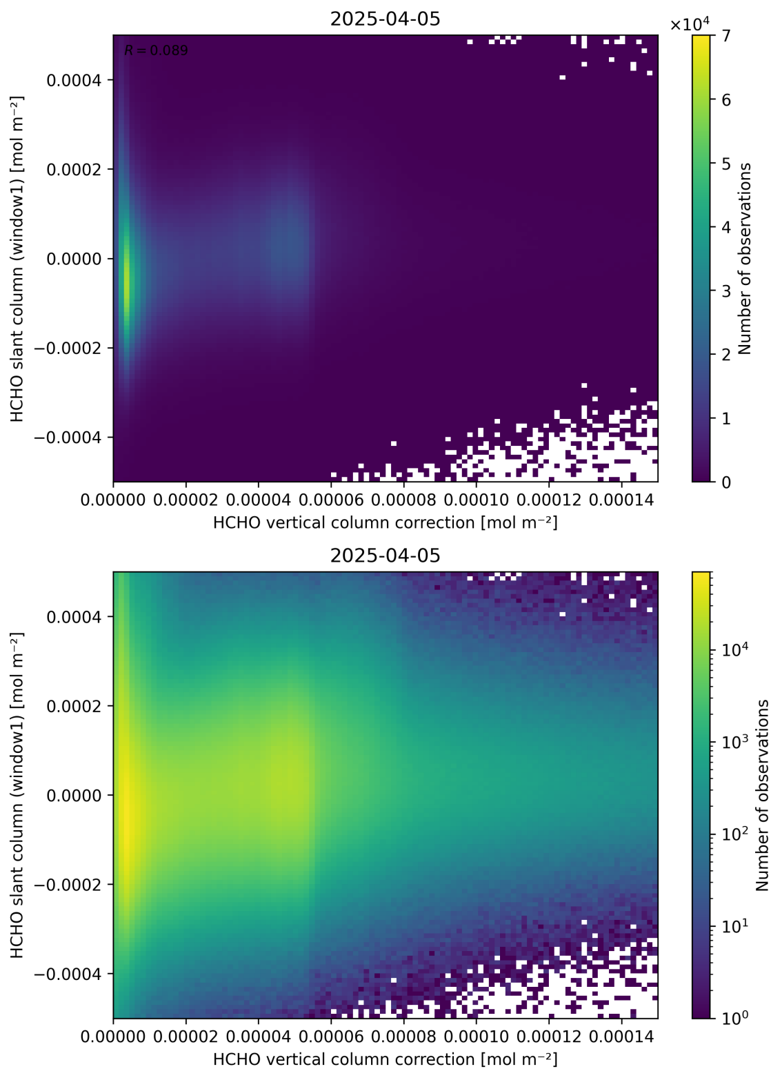
Figure 118: Scatter density plot of “HCHO vertical column correction” against “HCHO slant column (window1)” for 2025-04-04 to 2025-04-06.
