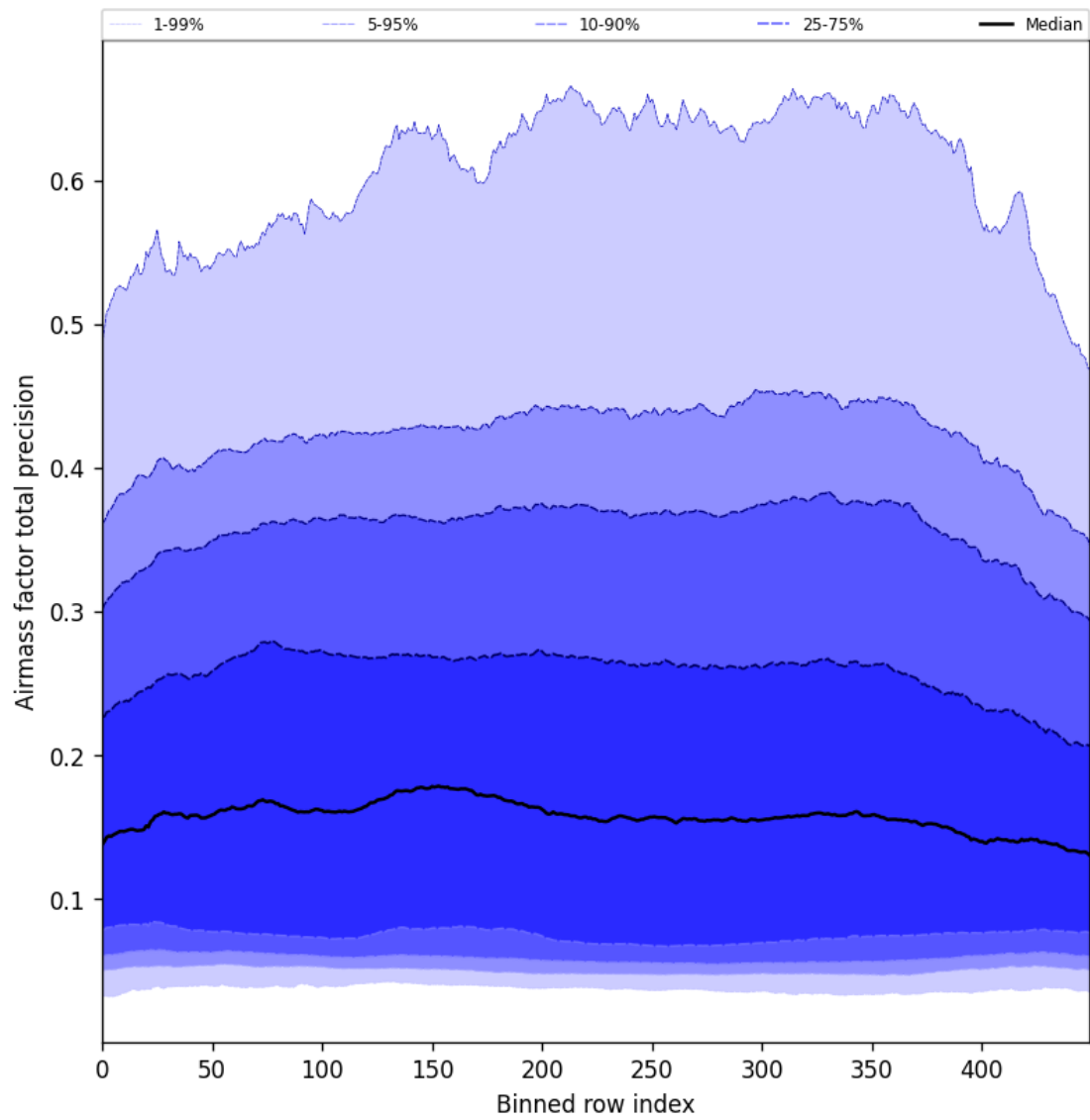
Figure 55: Along track statistics of “Airmass factor total precision” for 2025-04-04 to 2025-04-06
