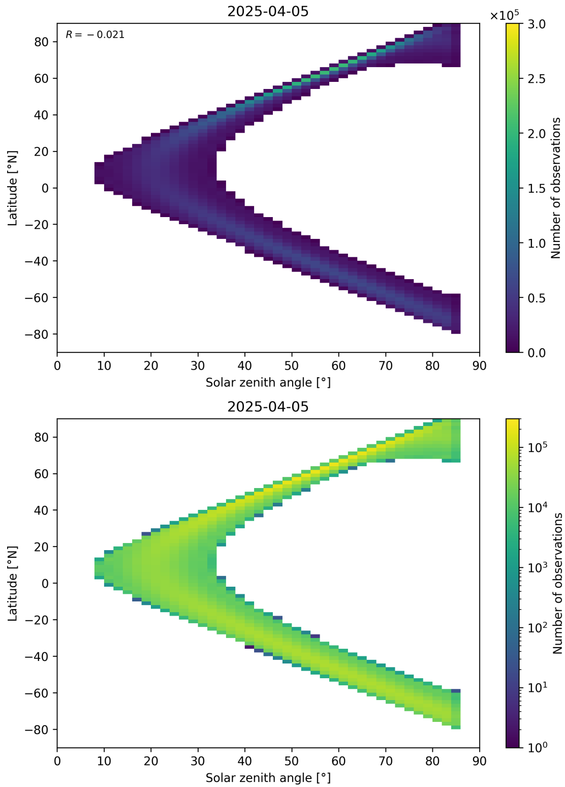
Figure 181: Scatter density plot of “Solar zenith angle” against “Latitude” for 2025-04-04 to 2025-04-06.
