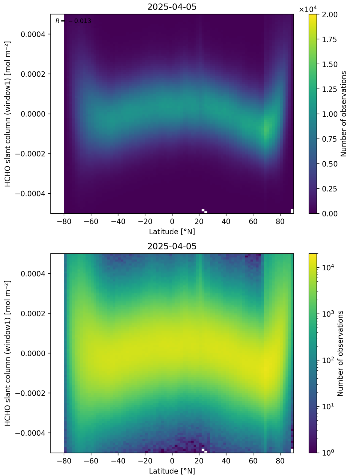
Figure 159: Scatter density plot of “Latitude” against “HCHO slant column (window1)” for 2025-04-04 to 2025-04-06.
