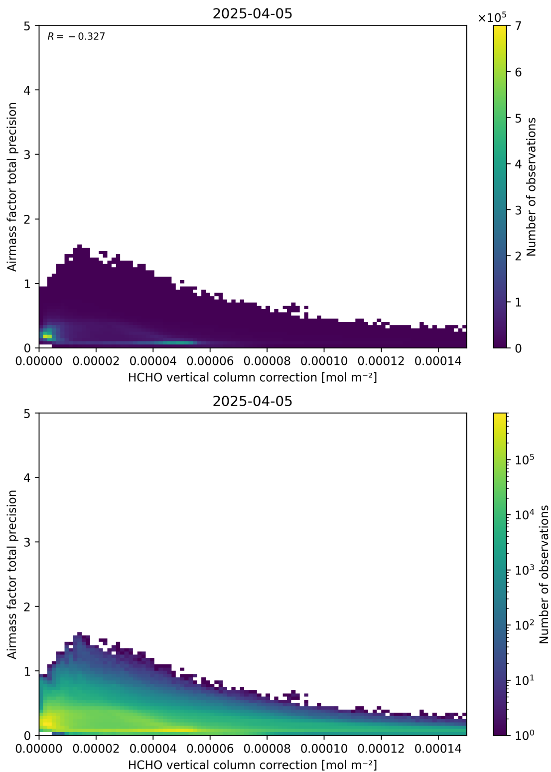
Figure 121: Scatter density plot of “HCHO vertical column correction” against “Airmass factor total precision” for 2025-04-04 to 2025-04-06.
