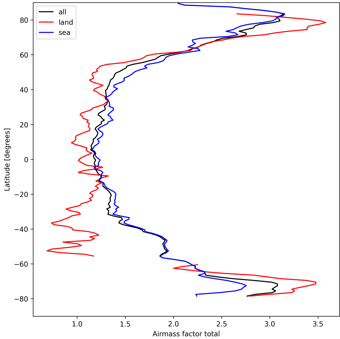
Figure 26: Zonal average of “Airmass factor total” for 2025-04-04 to 2025-04-06.
