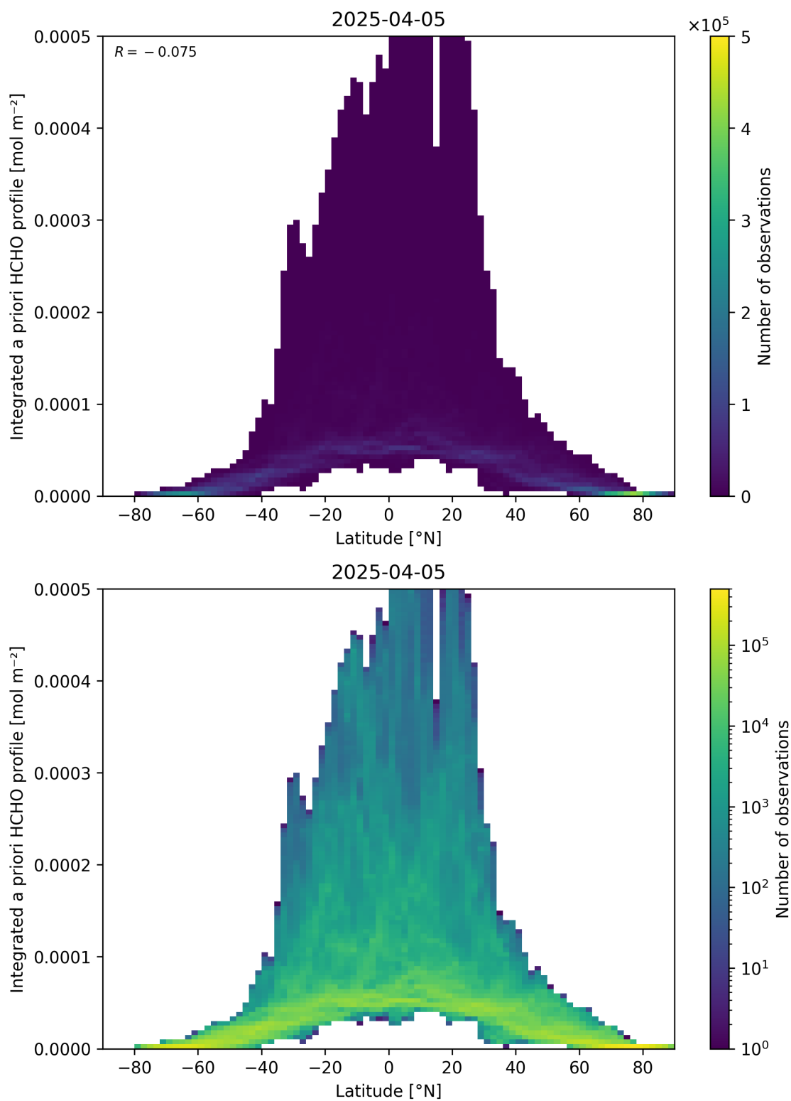
Figure 166: Scatter density plot of “Latitude” against “Integrated a priori HCHO profile” for 2025-04-04 to 2025-04-06.
