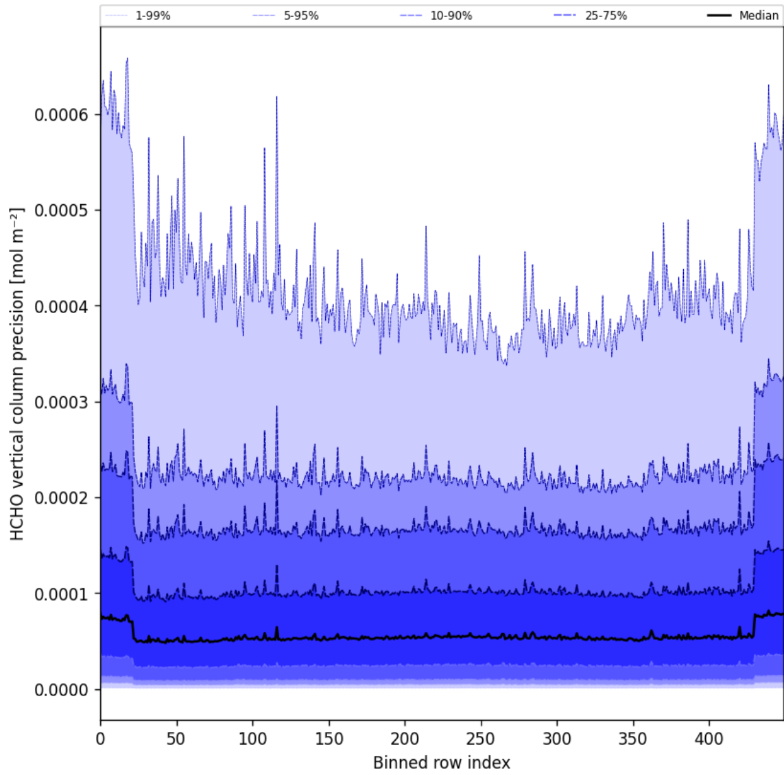
Figure 50: Along track statistics of “HCHO vertical column precision” for 2025-04-04 to 2025-04-06
