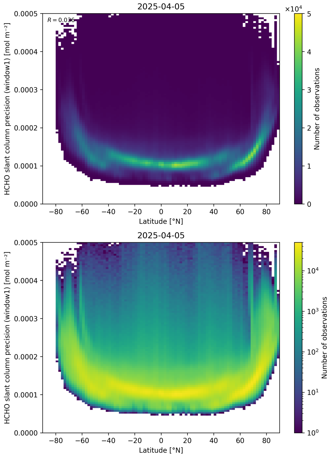
Figure 160: Scatter density plot of “Latitude” against “HCHO slant column precision (window1)” for 2025-04-04 to 2025-04-06.
