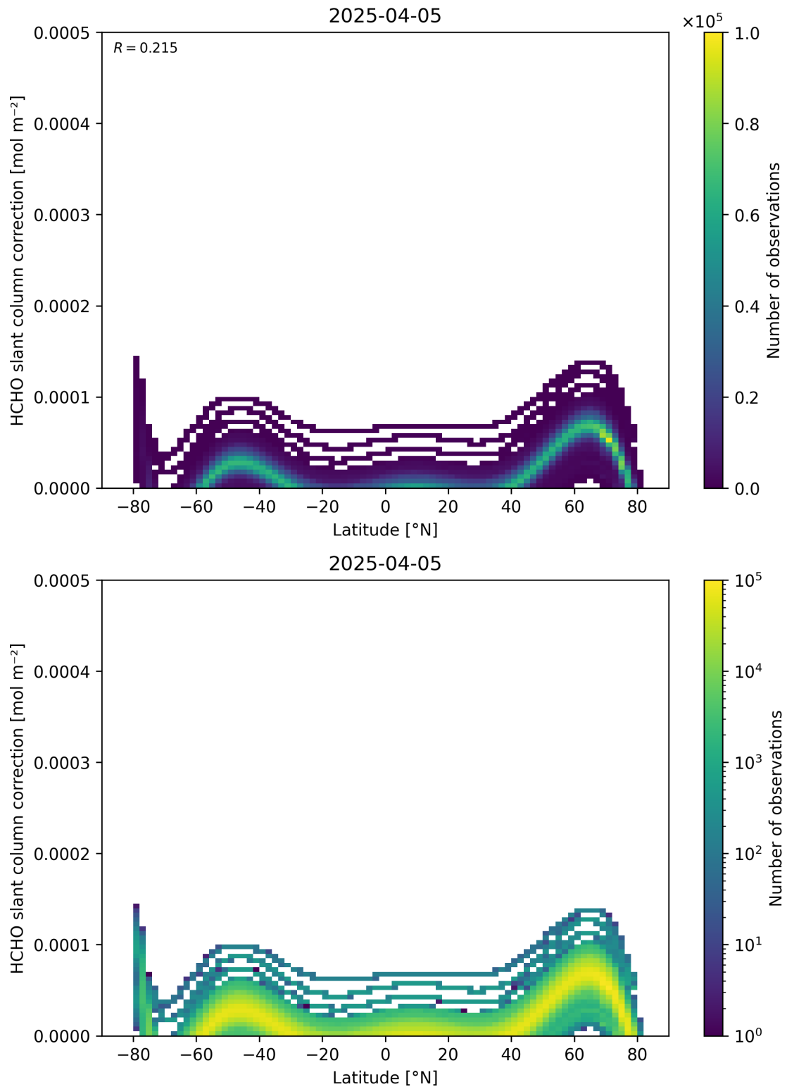
Figure 158: Scatter density plot of “Latitude” against “HCHO slant column correction” for 2025-04-04 to 2025-04-06.
