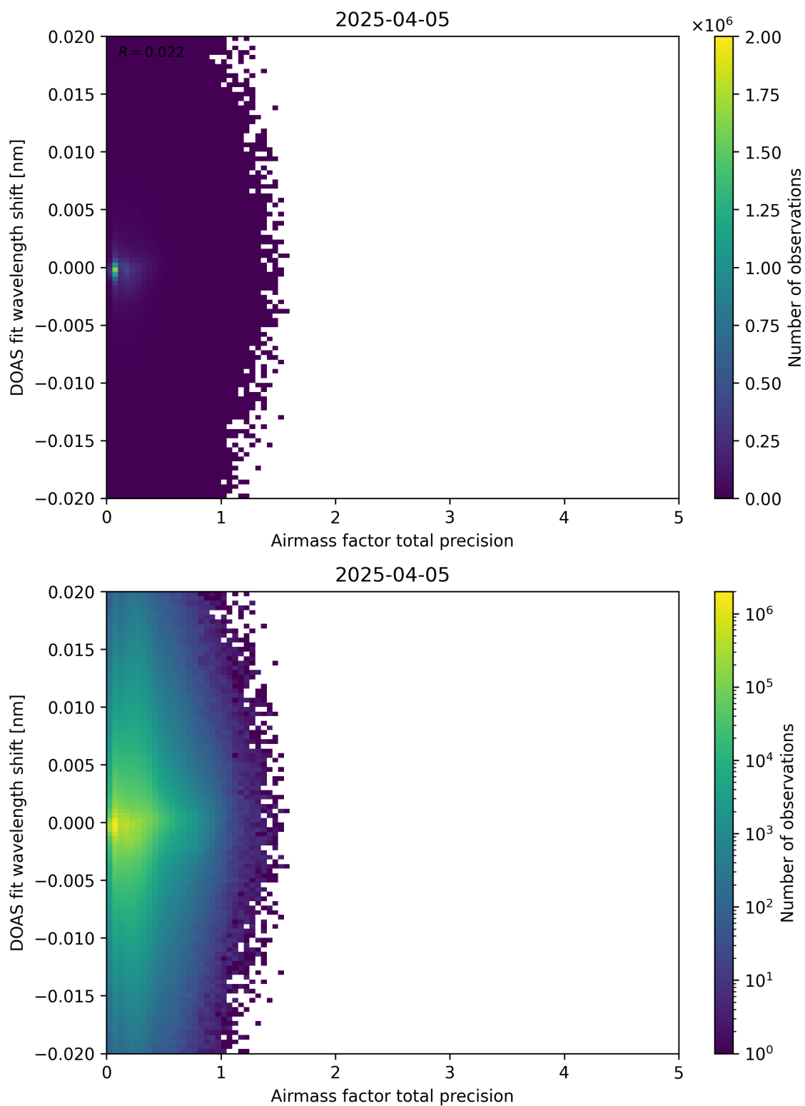
Figure 106: Scatter density plot of “Airmass factor total precision” against “DOAS fit wavelength shift” for 2025-04-04 to 2025-04-06.
