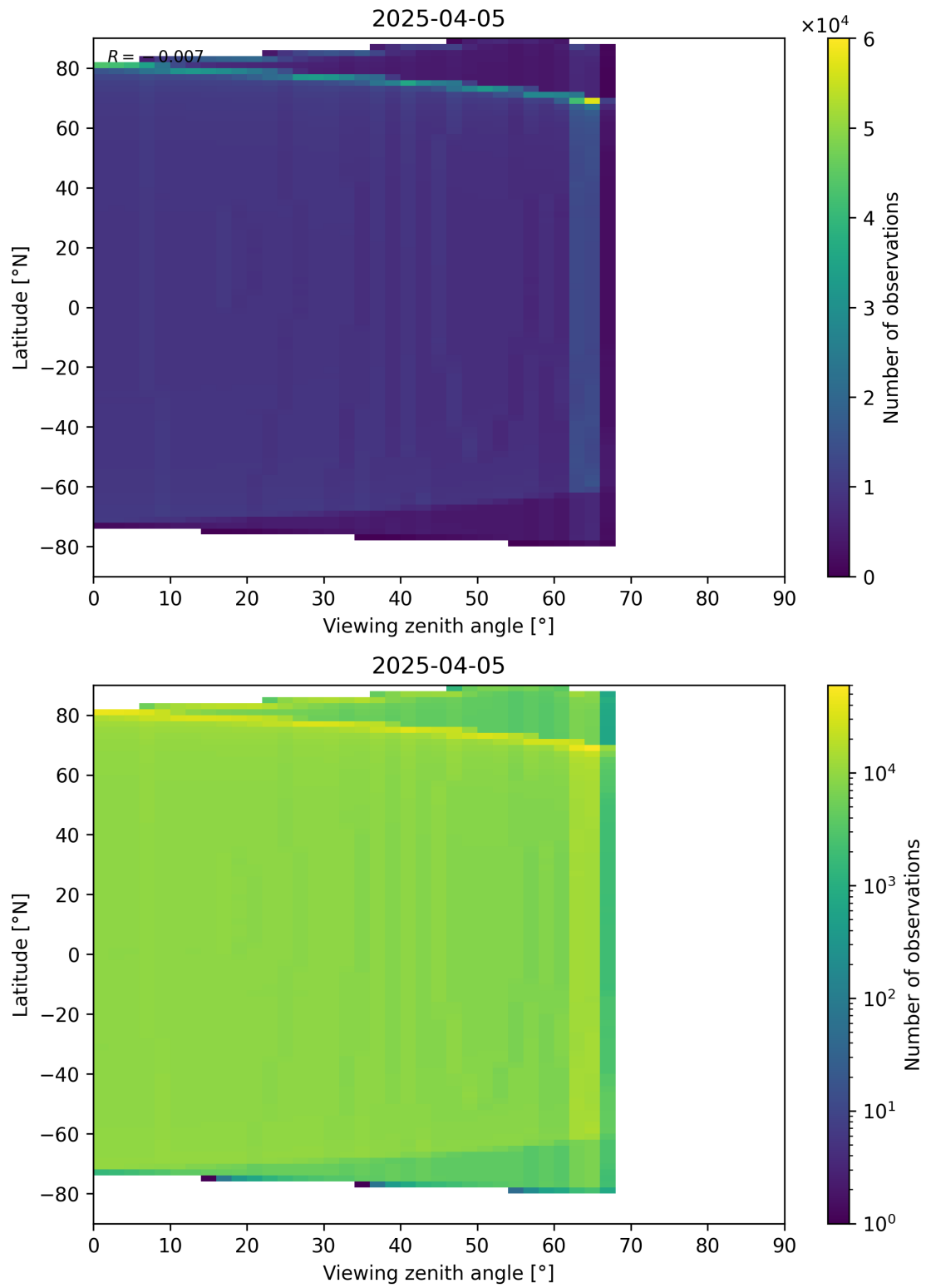
Figure 196: Scatter density plot of “Viewing zenith angle” against “Latitude” for 2025-04-04 to 2025-04-06.
