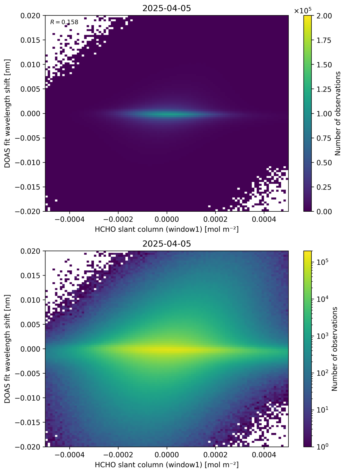
Figure 79: Scatter density plot of “HCHO slant column (window1)” against “DOAS fit wavelength shift” for 2025-04-04 to 2025-04-06.
