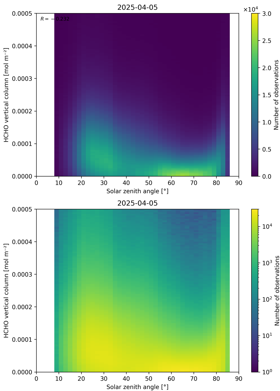
Figure 177: Scatter density plot of “Solar zenith angle” against “HCHO vertical column” for 2025-04-04 to 2025-04-06.
