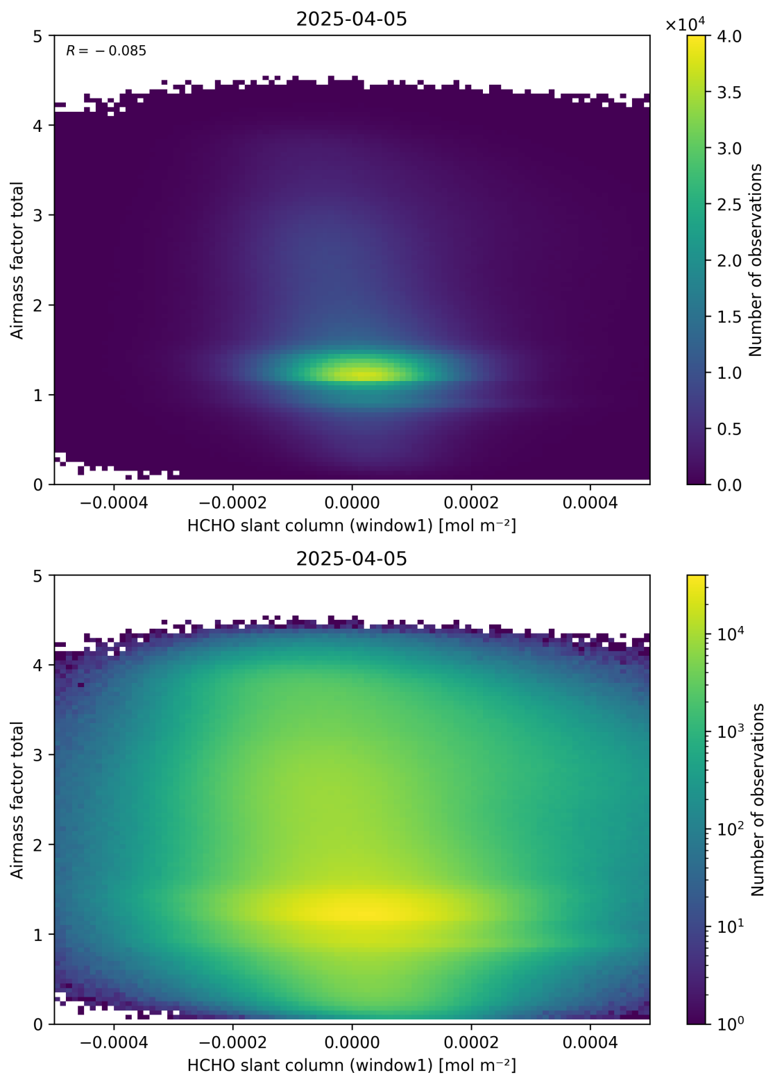
Figure 85: Scatter density plot of “HCHO slant column (window1)” against “Airmass factor total” for 2025-04-04 to 2025-04-06.
