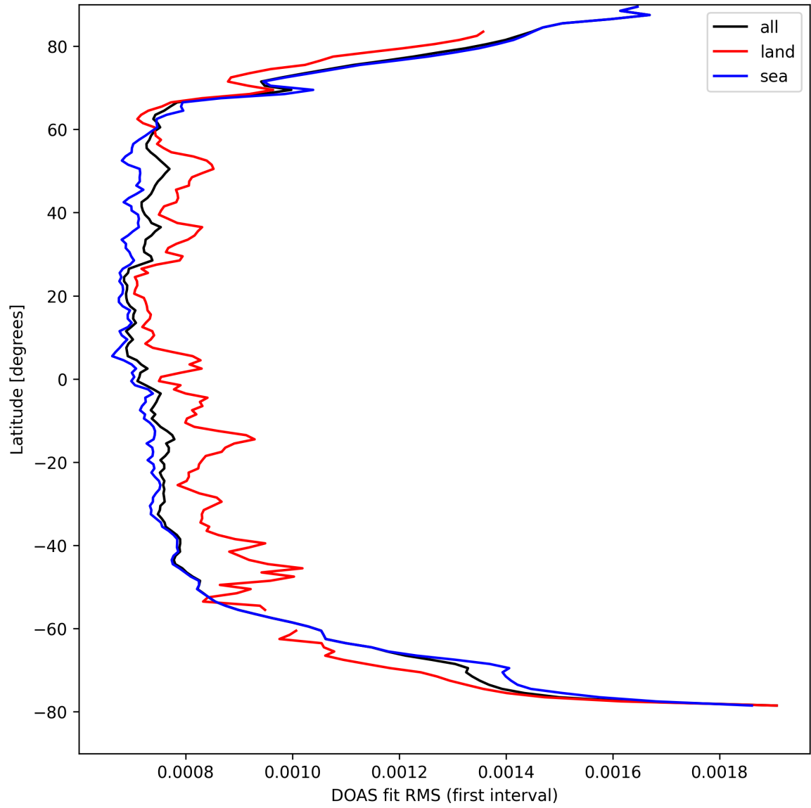
Figure 32: Zonal average of "DOAS fit RMS (first interval)" for 2025-04-04 to 2025-04-06.
