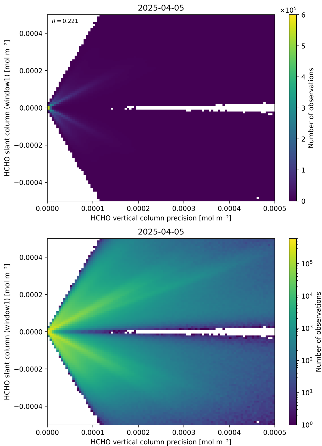
Figure 142: Scatter density plot of “HCHO vertical column precision” against “HCHO slant column (window1)” for 2025-04-04 to 2025-04-06.
