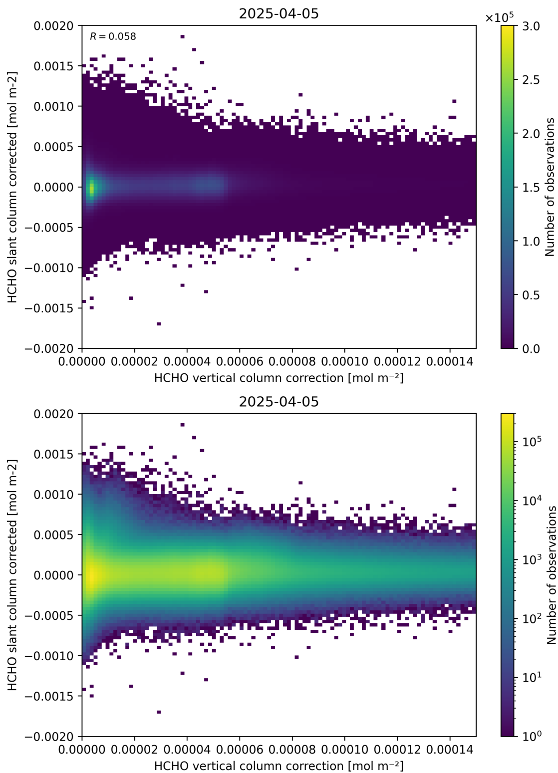
Figure 116: Scatter density plot of “HCHO vertical column correction” against “HCHO slant column corrected” for 2025-04-04 to 2025-04-06.
