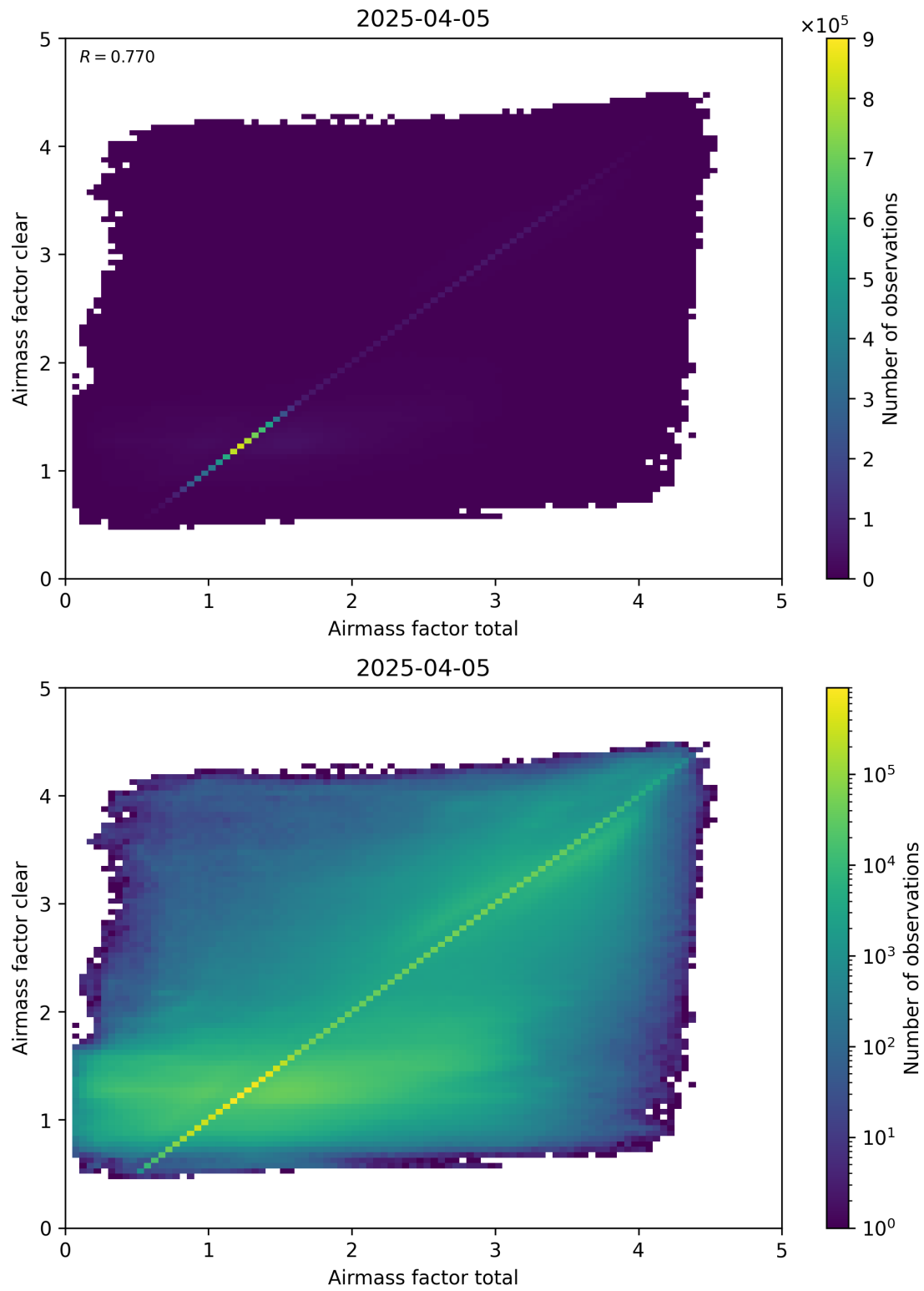
Figure 100: Scatter density plot of “Airmass factor total” against “Airmass factor clear” for 2025-04-04 to 2025-04-06.
