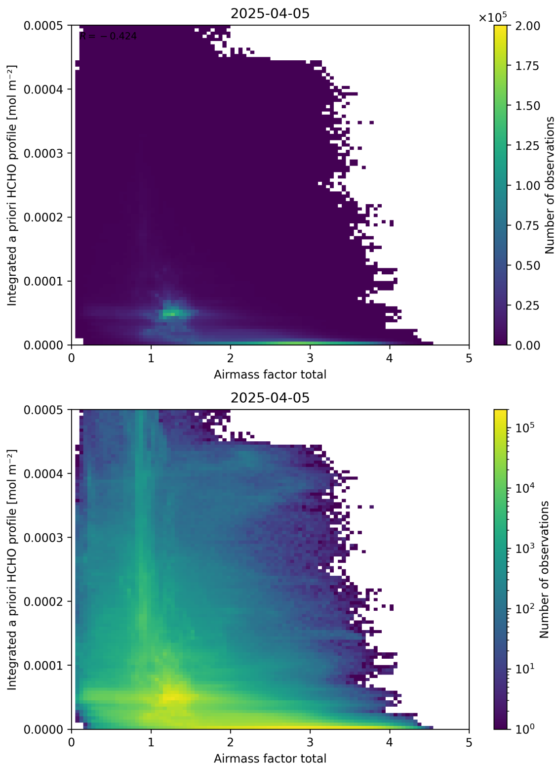
Figure 104: Scatter density plot of “Airmass factor total” against “Integrated a priori HCHO profile” for 2025-04-04 to 2025-04-06.
