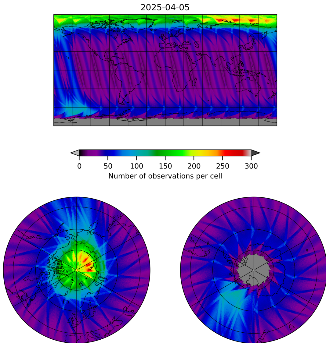
Figure 19: Map of the number of observations for 2025-04-04 to 2025-04-06
