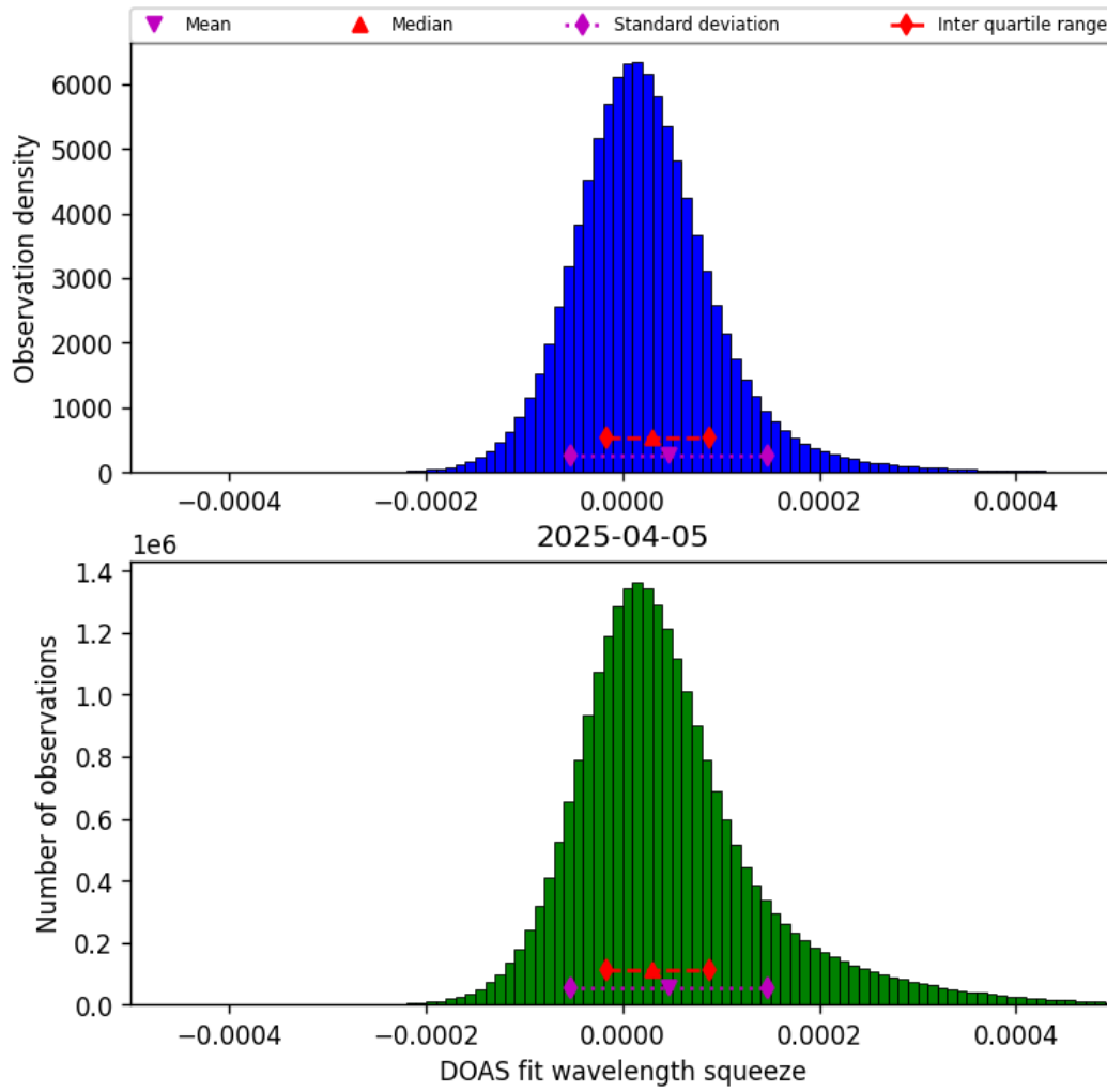
Figure 45: Histogram of “DOAS fit wavelength squeeze” for 2025-04-04 to 2025-04-06
