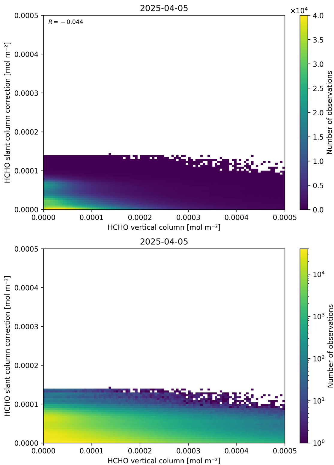
Figure 128: Scatter density plot of “HCHO vertical column” against “HCHO slant column correction” for 2025-04-04 to 2025-04-06.
