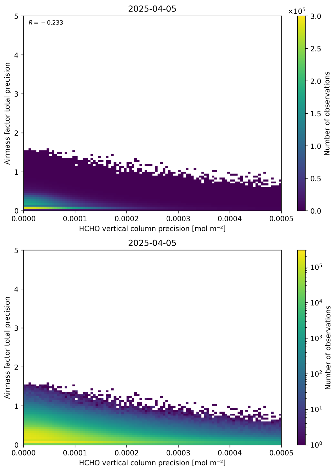
Figure 145: Scatter density plot of “HCHO vertical column precision” against “Airmass factor total precision” for 2025-04-04 to 2025-04-06.
