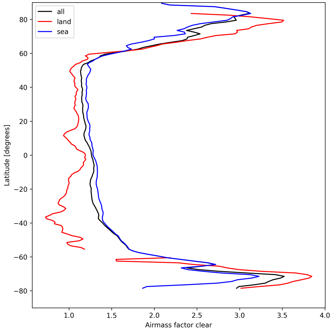
Figure 28: Zonal average of “Airmass factor clear” for 2025-04-04 to 2025-04-06.
