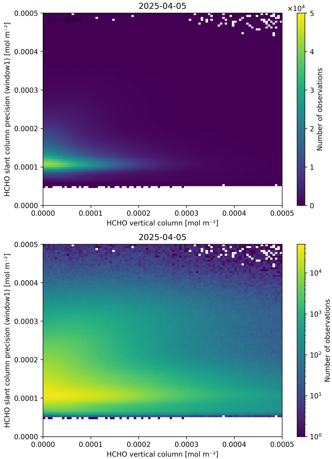
Figure 130: Scatter density plot of “HCHO vertical column” against “HCHO slant column precision (window1)” for 2025-04-04 to 2025-04-06.
