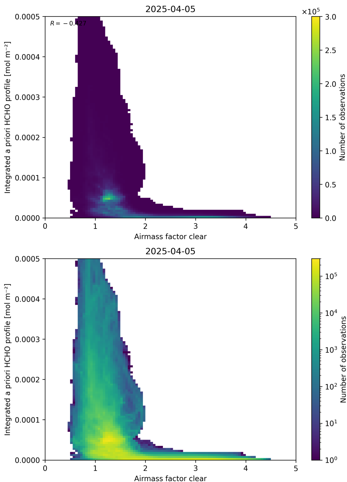
Figure 76: Scatter density plot of “Airmass factor clear” against “Integrated a priori HCHO profile” for 2025-04-04 to 2025-04-06.
