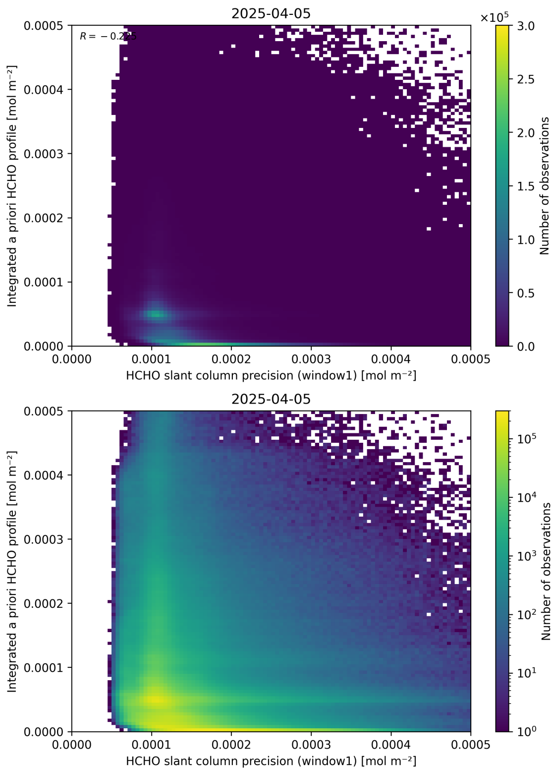
Figure 96: Scatter density plot of “HCHO slant column precision (window1)” against “Integrated a priori HCHO profile” for 2025-04-04 to 2025-04-06.
