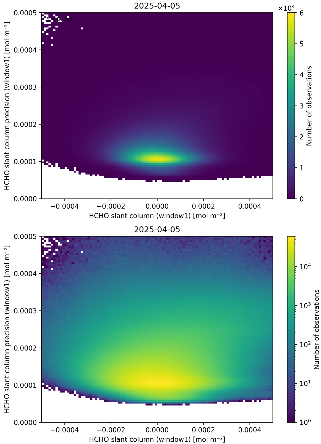
Figure 84: Scatter density plot of “HCHO slant column (window1)” against “HCHO slant column precision (window1)” for 2025-04-04 to 2025-04-06.
