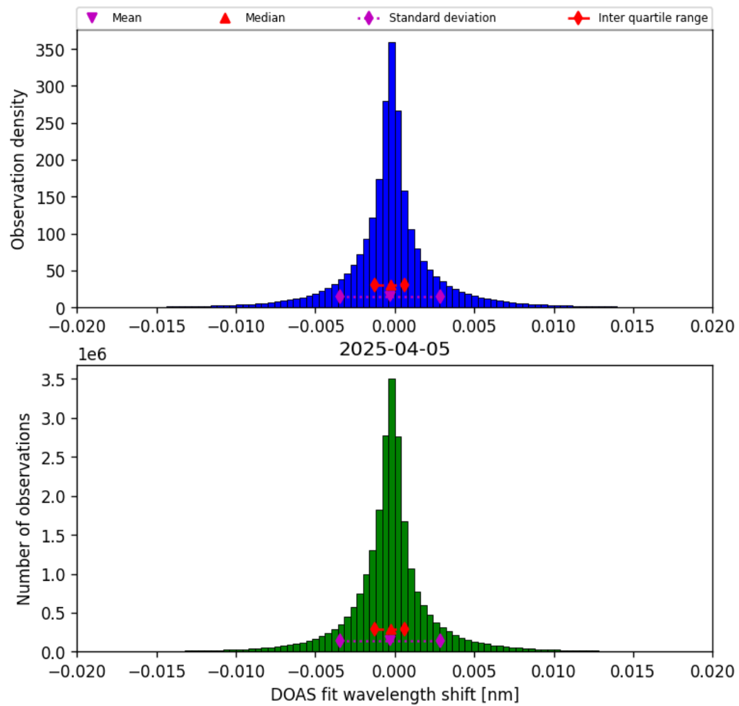
Figure 44: Histogram of “DOAS fit wavelength shift” for 2025-04-04 to 2025-04-06
