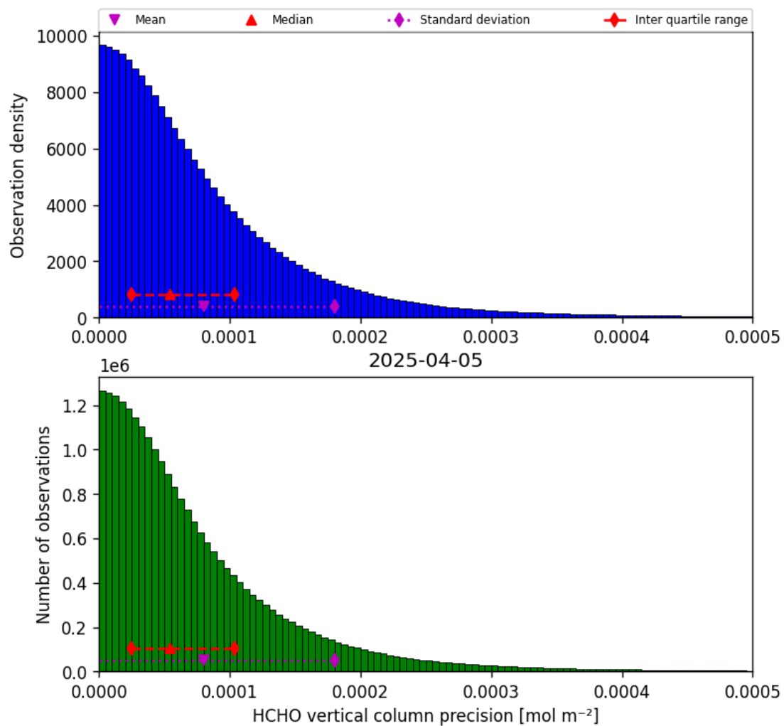
Figure 36: Histogram of “HCHO vertical column precision” for 2025-04-04 to 2025-04-06
