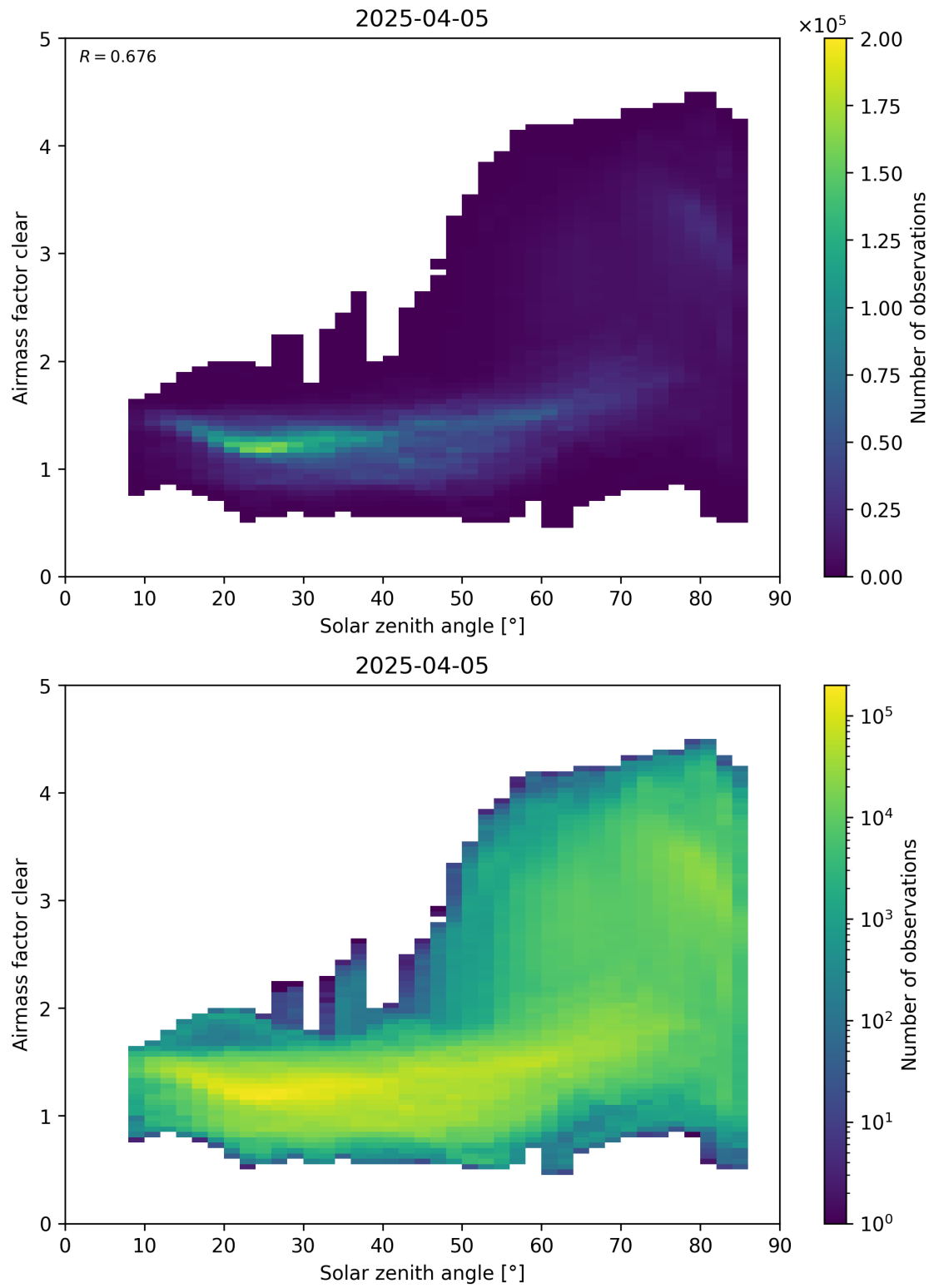
Figure 170: Scatter density plot of “Solar zenith angle” against “Airmass factor clear” for 2025-04-04 to 2025-04-06.
