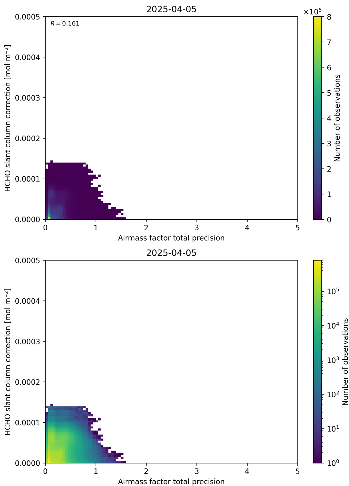
Figure 110: Scatter density plot of “Airmass factor total precision” against “HCHO slant column correction” for 2025-04-04 to 2025-04-06.
