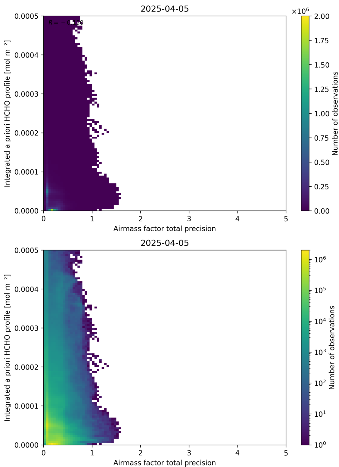
Figure 111: Scatter density plot of “Airmass factor total precision” against “Integrated a priori HCHO profile” for 2025-04-04 to 2025-04-06.
