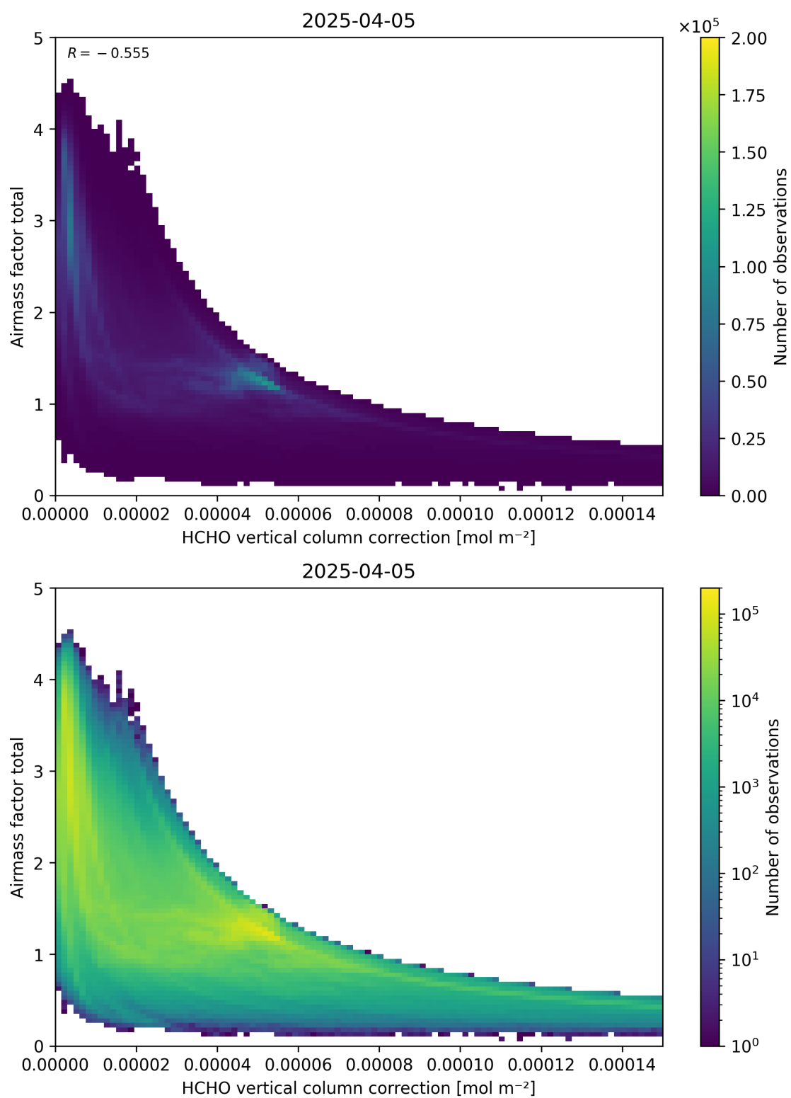
Figure 120: Scatter density plot of “HCHO vertical column correction” against “Airmass factor total” for 2025-04-04 to 2025-04-06.
