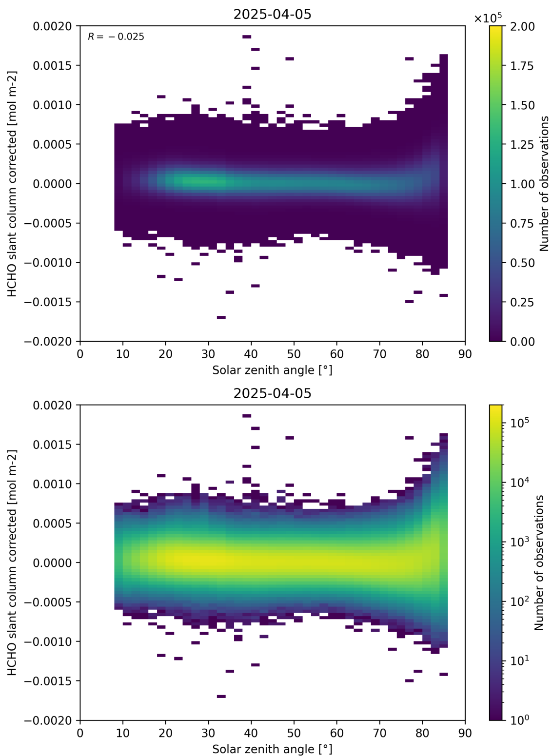
Figure 171: Scatter density plot of “Solar zenith angle” against “HCHO slant column corrected” for 2025-04-04 to 2025-04-06.
