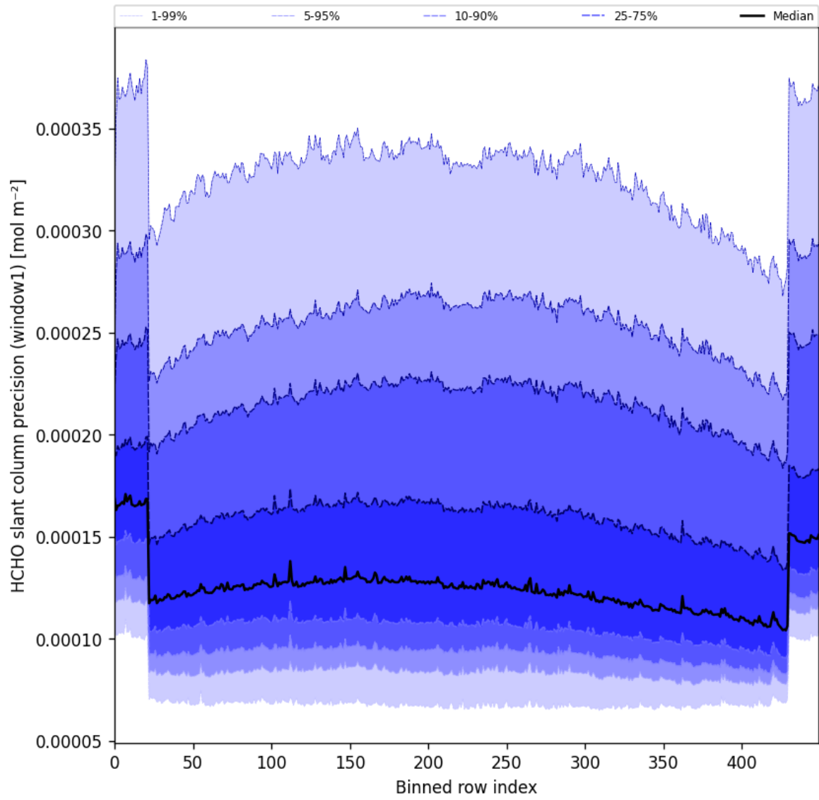
Figure 53: Along track statistics of “HCHO slant column precision (window1)” for 2025-04-04 to 2025-04-06
