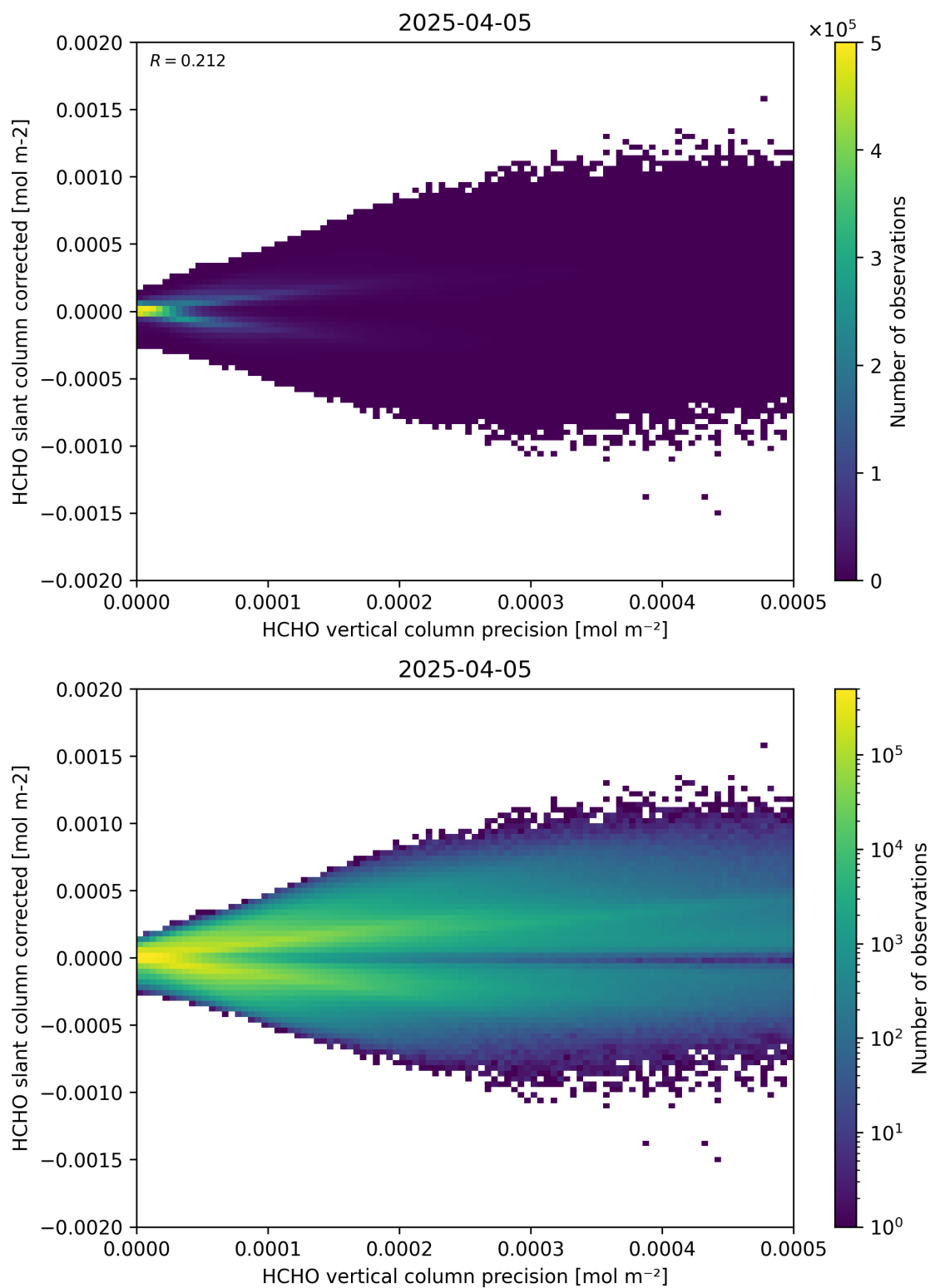
Figure 140: Scatter density plot of “HCHO vertical column precision” against “HCHO slant column corrected” for 2025-04-04 to 2025-04-06.
