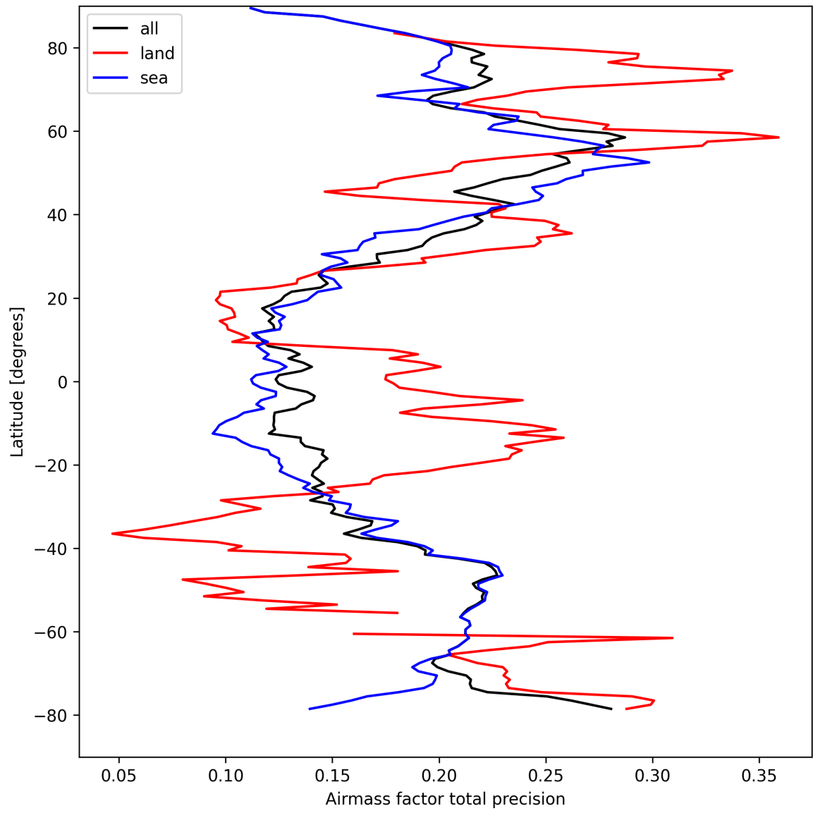
Figure 27: Zonal average of “Airmass factor total precision” for 2025-04-04 to 2025-04-06.
