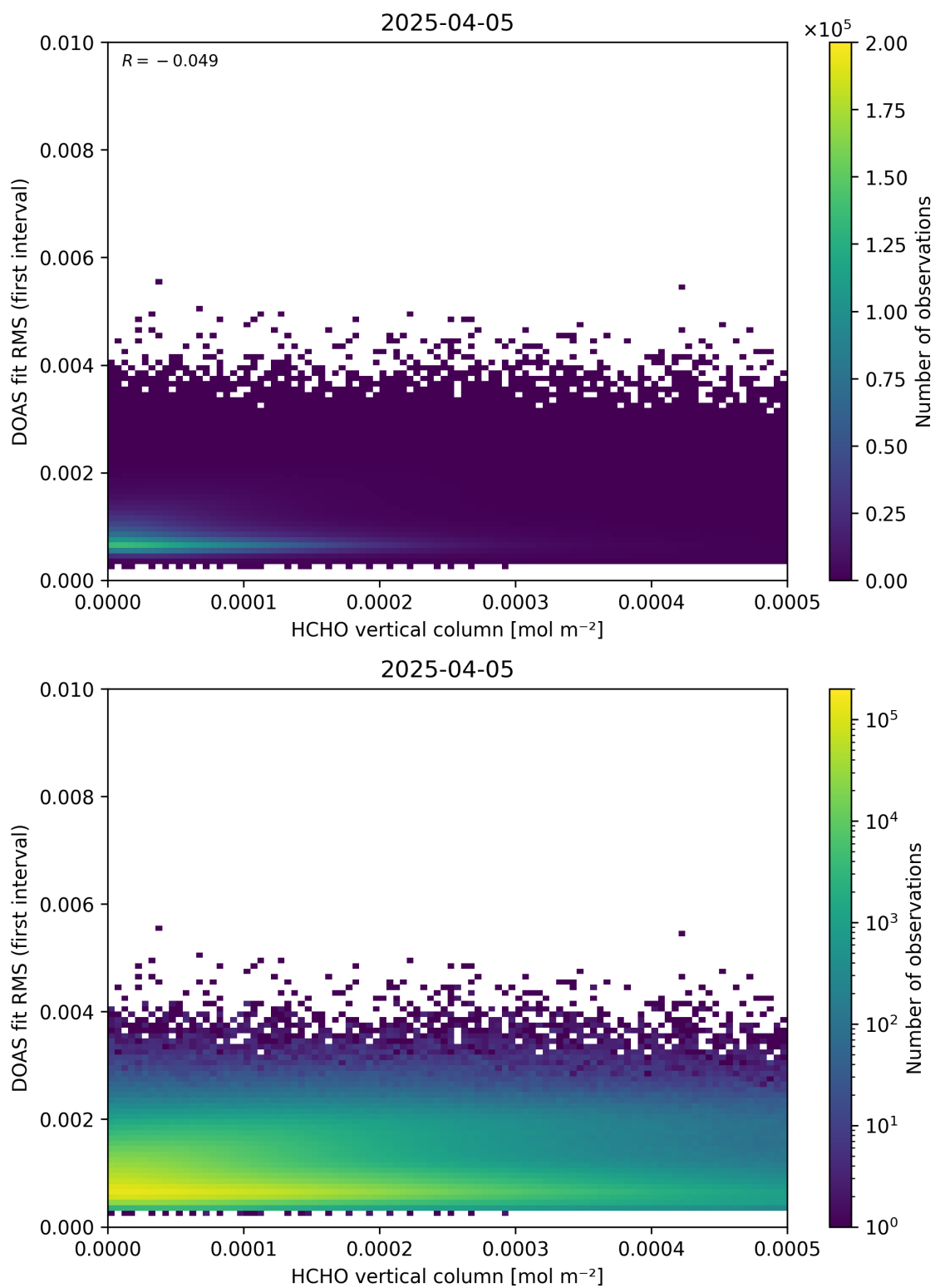
Figure 123: Scatter density plot of “HCHO vertical column” against “DOAS fit RMS (first interval)” for 2025-04-04 to 2025-04-06.
