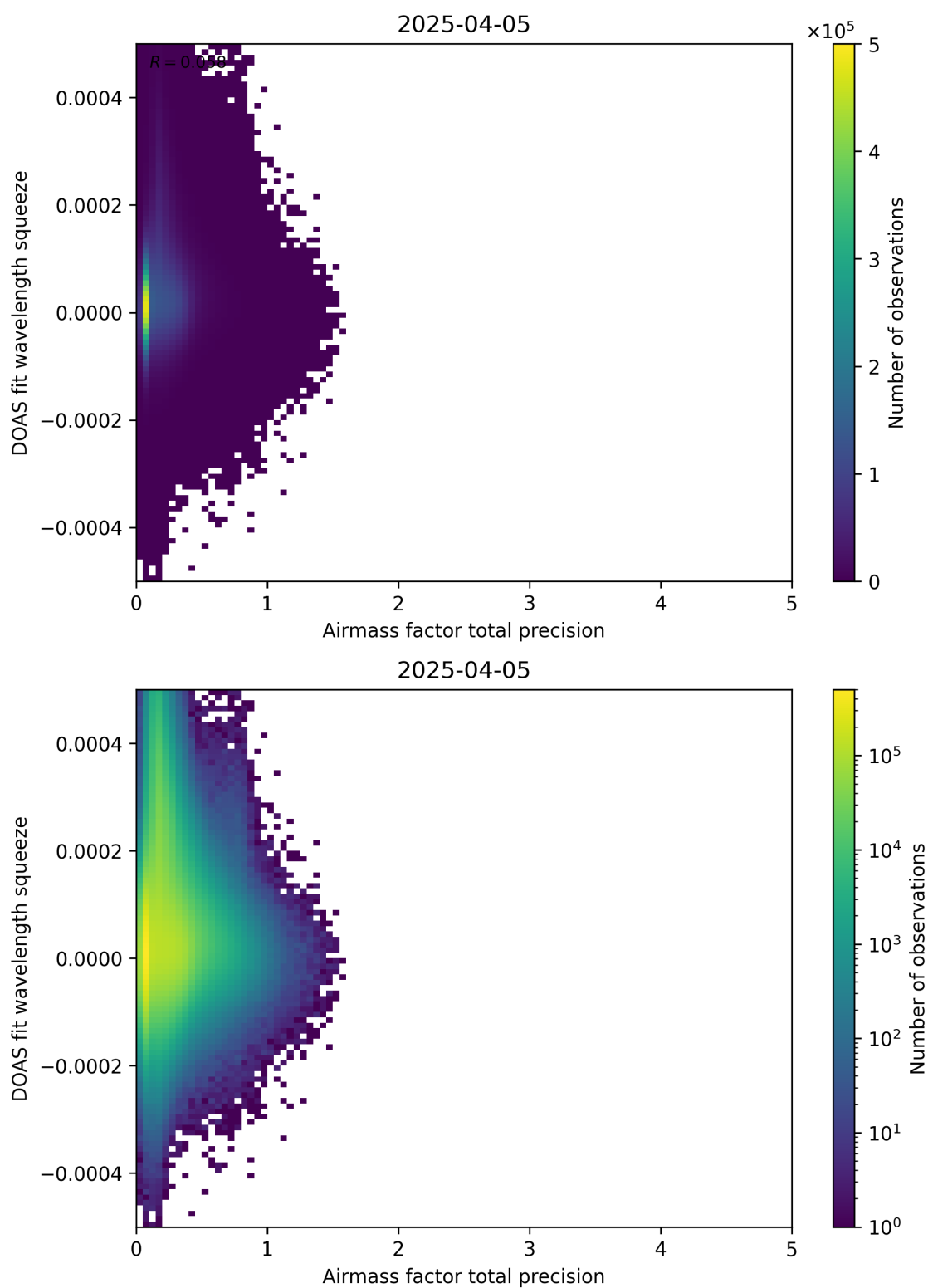
Figure 107: Scatter density plot of “Airmass factor total precision” against “DOAS fit wavelength squeeze” for 2025-04-04 to 2025-04-06.
