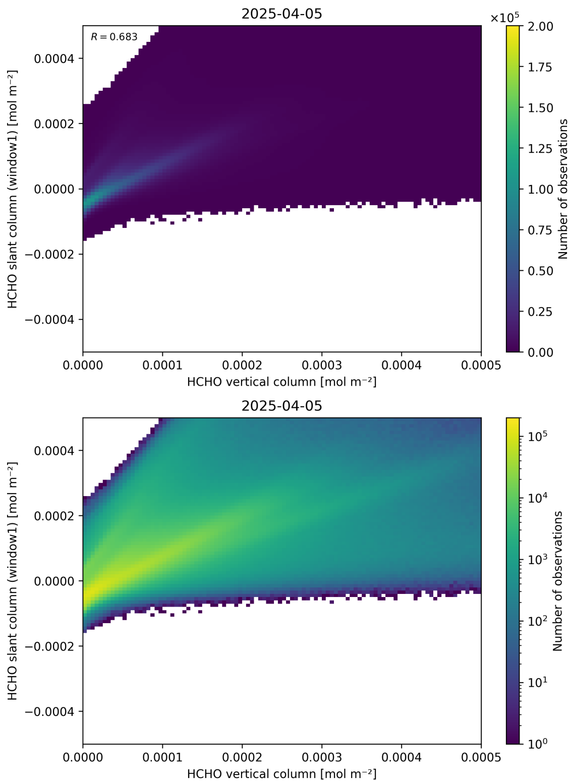
Figure 129: Scatter density plot of “HCHO vertical column” against “HCHO slant column (window1)” for 2025-04-04 to 2025-04-06.
