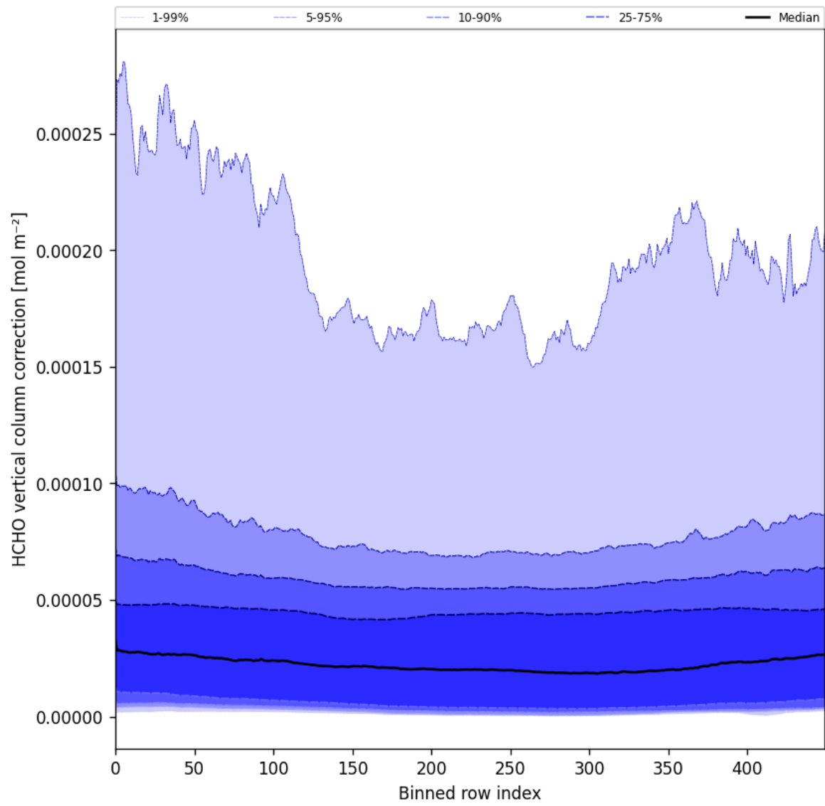
Figure 51: Along track statistics of “HCHO vertical column correction” for 2025-04-04 to 2025-04-06
