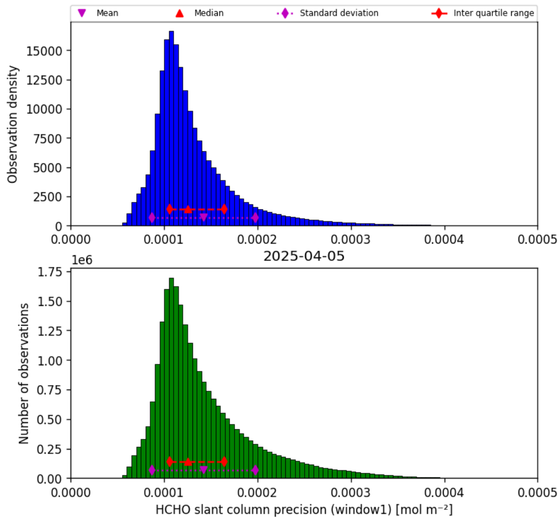
Figure 39: Histogram of “HCHO slant column precision (window1)” for 2025-04-04 to 2025-04-06
