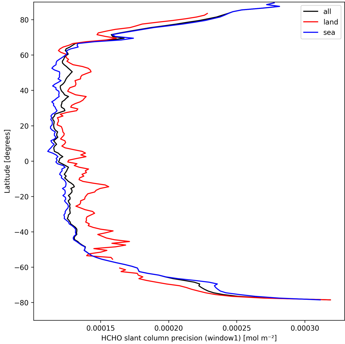
Figure 25: Zonal average of "HCHO slant column precision (window1)" for 2025-04-04 to 2025-04-06.
