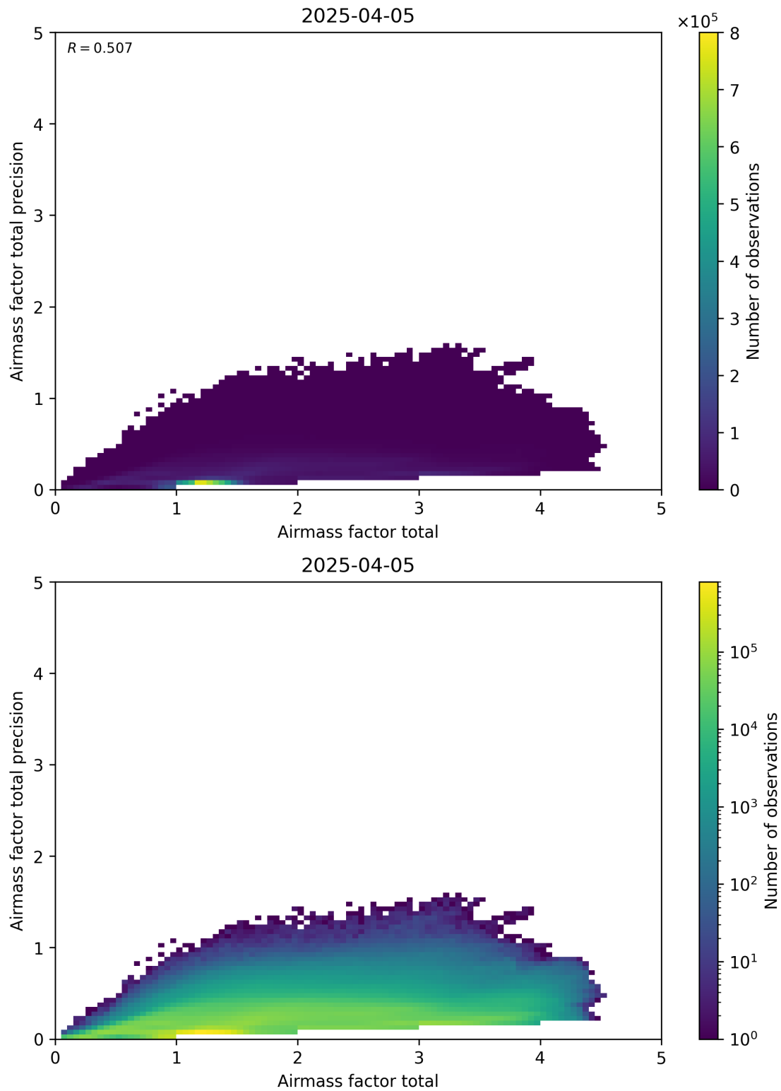
Figure 103: Scatter density plot of “Airmass factor total” against “Airmass factor total precision” for 2025-04-04 to 2025-04-06.
