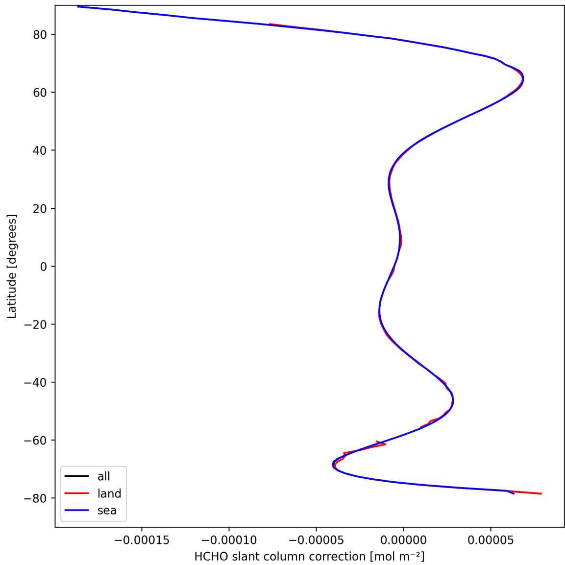
Figure 33: Zonal average of “HCHO slant column correction” for 2025-04-04 to 2025-04-06.
