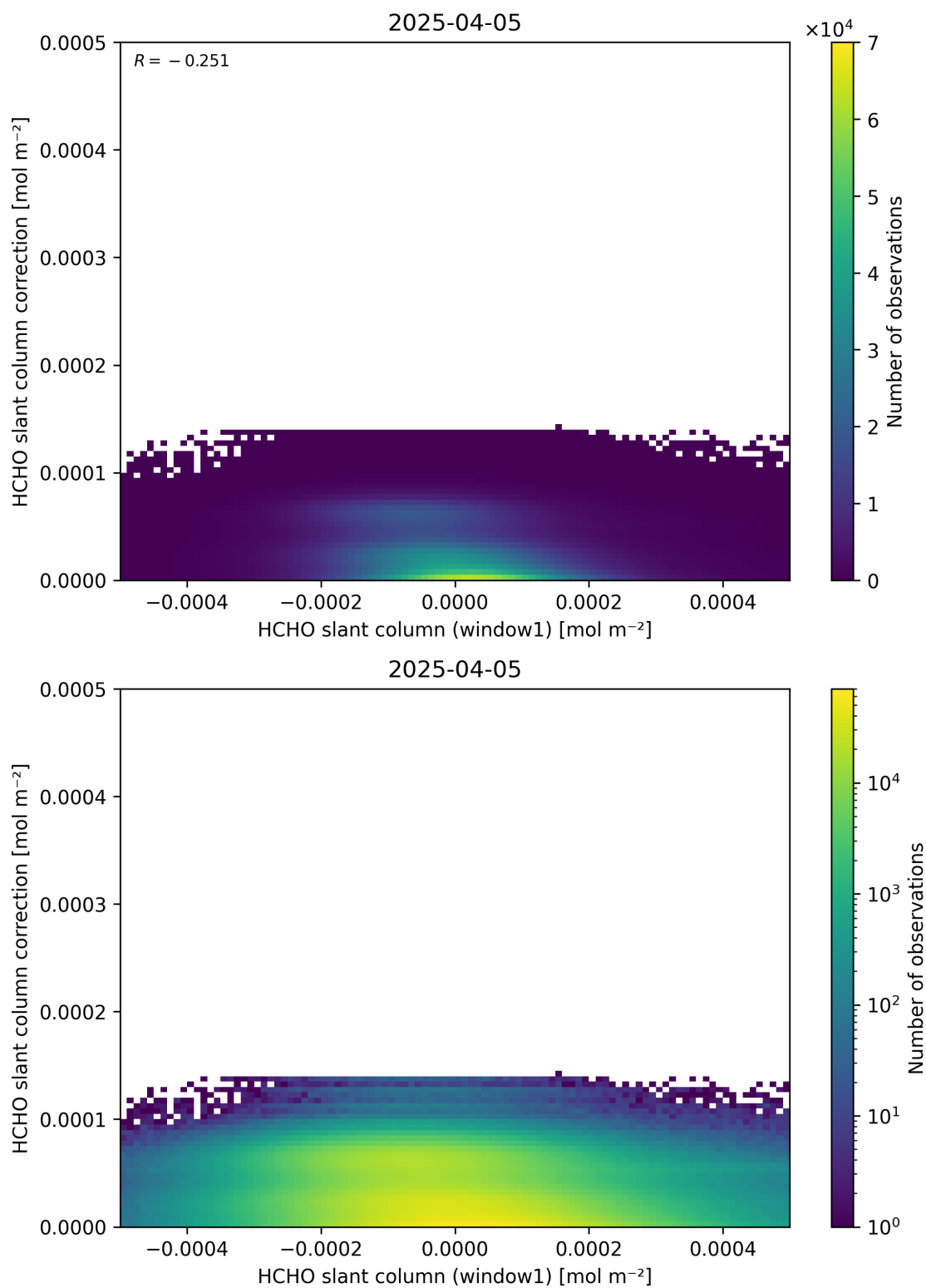
Figure 83: Scatter density plot of “HCHO slant column (window1)” against “HCHO slant column correction” for 2025-04-04 to 2025-04-06.
