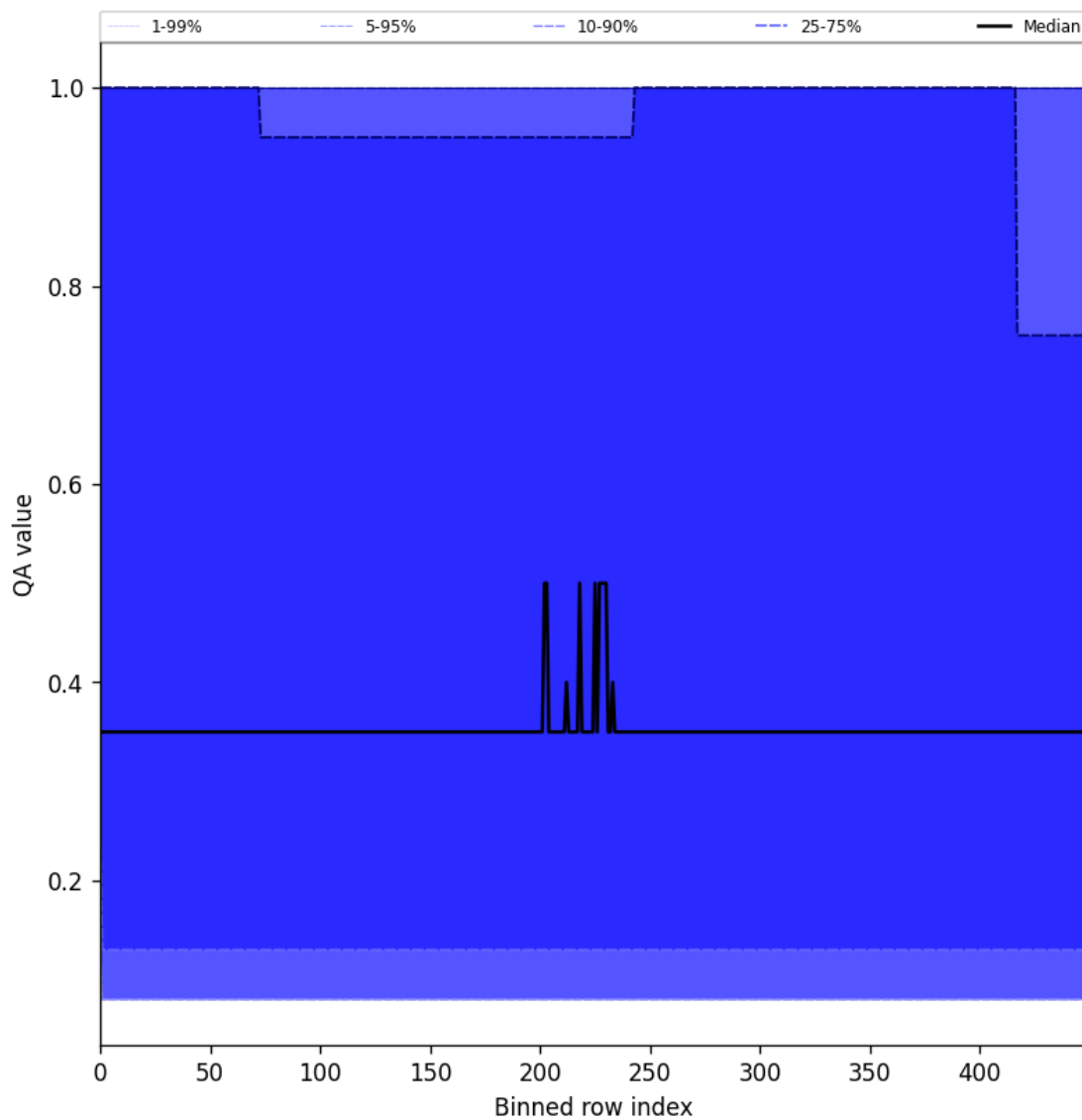
Figure 48: Along track statistics of “QA value” for 2025-04-04 to 2025-04-06
