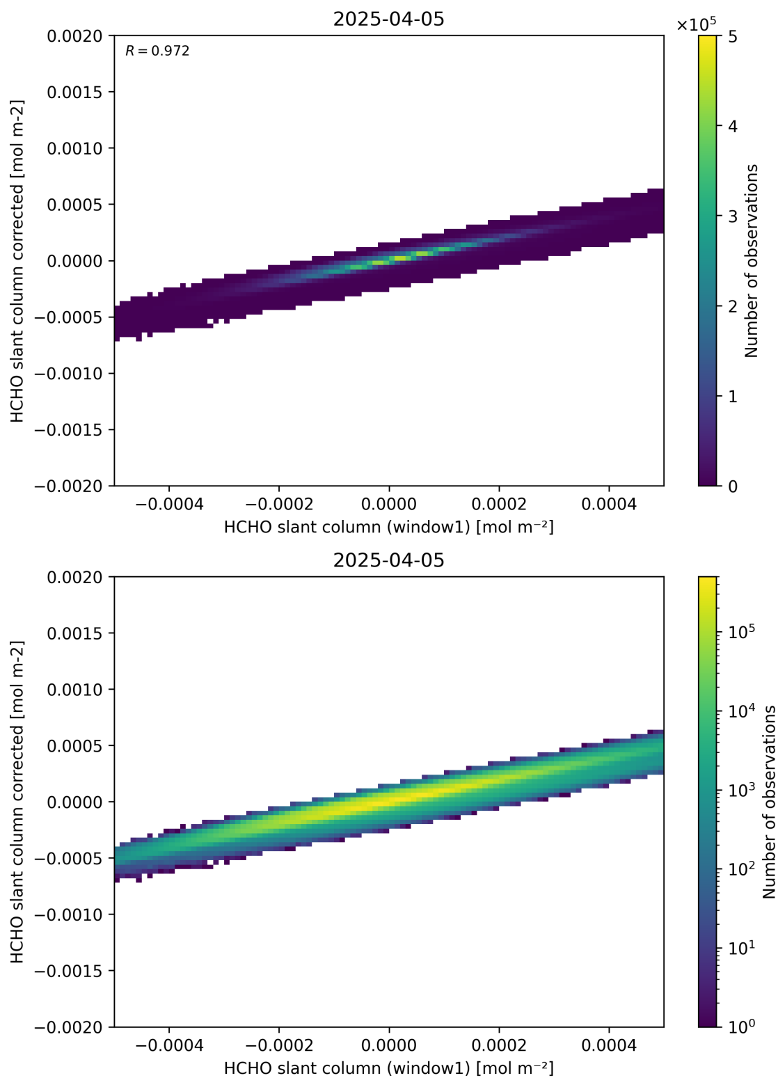
Figure 82: Scatter density plot of “HCHO slant column (window1)” against “HCHO slant column corrected” for 2025-04-04 to 2025-04-06.
