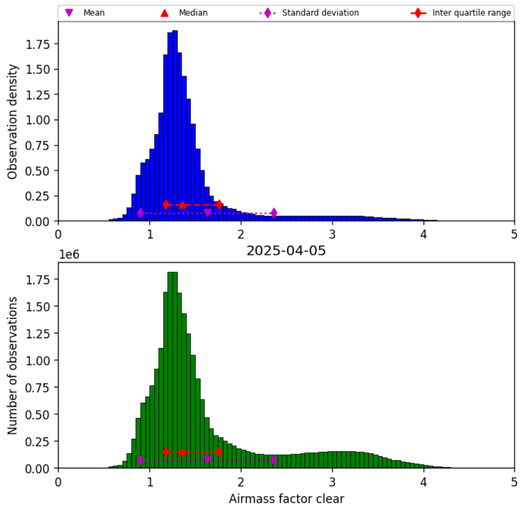
Figure 42: Histogram of “Airmass factor clear” for 2025-04-04 to 2025-04-06
