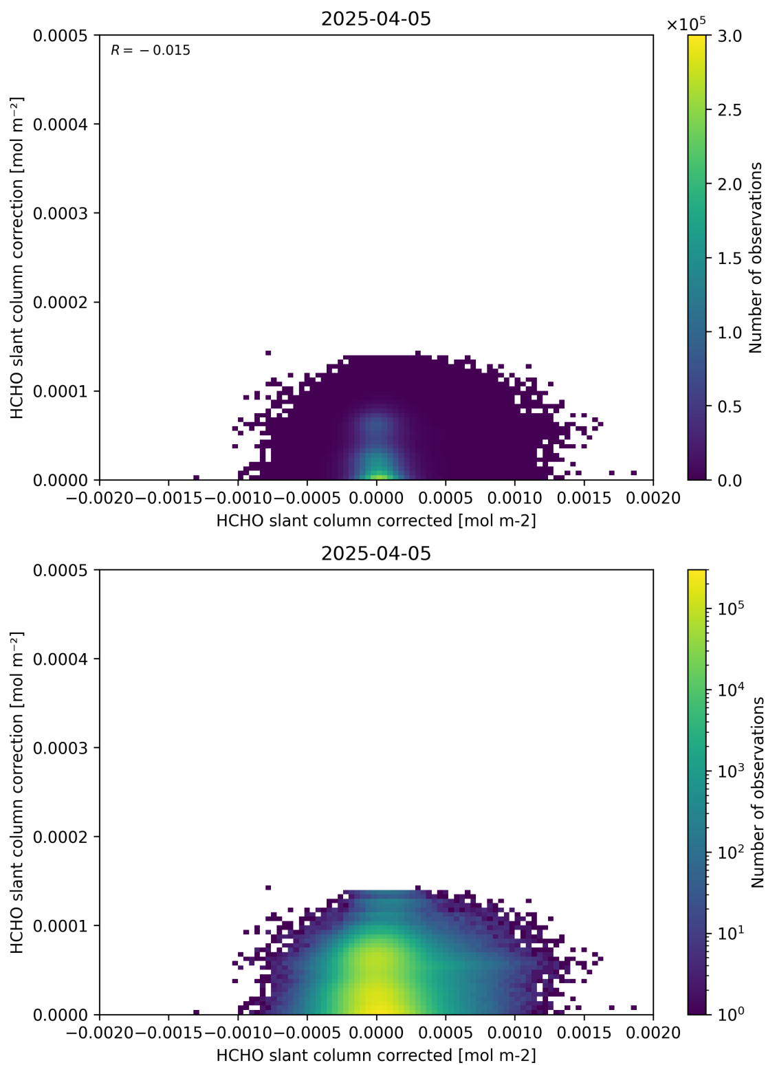
Figure 77: Scatter density plot of “HCHO slant column corrected” against “HCHO slant column correction” for 2025-04-04 to 2025-04-06.
