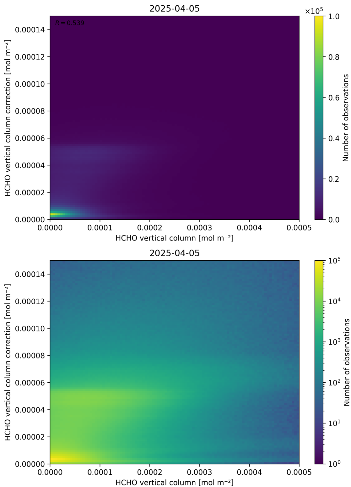
Figure 133: Scatter density plot of “HCHO vertical column” against “HCHO vertical column correction” for 2025-04-04 to 2025-04-06.
