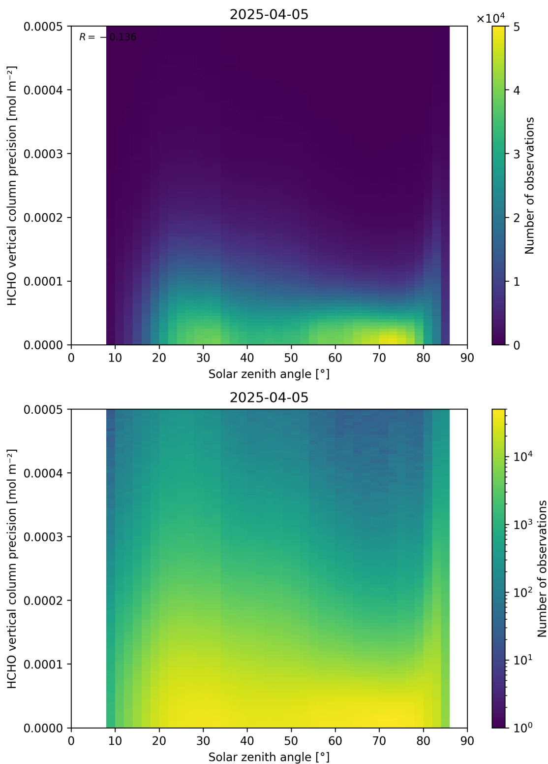
Figure 179: Scatter density plot of “Solar zenith angle” against “HCHO vertical column precision” for 2025-04-04 to 2025-04-06.
