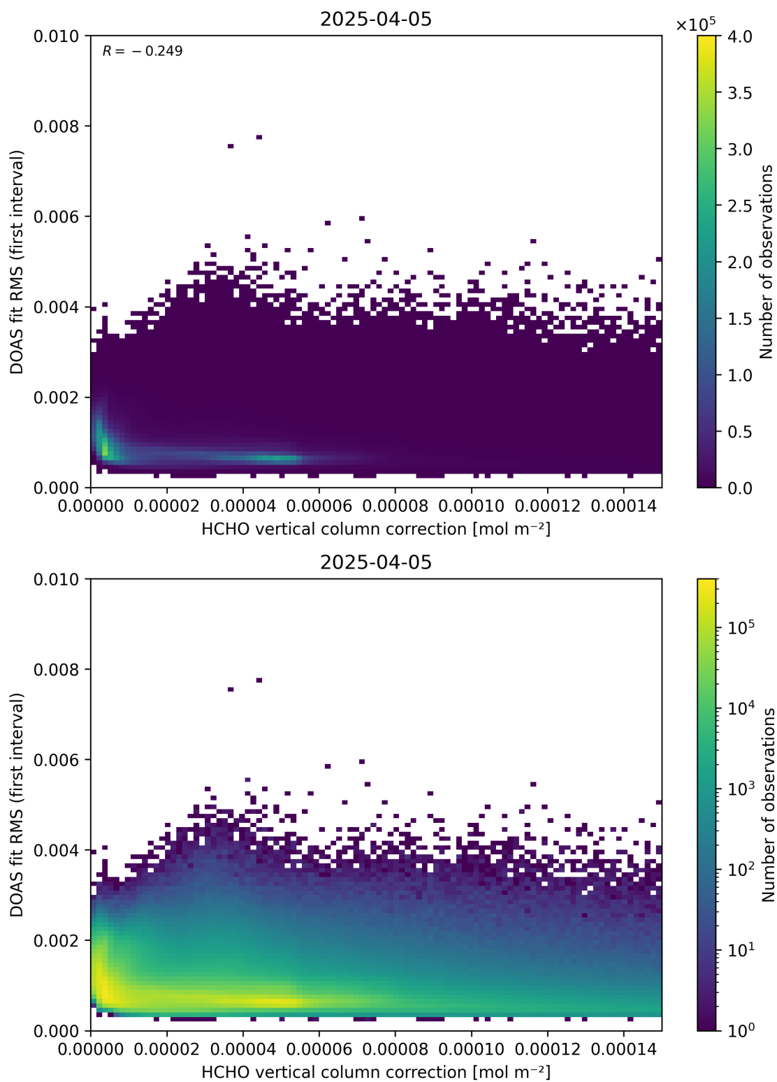
Figure 112: Scatter density plot of “HCHO vertical column correction” against “DOAS fit RMS (first interval)” for 2025-04-04 to 2025-04-06.
