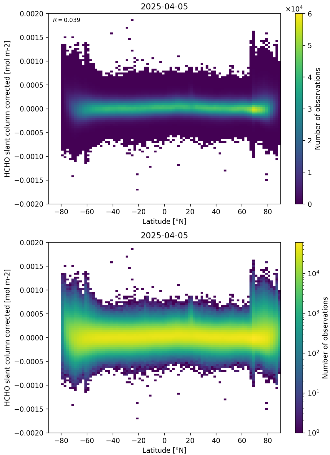
Figure 157: Scatter density plot of “Latitude” against “HCHO slant column corrected” for 2025-04-04 to 2025-04-06.
