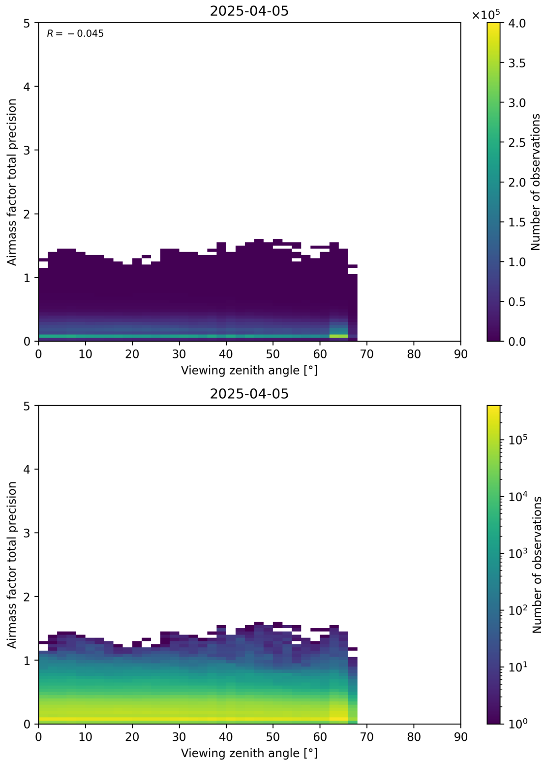
Figure 191: Scatter density plot of “Viewing zenith angle” against “Airmass factor total precision” for 2025-04-04 to 2025-04-06.
