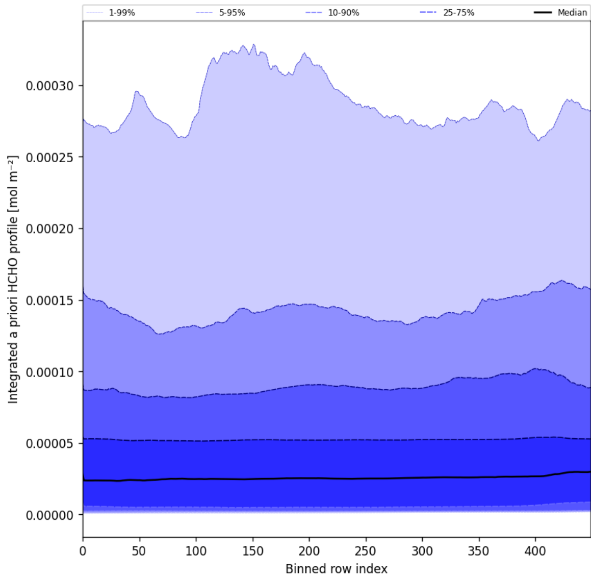
Figure 57: Along track statistics of "Integrated a priori HCHO profile" for 2025-04-04 to 2025-04-06
