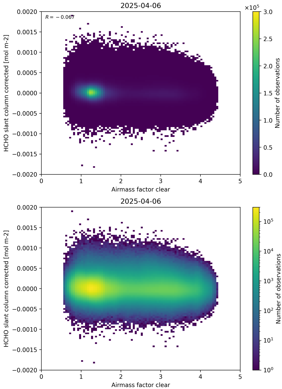
Figure 74: Scatter density plot of “Airmass factor clear” against “HCHO slant column corrected” for 2025-04-05 to 2025-04-07.
