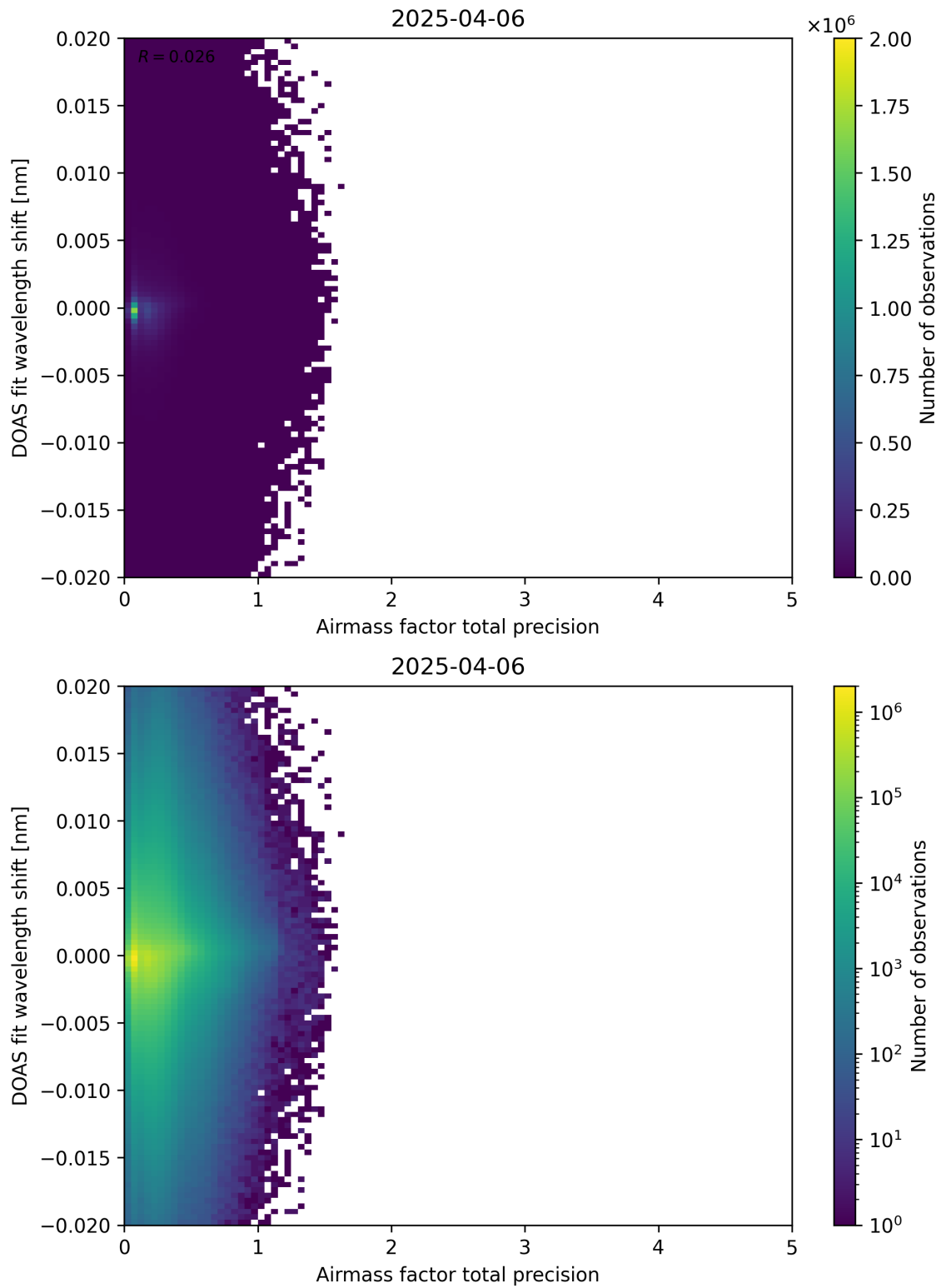
Figure 106: Scatter density plot of “Airmass factor total precision” against “DOAS fit wavelength shift” for 2025-04-05 to 2025-04-07.
