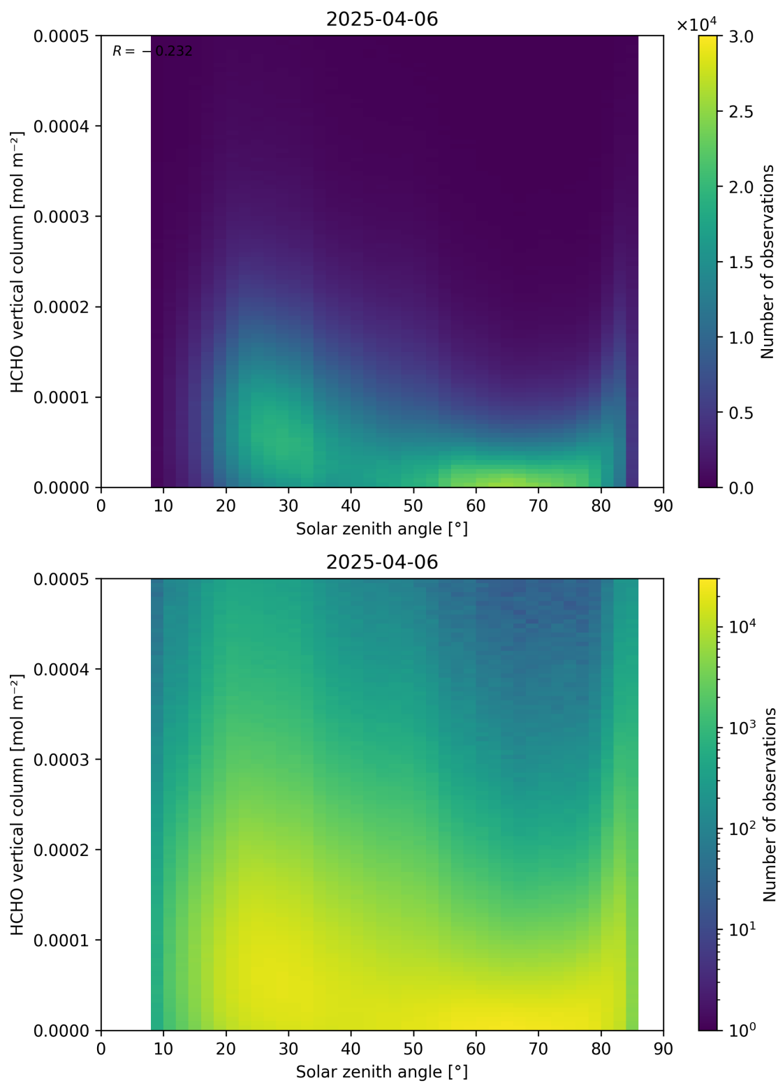
Figure 177: Scatter density plot of “Solar zenith angle” against “HCHO vertical column” for 2025-04-05 to 2025-04-07.
