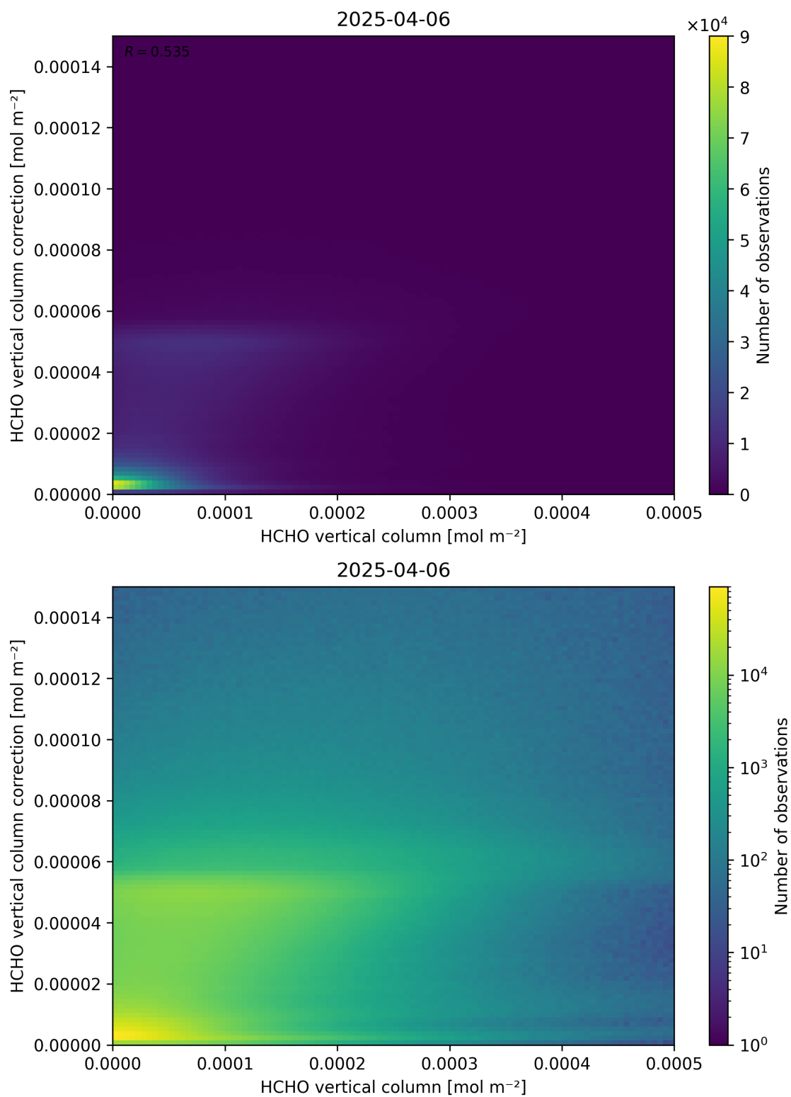
Figure 133: Scatter density plot of “HCHO vertical column” against “HCHO vertical column correction” for 2025-04-05 to 2025-04-07.
