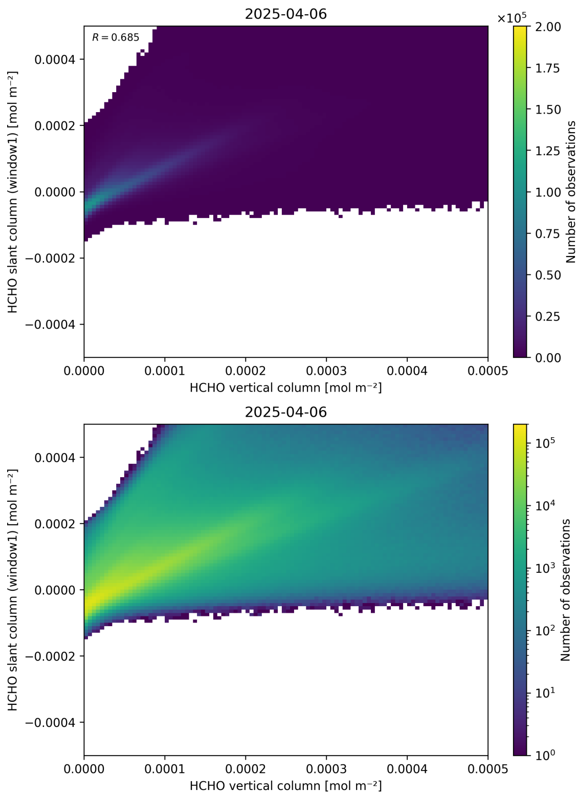
Figure 129: Scatter density plot of “HCHO vertical column” against “HCHO slant column (window1)” for 2025-04-05 to 2025-04-07.
