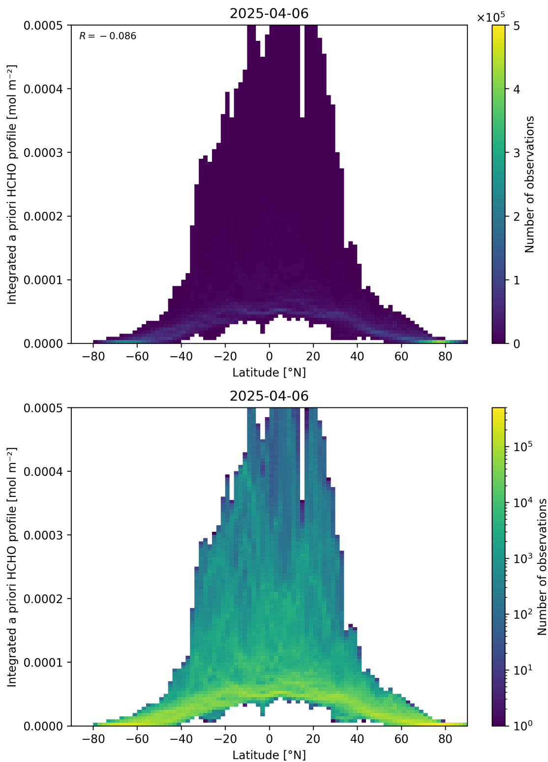
Figure 166: Scatter density plot of “Latitude” against “Integrated a priori HCHO profile” for 2025-04-05 to 2025-04-07.
