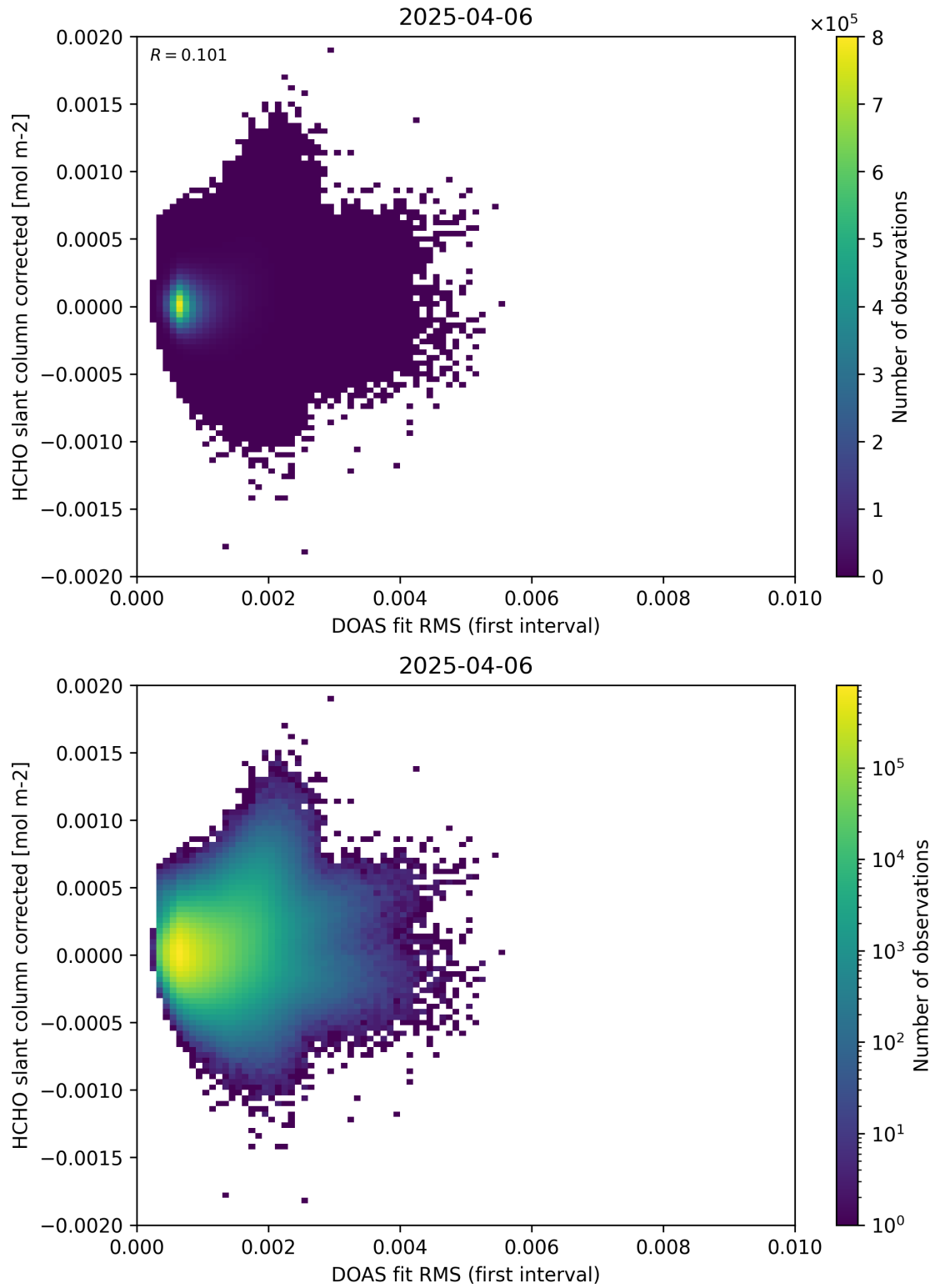
Figure 62: Scatter density plot of “DOAS fit RMS (first interval)” against “HCHO slant column corrected” for 2025-04-05 to 2025-04-07.
