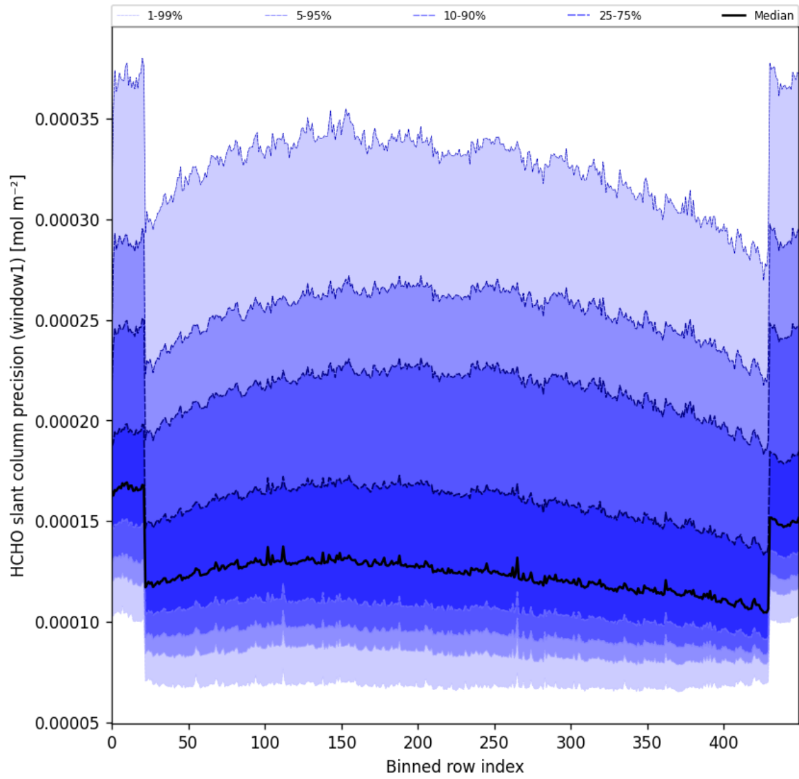
Figure 53: Along track statistics of “HCHO slant column precision (window1)” for 2025-04-05 to 2025-04-07
