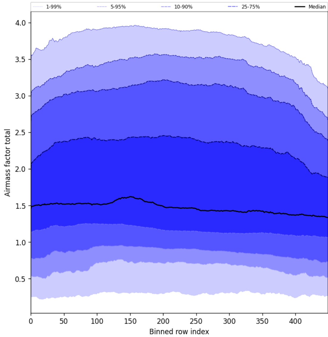
Figure 54: Along track statistics of “Airmass factor total” for 2025-04-05 to 2025-04-07
