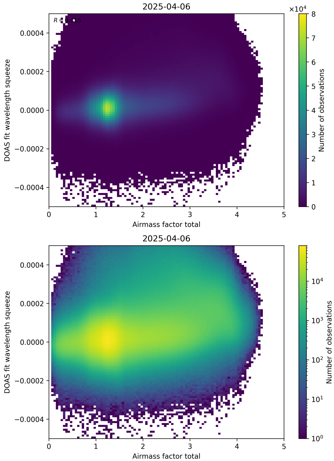
Figure 99: Scatter density plot of “Airmass factor total” against “DOAS fit wavelength squeeze” for 2025-04-05 to 2025-04-07.
