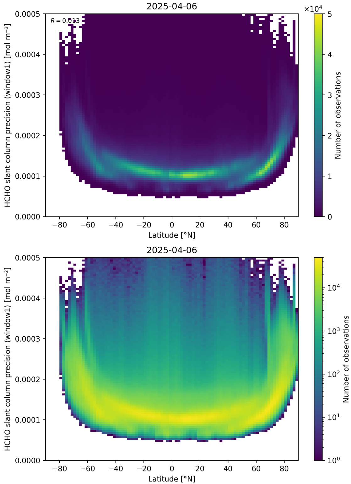
Figure 160: Scatter density plot of “Latitude” against “HCHO slant column precision (window1)” for 2025-04-05 to 2025-04-07.
