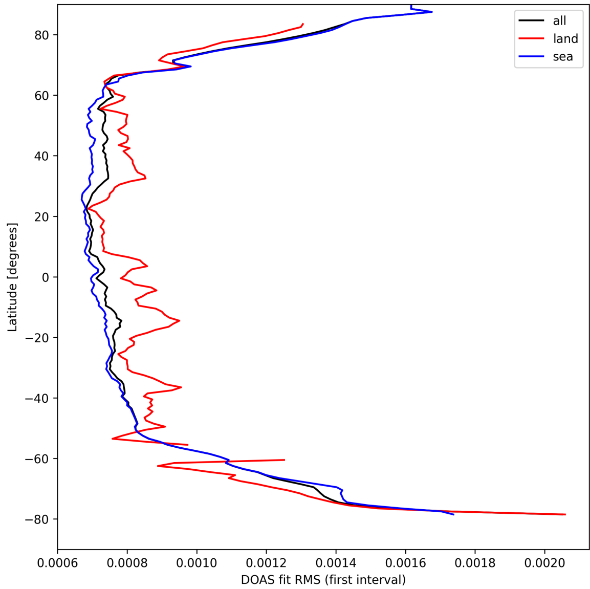
Figure 32: Zonal average of "DOAS fit RMS (first interval)" for 2025-04-05 to 2025-04-07.
