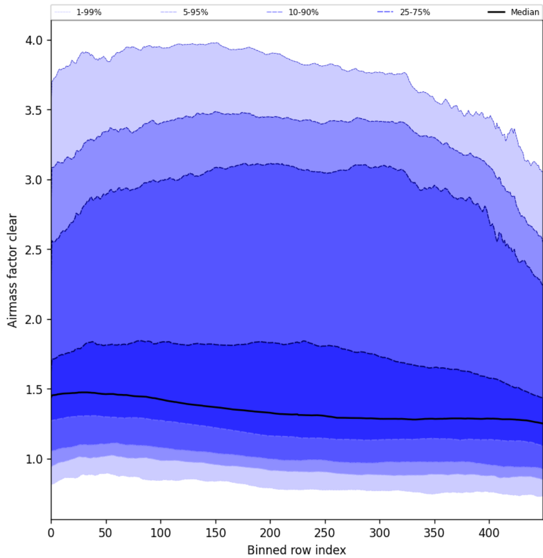
Figure 56: Along track statistics of “Airmass factor clear” for 2025-04-05 to 2025-04-07
