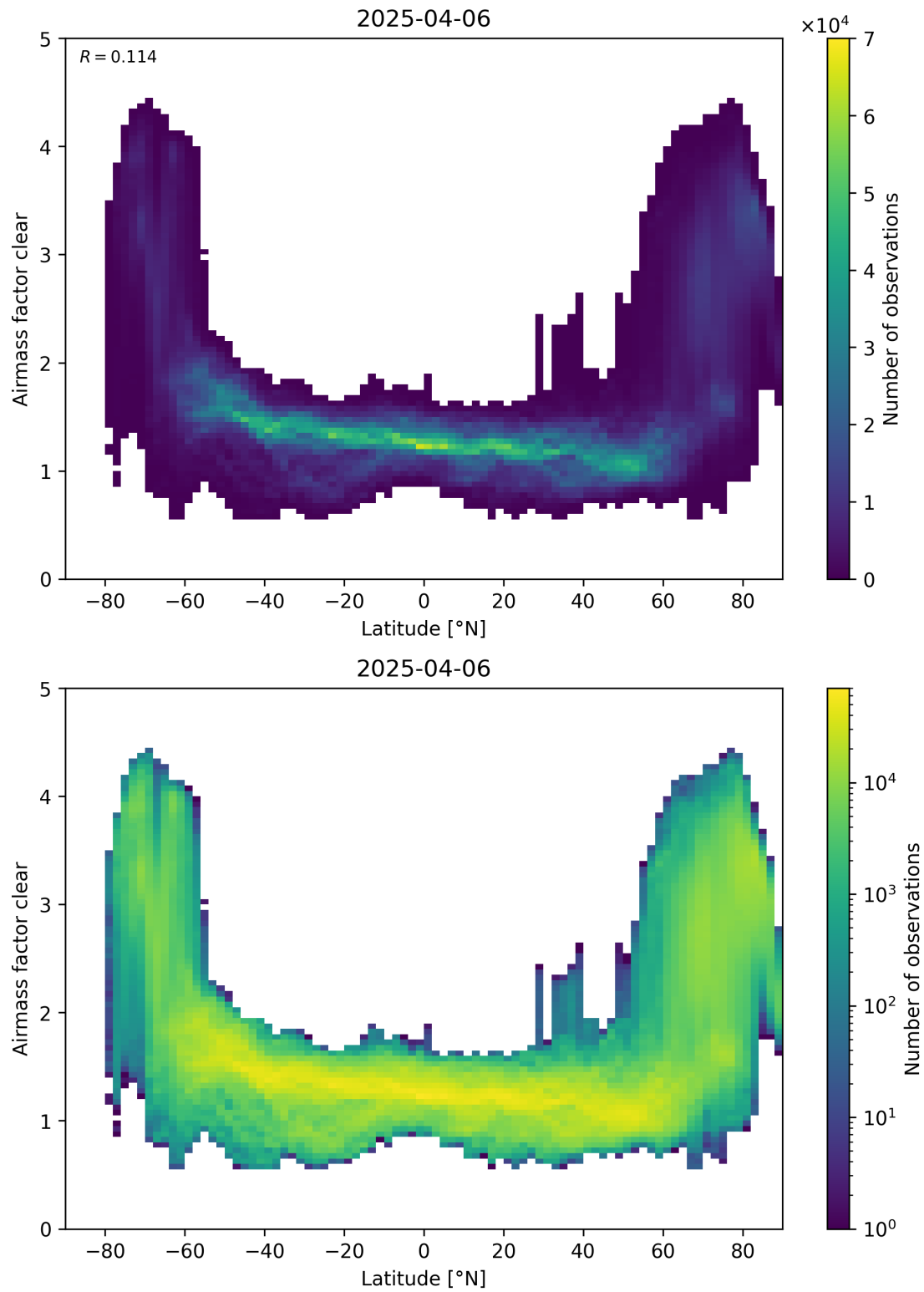
Figure 156: Scatter density plot of “Latitude” against “Airmass factor clear” for 2025-04-05 to 2025-04-07.
