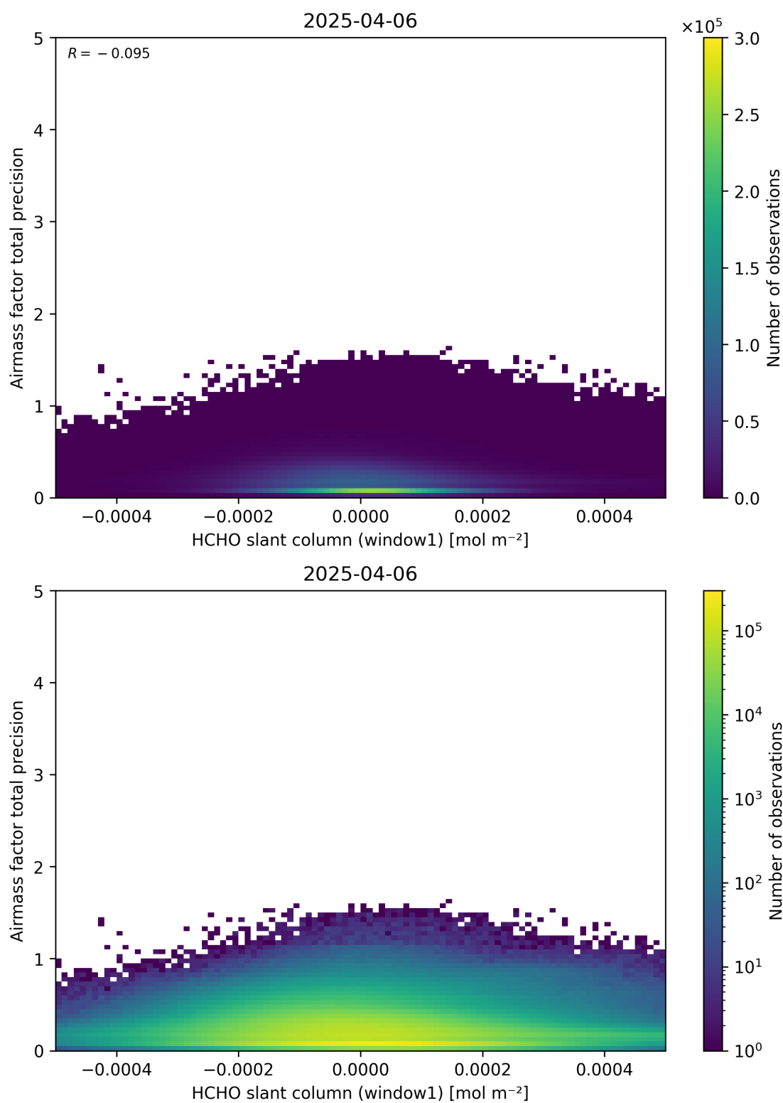
Figure 86: Scatter density plot of “HCHO slant column (window1)” against “Airmass factor total precision” for 2025-04-05 to 2025-04-07.
