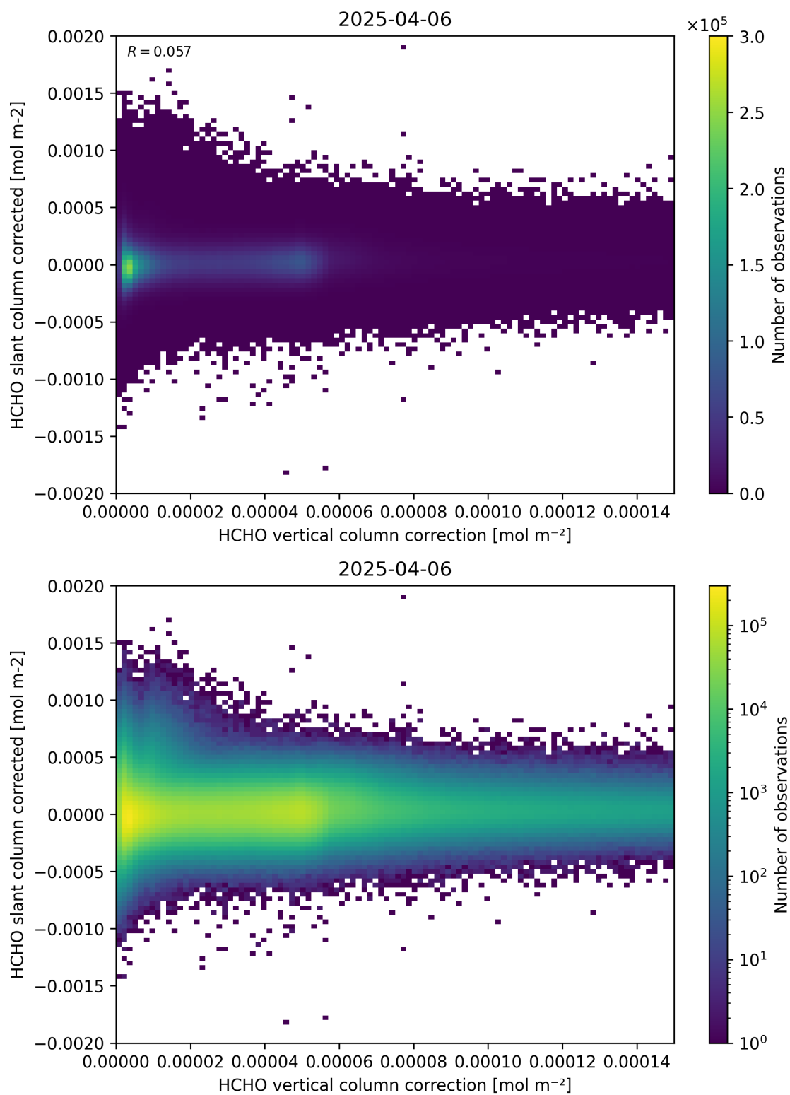
Figure 116: Scatter density plot of “HCHO vertical column correction” against “HCHO slant column corrected” for 2025-04-05 to 2025-04-07.
