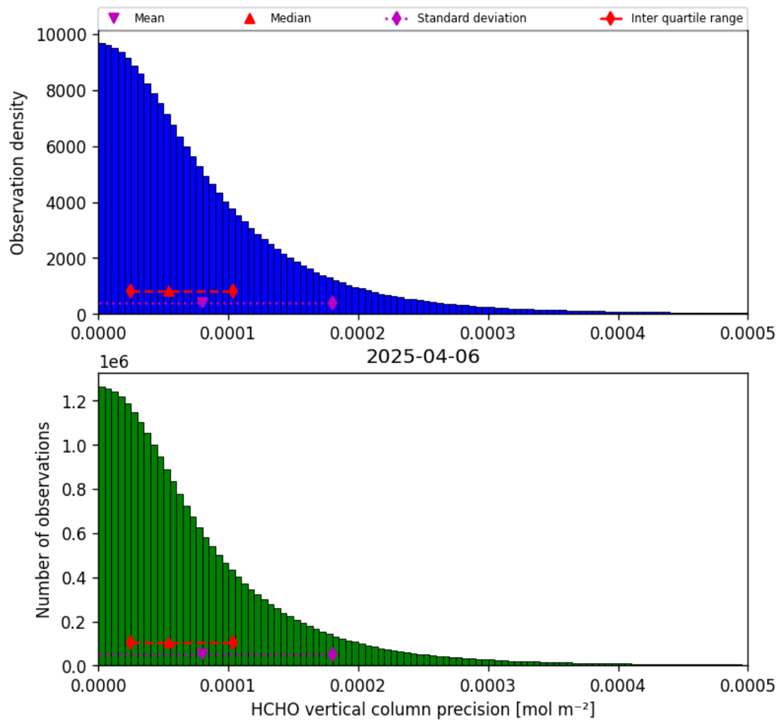
Figure 36: Histogram of “HCHO vertical column precision” for 2025-04-05 to 2025-04-07
