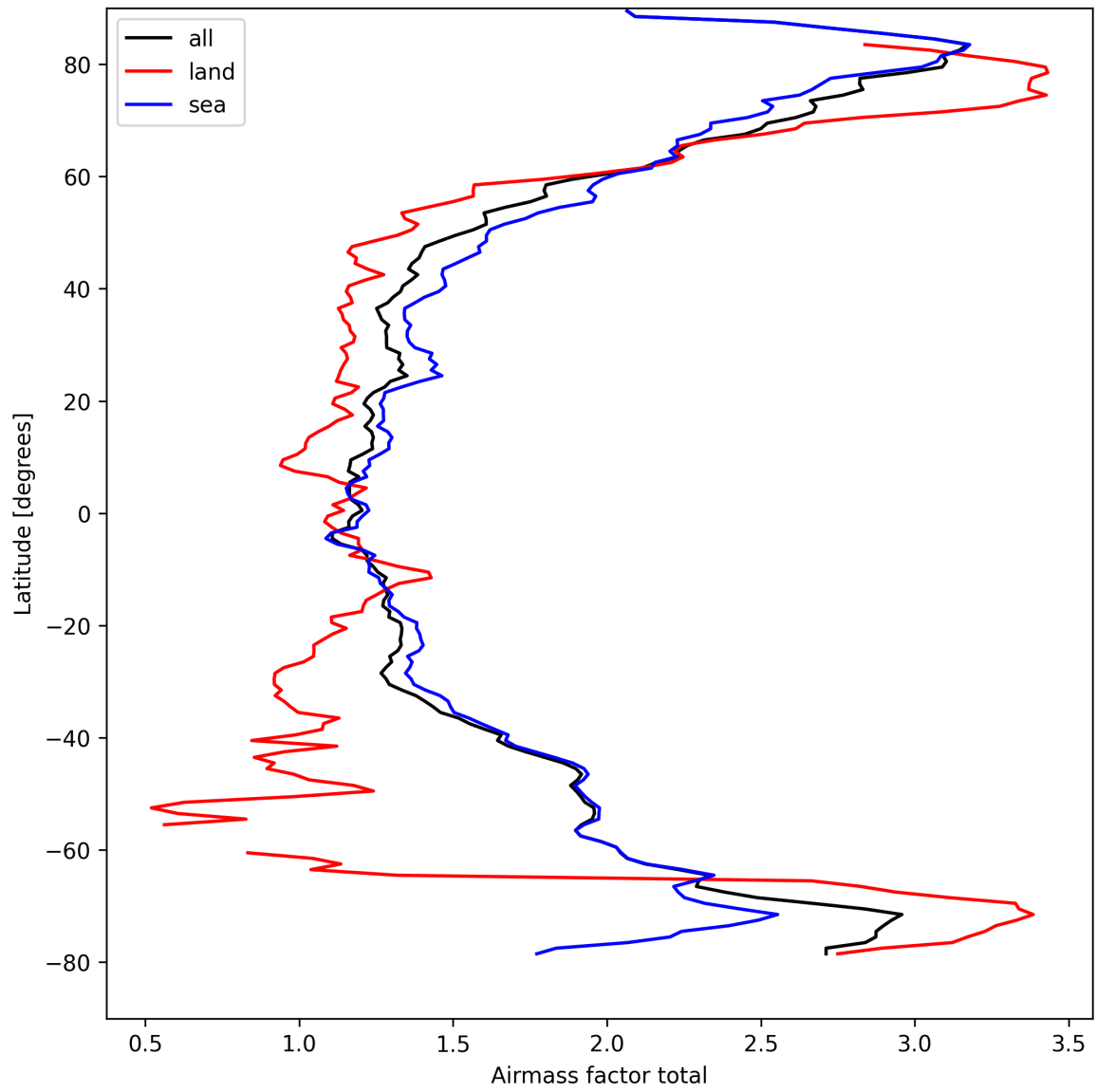
Figure 26: Zonal average of “Airmass factor total” for 2025-04-05 to 2025-04-07.
