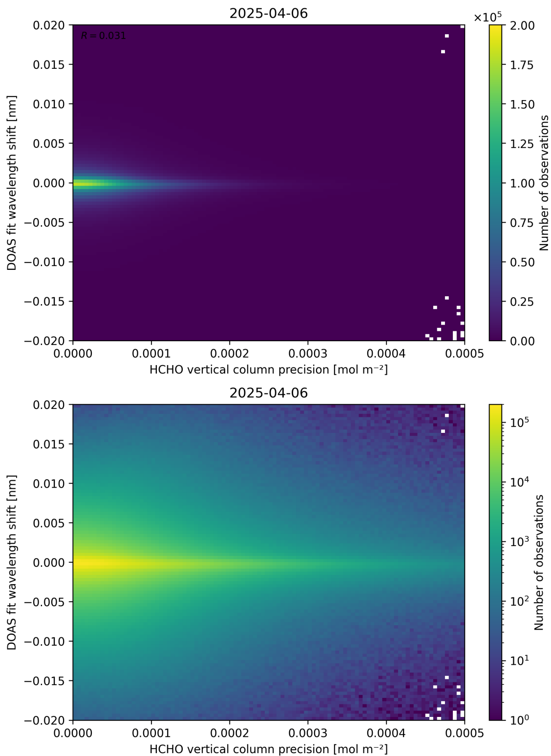
Figure 137: Scatter density plot of “HCHO vertical column precision” against “DOAS fit wavelength shift” for 2025-04-05 to 2025-04-07.
