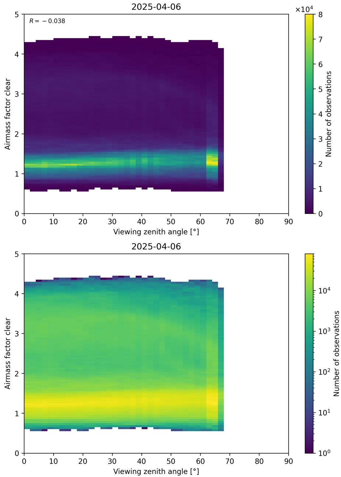
Figure 185: Scatter density plot of “Viewing zenith angle” against “Airmass factor clear” for 2025-04-05 to 2025-04-07.
