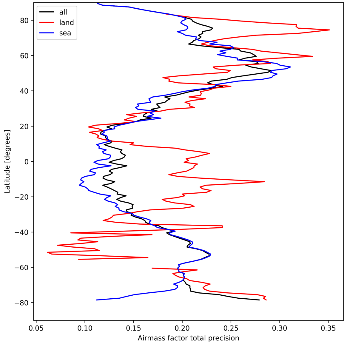
Figure 27: Zonal average of “Airmass factor total precision” for 2025-04-05 to 2025-04-07.
