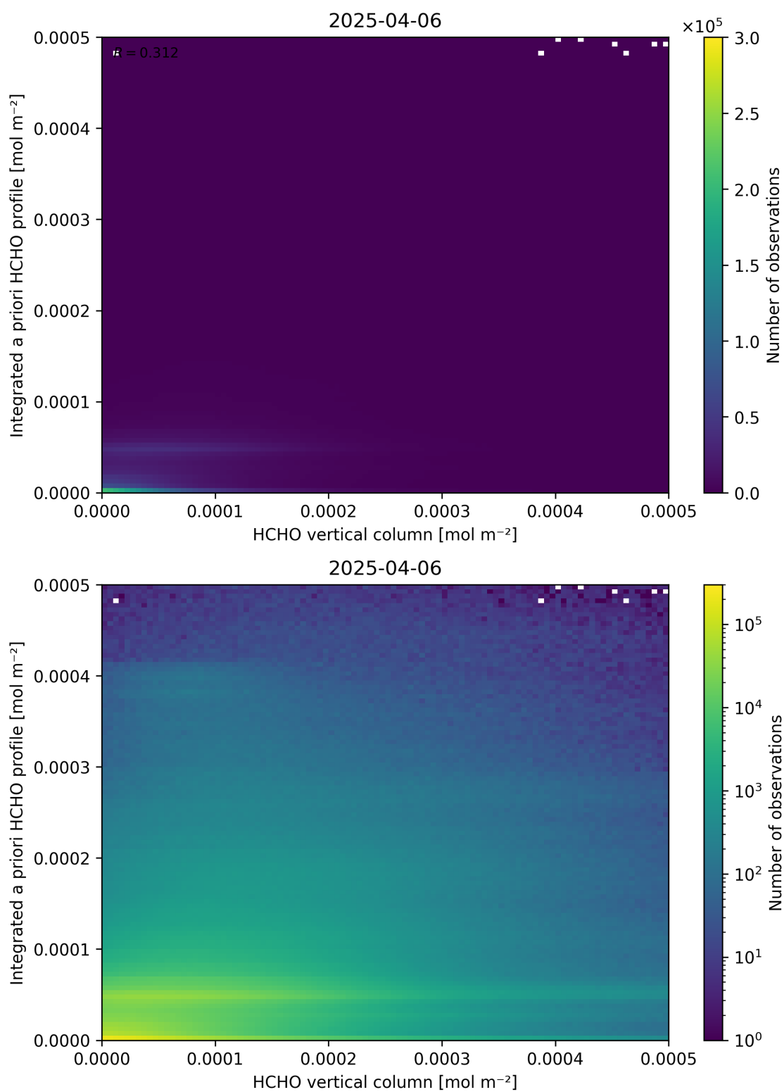
Figure 135: Scatter density plot of “HCHO vertical column” against “Integrated a priori HCHO profile” for 2025-04-05 to 2025-04-07.
