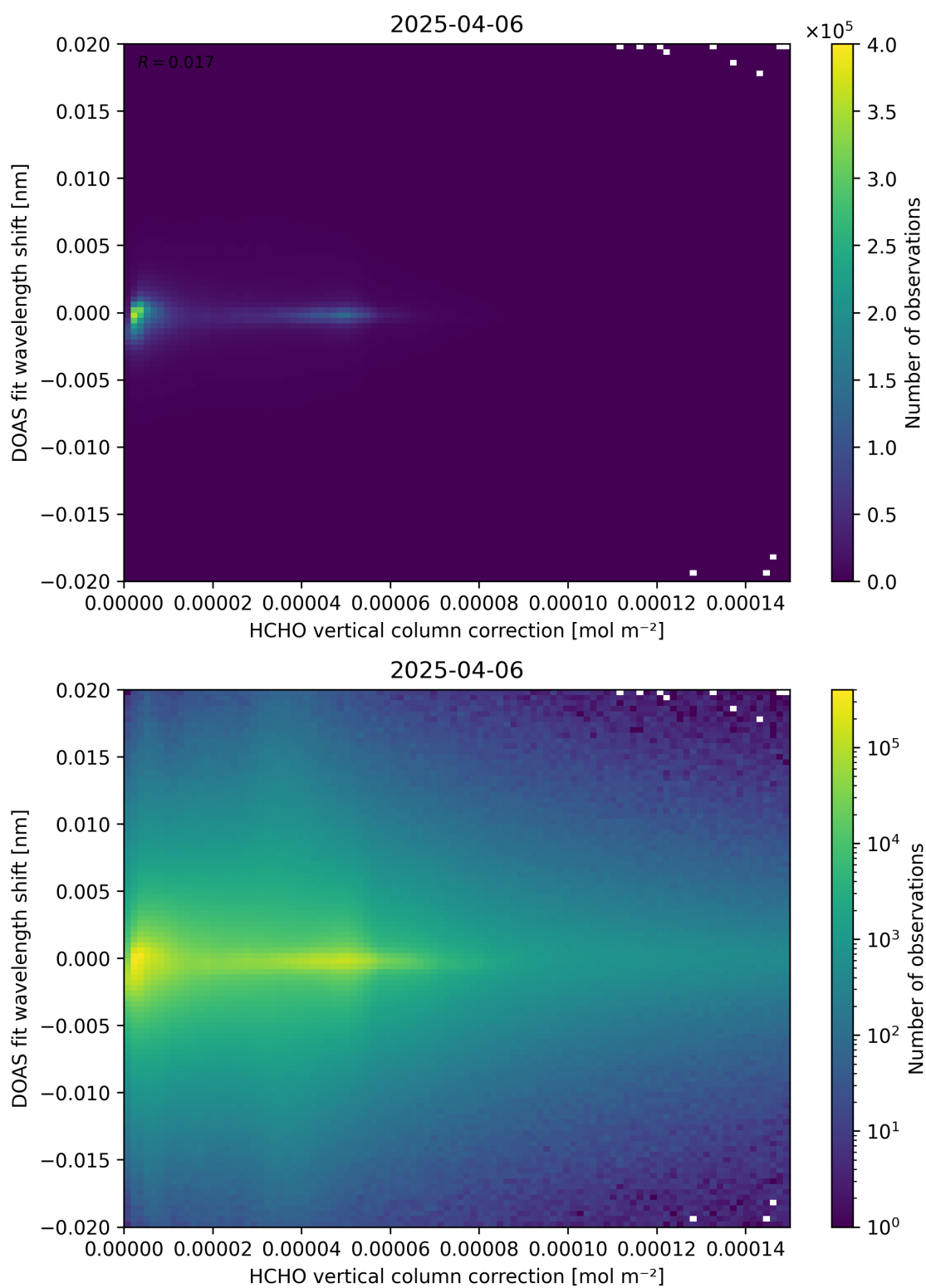
Figure 113: Scatter density plot of “HCHO vertical column correction” against “DOAS fit wavelength shift” for 2025-04-05 to 2025-04-07.
