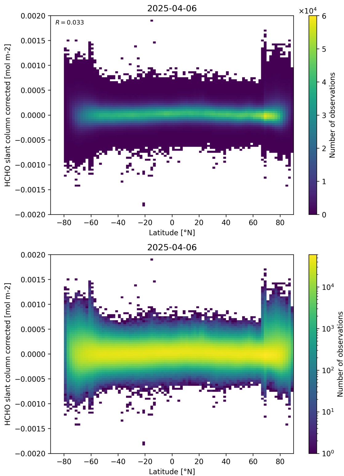
Figure 157: Scatter density plot of “Latitude” against “HCHO slant column corrected” for 2025-04-05 to 2025-04-07.
