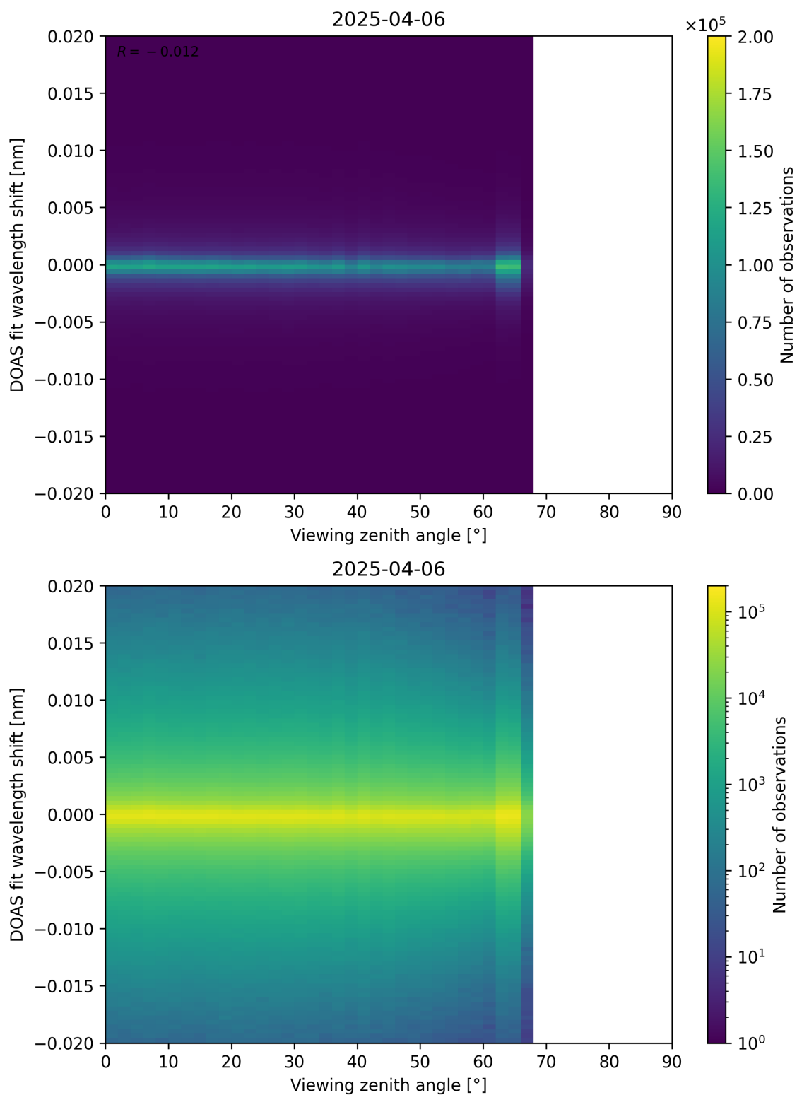
Figure 183: Scatter density plot of “Viewing zenith angle” against “DOAS fit wavelength shift” for 2025-04-05 to 2025-04-07.
