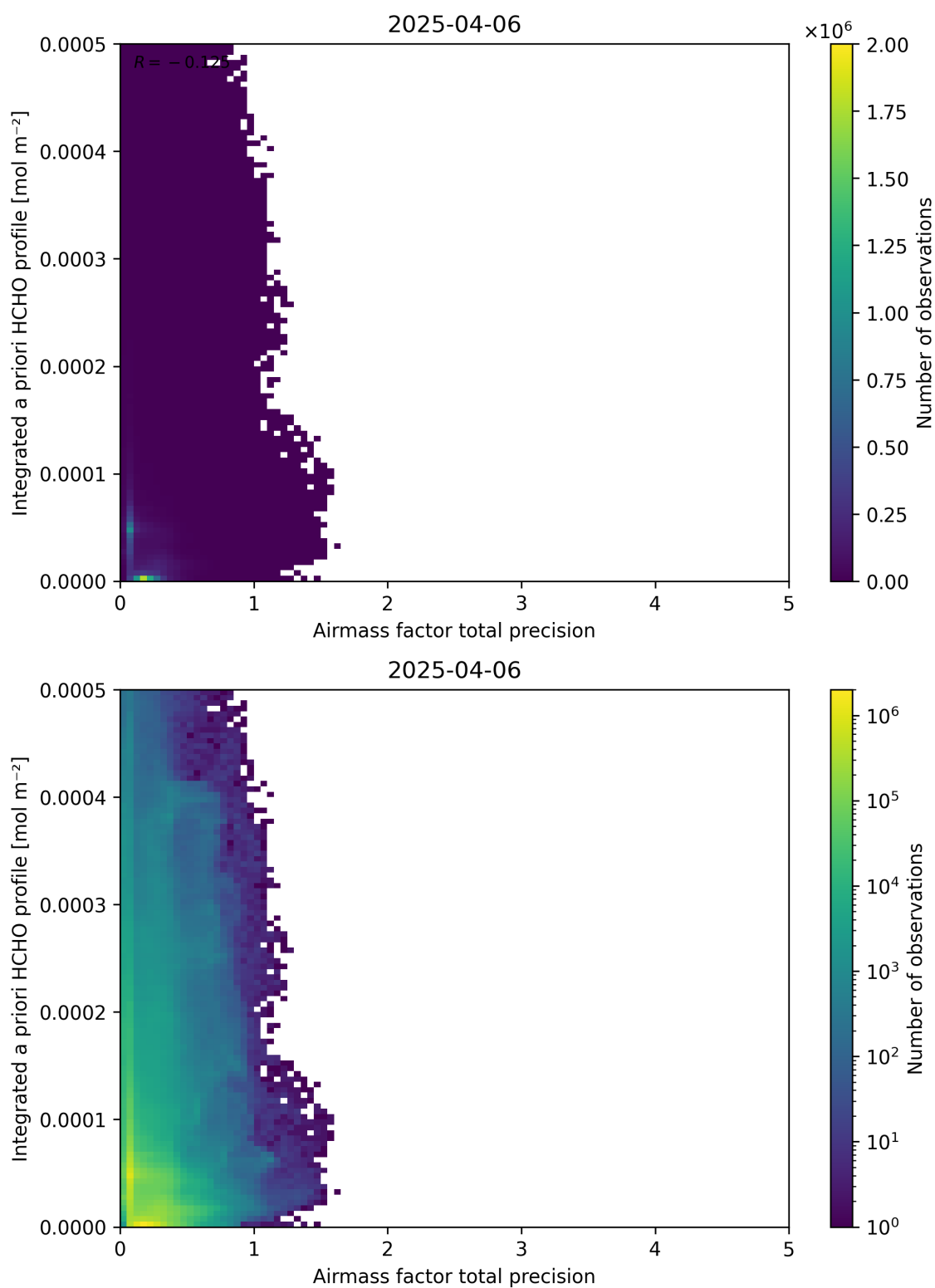
Figure 111: Scatter density plot of “Airmass factor total precision” against “Integrated a priori HCHO profile” for 2025-04-05 to 2025-04-07.
