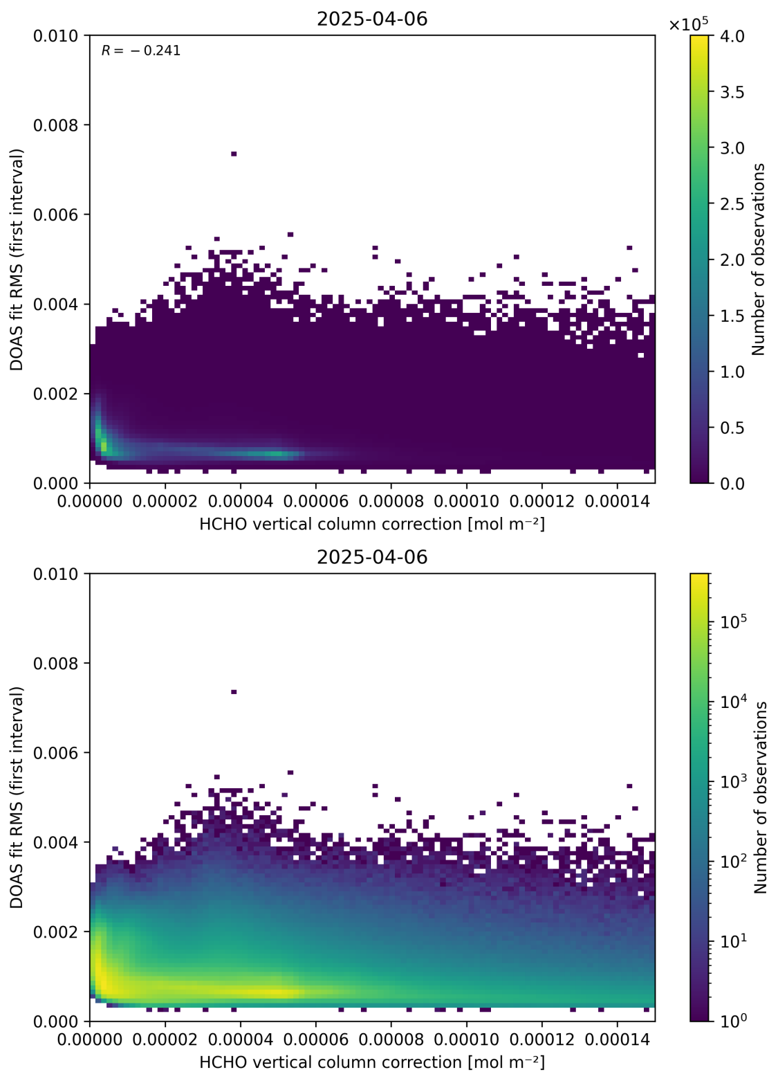
Figure 112: Scatter density plot of “HCHO vertical column correction” against “DOAS fit RMS (first interval)” for 2025-04-05 to 2025-04-07.
