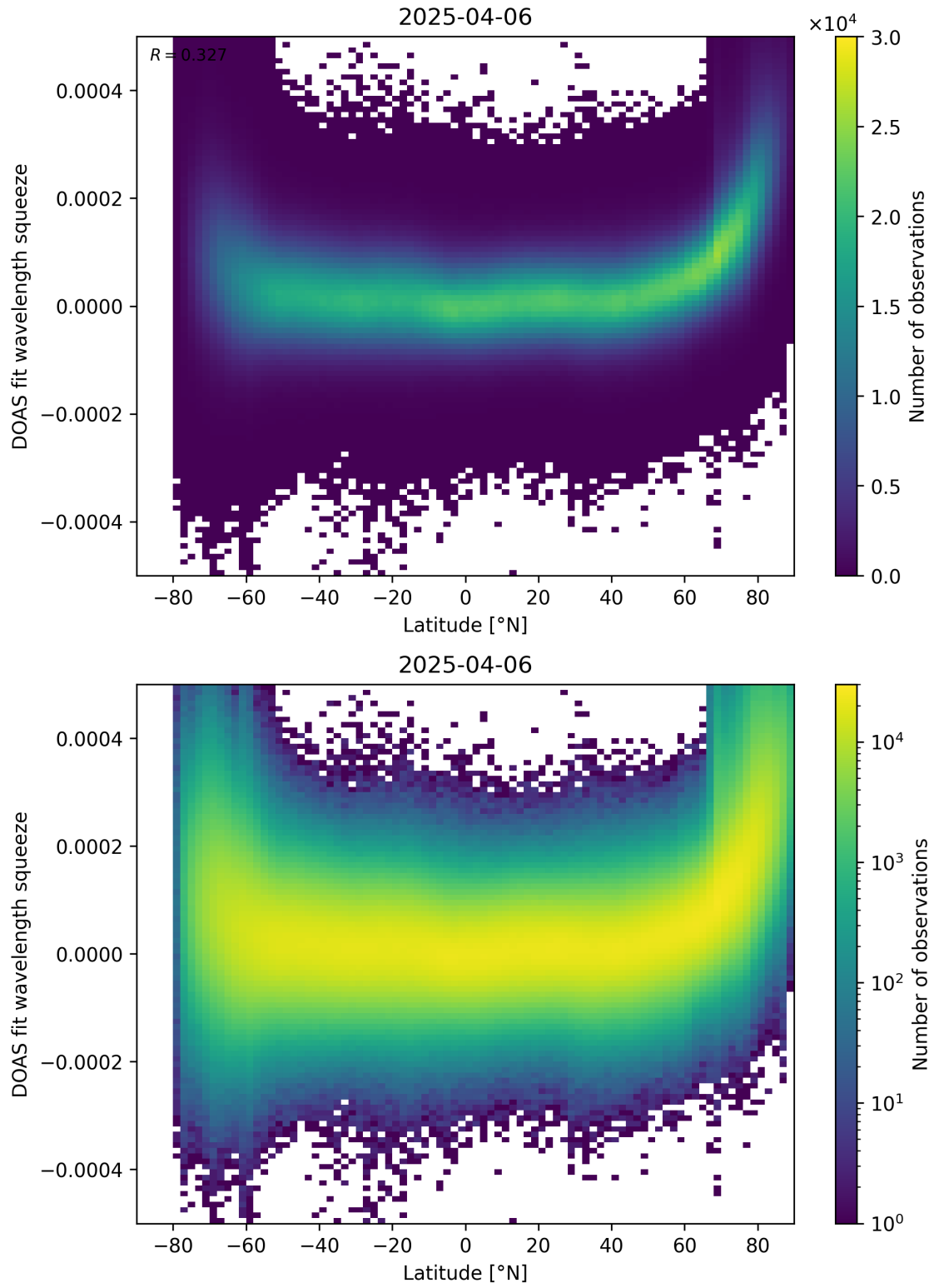
Figure 155: Scatter density plot of “Latitude” against “DOAS fit wavelength squeeze” for 2025-04-05 to 2025-04-07.
