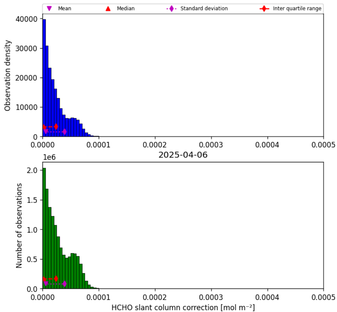
Figure 47: Histogram of “HCHO slant column correction” for 2025-04-05 to 2025-04-07
