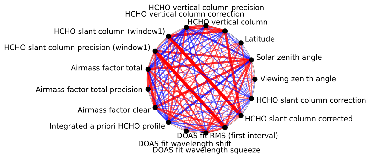
Figure 1: Map of correlation graph for 2025-04-05 to 2025-04-07.
