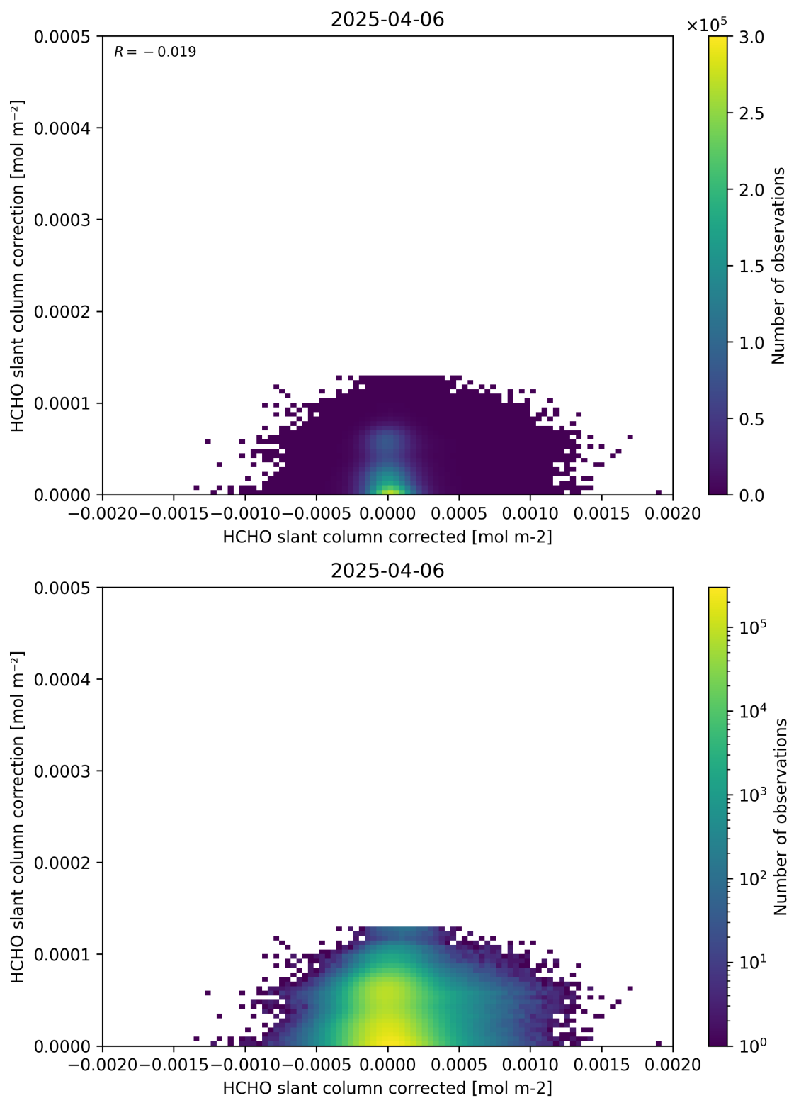
Figure 77: Scatter density plot of “HCHO slant column corrected” against “HCHO slant column correction” for 2025-04-05 to 2025-04-07.
