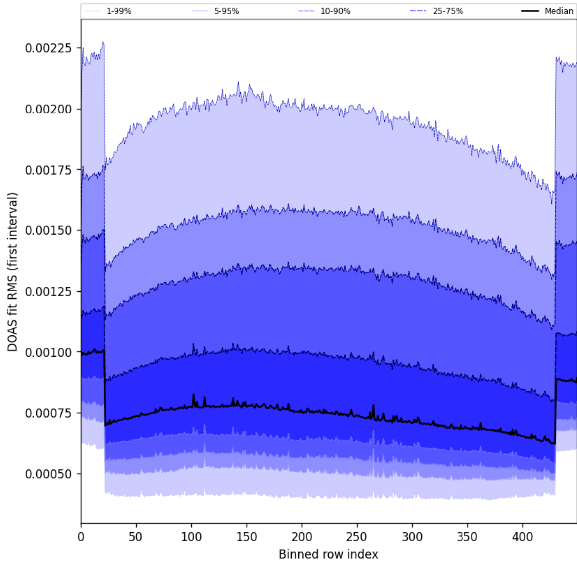
Figure 60: Along track statistics of “DOAS fit RMS (first interval)” for 2025-04-05 to 2025-04-07
