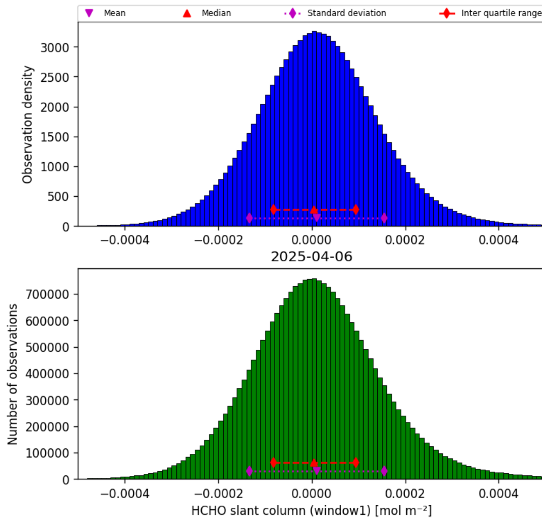
Figure 38: Histogram of “HCHO slant column (window1)” for 2025-04-05 to 2025-04-07
