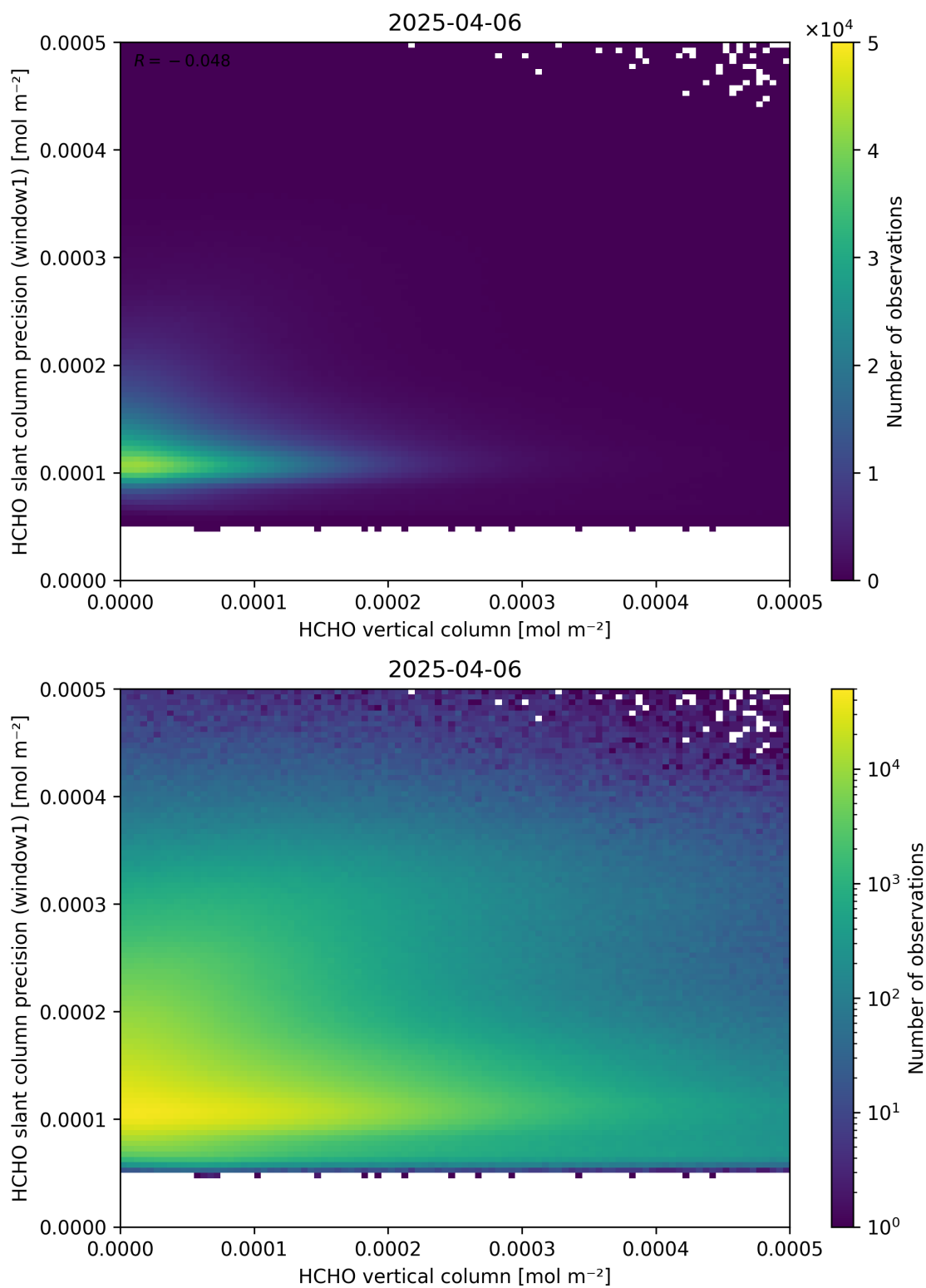
Figure 130: Scatter density plot of “HCHO vertical column” against “HCHO slant column precision (window1)” for 2025-04-05 to 2025-04-07.
