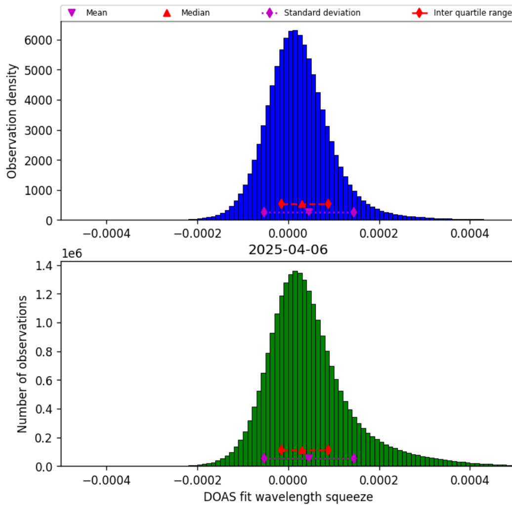
Figure 45: Histogram of “DOAS fit wavelength squeeze” for 2025-04-05 to 2025-04-07
