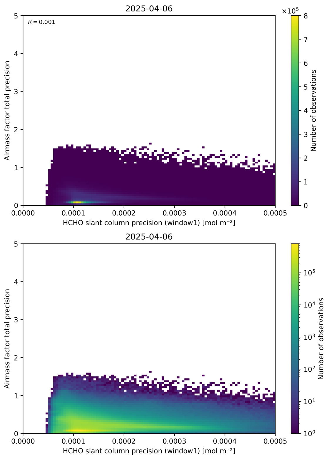
Figure 95: Scatter density plot of “HCHO slant column precision (window1)” against “Airmass factor total precision” for 2025-04-05 to 2025-04-07.
