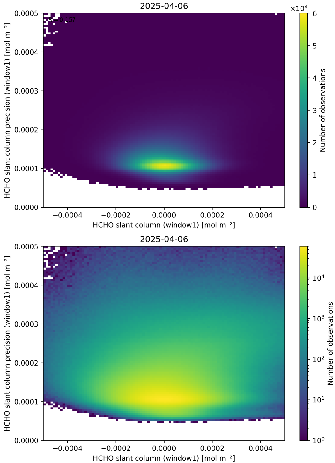
Figure 84: Scatter density plot of “HCHO slant column (window1)” against “HCHO slant column precision (window1)” for 2025-04-05 to 2025-04-07.
