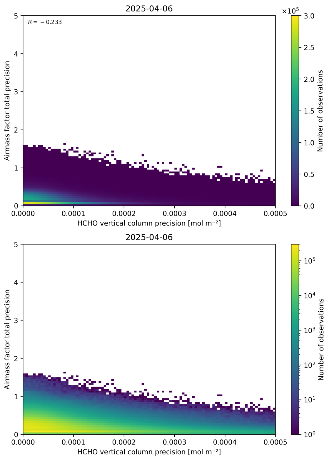
Figure 145: Scatter density plot of “HCHO vertical column precision” against “Airmass factor total precision” for 2025-04-05 to 2025-04-07.
