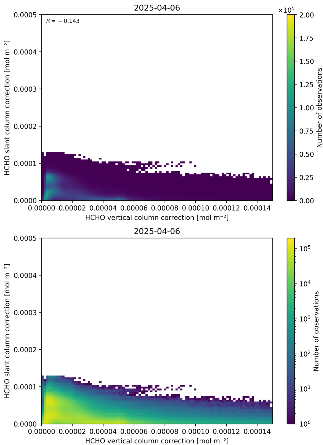
Figure 117: Scatter density plot of “HCHO vertical column correction” against “HCHO slant column correction” for 2025-04-05 to 2025-04-07.
