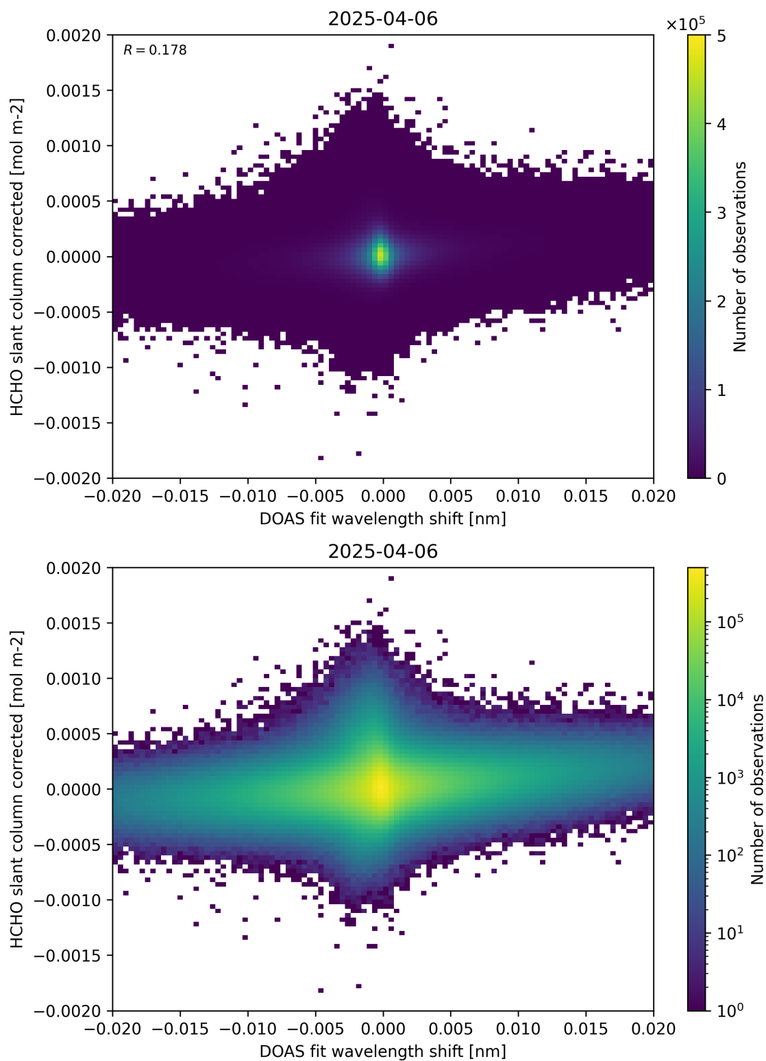
Figure 66: Scatter density plot of “DOAS fit wavelength shift” against “HCHO slant column corrected” for 2025-04-05 to 2025-04-07.
