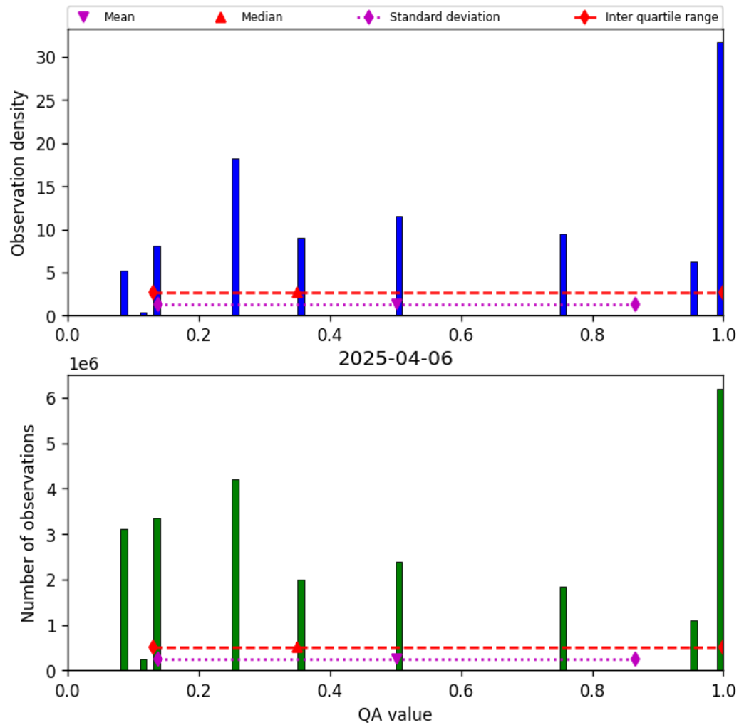
Figure 34: Histogram of “QA value” for 2025-04-05 to 2025-04-07
