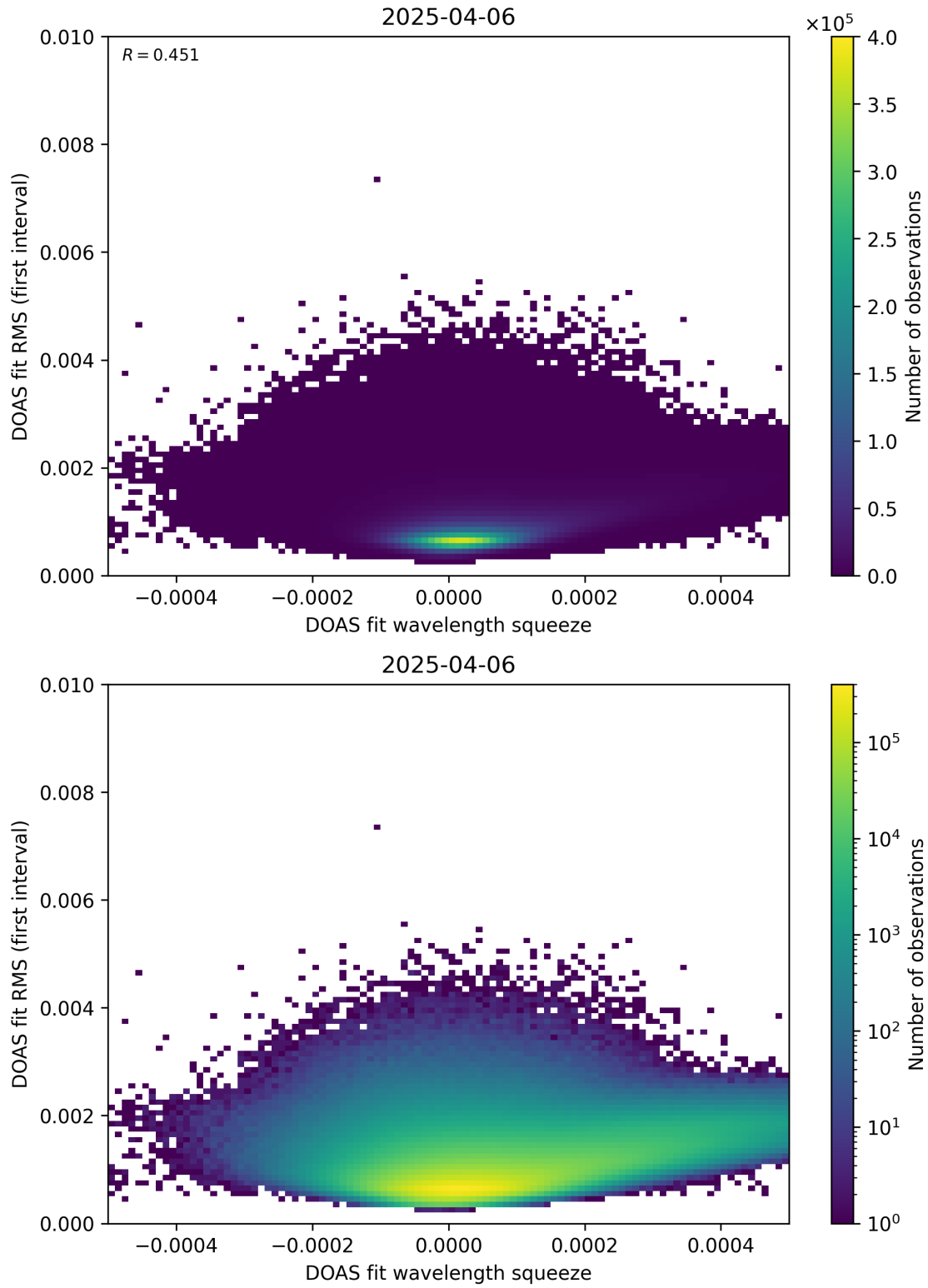
Figure 68: Scatter density plot of “DOAS fit wavelength squeeze” against “DOAS fit RMS (first interval)” for 2025-04-05 to 2025-04-07.
