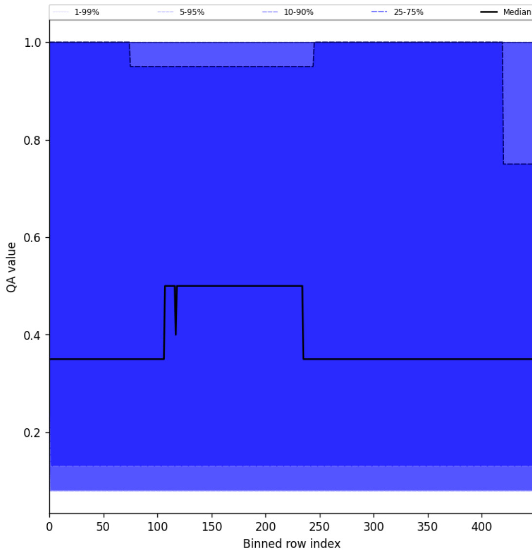
Figure 48: Along track statistics of “QA value” for 2025-04-05 to 2025-04-07
