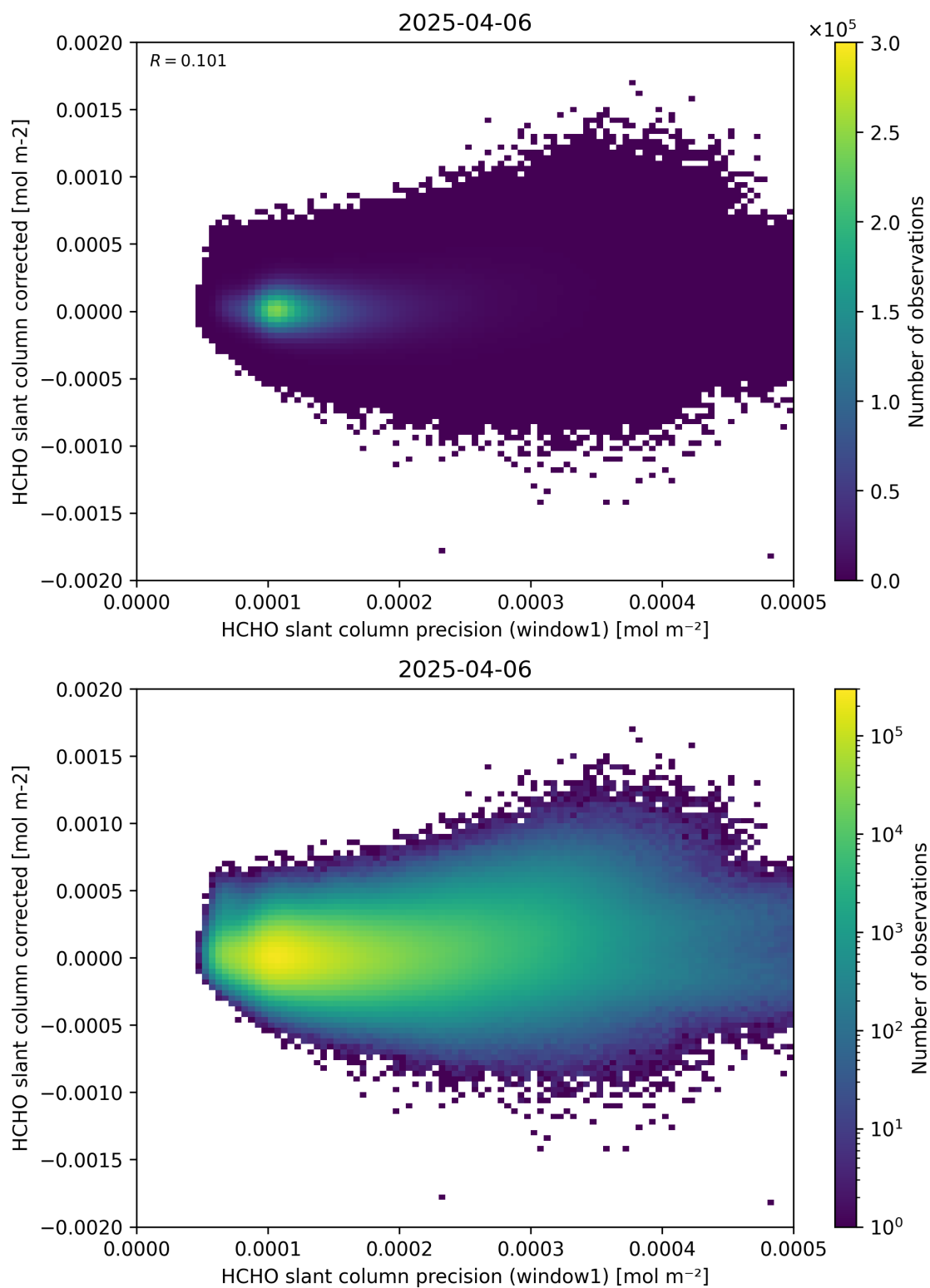
Figure 92: Scatter density plot of “HCHO slant column precision (window1)” against “HCHO slant column corrected” for 2025-04-05 to 2025-04-07.
