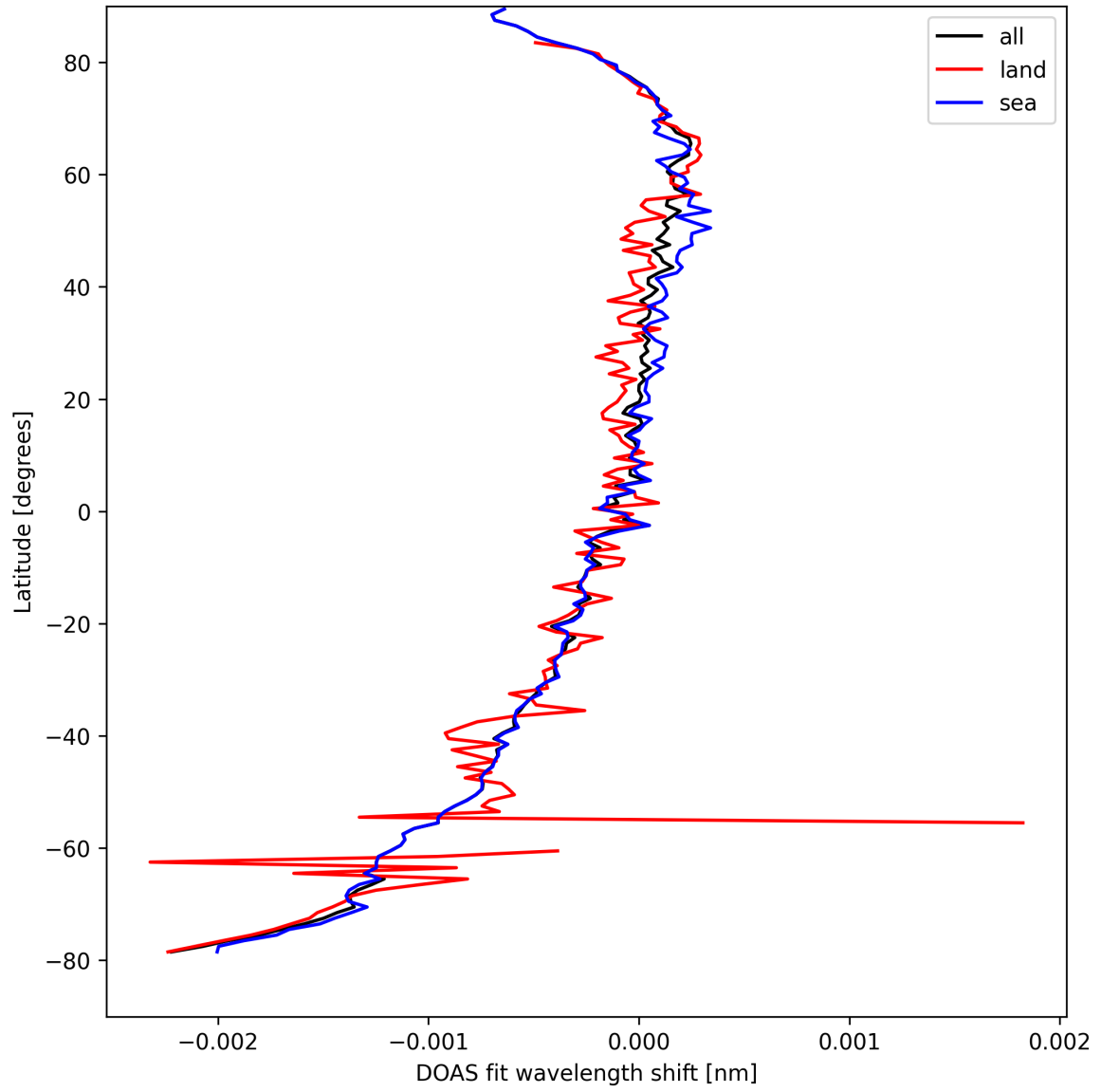
Figure 30: Zonal average of “DOAS fit wavelength shift” for 2025-04-05 to 2025-04-07.
