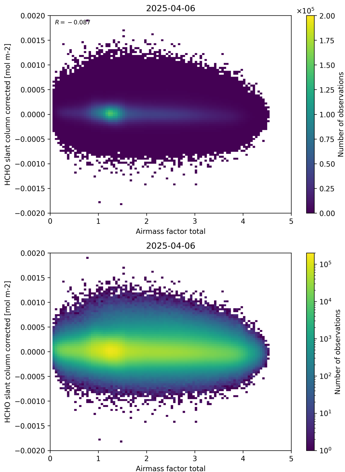
Figure 101: Scatter density plot of “Airmass factor total” against “HCHO slant column corrected” for 2025-04-05 to 2025-04-07.
