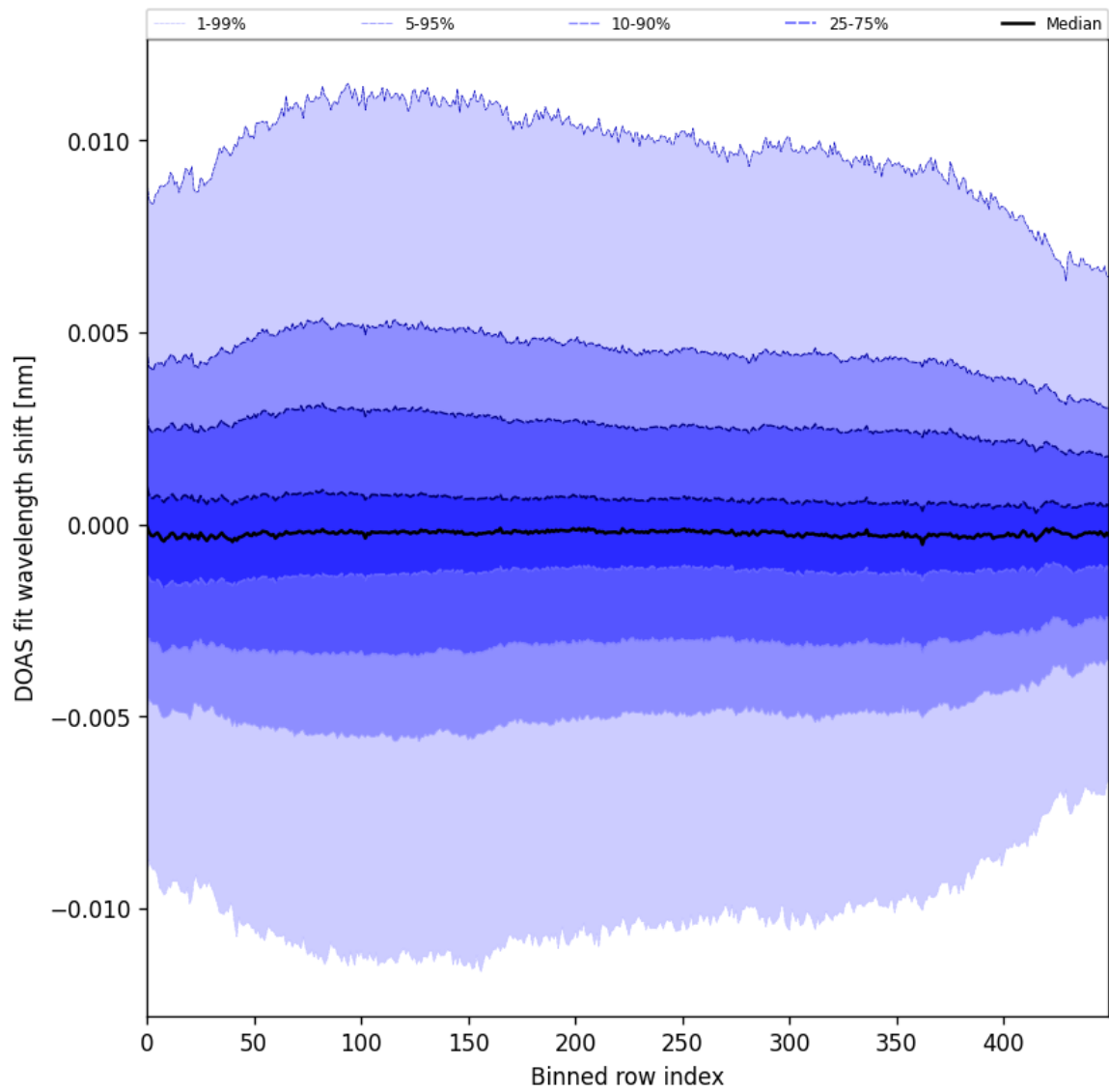
Figure 58: Along track statistics of “DOAS fit wavelength shift” for 2025-04-05 to 2025-04-07
