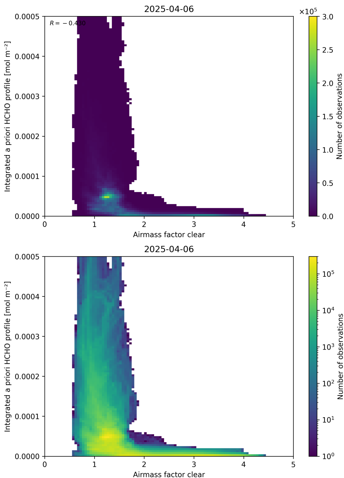
Figure 76: Scatter density plot of “Airmass factor clear” against “Integrated a priori HCHO profile” for 2025-04-05 to 2025-04-07.
