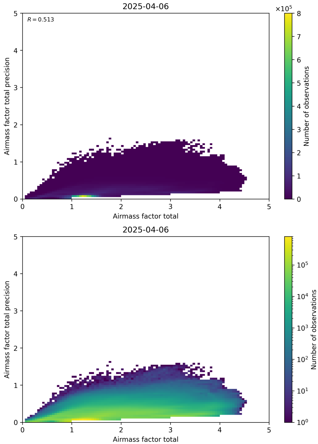
Figure 103: Scatter density plot of “Airmass factor total” against “Airmass factor total precision” for 2025-04-05 to 2025-04-07.
