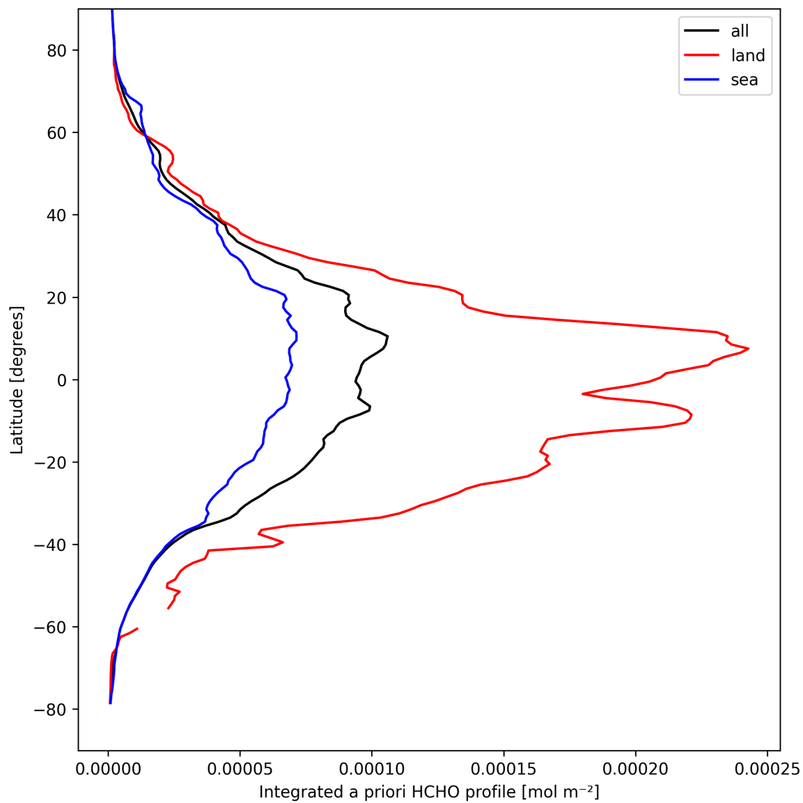
Figure 29: Zonal average of “Integrated a priori HCHO profile” for 2025-04-05 to 2025-04-07.
