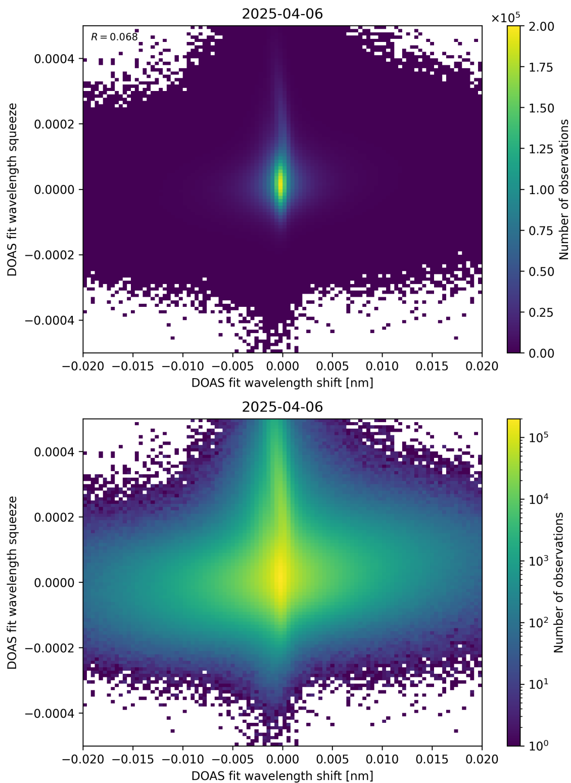
Figure 65: Scatter density plot of “DOAS fit wavelength shift” against “DOAS fit wavelength squeeze” for 2025-04-05 to 2025-04-07.
