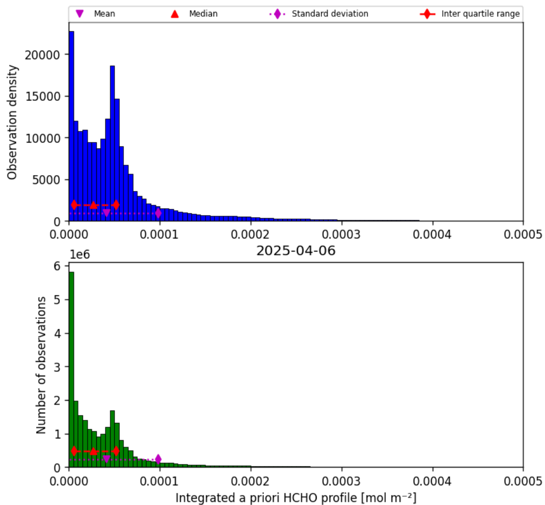
Figure 43: Histogram of “Integrated a priori HCHO profile” for 2025-04-05 to 2025-04-07
