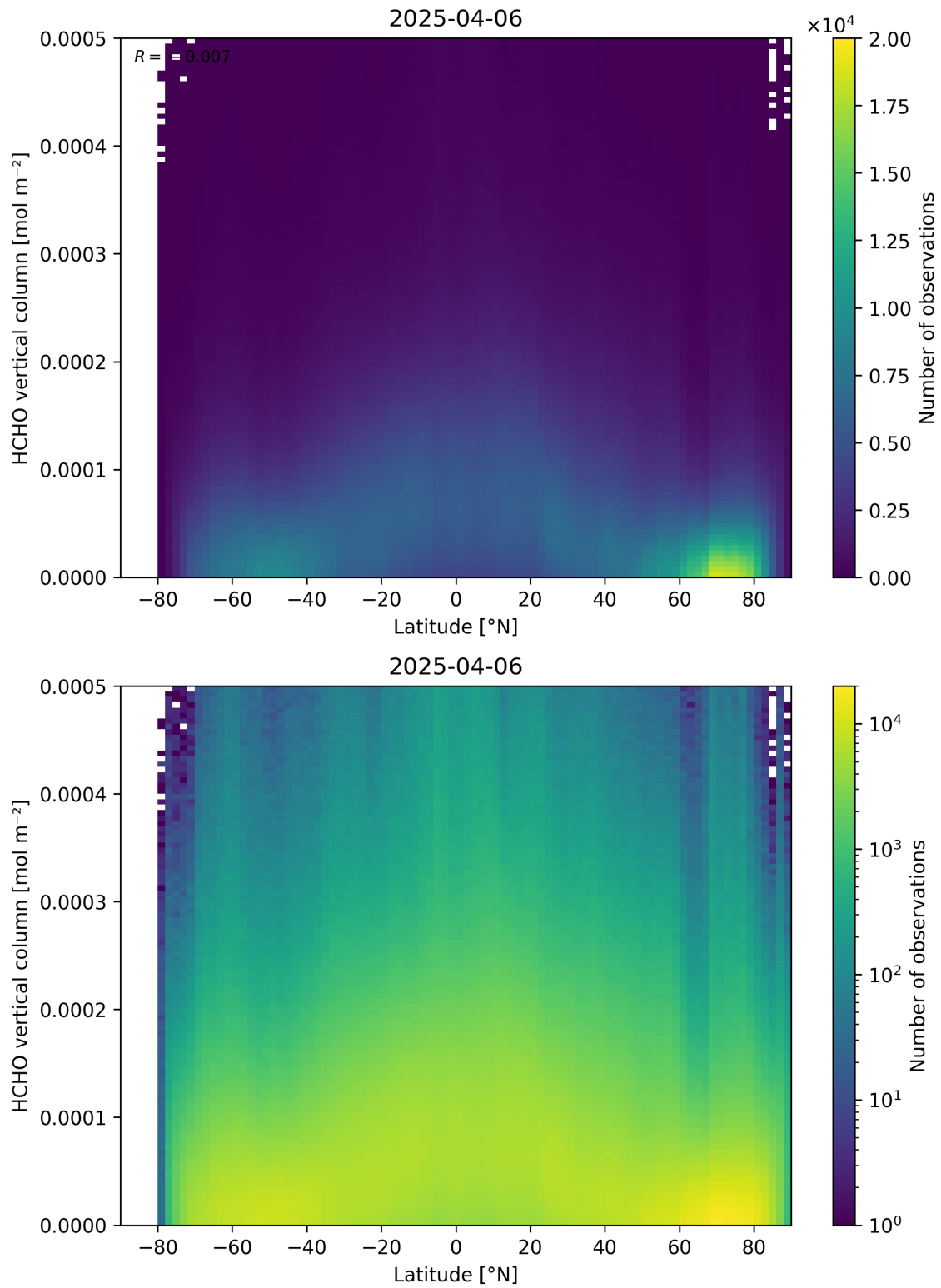
Figure 163: Scatter density plot of “Latitude” against “HCHO vertical column” for 2025-04-05 to 2025-04-07.
