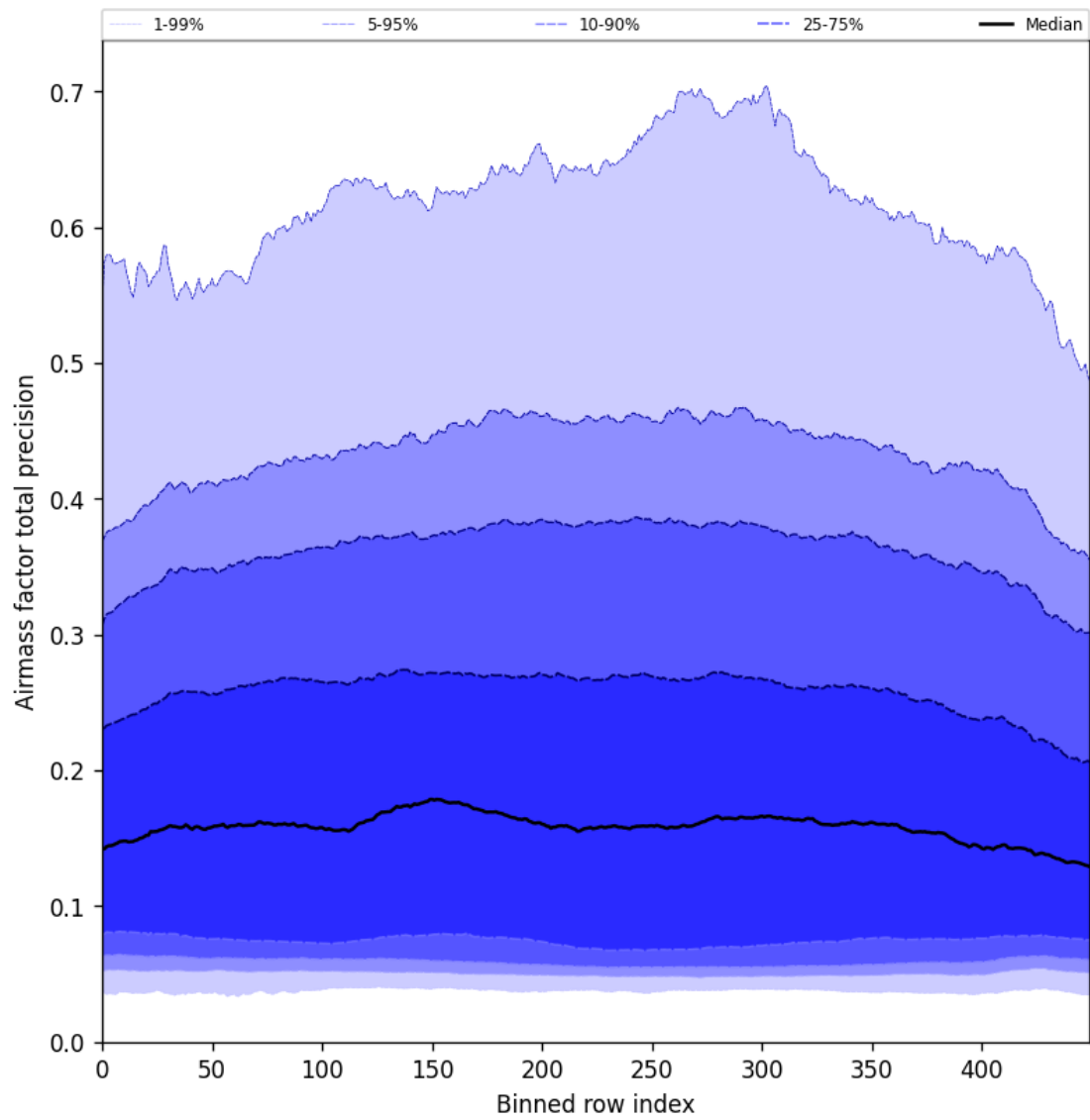
Figure 55: Along track statistics of “Airmass factor total precision” for 2025-04-05 to 2025-04-07
