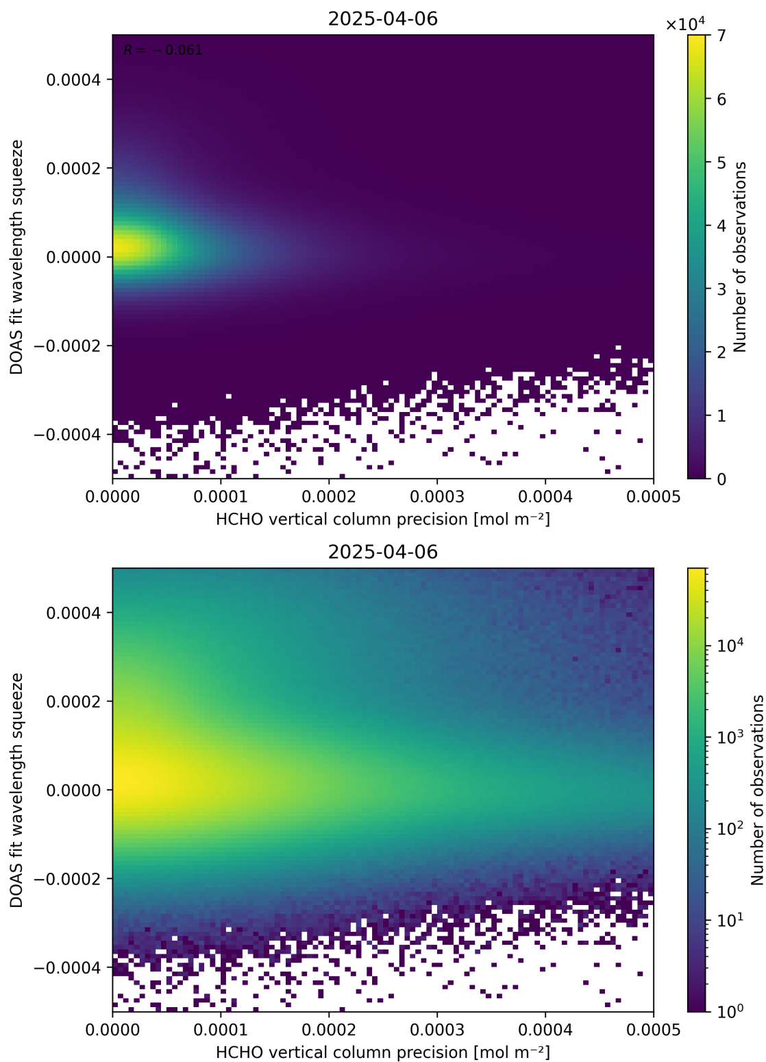
Figure 138: Scatter density plot of “HCHO vertical column precision” against “DOAS fit wavelength squeeze” for 2025-04-05 to 2025-04-07.
