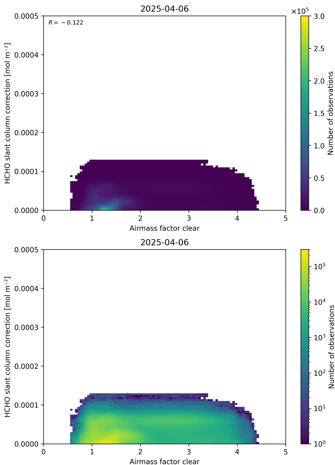
Figure 75: Scatter density plot of “Airmass factor clear” against “HCHO slant column correction” for 2025-04-05 to 2025-04-07.
