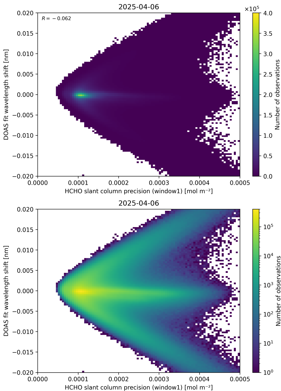
Figure 89: Scatter density plot of “HCHO slant column precision (window1)” against “DOAS fit wavelength shift” for 2025-04-05 to 2025-04-07.
