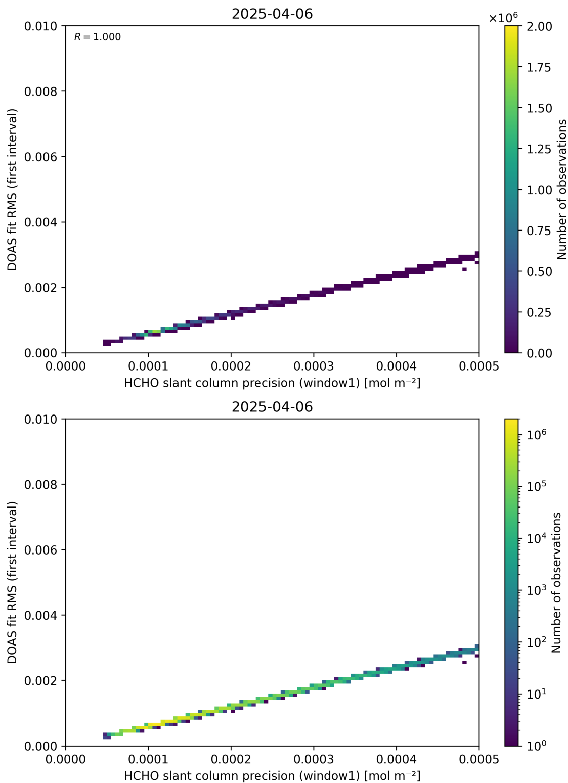
Figure 88: Scatter density plot of “HCHO slant column precision (window1)” against “DOAS fit RMS (first interval)” for 2025-04-05 to 2025-04-07.
