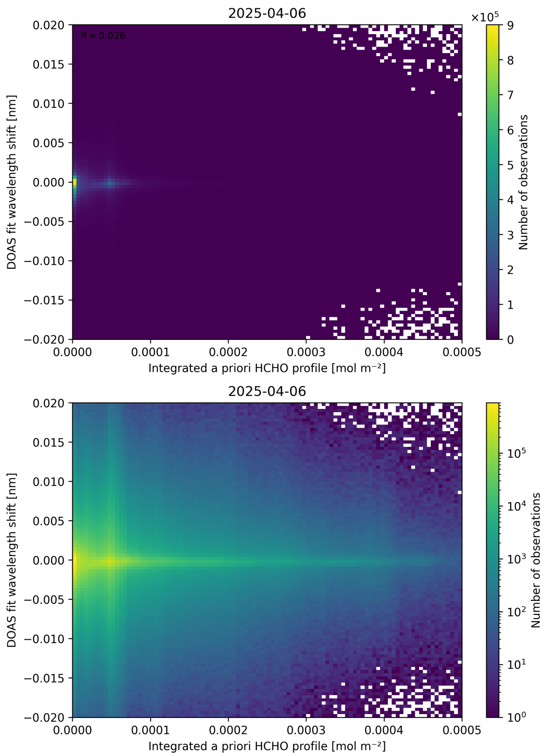
Figure 149: Scatter density plot of “Integrated a priori HCHO profile” against “DOAS fit wavelength shift” for 2025-04-05 to 2025-04-07.
