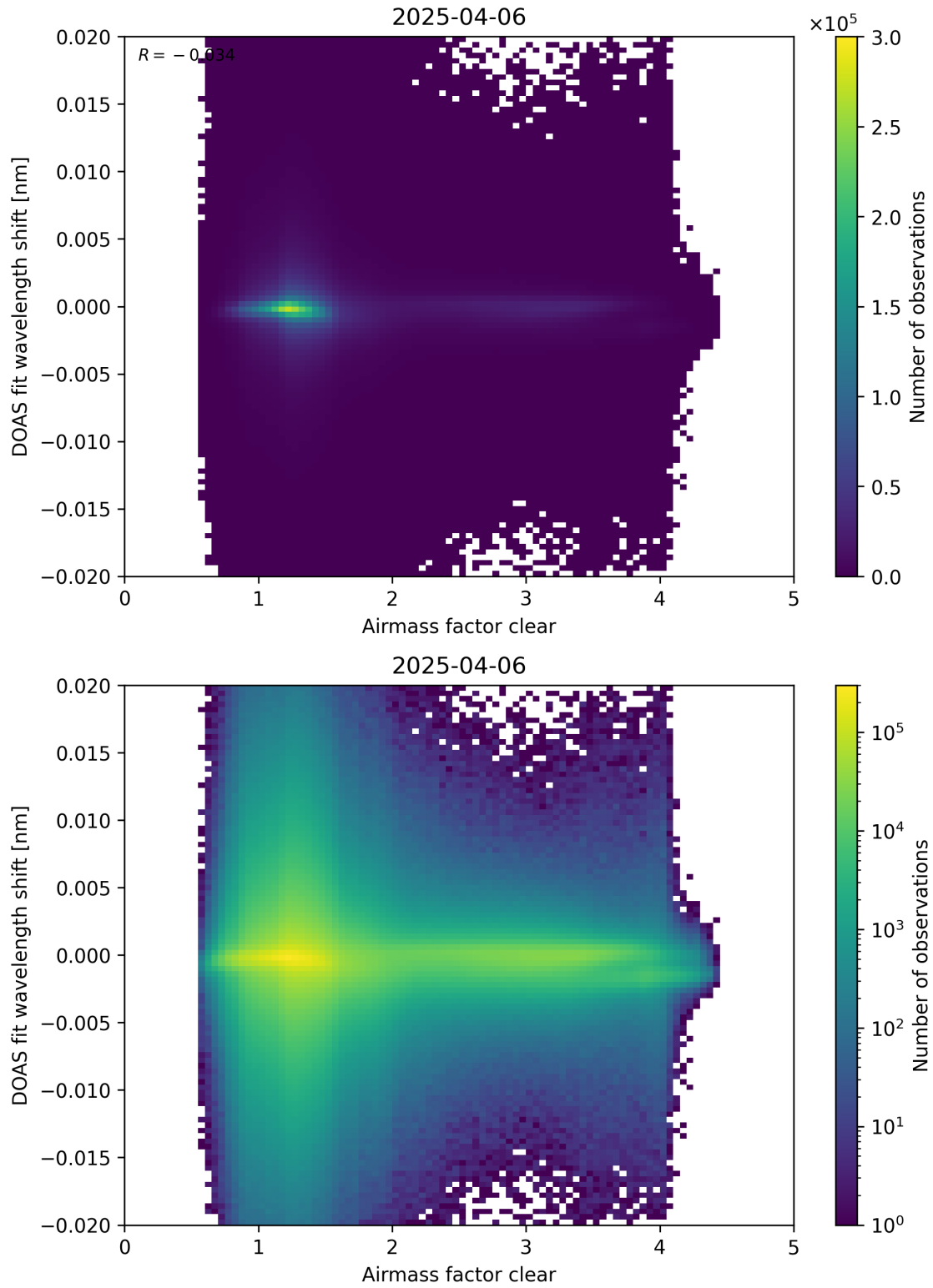
Figure 72: Scatter density plot of “Airmass factor clear” against “DOAS fit wavelength shift” for 2025-04-05 to 2025-04-07.
