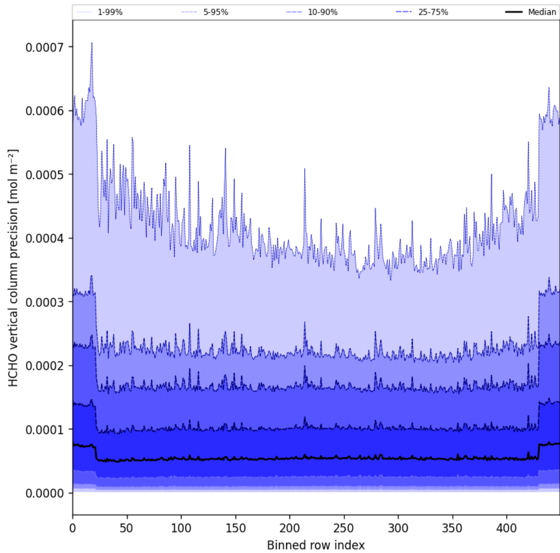
Figure 50: Along track statistics of “HCHO vertical column precision” for 2025-04-05 to 2025-04-07
