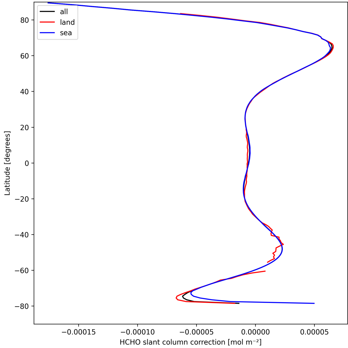
Figure 33: Zonal average of “HCHO slant column correction” for 2025-04-05 to 2025-04-07.
