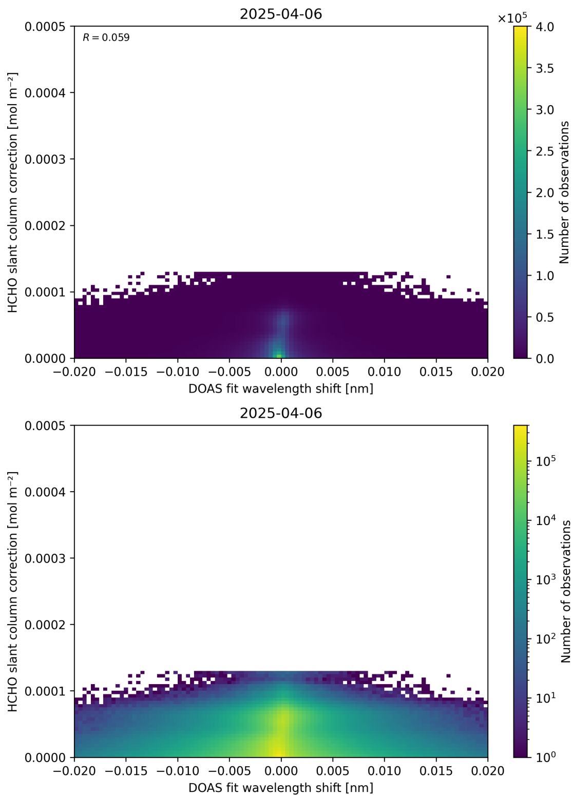
Figure 67: Scatter density plot of “DOAS fit wavelength shift” against “HCHO slant column correction” for 2025-04-05 to 2025-04-07.
