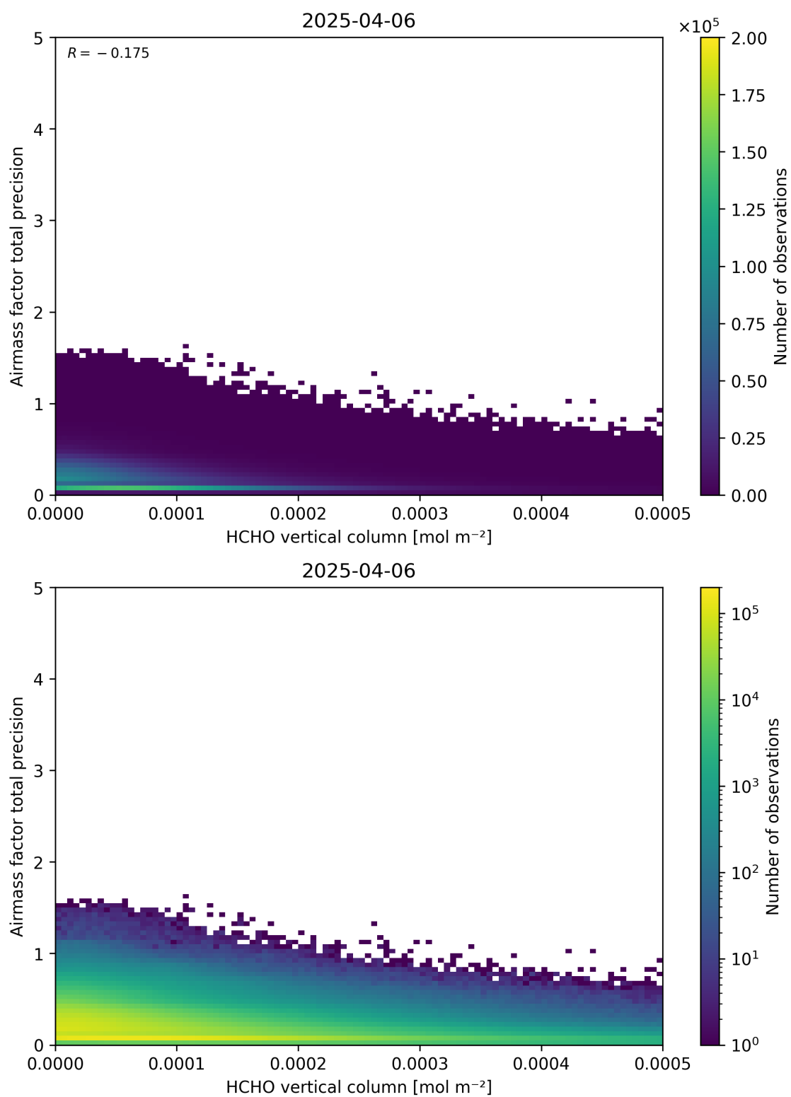
Figure 132: Scatter density plot of “HCHO vertical column” against “Airmass factor total precision” for 2025-04-05 to 2025-04-07.
