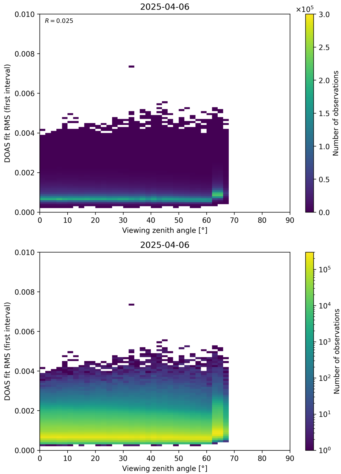
Figure 182: Scatter density plot of “Viewing zenith angle” against “DOAS fit RMS (first interval)” for 2025-04-05 to 2025-04-07.
