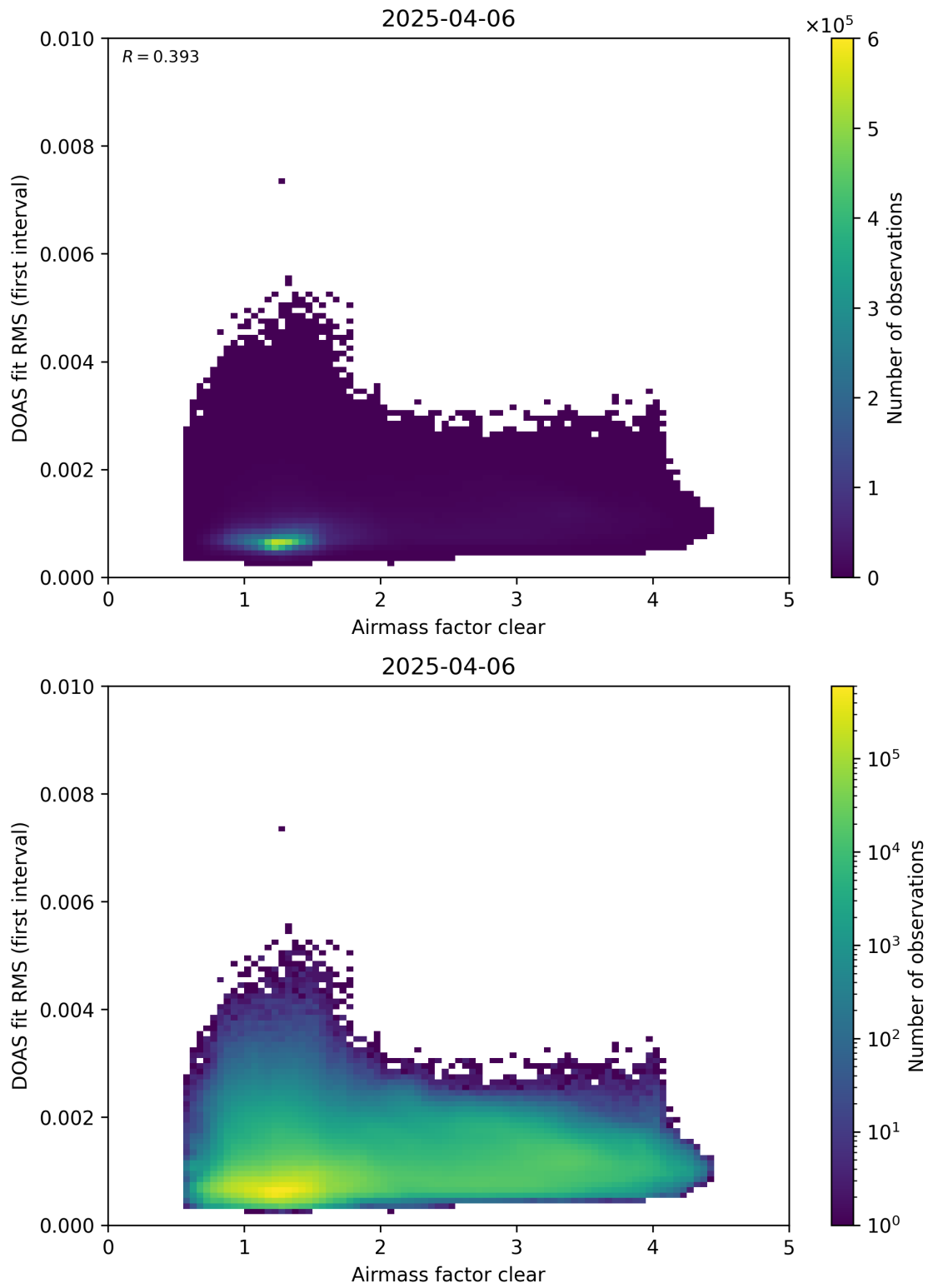
Figure 71: Scatter density plot of “Airmass factor clear” against “DOAS fit RMS (first interval)” for 2025-04-05 to 2025-04-07.
