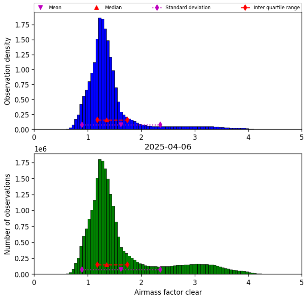
Figure 42: Histogram of “Airmass factor clear” for 2025-04-05 to 2025-04-07
