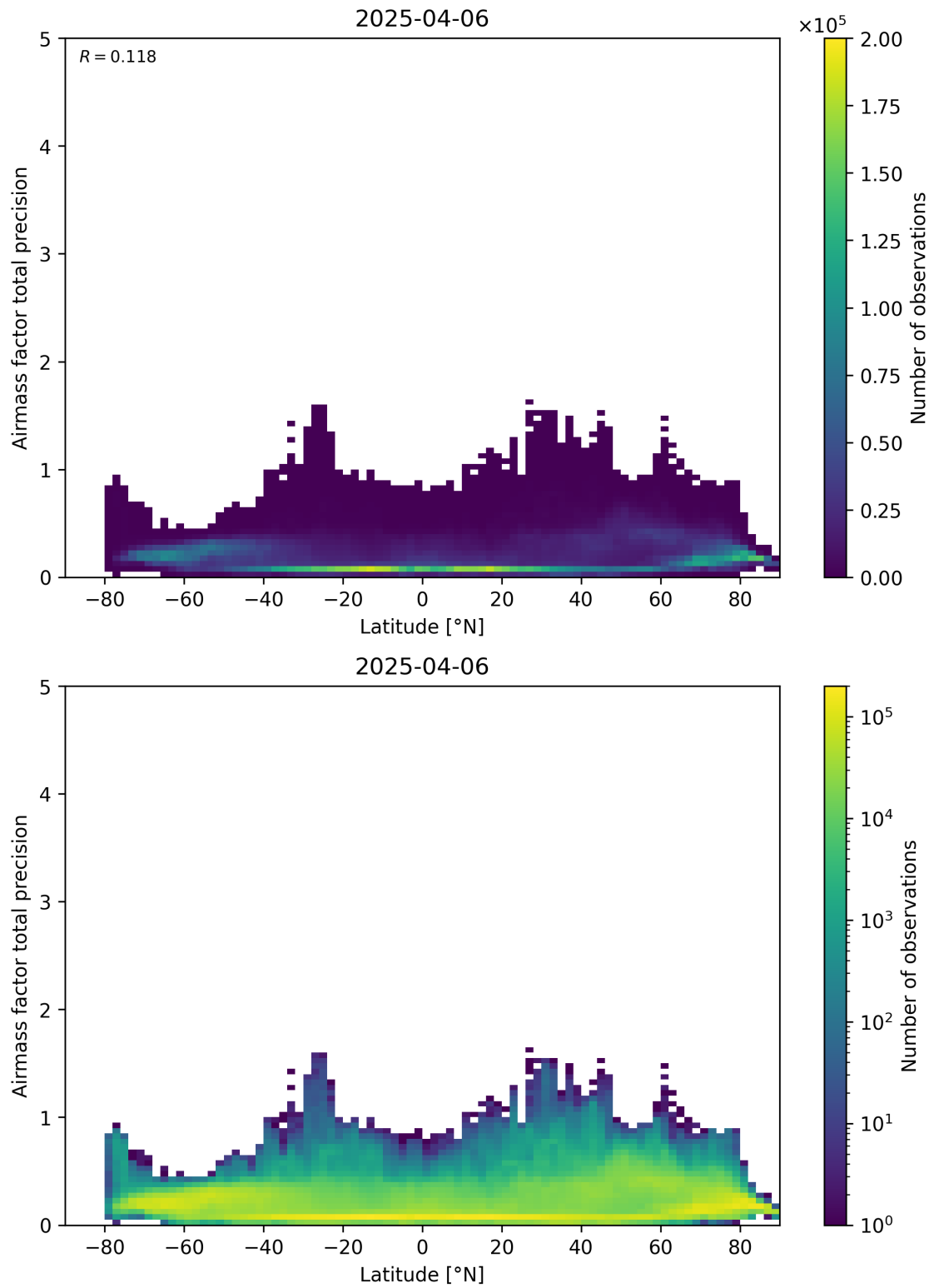
Figure 162: Scatter density plot of “Latitude” against “Airmass factor total precision” for 2025-04-05 to 2025-04-07.
