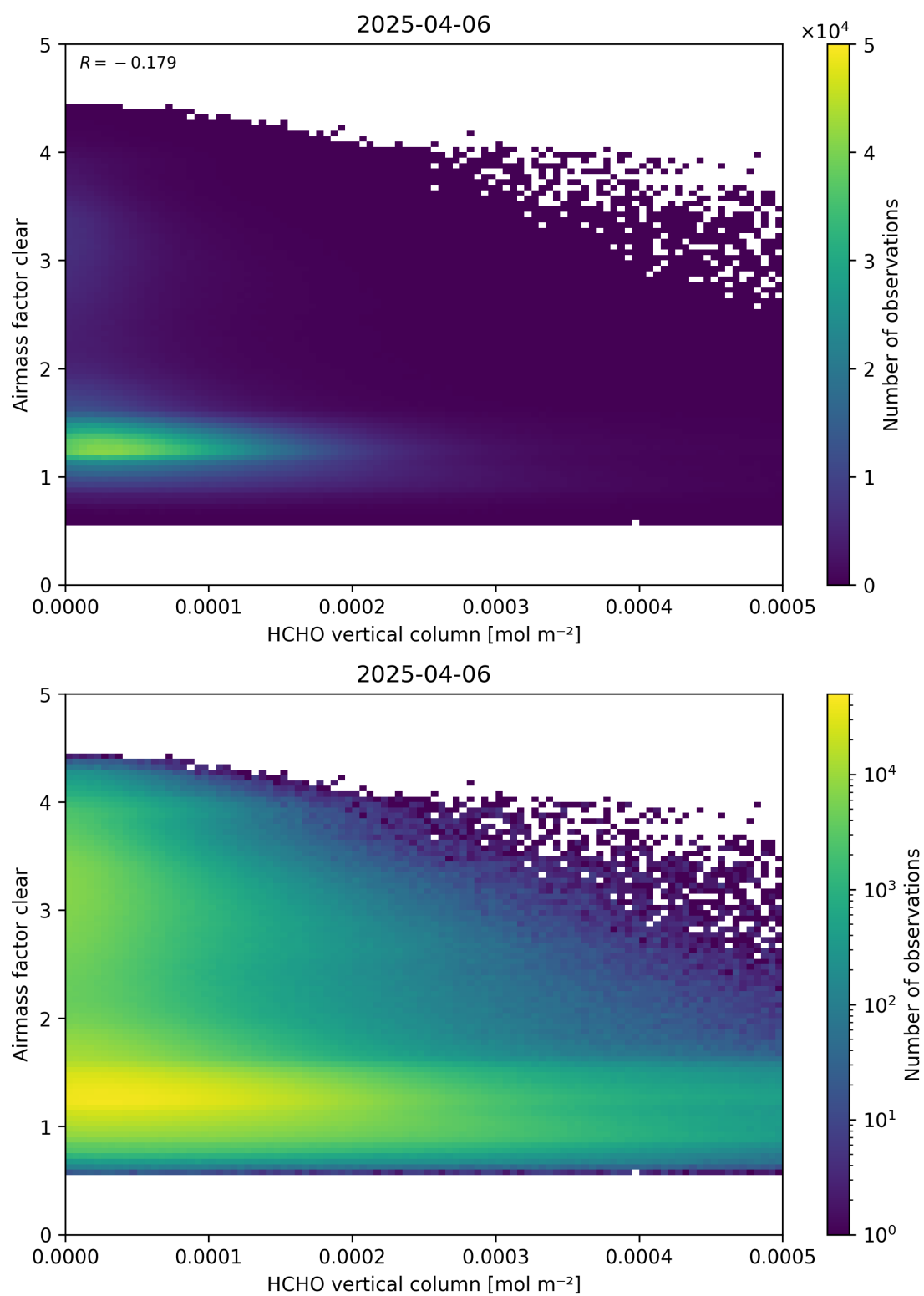
Figure 126: Scatter density plot of “HCHO vertical column” against “Airmass factor clear” for 2025-04-05 to 2025-04-07.
