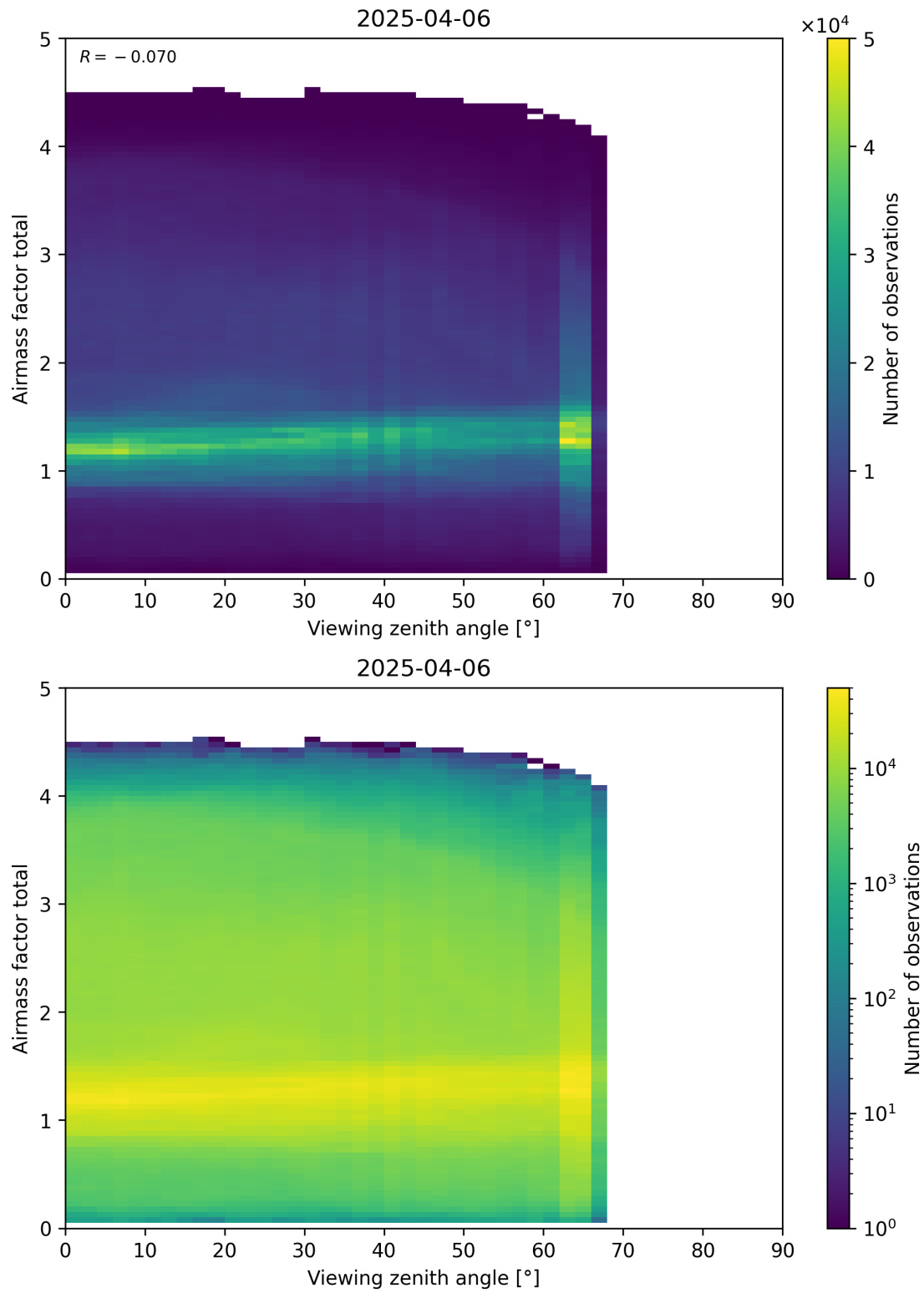
Figure 190: Scatter density plot of “Viewing zenith angle” against “Airmass factor total” for 2025-04-05 to 2025-04-07.
