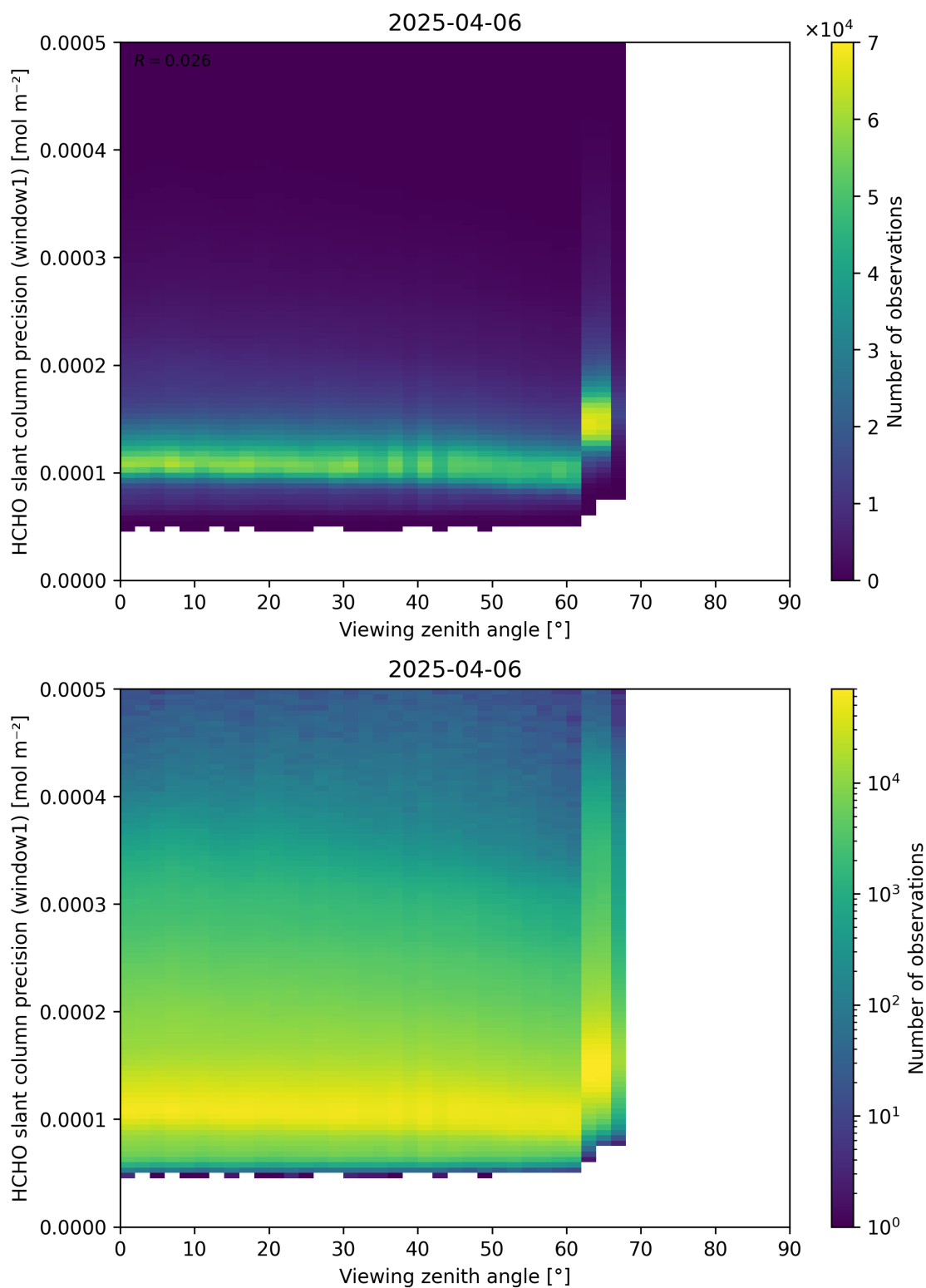
Figure 189: Scatter density plot of “Viewing zenith angle” against “HCHO slant column precision (window1)” for 2025-04-05 to 2025-04-07.
