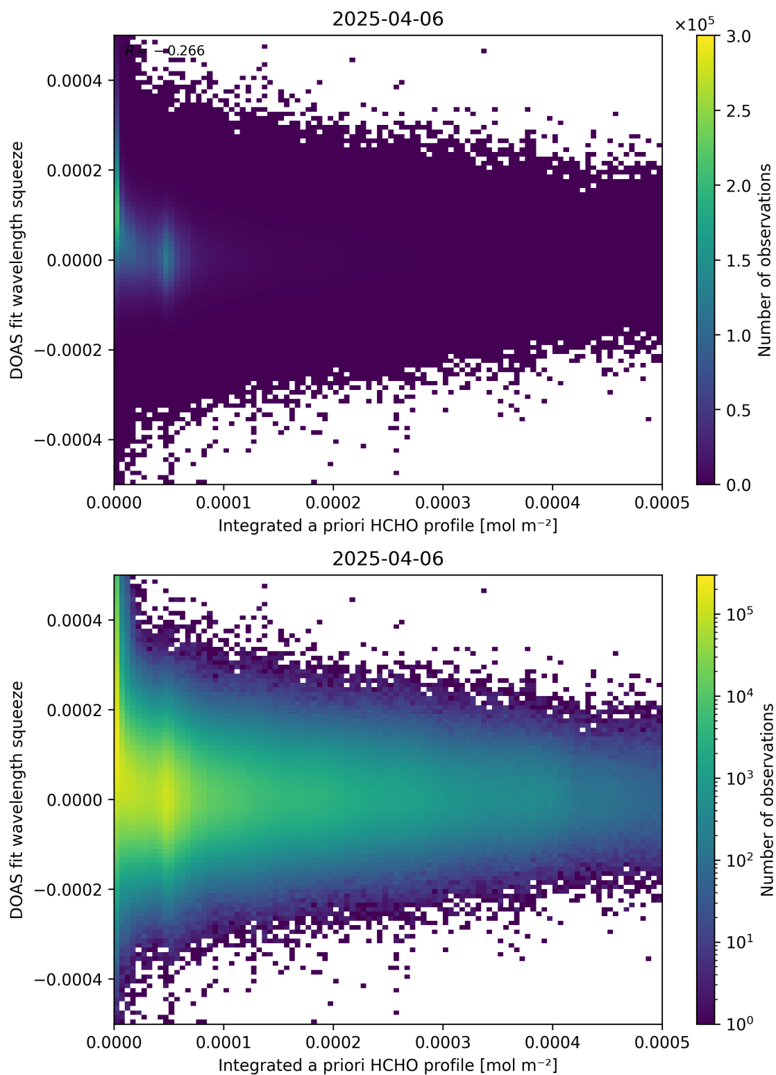
Figure 150: Scatter density plot of “Integrated a priori HCHO profile” against “DOAS fit wavelength squeeze” for 2025-04-05 to 2025-04-07.
