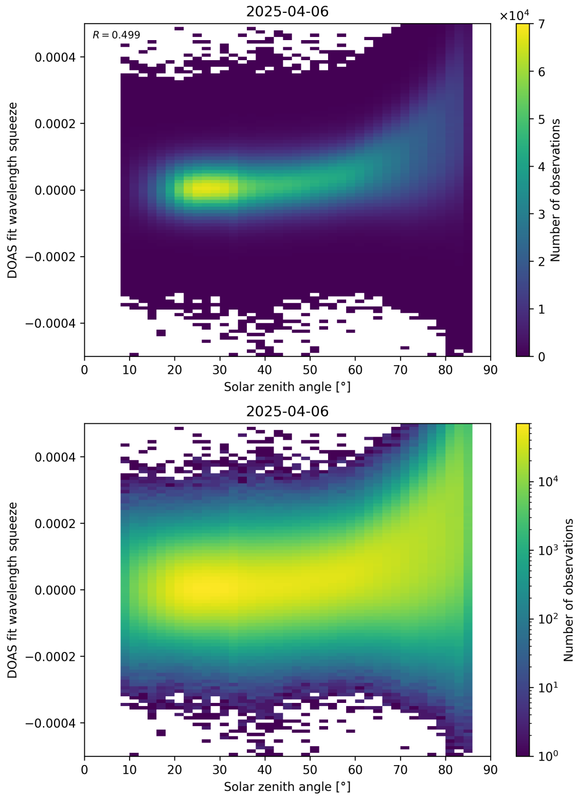
Figure 169: Scatter density plot of “Solar zenith angle” against “DOAS fit wavelength squeeze” for 2025-04-05 to 2025-04-07.
