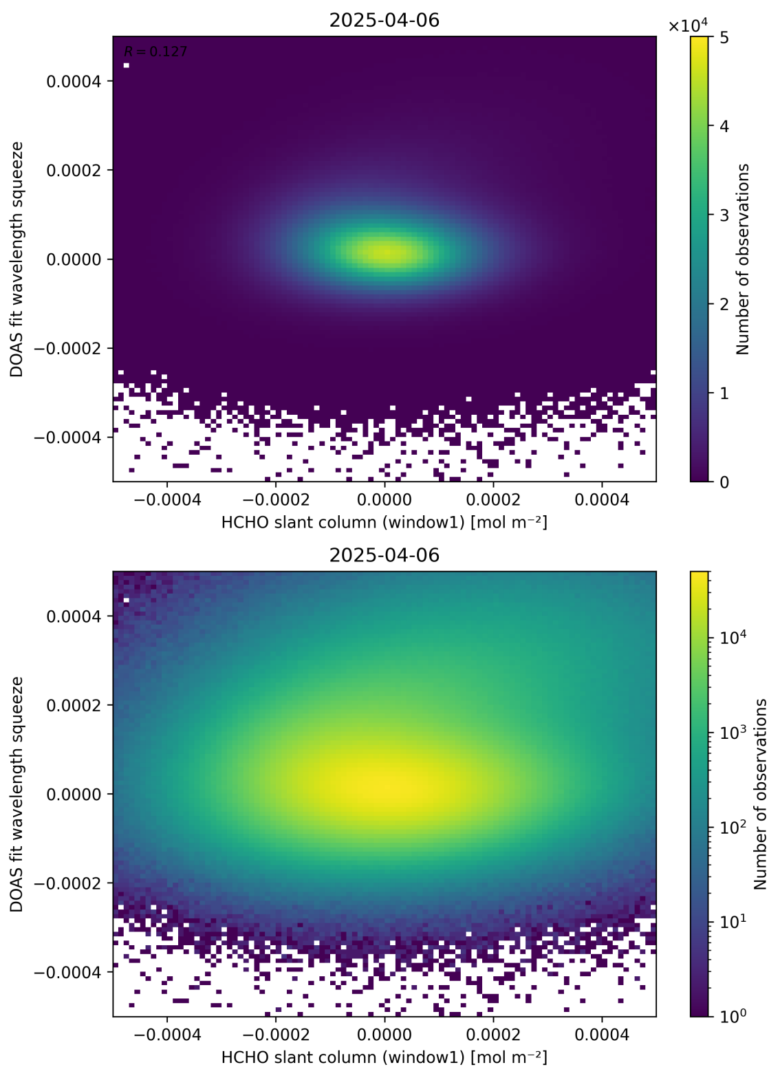
Figure 80: Scatter density plot of “HCHO slant column (window1)” against “DOAS fit wavelength squeeze” for 2025-04-05 to 2025-04-07.
