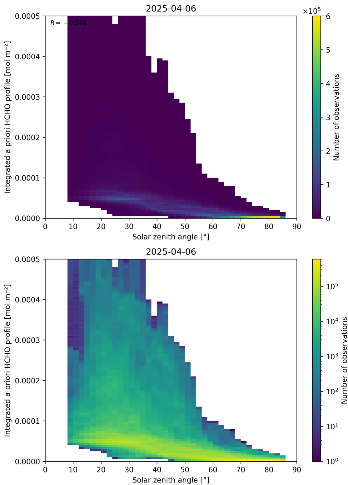
Figure 180: Scatter density plot of “Solar zenith angle” against “Integrated a priori HCHO profile” for 2025-04-05 to 2025-04-07.
