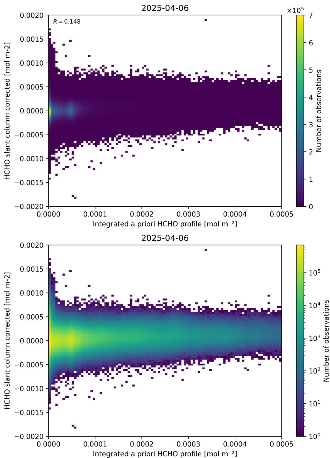
Figure 151: Scatter density plot of “Integrated a priori HCHO profile” against “HCHO slant column corrected” for 2025-04-05 to 2025-04-07.
