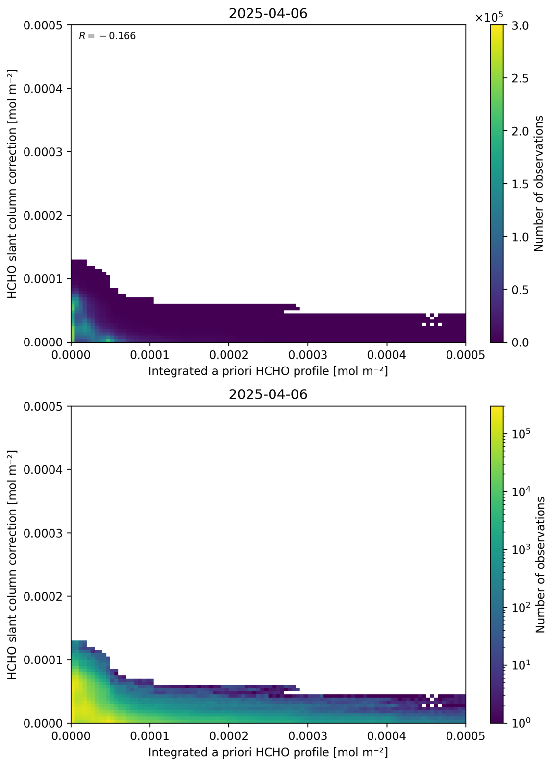
Figure 152: Scatter density plot of “Integrated a priori HCHO profile” against “HCHO slant column correction” for 2025-04-05 to 2025-04-07.
