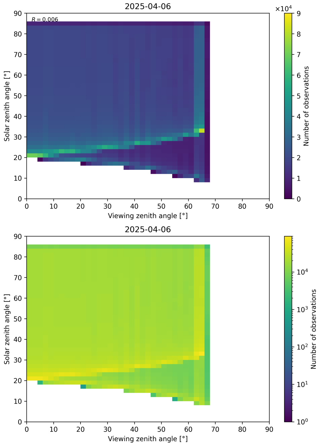
Figure 197: Scatter density plot of “Viewing zenith angle” against “Solar zenith angle” for 2025-04-05 to 2025-04-07.
