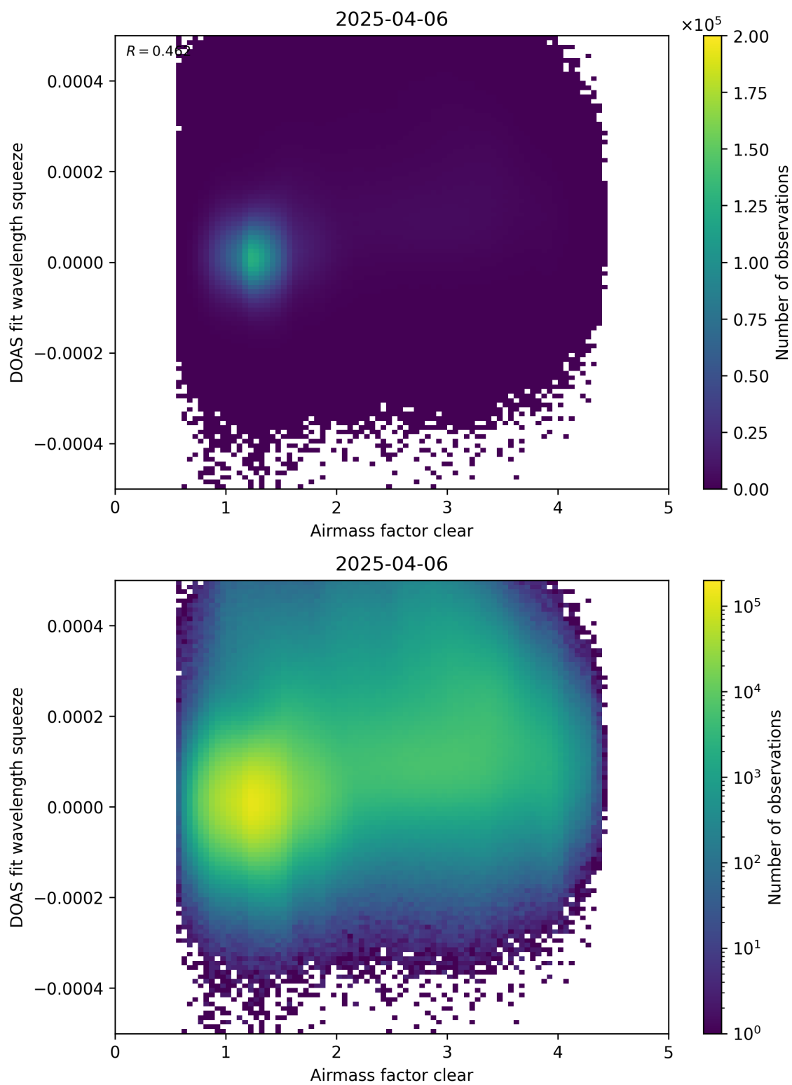
Figure 73: Scatter density plot of “Airmass factor clear” against “DOAS fit wavelength squeeze” for 2025-04-05 to 2025-04-07.
