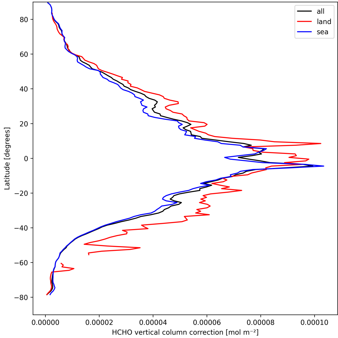
Figure 23: Zonal average of “HCHO vertical column correction” for 2025-04-05 to 2025-04-07.
