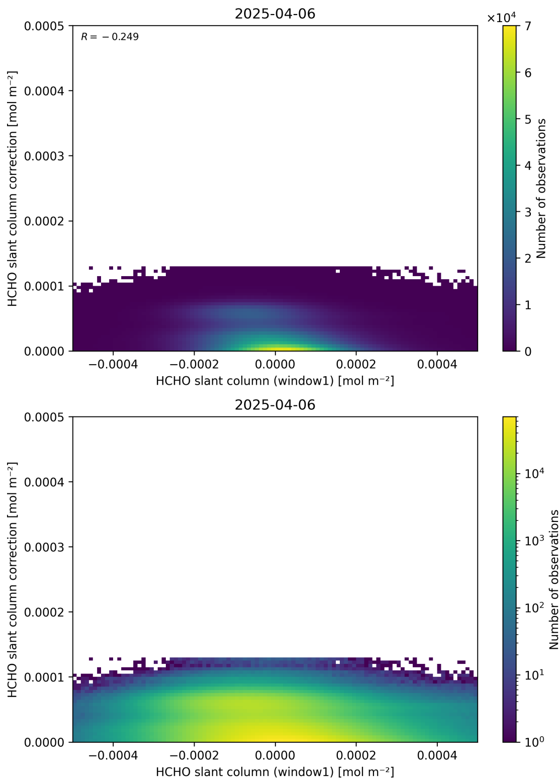
Figure 83: Scatter density plot of “HCHO slant column (window1)” against “HCHO slant column correction” for 2025-04-05 to 2025-04-07.
