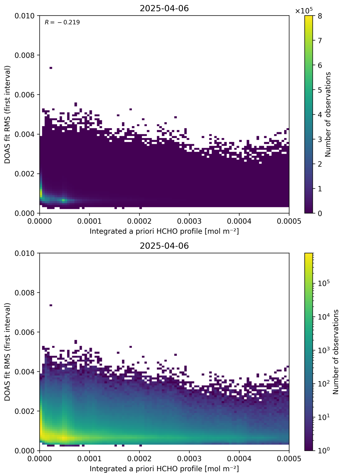
Figure 148: Scatter density plot of “Integrated a priori HCHO profile” against “DOAS fit RMS (first interval)” for 2025-04-05 to 2025-04-07.
