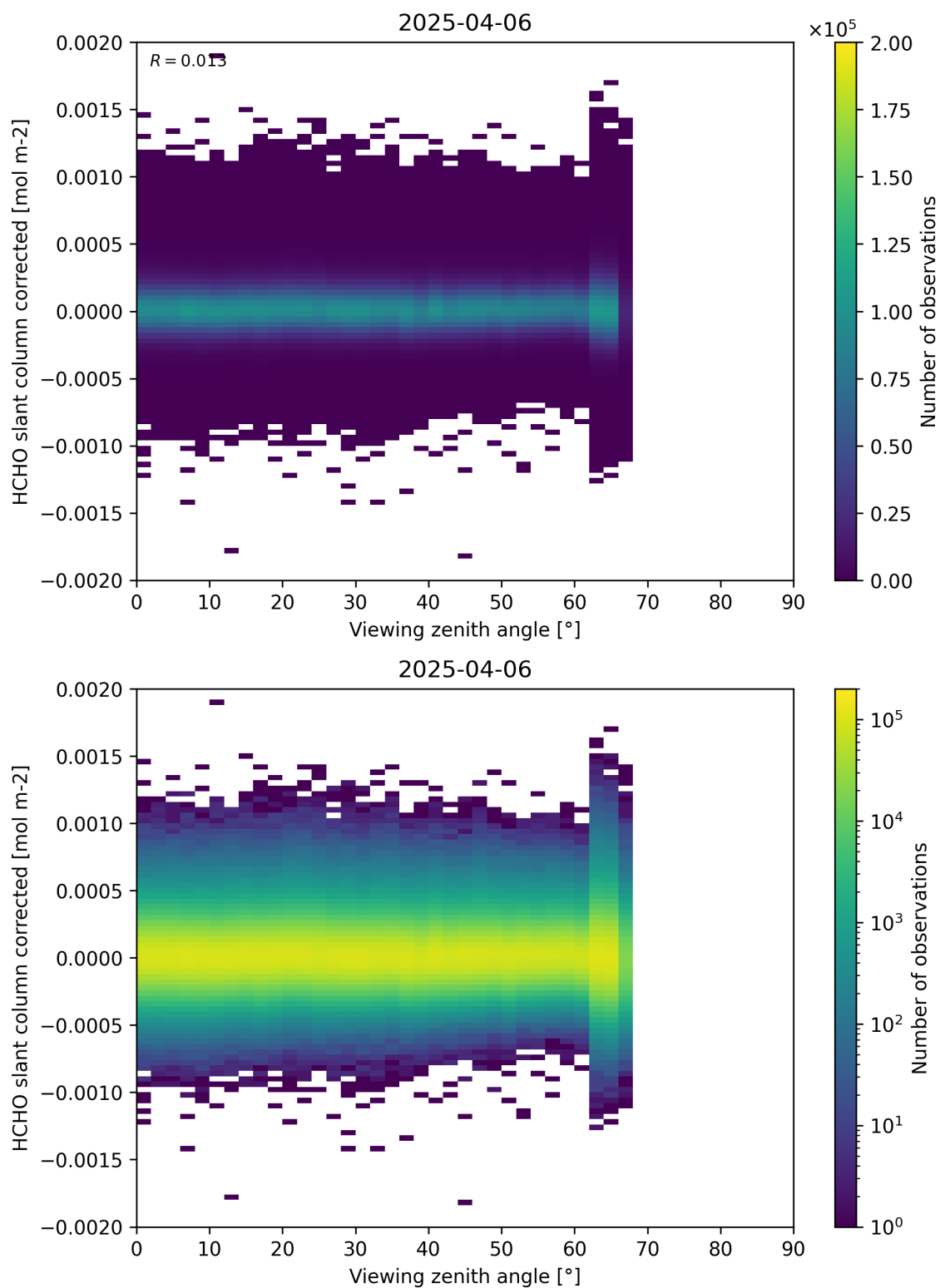
Figure 186: Scatter density plot of “Viewing zenith angle” against “HCHO slant column corrected” for 2025-04-05 to 2025-04-07.
