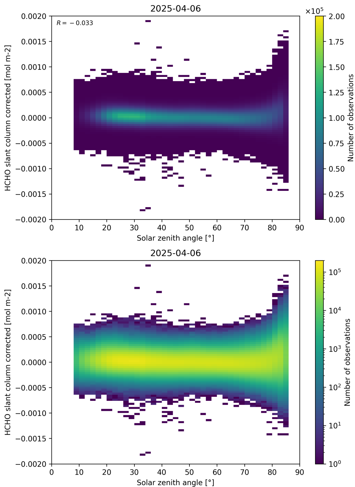
Figure 171: Scatter density plot of “Solar zenith angle” against “HCHO slant column corrected” for 2025-04-05 to 2025-04-07.
