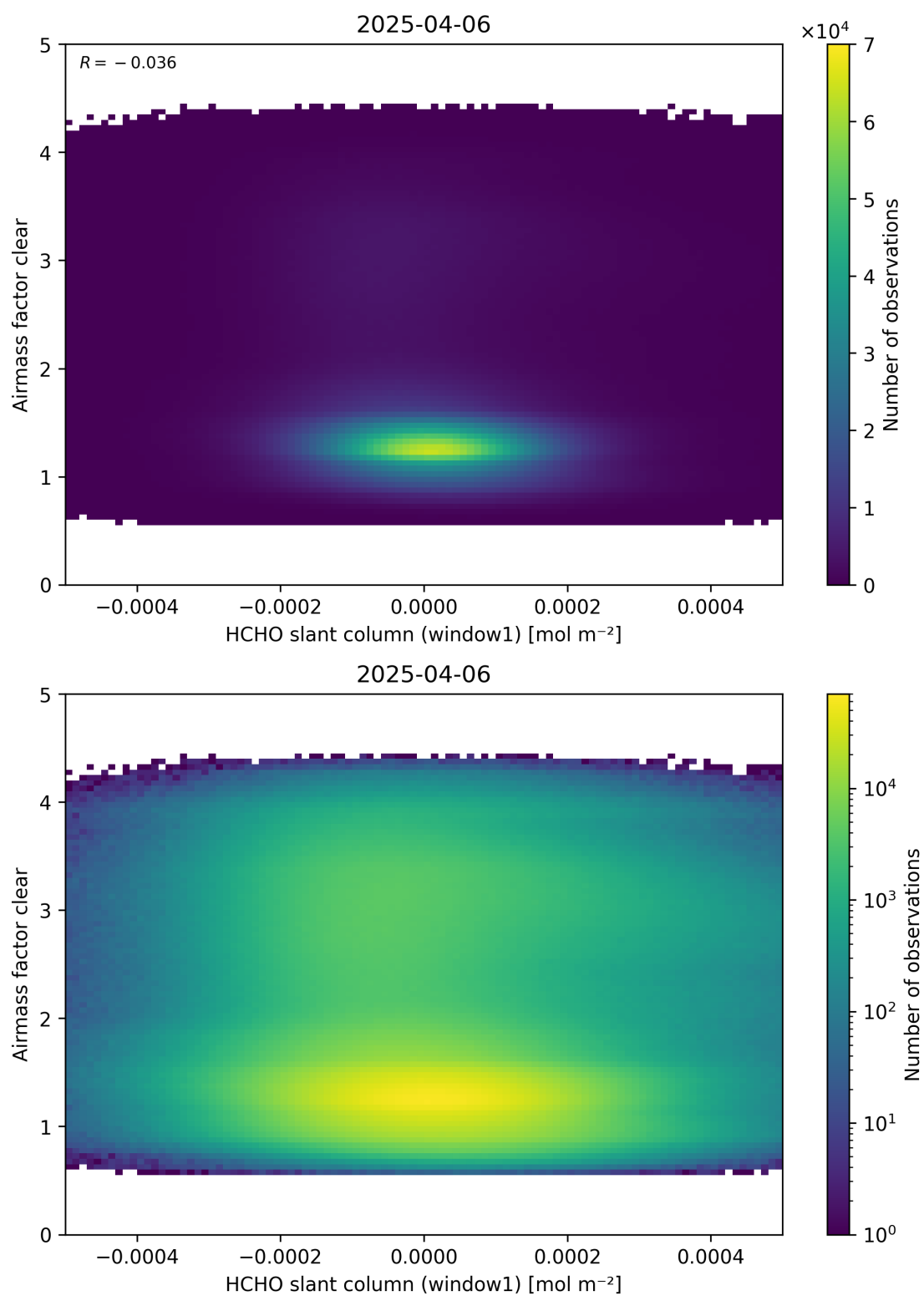
Figure 81: Scatter density plot of “HCHO slant column (window1)” against “Airmass factor clear” for 2025-04-05 to 2025-04-07.
