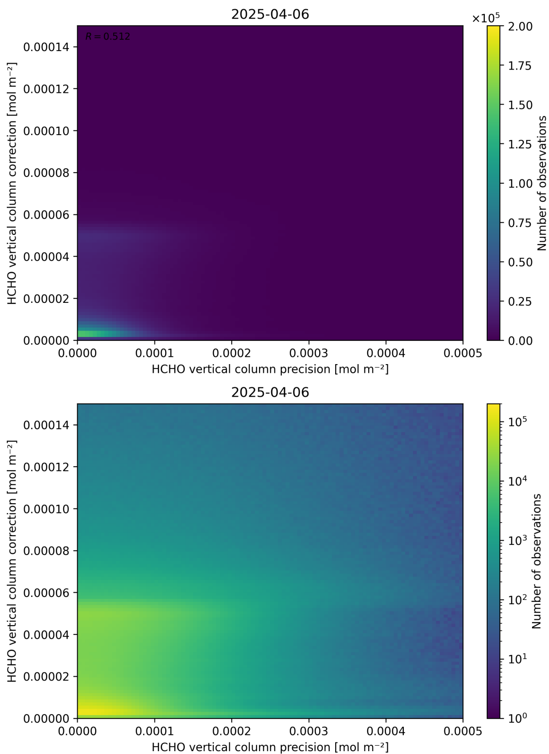
Figure 146: Scatter density plot of “HCHO vertical column precision” against “HCHO vertical column correction” for 2025-04-05 to 2025-04-07.
