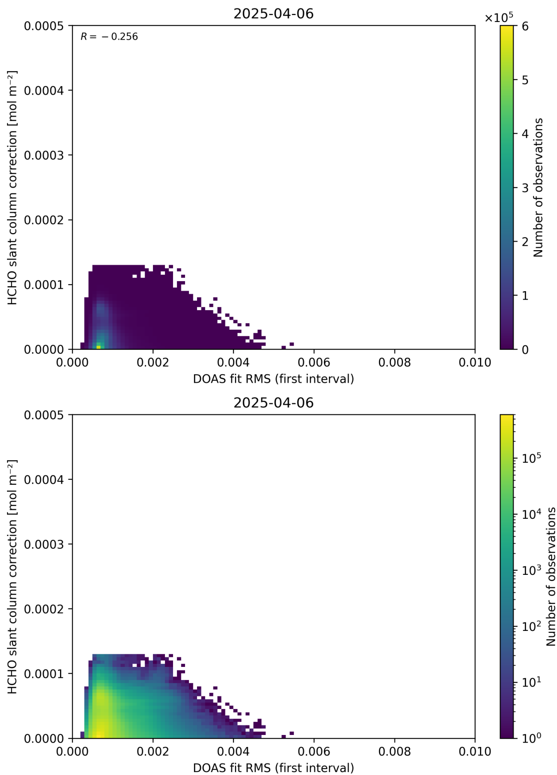
Figure 63: Scatter density plot of “DOAS fit RMS (first interval)” against “HCHO slant column correction” for 2025-04-05 to 2025-04-07.
