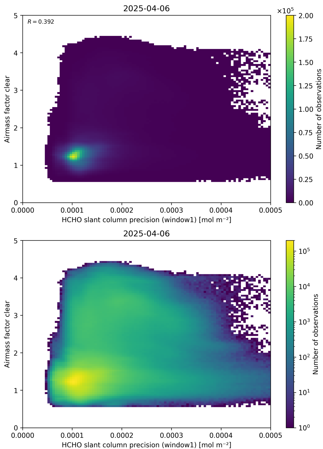
Figure 91: Scatter density plot of “HCHO slant column precision (window1)” against “Airmass factor clear” for 2025-04-05 to 2025-04-07.
