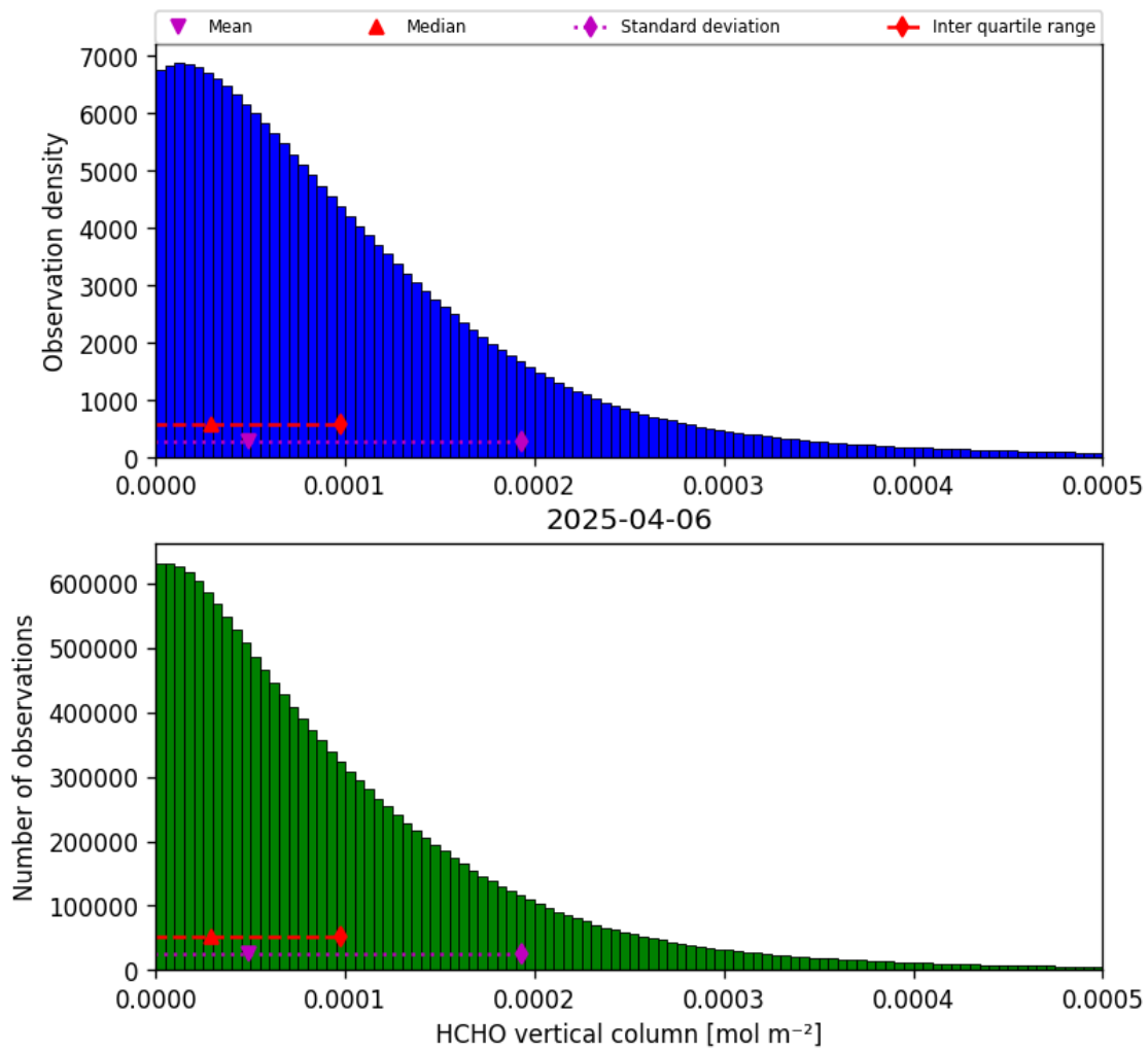
Figure 35: Histogram of “HCHO vertical column” for 2025-04-05 to 2025-04-07
