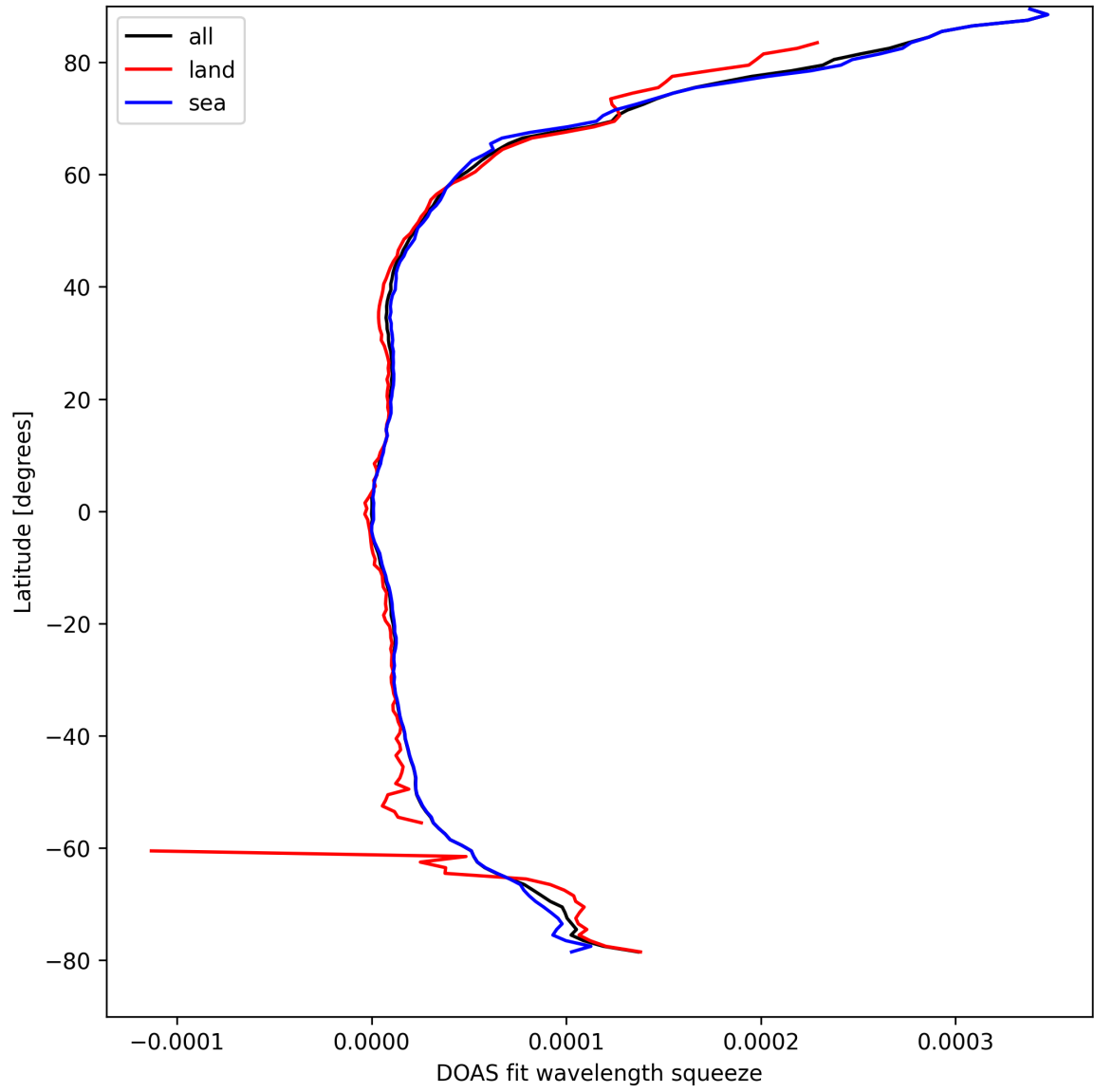
Figure 31: Zonal average of “DOAS fit wavelength squeeze” for 2025-04-05 to 2025-04-07.
