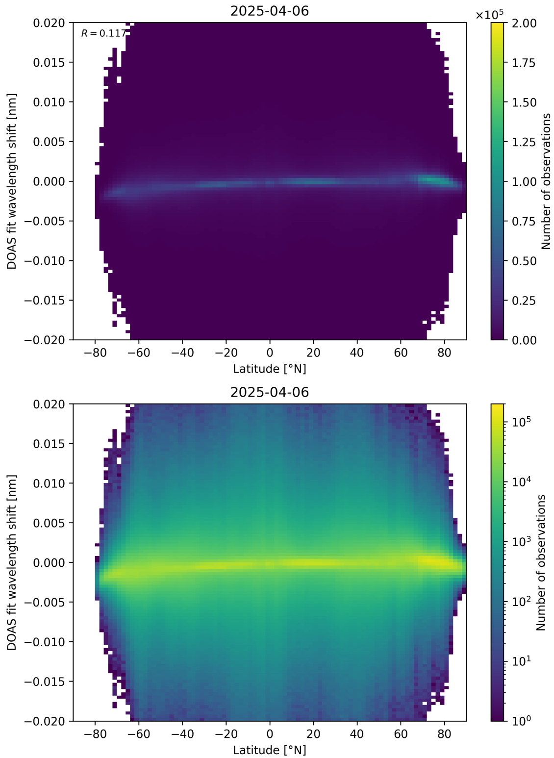
Figure 154: Scatter density plot of “Latitude” against “DOAS fit wavelength shift” for 2025-04-05 to 2025-04-07.
