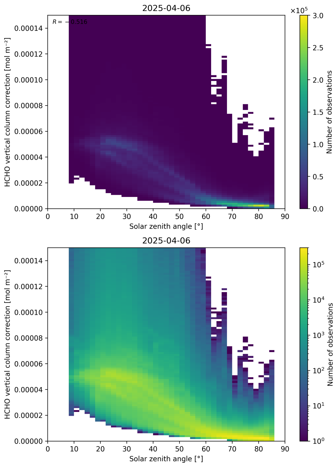
Figure 178: Scatter density plot of “Solar zenith angle” against “HCHO vertical column correction” for 2025-04-05 to 2025-04-07.
