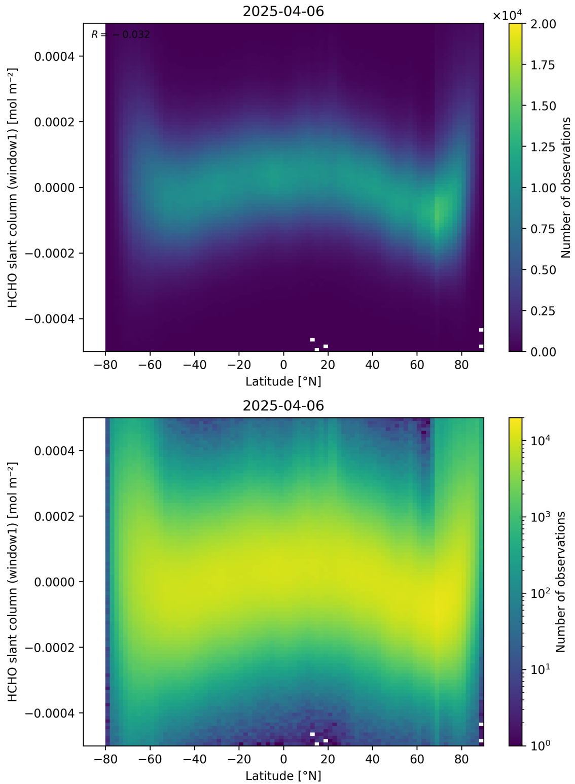
Figure 159: Scatter density plot of “Latitude” against “HCHO slant column (window1)” for 2025-04-05 to 2025-04-07.
