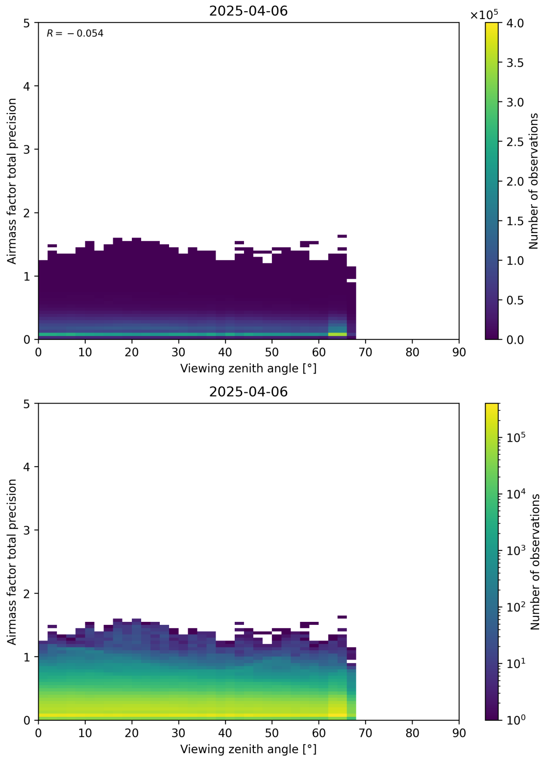
Figure 191: Scatter density plot of “Viewing zenith angle” against “Airmass factor total precision” for 2025-04-05 to 2025-04-07.
