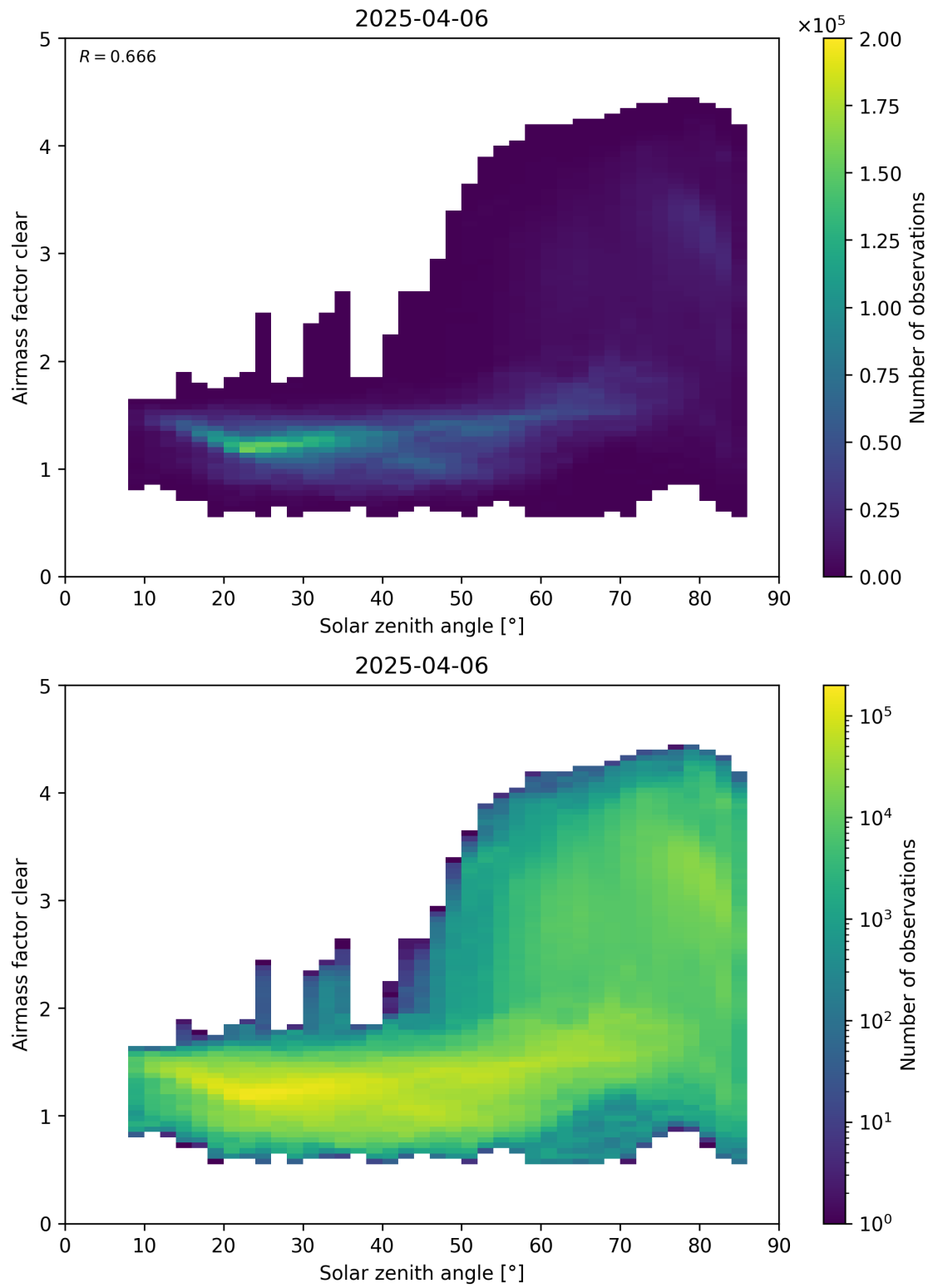
Figure 170: Scatter density plot of “Solar zenith angle” against “Airmass factor clear” for 2025-04-05 to 2025-04-07.
