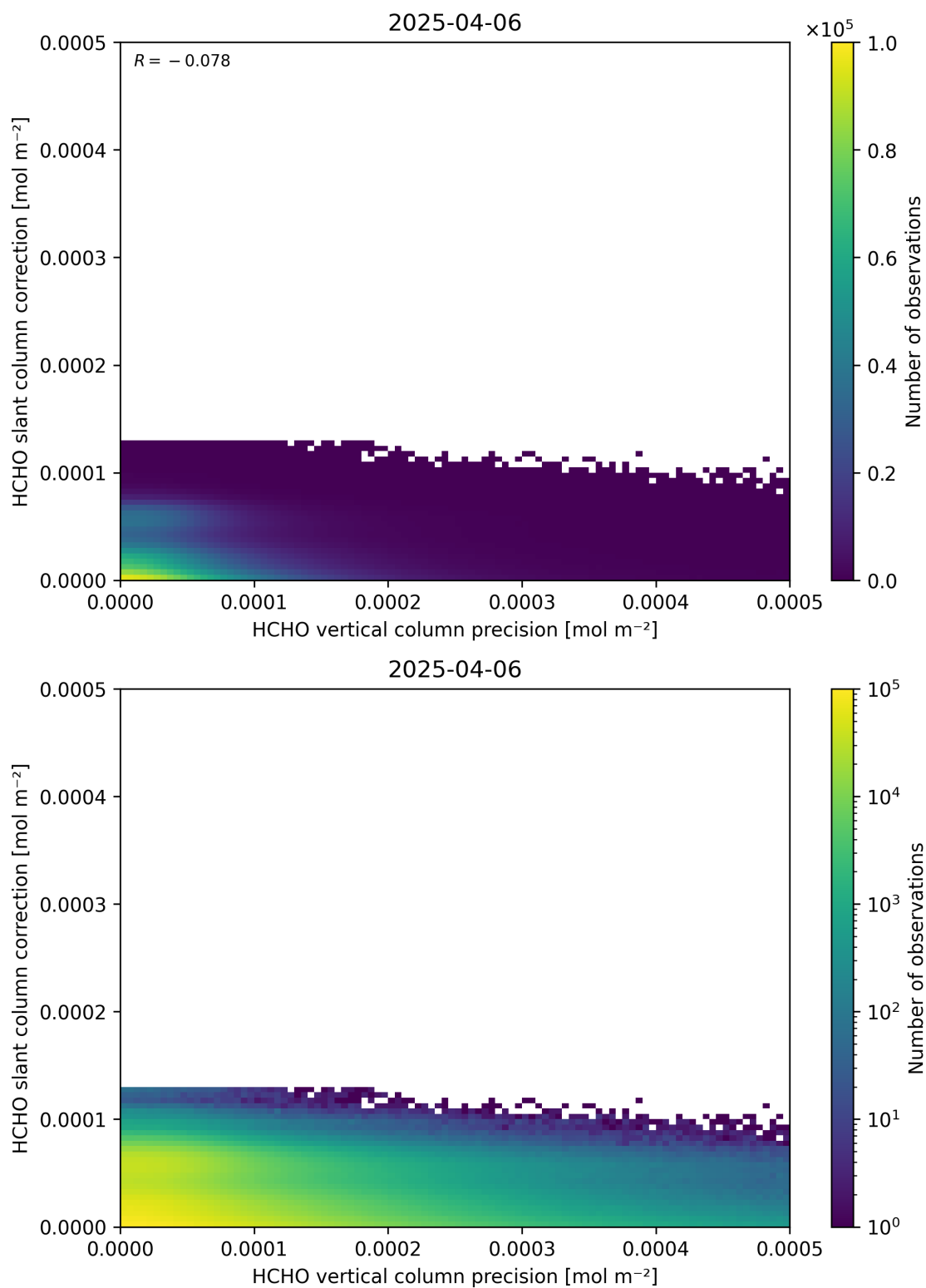
Figure 141: Scatter density plot of “HCHO vertical column precision” against “HCHO slant column correction” for 2025-04-05 to 2025-04-07.
