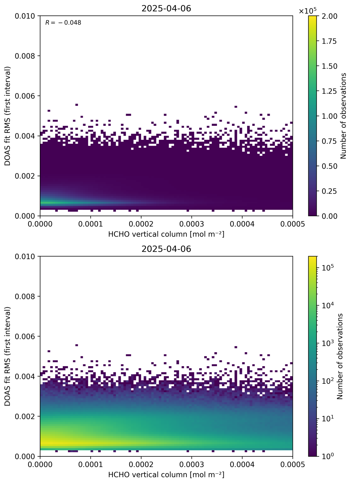
Figure 123: Scatter density plot of “HCHO vertical column” against “DOAS fit RMS (first interval)” for 2025-04-05 to 2025-04-07.
