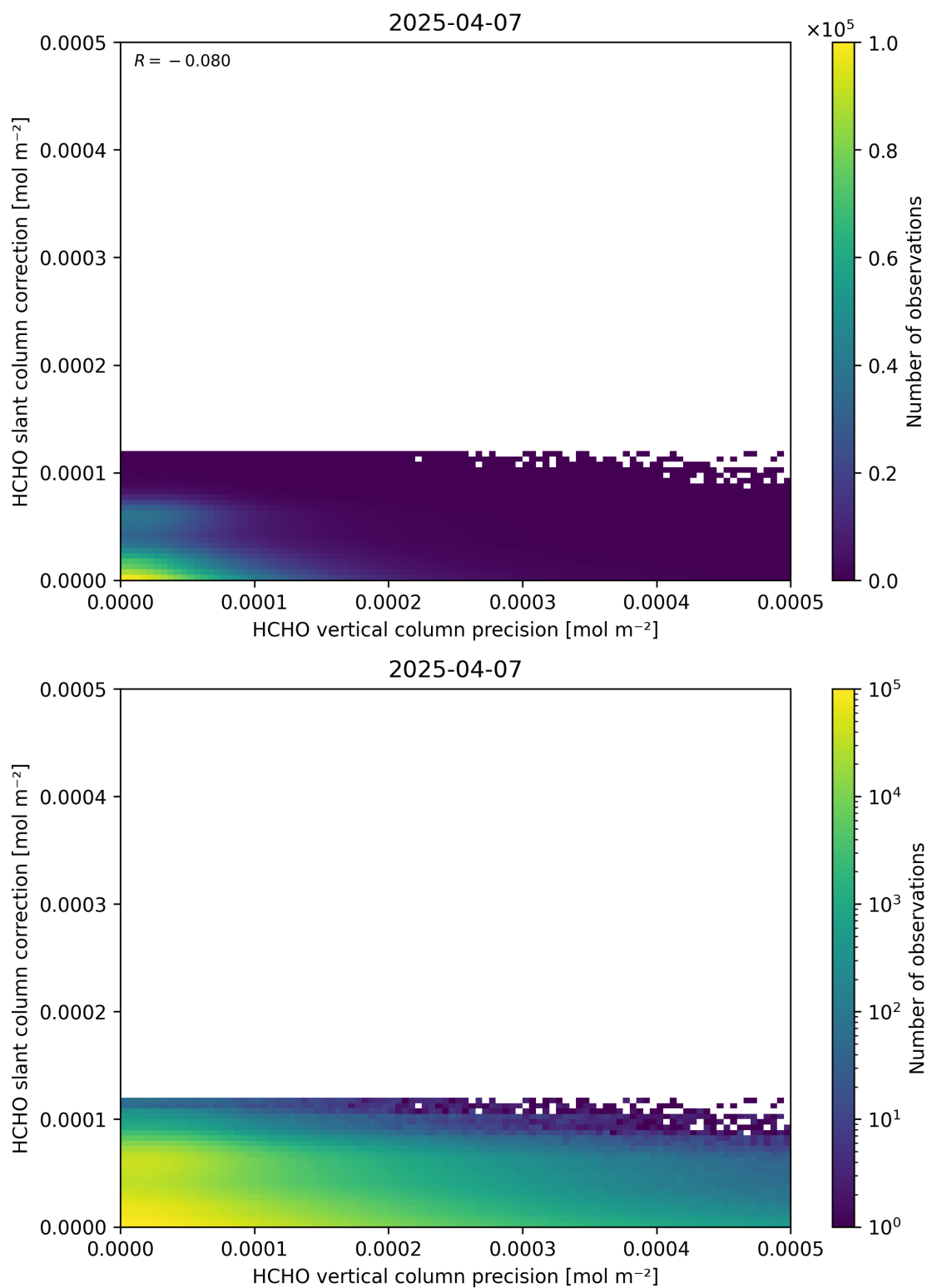
Figure 141: Scatter density plot of “HCHO vertical column precision” against “HCHO slant column correction” for 2025-04-06 to 2025-04-08.
