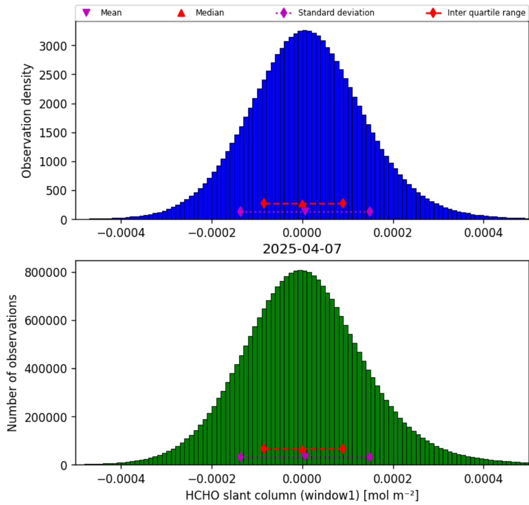
Figure 38: Histogram of “HCHO slant column (window1)” for 2025-04-06 to 2025-04-08
