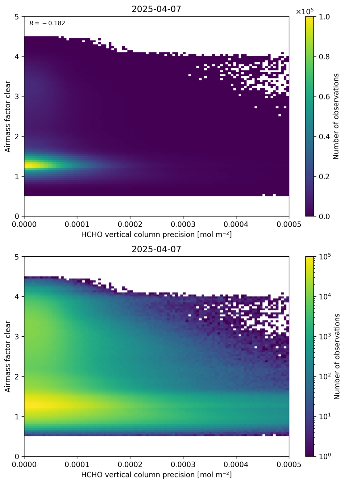
Figure 139: Scatter density plot of “HCHO vertical column precision” against “Airmass factor clear” for 2025-04-06 to 2025-04-08.
