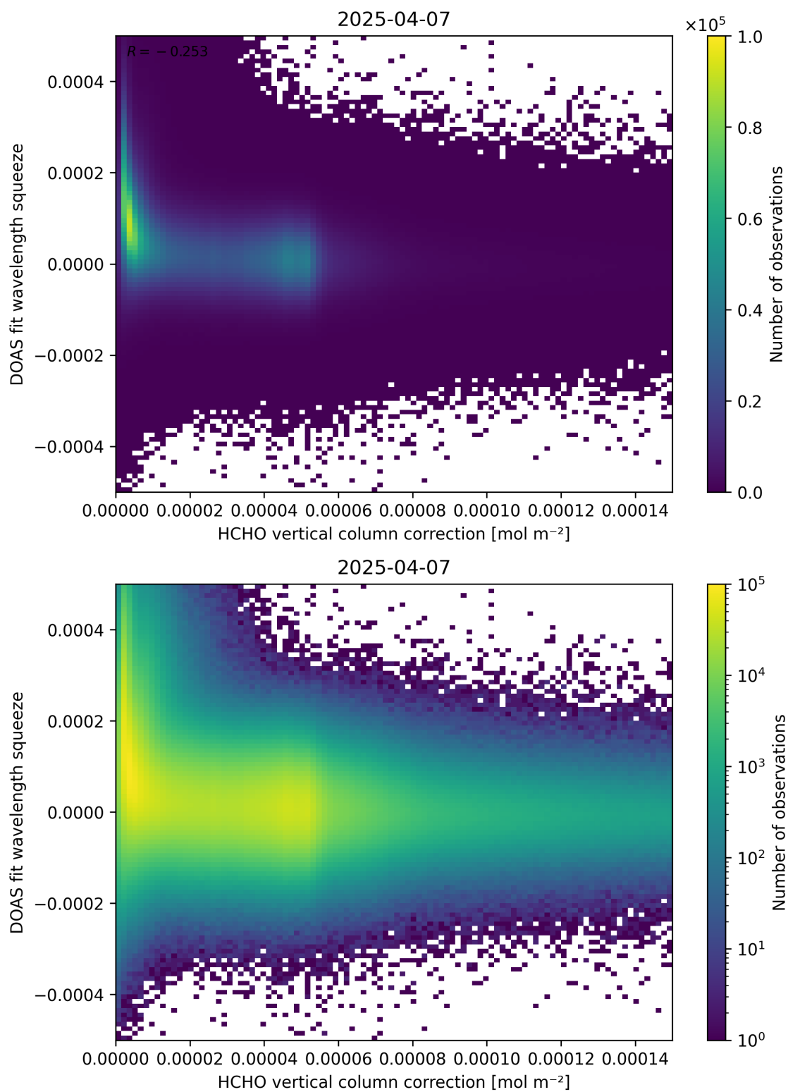
Figure 114: Scatter density plot of “HCHO vertical column correction” against “DOAS fit wavelength squeeze” for 2025-04-06 to 2025-04-08.
