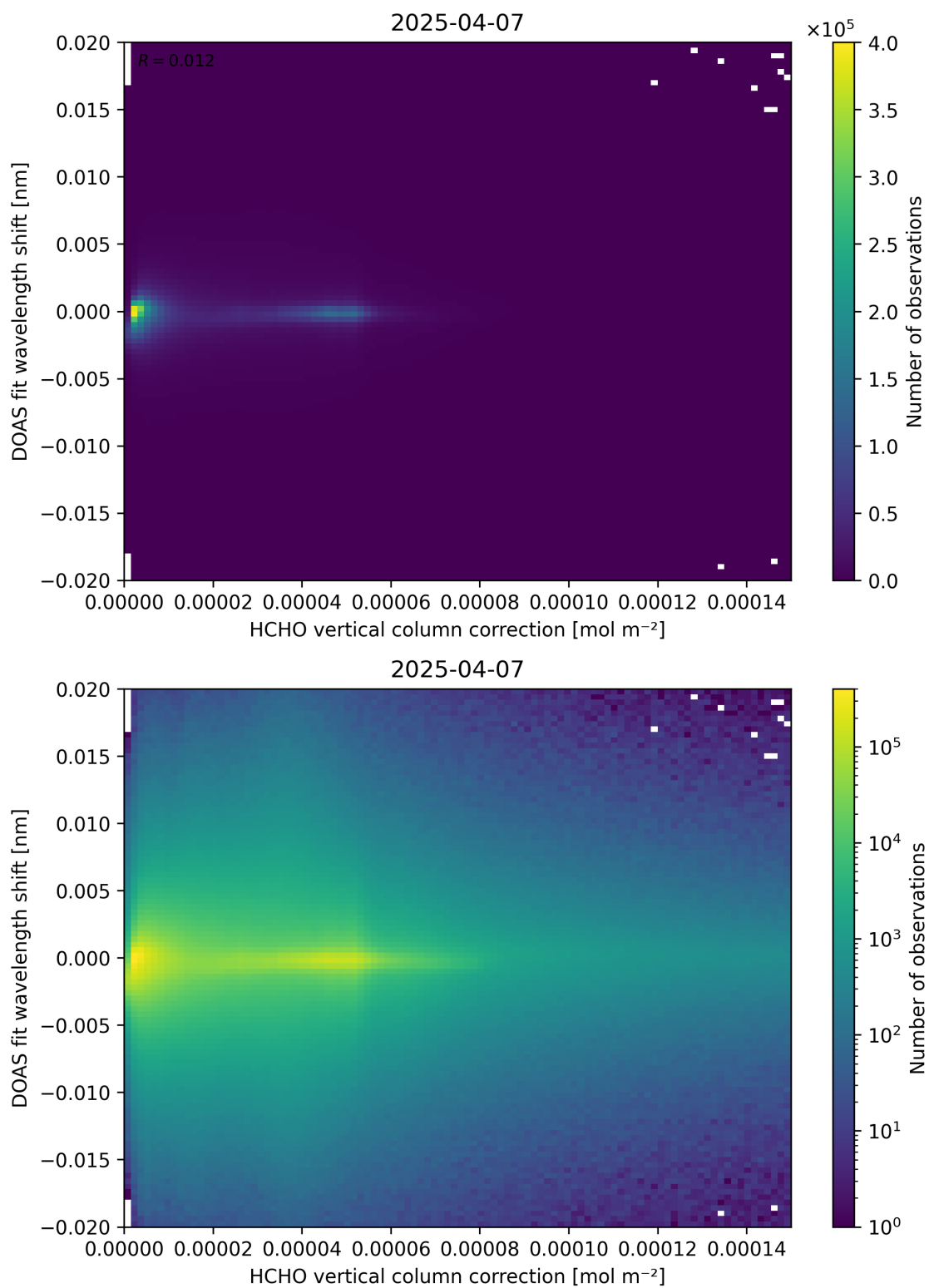
Figure 113: Scatter density plot of “HCHO vertical column correction” against “DOAS fit wavelength shift” for 2025-04-06 to 2025-04-08.
