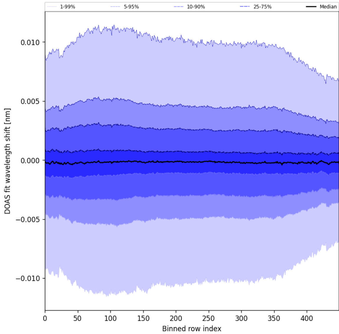
Figure 58: Along track statistics of “DOAS fit wavelength shift” for 2025-04-06 to 2025-04-08
