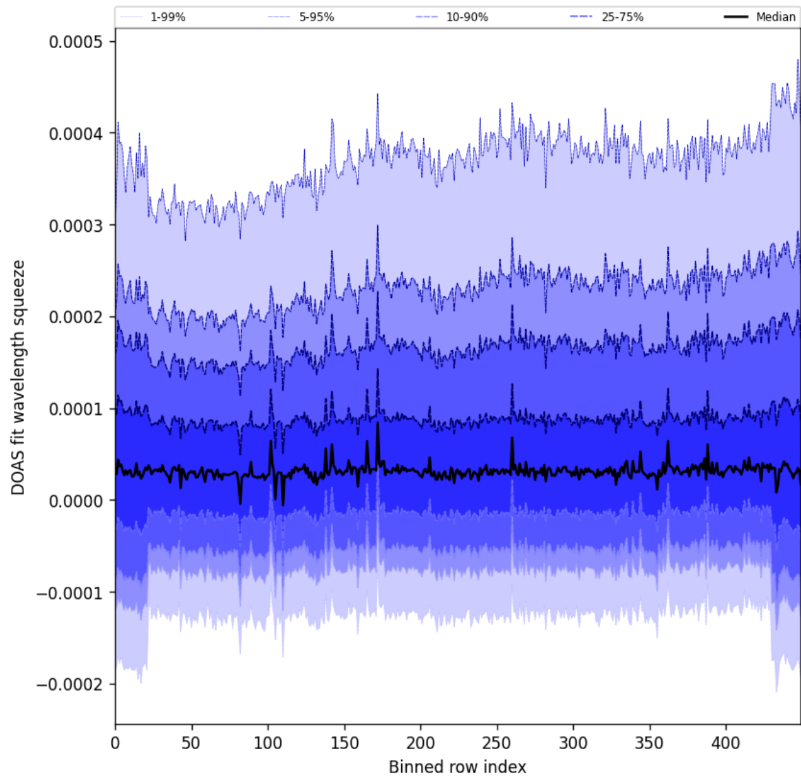
Figure 59: Along track statistics of “DOAS fit wavelength squeeze” for 2025-04-06 to 2025-04-08
