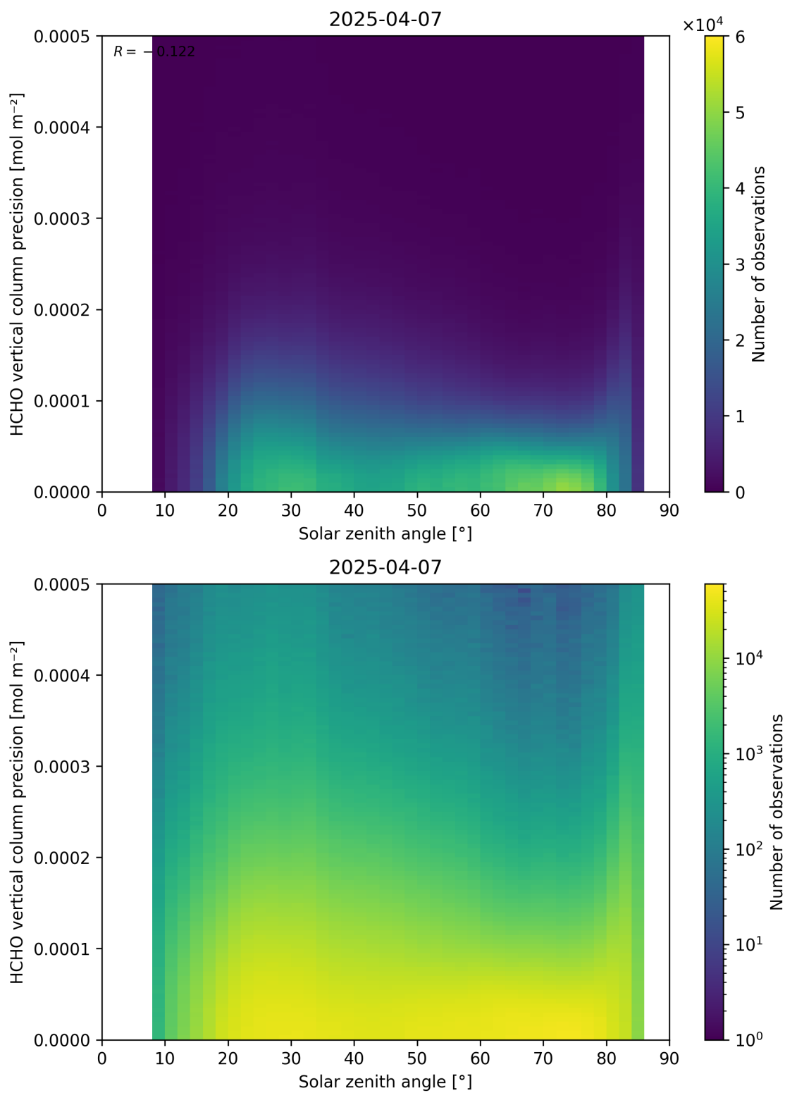
Figure 179: Scatter density plot of “Solar zenith angle” against “HCHO vertical column precision” for 2025-04-06 to 2025-04-08.
