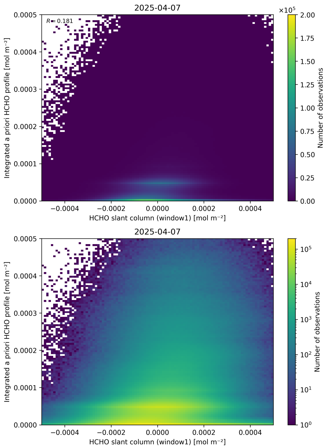
Figure 87: Scatter density plot of “HCHO slant column (window1)” against “Integrated a priori HCHO profile” for 2025-04-06 to 2025-04-08.
