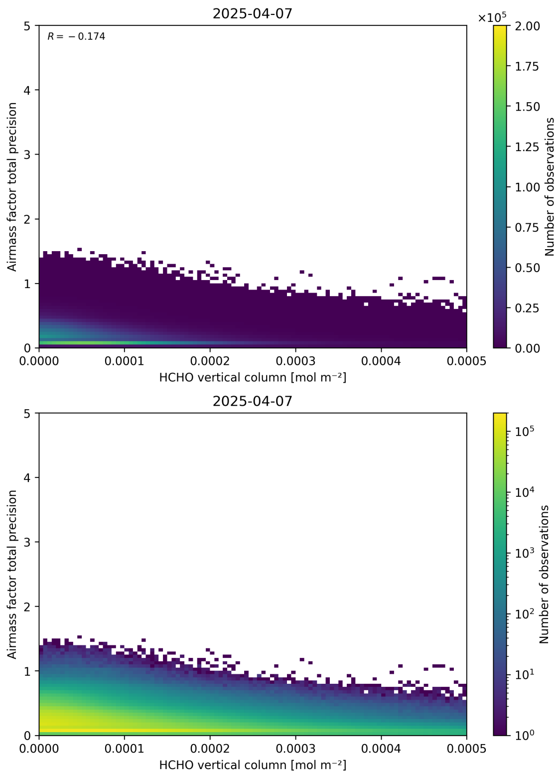
Figure 132: Scatter density plot of “HCHO vertical column” against “Airmass factor total precision” for 2025-04-06 to 2025-04-08.
