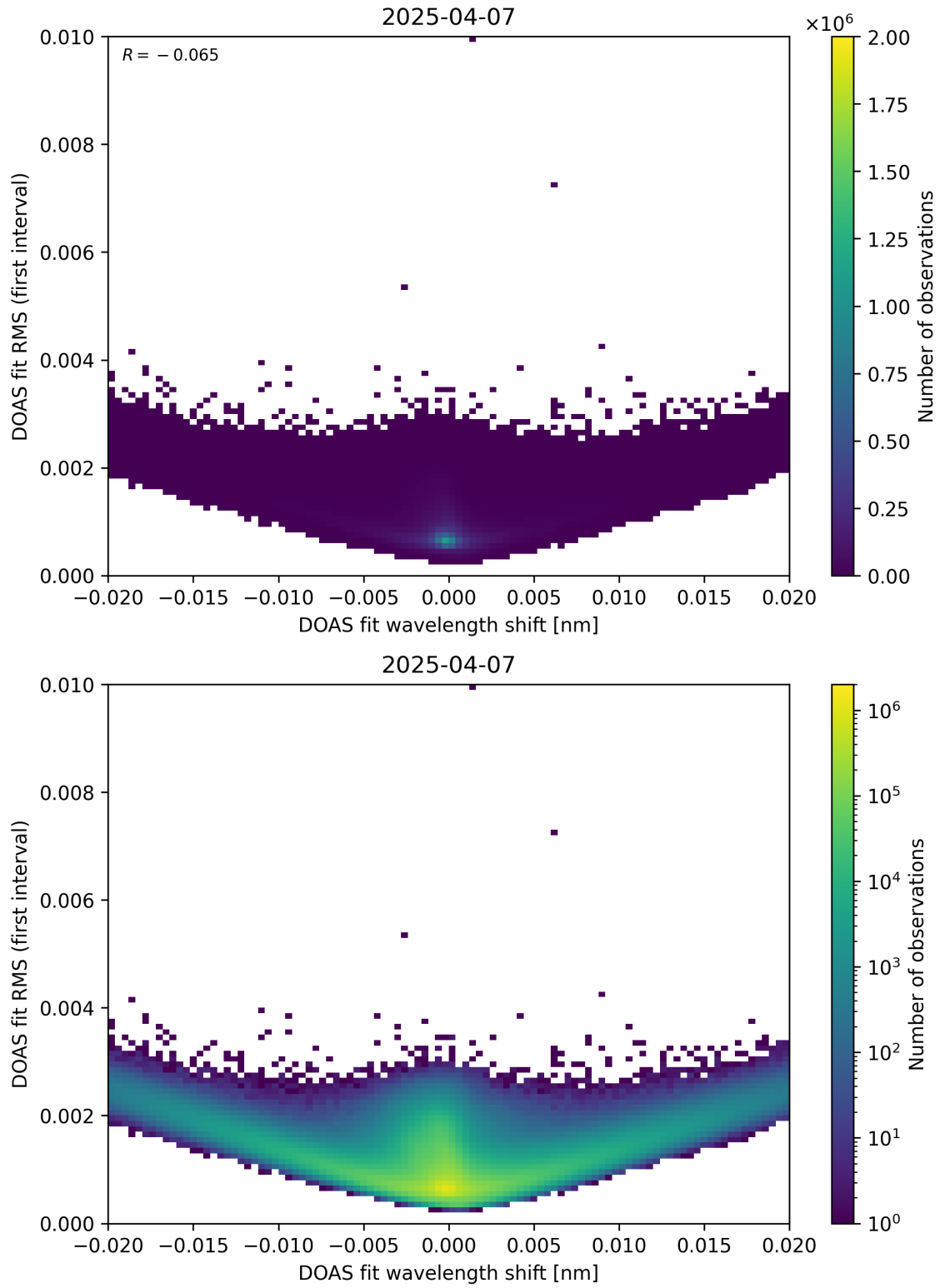
Figure 64: Scatter density plot of “DOAS fit wavelength shift” against “DOAS fit RMS (first interval)” for 2025-04-06 to 2025-04-08.
