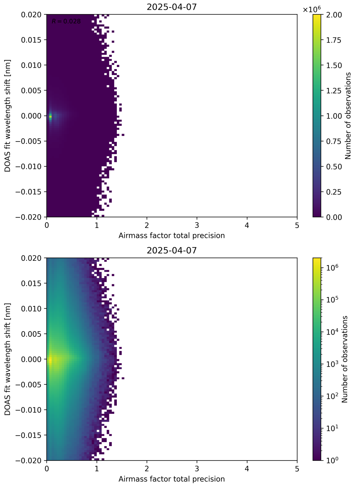
Figure 106: Scatter density plot of “Airmass factor total precision” against “DOAS fit wavelength shift” for 2025-04-06 to 2025-04-08.
