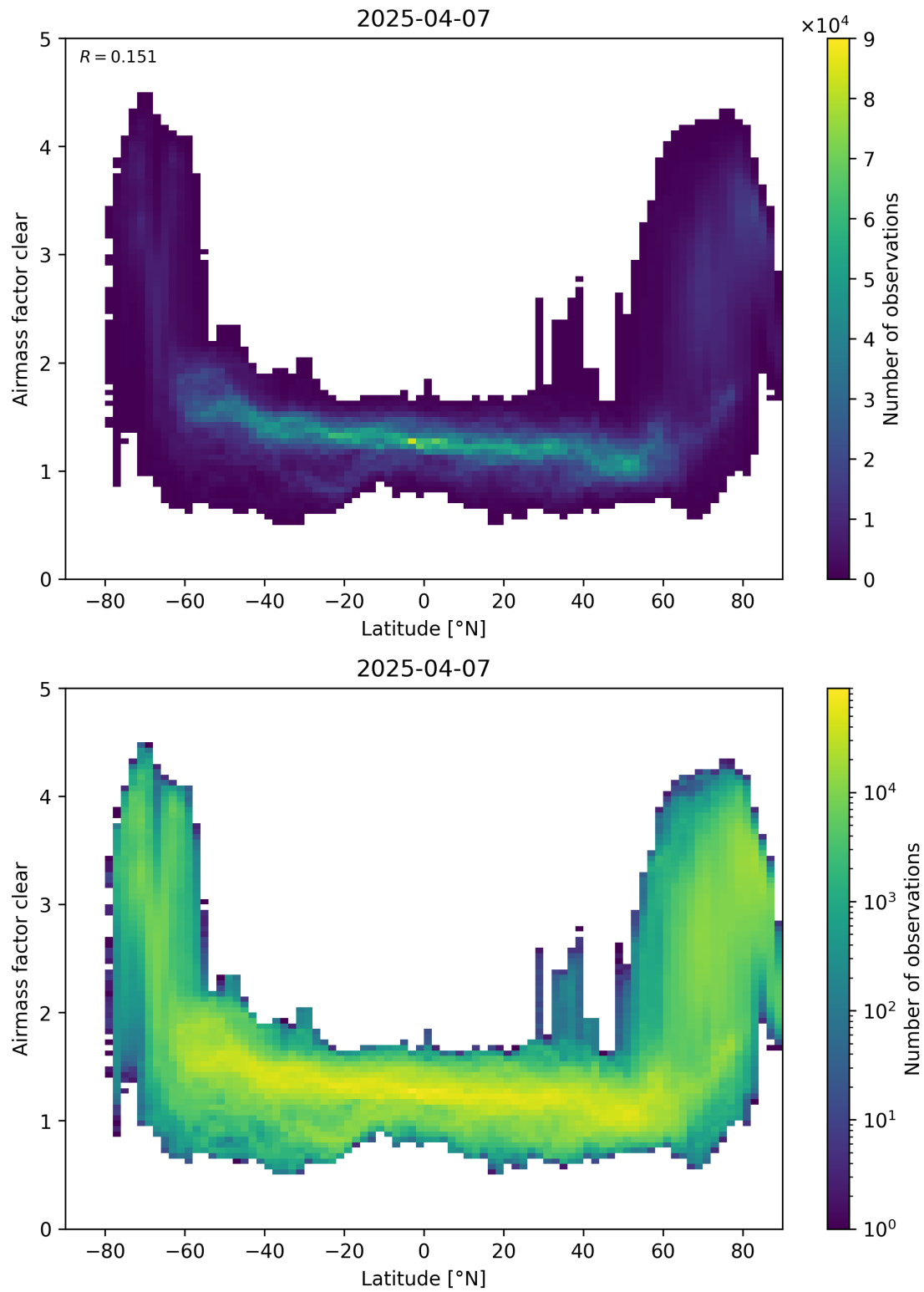
Figure 156: Scatter density plot of “Latitude” against “Airmass factor clear” for 2025-04-06 to 2025-04-08.
