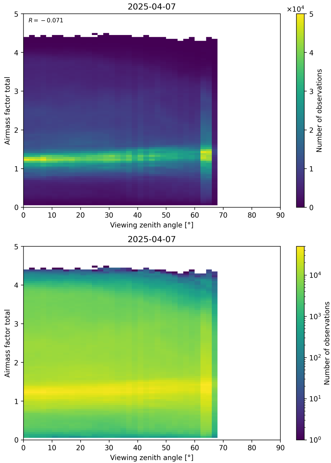
Figure 190: Scatter density plot of “Viewing zenith angle” against “Airmass factor total” for 2025-04-06 to 2025-04-08.
