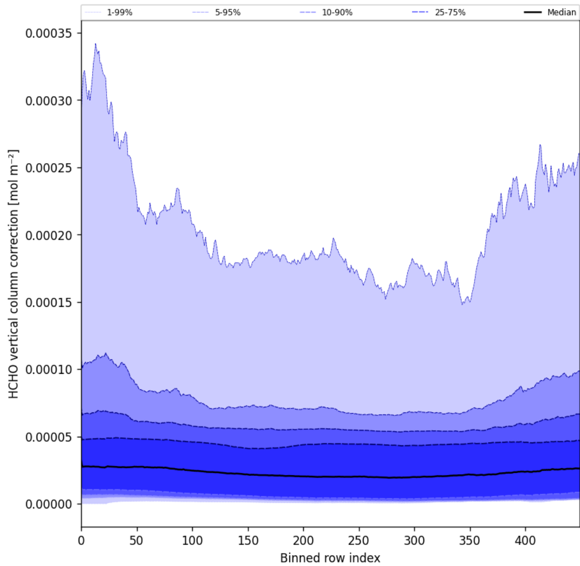
Figure 51: Along track statistics of “HCHO vertical column correction” for 2025-04-06 to 2025-04-08
