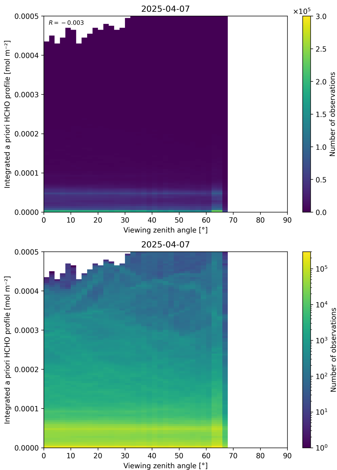
Figure 195: Scatter density plot of “Viewing zenith angle” against “Integrated a priori HCHO profile” for 2025-04-06 to 2025-04-08.
