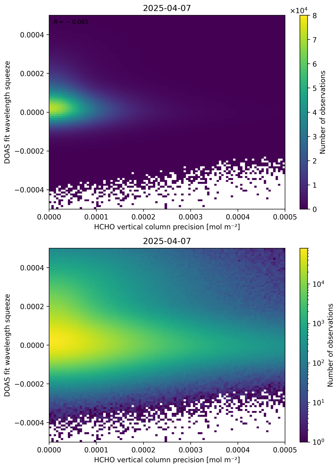
Figure 138: Scatter density plot of “HCHO vertical column precision” against “DOAS fit wavelength squeeze” for 2025-04-06 to 2025-04-08.
