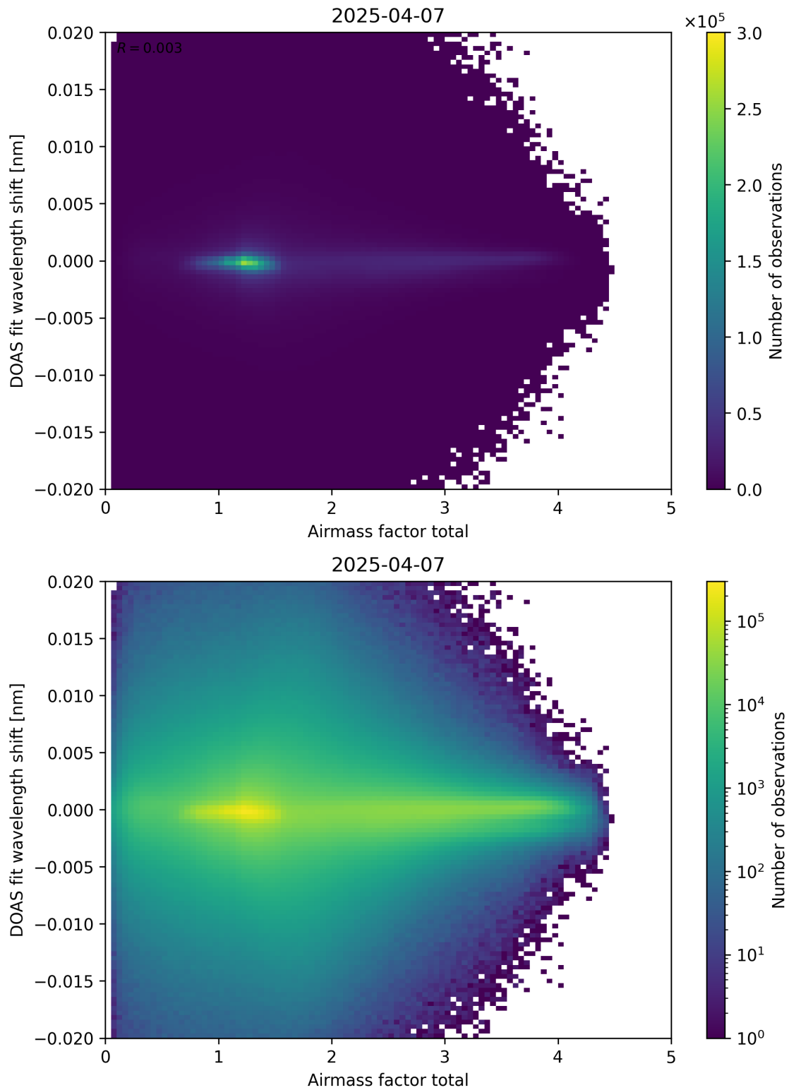
Figure 98: Scatter density plot of “Airmass factor total” against “DOAS fit wavelength shift” for 2025-04-06 to 2025-04-08.
