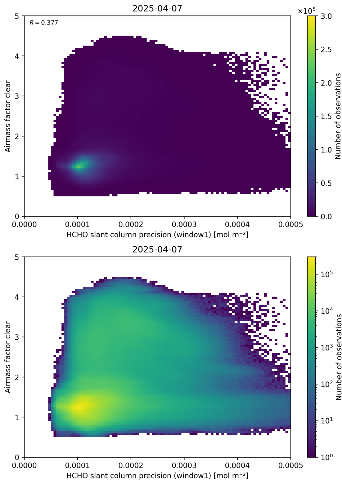
Figure 91: Scatter density plot of “HCHO slant column precision (window1)” against “Airmass factor clear” for 2025-04-06 to 2025-04-08.
