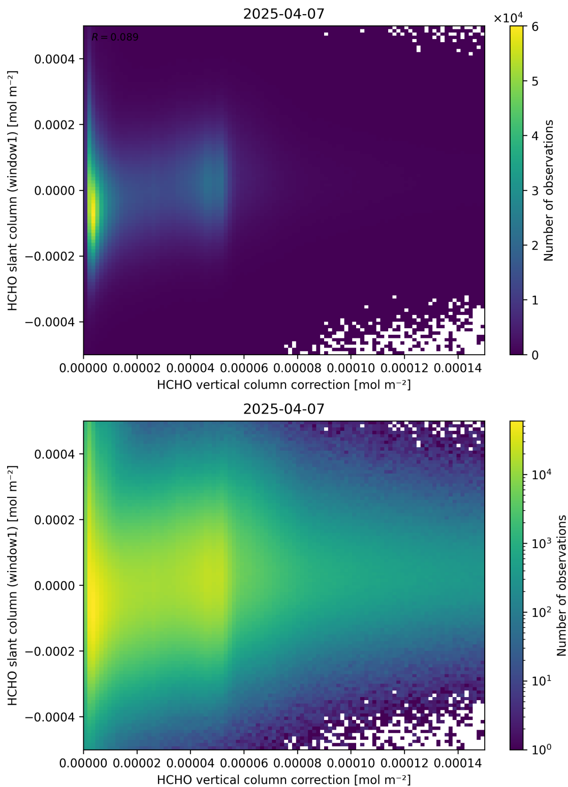
Figure 118: Scatter density plot of “HCHO vertical column correction” against “HCHO slant column (window1)” for 2025-04-06 to 2025-04-08.
