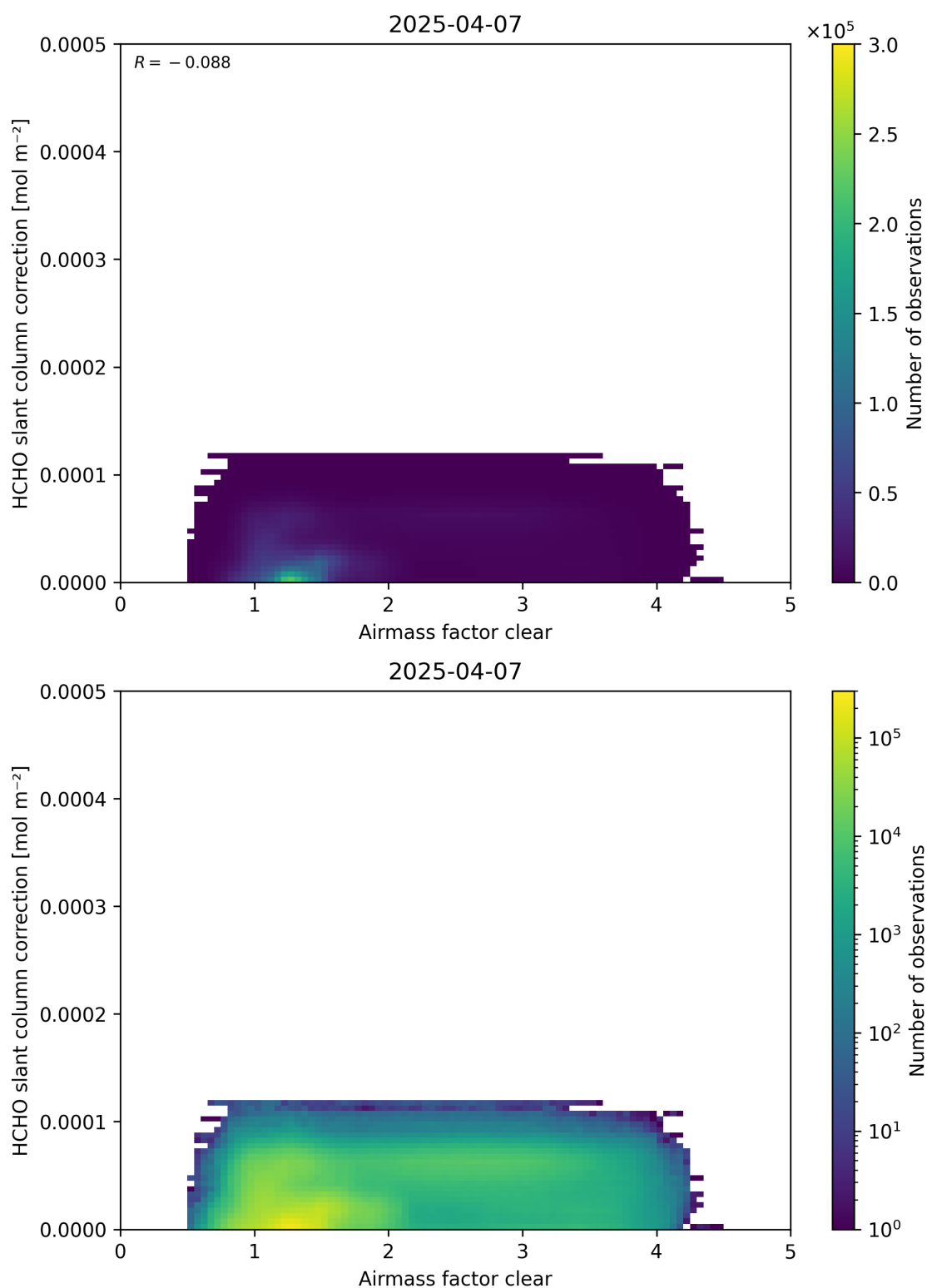
Figure 75: Scatter density plot of “Airmass factor clear” against “HCHO slant column correction” for 2025-04-06 to 2025-04-08.
