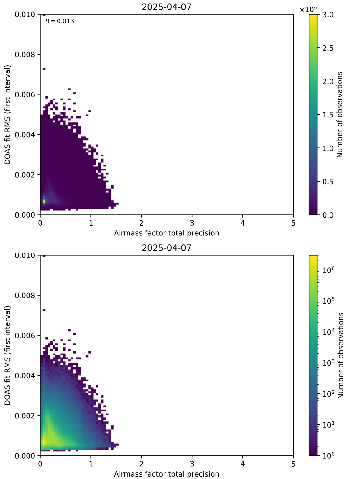
Figure 105: Scatter density plot of “Airmass factor total precision” against “DOAS fit RMS (first interval)” for 2025-04-06 to 2025-04-08.
