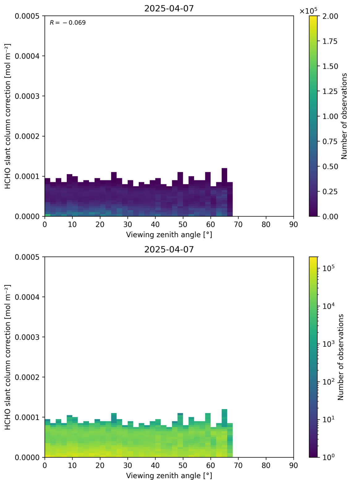
Figure 187: Scatter density plot of “Viewing zenith angle” against “HCHO slant column correction” for 2025-04-06 to 2025-04-08.
