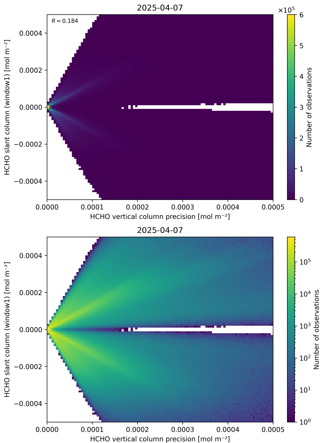
Figure 142: Scatter density plot of “HCHO vertical column precision” against “HCHO slant column (window1)” for 2025-04-06 to 2025-04-08.
