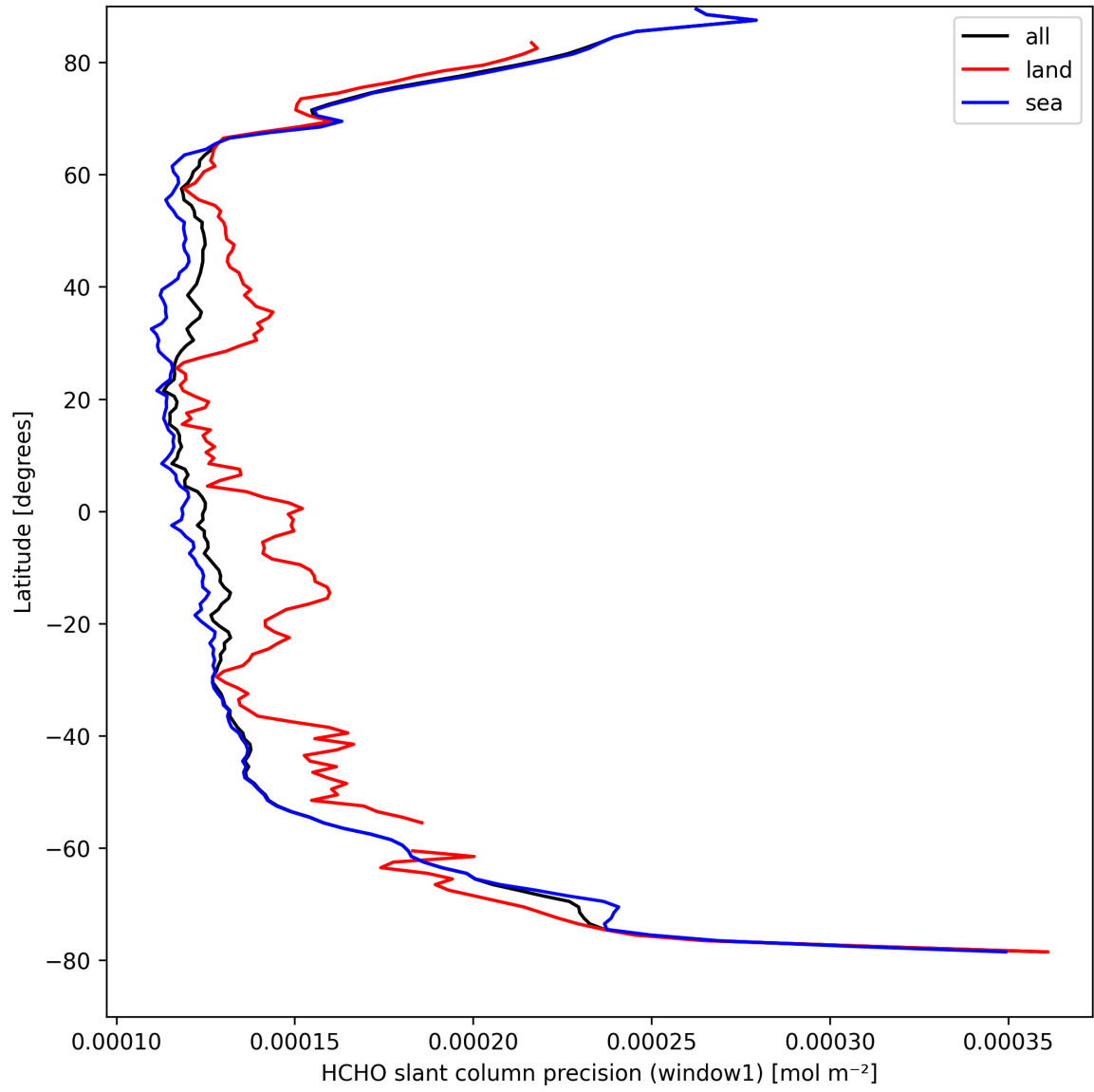
Figure 25: Zonal average of “HCHO slant column precision (window1)” for 2025-04-06 to 2025-04-08.
