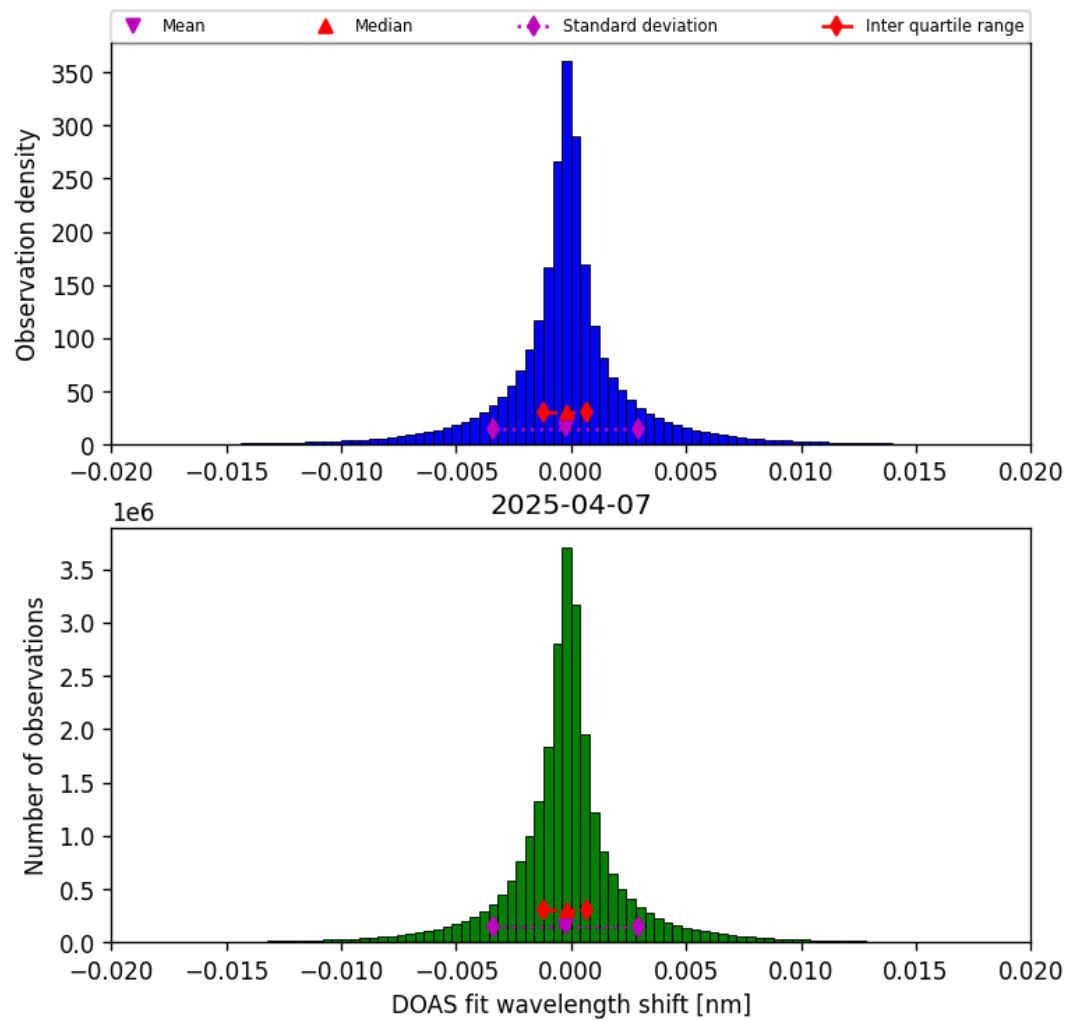
Figure 44: Histogram of “DOAS fit wavelength shift” for 2025-04-06 to 2025-04-08
