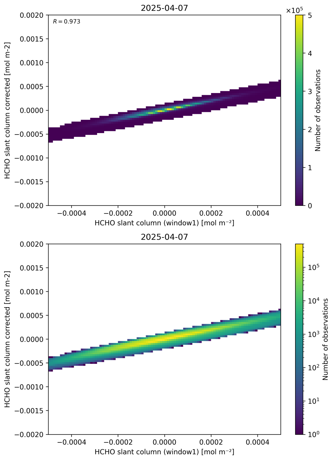
Figure 82: Scatter density plot of “HCHO slant column (window1)” against “HCHO slant column corrected” for 2025-04-06 to 2025-04-08.
