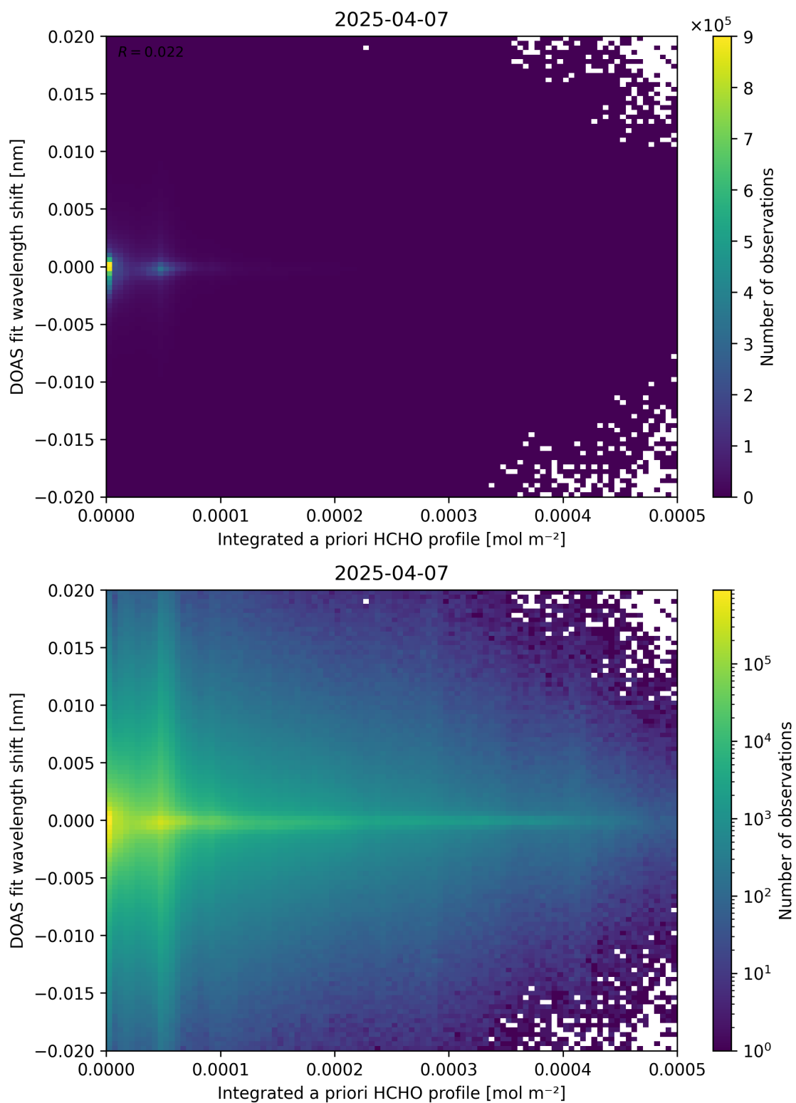
Figure 149: Scatter density plot of “Integrated a priori HCHO profile” against “DOAS fit wavelength shift” for 2025-04-06 to 2025-04-08.
