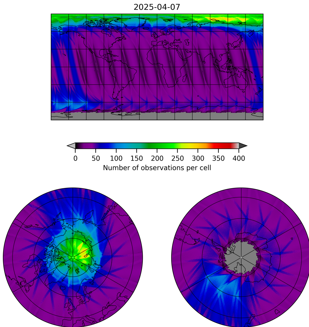
Figure 19: Map of the number of observations for 2025-04-06 to 2025-04-08
