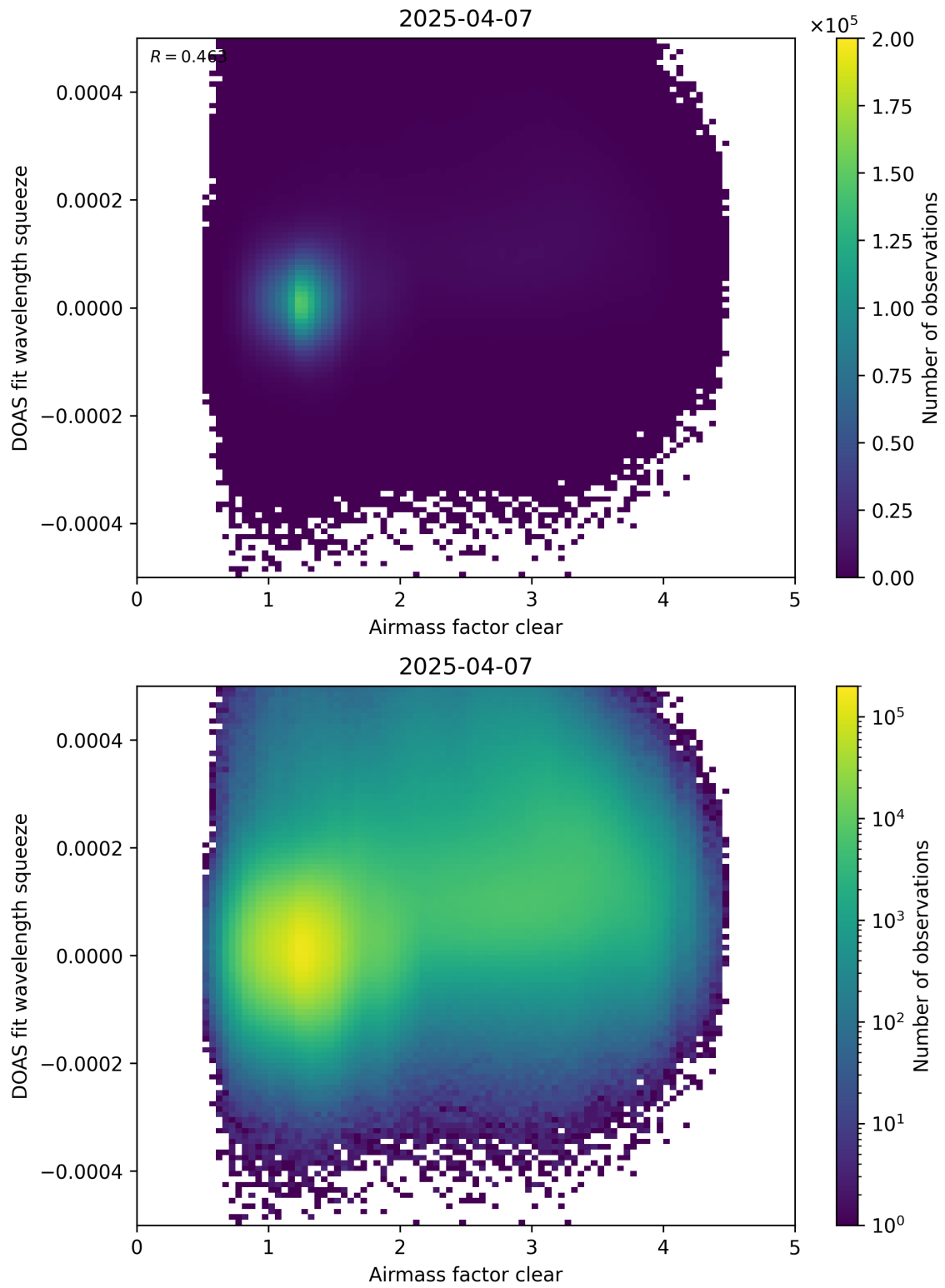
Figure 73: Scatter density plot of “Airmass factor clear” against “DOAS fit wavelength squeeze” for 2025-04-06 to 2025-04-08.
