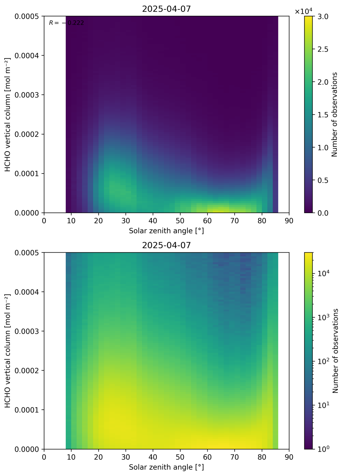
Figure 177: Scatter density plot of “Solar zenith angle” against “HCHO vertical column” for 2025-04-06 to 2025-04-08.
