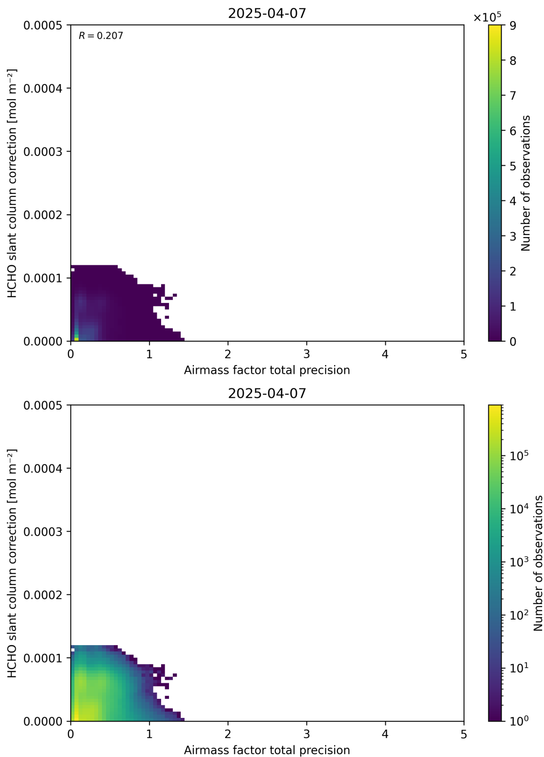
Figure 110: Scatter density plot of “Airmass factor total precision” against “HCHO slant column correction” for 2025-04-06 to 2025-04-08.
