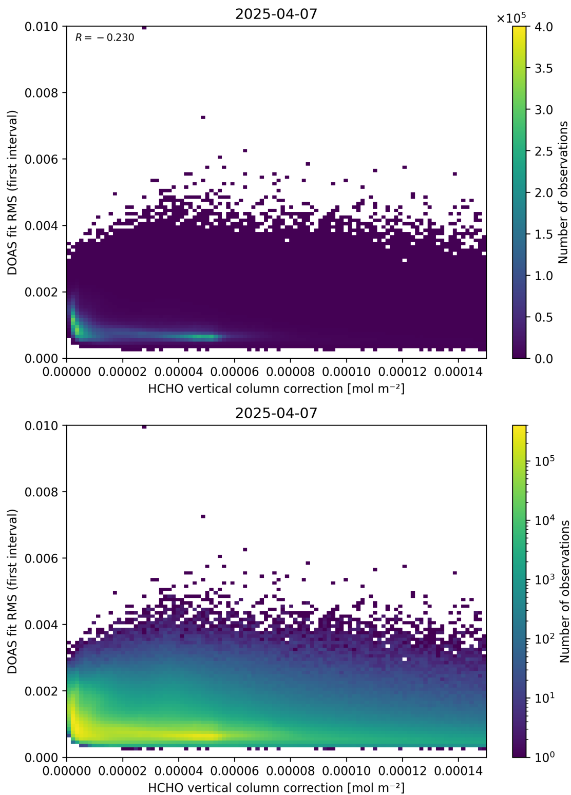
Figure 112: Scatter density plot of “HCHO vertical column correction” against “DOAS fit RMS (first interval)” for 2025-04-06 to 2025-04-08.
