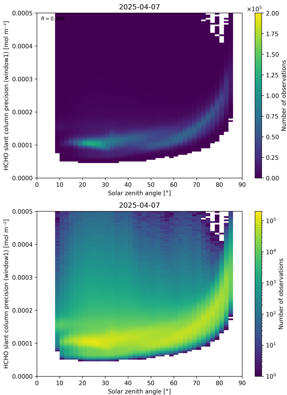
Figure 174: Scatter density plot of “Solar zenith angle” against “HCHO slant column precision (window1)” for 2025-04-06 to 2025-04-08.
