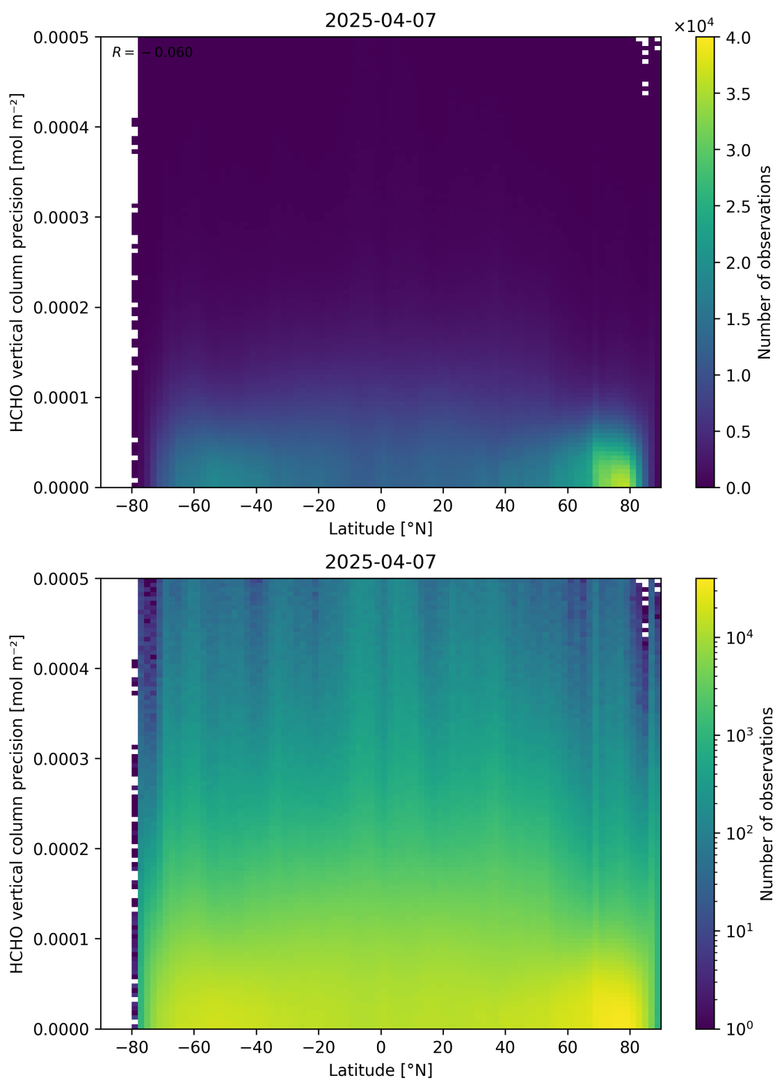
Figure 165: Scatter density plot of “Latitude” against “HCHO vertical column precision” for 2025-04-06 to 2025-04-08.
