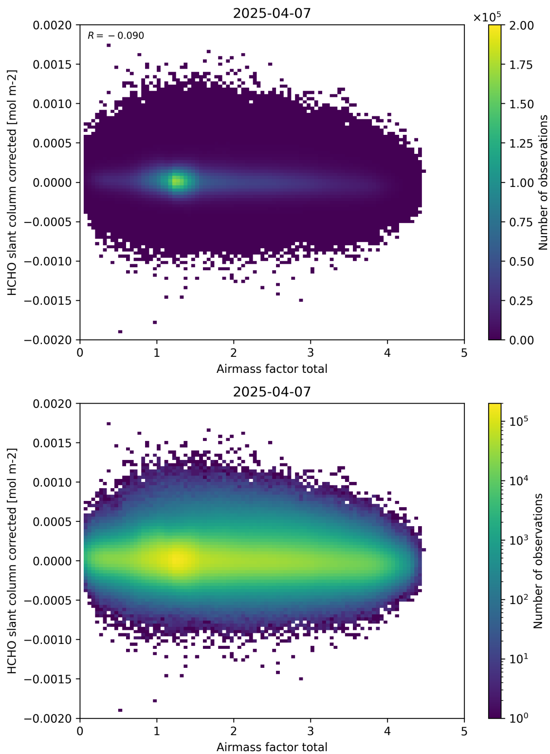
Figure 101: Scatter density plot of “Airmass factor total” against “HCHO slant column corrected” for 2025-04-06 to 2025-04-08.
