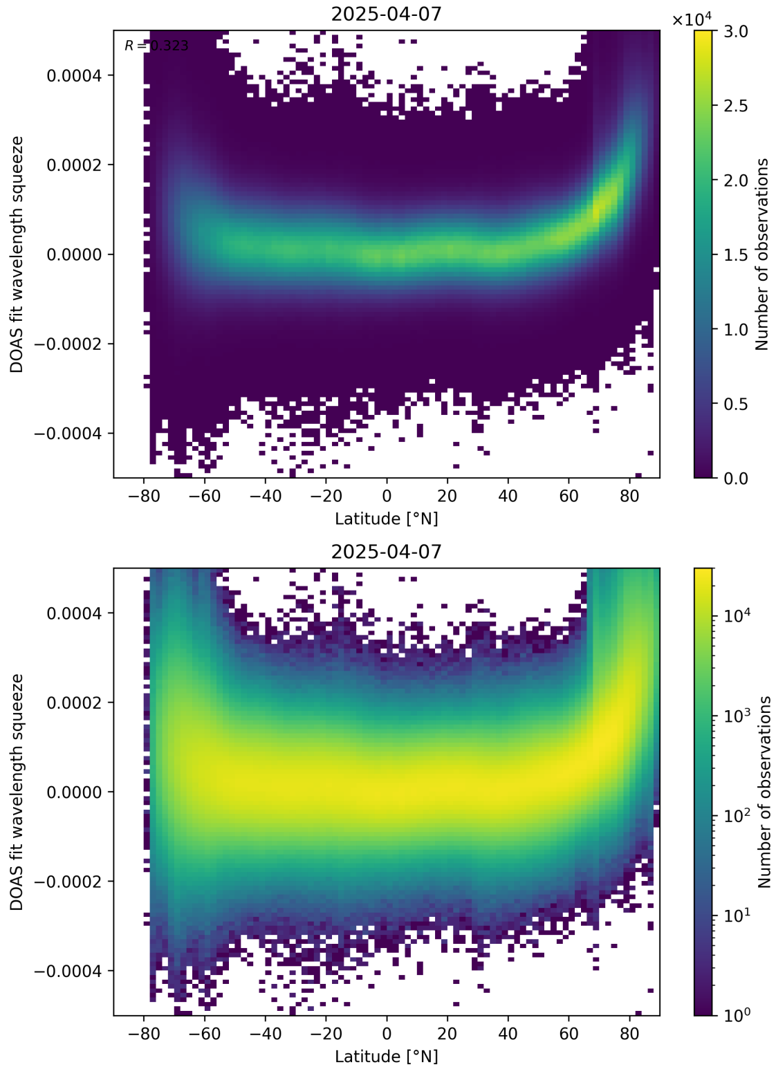
Figure 155: Scatter density plot of “Latitude” against “DOAS fit wavelength squeeze” for 2025-04-06 to 2025-04-08.
