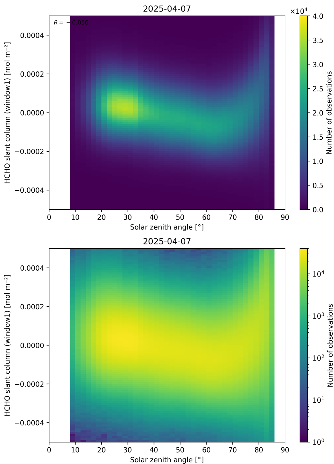
Figure 173: Scatter density plot of “Solar zenith angle” against “HCHO slant column (window1)” for 2025-04-06 to 2025-04-08.
