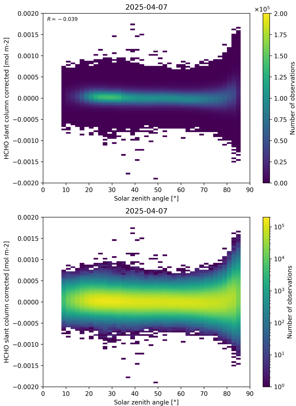
Figure 171: Scatter density plot of “Solar zenith angle” against “HCHO slant column corrected” for 2025-04-06 to 2025-04-08.
