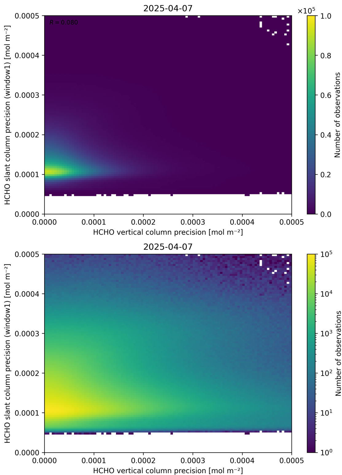
Figure 143: Scatter density plot of “HCHO vertical column precision” against “HCHO slant column precision (window1)” for 2025-04-06 to 2025-04-08.
