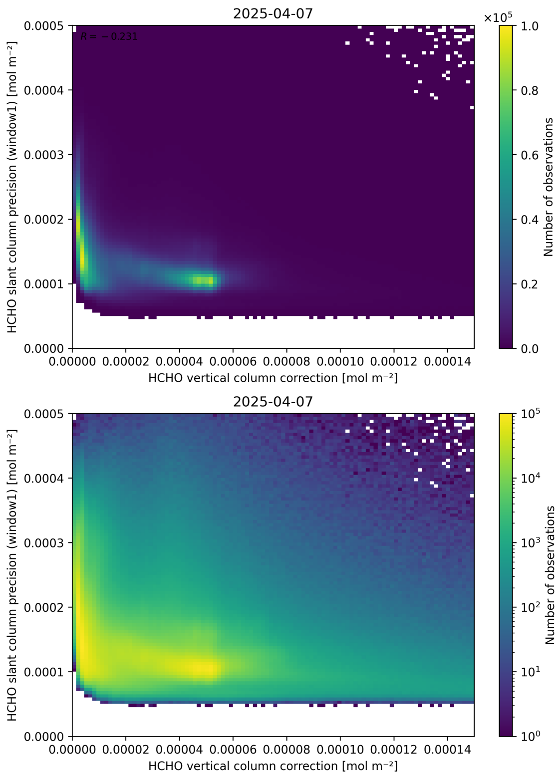
Figure 119: Scatter density plot of “HCHO vertical column correction” against “HCHO slant column precision (window1)” for 2025-04-06 to 2025-04-08.
