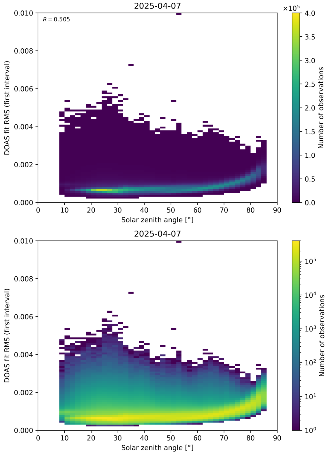
Figure 167: Scatter density plot of “Solar zenith angle” against “DOAS fit RMS (first interval)” for 2025-04-06 to 2025-04-08.
