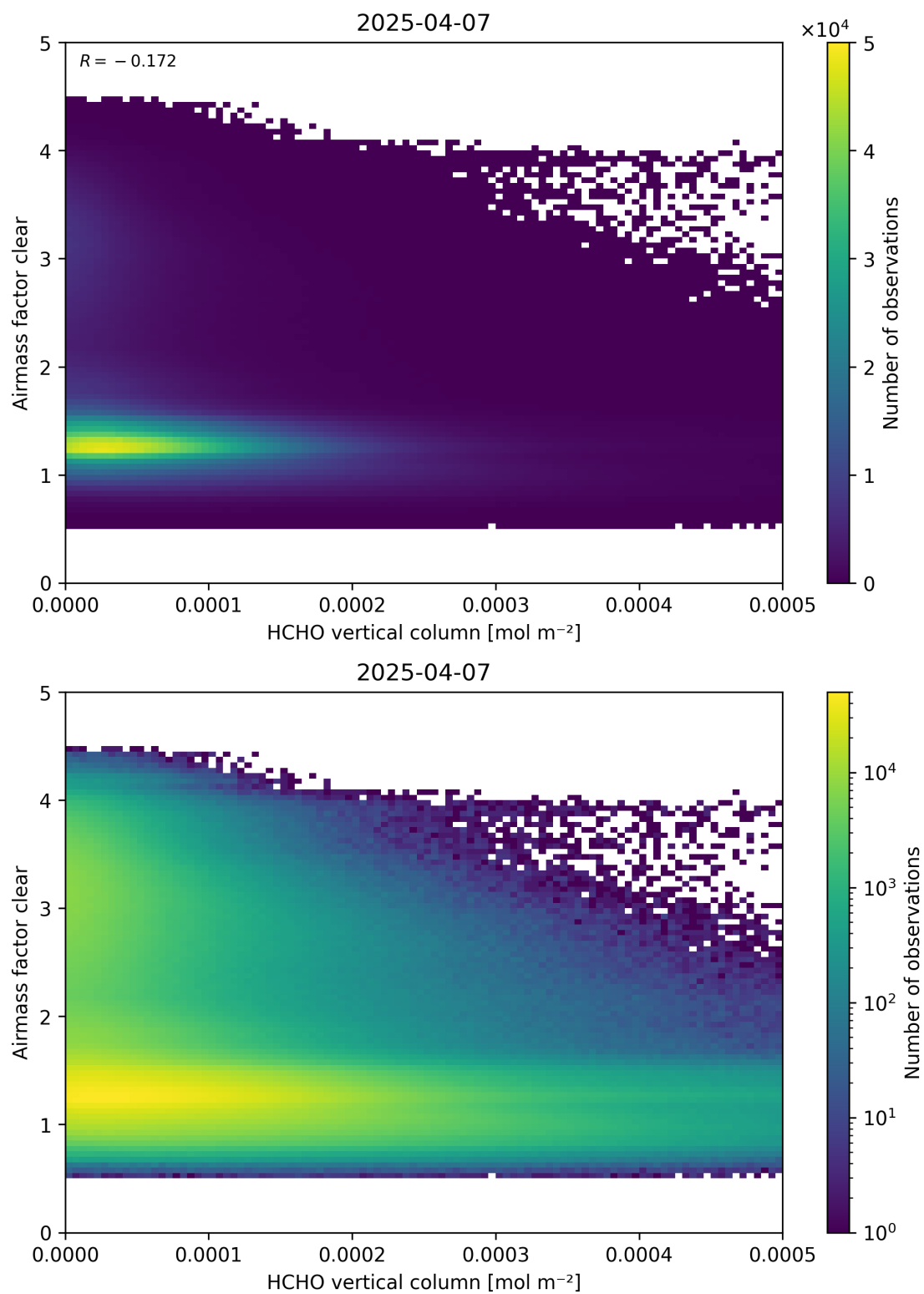
Figure 126: Scatter density plot of “HCHO vertical column” against “Airmass factor clear” for 2025-04-06 to 2025-04-08.
