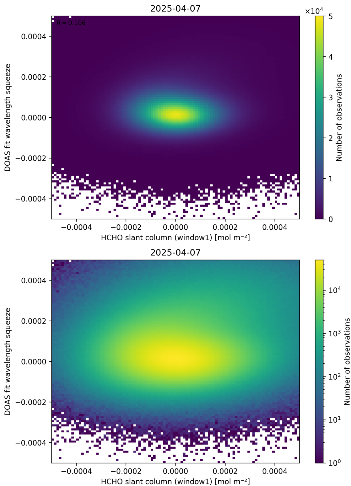
Figure 80: Scatter density plot of “HCHO slant column (window1)” against “DOAS fit wavelength squeeze” for 2025-04-06 to 2025-04-08.
