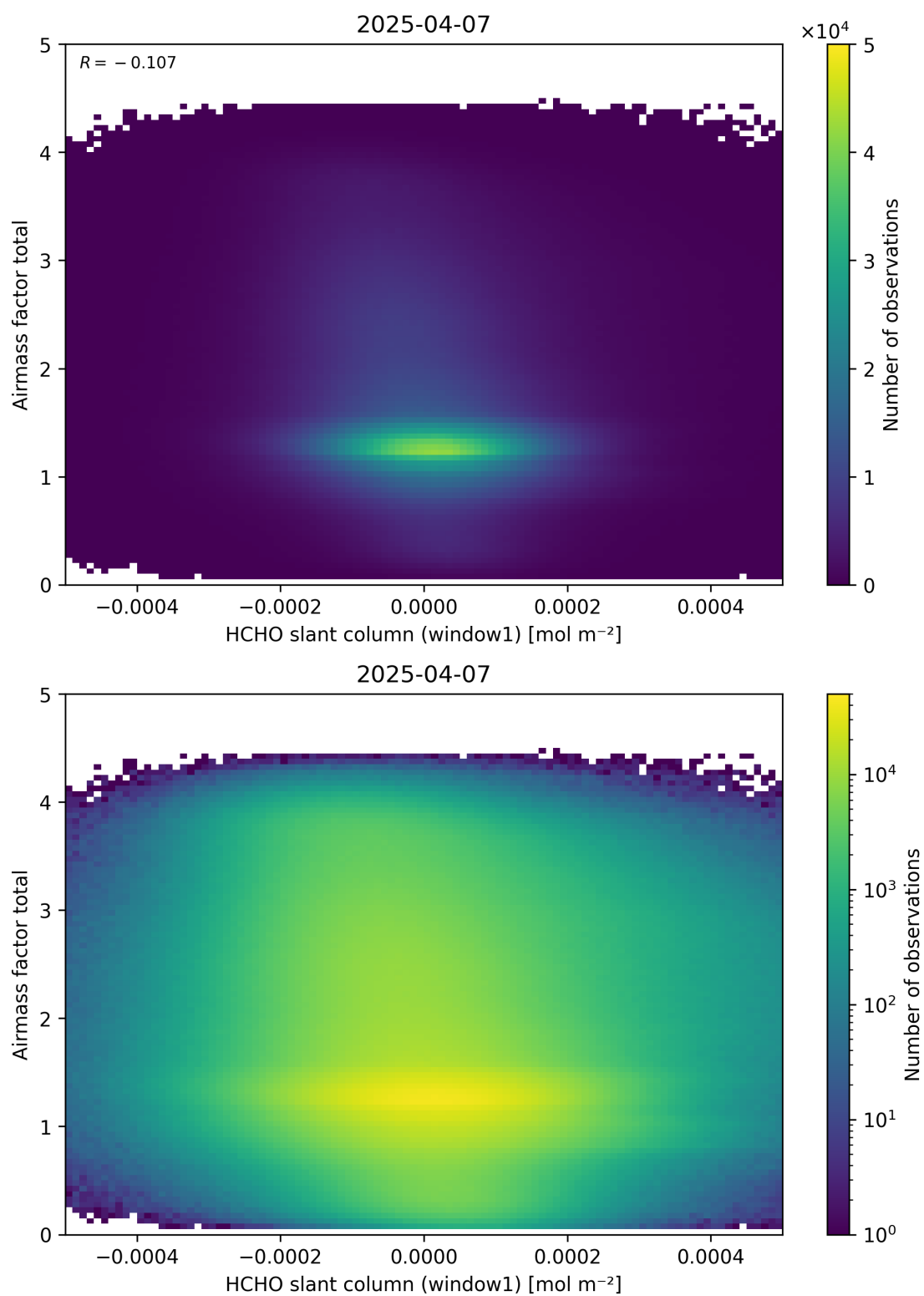
Figure 85: Scatter density plot of “HCHO slant column (window1)” against “Airmass factor total” for 2025-04-06 to 2025-04-08.
