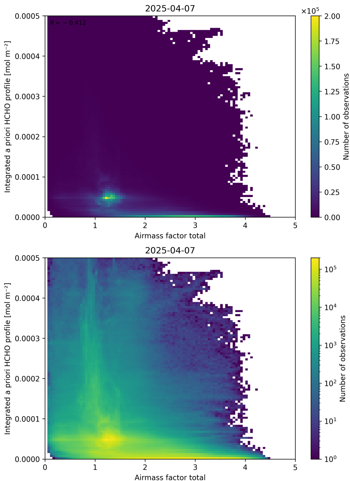
Figure 104: Scatter density plot of “Airmass factor total” against “Integrated a priori HCHO profile” for 2025-04-06 to 2025-04-08.
