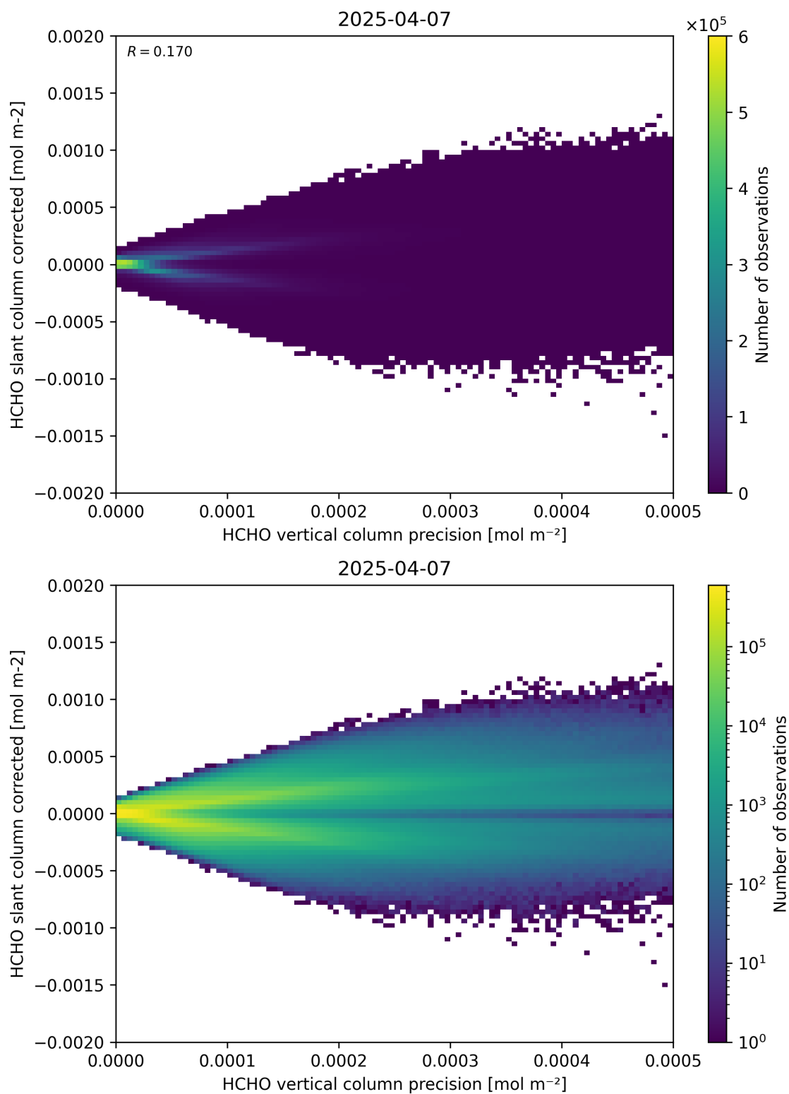
Figure 140: Scatter density plot of “HCHO vertical column precision” against “HCHO slant column corrected” for 2025-04-06 to 2025-04-08.
