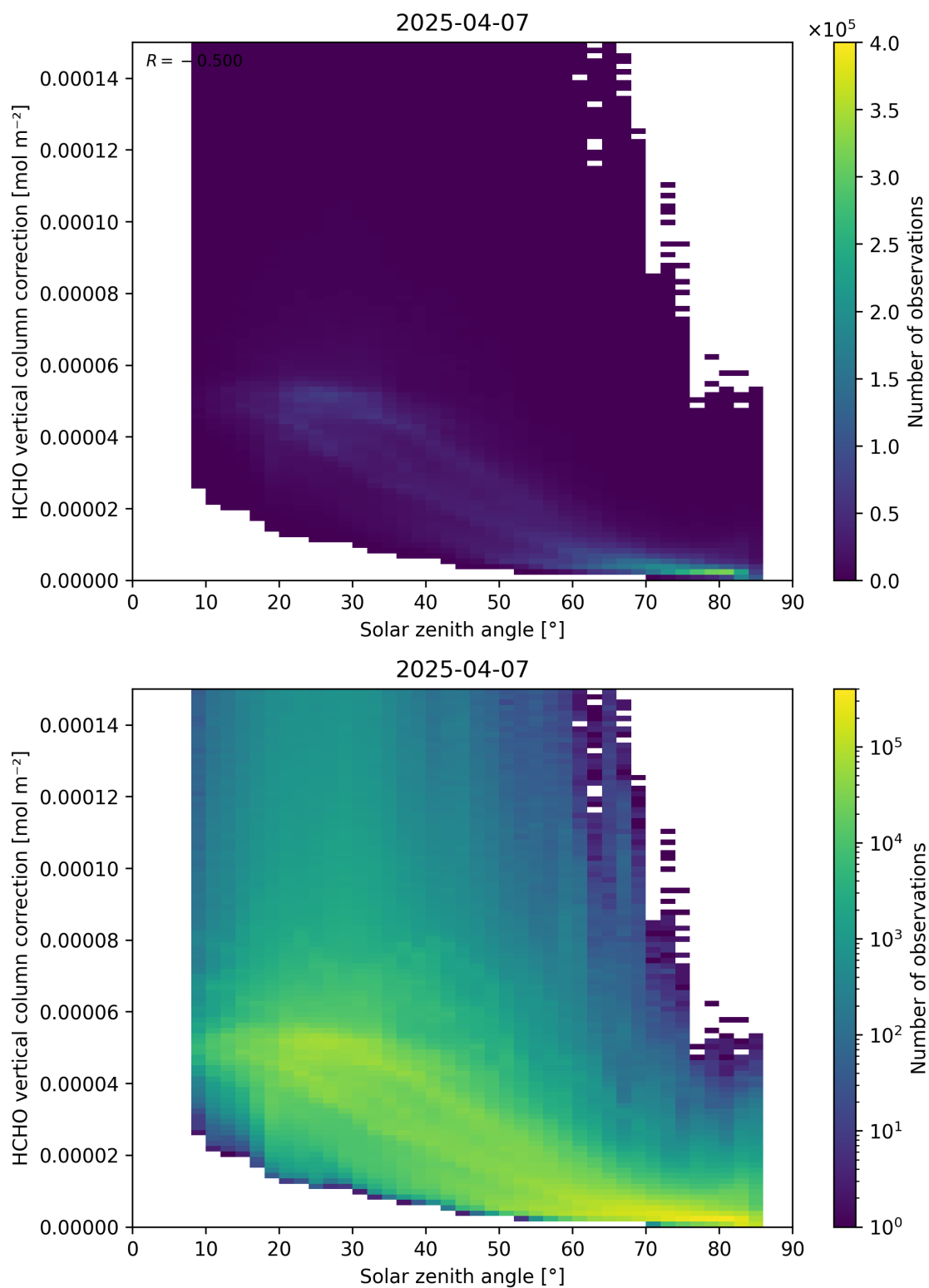
Figure 178: Scatter density plot of “Solar zenith angle” against “HCHO vertical column correction” for 2025-04-06 to 2025-04-08.
