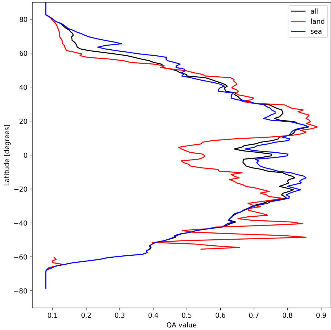
Figure 20: Zonal average of “QA value” for 2025-04-06 to 2025-04-08.
