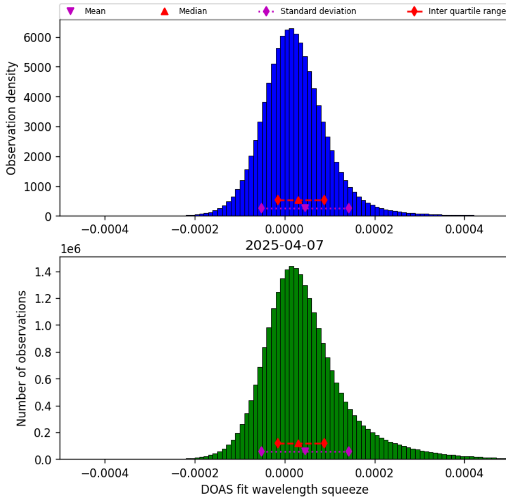
Figure 45: Histogram of “DOAS fit wavelength squeeze” for 2025-04-06 to 2025-04-08
