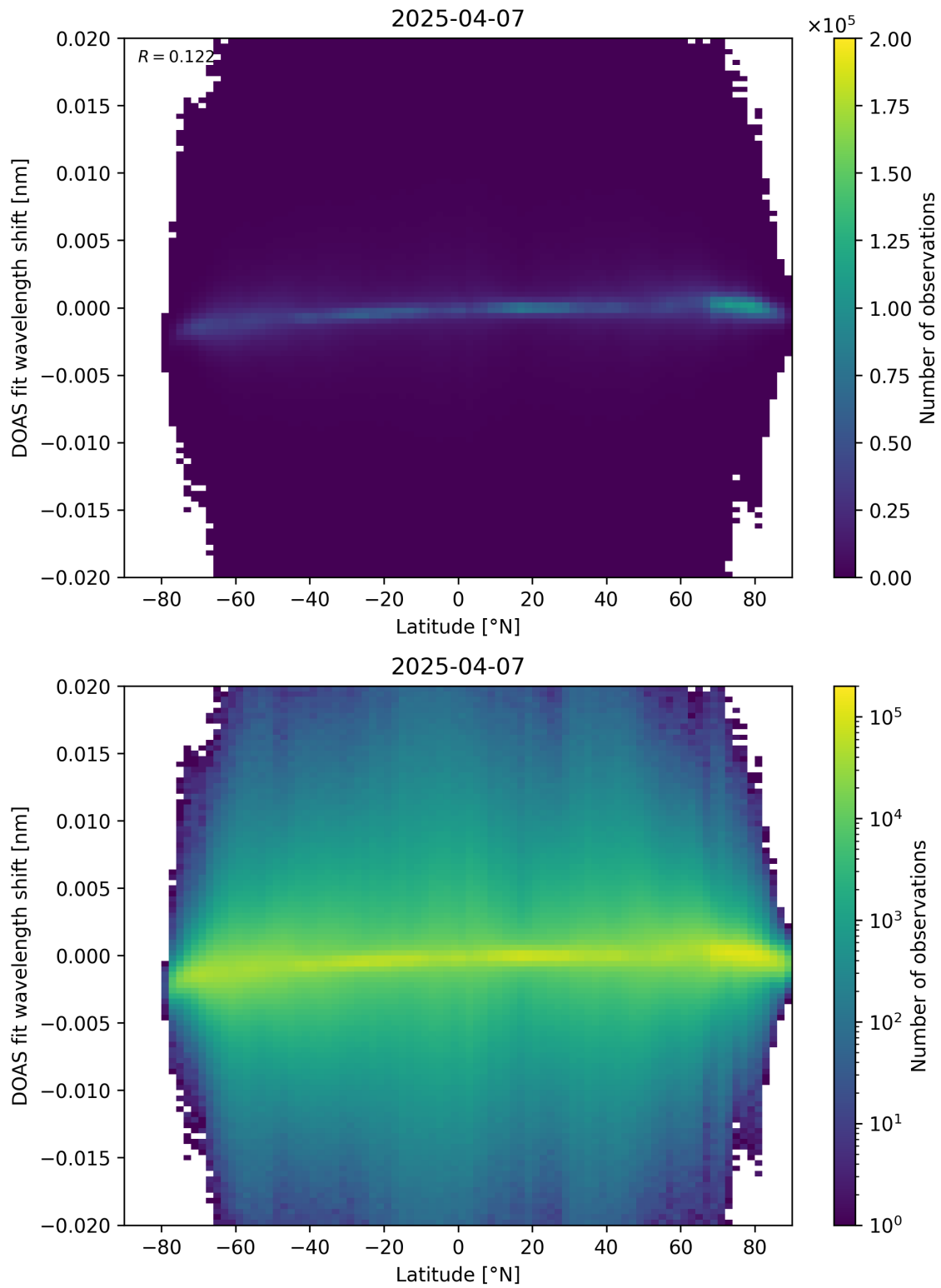
Figure 154: Scatter density plot of “Latitude” against “DOAS fit wavelength shift” for 2025-04-06 to 2025-04-08.
