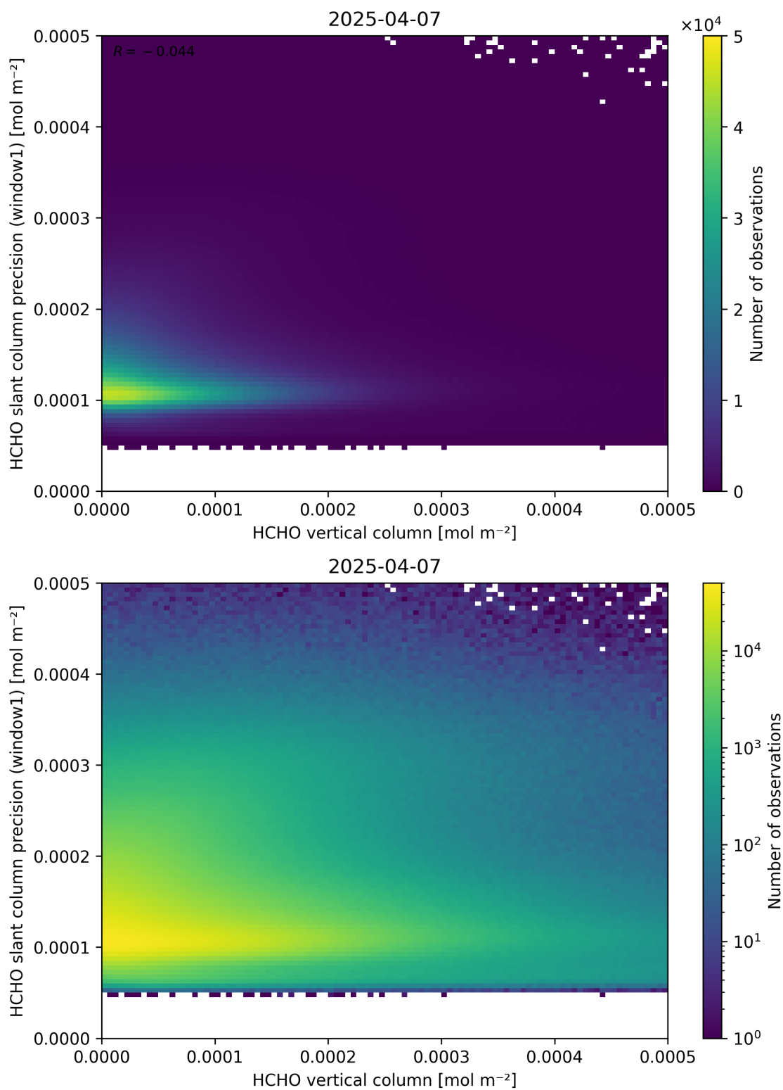
Figure 130: Scatter density plot of “HCHO vertical column” against “HCHO slant column precision (window1)” for 2025-04-06 to 2025-04-08.
