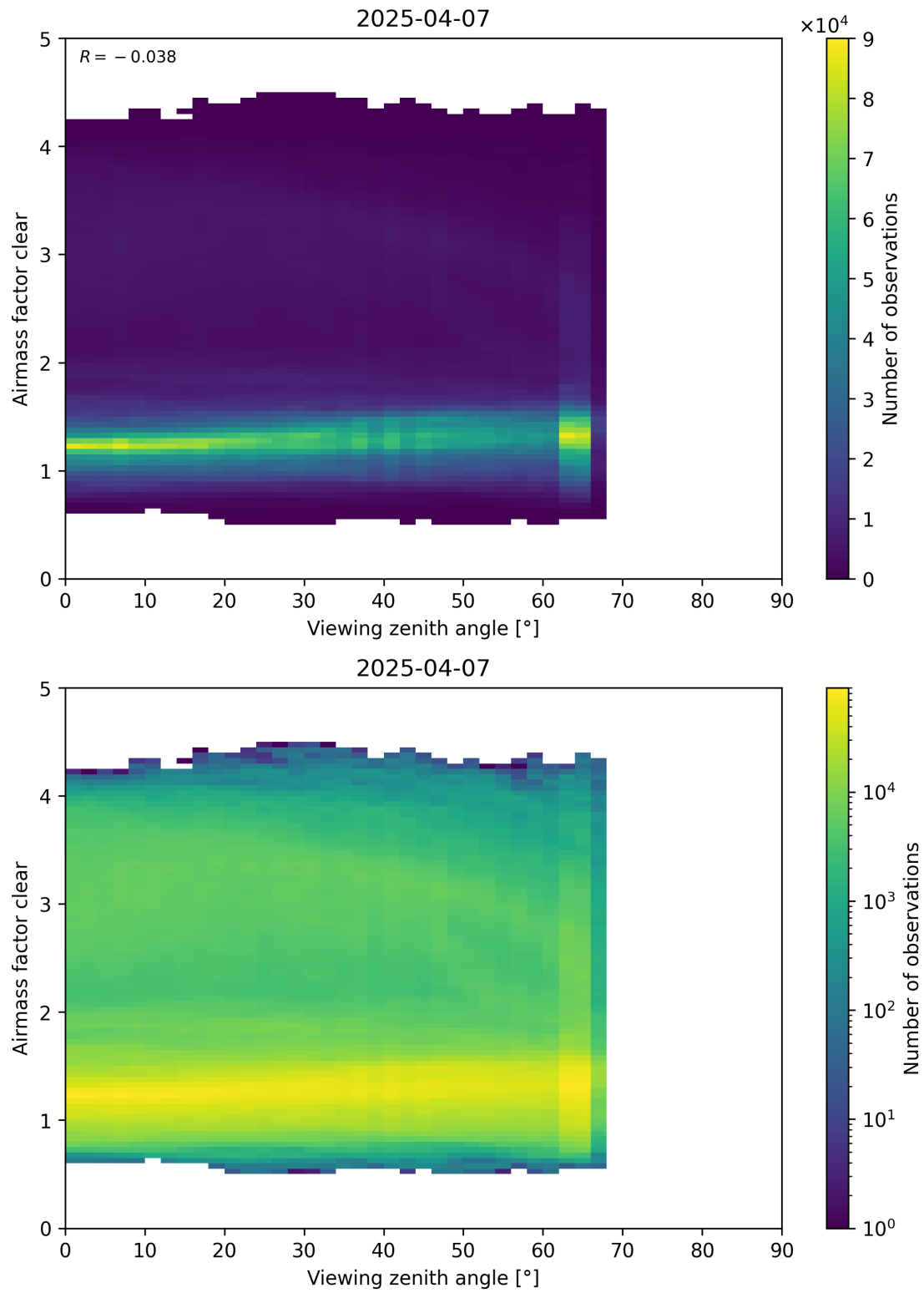
Figure 185: Scatter density plot of “Viewing zenith angle” against “Airmass factor clear” for 2025-04-06 to 2025-04-08.
