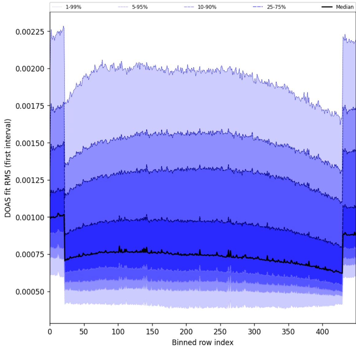
Figure 60: Along track statistics of “DOAS fit RMS (first interval)” for 2025-04-06 to 2025-04-08
