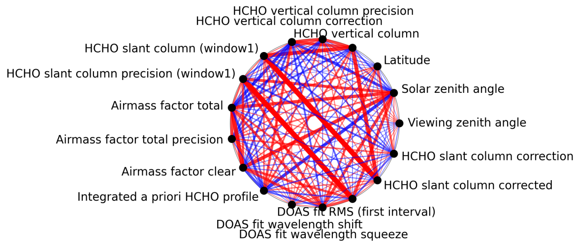
Figure 1: Map of correlation graph for 2025-04-06 to 2025-04-08.
