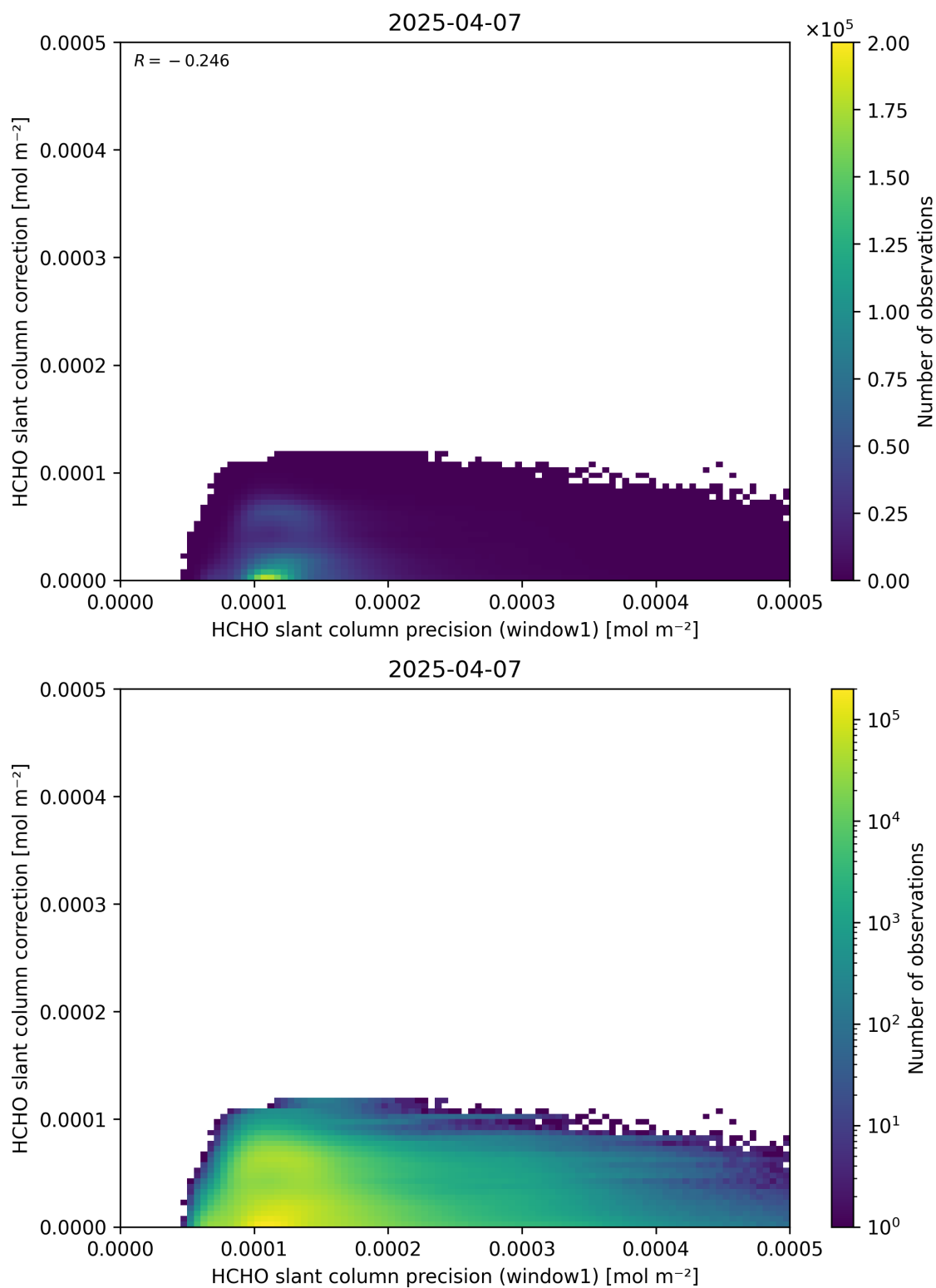
Figure 93: Scatter density plot of “HCHO slant column precision (window1)” against “HCHO slant column correction” for 2025-04-06 to 2025-04-08.
