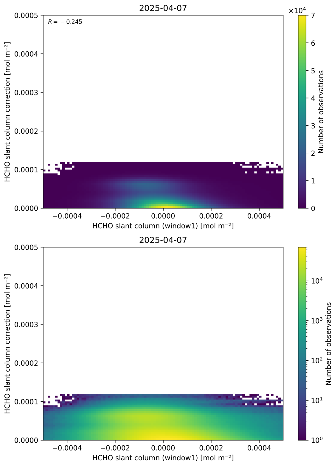
Figure 83: Scatter density plot of “HCHO slant column (window1)” against “HCHO slant column correction” for 2025-04-06 to 2025-04-08.
