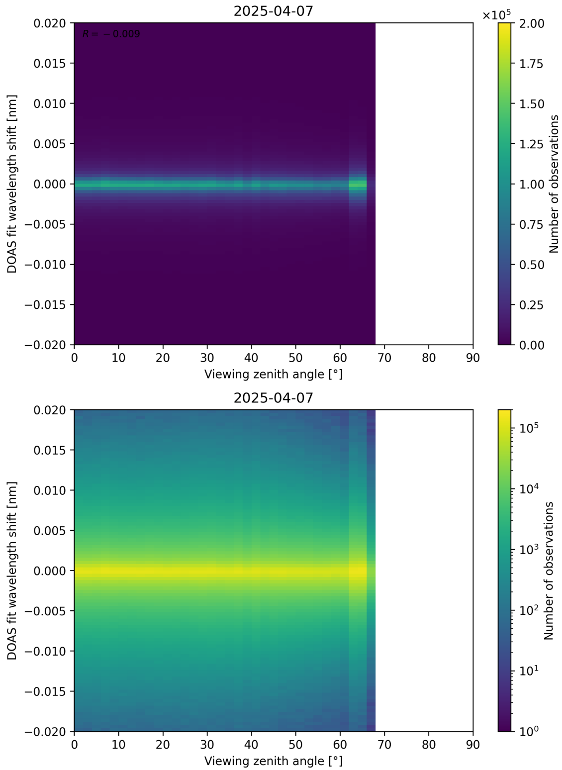
Figure 183: Scatter density plot of “Viewing zenith angle” against “DOAS fit wavelength shift” for 2025-04-06 to 2025-04-08.
