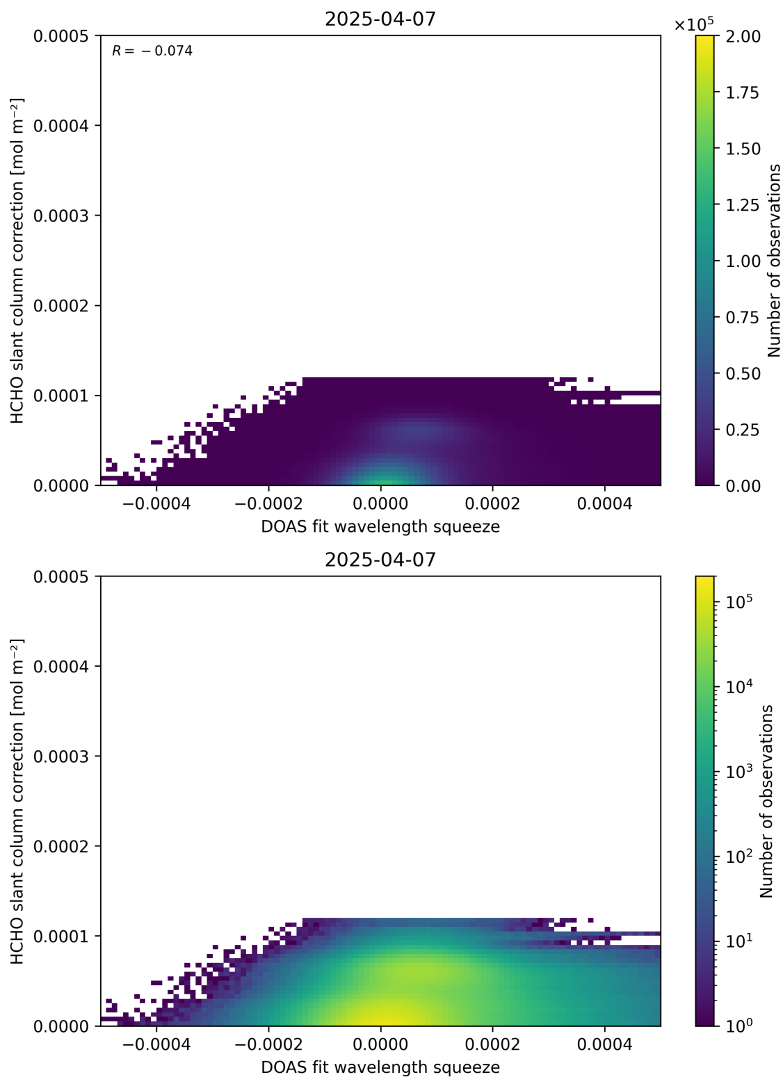
Figure 70: Scatter density plot of “DOAS fit wavelength squeeze” against “HCHO slant column correction” for 2025-04-06 to 2025-04-08.
