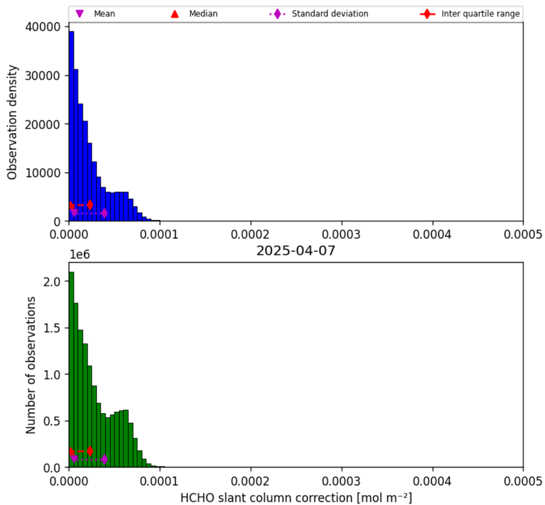
Figure 47: Histogram of “HCHO slant column correction” for 2025-04-06 to 2025-04-08
