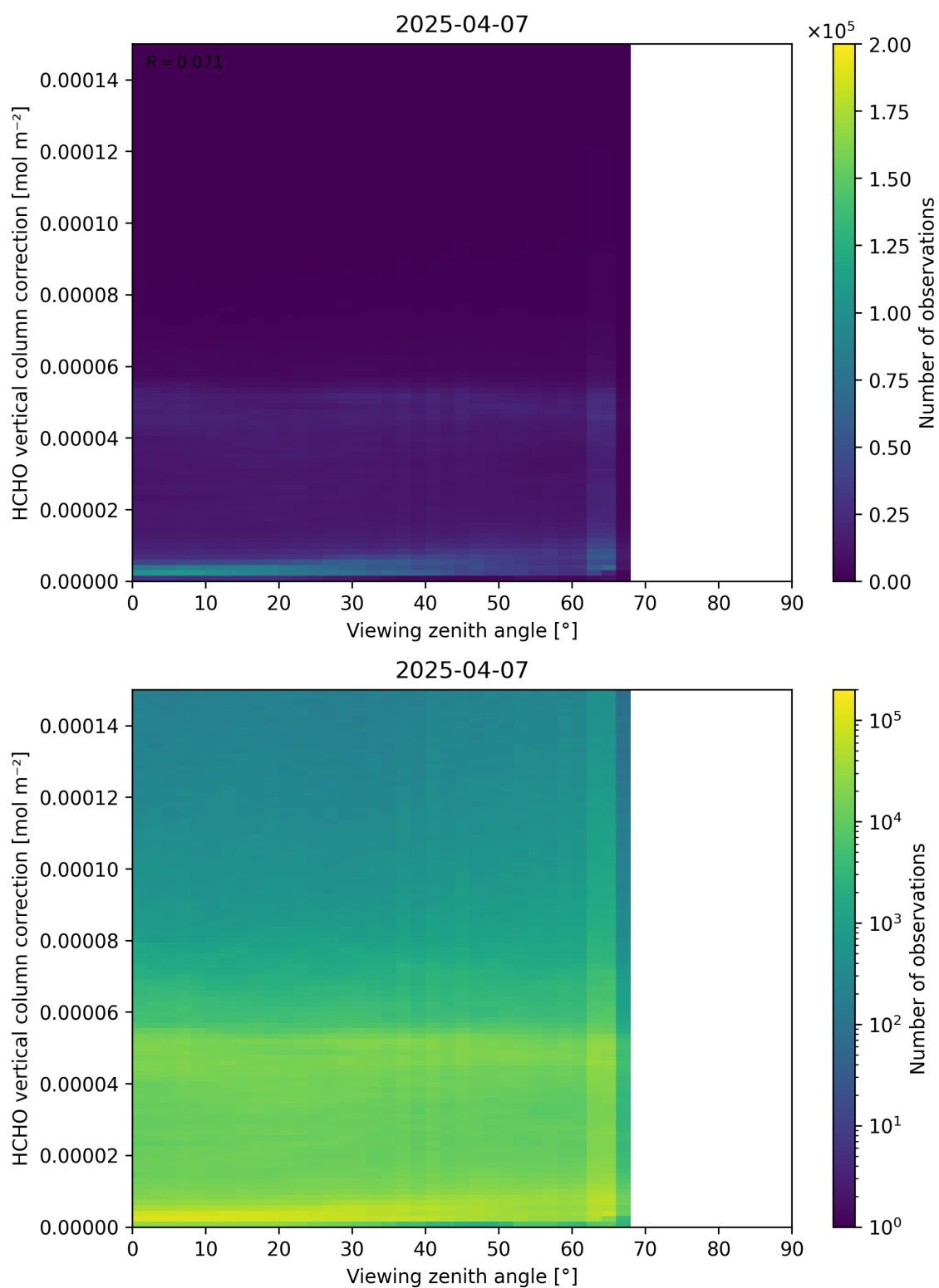
Figure 193: Scatter density plot of “Viewing zenith angle” against “HCHO vertical column correction” for 2025-04-06 to 2025-04-08.
