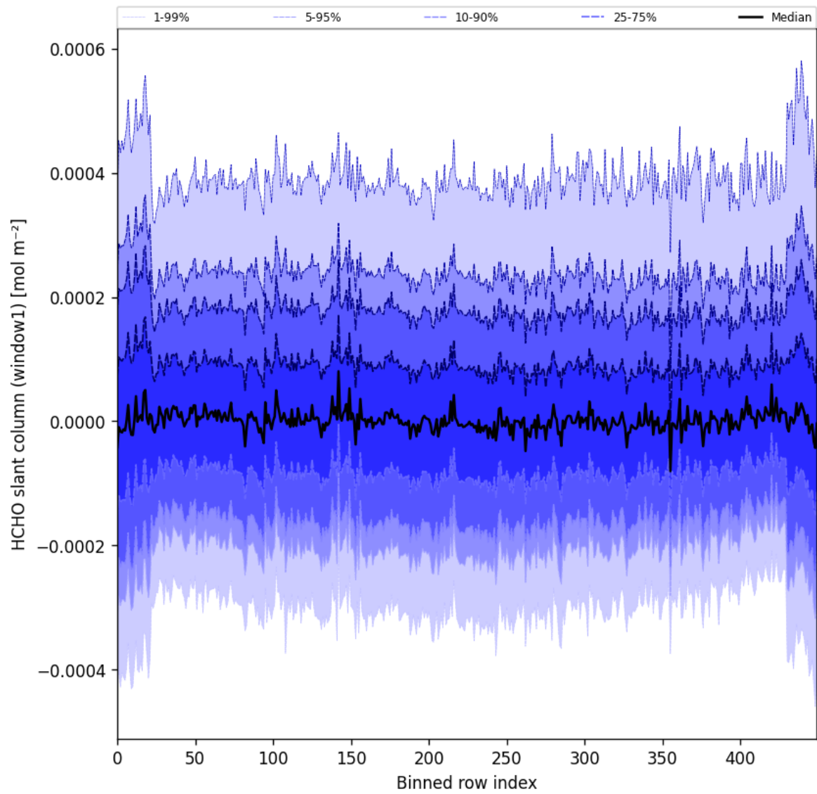
Figure 52: Along track statistics of “HCHO slant column (window1)” for 2025-04-06 to 2025-04-08
