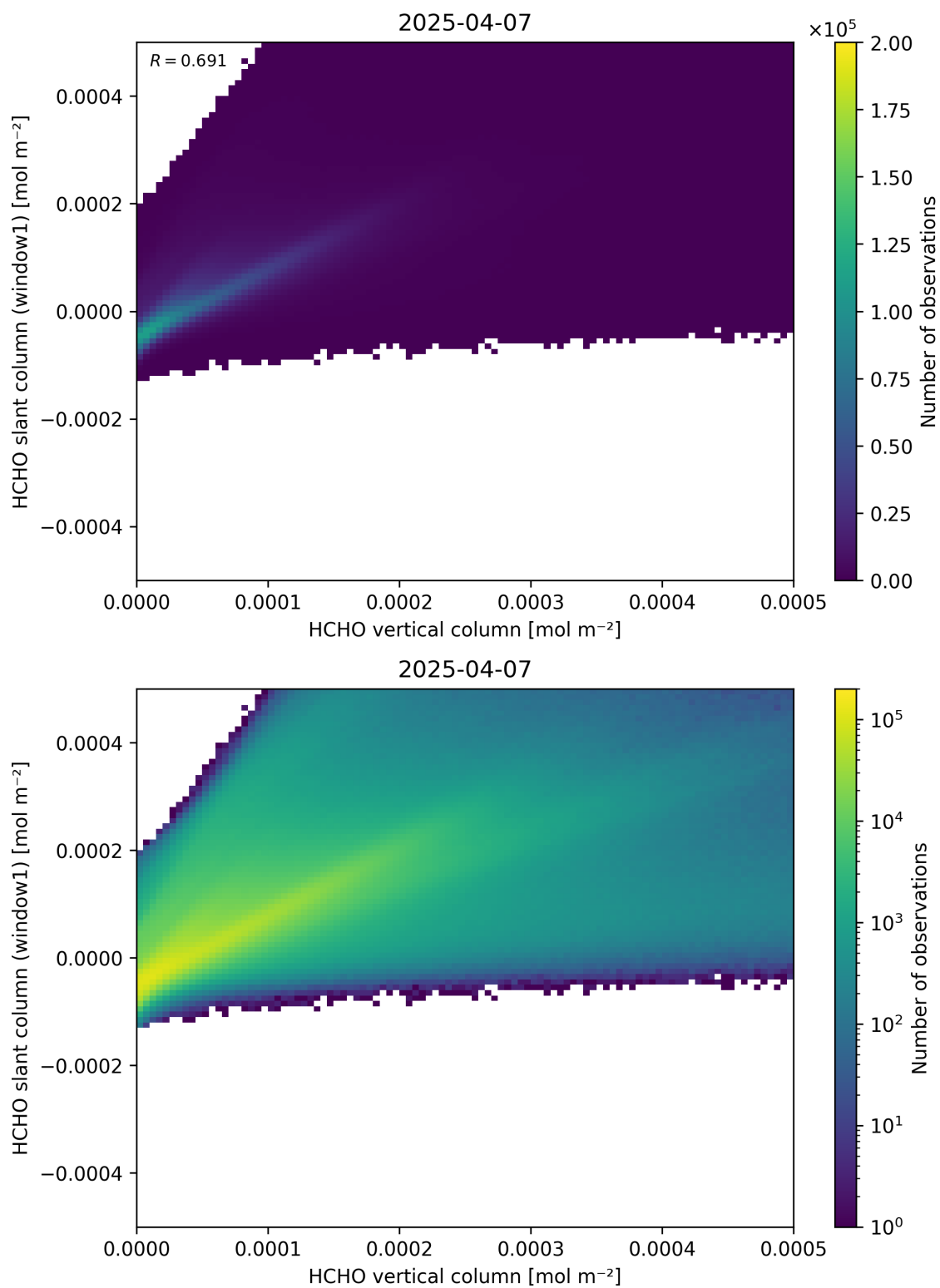
Figure 129: Scatter density plot of “HCHO vertical column” against “HCHO slant column (window1)” for 2025-04-06 to 2025-04-08.
