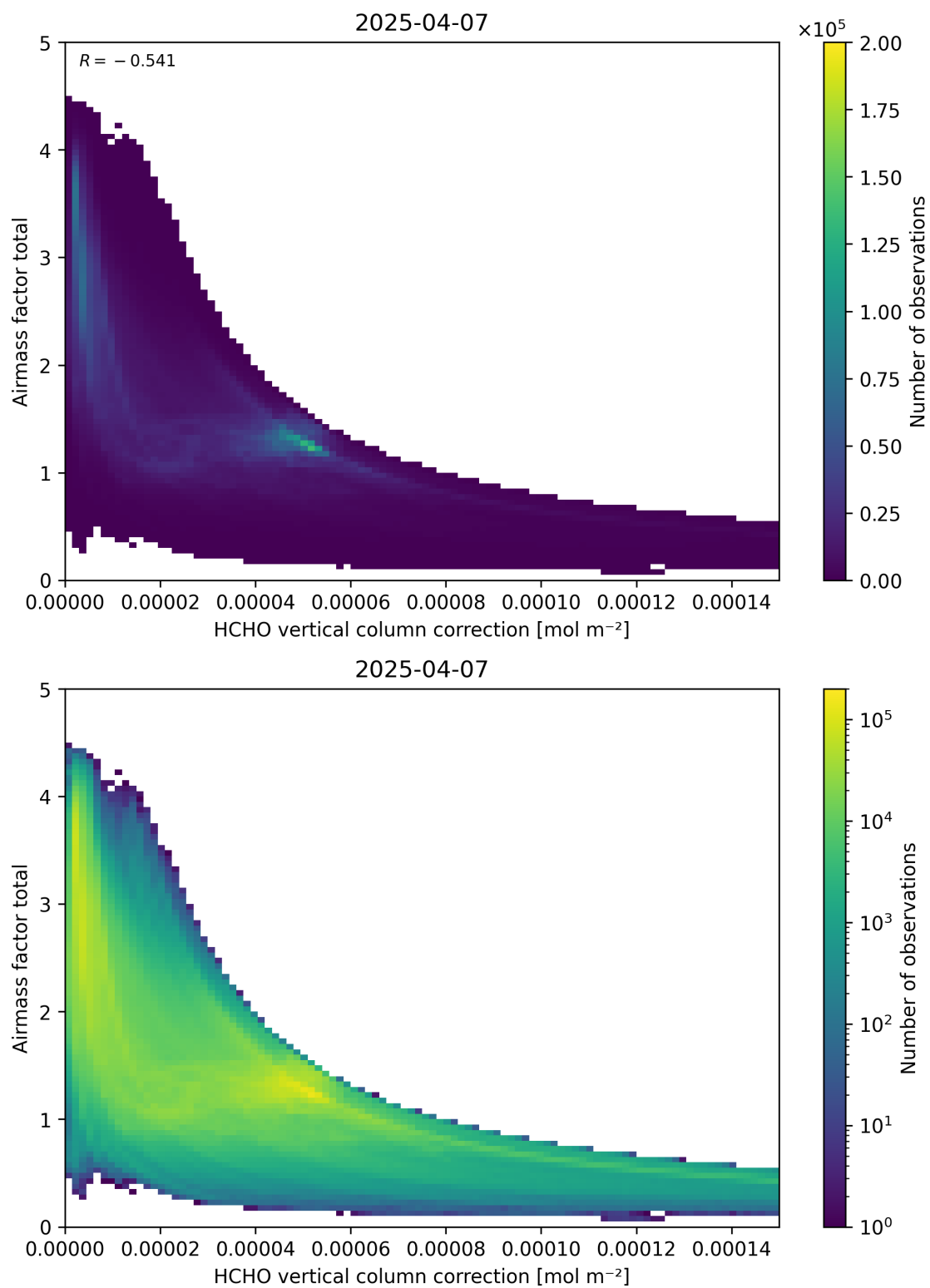
Figure 120: Scatter density plot of “HCHO vertical column correction” against “Airmass factor total” for 2025-04-06 to 2025-04-08.
