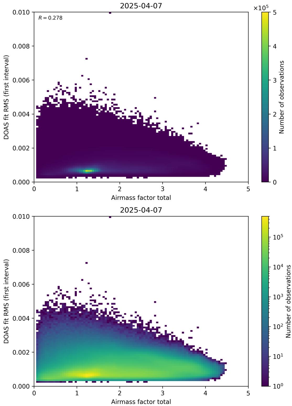
Figure 97: Scatter density plot of “Airmass factor total” against “DOAS fit RMS (first interval)” for 2025-04-06 to 2025-04-08.
