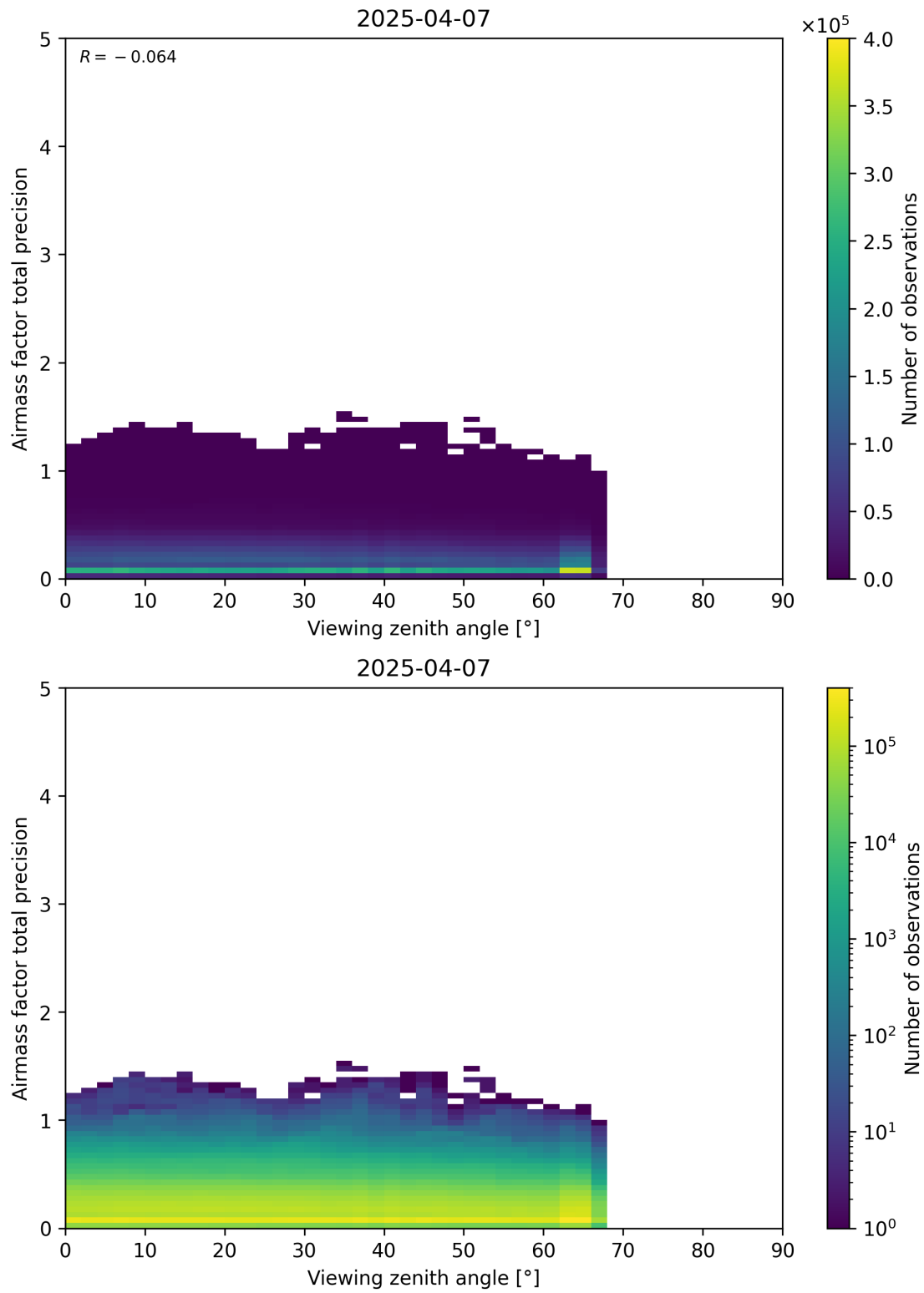
Figure 191: Scatter density plot of “Viewing zenith angle” against “Airmass factor total precision” for 2025-04-06 to 2025-04-08.
