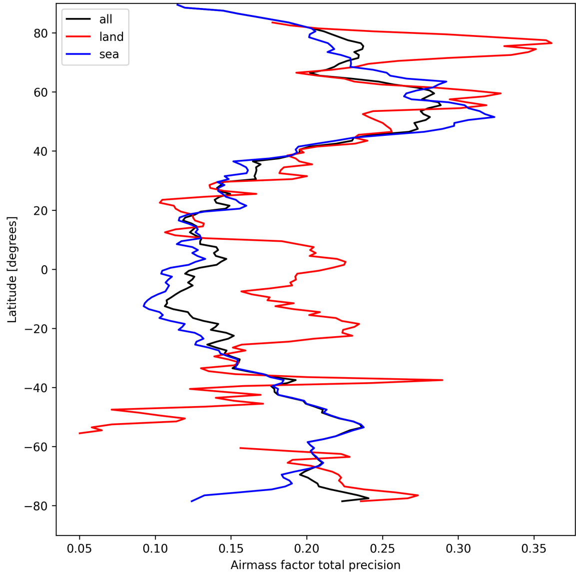
Figure 27: Zonal average of “Airmass factor total precision” for 2025-04-06 to 2025-04-08.
