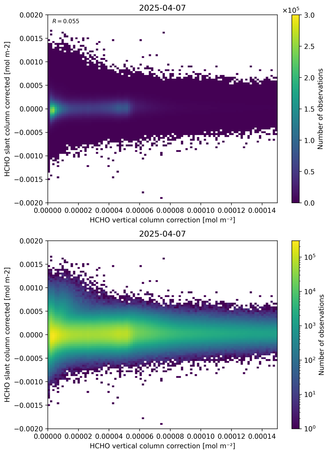
Figure 116: Scatter density plot of “HCHO vertical column correction” against “HCHO slant column corrected” for 2025-04-06 to 2025-04-08.
