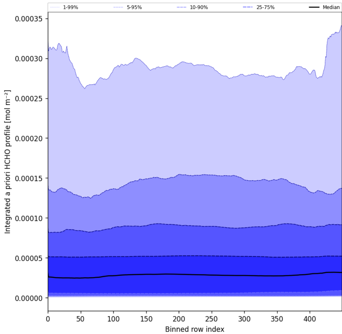
Figure 57: Along track statistics of “Integrated a priori HCHO profile” for 2025-04-06 to 2025-04-08
