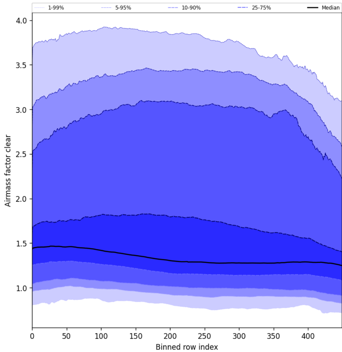
Figure 56: Along track statistics of “Airmass factor clear” for 2025-04-06 to 2025-04-08
