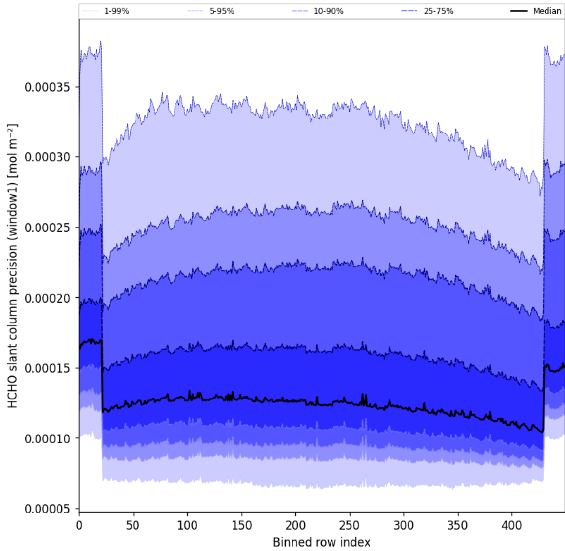
Figure 53: Along track statistics of “HCHO slant column precision (window1)” for 2025-04-06 to 2025-04-08
