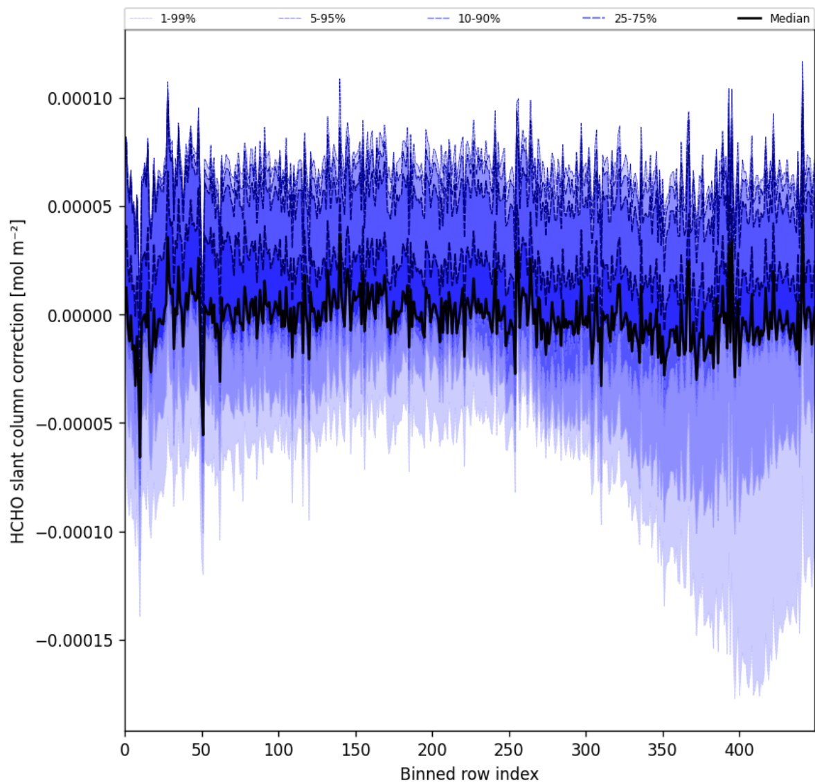
Figure 61: Along track statistics of “HCHO slant column correction” for 2025-04-06 to 2025-04-08
