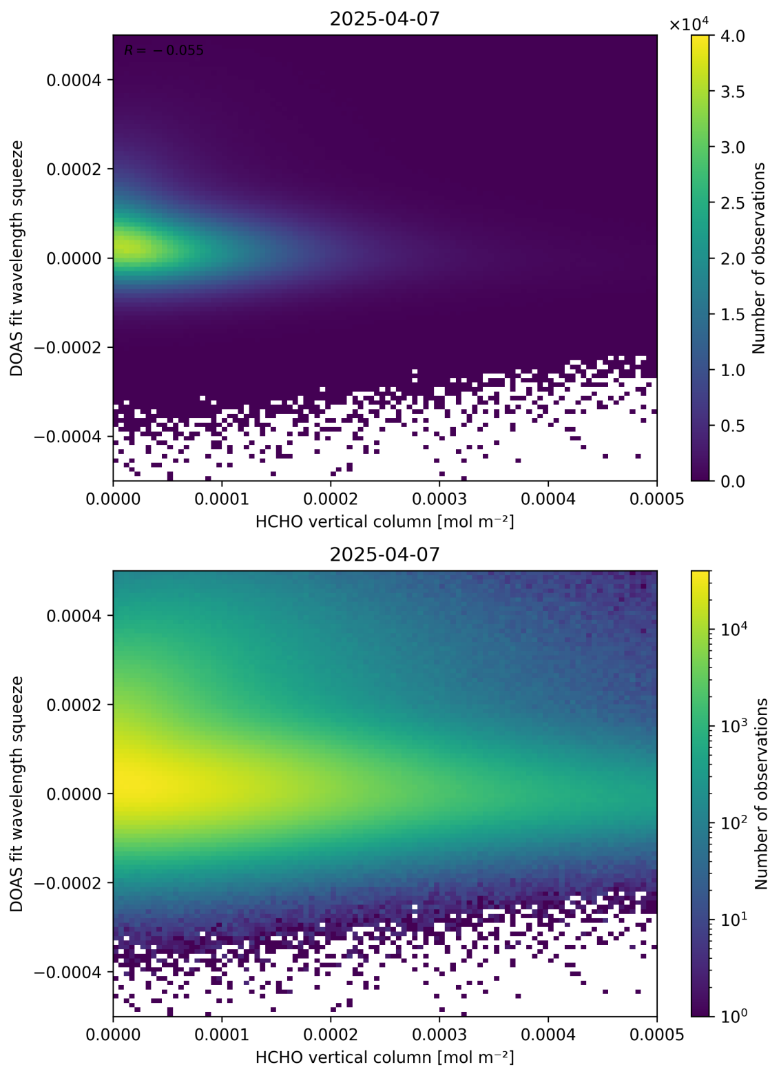
Figure 125: Scatter density plot of “HCHO vertical column” against “DOAS fit wavelength squeeze” for 2025-04-06 to 2025-04-08.
