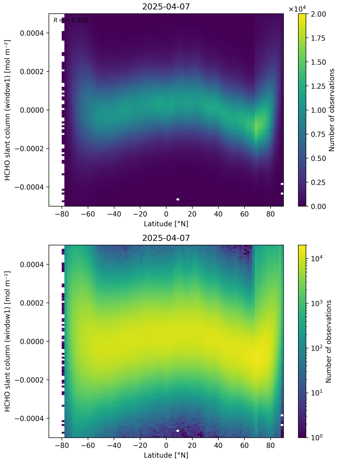
Figure 159: Scatter density plot of “Latitude” against “HCHO slant column (window1)” for 2025-04-06 to 2025-04-08.
