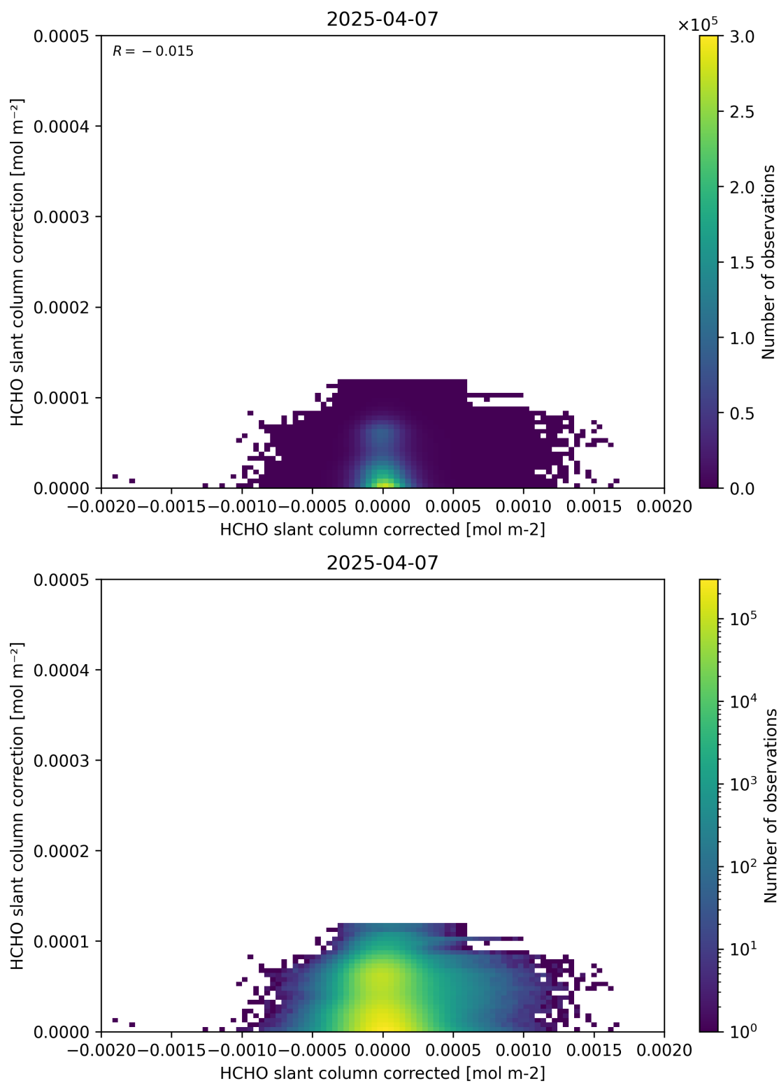
Figure 77: Scatter density plot of “HCHO slant column corrected” against “HCHO slant column correction” for 2025-04-06 to 2025-04-08.
