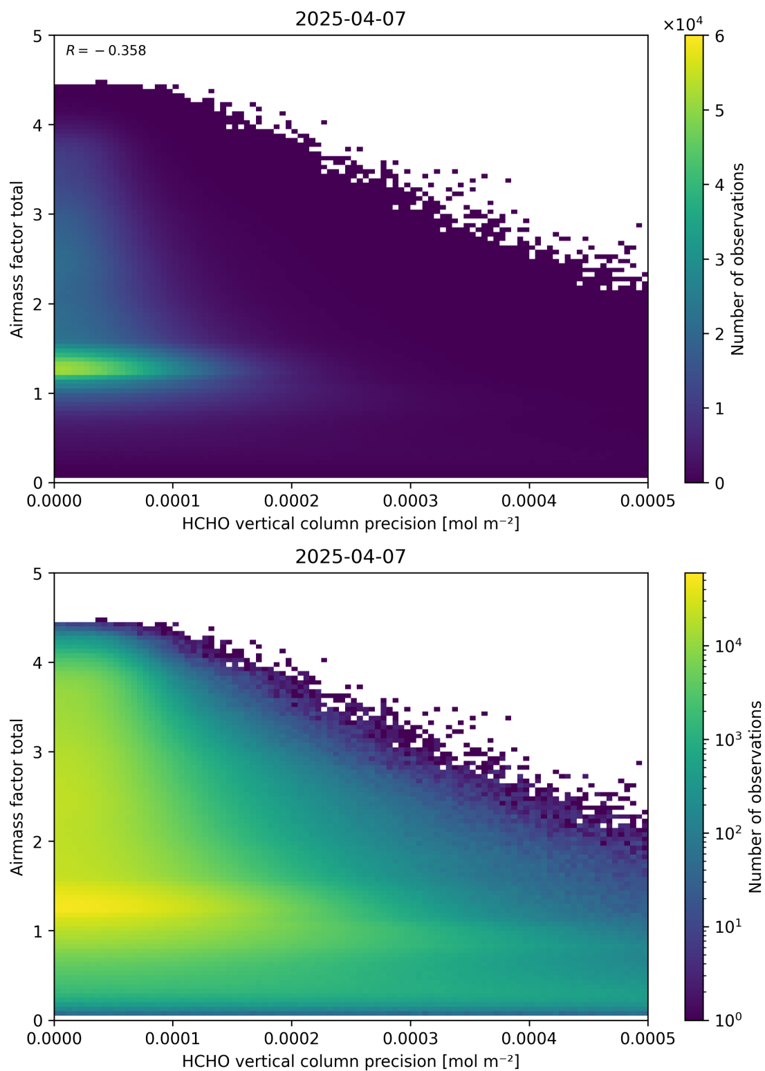
Figure 144: Scatter density plot of “HCHO vertical column precision” against “Airmass factor total” for 2025-04-06 to 2025-04-08.
