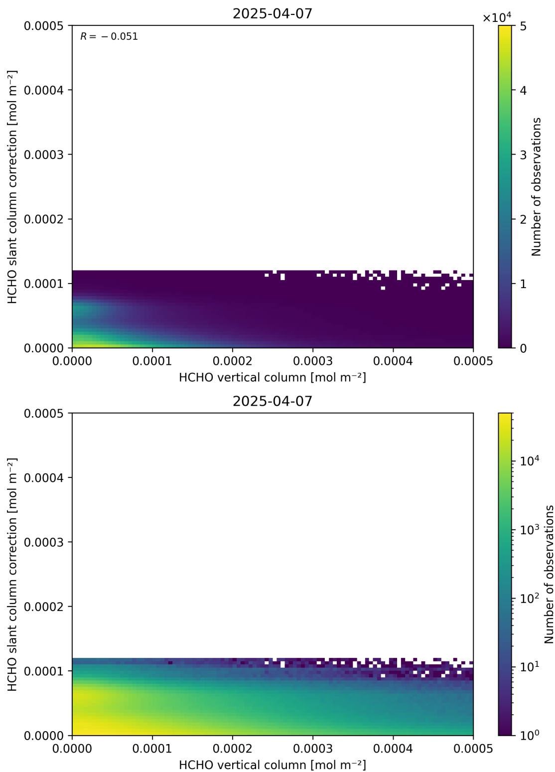
Figure 128: Scatter density plot of “HCHO vertical column” against “HCHO slant column correction” for 2025-04-06 to 2025-04-08.
