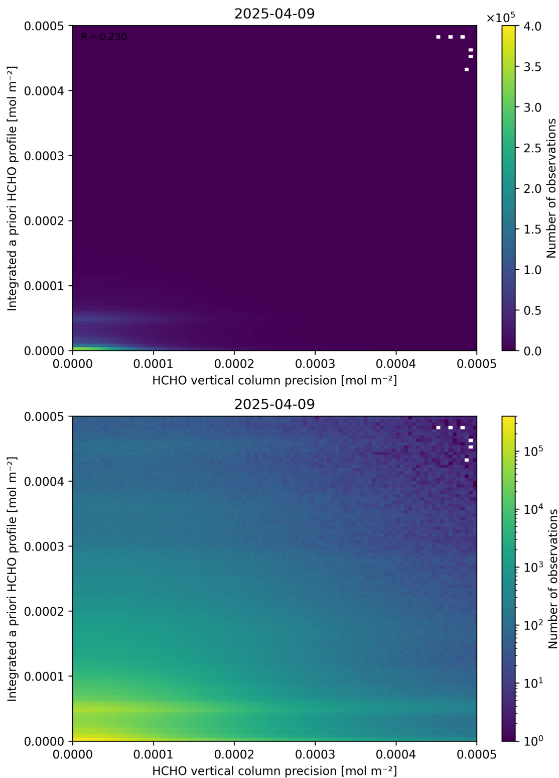
Figure 147: Scatter density plot of “HCHO vertical column precision” against “Integrated a priori HCHO profile” for 2025-04-08 to 2025-04-10.
