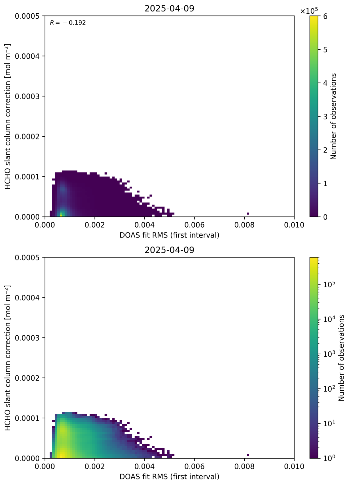
Figure 63: Scatter density plot of “DOAS fit RMS (first interval)” against “HCHO slant column correction” for 2025-04-08 to 2025-04-10.
