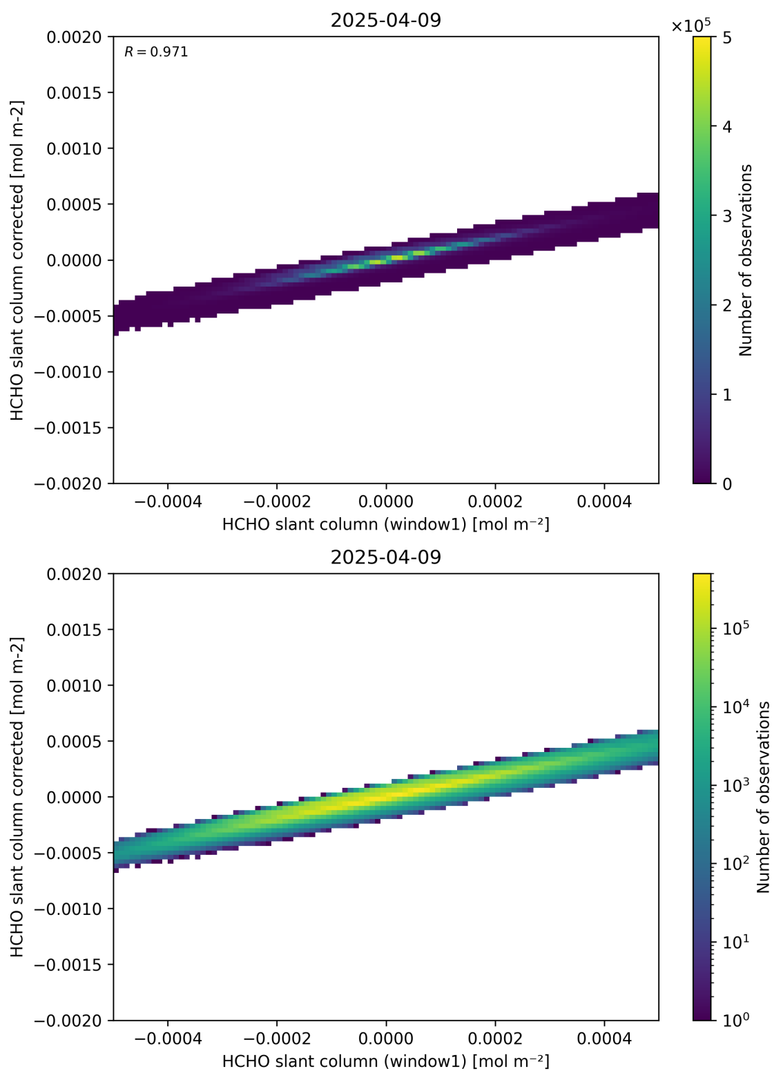
Figure 82: Scatter density plot of “HCHO slant column (window1)” against “HCHO slant column corrected” for 2025-04-08 to 2025-04-10.
