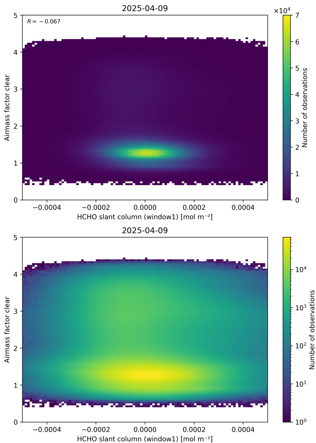
Figure 81: Scatter density plot of “HCHO slant column (window1)” against “Airmass factor clear” for 2025-04-08 to 2025-04-10.
