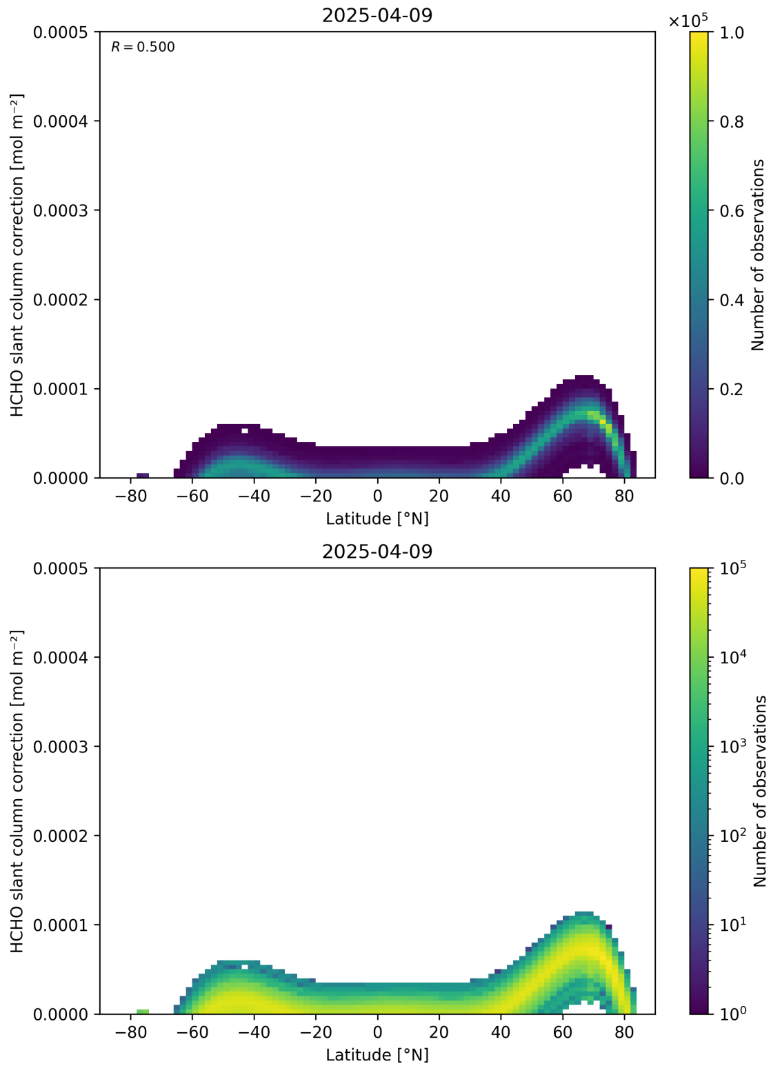
Figure 158: Scatter density plot of “Latitude” against “HCHO slant column correction” for 2025-04-08 to 2025-04-10.
