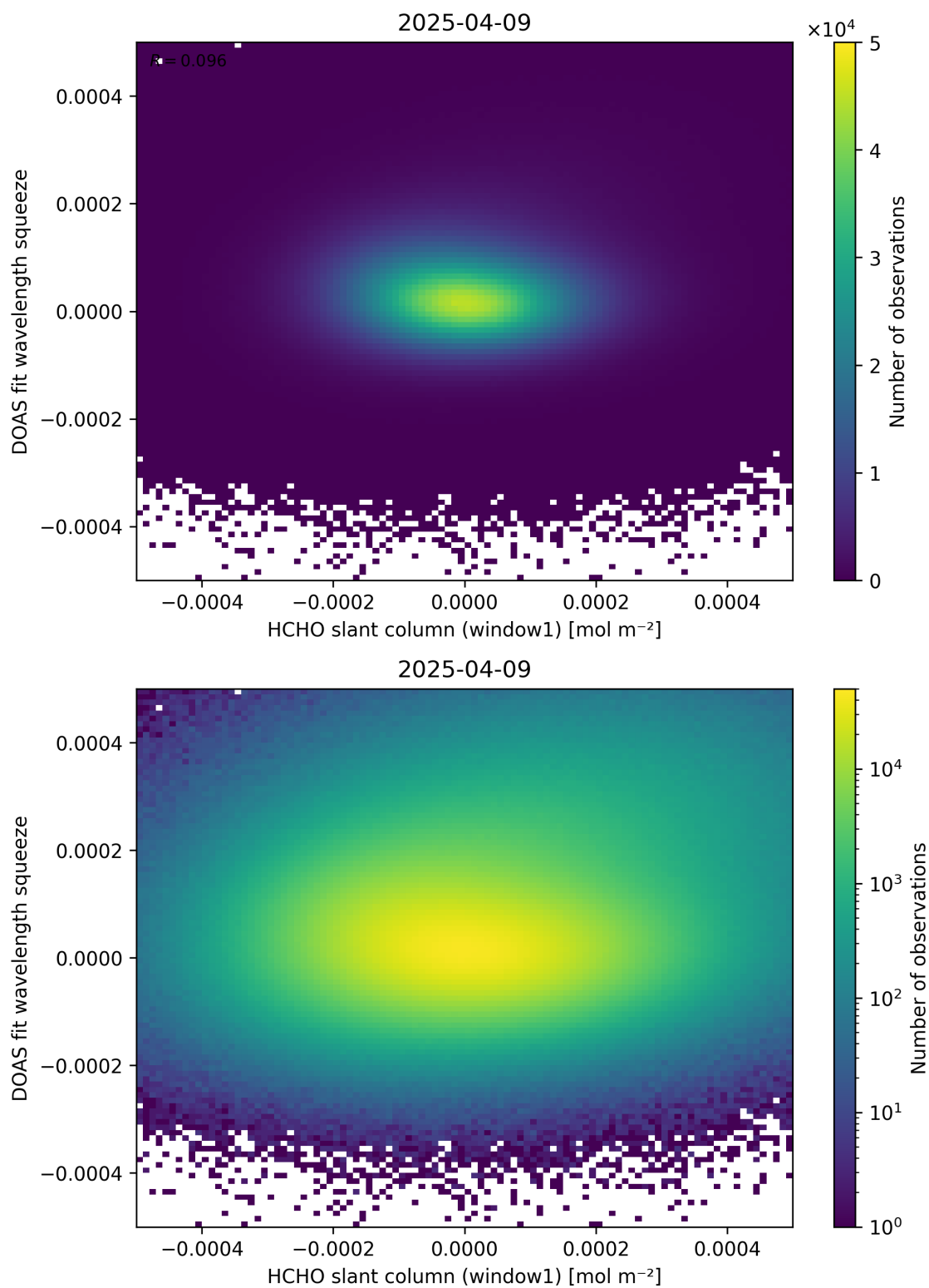
Figure 80: Scatter density plot of “HCHO slant column (window1)” against “DOAS fit wavelength squeeze” for 2025-04-08 to 2025-04-10.
