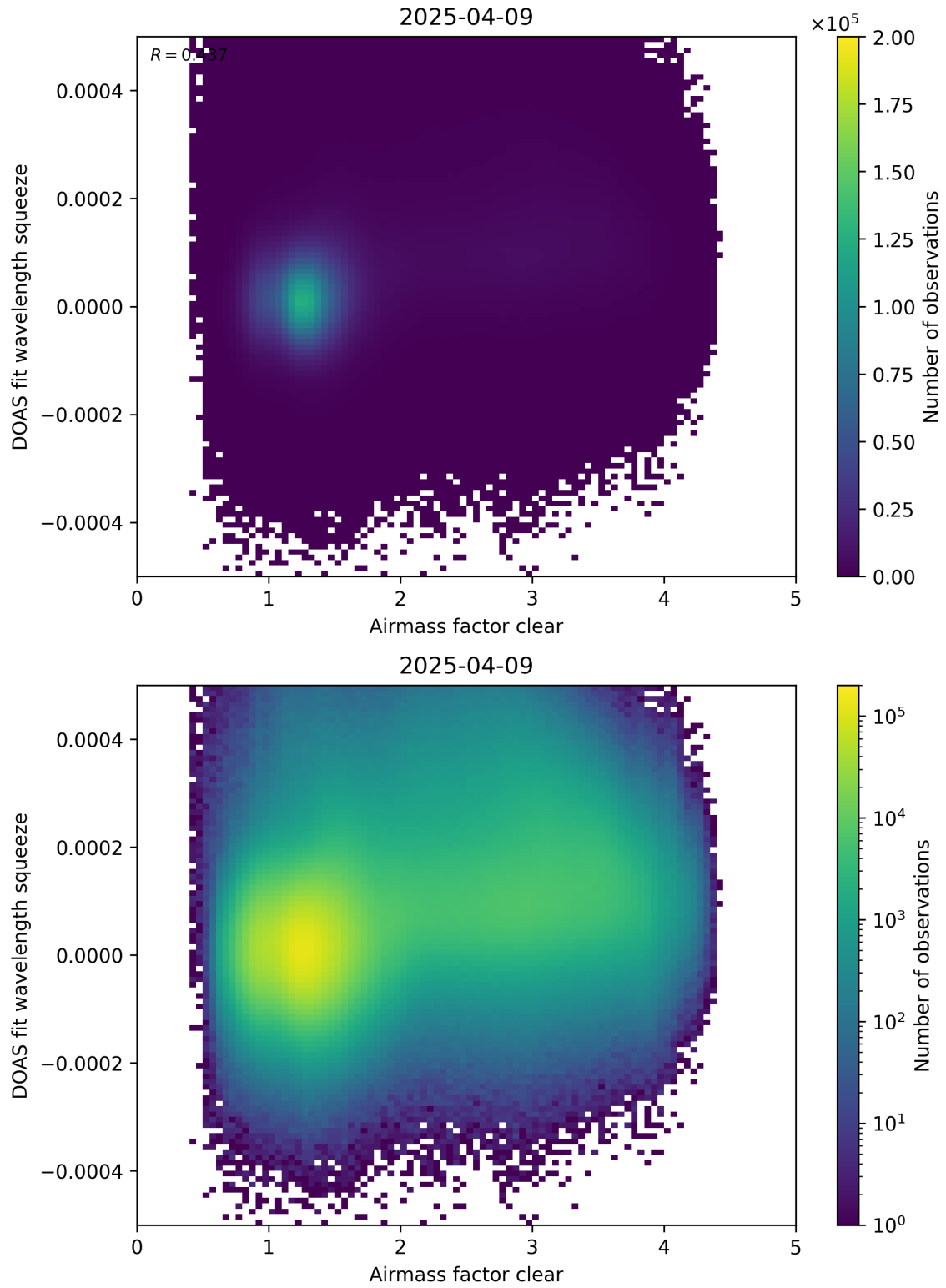
Figure 73: Scatter density plot of “Airmass factor clear” against “DOAS fit wavelength squeeze” for 2025-04-08 to 2025-04-10.
