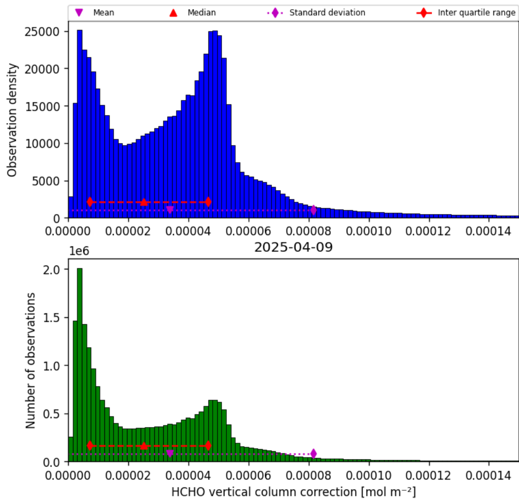
Figure 37: Histogram of “HCHO vertical column correction” for 2025-04-08 to 2025-04-10
