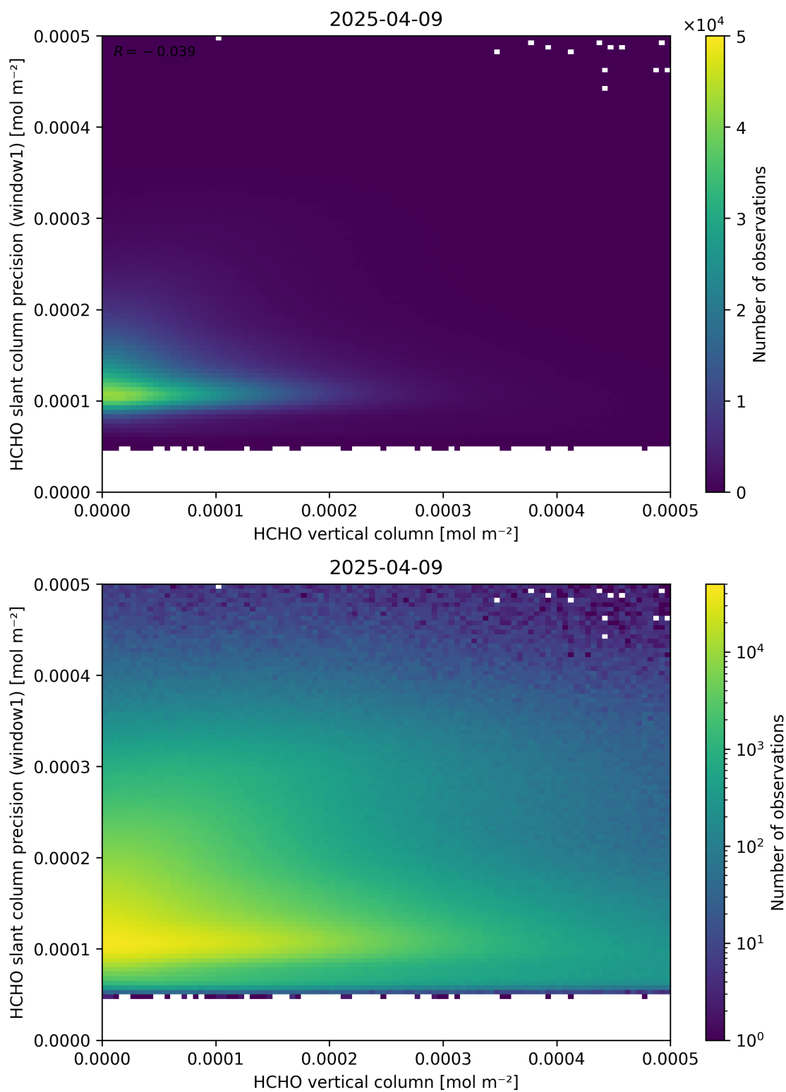
Figure 130: Scatter density plot of “HCHO vertical column” against “HCHO slant column precision (window1)” for 2025-04-08 to 2025-04-10.
