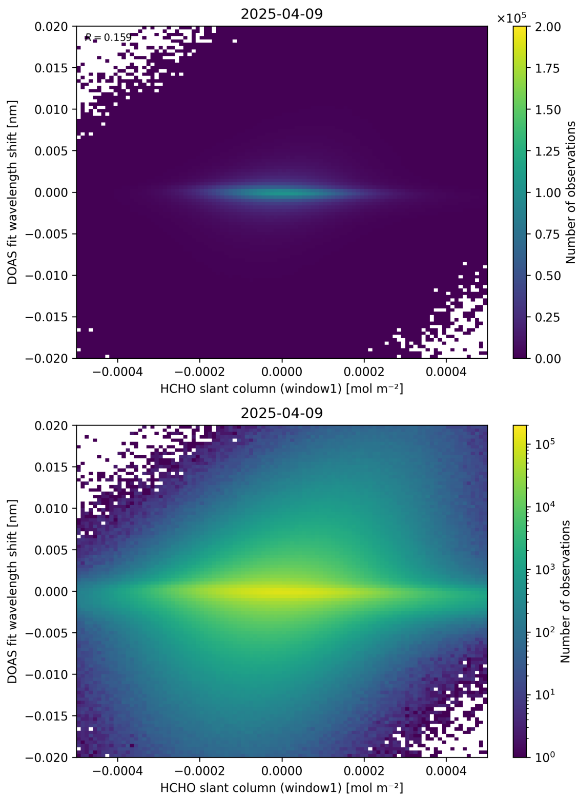
Figure 79: Scatter density plot of “HCHO slant column (window1)” against “DOAS fit wavelength shift” for 2025-04-08 to 2025-04-10.
