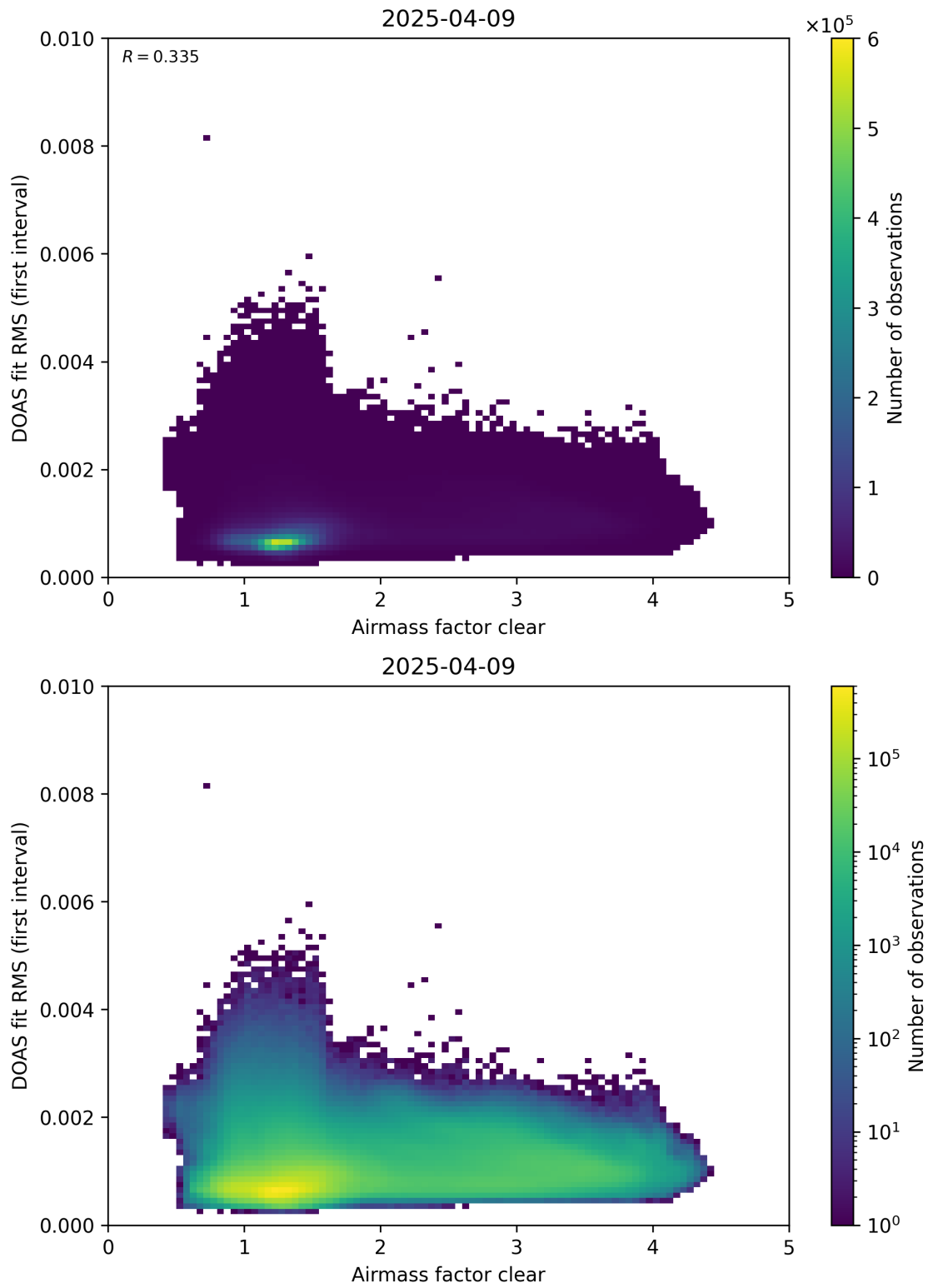
Figure 71: Scatter density plot of “Airmass factor clear” against “DOAS fit RMS (first interval)” for 2025-04-08 to 2025-04-10.
