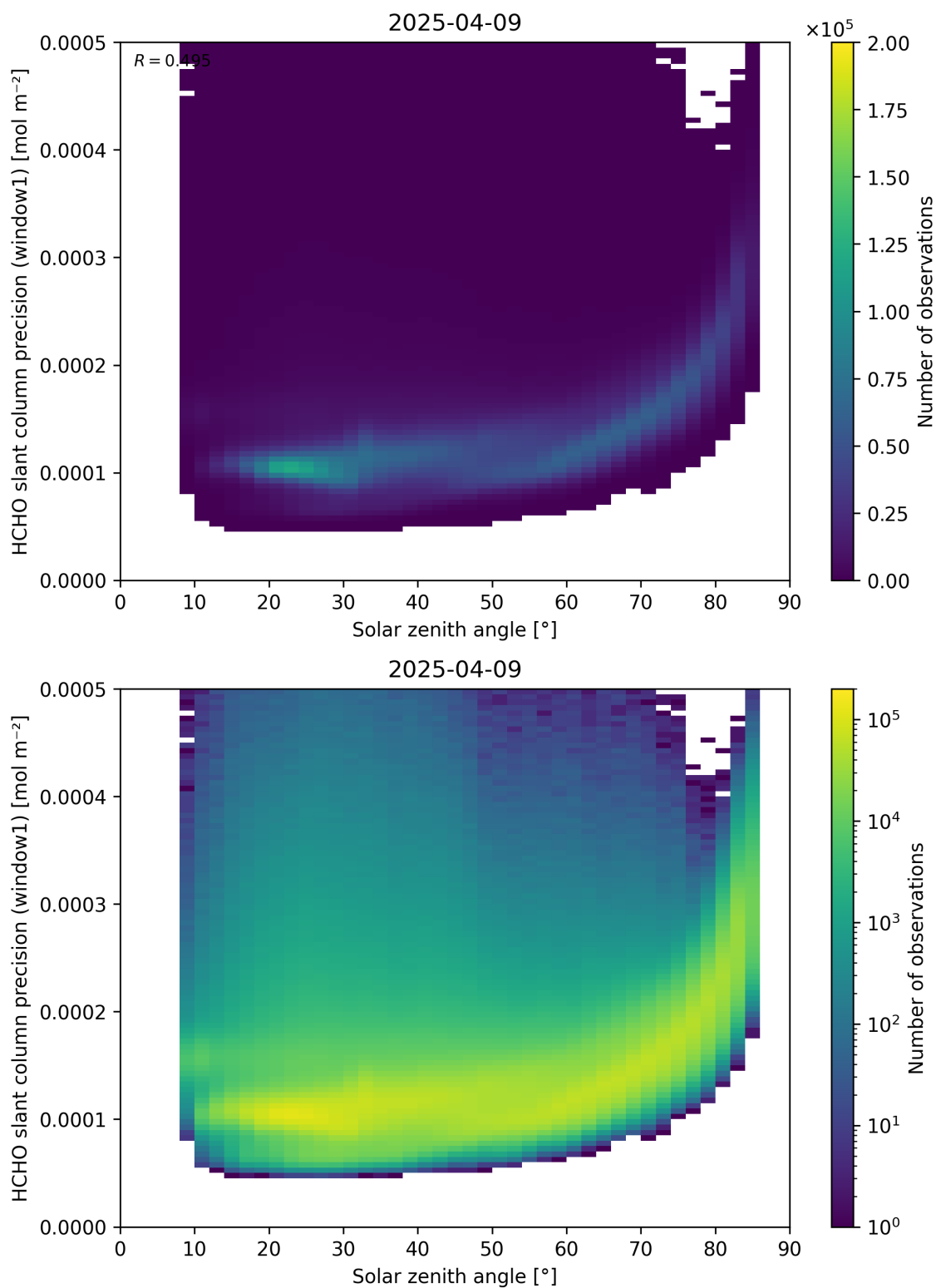
Figure 174: Scatter density plot of “Solar zenith angle” against “HCHO slant column precision (window1)” for 2025-04-08 to 2025-04-10.
