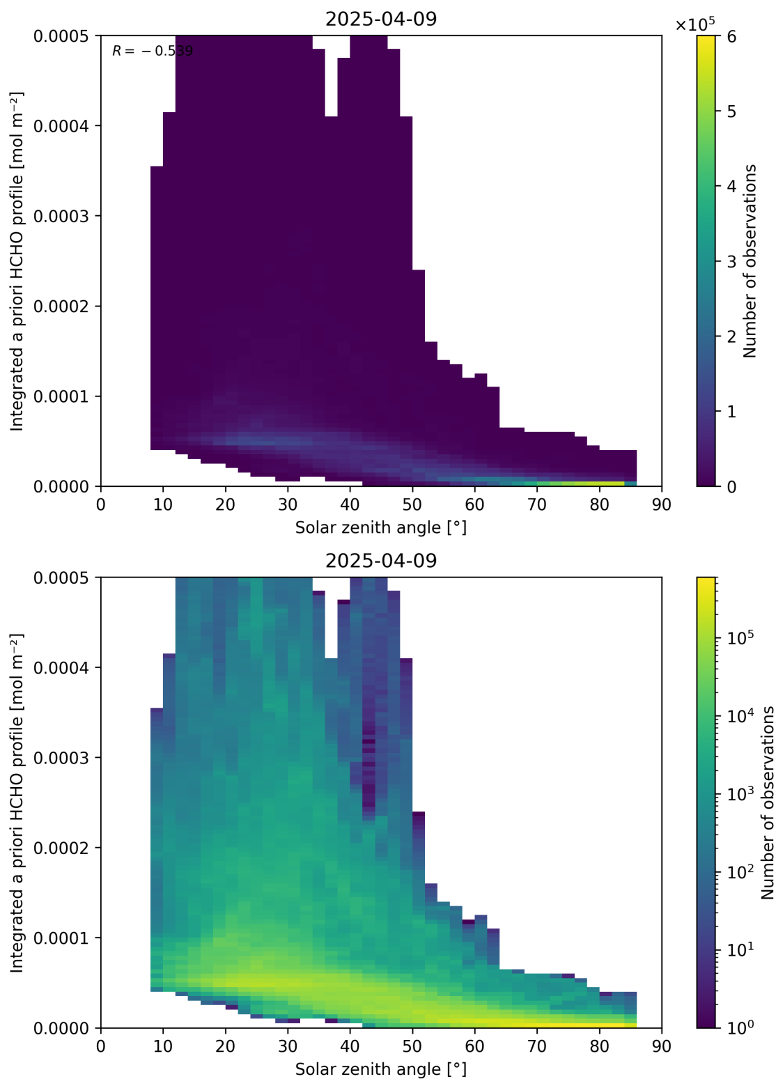
Figure 180: Scatter density plot of “Solar zenith angle” against “Integrated a priori HCHO profile” for 2025-04-08 to 2025-04-10.
