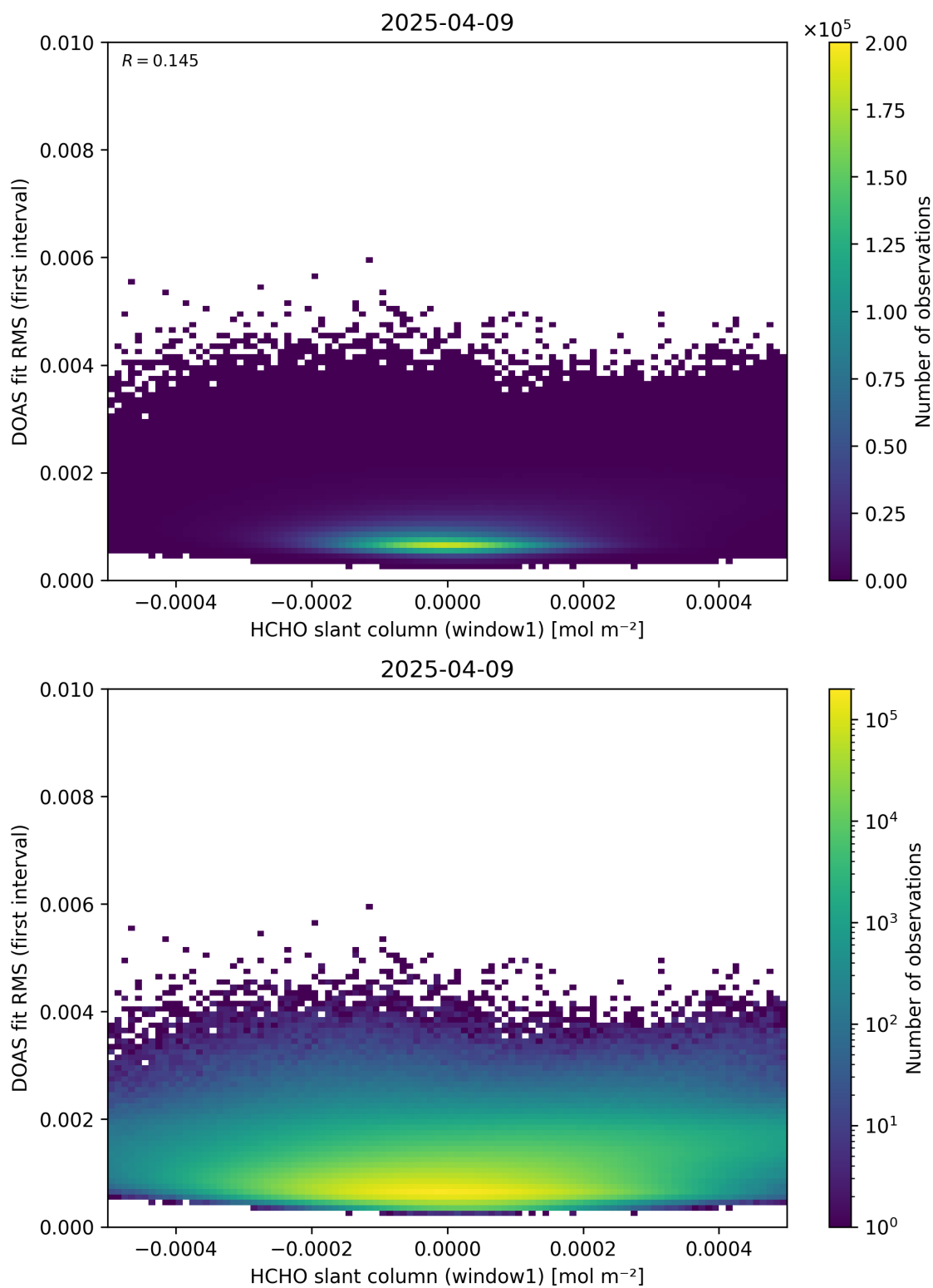
Figure 78: Scatter density plot of “HCHO slant column (window1)” against “DOAS fit RMS (first interval)” for 2025-04-08 to 2025-04-10.
