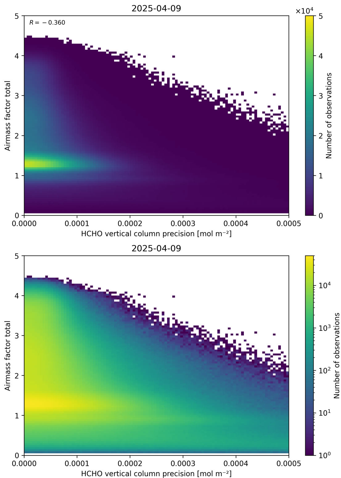
Figure 144: Scatter density plot of “HCHO vertical column precision” against “Airmass factor total” for 2025-04-08 to 2025-04-10.
