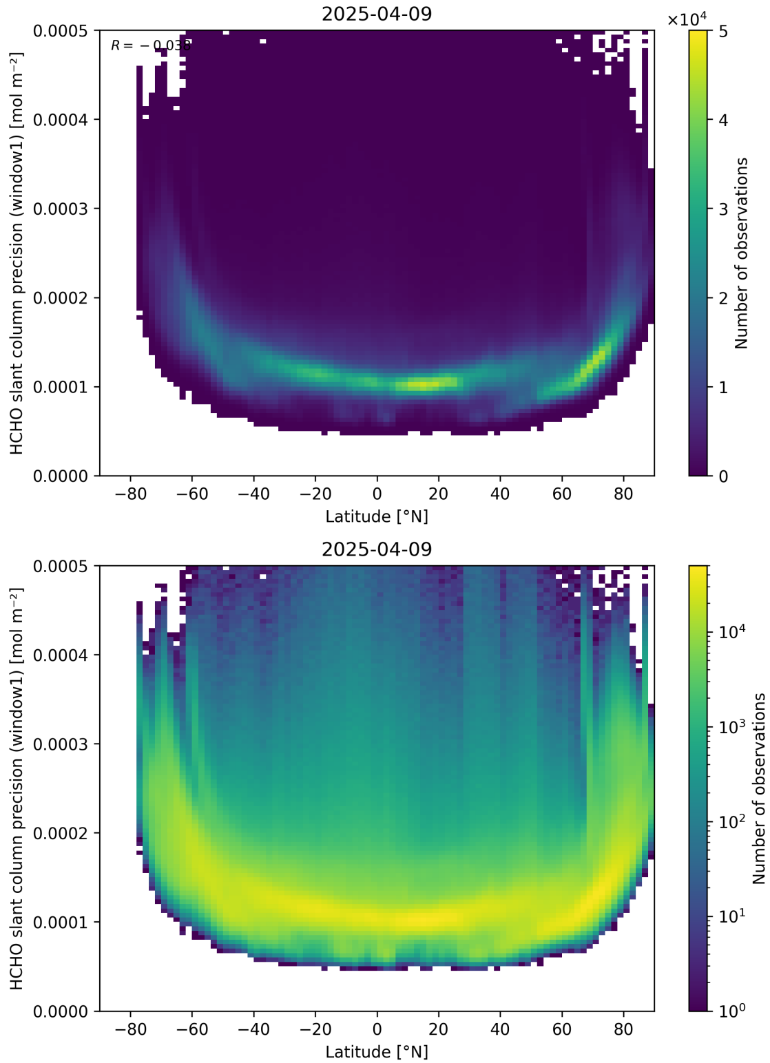
Figure 160: Scatter density plot of “Latitude” against “HCHO slant column precision (window1)” for 2025-04-08 to 2025-04-10.
