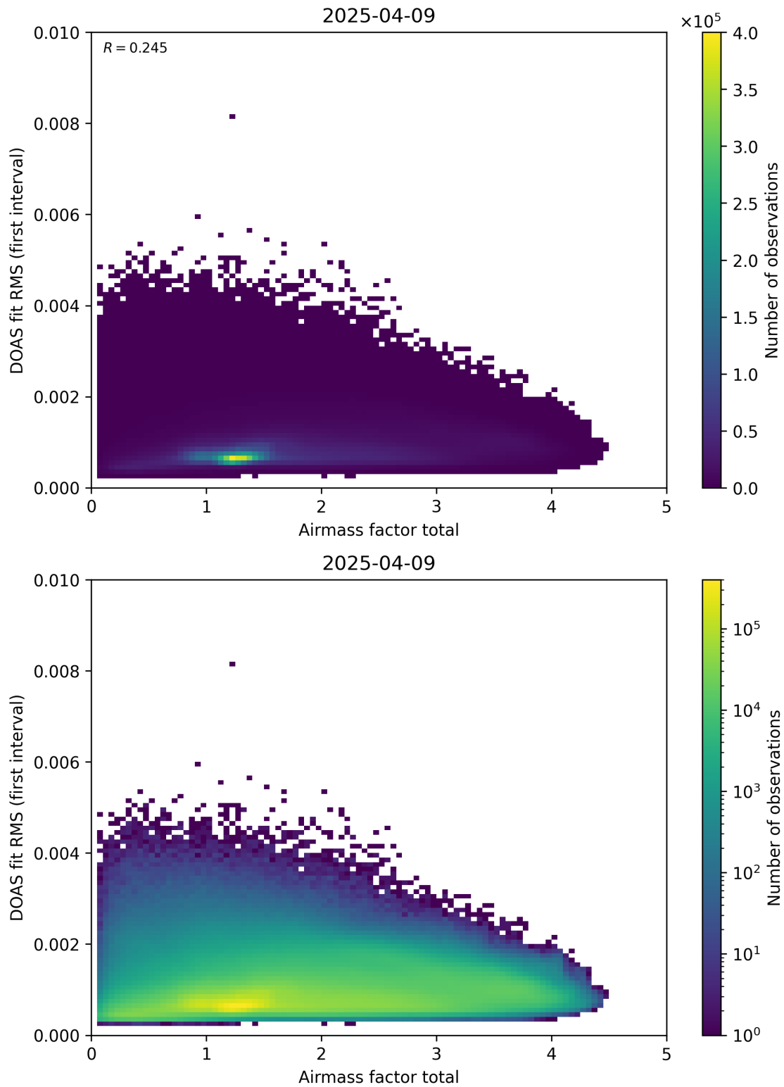
Figure 97: Scatter density plot of “Airmass factor total” against “DOAS fit RMS (first interval)” for 2025-04-08 to 2025-04-10.
