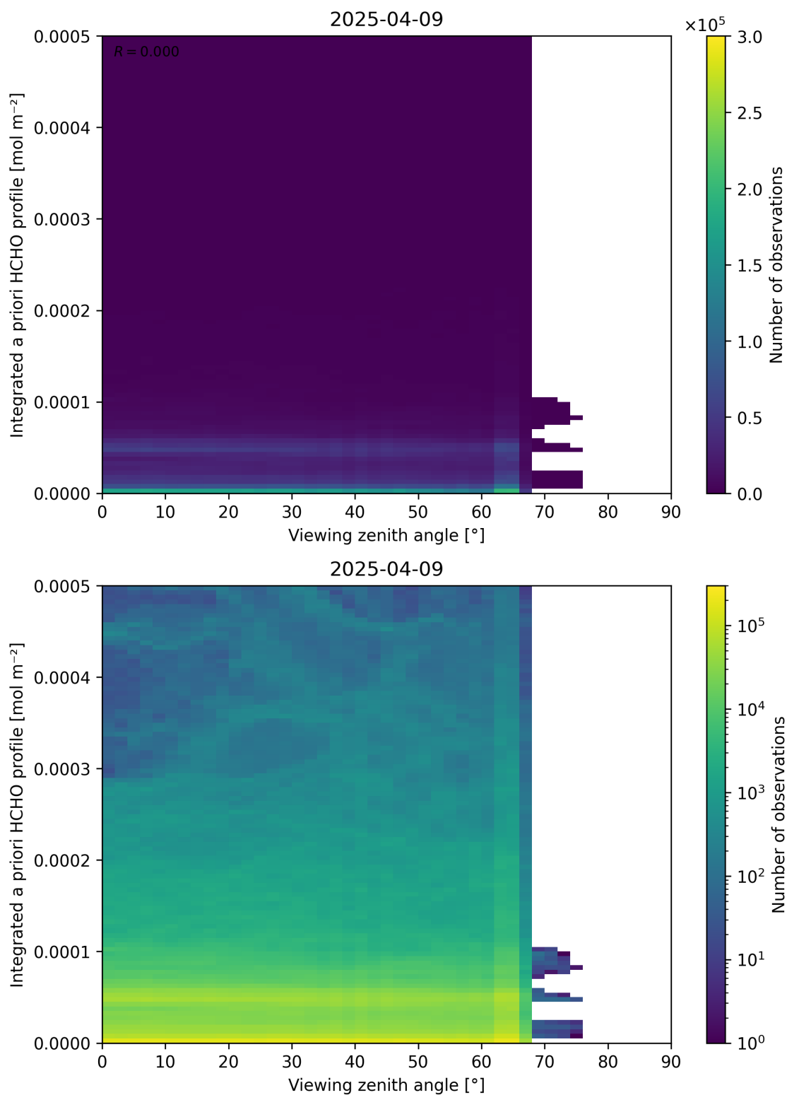
Figure 195: Scatter density plot of “Viewing zenith angle” against “Integrated a priori HCHO profile” for 2025-04-08 to 2025-04-10.
