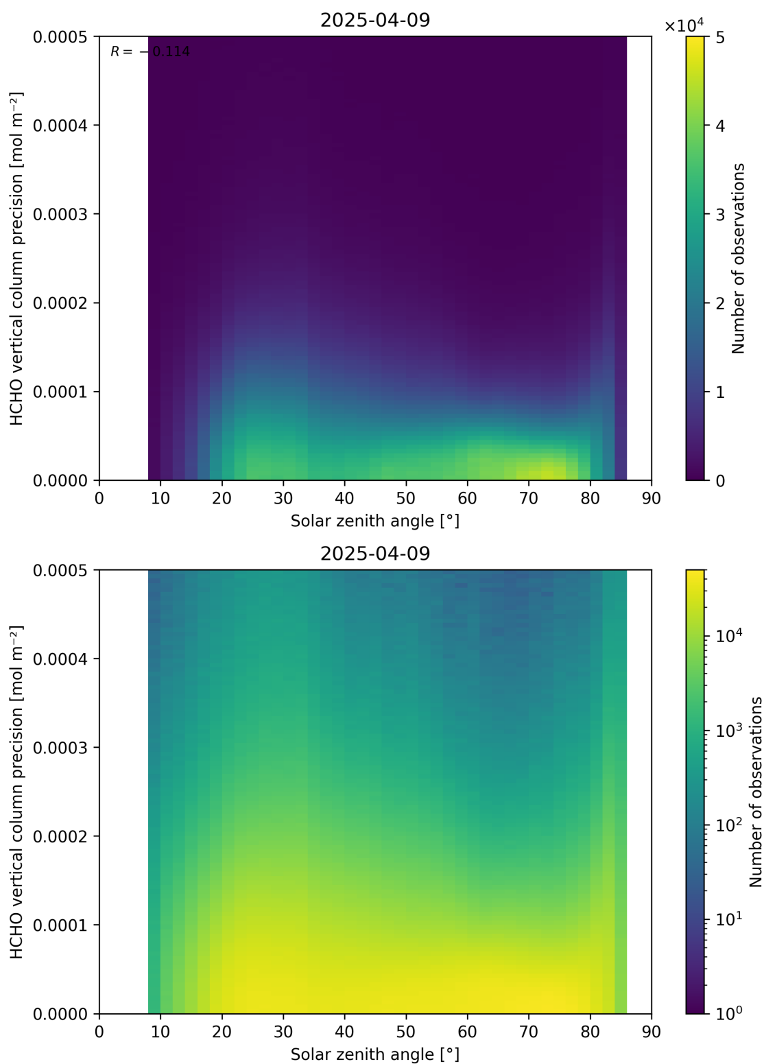
Figure 179: Scatter density plot of “Solar zenith angle” against “HCHO vertical column precision” for 2025-04-08 to 2025-04-10.
