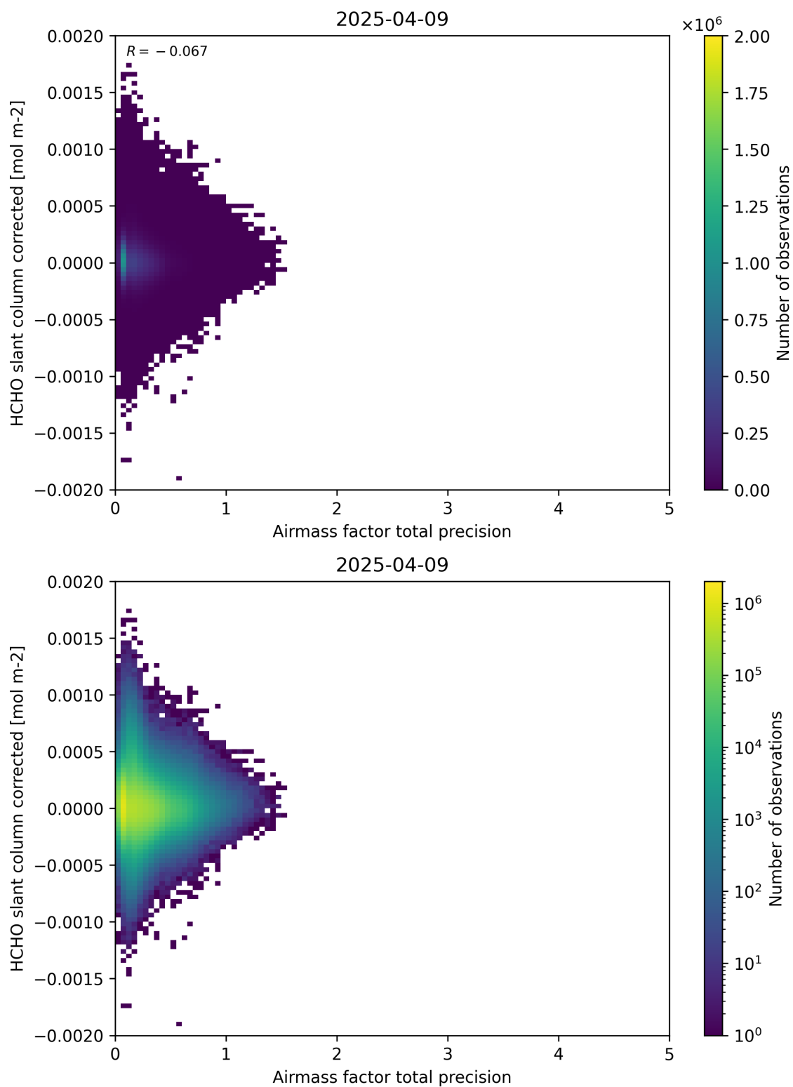
Figure 109: Scatter density plot of “Airmass factor total precision” against “HCHO slant column corrected” for 2025-04-08 to 2025-04-10.
