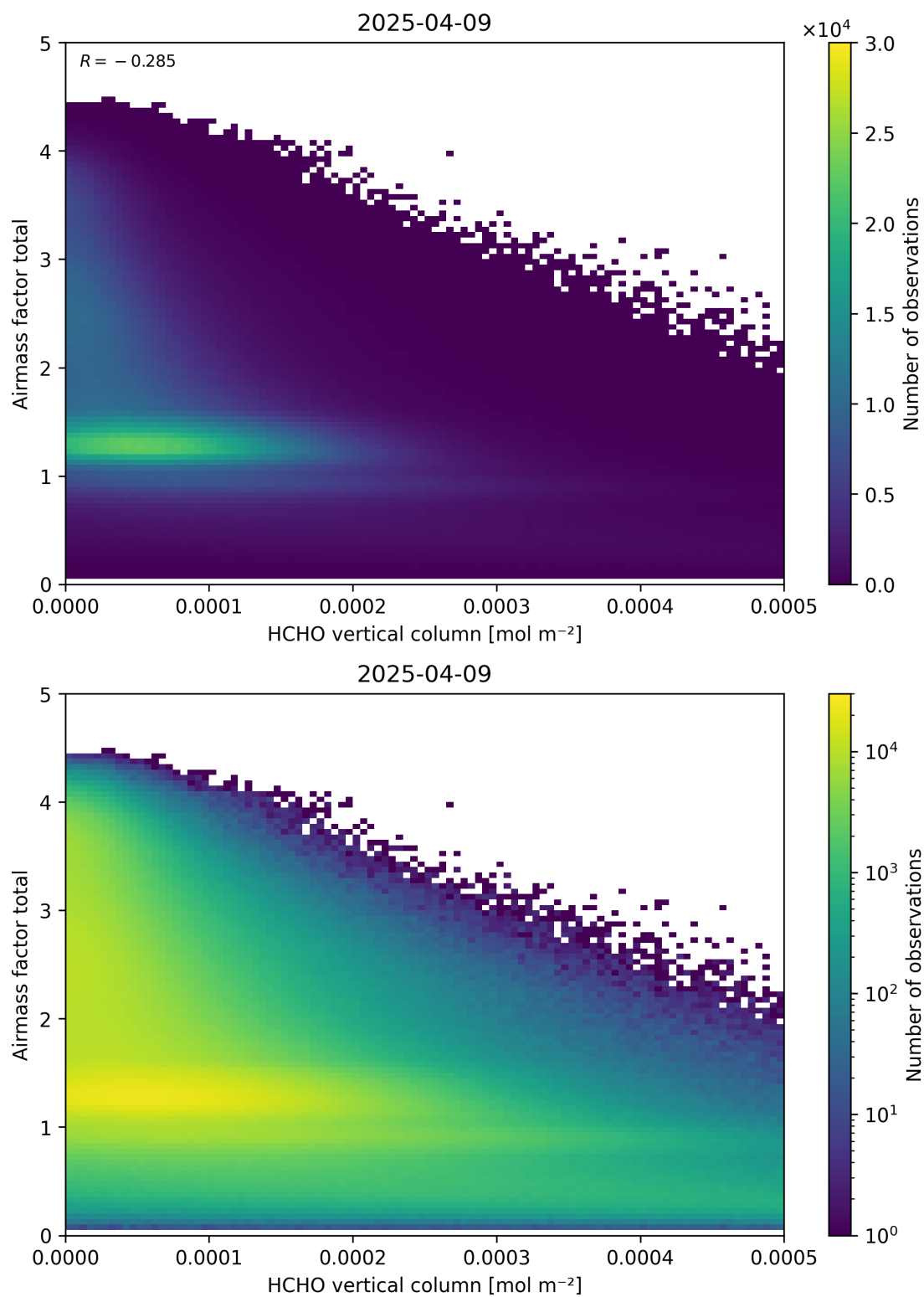
Figure 131: Scatter density plot of “HCHO vertical column” against “Airmass factor total” for 2025-04-08 to 2025-04-10.
