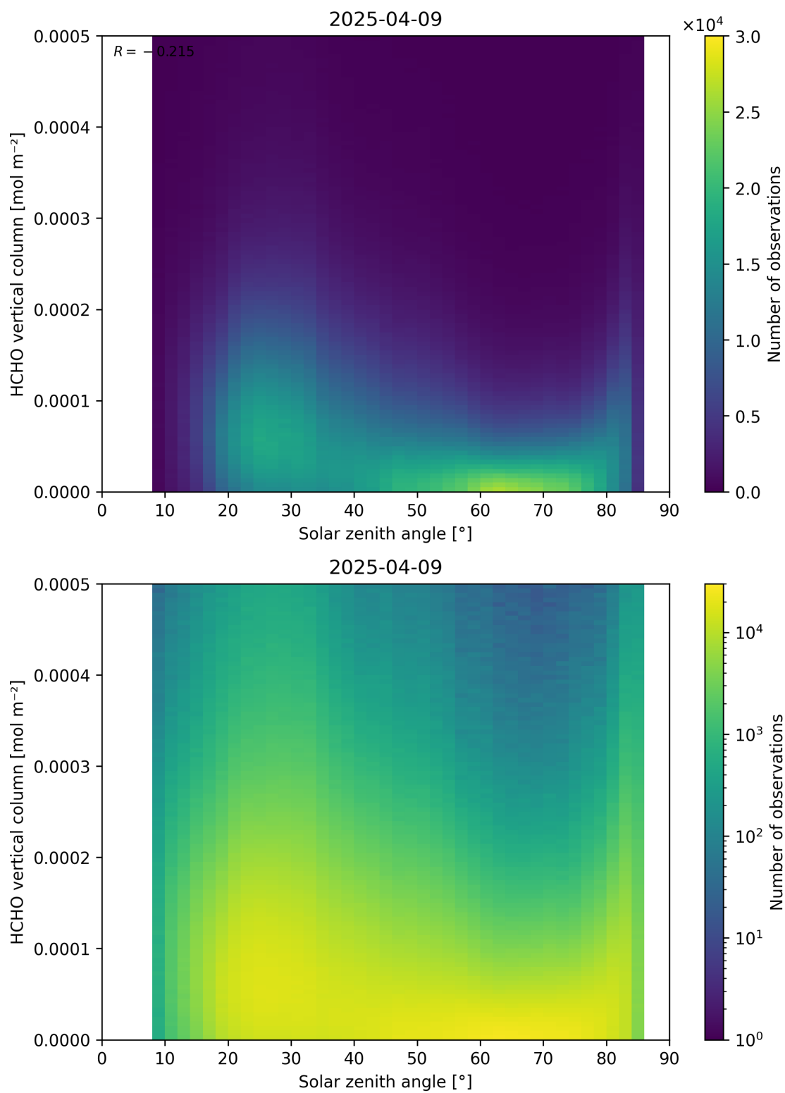
Figure 177: Scatter density plot of “Solar zenith angle” against “HCHO vertical column” for 2025-04-08 to 2025-04-10.
