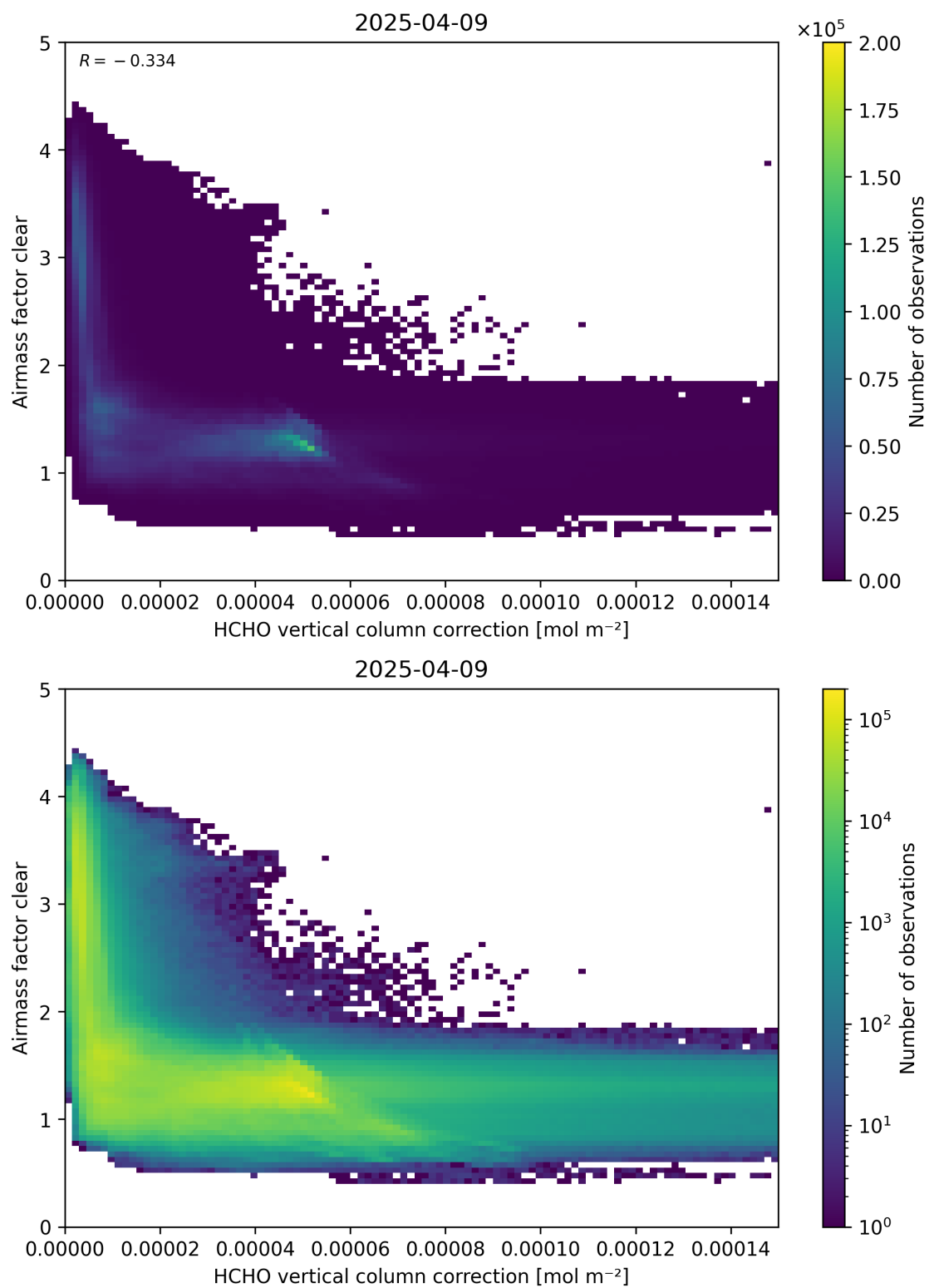
Figure 115: Scatter density plot of “HCHO vertical column correction” against “Airmass factor clear” for 2025-04-08 to 2025-04-10.
