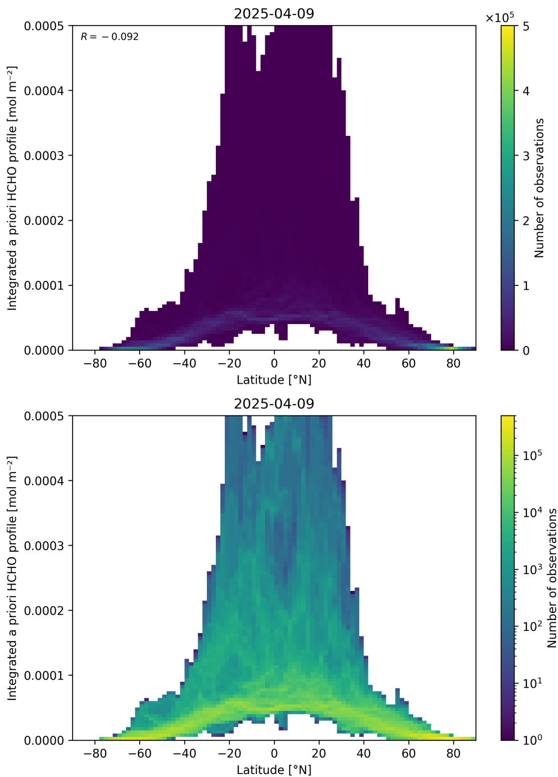
Figure 166: Scatter density plot of “Latitude” against “Integrated a priori HCHO profile” for 2025-04-08 to 2025-04-10.
