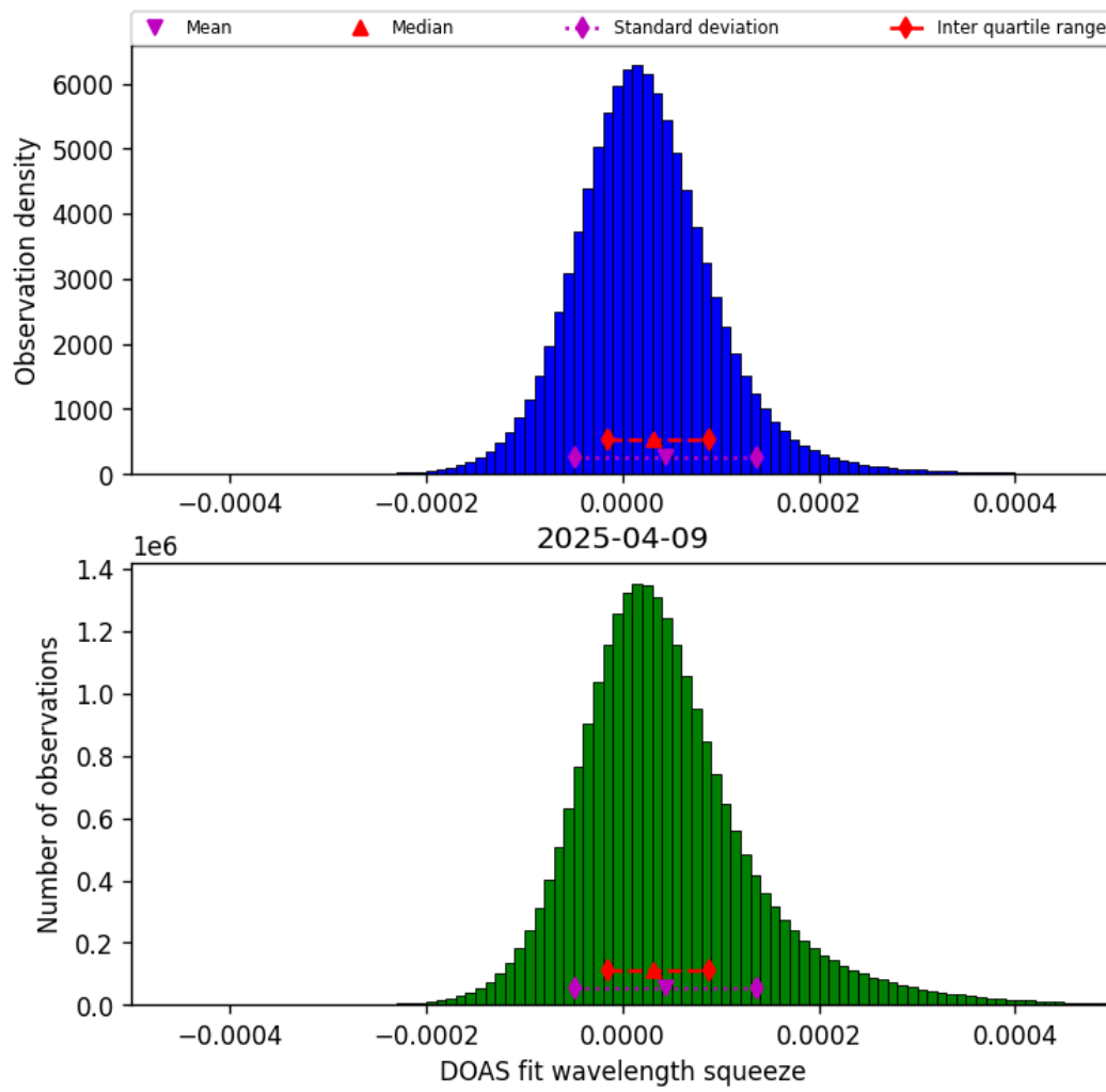
Figure 45: Histogram of “DOAS fit wavelength squeeze” for 2025-04-08 to 2025-04-10
