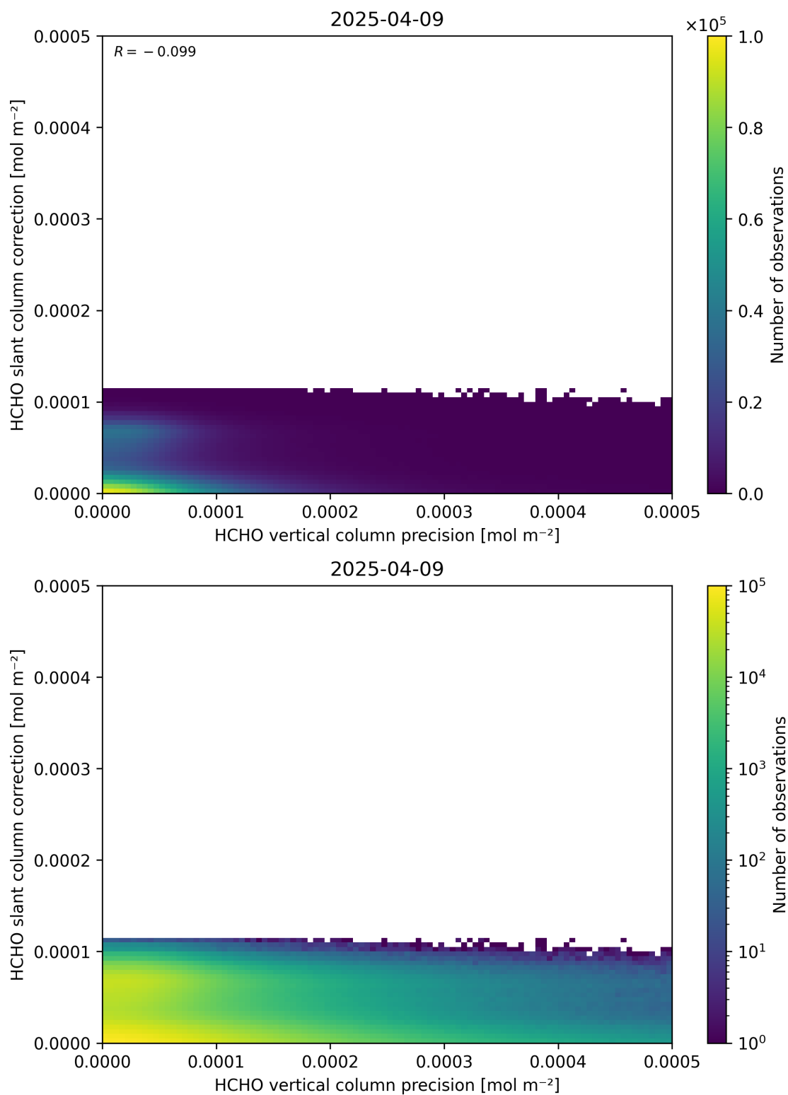
Figure 141: Scatter density plot of “HCHO vertical column precision” against “HCHO slant column correction” for 2025-04-08 to 2025-04-10.
