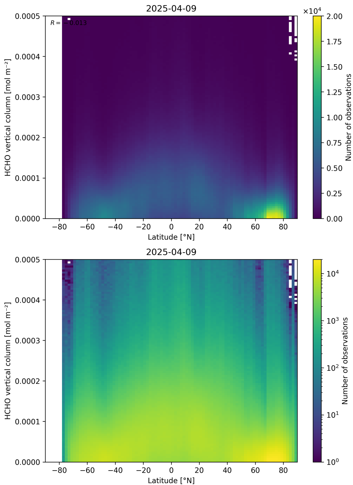
Figure 163: Scatter density plot of “Latitude” against “HCHO vertical column” for 2025-04-08 to 2025-04-10.
