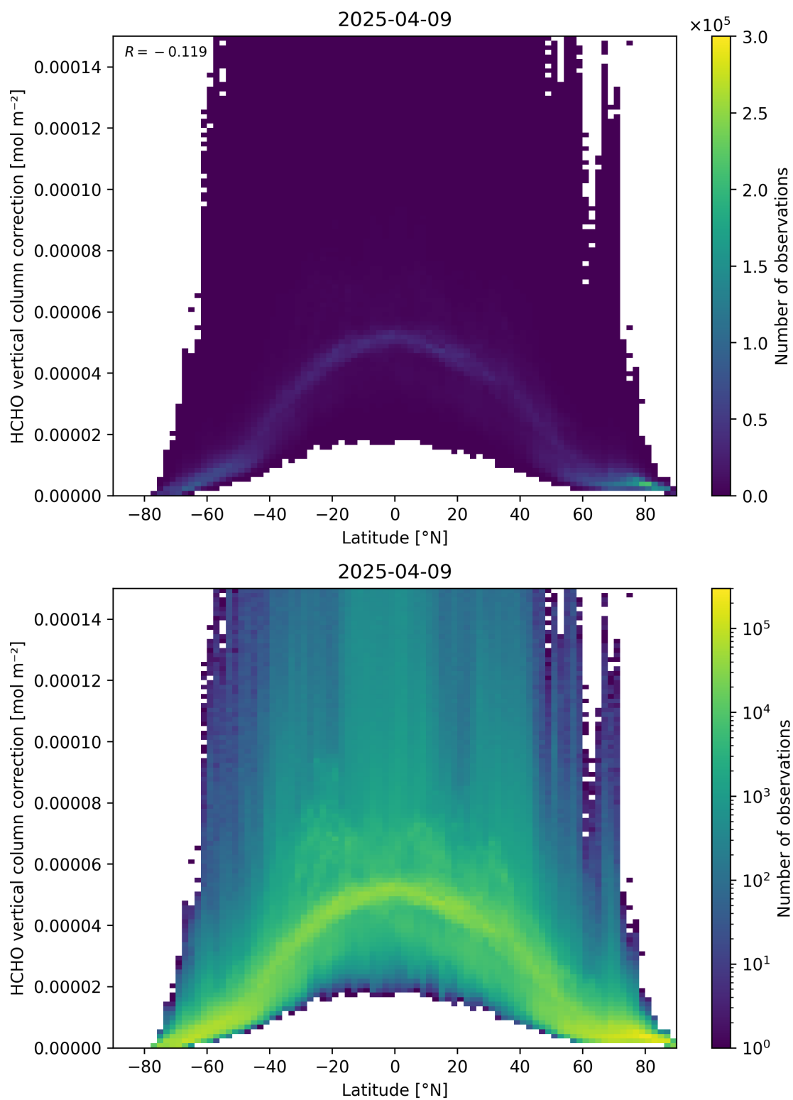
Figure 164: Scatter density plot of “Latitude” against “HCHO vertical column correction” for 2025-04-08 to 2025-04-10.
