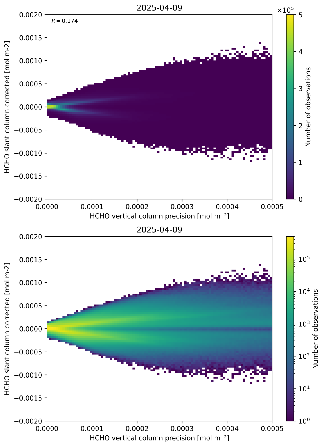
Figure 140: Scatter density plot of “HCHO vertical column precision” against “HCHO slant column corrected” for 2025-04-08 to 2025-04-10.
