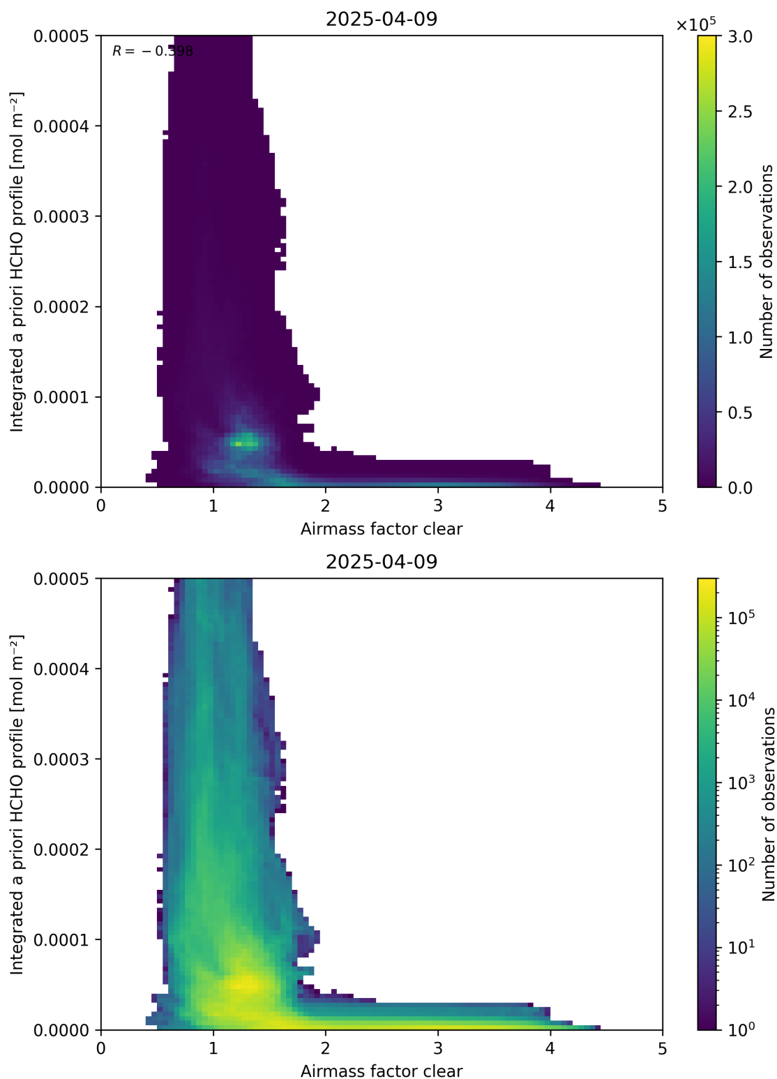
Figure 76: Scatter density plot of “Airmass factor clear” against “Integrated a priori HCHO profile” for 2025-04-08 to 2025-04-10.
