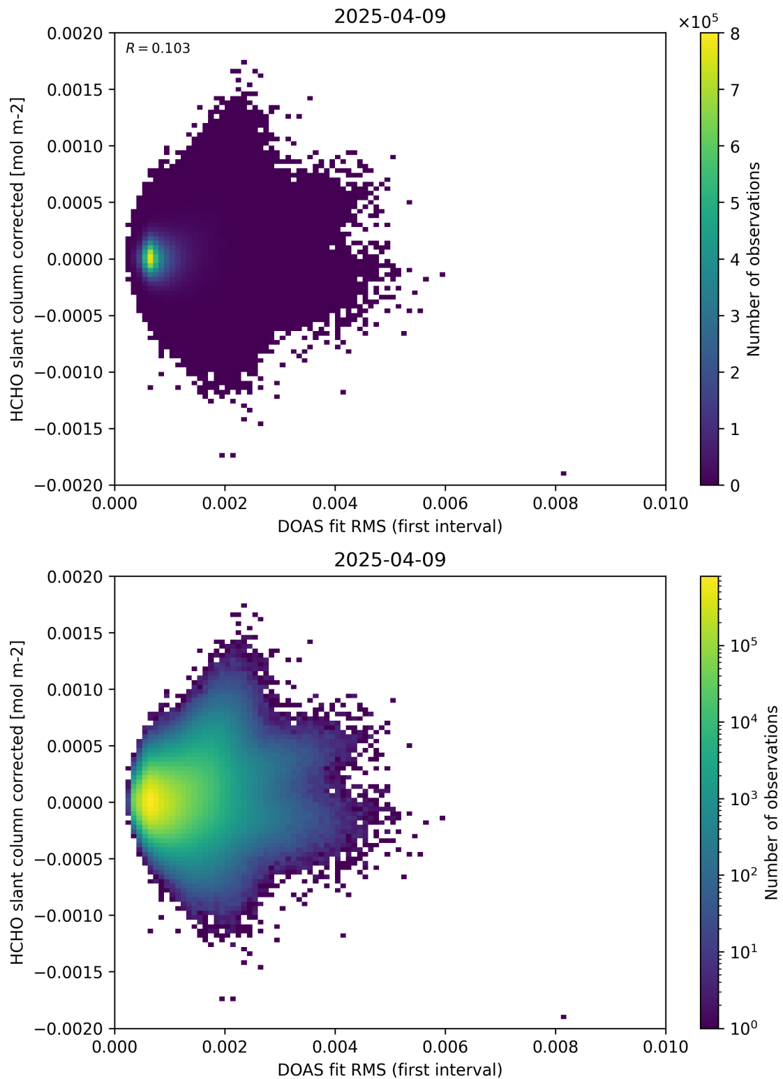
Figure 62: Scatter density plot of “DOAS fit RMS (first interval)” against “HCHO slant column corrected” for 2025-04-08 to 2025-04-10.
