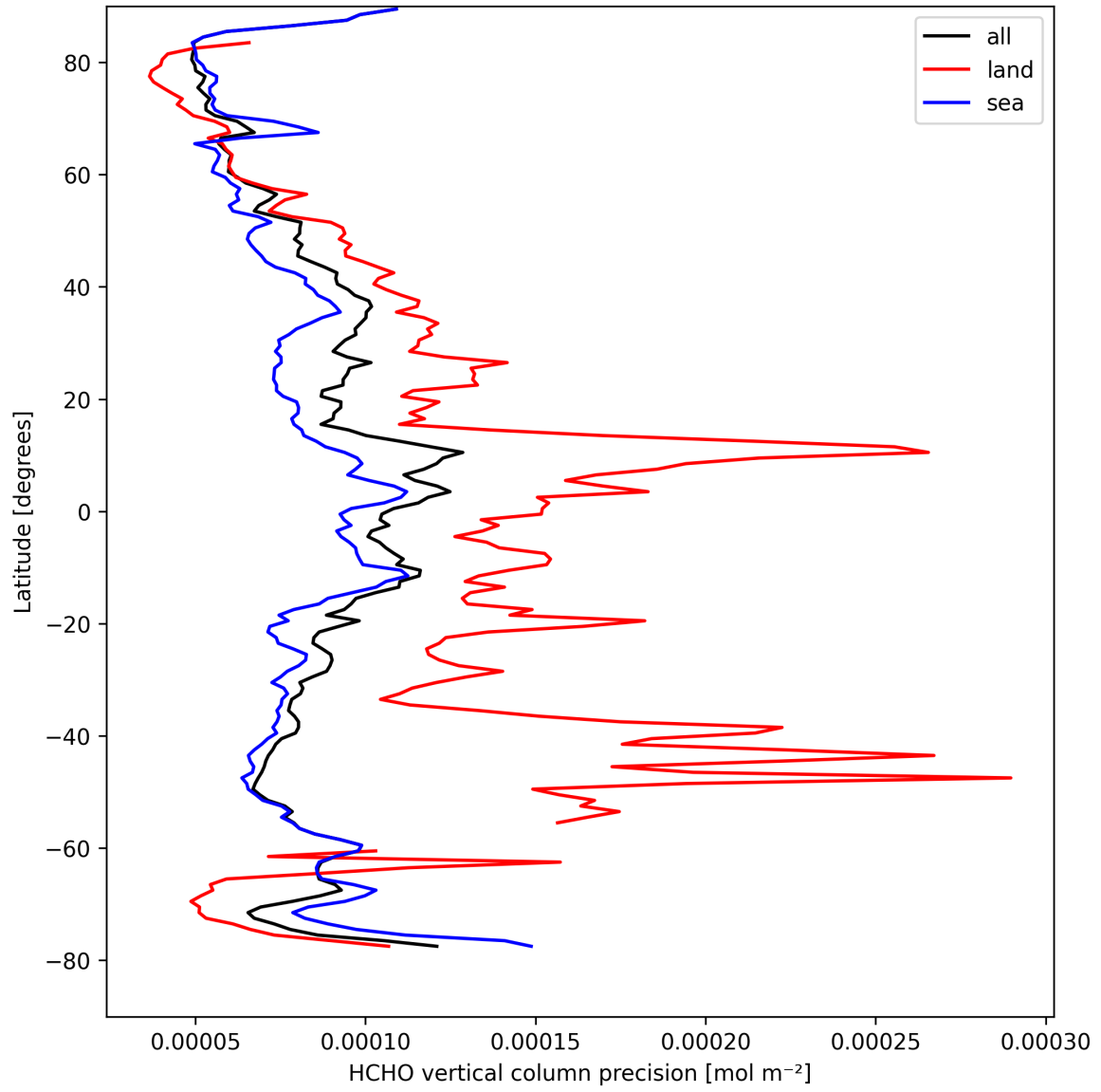
Figure 22: Zonal average of “HCHO vertical column precision” for 2025-04-08 to 2025-04-10.
