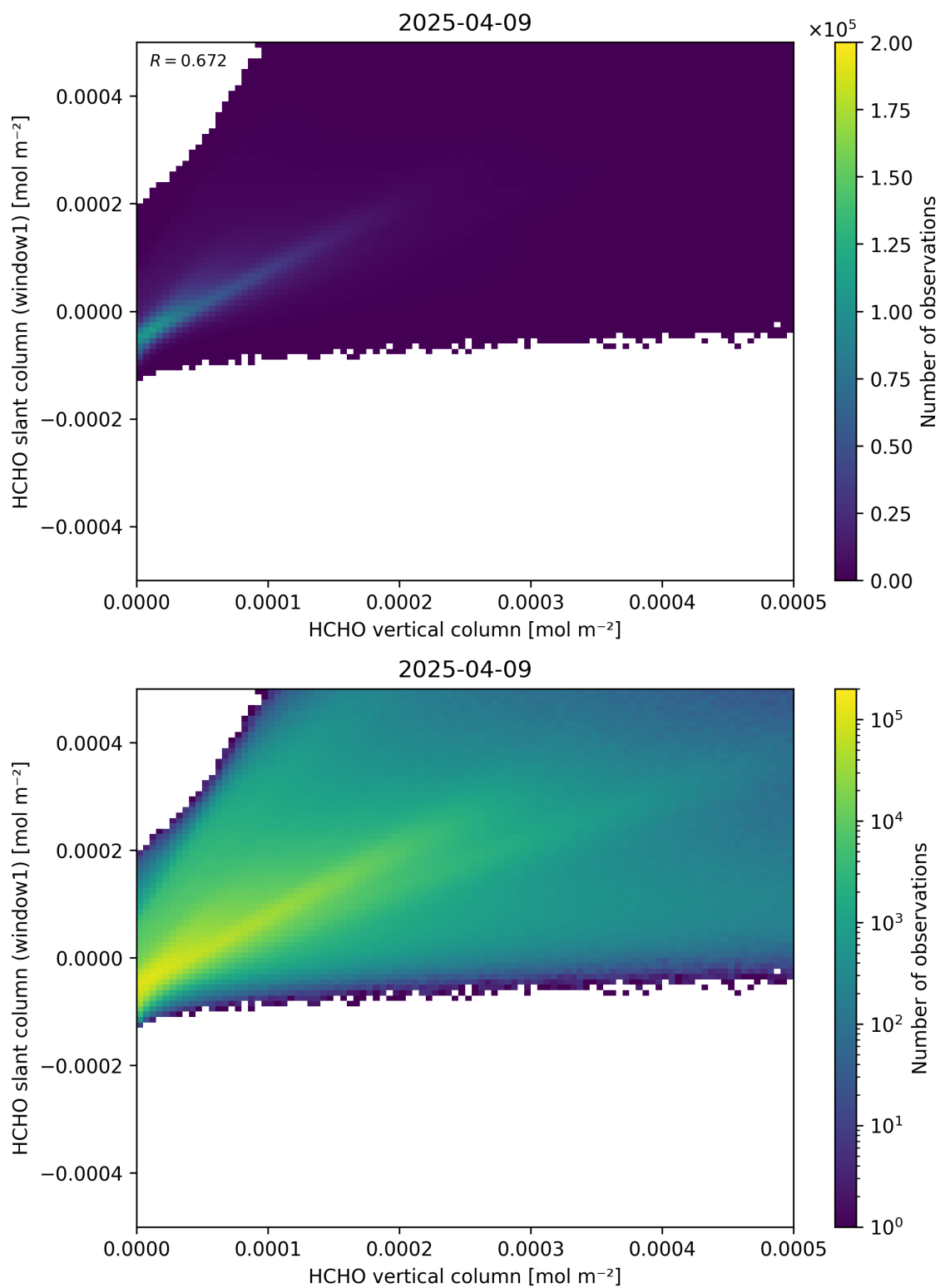
Figure 129: Scatter density plot of “HCHO vertical column” against “HCHO slant column (window1)” for 2025-04-08 to 2025-04-10.
