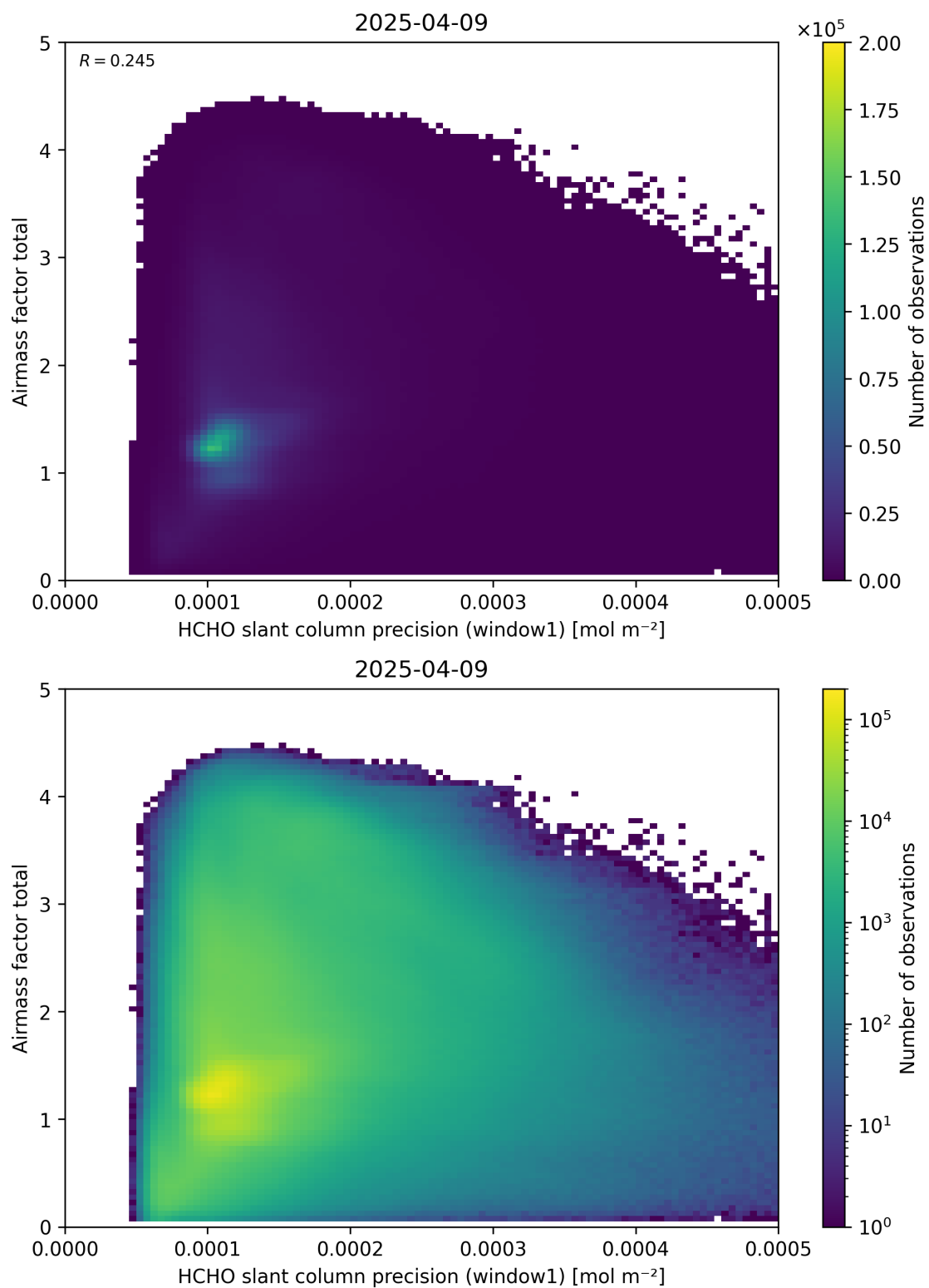
Figure 94: Scatter density plot of “HCHO slant column precision (window1)” against “Airmass factor total” for 2025-04-08 to 2025-04-10.
