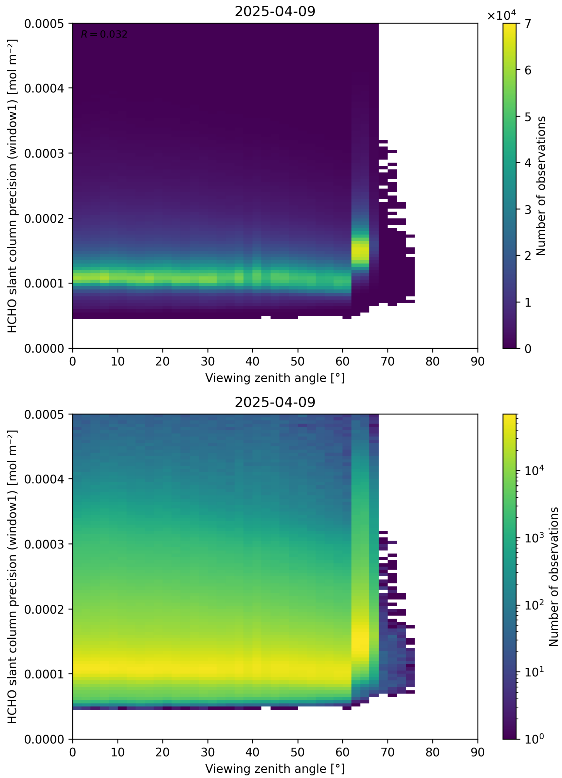
Figure 189: Scatter density plot of “Viewing zenith angle” against “HCHO slant column precision (window1)” for 2025-04-08 to 2025-04-10.
