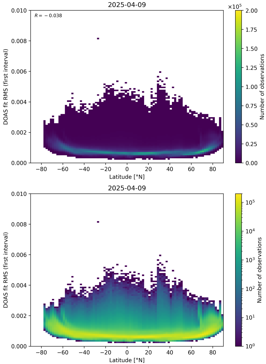
Figure 153: Scatter density plot of “Latitude” against “DOAS fit RMS (first interval)” for 2025-04-08 to 2025-04-10.
