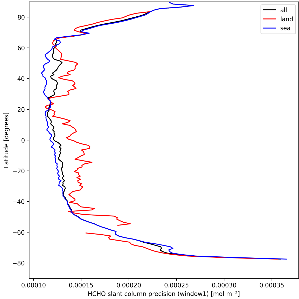
Figure 25: Zonal average of “HCHO slant column precision (window1)” for 2025-04-08 to 2025-04-10.
