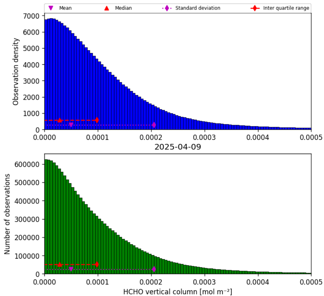
Figure 35: Histogram of “HCHO vertical column” for 2025-04-08 to 2025-04-10
