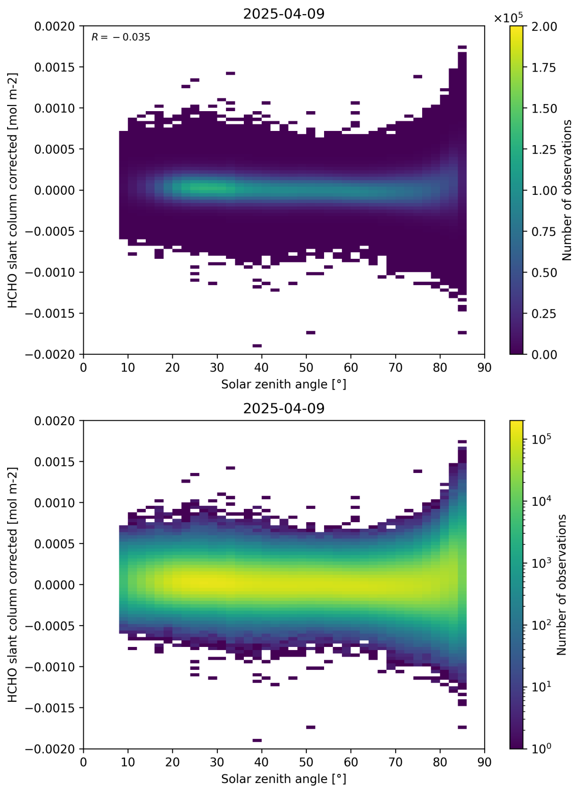
Figure 171: Scatter density plot of “Solar zenith angle” against “HCHO slant column corrected” for 2025-04-08 to 2025-04-10.
