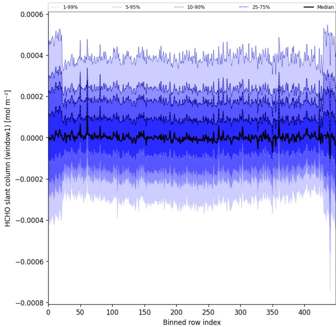
Figure 52: Along track statistics of “HCHO slant column (window1)” for 2025-04-08 to 2025-04-10
