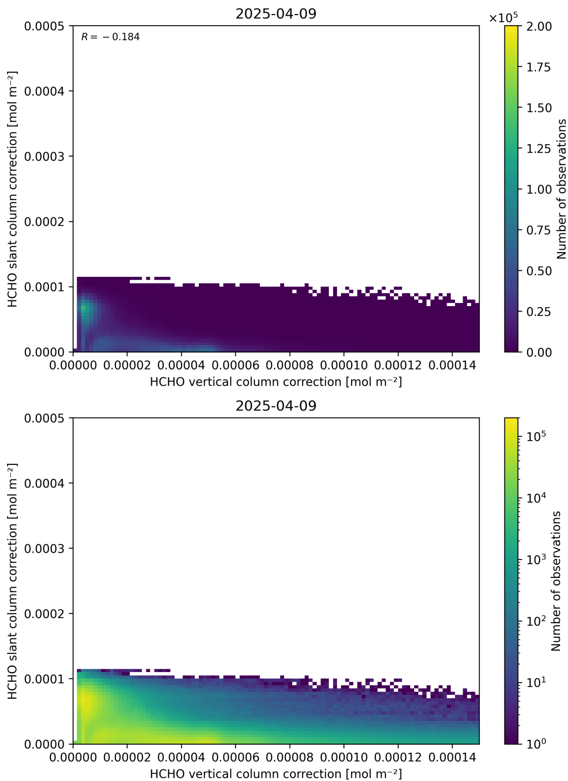
Figure 117: Scatter density plot of “HCHO vertical column correction” against “HCHO slant column correction” for 2025-04-08 to 2025-04-10.
