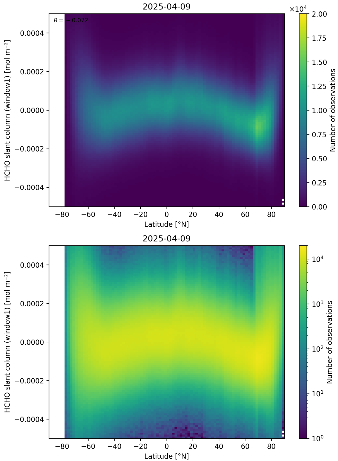
Figure 159: Scatter density plot of “Latitude” against “HCHO slant column (window1)” for 2025-04-08 to 2025-04-10.
