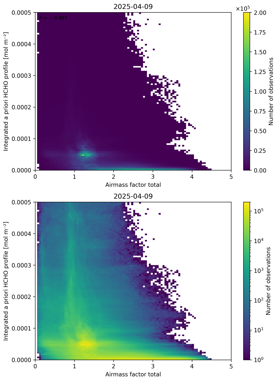
Figure 104: Scatter density plot of “Airmass factor total” against “Integrated a priori HCHO profile” for 2025-04-08 to 2025-04-10.
