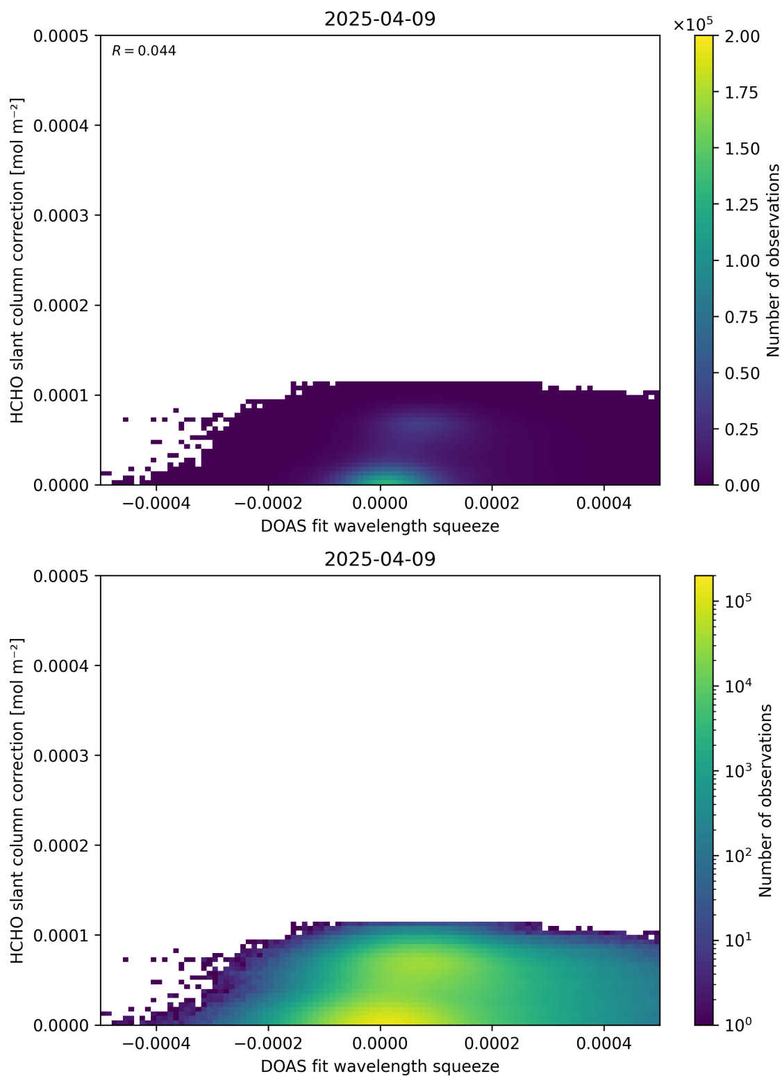
Figure 70: Scatter density plot of “DOAS fit wavelength squeeze” against “HCHO slant column correction” for 2025-04-08 to 2025-04-10.
