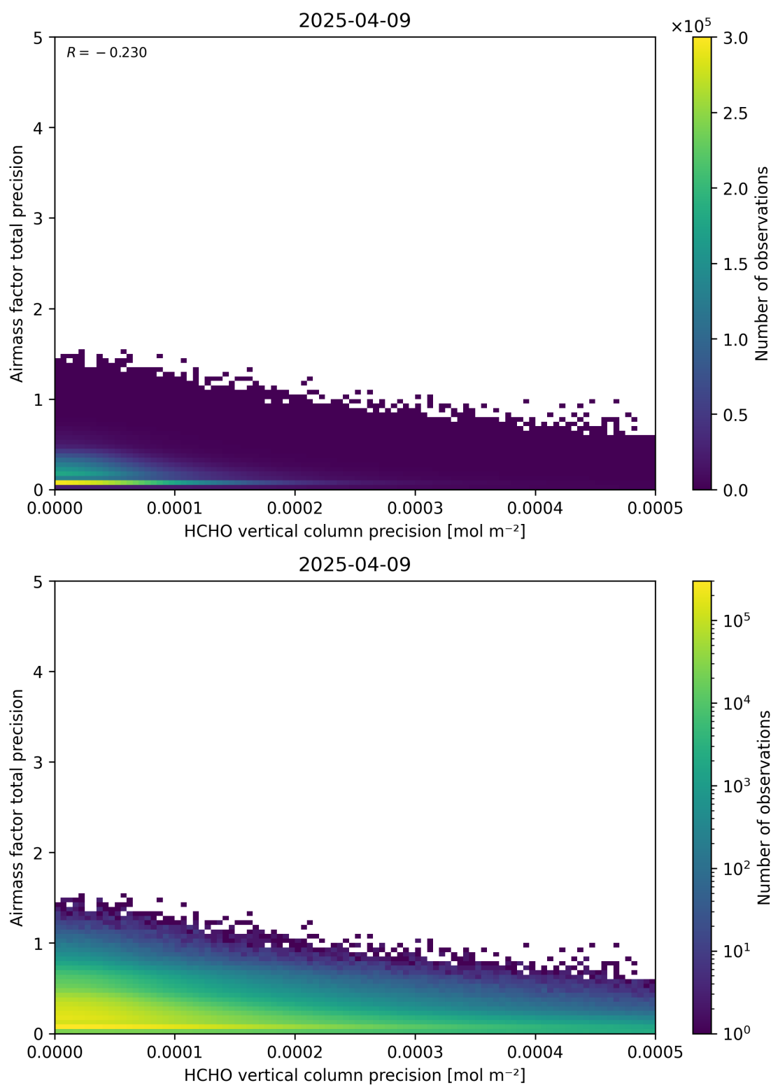
Figure 145: Scatter density plot of “HCHO vertical column precision” against “Airmass factor total precision” for 2025-04-08 to 2025-04-10.
