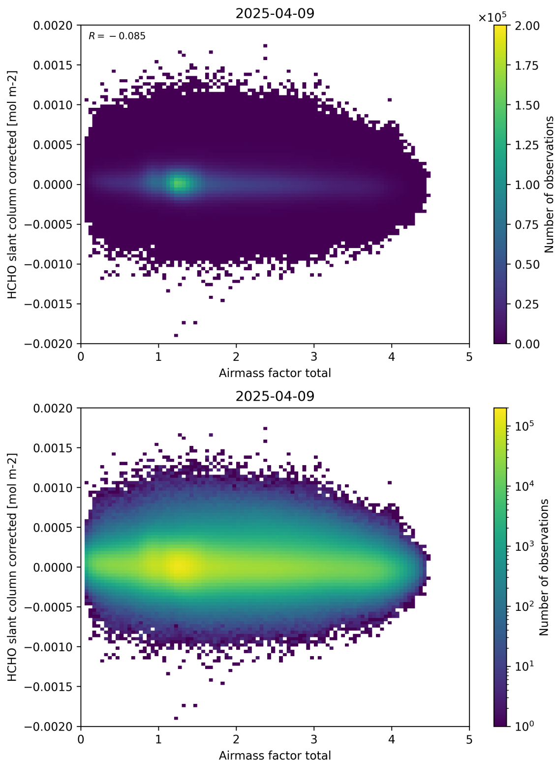
Figure 101: Scatter density plot of “Airmass factor total” against “HCHO slant column corrected” for 2025-04-08 to 2025-04-10.
