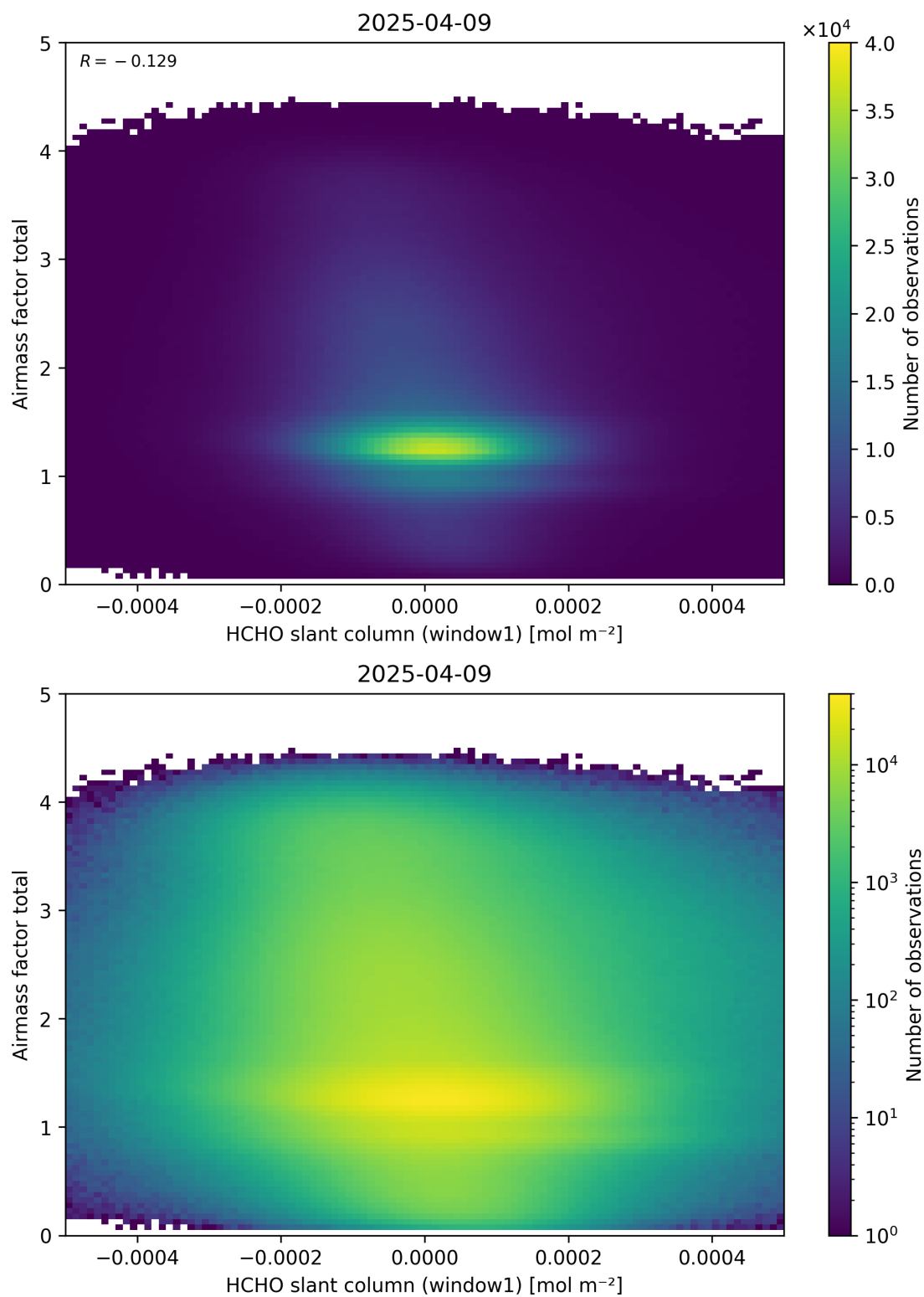
Figure 85: Scatter density plot of “HCHO slant column (window1)” against “Airmass factor total” for 2025-04-08 to 2025-04-10.
