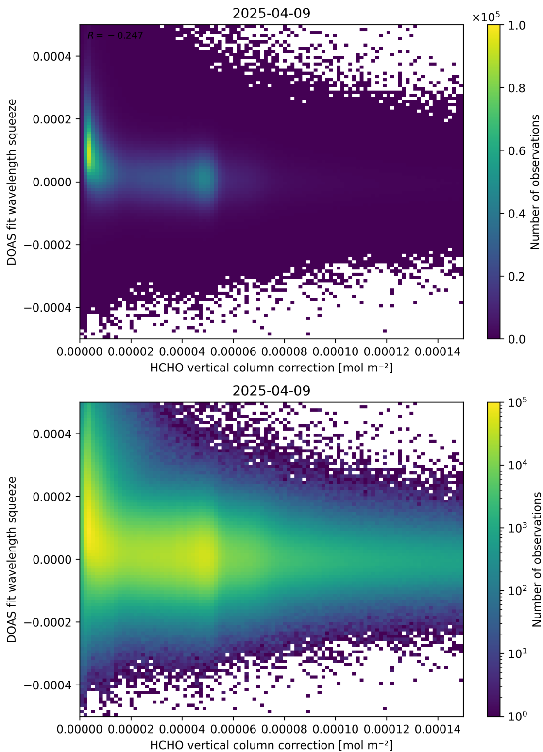
Figure 114: Scatter density plot of “HCHO vertical column correction” against “DOAS fit wavelength squeeze” for 2025-04-08 to 2025-04-10.
