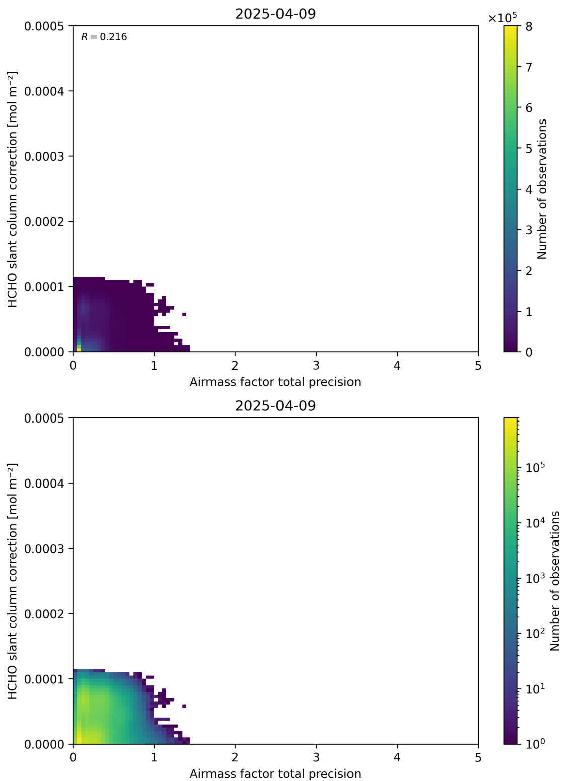
Figure 110: Scatter density plot of “Airmass factor total precision” against “HCHO slant column correction” for 2025-04-08 to 2025-04-10.
