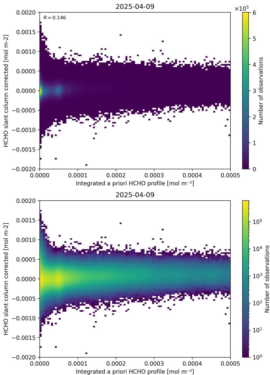
Figure 151: Scatter density plot of “Integrated a priori HCHO profile” against “HCHO slant column corrected” for 2025-04-08 to 2025-04-10.
