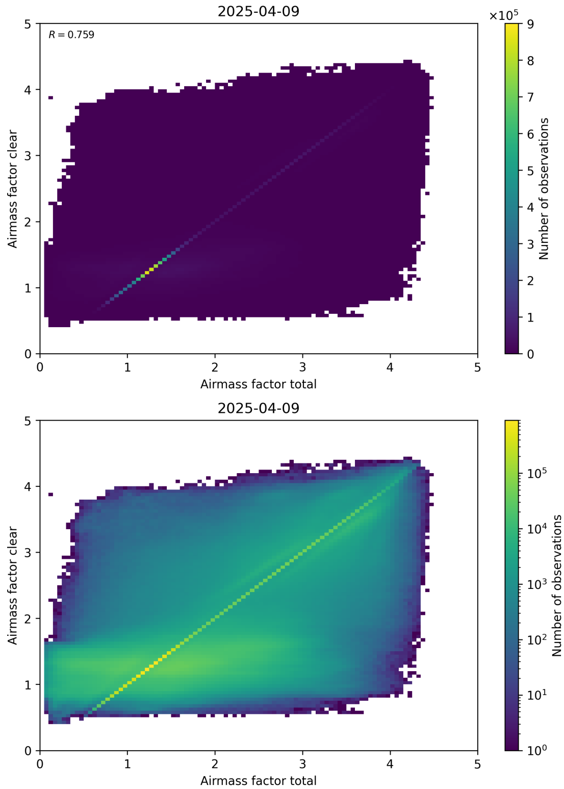
Figure 100: Scatter density plot of “Airmass factor total” against “Airmass factor clear” for 2025-04-08 to 2025-04-10.
