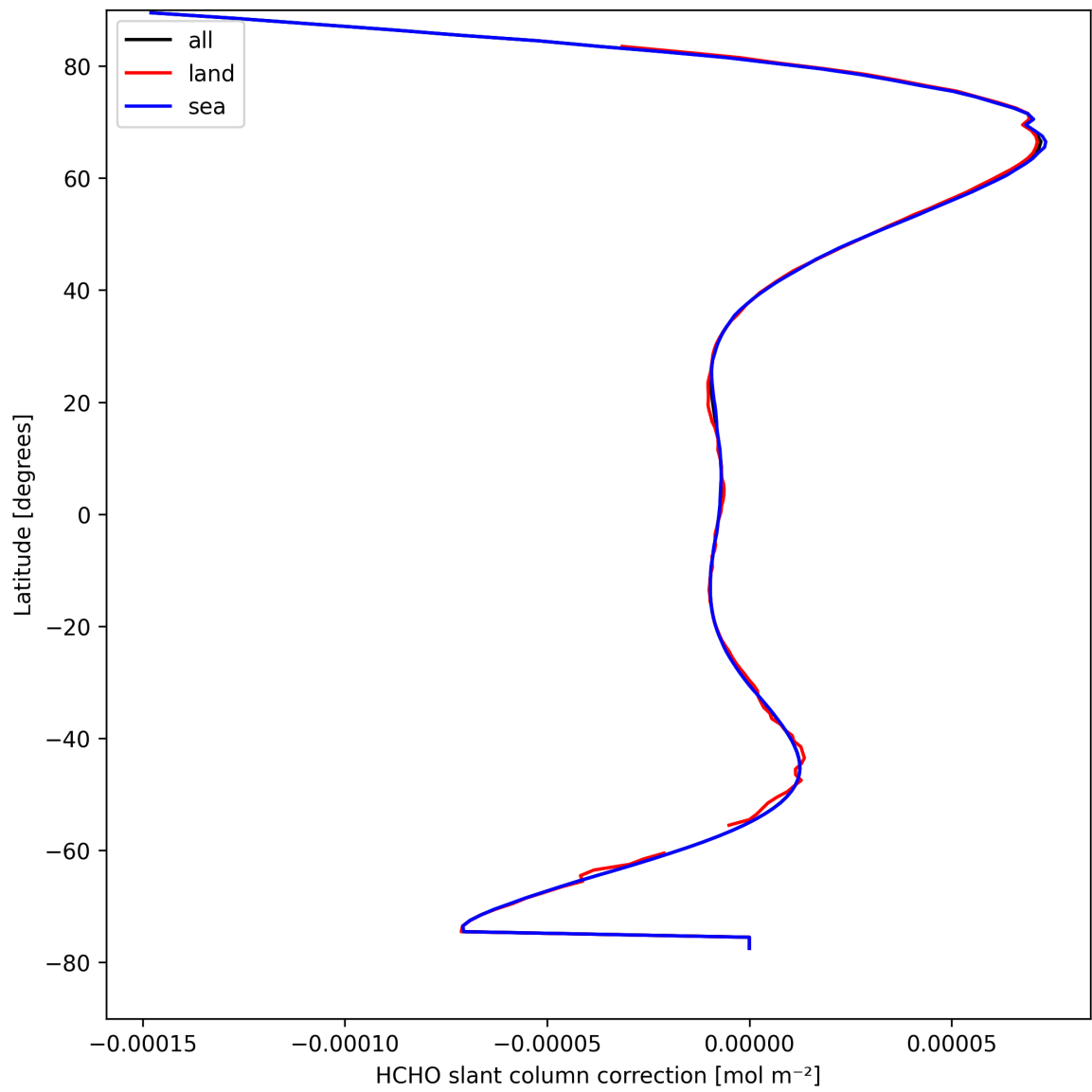
Figure 33: Zonal average of “HCHO slant column correction” for 2025-04-08 to 2025-04-10.
