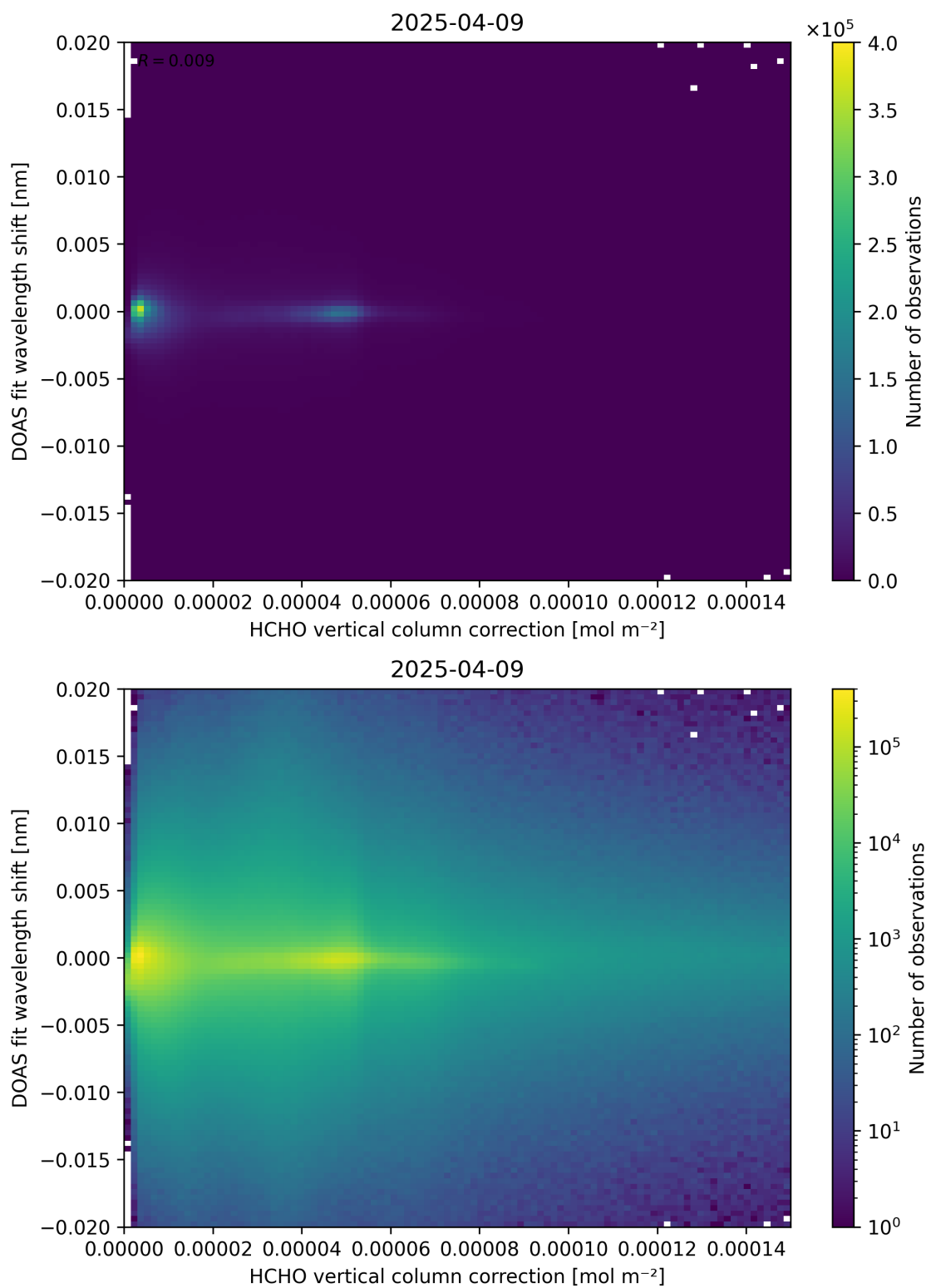
Figure 113: Scatter density plot of “HCHO vertical column correction” against “DOAS fit wavelength shift” for 2025-04-08 to 2025-04-10.
