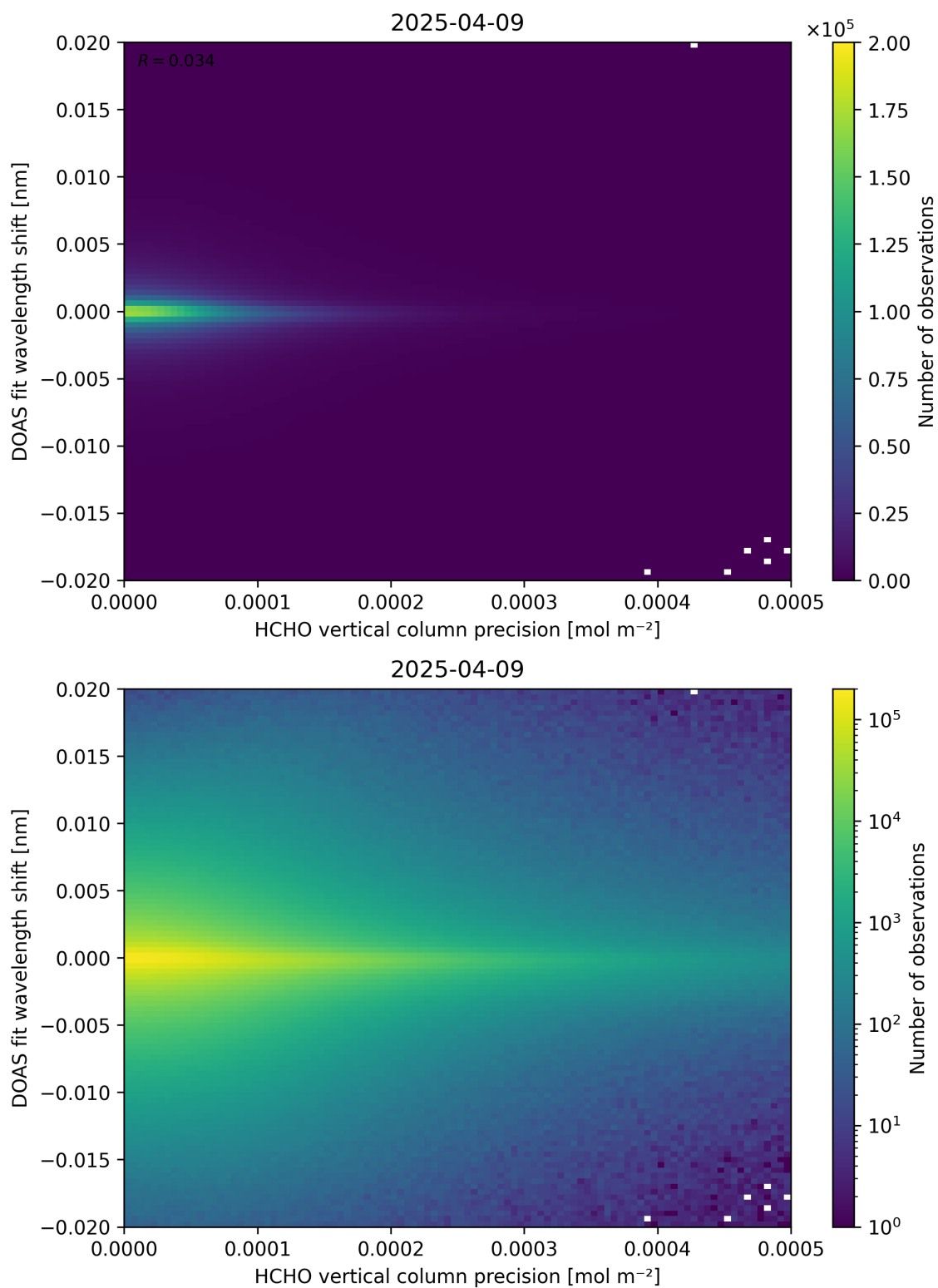
Figure 137: Scatter density plot of “HCHO vertical column precision” against “DOAS fit wavelength shift” for 2025-04-08 to 2025-04-10.
