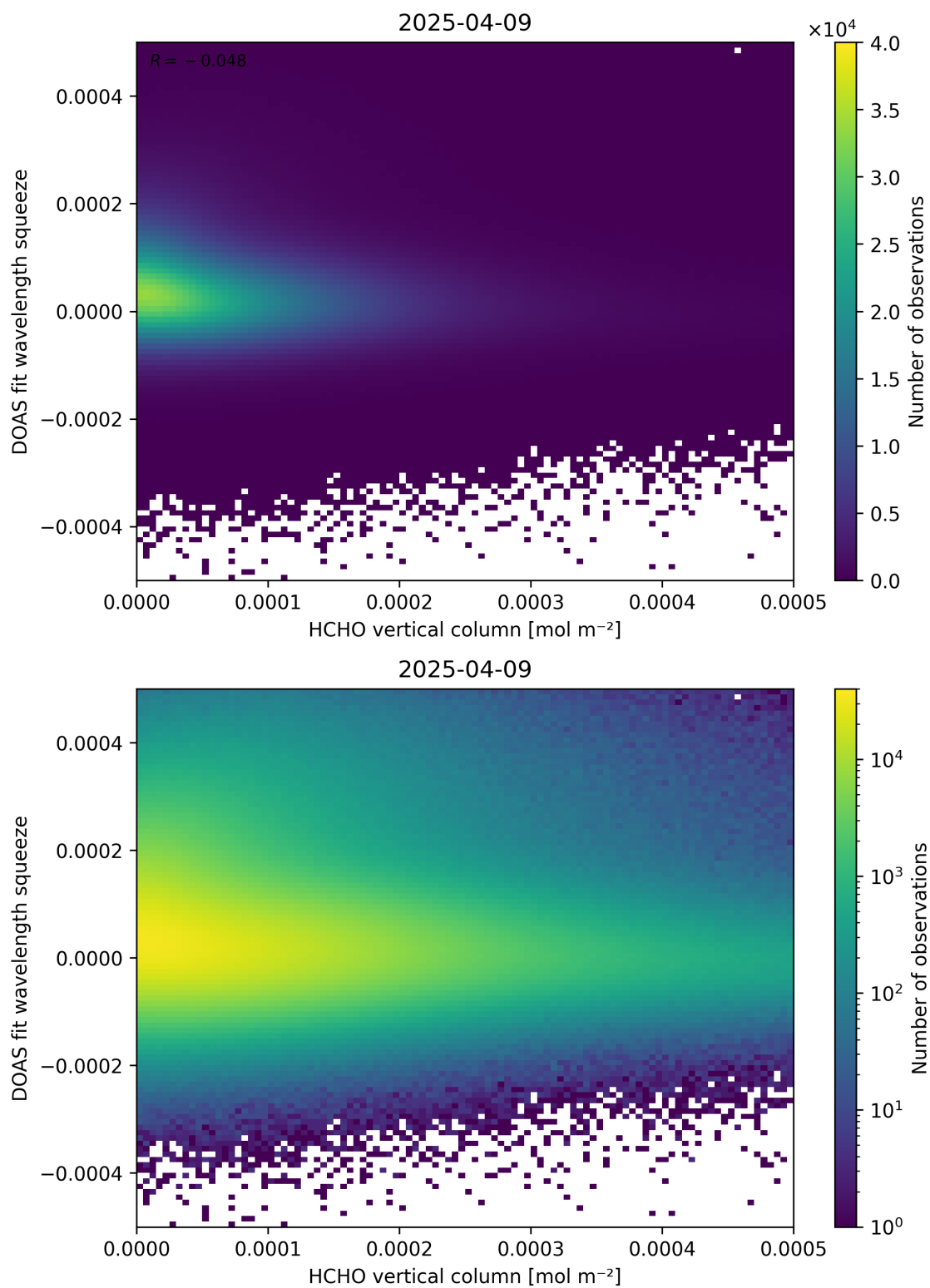
Figure 125: Scatter density plot of “HCHO vertical column” against “DOAS fit wavelength squeeze” for 2025-04-08 to 2025-04-10.
