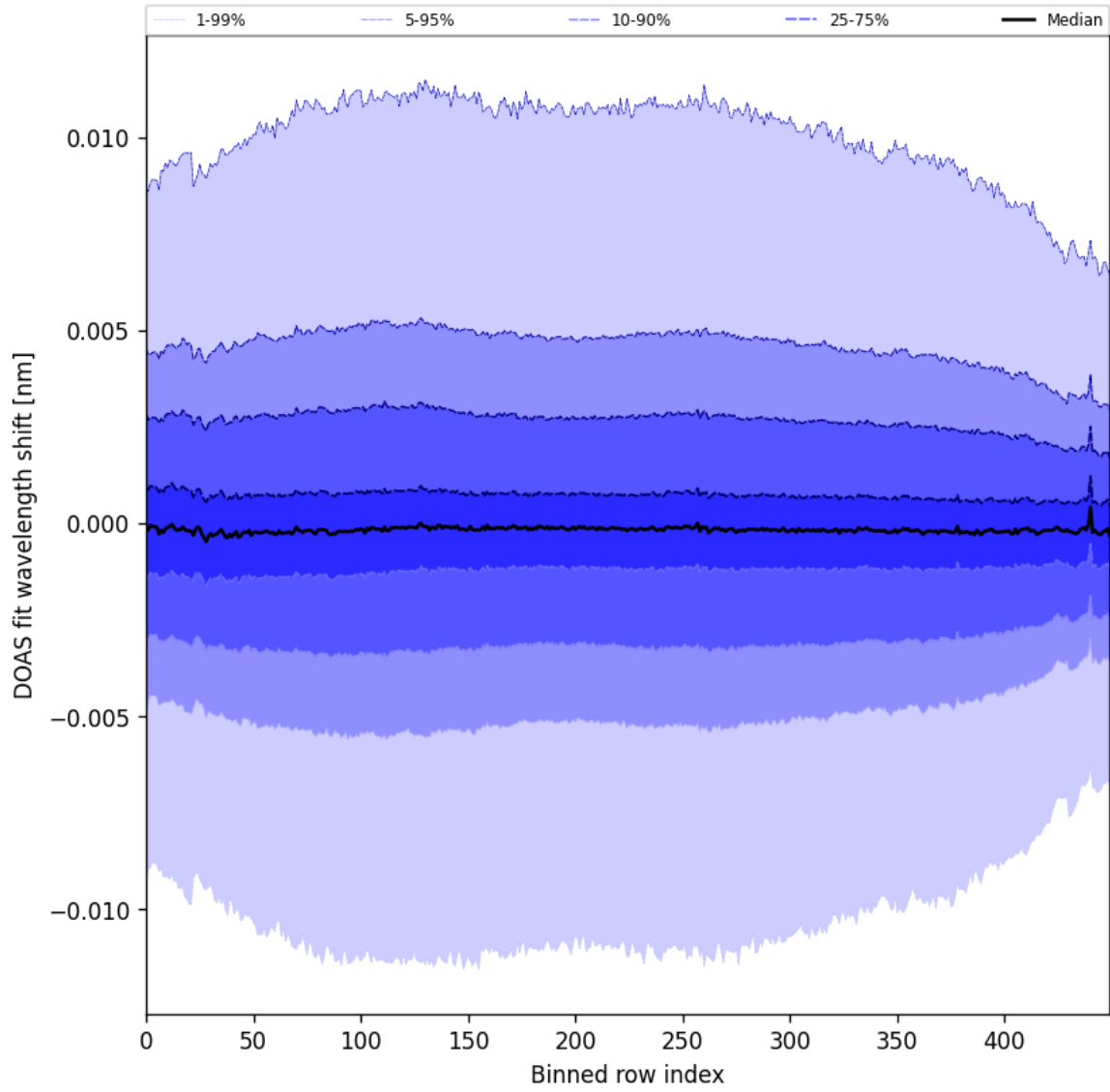
Figure 58: Along track statistics of “DOAS fit wavelength shift” for 2025-04-08 to 2025-04-10
