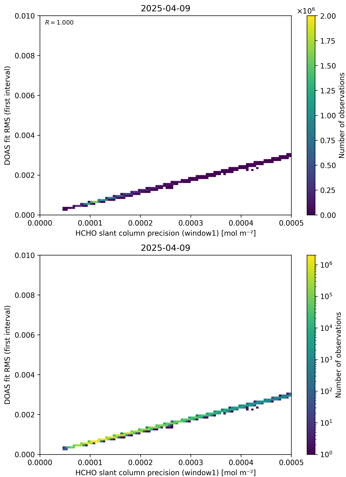
Figure 88: Scatter density plot of “HCHO slant column precision (window1)” against “DOAS fit RMS (first interval)” for 2025-04-08 to 2025-04-10.
