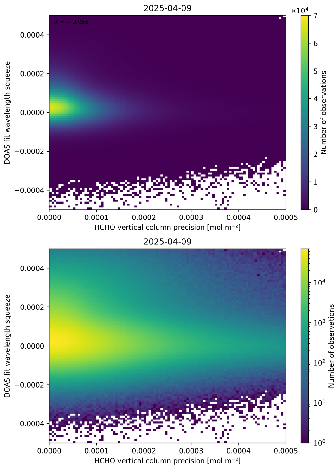
Figure 138: Scatter density plot of “HCHO vertical column precision” against “DOAS fit wavelength squeeze” for 2025-04-08 to 2025-04-10.
