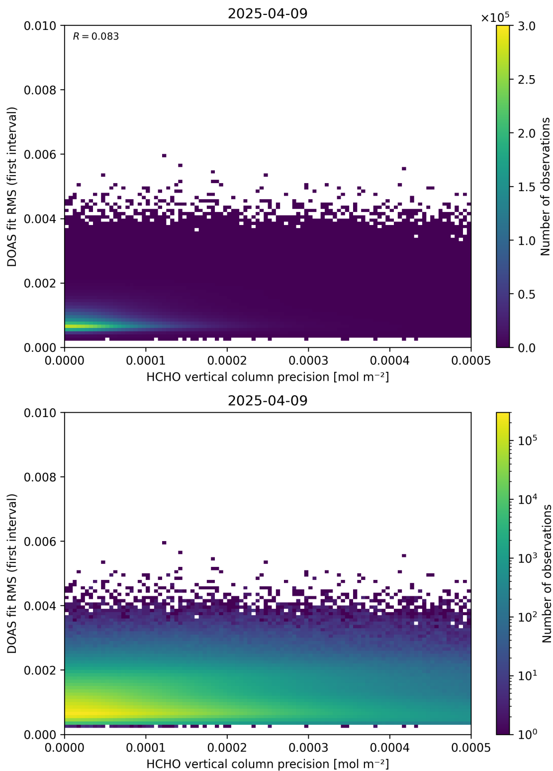
Figure 136: Scatter density plot of “HCHO vertical column precision” against “DOAS fit RMS (first interval)” for 2025-04-08 to 2025-04-10.
