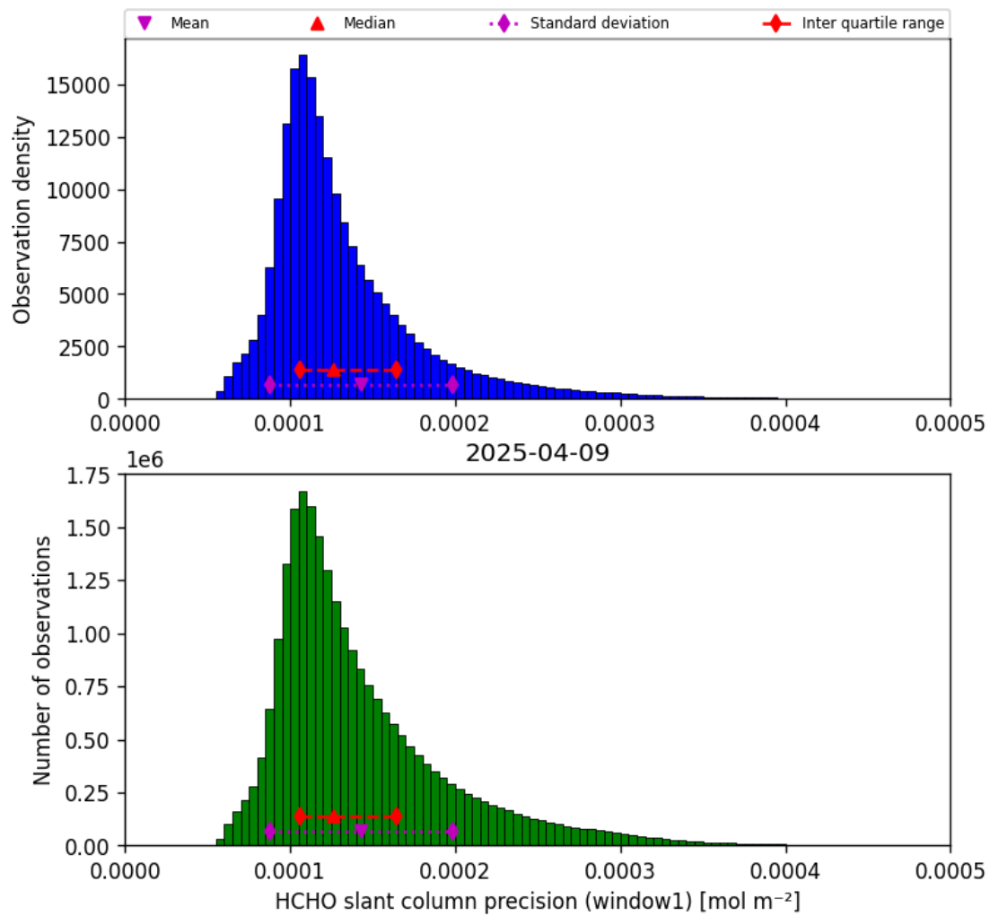
Figure 39: Histogram of “HCHO slant column precision (window1)” for 2025-04-08 to 2025-04-10
