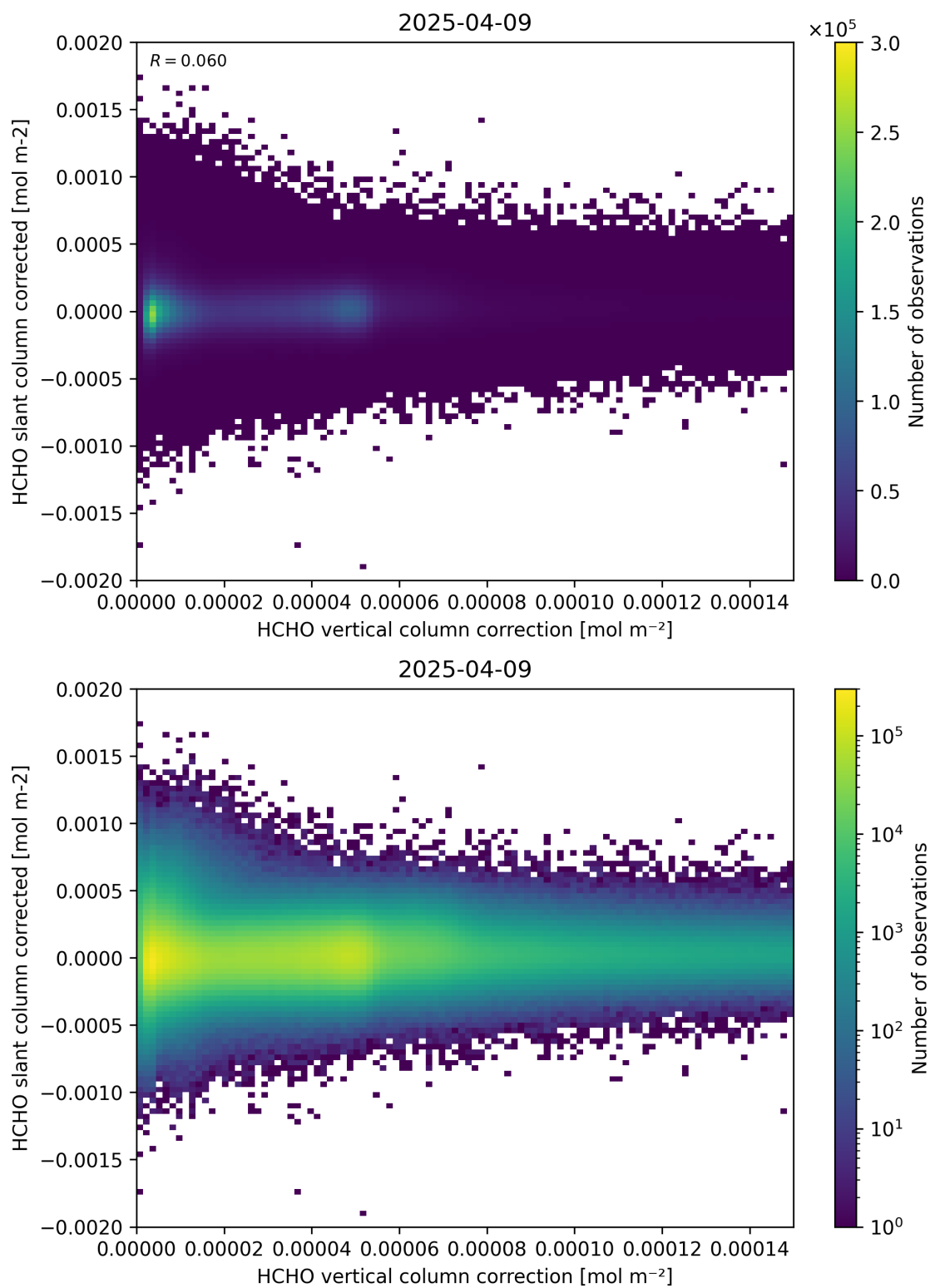
Figure 116: Scatter density plot of “HCHO vertical column correction” against “HCHO slant column corrected” for 2025-04-08 to 2025-04-10.
