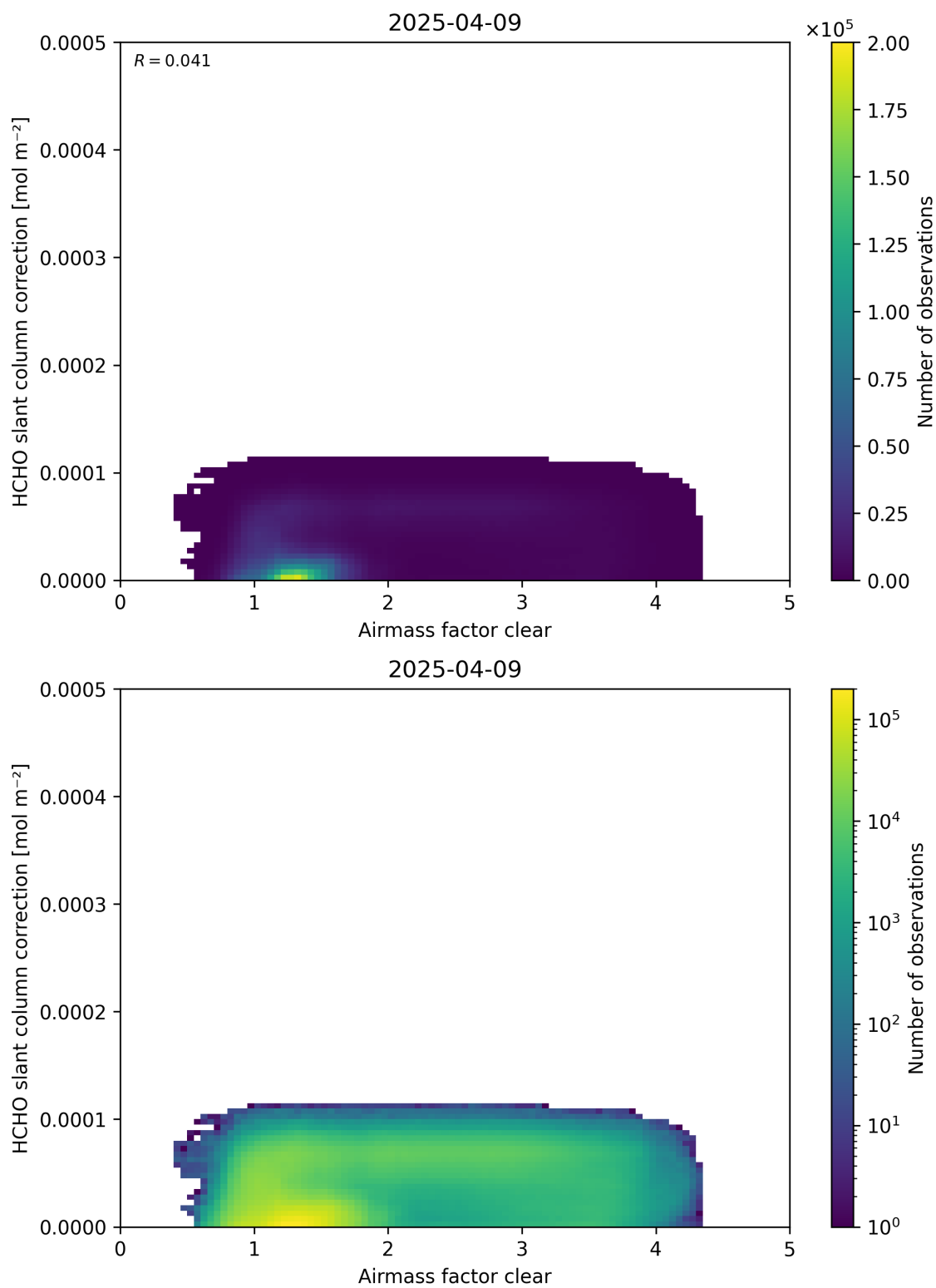
Figure 75: Scatter density plot of “Airmass factor clear” against “HCHO slant column correction” for 2025-04-08 to 2025-04-10.
