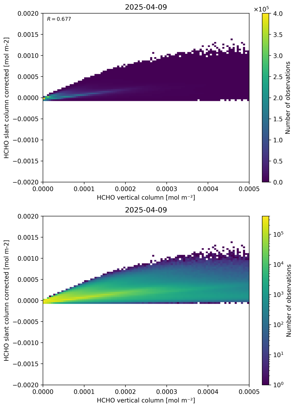
Figure 127: Scatter density plot of “HCHO vertical column” against “HCHO slant column corrected” for 2025-04-08 to 2025-04-10.
