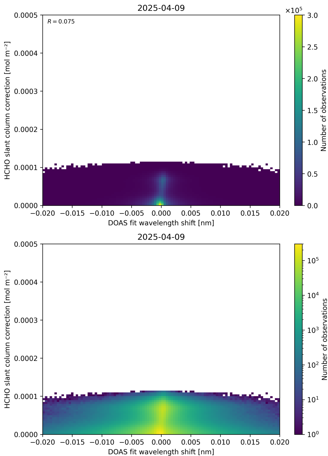
Figure 67: Scatter density plot of “DOAS fit wavelength shift” against “HCHO slant column correction” for 2025-04-08 to 2025-04-10.
