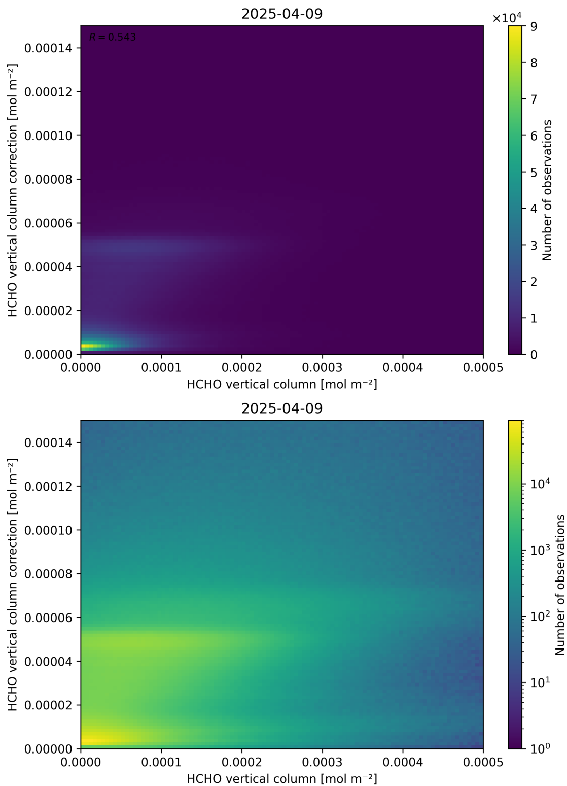
Figure 133: Scatter density plot of “HCHO vertical column” against “HCHO vertical column correction” for 2025-04-08 to 2025-04-10.
