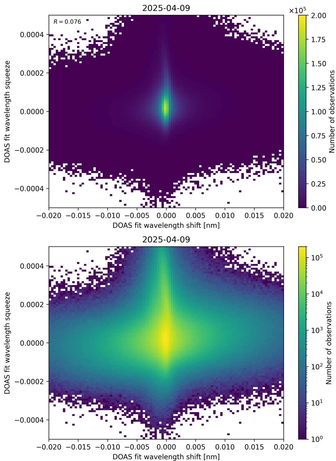
Figure 65: Scatter density plot of “DOAS fit wavelength shift” against “DOAS fit wavelength squeeze” for 2025-04-08 to 2025-04-10.
