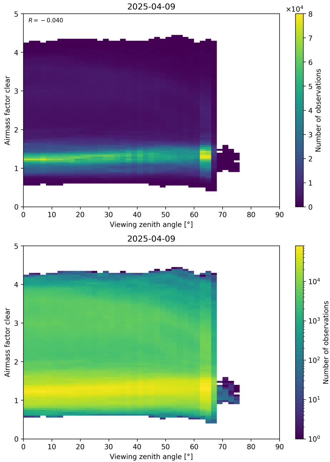
Figure 185: Scatter density plot of “Viewing zenith angle” against “Airmass factor clear” for 2025-04-08 to 2025-04-10.
