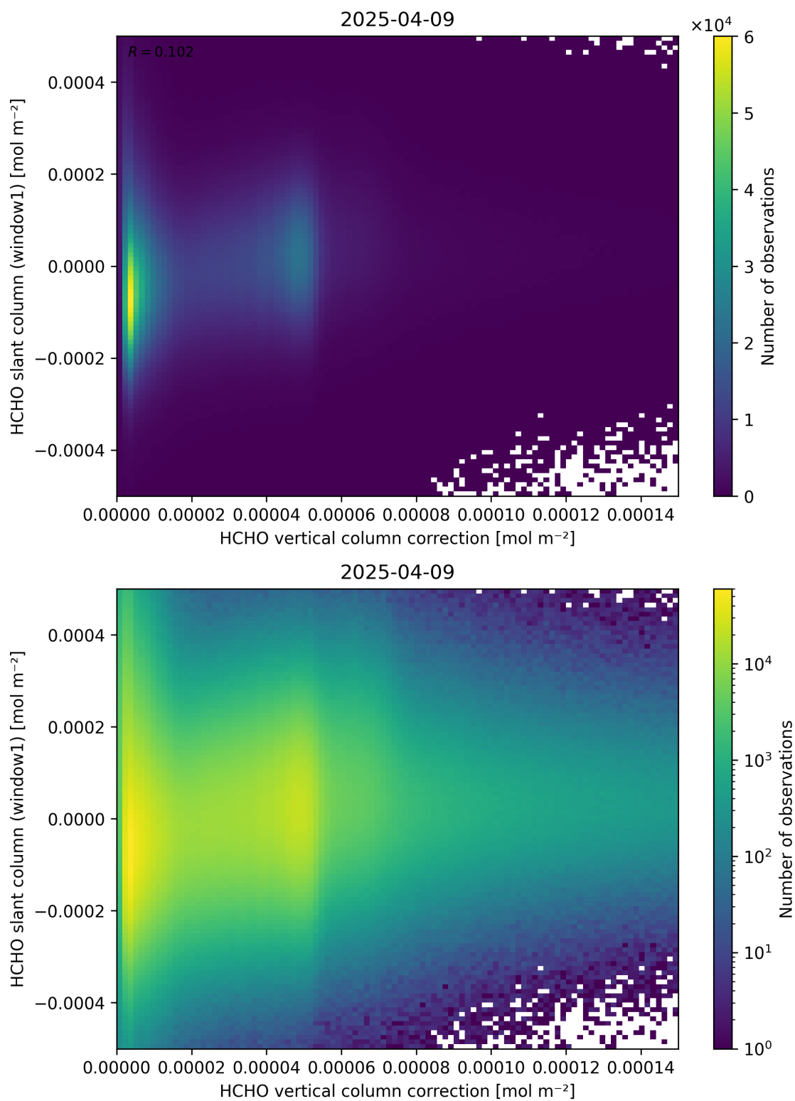
Figure 118: Scatter density plot of “HCHO vertical column correction” against “HCHO slant column (window1)” for 2025-04-08 to 2025-04-10.
