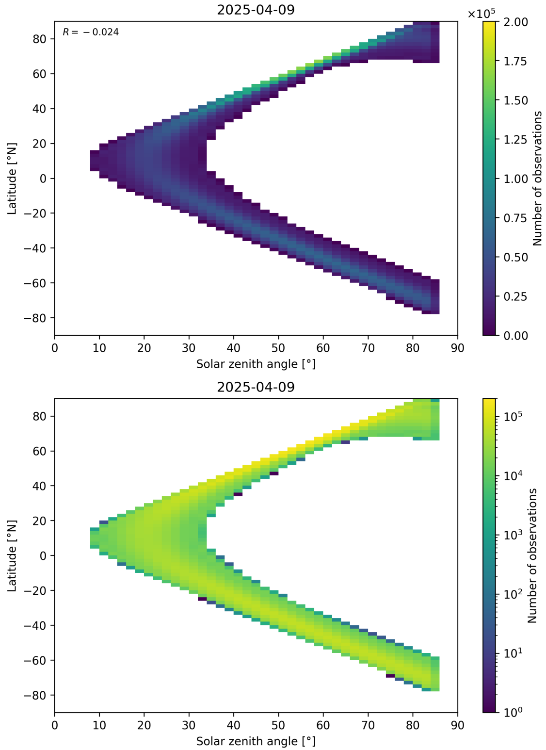
Figure 181: Scatter density plot of “Solar zenith angle” against “Latitude” for 2025-04-08 to 2025-04-10.
