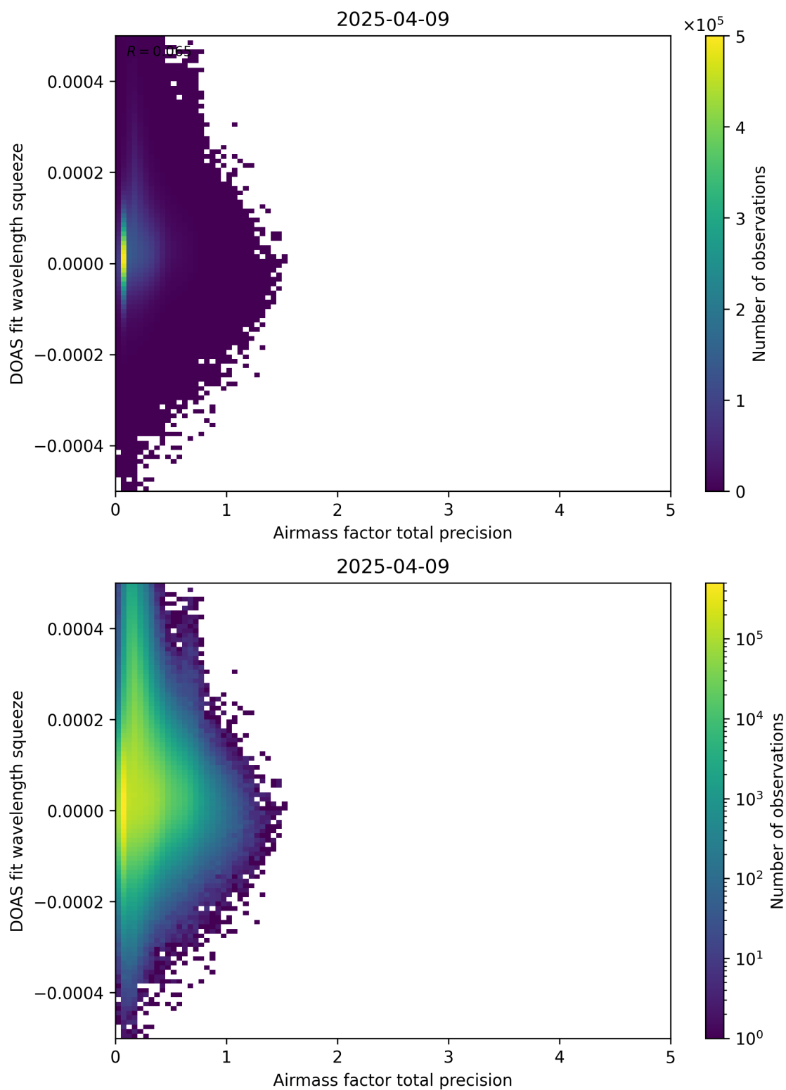
Figure 107: Scatter density plot of “Airmass factor total precision” against “DOAS fit wavelength squeeze” for 2025-04-08 to 2025-04-10.
