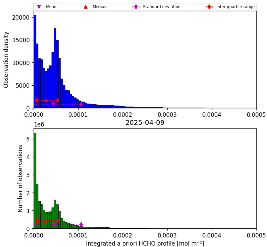
Figure 43: Histogram of “Integrated a priori HCHO profile” for 2025-04-08 to 2025-04-10
