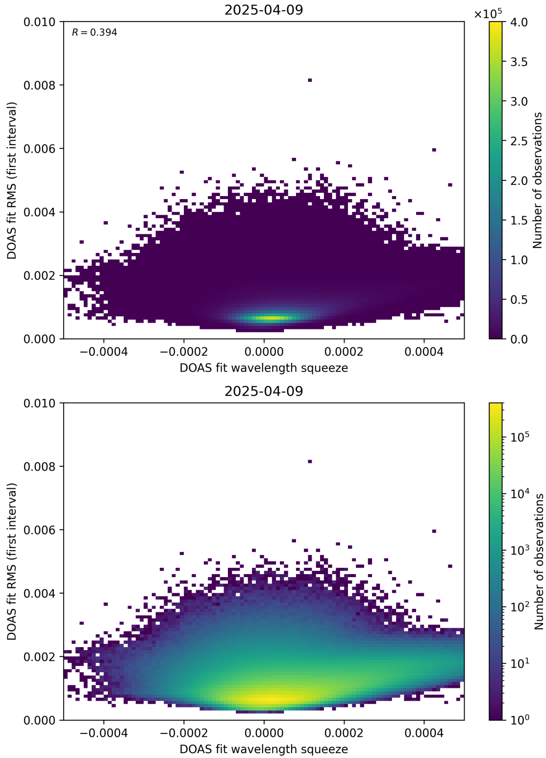
Figure 68: Scatter density plot of “DOAS fit wavelength squeeze” against “DOAS fit RMS (first interval)” for 2025-04-08 to 2025-04-10.
