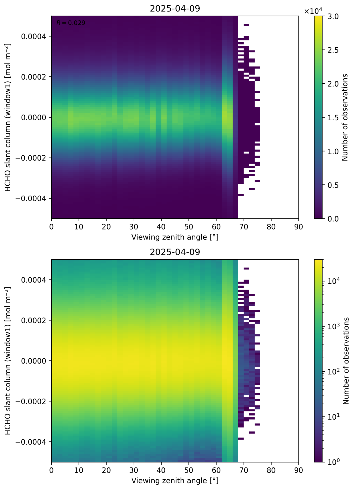
Figure 188: Scatter density plot of “Viewing zenith angle” against “HCHO slant column (window1)” for 2025-04-08 to 2025-04-10.
