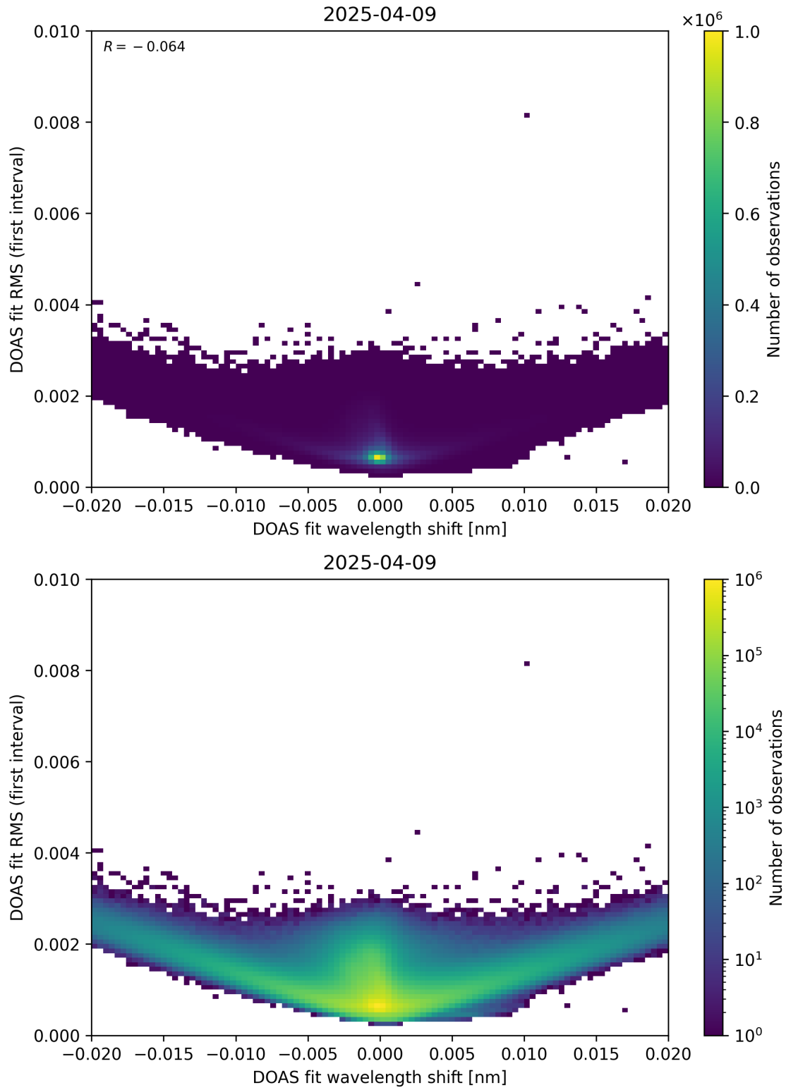
Figure 64: Scatter density plot of “DOAS fit wavelength shift” against “DOAS fit RMS (first interval)” for 2025-04-08 to 2025-04-10.
