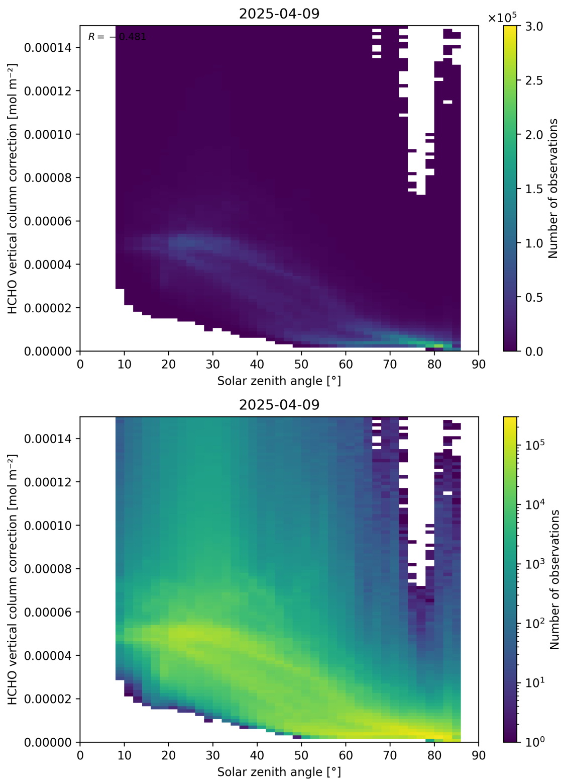
Figure 178: Scatter density plot of “Solar zenith angle” against “HCHO vertical column correction” for 2025-04-08 to 2025-04-10.
