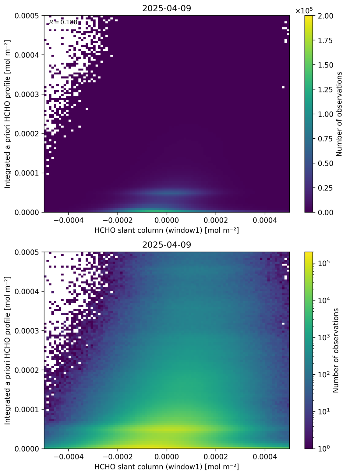
Figure 87: Scatter density plot of “HCHO slant column (window1)” against “Integrated a priori HCHO profile” for 2025-04-08 to 2025-04-10.
