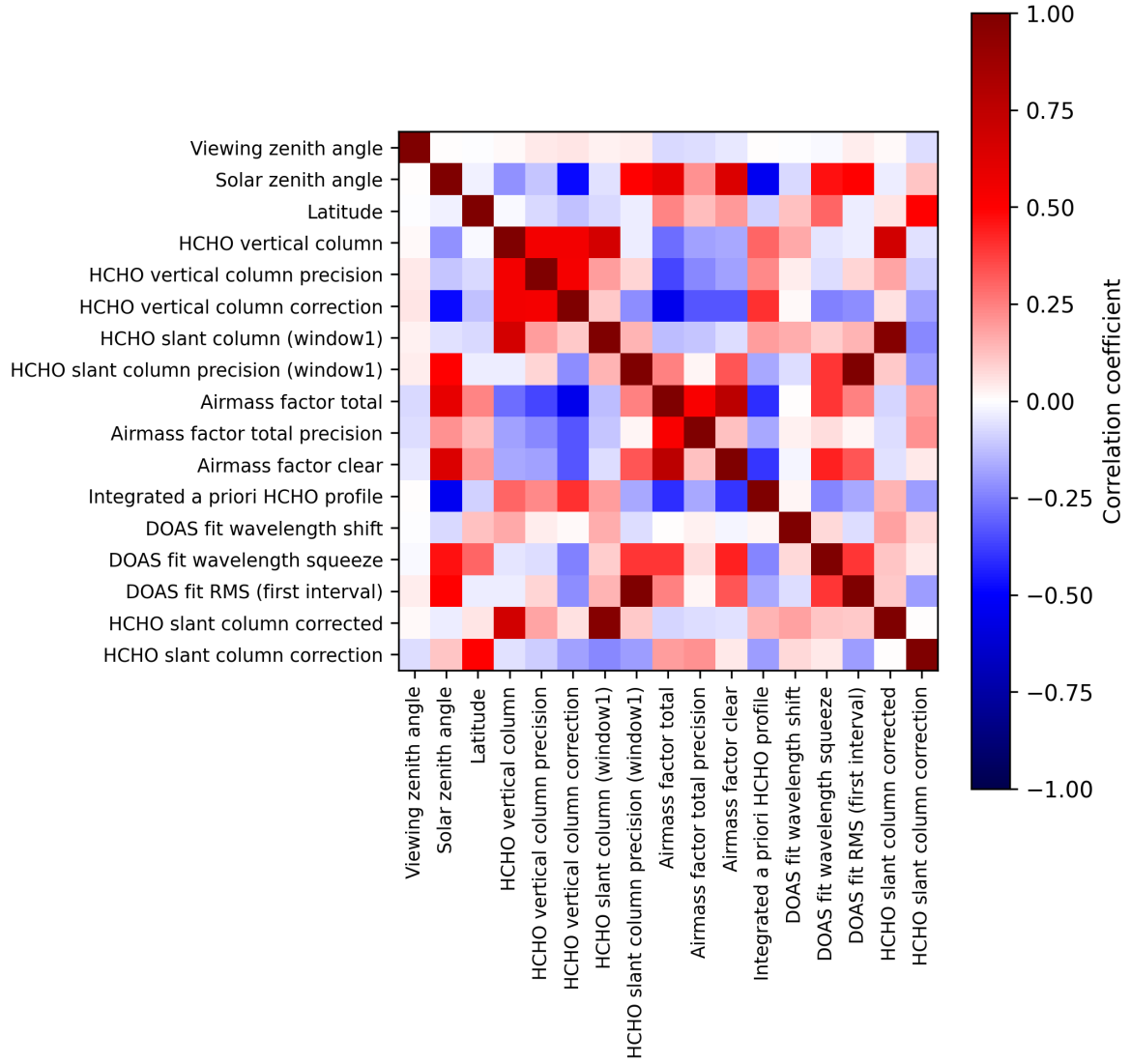
Figure 2: Map of correlation matrix for 2025-04-08 to 2025-04-10.
