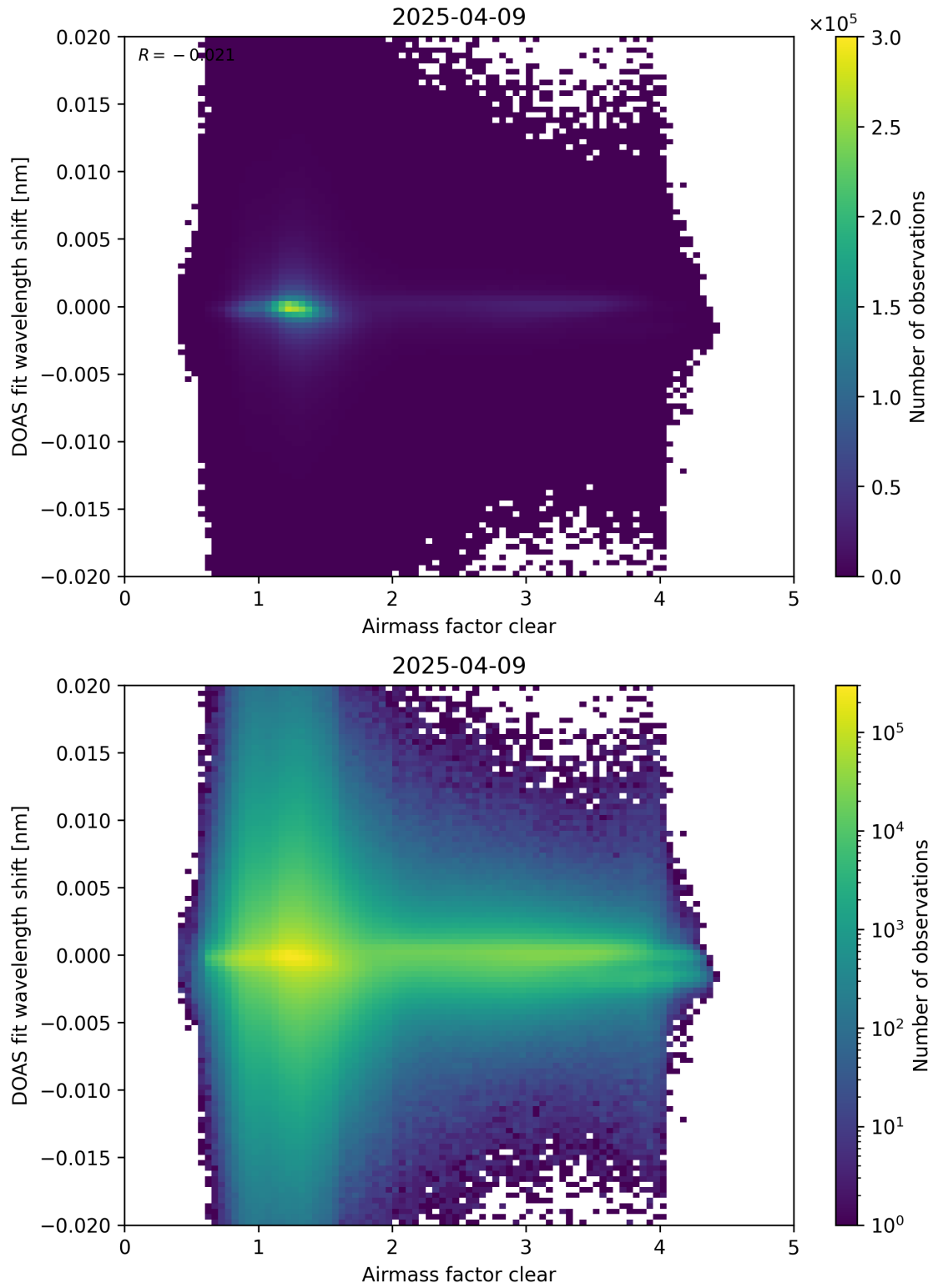
Figure 72: Scatter density plot of “Airmass factor clear” against “DOAS fit wavelength shift” for 2025-04-08 to 2025-04-10.
