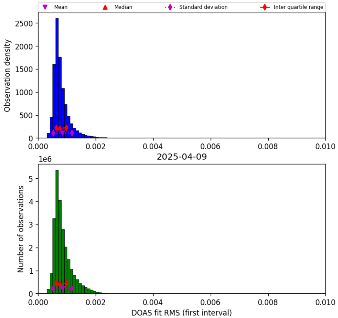
Figure 46: Histogram of “DOAS fit RMS (first interval)” for 2025-04-08 to 2025-04-10
