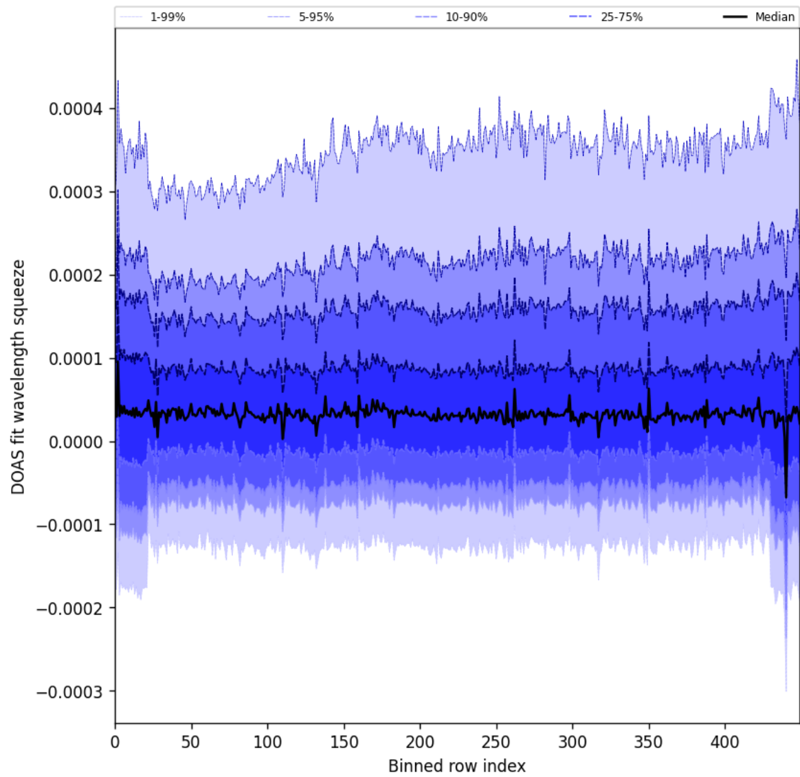
Figure 59: Along track statistics of “DOAS fit wavelength squeeze” for 2025-04-08 to 2025-04-10
