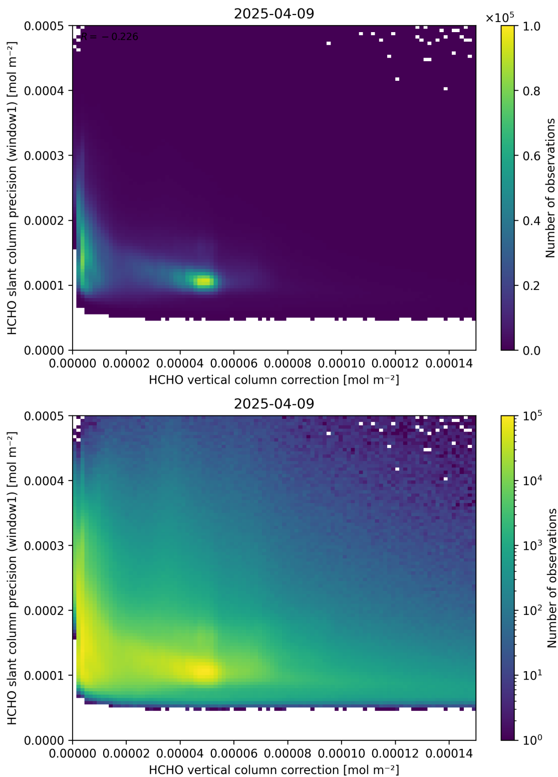
Figure 119: Scatter density plot of “HCHO vertical column correction” against “HCHO slant column precision (window1)” for 2025-04-08 to 2025-04-10.
