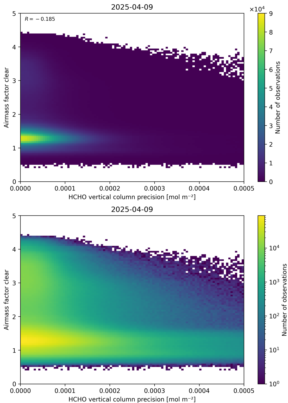
Figure 139: Scatter density plot of “HCHO vertical column precision” against “Airmass factor clear” for 2025-04-08 to 2025-04-10.
