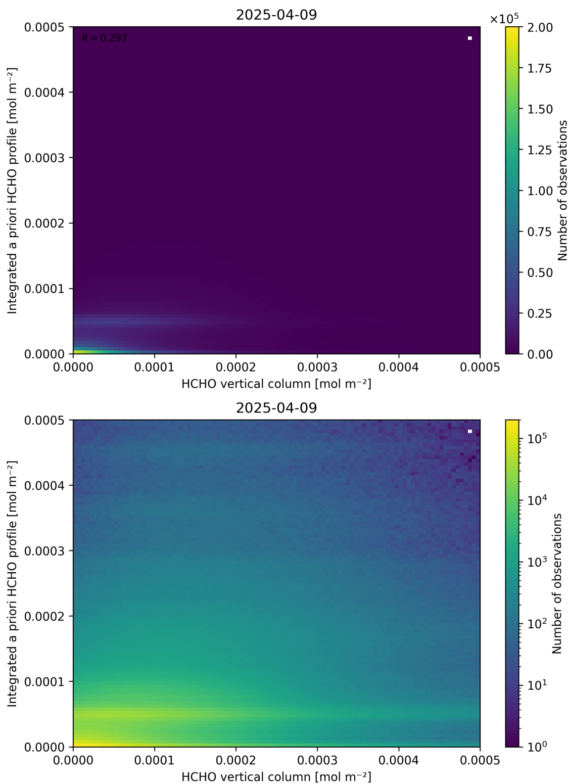
Figure 135: Scatter density plot of “HCHO vertical column” against “Integrated a priori HCHO profile” for 2025-04-08 to 2025-04-10.
