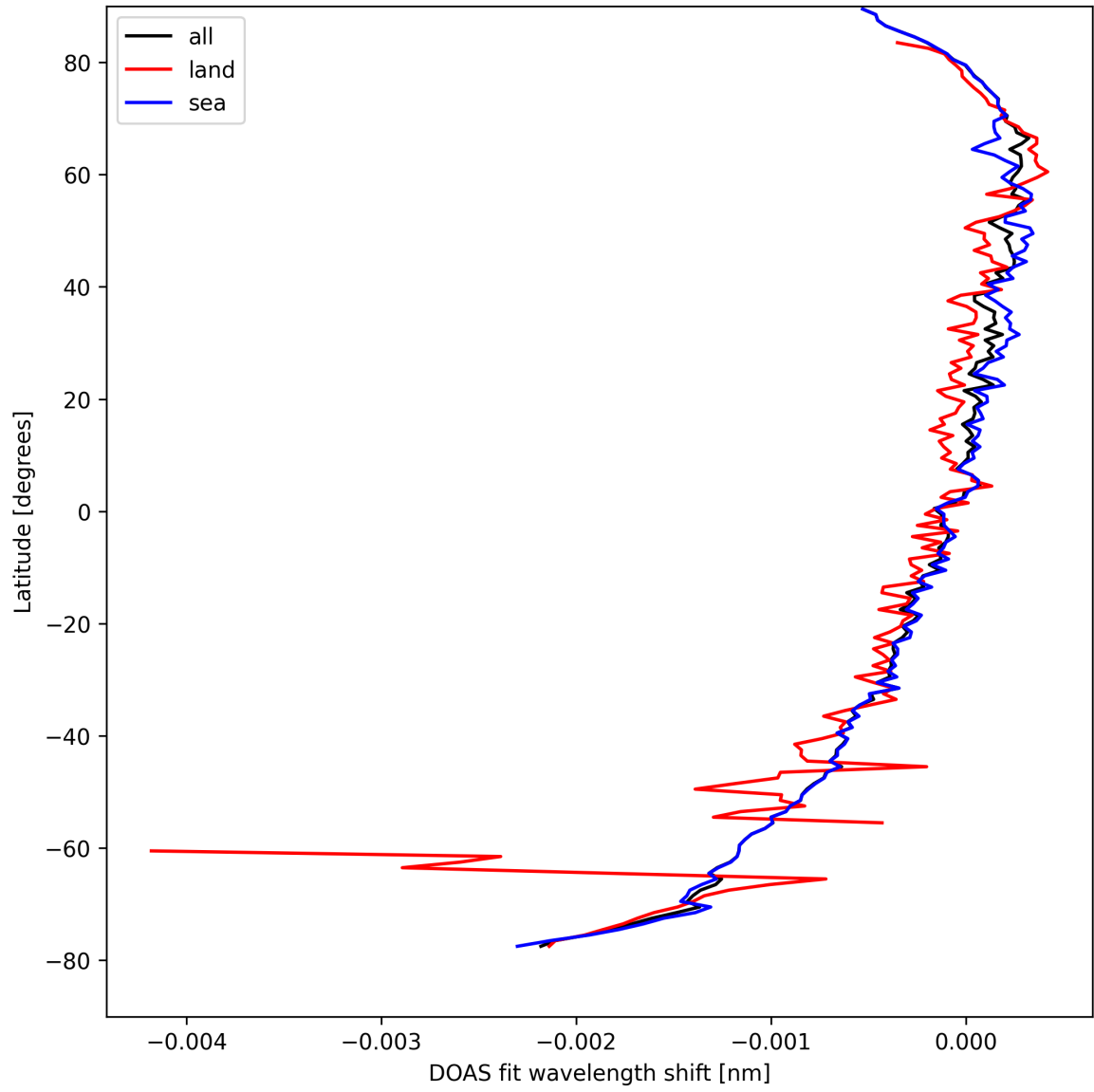
Figure 30: Zonal average of “DOAS fit wavelength shift” for 2025-04-08 to 2025-04-10.
