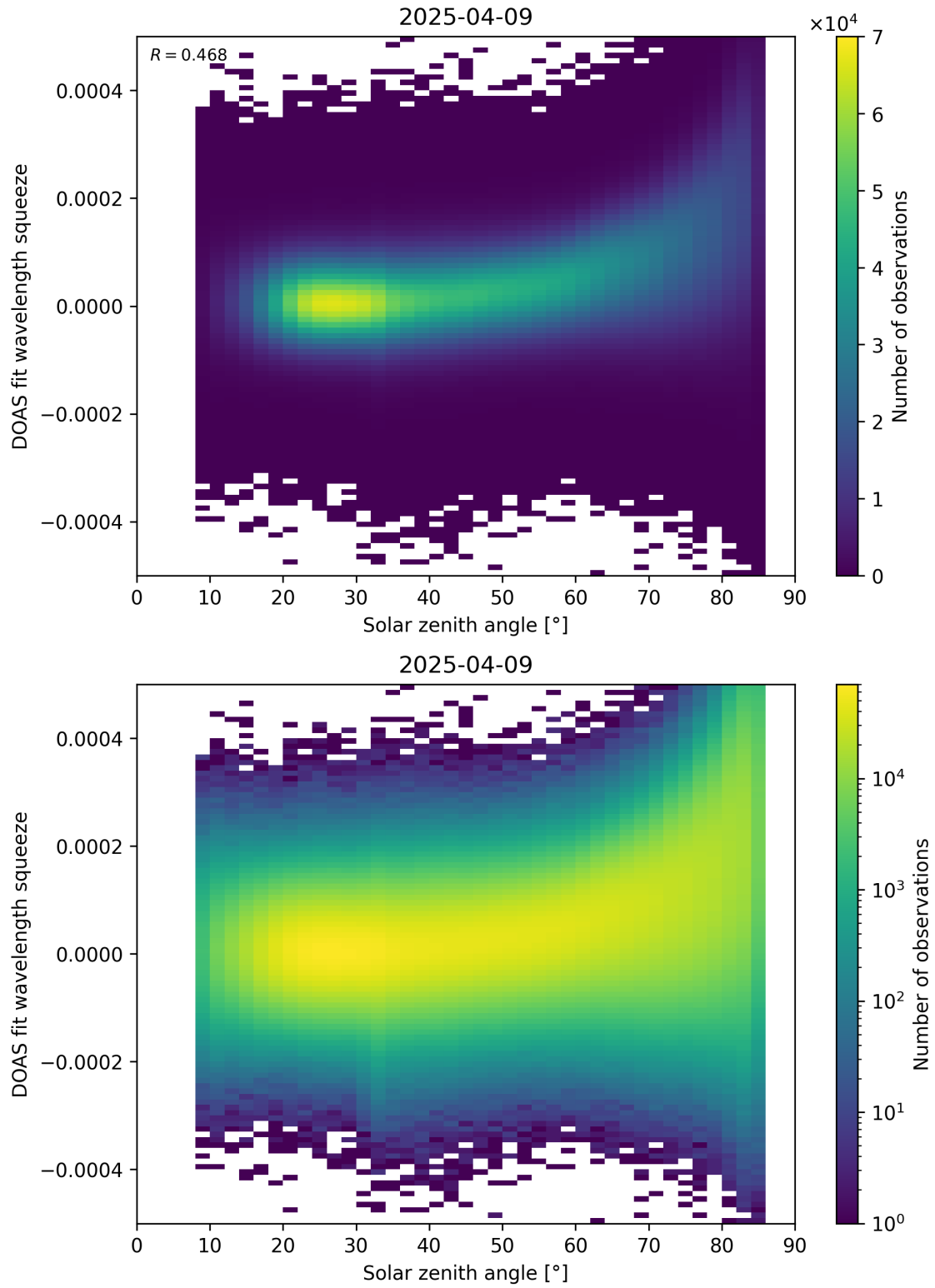
Figure 169: Scatter density plot of “Solar zenith angle” against “DOAS fit wavelength squeeze” for 2025-04-08 to 2025-04-10.
