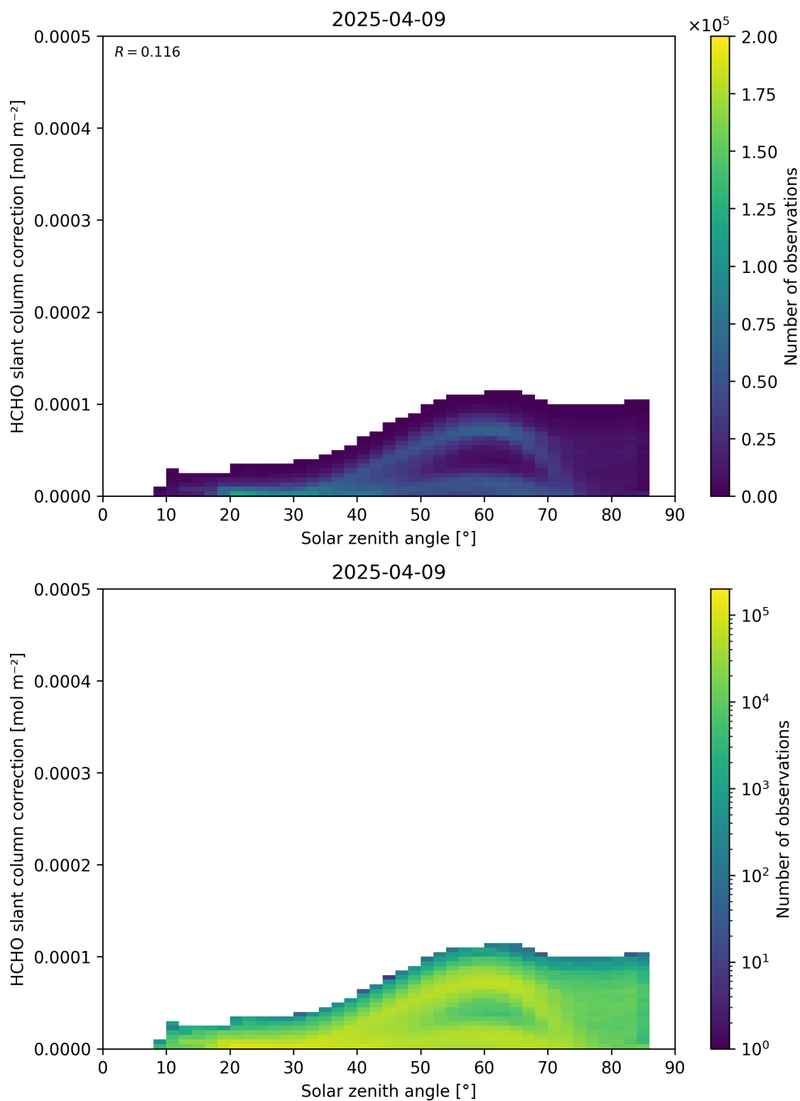
Figure 172: Scatter density plot of “Solar zenith angle” against “HCHO slant column correction” for 2025-04-08 to 2025-04-10.
