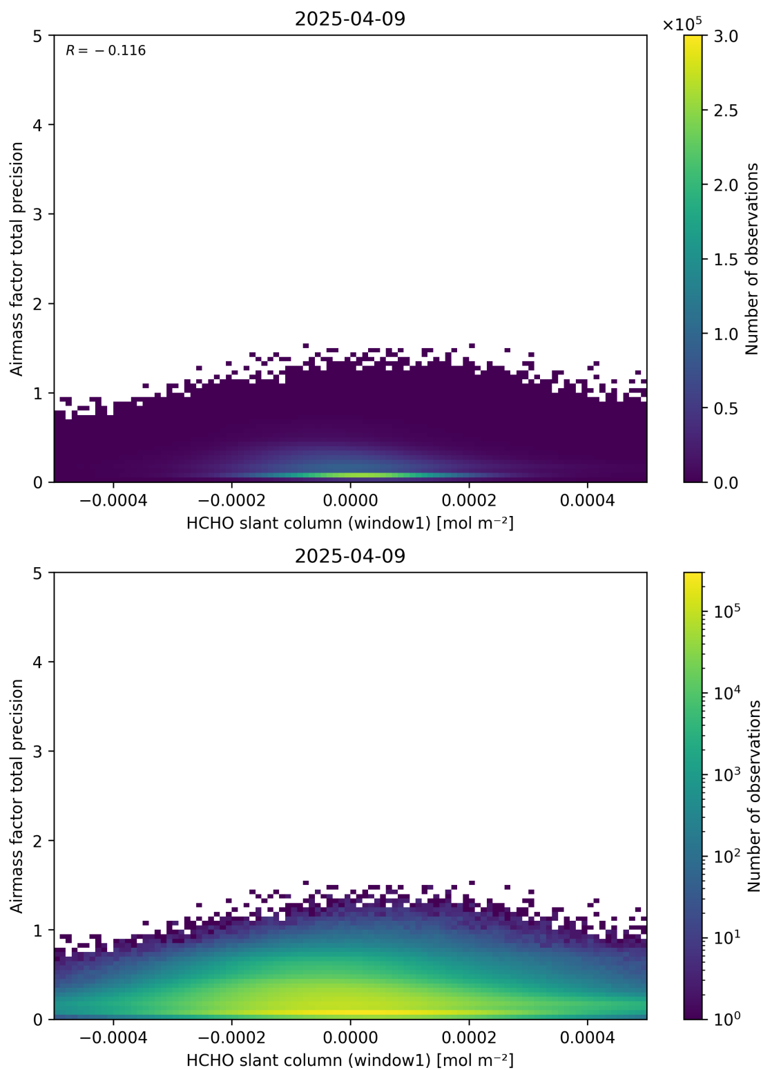
Figure 86: Scatter density plot of “HCHO slant column (window1)” against “Airmass factor total precision” for 2025-04-08 to 2025-04-10.
