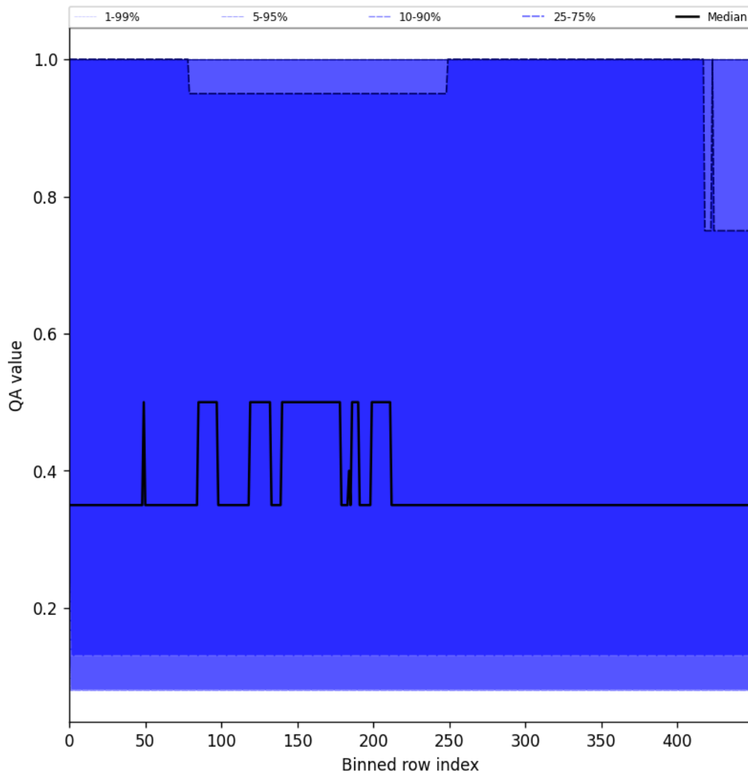
Figure 48: Along track statistics of “QA value” for 2025-04-08 to 2025-04-10
