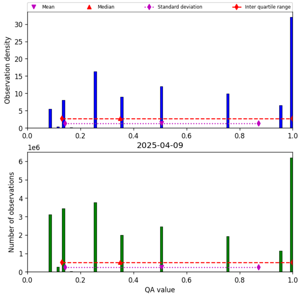
Figure 34: Histogram of “QA value” for 2025-04-08 to 2025-04-10
