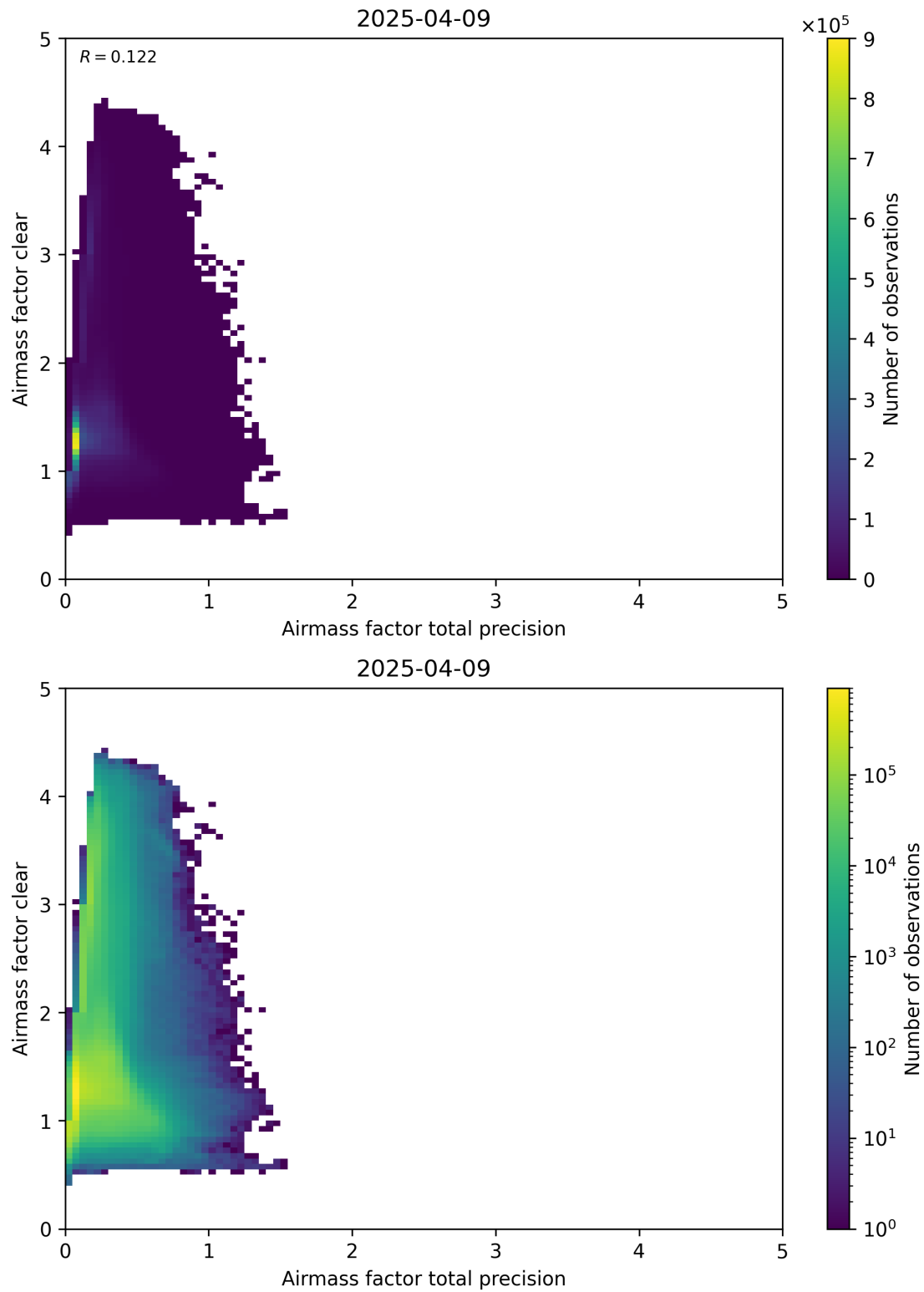
Figure 108: Scatter density plot of “Airmass factor total precision” against “Airmass factor clear” for 2025-04-08 to 2025-04-10.
