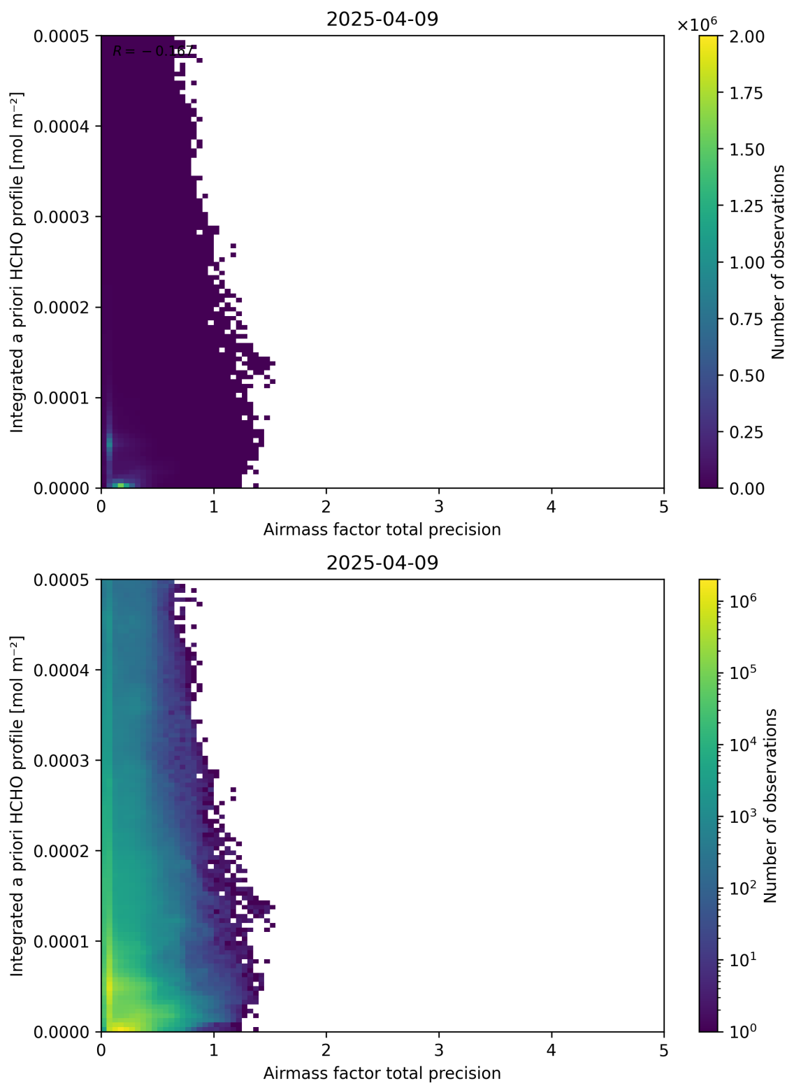
Figure 111: Scatter density plot of “Airmass factor total precision” against “Integrated a priori HCHO profile” for 2025-04-08 to 2025-04-10.
