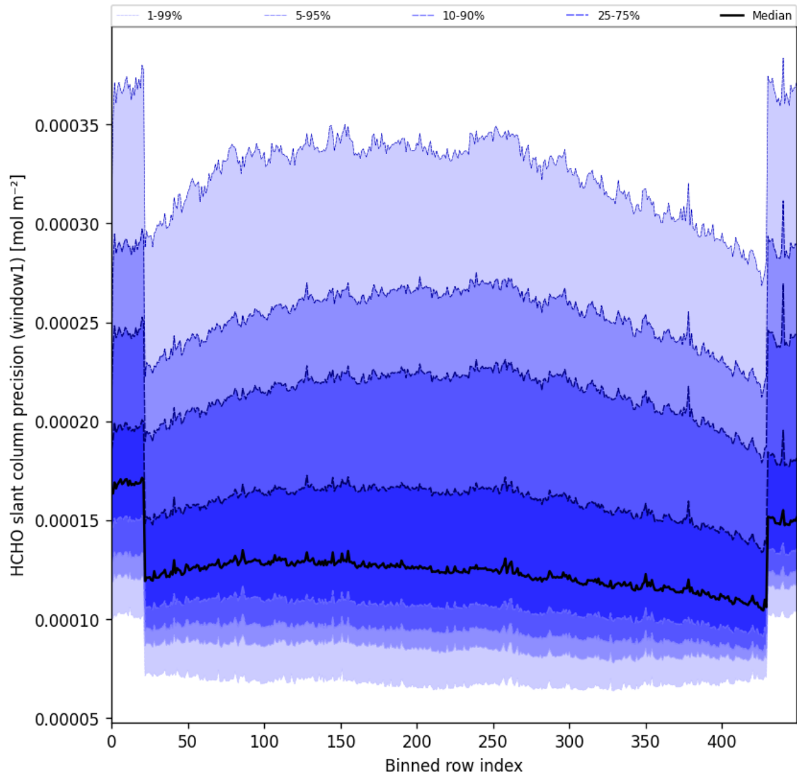
Figure 53: Along track statistics of “HCHO slant column precision (window1)” for 2025-04-08 to 2025-04-10
