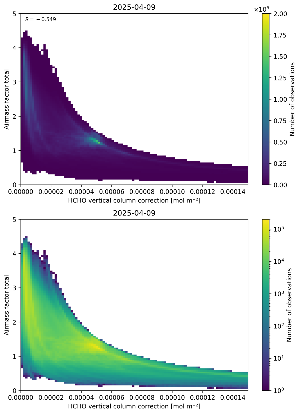
Figure 120: Scatter density plot of “HCHO vertical column correction” against “Airmass factor total” for 2025-04-08 to 2025-04-10.
