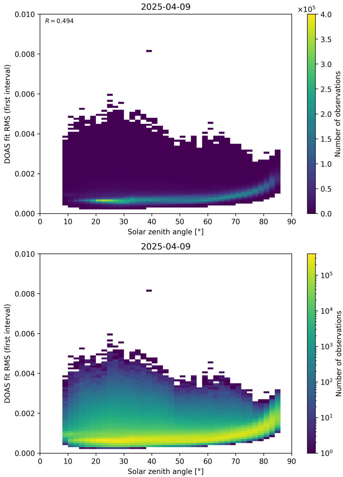
Figure 167: Scatter density plot of “Solar zenith angle” against “DOAS fit RMS (first interval)” for 2025-04-08 to 2025-04-10.
