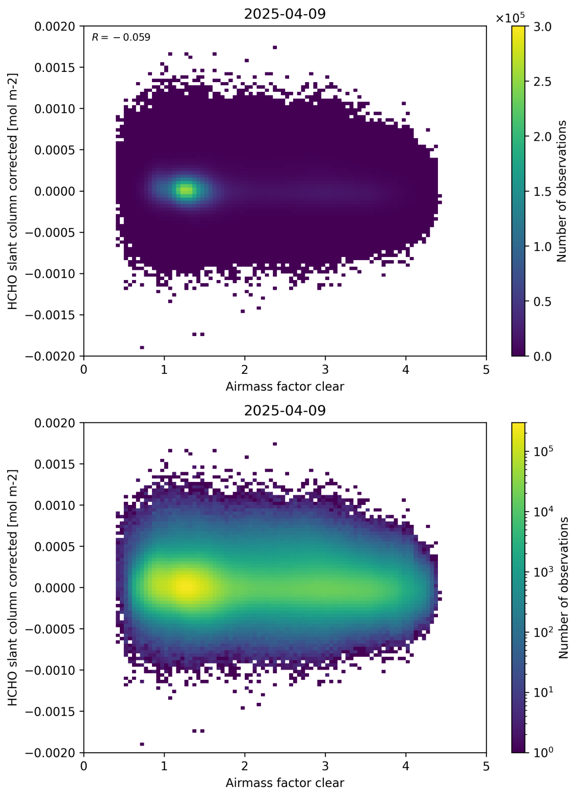
Figure 74: Scatter density plot of “Airmass factor clear” against “HCHO slant column corrected” for 2025-04-08 to 2025-04-10.
