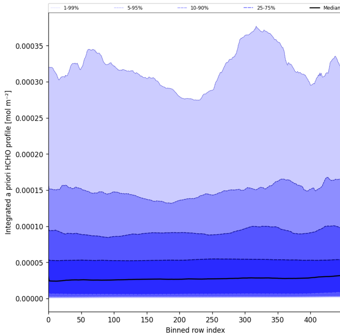
Figure 57: Along track statistics of “Integrated a priori HCHO profile” for 2025-04-08 to 2025-04-10
