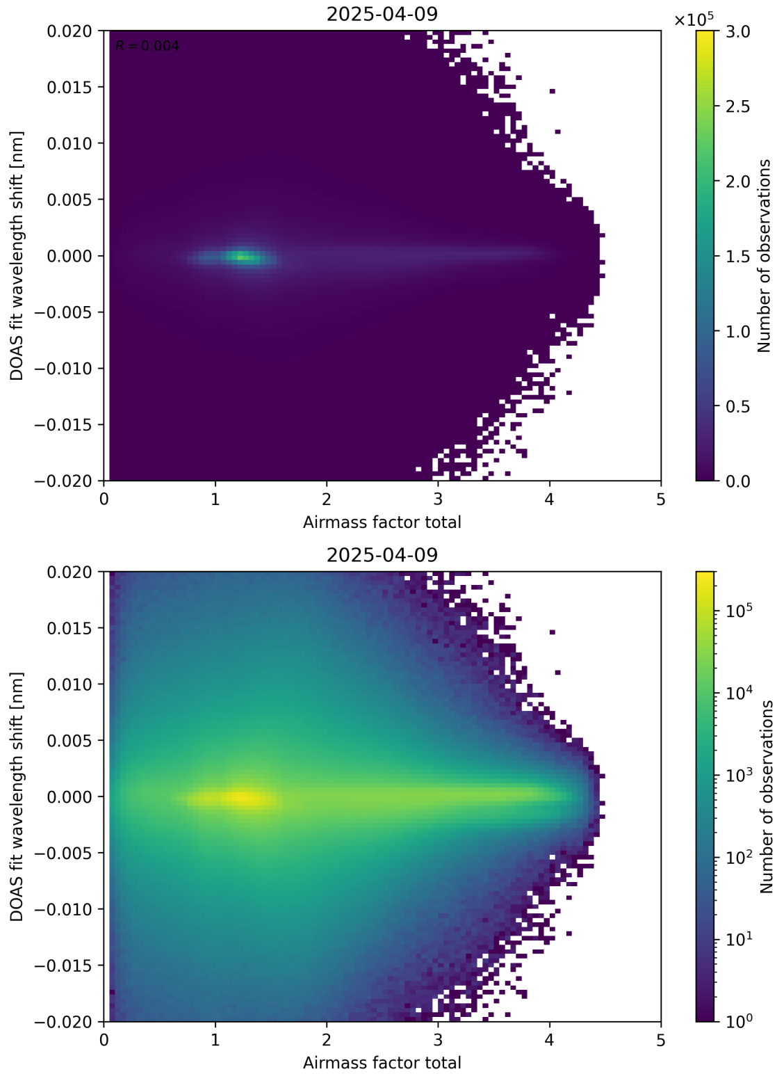
Figure 98: Scatter density plot of “Airmass factor total” against “DOAS fit wavelength shift” for 2025-04-08 to 2025-04-10.
