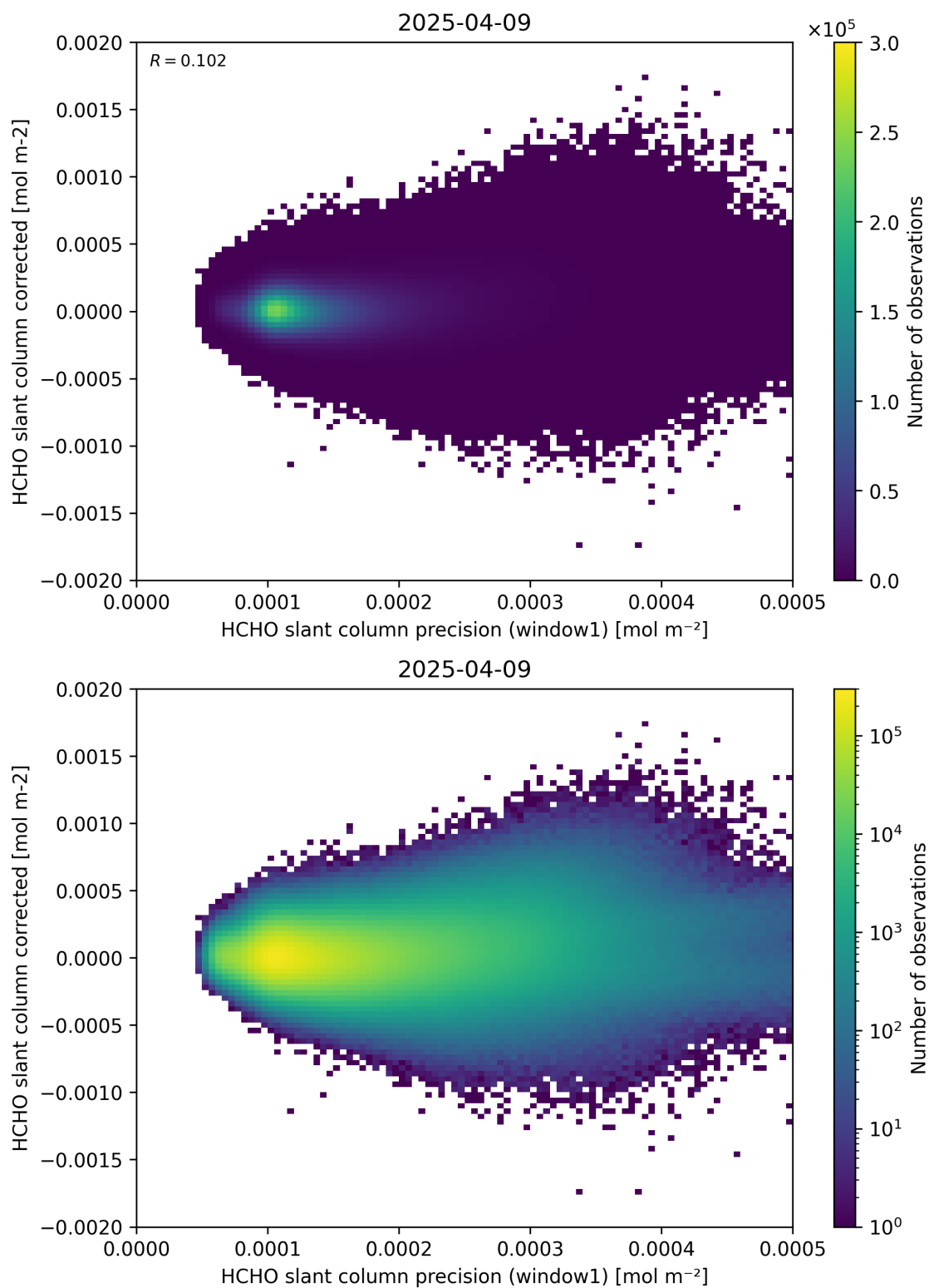
Figure 92: Scatter density plot of “HCHO slant column precision (window1)” against “HCHO slant column corrected” for 2025-04-08 to 2025-04-10.
