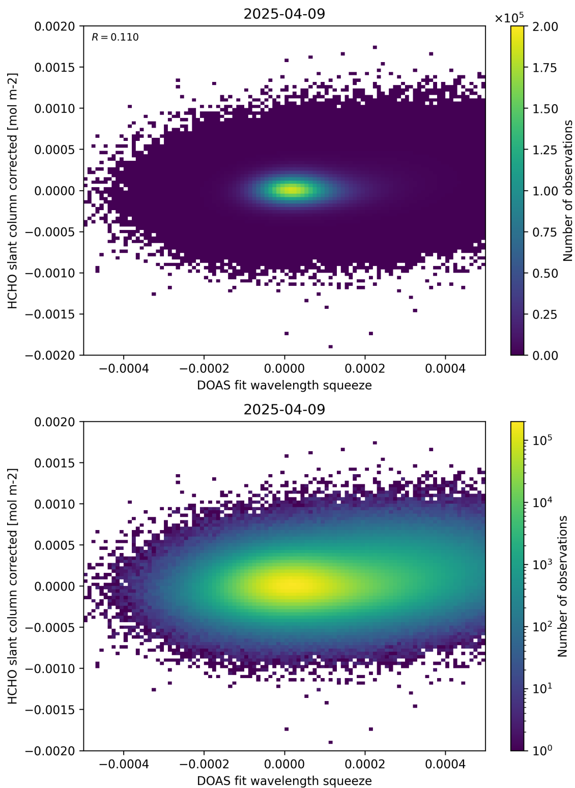
Figure 69: Scatter density plot of “DOAS fit wavelength squeeze” against “HCHO slant column corrected” for 2025-04-08 to 2025-04-10.
