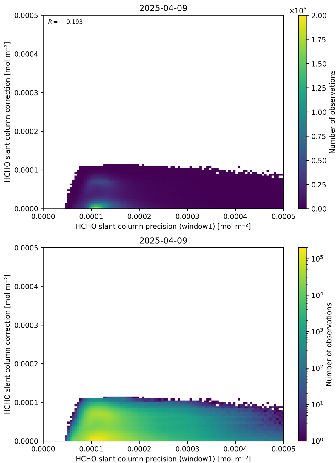
Figure 93: Scatter density plot of “HCHO slant column precision (window1)” against “HCHO slant column correction” for 2025-04-08 to 2025-04-10.
