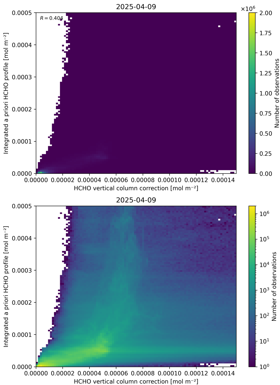
Figure 122: Scatter density plot of “HCHO vertical column correction” against “Integrated a priori HCHO profile” for 2025-04-08 to 2025-04-10.
