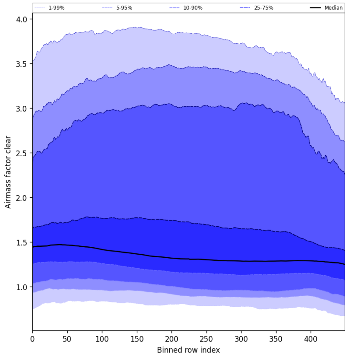
Figure 56: Along track statistics of “Air mass factor clear” for 2025-04-08 to 2025-04-10
