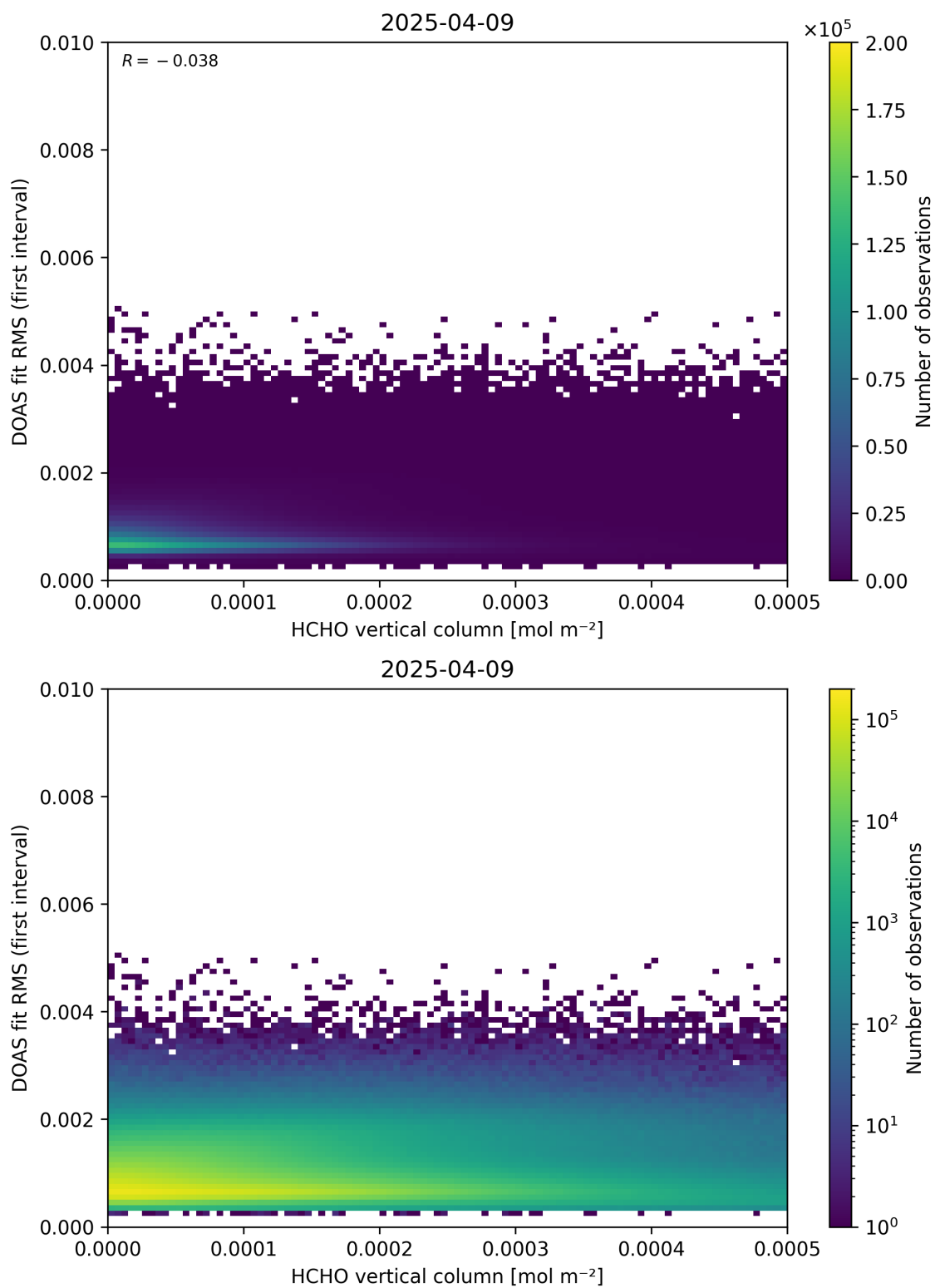
Figure 123: Scatter density plot of “HCHO vertical column” against “DOAS fit RMS (first interval)” for 2025-04-08 to 2025-04-10.
