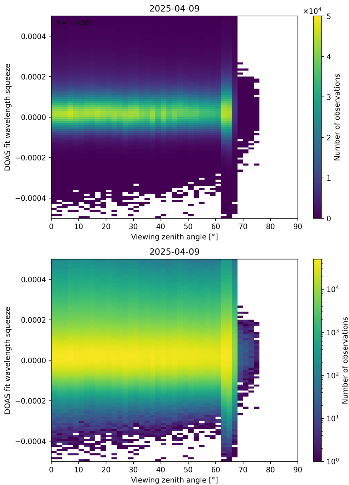
Figure 184: Scatter density plot of “Viewing zenith angle” against “DOAS fit wavelength squeeze” for 2025-04-08 to 2025-04-10.
