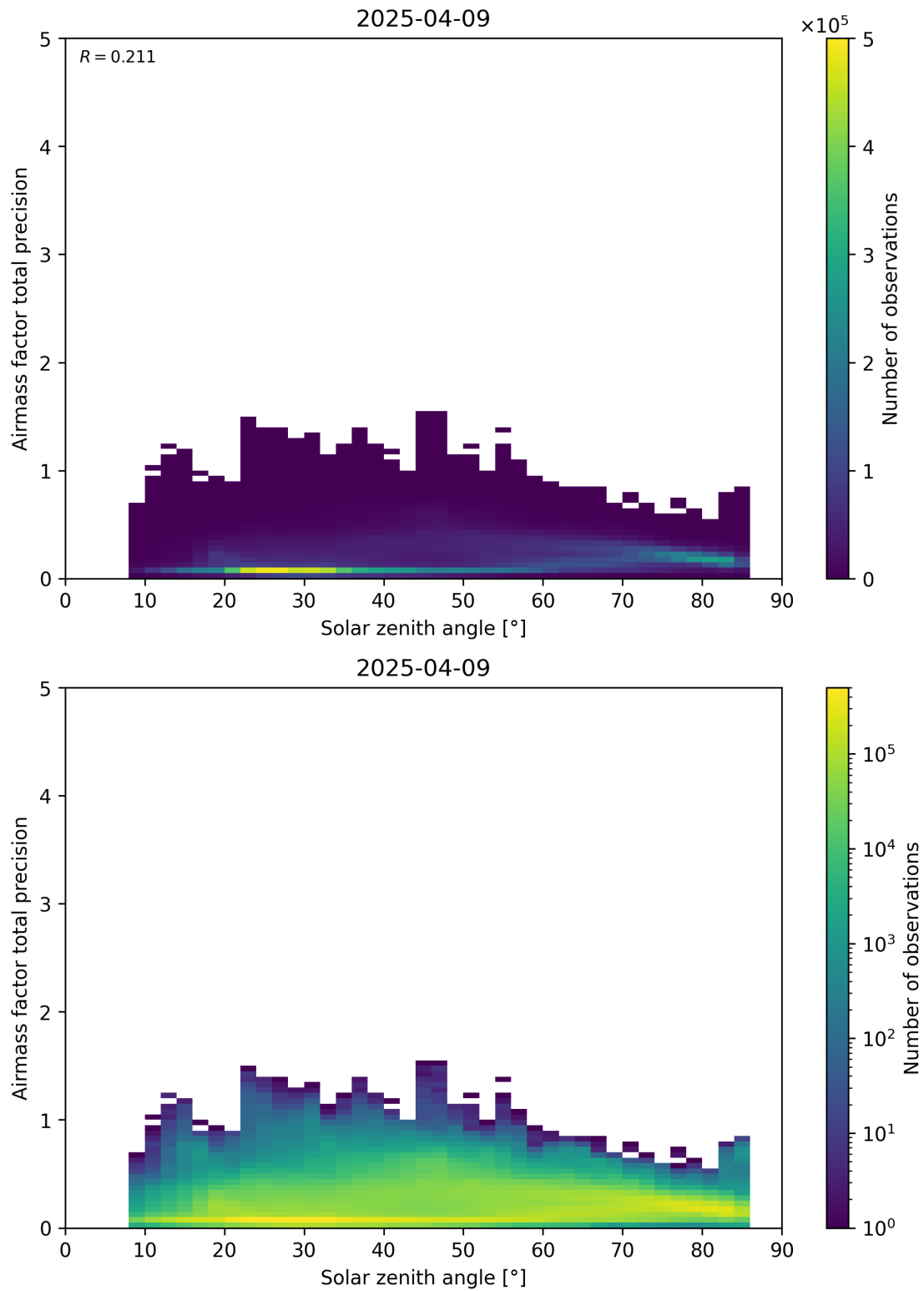
Figure 176: Scatter density plot of “Solar zenith angle” against “Airmass factor total precision” for 2025-04-08 to 2025-04-10.
