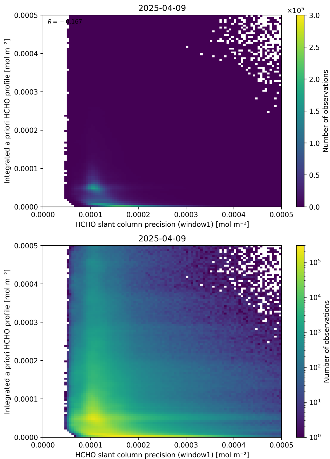
Figure 96: Scatter density plot of “HCHO slant column precision (window1)” against “Integrated a priori HCHO profile” for 2025-04-08 to 2025-04-10.
