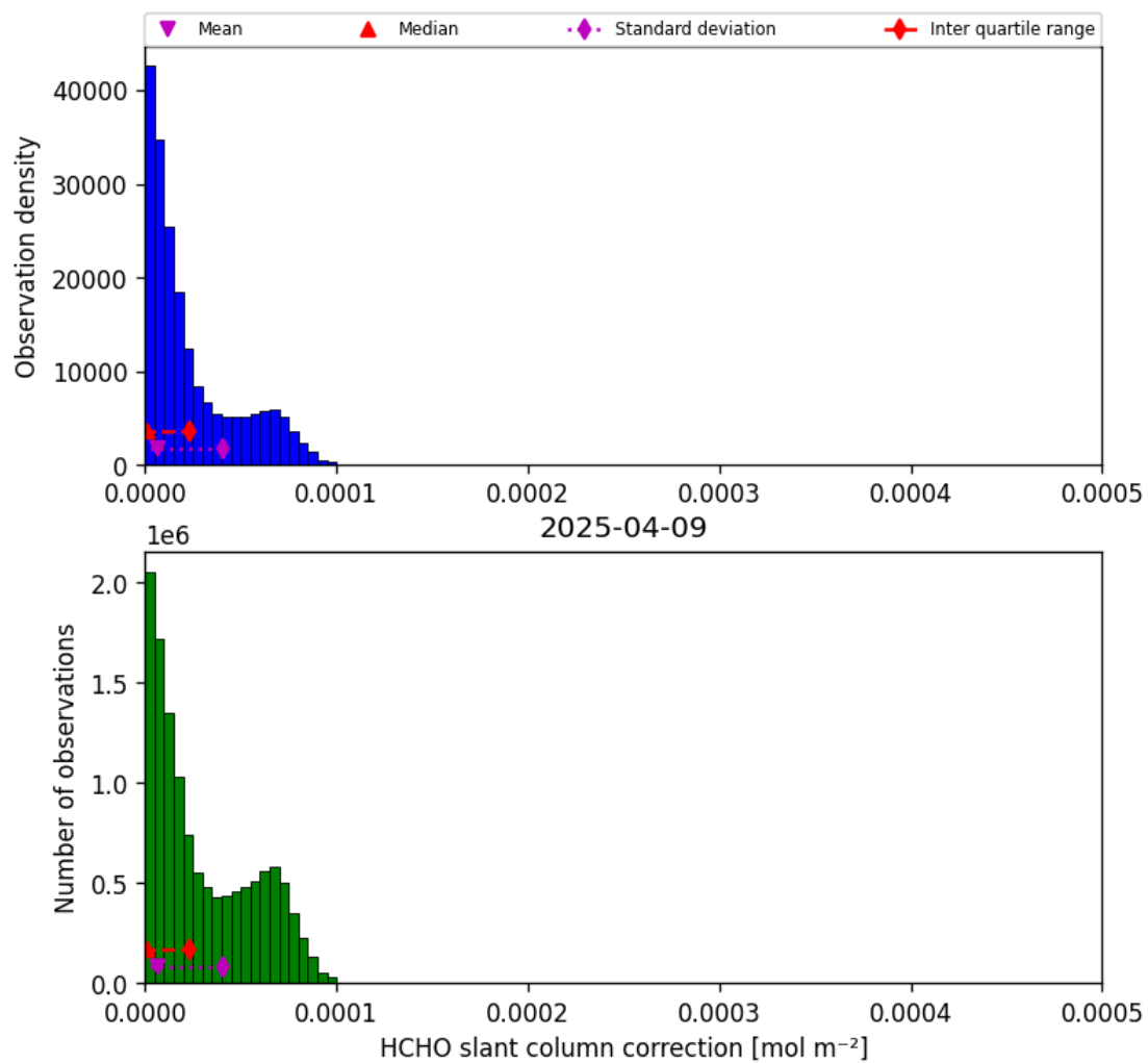
Figure 47: Histogram of “HCHO slant column correction” for 2025-04-08 to 2025-04-10
