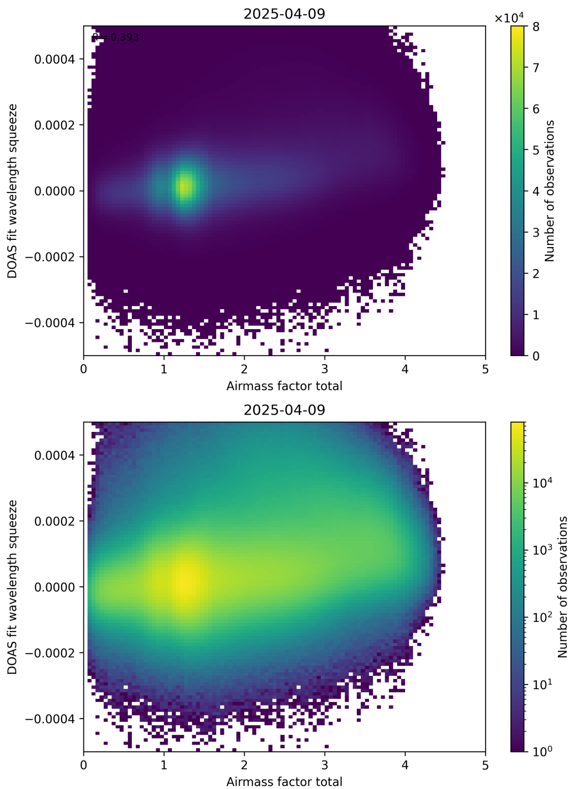
Figure 99: Scatter density plot of “Airmass factor total” against “DOAS fit wavelength squeeze” for 2025-04-08 to 2025-04-10.
