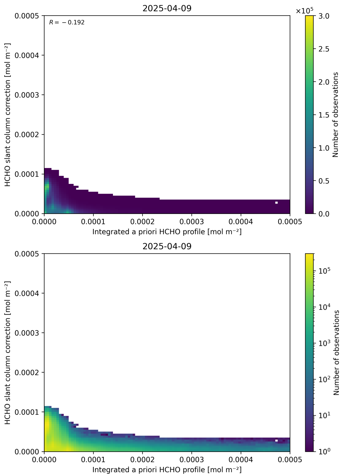
Figure 152: Scatter density plot of “Integrated a priori HCHO profile” against “HCHO slant column correction” for 2025-04-08 to 2025-04-10.
