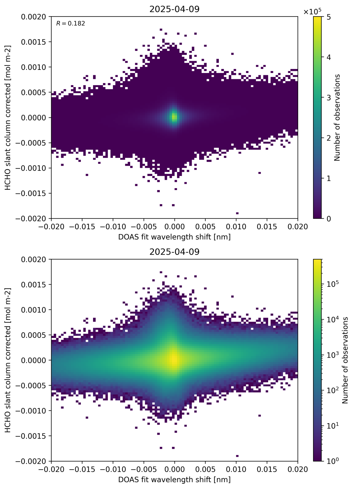
Figure 66: Scatter density plot of “DOAS fit wavelength shift” against “HCHO slant column corrected” for 2025-04-08 to 2025-04-10.
