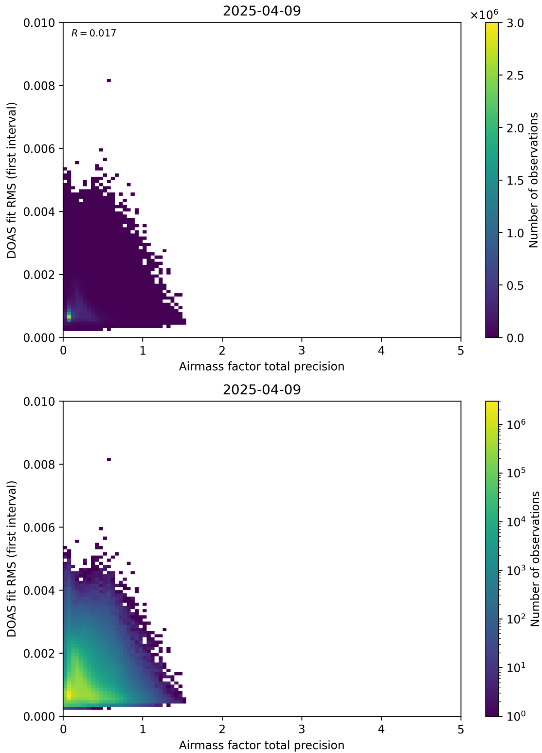
Figure 105: Scatter density plot of “Airmass factor total precision” against “DOAS fit RMS (first interval)” for 2025-04-08 to 2025-04-10.
