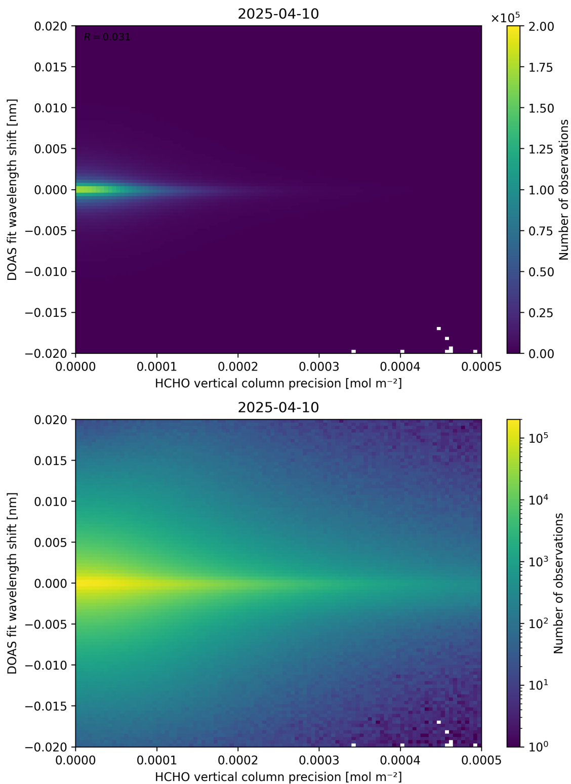
Figure 137: Scatter density plot of “HCHO vertical column precision” against “DOAS fit wavelength shift” for 2025-04-09 to 2025-04-11.
