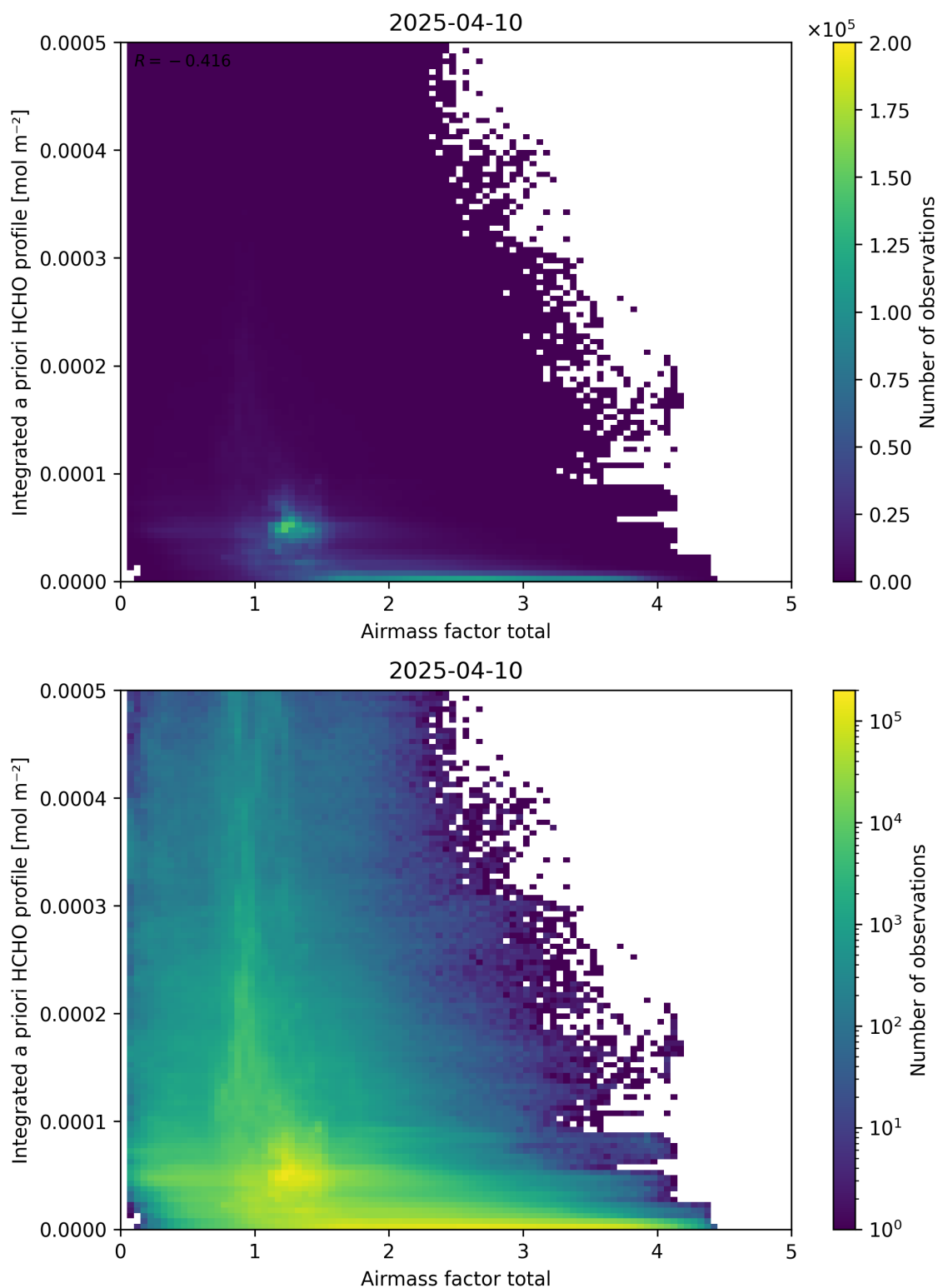
Figure 104: Scatter density plot of “Airmass factor total” against “Integrated a priori HCHO profile” for 2025-04-09 to 2025-04-11.
