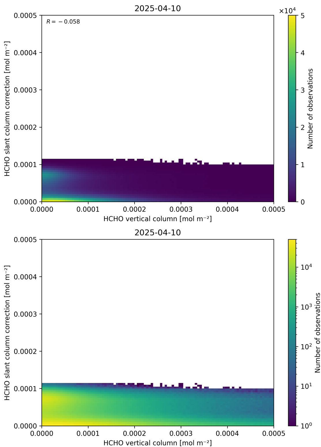
Figure 128: Scatter density plot of “HCHO vertical column” against “HCHO slant column correction” for 2025-04-09 to 2025-04-11.
