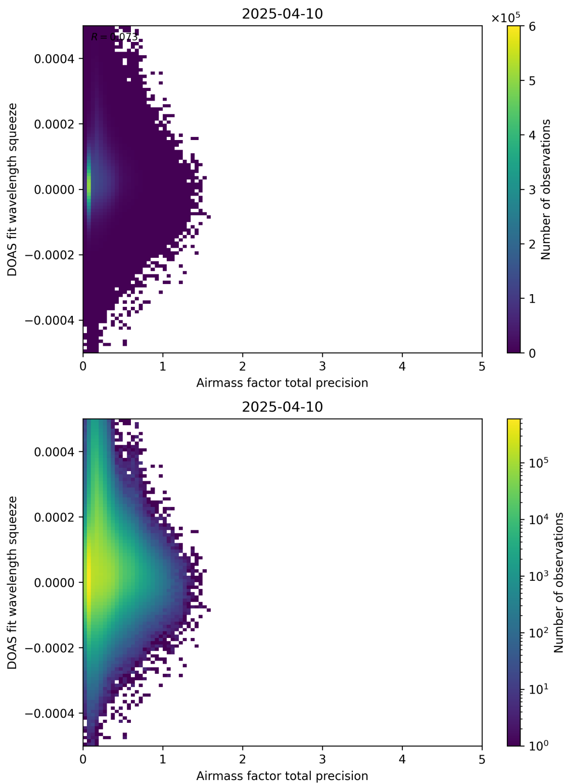
Figure 107: Scatter density plot of “Airmass factor total precision” against “DOAS fit wavelength squeeze” for 2025-04-09 to 2025-04-11.
