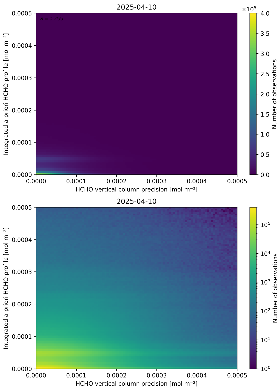
Figure 147: Scatter density plot of “HCHO vertical column precision” against “Integrated a priori HCHO profile” for 2025-04-09 to 2025-04-11.
