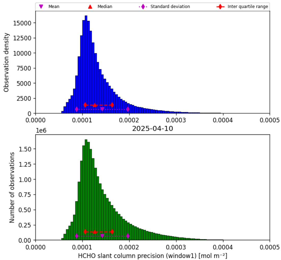
Figure 39: Histogram of “HCHO slant column precision (window1)” for 2025-04-09 to 2025-04-11
