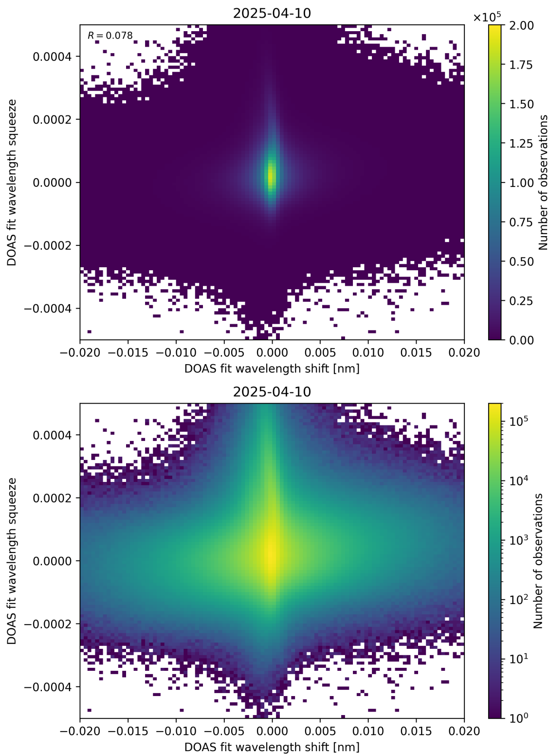
Figure 65: Scatter density plot of “DOAS fit wavelength shift” against “DOAS fit wavelength squeeze” for 2025-04-09 to 2025-04-11.
