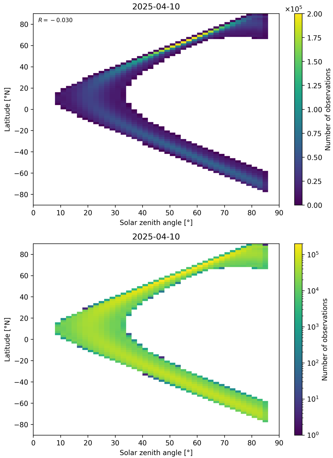
Figure 181: Scatter density plot of “Solar zenith angle” against “Latitude” for 2025-04-09 to 2025-04-11.
