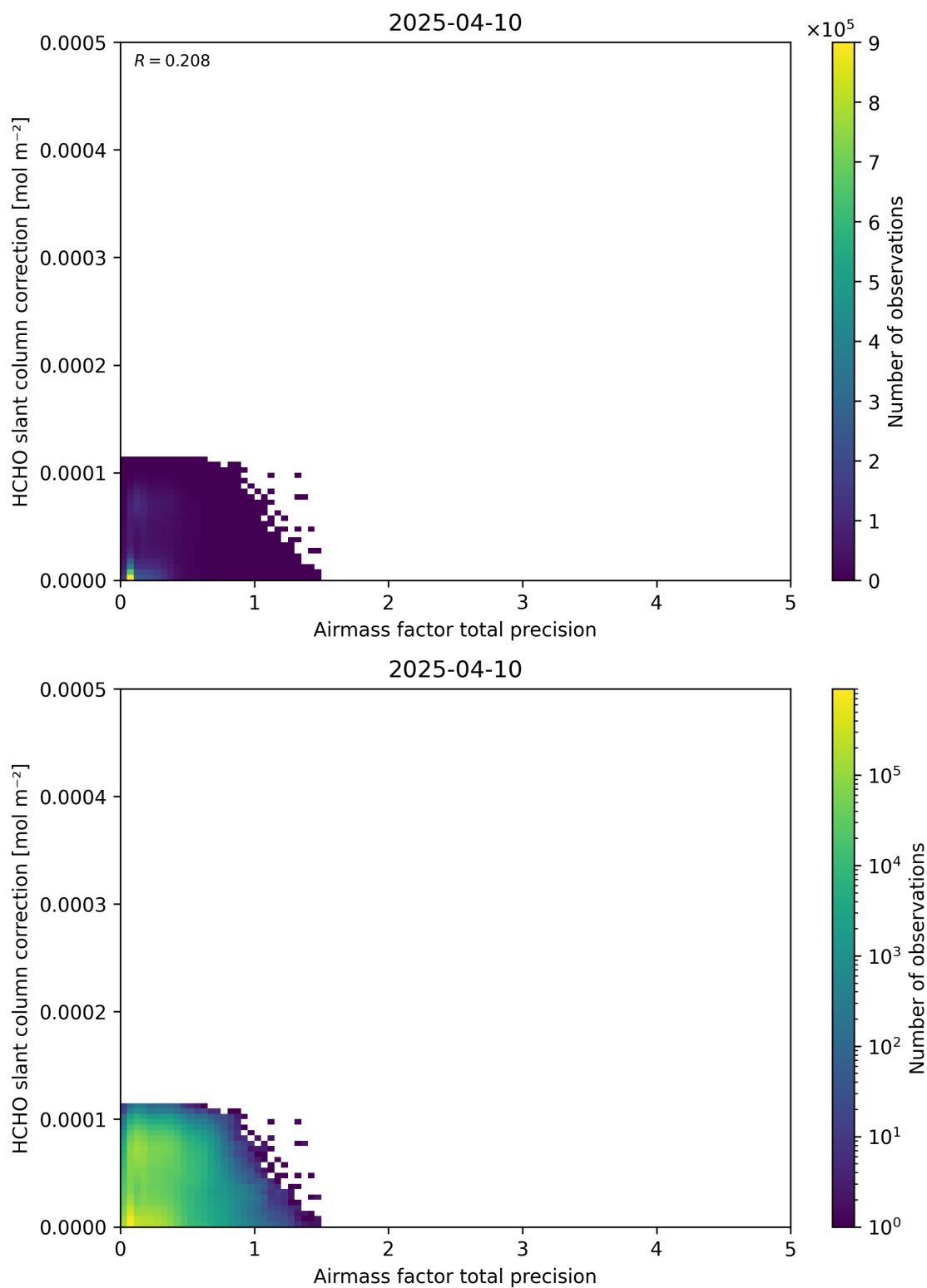
Figure 110: Scatter density plot of “Airmass factor total precision” against “HCHO slant column correction” for 2025-04-09 to 2025-04-11.
