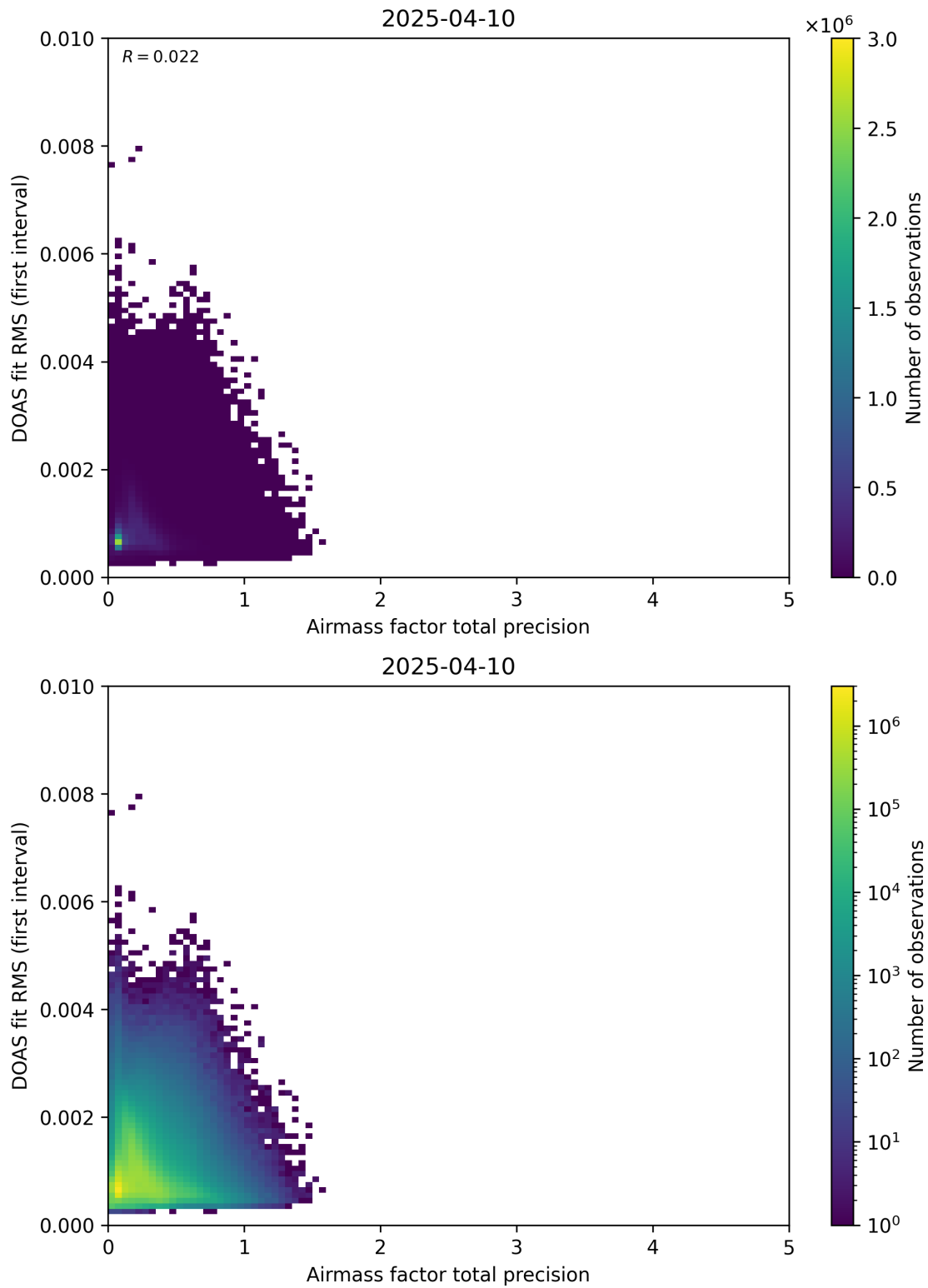
Figure 105: Scatter density plot of “Airmass factor total precision” against “DOAS fit RMS (first interval)” for 2025-04-09 to 2025-04-11.
