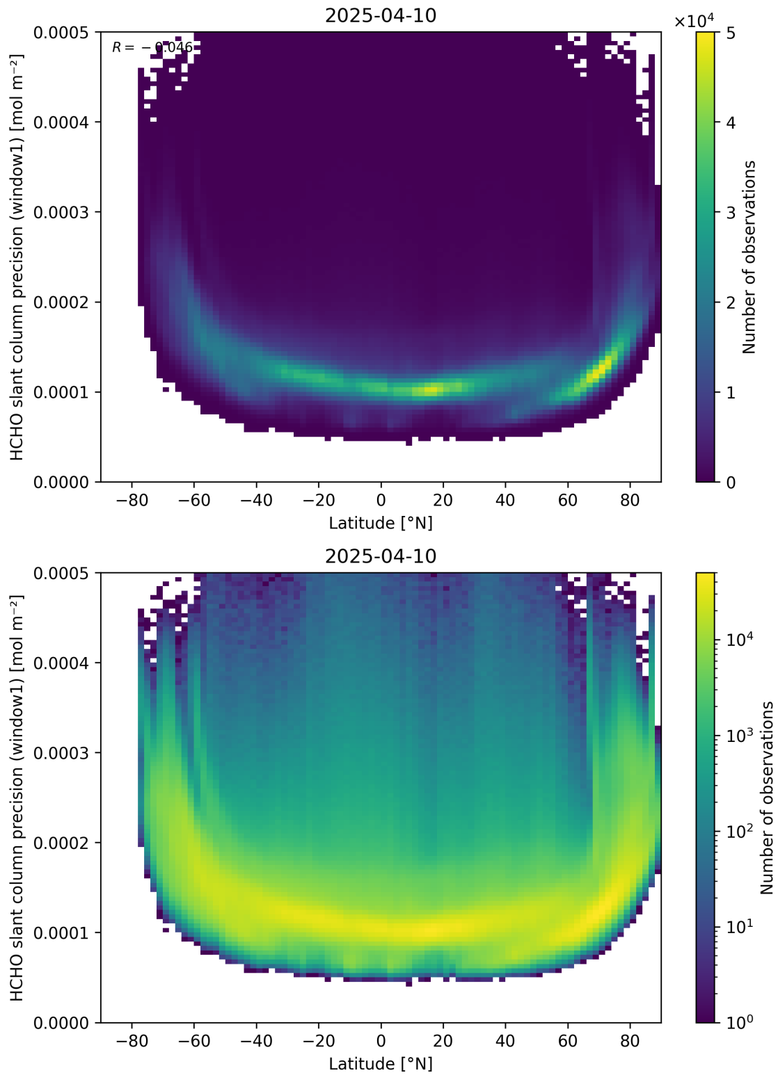
Figure 160: Scatter density plot of “Latitude” against “HCHO slant column precision (window1)” for 2025-04-09 to 2025-04-11.
