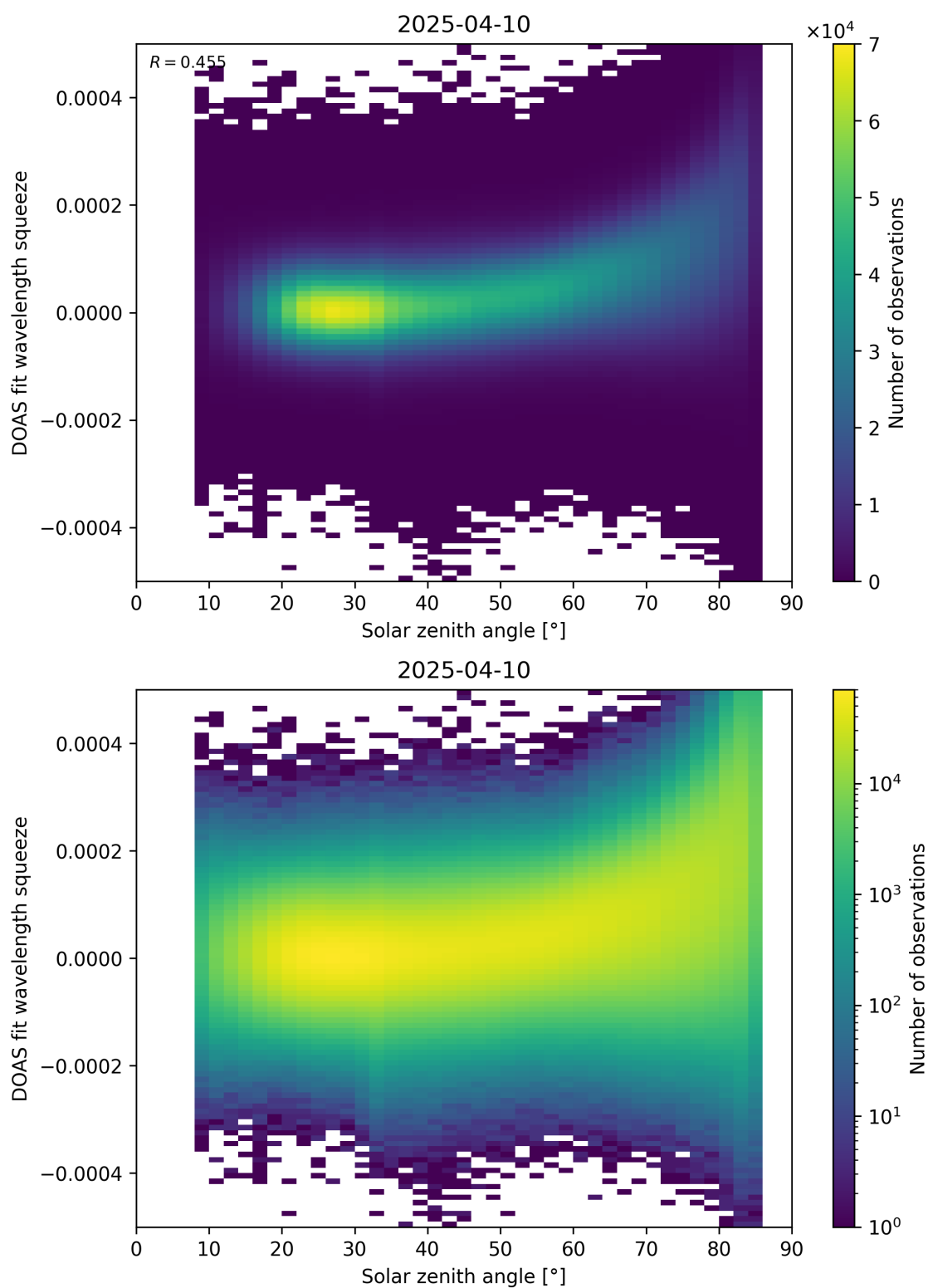
Figure 169: Scatter density plot of “Solar zenith angle” against “DOAS fit wavelength squeeze” for 2025-04-09 to 2025-04-11.
