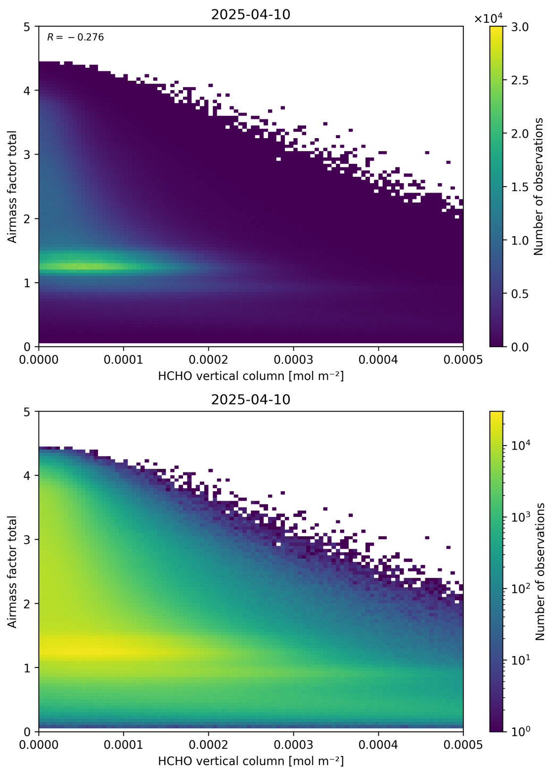
Figure 131: Scatter density plot of “HCHO vertical column” against “Airmass factor total” for 2025-04-09 to 2025-04-11.
