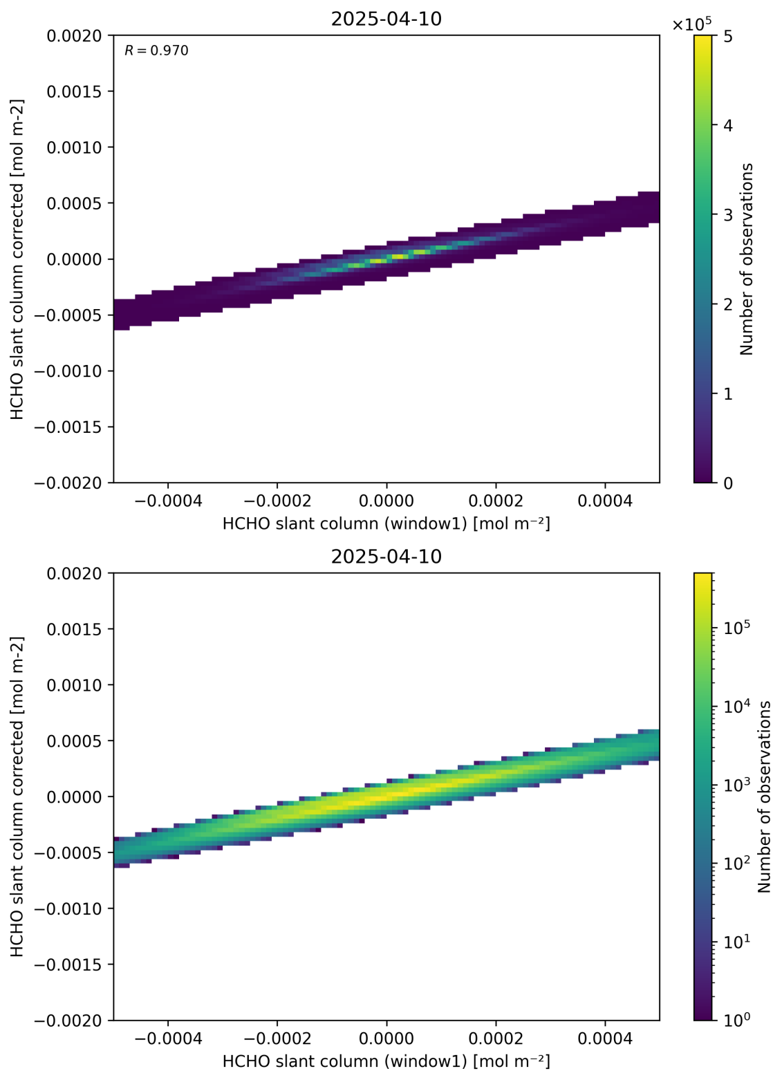
Figure 82: Scatter density plot of “HCHO slant column (window1)” against “HCHO slant column corrected” for 2025-04-09 to 2025-04-11.
