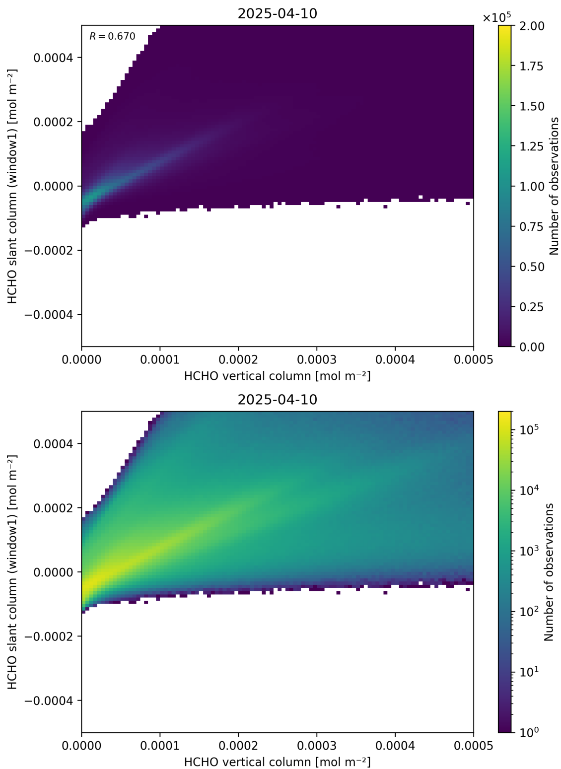
Figure 129: Scatter density plot of “HCHO vertical column” against “HCHO slant column (window1)” for 2025-04-09 to 2025-04-11.
