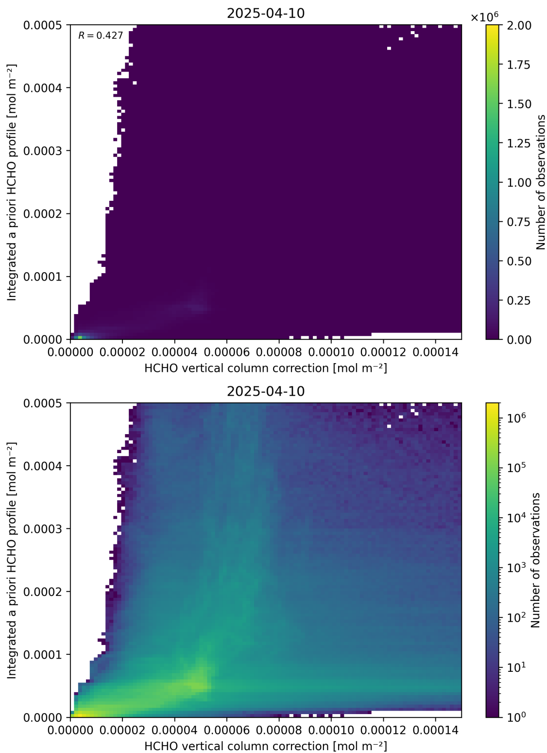
Figure 122: Scatter density plot of “HCHO vertical column correction” against “Integrated a priori HCHO profile” for 2025-04-09 to 2025-04-11.
