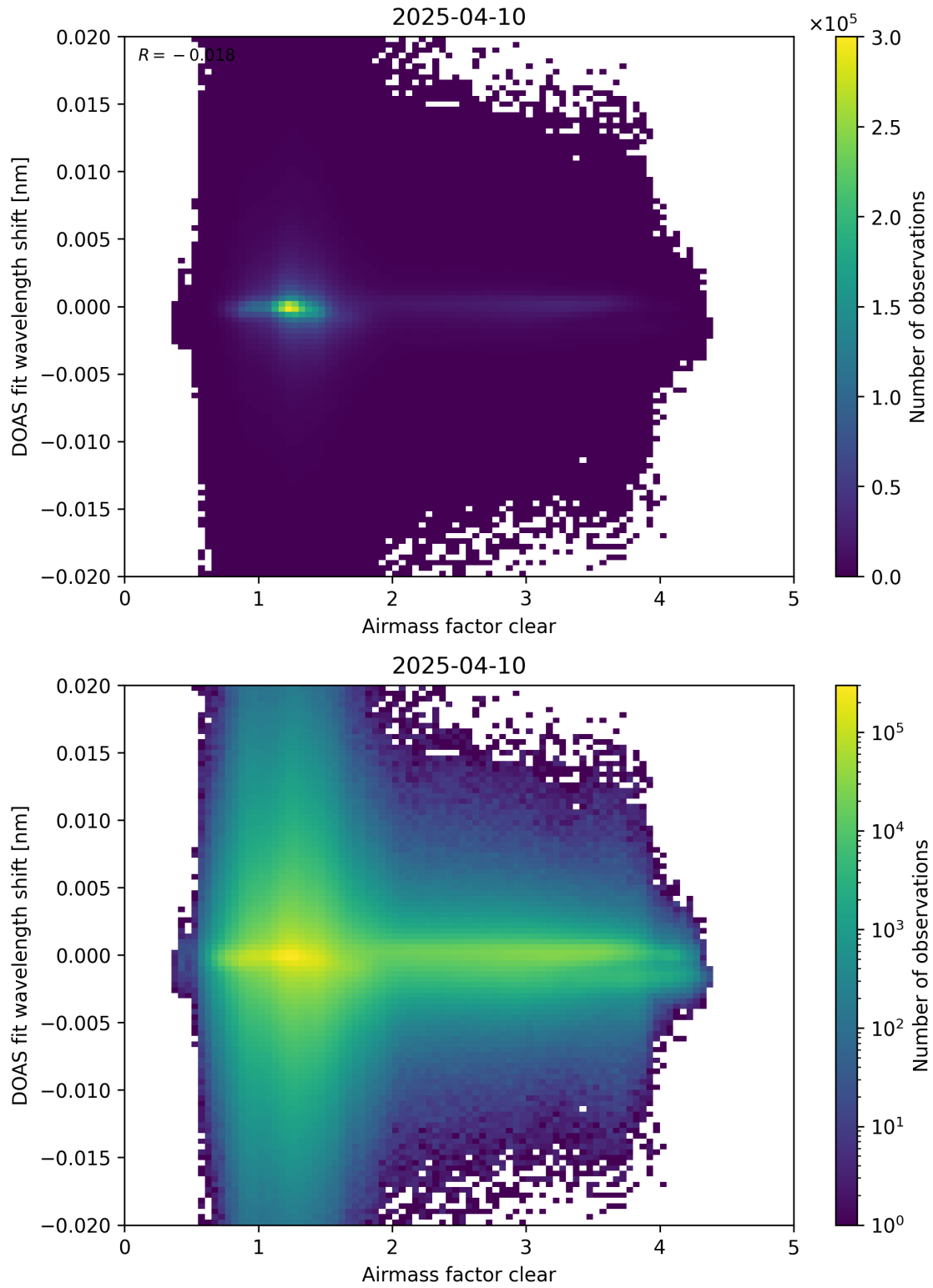
Figure 72: Scatter density plot of “Airmass factor clear” against “DOAS fit wavelength shift” for 2025-04-09 to 2025-04-11.
