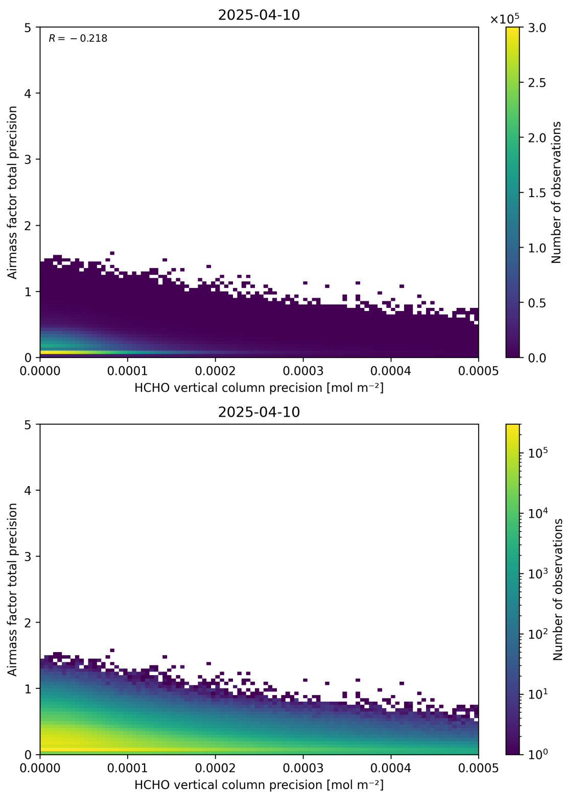
Figure 145: Scatter density plot of “HCHO vertical column precision” against “Airmass factor total precision” for 2025-04-09 to 2025-04-11.
