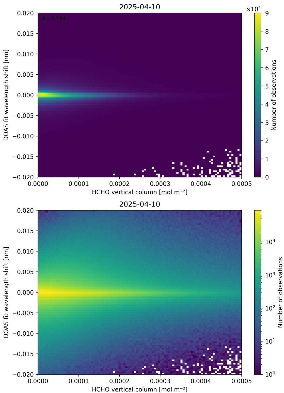
Figure 124: Scatter density plot of “HCHO vertical column” against “DOAS fit wavelength shift” for 2025-04-09 to 2025-04-11.
