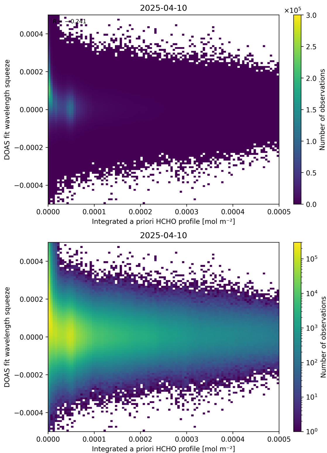
Figure 150: Scatter density plot of “Integrated a priori HCHO profile” against “DOAS fit wavelength squeeze” for 2025-04-09 to 2025-04-11.
