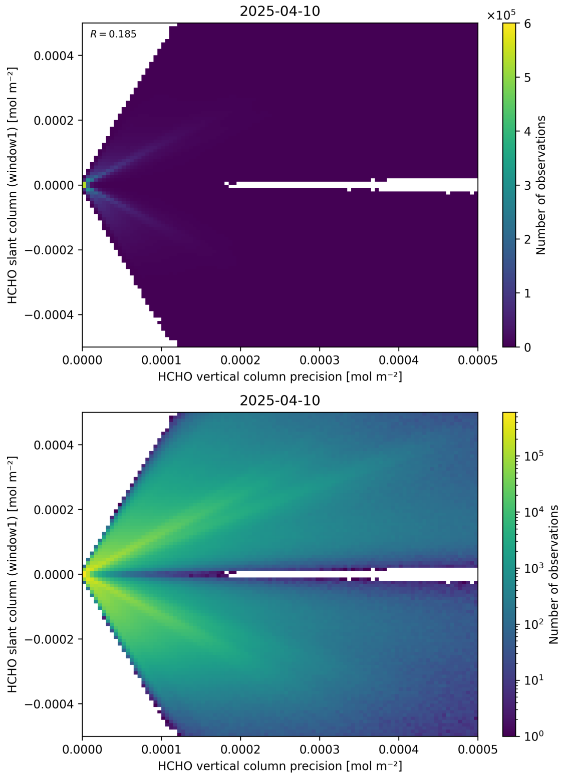
Figure 142: Scatter density plot of “HCHO vertical column precision” against “HCHO slant column (window1)” for 2025-04-09 to 2025-04-11.
