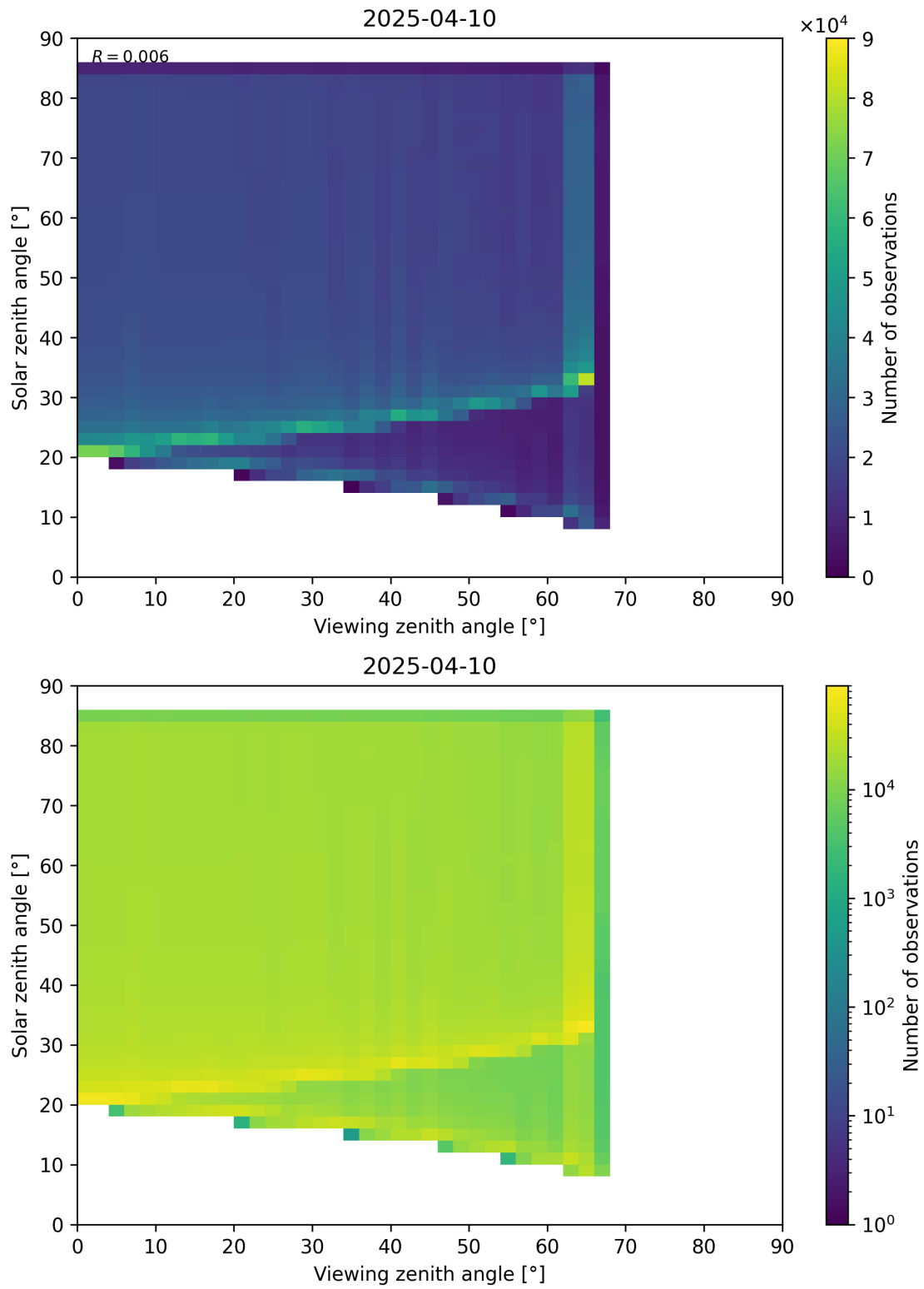
Figure 197: Scatter density plot of “Viewing zenith angle” against “Solar zenith angle” for 2025-04-09 to 2025-04-11.
