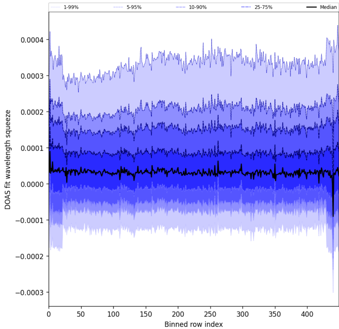
Figure 59: Along track statistics of “DOAS fit wavelength squeeze” for 2025-04-09 to 2025-04-11
