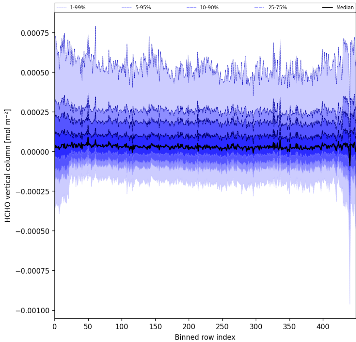
Figure 49: Along track statistics of “HCHO vertical column” for 2025-04-09 to 2025-04-11
