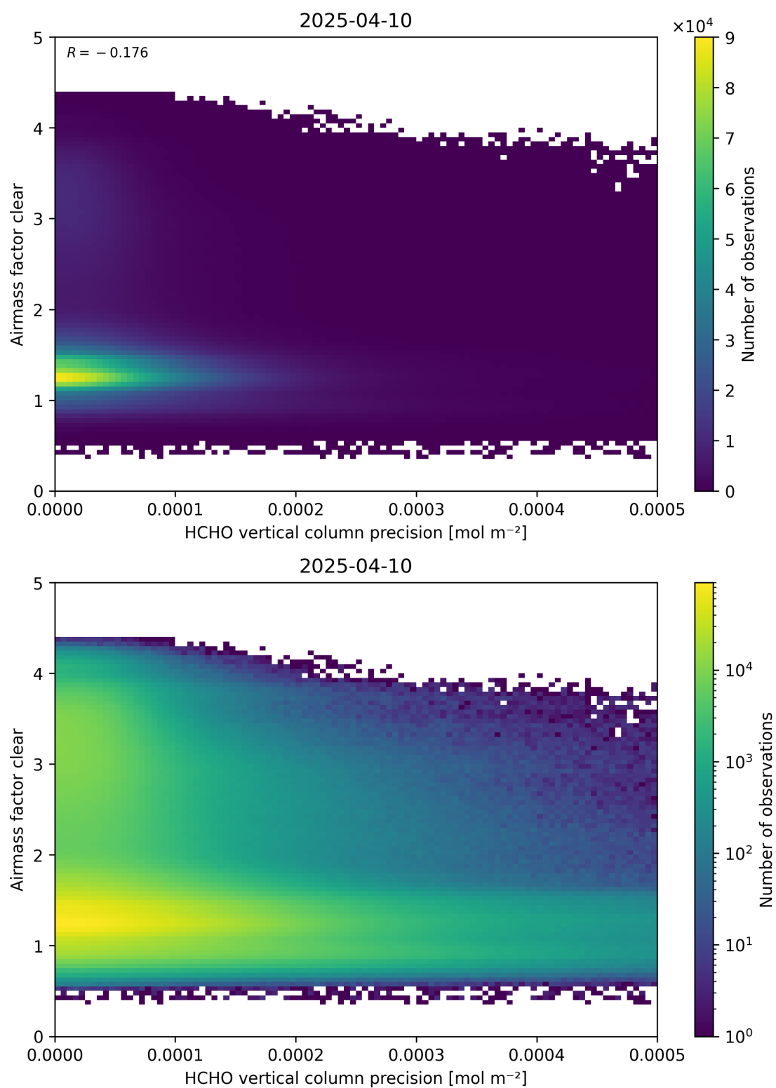
Figure 139: Scatter density plot of “HCHO vertical column precision” against “Airmass factor clear” for 2025-04-09 to 2025-04-11.
