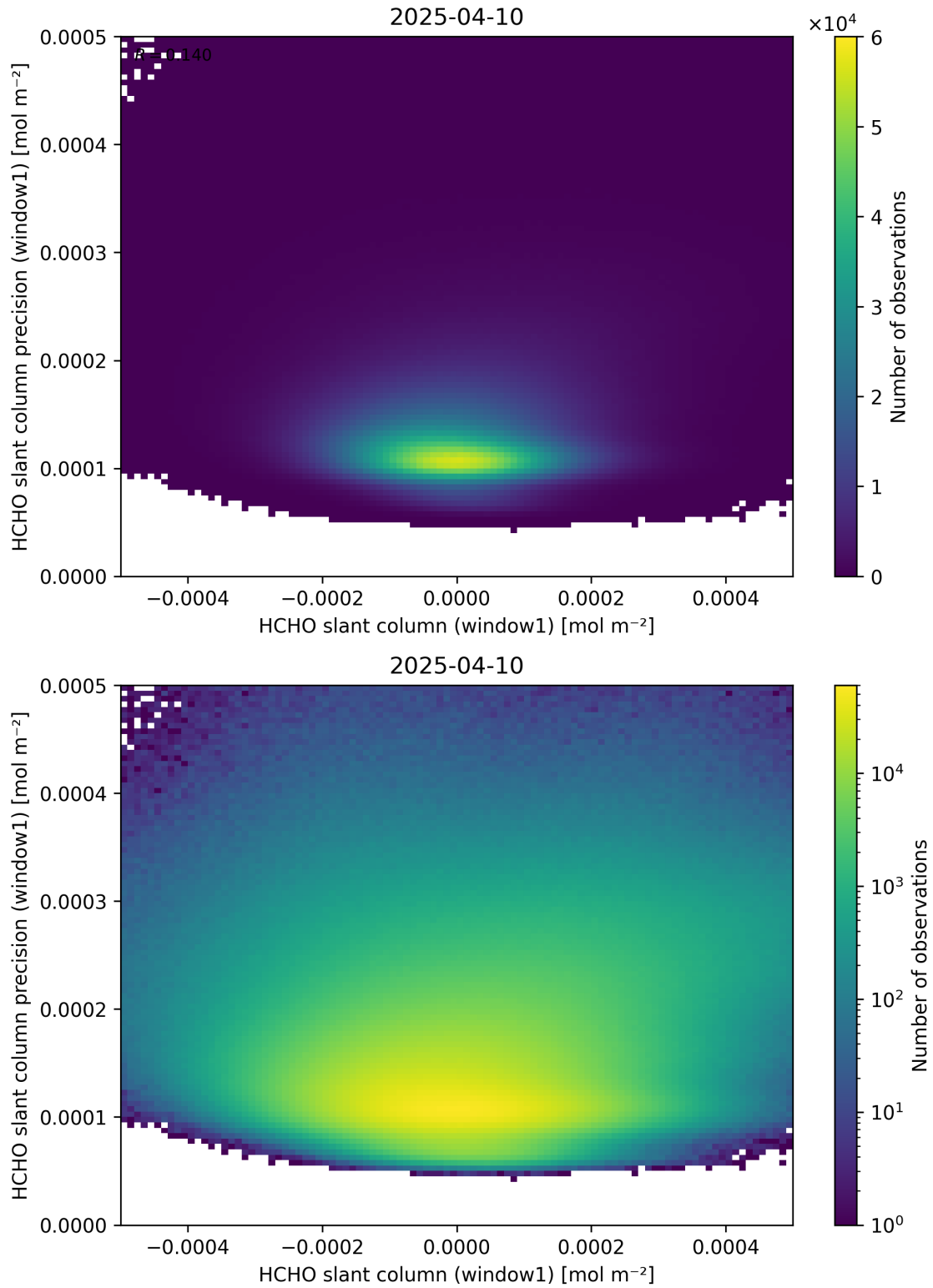
Figure 84: Scatter density plot of “HCHO slant column (window1)” against “HCHO slant column precision (window1)” for 2025-04-09 to 2025-04-11.
