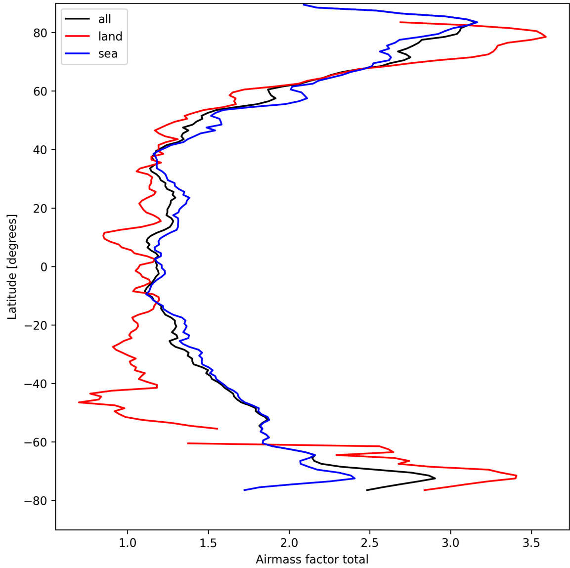
Figure 26: Zonal average of “Airmass factor total” for 2025-04-09 to 2025-04-11.
