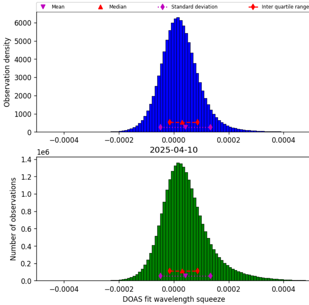
Figure 45: Histogram of “DOAS fit wavelength squeeze” for 2025-04-09 to 2025-04-11
