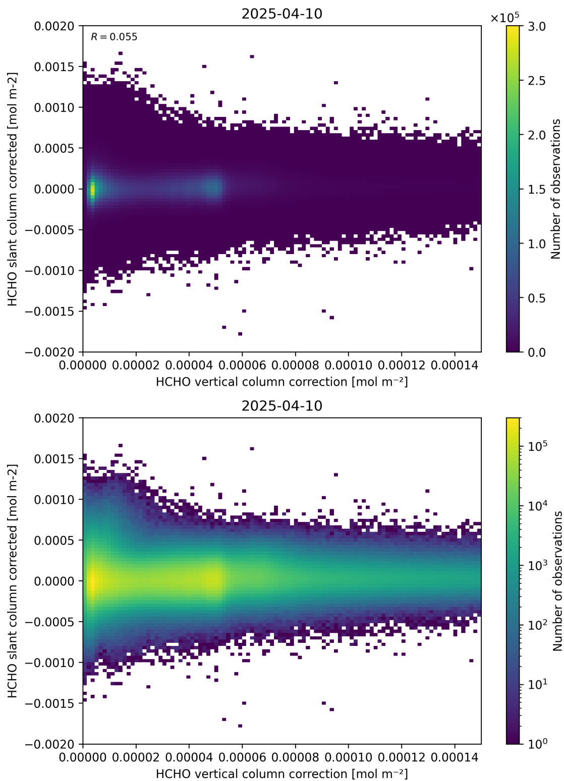
Figure 116: Scatter density plot of “HCHO vertical column correction” against “HCHO slant column corrected” for 2025-04-09 to 2025-04-11.
