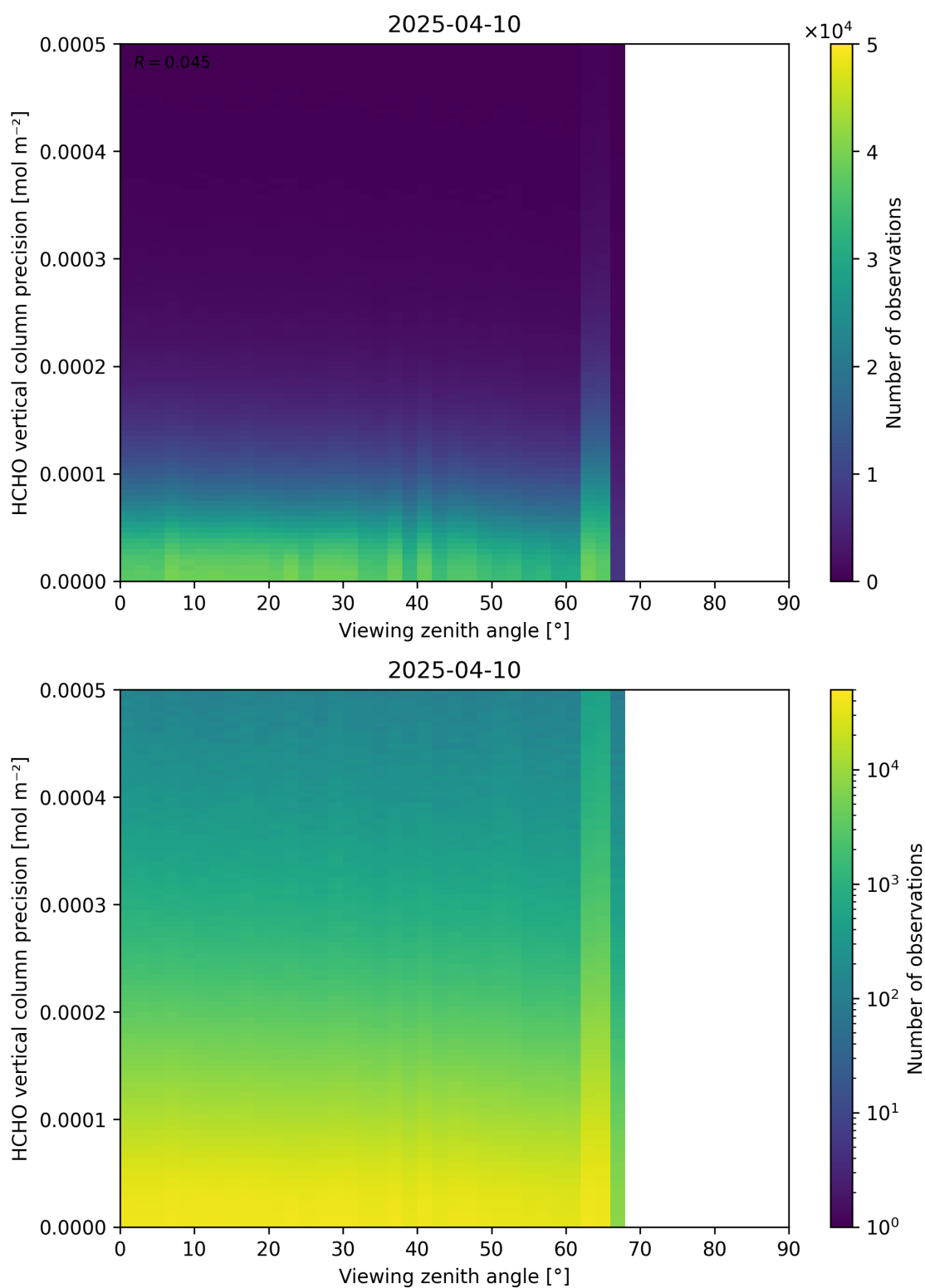
Figure 194: Scatter density plot of “Viewing zenith angle” against “HCHO vertical column precision” for 2025-04-09 to 2025-04-11.
