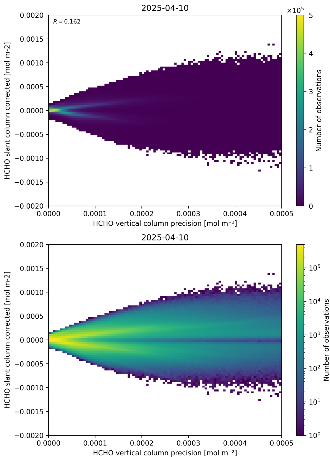
Figure 140: Scatter density plot of “HCHO vertical column precision” against “HCHO slant column corrected” for 2025-04-09 to 2025-04-11.
