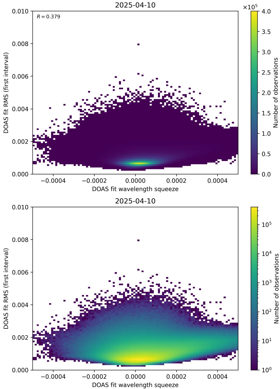
Figure 68: Scatter density plot of “DOAS fit wavelength squeeze” against “DOAS fit RMS (first interval)” for 2025-04-09 to 2025-04-11.
