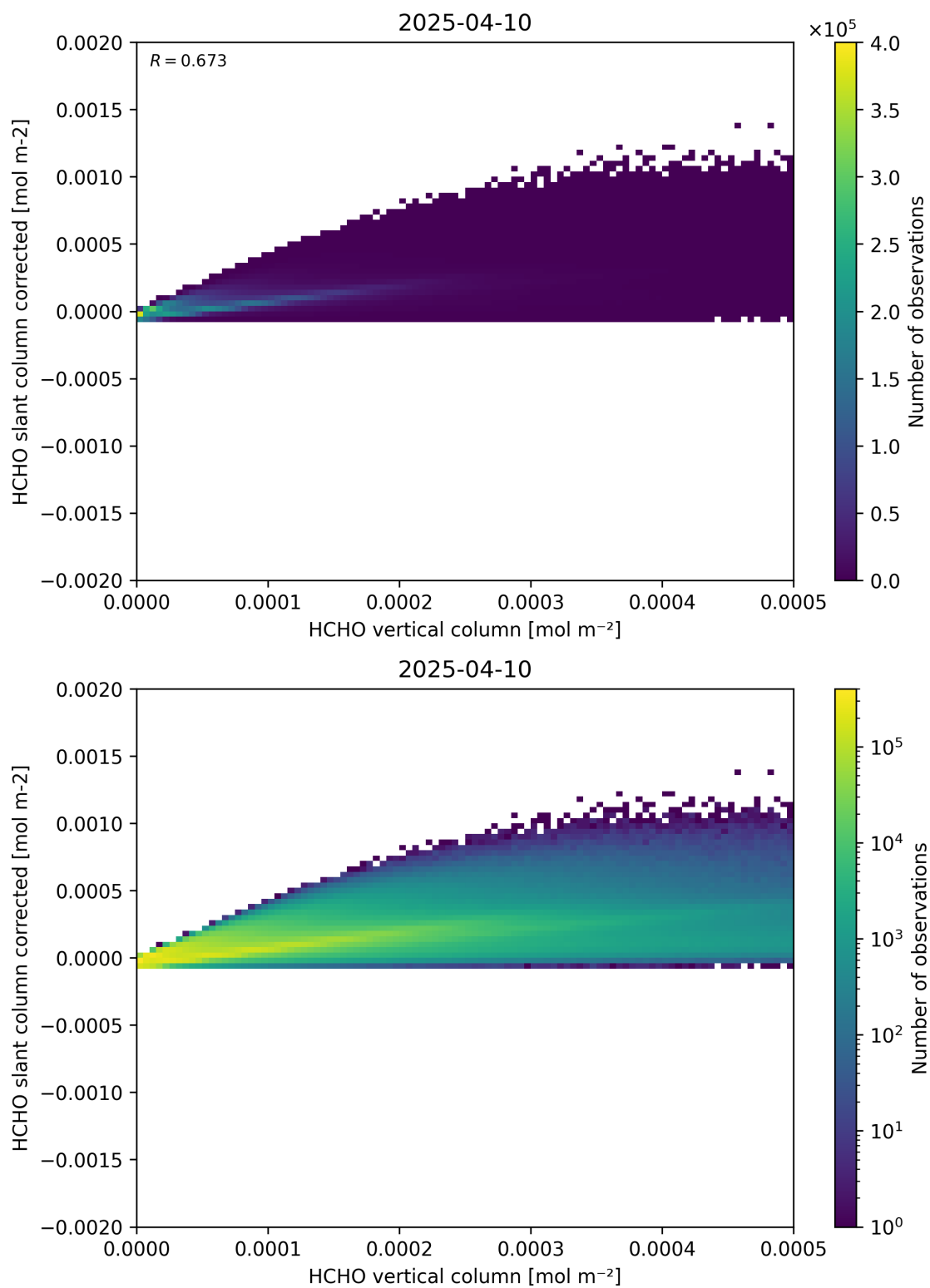
Figure 127: Scatter density plot of “HCHO vertical column” against “HCHO slant column corrected” for 2025-04-09 to 2025-04-11.
