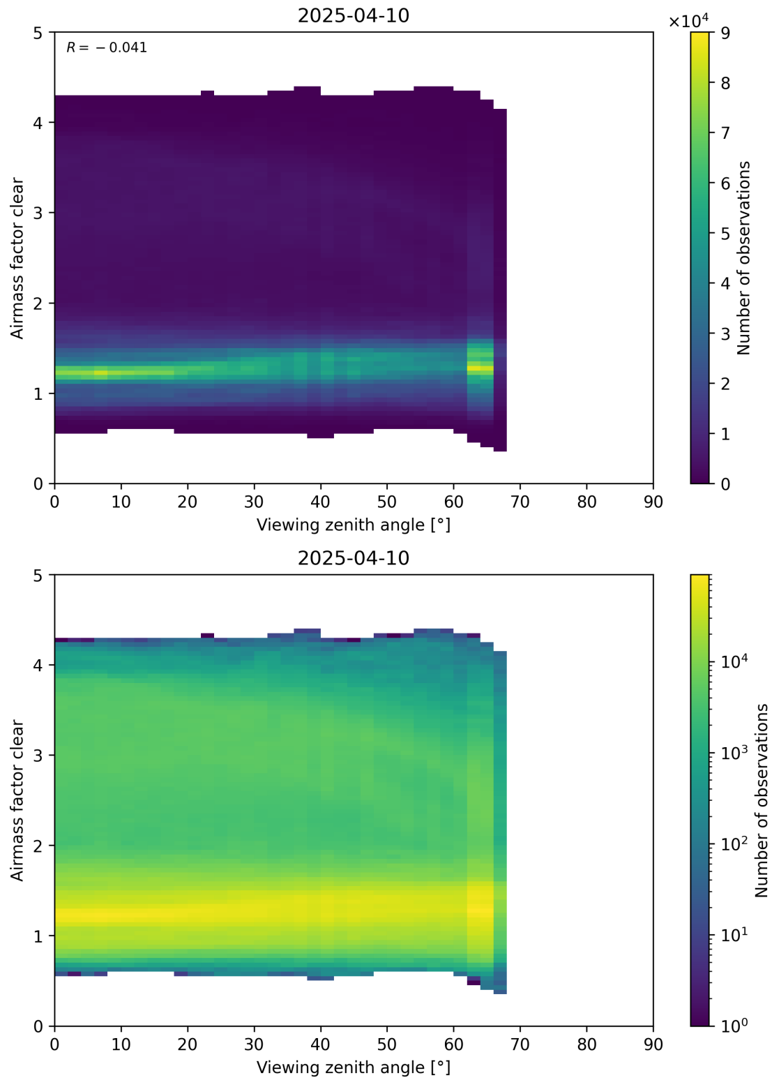
Figure 185: Scatter density plot of “Viewing zenith angle” against “Airmass factor clear” for 2025-04-09 to 2025-04-11.
