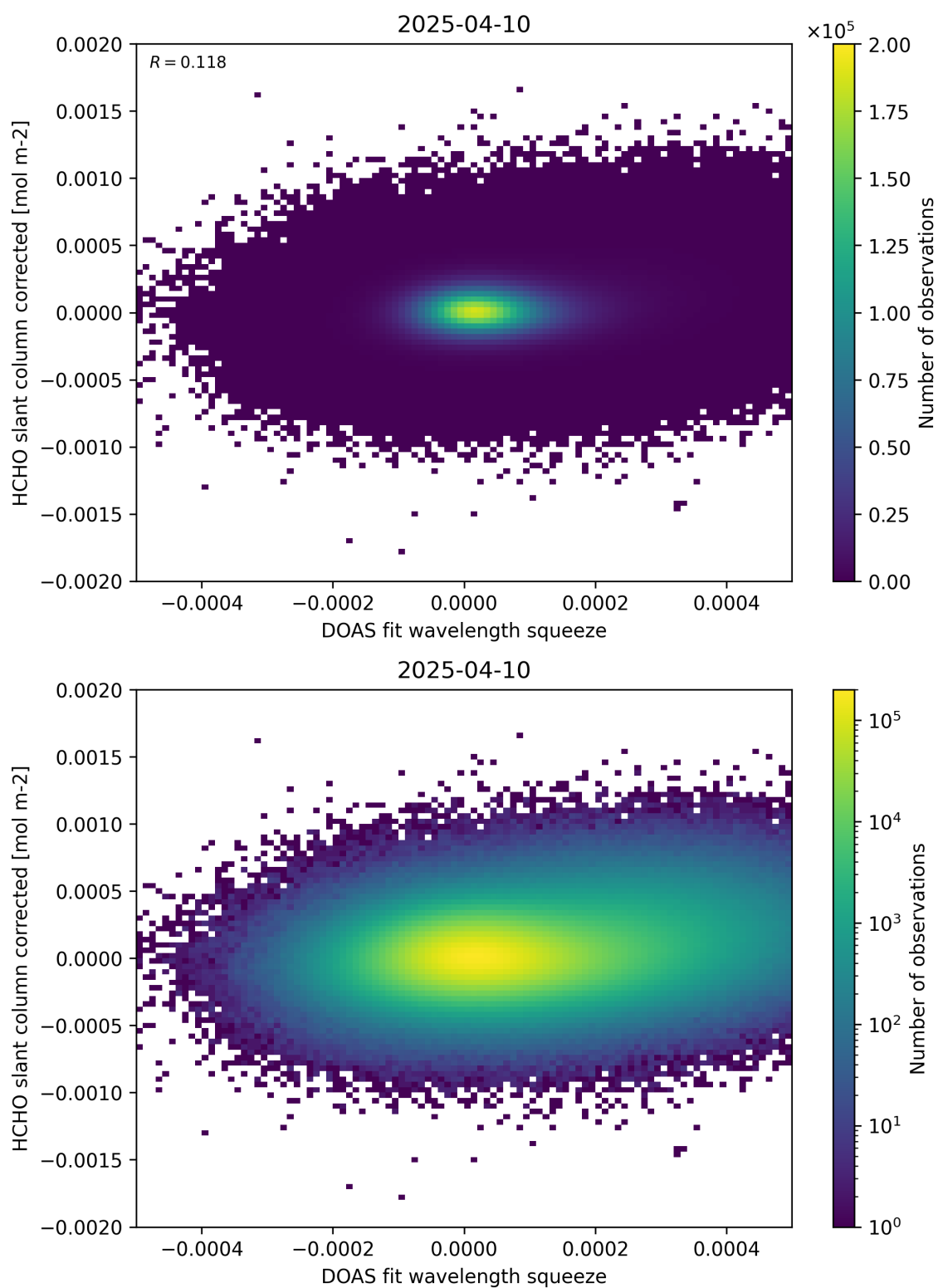
Figure 69: Scatter density plot of “DOAS fit wavelength squeeze” against “HCHO slant column corrected” for 2025-04-09 to 2025-04-11.
