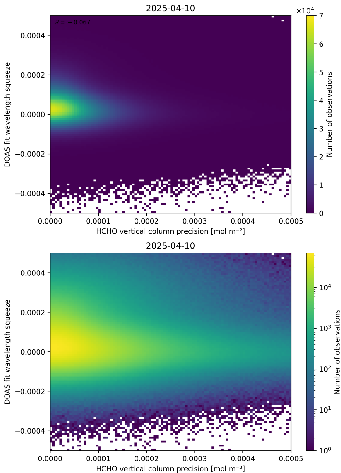
Figure 138: Scatter density plot of “HCHO vertical column precision” against “DOAS fit wavelength squeeze” for 2025-04-09 to 2025-04-11.
