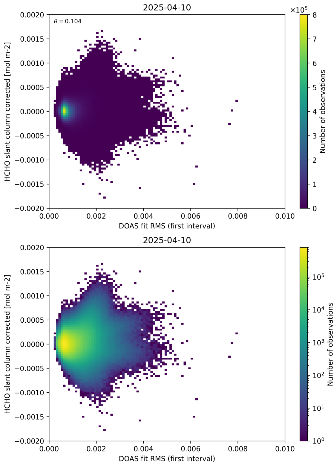
Figure 62: Scatter density plot of “DOAS fit RMS (first interval)” against “HCHO slant column corrected” for 2025-04-09 to 2025-04-11.
