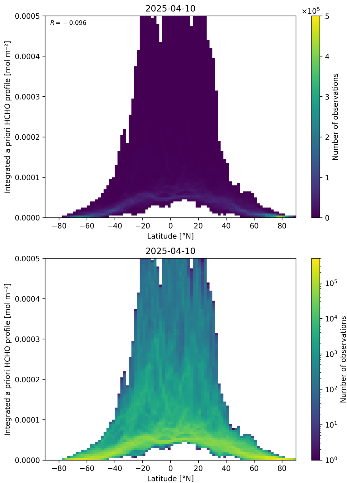
Figure 166: Scatter density plot of “Latitude” against “Integrated a priori HCHO profile” for 2025-04-09 to 2025-04-11.
