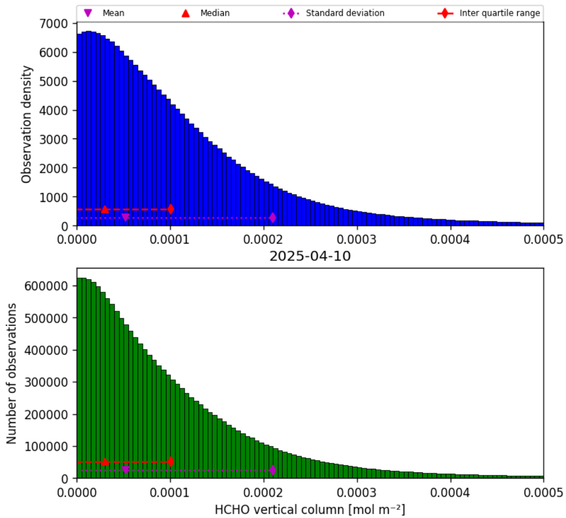
Figure 35: Histogram of “HCHO vertical column” for 2025-04-09 to 2025-04-11
