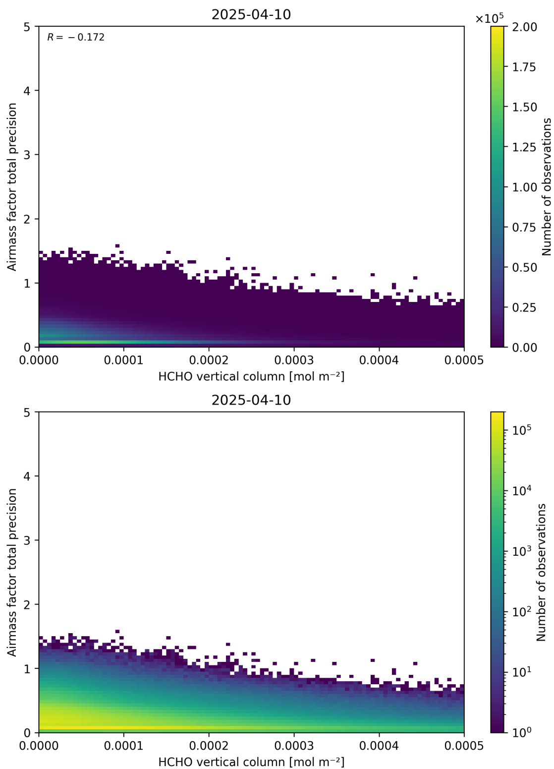
Figure 132: Scatter density plot of “HCHO vertical column” against “Airmass factor total precision” for 2025-04-09 to 2025-04-11.
