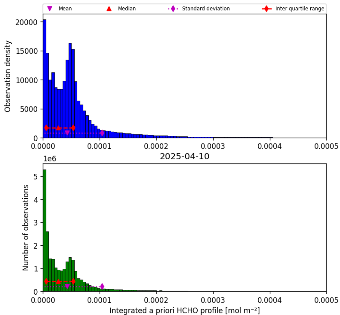
Figure 43: Histogram of “Integrated a priori HCHO profile” for 2025-04-09 to 2025-04-11
