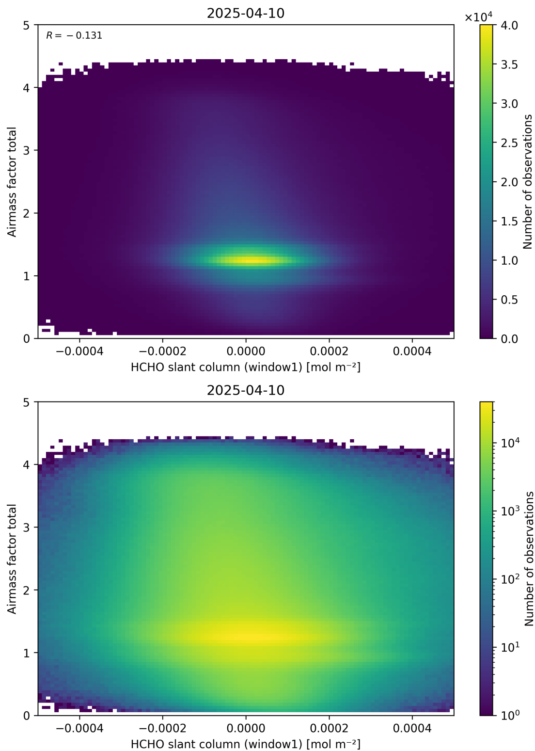
Figure 85: Scatter density plot of “HCHO slant column (window1)” against “Airmass factor total” for 2025-04-09 to 2025-04-11.
