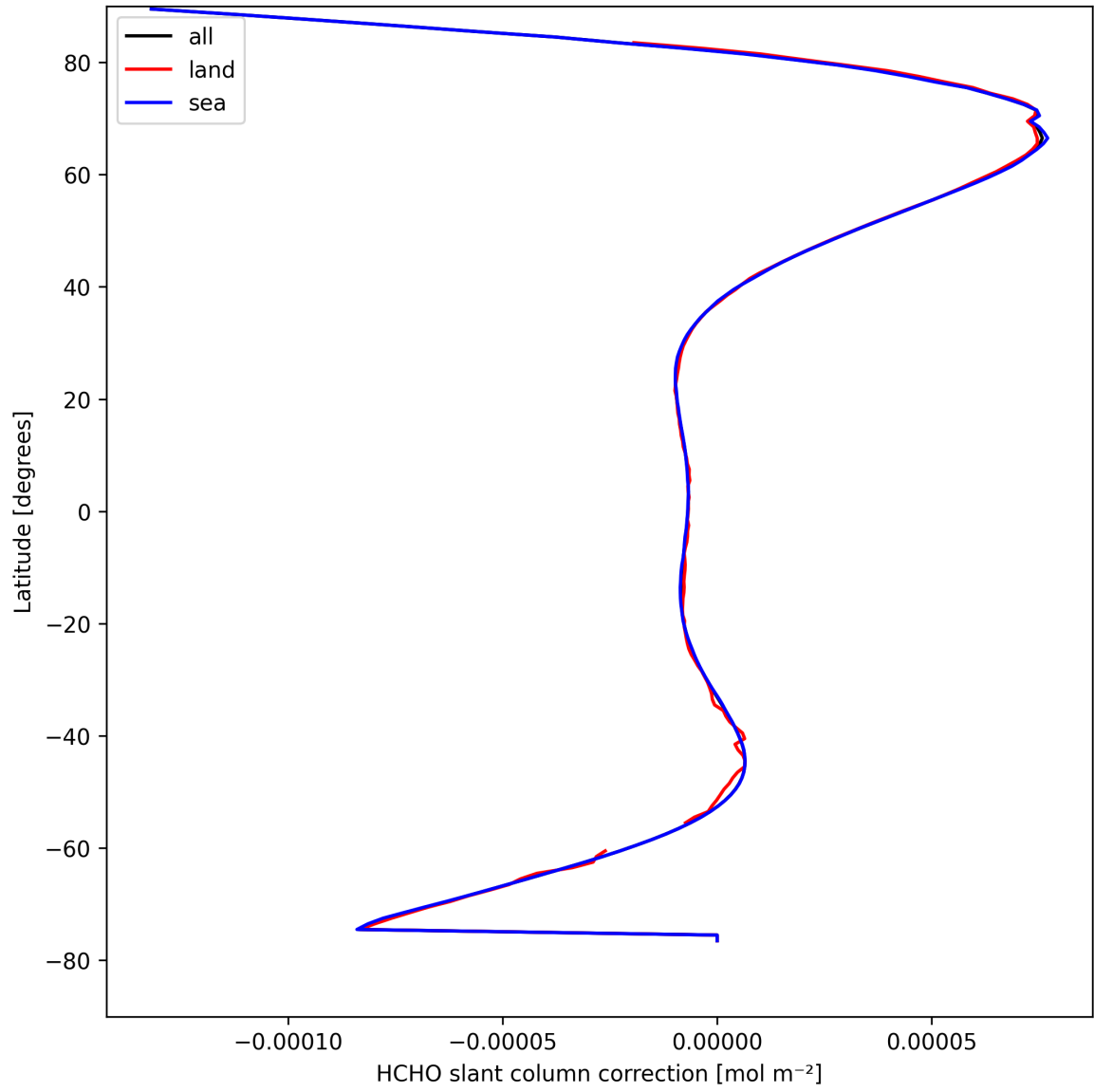
Figure 33: Zonal average of “HCHO slant column correction” for 2025-04-09 to 2025-04-11.
