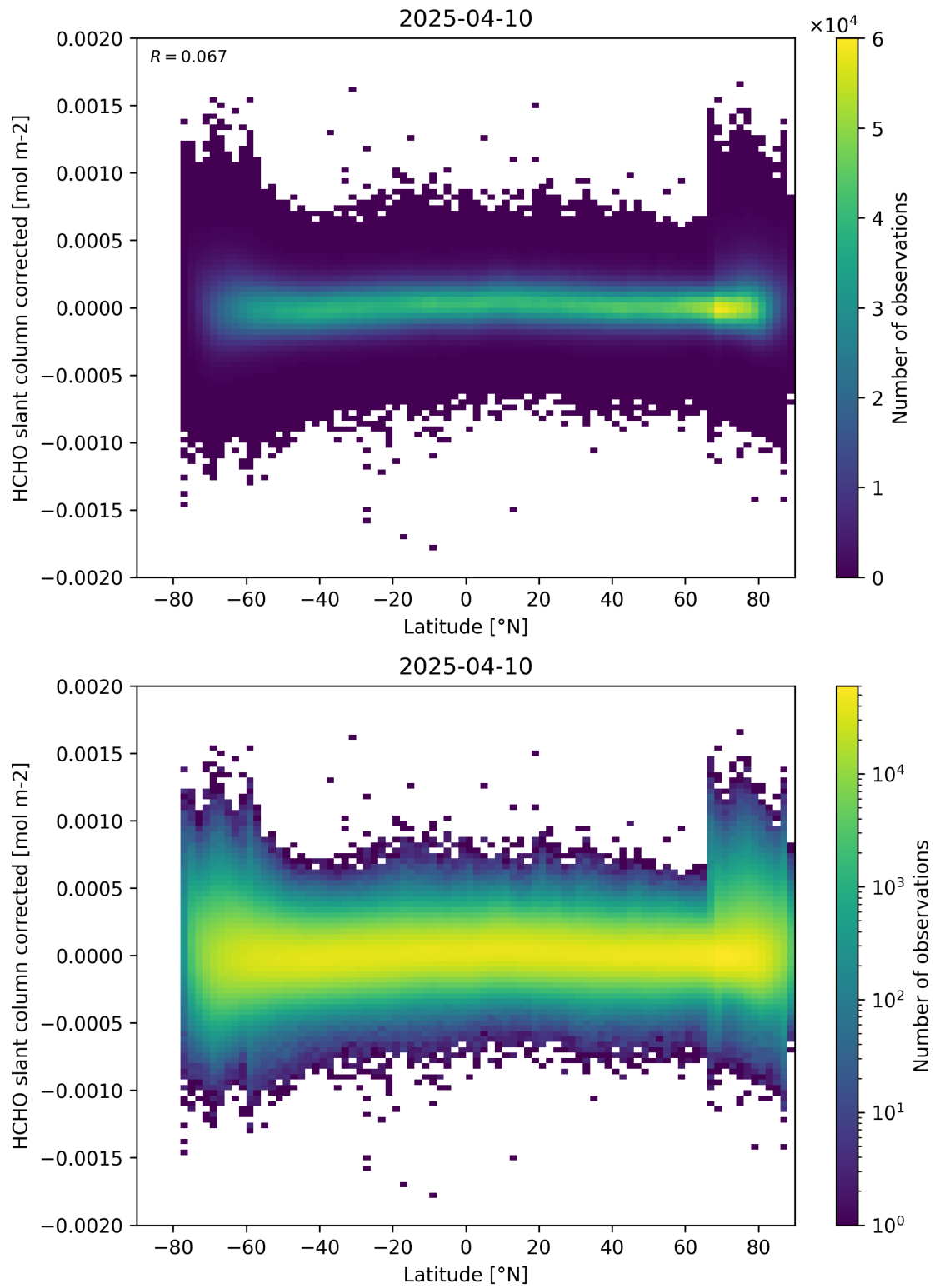
Figure 157: Scatter density plot of “Latitude” against “HCHO slant column corrected” for 2025-04-09 to 2025-04-11.
