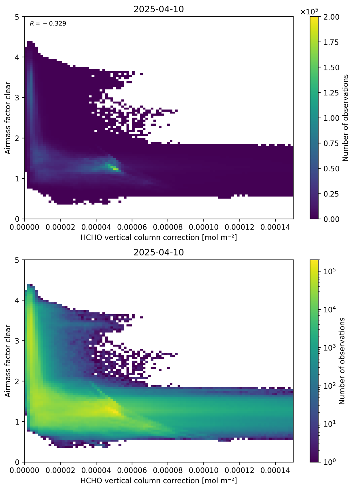
Figure 115: Scatter density plot of “HCHO vertical column correction” against “Airmass factor clear” for 2025-04-09 to 2025-04-11.
