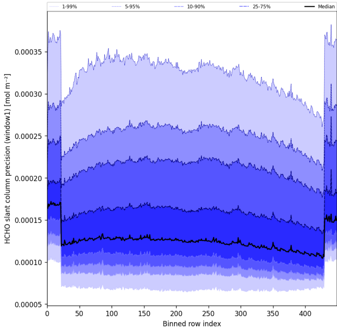
Figure 53: Along track statistics of “HCHO slant column precision (window1)” for 2025-04-09 to 2025-04-11
