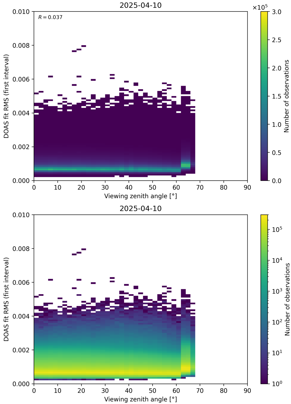
Figure 182: Scatter density plot of “Viewing zenith angle” against “DOAS fit RMS (first interval)” for 2025-04-09 to 2025-04-11.
