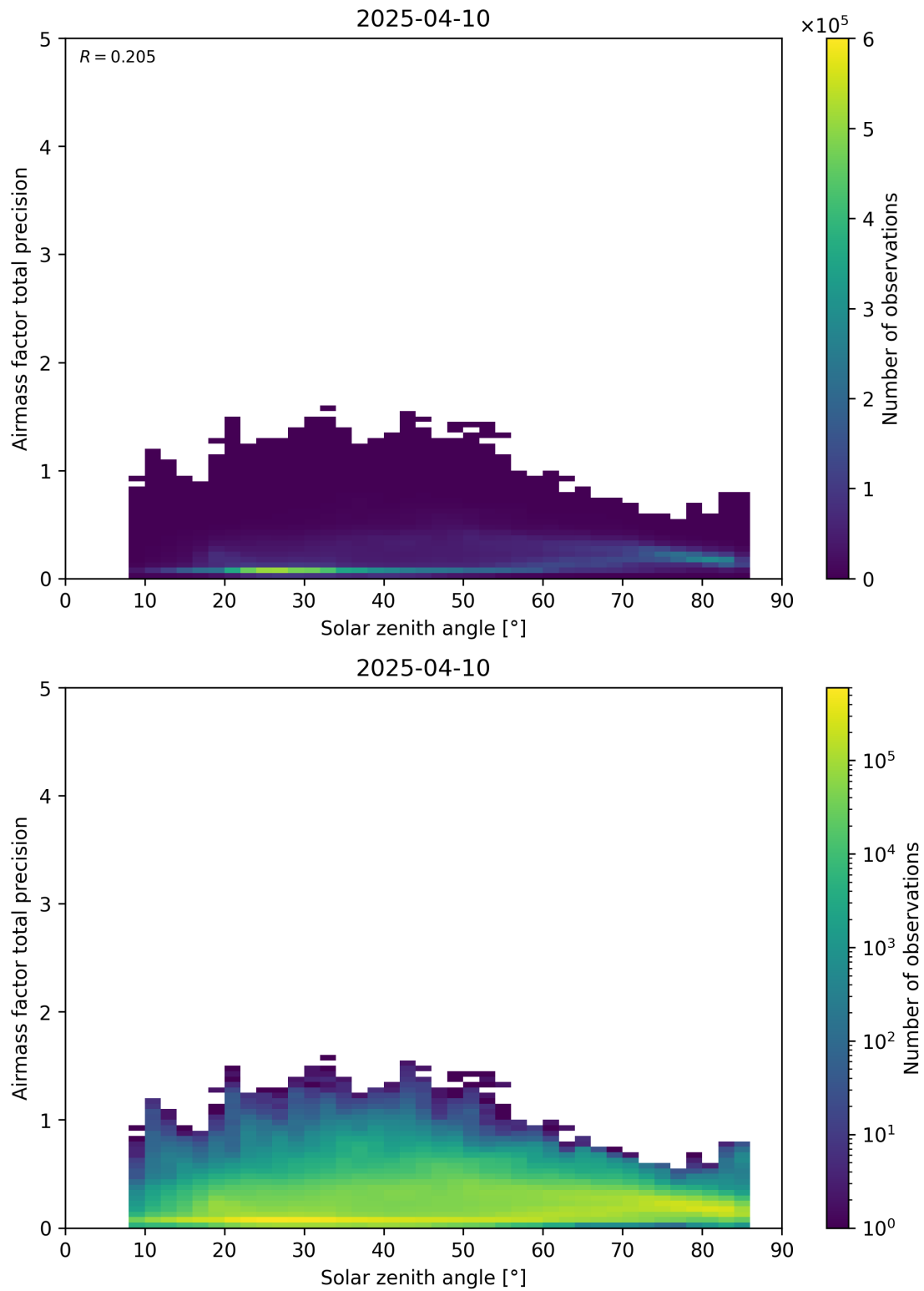
Figure 176: Scatter density plot of “Solar zenith angle” against “Airmass factor total precision” for 2025-04-09 to 2025-04-11.
