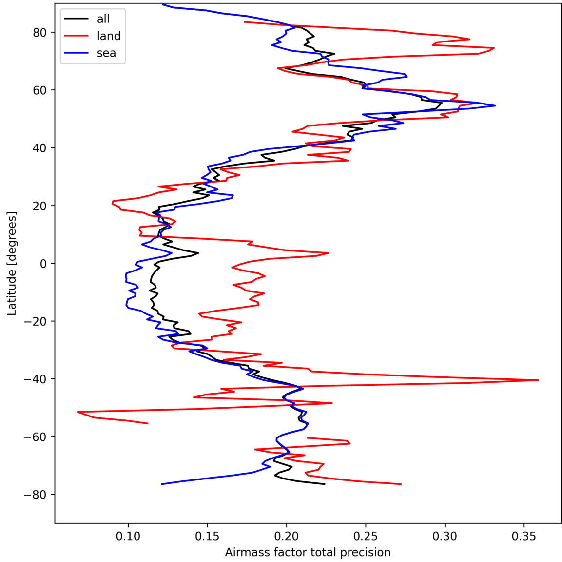
Figure 27: Zonal average of “Airmass factor total precision” for 2025-04-09 to 2025-04-11.
