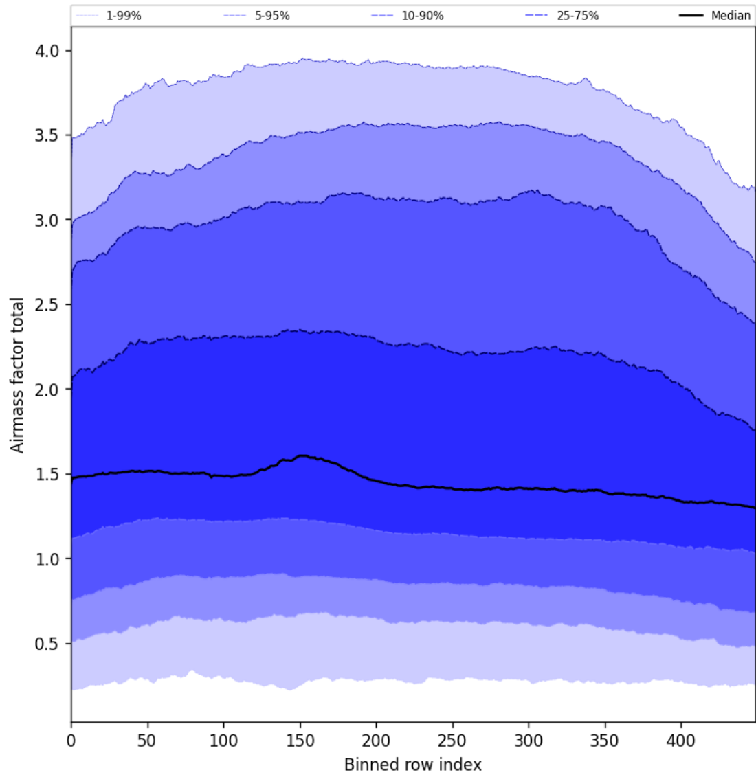
Figure 54: Along track statistics of “Airmass factor total” for 2025-04-09 to 2025-04-11
