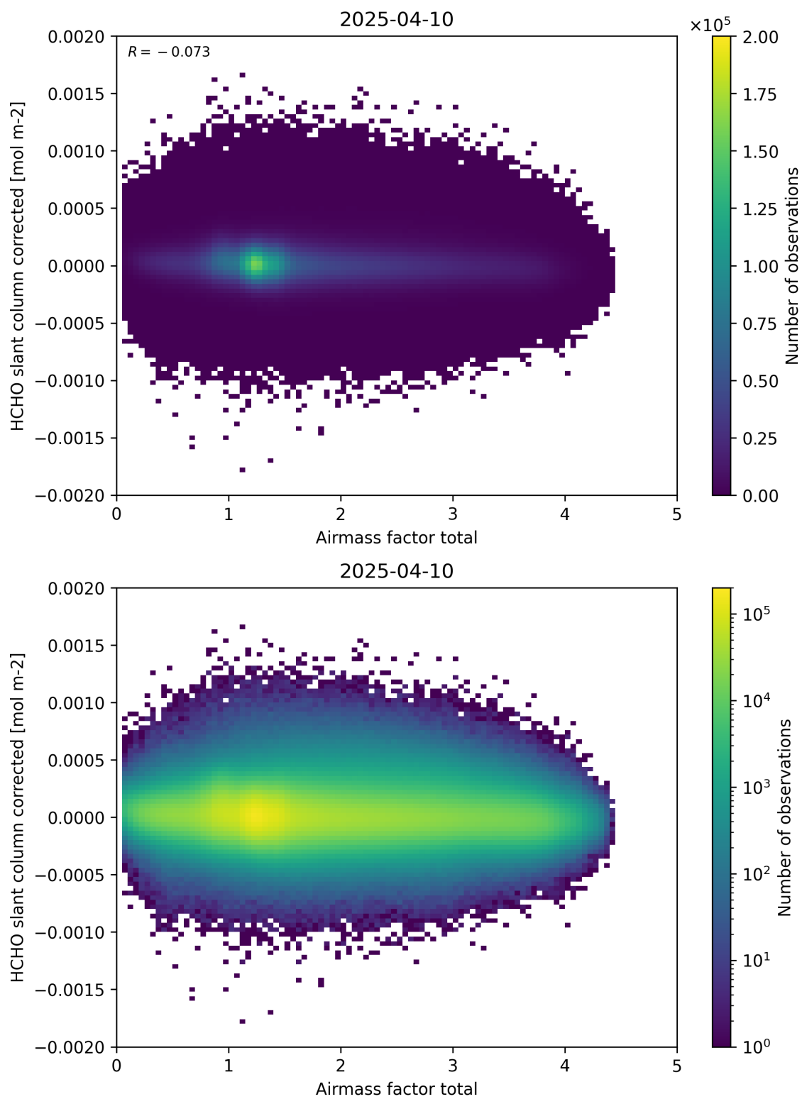
Figure 101: Scatter density plot of “Airmass factor total” against “HCHO slant column corrected” for 2025-04-09 to 2025-04-11.
