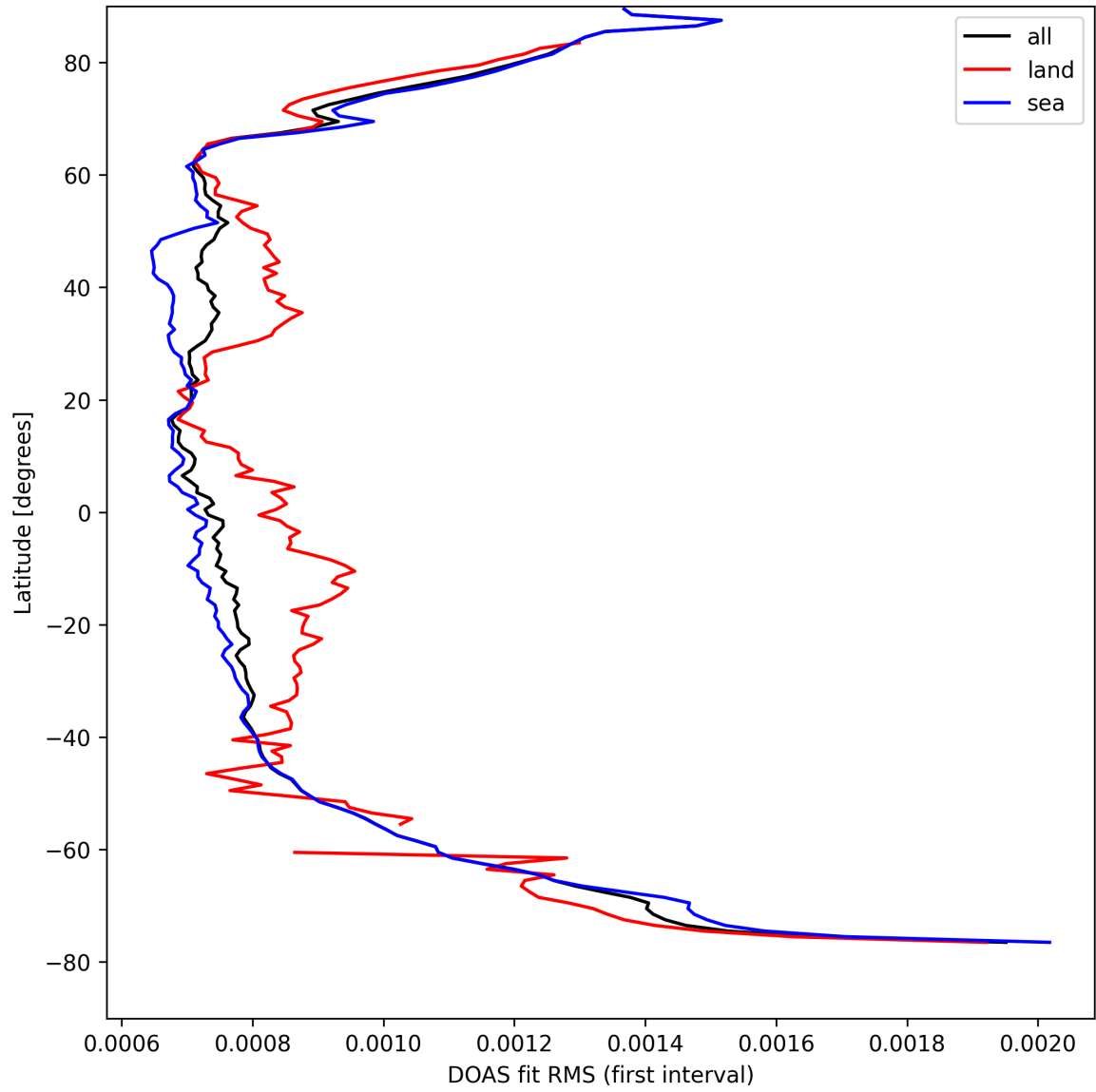
Figure 32: Zonal average of “DOAS fit RMS (first interval)” for 2025-04-09 to 2025-04-11.
