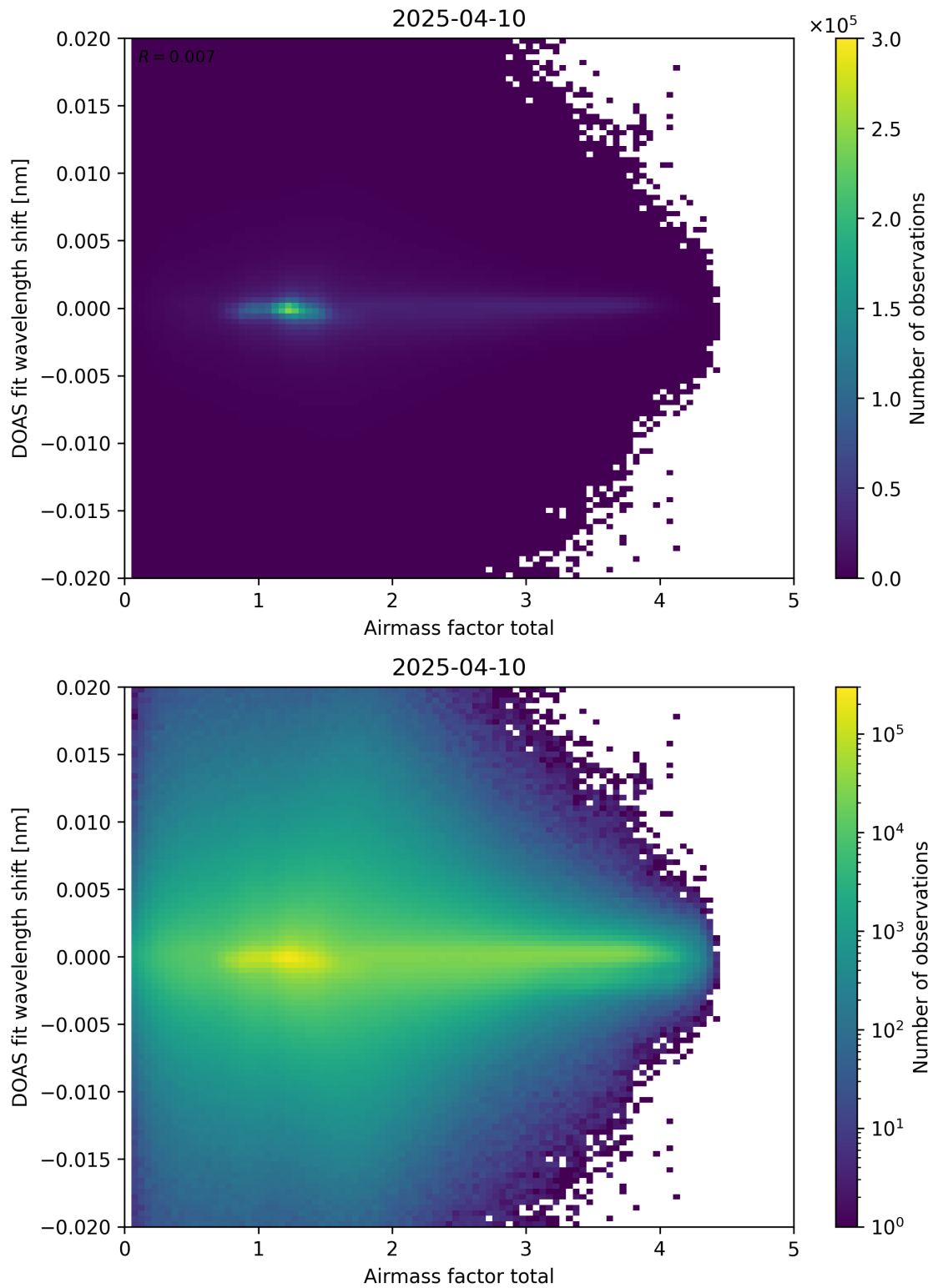
Figure 98: Scatter density plot of “Airmass factor total” against “DOAS fit wavelength shift” for 2025-04-09 to 2025-04-11.
