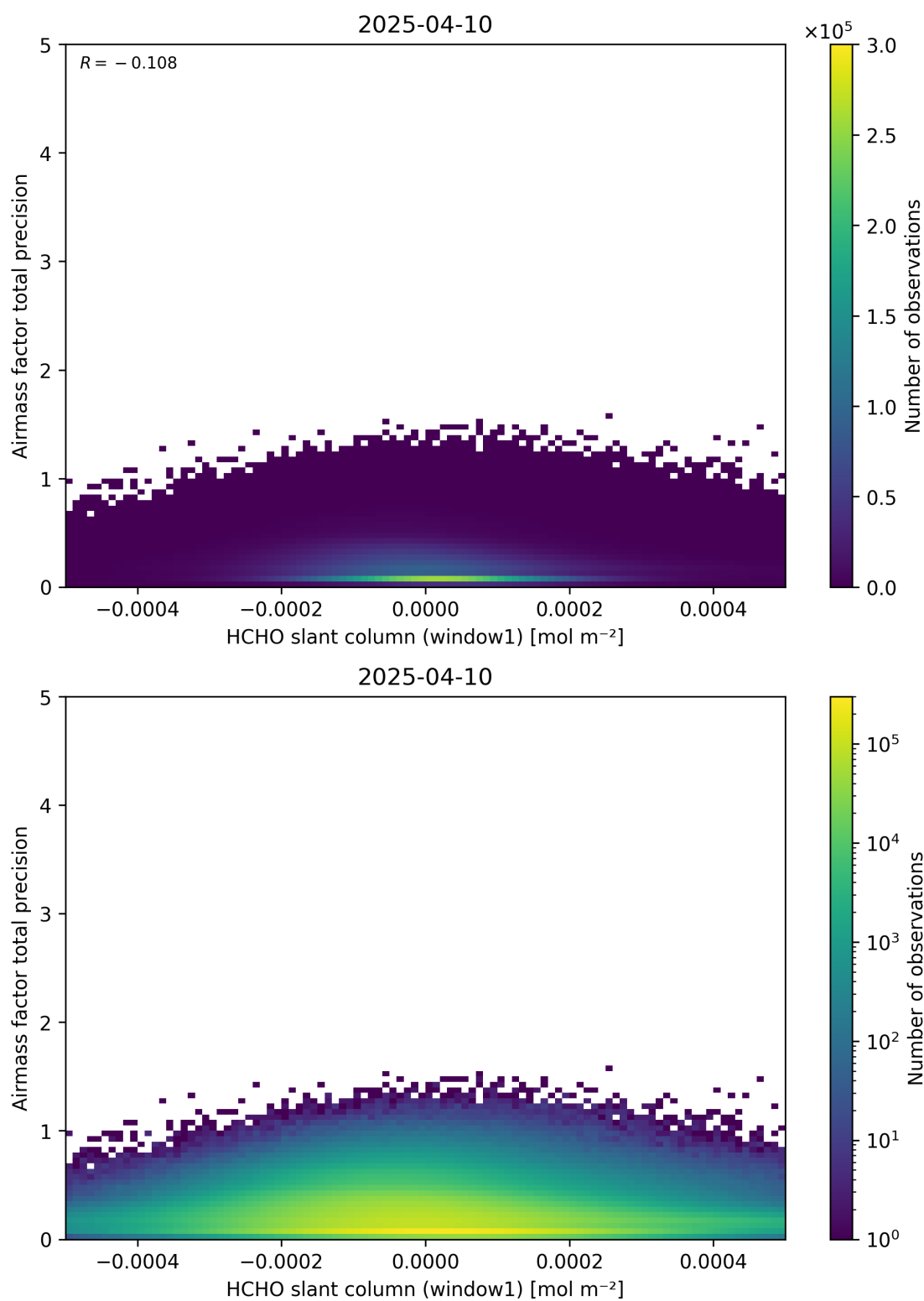
Figure 86: Scatter density plot of “HCHO slant column (window1)” against “Airmass factor total precision” for 2025-04-09 to 2025-04-11.
