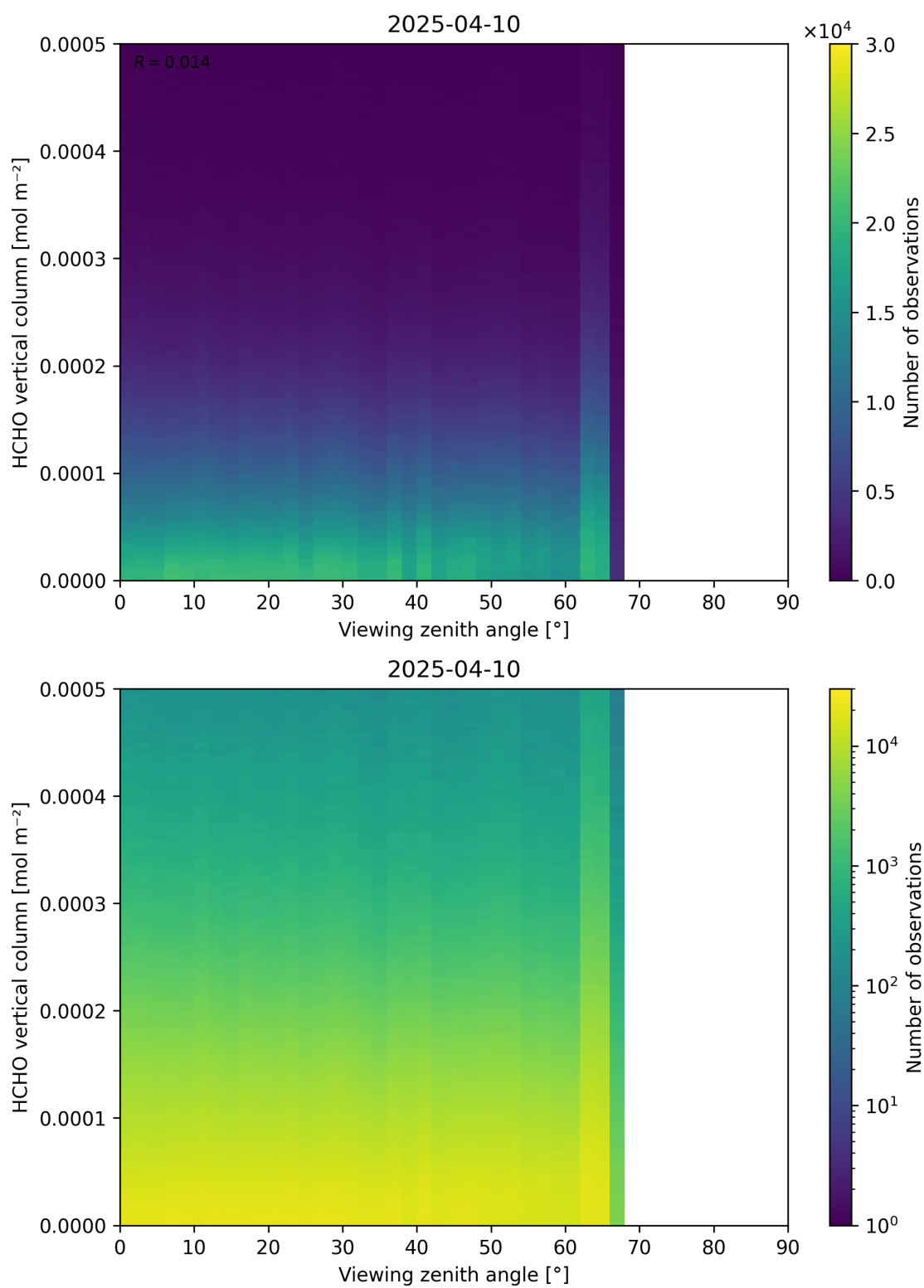
Figure 192: Scatter density plot of “Viewing zenith angle” against “HCHO vertical column” for 2025-04-09 to 2025-04-11.
