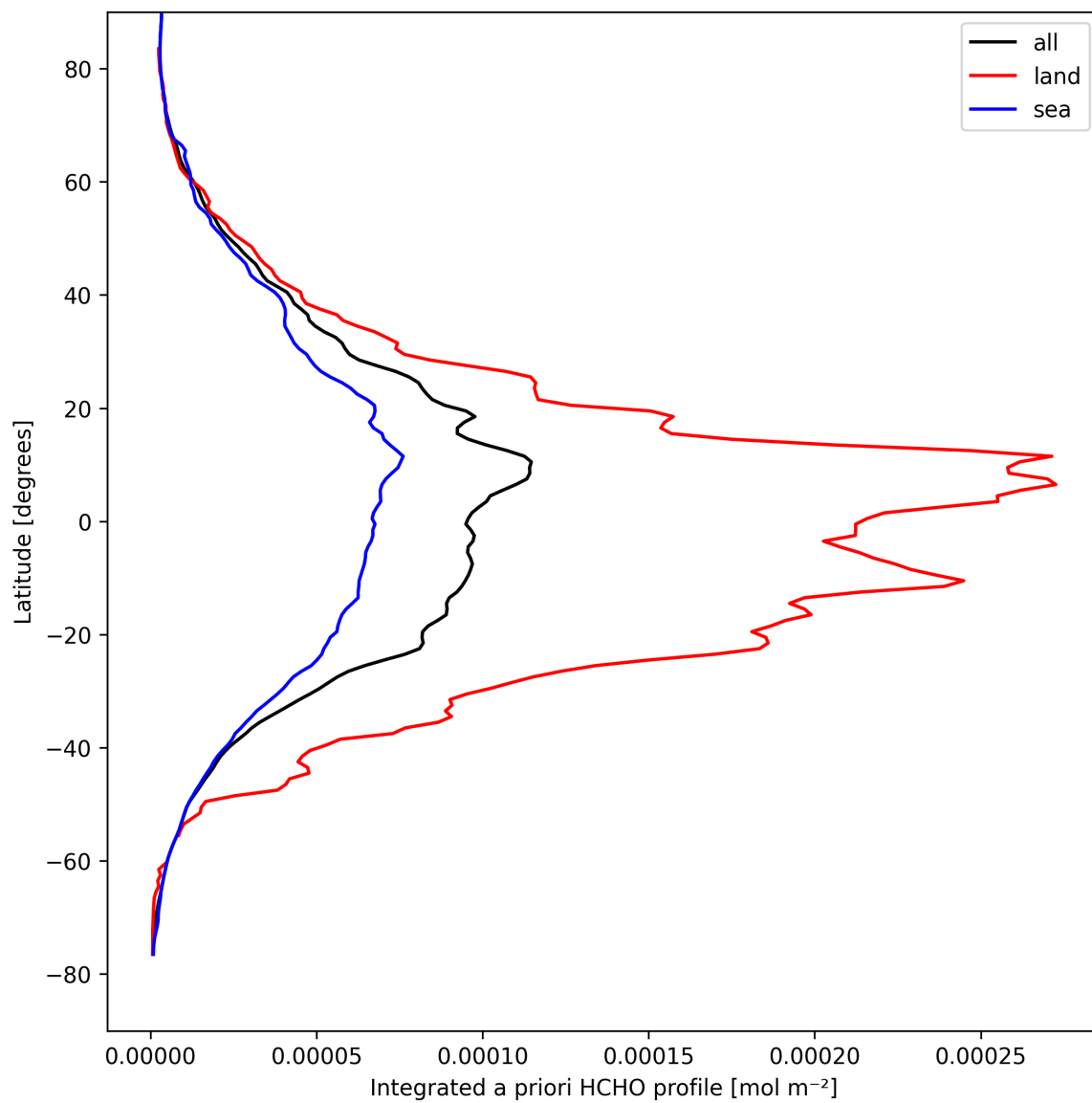
Figure 29: Zonal average of “Integrated a priori HCHO profile” for 2025-04-09 to 2025-04-11.
