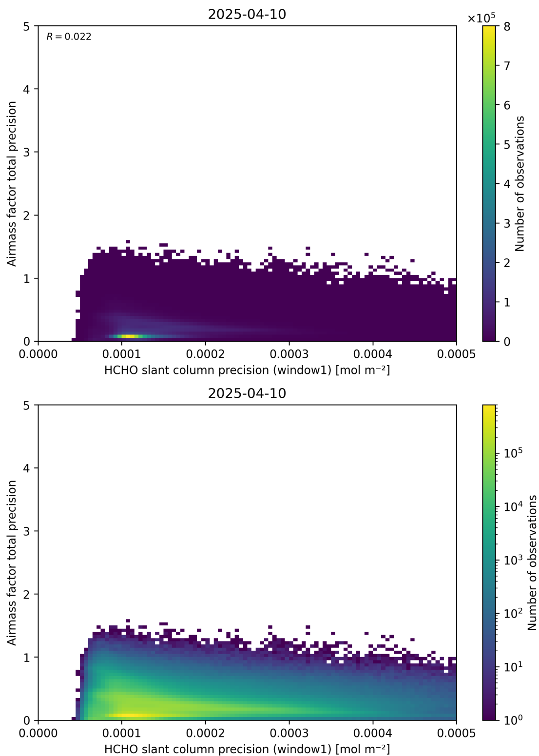
Figure 95: Scatter density plot of “HCHO slant column precision (window1)” against “Airmass factor total precision” for 2025-04-09 to 2025-04-11.
