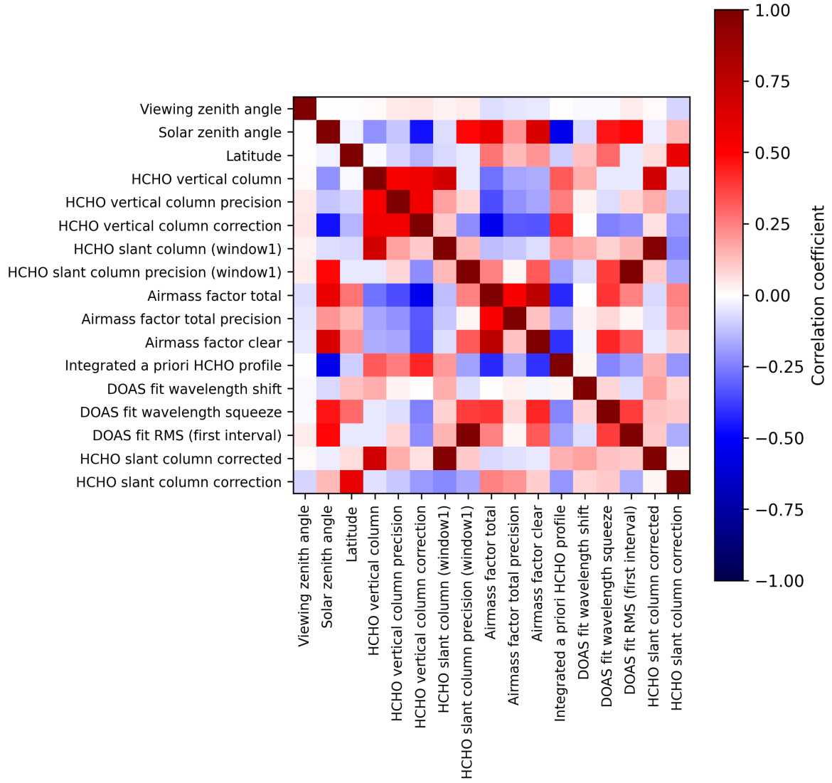
Figure 2: Map of correlation matrix for 2025-04-09 to 2025-04-11.
