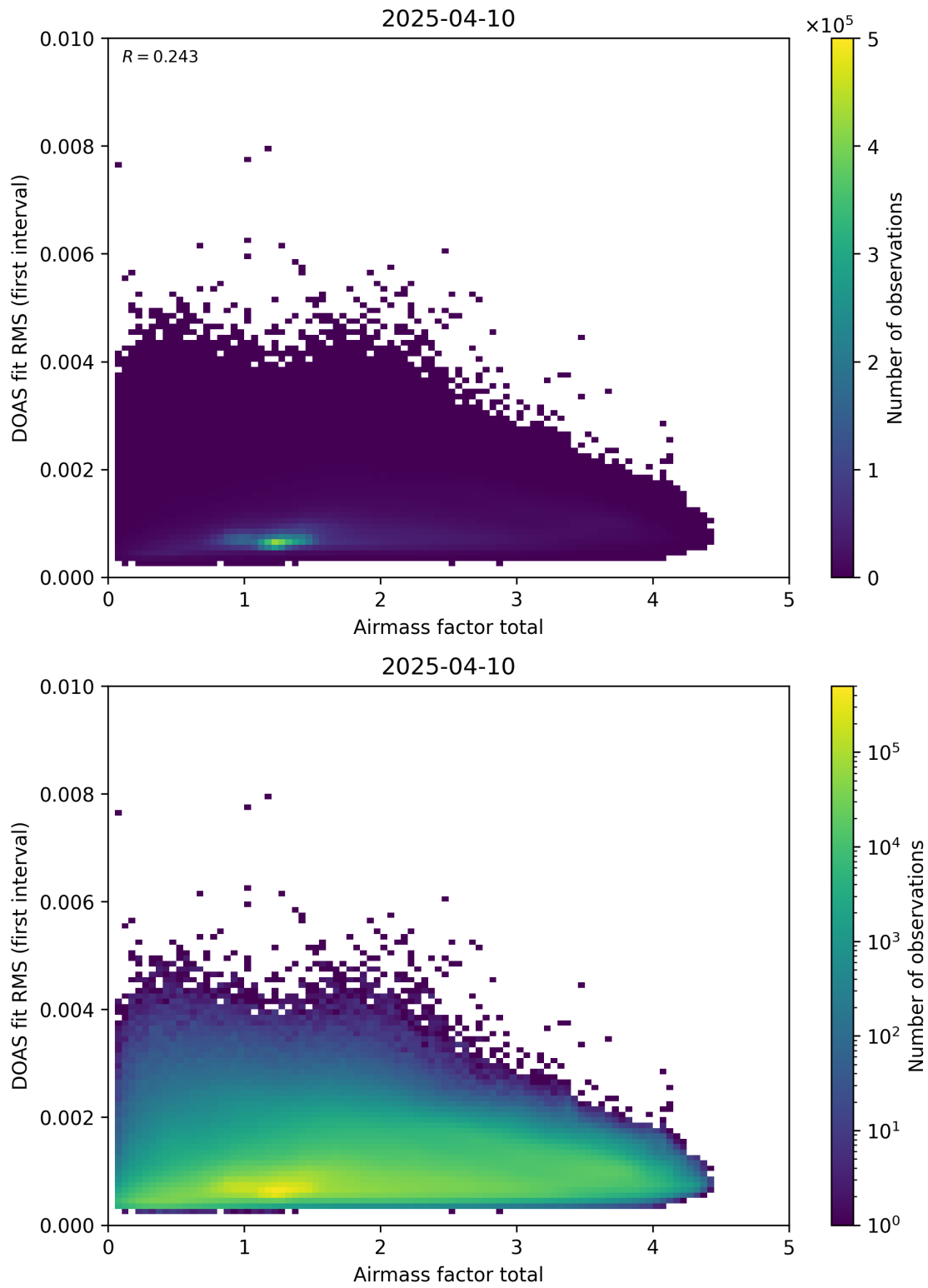
Figure 97: Scatter density plot of “Airmass factor total” against “DOAS fit RMS (first interval)” for 2025-04-09 to 2025-04-11.
