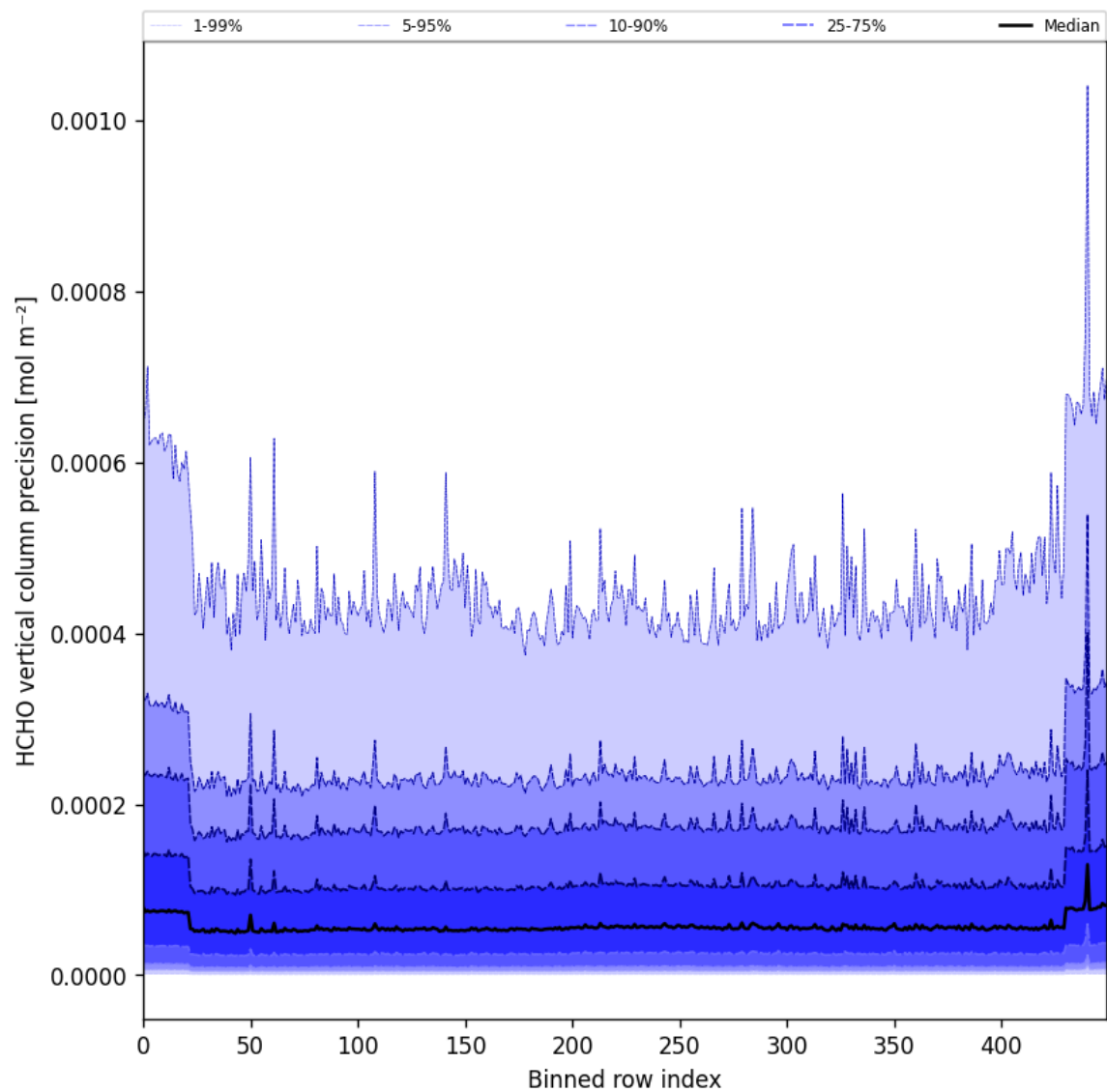
Figure 50: Along track statistics of “HCHO vertical column precision” for 2025-04-09 to 2025-04-11
