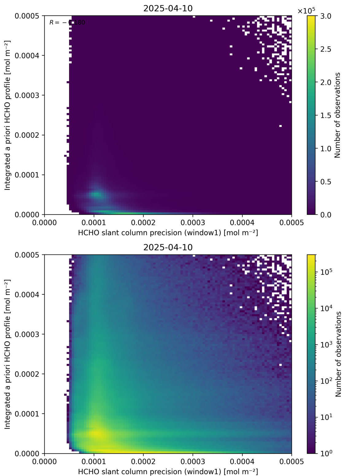
Figure 96: Scatter density plot of “HCHO slant column precision (window1)” against “Integrated a priori HCHO profile” for 2025-04-09 to 2025-04-11.
