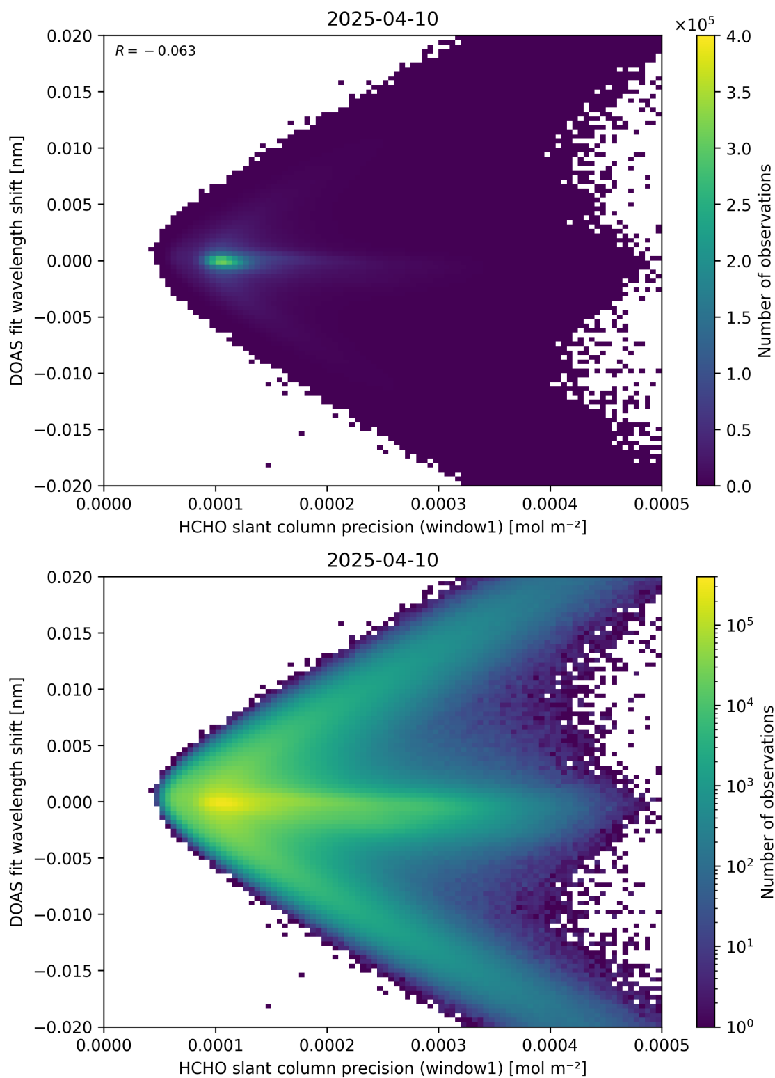
Figure 89: Scatter density plot of “HCHO slant column precision (window1)” against “DOAS fit wavelength shift” for 2025-04-09 to 2025-04-11.
