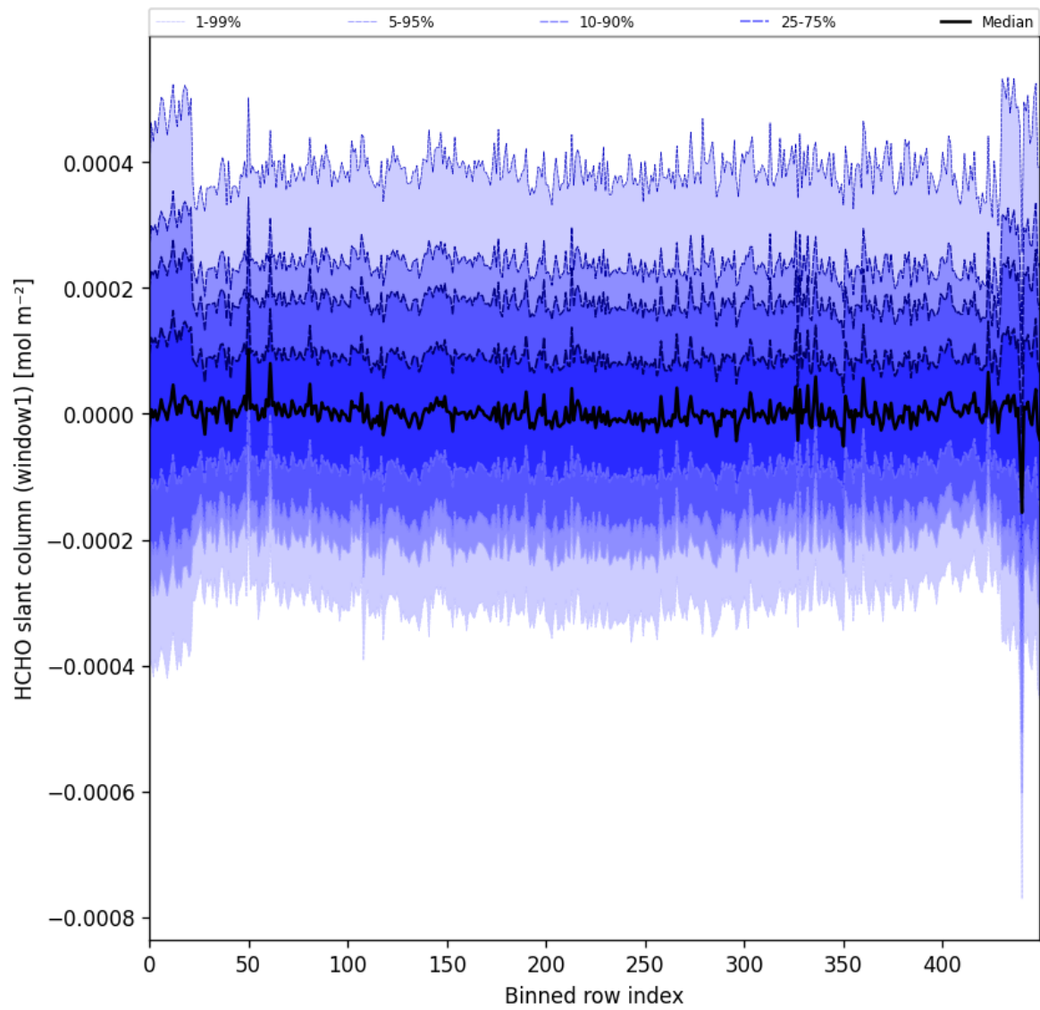
Figure 52: Along track statistics of “HCHO slant column (window1)” for 2025-04-09 to 2025-04-11
