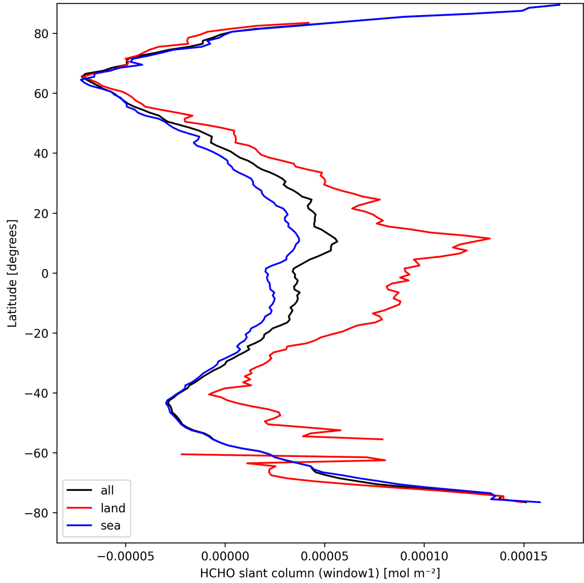
Figure 24: Zonal average of “HCHO slant column (window1)” for 2025-04-09 to 2025-04-11.
