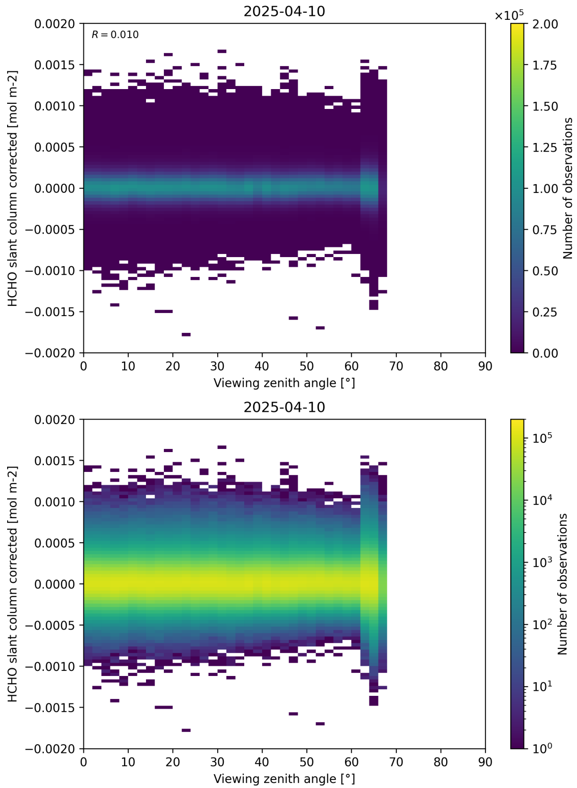
Figure 186: Scatter density plot of “Viewing zenith angle” against “HCHO slant column corrected” for 2025-04-09 to 2025-04-11.
