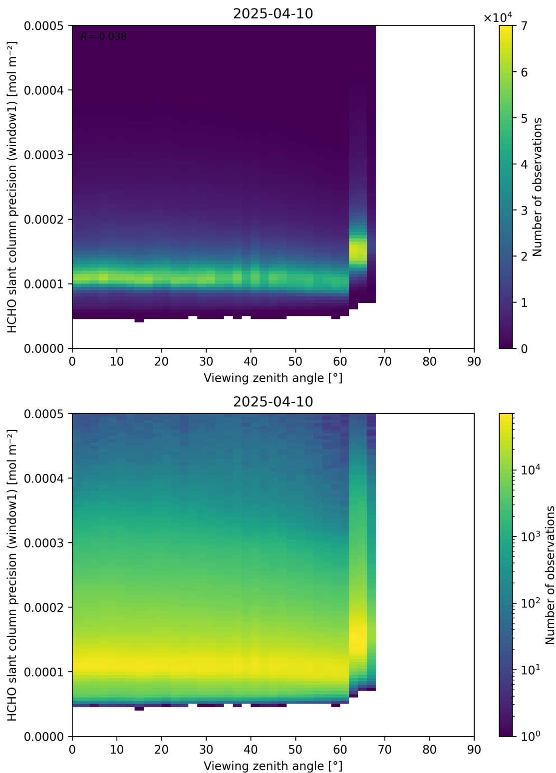
Figure 189: Scatter density plot of “Viewing zenith angle” against “HCHO slant column precision (window1)” for 2025-04-09 to 2025-04-11.
