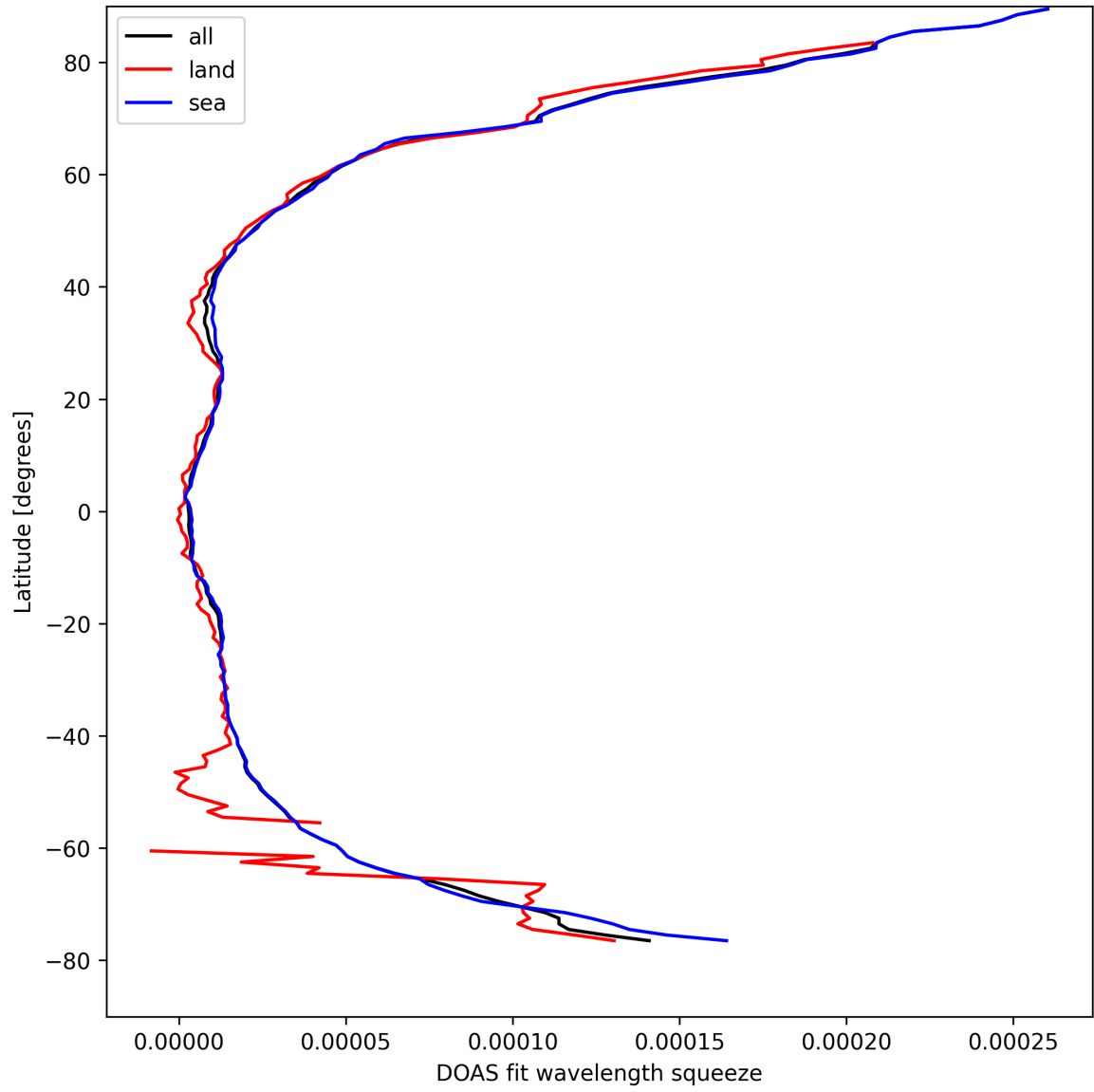
Figure 31: Zonal average of “DOAS fit wavelength squeeze” for 2025-04-09 to 2025-04-11.
