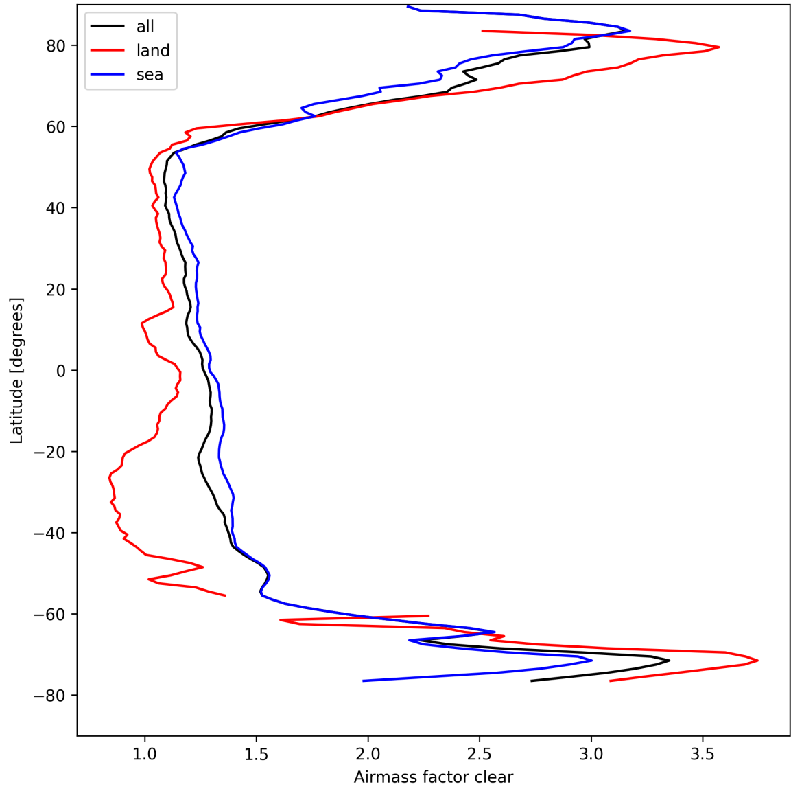
Figure 28: Zonal average of “Airmass factor clear” for 2025-04-09 to 2025-04-11.
