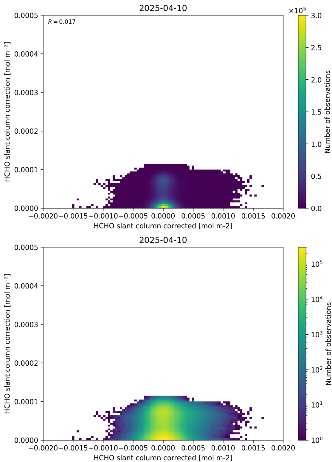
Figure 77: Scatter density plot of “HCHO slant column corrected” against “HCHO slant column correction” for 2025-04-09 to 2025-04-11.
