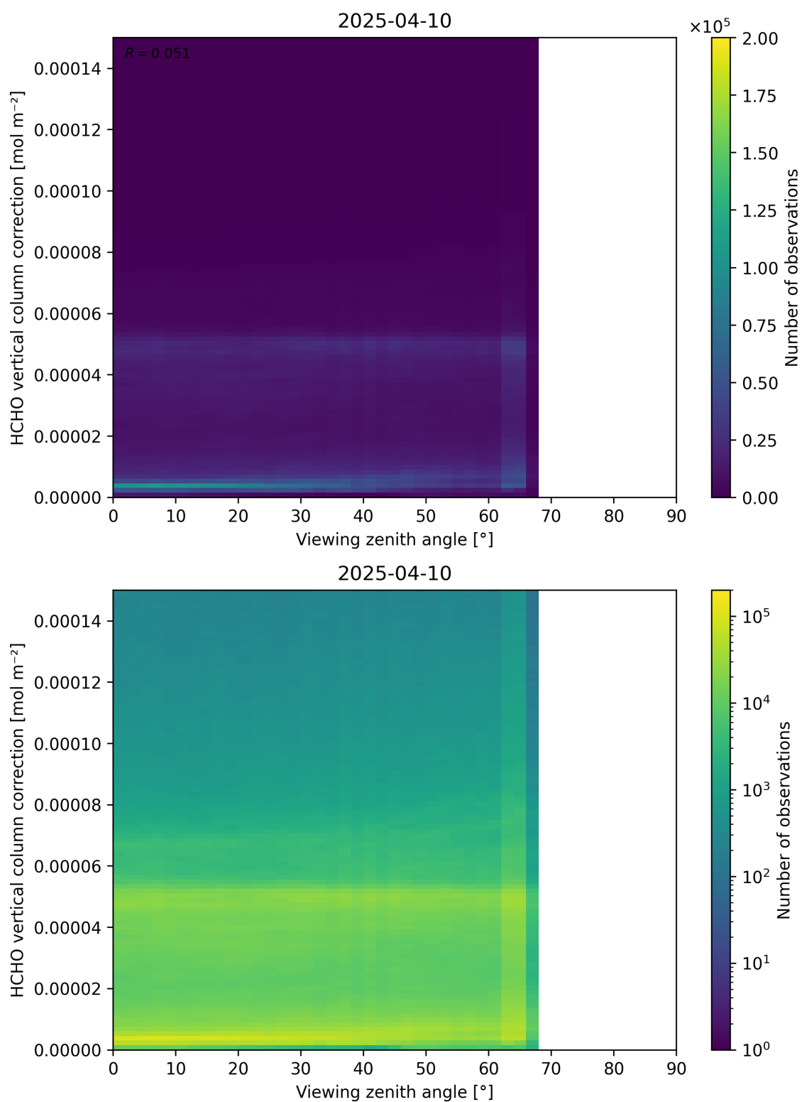
Figure 193: Scatter density plot of “Viewing zenith angle” against “HCHO vertical column correction” for 2025-04-09 to 2025-04-11.
