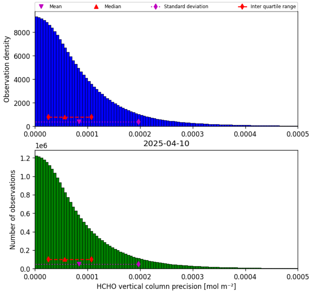
Figure 36: Histogram of “HCHO vertical column precision” for 2025-04-09 to 2025-04-11
