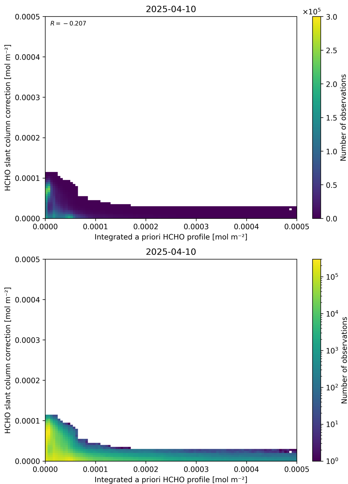
Figure 152: Scatter density plot of “Integrated a priori HCHO profile” against “HCHO slant column correction” for 2025-04-09 to 2025-04-11.
