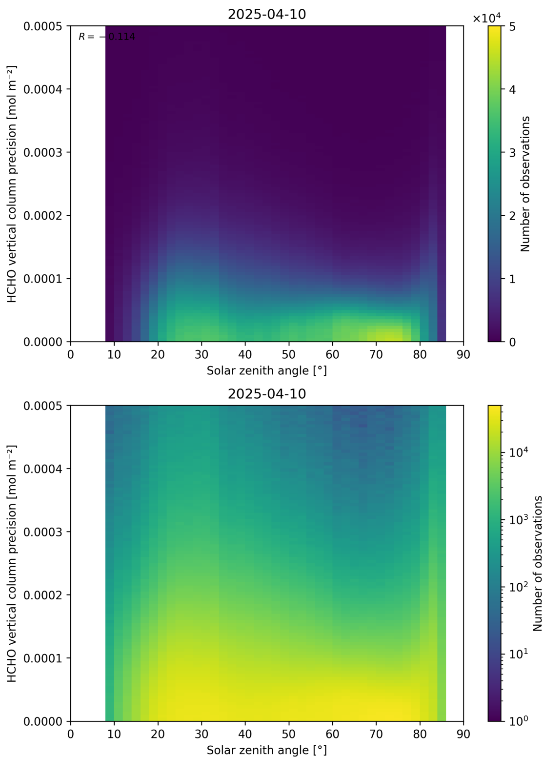
Figure 179: Scatter density plot of “Solar zenith angle” against “HCHO vertical column precision” for 2025-04-09 to 2025-04-11.
