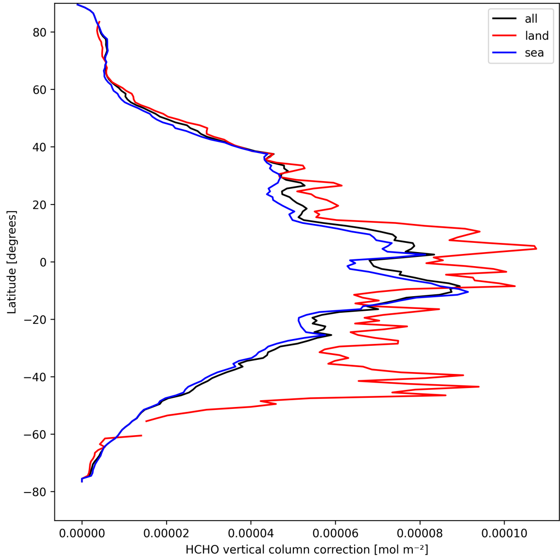
Figure 23: Zonal average of “HCHO vertical column correction” for 2025-04-09 to 2025-04-11.
