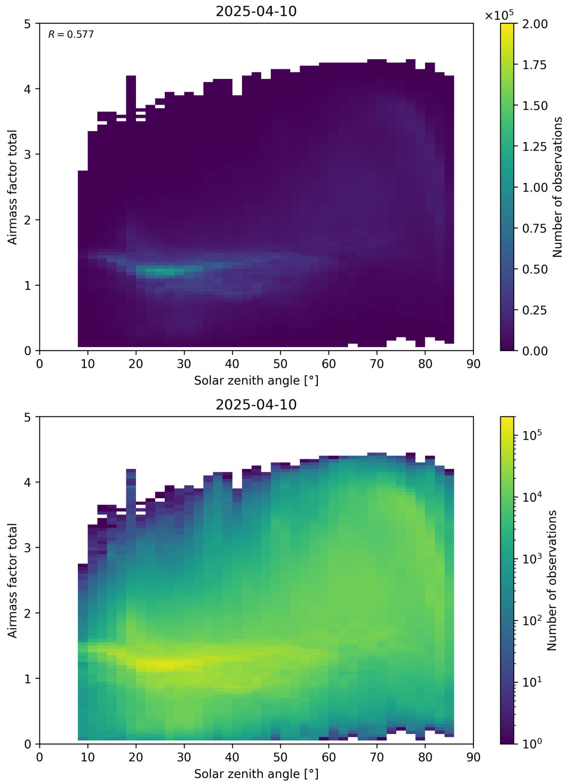
Figure 175: Scatter density plot of “Solar zenith angle” against “Airmass factor total” for 2025-04-09 to 2025-04-11.
