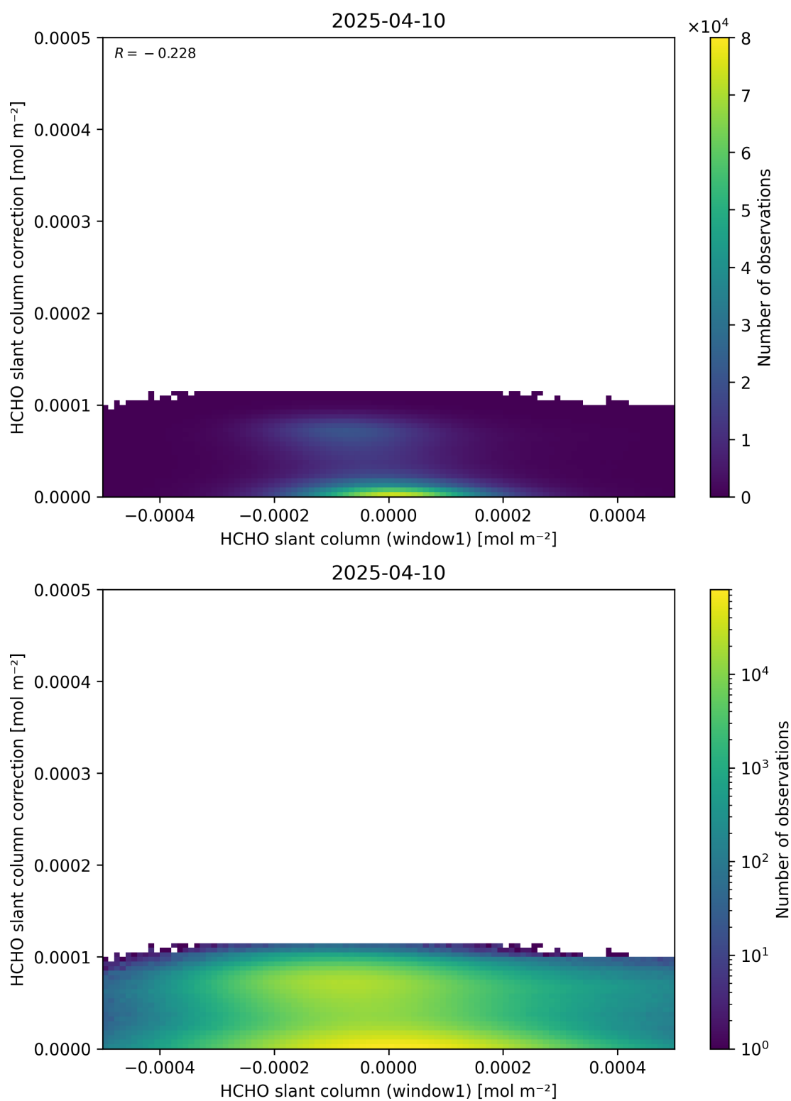
Figure 83: Scatter density plot of “HCHO slant column (window1)” against “HCHO slant column correction” for 2025-04-09 to 2025-04-11.
