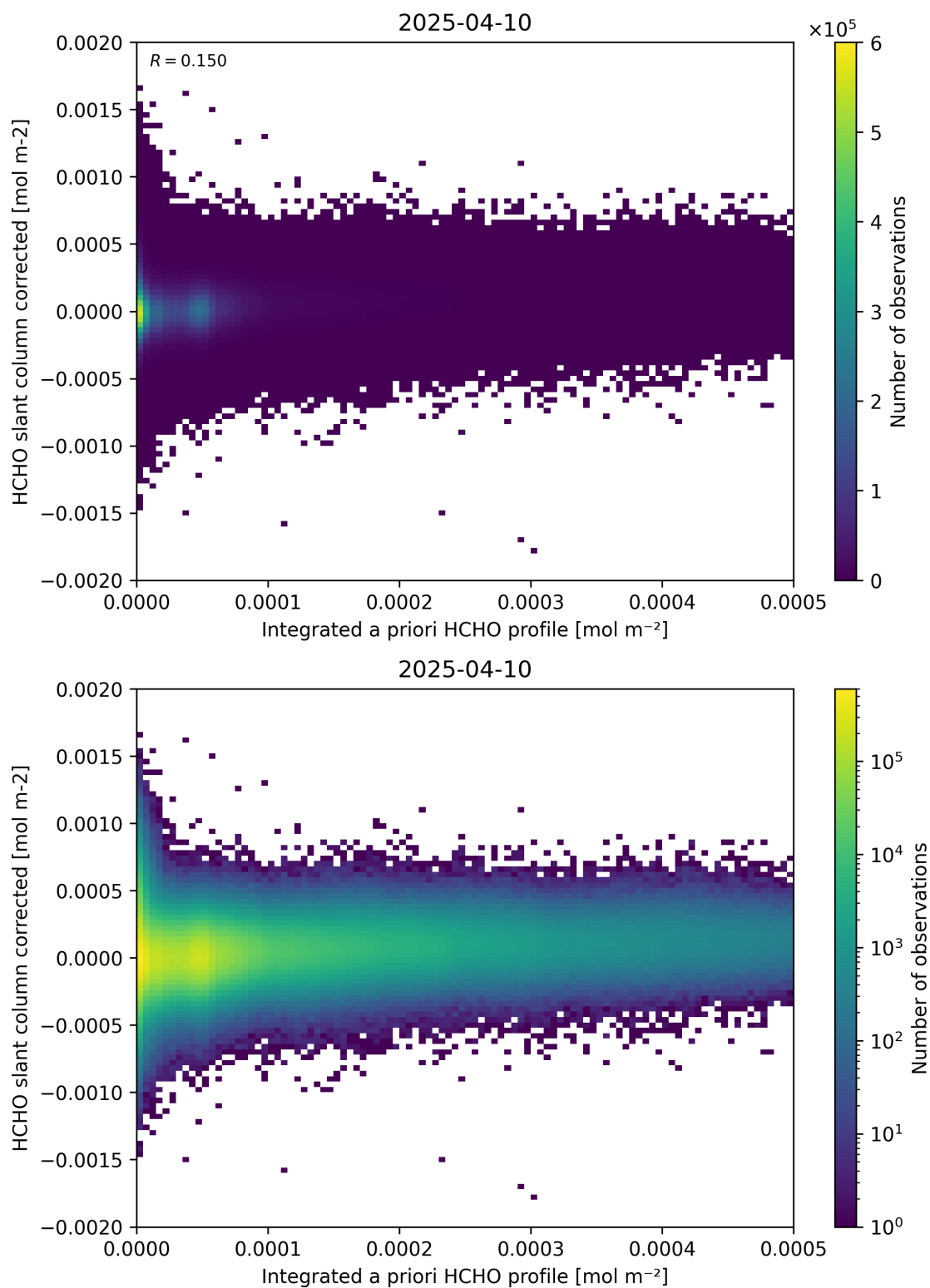
Figure 151: Scatter density plot of “Integrated a priori HCHO profile” against “HCHO slant column corrected” for 2025-04-09 to 2025-04-11.
