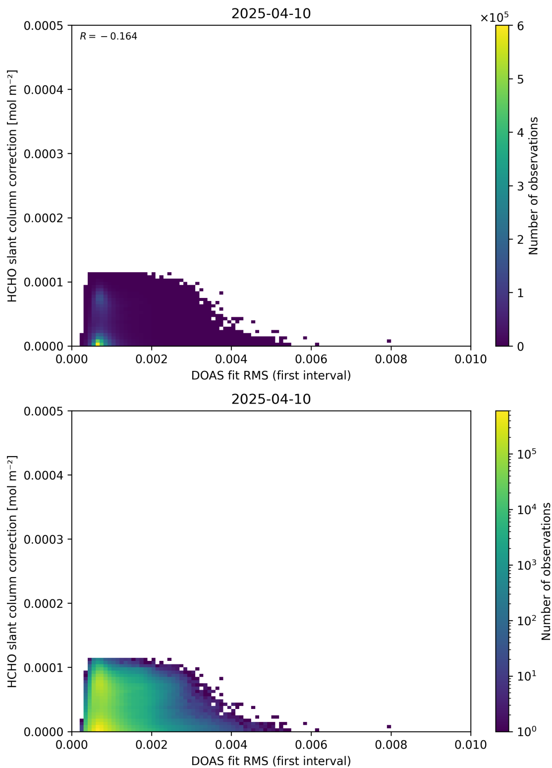
Figure 63: Scatter density plot of “DOAS fit RMS (first interval)” against “HCHO slant column correction” for 2025-04-09 to 2025-04-11.
