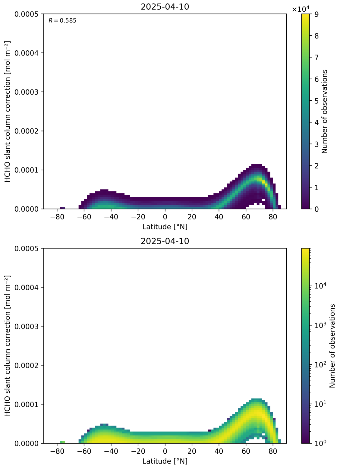
Figure 158: Scatter density plot of “Latitude” against “HCHO slant column correction” for 2025-04-09 to 2025-04-11.
