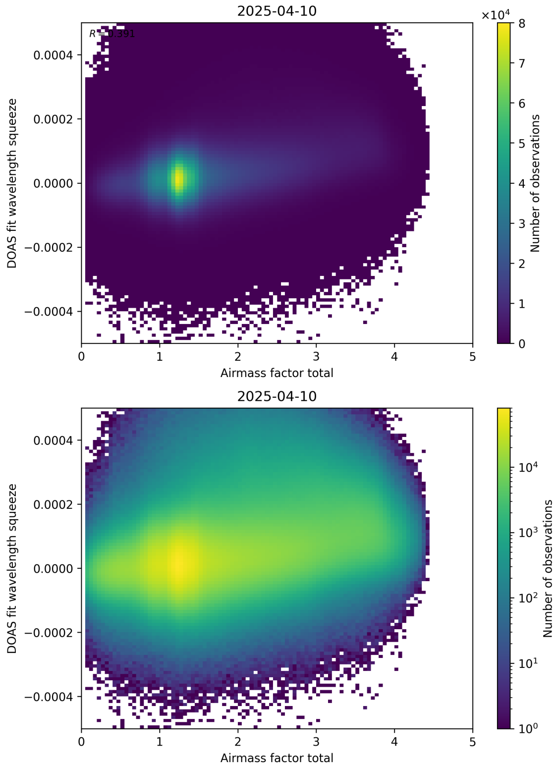
Figure 99: Scatter density plot of “Airmass factor total” against “DOAS fit wavelength squeeze” for 2025-04-09 to 2025-04-11.
