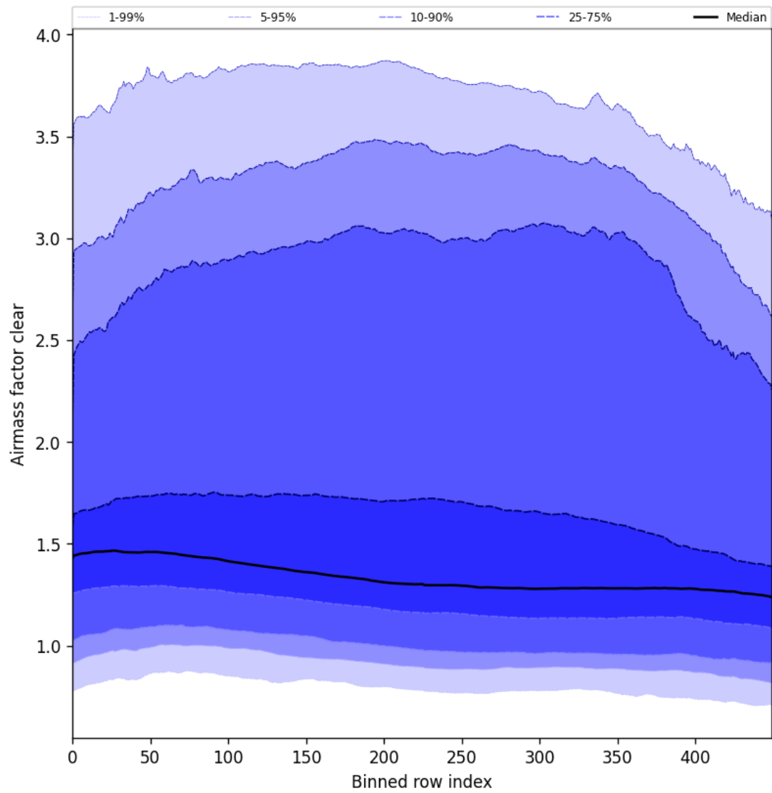
Figure 56: Along track statistics of “Air mass factor clear” for 2025-04-09 to 2025-04-11
