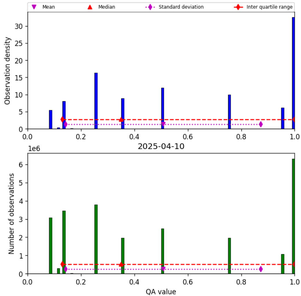
Figure 34: Histogram of “QA value” for 2025-04-09 to 2025-04-11
