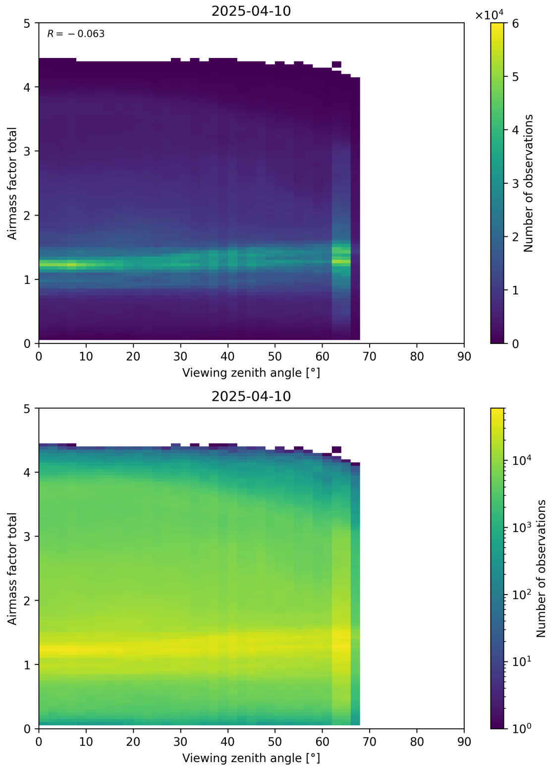
Figure 190: Scatter density plot of “Viewing zenith angle” against “Airmass factor total” for 2025-04-09 to 2025-04-11.
