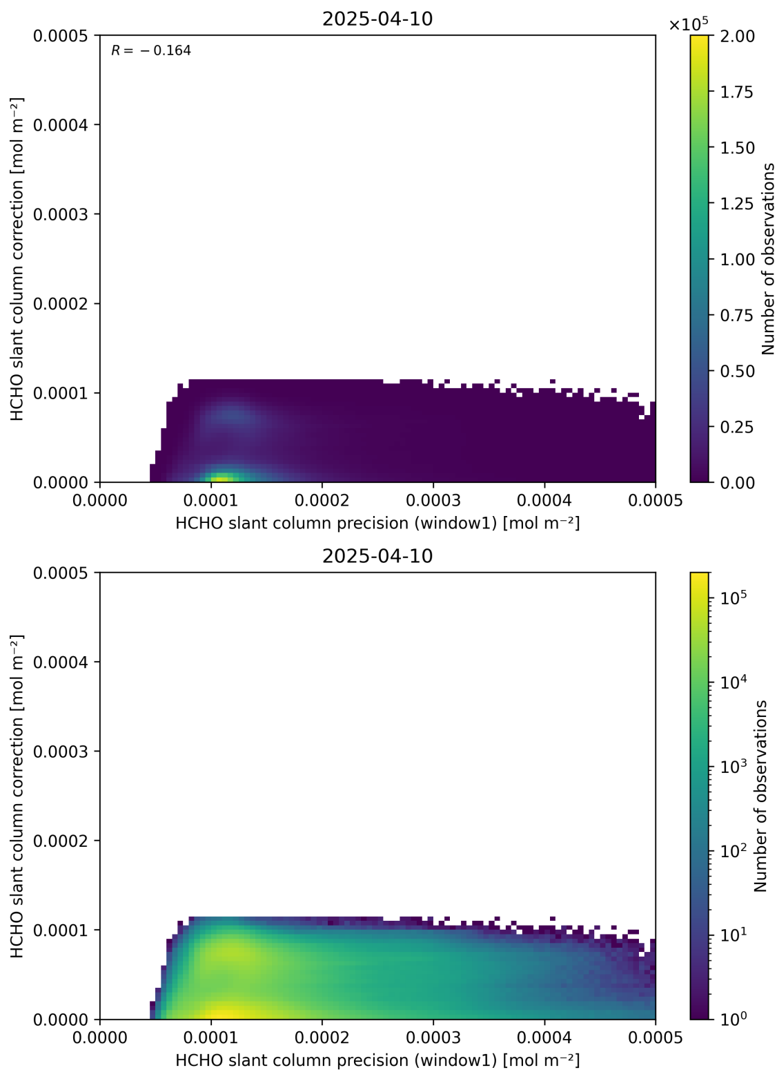
Figure 93: Scatter density plot of “HCHO slant column precision (window1)” against “HCHO slant column correction” for 2025-04-09 to 2025-04-11.
