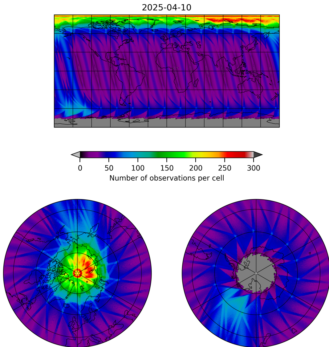
Figure 19: Map of the number of observations for 2025-04-09 to 2025-04-11
