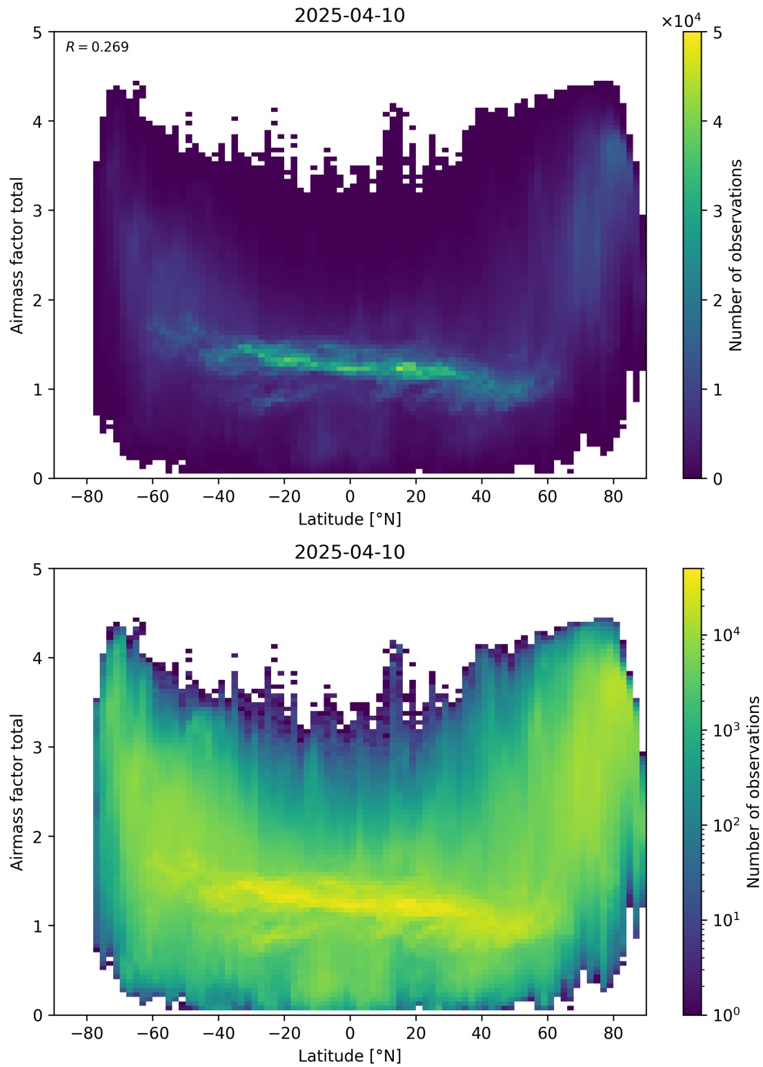
Figure 161: Scatter density plot of “Latitude” against “Airmass factor total” for 2025-04-09 to 2025-04-11.
