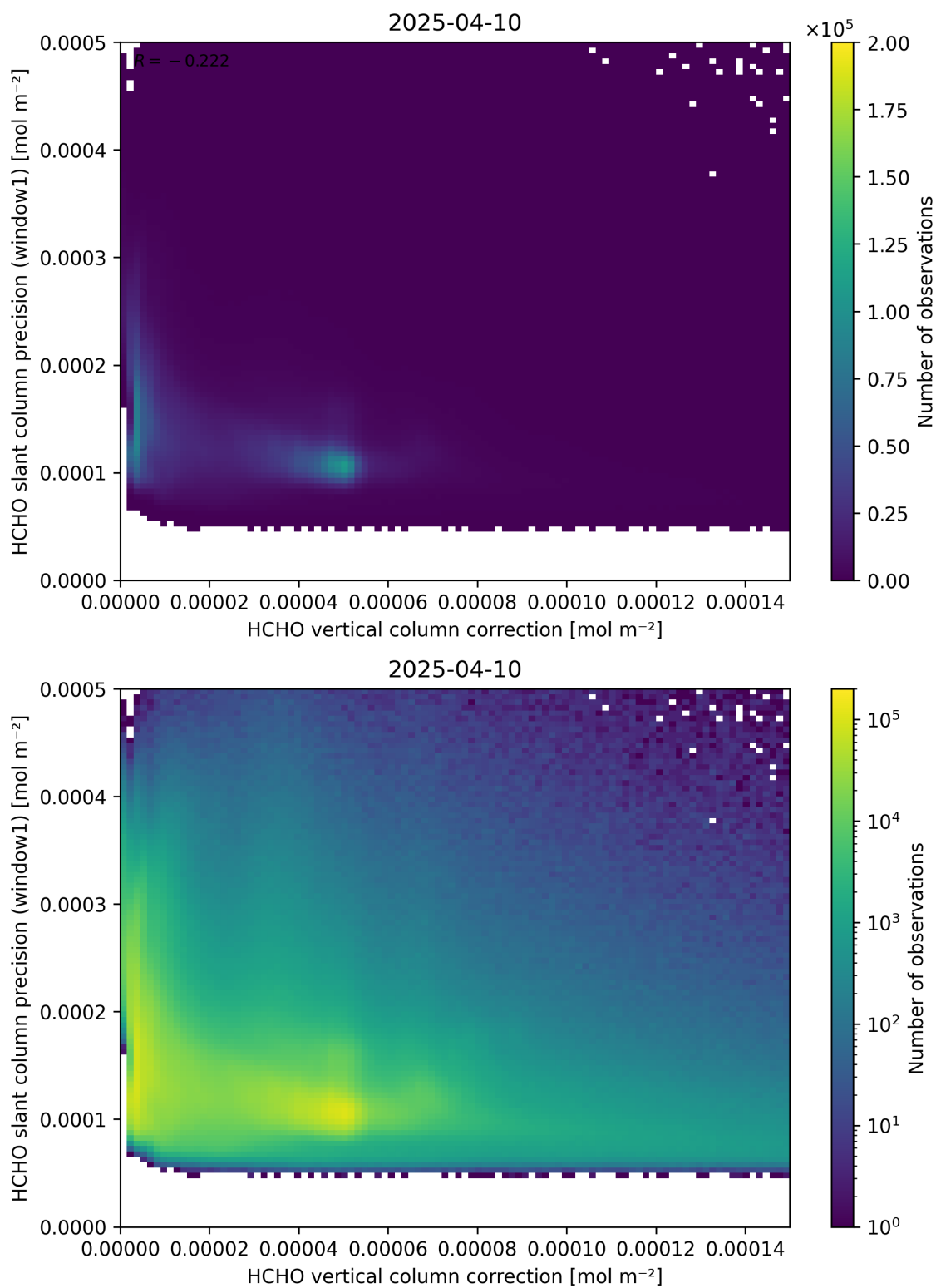
Figure 119: Scatter density plot of “HCHO vertical column correction” against “HCHO slant column precision (window1)” for 2025-04-09 to 2025-04-11.
