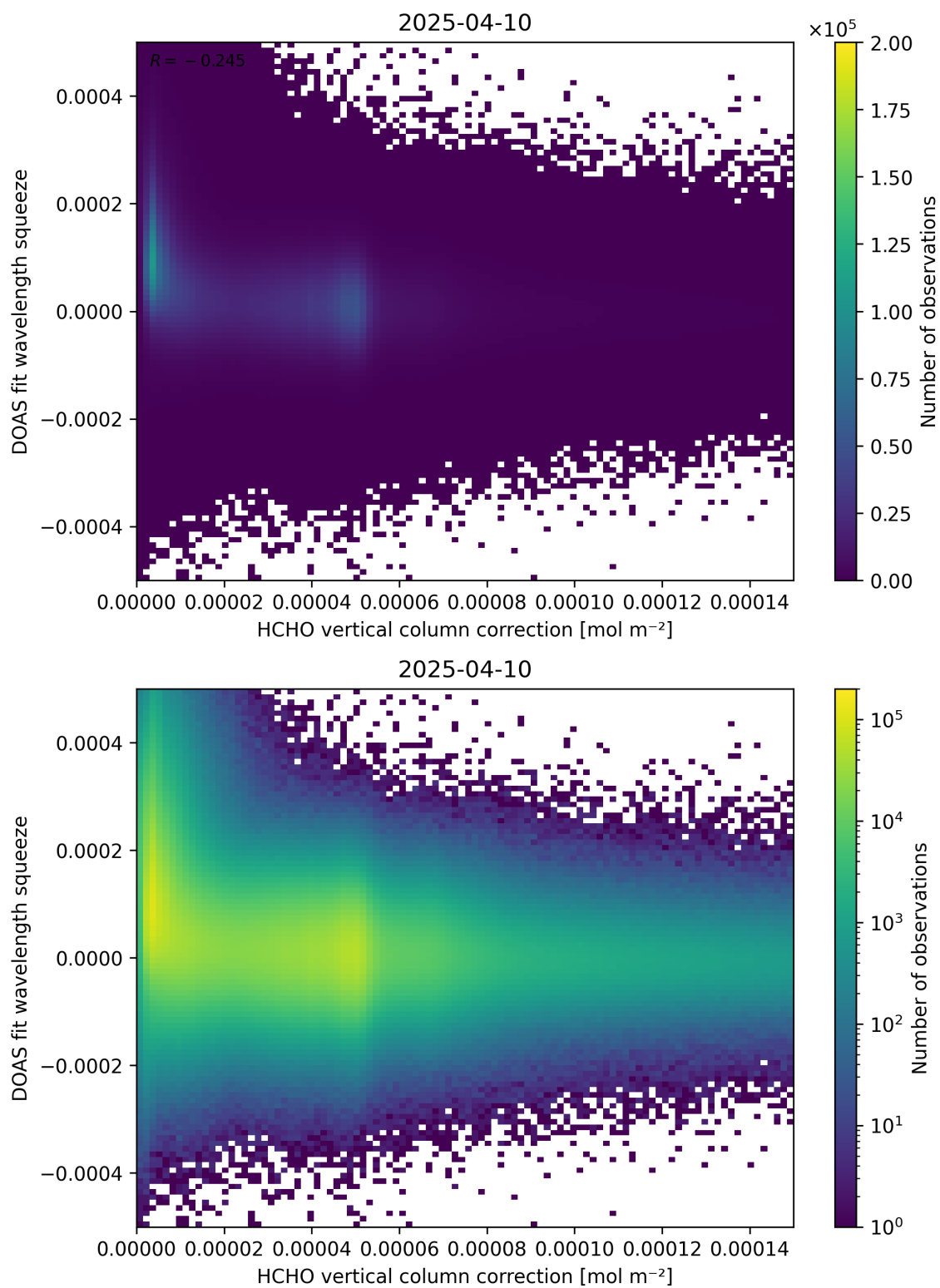
Figure 114: Scatter density plot of “HCHO vertical column correction” against “DOAS fit wavelength squeeze” for 2025-04-09 to 2025-04-11.
