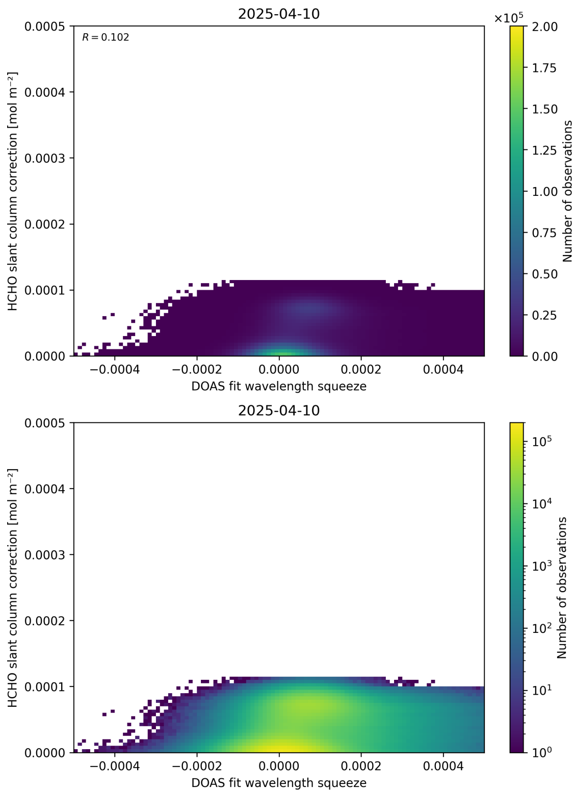
Figure 70: Scatter density plot of “DOAS fit wavelength squeeze” against “HCHO slant column correction” for 2025-04-09 to 2025-04-11.
