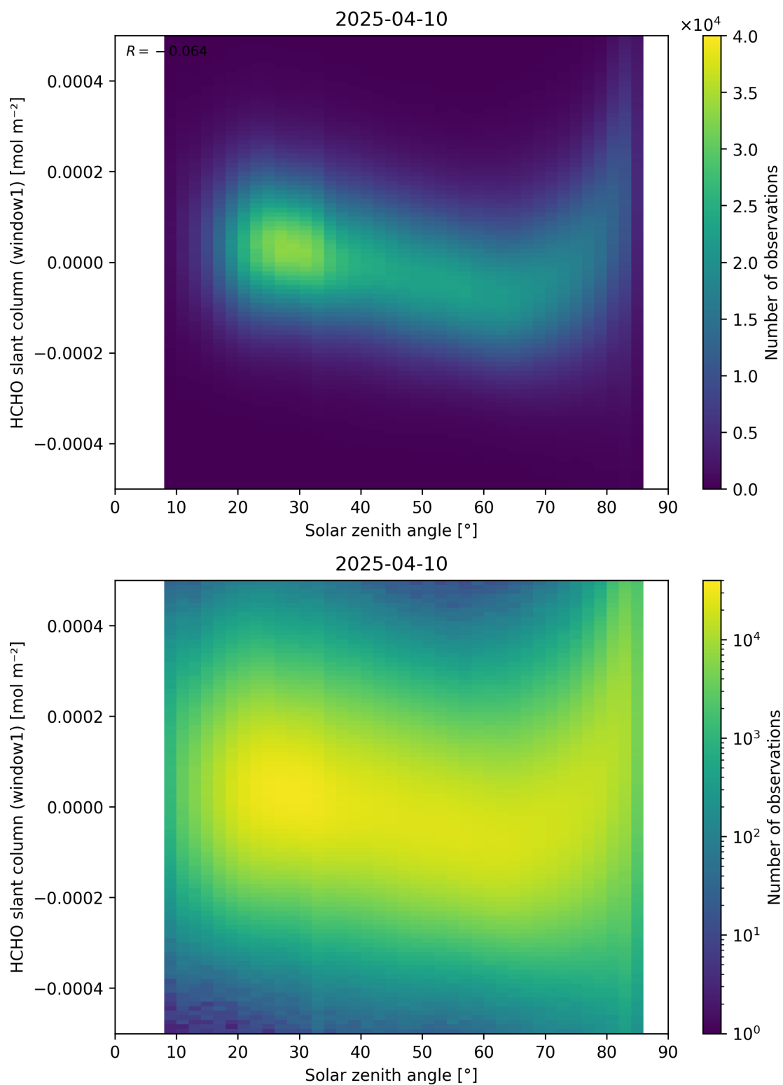
Figure 173: Scatter density plot of “Solar zenith angle” against “HCHO slant column (window1)” for 2025-04-09 to 2025-04-11.
