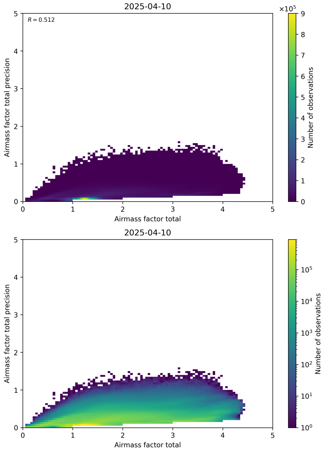
Figure 103: Scatter density plot of “Airmass factor total” against “Airmass factor total precision” for 2025-04-09 to 2025-04-11.
