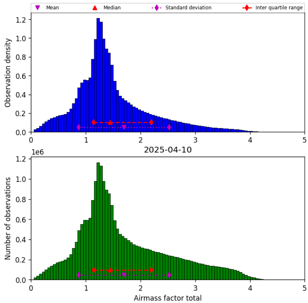
Figure 40: Histogram of “Airmass factor total” for 2025-04-09 to 2025-04-11
