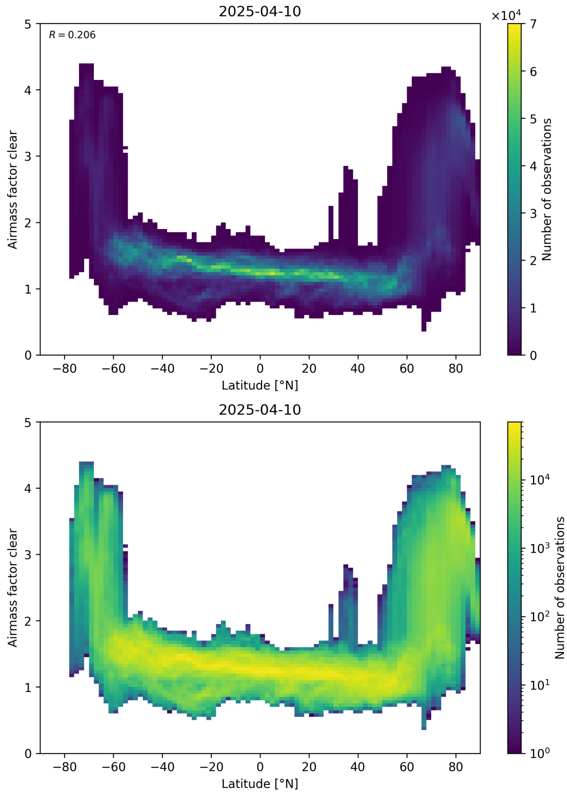
Figure 156: Scatter density plot of “Latitude” against “Airmass factor clear” for 2025-04-09 to 2025-04-11.
