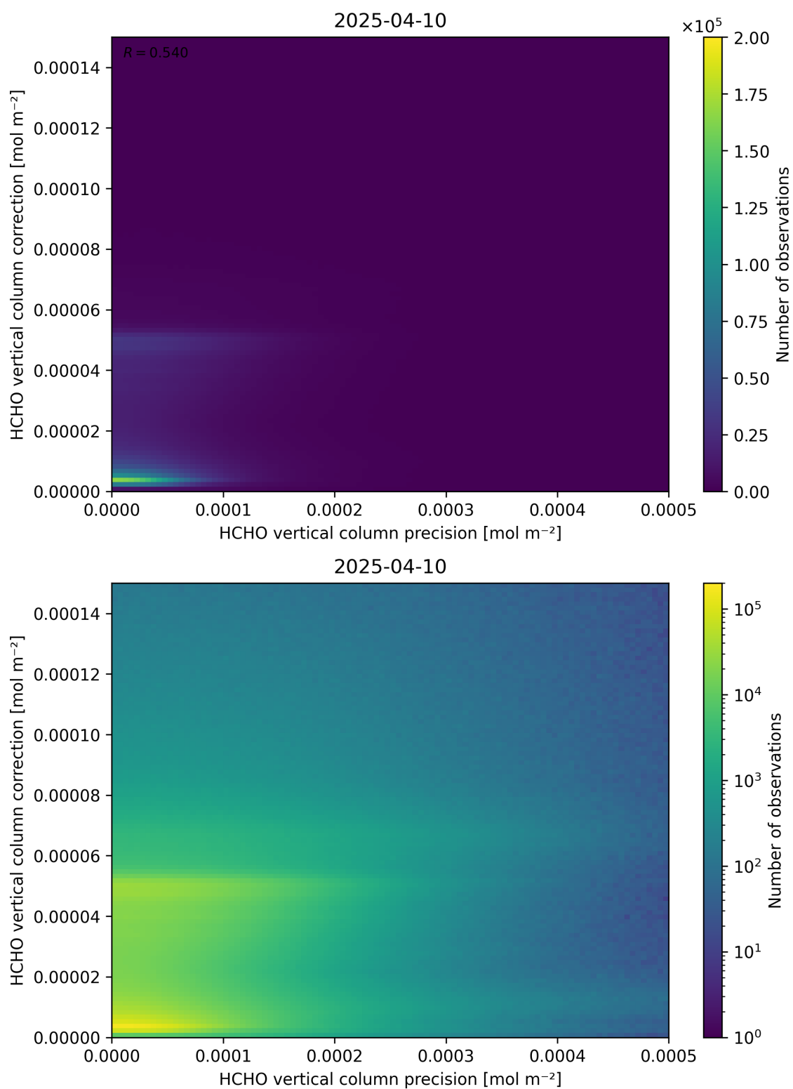
Figure 146: Scatter density plot of “HCHO vertical column precision” against “HCHO vertical column correction” for 2025-04-09 to 2025-04-11.
