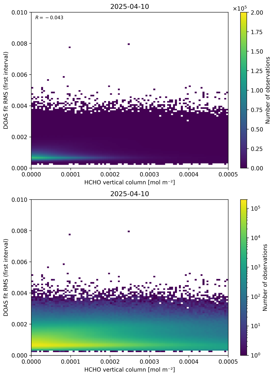
Figure 123: Scatter density plot of “HCHO vertical column” against “DOAS fit RMS (first interval)” for 2025-04-09 to 2025-04-11.
