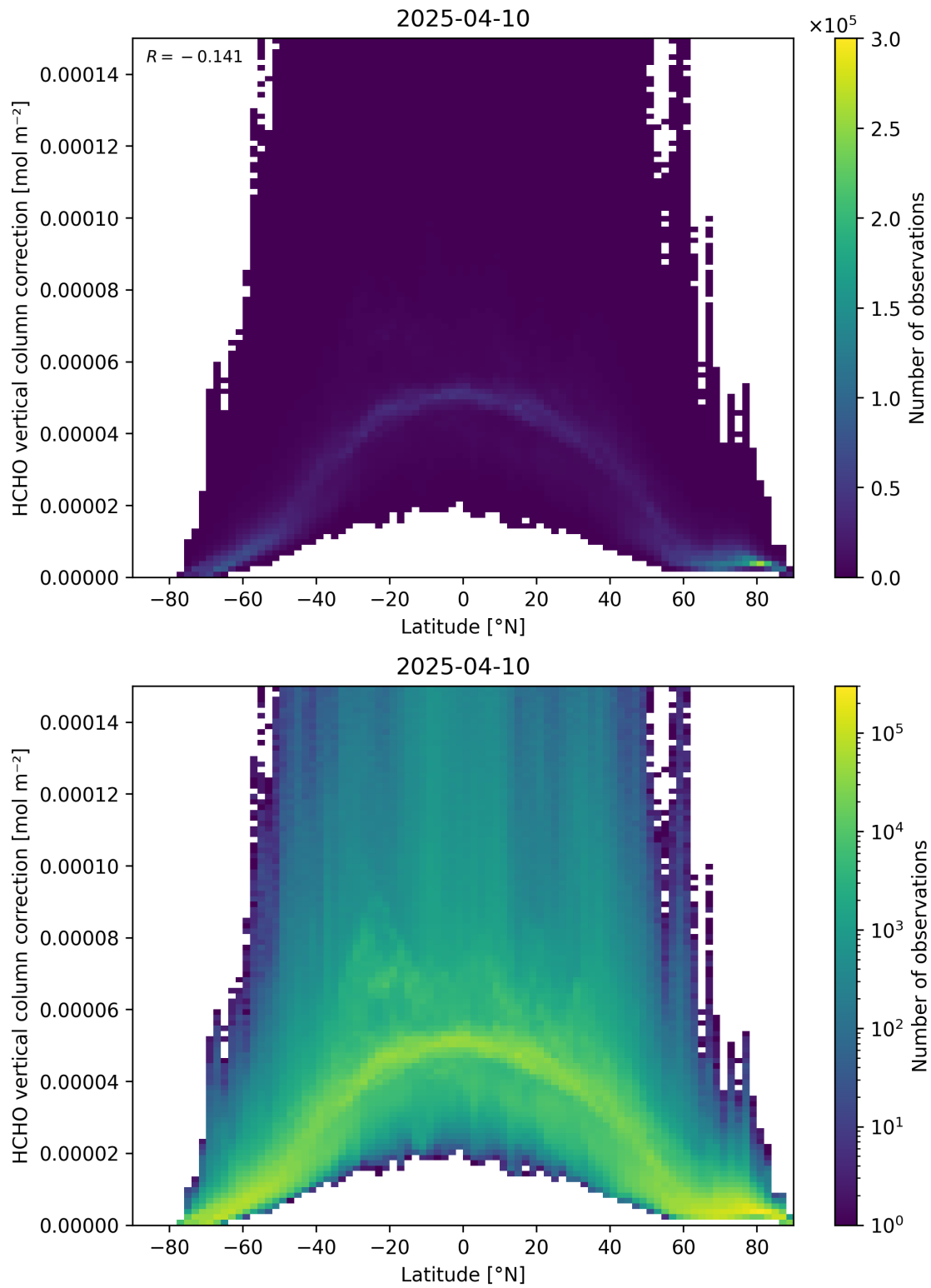
Figure 164: Scatter density plot of “Latitude” against “HCHO vertical column correction” for 2025-04-09 to 2025-04-11.
