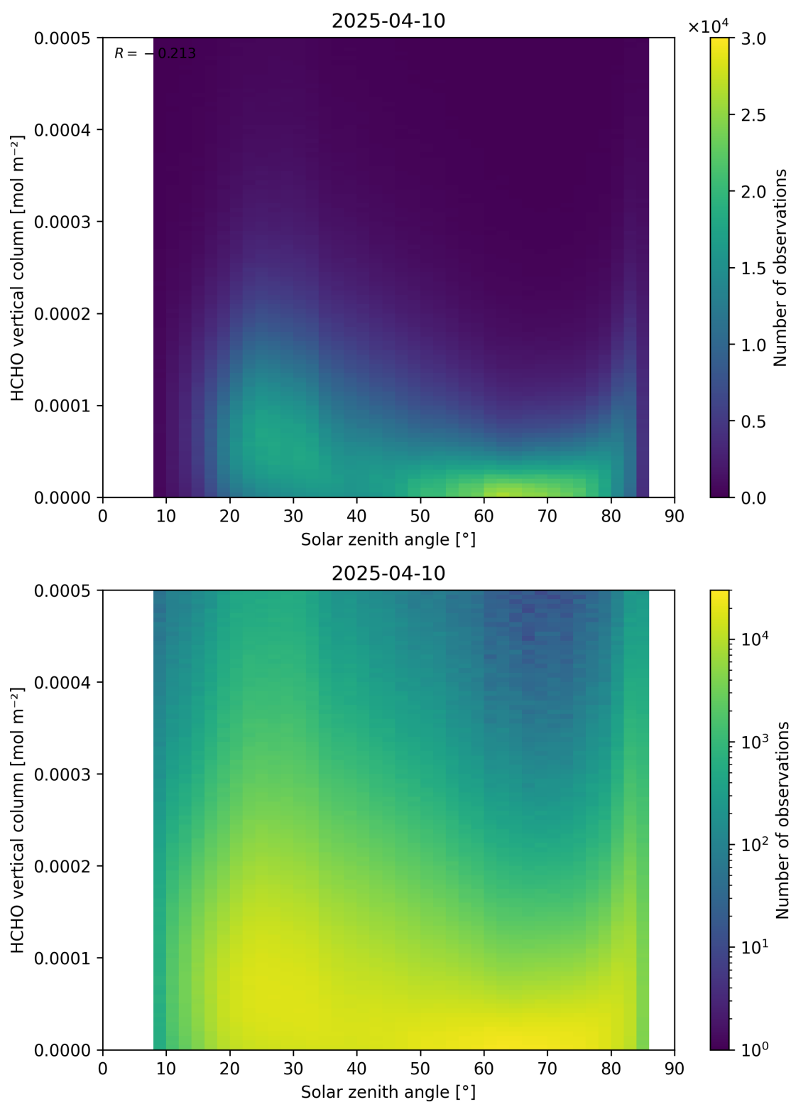
Figure 177: Scatter density plot of “Solar zenith angle” against “HCHO vertical column” for 2025-04-09 to 2025-04-11.
