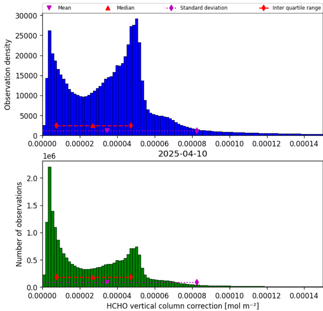
Figure 37: Histogram of “HCHO vertical column correction” for 2025-04-09 to 2025-04-11
