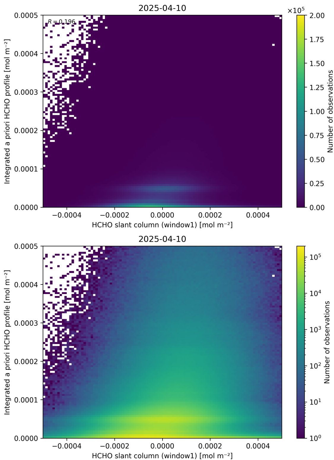
Figure 87: Scatter density plot of “HCHO slant column (window1)” against “Integrated a priori HCHO profile” for 2025-04-09 to 2025-04-11.
