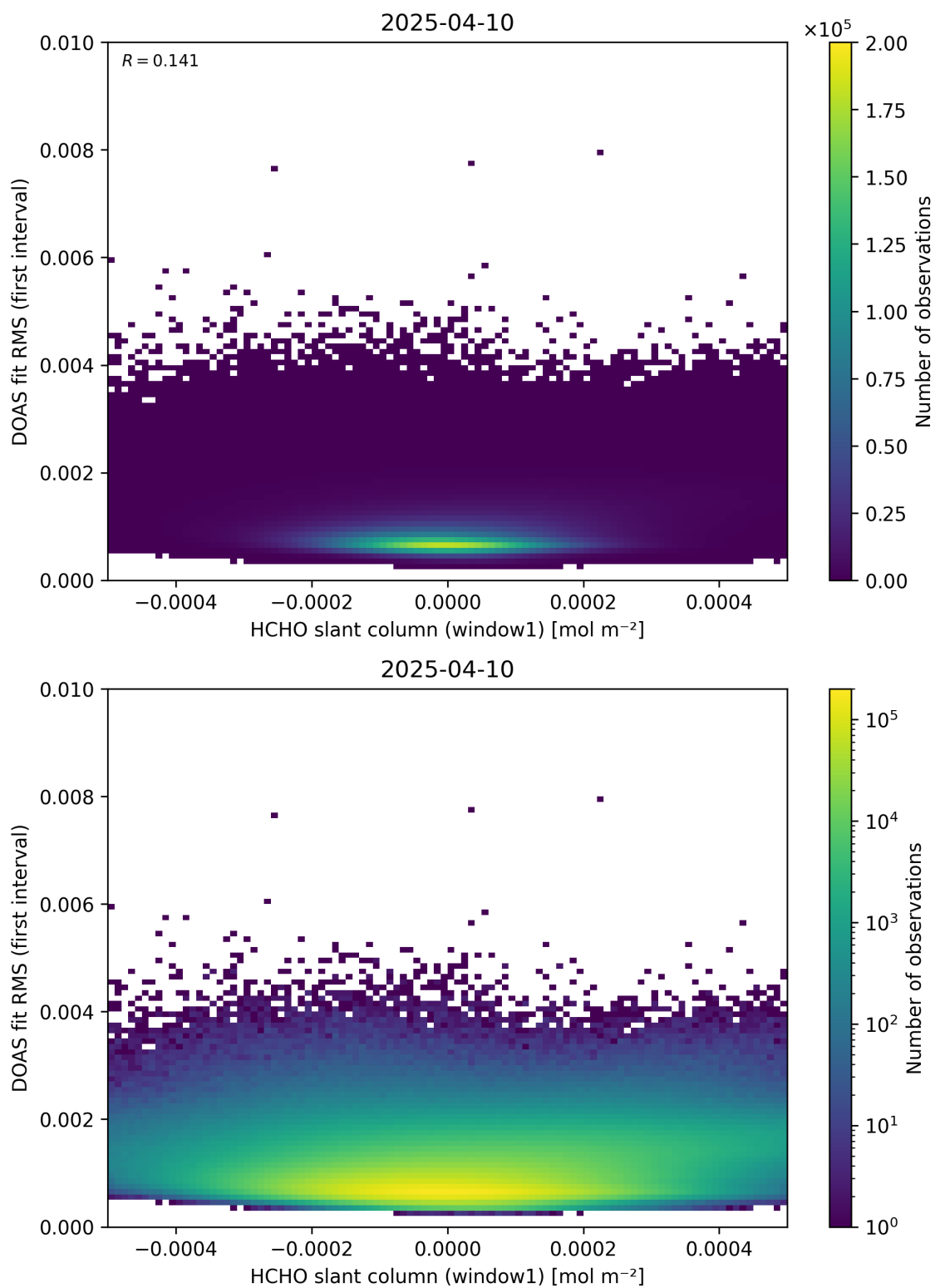
Figure 78: Scatter density plot of “HCHO slant column (window1)” against “DOAS fit RMS (first interval)” for 2025-04-09 to 2025-04-11.
