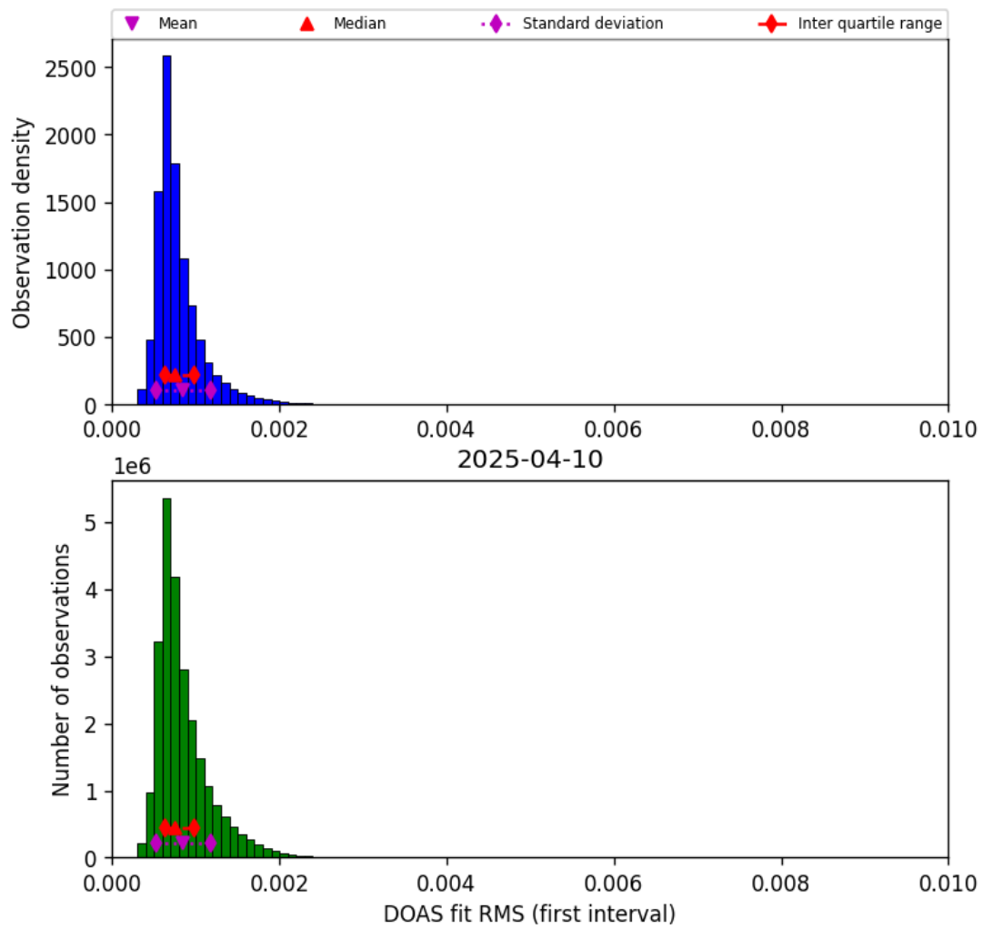
Figure 46: Histogram of “DOAS fit RMS (first interval)” for 2025-04-09 to 2025-04-11
