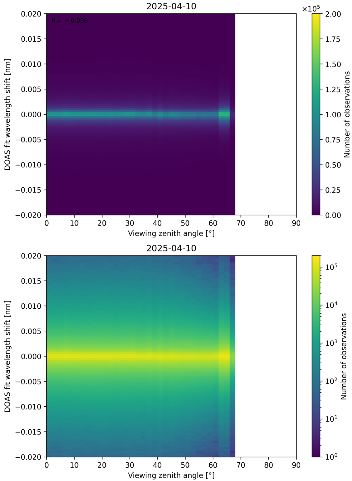
Figure 183: Scatter density plot of “Viewing zenith angle” against “DOAS fit wavelength shift” for 2025-04-09 to 2025-04-11.
