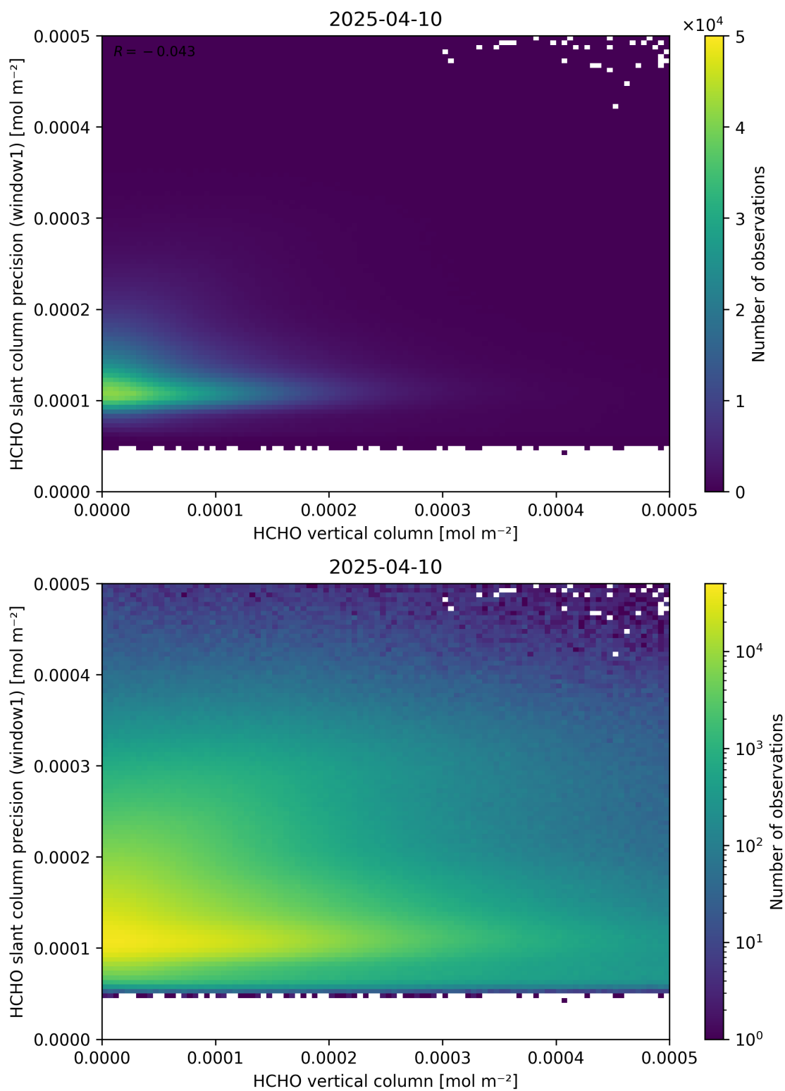
Figure 130: Scatter density plot of “HCHO vertical column” against “HCHO slant column precision (window1)” for 2025-04-09 to 2025-04-11.
