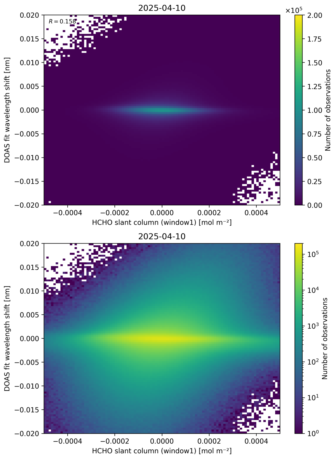
Figure 79: Scatter density plot of “HCHO slant column (window1)” against “DOAS fit wavelength shift” for 2025-04-09 to 2025-04-11.
