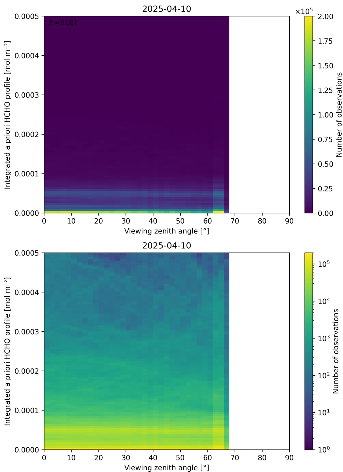
Figure 195: Scatter density plot of “Viewing zenith angle” against “Integrated a priori HCHO profile” for 2025-04-09 to 2025-04-11.
