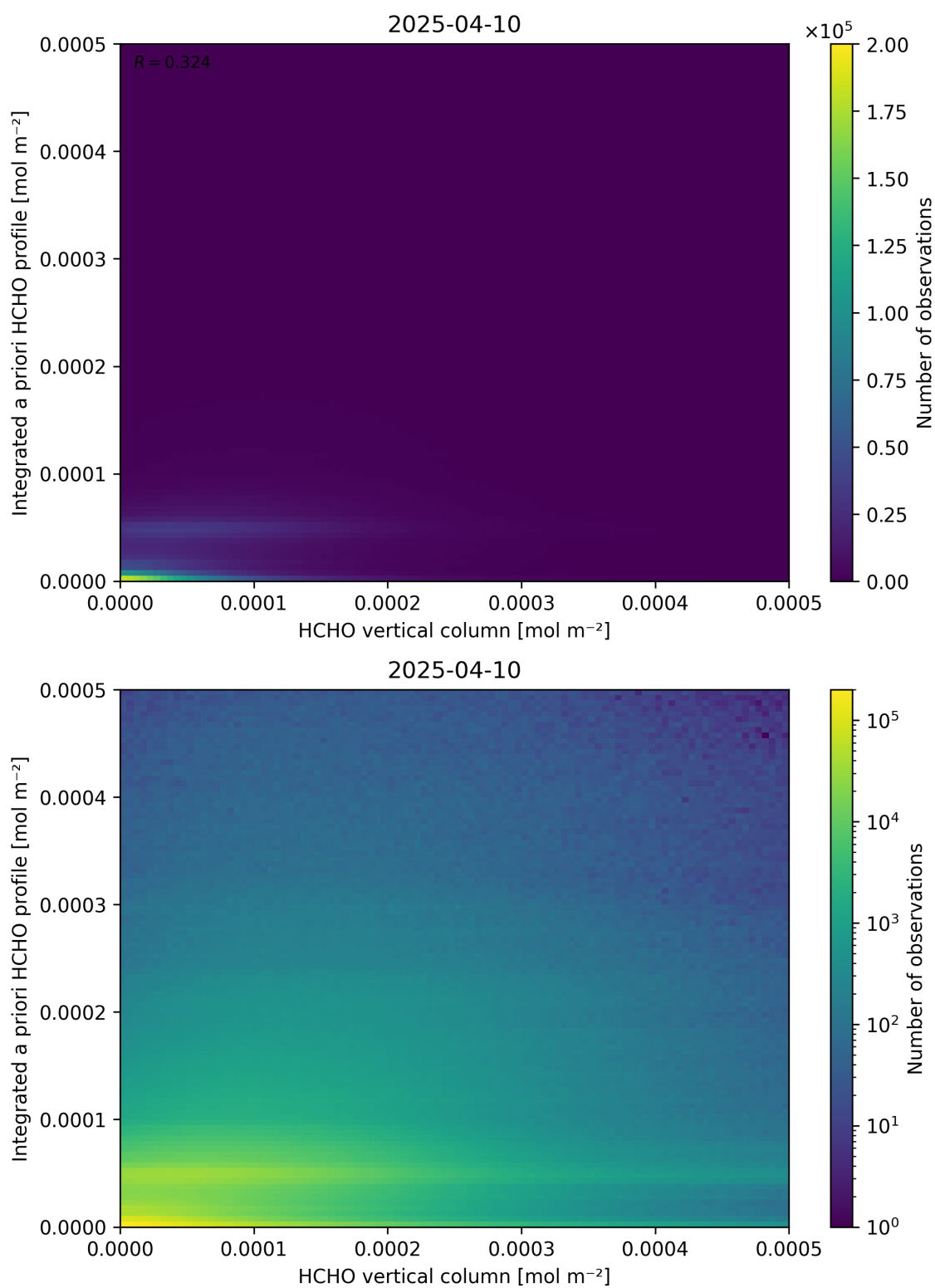
Figure 135: Scatter density plot of “HCHO vertical column” against “Integrated a priori HCHO profile” for 2025-04-09 to 2025-04-11.
