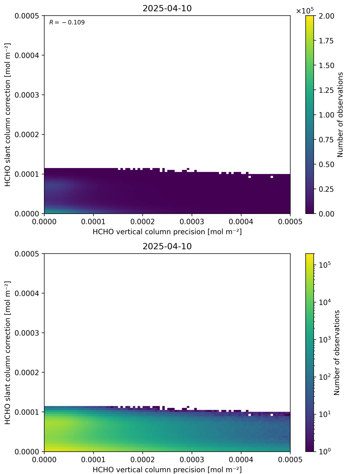
Figure 141: Scatter density plot of “HCHO vertical column precision” against “HCHO slant column correction” for 2025-04-09 to 2025-04-11.
