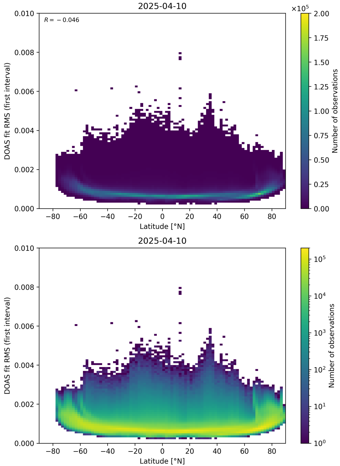
Figure 153: Scatter density plot of “Latitude” against “DOAS fit RMS (first interval)” for 2025-04-09 to 2025-04-11.
