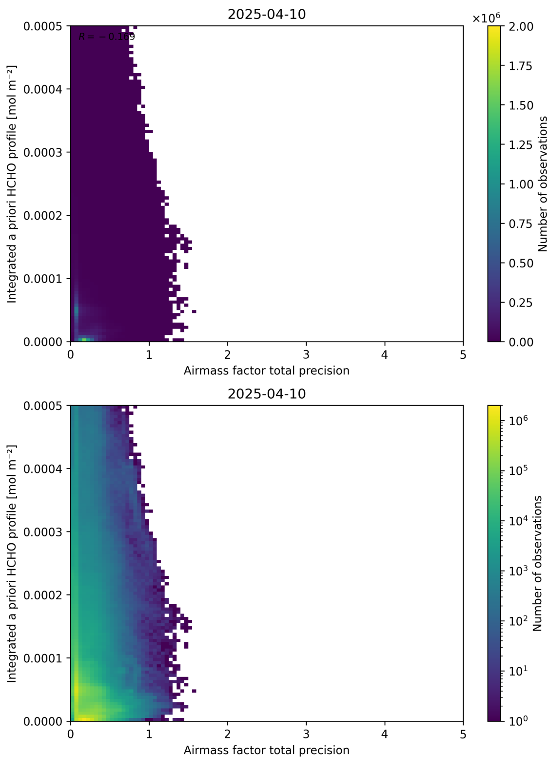
Figure 111: Scatter density plot of “Airmass factor total precision” against “Integrated a priori HCHO profile” for 2025-04-09 to 2025-04-11.
