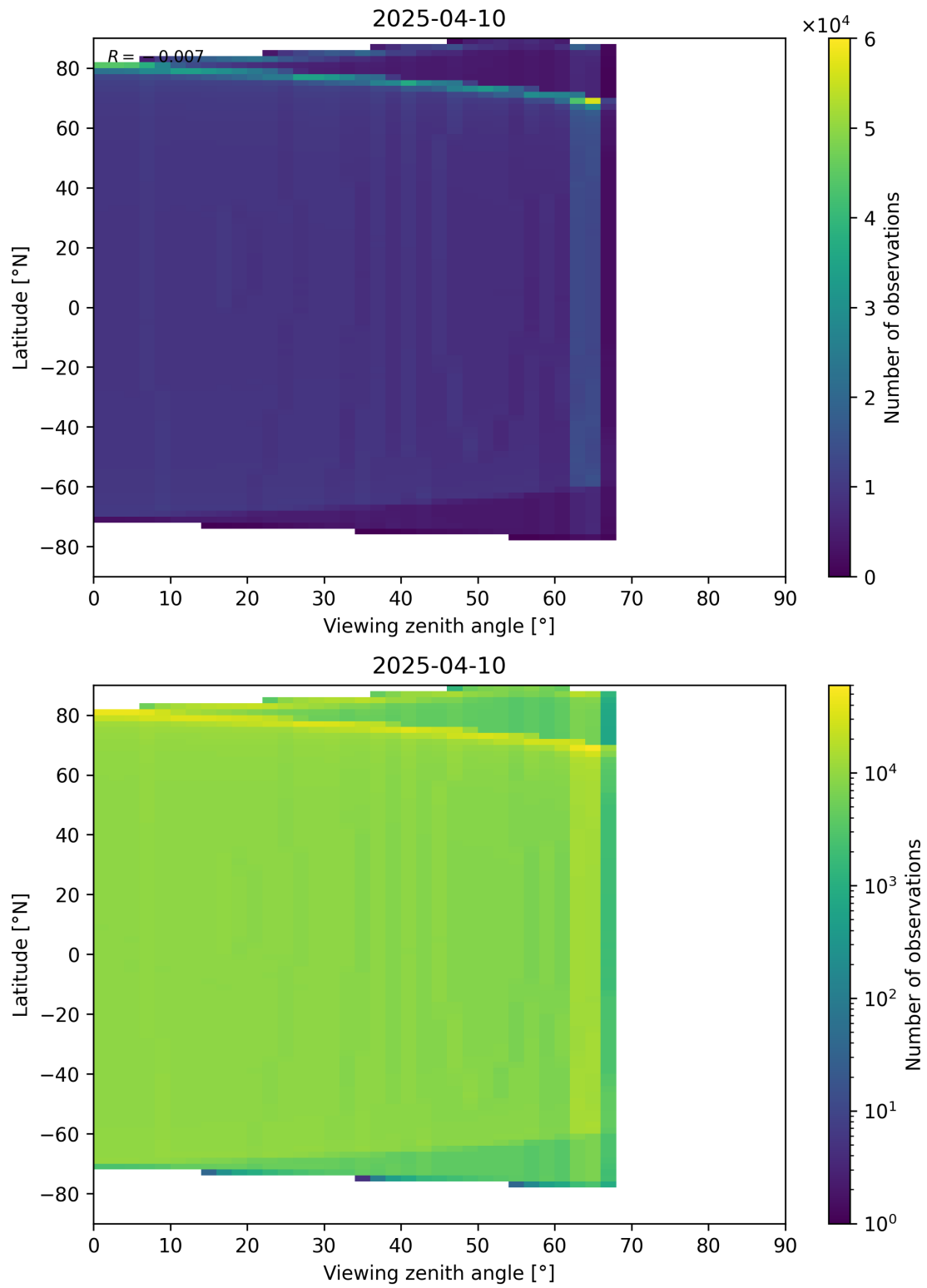
Figure 196: Scatter density plot of “Viewing zenith angle” against “Latitude” for 2025-04-09 to 2025-04-11.
