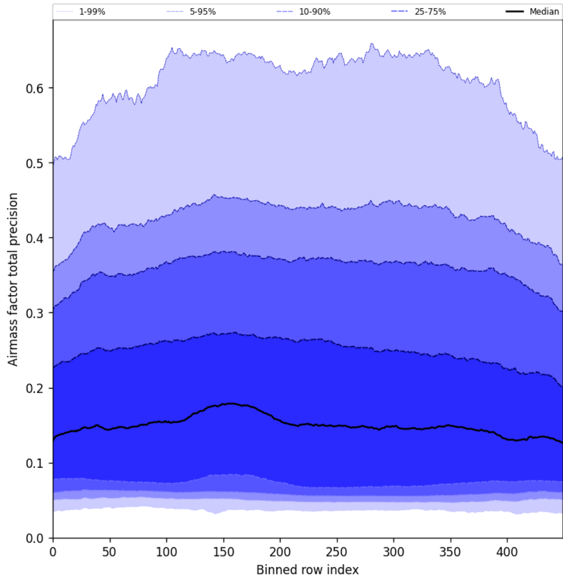
Figure 55: Along track statistics of “Airmass factor total precision” for 2025-04-09 to 2025-04-11
