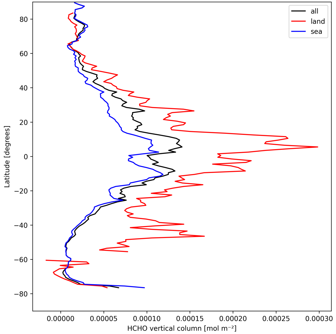
Figure 21: Zonal average of “HCHO vertical column” for 2025-04-09 to 2025-04-11.
