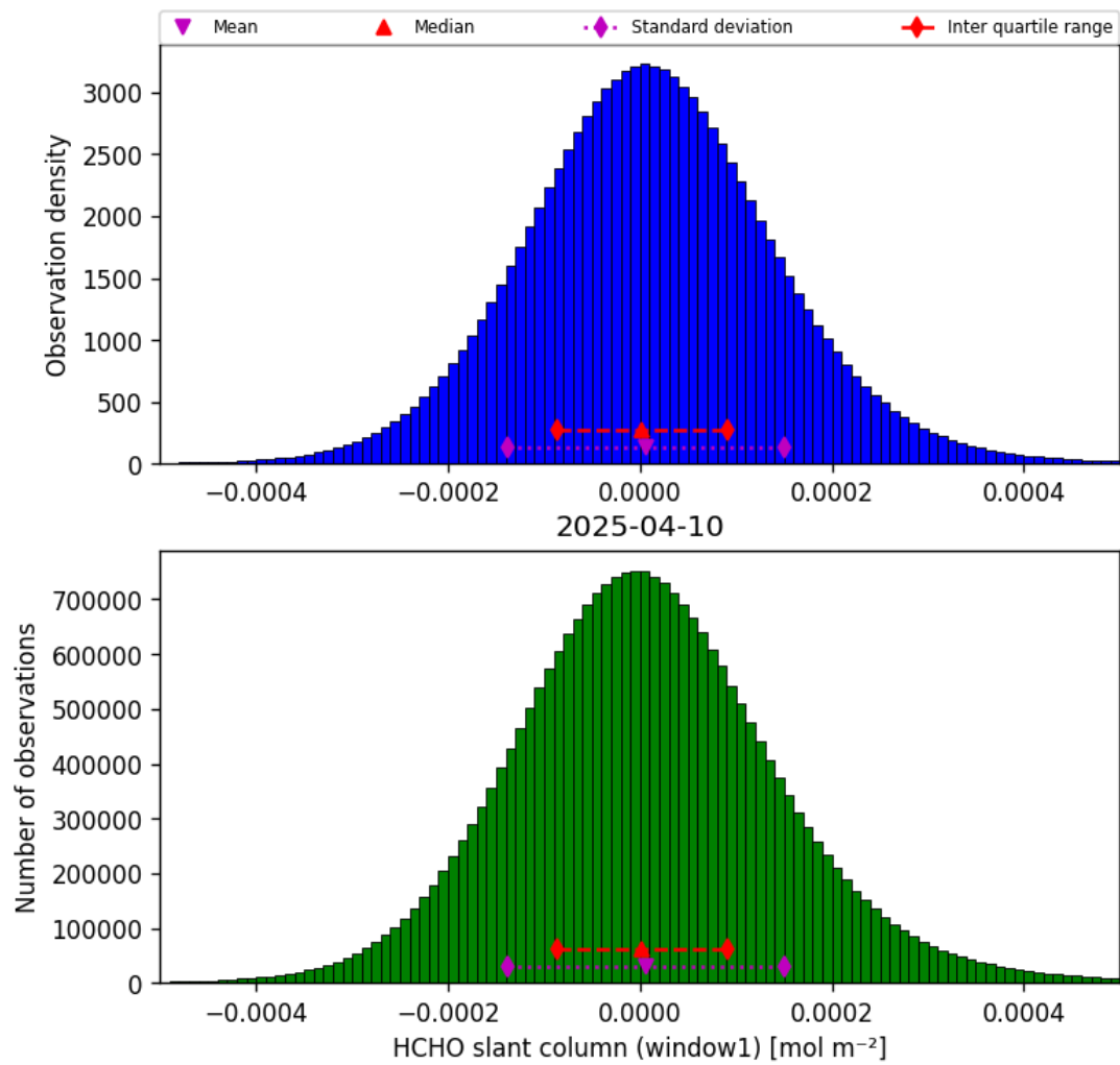
Figure 38: Histogram of “HCHO slant column (window1)” for 2025-04-09 to 2025-04-11
