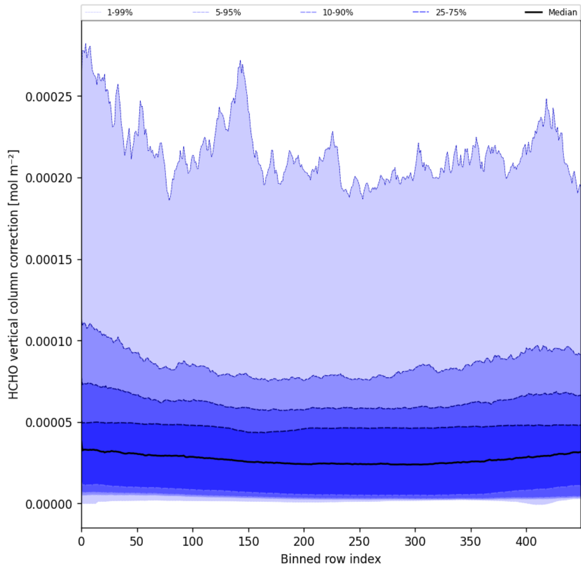
Figure 51: Along track statistics of “HCHO vertical column correction” for 2025-04-09 to 2025-04-11
