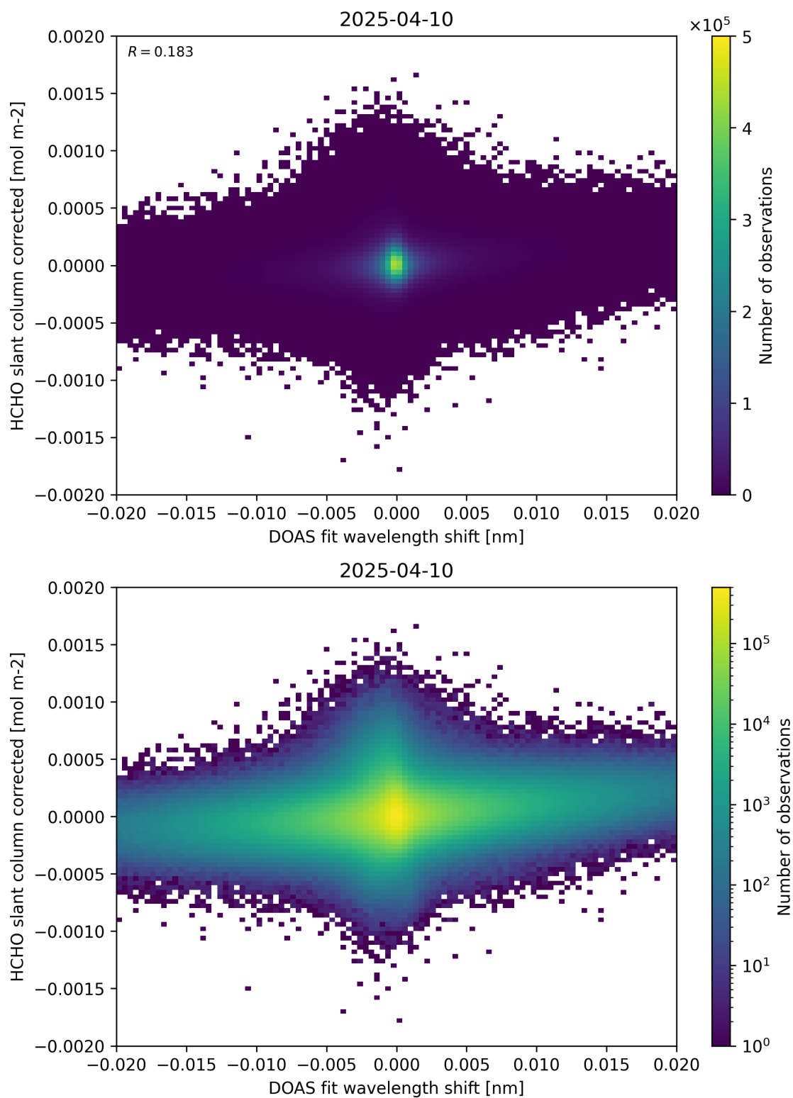
Figure 66: Scatter density plot of “DOAS fit wavelength shift” against “HCHO slant column corrected” for 2025-04-09 to 2025-04-11.
