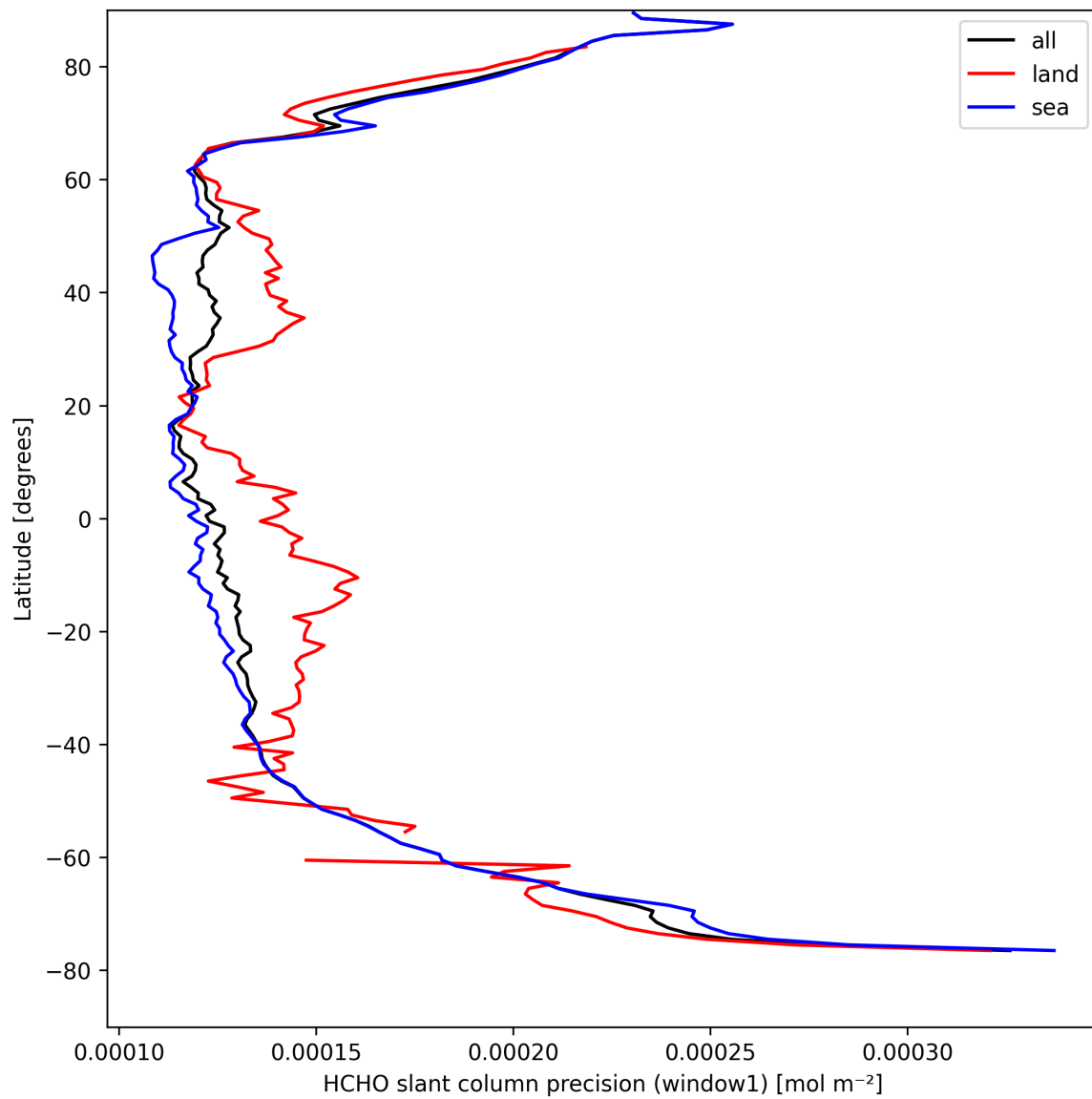
Figure 25: Zonal average of “HCHO slant column precision (window1)” for 2025-04-09 to 2025-04-11.
