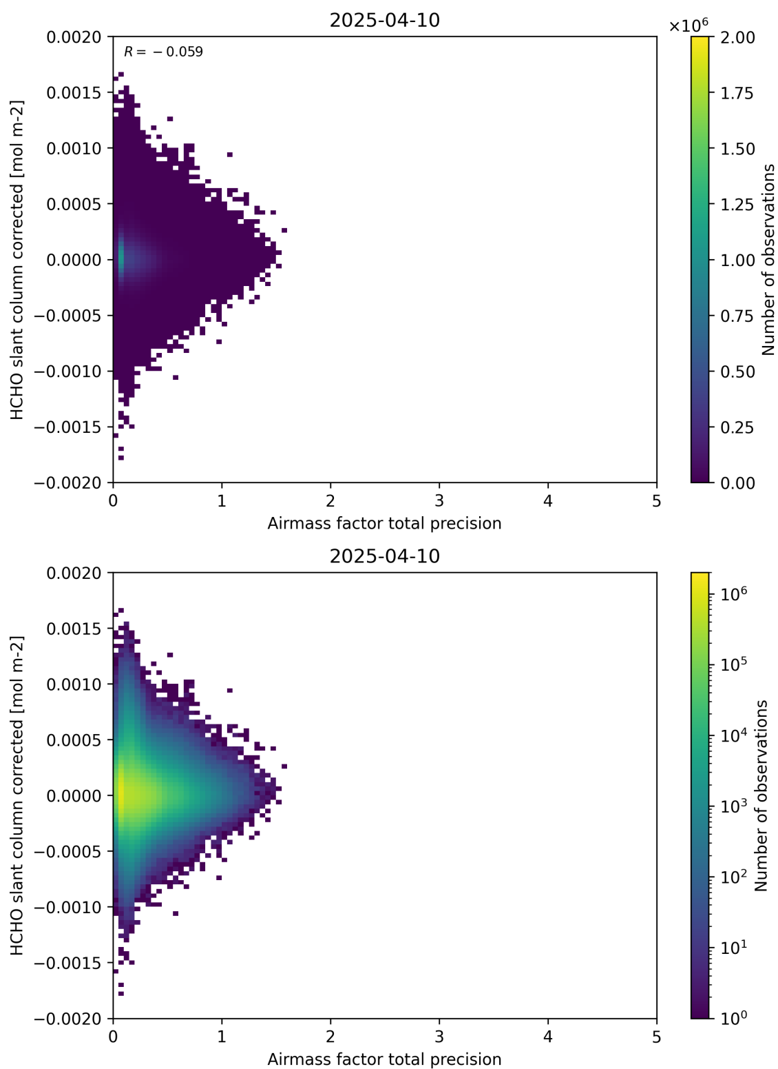
Figure 109: Scatter density plot of “Airmass factor total precision” against “HCHO slant column corrected” for 2025-04-09 to 2025-04-11.
