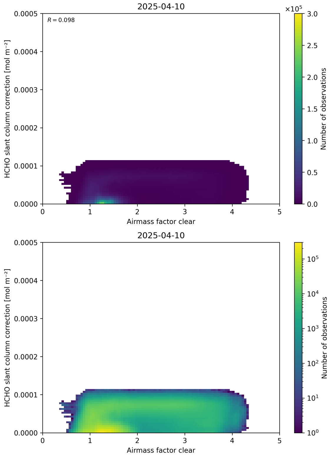
Figure 75: Scatter density plot of “Airmass factor clear” against “HCHO slant column correction” for 2025-04-09 to 2025-04-11.
