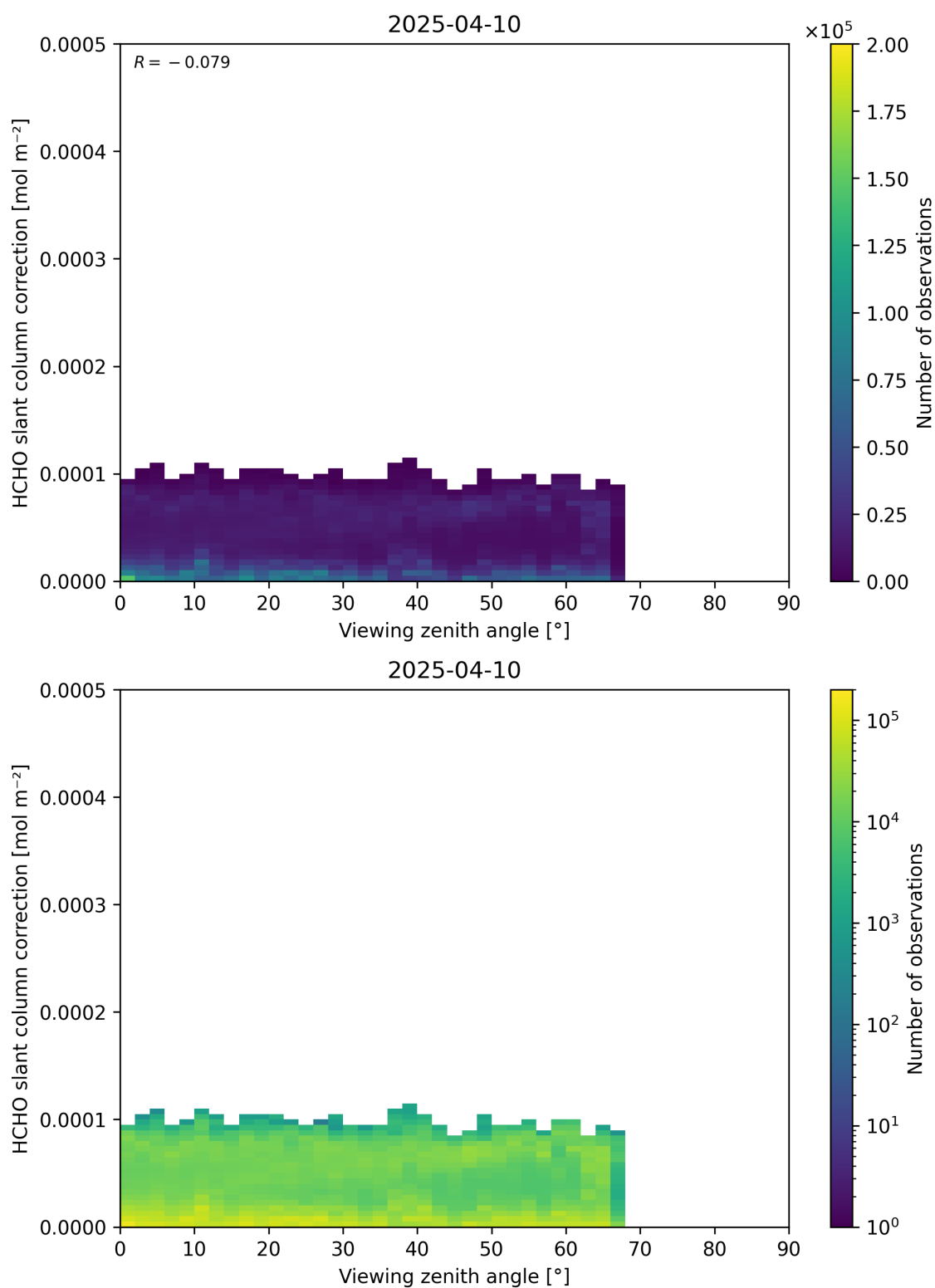
Figure 187: Scatter density plot of “Viewing zenith angle” against “HCHO slant column correction” for 2025-04-09 to 2025-04-11.
