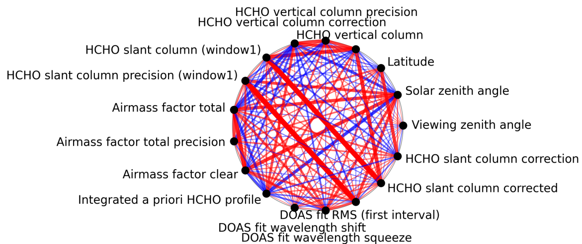
Figure 1: Map of correlation graph for 2025-04-09 to 2025-04-11.
