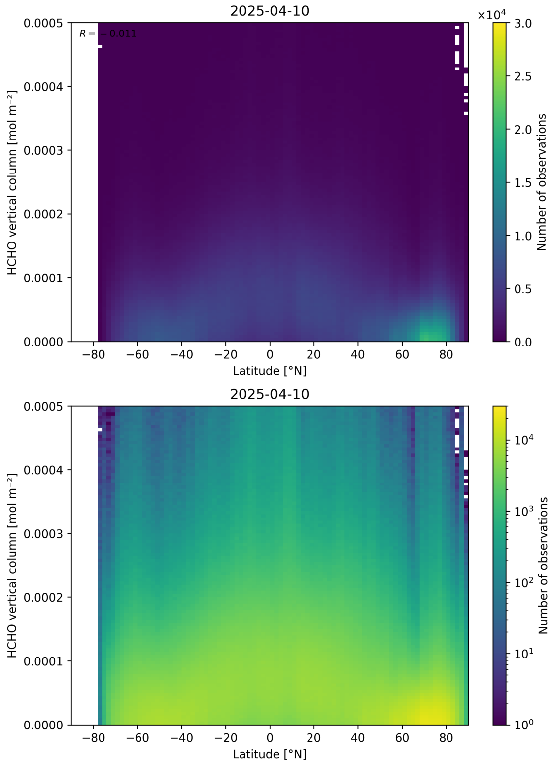
Figure 163: Scatter density plot of “Latitude” against “HCHO vertical column” for 2025-04-09 to 2025-04-11.
