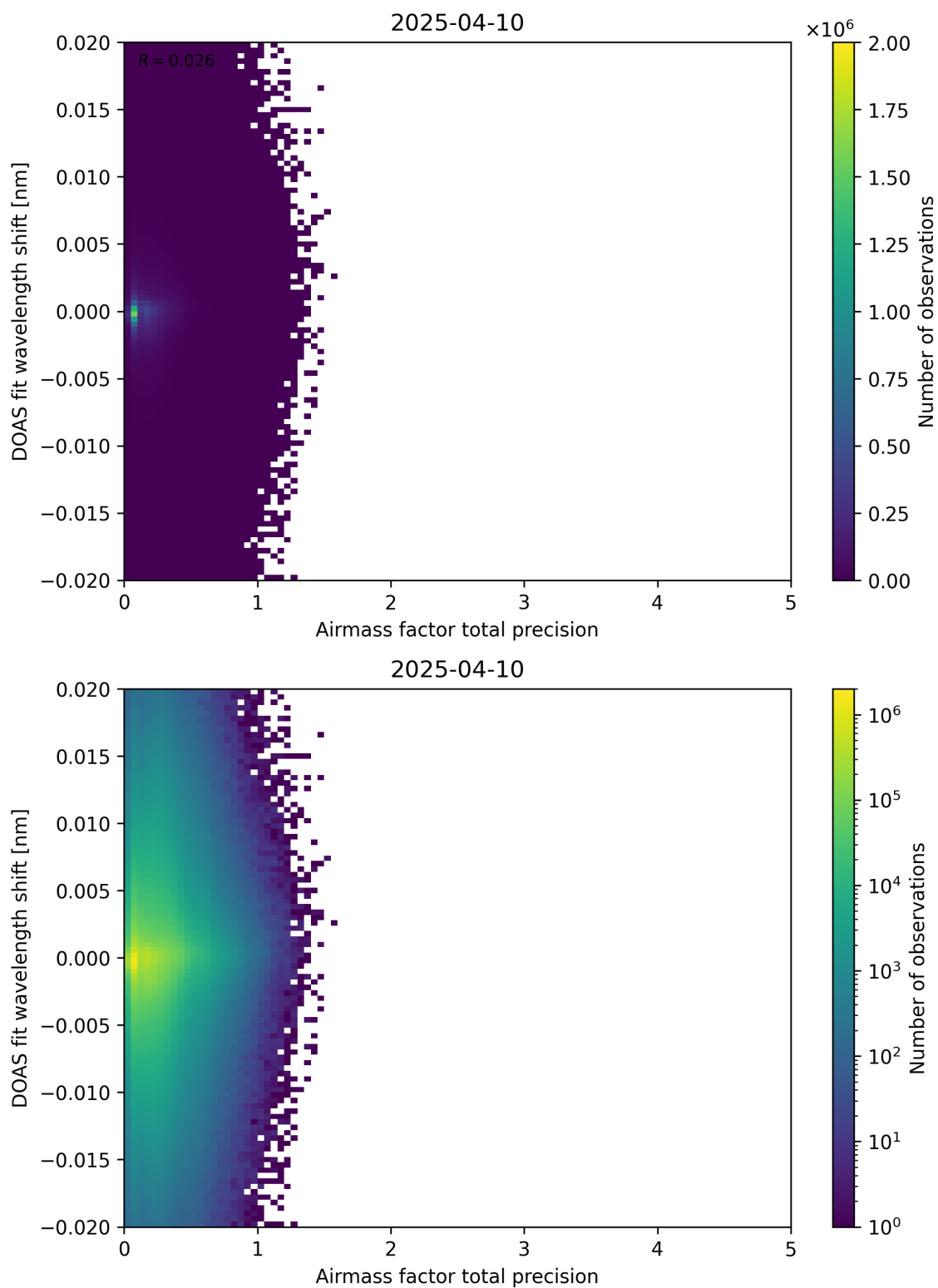
Figure 106: Scatter density plot of “Airmass factor total precision” against “DOAS fit wavelength shift” for 2025-04-09 to 2025-04-11.
