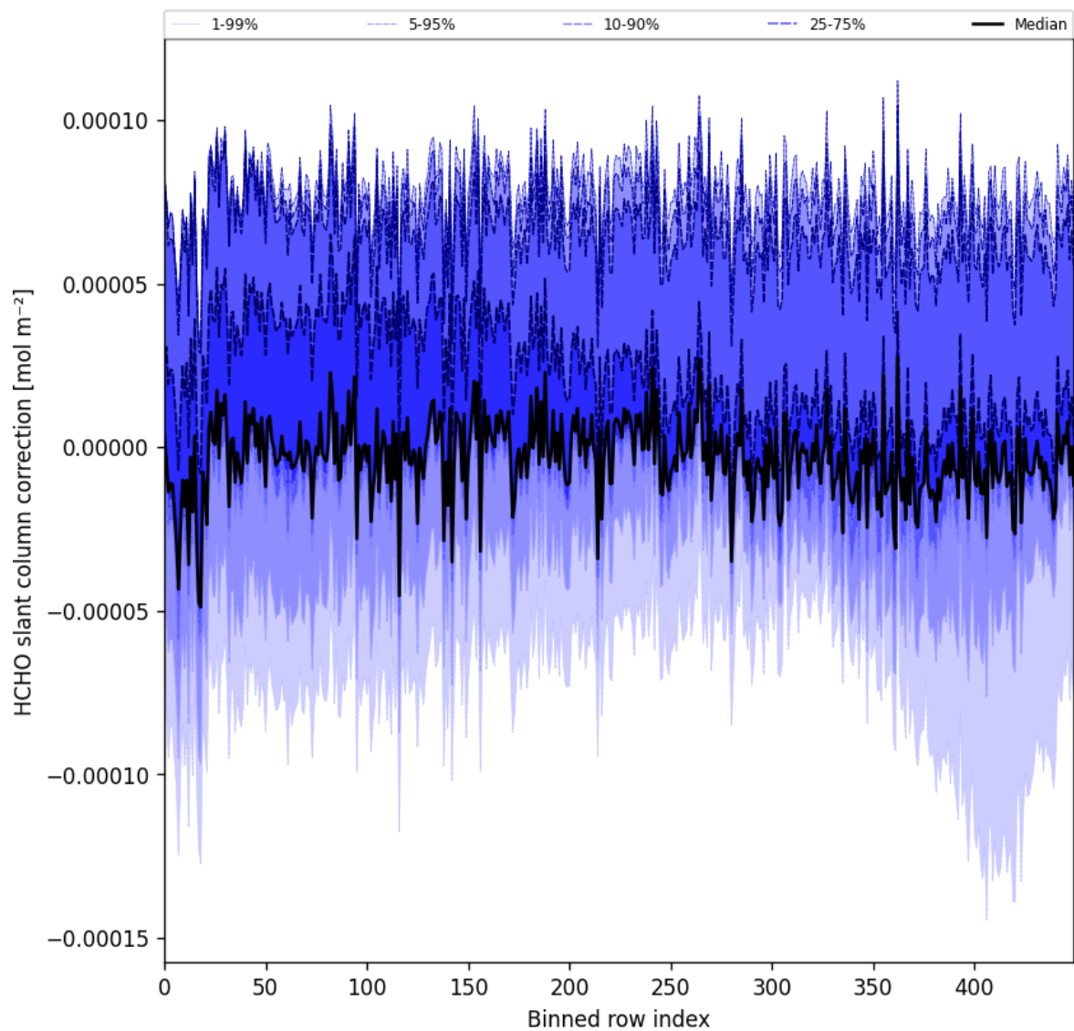
Figure 61: Along track statistics of “HCHO slant column correction” for 2025-04-09 to 2025-04-11
