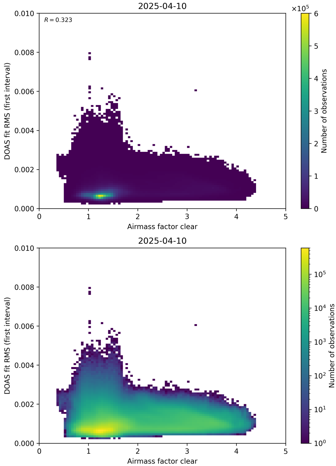
Figure 71: Scatter density plot of “Airmass factor clear” against “DOAS fit RMS (first interval)” for 2025-04-09 to 2025-04-11.
