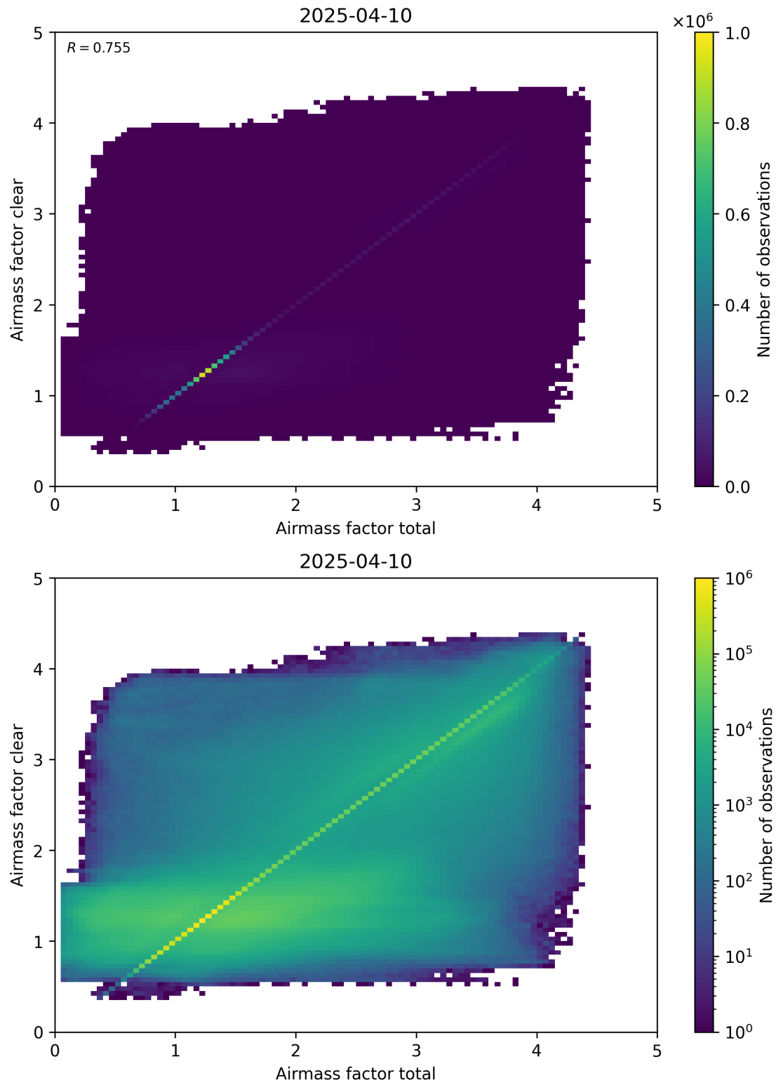
Figure 100: Scatter density plot of “Airmass factor total” against “Airmass factor clear” for 2025-04-09 to 2025-04-11.
