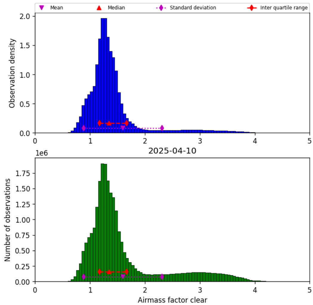
Figure 42: Histogram of “Airmass factor clear” for 2025-04-09 to 2025-04-11
