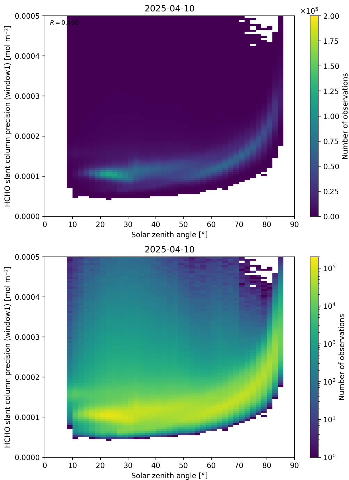
Figure 174: Scatter density plot of “Solar zenith angle” against “HCHO slant column precision (window1)” for 2025-04-09 to 2025-04-11.
