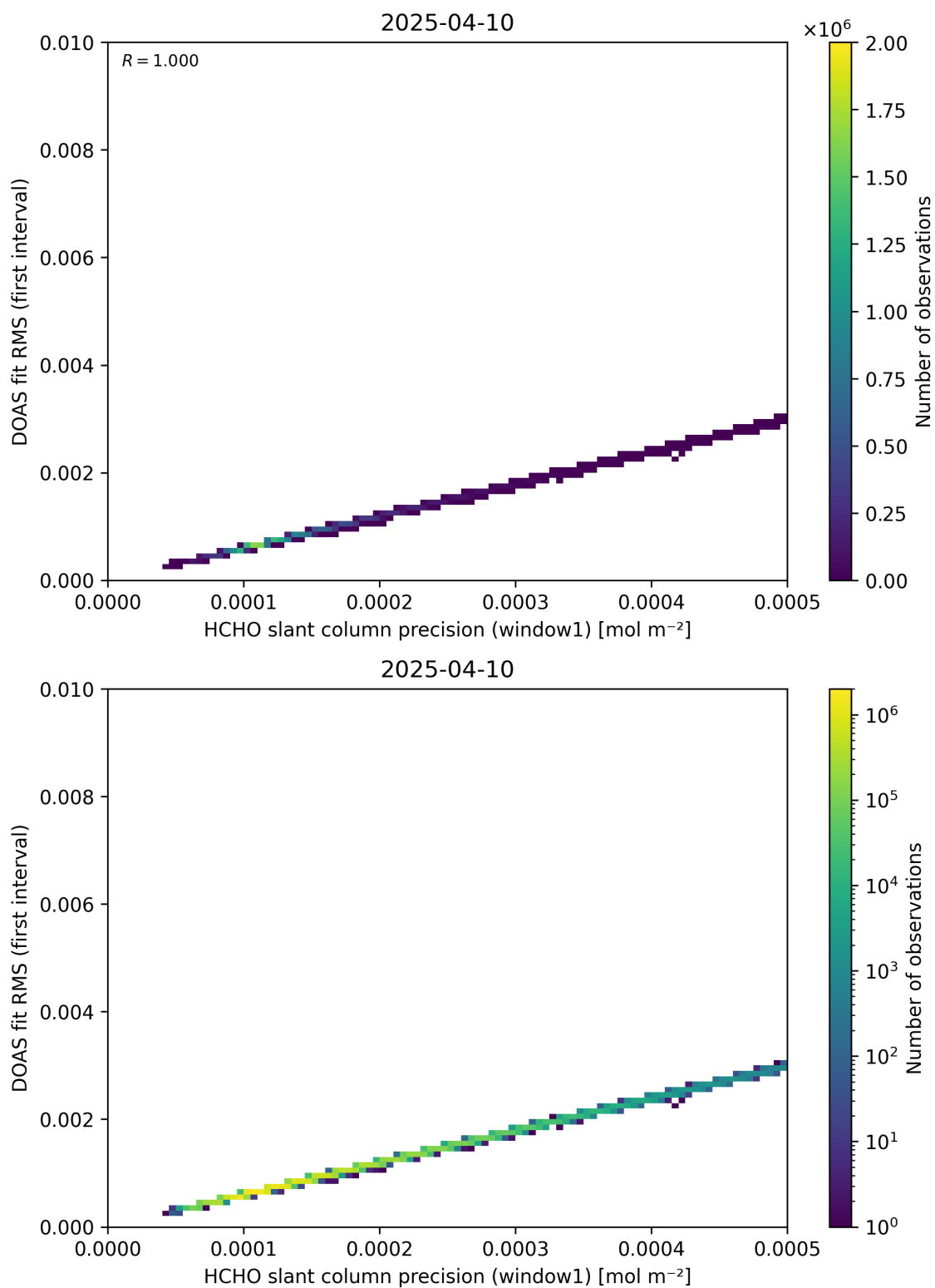
Figure 88: Scatter density plot of “HCHO slant column precision (window1)” against “DOAS fit RMS (first interval)” for 2025-04-09 to 2025-04-11.
