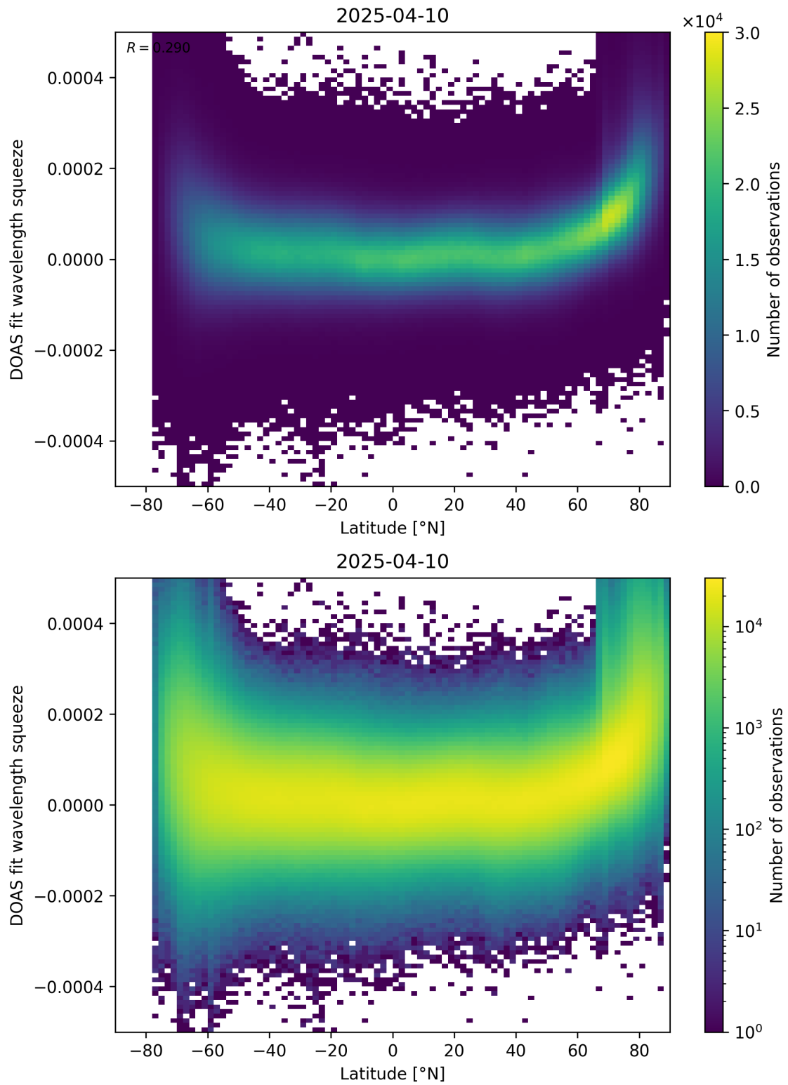
Figure 155: Scatter density plot of “Latitude” against “DOAS fit wavelength squeeze” for 2025-04-09 to 2025-04-11.
