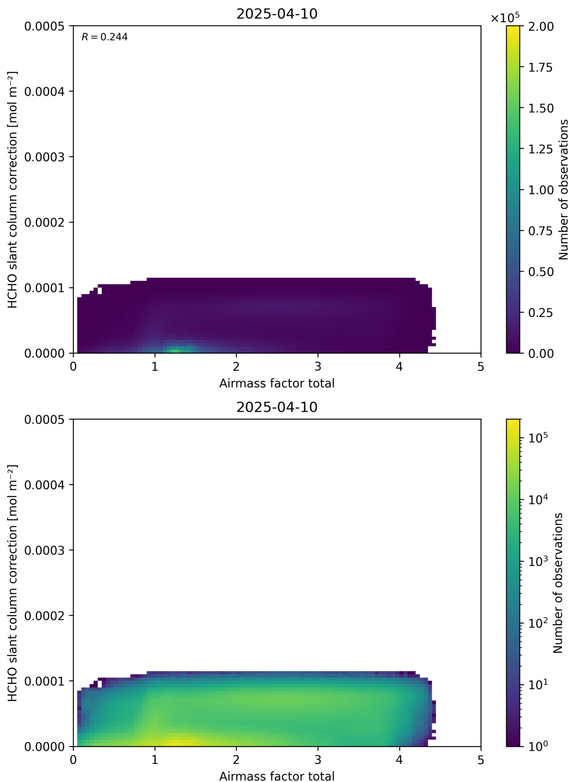
Figure 102: Scatter density plot of “Airmass factor total” against “HCHO slant column correction” for 2025-04-09 to 2025-04-11.
