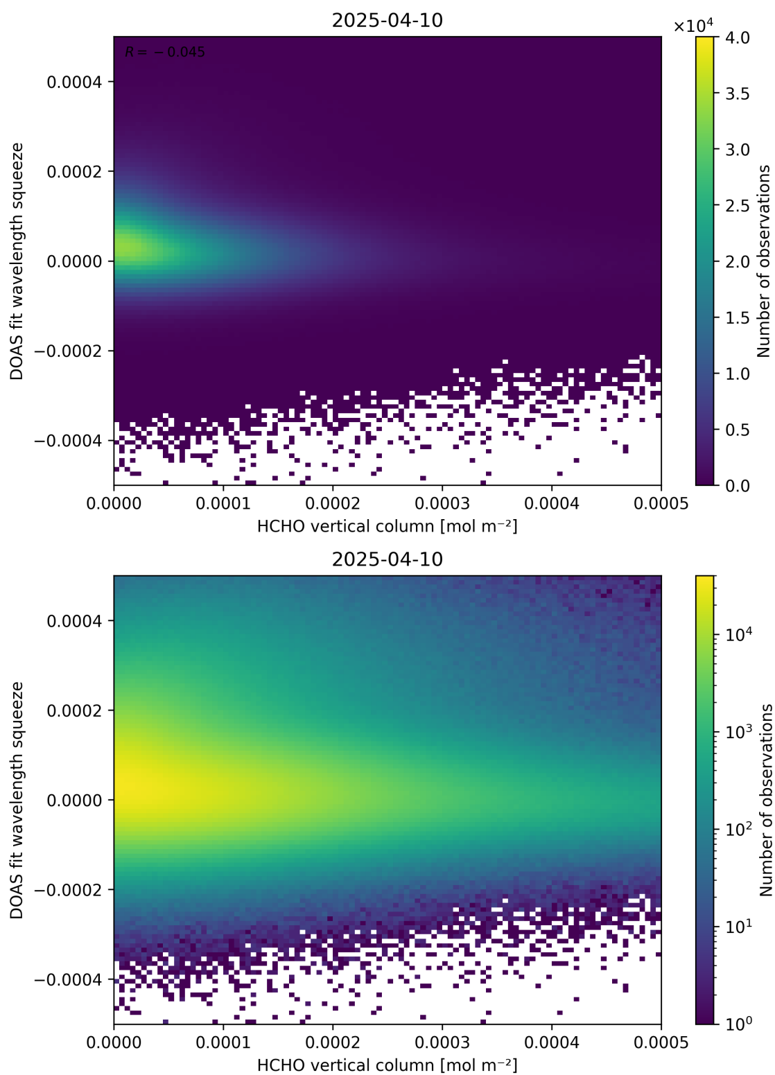
Figure 125: Scatter density plot of “HCHO vertical column” against “DOAS fit wavelength squeeze” for 2025-04-09 to 2025-04-11.
