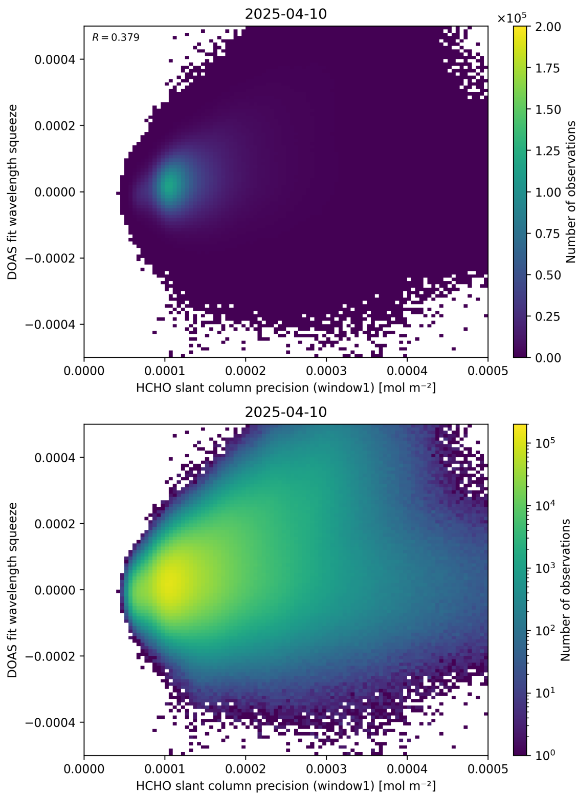
Figure 90: Scatter density plot of “HCHO slant column precision (window1)” against “DOAS fit wavelength squeeze” for 2025-04-09 to 2025-04-11.
