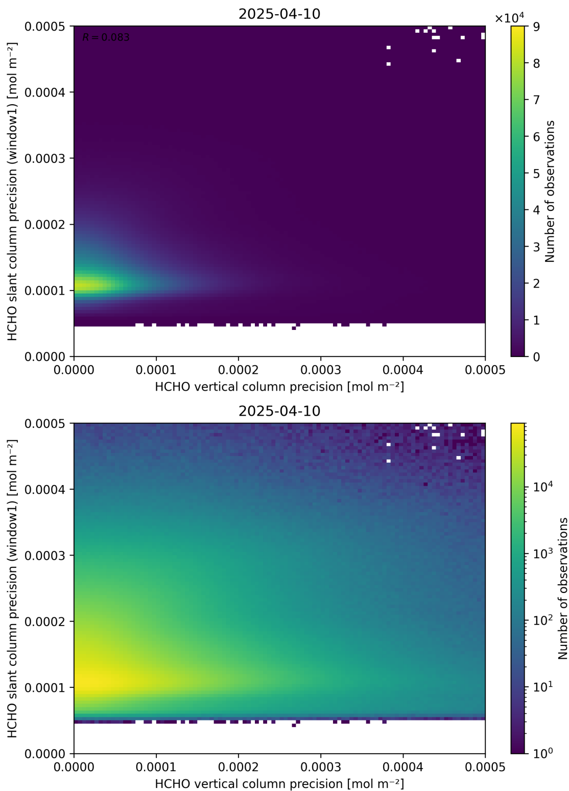
Figure 143: Scatter density plot of “HCHO vertical column precision” against “HCHO slant column precision (window1)” for 2025-04-09 to 2025-04-11.
