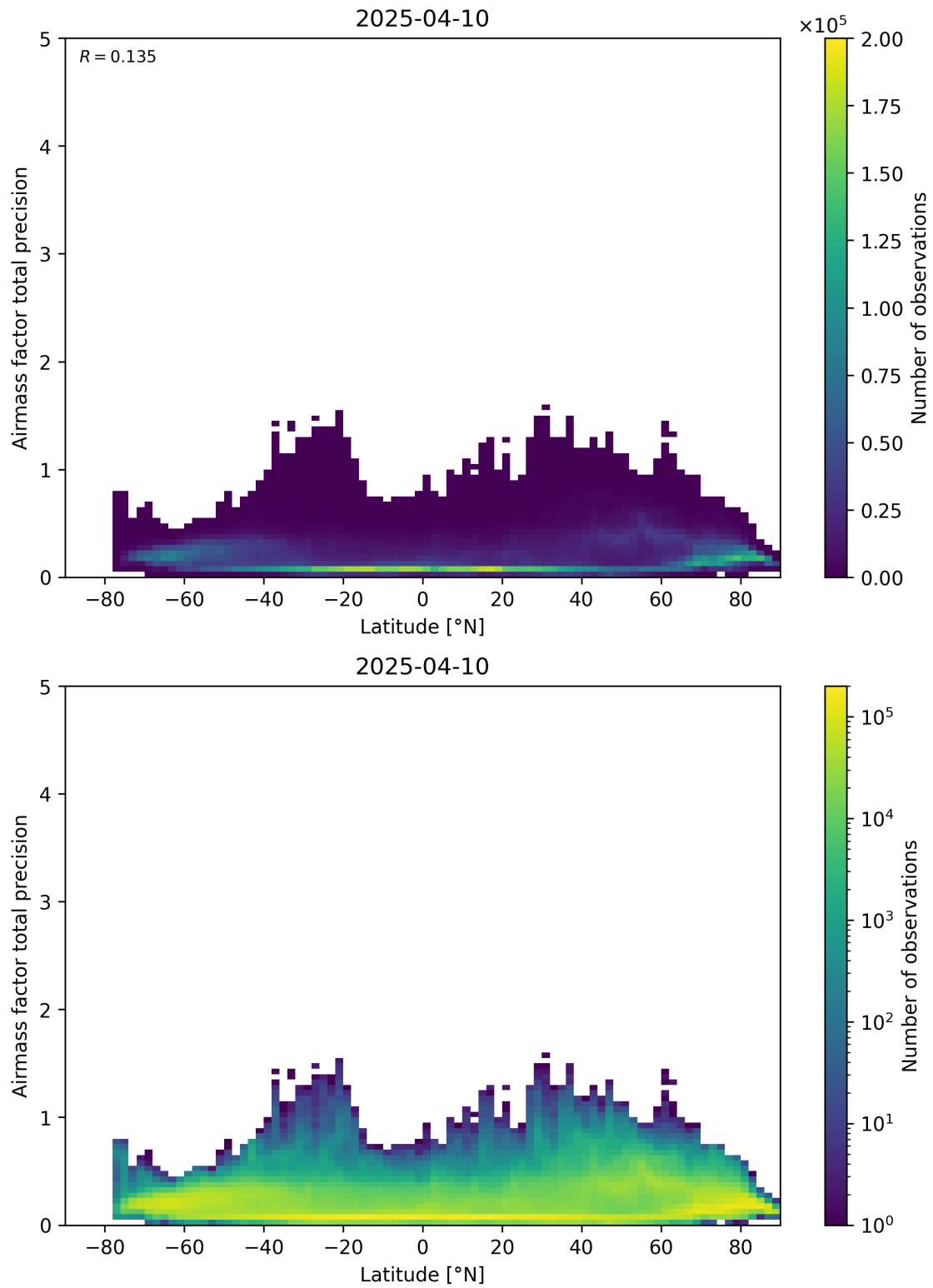
Figure 162: Scatter density plot of “Latitude” against “Airmass factor total precision” for 2025-04-09 to 2025-04-11.
