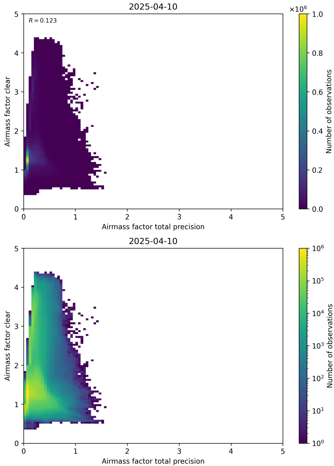
Figure 108: Scatter density plot of “Airmass factor total precision” against “Airmass factor clear” for 2025-04-09 to 2025-04-11.
