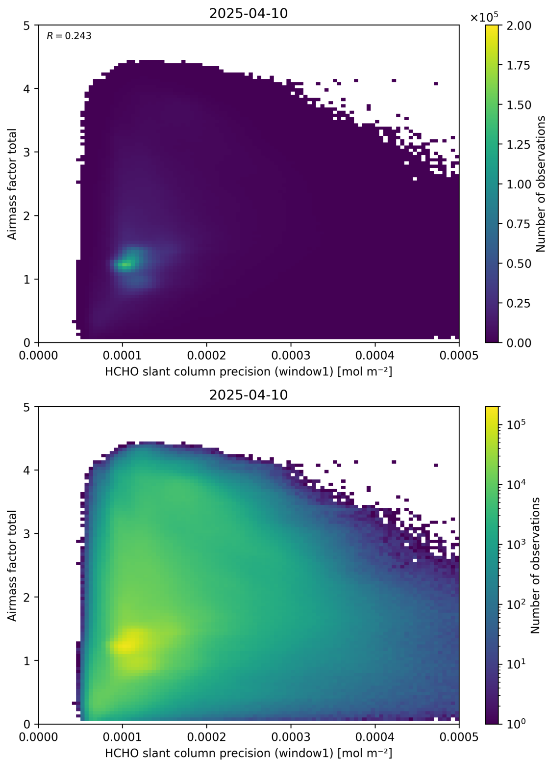
Figure 94: Scatter density plot of “HCHO slant column precision (window1)” against “Airmass factor total” for 2025-04-09 to 2025-04-11.
