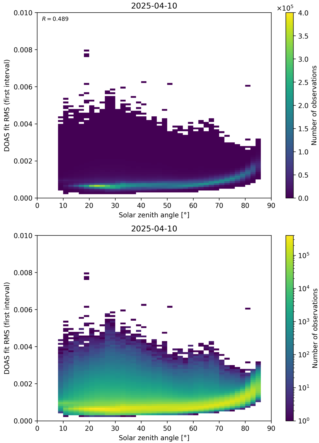
Figure 167: Scatter density plot of “Solar zenith angle” against “DOAS fit RMS (first interval)” for 2025-04-09 to 2025-04-11.
