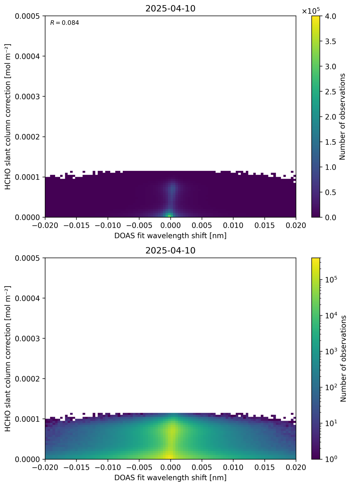
Figure 67: Scatter density plot of “DOAS fit wavelength shift” against “HCHO slant column correction” for 2025-04-09 to 2025-04-11.
