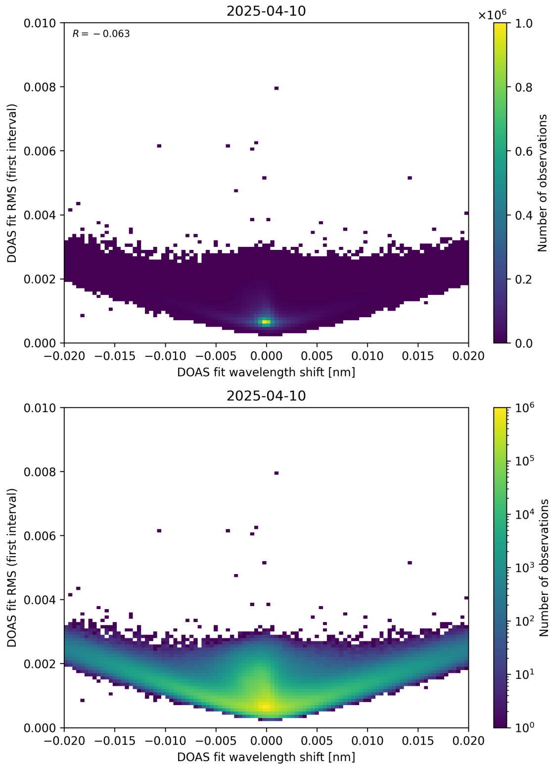
Figure 64: Scatter density plot of “DOAS fit wavelength shift” against “DOAS fit RMS (first interval)” for 2025-04-09 to 2025-04-11.
