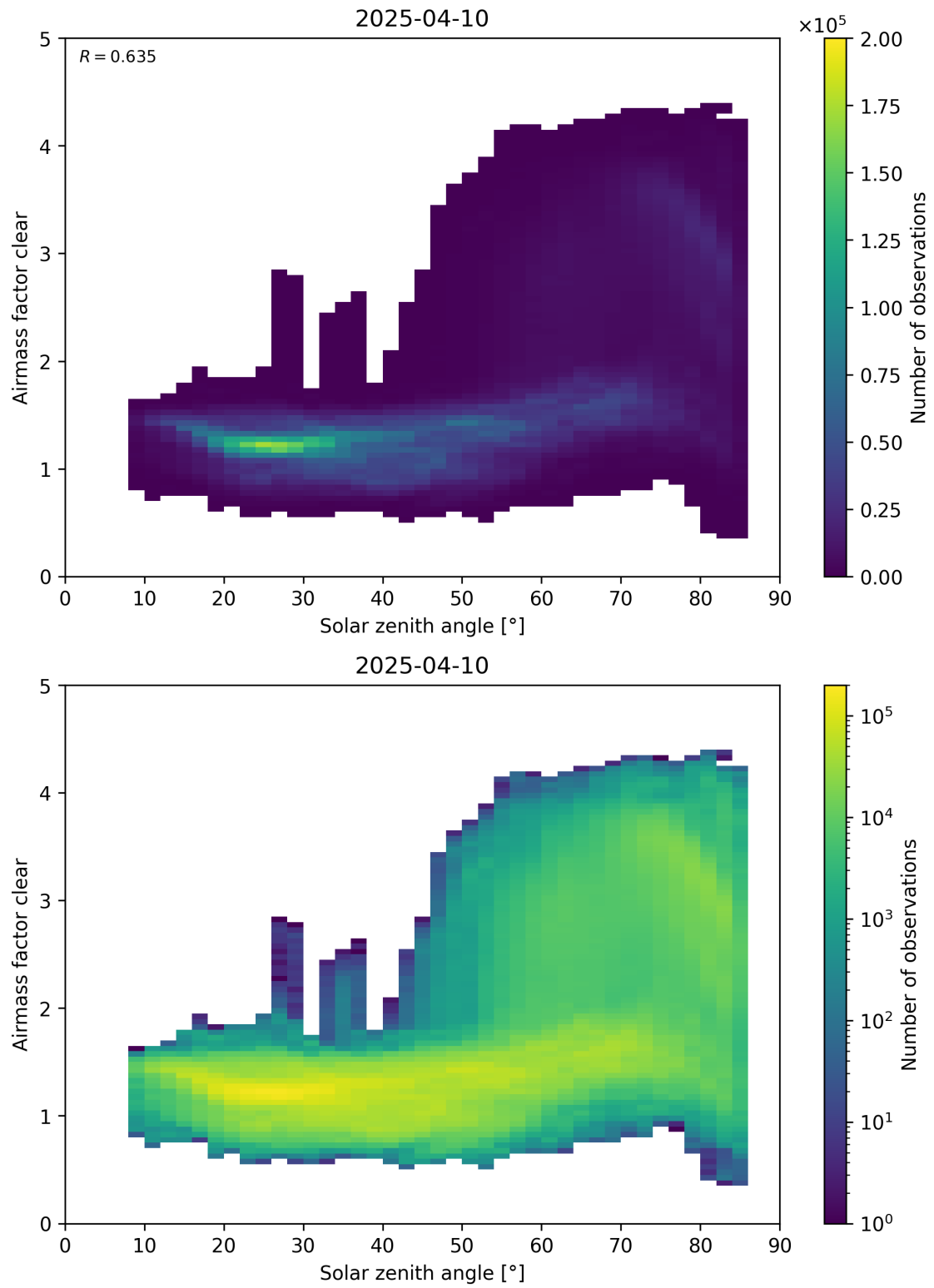
Figure 170: Scatter density plot of “Solar zenith angle” against “Airmass factor clear” for 2025-04-09 to 2025-04-11.
