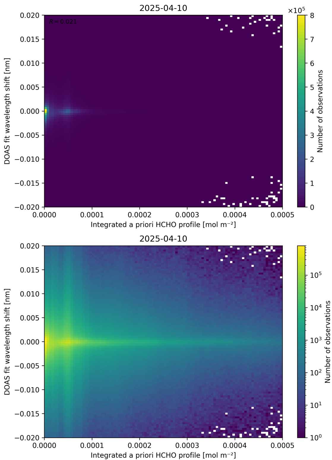
Figure 149: Scatter density plot of “Integrated a priori HCHO profile” against “DOAS fit wavelength shift” for 2025-04-09 to 2025-04-11.
