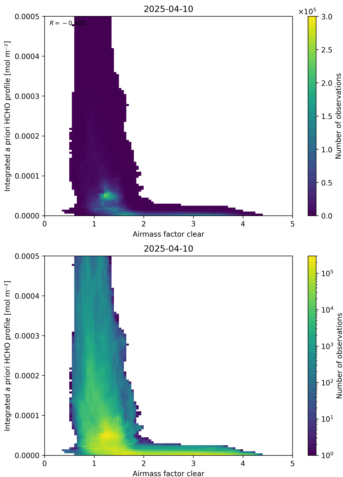
Figure 76: Scatter density plot of “Airmass factor clear” against “Integrated a priori HCHO profile” for 2025-04-09 to 2025-04-11.
