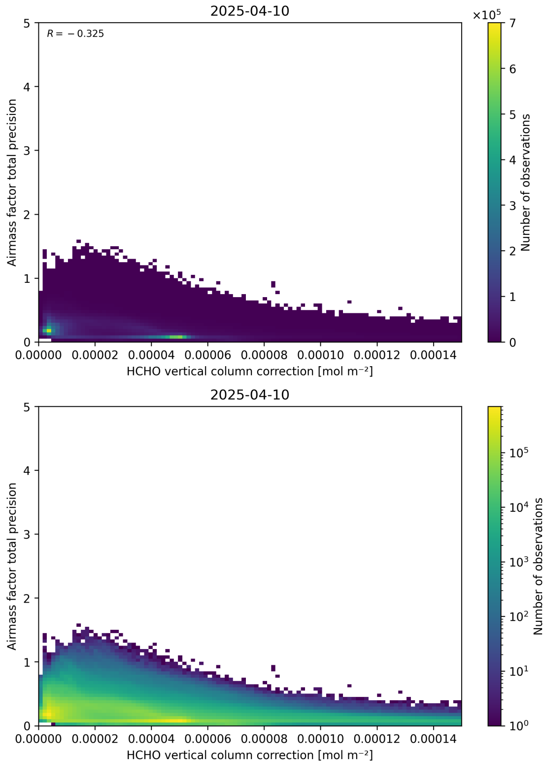
Figure 121: Scatter density plot of “HCHO vertical column correction” against “Airmass factor total precision” for 2025-04-09 to 2025-04-11.
