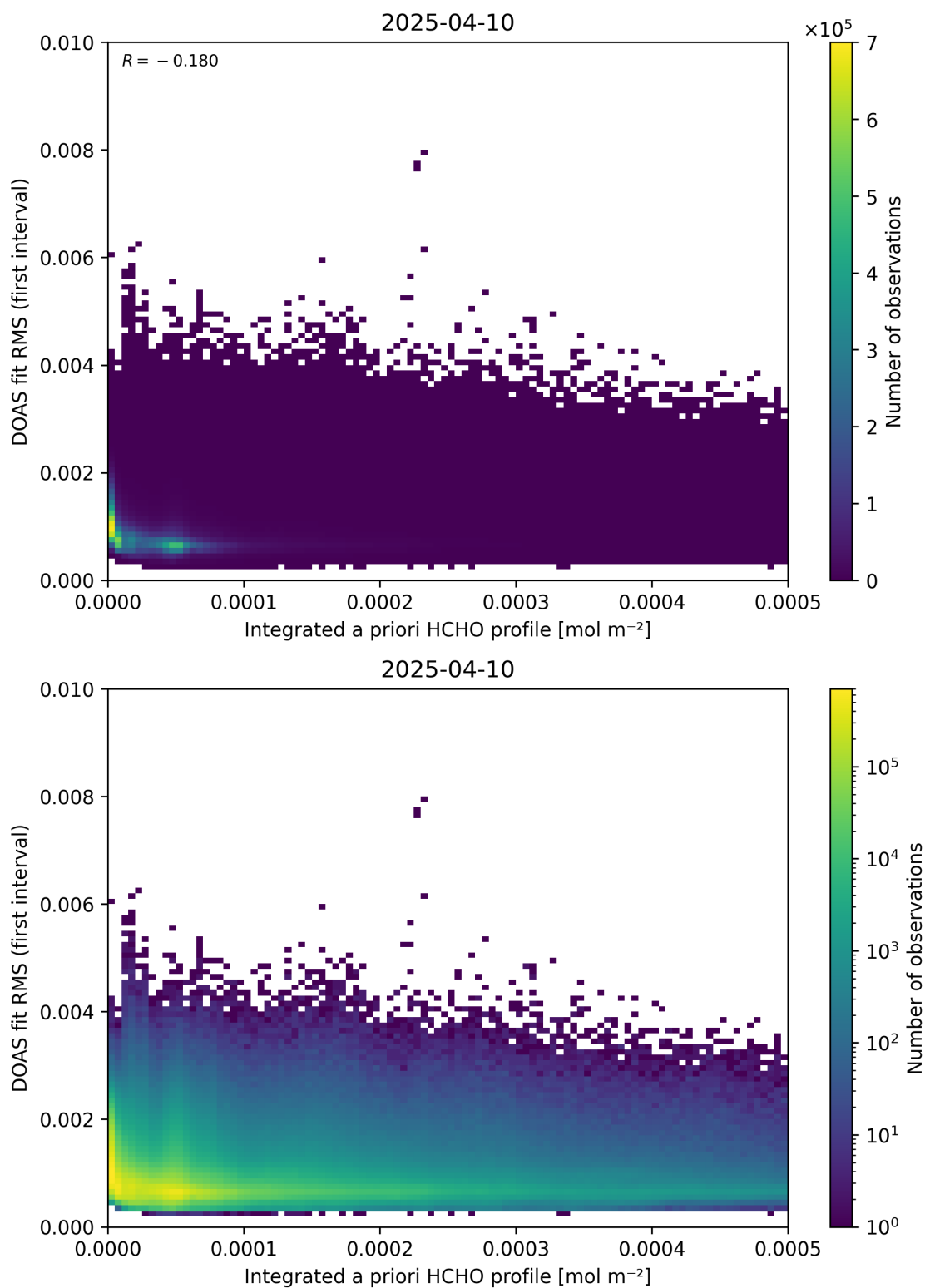
Figure 148: Scatter density plot of “Integrated a priori HCHO profile” against “DOAS fit RMS (first interval)” for 2025-04-09 to 2025-04-11.
