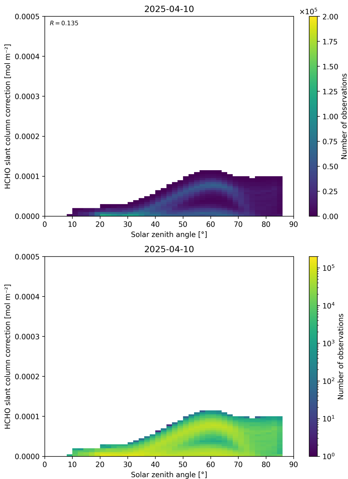
Figure 172: Scatter density plot of “Solar zenith angle” against “HCHO slant column correction” for 2025-04-09 to 2025-04-11.
