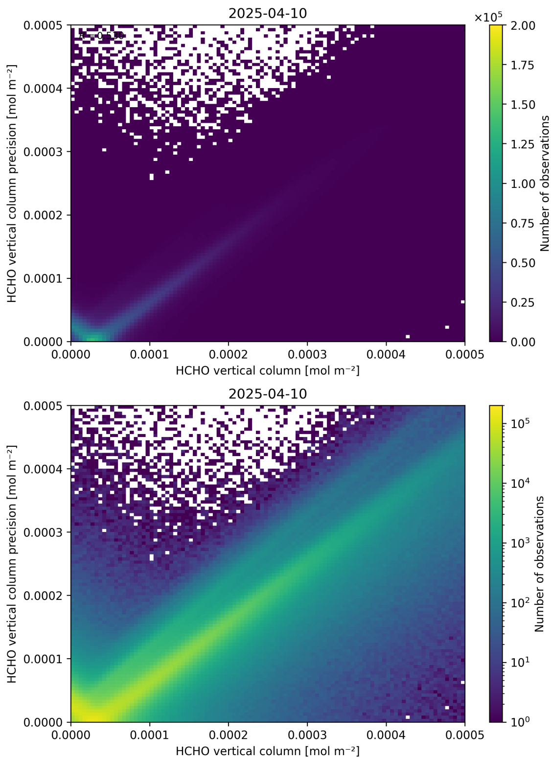
Figure 134: Scatter density plot of “HCHO vertical column” against “HCHO vertical column precision” for 2025-04-09 to 2025-04-11.
