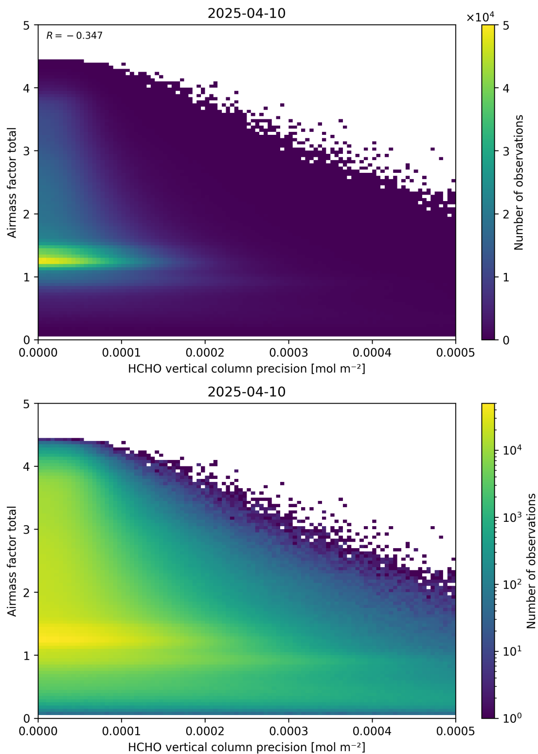
Figure 144: Scatter density plot of “HCHO vertical column precision” against “Airmass factor total” for 2025-04-09 to 2025-04-11.
