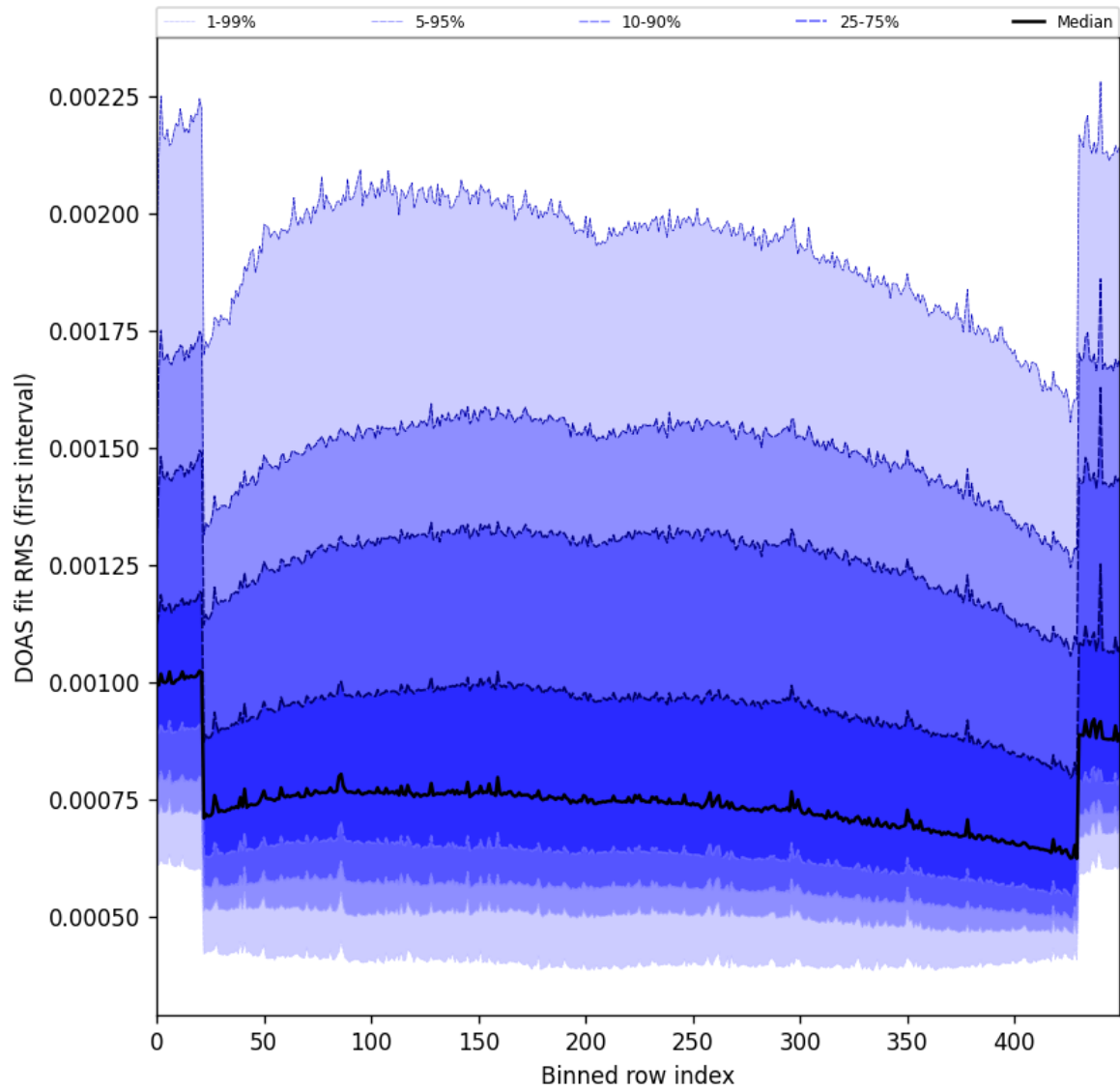
Figure 60: Along track statistics of “DOAS fit RMS (first interval)” for 2025-04-09 to 2025-04-11
