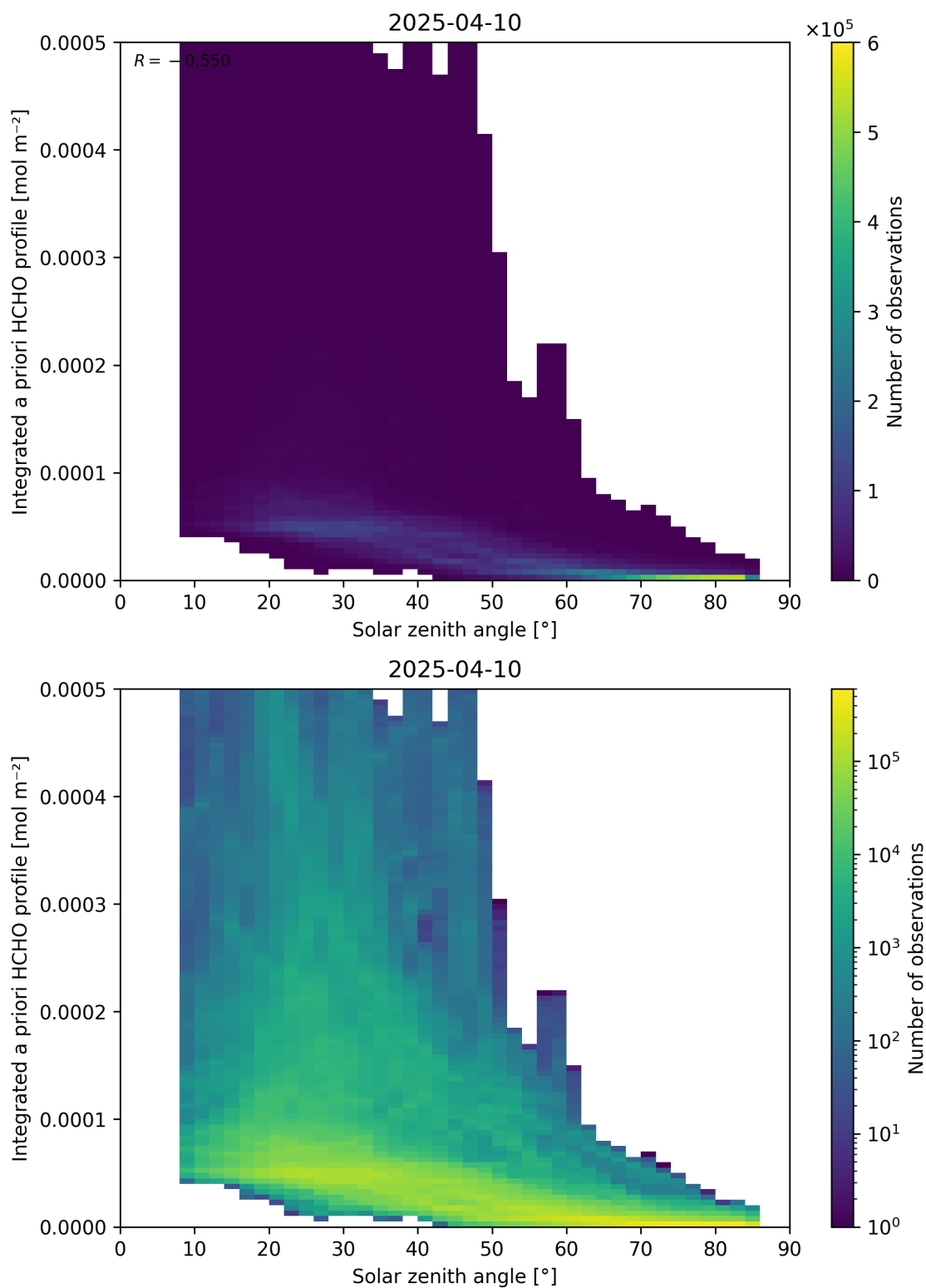
Figure 180: Scatter density plot of “Solar zenith angle” against “Integrated a priori HCHO profile” for 2025-04-09 to 2025-04-11.
