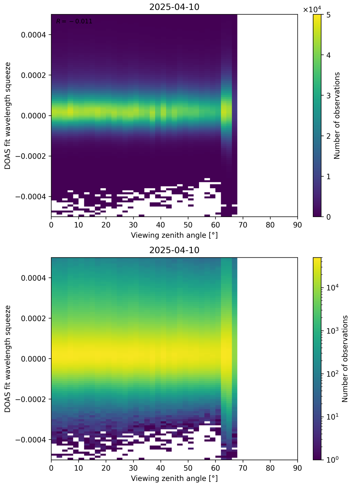
Figure 184: Scatter density plot of “Viewing zenith angle” against “DOAS fit wavelength squeeze” for 2025-04-09 to 2025-04-11.
