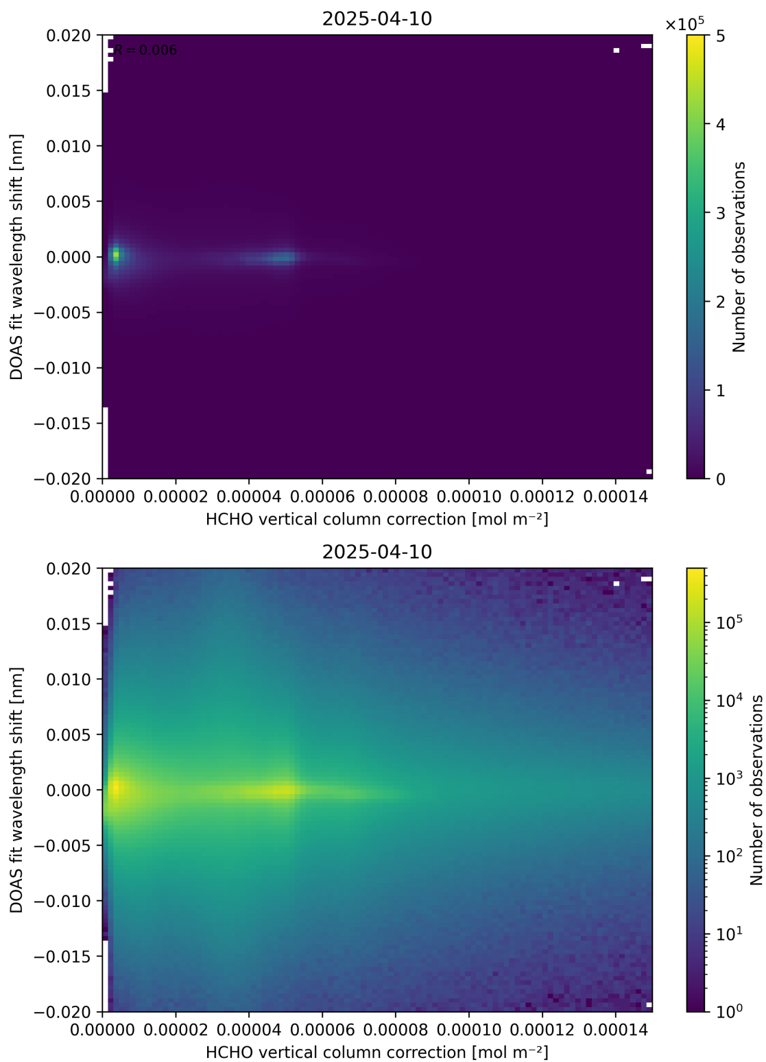
Figure 113: Scatter density plot of “HCHO vertical column correction” against “DOAS fit wavelength shift” for 2025-04-09 to 2025-04-11.
