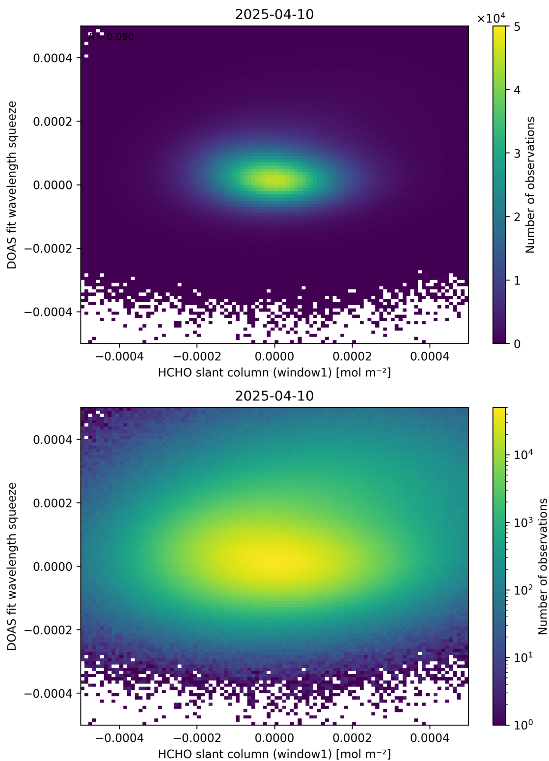
Figure 80: Scatter density plot of “HCHO slant column (window1)” against “DOAS fit wavelength squeeze” for 2025-04-09 to 2025-04-11.
