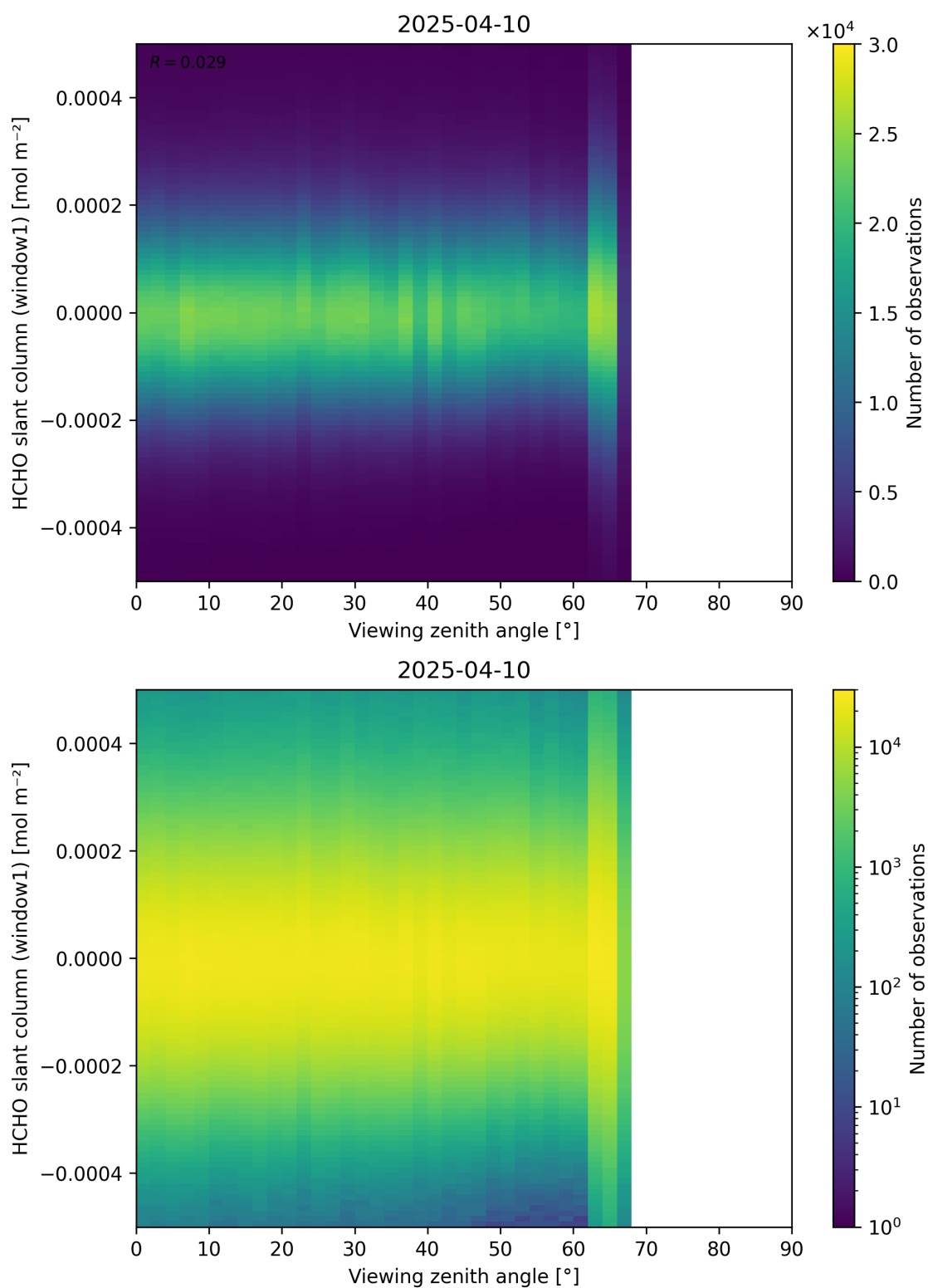
Figure 188: Scatter density plot of “Viewing zenith angle” against “HCHO slant column (window1)” for 2025-04-09 to 2025-04-11.
