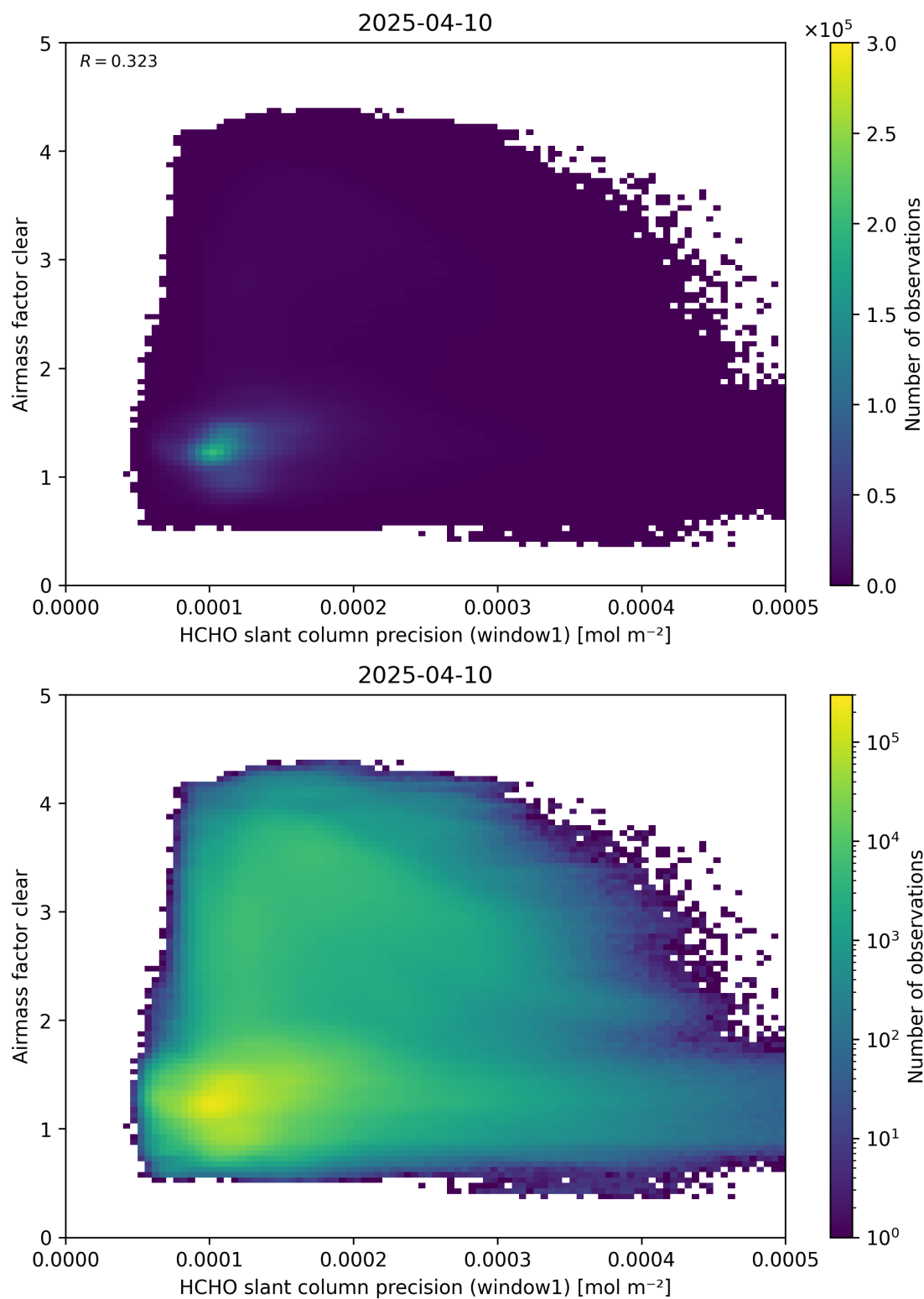
Figure 91: Scatter density plot of “HCHO slant column precision (window1)” against “Airmass factor clear” for 2025-04-09 to 2025-04-11.
