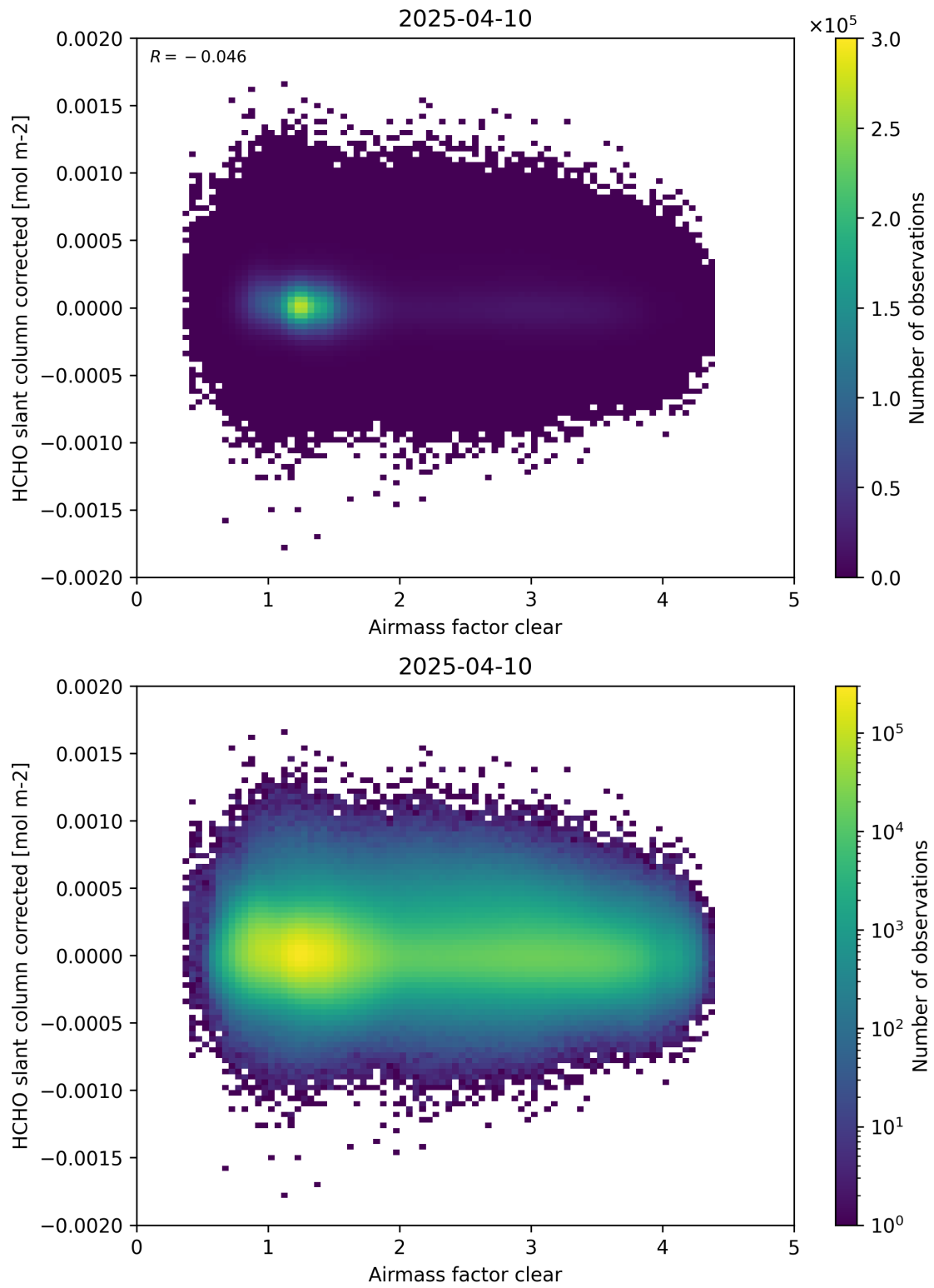
Figure 74: Scatter density plot of “Airmass factor clear” against “HCHO slant column corrected” for 2025-04-09 to 2025-04-11.
