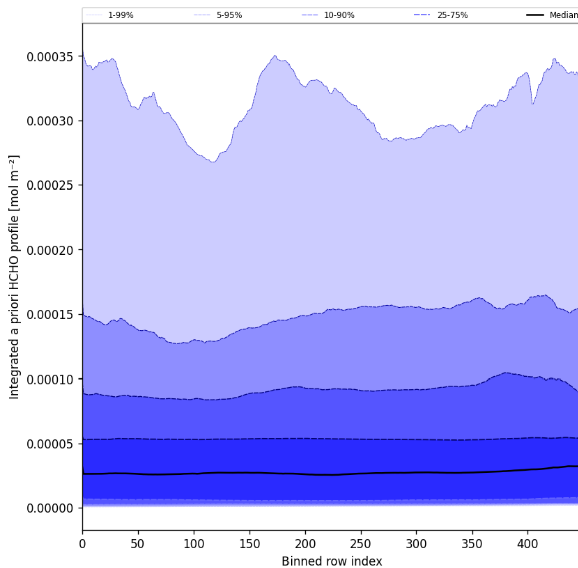
Figure 57: Along track statistics of "Integrated a priori HCHO profile" for 2025-04-09 to 2025-04-11
