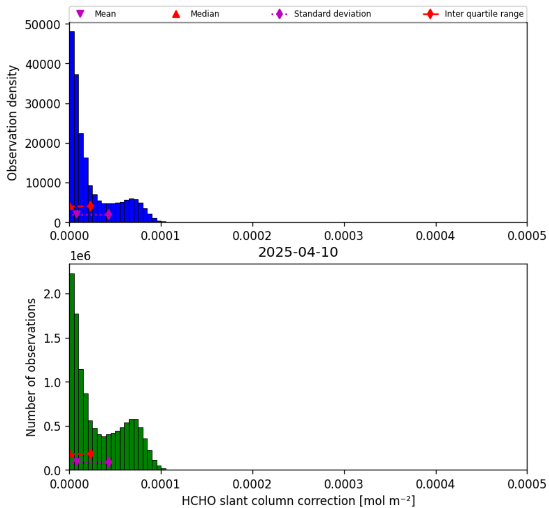
Figure 47: Histogram of “HCHO slant column correction” for 2025-04-09 to 2025-04-11
