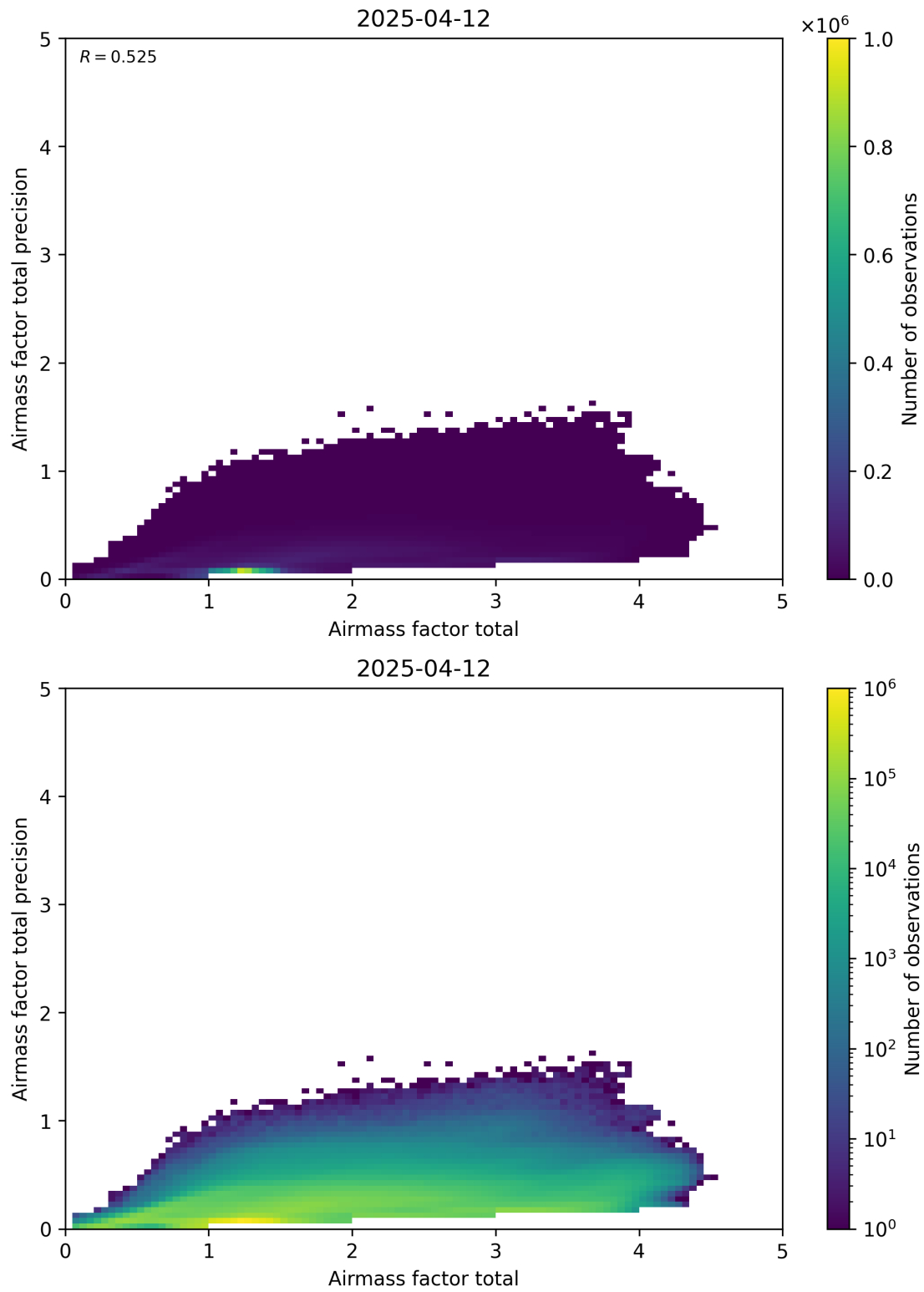
Figure 103: Scatter density plot of “Airmass factor total” against “Airmass factor total precision” for 2025-04-11 to 2025-04-13.
