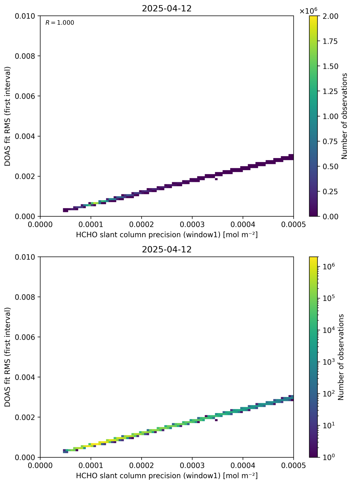
Figure 88: Scatter density plot of “HCHO slant column precision (window1)” against “DOAS fit RMS (first interval)” for 2025-04-11 to 2025-04-13.
