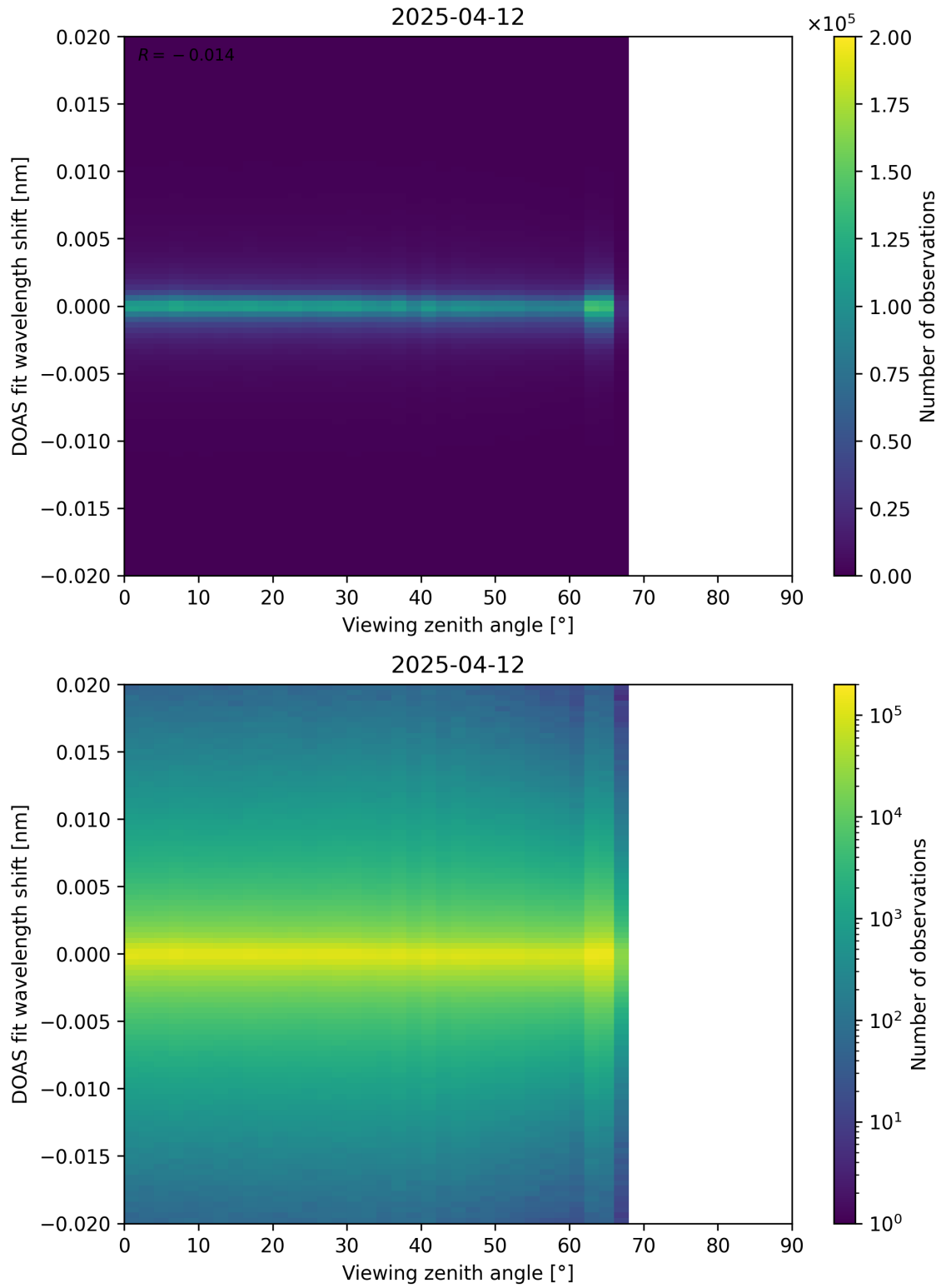
Figure 183: Scatter density plot of “Viewing zenith angle” against “DOAS fit wavelength shift” for 2025-04-11 to 2025-04-13.
