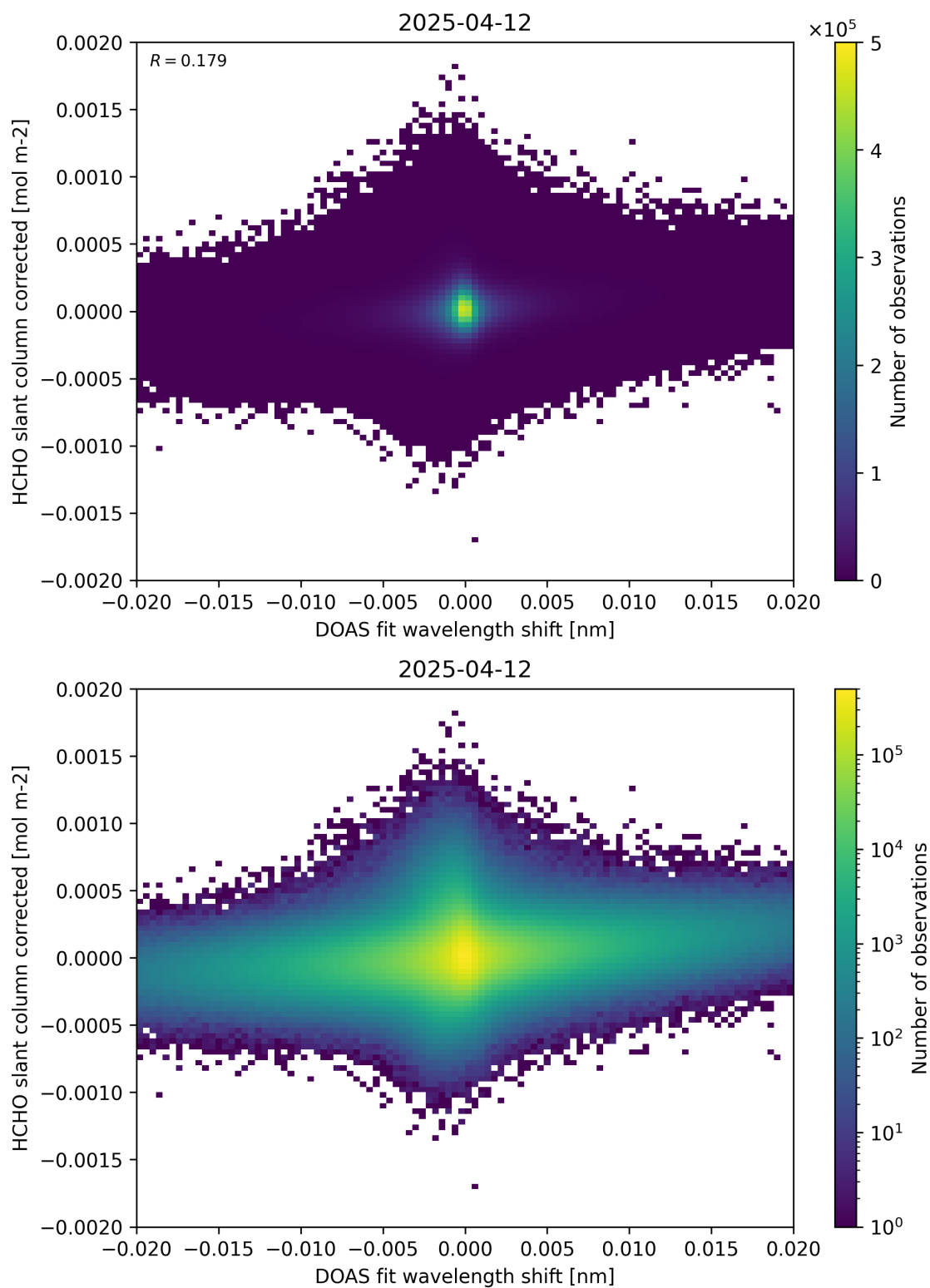
Figure 66: Scatter density plot of “DOAS fit wavelength shift” against “HCHO slant column corrected” for 2025-04-11 to 2025-04-13.
