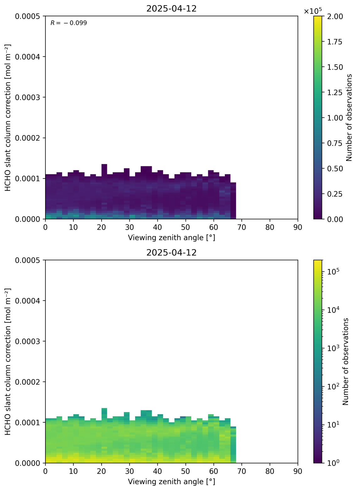
Figure 187: Scatter density plot of “Viewing zenith angle” against “HCHO slant column correction” for 2025-04-11 to 2025-04-13.
