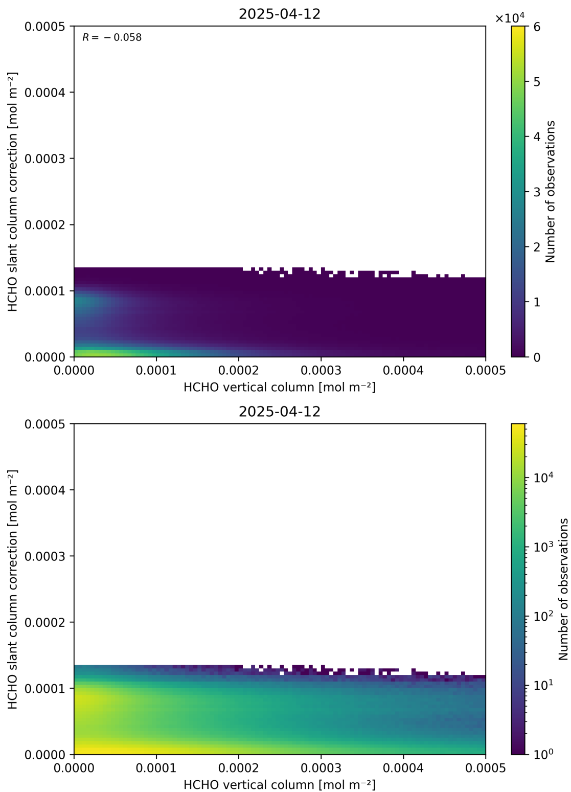
Figure 128: Scatter density plot of “HCHO vertical column” against “HCHO slant column correction” for 2025-04-11 to 2025-04-13.
