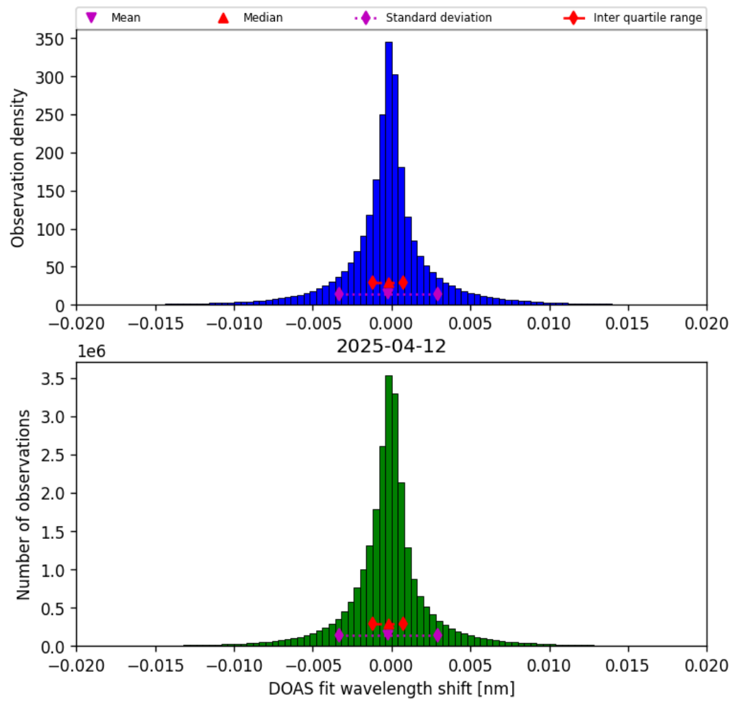
Figure 44: Histogram of “DOAS fit wavelength shift” for 2025-04-11 to 2025-04-13
