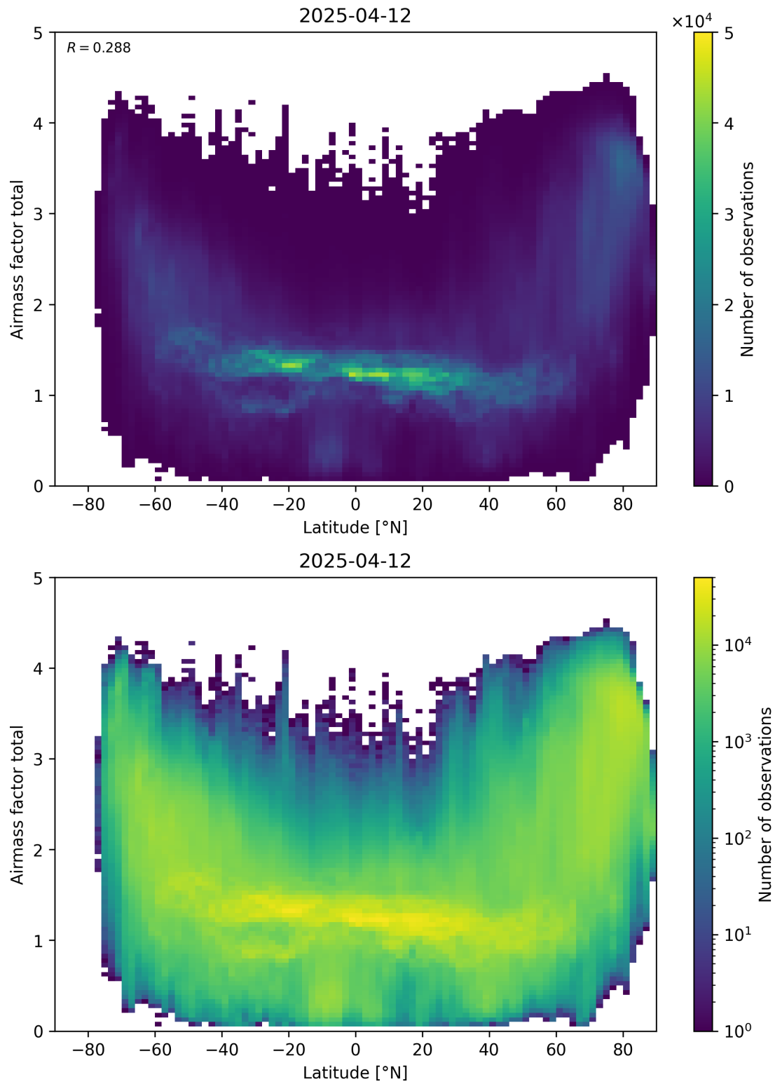
Figure 161: Scatter density plot of “Latitude” against “Airmass factor total” for 2025-04-11 to 2025-04-13.
