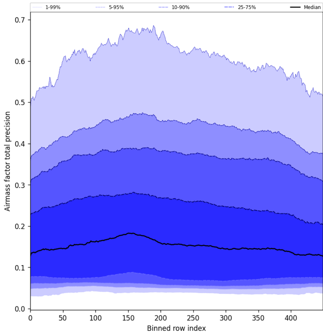
Figure 55: Along track statistics of “Airmass factor total precision” for 2025-04-11 to 2025-04-13
