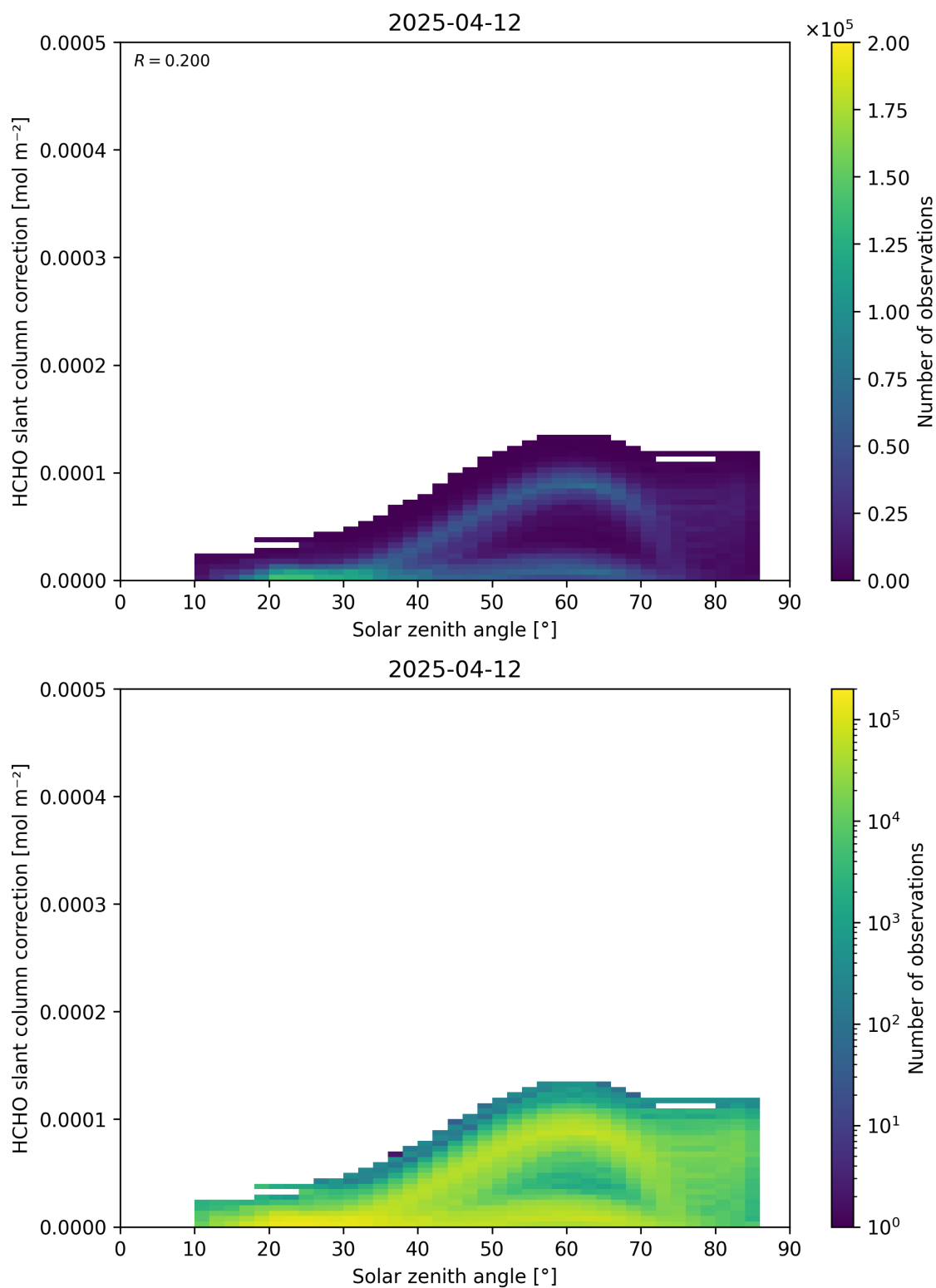
Figure 172: Scatter density plot of “Solar zenith angle” against “HCHO slant column correction” for 2025-04-11 to 2025-04-13.
