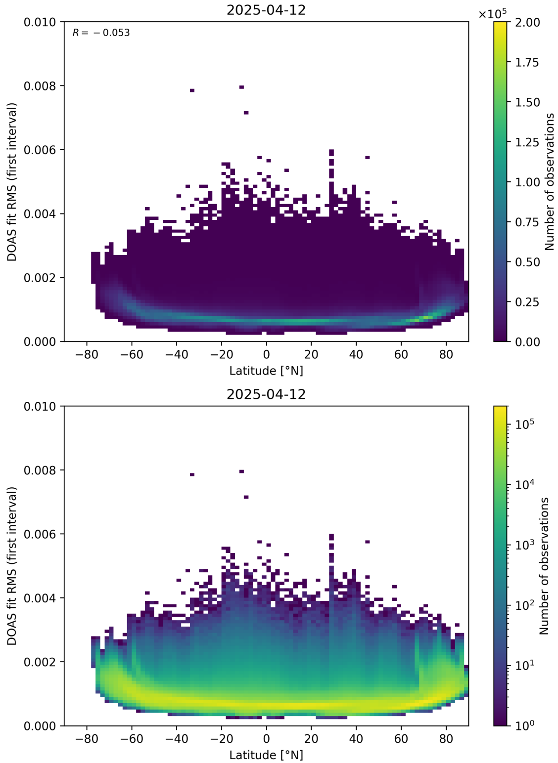
Figure 153: Scatter density plot of “Latitude” against “DOAS fit RMS (first interval)” for 2025-04-11 to 2025-04-13.
