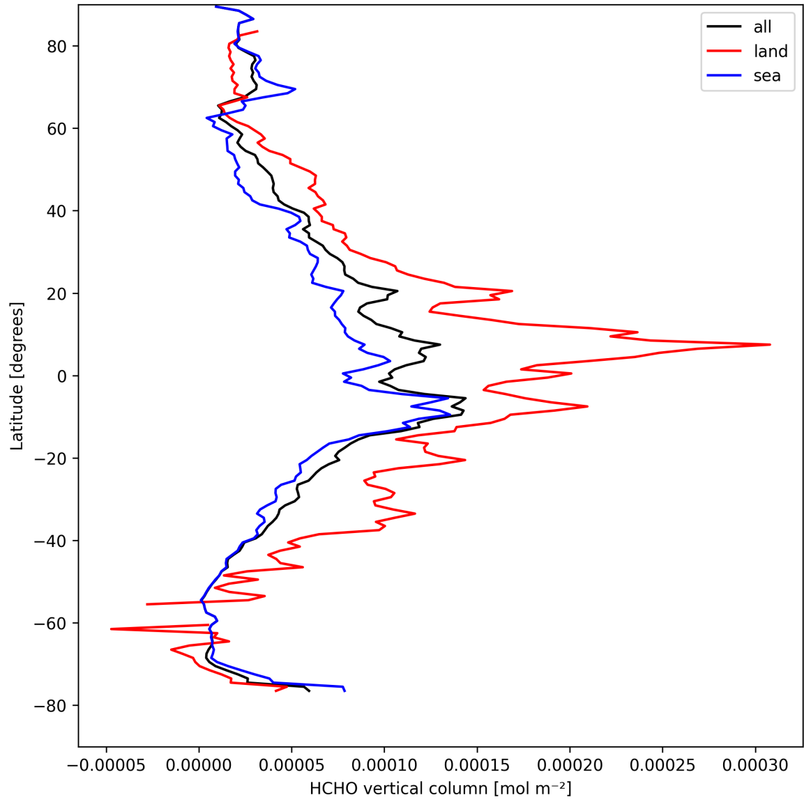
Figure 21: Zonal average of “HCHO vertical column” for 2025-04-11 to 2025-04-13.
