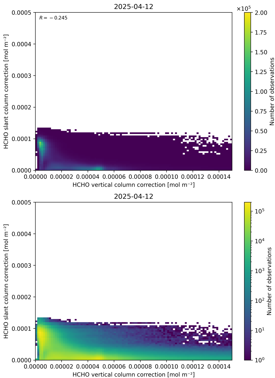
Figure 117: Scatter density plot of “HCHO vertical column correction” against “HCHO slant column correction” for 2025-04-11 to 2025-04-13.
