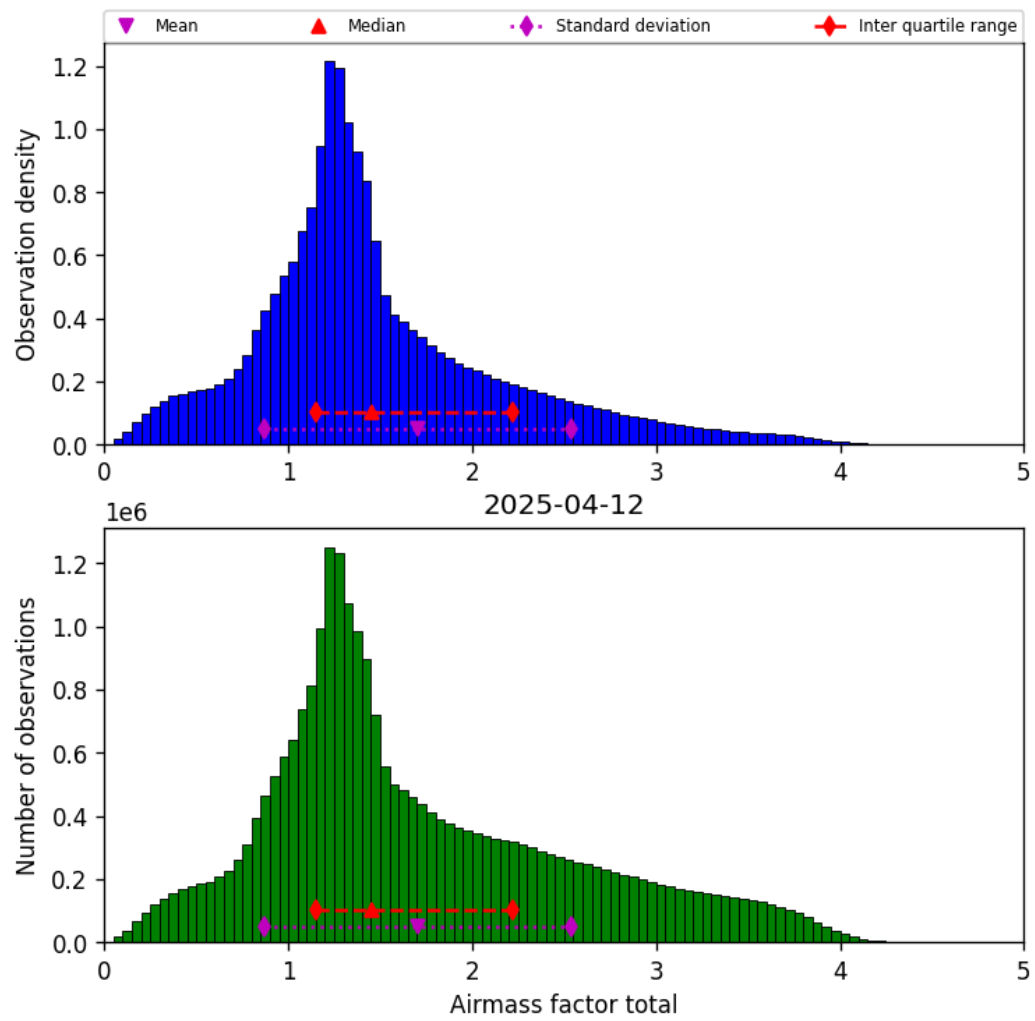
Figure 40: Histogram of “Airmass factor total” for 2025-04-11 to 2025-04-13
