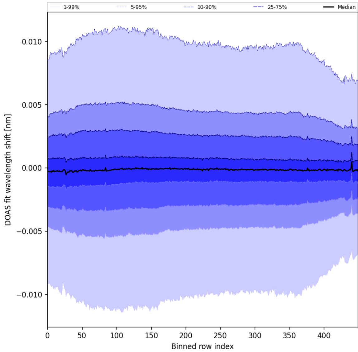
Figure 58: Along track statistics of “DOAS fit wavelength shift” for 2025-04-11 to 2025-04-13
