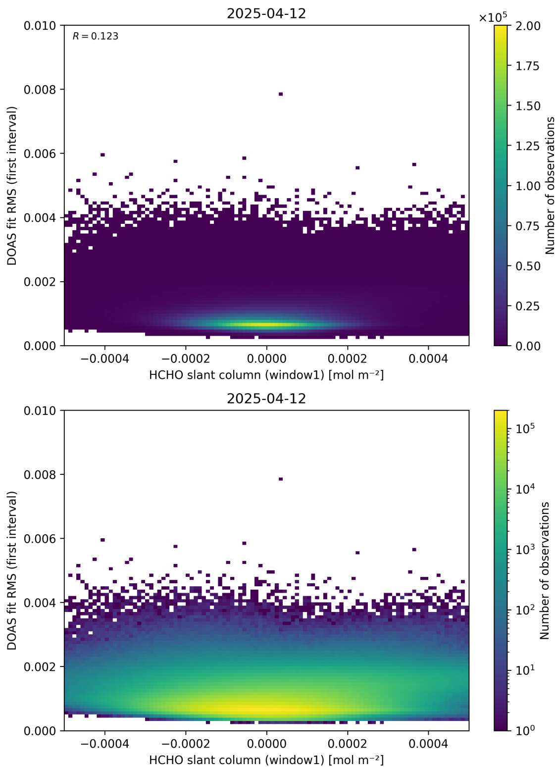
Figure 78: Scatter density plot of “HCHO slant column (window1)” against “DOAS fit RMS (first interval)” for 2025-04-11 to 2025-04-13.
