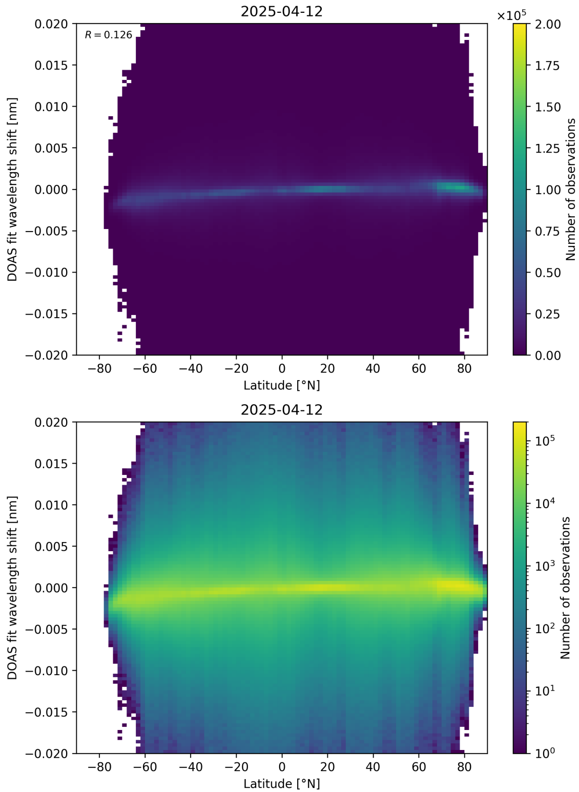
Figure 154: Scatter density plot of “Latitude” against “DOAS fit wavelength shift” for 2025-04-11 to 2025-04-13.
