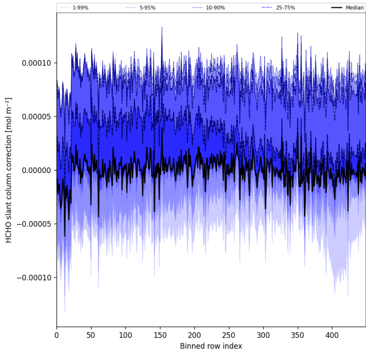
Figure 61: Along track statistics of “HCHO slant column correction” for 2025-04-11 to 2025-04-13
