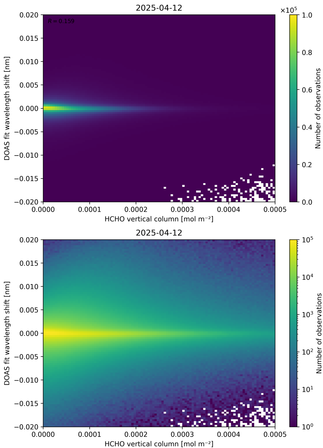
Figure 124: Scatter density plot of “HCHO vertical column” against “DOAS fit wavelength shift” for 2025-04-11 to 2025-04-13.
