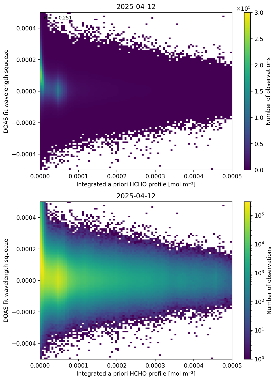
Figure 150: Scatter density plot of “Integrated a priori HCHO profile” against “DOAS fit wavelength squeeze” for 2025-04-11 to 2025-04-13.
