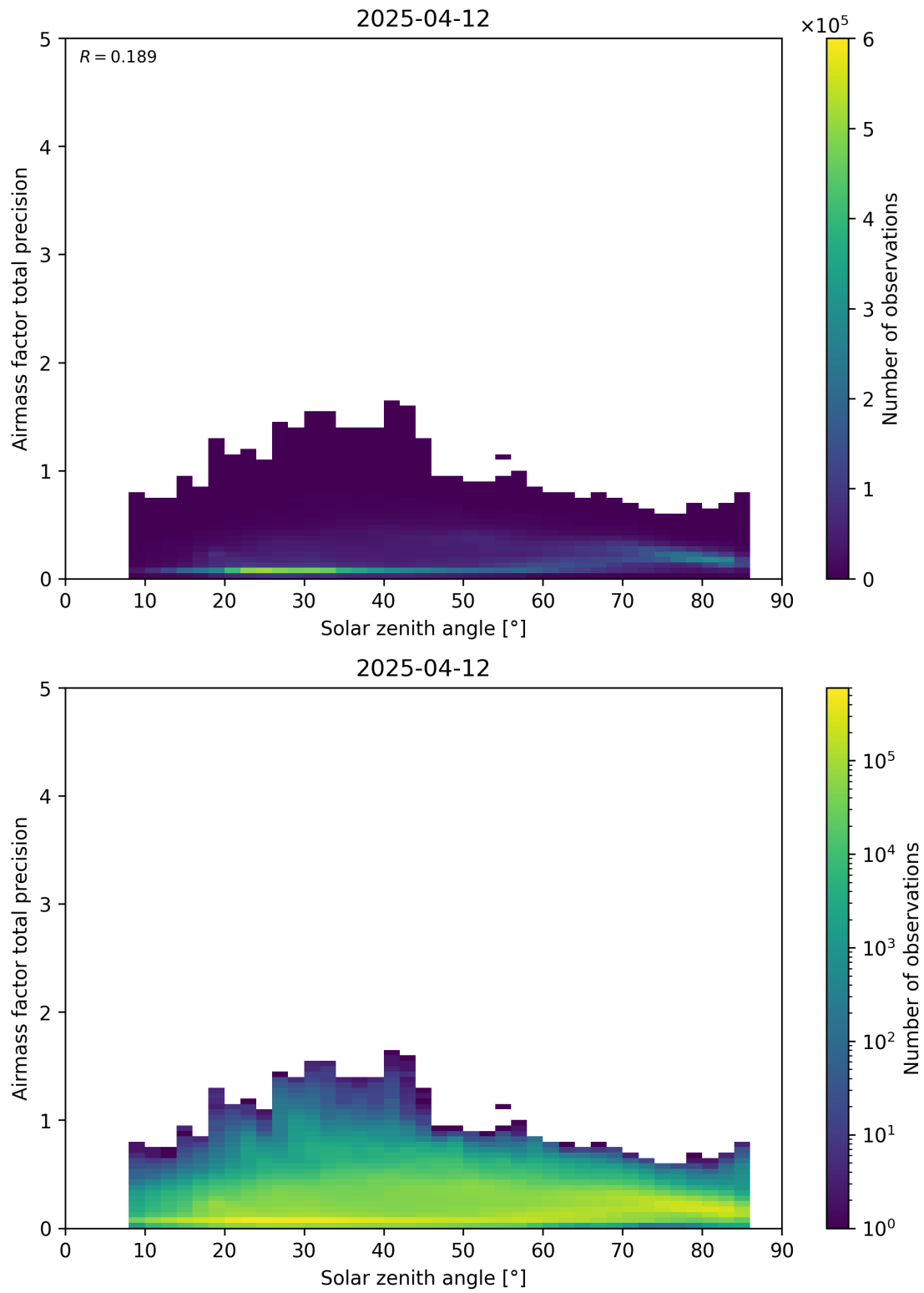
Figure 176: Scatter density plot of “Solar zenith angle” against “Airmass factor total precision” for 2025-04-11 to 2025-04-13.
