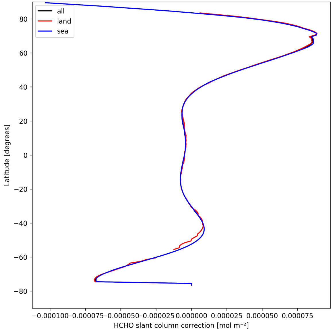
Figure 33: Zonal average of “HCHO slant column correction” for 2025-04-11 to 2025-04-13.
