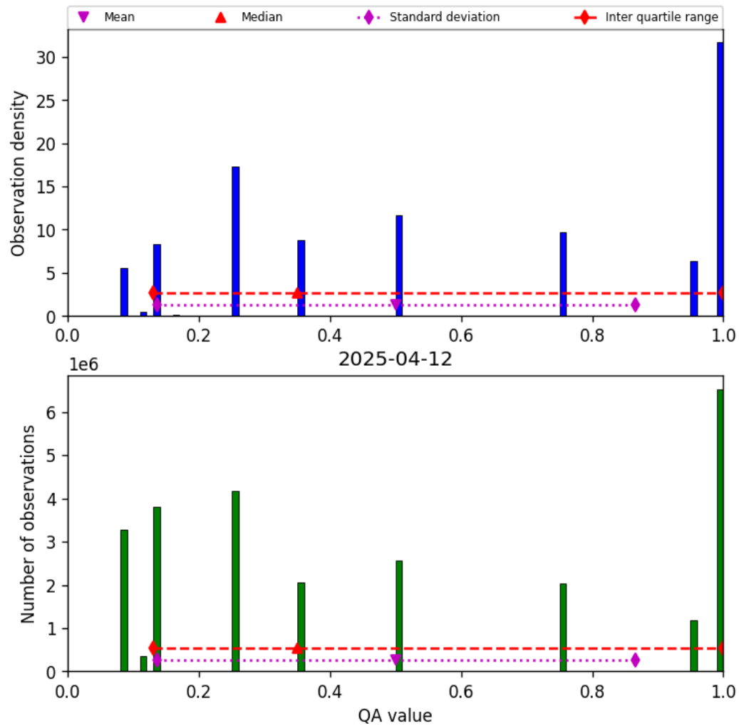
Figure 34: Histogram of “QA value” for 2025-04-11 to 2025-04-13
