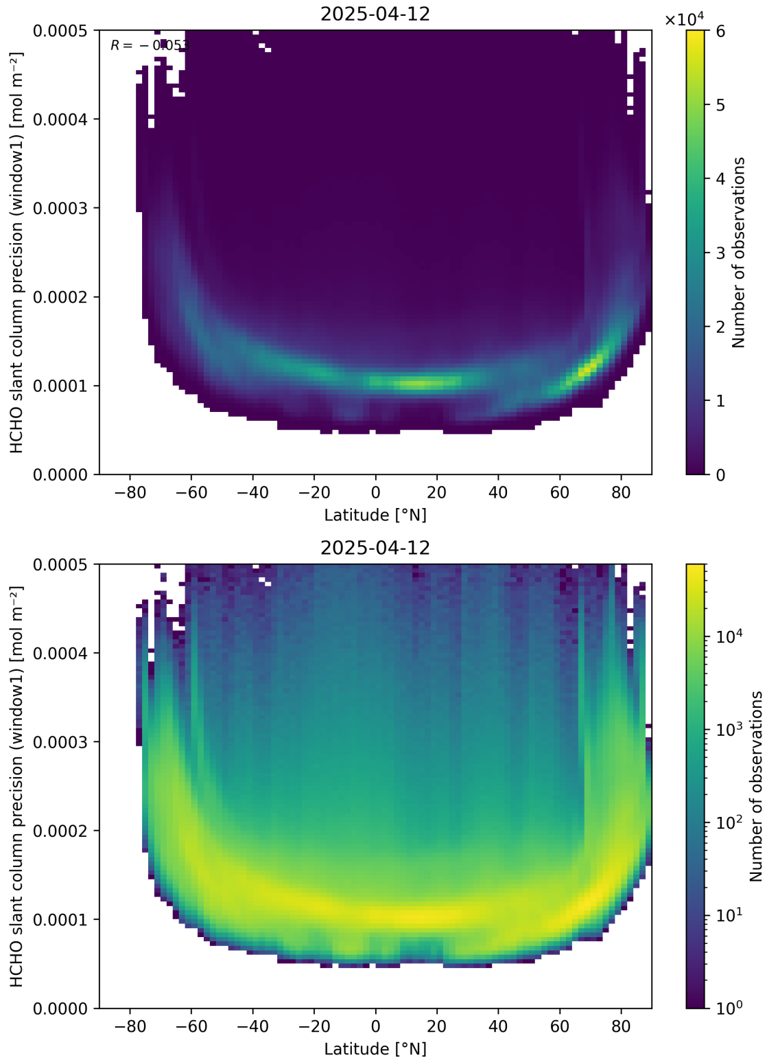
Figure 160: Scatter density plot of “Latitude” against “HCHO slant column precision (window1)” for 2025-04-11 to 2025-04-13.
