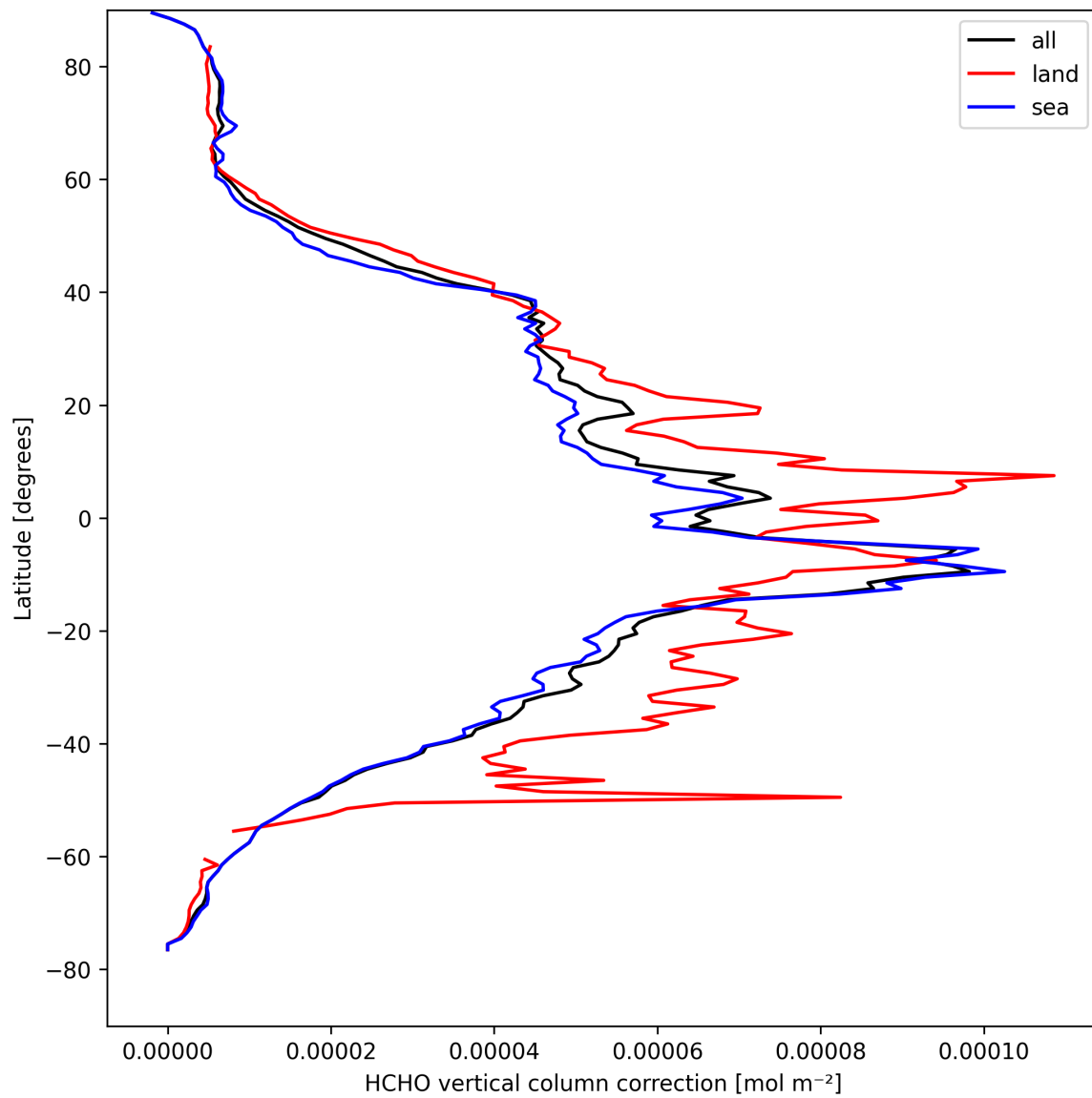
Figure 23: Zonal average of “HCHO vertical column correction” for 2025-04-11 to 2025-04-13.
