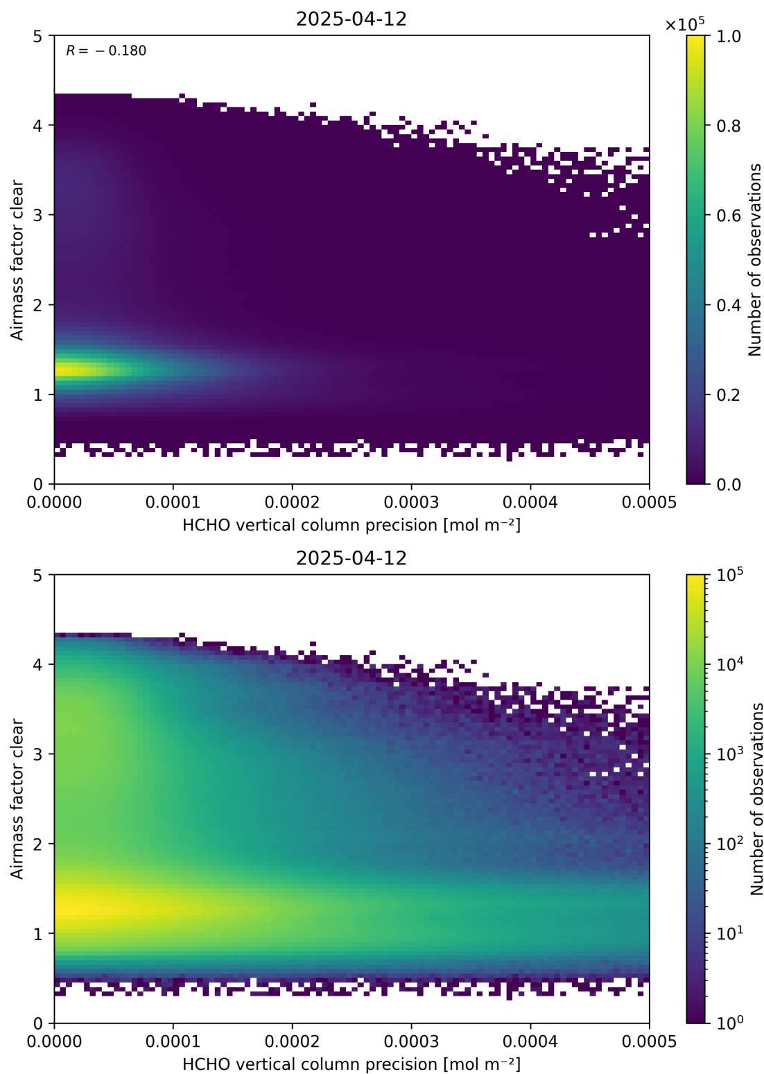
Figure 139: Scatter density plot of “HCHO vertical column precision” against “Airmass factor clear” for 2025-04-11 to 2025-04-13.
