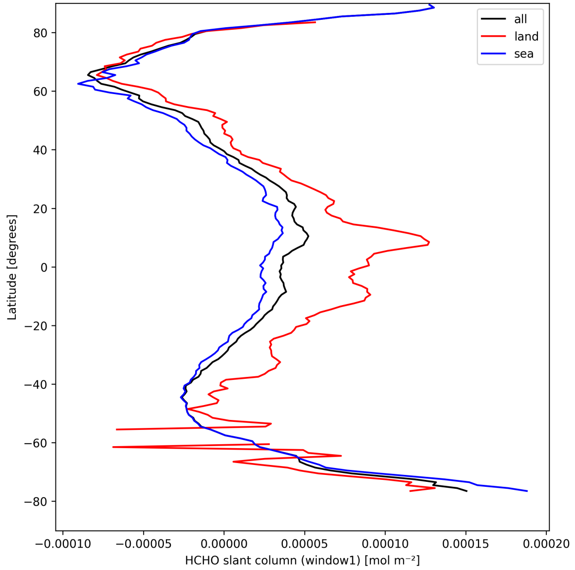
Figure 24: Zonal average of “HCHO slant column (window1)” for 2025-04-11 to 2025-04-13.
