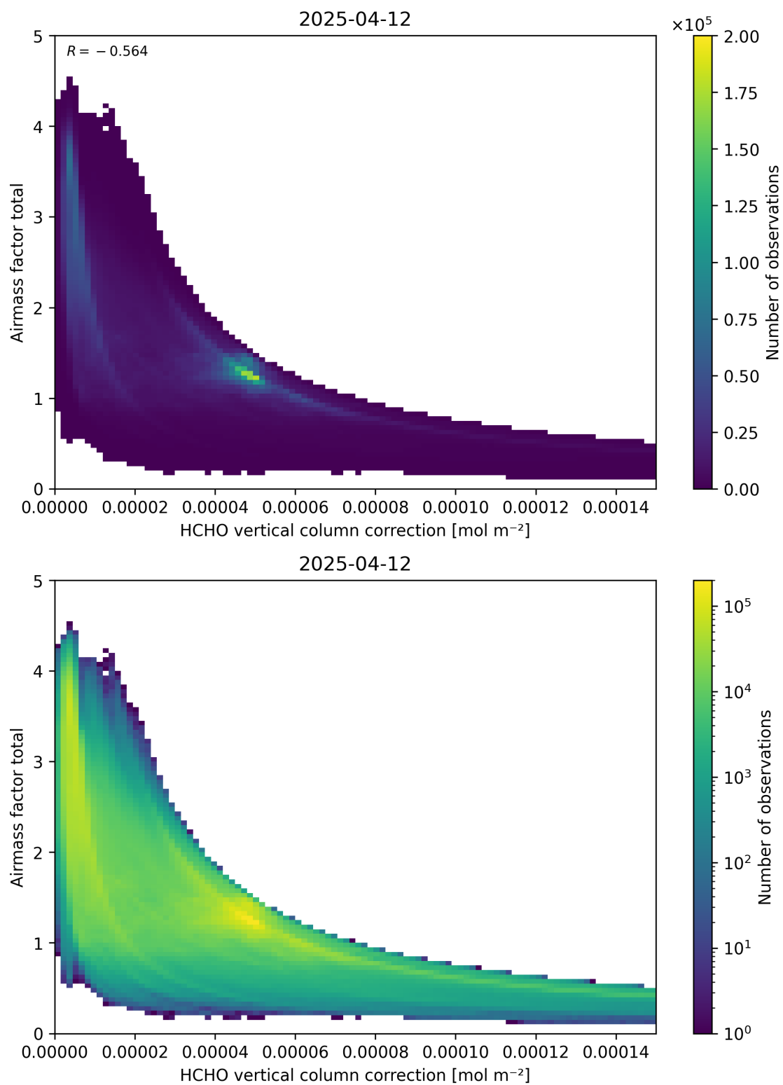
Figure 120: Scatter density plot of “HCHO vertical column correction” against “Airmass factor total” for 2025-04-11 to 2025-04-13.
