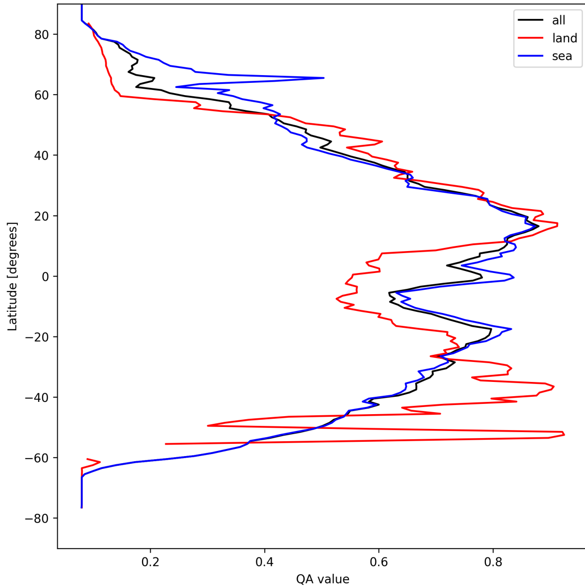
Figure 20: Zonal average of “QA value” for 2025-04-11 to 2025-04-13.
