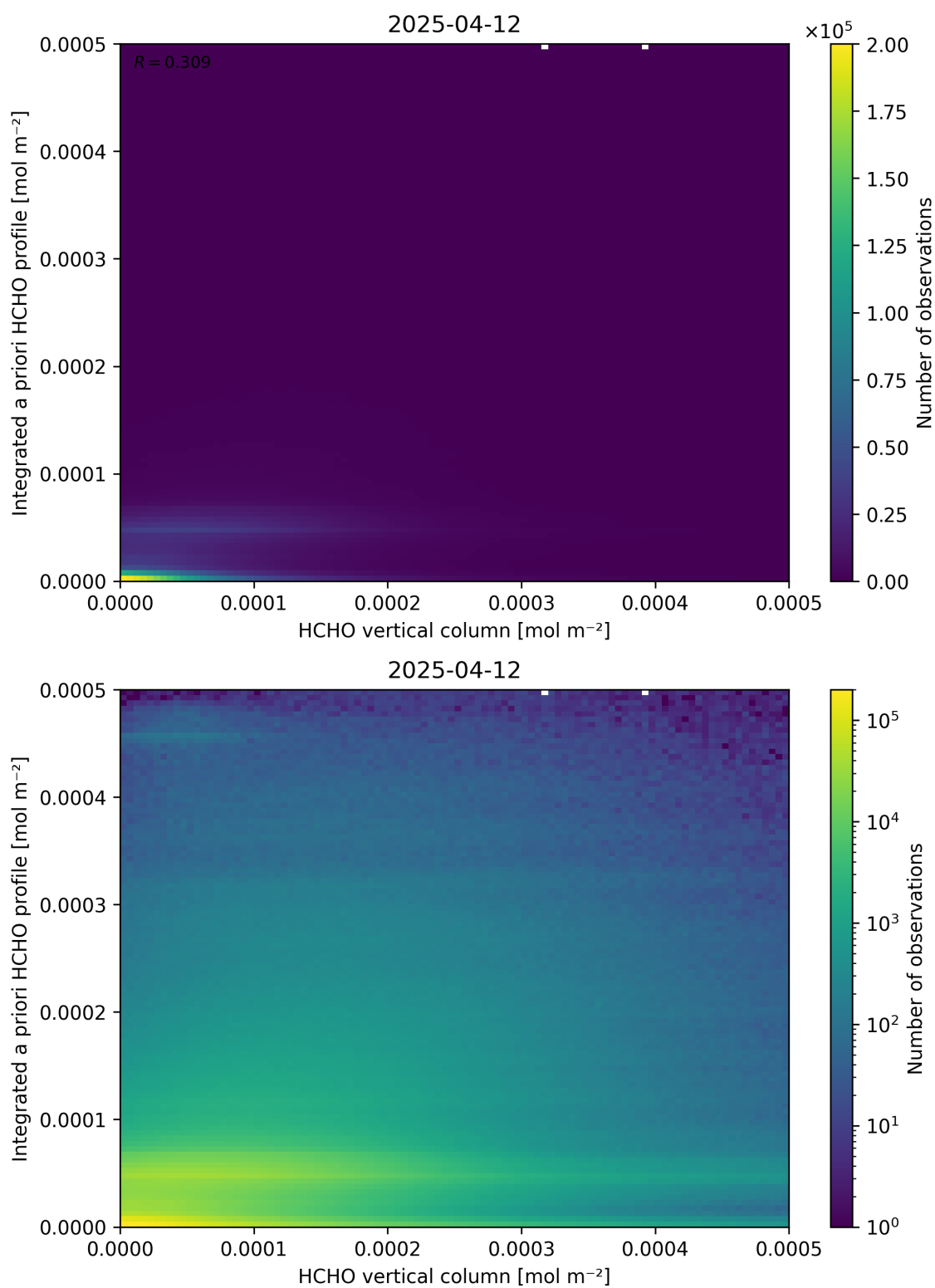
Figure 135: Scatter density plot of “HCHO vertical column” against “Integrated a priori HCHO profile” for 2025-04-11 to 2025-04-13.
