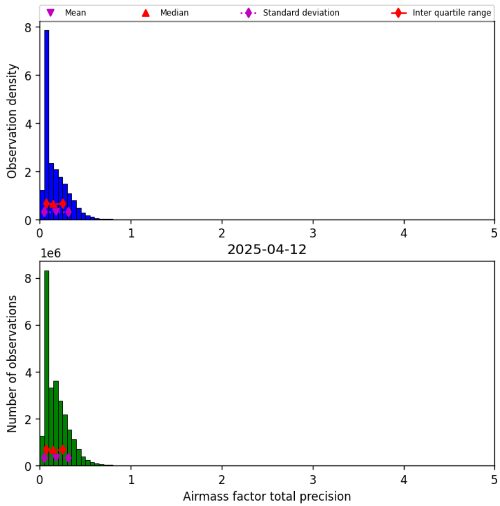
Figure 41: Histogram of “Airmass factor total precision” for 2025-04-11 to 2025-04-13
