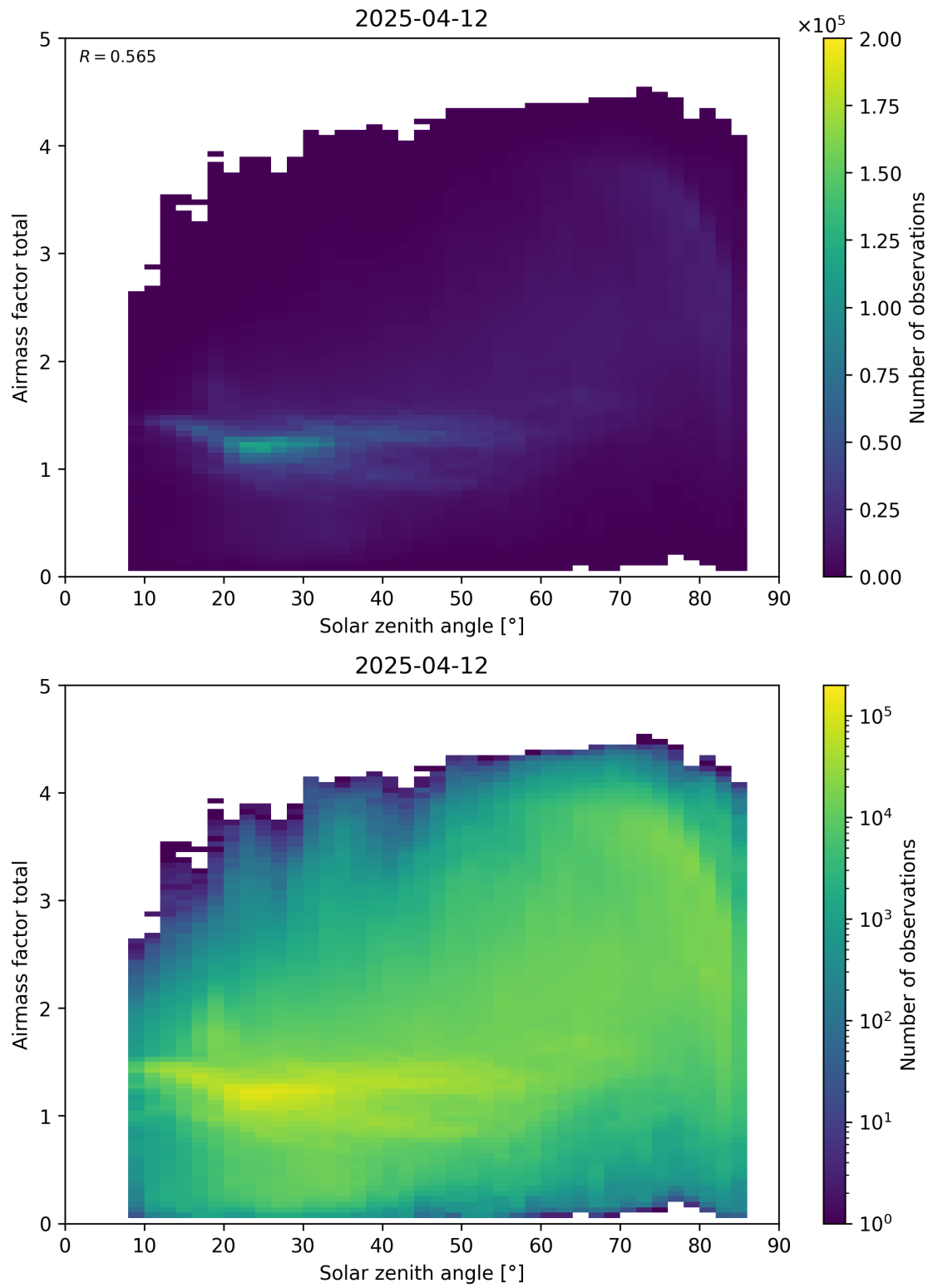
Figure 175: Scatter density plot of “Solar zenith angle” against “Airmass factor total” for 2025-04-11 to 2025-04-13.
