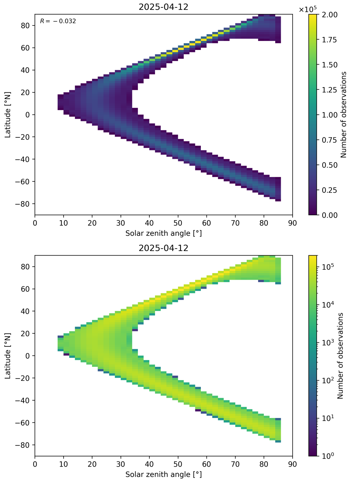
Figure 181: Scatter density plot of “Solar zenith angle” against “Latitude” for 2025-04-11 to 2025-04-13.
