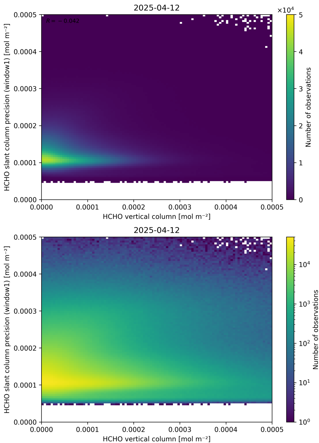
Figure 130: Scatter density plot of “HCHO vertical column” against “HCHO slant column precision (window1)” for 2025-04-11 to 2025-04-13.
