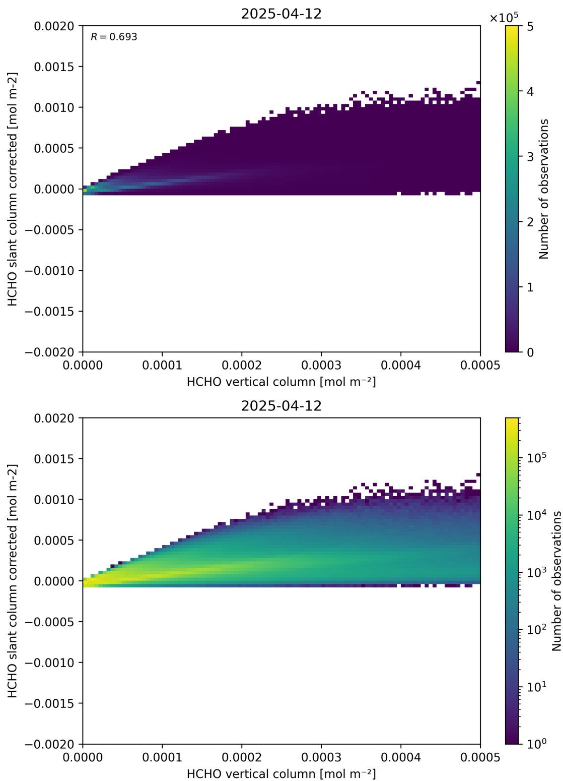
Figure 127: Scatter density plot of “HCHO vertical column” against “HCHO slant column corrected” for 2025-04-11 to 2025-04-13.
