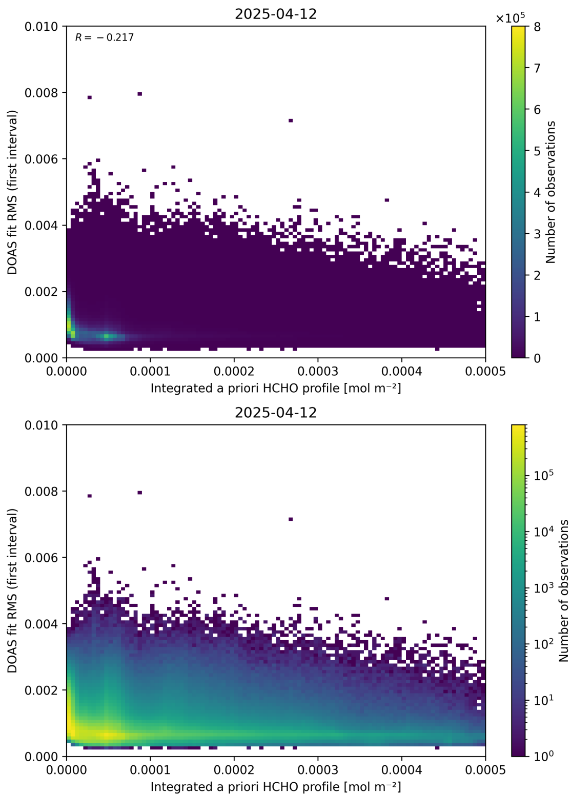
Figure 148: Scatter density plot of “Integrated a priori HCHO profile” against “DOAS fit RMS (first interval)” for 2025-04-11 to 2025-04-13.
