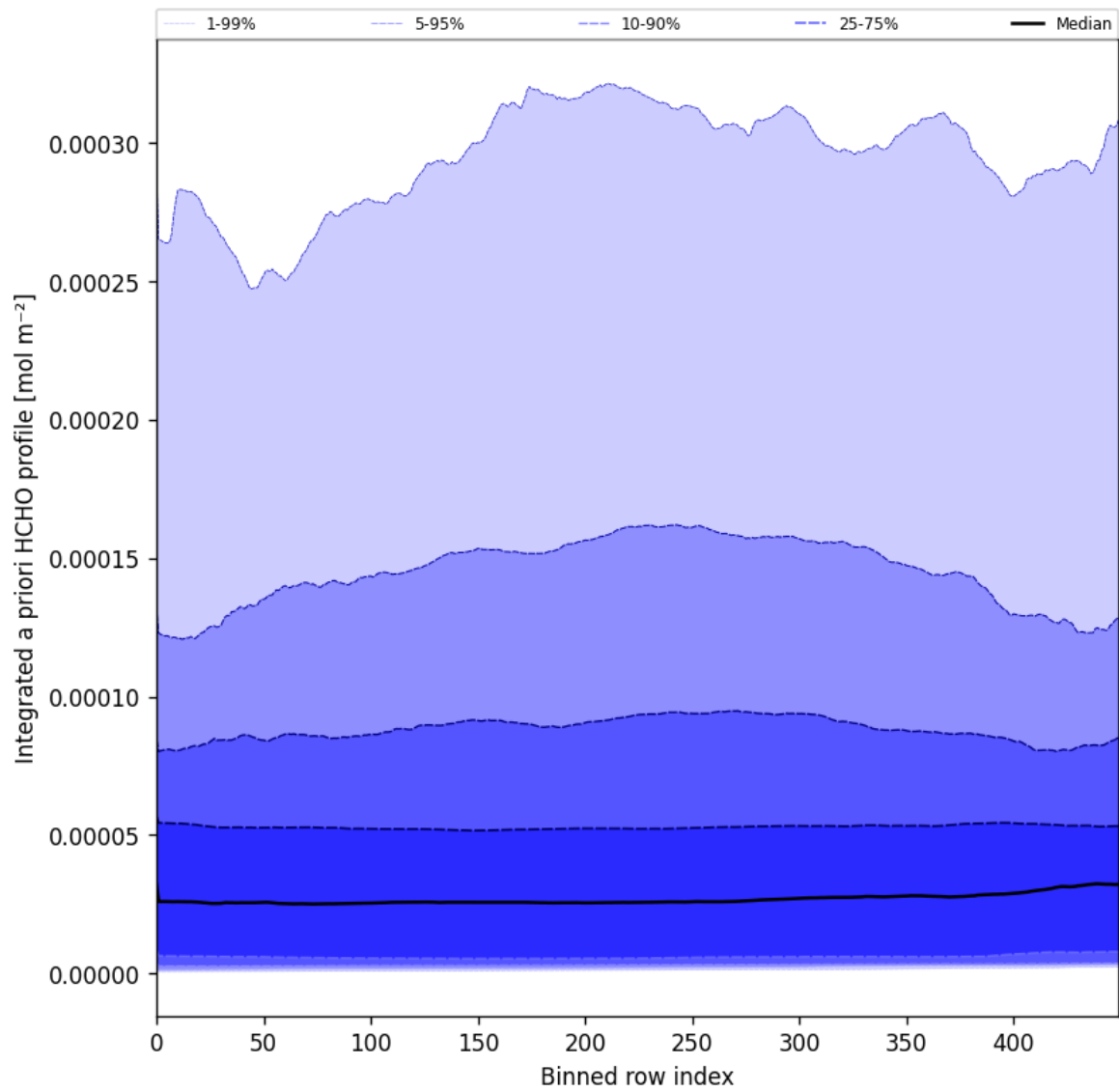
Figure 57: Along track statistics of “Integrated a priori HCHO profile” for 2025-04-11 to 2025-04-13
