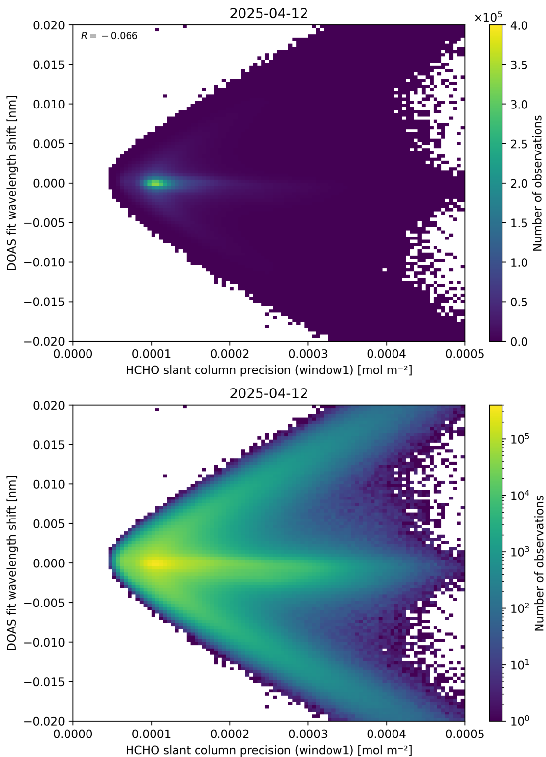
Figure 89: Scatter density plot of “HCHO slant column precision (window1)” against “DOAS fit wavelength shift” for 2025-04-11 to 2025-04-13.
