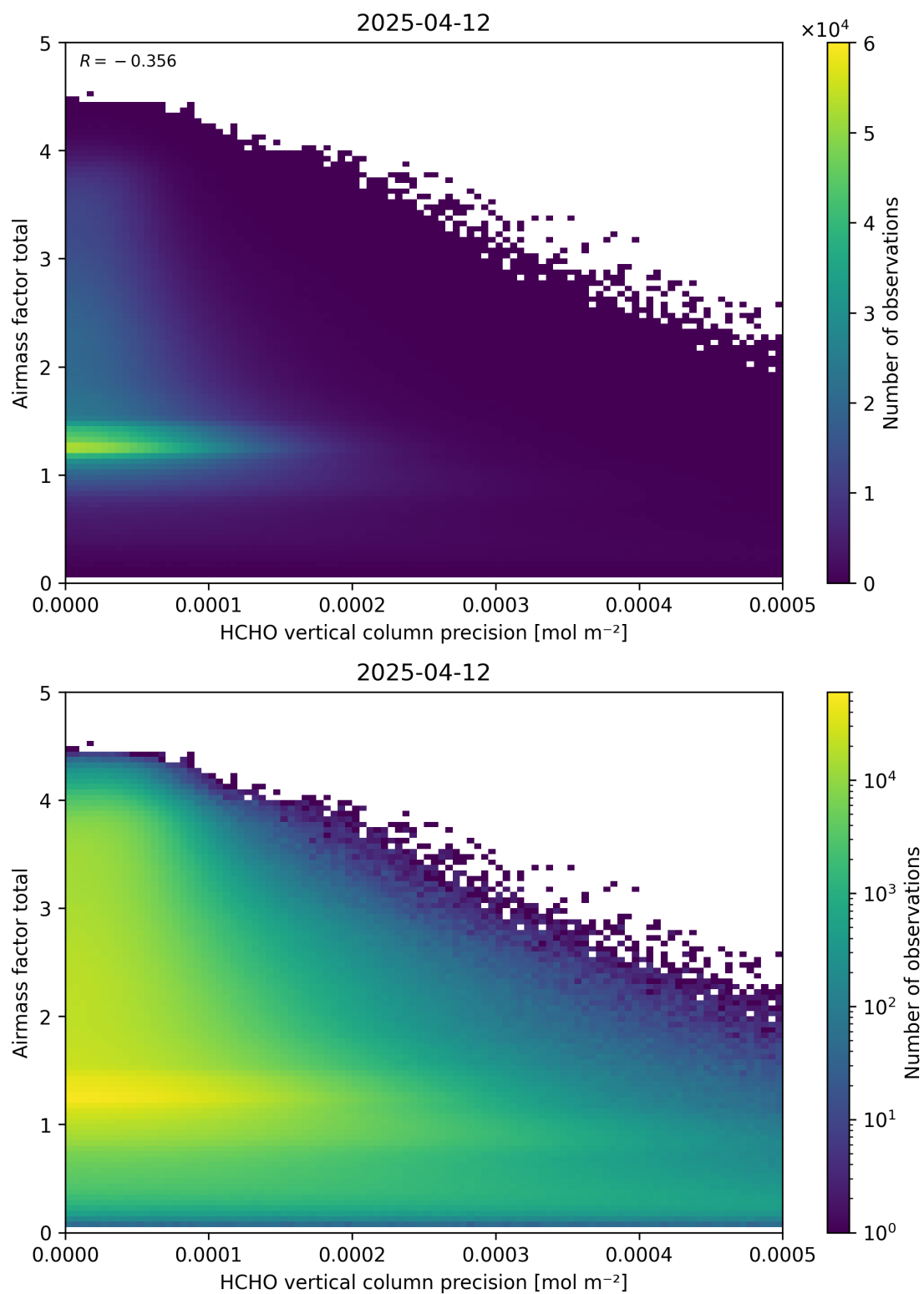
Figure 144: Scatter density plot of “HCHO vertical column precision” against “Airmass factor total” for 2025-04-11 to 2025-04-13.
