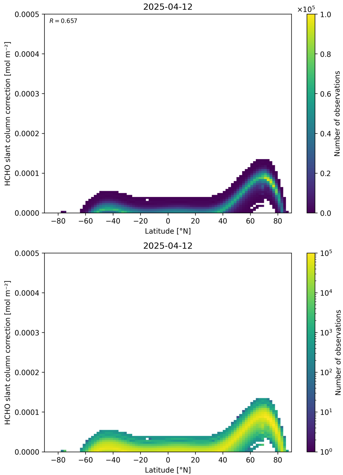
Figure 158: Scatter density plot of “Latitude” against “HCHO slant column correction” for 2025-04-11 to 2025-04-13.
