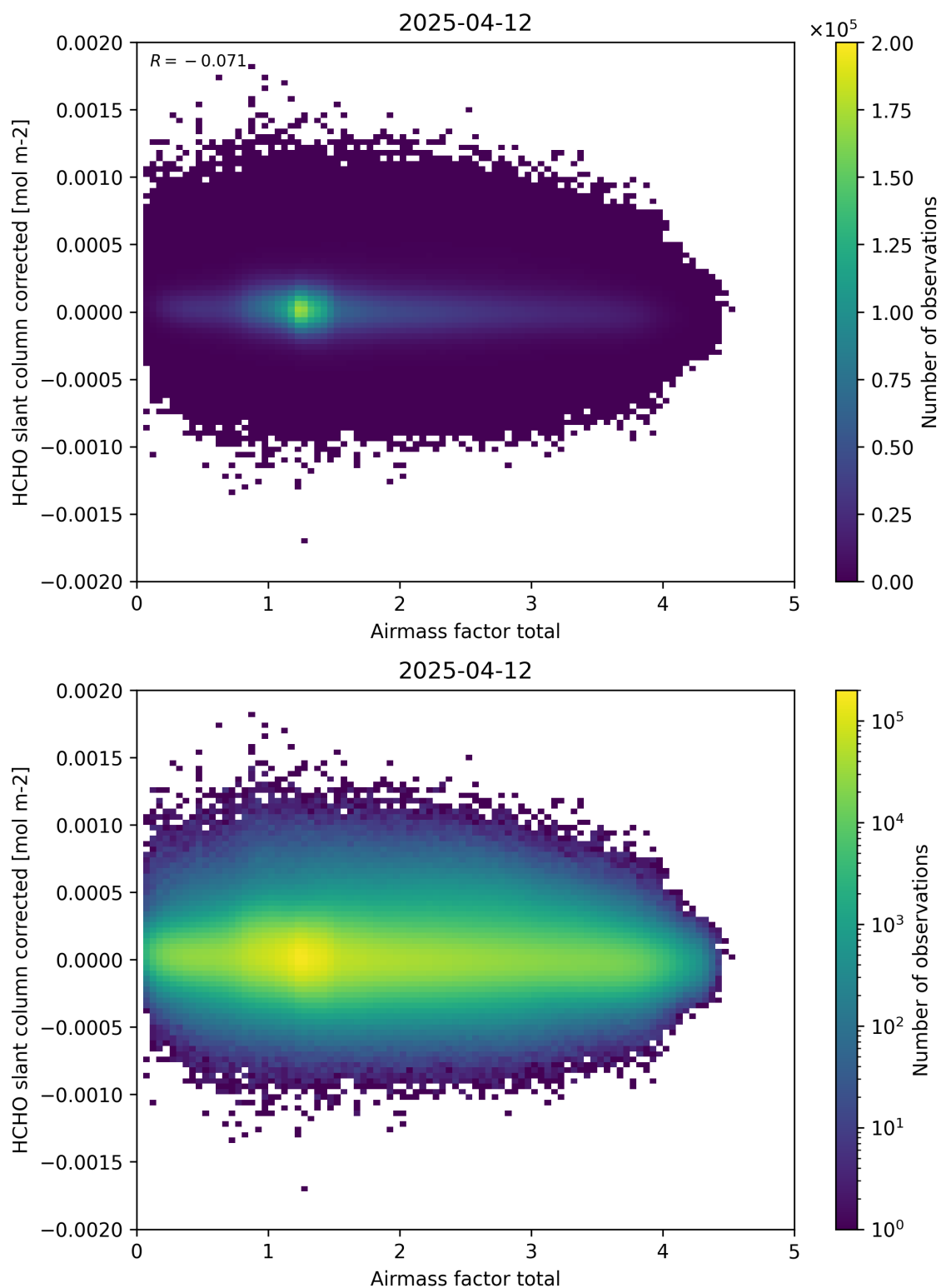
Figure 101: Scatter density plot of “Airmass factor total” against “HCHO slant column corrected” for 2025-04-11 to 2025-04-13.
