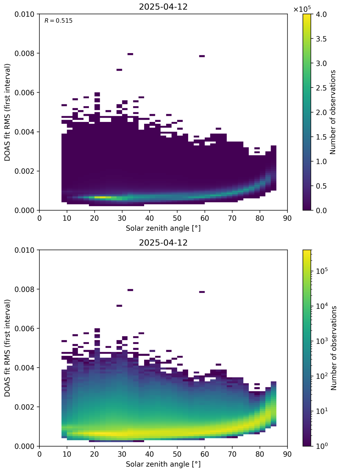
Figure 167: Scatter density plot of “Solar zenith angle” against “DOAS fit RMS (first interval)” for 2025-04-11 to 2025-04-13.
