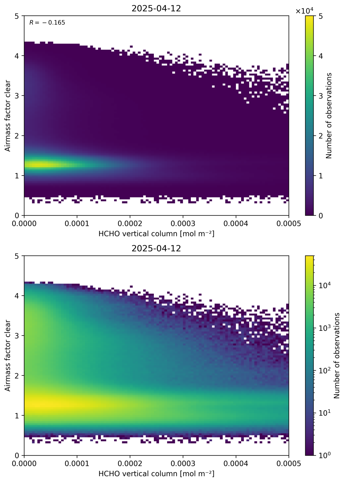
Figure 126: Scatter density plot of “HCHO vertical column” against “Airmass factor clear” for 2025-04-11 to 2025-04-13.
