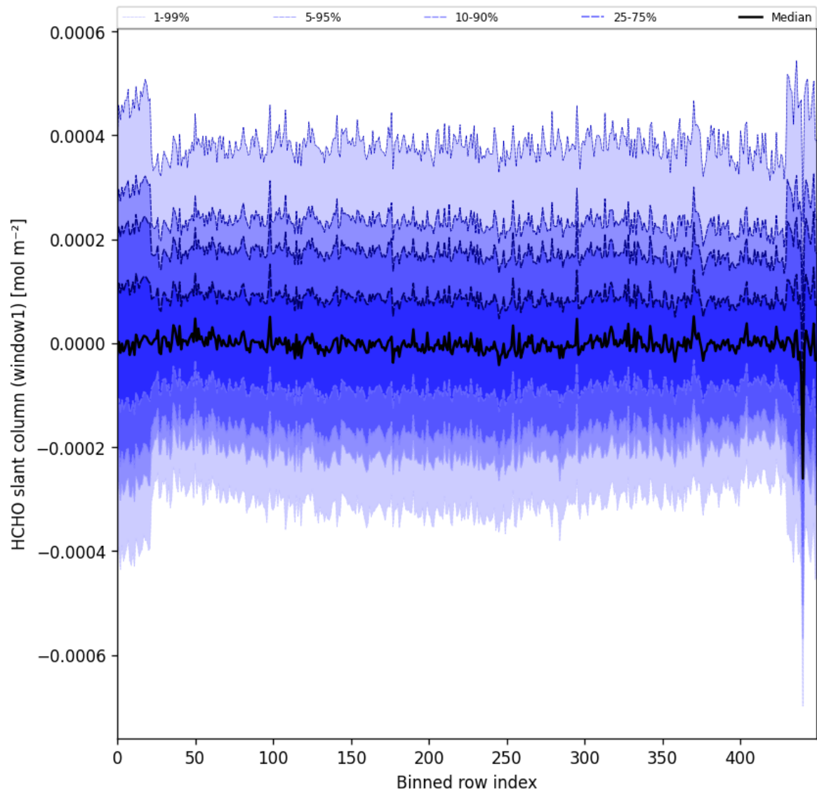
Figure 52: Along track statistics of “HCHO slant column (window1)” for 2025-04-11 to 2025-04-13
