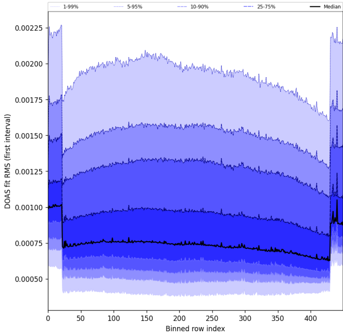
Figure 60: Along track statistics of “DOAS fit RMS (first interval)” for 2025-04-11 to 2025-04-13
