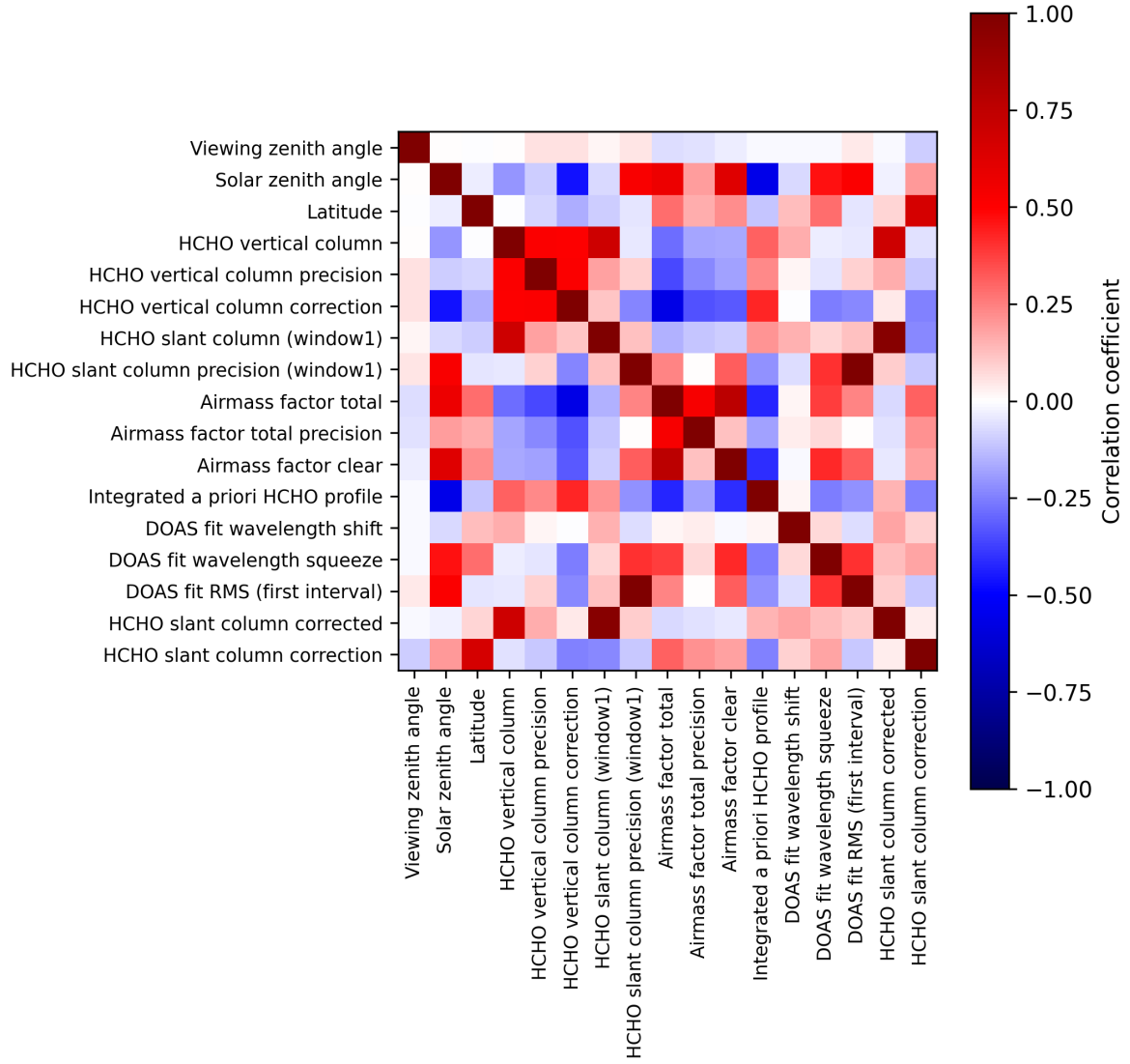
Figure 2: Map of correlation matrix for 2025-04-11 to 2025-04-13.
