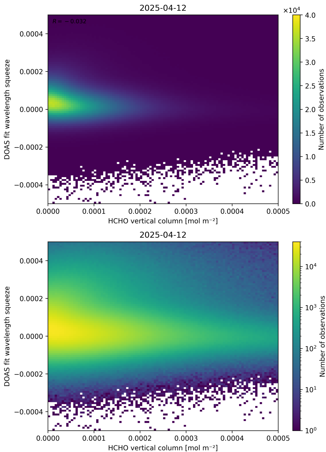
Figure 125: Scatter density plot of “HCHO vertical column” against “DOAS fit wavelength squeeze” for 2025-04-11 to 2025-04-13.
