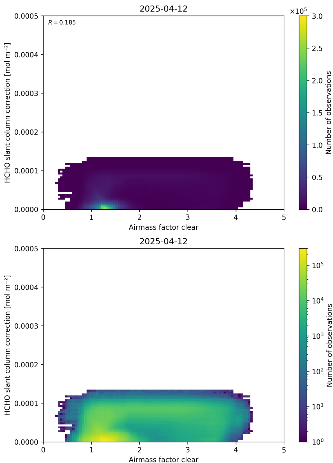
Figure 75: Scatter density plot of “Airmass factor clear” against “HCHO slant column correction” for 2025-04-11 to 2025-04-13.
