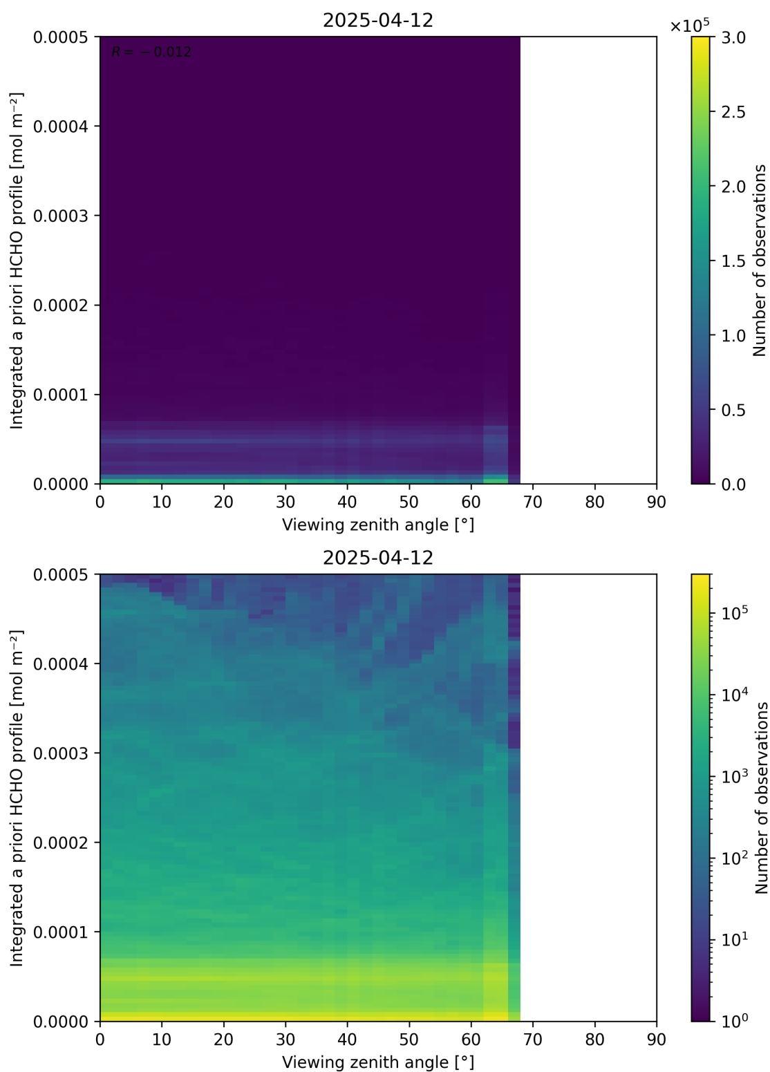
Figure 195: Scatter density plot of “Viewing zenith angle” against “Integrated a priori HCHO profile” for 2025-04-11 to 2025-04-13.
