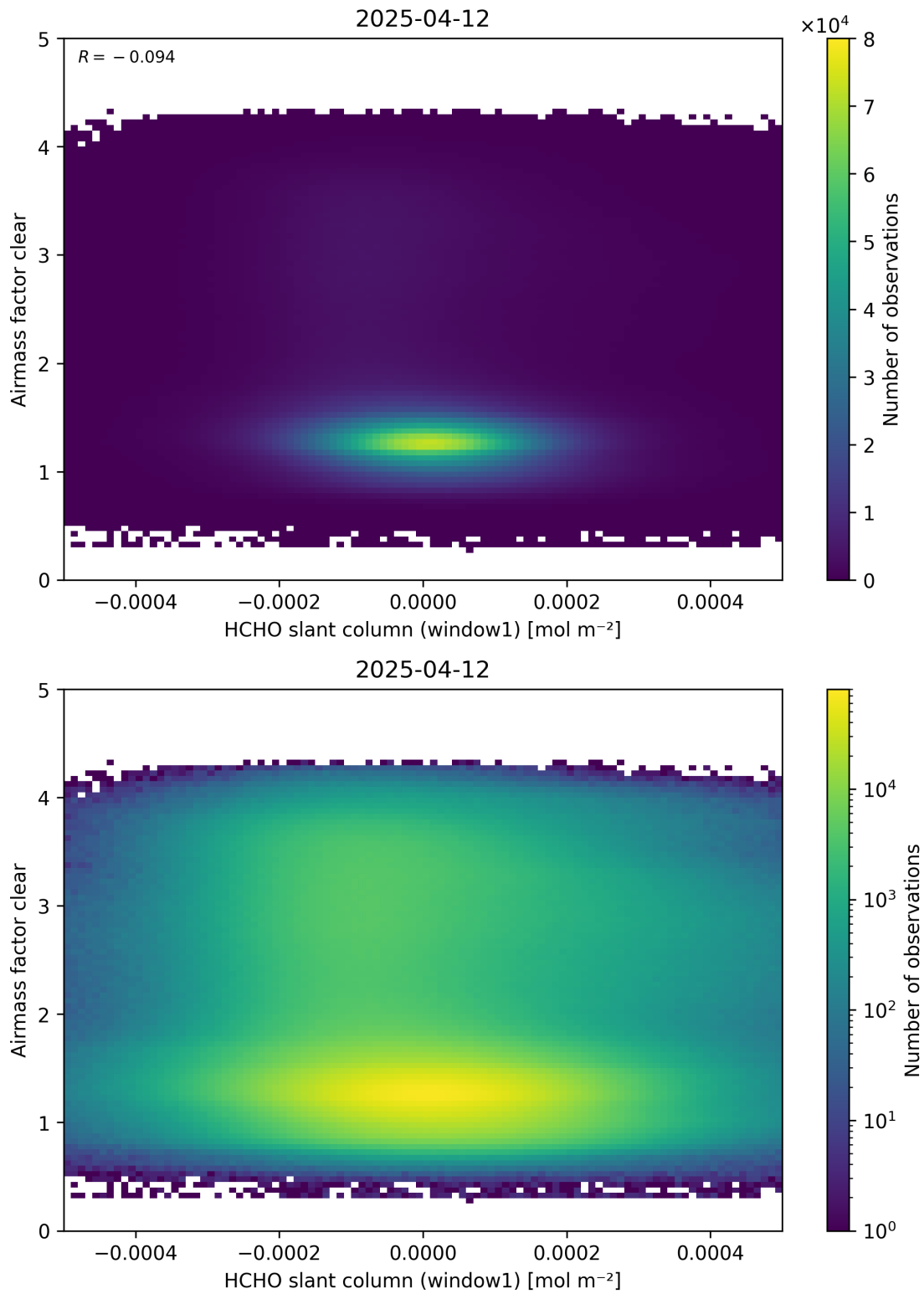
Figure 81: Scatter density plot of “HCHO slant column (window1)” against “Airmass factor clear” for 2025-04-11 to 2025-04-13.
