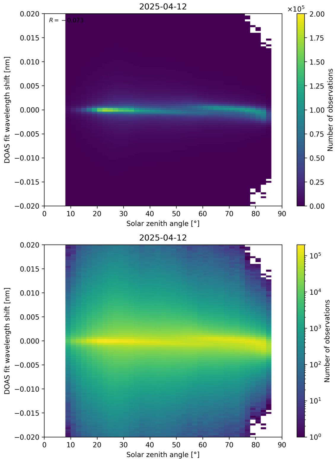
Figure 168: Scatter density plot of “Solar zenith angle” against “DOAS fit wavelength shift” for 2025-04-11 to 2025-04-13.
