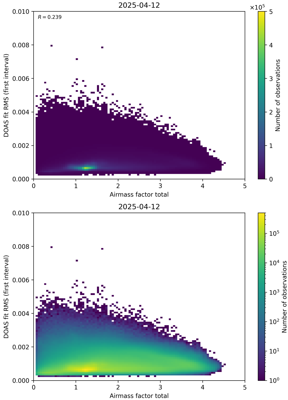
Figure 97: Scatter density plot of “Airmass factor total” against “DOAS fit RMS (first interval)” for 2025-04-11 to 2025-04-13.
