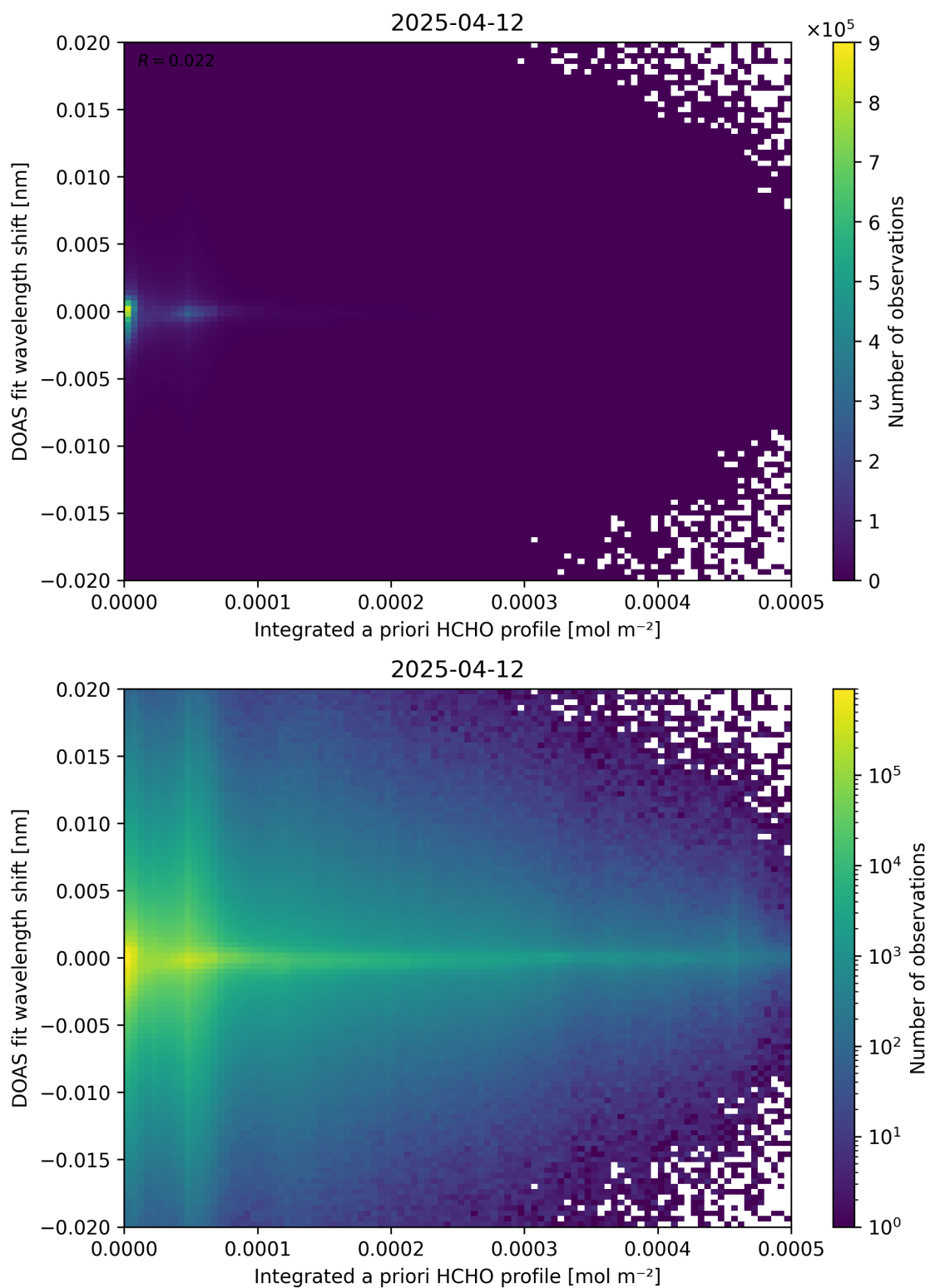
Figure 149: Scatter density plot of “Integrated a priori HCHO profile” against “DOAS fit wavelength shift” for 2025-04-11 to 2025-04-13.
