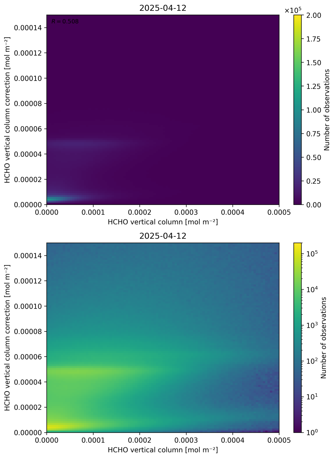
Figure 133: Scatter density plot of “HCHO vertical column” against “HCHO vertical column correction” for 2025-04-11 to 2025-04-13.
