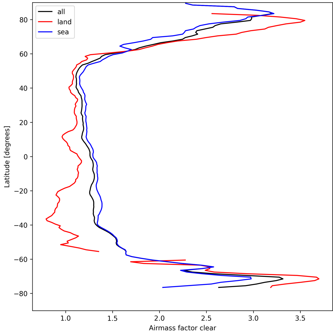
Figure 28: Zonal average of “Airmass factor clear” for 2025-04-11 to 2025-04-13.
