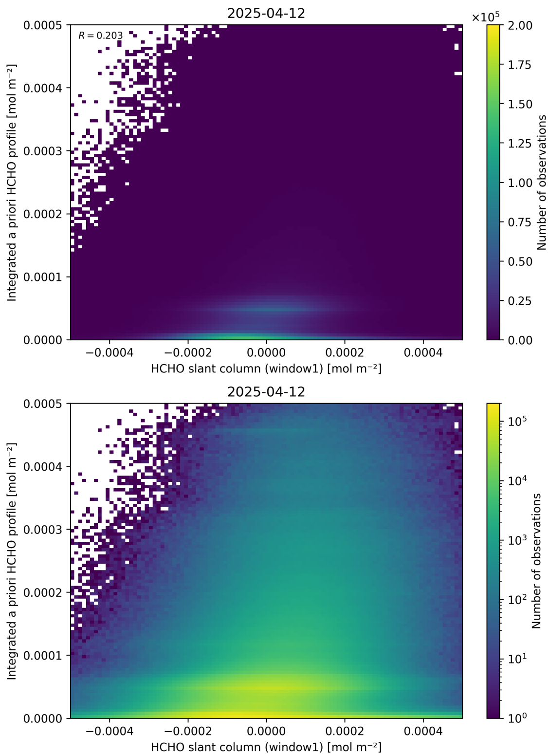
Figure 87: Scatter density plot of “HCHO slant column (window1)” against “Integrated a priori HCHO profile” for 2025-04-11 to 2025-04-13.
