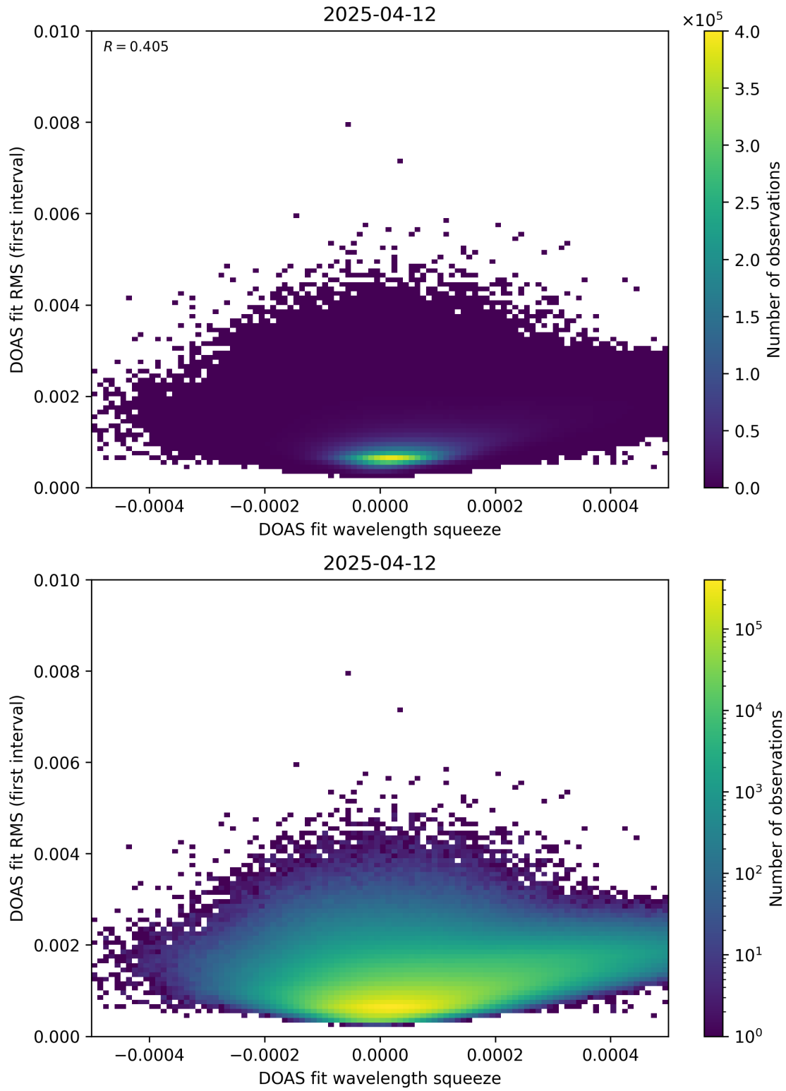
Figure 68: Scatter density plot of “DOAS fit wavelength squeeze” against “DOAS fit RMS (first interval)” for 2025-04-11 to 2025-04-13.
