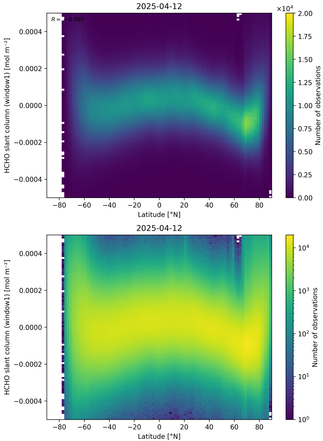
Figure 159: Scatter density plot of “Latitude” against “HCHO slant column (window1)” for 2025-04-11 to 2025-04-13.
