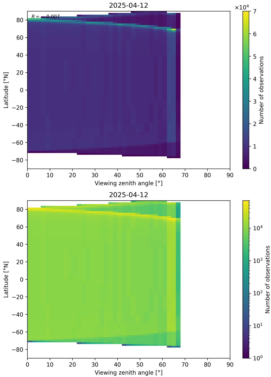
Figure 196: Scatter density plot of “Viewing zenith angle” against “Latitude” for 2025-04-11 to 2025-04-13.
