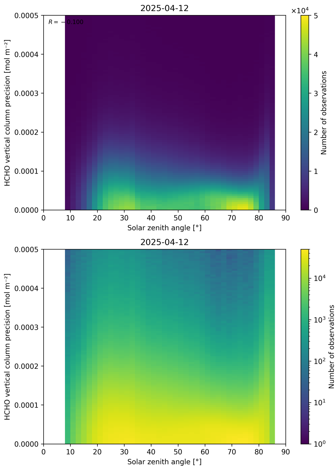
Figure 179: Scatter density plot of “Solar zenith angle” against “HCHO vertical column precision” for 2025-04-11 to 2025-04-13.
