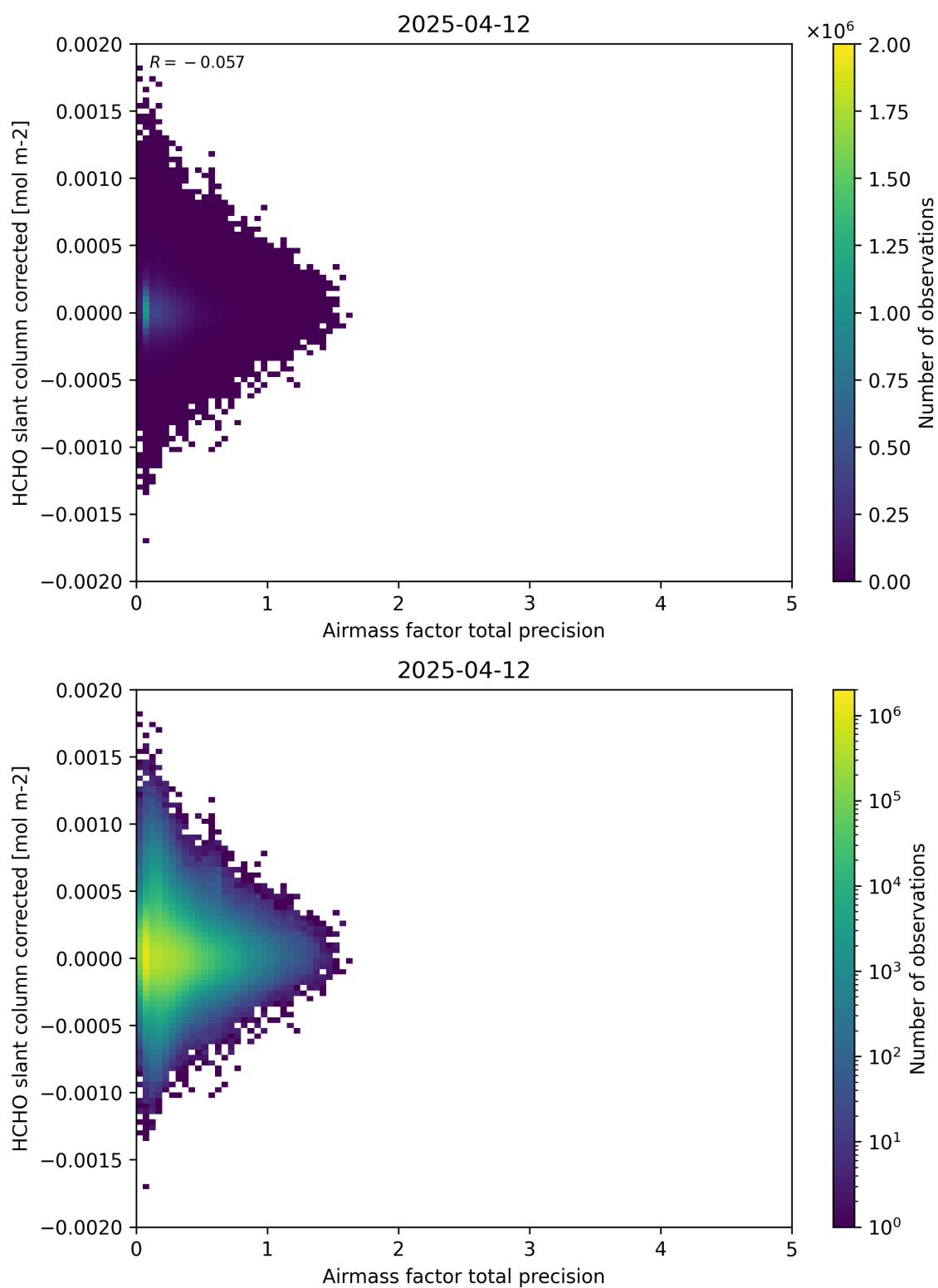
Figure 109: Scatter density plot of “Airmass factor total precision” against “HCHO slant column corrected” for 2025-04-11 to 2025-04-13.
