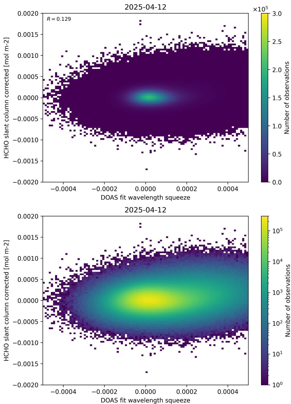
Figure 69: Scatter density plot of “DOAS fit wavelength squeeze” against “HCHO slant column corrected” for 2025-04-11 to 2025-04-13.
