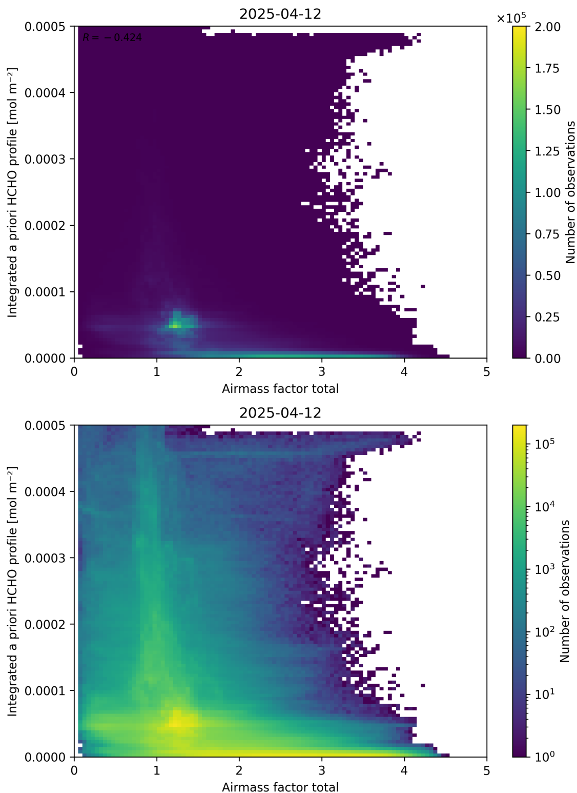
Figure 104: Scatter density plot of “Airmass factor total” against “Integrated a priori HCHO profile” for 2025-04-11 to 2025-04-13.
