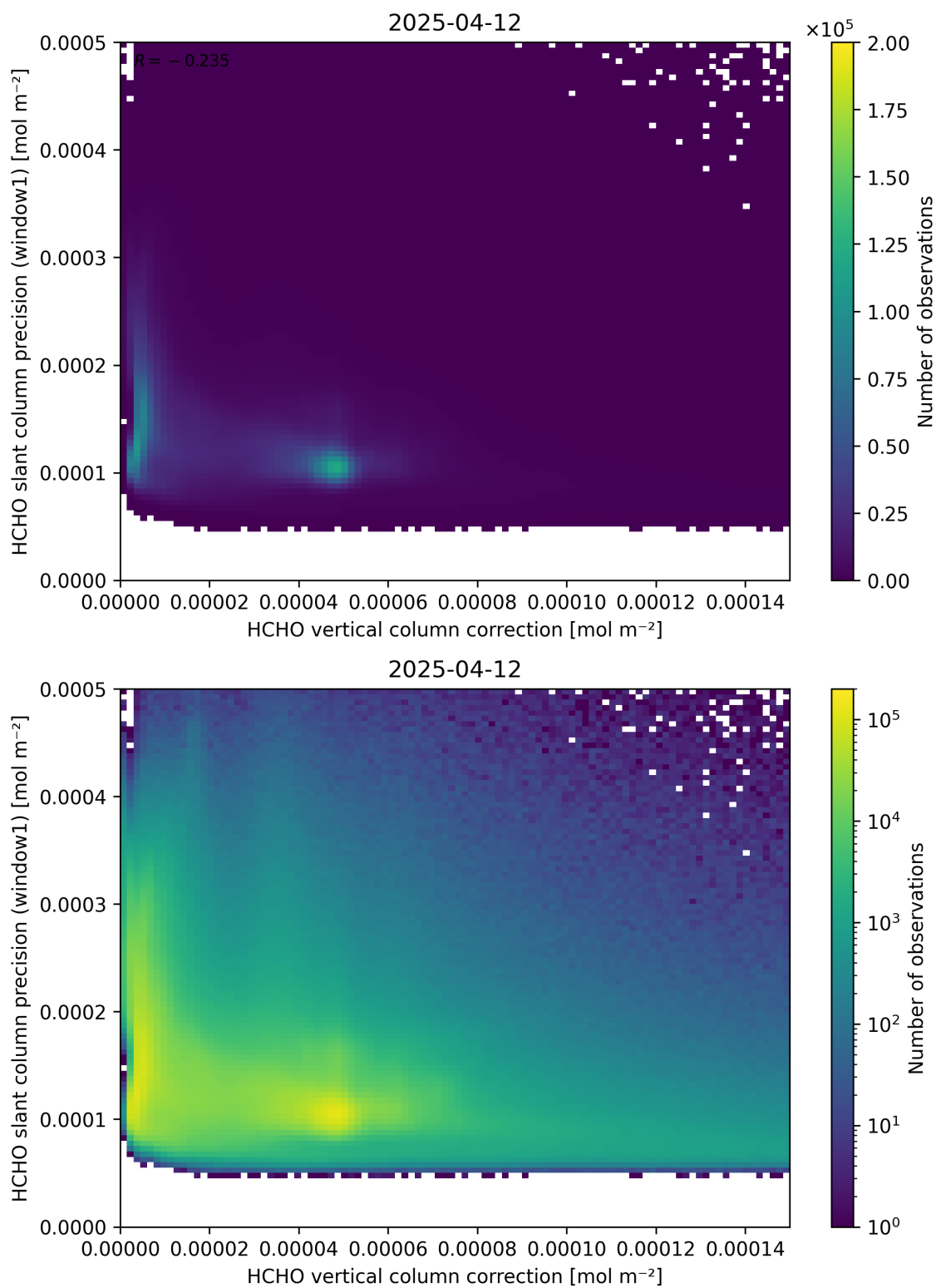
Figure 119: Scatter density plot of “HCHO vertical column correction” against “HCHO slant column precision (window1)” for 2025-04-11 to 2025-04-13.
