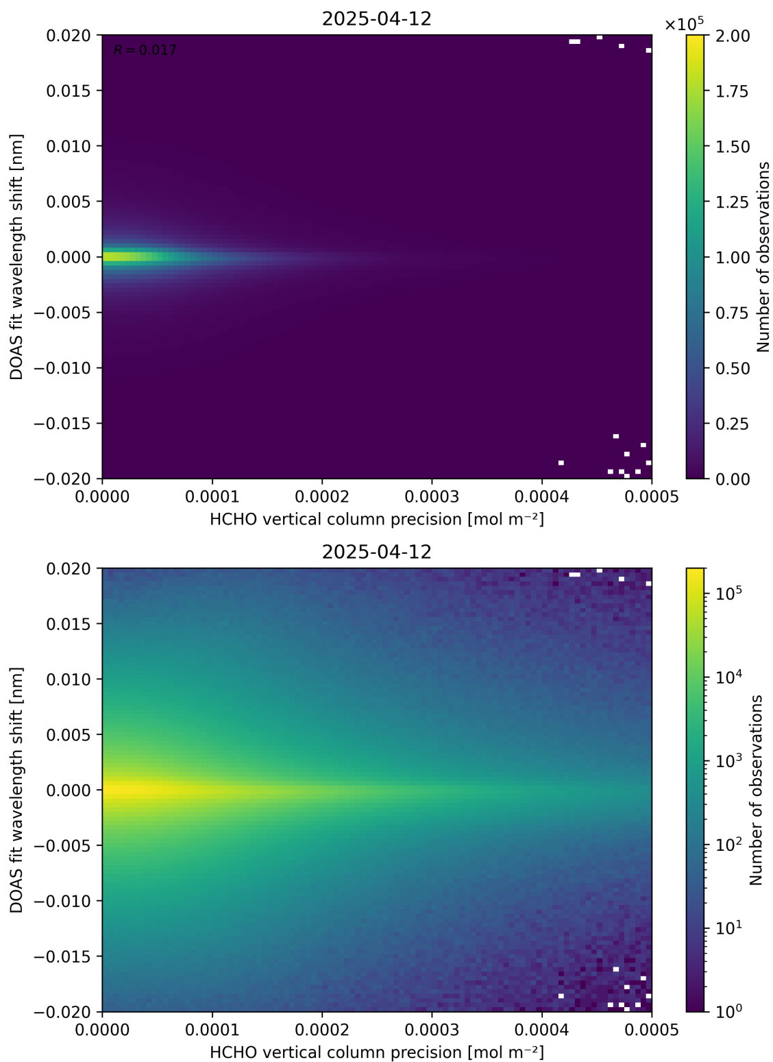
Figure 137: Scatter density plot of “HCHO vertical column precision” against “DOAS fit wavelength shift” for 2025-04-11 to 2025-04-13.
