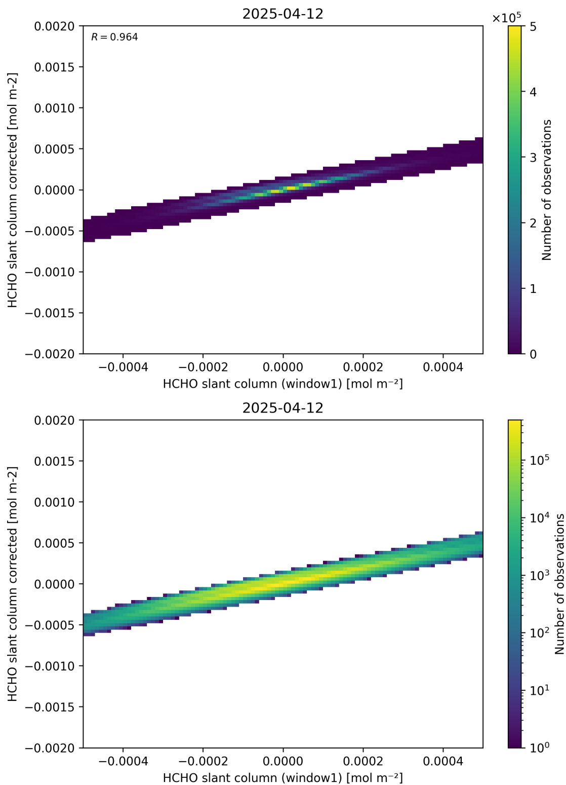
Figure 82: Scatter density plot of “HCHO slant column (window1)” against “HCHO slant column corrected” for 2025-04-11 to 2025-04-13.
