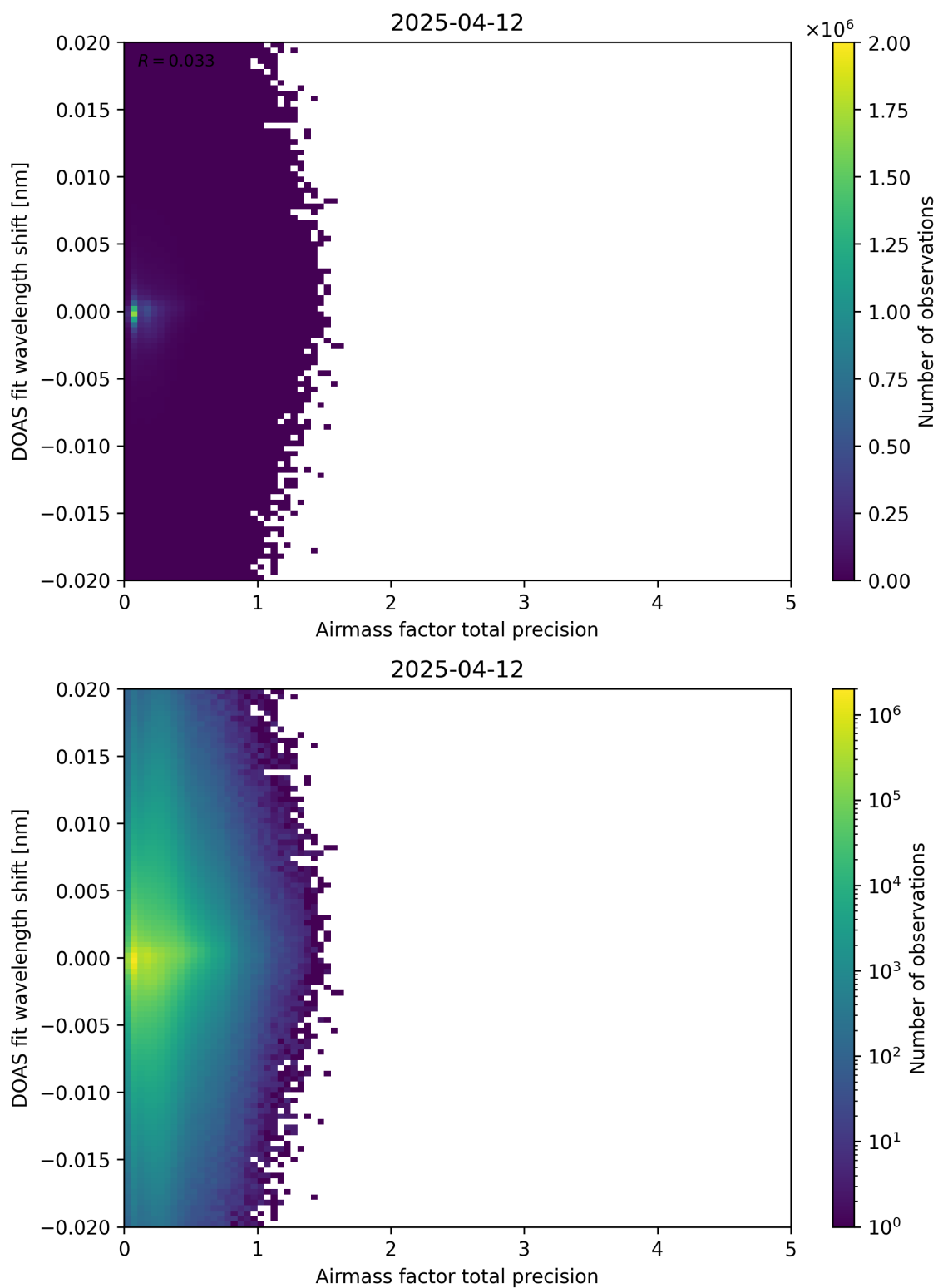
Figure 106: Scatter density plot of “Airmass factor total precision” against “DOAS fit wavelength shift” for 2025-04-11 to 2025-04-13.
