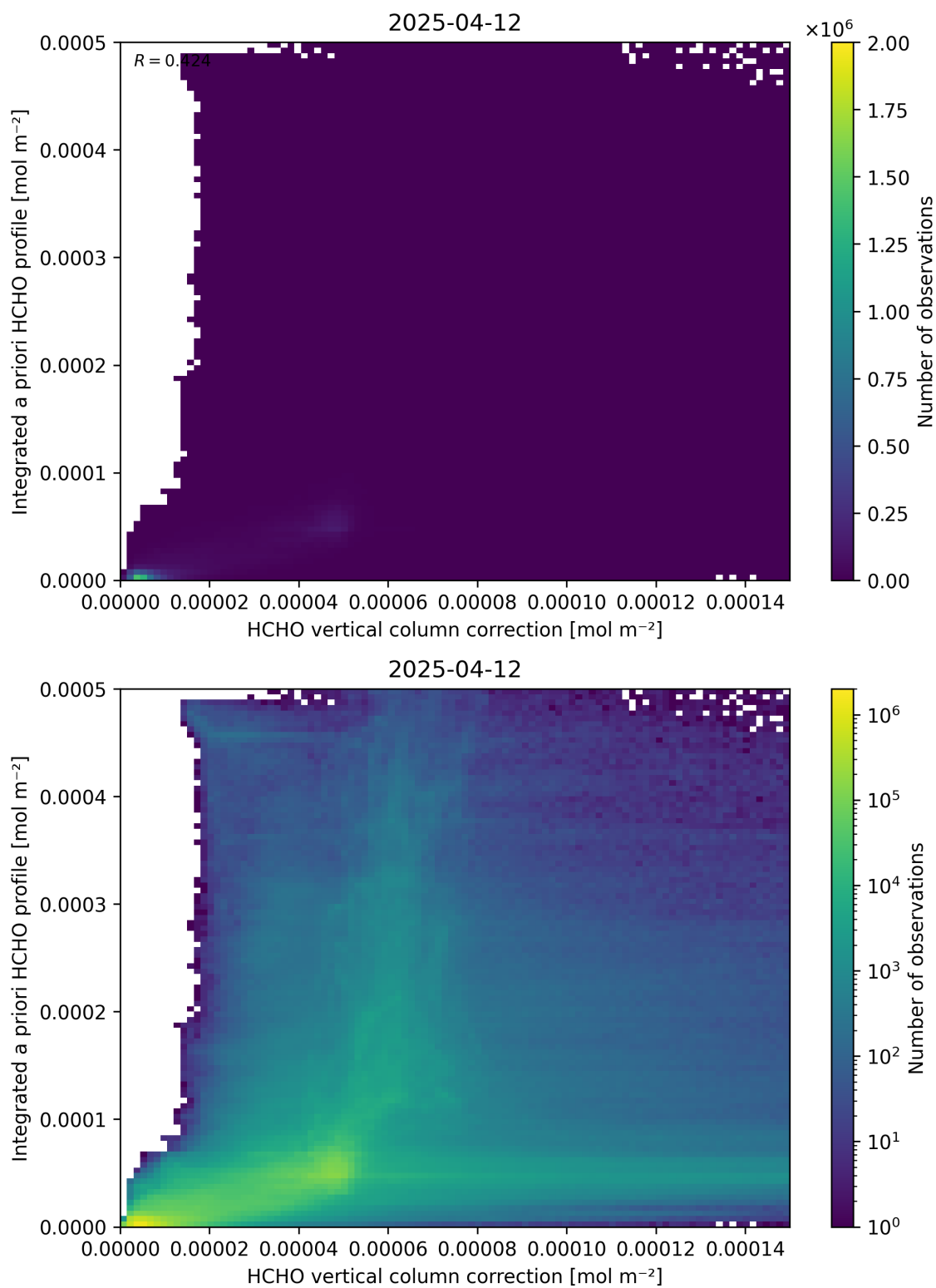
Figure 122: Scatter density plot of “HCHO vertical column correction” against “Integrated a priori HCHO profile” for 2025-04-11 to 2025-04-13.
