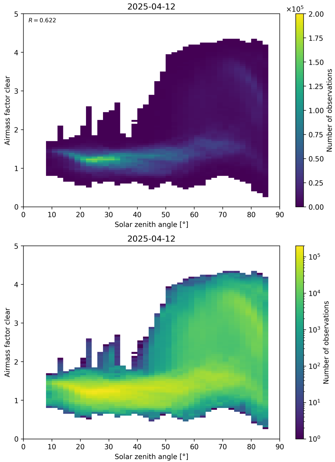
Figure 170: Scatter density plot of “Solar zenith angle” against “Airmass factor clear” for 2025-04-11 to 2025-04-13.
