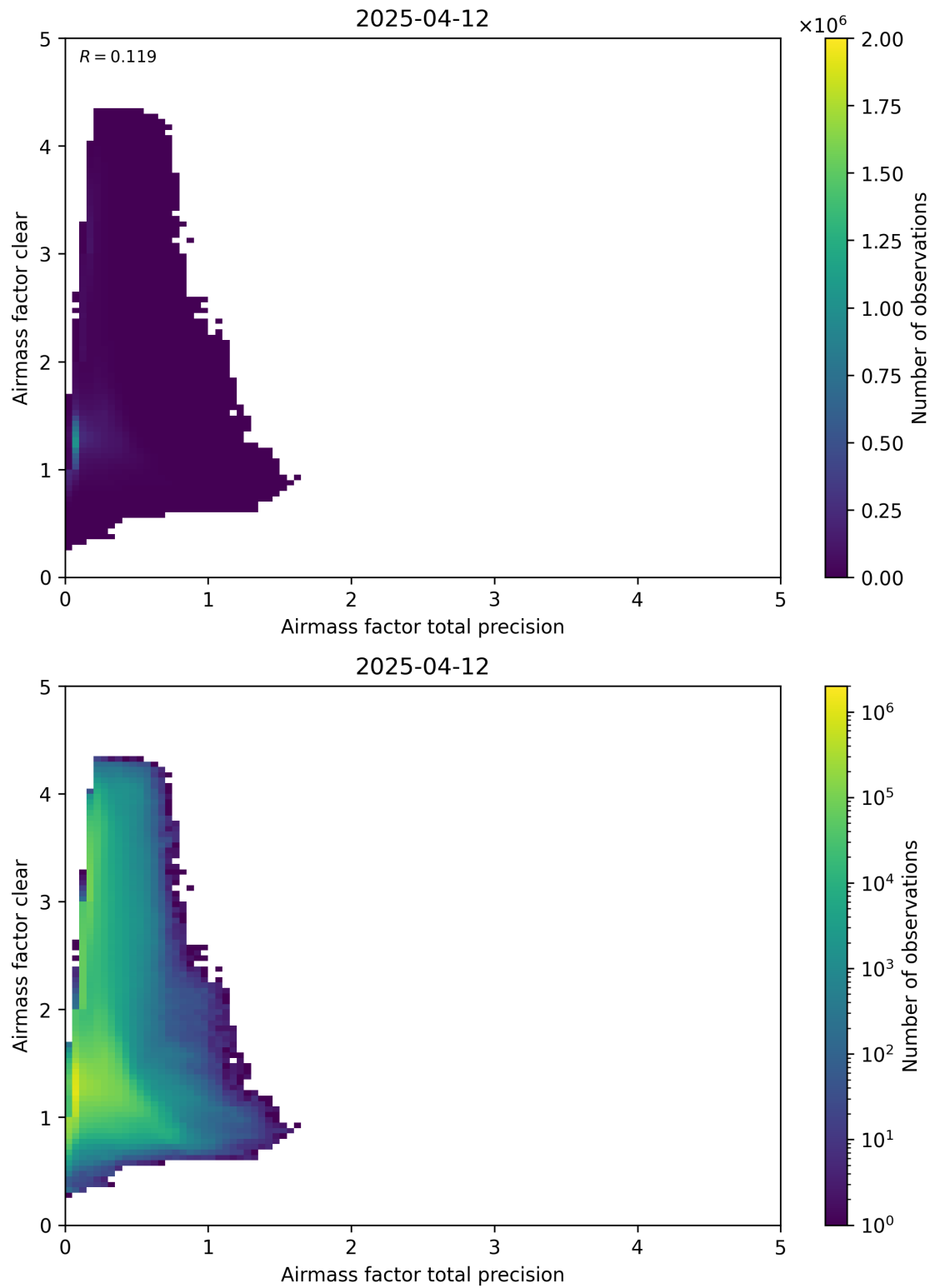
Figure 108: Scatter density plot of “Airmass factor total precision” against “Airmass factor clear” for 2025-04-11 to 2025-04-13.
