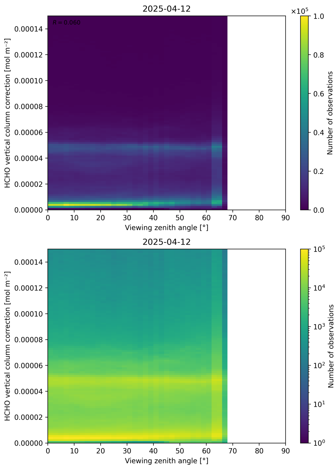
Figure 193: Scatter density plot of “Viewing zenith angle” against “HCHO vertical column correction” for 2025-04-11 to 2025-04-13.
