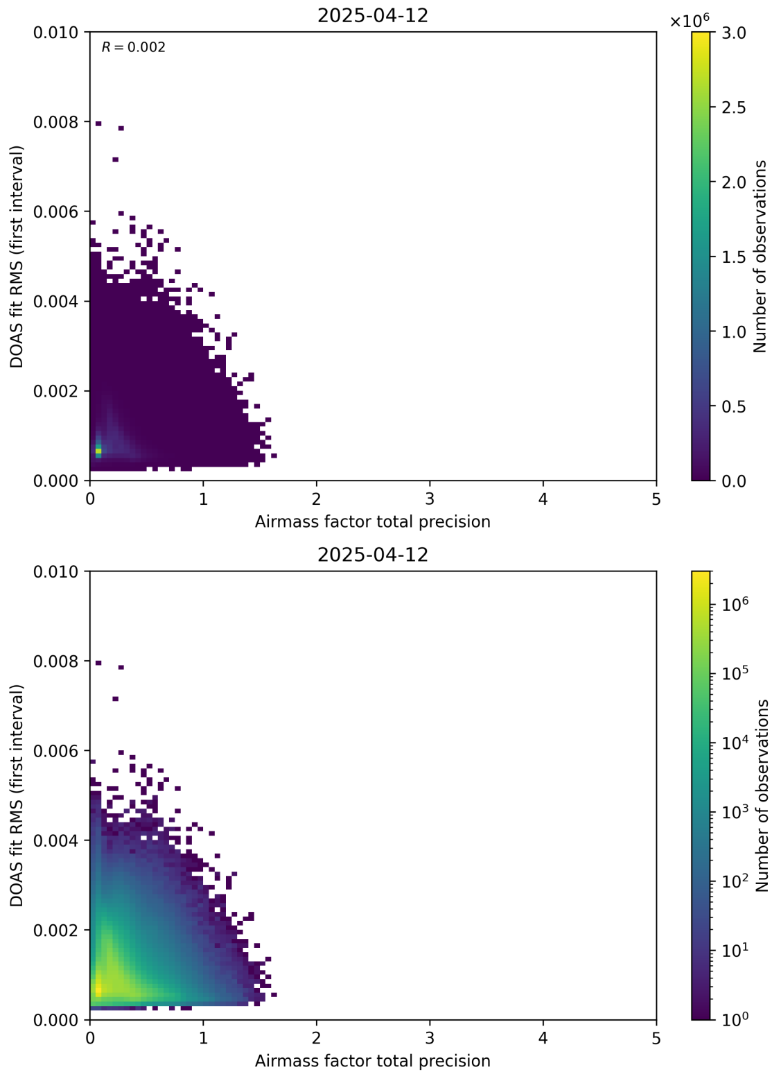
Figure 105: Scatter density plot of “Airmass factor total precision” against “DOAS fit RMS (first interval)” for 2025-04-11 to 2025-04-13.
