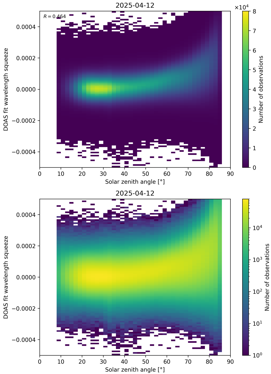
Figure 169: Scatter density plot of “Solar zenith angle” against “DOAS fit wavelength squeeze” for 2025-04-11 to 2025-04-13.
