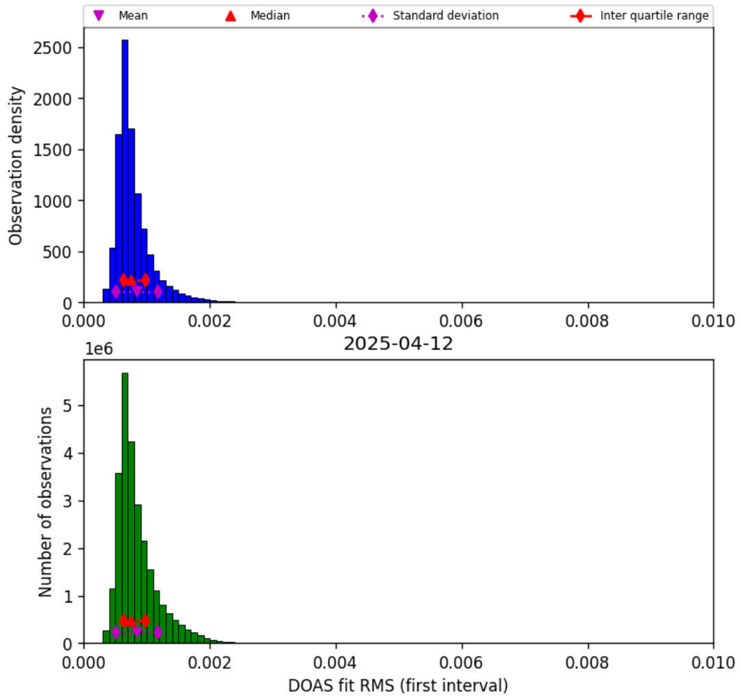
Figure 46: Histogram of “DOAS fit RMS (first interval)” for 2025-04-11 to 2025-04-13
