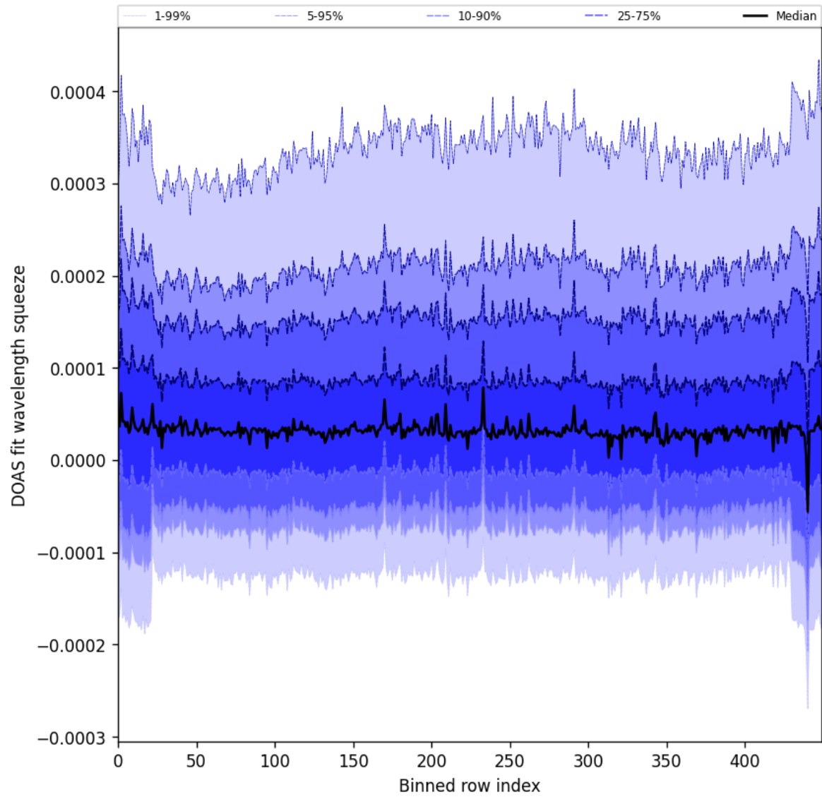
Figure 59: Along track statistics of “DOAS fit wavelength squeeze” for 2025-04-11 to 2025-04-13
