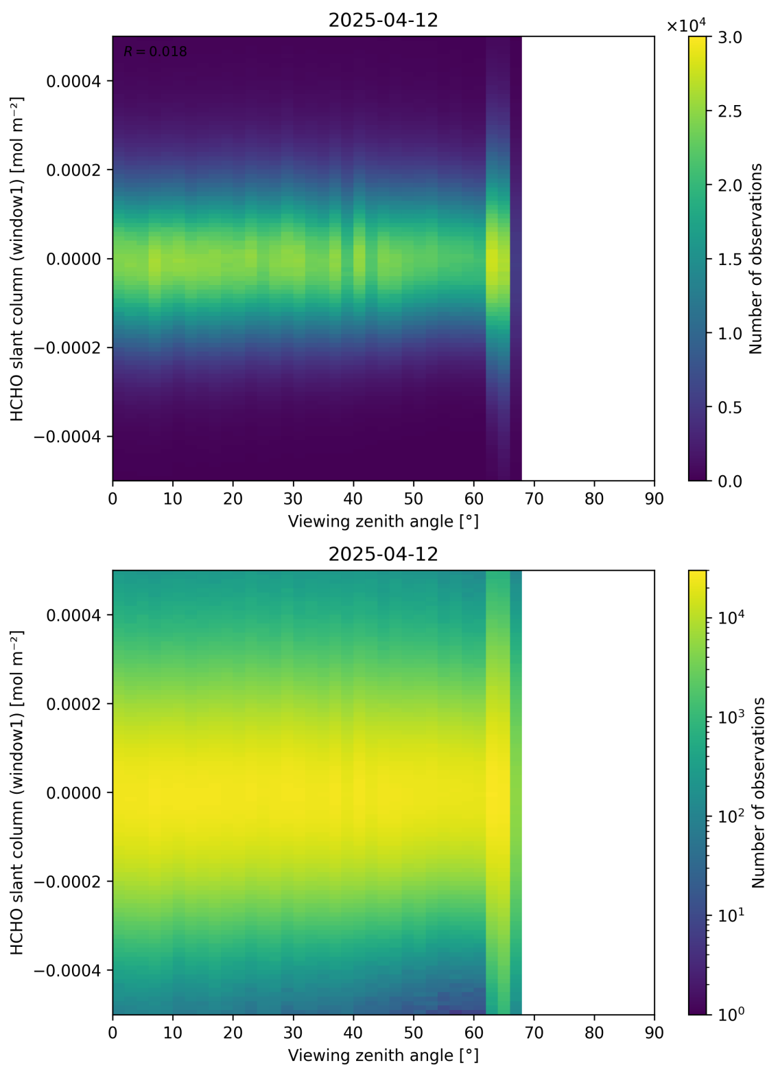
Figure 188: Scatter density plot of “Viewing zenith angle” against “HCHO slant column (window1)” for 2025-04-11 to 2025-04-13.
