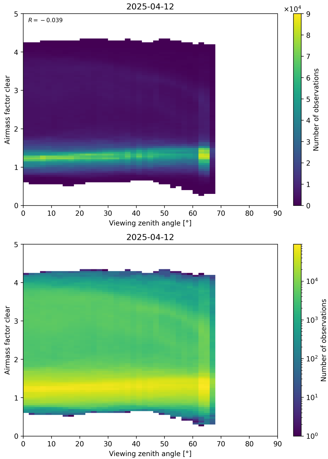
Figure 185: Scatter density plot of “Viewing zenith angle” against “Airmass factor clear” for 2025-04-11 to 2025-04-13.
