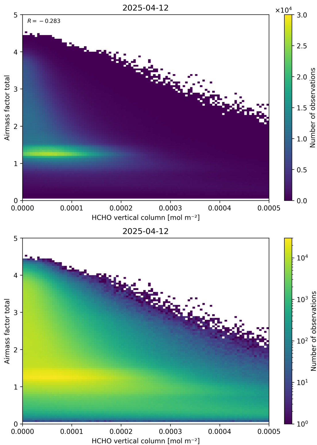
Figure 131: Scatter density plot of “HCHO vertical column” against “Airmass factor total” for 2025-04-11 to 2025-04-13.
