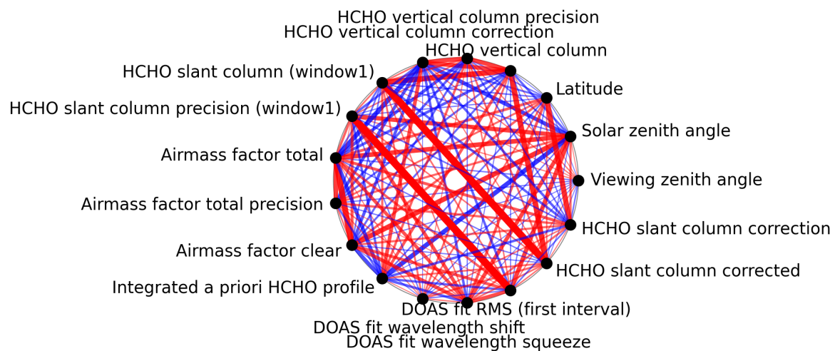
Figure 1: Map of correlation graph for 2025-04-11 to 2025-04-13.
