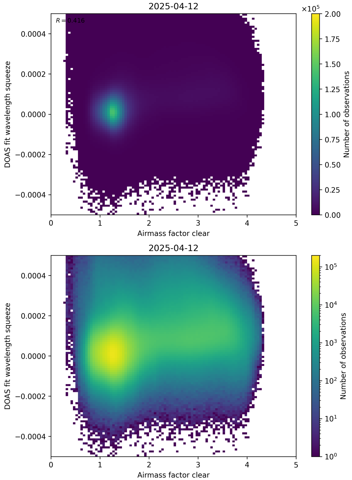
Figure 73: Scatter density plot of “Airmass factor clear” against “DOAS fit wavelength squeeze” for 2025-04-11 to 2025-04-13.
