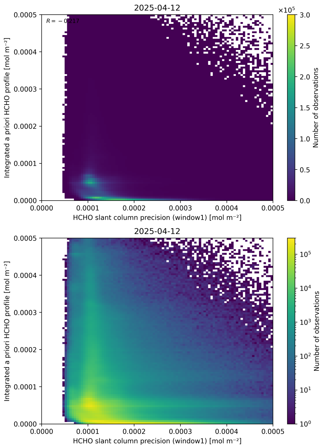
Figure 96: Scatter density plot of “HCHO slant column precision (window1)” against “Integrated a priori HCHO profile” for 2025-04-11 to 2025-04-13.
