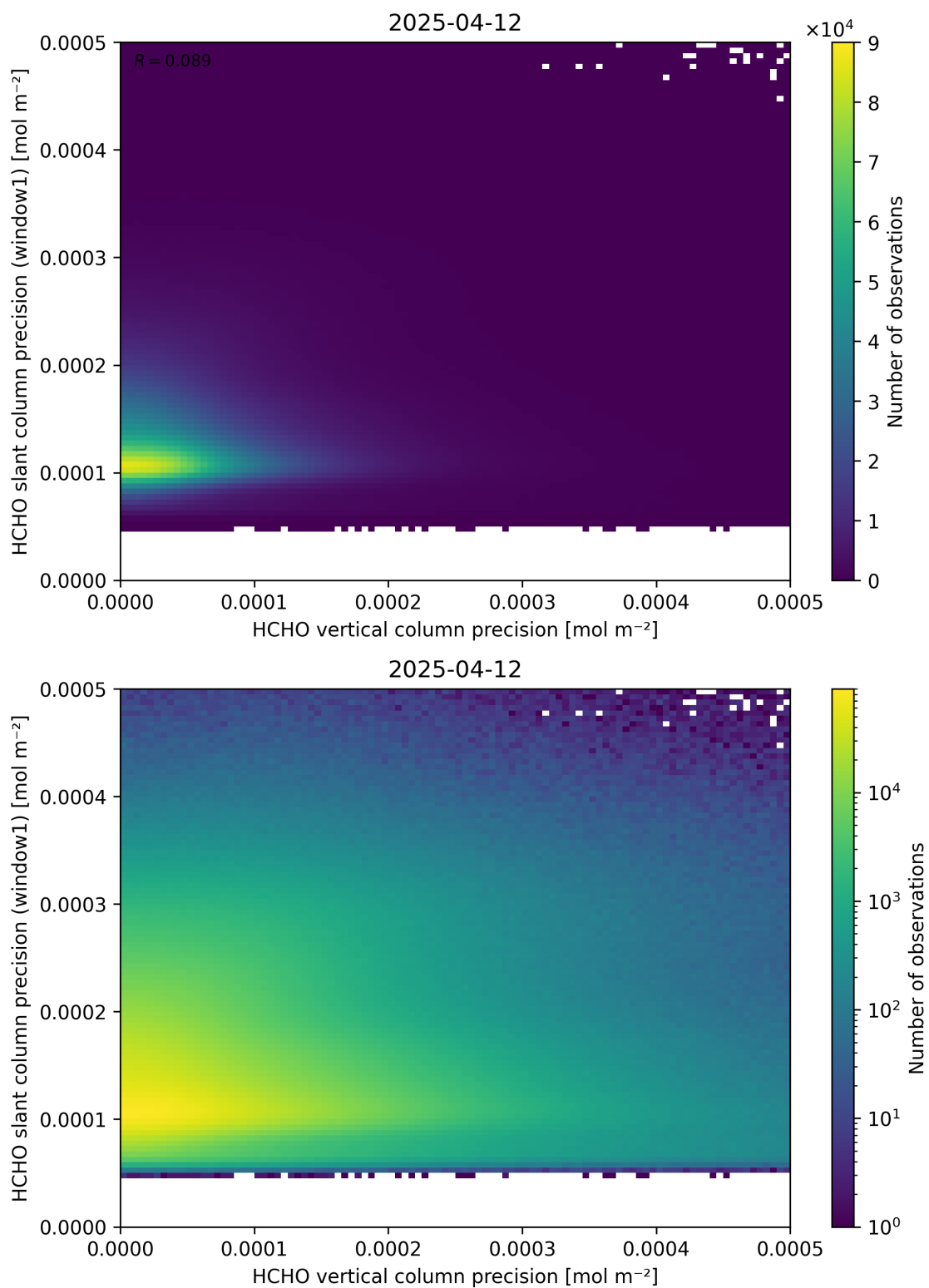
Figure 143: Scatter density plot of “HCHO vertical column precision” against “HCHO slant column precision (window1)” for 2025-04-11 to 2025-04-13.
