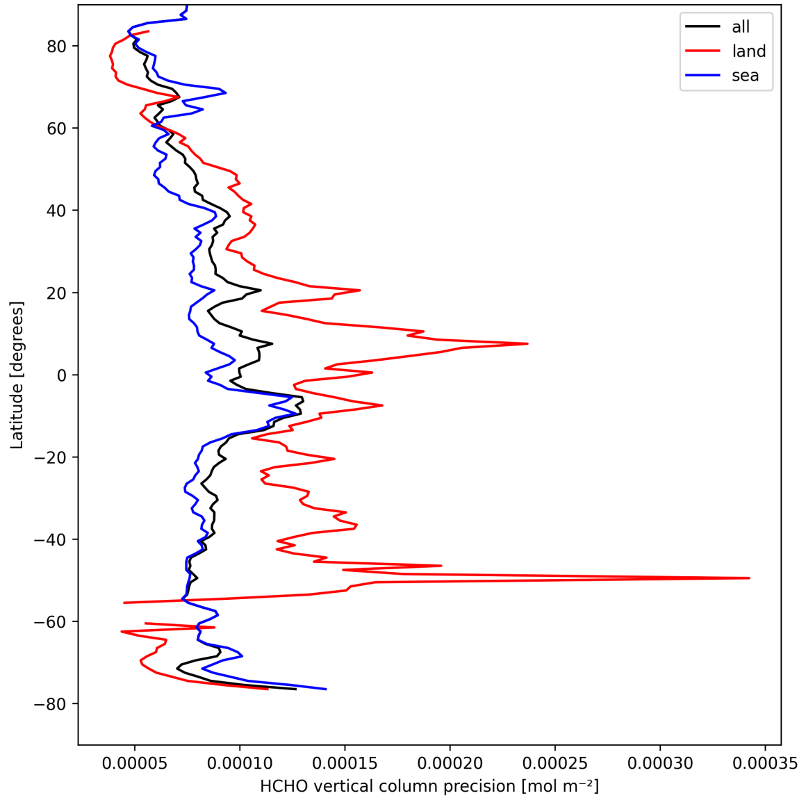
Figure 22: Zonal average of “HCHO vertical column precision” for 2025-04-11 to 2025-04-13.
