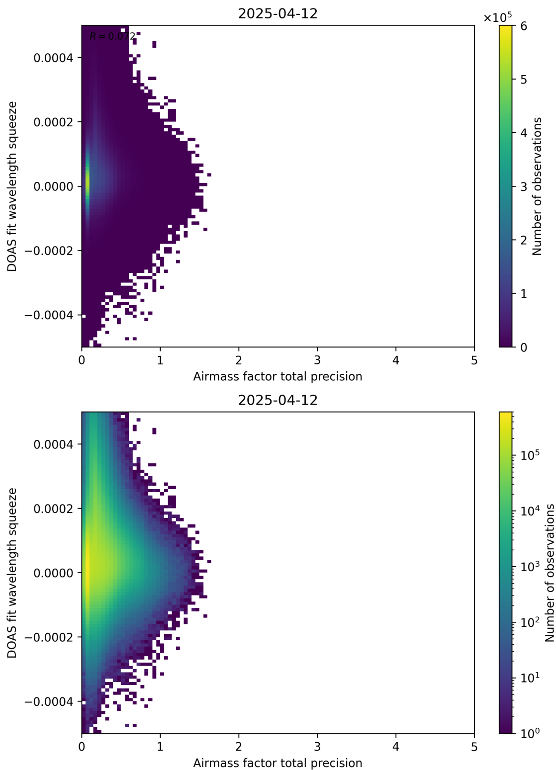
Figure 107: Scatter density plot of “Airmass factor total precision” against “DOAS fit wavelength squeeze” for 2025-04-11 to 2025-04-13.
