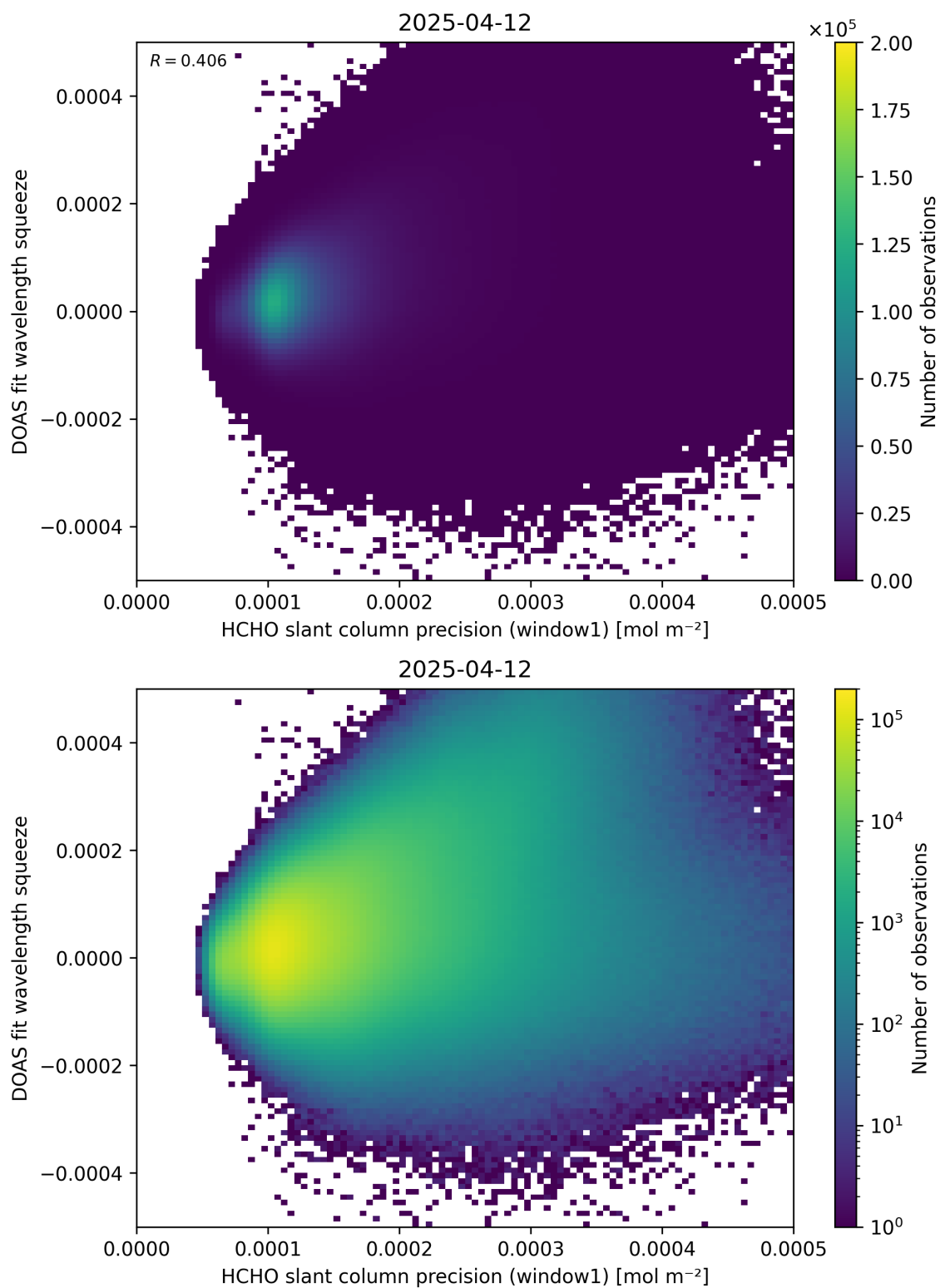
Figure 90: Scatter density plot of “HCHO slant column precision (window1)” against “DOAS fit wavelength squeeze” for 2025-04-11 to 2025-04-13.
