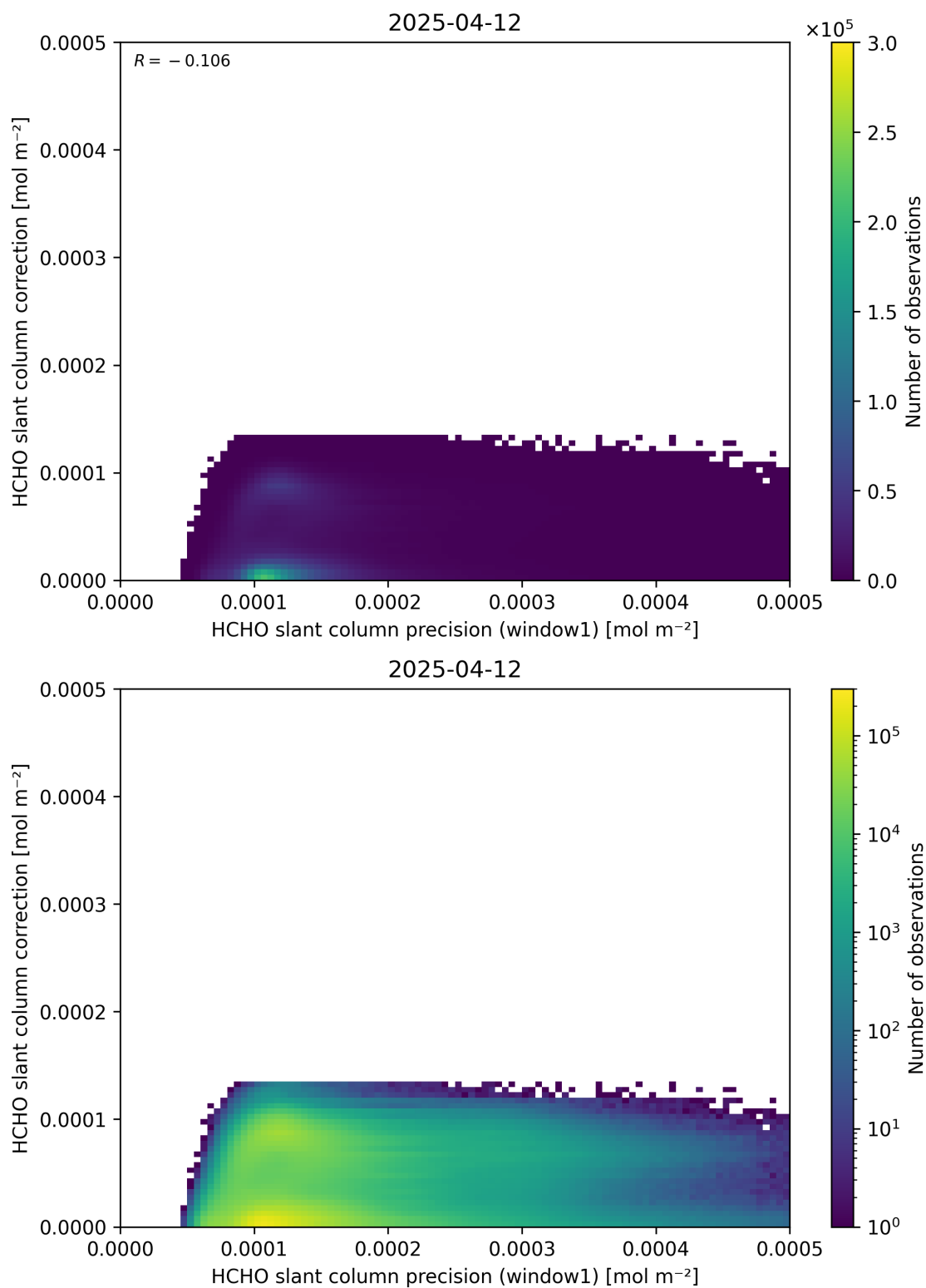
Figure 93: Scatter density plot of “HCHO slant column precision (window1)” against “HCHO slant column correction” for 2025-04-11 to 2025-04-13.
