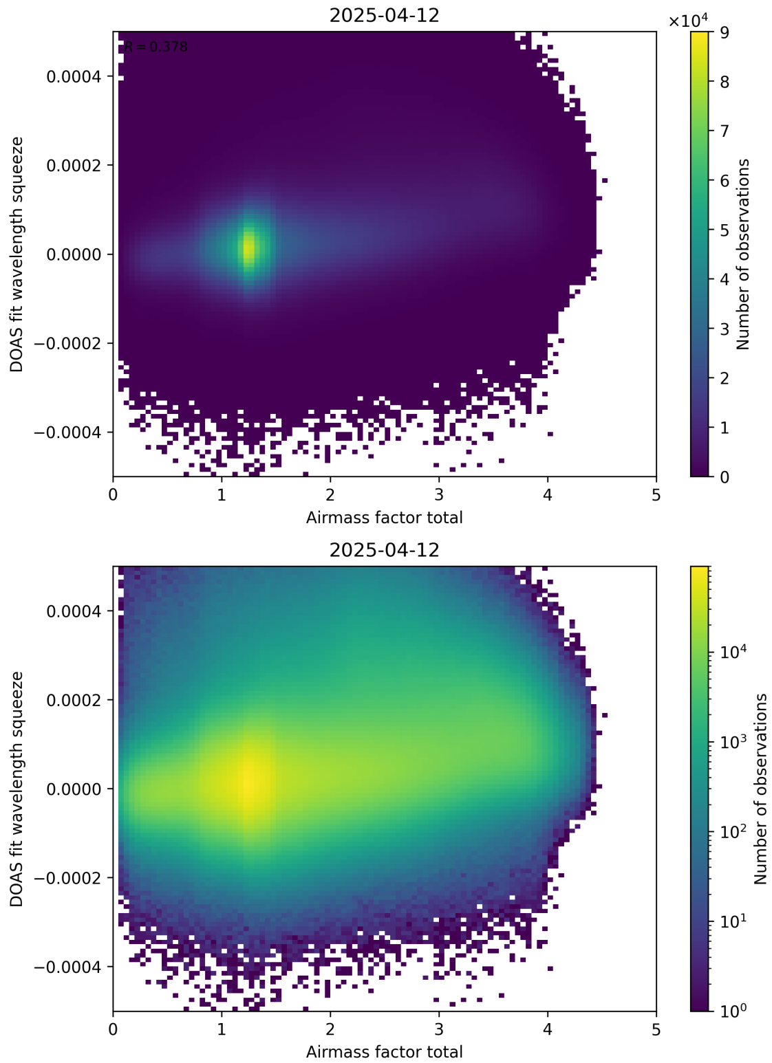
Figure 99: Scatter density plot of “Airmass factor total” against “DOAS fit wavelength squeeze” for 2025-04-11 to 2025-04-13.
