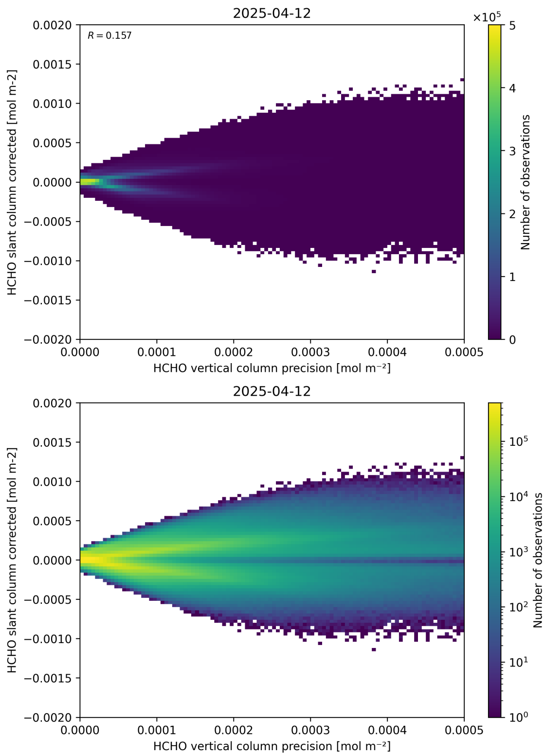
Figure 140: Scatter density plot of “HCHO vertical column precision” against “HCHO slant column corrected” for 2025-04-11 to 2025-04-13.
