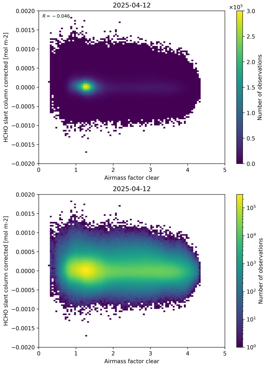
Figure 74: Scatter density plot of “Airmass factor clear” against “HCHO slant column corrected” for 2025-04-11 to 2025-04-13.
