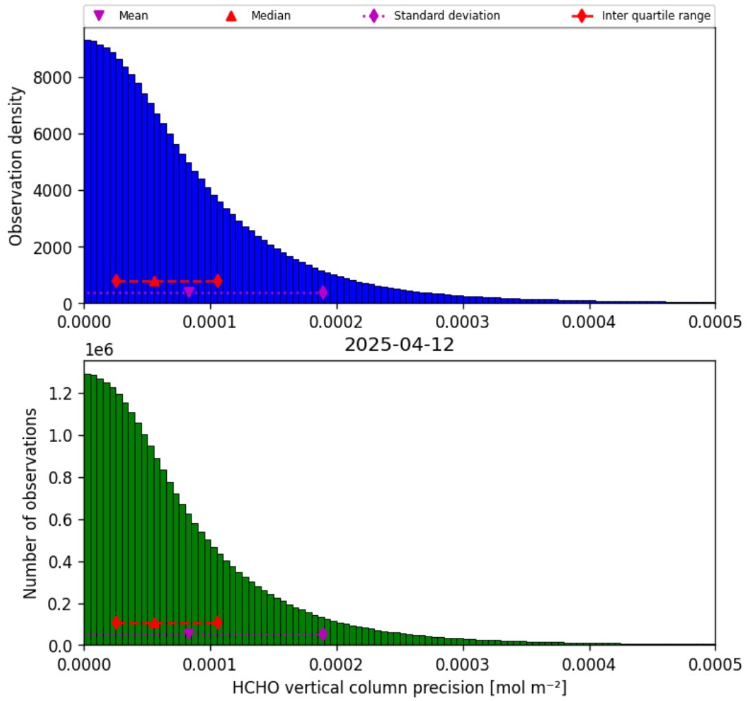
Figure 36: Histogram of “HCHO vertical column precision” for 2025-04-11 to 2025-04-13
