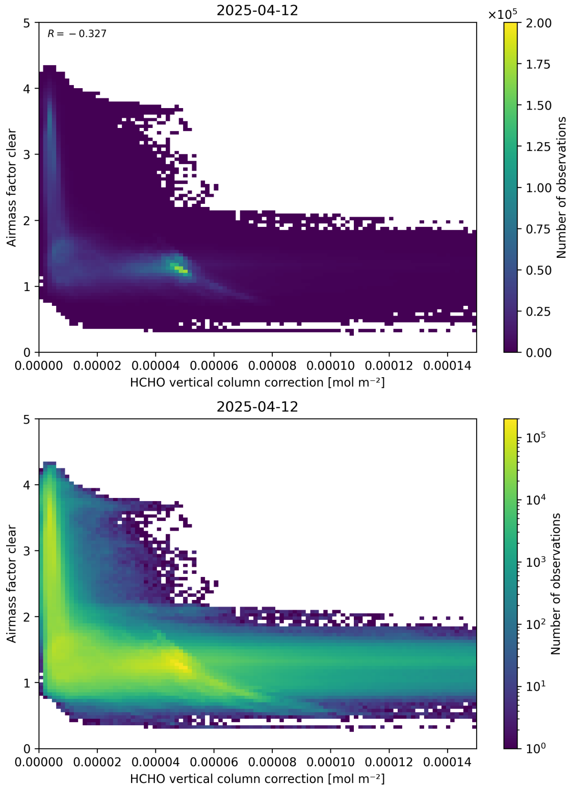
Figure 115: Scatter density plot of “HCHO vertical column correction” against “Airmass factor clear” for 2025-04-11 to 2025-04-13.
