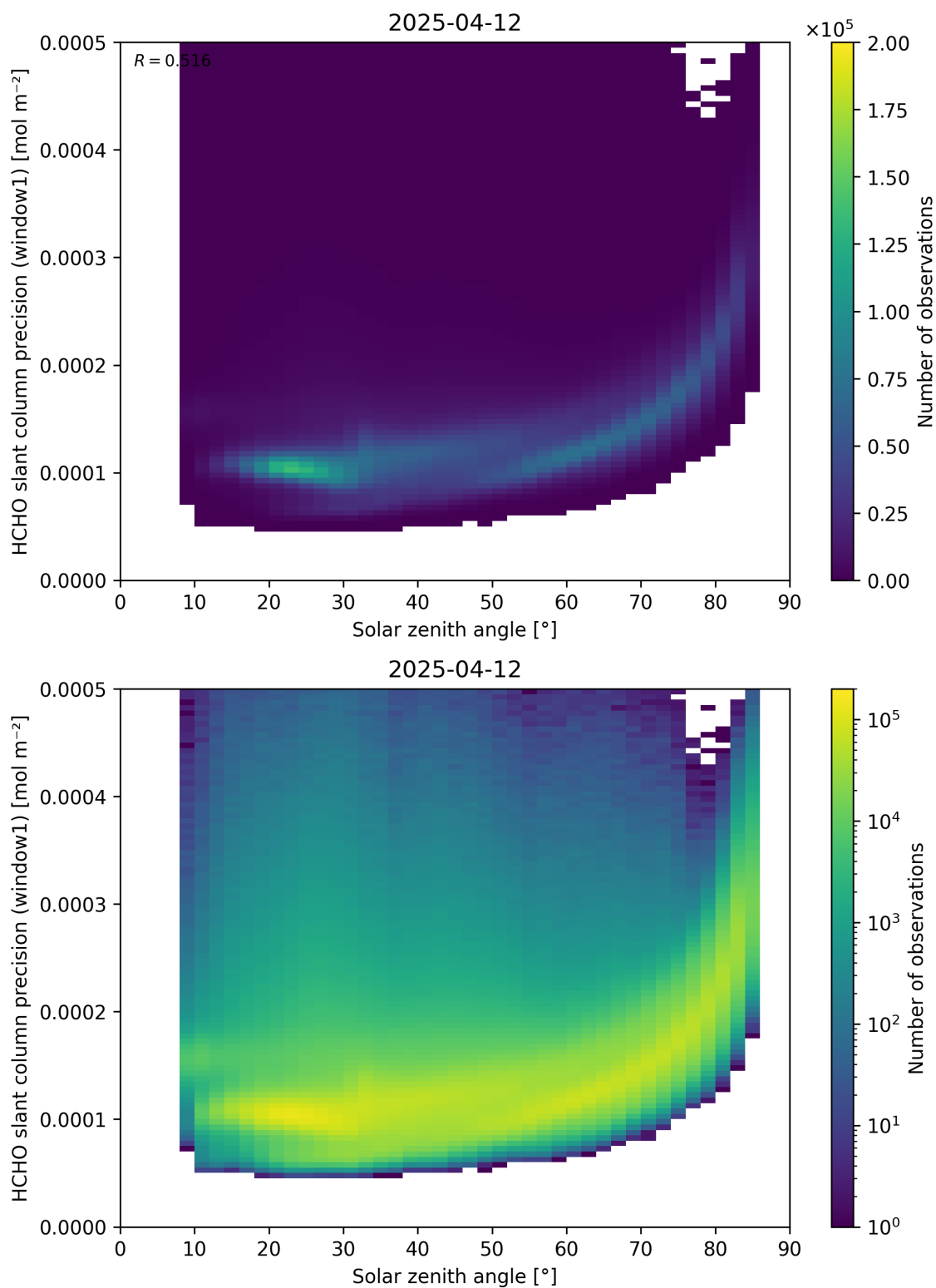
Figure 174: Scatter density plot of “Solar zenith angle” against “HCHO slant column precision (window1)” for 2025-04-11 to 2025-04-13.
