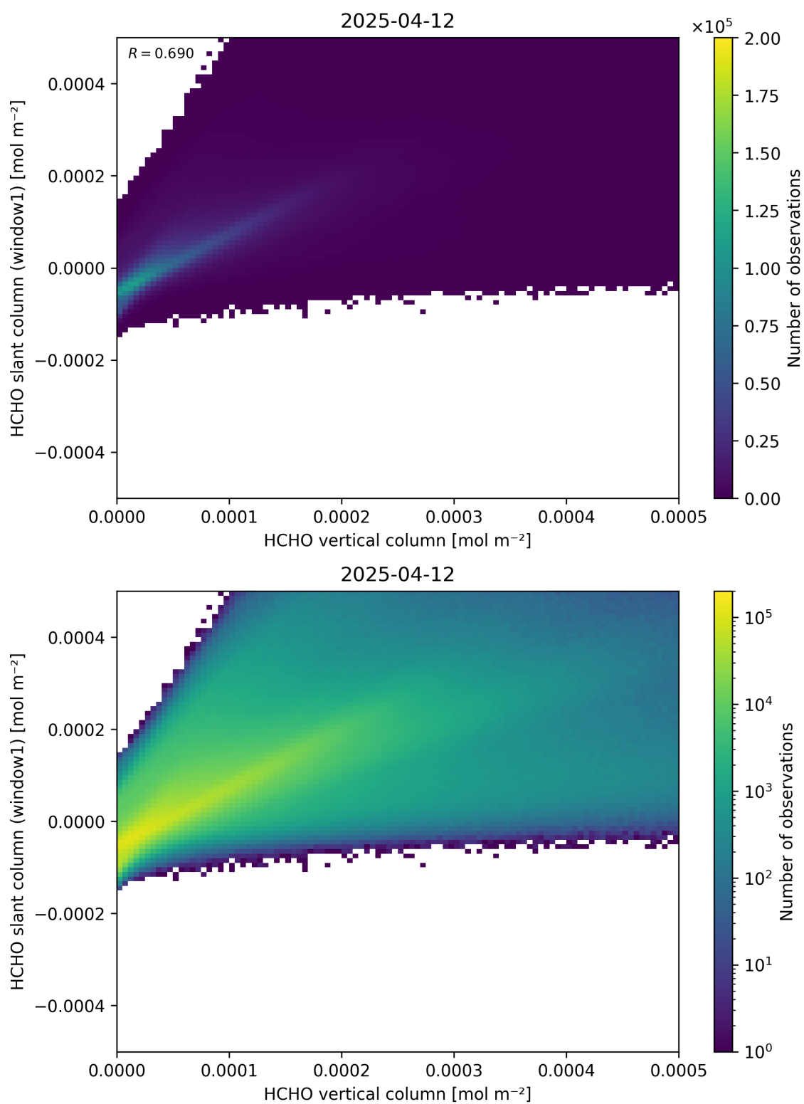
Figure 129: Scatter density plot of “HCHO vertical column” against “HCHO slant column (window1)” for 2025-04-11 to 2025-04-13.
