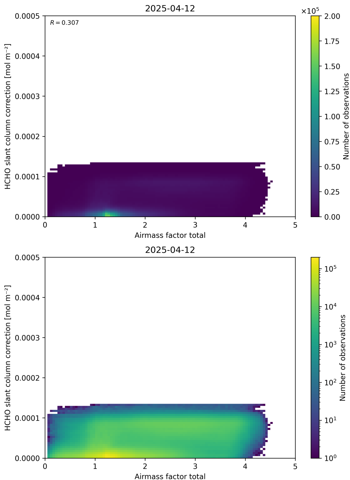
Figure 102: Scatter density plot of “Airmass factor total” against “HCHO slant column correction” for 2025-04-11 to 2025-04-13.
