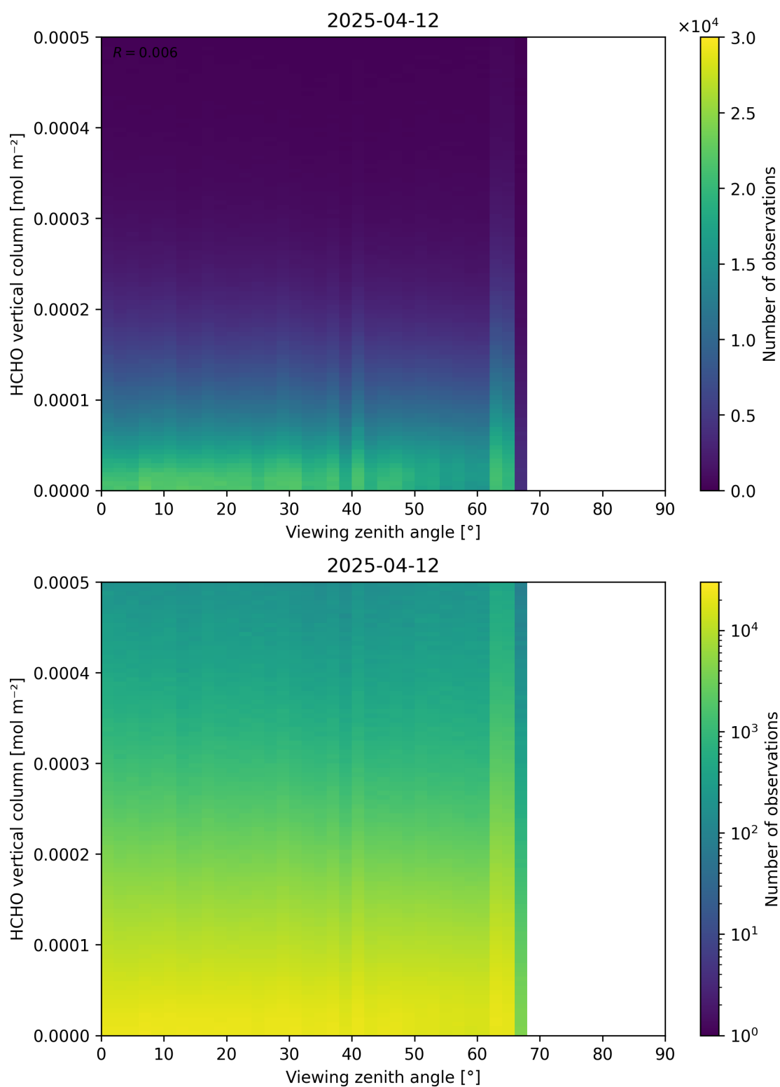
Figure 192: Scatter density plot of “Viewing zenith angle” against “HCHO vertical column” for 2025-04-11 to 2025-04-13.
