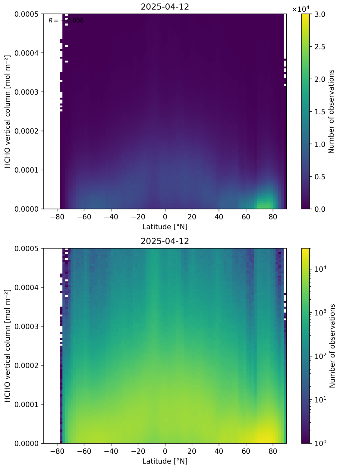
Figure 163: Scatter density plot of “Latitude” against “HCHO vertical column” for 2025-04-11 to 2025-04-13.
