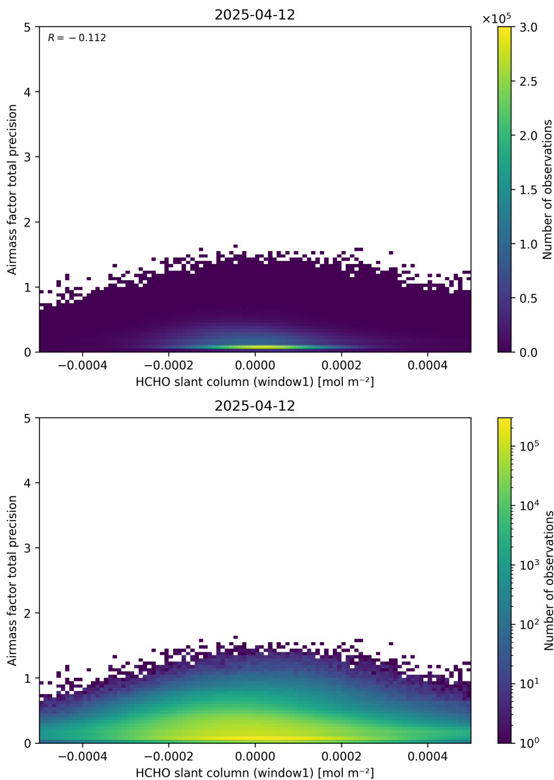
Figure 86: Scatter density plot of “HCHO slant column (window1)” against “Airmass factor total precision” for 2025-04-11 to 2025-04-13.
