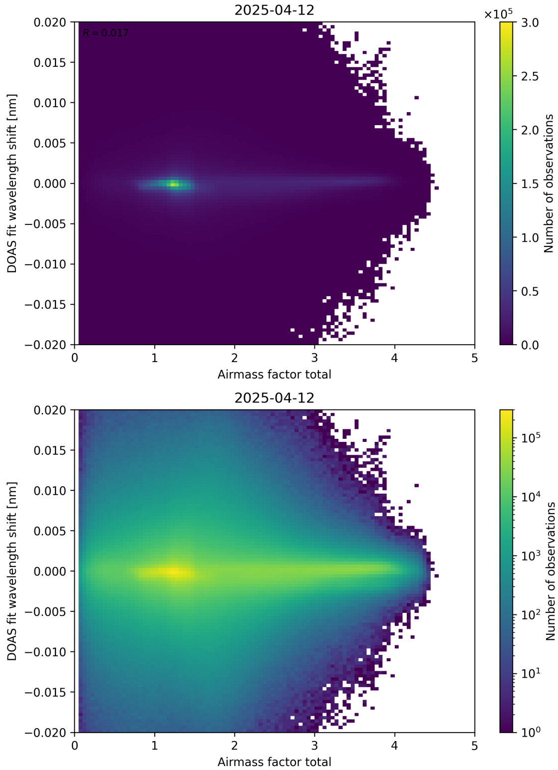
Figure 98: Scatter density plot of “Airmass factor total” against “DOAS fit wavelength shift” for 2025-04-11 to 2025-04-13.
