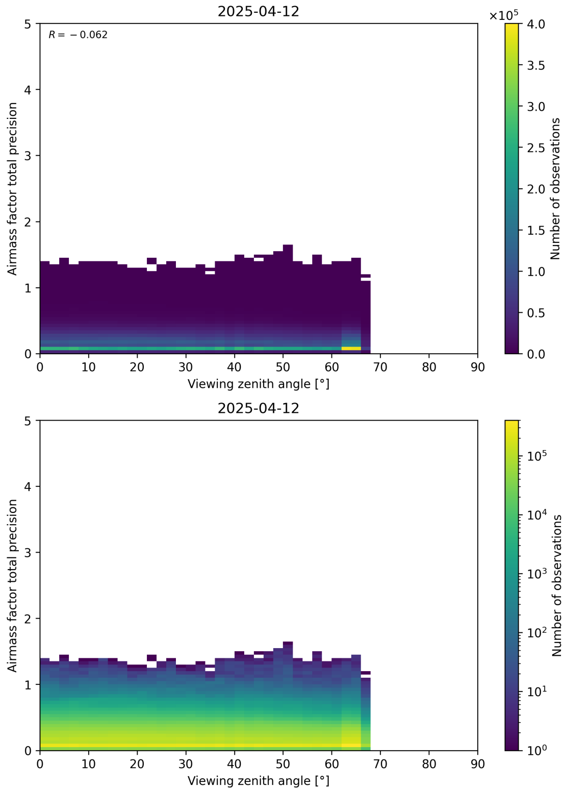
Figure 191: Scatter density plot of “Viewing zenith angle” against “Airmass factor total precision” for 2025-04-11 to 2025-04-13.
