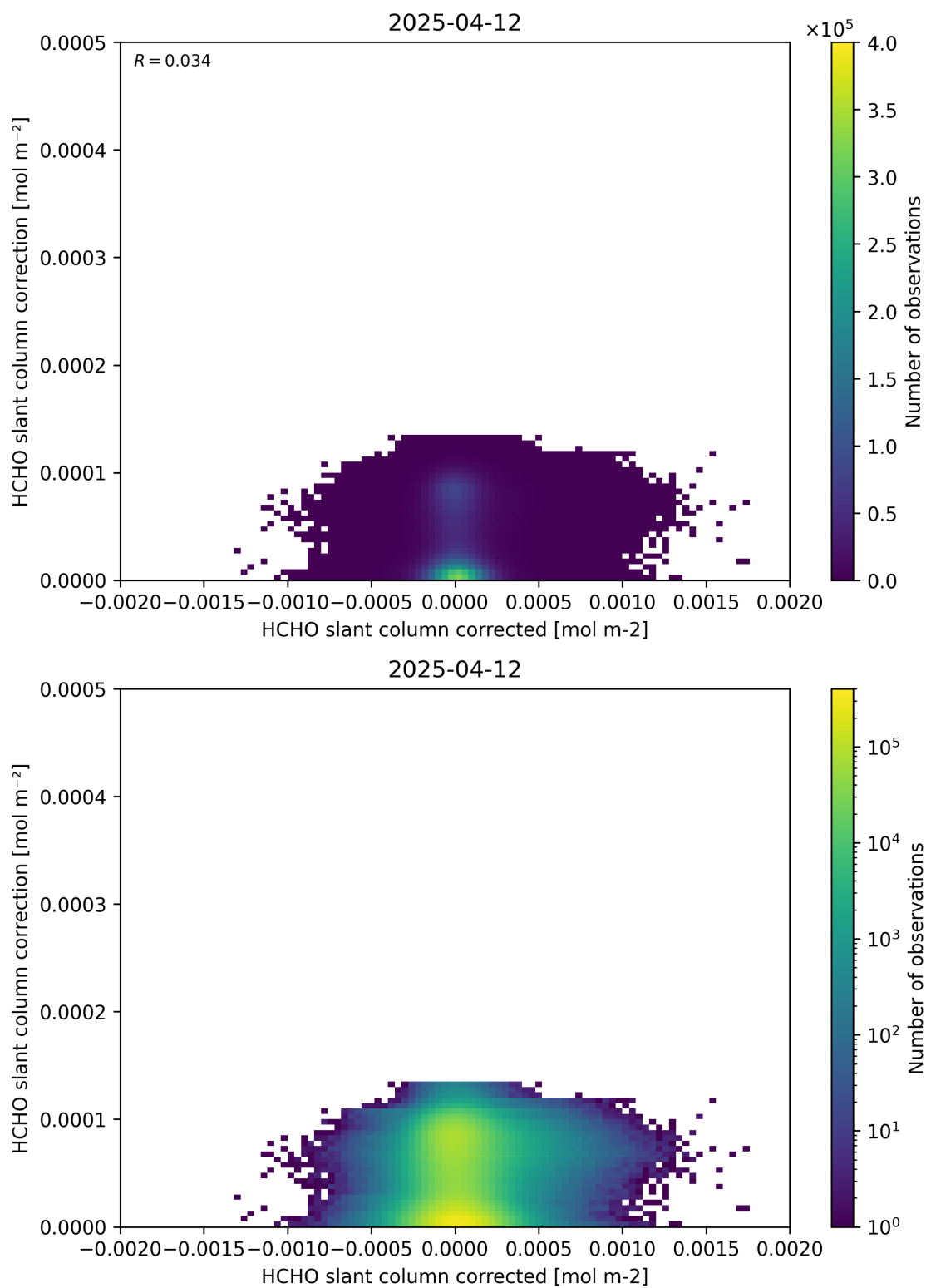
Figure 77: Scatter density plot of “HCHO slant column corrected” against “HCHO slant column correction” for 2025-04-11 to 2025-04-13.
