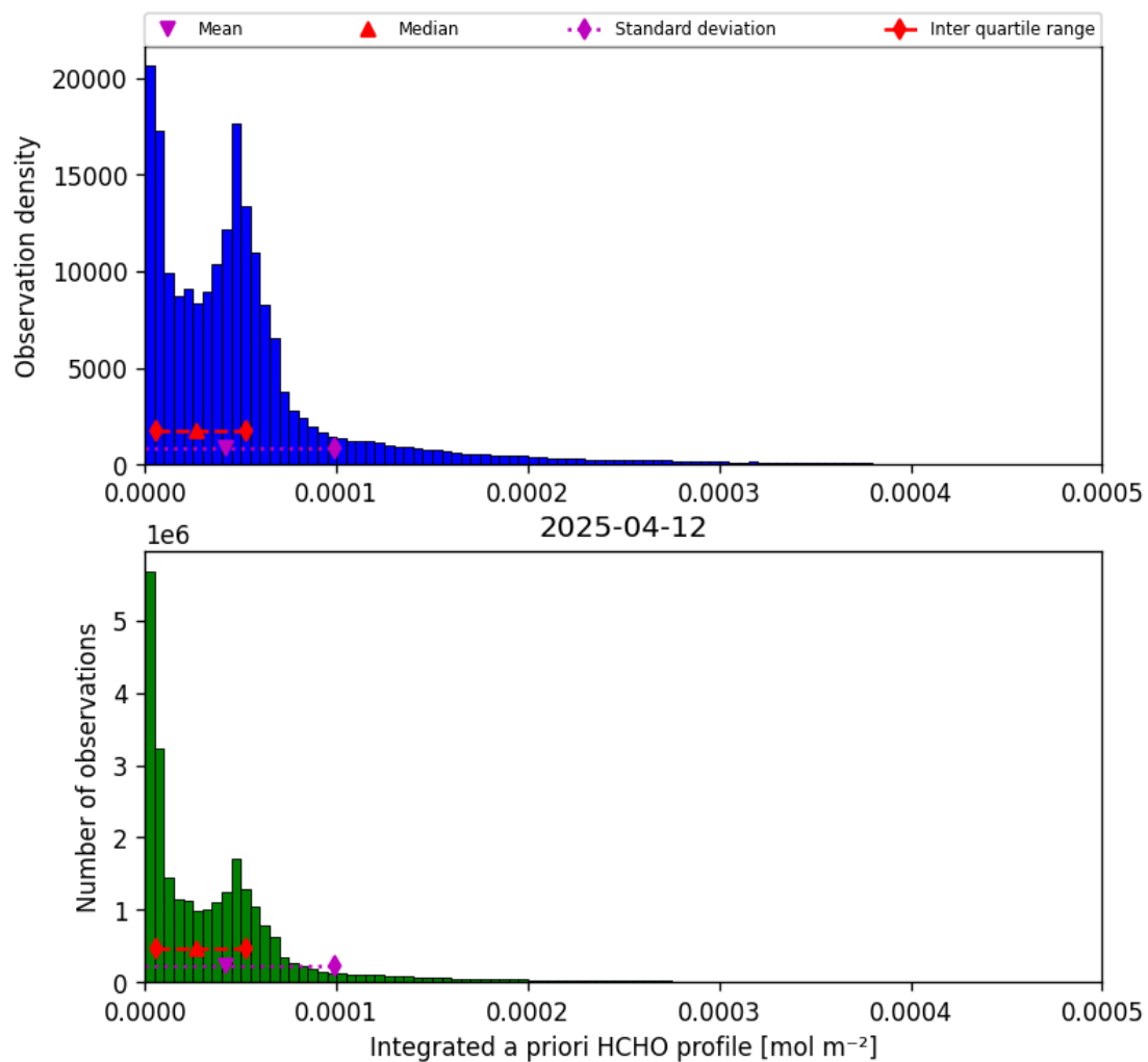
Figure 43: Histogram of “Integrated a priori HCHO profile” for 2025-04-11 to 2025-04-13
