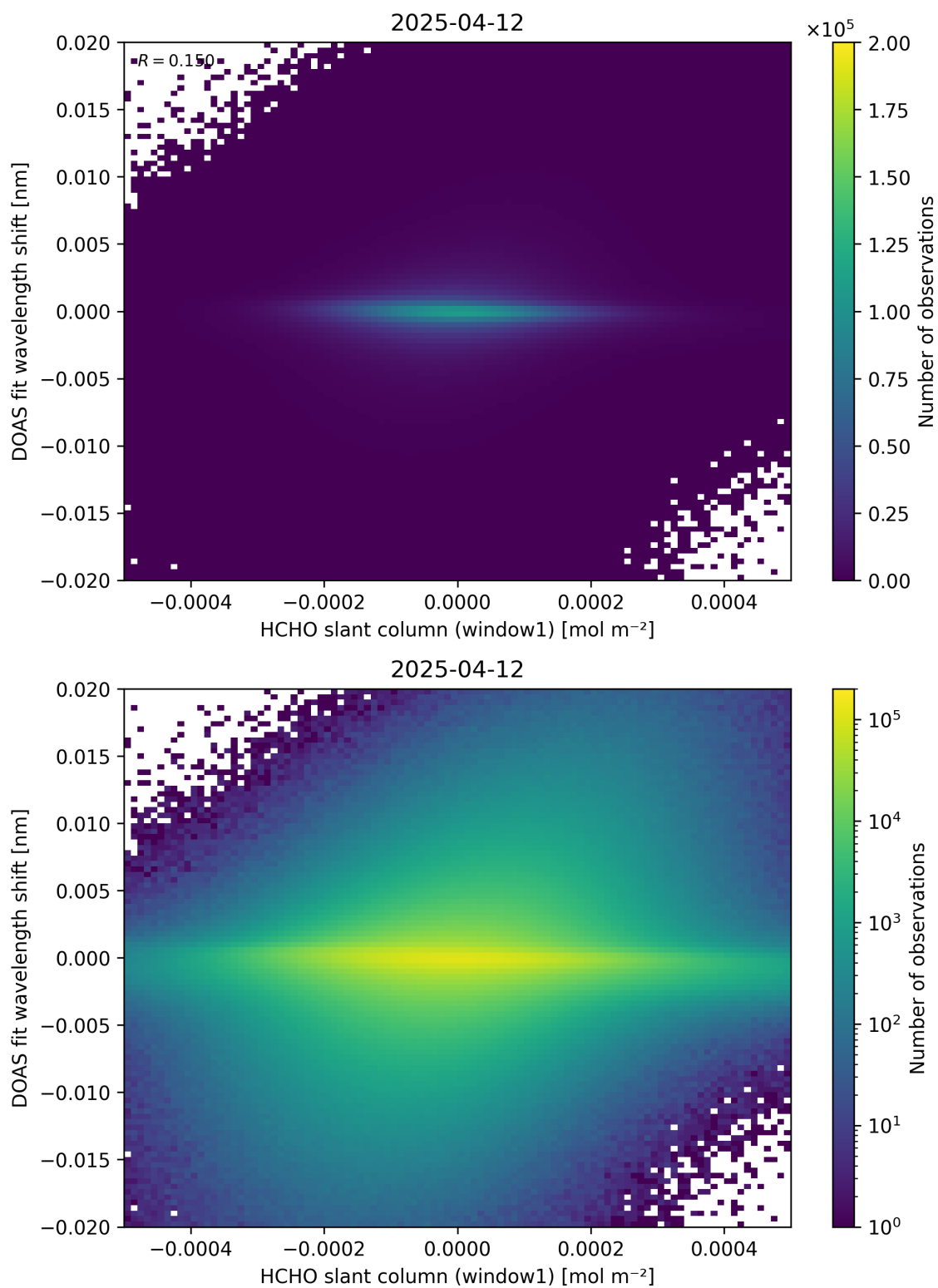
Figure 79: Scatter density plot of “HCHO slant column (window1)” against “DOAS fit wavelength shift” for 2025-04-11 to 2025-04-13.
