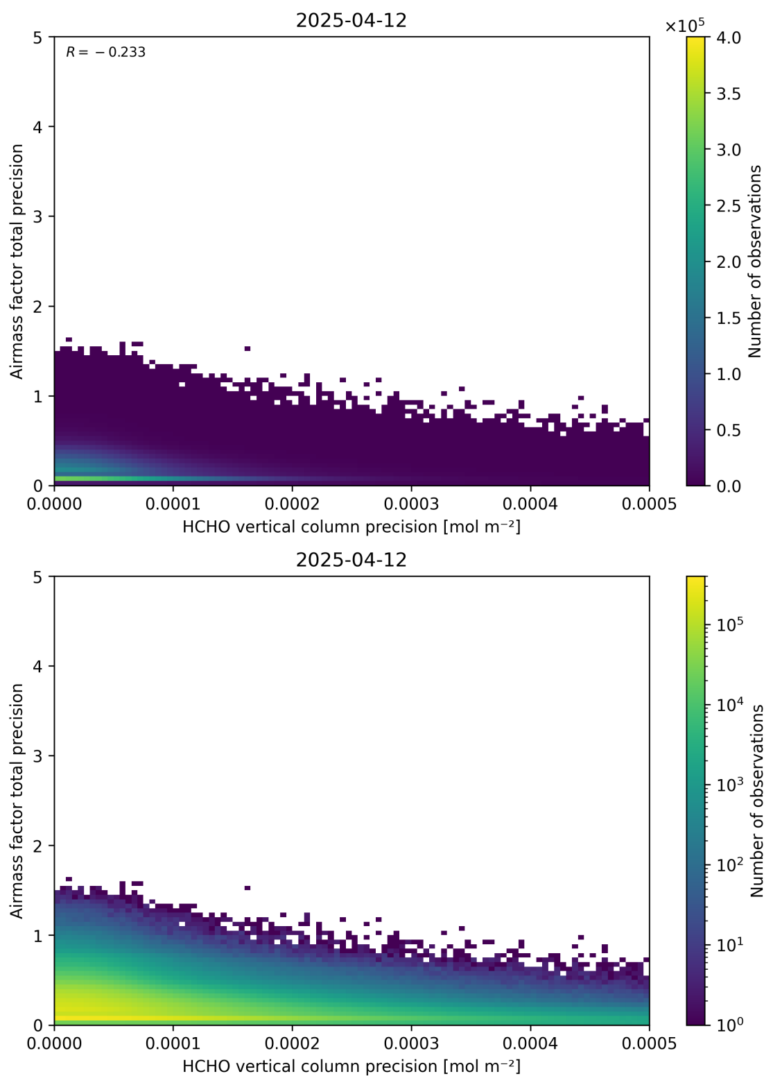
Figure 145: Scatter density plot of “HCHO vertical column precision” against “Airmass factor total precision” for 2025-04-11 to 2025-04-13.
