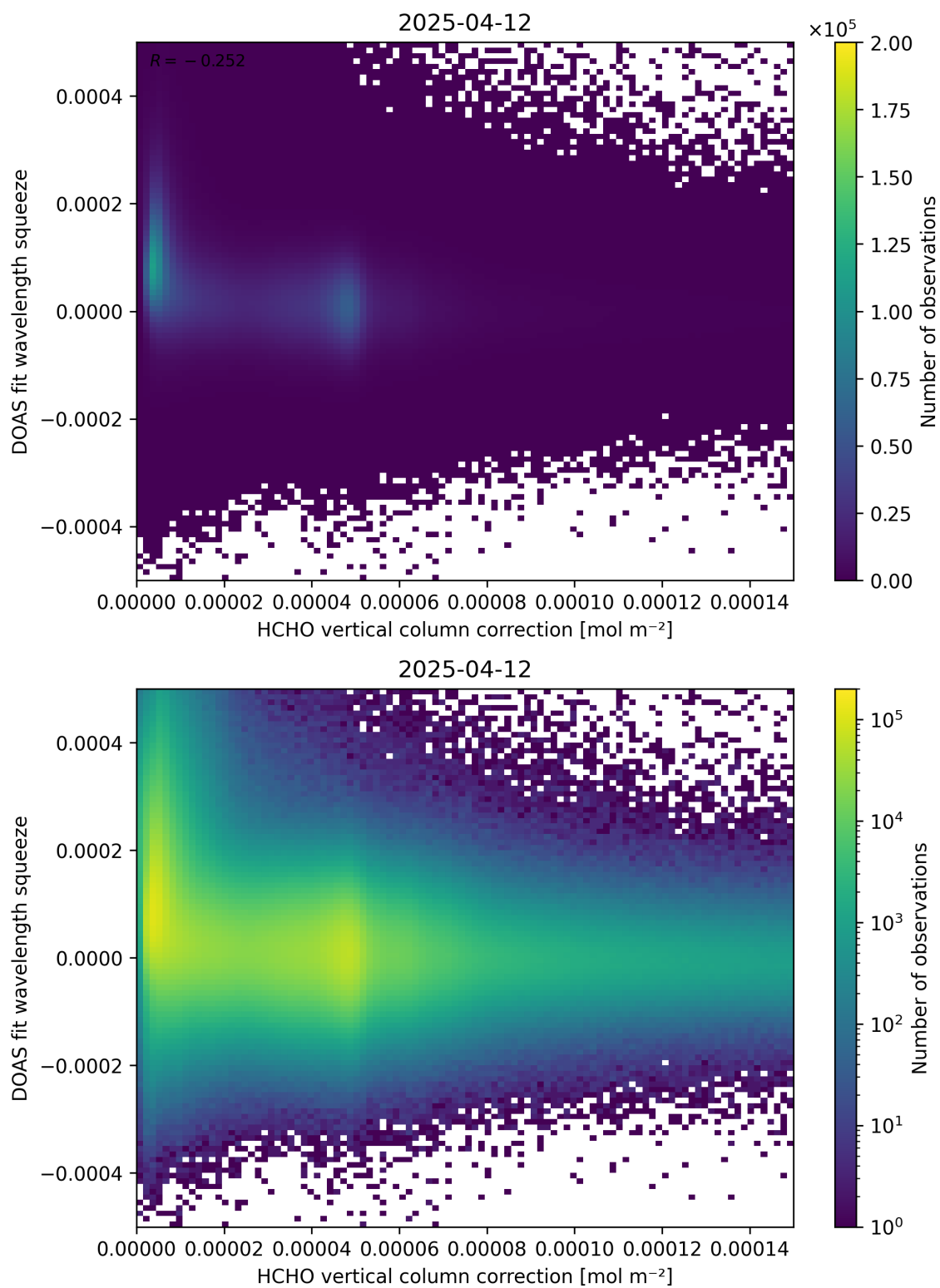
Figure 114: Scatter density plot of “HCHO vertical column correction” against “DOAS fit wavelength squeeze” for 2025-04-11 to 2025-04-13.
