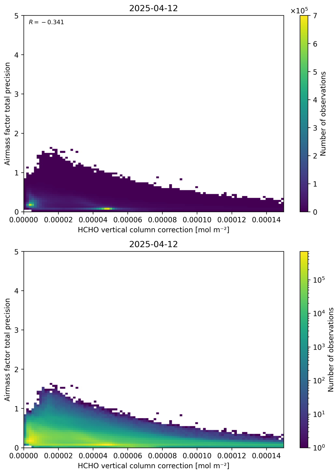
Figure 121: Scatter density plot of “HCHO vertical column correction” against “Airmass factor total precision” for 2025-04-11 to 2025-04-13.
