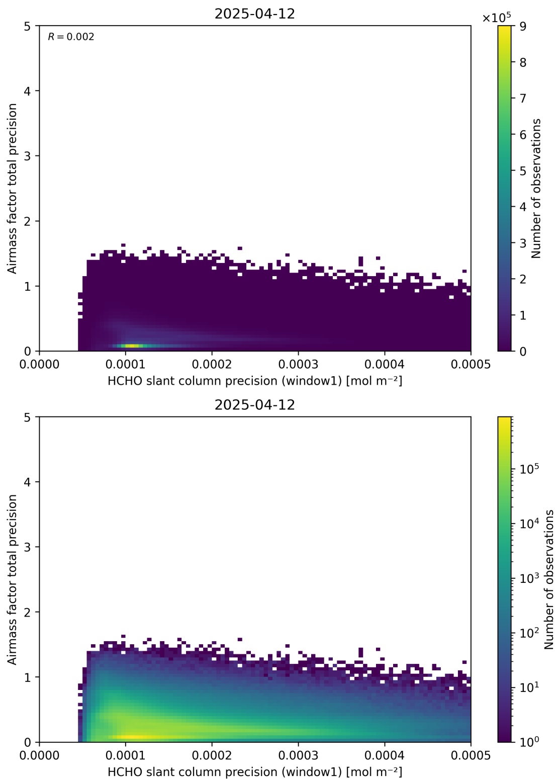
Figure 95: Scatter density plot of “HCHO slant column precision (window1)” against “Airmass factor total precision” for 2025-04-11 to 2025-04-13.
