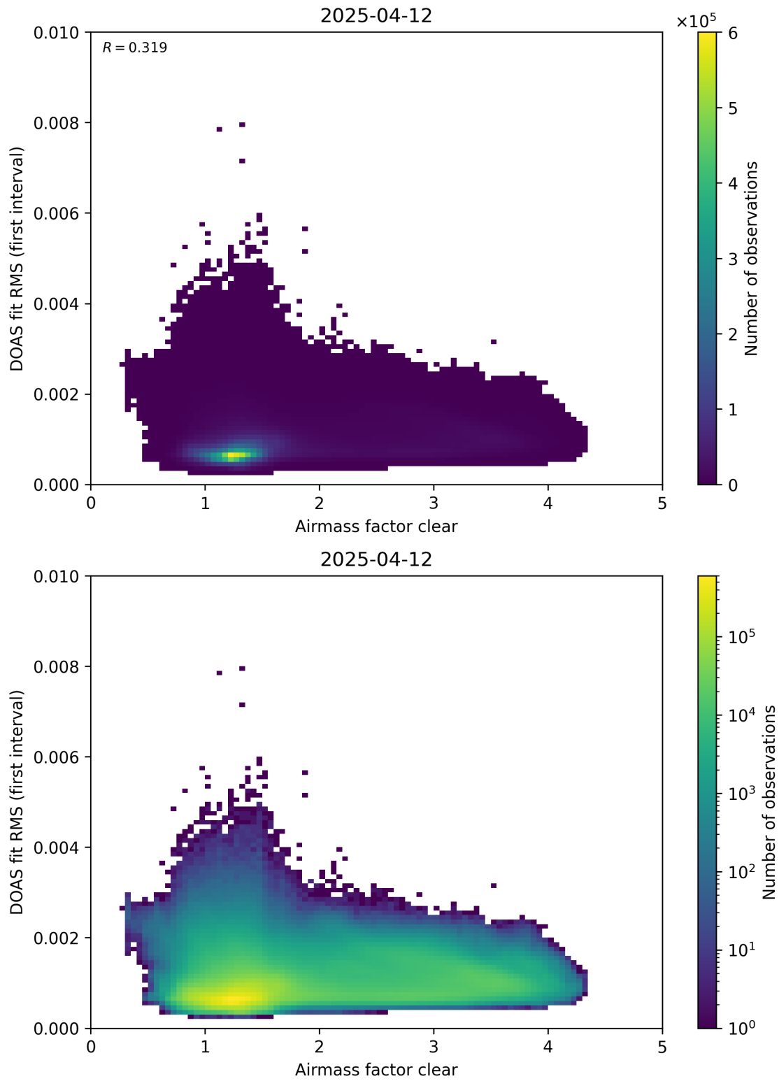
Figure 71: Scatter density plot of “Airmass factor clear” against “DOAS fit RMS (first interval)” for 2025-04-11 to 2025-04-13.
