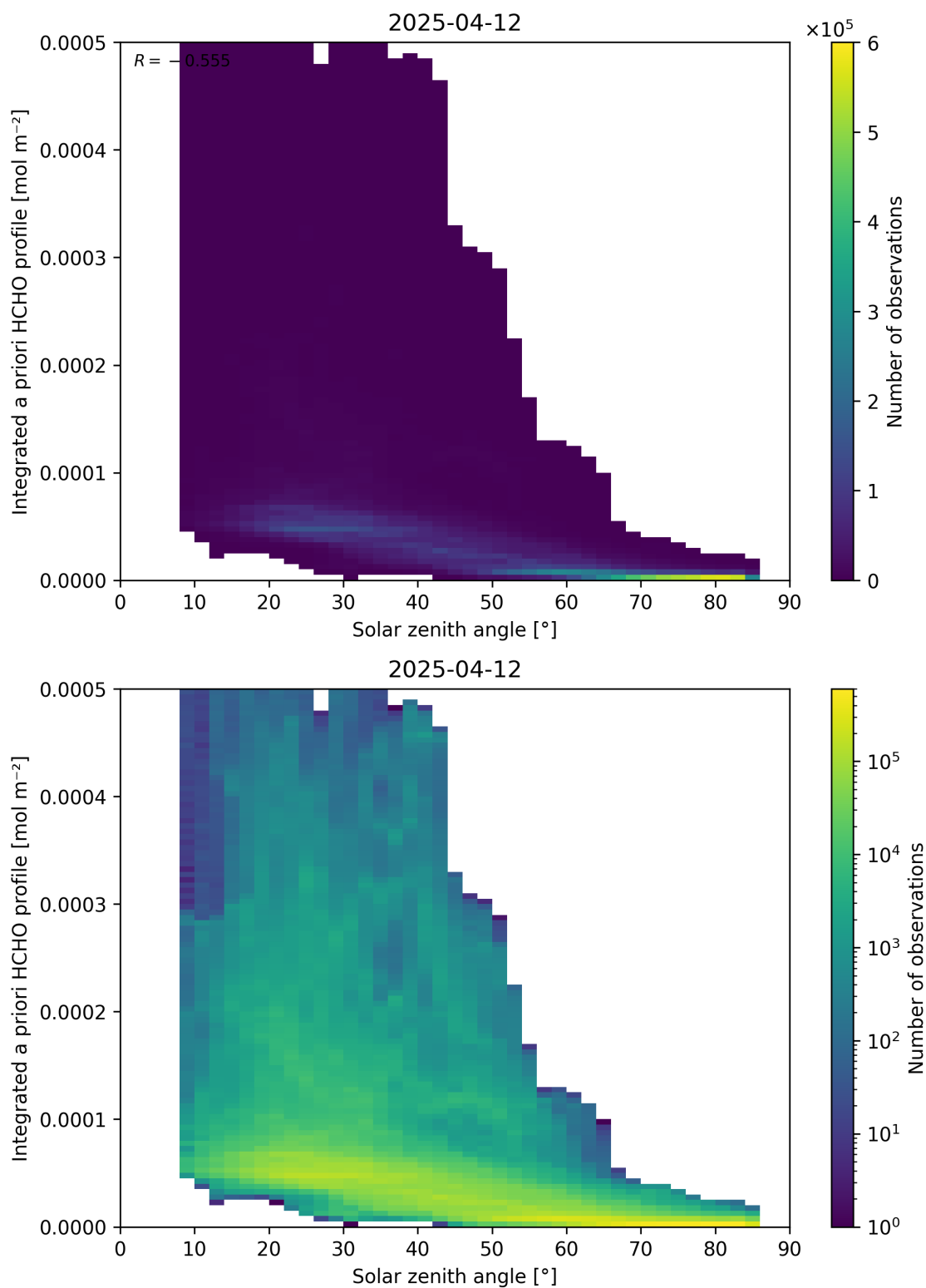
Figure 180: Scatter density plot of “Solar zenith angle” against “Integrated a priori HCHO profile” for 2025-04-11 to 2025-04-13.
