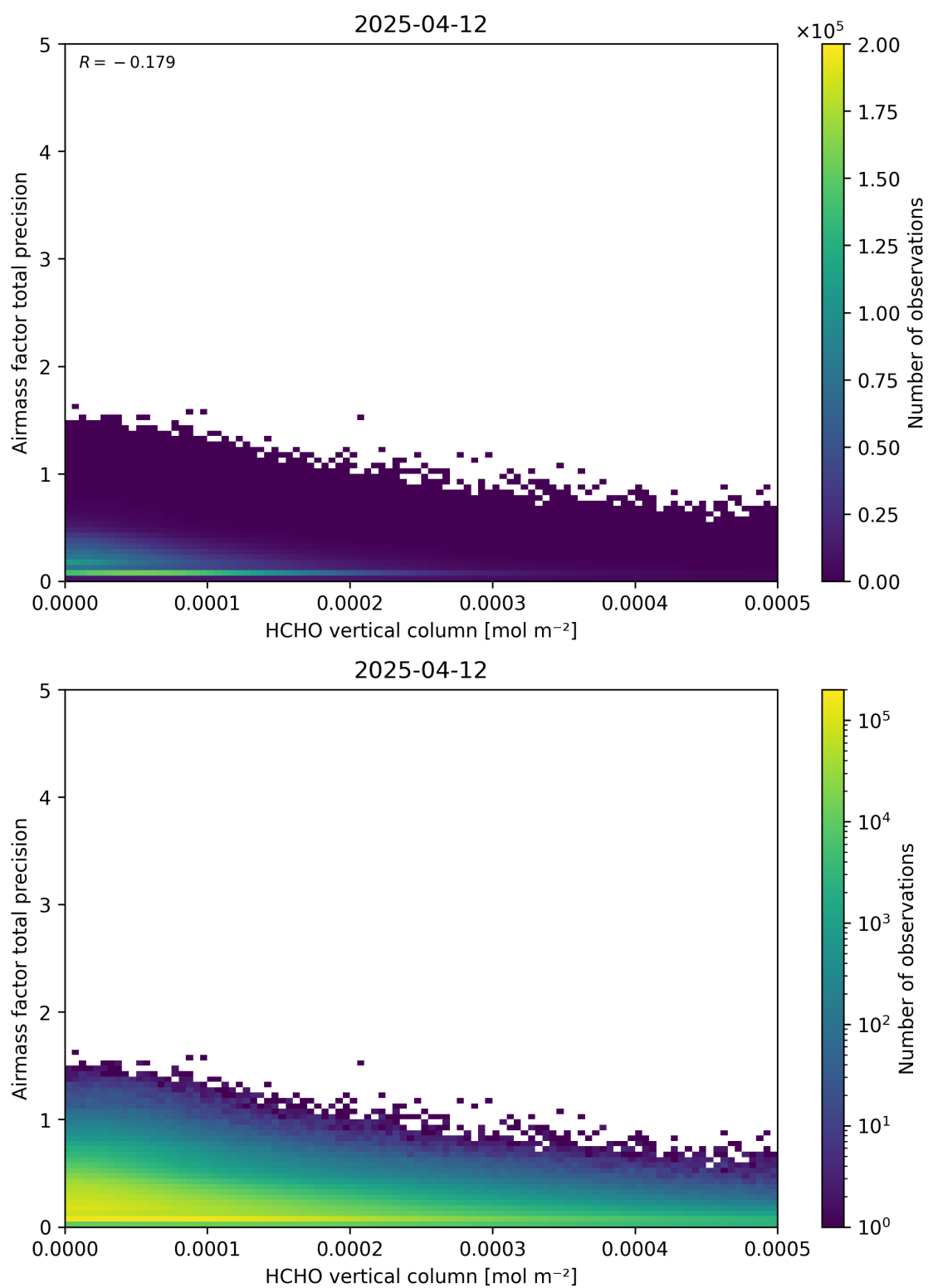
Figure 132: Scatter density plot of “HCHO vertical column” against “Airmass factor total precision” for 2025-04-11 to 2025-04-13.
