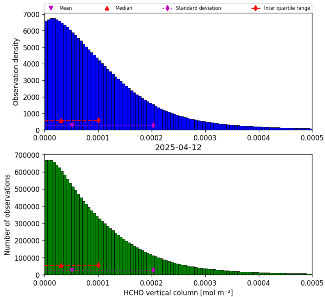
Figure 35: Histogram of “HCHO vertical column” for 2025-04-11 to 2025-04-13
