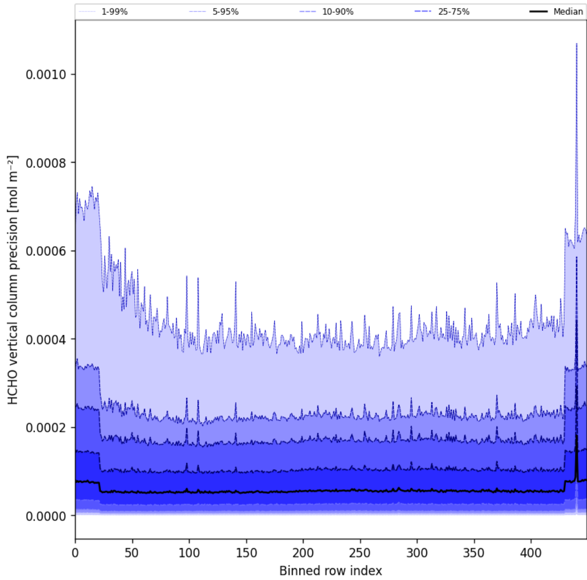
Figure 50: Along track statistics of “HCHO vertical column precision” for 2025-04-11 to 2025-04-13
