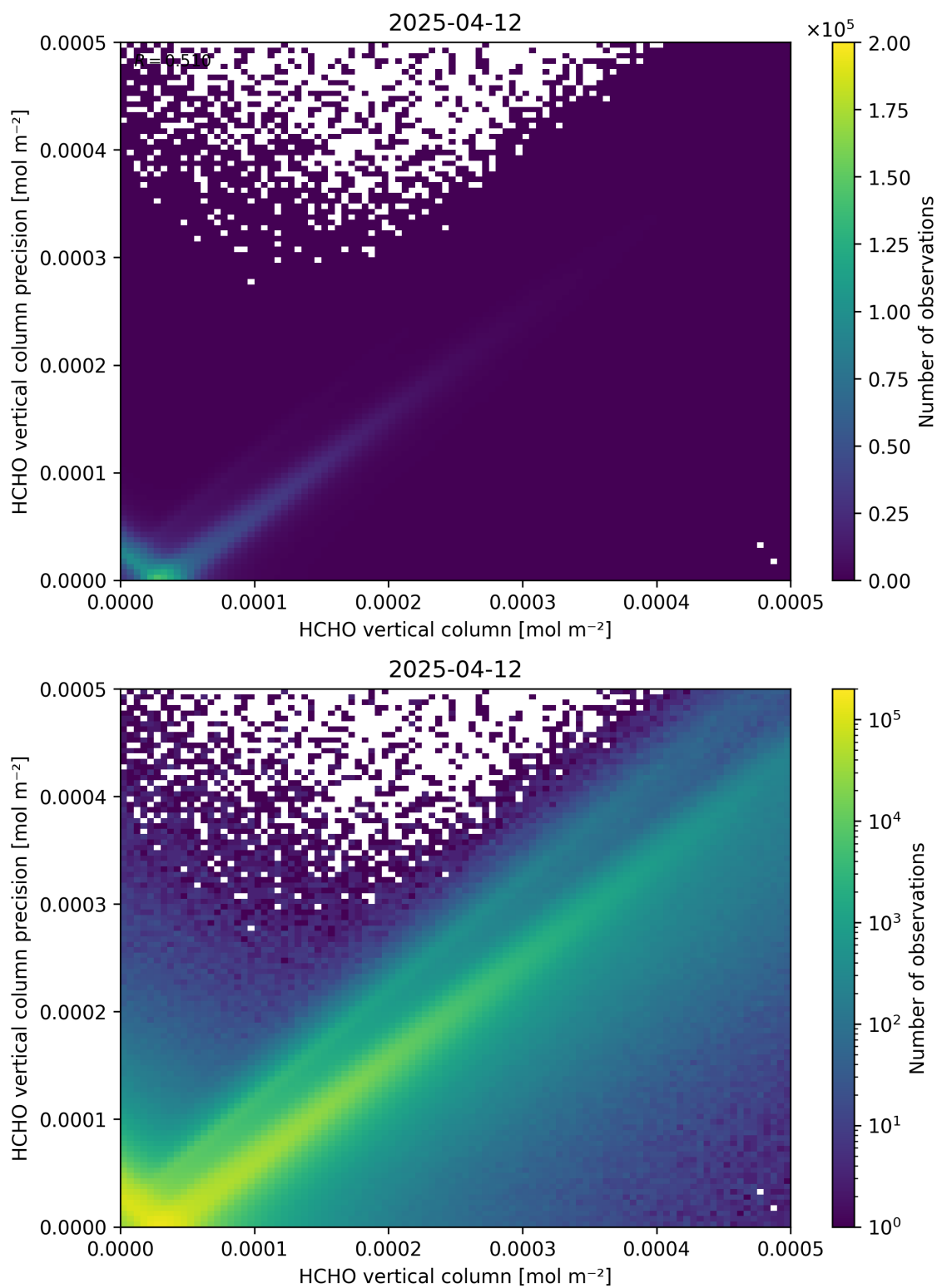
Figure 134: Scatter density plot of “HCHO vertical column” against “HCHO vertical column precision” for 2025-04-11 to 2025-04-13.
