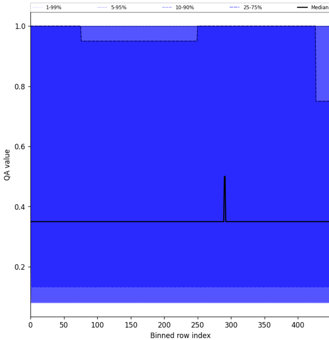
Figure 48: Along track statistics of "QA value" for 2025-04-11 to 2025-04-13
