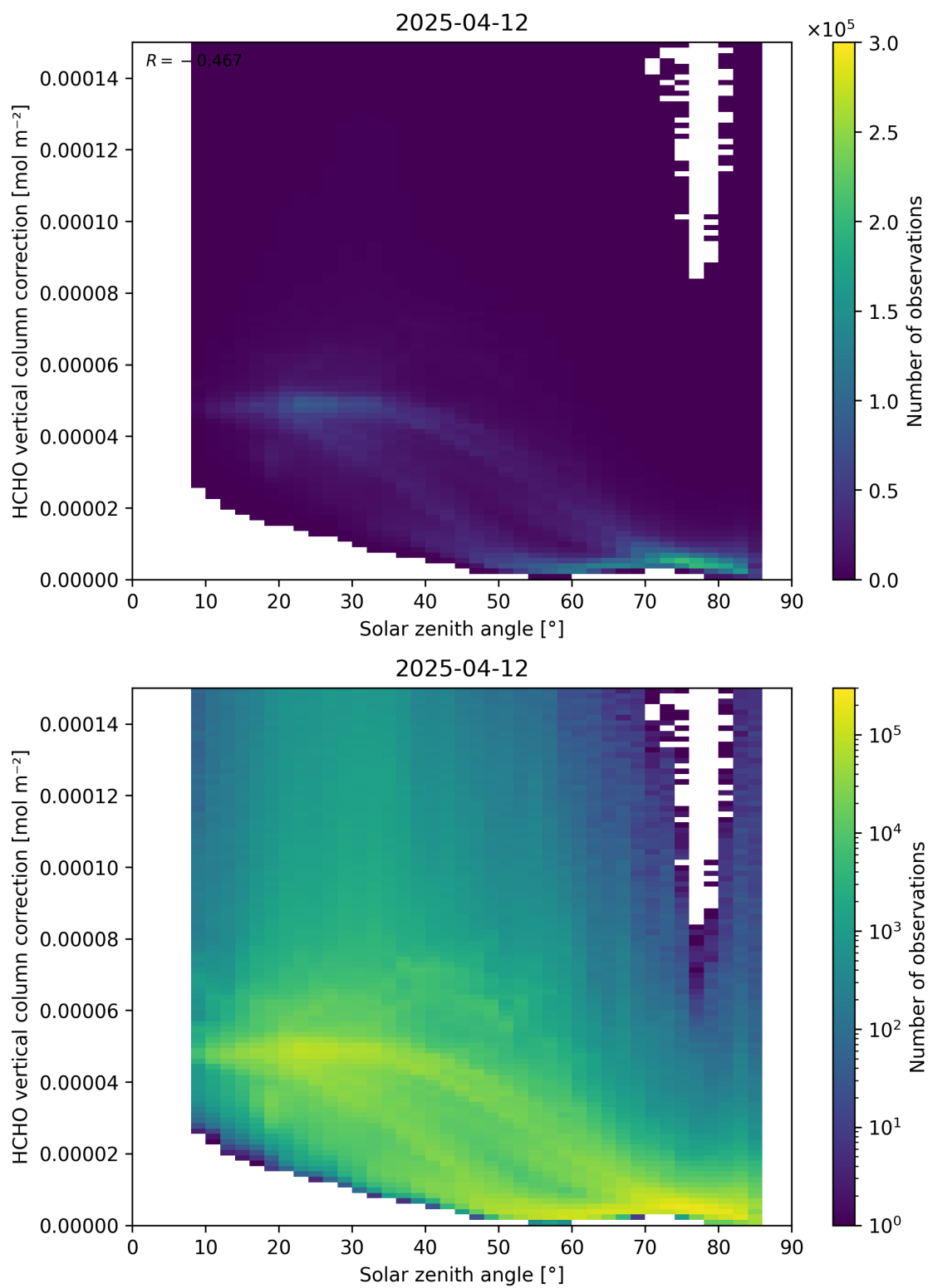
Figure 178: Scatter density plot of “Solar zenith angle” against “HCHO vertical column correction” for 2025-04-11 to 2025-04-13.
