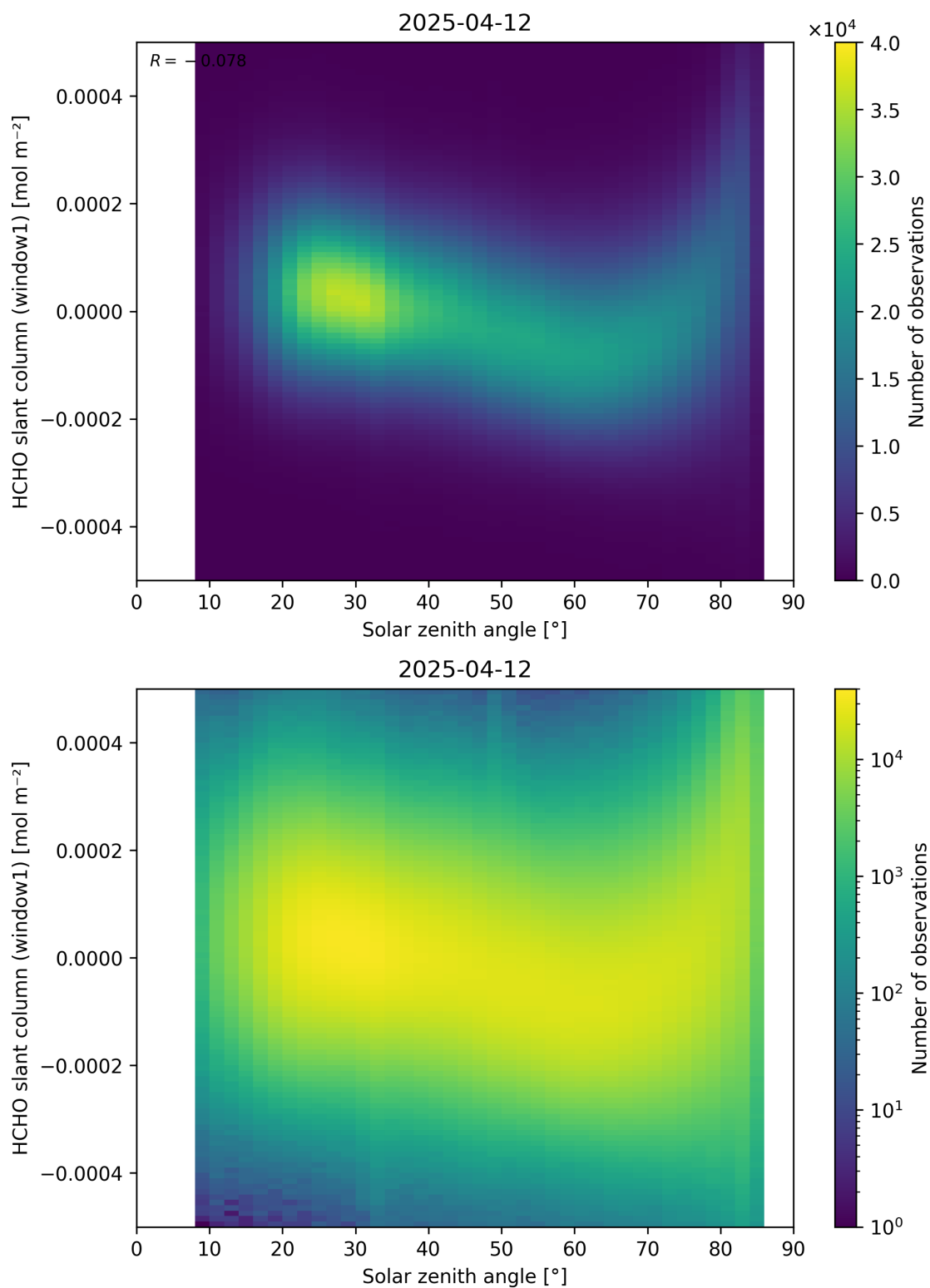
Figure 173: Scatter density plot of “Solar zenith angle” against “HCHO slant column (window1)” for 2025-04-11 to 2025-04-13.
