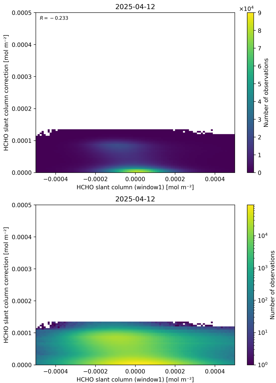
Figure 83: Scatter density plot of “HCHO slant column (window1)” against “HCHO slant column correction” for 2025-04-11 to 2025-04-13.
