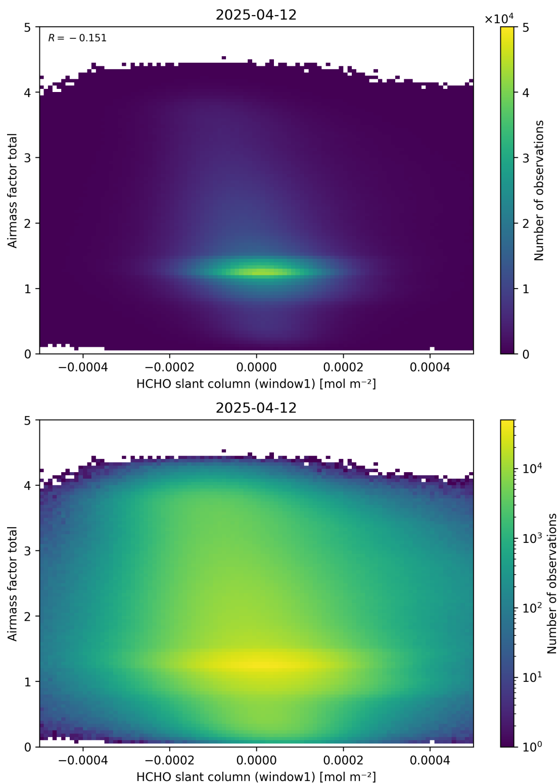
Figure 85: Scatter density plot of “HCHO slant column (window1)” against “Airmass factor total” for 2025-04-11 to 2025-04-13.
