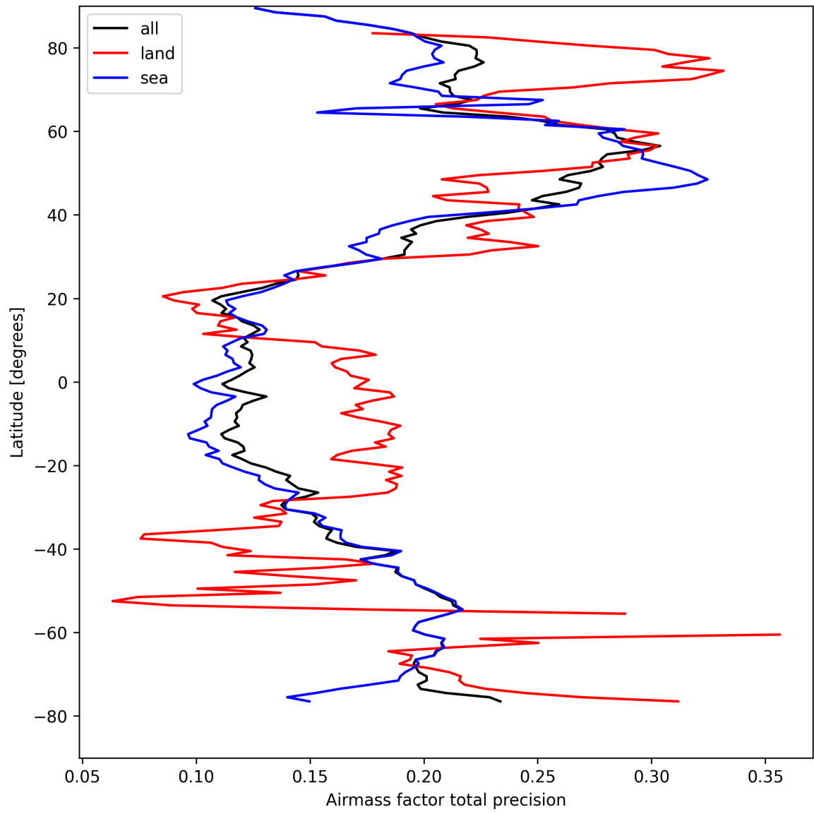
Figure 27: Zonal average of “Airmass factor total precision” for 2025-04-11 to 2025-04-13.
