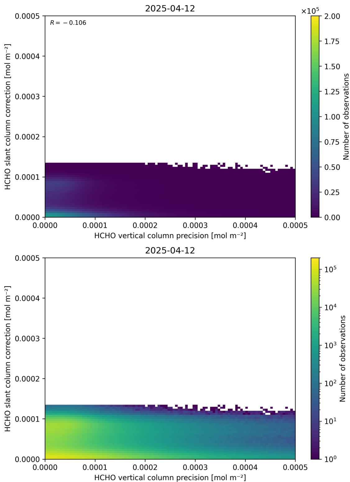
Figure 141: Scatter density plot of “HCHO vertical column precision” against “HCHO slant column correction” for 2025-04-11 to 2025-04-13.
