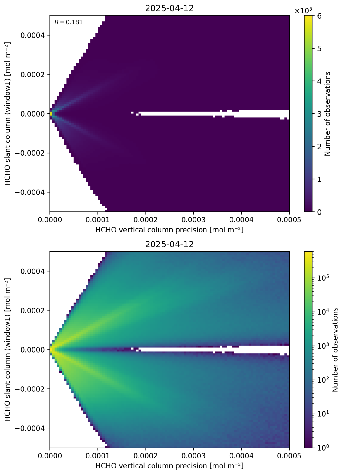
Figure 142: Scatter density plot of “HCHO vertical column precision” against “HCHO slant column (window1)” for 2025-04-11 to 2025-04-13.
