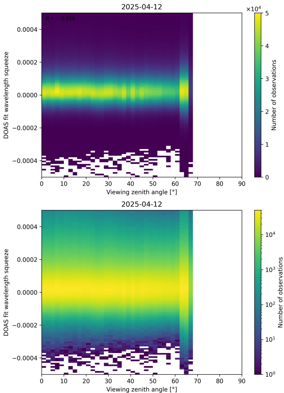
Figure 184: Scatter density plot of “Viewing zenith angle” against “DOAS fit wavelength squeeze” for 2025-04-11 to 2025-04-13.
