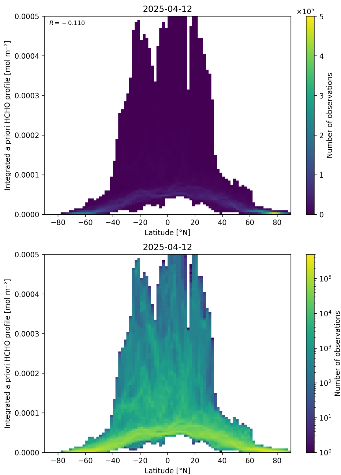
Figure 166: Scatter density plot of “Latitude” against “Integrated a priori HCHO profile” for 2025-04-11 to 2025-04-13.
