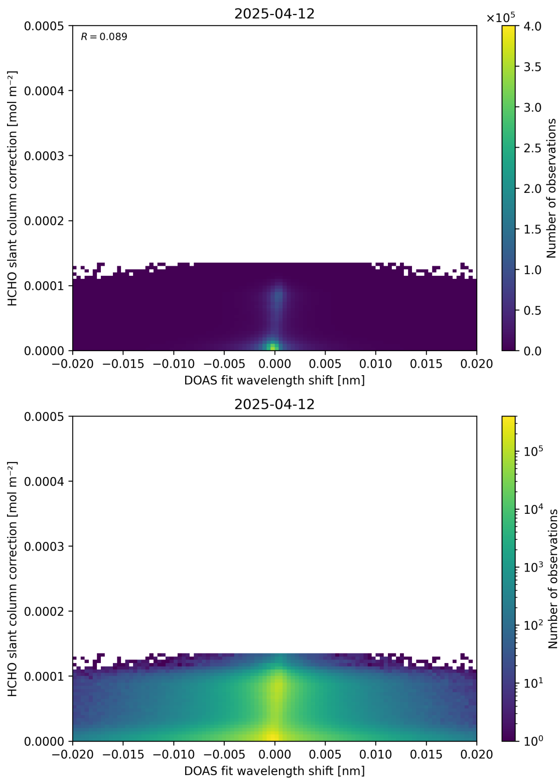
Figure 67: Scatter density plot of “DOAS fit wavelength shift” against “HCHO slant column correction” for 2025-04-11 to 2025-04-13.
