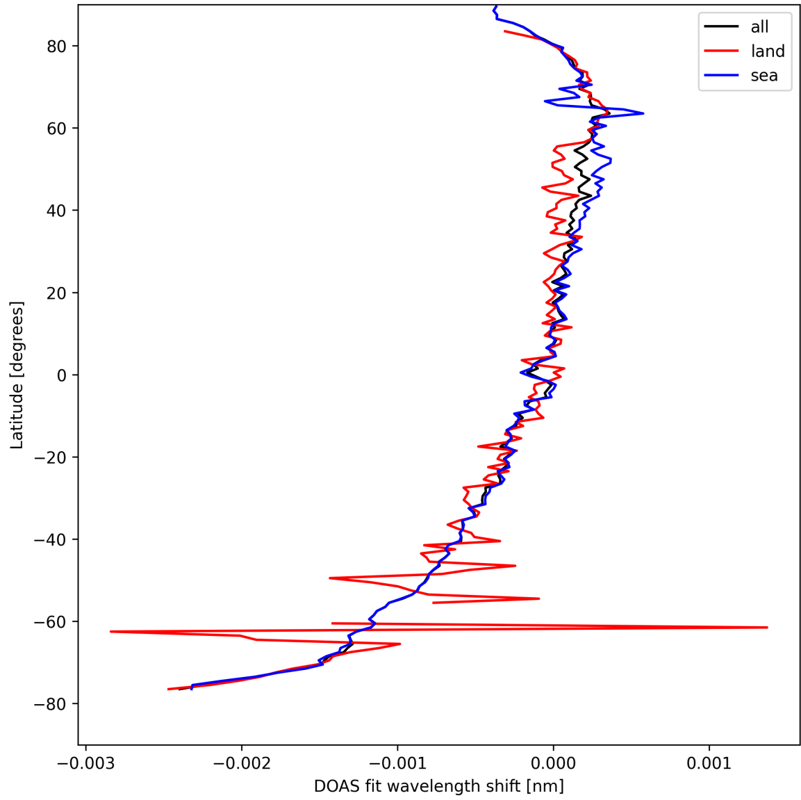
Figure 30: Zonal average of "DOAS fit wavelength shift" for 2025-04-11 to 2025-04-13.
