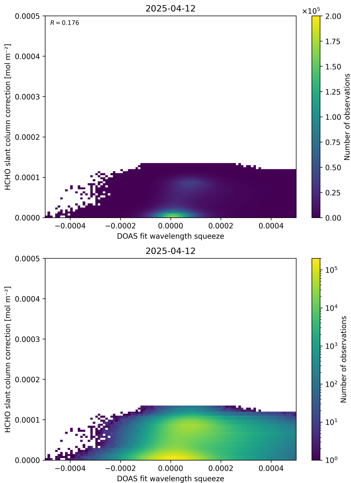
Figure 70: Scatter density plot of “DOAS fit wavelength squeeze” against “HCHO slant column correction” for 2025-04-11 to 2025-04-13.
