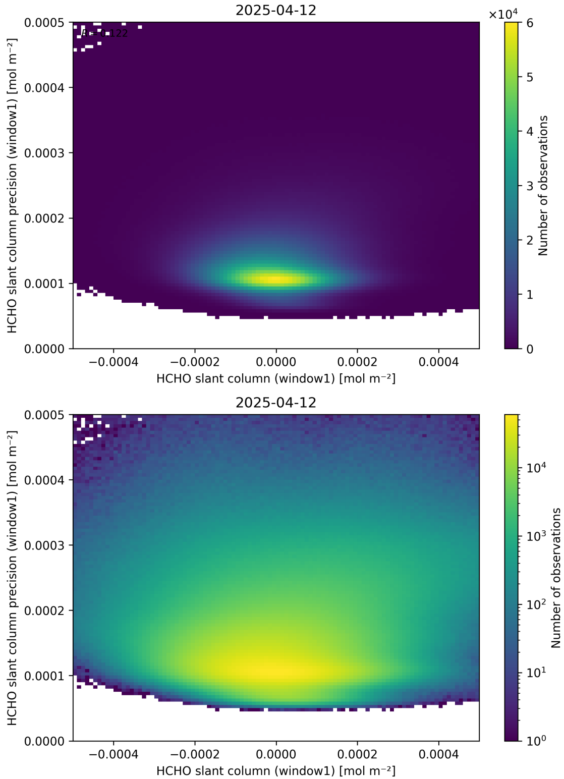
Figure 84: Scatter density plot of “HCHO slant column (window1)” against “HCHO slant column precision (window1)” for 2025-04-11 to 2025-04-13.
