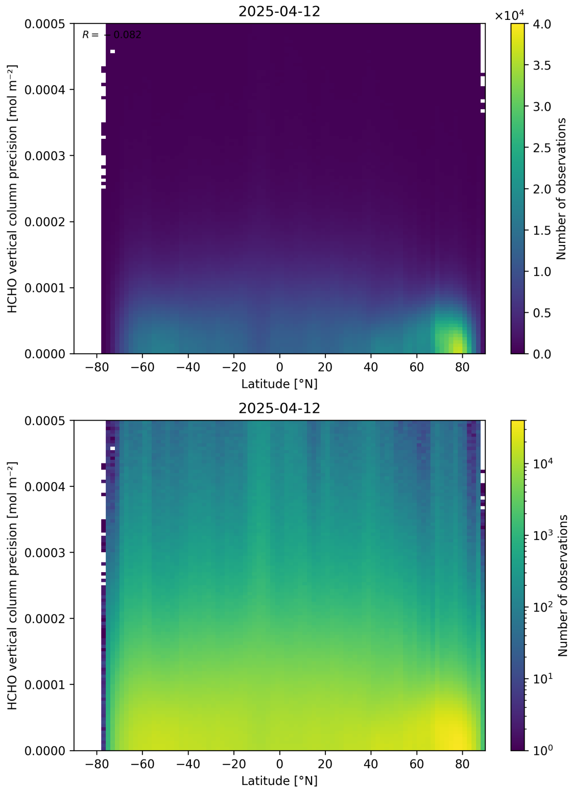
Figure 165: Scatter density plot of “Latitude” against “HCHO vertical column precision” for 2025-04-11 to 2025-04-13.
