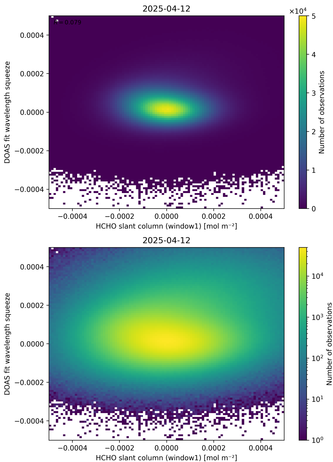
Figure 80: Scatter density plot of “HCHO slant column (window1)” against “DOAS fit wavelength squeeze” for 2025-04-11 to 2025-04-13.
