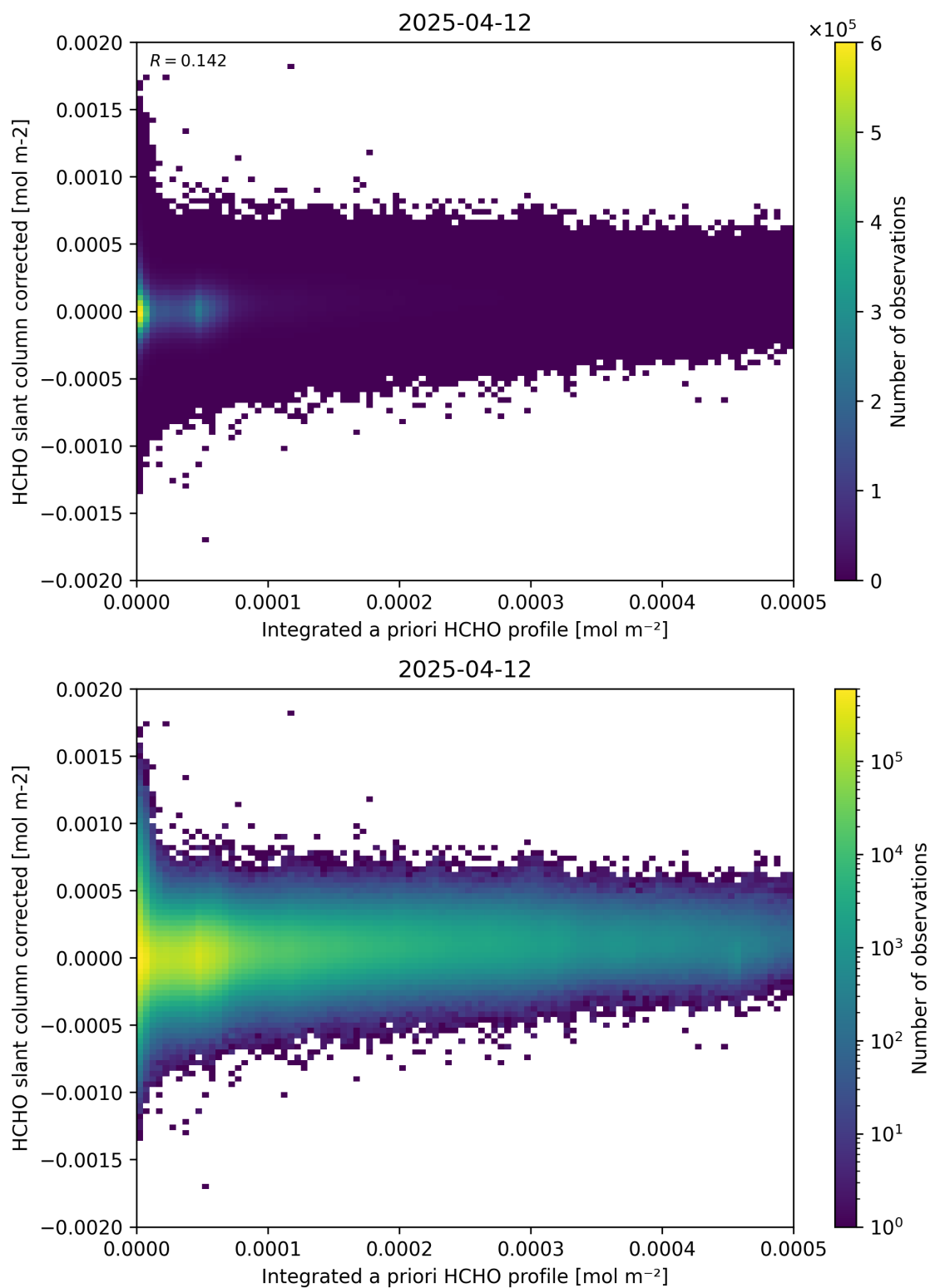
Figure 151: Scatter density plot of “Integrated a priori HCHO profile” against “HCHO slant column corrected” for 2025-04-11 to 2025-04-13.
