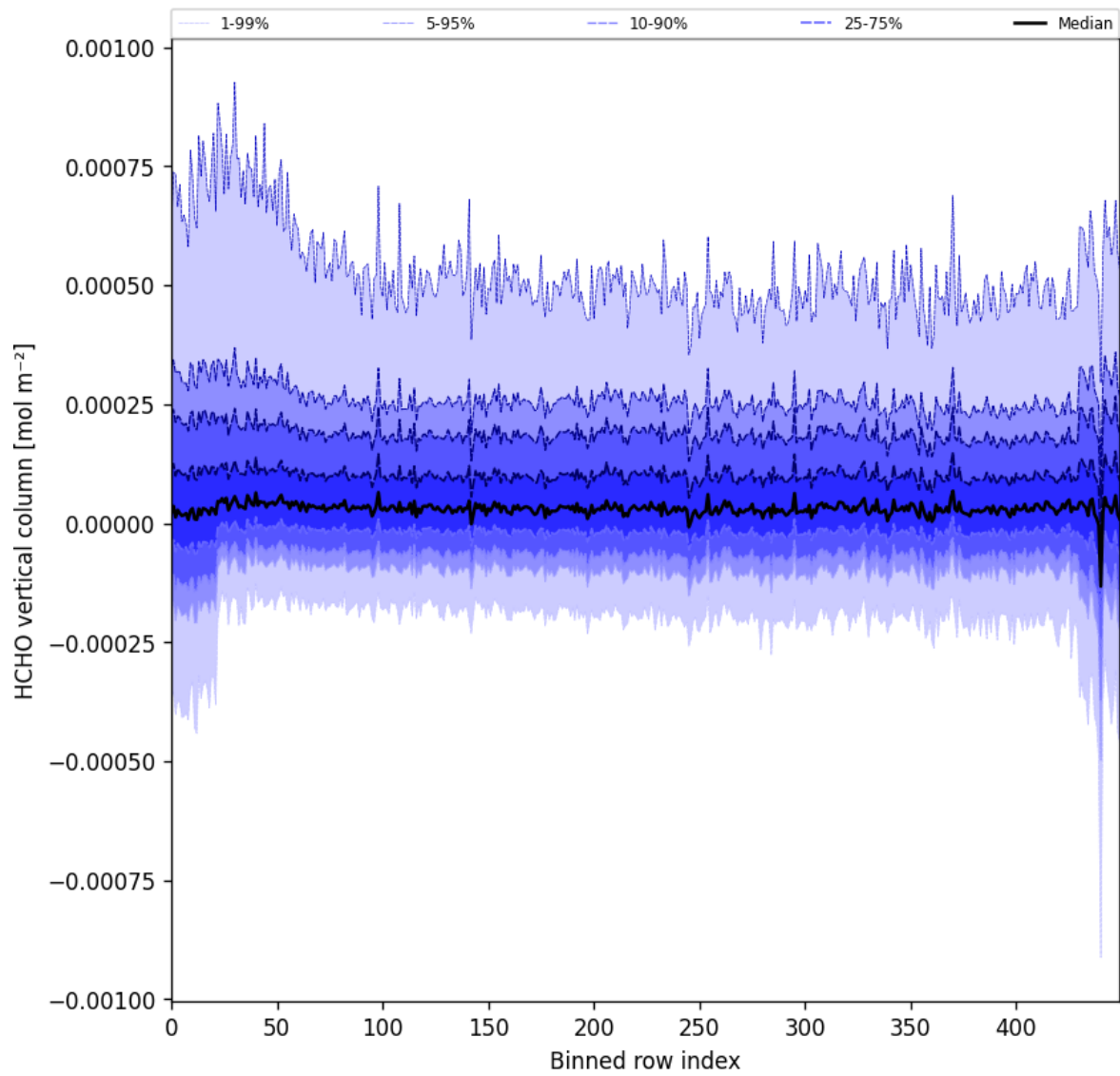
Figure 49: Along track statistics of “HCHO vertical column” for 2025-04-11 to 2025-04-13
