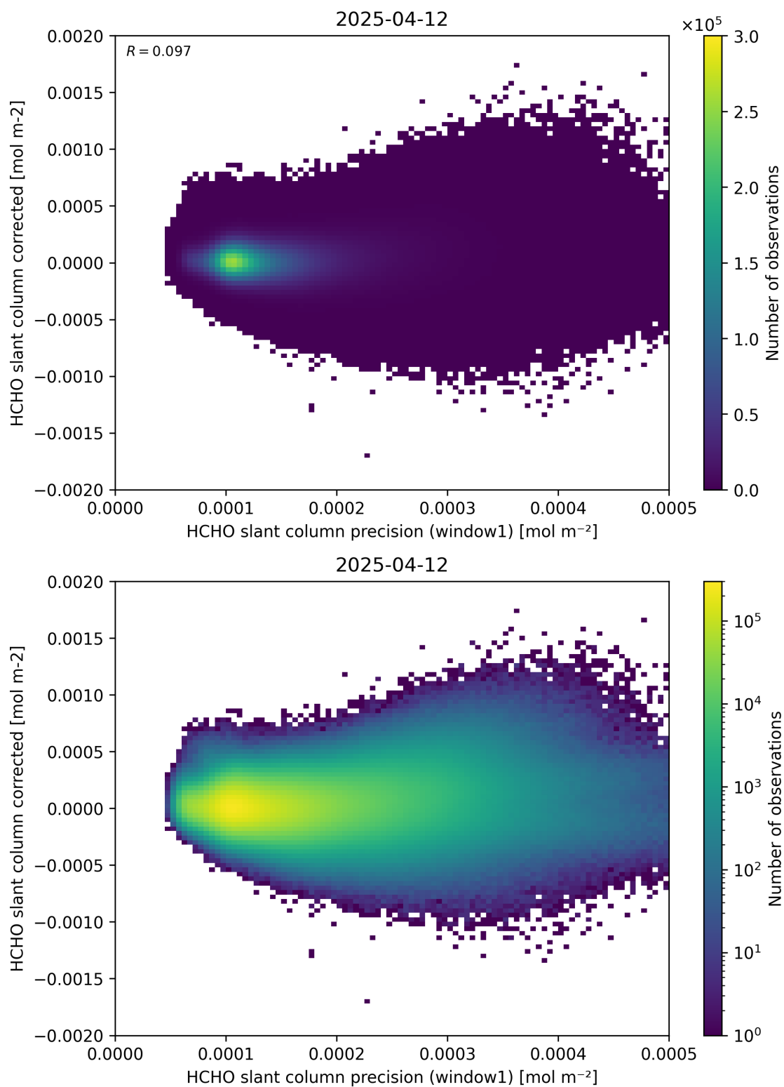
Figure 92: Scatter density plot of “HCHO slant column precision (window1)” against “HCHO slant column corrected” for 2025-04-11 to 2025-04-13.
