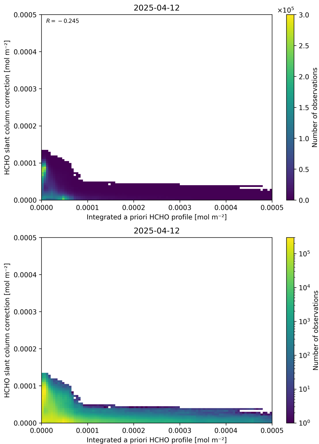
Figure 152: Scatter density plot of “Integrated a priori HCHO profile” against “HCHO slant column correction” for 2025-04-11 to 2025-04-13.
