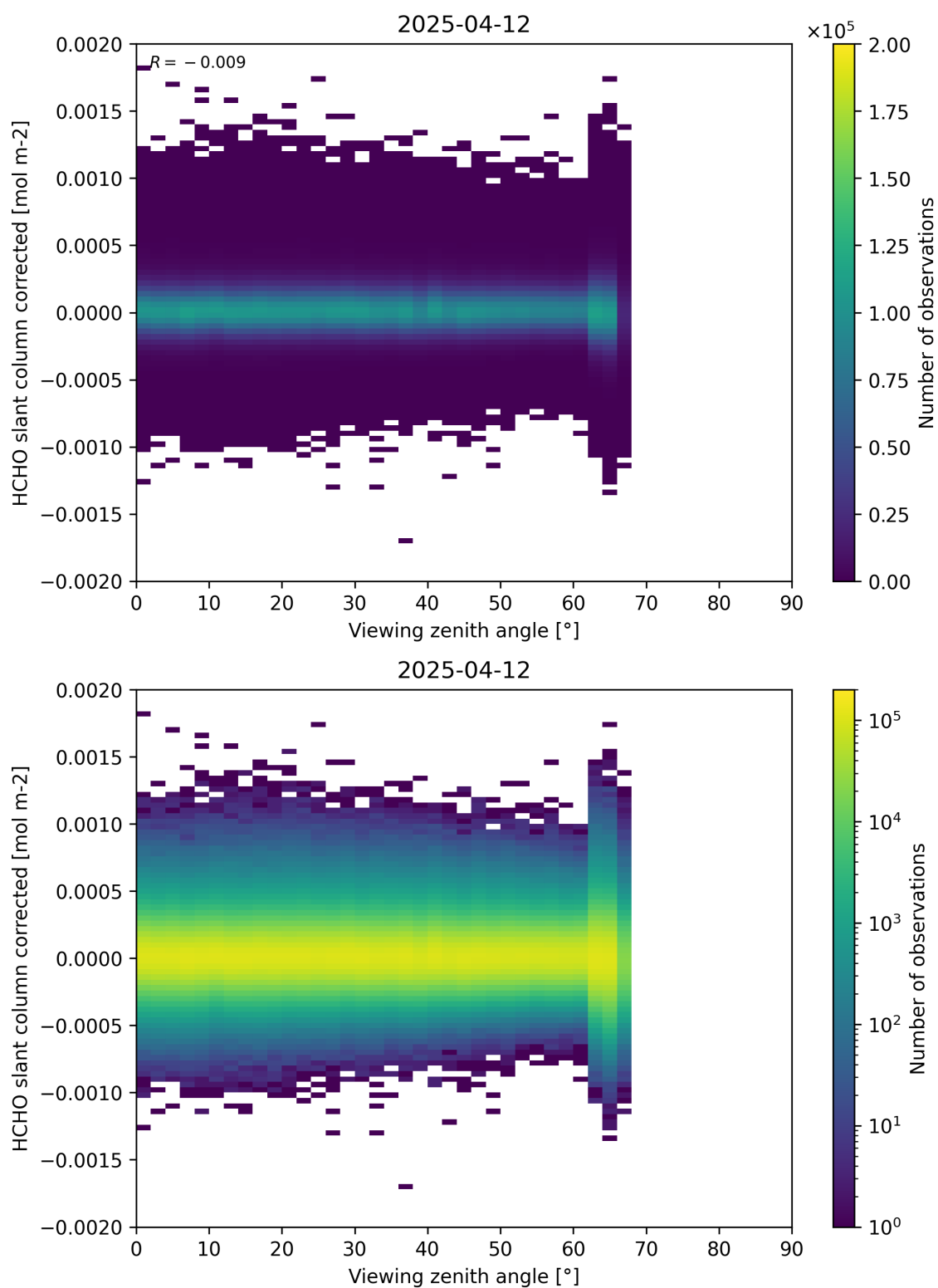
Figure 186: Scatter density plot of “Viewing zenith angle” against “HCHO slant column corrected” for 2025-04-11 to 2025-04-13.
