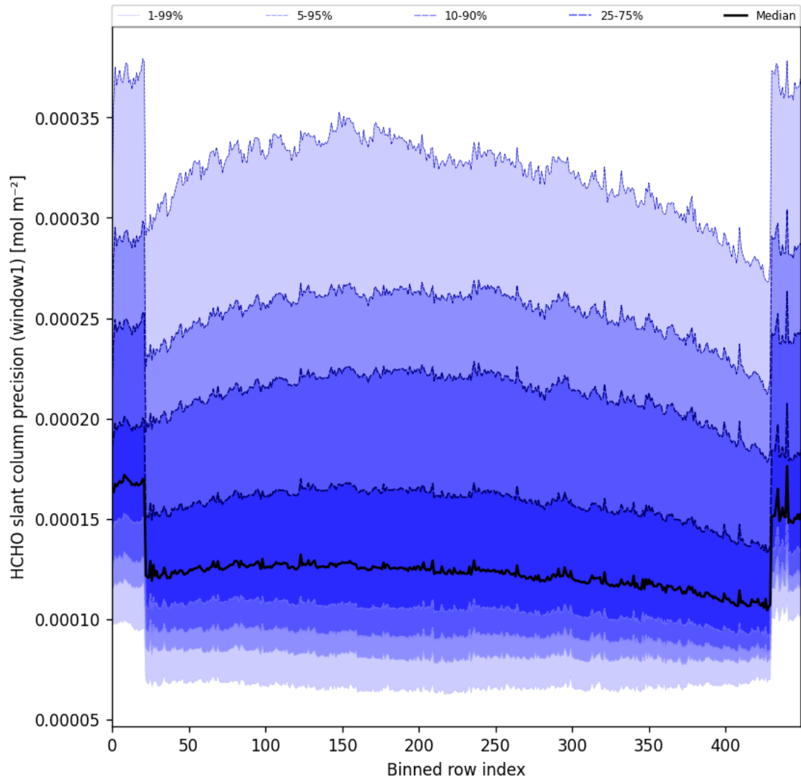
Figure 53: Along track statistics of “HCHO slant column precision (window1)” for 2025-04-11 to 2025-04-13
