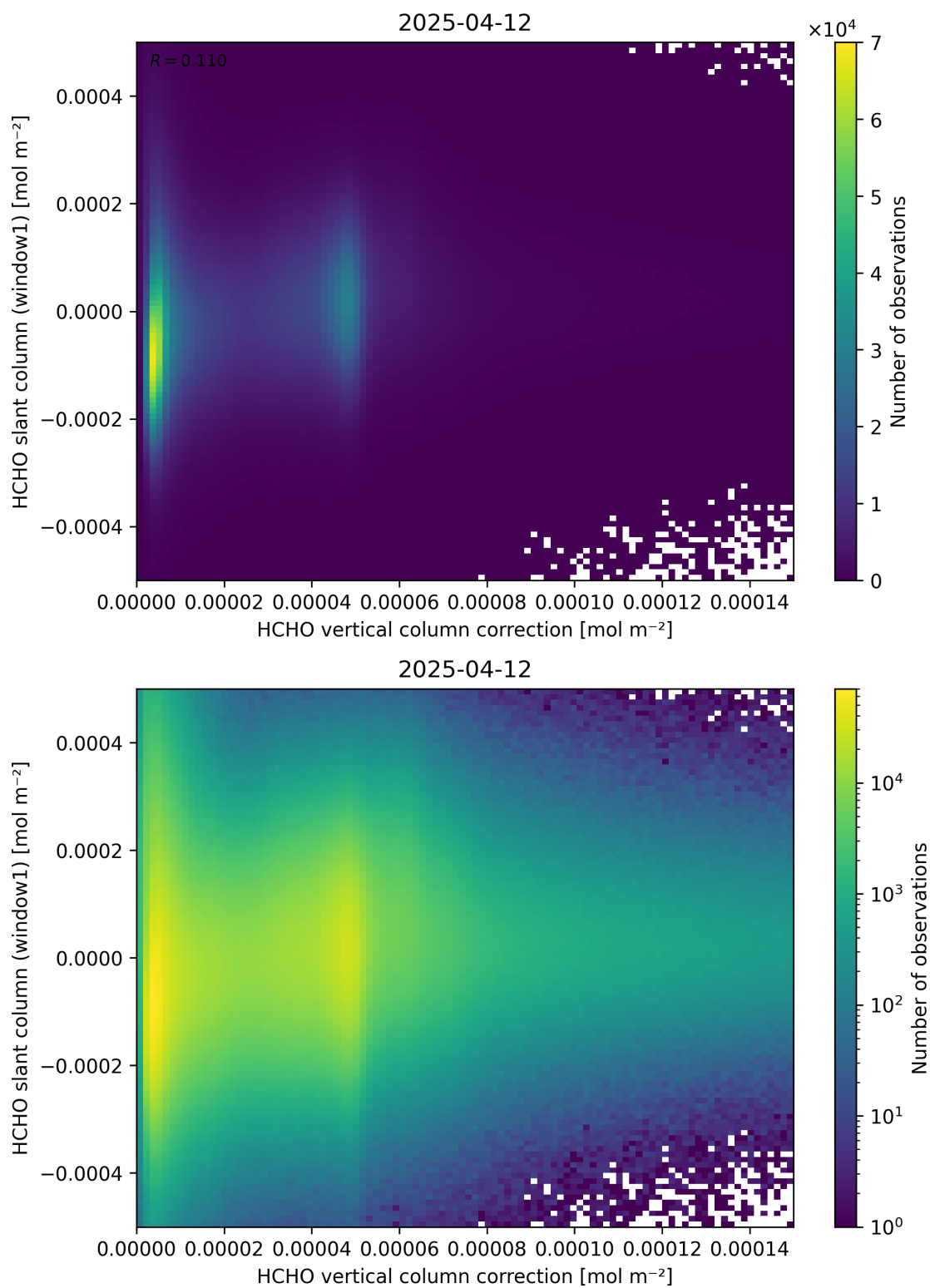
Figure 118: Scatter density plot of “HCHO vertical column correction” against “HCHO slant column (window1)” for 2025-04-11 to 2025-04-13.
