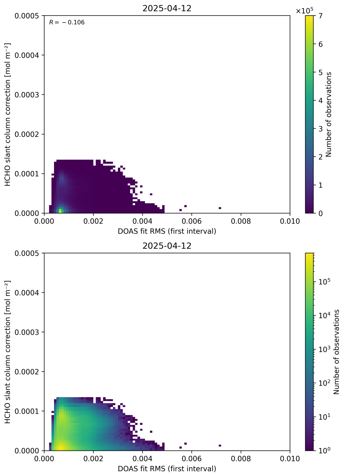
Figure 63: Scatter density plot of “DOAS fit RMS (first interval)” against “HCHO slant column correction” for 2025-04-11 to 2025-04-13.
