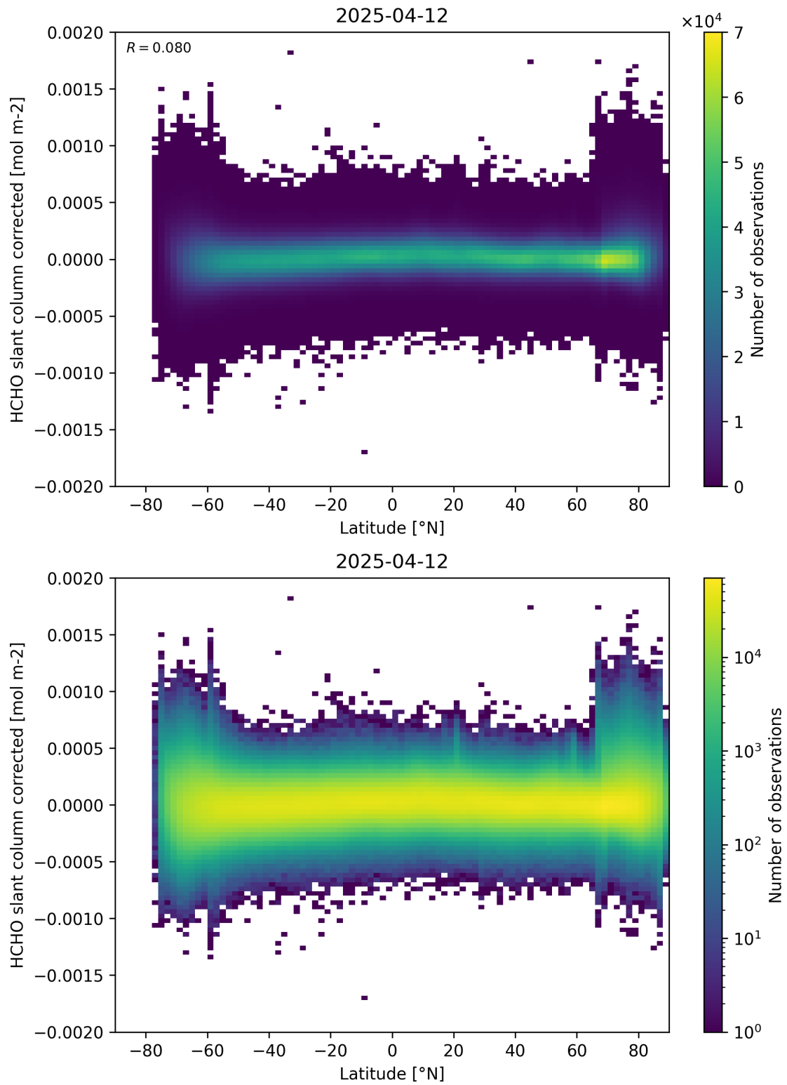
Figure 157: Scatter density plot of “Latitude” against “HCHO slant column corrected” for 2025-04-11 to 2025-04-13.
