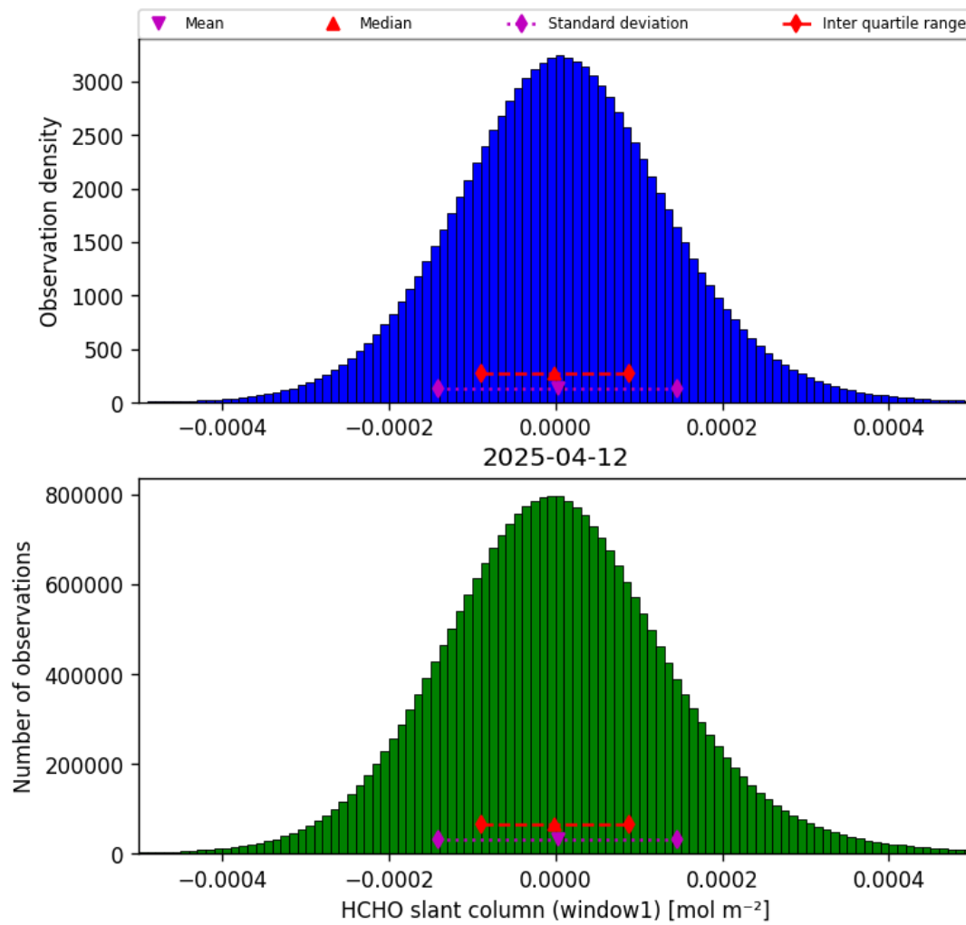
Figure 38: Histogram of “HCHO slant column (window1)” for 2025-04-11 to 2025-04-13
