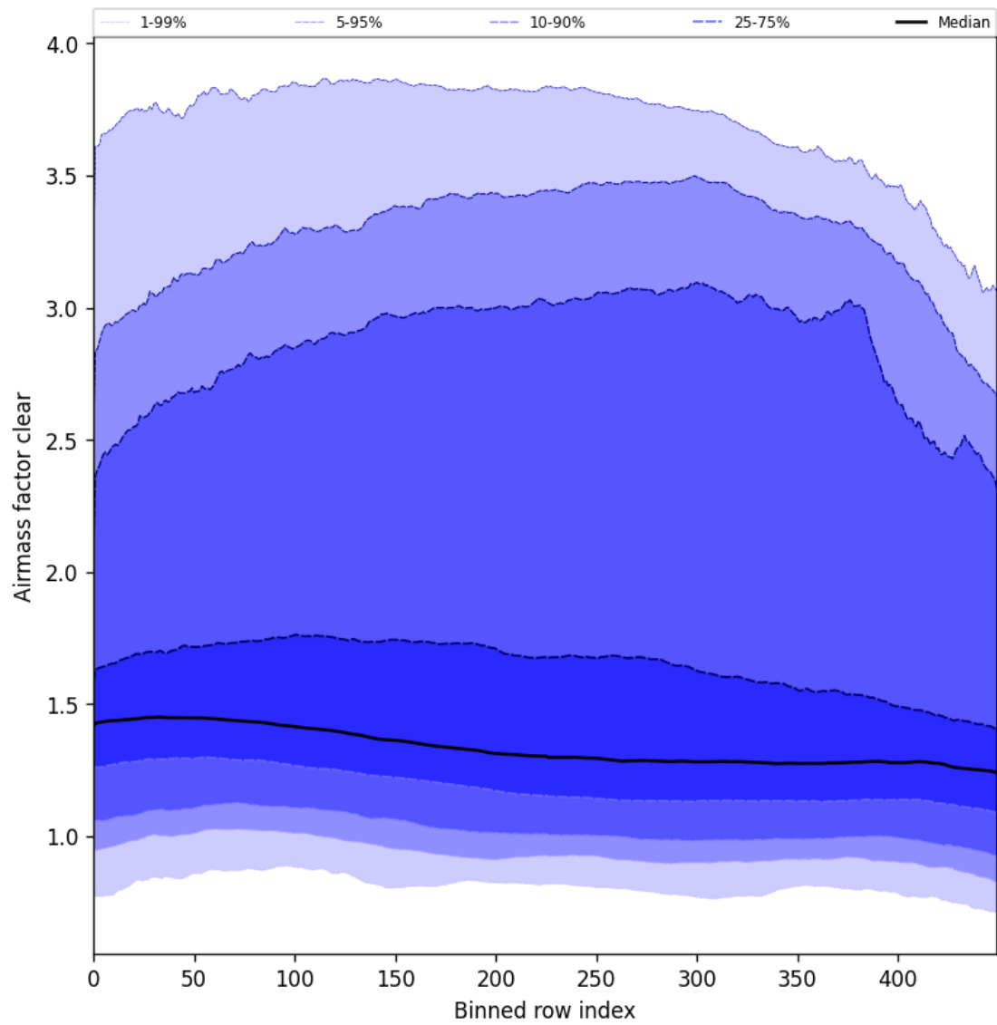
Figure 56: Along track statistics of “Air mass factor clear” for 2025-04-11 to 2025-04-13
