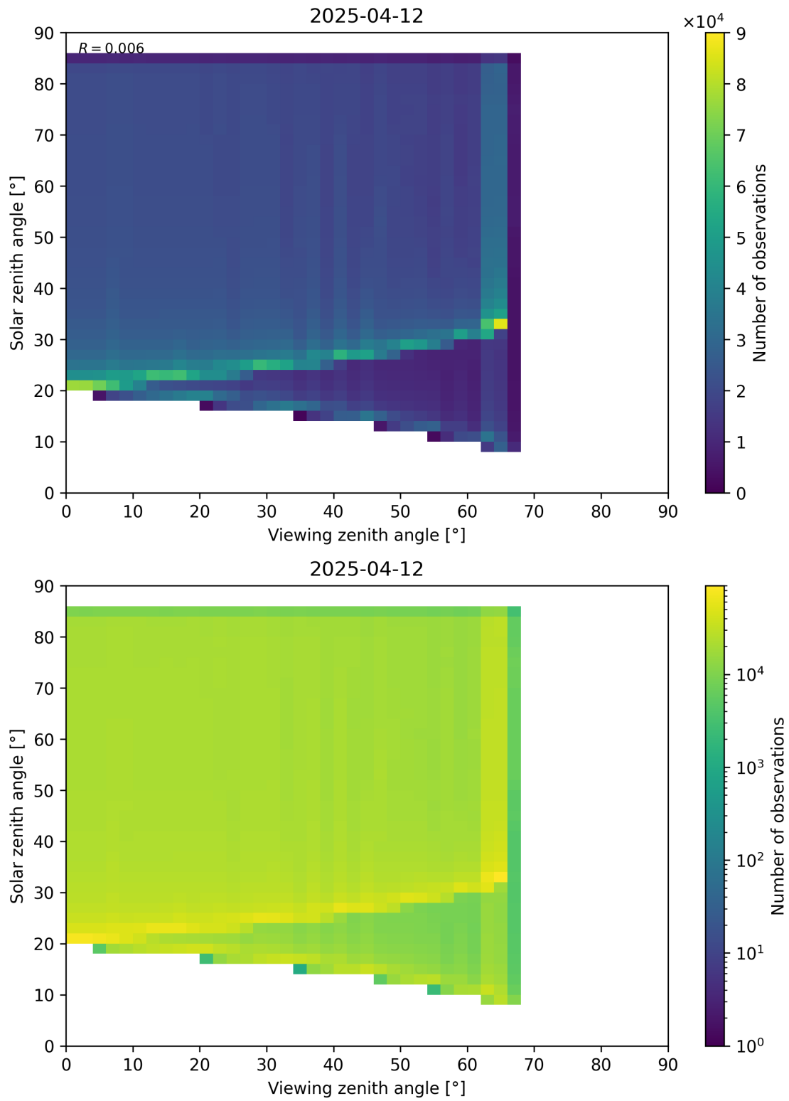
Figure 197: Scatter density plot of “Viewing zenith angle” against “Solar zenith angle” for 2025-04-11 to 2025-04-13.
