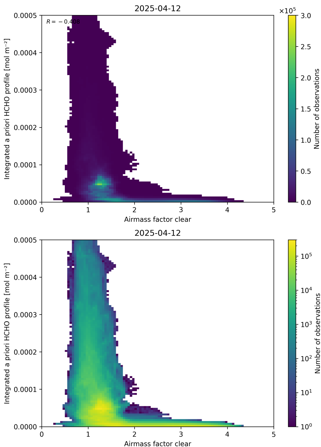
Figure 76: Scatter density plot of “Airmass factor clear” against “Integrated a priori HCHO profile” for 2025-04-11 to 2025-04-13.
