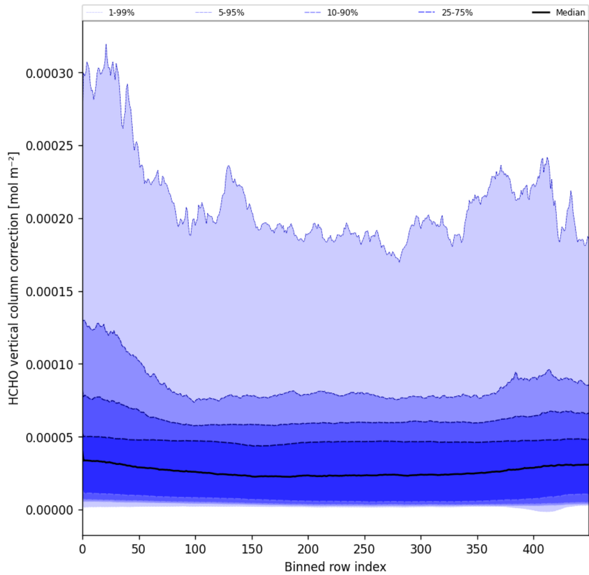
Figure 51: Along track statistics of “HCHO vertical column correction” for 2025-04-11 to 2025-04-13
