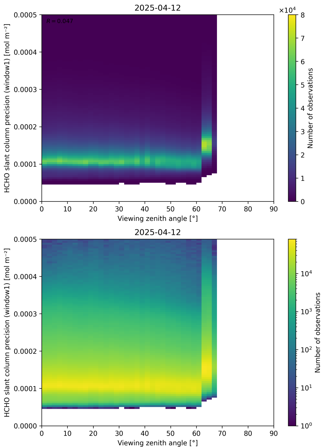
Figure 189: Scatter density plot of “Viewing zenith angle” against “HCHO slant column precision (window1)” for 2025-04-11 to 2025-04-13.
