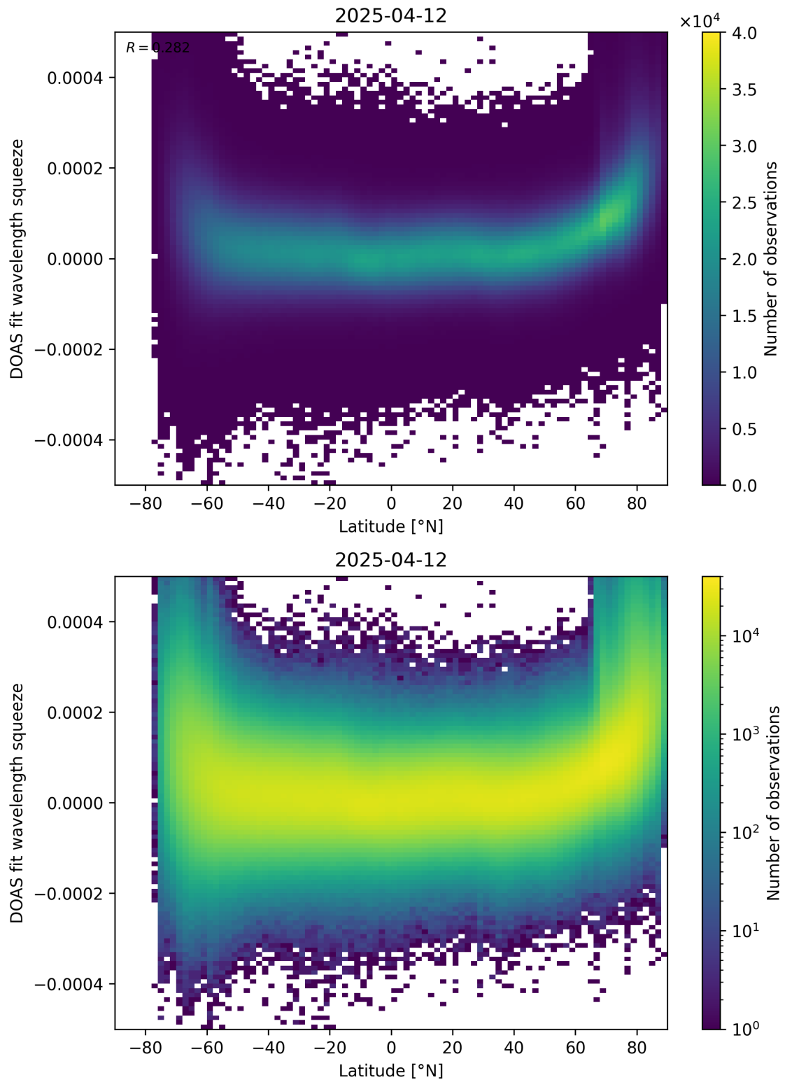
Figure 155: Scatter density plot of “Latitude” against “DOAS fit wavelength squeeze” for 2025-04-11 to 2025-04-13.
