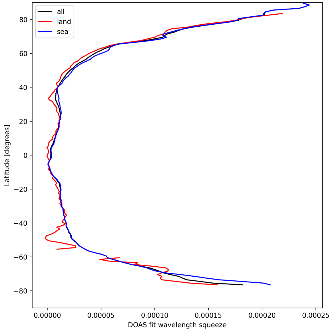
Figure 31: Zonal average of “DOAS fit wavelength squeeze” for 2025-04-11 to 2025-04-13.
