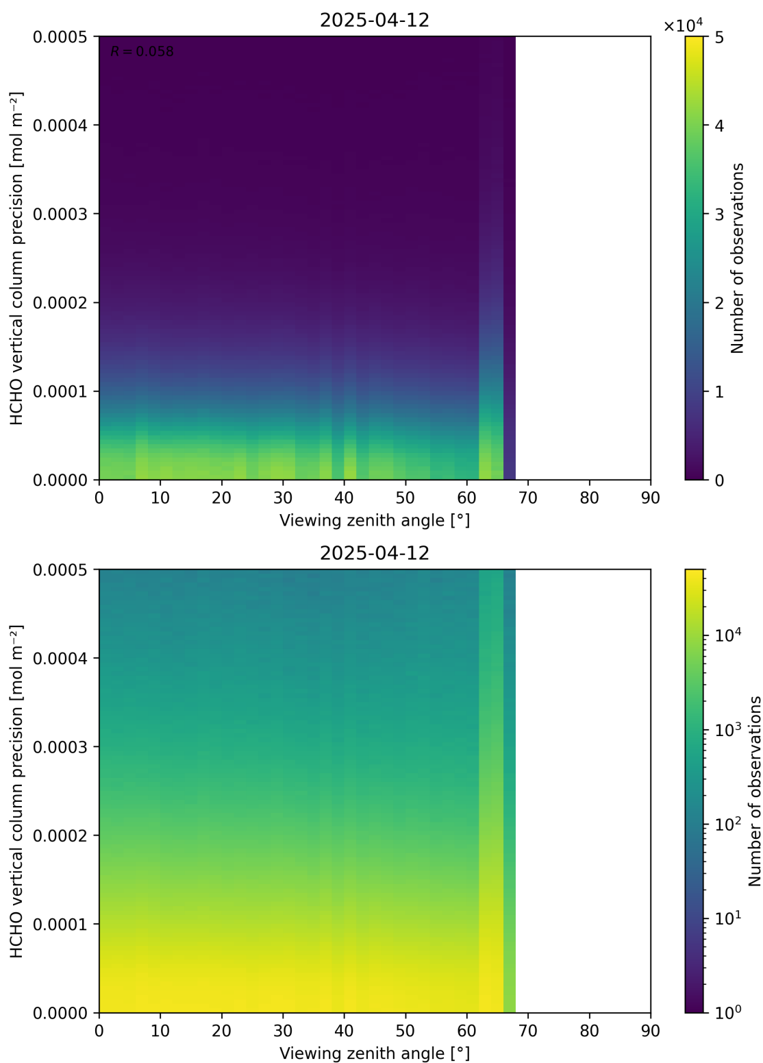
Figure 194: Scatter density plot of “Viewing zenith angle” against “HCHO vertical column precision” for 2025-04-11 to 2025-04-13.
