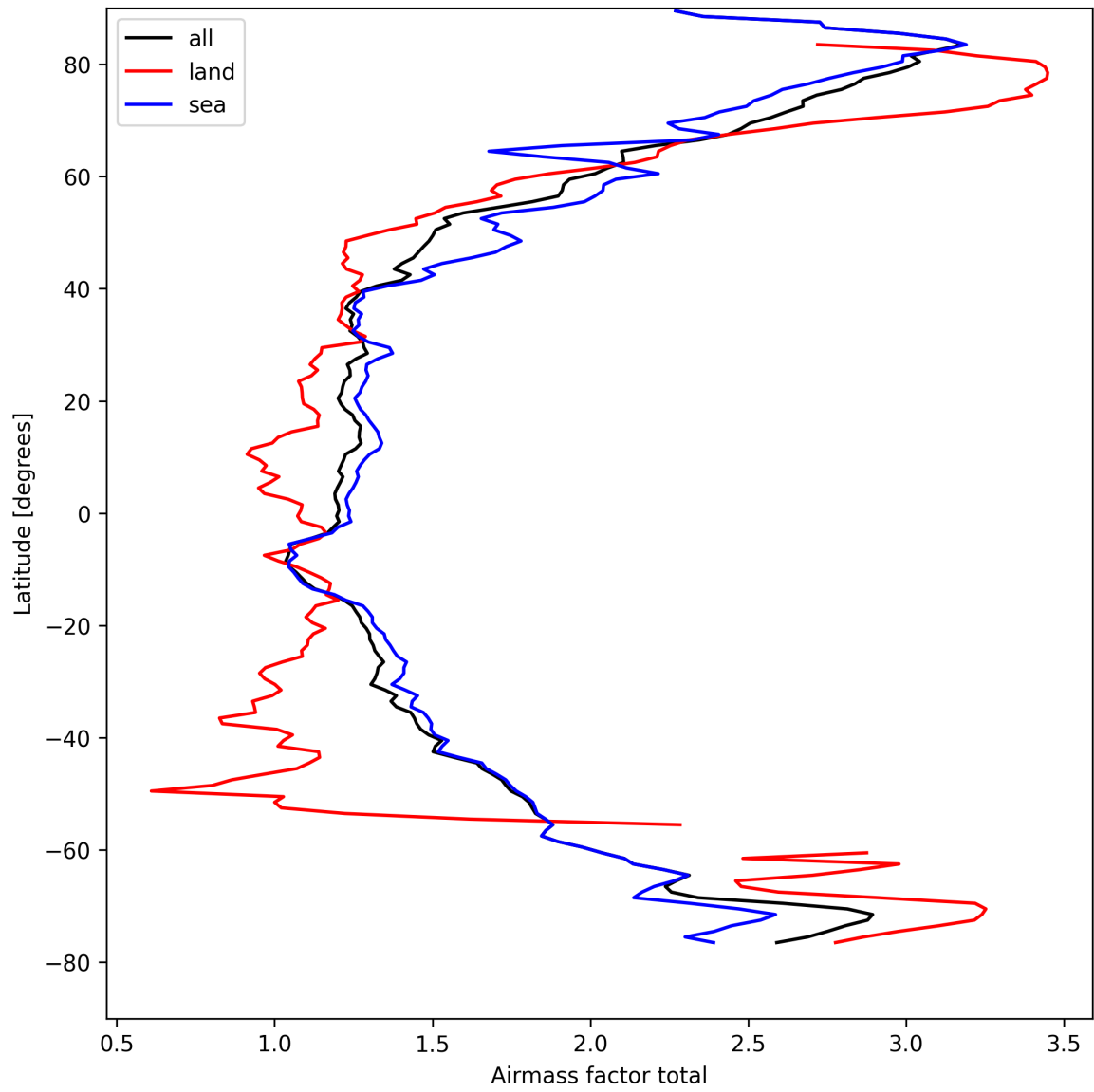
Figure 26: Zonal average of “Airmass factor total” for 2025-04-11 to 2025-04-13.
