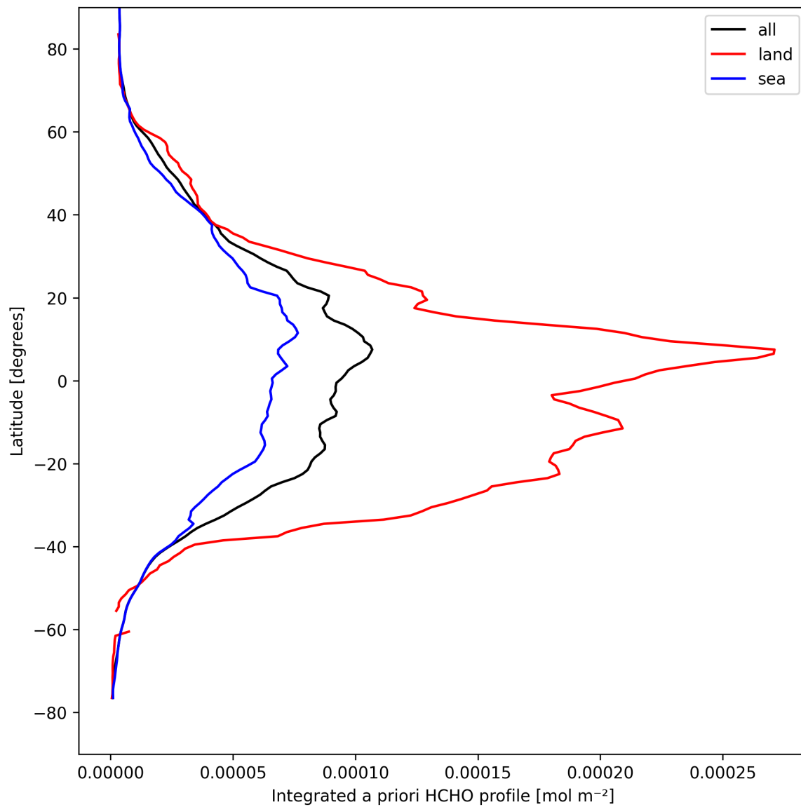
Figure 29: Zonal average of “Integrated a priori HCHO profile” for 2025-04-11 to 2025-04-13.
