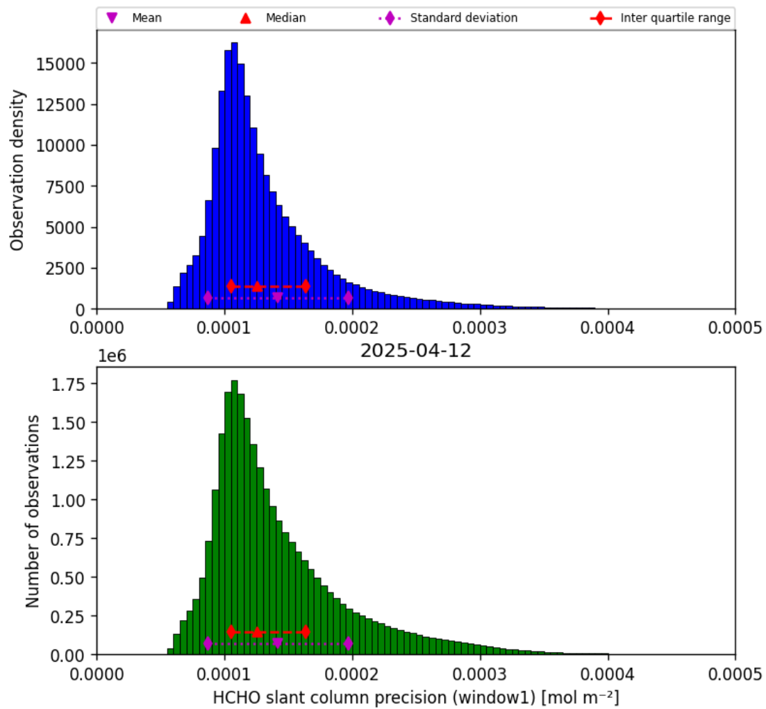
Figure 39: Histogram of “HCHO slant column precision (window1)” for 2025-04-11 to 2025-04-13
