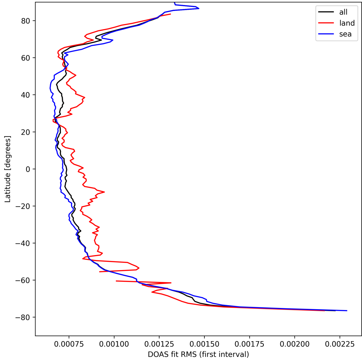
Figure 32: Zonal average of “DOAS fit RMS (first interval)” for 2025-04-11 to 2025-04-13.
