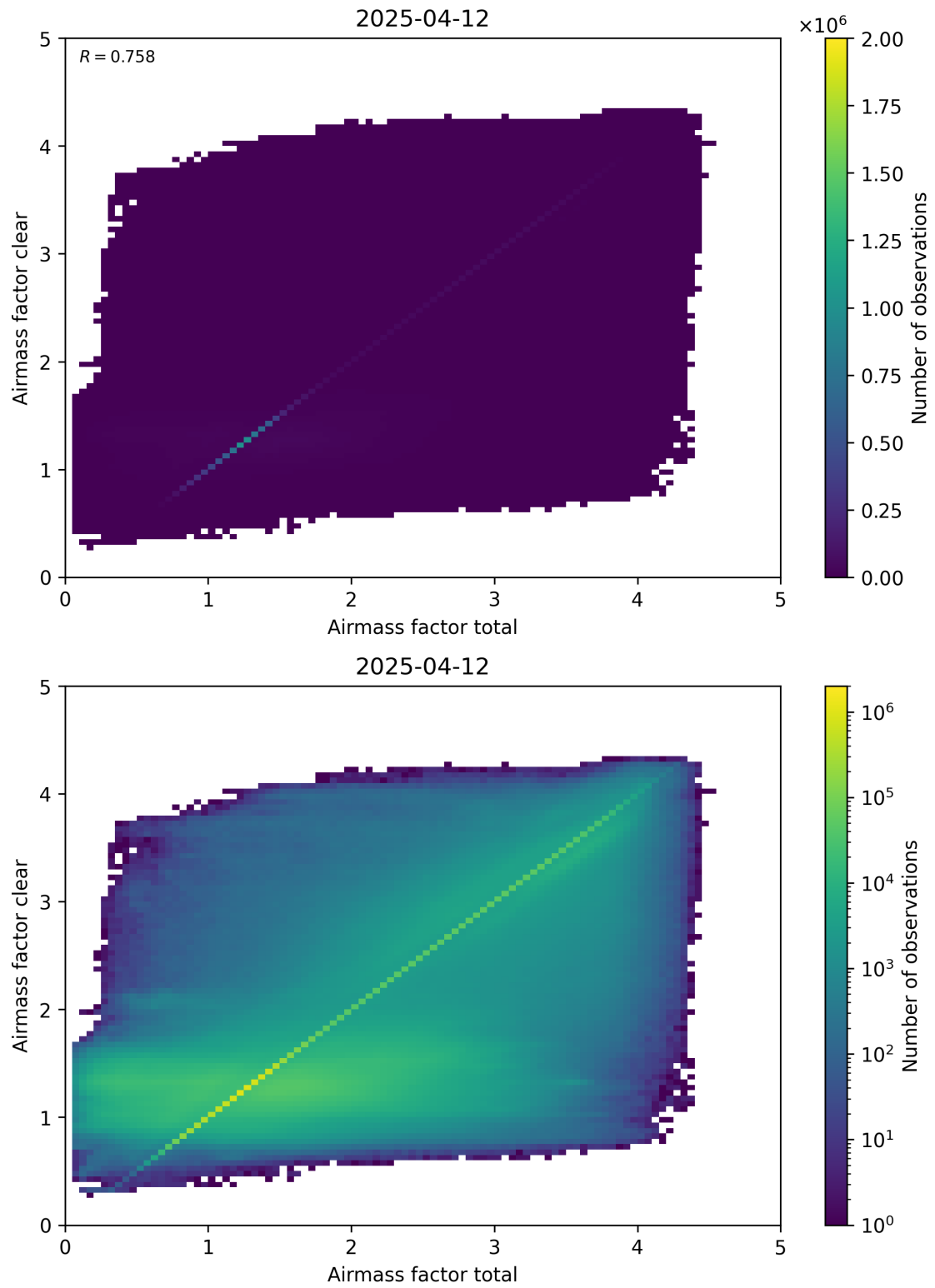
Figure 100: Scatter density plot of “Airmass factor total” against “Airmass factor clear” for 2025-04-11 to 2025-04-13.
