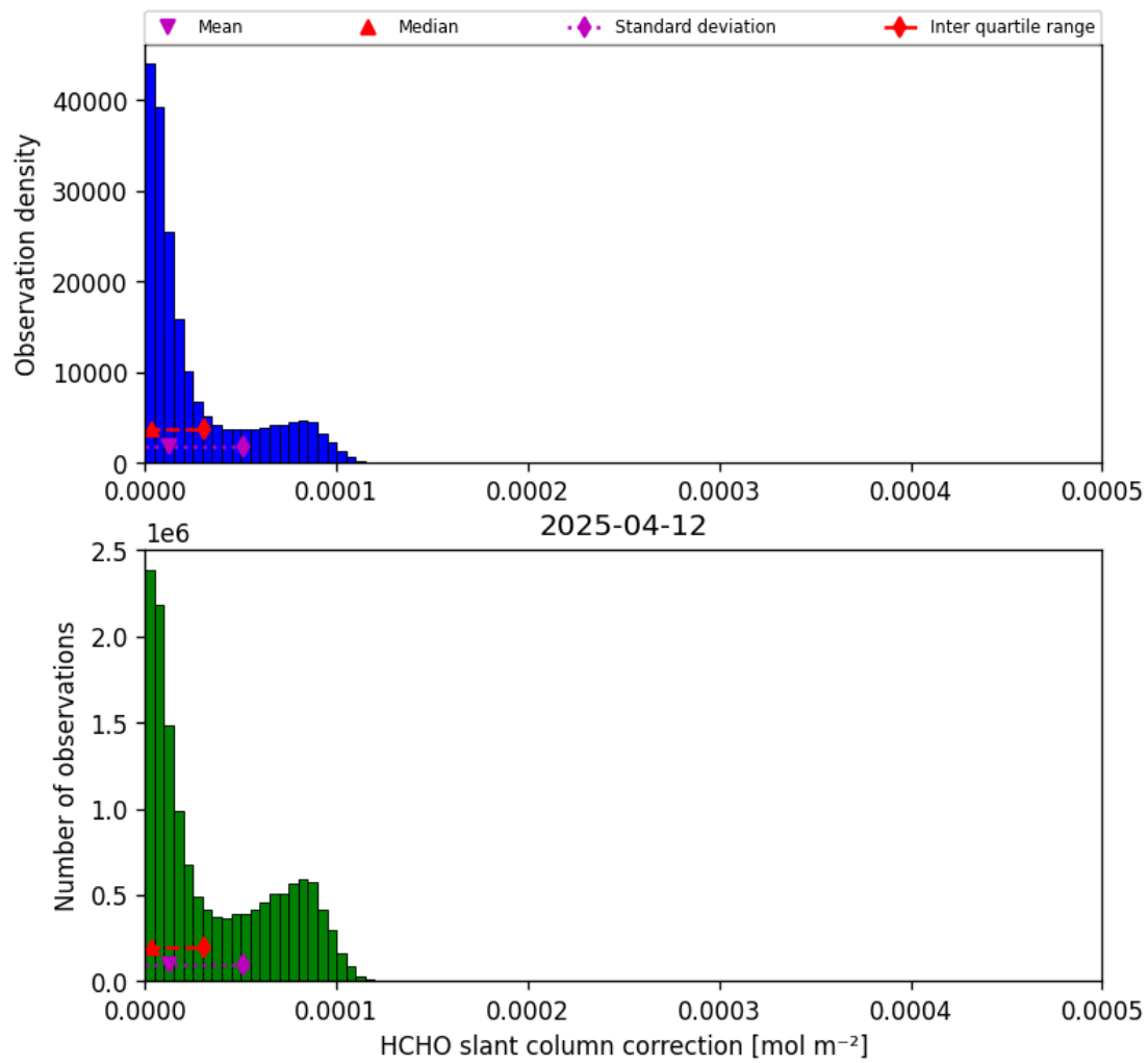
Figure 47: Histogram of “HCHO slant column correction” for 2025-04-11 to 2025-04-13
