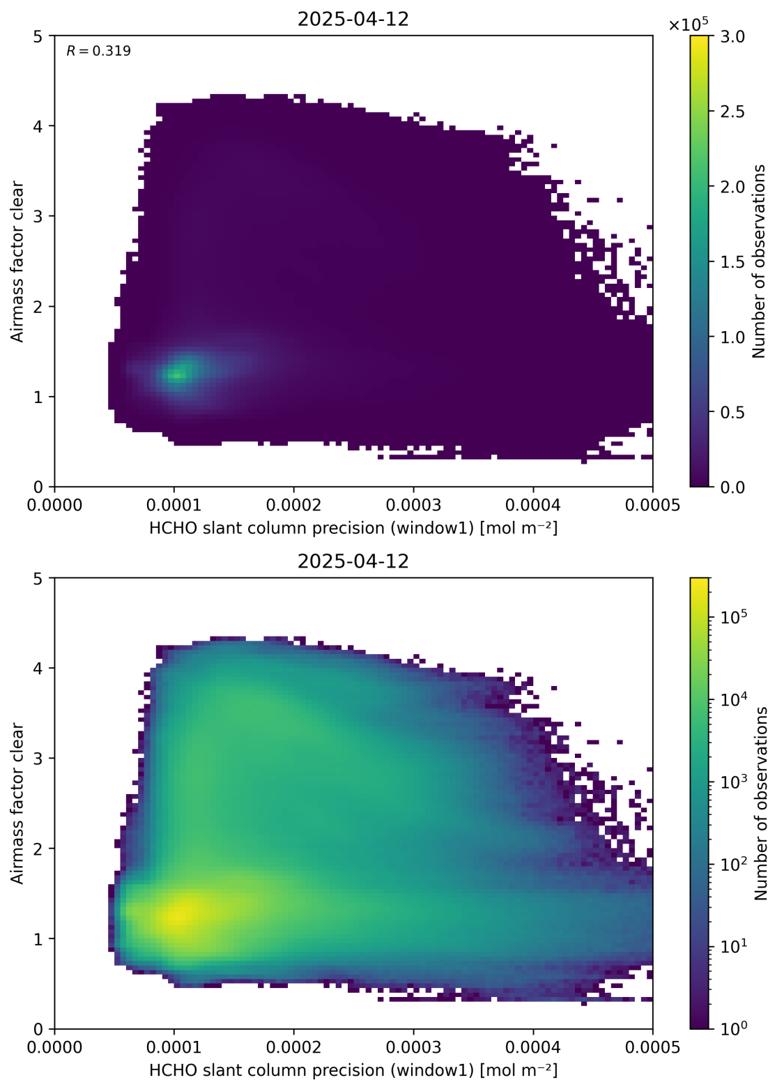
Figure 91: Scatter density plot of “HCHO slant column precision (window1)” against “Airmass factor clear” for 2025-04-11 to 2025-04-13.
