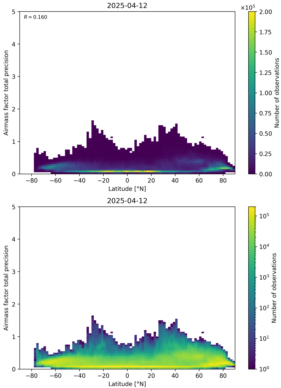
Figure 162: Scatter density plot of “Latitude” against “Airmass factor total precision” for 2025-04-11 to 2025-04-13.
