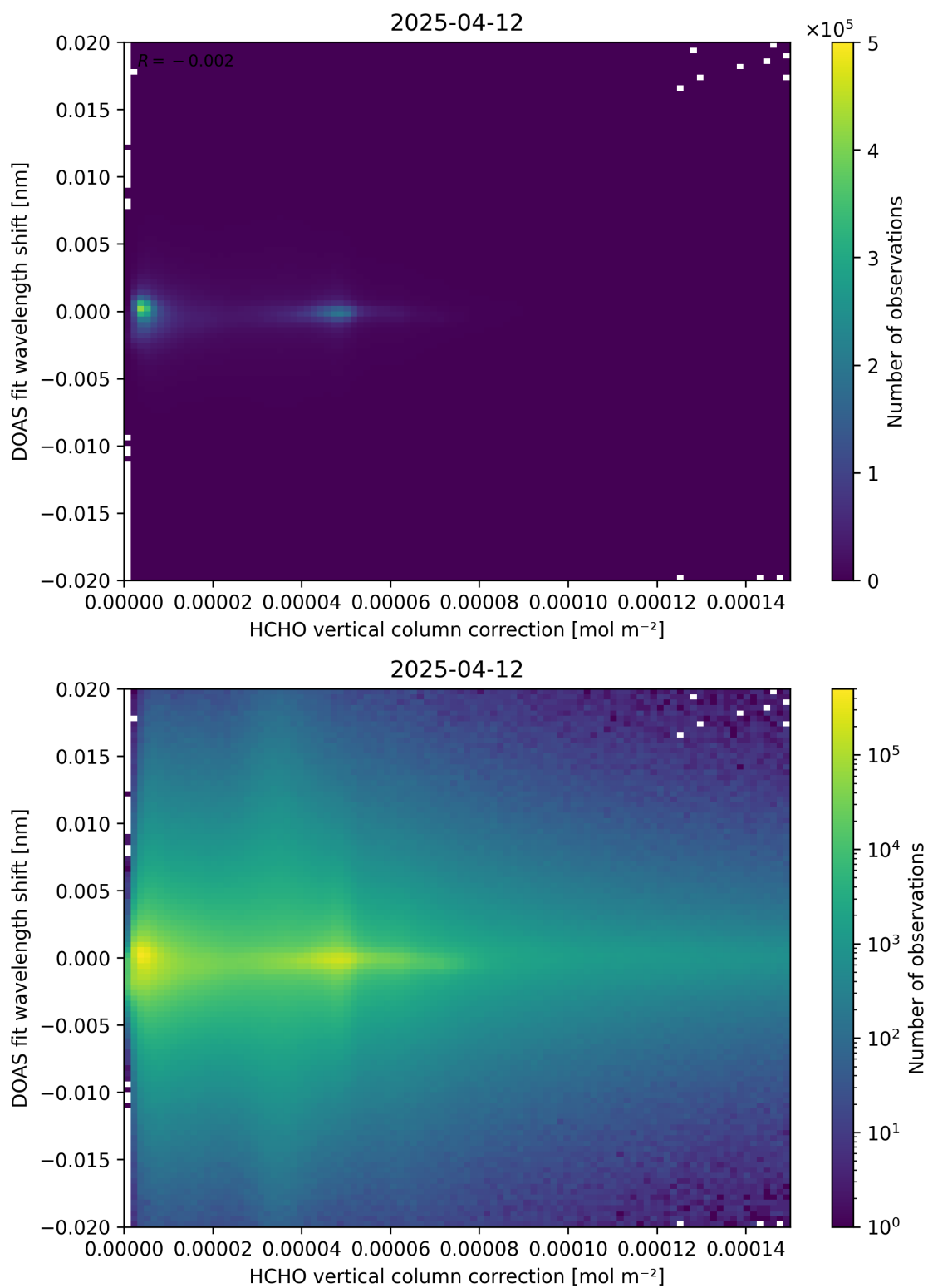
Figure 113: Scatter density plot of “HCHO vertical column correction” against “DOAS fit wavelength shift” for 2025-04-11 to 2025-04-13.
