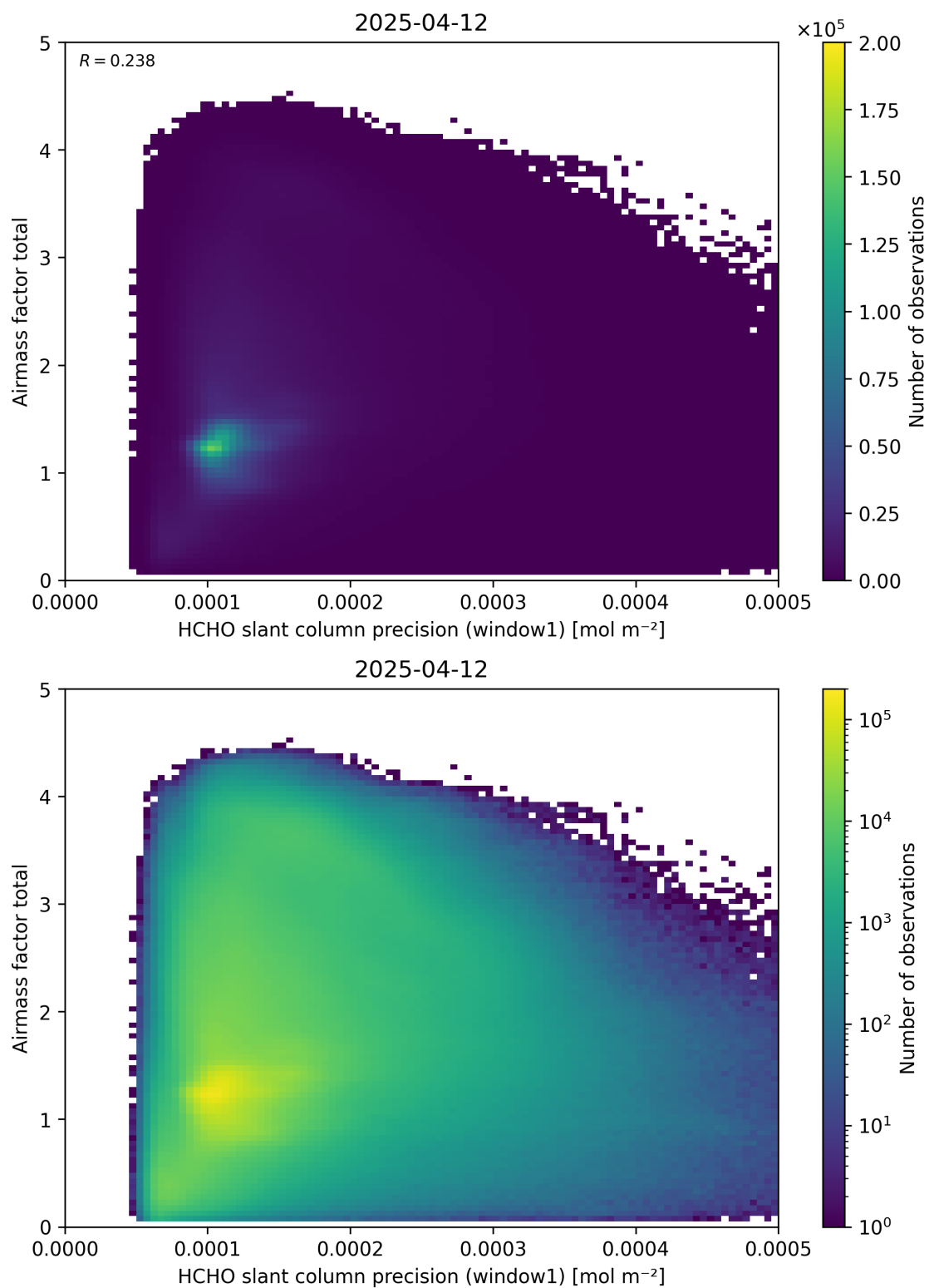
Figure 94: Scatter density plot of “HCHO slant column precision (window1)” against “Airmass factor total” for 2025-04-11 to 2025-04-13.
