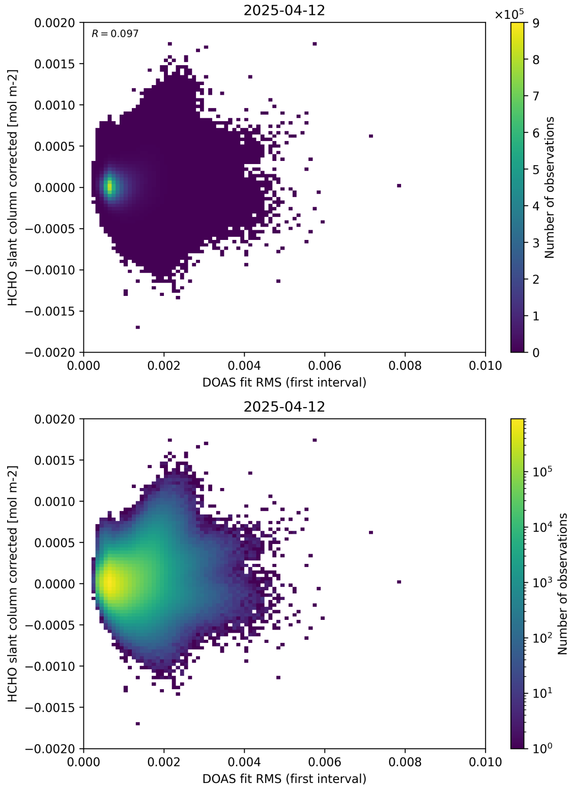
Figure 62: Scatter density plot of “DOAS fit RMS (first interval)” against “HCHO slant column corrected” for 2025-04-11 to 2025-04-13.
