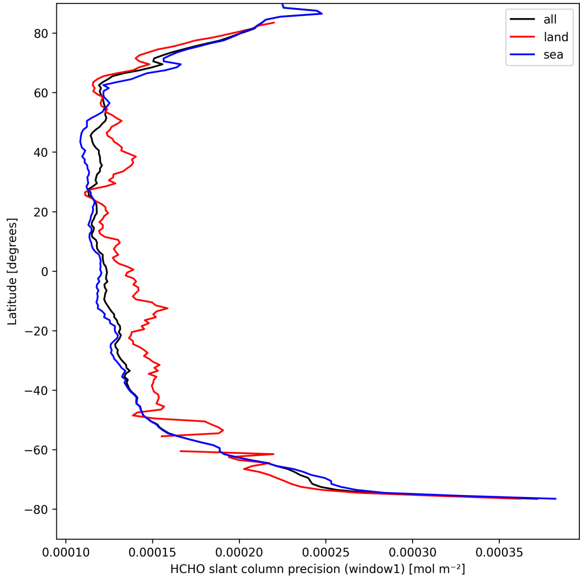
Figure 25: Zonal average of “HCHO slant column precision (window1)” for 2025-04-11 to 2025-04-13.
