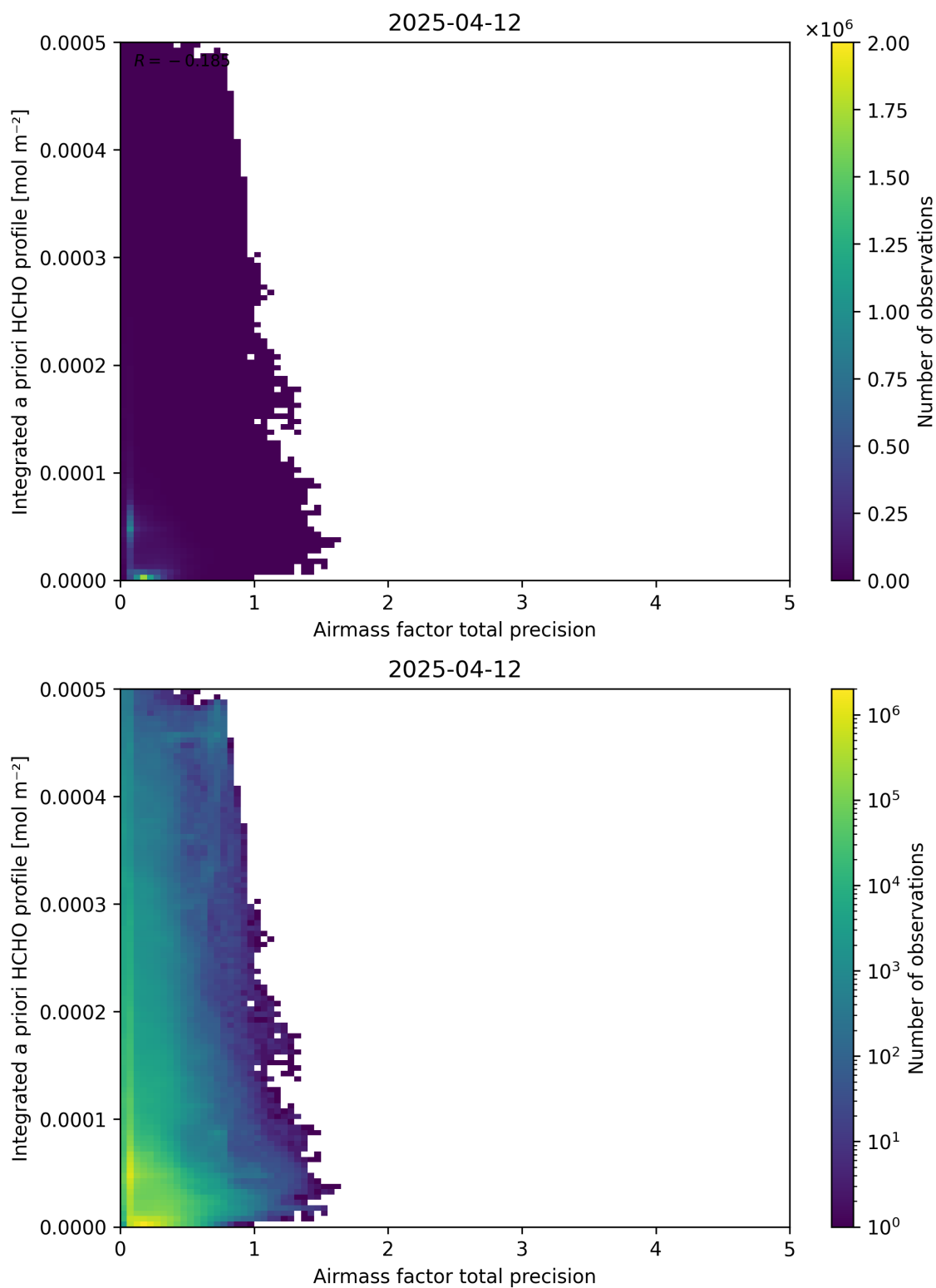
Figure 111: Scatter density plot of “Airmass factor total precision” against “Integrated a priori HCHO profile” for 2025-04-11 to 2025-04-13.
