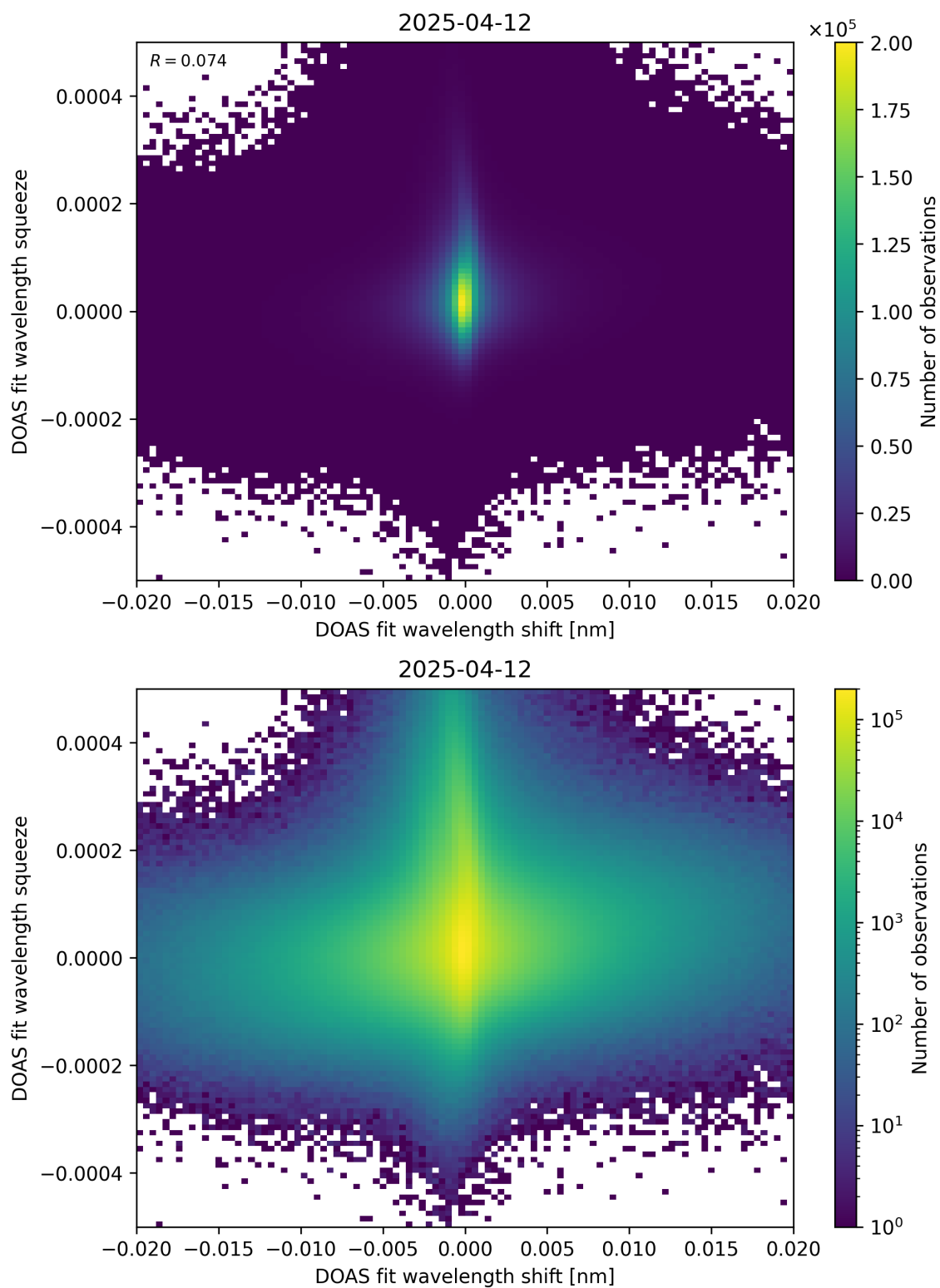
Figure 65: Scatter density plot of “DOAS fit wavelength shift” against “DOAS fit wavelength squeeze” for 2025-04-11 to 2025-04-13.
