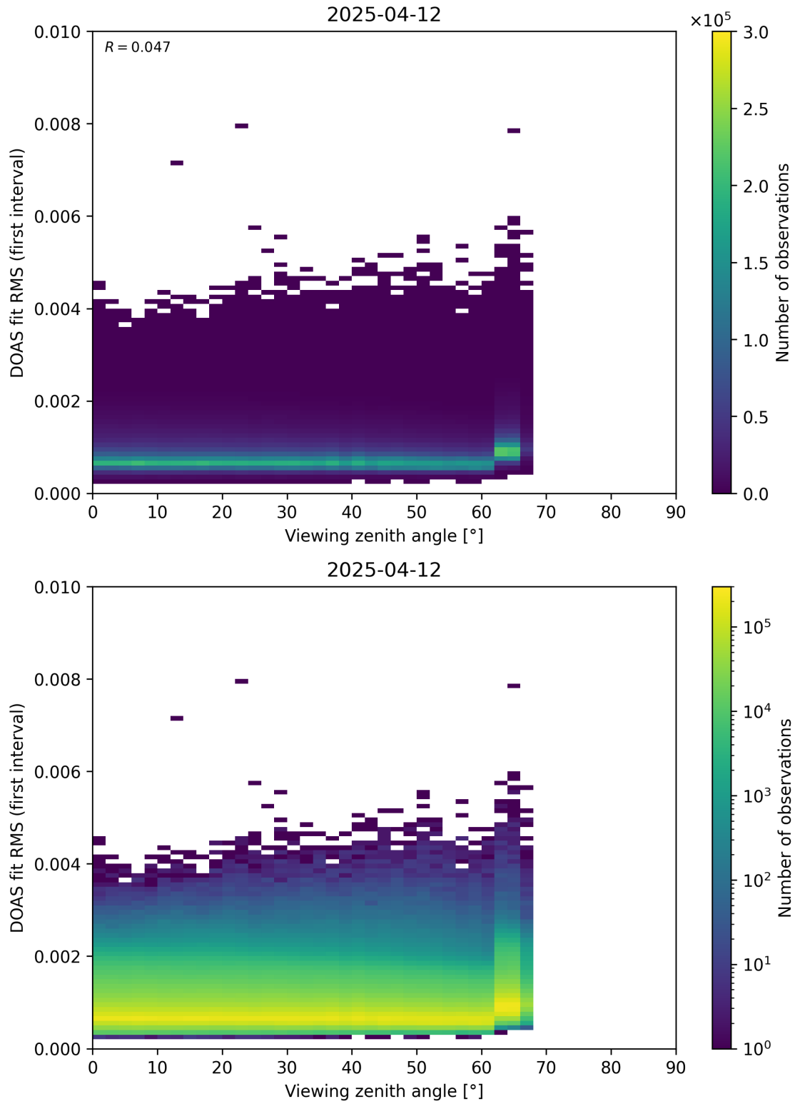
Figure 182: Scatter density plot of “Viewing zenith angle” against “DOAS fit RMS (first interval)” for 2025-04-11 to 2025-04-13.
