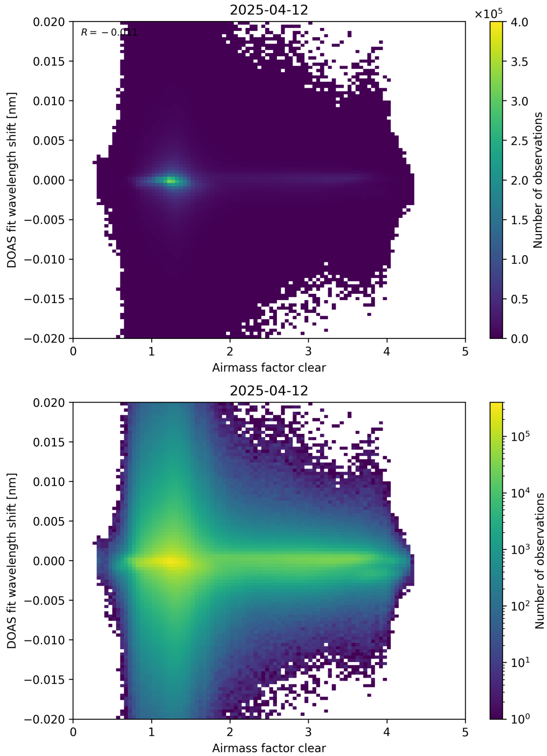
Figure 72: Scatter density plot of “Airmass factor clear” against “DOAS fit wavelength shift” for 2025-04-11 to 2025-04-13.
