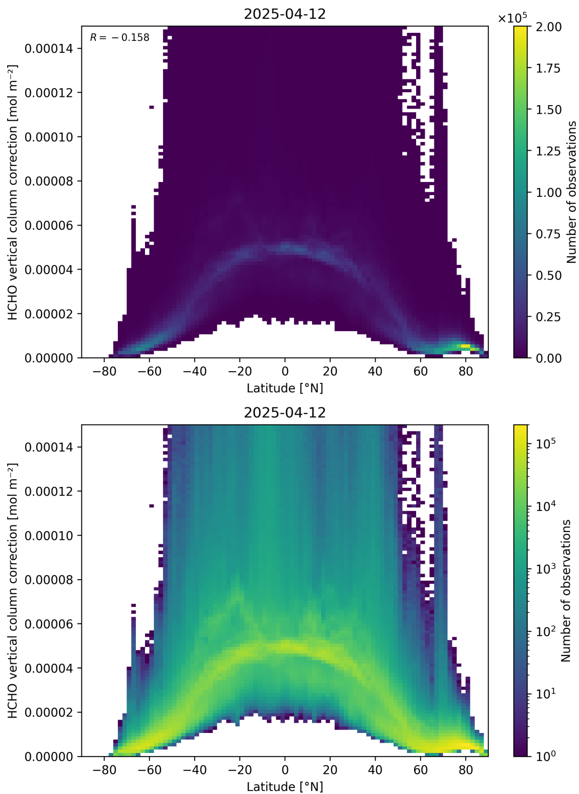
Figure 164: Scatter density plot of “Latitude” against “HCHO vertical column correction” for 2025-04-11 to 2025-04-13.
