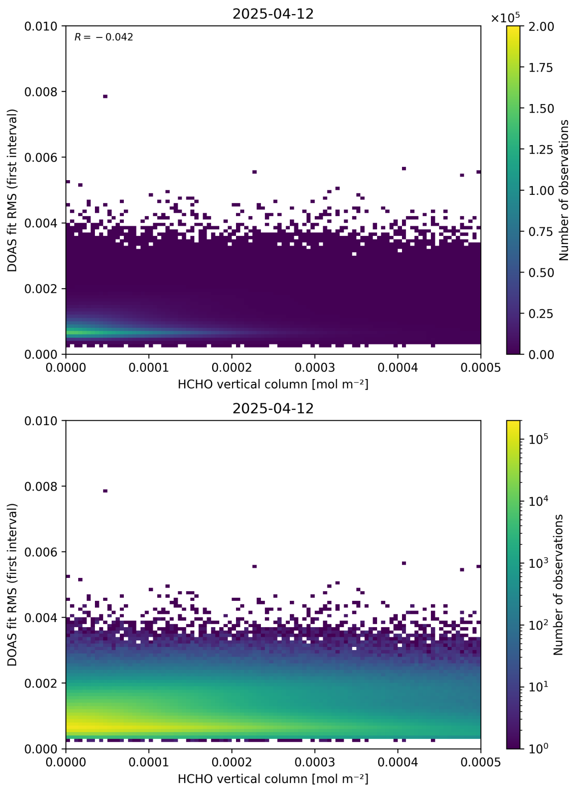
Figure 123: Scatter density plot of “HCHO vertical column” against “DOAS fit RMS (first interval)” for 2025-04-11 to 2025-04-13.
