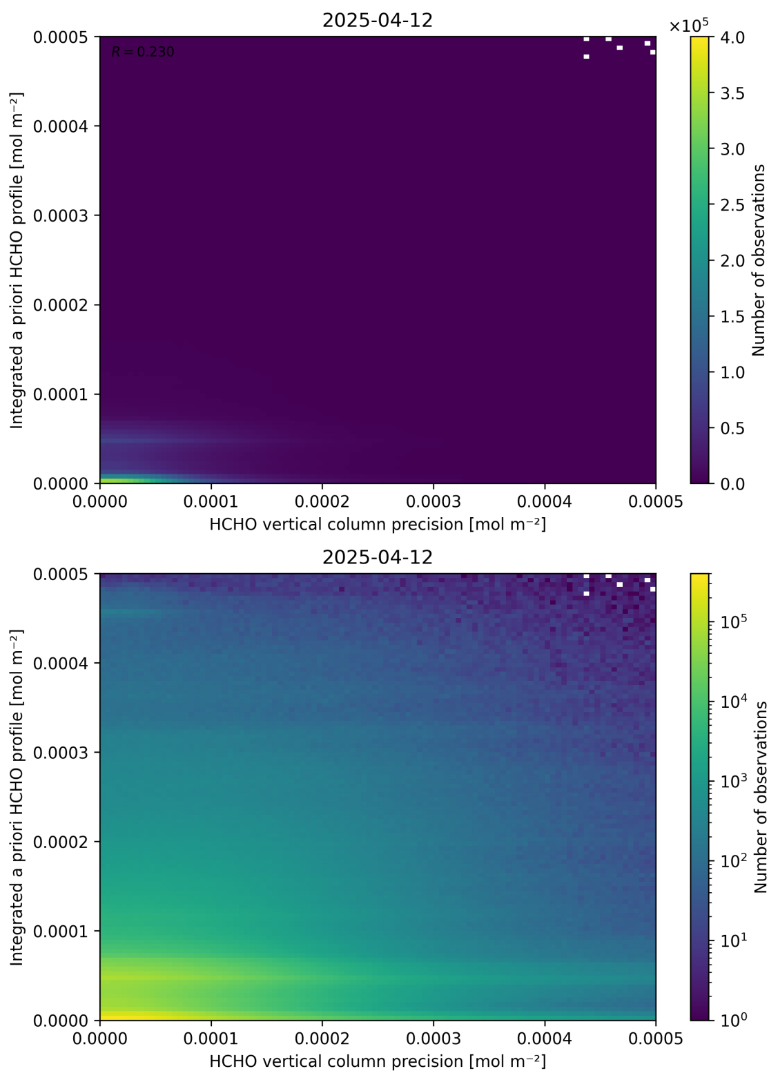
Figure 147: Scatter density plot of “HCHO vertical column precision” against “Integrated a priori HCHO profile” for 2025-04-11 to 2025-04-13.
