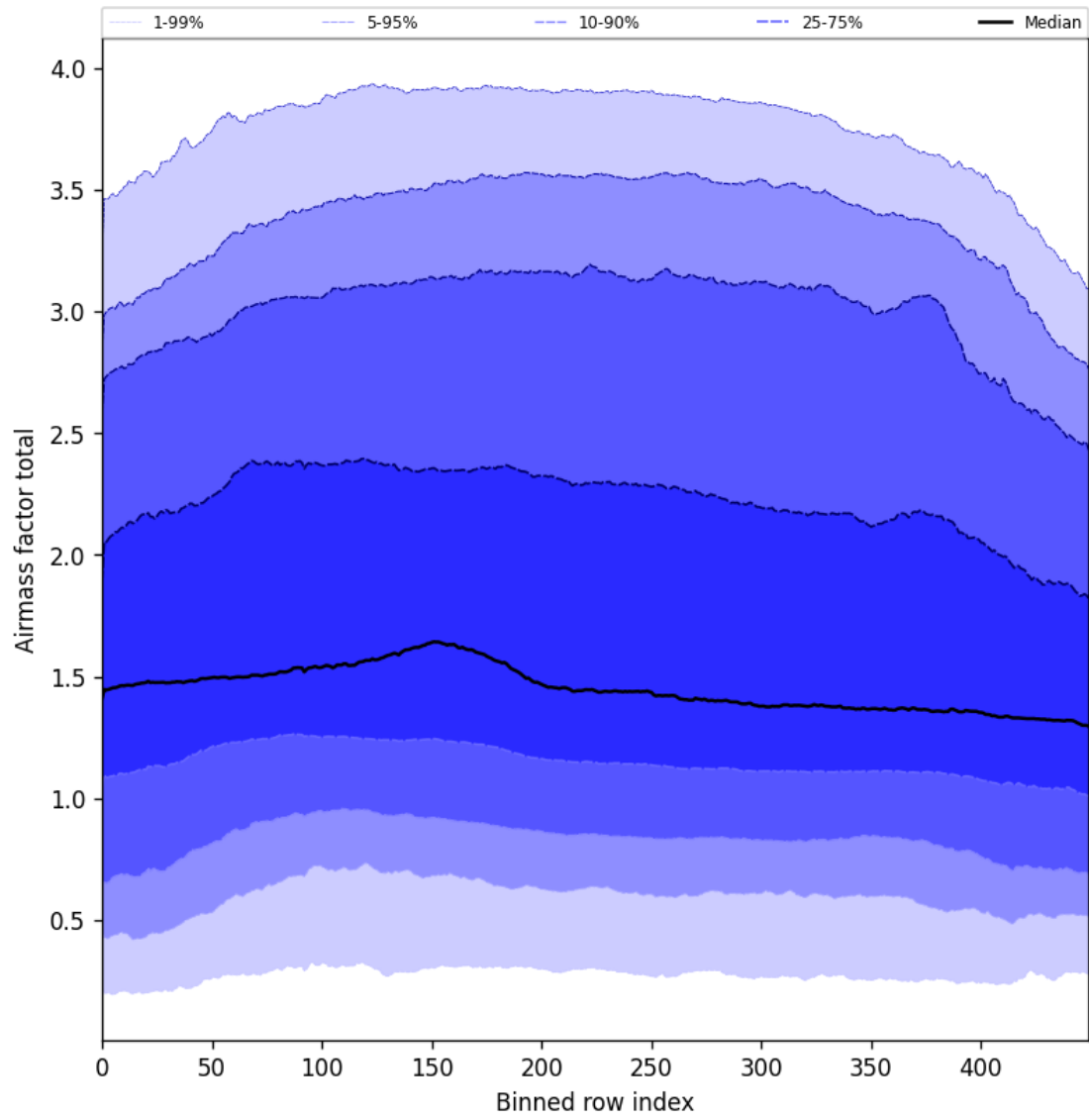
Figure 54: Along track statistics of “Airmass factor total” for 2025-04-11 to 2025-04-13
