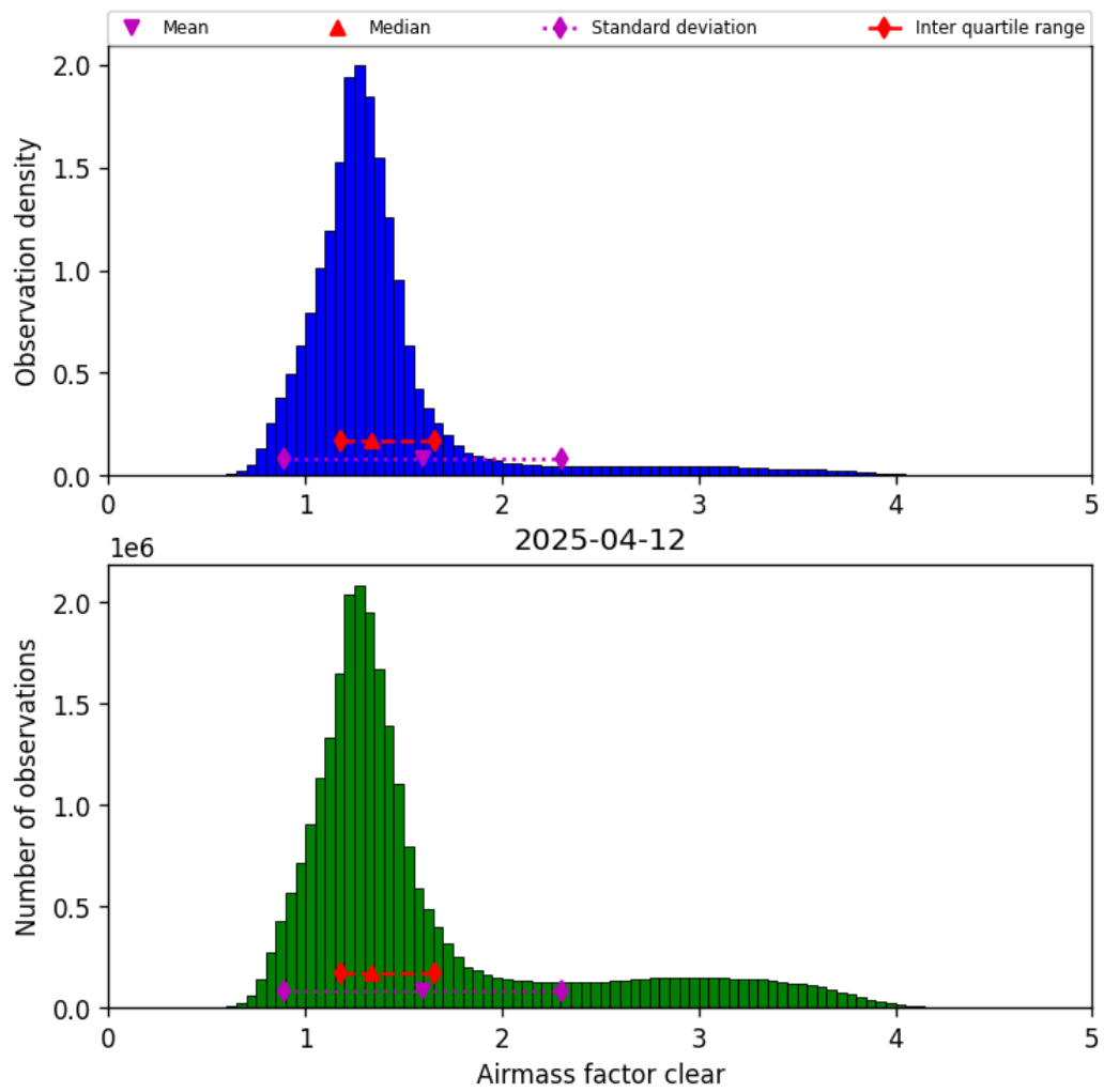
Figure 42: Histogram of “Airmass factor clear” for 2025-04-11 to 2025-04-13
