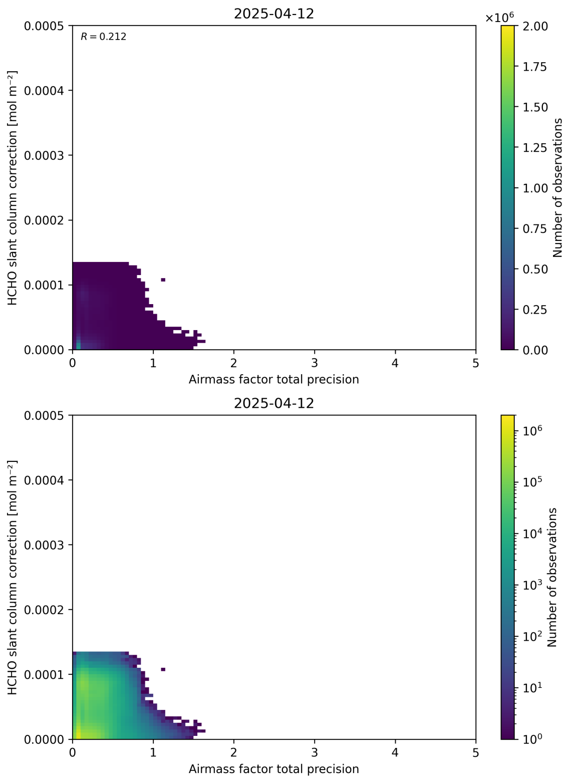
Figure 110: Scatter density plot of “Airmass factor total precision” against “HCHO slant column correction” for 2025-04-11 to 2025-04-13.
