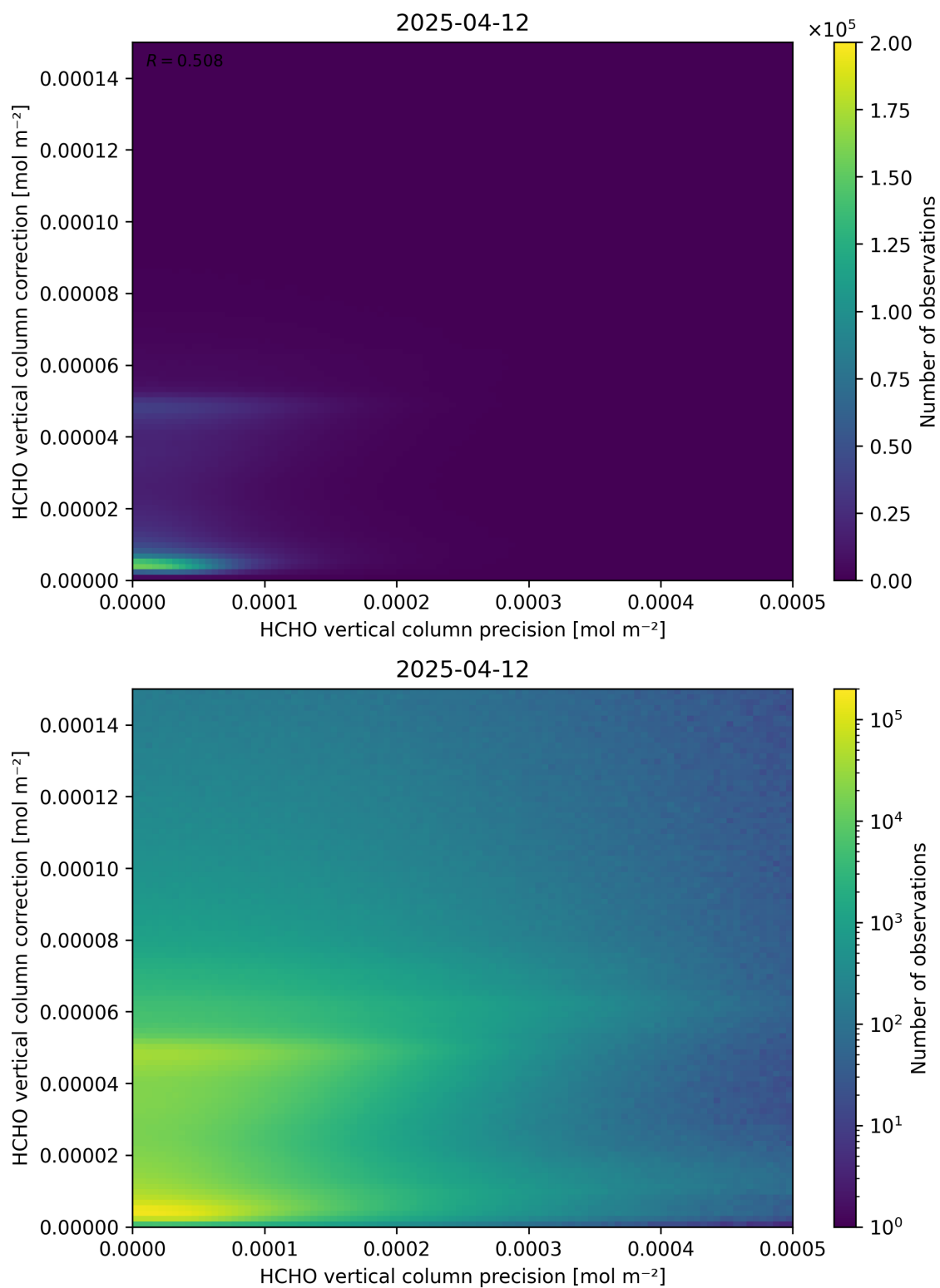
Figure 146: Scatter density plot of “HCHO vertical column precision” against “HCHO vertical column correction” for 2025-04-11 to 2025-04-13.
