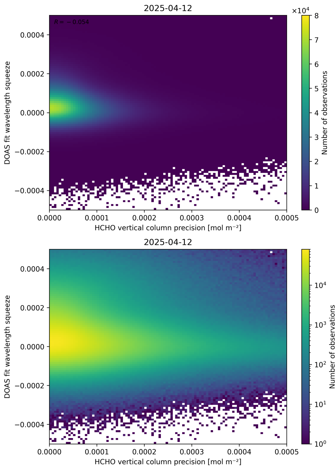
Figure 138: Scatter density plot of “HCHO vertical column precision” against “DOAS fit wavelength squeeze” for 2025-04-11 to 2025-04-13.
