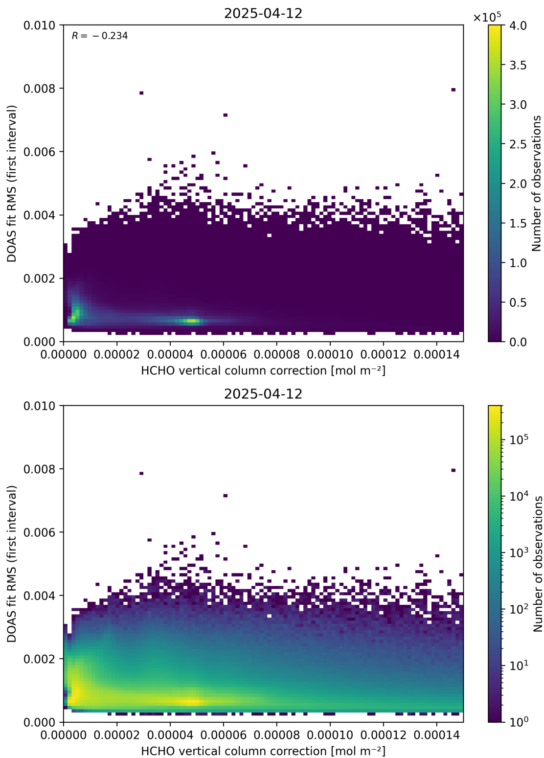
Figure 112: Scatter density plot of “HCHO vertical column correction” against “DOAS fit RMS (first interval)” for 2025-04-11 to 2025-04-13.
