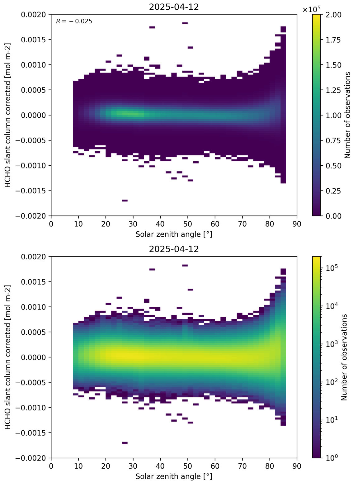
Figure 171: Scatter density plot of “Solar zenith angle” against “HCHO slant column corrected” for 2025-04-11 to 2025-04-13.
