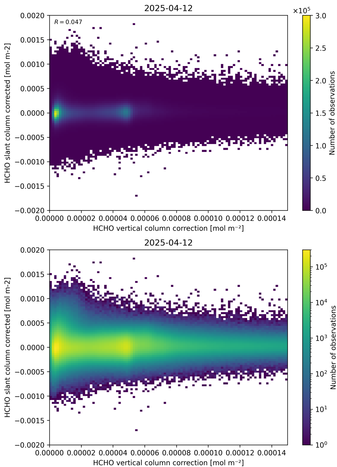
Figure 116: Scatter density plot of “HCHO vertical column correction” against “HCHO slant column corrected” for 2025-04-11 to 2025-04-13.
