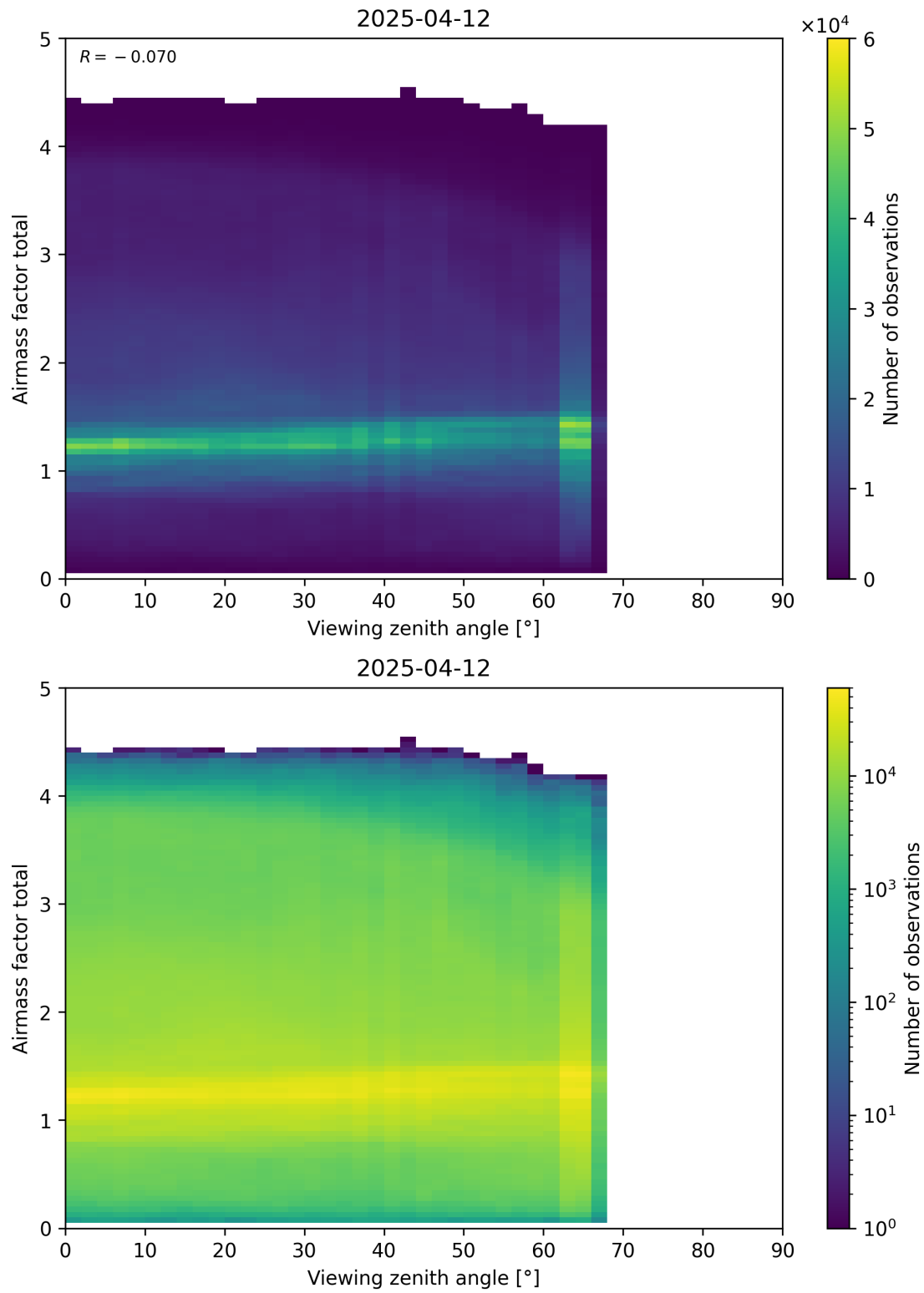
Figure 190: Scatter density plot of “Viewing zenith angle” against “Airmass factor total” for 2025-04-11 to 2025-04-13.
