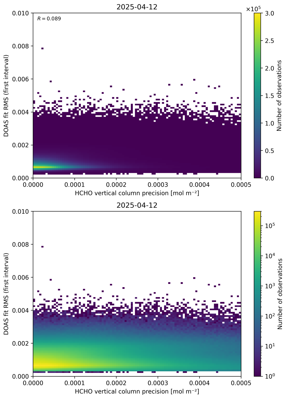
Figure 136: Scatter density plot of “HCHO vertical column precision” against “DOAS fit RMS (first interval)” for 2025-04-11 to 2025-04-13.
