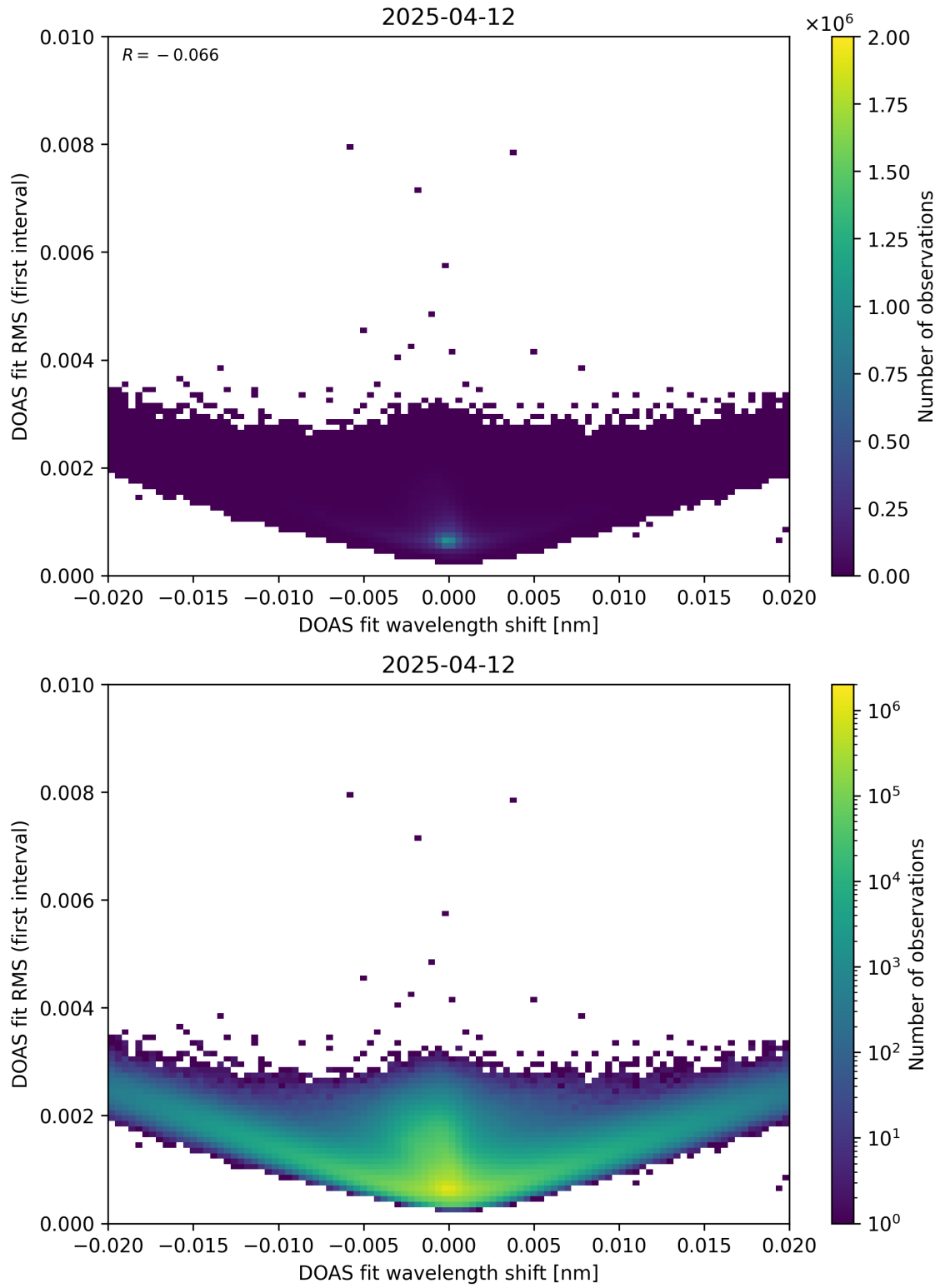
Figure 64: Scatter density plot of “DOAS fit wavelength shift” against “DOAS fit RMS (first interval)” for 2025-04-11 to 2025-04-13.
