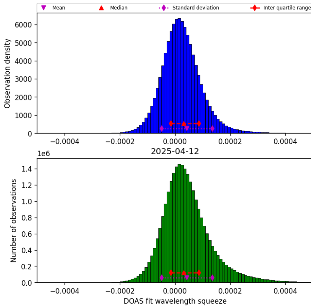
Figure 45: Histogram of “DOAS fit wavelength squeeze” for 2025-04-11 to 2025-04-13
