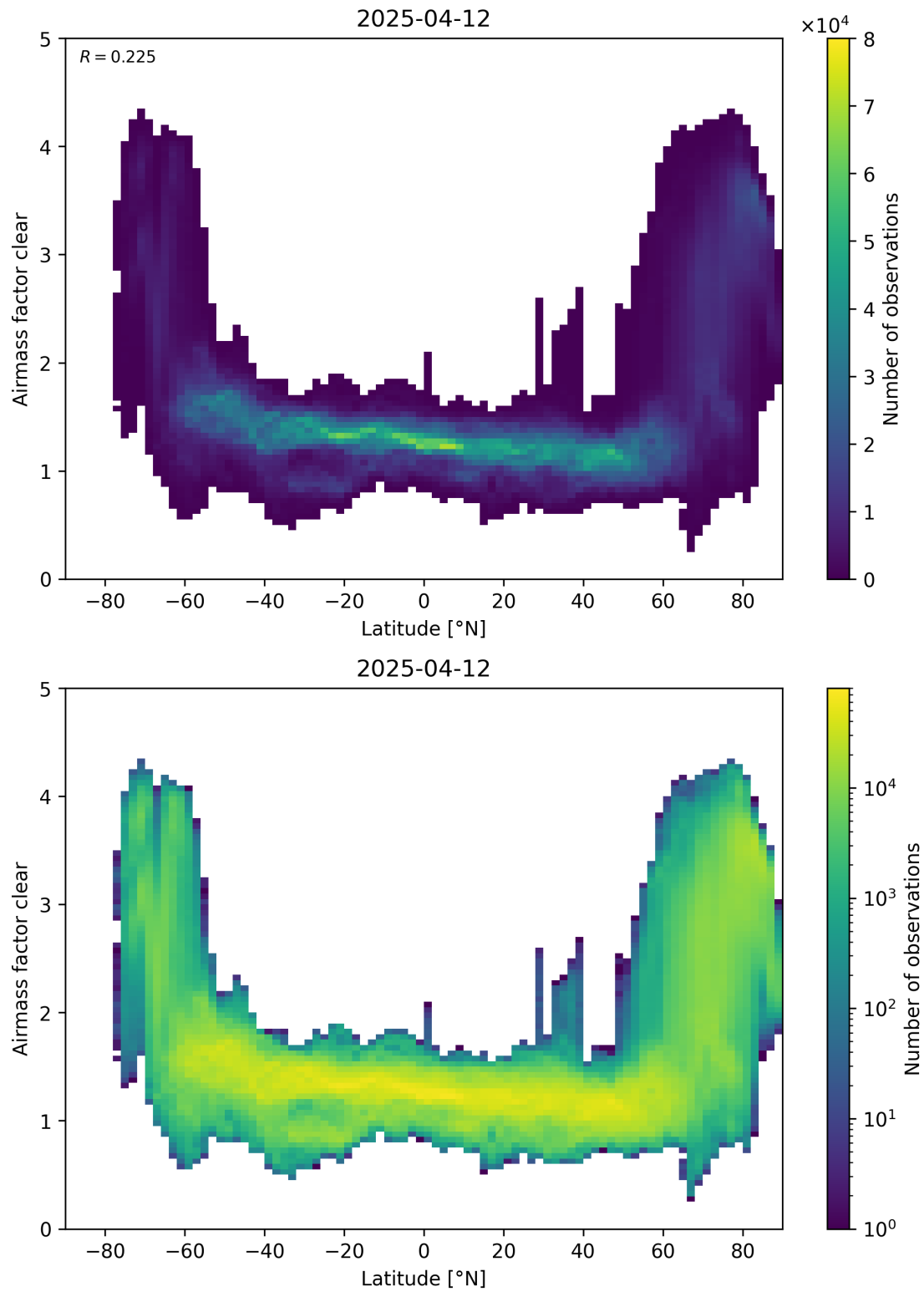
Figure 156: Scatter density plot of “Latitude” against “Airmass factor clear” for 2025-04-11 to 2025-04-13.
