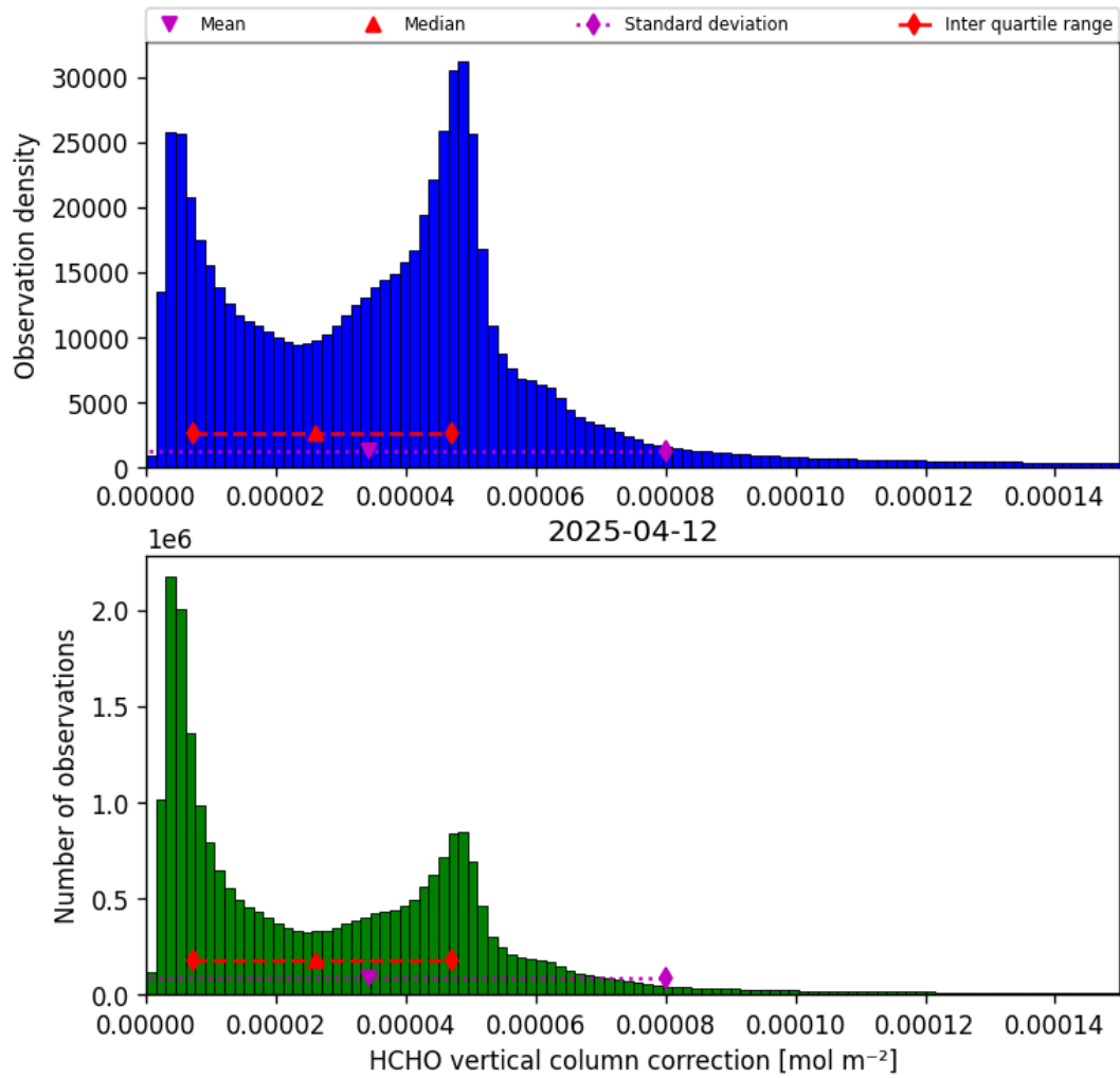
Figure 37: Histogram of “HCHO vertical column correction” for 2025-04-11 to 2025-04-13
