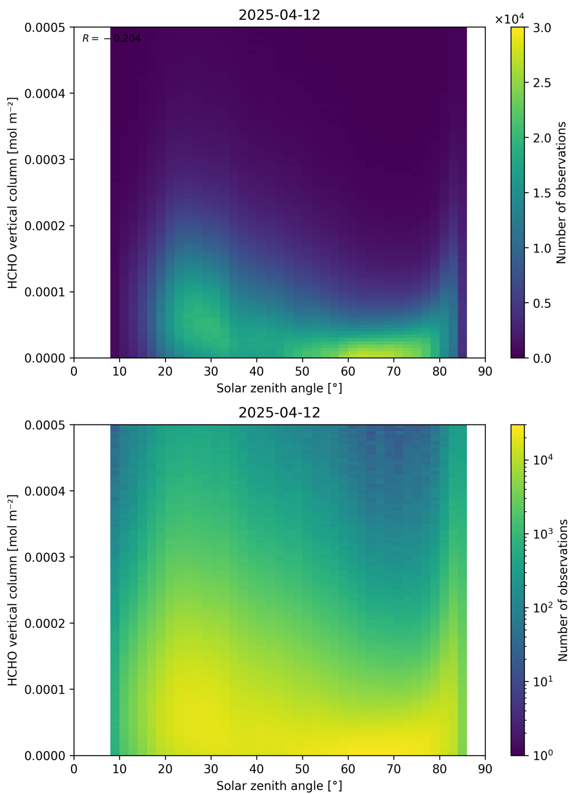
Figure 177: Scatter density plot of “Solar zenith angle” against “HCHO vertical column” for 2025-04-11 to 2025-04-13.
