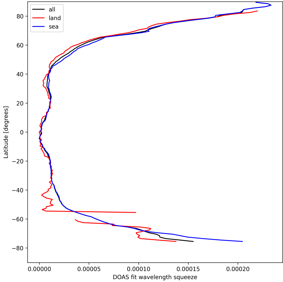
Figure 31: Zonal average of “DOAS fit wavelength squeeze” for 2025-04-13 to 2025-04-14.
