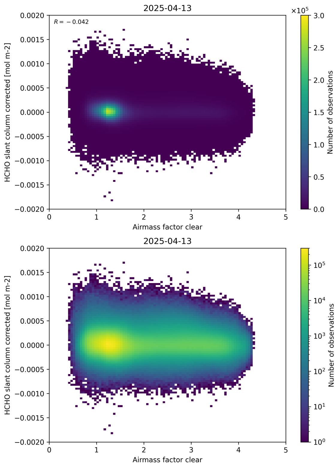
Figure 74: Scatter density plot of “Airmass factor clear” against “HCHO slant column corrected” for 2025-04-13 to 2025-04-14.
