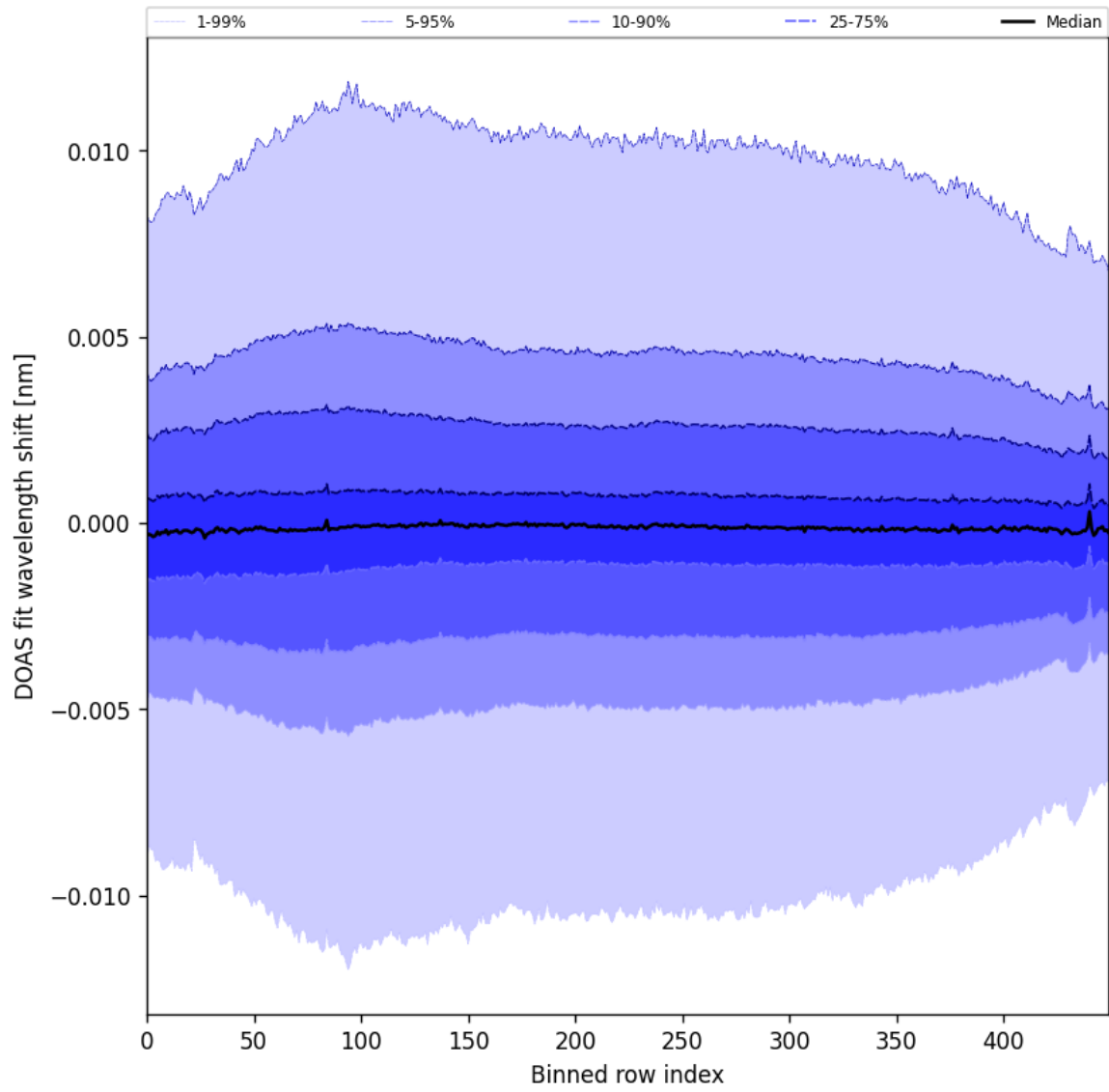
Figure 58: Along track statistics of “DOAS fit wavelength shift” for 2025-04-13 to 2025-04-14
