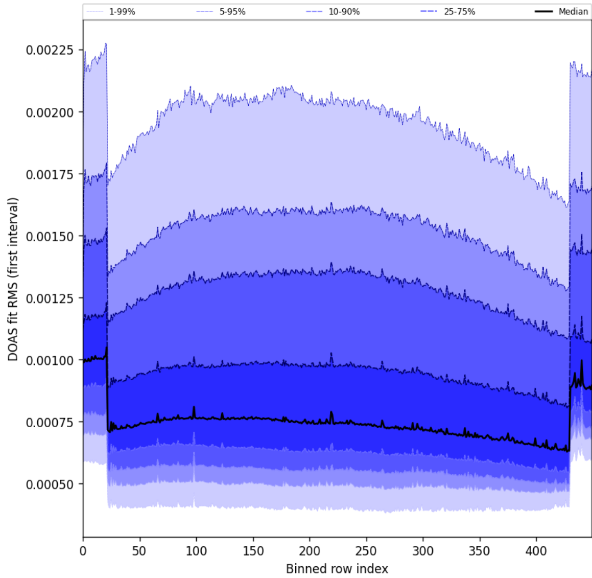
Figure 60: Along track statistics of “DOAS fit RMS (first interval)” for 2025-04-13 to 2025-04-14
