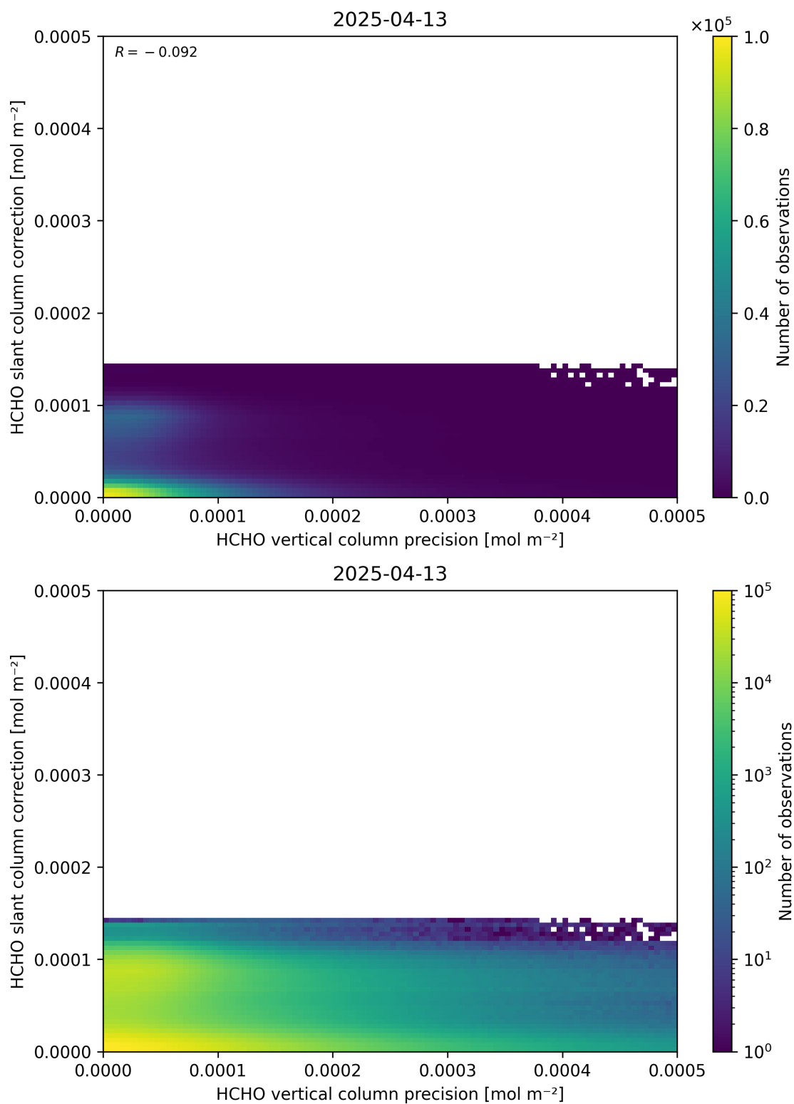
Figure 141: Scatter density plot of “HCHO vertical column precision” against “HCHO slant column correction” for 2025-04-13 to 2025-04-14.
