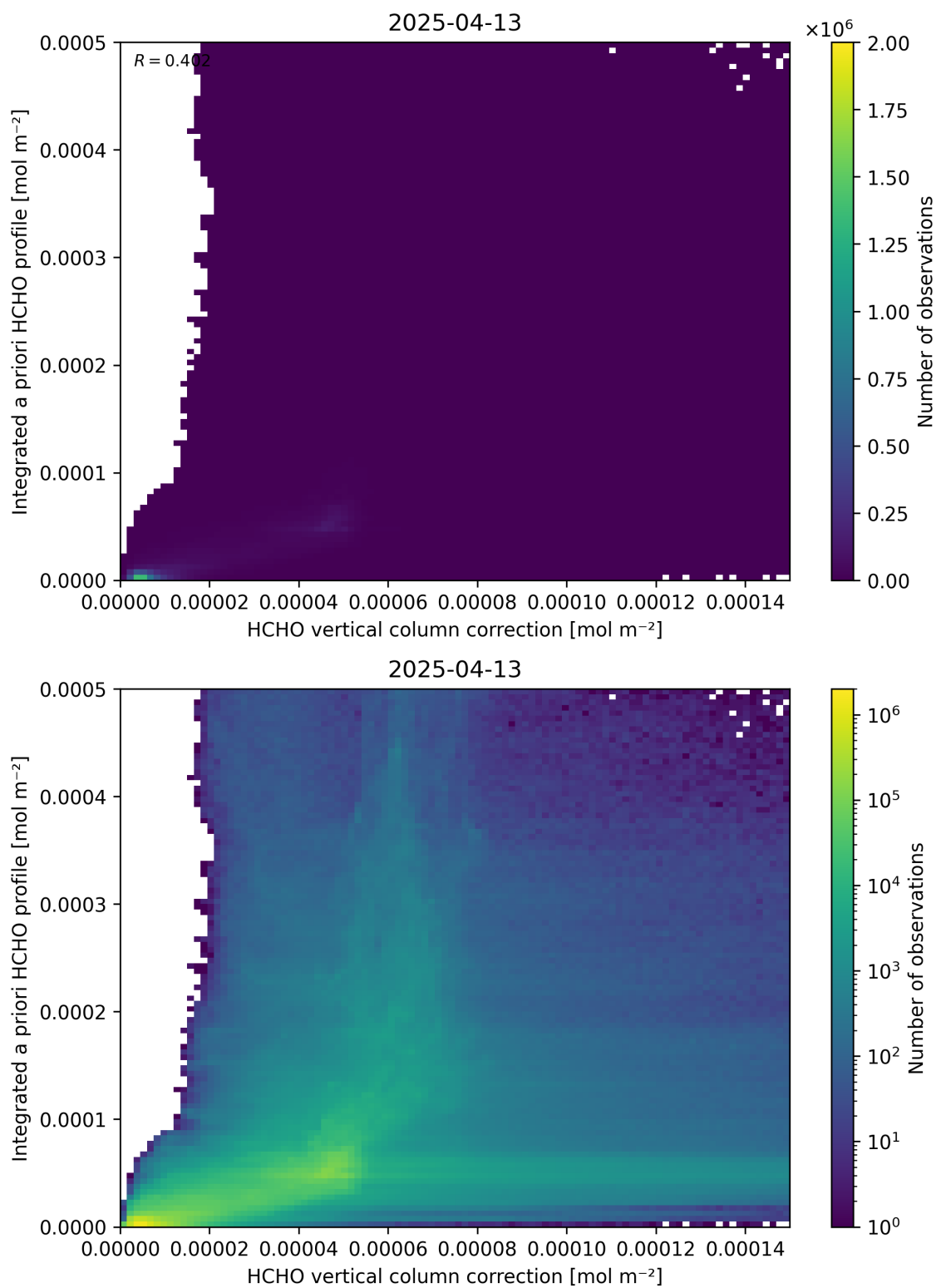
Figure 122: Scatter density plot of “HCHO vertical column correction” against “Integrated a priori HCHO profile” for 2025-04-13 to 2025-04-14.
