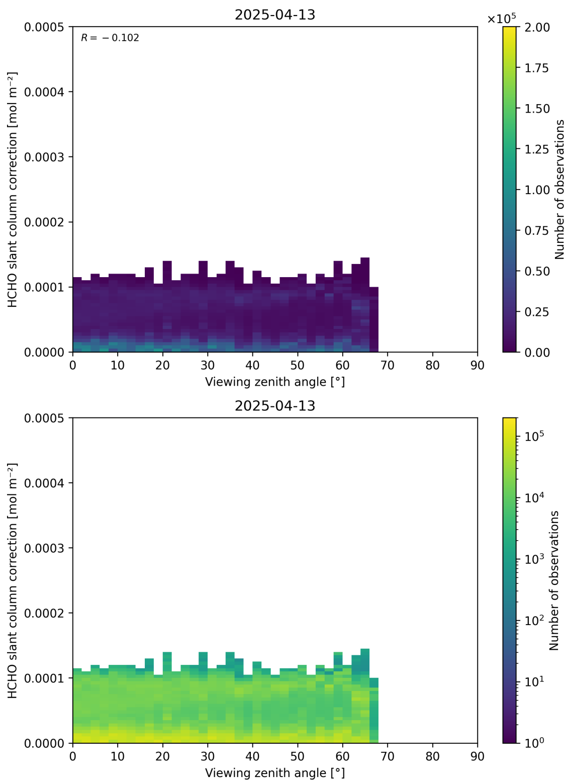
Figure 187: Scatter density plot of “Viewing zenith angle” against “HCHO slant column correction” for 2025-04-13 to 2025-04-14.
