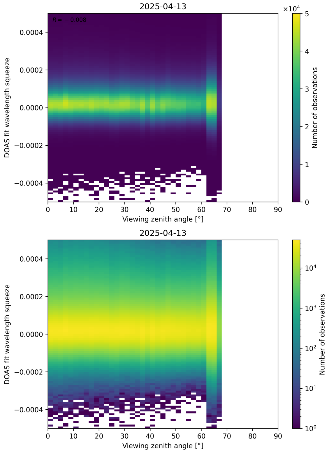
Figure 184: Scatter density plot of “Viewing zenith angle” against “DOAS fit wavelength squeeze” for 2025-04-13 to 2025-04-14.
