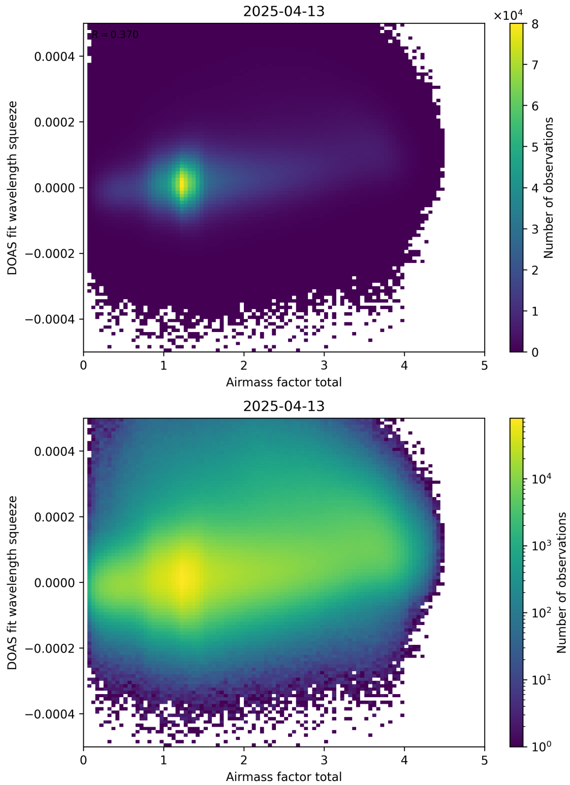
Figure 99: Scatter density plot of “Airmass factor total” against “DOAS fit wavelength squeeze” for 2025-04-13 to 2025-04-14.
