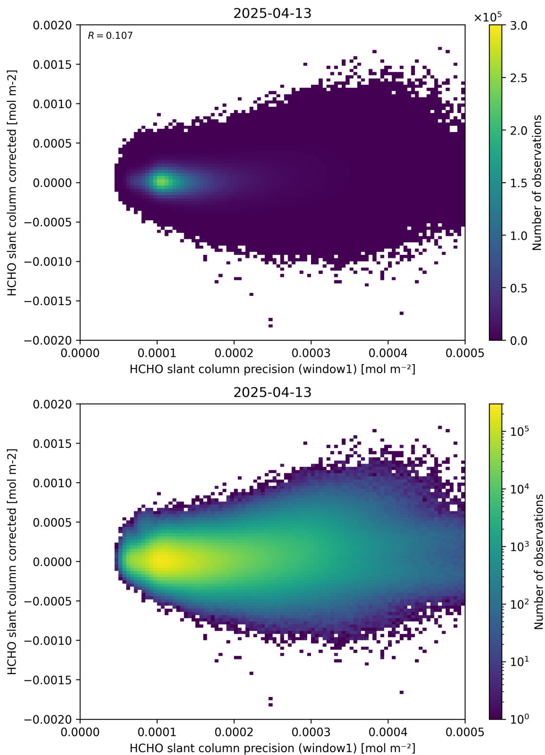
Figure 92: Scatter density plot of “HCHO slant column precision (window1)” against “HCHO slant column corrected” for 2025-04-13 to 2025-04-14.
