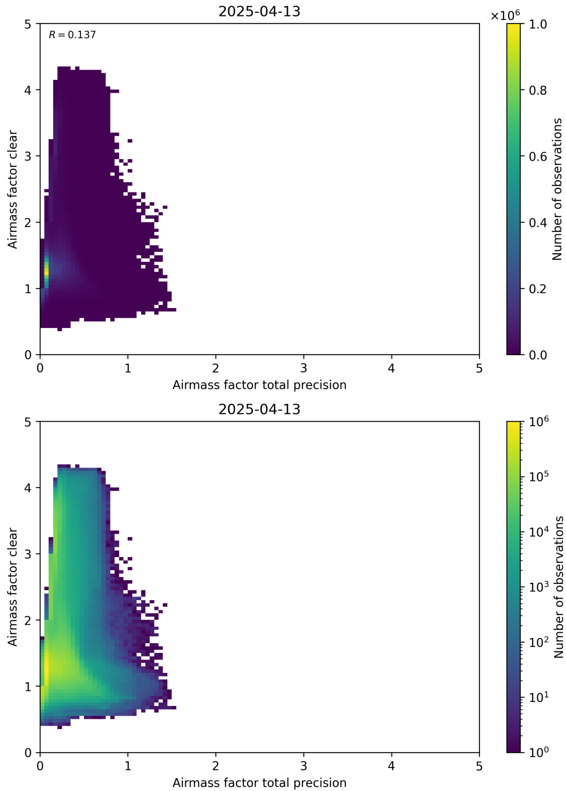
Figure 108: Scatter density plot of “Airmass factor total precision” against “Airmass factor clear” for 2025-04-13 to 2025-04-14.
