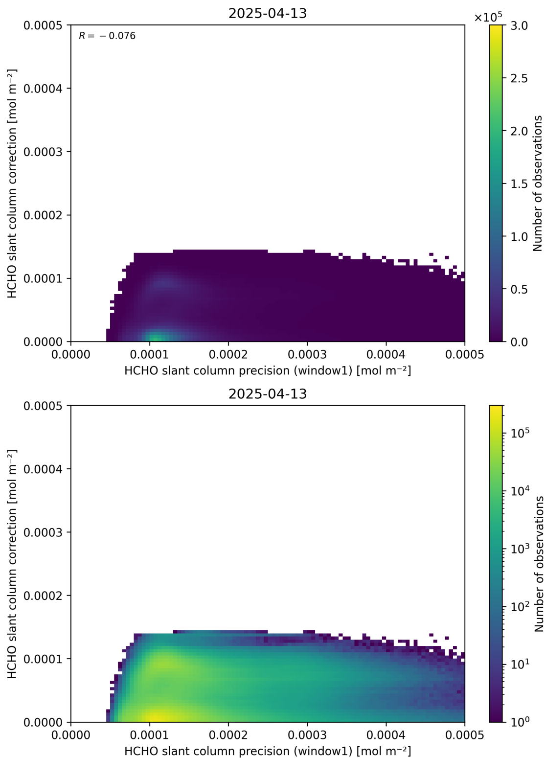
Figure 93: Scatter density plot of “HCHO slant column precision (window1)” against “HCHO slant column correction” for 2025-04-13 to 2025-04-14.
