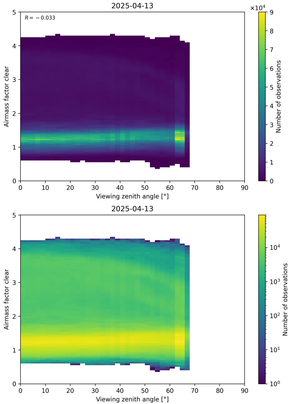
Figure 185: Scatter density plot of “Viewing zenith angle” against “Airmass factor clear” for 2025-04-13 to 2025-04-14.
