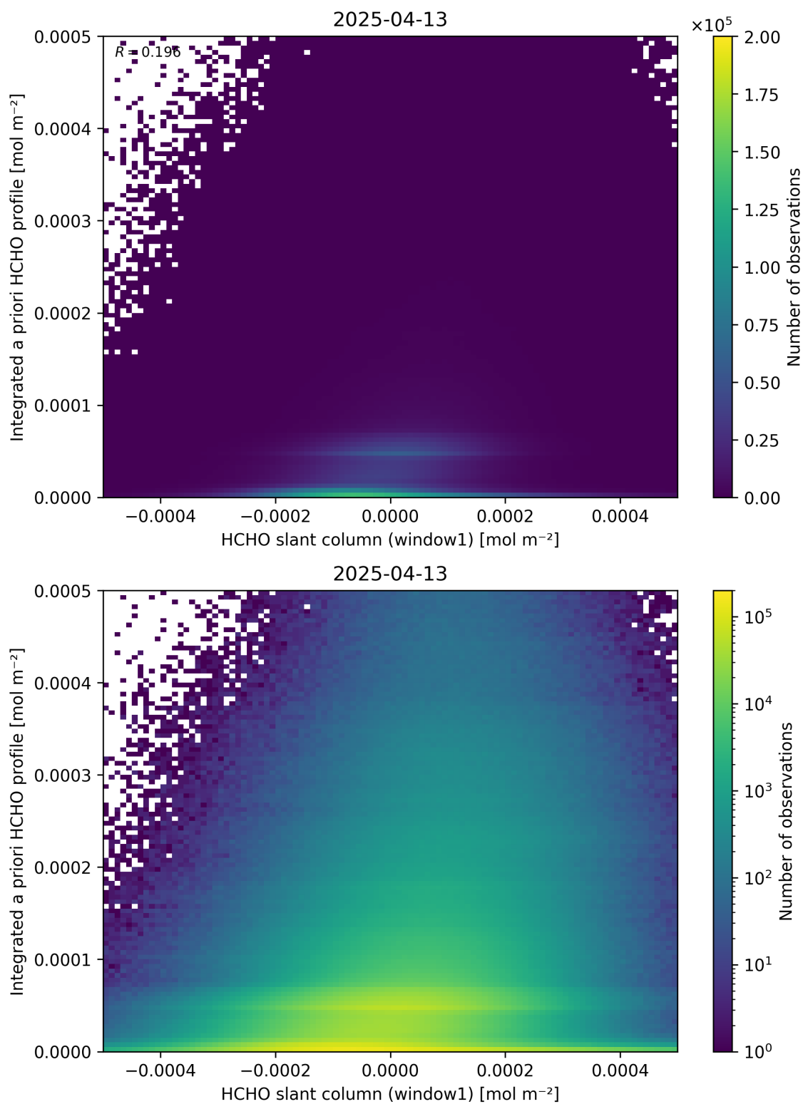
Figure 87: Scatter density plot of “HCHO slant column (window1)” against “Integrated a priori HCHO profile” for 2025-04-13 to 2025-04-14.
