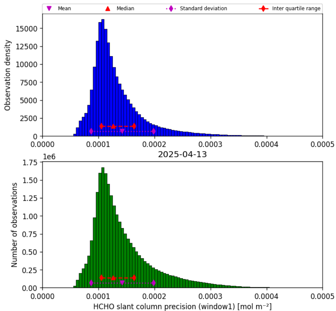
Figure 39: Histogram of “HCHO slant column precision (window1)” for 2025-04-13 to 2025-04-14
