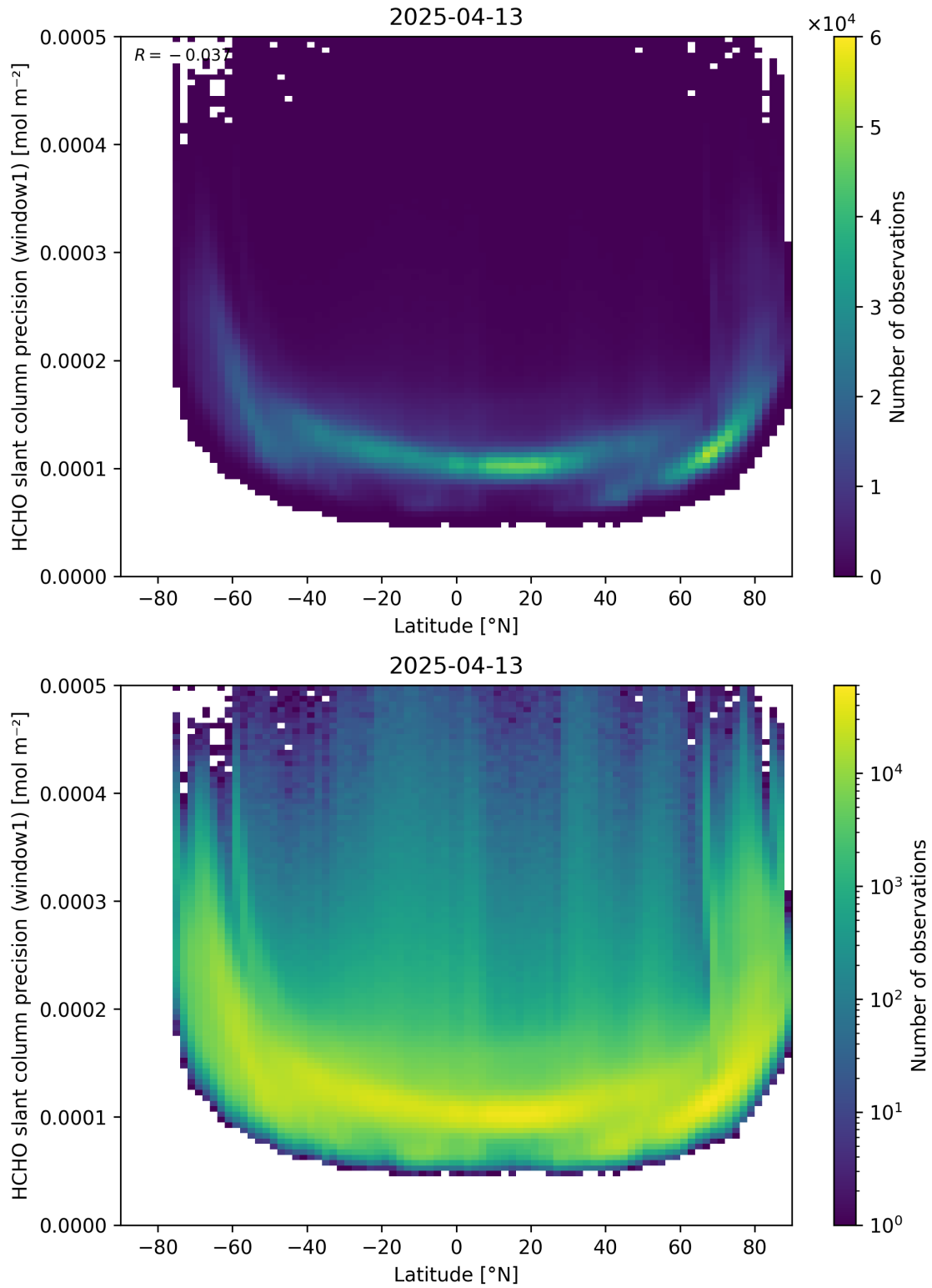
Figure 160: Scatter density plot of “Latitude” against “HCHO slant column precision (window1)” for 2025-04-13 to 2025-04-14.
