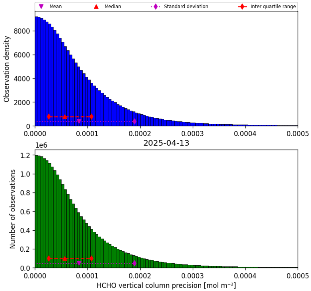
Figure 36: Histogram of “HCHO vertical column precision” for 2025-04-13 to 2025-04-14
