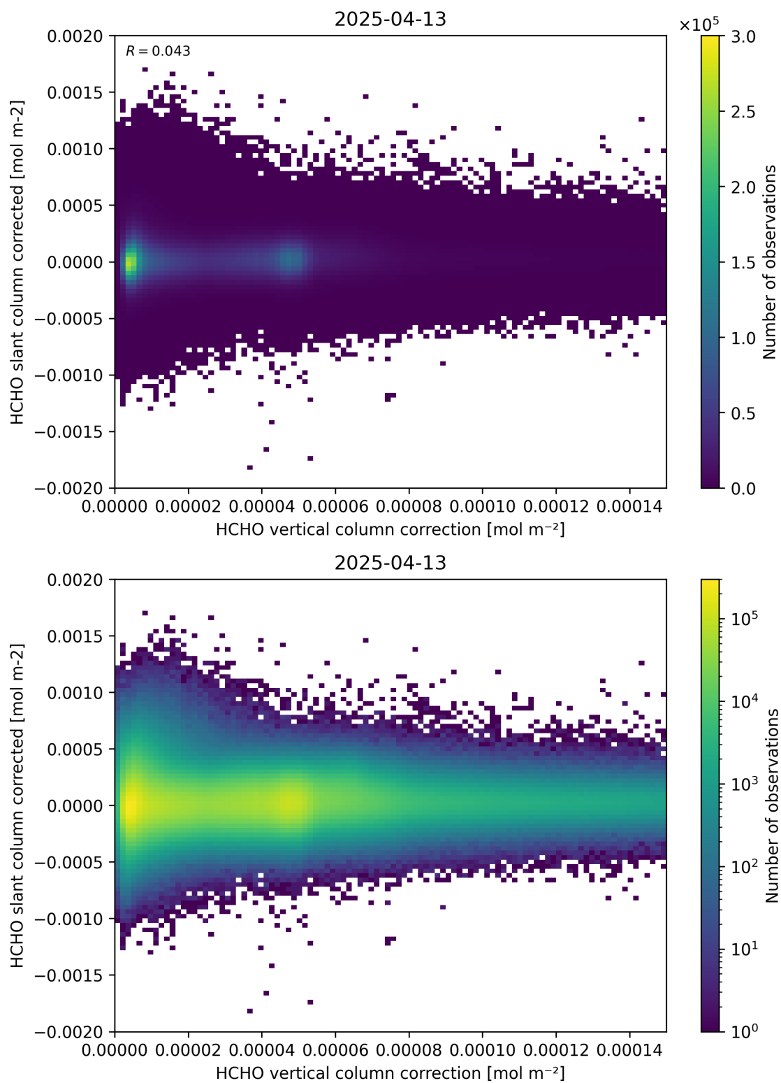
Figure 116: Scatter density plot of “HCHO vertical column correction” against “HCHO slant column corrected” for 2025-04-13 to 2025-04-14.
