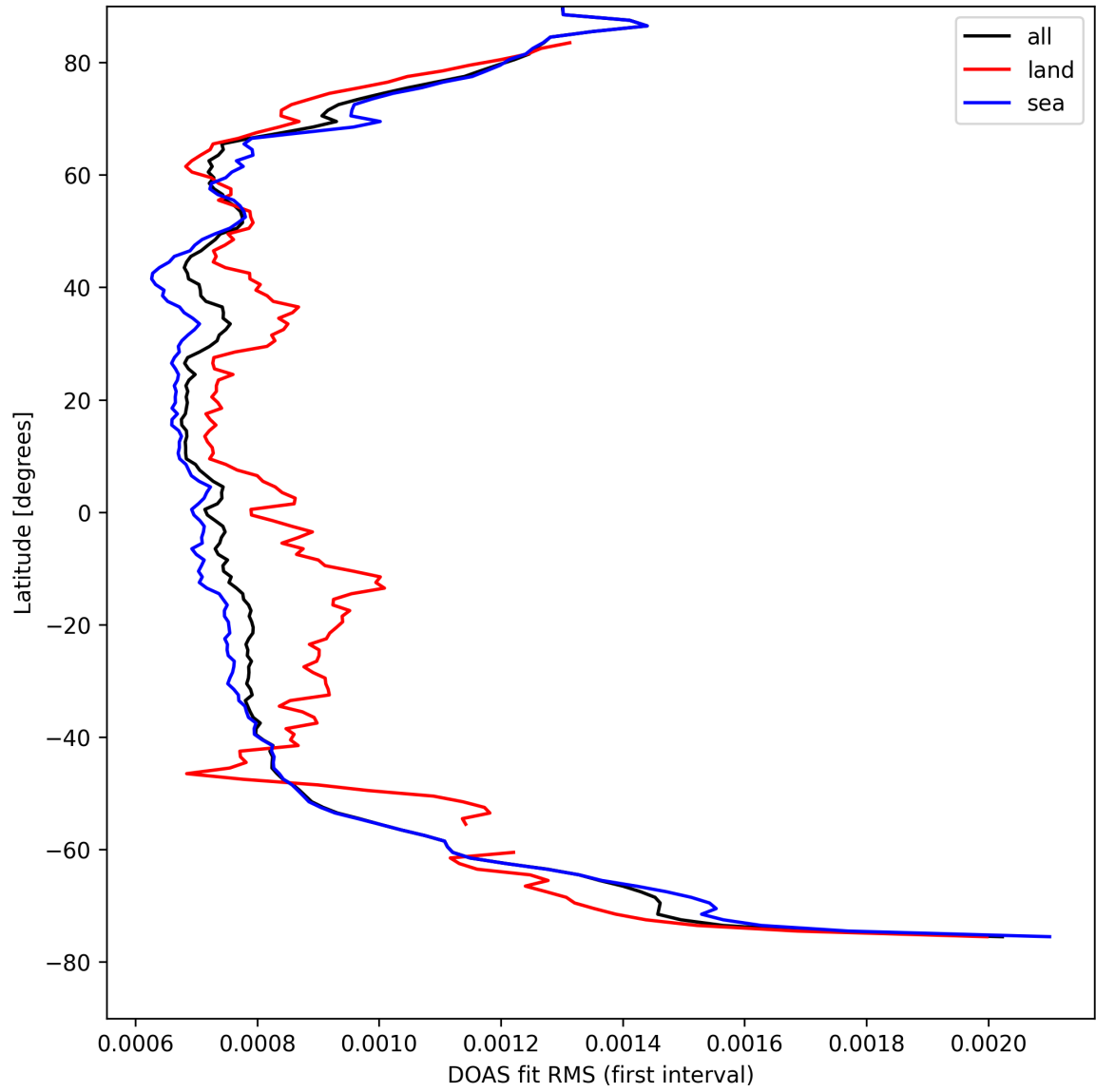
Figure 32: Zonal average of “DOAS fit RMS (first interval)” for 2025-04-13 to 2025-04-14.
