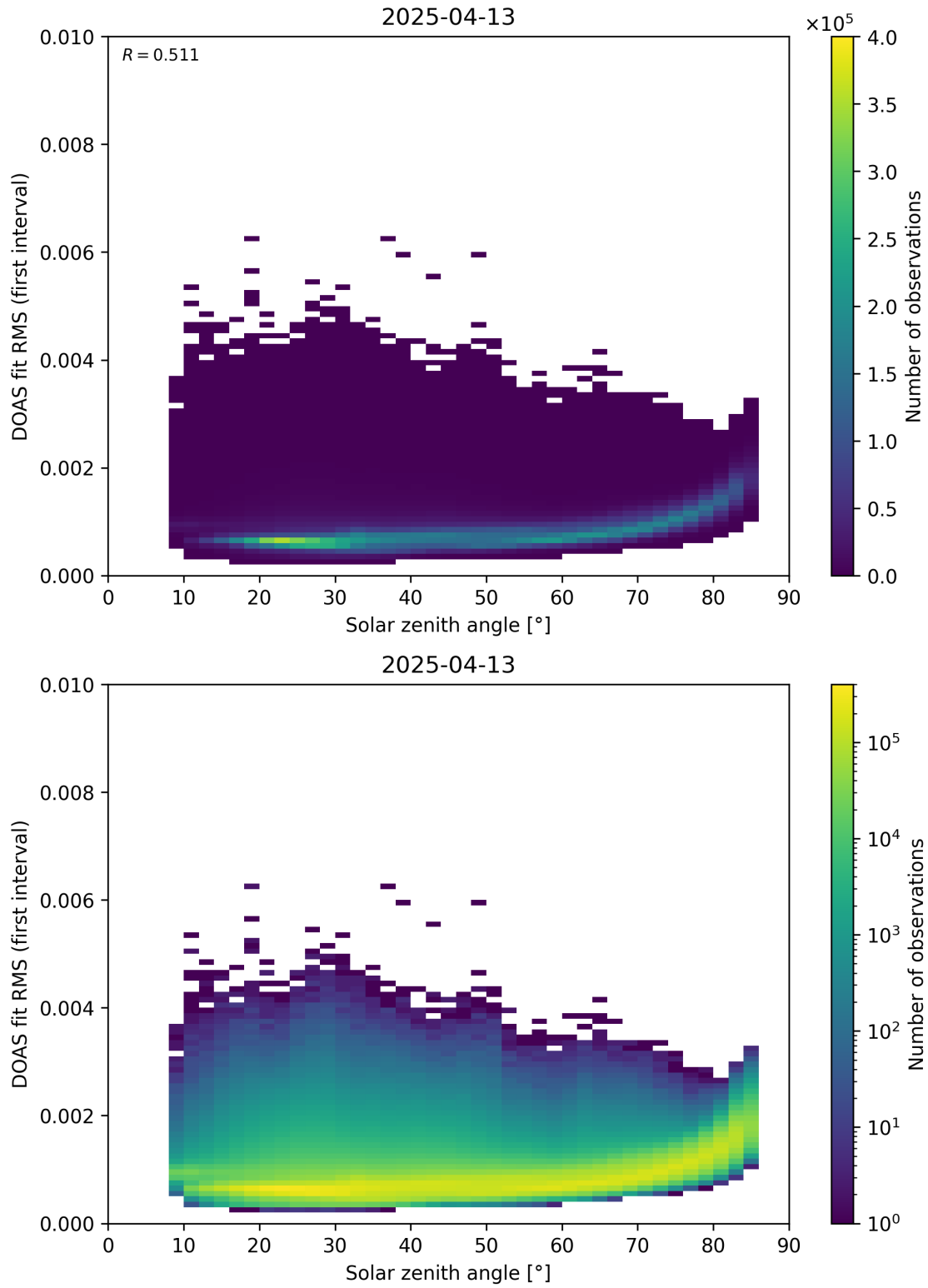
Figure 167: Scatter density plot of “Solar zenith angle” against “DOAS fit RMS (first interval)” for 2025-04-13 to 2025-04-14.
