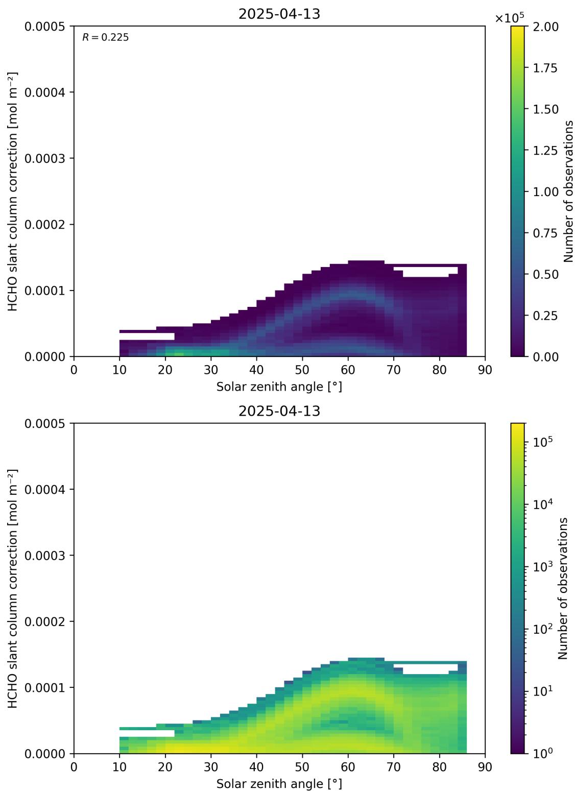
Figure 172: Scatter density plot of “Solar zenith angle” against “HCHO slant column correction” for 2025-04-13 to 2025-04-14.
