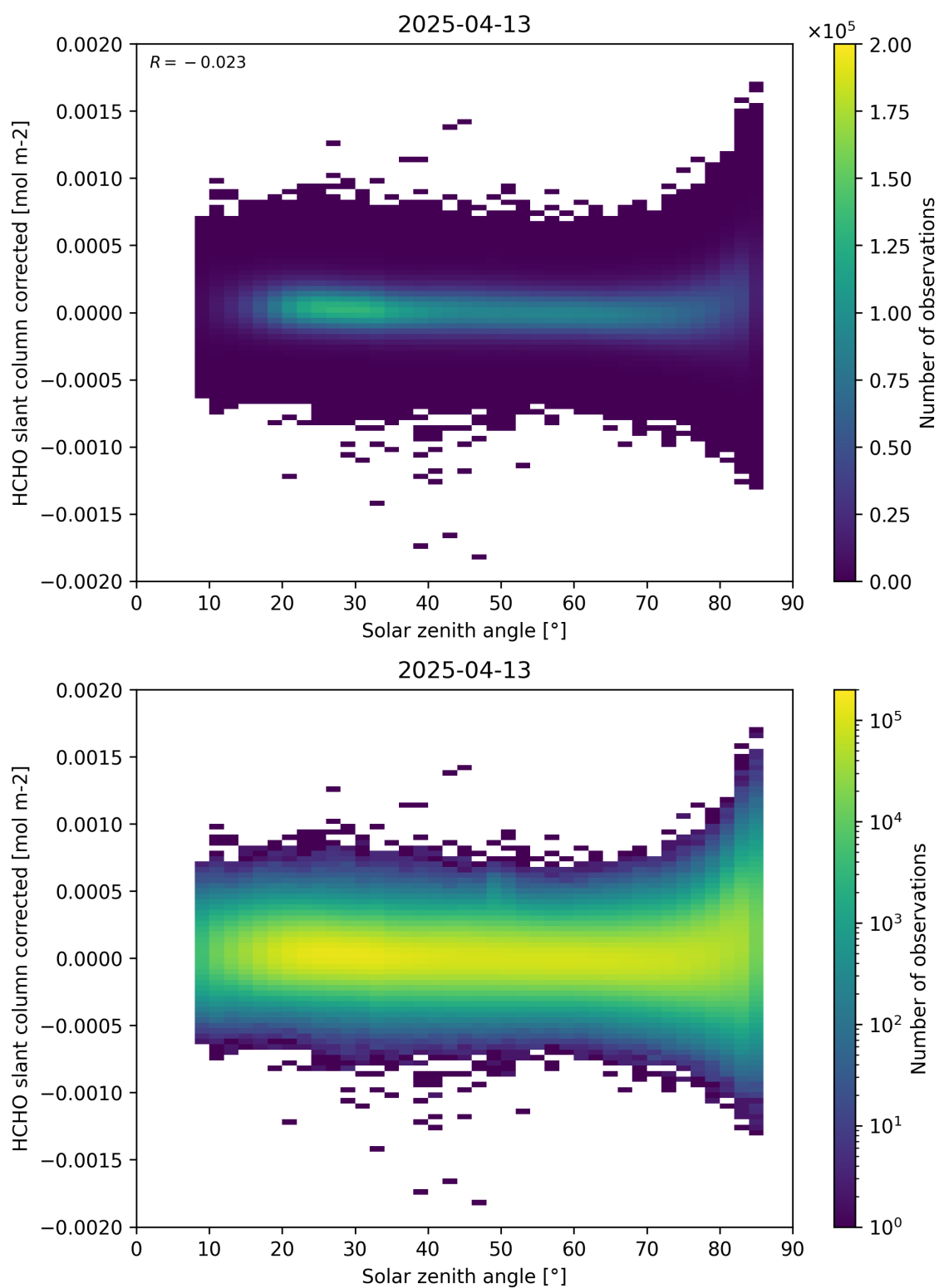
Figure 171: Scatter density plot of “Solar zenith angle” against “HCHO slant column corrected” for 2025-04-13 to 2025-04-14.
