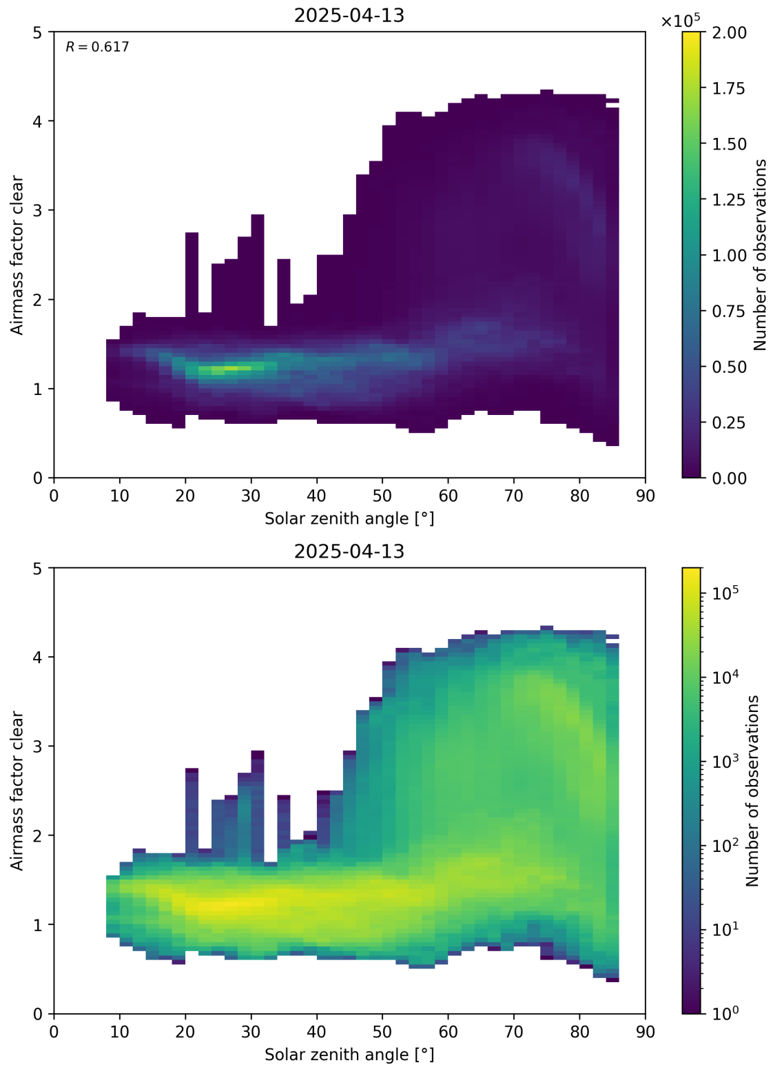
Figure 170: Scatter density plot of “Solar zenith angle” against “Airmass factor clear” for 2025-04-13 to 2025-04-14.
