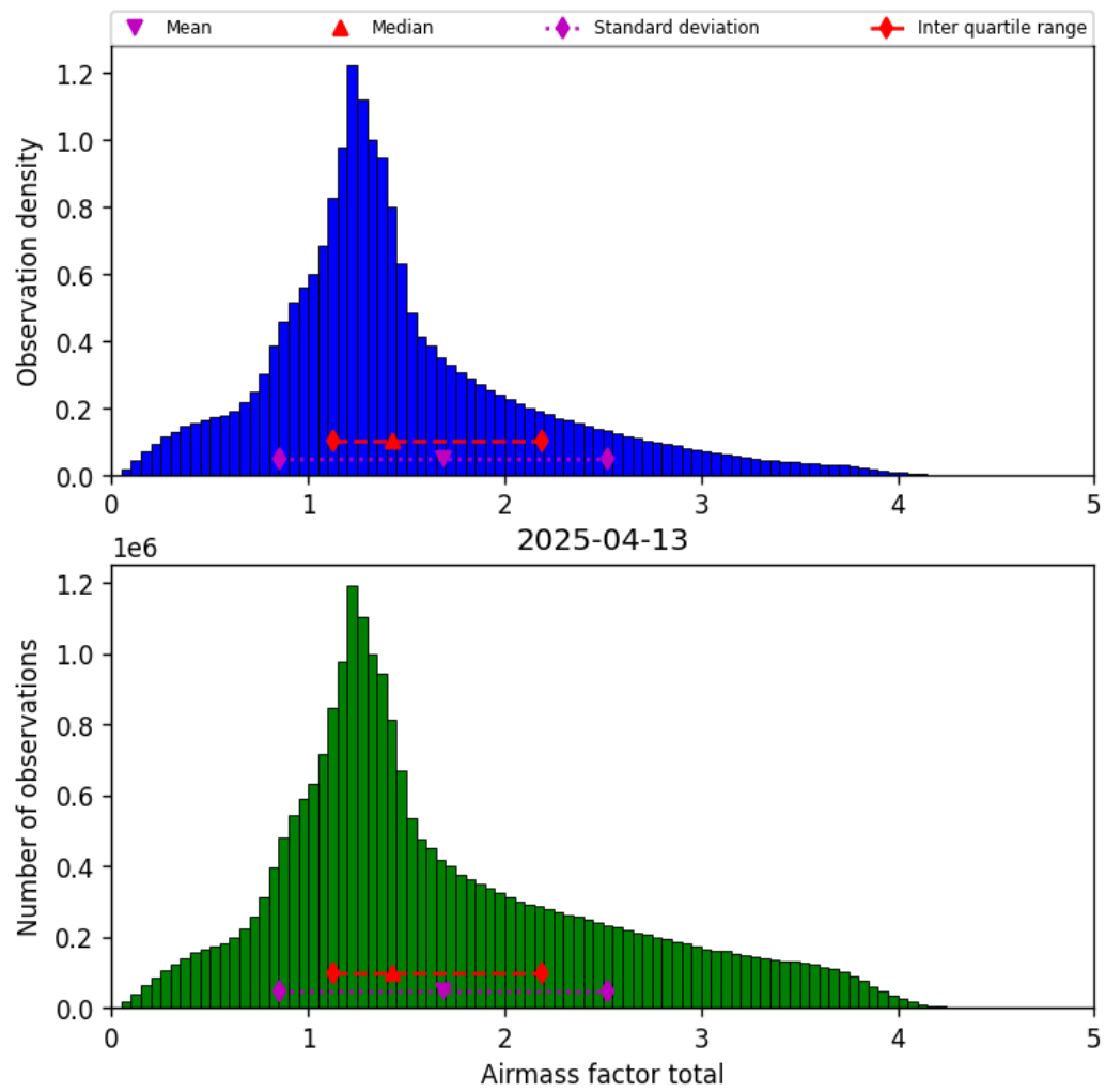
Figure 40: Histogram of “Airmass factor total” for 2025-04-13 to 2025-04-14
