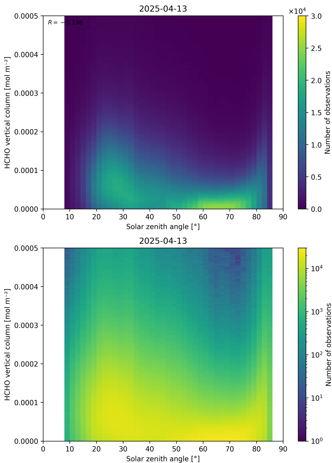
Figure 177: Scatter density plot of “Solar zenith angle” against “HCHO vertical column” for 2025-04-13 to 2025-04-14.
