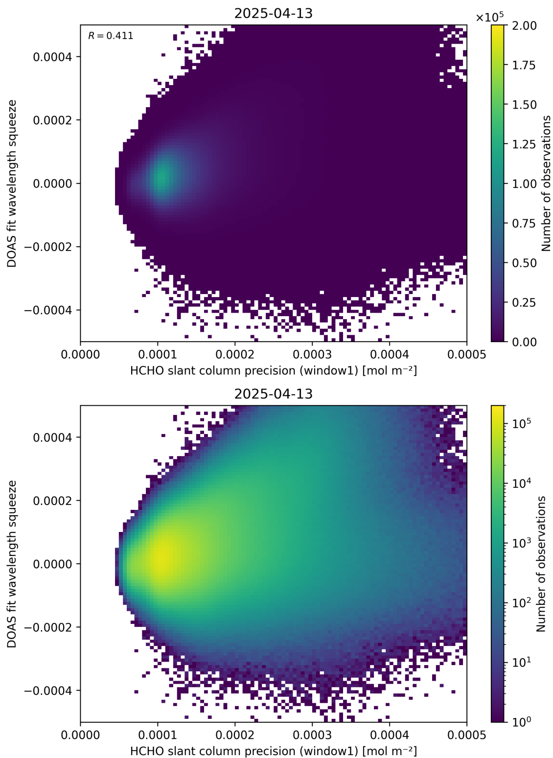
Figure 90: Scatter density plot of “HCHO slant column precision (window1)” against “DOAS fit wavelength squeeze” for 2025-04-13 to 2025-04-14.
