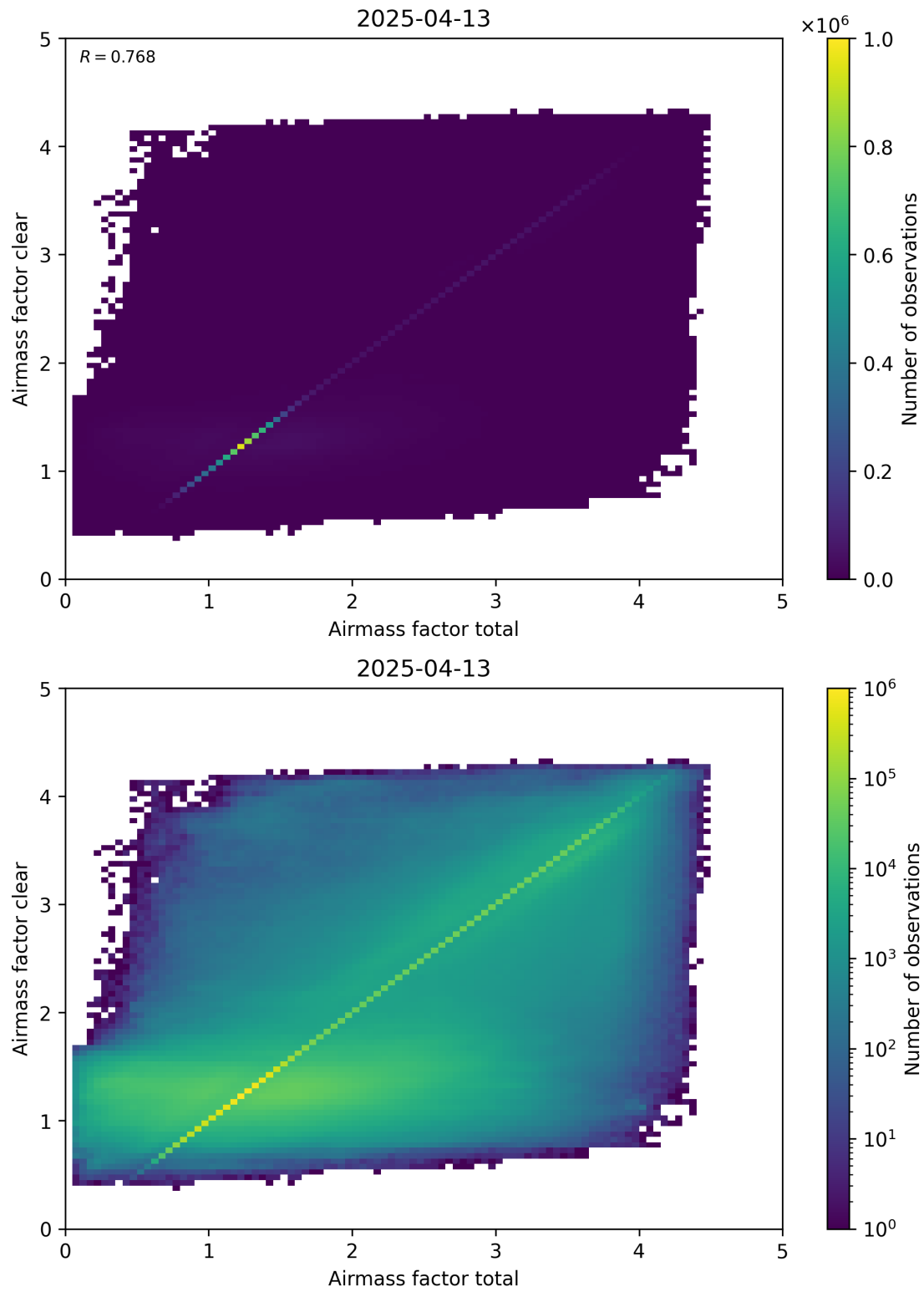
Figure 100: Scatter density plot of “Airmass factor total” against “Airmass factor clear” for 2025-04-13 to 2025-04-14.
