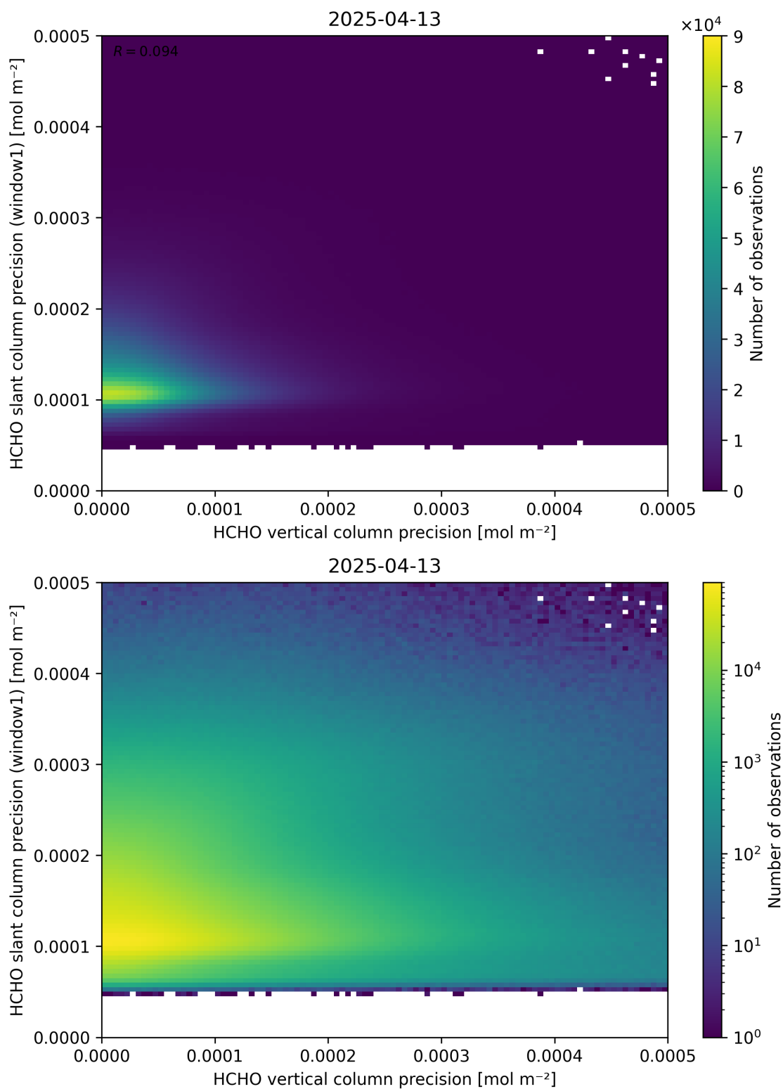
Figure 143: Scatter density plot of “HCHO vertical column precision” against “HCHO slant column precision (window1)” for 2025-04-13 to 2025-04-14.
