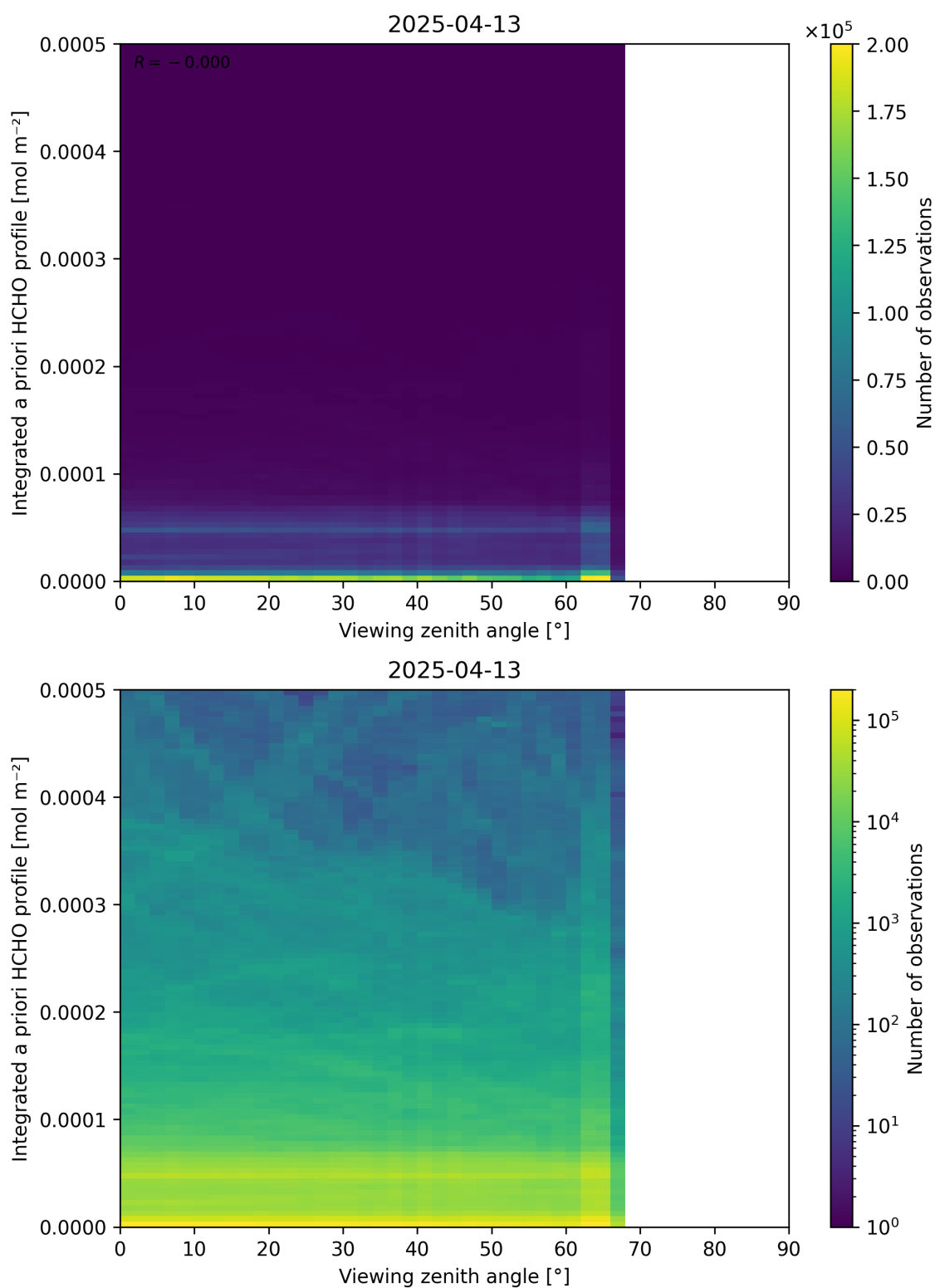
Figure 195: Scatter density plot of “Viewing zenith angle” against “Integrated a priori HCHO profile” for 2025-04-13 to 2025-04-14.
