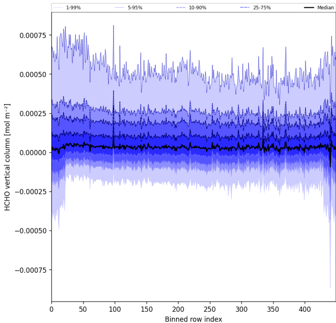
Figure 49: Along track statistics of “HCHO vertical column” for 2025-04-13 to 2025-04-14
