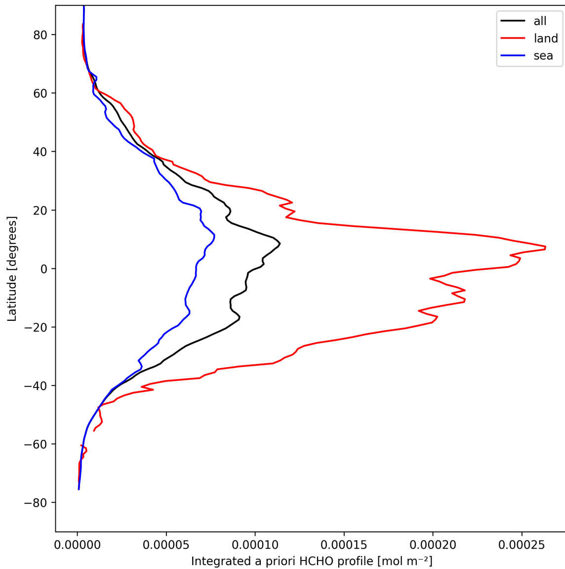
Figure 29: Zonal average of “Integrated a priori HCHO profile” for 2025-04-13 to 2025-04-14.
