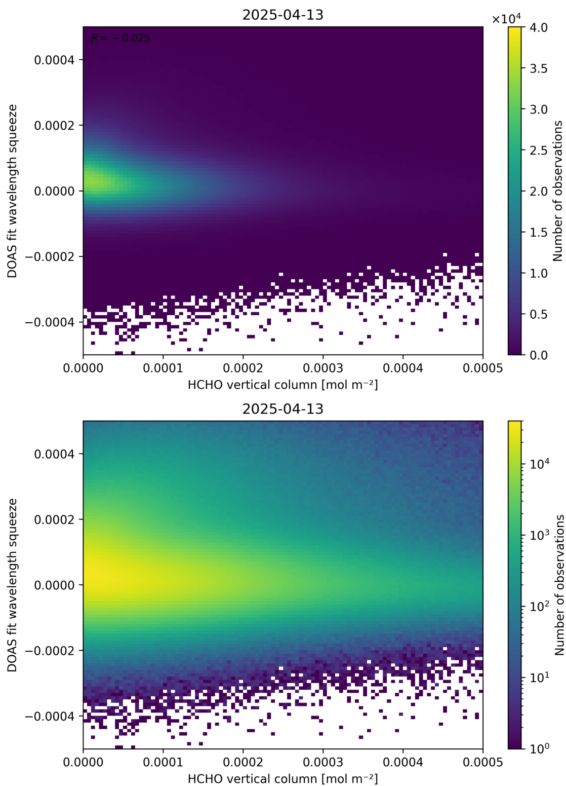
Figure 125: Scatter density plot of “HCHO vertical column” against “DOAS fit wavelength squeeze” for 2025-04-13 to 2025-04-14.
