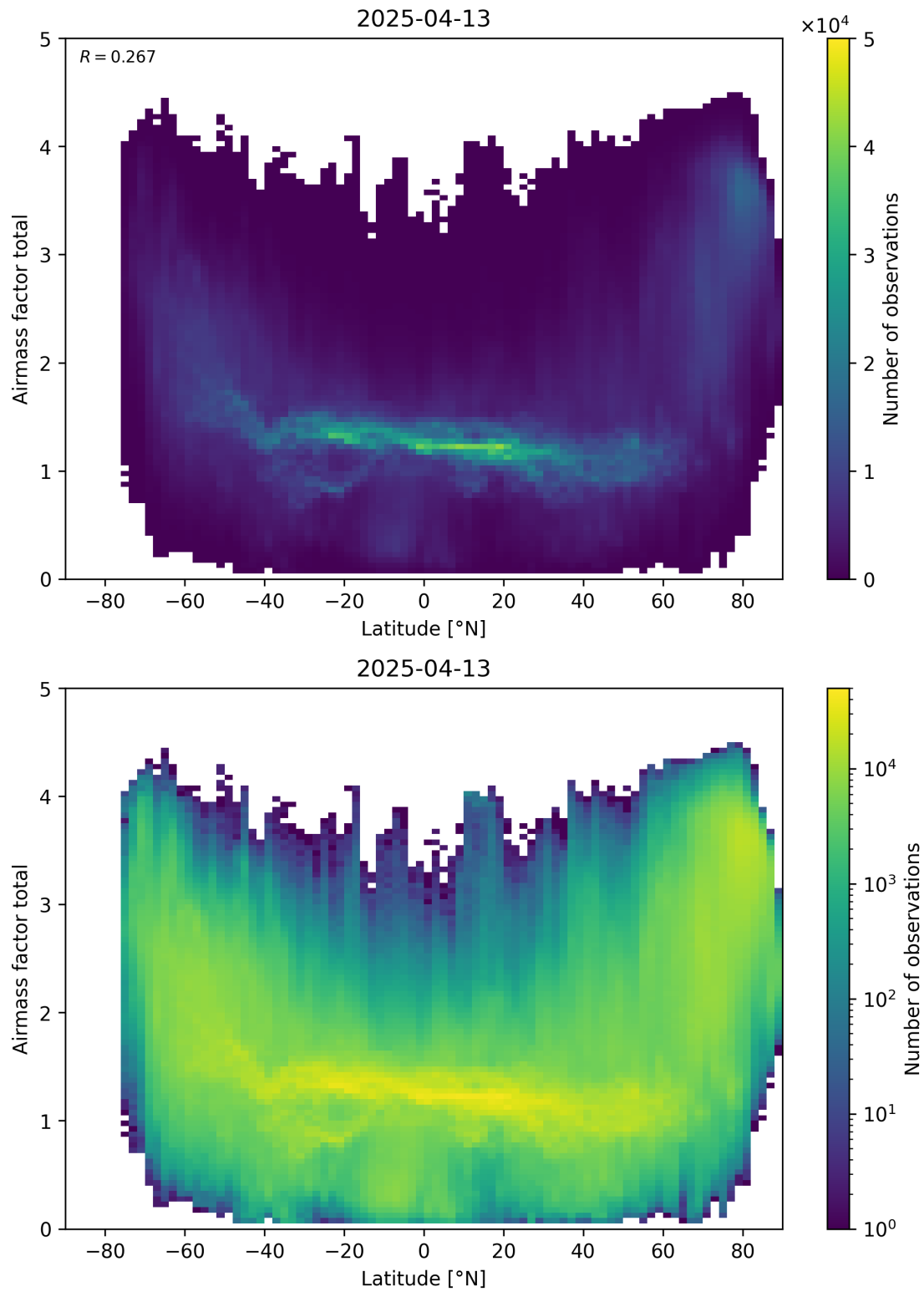
Figure 161: Scatter density plot of “Latitude” against “Airmass factor total” for 2025-04-13 to 2025-04-14.
