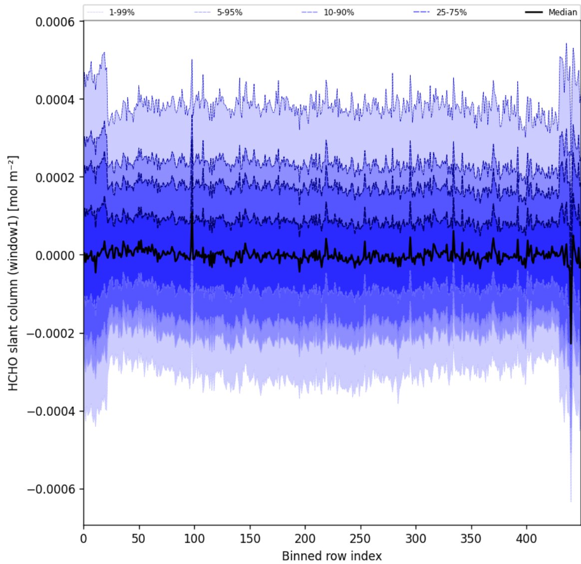
Figure 52: Along track statistics of “HCHO slant column (window1)” for 2025-04-13 to 2025-04-14
