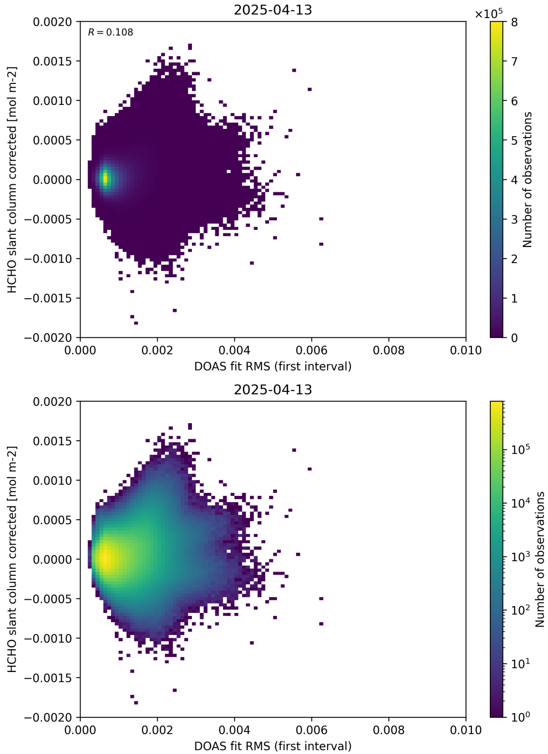
Figure 62: Scatter density plot of “DOAS fit RMS (first interval)” against “HCHO slant column corrected” for 2025-04-13 to 2025-04-14.
