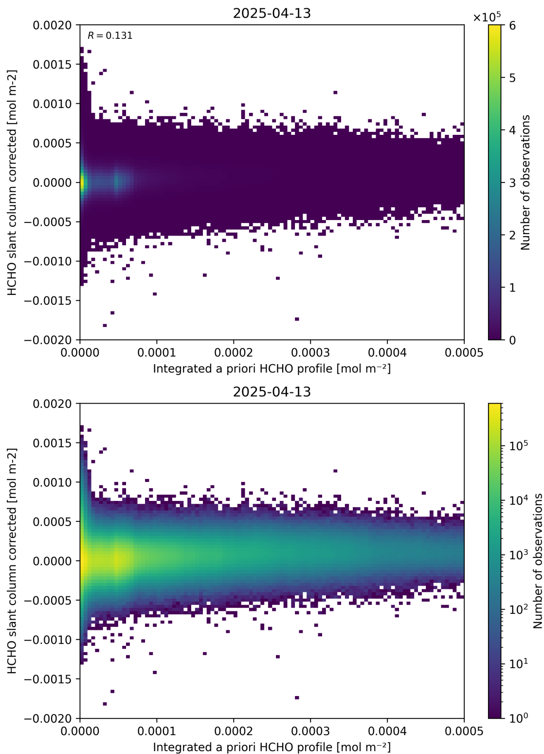
Figure 151: Scatter density plot of “Integrated a priori HCHO profile” against “HCHO slant column corrected” for 2025-04-13 to 2025-04-14.
