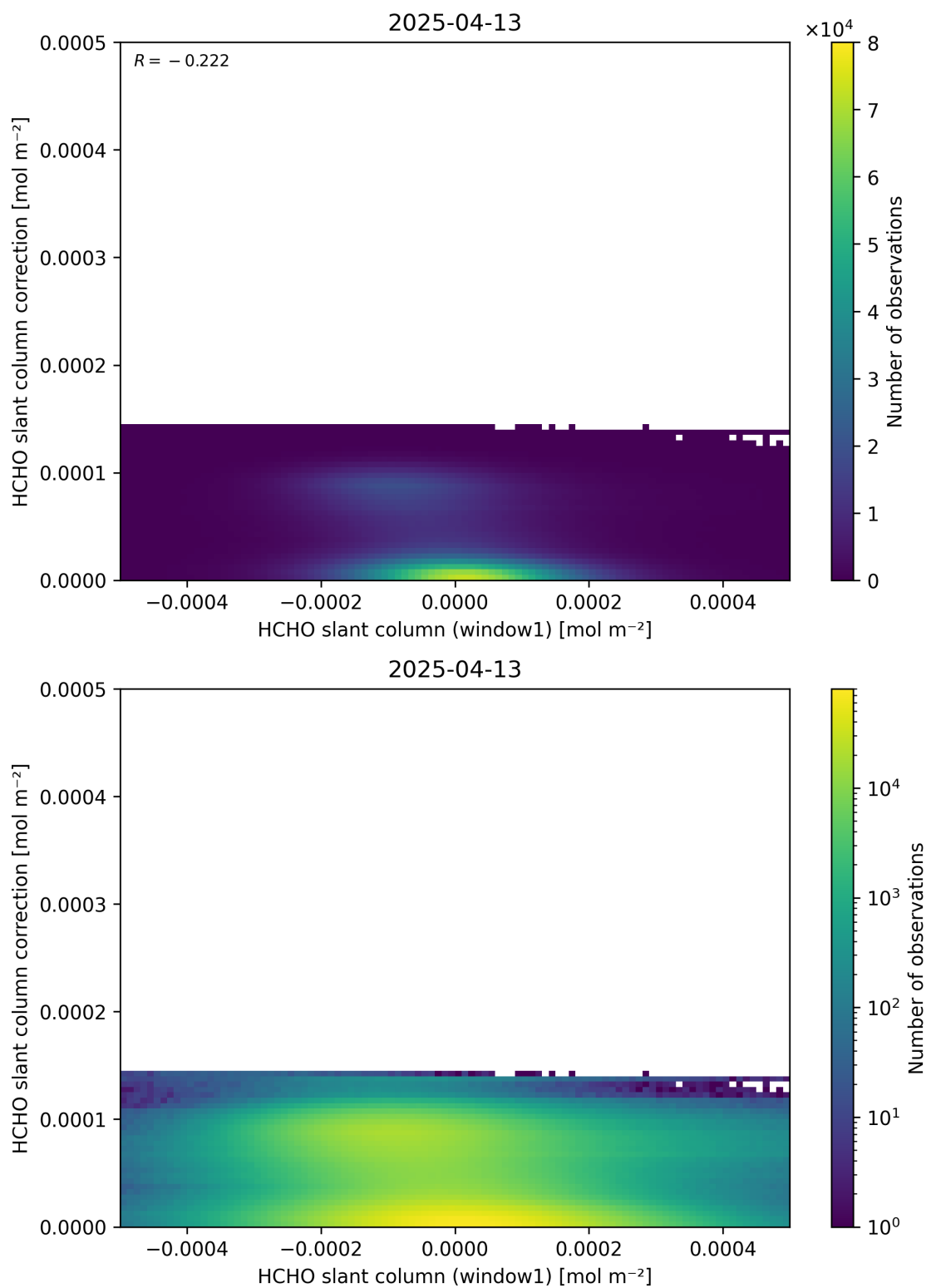
Figure 83: Scatter density plot of “HCHO slant column (window1)” against “HCHO slant column correction” for 2025-04-13 to 2025-04-14.
