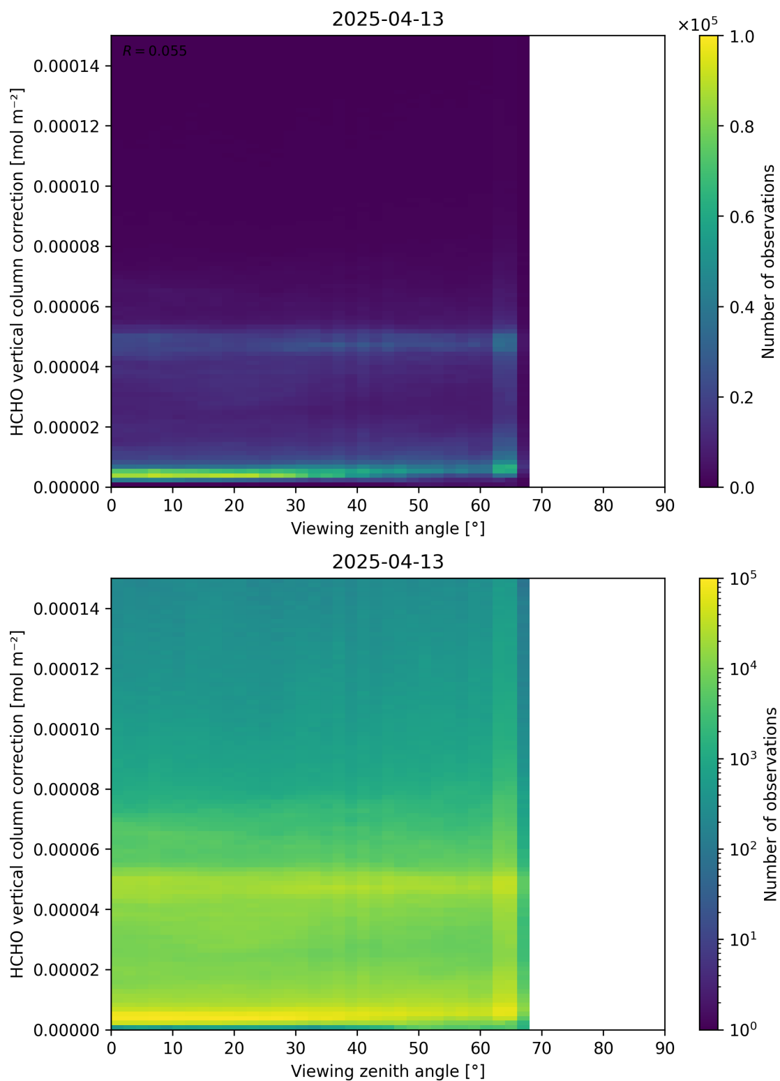
Figure 193: Scatter density plot of “Viewing zenith angle” against “HCHO vertical column correction” for 2025-04-13 to 2025-04-14.
