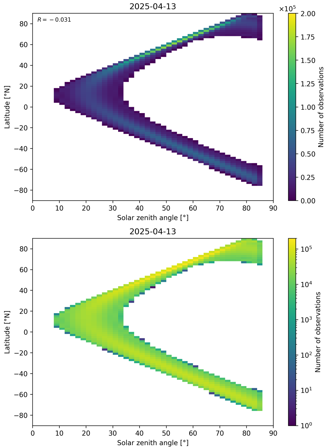
Figure 181: Scatter density plot of “Solar zenith angle” against “Latitude” for 2025-04-13 to 2025-04-14.
