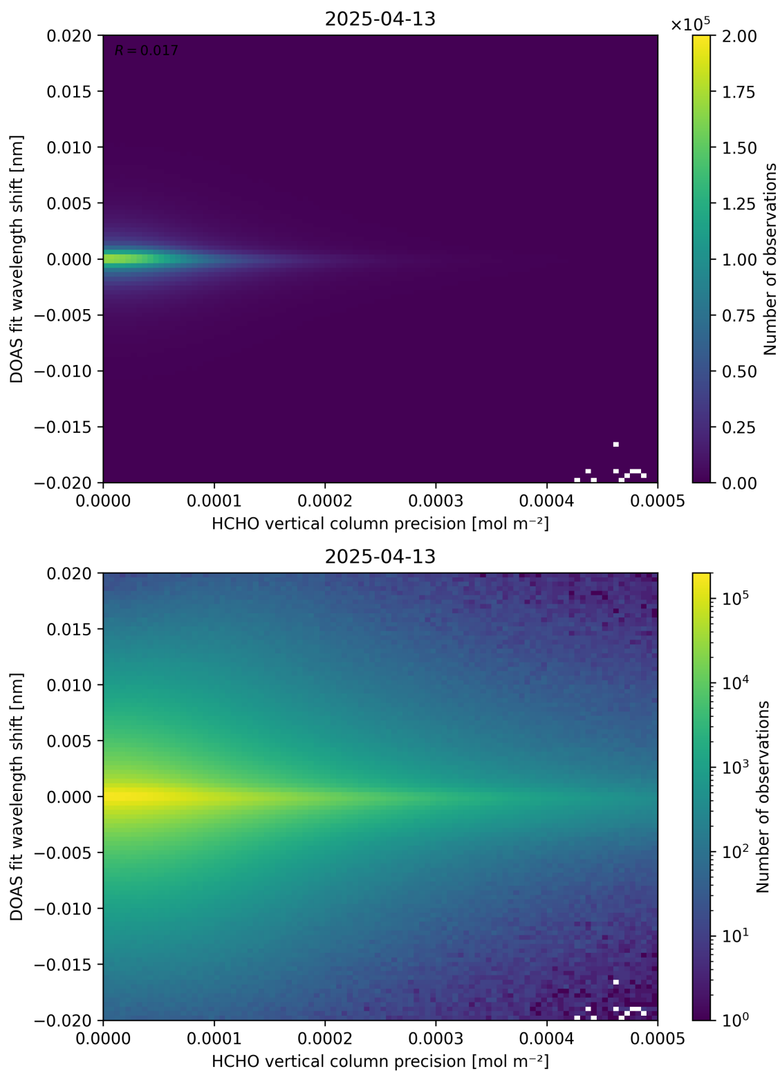
Figure 137: Scatter density plot of “HCHO vertical column precision” against “DOAS fit wavelength shift” for 2025-04-13 to 2025-04-14.
