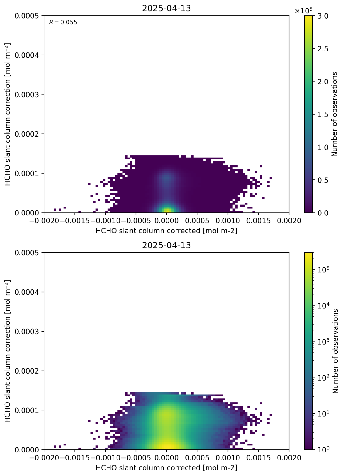
Figure 77: Scatter density plot of “HCHO slant column corrected” against “HCHO slant column correction” for 2025-04-13 to 2025-04-14.
