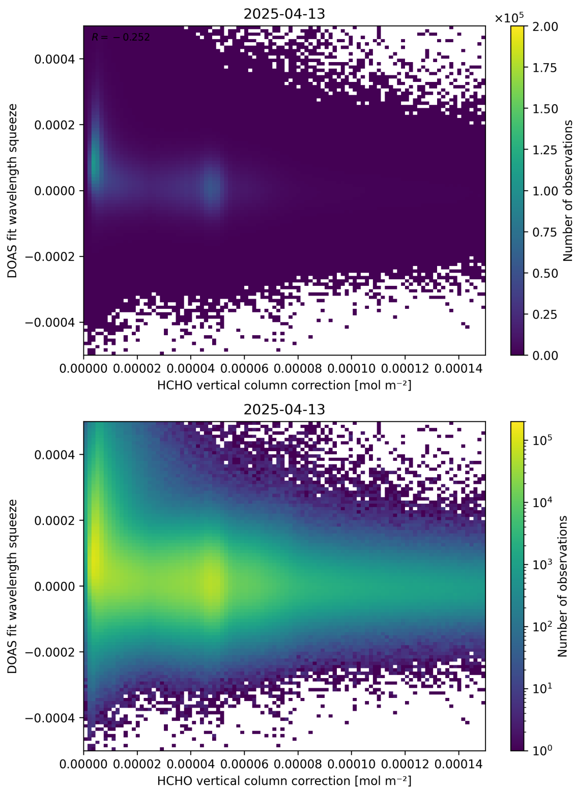
Figure 114: Scatter density plot of “HCHO vertical column correction” against “DOAS fit wavelength squeeze” for 2025-04-13 to 2025-04-14.
