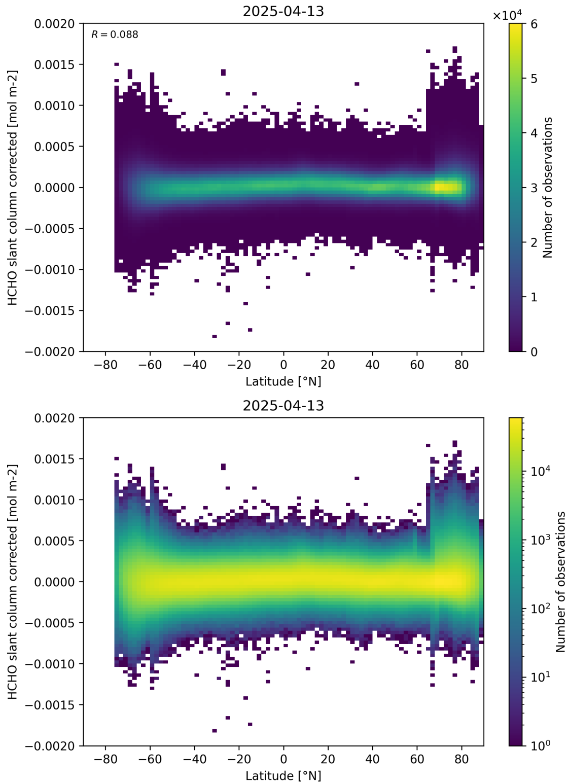
Figure 157: Scatter density plot of “Latitude” against “HCHO slant column corrected” for 2025-04-13 to 2025-04-14.
