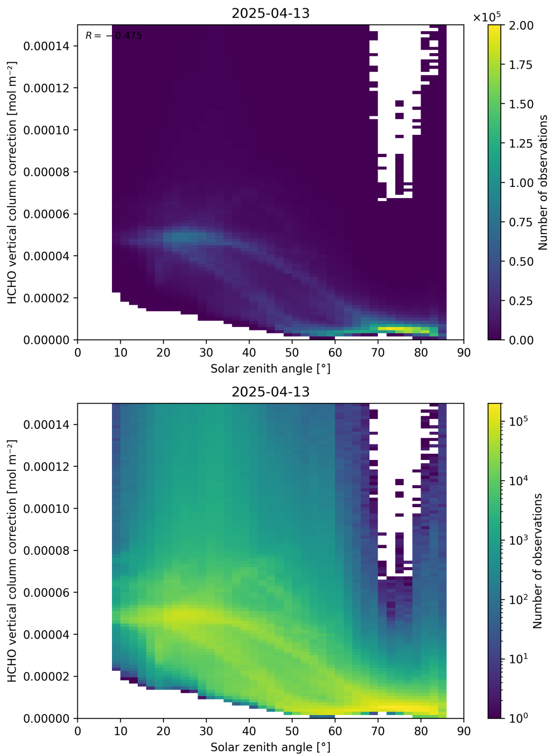
Figure 178: Scatter density plot of “Solar zenith angle” against “HCHO vertical column correction” for 2025-04-13 to 2025-04-14.
