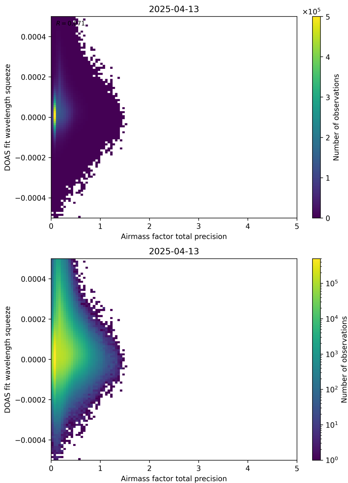
Figure 107: Scatter density plot of “Airmass factor total precision” against “DOAS fit wavelength squeeze” for 2025-04-13 to 2025-04-14.
