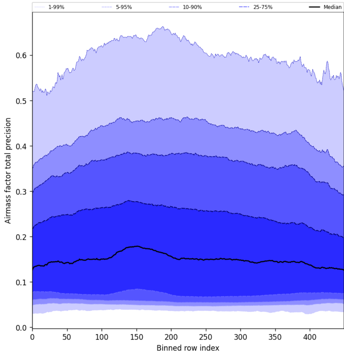
Figure 55: Along track statistics of “Airmass factor total precision” for 2025-04-13 to 2025-04-14
