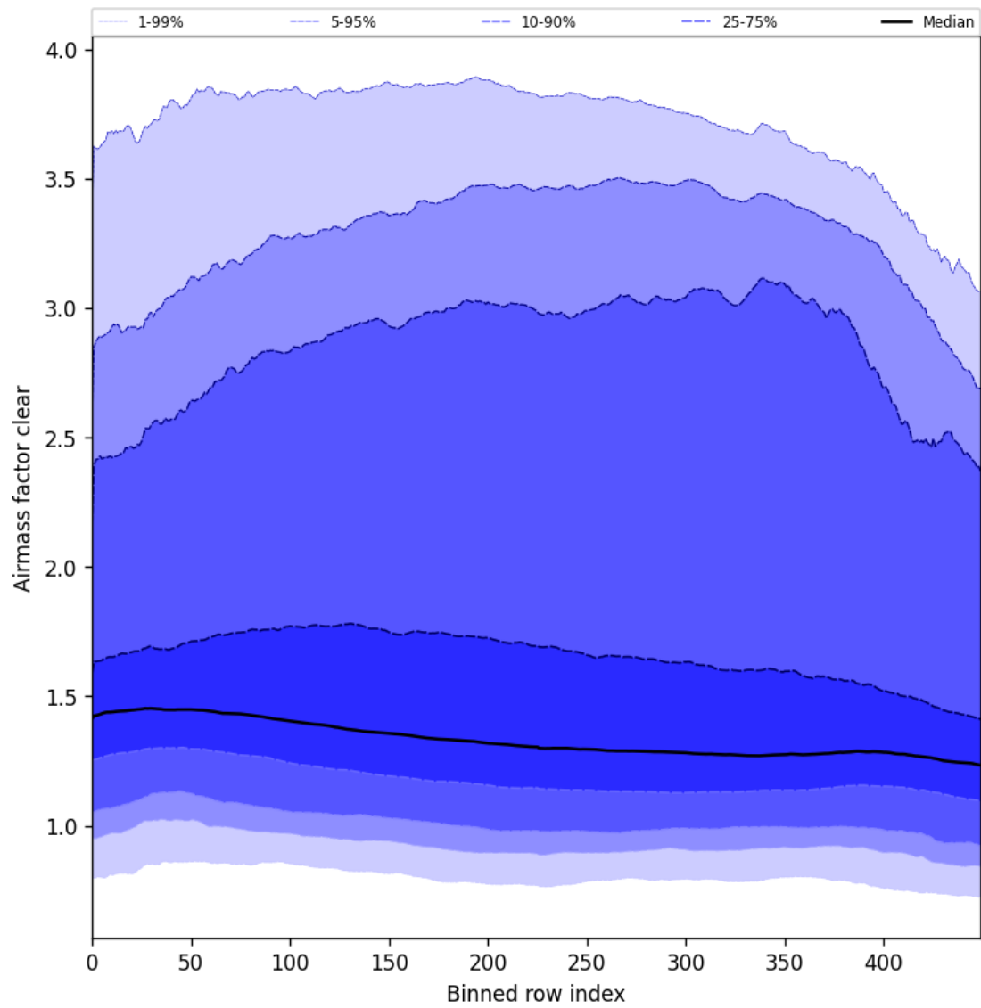
Figure 56: Along track statistics of “Air mass factor clear” for 2025-04-13 to 2025-04-14
