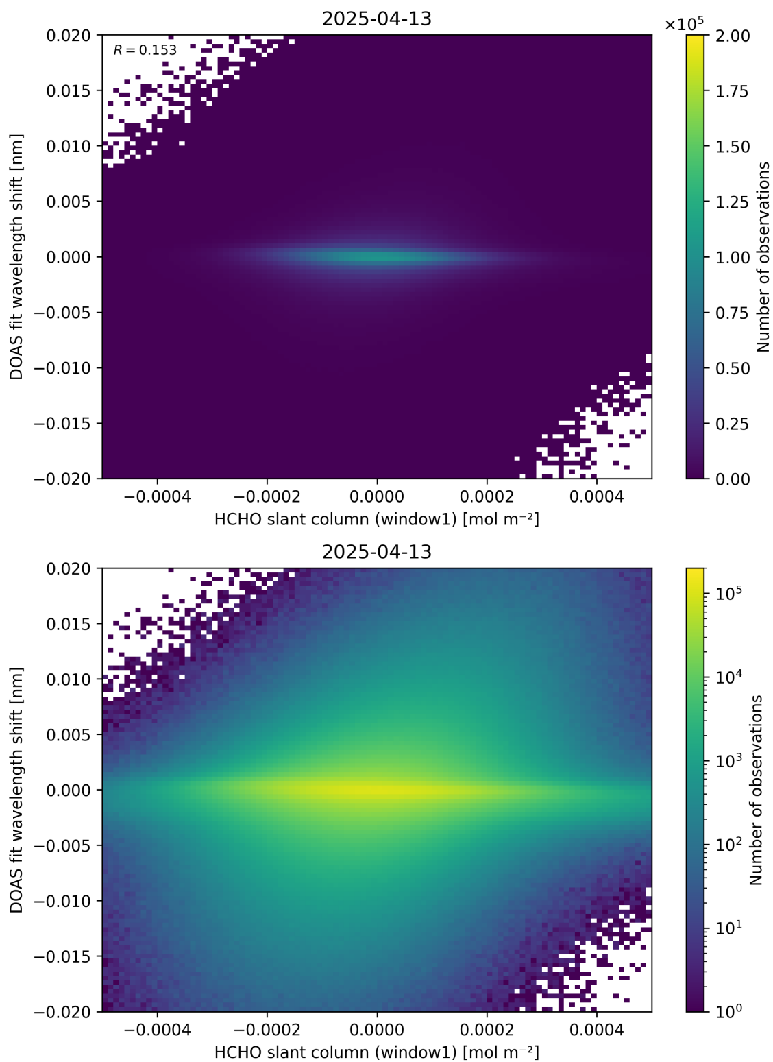
Figure 79: Scatter density plot of “HCHO slant column (window1)” against “DOAS fit wavelength shift” for 2025-04-13 to 2025-04-14.
