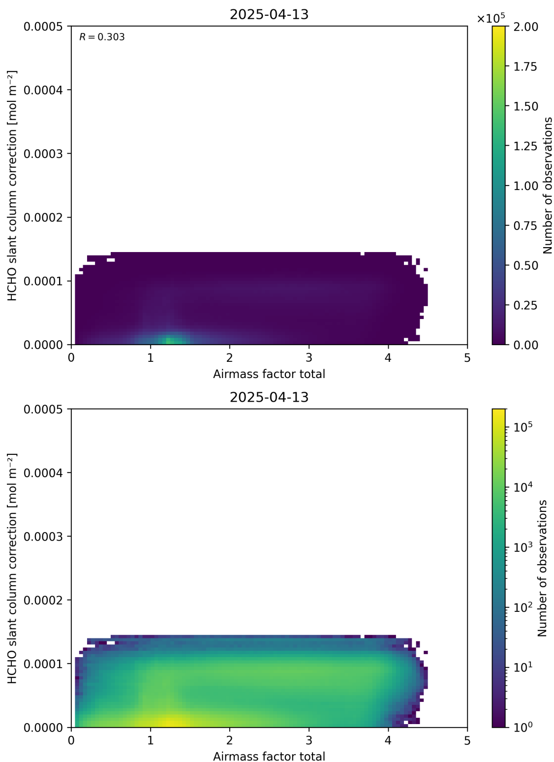
Figure 102: Scatter density plot of “Airmass factor total” against “HCHO slant column correction” for 2025-04-13 to 2025-04-14.
