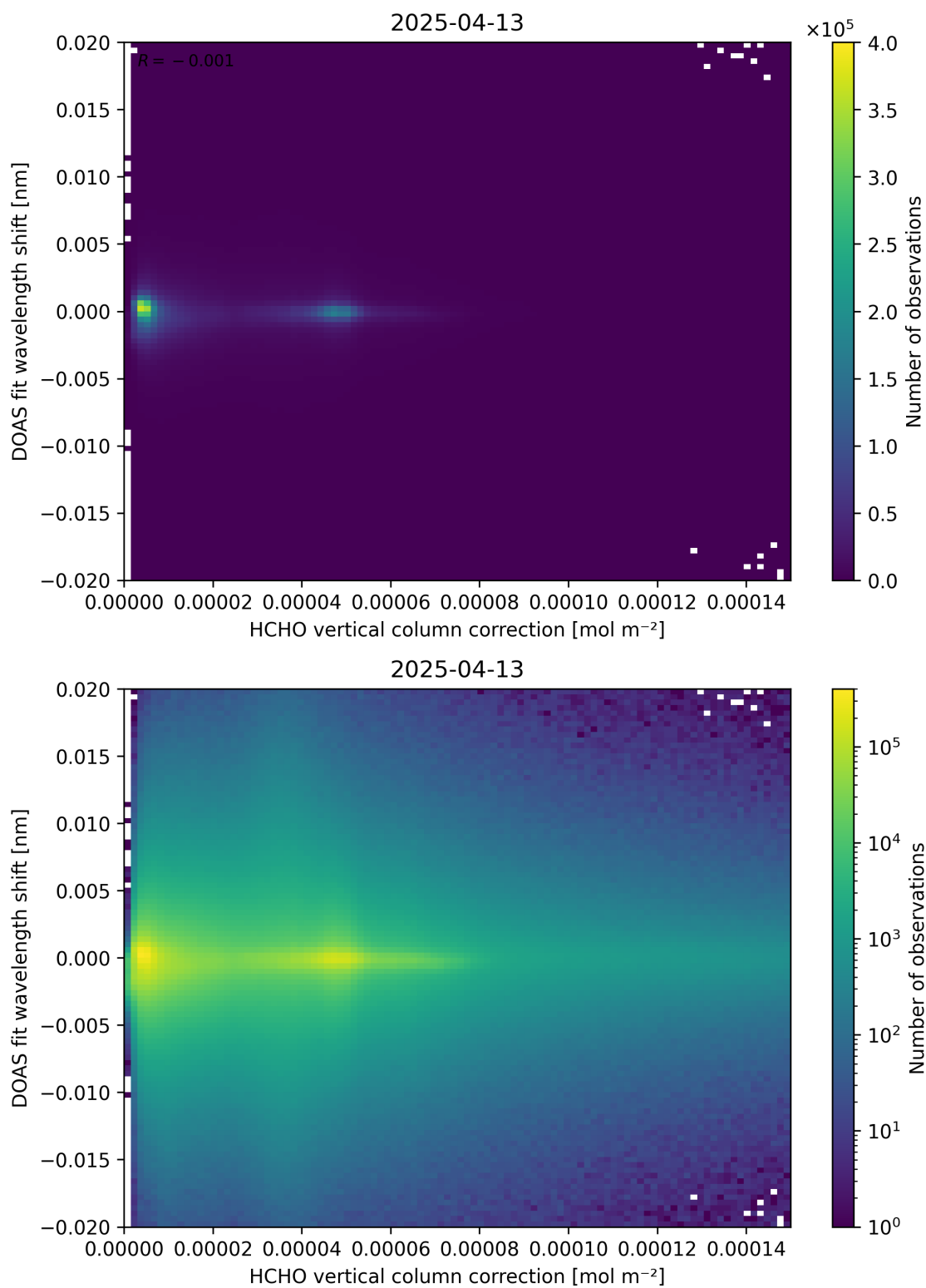
Figure 113: Scatter density plot of “HCHO vertical column correction” against “DOAS fit wavelength shift” for 2025-04-13 to 2025-04-14.
