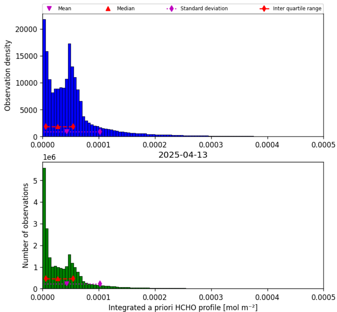
Figure 43: Histogram of “Integrated a priori HCHO profile” for 2025-04-13 to 2025-04-14
