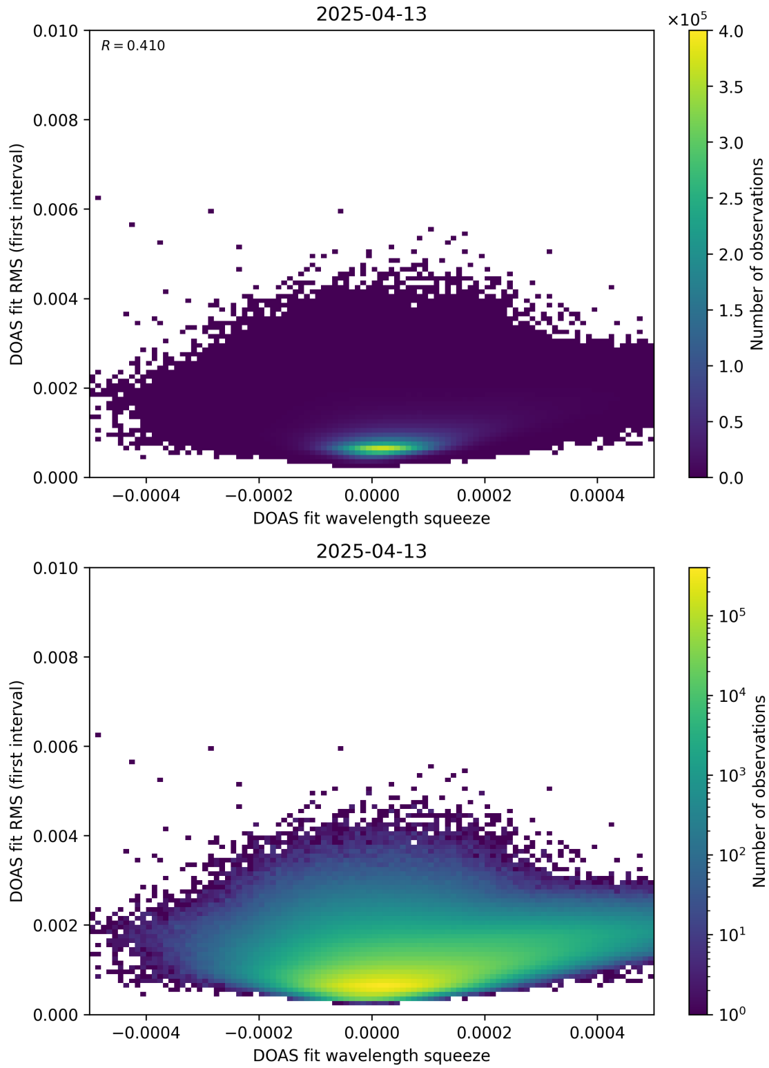
Figure 68: Scatter density plot of “DOAS fit wavelength squeeze” against “DOAS fit RMS (first interval)” for 2025-04-13 to 2025-04-14.
