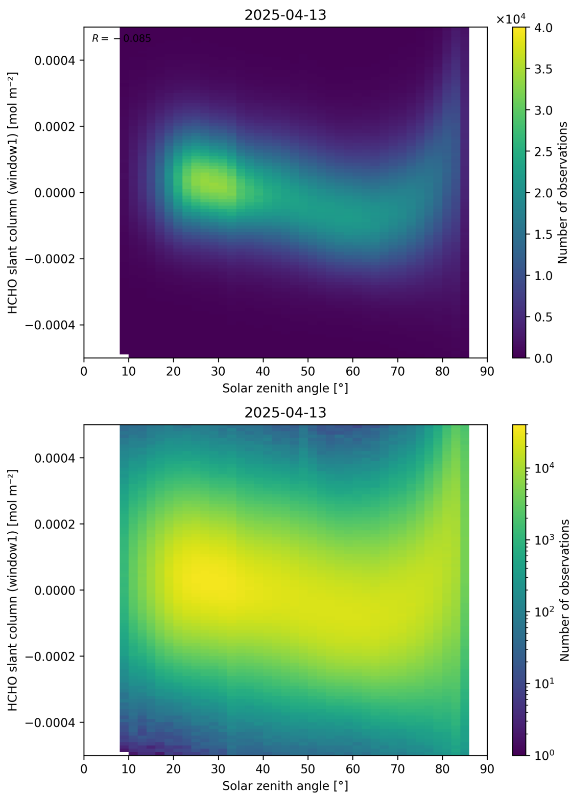
Figure 173: Scatter density plot of “Solar zenith angle” against “HCHO slant column (window1)” for 2025-04-13 to 2025-04-14.
