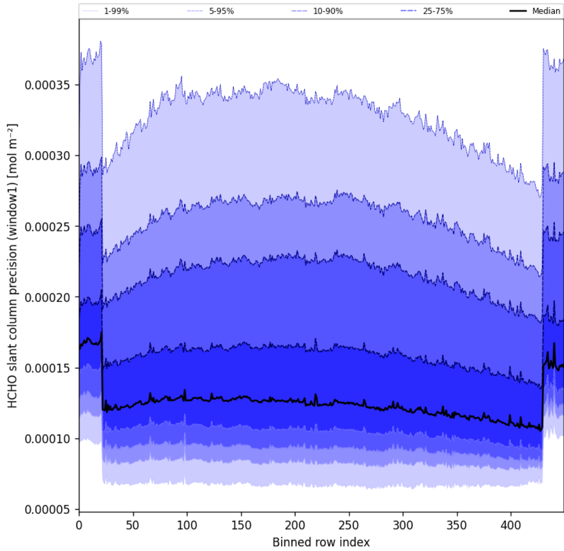
Figure 53: Along track statistics of “HCHO slant column precision (window1)” for 2025-04-13 to 2025-04-14
