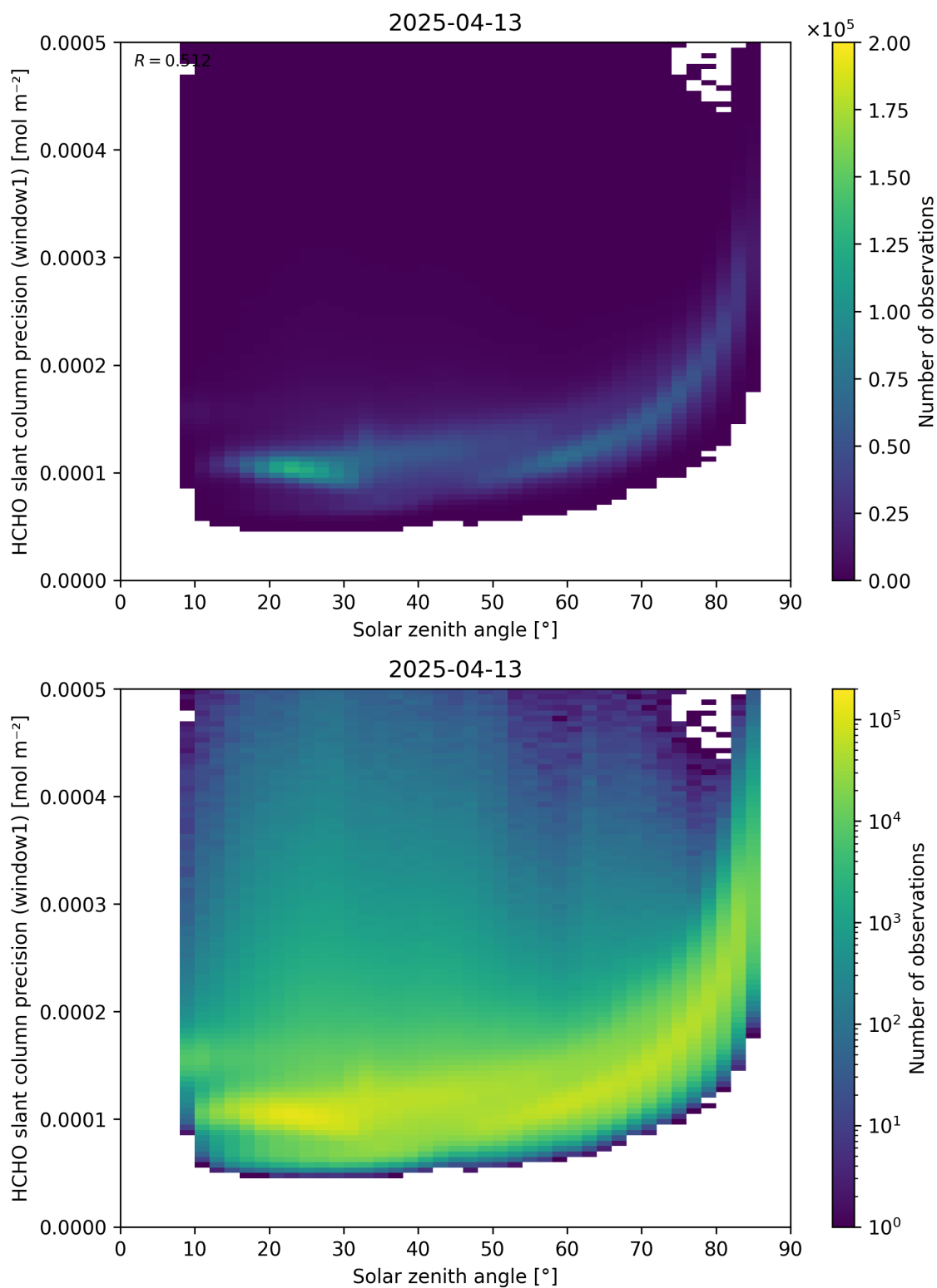
Figure 174: Scatter density plot of “Solar zenith angle” against “HCHO slant column precision (window1)” for 2025-04-13 to 2025-04-14.
