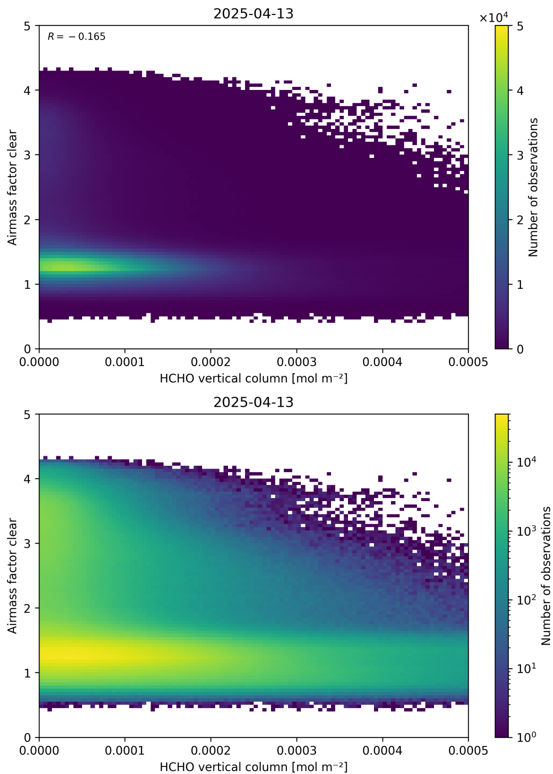
Figure 126: Scatter density plot of “HCHO vertical column” against “Airmass factor clear” for 2025-04-13 to 2025-04-14.
