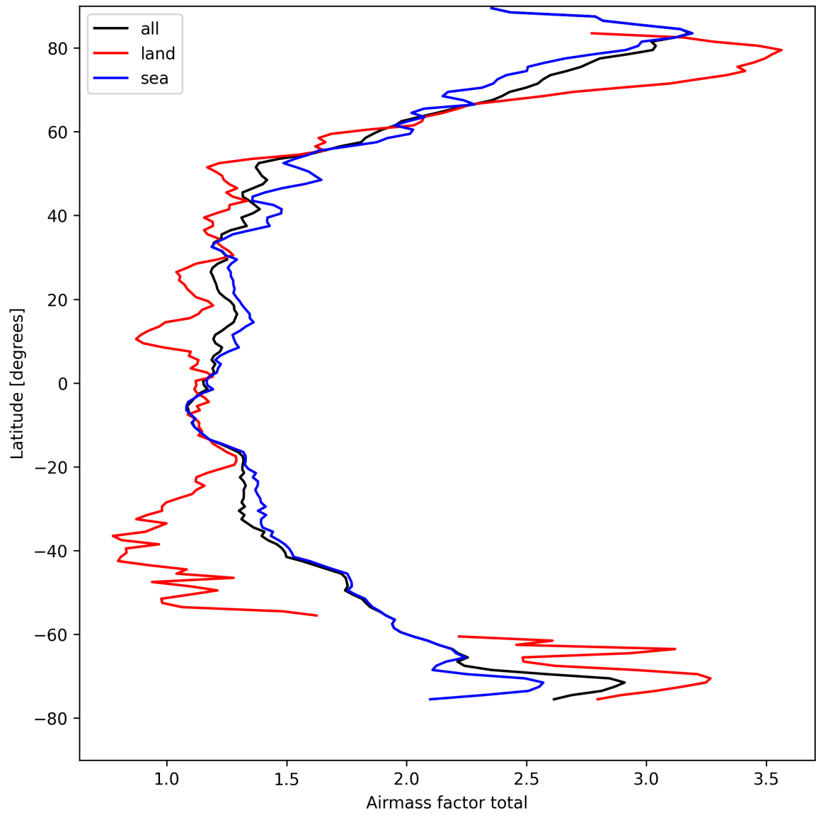
Figure 26: Zonal average of “Airmass factor total” for 2025-04-13 to 2025-04-14.
