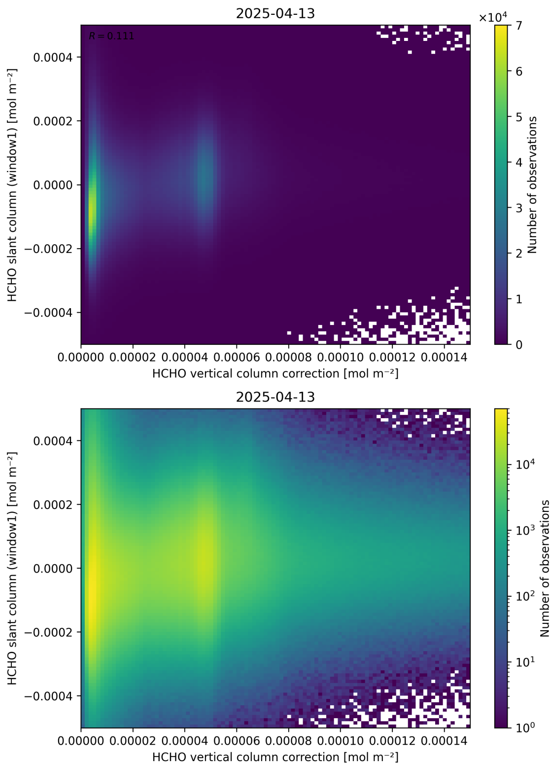
Figure 118: Scatter density plot of “HCHO vertical column correction” against “HCHO slant column (window1)” for 2025-04-13 to 2025-04-14.
