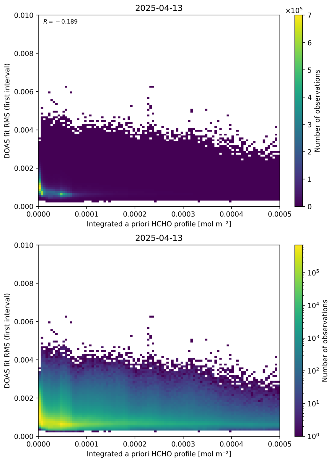
Figure 148: Scatter density plot of “Integrated a priori HCHO profile” against “DOAS fit RMS (first interval)” for 2025-04-13 to 2025-04-14.
