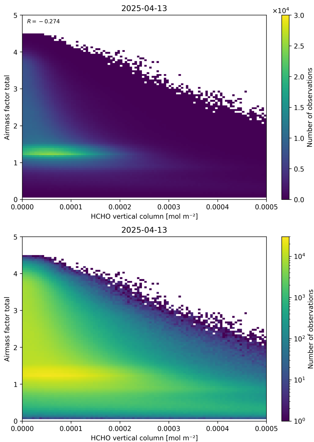
Figure 131: Scatter density plot of “HCHO vertical column” against “Airmass factor total” for 2025-04-13 to 2025-04-14.
