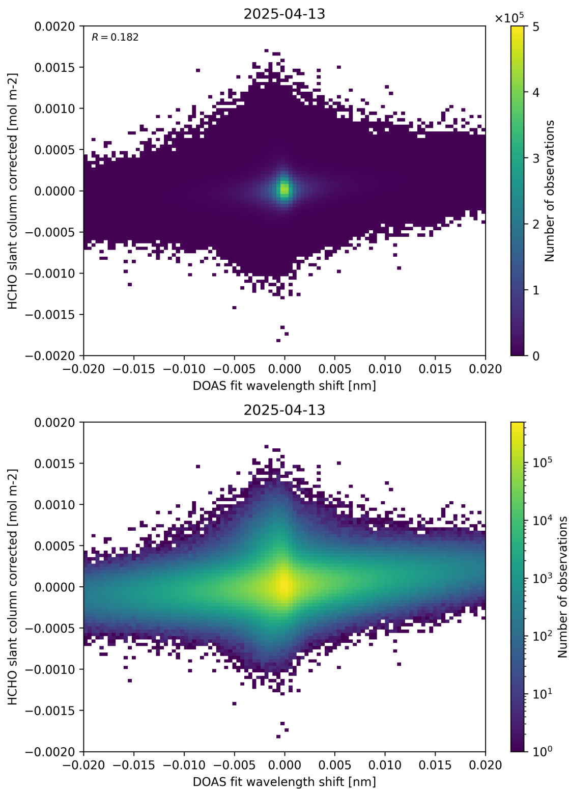
Figure 66: Scatter density plot of “DOAS fit wavelength shift” against “HCHO slant column corrected” for 2025-04-13 to 2025-04-14.
