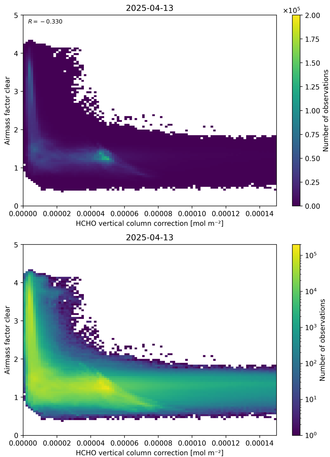
Figure 115: Scatter density plot of “HCHO vertical column correction” against “Airmass factor clear” for 2025-04-13 to 2025-04-14.
