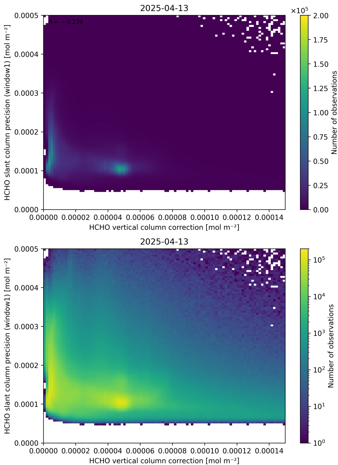
Figure 119: Scatter density plot of “HCHO vertical column correction” against “HCHO slant column precision (window1)” for 2025-04-13 to 2025-04-14.
