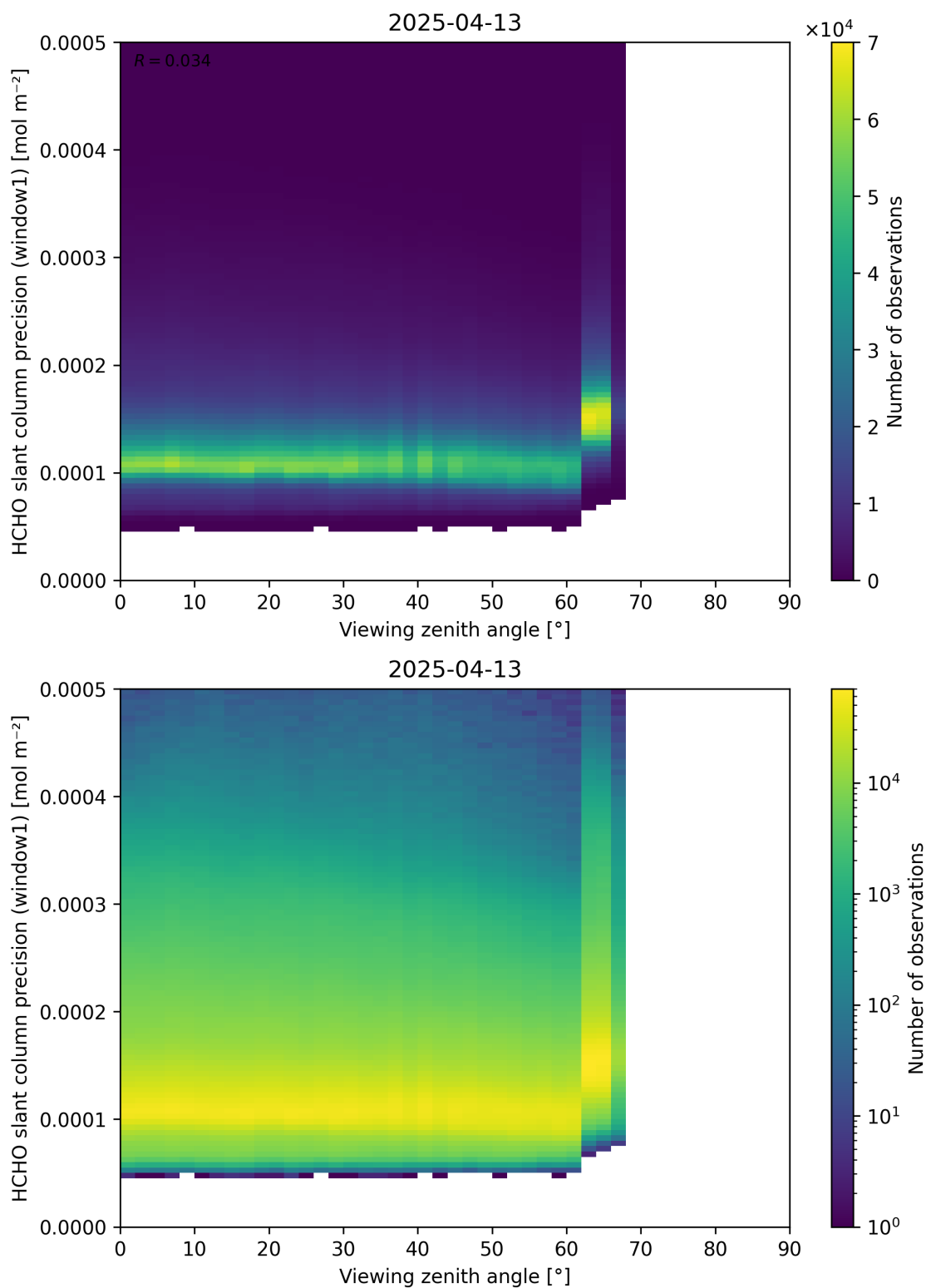
Figure 189: Scatter density plot of “Viewing zenith angle” against “HCHO slant column precision (window1)” for 2025-04-13 to 2025-04-14.
