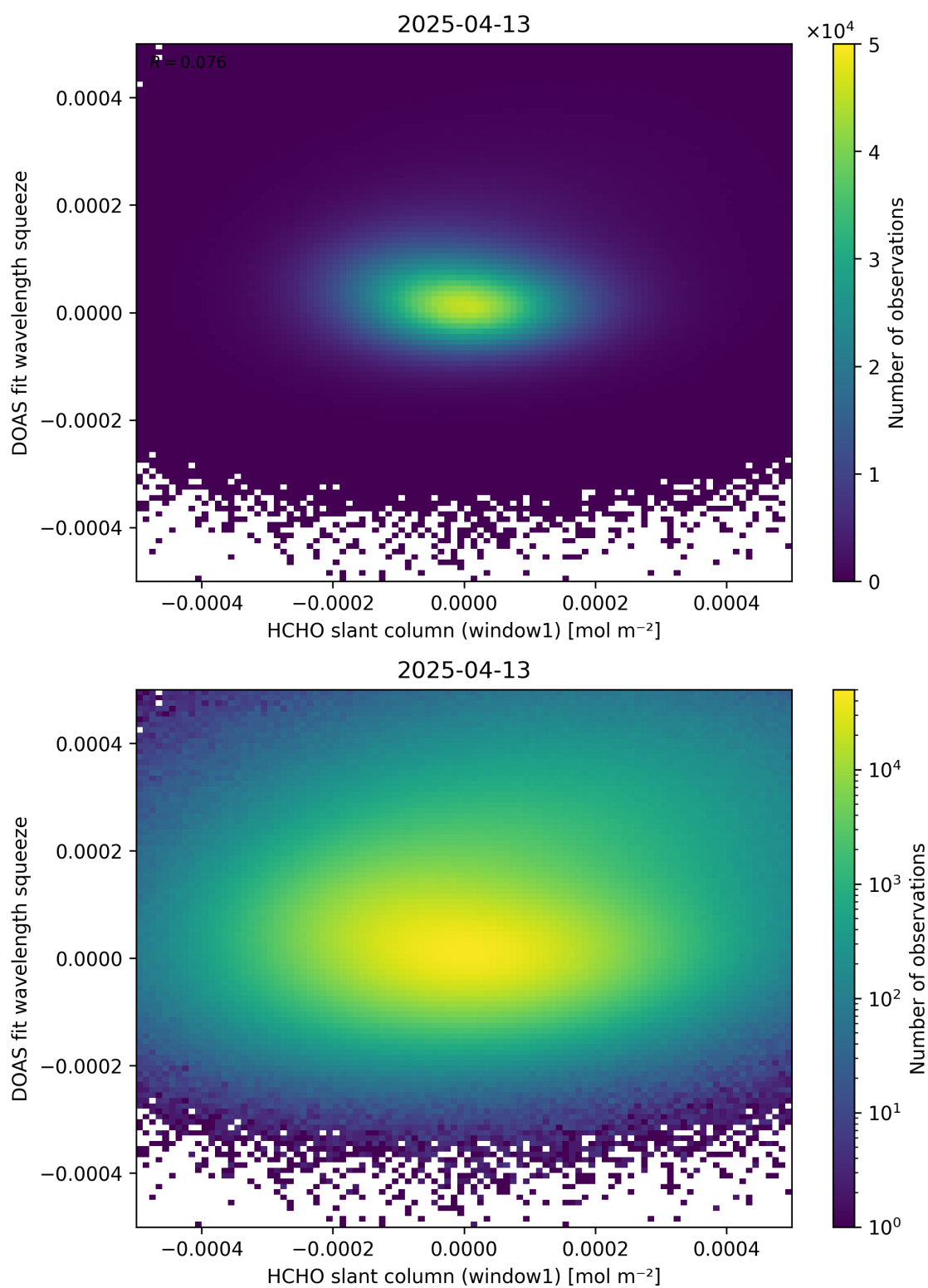
Figure 80: Scatter density plot of “HCHO slant column (window1)” against “DOAS fit wavelength squeeze” for 2025-04-13 to 2025-04-14.
