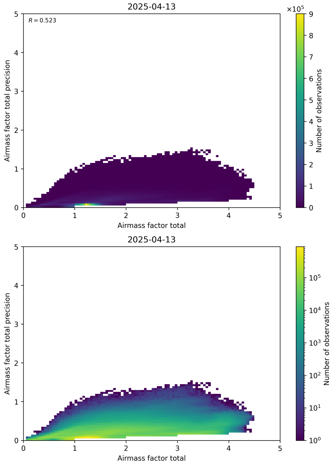
Figure 103: Scatter density plot of “Airmass factor total” against “Airmass factor total precision” for 2025-04-13 to 2025-04-14.
