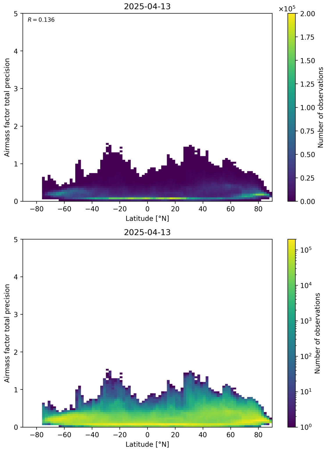
Figure 162: Scatter density plot of “Latitude” against “Airmass factor total precision” for 2025-04-13 to 2025-04-14.
