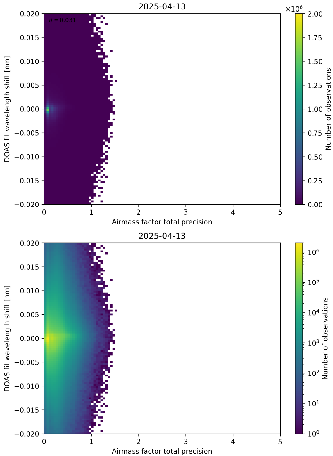
Figure 106: Scatter density plot of “Airmass factor total precision” against “DOAS fit wavelength shift” for 2025-04-13 to 2025-04-14.
