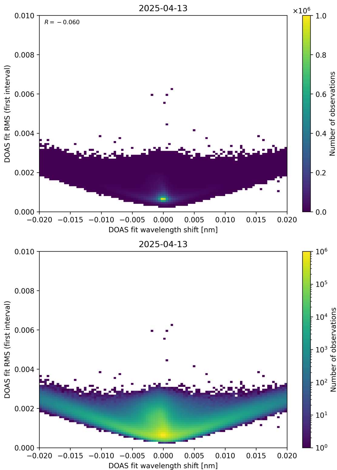
Figure 64: Scatter density plot of “DOAS fit wavelength shift” against “DOAS fit RMS (first interval)” for 2025-04-13 to 2025-04-14.
