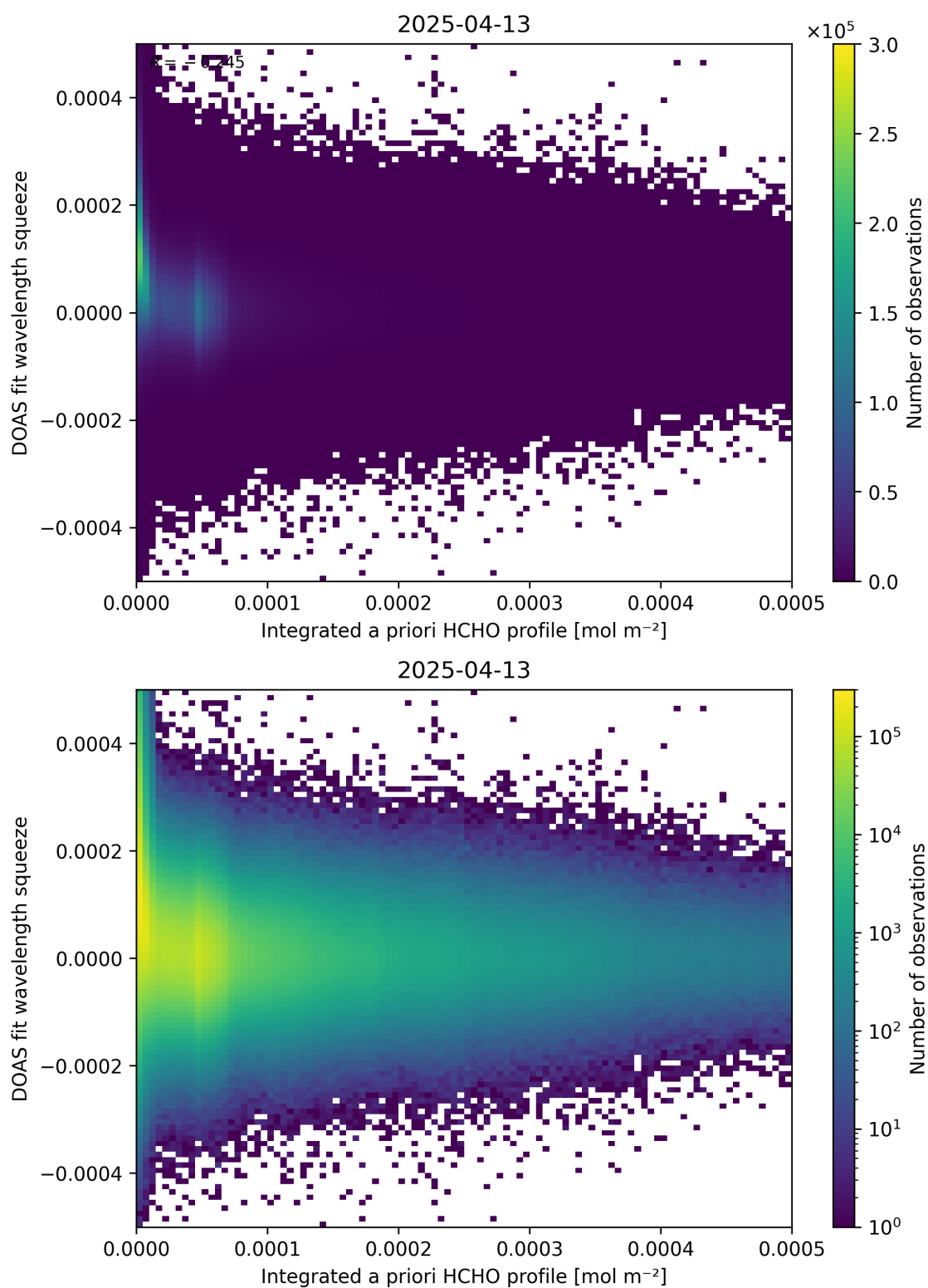
Figure 150: Scatter density plot of “Integrated a priori HCHO profile” against “DOAS fit wavelength squeeze” for 2025-04-13 to 2025-04-14.
