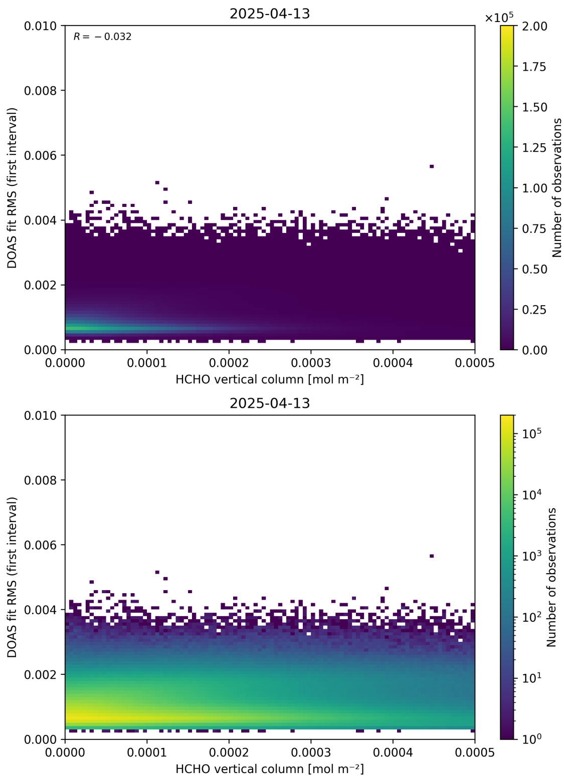
Figure 123: Scatter density plot of “HCHO vertical column” against “DOAS fit RMS (first interval)” for 2025-04-13 to 2025-04-14.
