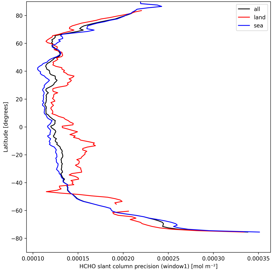
Figure 25: Zonal average of “HCHO slant column precision (window1)” for 2025-04-13 to 2025-04-14.
