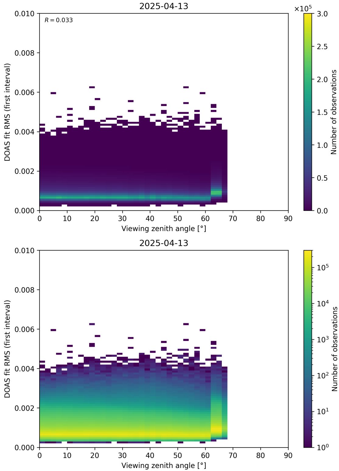
Figure 182: Scatter density plot of “Viewing zenith angle” against “DOAS fit RMS (first interval)” for 2025-04-13 to 2025-04-14.
