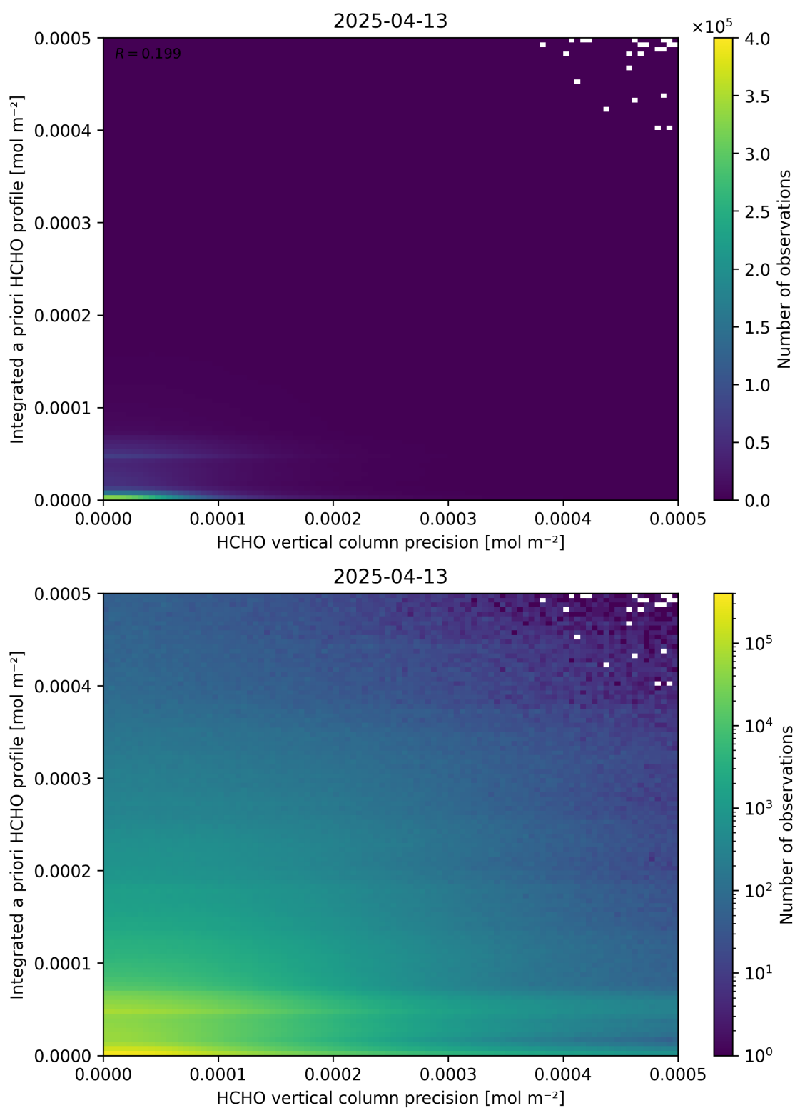
Figure 147: Scatter density plot of “HCHO vertical column precision” against “Integrated a priori HCHO profile” for 2025-04-13 to 2025-04-14.
