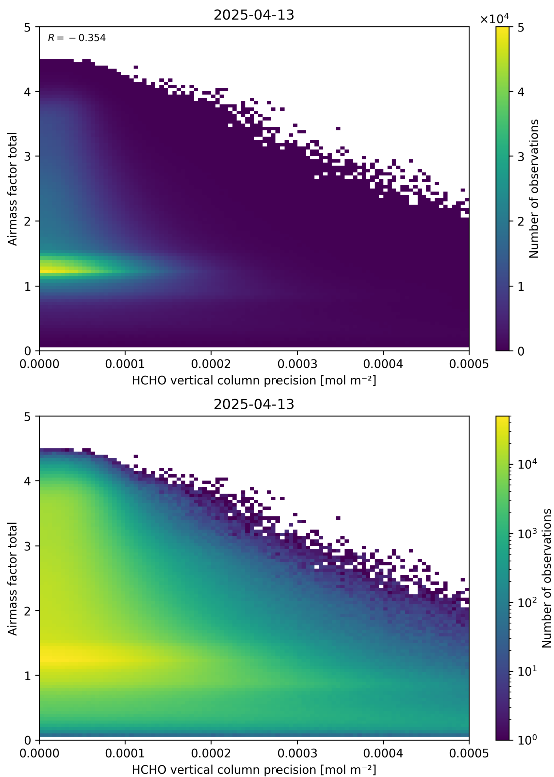
Figure 144: Scatter density plot of “HCHO vertical column precision” against “Airmass factor total” for 2025-04-13 to 2025-04-14.
