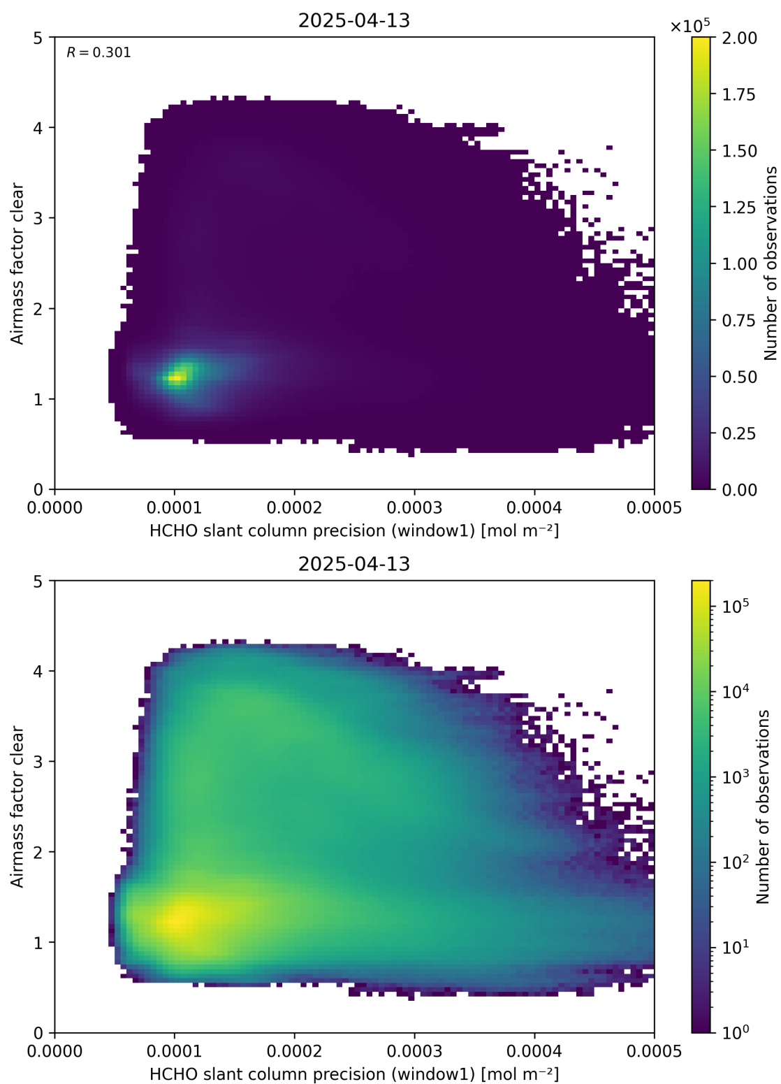
Figure 91: Scatter density plot of “HCHO slant column precision (window1)” against “Airmass factor clear” for 2025-04-13 to 2025-04-14.
