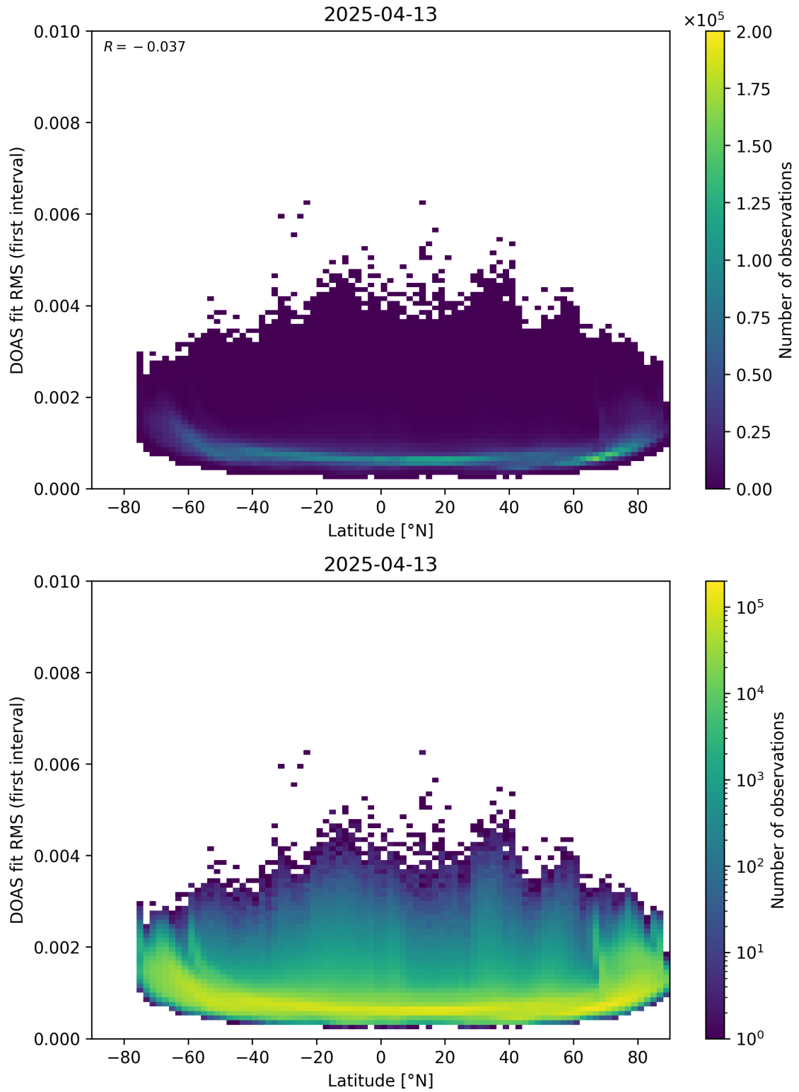
Figure 153: Scatter density plot of “Latitude” against “DOAS fit RMS (first interval)” for 2025-04-13 to 2025-04-14.
