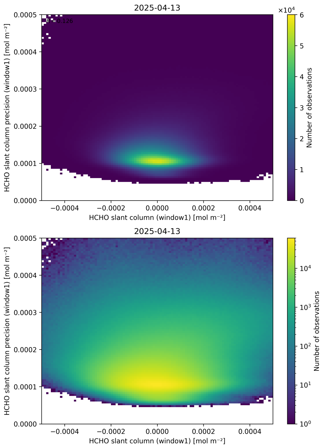
Figure 84: Scatter density plot of “HCHO slant column (window1)” against “HCHO slant column precision (window1)” for 2025-04-13 to 2025-04-14.
