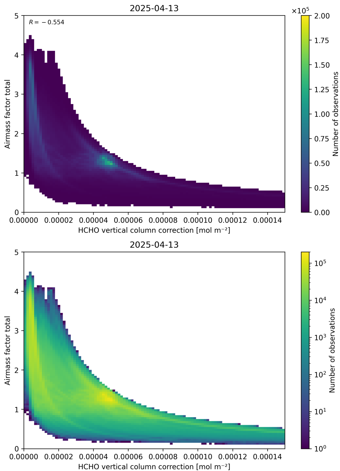
Figure 120: Scatter density plot of “HCHO vertical column correction” against “Airmass factor total” for 2025-04-13 to 2025-04-14.
