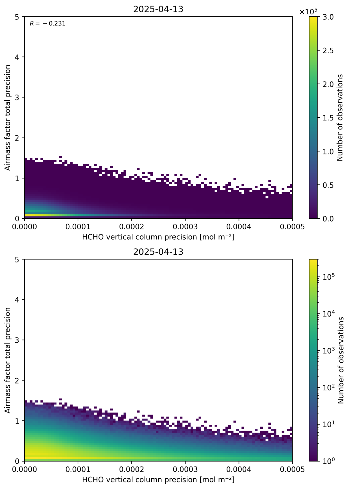
Figure 145: Scatter density plot of “HCHO vertical column precision” against “Airmass factor total precision” for 2025-04-13 to 2025-04-14.
