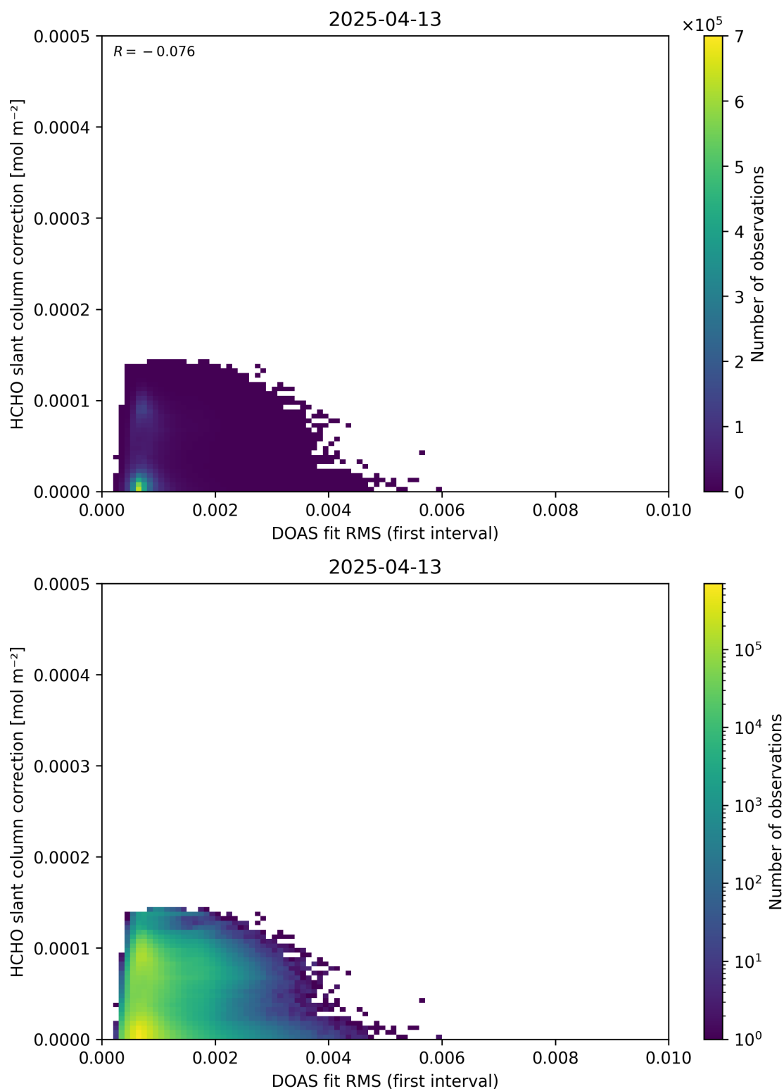
Figure 63: Scatter density plot of “DOAS fit RMS (first interval)” against “HCHO slant column correction” for 2025-04-13 to 2025-04-14.
