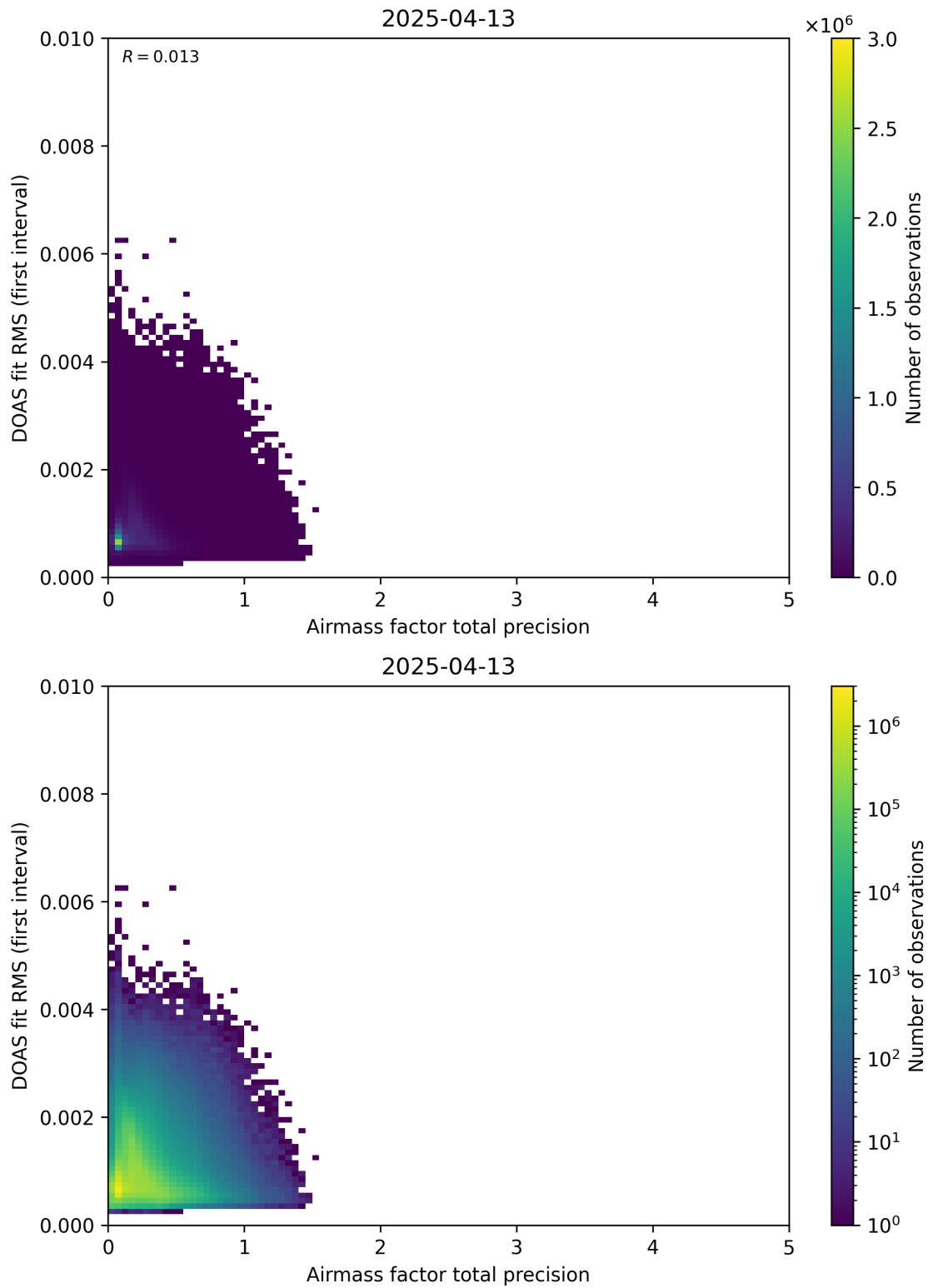
Figure 105: Scatter density plot of “Airmass factor total precision” against “DOAS fit RMS (first interval)” for 2025-04-13 to 2025-04-14.
