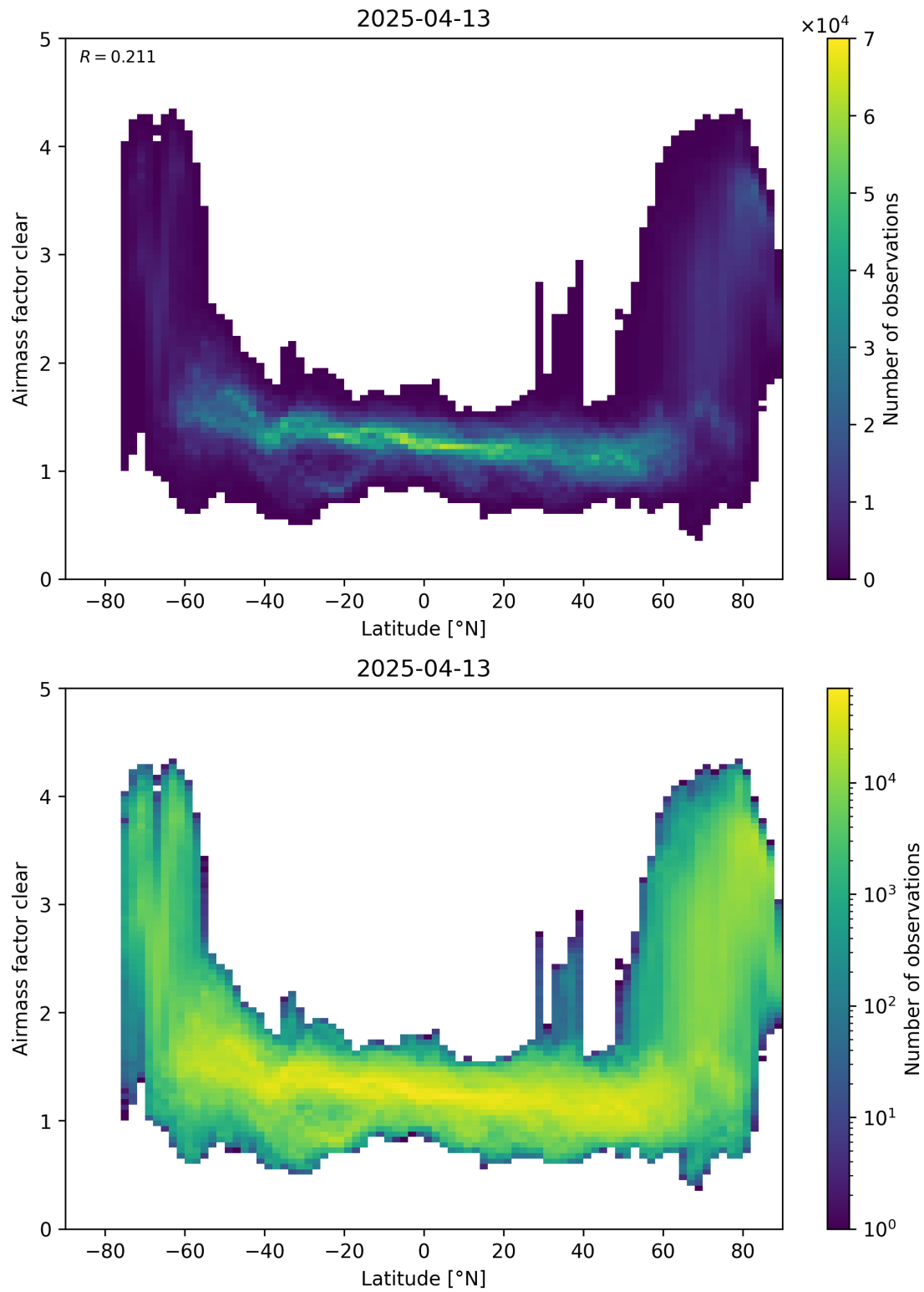
Figure 156: Scatter density plot of “Latitude” against “Airmass factor clear” for 2025-04-13 to 2025-04-14.
