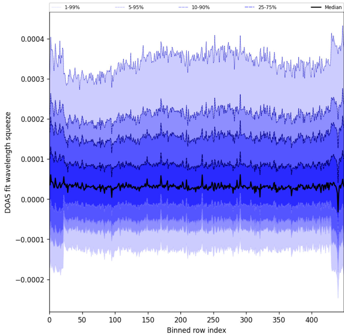
Figure 59: Along track statistics of “DOAS fit wavelength squeeze” for 2025-04-13 to 2025-04-14
