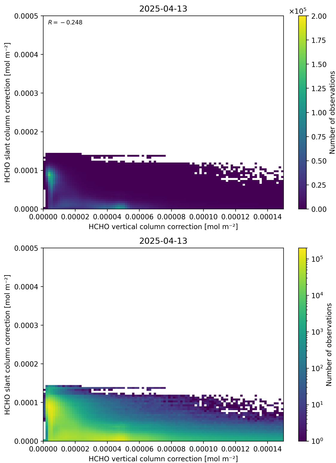
Figure 117: Scatter density plot of “HCHO vertical column correction” against “HCHO slant column correction” for 2025-04-13 to 2025-04-14.
