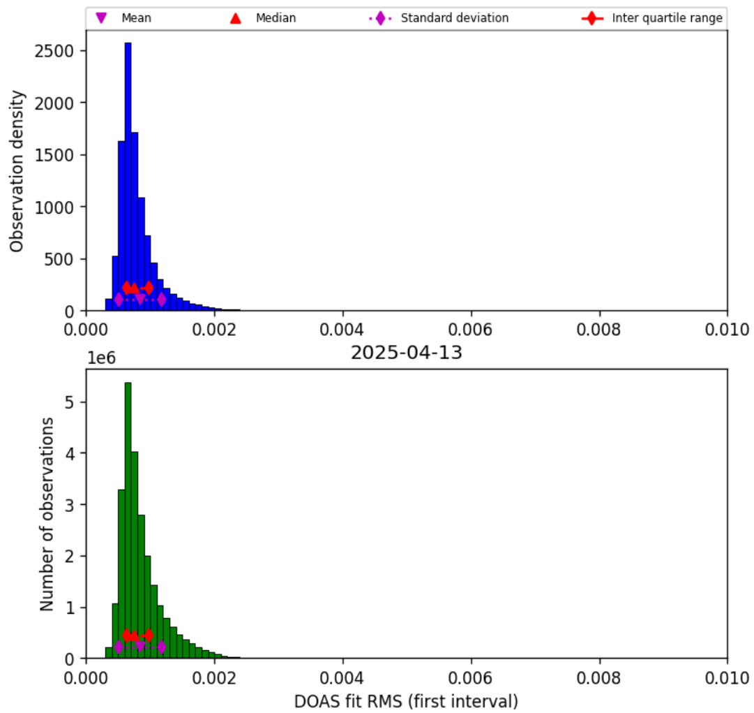
Figure 46: Histogram of “DOAS fit RMS (first interval)” for 2025-04-13 to 2025-04-14
