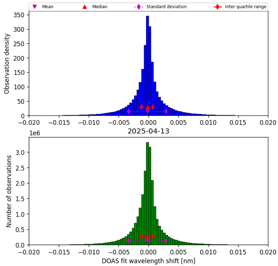
Figure 44: Histogram of “DOAS fit wavelength shift” for 2025-04-13 to 2025-04-14
