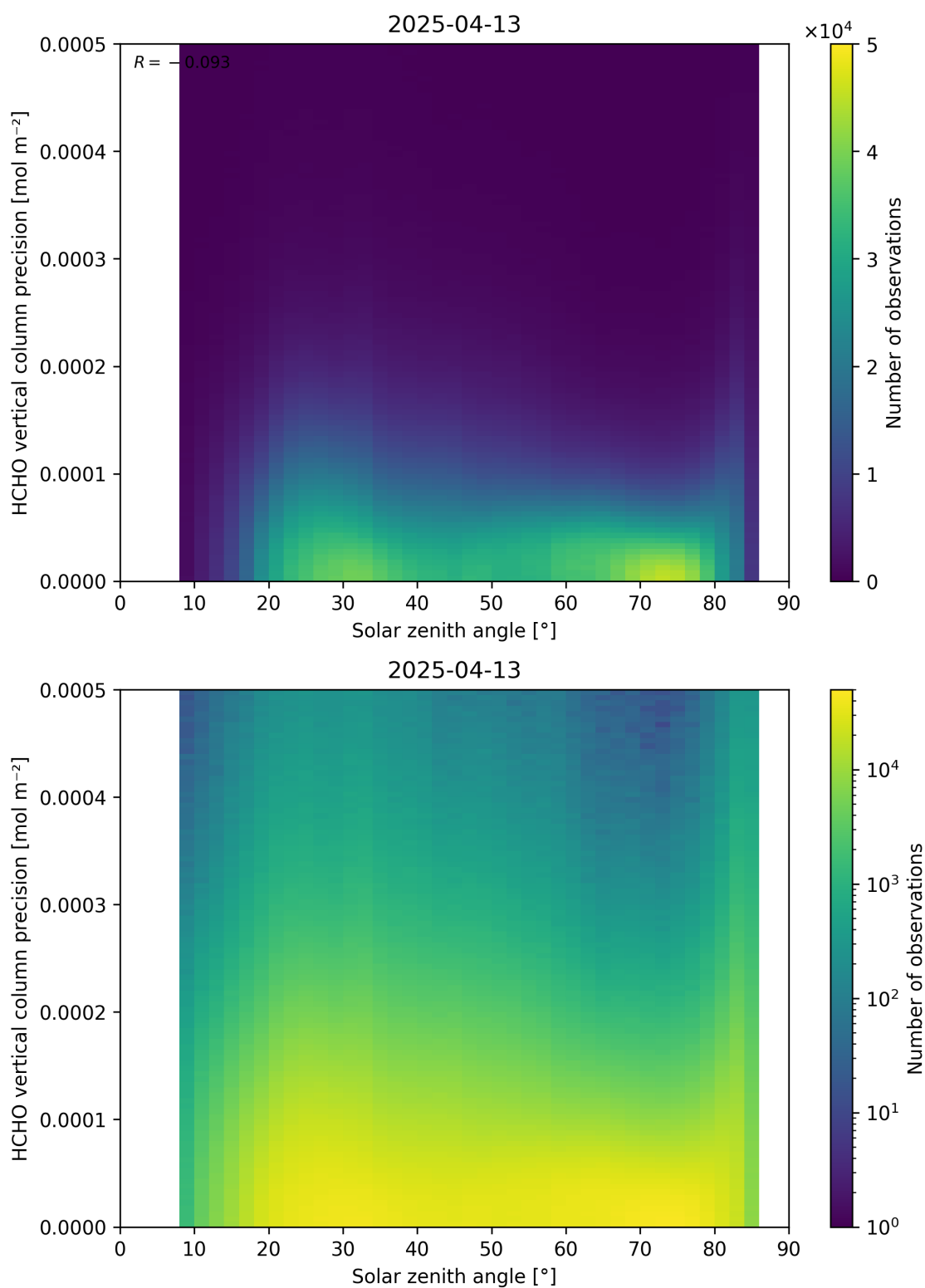
Figure 179: Scatter density plot of “Solar zenith angle” against “HCHO vertical column precision” for 2025-04-13 to 2025-04-14.
