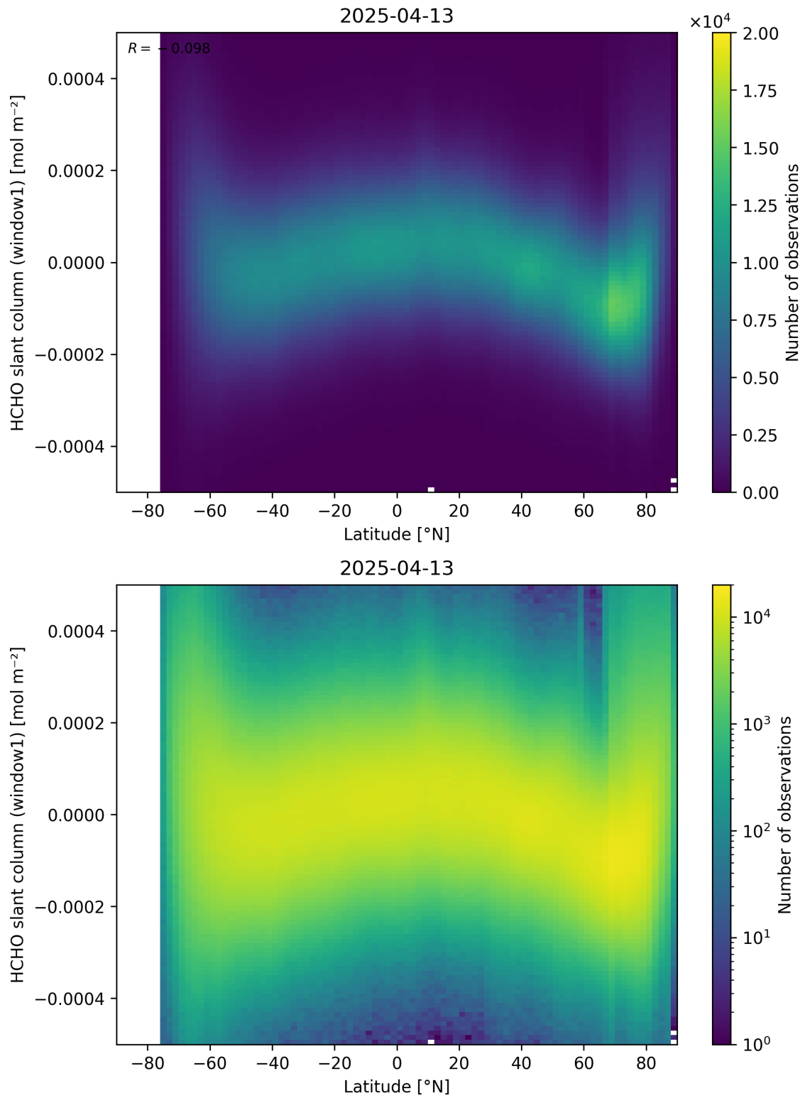
Figure 159: Scatter density plot of “Latitude” against “HCHO slant column (window1)” for 2025-04-13 to 2025-04-14.
