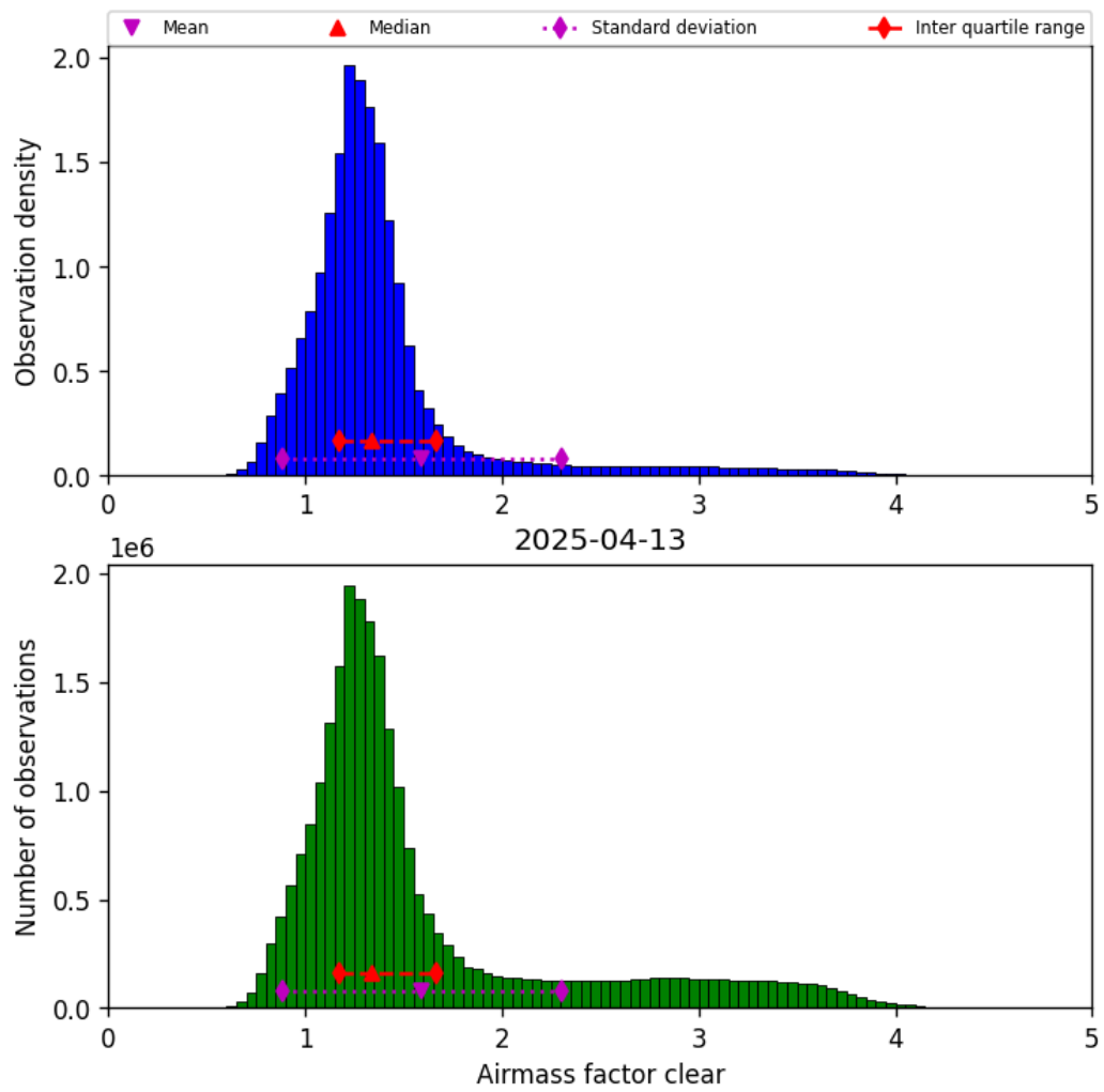
Figure 42: Histogram of “Airmass factor clear” for 2025-04-13 to 2025-04-14
