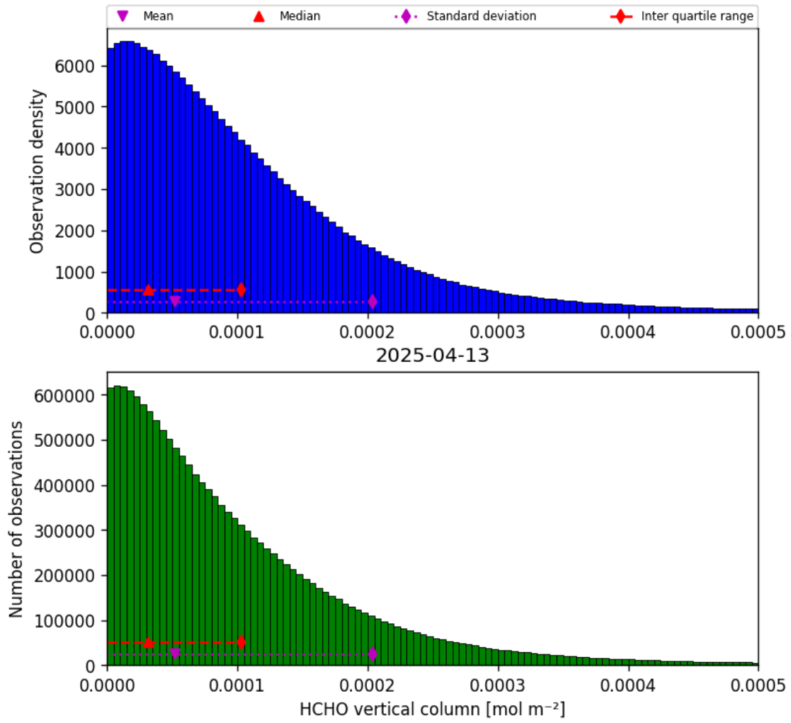
Figure 35: Histogram of “HCHO vertical column” for 2025-04-13 to 2025-04-14
