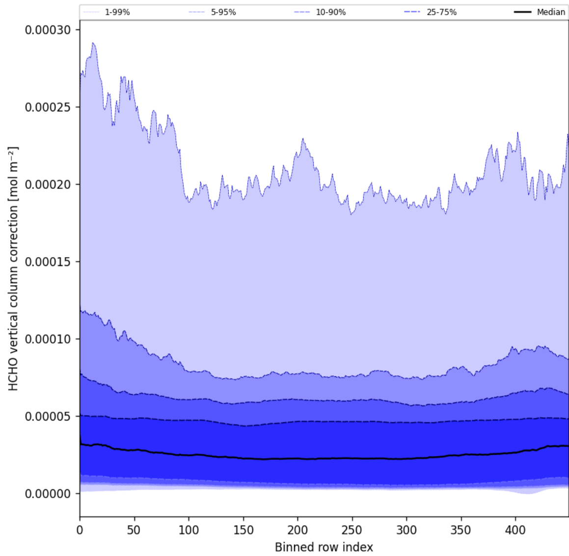
Figure 51: Along track statistics of “HCHO vertical column correction” for 2025-04-13 to 2025-04-14
