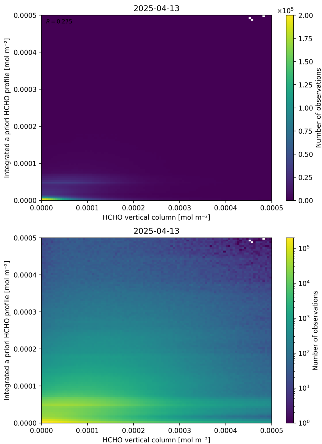
Figure 135: Scatter density plot of “HCHO vertical column” against “Integrated a priori HCHO profile” for 2025-04-13 to 2025-04-14.
