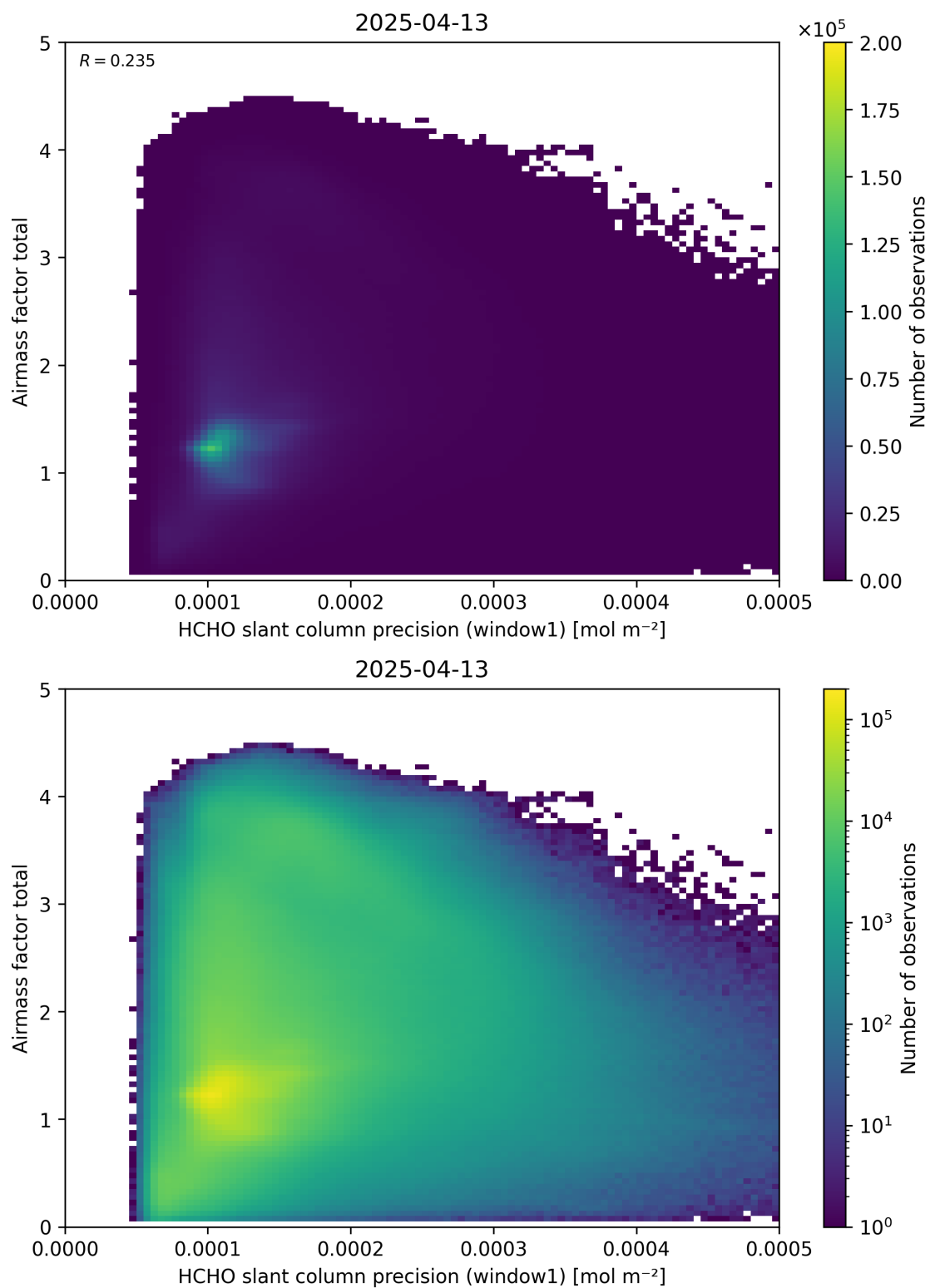
Figure 94: Scatter density plot of “HCHO slant column precision (window1)” against “Airmass factor total” for 2025-04-13 to 2025-04-14.
