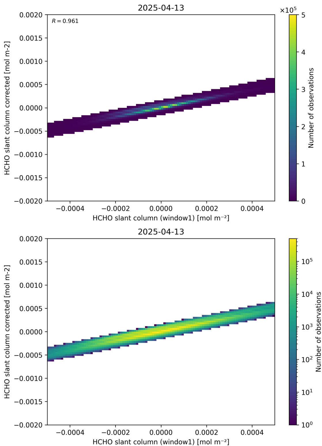
Figure 82: Scatter density plot of “HCHO slant column (window1)” against “HCHO slant column corrected” for 2025-04-13 to 2025-04-14.
