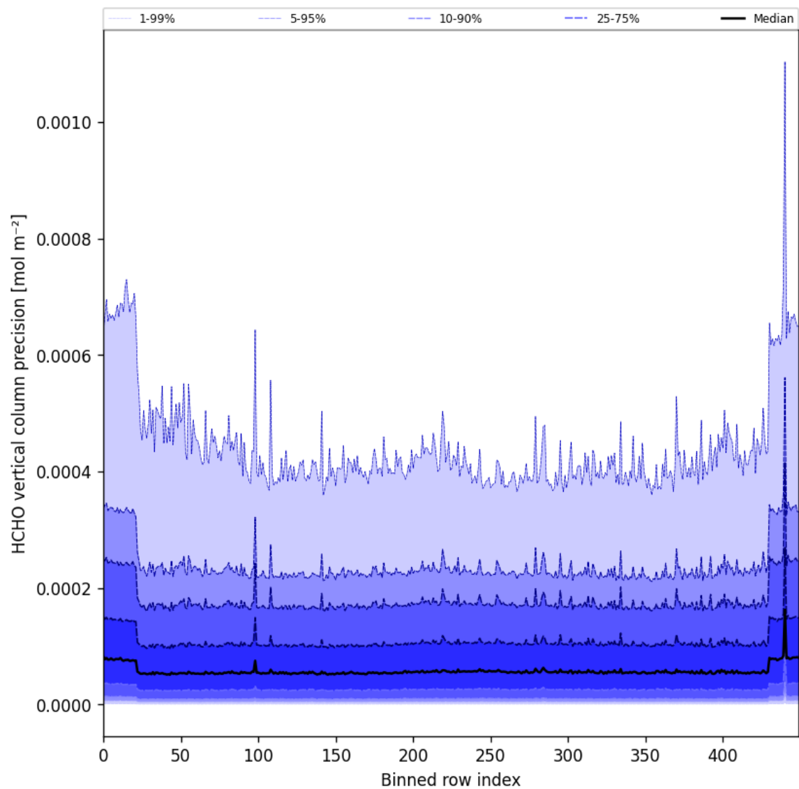
Figure 50: Along track statistics of “HCHO vertical column precision” for 2025-04-13 to 2025-04-14
