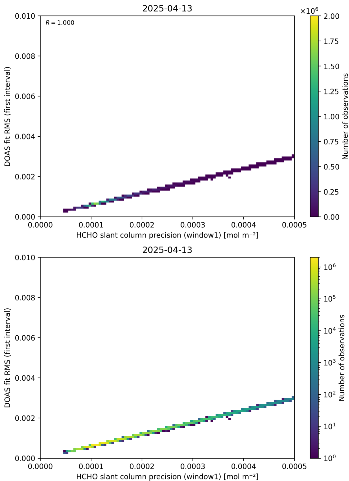
Figure 88: Scatter density plot of “HCHO slant column precision (window1)” against “DOAS fit RMS (first interval)” for 2025-04-13 to 2025-04-14.
