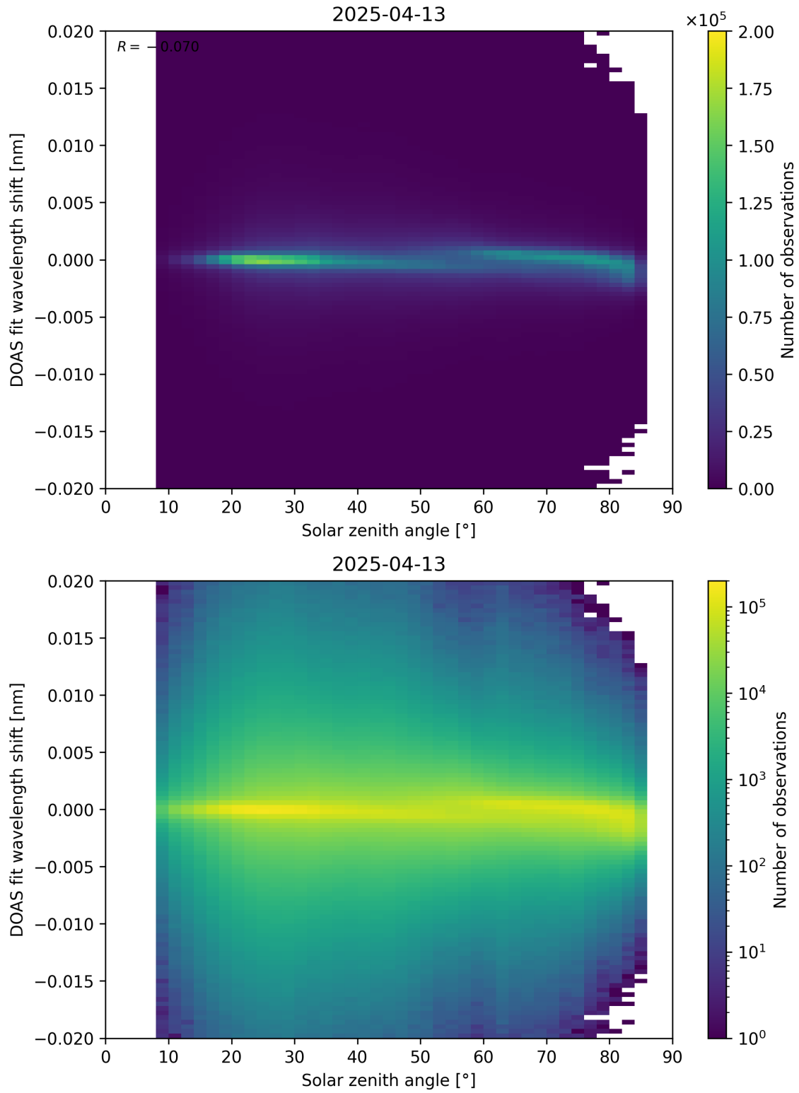
Figure 168: Scatter density plot of “Solar zenith angle” against “DOAS fit wavelength shift” for 2025-04-13 to 2025-04-14.
