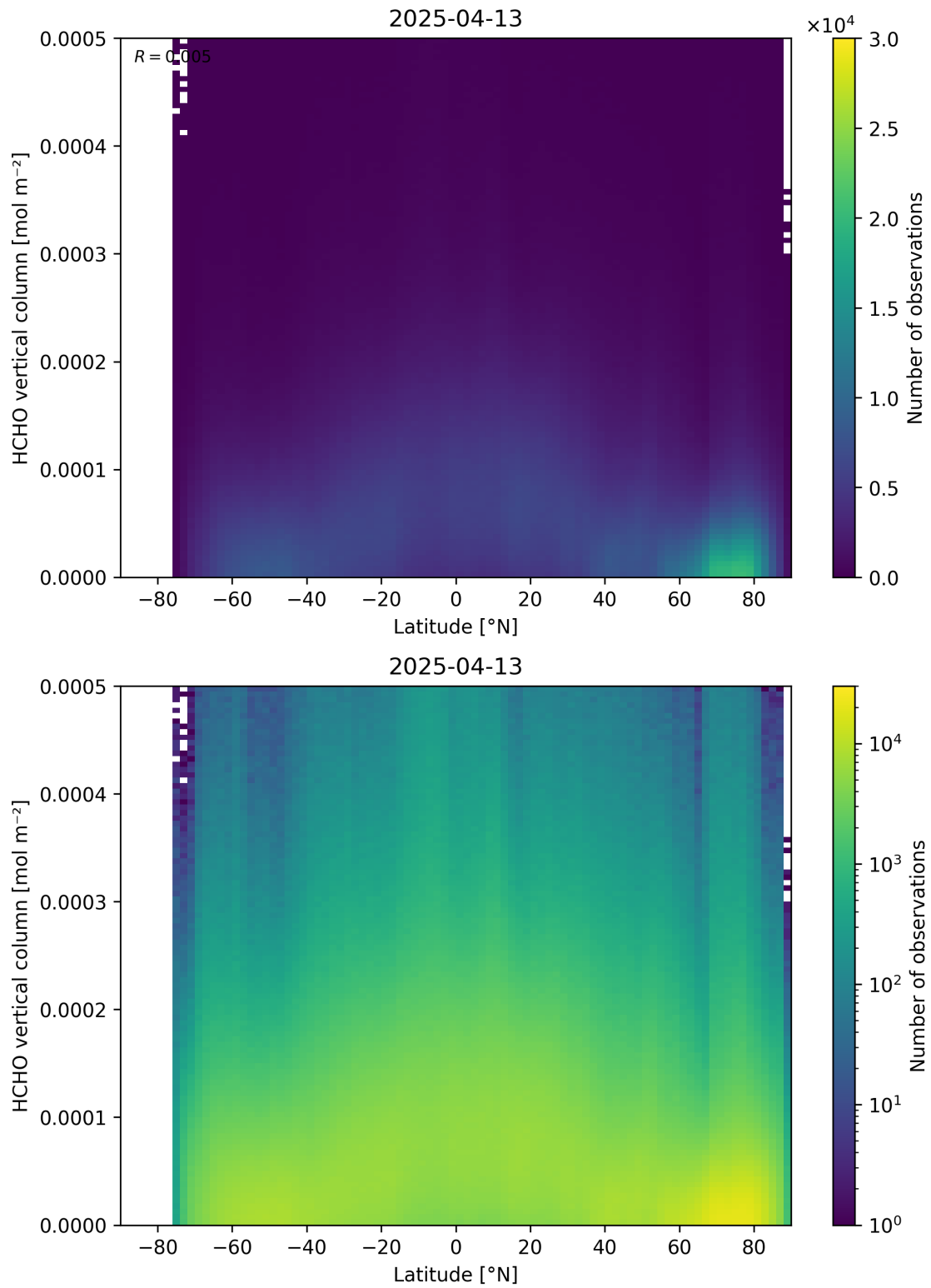
Figure 163: Scatter density plot of “Latitude” against “HCHO vertical column” for 2025-04-13 to 2025-04-14.
