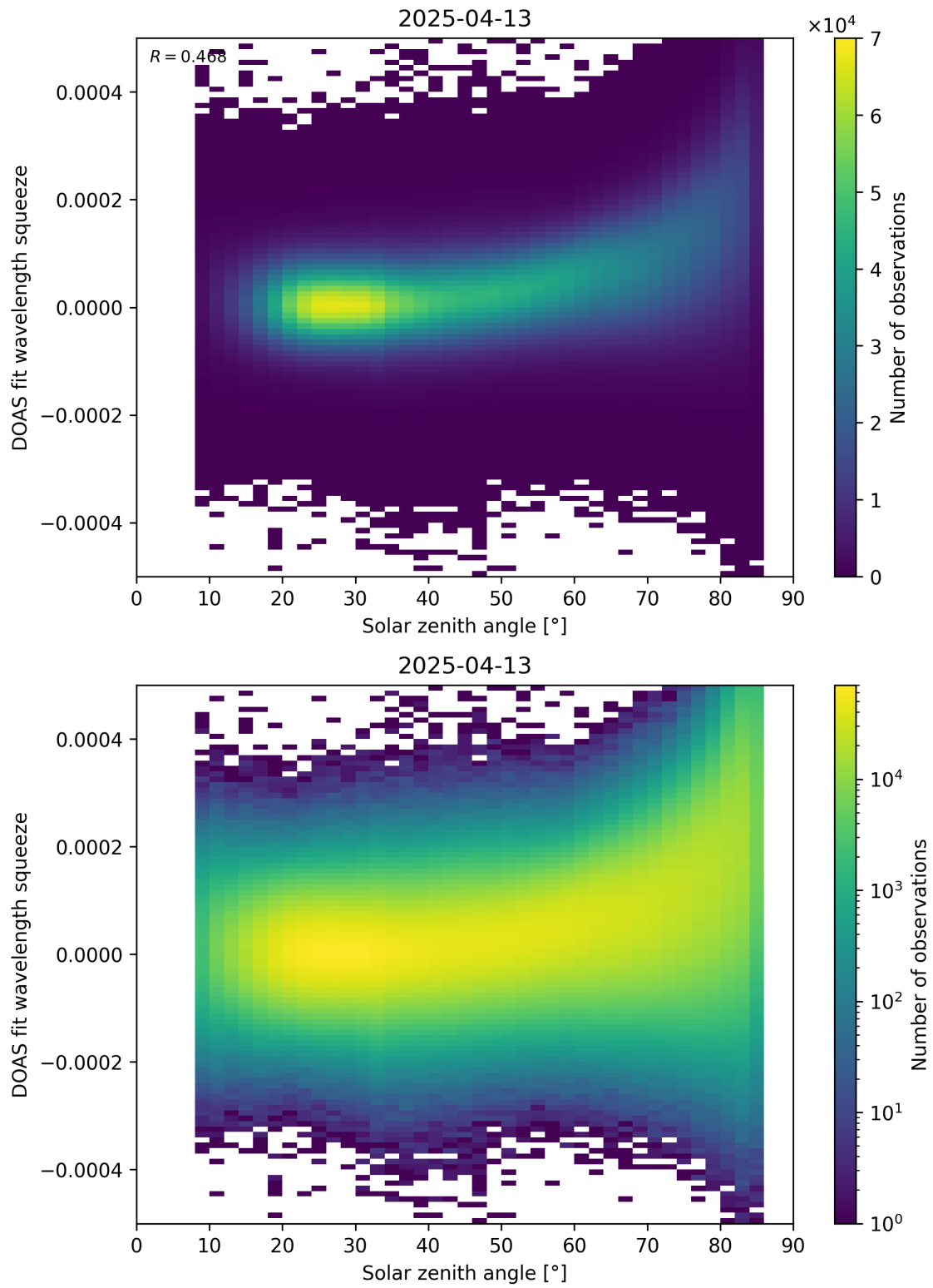
Figure 169: Scatter density plot of “Solar zenith angle” against “DOAS fit wavelength squeeze” for 2025-04-13 to 2025-04-14.
