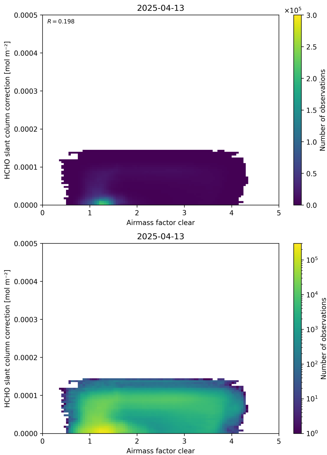
Figure 75: Scatter density plot of “Airmass factor clear” against “HCHO slant column correction” for 2025-04-13 to 2025-04-14.
