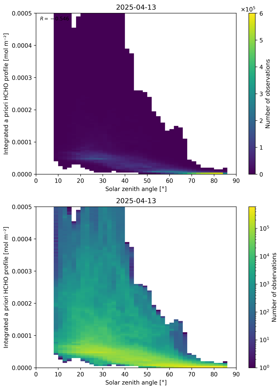
Figure 180: Scatter density plot of “Solar zenith angle” against “Integrated a priori HCHO profile” for 2025-04-13 to 2025-04-14.
