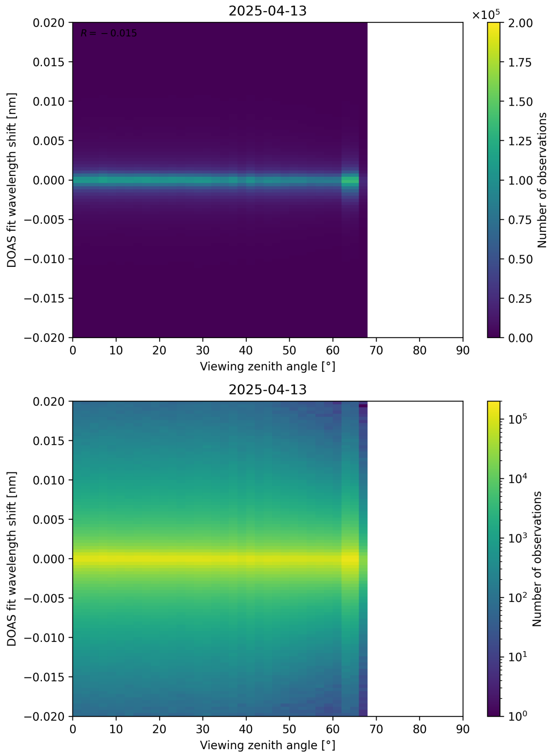
Figure 183: Scatter density plot of “Viewing zenith angle” against “DOAS fit wavelength shift” for 2025-04-13 to 2025-04-14.
