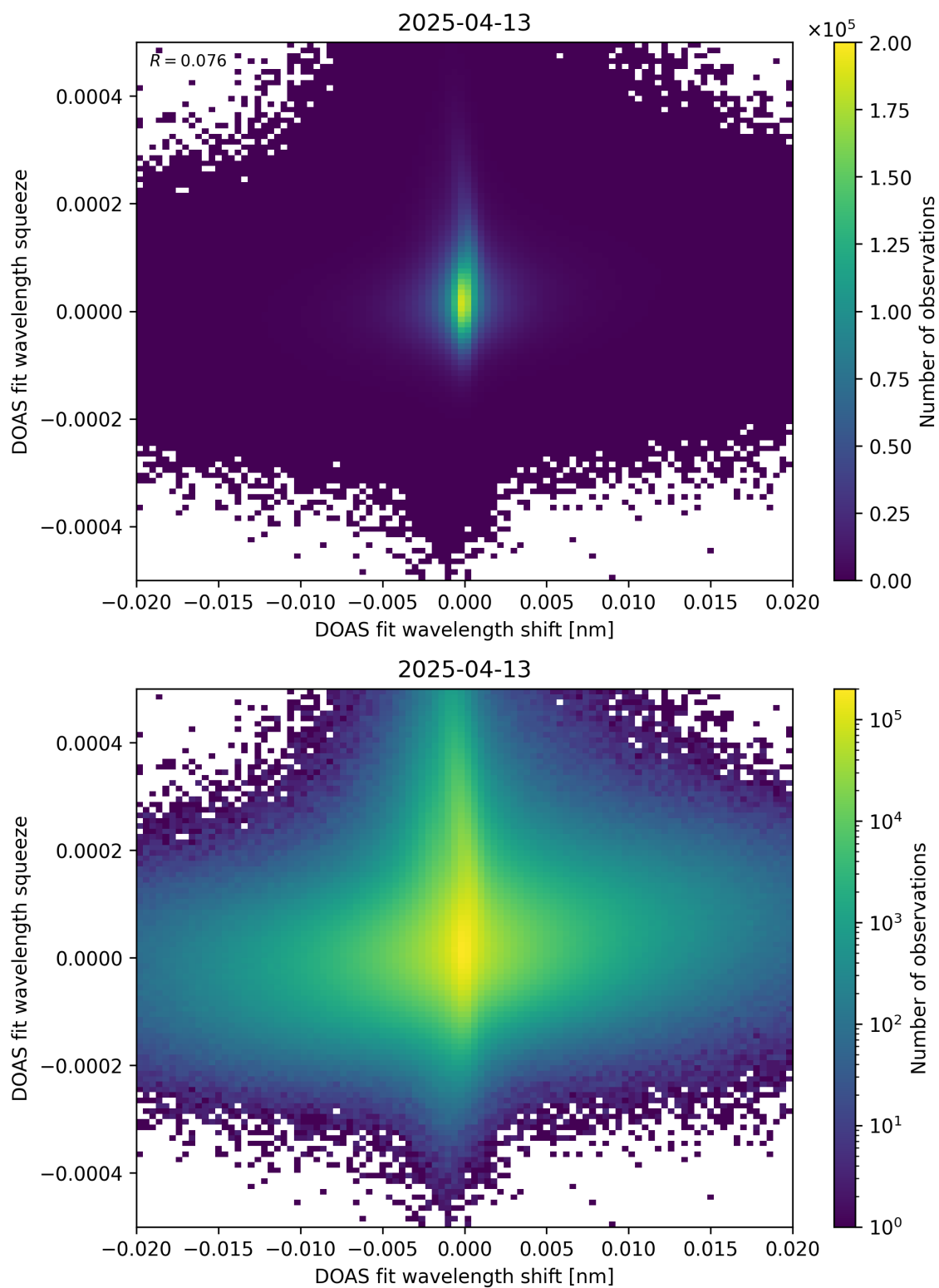
Figure 65: Scatter density plot of “DOAS fit wavelength shift” against “DOAS fit wavelength squeeze” for 2025-04-13 to 2025-04-14.
