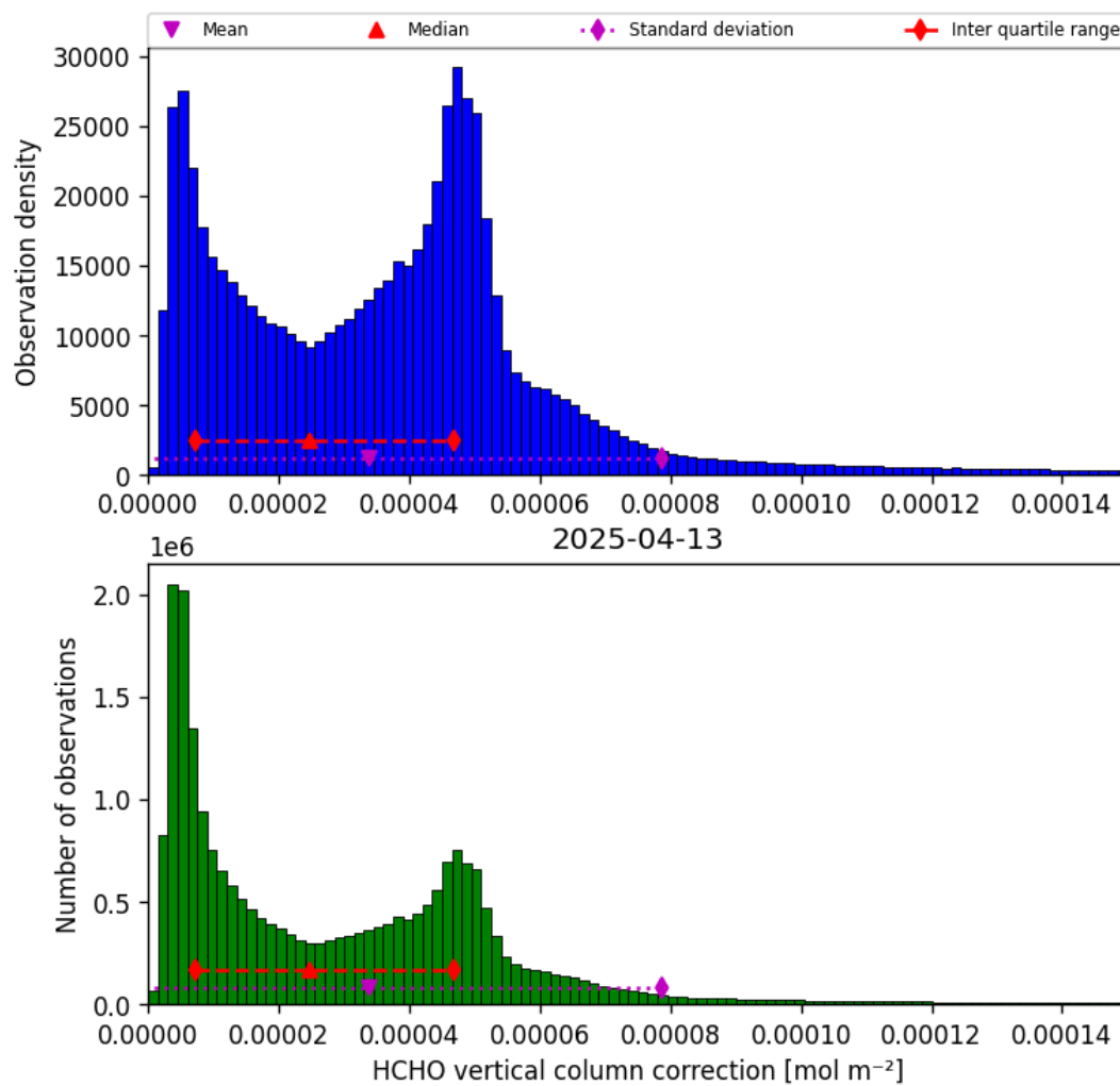
Figure 37: Histogram of “HCHO vertical column correction” for 2025-04-13 to 2025-04-14
