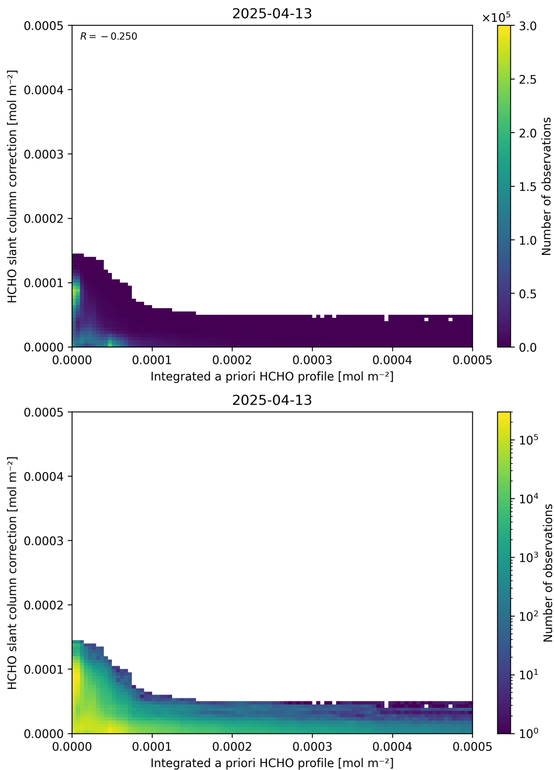
Figure 152: Scatter density plot of “Integrated a priori HCHO profile” against “HCHO slant column correction” for 2025-04-13 to 2025-04-14.
