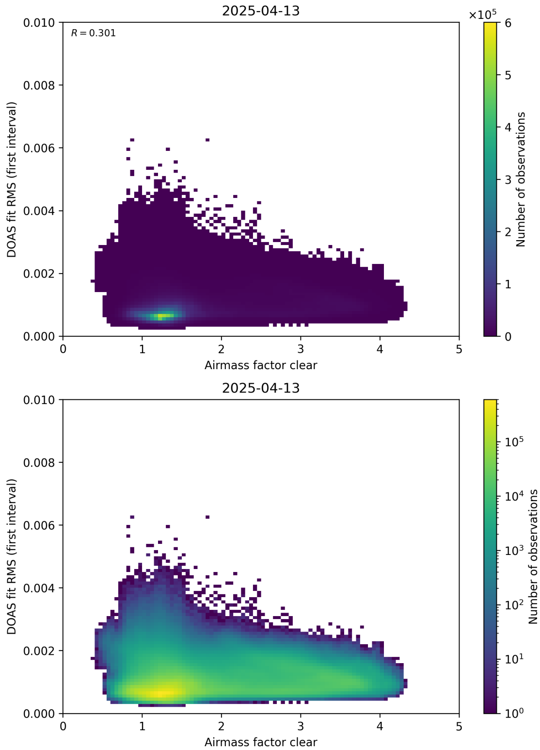
Figure 71: Scatter density plot of “Airmass factor clear” against “DOAS fit RMS (first interval)” for 2025-04-13 to 2025-04-14.
