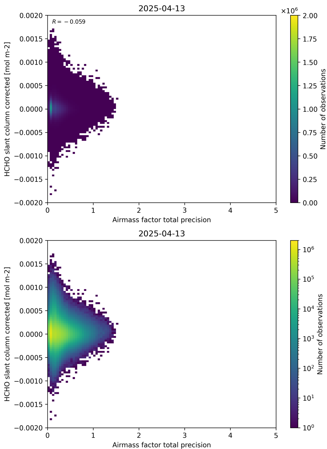
Figure 109: Scatter density plot of “Airmass factor total precision” against “HCHO slant column corrected” for 2025-04-13 to 2025-04-14.
