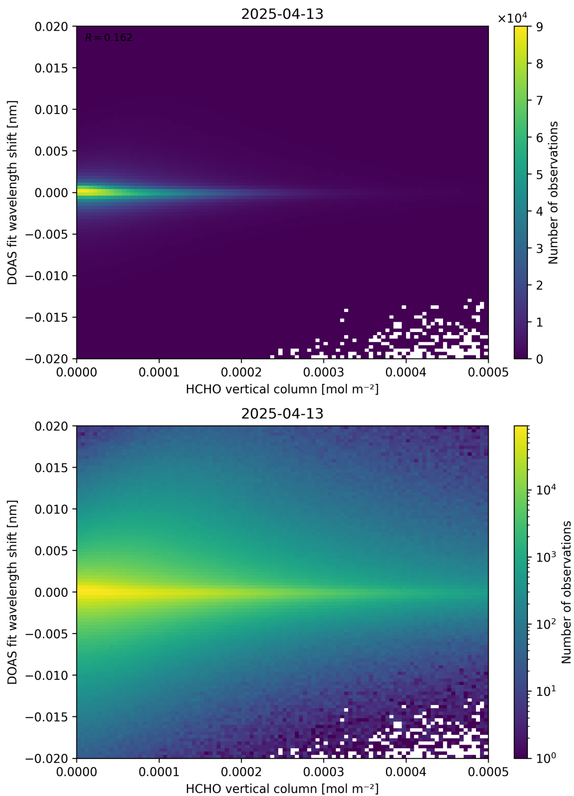
Figure 124: Scatter density plot of “HCHO vertical column” against “DOAS fit wavelength shift” for 2025-04-13 to 2025-04-14.
