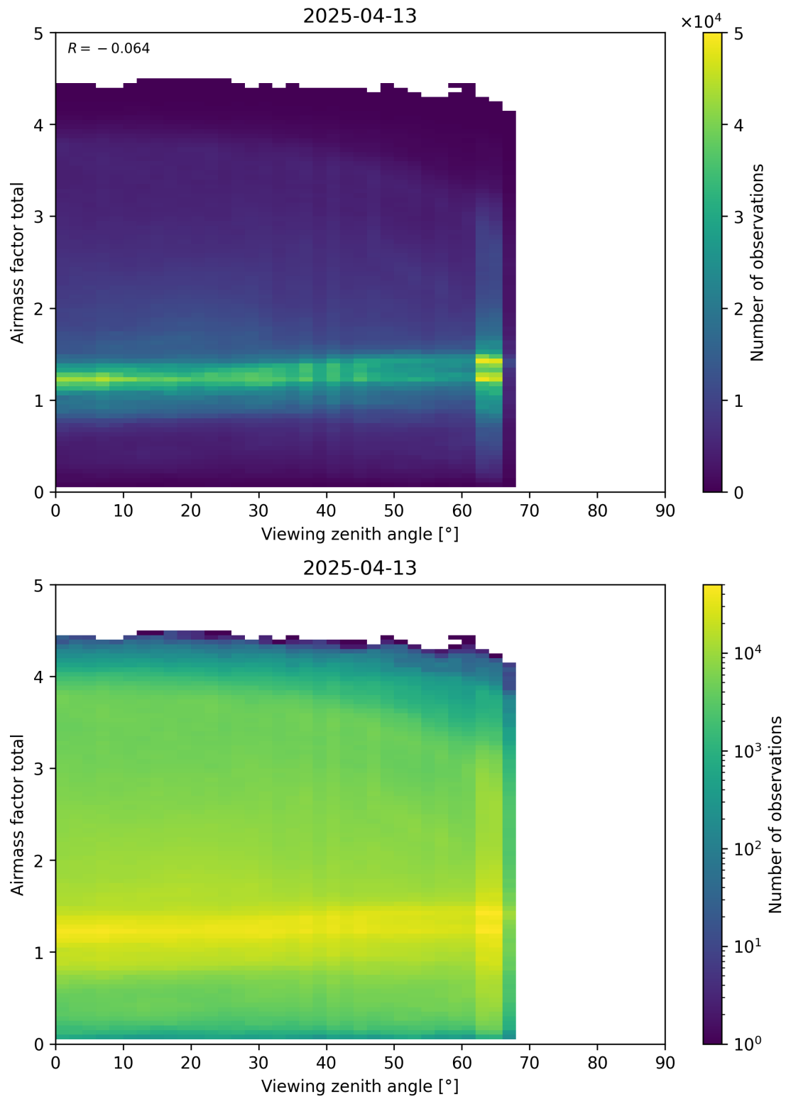
Figure 190: Scatter density plot of “Viewing zenith angle” against “Airmass factor total” for 2025-04-13 to 2025-04-14.
