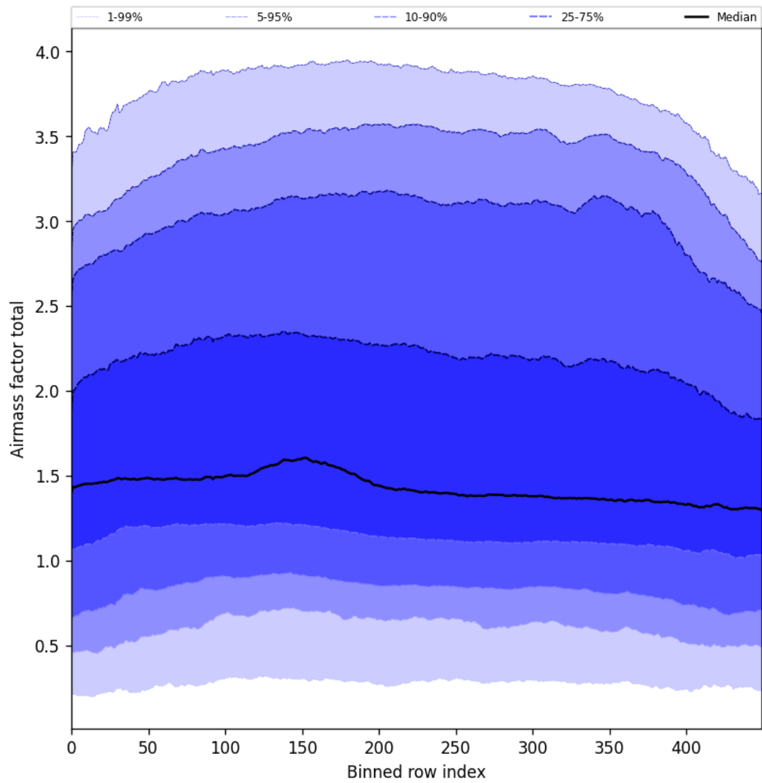
Figure 54: Along track statistics of “Airmass factor total” for 2025-04-13 to 2025-04-14
