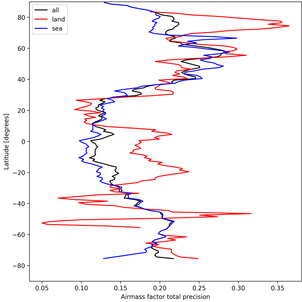
Figure 27: Zonal average of “Airmass factor total precision” for 2025-04-13 to 2025-04-14.
