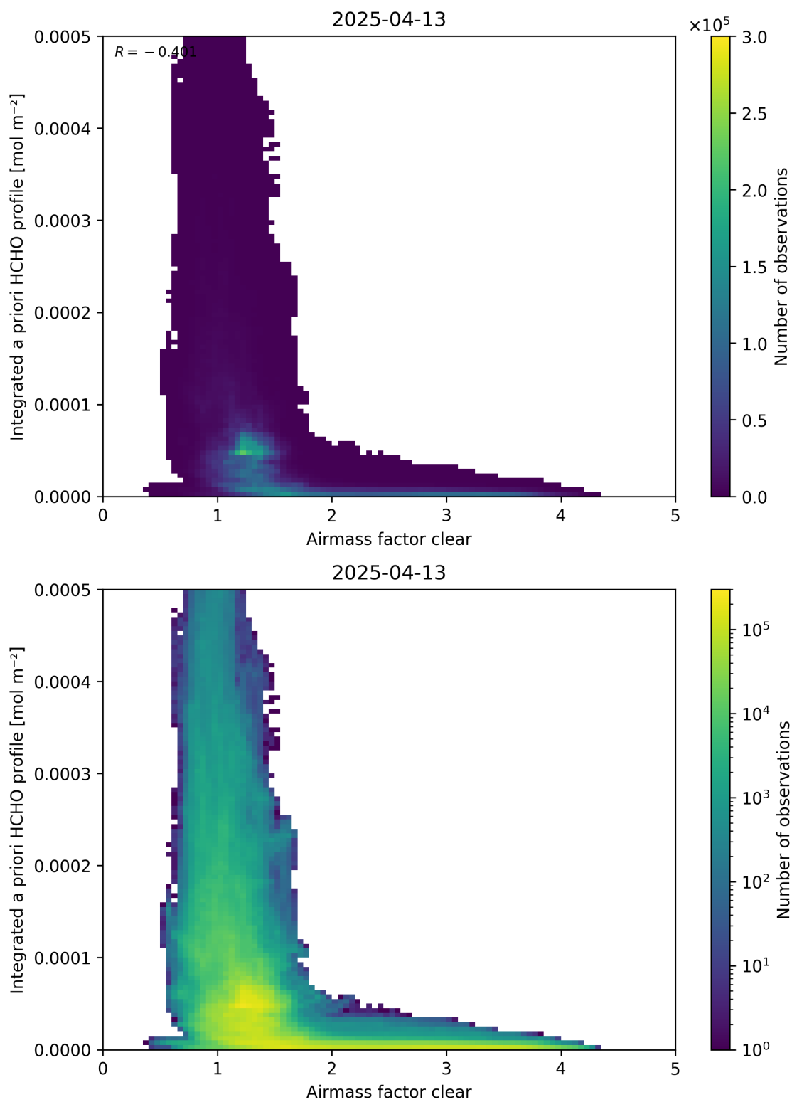
Figure 76: Scatter density plot of “Airmass factor clear” against “Integrated a priori HCHO profile” for 2025-04-13 to 2025-04-14.
