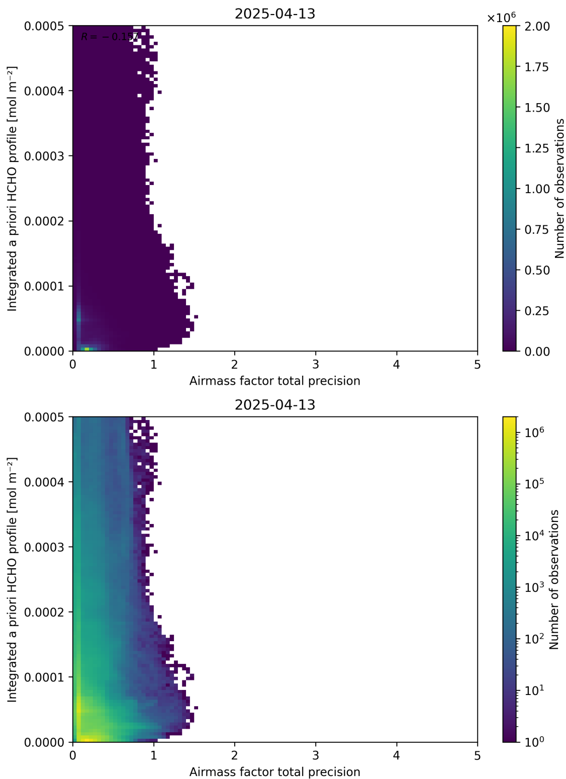
Figure 111: Scatter density plot of “Airmass factor total precision” against “Integrated a priori HCHO profile” for 2025-04-13 to 2025-04-14.
