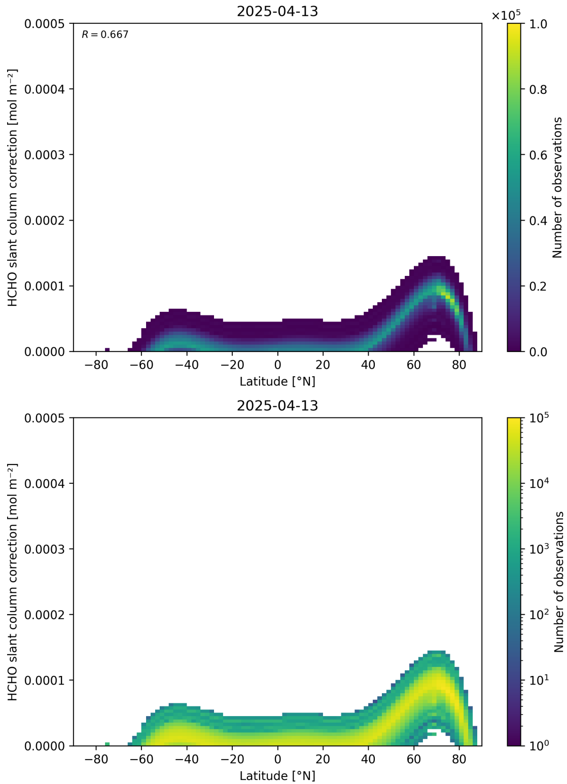
Figure 158: Scatter density plot of “Latitude” against “HCHO slant column correction” for 2025-04-13 to 2025-04-14.
