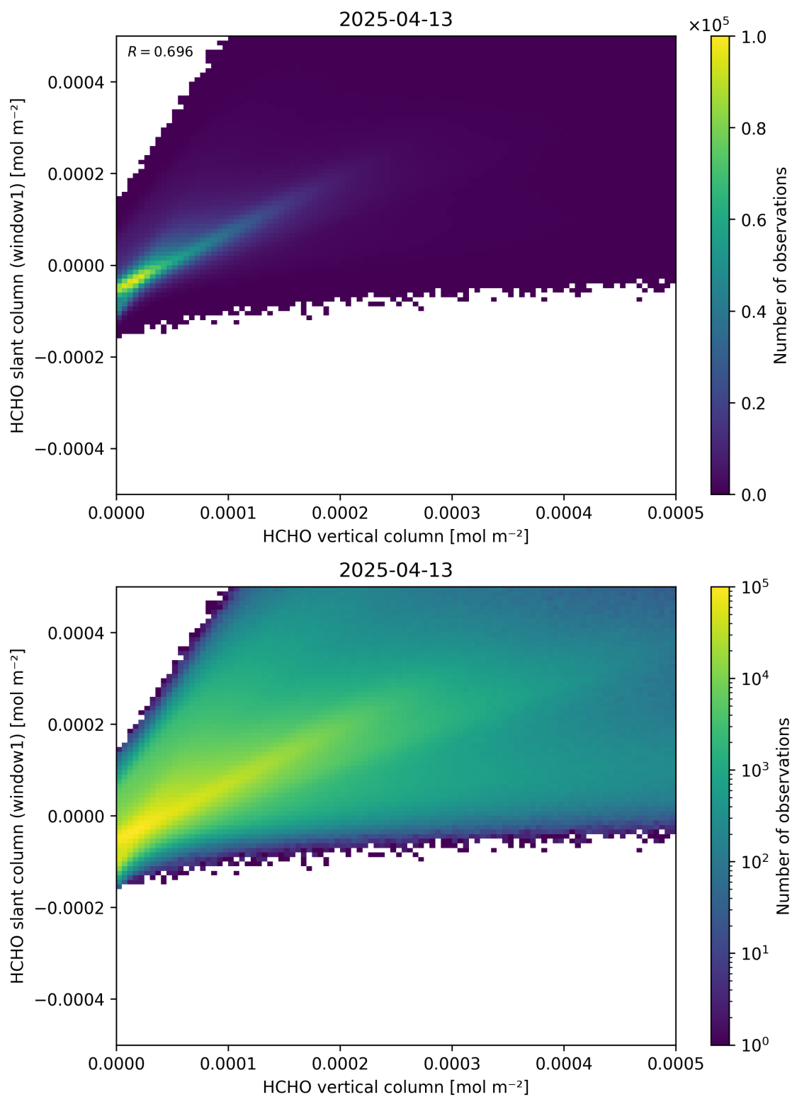
Figure 129: Scatter density plot of “HCHO vertical column” against “HCHO slant column (window1)” for 2025-04-13 to 2025-04-14.
