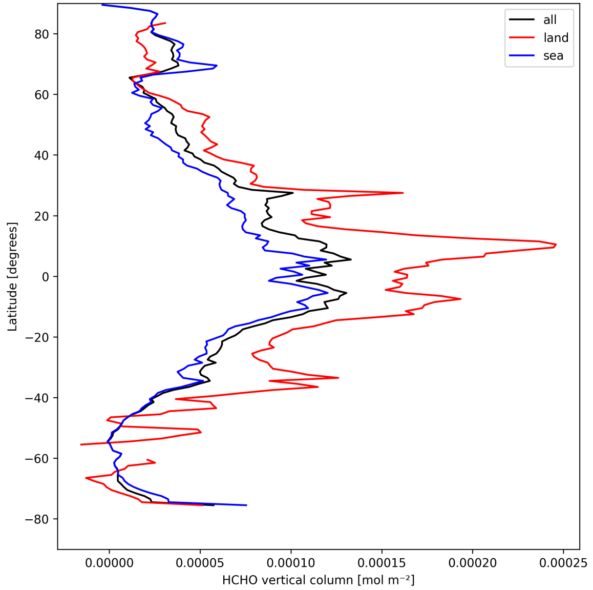
Figure 21: Zonal average of “HCHO vertical column” for 2025-04-13 to 2025-04-14.
