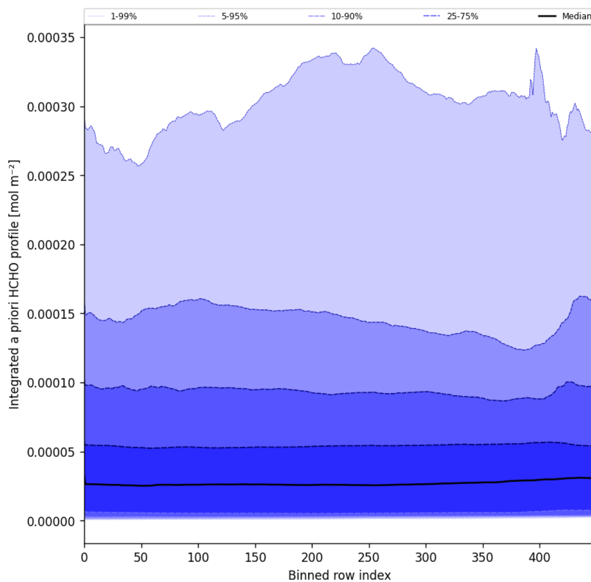
Figure 57: Along track statistics of "Integrated a priori HCHO profile" for 2025-04-13 to 2025-04-14
