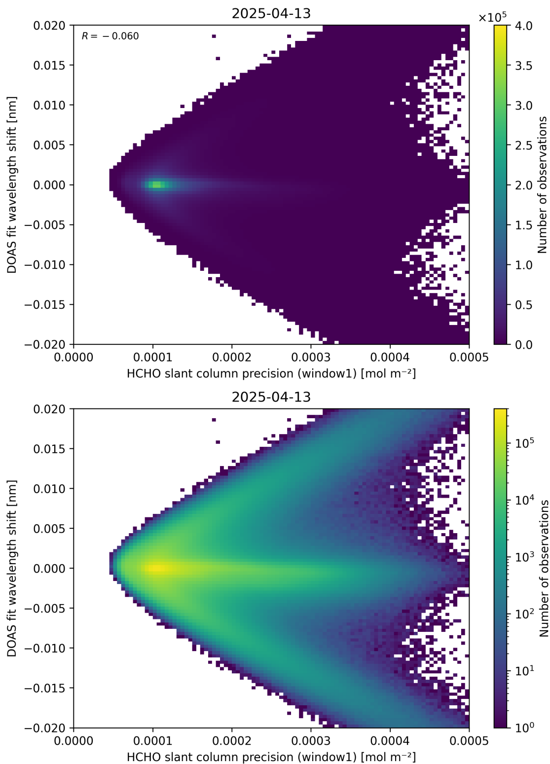
Figure 89: Scatter density plot of “HCHO slant column precision (window1)” against “DOAS fit wavelength shift” for 2025-04-13 to 2025-04-14.
