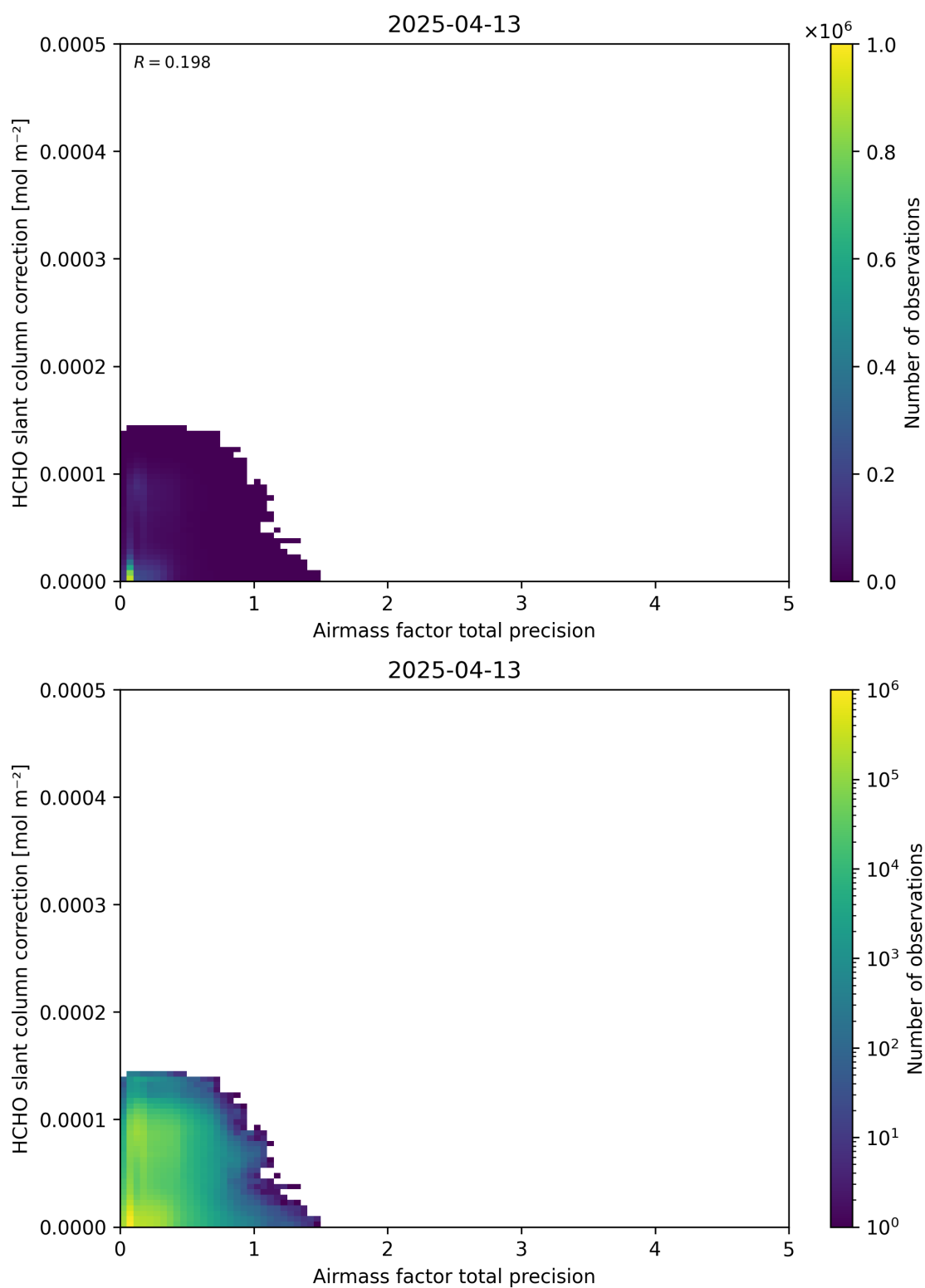
Figure 110: Scatter density plot of “Airmass factor total precision” against “HCHO slant column correction” for 2025-04-13 to 2025-04-14.
