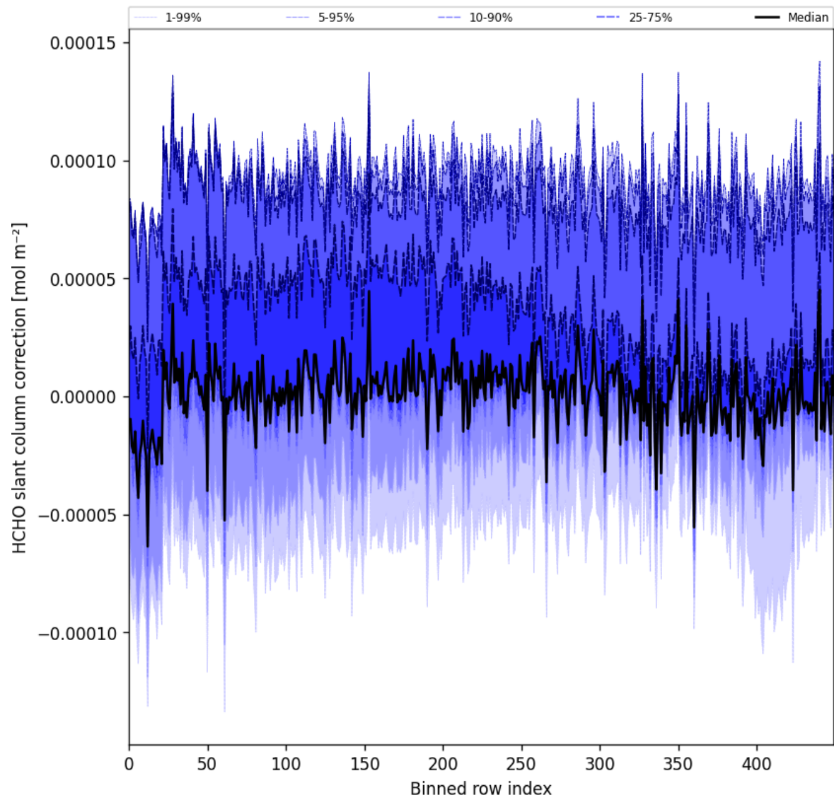
Figure 61: Along track statistics of “HCHO slant column correction” for 2025-04-13 to 2025-04-14
