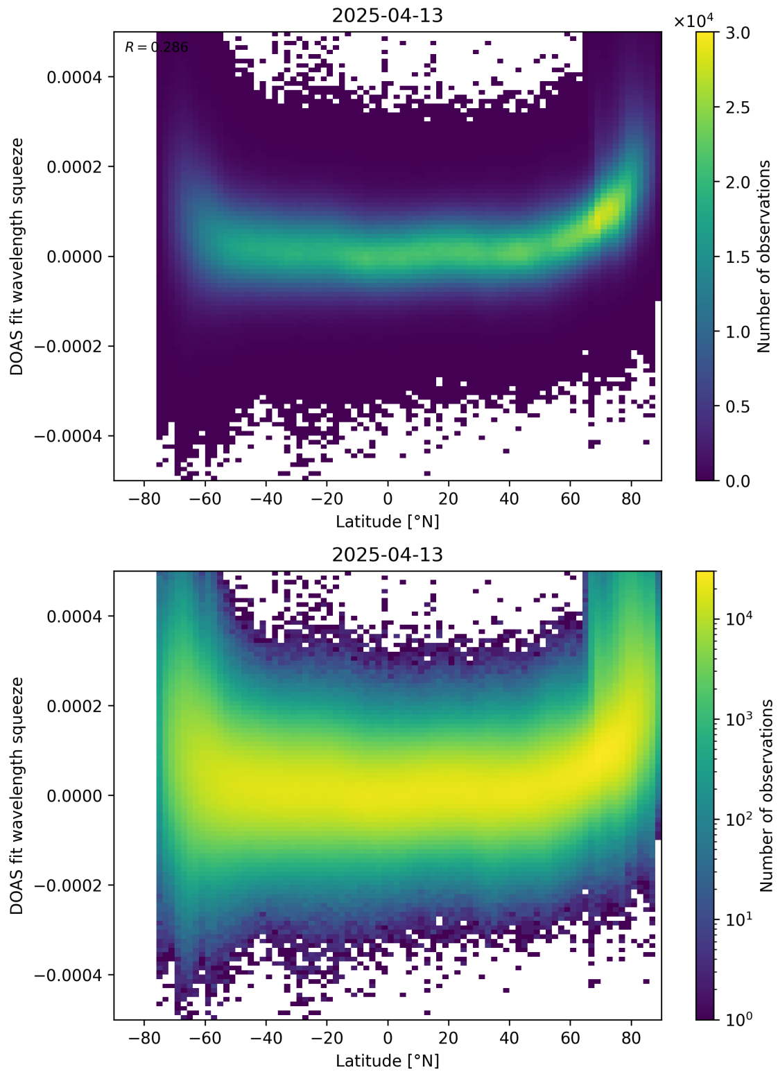
Figure 155: Scatter density plot of “Latitude” against “DOAS fit wavelength squeeze” for 2025-04-13 to 2025-04-14.
