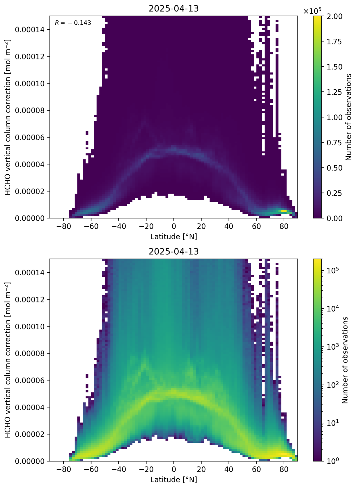
Figure 164: Scatter density plot of “Latitude” against “HCHO vertical column correction” for 2025-04-13 to 2025-04-14.
