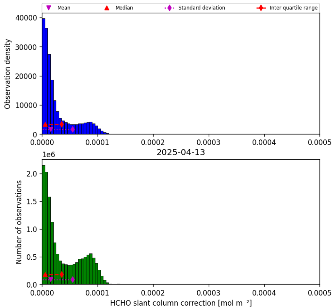
Figure 47: Histogram of “HCHO slant column correction” for 2025-04-13 to 2025-04-14
