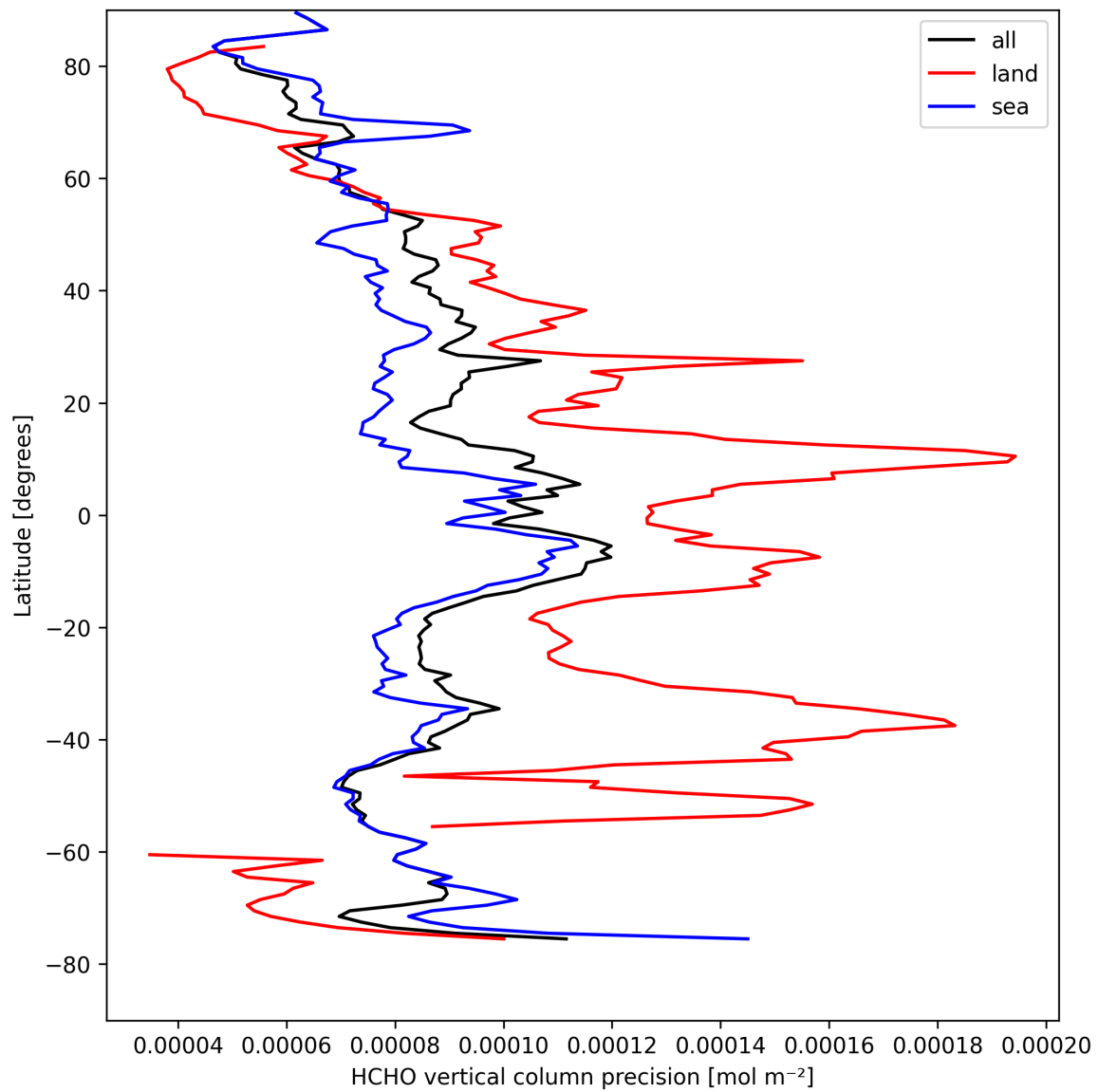
Figure 22: Zonal average of “HCHO vertical column precision” for 2025-04-13 to 2025-04-14.
