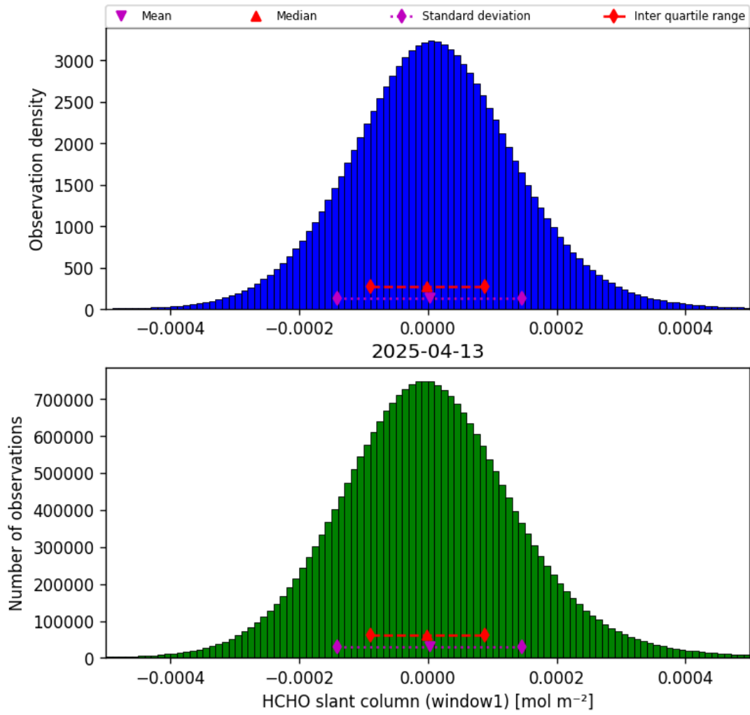
Figure 38: Histogram of “HCHO slant column (window1)” for 2025-04-13 to 2025-04-14
