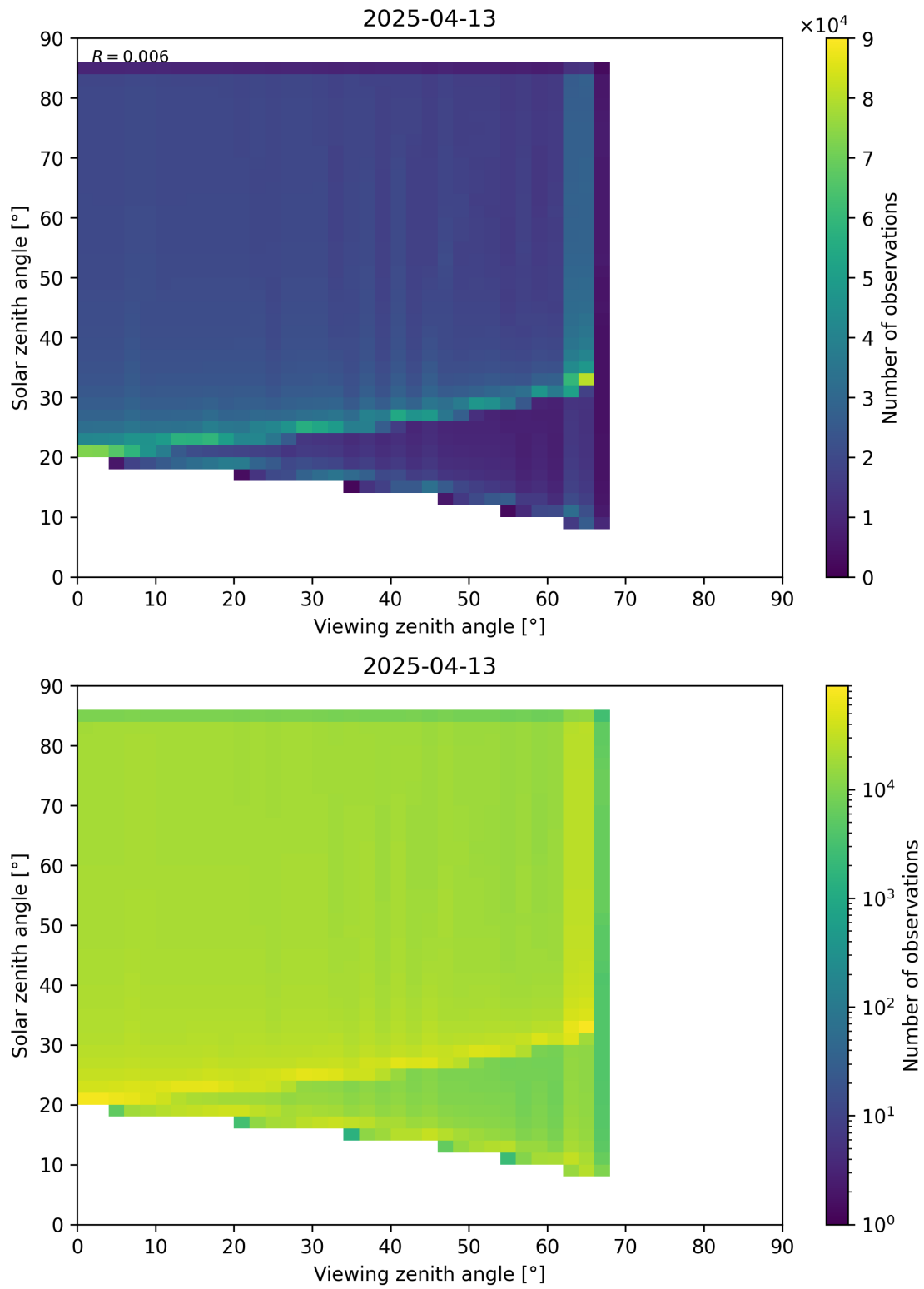
Figure 197: Scatter density plot of “Viewing zenith angle” against “Solar zenith angle” for 2025-04-13 to 2025-04-14.
