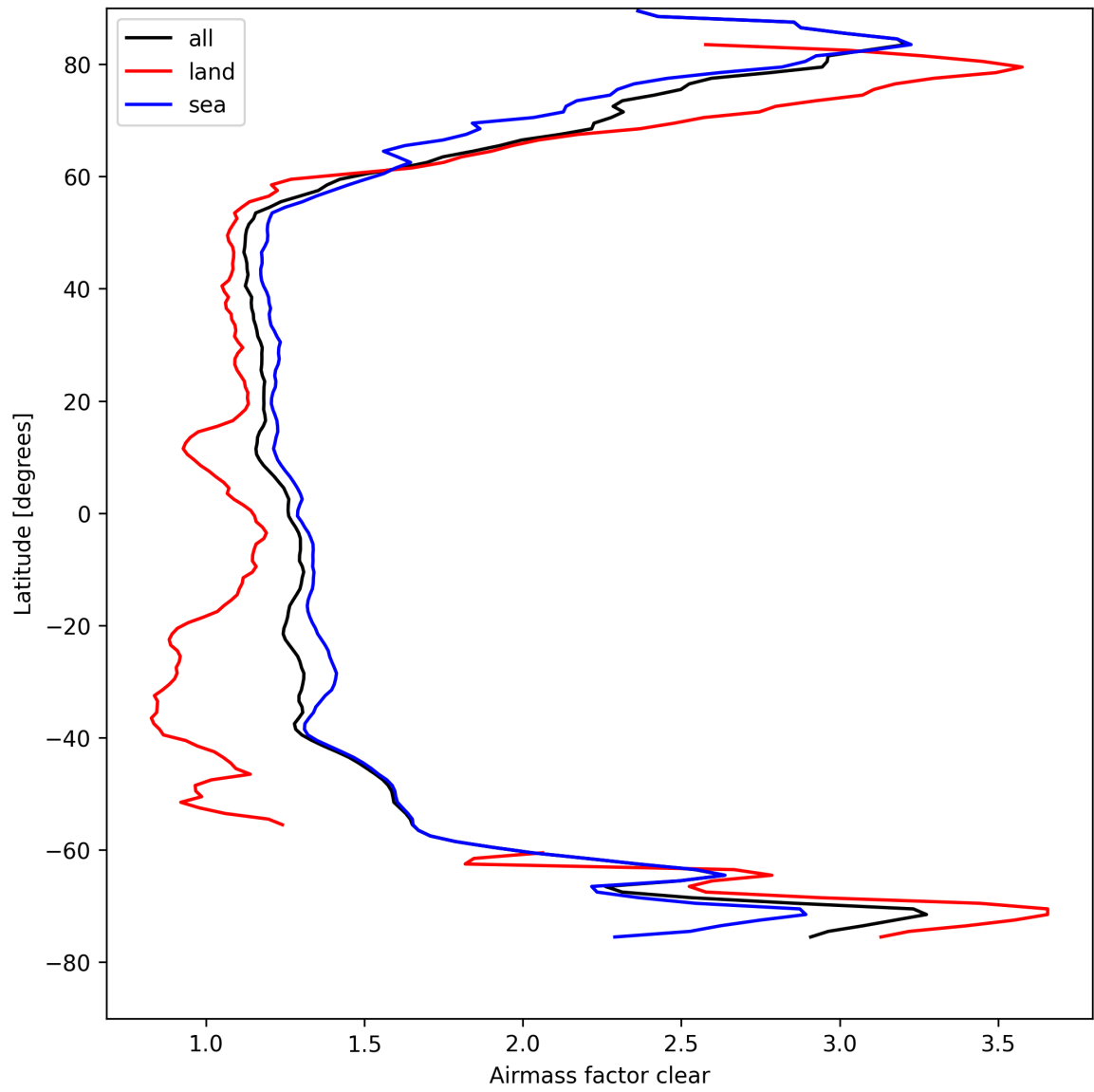
Figure 28: Zonal average of “Airmass factor clear” for 2025-04-13 to 2025-04-14.
