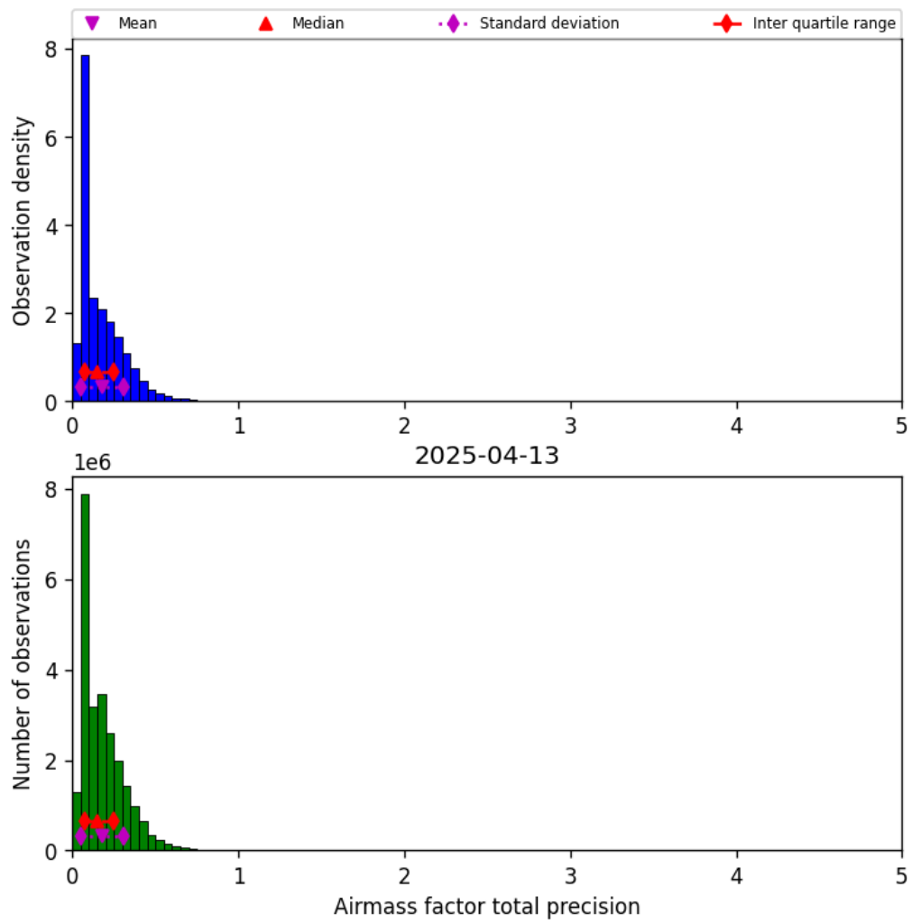
Figure 41: Histogram of “Airmass factor total precision” for 2025-04-13 to 2025-04-14
