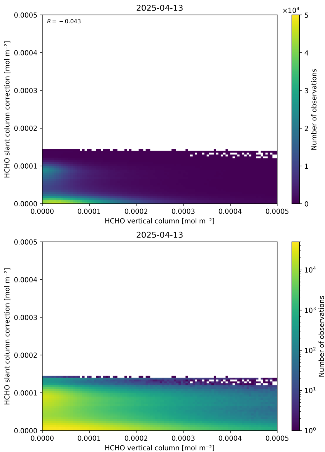
Figure 128: Scatter density plot of “HCHO vertical column” against “HCHO slant column correction” for 2025-04-13 to 2025-04-14.
