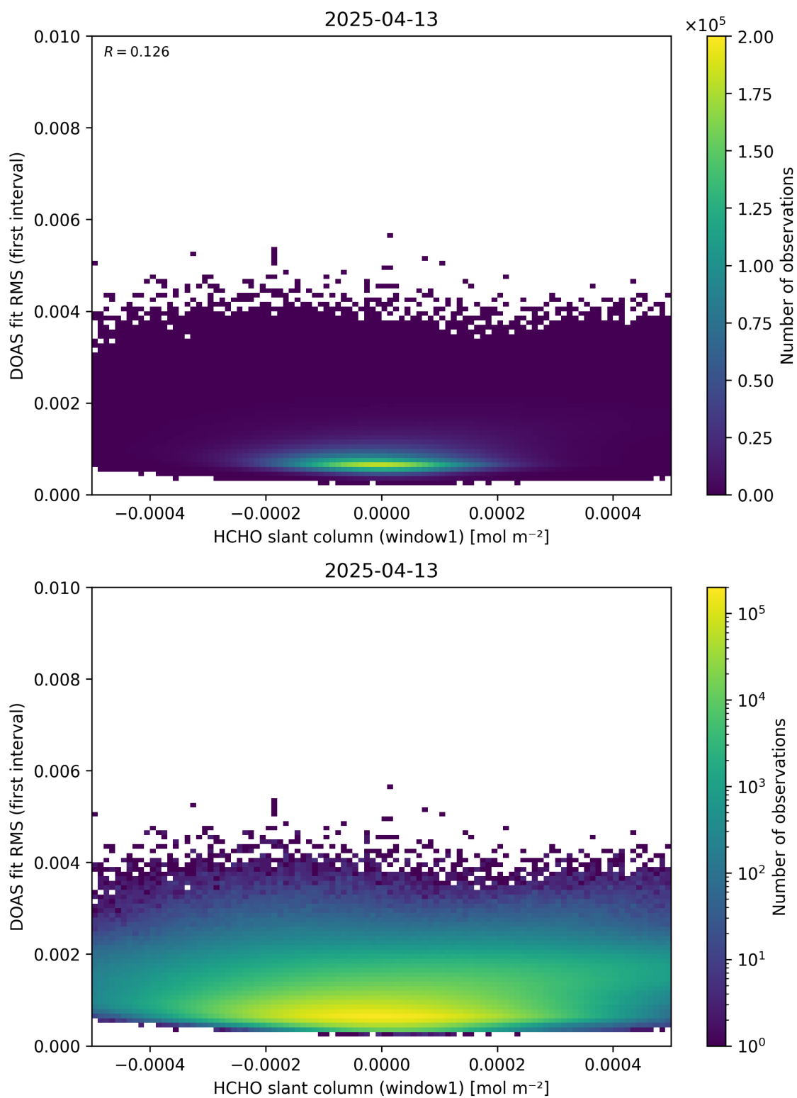
Figure 78: Scatter density plot of “HCHO slant column (window1)” against “DOAS fit RMS (first interval)” for 2025-04-13 to 2025-04-14.
