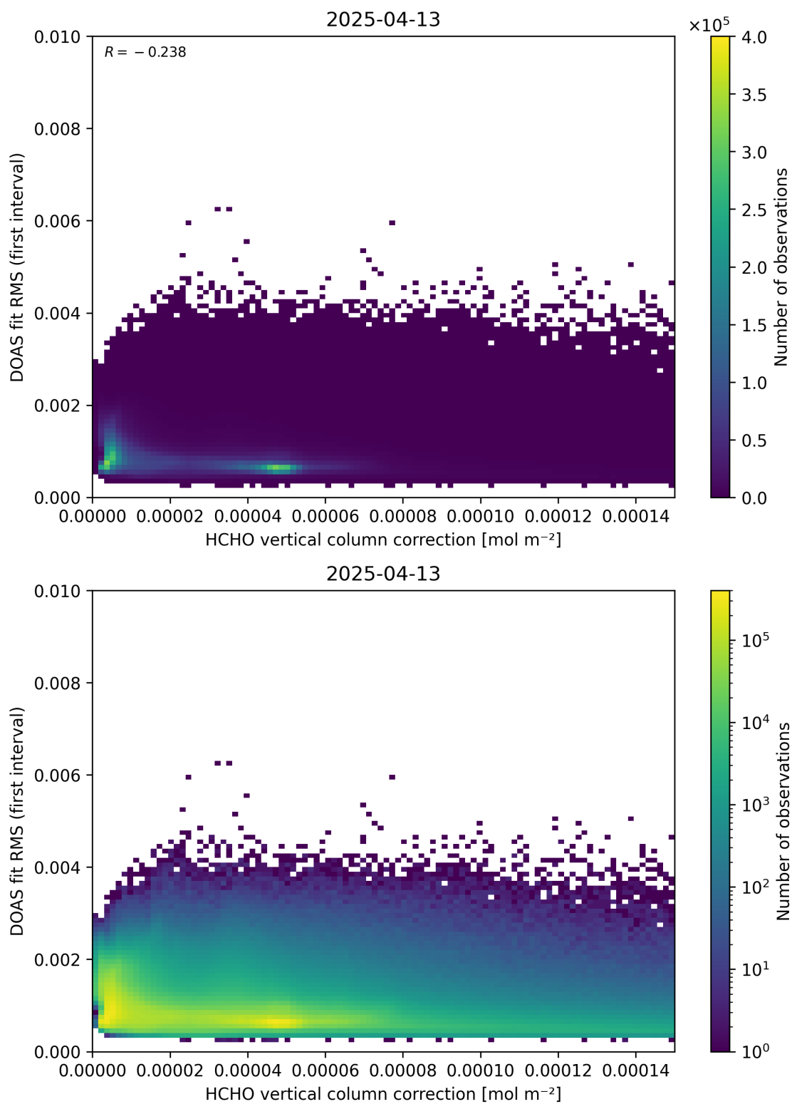
Figure 112: Scatter density plot of “HCHO vertical column correction” against “DOAS fit RMS (first interval)” for 2025-04-13 to 2025-04-14.
