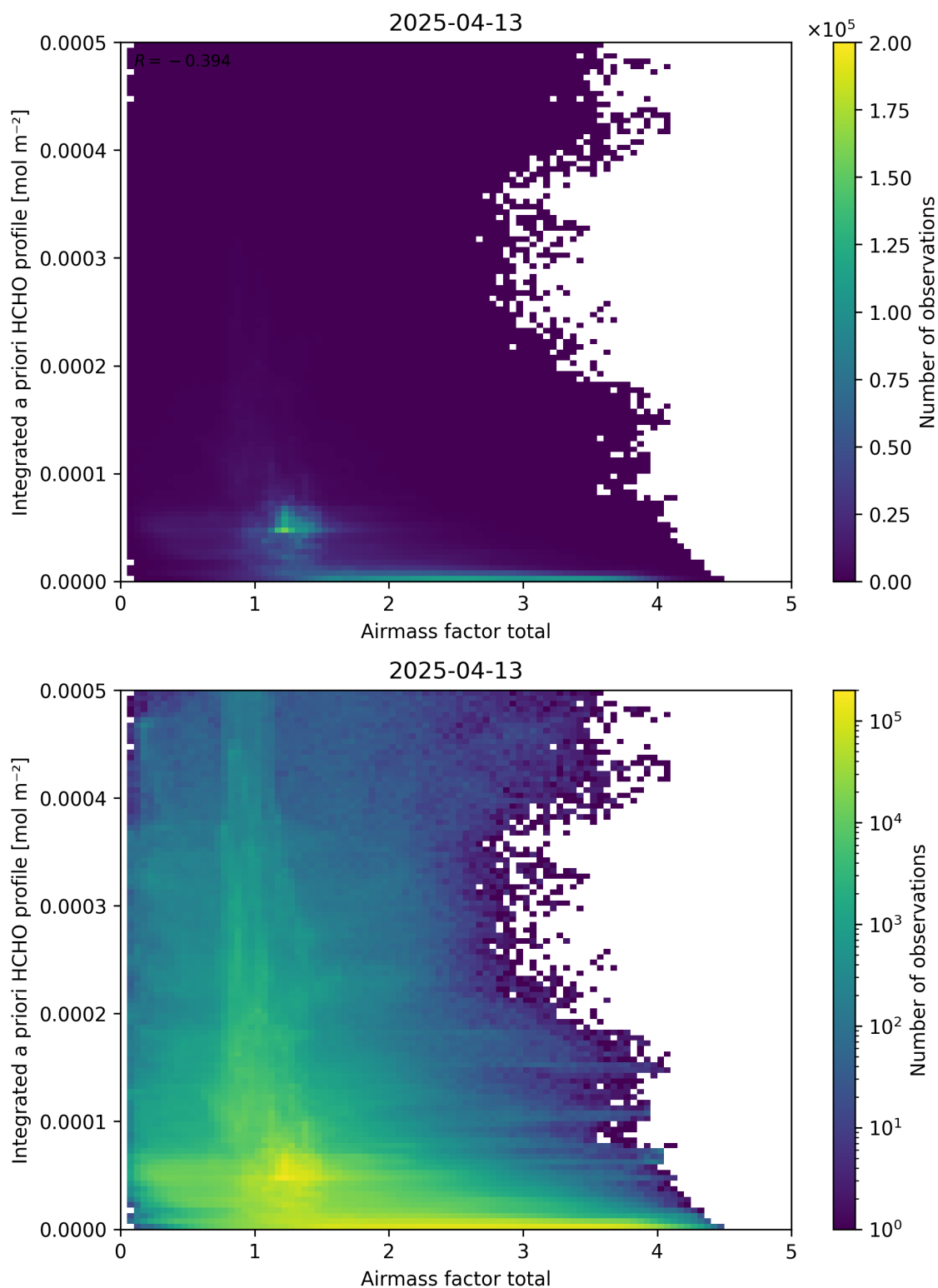
Figure 104: Scatter density plot of “Airmass factor total” against “Integrated a priori HCHO profile” for 2025-04-13 to 2025-04-14.
