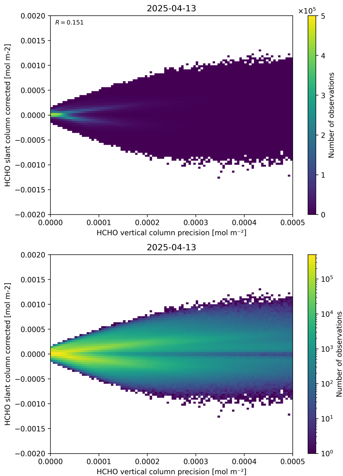
Figure 140: Scatter density plot of “HCHO vertical column precision” against “HCHO slant column corrected” for 2025-04-13 to 2025-04-14.
