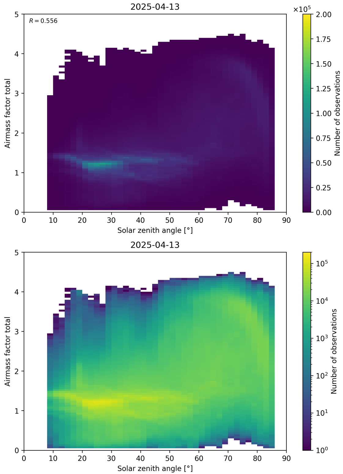
Figure 175: Scatter density plot of “Solar zenith angle” against “Airmass factor total” for 2025-04-13 to 2025-04-14.
