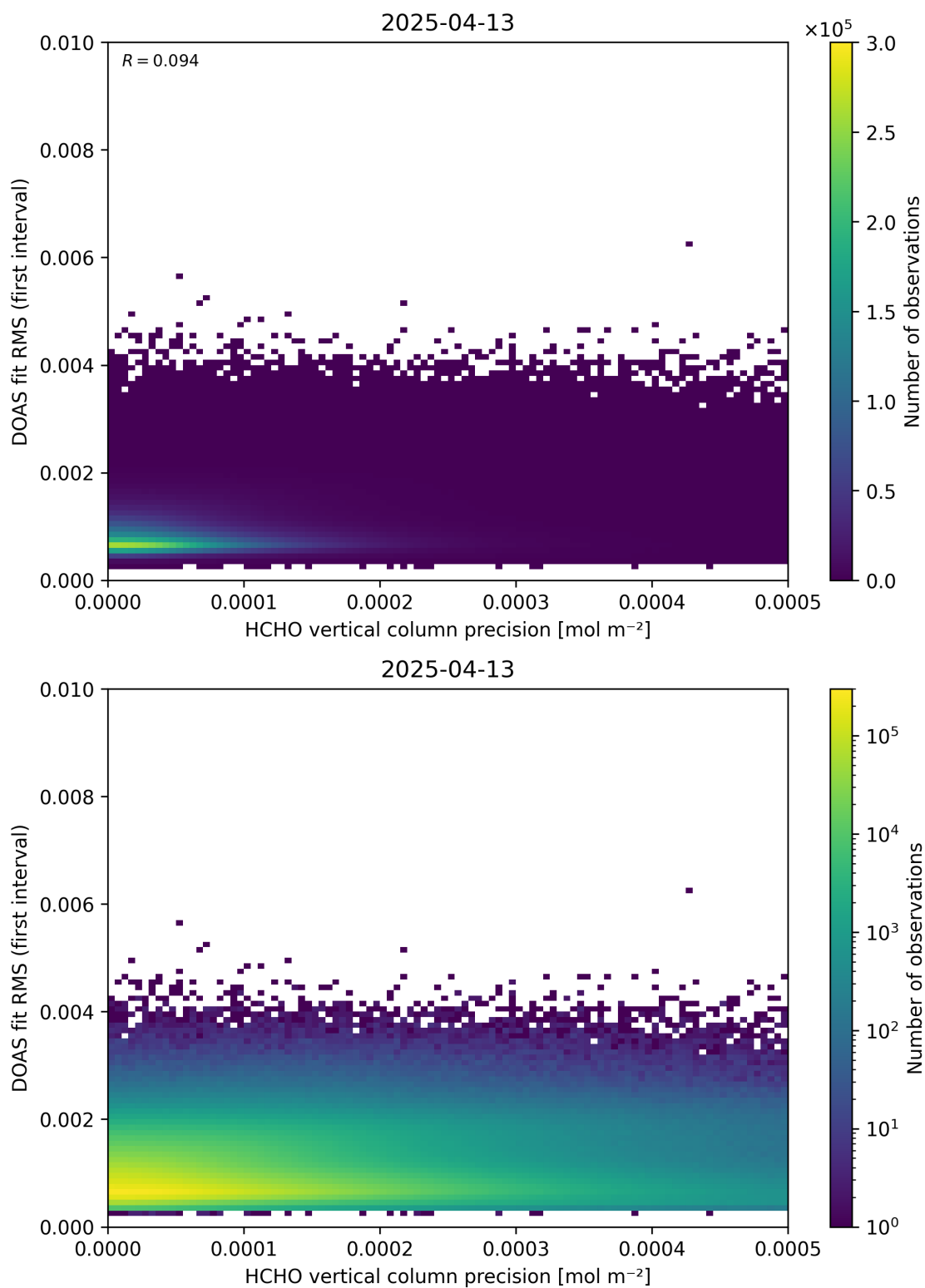
Figure 136: Scatter density plot of “HCHO vertical column precision” against “DOAS fit RMS (first interval)” for 2025-04-13 to 2025-04-14.
