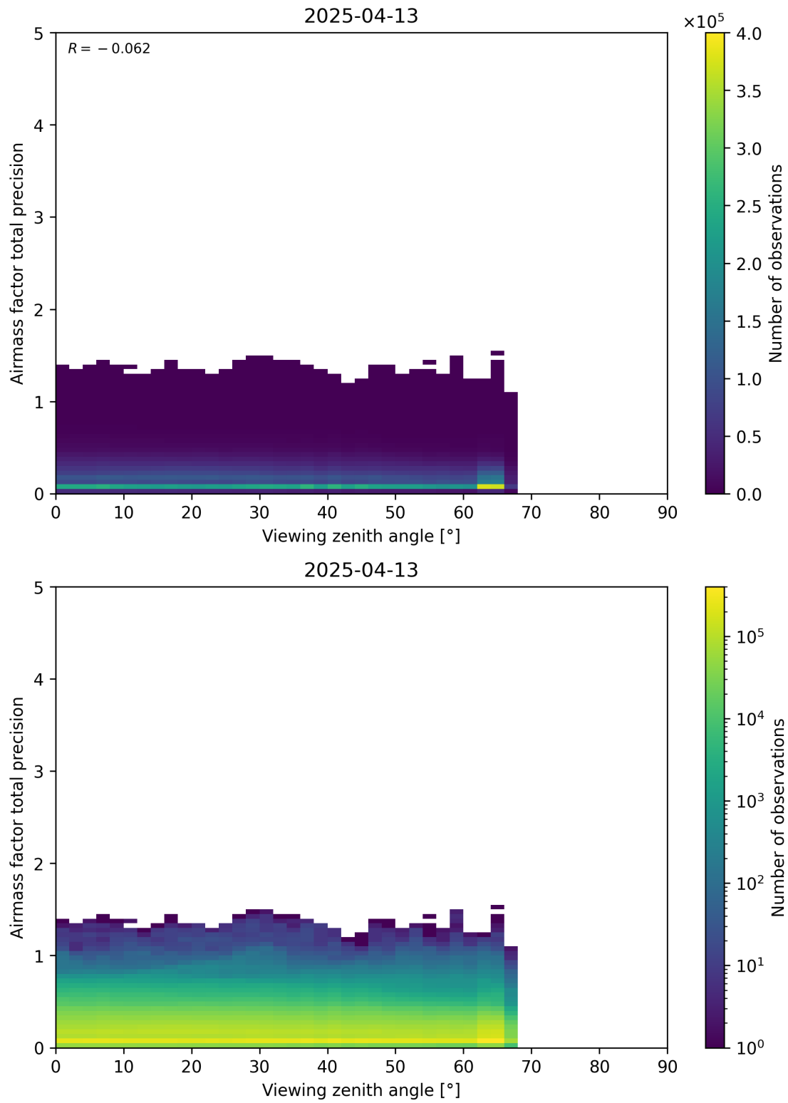
Figure 191: Scatter density plot of “Viewing zenith angle” against “Airmass factor total precision” for 2025-04-13 to 2025-04-14.
