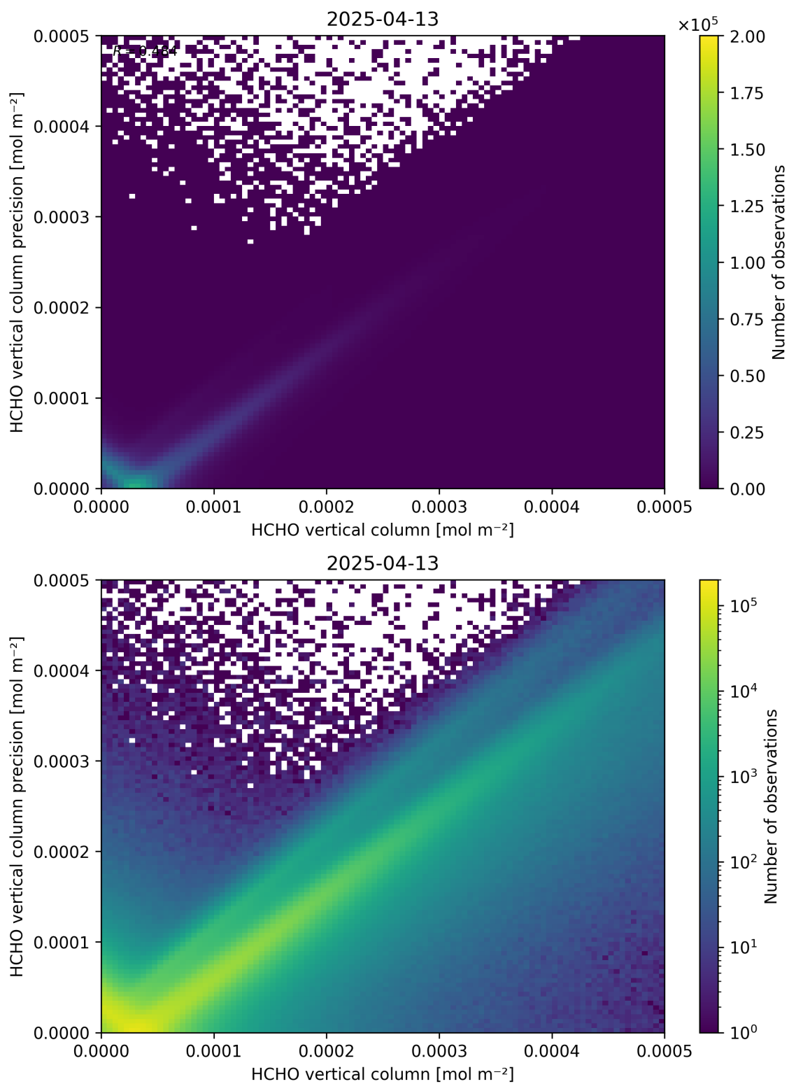
Figure 134: Scatter density plot of “HCHO vertical column” against “HCHO vertical column precision” for 2025-04-13 to 2025-04-14.
