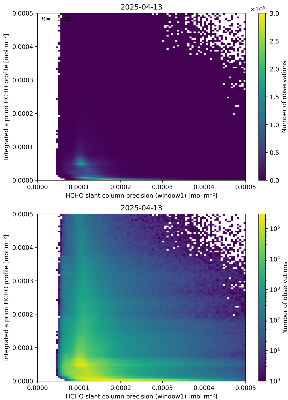
Figure 96: Scatter density plot of “HCHO slant column precision (window1)” against “Integrated a priori HCHO profile” for 2025-04-13 to 2025-04-14.
