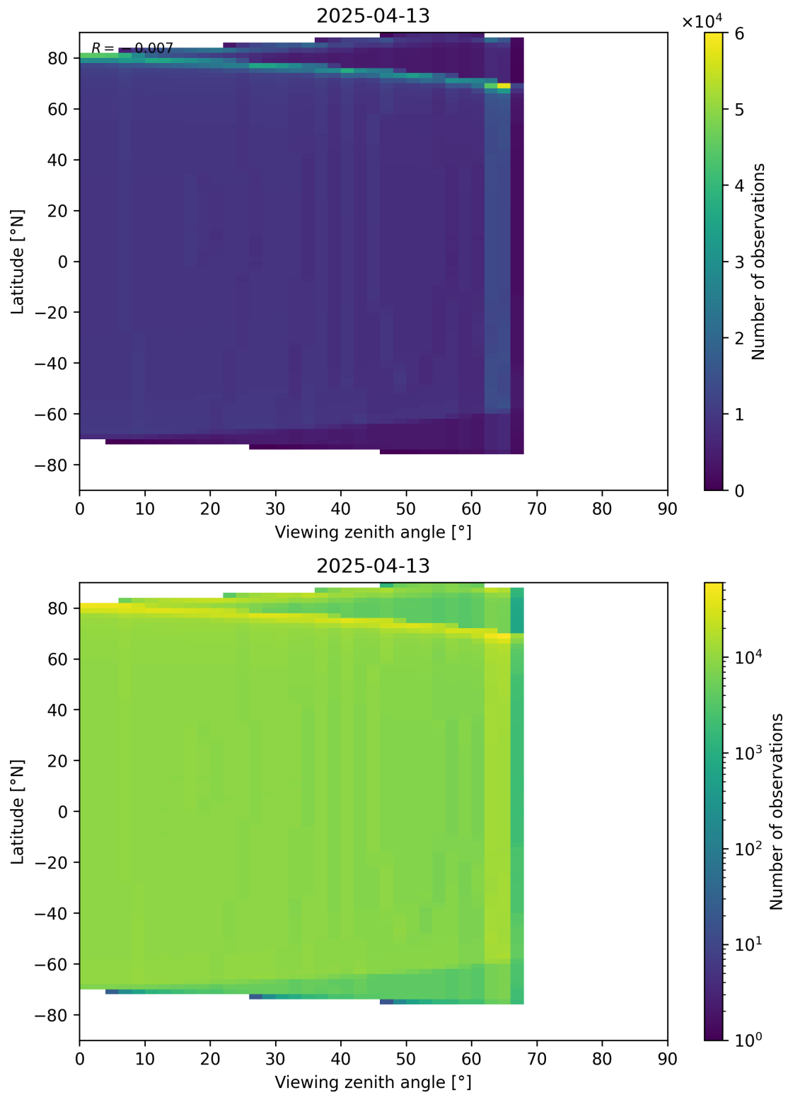
Figure 196: Scatter density plot of “Viewing zenith angle” against “Latitude” for 2025-04-13 to 2025-04-14.
