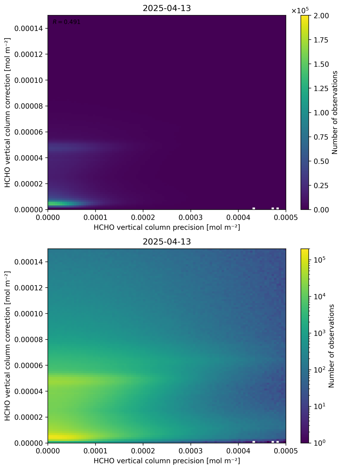
Figure 146: Scatter density plot of “HCHO vertical column precision” against “HCHO vertical column correction” for 2025-04-13 to 2025-04-14.
