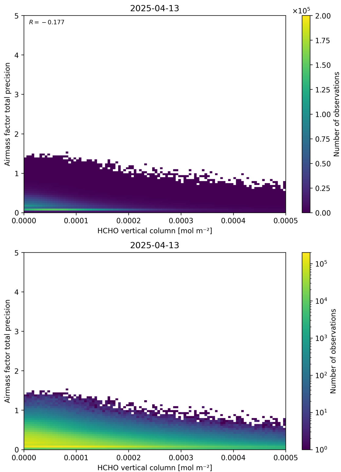
Figure 132: Scatter density plot of “HCHO vertical column” against “Airmass factor total precision” for 2025-04-13 to 2025-04-14.
