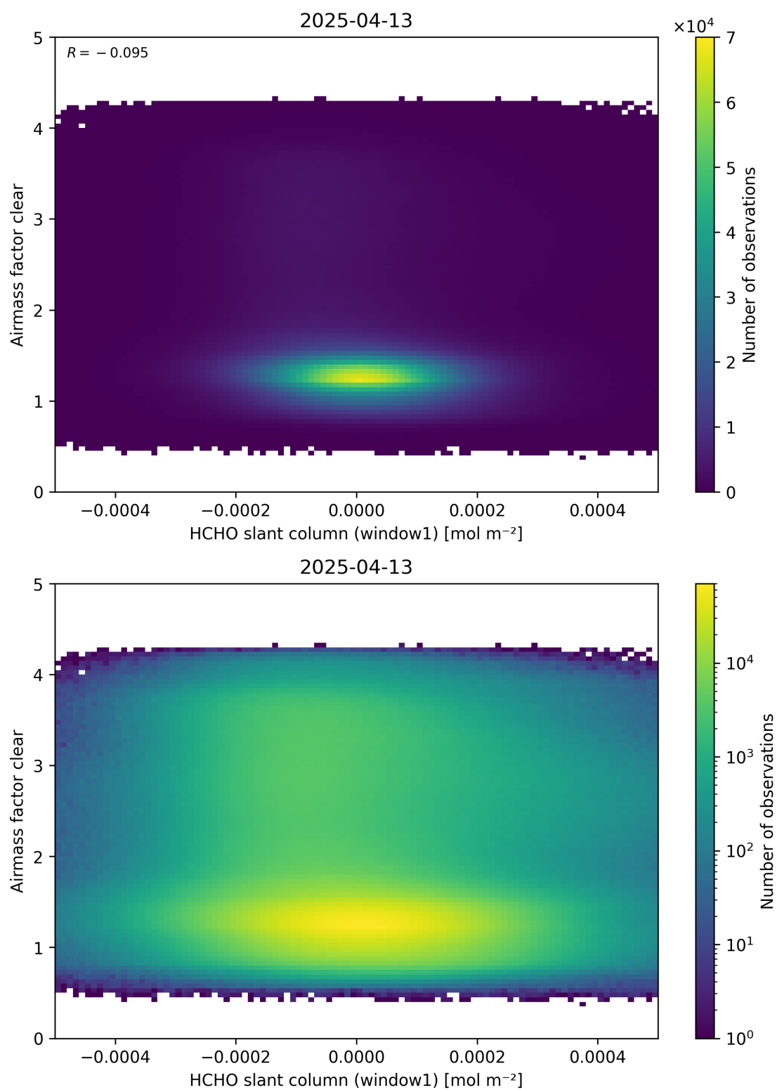
Figure 81: Scatter density plot of “HCHO slant column (window1)” against “Airmass factor clear” for 2025-04-13 to 2025-04-14.
