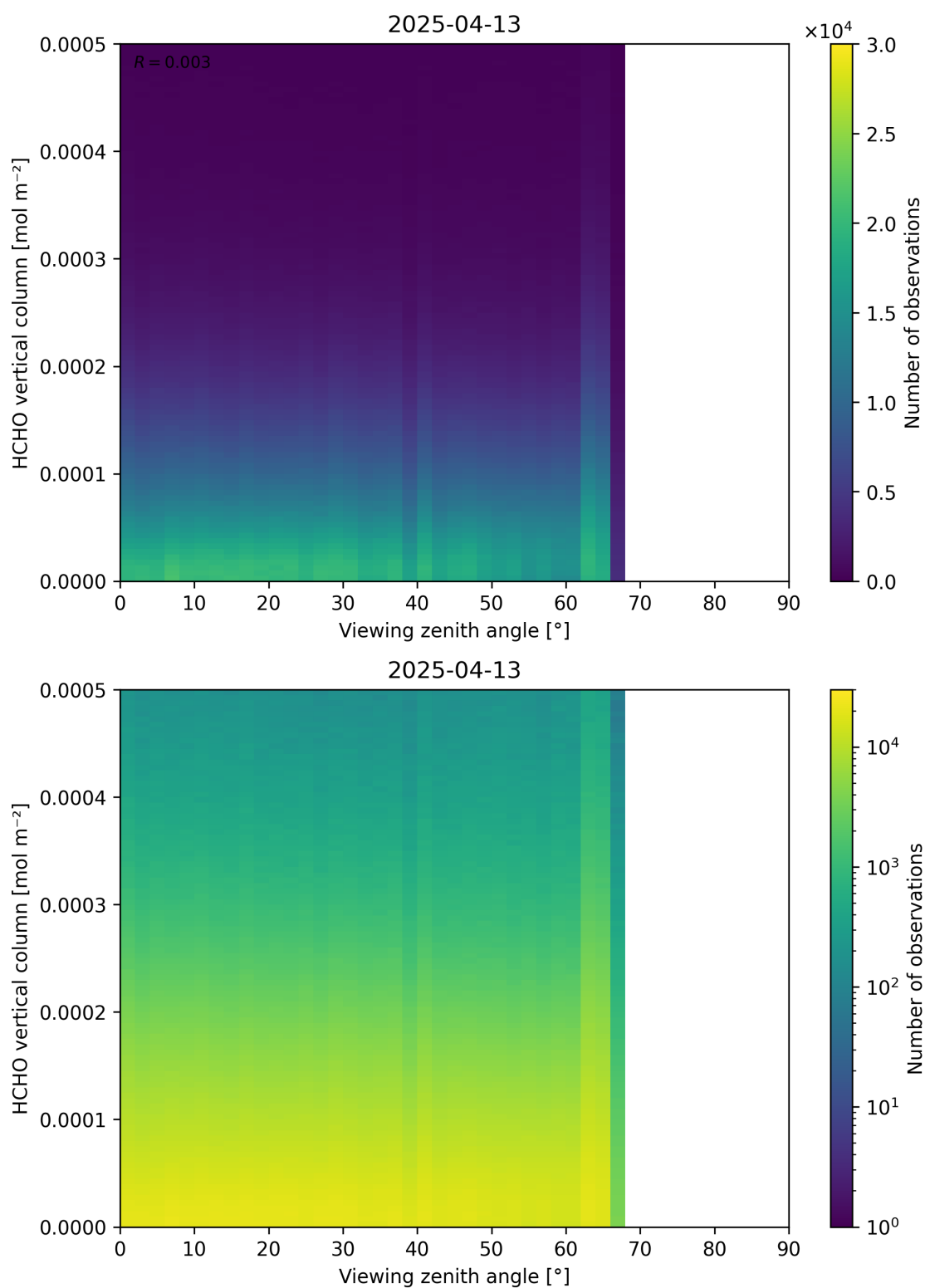
Figure 192: Scatter density plot of “Viewing zenith angle” against “HCHO vertical column” for 2025-04-13 to 2025-04-14.
