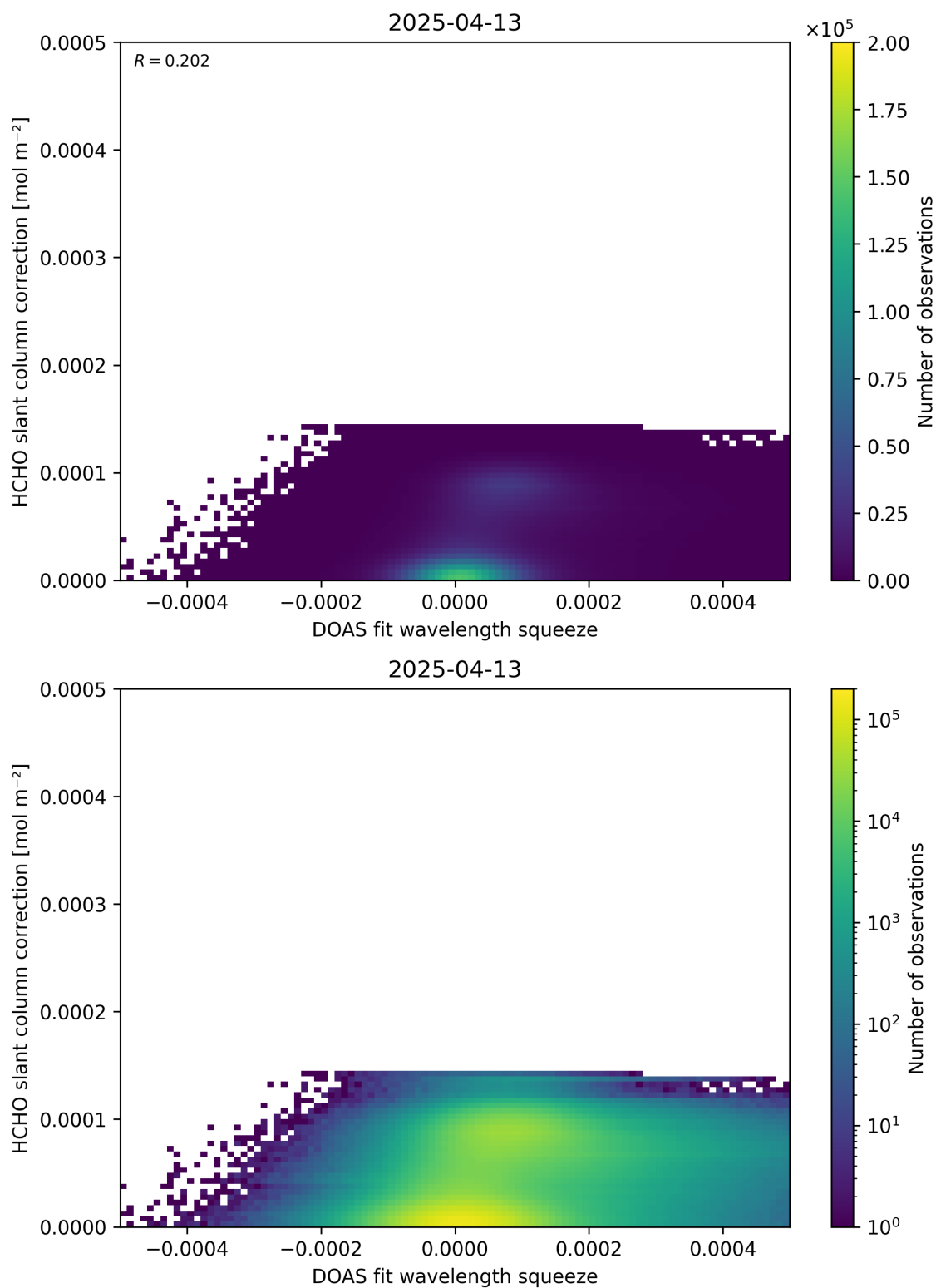
Figure 70: Scatter density plot of “DOAS fit wavelength squeeze” against “HCHO slant column correction” for 2025-04-13 to 2025-04-14.
