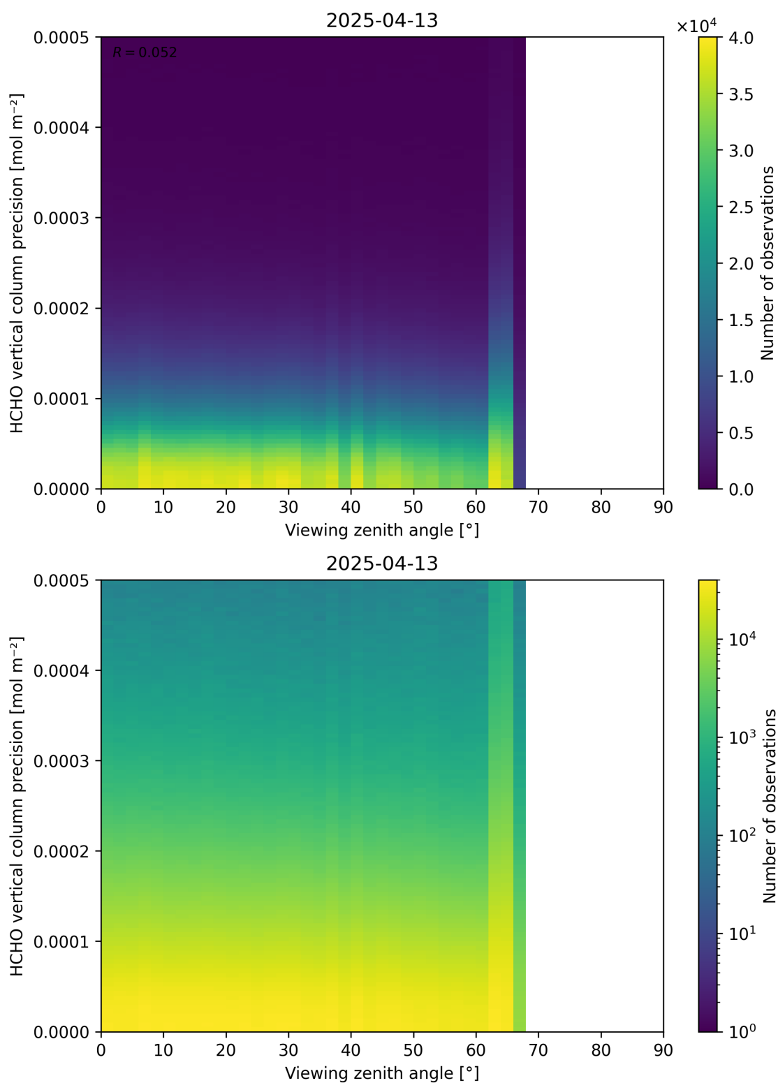
Figure 194: Scatter density plot of “Viewing zenith angle” against “HCHO vertical column precision” for 2025-04-13 to 2025-04-14.
