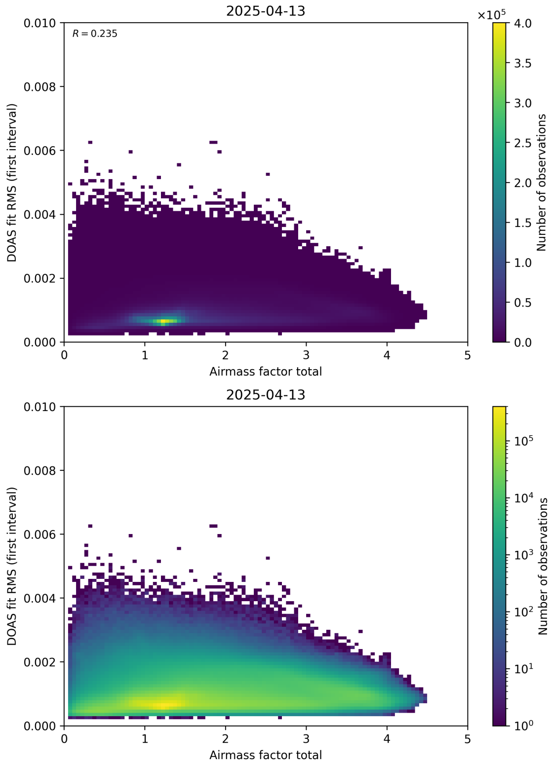
Figure 97: Scatter density plot of “Airmass factor total” against “DOAS fit RMS (first interval)” for 2025-04-13 to 2025-04-14.
