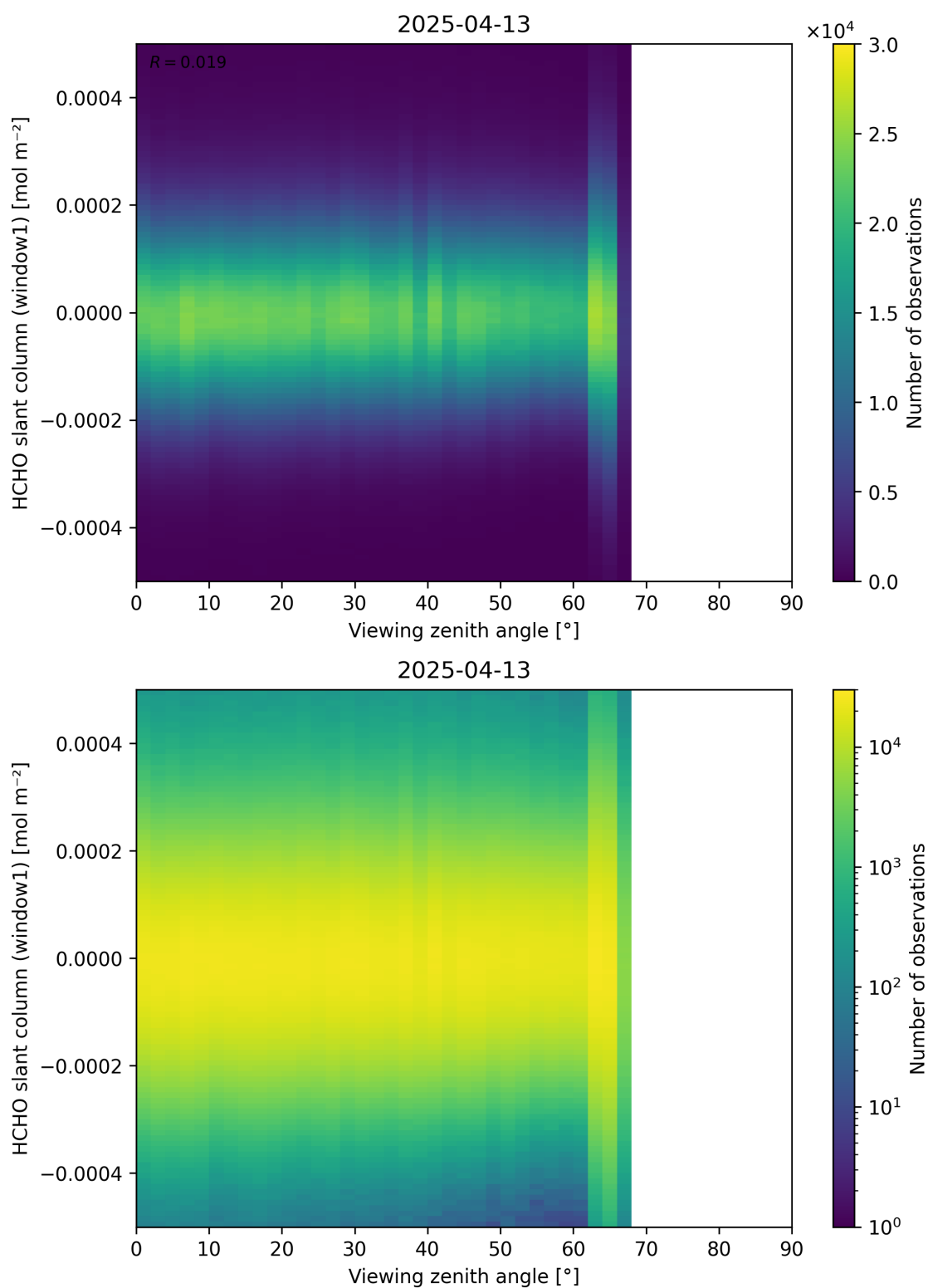
Figure 188: Scatter density plot of “Viewing zenith angle” against “HCHO slant column (window1)” for 2025-04-13 to 2025-04-14.
