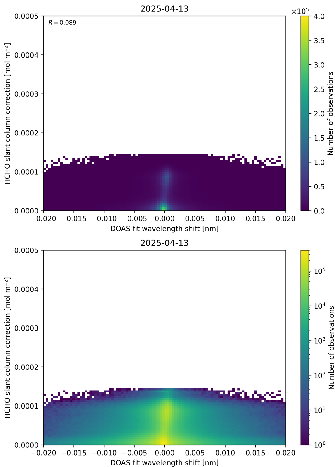
Figure 67: Scatter density plot of “DOAS fit wavelength shift” against “HCHO slant column correction” for 2025-04-13 to 2025-04-14.
