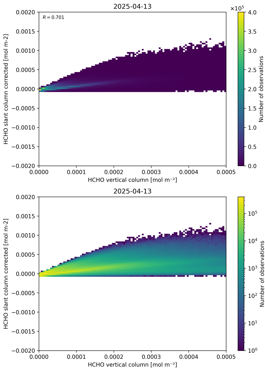
Figure 127: Scatter density plot of “HCHO vertical column” against “HCHO slant column corrected” for 2025-04-13 to 2025-04-14.
