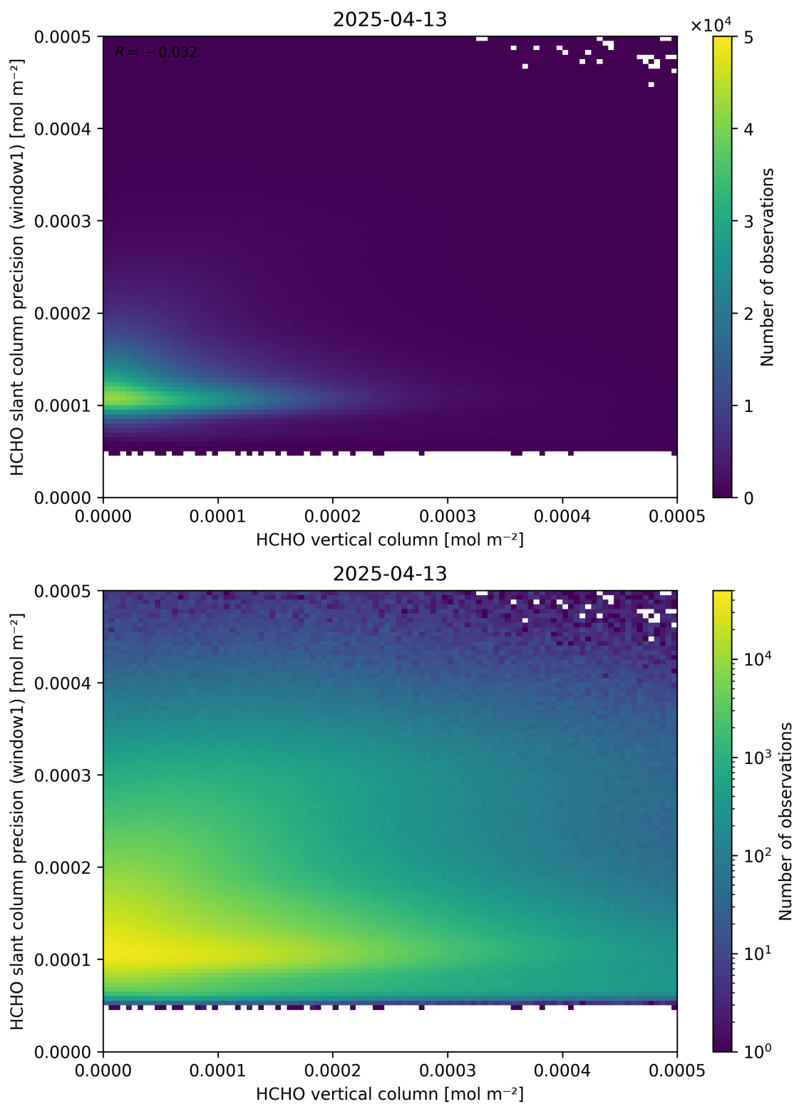
Figure 130: Scatter density plot of “HCHO vertical column” against “HCHO slant column precision (window1)” for 2025-04-13 to 2025-04-14.
