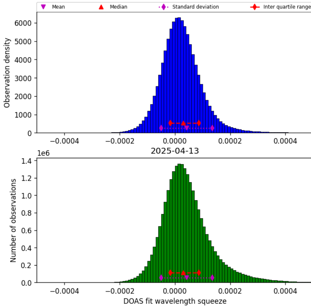
Figure 45: Histogram of “DOAS fit wavelength squeeze” for 2025-04-13 to 2025-04-14
