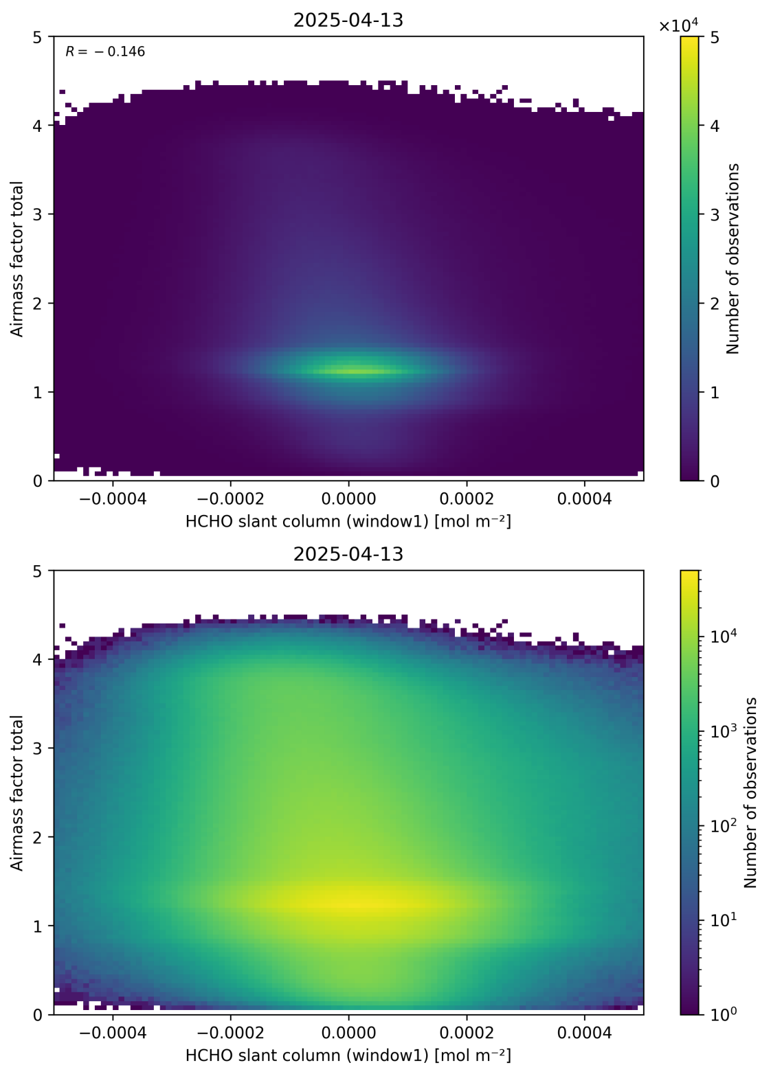
Figure 85: Scatter density plot of “HCHO slant column (window1)” against “Airmass factor total” for 2025-04-13 to 2025-04-14.
