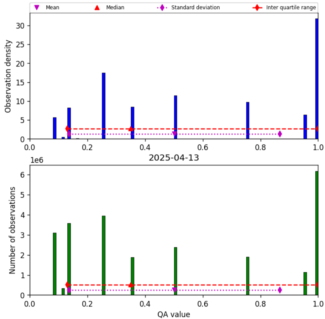
Figure 34: Histogram of “QA value” for 2025-04-13 to 2025-04-14
