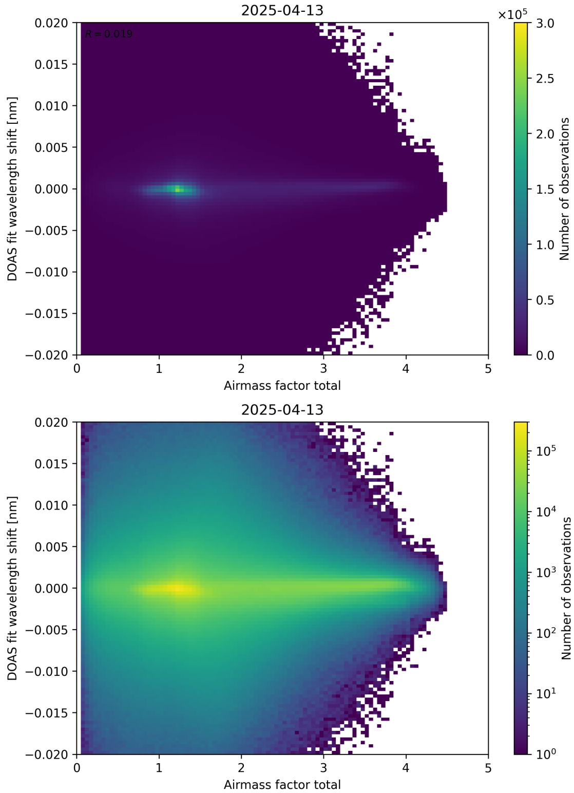
Figure 98: Scatter density plot of “Airmass factor total” against “DOAS fit wavelength shift” for 2025-04-13 to 2025-04-14.
