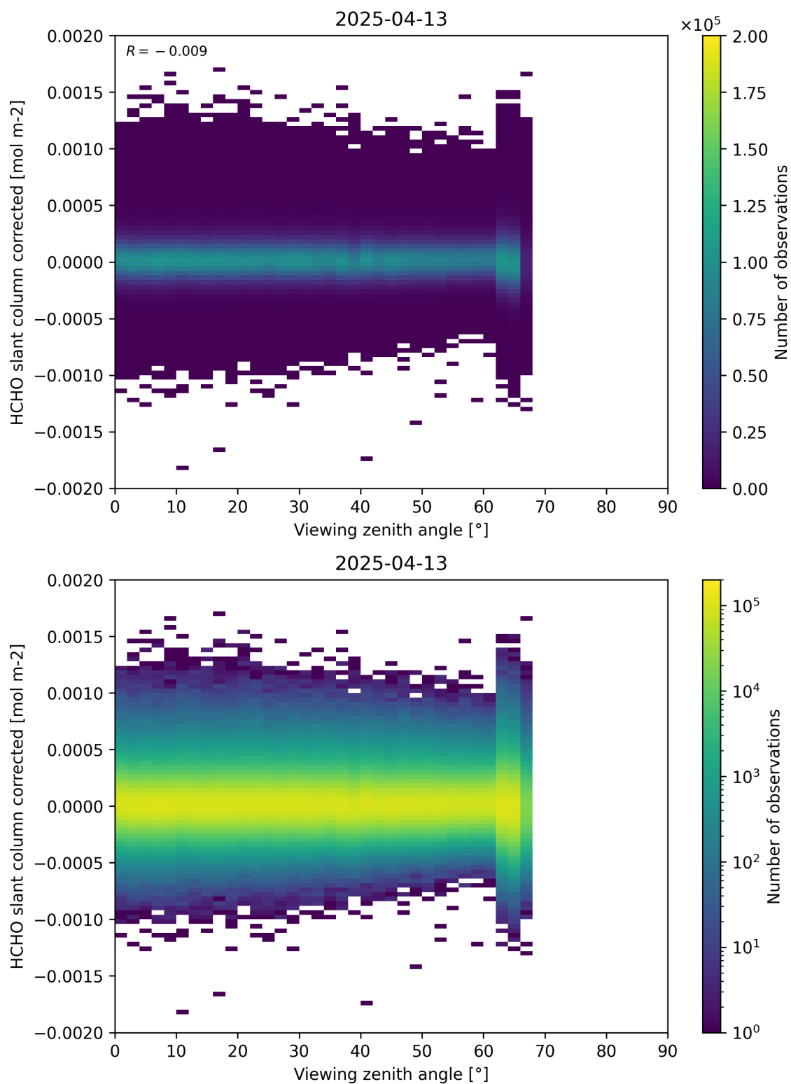
Figure 186: Scatter density plot of “Viewing zenith angle” against “HCHO slant column corrected” for 2025-04-13 to 2025-04-14.
