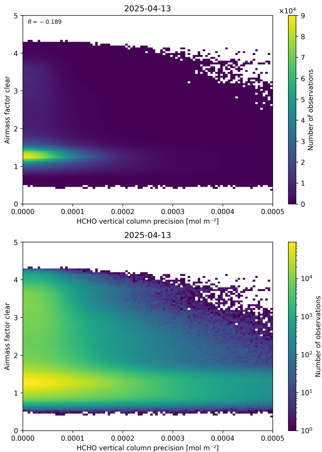
Figure 139: Scatter density plot of “HCHO vertical column precision” against “Airmass factor clear” for 2025-04-13 to 2025-04-14.
