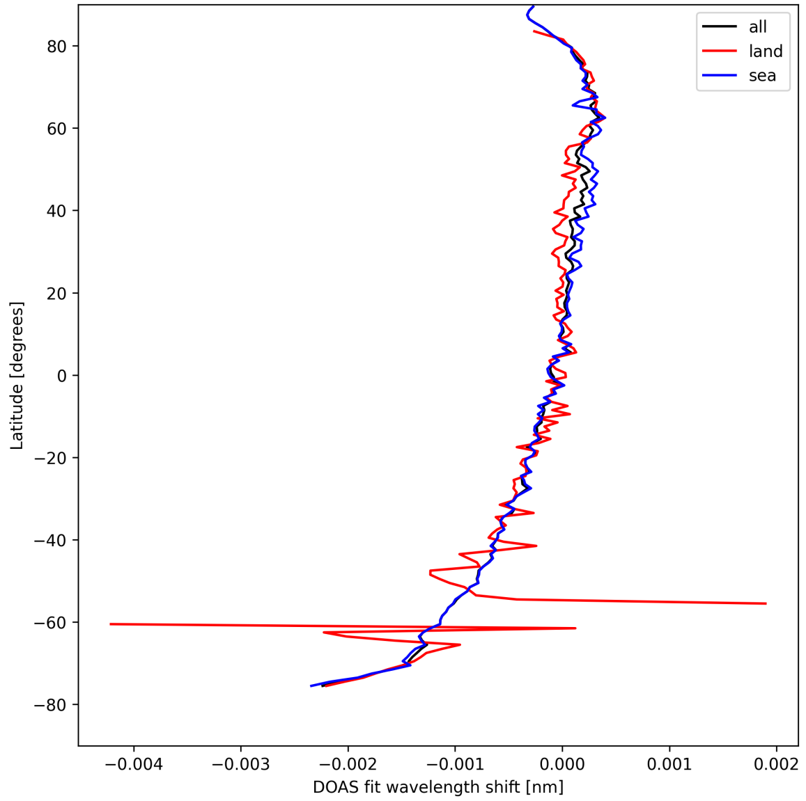
Figure 30: Zonal average of “DOAS fit wavelength shift” for 2025-04-13 to 2025-04-14.
