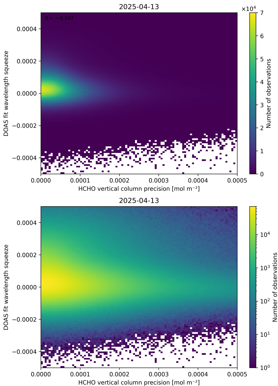
Figure 138: Scatter density plot of “HCHO vertical column precision” against “DOAS fit wavelength squeeze” for 2025-04-13 to 2025-04-14.
