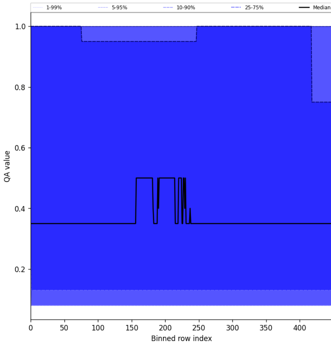
Figure 48: Along track statistics of “QA value” for 2025-04-13 to 2025-04-14
