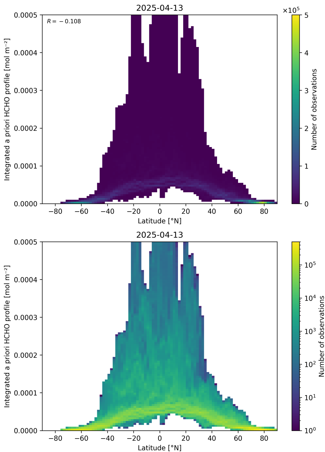
Figure 166: Scatter density plot of “Latitude” against “Integrated a priori HCHO profile” for 2025-04-13 to 2025-04-14.
