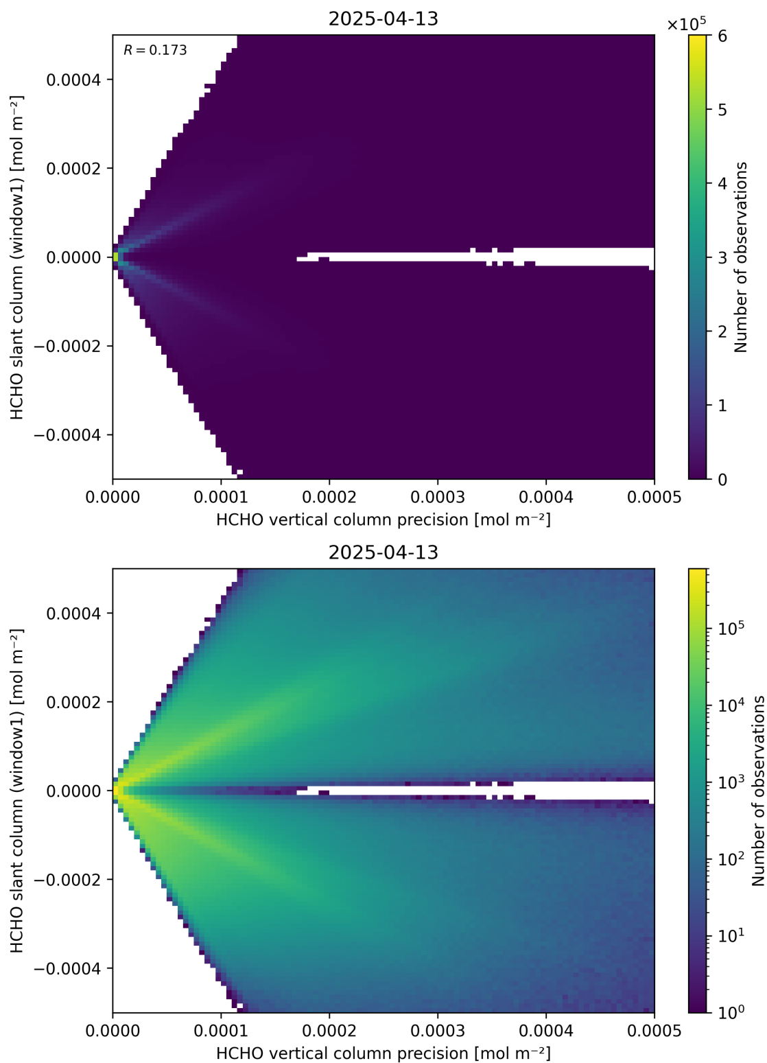
Figure 142: Scatter density plot of “HCHO vertical column precision” against “HCHO slant column (window1)” for 2025-04-13 to 2025-04-14.
