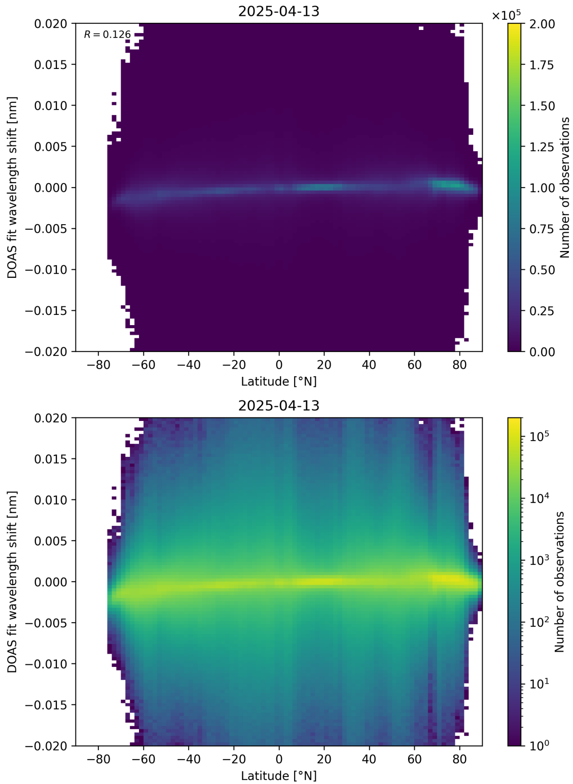
Figure 154: Scatter density plot of “Latitude” against “DOAS fit wavelength shift” for 2025-04-13 to 2025-04-14.
