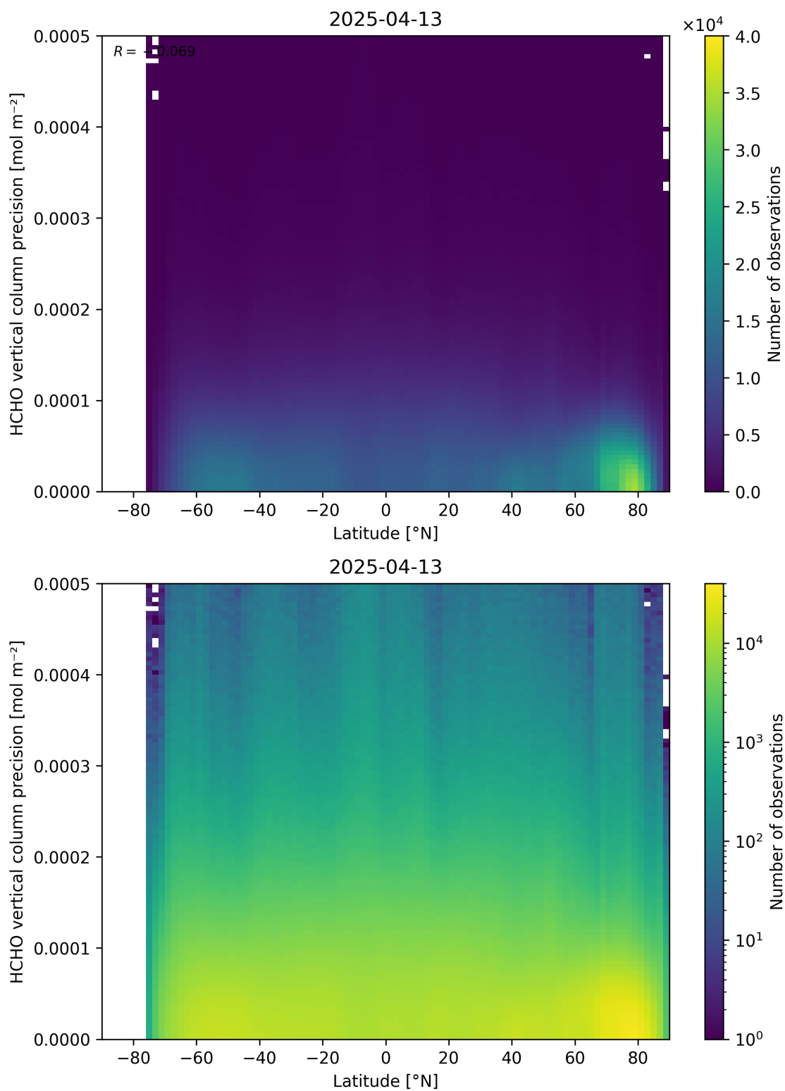
Figure 165: Scatter density plot of “Latitude” against “HCHO vertical column precision” for 2025-04-13 to 2025-04-14.
