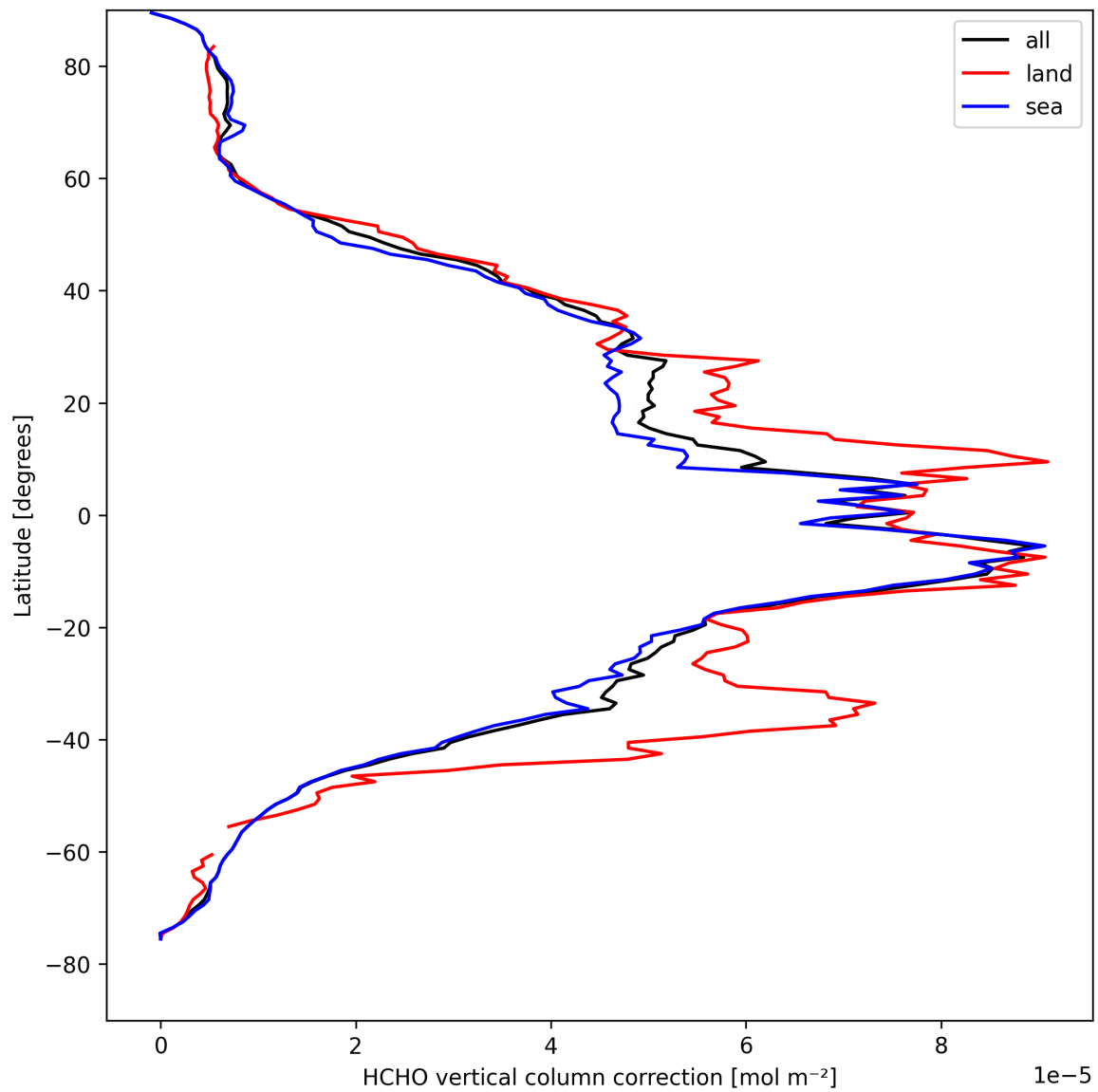
Figure 23: Zonal average of “HCHO vertical column correction” for 2025-04-13 to 2025-04-14.
