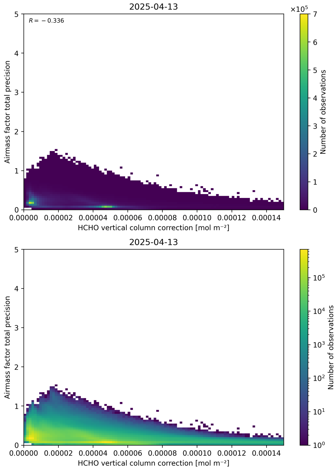
Figure 121: Scatter density plot of “HCHO vertical column correction” against “Airmass factor total precision” for 2025-04-13 to 2025-04-14.
