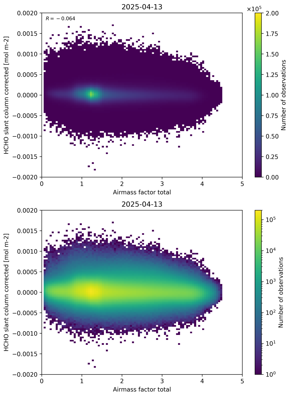
Figure 101: Scatter density plot of “Airmass factor total” against “HCHO slant column corrected” for 2025-04-13 to 2025-04-14.
