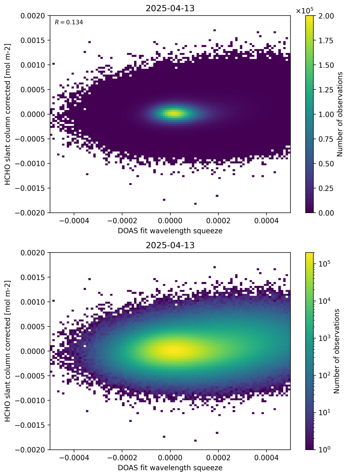
Figure 69: Scatter density plot of “DOAS fit wavelength squeeze” against “HCHO slant column corrected” for 2025-04-13 to 2025-04-14.
