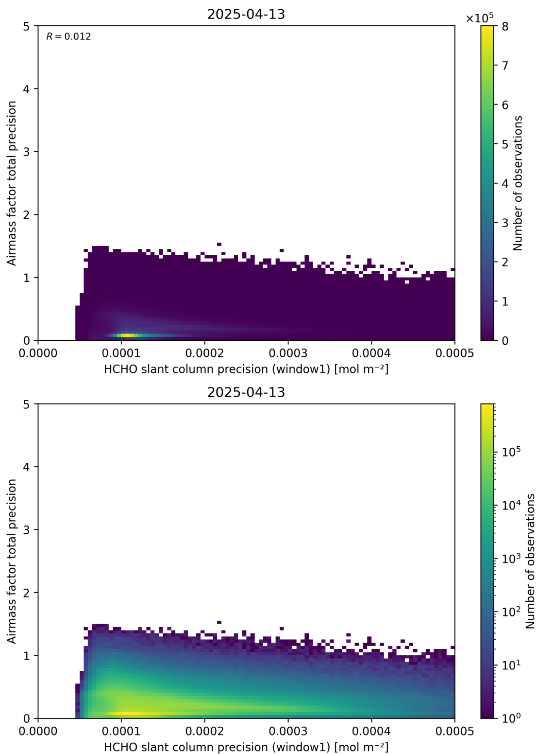
Figure 95: Scatter density plot of “HCHO slant column precision (window1)” against “Airmass factor total precision” for 2025-04-13 to 2025-04-14.
