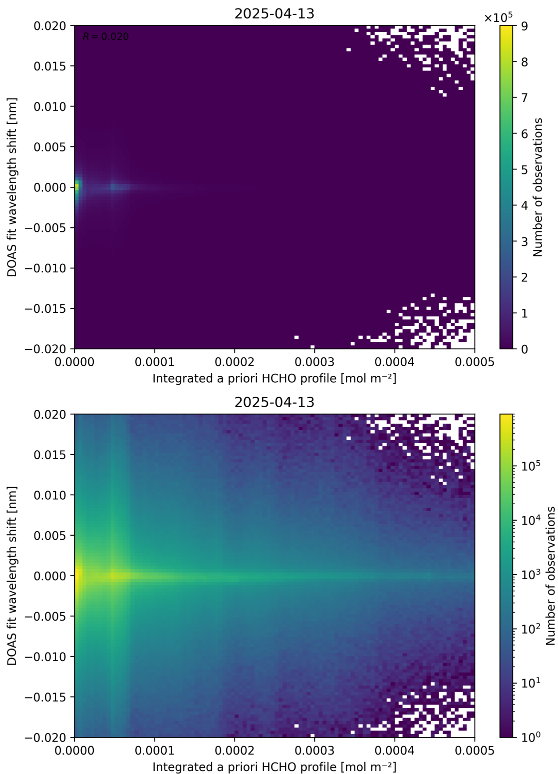
Figure 149: Scatter density plot of “Integrated a priori HCHO profile” against “DOAS fit wavelength shift” for 2025-04-13 to 2025-04-14.
