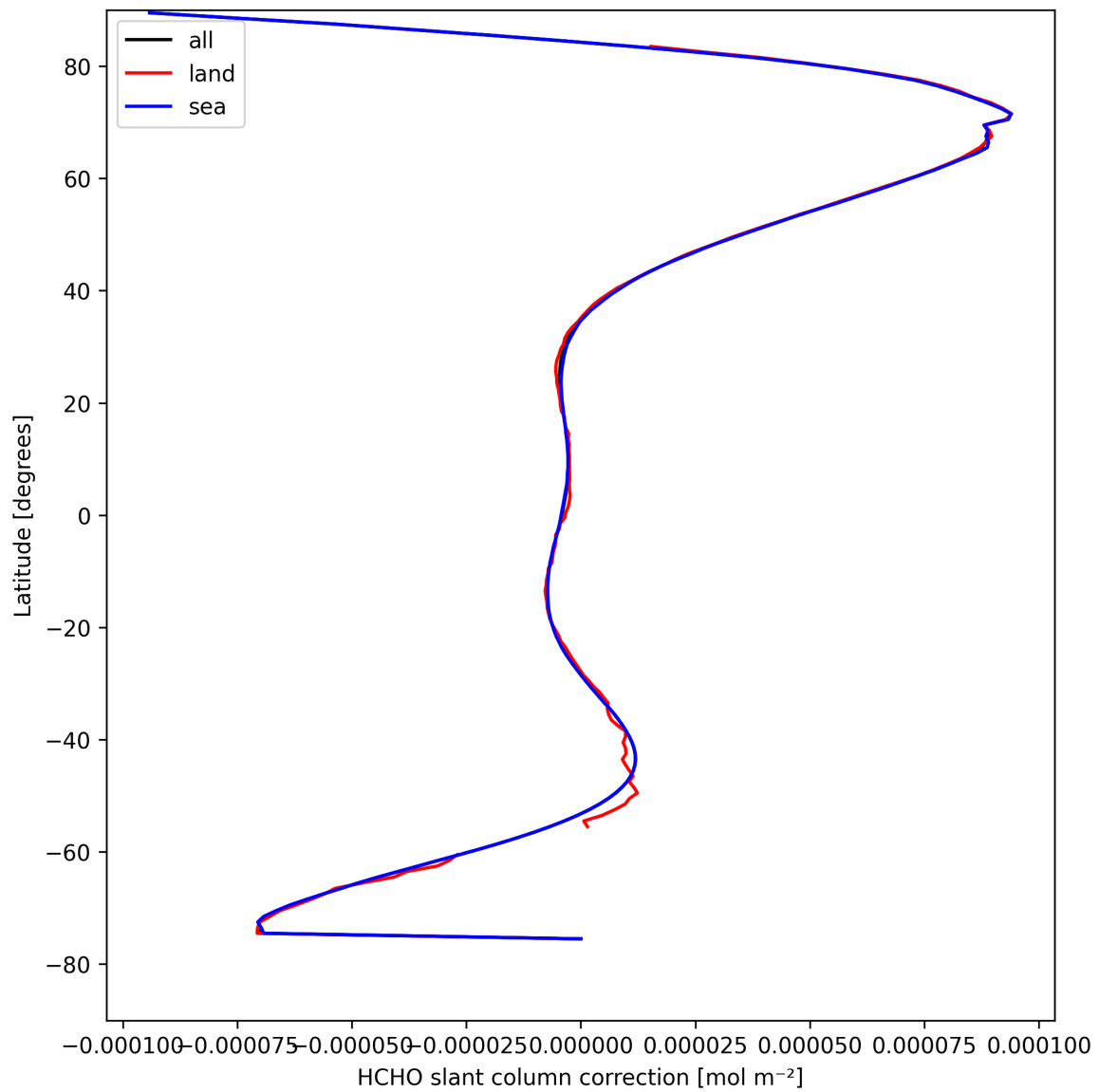
Figure 33: Zonal average of “HCHO slant column correction” for 2025-04-13 to 2025-04-14.
