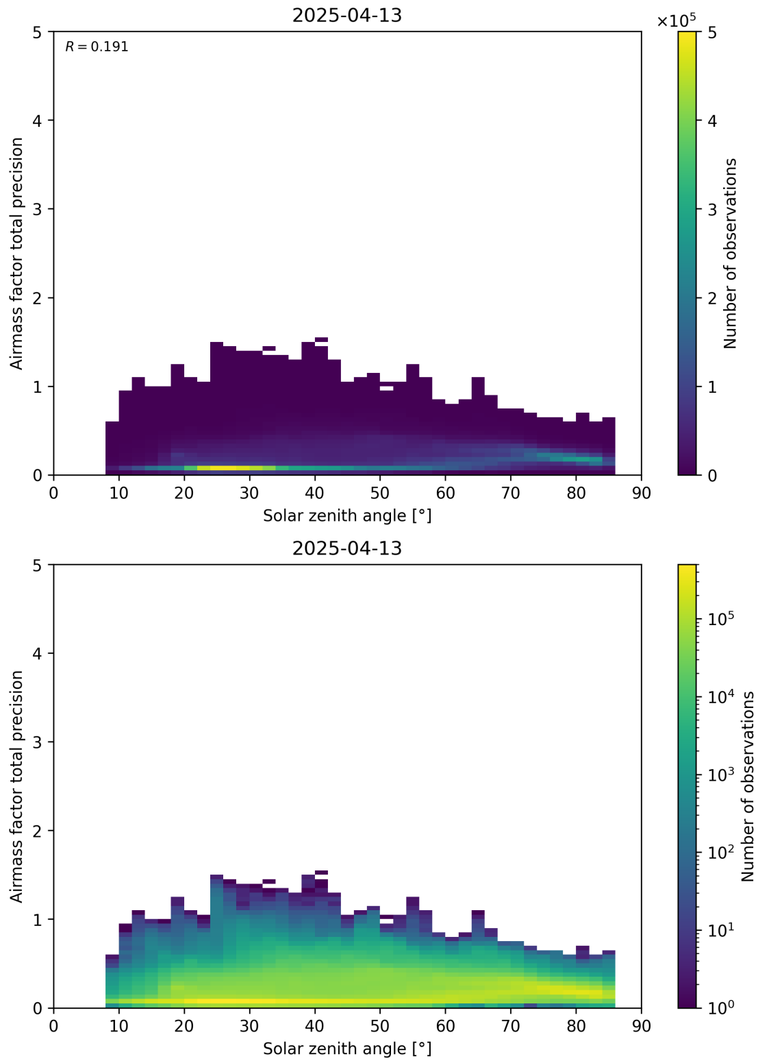
Figure 176: Scatter density plot of “Solar zenith angle” against “Airmass factor total precision” for 2025-04-13 to 2025-04-14.
