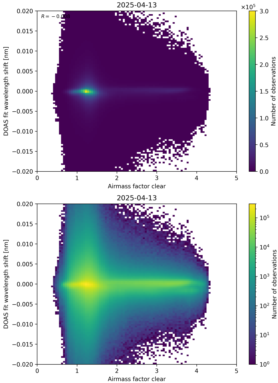
Figure 72: Scatter density plot of “Airmass factor clear” against “DOAS fit wavelength shift” for 2025-04-13 to 2025-04-14.
