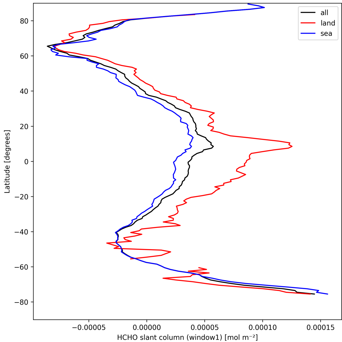
Figure 24: Zonal average of “HCHO slant column (window1)” for 2025-04-13 to 2025-04-14.
