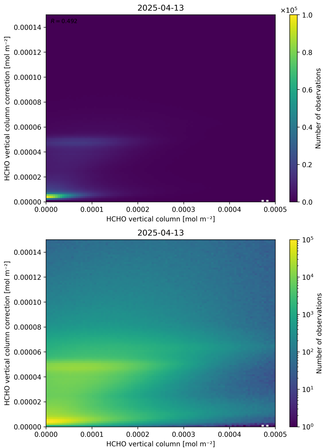
Figure 133: Scatter density plot of “HCHO vertical column” against “HCHO vertical column correction” for 2025-04-13 to 2025-04-14.
