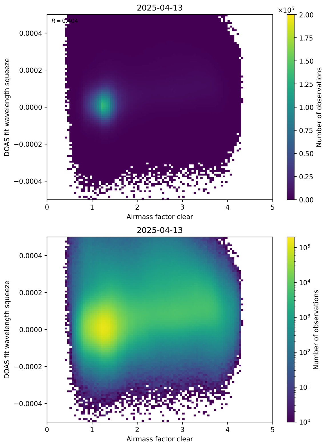
Figure 73: Scatter density plot of “Airmass factor clear” against “DOAS fit wavelength squeeze” for 2025-04-13 to 2025-04-14.
