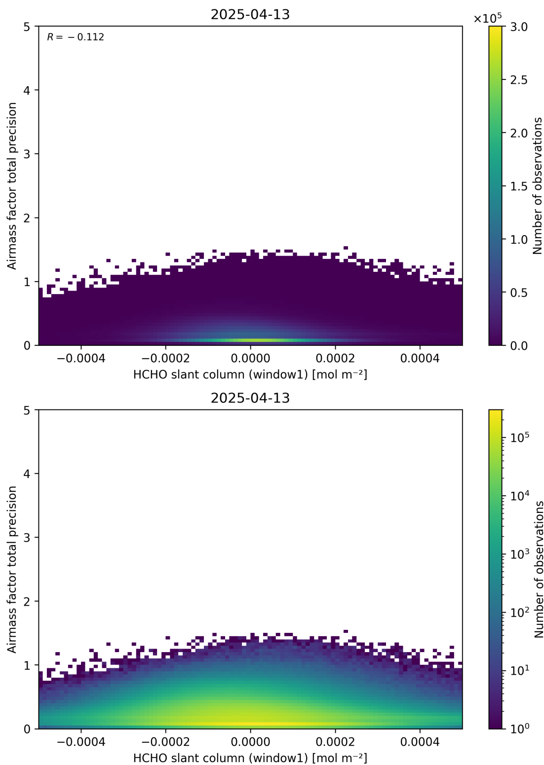
Figure 86: Scatter density plot of “HCHO slant column (window1)” against “Airmass factor total precision” for 2025-04-13 to 2025-04-14.
