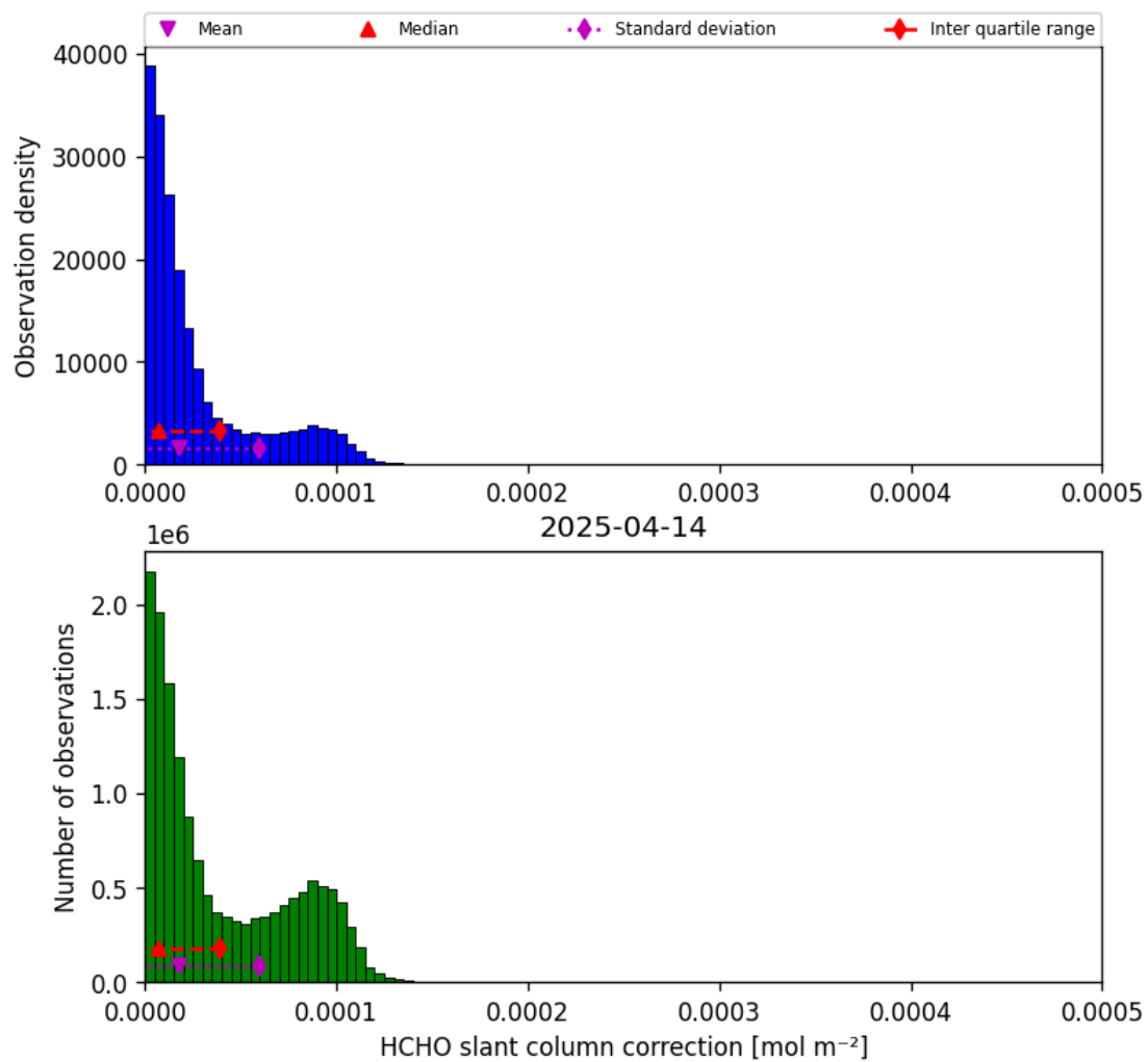
Figure 47: Histogram of “HCHO slant column correction” for 2025-04-13 to 2025-04-15
