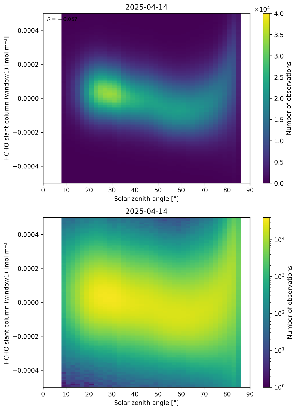
Figure 173: Scatter density plot of “Solar zenith angle” against “HCHO slant column (window1)” for 2025-04-13 to 2025-04-15.
