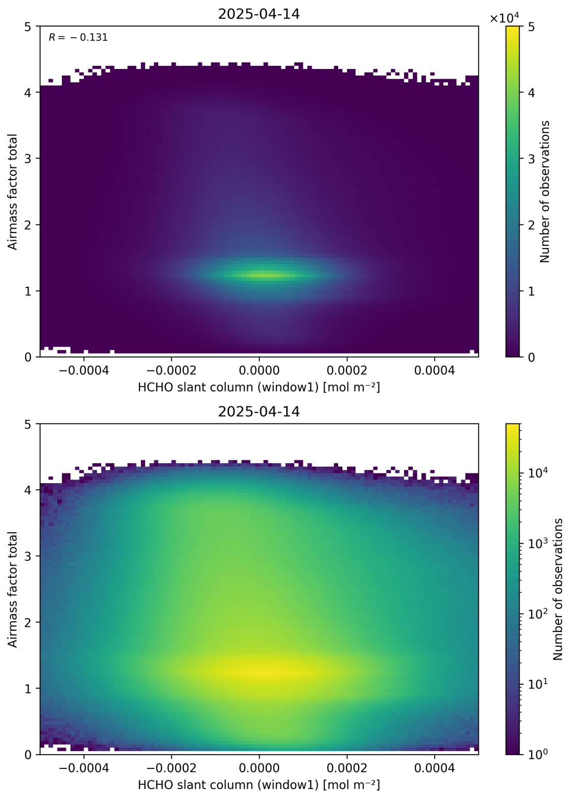
Figure 85: Scatter density plot of “HCHO slant column (window1)” against “Airmass factor total” for 2025-04-13 to 2025-04-15.
