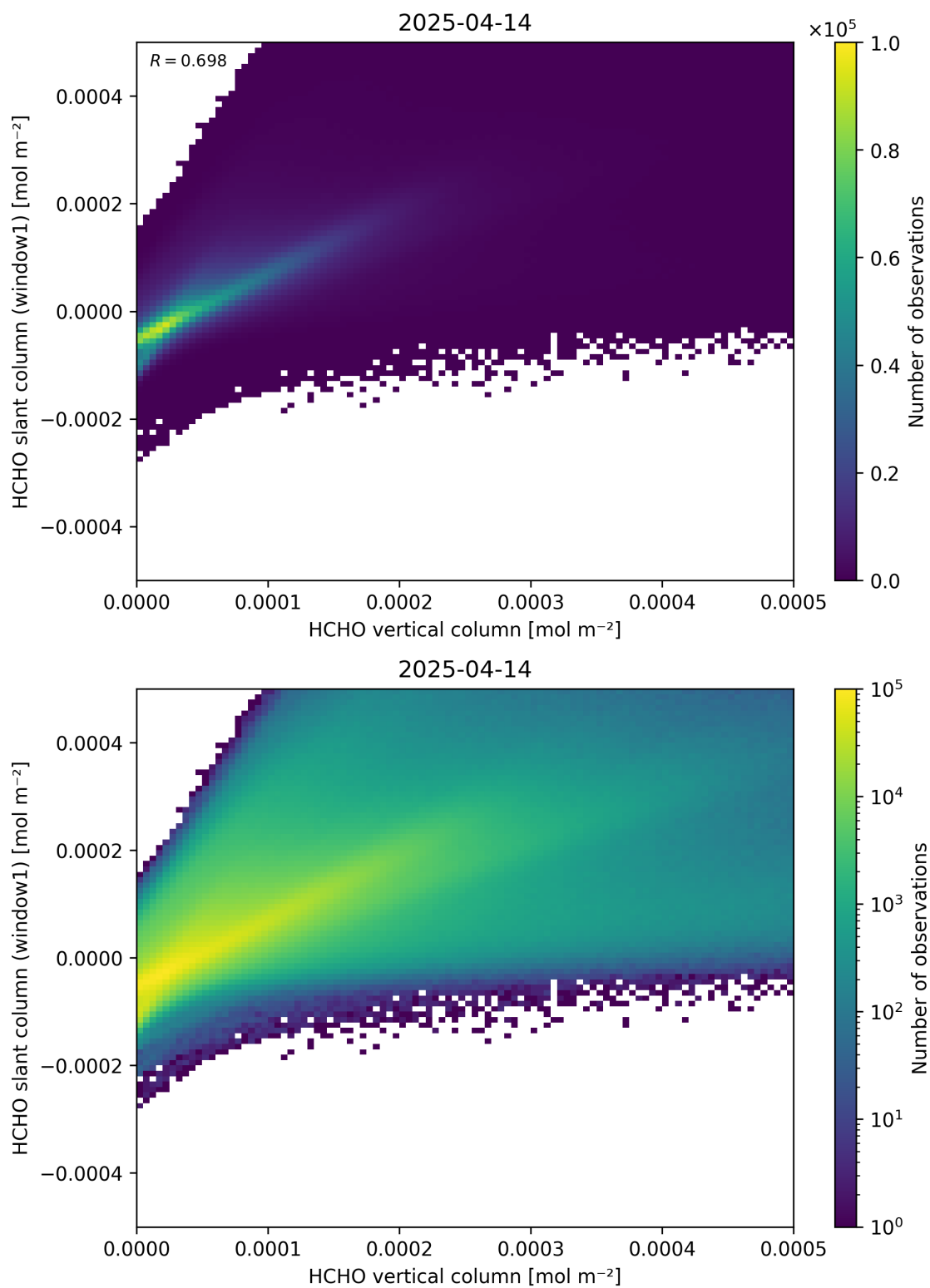
Figure 129: Scatter density plot of “HCHO vertical column” against “HCHO slant column (window1)” for 2025-04-13 to 2025-04-15.
