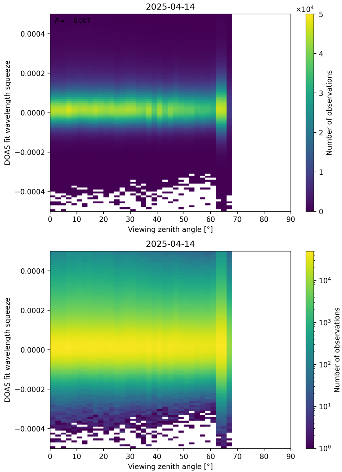
Figure 184: Scatter density plot of “Viewing zenith angle” against “DOAS fit wavelength squeeze” for 2025-04-13 to 2025-04-15.
