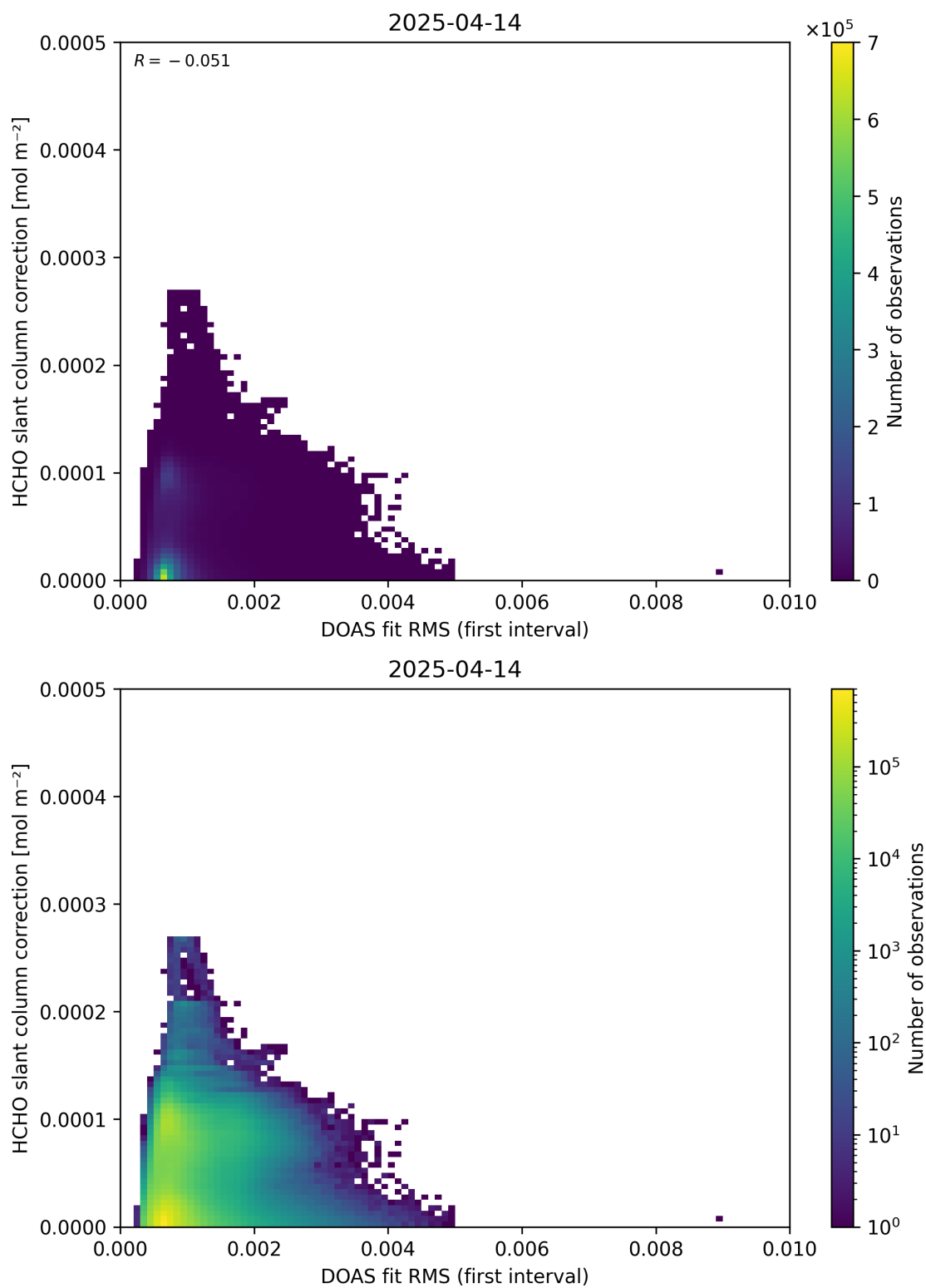
Figure 63: Scatter density plot of “DOAS fit RMS (first interval)” against “HCHO slant column correction” for 2025-04-13 to 2025-04-15.
