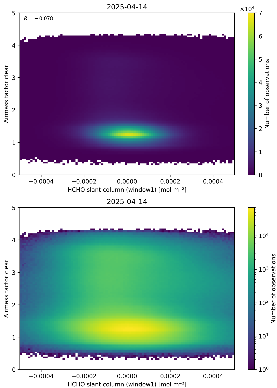
Figure 81: Scatter density plot of “HCHO slant column (window1)” against “Airmass factor clear” for 2025-04-13 to 2025-04-15.
