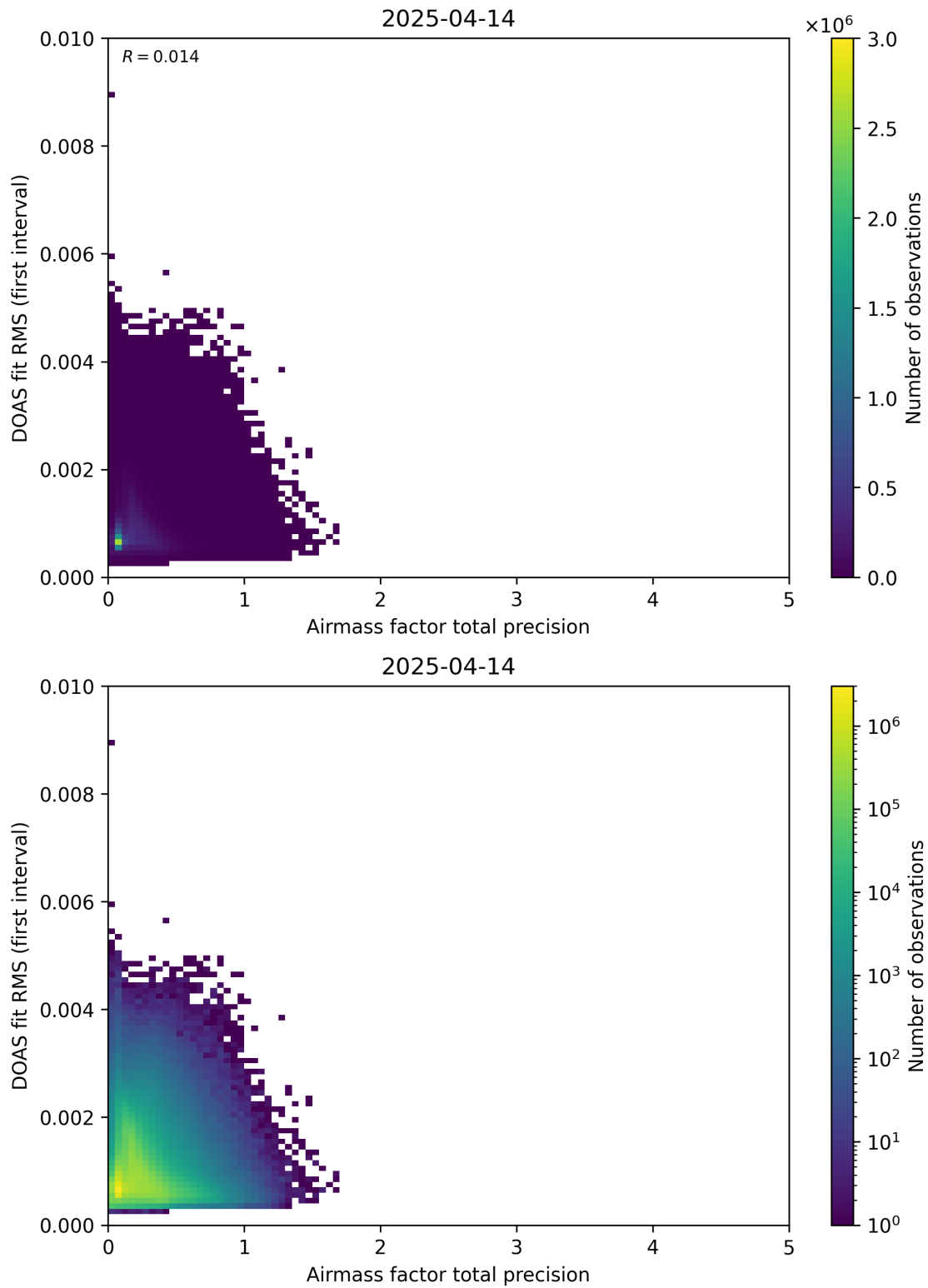
Figure 105: Scatter density plot of “Airmass factor total precision” against “DOAS fit RMS (first interval)” for 2025-04-13 to 2025-04-15.
