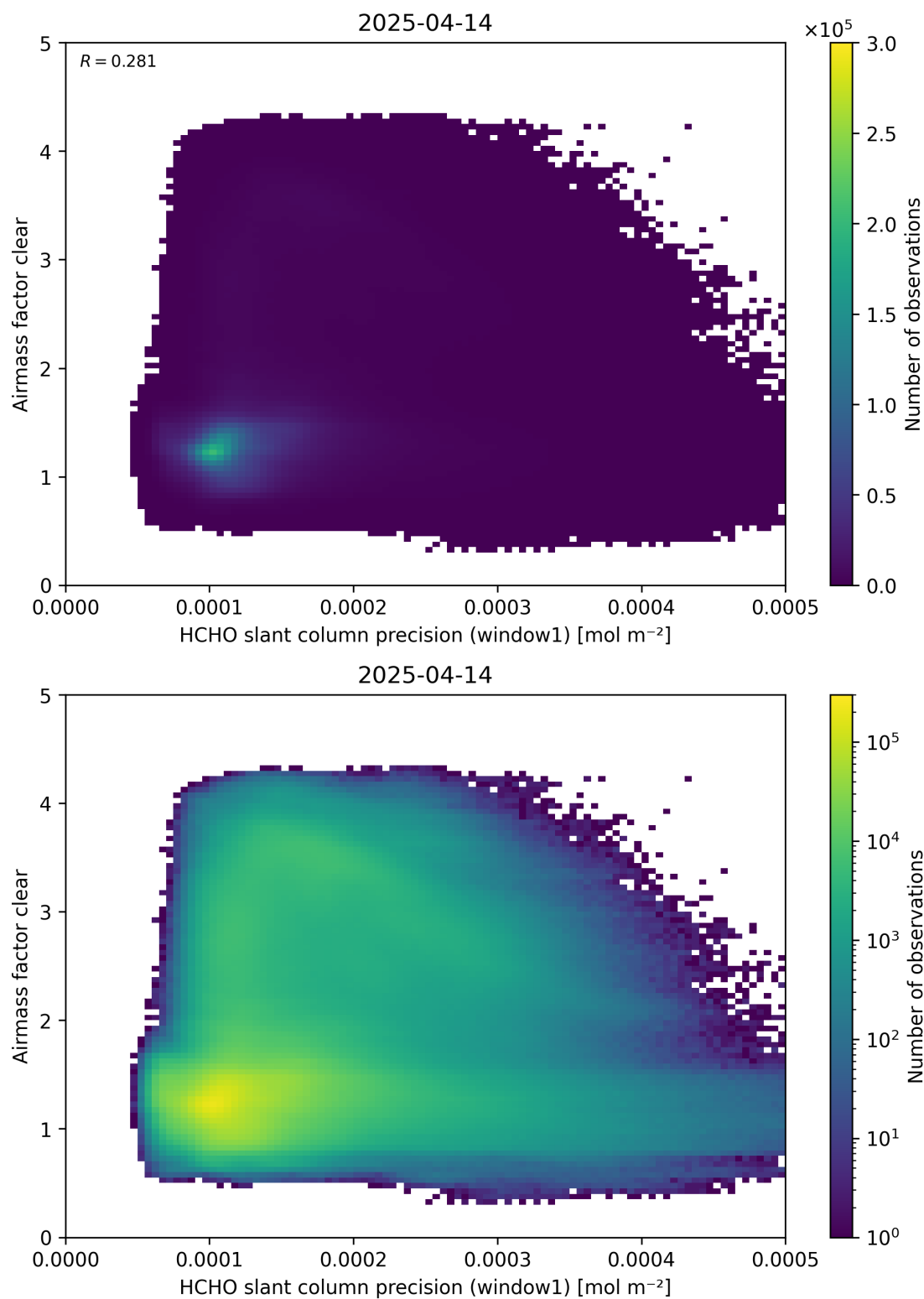
Figure 91: Scatter density plot of “HCHO slant column precision (window1)” against “Airmass factor clear” for 2025-04-13 to 2025-04-15.
