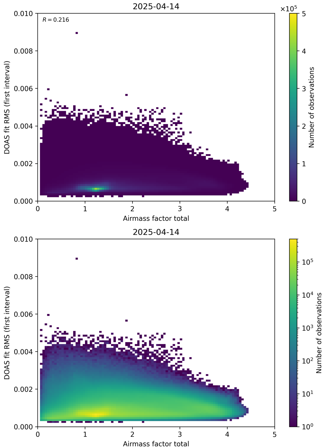
Figure 97: Scatter density plot of “Airmass factor total” against “DOAS fit RMS (first interval)” for 2025-04-13 to 2025-04-15.
