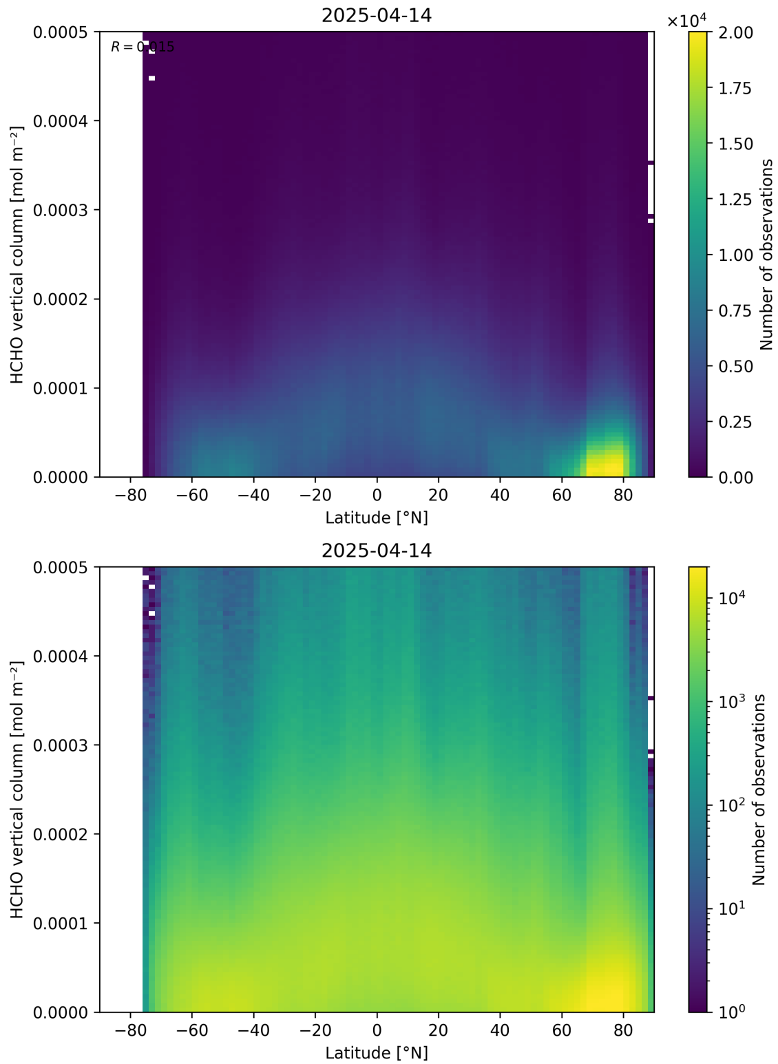
Figure 163: Scatter density plot of “Latitude” against “HCHO vertical column” for 2025-04-13 to 2025-04-15.
