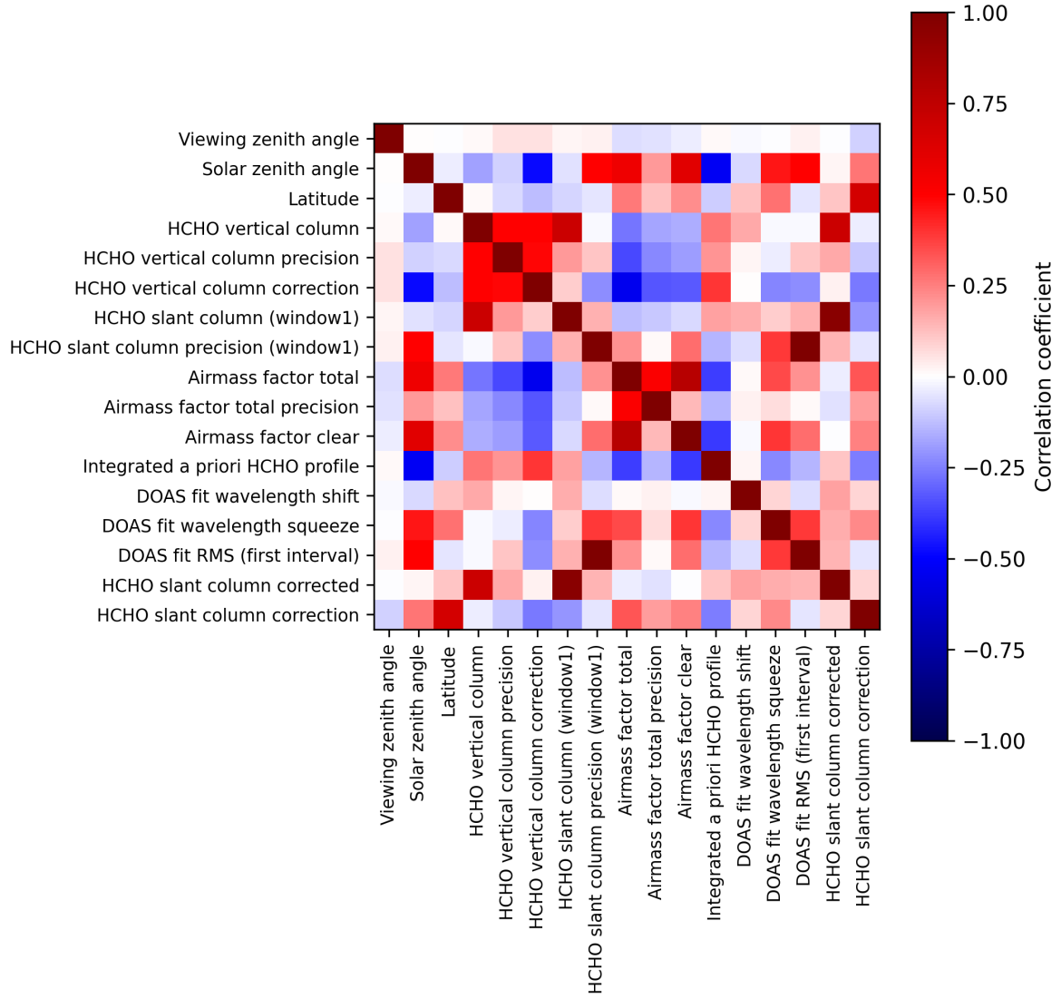
Figure 2: Map of correlation matrix for 2025-04-13 to 2025-04-15.
