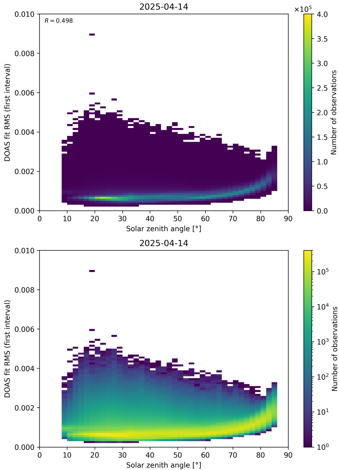
Figure 167: Scatter density plot of “Solar zenith angle” against “DOAS fit RMS (first interval)” for 2025-04-13 to 2025-04-15.
