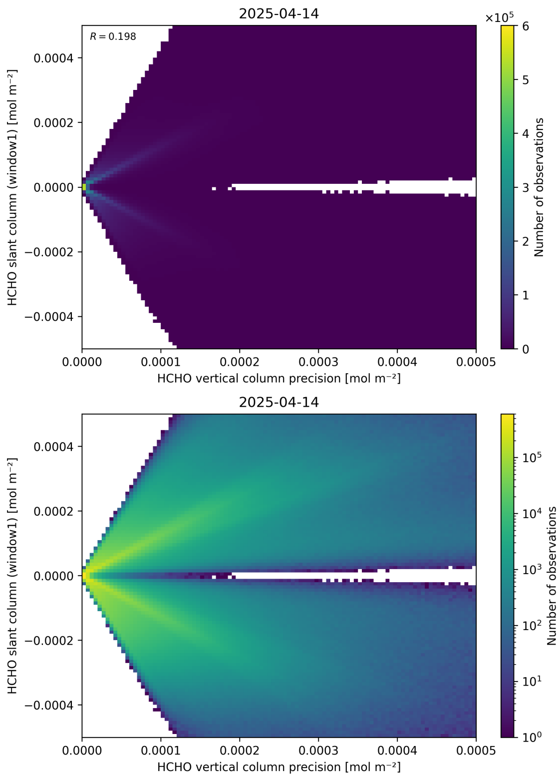
Figure 142: Scatter density plot of “HCHO vertical column precision” against “HCHO slant column (window1)” for 2025-04-13 to 2025-04-15.
