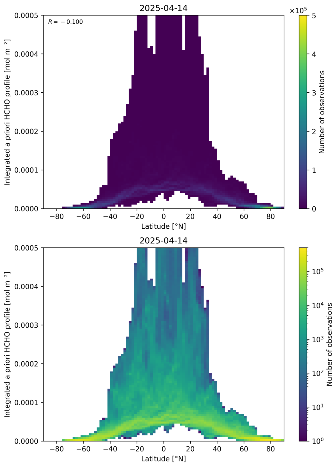
Figure 166: Scatter density plot of “Latitude” against “Integrated a priori HCHO profile” for 2025-04-13 to 2025-04-15.
