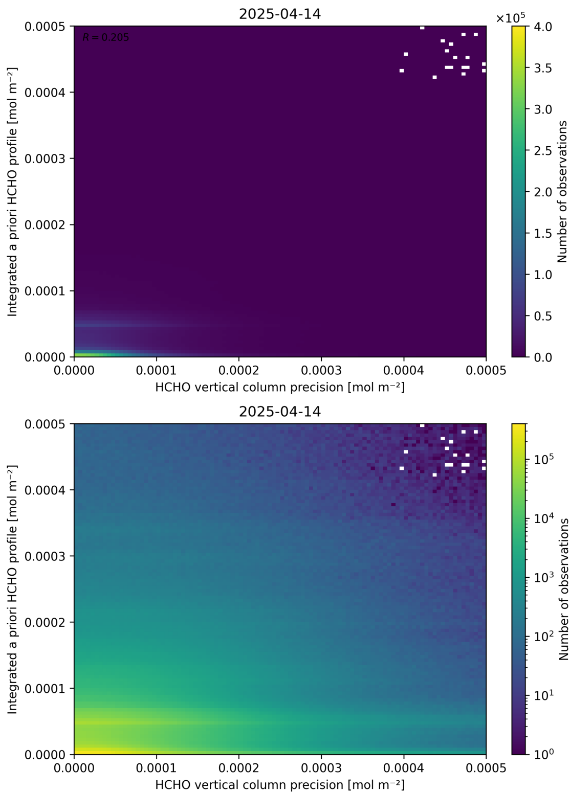
Figure 147: Scatter density plot of “HCHO vertical column precision” against “Integrated a priori HCHO profile” for 2025-04-13 to 2025-04-15.
