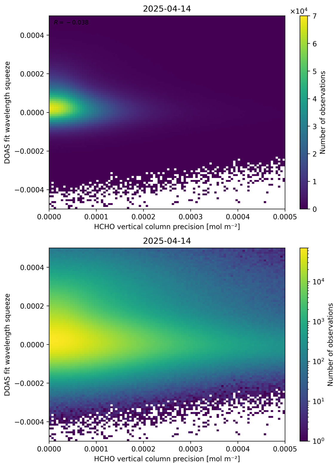
Figure 138: Scatter density plot of “HCHO vertical column precision” against “DOAS fit wavelength squeeze” for 2025-04-13 to 2025-04-15.
