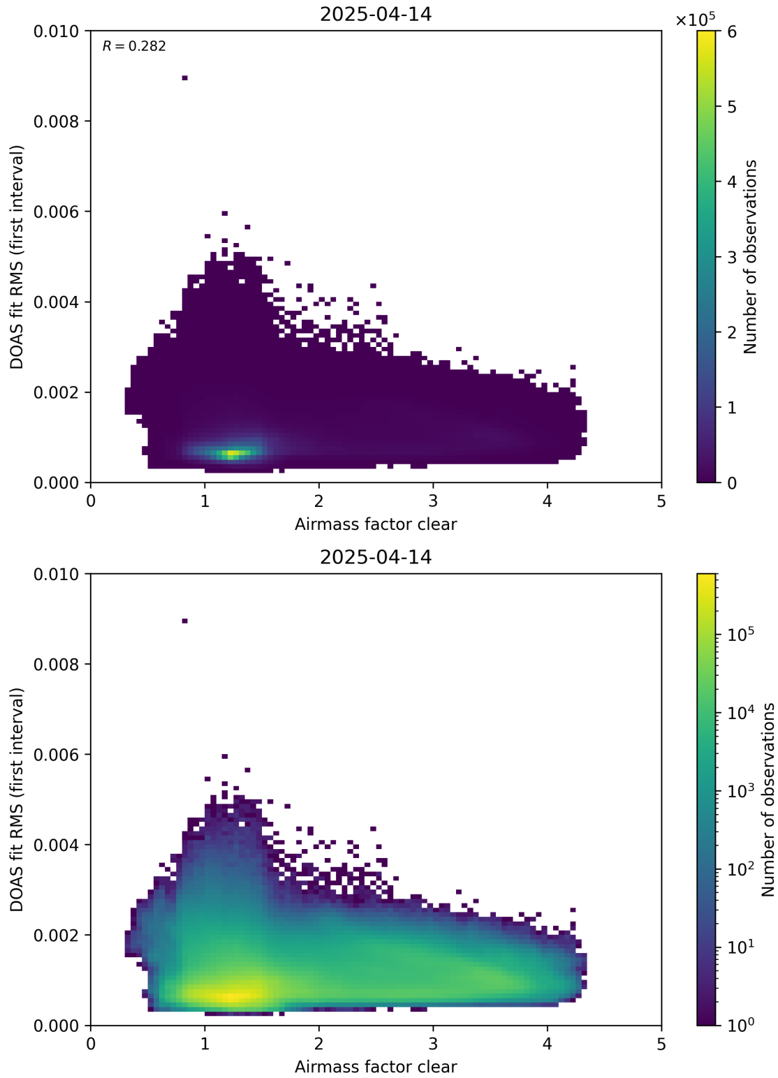
Figure 71: Scatter density plot of “Airmass factor clear” against “DOAS fit RMS (first interval)” for 2025-04-13 to 2025-04-15.
