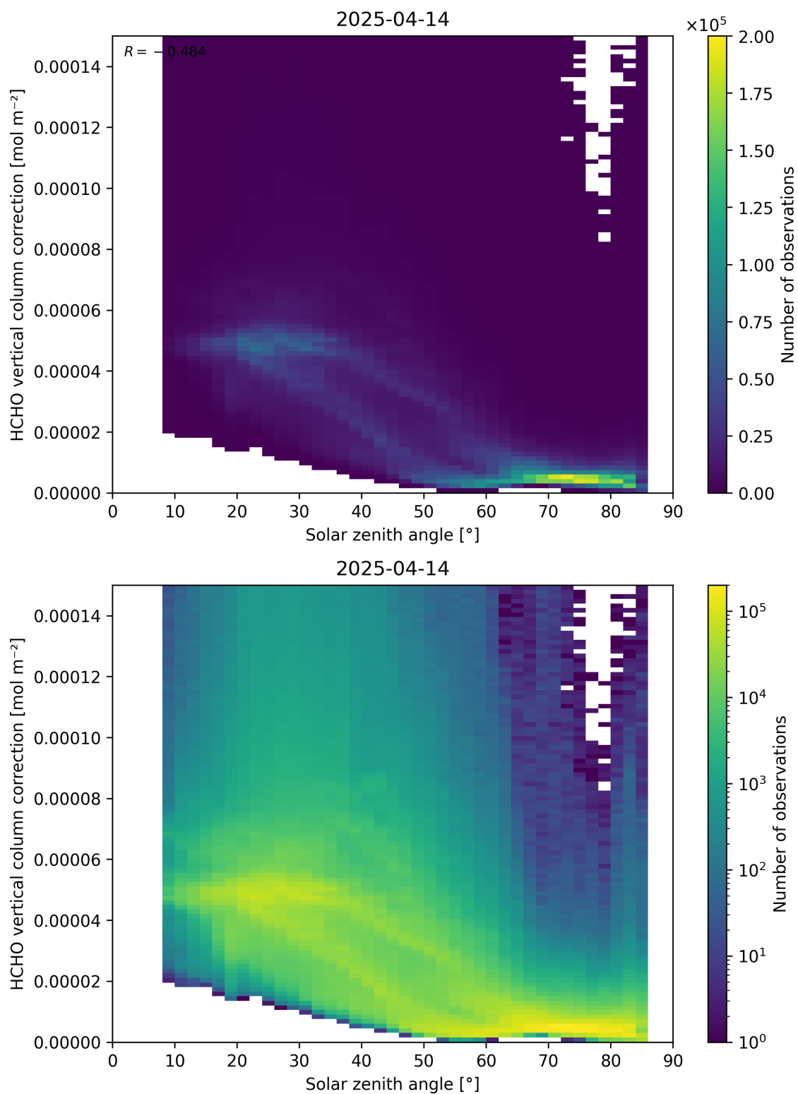
Figure 178: Scatter density plot of “Solar zenith angle” against “HCHO vertical column correction” for 2025-04-13 to 2025-04-15.
