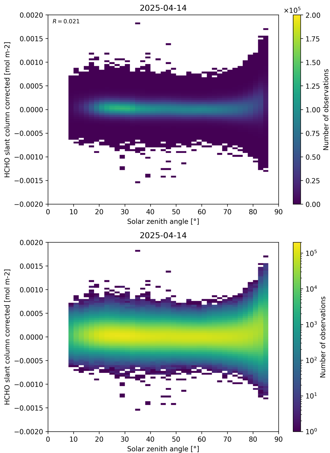
Figure 171: Scatter density plot of “Solar zenith angle” against “HCHO slant column corrected” for 2025-04-13 to 2025-04-15.
