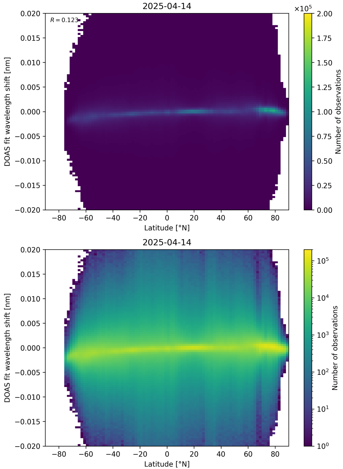
Figure 154: Scatter density plot of “Latitude” against “DOAS fit wavelength shift” for 2025-04-13 to 2025-04-15.
