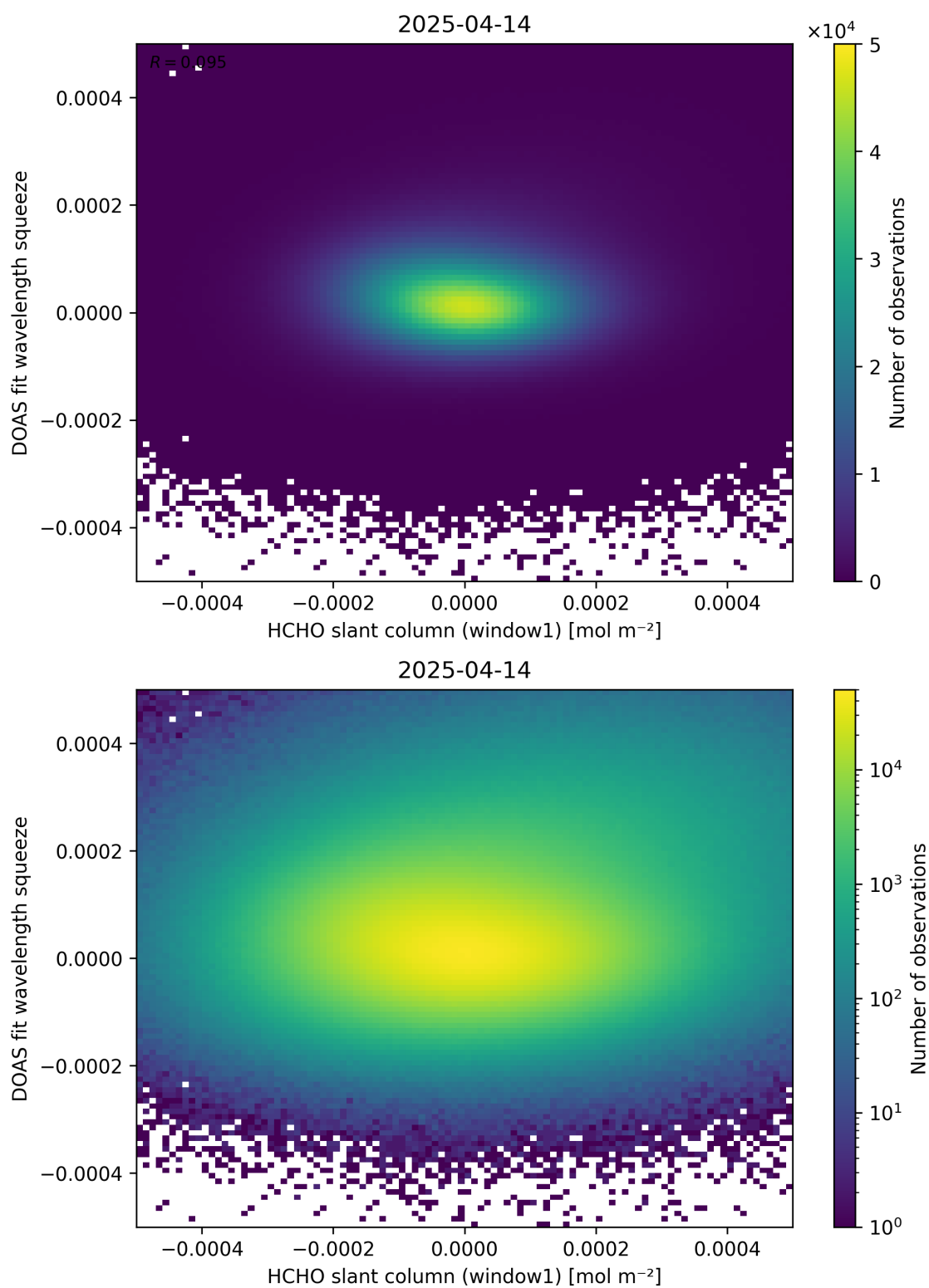
Figure 80: Scatter density plot of “HCHO slant column (window1)” against “DOAS fit wavelength squeeze” for 2025-04-13 to 2025-04-15.
