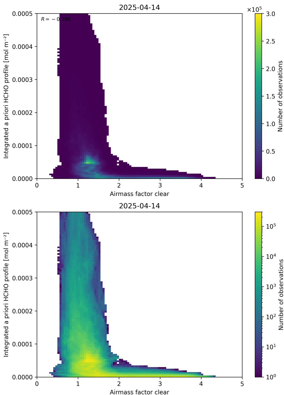
Figure 76: Scatter density plot of “Airmass factor clear” against “Integrated a priori HCHO profile” for 2025-04-13 to 2025-04-15.
