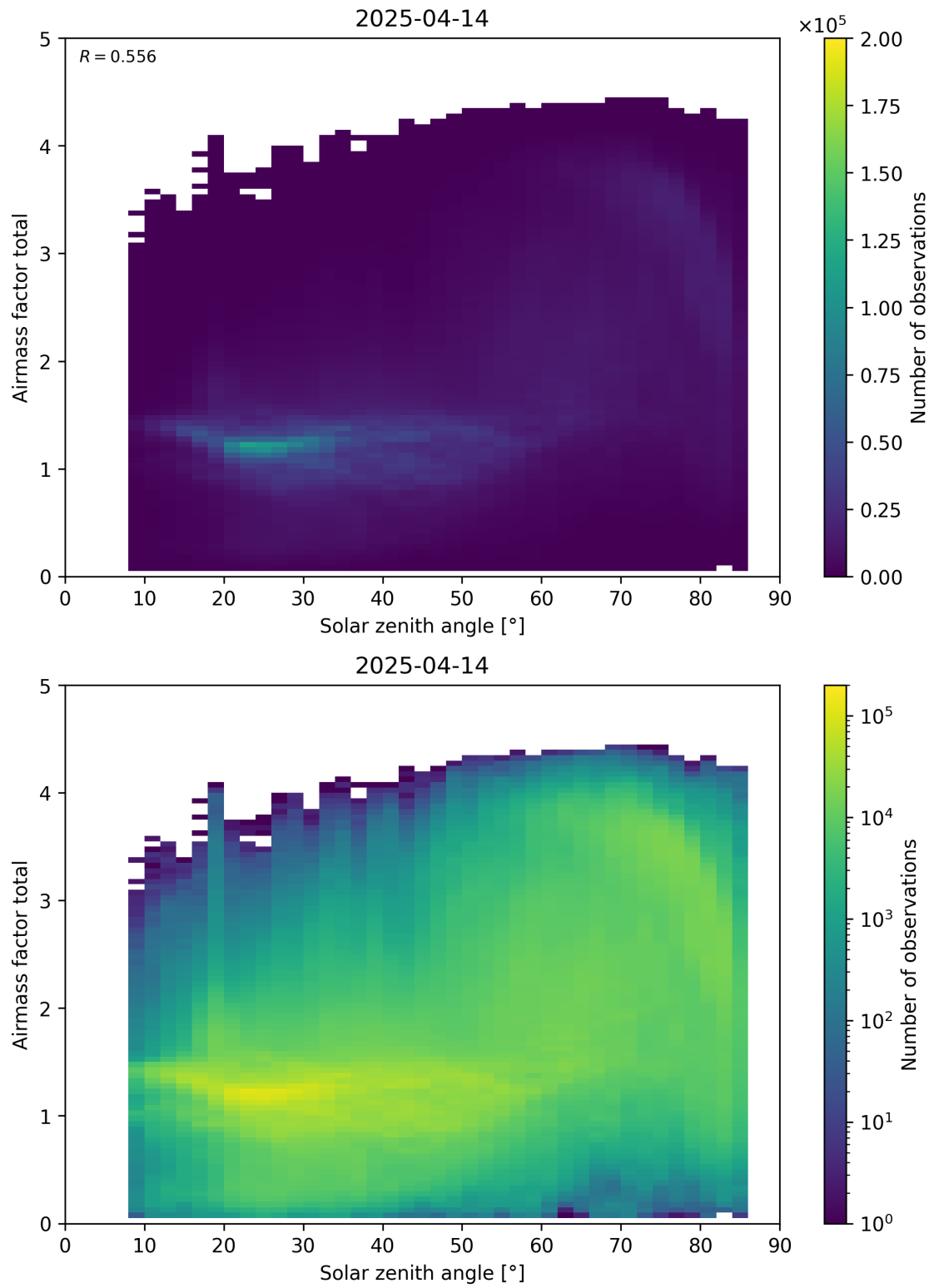
Figure 175: Scatter density plot of “Solar zenith angle” against “Airmass factor total” for 2025-04-13 to 2025-04-15.
