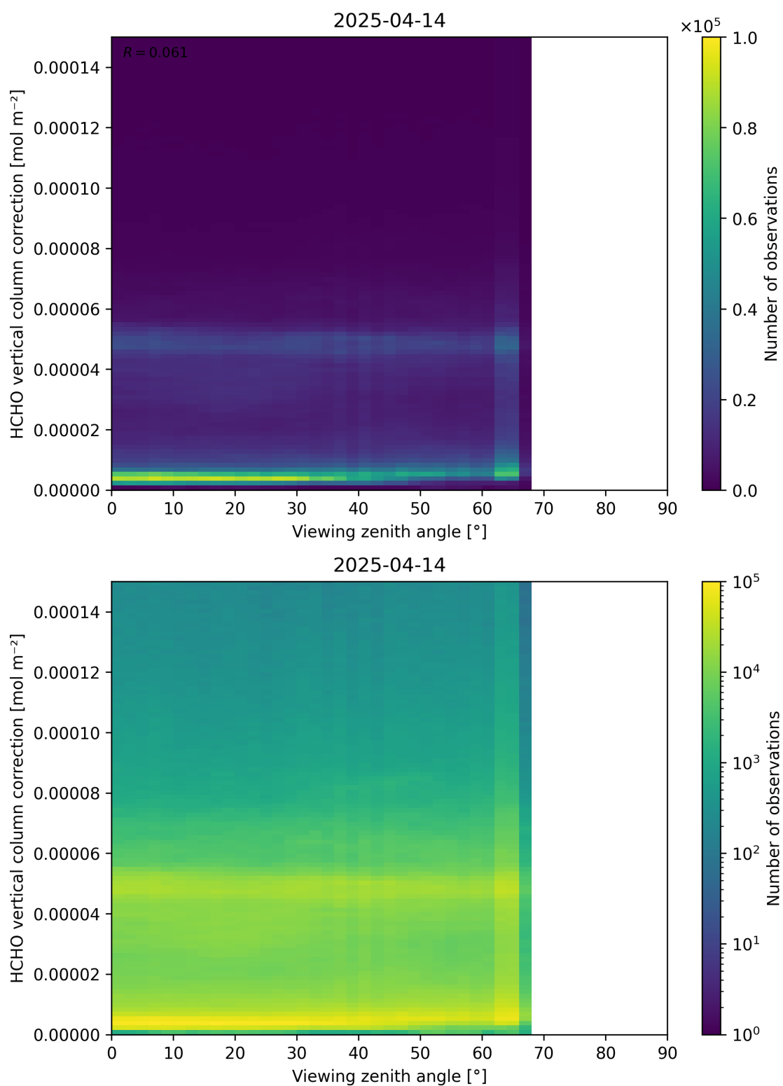
Figure 193: Scatter density plot of “Viewing zenith angle” against “HCHO vertical column correction” for 2025-04-13 to 2025-04-15.
