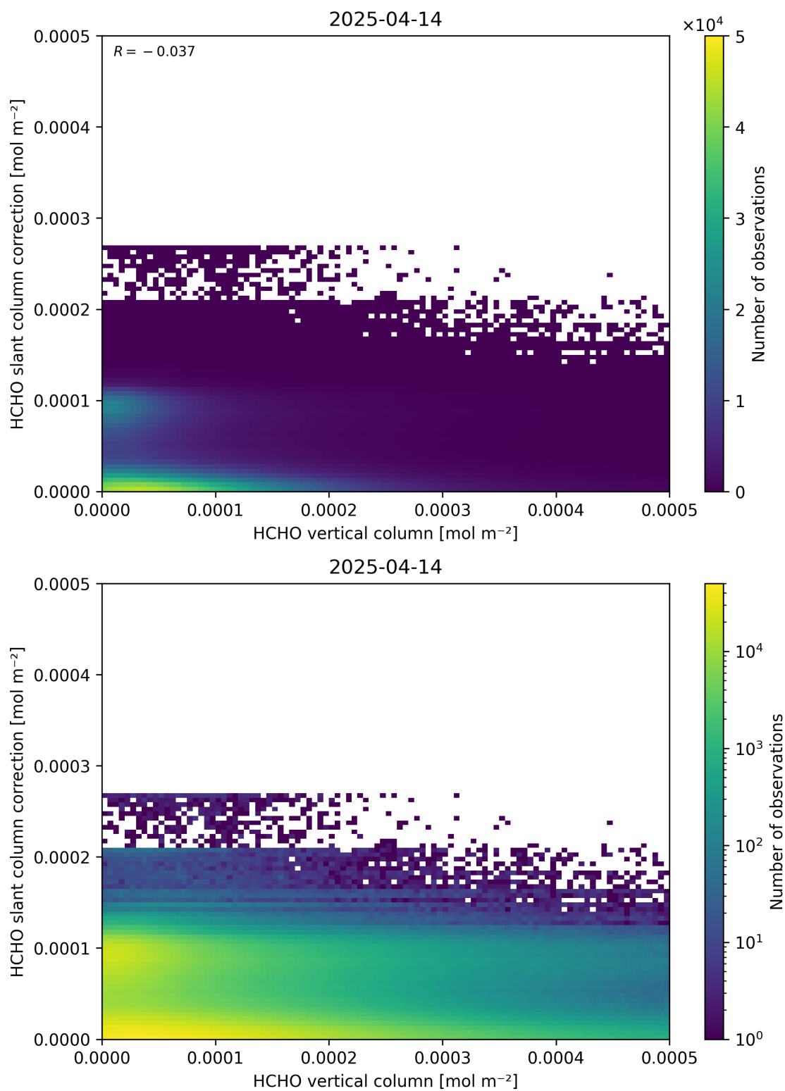
Figure 128: Scatter density plot of “HCHO vertical column” against “HCHO slant column correction” for 2025-04-13 to 2025-04-15.
