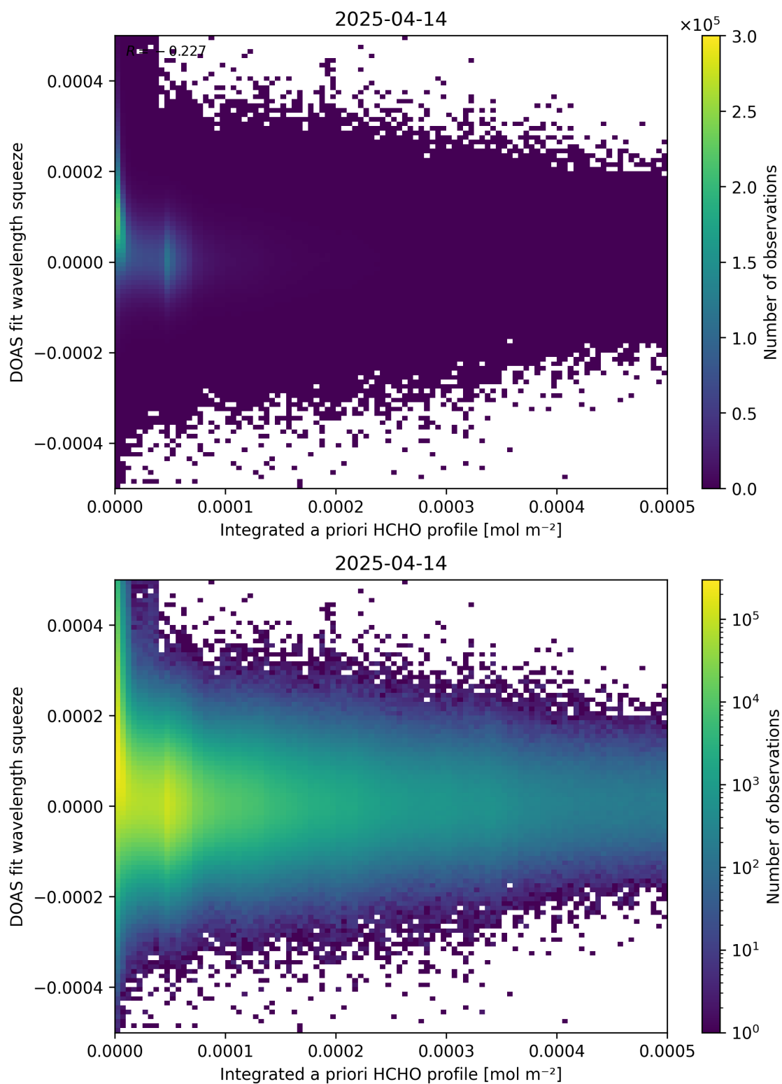
Figure 150: Scatter density plot of “Integrated a priori HCHO profile” against “DOAS fit wavelength squeeze” for 2025-04-13 to 2025-04-15.
