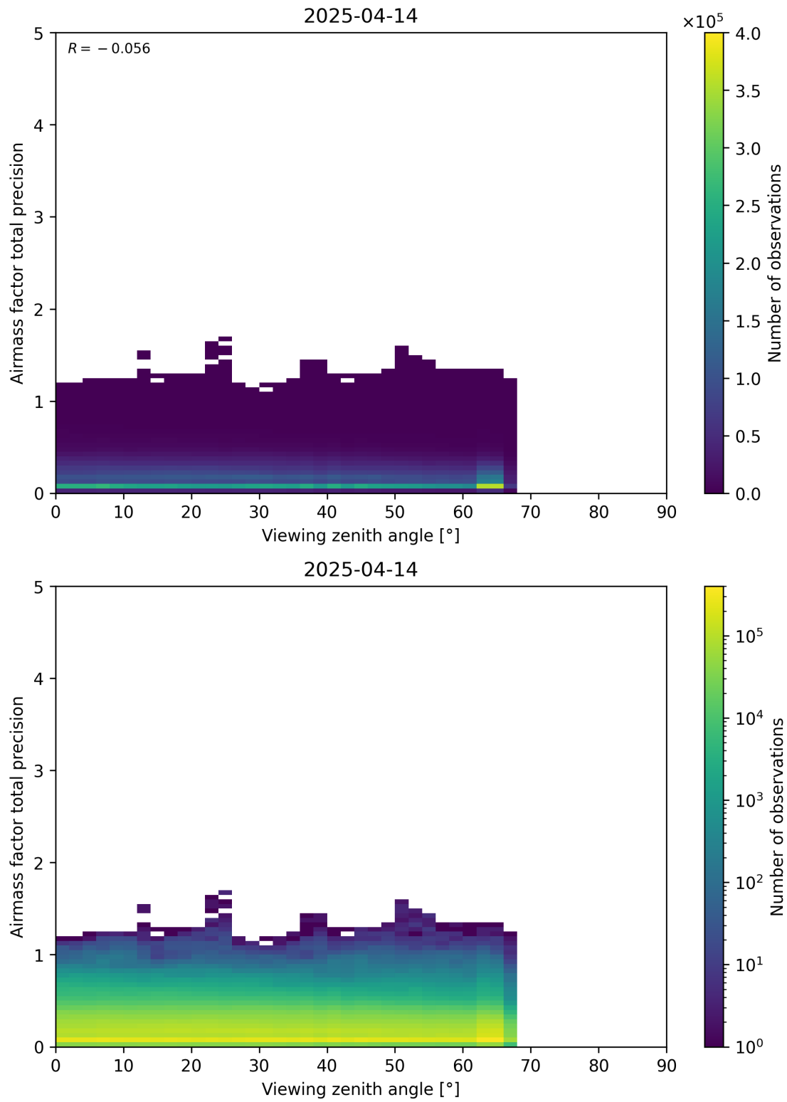
Figure 191: Scatter density plot of “Viewing zenith angle” against “Airmass factor total precision” for 2025-04-13 to 2025-04-15.
