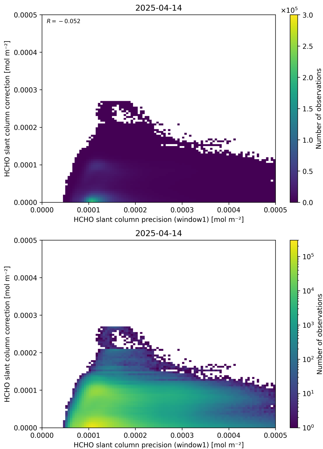
Figure 93: Scatter density plot of “HCHO slant column precision (window1)” against “HCHO slant column correction” for 2025-04-13 to 2025-04-15.
