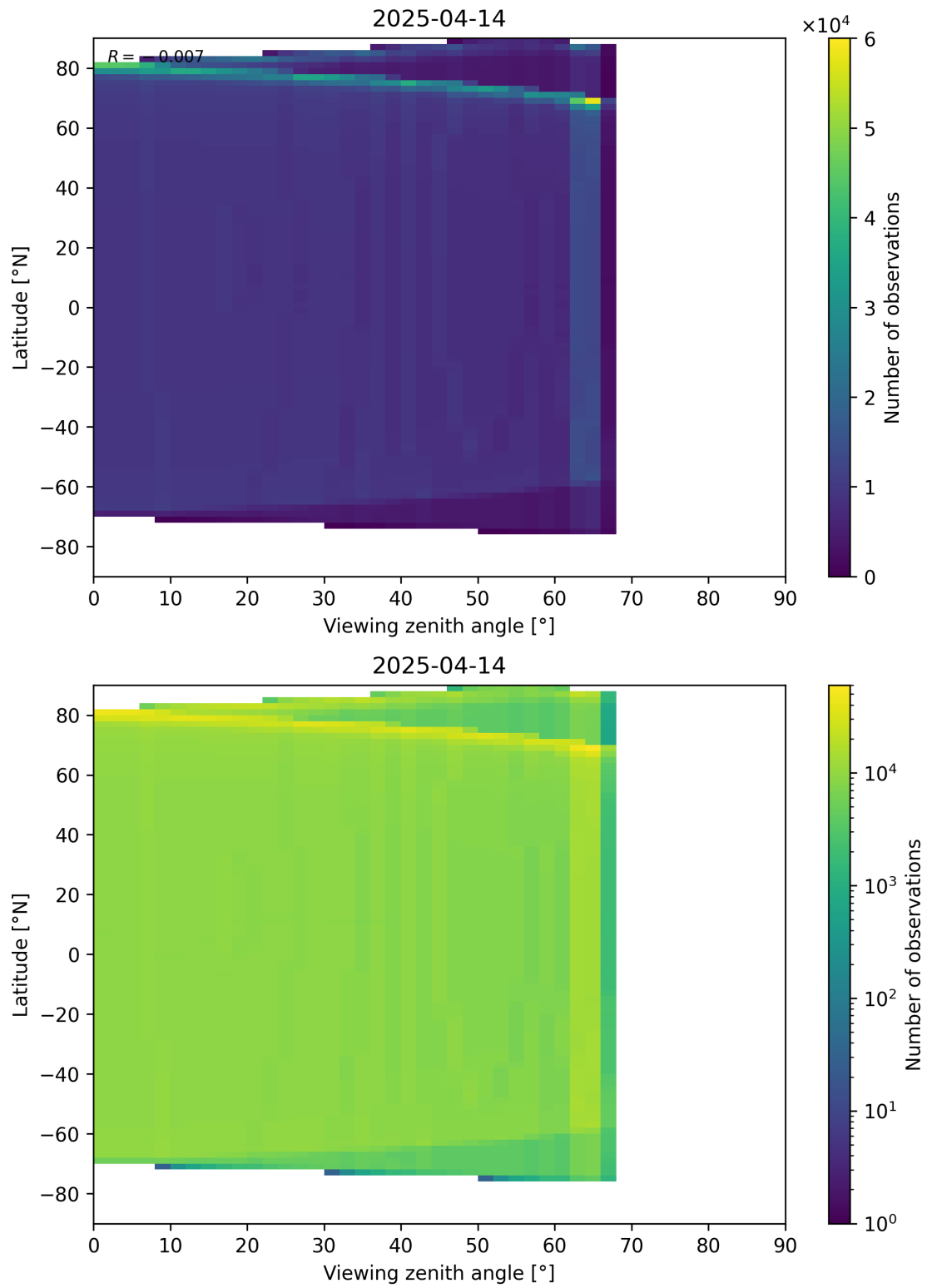
Figure 196: Scatter density plot of “Viewing zenith angle” against “Latitude” for 2025-04-13 to 2025-04-15.
