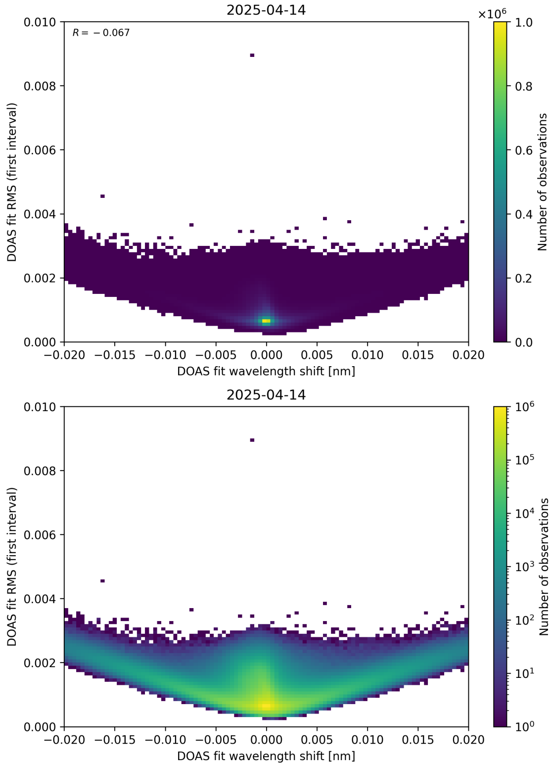
Figure 64: Scatter density plot of “DOAS fit wavelength shift” against “DOAS fit RMS (first interval)” for 2025-04-13 to 2025-04-15.
