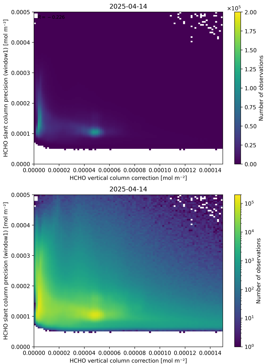
Figure 119: Scatter density plot of “HCHO vertical column correction” against “HCHO slant column precision (window1)” for 2025-04-13 to 2025-04-15.
