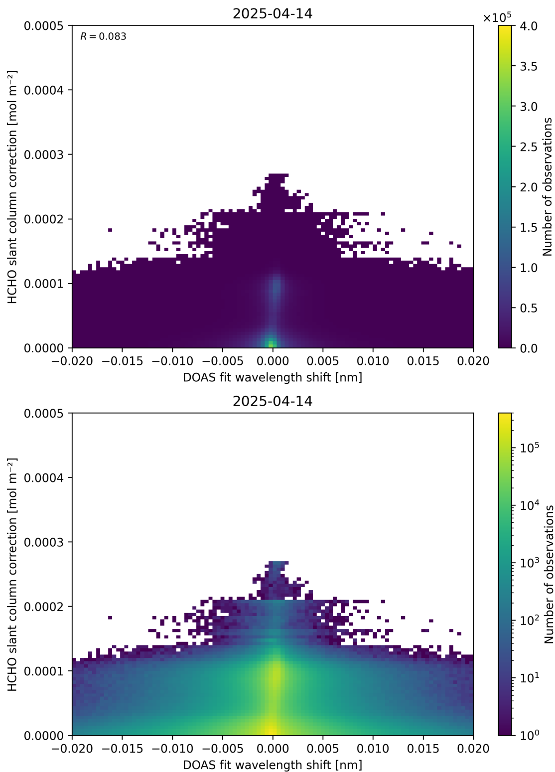
Figure 67: Scatter density plot of “DOAS fit wavelength shift” against “HCHO slant column correction” for 2025-04-13 to 2025-04-15.
