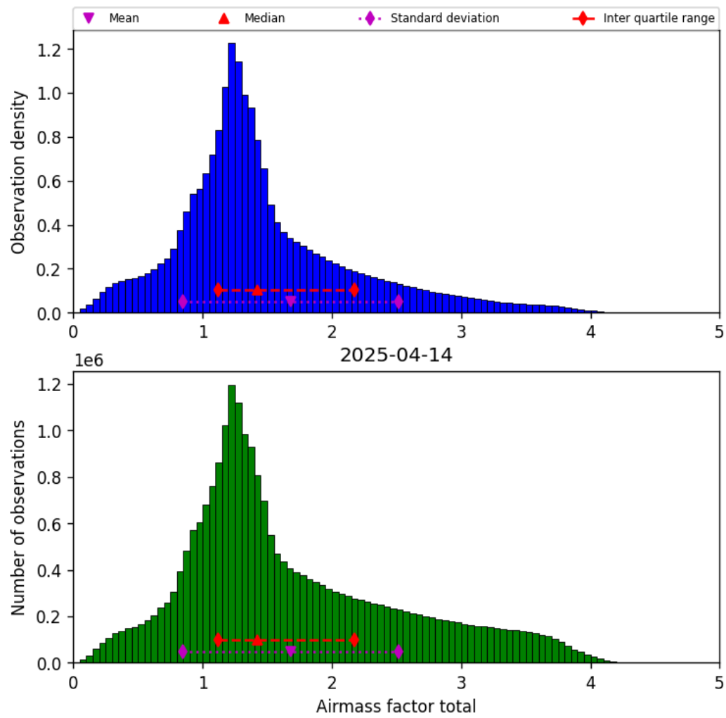
Figure 40: Histogram of “Airmass factor total” for 2025-04-13 to 2025-04-15
