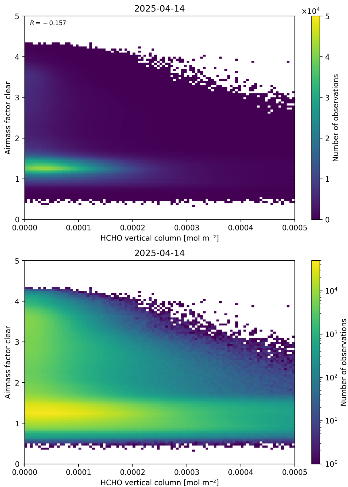
Figure 126: Scatter density plot of “HCHO vertical column” against “Airmass factor clear” for 2025-04-13 to 2025-04-15.
