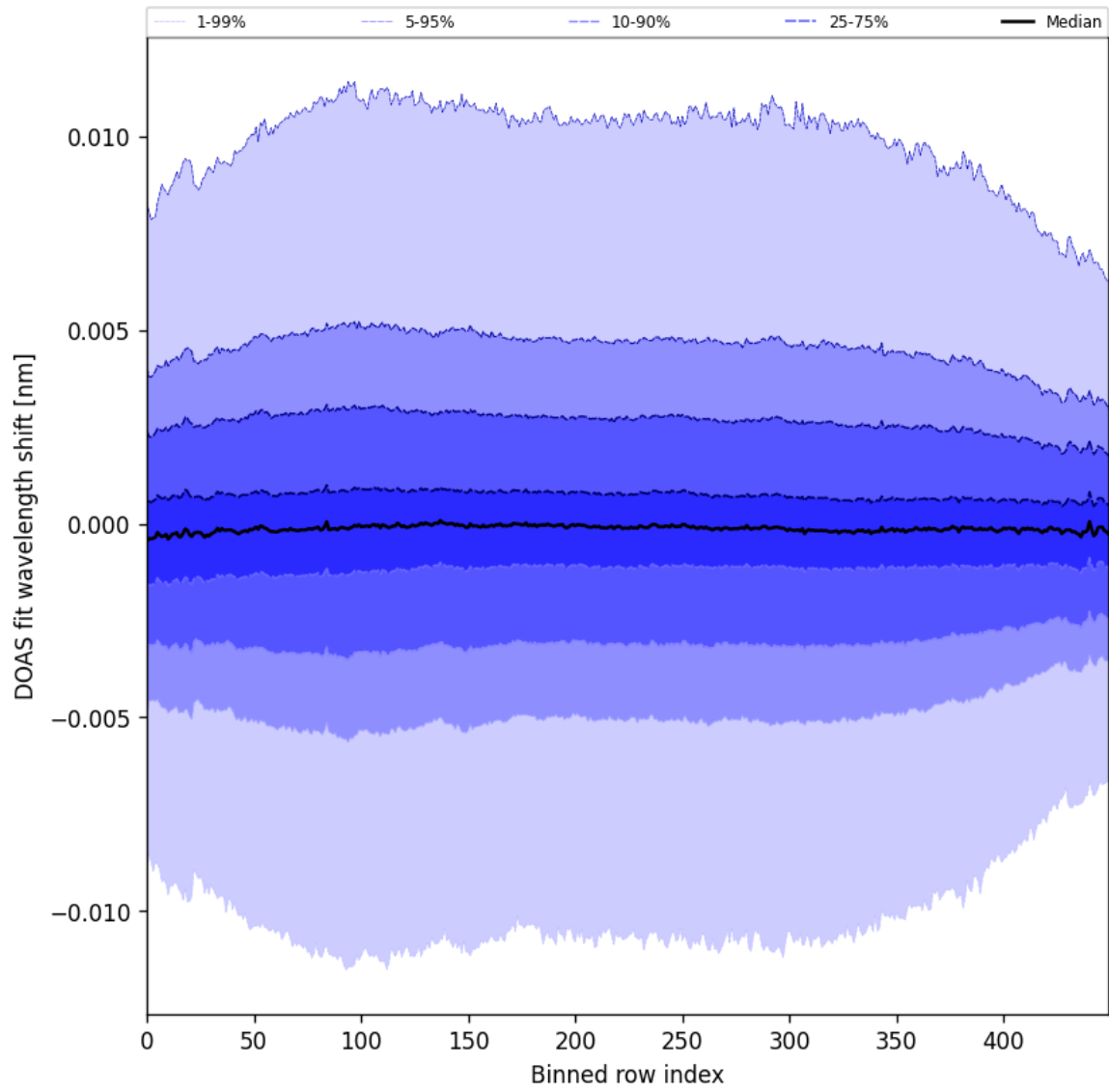
Figure 58: Along track statistics of “DOAS fit wavelength shift” for 2025-04-13 to 2025-04-15
