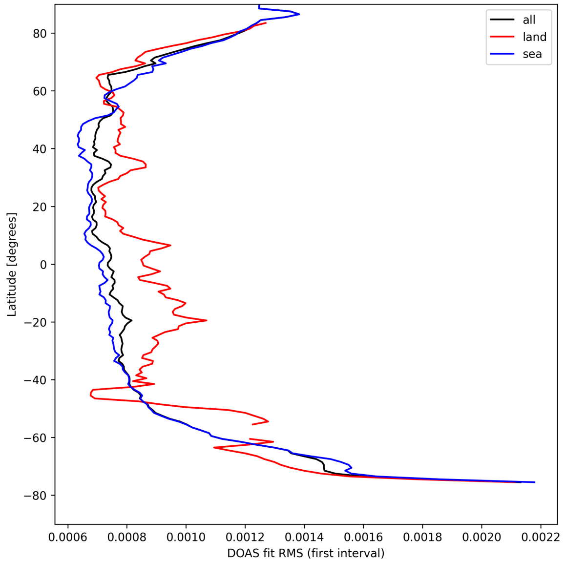
Figure 32: Zonal average of “DOAS fit RMS (first interval)” for 2025-04-13 to 2025-04-15.
