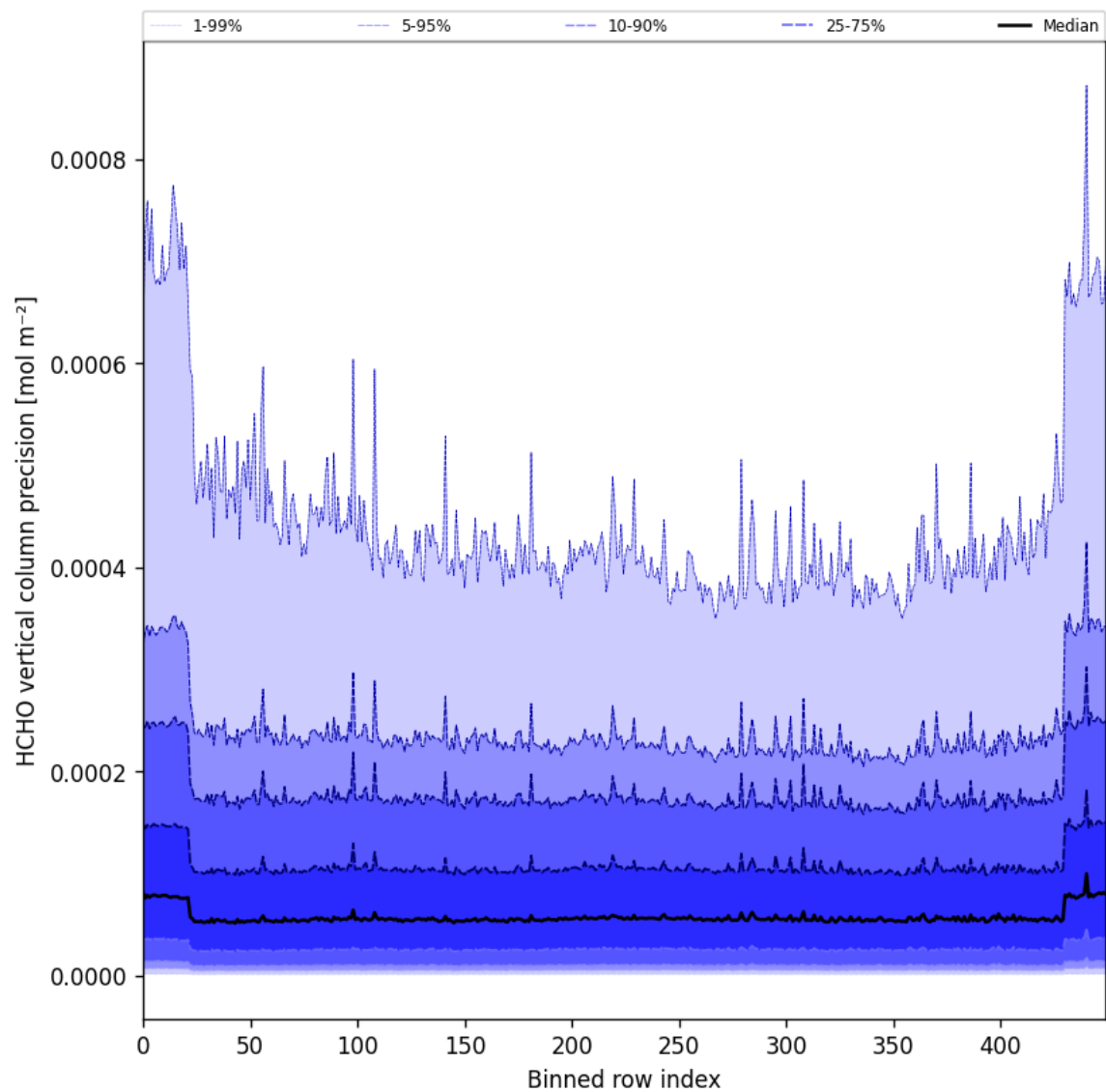
Figure 50: Along track statistics of “HCHO vertical column precision” for 2025-04-13 to 2025-04-15
