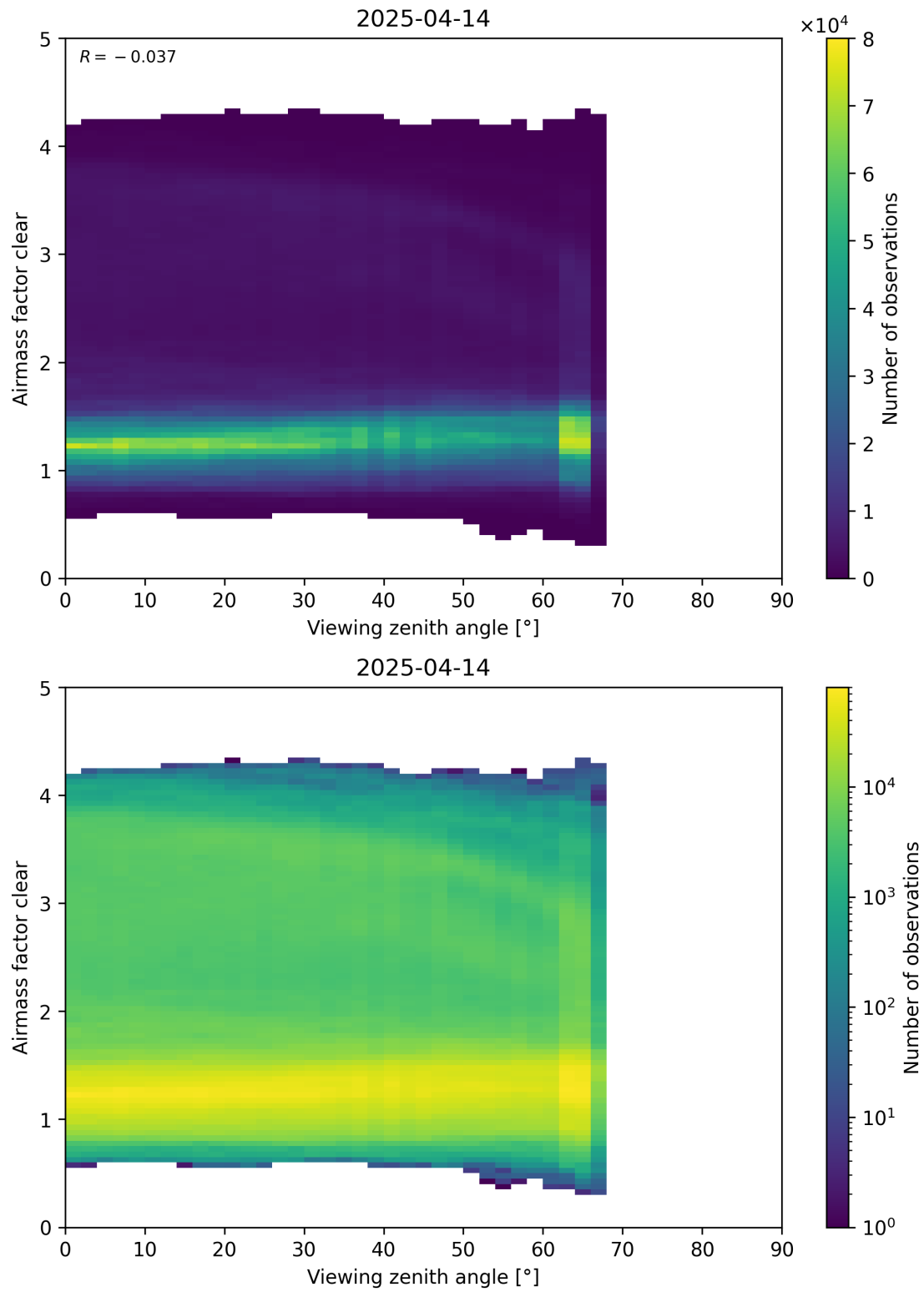
Figure 185: Scatter density plot of “Viewing zenith angle” against “Airmass factor clear” for 2025-04-13 to 2025-04-15.
