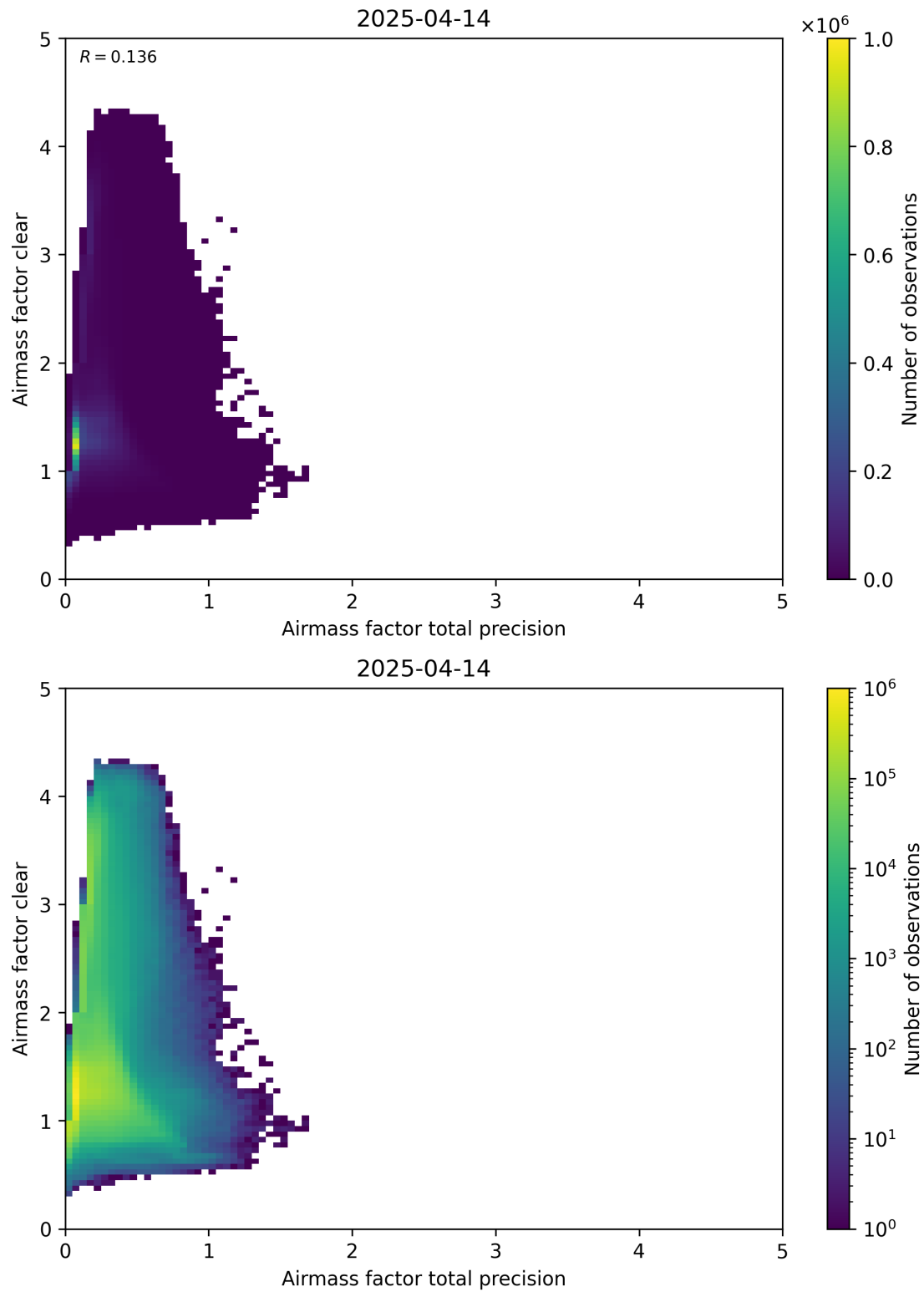
Figure 108: Scatter density plot of “Airmass factor total precision” against “Airmass factor clear” for 2025-04-13 to 2025-04-15.
