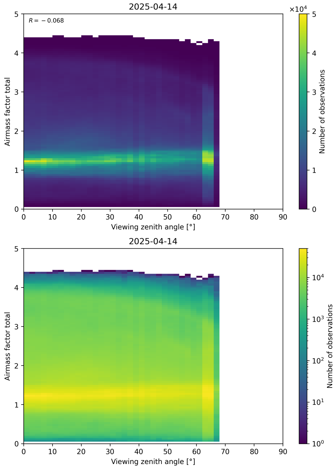
Figure 190: Scatter density plot of “Viewing zenith angle” against “Airmass factor total” for 2025-04-13 to 2025-04-15.
