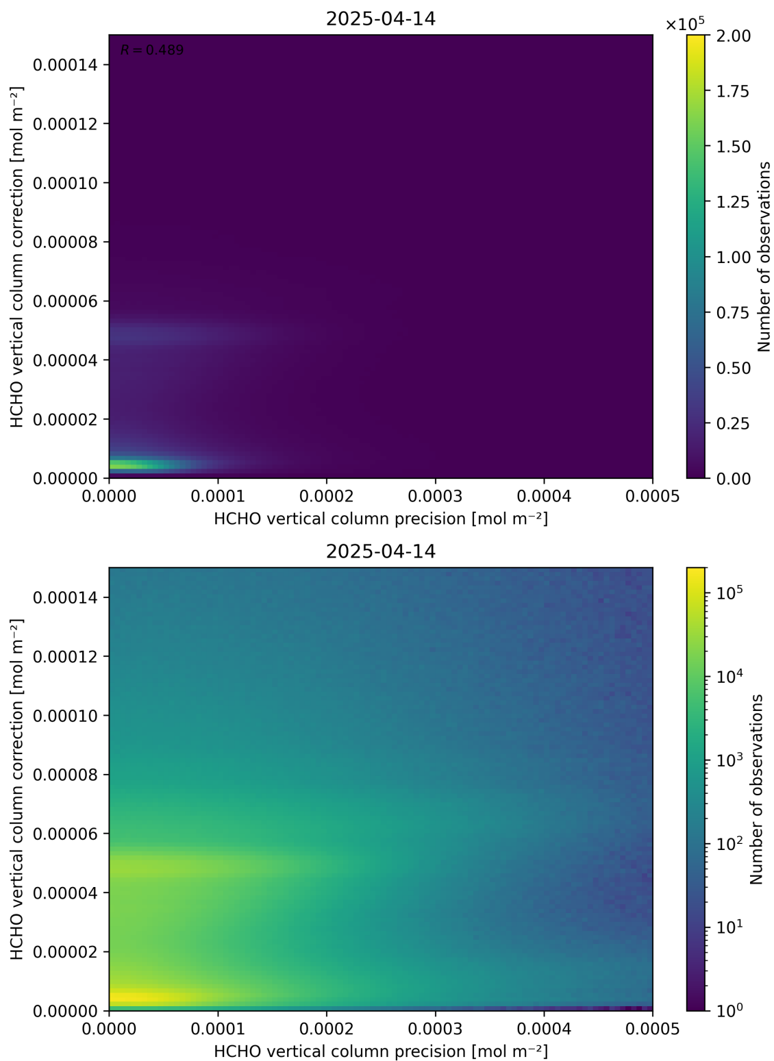
Figure 146: Scatter density plot of “HCHO vertical column precision” against “HCHO vertical column correction” for 2025-04-13 to 2025-04-15.
