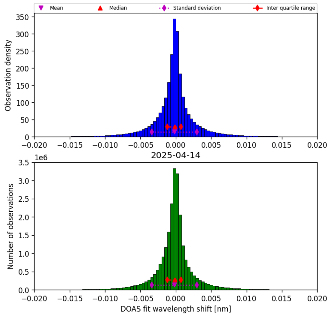
Figure 44: Histogram of “DOAS fit wavelength shift” for 2025-04-13 to 2025-04-15
