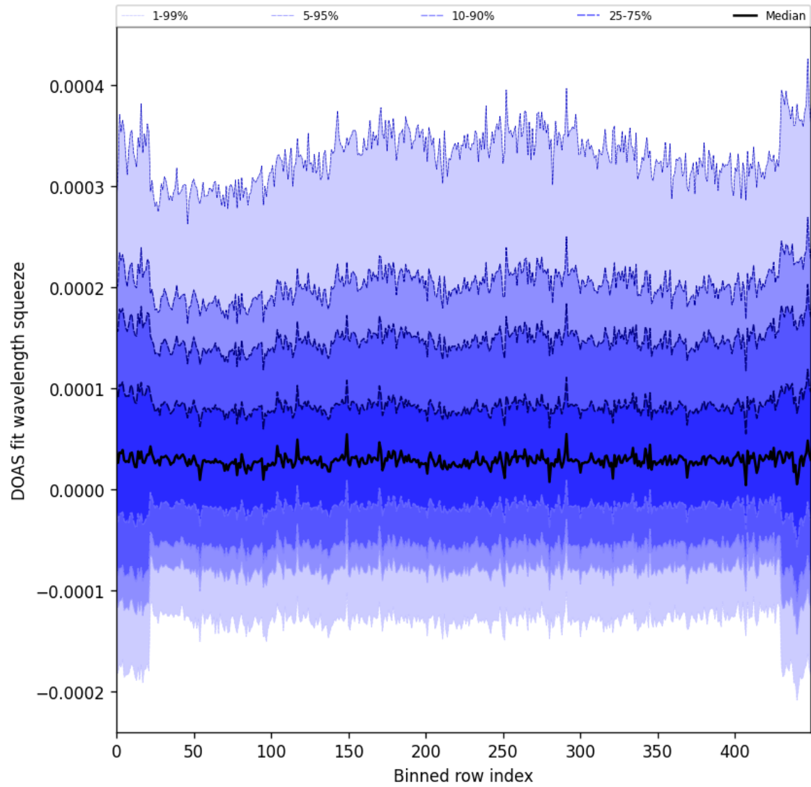
Figure 59: Along track statistics of “DOAS fit wavelength squeeze” for 2025-04-13 to 2025-04-15
