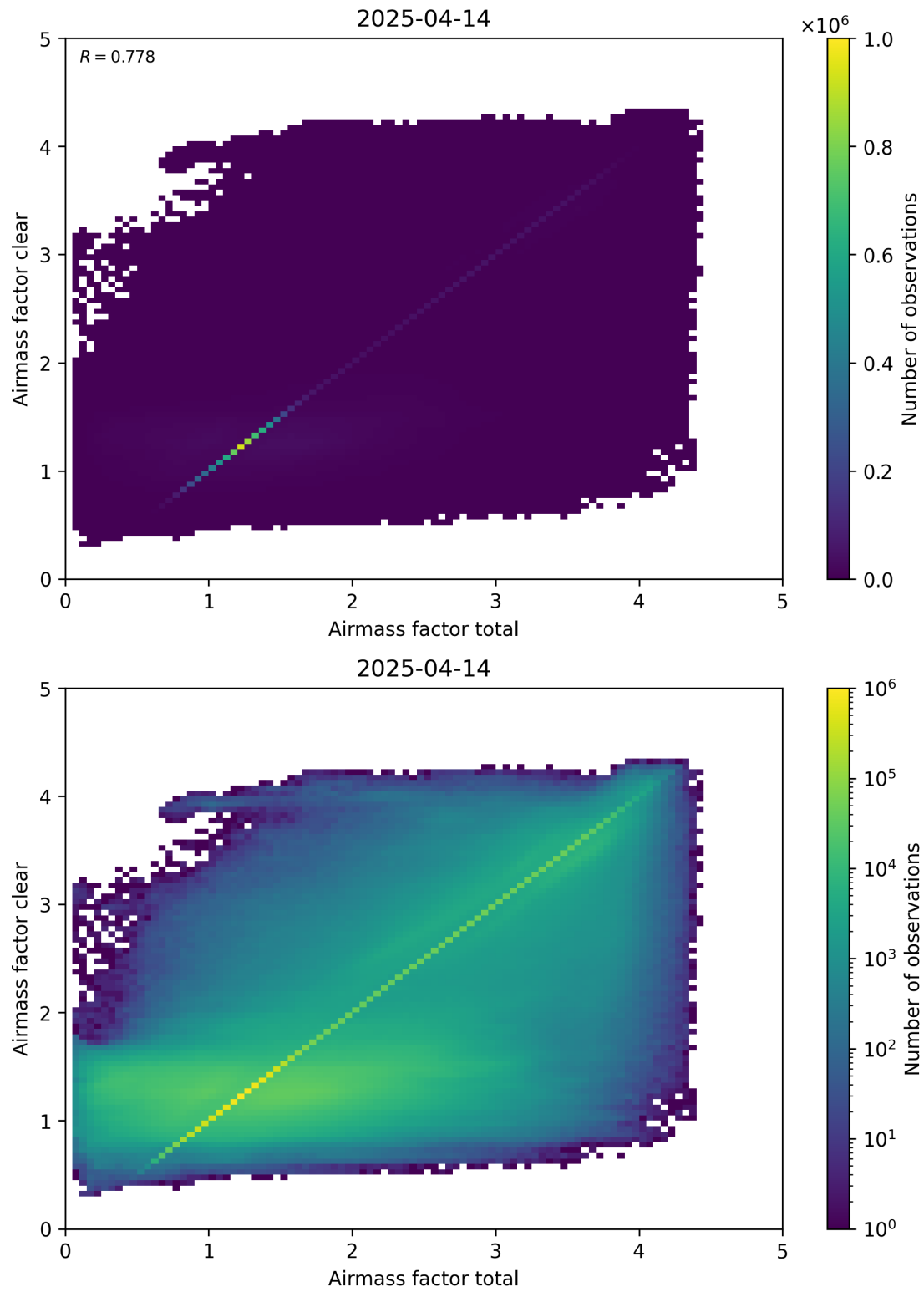
Figure 100: Scatter density plot of “Airmass factor total” against “Airmass factor clear” for 2025-04-13 to 2025-04-15.
