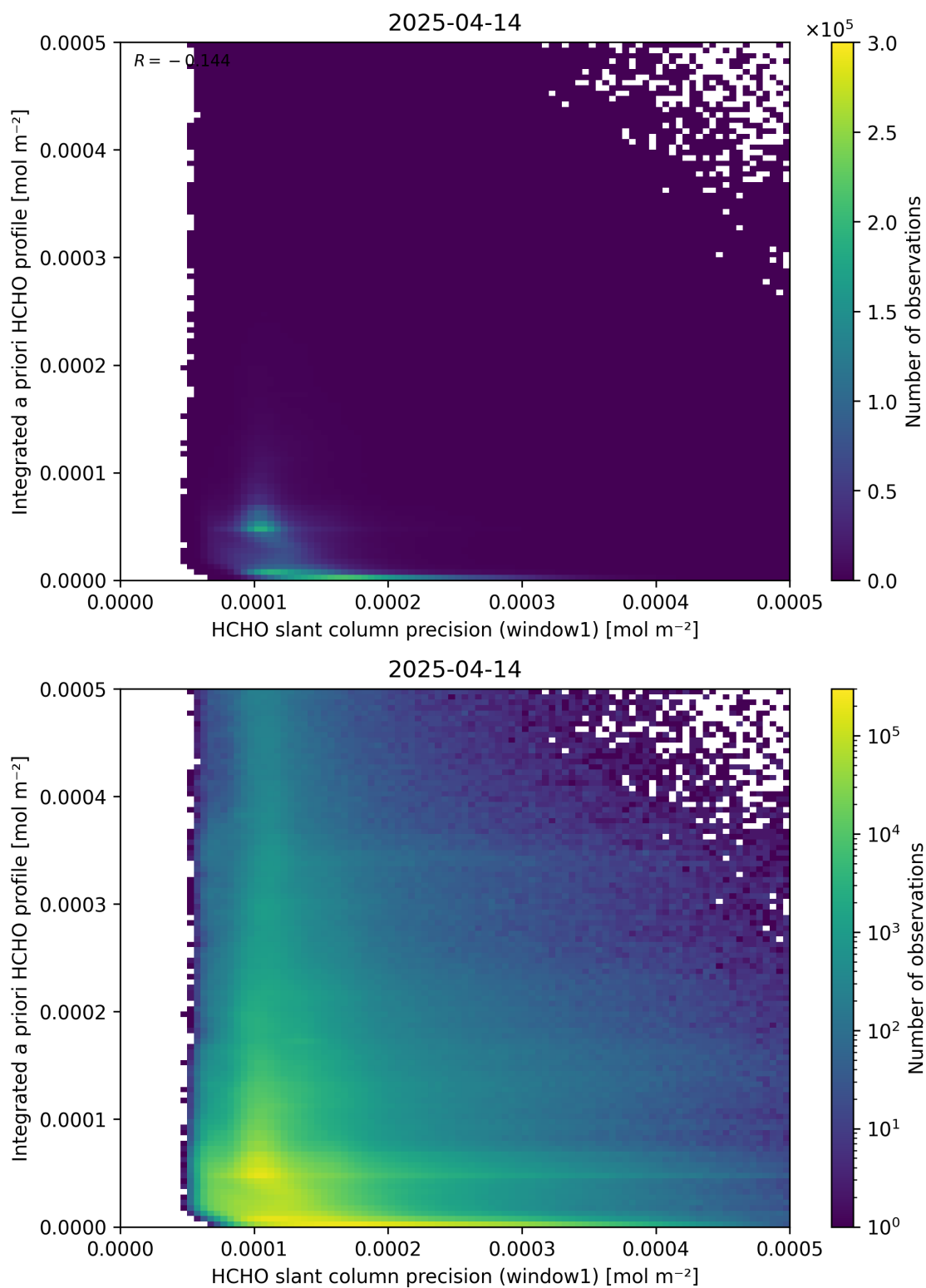
Figure 96: Scatter density plot of “HCHO slant column precision (window1)” against “Integrated a priori HCHO profile” for 2025-04-13 to 2025-04-15.
