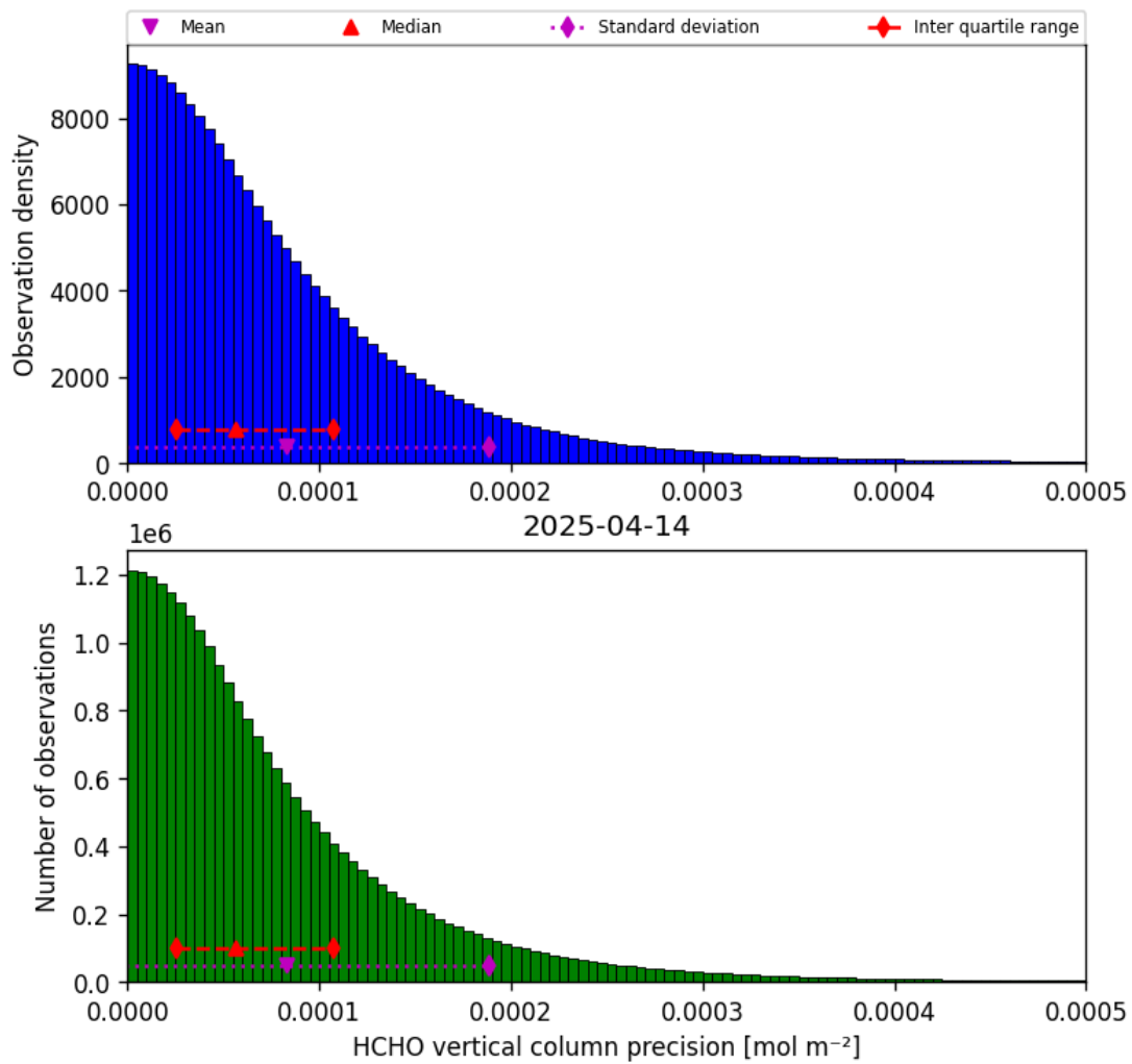
Figure 36: Histogram of “HCHO vertical column precision” for 2025-04-13 to 2025-04-15
