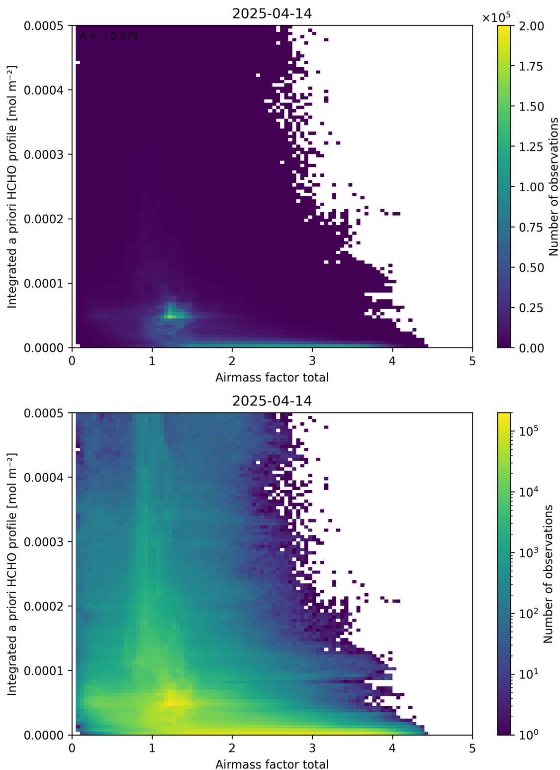
Figure 104: Scatter density plot of “Airmass factor total” against “Integrated a priori HCHO profile” for 2025-04-13 to 2025-04-15.
