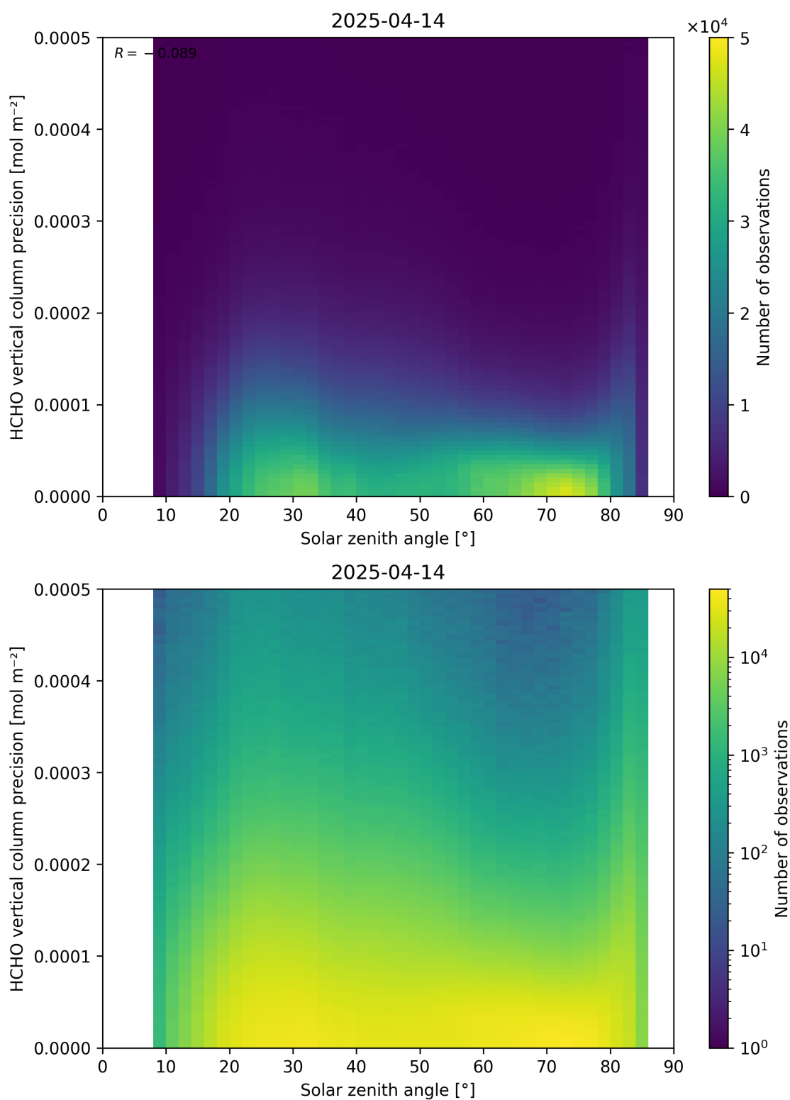
Figure 179: Scatter density plot of “Solar zenith angle” against “HCHO vertical column precision” for 2025-04-13 to 2025-04-15.
