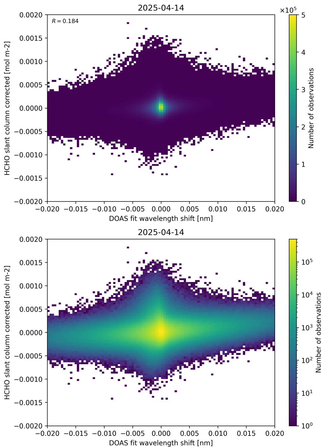
Figure 66: Scatter density plot of “DOAS fit wavelength shift” against “HCHO slant column corrected” for 2025-04-13 to 2025-04-15.
