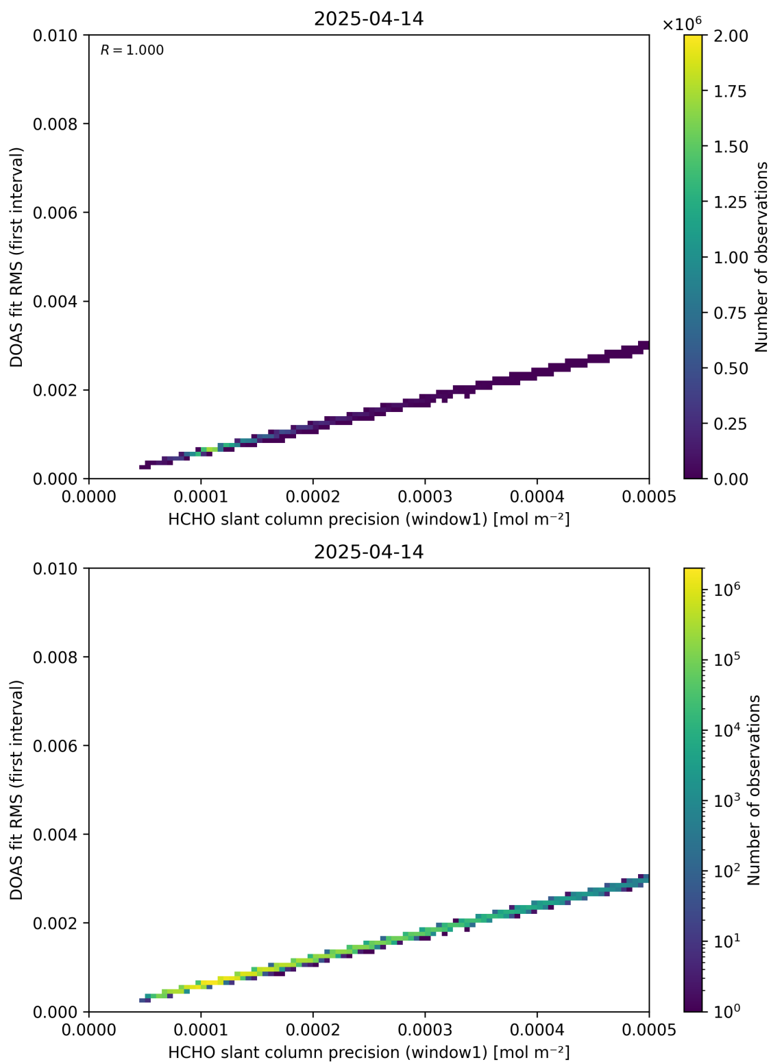
Figure 88: Scatter density plot of “HCHO slant column precision (window1)” against “DOAS fit RMS (first interval)” for 2025-04-13 to 2025-04-15.
