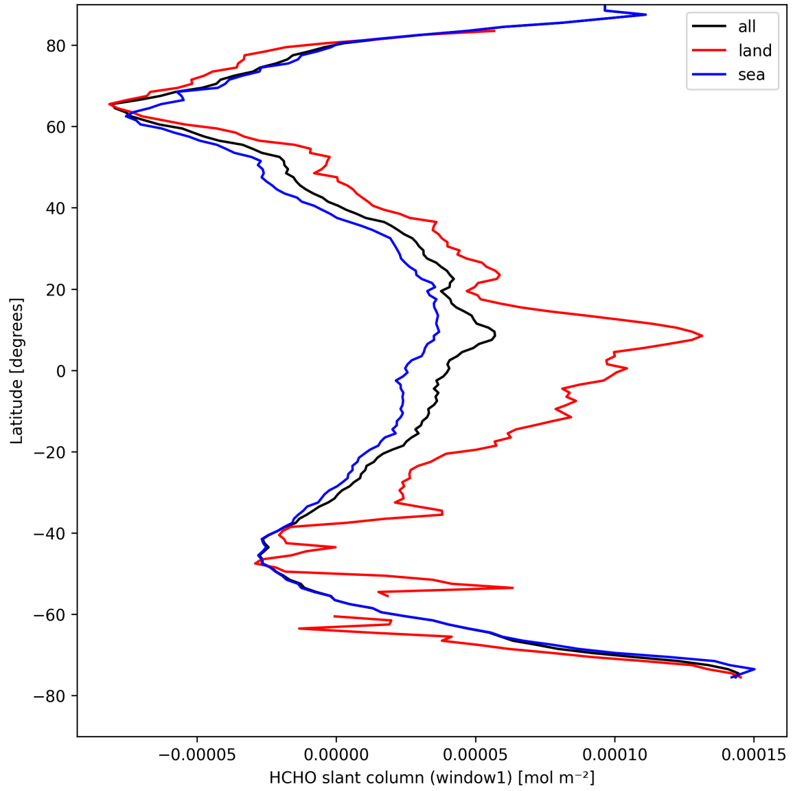
Figure 24: Zonal average of “HCHO slant column (window1)” for 2025-04-13 to 2025-04-15.
