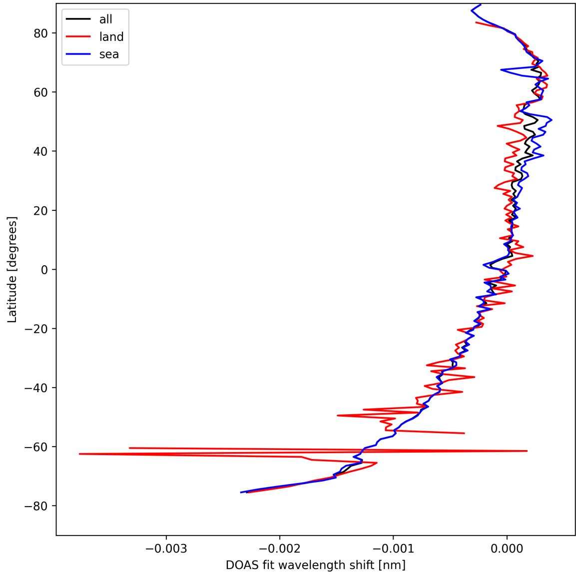
Figure 30: Zonal average of “DOAS fit wavelength shift” for 2025-04-13 to 2025-04-15.
