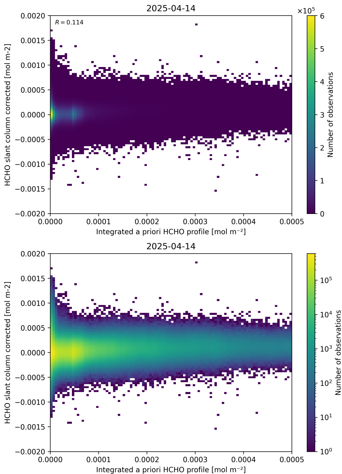
Figure 151: Scatter density plot of “Integrated a priori HCHO profile” against “HCHO slant column corrected” for 2025-04-13 to 2025-04-15.
