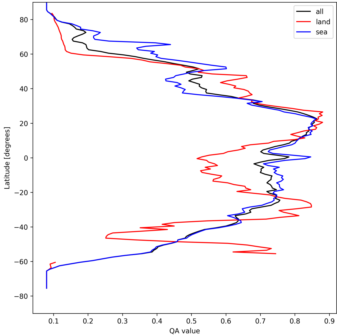
Figure 20: Zonal average of “QA value” for 2025-04-13 to 2025-04-15.
