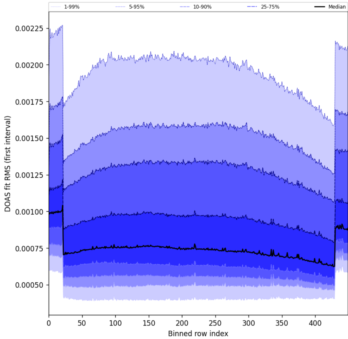
Figure 60: Along track statistics of “DOAS fit RMS (first interval)” for 2025-04-13 to 2025-04-15
