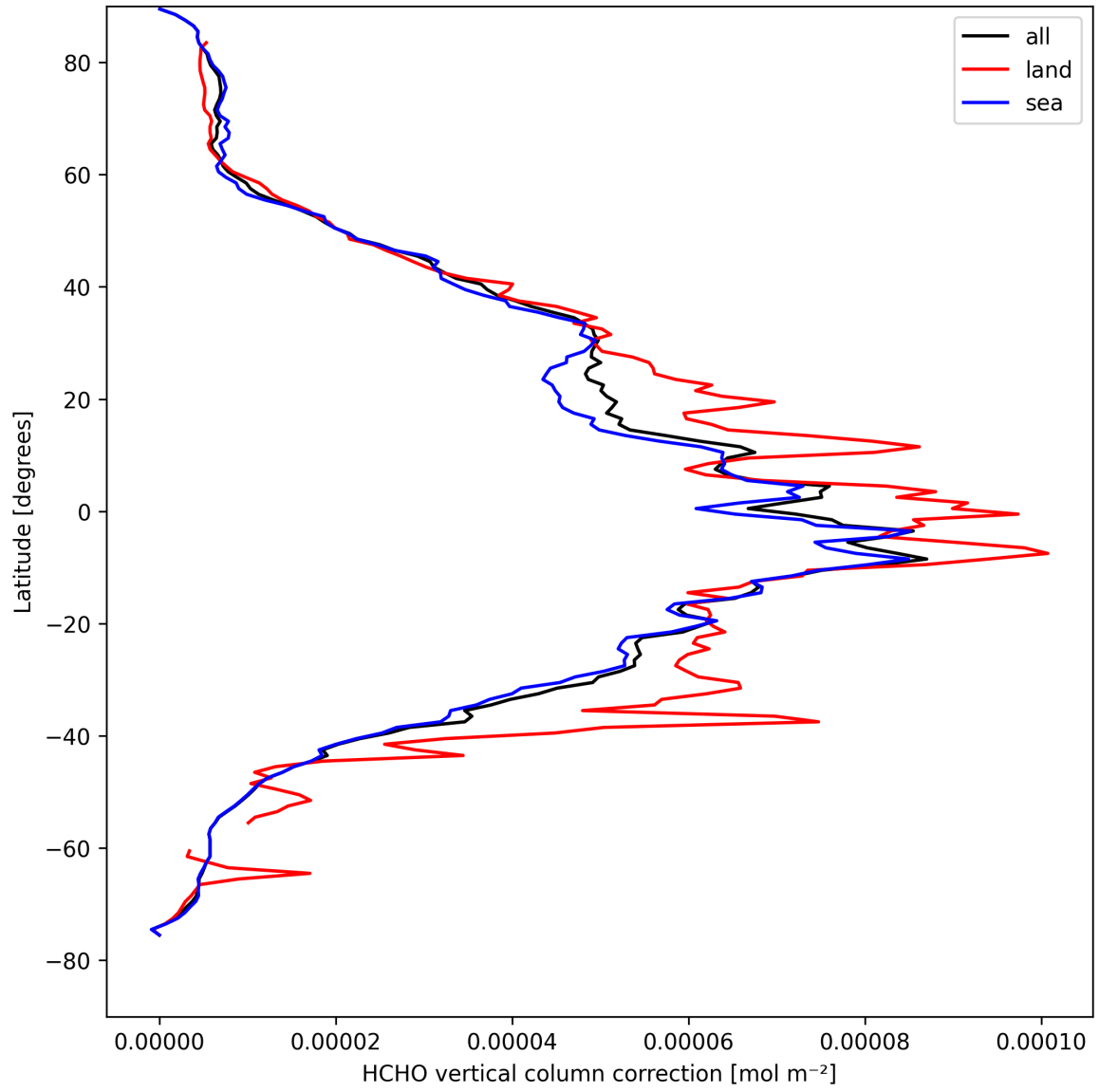
Figure 23: Zonal average of “HCHO vertical column correction” for 2025-04-13 to 2025-04-15.
