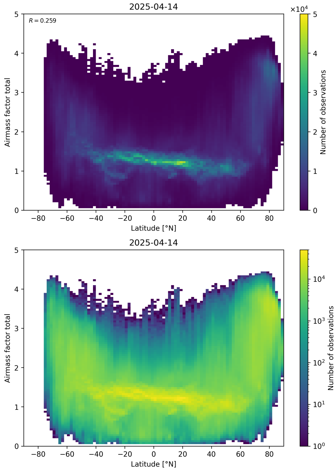
Figure 161: Scatter density plot of “Latitude” against “Airmass factor total” for 2025-04-13 to 2025-04-15.
