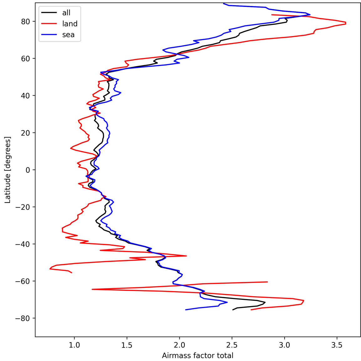
Figure 26: Zonal average of “Airmass factor total” for 2025-04-13 to 2025-04-15.
