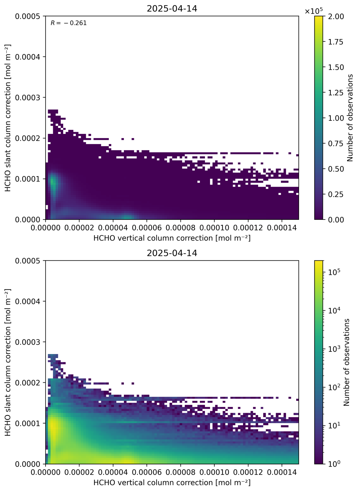
Figure 117: Scatter density plot of “HCHO vertical column correction” against “HCHO slant column correction” for 2025-04-13 to 2025-04-15.
