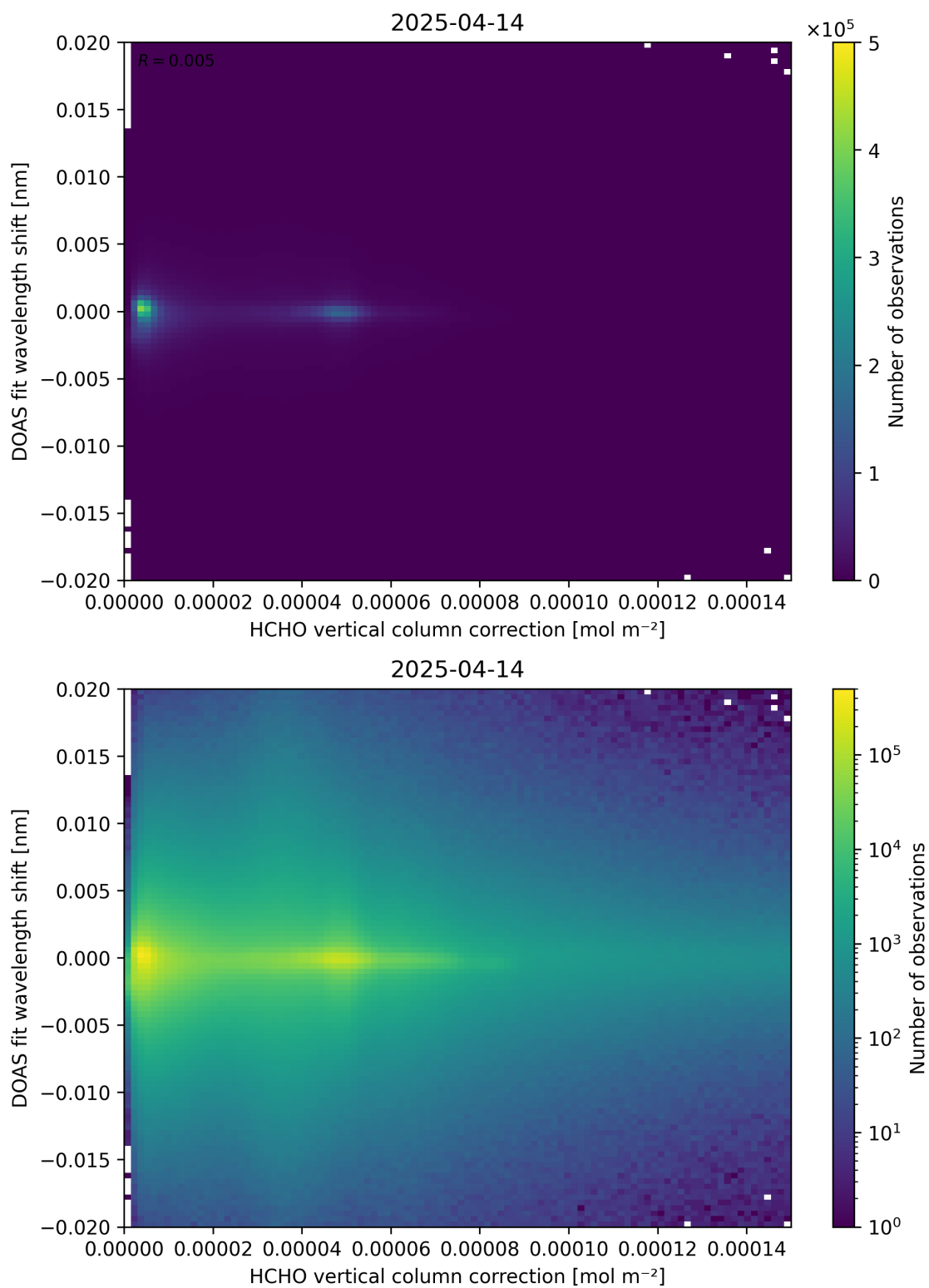
Figure 113: Scatter density plot of “HCHO vertical column correction” against “DOAS fit wavelength shift” for 2025-04-13 to 2025-04-15.
