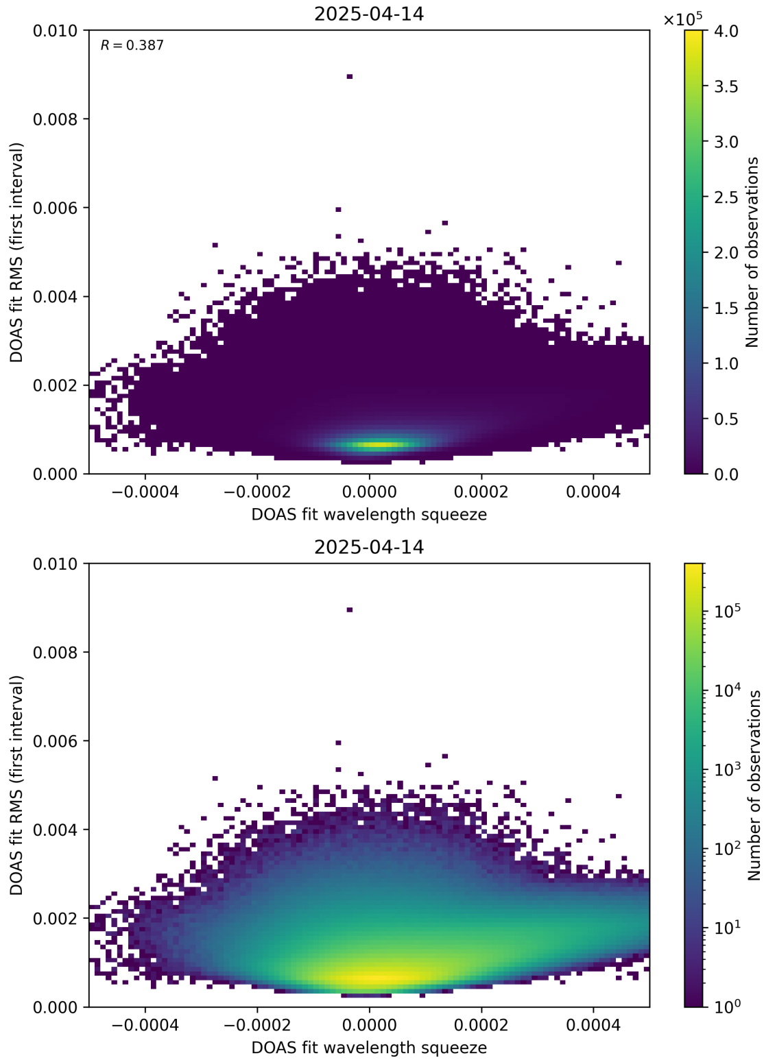
Figure 68: Scatter density plot of “DOAS fit wavelength squeeze” against “DOAS fit RMS (first interval)” for 2025-04-13 to 2025-04-15.
