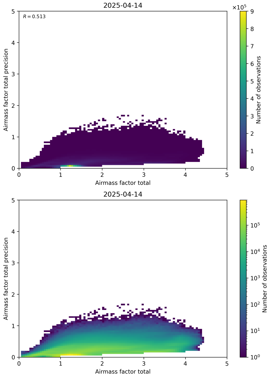
Figure 103: Scatter density plot of “Airmass factor total” against “Airmass factor total precision” for 2025-04-13 to 2025-04-15.
