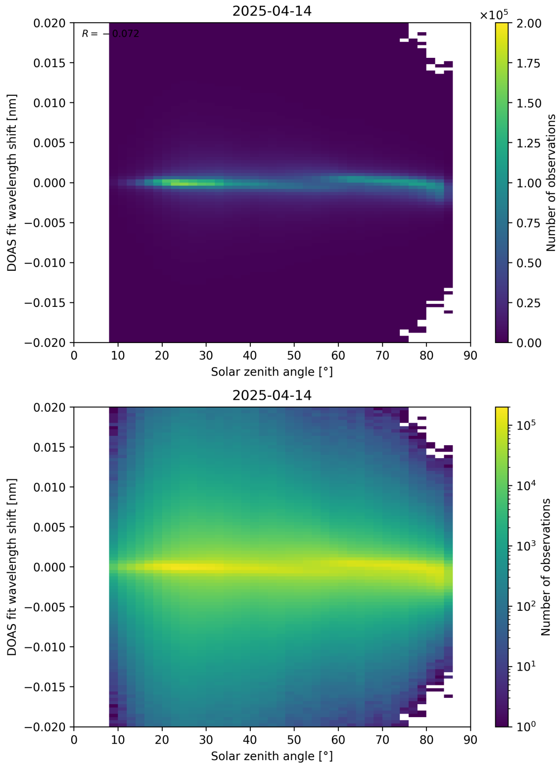
Figure 168: Scatter density plot of “Solar zenith angle” against “DOAS fit wavelength shift” for 2025-04-13 to 2025-04-15.
