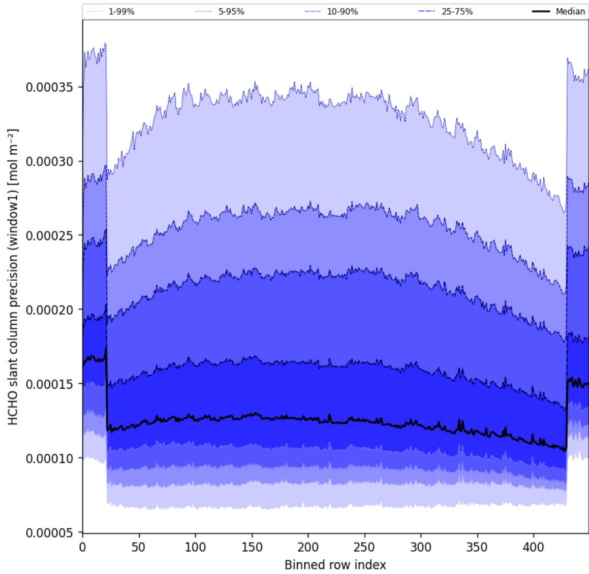
Figure 53: Along track statistics of “HCHO slant column precision (window1)” for 2025-04-13 to 2025-04-15
