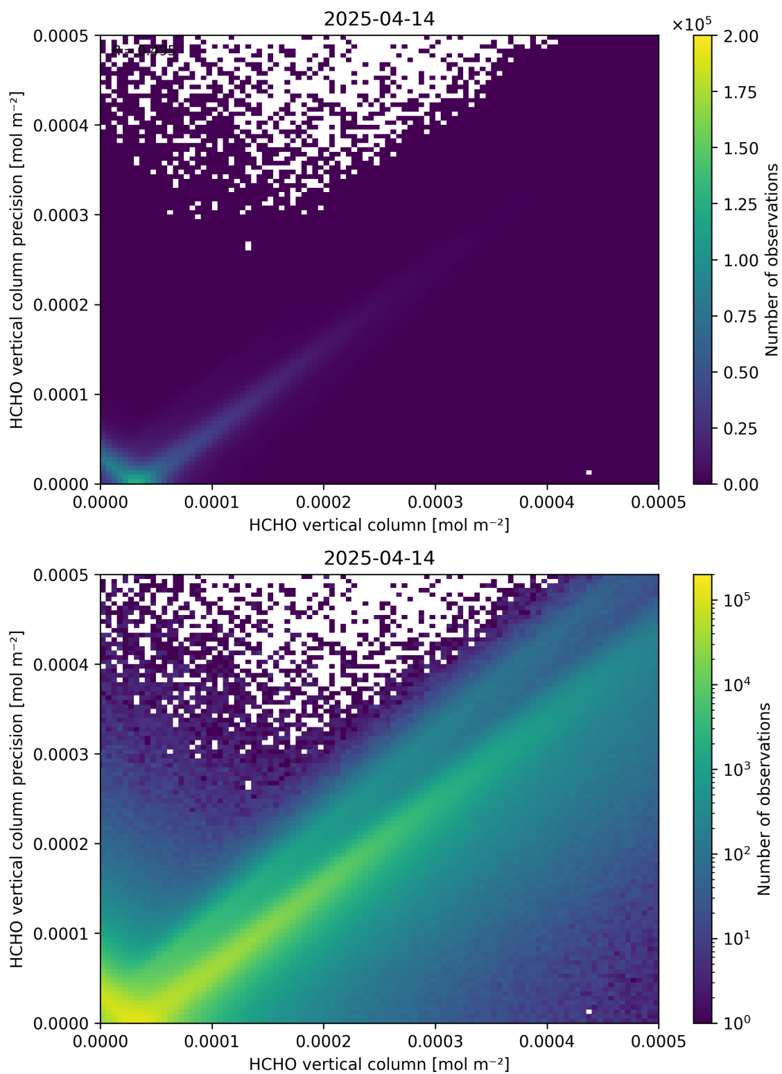
Figure 134: Scatter density plot of “HCHO vertical column” against “HCHO vertical column precision” for 2025-04-13 to 2025-04-15.
