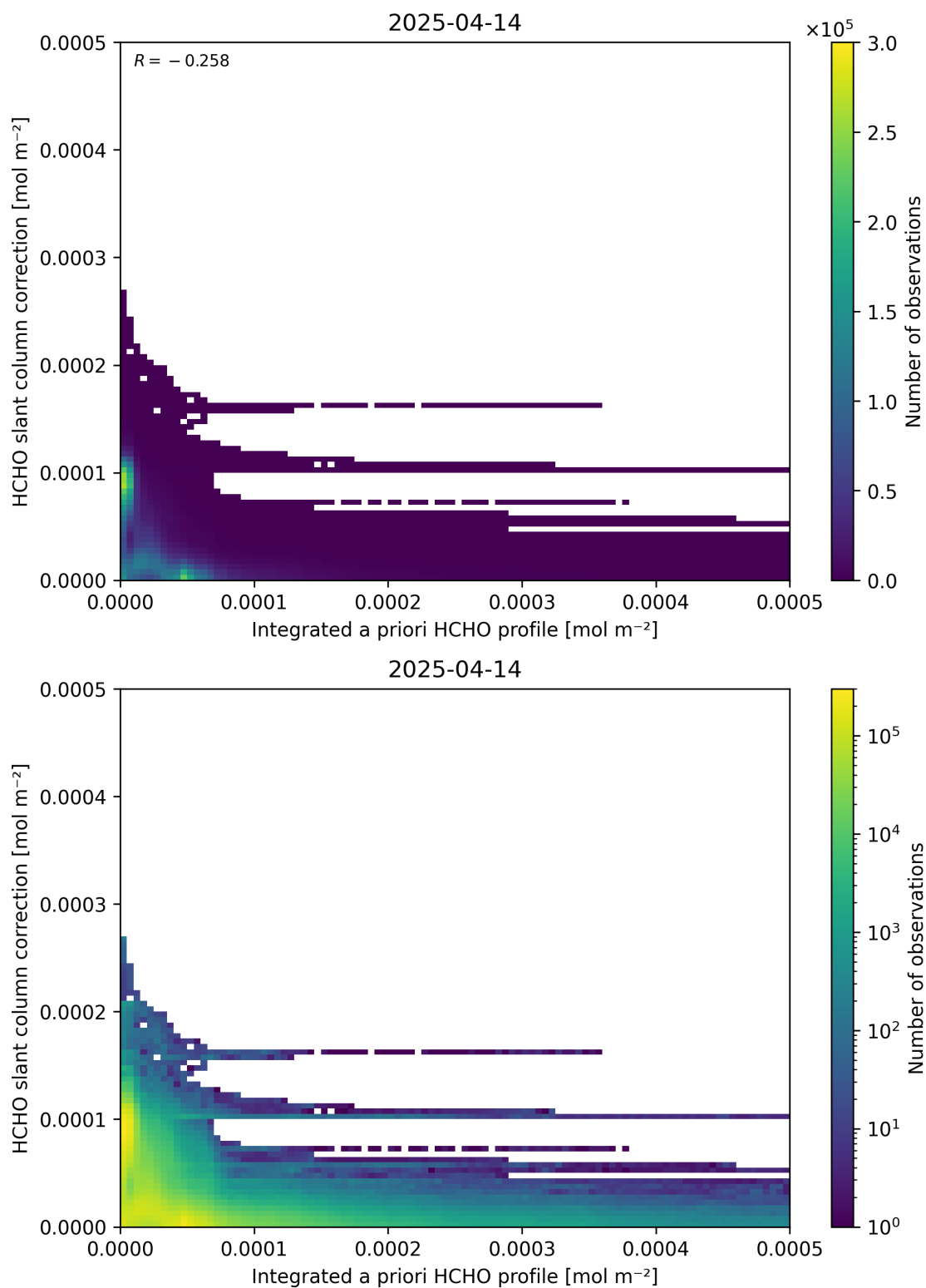
Figure 152: Scatter density plot of “Integrated a priori HCHO profile” against “HCHO slant column correction” for 2025-04-13 to 2025-04-15.
