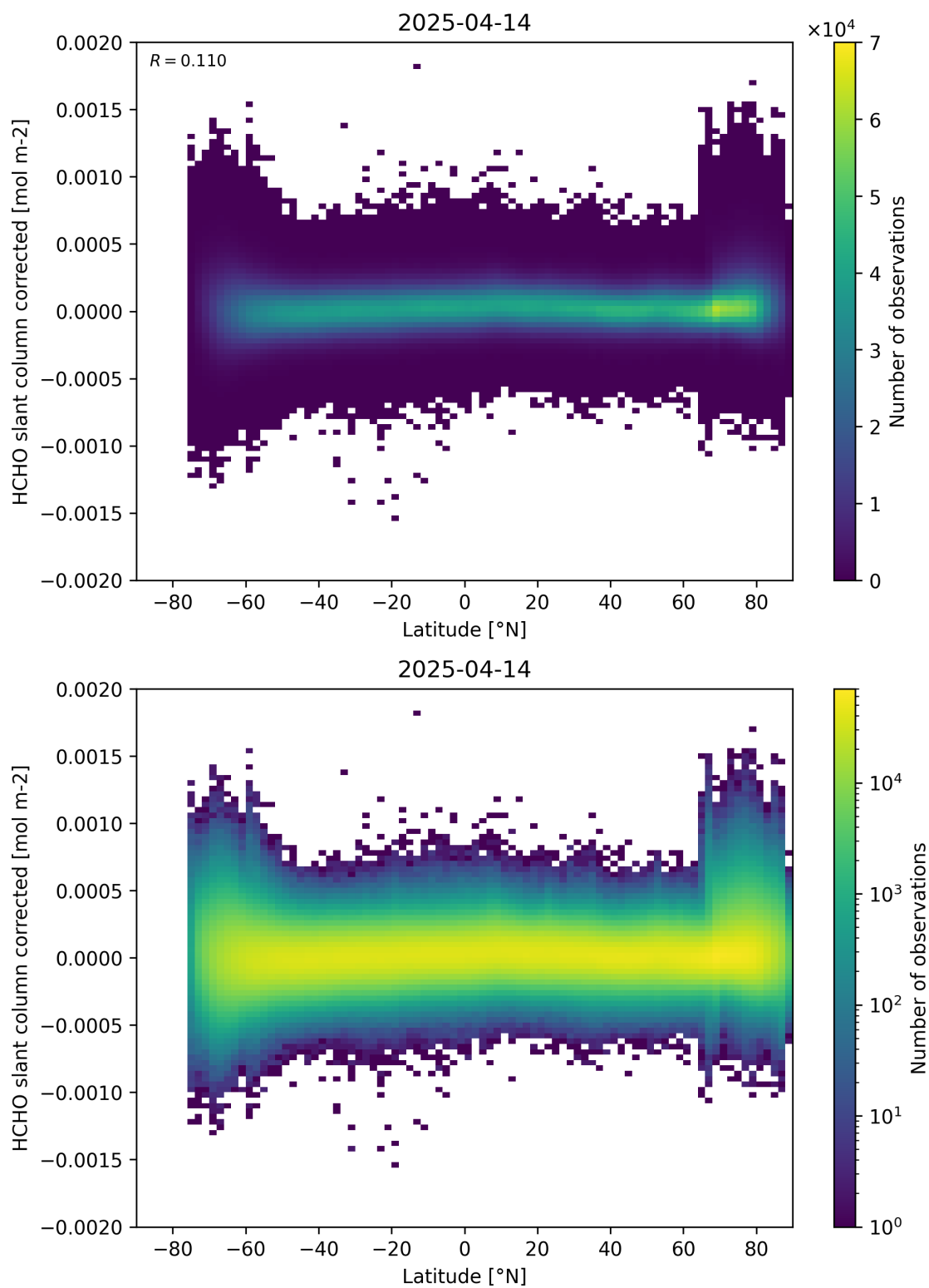
Figure 157: Scatter density plot of “Latitude” against “HCHO slant column corrected” for 2025-04-13 to 2025-04-15.
