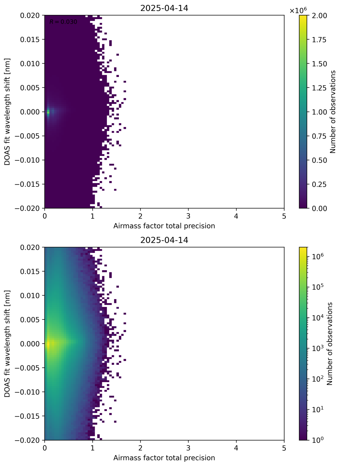
Figure 106: Scatter density plot of “Airmass factor total precision” against “DOAS fit wavelength shift” for 2025-04-13 to 2025-04-15.
