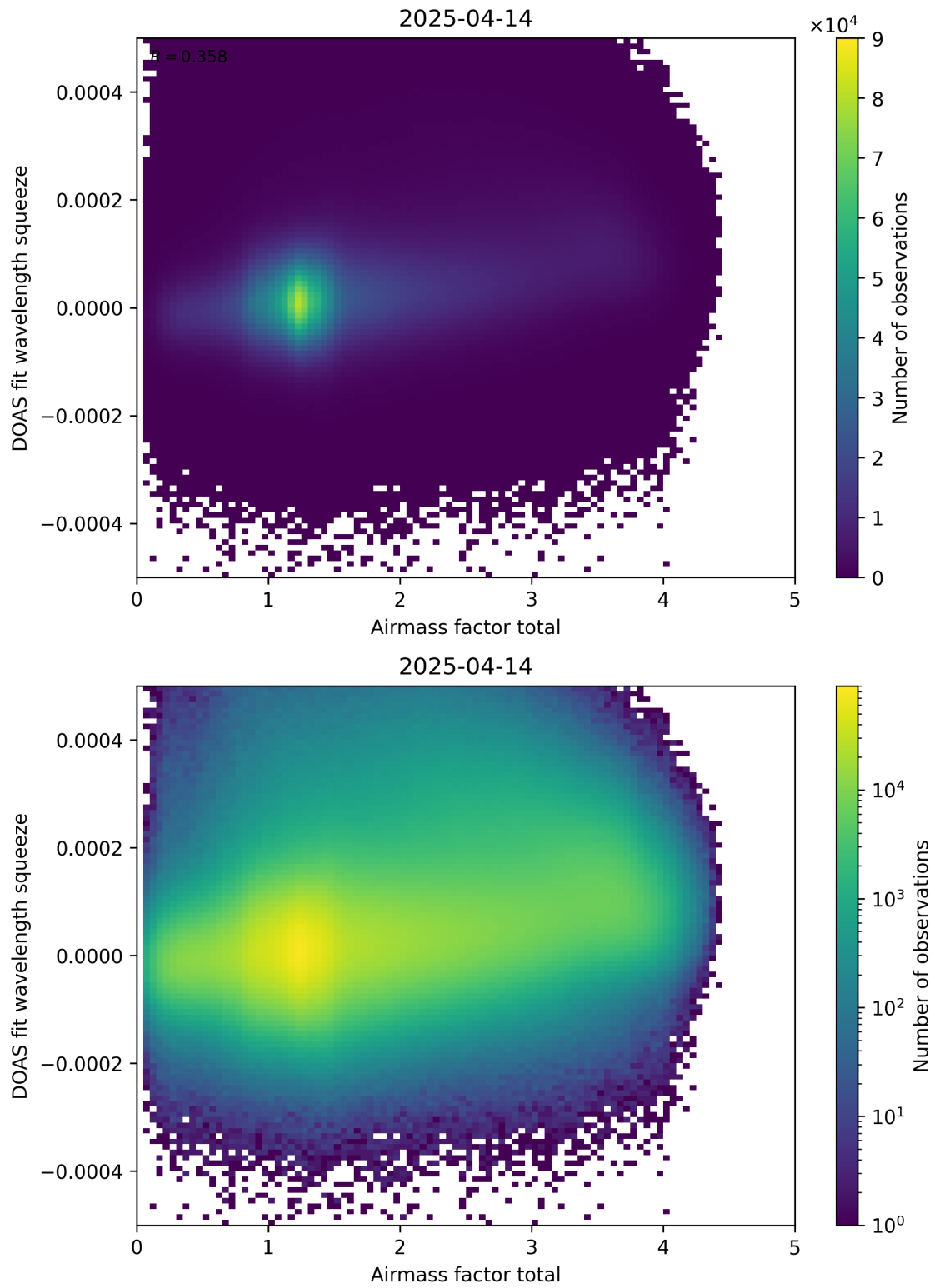
Figure 99: Scatter density plot of “Airmass factor total” against “DOAS fit wavelength squeeze” for 2025-04-13 to 2025-04-15.
