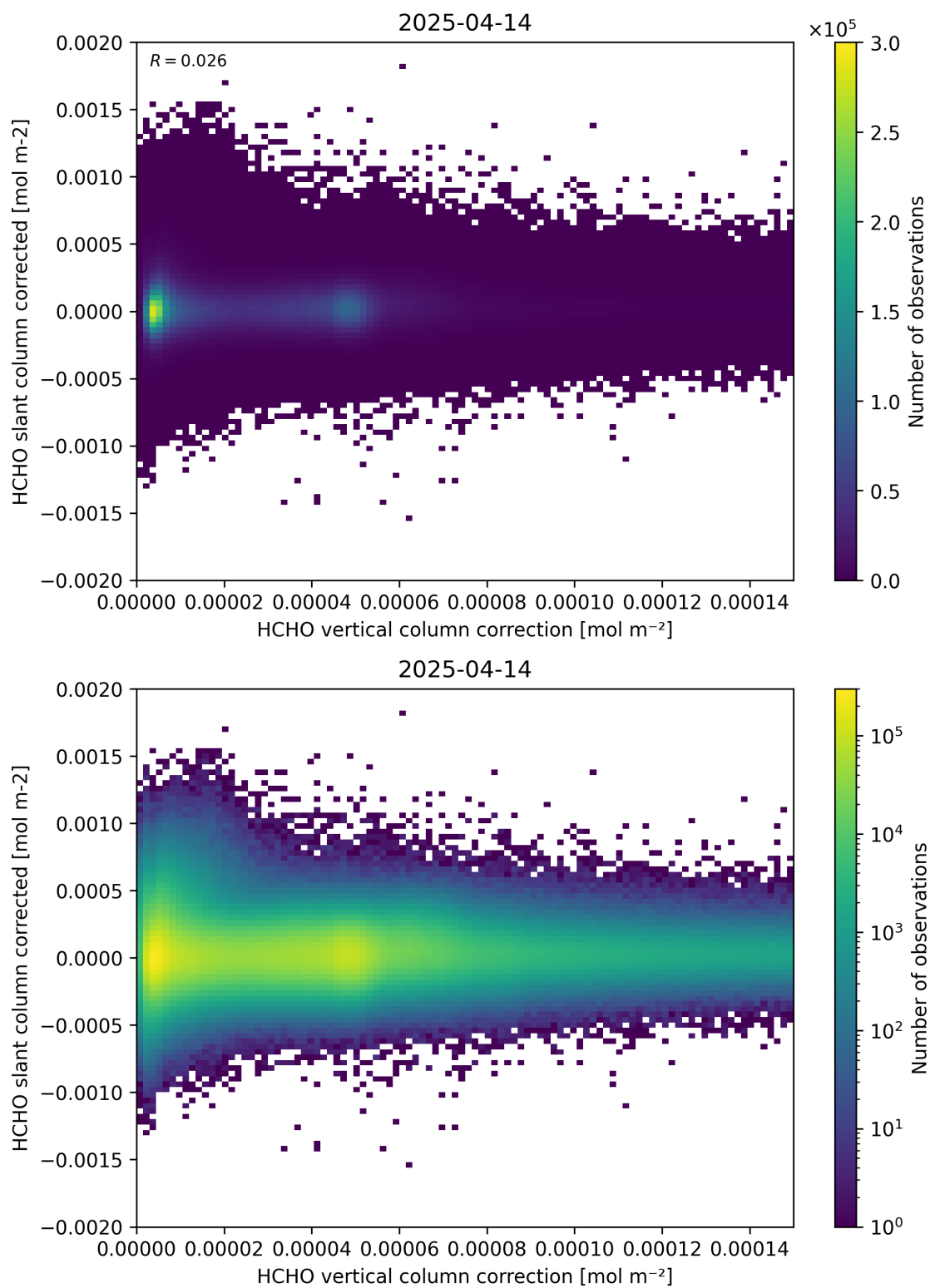
Figure 116: Scatter density plot of “HCHO vertical column correction” against “HCHO slant column corrected” for 2025-04-13 to 2025-04-15.
