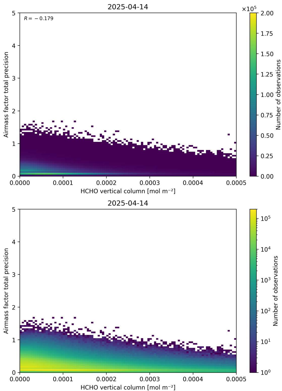
Figure 132: Scatter density plot of “HCHO vertical column” against “Airmass factor total precision” for 2025-04-13 to 2025-04-15.
