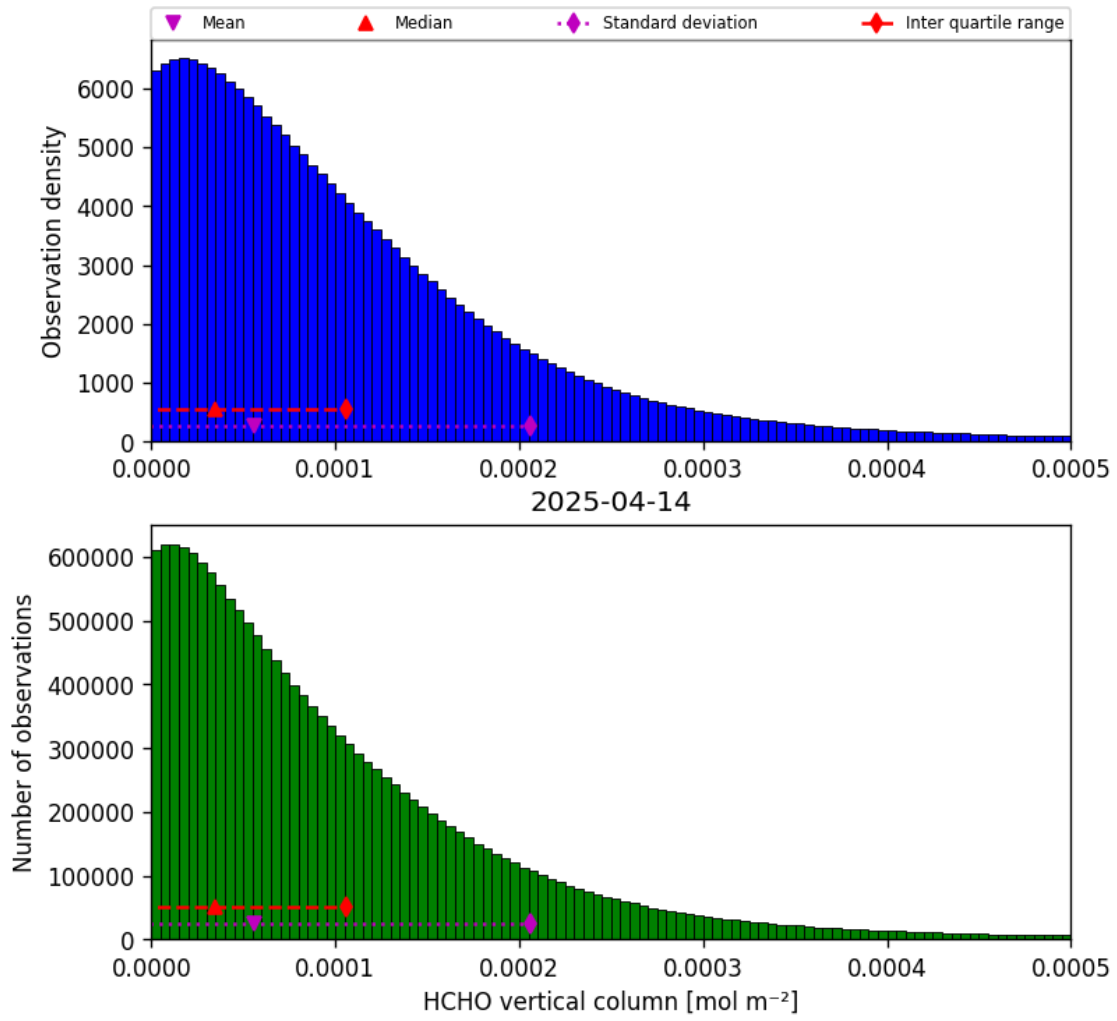
Figure 35: Histogram of “HCHO vertical column” for 2025-04-13 to 2025-04-15
