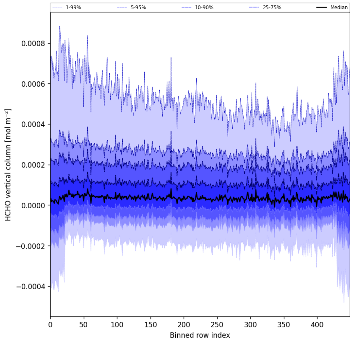
Figure 49: Along track statistics of “HCHO vertical column” for 2025-04-13 to 2025-04-15
