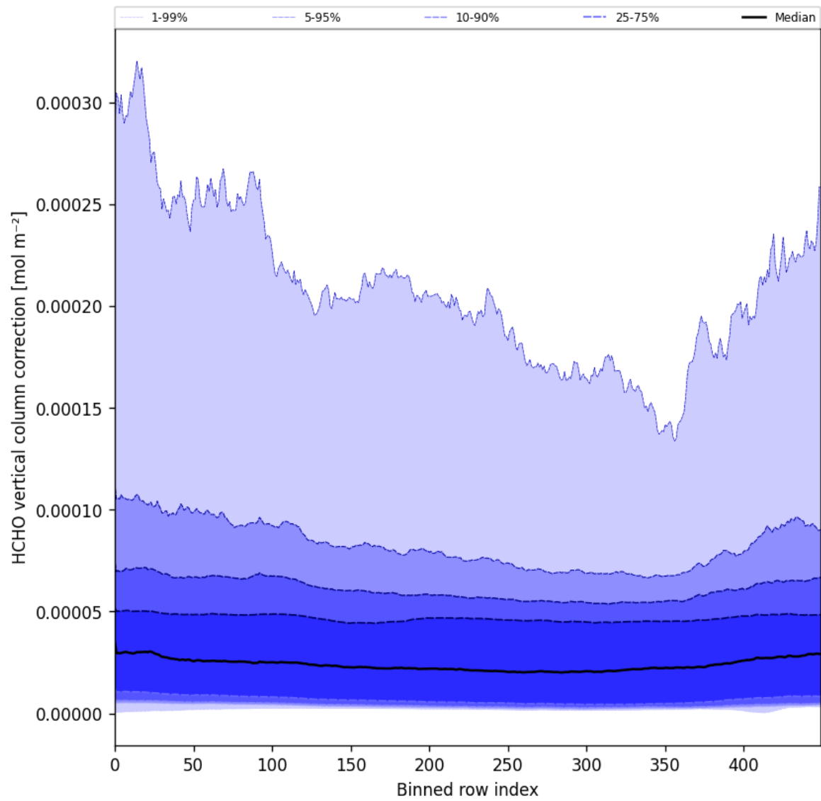
Figure 51: Along track statistics of “HCHO vertical column correction” for 2025-04-13 to 2025-04-15
