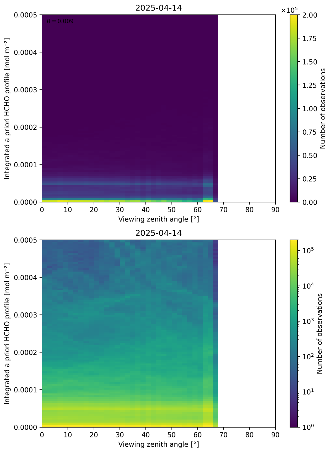
Figure 195: Scatter density plot of “Viewing zenith angle” against “Integrated a priori HCHO profile” for 2025-04-13 to 2025-04-15.
