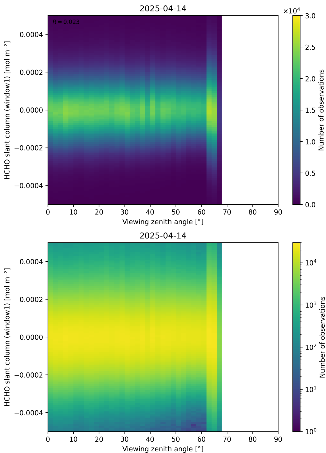
Figure 188: Scatter density plot of “Viewing zenith angle” against “HCHO slant column (window1)” for 2025-04-13 to 2025-04-15.
