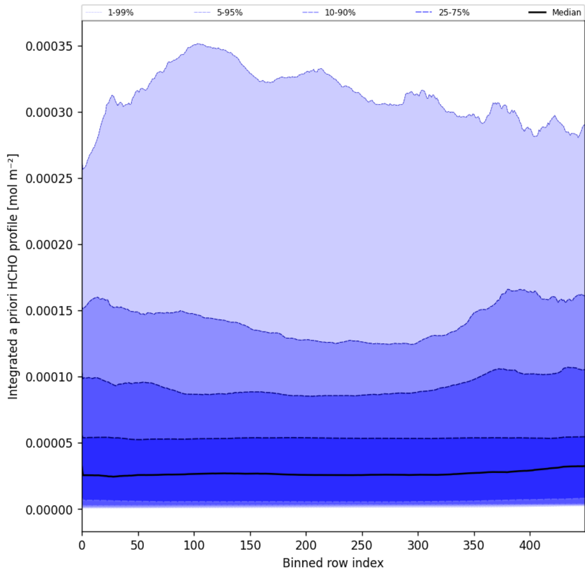
Figure 57: Along track statistics of "Integrated a priori HCHO profile" for 2025-04-13 to 2025-04-15
