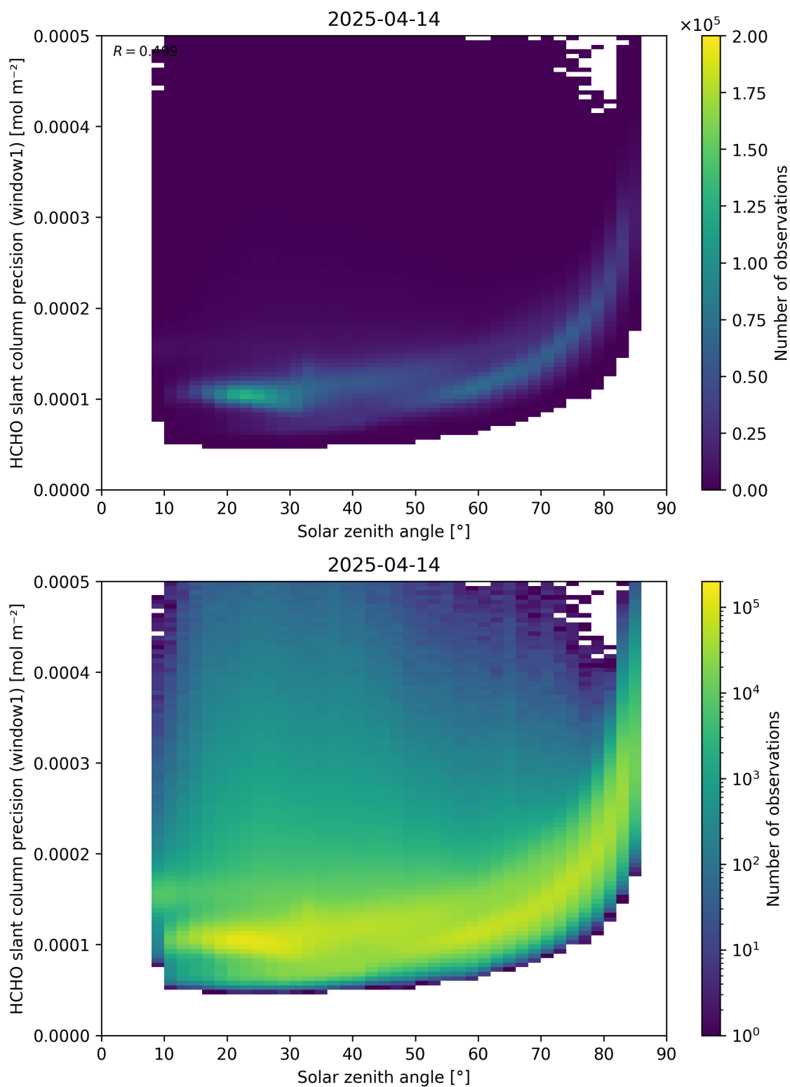
Figure 174: Scatter density plot of “Solar zenith angle” against “HCHO slant column precision (window1)” for 2025-04-13 to 2025-04-15.
