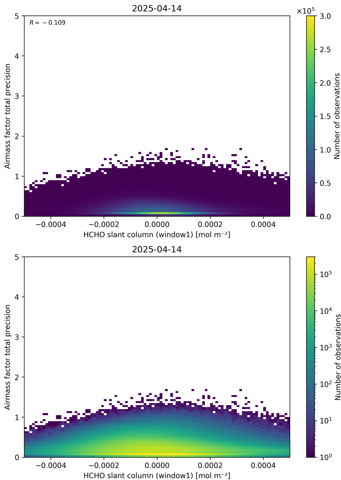
Figure 86: Scatter density plot of “HCHO slant column (window1)” against “Airmass factor total precision” for 2025-04-13 to 2025-04-15.
