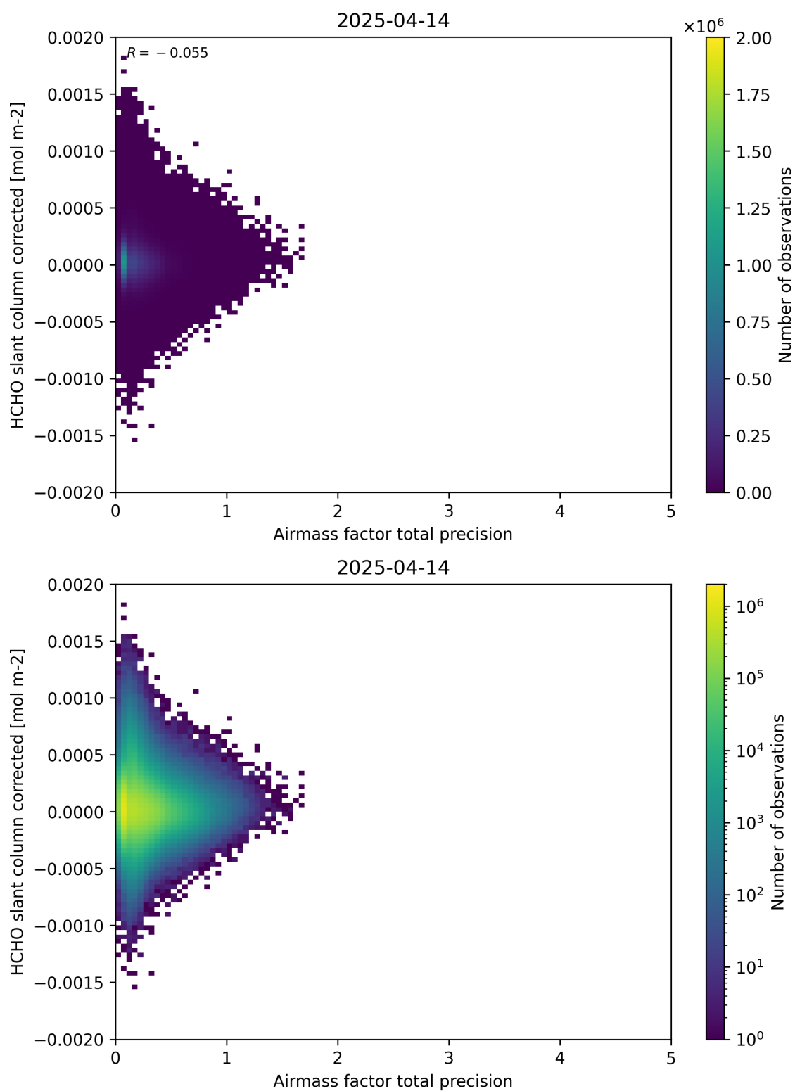
Figure 109: Scatter density plot of “Airmass factor total precision” against “HCHO slant column corrected” for 2025-04-13 to 2025-04-15.
