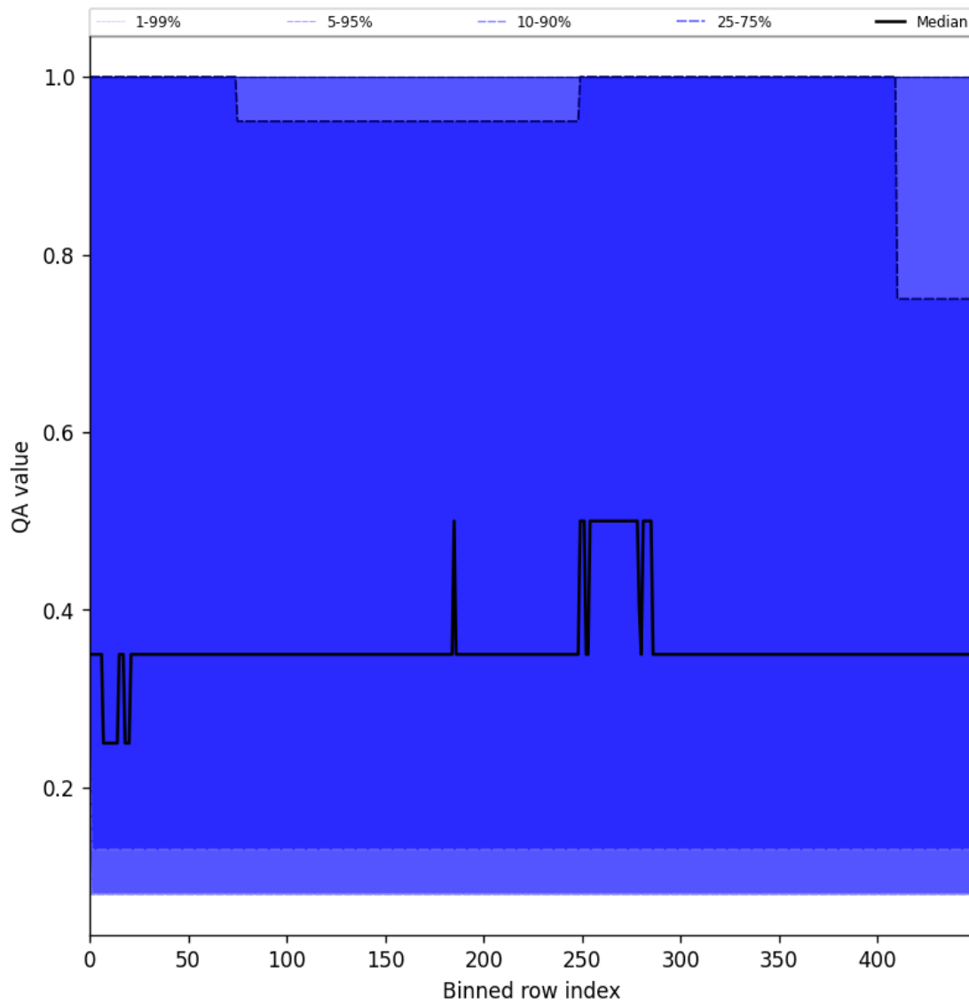
Figure 48: Along track statistics of “QA value” for 2025-04-13 to 2025-04-15
