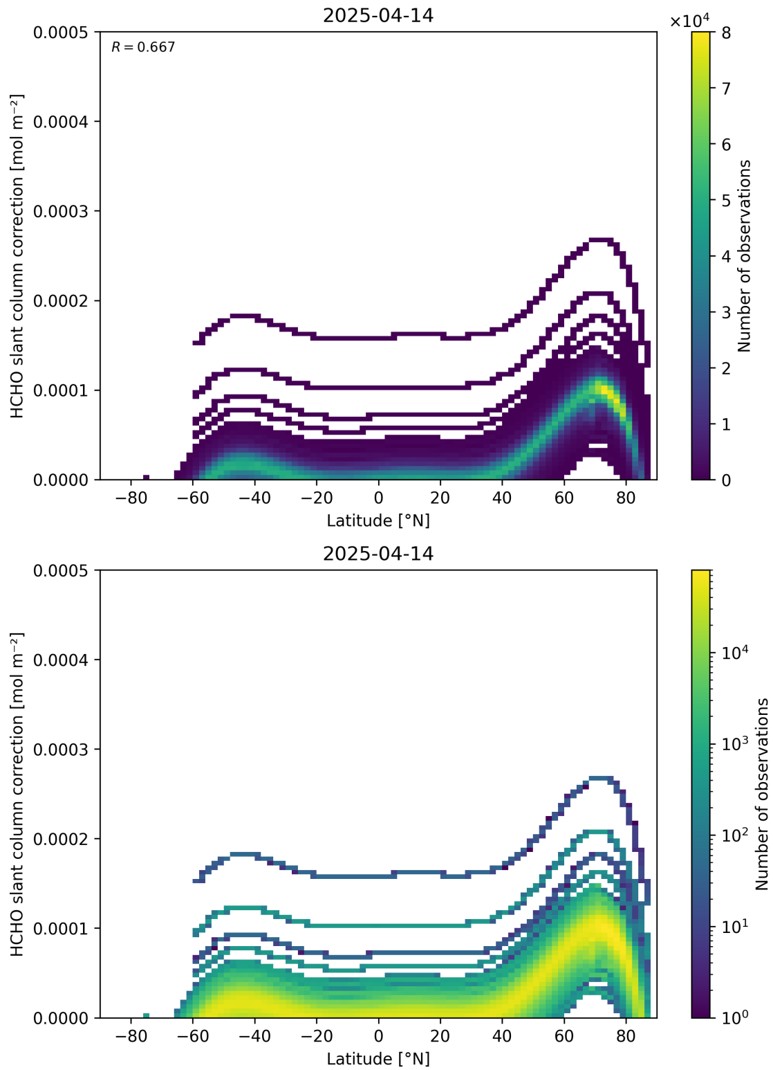
Figure 158: Scatter density plot of “Latitude” against “HCHO slant column correction” for 2025-04-13 to 2025-04-15.
