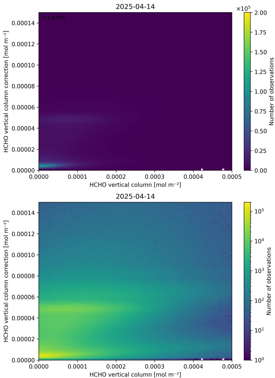
Figure 133: Scatter density plot of “HCHO vertical column” against “HCHO vertical column correction” for 2025-04-13 to 2025-04-15.
