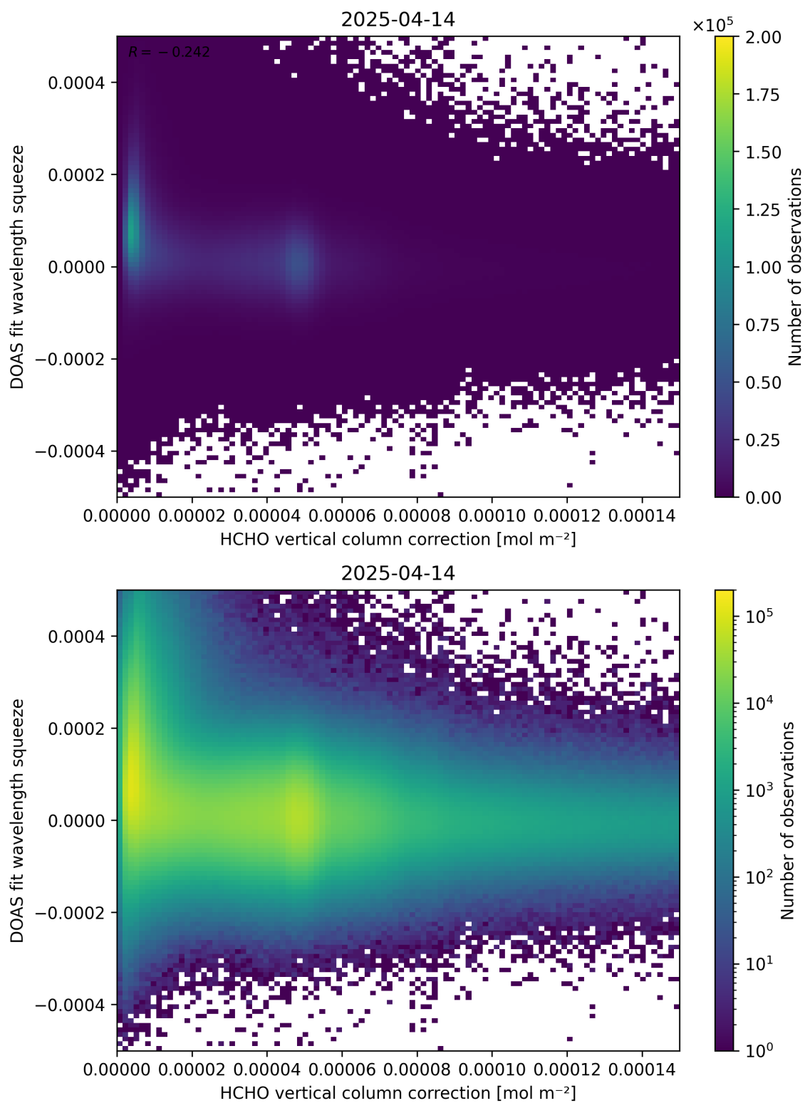
Figure 114: Scatter density plot of “HCHO vertical column correction” against “DOAS fit wavelength squeeze” for 2025-04-13 to 2025-04-15.
