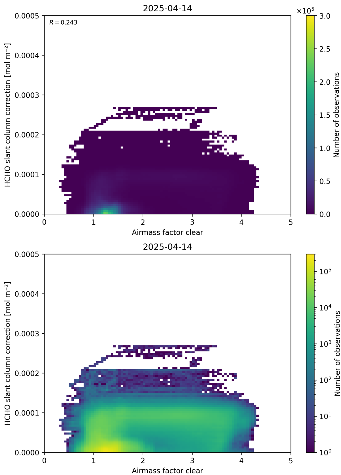
Figure 75: Scatter density plot of “Airmass factor clear” against “HCHO slant column correction” for 2025-04-13 to 2025-04-15.
