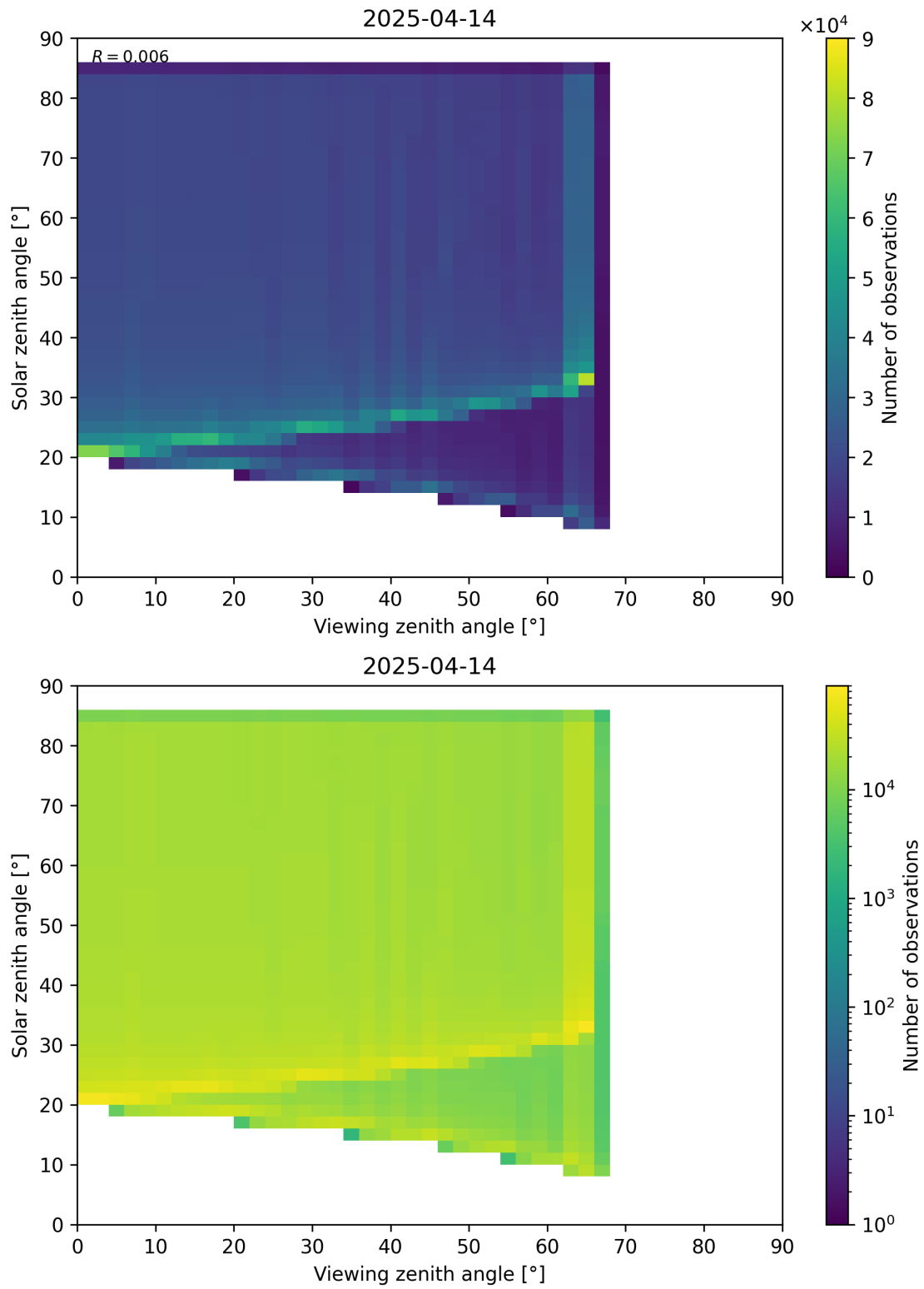
Figure 197: Scatter density plot of “Viewing zenith angle” against “Solar zenith angle” for 2025-04-13 to 2025-04-15.
