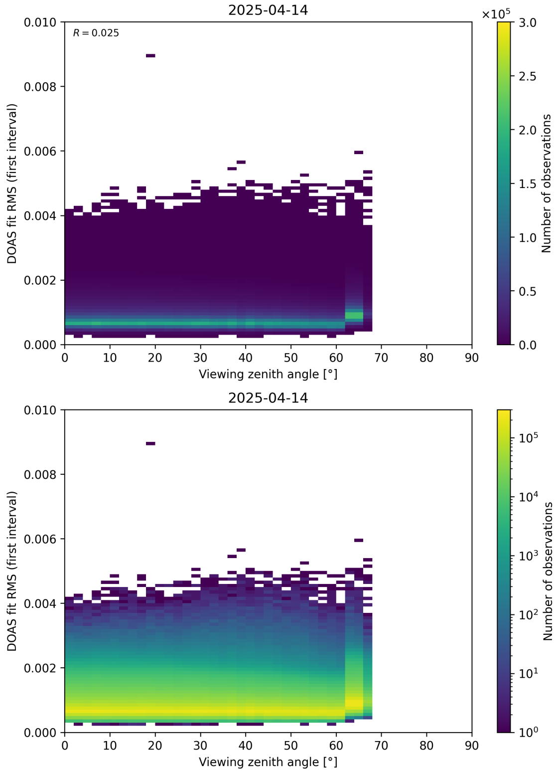
Figure 182: Scatter density plot of “Viewing zenith angle” against “DOAS fit RMS (first interval)” for 2025-04-13 to 2025-04-15.
