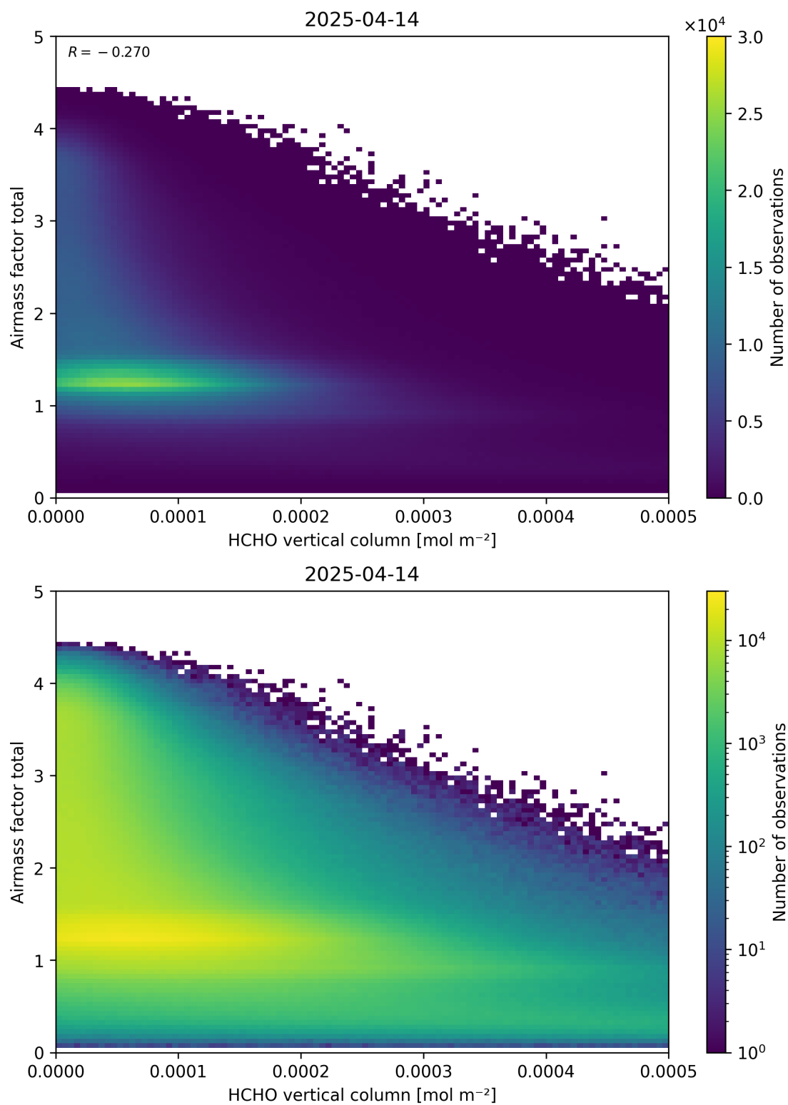
Figure 131: Scatter density plot of “HCHO vertical column” against “Airmass factor total” for 2025-04-13 to 2025-04-15.
