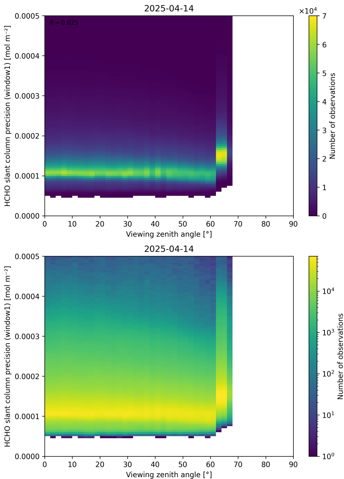
Figure 189: Scatter density plot of “Viewing zenith angle” against “HCHO slant column precision (window1)” for 2025-04-13 to 2025-04-15.
