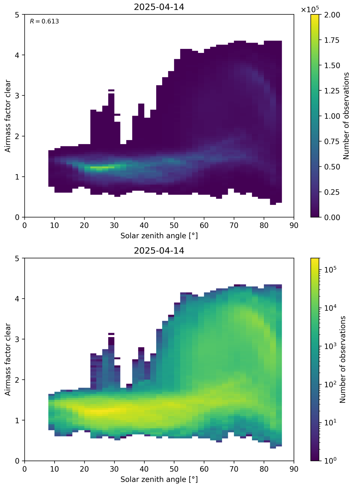
Figure 170: Scatter density plot of “Solar zenith angle” against “Airmass factor clear” for 2025-04-13 to 2025-04-15.
