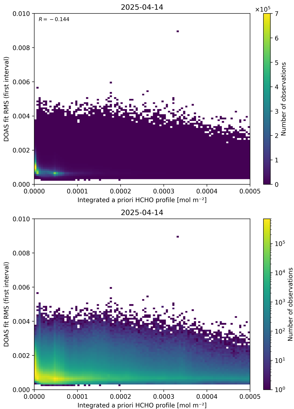
Figure 148: Scatter density plot of “Integrated a priori HCHO profile” against “DOAS fit RMS (first interval)” for 2025-04-13 to 2025-04-15.
