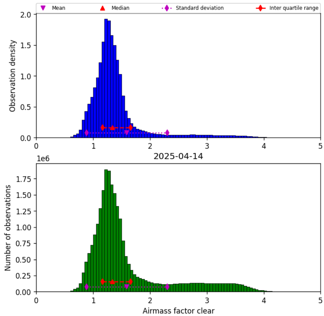
Figure 42: Histogram of “Airmass factor clear” for 2025-04-13 to 2025-04-15
