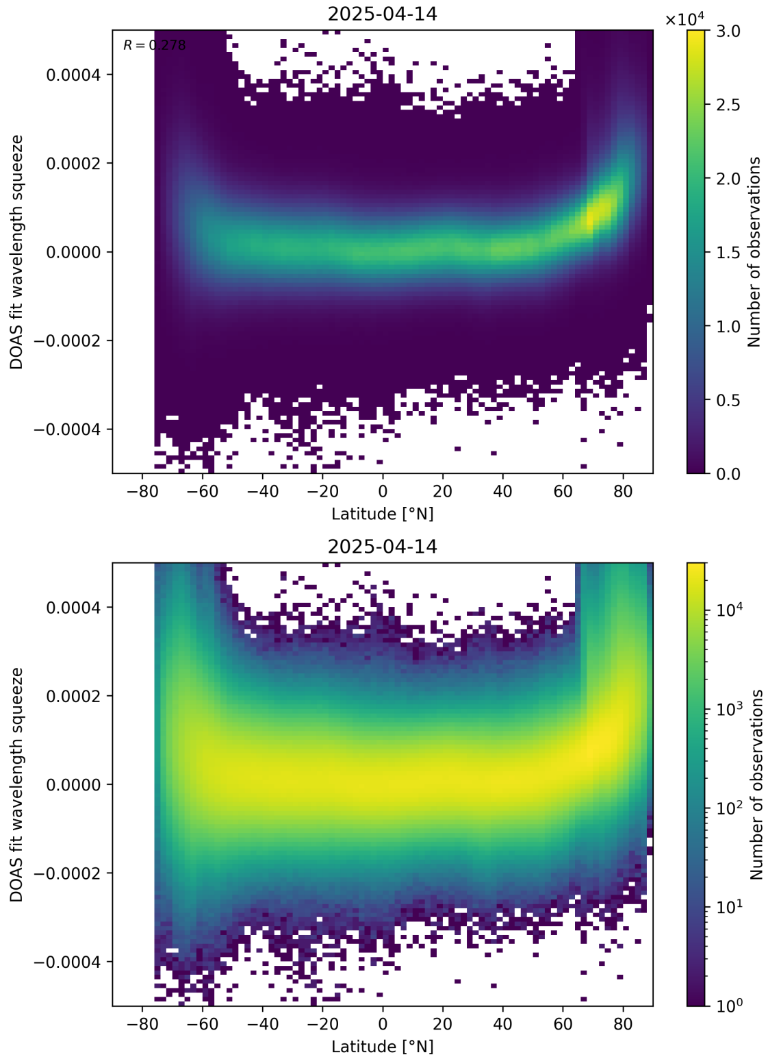
Figure 155: Scatter density plot of “Latitude” against “DOAS fit wavelength squeeze” for 2025-04-13 to 2025-04-15.
