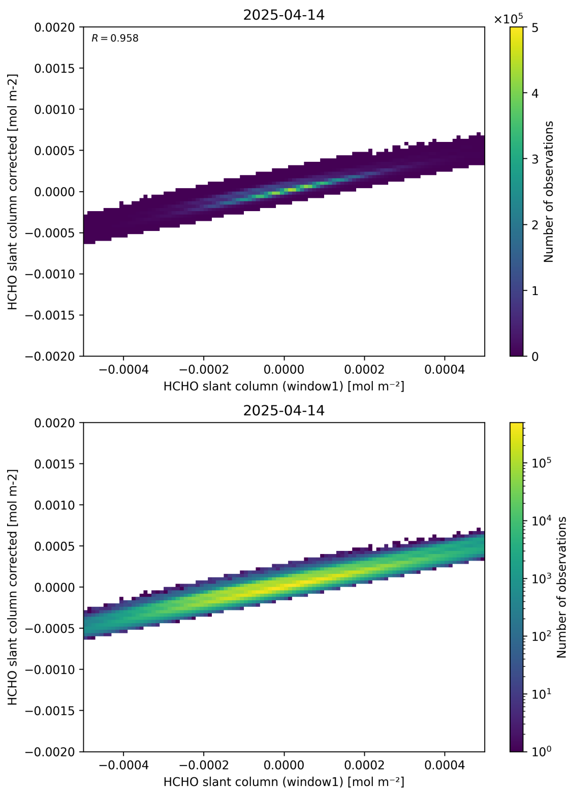
Figure 82: Scatter density plot of “HCHO slant column (window1)” against “HCHO slant column corrected” for 2025-04-13 to 2025-04-15.
