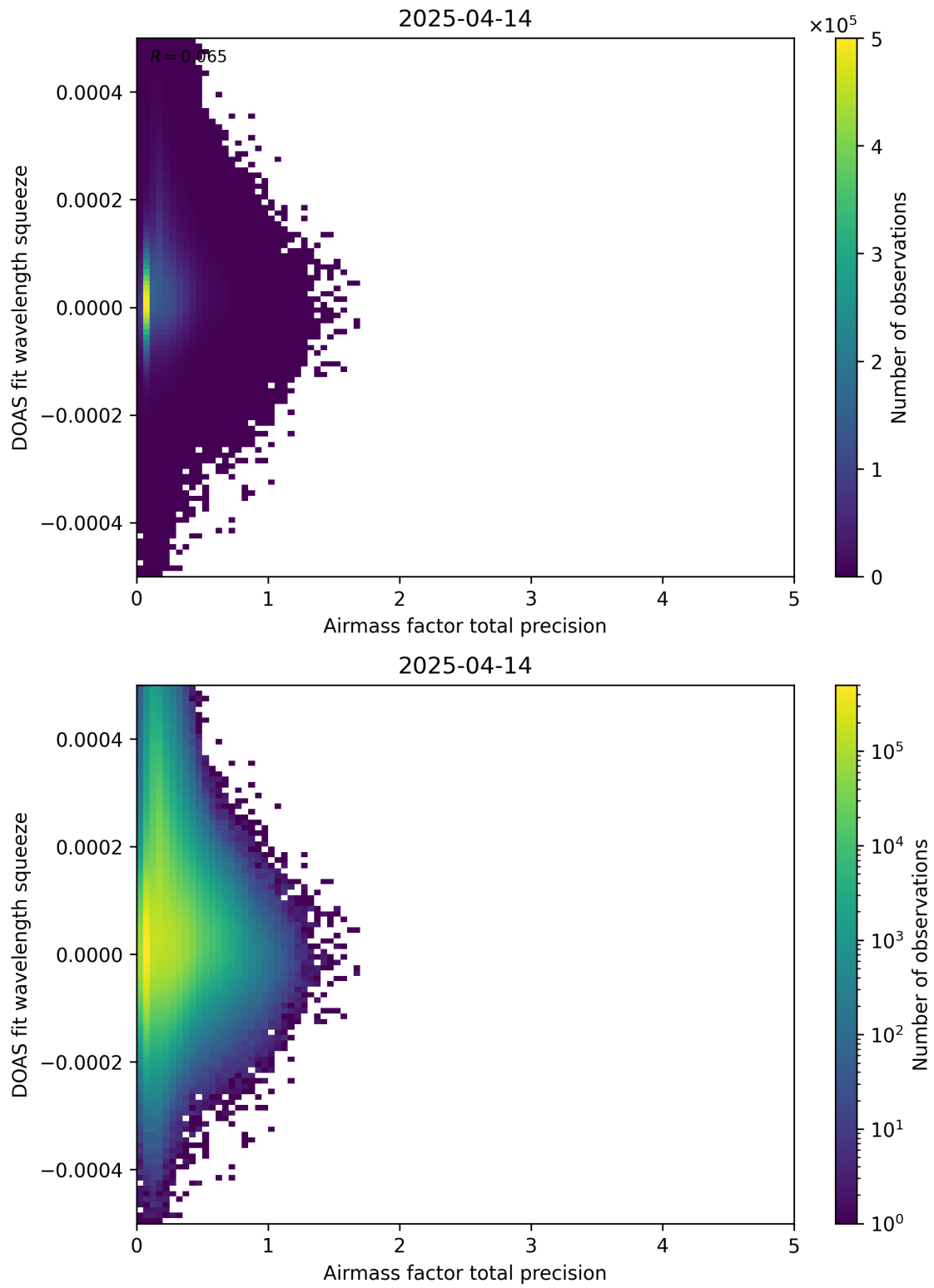
Figure 107: Scatter density plot of “Airmass factor total precision” against “DOAS fit wavelength squeeze” for 2025-04-13 to 2025-04-15.
