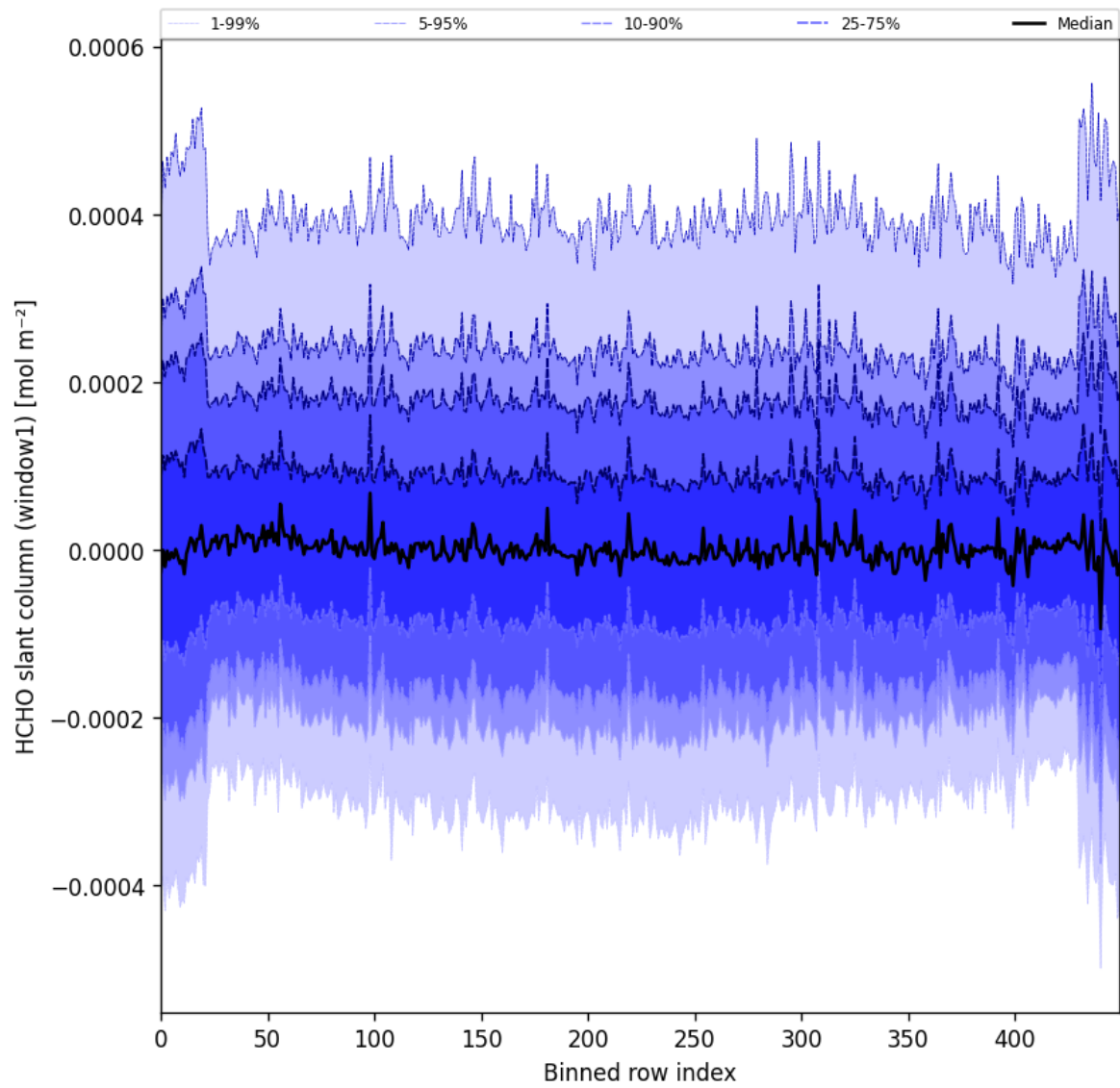
Figure 52: Along track statistics of “HCHO slant column (window1)” for 2025-04-13 to 2025-04-15
