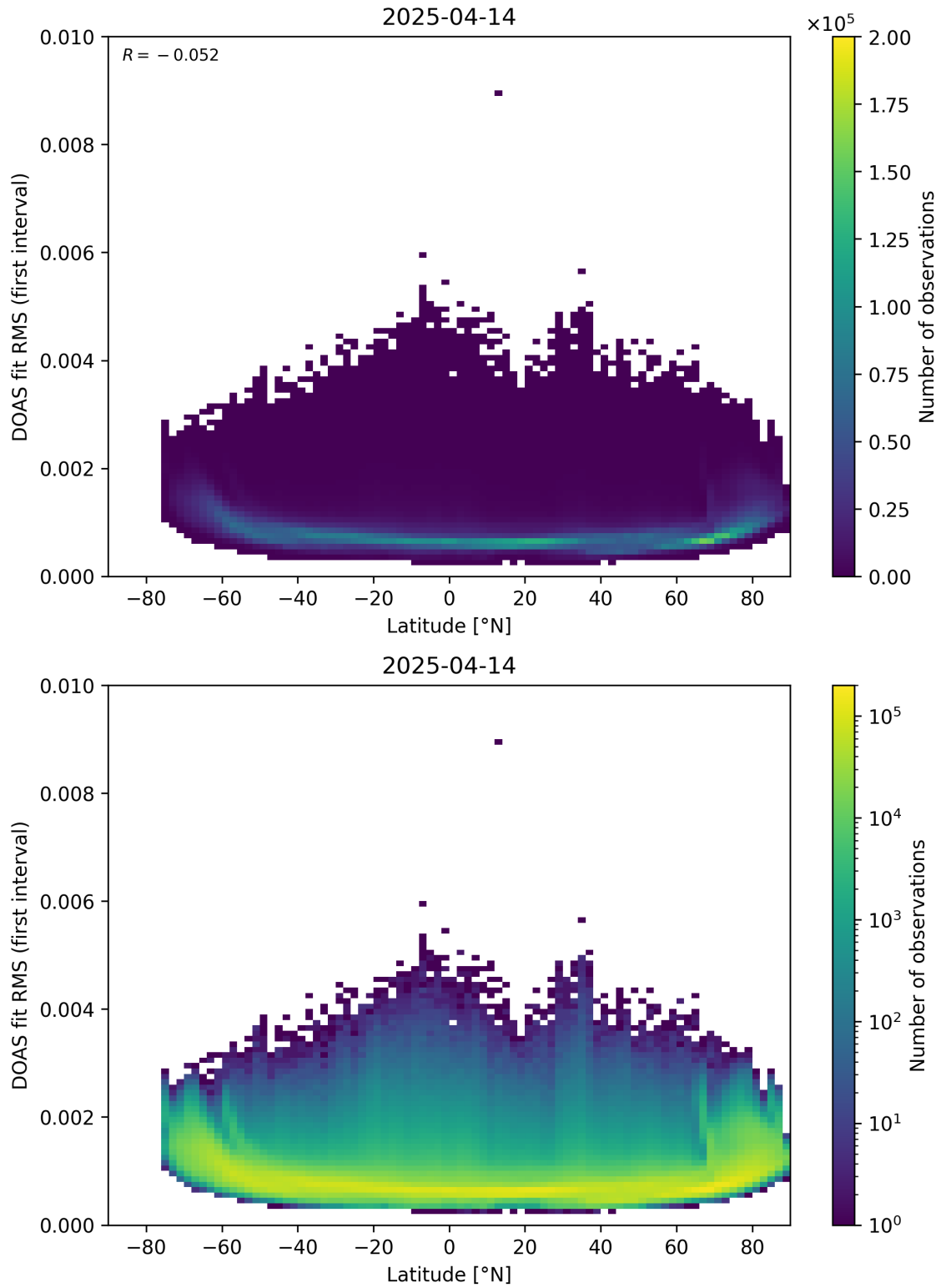
Figure 153: Scatter density plot of “Latitude” against “DOAS fit RMS (first interval)” for 2025-04-13 to 2025-04-15.
