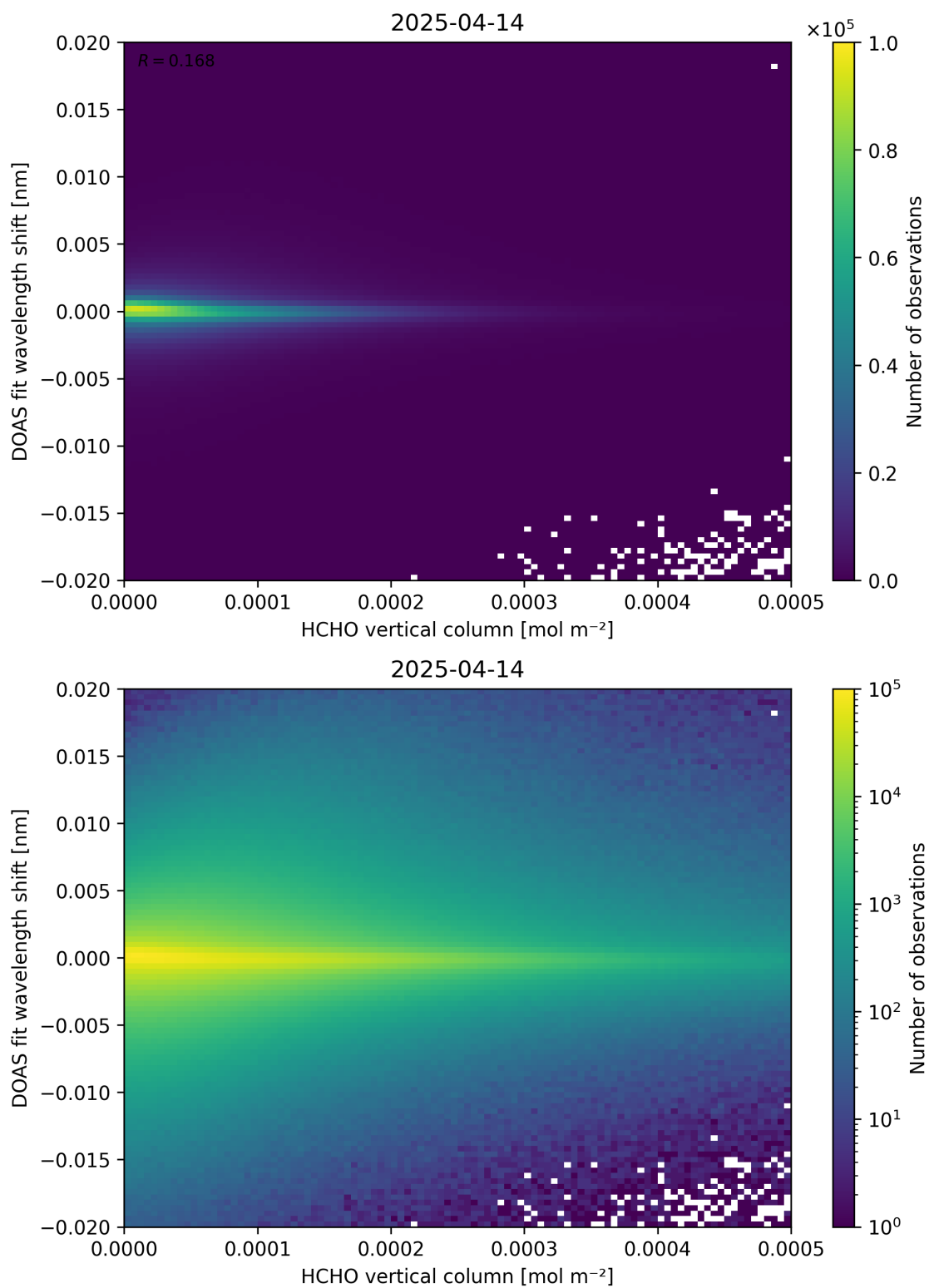
Figure 124: Scatter density plot of “HCHO vertical column” against “DOAS fit wavelength shift” for 2025-04-13 to 2025-04-15.
