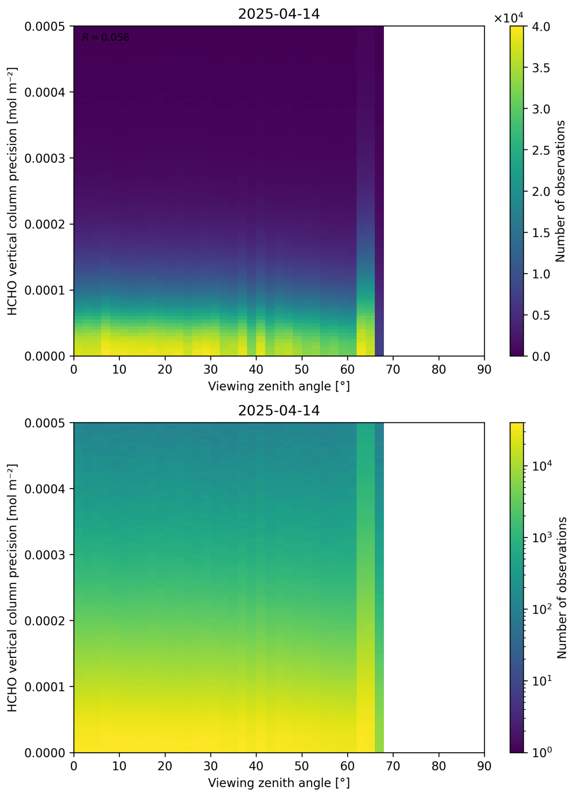
Figure 194: Scatter density plot of “Viewing zenith angle” against “HCHO vertical column precision” for 2025-04-13 to 2025-04-15.
