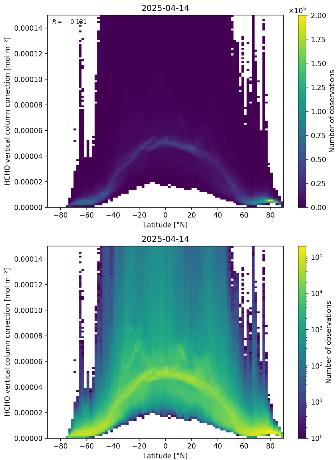
Figure 164: Scatter density plot of “Latitude” against “HCHO vertical column correction” for 2025-04-13 to 2025-04-15.
