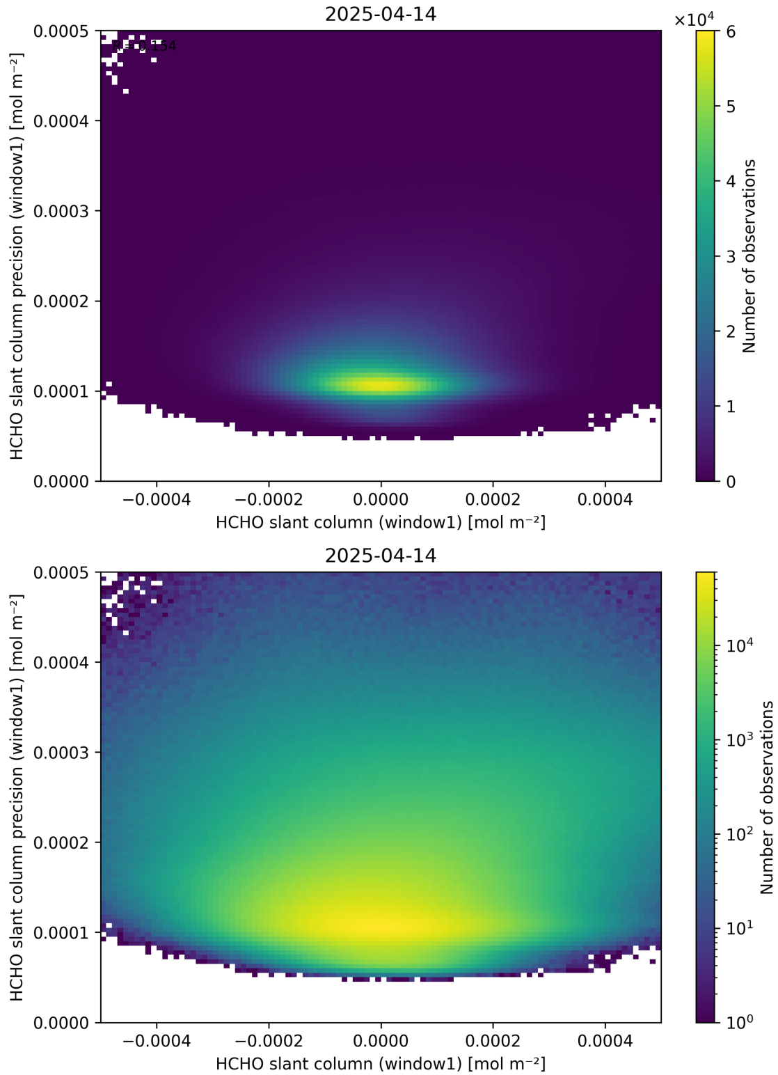
Figure 84: Scatter density plot of “HCHO slant column (window1)” against “HCHO slant column precision (window1)” for 2025-04-13 to 2025-04-15.
