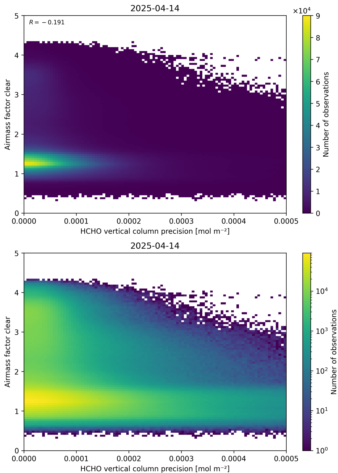
Figure 139: Scatter density plot of “HCHO vertical column precision” against “Airmass factor clear” for 2025-04-13 to 2025-04-15.
