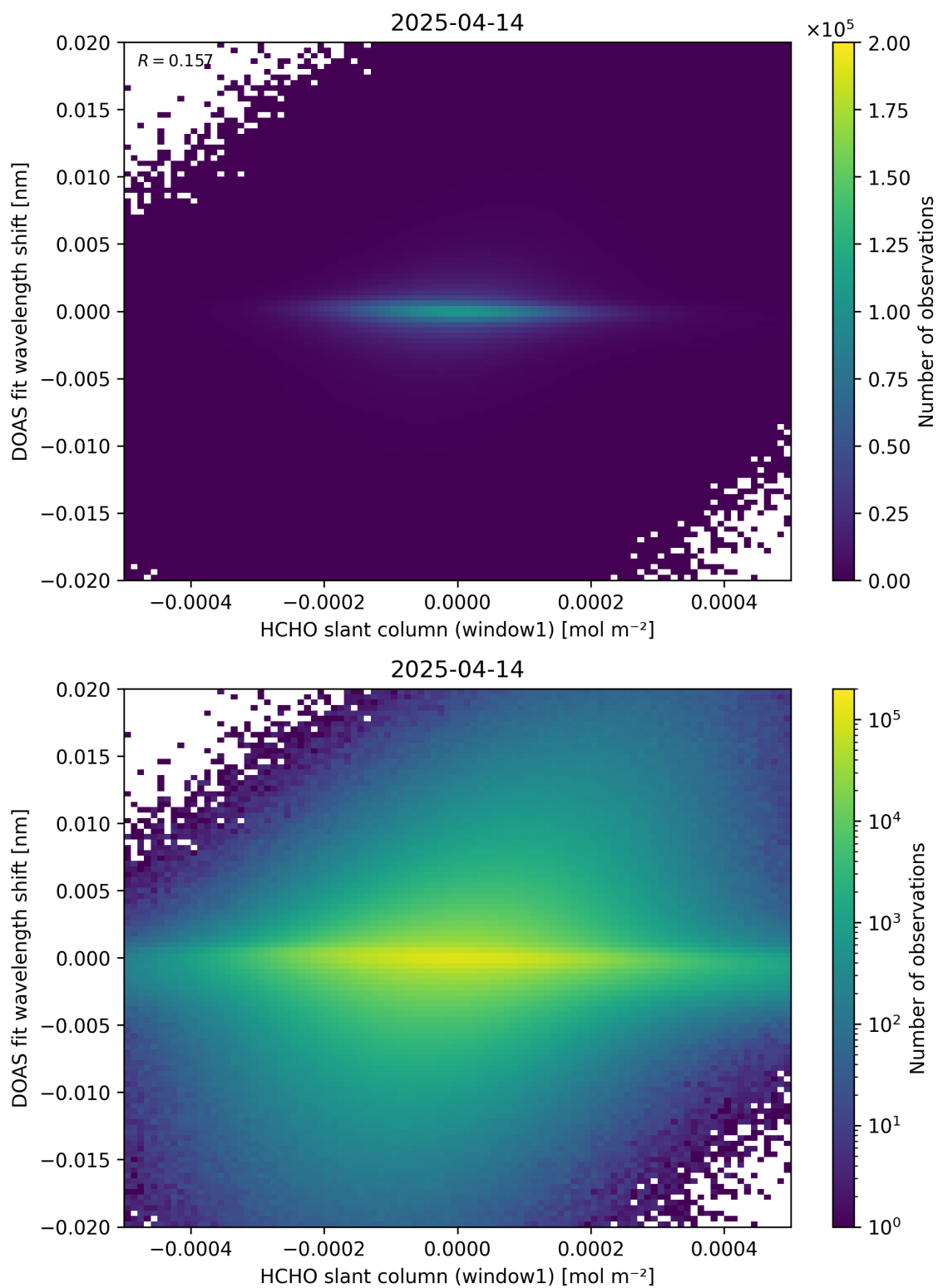
Figure 79: Scatter density plot of “HCHO slant column (window1)” against “DOAS fit wavelength shift” for 2025-04-13 to 2025-04-15.
