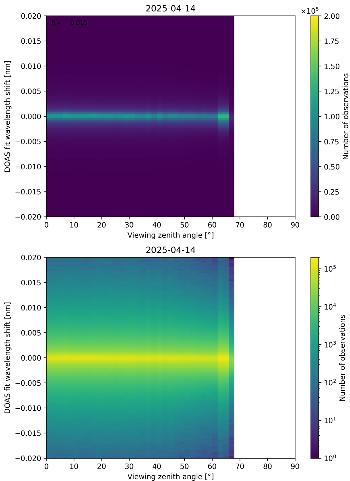
Figure 183: Scatter density plot of “Viewing zenith angle” against “DOAS fit wavelength shift” for 2025-04-13 to 2025-04-15.
