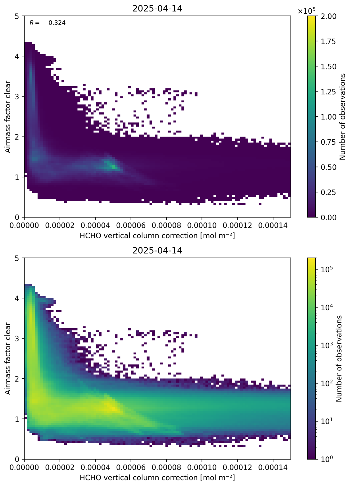
Figure 115: Scatter density plot of “HCHO vertical column correction” against “Airmass factor clear” for 2025-04-13 to 2025-04-15.
