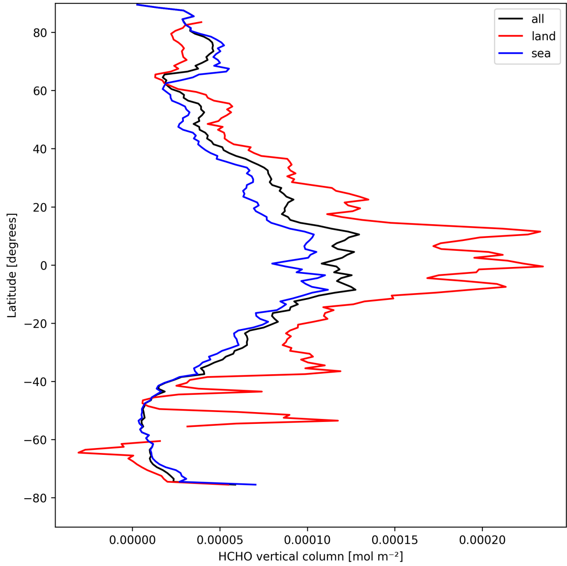
Figure 21: Zonal average of “HCHO vertical column” for 2025-04-13 to 2025-04-15.
