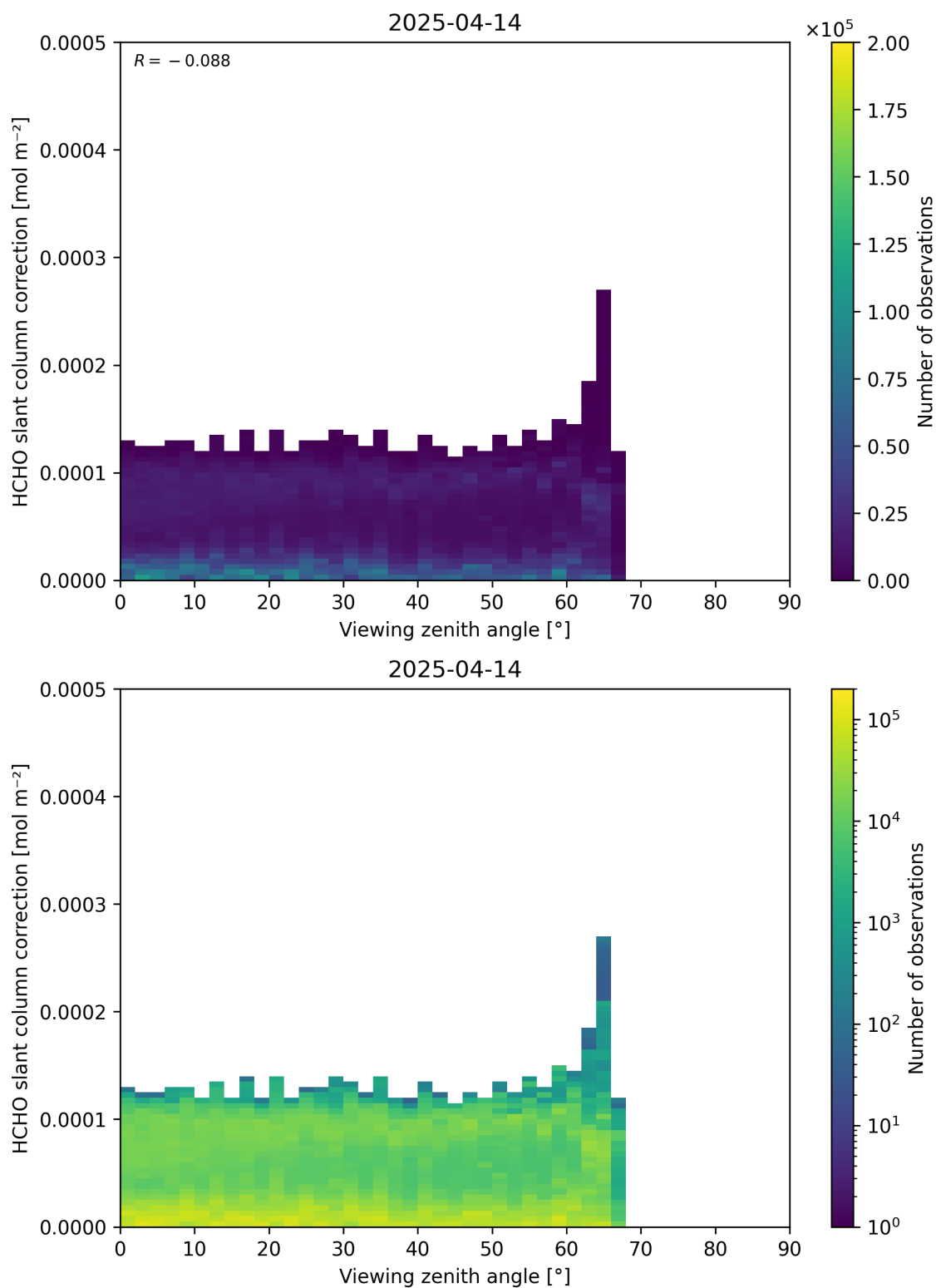
Figure 187: Scatter density plot of “Viewing zenith angle” against “HCHO slant column correction” for 2025-04-13 to 2025-04-15.
