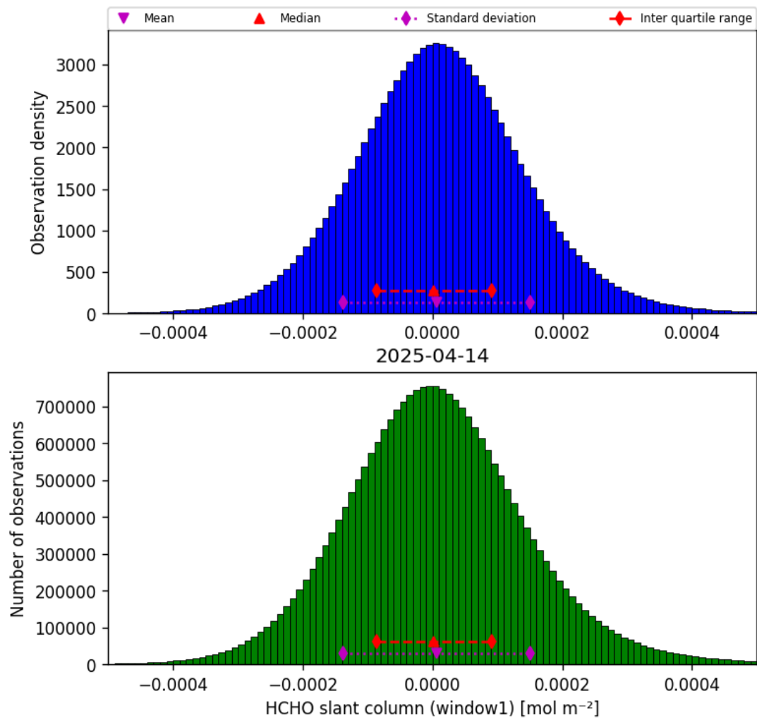
Figure 38: Histogram of “HCHO slant column (window1)” for 2025-04-13 to 2025-04-15
