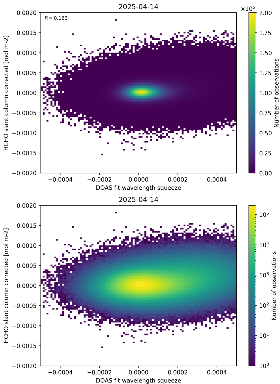
Figure 69: Scatter density plot of “DOAS fit wavelength squeeze” against “HCHO slant column corrected” for 2025-04-13 to 2025-04-15.
