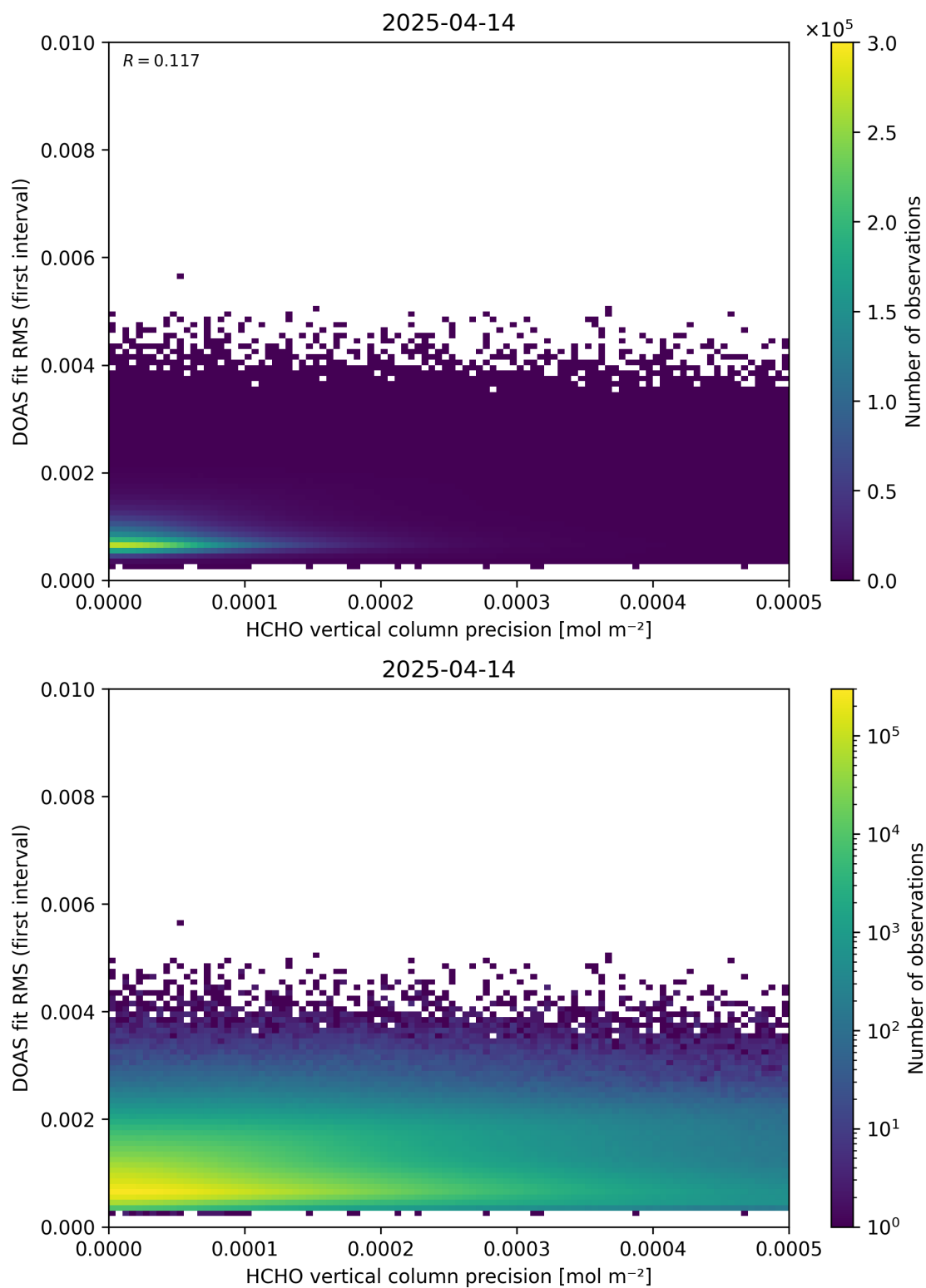
Figure 136: Scatter density plot of “HCHO vertical column precision” against “DOAS fit RMS (first interval)” for 2025-04-13 to 2025-04-15.
