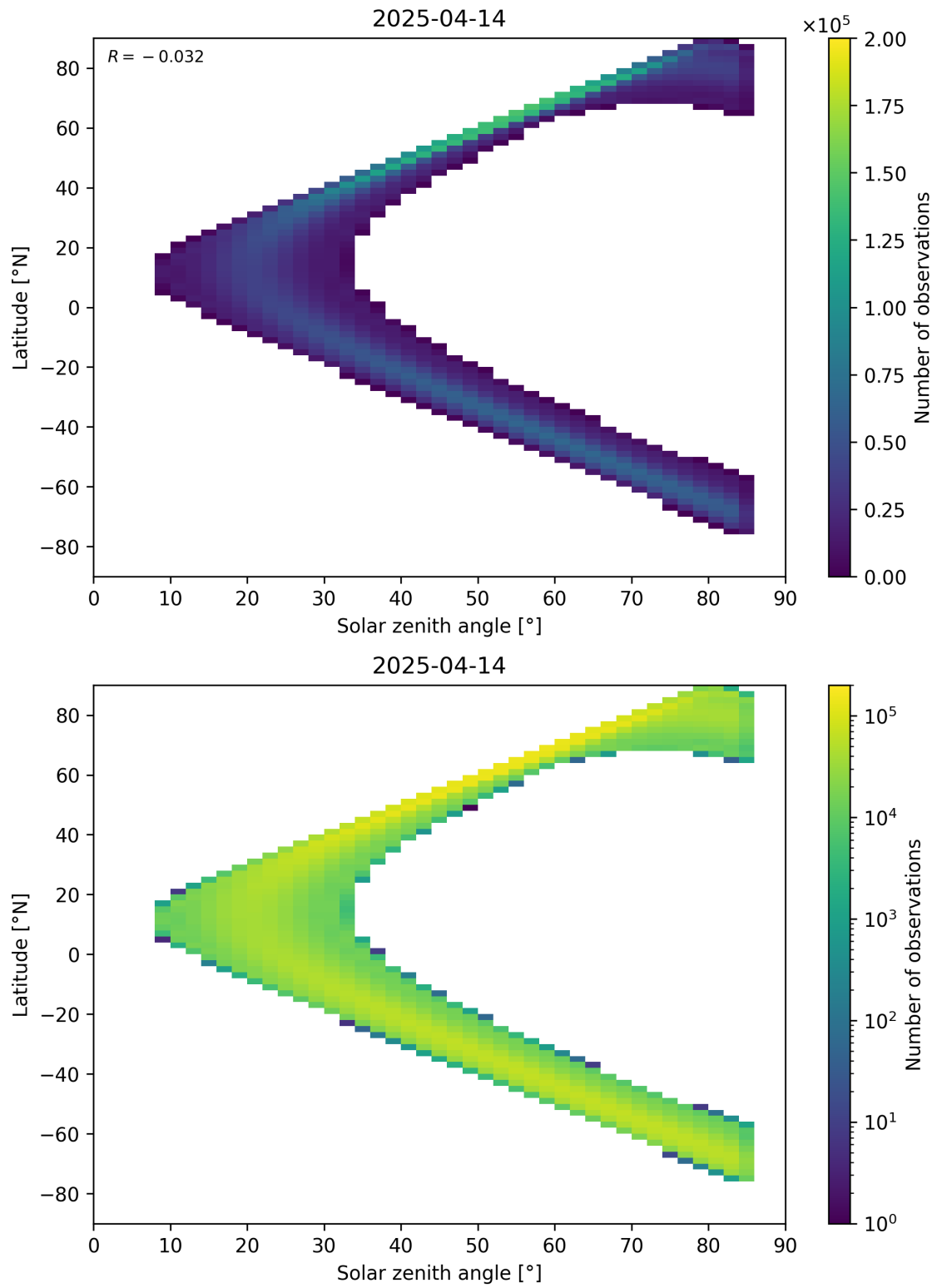
Figure 181: Scatter density plot of “Solar zenith angle” against “Latitude” for 2025-04-13 to 2025-04-15.
