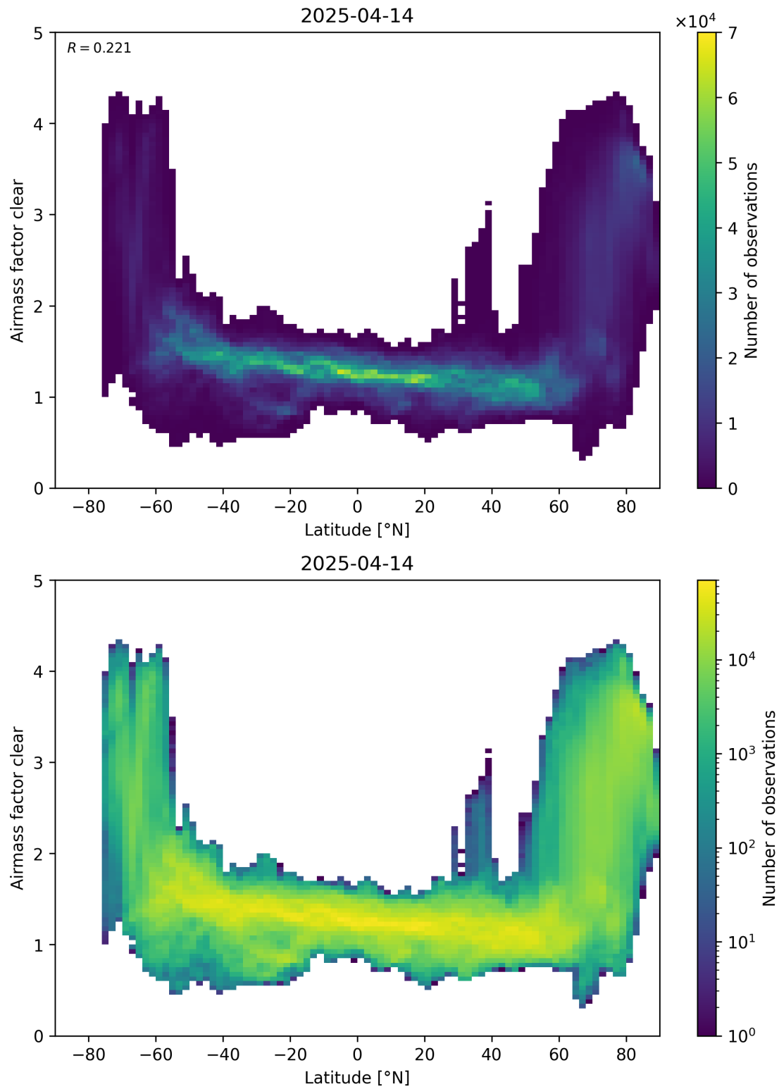
Figure 156: Scatter density plot of “Latitude” against “Airmass factor clear” for 2025-04-13 to 2025-04-15.
