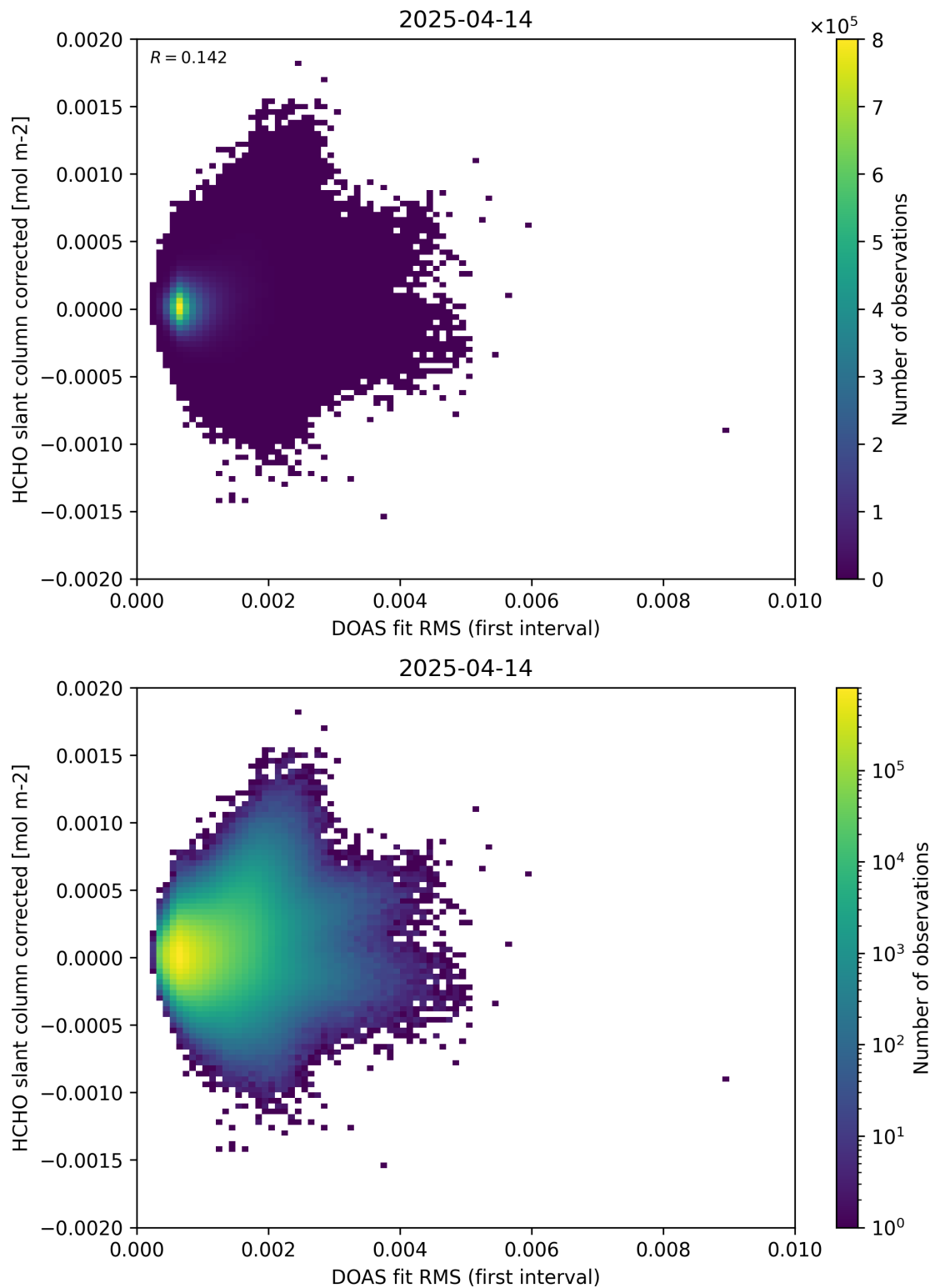
Figure 62: Scatter density plot of “DOAS fit RMS (first interval)” against “HCHO slant column corrected” for 2025-04-13 to 2025-04-15.
