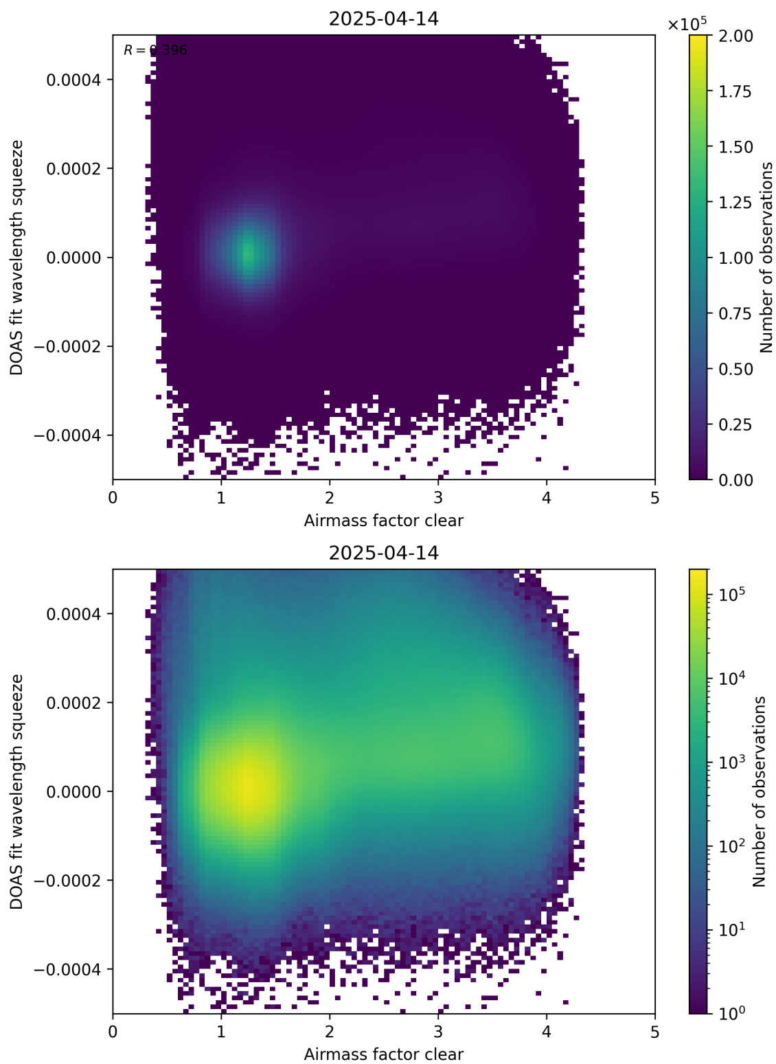
Figure 73: Scatter density plot of “Airmass factor clear” against “DOAS fit wavelength squeeze” for 2025-04-13 to 2025-04-15.
