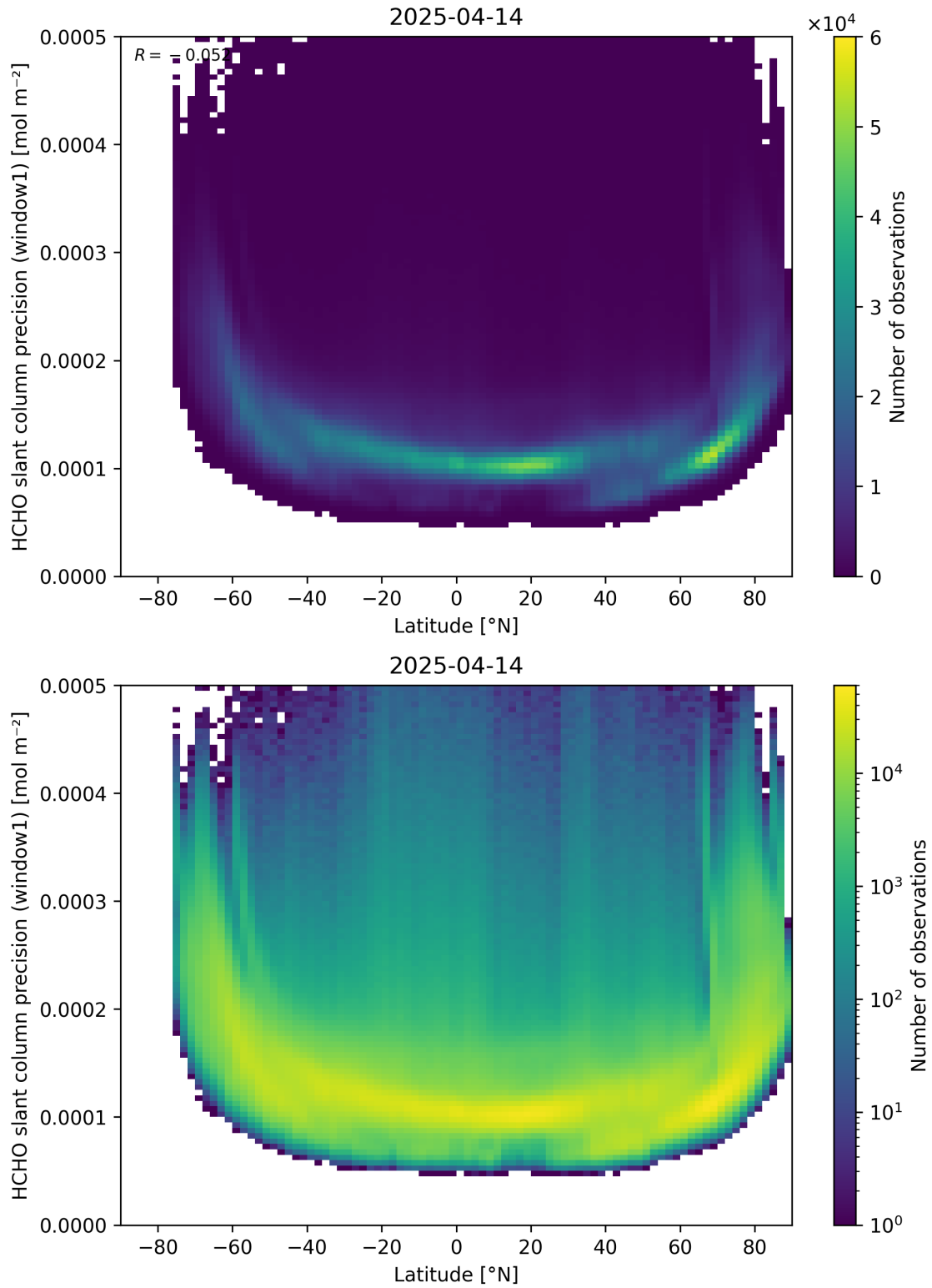
Figure 160: Scatter density plot of “Latitude” against “HCHO slant column precision (window1)” for 2025-04-13 to 2025-04-15.
