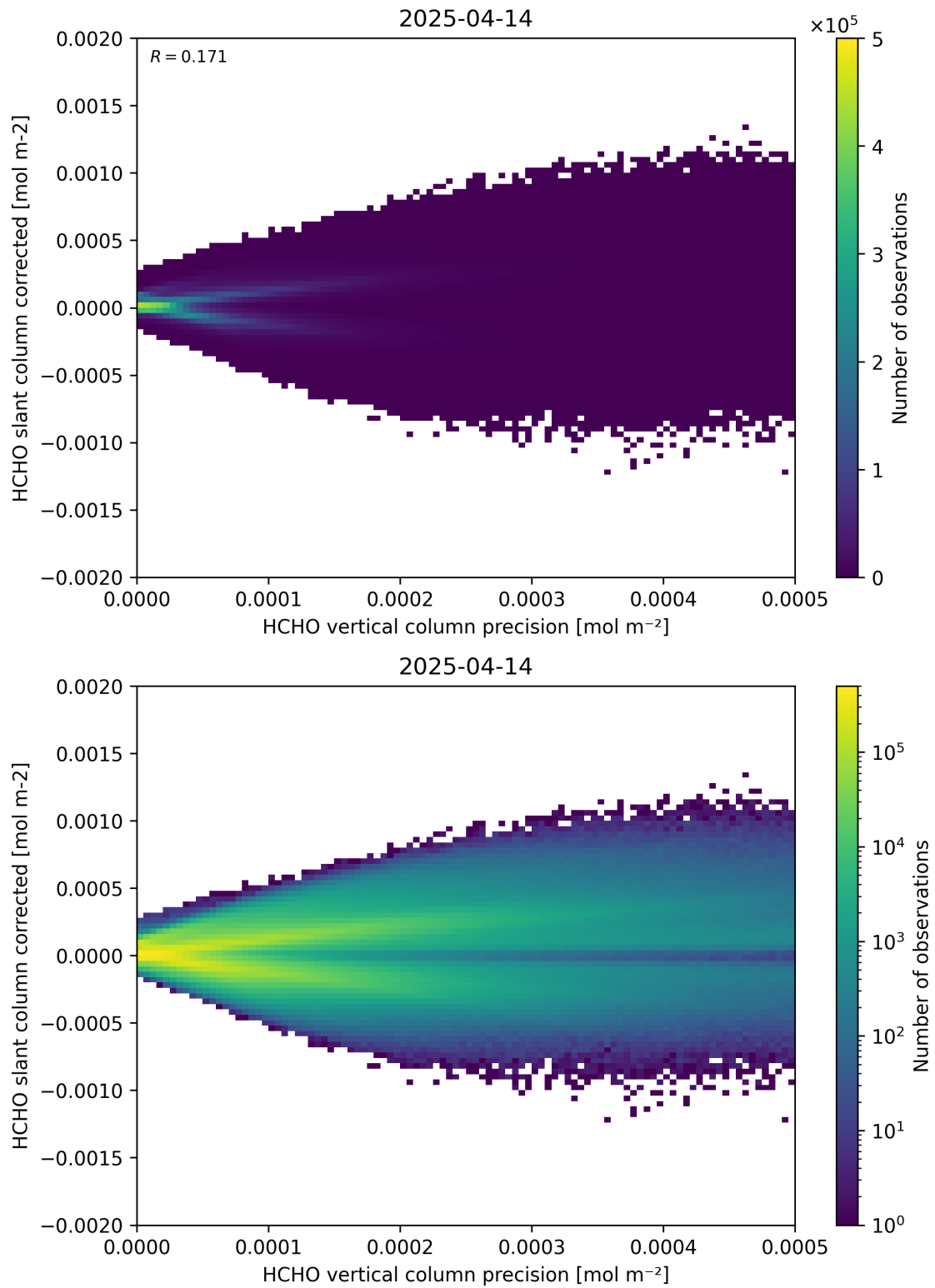
Figure 140: Scatter density plot of “HCHO vertical column precision” against “HCHO slant column corrected” for 2025-04-13 to 2025-04-15.
