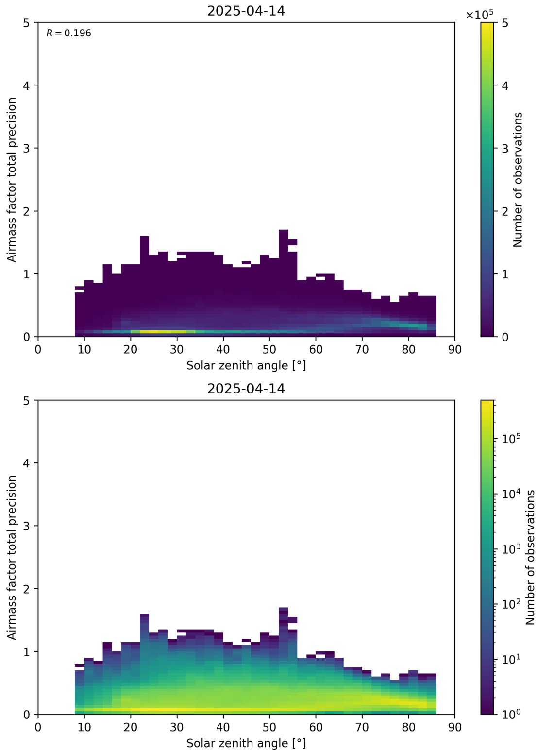
Figure 176: Scatter density plot of “Solar zenith angle” against “Airmass factor total precision” for 2025-04-13 to 2025-04-15.
