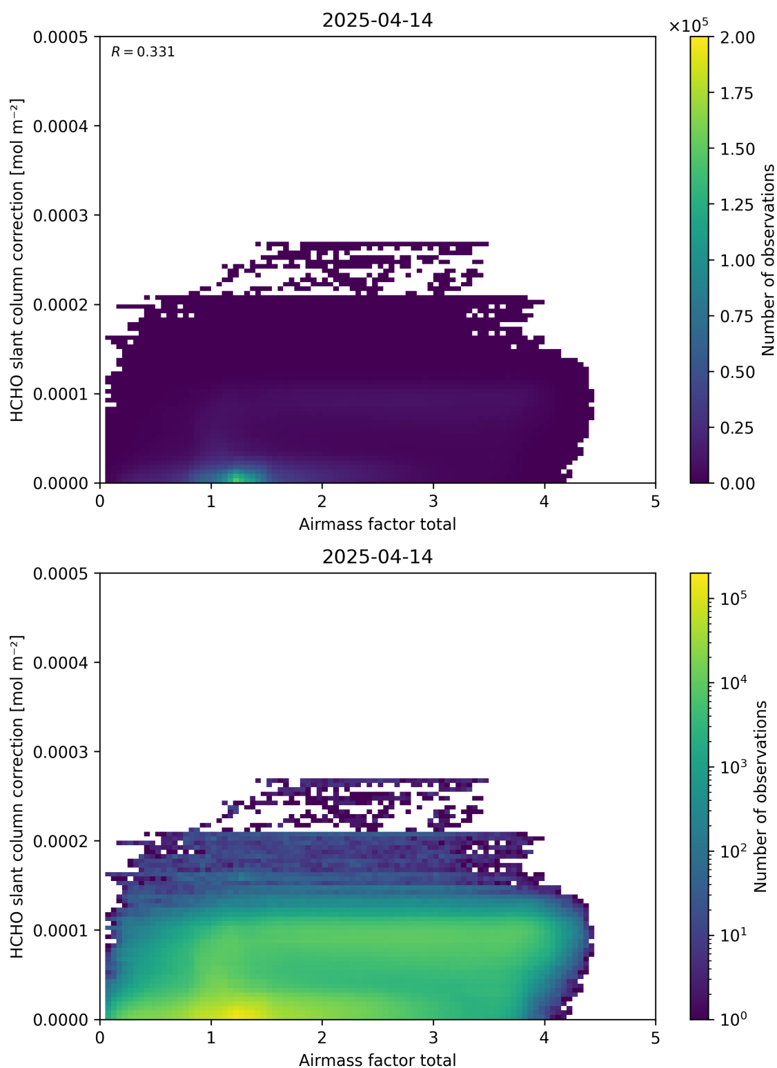
Figure 102: Scatter density plot of “Airmass factor total” against “HCHO slant column correction” for 2025-04-13 to 2025-04-15.
