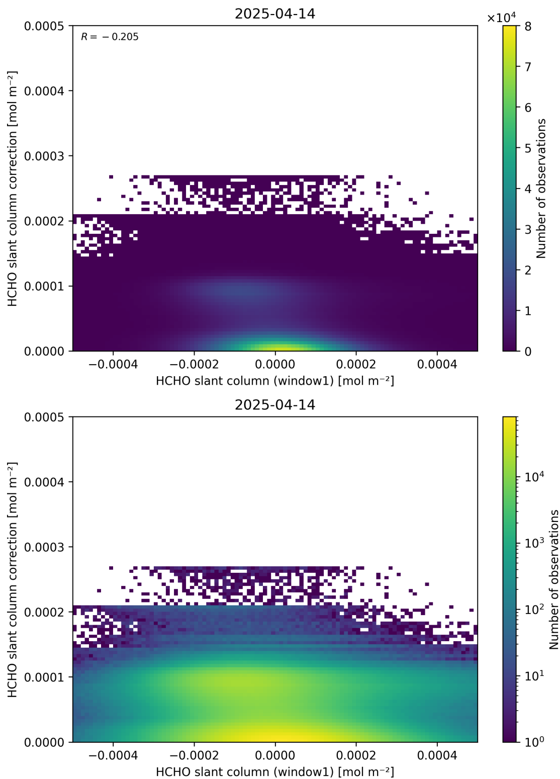
Figure 83: Scatter density plot of “HCHO slant column (window1)” against “HCHO slant column correction” for 2025-04-13 to 2025-04-15.
