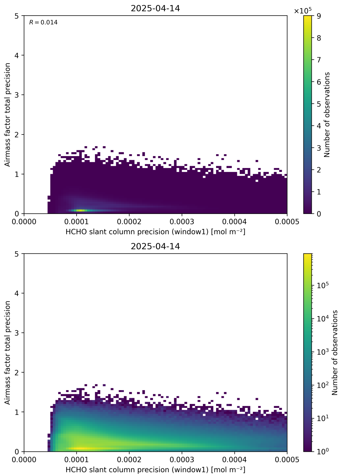
Figure 95: Scatter density plot of “HCHO slant column precision (window1)” against “Airmass factor total precision” for 2025-04-13 to 2025-04-15.
