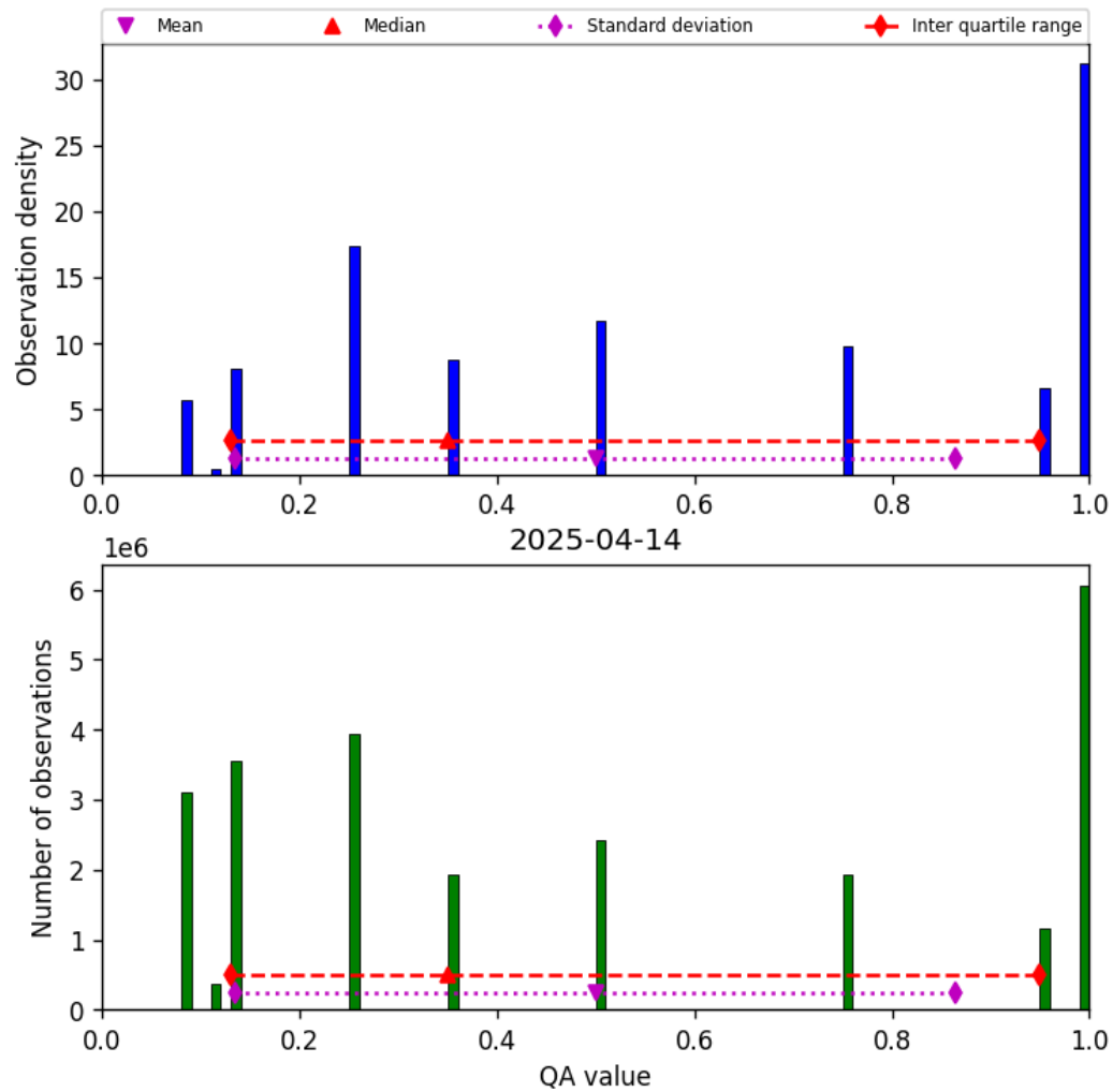
Figure 34: Histogram of “QA value” for 2025-04-13 to 2025-04-15
