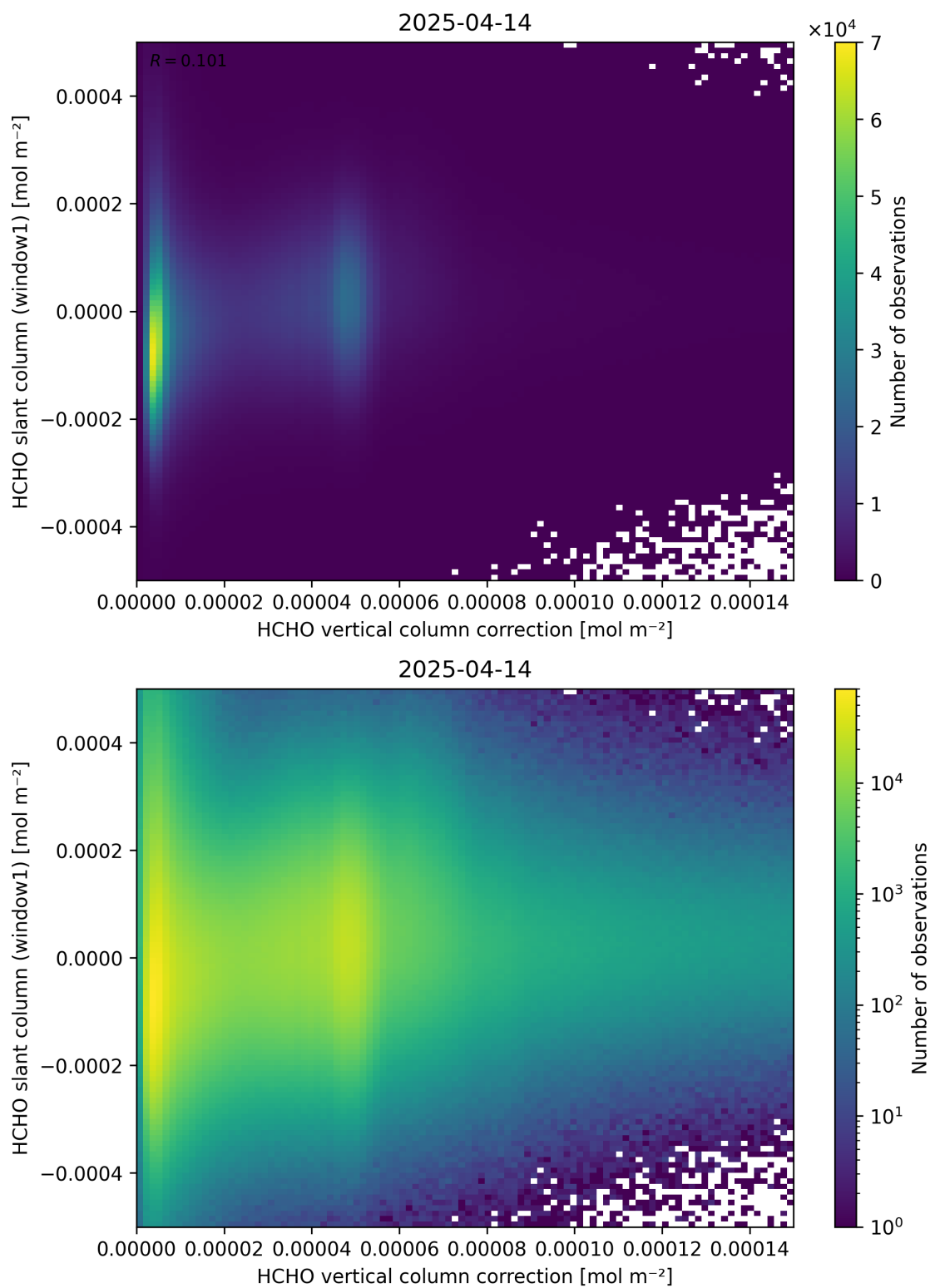
Figure 118: Scatter density plot of “HCHO vertical column correction” against “HCHO slant column (window1)” for 2025-04-13 to 2025-04-15.
