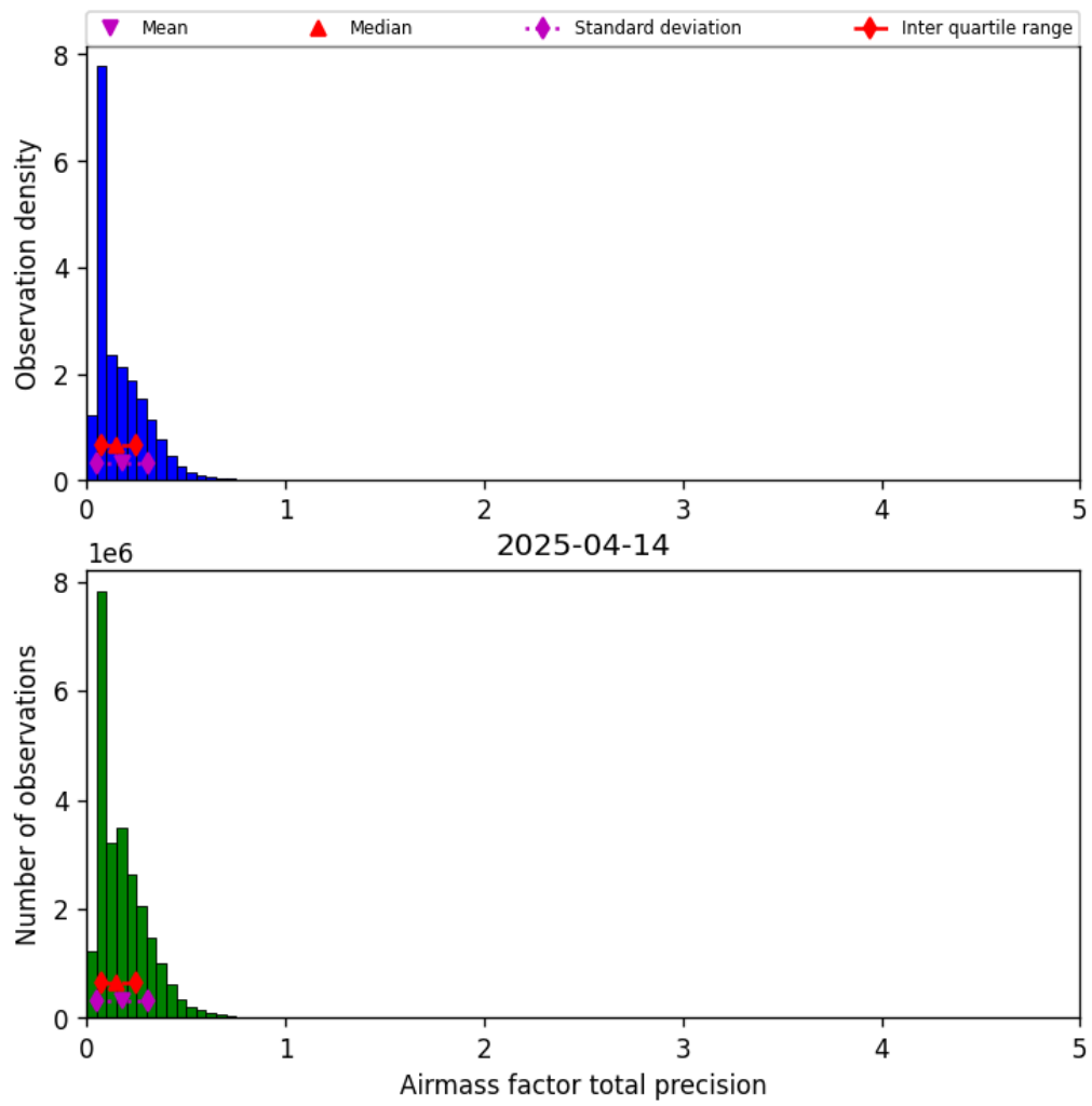
Figure 41: Histogram of “Airmass factor total precision” for 2025-04-13 to 2025-04-15
