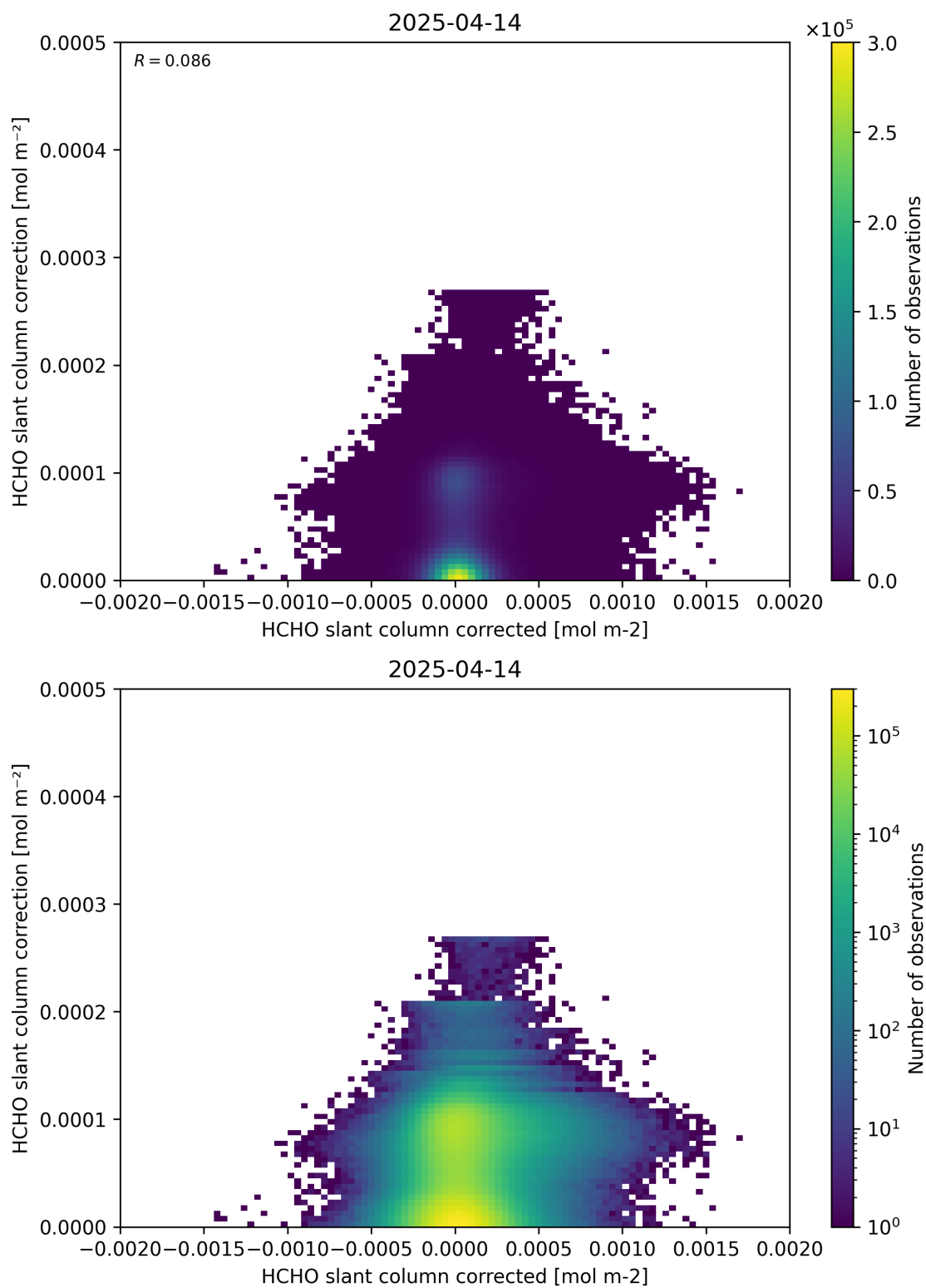
Figure 77: Scatter density plot of “HCHO slant column corrected” against “HCHO slant column correction” for 2025-04-13 to 2025-04-15.
