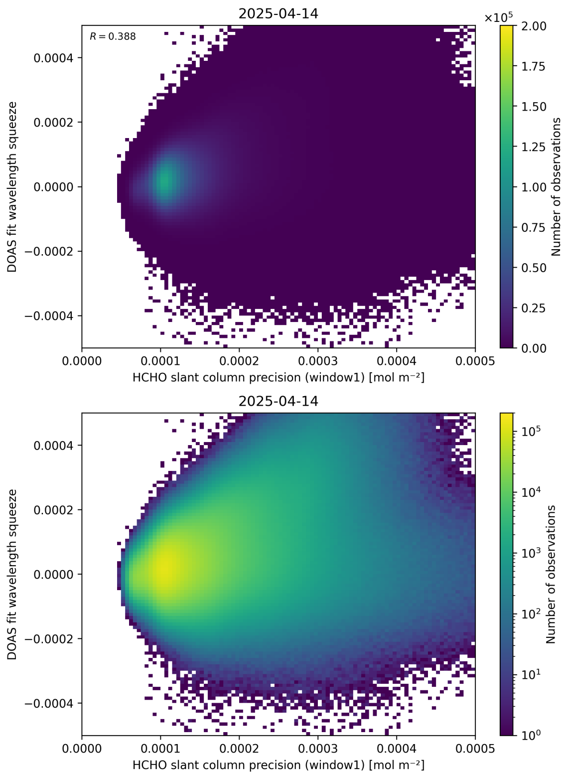
Figure 90: Scatter density plot of “HCHO slant column precision (window1)” against “DOAS fit wavelength squeeze” for 2025-04-13 to 2025-04-15.
