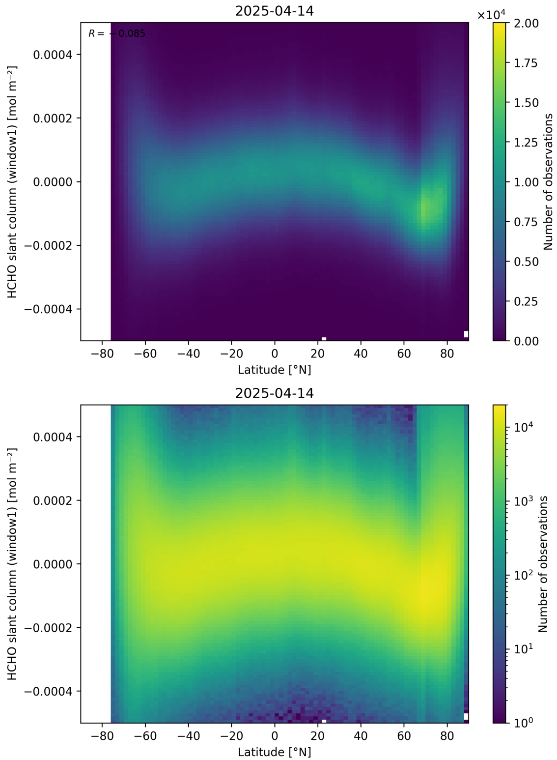
Figure 159: Scatter density plot of “Latitude” against “HCHO slant column (window1)” for 2025-04-13 to 2025-04-15.
