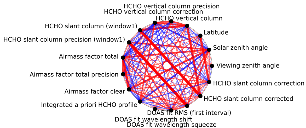
Figure 1: Map of correlation graph for 2025-04-13 to 2025-04-15.
