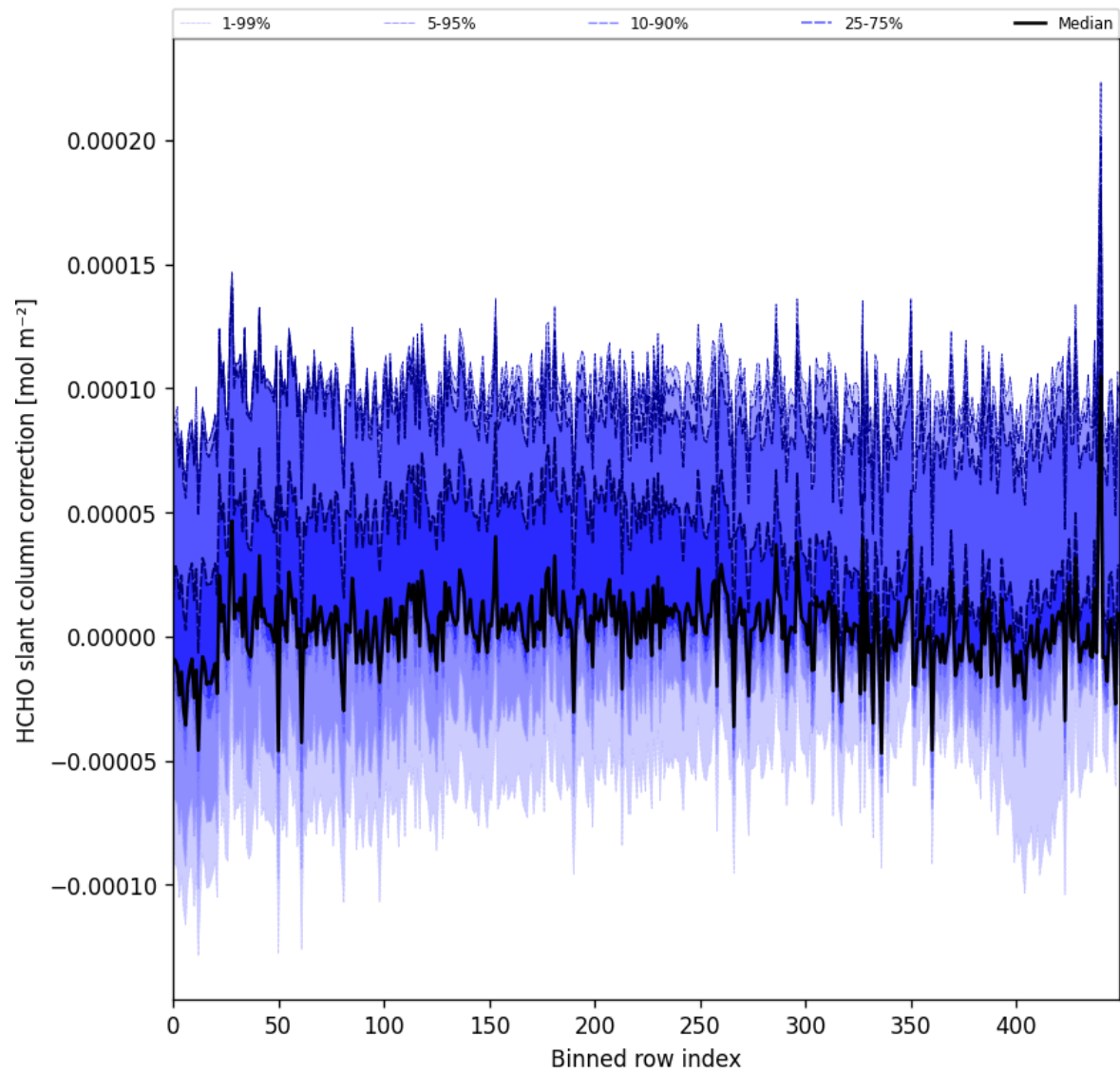
Figure 61: Along track statistics of “HCHO slant column correction” for 2025-04-13 to 2025-04-15
