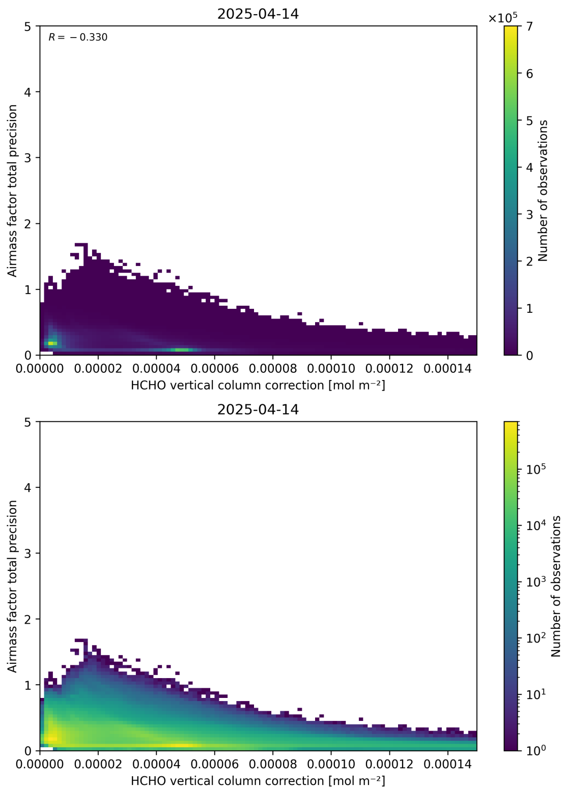
Figure 121: Scatter density plot of “HCHO vertical column correction” against “Airmass factor total precision” for 2025-04-13 to 2025-04-15.
