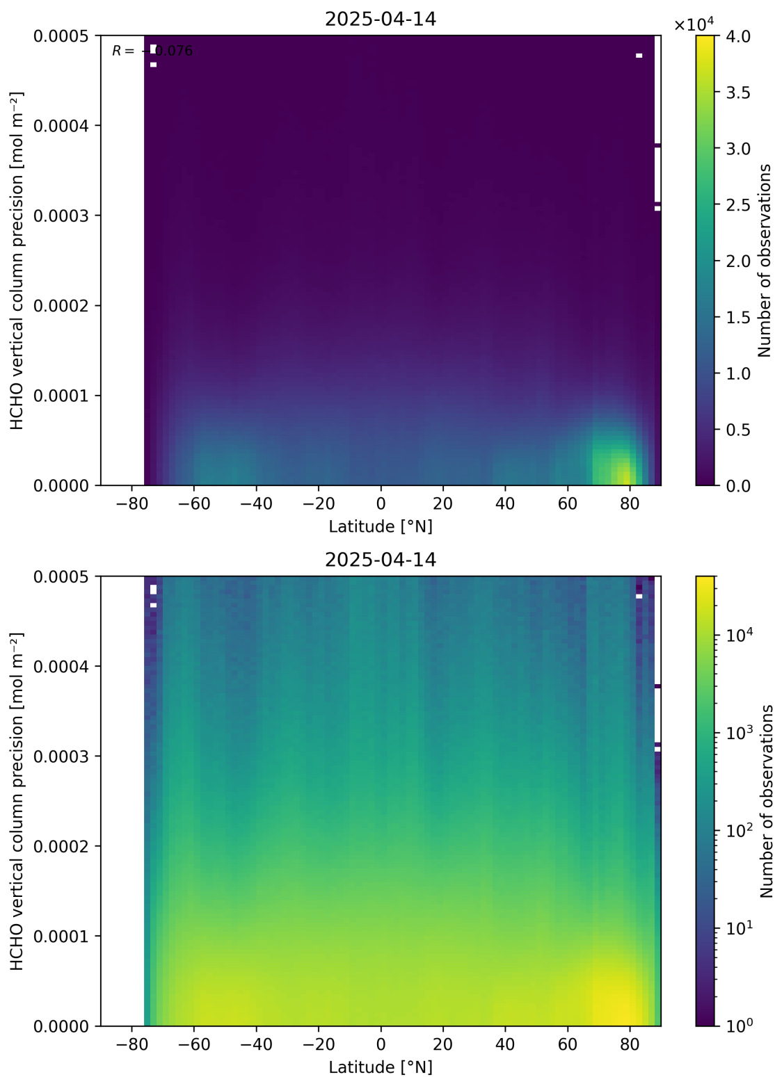
Figure 165: Scatter density plot of “Latitude” against “HCHO vertical column precision” for 2025-04-13 to 2025-04-15.
