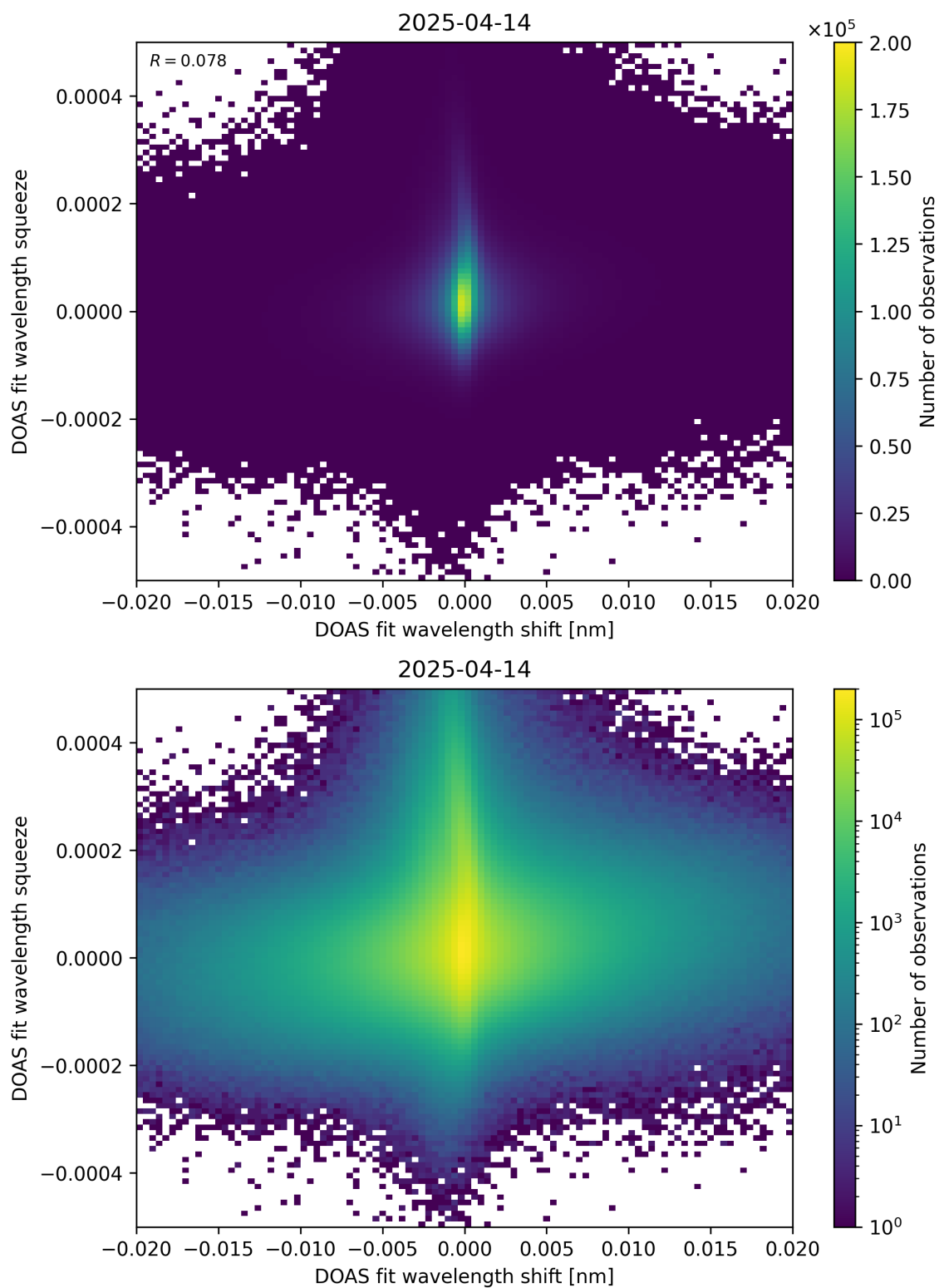
Figure 65: Scatter density plot of “DOAS fit wavelength shift” against “DOAS fit wavelength squeeze” for 2025-04-13 to 2025-04-15.
