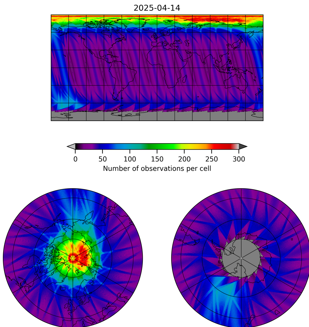
Figure 19: Map of the number of observations for 2025-04-13 to 2025-04-15
