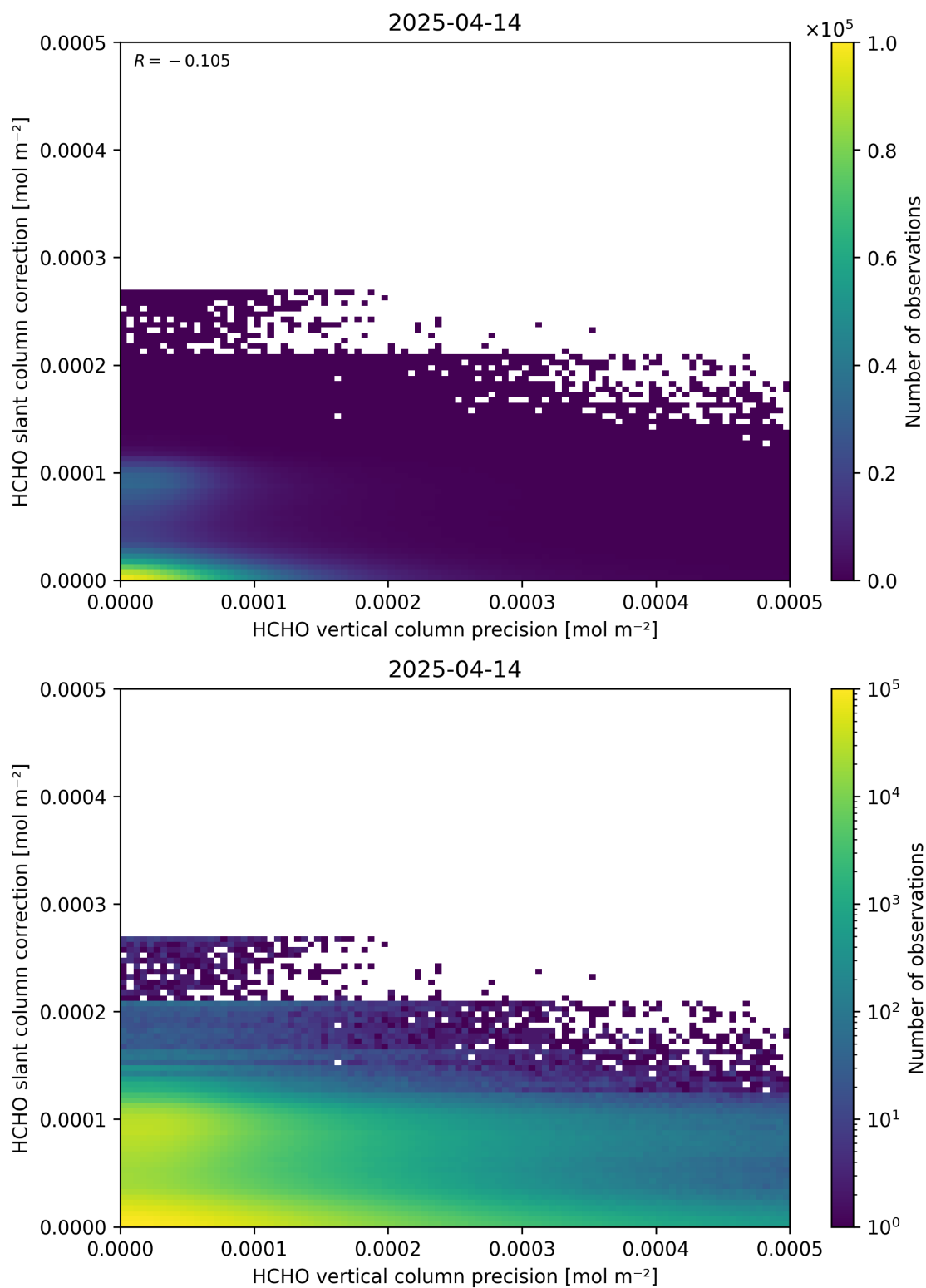
Figure 141: Scatter density plot of “HCHO vertical column precision” against “HCHO slant column correction” for 2025-04-13 to 2025-04-15.
