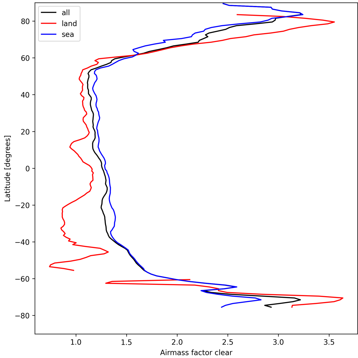
Figure 28: Zonal average of “Airmass factor clear” for 2025-04-13 to 2025-04-15.
