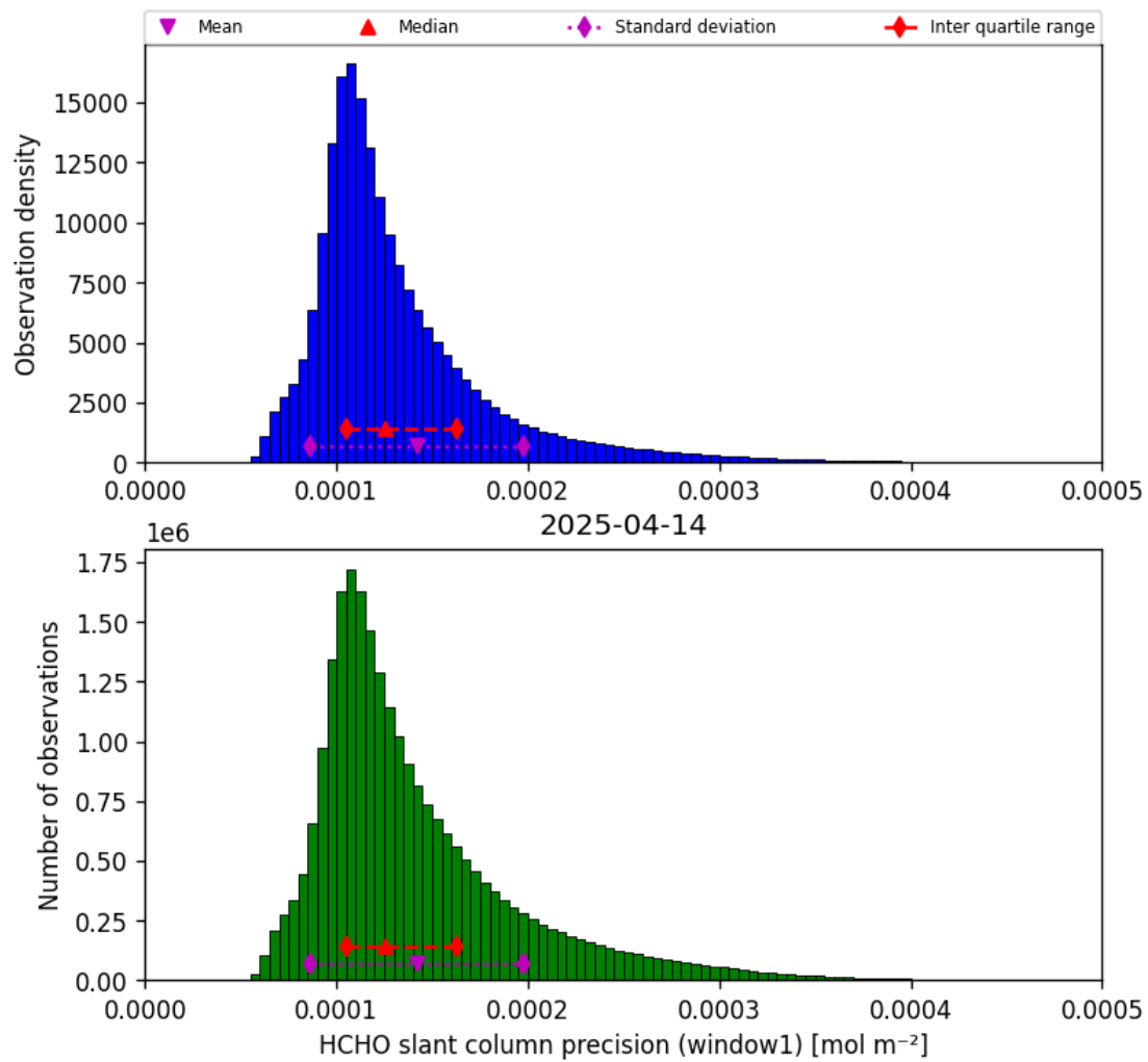
Figure 39: Histogram of “HCHO slant column precision (window1)” for 2025-04-13 to 2025-04-15
