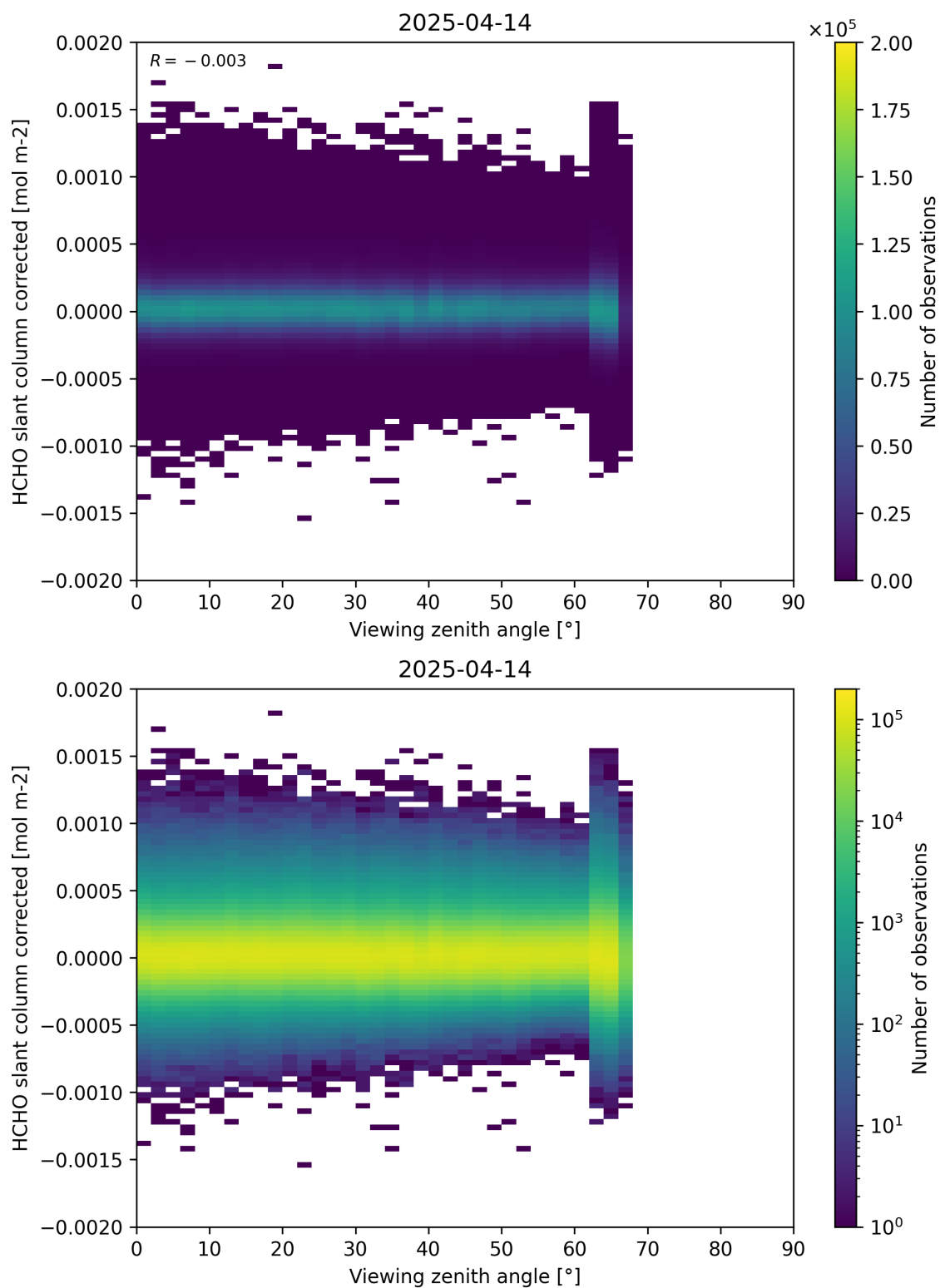
Figure 186: Scatter density plot of “Viewing zenith angle” against “HCHO slant column corrected” for 2025-04-13 to 2025-04-15.
