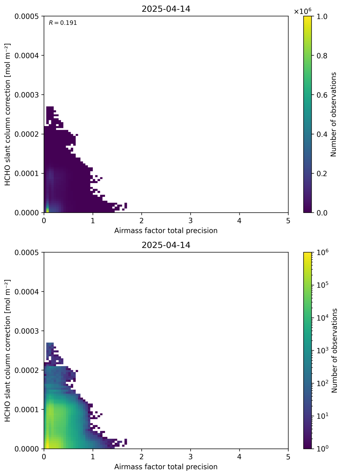
Figure 110: Scatter density plot of “Airmass factor total precision” against “HCHO slant column correction” for 2025-04-13 to 2025-04-15.
