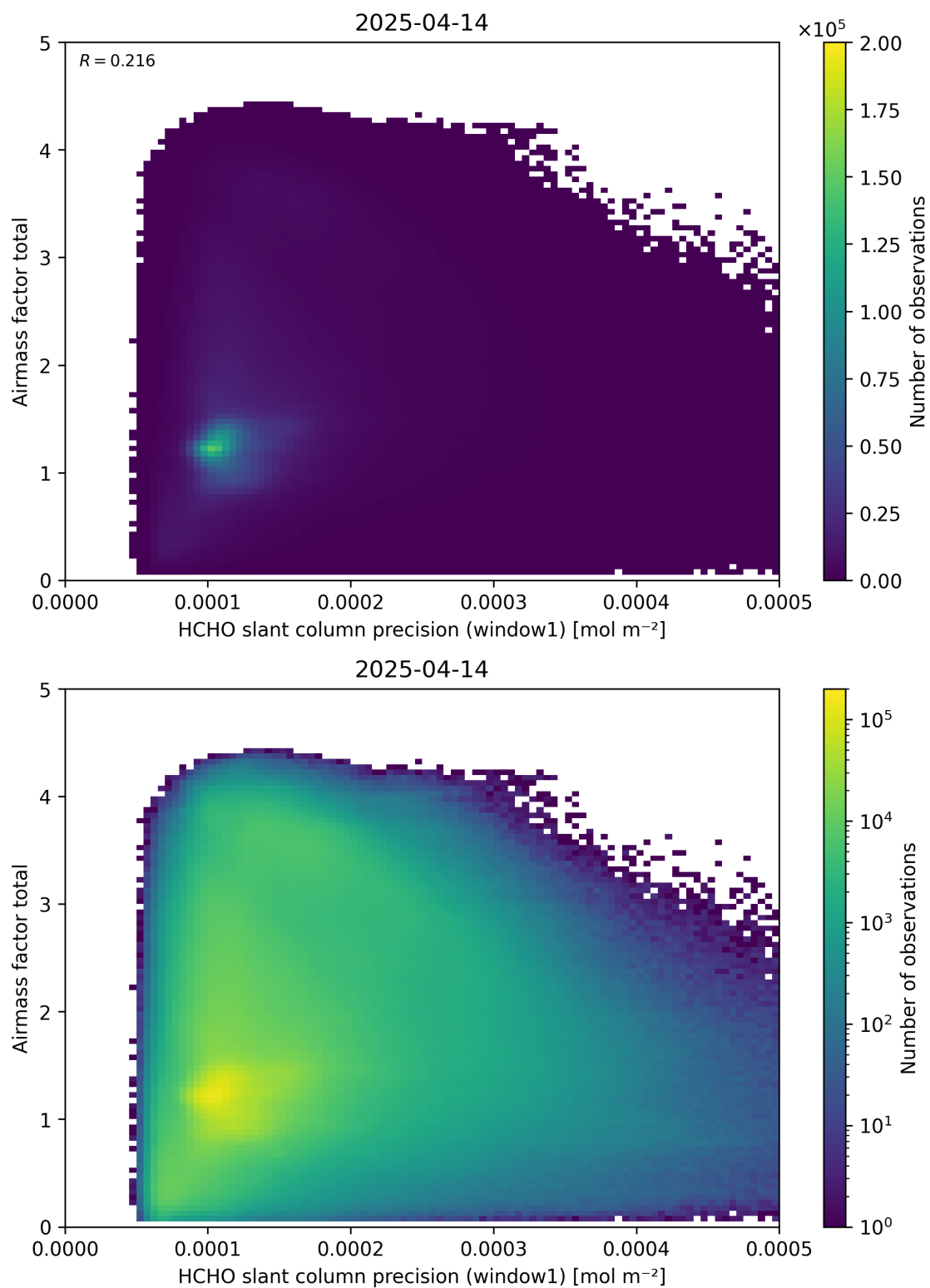
Figure 94: Scatter density plot of “HCHO slant column precision (window1)” against “Airmass factor total” for 2025-04-13 to 2025-04-15.
