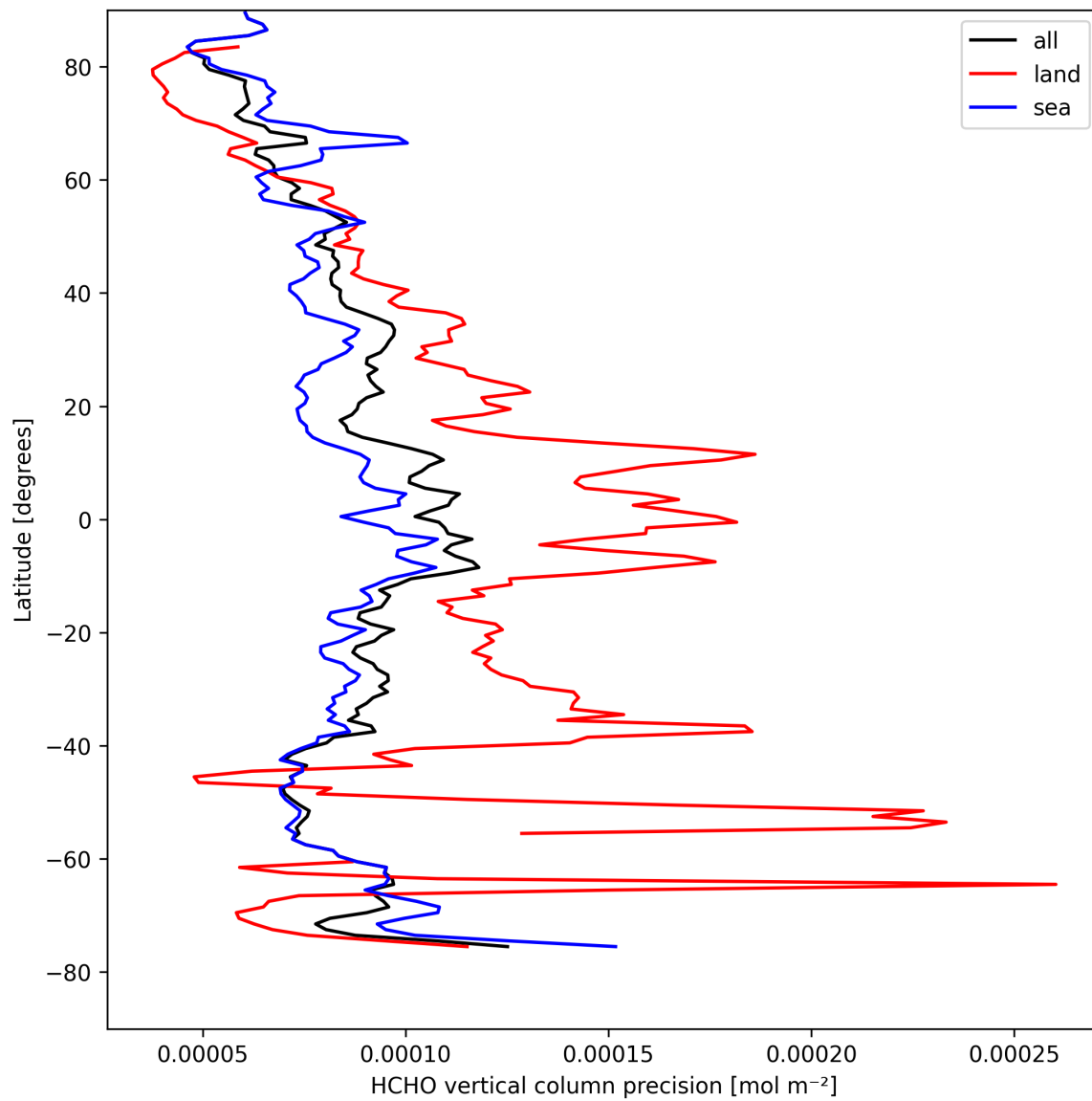
Figure 22: Zonal average of “HCHO vertical column precision” for 2025-04-13 to 2025-04-15.
