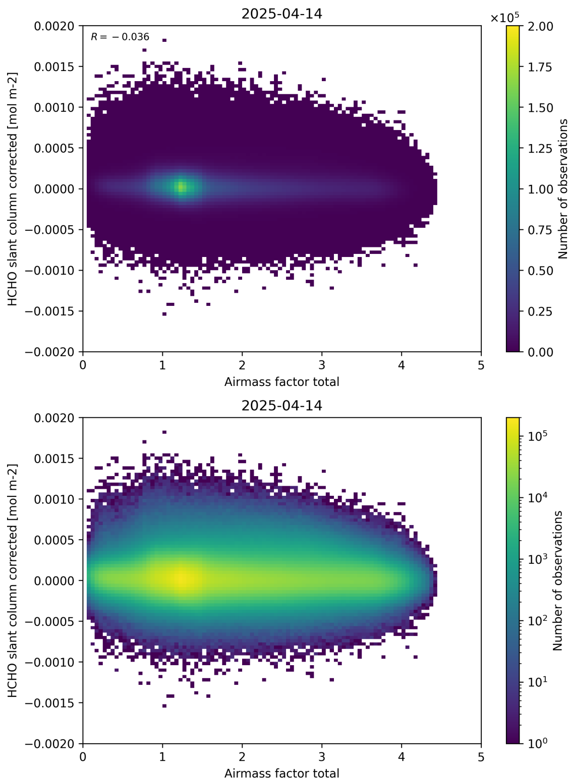
Figure 101: Scatter density plot of “Airmass factor total” against “HCHO slant column corrected” for 2025-04-13 to 2025-04-15.
