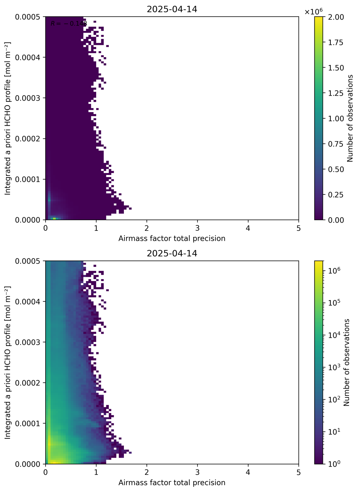
Figure 111: Scatter density plot of “Airmass factor total precision” against “Integrated a priori HCHO profile” for 2025-04-13 to 2025-04-15.
