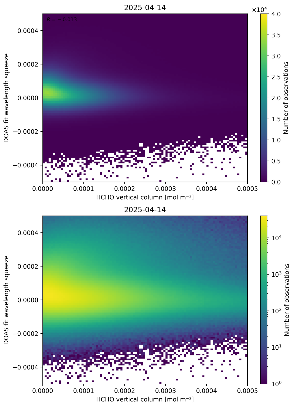
Figure 125: Scatter density plot of “HCHO vertical column” against “DOAS fit wavelength squeeze” for 2025-04-13 to 2025-04-15.
