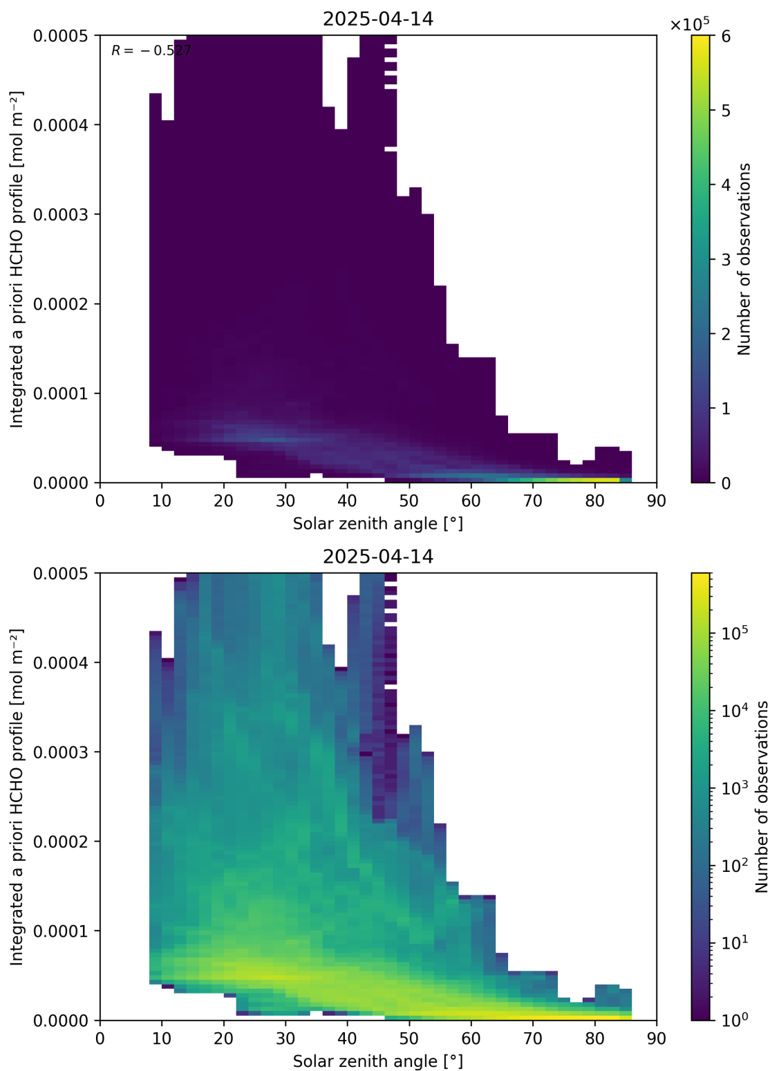
Figure 180: Scatter density plot of “Solar zenith angle” against “Integrated a priori HCHO profile” for 2025-04-13 to 2025-04-15.
