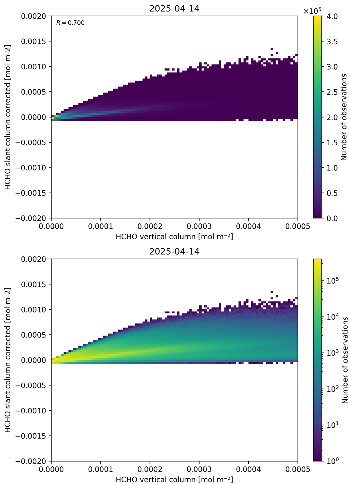
Figure 127: Scatter density plot of “HCHO vertical column” against “HCHO slant column corrected” for 2025-04-13 to 2025-04-15.
