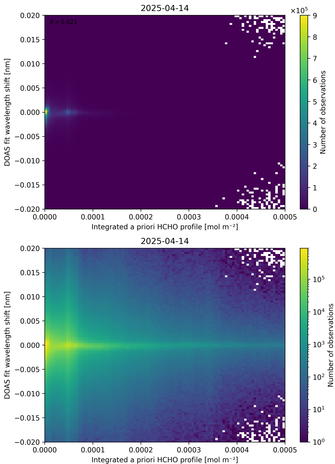
Figure 149: Scatter density plot of “Integrated a priori HCHO profile” against “DOAS fit wavelength shift” for 2025-04-13 to 2025-04-15.
