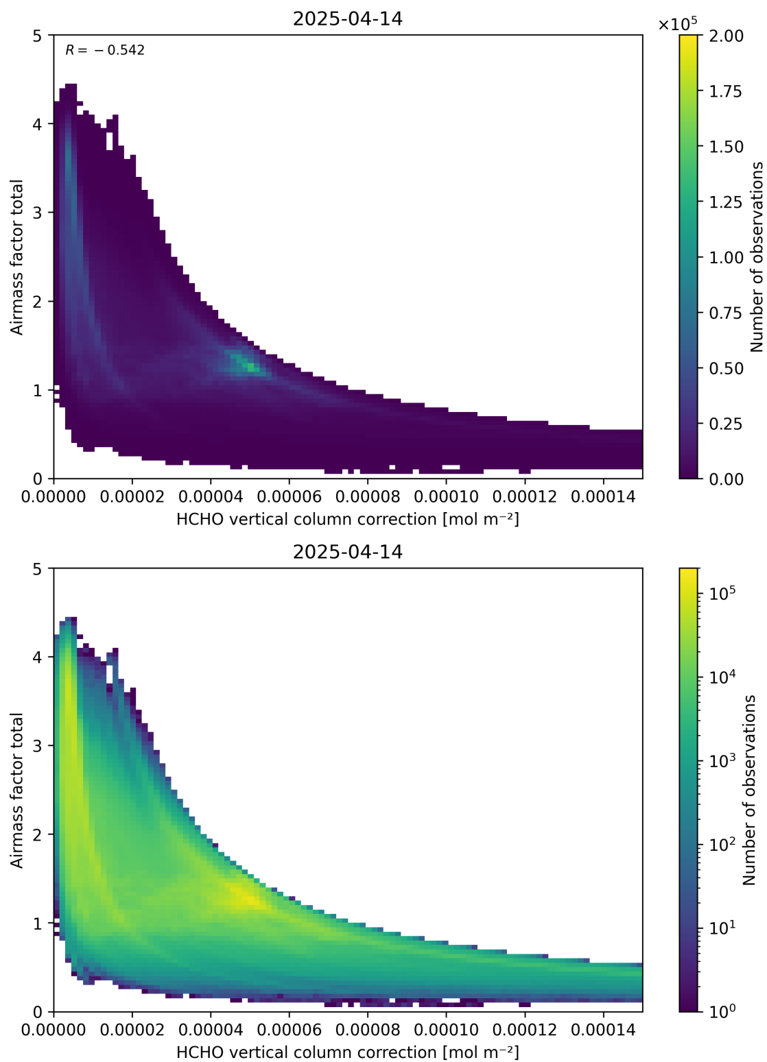
Figure 120: Scatter density plot of “HCHO vertical column correction” against “Airmass factor total” for 2025-04-13 to 2025-04-15.
