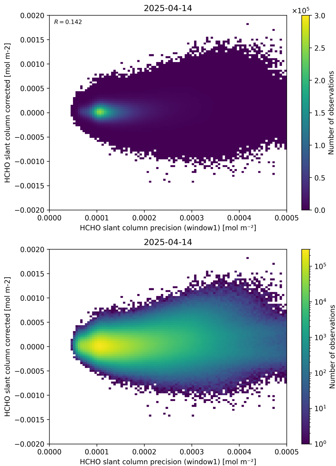
Figure 92: Scatter density plot of “HCHO slant column precision (window1)” against “HCHO slant column corrected” for 2025-04-13 to 2025-04-15.
