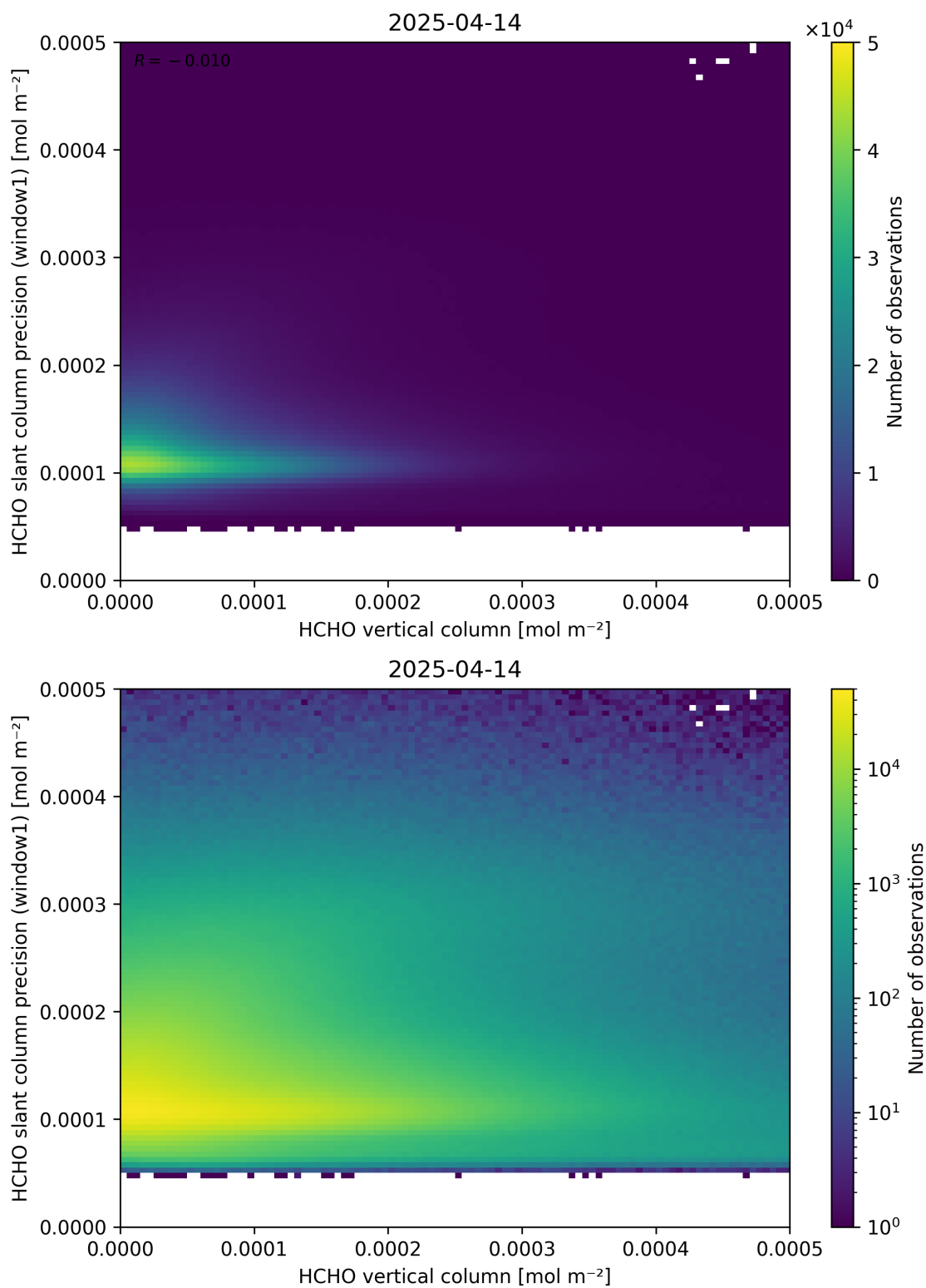
Figure 130: Scatter density plot of “HCHO vertical column” against “HCHO slant column precision (window1)” for 2025-04-13 to 2025-04-15.
