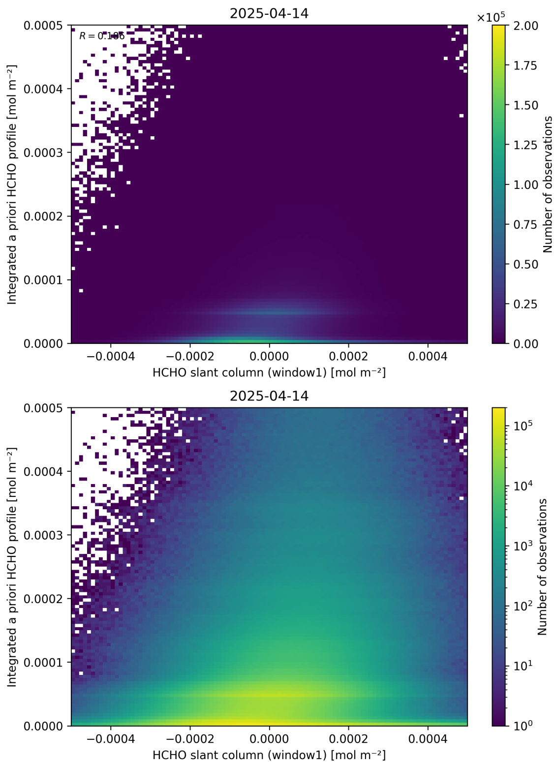
Figure 87: Scatter density plot of “HCHO slant column (window1)” against “Integrated a priori HCHO profile” for 2025-04-13 to 2025-04-15.
