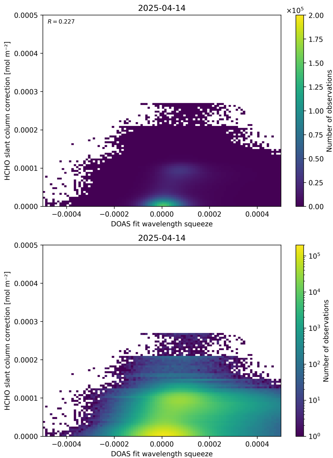
Figure 70: Scatter density plot of “DOAS fit wavelength squeeze” against “HCHO slant column correction” for 2025-04-13 to 2025-04-15.
