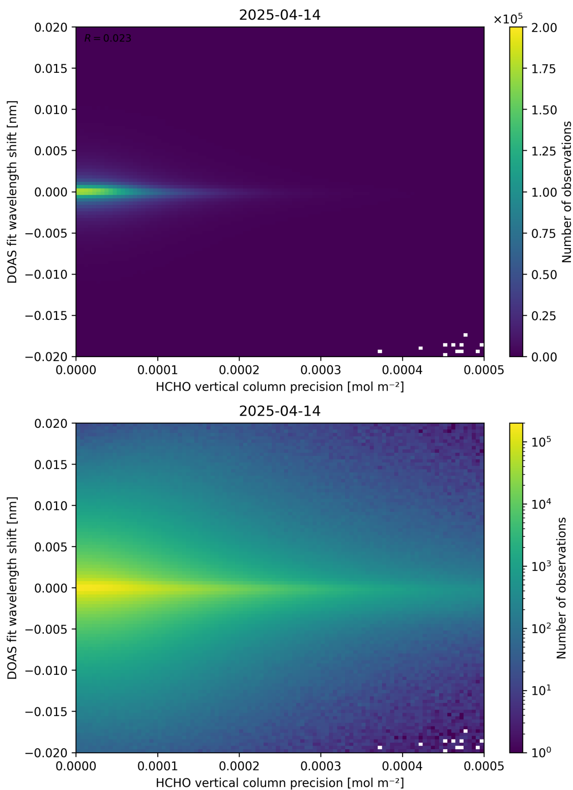
Figure 137: Scatter density plot of “HCHO vertical column precision” against “DOAS fit wavelength shift” for 2025-04-13 to 2025-04-15.
