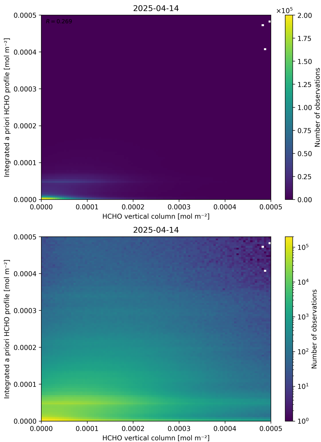
Figure 135: Scatter density plot of “HCHO vertical column” against “Integrated a priori HCHO profile” for 2025-04-13 to 2025-04-15.
