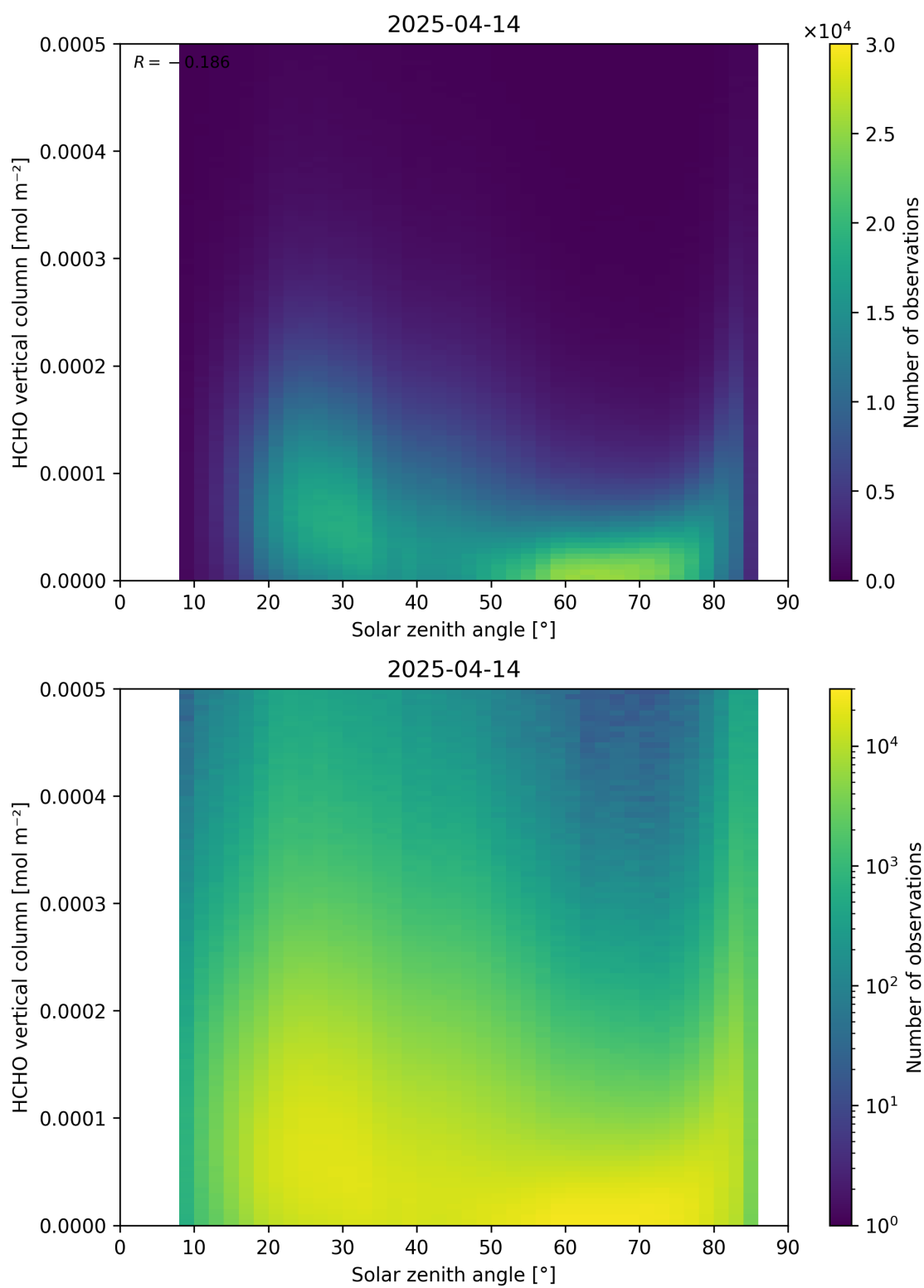
Figure 177: Scatter density plot of “Solar zenith angle” against “HCHO vertical column” for 2025-04-13 to 2025-04-15.
