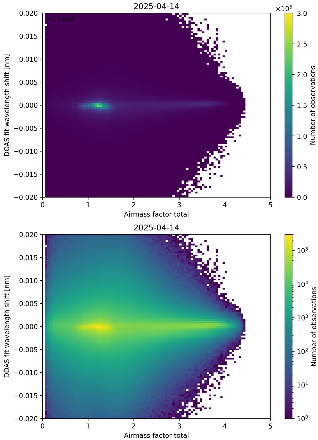
Figure 98: Scatter density plot of “Airmass factor total” against “DOAS fit wavelength shift” for 2025-04-13 to 2025-04-15.
