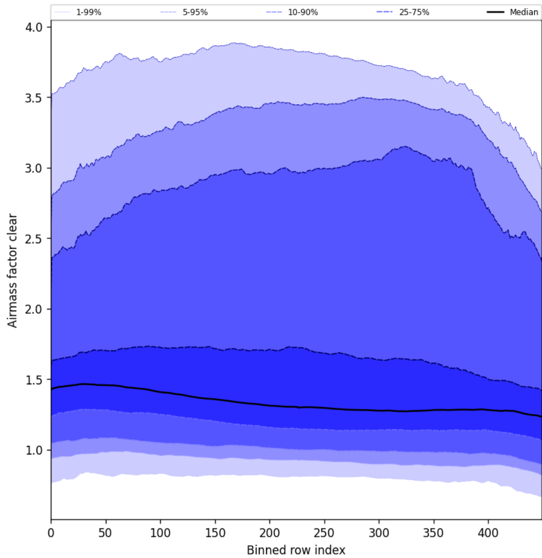
Figure 56: Along track statistics of “Airmass factor clear” for 2025-04-13 to 2025-04-15
