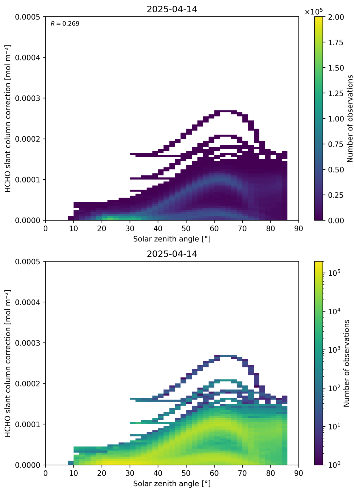
Figure 172: Scatter density plot of “Solar zenith angle” against “HCHO slant column correction” for 2025-04-13 to 2025-04-15.
