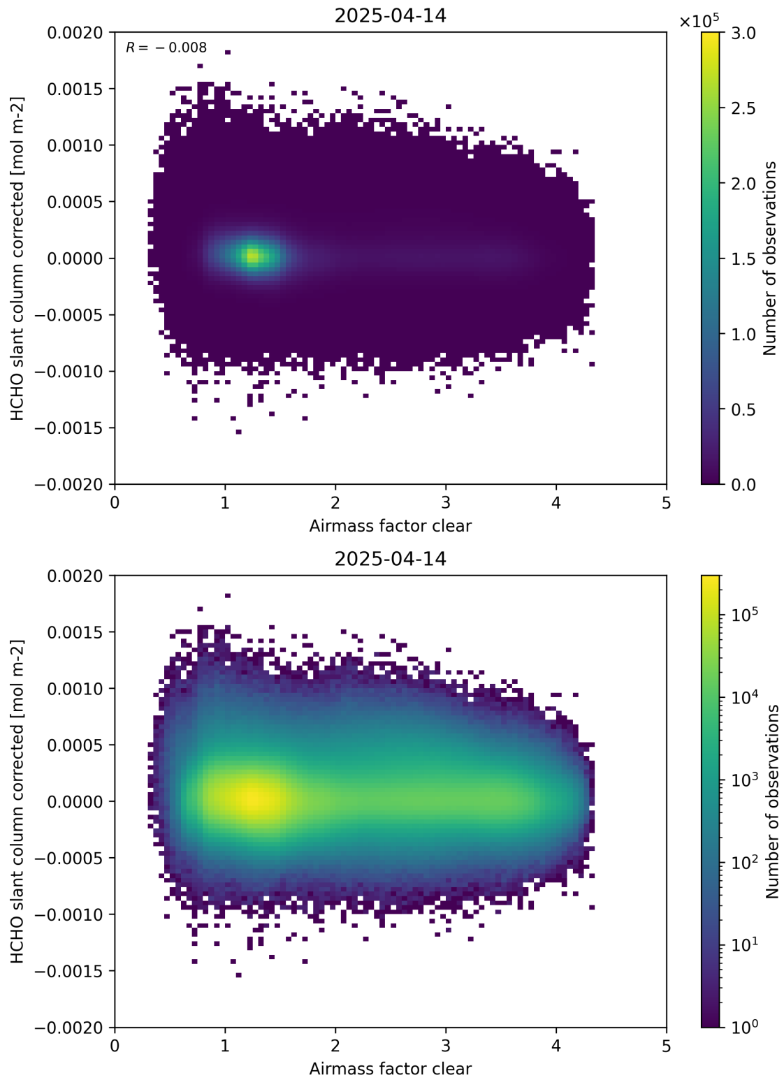
Figure 74: Scatter density plot of “Airmass factor clear” against “HCHO slant column corrected” for 2025-04-13 to 2025-04-15.
