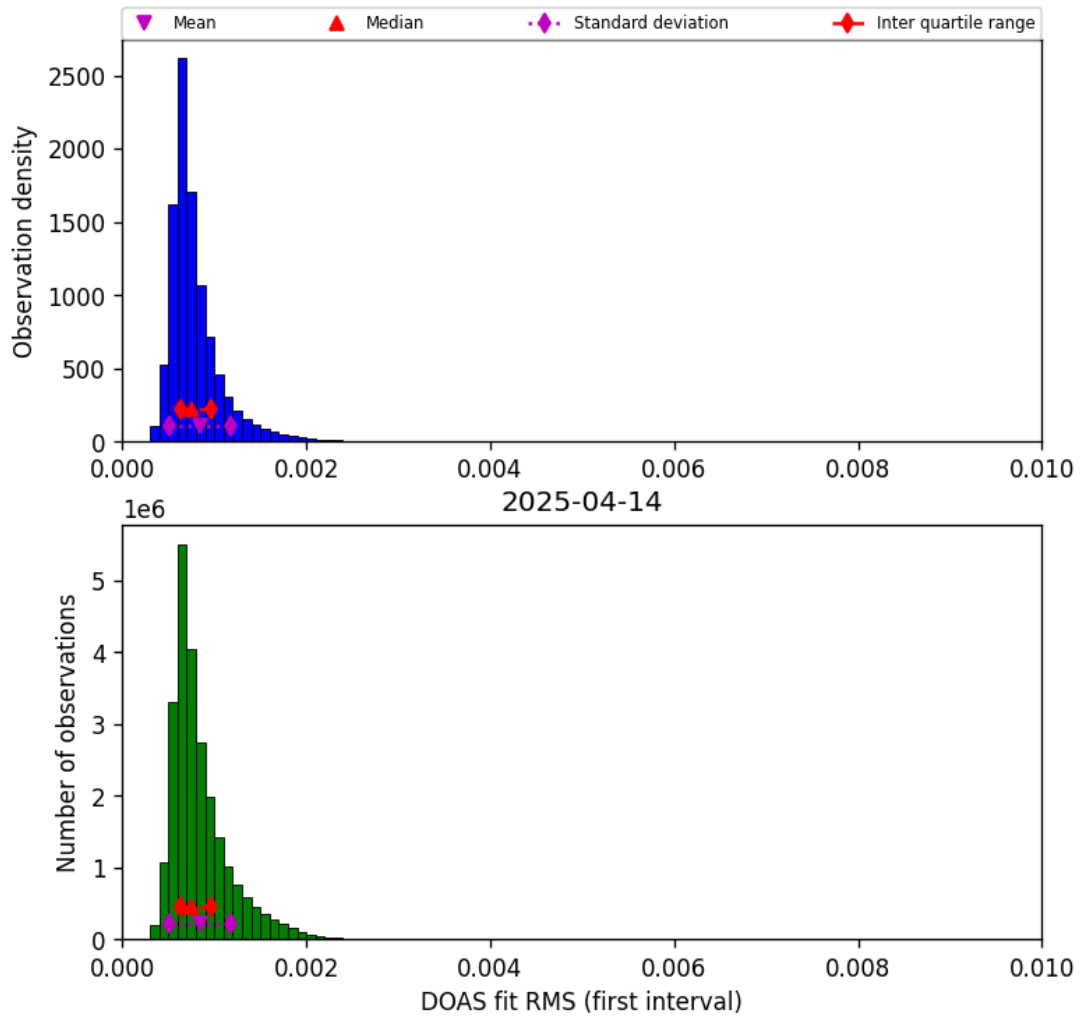
Figure 46: Histogram of “DOAS fit RMS (first interval)” for 2025-04-13 to 2025-04-15
