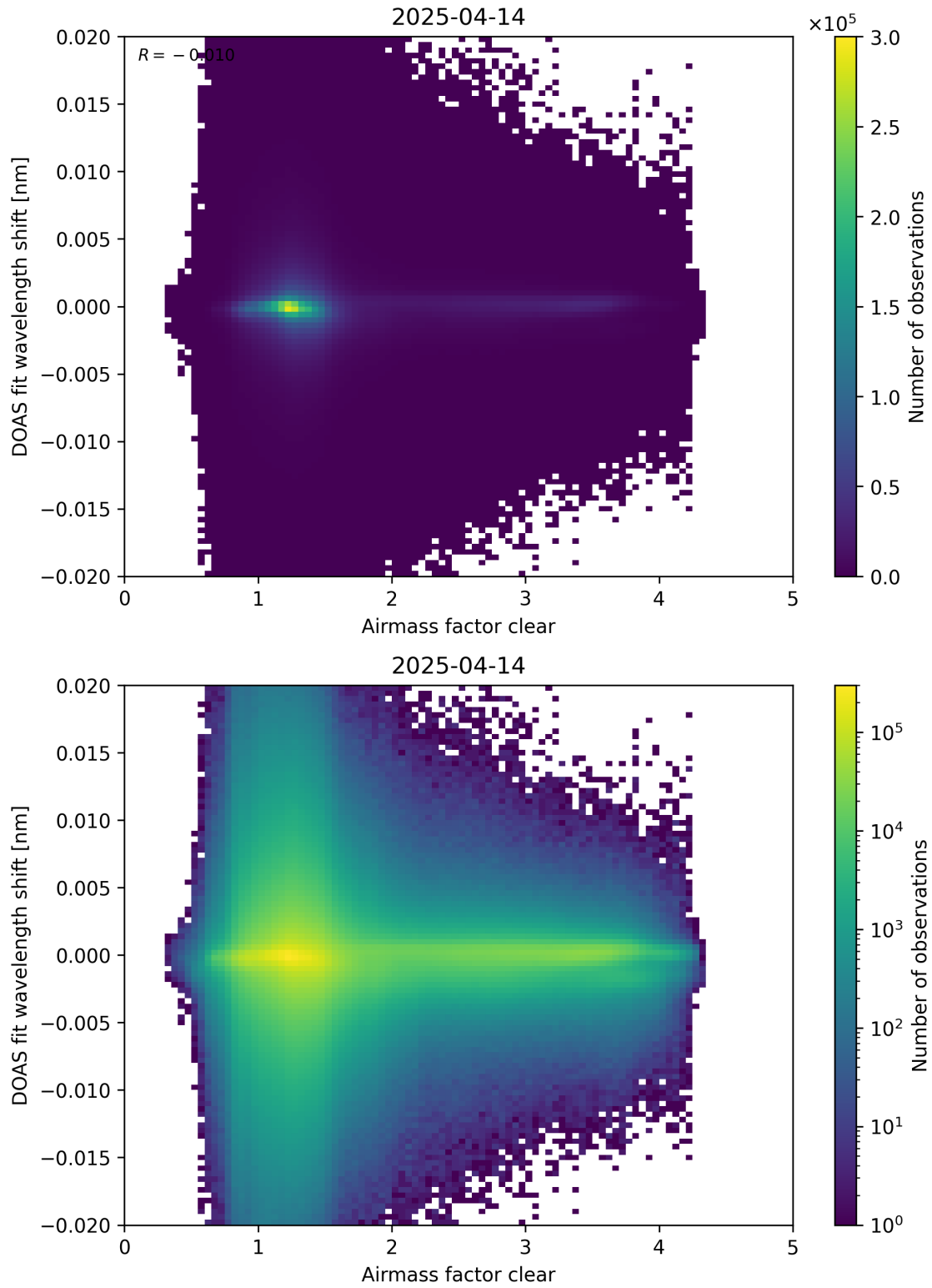
Figure 72: Scatter density plot of “Airmass factor clear” against “DOAS fit wavelength shift” for 2025-04-13 to 2025-04-15.
