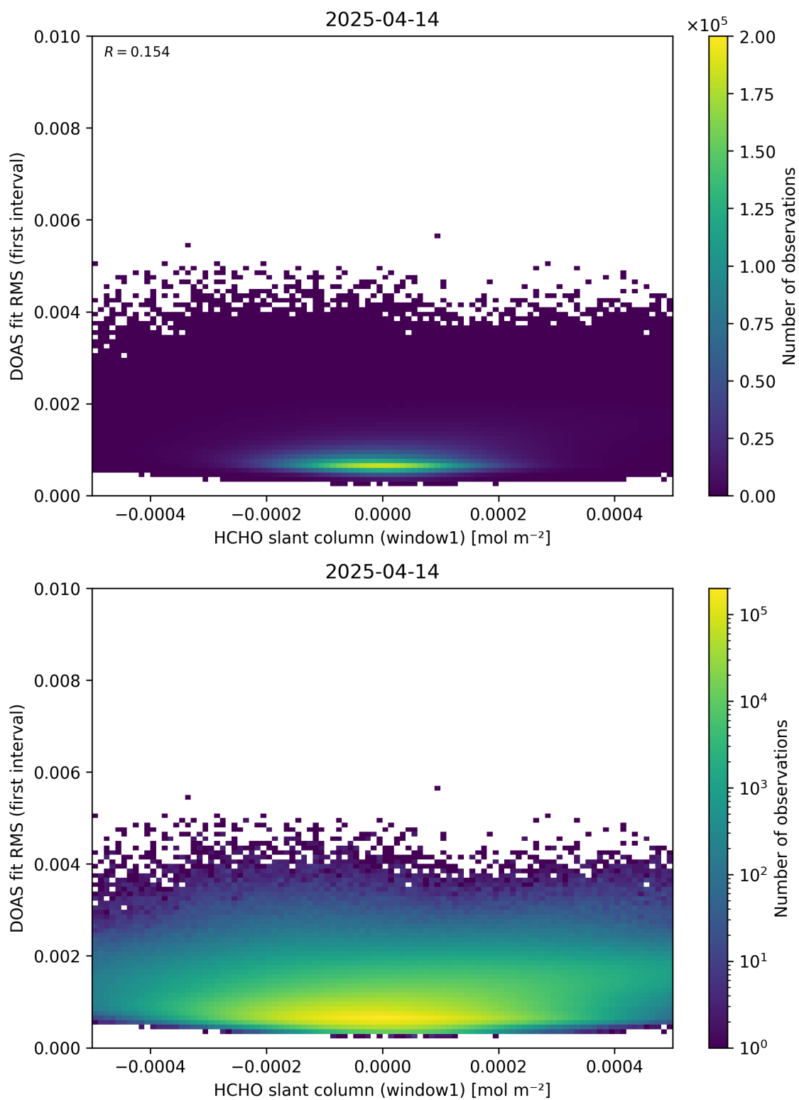
Figure 78: Scatter density plot of “HCHO slant column (window1)” against “DOAS fit RMS (first interval)” for 2025-04-13 to 2025-04-15.
