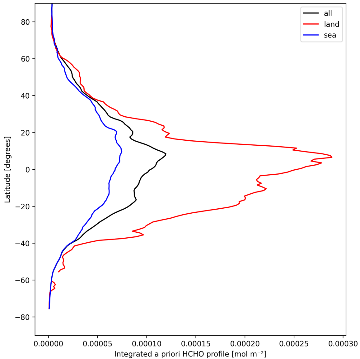
Figure 29: Zonal average of “Integrated a priori HCHO profile” for 2025-04-13 to 2025-04-15.
