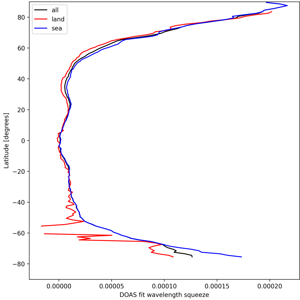
Figure 31: Zonal average of “DOAS fit wavelength squeeze” for 2025-04-13 to 2025-04-15.
