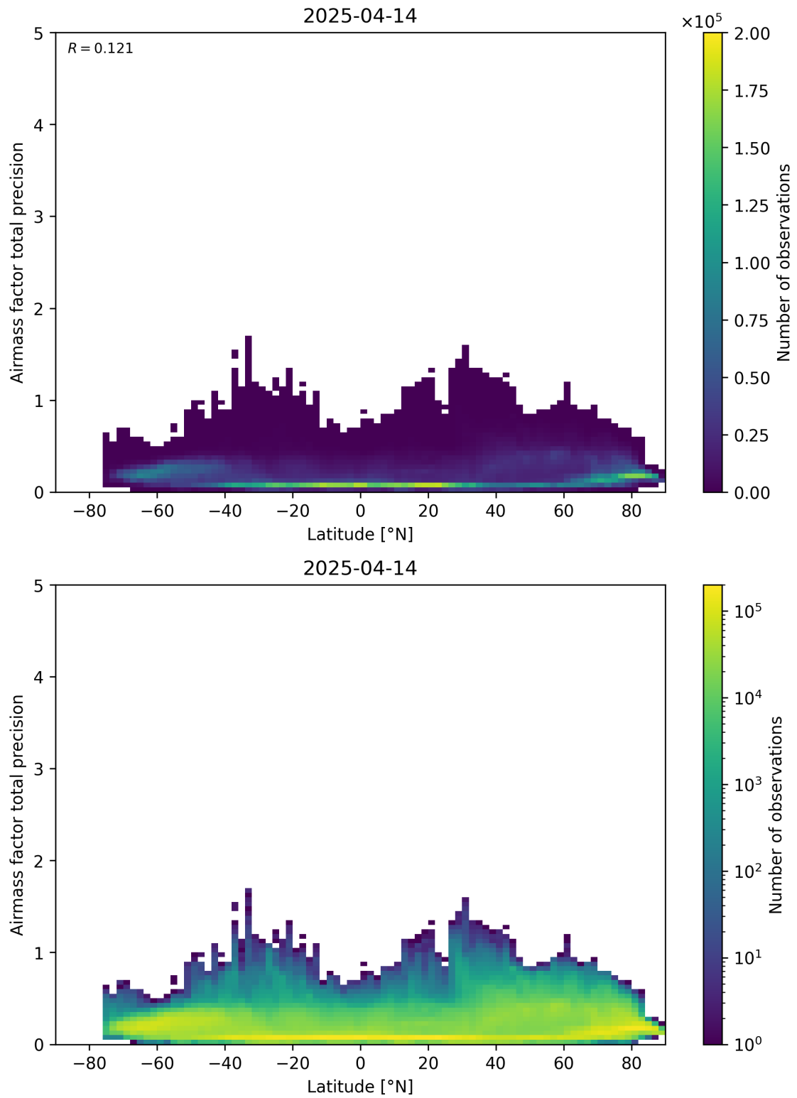
Figure 162: Scatter density plot of “Latitude” against “Airmass factor total precision” for 2025-04-13 to 2025-04-15.
