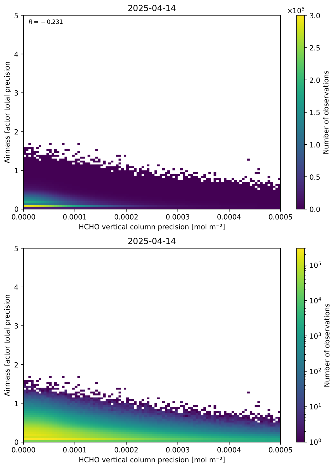
Figure 145: Scatter density plot of “HCHO vertical column precision” against “Airmass factor total precision” for 2025-04-13 to 2025-04-15.
