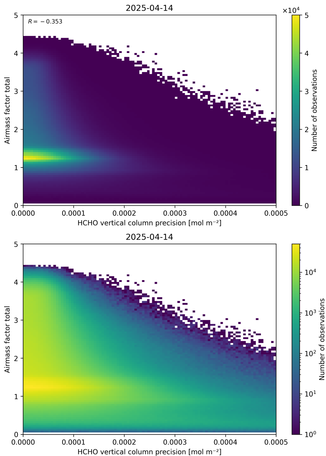
Figure 144: Scatter density plot of “HCHO vertical column precision” against “Airmass factor total” for 2025-04-13 to 2025-04-15.
