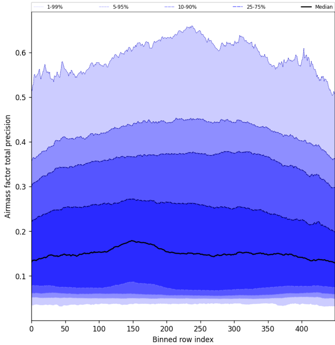
Figure 55: Along track statistics of “Airmass factor total precision” for 2025-04-13 to 2025-04-15
