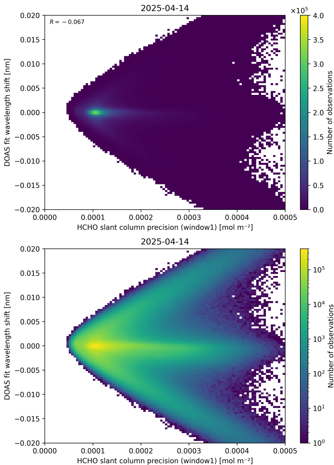
Figure 89: Scatter density plot of “HCHO slant column precision (window1)” against “DOAS fit wavelength shift” for 2025-04-13 to 2025-04-15.
