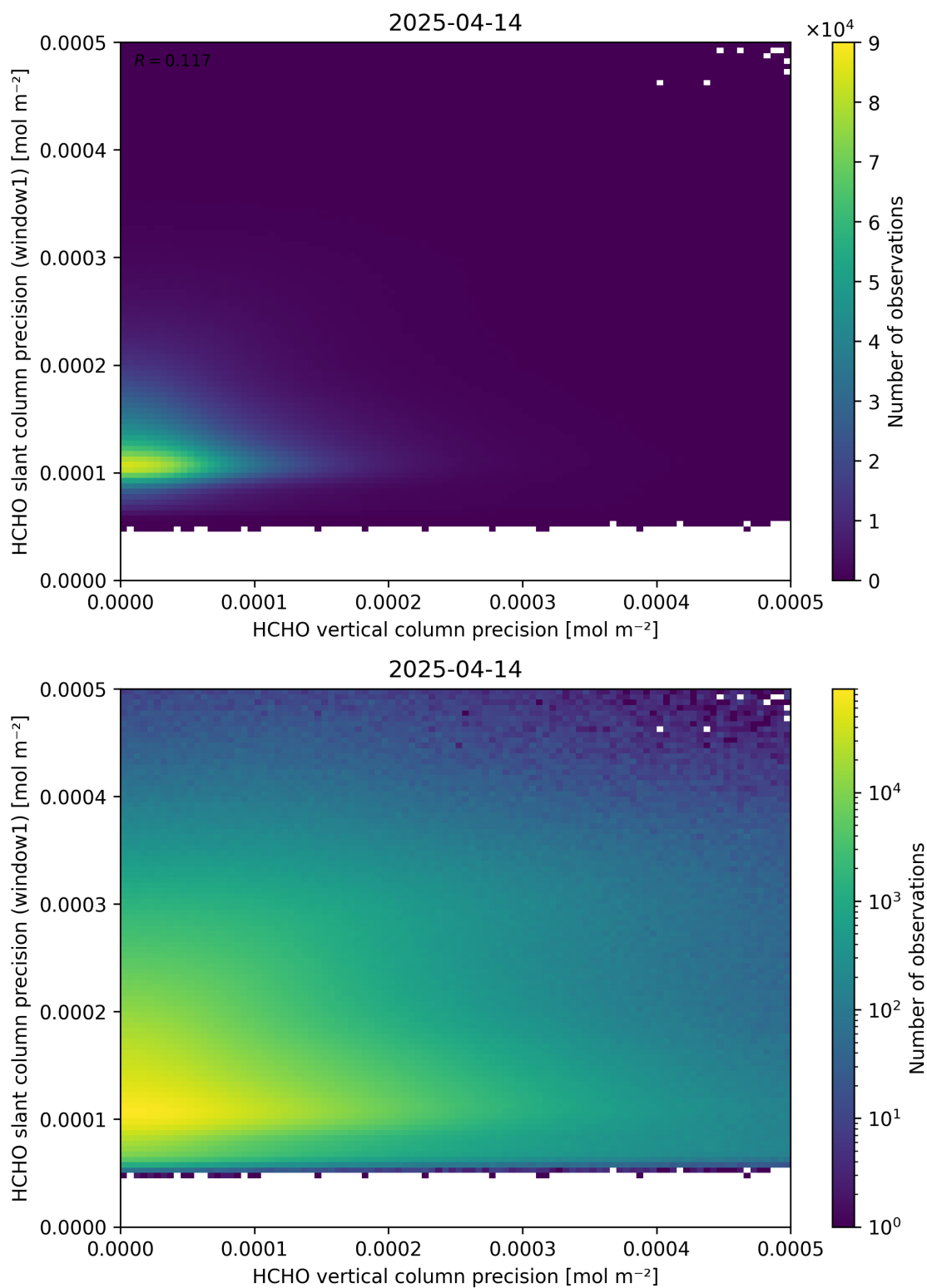
Figure 143: Scatter density plot of “HCHO vertical column precision” against “HCHO slant column precision (window1)” for 2025-04-13 to 2025-04-15.
