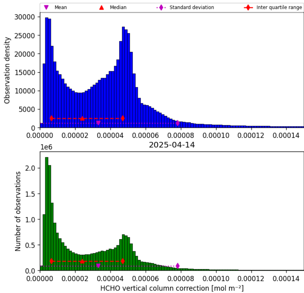
Figure 37: Histogram of “HCHO vertical column correction” for 2025-04-13 to 2025-04-15
