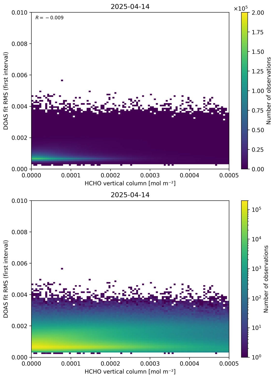
Figure 123: Scatter density plot of “HCHO vertical column” against “DOAS fit RMS (first interval)” for 2025-04-13 to 2025-04-15.
