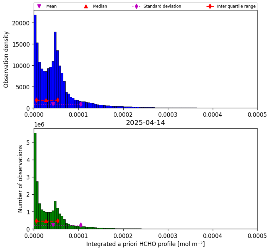
Figure 43: Histogram of “Integrated a priori HCHO profile” for 2025-04-13 to 2025-04-15
