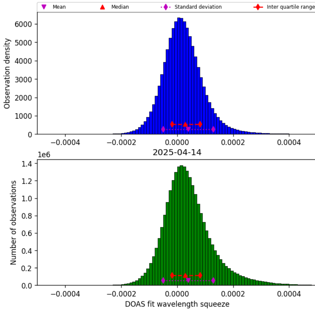
Figure 45: Histogram of “DOAS fit wavelength squeeze” for 2025-04-13 to 2025-04-15
