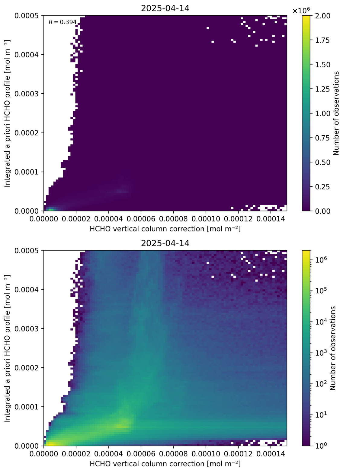
Figure 122: Scatter density plot of “HCHO vertical column correction” against “Integrated a priori HCHO profile” for 2025-04-13 to 2025-04-15.
