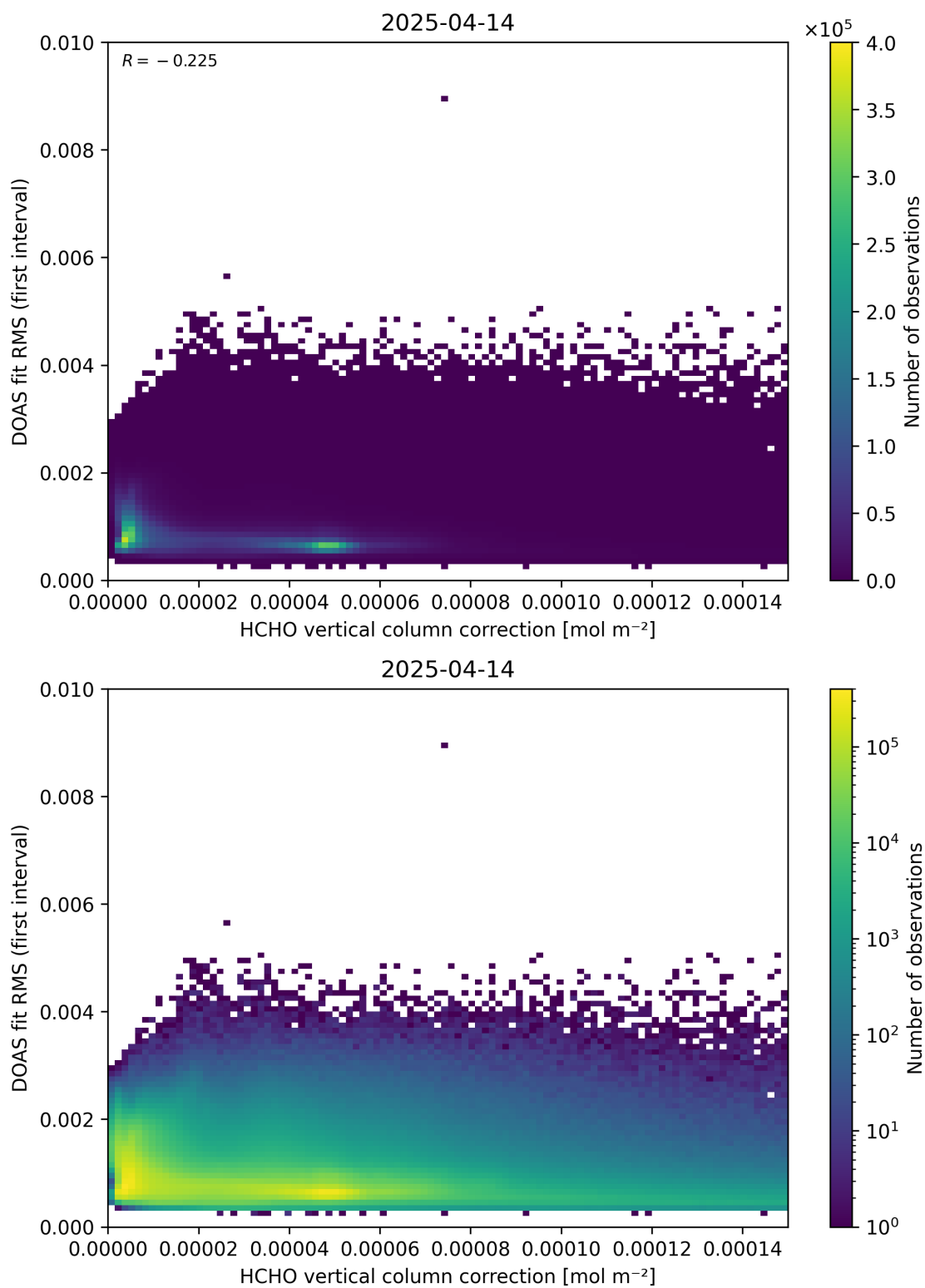
Figure 112: Scatter density plot of “HCHO vertical column correction” against “DOAS fit RMS (first interval)” for 2025-04-13 to 2025-04-15.
