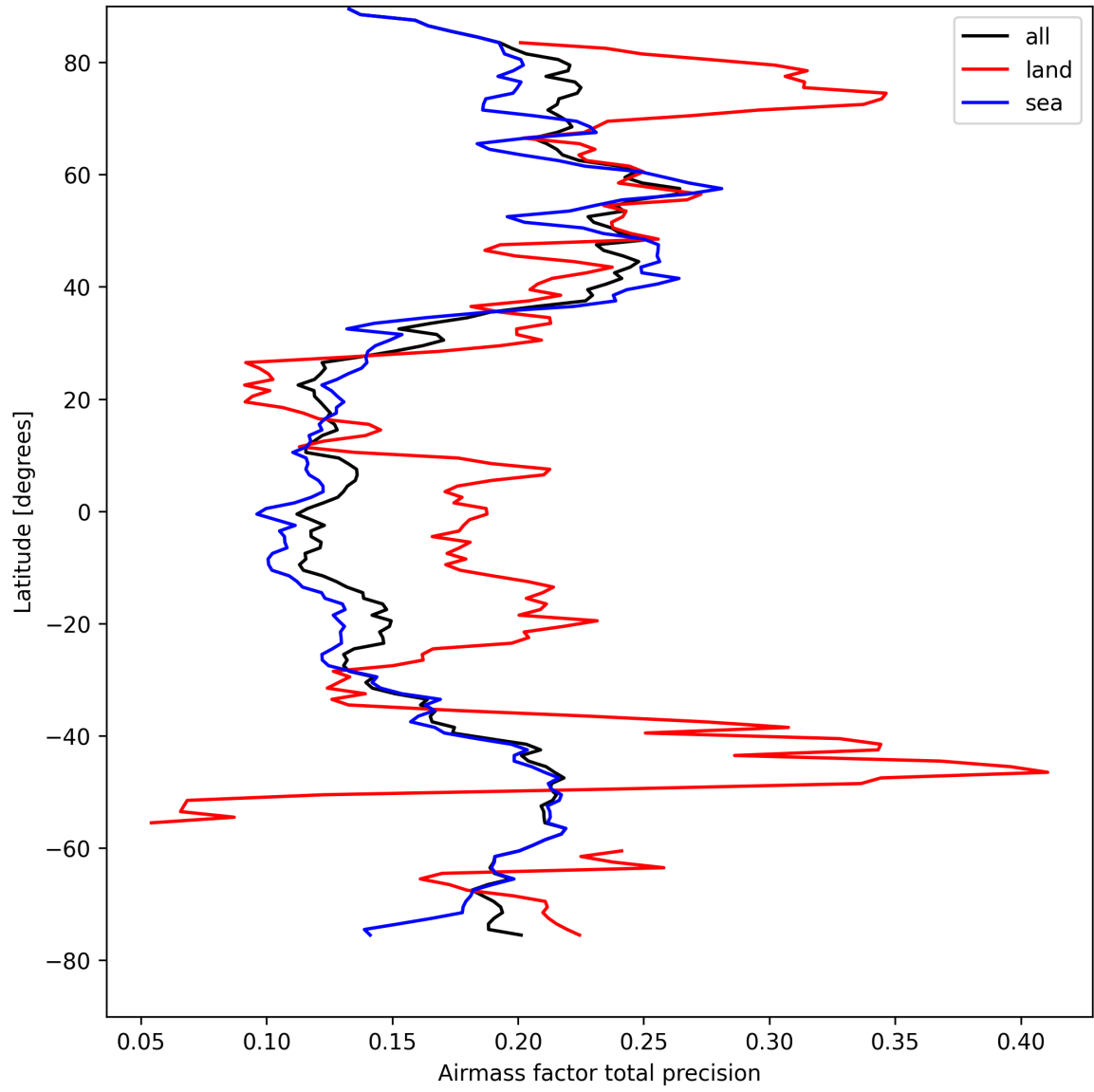
Figure 27: Zonal average of “Airmass factor total precision” for 2025-04-13 to 2025-04-15.
