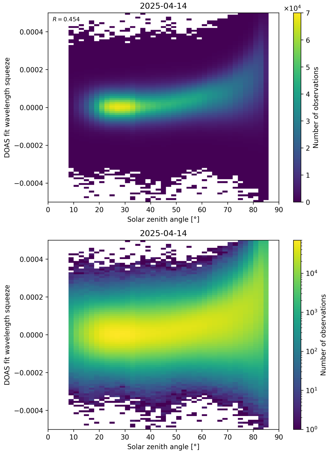
Figure 169: Scatter density plot of “Solar zenith angle” against “DOAS fit wavelength squeeze” for 2025-04-13 to 2025-04-15.
