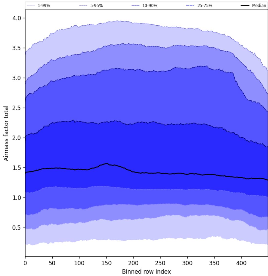
Figure 54: Along track statistics of “Airmass factor total” for 2025-04-13 to 2025-04-15
