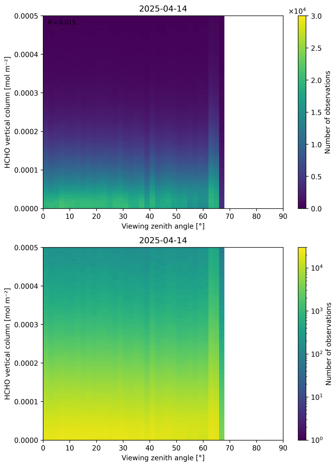
Figure 192: Scatter density plot of “Viewing zenith angle” against “HCHO vertical column” for 2025-04-13 to 2025-04-15.
