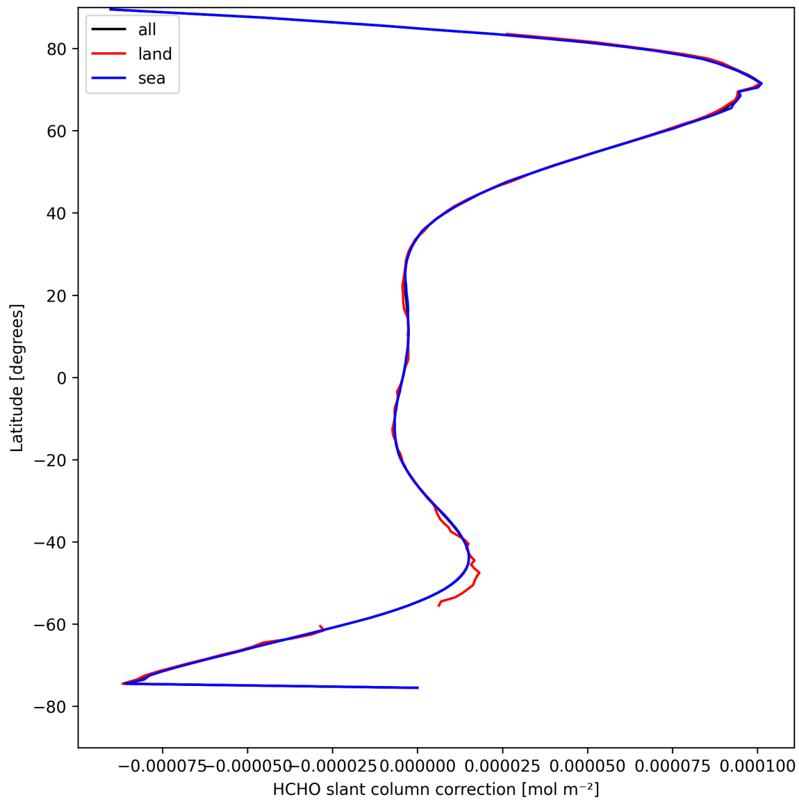
Figure 33: Zonal average of “HCHO slant column correction” for 2025-04-13 to 2025-04-15.
