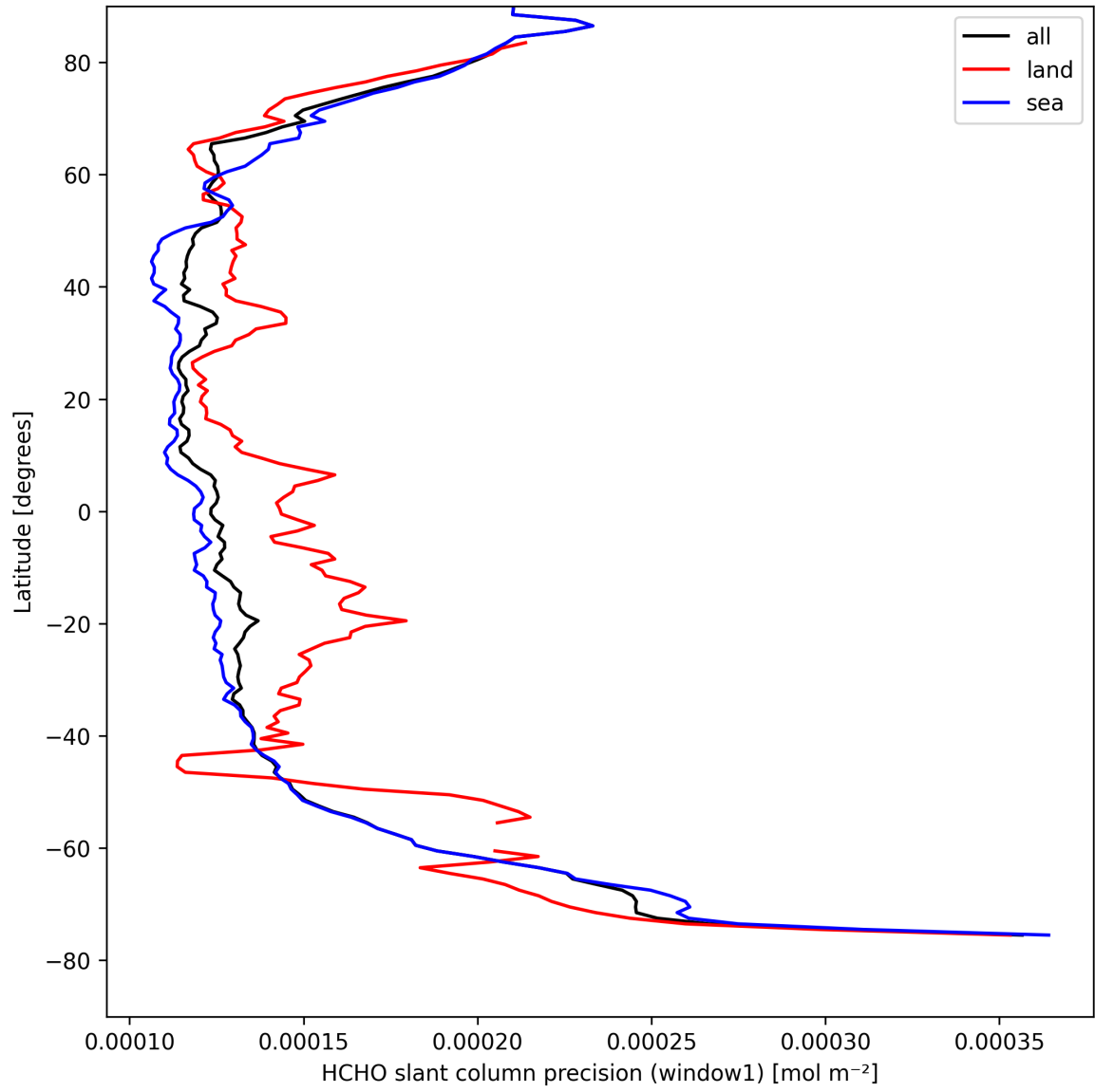
Figure 25: Zonal average of “HCHO slant column precision (window1)” for 2025-04-13 to 2025-04-15.
