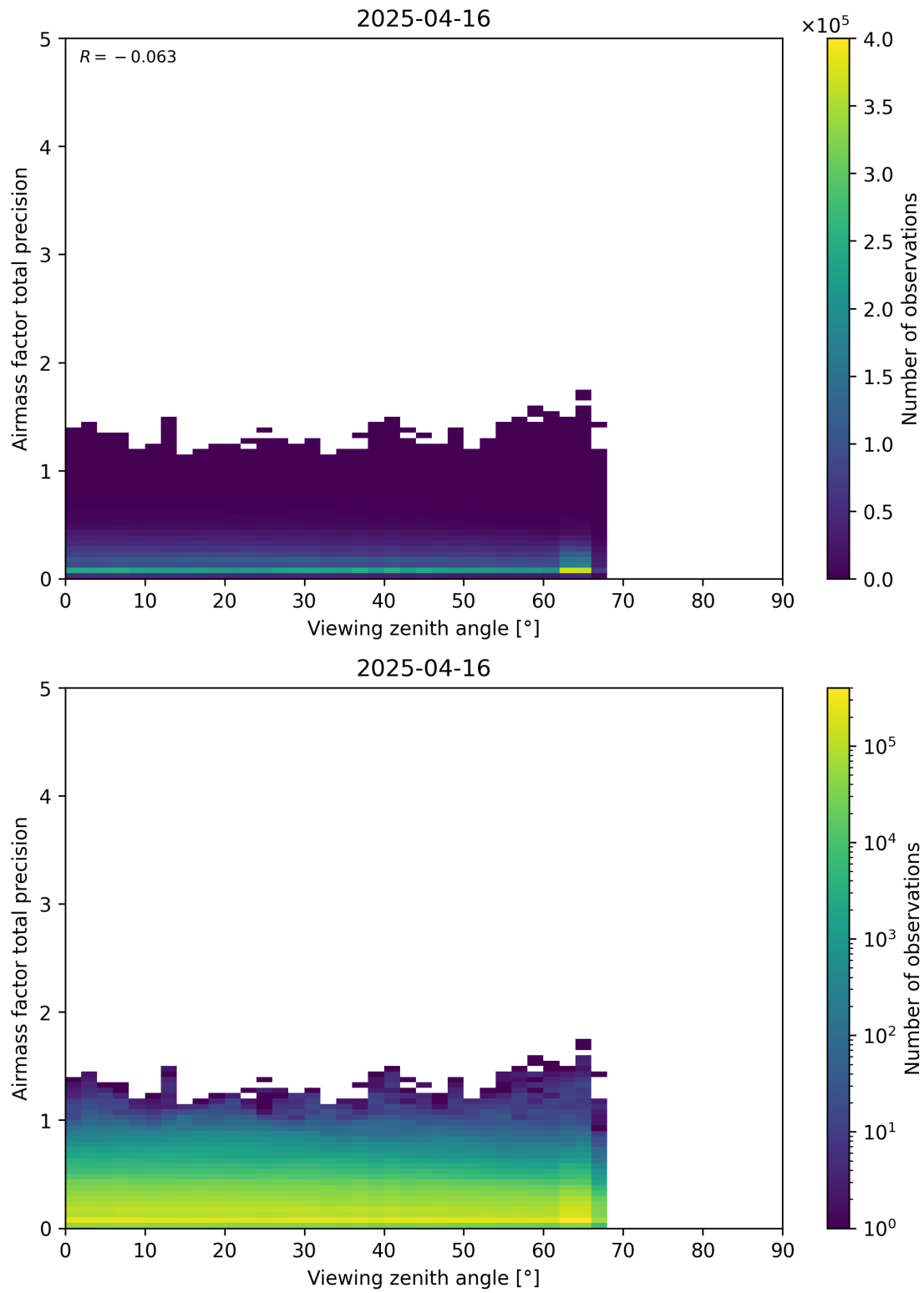
Figure 191: Scatter density plot of “Viewing zenith angle” against “Airmass factor total precision” for 2025-04-15 to 2025-04-17.
