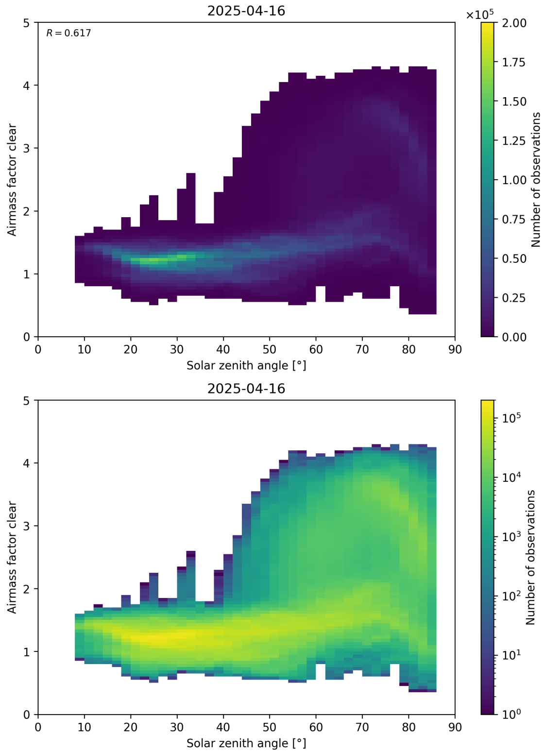
Figure 170: Scatter density plot of “Solar zenith angle” against “Airmass factor clear” for 2025-04-15 to 2025-04-17.
