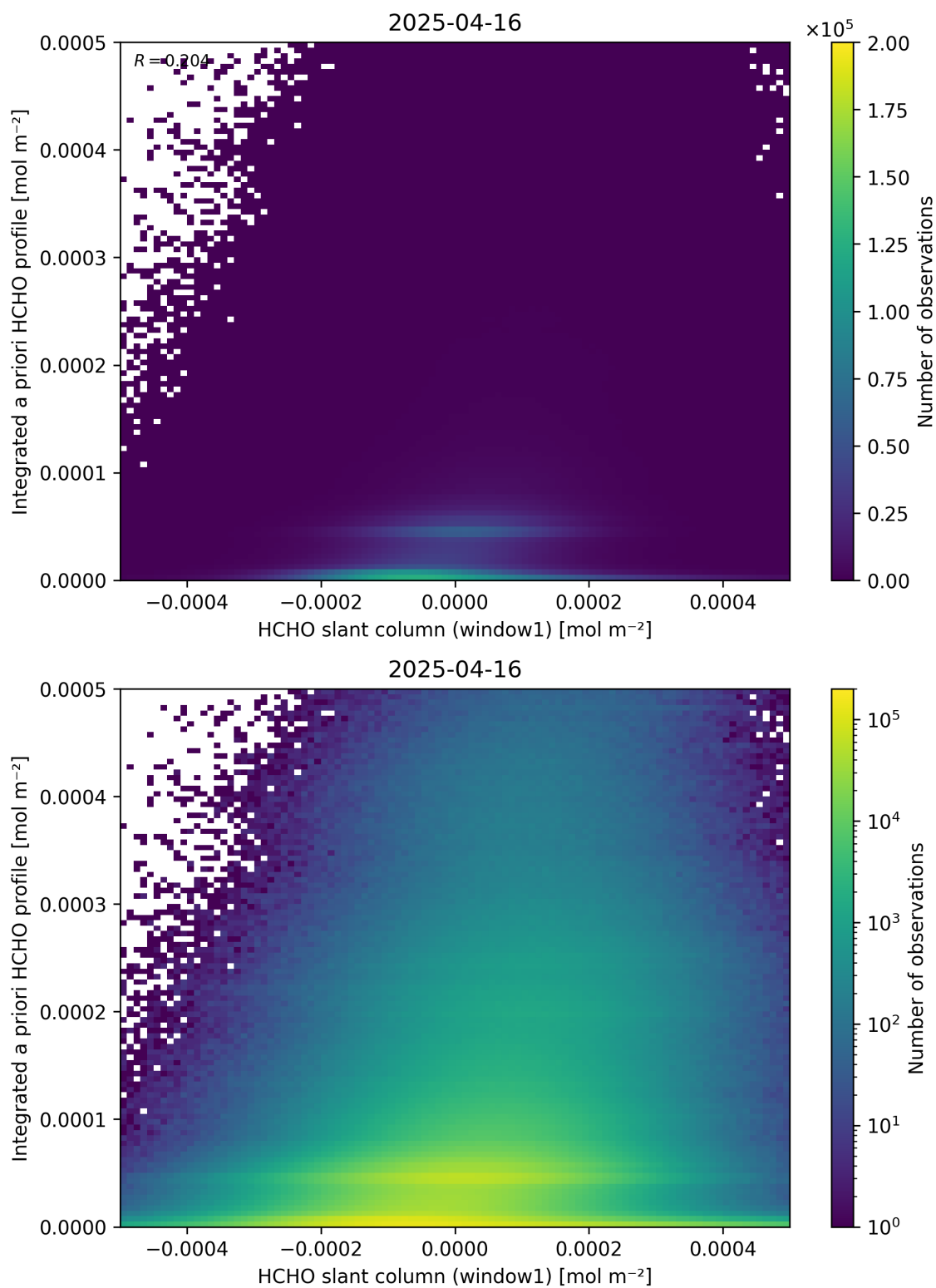
Figure 87: Scatter density plot of “HCHO slant column (window1)” against “Integrated a priori HCHO profile” for 2025-04-15 to 2025-04-17.
