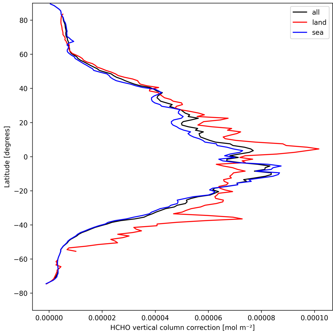
Figure 23: Zonal average of “HCHO vertical column correction” for 2025-04-15 to 2025-04-17.
