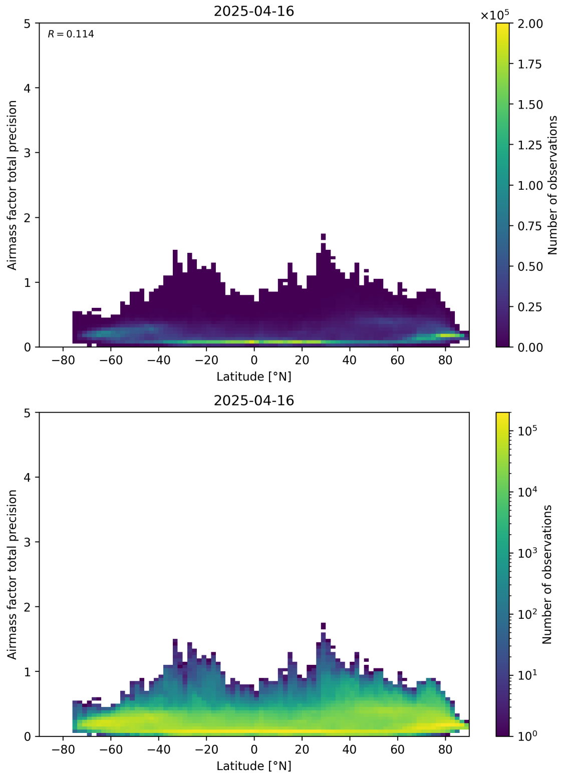
Figure 162: Scatter density plot of “Latitude” against “Airmass factor total precision” for 2025-04-15 to 2025-04-17.
