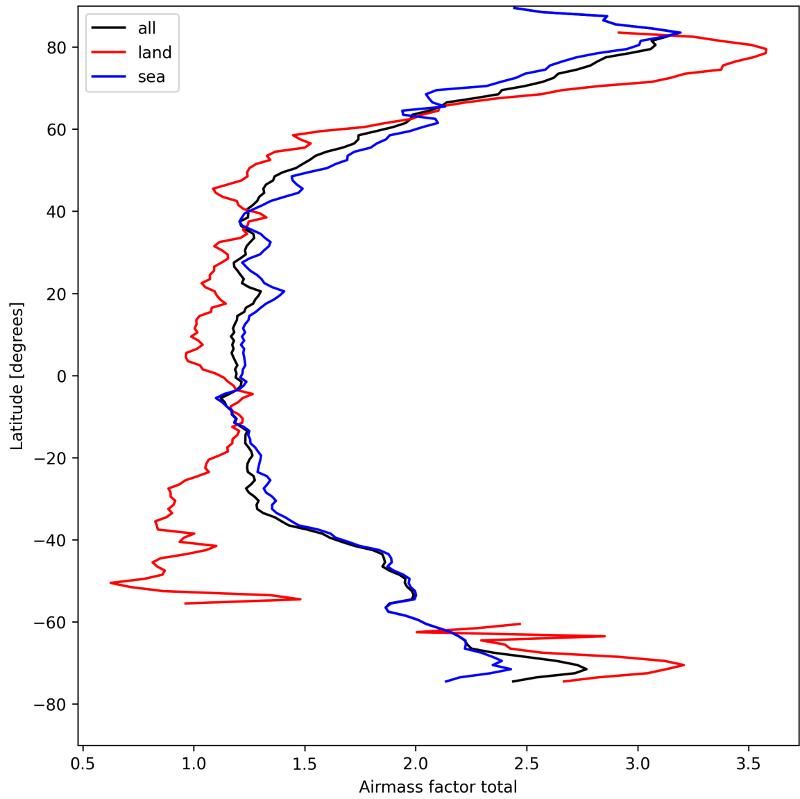
Figure 26: Zonal average of “Airmass factor total” for 2025-04-15 to 2025-04-17.
