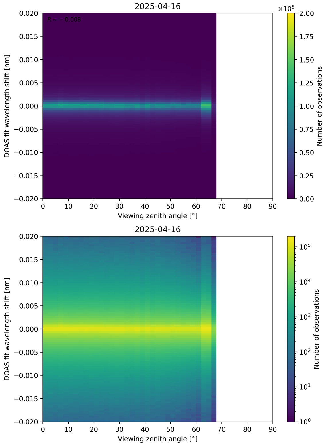
Figure 183: Scatter density plot of “Viewing zenith angle” against “DOAS fit wavelength shift” for 2025-04-15 to 2025-04-17.
