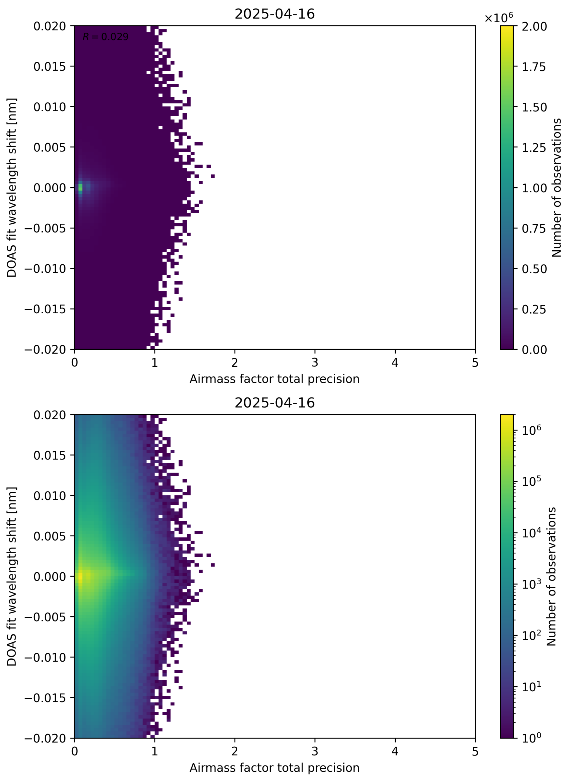
Figure 106: Scatter density plot of “Airmass factor total precision” against “DOAS fit wavelength shift” for 2025-04-15 to 2025-04-17.
