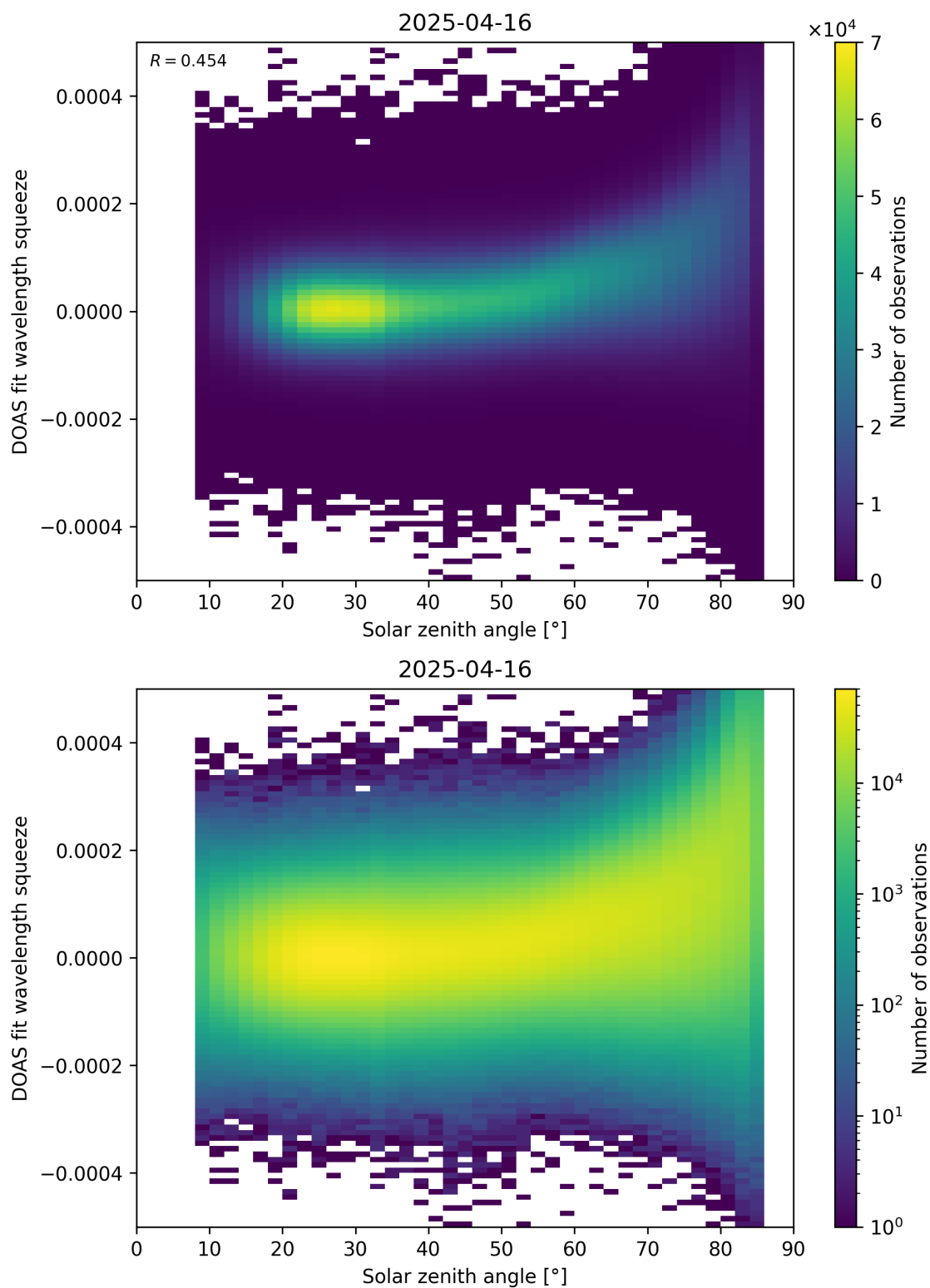
Figure 169: Scatter density plot of “Solar zenith angle” against “DOAS fit wavelength squeeze” for 2025-04-15 to 2025-04-17.
