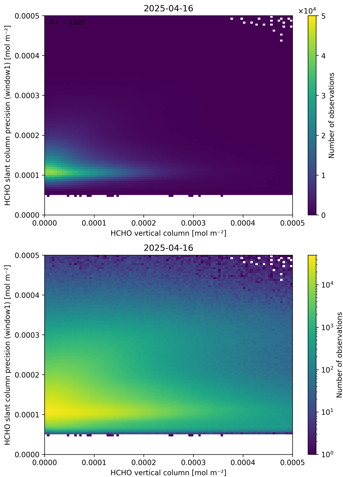
Figure 130: Scatter density plot of “HCHO vertical column” against “HCHO slant column precision (window1)” for 2025-04-15 to 2025-04-17.
