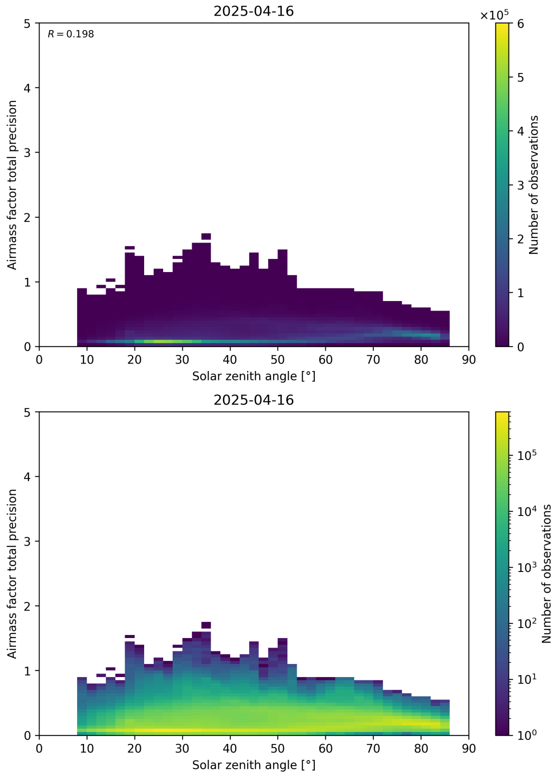
Figure 176: Scatter density plot of “Solar zenith angle” against “Airmass factor total precision” for 2025-04-15 to 2025-04-17.
