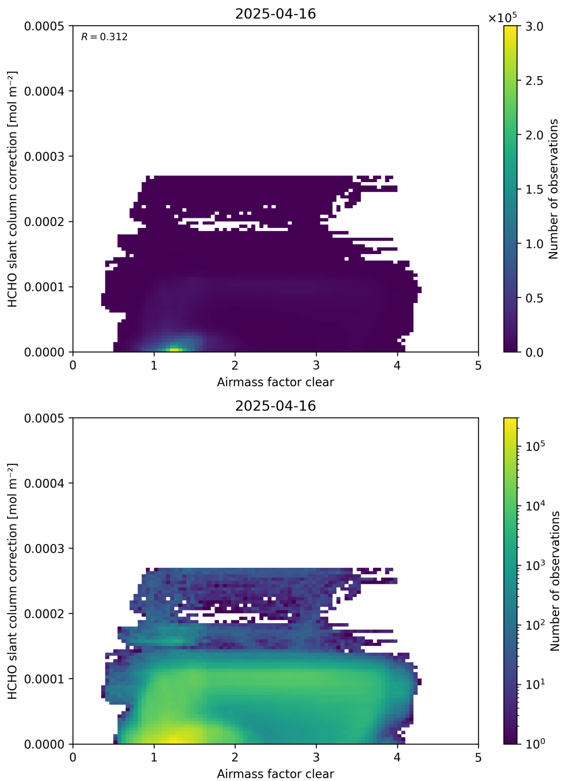
Figure 75: Scatter density plot of “Airmass factor clear” against “HCHO slant column correction” for 2025-04-15 to 2025-04-17.
