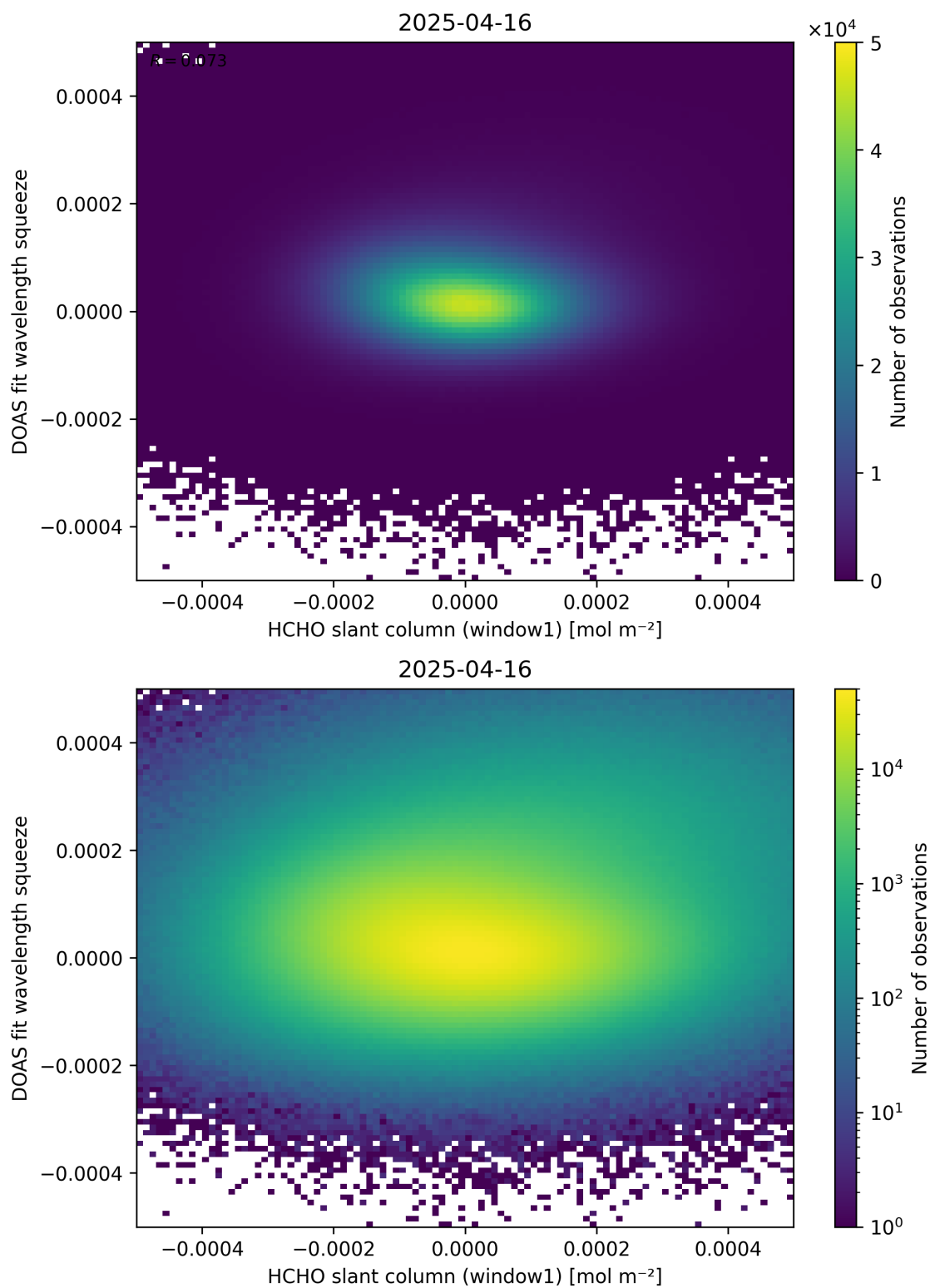
Figure 80: Scatter density plot of “HCHO slant column (window1)” against “DOAS fit wavelength squeeze” for 2025-04-15 to 2025-04-17.
