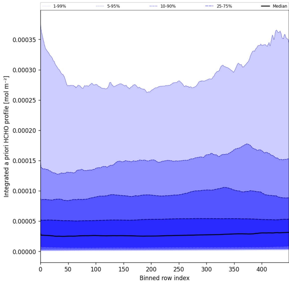
Figure 57: Along track statistics of “Integrated a priori HCHO profile” for 2025-04-15 to 2025-04-17
