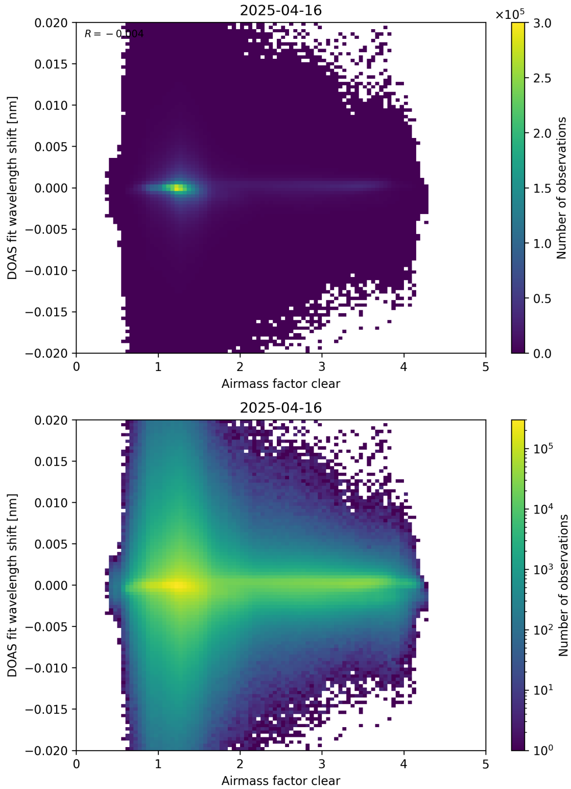
Figure 72: Scatter density plot of “Airmass factor clear” against “DOAS fit wavelength shift” for 2025-04-15 to 2025-04-17.
