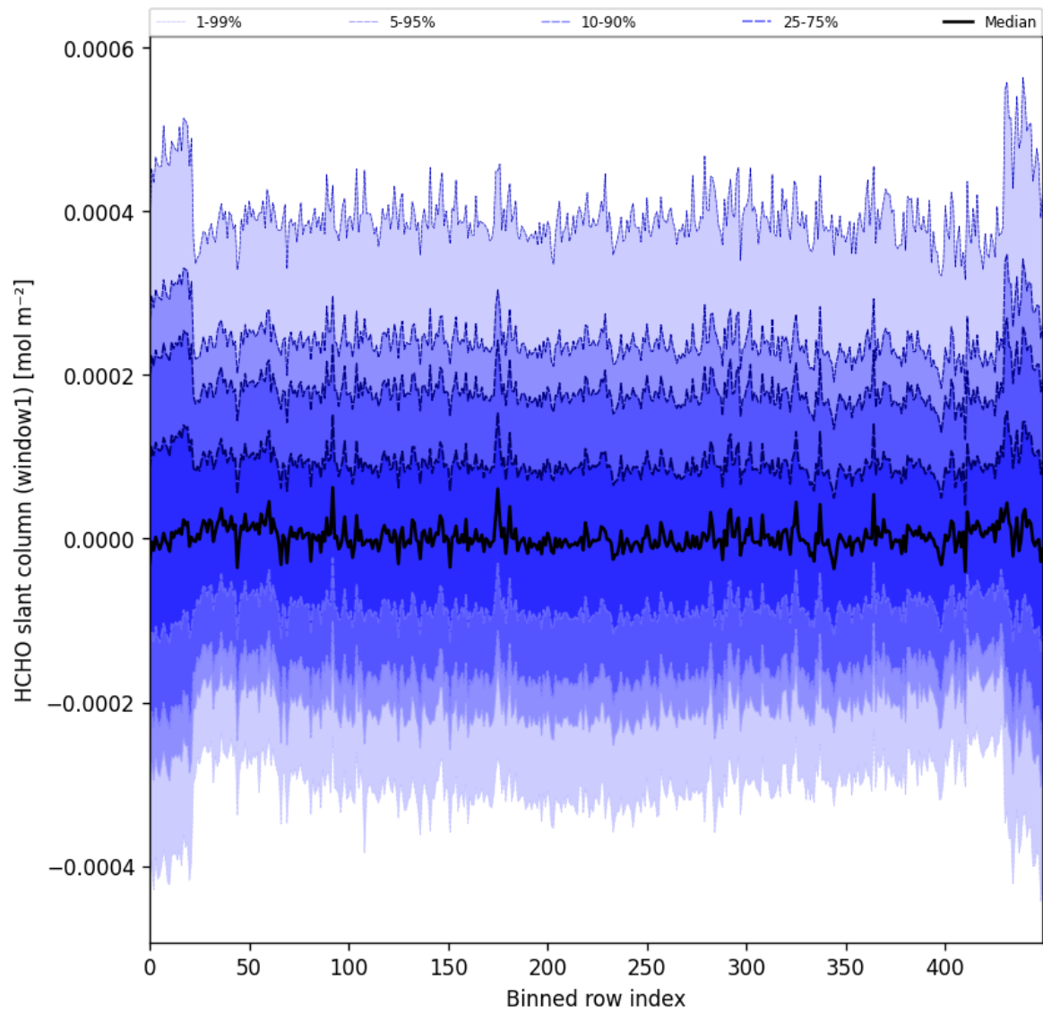
Figure 52: Along track statistics of “HCHO slant column (window1)” for 2025-04-15 to 2025-04-17
