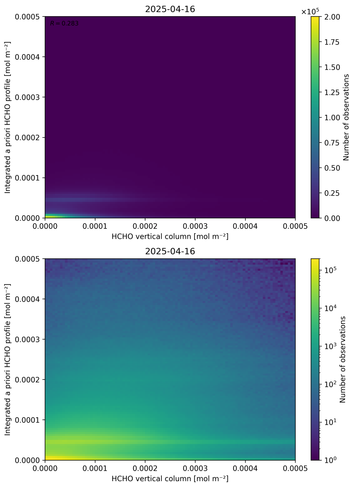
Figure 135: Scatter density plot of “HCHO vertical column” against “Integrated a priori HCHO profile” for 2025-04-15 to 2025-04-17.
