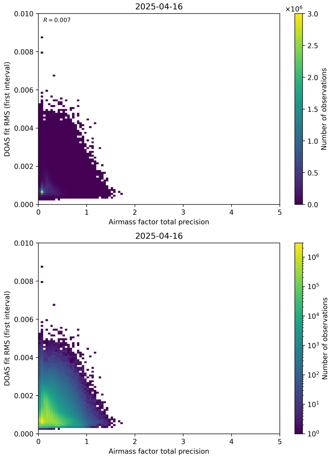
Figure 105: Scatter density plot of “Airmass factor total precision” against “DOAS fit RMS (first interval)” for 2025-04-15 to 2025-04-17.
