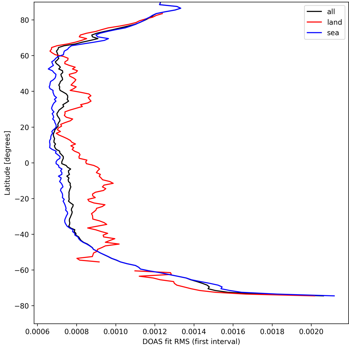
Figure 32: Zonal average of "DOAS fit RMS (first interval)" for 2025-04-15 to 2025-04-17.
