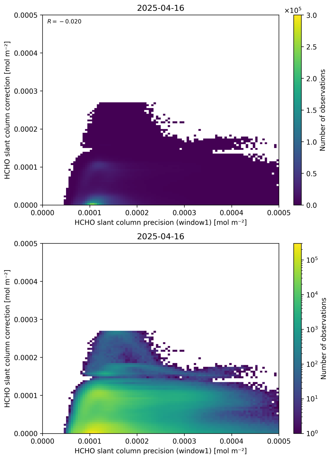
Figure 93: Scatter density plot of “HCHO slant column precision (window1)” against “HCHO slant column correction” for 2025-04-15 to 2025-04-17.
