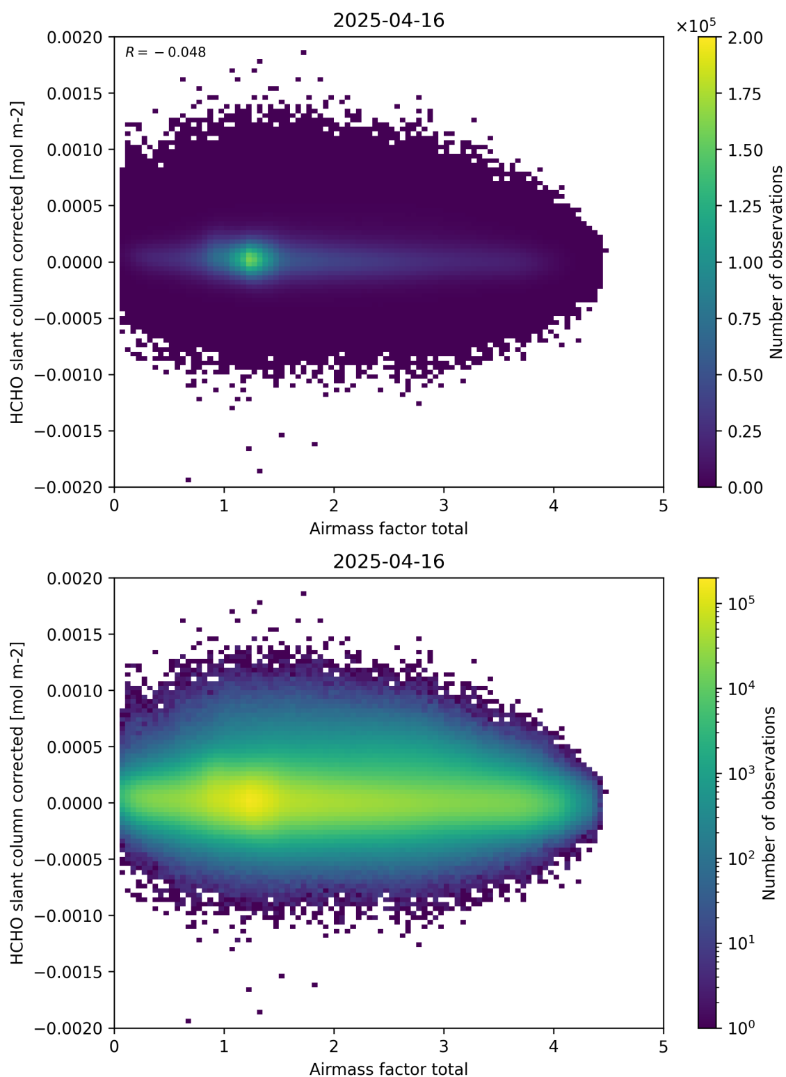
Figure 101: Scatter density plot of “Airmass factor total” against “HCHO slant column corrected” for 2025-04-15 to 2025-04-17.
