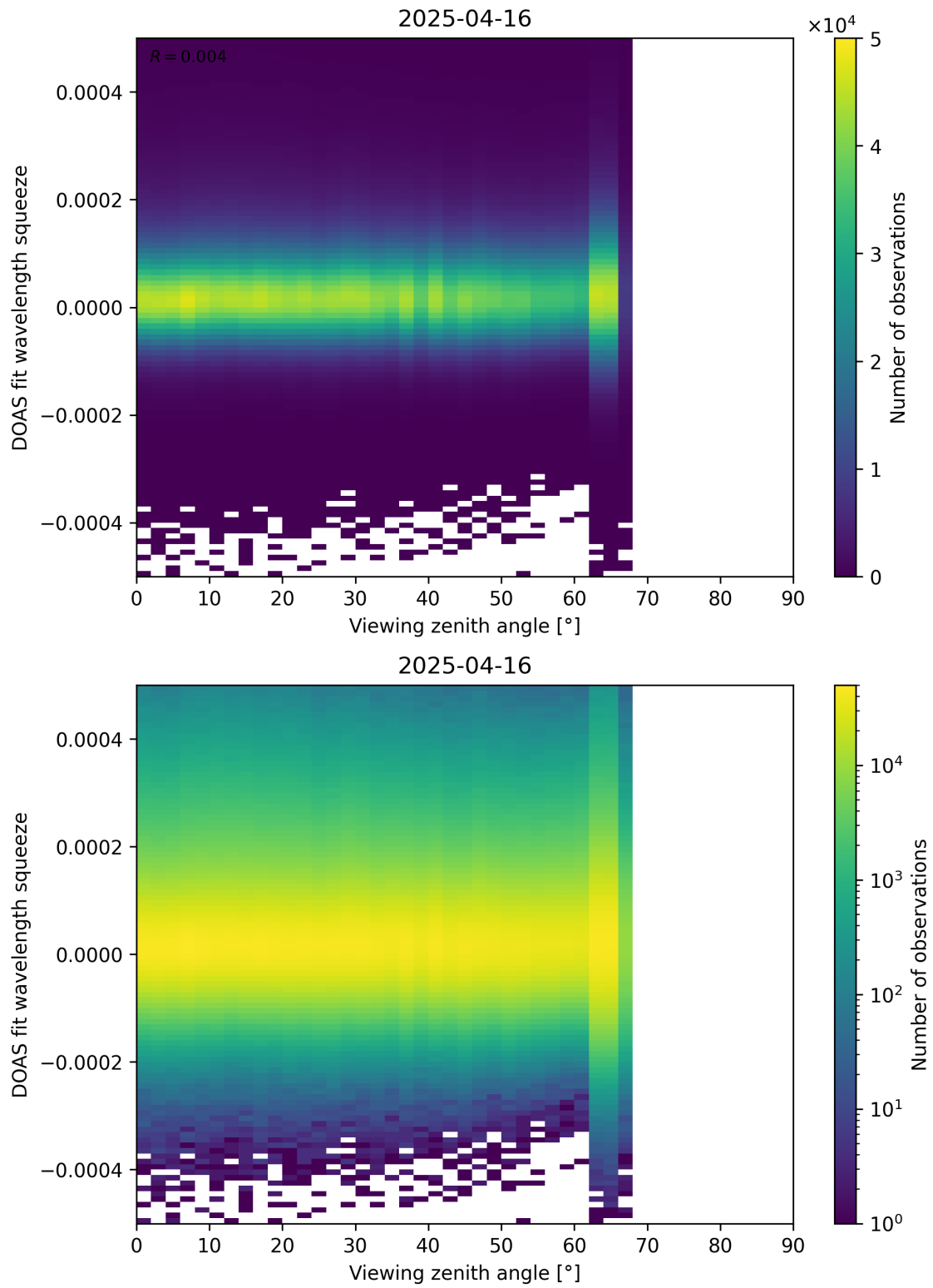
Figure 184: Scatter density plot of “Viewing zenith angle” against “DOAS fit wavelength squeeze” for 2025-04-15 to 2025-04-17.
