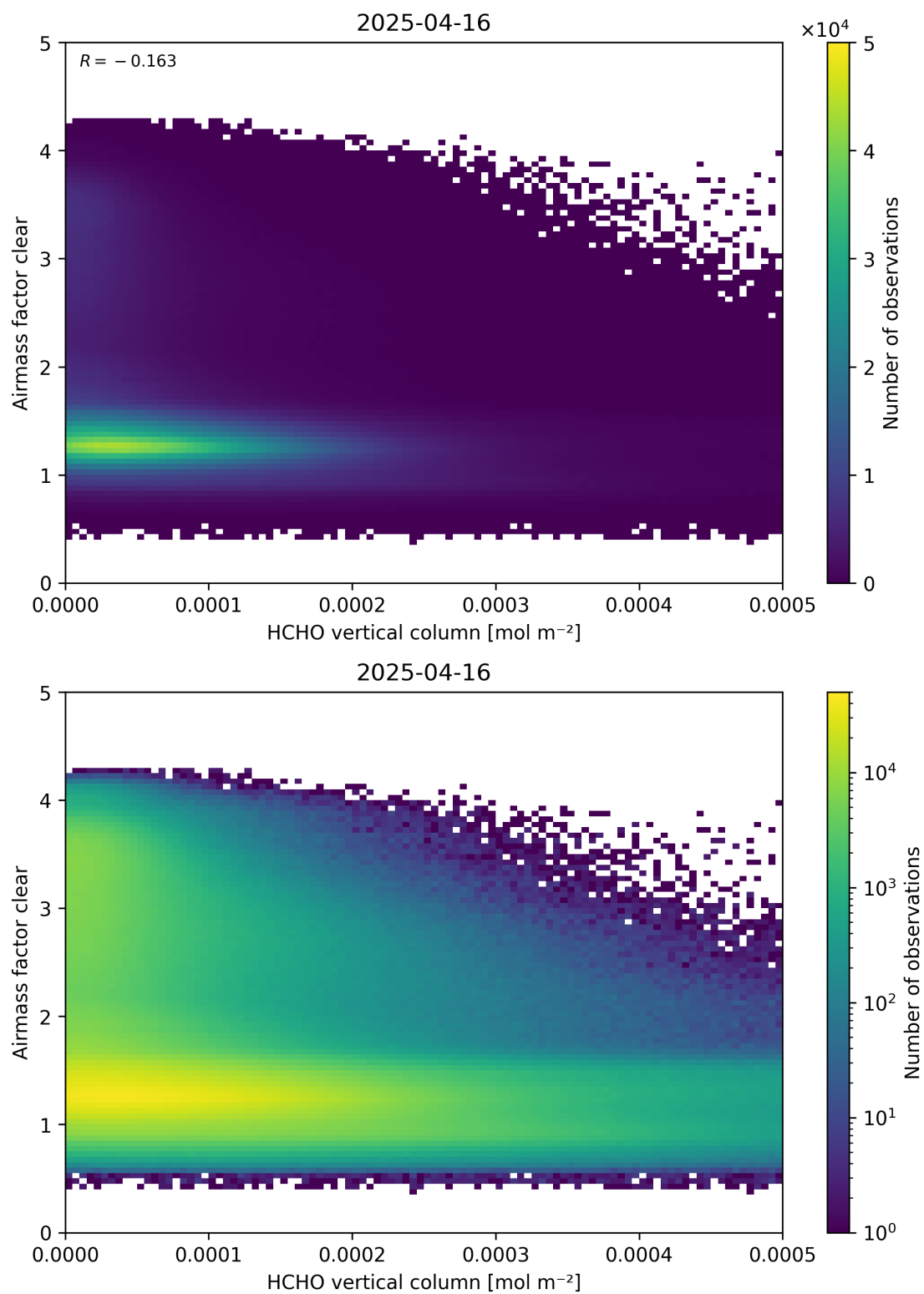
Figure 126: Scatter density plot of “HCHO vertical column” against “Airmass factor clear” for 2025-04-15 to 2025-04-17.
