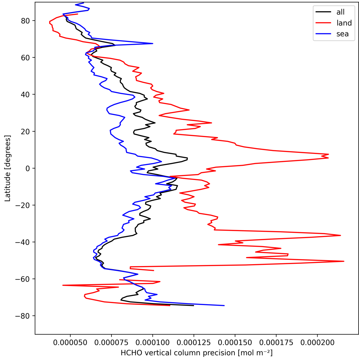
Figure 22: Zonal average of “HCHO vertical column precision” for 2025-04-15 to 2025-04-17.
