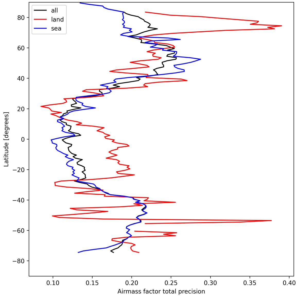
Figure 27: Zonal average of “Airmass factor total precision” for 2025-04-15 to 2025-04-17.
