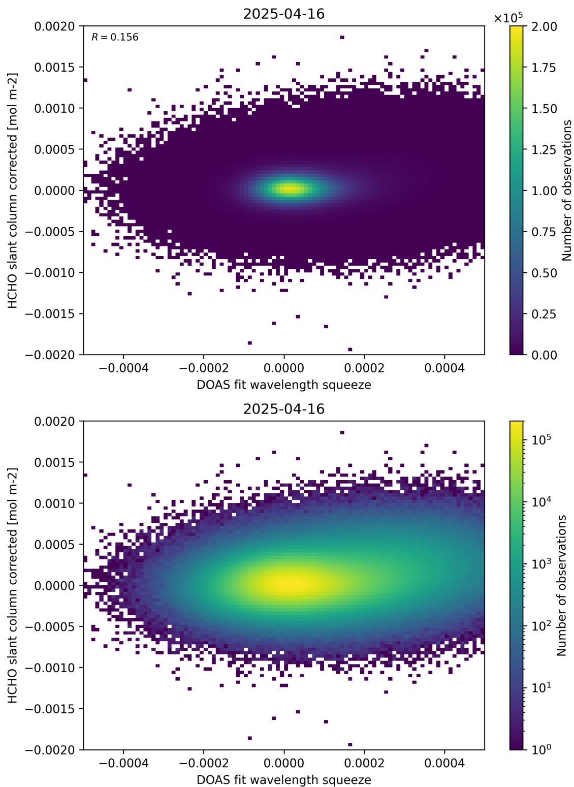
Figure 69: Scatter density plot of “DOAS fit wavelength squeeze” against “HCHO slant column corrected” for 2025-04-15 to 2025-04-17.
