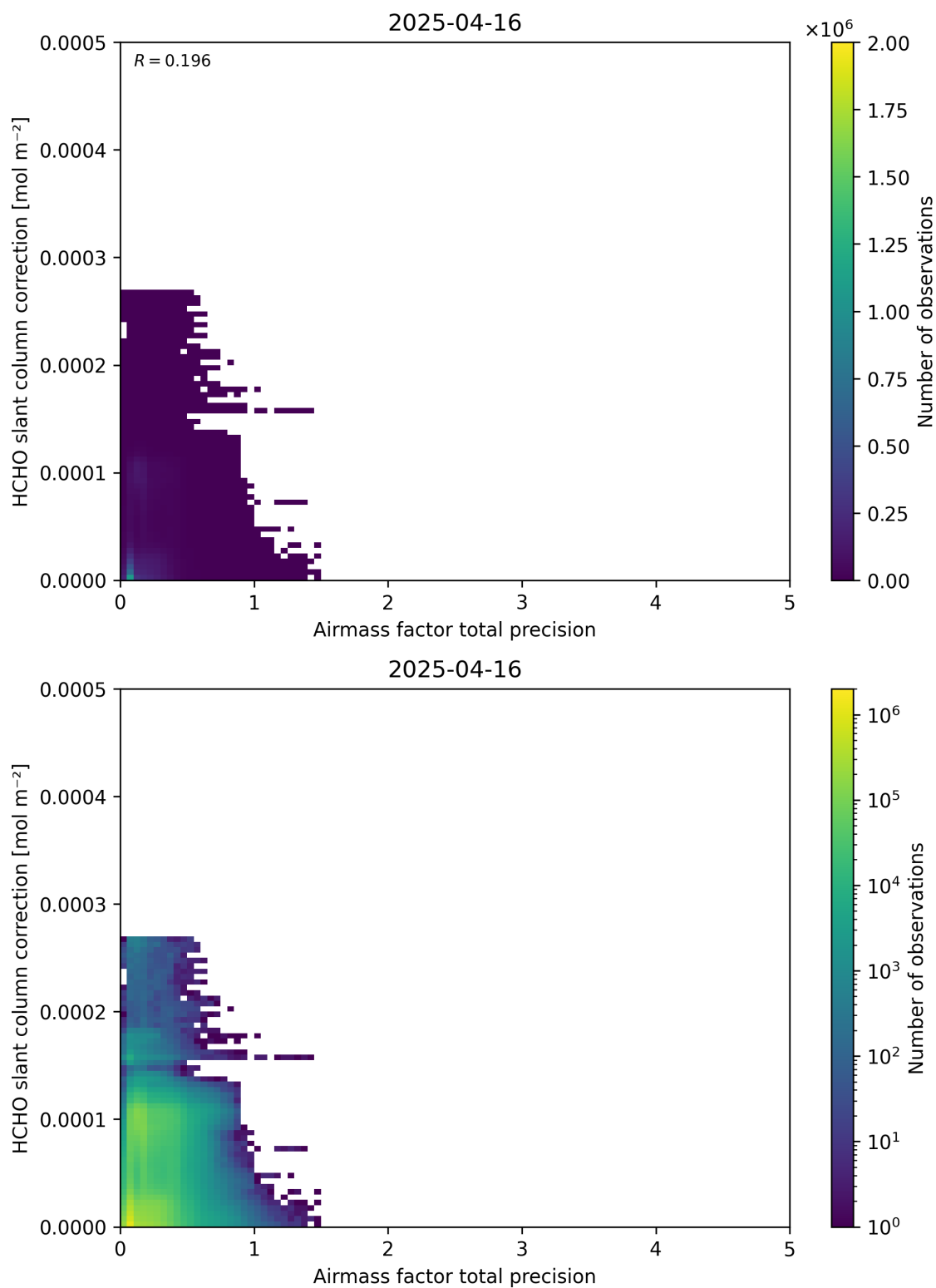
Figure 110: Scatter density plot of “Airmass factor total precision” against “HCHO slant column correction” for 2025-04-15 to 2025-04-17.
