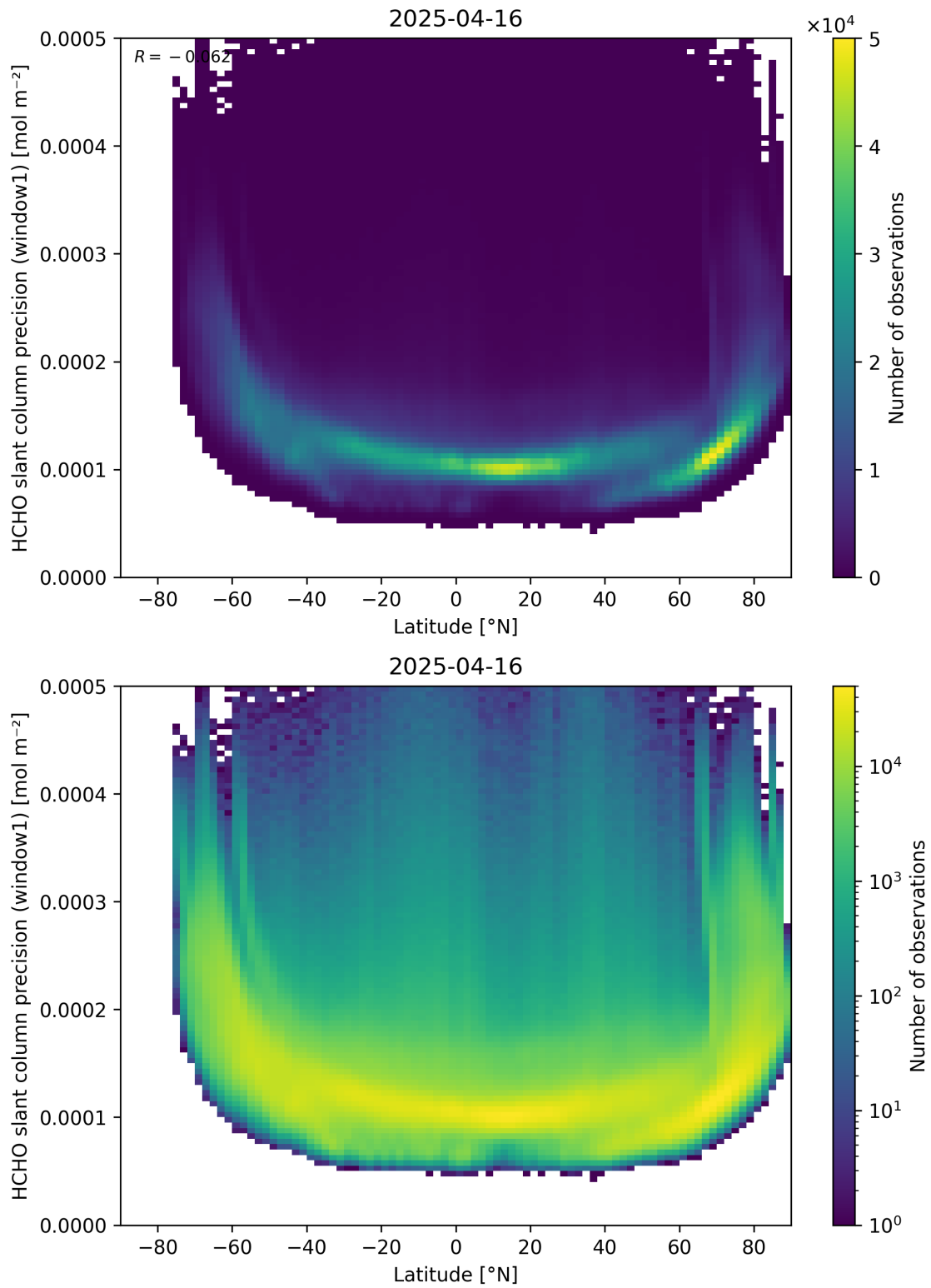
Figure 160: Scatter density plot of “Latitude” against “HCHO slant column precision (window1)” for 2025-04-15 to 2025-04-17.
