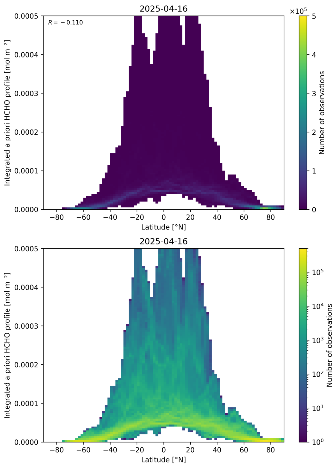
Figure 166: Scatter density plot of “Latitude” against “Integrated a priori HCHO profile” for 2025-04-15 to 2025-04-17.
