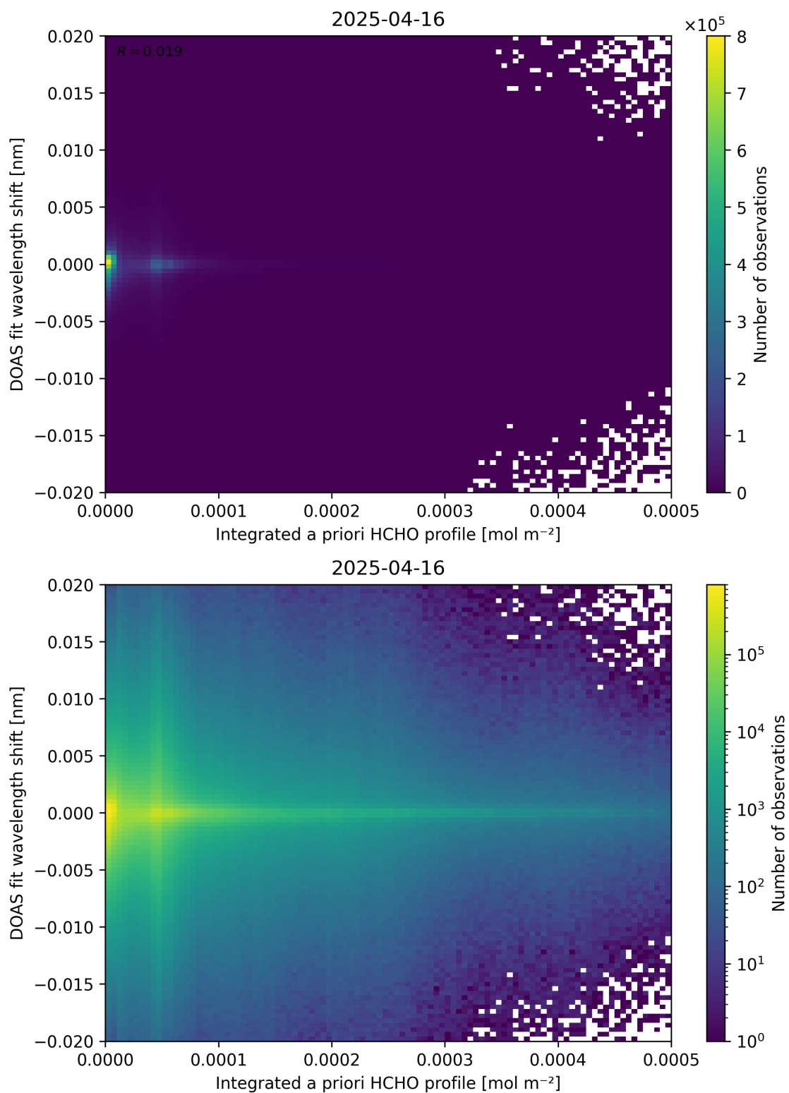
Figure 149: Scatter density plot of “Integrated a priori HCHO profile” against “DOAS fit wavelength shift” for 2025-04-15 to 2025-04-17.
