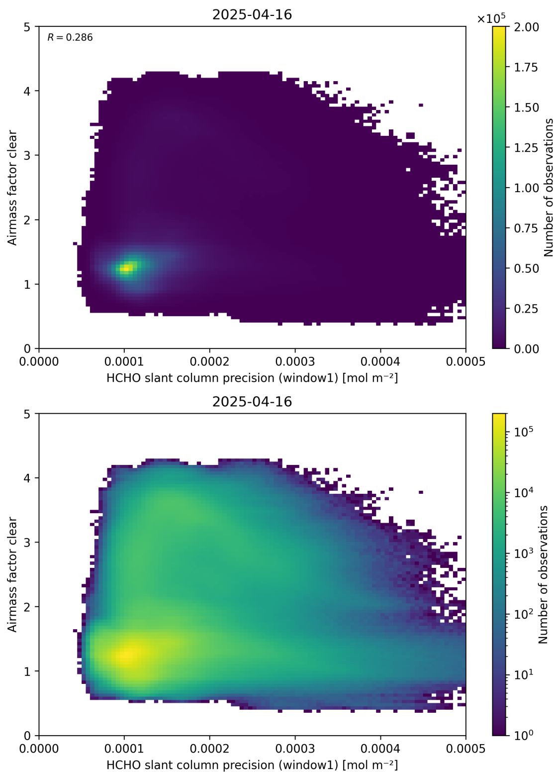
Figure 91: Scatter density plot of “HCHO slant column precision (window1)” against “Airmass factor clear” for 2025-04-15 to 2025-04-17.
