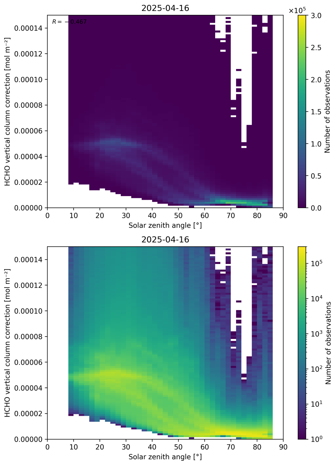
Figure 178: Scatter density plot of “Solar zenith angle” against “HCHO vertical column correction” for 2025-04-15 to 2025-04-17.
