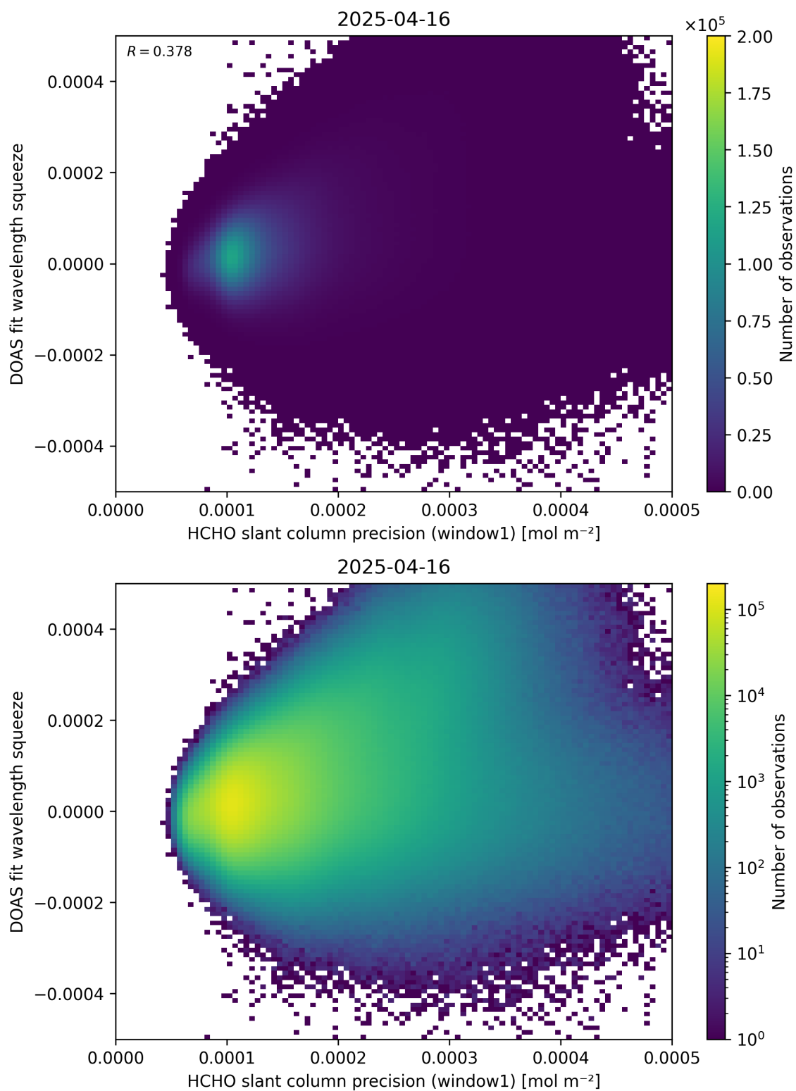
Figure 90: Scatter density plot of “HCHO slant column precision (window1)” against “DOAS fit wavelength squeeze” for 2025-04-15 to 2025-04-17.
