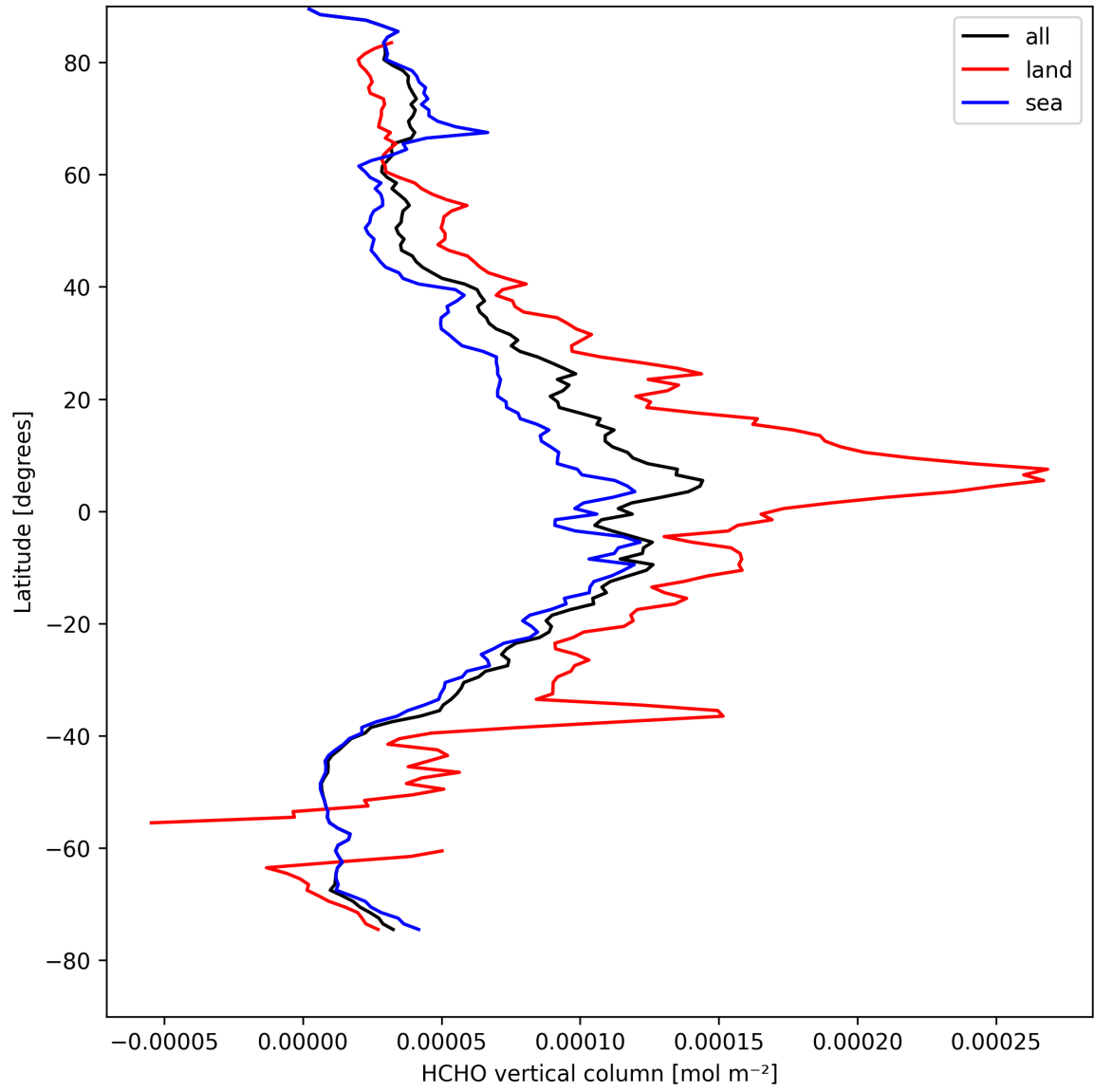
Figure 21: Zonal average of “HCHO vertical column” for 2025-04-15 to 2025-04-17.
