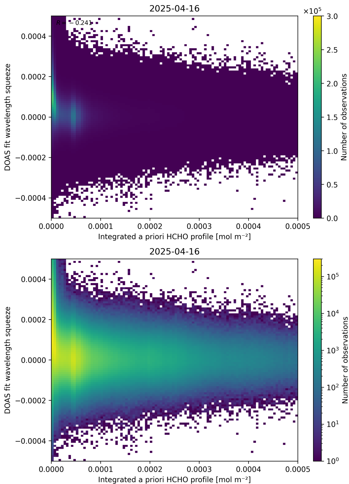
Figure 150: Scatter density plot of “Integrated a priori HCHO profile” against “DOAS fit wavelength squeeze” for 2025-04-15 to 2025-04-17.
