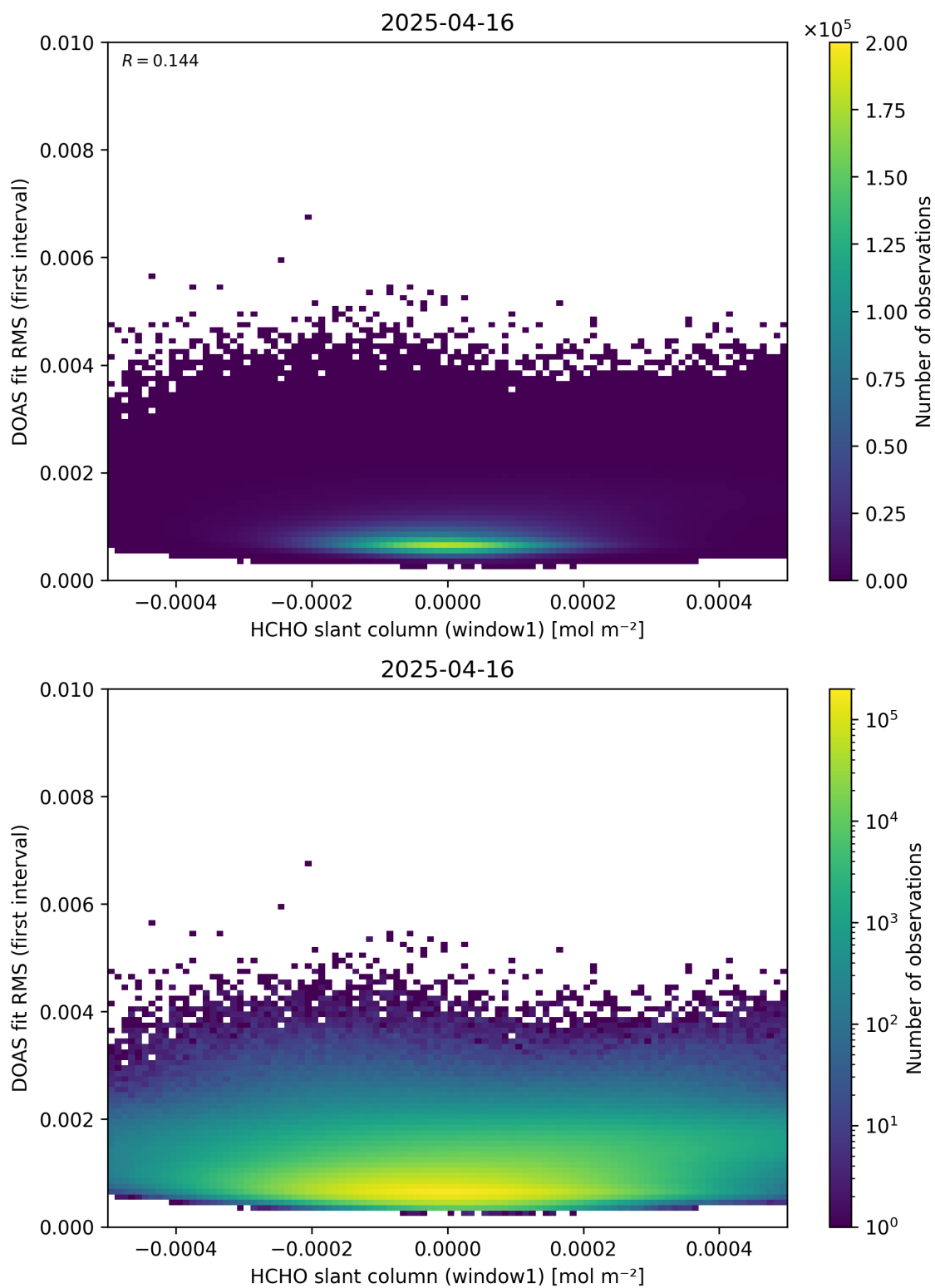
Figure 78: Scatter density plot of “HCHO slant column (window1)” against “DOAS fit RMS (first interval)” for 2025-04-15 to 2025-04-17.
