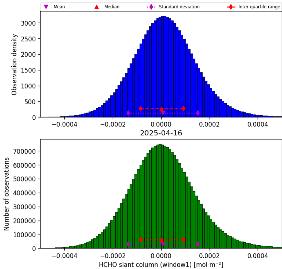
Figure 38: Histogram of “HCHO slant column (window1)” for 2025-04-15 to 2025-04-17
