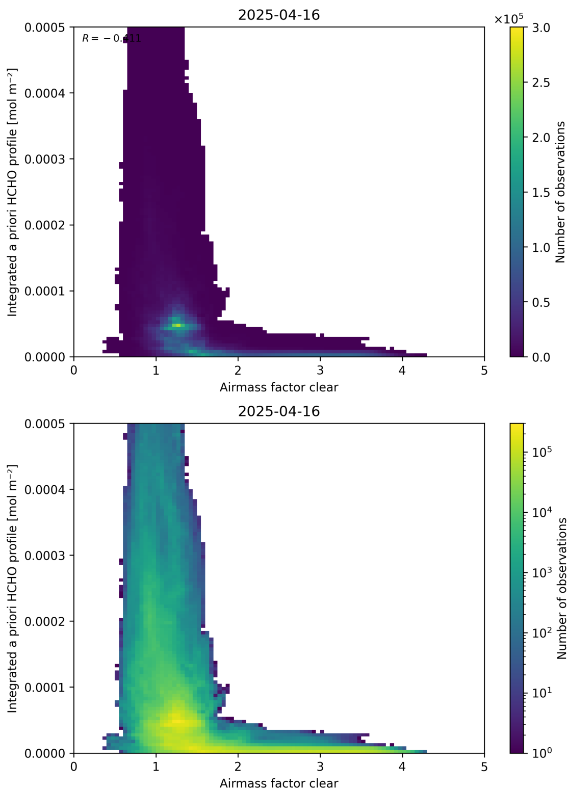
Figure 76: Scatter density plot of “Airmass factor clear” against “Integrated a priori HCHO profile” for 2025-04-15 to 2025-04-17.
