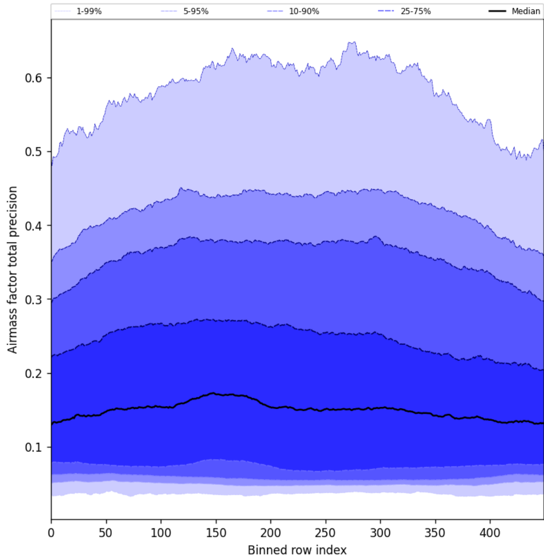
Figure 55: Along track statistics of “Airmass factor total precision” for 2025-04-15 to 2025-04-17
