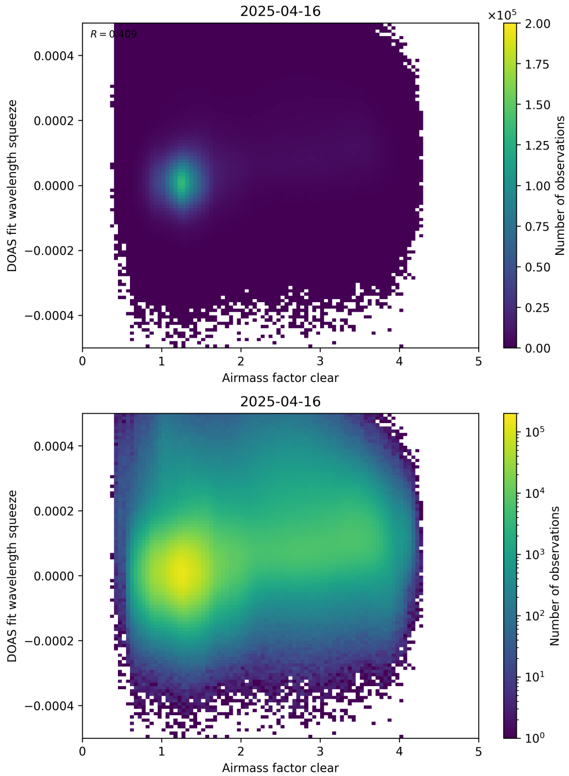
Figure 73: Scatter density plot of “Airmass factor clear” against “DOAS fit wavelength squeeze” for 2025-04-15 to 2025-04-17.
