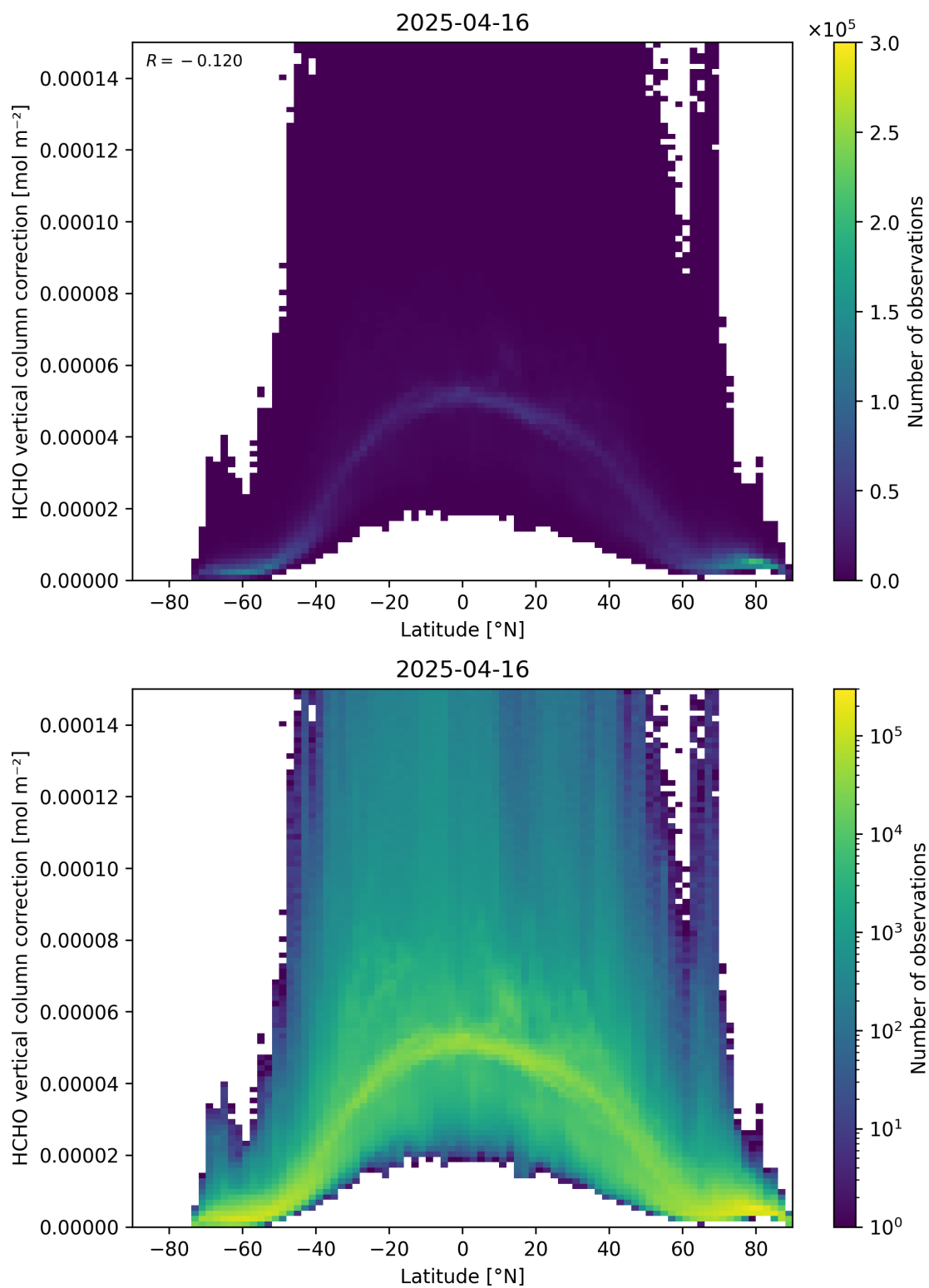
Figure 164: Scatter density plot of “Latitude” against “HCHO vertical column correction” for 2025-04-15 to 2025-04-17.
