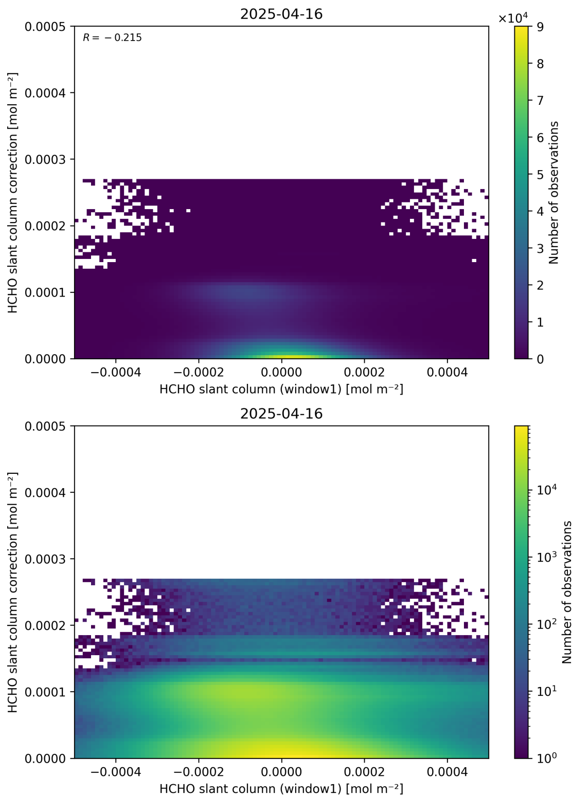
Figure 83: Scatter density plot of “HCHO slant column (window1)” against “HCHO slant column correction” for 2025-04-15 to 2025-04-17.
