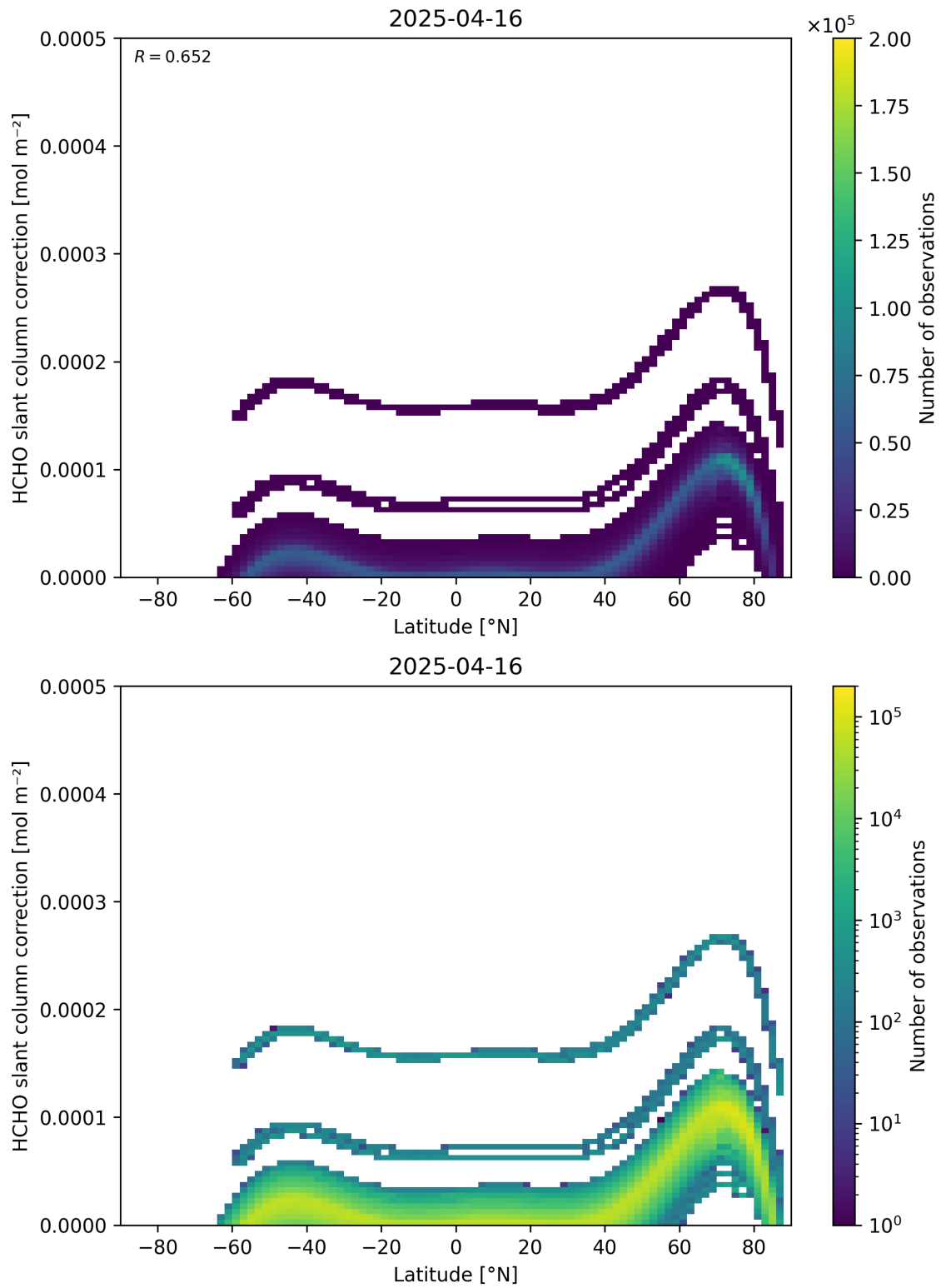
Figure 158: Scatter density plot of “Latitude” against “HCHO slant column correction” for 2025-04-15 to 2025-04-17.
