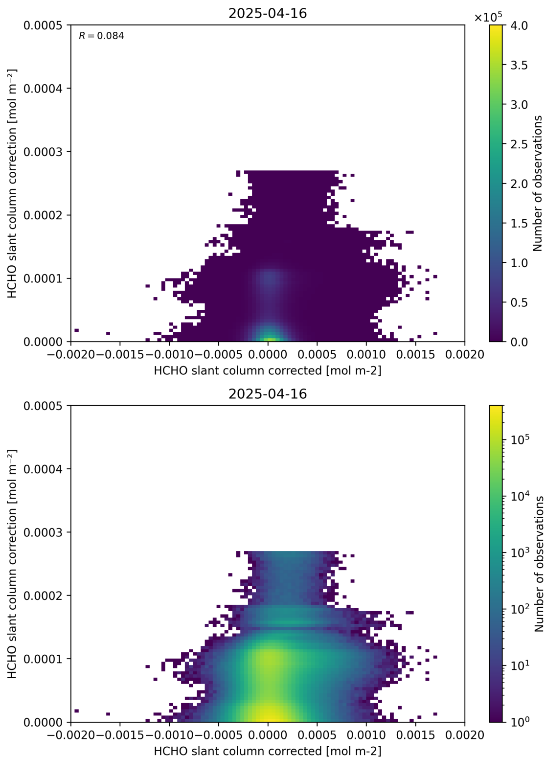
Figure 77: Scatter density plot of “HCHO slant column corrected” against “HCHO slant column correction” for 2025-04-15 to 2025-04-17.
