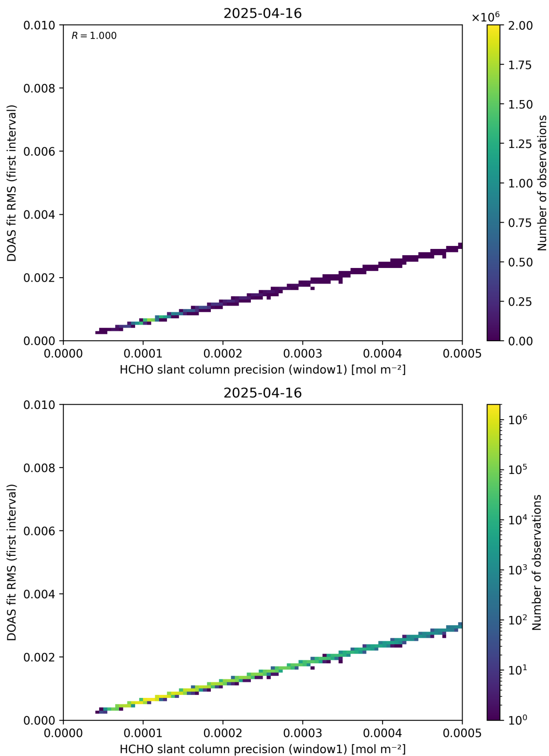
Figure 88: Scatter density plot of “HCHO slant column precision (window1)” against “DOAS fit RMS (first interval)” for 2025-04-15 to 2025-04-17.
