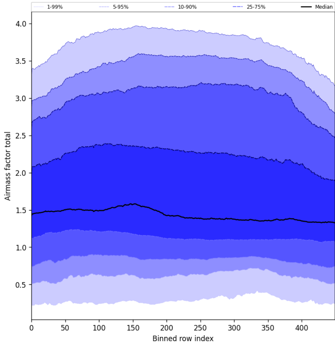
Figure 54: Along track statistics of “Airmass factor total” for 2025-04-15 to 2025-04-17
