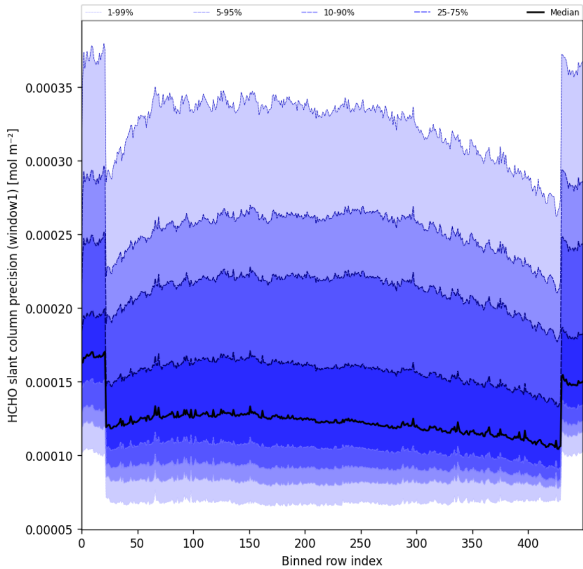
Figure 53: Along track statistics of "HCHO slant column precision (window1)" for 2025-04-15 to 2025-04-17
