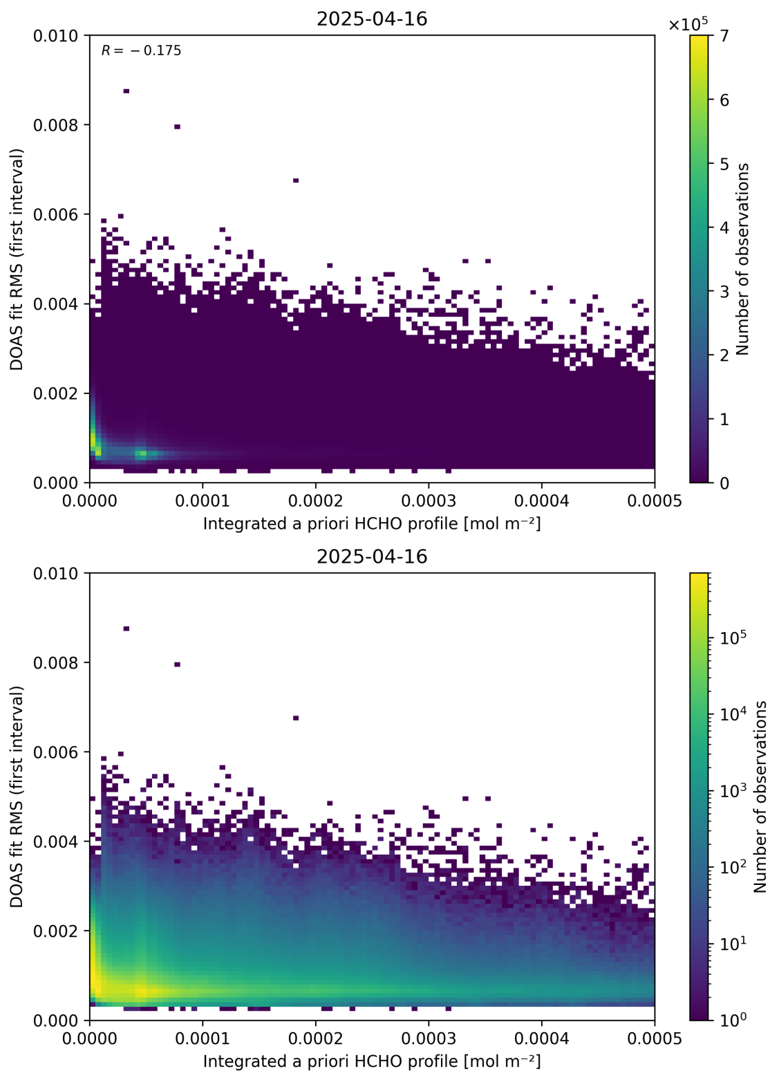
Figure 148: Scatter density plot of “Integrated a priori HCHO profile” against “DOAS fit RMS (first interval)” for 2025-04-15 to 2025-04-17.
