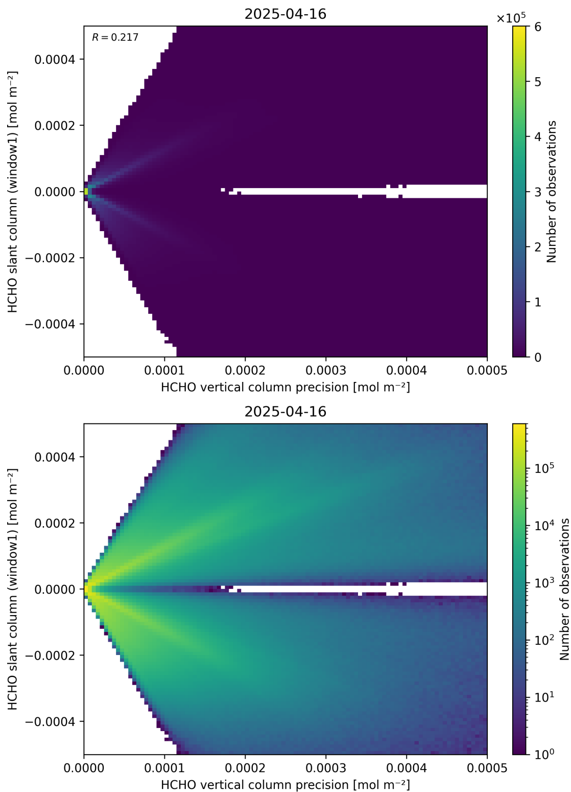
Figure 142: Scatter density plot of “HCHO vertical column precision” against “HCHO slant column (window1)” for 2025-04-15 to 2025-04-17.
