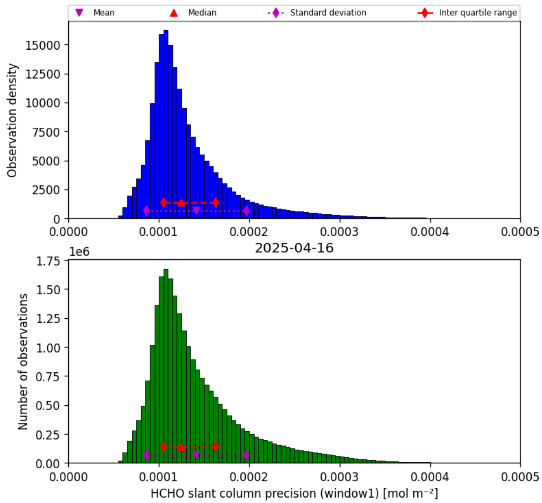
Figure 39: Histogram of “HCHO slant column precision (window1)” for 2025-04-15 to 2025-04-17
