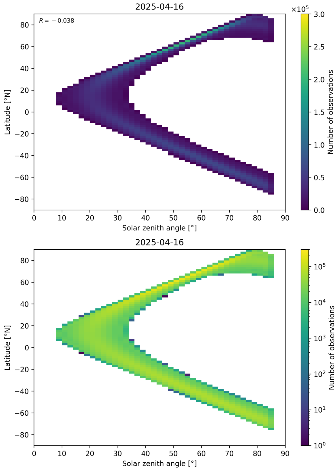
Figure 181: Scatter density plot of “Solar zenith angle” against “Latitude” for 2025-04-15 to 2025-04-17.
