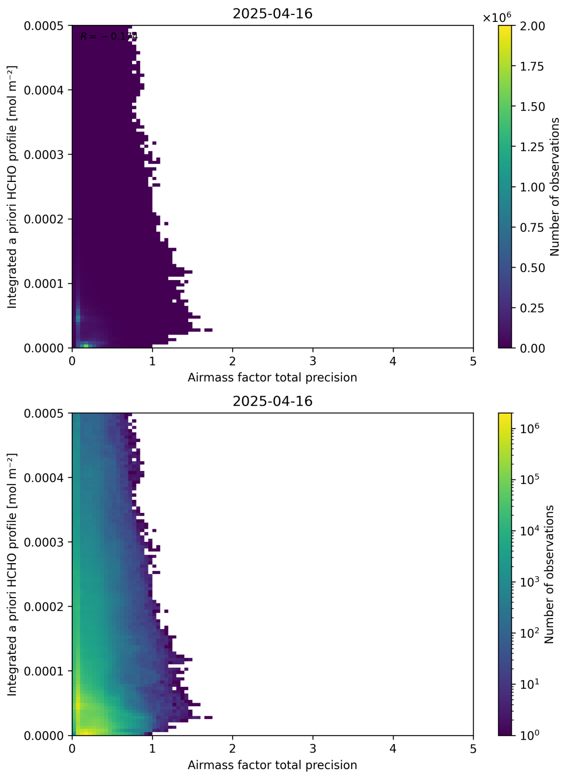
Figure 111: Scatter density plot of “Airmass factor total precision” against “Integrated a priori HCHO profile” for 2025-04-15 to 2025-04-17.
