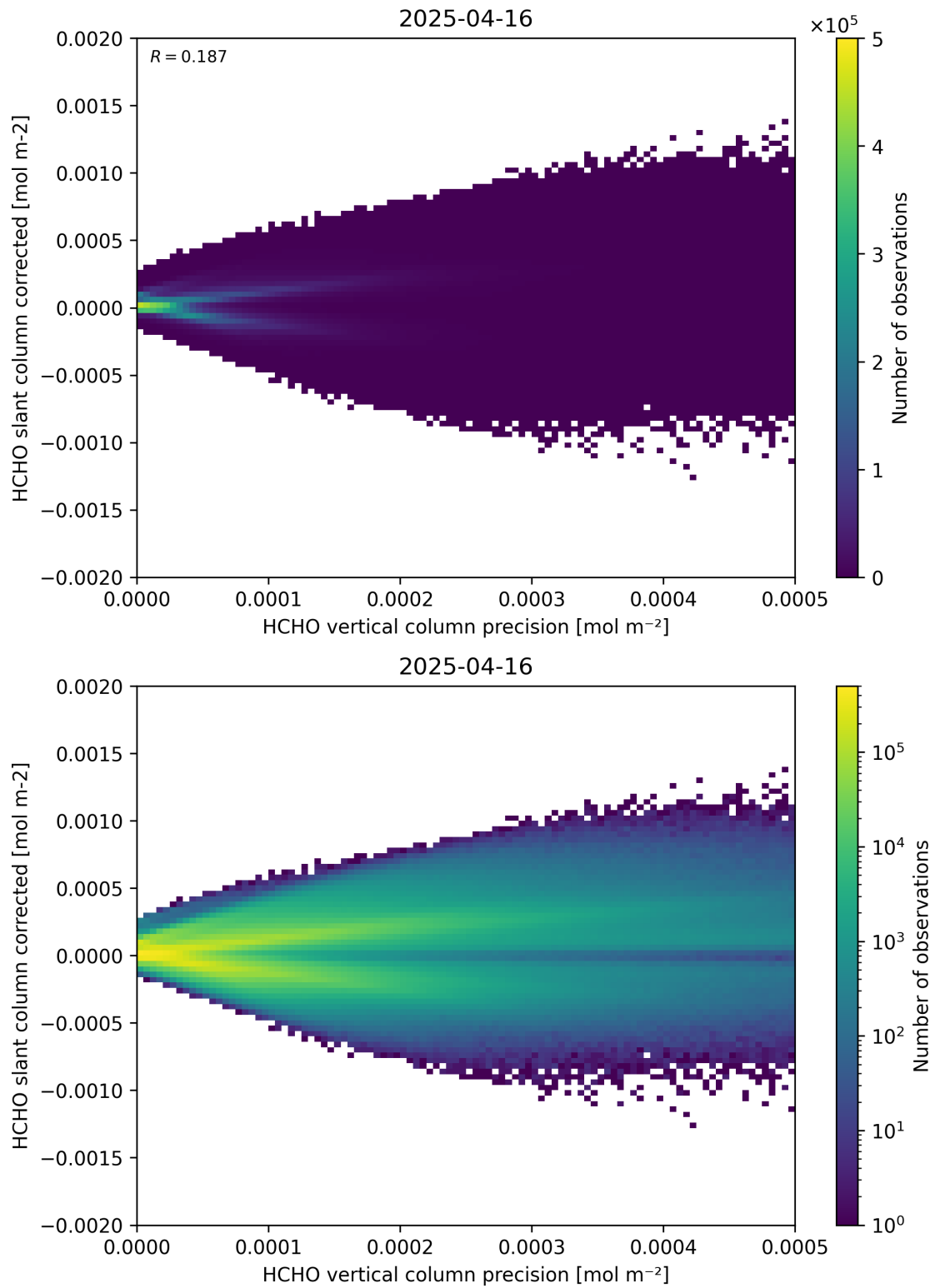
Figure 140: Scatter density plot of “HCHO vertical column precision” against “HCHO slant column corrected” for 2025-04-15 to 2025-04-17.
