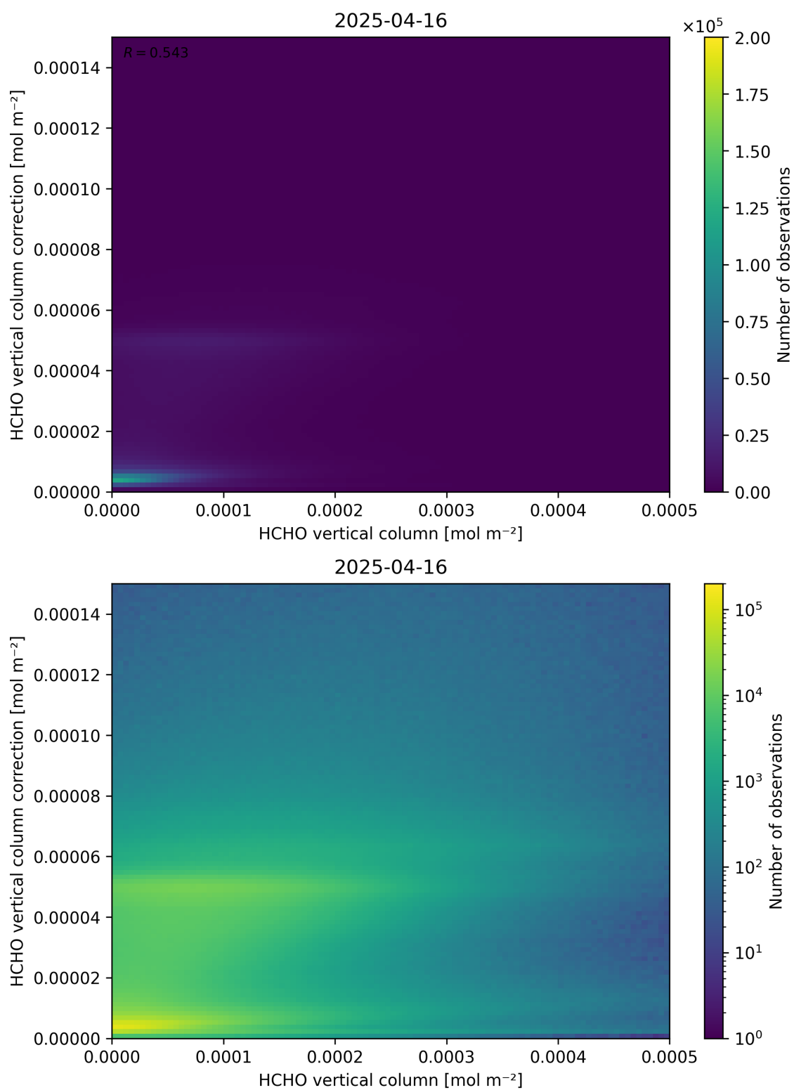
Figure 133: Scatter density plot of “HCHO vertical column” against “HCHO vertical column correction” for 2025-04-15 to 2025-04-17.
