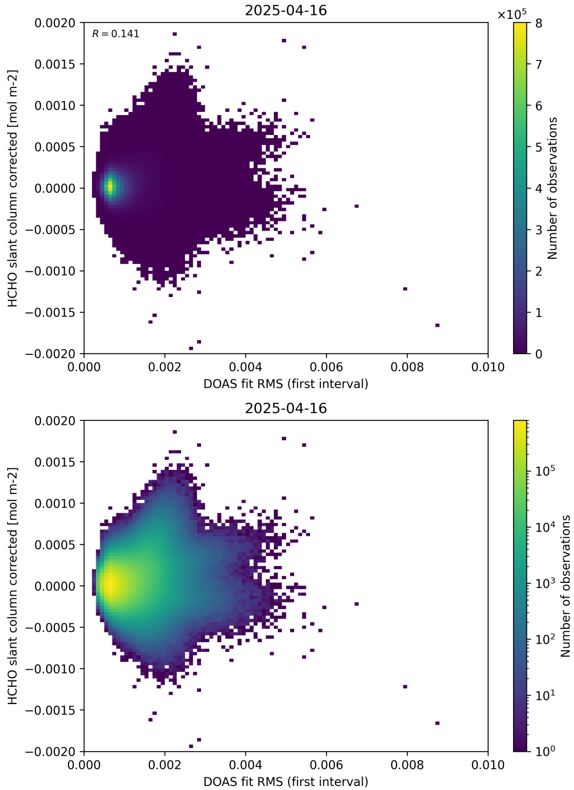
Figure 62: Scatter density plot of “DOAS fit RMS (first interval)” against “HCHO slant column corrected” for 2025-04-15 to 2025-04-17.
