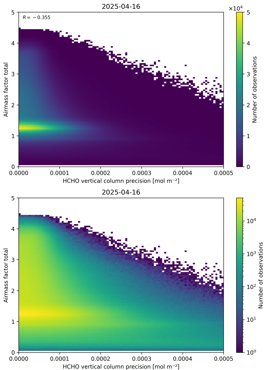
Figure 144: Scatter density plot of “HCHO vertical column precision” against “Airmass factor total” for 2025-04-15 to 2025-04-17.
