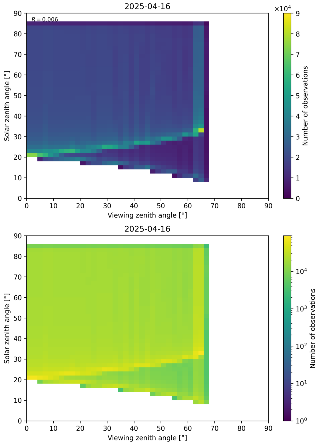
Figure 197: Scatter density plot of “Viewing zenith angle” against “Solar zenith angle” for 2025-04-15 to 2025-04-17.
