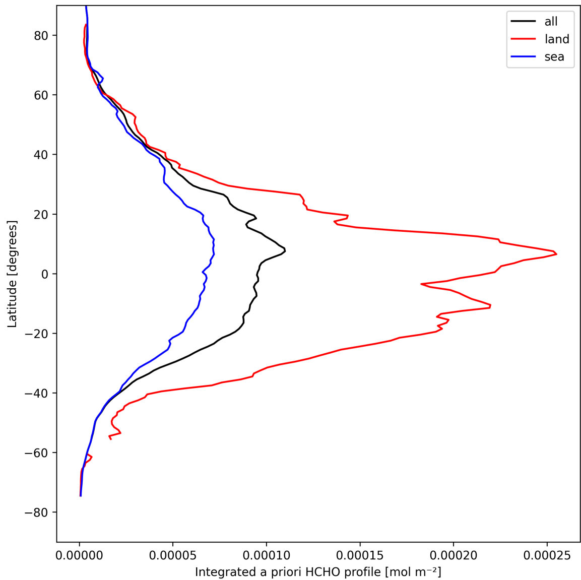
Figure 29: Zonal average of “Integrated a priori HCHO profile” for 2025-04-15 to 2025-04-17.
