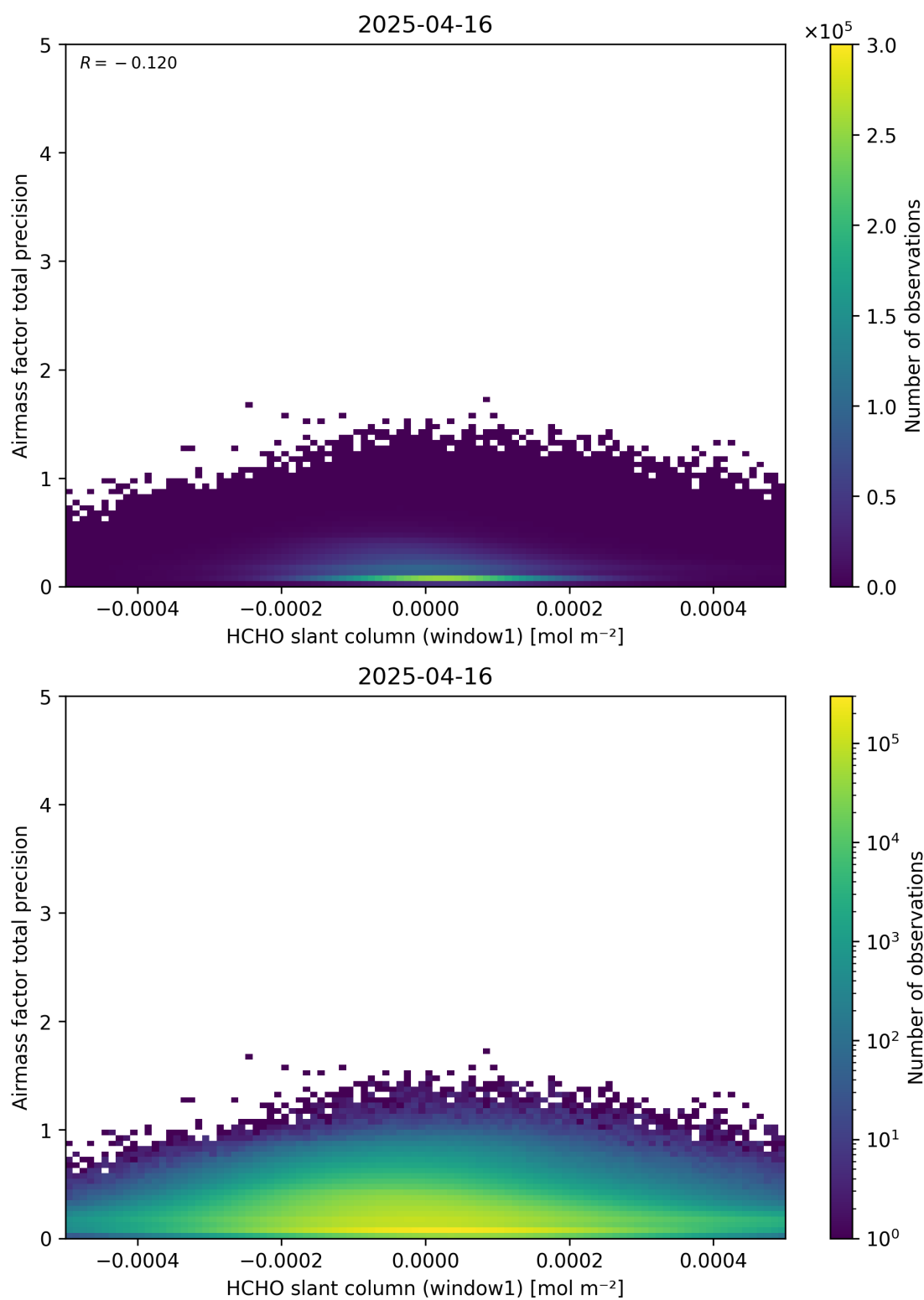
Figure 86: Scatter density plot of “HCHO slant column (window1)” against “Airmass factor total precision” for 2025-04-15 to 2025-04-17.
