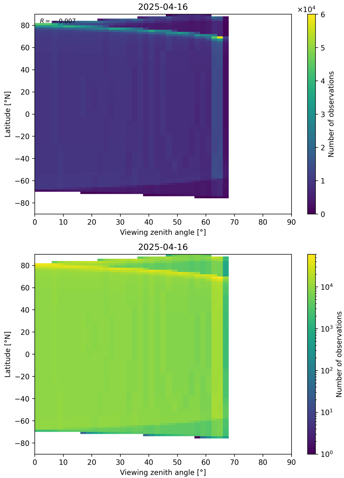
Figure 196: Scatter density plot of “Viewing zenith angle” against “Latitude” for 2025-04-15 to 2025-04-17.
