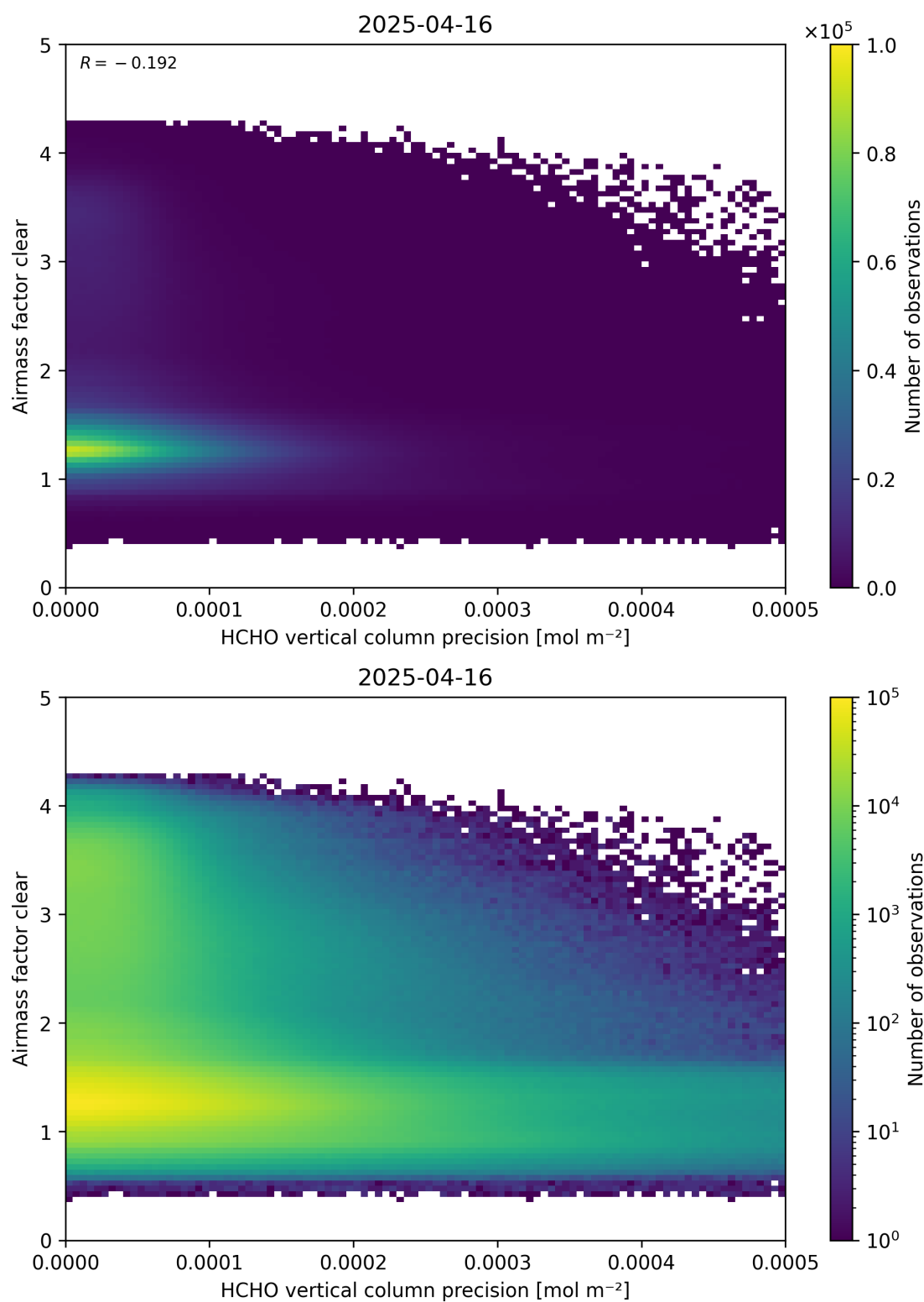
Figure 139: Scatter density plot of “HCHO vertical column precision” against “Airmass factor clear” for 2025-04-15 to 2025-04-17.
