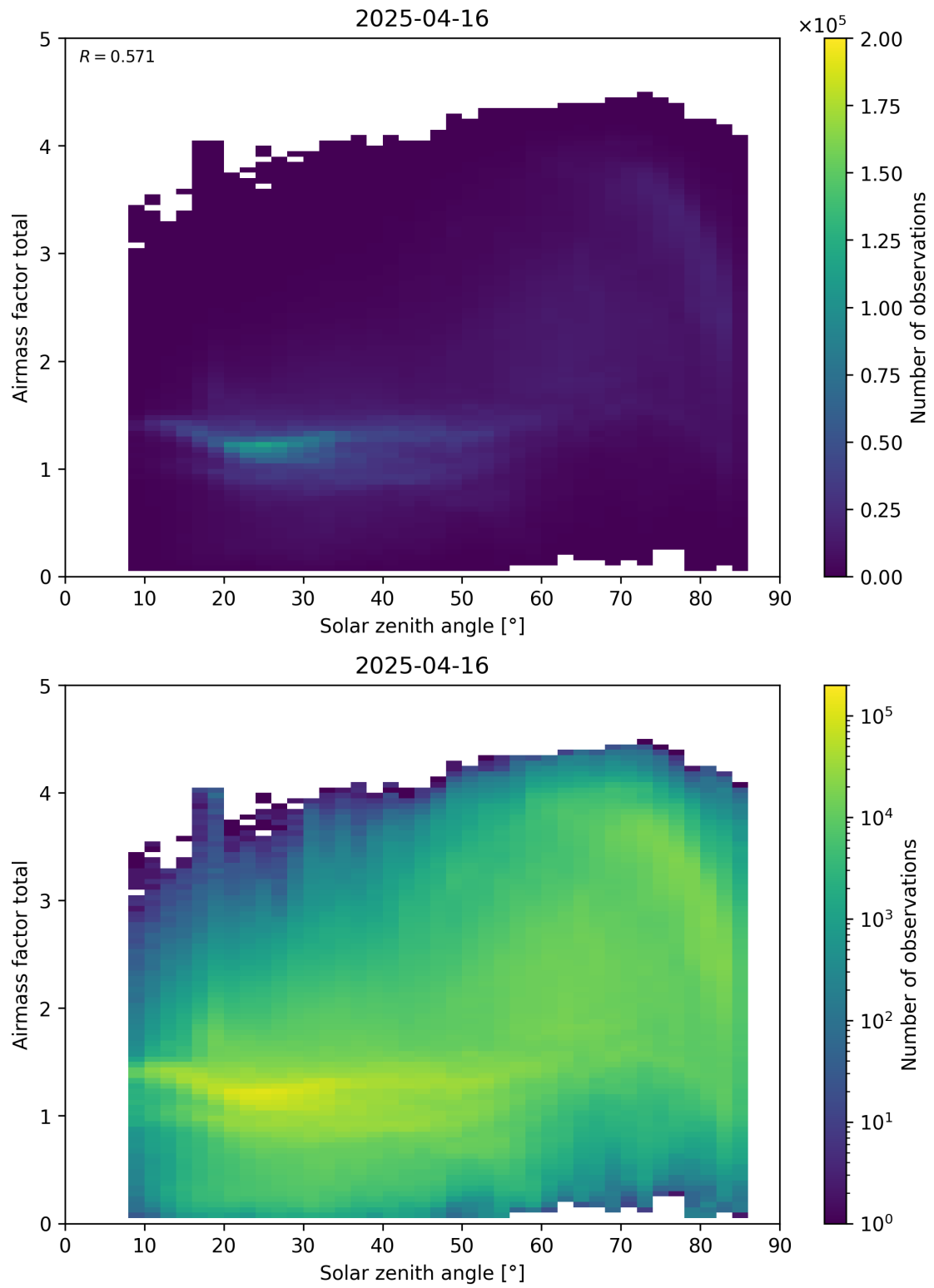
Figure 175: Scatter density plot of “Solar zenith angle” against “Airmass factor total” for 2025-04-15 to 2025-04-17.
