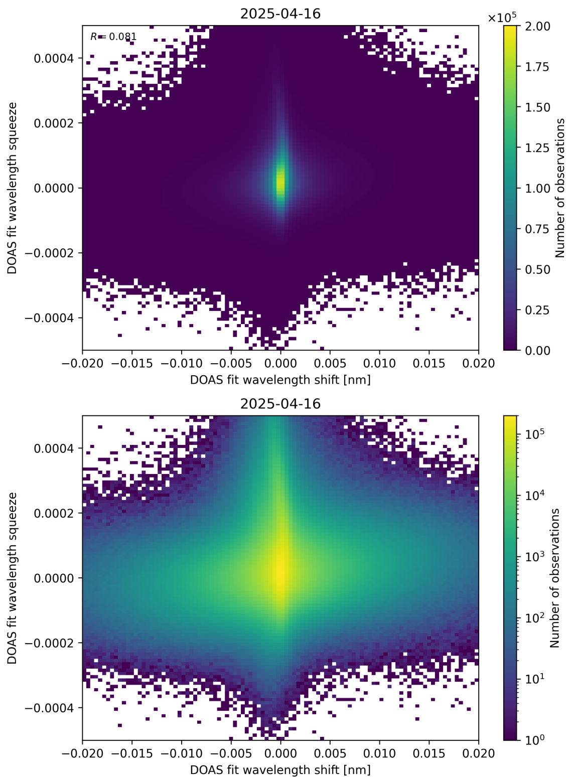
Figure 65: Scatter density plot of “DOAS fit wavelength shift” against “DOAS fit wavelength squeeze” for 2025-04-15 to 2025-04-17.
