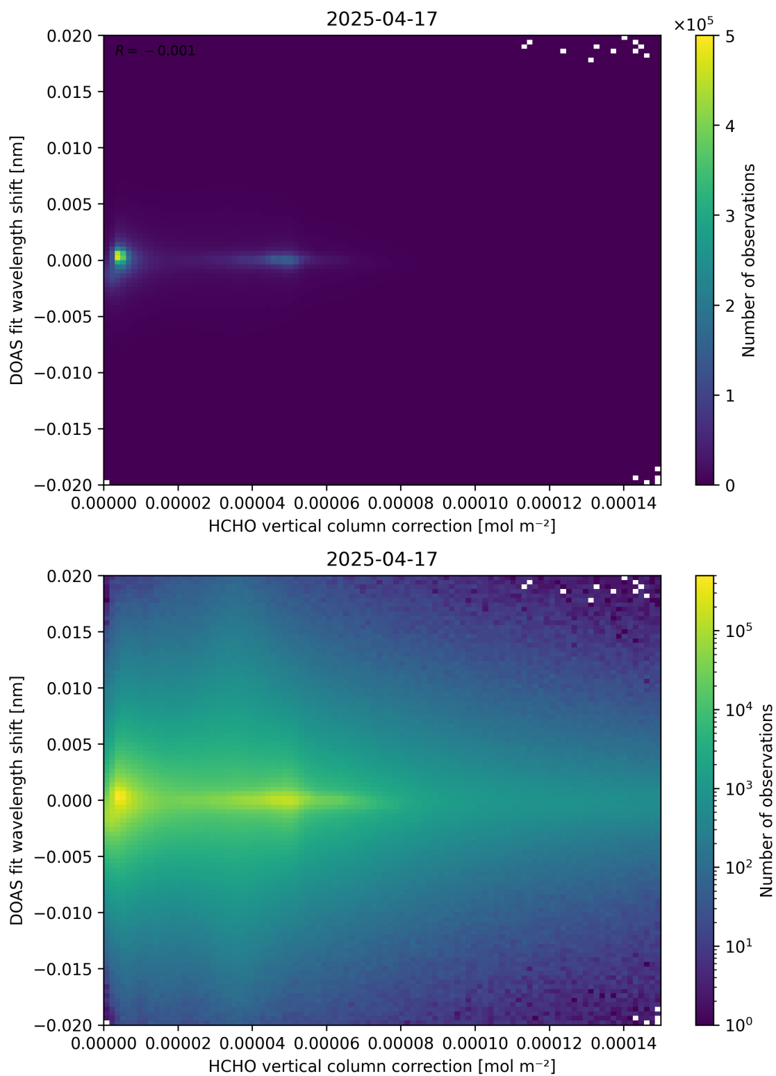
Figure 113: Scatter density plot of “HCHO vertical column correction” against “DOAS fit wavelength shift” for 2025-04-16 to 2025-04-18.
