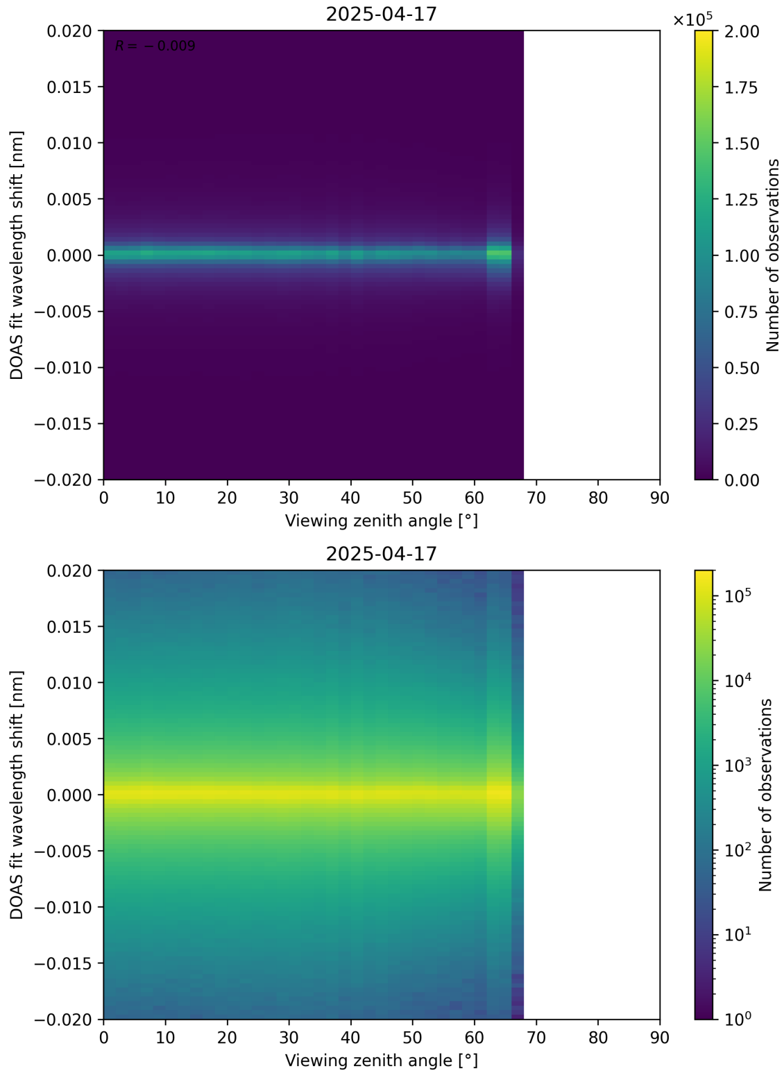
Figure 183: Scatter density plot of “Viewing zenith angle” against “DOAS fit wavelength shift” for 2025-04-16 to 2025-04-18.
