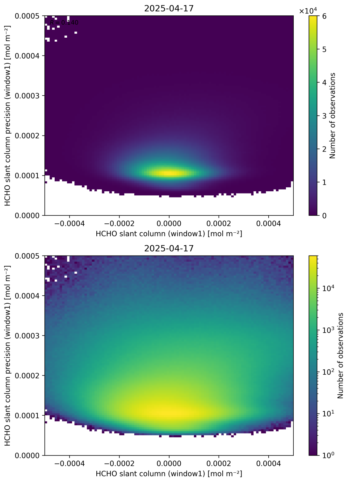
Figure 84: Scatter density plot of “HCHO slant column (window1)” against “HCHO slant column precision (window1)” for 2025-04-16 to 2025-04-18.
