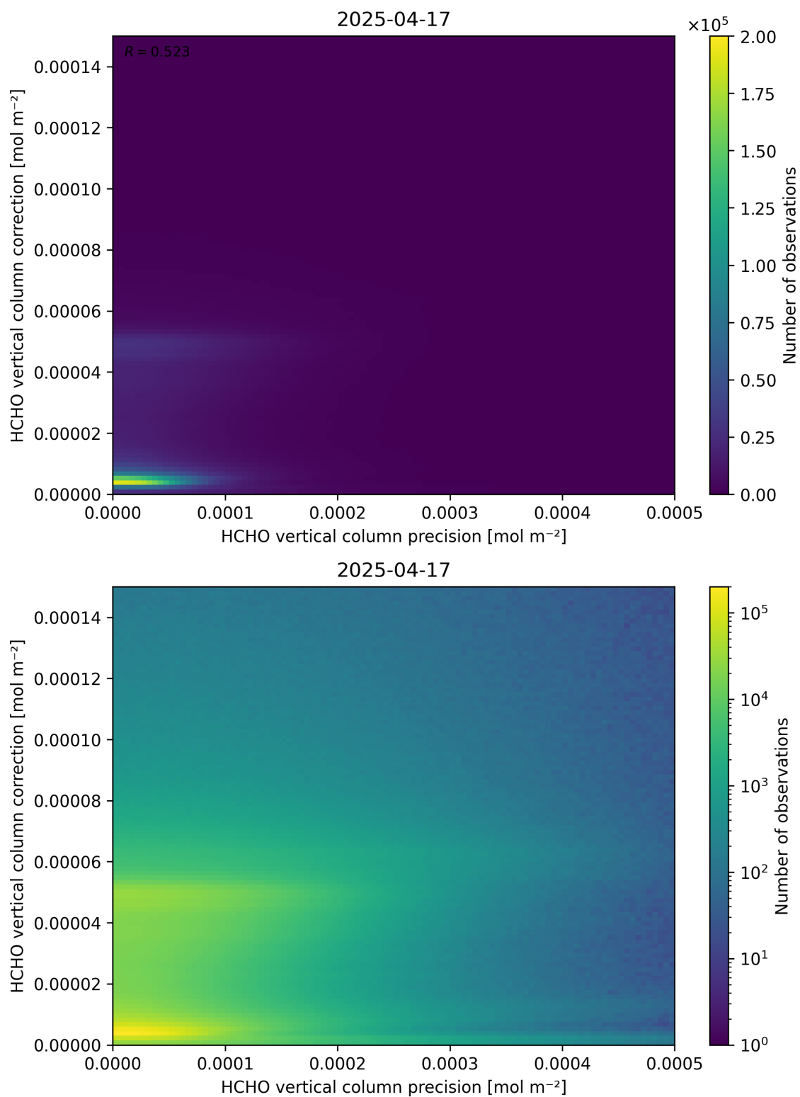
Figure 146: Scatter density plot of “HCHO vertical column precision” against “HCHO vertical column correction” for 2025-04-16 to 2025-04-18.
