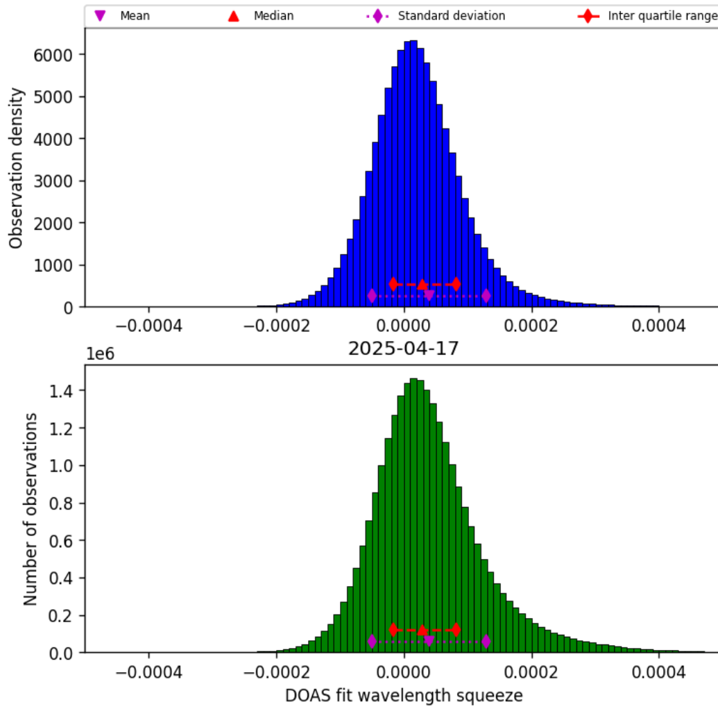
Figure 45: Histogram of “DOAS fit wavelength squeeze” for 2025-04-16 to 2025-04-18
