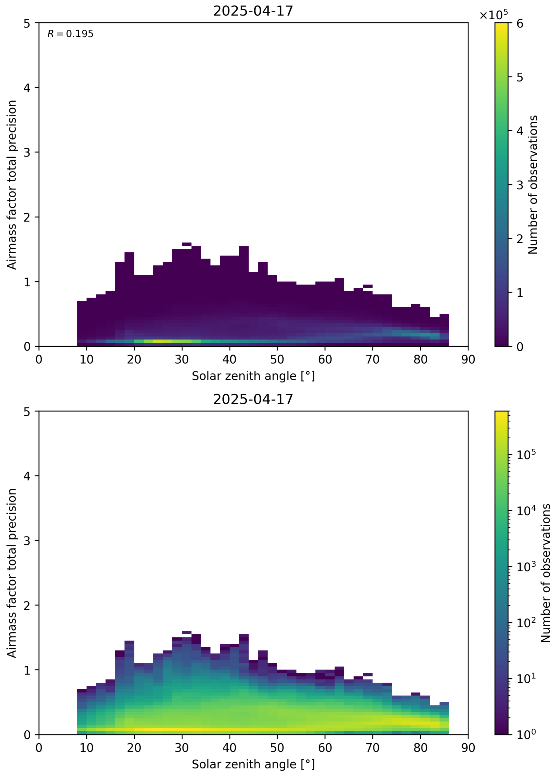
Figure 176: Scatter density plot of “Solar zenith angle” against “Airmass factor total precision” for 2025-04-16 to 2025-04-18.
