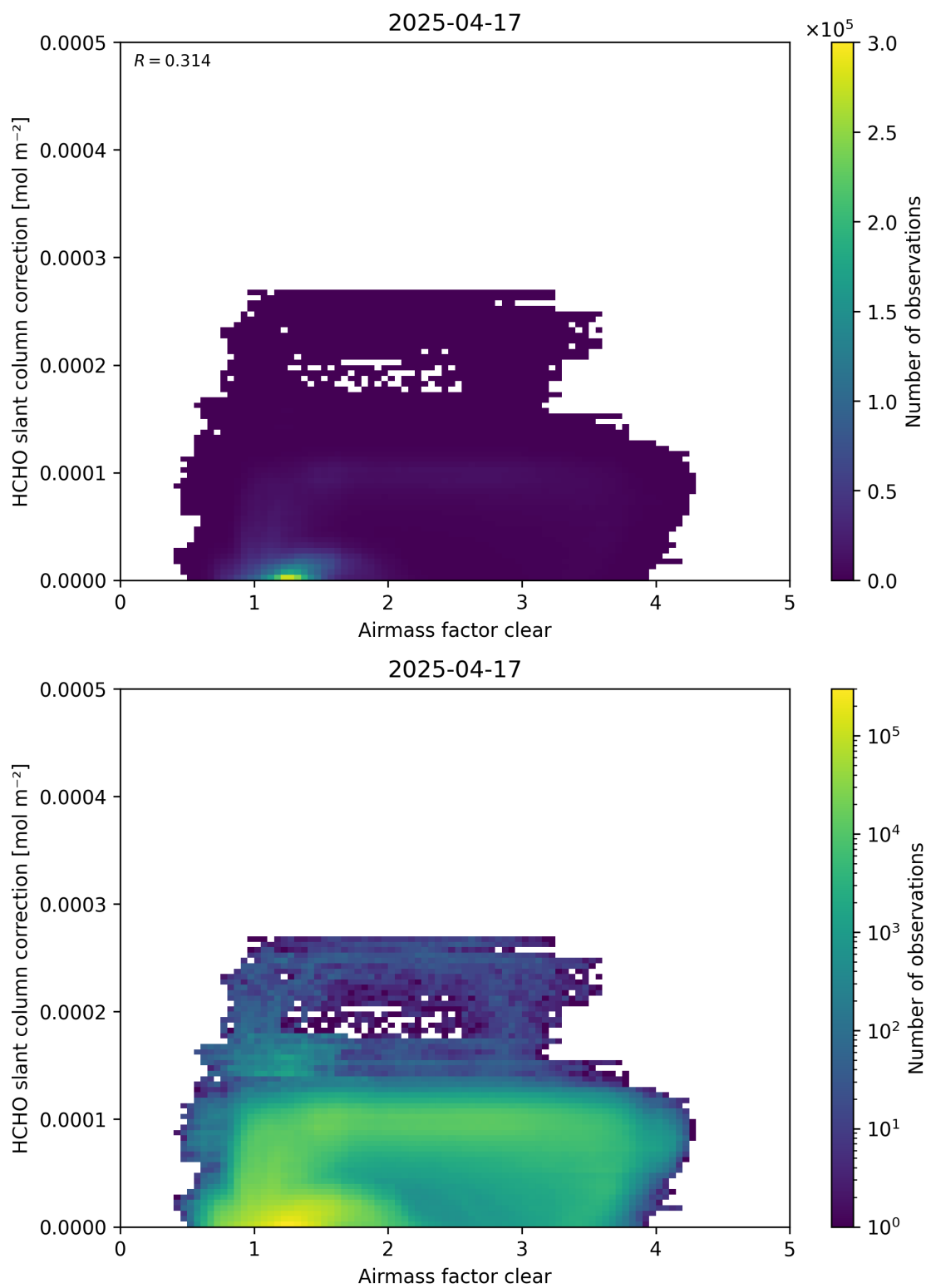
Figure 75: Scatter density plot of “Air mass factor clear” against “HCHO slant column correction” for 2025-04-16 to 2025-04-18.
