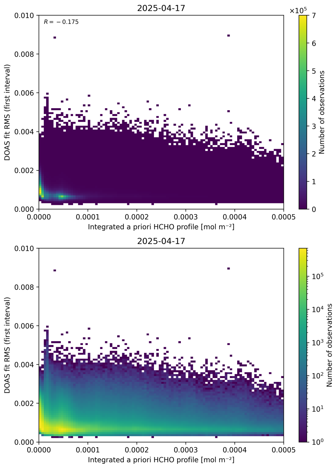
Figure 148: Scatter density plot of “Integrated a priori HCHO profile” against “DOAS fit RMS (first interval)” for 2025-04-16 to 2025-04-18.
