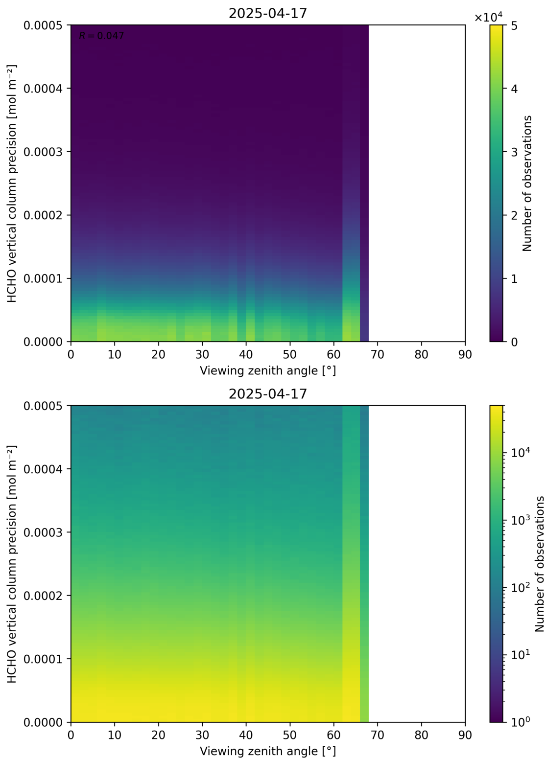
Figure 194: Scatter density plot of “Viewing zenith angle” against “HCHO vertical column precision” for 2025-04-16 to 2025-04-18.
