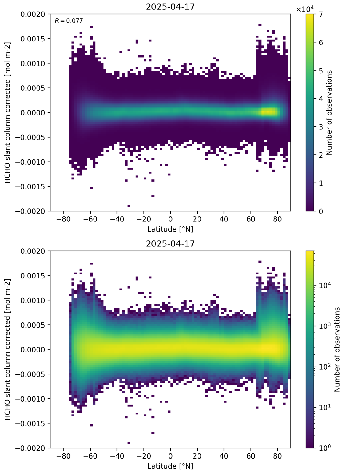
Figure 157: Scatter density plot of “Latitude” against “HCHO slant column corrected” for 2025-04-16 to 2025-04-18.
