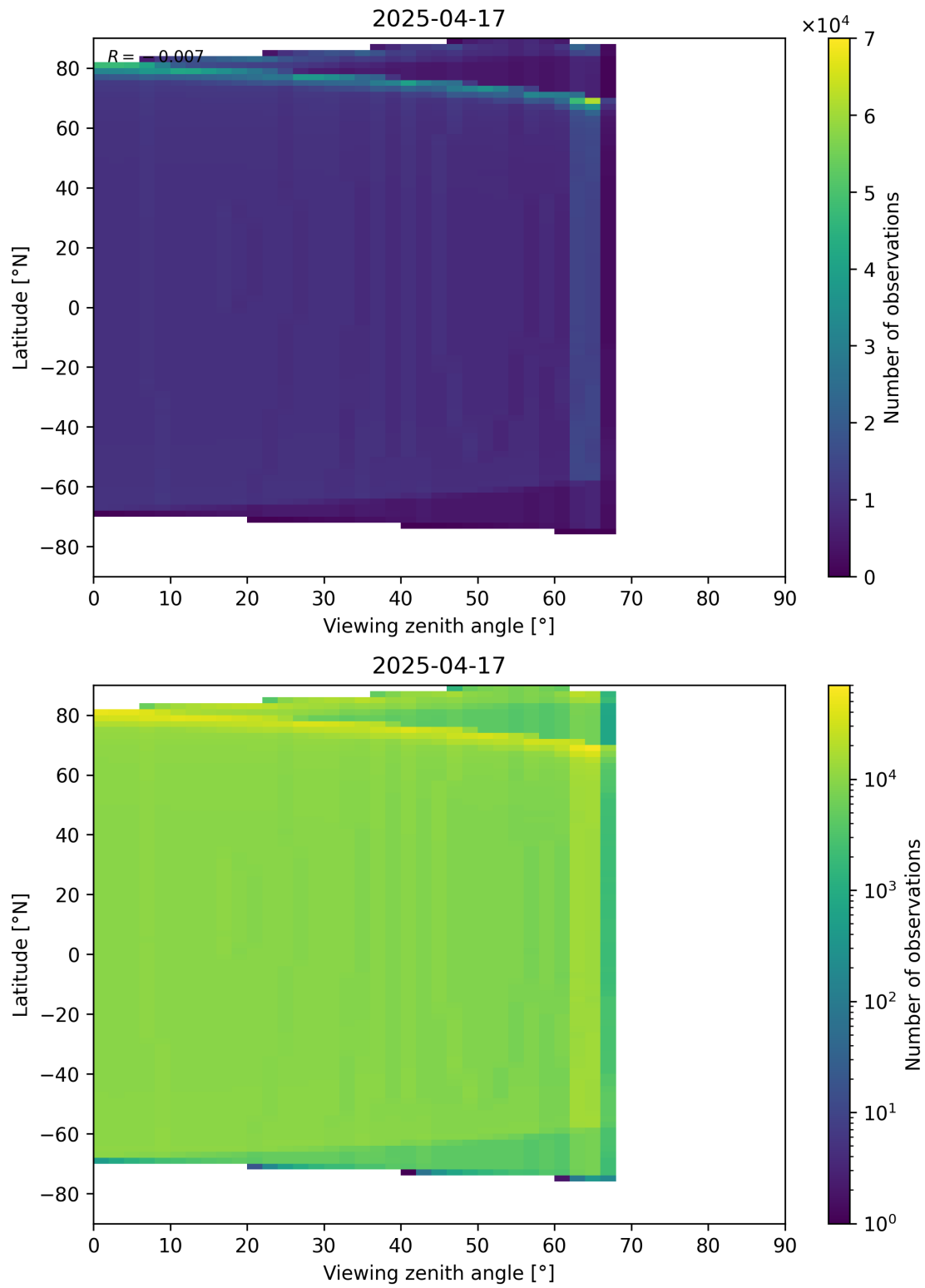
Figure 196: Scatter density plot of “Viewing zenith angle” against “Latitude” for 2025-04-16 to 2025-04-18.
