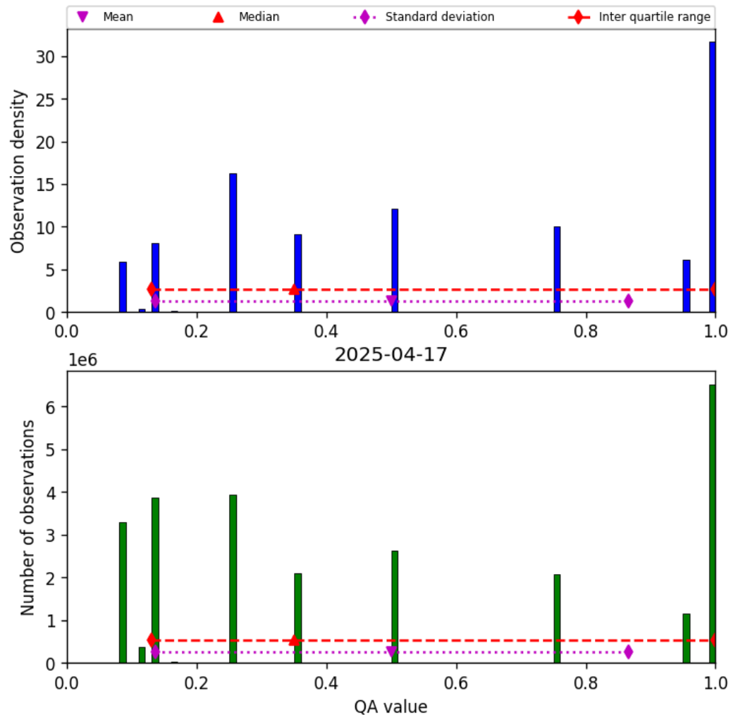
Figure 34: Histogram of “QA value” for 2025-04-16 to 2025-04-18
