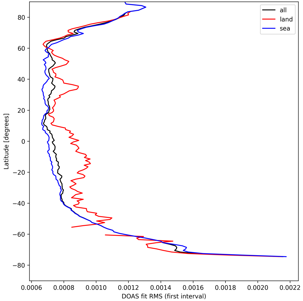
Figure 32: Zonal average of “DOAS fit RMS (first interval)” for 2025-04-16 to 2025-04-18.
