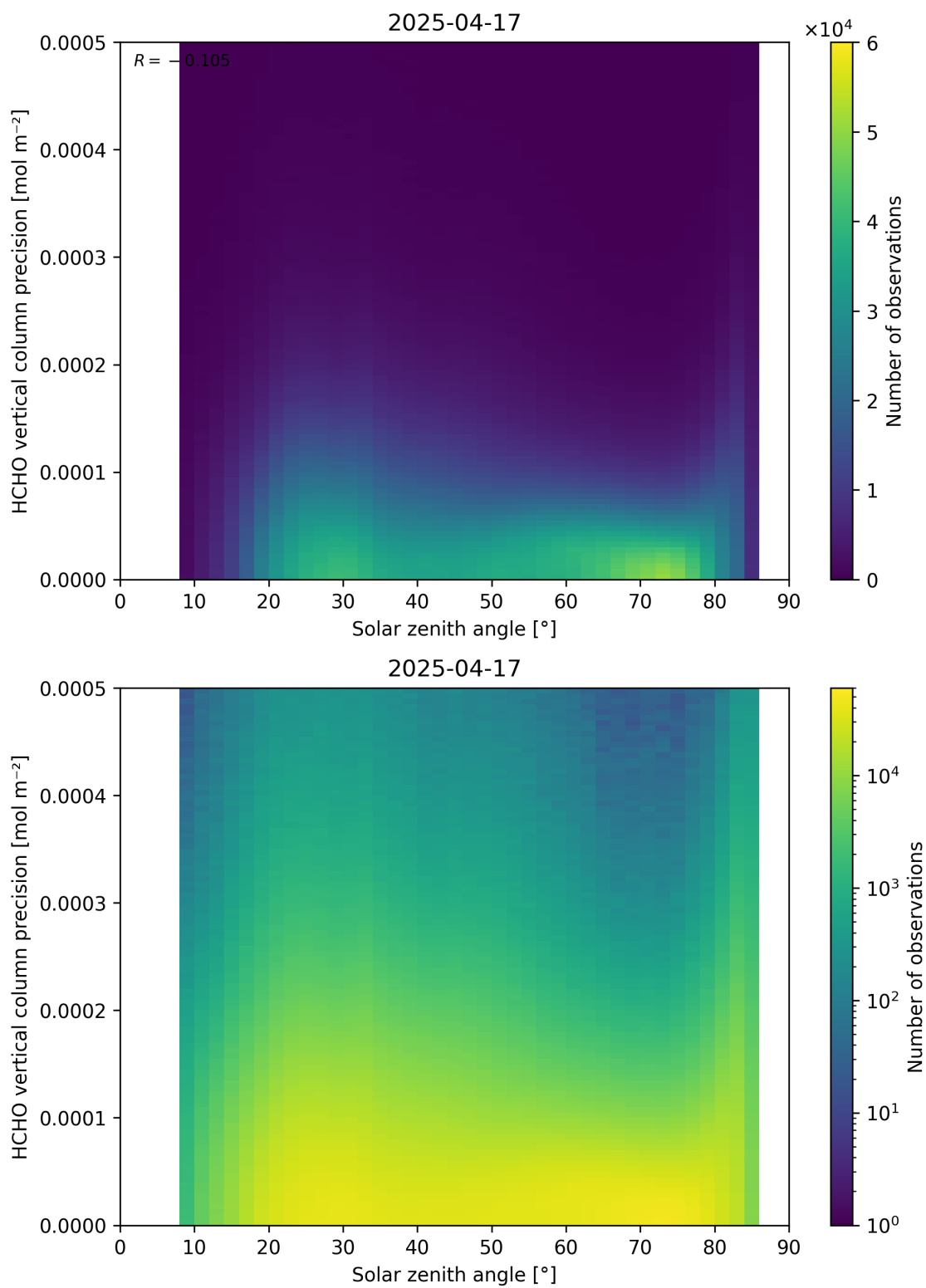
Figure 179: Scatter density plot of “Solar zenith angle” against “HCHO vertical column precision” for 2025-04-16 to 2025-04-18.
