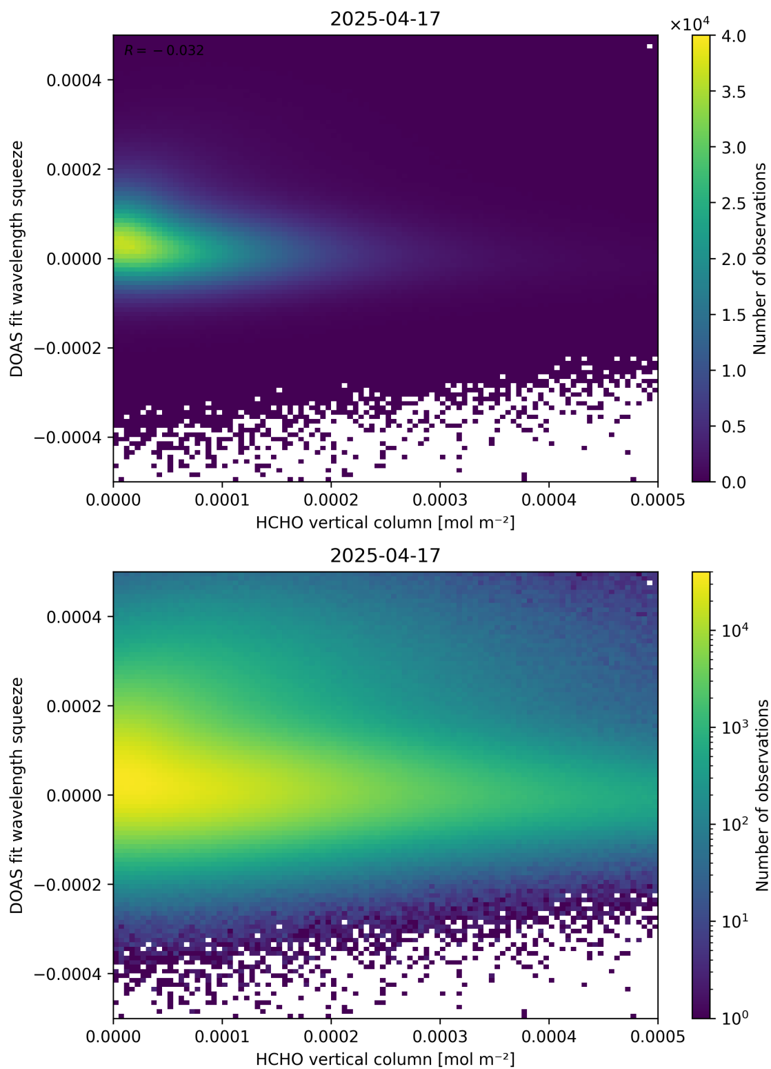
Figure 125: Scatter density plot of “HCHO vertical column” against “DOAS fit wavelength squeeze” for 2025-04-16 to 2025-04-18.
