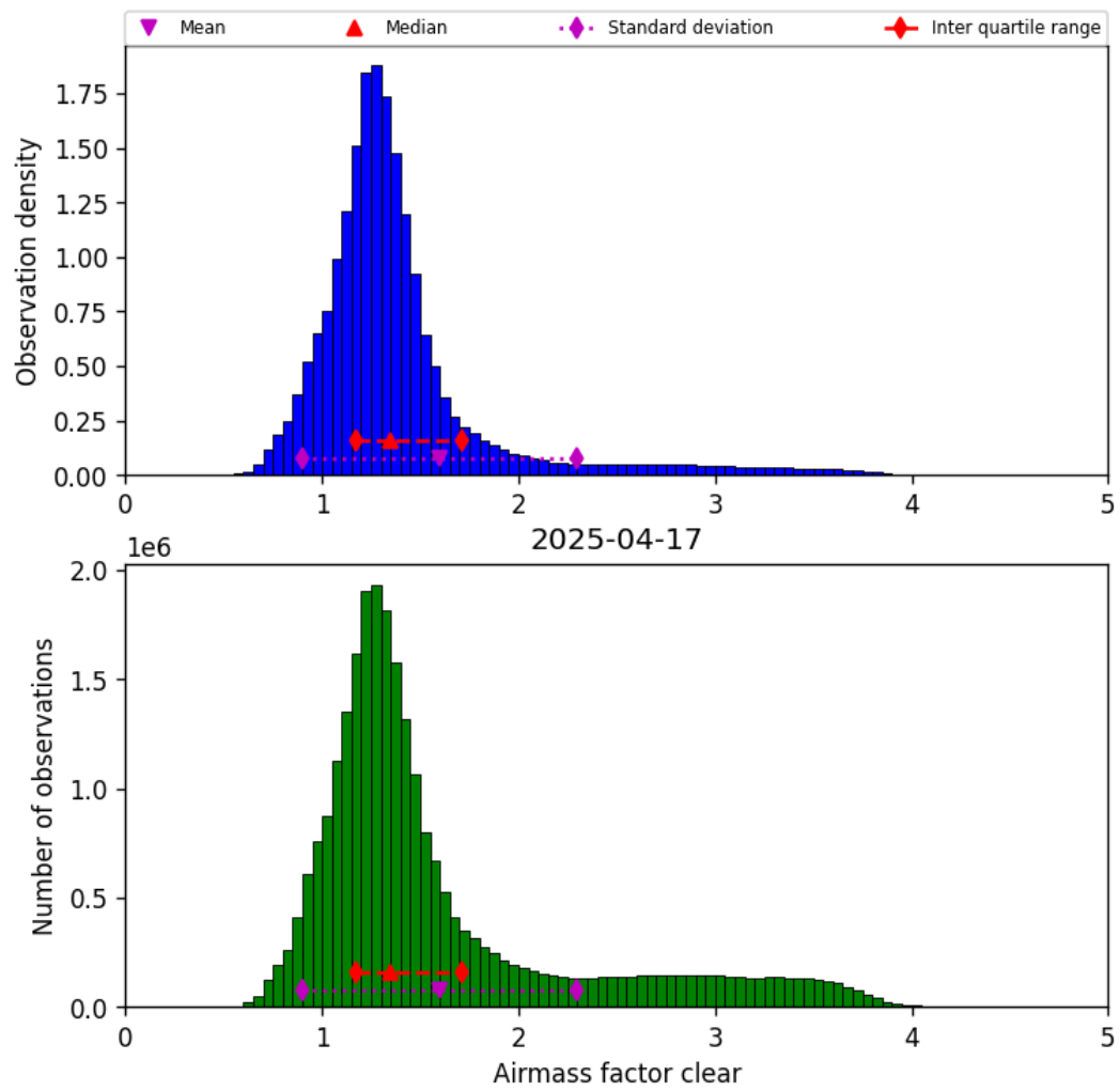
Figure 42: Histogram of “Airmass factor clear” for 2025-04-16 to 2025-04-18
