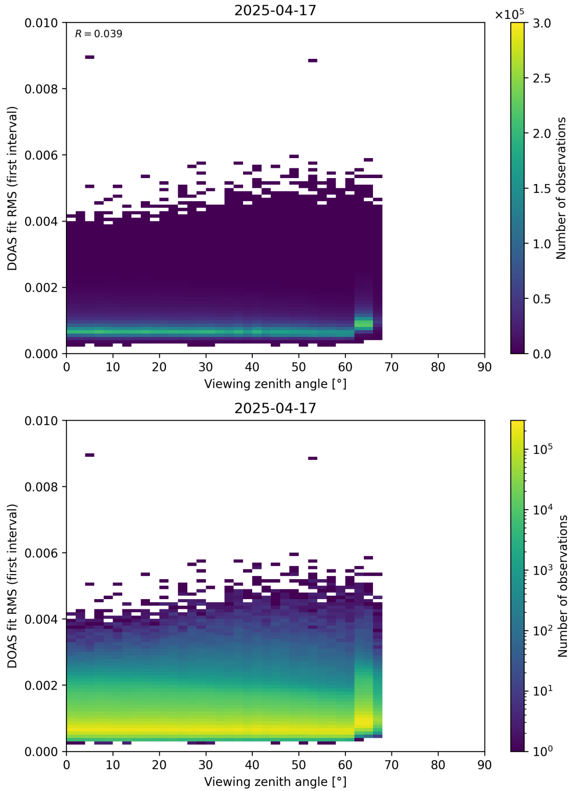
Figure 182: Scatter density plot of “Viewing zenith angle” against “DOAS fit RMS (first interval)” for 2025-04-16 to 2025-04-18.
