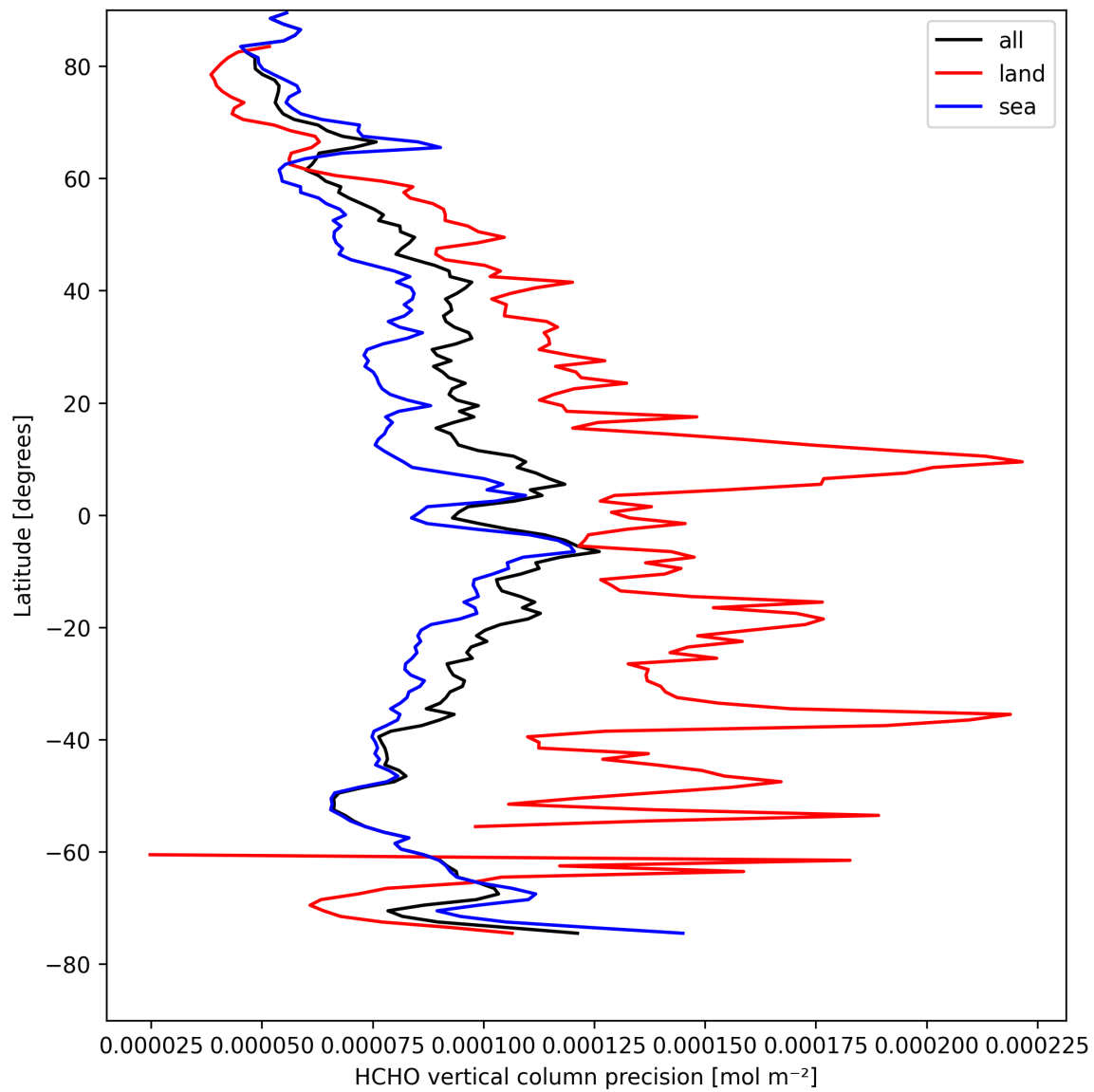
Figure 22: Zonal average of “HCHO vertical column precision” for 2025-04-16 to 2025-04-18.
