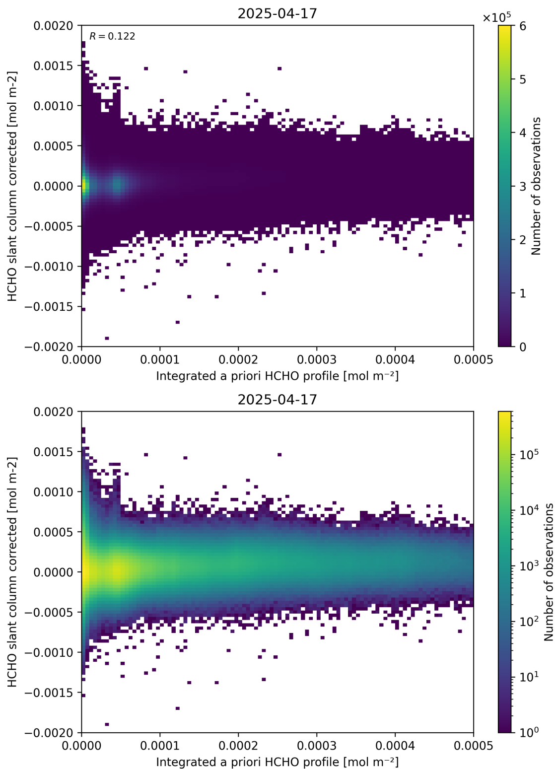
Figure 151: Scatter density plot of “Integrated a priori HCHO profile” against “HCHO slant column corrected” for 2025-04-16 to 2025-04-18.
