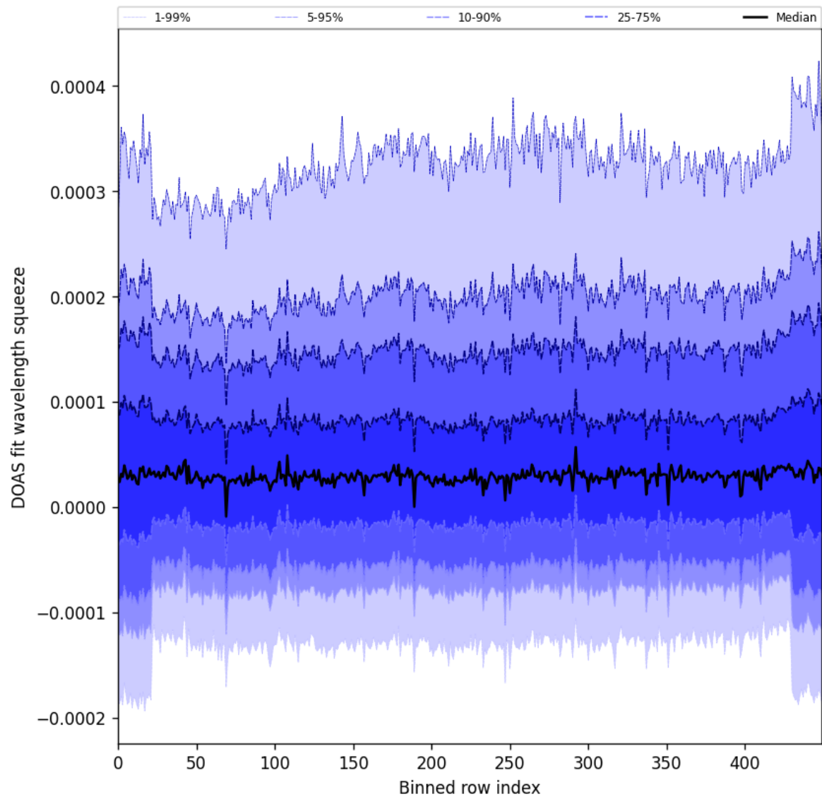
Figure 59: Along track statistics of “DOAS fit wavelength squeeze” for 2025-04-16 to 2025-04-18
