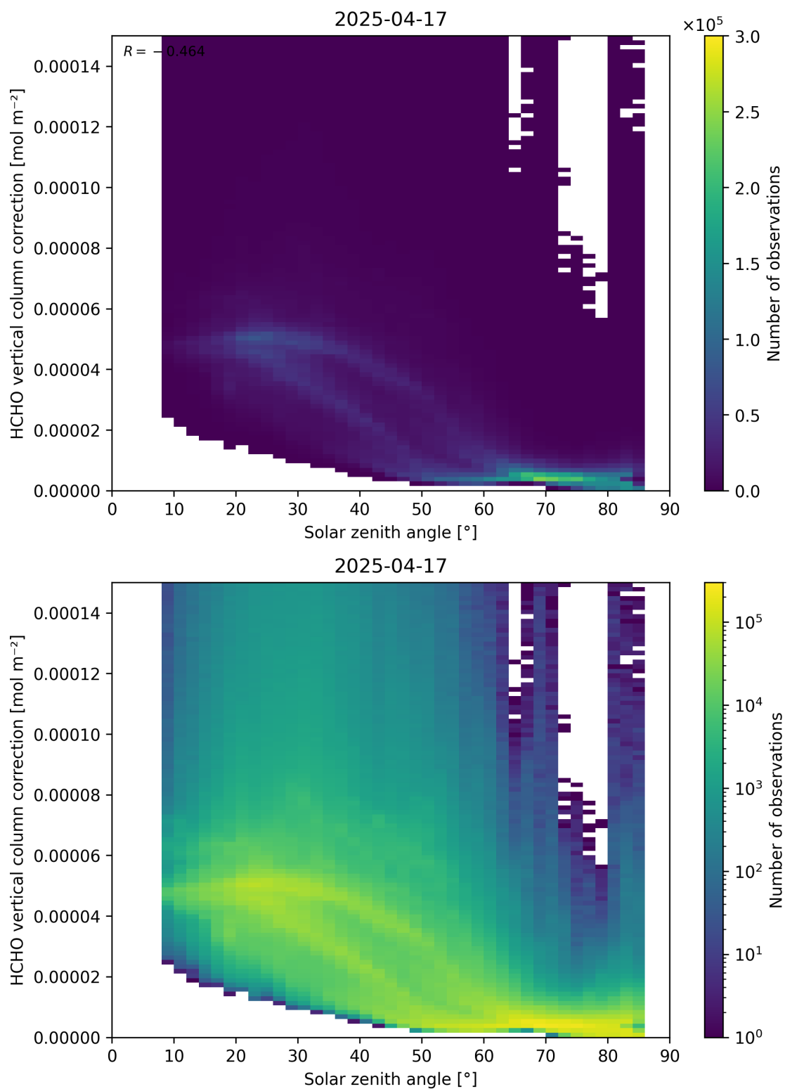
Figure 178: Scatter density plot of “Solar zenith angle” against “HCHO vertical column correction” for 2025-04-16 to 2025-04-18.
