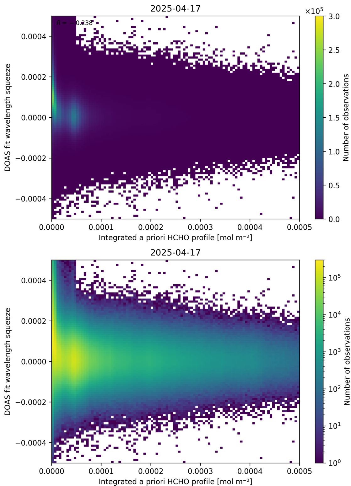
Figure 150: Scatter density plot of “Integrated a priori HCHO profile” against “DOAS fit wavelength squeeze” for 2025-04-16 to 2025-04-18.
