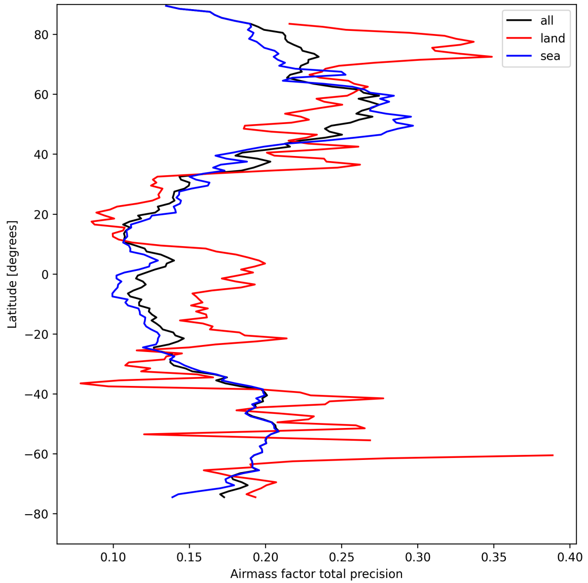
Figure 27: Zonal average of “Airmass factor total precision” for 2025-04-16 to 2025-04-18.
