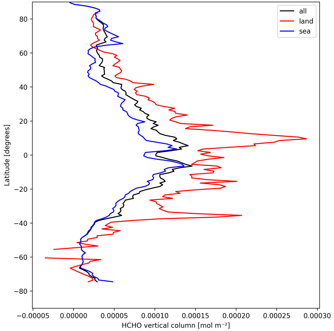
Figure 21: Zonal average of “HCHO vertical column” for 2025-04-16 to 2025-04-18.
