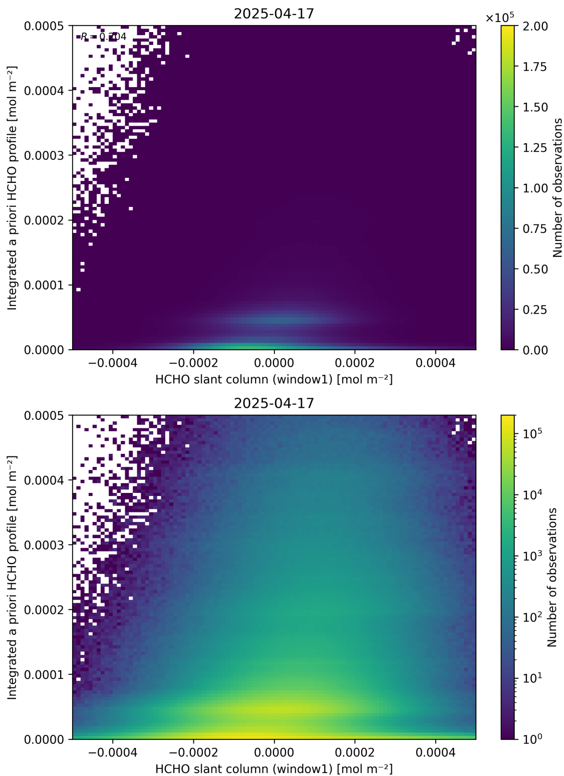
Figure 87: Scatter density plot of “HCHO slant column (window1)” against “Integrated a priori HCHO profile” for 2025-04-16 to 2025-04-18.
