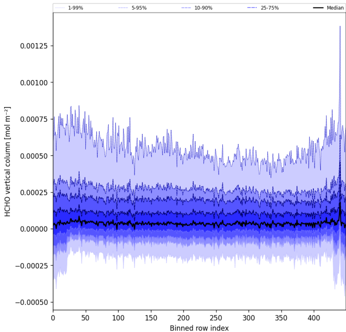
Figure 49: Along track statistics of “HCHO vertical column” for 2025-04-16 to 2025-04-18
