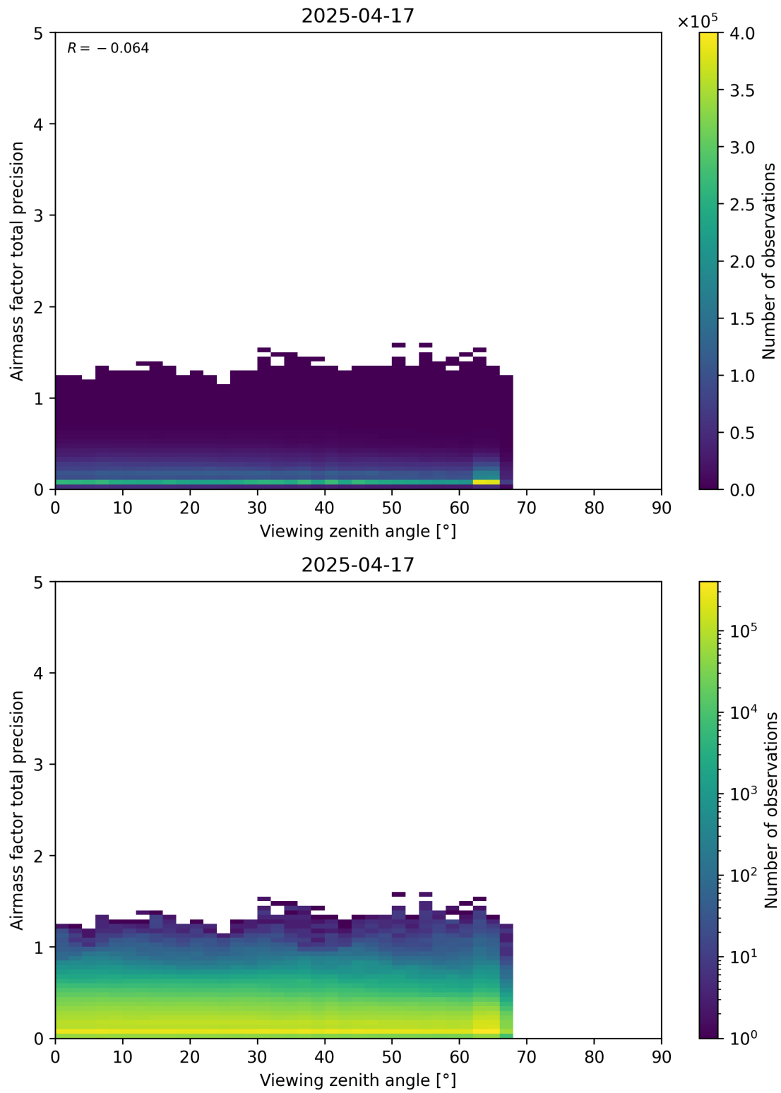
Figure 191: Scatter density plot of “Viewing zenith angle” against “Airmass factor total precision” for 2025-04-16 to 2025-04-18.
