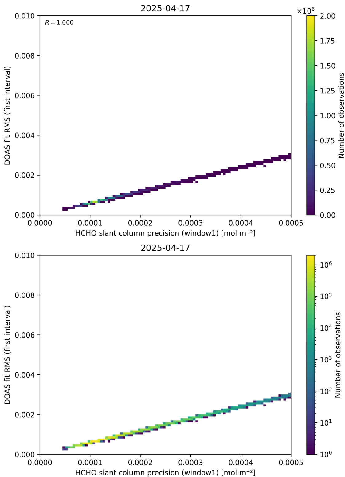
Figure 88: Scatter density plot of “HCHO slant column precision (window1)” against “DOAS fit RMS (first interval)” for 2025-04-16 to 2025-04-18.
