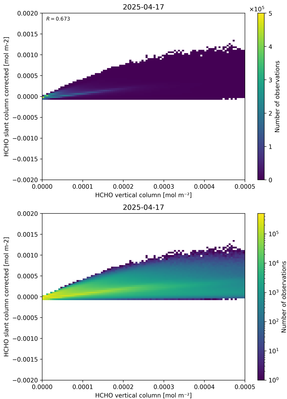
Figure 127: Scatter density plot of “HCHO vertical column” against “HCHO slant column corrected” for 2025-04-16 to 2025-04-18.
