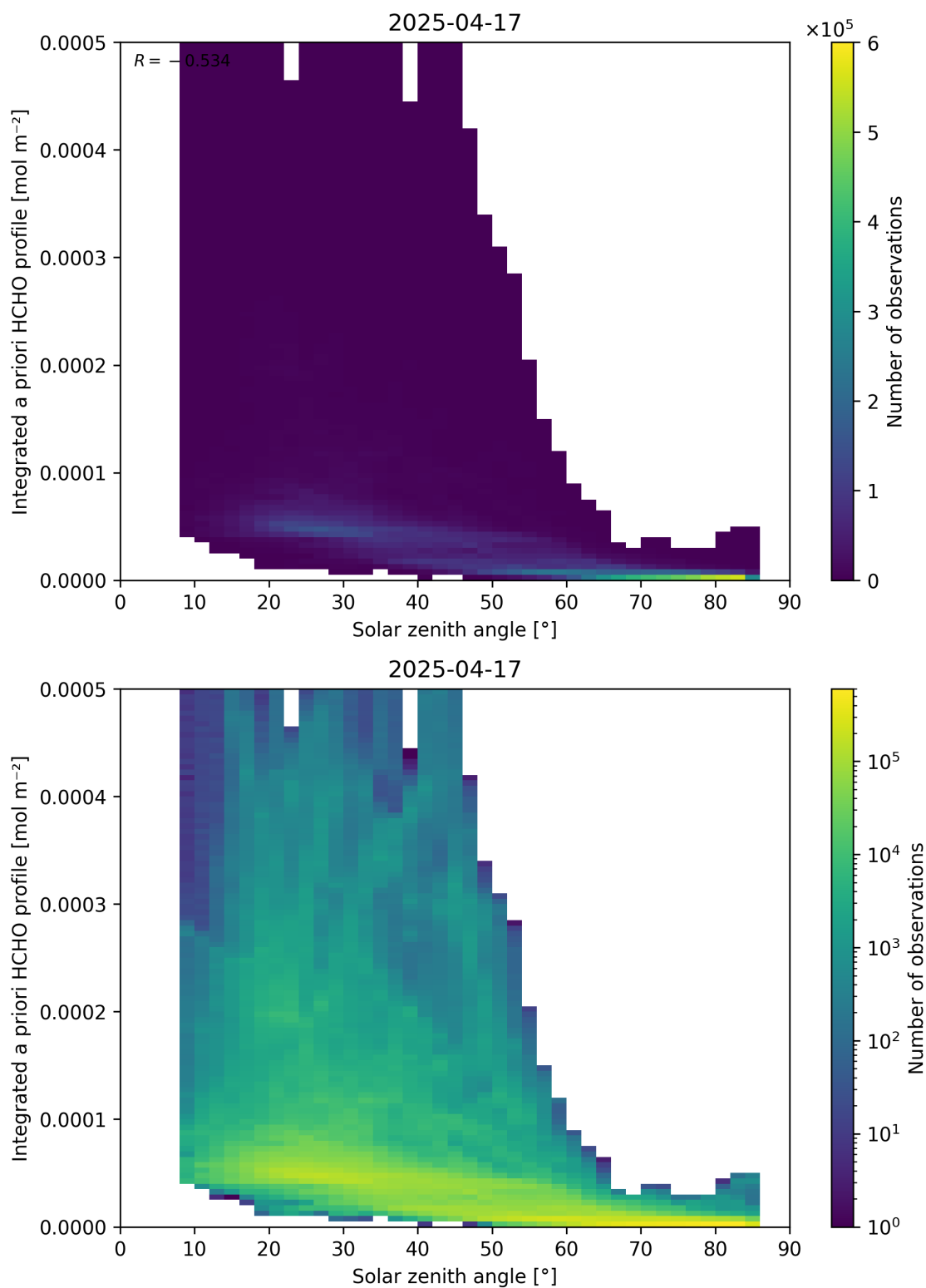
Figure 180: Scatter density plot of “Solar zenith angle” against “Integrated a priori HCHO profile” for 2025-04-16 to 2025-04-18.
