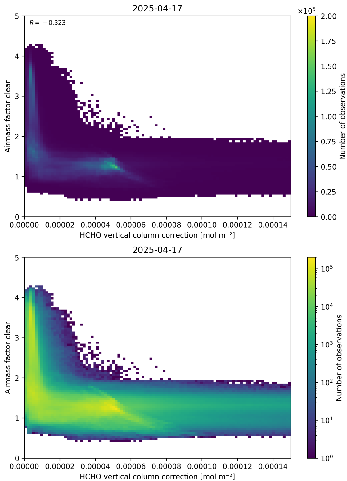
Figure 115: Scatter density plot of “HCHO vertical column correction” against “Airmass factor clear” for 2025-04-16 to 2025-04-18.
