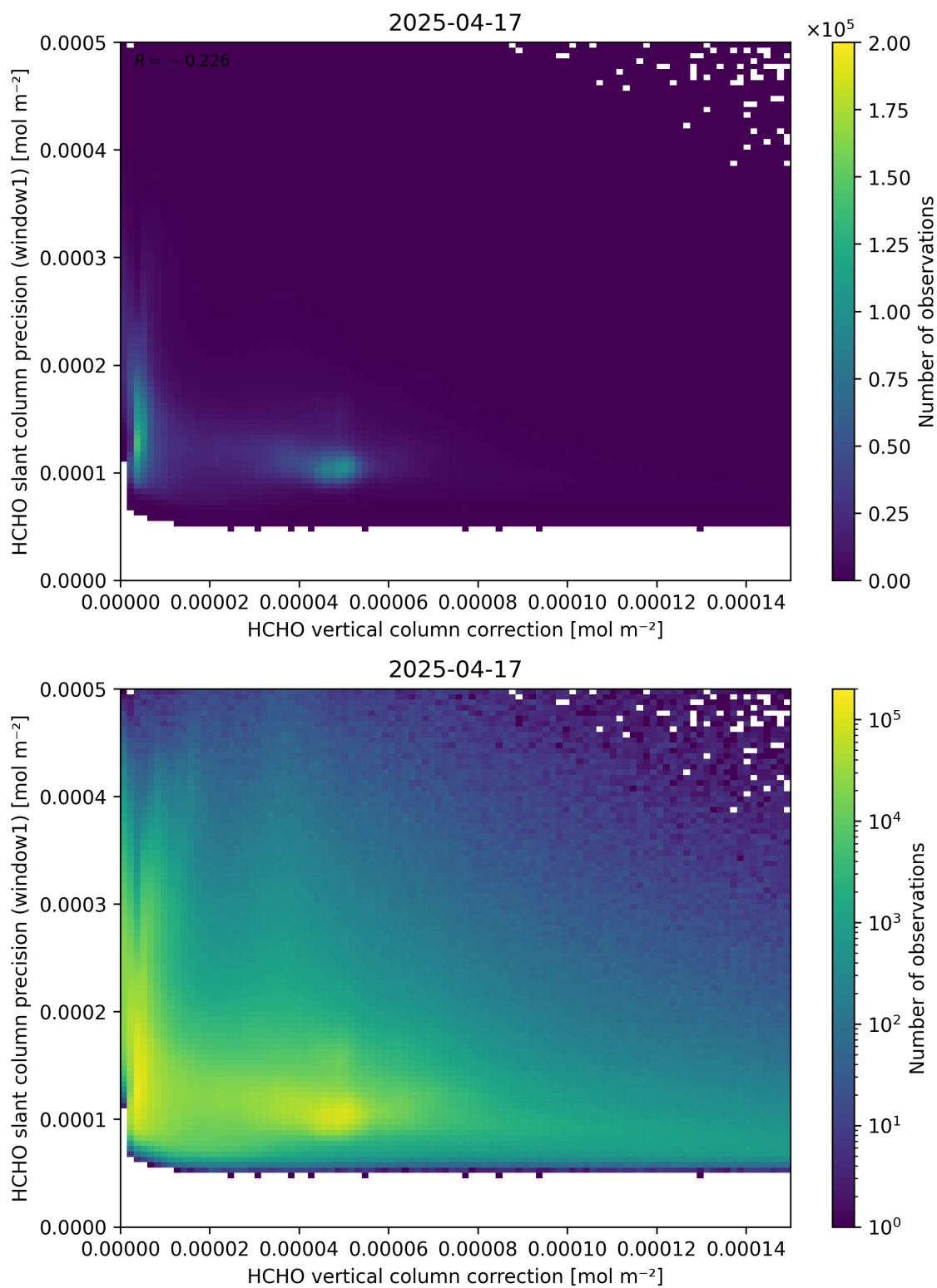
Figure 119: Scatter density plot of “HCHO vertical column correction” against “HCHO slant column precision (window1)” for 2025-04-16 to 2025-04-18.
