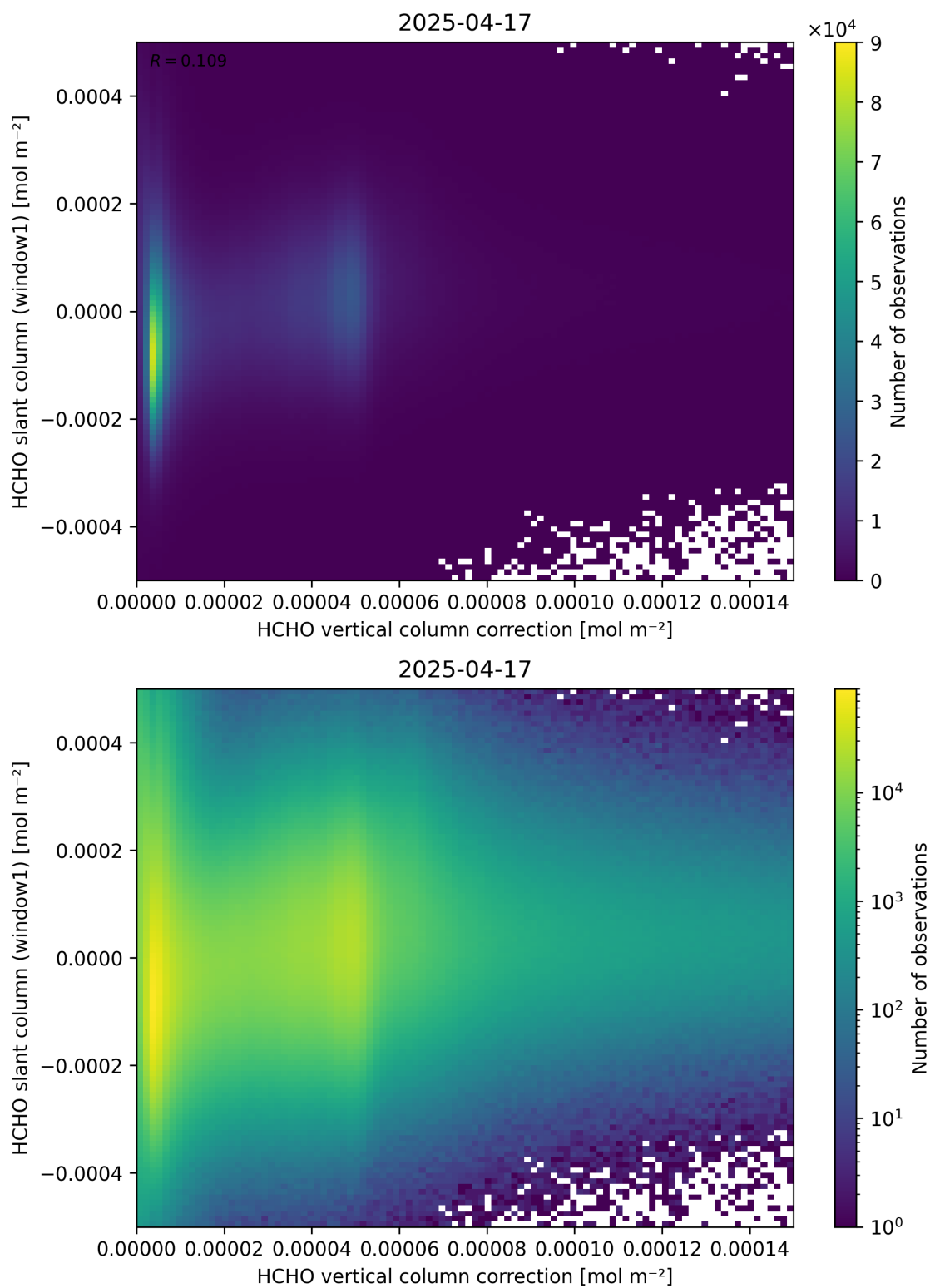
Figure 118: Scatter density plot of “HCHO vertical column correction” against “HCHO slant column (window1)” for 2025-04-16 to 2025-04-18.
