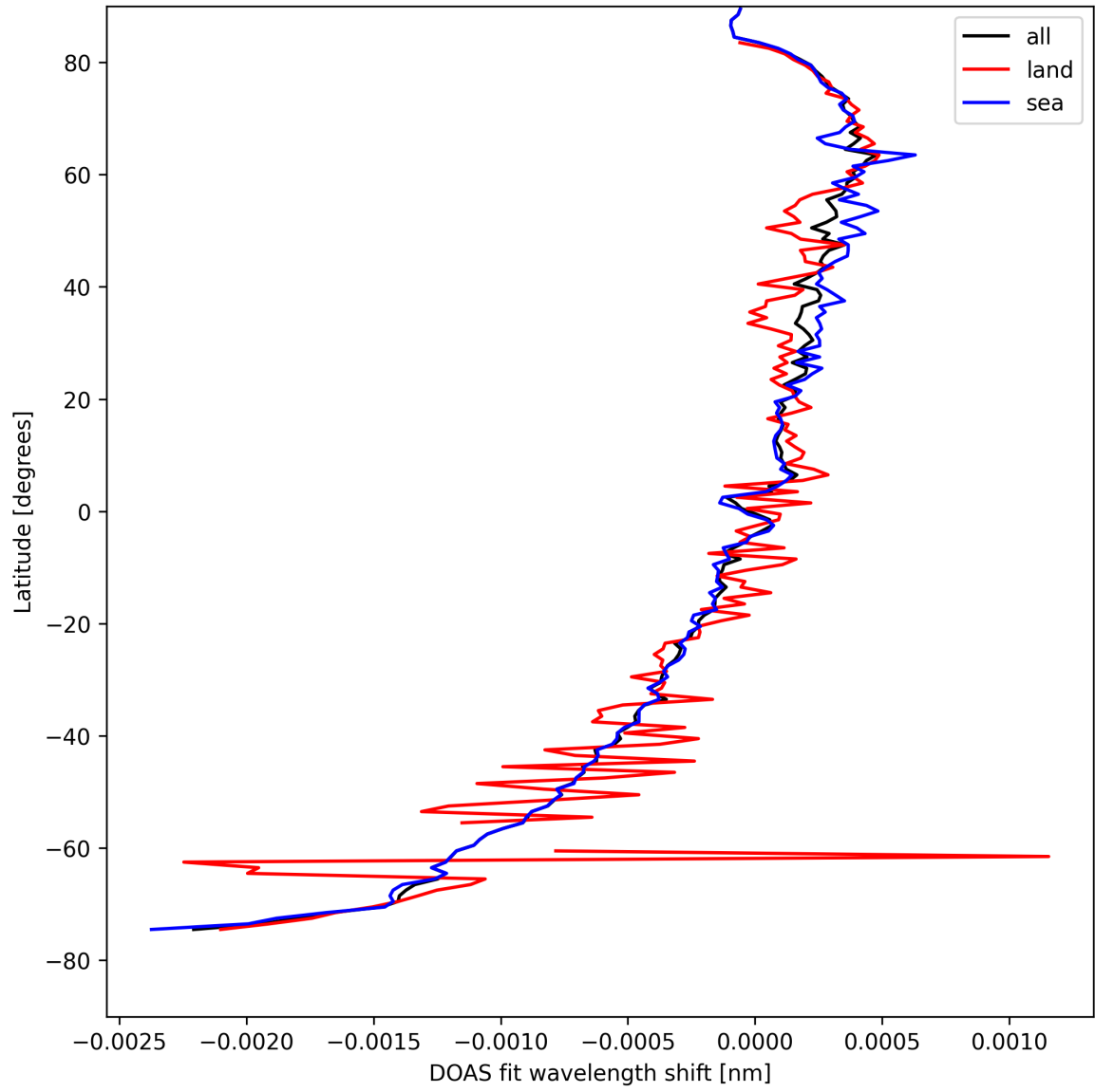
Figure 30: Zonal average of “DOAS fit wavelength shift” for 2025-04-16 to 2025-04-18.
