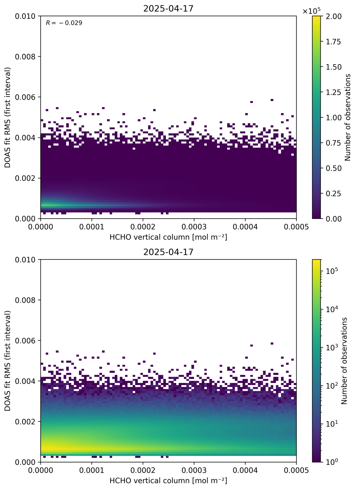
Figure 123: Scatter density plot of “HCHO vertical column” against “DOAS fit RMS (first interval)” for 2025-04-16 to 2025-04-18.
