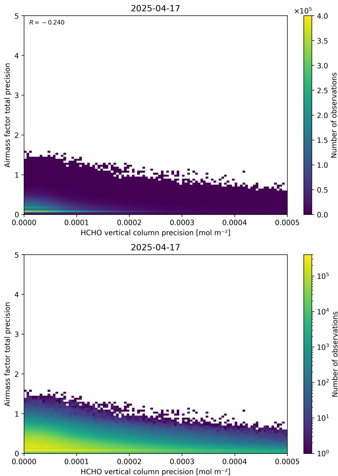
Figure 145: Scatter density plot of “HCHO vertical column precision” against “Airmass factor total precision” for 2025-04-16 to 2025-04-18.
