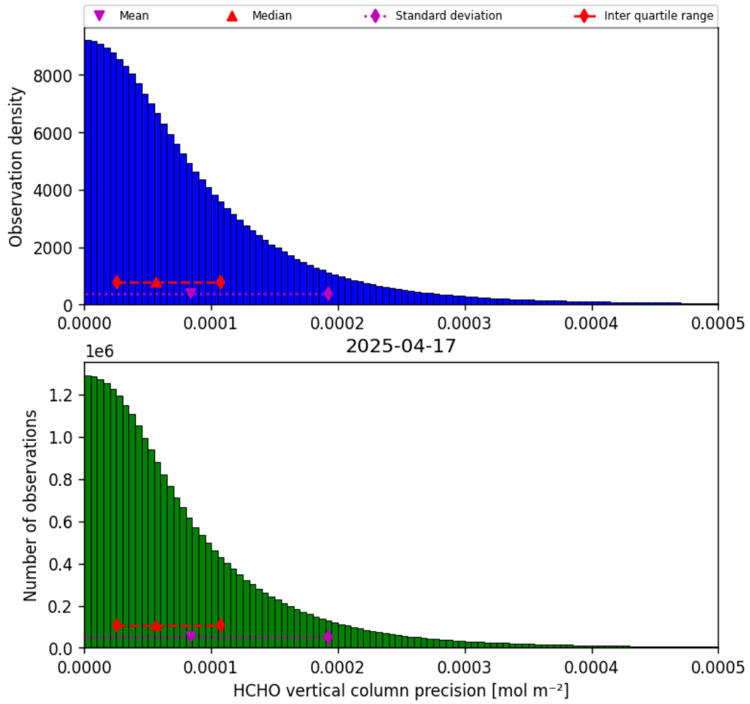
Figure 36: Histogram of “HCHO vertical column precision” for 2025-04-16 to 2025-04-18
