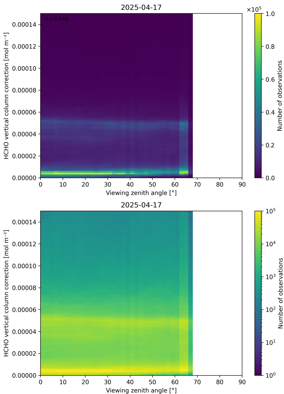
Figure 193: Scatter density plot of “Viewing zenith angle” against “HCHO vertical column correction” for 2025-04-16 to 2025-04-18.
