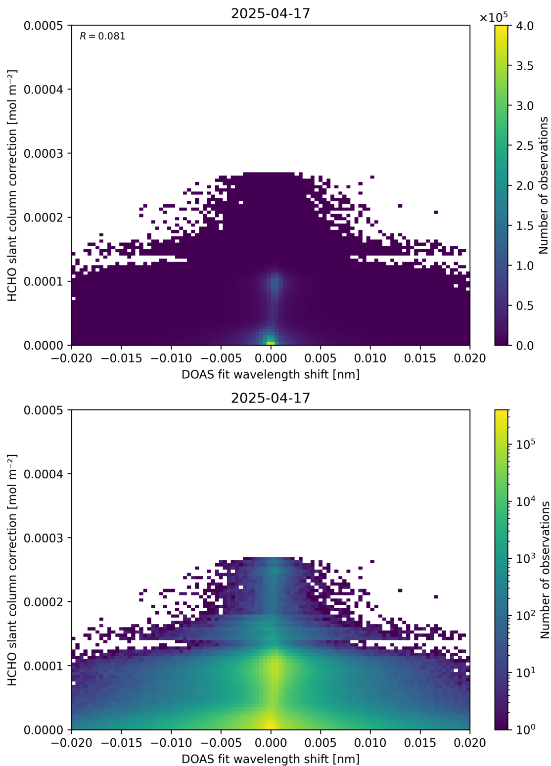
Figure 67: Scatter density plot of “DOAS fit wavelength shift” against “HCHO slant column correction” for 2025-04-16 to 2025-04-18.
