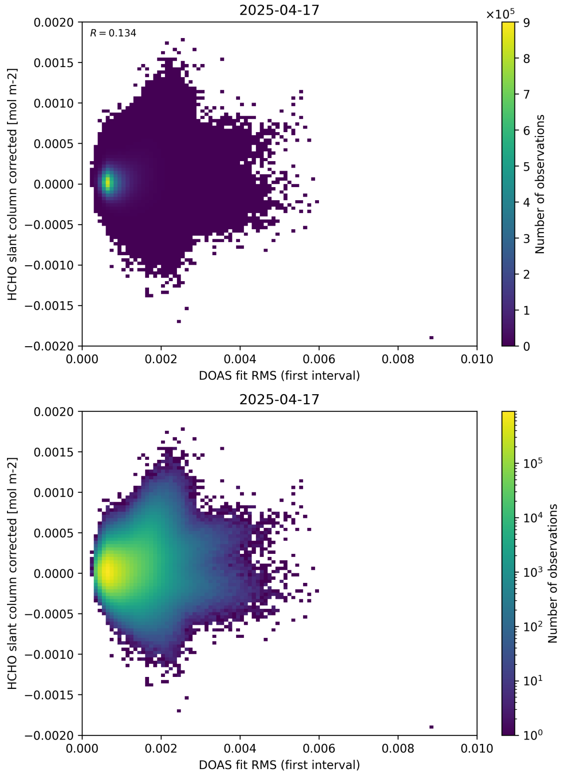
Figure 62: Scatter density plot of “DOAS fit RMS (first interval)” against “HCHO slant column corrected” for 2025-04-16 to 2025-04-18.
