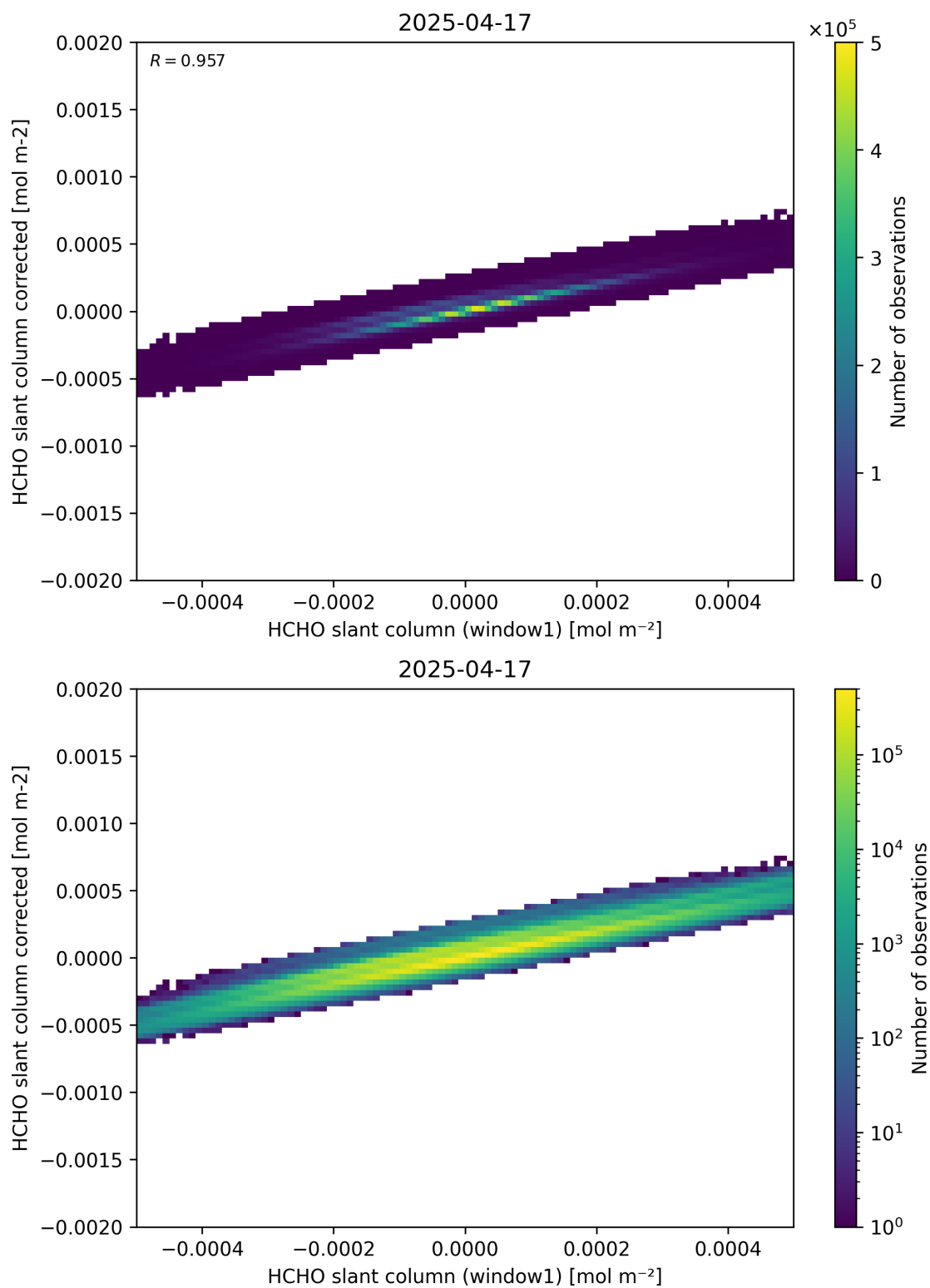
Figure 82: Scatter density plot of “HCHO slant column (window1)” against “HCHO slant column corrected” for 2025-04-16 to 2025-04-18.
