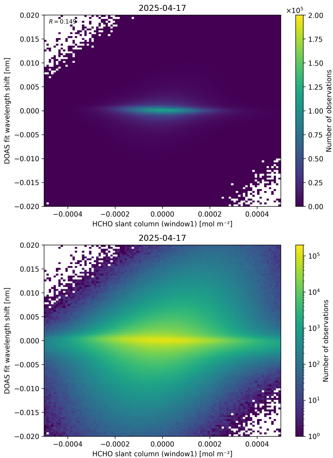
Figure 79: Scatter density plot of “HCHO slant column (window1)” against “DOAS fit wavelength shift” for 2025-04-16 to 2025-04-18.
