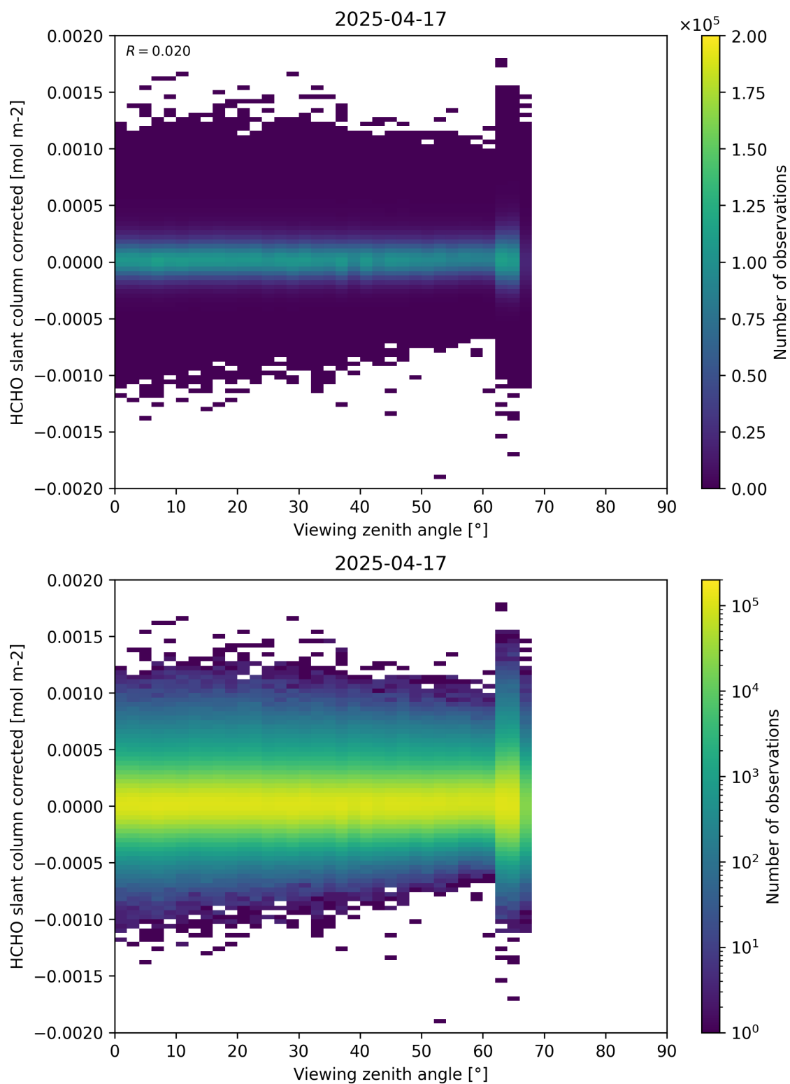
Figure 186: Scatter density plot of “Viewing zenith angle” against “HCHO slant column corrected” for 2025-04-16 to 2025-04-18.
