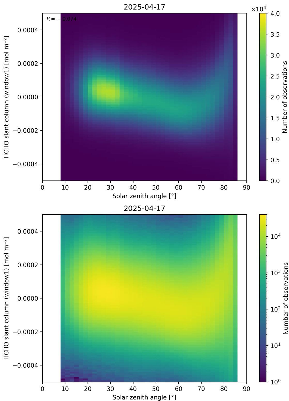
Figure 173: Scatter density plot of “Solar zenith angle” against “HCHO slant column (window1)” for 2025-04-16 to 2025-04-18.
