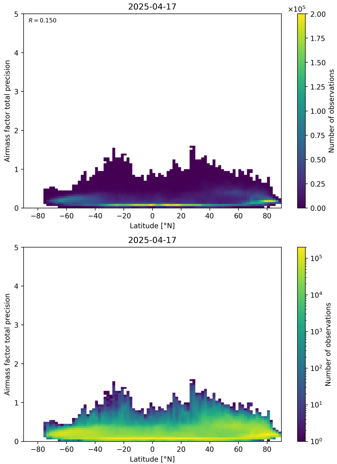
Figure 162: Scatter density plot of “Latitude” against “Airmass factor total precision” for 2025-04-16 to 2025-04-18.
