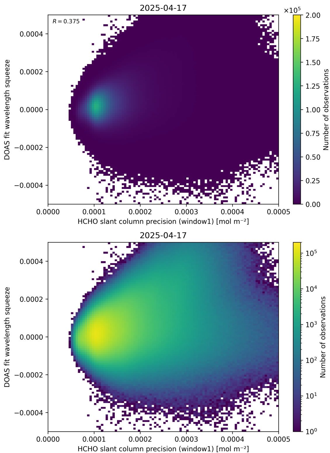
Figure 90: Scatter density plot of “HCHO slant column precision (window1)” against “DOAS fit wavelength squeeze” for 2025-04-16 to 2025-04-18.
