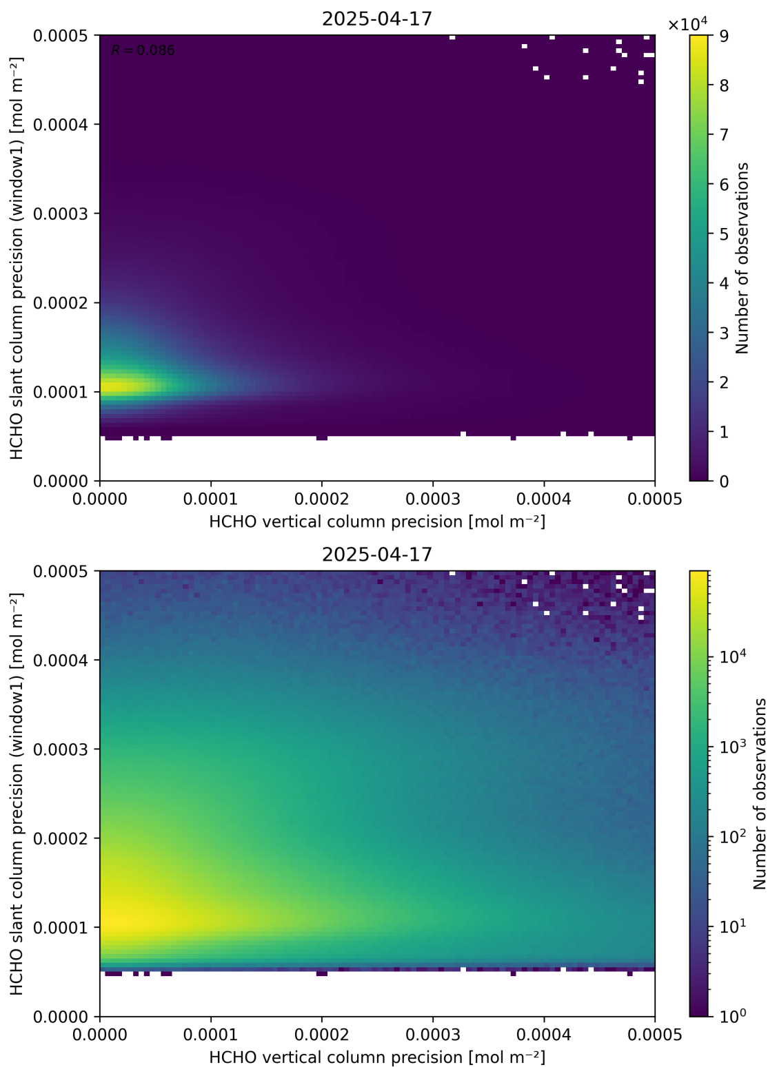
Figure 143: Scatter density plot of “HCHO vertical column precision” against “HCHO slant column precision (window1)” for 2025-04-16 to 2025-04-18.
