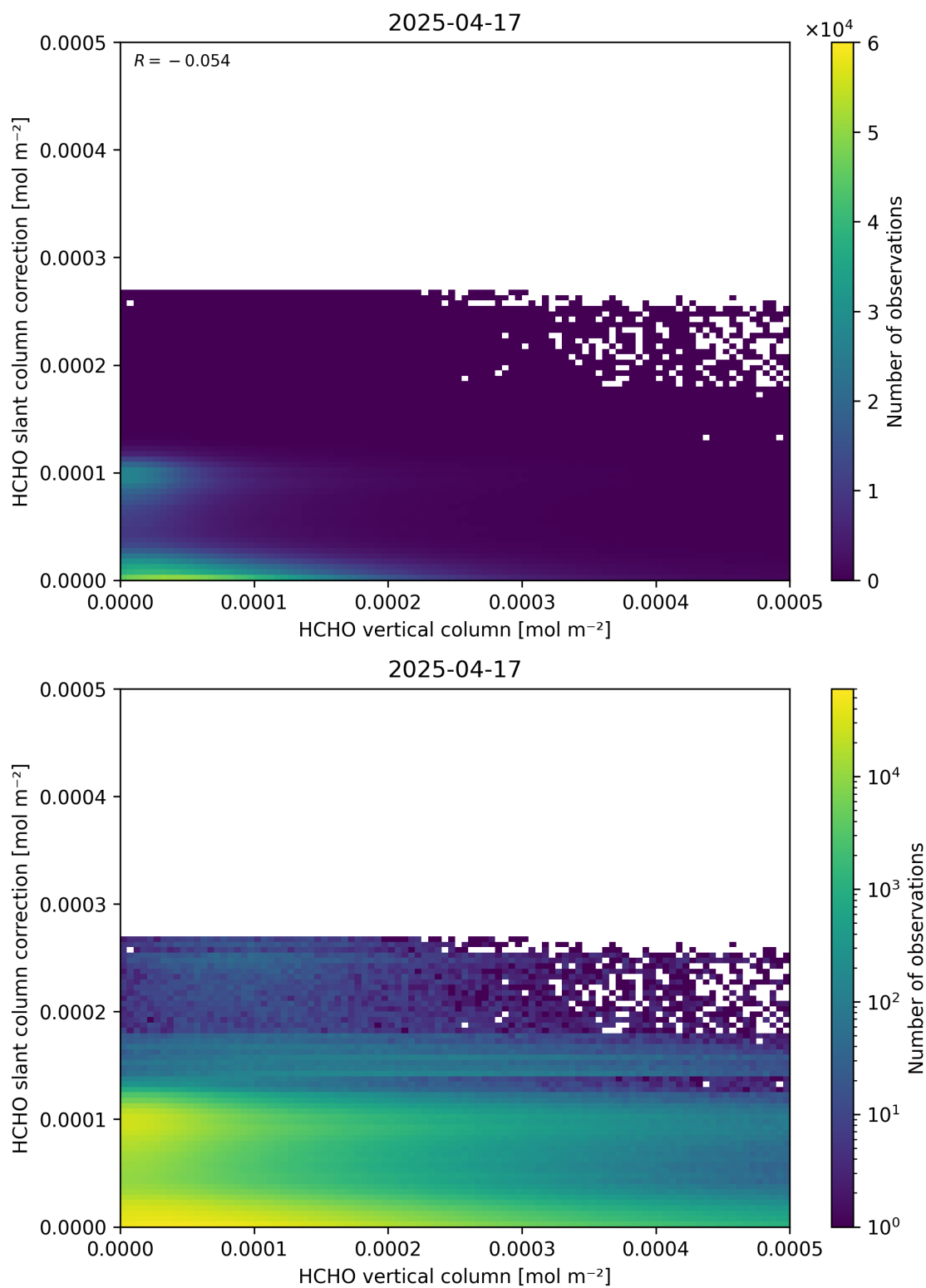
Figure 128: Scatter density plot of “HCHO vertical column” against “HCHO slant column correction” for 2025-04-16 to 2025-04-18.
