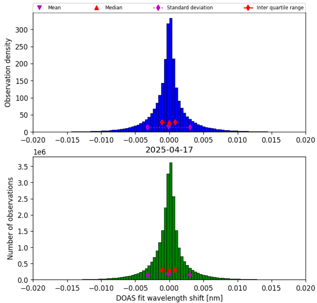
Figure 44: Histogram of “DOAS fit wavelength shift” for 2025-04-16 to 2025-04-18
