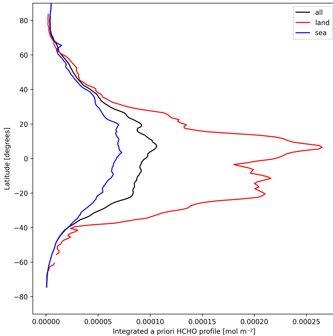
Figure 29: Zonal average of “Integrated a priori HCHO profile” for 2025-04-16 to 2025-04-18.
