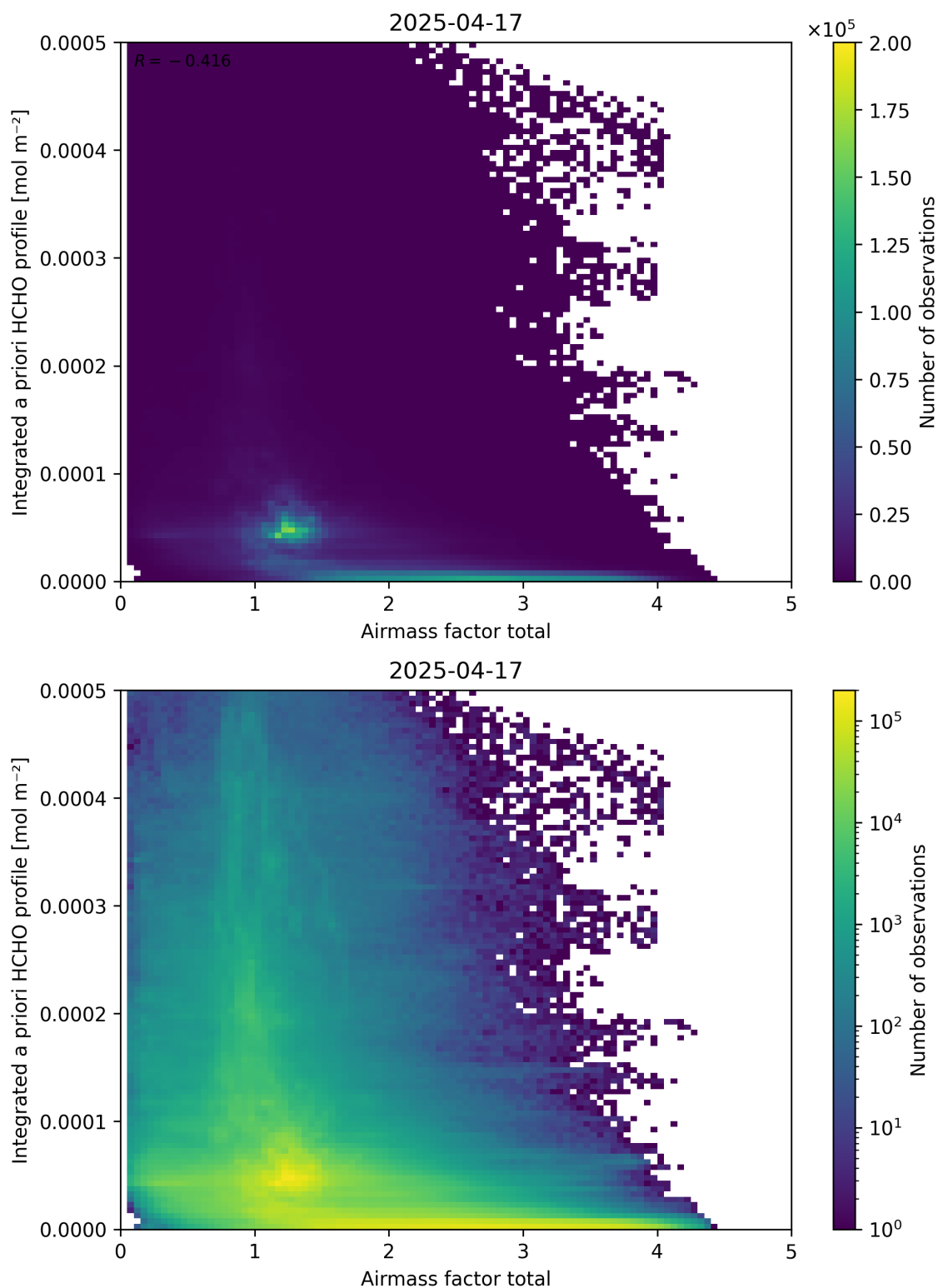
Figure 104: Scatter density plot of “Airmass factor total” against “Integrated a priori HCHO profile” for 2025-04-16 to 2025-04-18.
