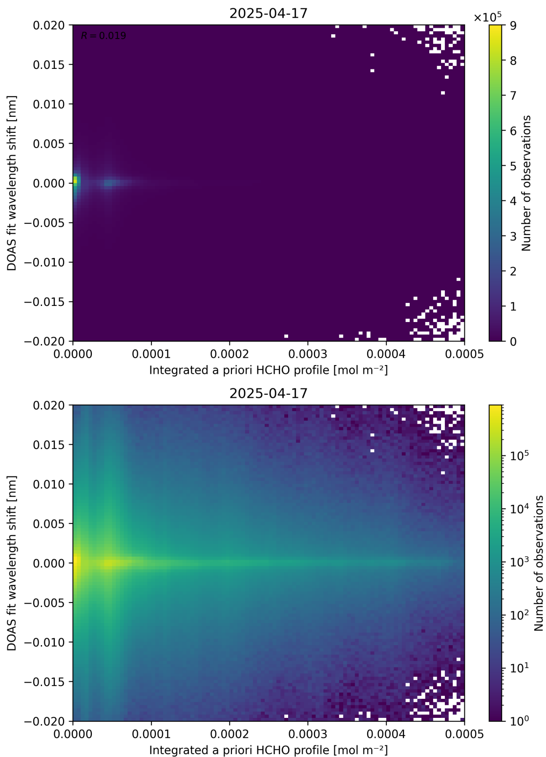
Figure 149: Scatter density plot of “Integrated a priori HCHO profile” against “DOAS fit wavelength shift” for 2025-04-16 to 2025-04-18.
