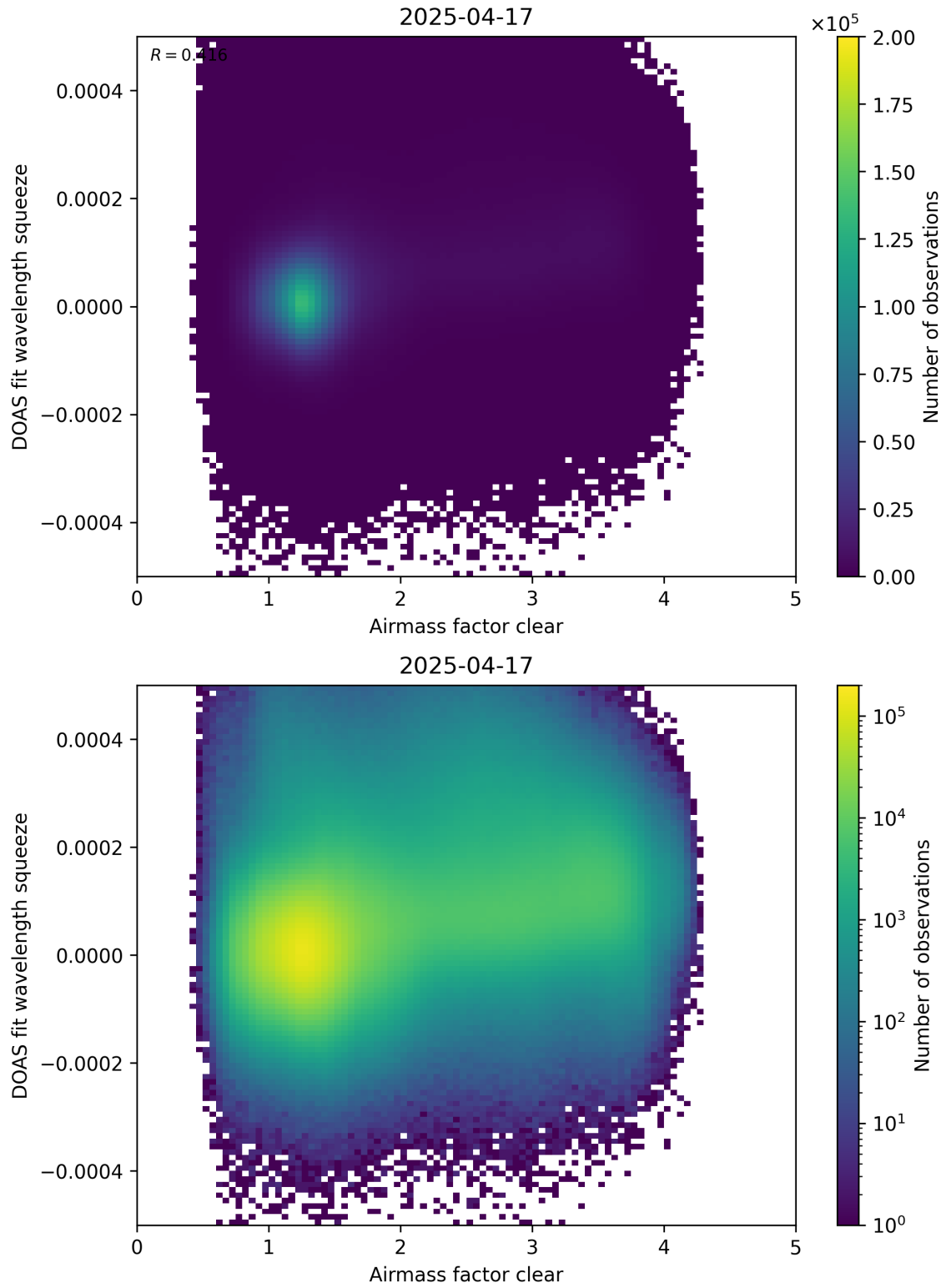
Figure 73: Scatter density plot of “Airmass factor clear” against “DOAS fit wavelength squeeze” for 2025-04-16 to 2025-04-18.
