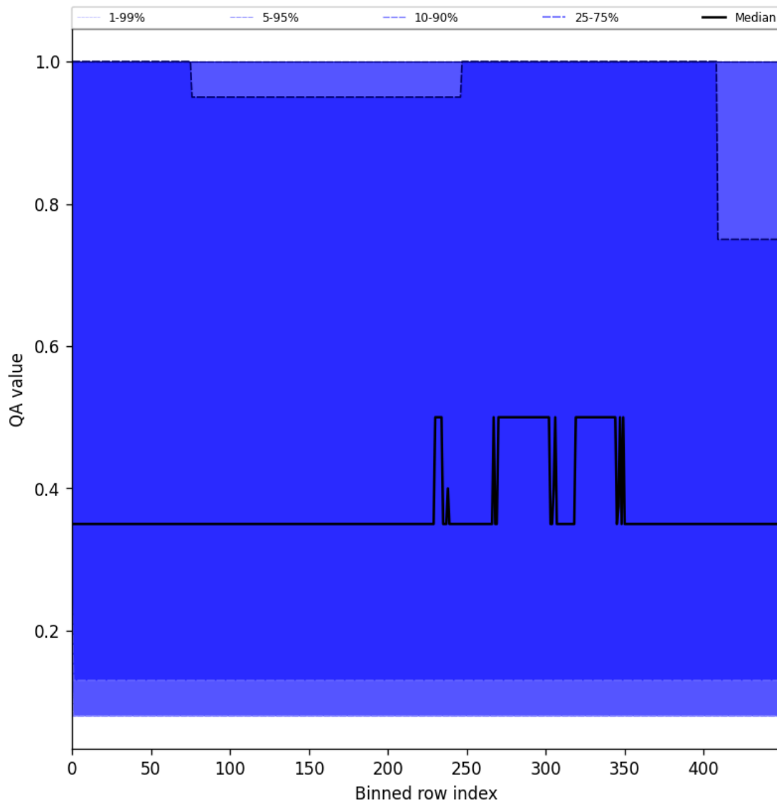
Figure 48: Along track statistics of “QA value” for 2025-04-16 to 2025-04-18
