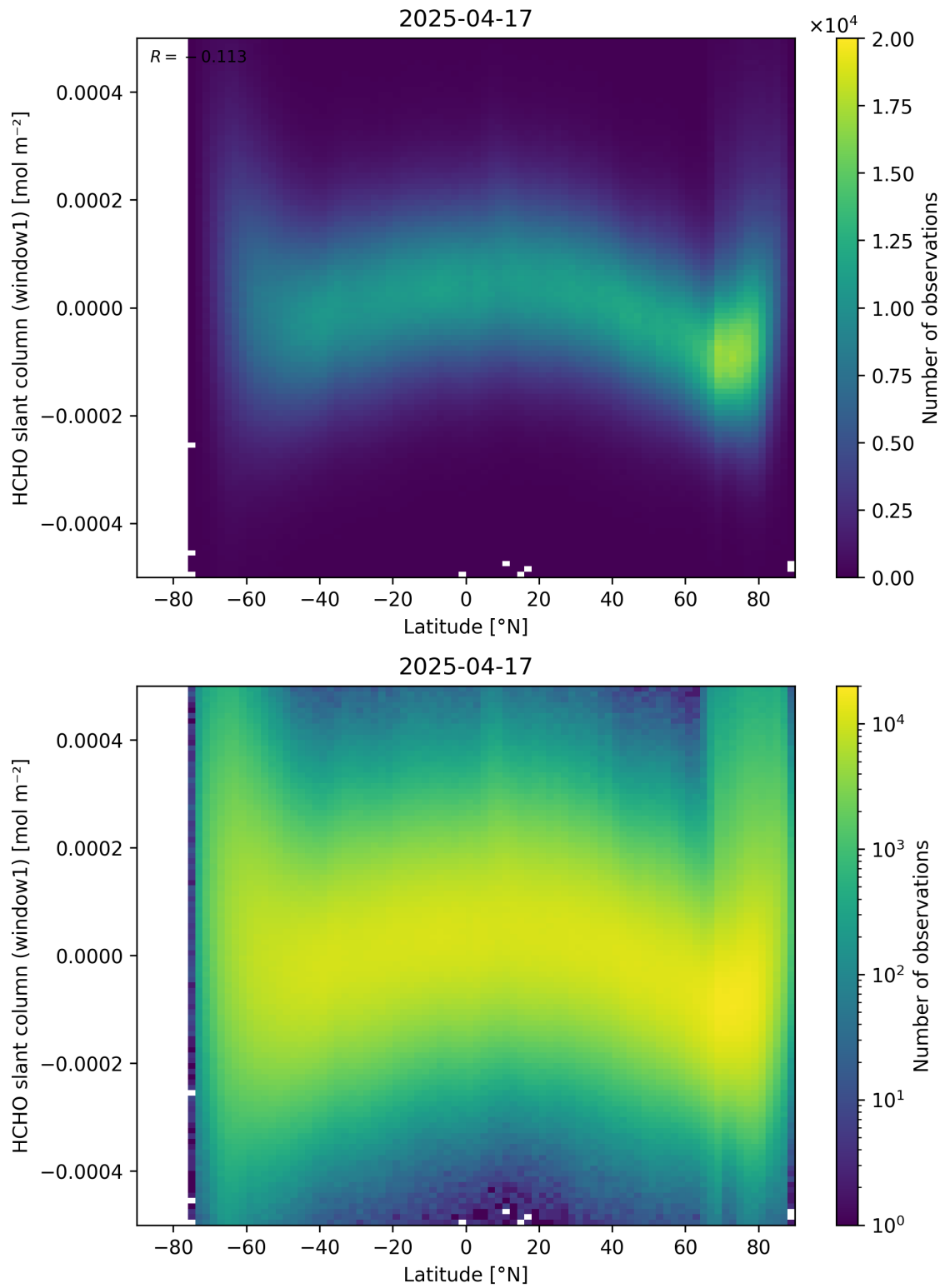
Figure 159: Scatter density plot of “Latitude” against “HCHO slant column (window1)” for 2025-04-16 to 2025-04-18.
