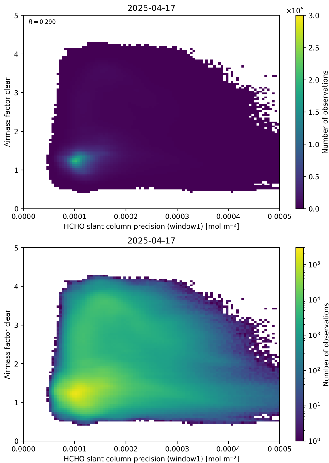
Figure 91: Scatter density plot of “HCHO slant column precision (window1)” against “Airmass factor clear” for 2025-04-16 to 2025-04-18.
