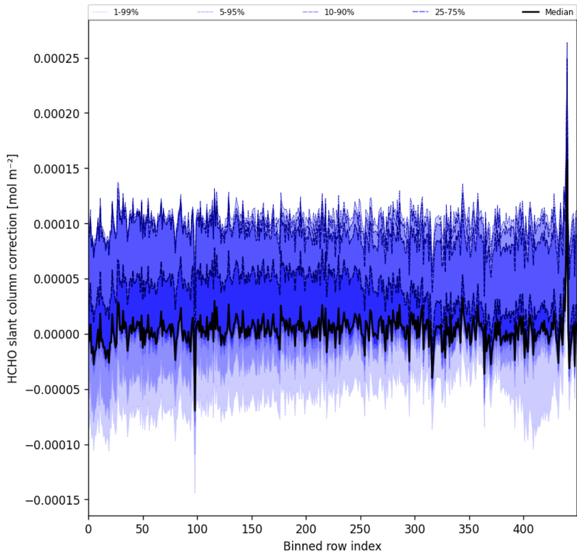
Figure 61: Along track statistics of “HCHO slant column correction” for 2025-04-16 to 2025-04-18
