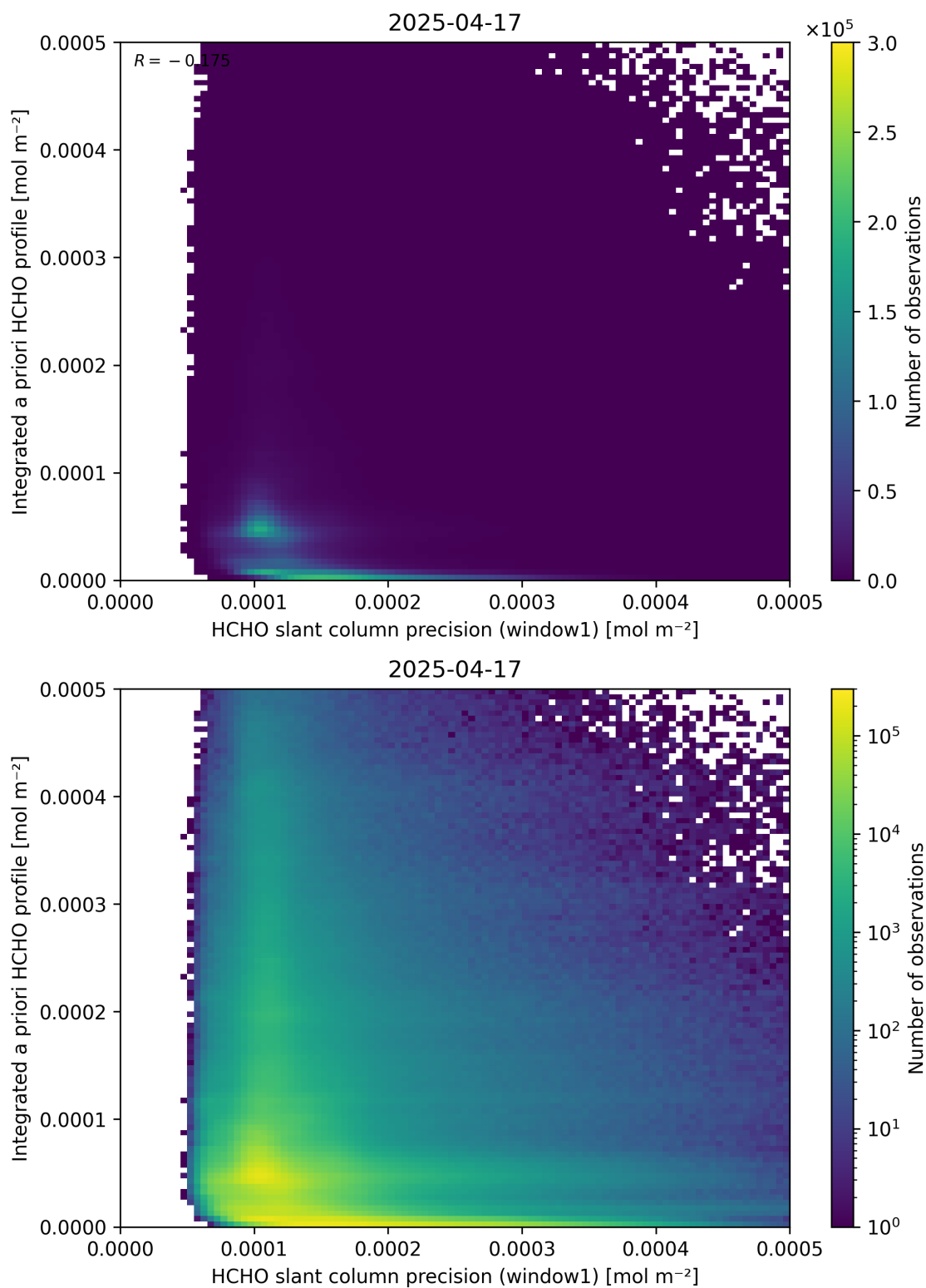
Figure 96: Scatter density plot of “HCHO slant column precision (window1)” against “Integrated a priori HCHO profile” for 2025-04-16 to 2025-04-18.
