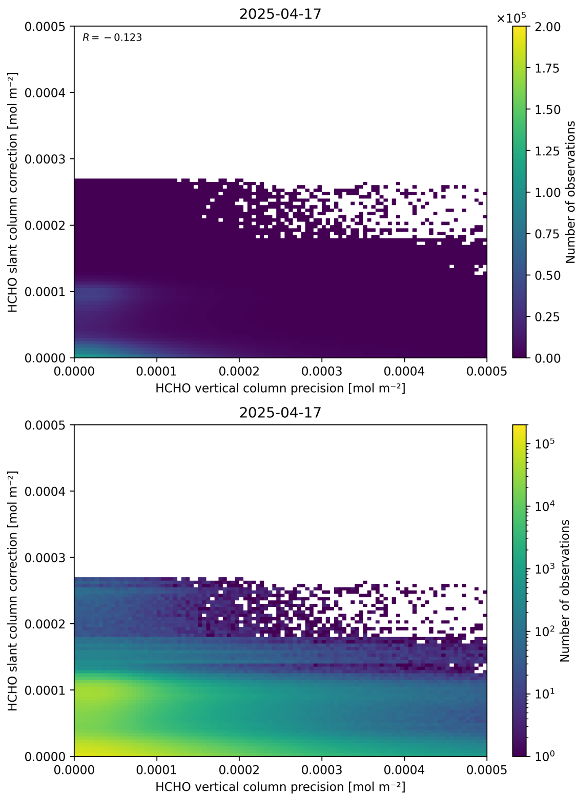
Figure 141: Scatter density plot of “HCHO vertical column precision” against “HCHO slant column correction” for 2025-04-16 to 2025-04-18.
