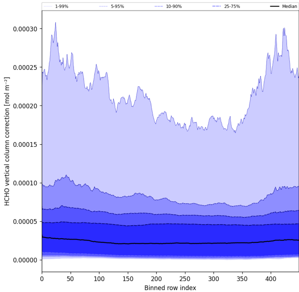
Figure 51: Along track statistics of “HCHO vertical column correction” for 2025-04-16 to 2025-04-18
