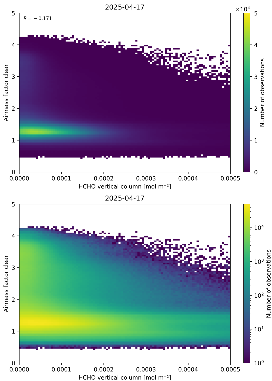
Figure 126: Scatter density plot of “HCHO vertical column” against “Airmass factor clear” for 2025-04-16 to 2025-04-18.
