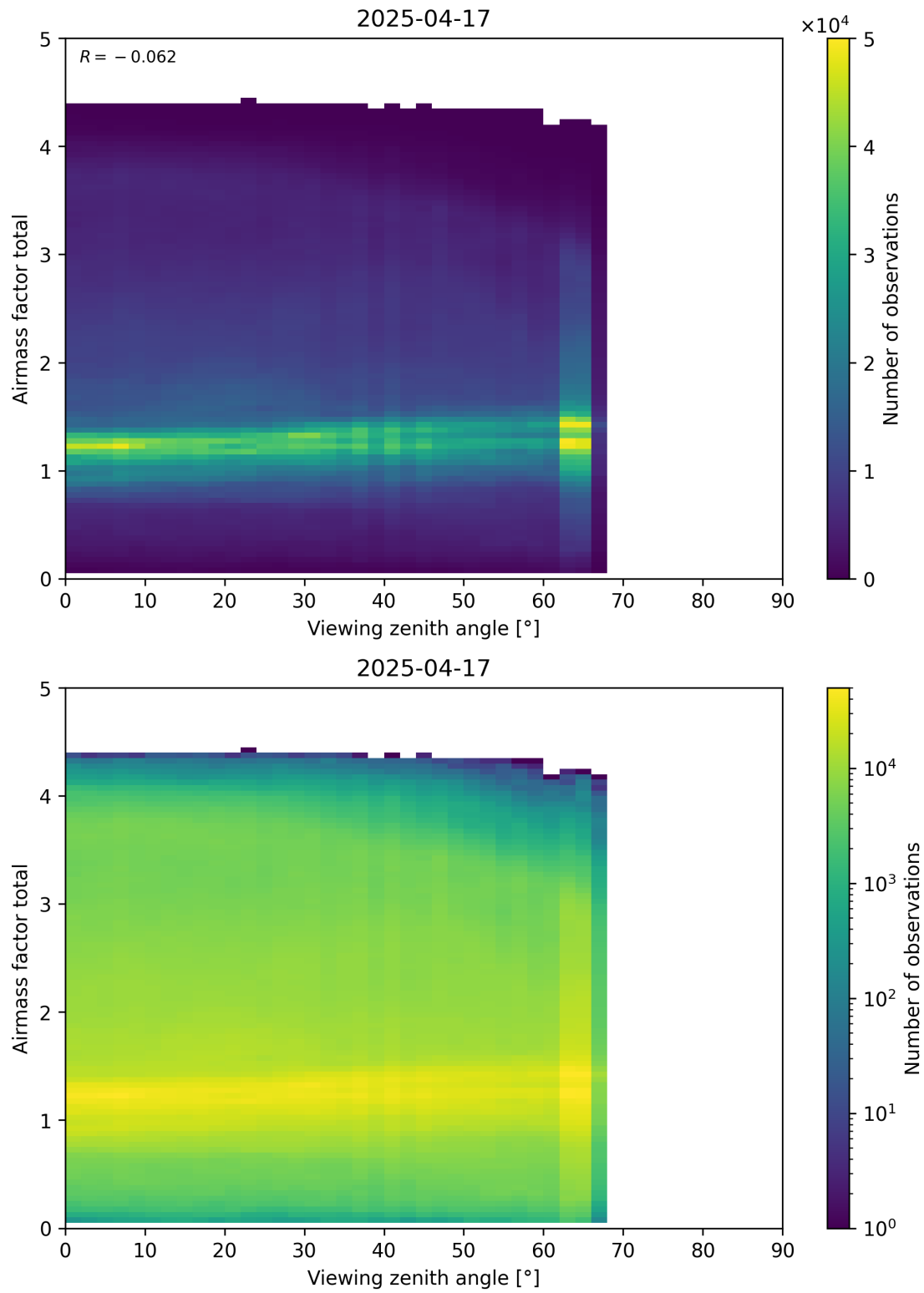
Figure 190: Scatter density plot of “Viewing zenith angle” against “Airmass factor total” for 2025-04-16 to 2025-04-18.
