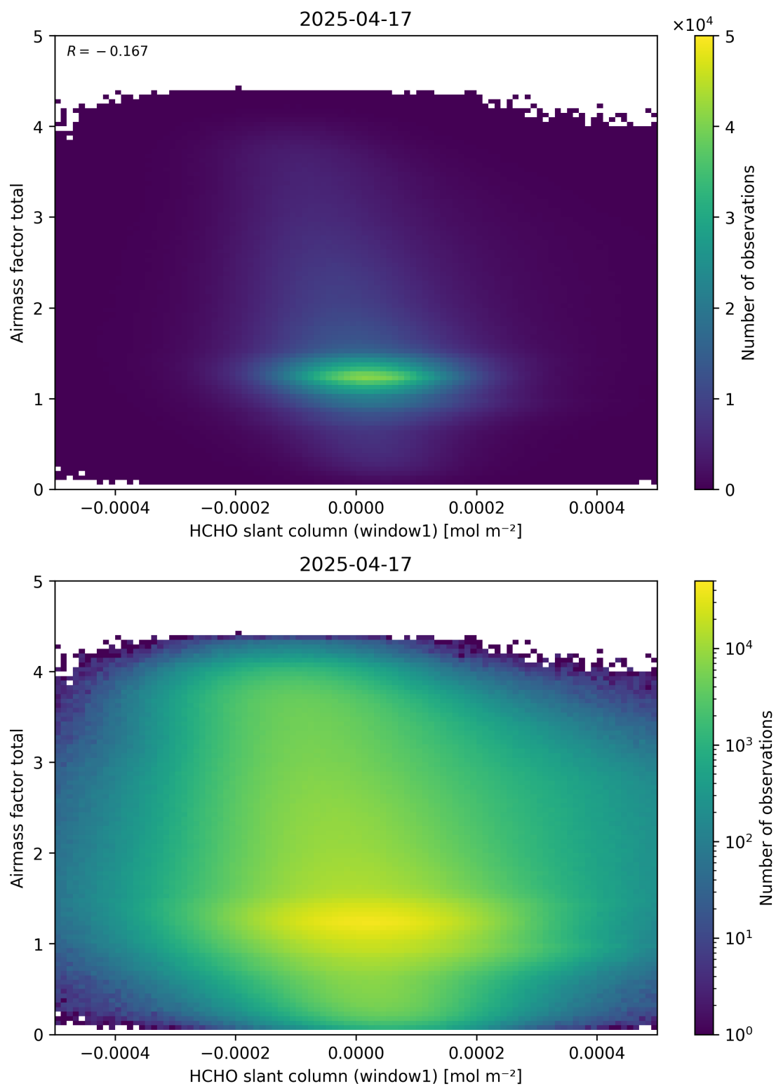
Figure 85: Scatter density plot of “HCHO slant column (window1)” against “Airmass factor total” for 2025-04-16 to 2025-04-18.
