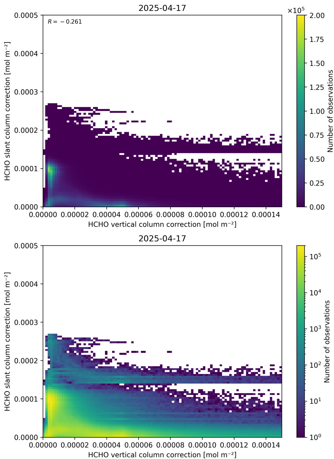
Figure 117: Scatter density plot of “HCHO vertical column correction” against “HCHO slant column correction” for 2025-04-16 to 2025-04-18.
