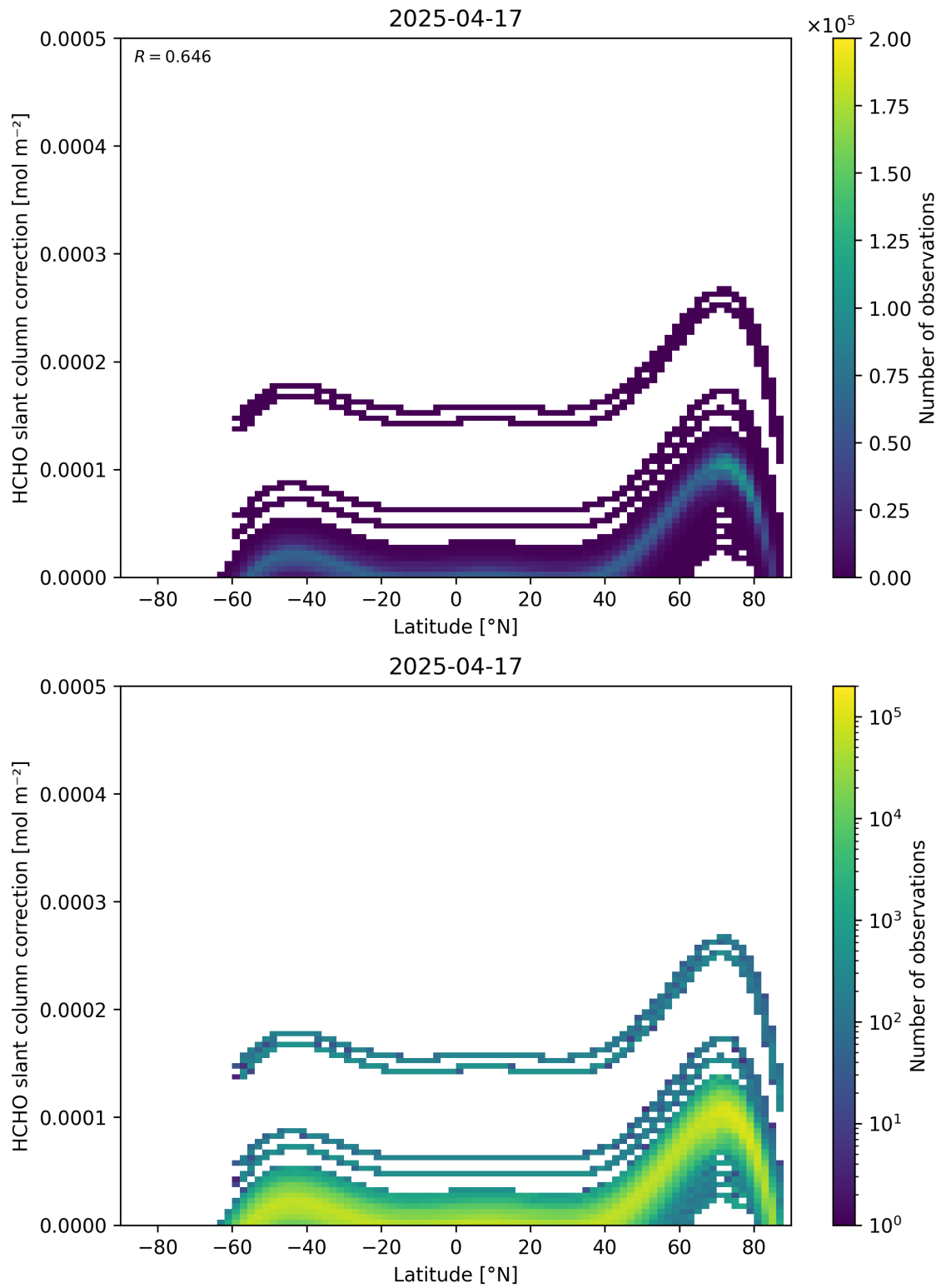
Figure 158: Scatter density plot of “Latitude” against “HCHO slant column correction” for 2025-04-16 to 2025-04-18.
