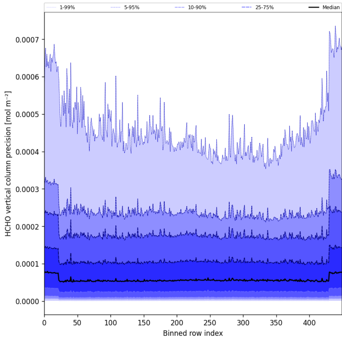
Figure 50: Along track statistics of “HCHO vertical column precision” for 2025-04-16 to 2025-04-18
