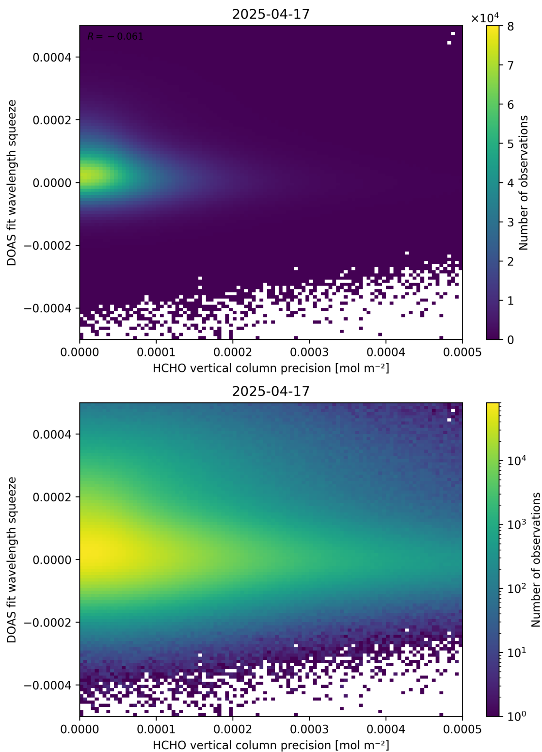
Figure 138: Scatter density plot of “HCHO vertical column precision” against “DOAS fit wavelength squeeze” for 2025-04-16 to 2025-04-18.
