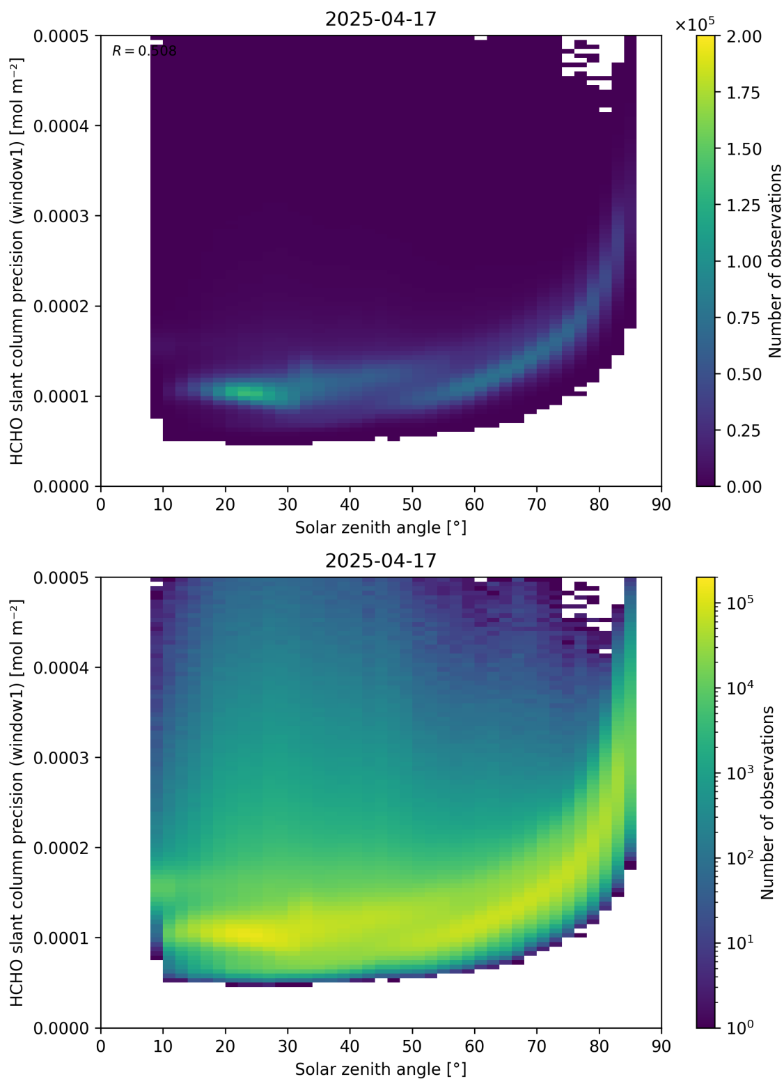
Figure 174: Scatter density plot of “Solar zenith angle” against “HCHO slant column precision (window1)” for 2025-04-16 to 2025-04-18.
