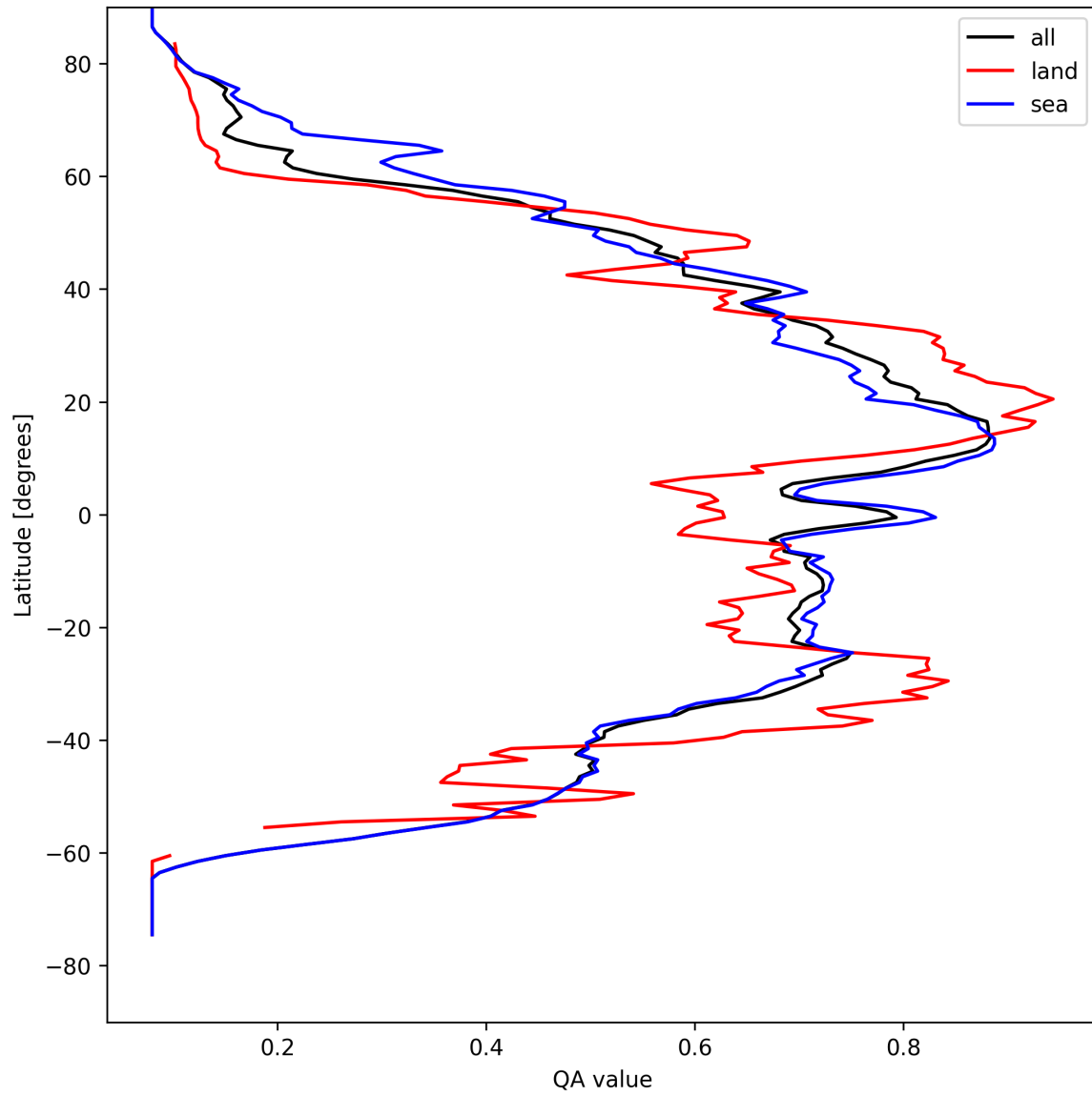
Figure 20: Zonal average of “QA value” for 2025-04-16 to 2025-04-18.
