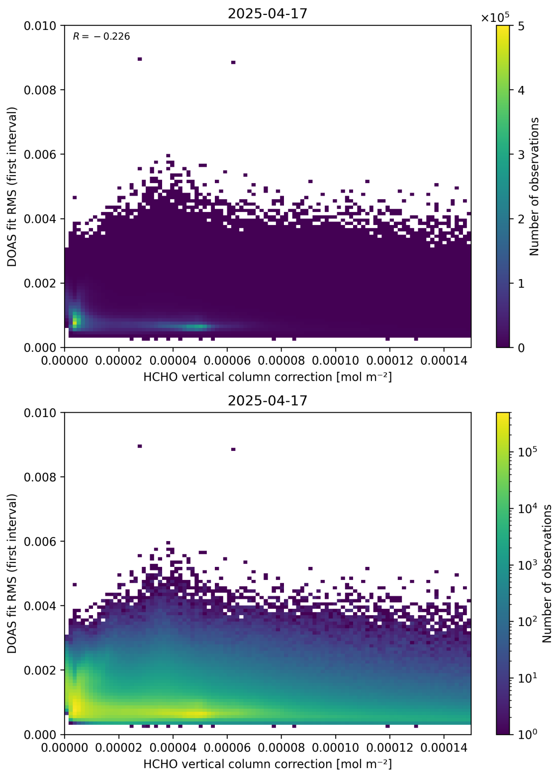
Figure 112: Scatter density plot of “HCHO vertical column correction” against “DOAS fit RMS (first interval)” for 2025-04-16 to 2025-04-18.
