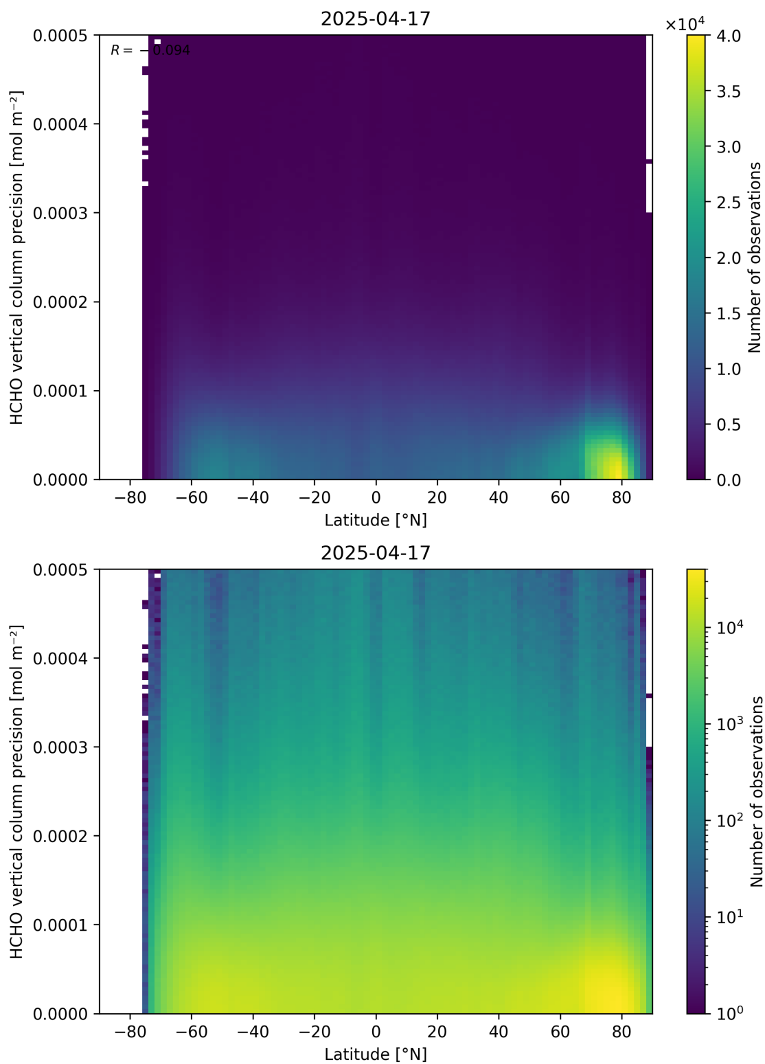
Figure 165: Scatter density plot of “Latitude” against “HCHO vertical column precision” for 2025-04-16 to 2025-04-18.
