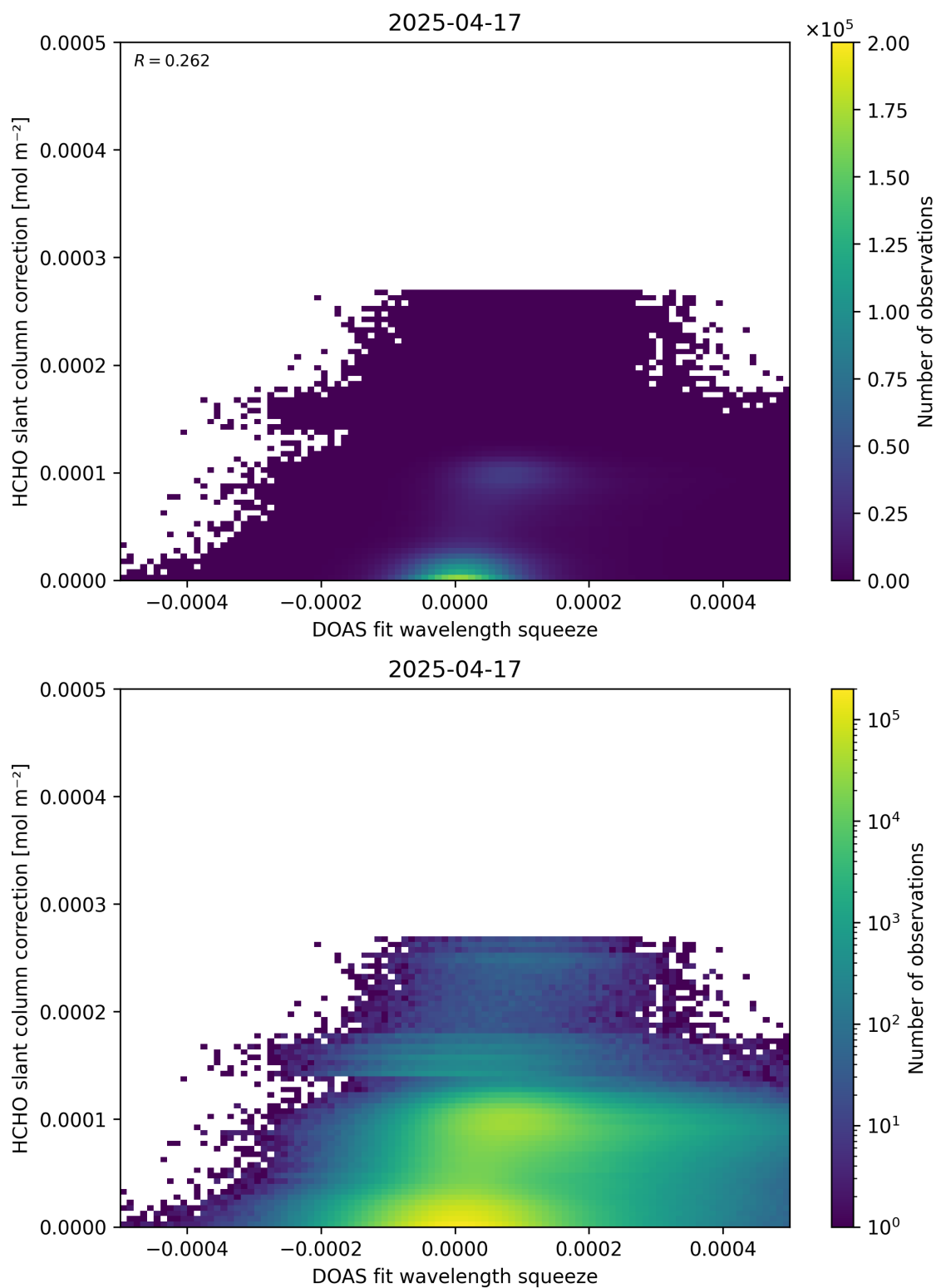
Figure 70: Scatter density plot of “DOAS fit wavelength squeeze” against “HCHO slant column correction” for 2025-04-16 to 2025-04-18.
