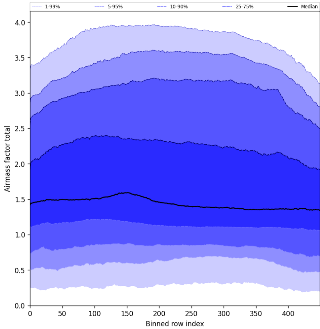
Figure 54: Along track statistics of “Airmass factor total” for 2025-04-16 to 2025-04-18
