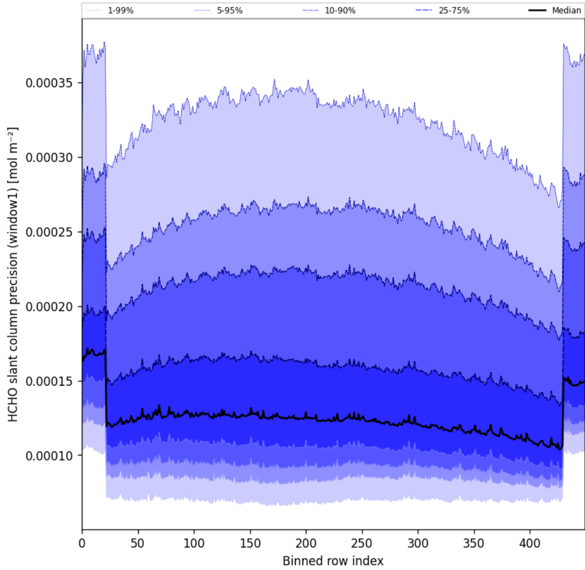
Figure 53: Along track statistics of “HCHO slant column precision (window1)” for 2025-04-16 to 2025-04-18
