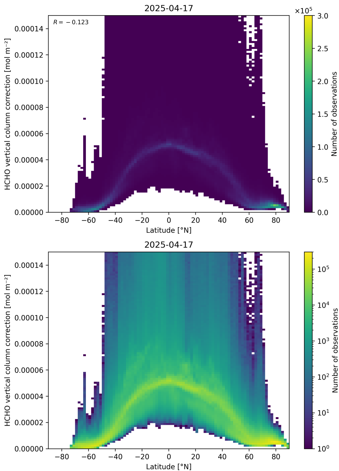
Figure 164: Scatter density plot of “Latitude” against “HCHO vertical column correction” for 2025-04-16 to 2025-04-18.
