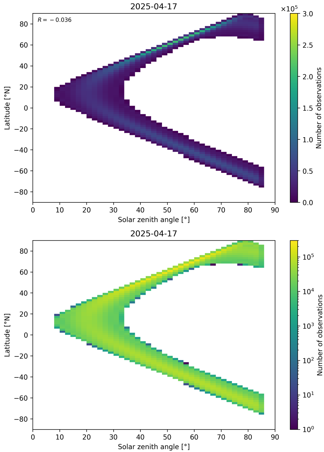
Figure 181: Scatter density plot of “Solar zenith angle” against “Latitude” for 2025-04-16 to 2025-04-18.
