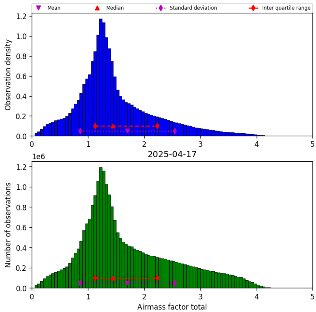
Figure 40: Histogram of “Airmass factor total” for 2025-04-16 to 2025-04-18
