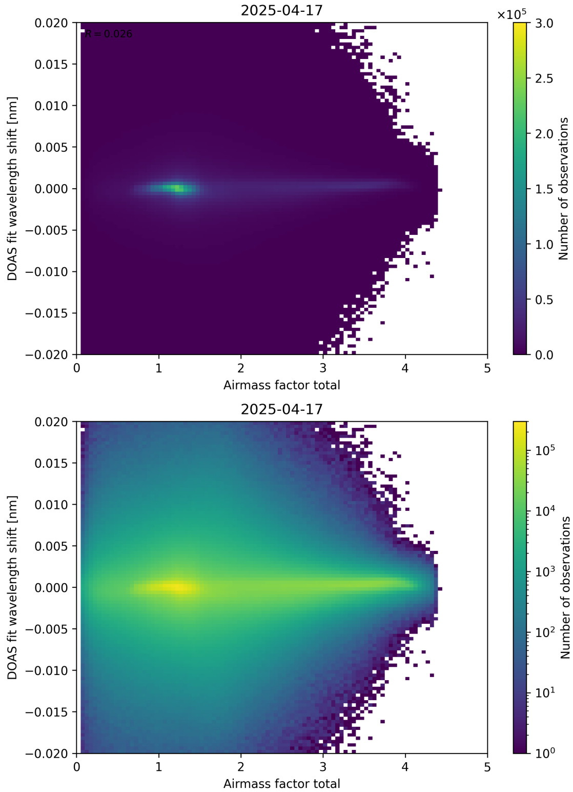
Figure 98: Scatter density plot of “Airmass factor total” against “DOAS fit wavelength shift” for 2025-04-16 to 2025-04-18.
