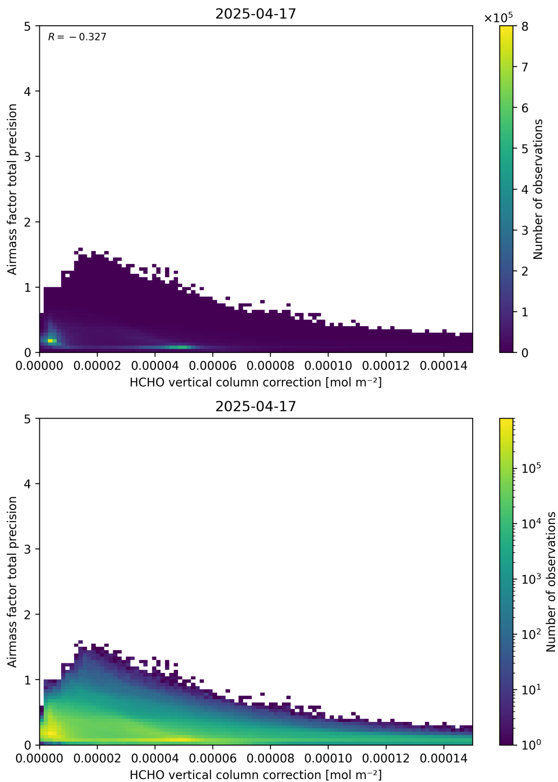
Figure 121: Scatter density plot of “HCHO vertical column correction” against “Airmass factor total precision” for 2025-04-16 to 2025-04-18.
