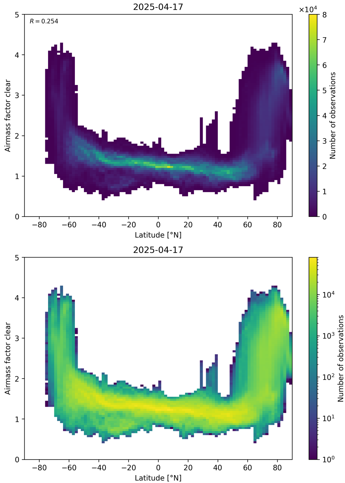
Figure 156: Scatter density plot of “Latitude” against “Airmass factor clear” for 2025-04-16 to 2025-04-18.
