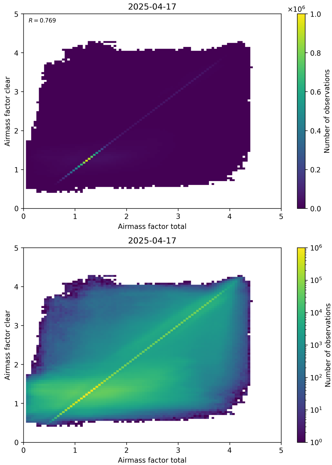
Figure 100: Scatter density plot of “Airmass factor total” against “Airmass factor clear” for 2025-04-16 to 2025-04-18.
