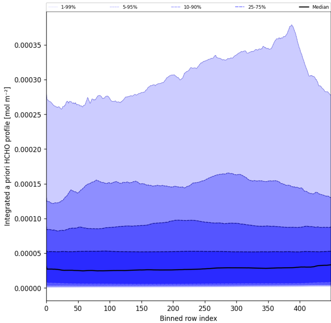
Figure 57: Along track statistics of “Integrated a priori HCHO profile” for 2025-04-16 to 2025-04-18
