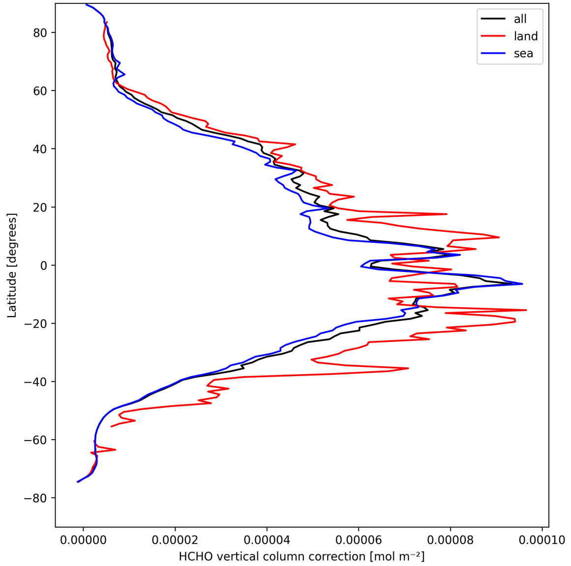
Figure 23: Zonal average of “HCHO vertical column correction” for 2025-04-16 to 2025-04-18.
