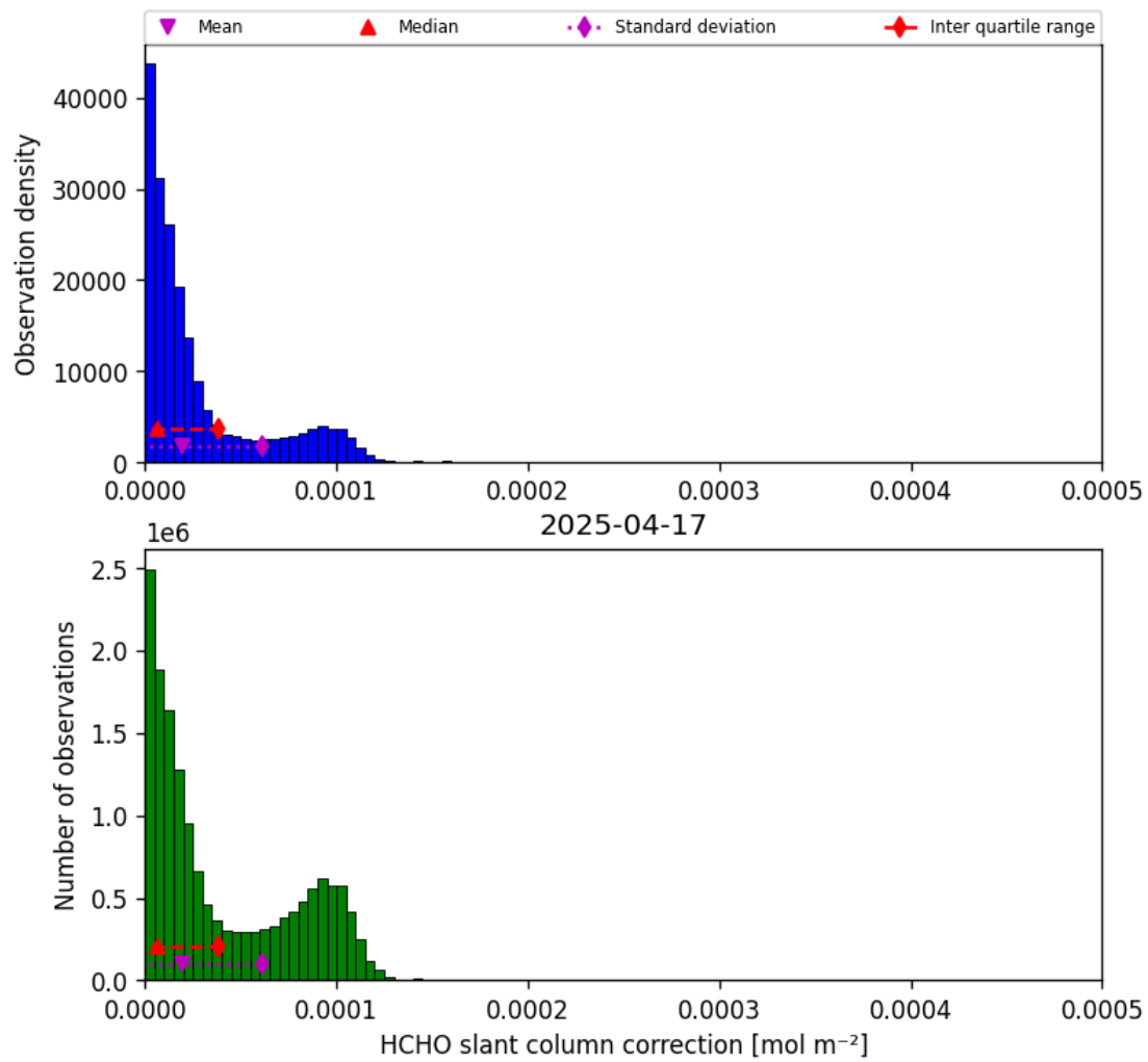
Figure 47: Histogram of “HCHO slant column correction” for 2025-04-16 to 2025-04-18
