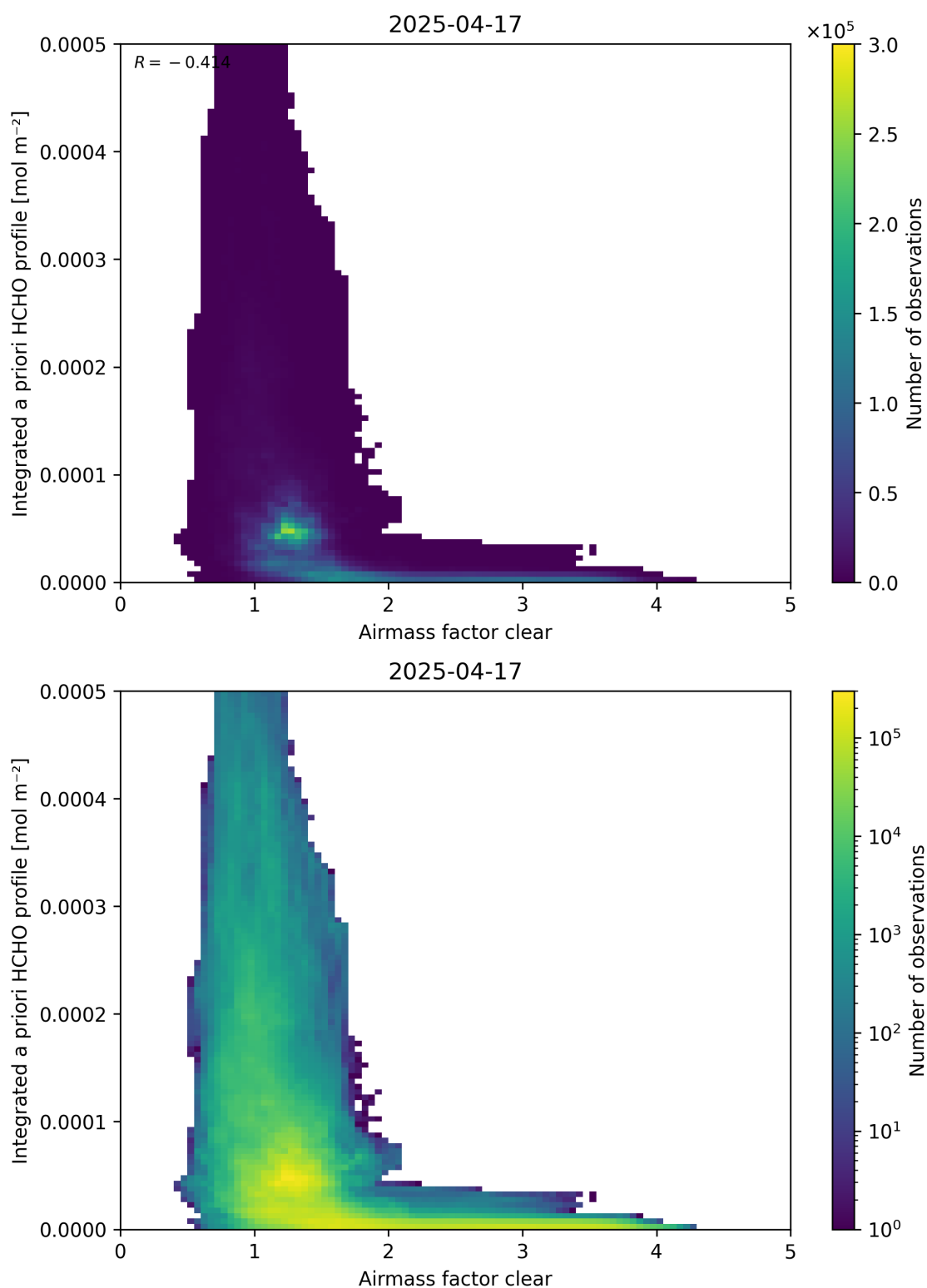
Figure 76: Scatter density plot of “Airmass factor clear” against “Integrated a priori HCHO profile” for 2025-04-16 to 2025-04-18.
