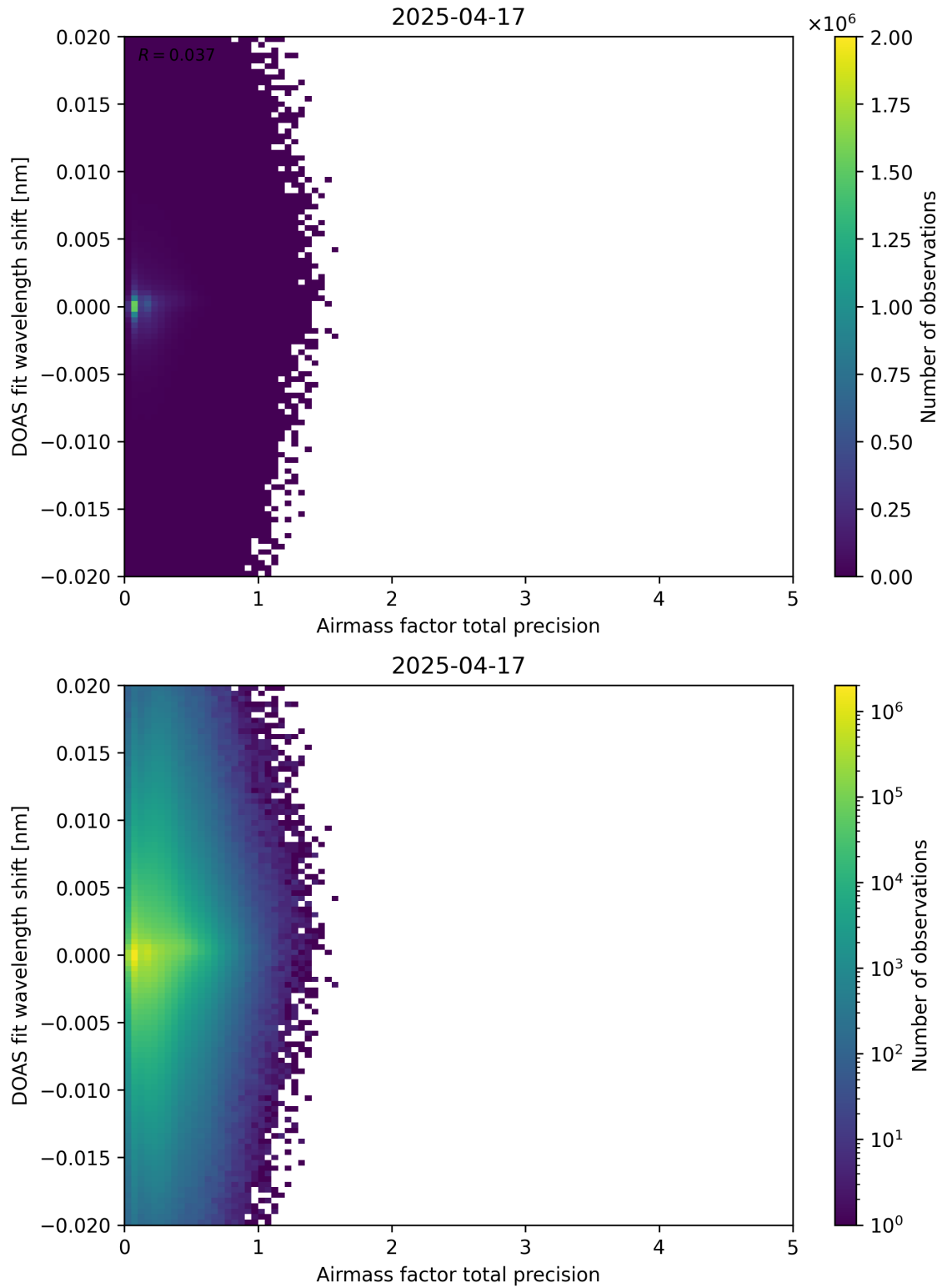
Figure 106: Scatter density plot of “Airmass factor total precision” against “DOAS fit wavelength shift” for 2025-04-16 to 2025-04-18.
