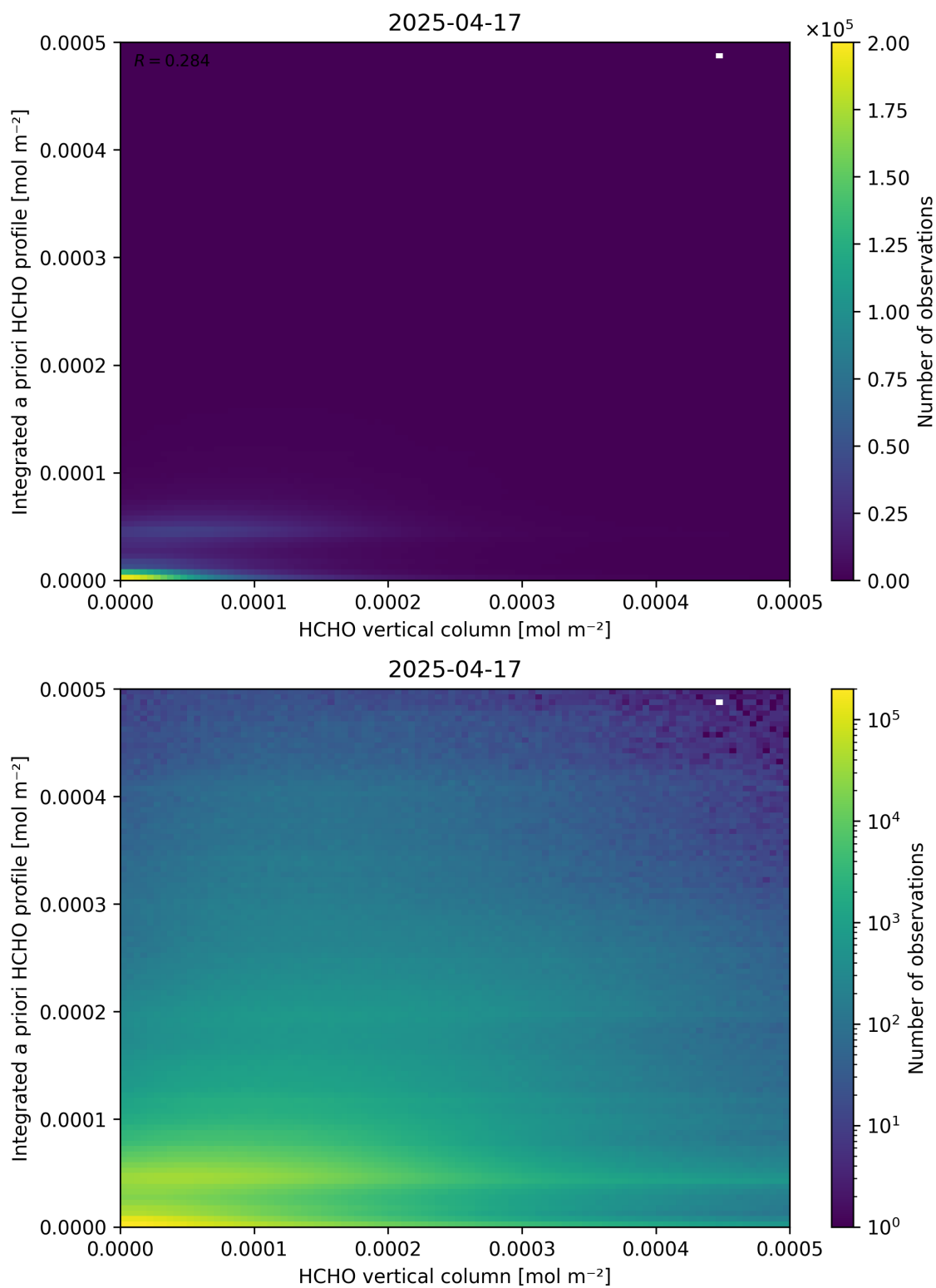
Figure 135: Scatter density plot of “HCHO vertical column” against “Integrated a priori HCHO profile” for 2025-04-16 to 2025-04-18.
