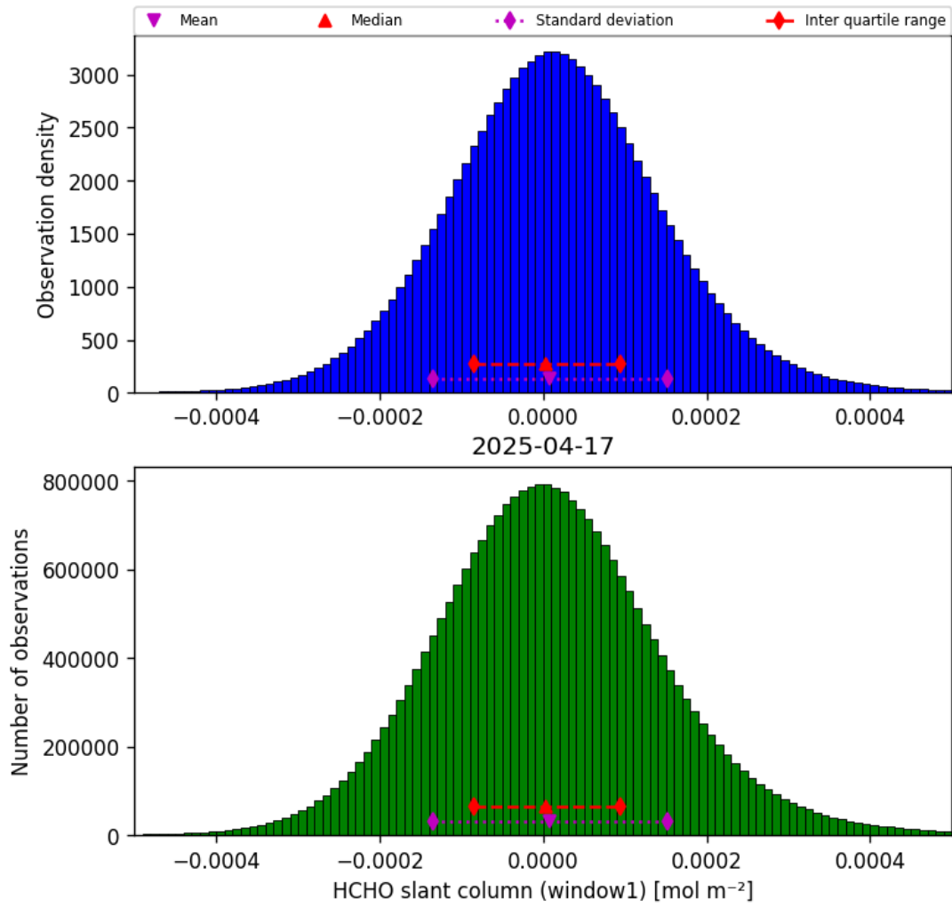
Figure 38: Histogram of “HCHO slant column (window1)” for 2025-04-16 to 2025-04-18
