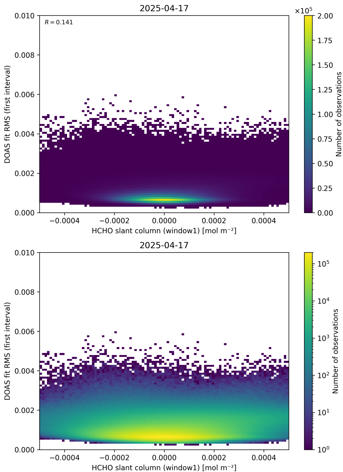
Figure 78: Scatter density plot of “HCHO slant column (window1)” against “DOAS fit RMS (first interval)” for 2025-04-16 to 2025-04-18.
