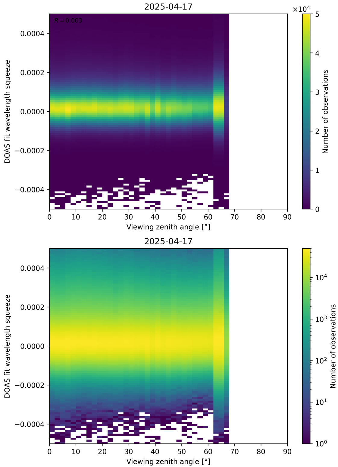
Figure 184: Scatter density plot of “Viewing zenith angle” against “DOAS fit wavelength squeeze” for 2025-04-16 to 2025-04-18.
