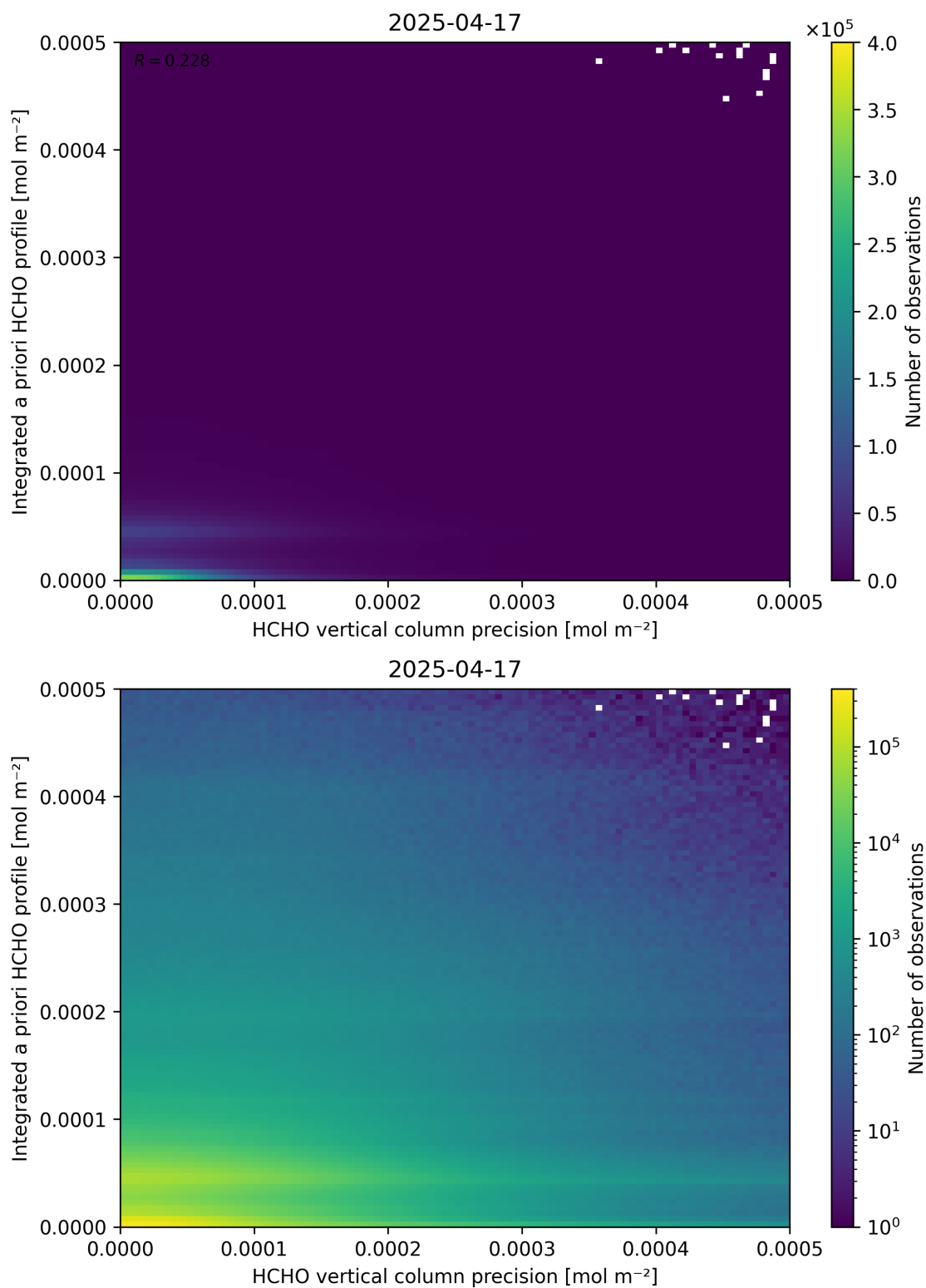
Figure 147: Scatter density plot of “HCHO vertical column precision” against “Integrated a priori HCHO profile” for 2025-04-16 to 2025-04-18.
