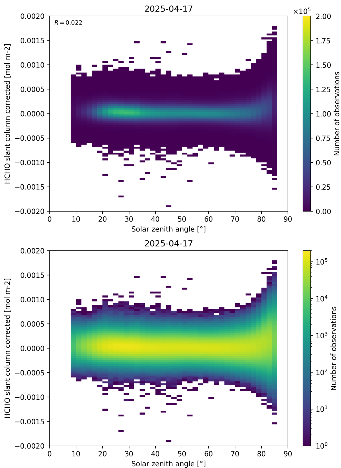
Figure 171: Scatter density plot of “Solar zenith angle” against “HCHO slant column corrected” for 2025-04-16 to 2025-04-18.
