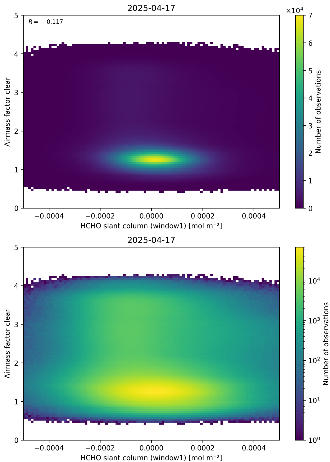
Figure 81: Scatter density plot of “HCHO slant column (window1)” against “Airmass factor clear” for 2025-04-16 to 2025-04-18.
