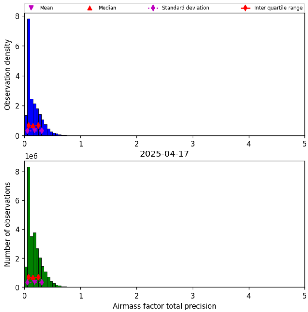
Figure 41: Histogram of “Airmass factor total precision” for 2025-04-16 to 2025-04-18
