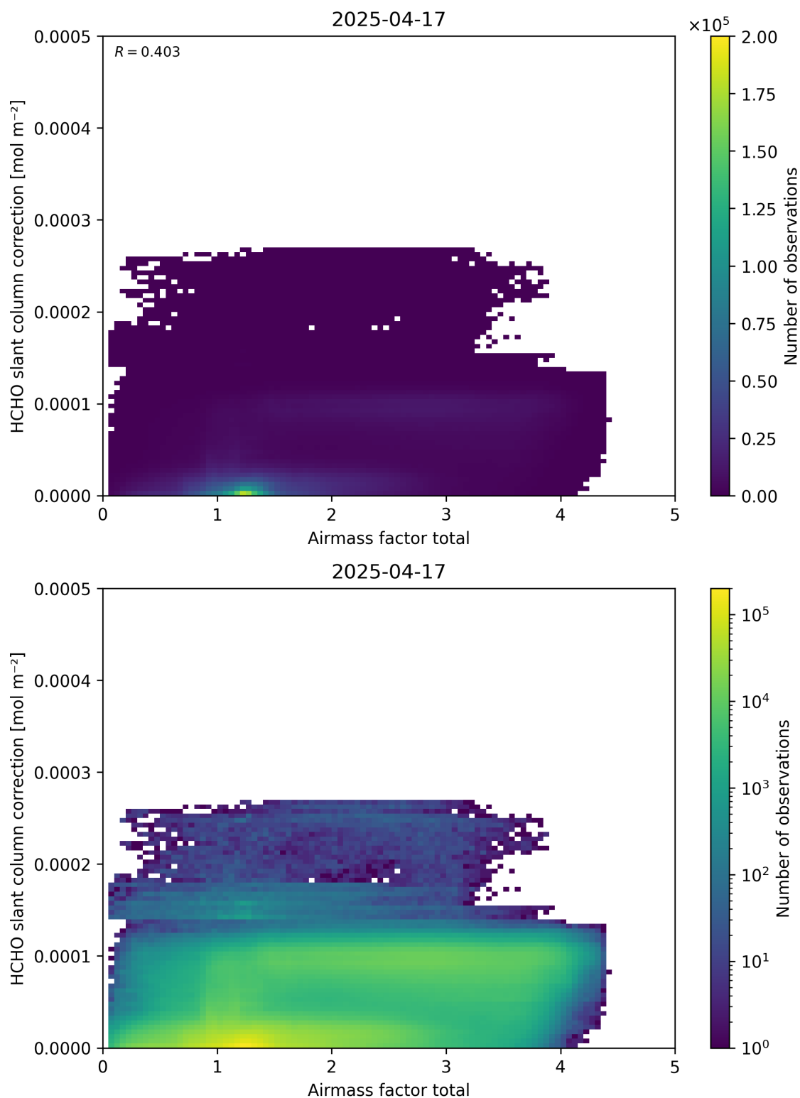
Figure 102: Scatter density plot of “Airmass factor total” against “HCHO slant column correction” for 2025-04-16 to 2025-04-18.
