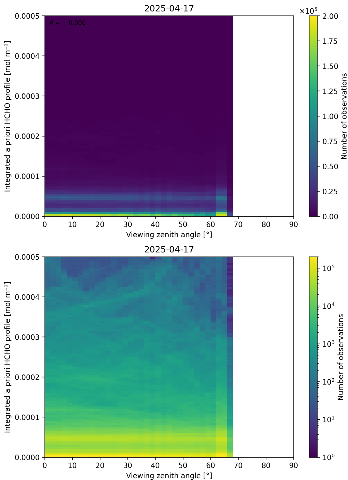
Figure 195: Scatter density plot of “Viewing zenith angle” against “Integrated a priori HCHO profile” for 2025-04-16 to 2025-04-18.
