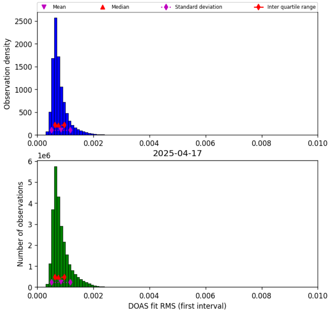
Figure 46: Histogram of “DOAS fit RMS (first interval)” for 2025-04-16 to 2025-04-18
