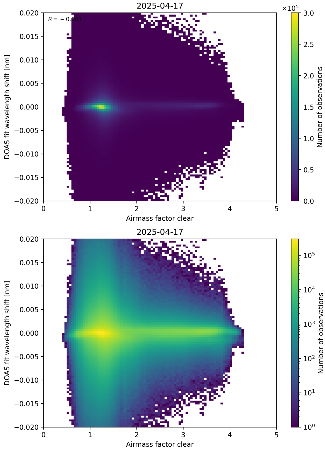
Figure 72: Scatter density plot of “Airmass factor clear” against “DOAS fit wavelength shift” for 2025-04-16 to 2025-04-18.
