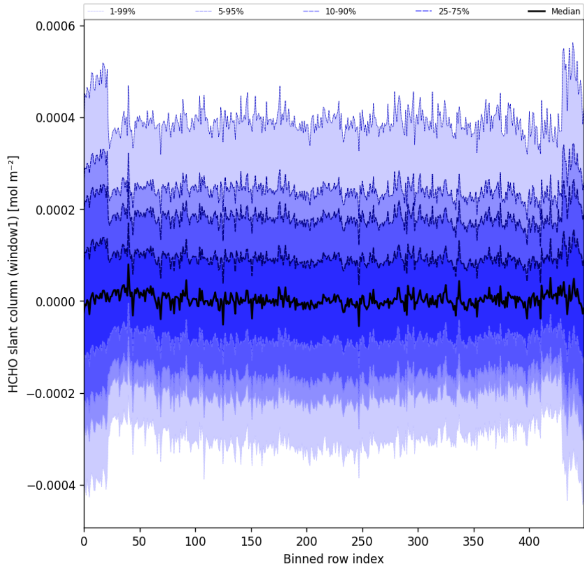
Figure 52: Along track statistics of “HCHO slant column (window1)” for 2025-04-16 to 2025-04-18
