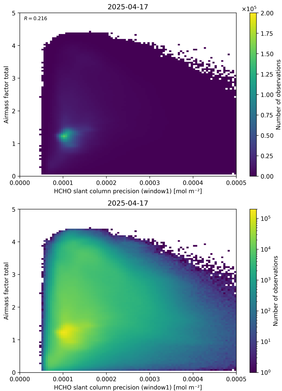
Figure 94: Scatter density plot of “HCHO slant column precision (window1)” against “Airmass factor total” for 2025-04-16 to 2025-04-18.
