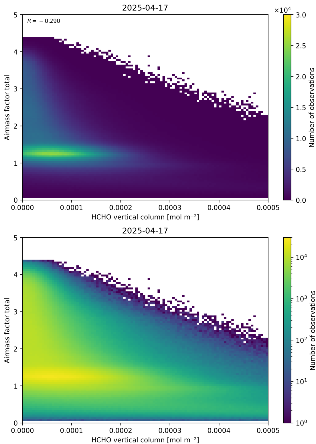
Figure 131: Scatter density plot of “HCHO vertical column” against “Airmass factor total” for 2025-04-16 to 2025-04-18.
