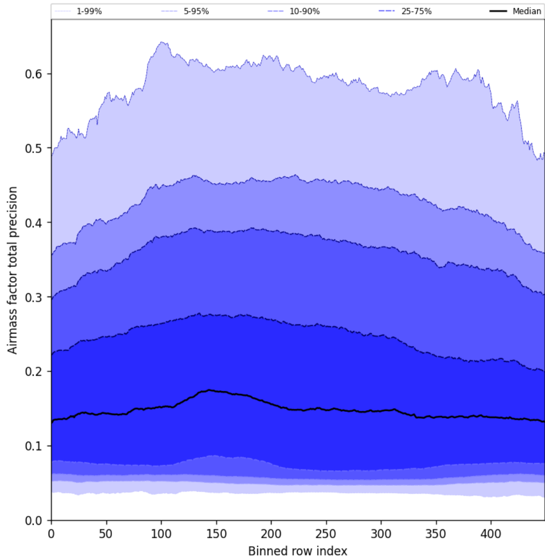
Figure 55: Along track statistics of “Airmass factor total precision” for 2025-04-16 to 2025-04-18
