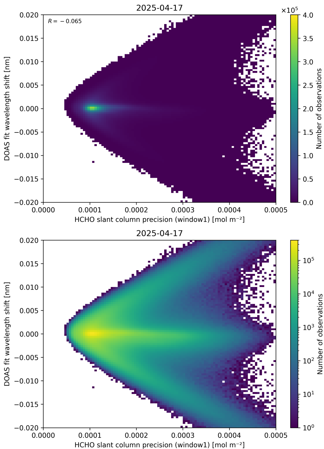
Figure 89: Scatter density plot of “HCHO slant column precision (window1)” against “DOAS fit wavelength shift” for 2025-04-16 to 2025-04-18.
