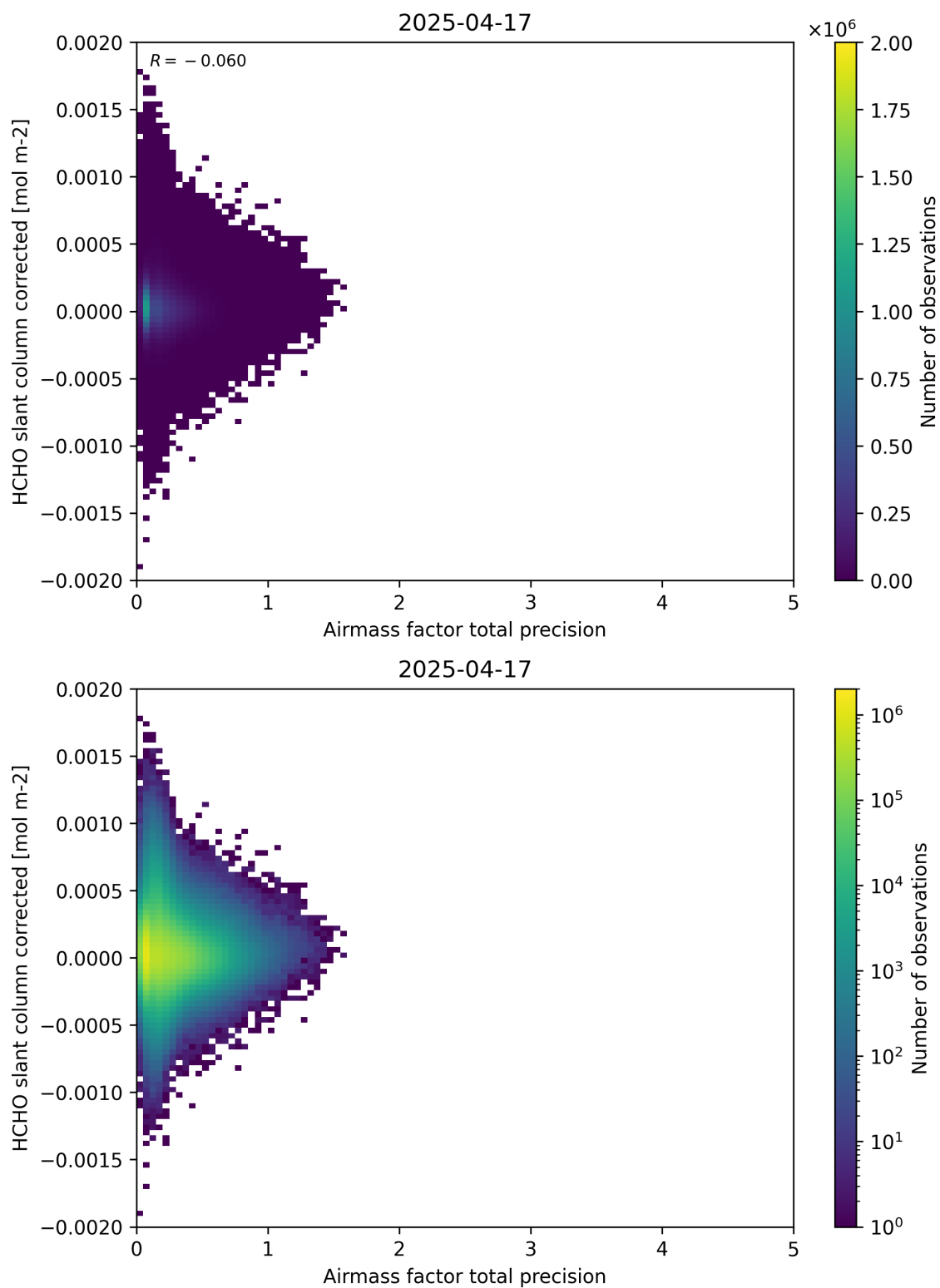
Figure 109: Scatter density plot of “Airmass factor total precision” against “HCHO slant column corrected” for 2025-04-16 to 2025-04-18.
