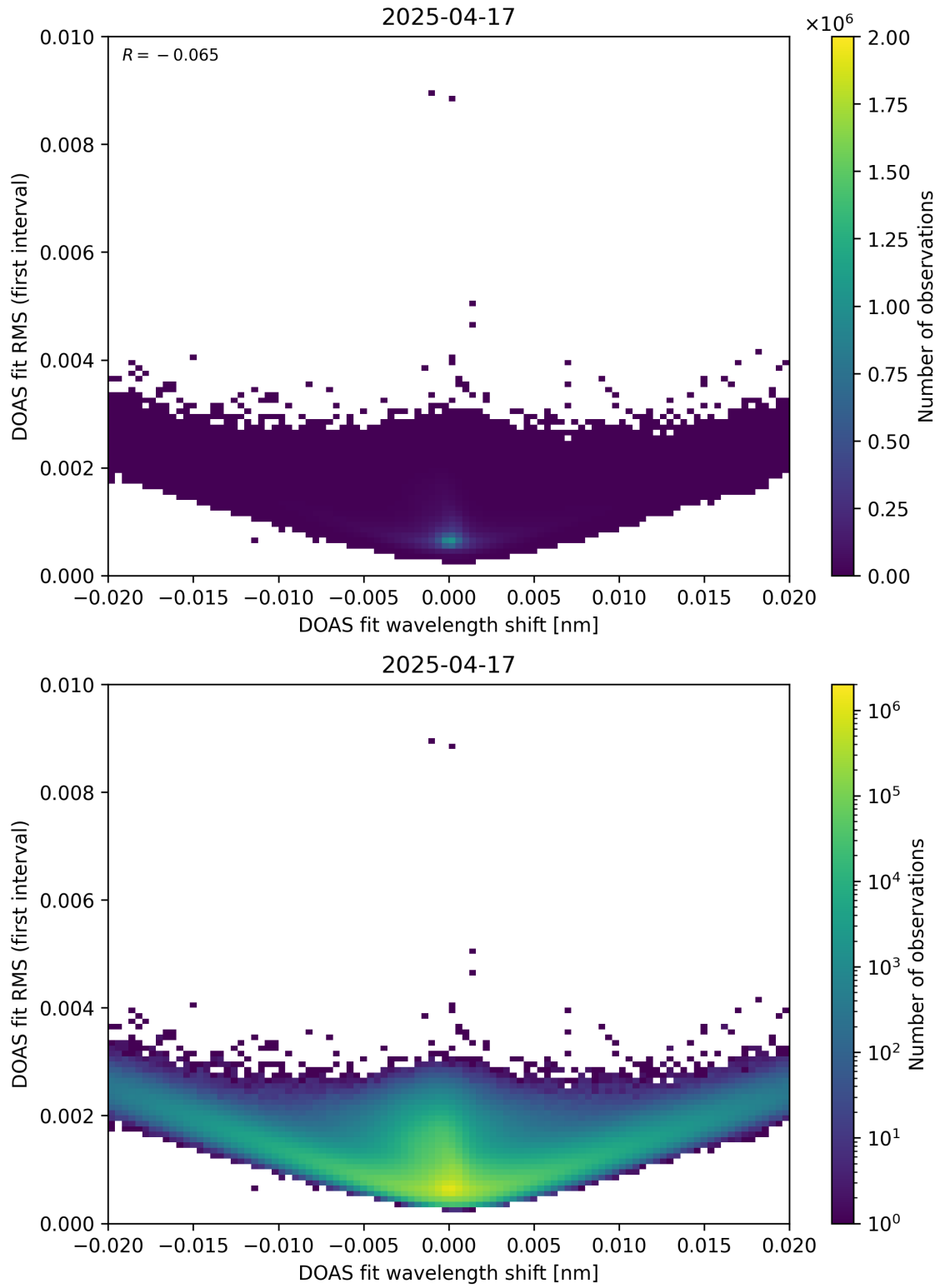
Figure 64: Scatter density plot of “DOAS fit wavelength shift” against “DOAS fit RMS (first interval)” for 2025-04-16 to 2025-04-18.
