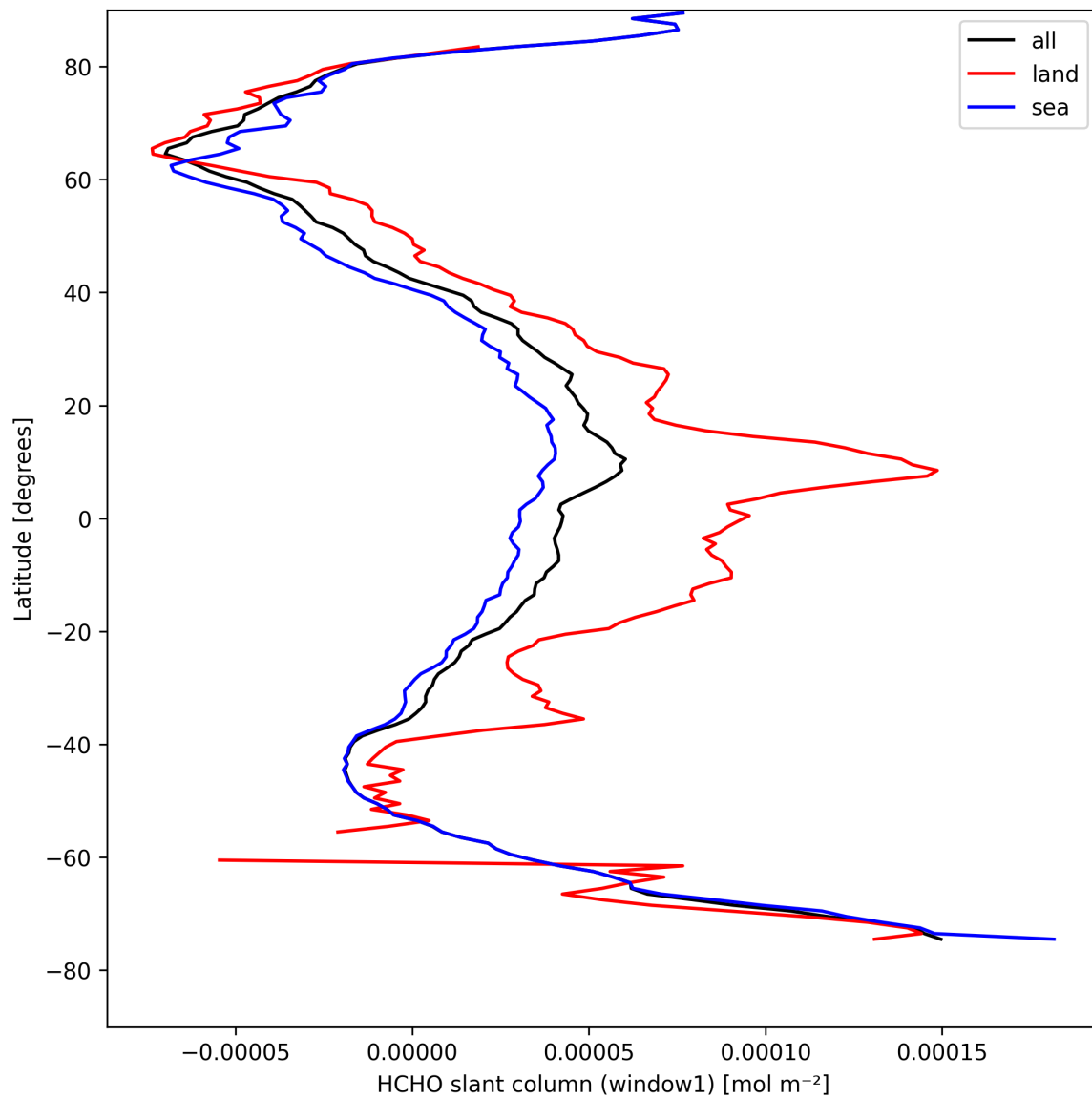
Figure 24: Zonal average of “HCHO slant column (window1)” for 2025-04-16 to 2025-04-18.
