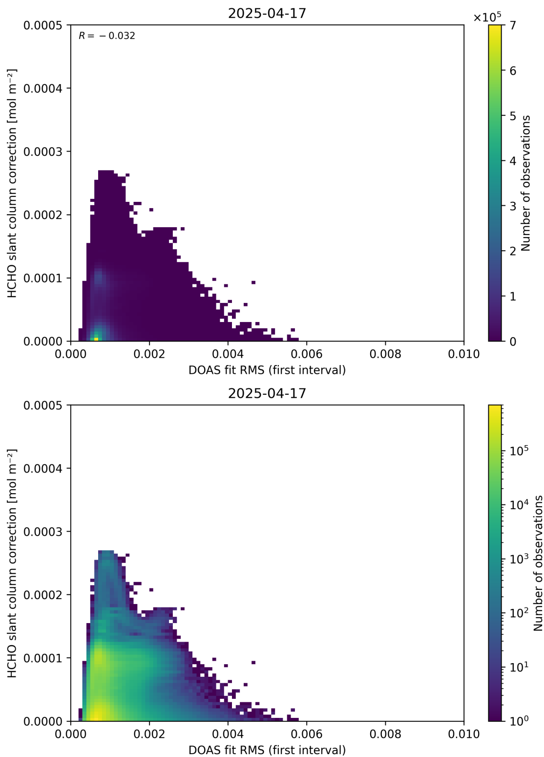
Figure 63: Scatter density plot of “DOAS fit RMS (first interval)” against “HCHO slant column correction” for 2025-04-16 to 2025-04-18.
