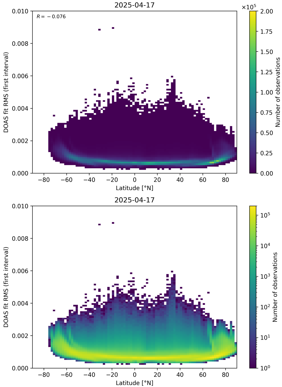
Figure 153: Scatter density plot of “Latitude” against “DOAS fit RMS (first interval)” for 2025-04-16 to 2025-04-18.
