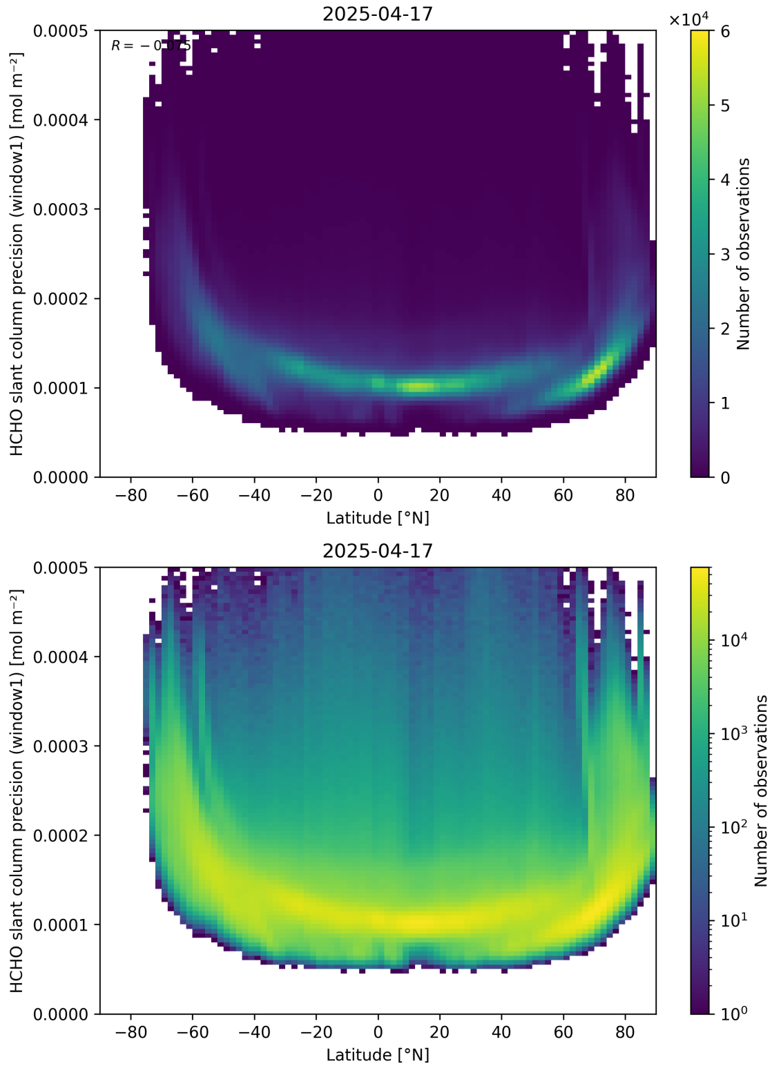
Figure 160: Scatter density plot of “Latitude” against “HCHO slant column precision (window1)” for 2025-04-16 to 2025-04-18.
