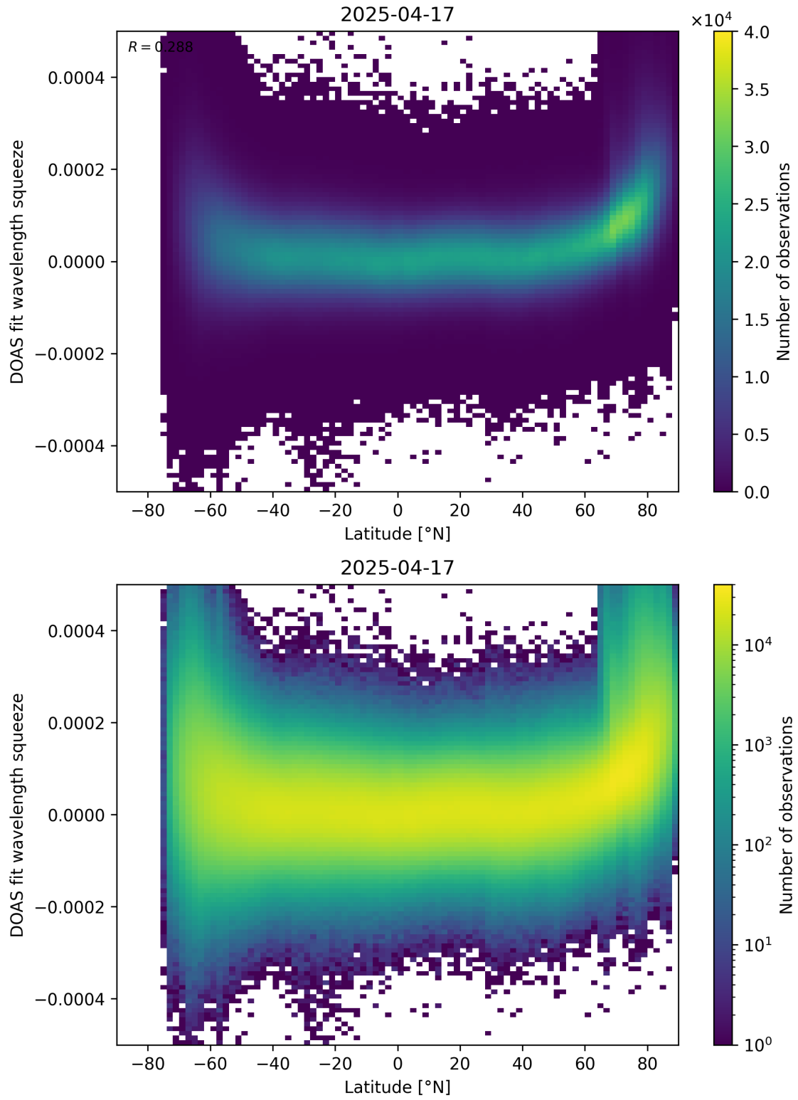
Figure 155: Scatter density plot of “Latitude” against “DOAS fit wavelength squeeze” for 2025-04-16 to 2025-04-18.
