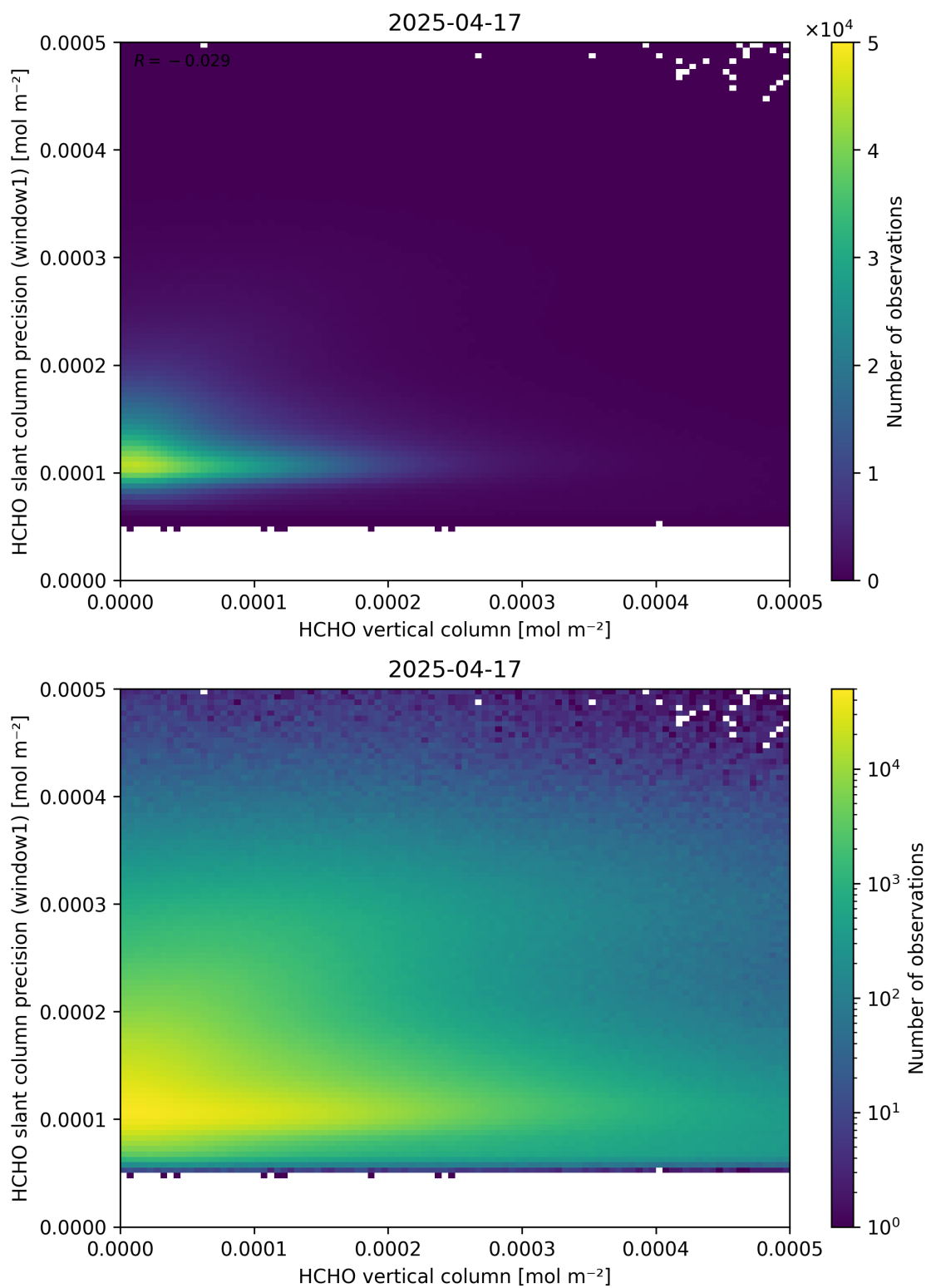
Figure 130: Scatter density plot of “HCHO vertical column” against “HCHO slant column precision (window1)” for 2025-04-16 to 2025-04-18.
