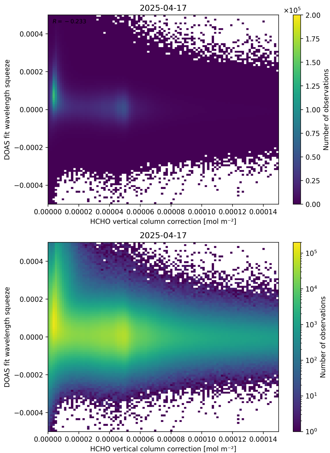
Figure 114: Scatter density plot of “HCHO vertical column correction” against “DOAS fit wavelength squeeze” for 2025-04-16 to 2025-04-18.
