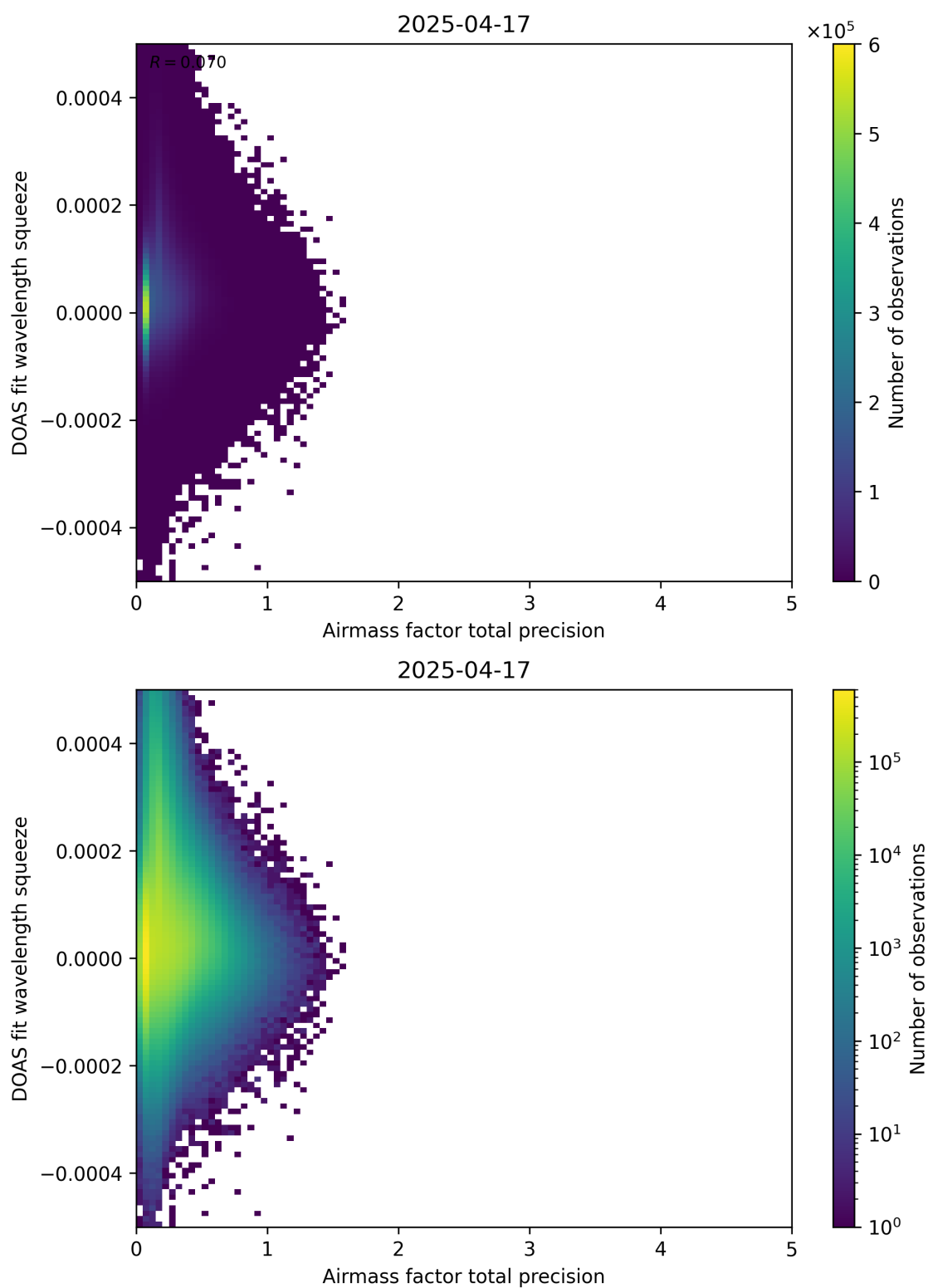
Figure 107: Scatter density plot of “Airmass factor total precision” against “DOAS fit wavelength squeeze” for 2025-04-16 to 2025-04-18.
