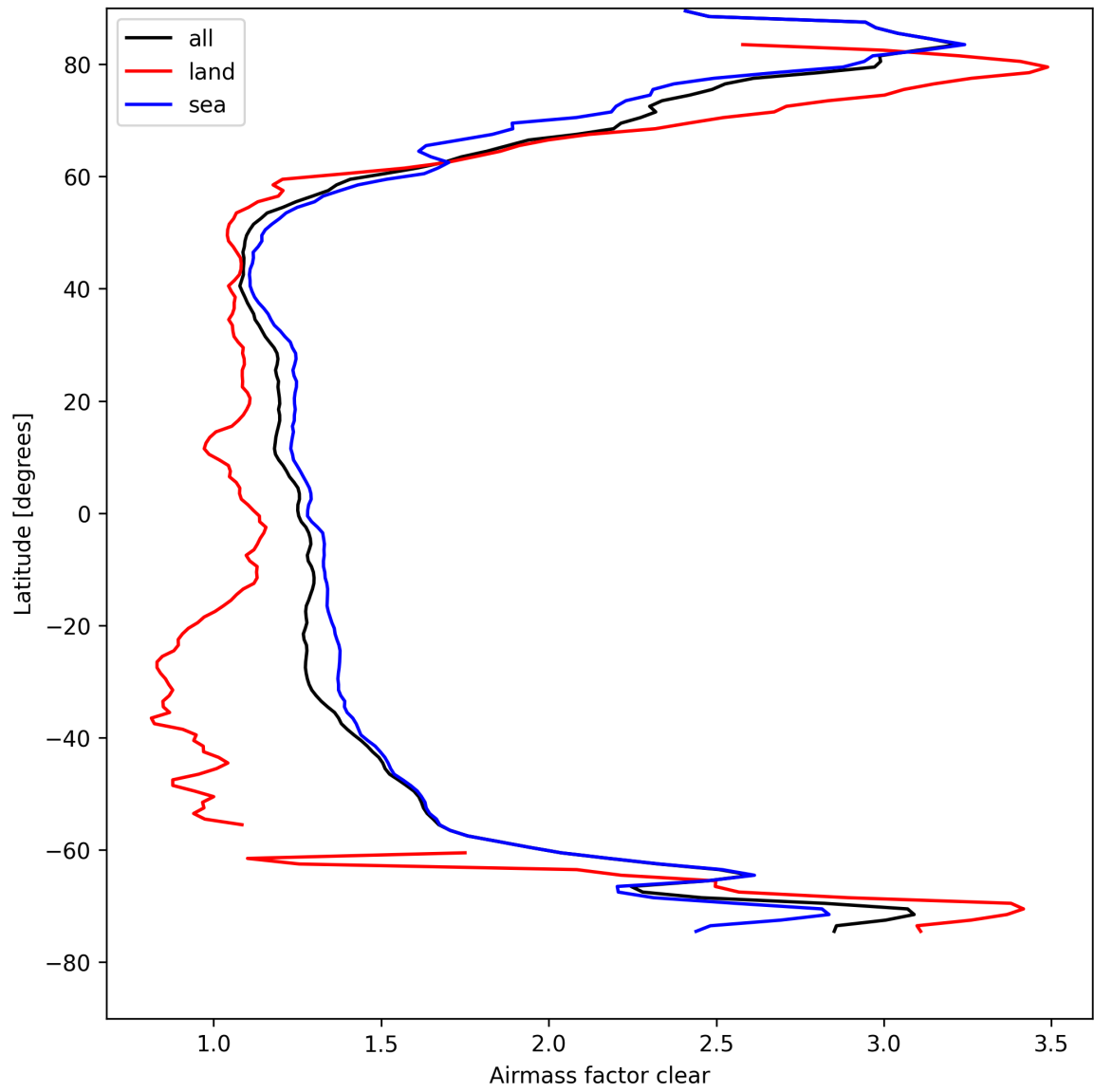
Figure 28: Zonal average of “Airmass factor clear” for 2025-04-16 to 2025-04-18.
