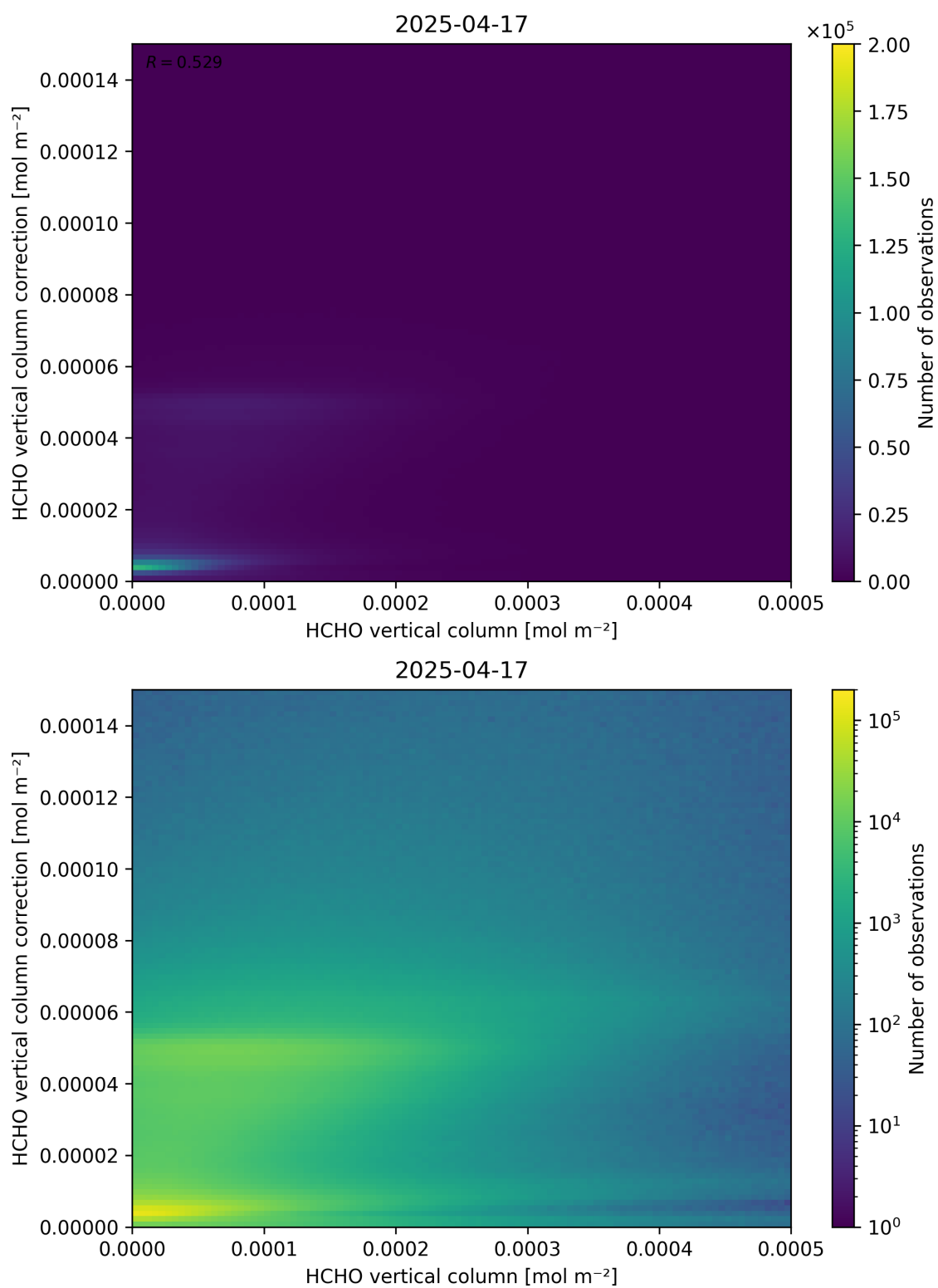
Figure 133: Scatter density plot of “HCHO vertical column” against “HCHO vertical column correction” for 2025-04-16 to 2025-04-18.
