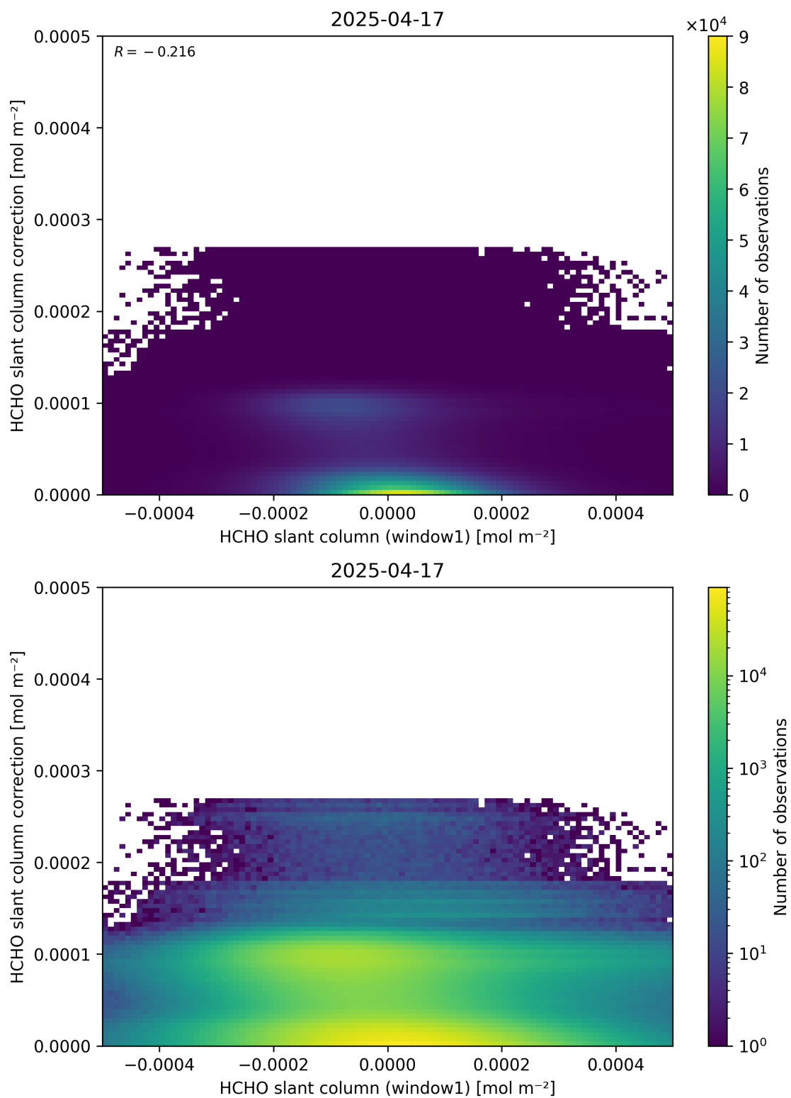
Figure 83: Scatter density plot of “HCHO slant column (window1)” against “HCHO slant column correction” for 2025-04-16 to 2025-04-18.
