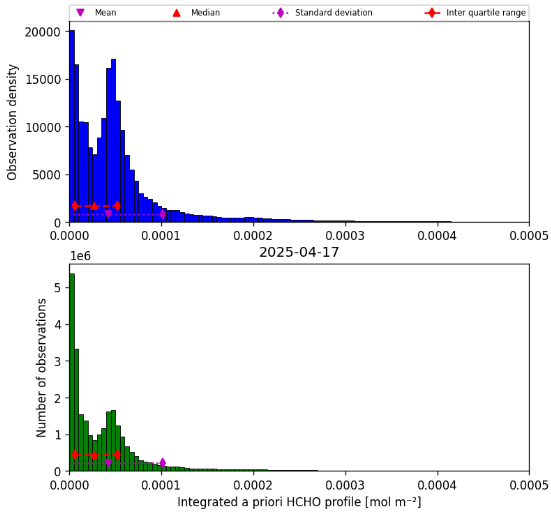
Figure 43: Histogram of “Integrated a priori HCHO profile” for 2025-04-16 to 2025-04-18
