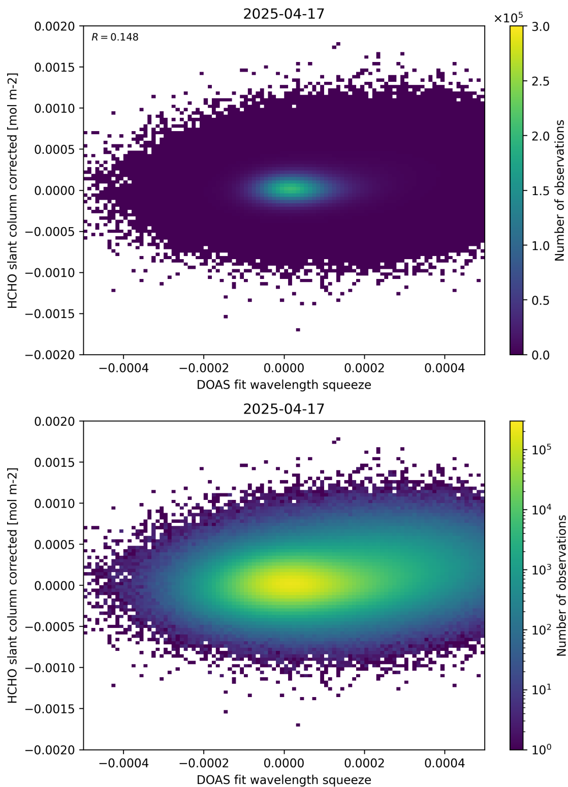
Figure 69: Scatter density plot of “DOAS fit wavelength squeeze” against “HCHO slant column corrected” for 2025-04-16 to 2025-04-18.
