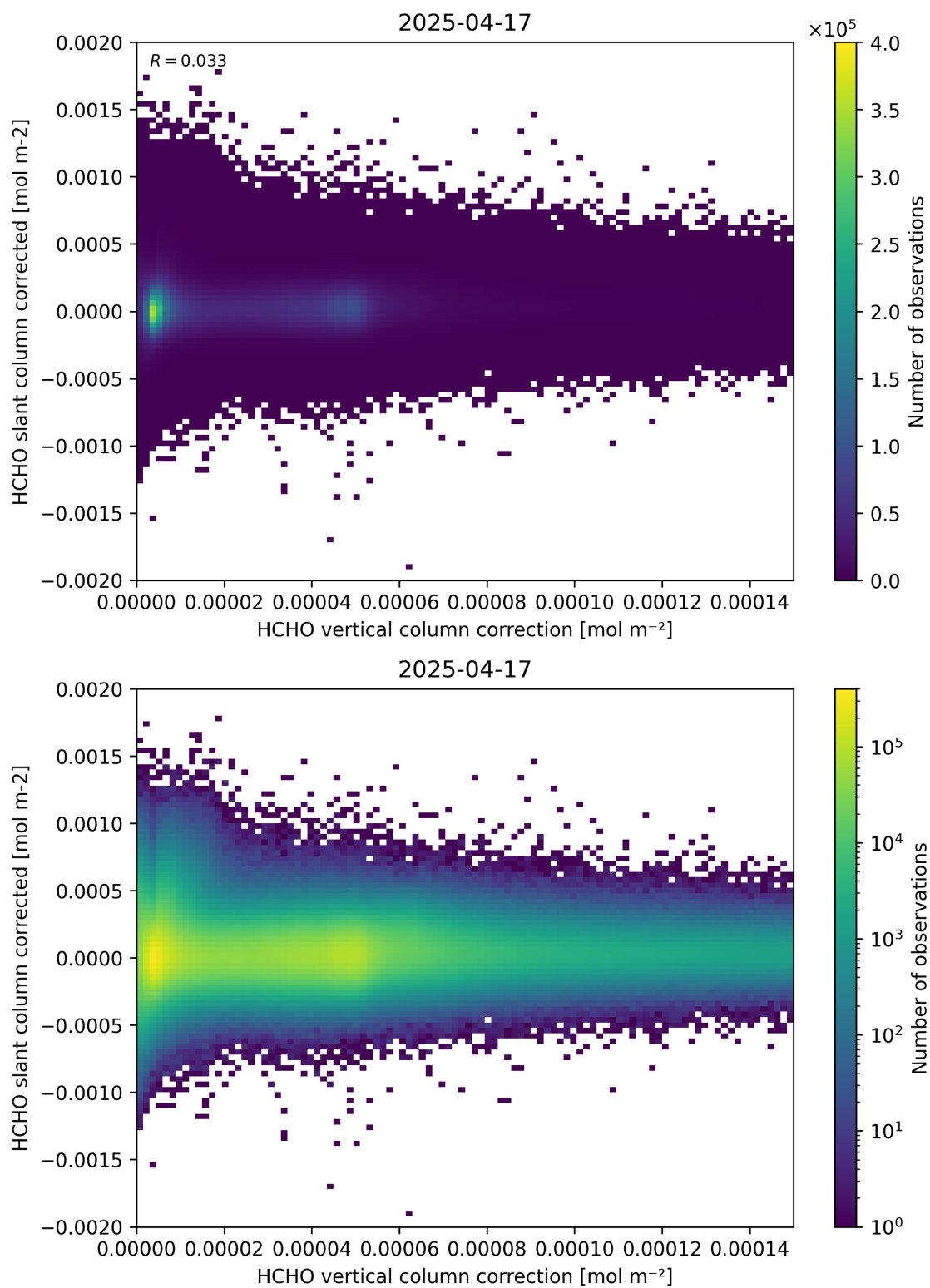
Figure 116: Scatter density plot of “HCHO vertical column correction” against “HCHO slant column corrected” for 2025-04-16 to 2025-04-18.
