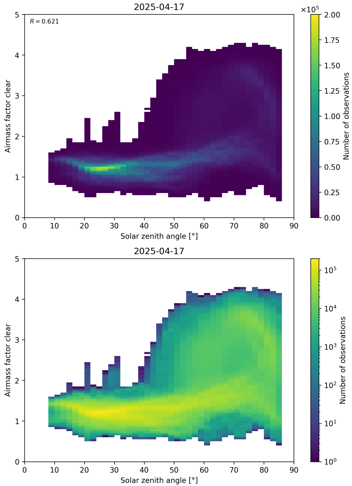
Figure 170: Scatter density plot of “Solar zenith angle” against “Airmass factor clear” for 2025-04-16 to 2025-04-18.
