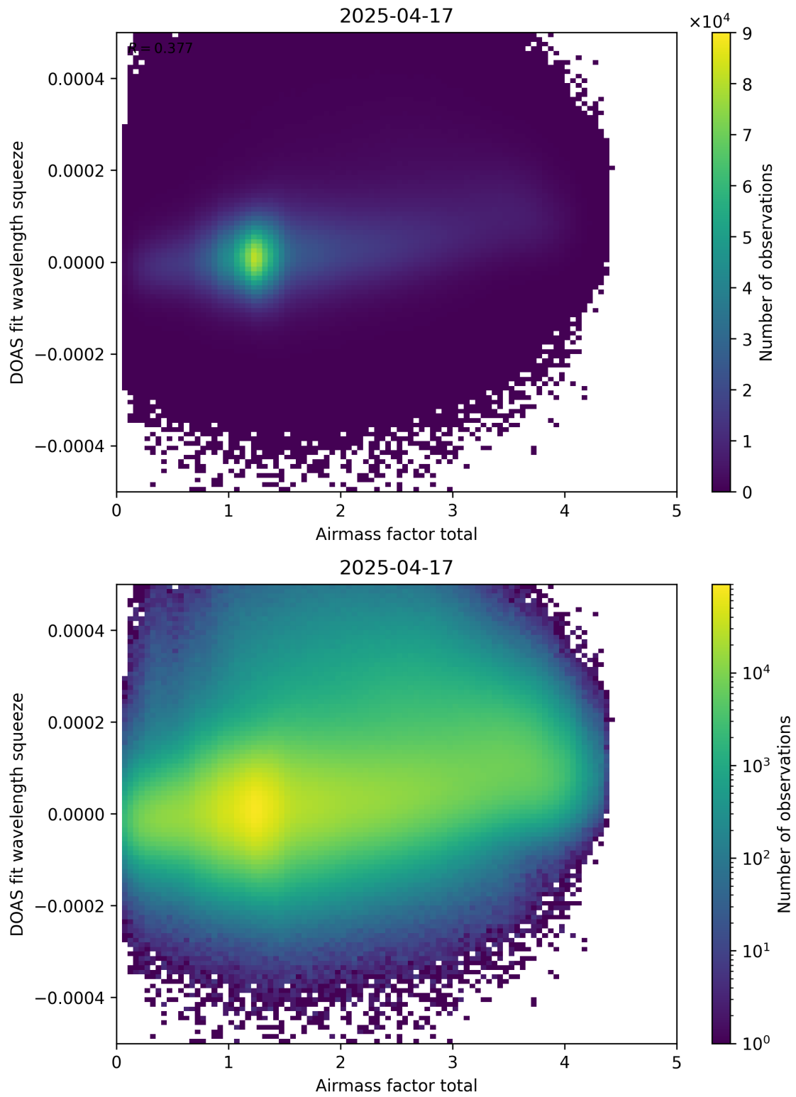
Figure 99: Scatter density plot of “Airmass factor total” against “DOAS fit wavelength squeeze” for 2025-04-16 to 2025-04-18.
