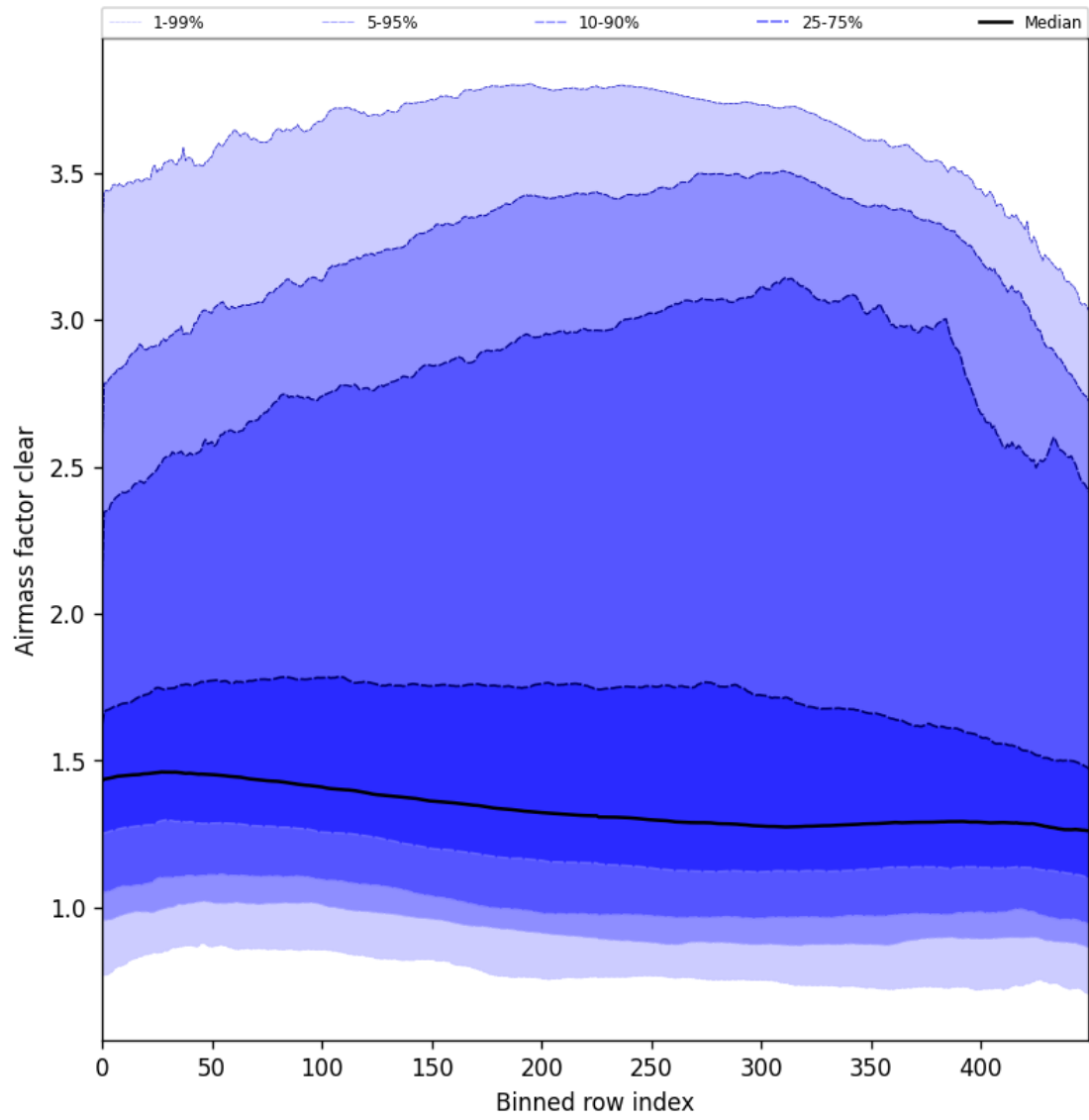
Figure 56: Along track statistics of “Airmass factor clear” for 2025-04-16 to 2025-04-18
