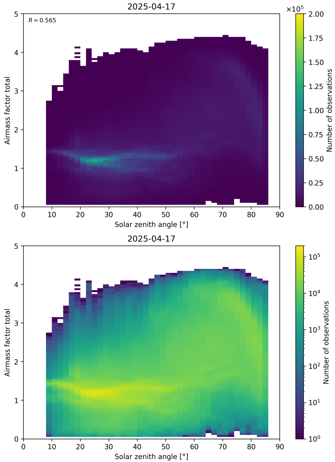
Figure 175: Scatter density plot of “Solar zenith angle” against “Airmass factor total” for 2025-04-16 to 2025-04-18.
