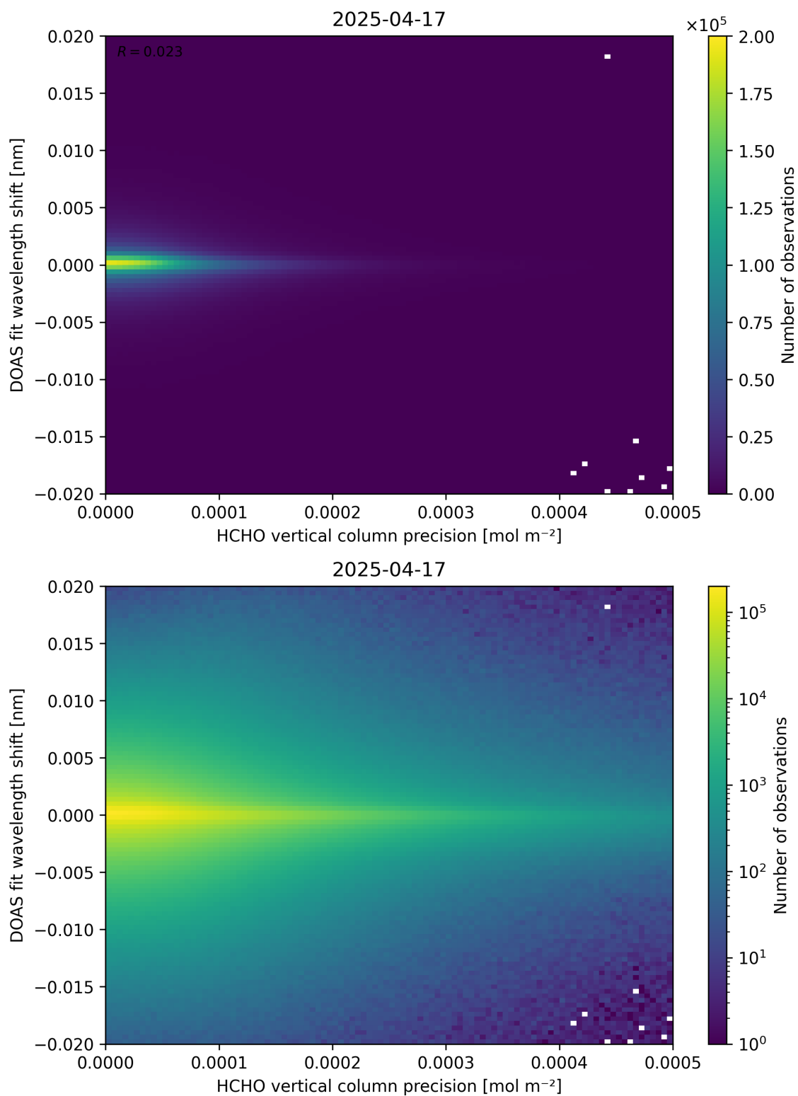
Figure 137: Scatter density plot of “HCHO vertical column precision” against “DOAS fit wavelength shift” for 2025-04-16 to 2025-04-18.
