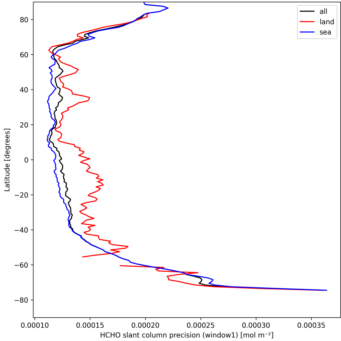
Figure 25: Zonal average of “HCHO slant column precision (window1)” for 2025-04-16 to 2025-04-18.
