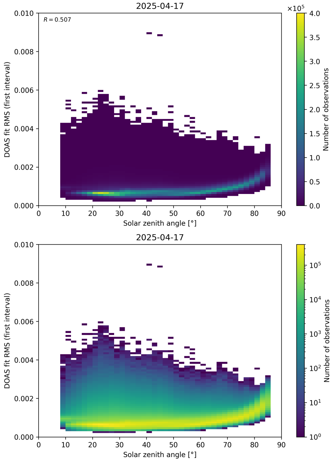
Figure 167: Scatter density plot of “Solar zenith angle” against “DOAS fit RMS (first interval)” for 2025-04-16 to 2025-04-18.
