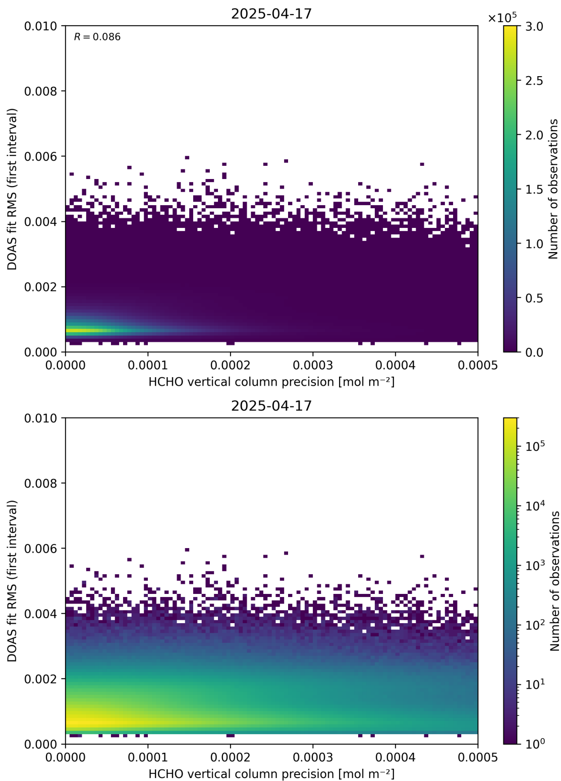
Figure 136: Scatter density plot of “HCHO vertical column precision” against “DOAS fit RMS (first interval)” for 2025-04-16 to 2025-04-18.
