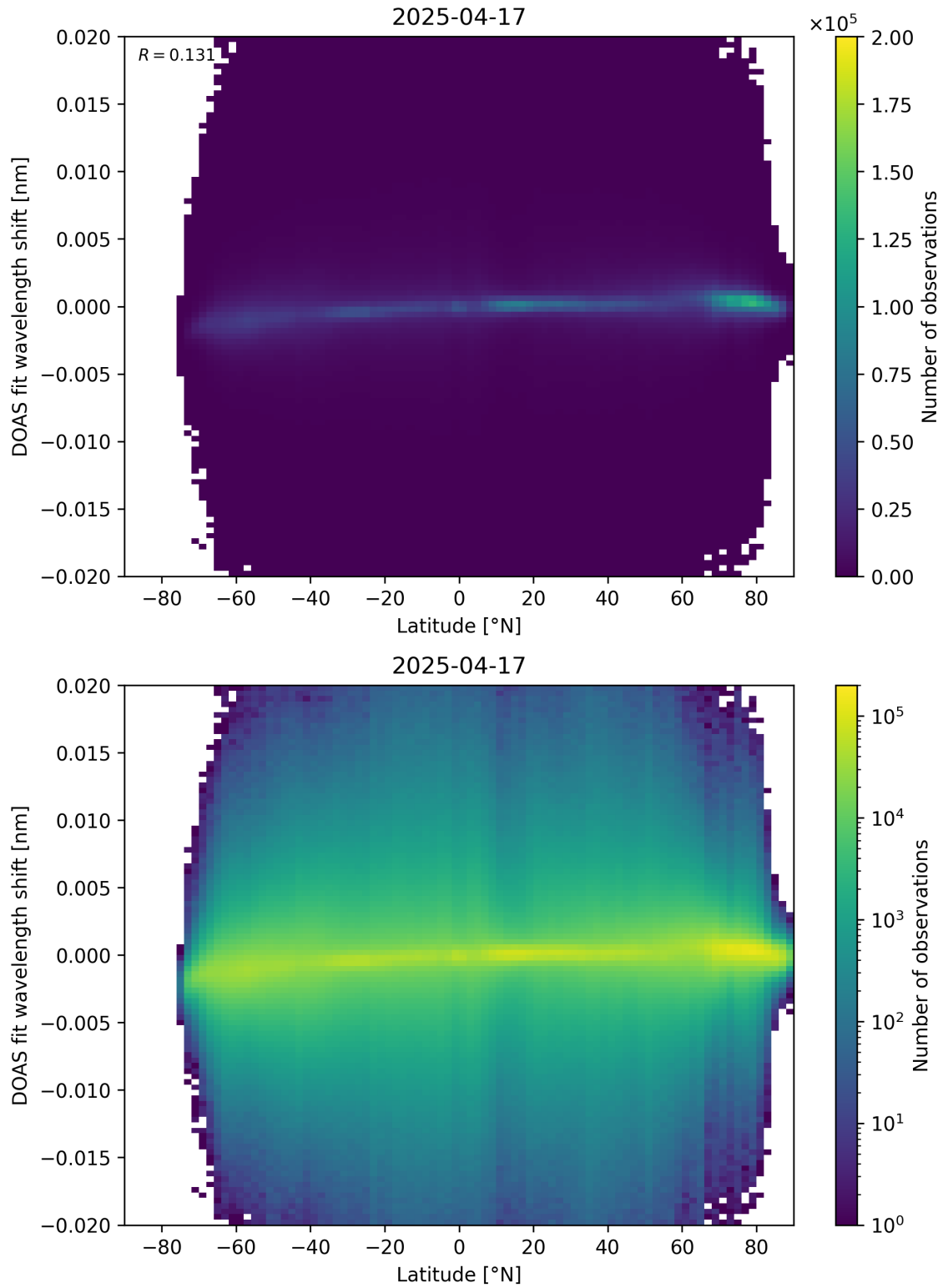
Figure 154: Scatter density plot of “Latitude” against “DOAS fit wavelength shift” for 2025-04-16 to 2025-04-18.
