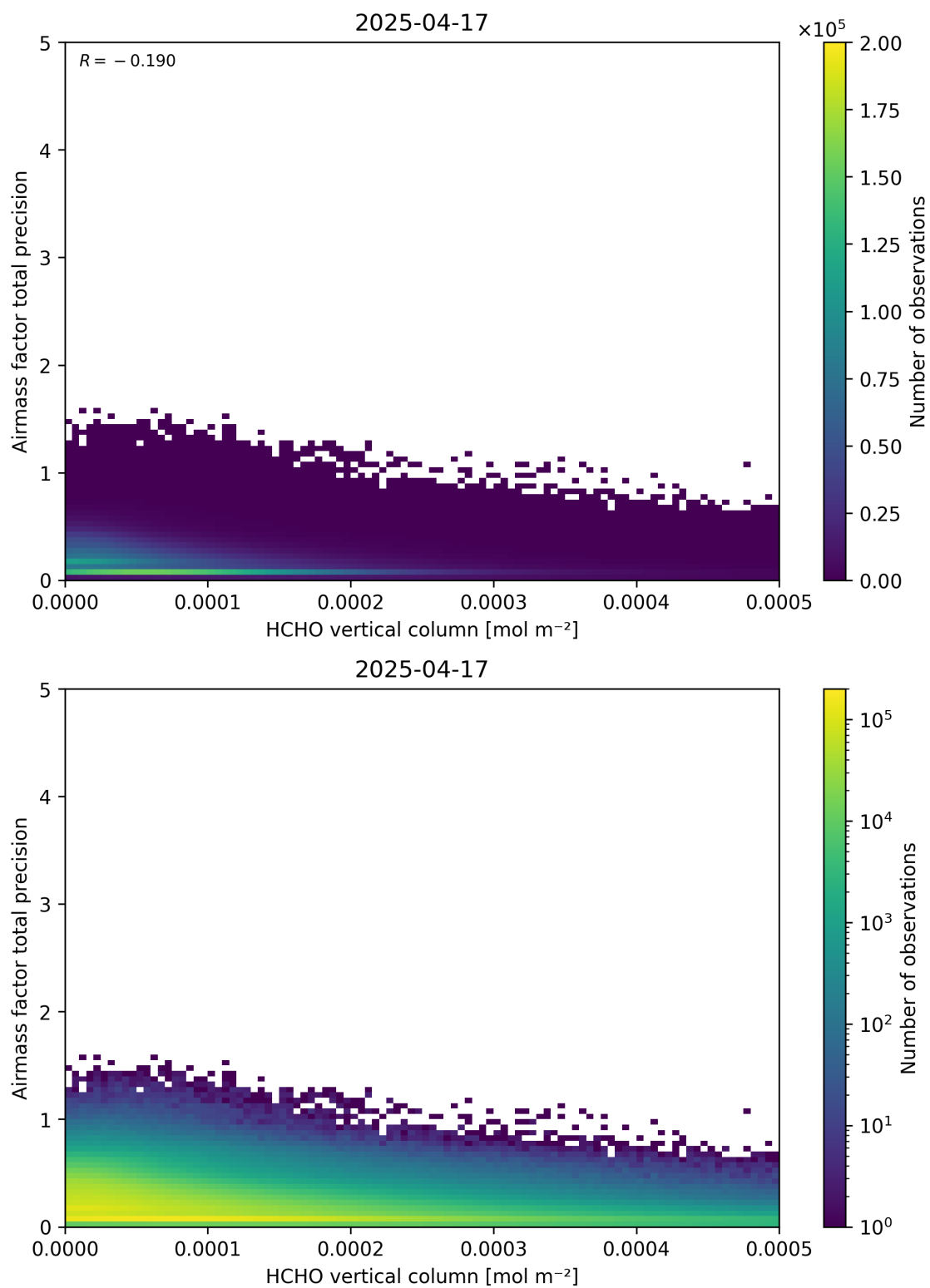
Figure 132: Scatter density plot of “HCHO vertical column” against “Airmass factor total precision” for 2025-04-16 to 2025-04-18.
