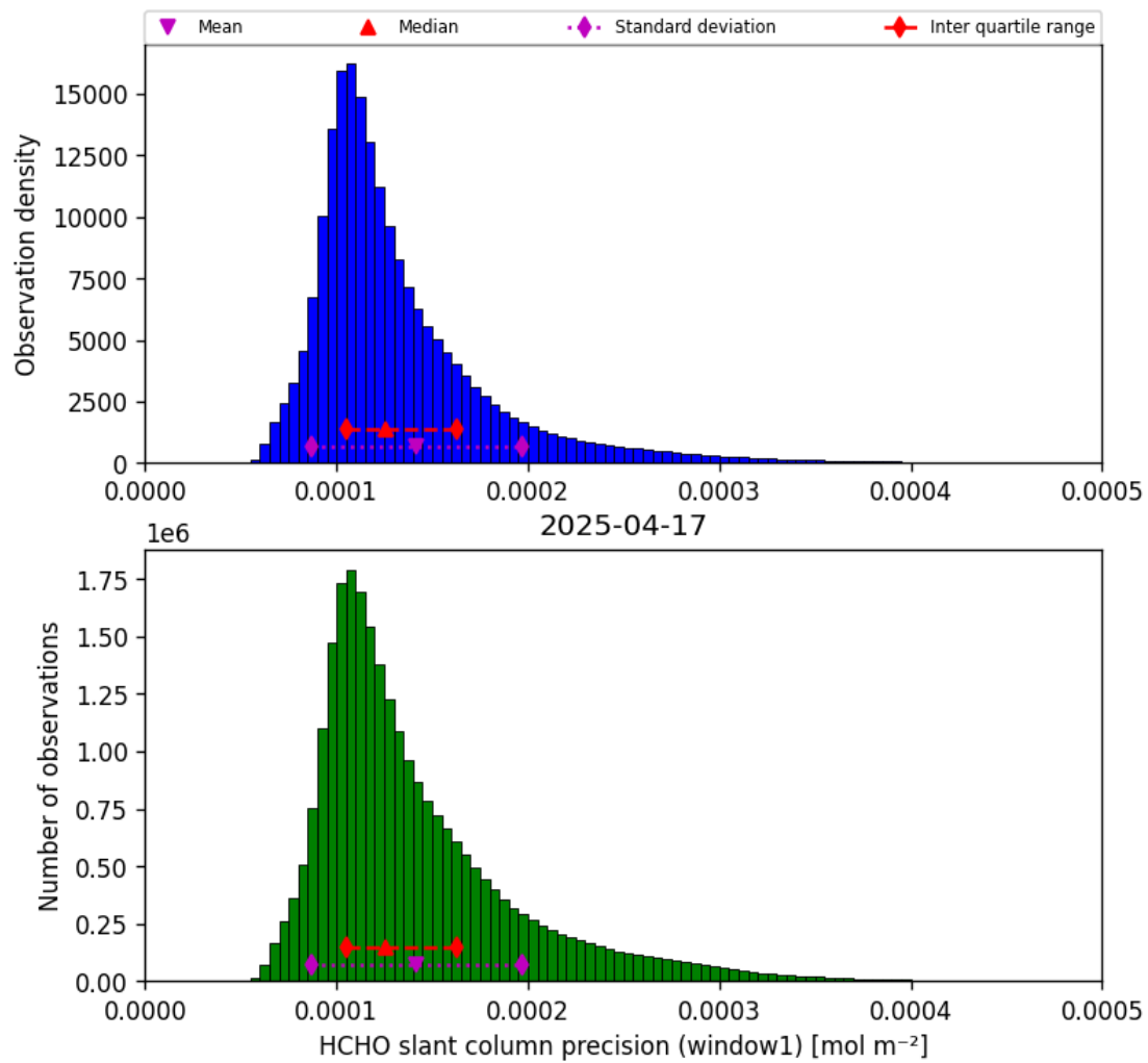
Figure 39: Histogram of “HCHO slant column precision (window1)” for 2025-04-16 to 2025-04-18
