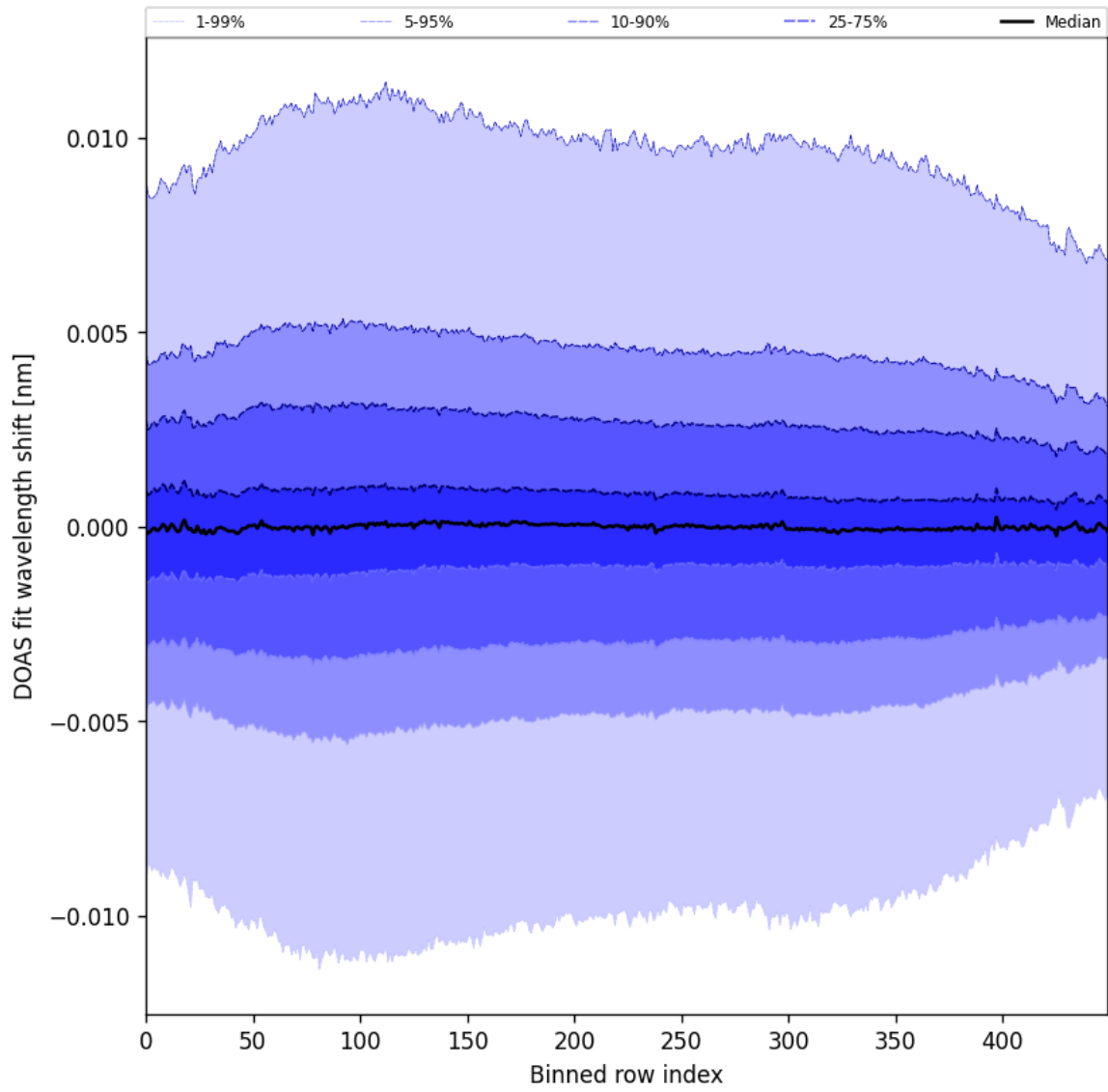
Figure 58: Along track statistics of “DOAS fit wavelength shift” for 2025-04-16 to 2025-04-18
