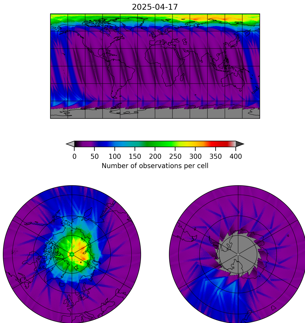
Figure 19: Map of the number of observations for 2025-04-16 to 2025-04-18
