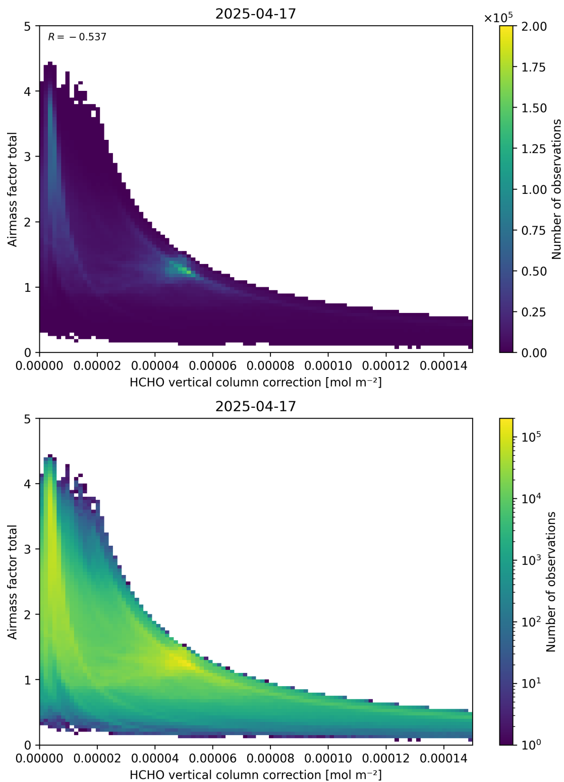
Figure 120: Scatter density plot of “HCHO vertical column correction” against “Airmass factor total” for 2025-04-16 to 2025-04-18.
