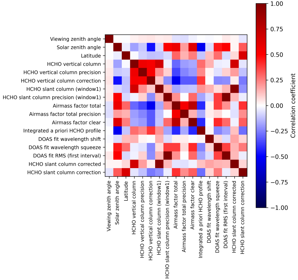
Figure 2: Map of correlation matrix for 2025-04-16 to 2025-04-18.
