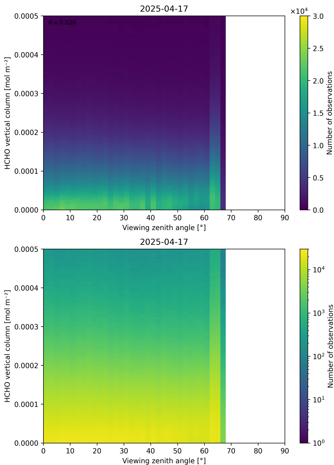
Figure 192: Scatter density plot of “Viewing zenith angle” against “HCHO vertical column” for 2025-04-16 to 2025-04-18.
