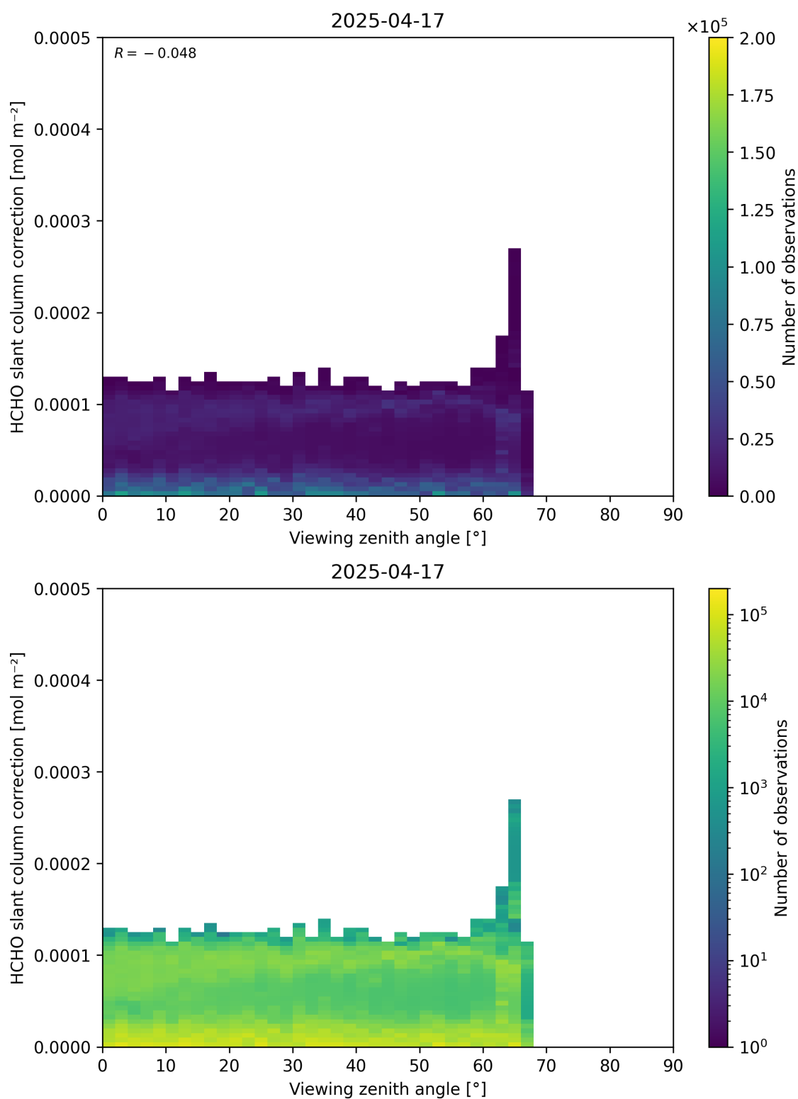
Figure 187: Scatter density plot of “Viewing zenith angle” against “HCHO slant column correction” for 2025-04-16 to 2025-04-18.
