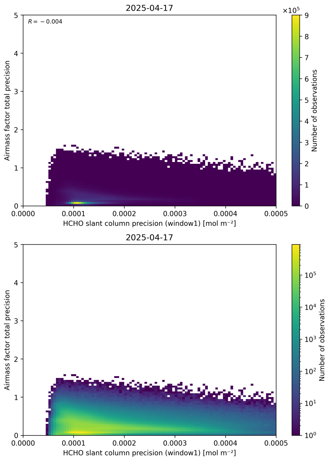
Figure 95: Scatter density plot of “HCHO slant column precision (window1)” against “Airmass factor total precision” for 2025-04-16 to 2025-04-18.
