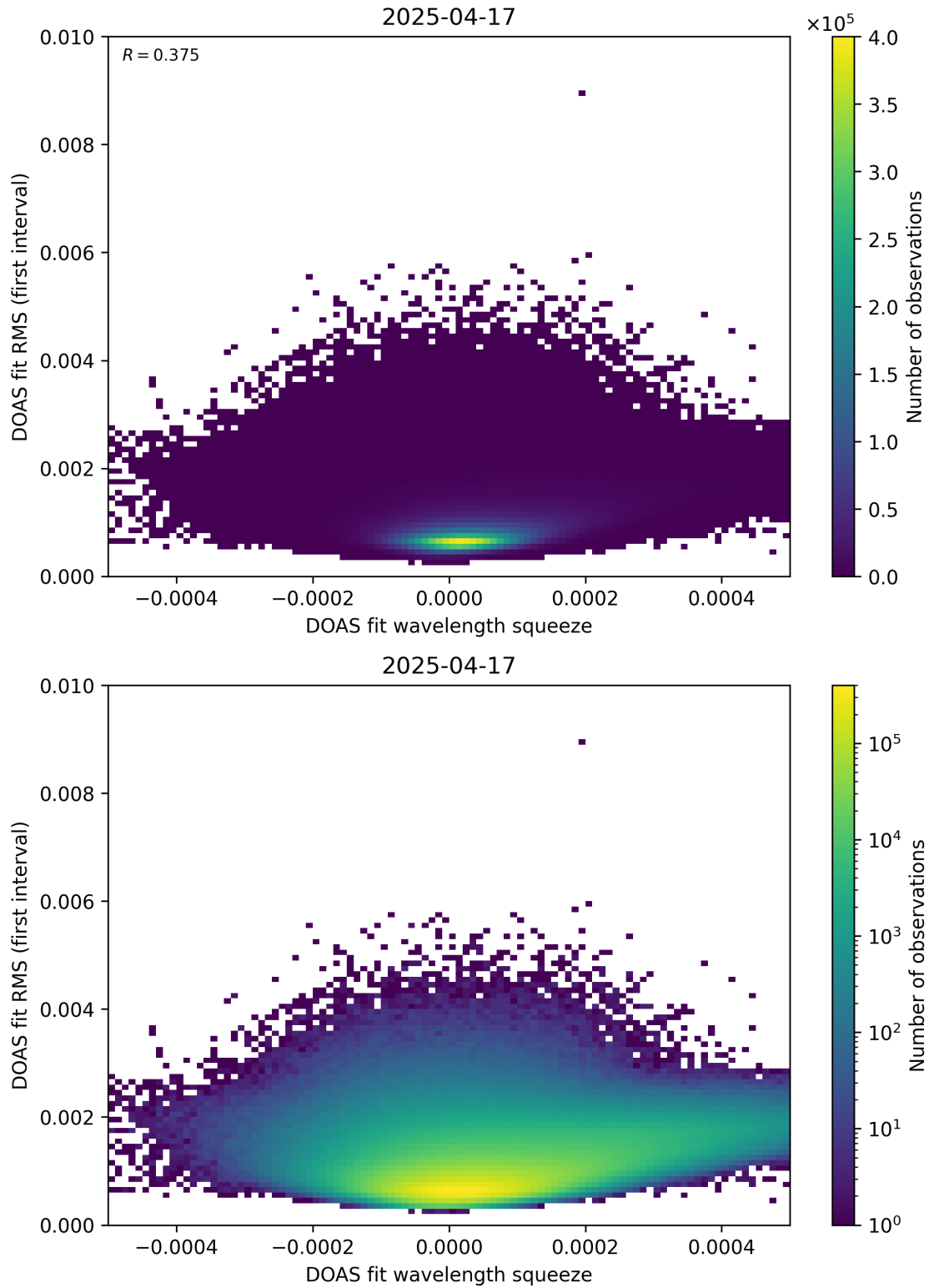
Figure 68: Scatter density plot of “DOAS fit wavelength squeeze” against “DOAS fit RMS (first interval)” for 2025-04-16 to 2025-04-18.
