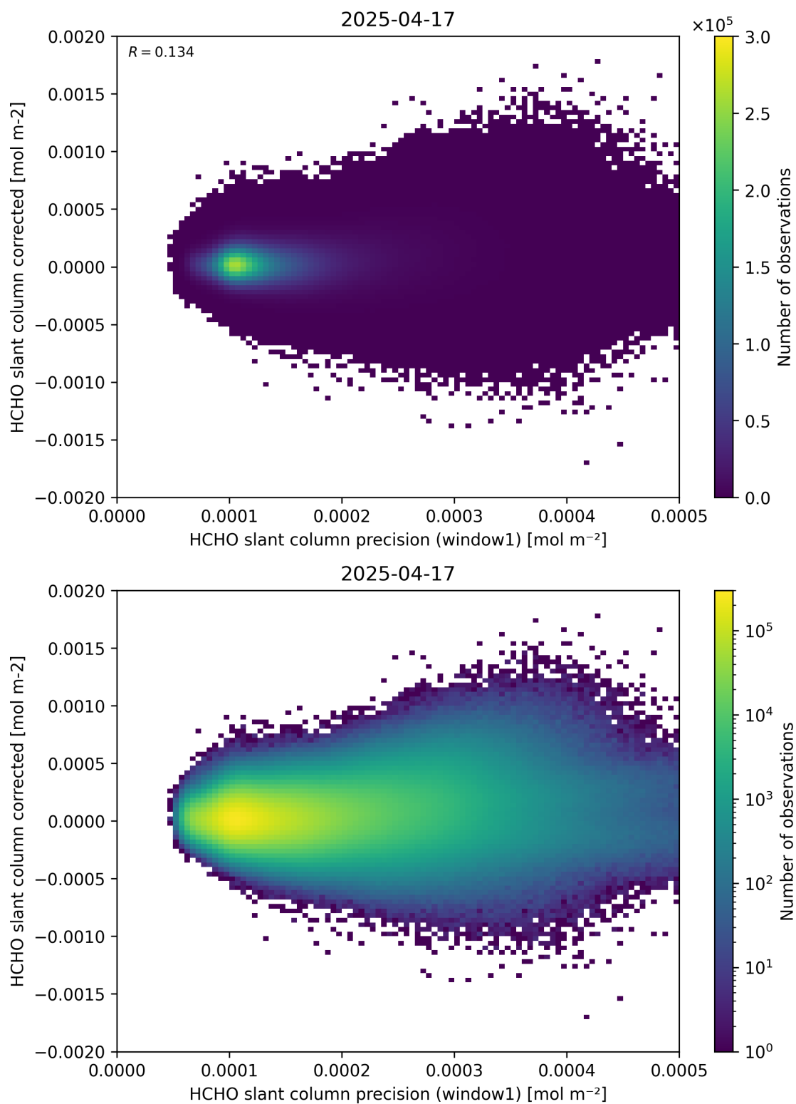
Figure 92: Scatter density plot of “HCHO slant column precision (window1)” against “HCHO slant column corrected” for 2025-04-16 to 2025-04-18.
