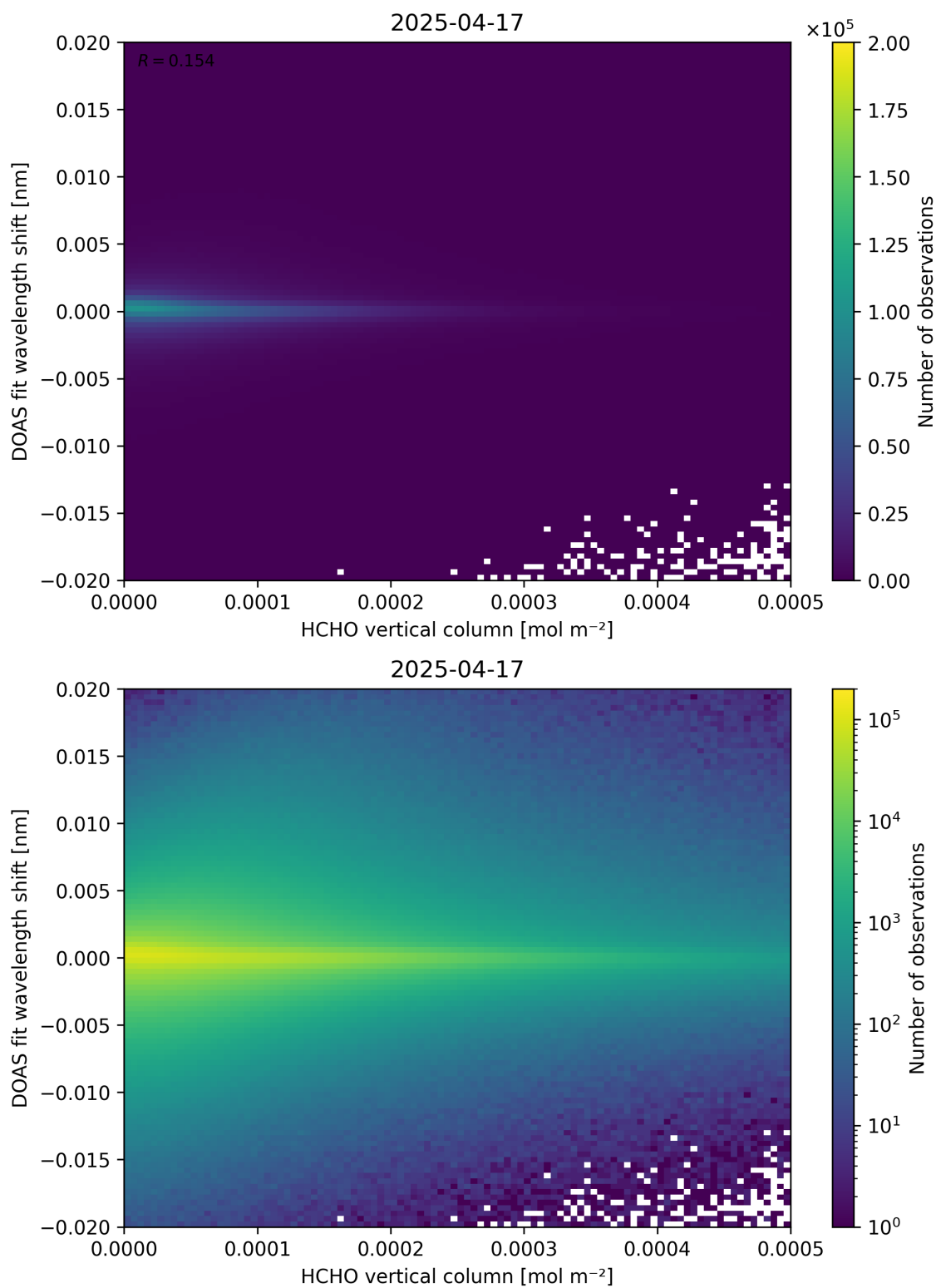
Figure 124: Scatter density plot of “HCHO vertical column” against “DOAS fit wavelength shift” for 2025-04-16 to 2025-04-18.
