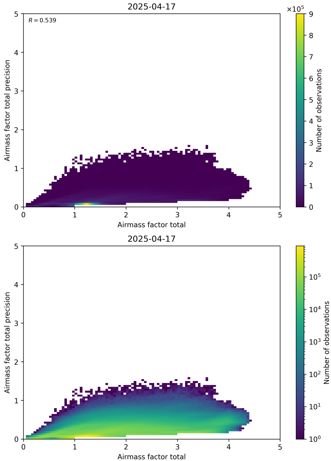
Figure 103: Scatter density plot of “Airmass factor total” against “Airmass factor total precision” for 2025-04-16 to 2025-04-18.
