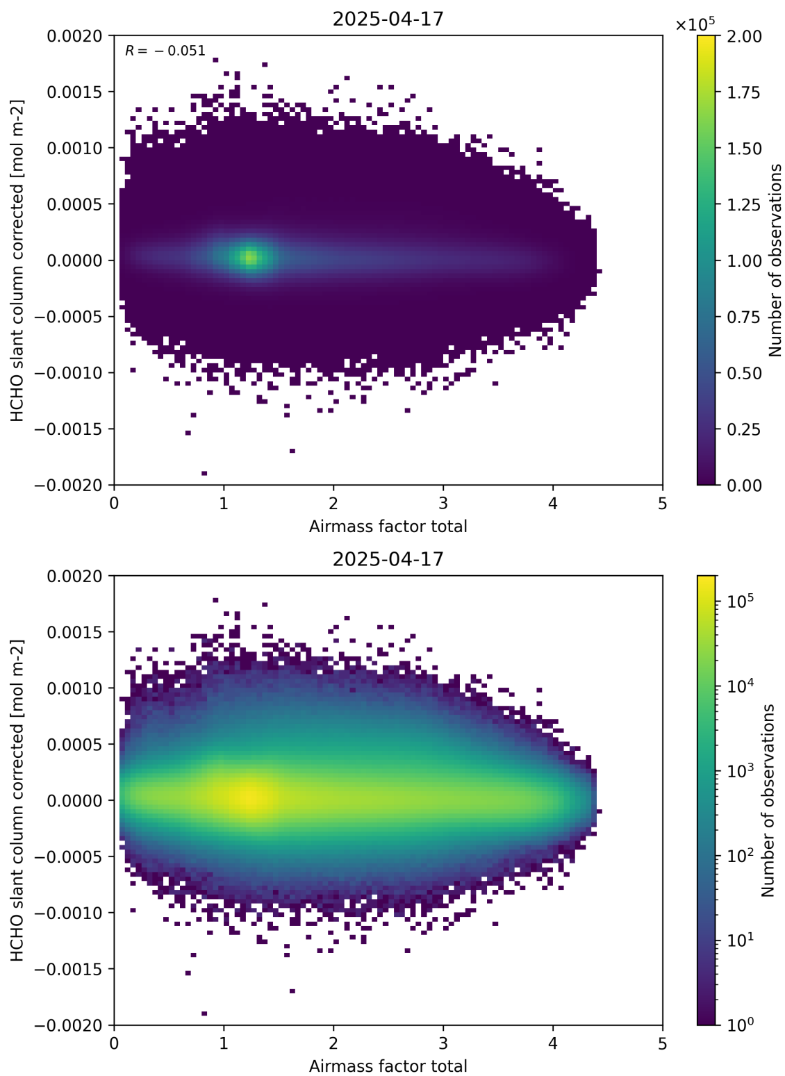
Figure 101: Scatter density plot of “Airmass factor total” against “HCHO slant column corrected” for 2025-04-16 to 2025-04-18.
