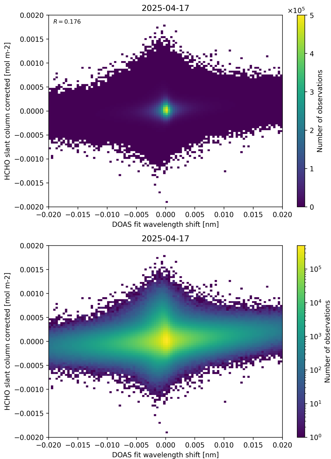
Figure 66: Scatter density plot of “DOAS fit wavelength shift” against “HCHO slant column corrected” for 2025-04-16 to 2025-04-18.
