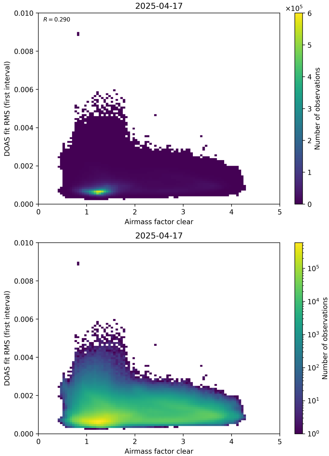
Figure 71: Scatter density plot of “Airmass factor clear” against “DOAS fit RMS (first interval)” for 2025-04-16 to 2025-04-18.
