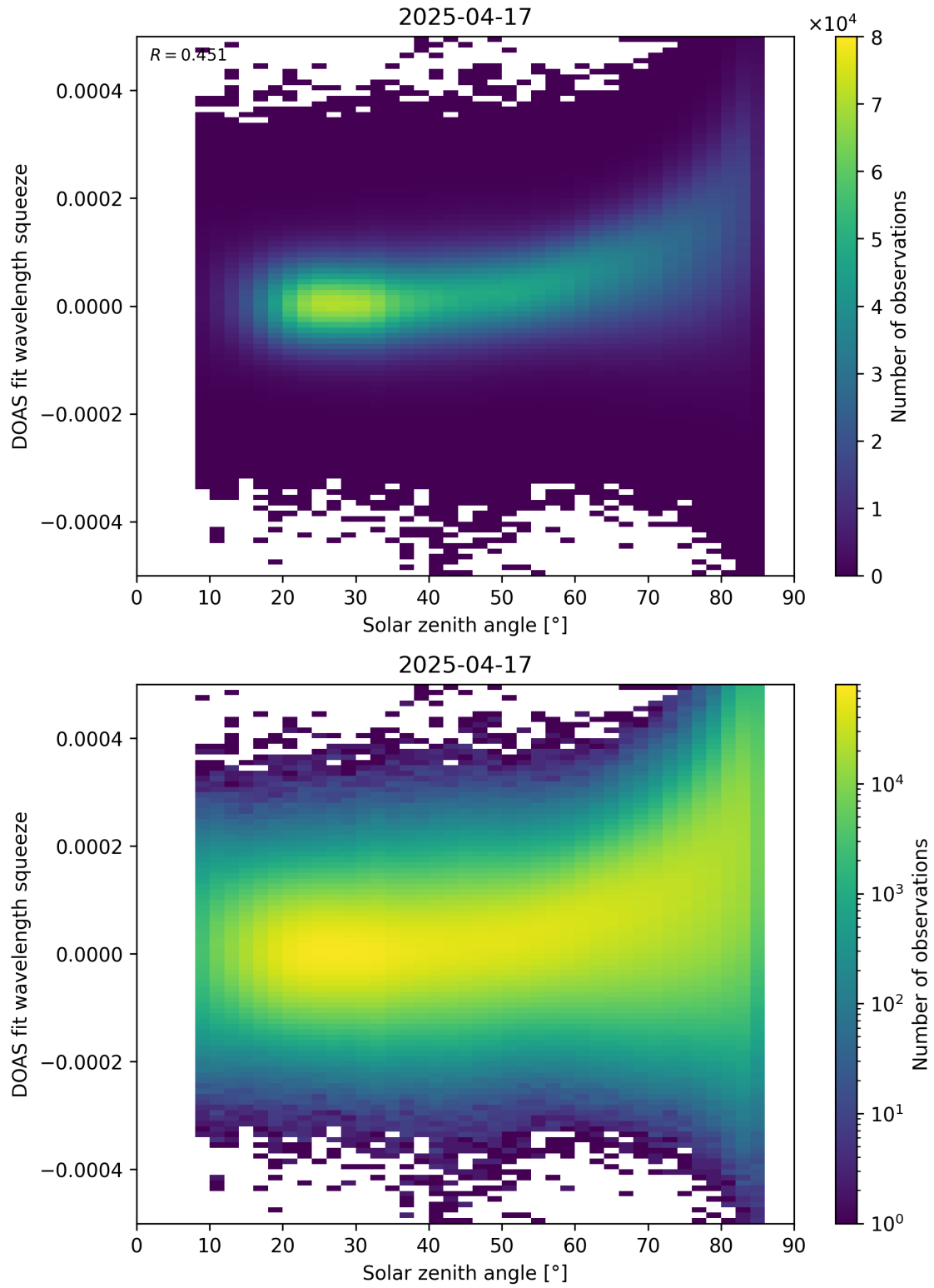
Figure 169: Scatter density plot of “Solar zenith angle” against “DOAS fit wavelength squeeze” for 2025-04-16 to 2025-04-18.
