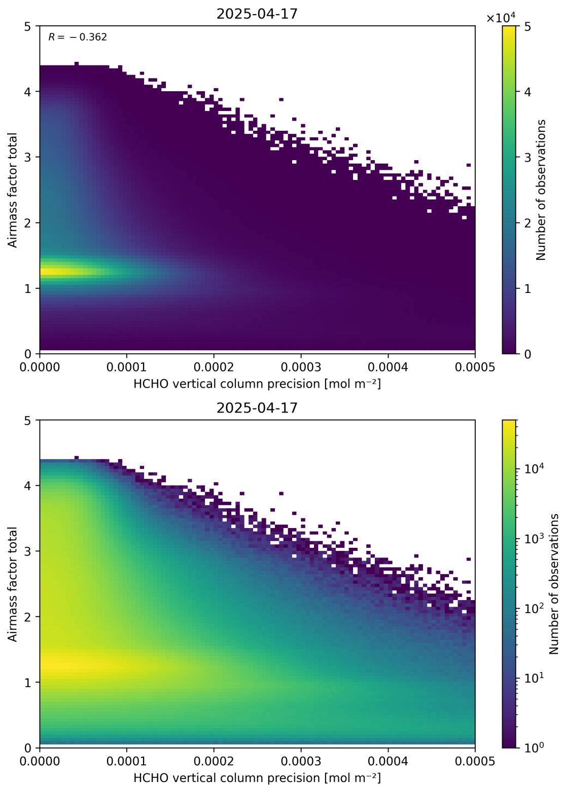
Figure 144: Scatter density plot of “HCHO vertical column precision” against “Airmass factor total” for 2025-04-16 to 2025-04-18.
