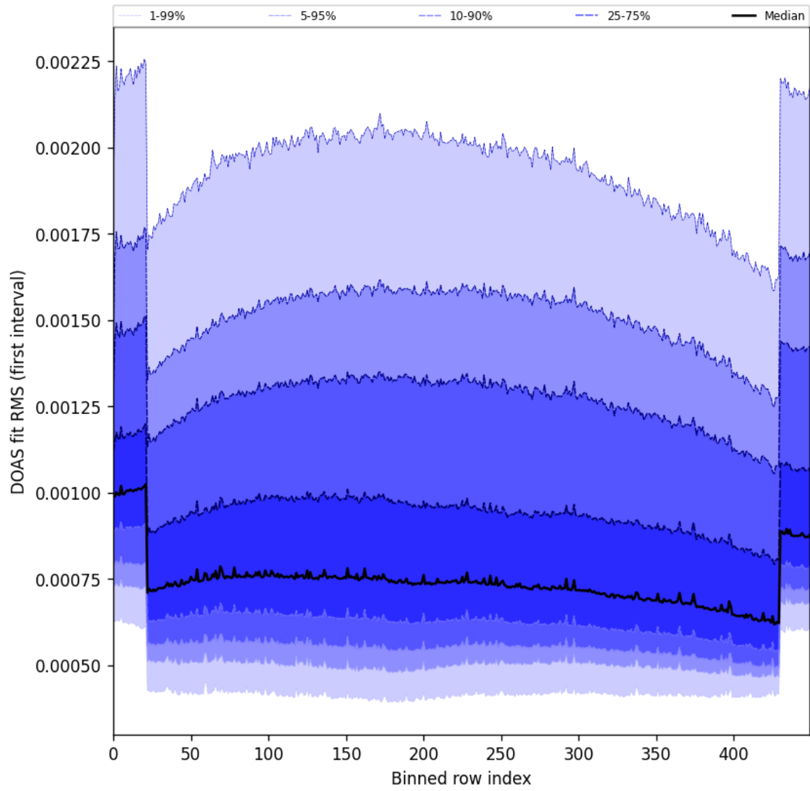
Figure 60: Along track statistics of “DOAS fit RMS (first interval)” for 2025-04-16 to 2025-04-18
