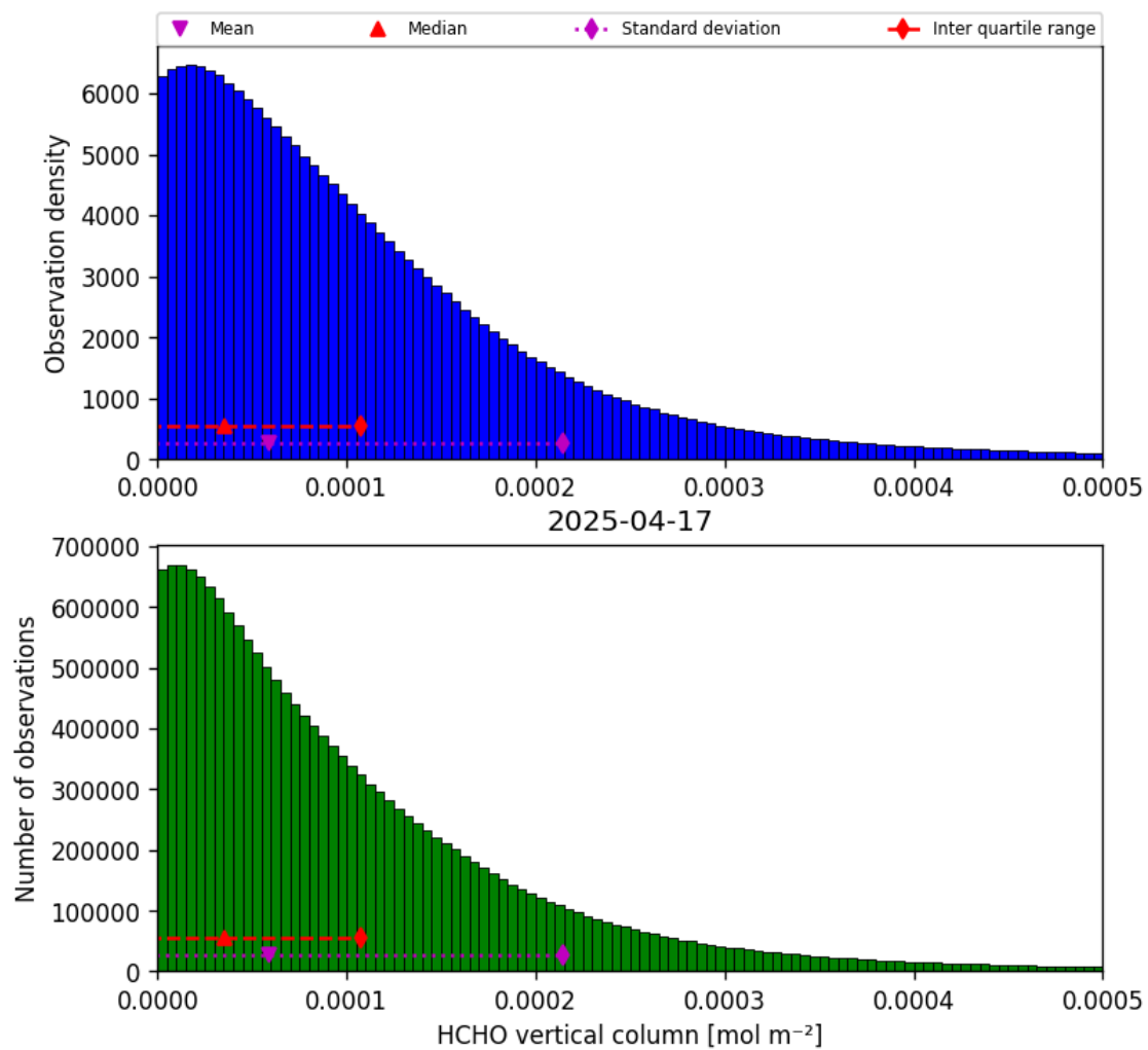
Figure 35: Histogram of “HCHO vertical column” for 2025-04-16 to 2025-04-18
