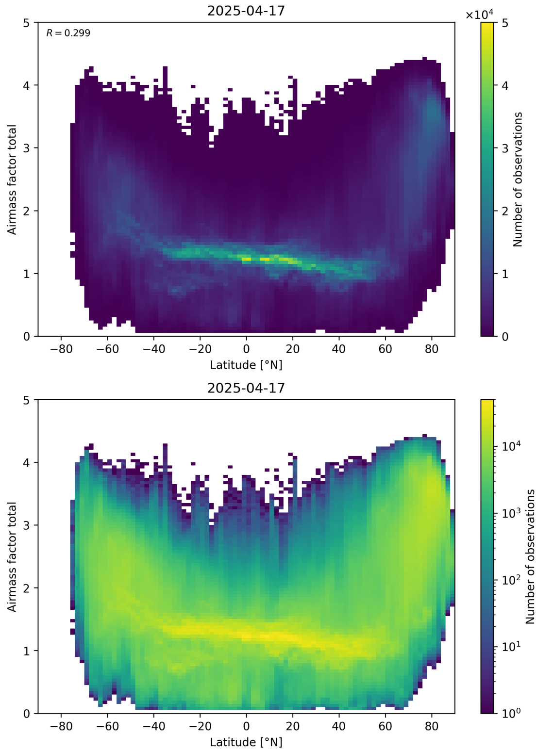
Figure 161: Scatter density plot of “Latitude” against “Airmass factor total” for 2025-04-16 to 2025-04-18.
