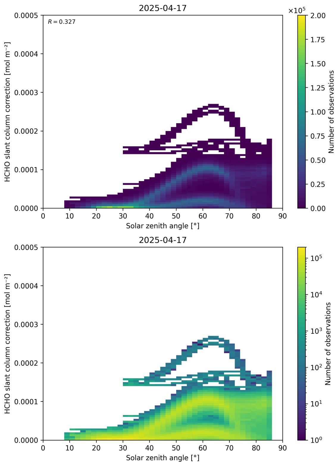
Figure 172: Scatter density plot of “Solar zenith angle” against “HCHO slant column correction” for 2025-04-16 to 2025-04-18.
