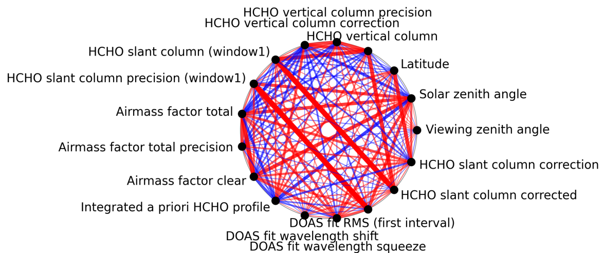
Figure 1: Map of correlation graph for 2025-04-16 to 2025-04-18.
