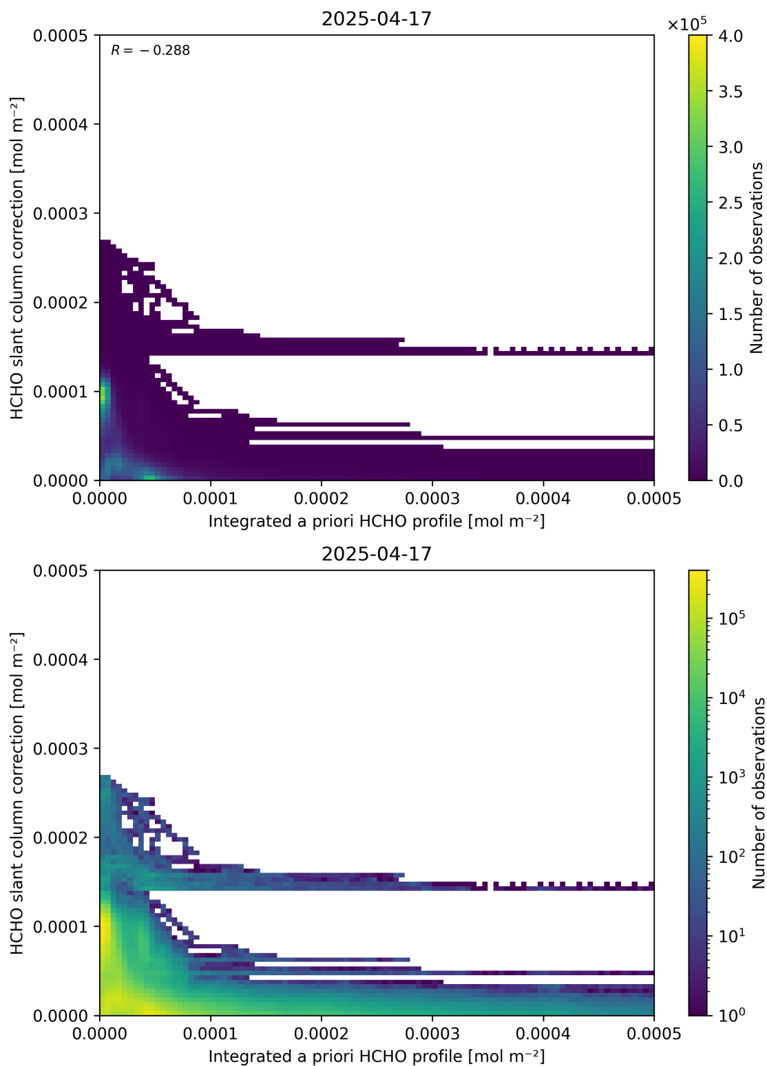
Figure 152: Scatter density plot of “Integrated a priori HCHO profile” against “HCHO slant column correction” for 2025-04-16 to 2025-04-18.
