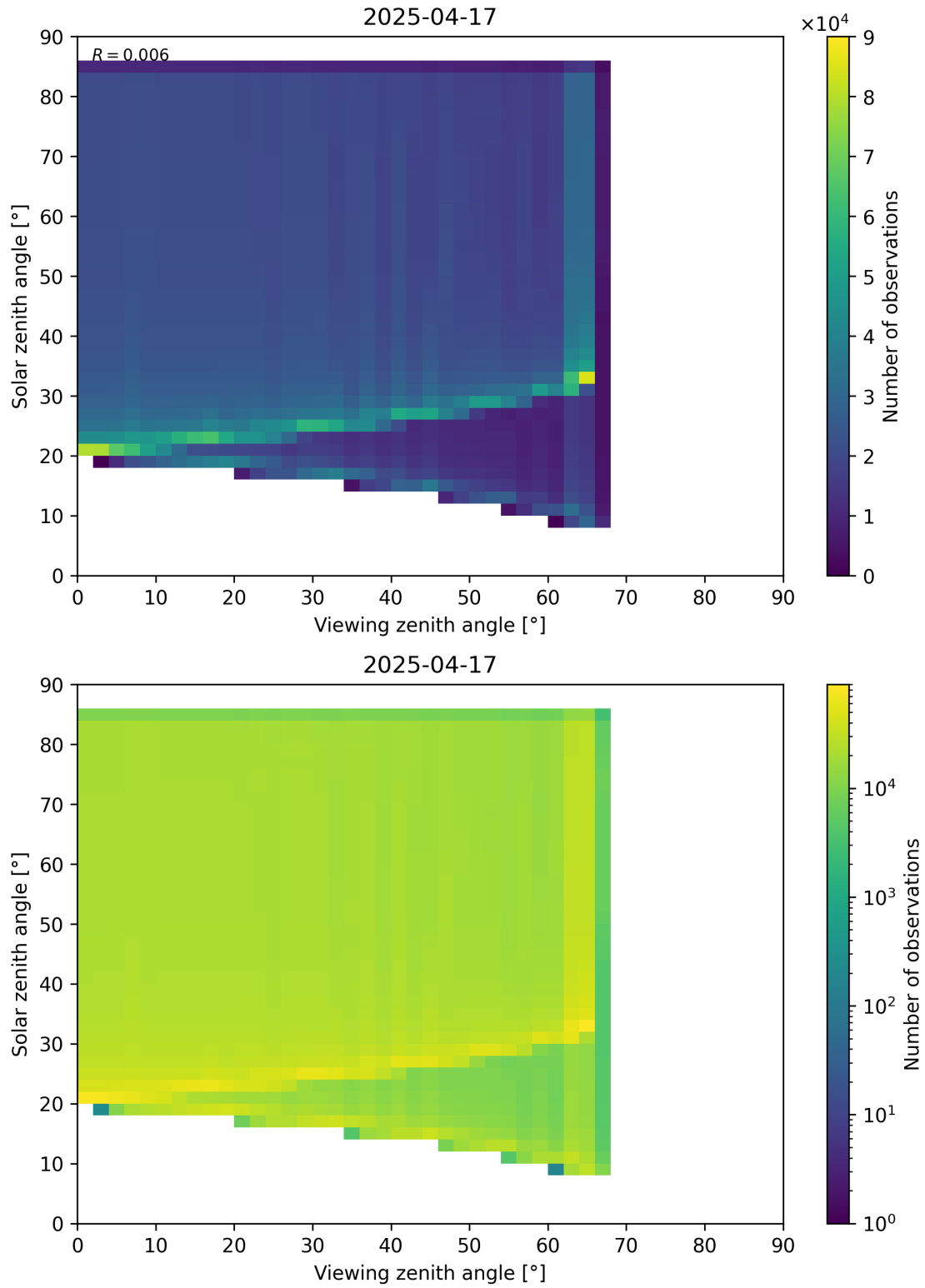
Figure 197: Scatter density plot of “Viewing zenith angle” against “Solar zenith angle” for 2025-04-16 to 2025-04-18.
