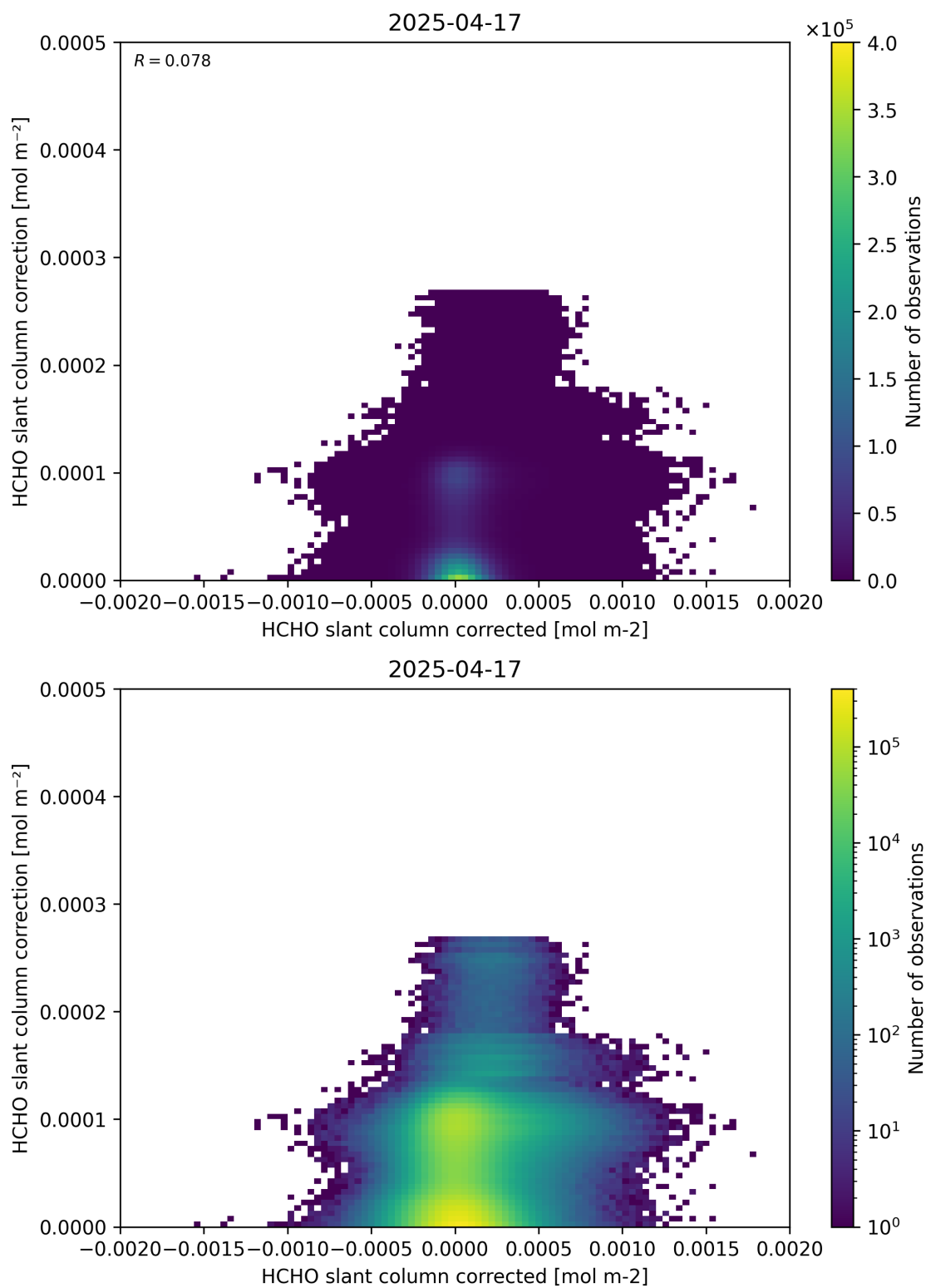
Figure 77: Scatter density plot of “HCHO slant column corrected” against “HCHO slant column correction” for 2025-04-16 to 2025-04-18.
