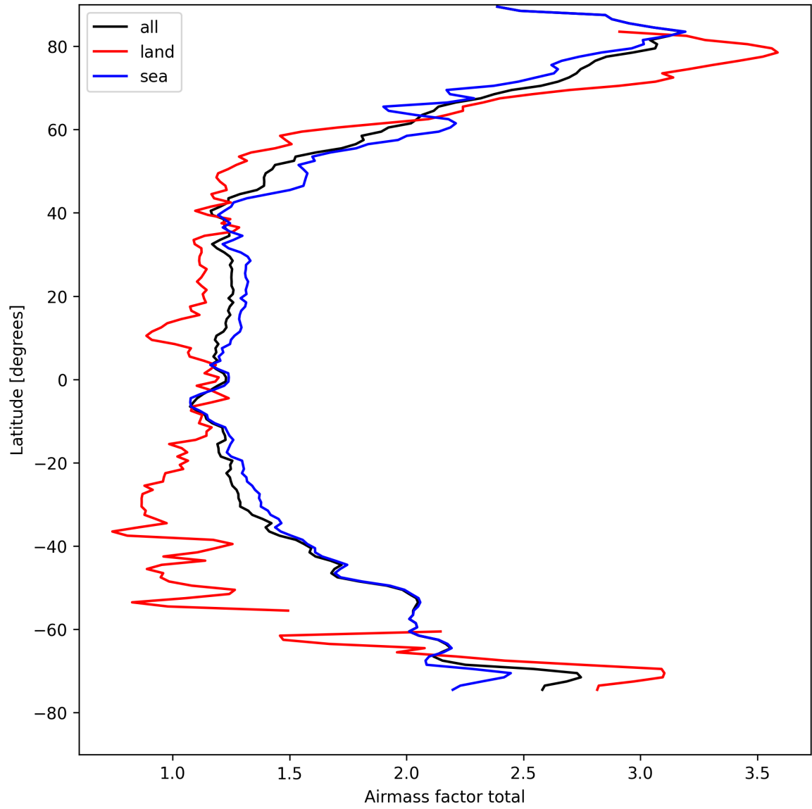
Figure 26: Zonal average of “Airmass factor total” for 2025-04-16 to 2025-04-18.
