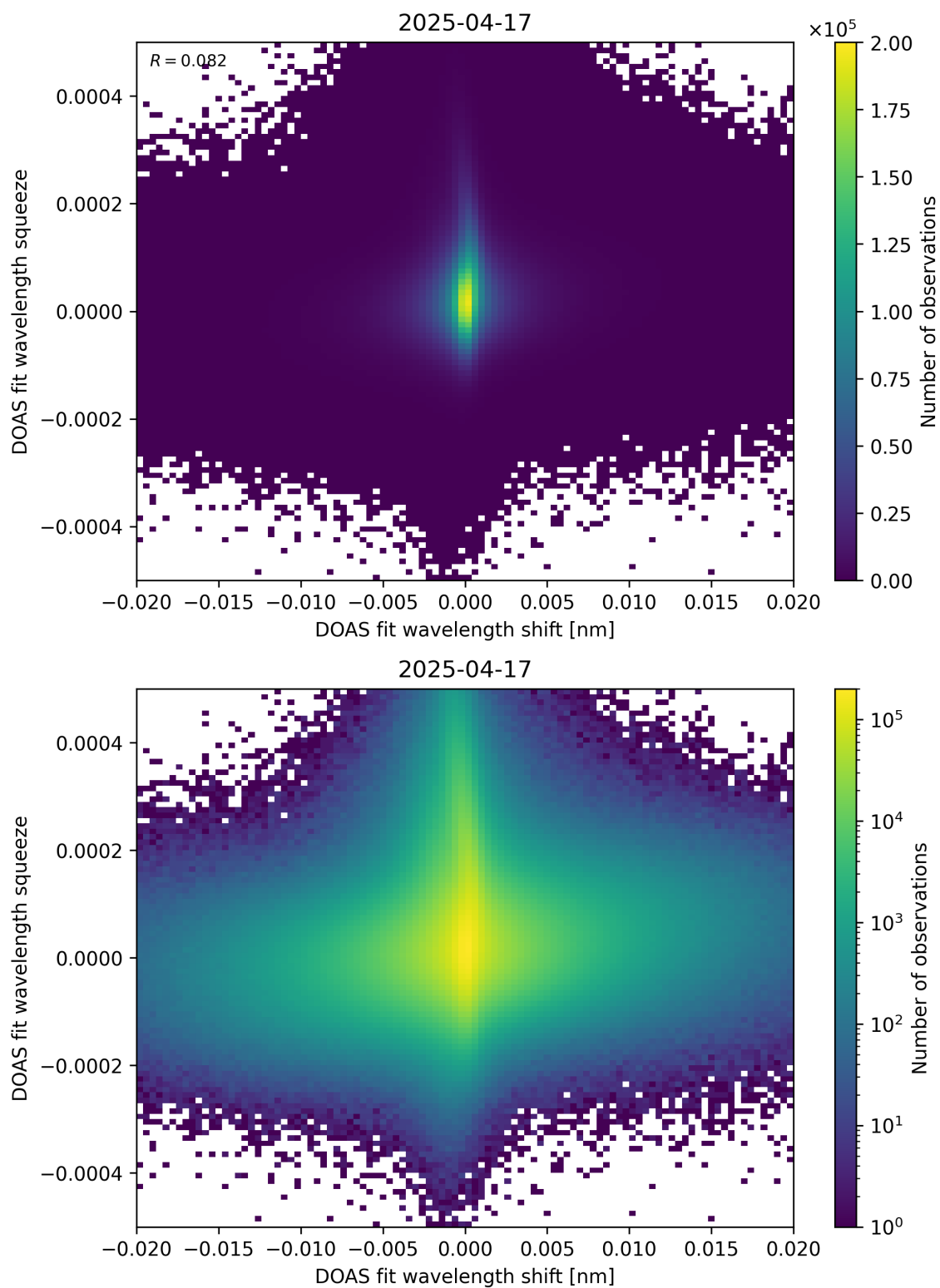
Figure 65: Scatter density plot of “DOAS fit wavelength shift” against “DOAS fit wavelength squeeze” for 2025-04-16 to 2025-04-18.
