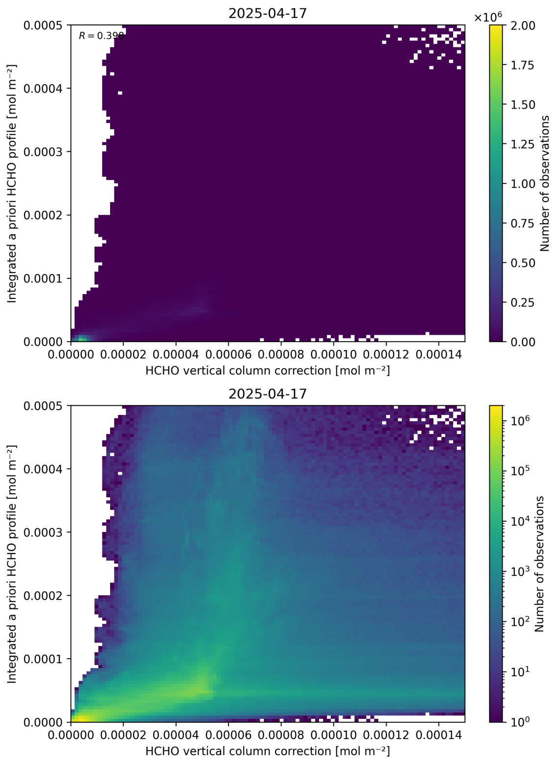
Figure 122: Scatter density plot of “HCHO vertical column correction” against “Integrated a priori HCHO profile” for 2025-04-16 to 2025-04-18.
