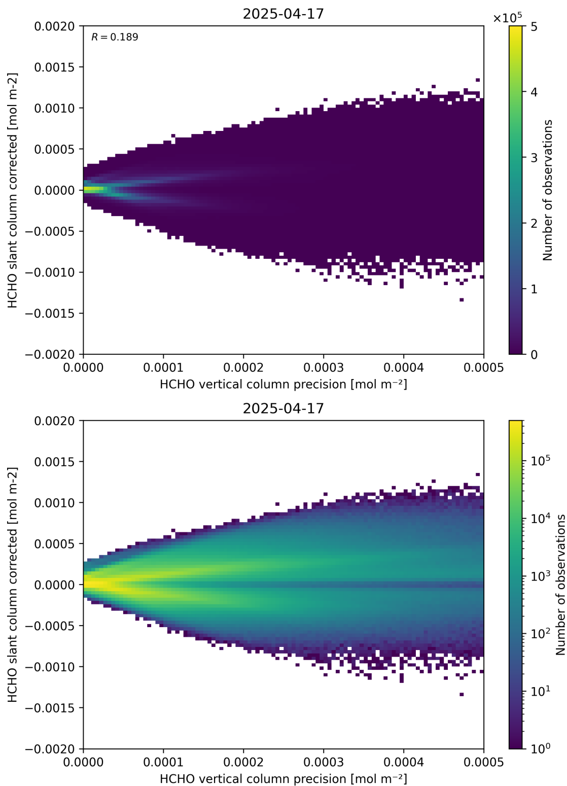
Figure 140: Scatter density plot of “HCHO vertical column precision” against “HCHO slant column corrected” for 2025-04-16 to 2025-04-18.
