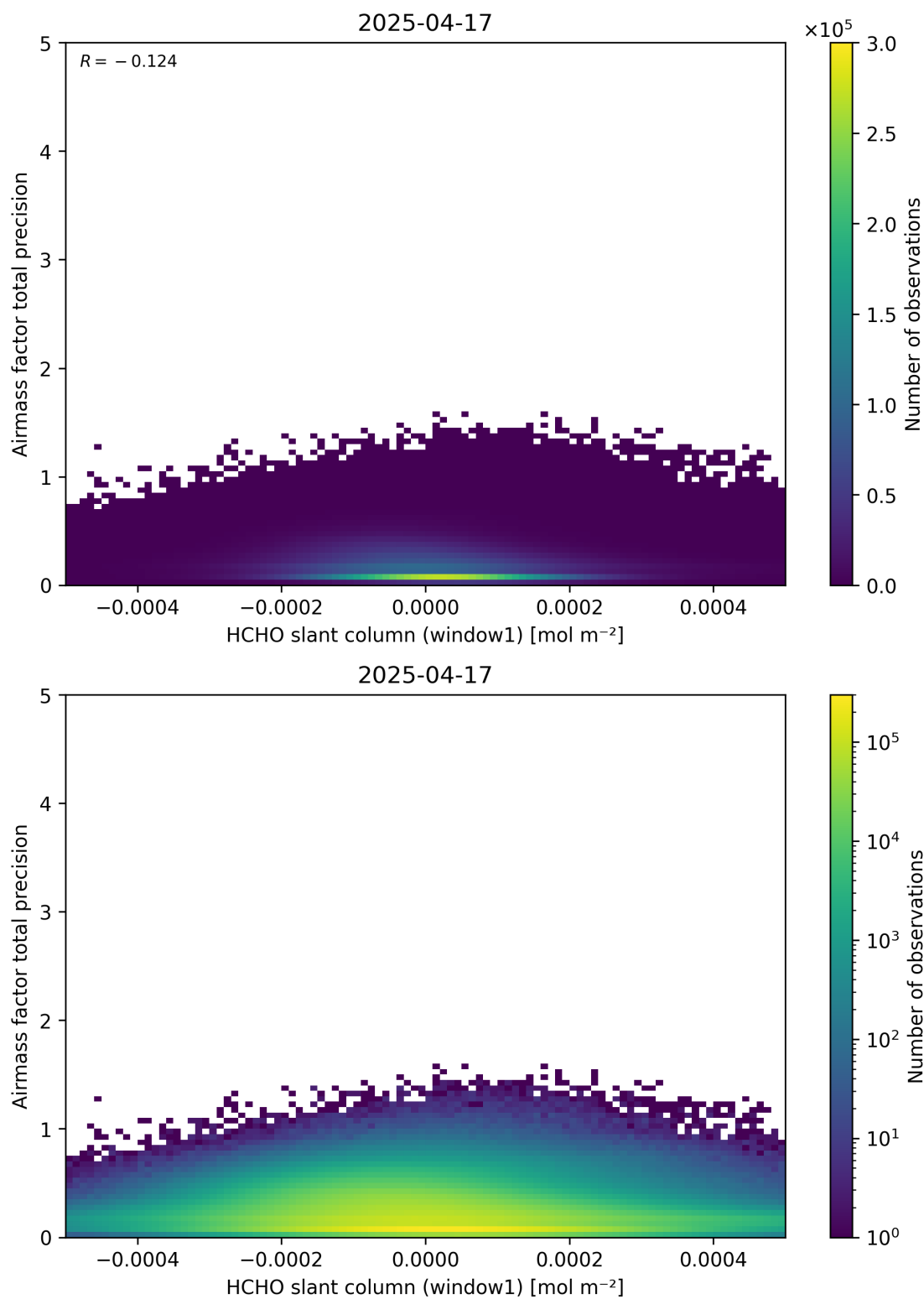
Figure 86: Scatter density plot of “HCHO slant column (window1)” against “Airmass factor total precision” for 2025-04-16 to 2025-04-18.
