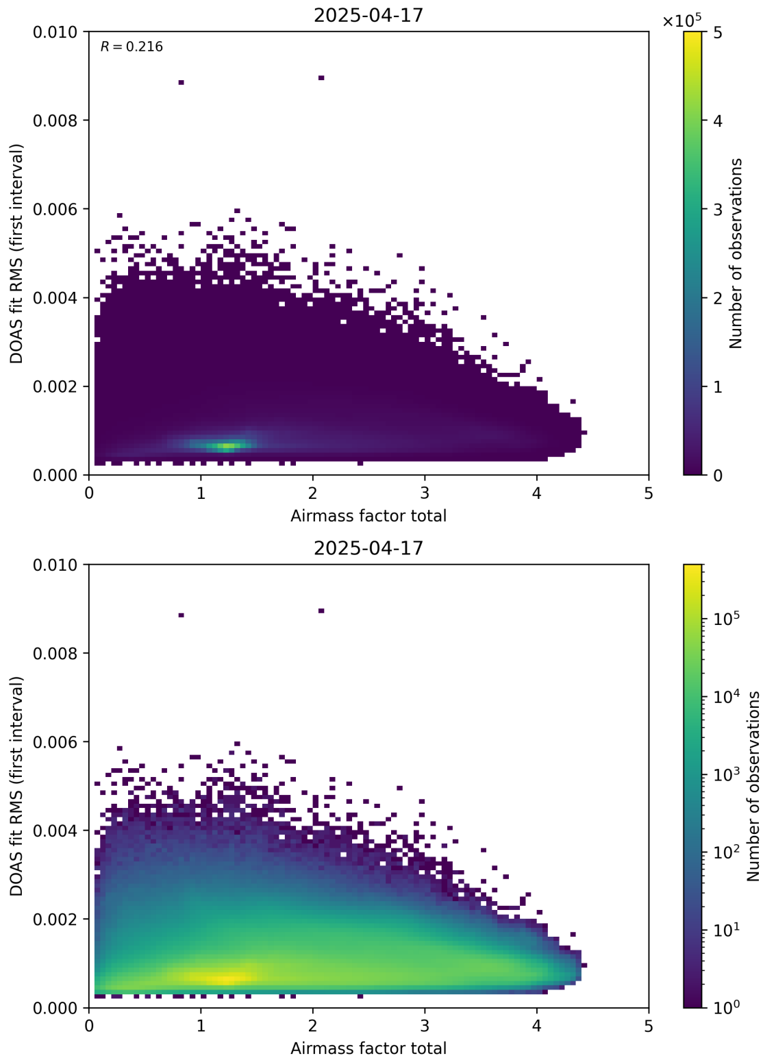
Figure 97: Scatter density plot of “Airmass factor total” against “DOAS fit RMS (first interval)” for 2025-04-16 to 2025-04-18.
