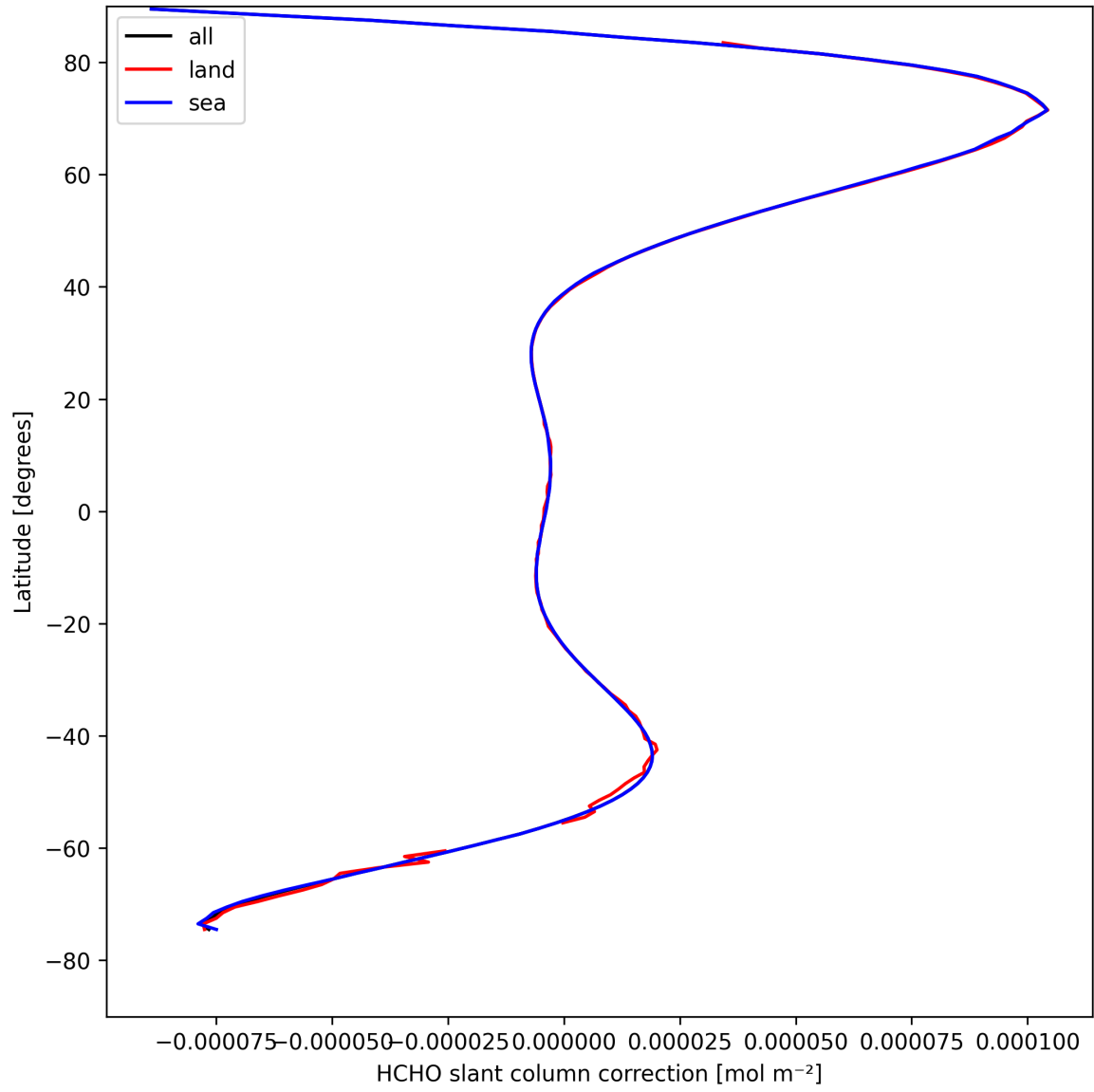
Figure 33: Zonal average of “HCHO slant column correction” for 2025-04-16 to 2025-04-18.
