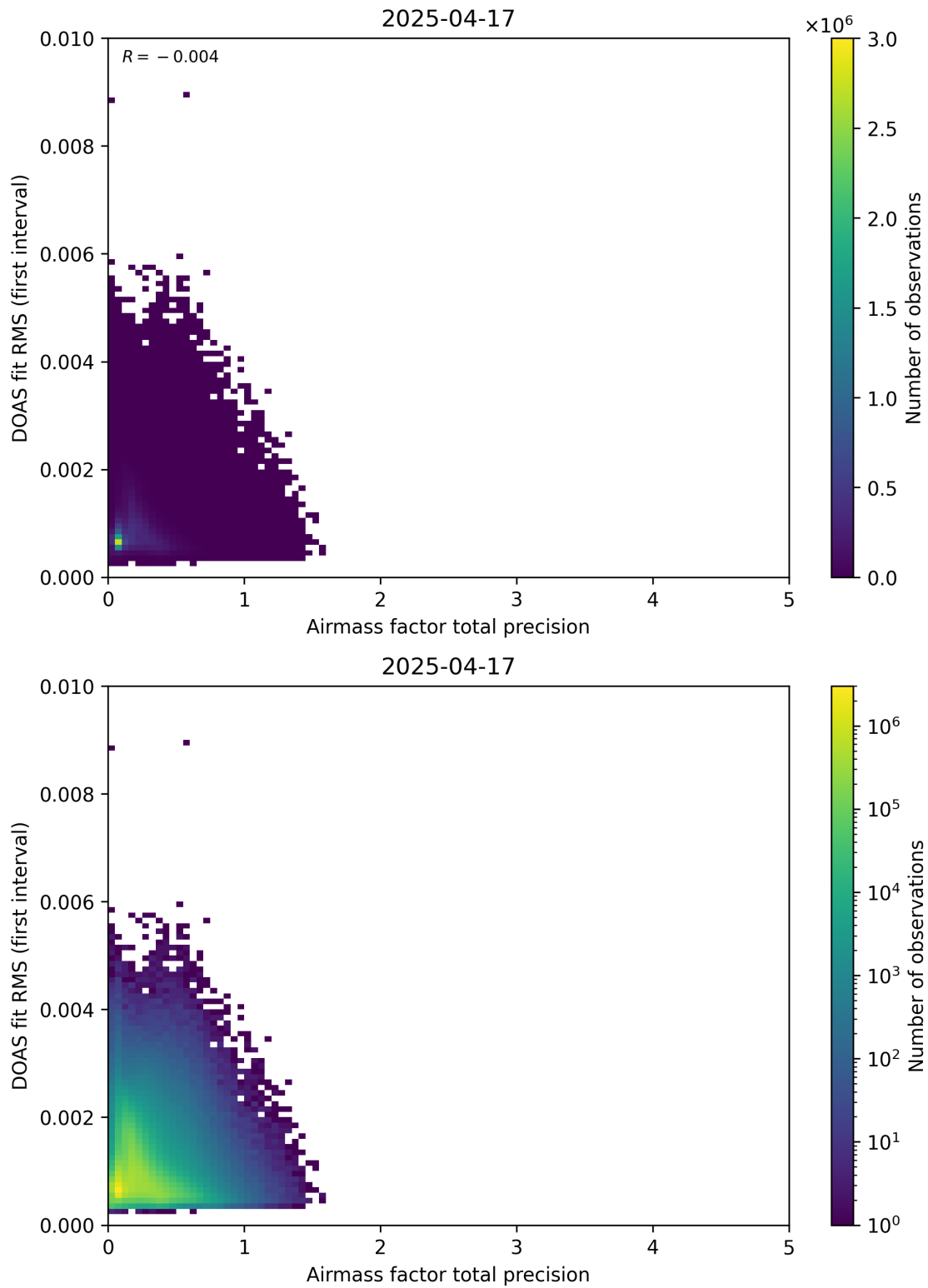
Figure 105: Scatter density plot of “Airmass factor total precision” against “DOAS fit RMS (first interval)” for 2025-04-16 to 2025-04-18.
