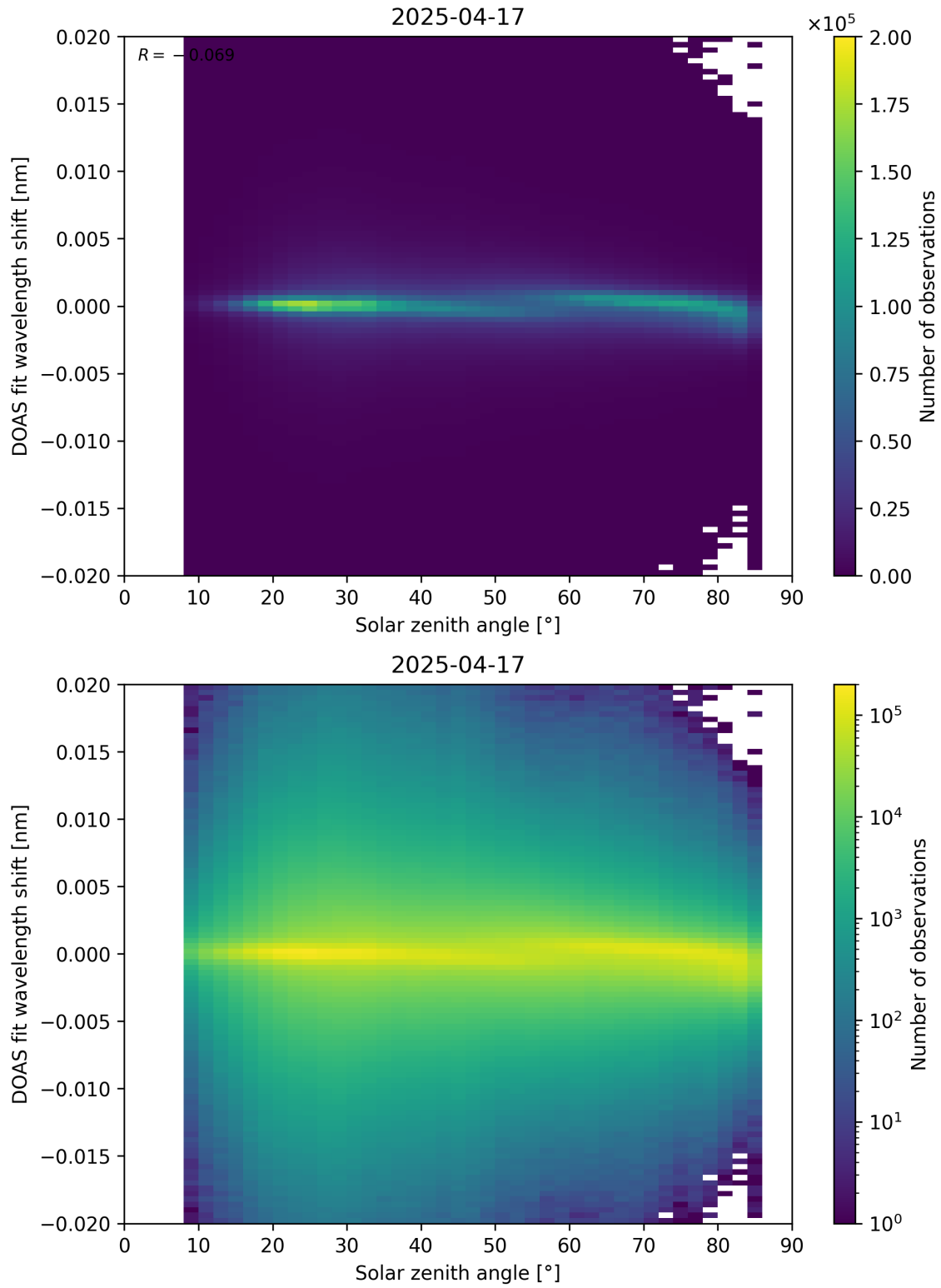
Figure 168: Scatter density plot of “Solar zenith angle” against “DOAS fit wavelength shift” for 2025-04-16 to 2025-04-18.
