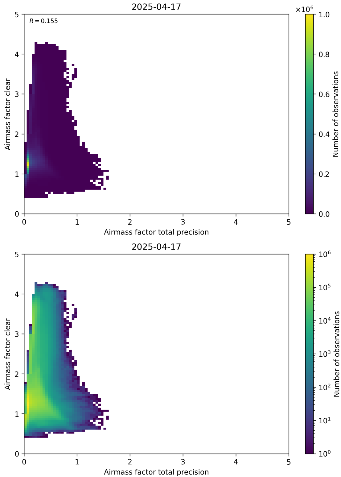
Figure 108: Scatter density plot of “Airmass factor total precision” against “Airmass factor clear” for 2025-04-16 to 2025-04-18.
