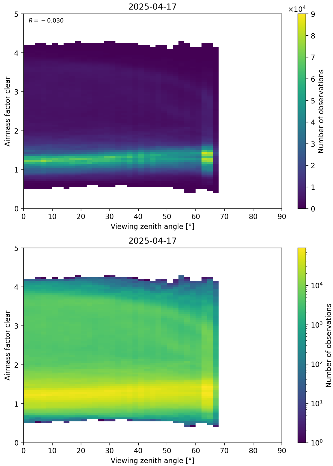
Figure 185: Scatter density plot of “Viewing zenith angle” against “Airmass factor clear” for 2025-04-16 to 2025-04-18.
