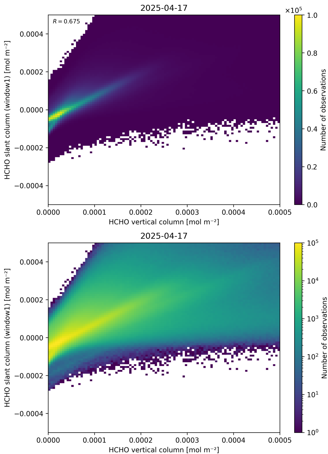
Figure 129: Scatter density plot of “HCHO vertical column” against “HCHO slant column (window1)” for 2025-04-16 to 2025-04-18.
