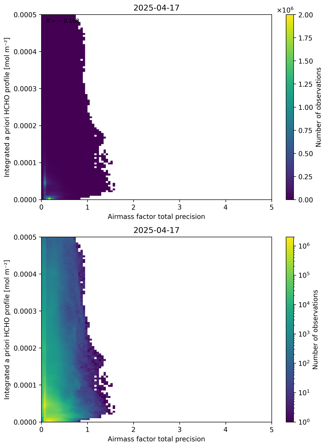
Figure 111: Scatter density plot of “Airmass factor total precision” against “Integrated a priori HCHO profile” for 2025-04-16 to 2025-04-18.
