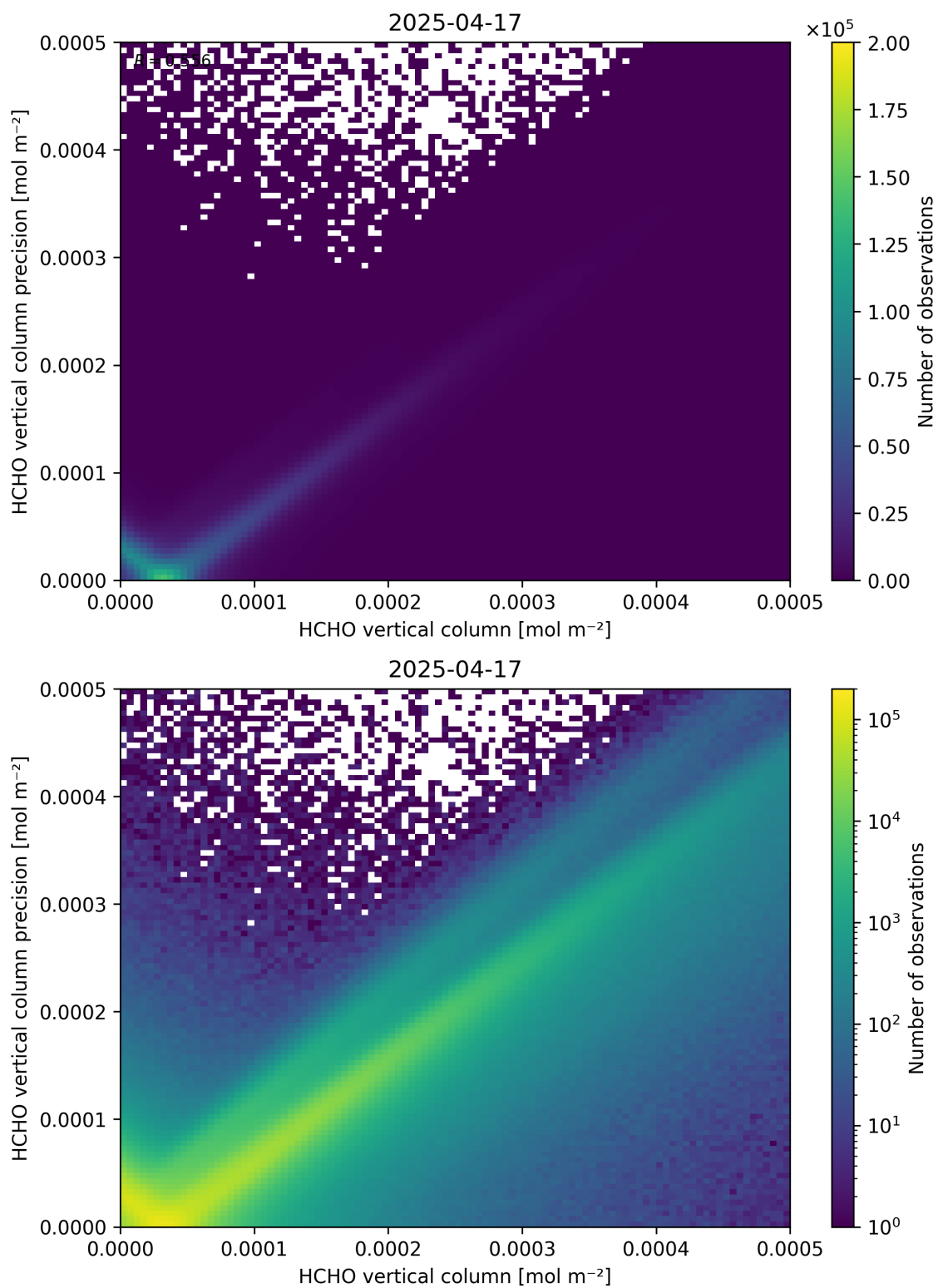
Figure 134: Scatter density plot of “HCHO vertical column” against “HCHO vertical column precision” for 2025-04-16 to 2025-04-18.
