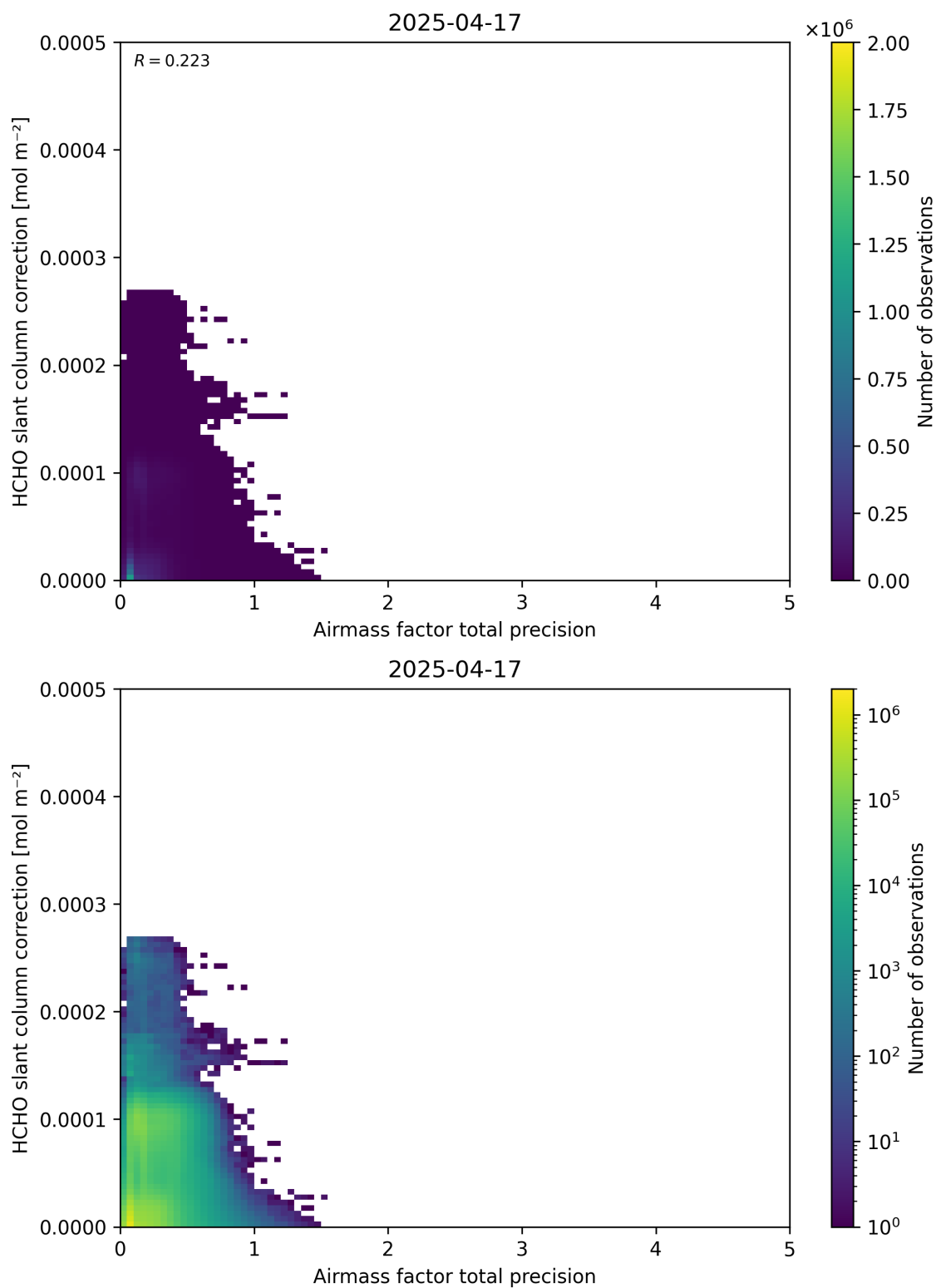
Figure 110: Scatter density plot of “Airmass factor total precision” against “HCHO slant column correction” for 2025-04-16 to 2025-04-18.
