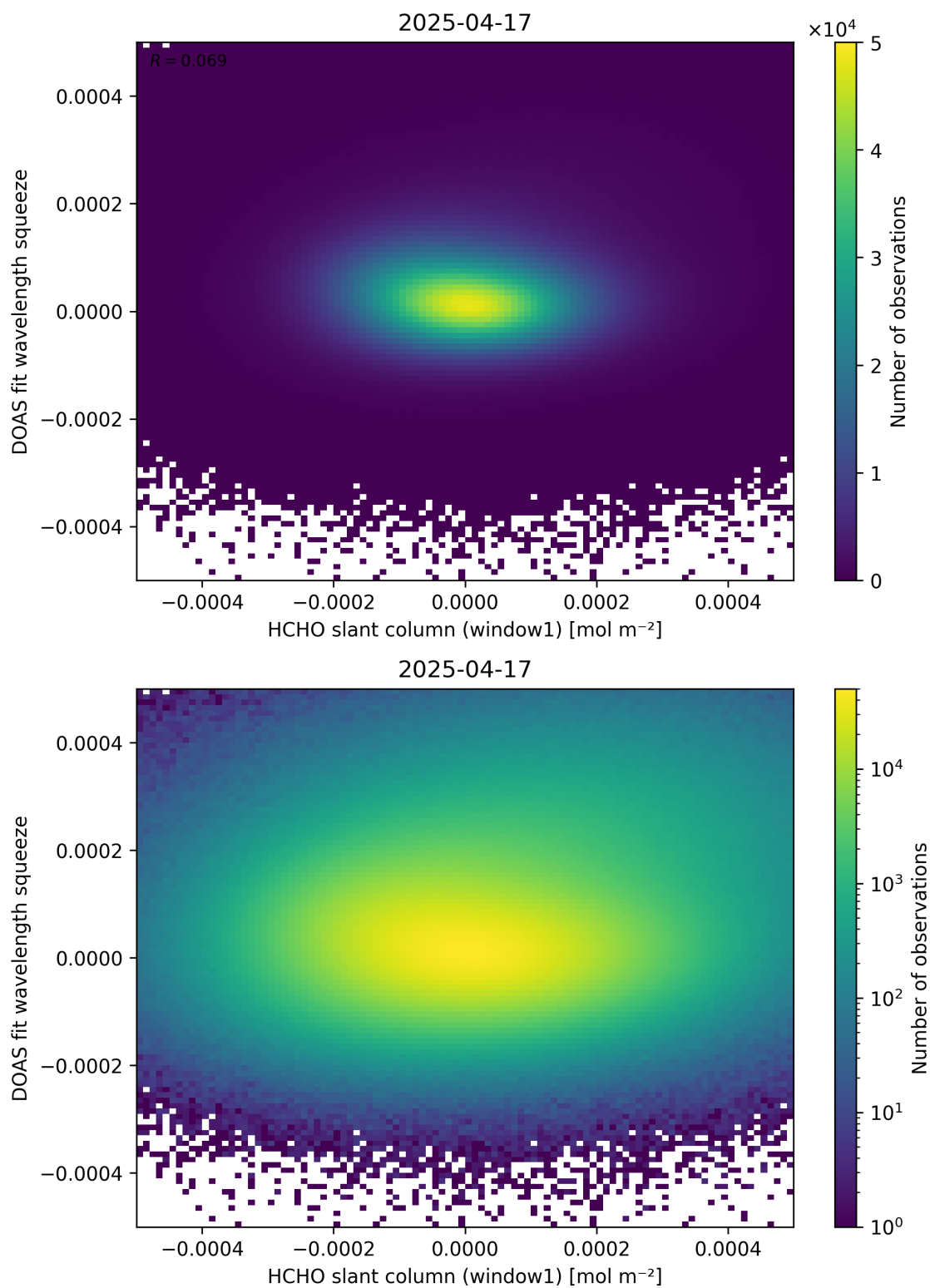
Figure 80: Scatter density plot of “HCHO slant column (window1)” against “DOAS fit wavelength squeeze” for 2025-04-16 to 2025-04-18.
