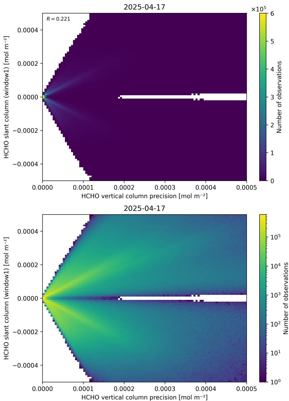
Figure 142: Scatter density plot of “HCHO vertical column precision” against “HCHO slant column (window1)” for 2025-04-16 to 2025-04-18.
