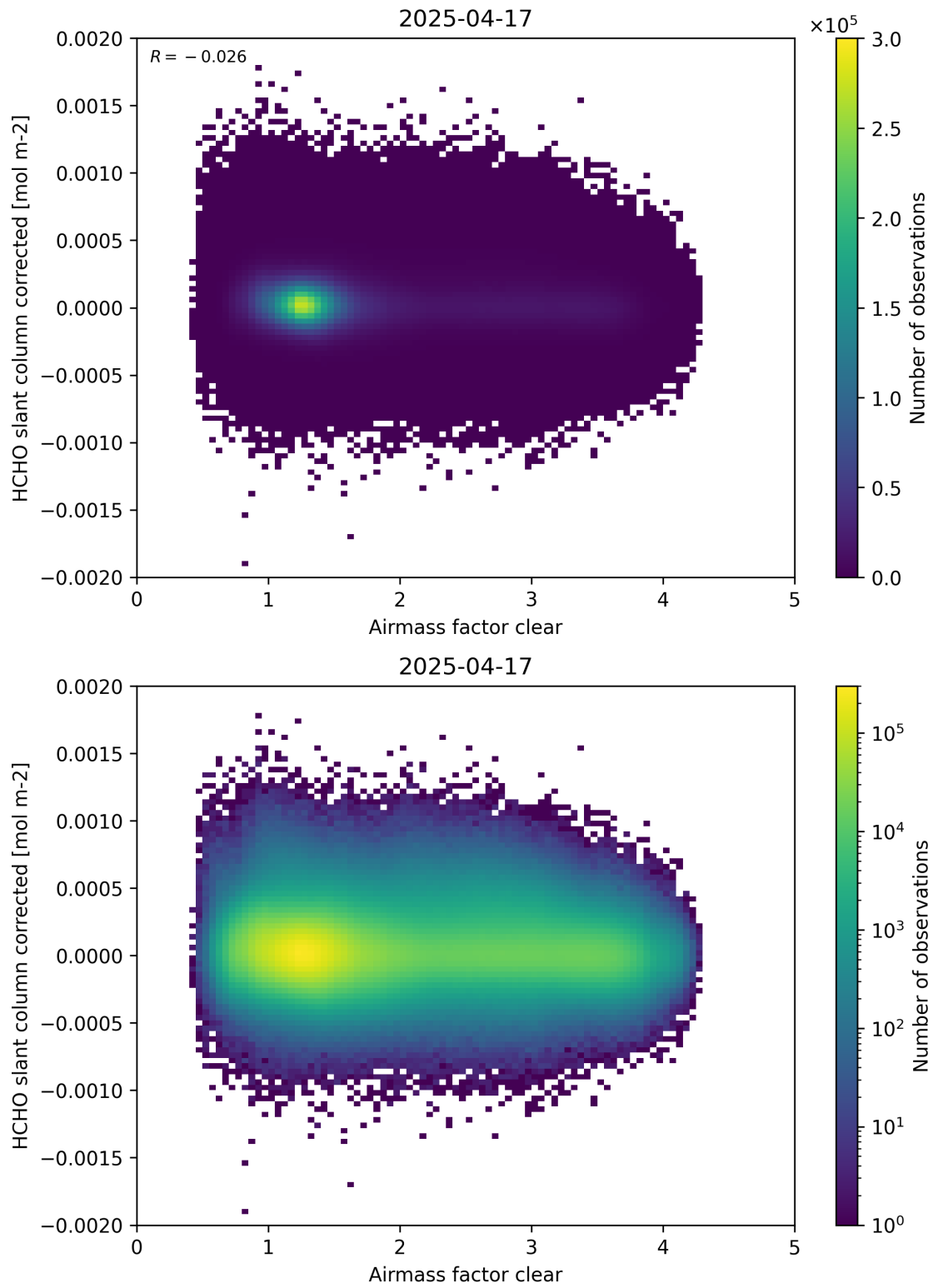
Figure 74: Scatter density plot of “Airmass factor clear” against “HCHO slant column corrected” for 2025-04-16 to 2025-04-18.
