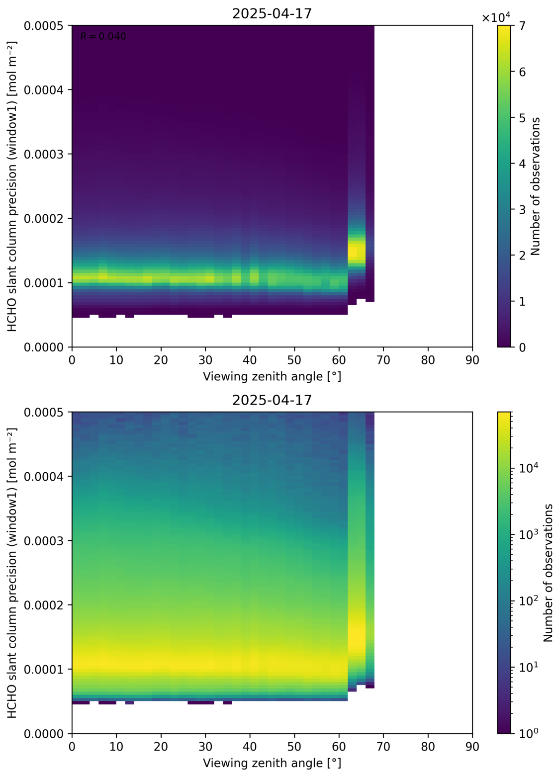
Figure 189: Scatter density plot of “Viewing zenith angle” against “HCHO slant column precision (window1)” for 2025-04-16 to 2025-04-18.
