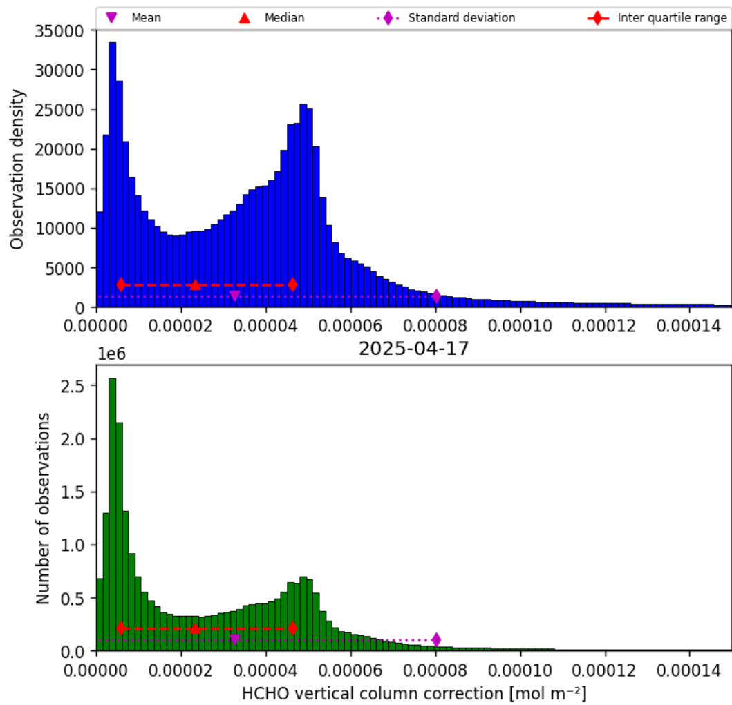
Figure 37: Histogram of “HCHO vertical column correction” for 2025-04-16 to 2025-04-18
