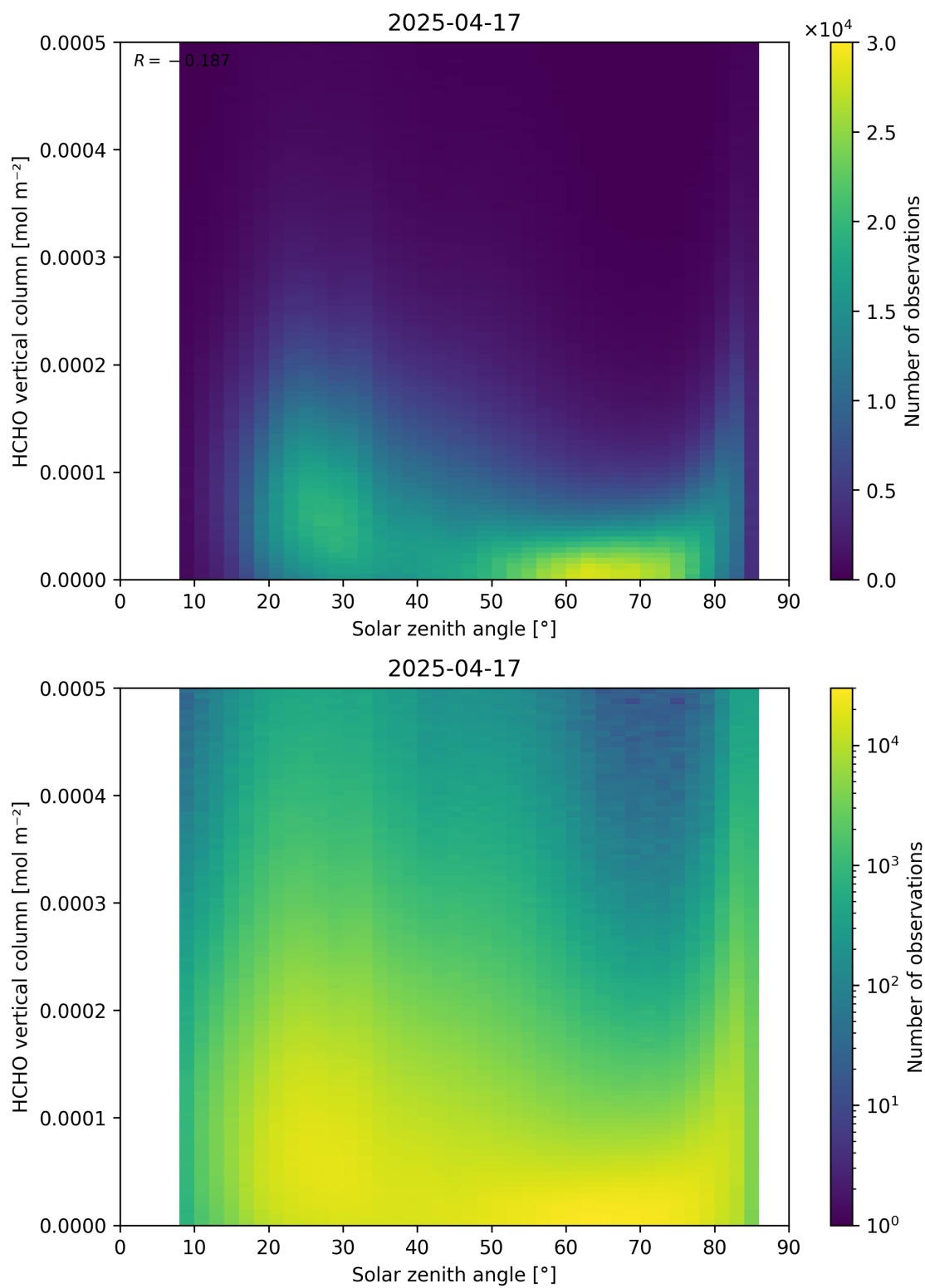
Figure 177: Scatter density plot of “Solar zenith angle” against “HCHO vertical column” for 2025-04-16 to 2025-04-18.
