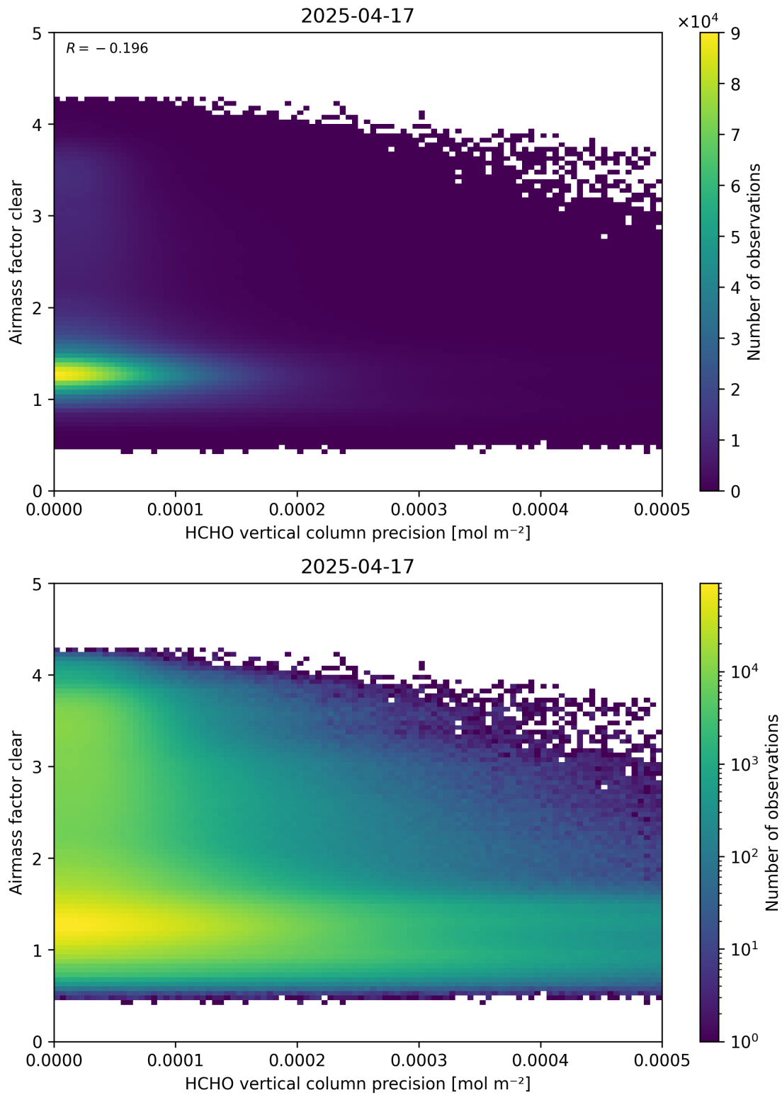
Figure 139: Scatter density plot of “HCHO vertical column precision” against “Airmass factor clear” for 2025-04-16 to 2025-04-18.
