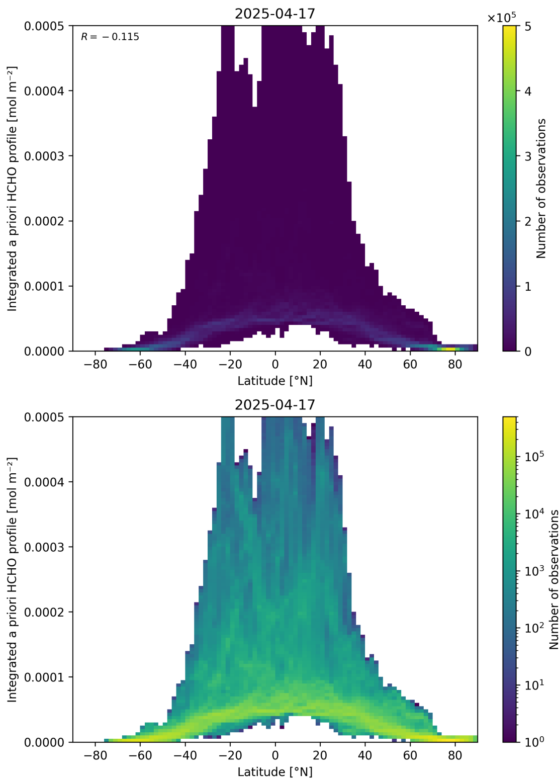
Figure 166: Scatter density plot of “Latitude” against “Integrated a priori HCHO profile” for 2025-04-16 to 2025-04-18.
