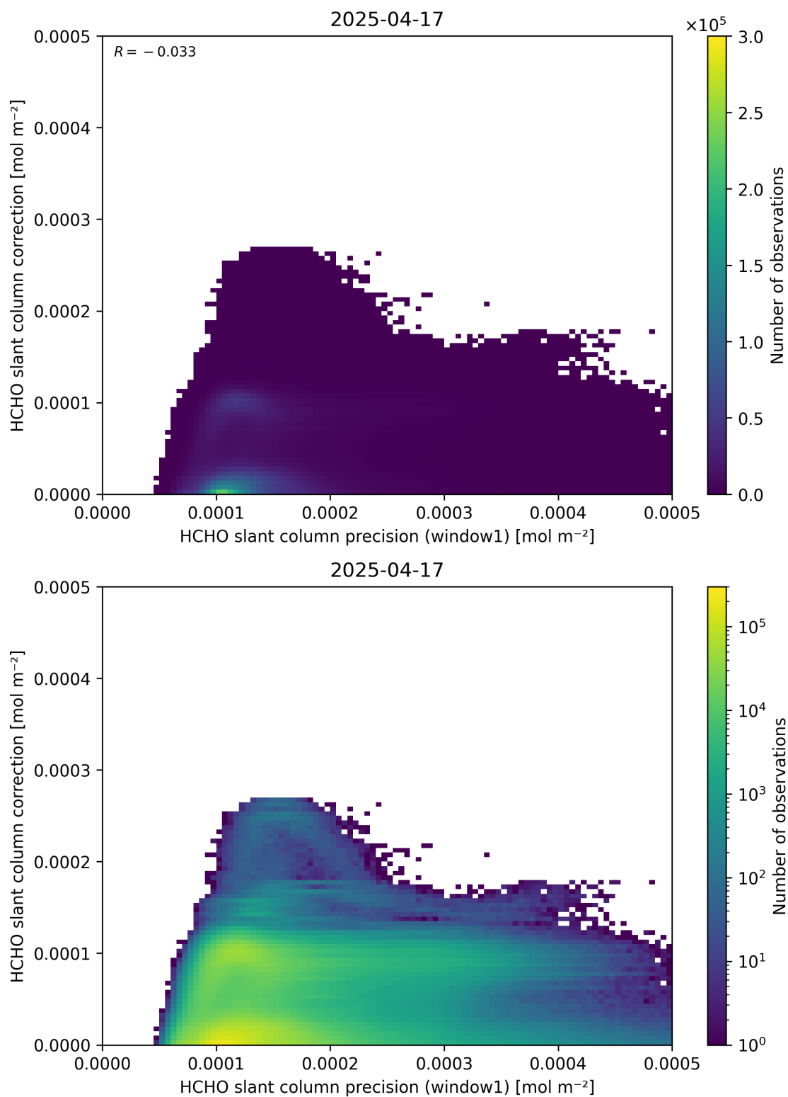
Figure 93: Scatter density plot of “HCHO slant column precision (window1)” against “HCHO slant column correction” for 2025-04-16 to 2025-04-18.
