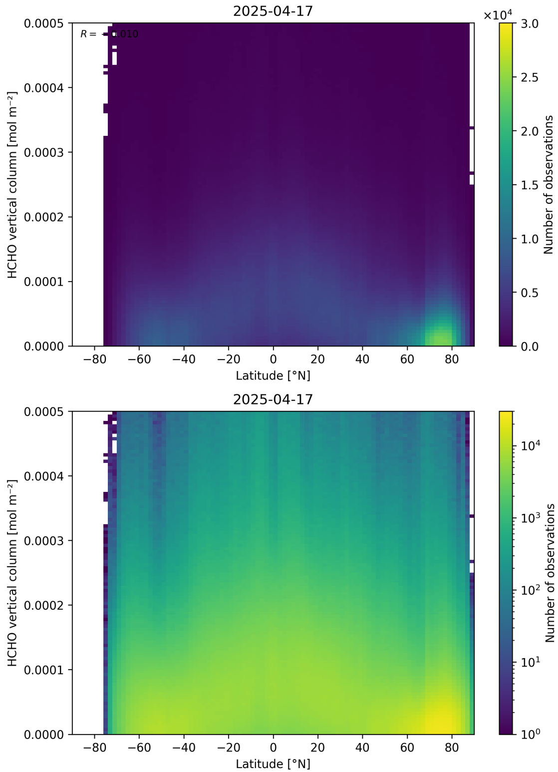
Figure 163: Scatter density plot of “Latitude” against “HCHO vertical column” for 2025-04-16 to 2025-04-18.
