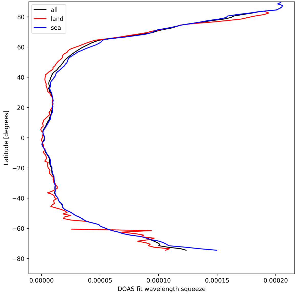
Figure 31: Zonal average of “DOAS fit wavelength squeeze” for 2025-04-16 to 2025-04-18.
