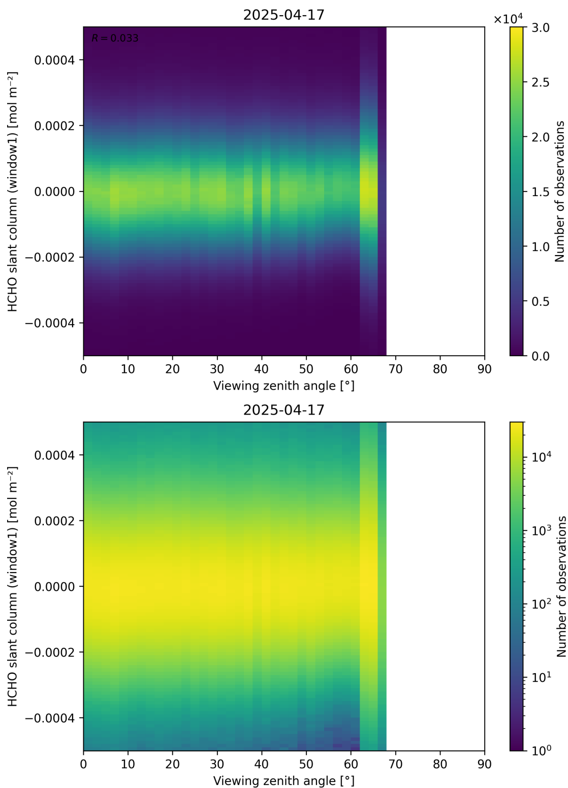
Figure 188: Scatter density plot of “Viewing zenith angle” against “HCHO slant column (window1)” for 2025-04-16 to 2025-04-18.
