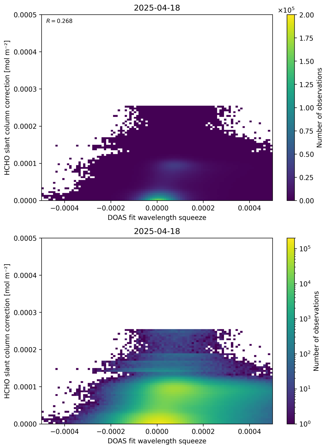
Figure 70: Scatter density plot of “DOAS fit wavelength squeeze” against “HCHO slant column correction” for 2025-04-18 to 2025-04-19.
