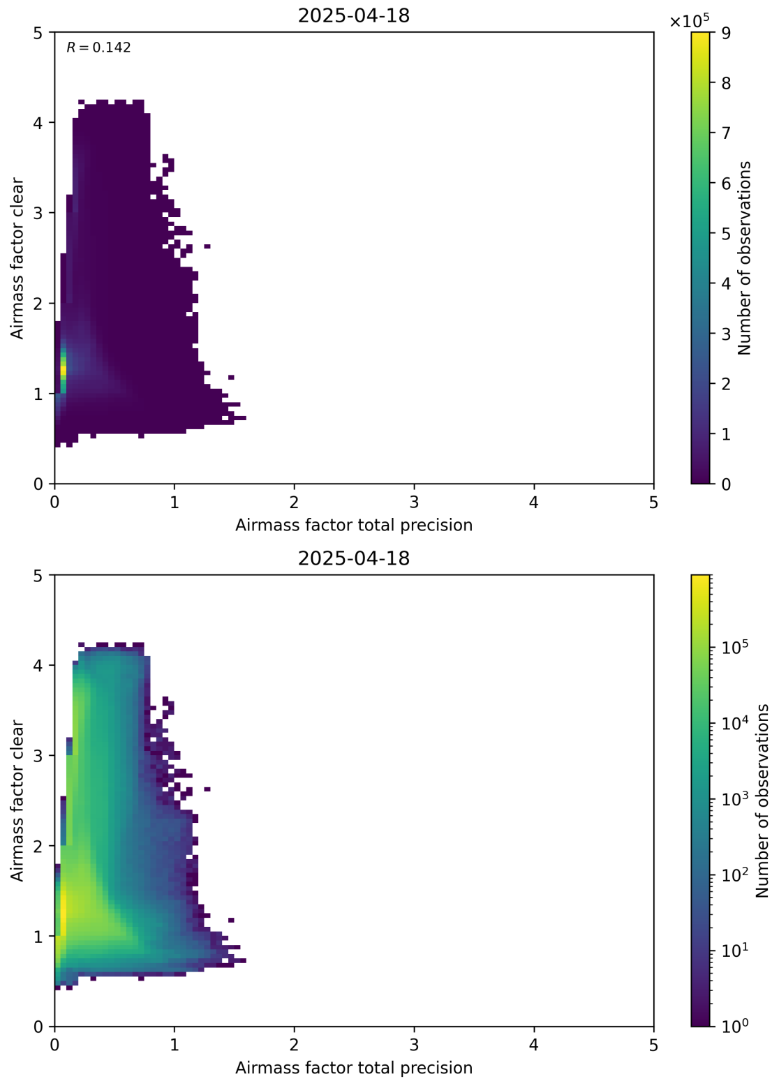
Figure 108: Scatter density plot of “Airmass factor total precision” against “Airmass factor clear” for 2025-04-18 to 2025-04-19.
