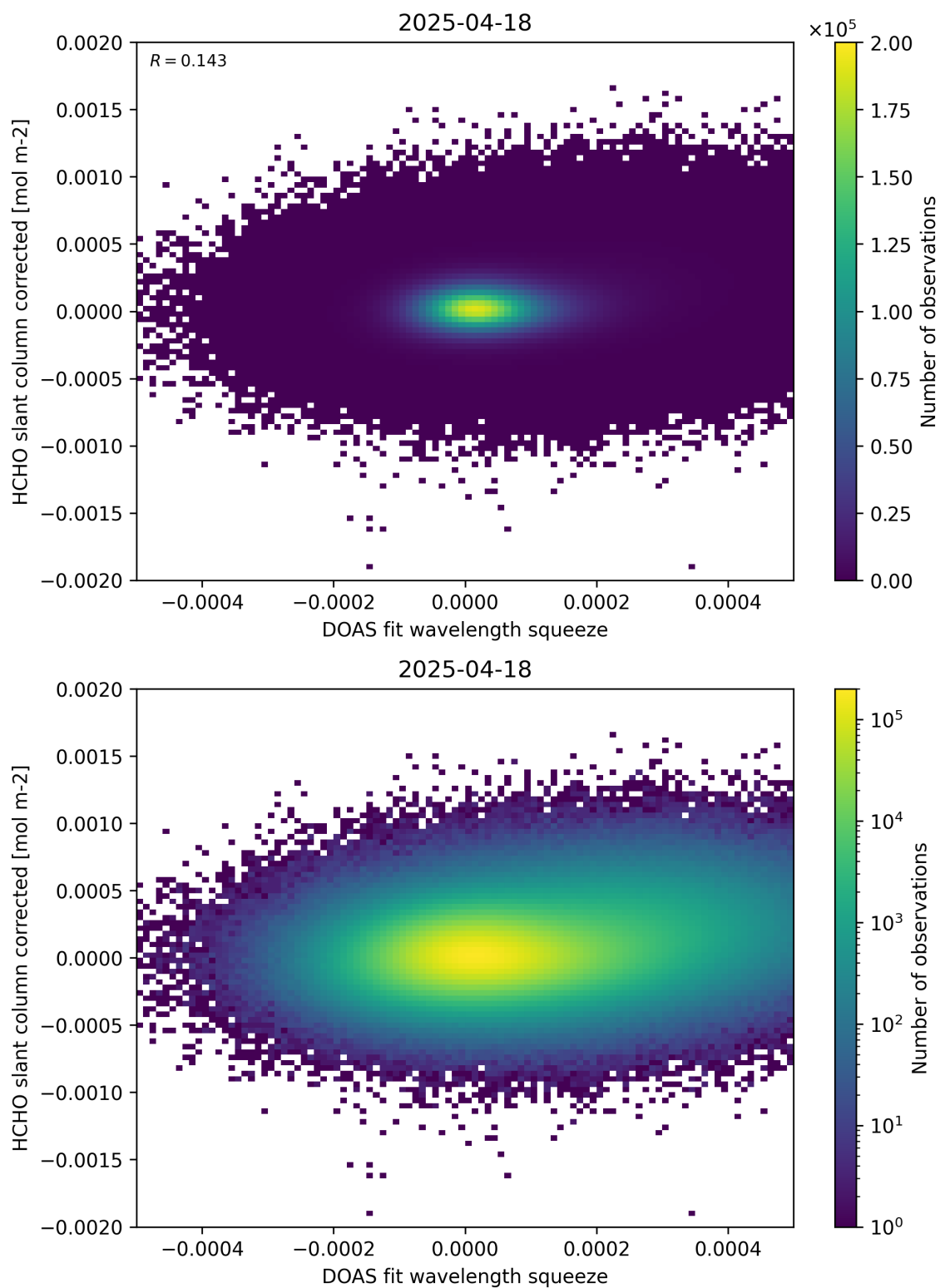
Figure 69: Scatter density plot of “DOAS fit wavelength squeeze” against “HCHO slant column corrected” for 2025-04-18 to 2025-04-19.
