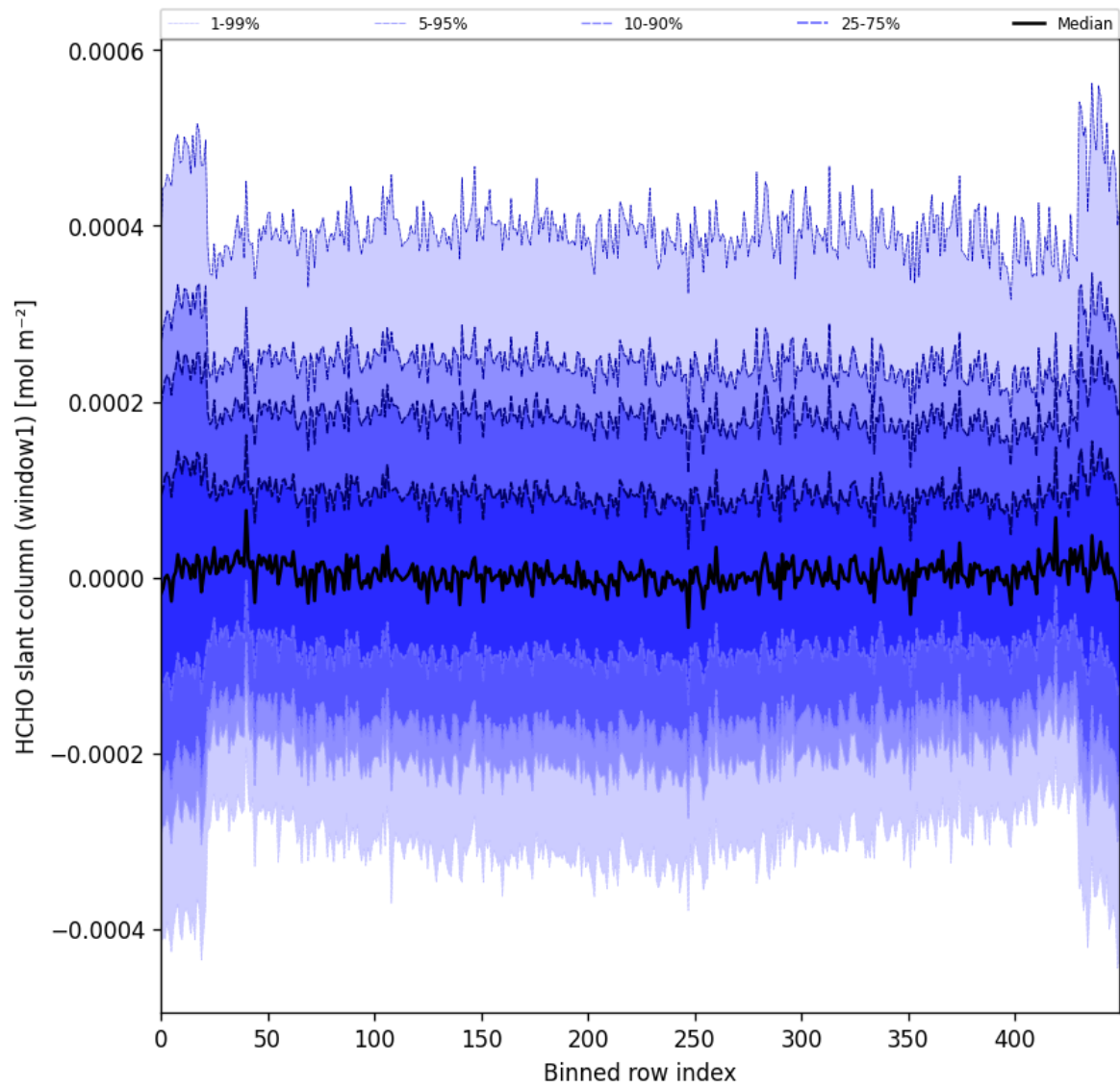
Figure 52: Along track statistics of “HCHO slant column (window1)” for 2025-04-18 to 2025-04-19
