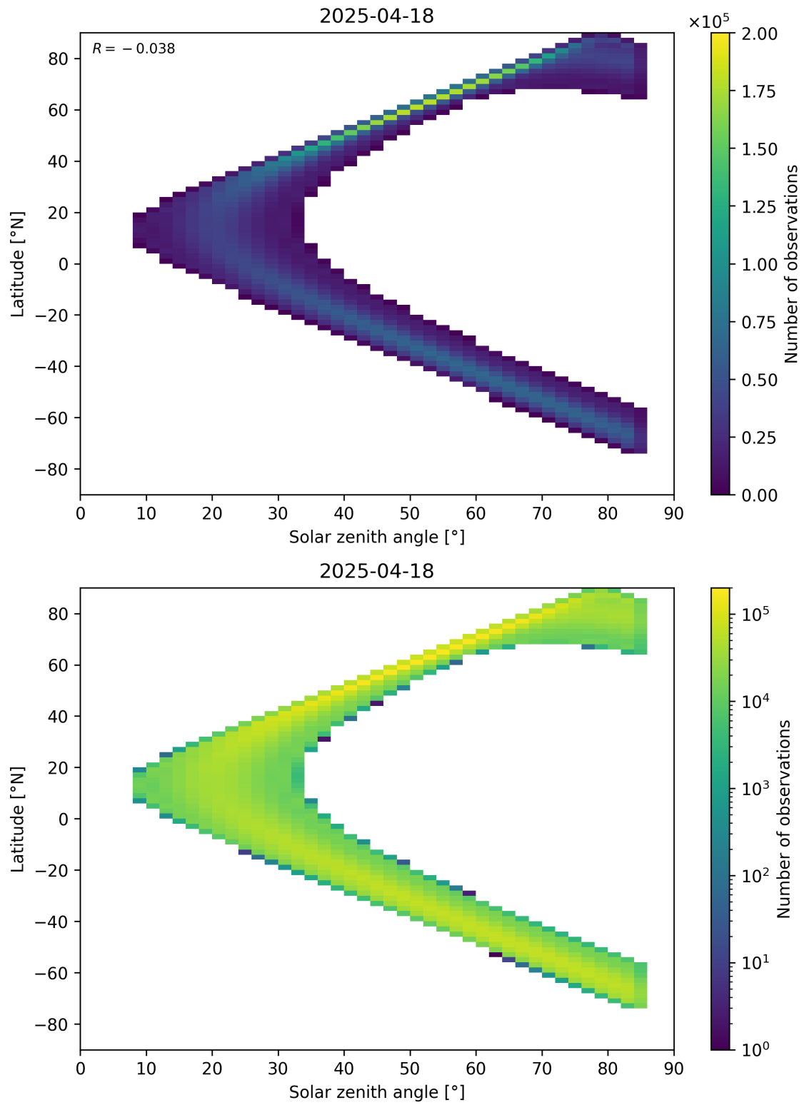
Figure 181: Scatter density plot of “Solar zenith angle” against “Latitude” for 2025-04-18 to 2025-04-19.
