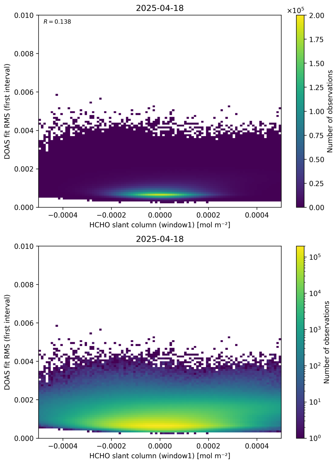
Figure 78: Scatter density plot of “HCHO slant column (window1)” against “DOAS fit RMS (first interval)” for 2025-04-18 to 2025-04-19.
