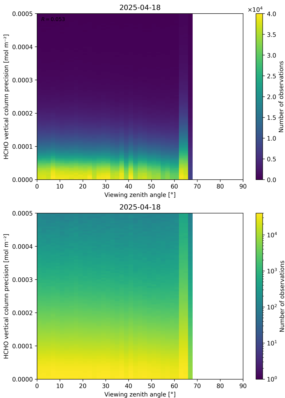
Figure 194: Scatter density plot of “Viewing zenith angle” against “HCHO vertical column precision” for 2025-04-18 to 2025-04-19.
