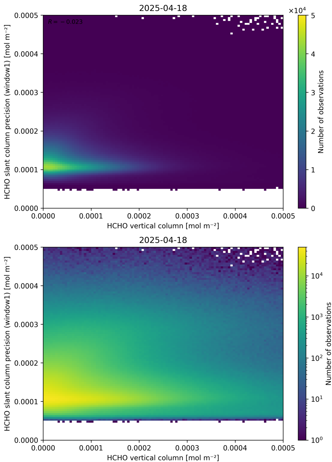
Figure 130: Scatter density plot of “HCHO vertical column” against “HCHO slant column precision (window1)” for 2025-04-18 to 2025-04-19.
