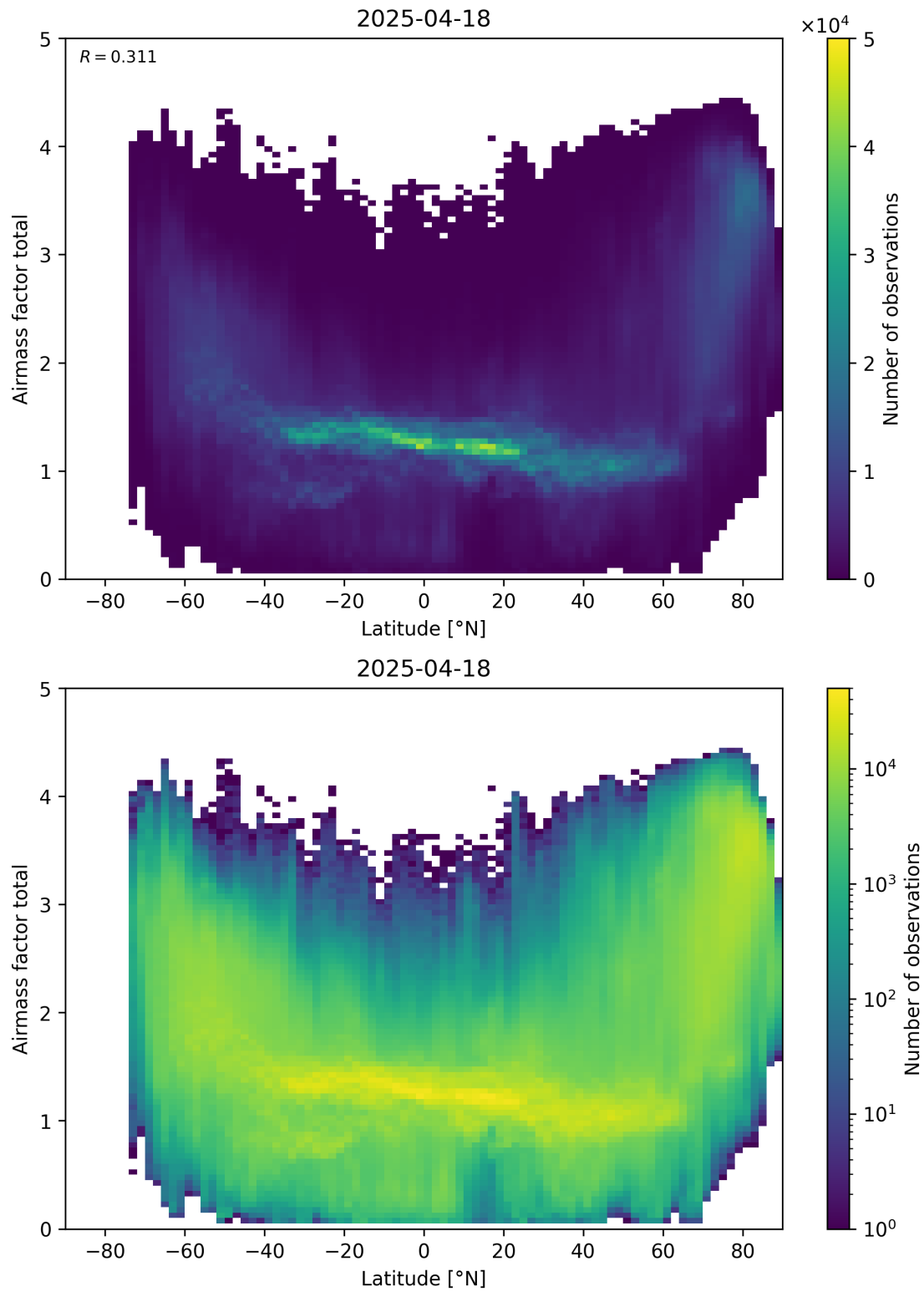
Figure 161: Scatter density plot of “Latitude” against “Airmass factor total” for 2025-04-18 to 2025-04-19.
