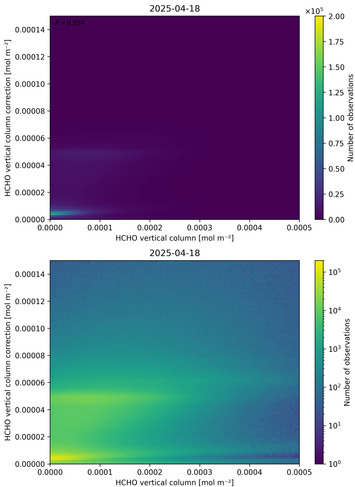
Figure 133: Scatter density plot of “HCHO vertical column” against “HCHO vertical column correction” for 2025-04-18 to 2025-04-19.
