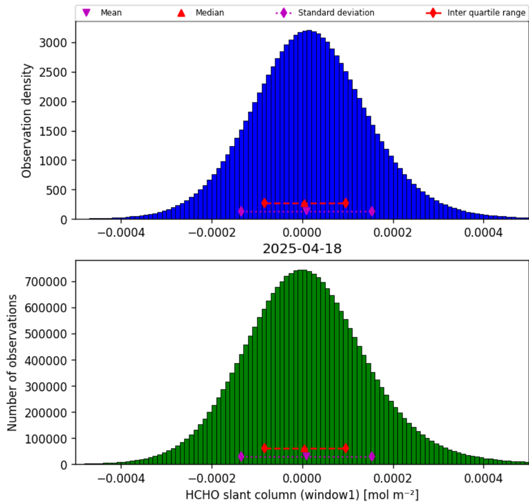
Figure 38: Histogram of “HCHO slant column (window1)” for 2025-04-18 to 2025-04-19
