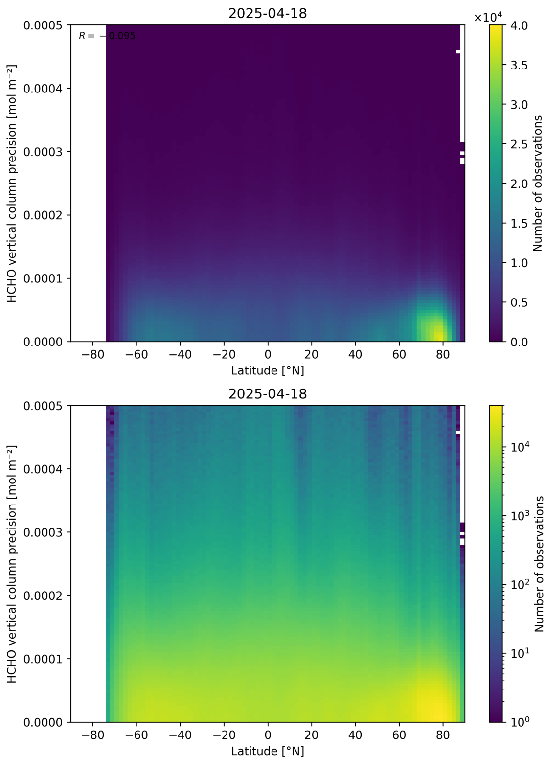
Figure 165: Scatter density plot of “Latitude” against “HCHO vertical column precision” for 2025-04-18 to 2025-04-19.
