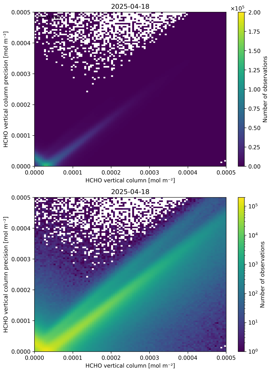
Figure 134: Scatter density plot of “HCHO vertical column” against “HCHO vertical column precision” for 2025-04-18 to 2025-04-19.
