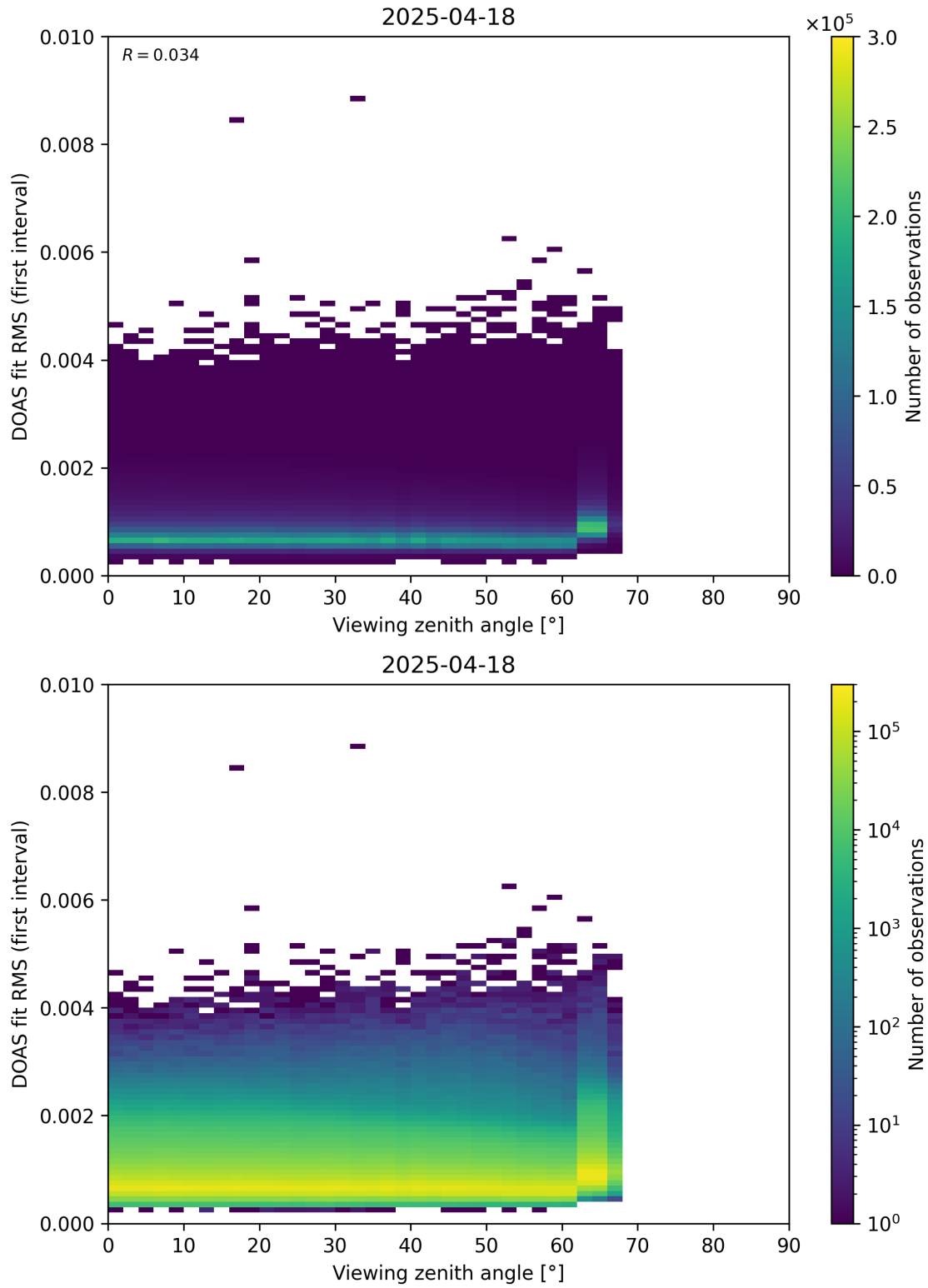
Figure 182: Scatter density plot of “Viewing zenith angle” against “DOAS fit RMS (first interval)” for 2025-04-18 to 2025-04-19.
