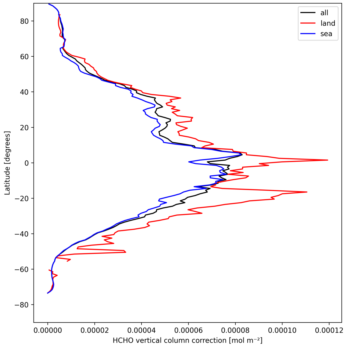
Figure 23: Zonal average of “HCHO vertical column correction” for 2025-04-18 to 2025-04-19.
