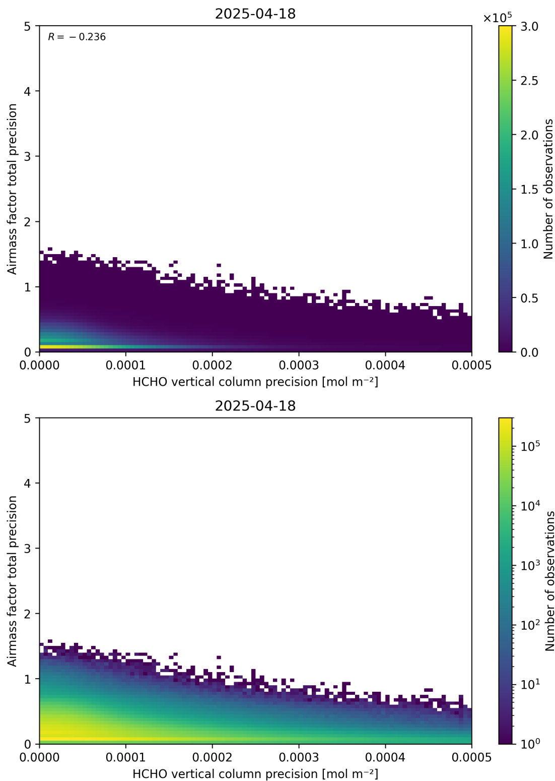
Figure 145: Scatter density plot of “HCHO vertical column precision” against “Airmass factor total precision” for 2025-04-18 to 2025-04-19.
