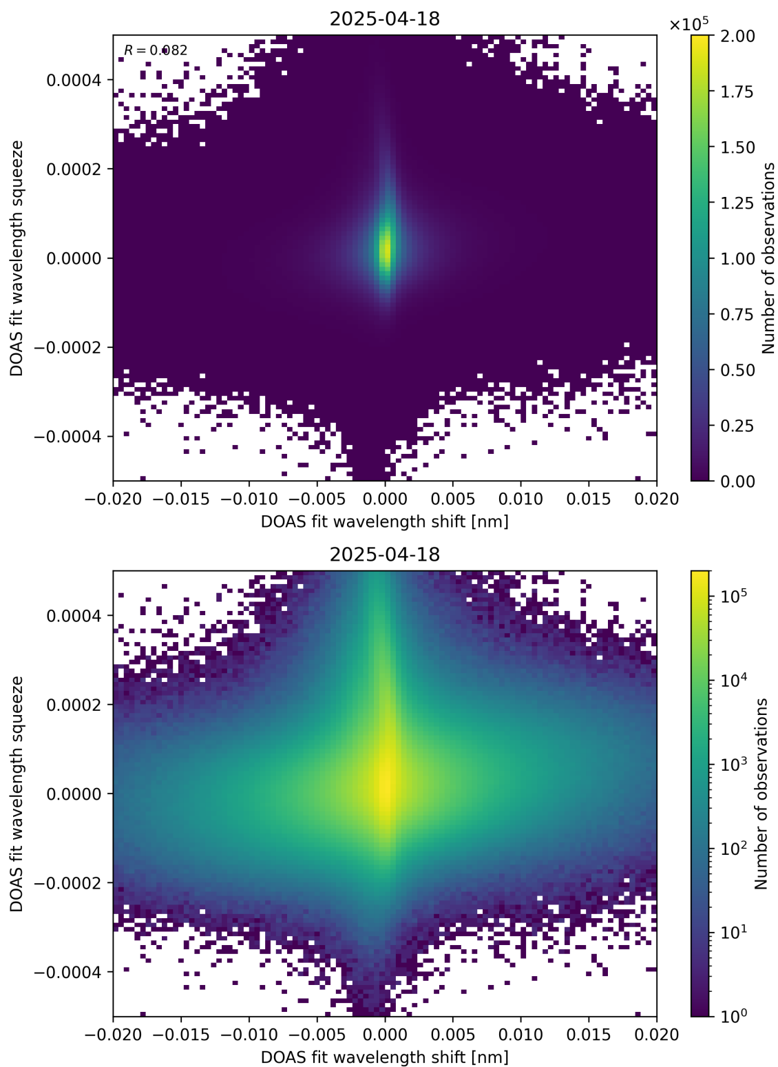
Figure 65: Scatter density plot of “DOAS fit wavelength shift” against “DOAS fit wavelength squeeze” for 2025-04-18 to 2025-04-19.
