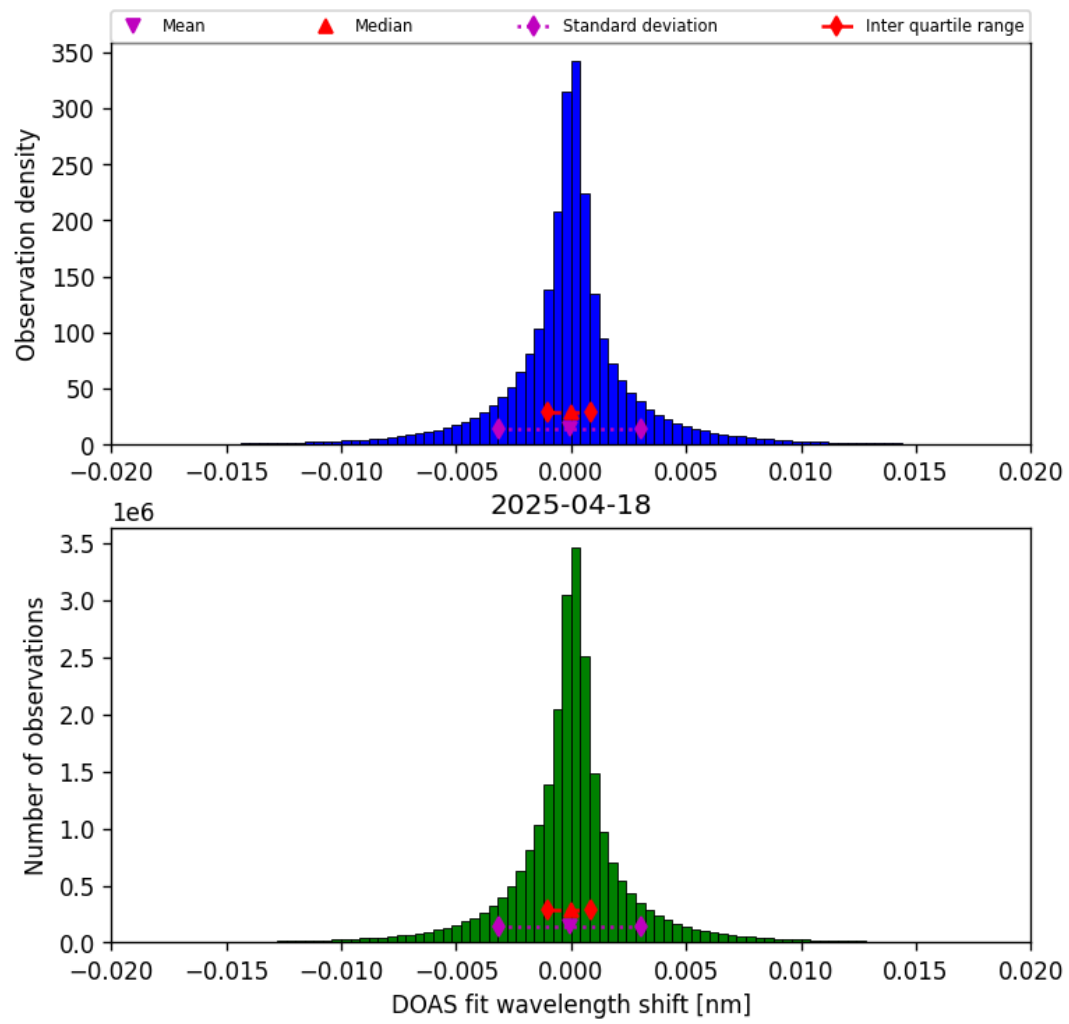
Figure 44: Histogram of “DOAS fit wavelength shift” for 2025-04-18 to 2025-04-19
