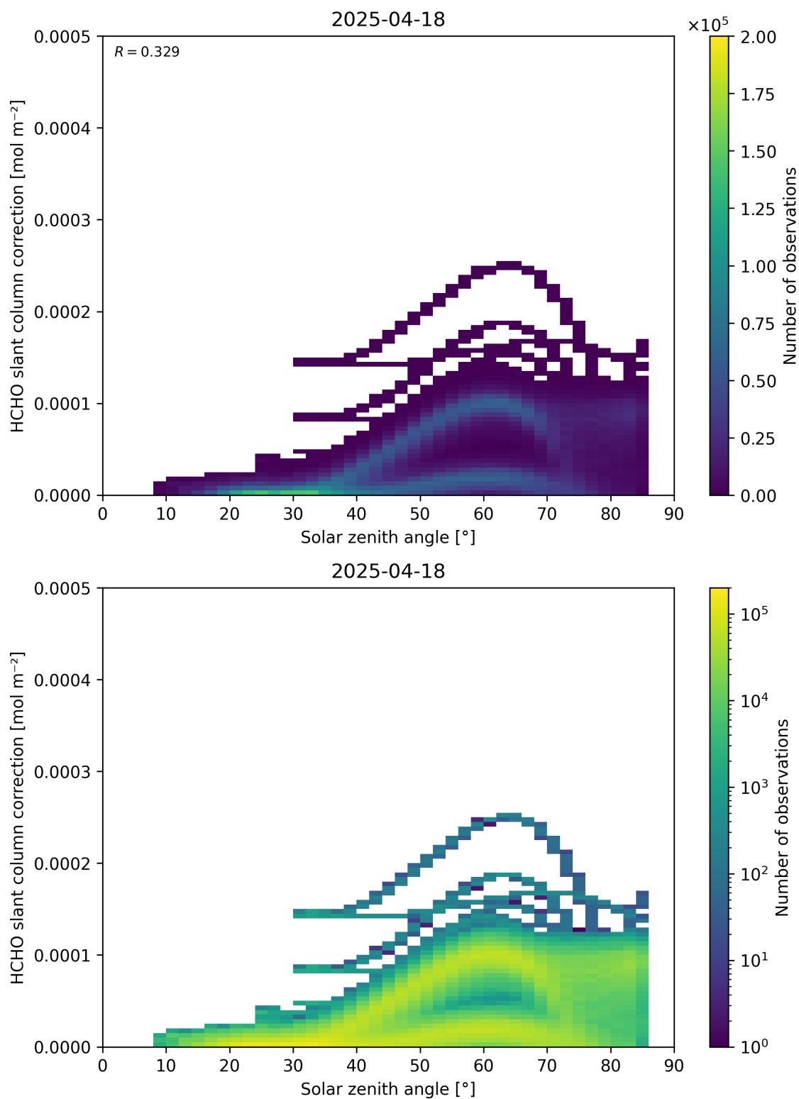
Figure 172: Scatter density plot of “Solar zenith angle” against “HCHO slant column correction” for 2025-04-18 to 2025-04-19.
