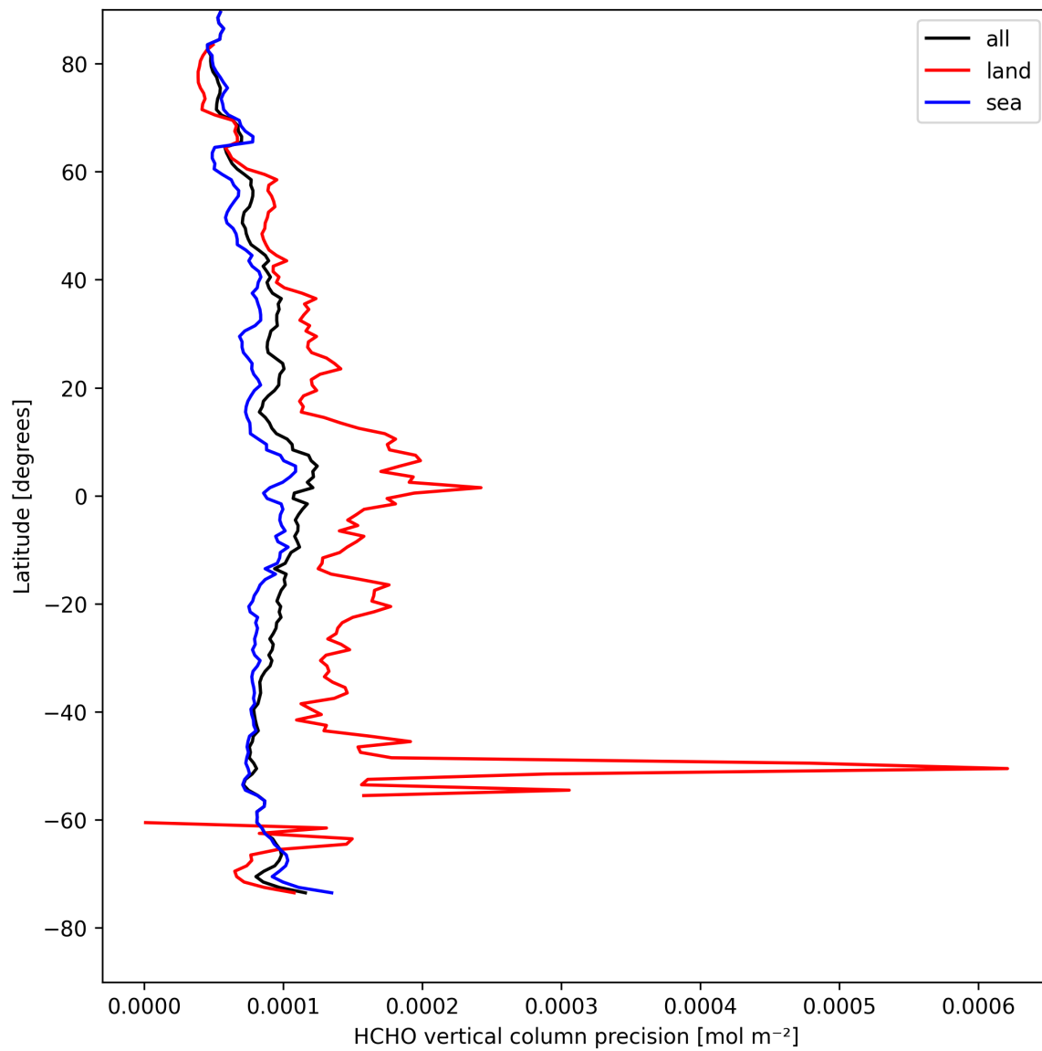
Figure 22: Zonal average of “HCHO vertical column precision” for 2025-04-18 to 2025-04-19.
