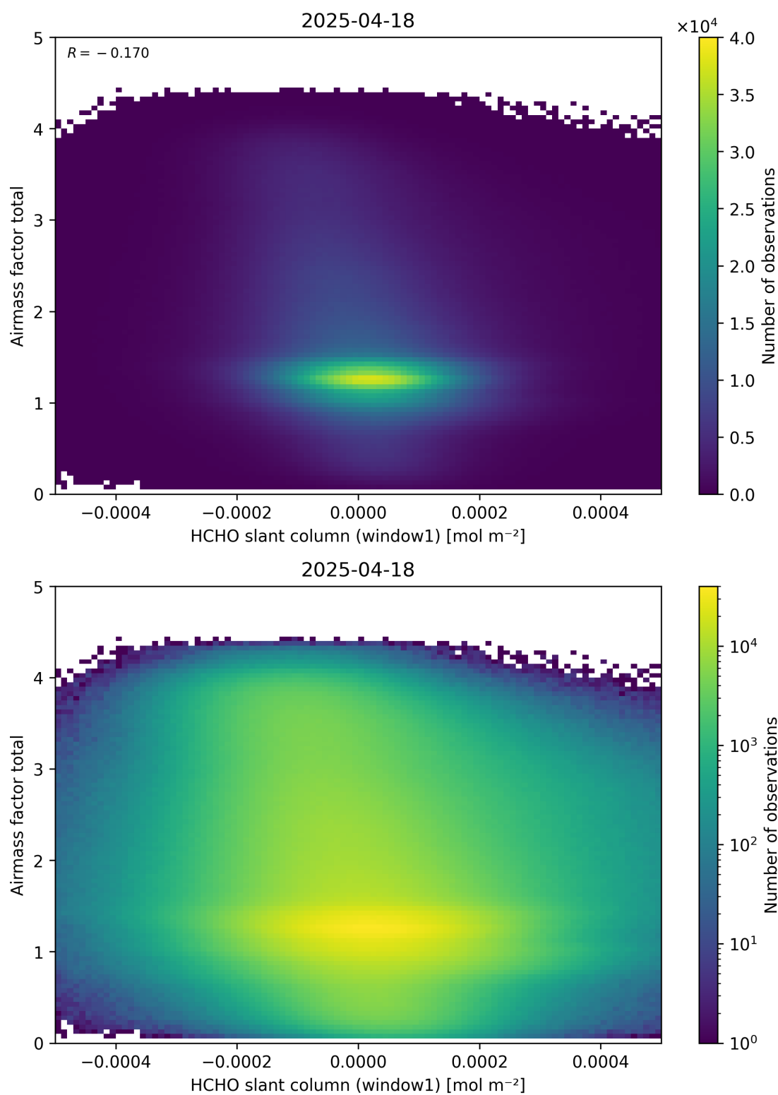
Figure 85: Scatter density plot of “HCHO slant column (window1)” against “Airmass factor total” for 2025-04-18 to 2025-04-19.
