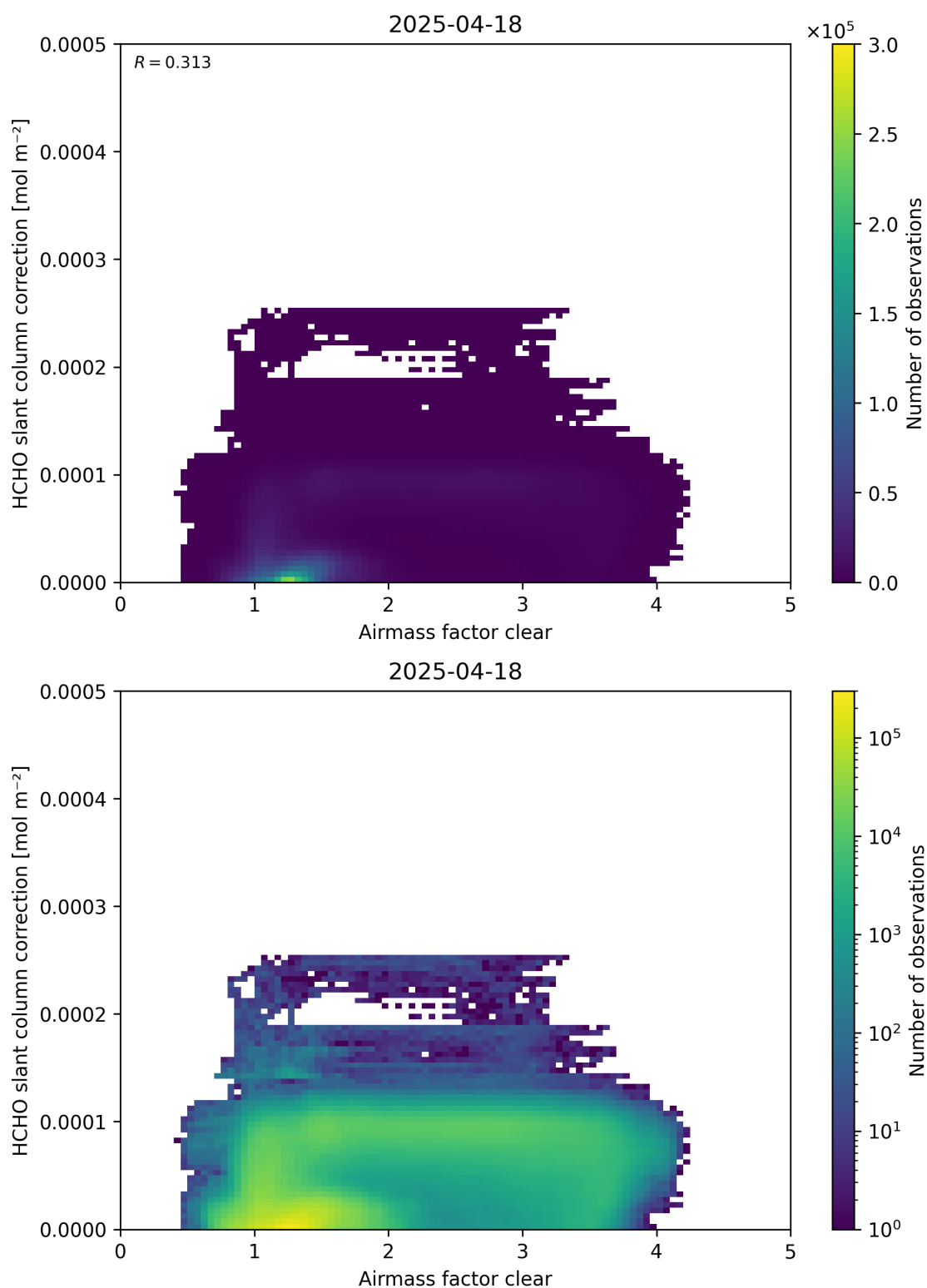
Figure 75: Scatter density plot of “Airmass factor clear” against “HCHO slant column correction” for 2025-04-18 to 2025-04-19.
