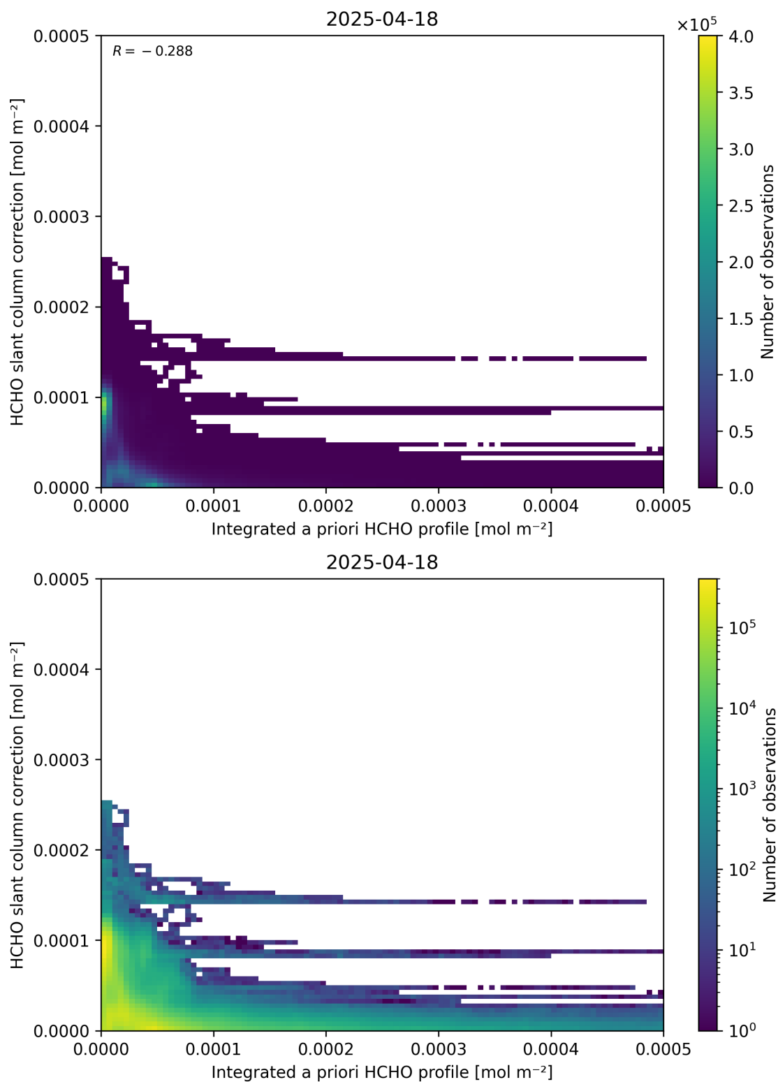
Figure 152: Scatter density plot of “Integrated a priori HCHO profile” against “HCHO slant column correction” for 2025-04-18 to 2025-04-19.
