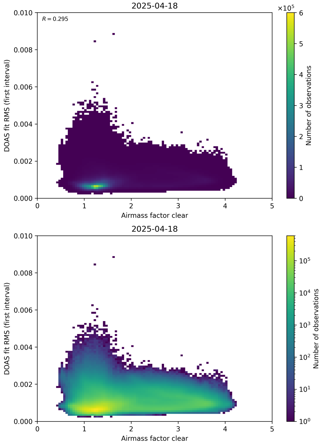
Figure 71: Scatter density plot of “Airmass factor clear” against “DOAS fit RMS (first interval)” for 2025-04-18 to 2025-04-19.
