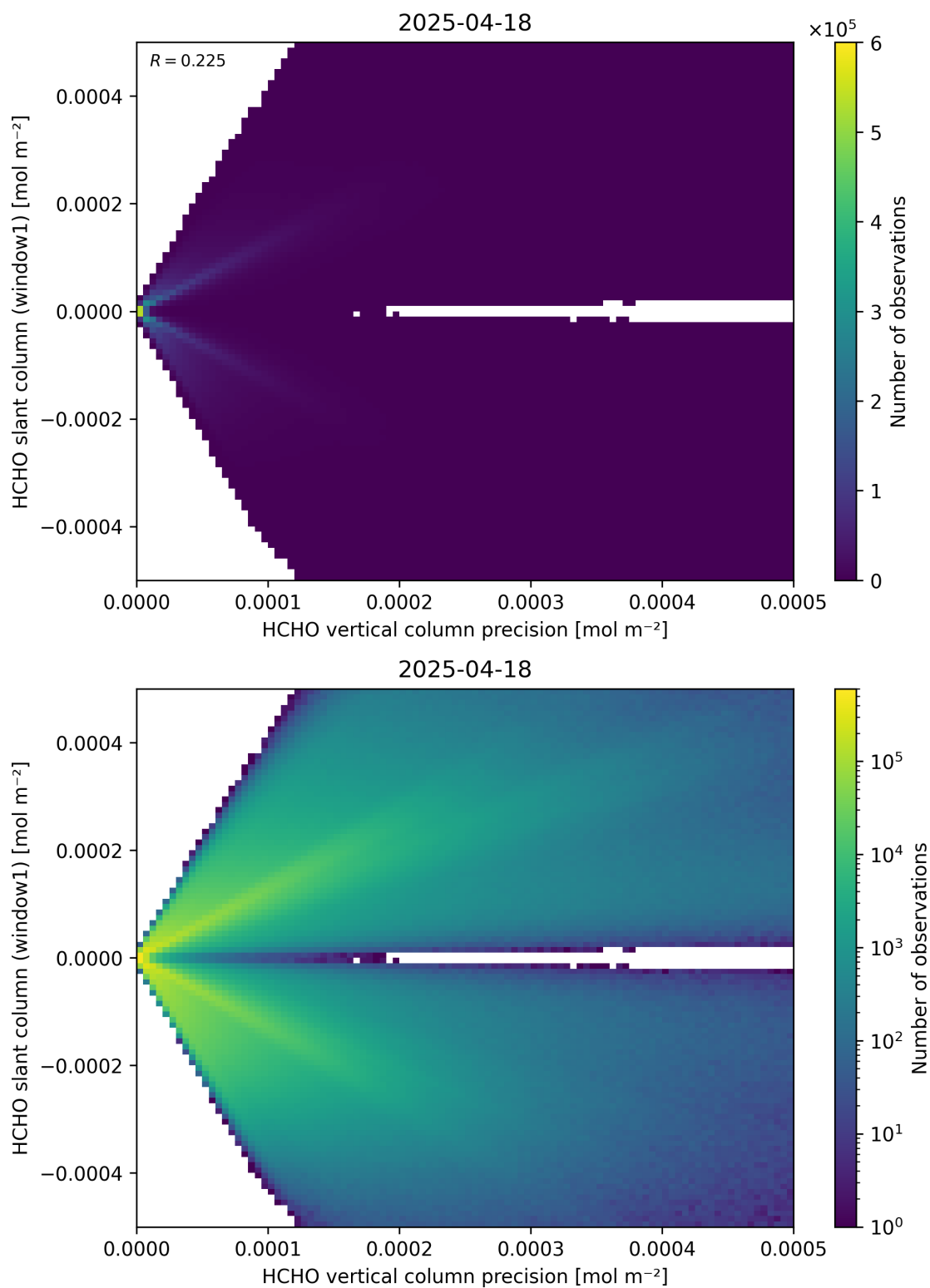
Figure 142: Scatter density plot of “HCHO vertical column precision” against “HCHO slant column (window1)” for 2025-04-18 to 2025-04-19.
