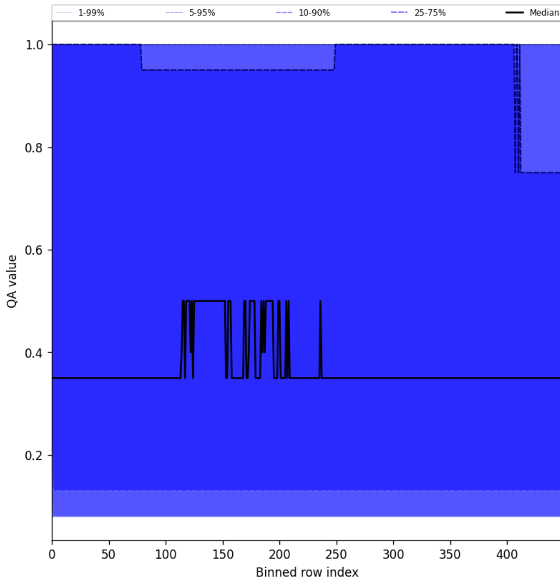
Figure 48: Along track statistics of “QA value” for 2025-04-18 to 2025-04-19
