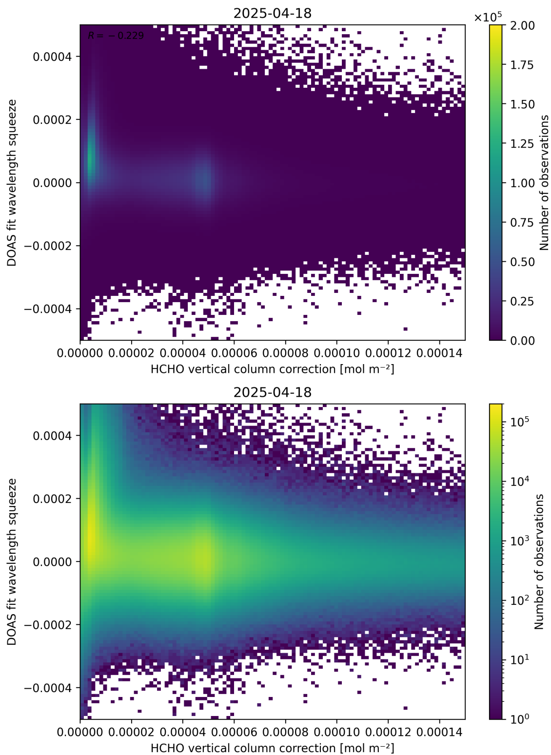
Figure 114: Scatter density plot of “HCHO vertical column correction” against “DOAS fit wavelength squeeze” for 2025-04-18 to 2025-04-19.
