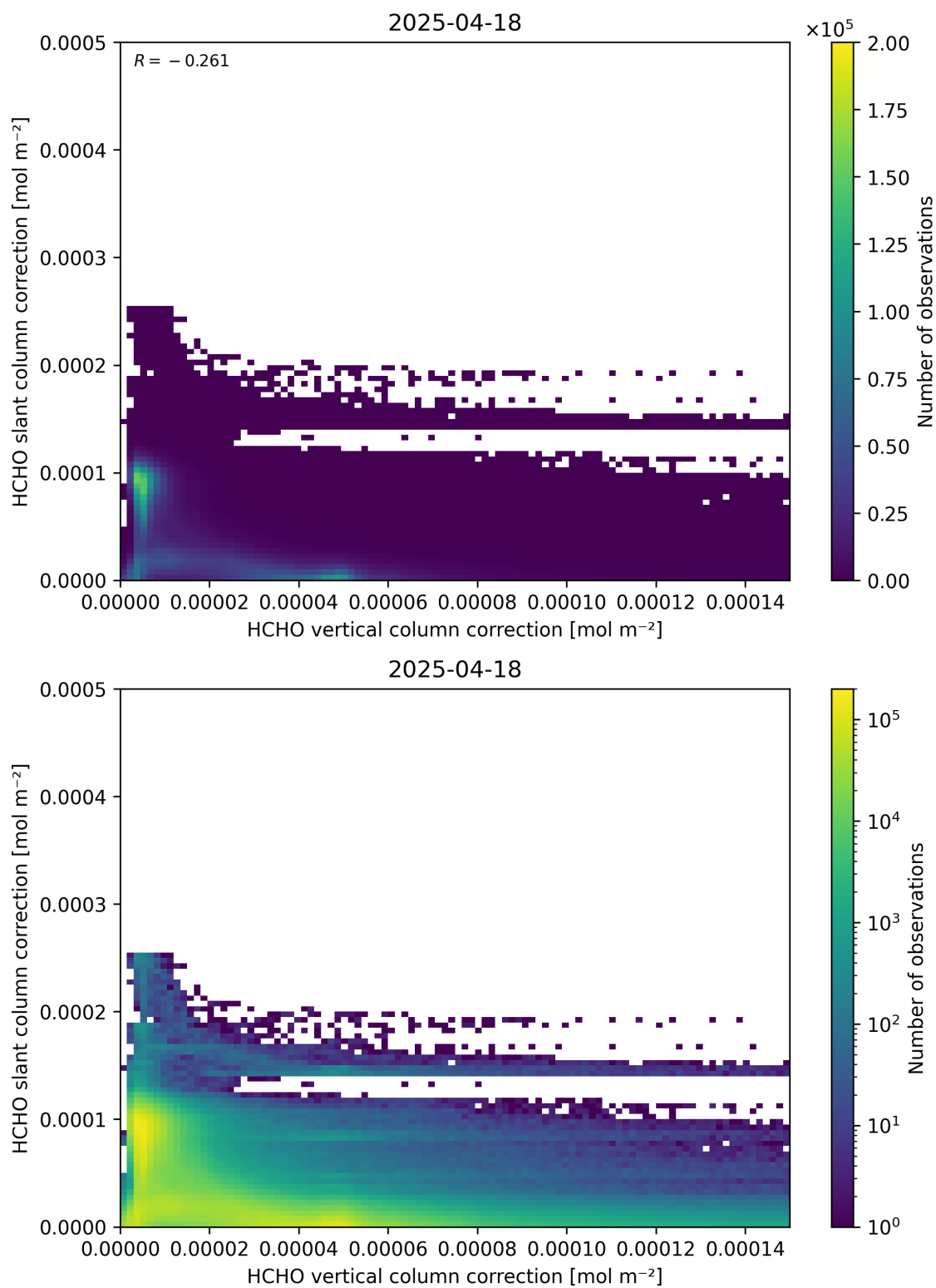
Figure 117: Scatter density plot of “HCHO vertical column correction” against “HCHO slant column correction” for 2025-04-18 to 2025-04-19.
