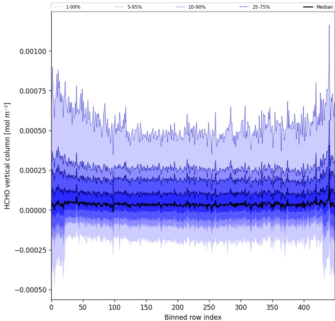
Figure 49: Along track statistics of “HCHO vertical column” for 2025-04-18 to 2025-04-19
