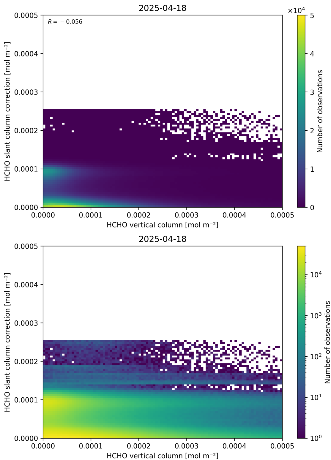
Figure 128: Scatter density plot of “HCHO vertical column” against “HCHO slant column correction” for 2025-04-18 to 2025-04-19.
