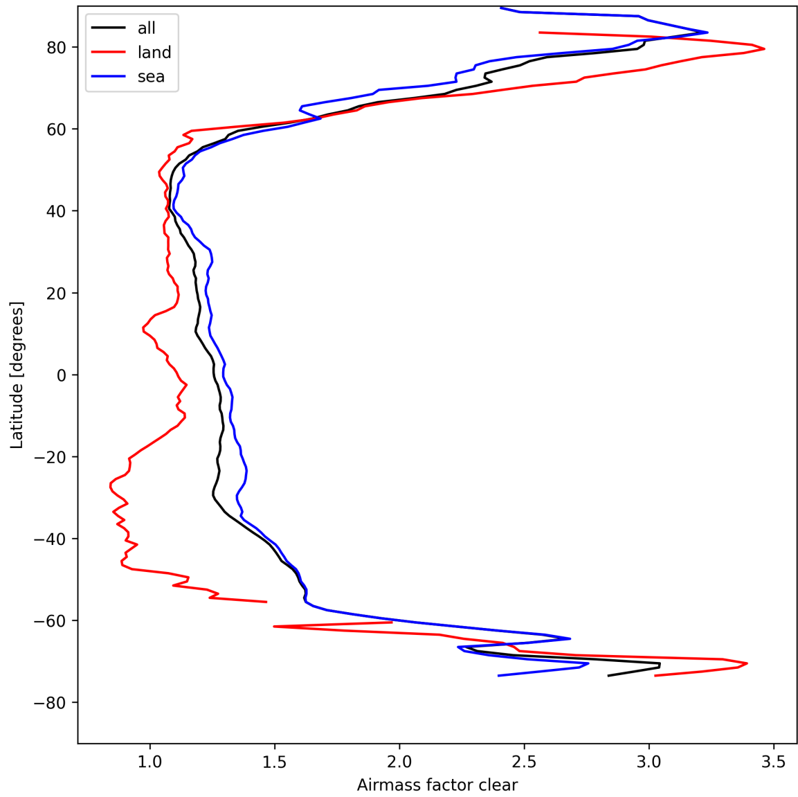
Figure 28: Zonal average of “Airmass factor clear” for 2025-04-18 to 2025-04-19.
