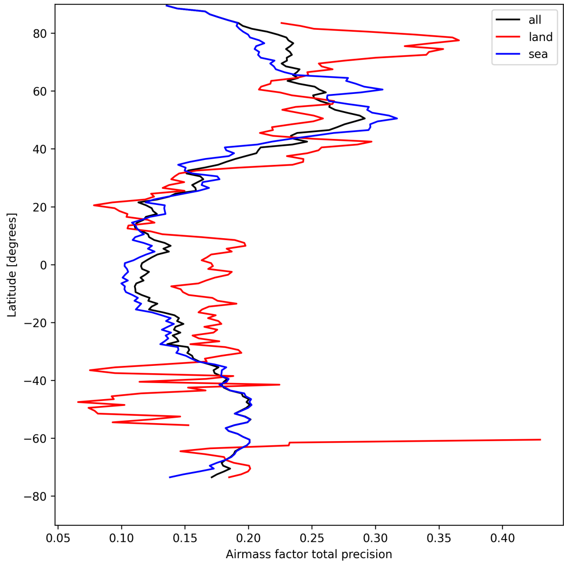
Figure 27: Zonal average of “Airmass factor total precision” for 2025-04-18 to 2025-04-19.
