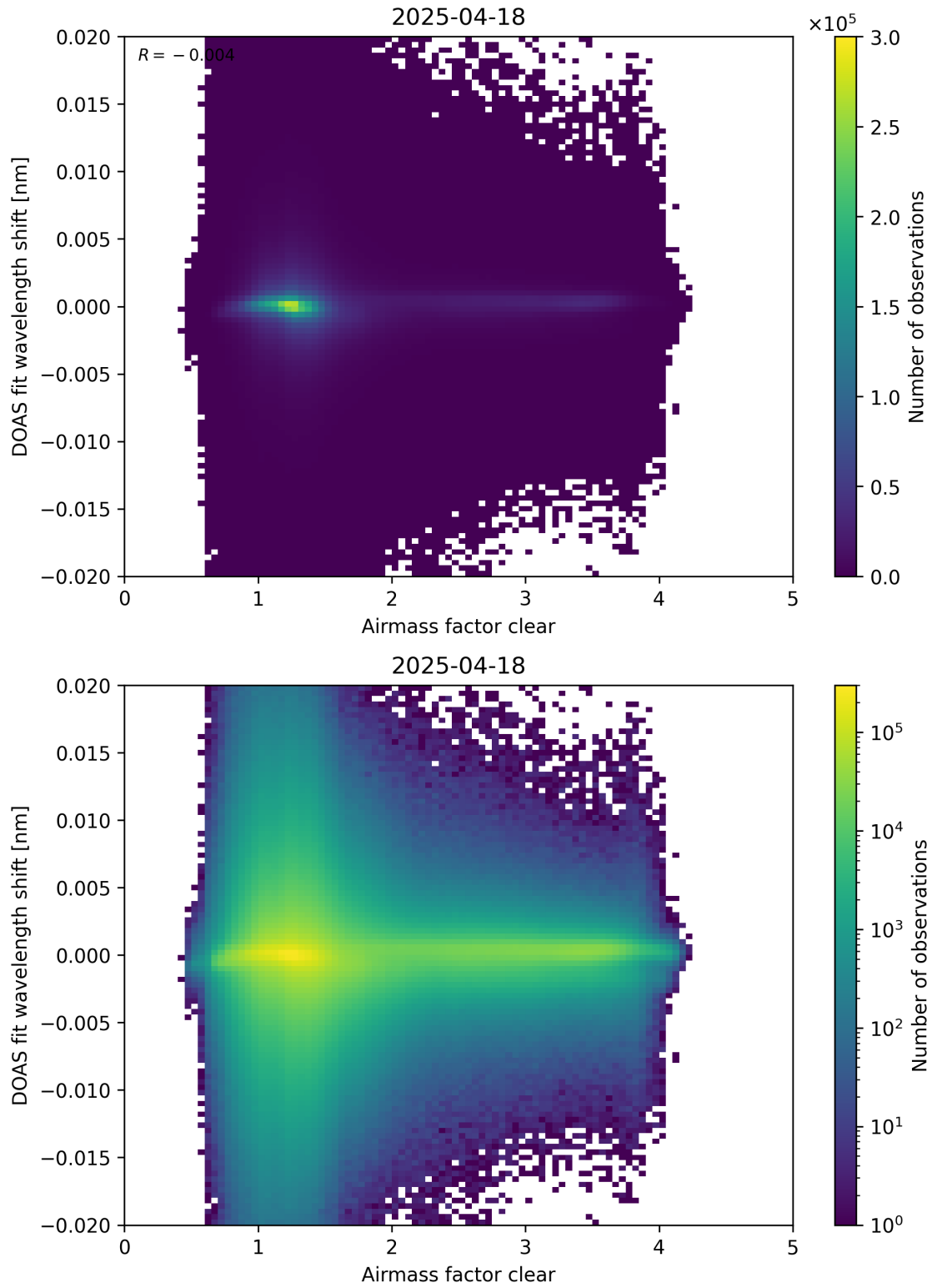
Figure 72: Scatter density plot of “Airmass factor clear” against “DOAS fit wavelength shift” for 2025-04-18 to 2025-04-19.
