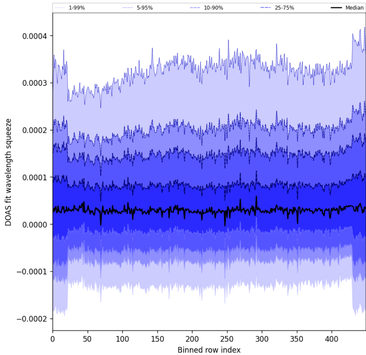
Figure 59: Along track statistics of “DOAS fit wavelength squeeze” for 2025-04-18 to 2025-04-19
