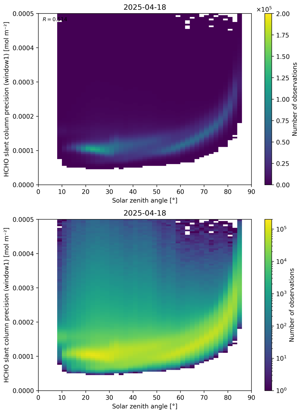
Figure 174: Scatter density plot of “Solar zenith angle” against “HCHO slant column precision (window1)” for 2025-04-18 to 2025-04-19.
