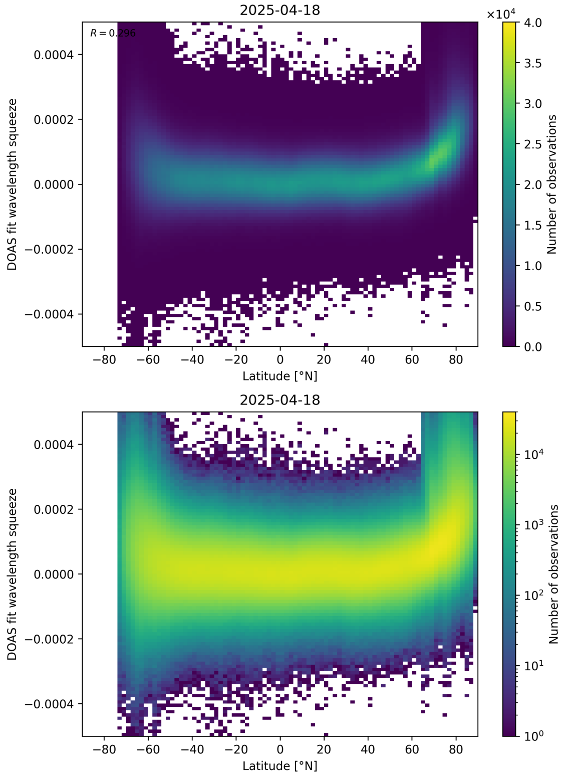
Figure 155: Scatter density plot of “Latitude” against “DOAS fit wavelength squeeze” for 2025-04-18 to 2025-04-19.
