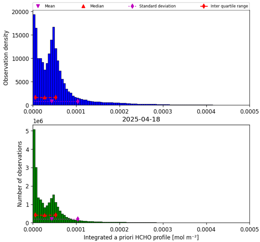
Figure 43: Histogram of “Integrated a priori HCHO profile” for 2025-04-18 to 2025-04-19
