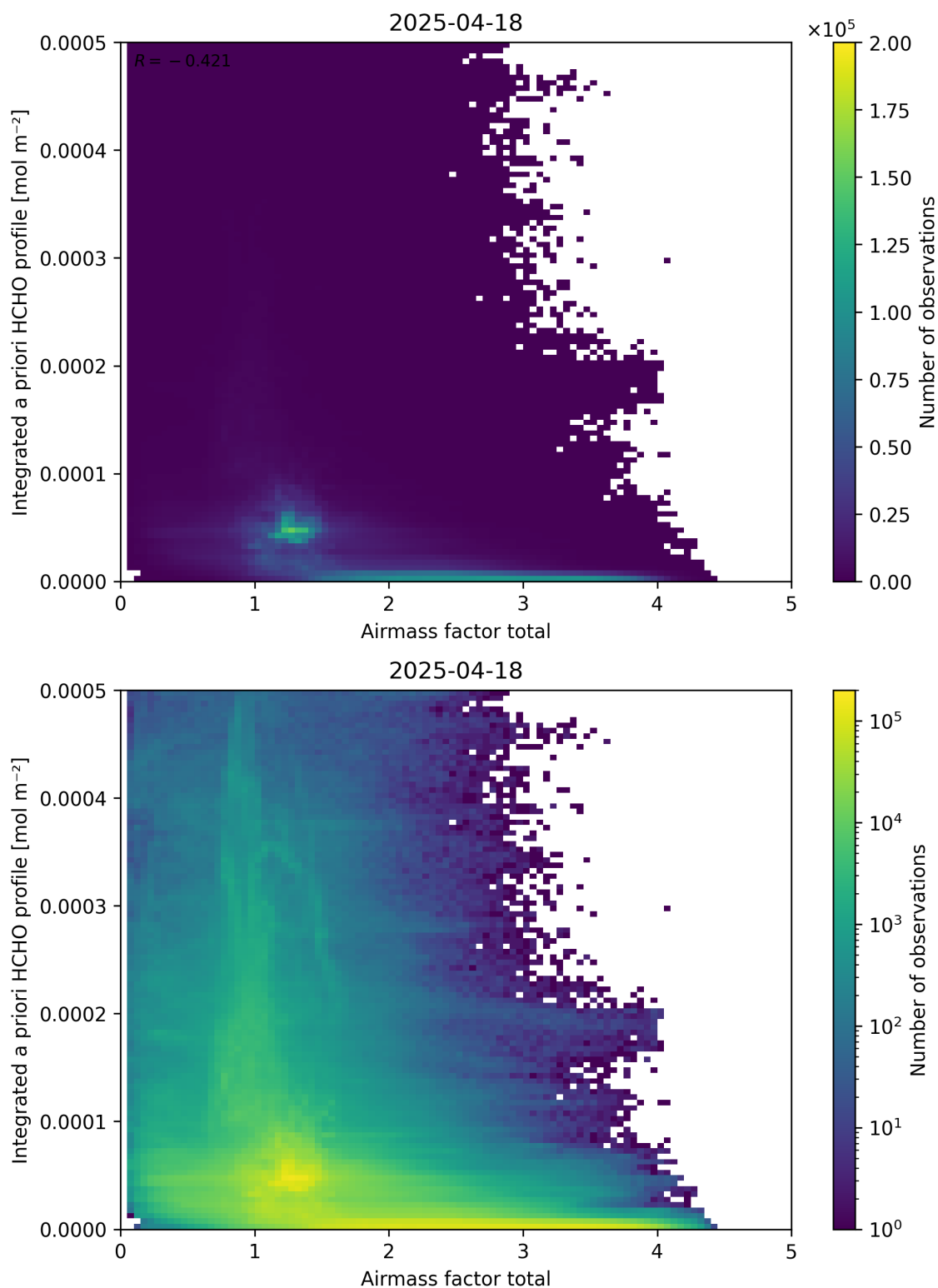
Figure 104: Scatter density plot of “Airmass factor total” against “Integrated a priori HCHO profile” for 2025-04-18 to 2025-04-19.
