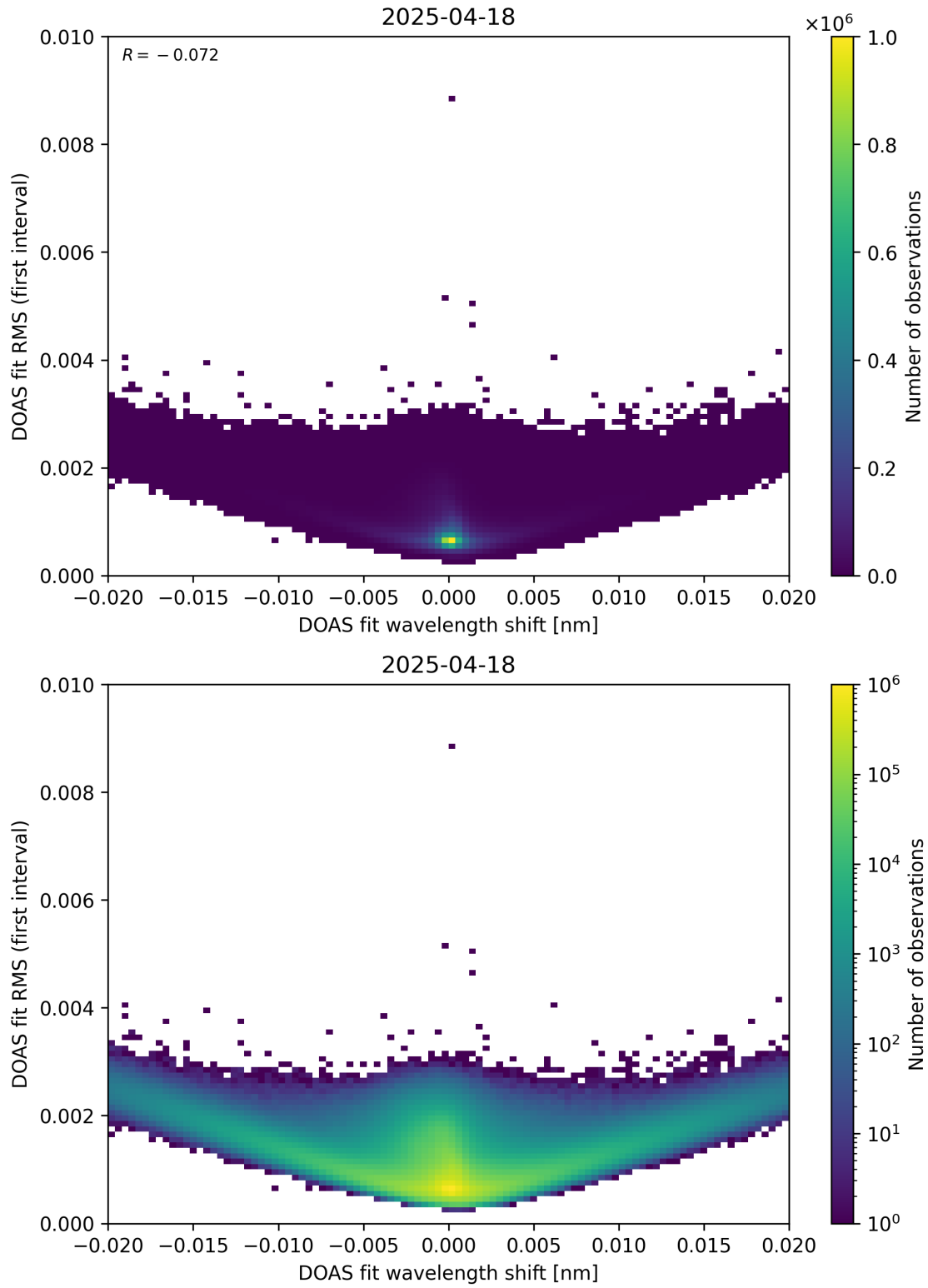
Figure 64: Scatter density plot of “DOAS fit wavelength shift” against “DOAS fit RMS (first interval)” for 2025-04-18 to 2025-04-19.
