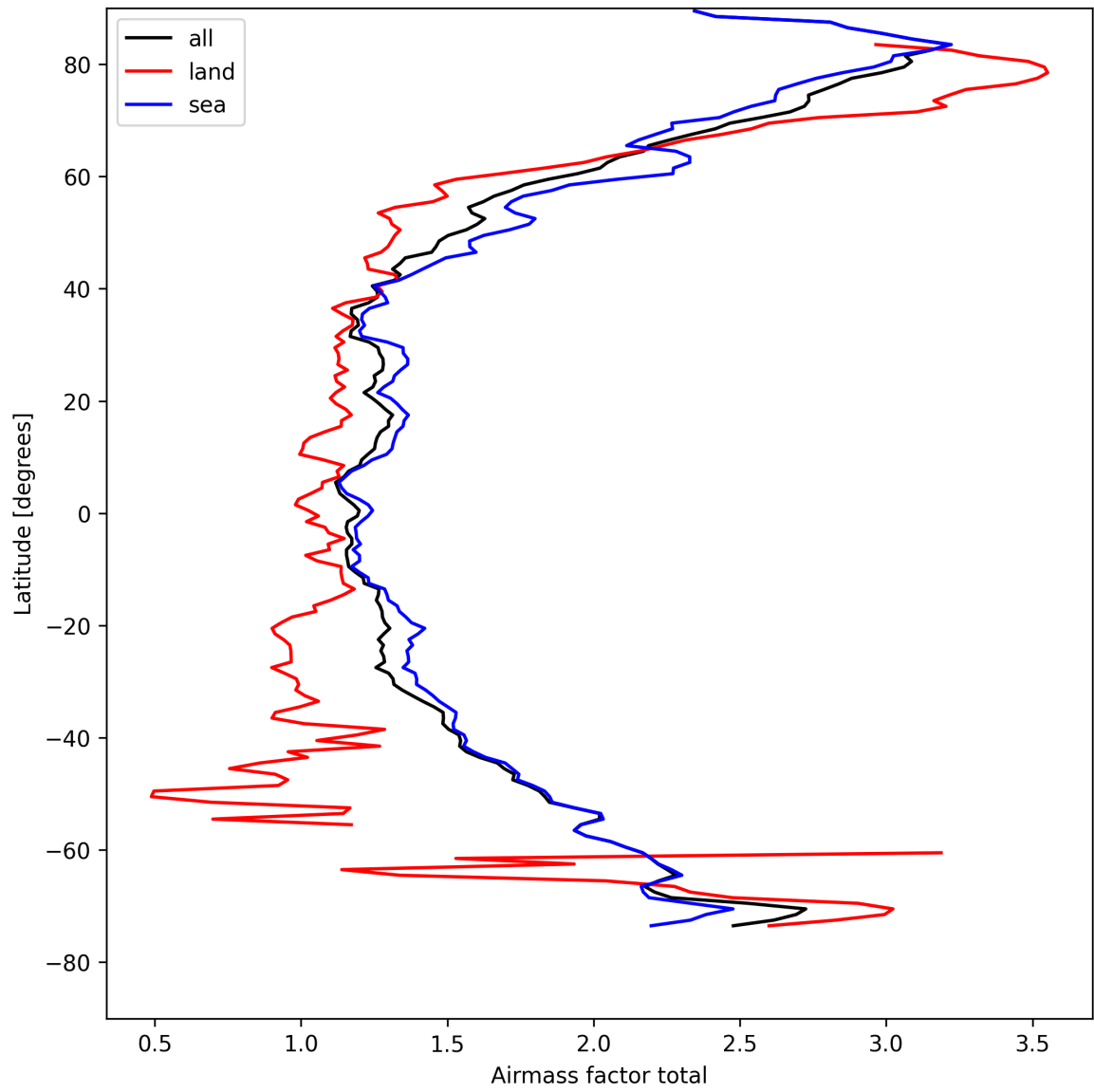
Figure 26: Zonal average of “Airmass factor total” for 2025-04-18 to 2025-04-19.
