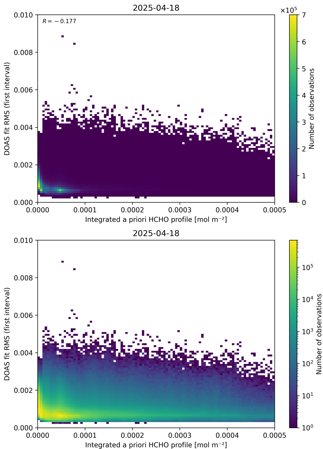
Figure 148: Scatter density plot of “Integrated a priori HCHO profile” against “DOAS fit RMS (first interval)” for 2025-04-18 to 2025-04-19.
