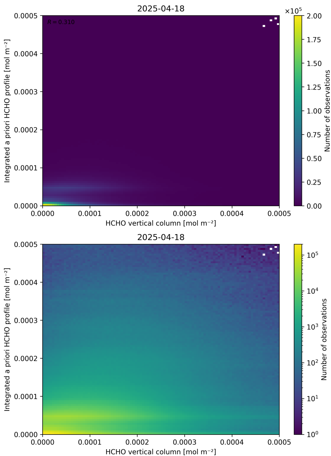
Figure 135: Scatter density plot of “HCHO vertical column” against “Integrated a priori HCHO profile” for 2025-04-18 to 2025-04-19.
