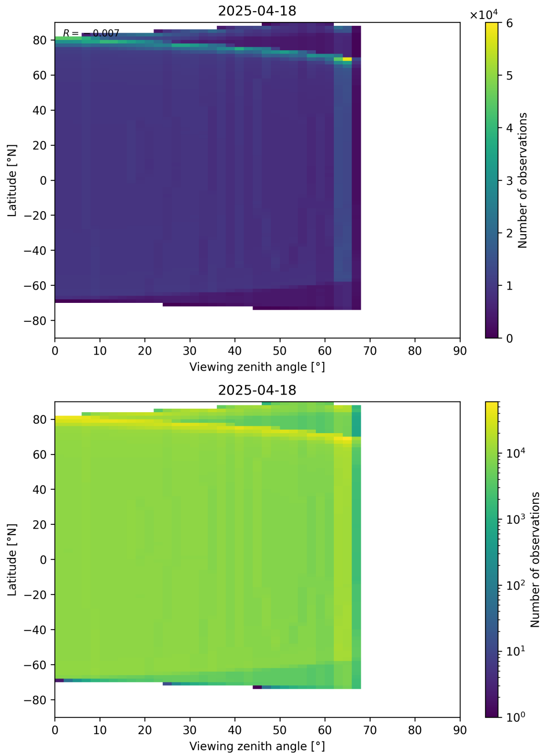
Figure 196: Scatter density plot of “Viewing zenith angle” against “Latitude” for 2025-04-18 to 2025-04-19.
