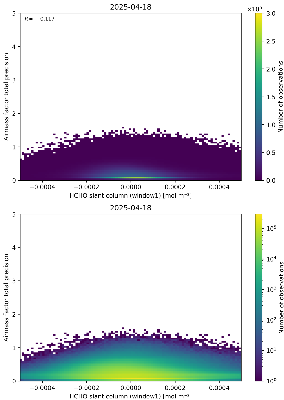
Figure 86: Scatter density plot of “HCHO slant column (window1)” against “Airmass factor total precision” for 2025-04-18 to 2025-04-19.
