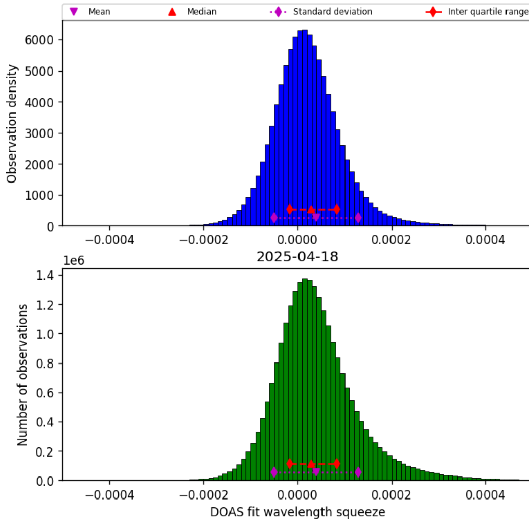
Figure 45: Histogram of “DOAS fit wavelength squeeze” for 2025-04-18 to 2025-04-19
