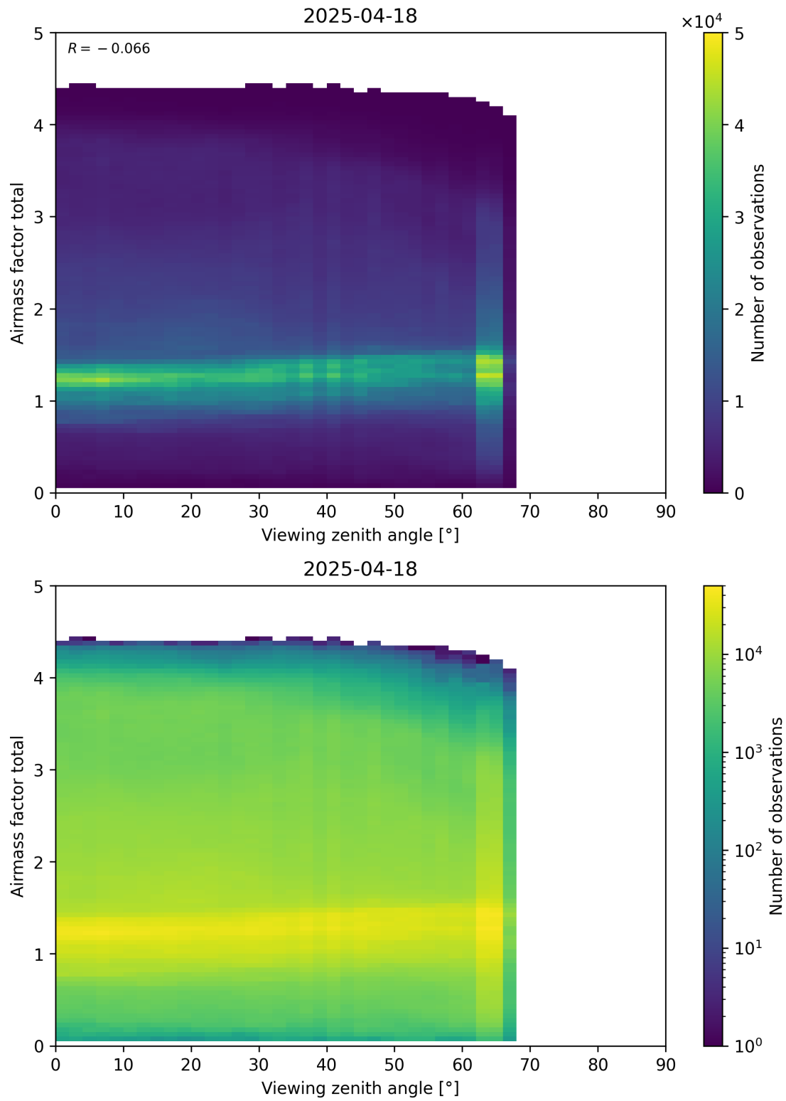
Figure 190: Scatter density plot of “Viewing zenith angle” against “Airmass factor total” for 2025-04-18 to 2025-04-19.
