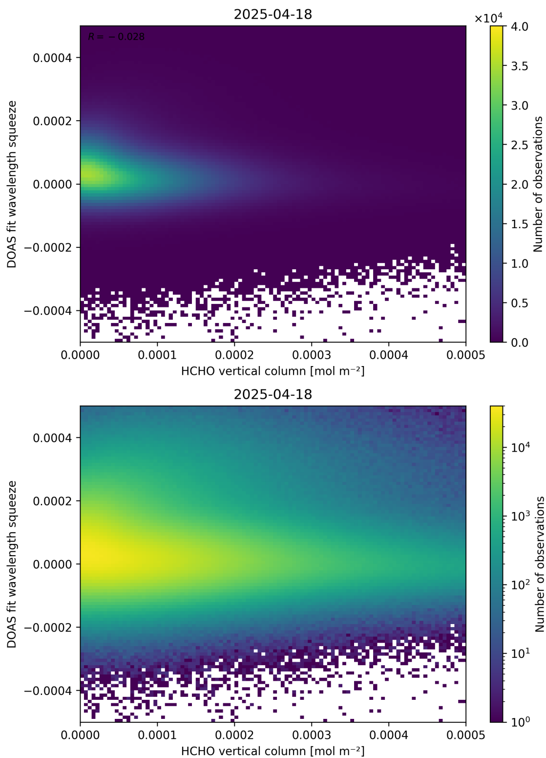
Figure 125: Scatter density plot of “HCHO vertical column” against “DOAS fit wavelength squeeze” for 2025-04-18 to 2025-04-19.
