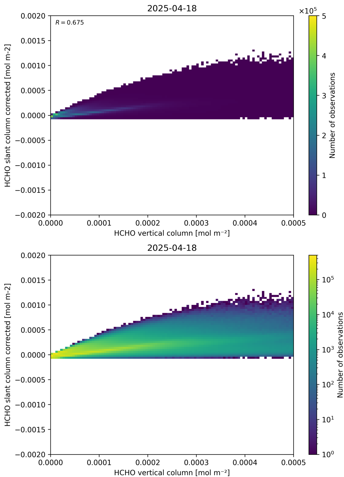
Figure 127: Scatter density plot of “HCHO vertical column” against “HCHO slant column corrected” for 2025-04-18 to 2025-04-19.
