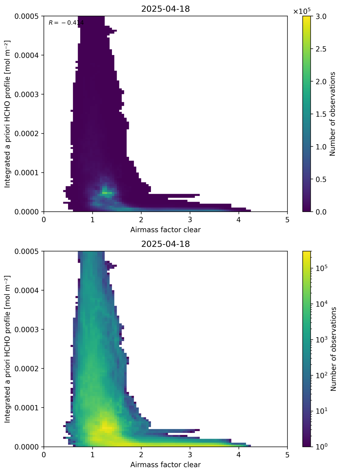
Figure 76: Scatter density plot of “Airmass factor clear” against “Integrated a priori HCHO profile” for 2025-04-18 to 2025-04-19.
