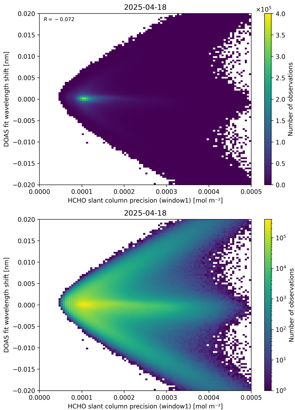
Figure 89: Scatter density plot of “HCHO slant column precision (window1)” against “DOAS fit wavelength shift” for 2025-04-18 to 2025-04-19.
