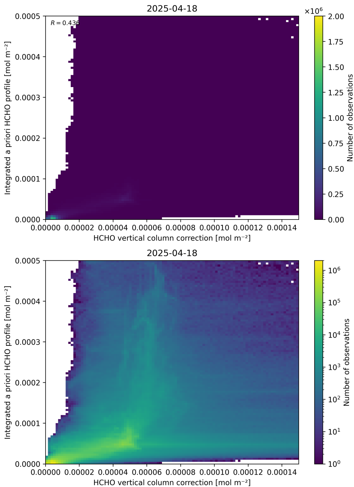
Figure 122: Scatter density plot of “HCHO vertical column correction” against “Integrated a priori HCHO profile” for 2025-04-18 to 2025-04-19.
