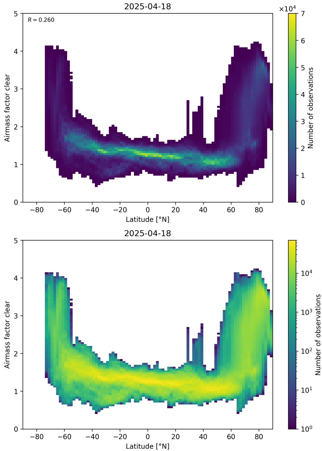
Figure 156: Scatter density plot of “Latitude” against “Airmass factor clear” for 2025-04-18 to 2025-04-19.
