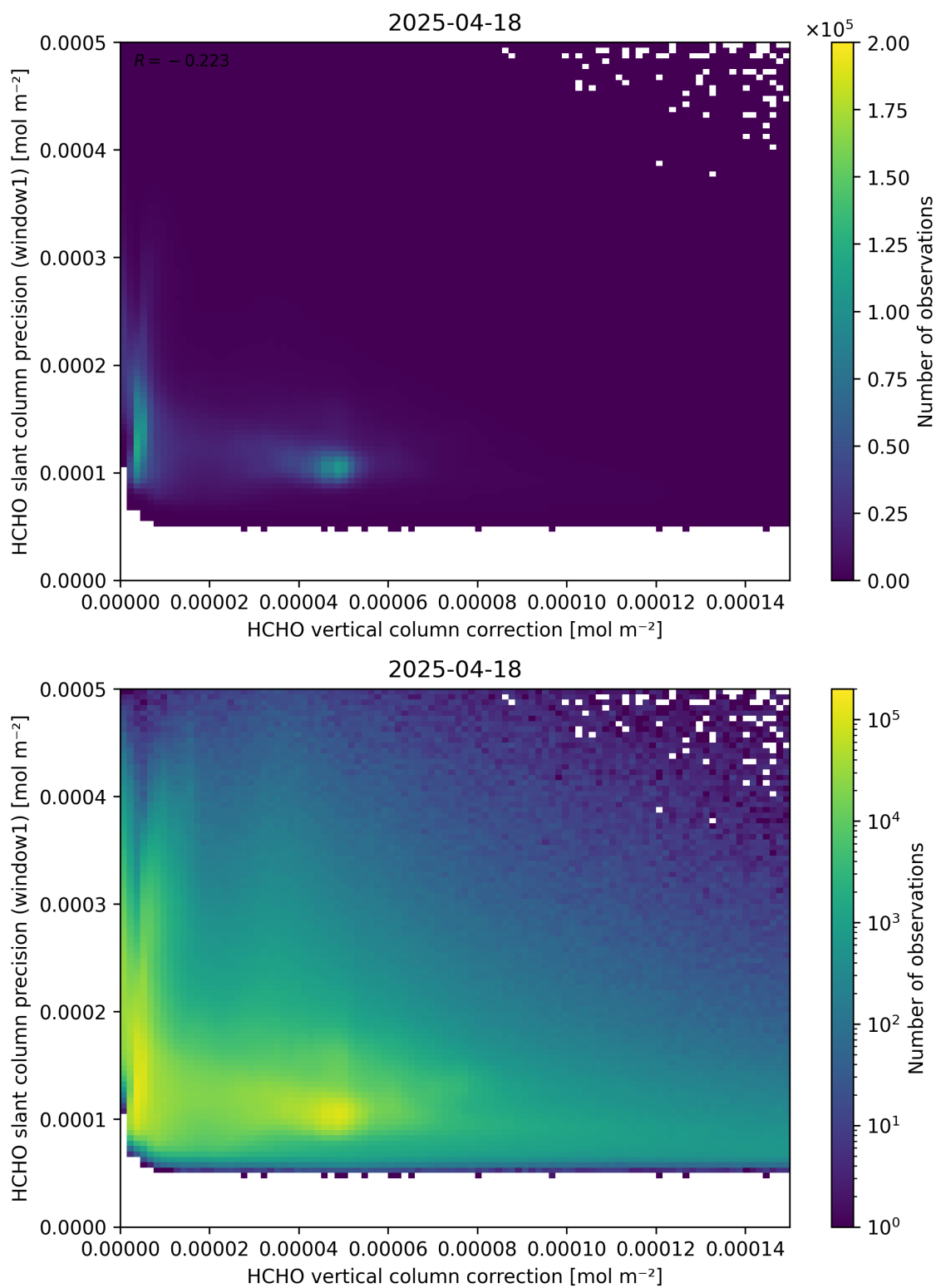
Figure 119: Scatter density plot of “HCHO vertical column correction” against “HCHO slant column precision (window1)” for 2025-04-18 to 2025-04-19.
