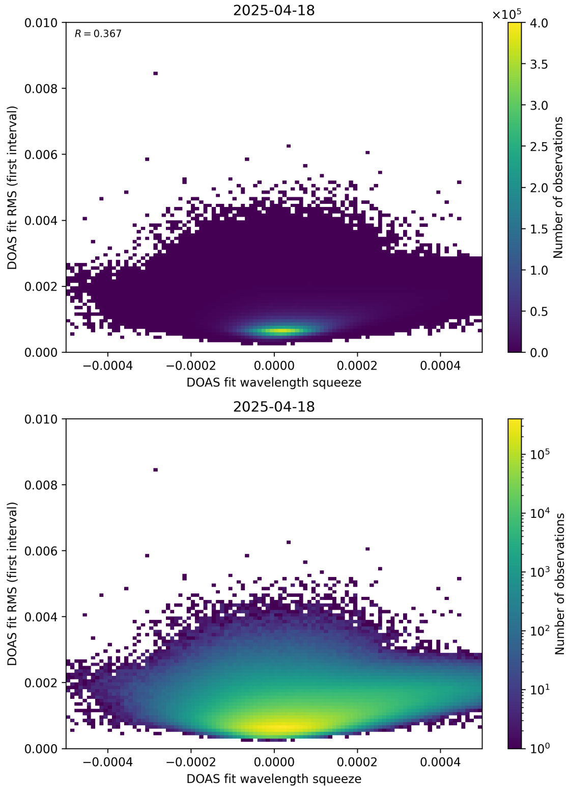
Figure 68: Scatter density plot of “DOAS fit wavelength squeeze” against “DOAS fit RMS (first interval)” for 2025-04-18 to 2025-04-19.
