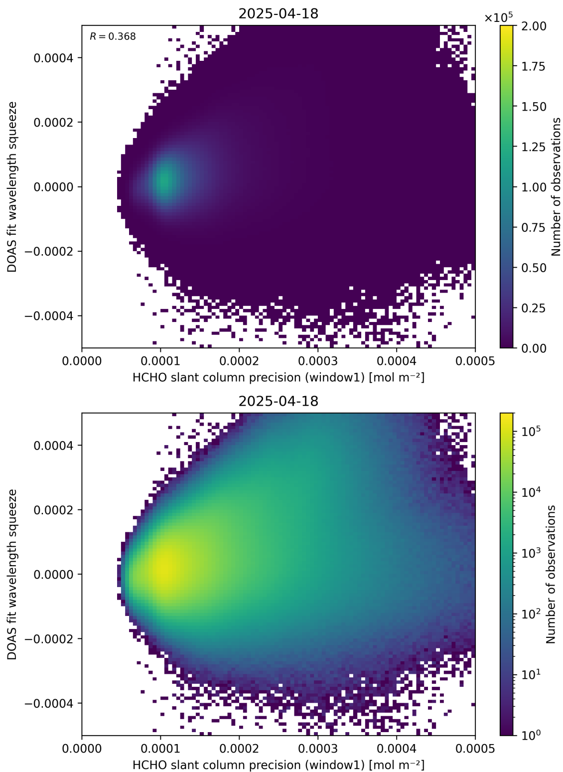
Figure 90: Scatter density plot of “HCHO slant column precision (window1)” against “DOAS fit wavelength squeeze” for 2025-04-18 to 2025-04-19.
