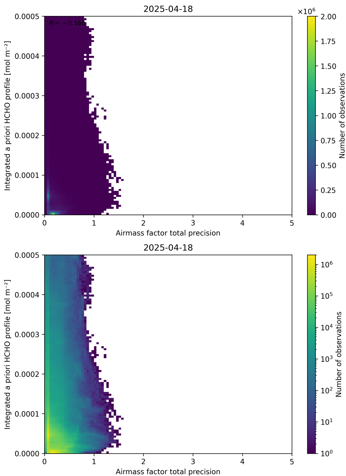
Figure 111: Scatter density plot of “Airmass factor total precision” against “Integrated a priori HCHO profile” for 2025-04-18 to 2025-04-19.
