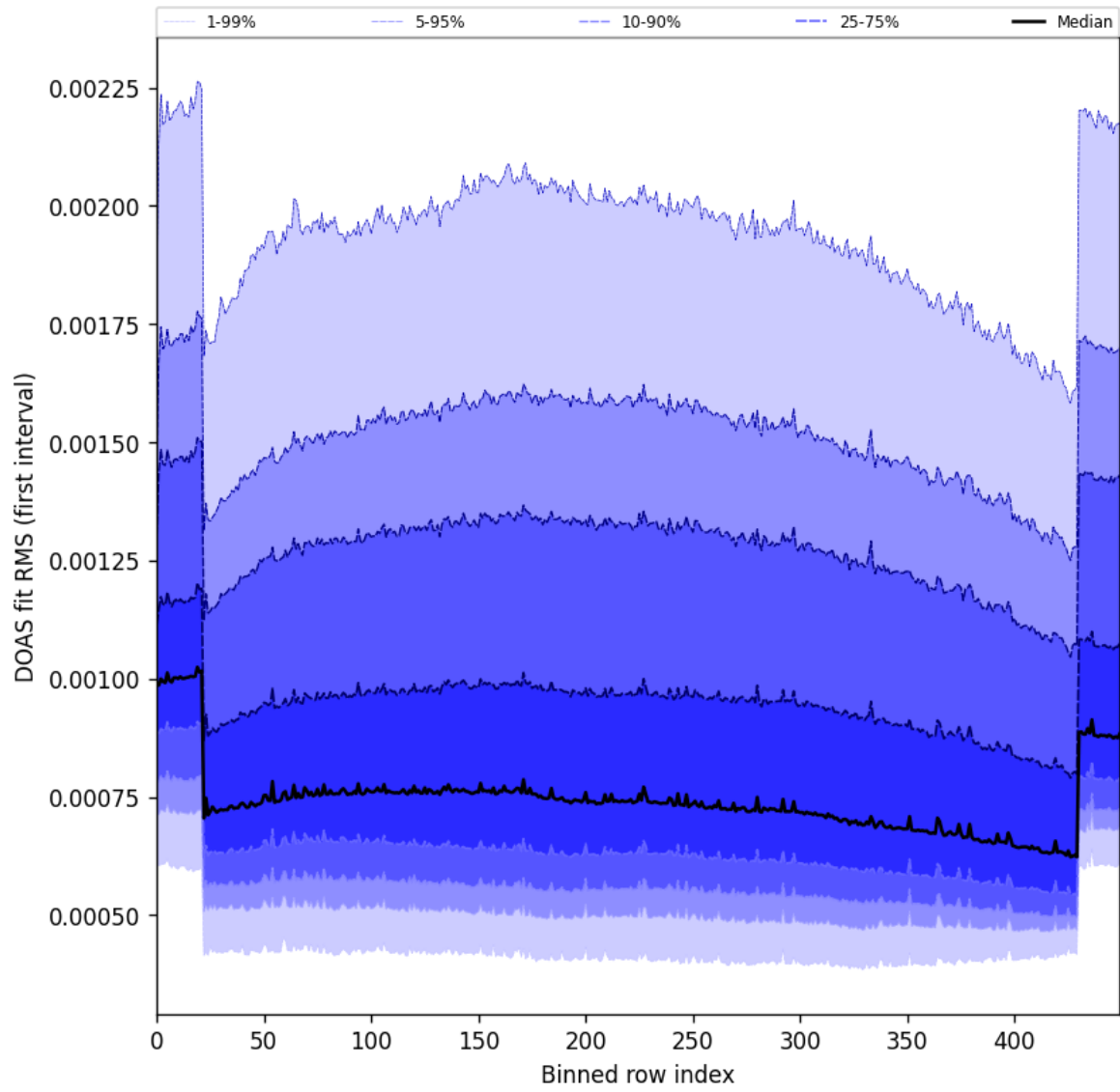
Figure 60: Along track statistics of “DOAS fit RMS (first interval)” for 2025-04-18 to 2025-04-19
