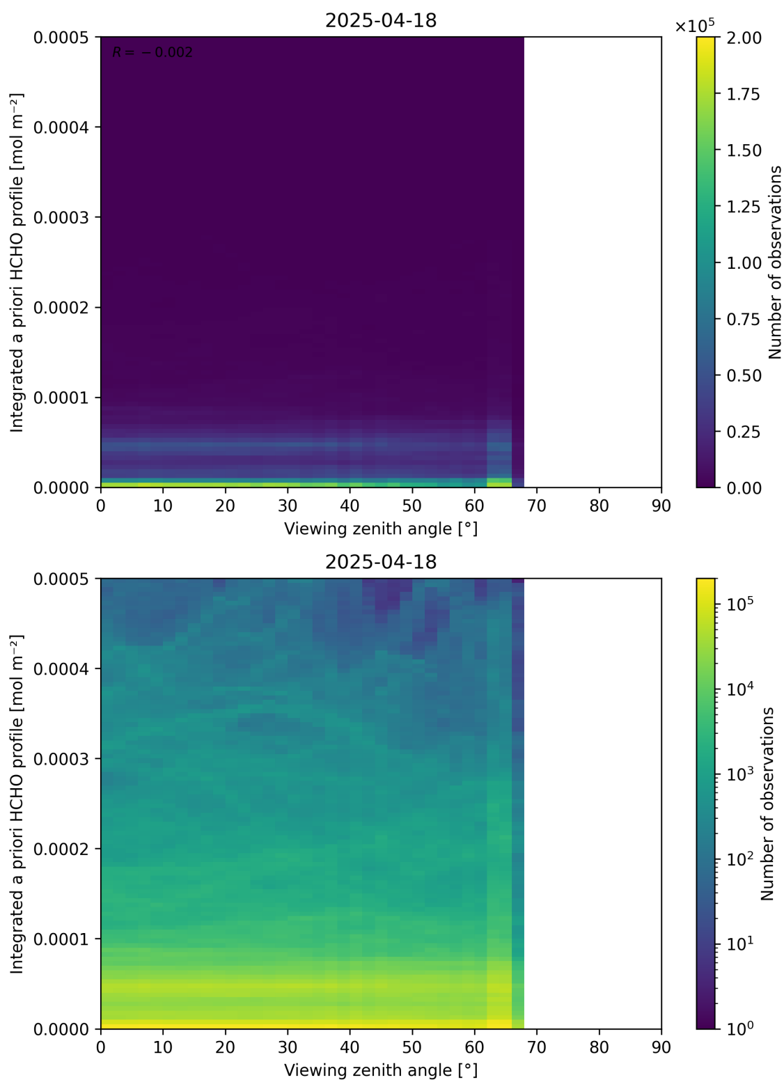
Figure 195: Scatter density plot of “Viewing zenith angle” against “Integrated a priori HCHO profile” for 2025-04-18 to 2025-04-19.
