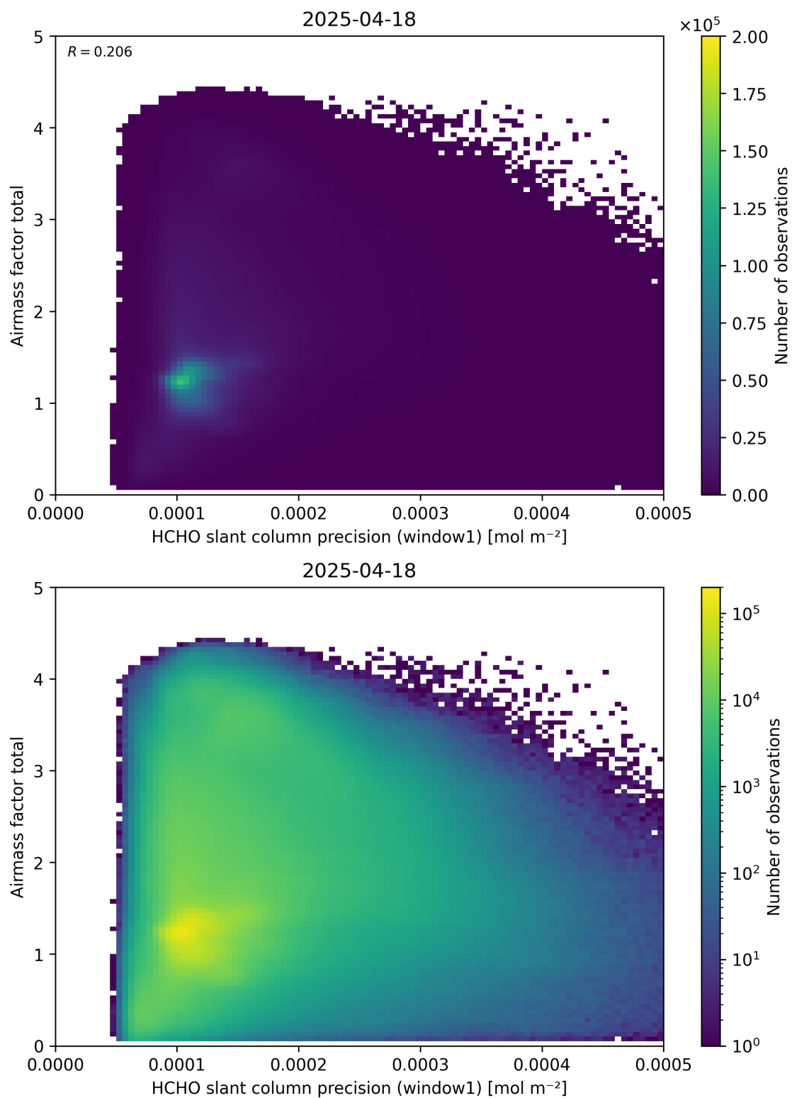
Figure 94: Scatter density plot of “HCHO slant column precision (window1)” against “Airmass factor total” for 2025-04-18 to 2025-04-19.
