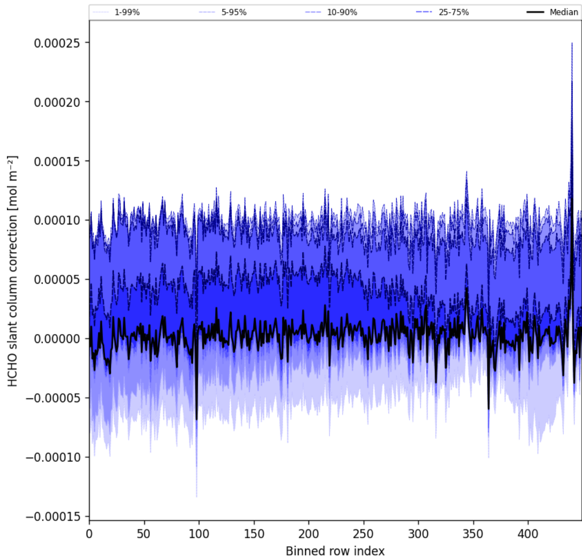
Figure 61: Along track statistics of “HCHO slant column correction” for 2025-04-18 to 2025-04-19
