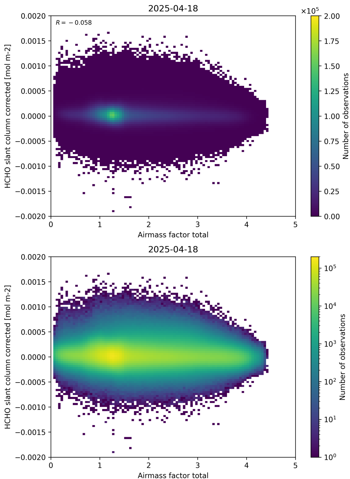
Figure 101: Scatter density plot of “Airmass factor total” against “HCHO slant column corrected” for 2025-04-18 to 2025-04-19.
