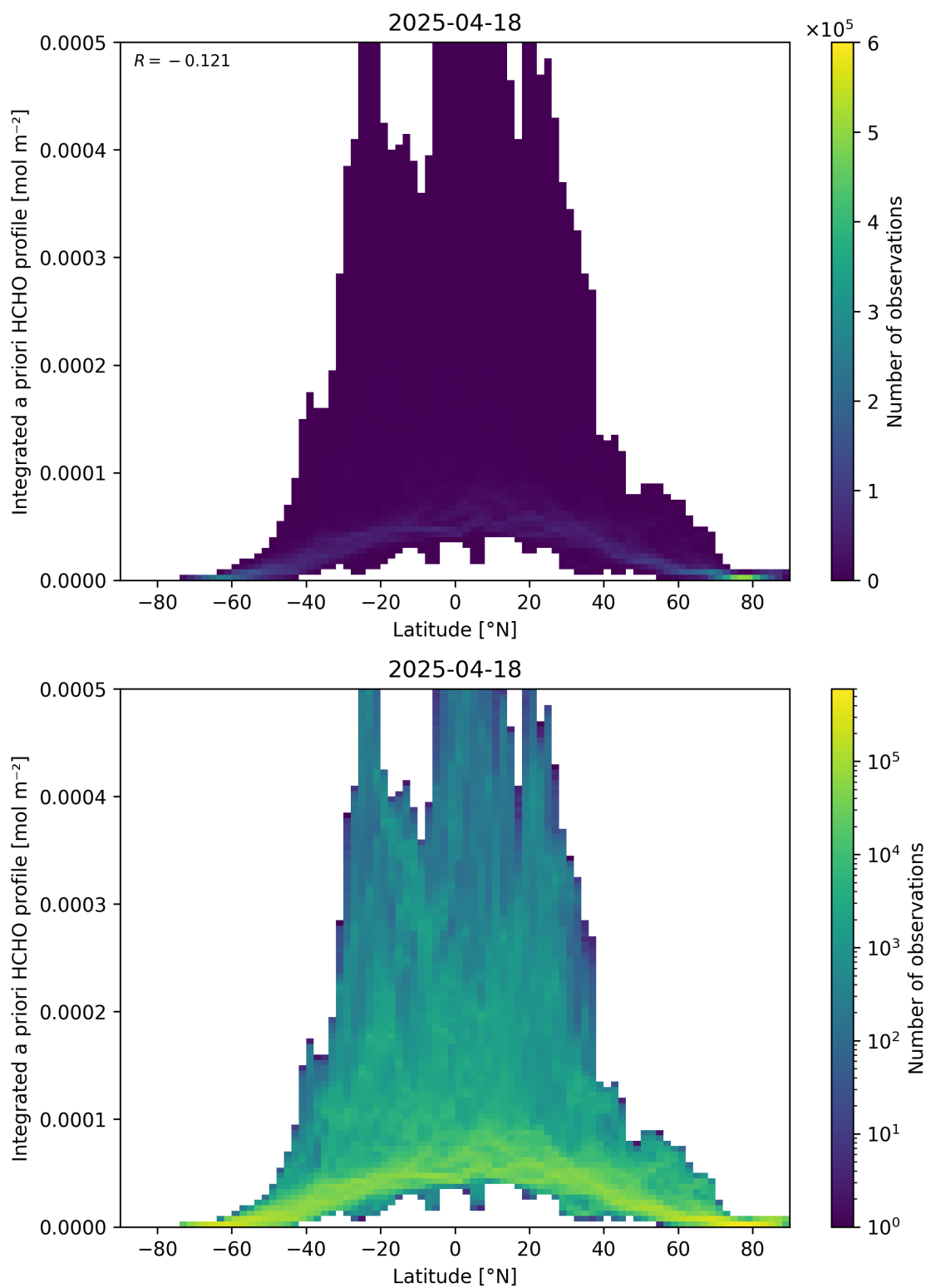
Figure 166: Scatter density plot of “Latitude” against “Integrated a priori HCHO profile” for 2025-04-18 to 2025-04-19.
