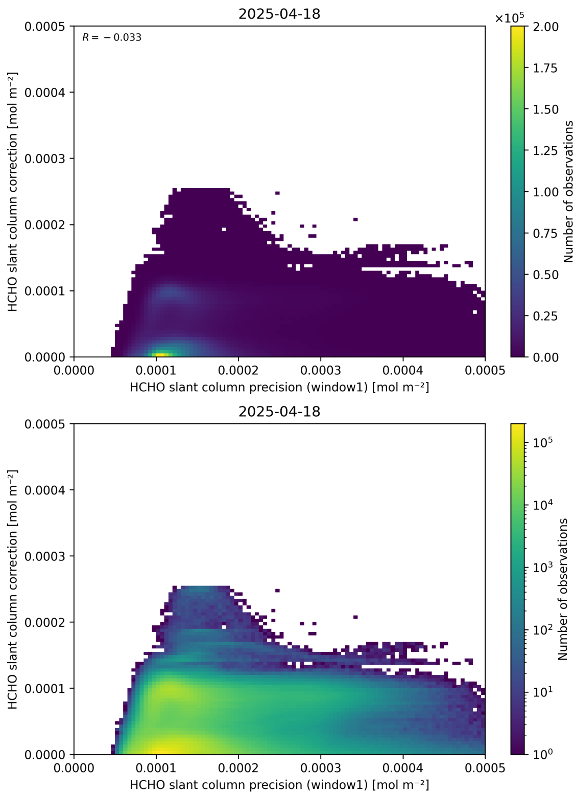
Figure 93: Scatter density plot of “HCHO slant column precision (window1)” against “HCHO slant column correction” for 2025-04-18 to 2025-04-19.
