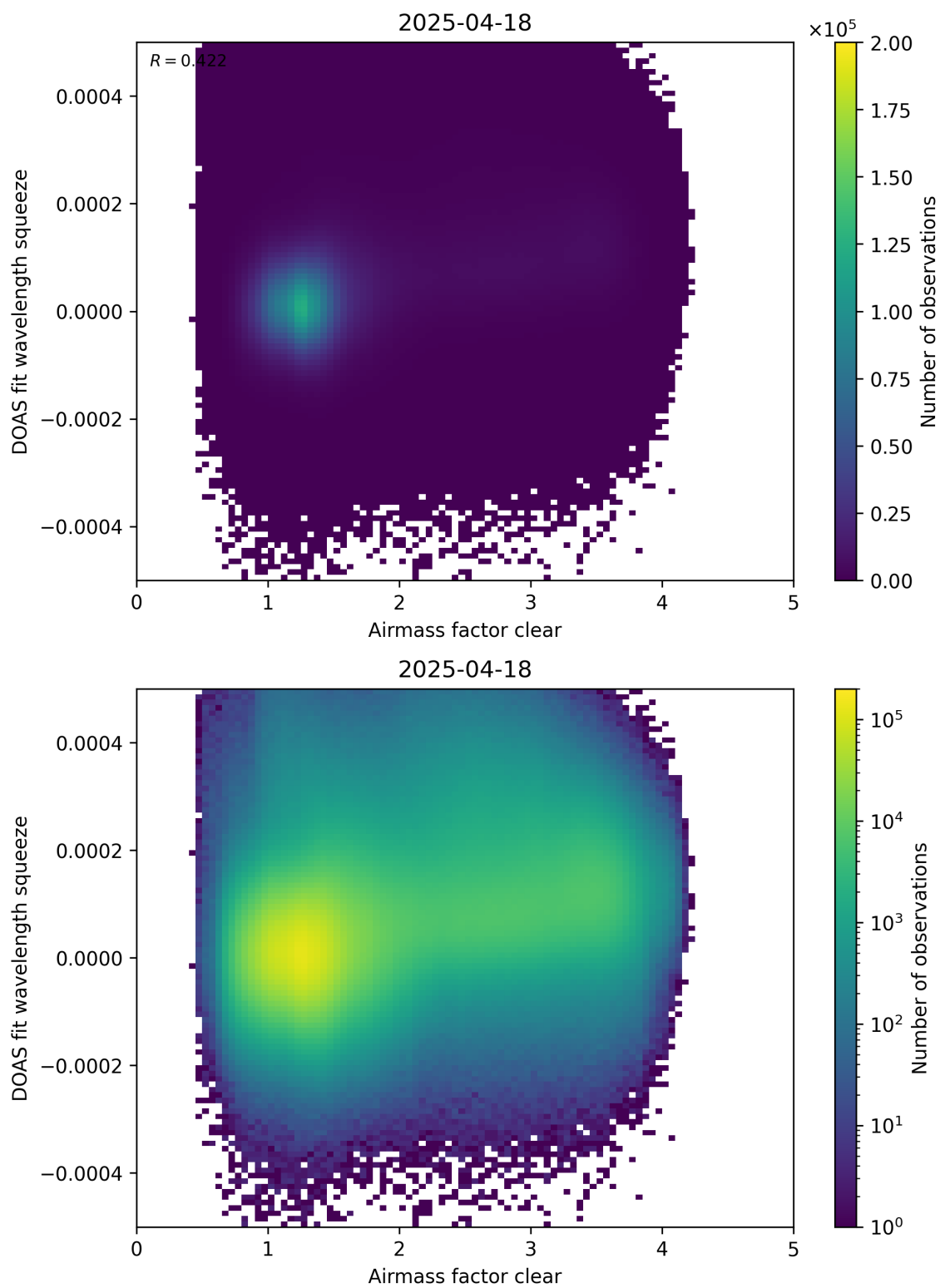
Figure 73: Scatter density plot of “Airmass factor clear” against “DOAS fit wavelength squeeze” for 2025-04-18 to 2025-04-19.
