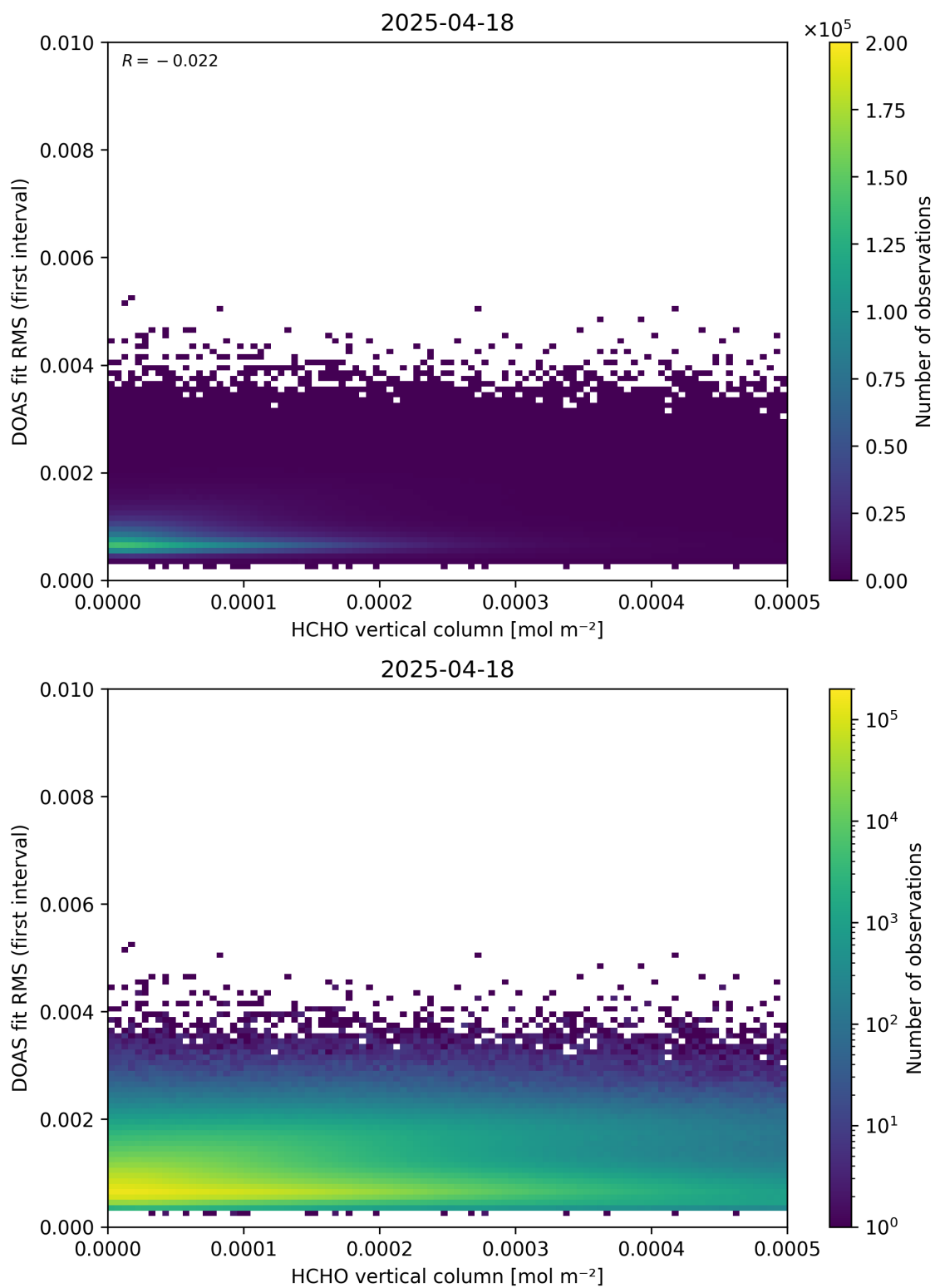
Figure 123: Scatter density plot of “HCHO vertical column” against “DOAS fit RMS (first interval)” for 2025-04-18 to 2025-04-19.
