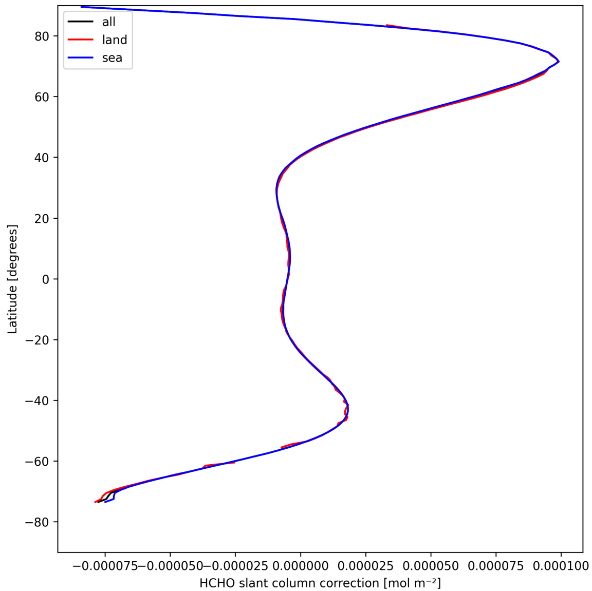
Figure 33: Zonal average of “HCHO slant column correction” for 2025-04-18 to 2025-04-19.
