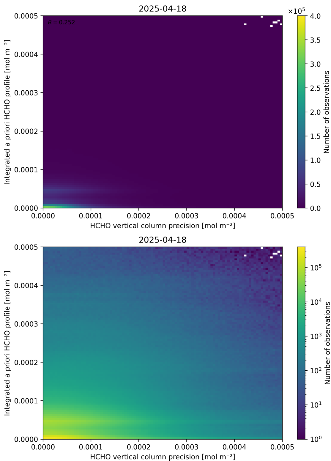
Figure 147: Scatter density plot of “HCHO vertical column precision” against “Integrated a priori HCHO profile” for 2025-04-18 to 2025-04-19.
