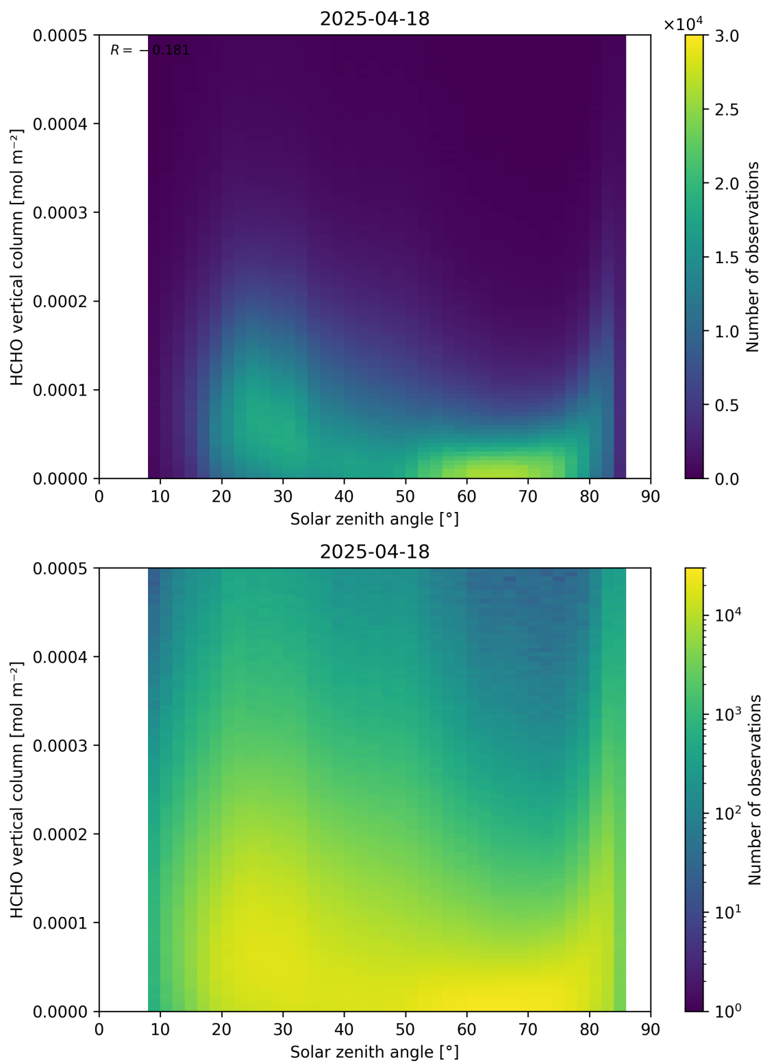
Figure 177: Scatter density plot of “Solar zenith angle” against “HCHO vertical column” for 2025-04-18 to 2025-04-19.
