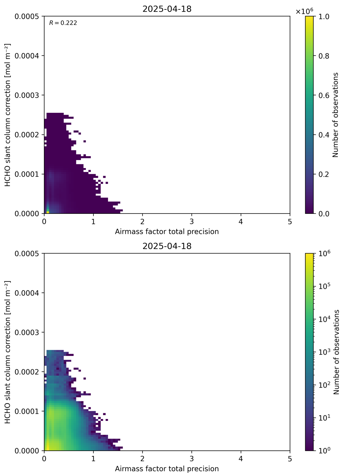
Figure 110: Scatter density plot of “Airmass factor total precision” against “HCHO slant column correction” for 2025-04-18 to 2025-04-19.
