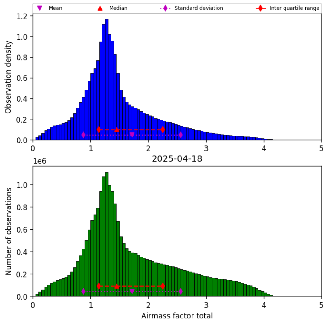
Figure 40: Histogram of “Airmass factor total” for 2025-04-18 to 2025-04-19
