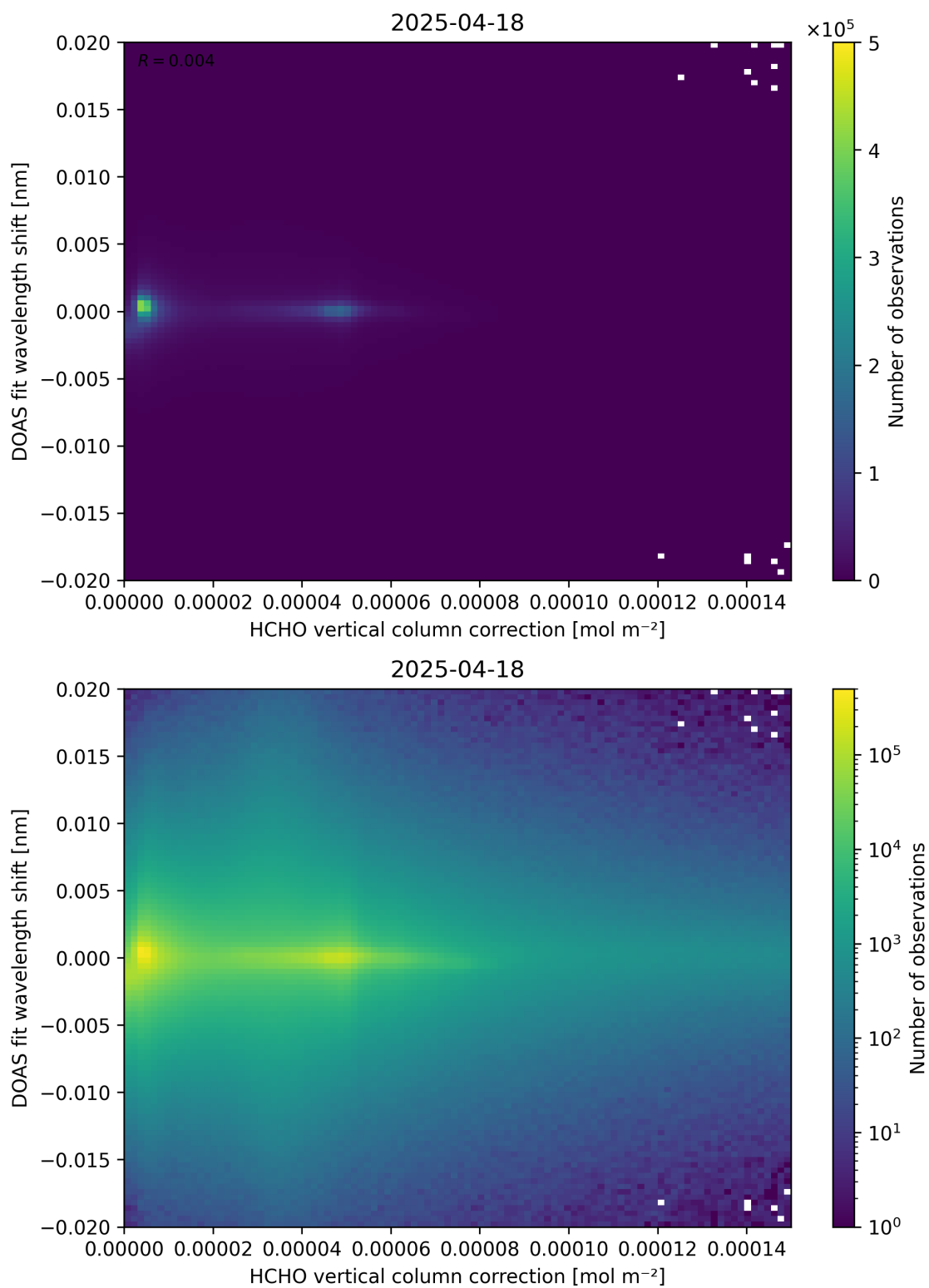
Figure 113: Scatter density plot of “HCHO vertical column correction” against “DOAS fit wavelength shift” for 2025-04-18 to 2025-04-19.
