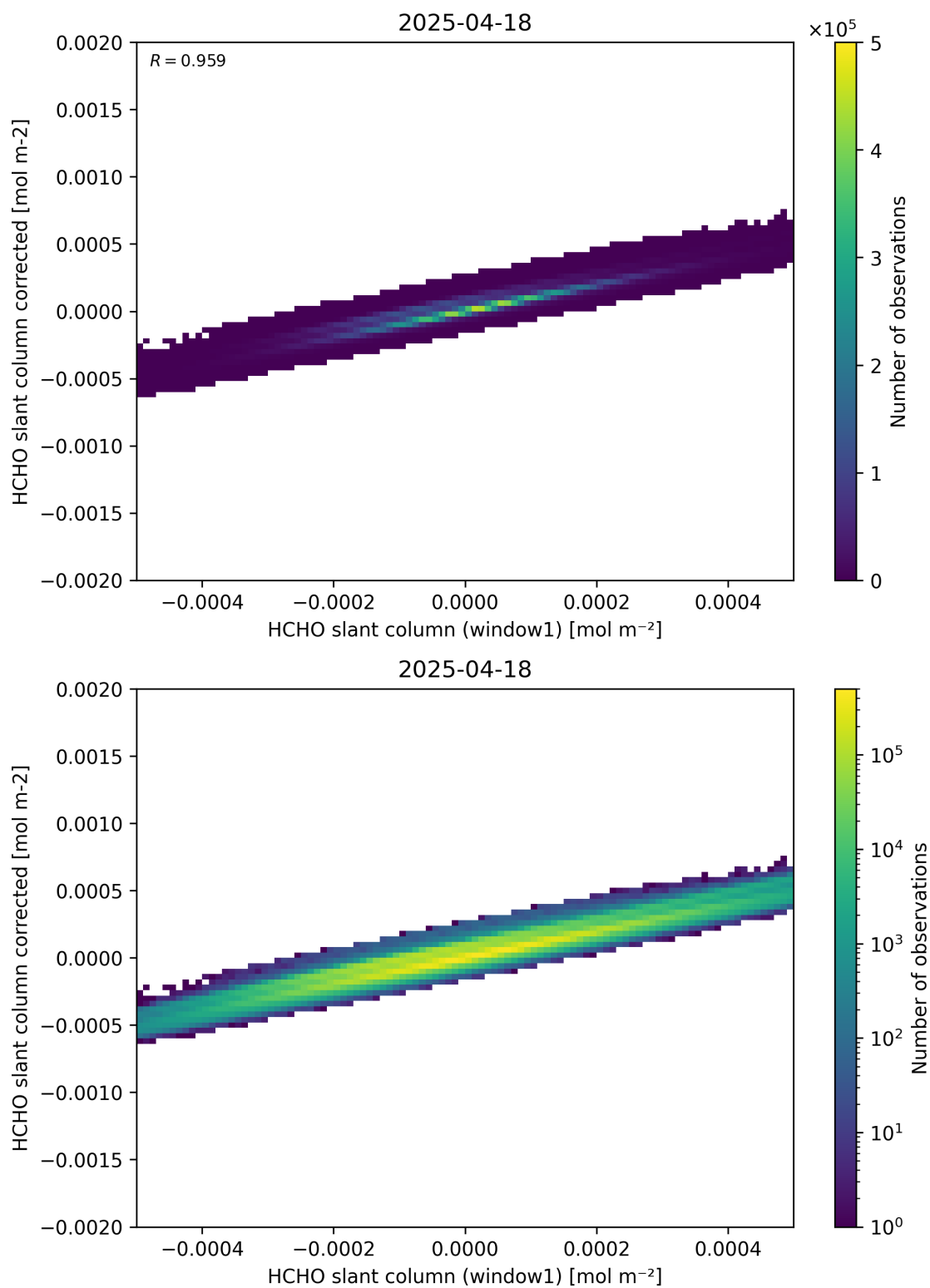
Figure 82: Scatter density plot of “HCHO slant column (window1)” against “HCHO slant column corrected” for 2025-04-18 to 2025-04-19.
