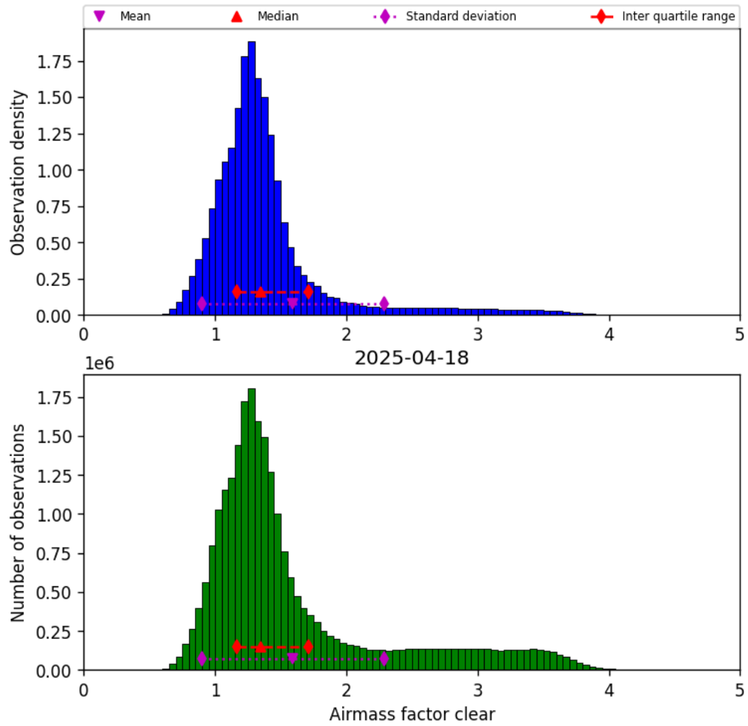
Figure 42: Histogram of “Airmass factor clear” for 2025-04-18 to 2025-04-19
