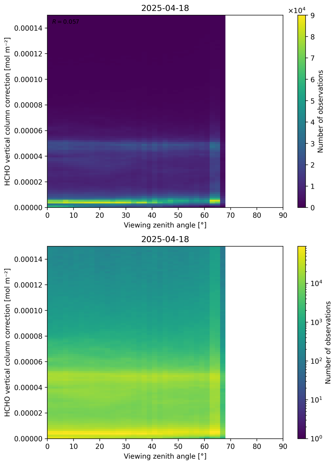
Figure 193: Scatter density plot of “Viewing zenith angle” against “HCHO vertical column correction” for 2025-04-18 to 2025-04-19.
