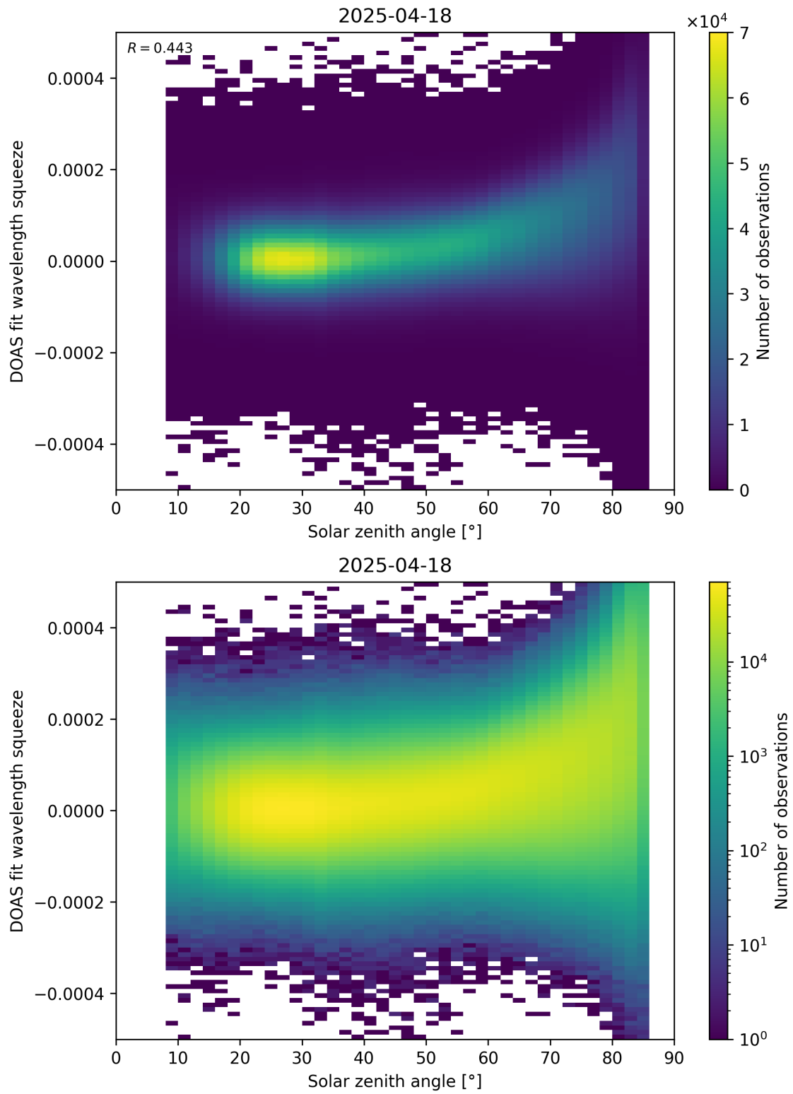
Figure 169: Scatter density plot of “Solar zenith angle” against “DOAS fit wavelength squeeze” for 2025-04-18 to 2025-04-19.
