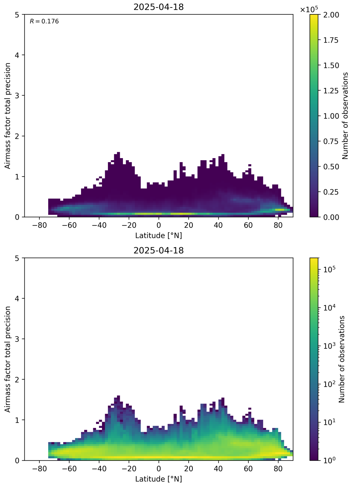
Figure 162: Scatter density plot of “Latitude” against “Airmass factor total precision” for 2025-04-18 to 2025-04-19.
