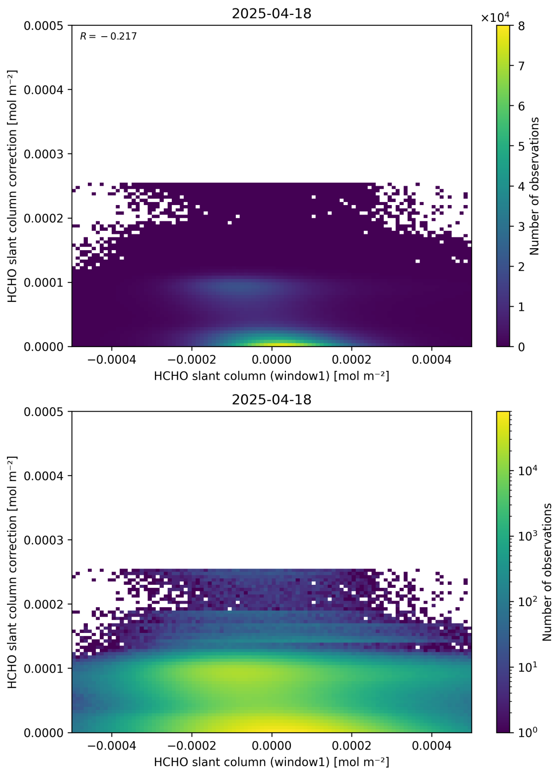
Figure 83: Scatter density plot of “HCHO slant column (window1)” against “HCHO slant column correction” for 2025-04-18 to 2025-04-19.
