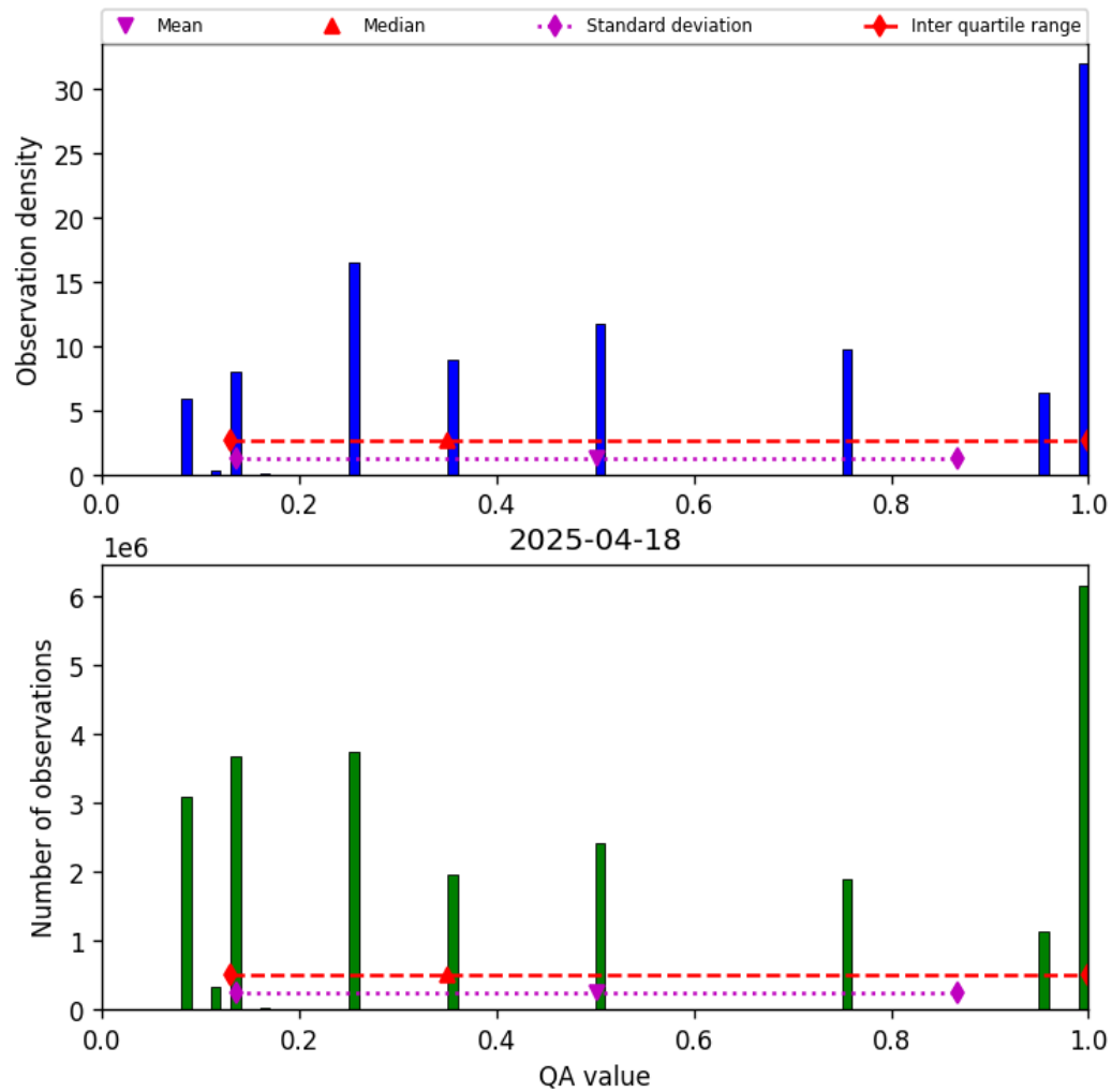
Figure 34: Histogram of “QA value” for 2025-04-18 to 2025-04-19
