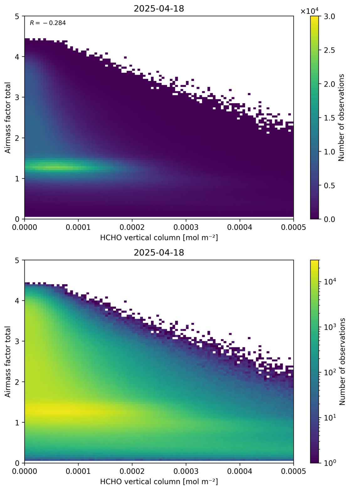
Figure 131: Scatter density plot of “HCHO vertical column” against “Airmass factor total” for 2025-04-18 to 2025-04-19.
