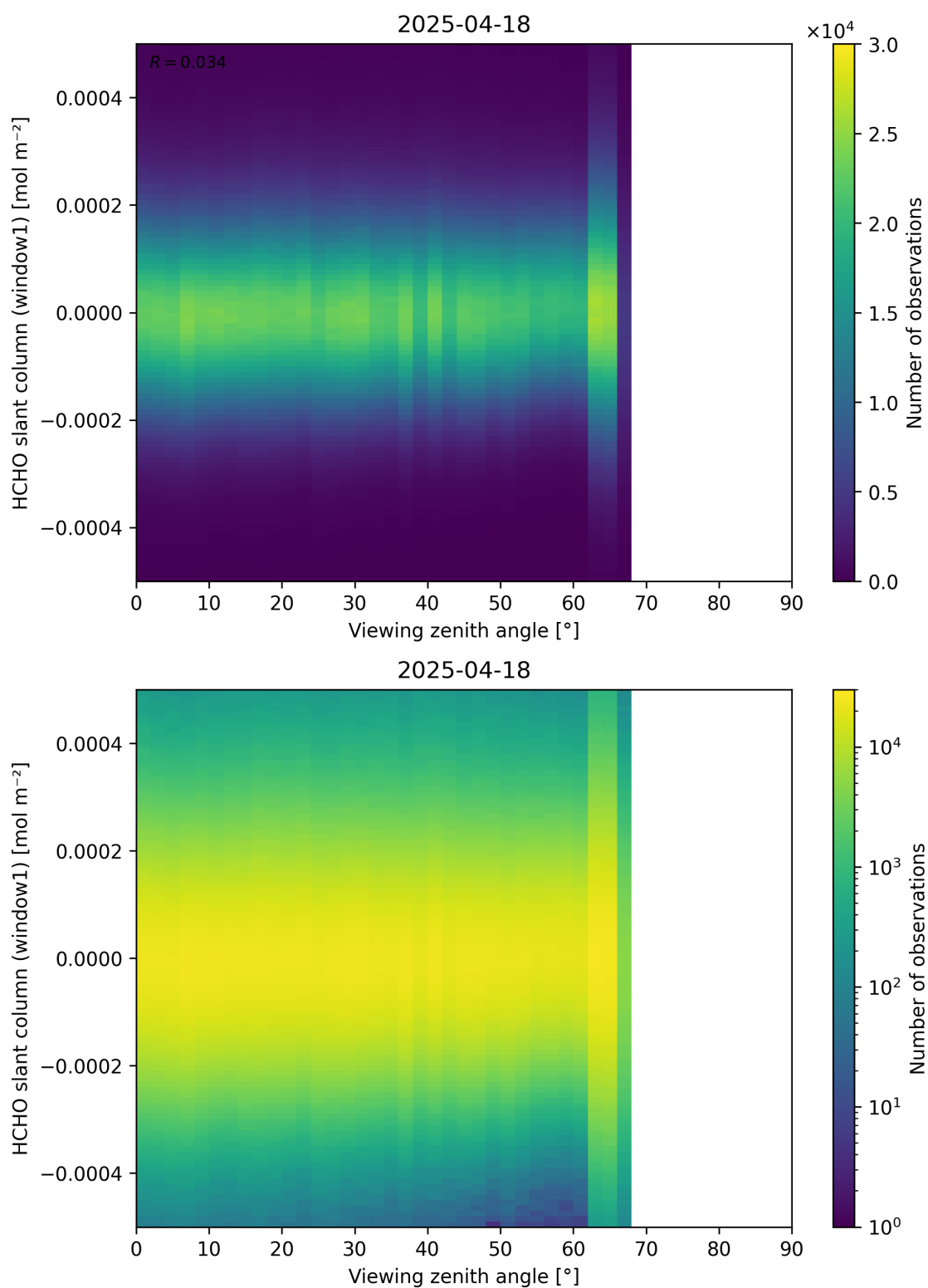
Figure 188: Scatter density plot of “Viewing zenith angle” against “HCHO slant column (window1)” for 2025-04-18 to 2025-04-19.
