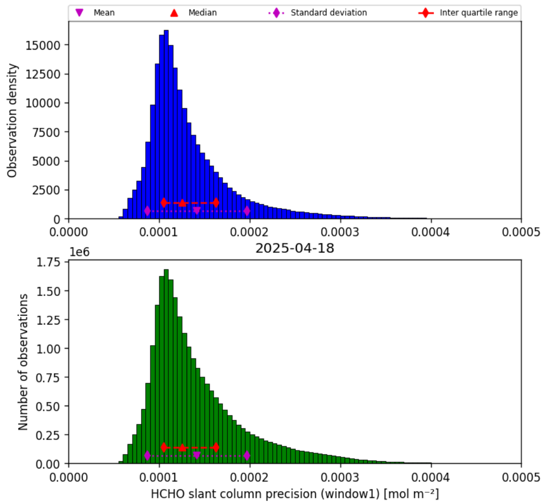
Figure 39: Histogram of “HCHO slant column precision (window1)” for 2025-04-18 to 2025-04-19
