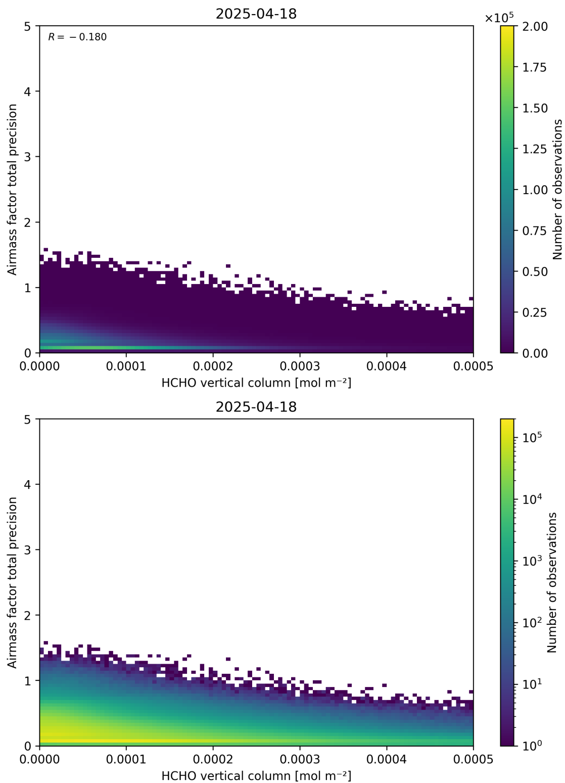
Figure 132: Scatter density plot of “HCHO vertical column” against “Airmass factor total precision” for 2025-04-18 to 2025-04-19.
