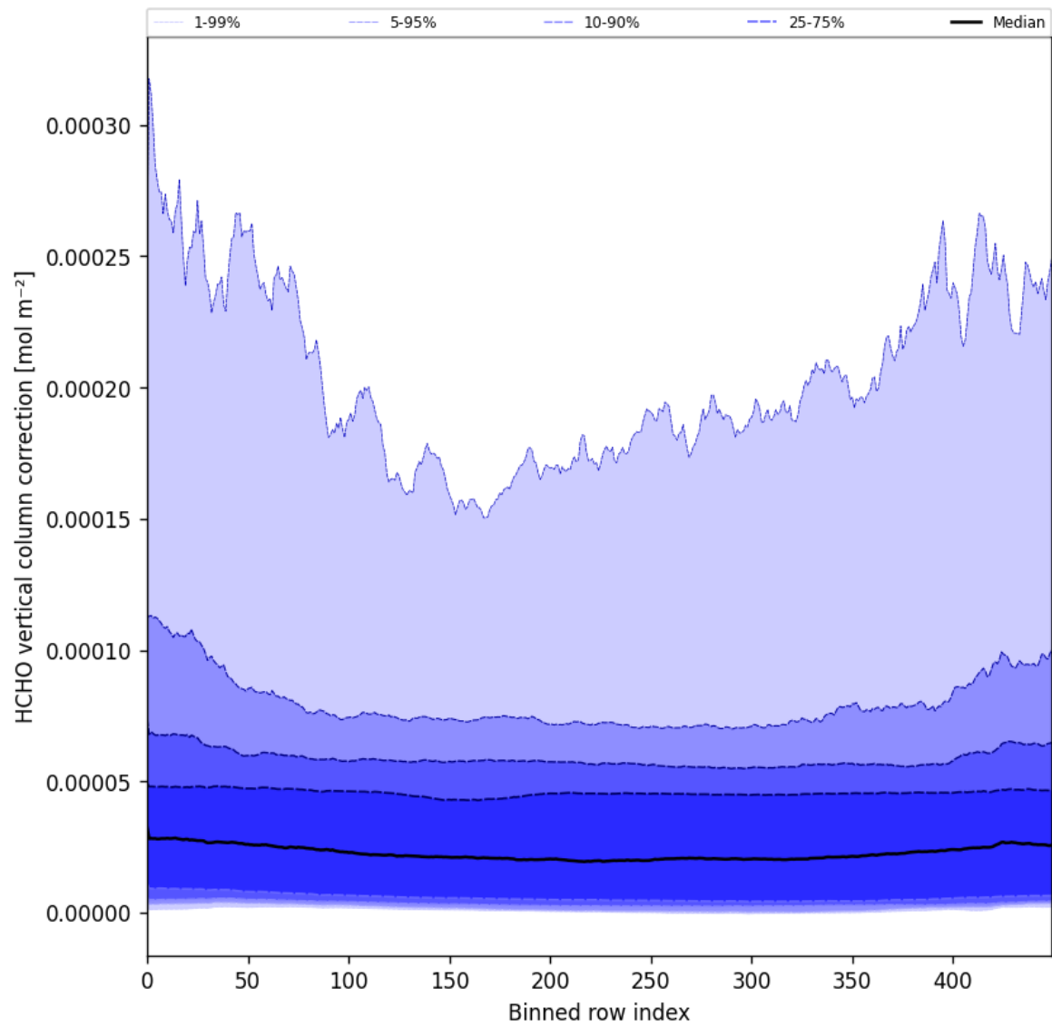
Figure 51: Along track statistics of “HCHO vertical column correction” for 2025-04-18 to 2025-04-19
