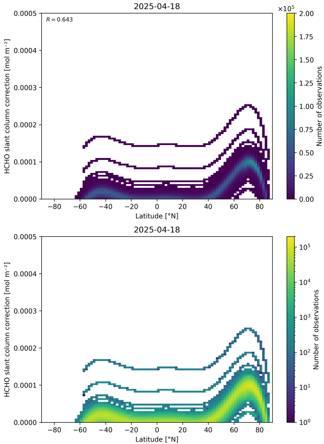
Figure 158: Scatter density plot of “Latitude” against “HCHO slant column correction” for 2025-04-18 to 2025-04-19.
