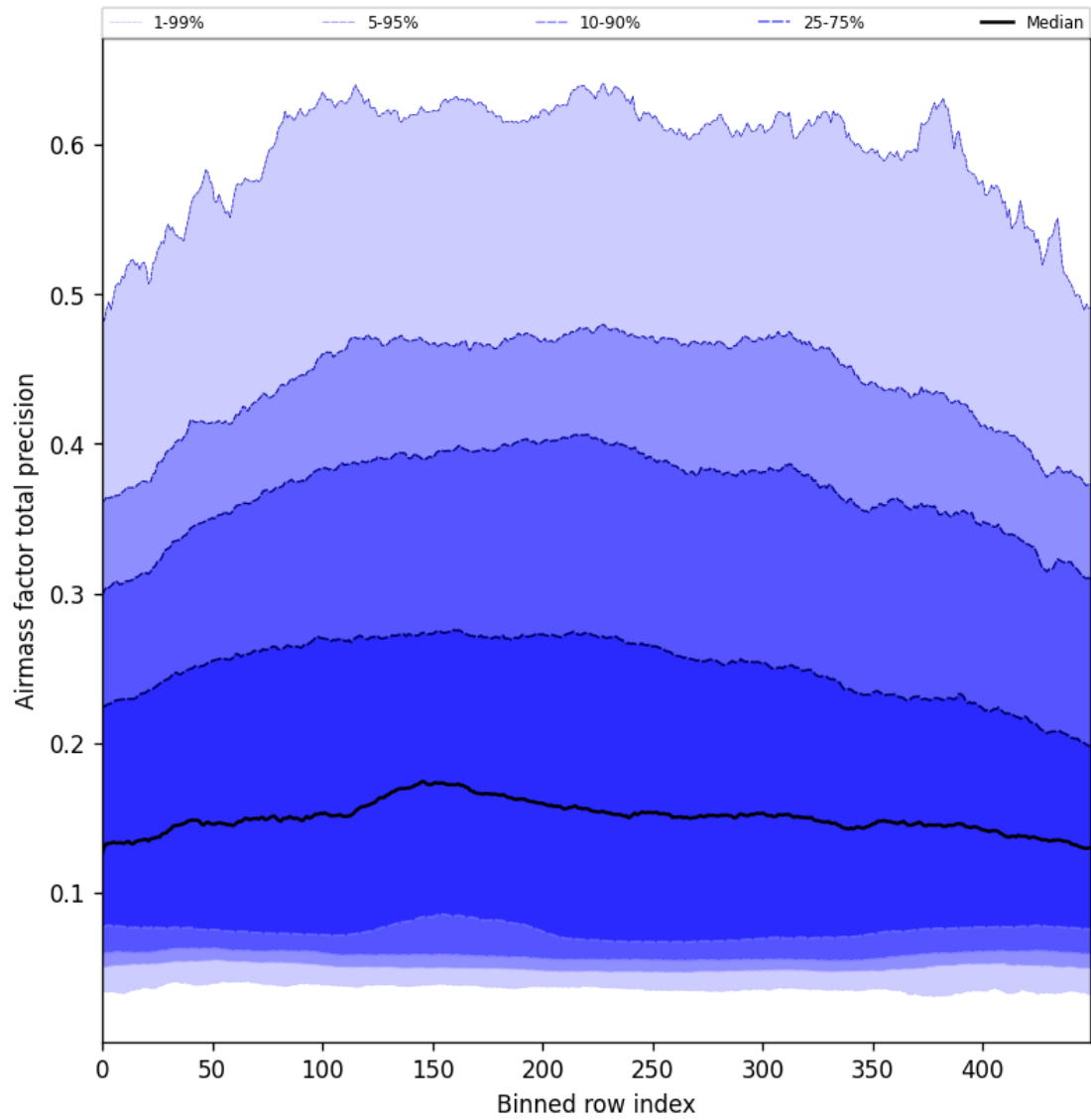
Figure 55: Along track statistics of “Airmass factor total precision” for 2025-04-18 to 2025-04-19
