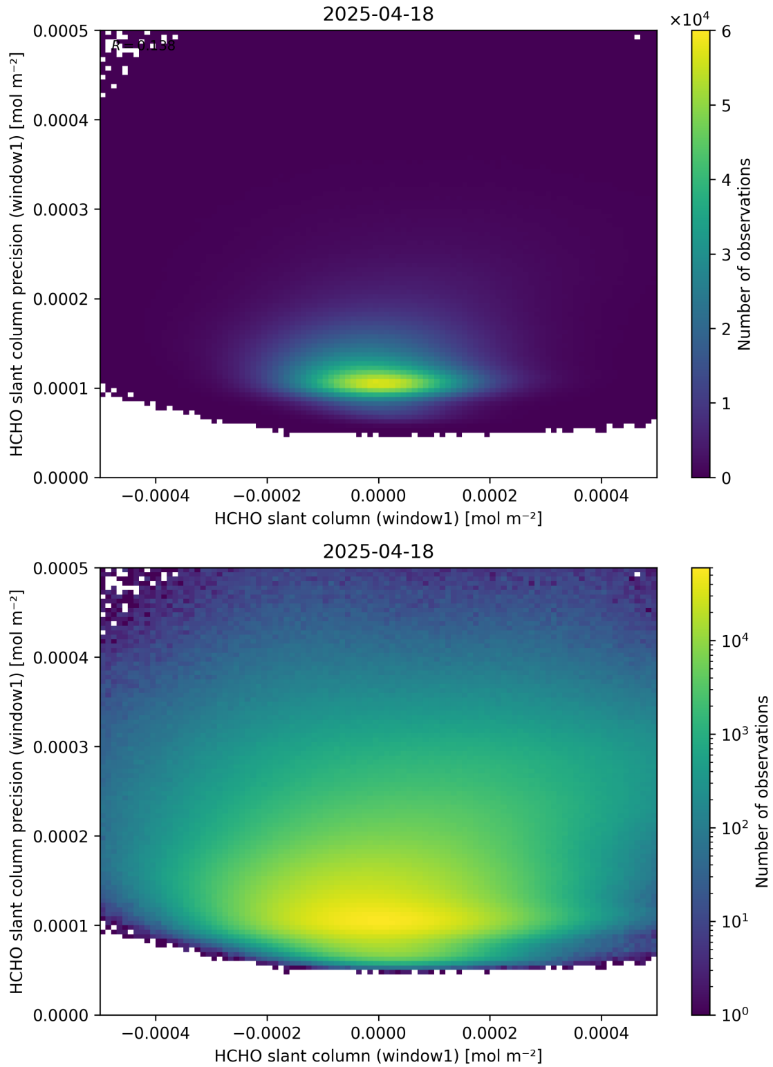
Figure 84: Scatter density plot of “HCHO slant column (window1)” against “HCHO slant column precision (window1)” for 2025-04-18 to 2025-04-19.
