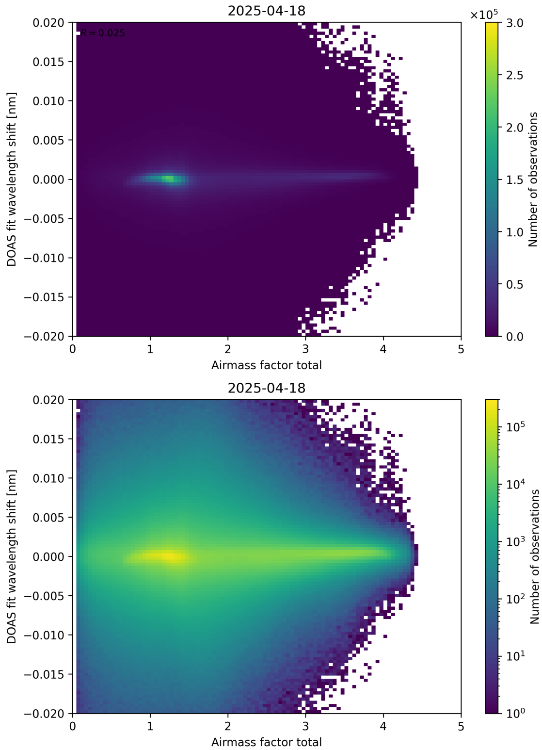
Figure 98: Scatter density plot of “Airmass factor total” against “DOAS fit wavelength shift” for 2025-04-18 to 2025-04-19.
