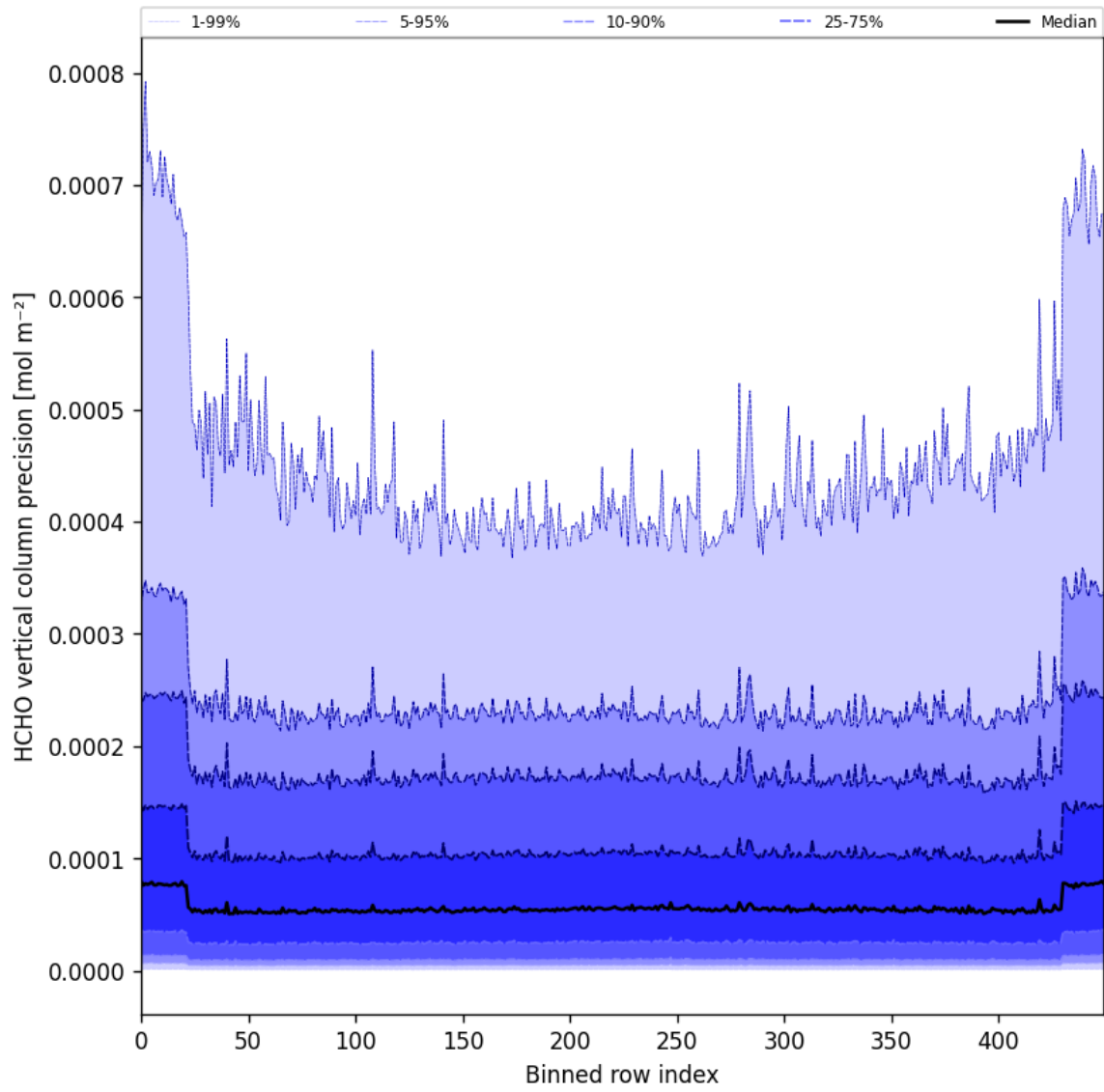
Figure 50: Along track statistics of “HCHO vertical column precision” for 2025-04-18 to 2025-04-19
