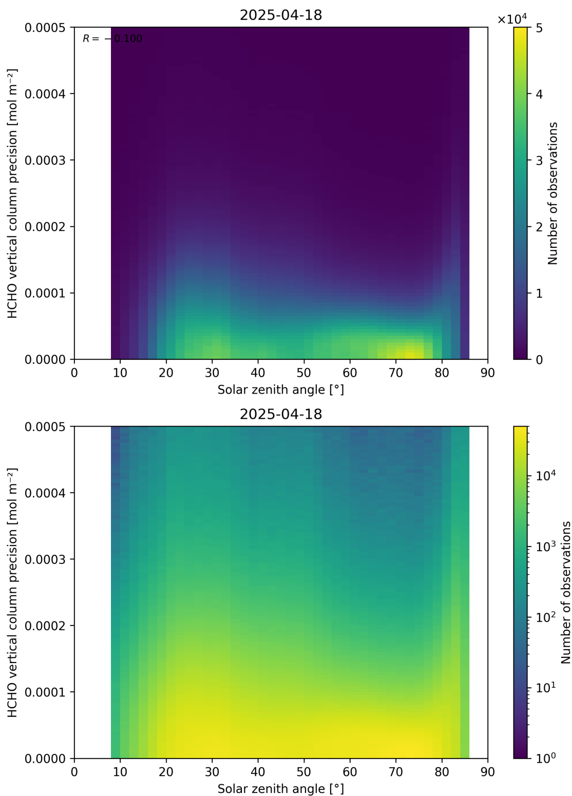
Figure 179: Scatter density plot of “Solar zenith angle” against “HCHO vertical column precision” for 2025-04-18 to 2025-04-19.
