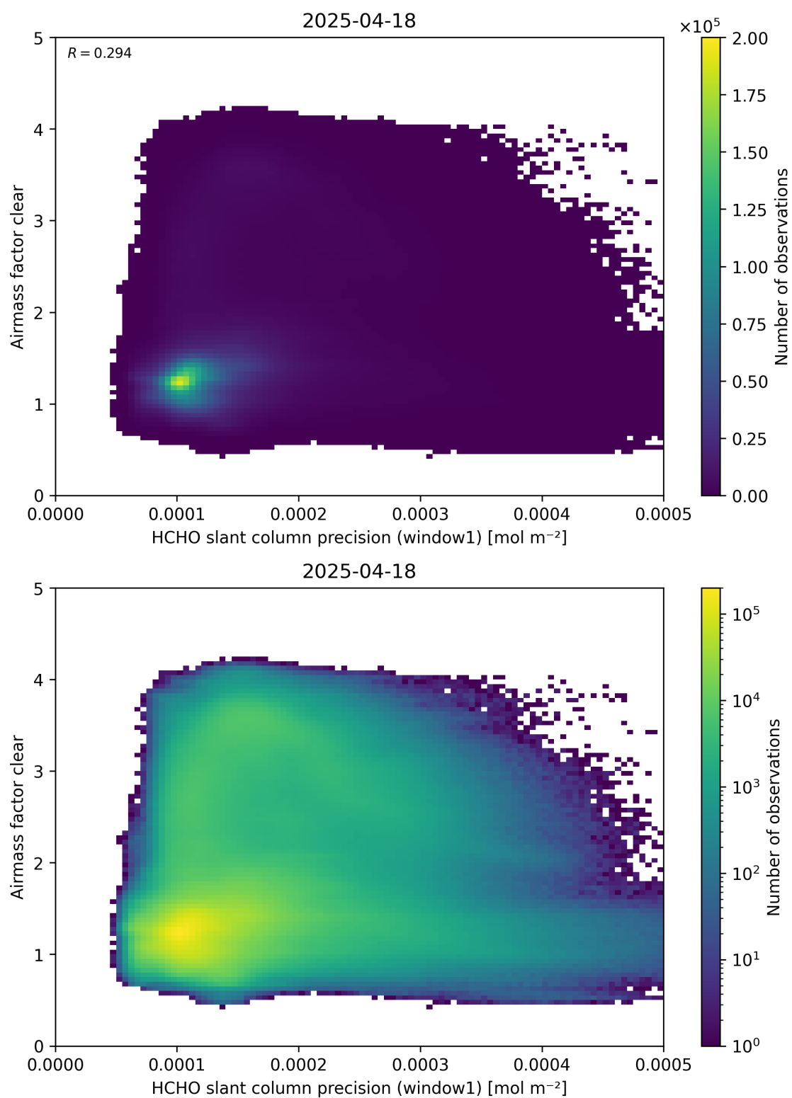
Figure 91: Scatter density plot of “HCHO slant column precision (window1)” against “Airmass factor clear” for 2025-04-18 to 2025-04-19.
