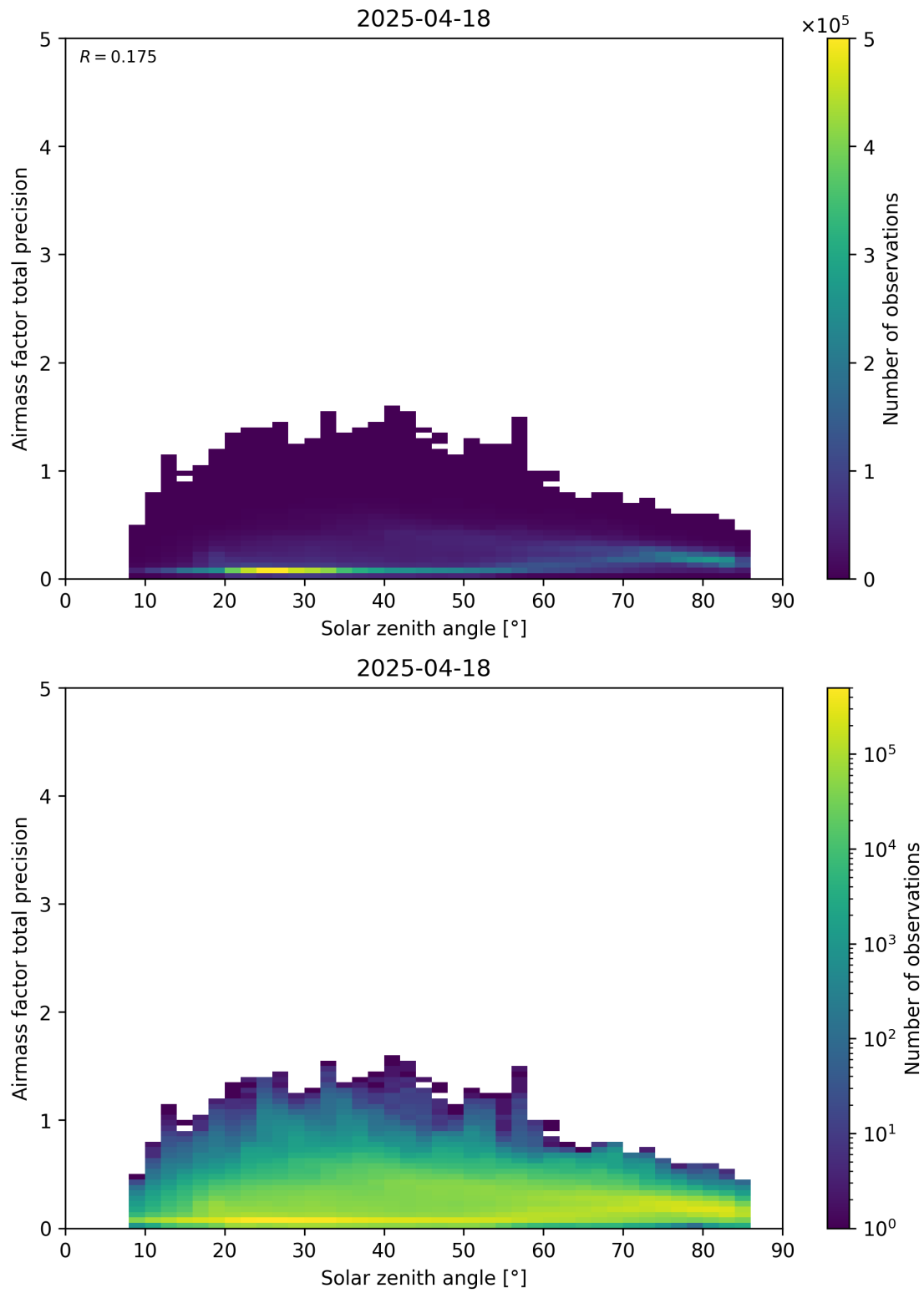
Figure 176: Scatter density plot of “Solar zenith angle” against “Airmass factor total precision” for 2025-04-18 to 2025-04-19.
