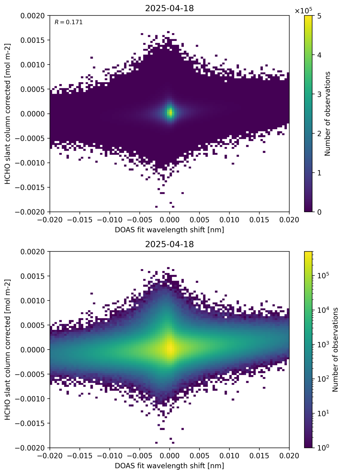
Figure 66: Scatter density plot of “DOAS fit wavelength shift” against “HCHO slant column corrected” for 2025-04-18 to 2025-04-19.
