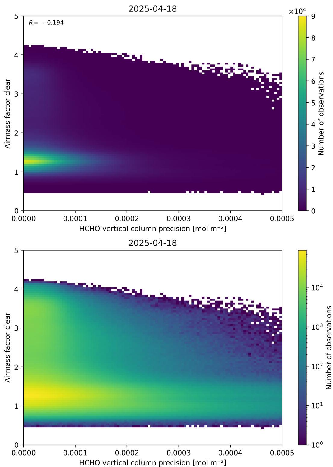
Figure 139: Scatter density plot of “HCHO vertical column precision” against “Airmass factor clear” for 2025-04-18 to 2025-04-19.
