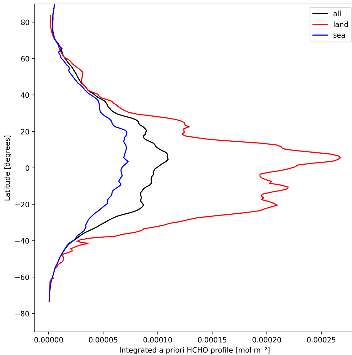
Figure 29: Zonal average of “Integrated a priori HCHO profile” for 2025-04-18 to 2025-04-19.
