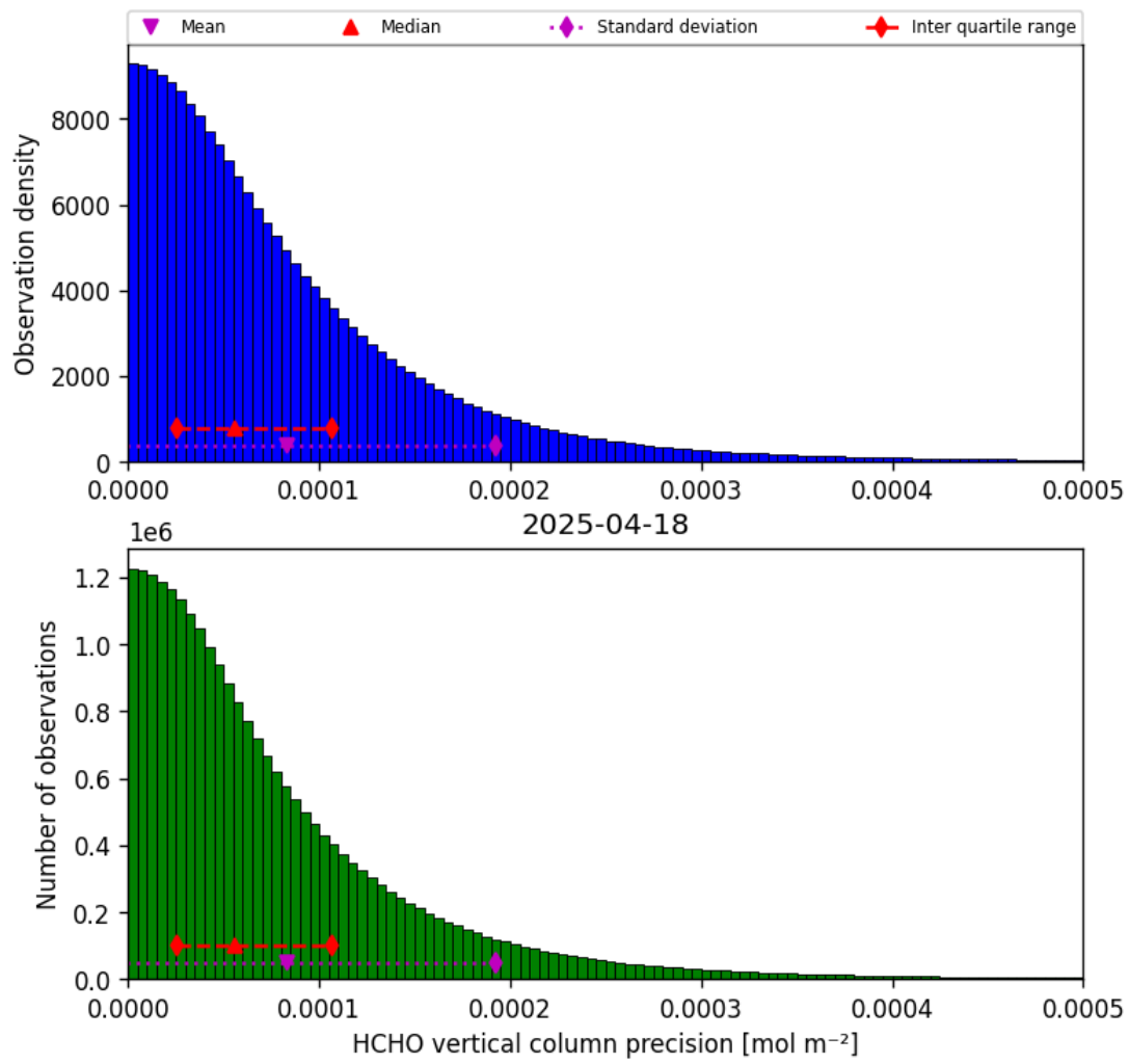
Figure 36: Histogram of “HCHO vertical column precision” for 2025-04-18 to 2025-04-19
