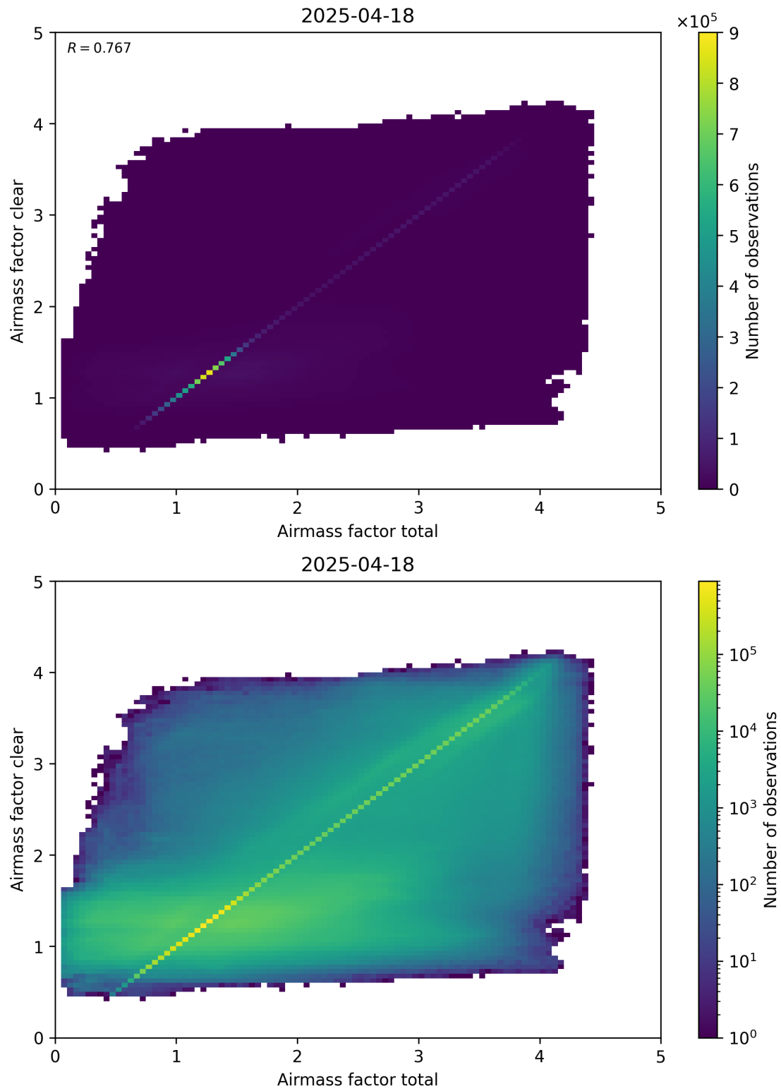
Figure 100: Scatter density plot of “Airmass factor total” against “Airmass factor clear” for 2025-04-18 to 2025-04-19.
