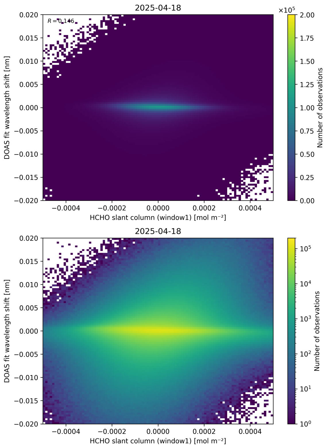
Figure 79: Scatter density plot of “HCHO slant column (window1)” against “DOAS fit wavelength shift” for 2025-04-18 to 2025-04-19.
