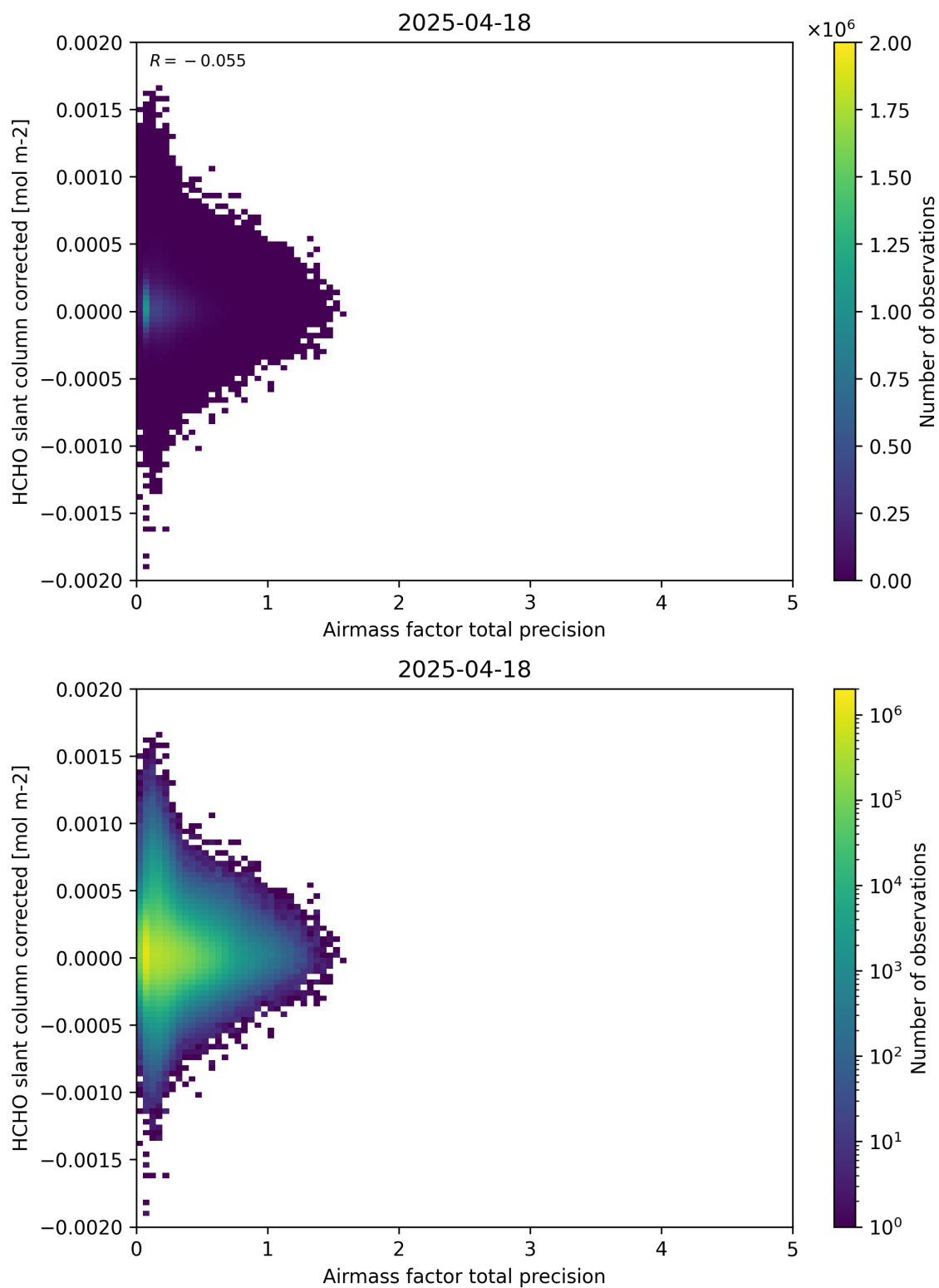
Figure 109: Scatter density plot of “Airmass factor total precision” against “HCHO slant column corrected” for 2025-04-18 to 2025-04-19.
