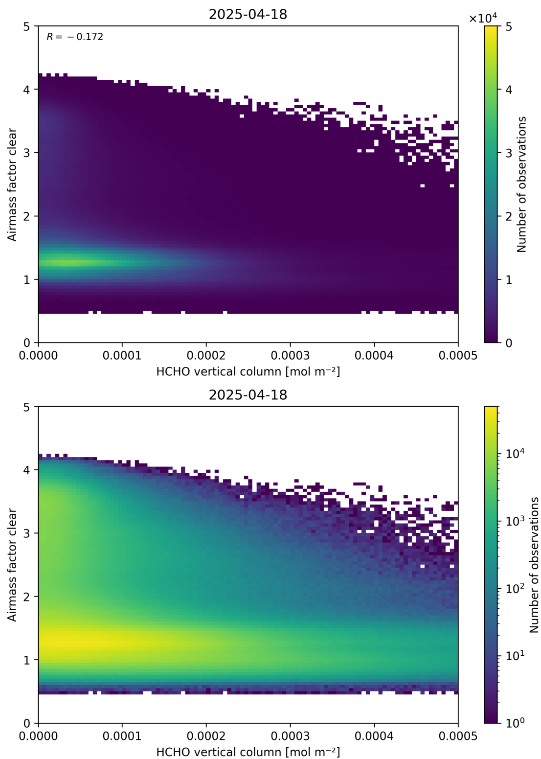
Figure 126: Scatter density plot of “HCHO vertical column” against “Airmass factor clear” for 2025-04-18 to 2025-04-19.
