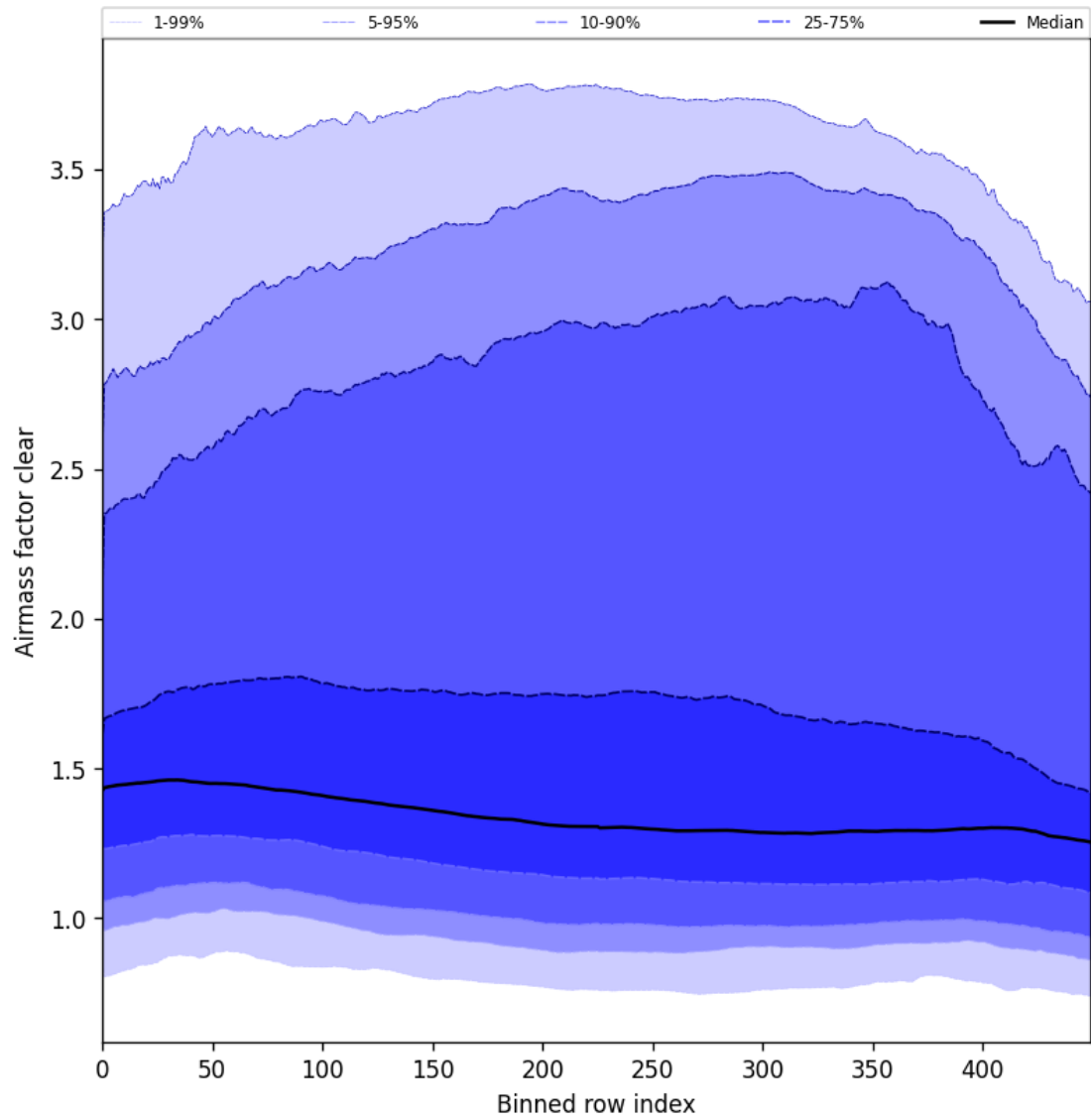
Figure 56: Along track statistics of “Airmass factor clear” for 2025-04-18 to 2025-04-19
