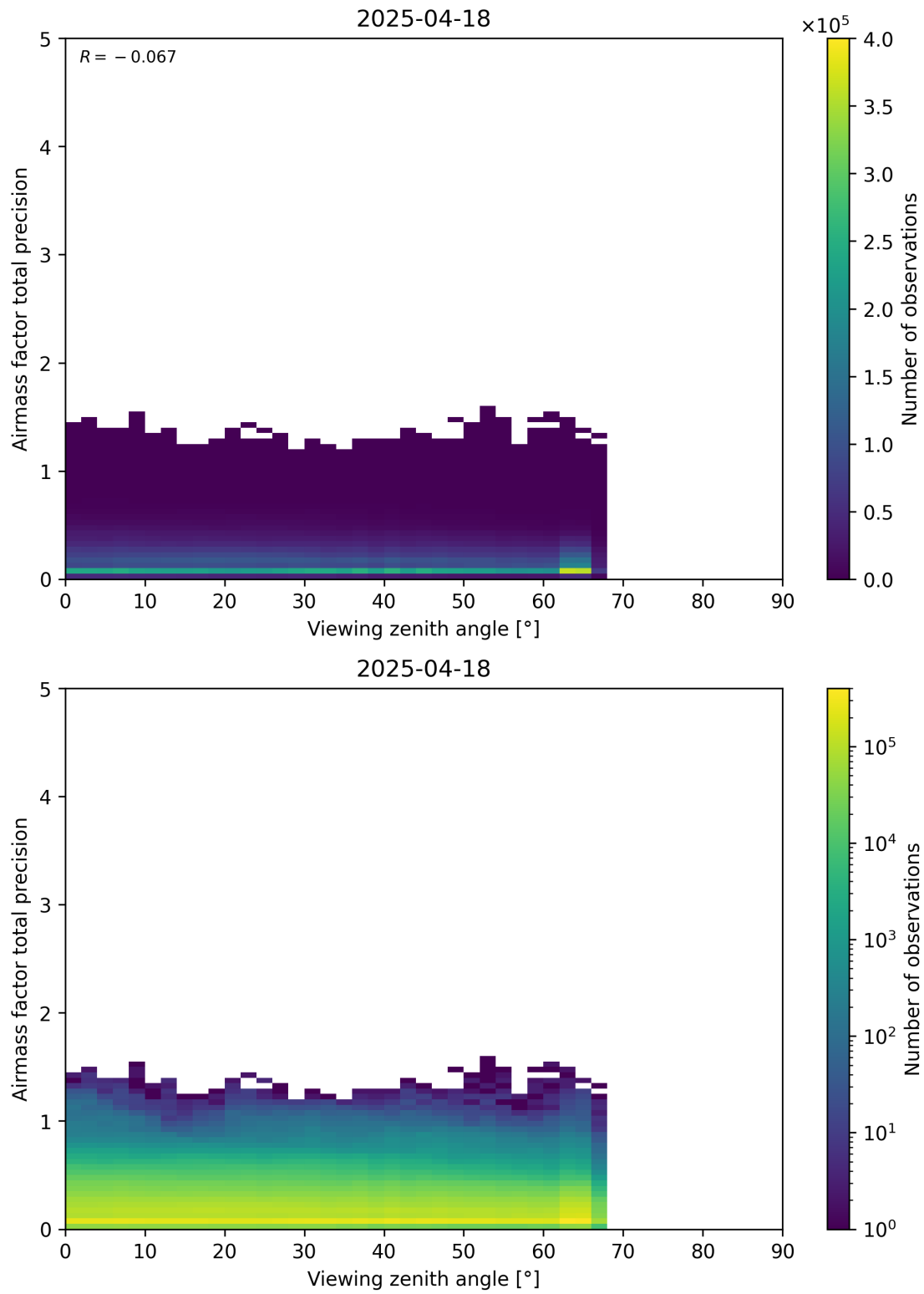
Figure 191: Scatter density plot of “Viewing zenith angle” against “Airmass factor total precision” for 2025-04-18 to 2025-04-19.
