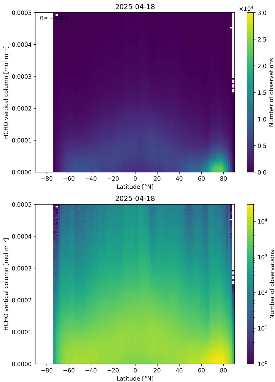
Figure 163: Scatter density plot of “Latitude” against “HCHO vertical column” for 2025-04-18 to 2025-04-19.
