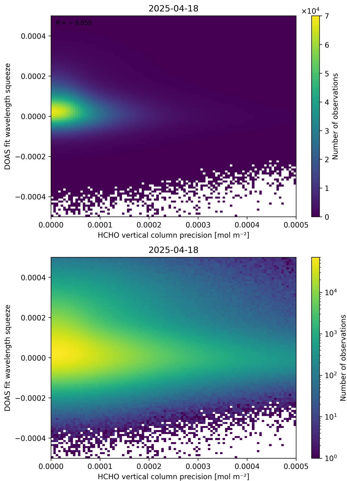
Figure 138: Scatter density plot of “HCHO vertical column precision” against “DOAS fit wavelength squeeze” for 2025-04-18 to 2025-04-19.
