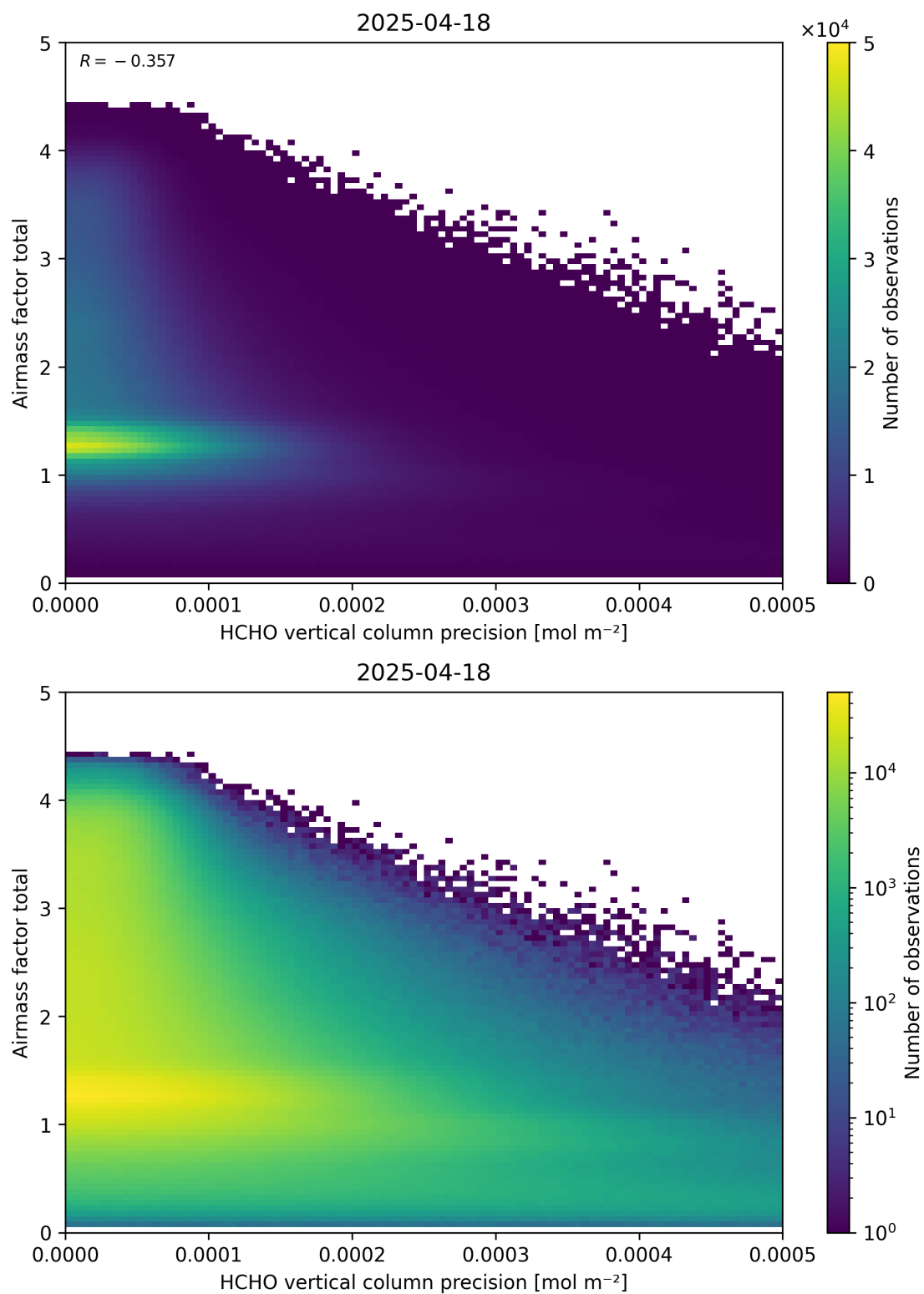
Figure 144: Scatter density plot of “HCHO vertical column precision” against “Airmass factor total” for 2025-04-18 to 2025-04-19.
