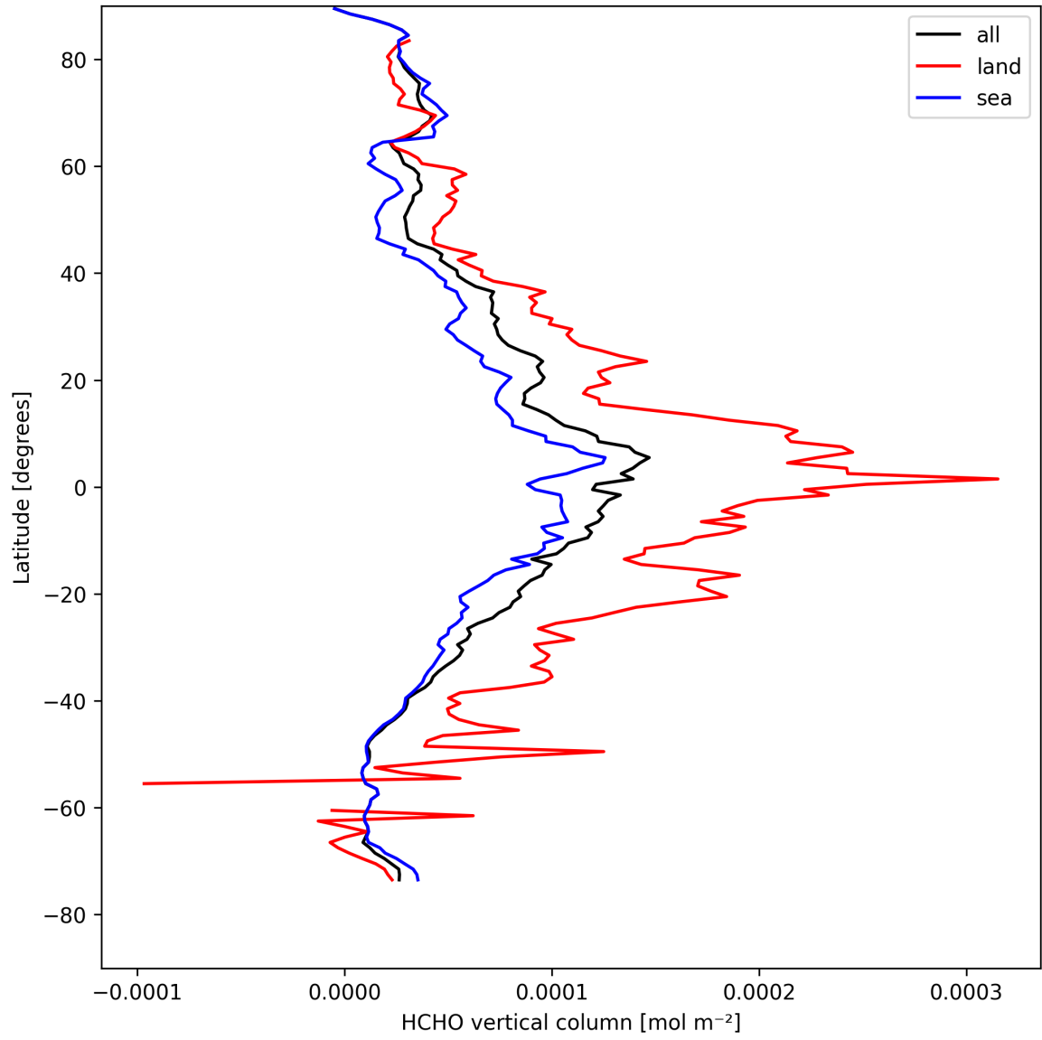
Figure 21: Zonal average of “HCHO vertical column” for 2025-04-18 to 2025-04-19.
