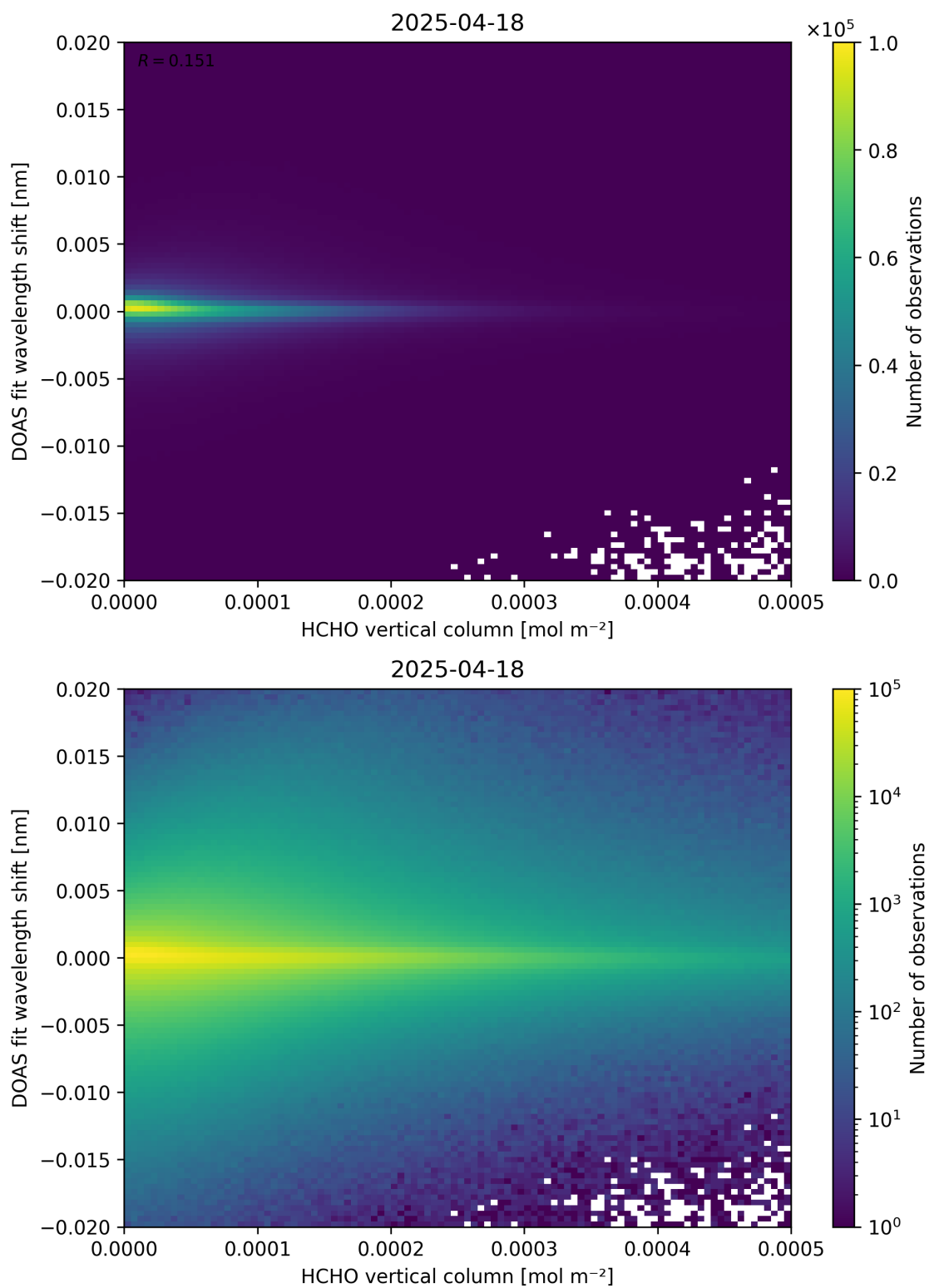
Figure 124: Scatter density plot of “HCHO vertical column” against “DOAS fit wavelength shift” for 2025-04-18 to 2025-04-19.
