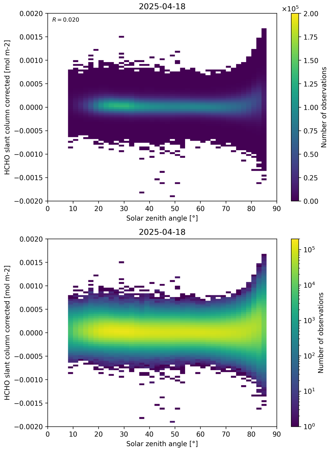
Figure 171: Scatter density plot of “Solar zenith angle” against “HCHO slant column corrected” for 2025-04-18 to 2025-04-19.
