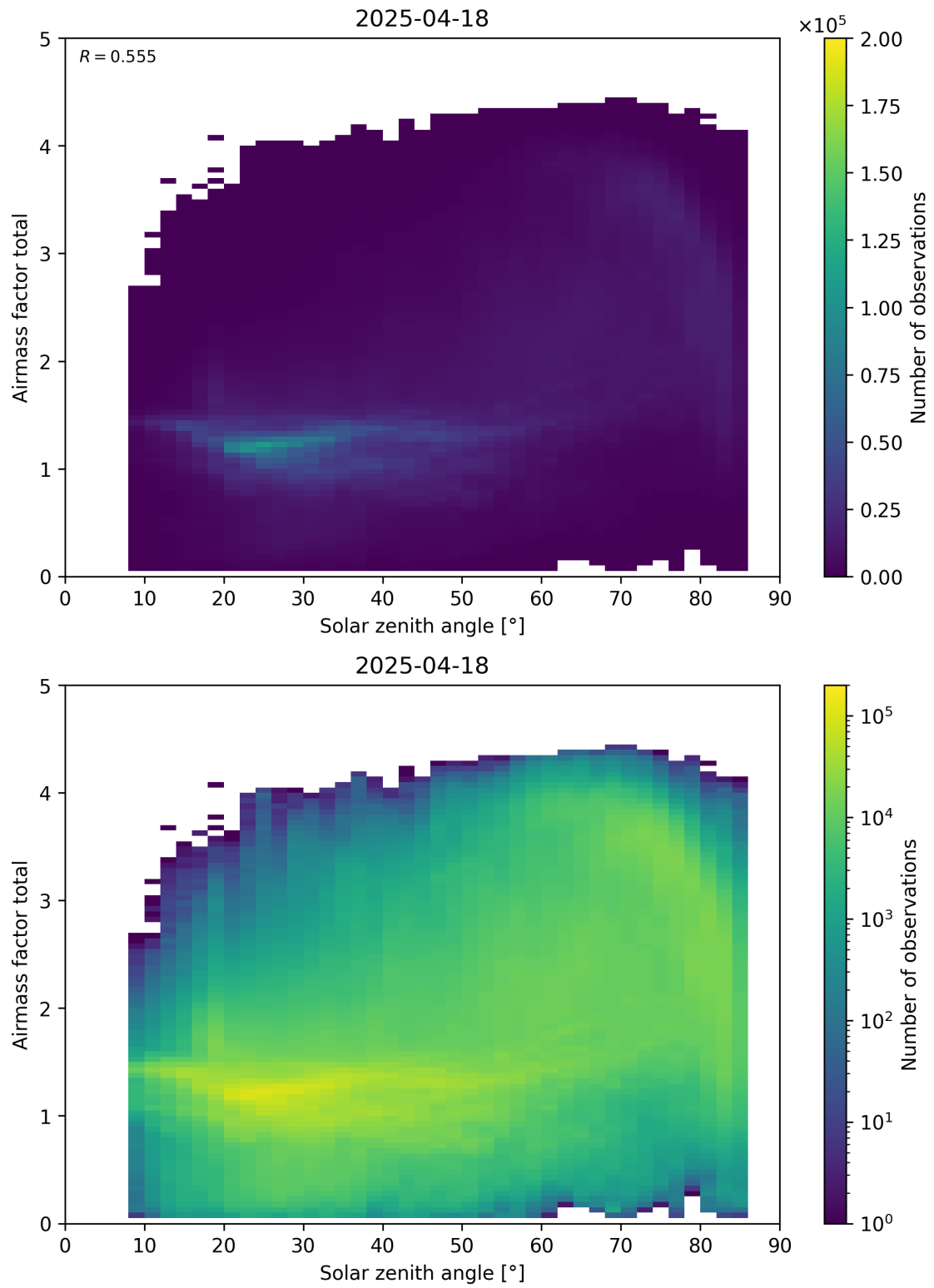
Figure 175: Scatter density plot of “Solar zenith angle” against “Airmass factor total” for 2025-04-18 to 2025-04-19.
