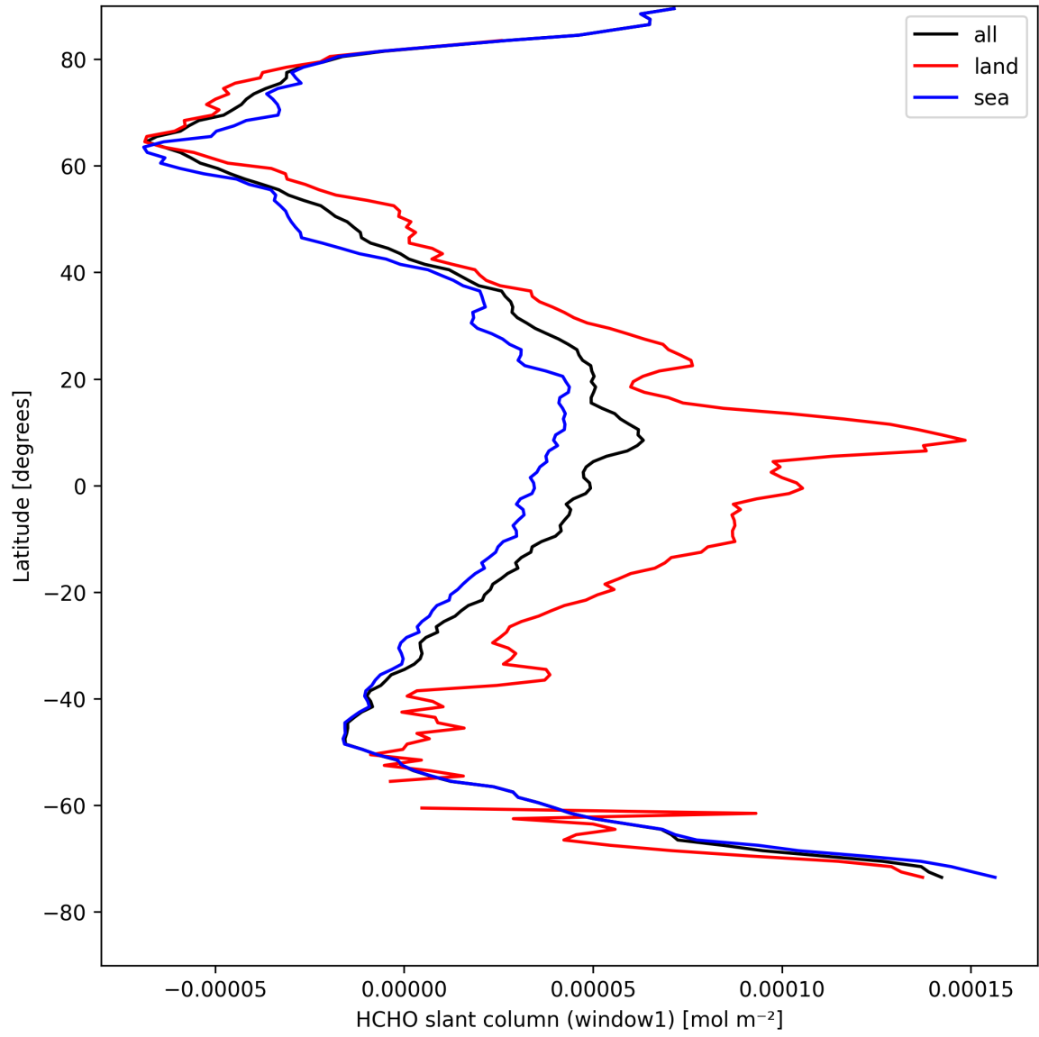
Figure 24: Zonal average of “HCHO slant column (window1)” for 2025-04-18 to 2025-04-19.
