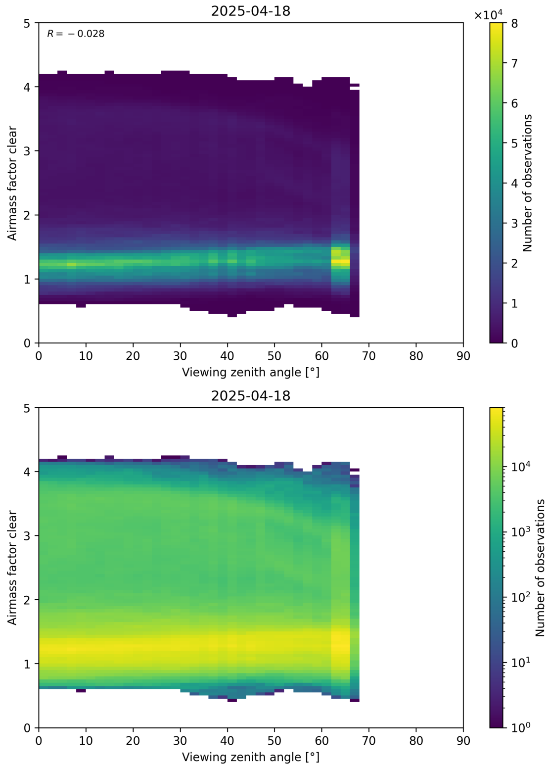
Figure 185: Scatter density plot of “Viewing zenith angle” against “Airmass factor clear” for 2025-04-18 to 2025-04-19.
