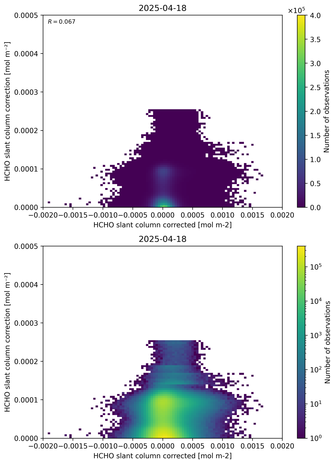
Figure 77: Scatter density plot of “HCHO slant column corrected” against “HCHO slant column correction” for 2025-04-18 to 2025-04-19.
