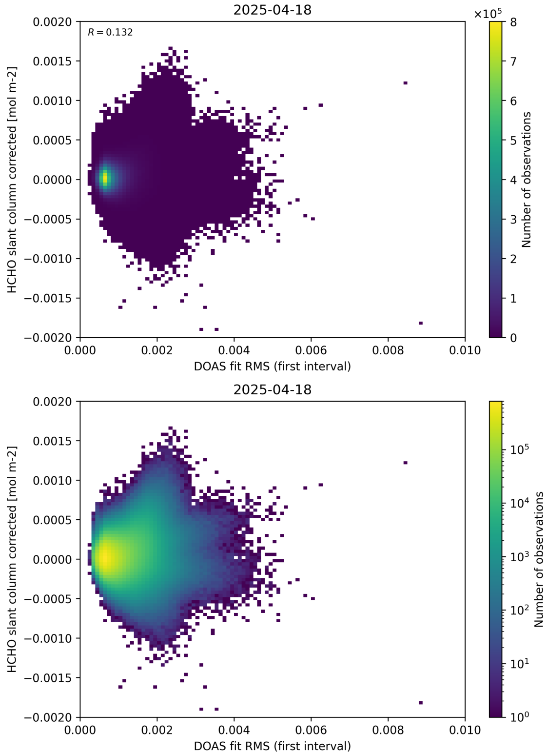
Figure 62: Scatter density plot of “DOAS fit RMS (first interval)” against “HCHO slant column corrected” for 2025-04-18 to 2025-04-19.
