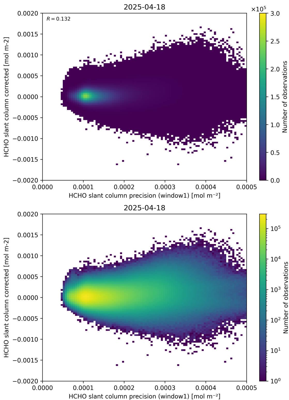
Figure 92: Scatter density plot of “HCHO slant column precision (window1)” against “HCHO slant column corrected” for 2025-04-18 to 2025-04-19.
