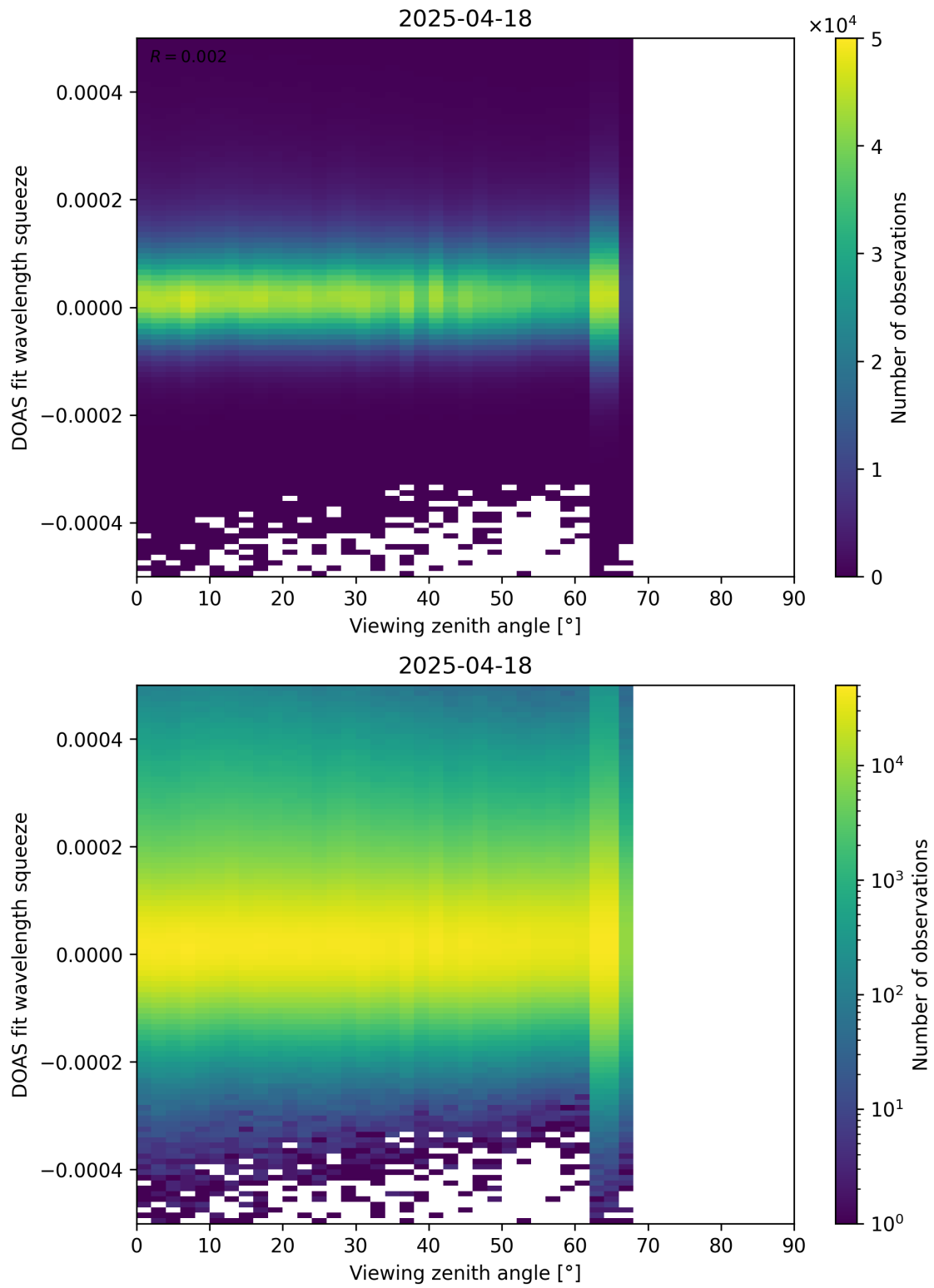
Figure 184: Scatter density plot of “Viewing zenith angle” against “DOAS fit wavelength squeeze” for 2025-04-18 to 2025-04-19.
