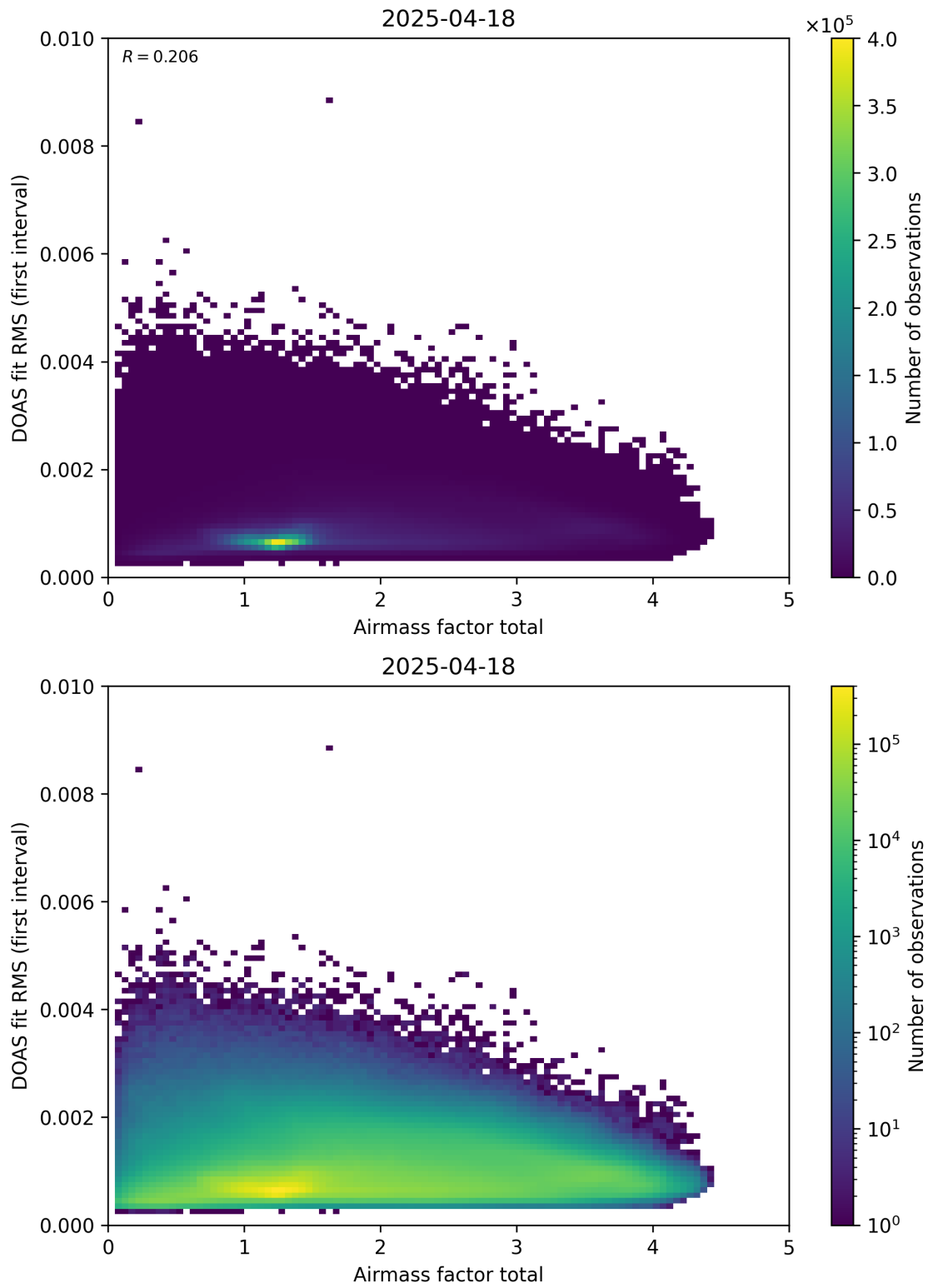
Figure 97: Scatter density plot of “Airmass factor total” against “DOAS fit RMS (first interval)” for 2025-04-18 to 2025-04-19.
