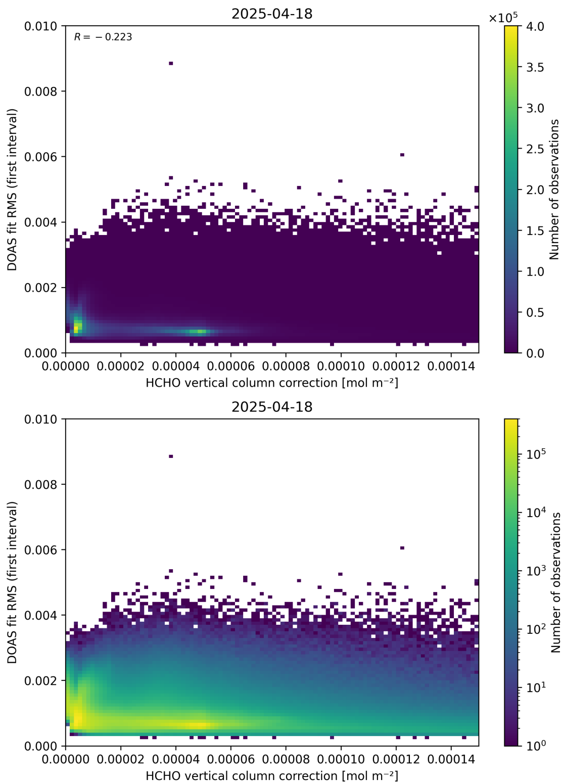
Figure 112: Scatter density plot of “HCHO vertical column correction” against “DOAS fit RMS (first interval)” for 2025-04-18 to 2025-04-19.
