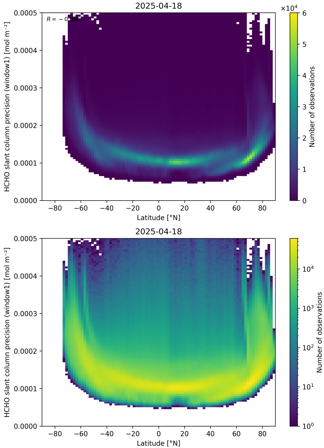
Figure 160: Scatter density plot of “Latitude” against “HCHO slant column precision (window1)” for 2025-04-18 to 2025-04-19.
