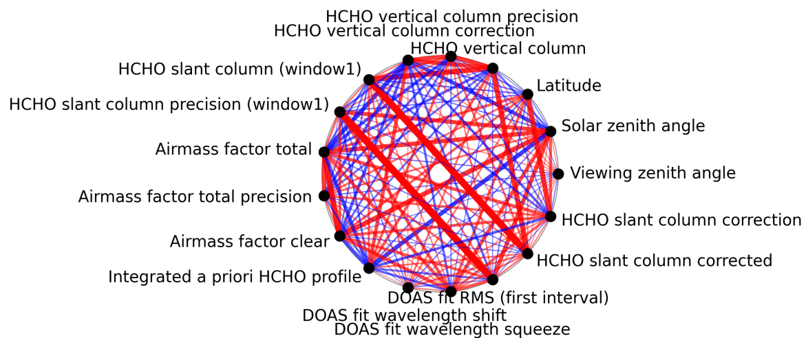
Figure 1: Map of correlation graph for 2025-04-18 to 2025-04-19.
