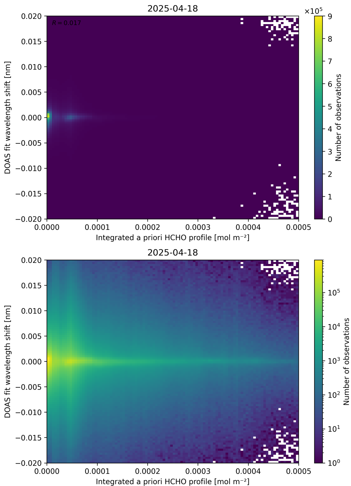
Figure 149: Scatter density plot of “Integrated a priori HCHO profile” against “DOAS fit wavelength shift” for 2025-04-18 to 2025-04-19.
