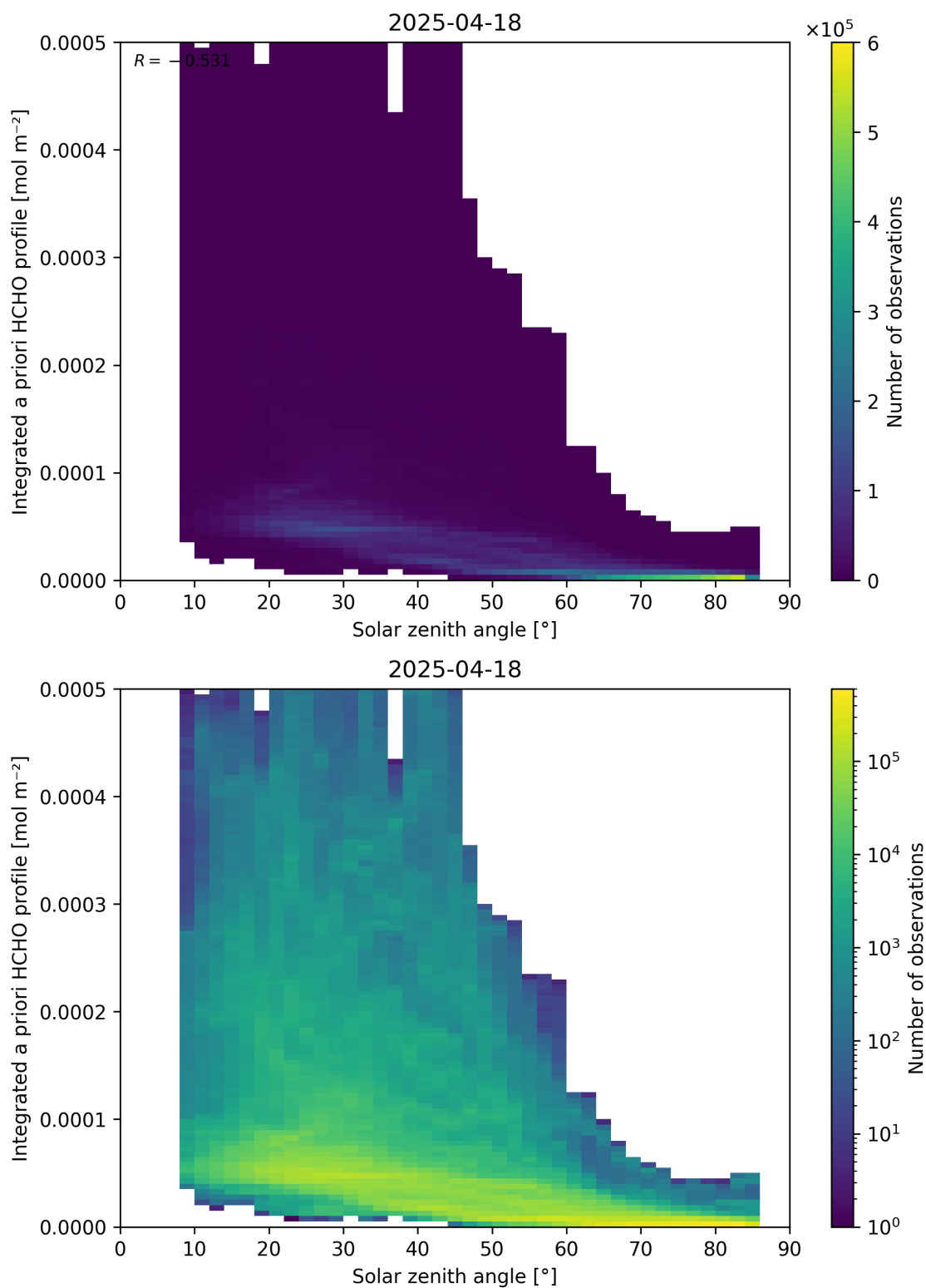
Figure 180: Scatter density plot of “Solar zenith angle” against “Integrated a priori HCHO profile” for 2025-04-18 to 2025-04-19.
