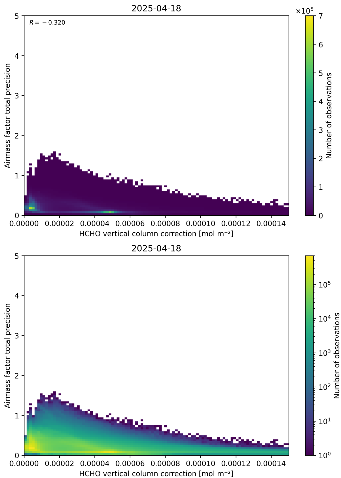
Figure 121: Scatter density plot of “HCHO vertical column correction” against “Airmass factor total precision” for 2025-04-18 to 2025-04-19.
