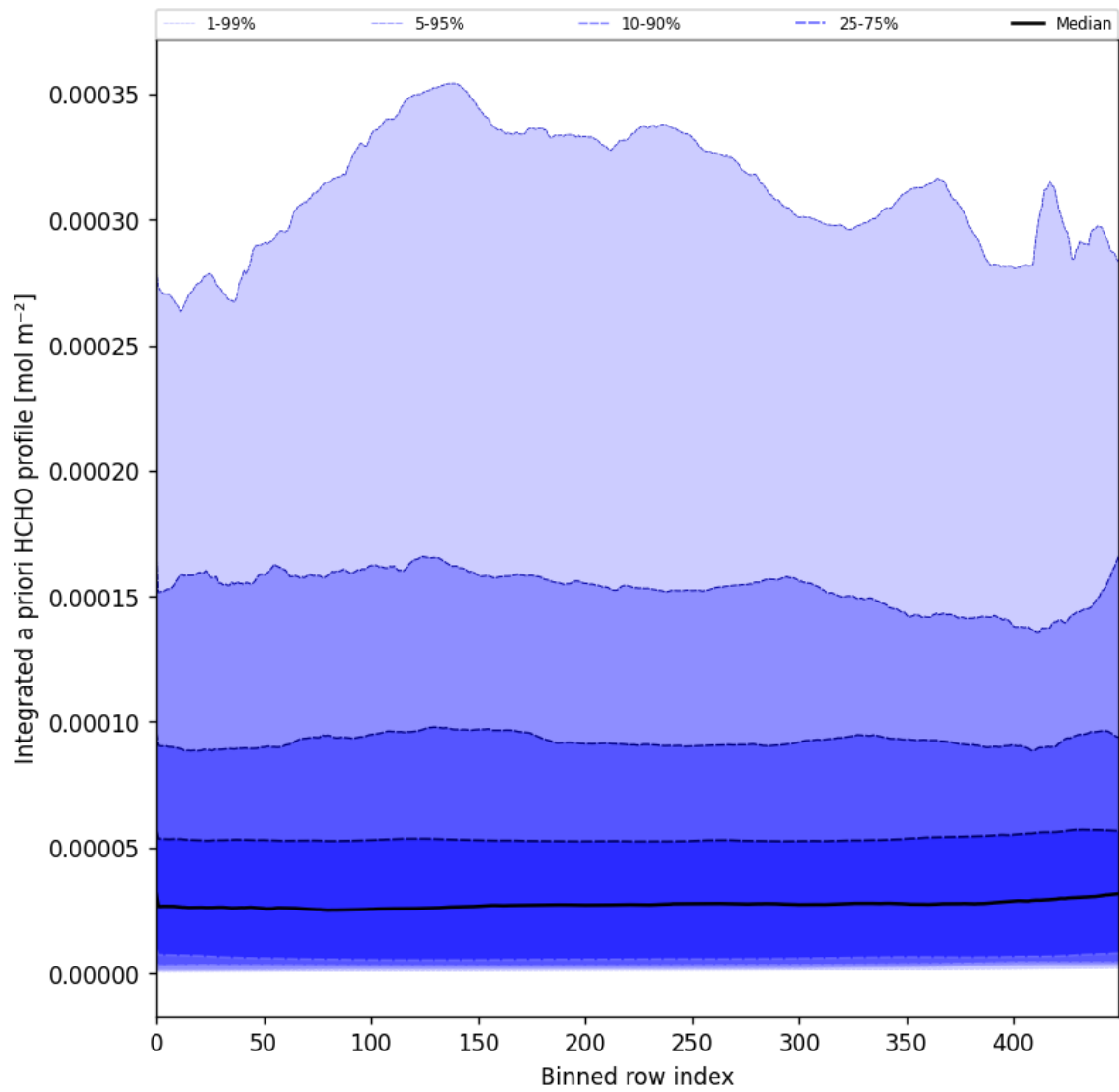
Figure 57: Along track statistics of "Integrated a priori HCHO profile" for 2025-04-18 to 2025-04-19
