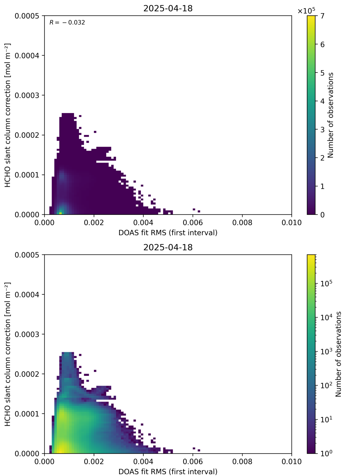
Figure 63: Scatter density plot of “DOAS fit RMS (first interval)” against “HCHO slant column correction” for 2025-04-18 to 2025-04-19.
