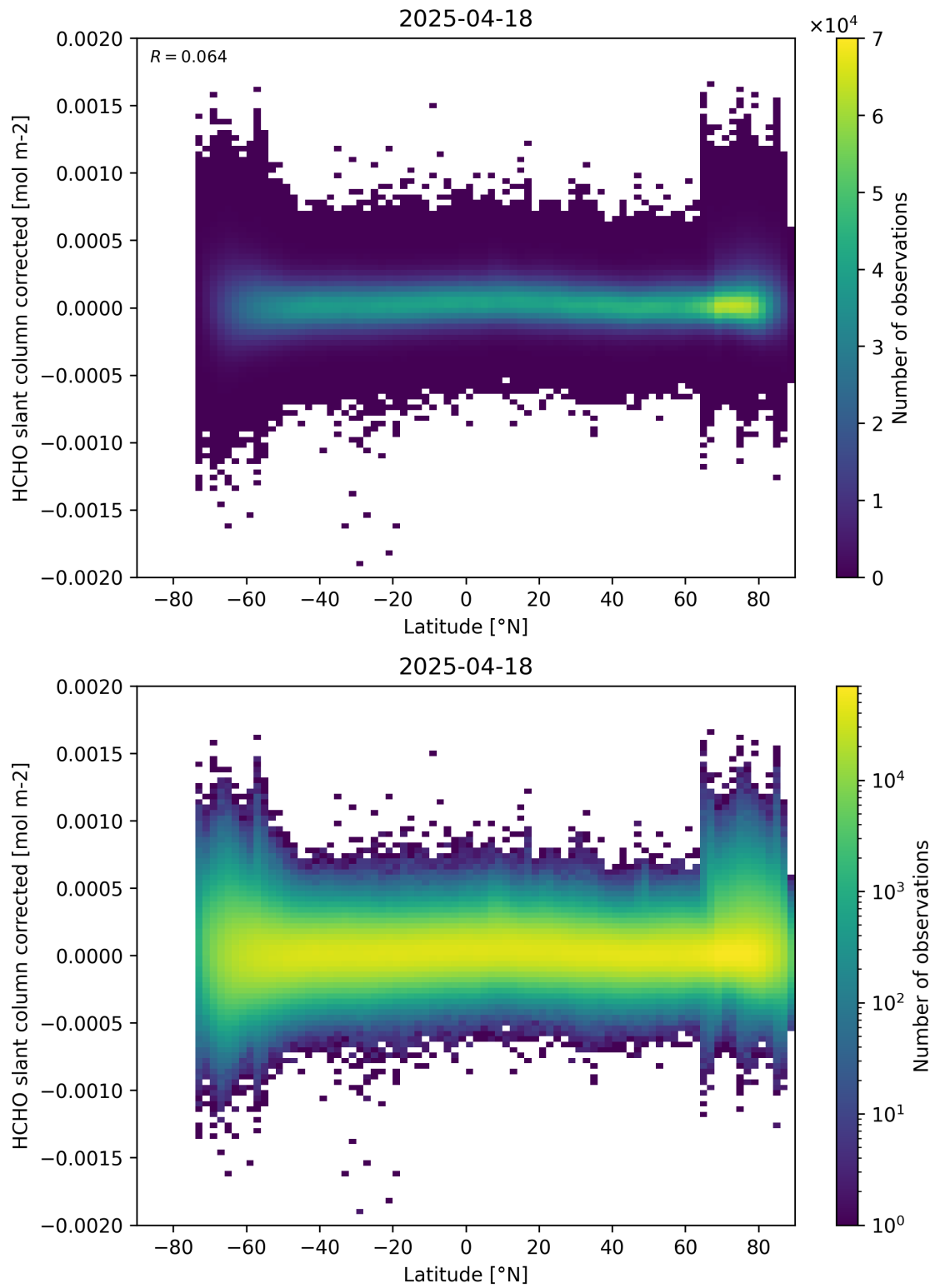
Figure 157: Scatter density plot of “Latitude” against “HCHO slant column corrected” for 2025-04-18 to 2025-04-19.
