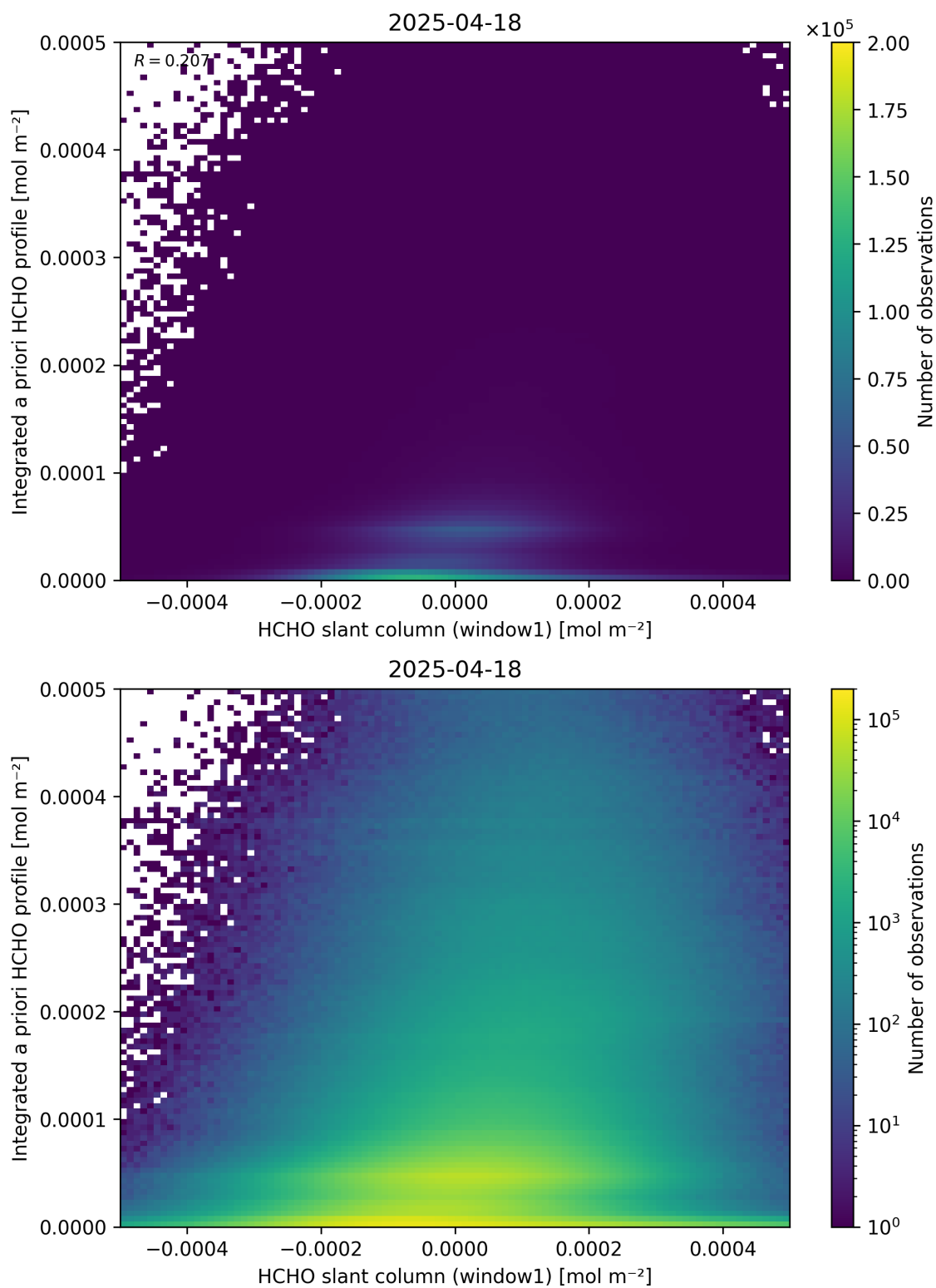
Figure 87: Scatter density plot of “HCHO slant column (window1)” against “Integrated a priori HCHO profile” for 2025-04-18 to 2025-04-19.
