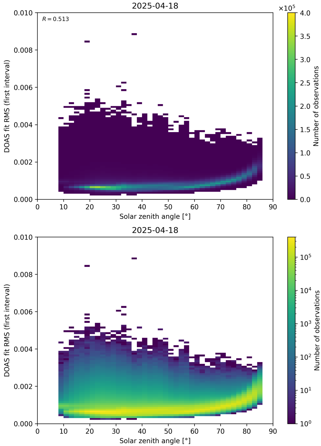
Figure 167: Scatter density plot of “Solar zenith angle” against “DOAS fit RMS (first interval)” for 2025-04-18 to 2025-04-19.
