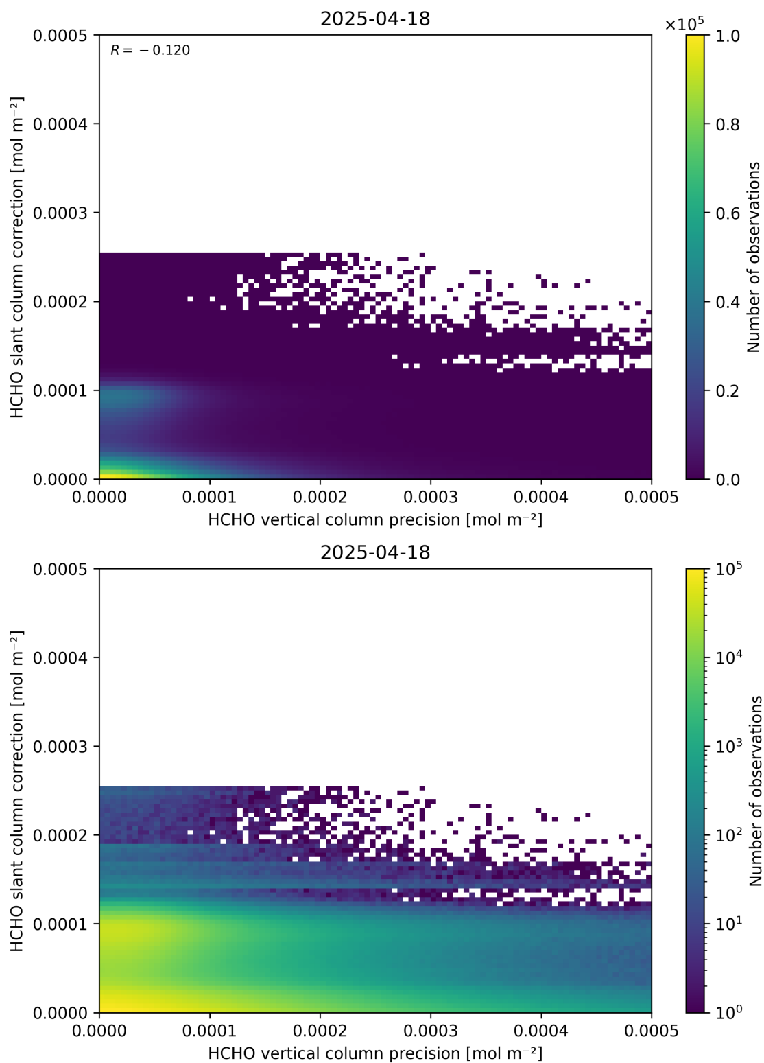
Figure 141: Scatter density plot of “HCHO vertical column precision” against “HCHO slant column correction” for 2025-04-18 to 2025-04-19.
