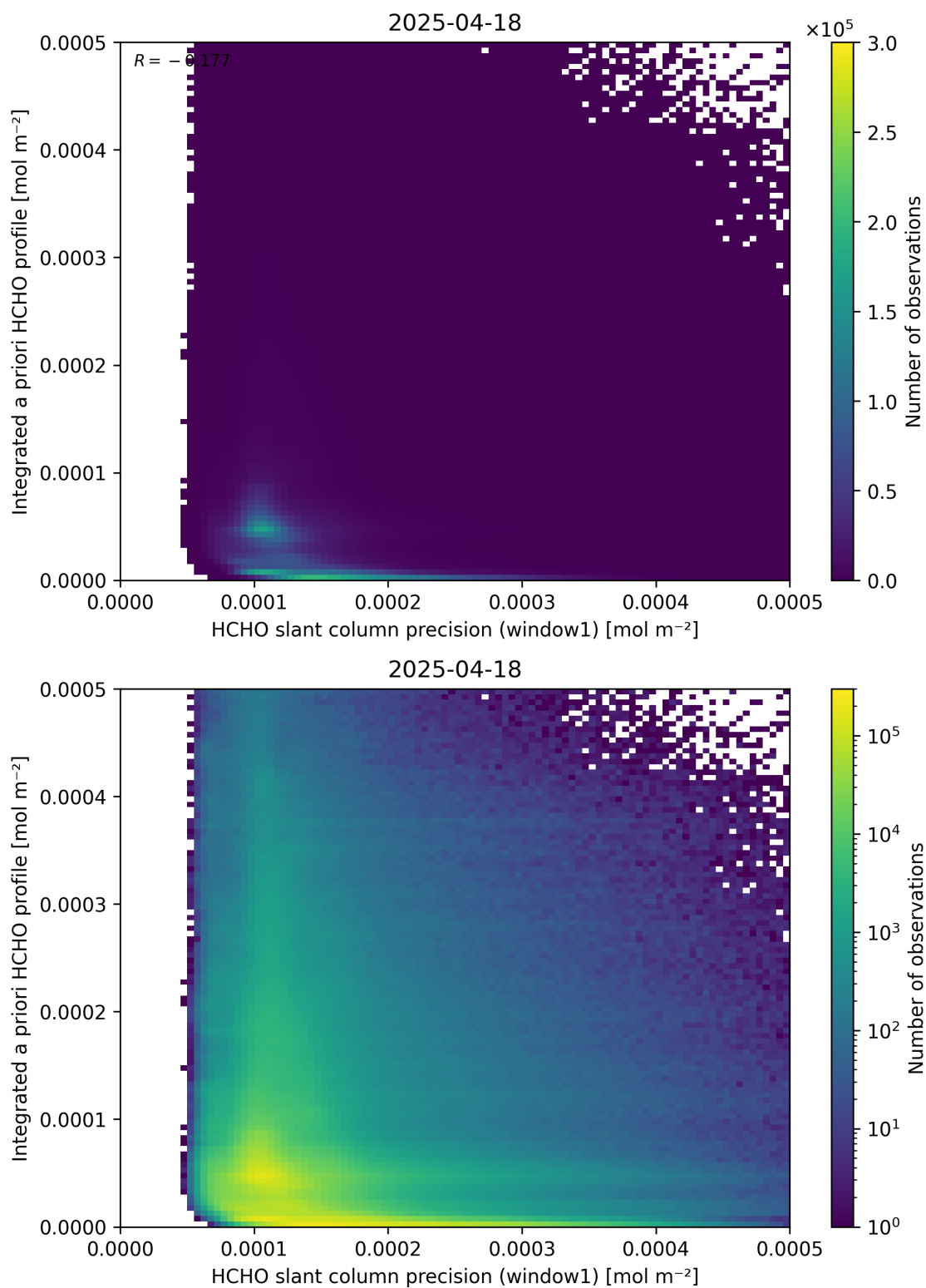
Figure 96: Scatter density plot of “HCHO slant column precision (window1)” against “Integrated a priori HCHO profile” for 2025-04-18 to 2025-04-19.
