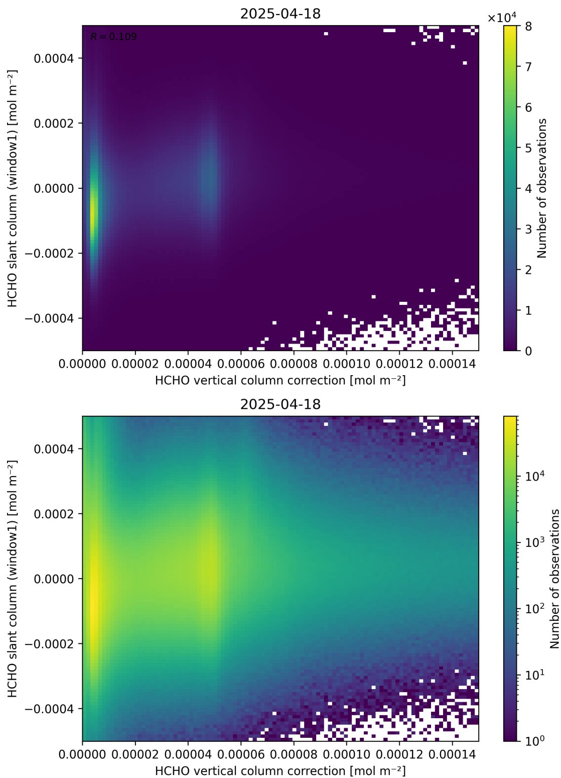
Figure 118: Scatter density plot of “HCHO vertical column correction” against “HCHO slant column (window1)” for 2025-04-18 to 2025-04-19.
