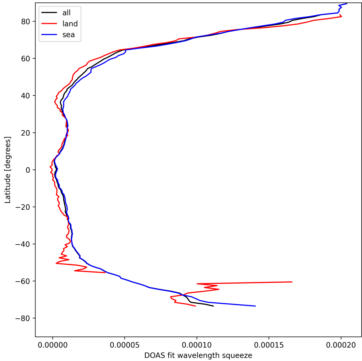
Figure 31: Zonal average of “DOAS fit wavelength squeeze” for 2025-04-18 to 2025-04-19.
