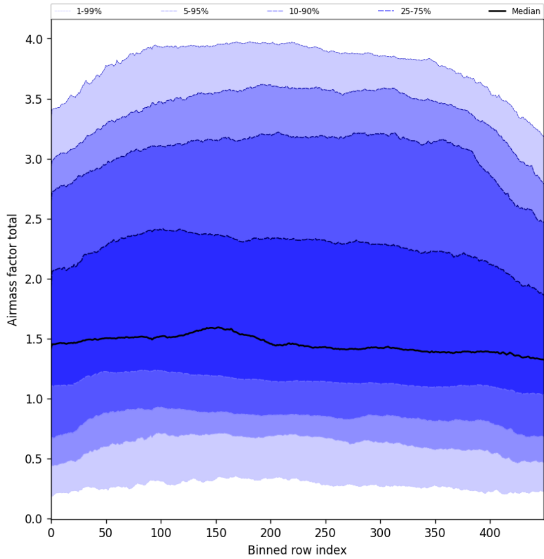
Figure 54: Along track statistics of “Airmass factor total” for 2025-04-18 to 2025-04-19
