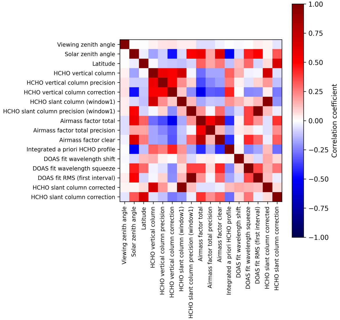
Figure 2: Map of correlation matrix for 2025-04-18 to 2025-04-19.
