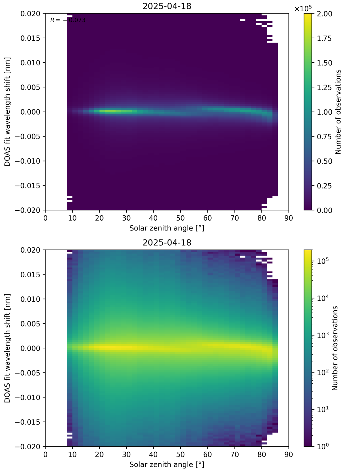
Figure 168: Scatter density plot of “Solar zenith angle” against “DOAS fit wavelength shift” for 2025-04-18 to 2025-04-19.
