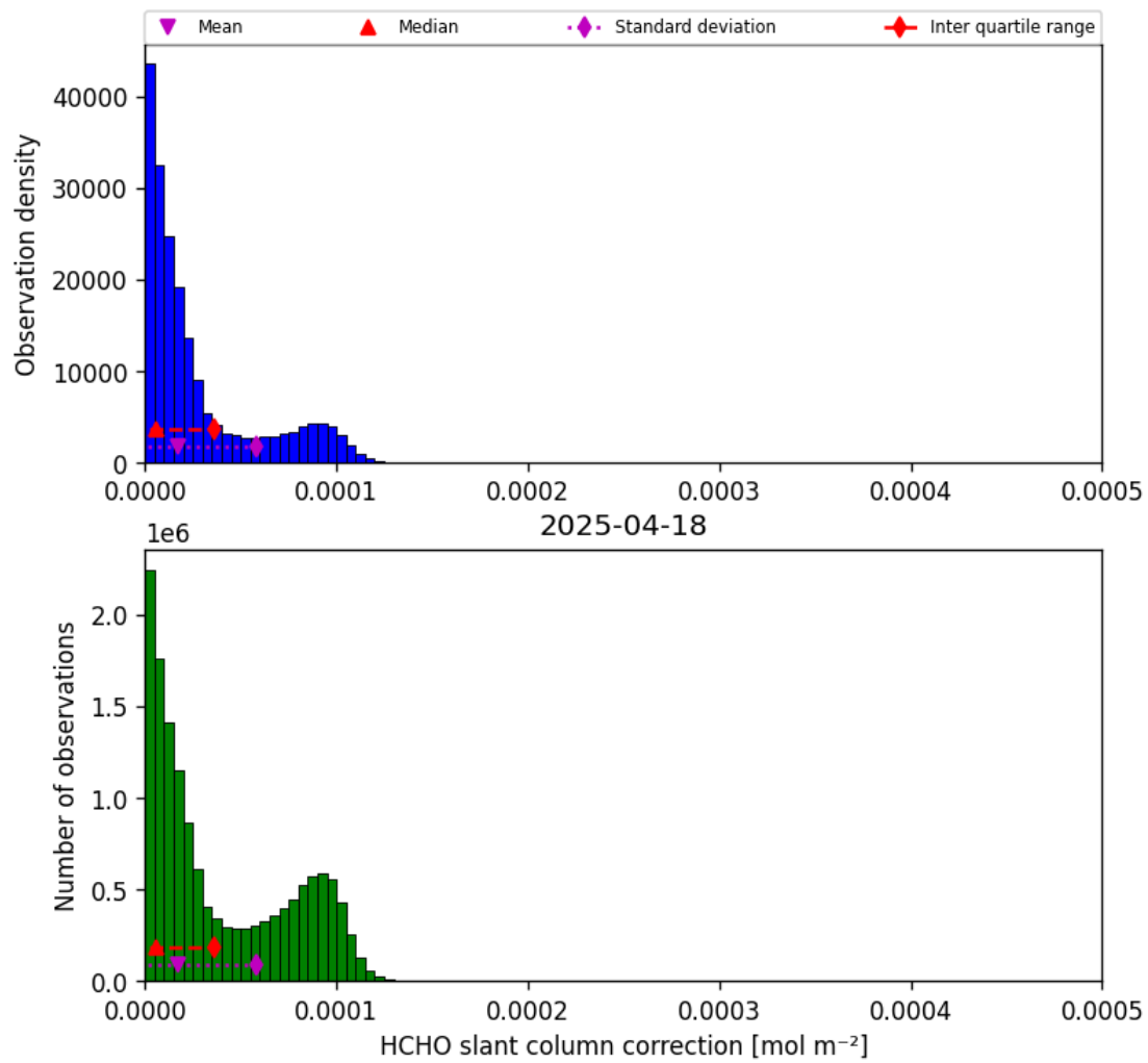
Figure 47: Histogram of “HCHO slant column correction” for 2025-04-18 to 2025-04-19
