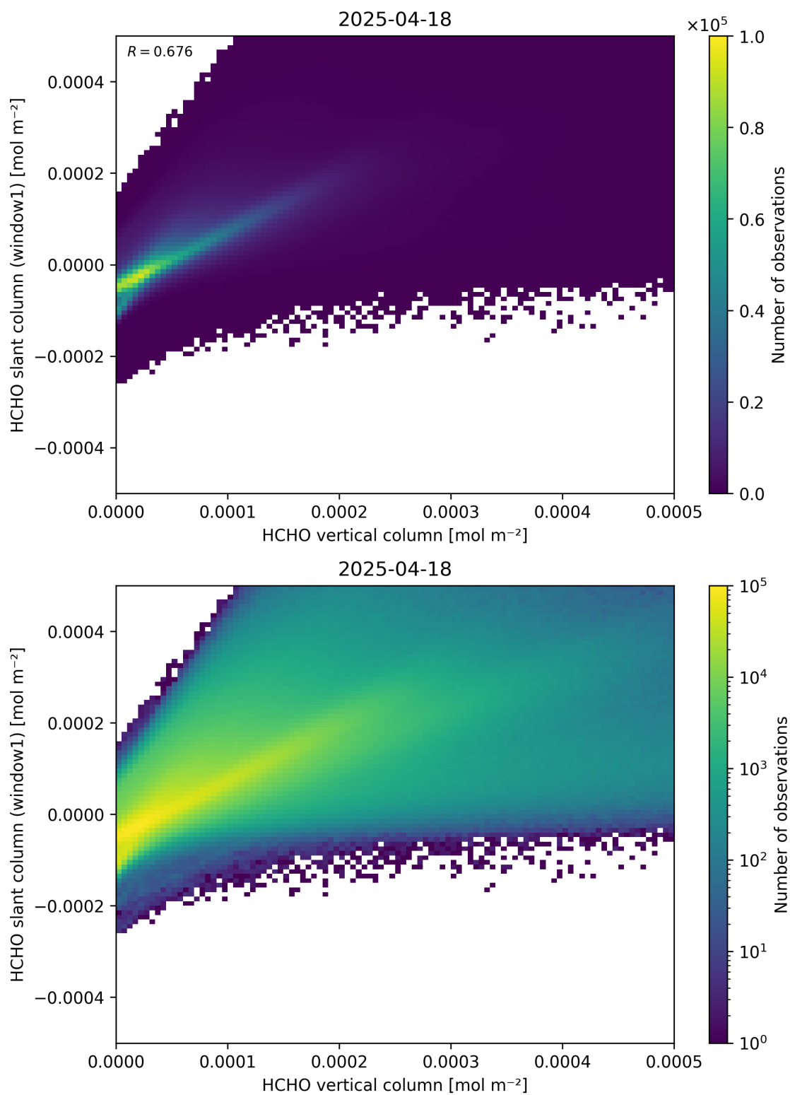
Figure 129: Scatter density plot of “HCHO vertical column” against “HCHO slant column (window1)” for 2025-04-18 to 2025-04-19.
