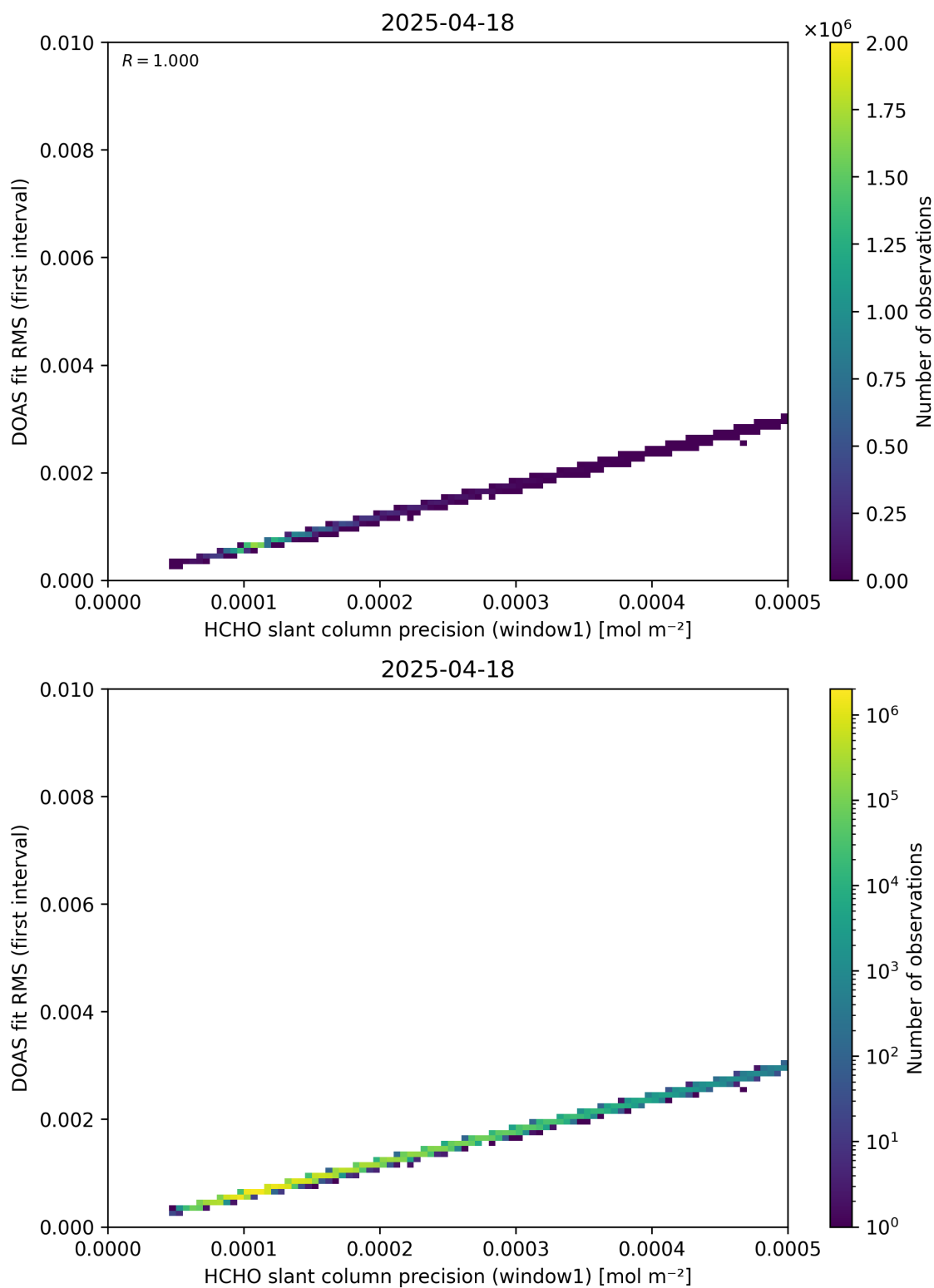
Figure 88: Scatter density plot of “HCHO slant column precision (window1)” against “DOAS fit RMS (first interval)” for 2025-04-18 to 2025-04-19.
