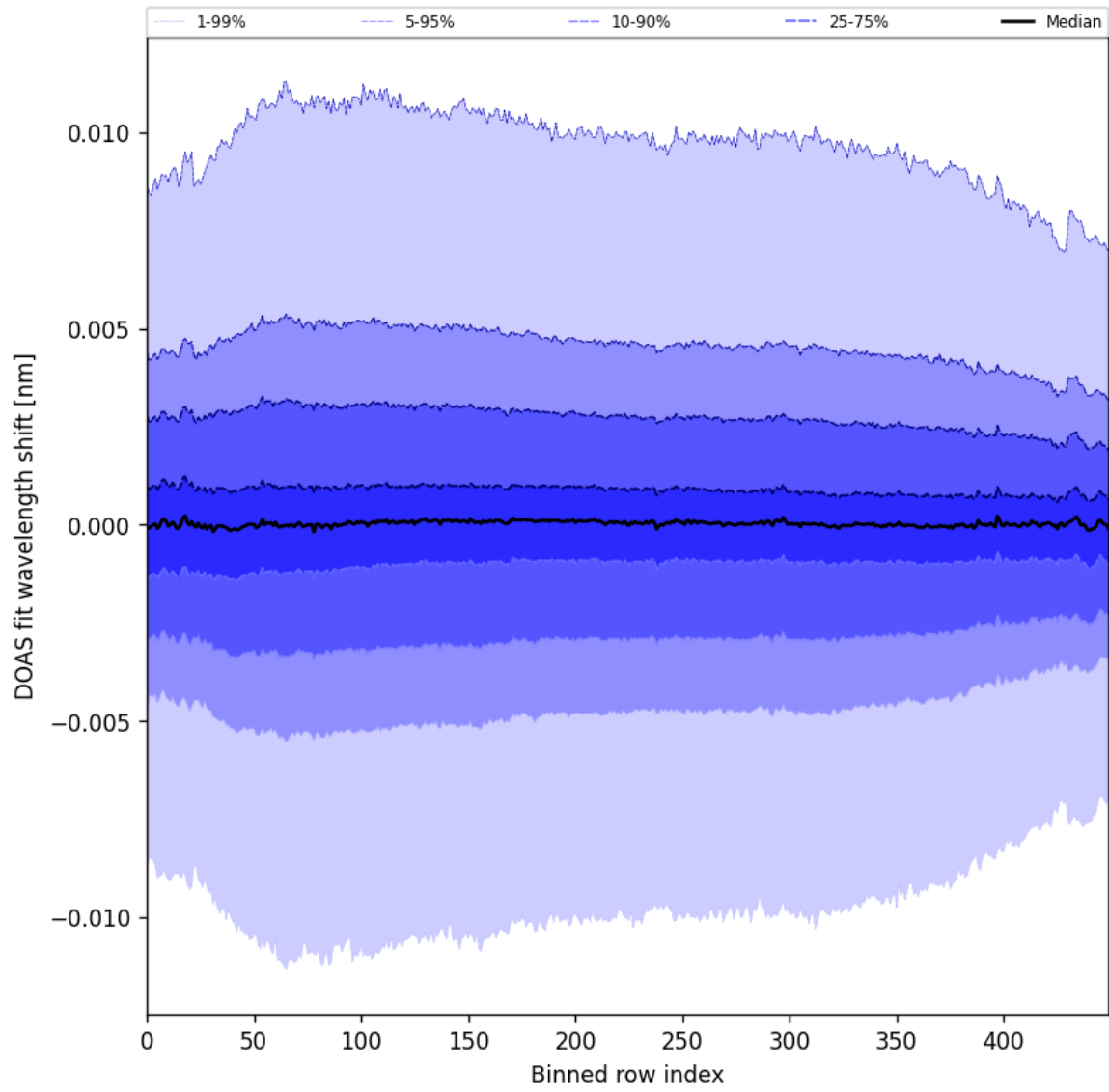
Figure 58: Along track statistics of “DOAS fit wavelength shift” for 2025-04-18 to 2025-04-19
