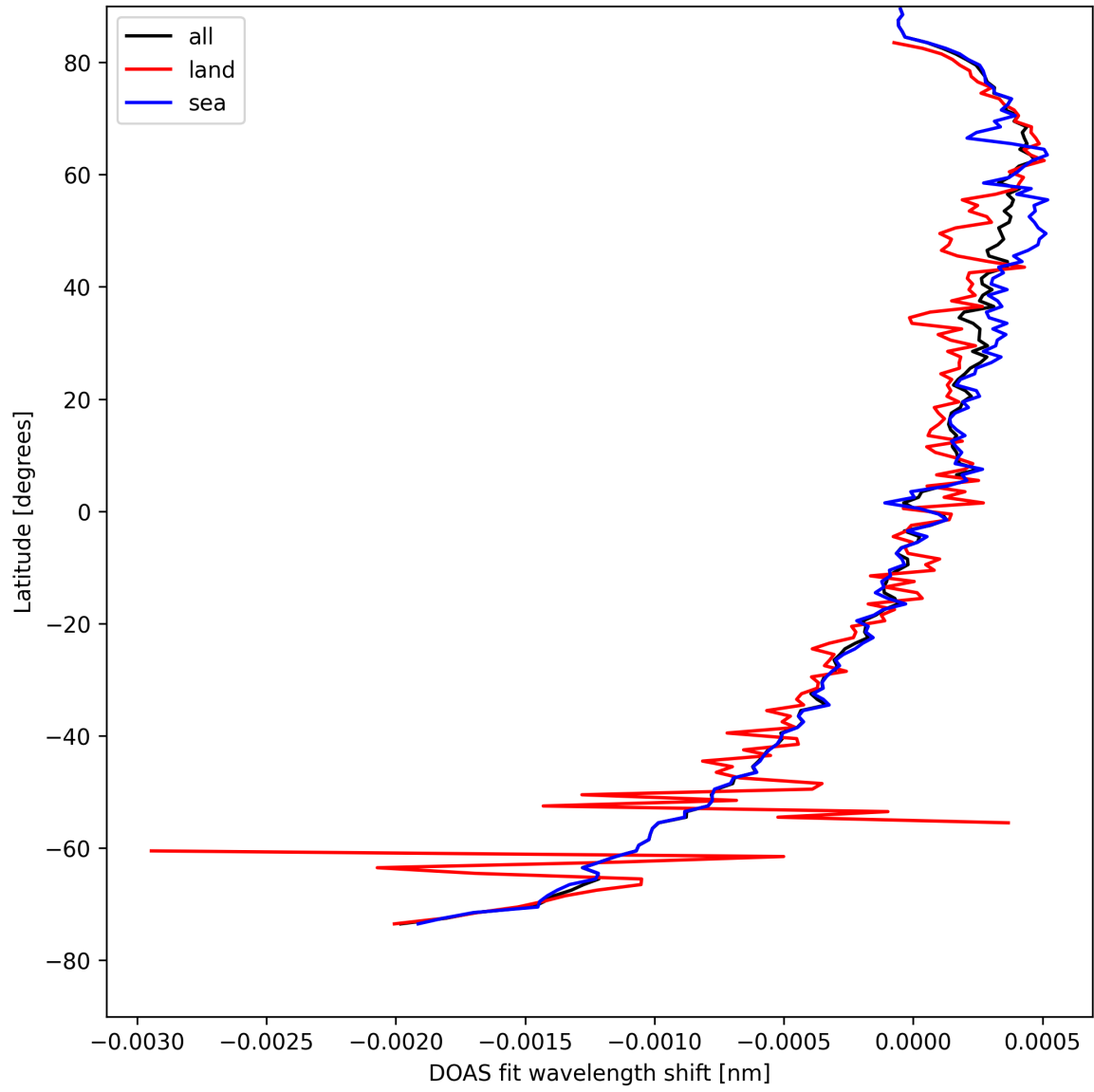
Figure 30: Zonal average of “DOAS fit wavelength shift” for 2025-04-18 to 2025-04-19.
