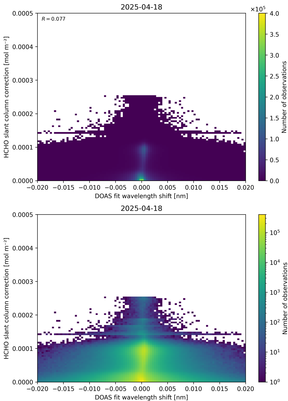
Figure 67: Scatter density plot of “DOAS fit wavelength shift” against “HCHO slant column correction” for 2025-04-18 to 2025-04-19.
