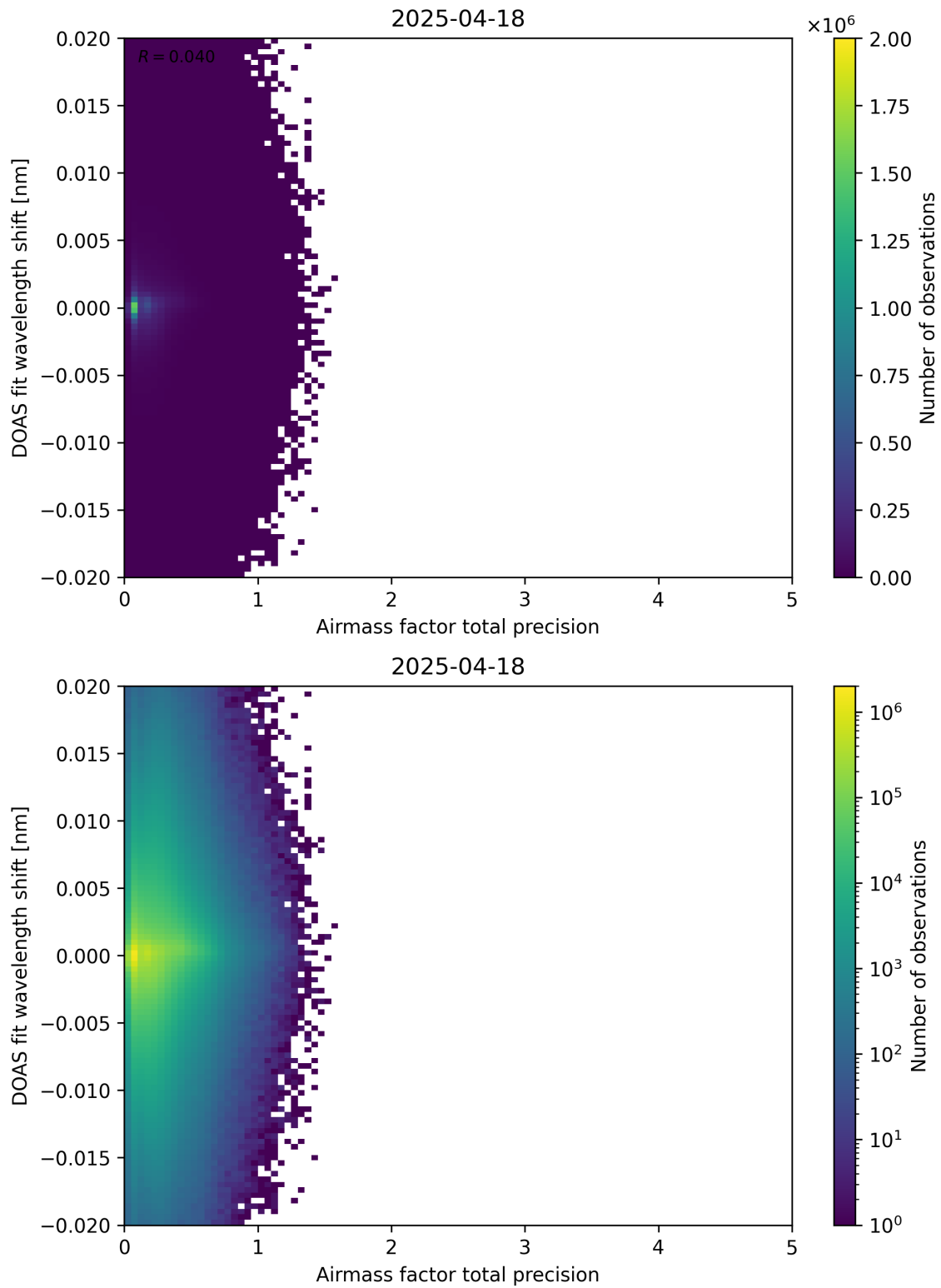
Figure 106: Scatter density plot of “Airmass factor total precision” against “DOAS fit wavelength shift” for 2025-04-18 to 2025-04-19.
