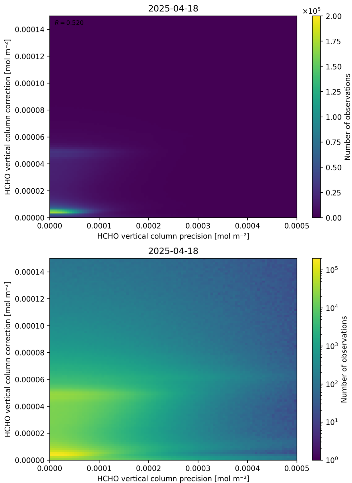
Figure 146: Scatter density plot of “HCHO vertical column precision” against “HCHO vertical column correction” for 2025-04-18 to 2025-04-19.
