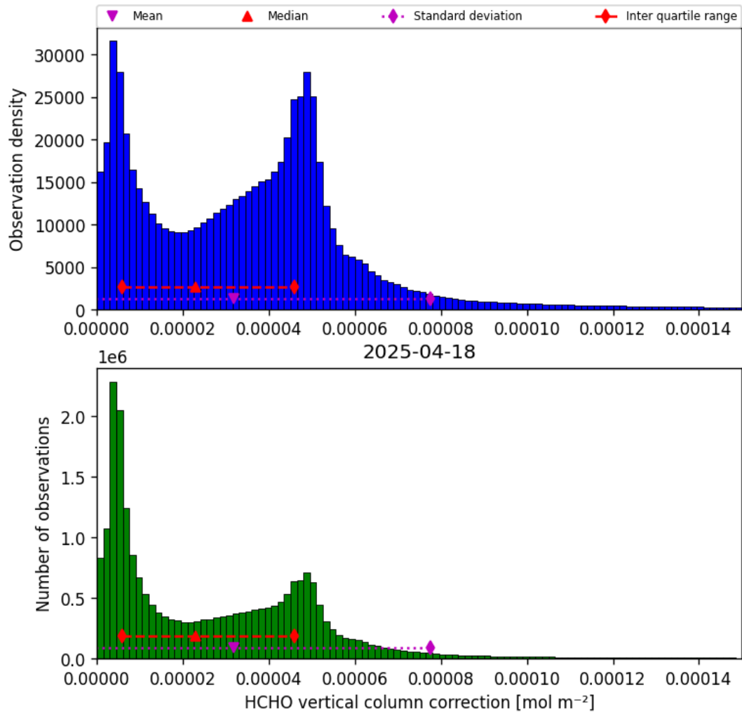
Figure 37: Histogram of “HCHO vertical column correction” for 2025-04-18 to 2025-04-19
