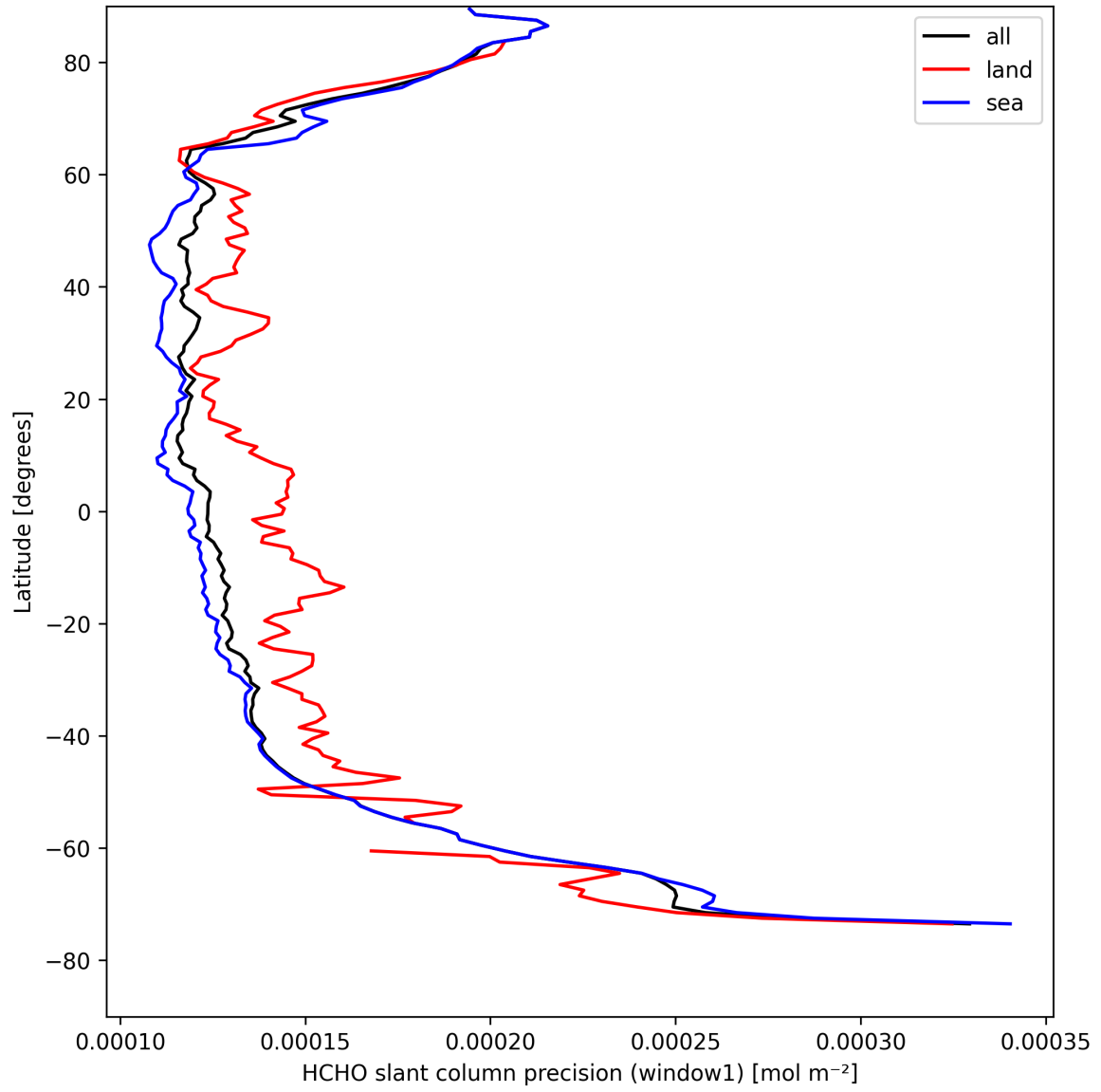
Figure 25: Zonal average of “HCHO slant column precision (window1)” for 2025-04-18 to 2025-04-19.
