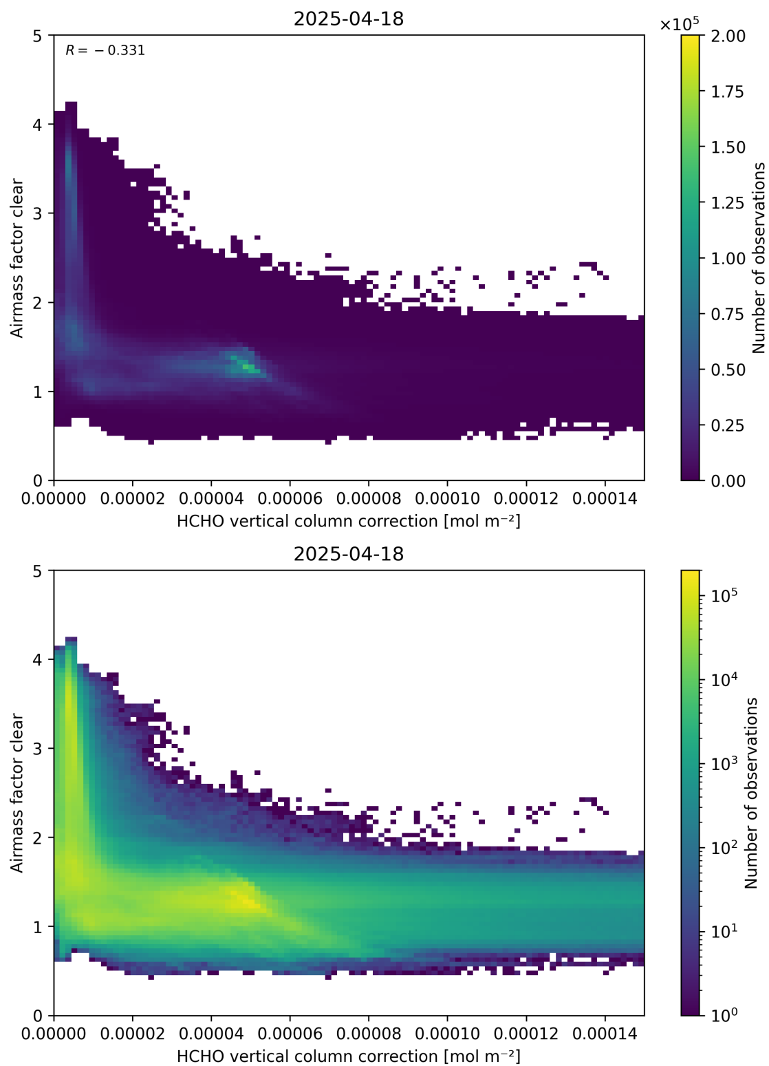
Figure 115: Scatter density plot of “HCHO vertical column correction” against “Airmass factor clear” for 2025-04-18 to 2025-04-19.
