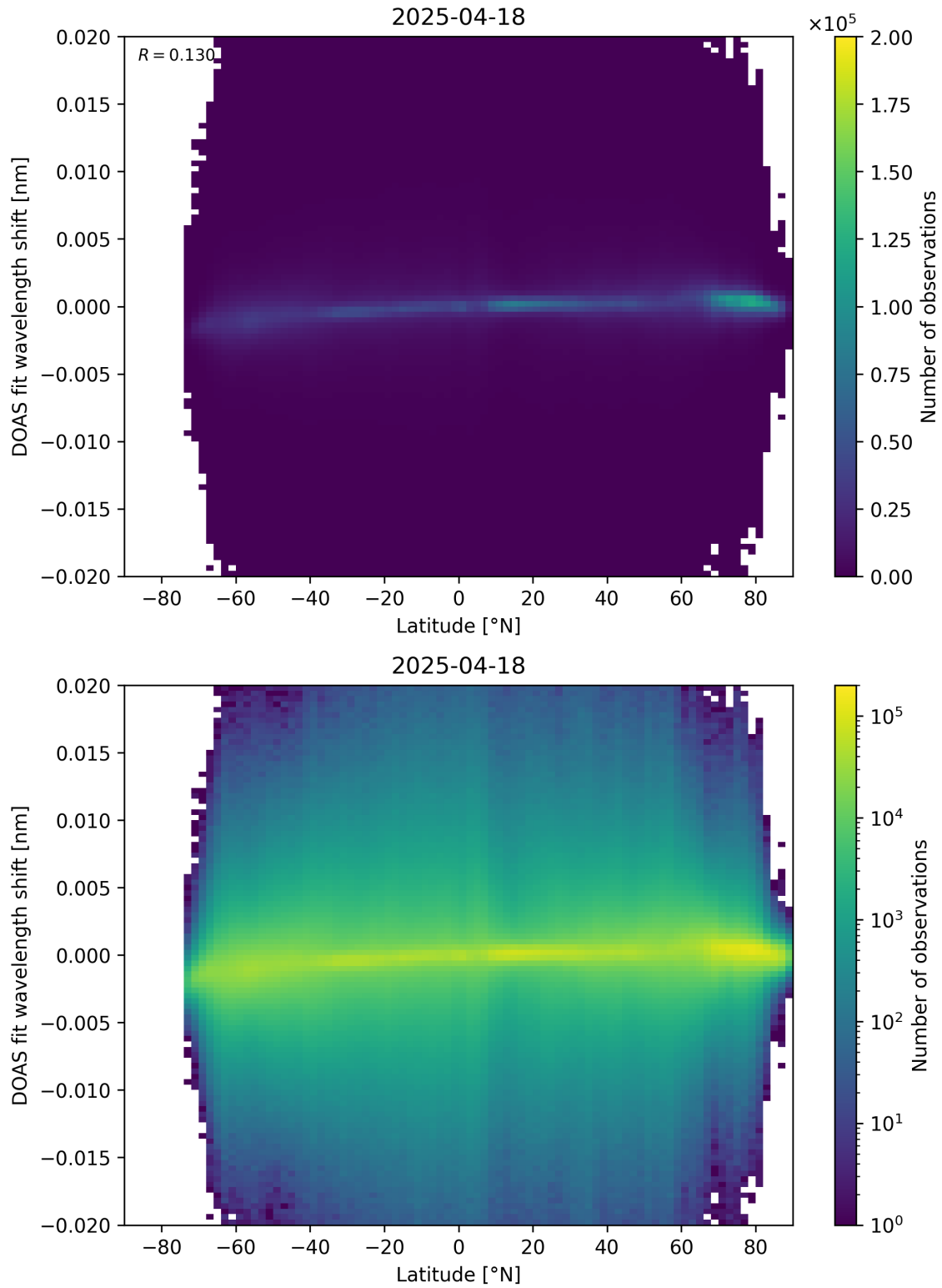
Figure 154: Scatter density plot of “Latitude” against “DOAS fit wavelength shift” for 2025-04-18 to 2025-04-19.
