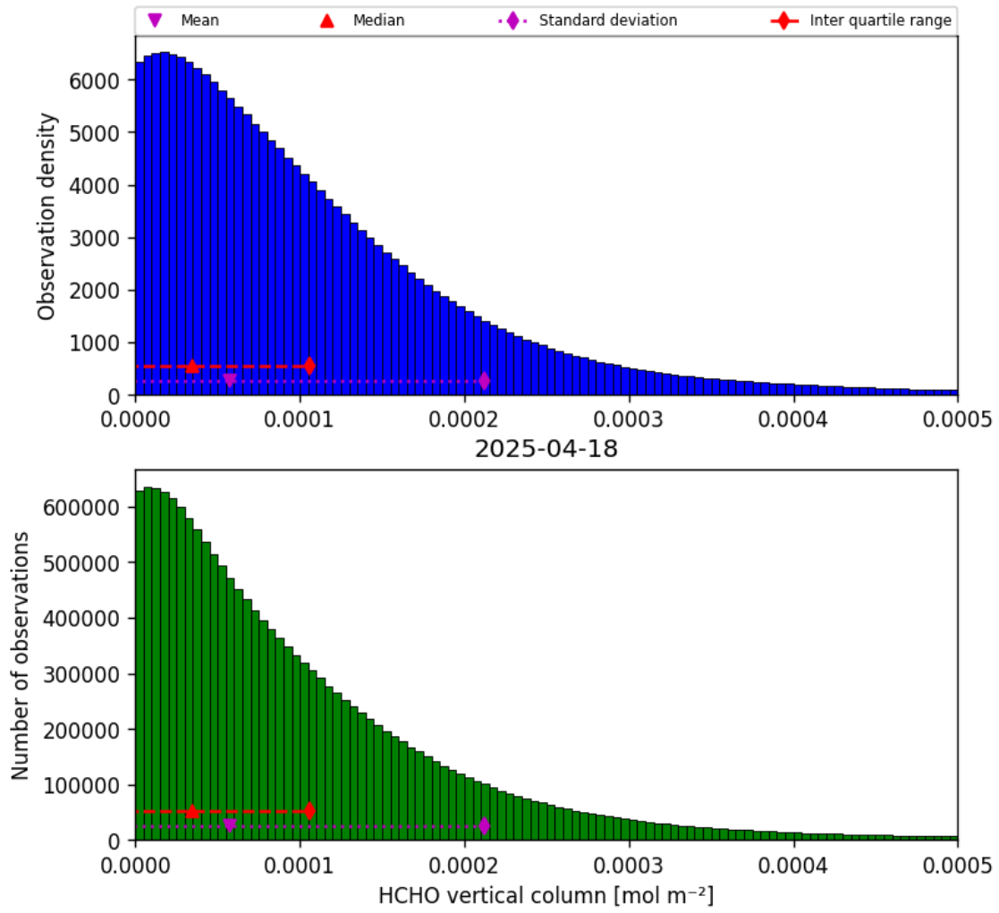
Figure 35: Histogram of “HCHO vertical column” for 2025-04-18 to 2025-04-19
