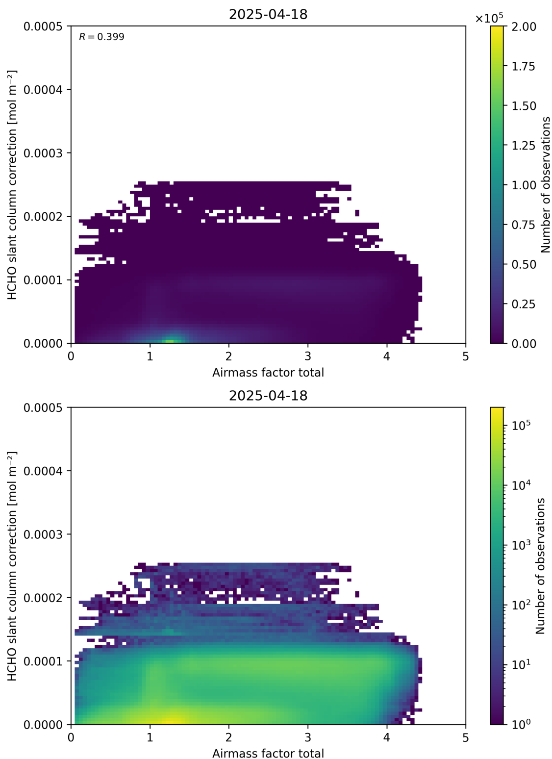
Figure 102: Scatter density plot of “Airmass factor total” against “HCHO slant column correction” for 2025-04-18 to 2025-04-19.
