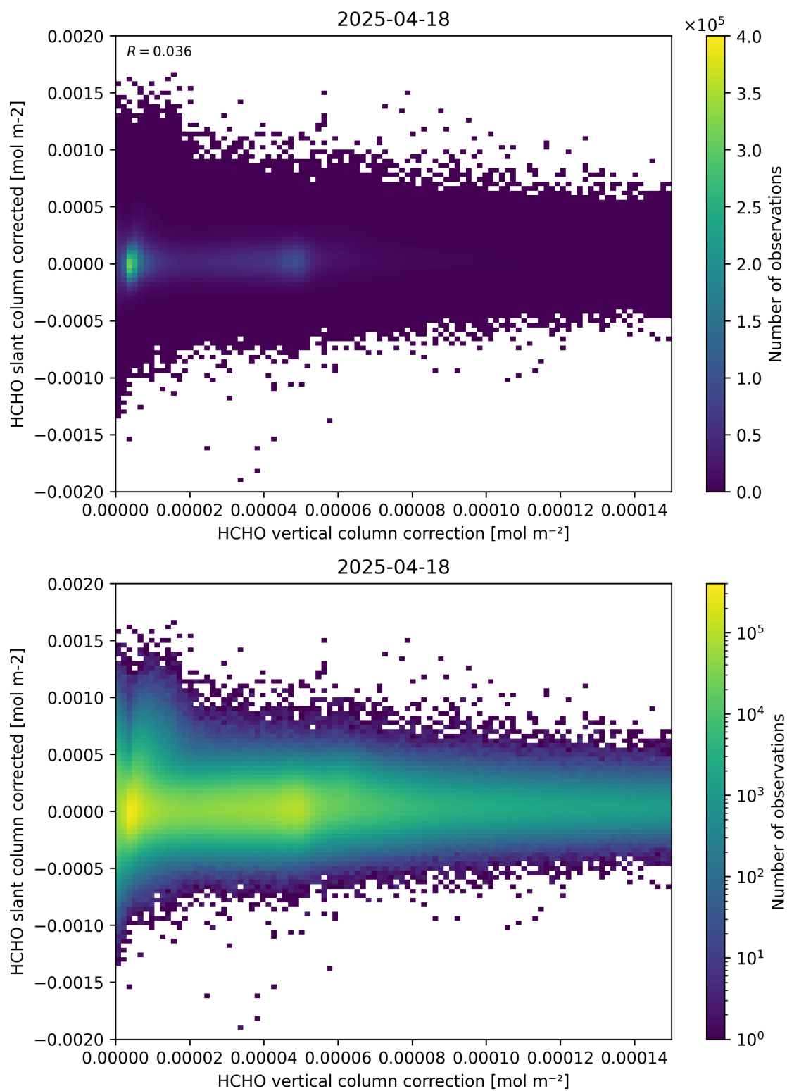
Figure 116: Scatter density plot of “HCHO vertical column correction” against “HCHO slant column corrected” for 2025-04-18 to 2025-04-19.
