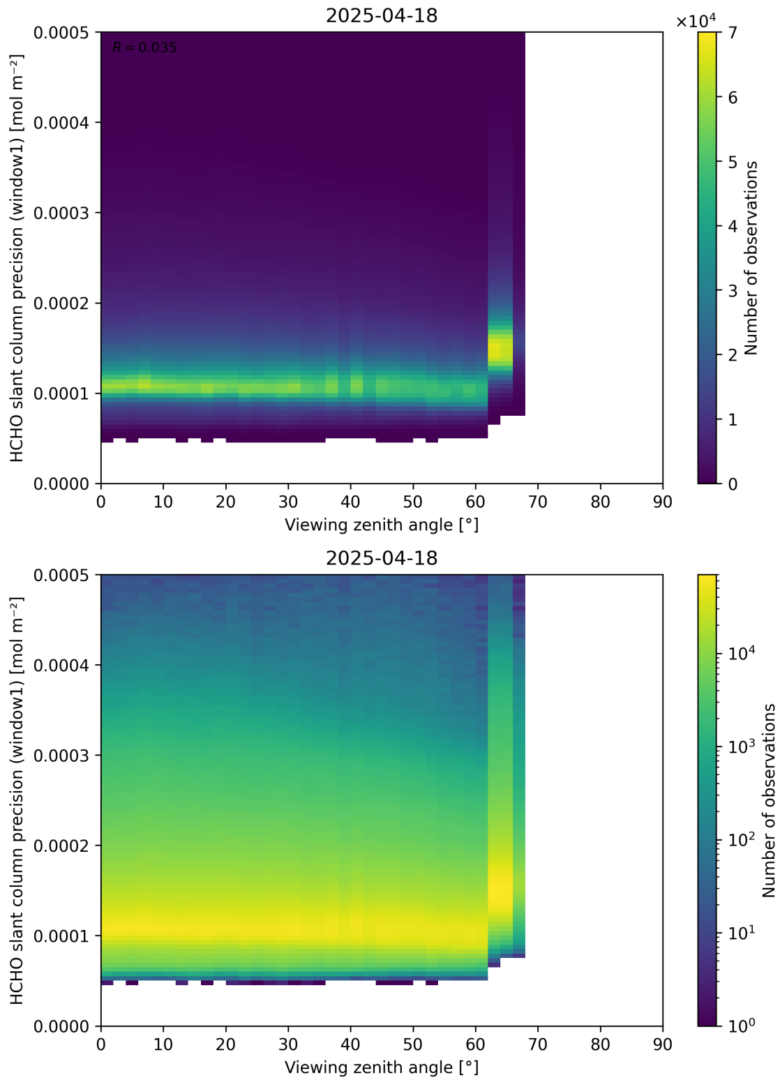
Figure 189: Scatter density plot of “Viewing zenith angle” against “HCHO slant column precision (window1)” for 2025-04-18 to 2025-04-19.
