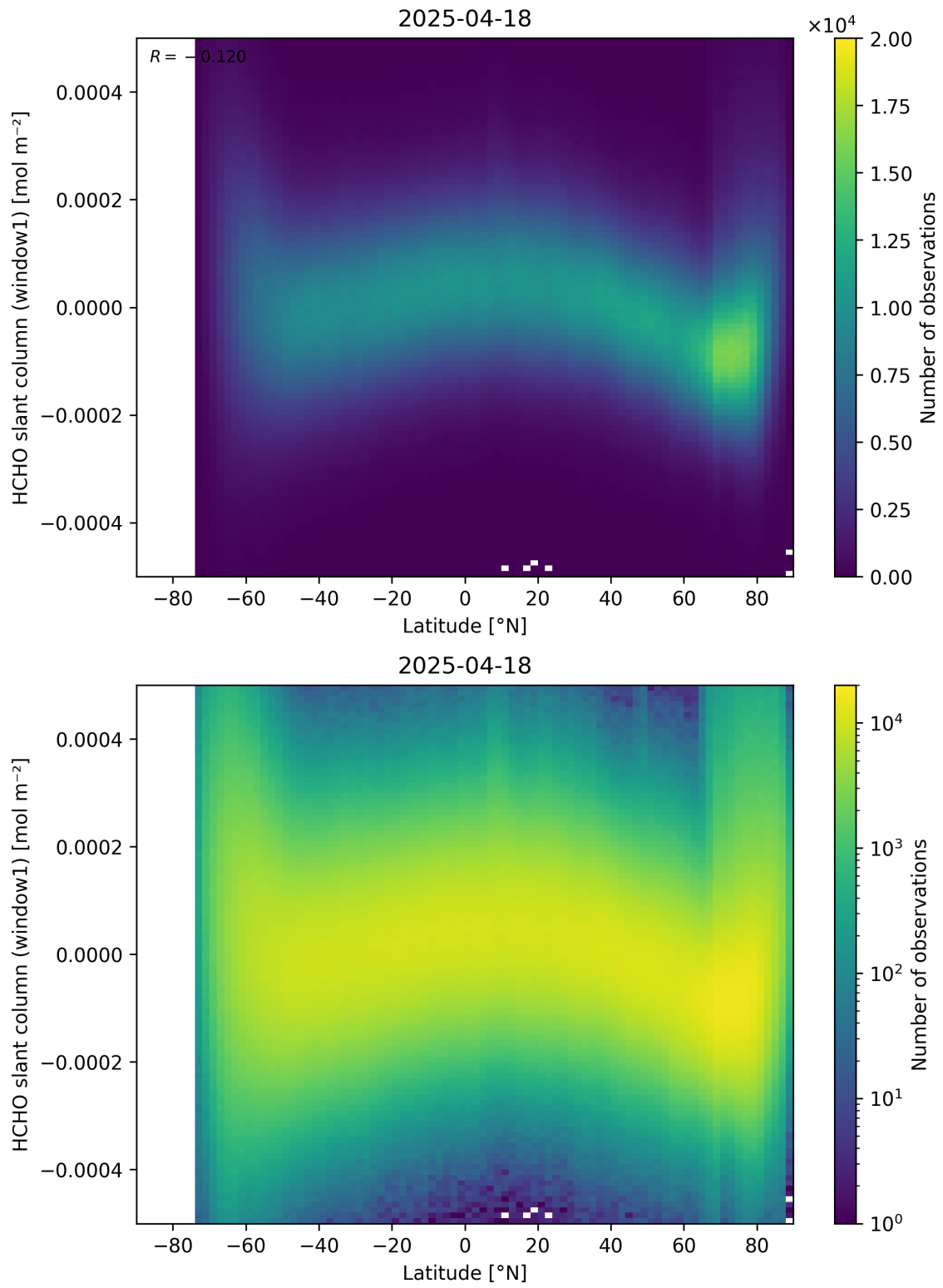
Figure 159: Scatter density plot of “Latitude” against “HCHO slant column (window1)” for 2025-04-18 to 2025-04-19.
