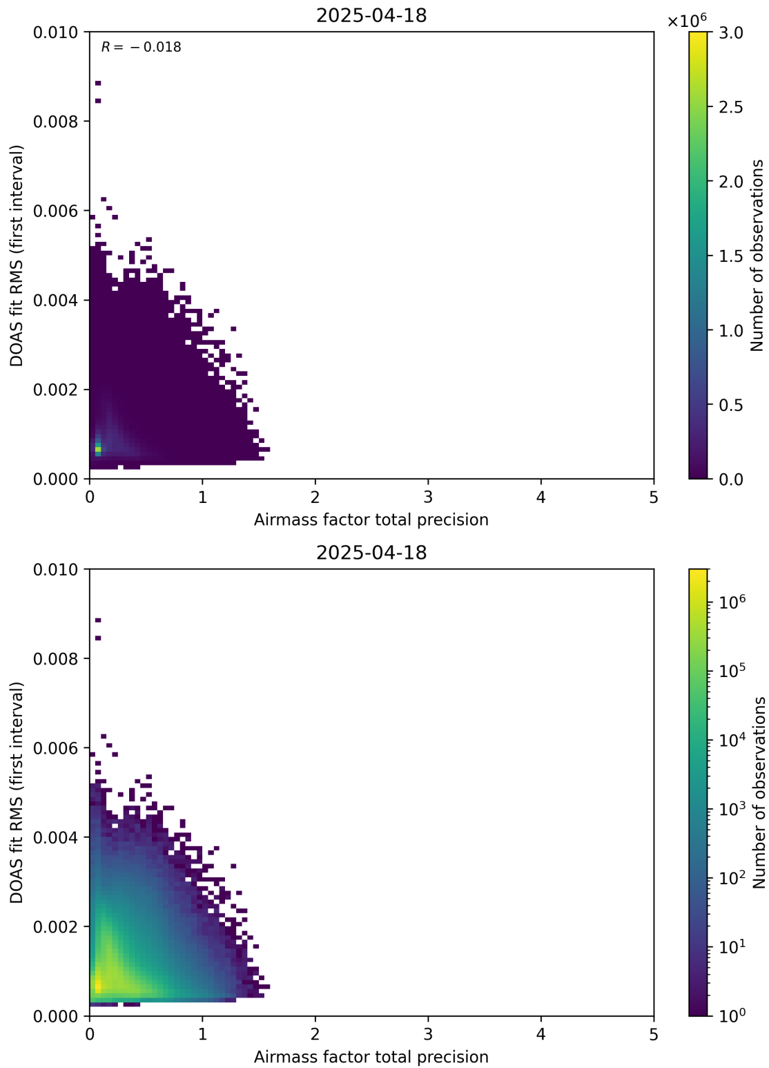
Figure 105: Scatter density plot of “Airmass factor total precision” against “DOAS fit RMS (first interval)” for 2025-04-18 to 2025-04-19.
