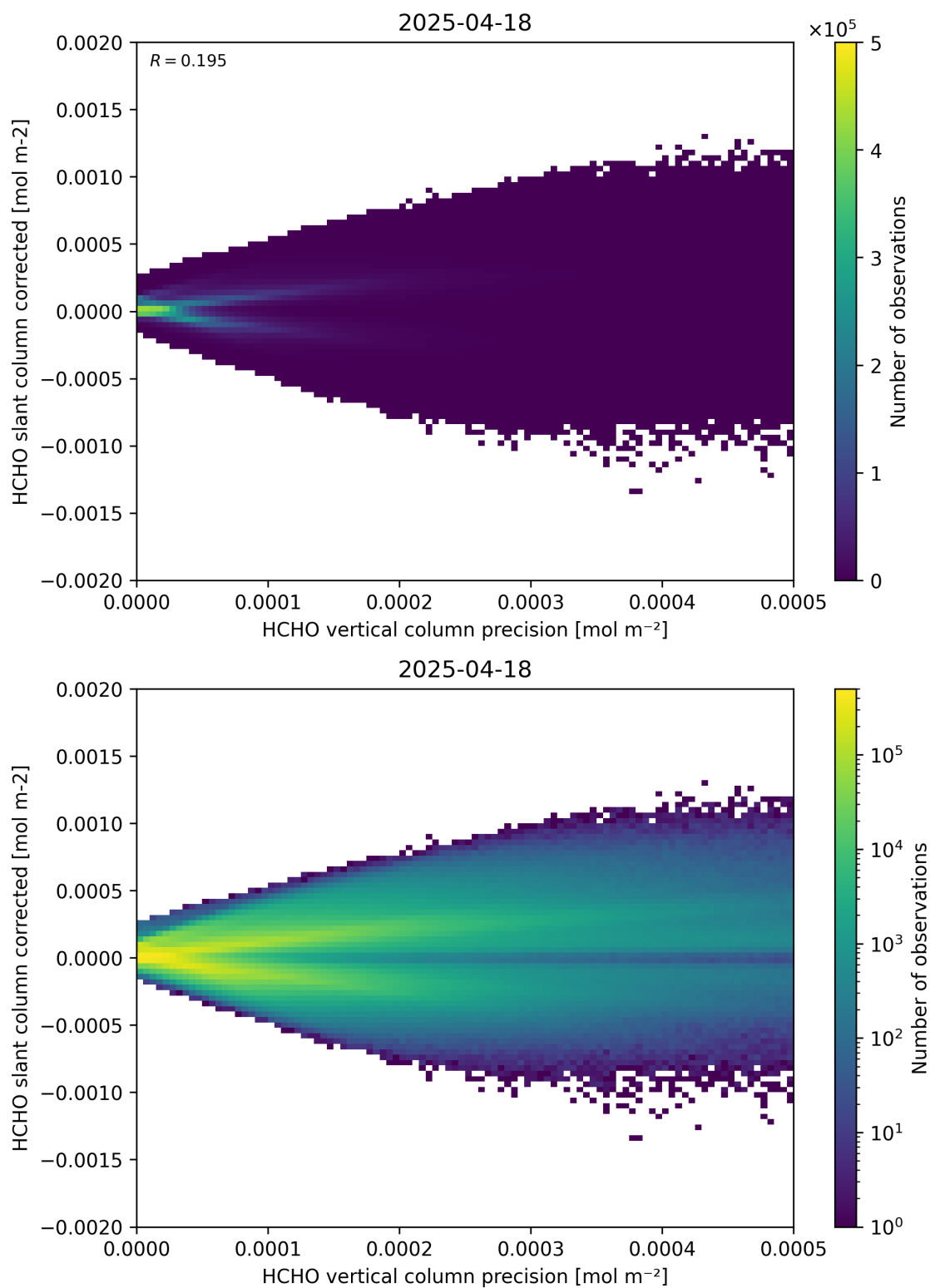
Figure 140: Scatter density plot of “HCHO vertical column precision” against “HCHO slant column corrected” for 2025-04-18 to 2025-04-19.
