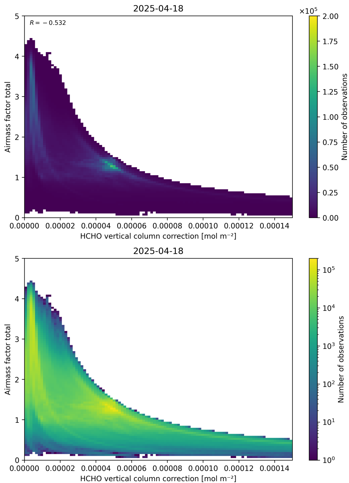
Figure 120: Scatter density plot of “HCHO vertical column correction” against “Airmass factor total” for 2025-04-18 to 2025-04-19.
