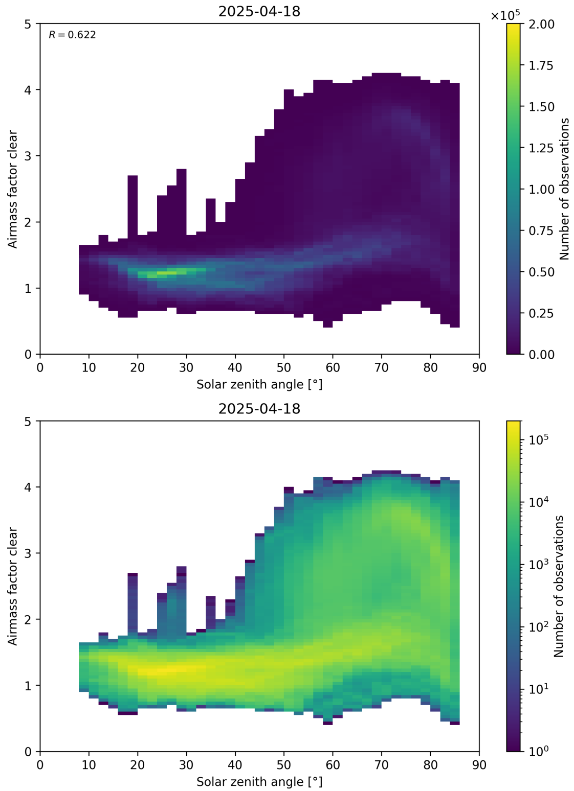
Figure 170: Scatter density plot of “Solar zenith angle” against “Airmass factor clear” for 2025-04-18 to 2025-04-19.
