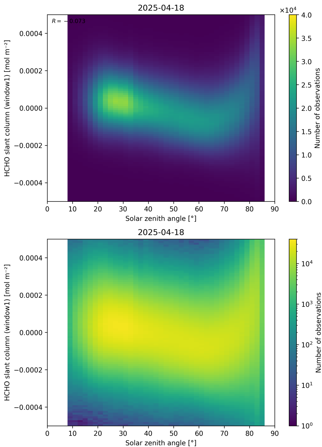
Figure 173: Scatter density plot of “Solar zenith angle” against “HCHO slant column (window1)” for 2025-04-18 to 2025-04-19.
