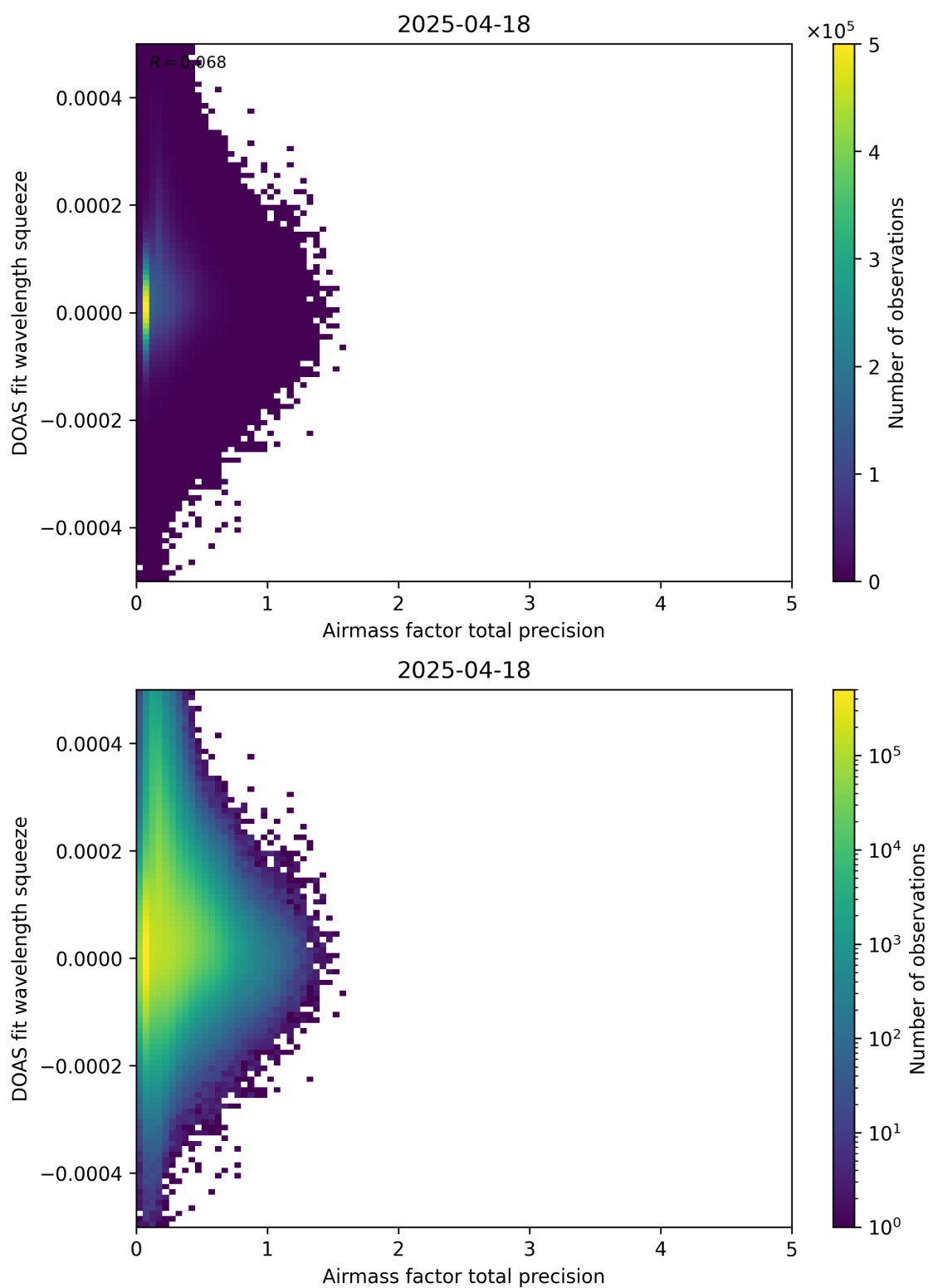
Figure 107: Scatter density plot of “Airmass factor total precision” against “DOAS fit wavelength squeeze” for 2025-04-18 to 2025-04-19.
