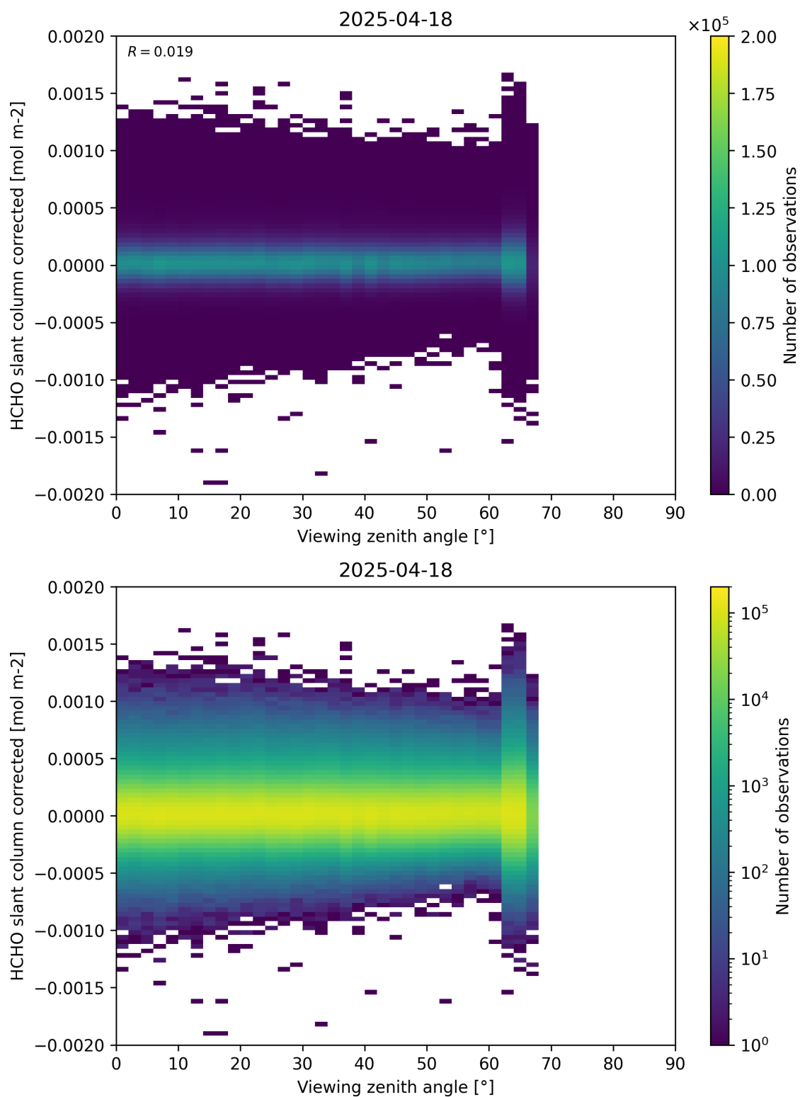
Figure 186: Scatter density plot of “Viewing zenith angle” against “HCHO slant column corrected” for 2025-04-18 to 2025-04-19.
