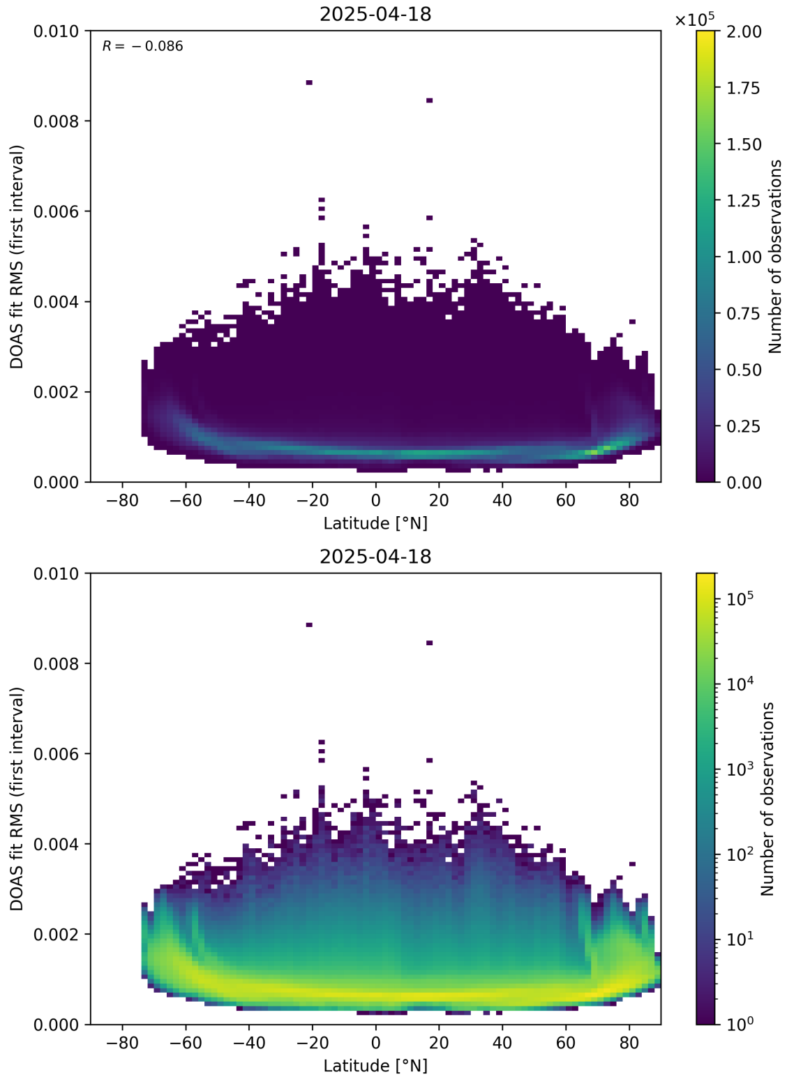
Figure 153: Scatter density plot of “Latitude” against “DOAS fit RMS (first interval)” for 2025-04-18 to 2025-04-19.
