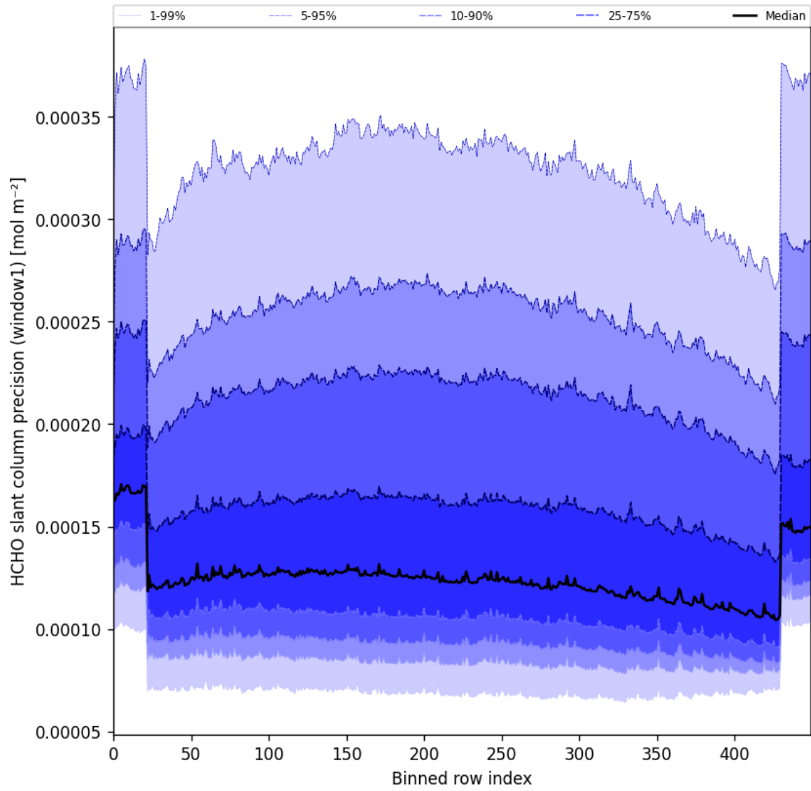
Figure 53: Along track statistics of “HCHO slant column precision (window1)” for 2025-04-18 to 2025-04-19
