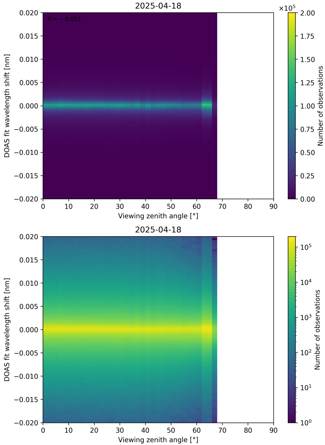
Figure 183: Scatter density plot of “Viewing zenith angle” against “DOAS fit wavelength shift” for 2025-04-18 to 2025-04-19.
