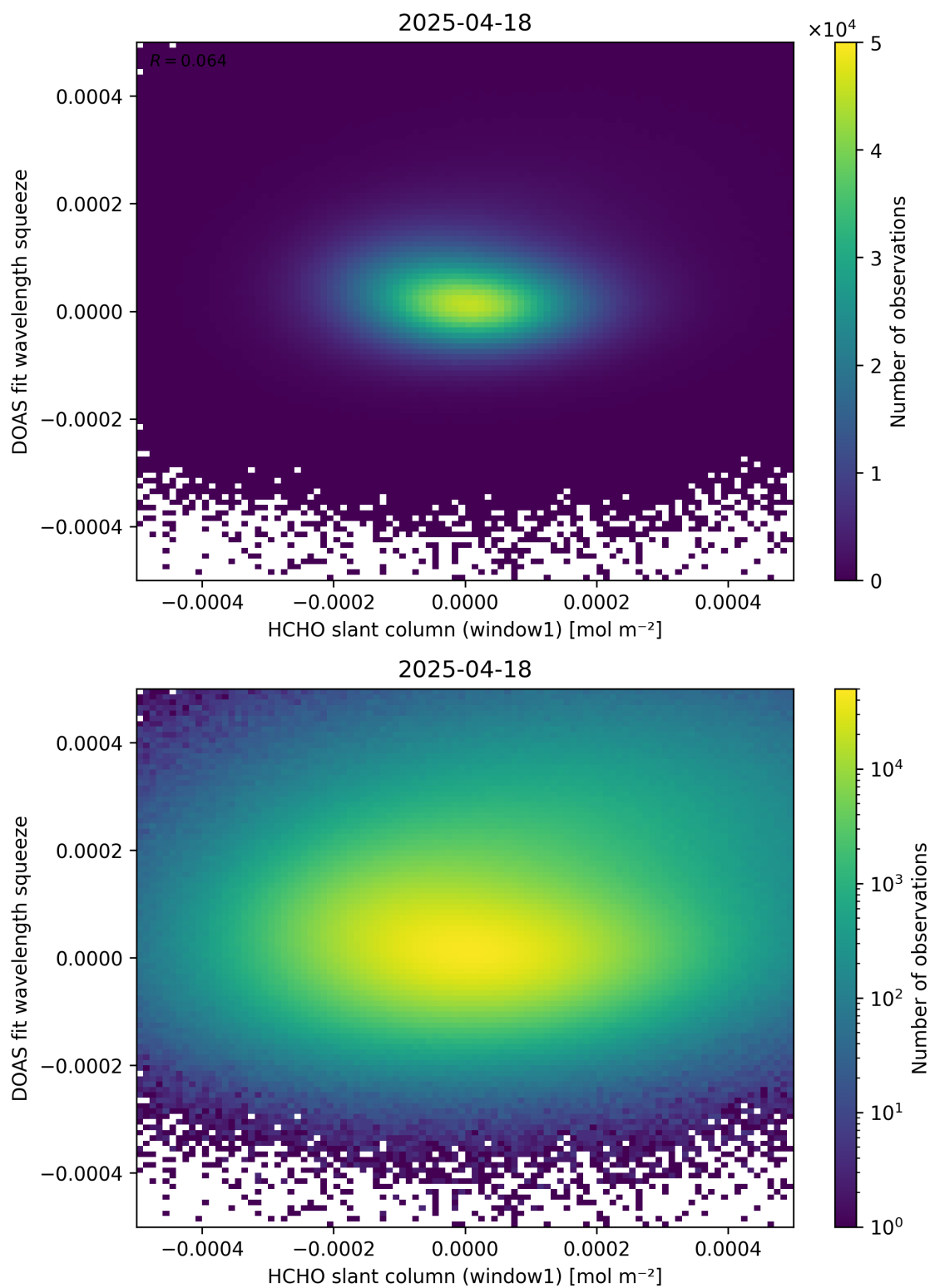
Figure 80: Scatter density plot of “HCHO slant column (window1)” against “DOAS fit wavelength squeeze” for 2025-04-18 to 2025-04-19.
