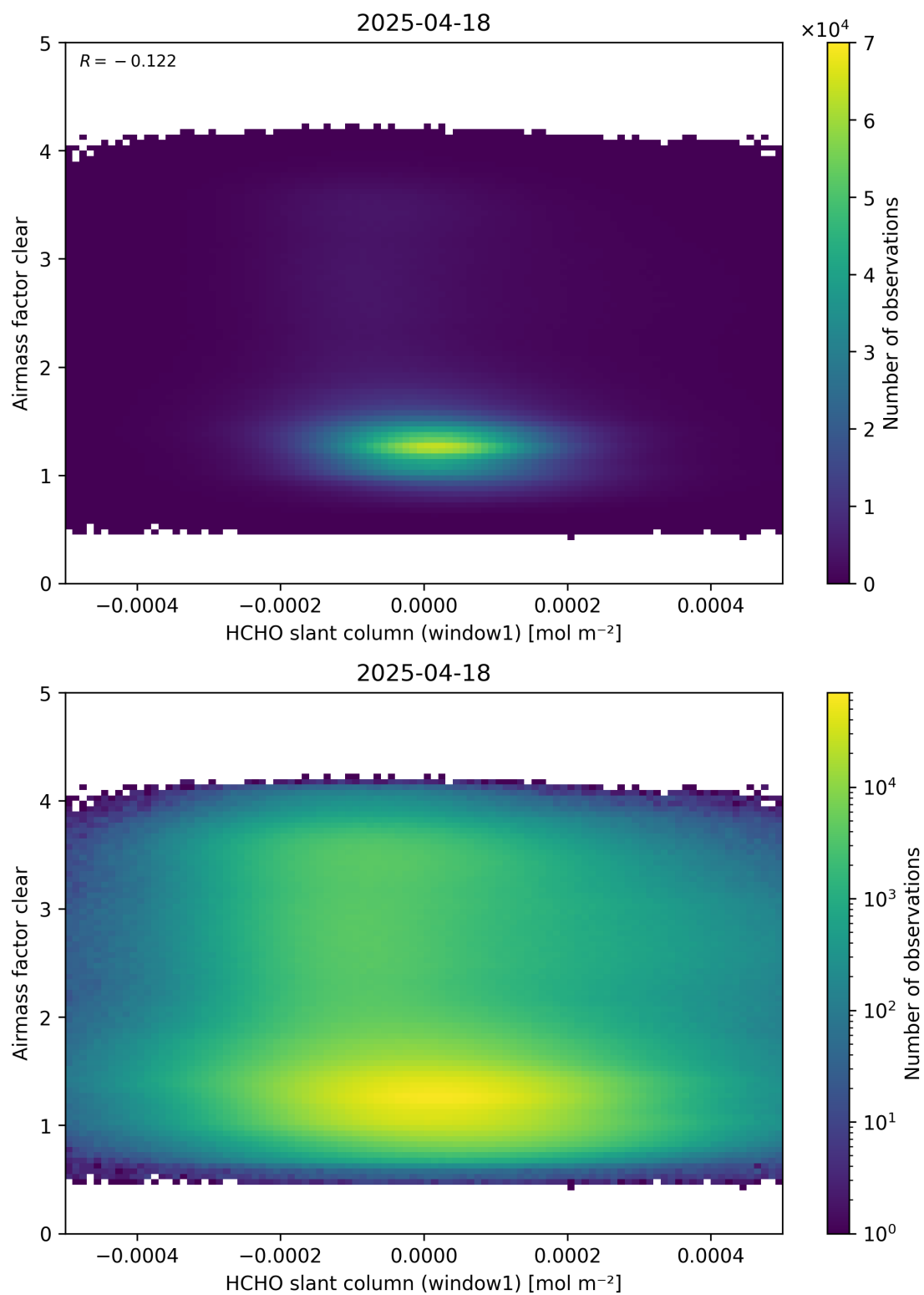
Figure 81: Scatter density plot of “HCHO slant column (window1)” against “Airmass factor clear” for 2025-04-18 to 2025-04-19.
