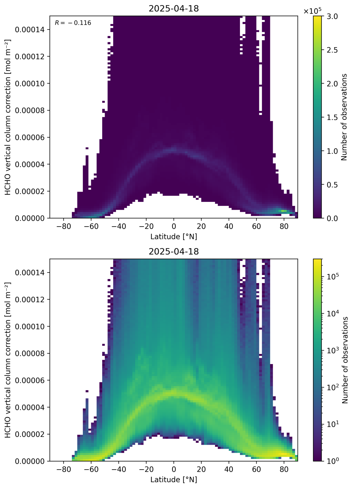
Figure 164: Scatter density plot of “Latitude” against “HCHO vertical column correction” for 2025-04-18 to 2025-04-19.
