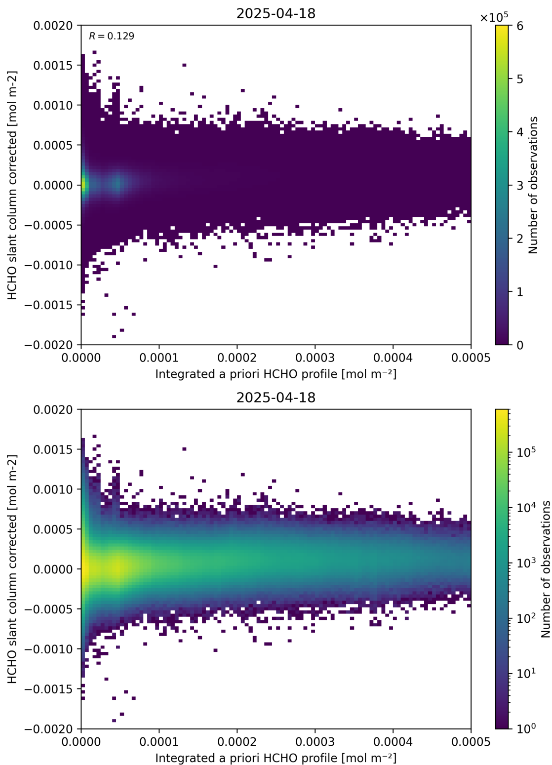
Figure 151: Scatter density plot of “Integrated a priori HCHO profile” against “HCHO slant column corrected” for 2025-04-18 to 2025-04-19.
