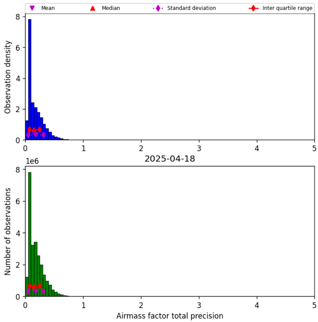
Figure 41: Histogram of “Airmass factor total precision” for 2025-04-18 to 2025-04-19
