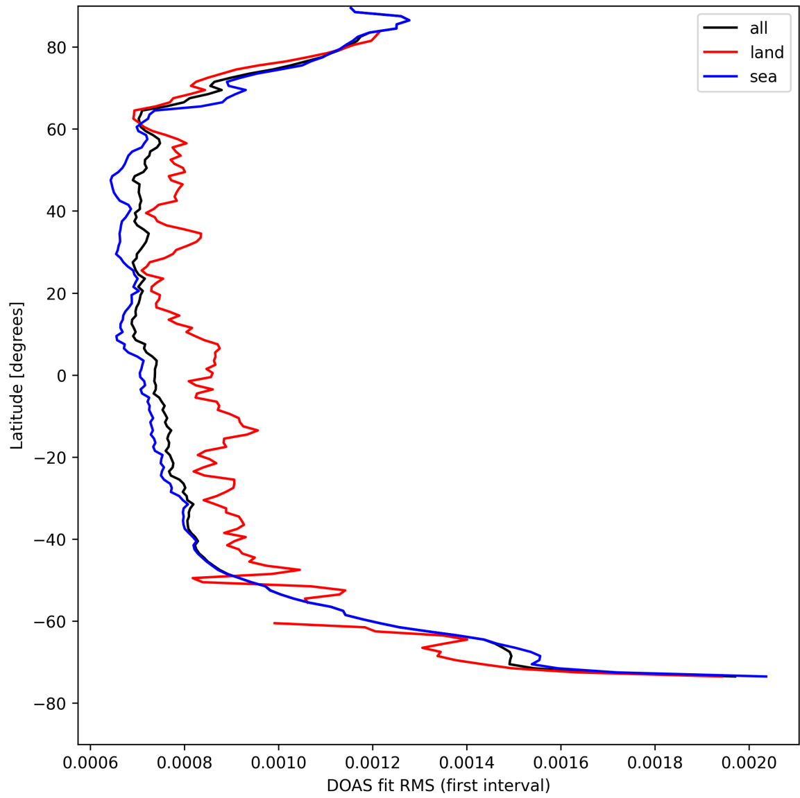
Figure 32: Zonal average of “DOAS fit RMS (first interval)” for 2025-04-18 to 2025-04-19.
