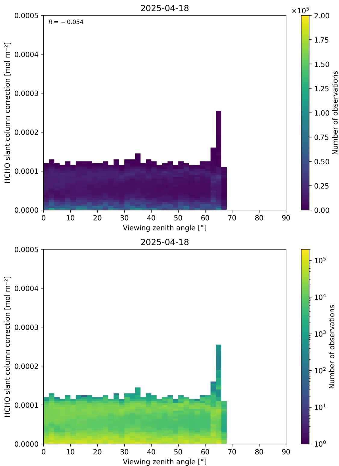
Figure 187: Scatter density plot of “Viewing zenith angle” against “HCHO slant column correction” for 2025-04-18 to 2025-04-19.
