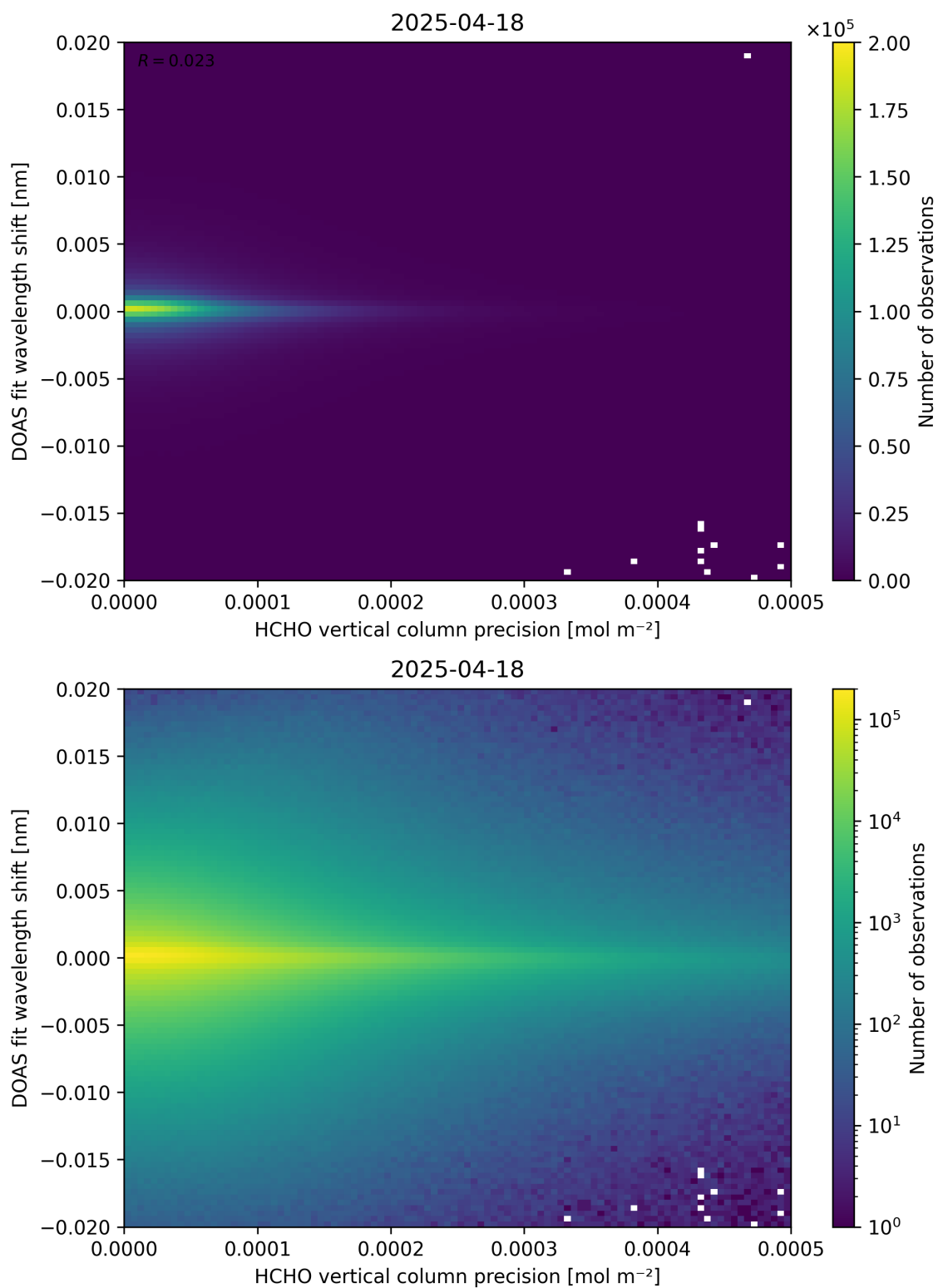
Figure 137: Scatter density plot of “HCHO vertical column precision” against “DOAS fit wavelength shift” for 2025-04-18 to 2025-04-19.
