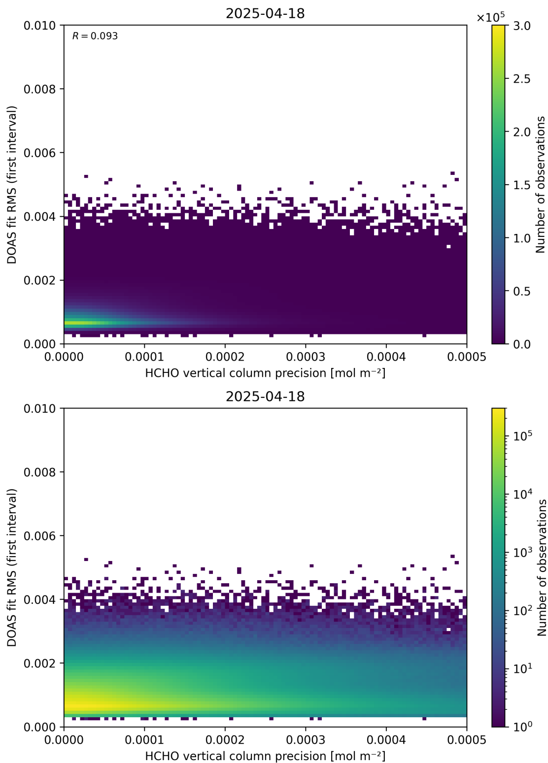
Figure 136: Scatter density plot of “HCHO vertical column precision” against “DOAS fit RMS (first interval)” for 2025-04-18 to 2025-04-19.
