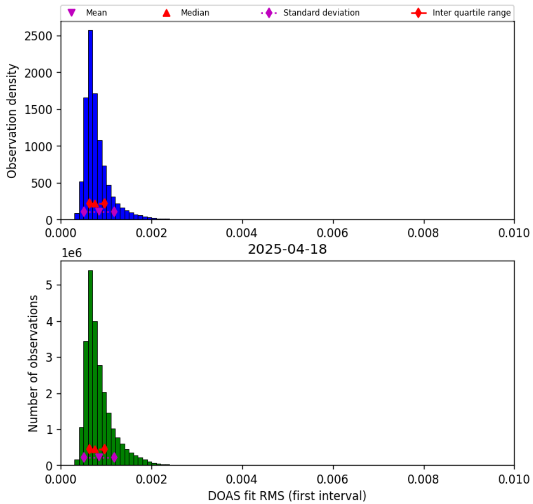
Figure 46: Histogram of “DOAS fit RMS (first interval)” for 2025-04-18 to 2025-04-19
