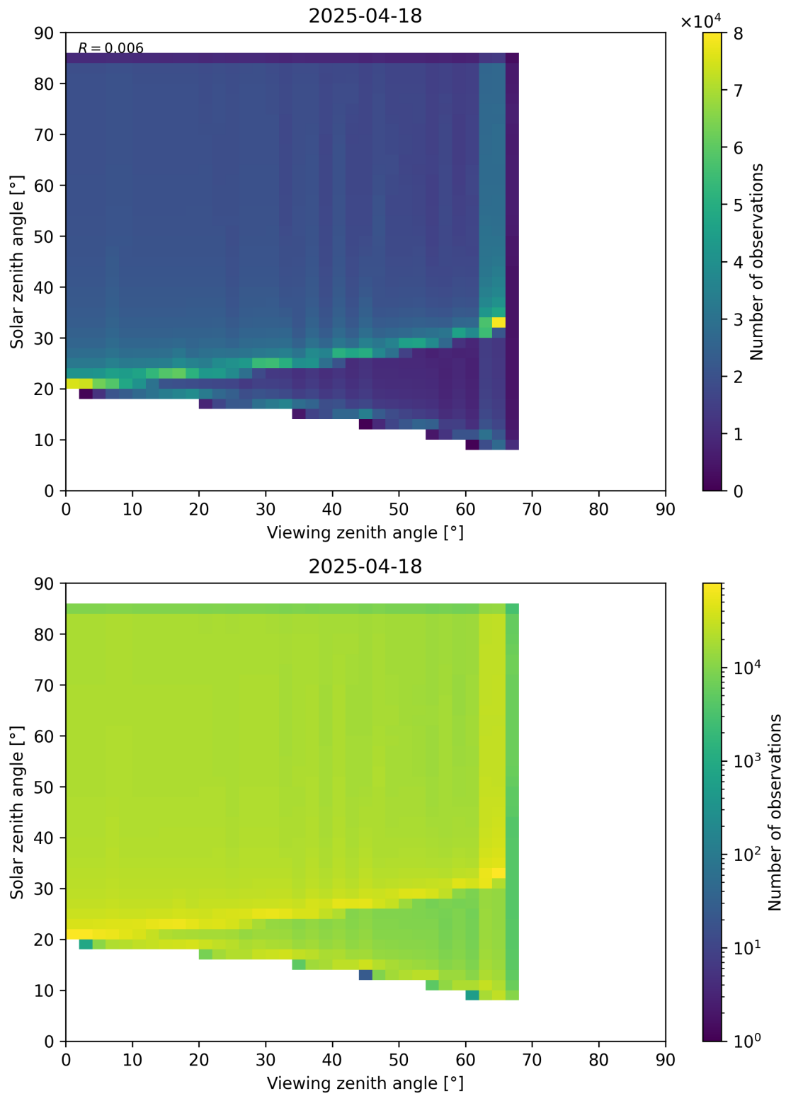
Figure 197: Scatter density plot of “Viewing zenith angle” against “Solar zenith angle” for 2025-04-18 to 2025-04-19.
