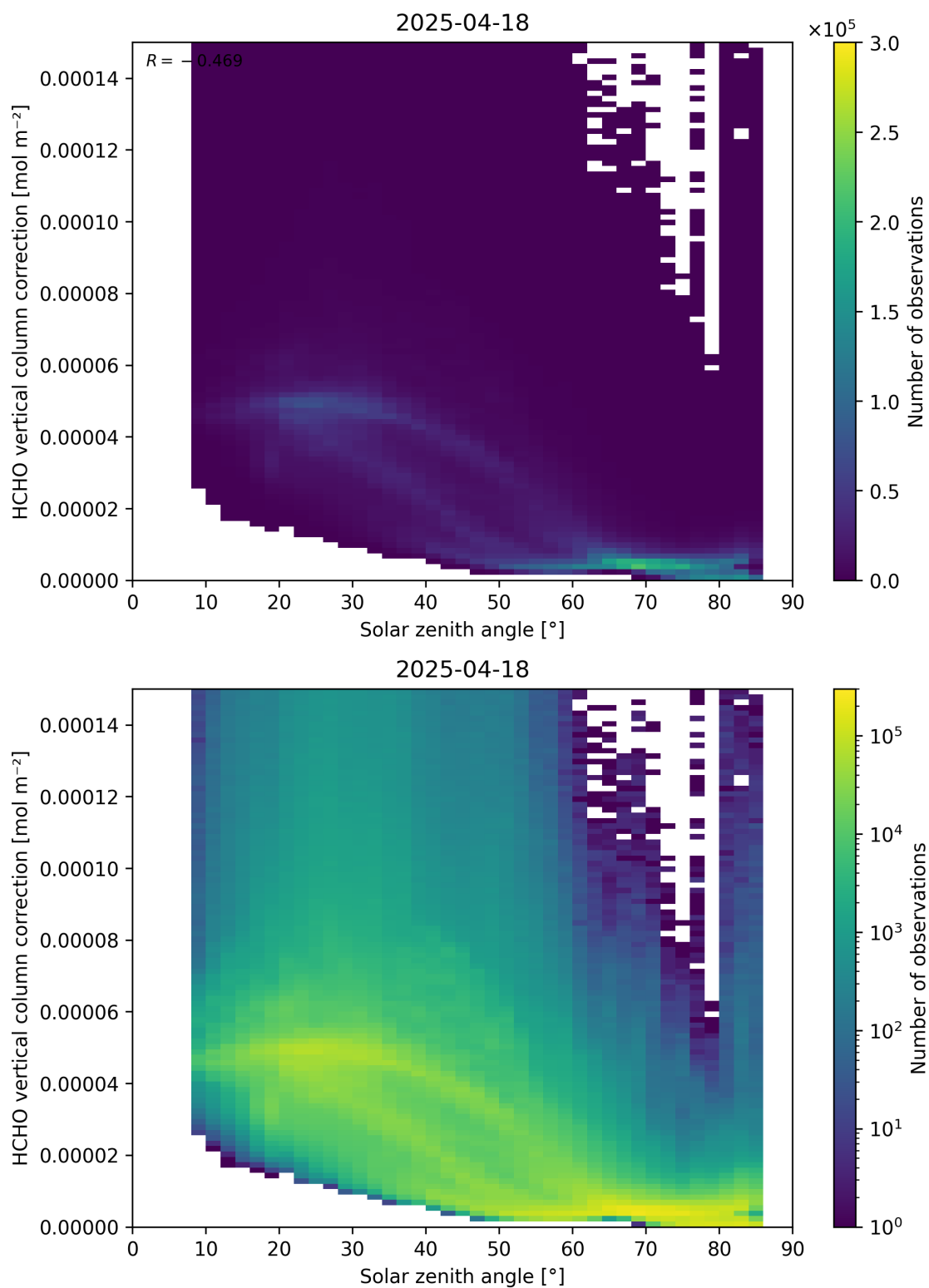
Figure 178: Scatter density plot of “Solar zenith angle” against “HCHO vertical column correction” for 2025-04-18 to 2025-04-19.
