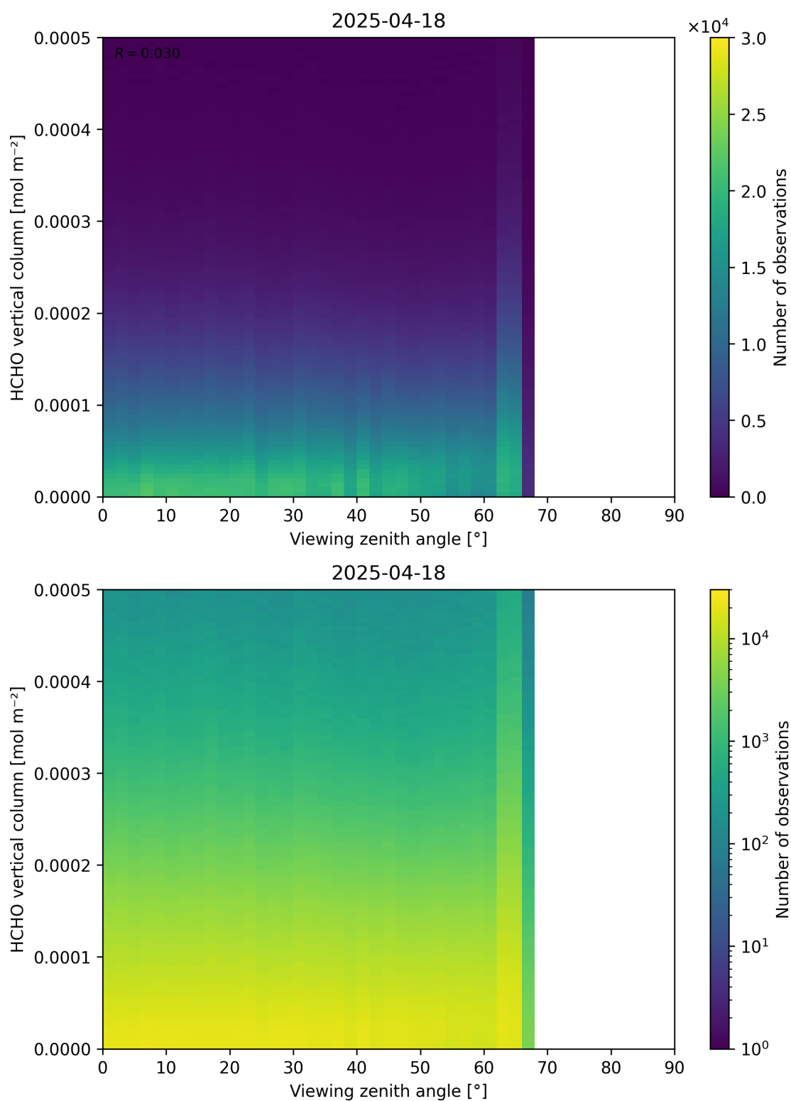
Figure 192: Scatter density plot of “Viewing zenith angle” against “HCHO vertical column” for 2025-04-18 to 2025-04-19.
