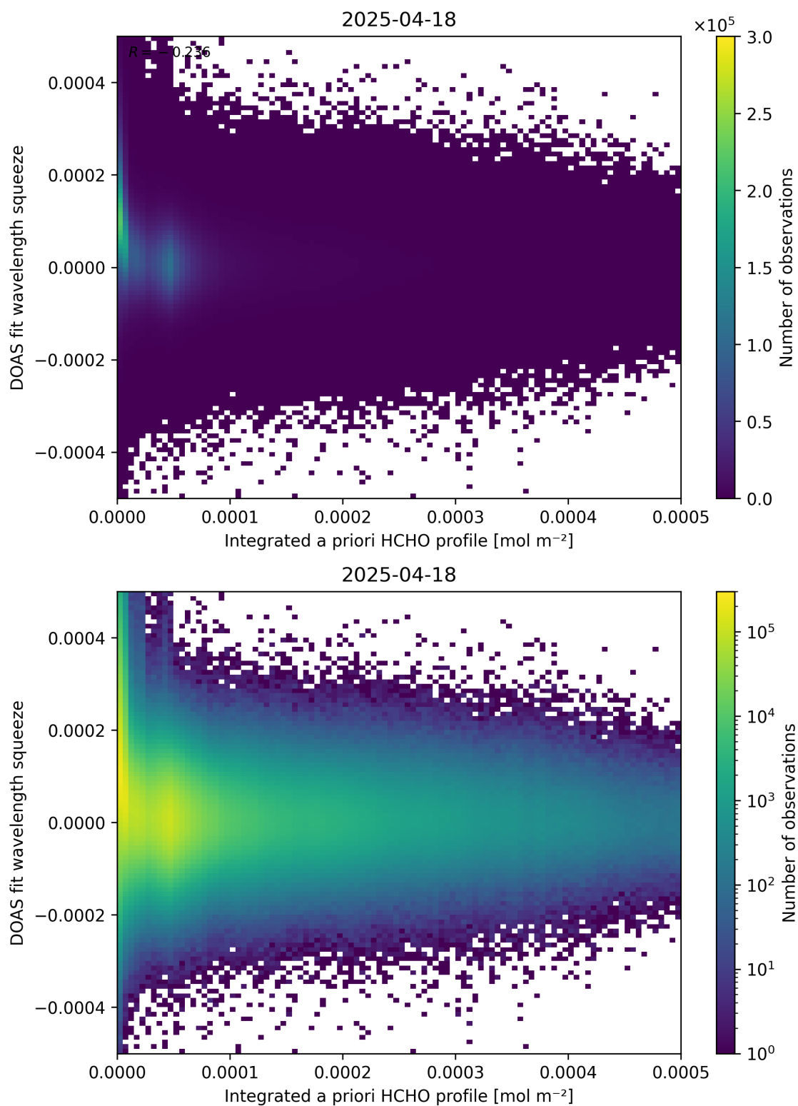
Figure 150: Scatter density plot of “Integrated a priori HCHO profile” against “DOAS fit wavelength squeeze” for 2025-04-18 to 2025-04-19.
