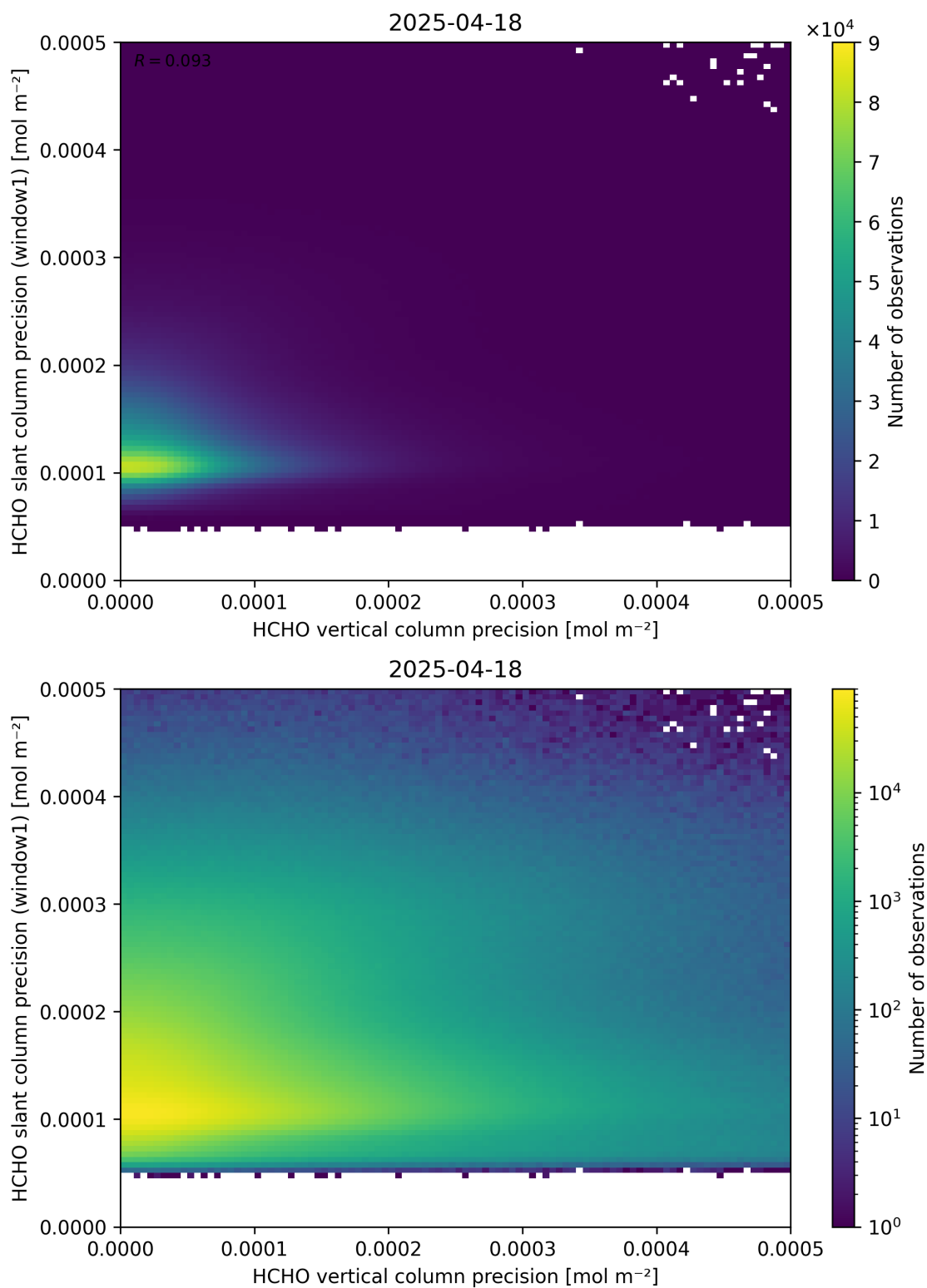
Figure 143: Scatter density plot of “HCHO vertical column precision” against “HCHO slant column precision (window1)” for 2025-04-18 to 2025-04-19.
