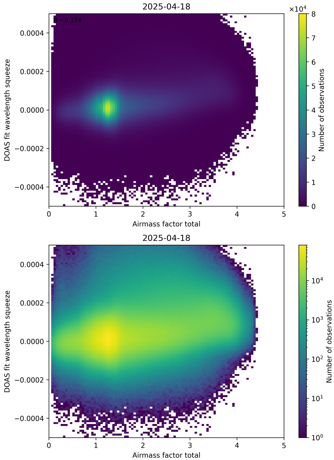
Figure 99: Scatter density plot of “Airmass factor total” against “DOAS fit wavelength squeeze” for 2025-04-18 to 2025-04-19.
