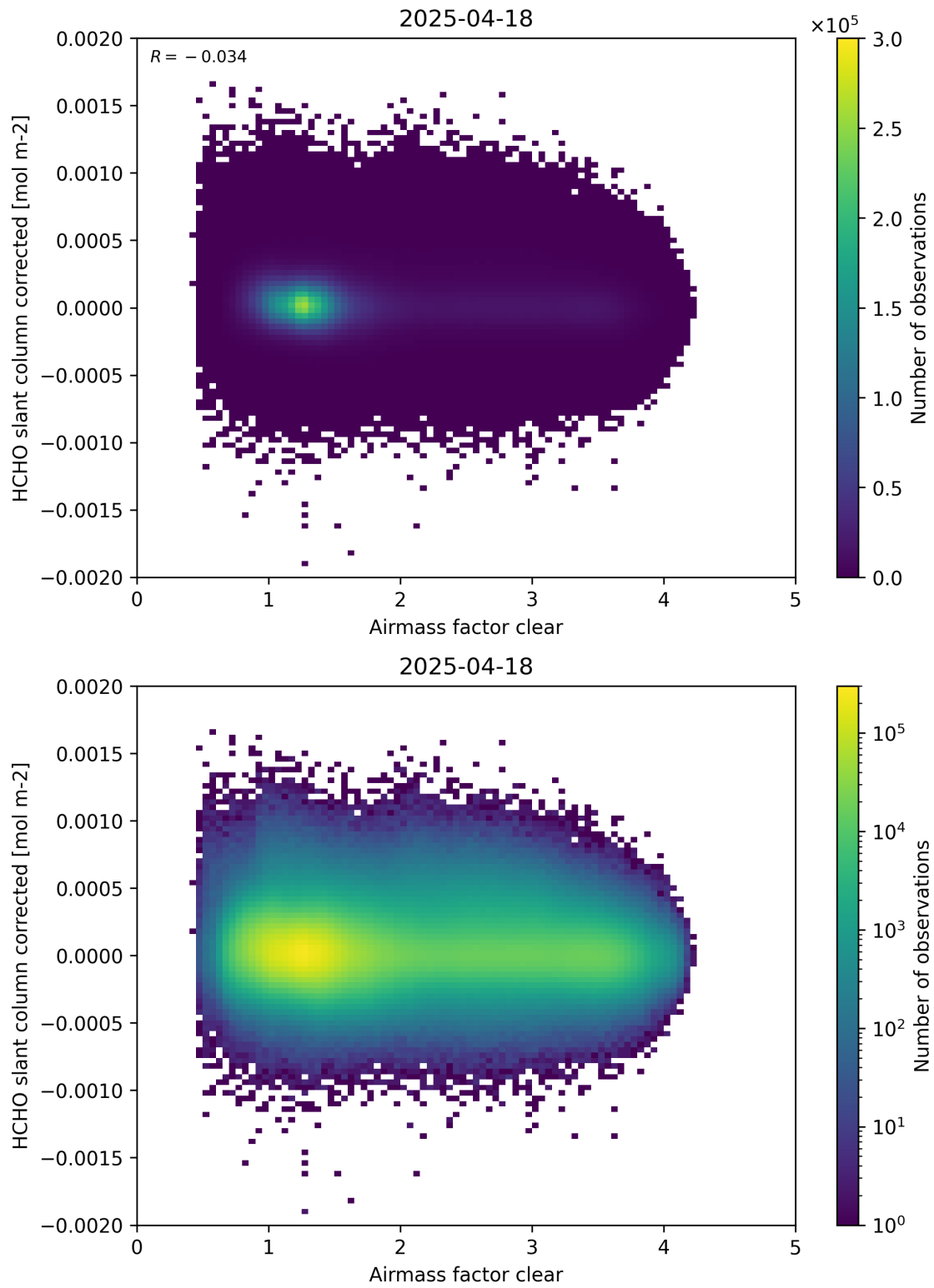
Figure 74: Scatter density plot of “Airmass factor clear” against “HCHO slant column corrected” for 2025-04-18 to 2025-04-19.
