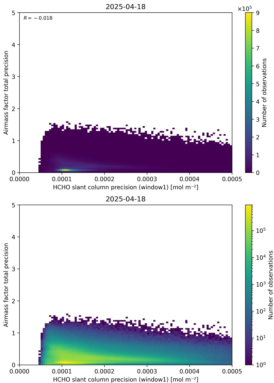
Figure 95: Scatter density plot of “HCHO slant column precision (window1)” against “Airmass factor total precision” for 2025-04-18 to 2025-04-19.
