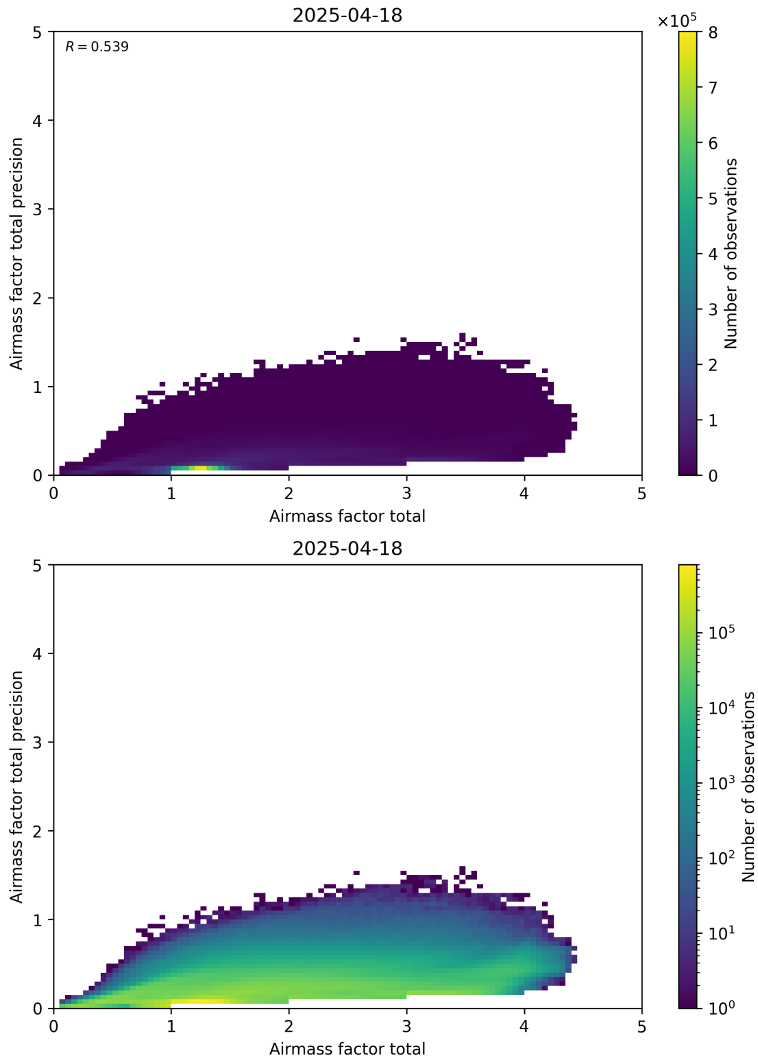
Figure 103: Scatter density plot of “Airmass factor total” against “Airmass factor total precision” for 2025-04-18 to 2025-04-19.
