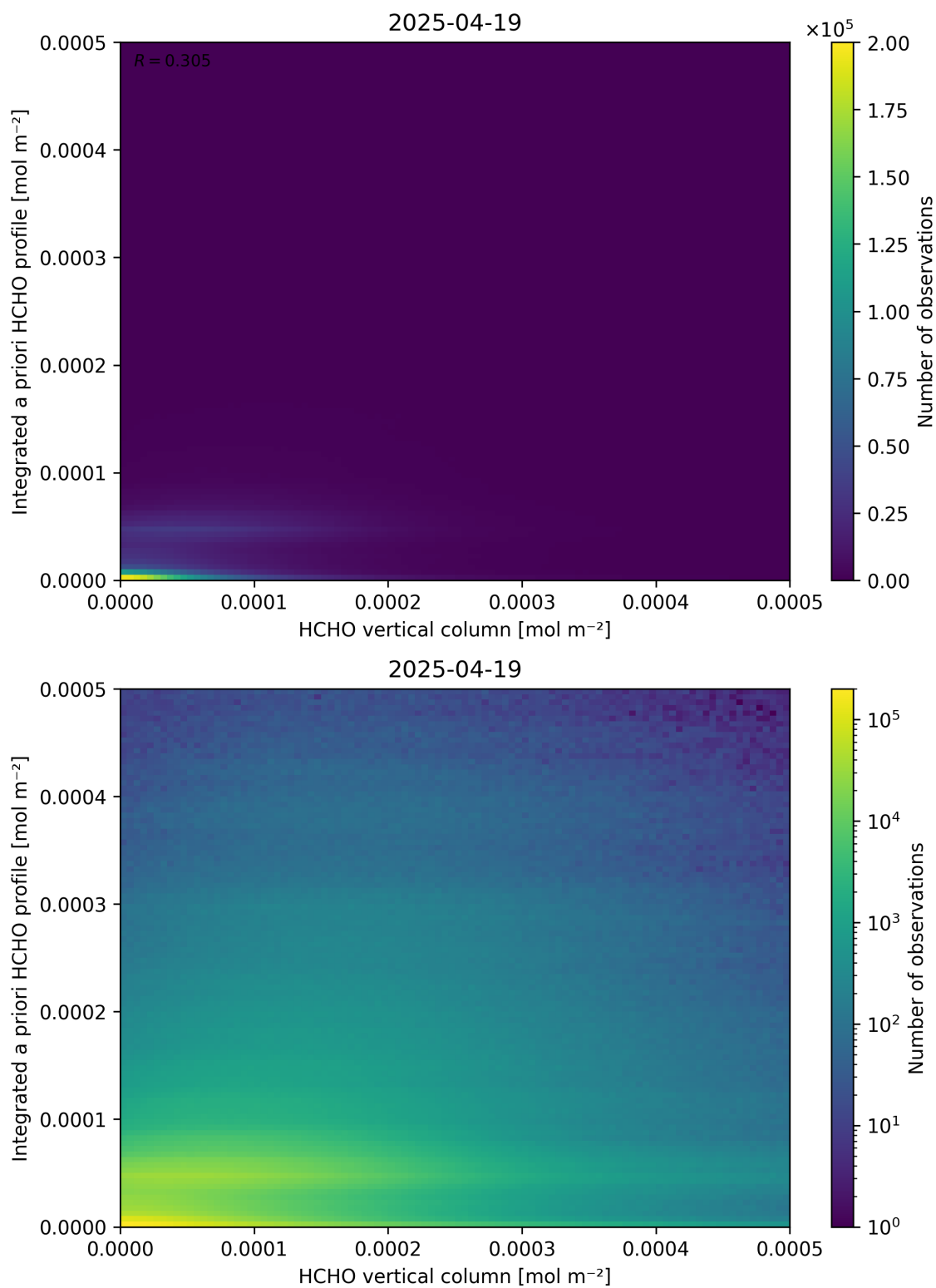
Figure 135: Scatter density plot of “HCHO vertical column” against “Integrated a priori HCHO profile” for 2025-04-19 to 2025-04-20.
