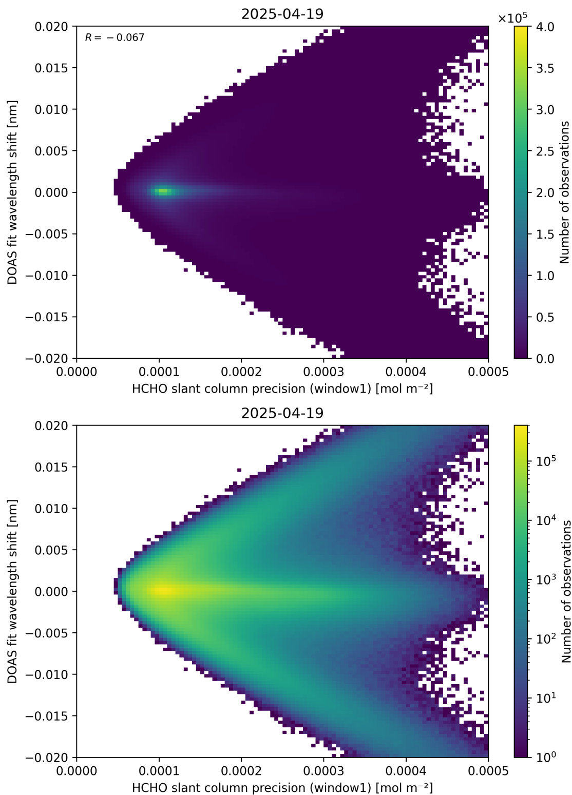
Figure 89: Scatter density plot of “HCHO slant column precision (window1)” against “DOAS fit wavelength shift” for 2025-04-19 to 2025-04-20.
