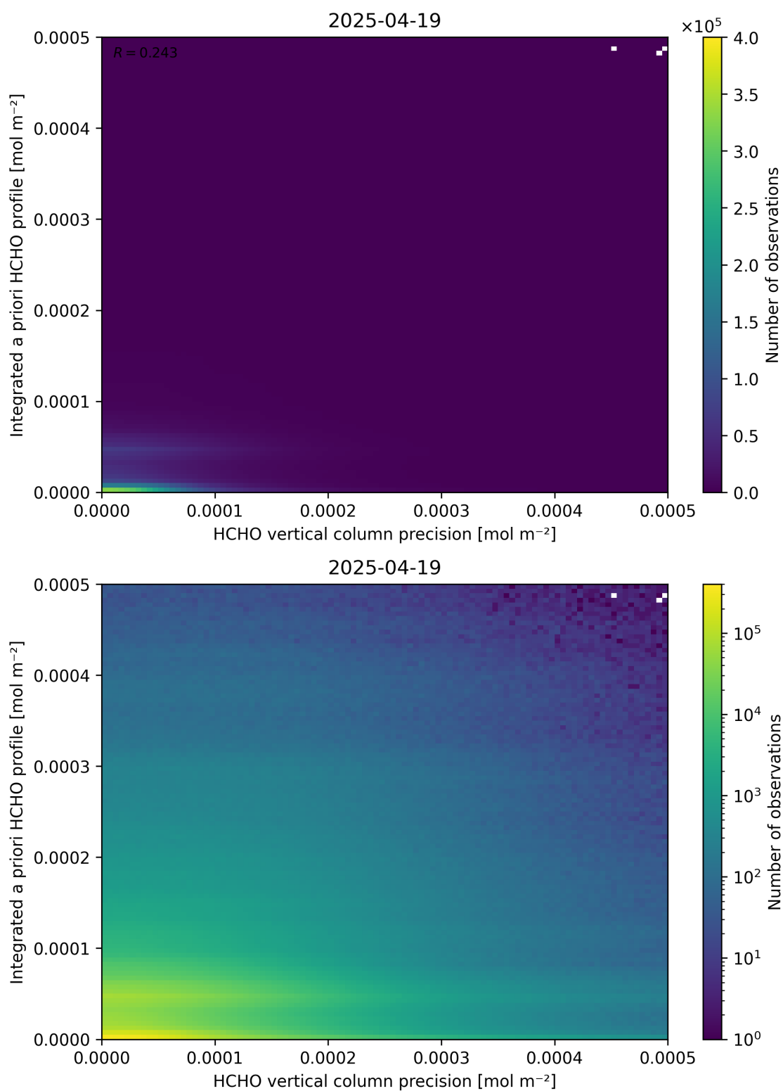
Figure 147: Scatter density plot of “HCHO vertical column precision” against “Integrated a priori HCHO profile” for 2025-04-19 to 2025-04-20.
