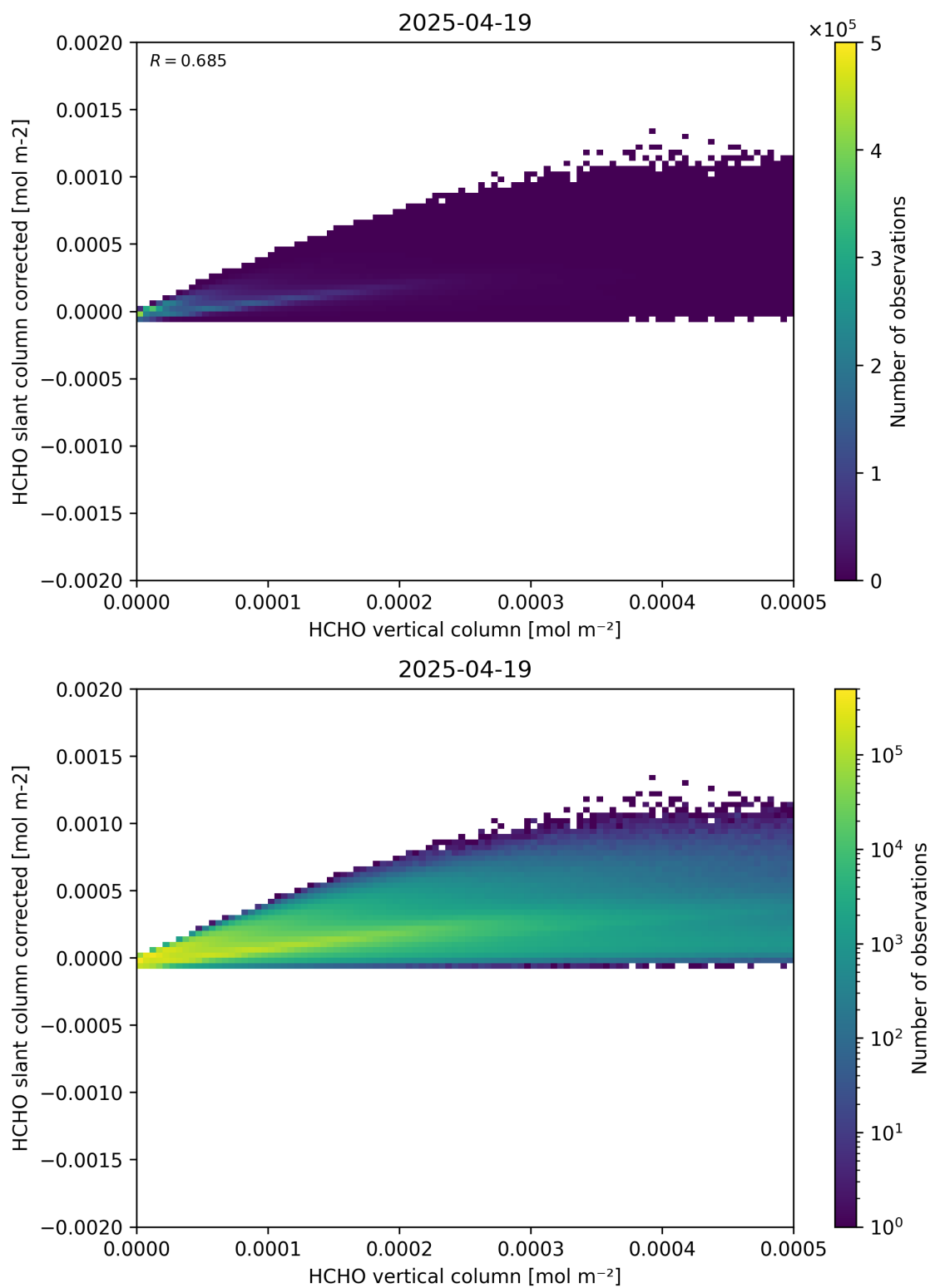
Figure 127: Scatter density plot of “HCHO vertical column” against “HCHO slant column corrected” for 2025-04-19 to 2025-04-20.
