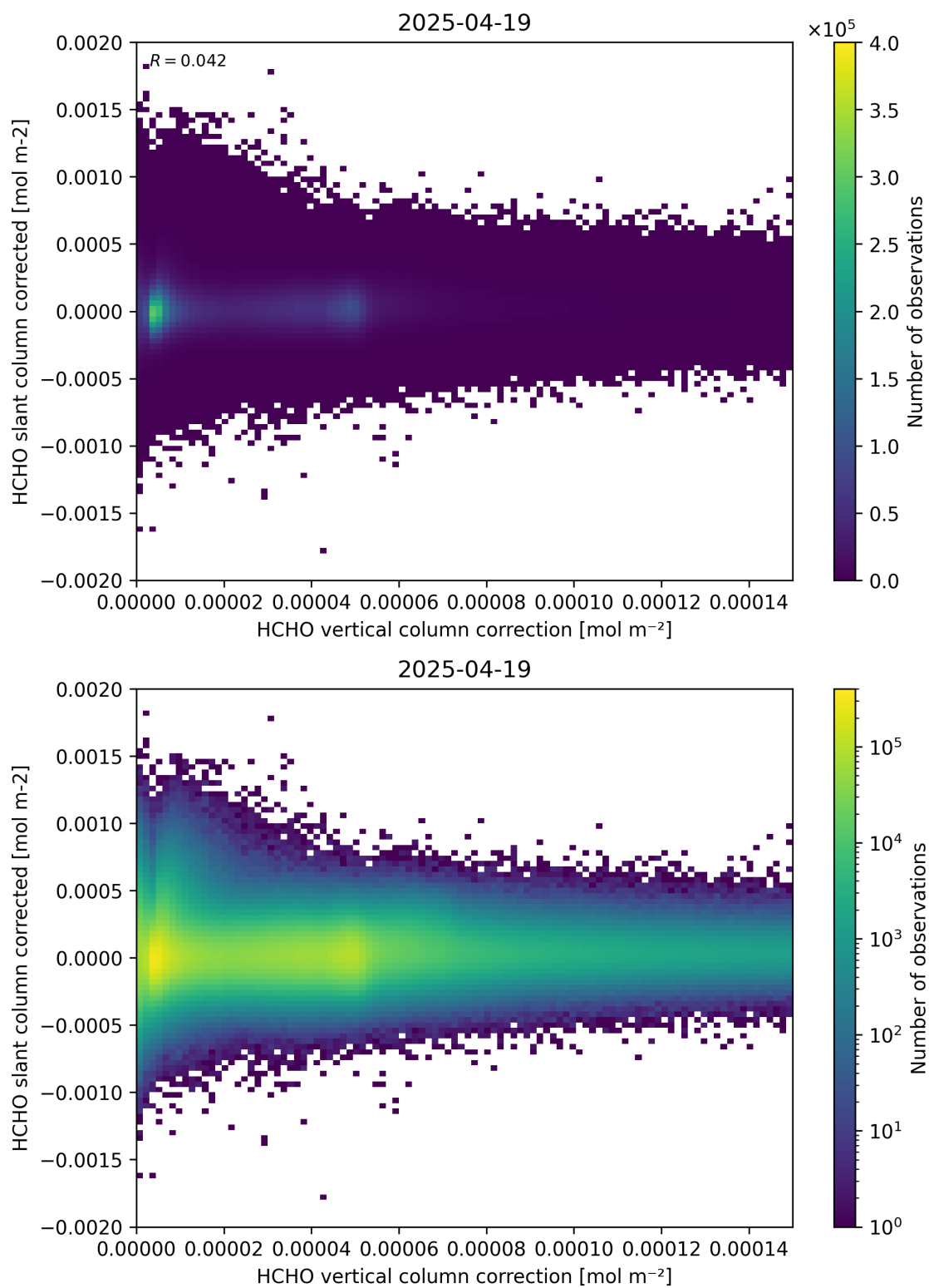
Figure 116: Scatter density plot of “HCHO vertical column correction” against “HCHO slant column corrected” for 2025-04-19 to 2025-04-20.
