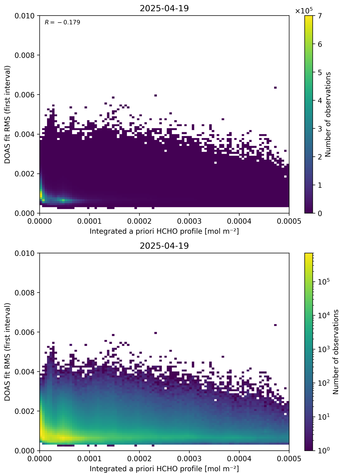
Figure 148: Scatter density plot of “Integrated a priori HCHO profile” against “DOAS fit RMS (first interval)” for 2025-04-19 to 2025-04-20.
