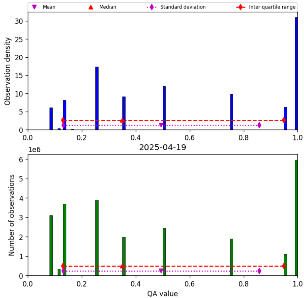
Figure 34: Histogram of “QA value” for 2025-04-19 to 2025-04-20
