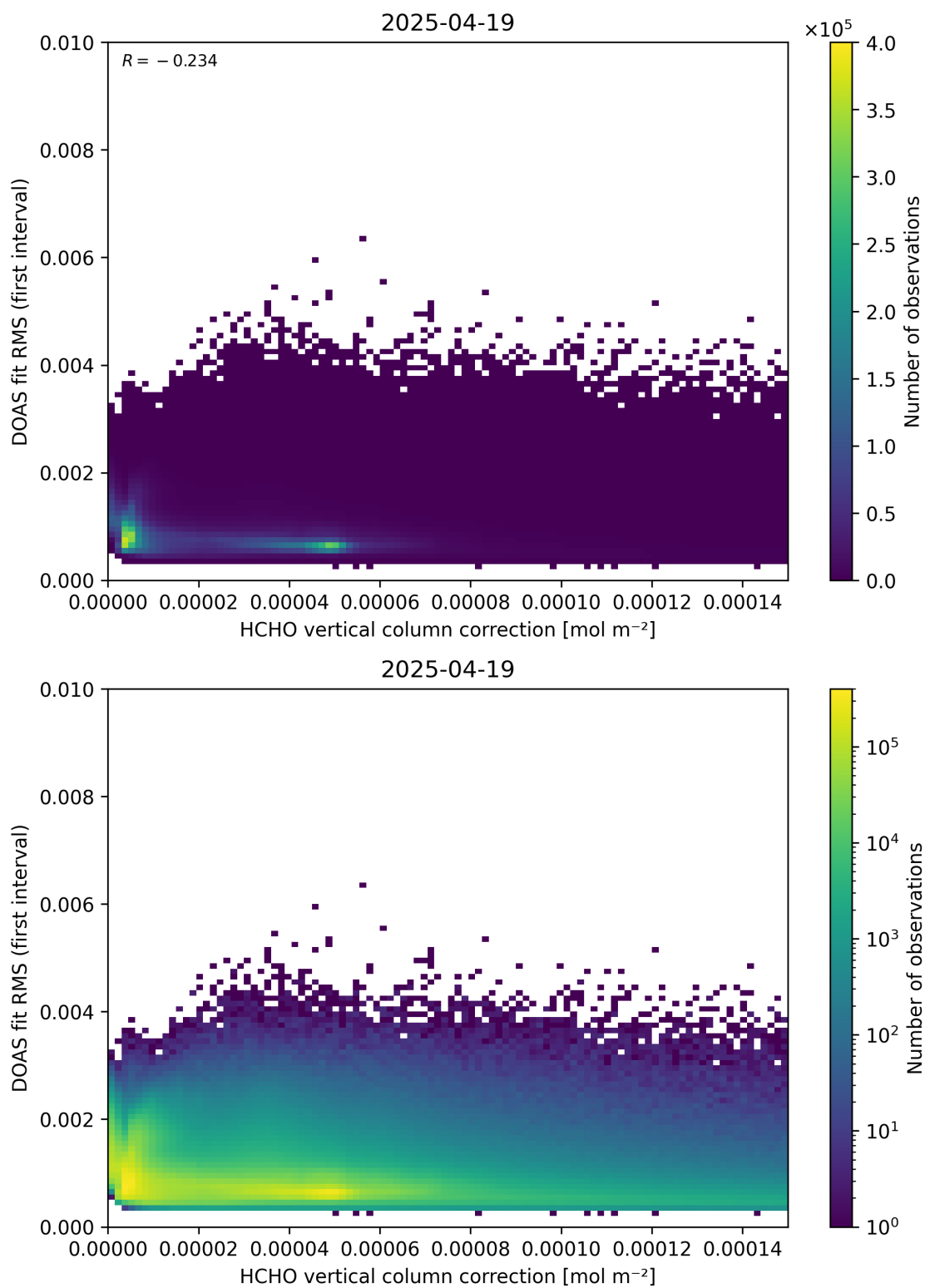
Figure 112: Scatter density plot of “HCHO vertical column correction” against “DOAS fit RMS (first interval)” for 2025-04-19 to 2025-04-20.
