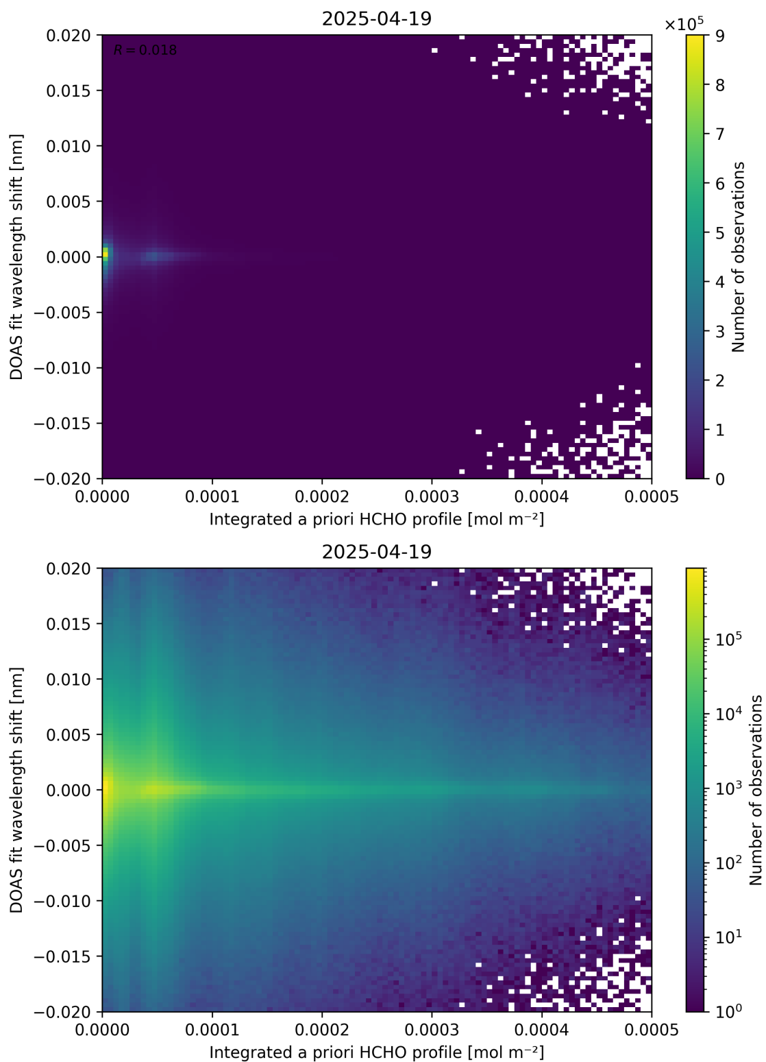
Figure 149: Scatter density plot of “Integrated a priori HCHO profile” against “DOAS fit wavelength shift” for 2025-04-19 to 2025-04-20.
