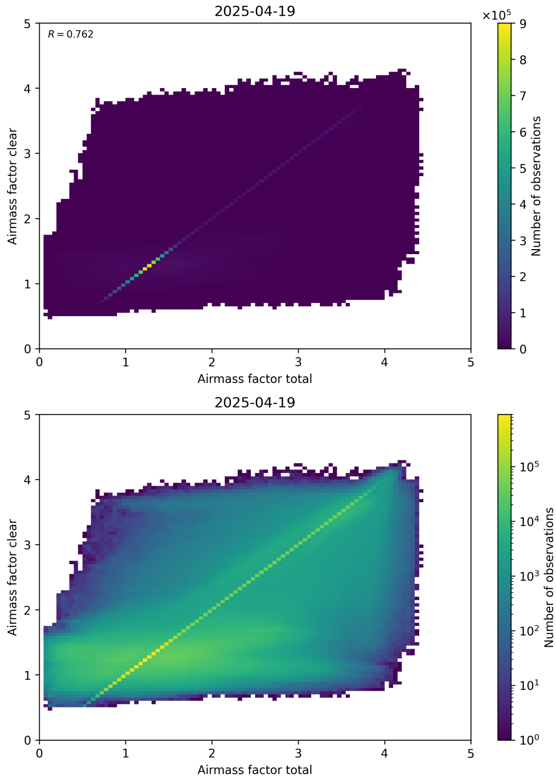
Figure 100: Scatter density plot of “Airmass factor total” against “Airmass factor clear” for 2025-04-19 to 2025-04-20.
