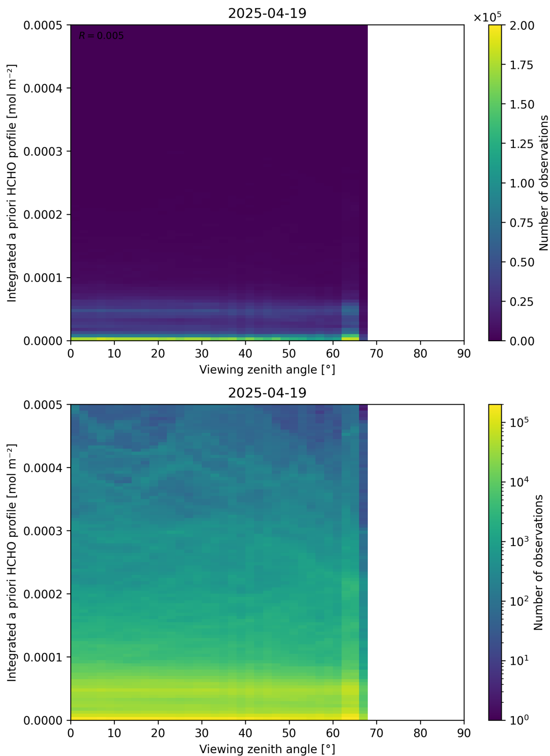
Figure 195: Scatter density plot of “Viewing zenith angle” against “Integrated a priori HCHO profile” for 2025-04-19 to 2025-04-20.
