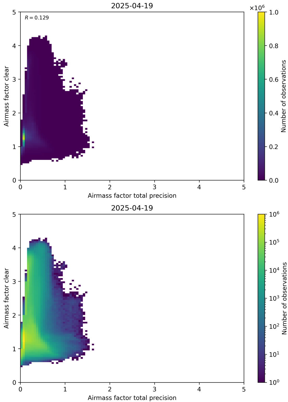
Figure 108: Scatter density plot of “Airmass factor total precision” against “Airmass factor clear” for 2025-04-19 to 2025-04-20.
