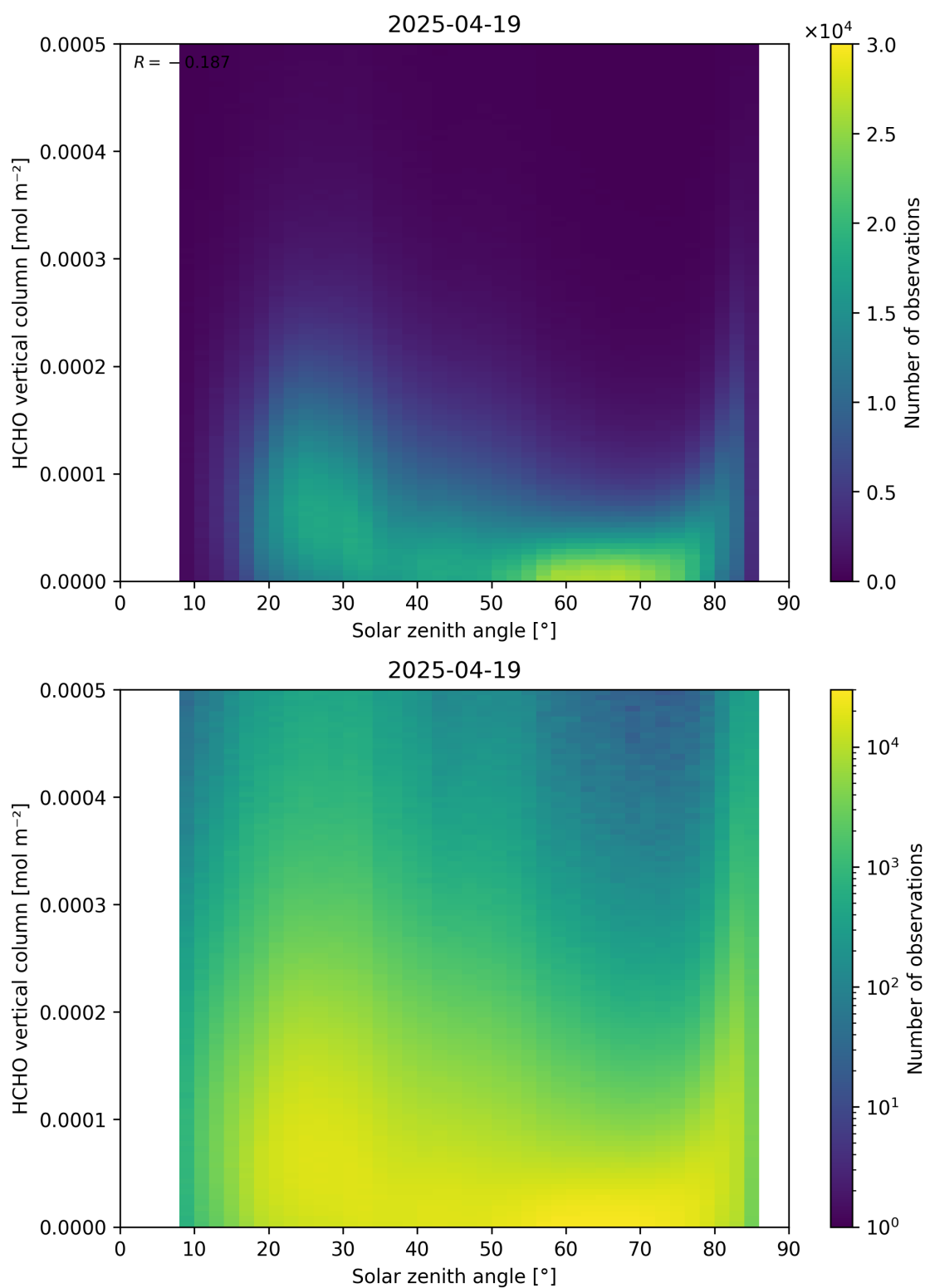
Figure 177: Scatter density plot of “Solar zenith angle” against “HCHO vertical column” for 2025-04-19 to 2025-04-20.
