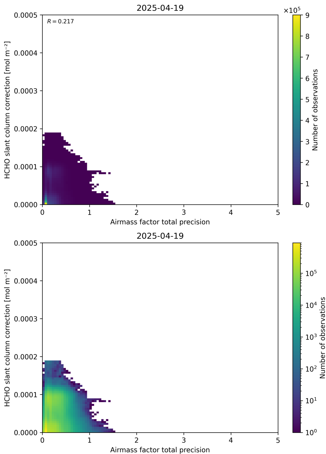
Figure 110: Scatter density plot of “Airmass factor total precision” against “HCHO slant column correction” for 2025-04-19 to 2025-04-20.
