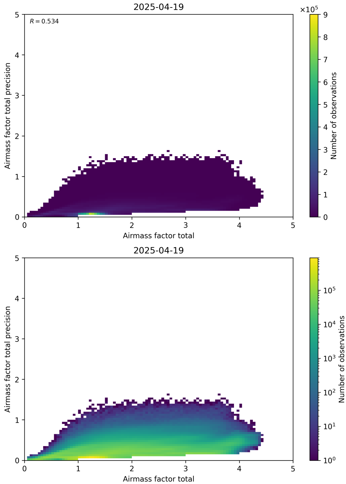
Figure 103: Scatter density plot of “Airmass factor total” against “Airmass factor total precision” for 2025-04-19 to 2025-04-20.
