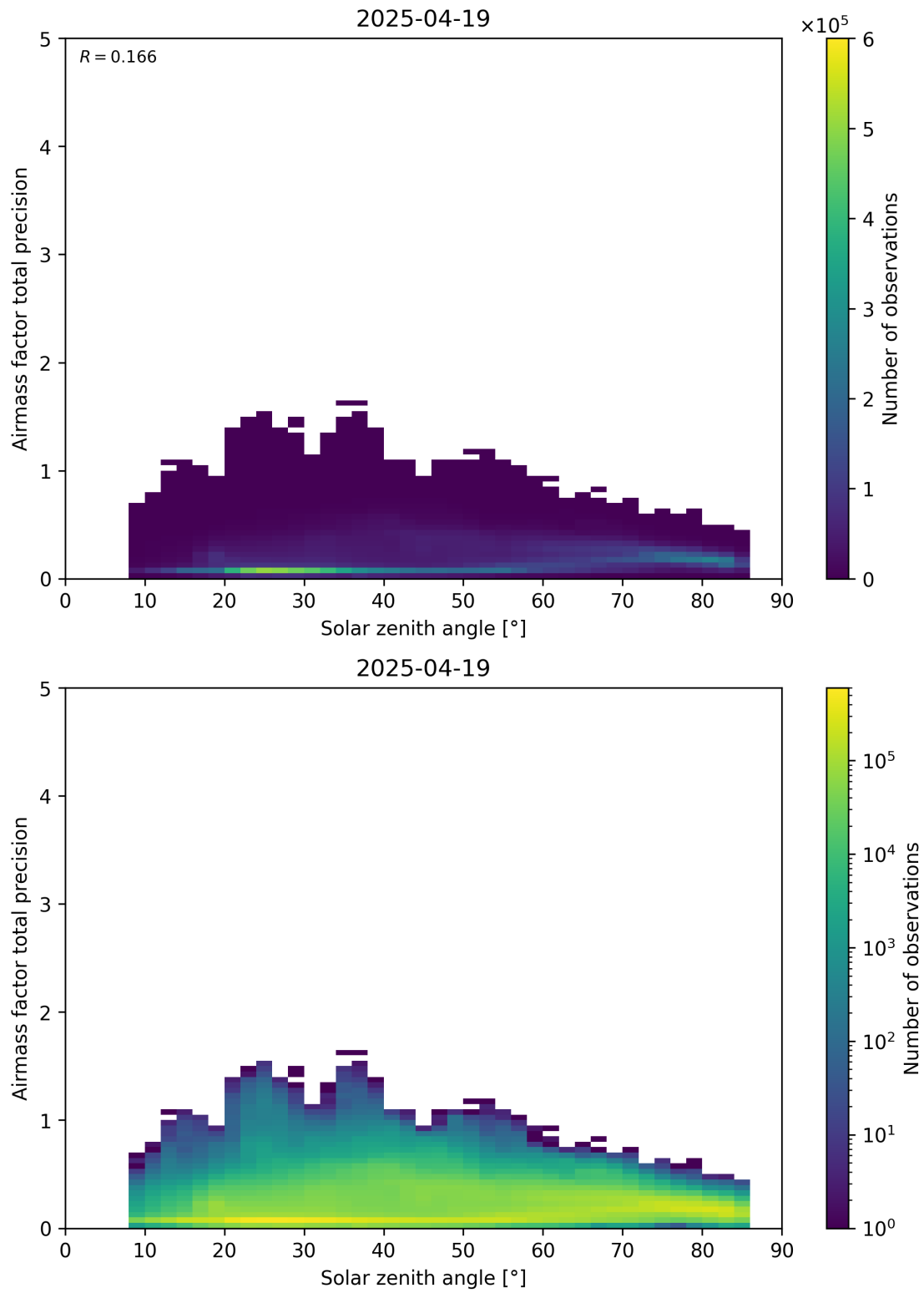
Figure 176: Scatter density plot of “Solar zenith angle” against “Airmass factor total precision” for 2025-04-19 to 2025-04-20.
