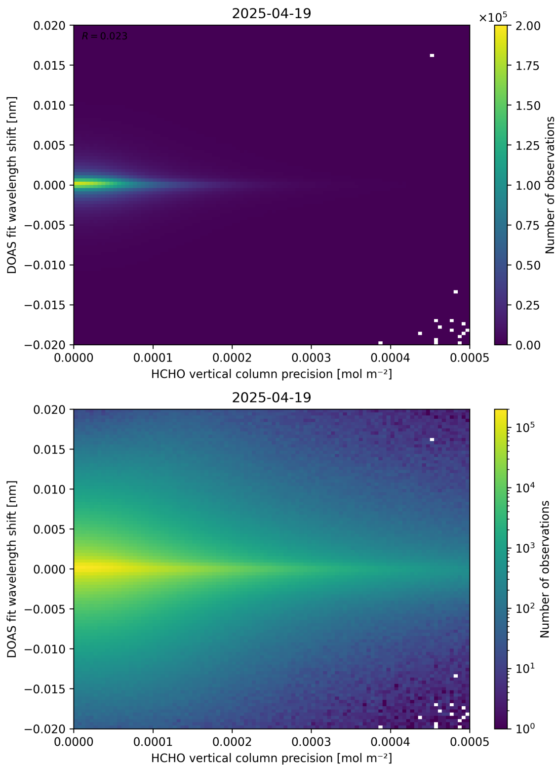
Figure 137: Scatter density plot of “HCHO vertical column precision” against “DOAS fit wavelength shift” for 2025-04-19 to 2025-04-20.
