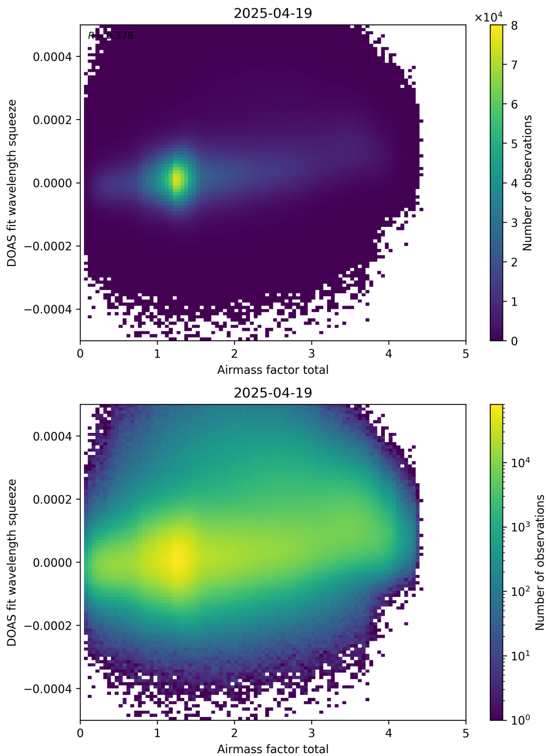
Figure 99: Scatter density plot of “Airmass factor total” against “DOAS fit wavelength squeeze” for 2025-04-19 to 2025-04-20.
