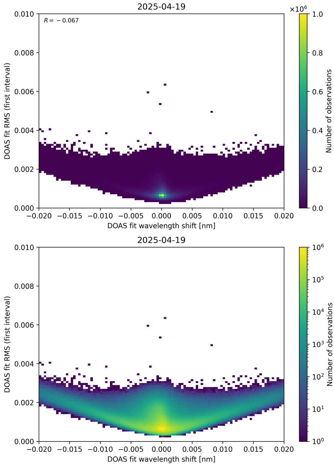
Figure 64: Scatter density plot of “DOAS fit wavelength shift” against “DOAS fit RMS (first interval)” for 2025-04-19 to 2025-04-20.
