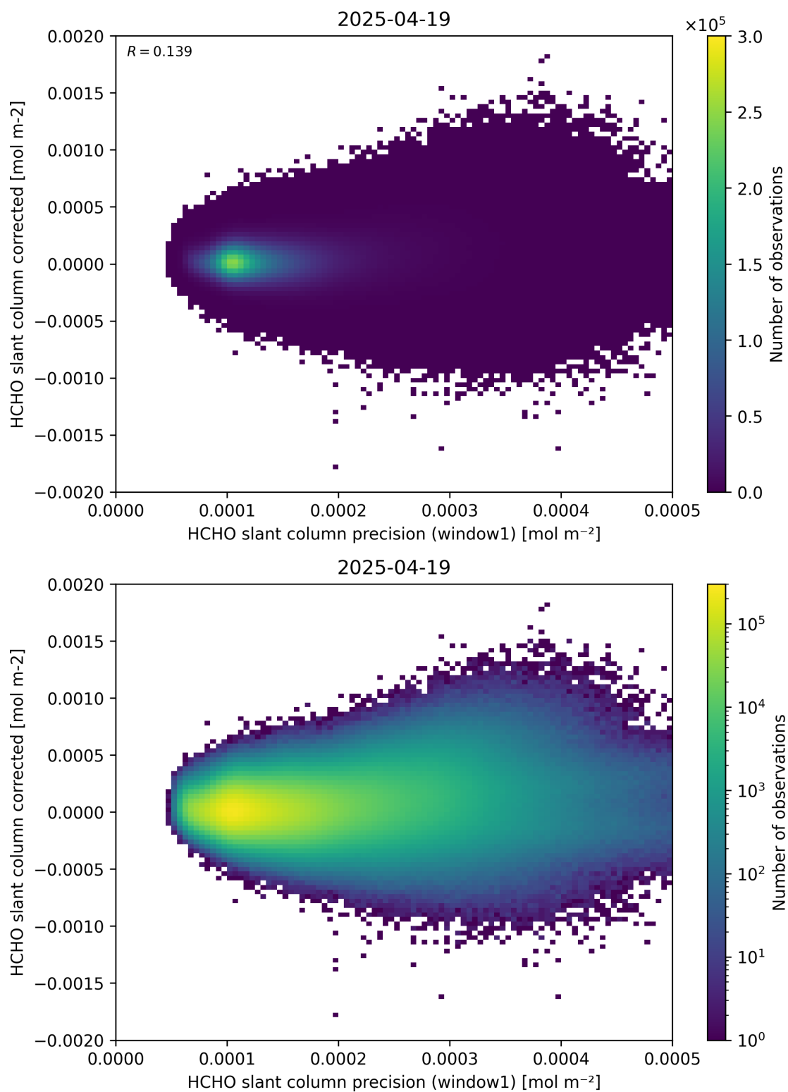
Figure 92: Scatter density plot of “HCHO slant column precision (window1)” against “HCHO slant column corrected” for 2025-04-19 to 2025-04-20.
