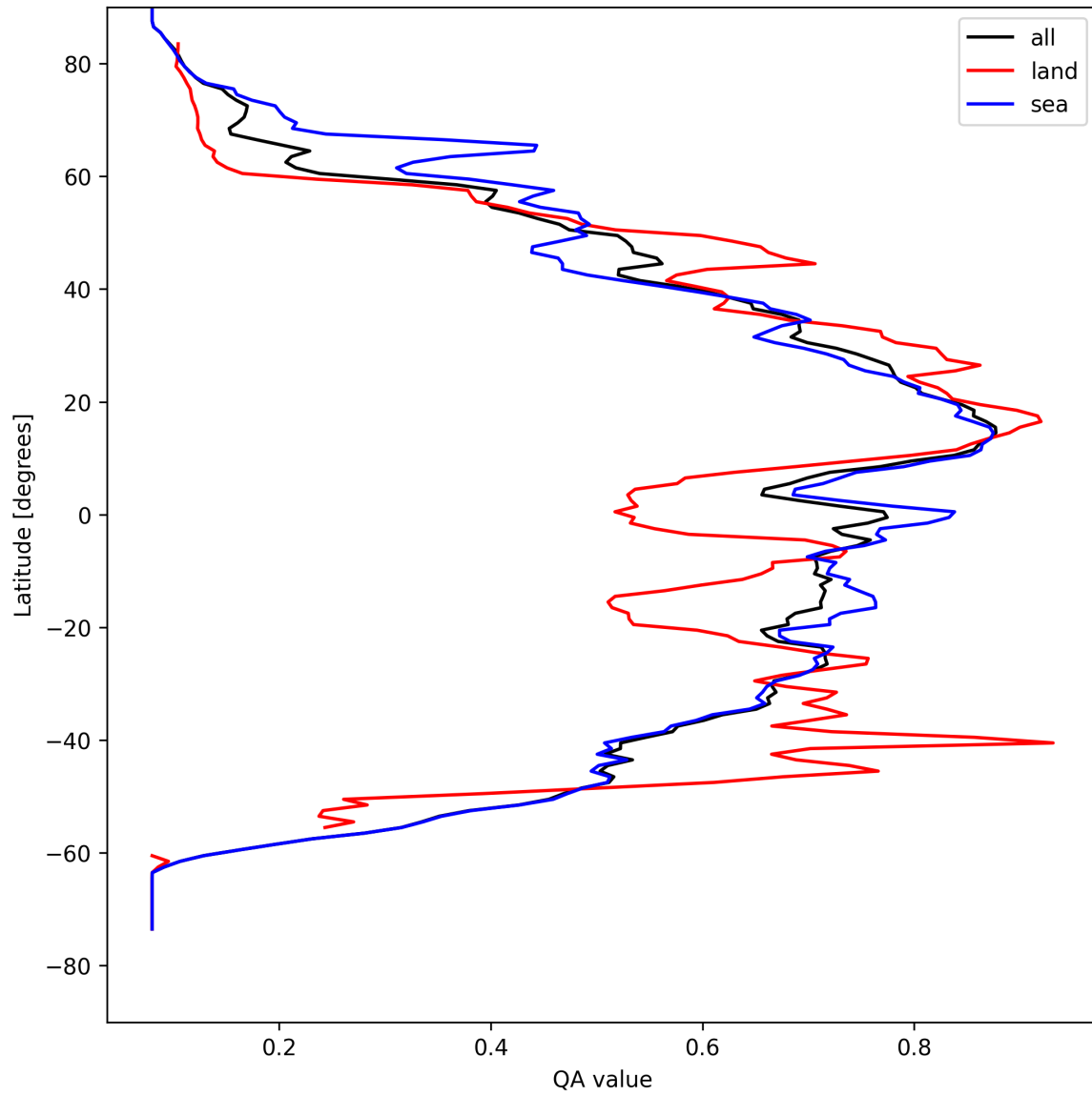
Figure 20: Zonal average of “QA value” for 2025-04-19 to 2025-04-20.
