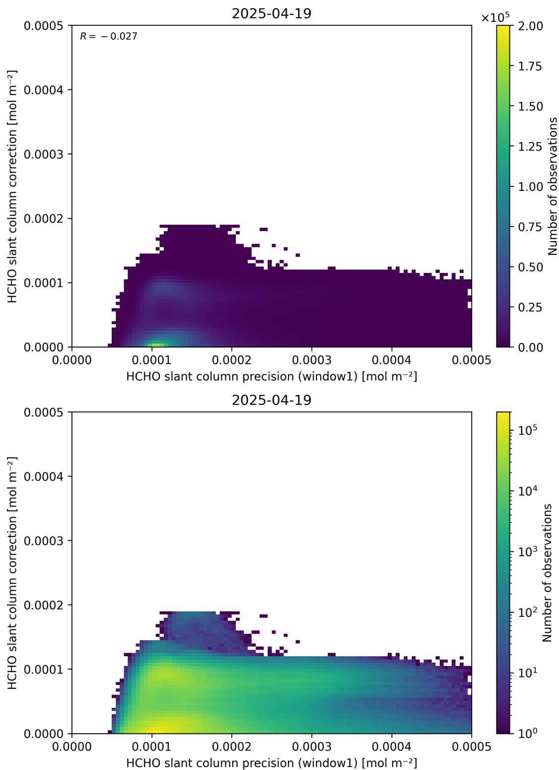
Figure 93: Scatter density plot of “HCHO slant column precision (window1)” against “HCHO slant column correction” for 2025-04-19 to 2025-04-20.
