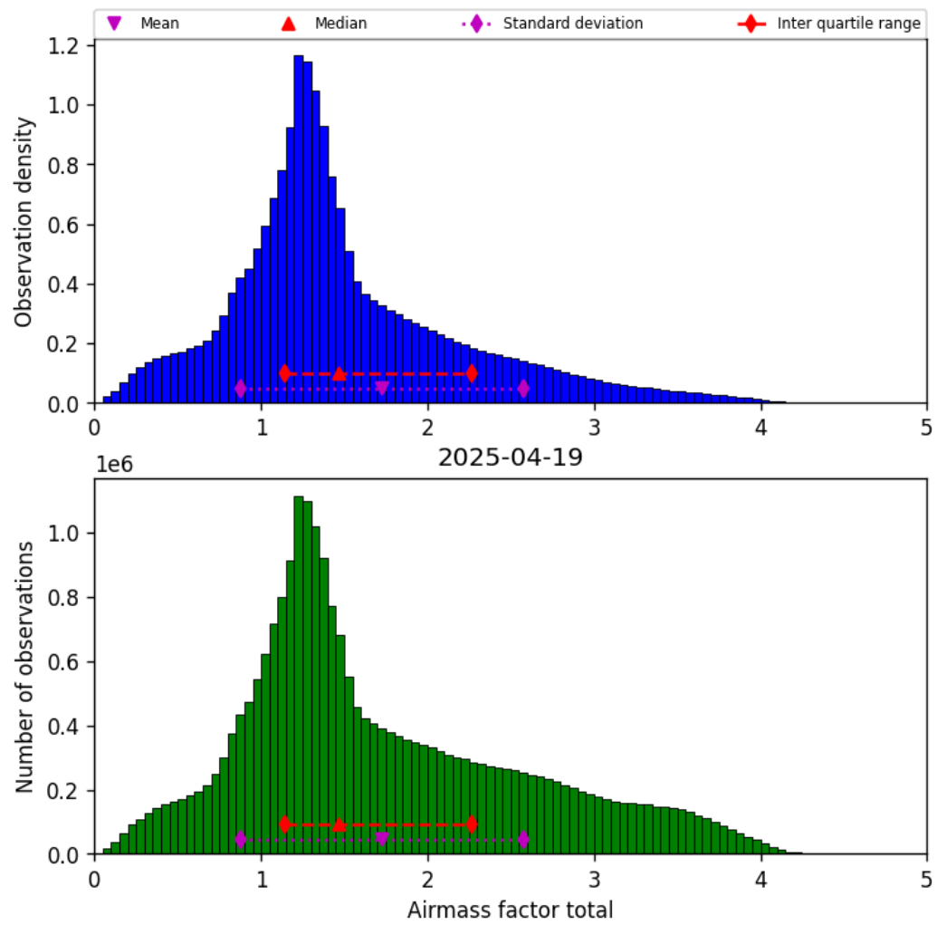
Figure 40: Histogram of “Airmass factor total” for 2025-04-19 to 2025-04-20
