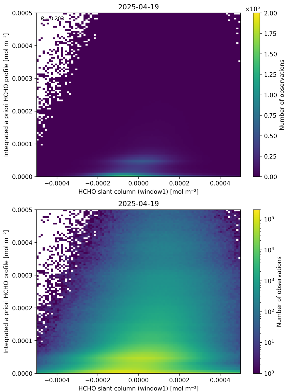
Figure 87: Scatter density plot of “HCHO slant column (window1)” against “Integrated a priori HCHO profile” for 2025-04-19 to 2025-04-20.
