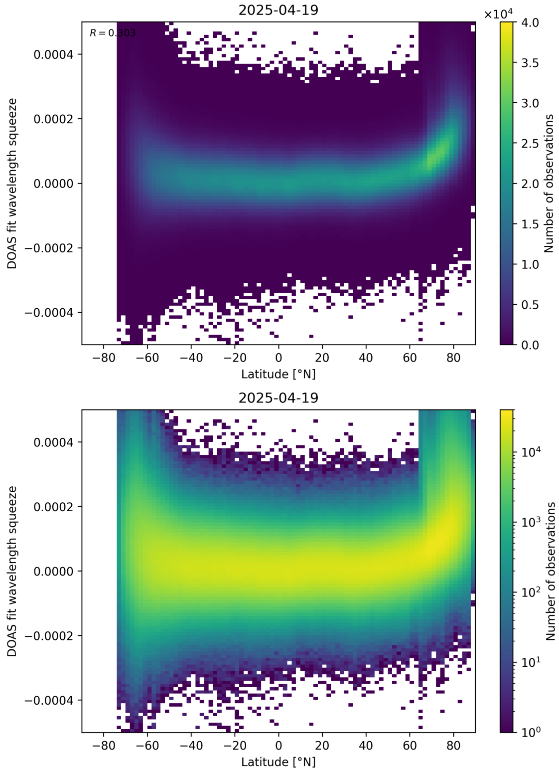
Figure 155: Scatter density plot of “Latitude” against “DOAS fit wavelength squeeze” for 2025-04-19 to 2025-04-20.
