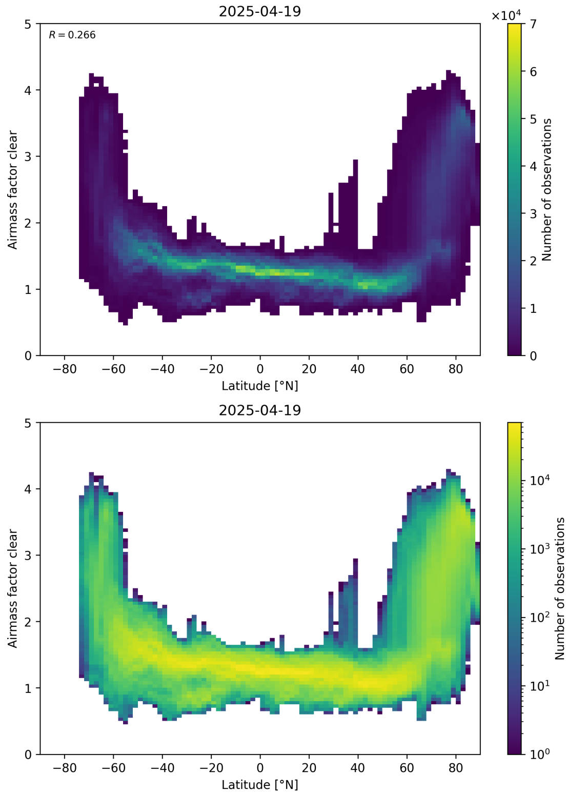
Figure 156: Scatter density plot of “Latitude” against “Airmass factor clear” for 2025-04-19 to 2025-04-20.
