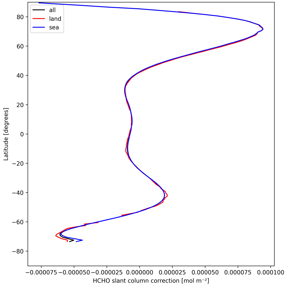
Figure 33: Zonal average of “HCHO slant column correction” for 2025-04-19 to 2025-04-20.
