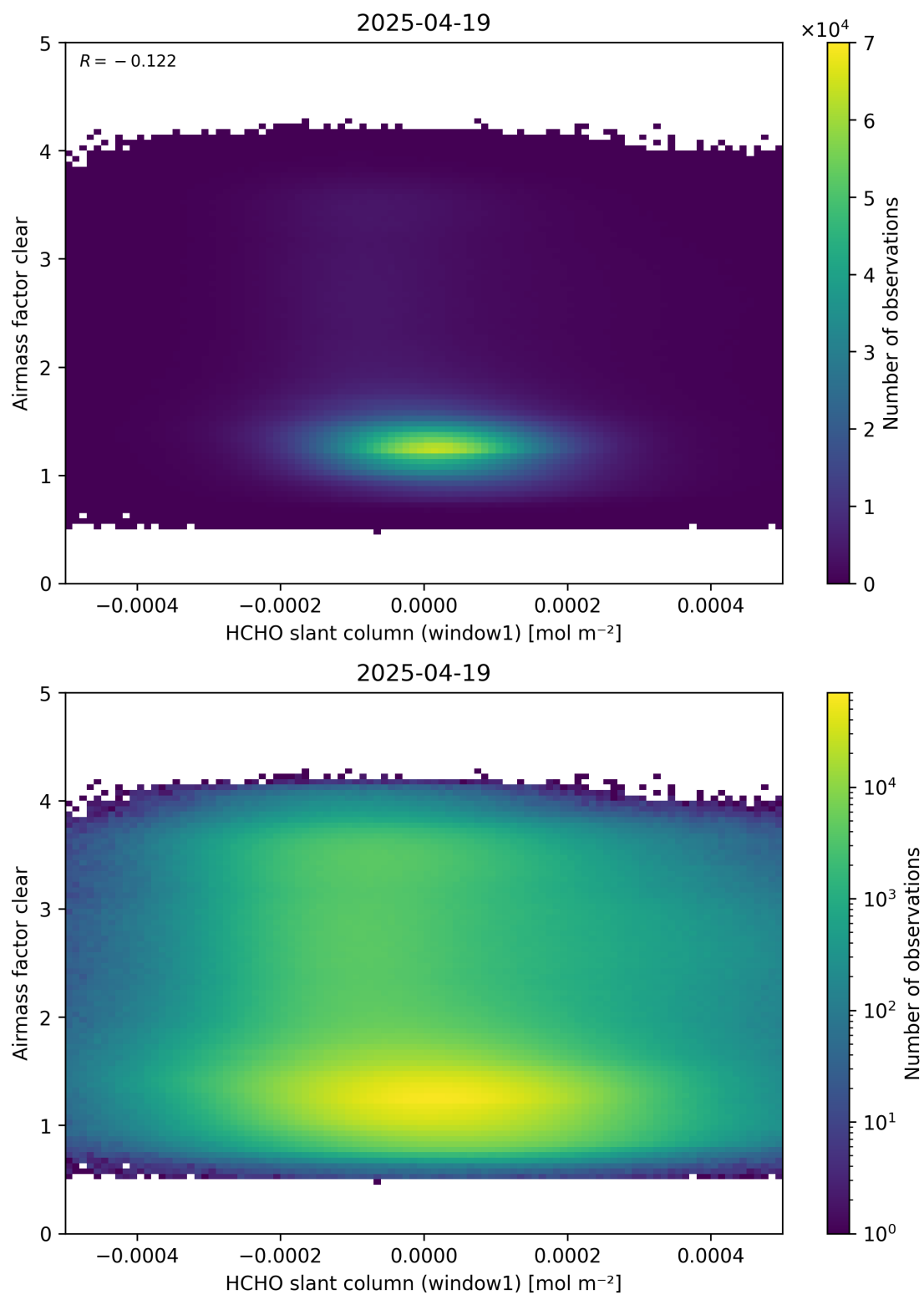
Figure 81: Scatter density plot of “HCHO slant column (window1)” against “Airmass factor clear” for 2025-04-19 to 2025-04-20.
