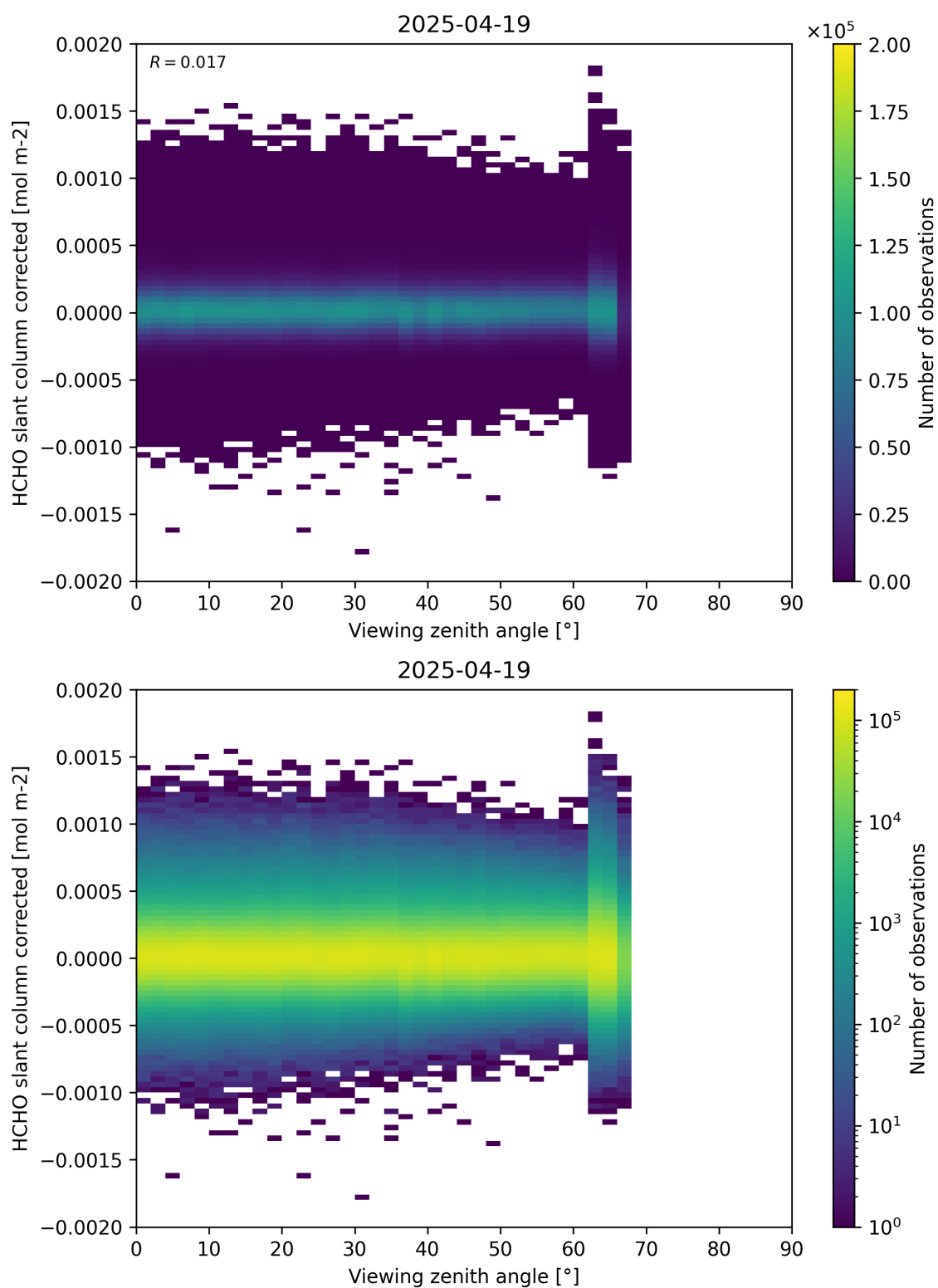
Figure 186: Scatter density plot of “Viewing zenith angle” against “HCHO slant column corrected” for 2025-04-19 to 2025-04-20.
