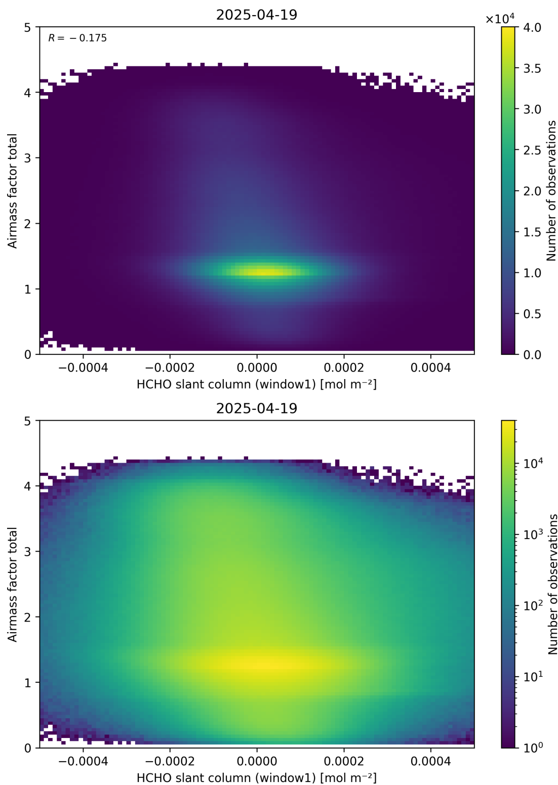
Figure 85: Scatter density plot of “HCHO slant column (window1)” against “Airmass factor total” for 2025-04-19 to 2025-04-20.
