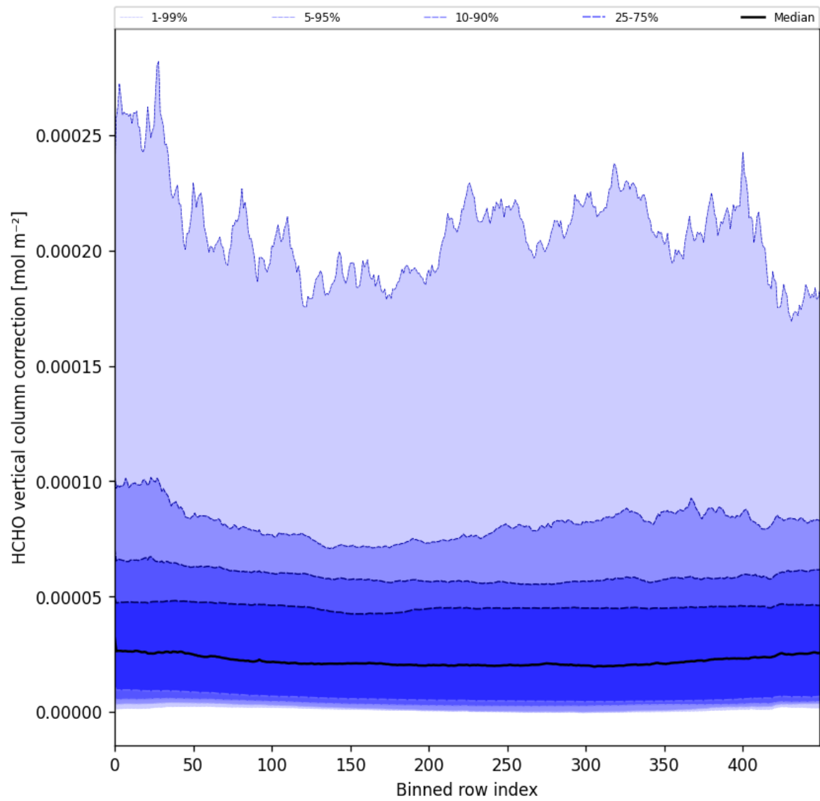
Figure 51: Along track statistics of “HCHO vertical column correction” for 2025-04-19 to 2025-04-20
