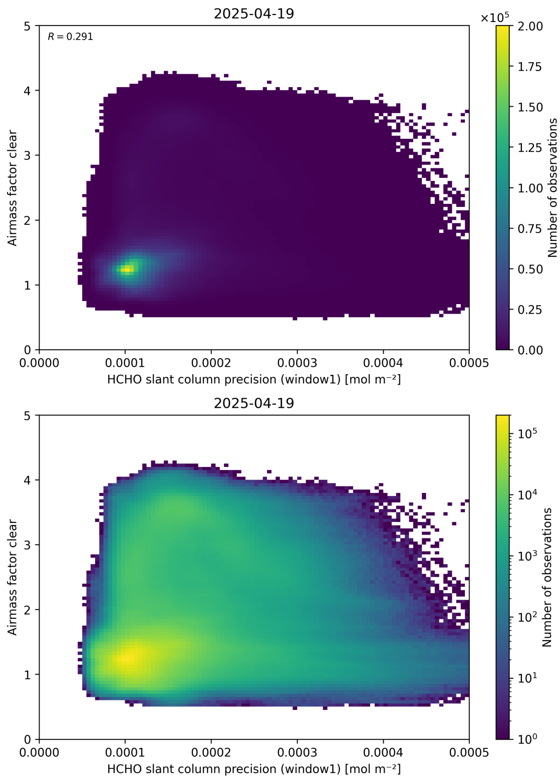
Figure 91: Scatter density plot of “HCHO slant column precision (window1)” against “Airmass factor clear” for 2025-04-19 to 2025-04-20.
