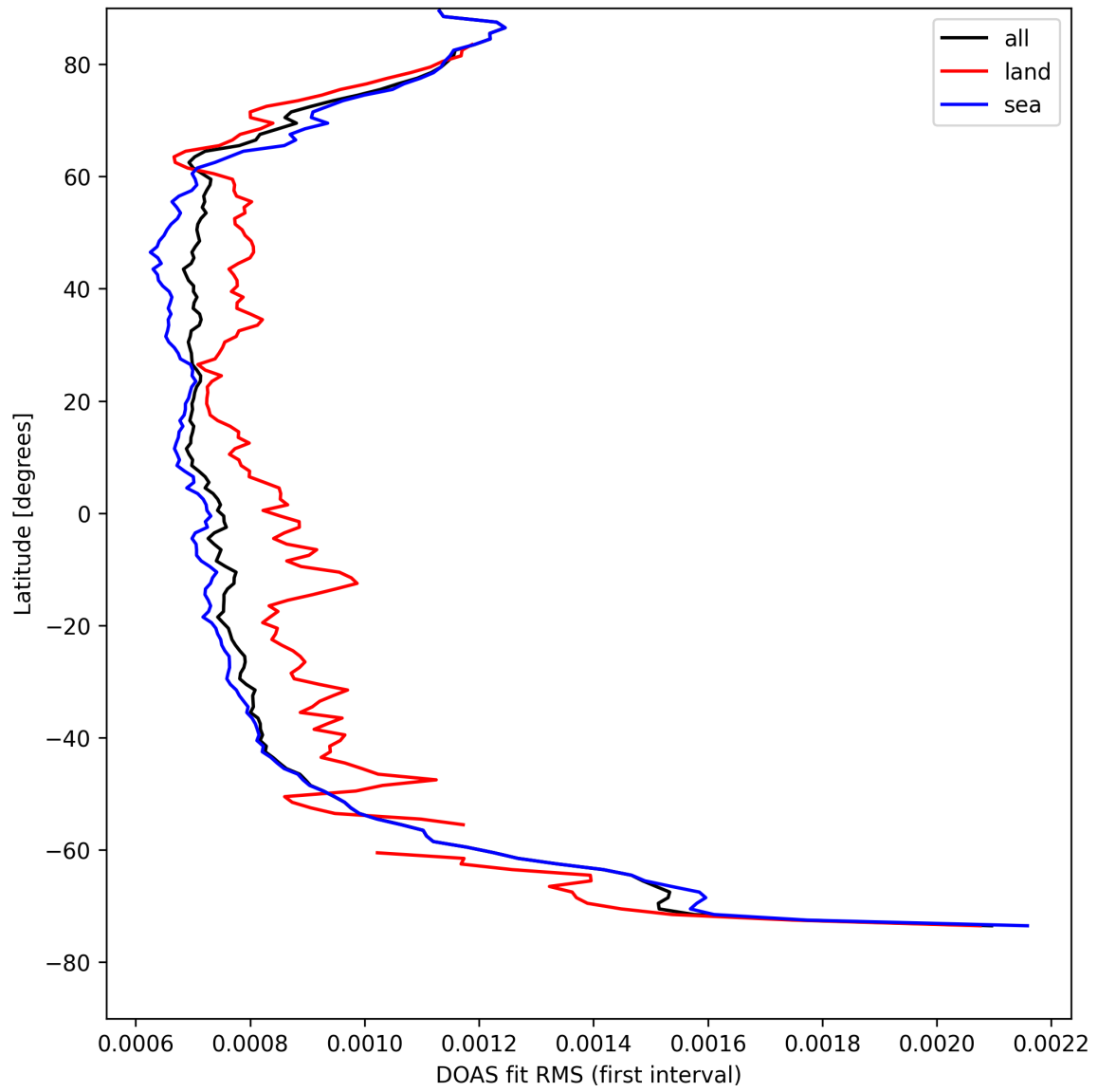
Figure 32: Zonal average of "DOAS fit RMS (first interval)" for 2025-04-19 to 2025-04-20.
