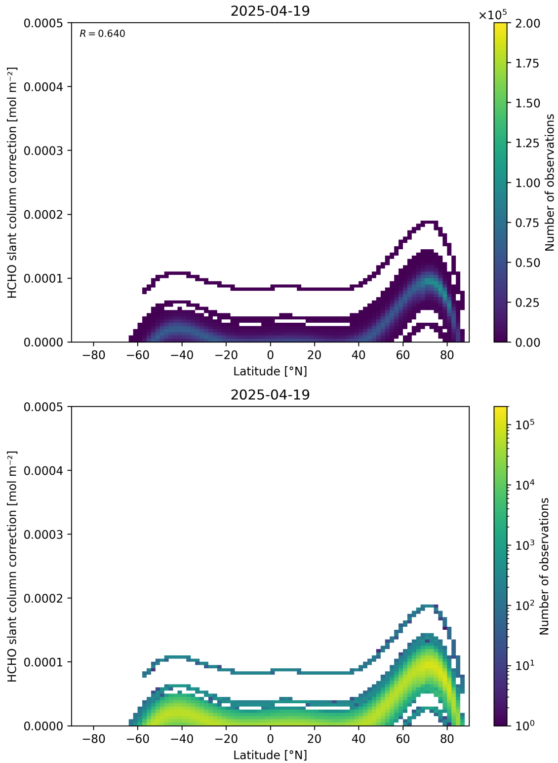
Figure 158: Scatter density plot of “Latitude” against “HCHO slant column correction” for 2025-04-19 to 2025-04-20.
