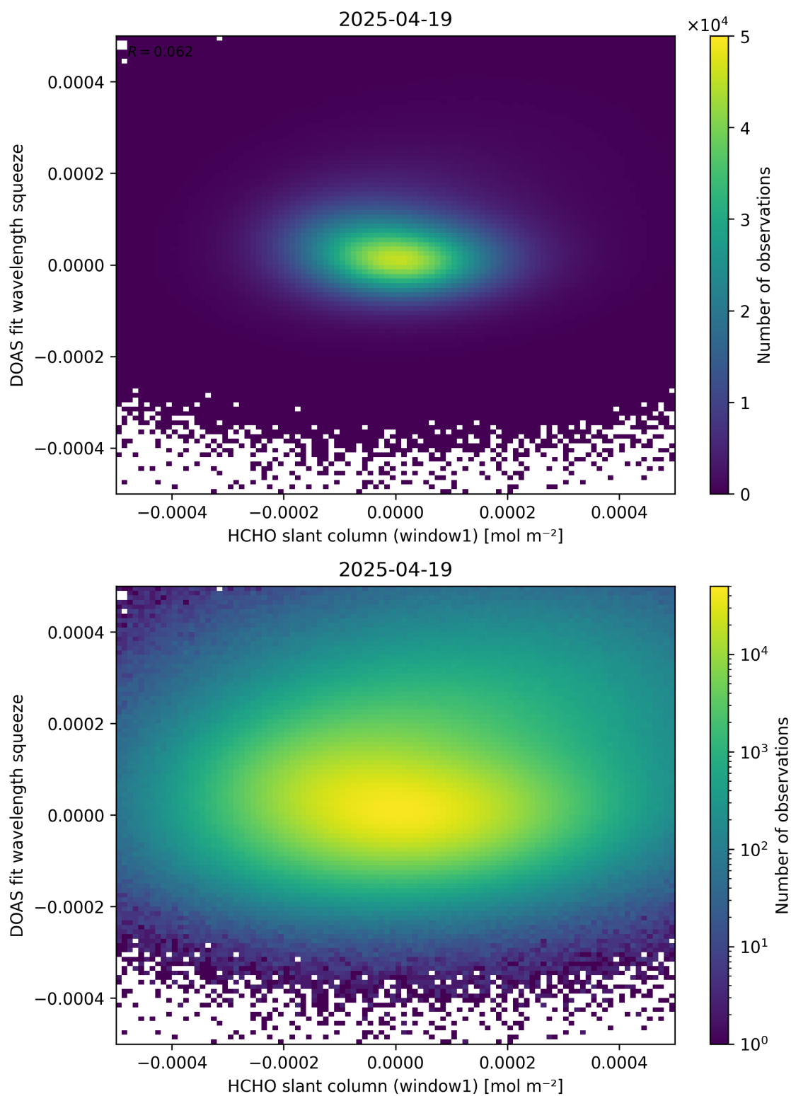
Figure 80: Scatter density plot of “HCHO slant column (window1)” against “DOAS fit wavelength squeeze” for 2025-04-19 to 2025-04-20.
