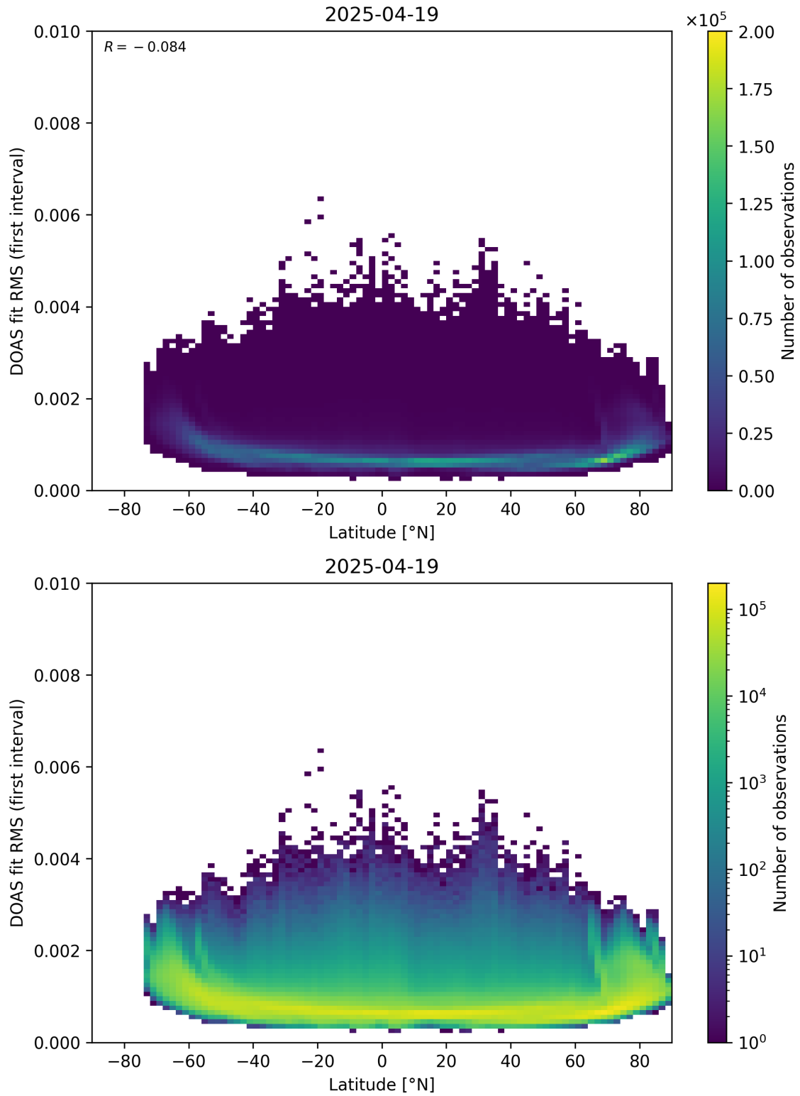
Figure 153: Scatter density plot of “Latitude” against “DOAS fit RMS (first interval)” for 2025-04-19 to 2025-04-20.
