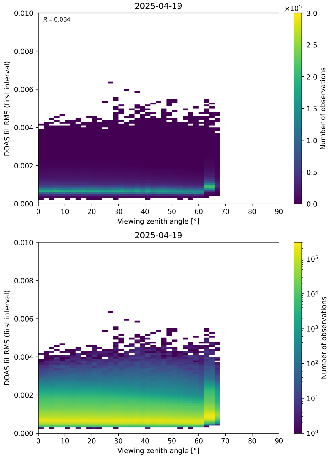
Figure 182: Scatter density plot of “Viewing zenith angle” against “DOAS fit RMS (first interval)” for 2025-04-19 to 2025-04-20.
