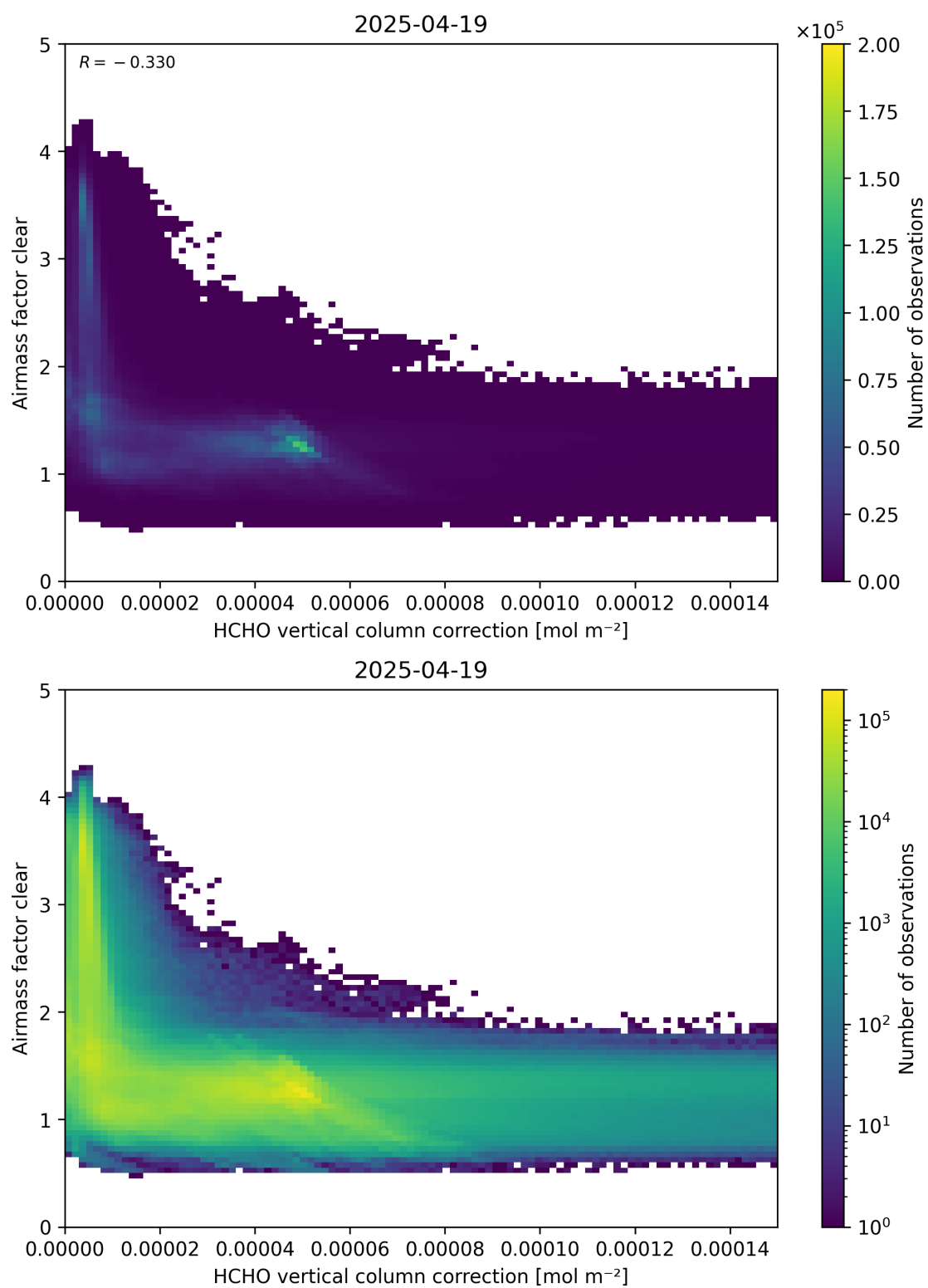
Figure 115: Scatter density plot of “HCHO vertical column correction” against “Airmass factor clear” for 2025-04-19 to 2025-04-20.
