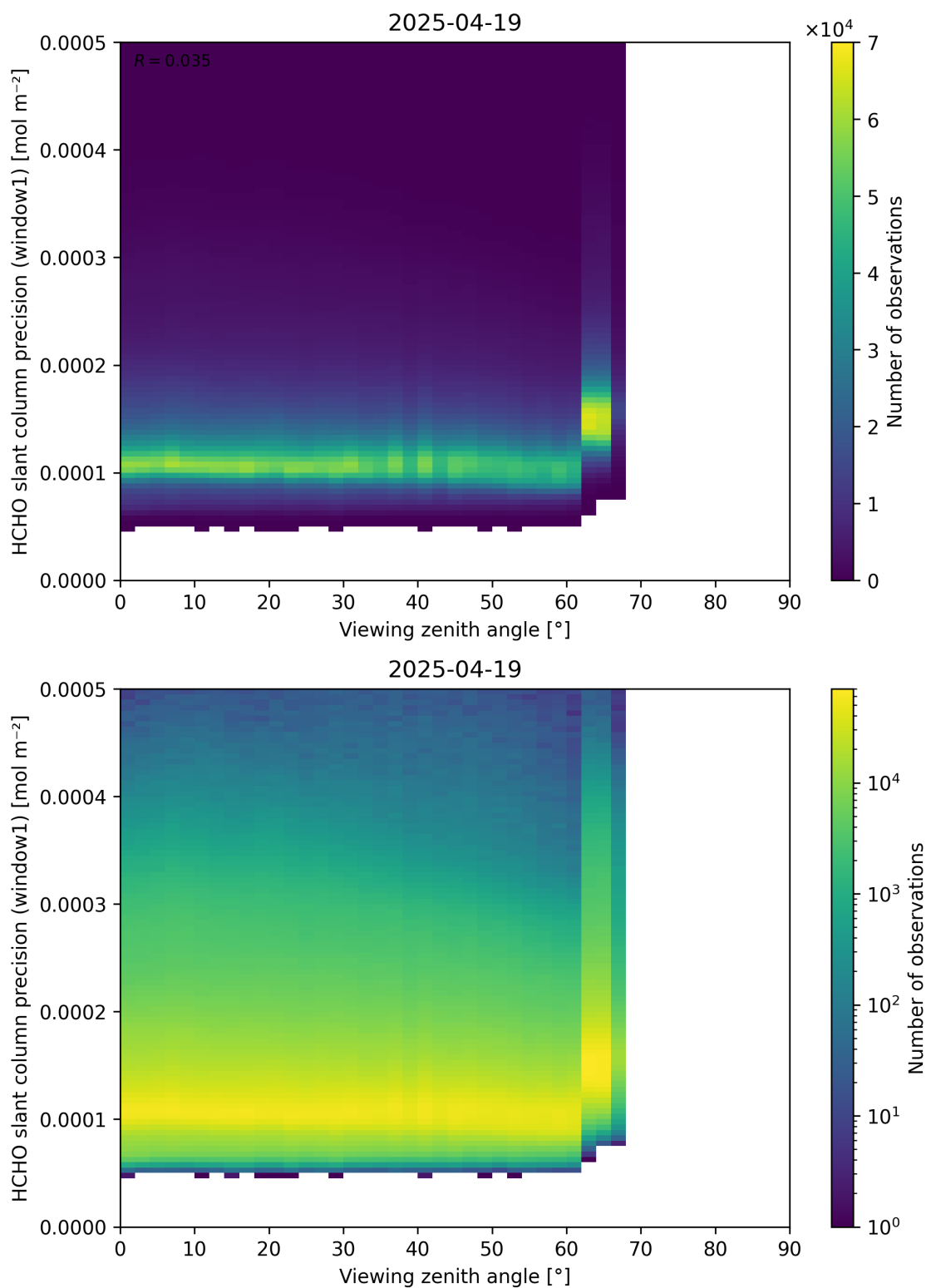
Figure 189: Scatter density plot of “Viewing zenith angle” against “HCHO slant column precision (window1)” for 2025-04-19 to 2025-04-20.
