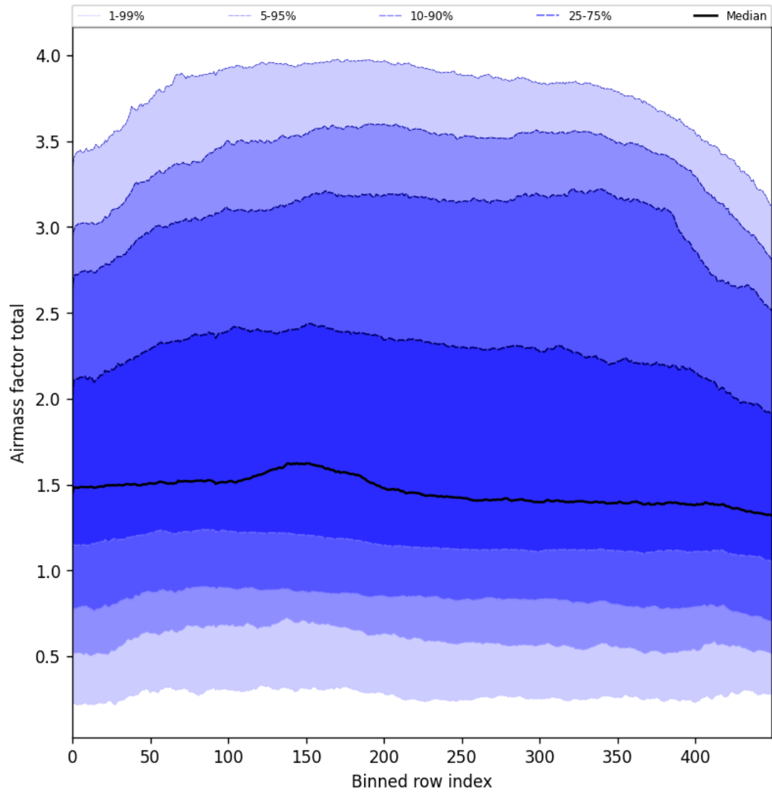
Figure 54: Along track statistics of “Airmass factor total” for 2025-04-19 to 2025-04-20
