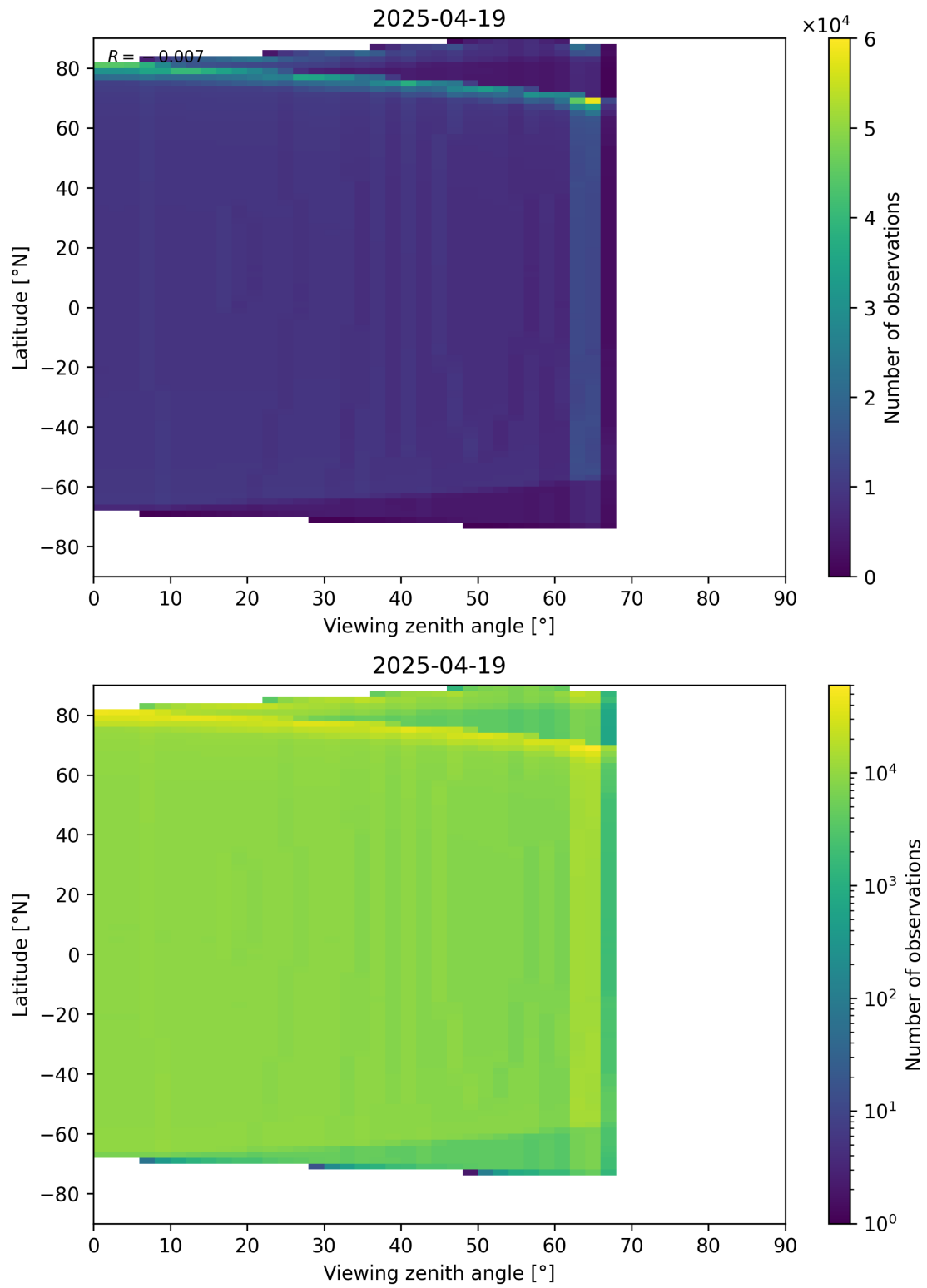
Figure 196: Scatter density plot of “Viewing zenith angle” against “Latitude” for 2025-04-19 to 2025-04-20.
