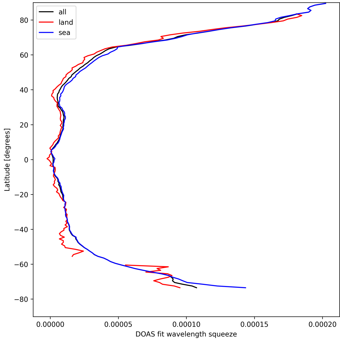
Figure 31: Zonal average of “DOAS fit wavelength squeeze” for 2025-04-19 to 2025-04-20.
