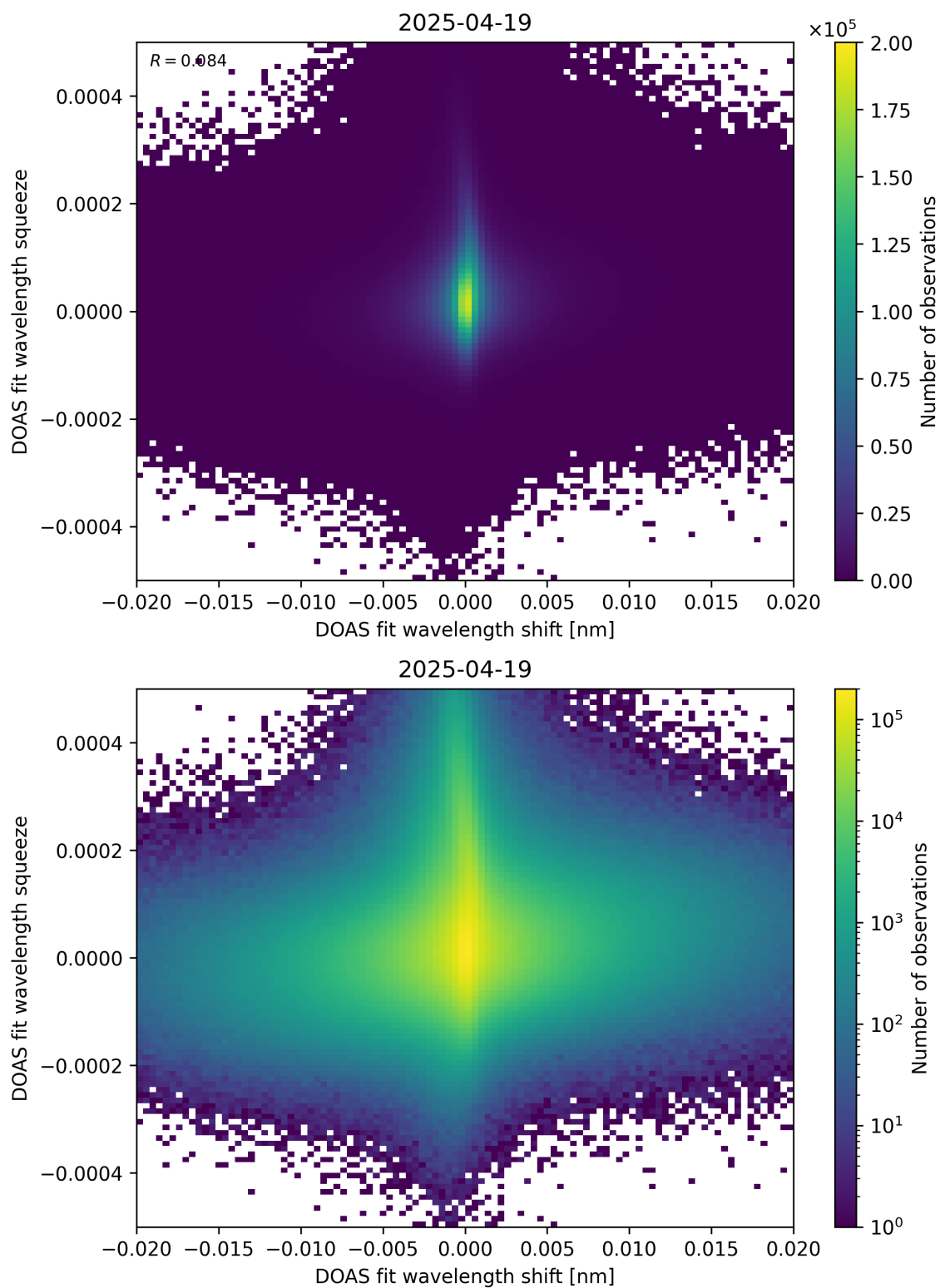
Figure 65: Scatter density plot of “DOAS fit wavelength shift” against “DOAS fit wavelength squeeze” for 2025-04-19 to 2025-04-20.
