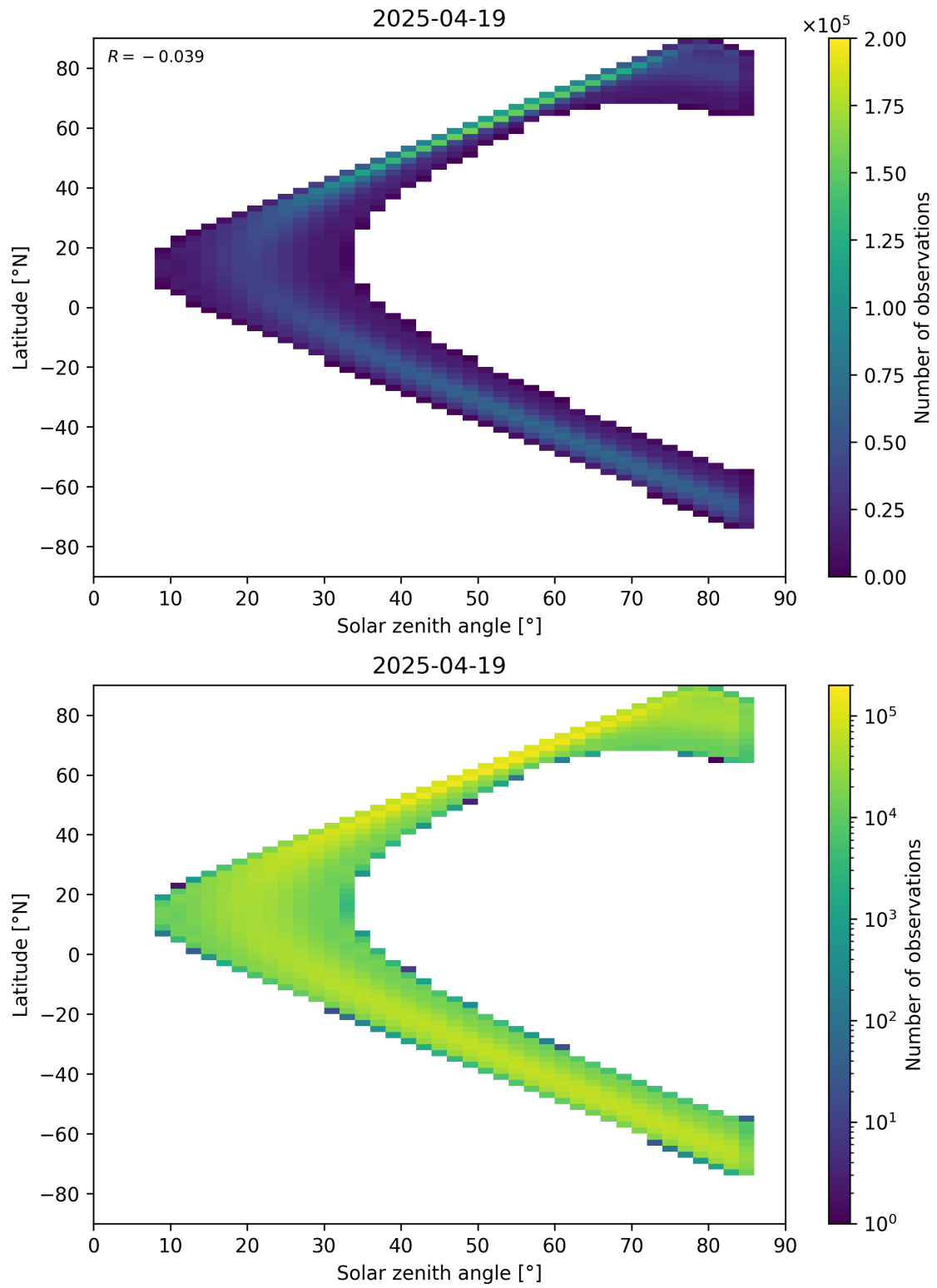
Figure 181: Scatter density plot of “Solar zenith angle” against “Latitude” for 2025-04-19 to 2025-04-20.
