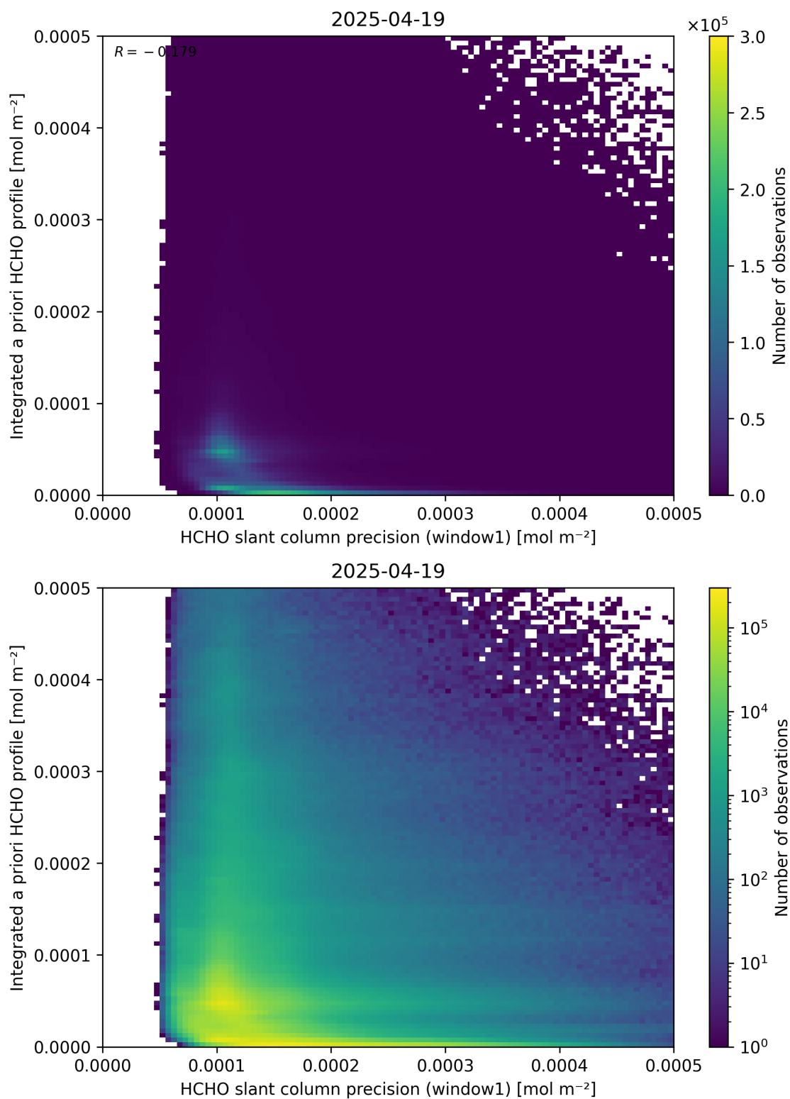
Figure 96: Scatter density plot of “HCHO slant column precision (window1)” against “Integrated a priori HCHO profile” for 2025-04-19 to 2025-04-20.
