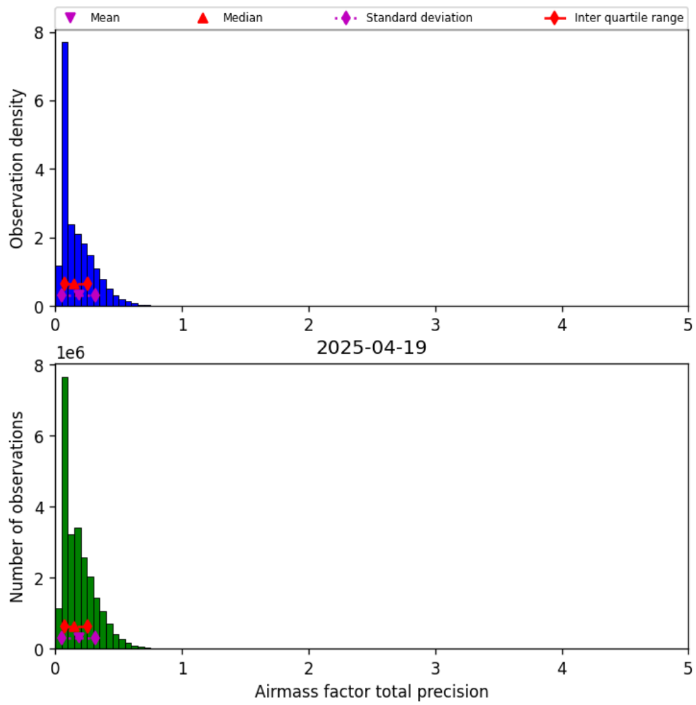
Figure 41: Histogram of “Airmass factor total precision” for 2025-04-19 to 2025-04-20
