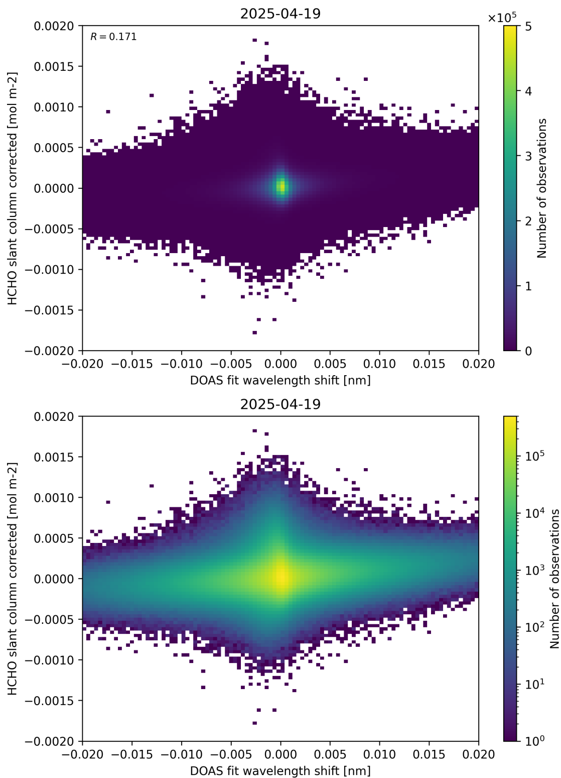
Figure 66: Scatter density plot of “DOAS fit wavelength shift” against “HCHO slant column corrected” for 2025-04-19 to 2025-04-20.
