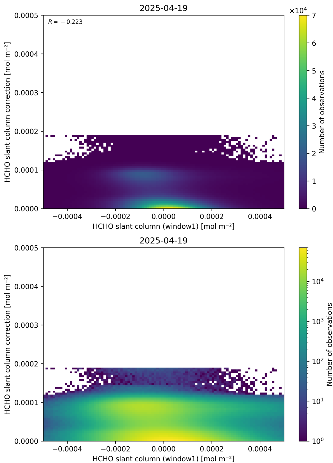
Figure 83: Scatter density plot of “HCHO slant column (window1)” against “HCHO slant column correction” for 2025-04-19 to 2025-04-20.
