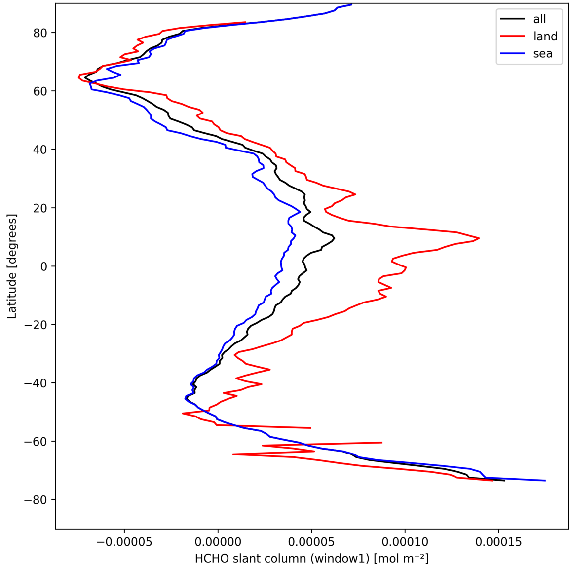
Figure 24: Zonal average of “HCHO slant column (window1)” for 2025-04-19 to 2025-04-20.
