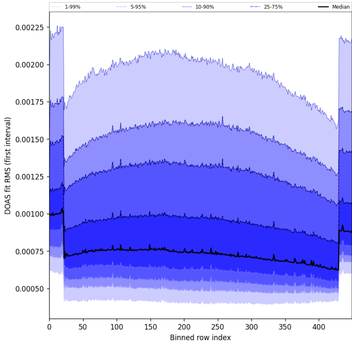
Figure 60: Along track statistics of “DOAS fit RMS (first interval)” for 2025-04-19 to 2025-04-20
