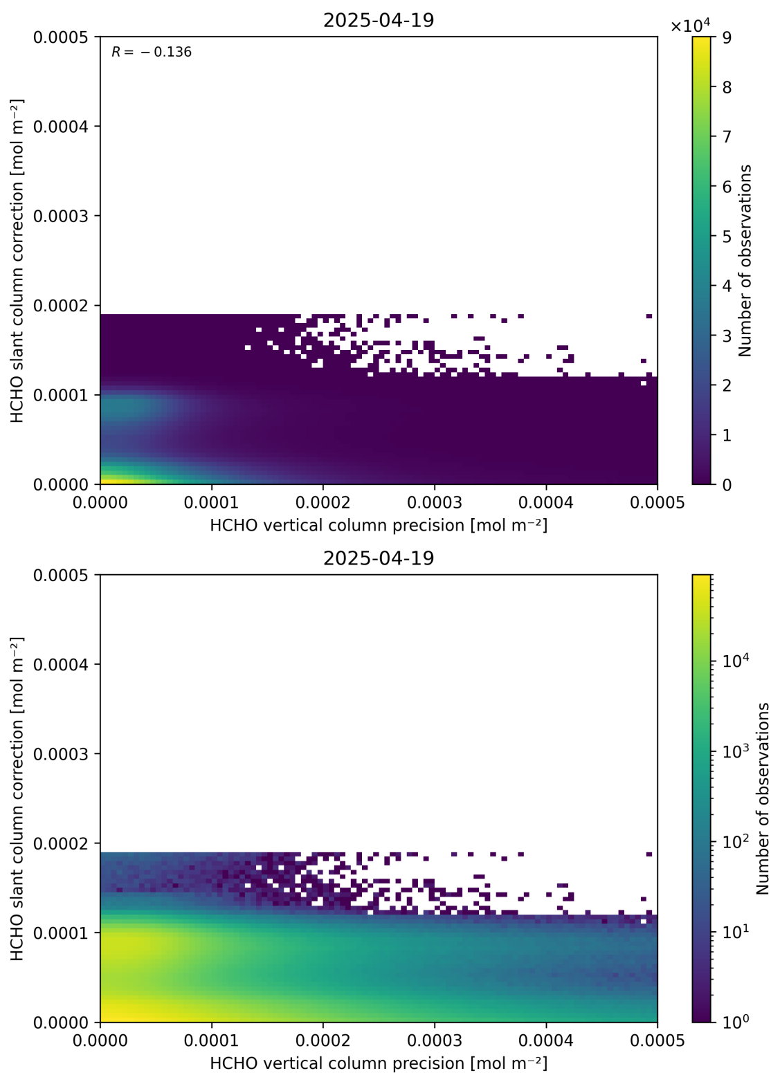
Figure 141: Scatter density plot of “HCHO vertical column precision” against “HCHO slant column correction” for 2025-04-19 to 2025-04-20.
