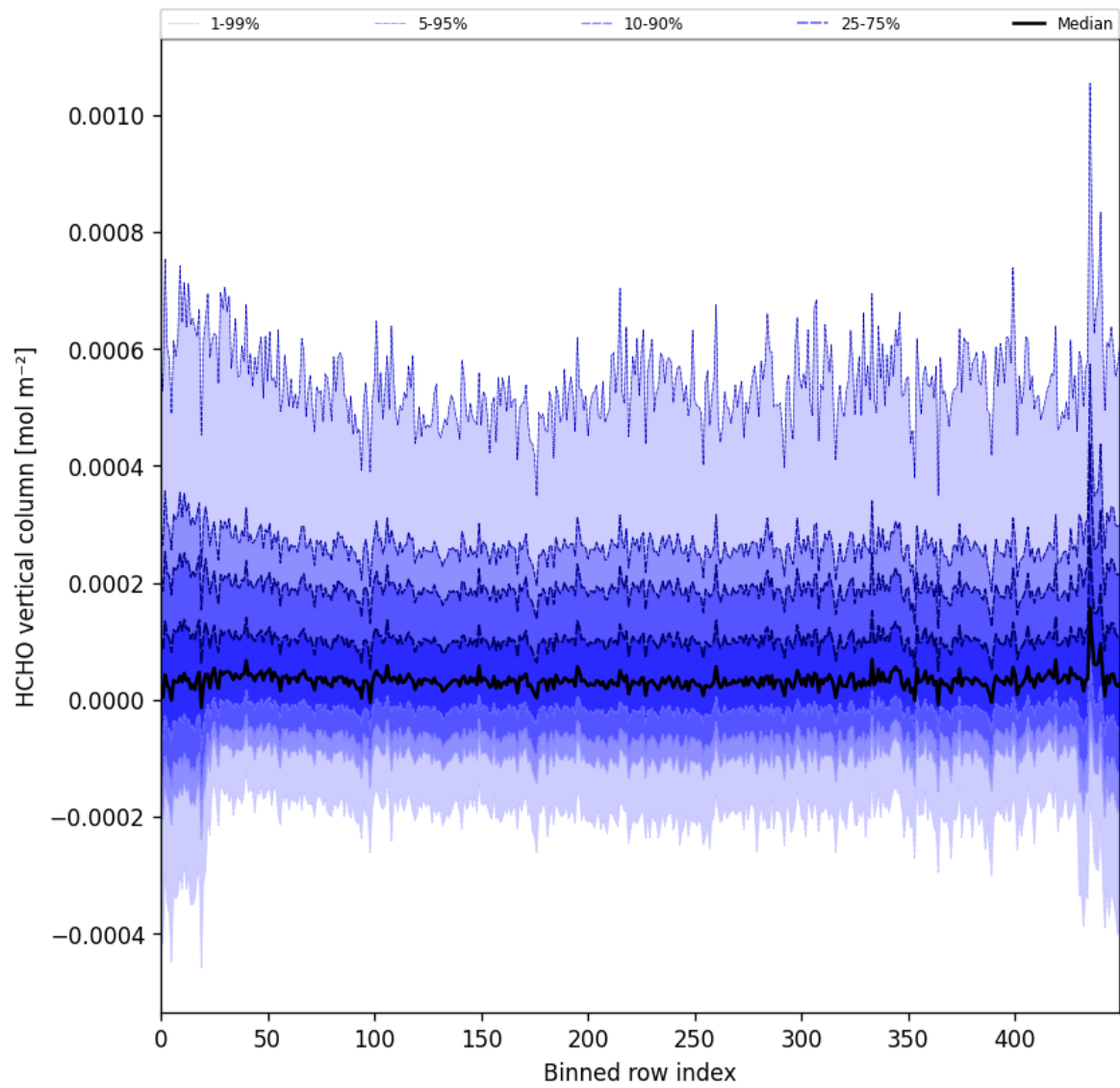
Figure 49: Along track statistics of “HCHO vertical column” for 2025-04-19 to 2025-04-20
