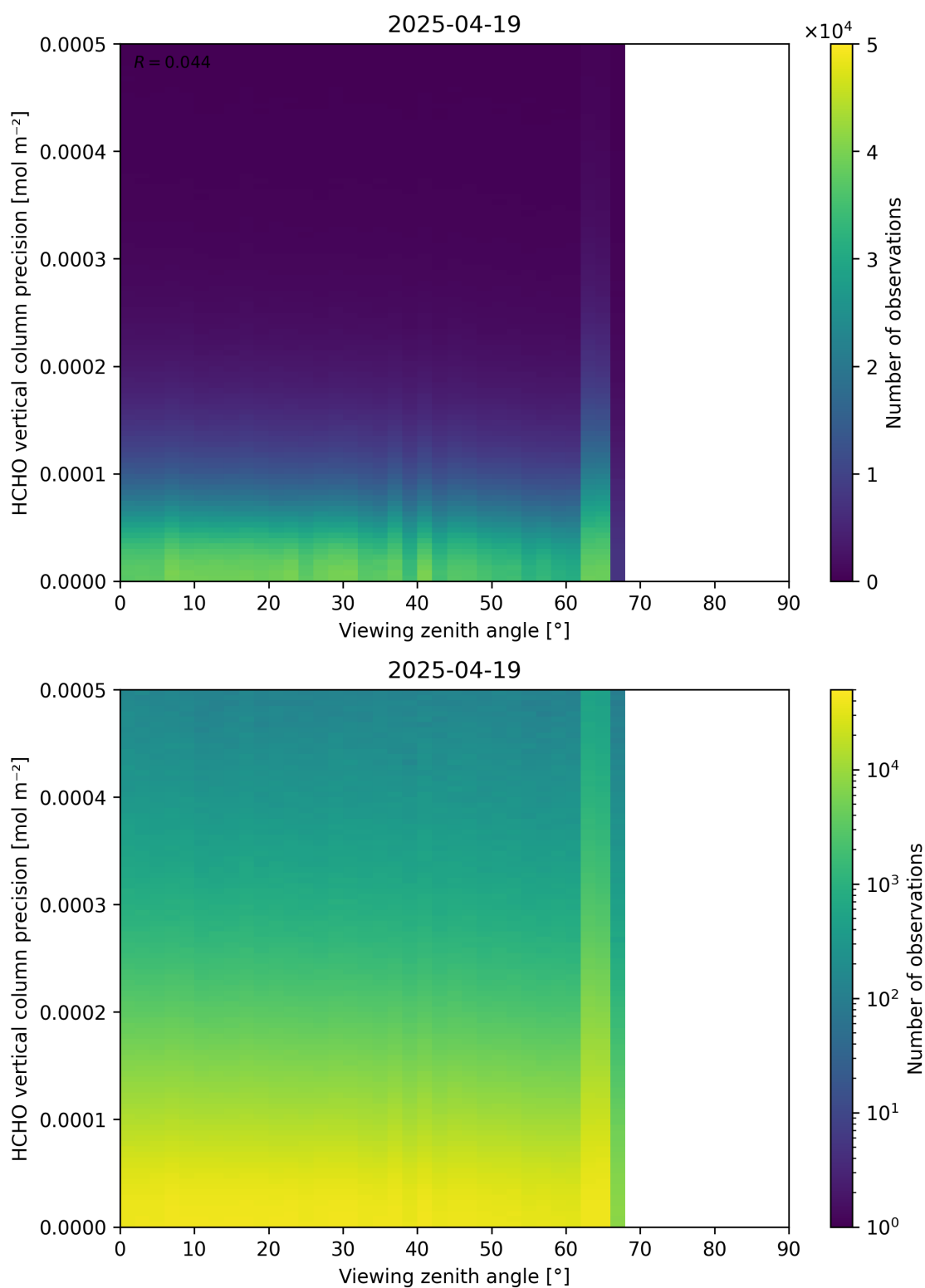
Figure 194: Scatter density plot of “Viewing zenith angle” against “HCHO vertical column precision” for 2025-04-19 to 2025-04-20.
