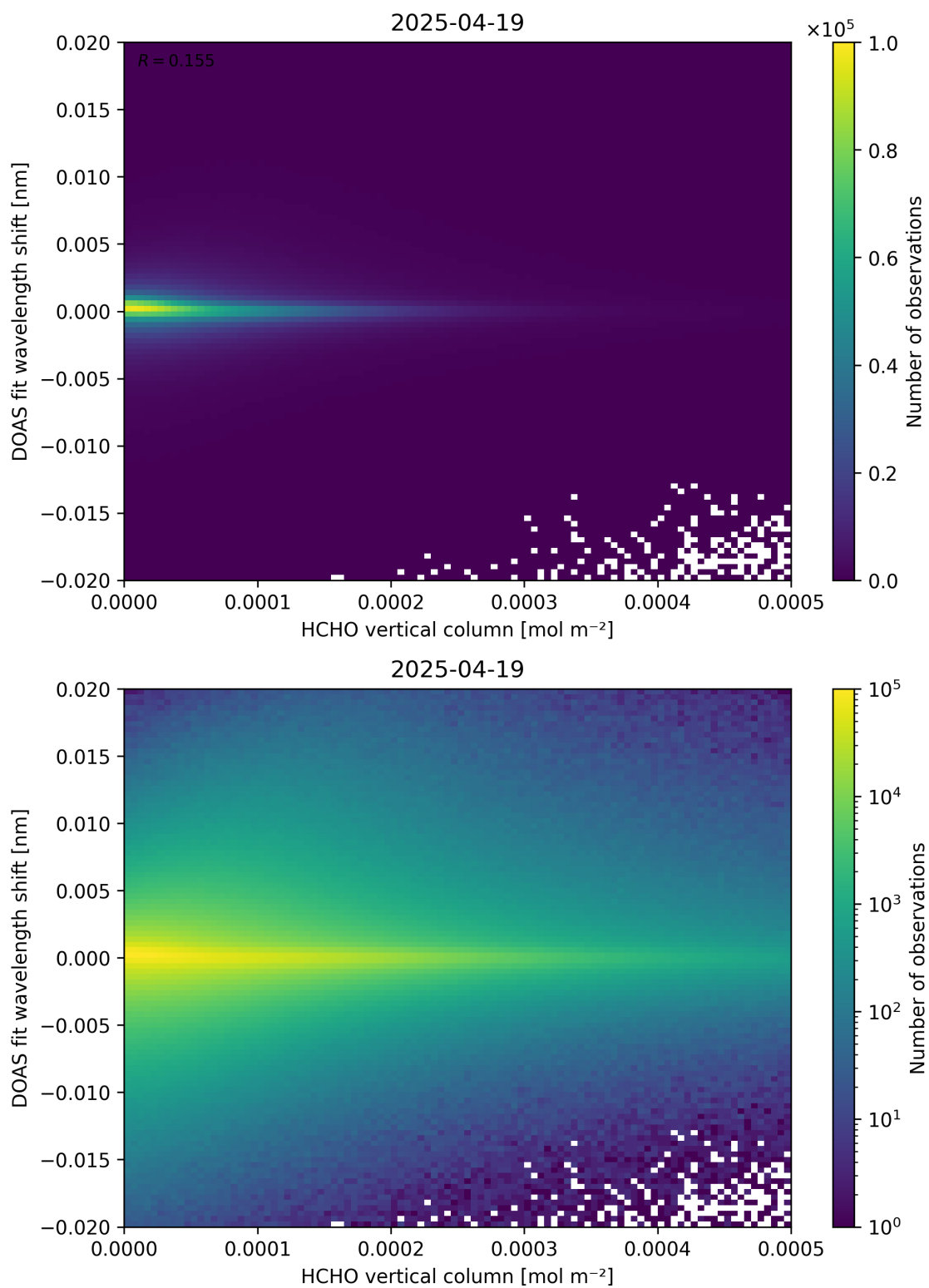
Figure 124: Scatter density plot of “HCHO vertical column” against “DOAS fit wavelength shift” for 2025-04-19 to 2025-04-20.
