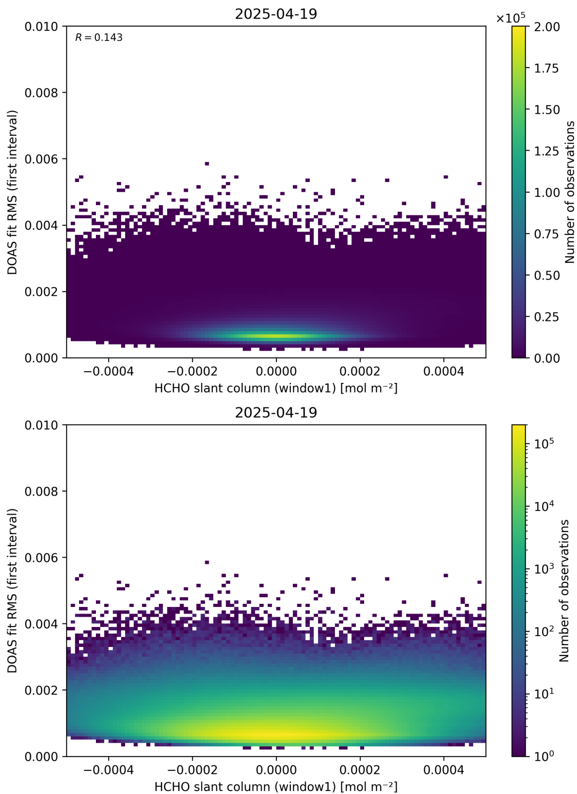
Figure 78: Scatter density plot of “HCHO slant column (window1)” against “DOAS fit RMS (first interval)” for 2025-04-19 to 2025-04-20.
