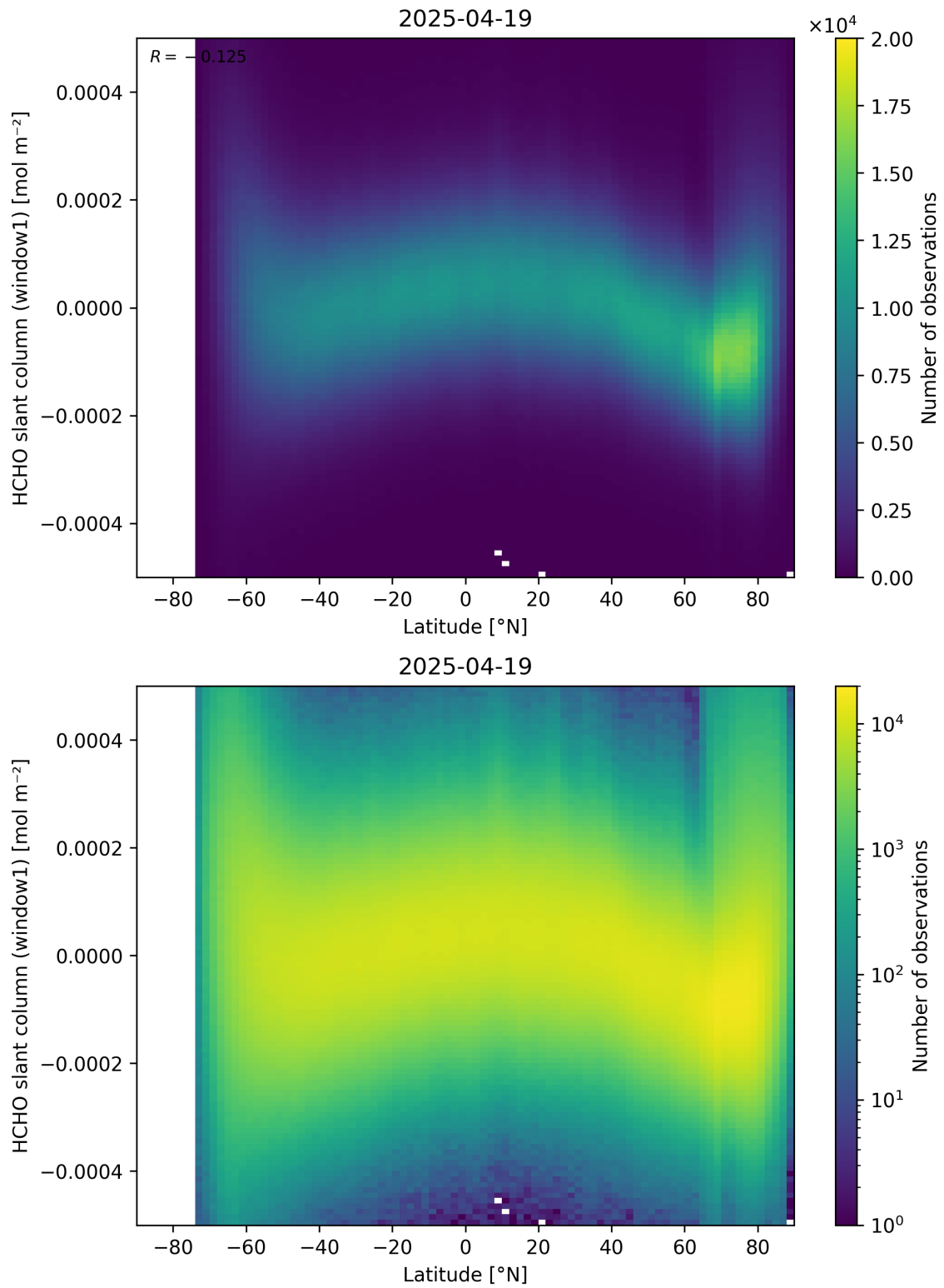
Figure 159: Scatter density plot of “Latitude” against “HCHO slant column (window1)” for 2025-04-19 to 2025-04-20.
