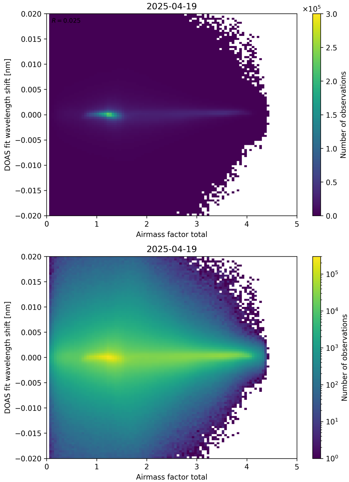
Figure 98: Scatter density plot of “Airmass factor total” against “DOAS fit wavelength shift” for 2025-04-19 to 2025-04-20.
