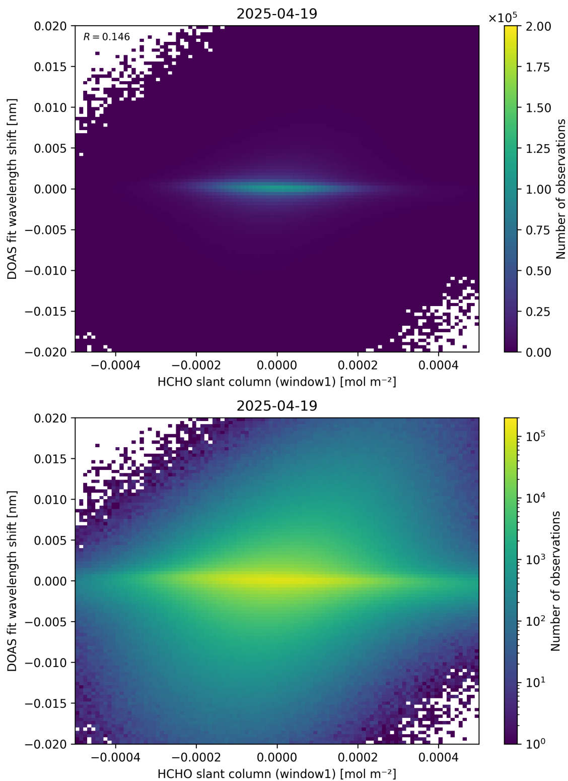
Figure 79: Scatter density plot of “HCHO slant column (window1)” against “DOAS fit wavelength shift” for 2025-04-19 to 2025-04-20.
