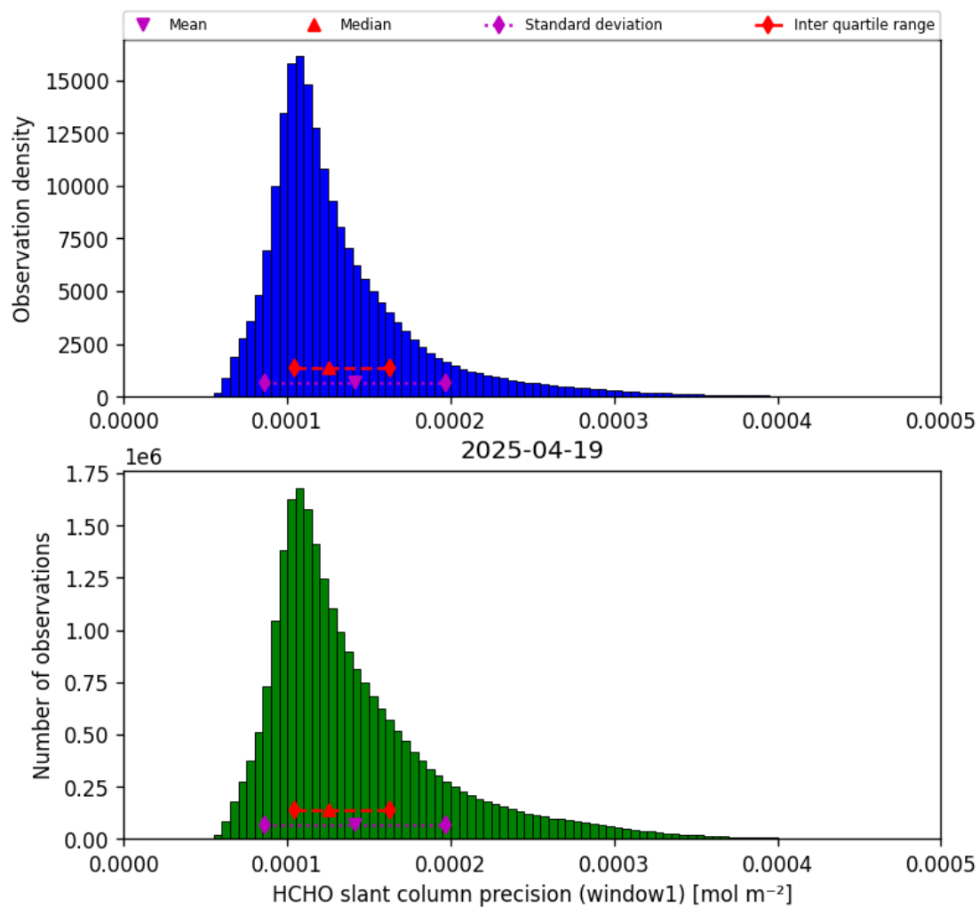
Figure 39: Histogram of “HCHO slant column precision (window1)” for 2025-04-19 to 2025-04-20
