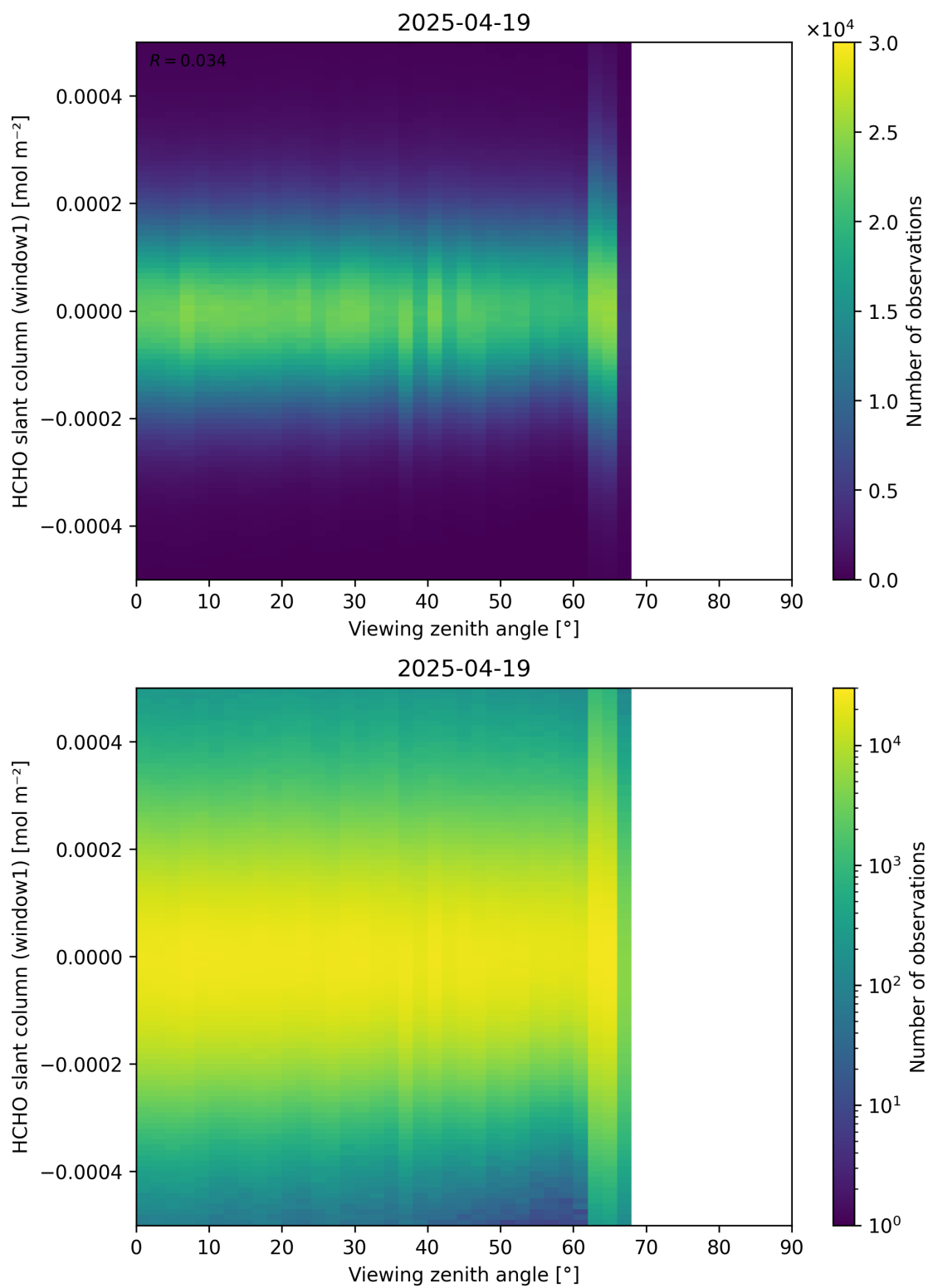
Figure 188: Scatter density plot of “Viewing zenith angle” against “HCHO slant column (window1)” for 2025-04-19 to 2025-04-20.
