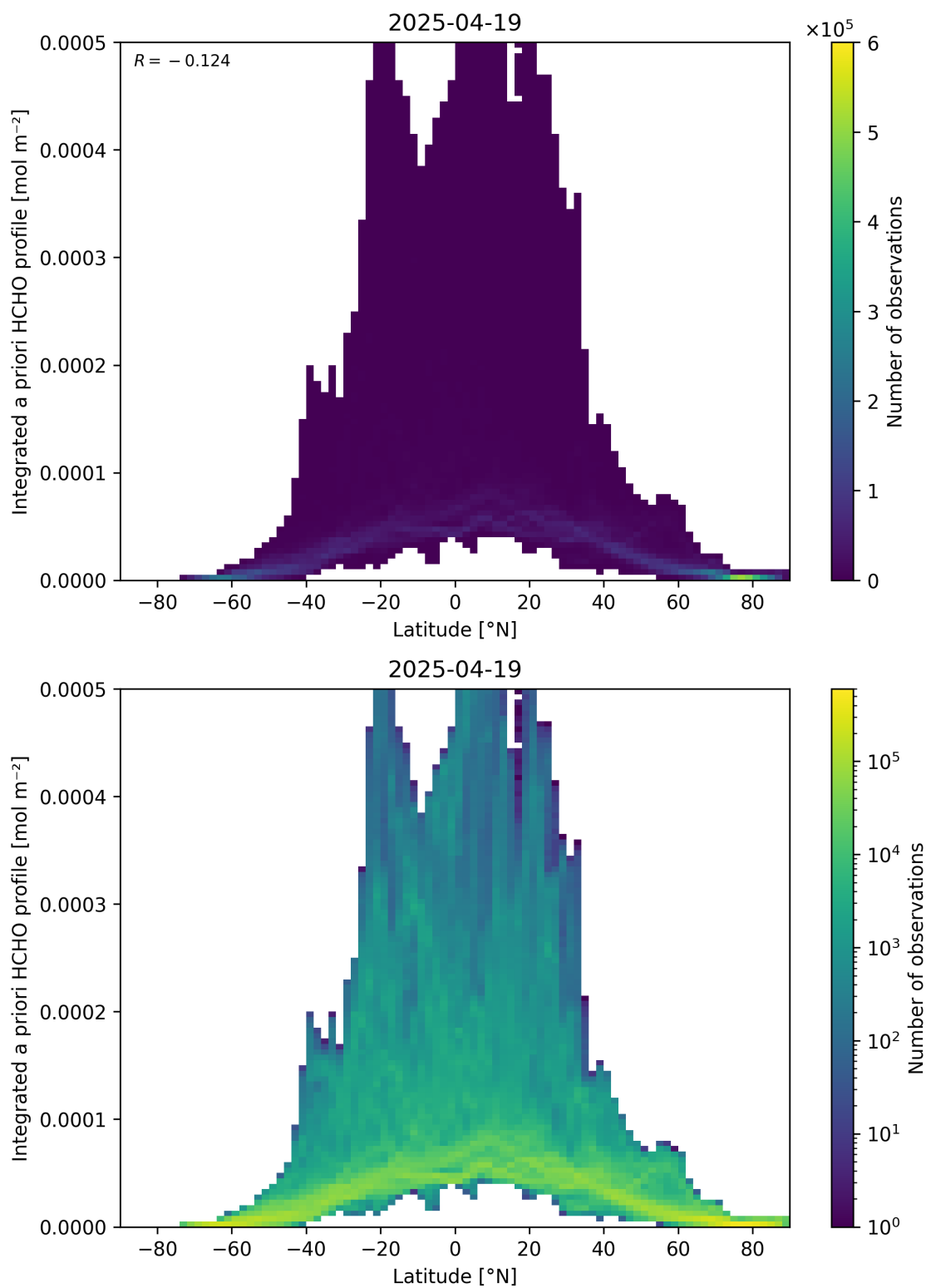
Figure 166: Scatter density plot of “Latitude” against “Integrated a priori HCHO profile” for 2025-04-19 to 2025-04-20.
