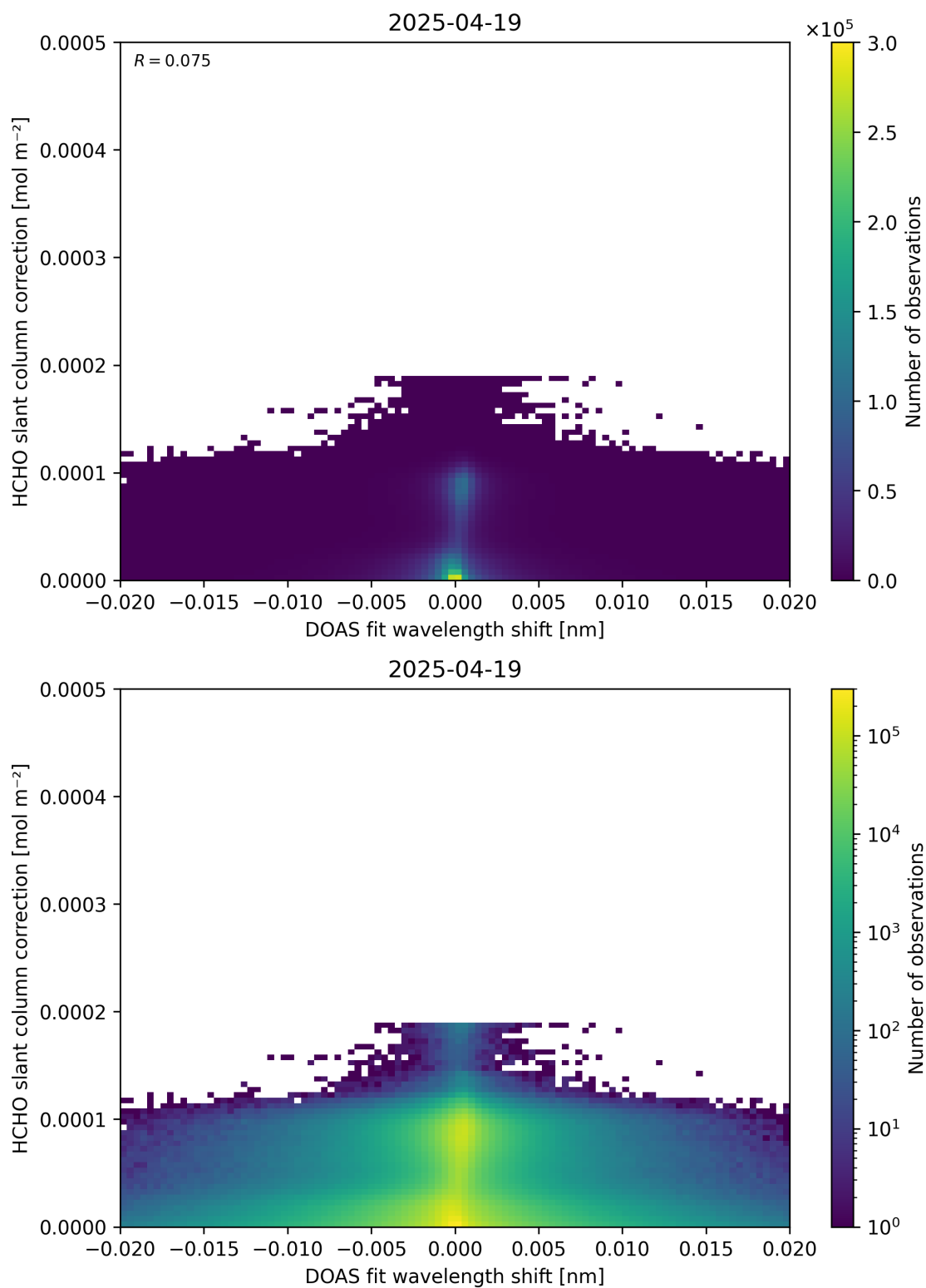
Figure 67: Scatter density plot of “DOAS fit wavelength shift” against “HCHO slant column correction” for 2025-04-19 to 2025-04-20.
