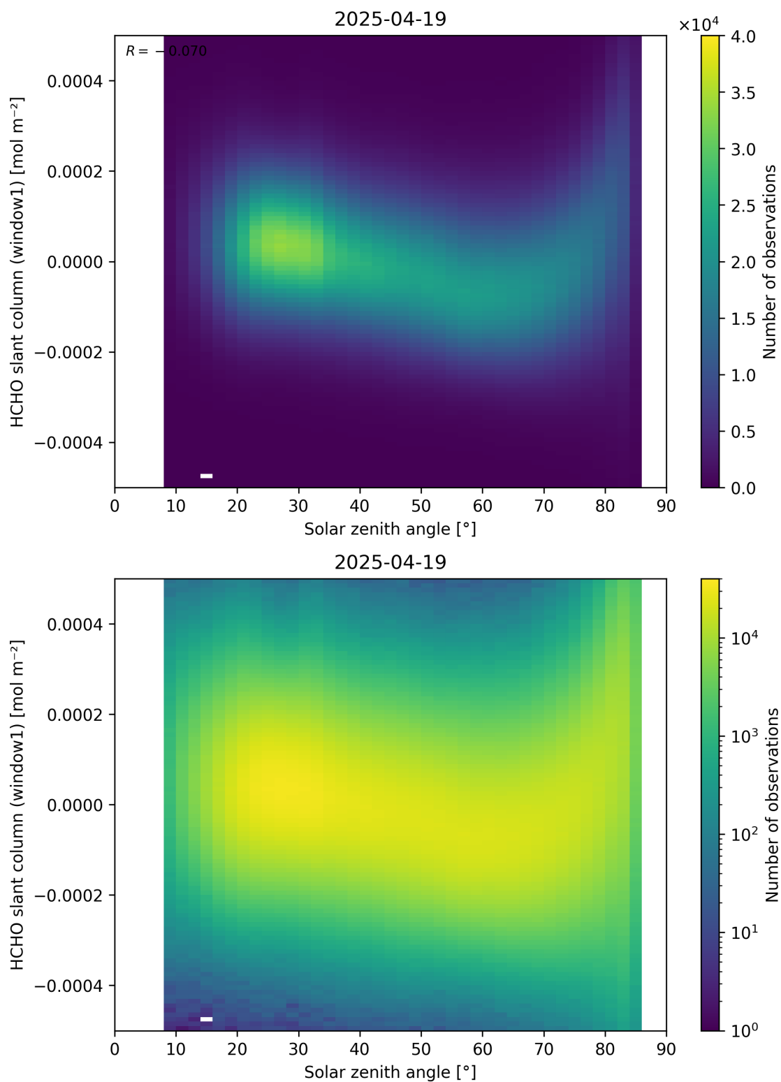
Figure 173: Scatter density plot of “Solar zenith angle” against “HCHO slant column (window1)” for 2025-04-19 to 2025-04-20.
