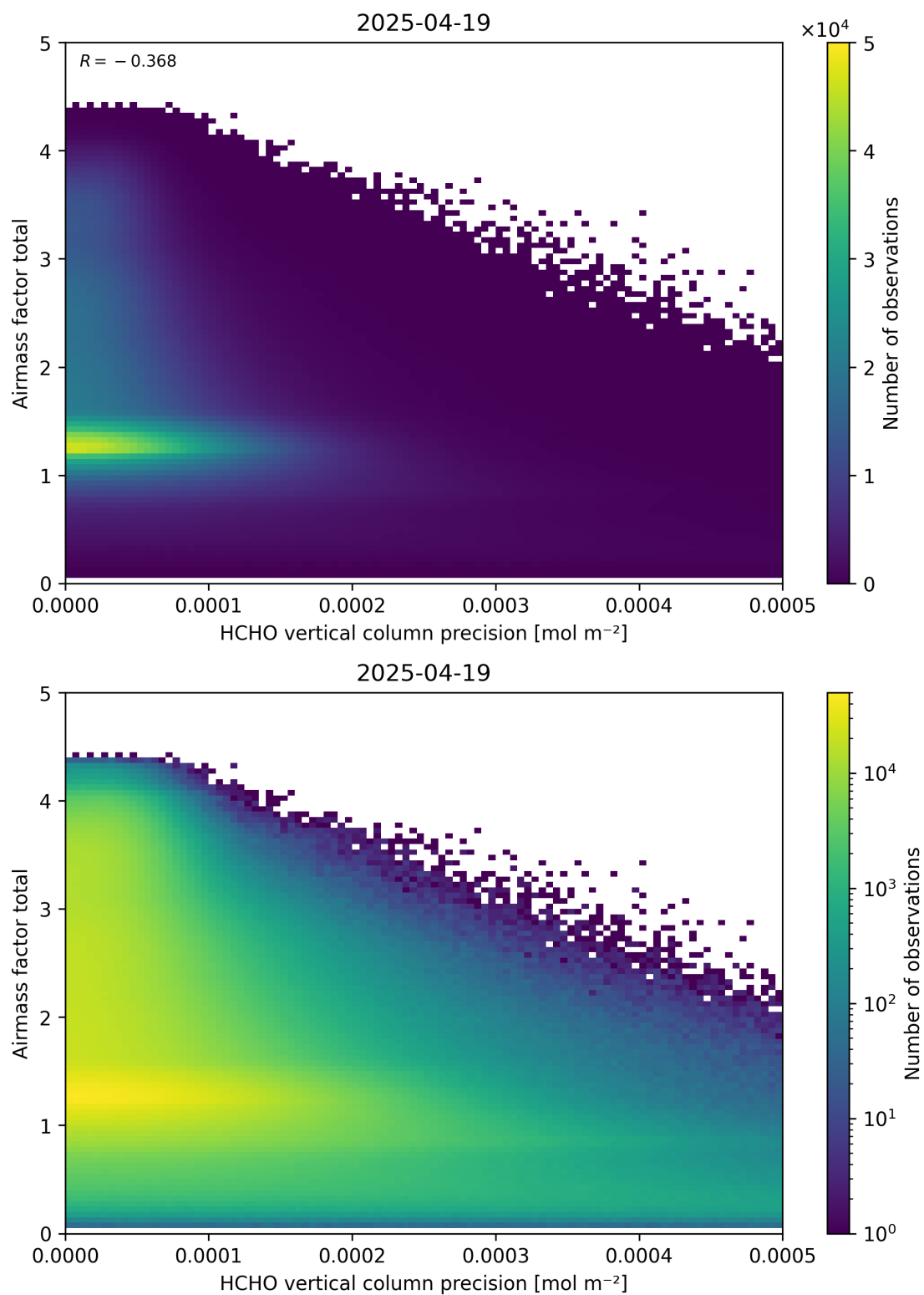
Figure 144: Scatter density plot of “HCHO vertical column precision” against “Airmass factor total” for 2025-04-19 to 2025-04-20.
