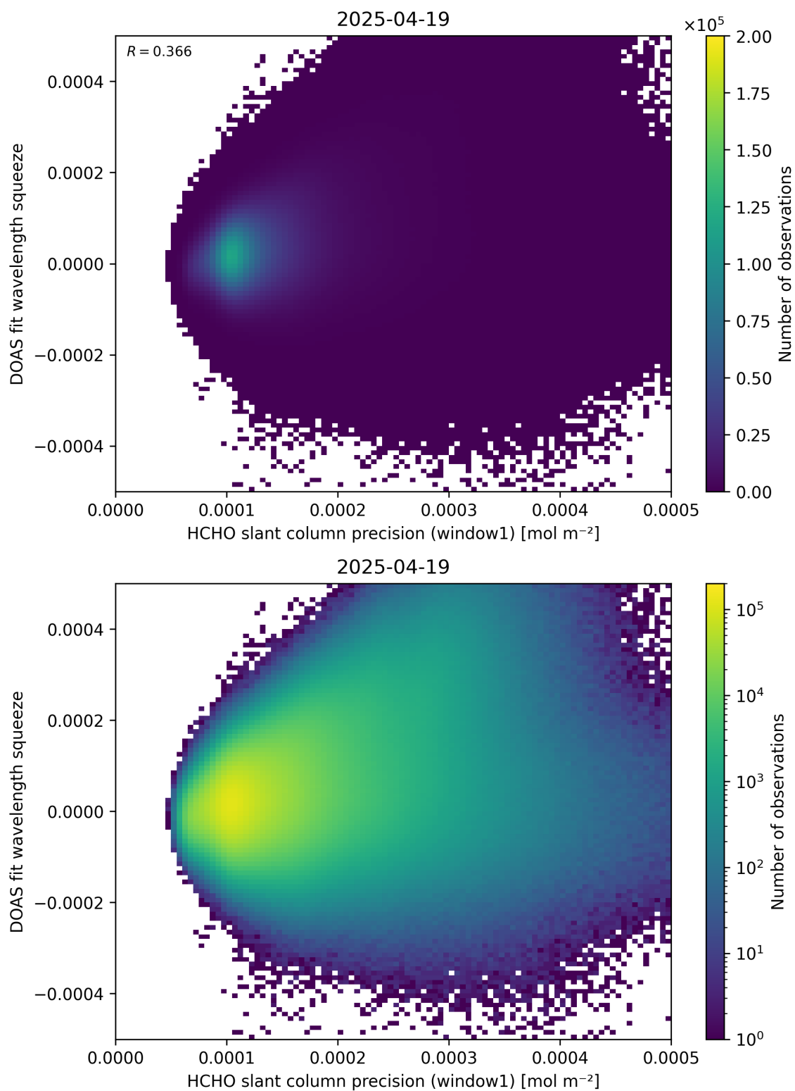
Figure 90: Scatter density plot of “HCHO slant column precision (window1)” against “DOAS fit wavelength squeeze” for 2025-04-19 to 2025-04-20.
