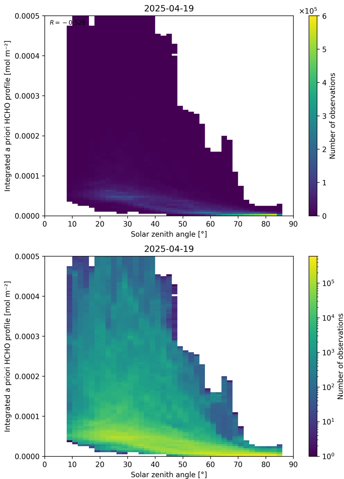
Figure 180: Scatter density plot of “Solar zenith angle” against “Integrated a priori HCHO profile” for 2025-04-19 to 2025-04-20.
