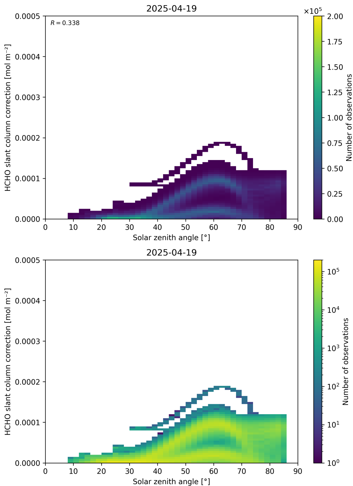
Figure 172: Scatter density plot of “Solar zenith angle” against “HCHO slant column correction” for 2025-04-19 to 2025-04-20.
