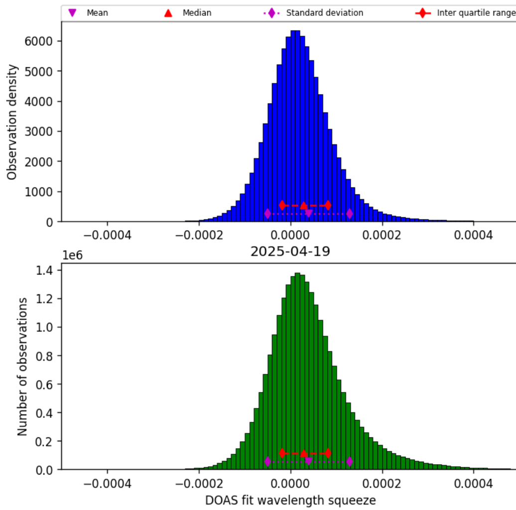
Figure 45: Histogram of “DOAS fit wavelength squeeze” for 2025-04-19 to 2025-04-20
