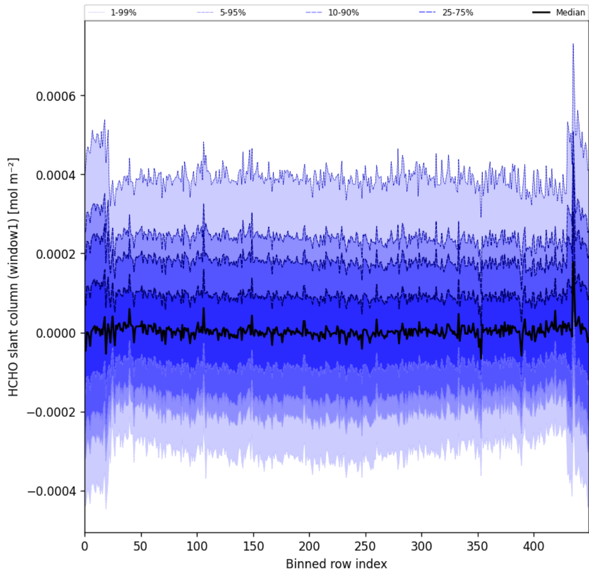
Figure 52: Along track statistics of “HCHO slant column (window1)” for 2025-04-19 to 2025-04-20
