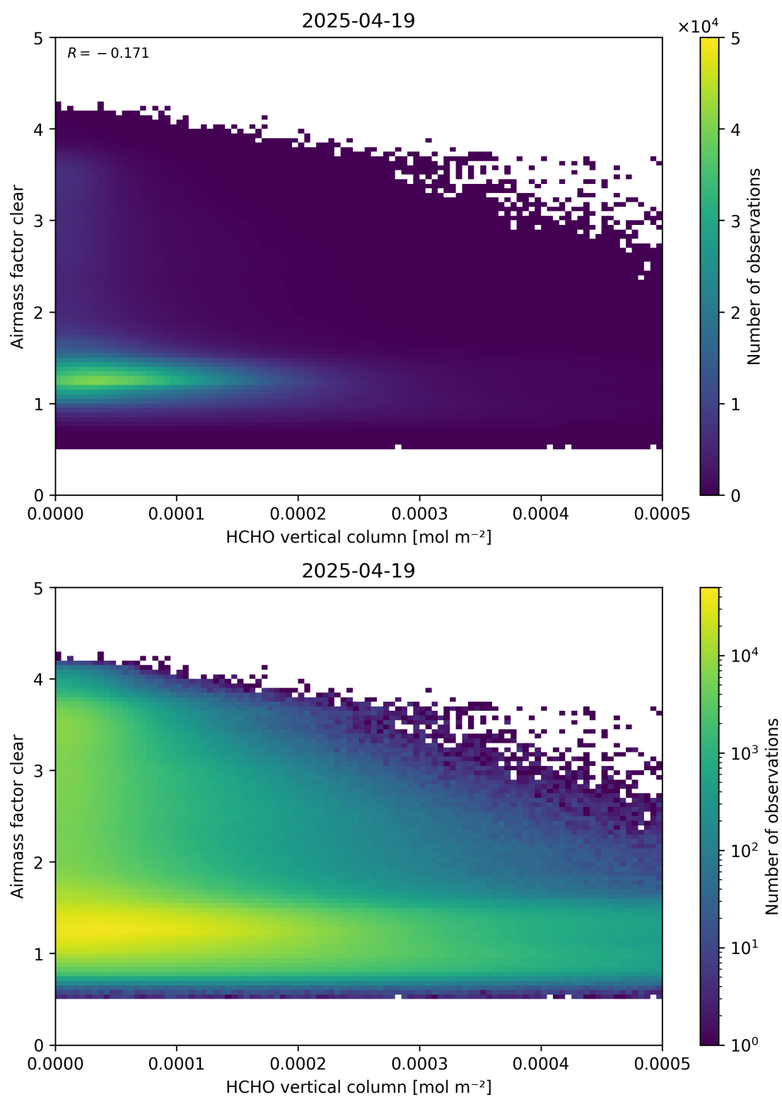
Figure 126: Scatter density plot of “HCHO vertical column” against “Airmass factor clear” for 2025-04-19 to 2025-04-20.
