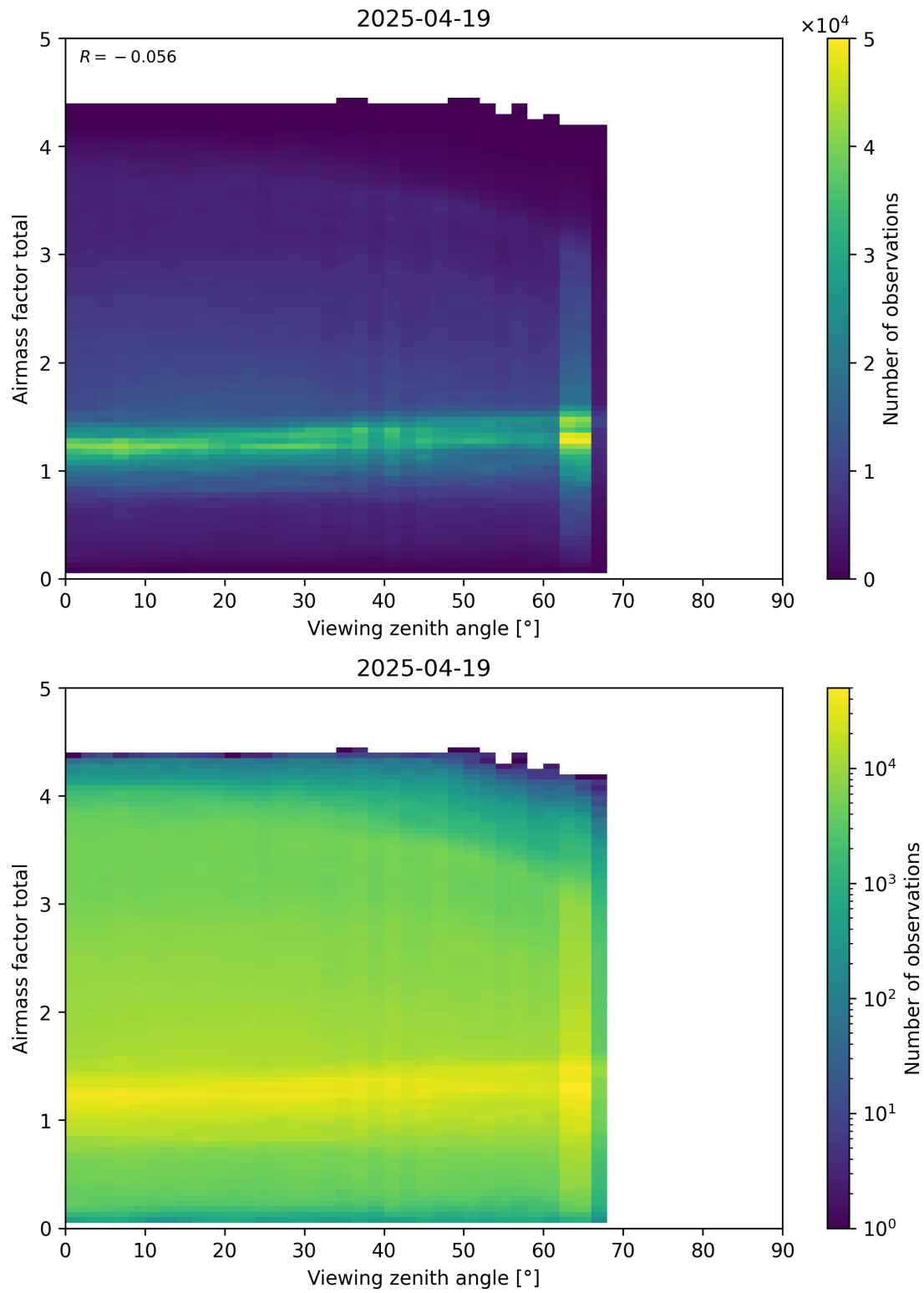
Figure 190: Scatter density plot of “Viewing zenith angle” against “Airmass factor total” for 2025-04-19 to 2025-04-20.
