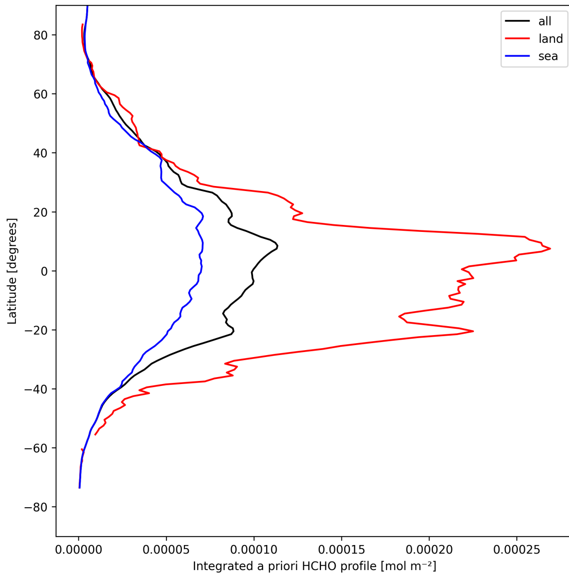
Figure 29: Zonal average of “Integrated a priori HCHO profile” for 2025-04-19 to 2025-04-20.
