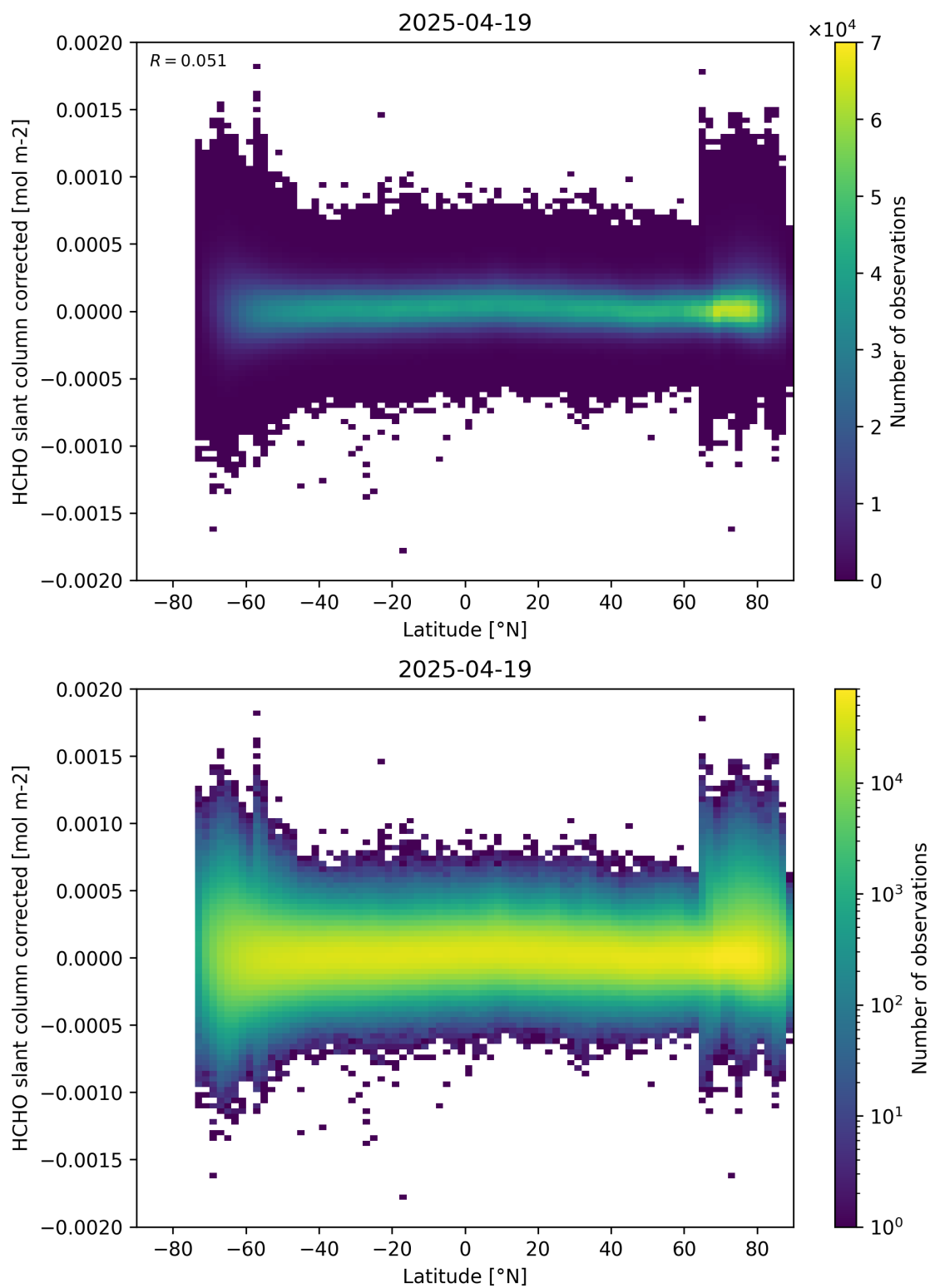
Figure 157: Scatter density plot of “Latitude” against “HCHO slant column corrected” for 2025-04-19 to 2025-04-20.
