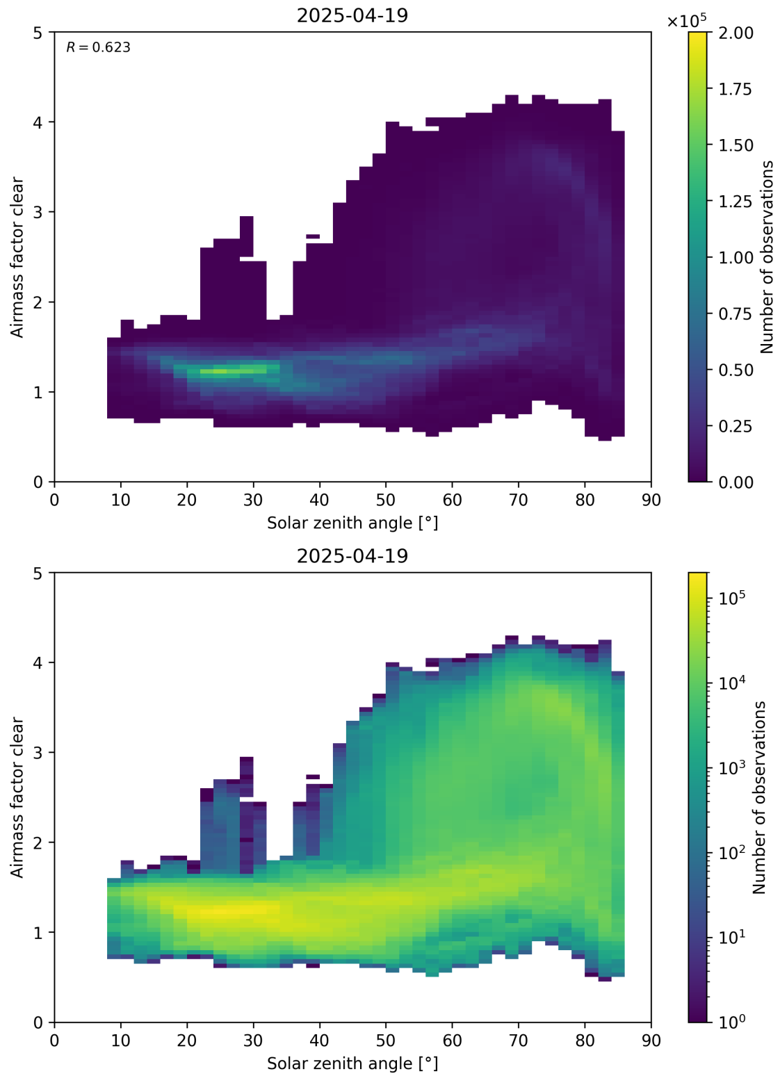
Figure 170: Scatter density plot of “Solar zenith angle” against “Airmass factor clear” for 2025-04-19 to 2025-04-20.
