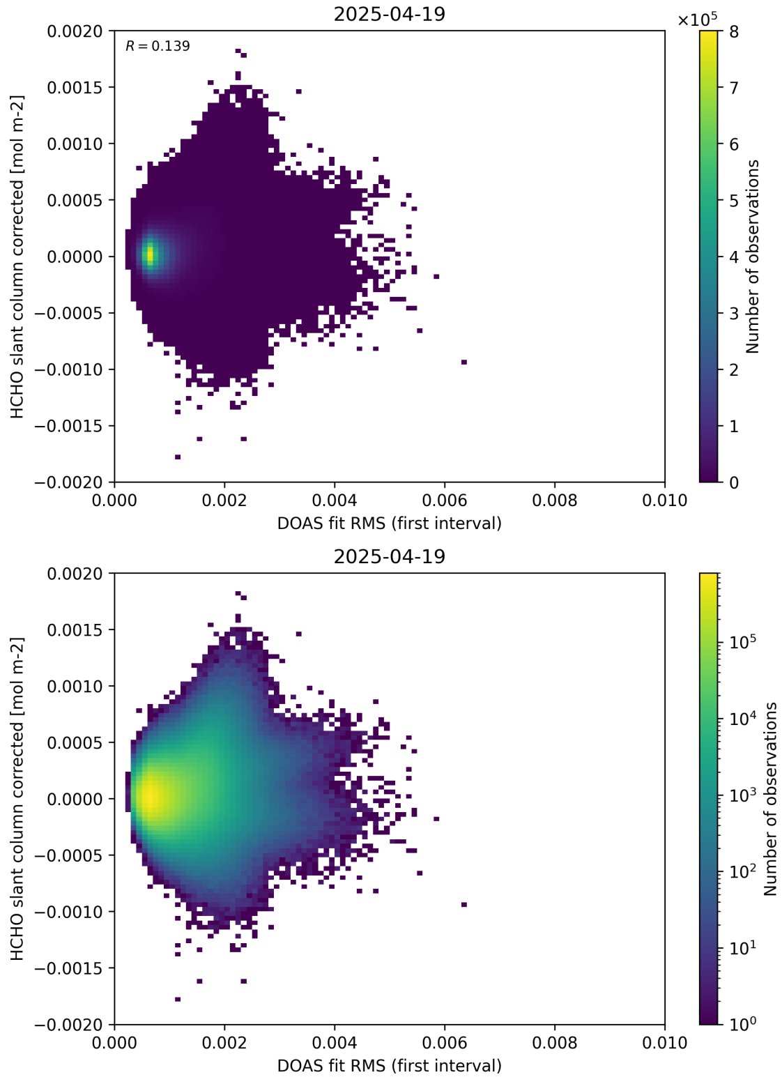
Figure 62: Scatter density plot of “DOAS fit RMS (first interval)” against “HCHO slant column corrected” for 2025-04-19 to 2025-04-20.
