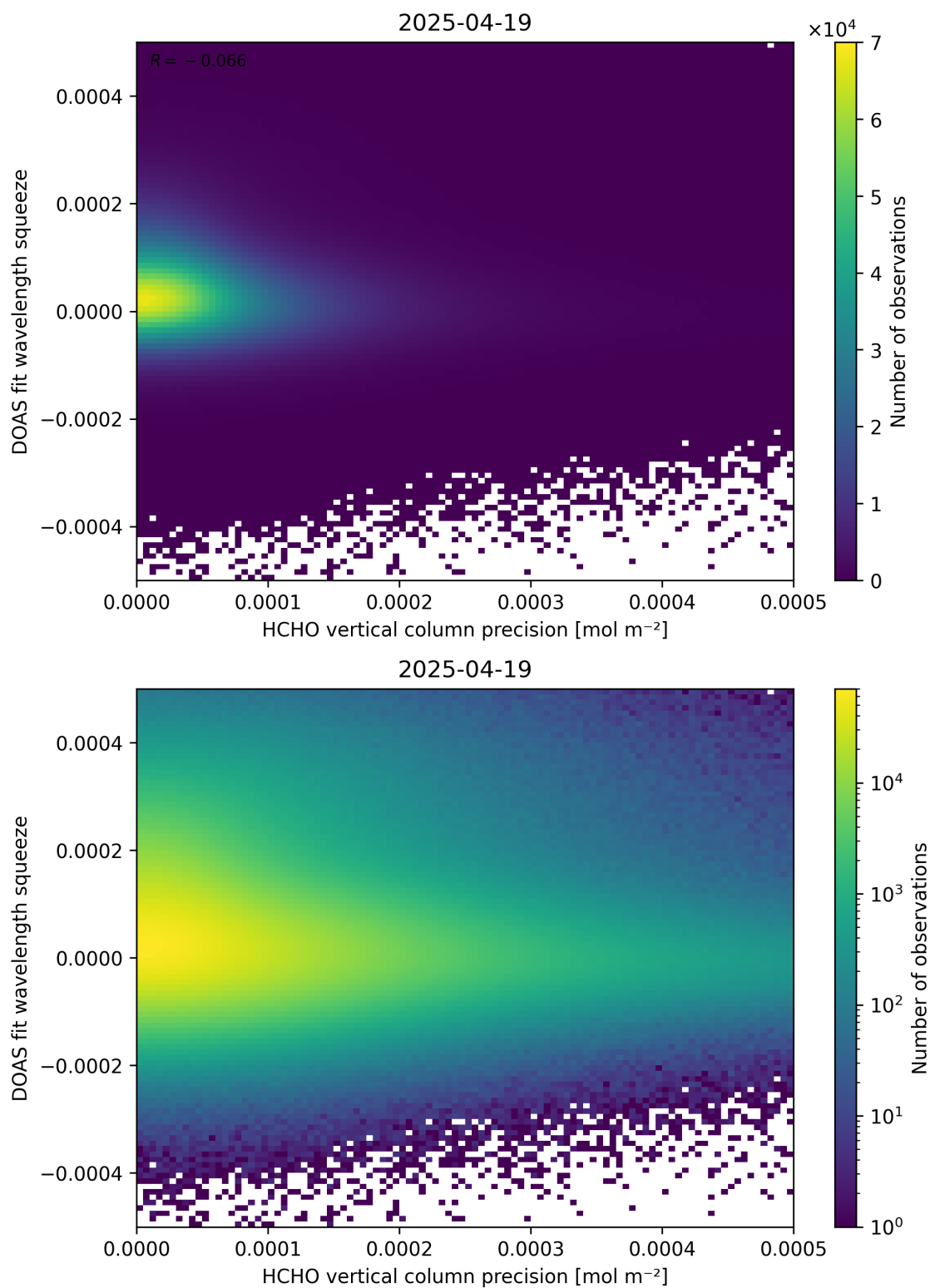
Figure 138: Scatter density plot of “HCHO vertical column precision” against “DOAS fit wavelength squeeze” for 2025-04-19 to 2025-04-20.
