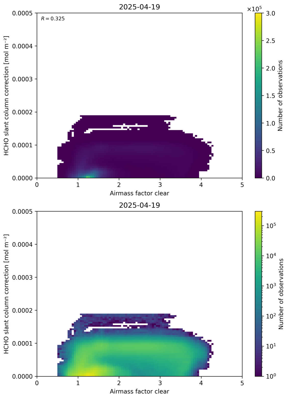
Figure 75: Scatter density plot of “Airmass factor clear” against “HCHO slant column correction” for 2025-04-19 to 2025-04-20.
