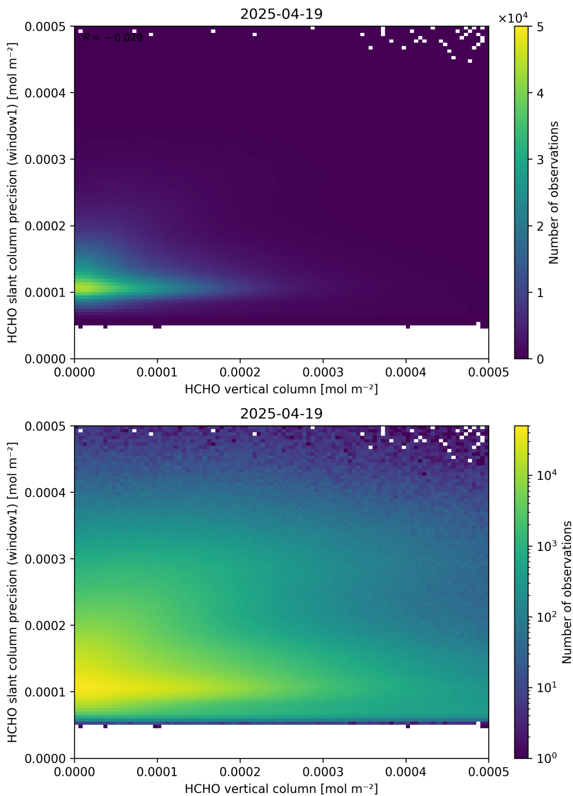
Figure 130: Scatter density plot of “HCHO vertical column” against “HCHO slant column precision (window1)” for 2025-04-19 to 2025-04-20.
