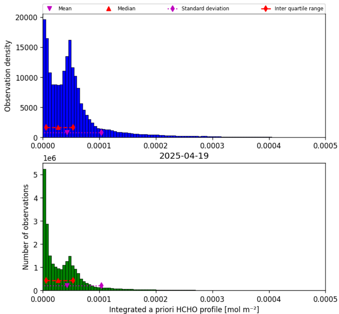
Figure 43: Histogram of “Integrated a priori HCHO profile” for 2025-04-19 to 2025-04-20
