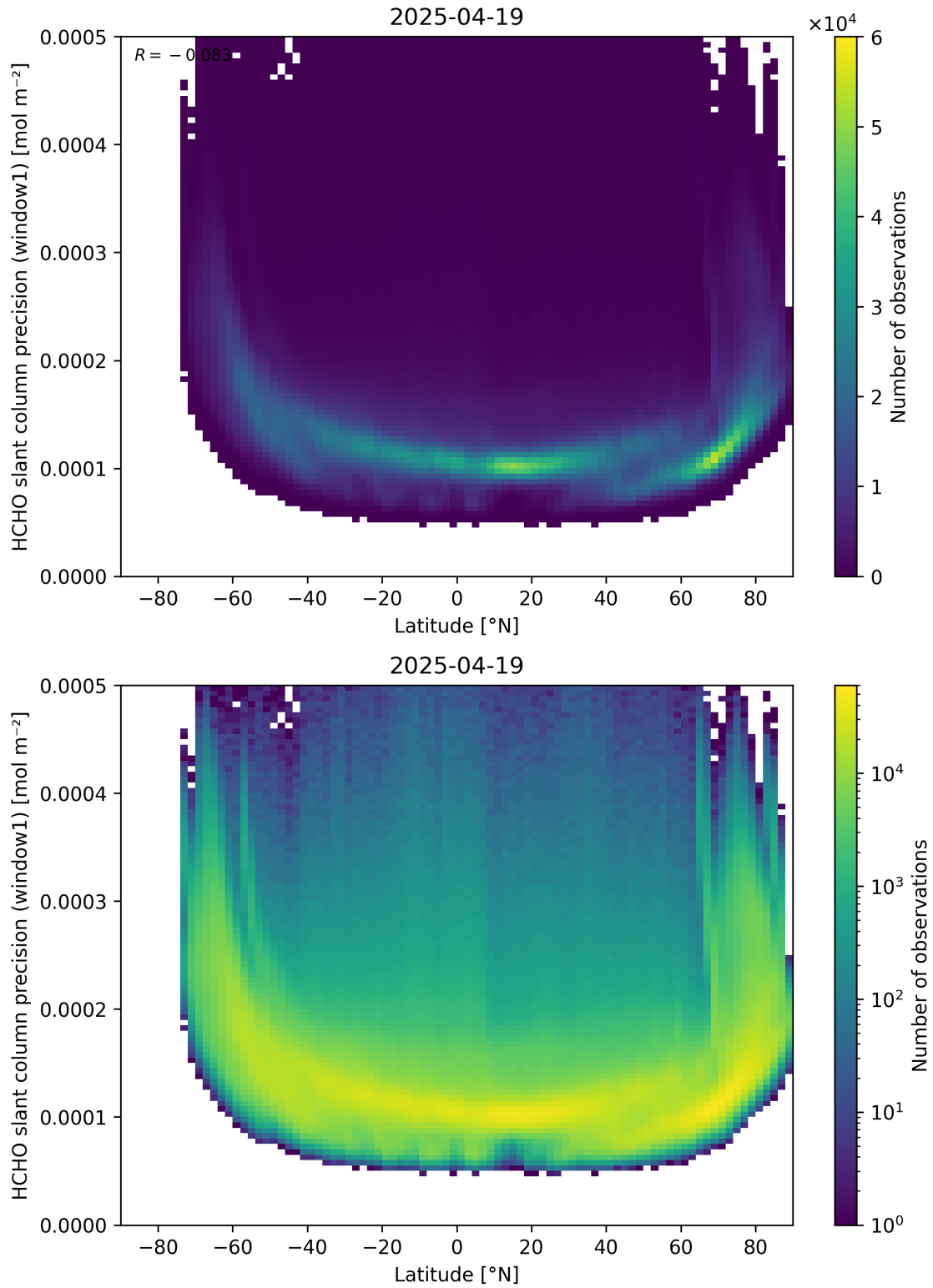
Figure 160: Scatter density plot of “Latitude” against “HCHO slant column precision (window1)” for 2025-04-19 to 2025-04-20.
