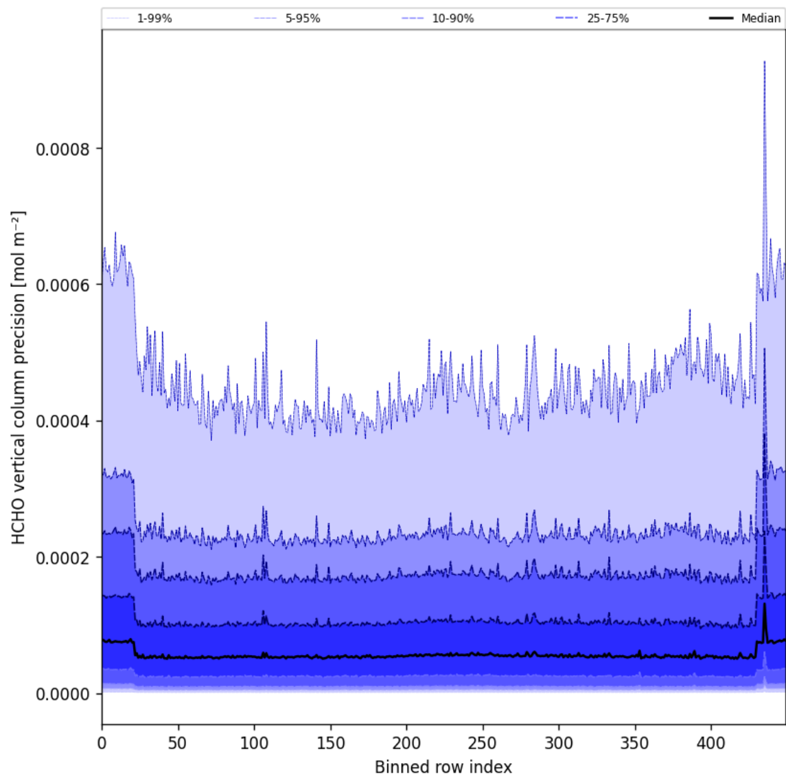
Figure 50: Along track statistics of “HCHO vertical column precision” for 2025-04-19 to 2025-04-20
