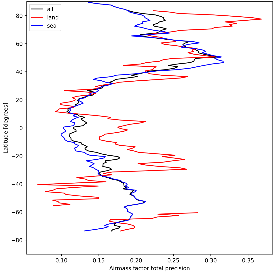
Figure 27: Zonal average of “Airmass factor total precision” for 2025-04-19 to 2025-04-20.
