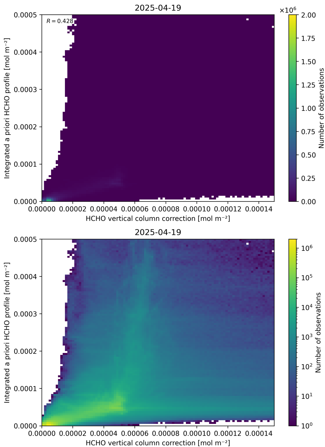
Figure 122: Scatter density plot of “HCHO vertical column correction” against “Integrated a priori HCHO profile” for 2025-04-19 to 2025-04-20.
