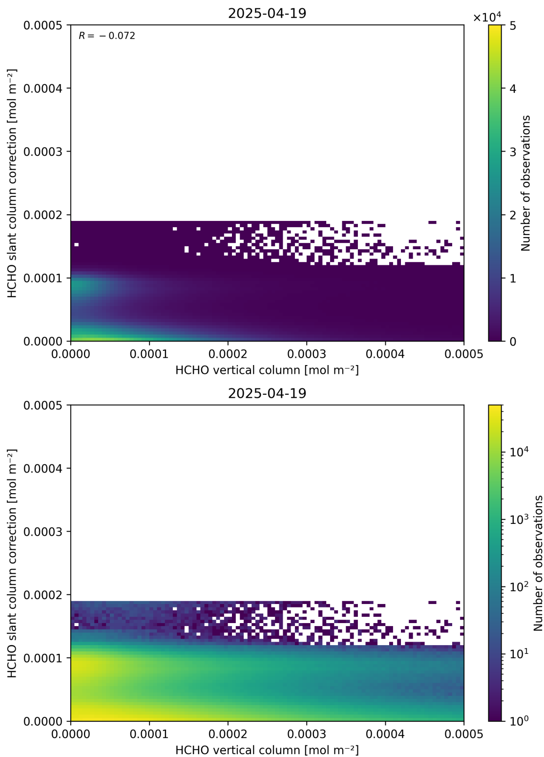
Figure 128: Scatter density plot of “HCHO vertical column” against “HCHO slant column correction” for 2025-04-19 to 2025-04-20.
