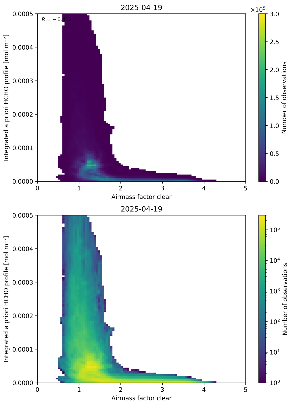
Figure 76: Scatter density plot of “Airmass factor clear” against “Integrated a priori HCHO profile” for 2025-04-19 to 2025-04-20.
