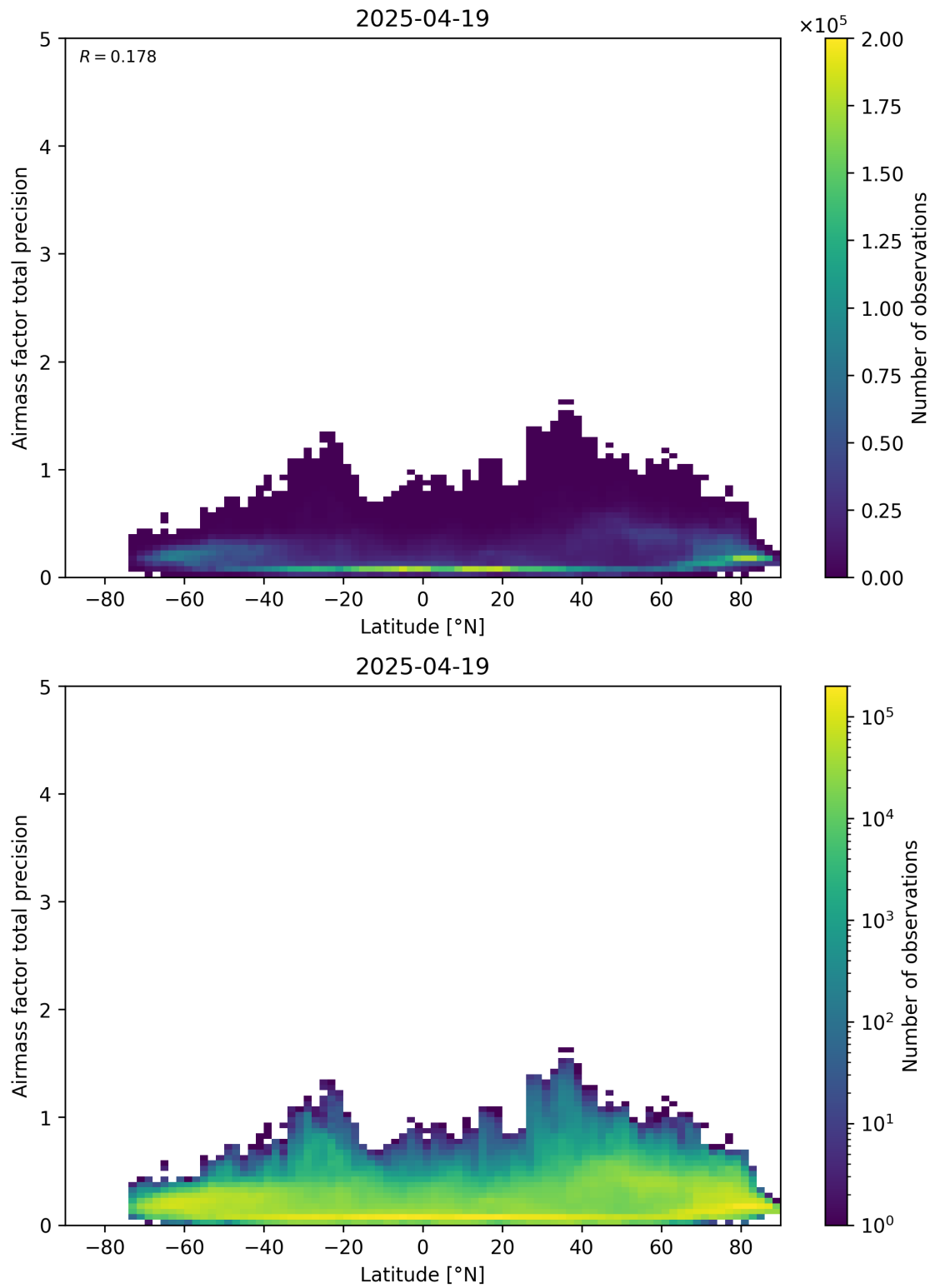
Figure 162: Scatter density plot of “Latitude” against “Airmass factor total precision” for 2025-04-19 to 2025-04-20.
