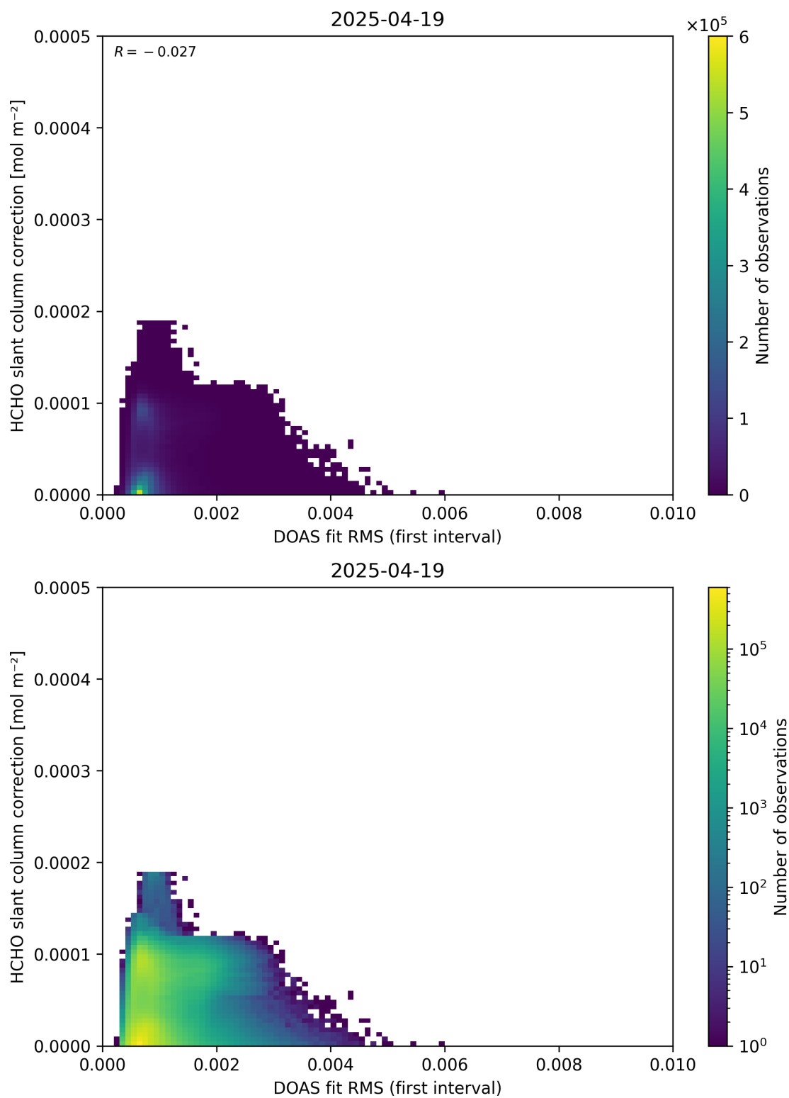
Figure 63: Scatter density plot of “DOAS fit RMS (first interval)” against “HCHO slant column correction” for 2025-04-19 to 2025-04-20.
