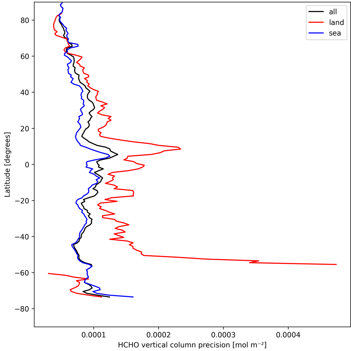
Figure 22: Zonal average of “HCHO vertical column precision” for 2025-04-19 to 2025-04-20.
