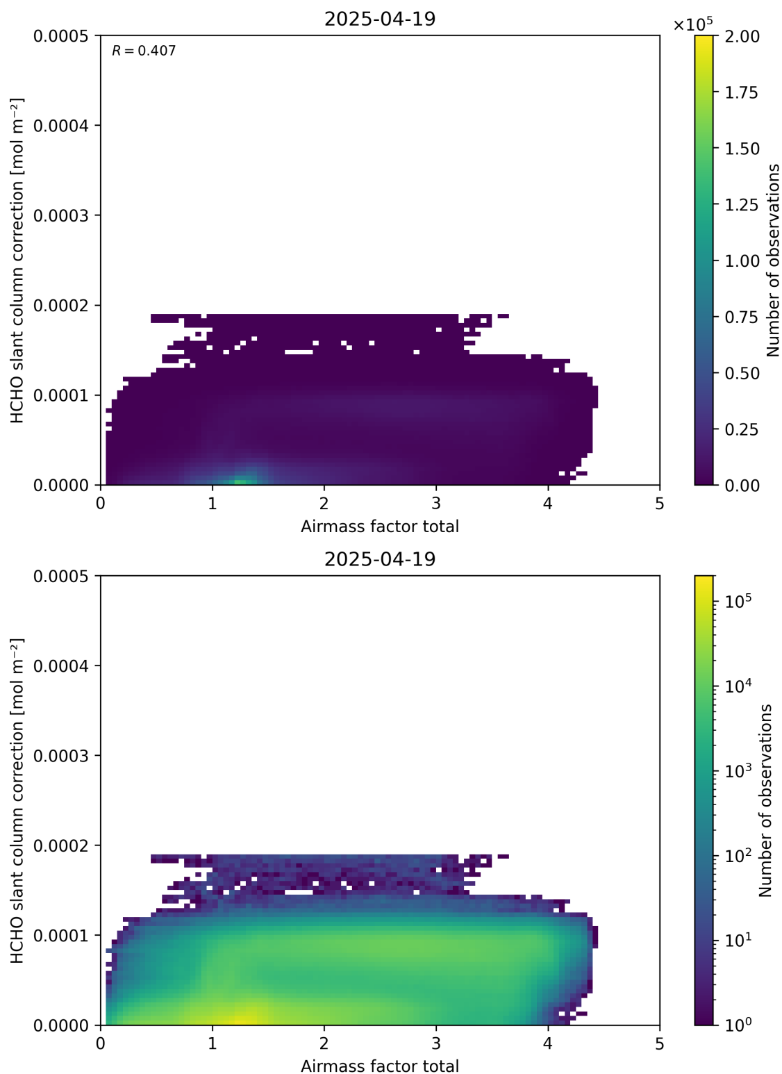
Figure 102: Scatter density plot of “Airmass factor total” against “HCHO slant column correction” for 2025-04-19 to 2025-04-20.
