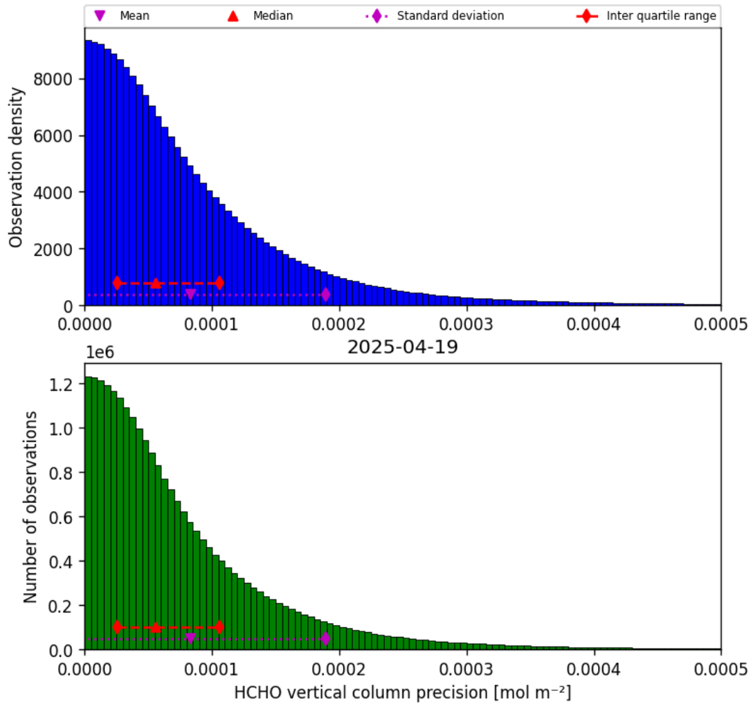
Figure 36: Histogram of “HCHO vertical column precision” for 2025-04-19 to 2025-04-20
