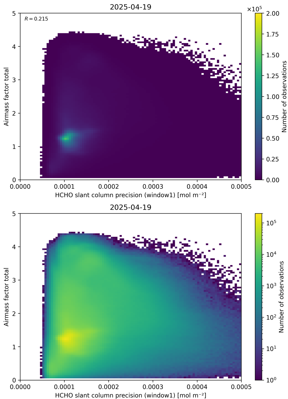
Figure 94: Scatter density plot of “HCHO slant column precision (window1)” against “Airmass factor total” for 2025-04-19 to 2025-04-20.
