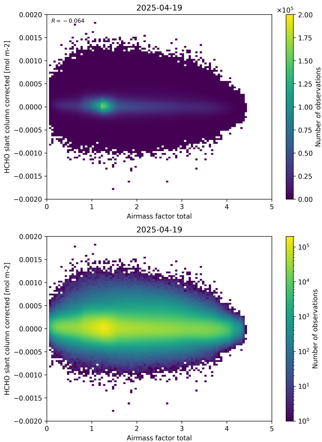
Figure 101: Scatter density plot of “Airmass factor total” against “HCHO slant column corrected” for 2025-04-19 to 2025-04-20.
