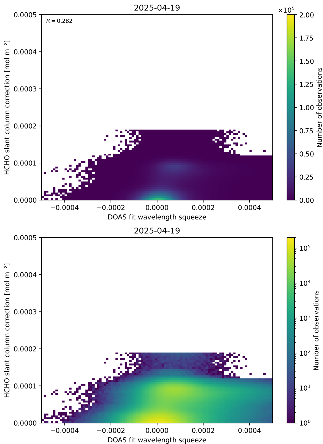
Figure 70: Scatter density plot of “DOAS fit wavelength squeeze” against “HCHO slant column correction” for 2025-04-19 to 2025-04-20.
