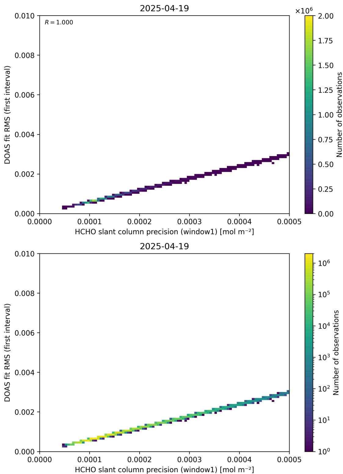
Figure 88: Scatter density plot of “HCHO slant column precision (window1)” against “DOAS fit RMS (first interval)” for 2025-04-19 to 2025-04-20.
