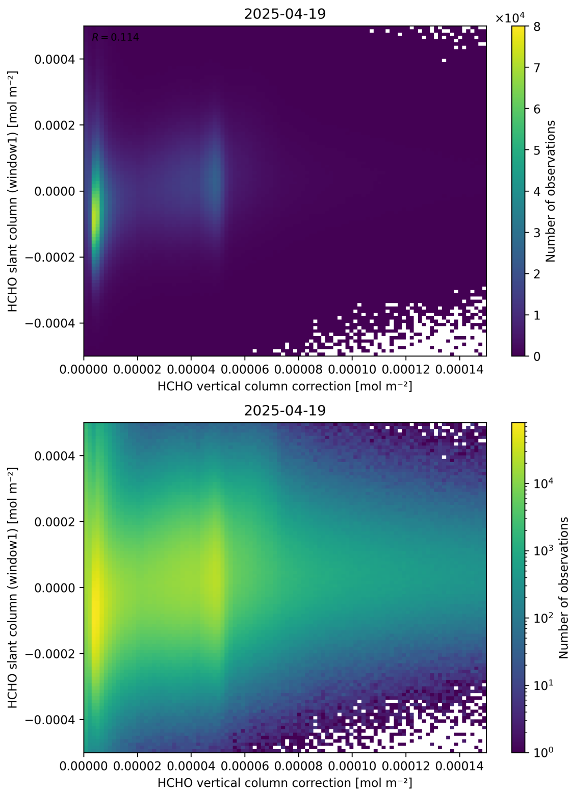
Figure 118: Scatter density plot of “HCHO vertical column correction” against “HCHO slant column (window1)” for 2025-04-19 to 2025-04-20.
