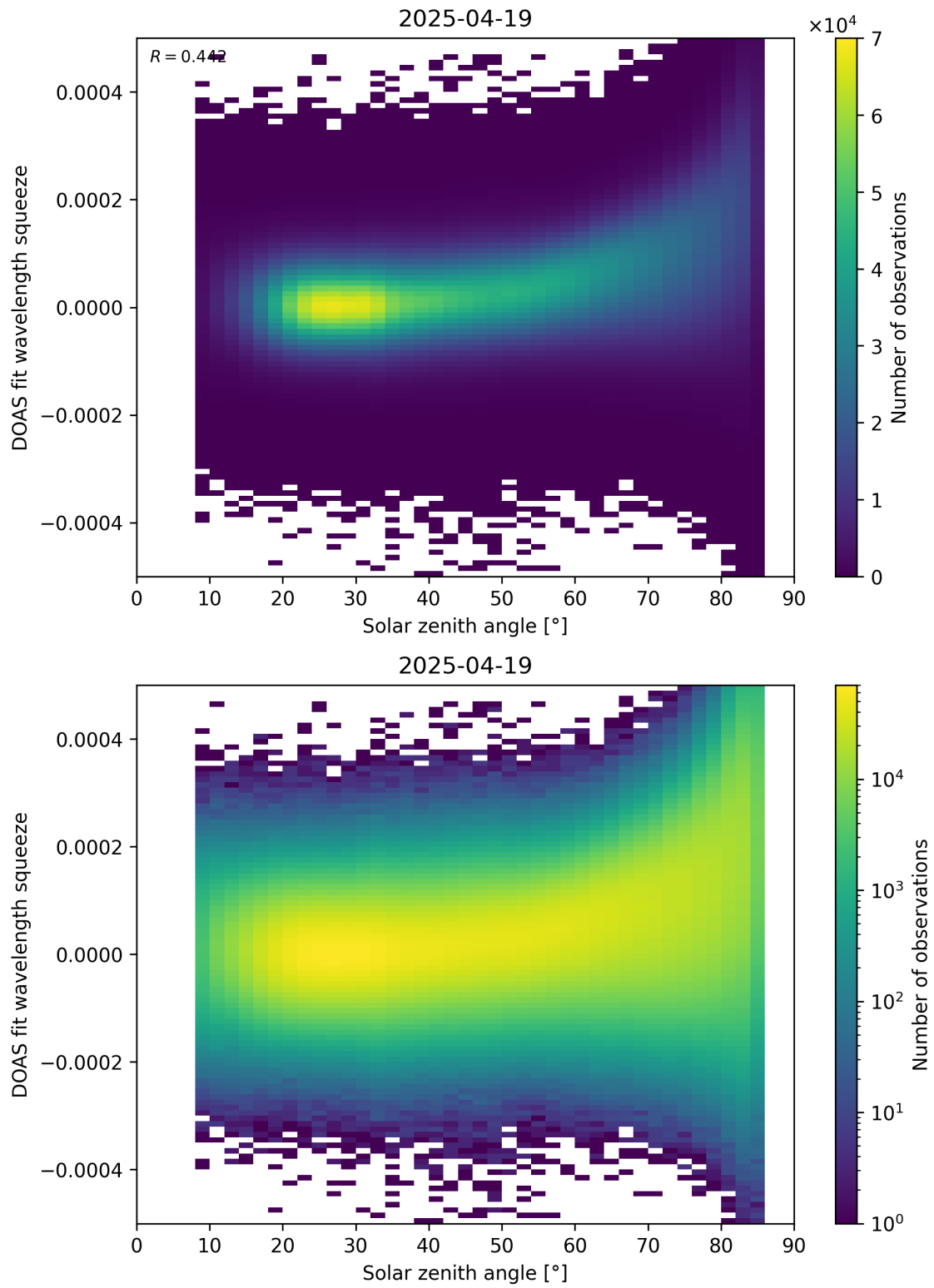
Figure 169: Scatter density plot of “Solar zenith angle” against “DOAS fit wavelength squeeze” for 2025-04-19 to 2025-04-20.
