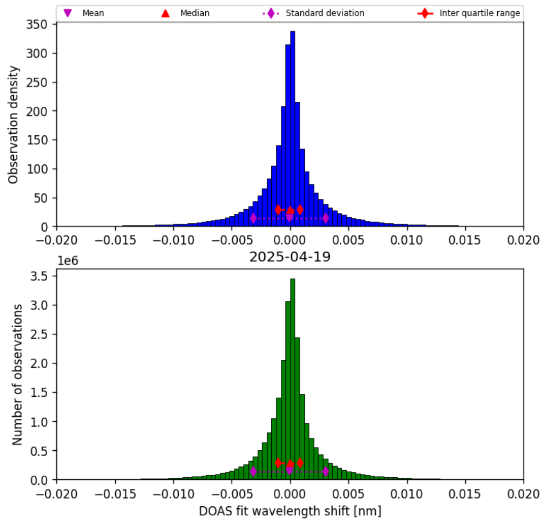
Figure 44: Histogram of “DOAS fit wavelength shift” for 2025-04-19 to 2025-04-20
