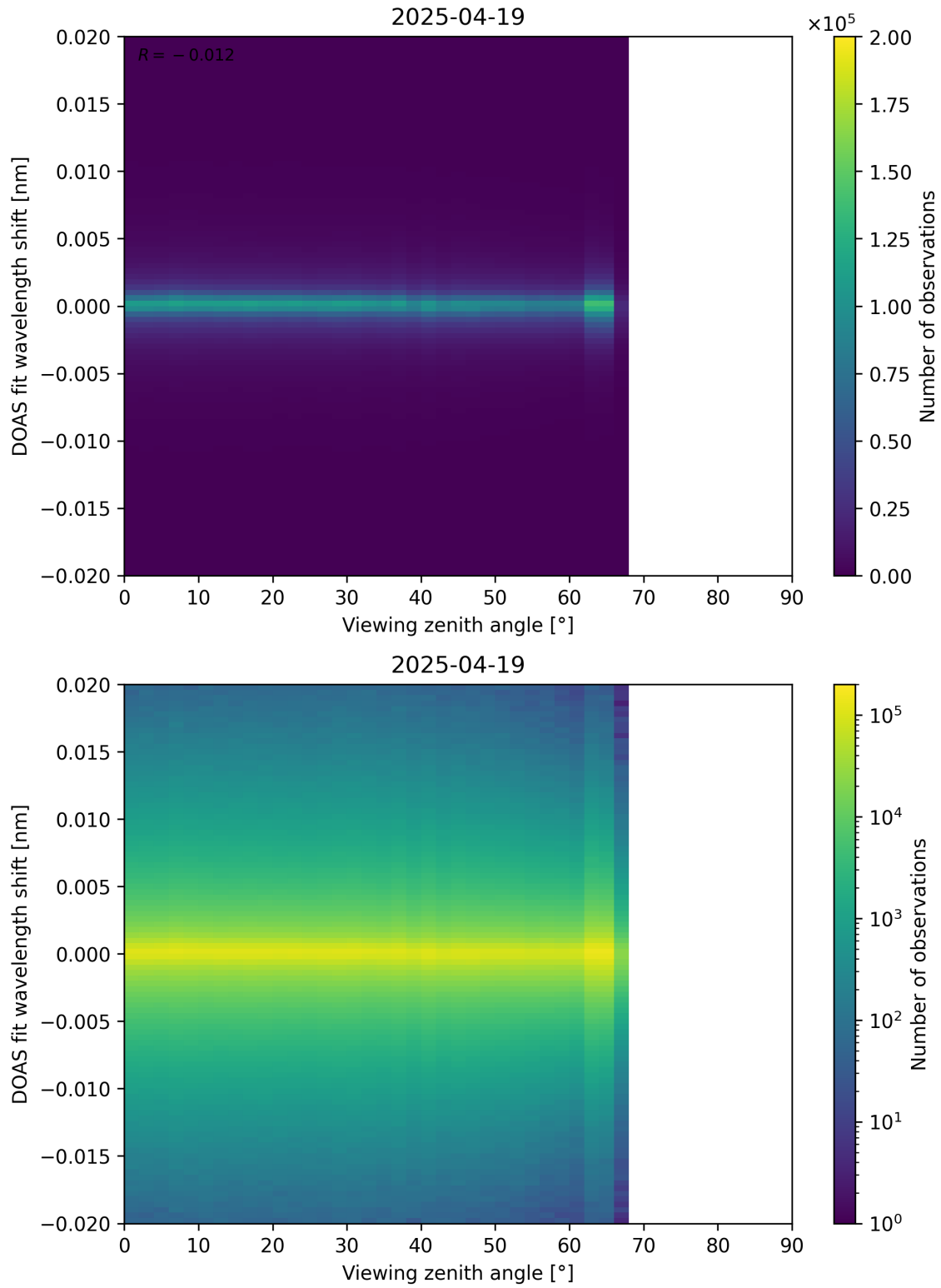
Figure 183: Scatter density plot of “Viewing zenith angle” against “DOAS fit wavelength shift” for 2025-04-19 to 2025-04-20.
