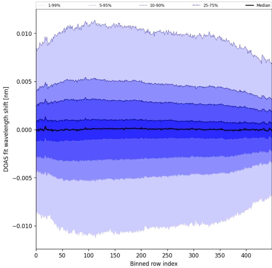
Figure 58: Along track statistics of “DOAS fit wavelength shift” for 2025-04-19 to 2025-04-20
