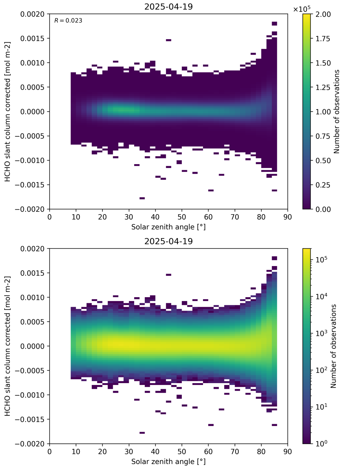
Figure 171: Scatter density plot of “Solar zenith angle” against “HCHO slant column corrected” for 2025-04-19 to 2025-04-20.
