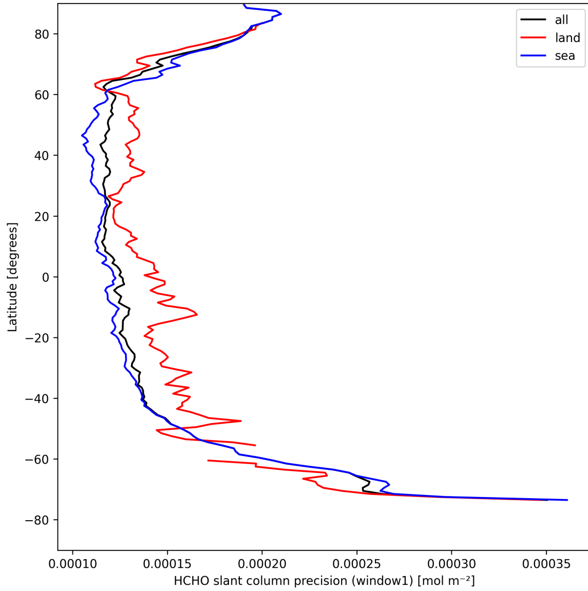
Figure 25: Zonal average of "HCHO slant column precision (window1)" for 2025-04-19 to 2025-04-20.
