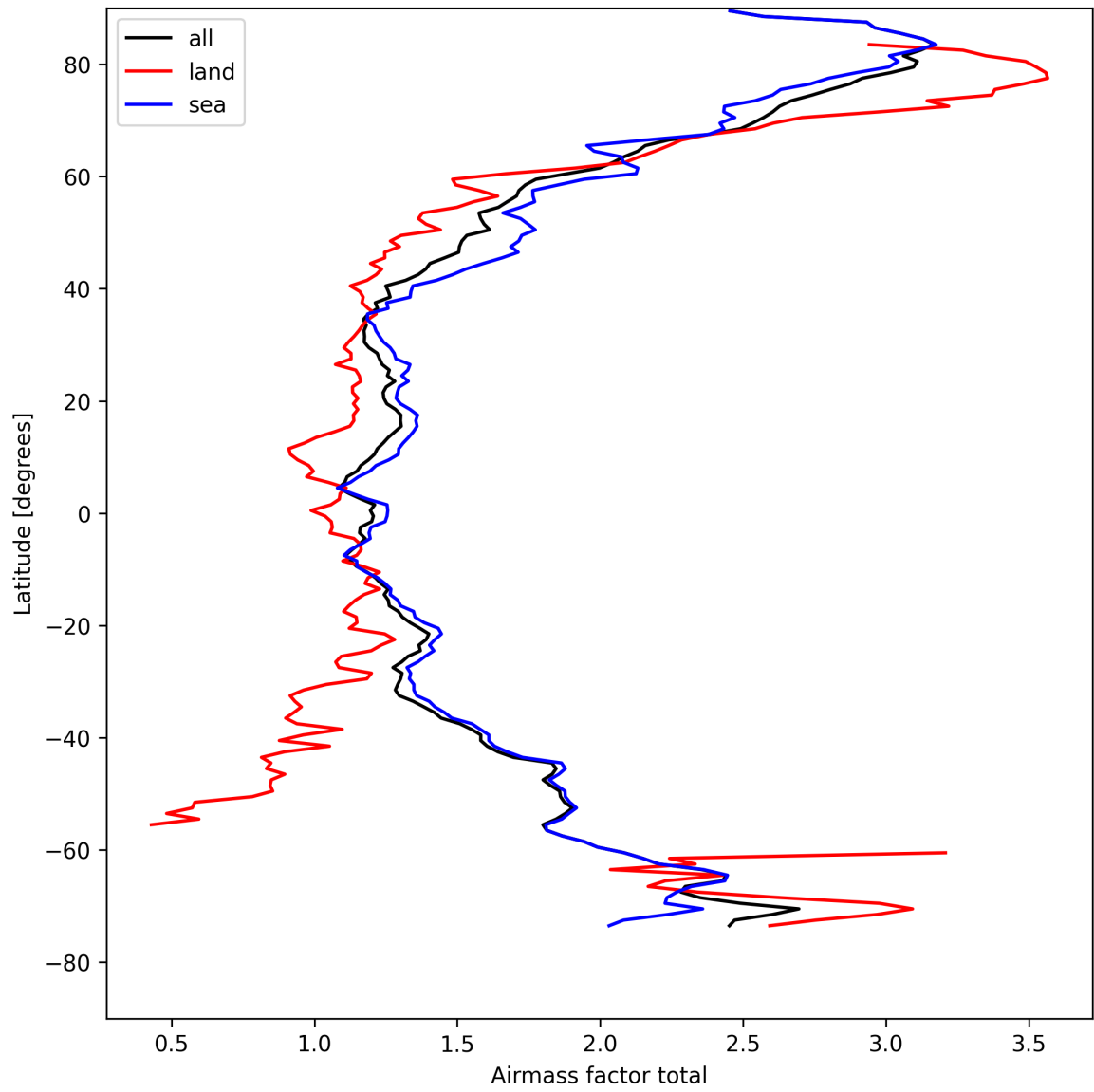
Figure 26: Zonal average of “Airmass factor total” for 2025-04-19 to 2025-04-20.
