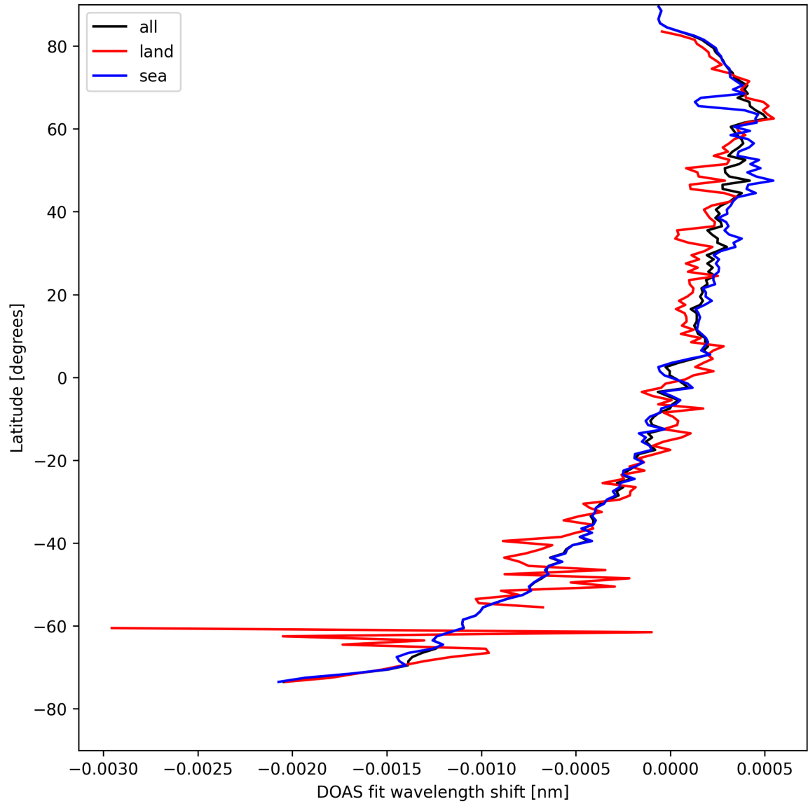
Figure 30: Zonal average of “DOAS fit wavelength shift” for 2025-04-19 to 2025-04-20.
