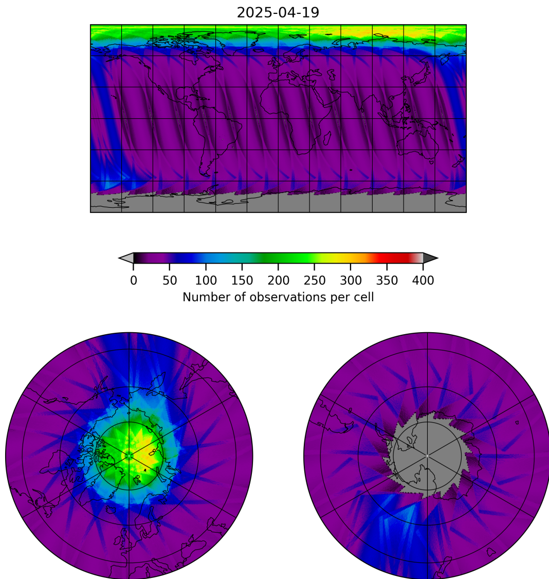
Figure 19: Map of the number of observations for 2025-04-19 to 2025-04-20
