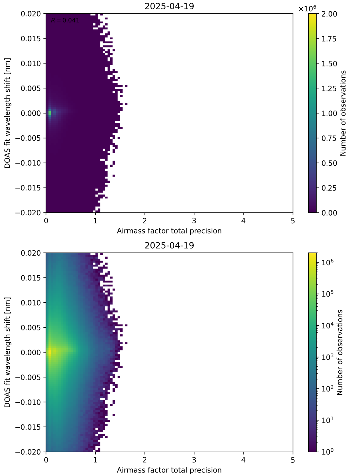
Figure 106: Scatter density plot of “Airmass factor total precision” against “DOAS fit wavelength shift” for 2025-04-19 to 2025-04-20.
