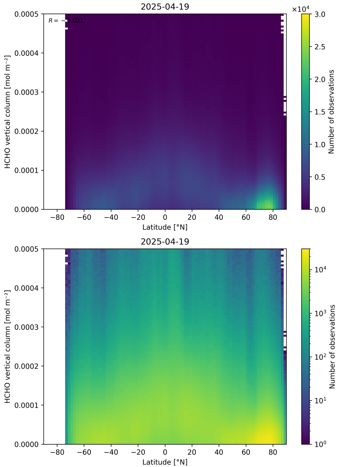
Figure 163: Scatter density plot of “Latitude” against “HCHO vertical column” for 2025-04-19 to 2025-04-20.
