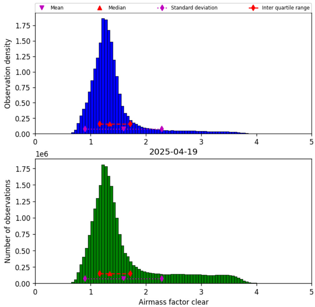
Figure 42: Histogram of “Airmass factor clear” for 2025-04-19 to 2025-04-20
