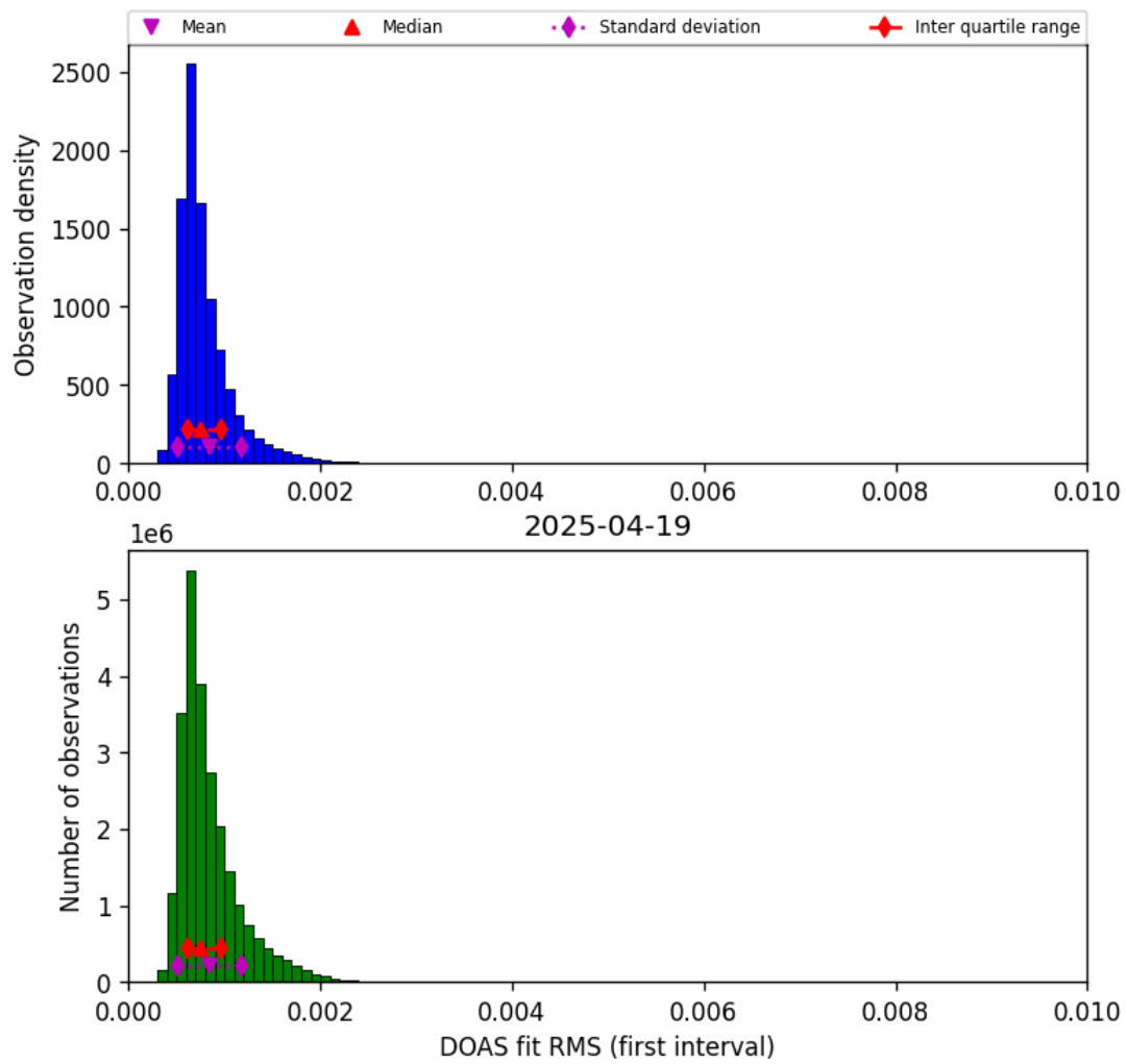
Figure 46: Histogram of “DOAS fit RMS (first interval)” for 2025-04-19 to 2025-04-20
