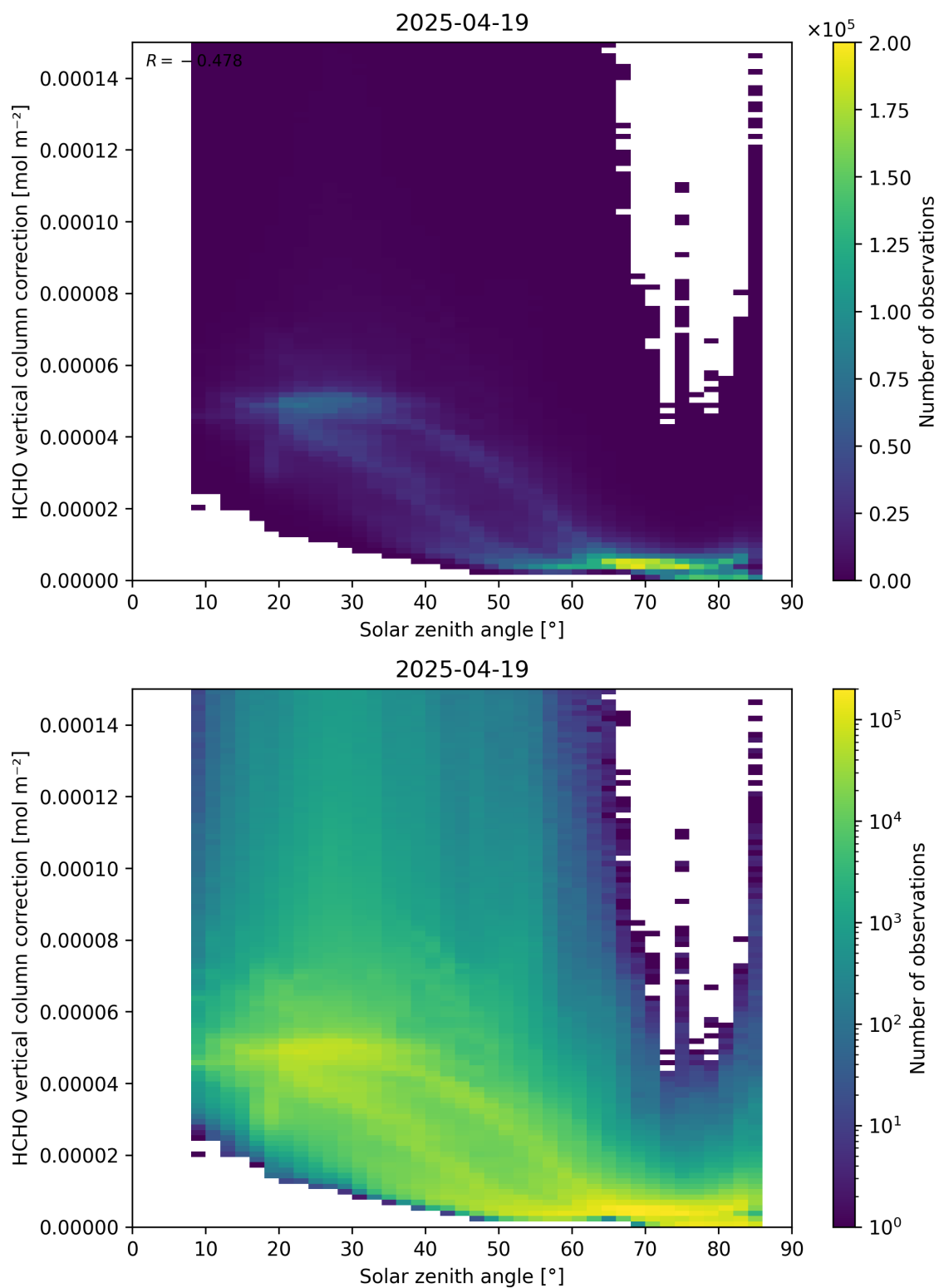
Figure 178: Scatter density plot of “Solar zenith angle” against “HCHO vertical column correction” for 2025-04-19 to 2025-04-20.
