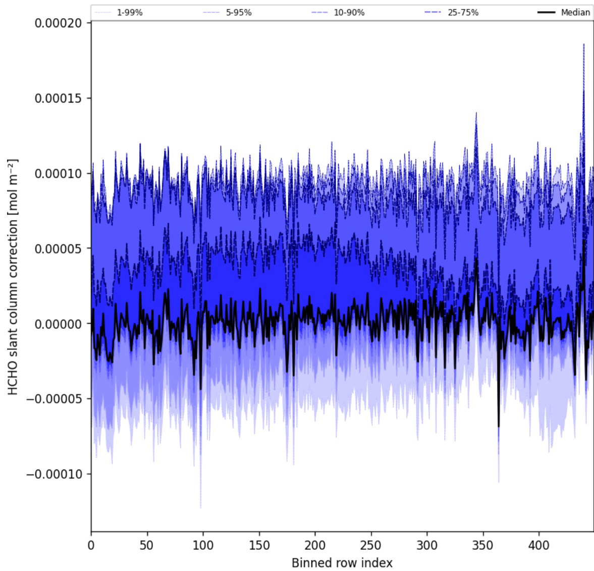
Figure 61: Along track statistics of “HCHO slant column correction” for 2025-04-19 to 2025-04-20
