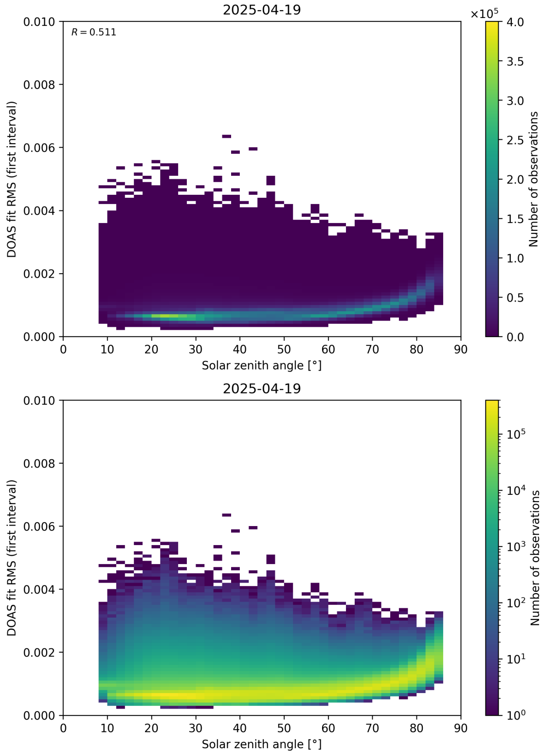
Figure 167: Scatter density plot of “Solar zenith angle” against “DOAS fit RMS (first interval)” for 2025-04-19 to 2025-04-20.
