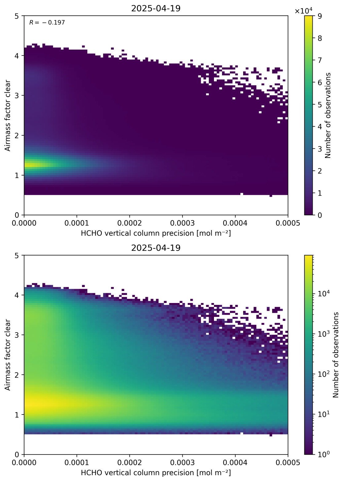
Figure 139: Scatter density plot of “HCHO vertical column precision” against “Airmass factor clear” for 2025-04-19 to 2025-04-20.
