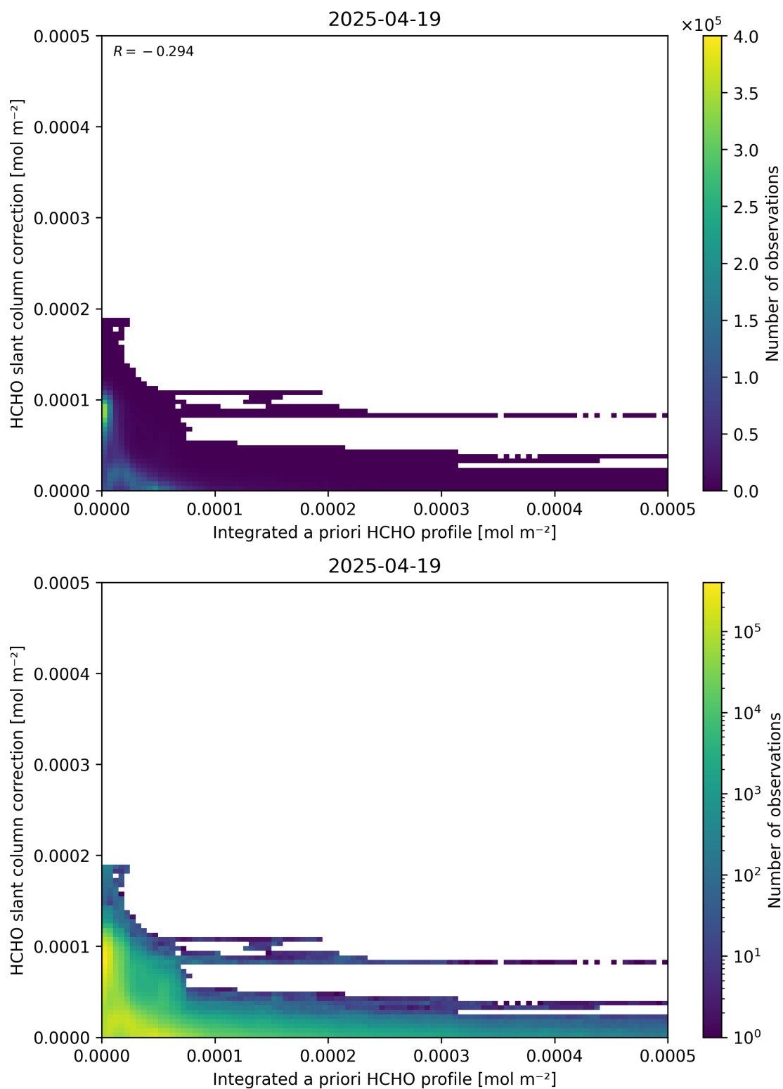
Figure 152: Scatter density plot of “Integrated a priori HCHO profile” against “HCHO slant column correction” for 2025-04-19 to 2025-04-20.
