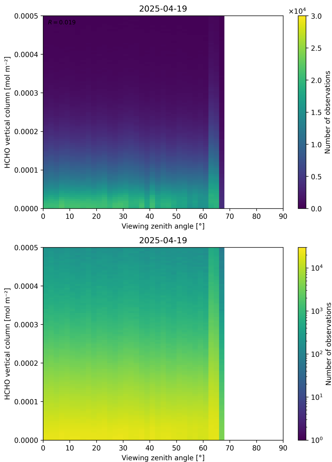
Figure 192: Scatter density plot of “Viewing zenith angle” against “HCHO vertical column” for 2025-04-19 to 2025-04-20.
