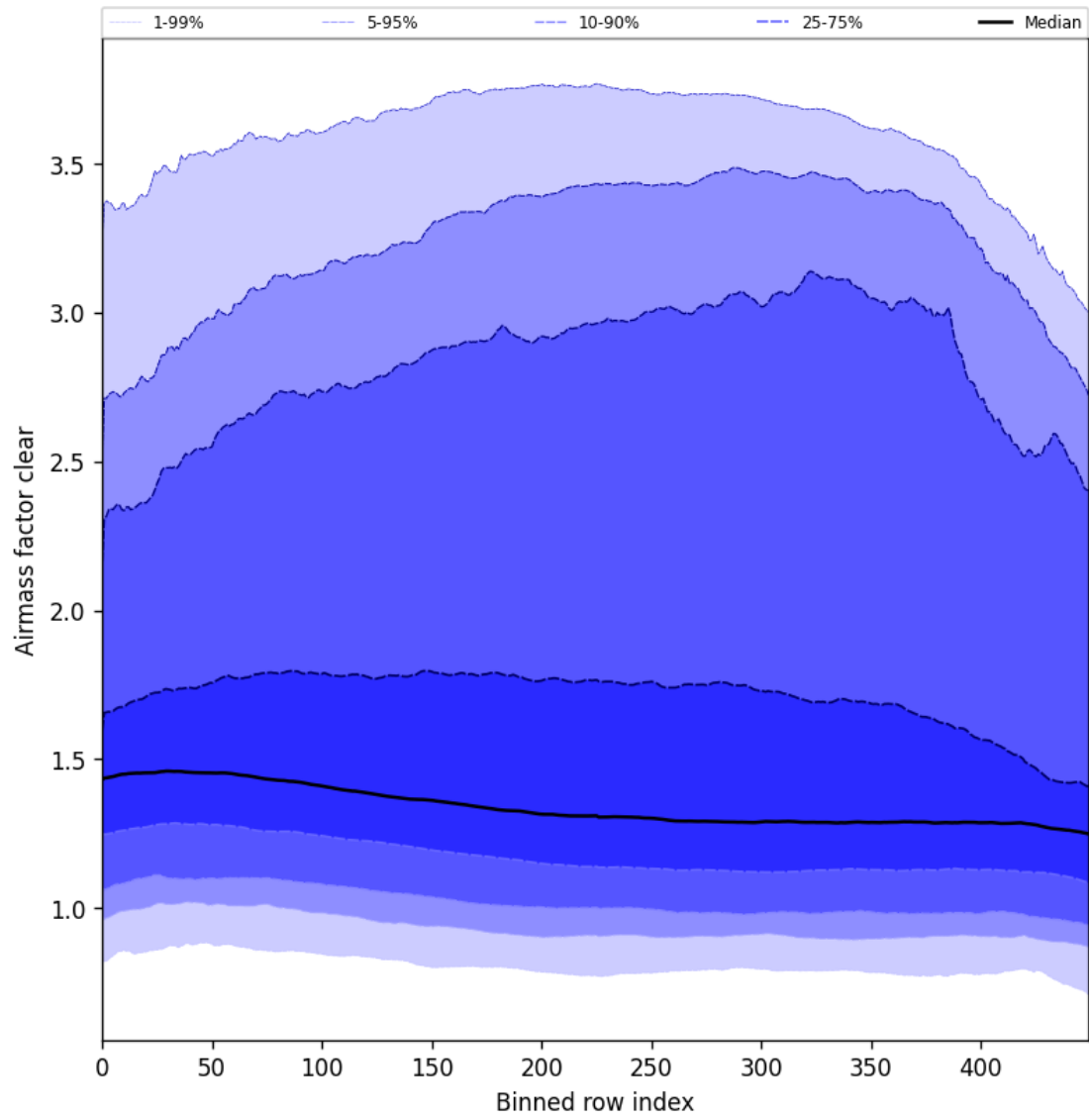
Figure 56: Along track statistics of “Airmass factor clear” for 2025-04-19 to 2025-04-20
