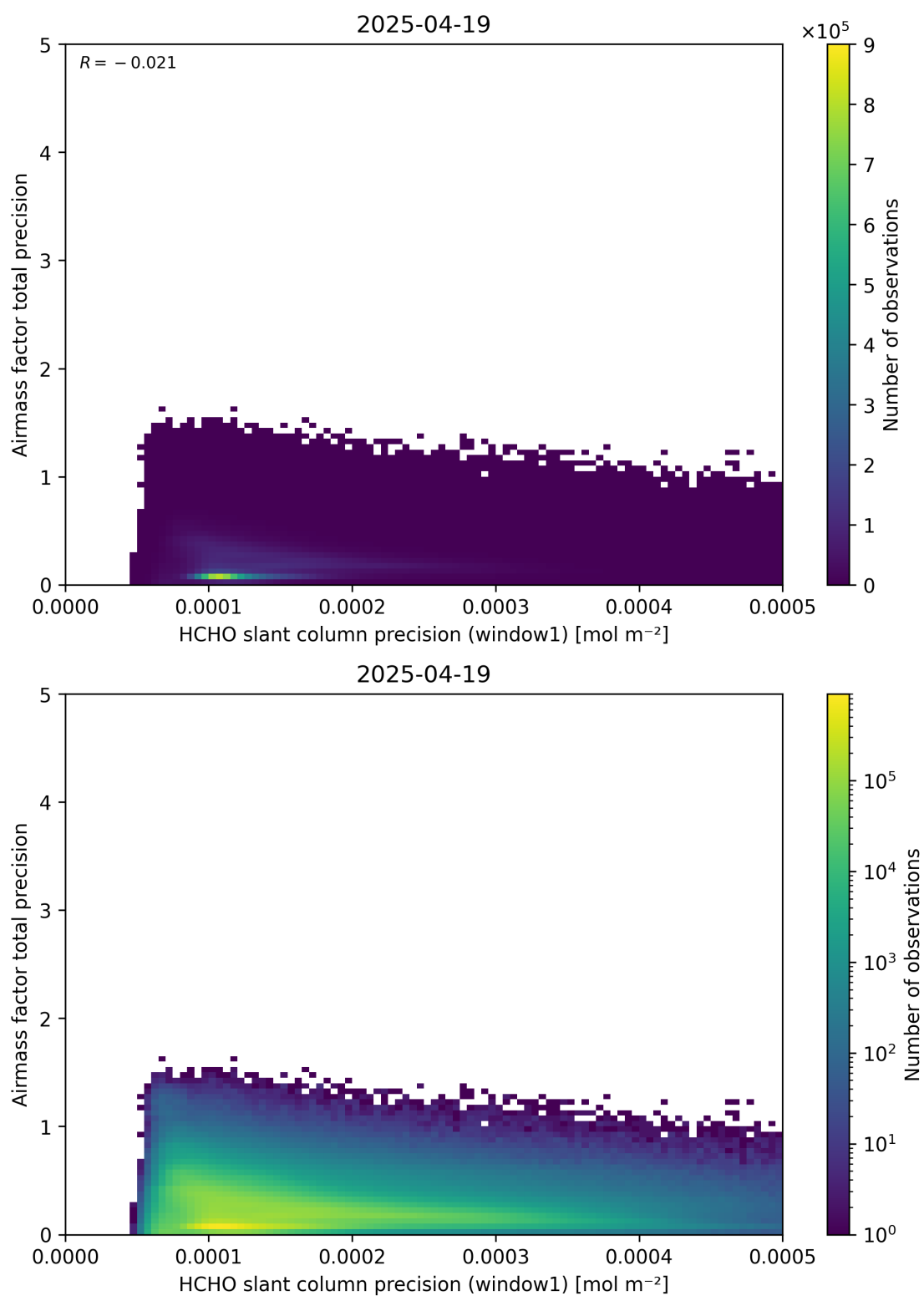
Figure 95: Scatter density plot of “HCHO slant column precision (window1)” against “Airmass factor total precision” for 2025-04-19 to 2025-04-20.
