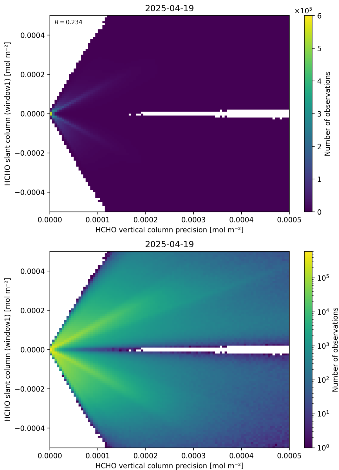
Figure 142: Scatter density plot of “HCHO vertical column precision” against “HCHO slant column (window1)” for 2025-04-19 to 2025-04-20.
