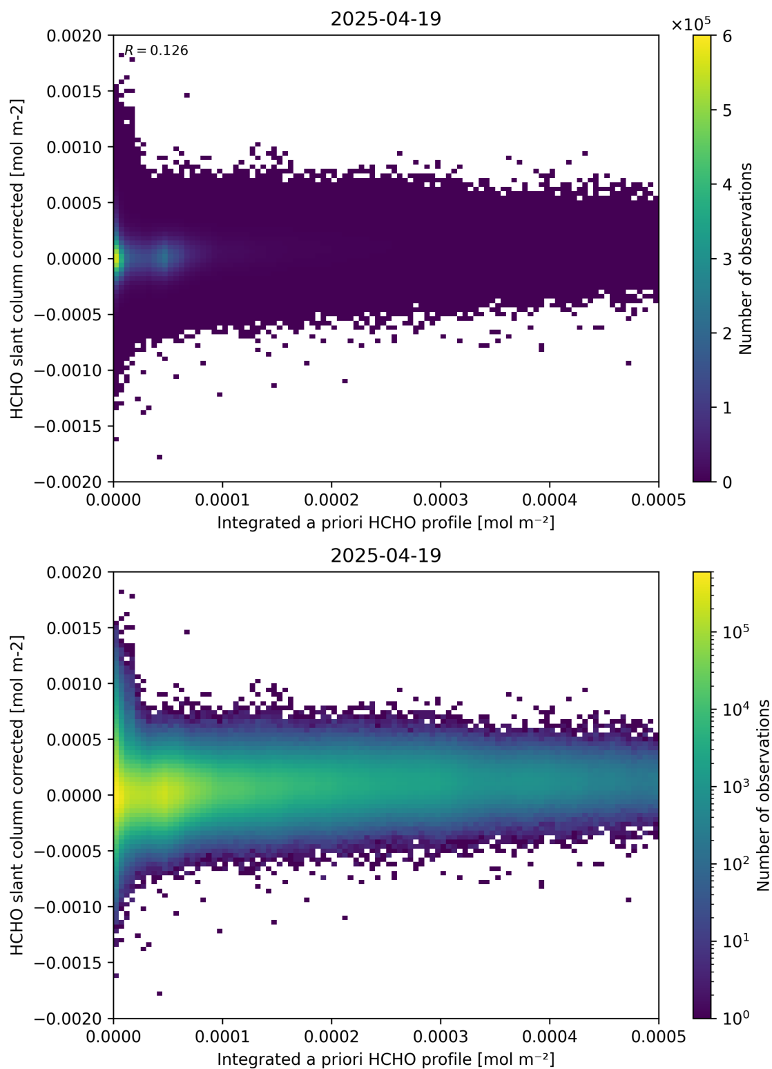
Figure 151: Scatter density plot of “Integrated a priori HCHO profile” against “HCHO slant column corrected” for 2025-04-19 to 2025-04-20.
