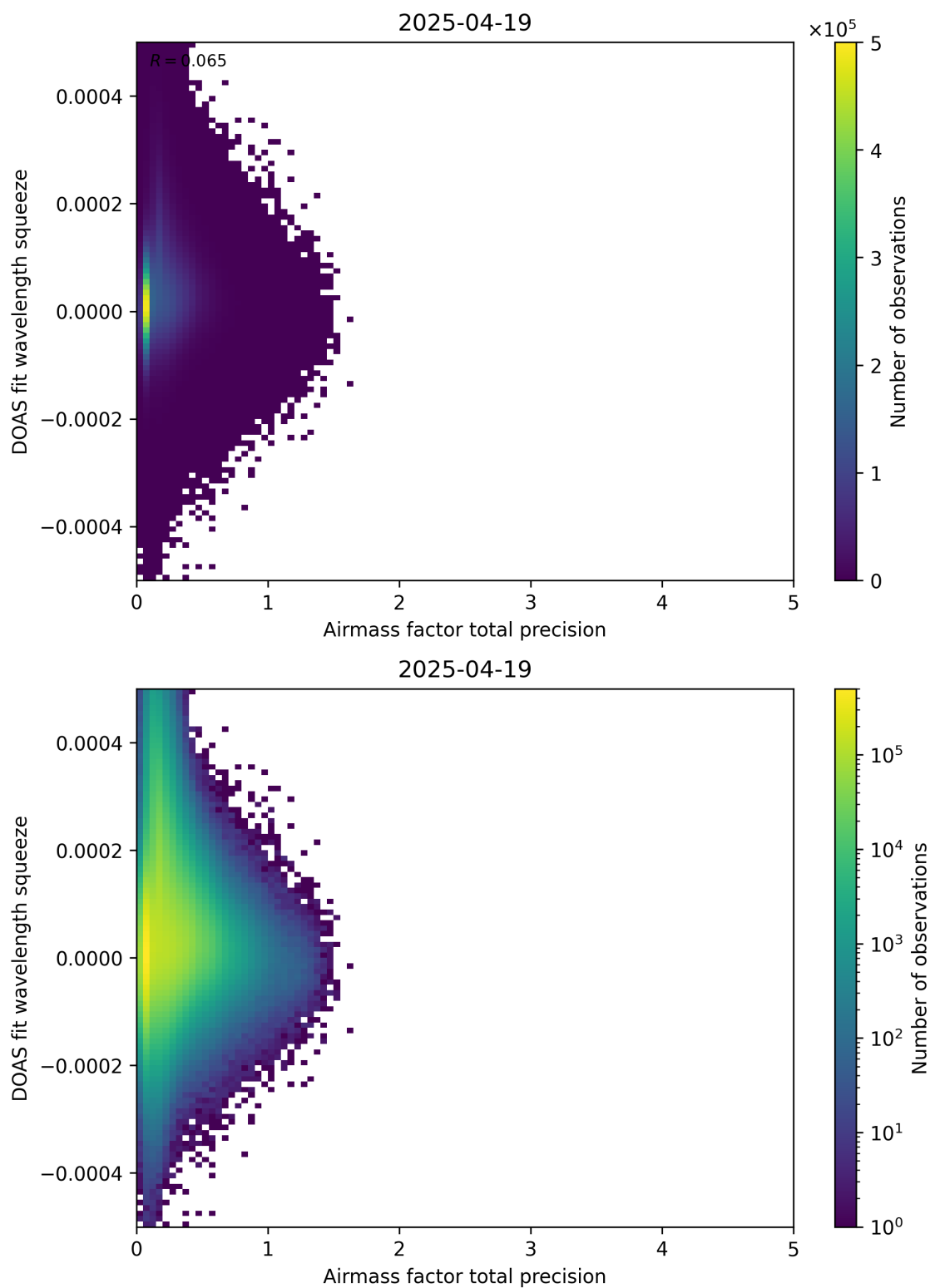
Figure 107: Scatter density plot of “Airmass factor total precision” against “DOAS fit wavelength squeeze” for 2025-04-19 to 2025-04-20.
