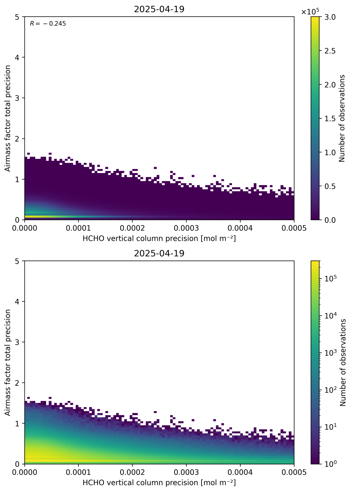
Figure 145: Scatter density plot of “HCHO vertical column precision” against “Airmass factor total precision” for 2025-04-19 to 2025-04-20.
