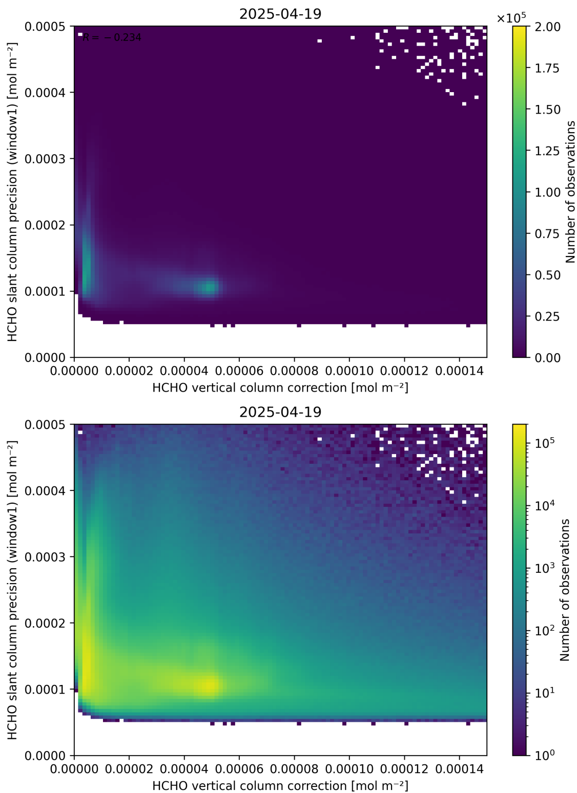
Figure 119: Scatter density plot of “HCHO vertical column correction” against “HCHO slant column precision (window1)” for 2025-04-19 to 2025-04-20.
