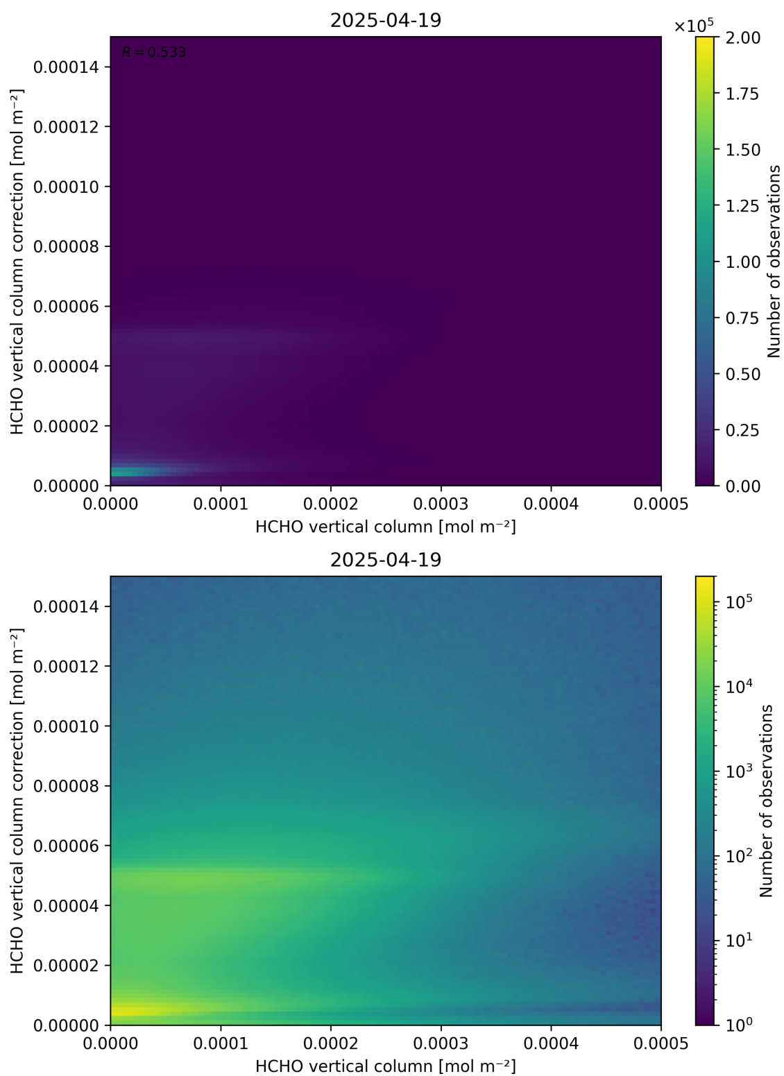
Figure 133: Scatter density plot of “HCHO vertical column” against “HCHO vertical column correction” for 2025-04-19 to 2025-04-20.
