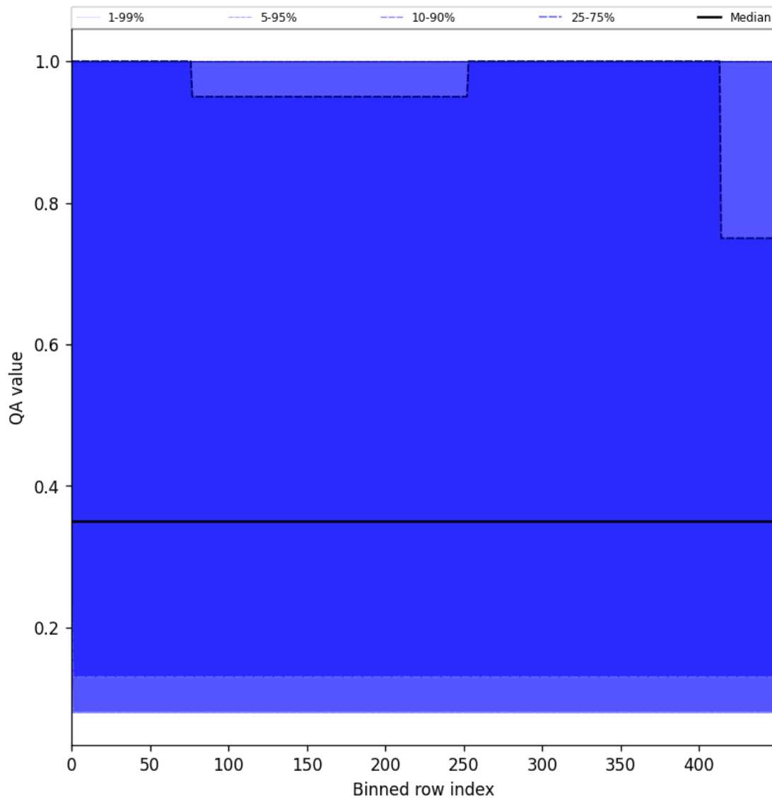
Figure 48: Along track statistics of "QA value" for 2025-04-19 to 2025-04-20
