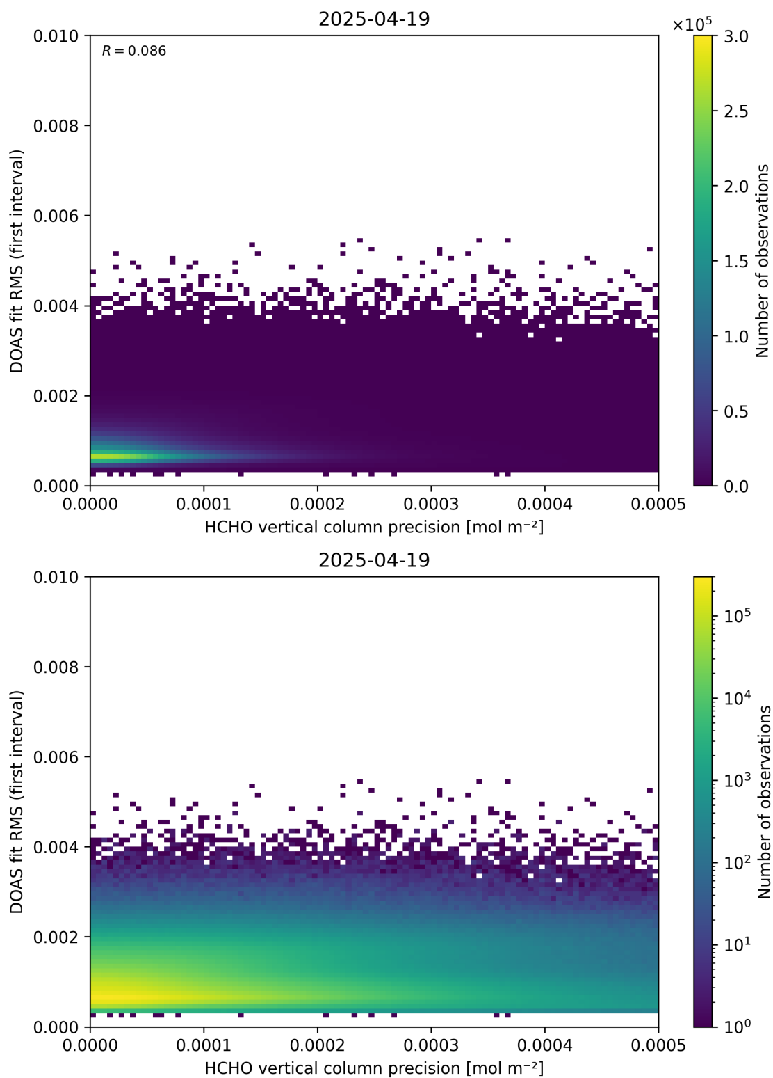
Figure 136: Scatter density plot of “HCHO vertical column precision” against “DOAS fit RMS (first interval)” for 2025-04-19 to 2025-04-20.
