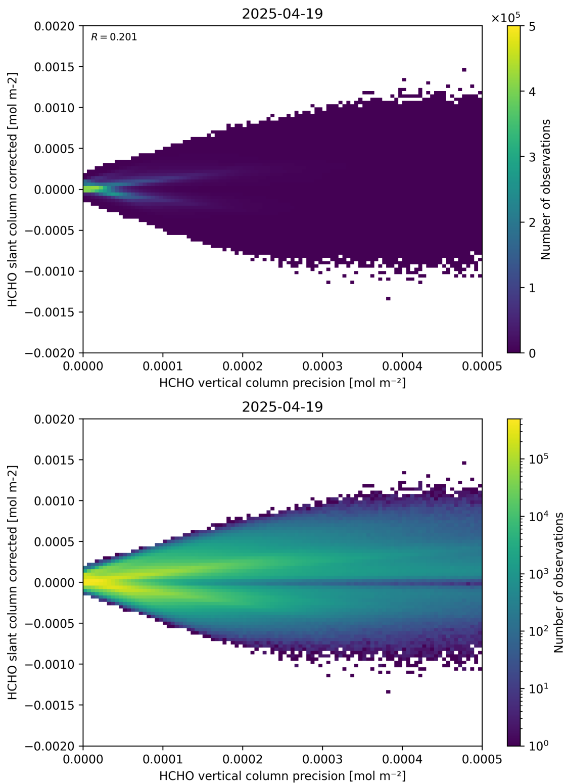
Figure 140: Scatter density plot of “HCHO vertical column precision” against “HCHO slant column corrected” for 2025-04-19 to 2025-04-20.
