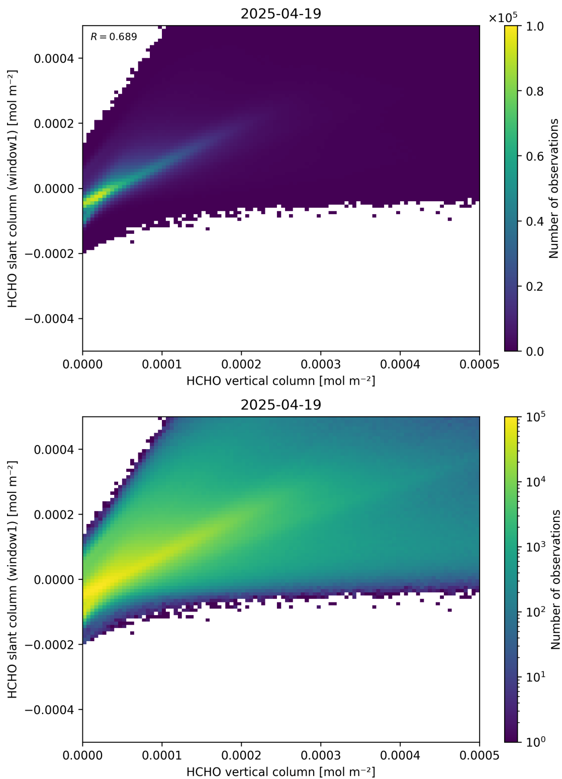
Figure 129: Scatter density plot of “HCHO vertical column” against “HCHO slant column (window1)” for 2025-04-19 to 2025-04-20.
