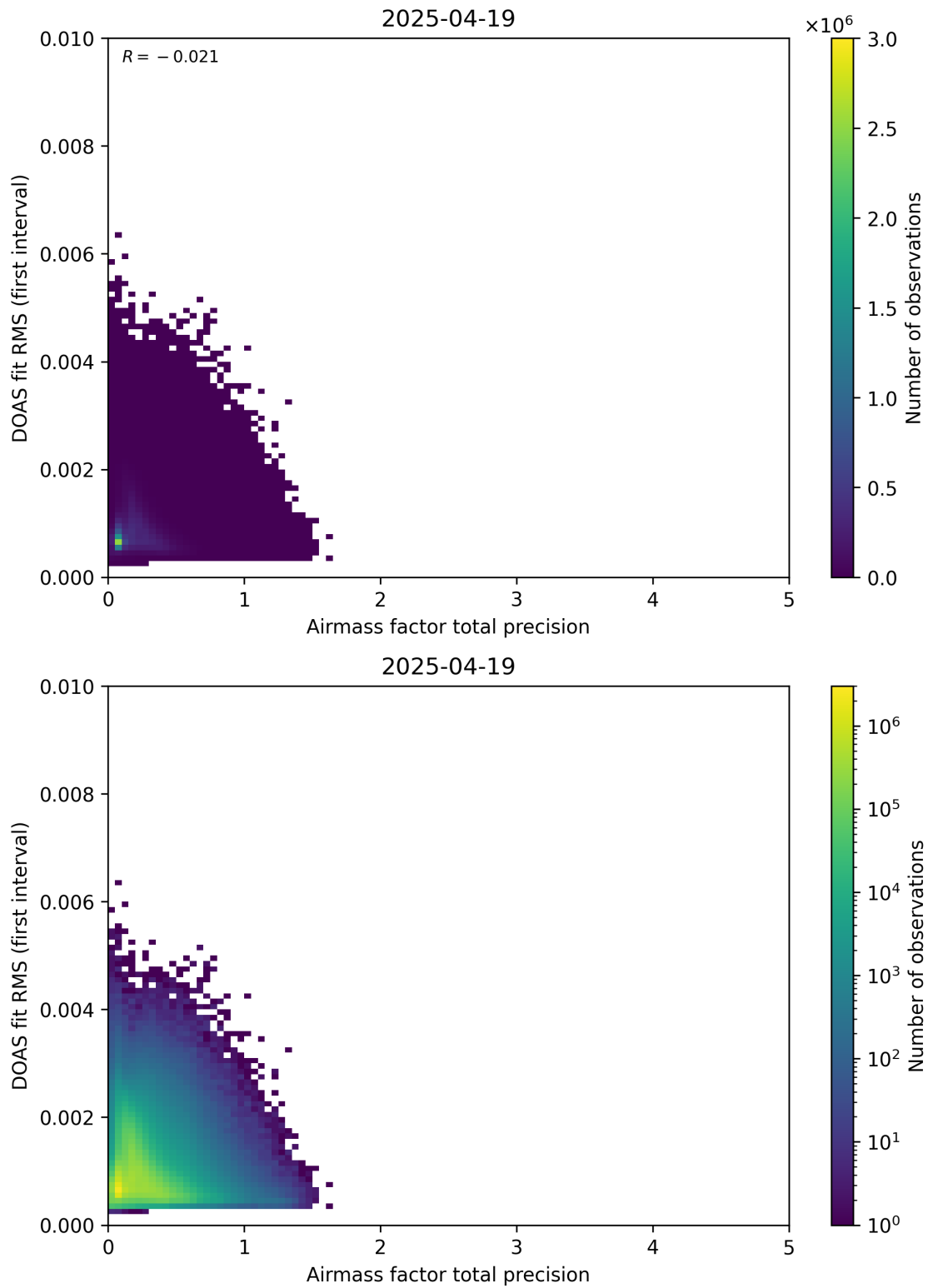
Figure 105: Scatter density plot of “Airmass factor total precision” against “DOAS fit RMS (first interval)” for 2025-04-19 to 2025-04-20.
