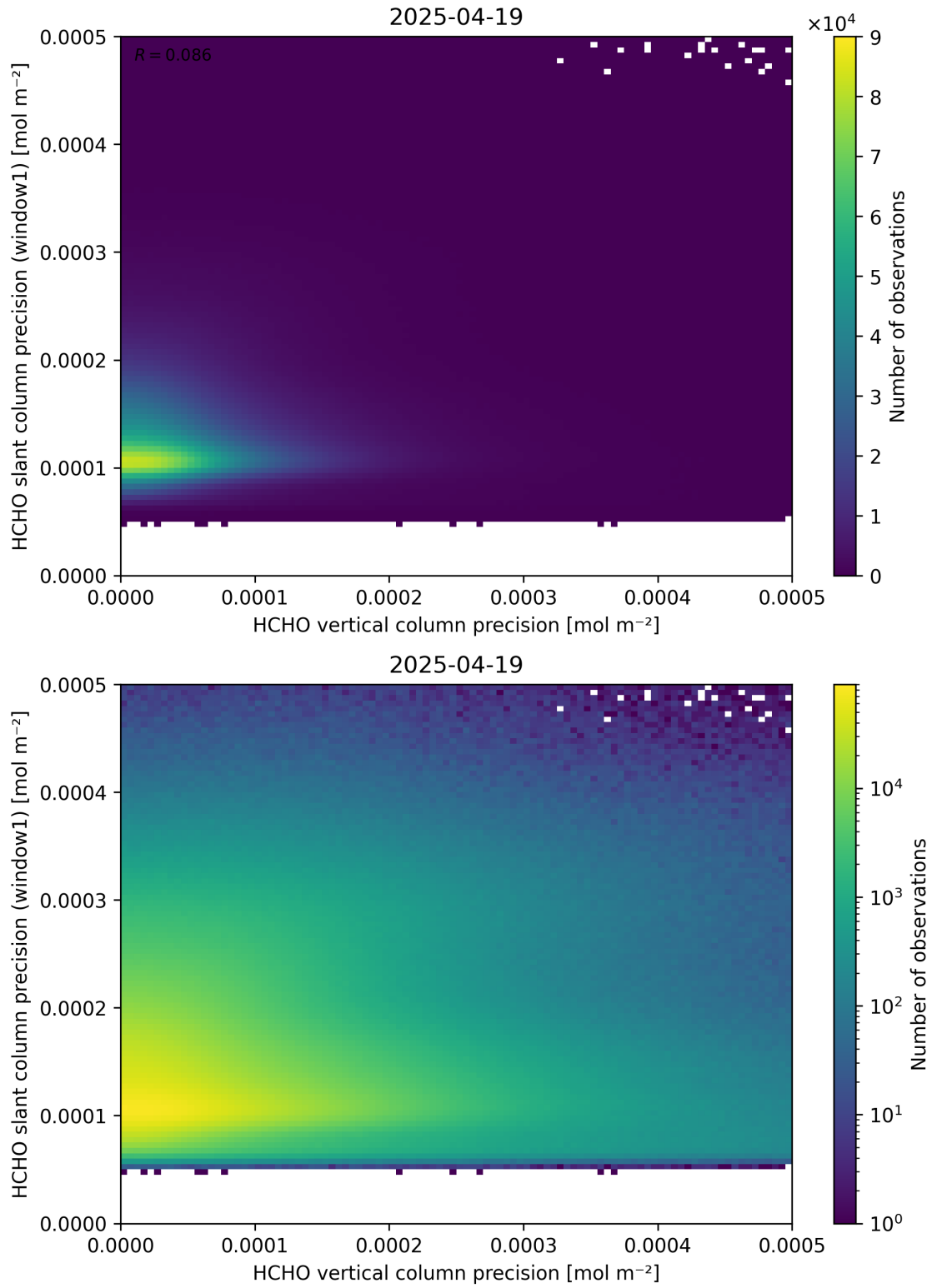
Figure 143: Scatter density plot of “HCHO vertical column precision” against “HCHO slant column precision (window1)” for 2025-04-19 to 2025-04-20.
