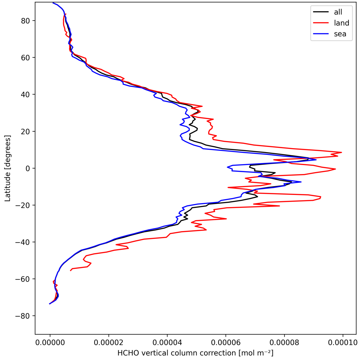
Figure 23: Zonal average of “HCHO vertical column correction” for 2025-04-19 to 2025-04-20.
