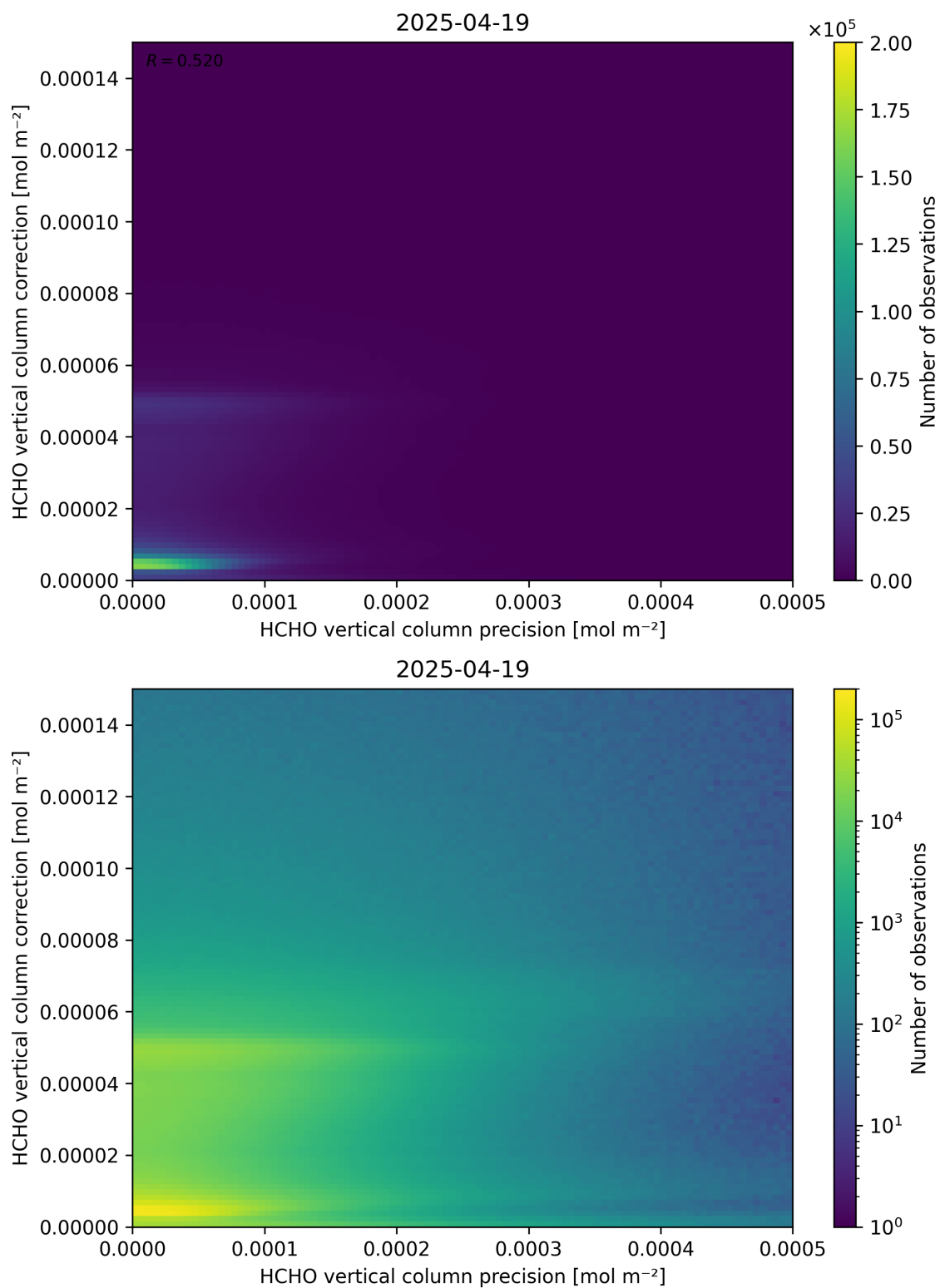
Figure 146: Scatter density plot of “HCHO vertical column precision” against “HCHO vertical column correction” for 2025-04-19 to 2025-04-20.
