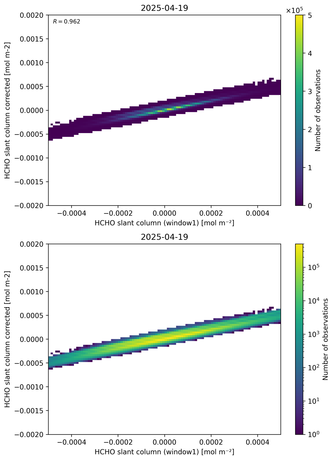
Figure 82: Scatter density plot of “HCHO slant column (window1)” against “HCHO slant column corrected” for 2025-04-19 to 2025-04-20.
