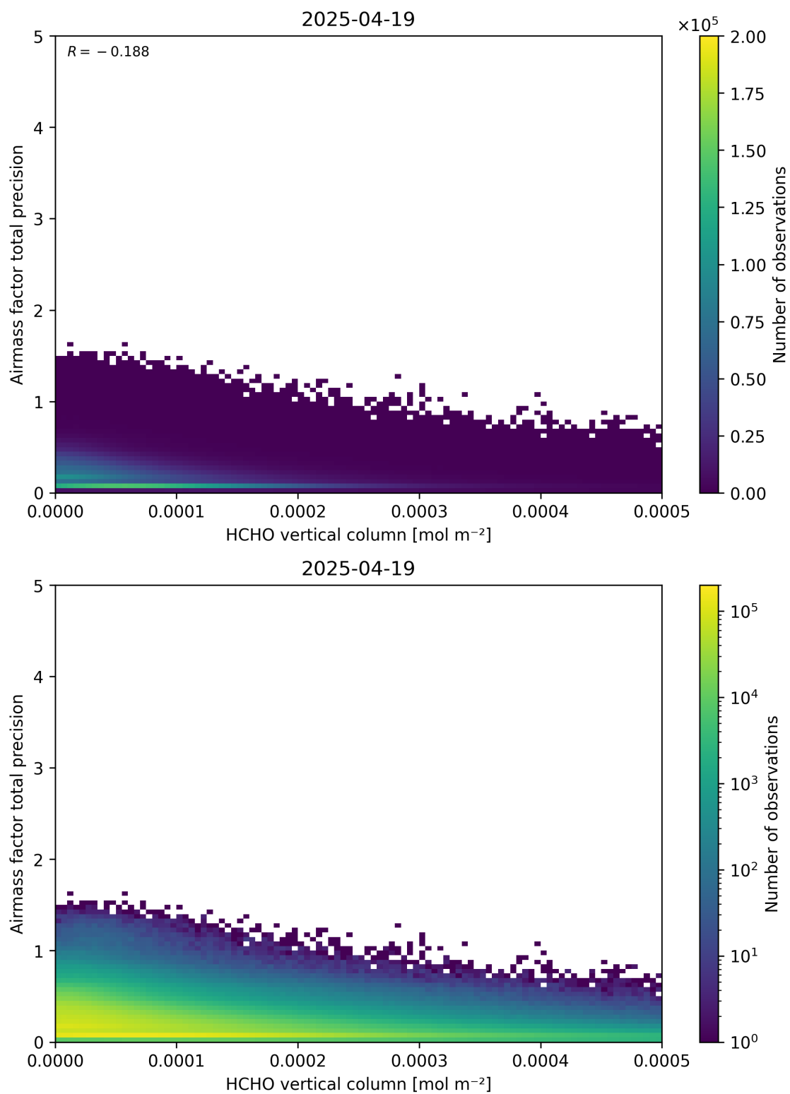
Figure 132: Scatter density plot of “HCHO vertical column” against “Airmass factor total precision” for 2025-04-19 to 2025-04-20.
