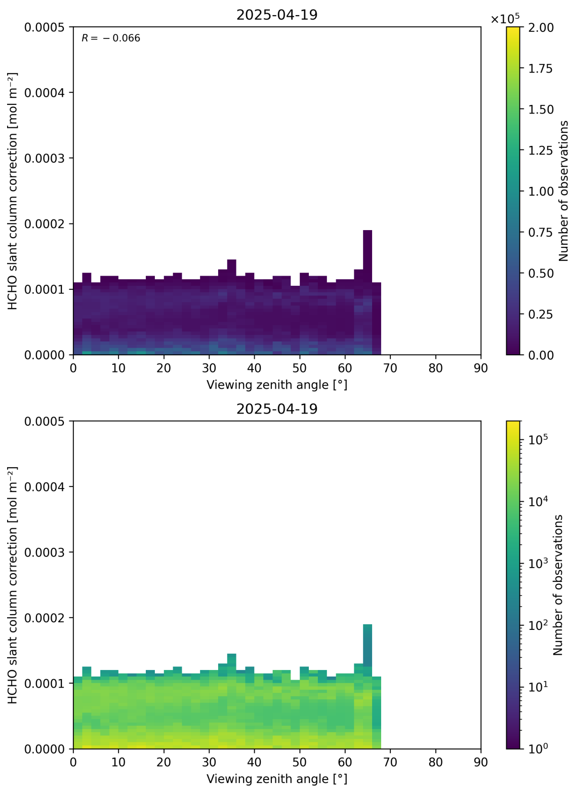
Figure 187: Scatter density plot of “Viewing zenith angle” against “HCHO slant column correction” for 2025-04-19 to 2025-04-20.
