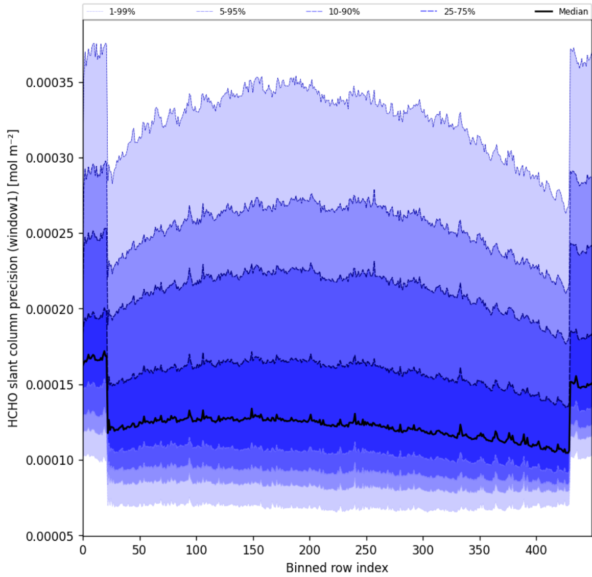
Figure 53: Along track statistics of “HCHO slant column precision (window1)” for 2025-04-19 to 2025-04-20
