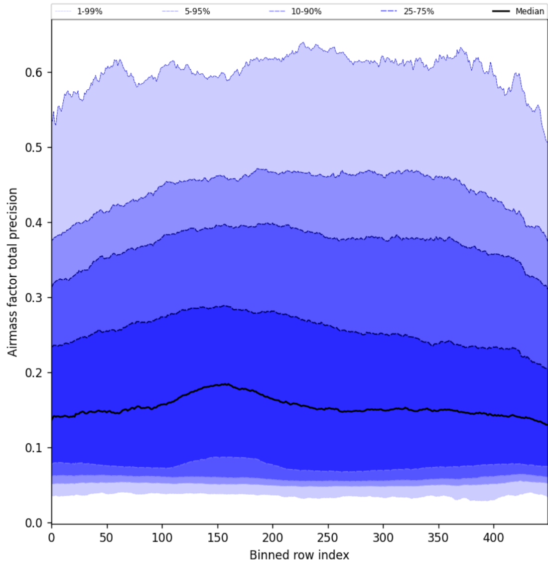
Figure 55: Along track statistics of “Airmass factor total precision” for 2025-04-19 to 2025-04-20
