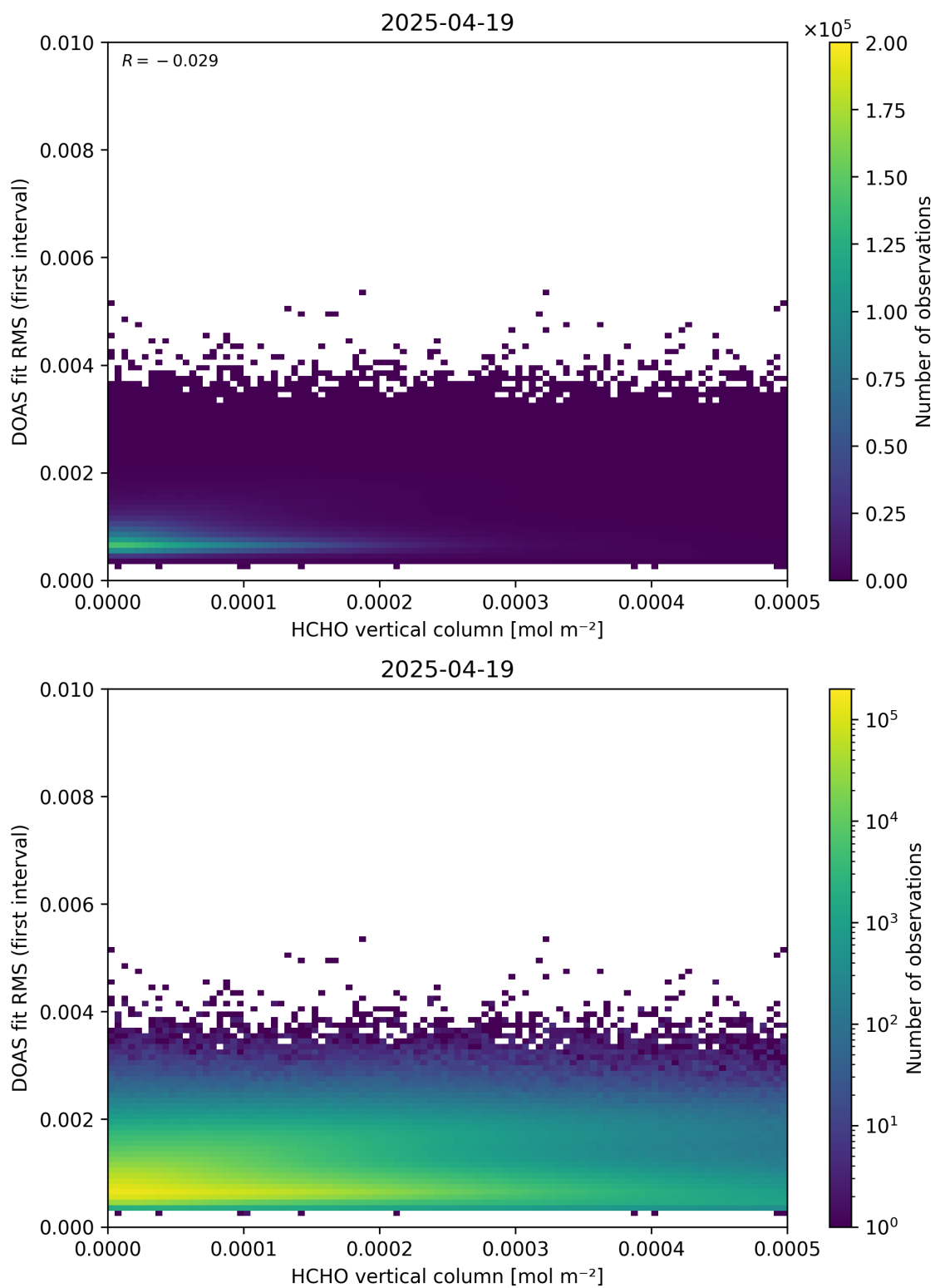
Figure 123: Scatter density plot of “HCHO vertical column” against “DOAS fit RMS (first interval)” for 2025-04-19 to 2025-04-20.
