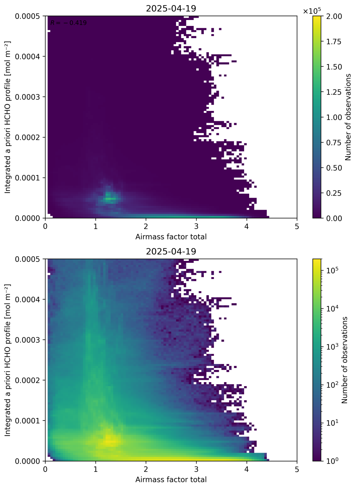
Figure 104: Scatter density plot of “Airmass factor total” against “Integrated a priori HCHO profile” for 2025-04-19 to 2025-04-20.
