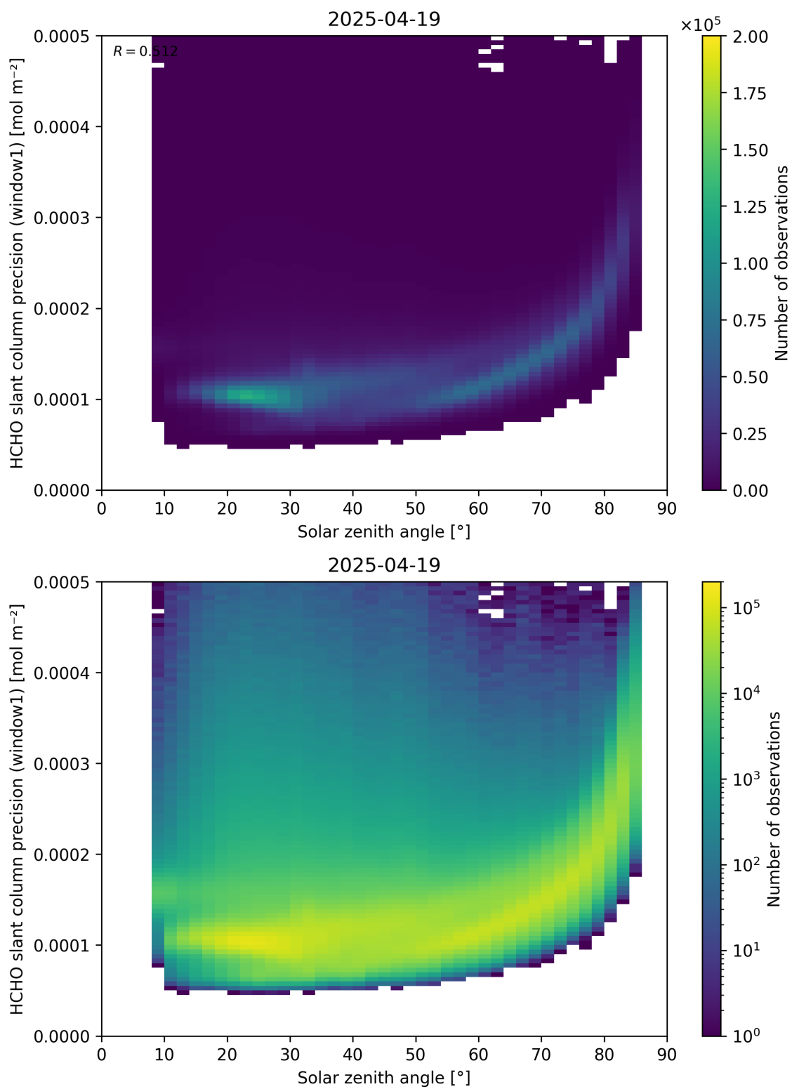
Figure 174: Scatter density plot of “Solar zenith angle” against “HCHO slant column precision (window1)” for 2025-04-19 to 2025-04-20.
