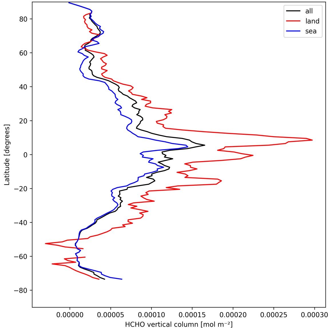
Figure 21: Zonal average of “HCHO vertical column” for 2025-04-19 to 2025-04-20.
