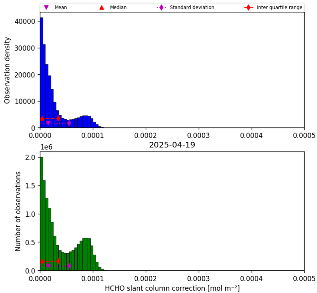
Figure 47: Histogram of “HCHO slant column correction” for 2025-04-19 to 2025-04-20
