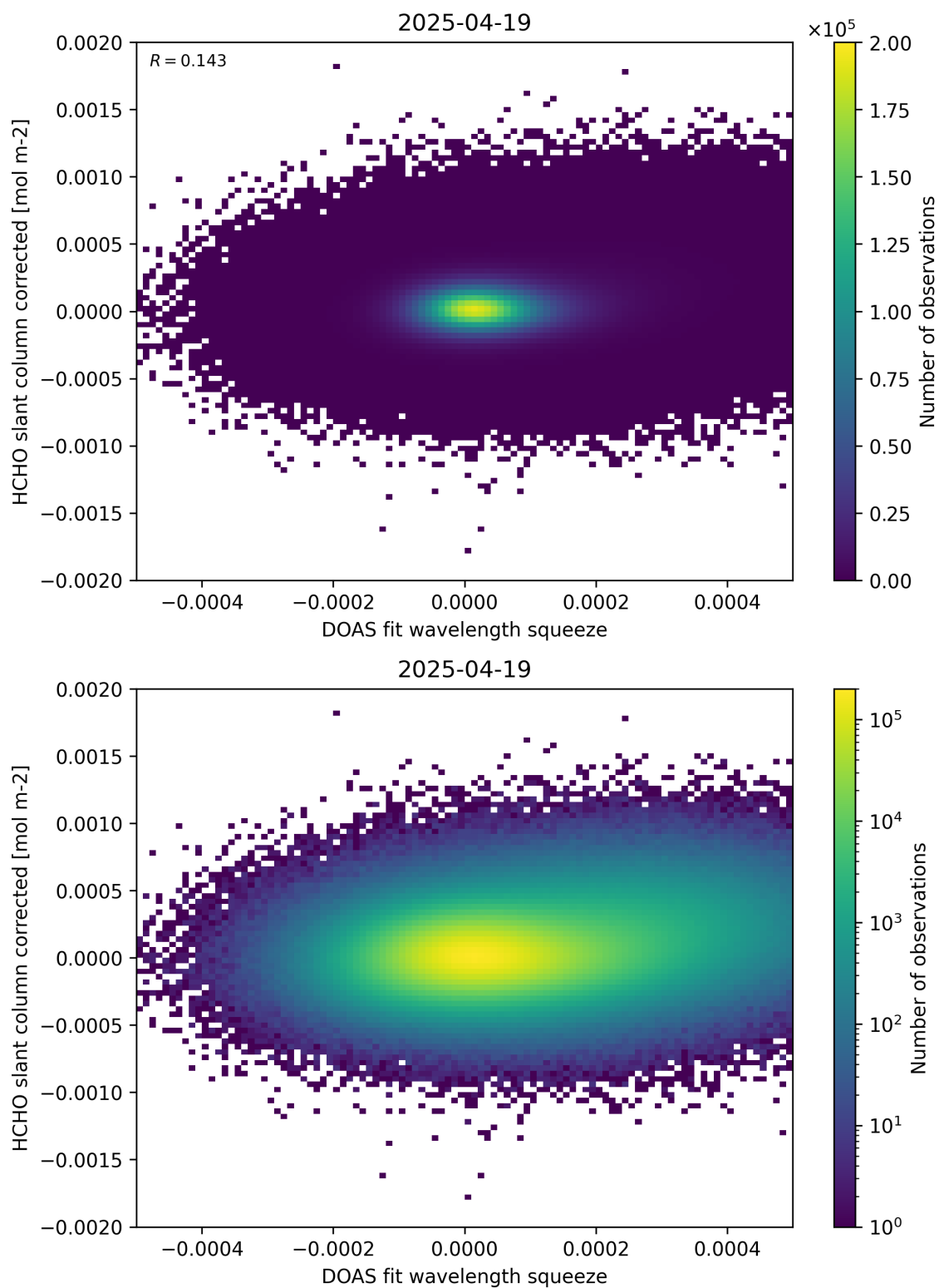
Figure 69: Scatter density plot of “DOAS fit wavelength squeeze” against “HCHO slant column corrected” for 2025-04-19 to 2025-04-20.
