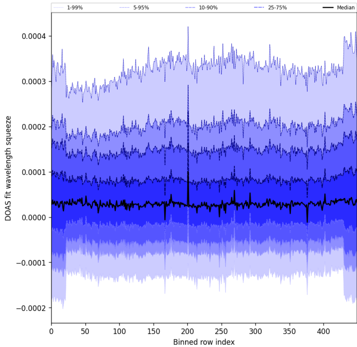
Figure 59: Along track statistics of “DOAS fit wavelength squeeze” for 2025-04-19 to 2025-04-20
