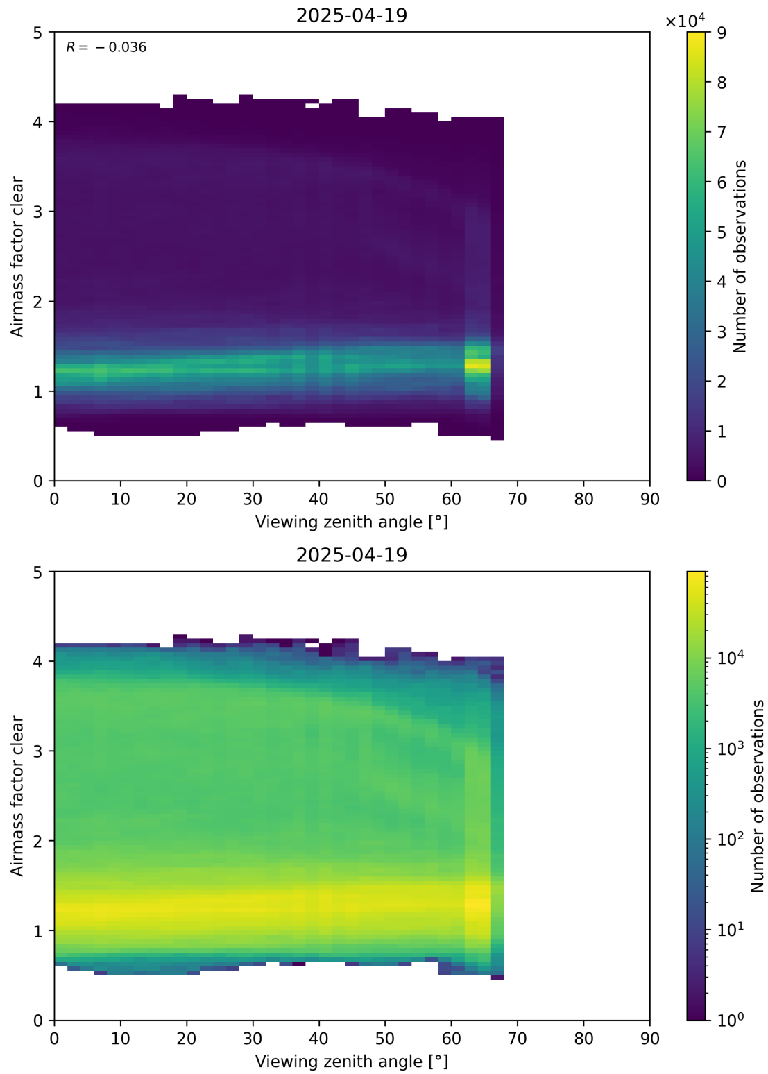
Figure 185: Scatter density plot of “Viewing zenith angle” against “Airmass factor clear” for 2025-04-19 to 2025-04-20.
