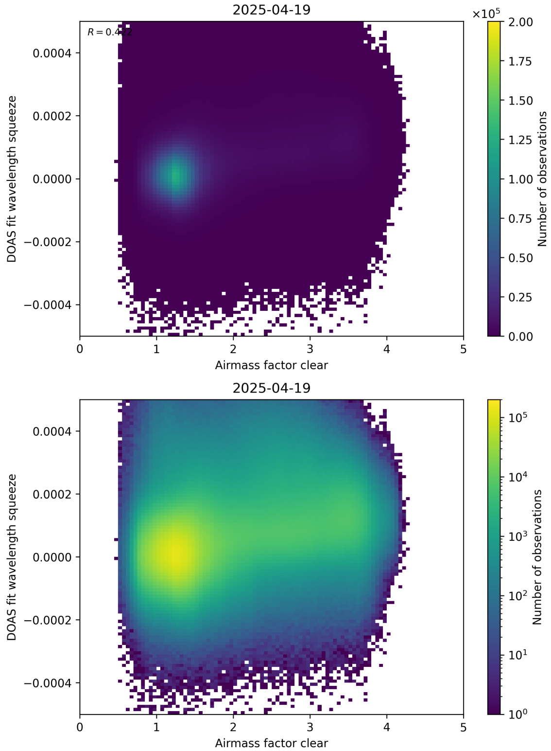
Figure 73: Scatter density plot of “Airmass factor clear” against “DOAS fit wavelength squeeze” for 2025-04-19 to 2025-04-20.
