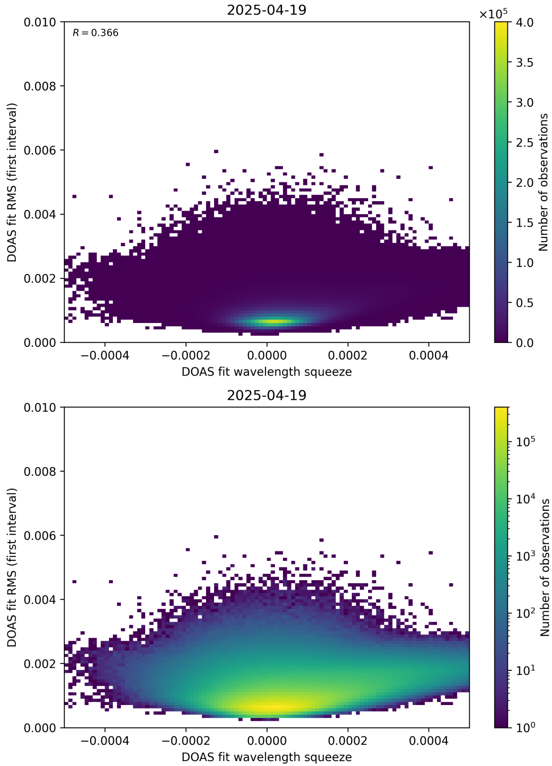
Figure 68: Scatter density plot of “DOAS fit wavelength squeeze” against “DOAS fit RMS (first interval)” for 2025-04-19 to 2025-04-20.
