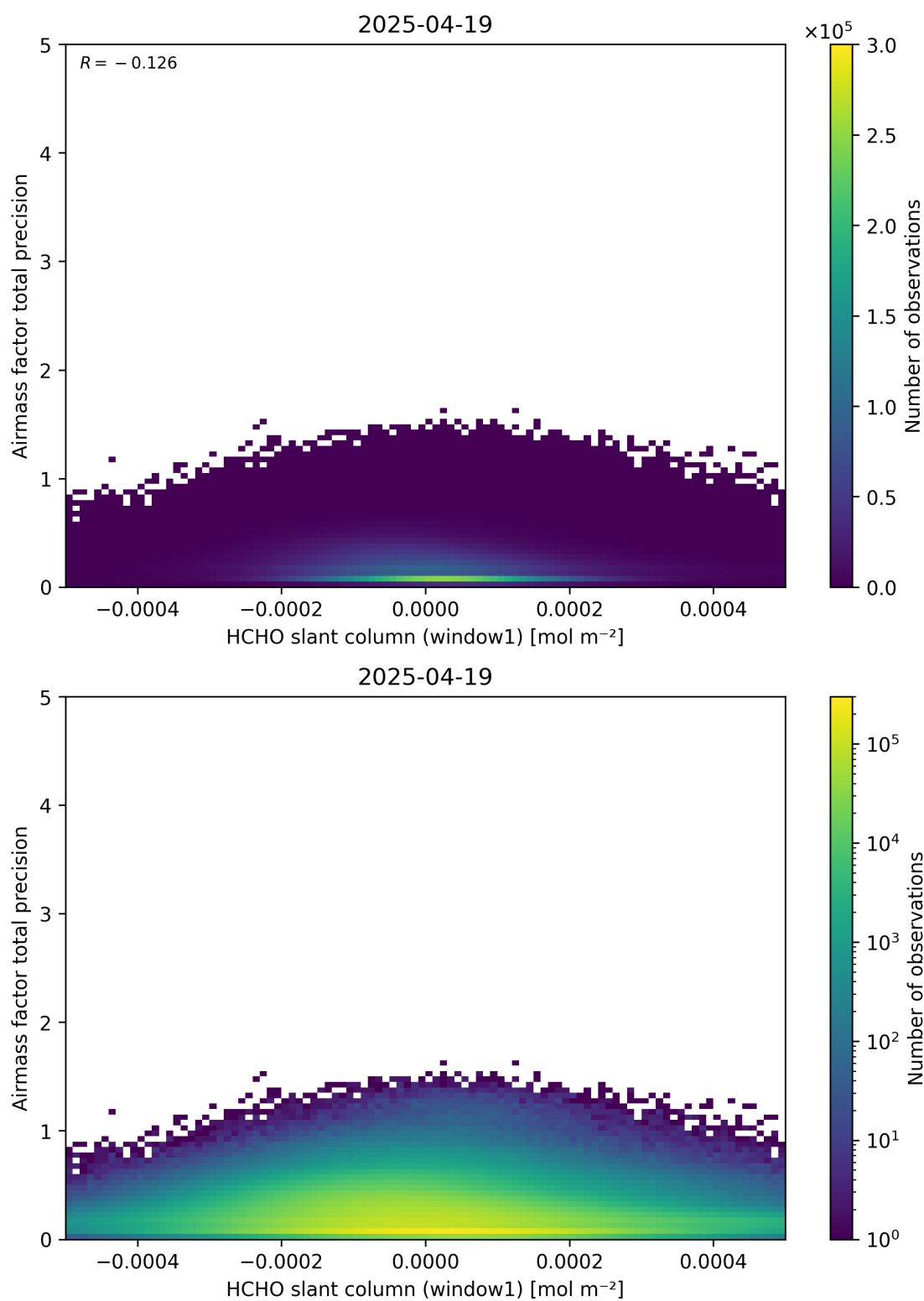
Figure 86: Scatter density plot of “HCHO slant column (window1)” against “Airmass factor total precision” for 2025-04-19 to 2025-04-20.
