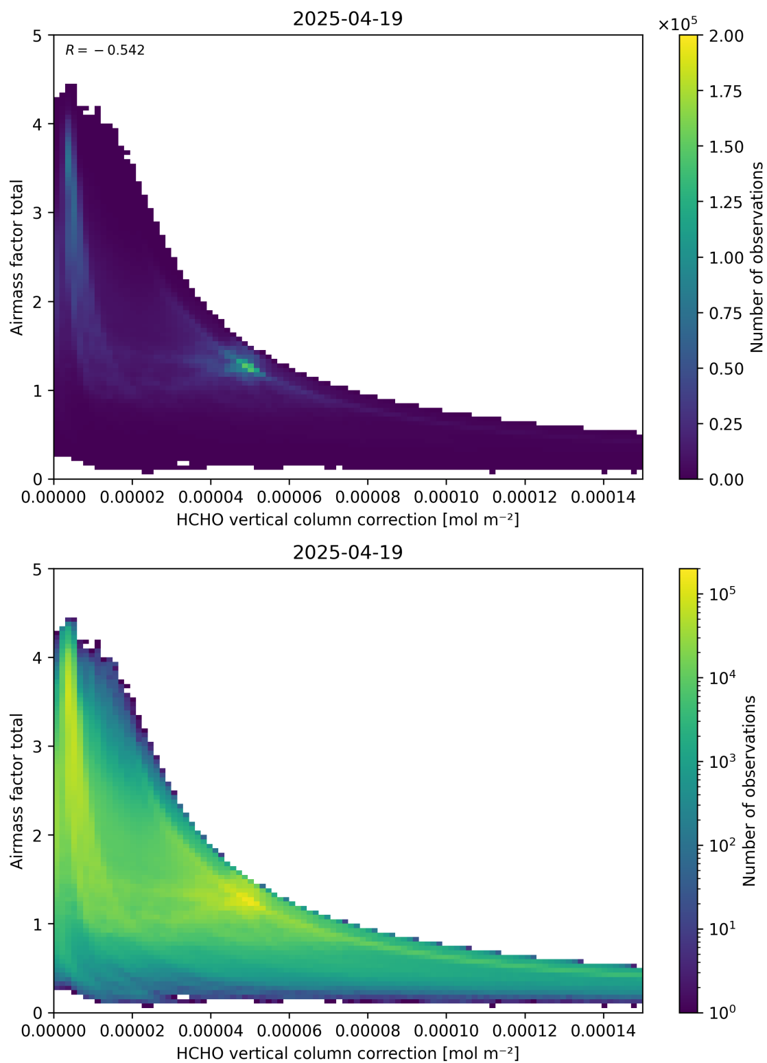
Figure 120: Scatter density plot of “HCHO vertical column correction” against “Airmass factor total” for 2025-04-19 to 2025-04-20.
