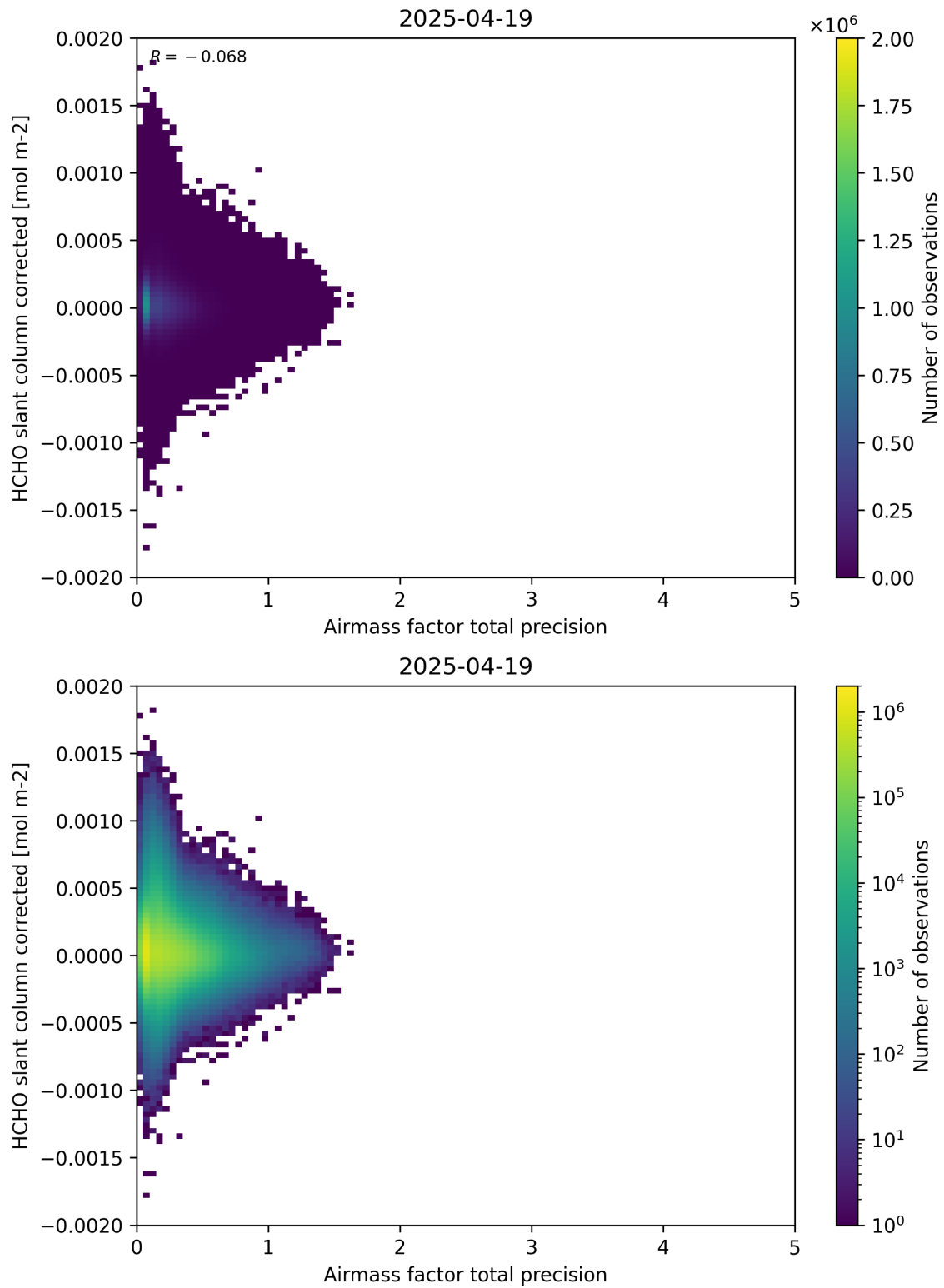
Figure 109: Scatter density plot of “Airmass factor total precision” against “HCHO slant column corrected” for 2025-04-19 to 2025-04-20.
