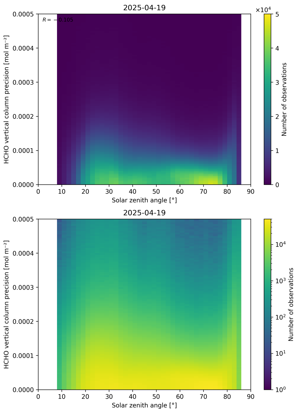
Figure 179: Scatter density plot of “Solar zenith angle” against “HCHO vertical column precision” for 2025-04-19 to 2025-04-20.
