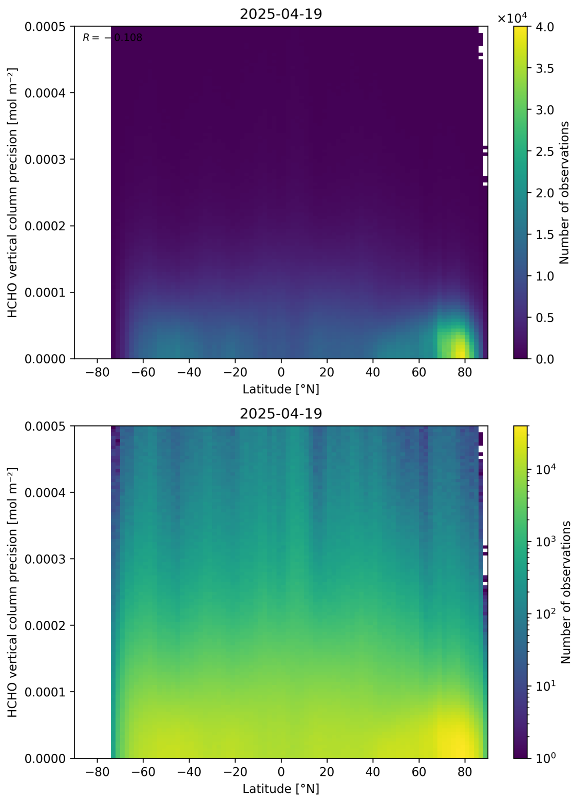
Figure 165: Scatter density plot of “Latitude” against “HCHO vertical column precision” for 2025-04-19 to 2025-04-20.
