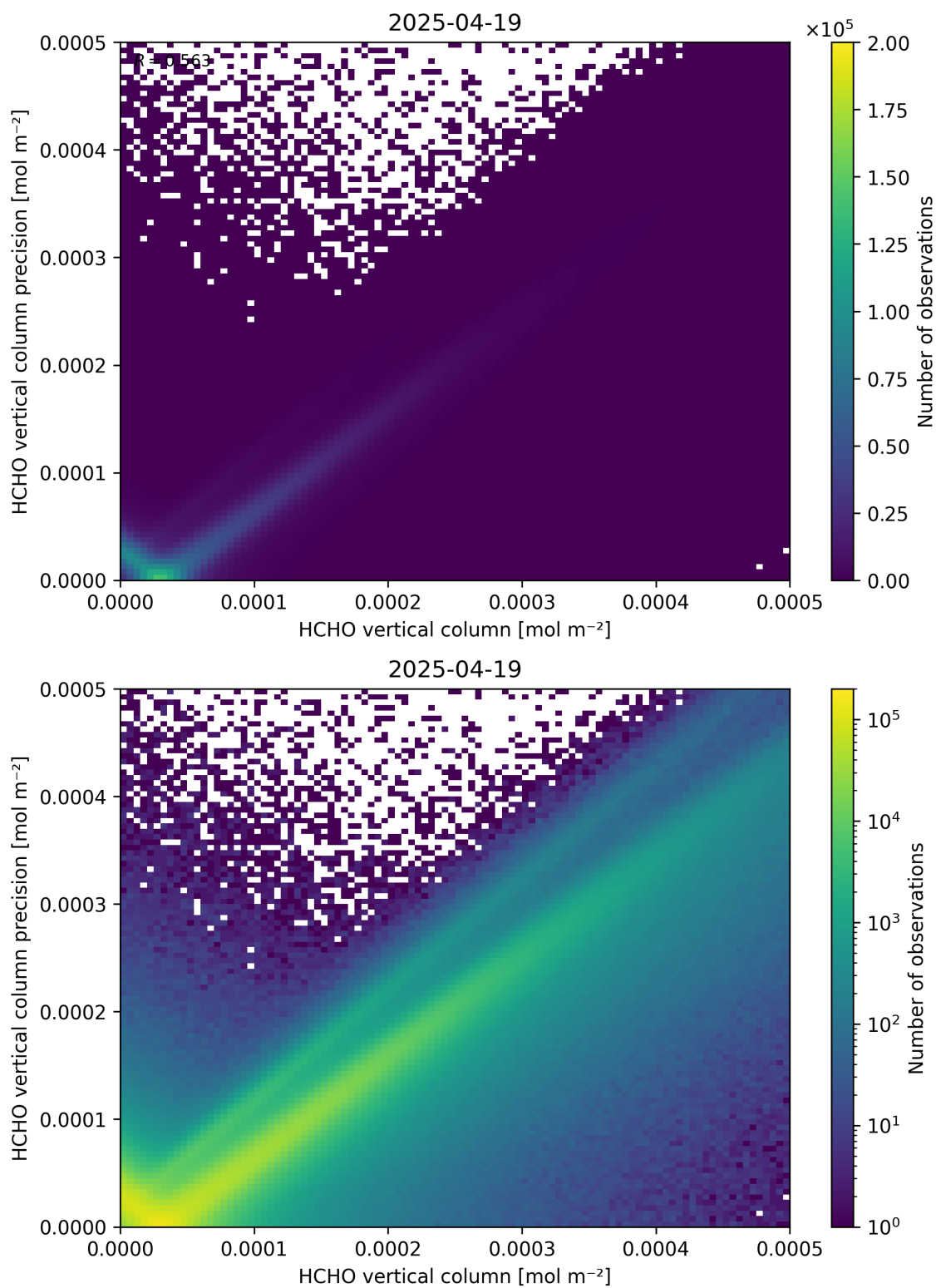
Figure 134: Scatter density plot of “HCHO vertical column” against “HCHO vertical column precision” for 2025-04-19 to 2025-04-20.
