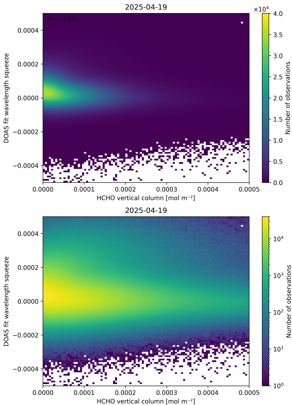
Figure 125: Scatter density plot of “HCHO vertical column” against “DOAS fit wavelength squeeze” for 2025-04-19 to 2025-04-20.
