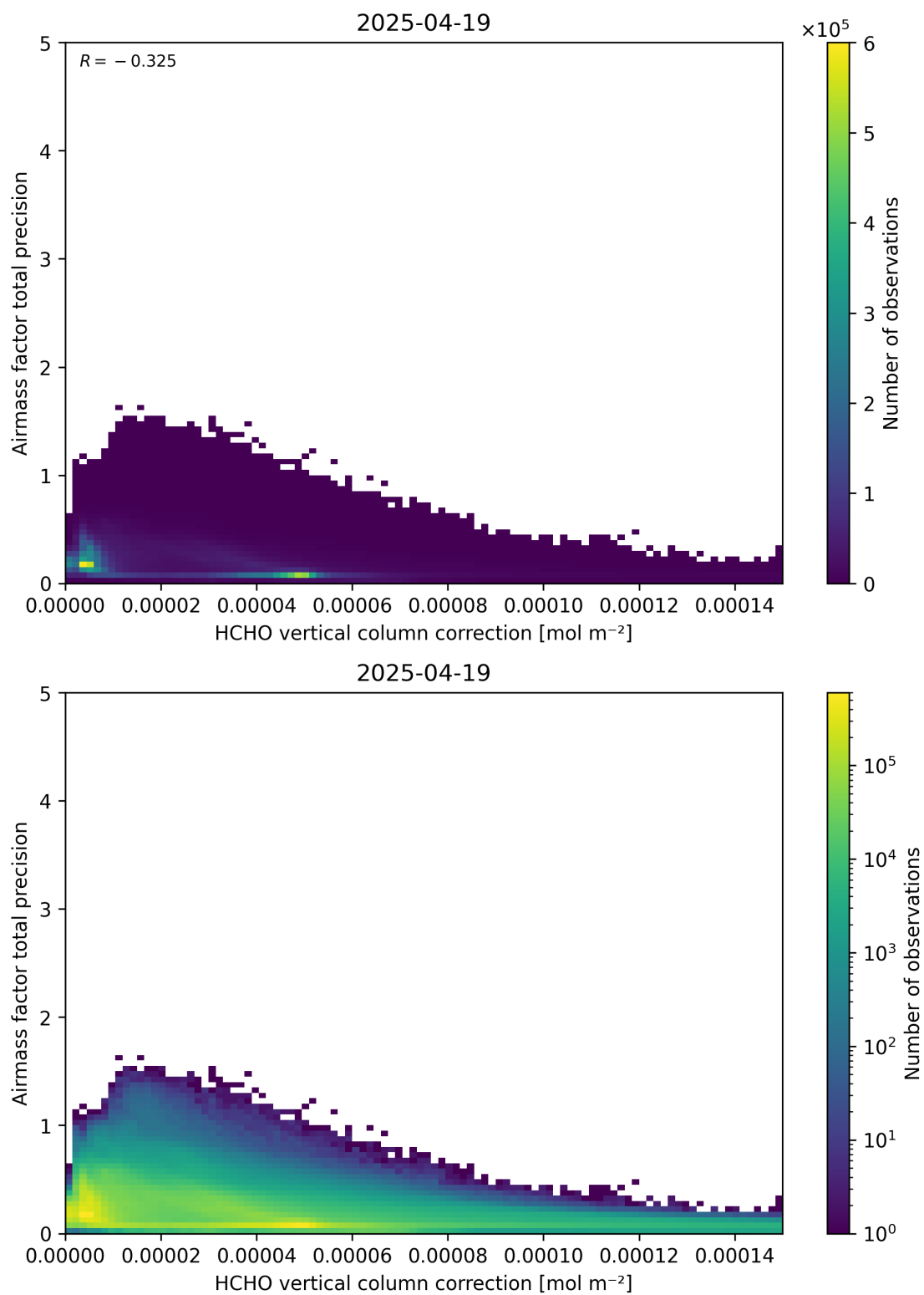
Figure 121: Scatter density plot of “HCHO vertical column correction” against “Airmass factor total precision” for 2025-04-19 to 2025-04-20.
