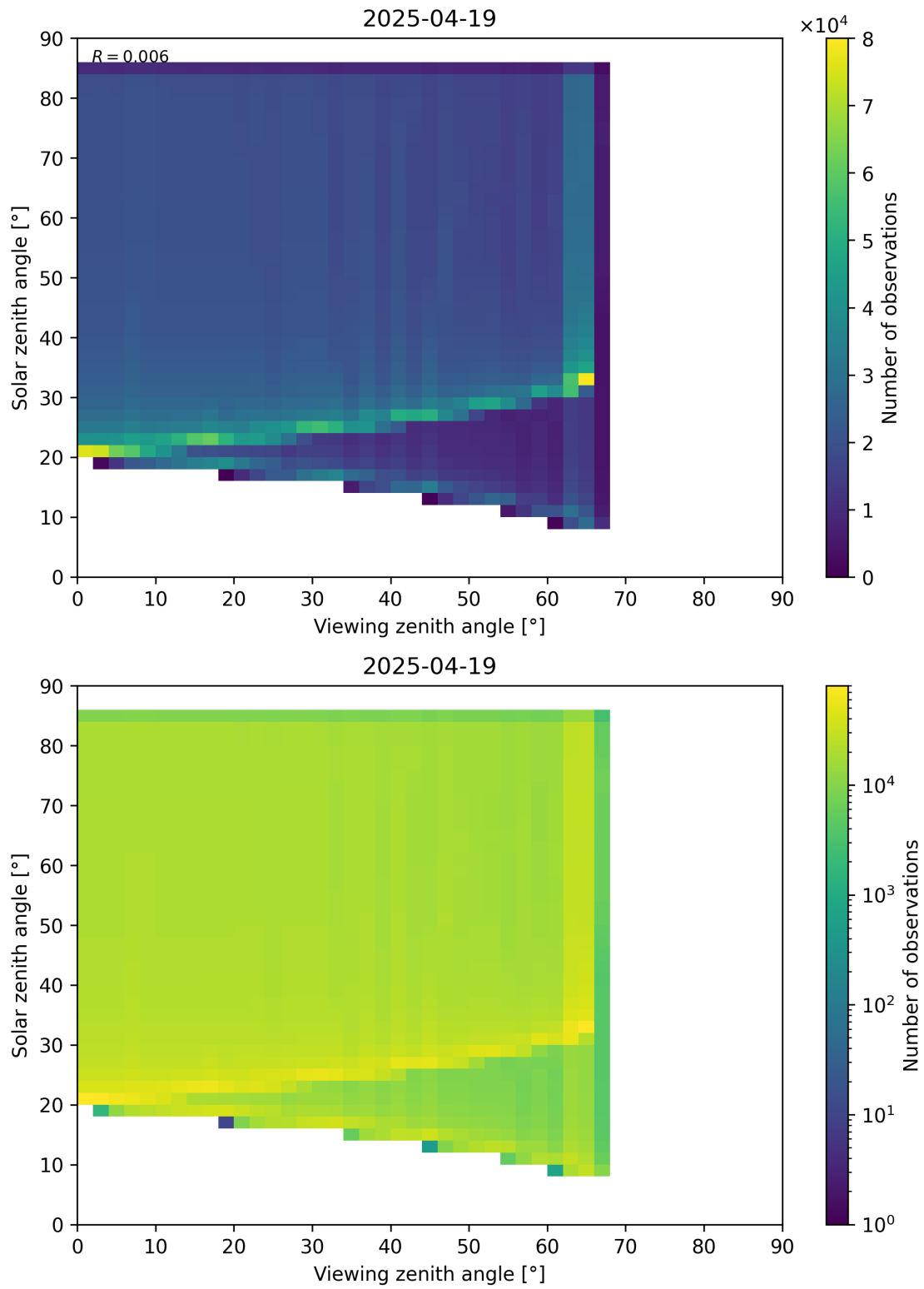
Figure 197: Scatter density plot of “Viewing zenith angle” against “Solar zenith angle” for 2025-04-19 to 2025-04-20.
