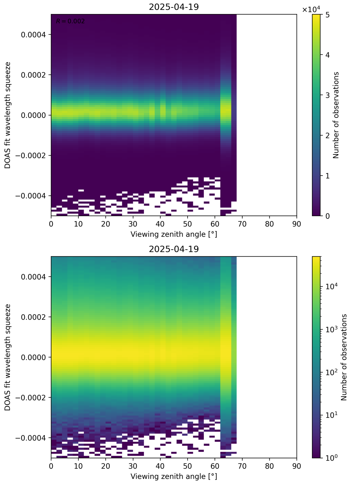
Figure 184: Scatter density plot of “Viewing zenith angle” against “DOAS fit wavelength squeeze” for 2025-04-19 to 2025-04-20.
