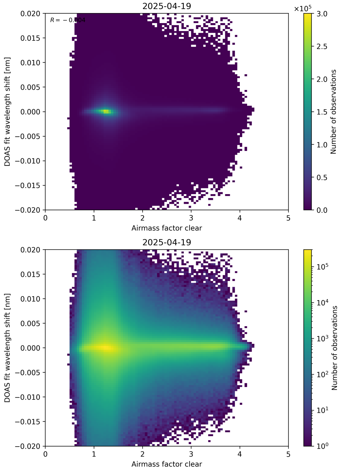
Figure 72: Scatter density plot of “Airmass factor clear” against “DOAS fit wavelength shift” for 2025-04-19 to 2025-04-20.
