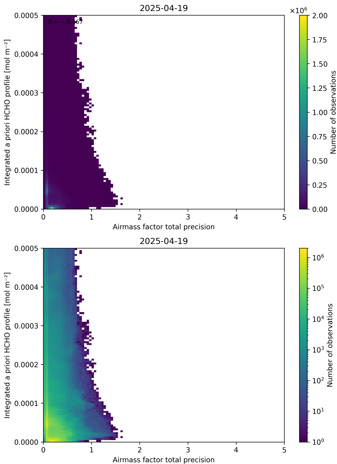
Figure 111: Scatter density plot of “Airmass factor total precision” against “Integrated a priori HCHO profile” for 2025-04-19 to 2025-04-20.
