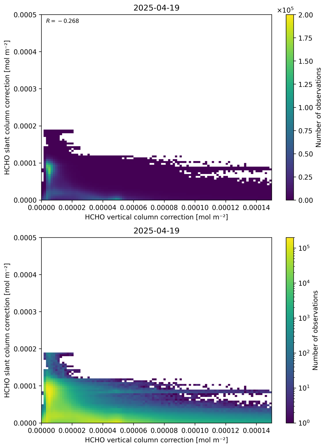
Figure 117: Scatter density plot of “HCHO vertical column correction” against “HCHO slant column correction” for 2025-04-19 to 2025-04-20.
