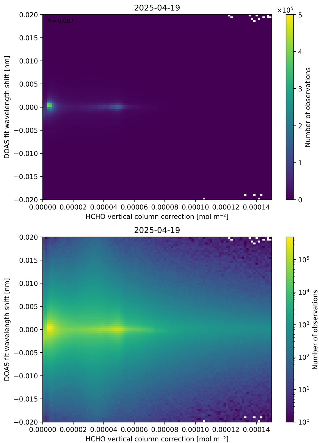
Figure 113: Scatter density plot of “HCHO vertical column correction” against “DOAS fit wavelength shift” for 2025-04-19 to 2025-04-20.
