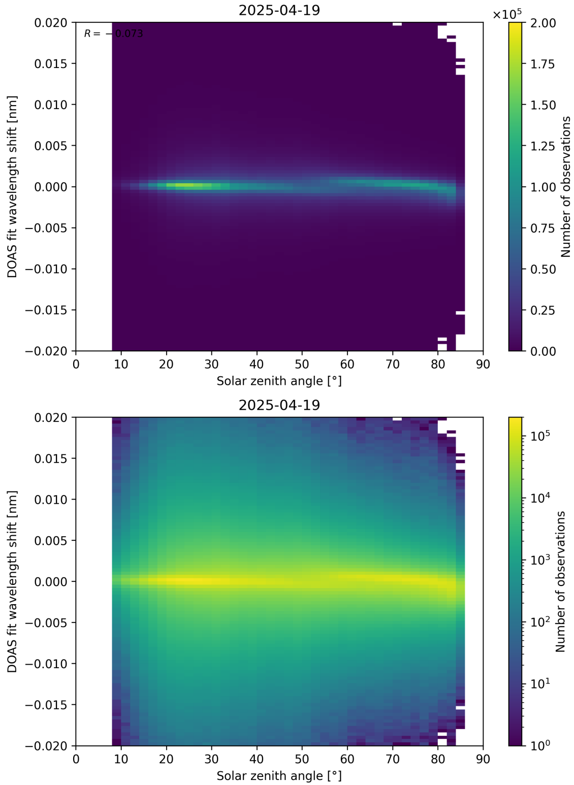
Figure 168: Scatter density plot of “Solar zenith angle” against “DOAS fit wavelength shift” for 2025-04-19 to 2025-04-20.
