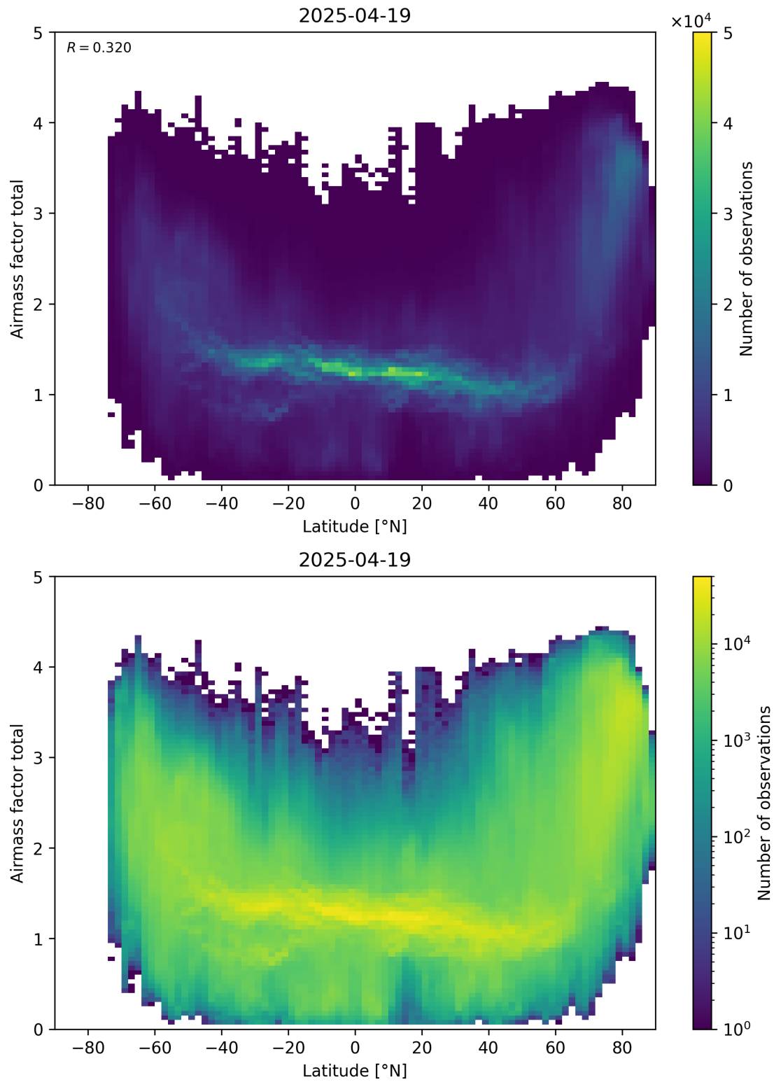
Figure 161: Scatter density plot of “Latitude” against “Airmass factor total” for 2025-04-19 to 2025-04-20.
