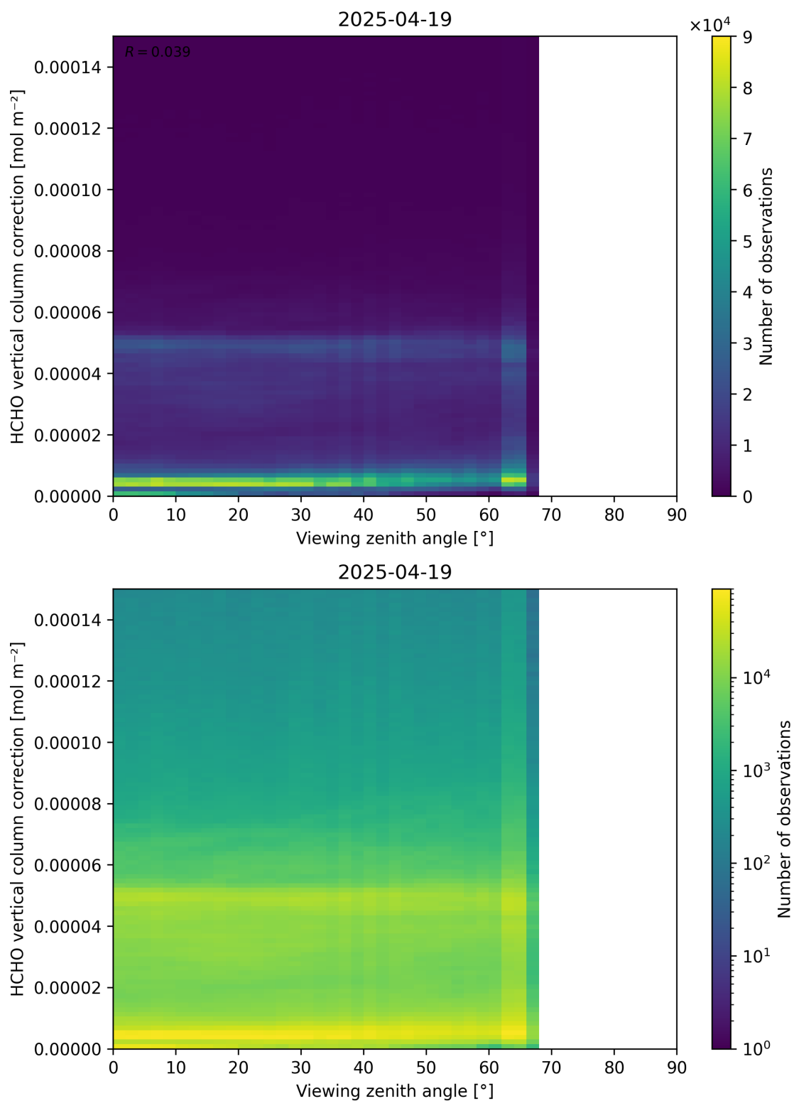
Figure 193: Scatter density plot of “Viewing zenith angle” against “HCHO vertical column correction” for 2025-04-19 to 2025-04-20.
