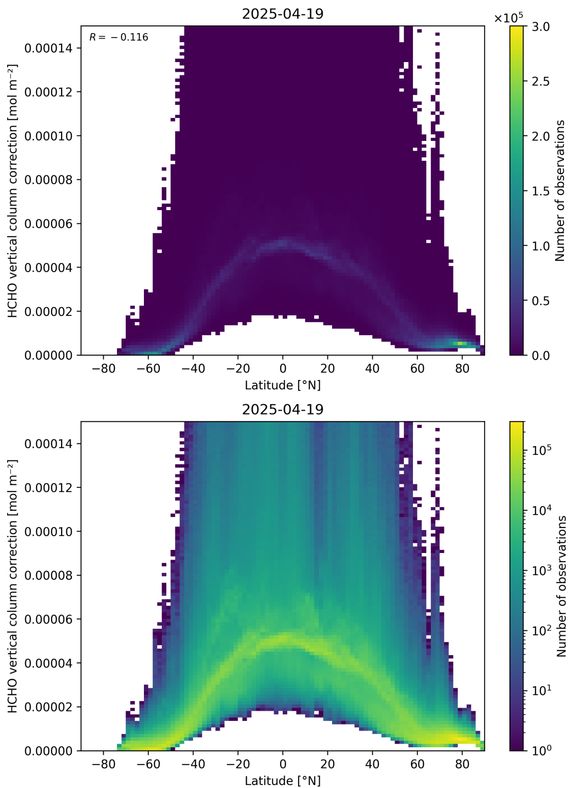
Figure 164: Scatter density plot of “Latitude” against “HCHO vertical column correction” for 2025-04-19 to 2025-04-20.
