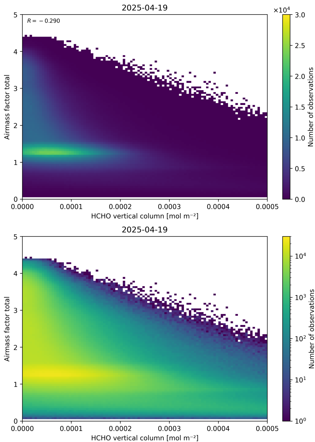
Figure 131: Scatter density plot of “HCHO vertical column” against “Airmass factor total” for 2025-04-19 to 2025-04-20.
