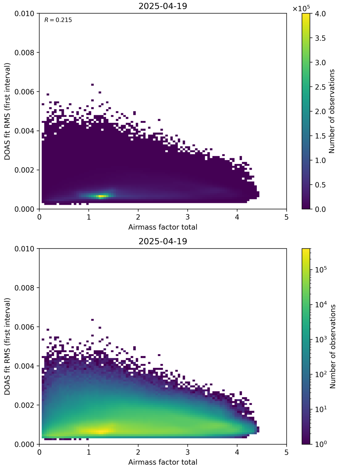
Figure 97: Scatter density plot of “Airmass factor total” against “DOAS fit RMS (first interval)” for 2025-04-19 to 2025-04-20.
