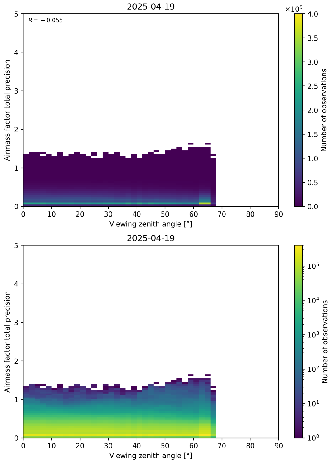
Figure 191: Scatter density plot of “Viewing zenith angle” against “Airmass factor total precision” for 2025-04-19 to 2025-04-20.
