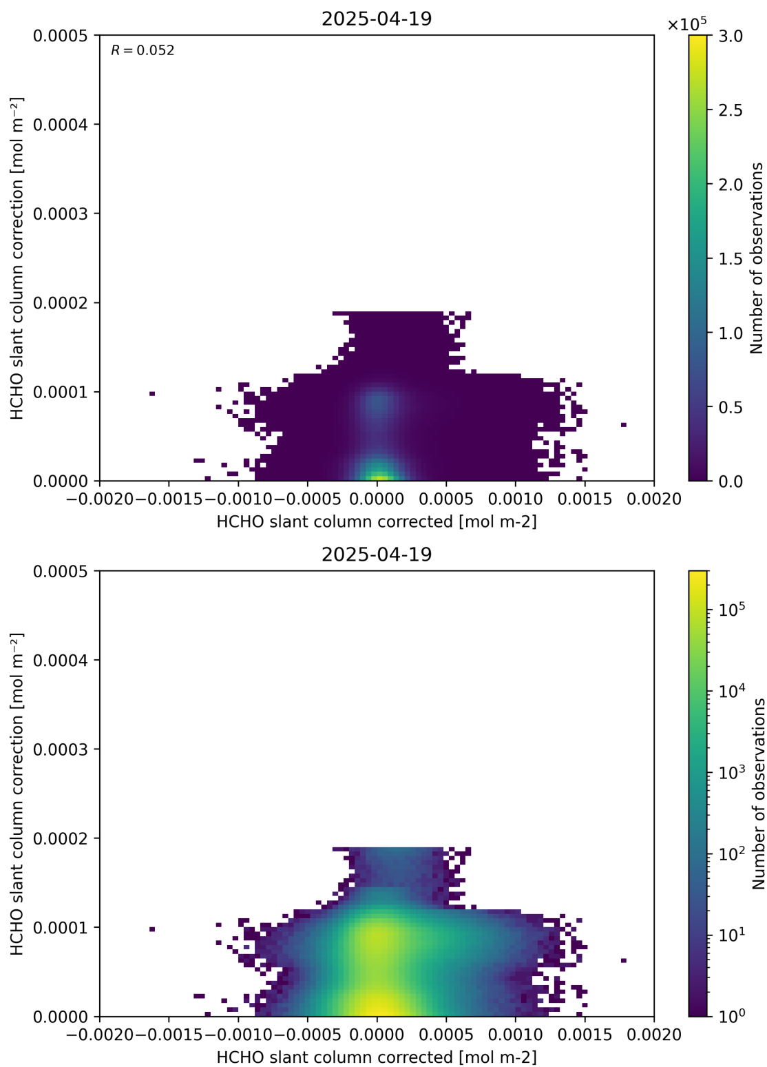
Figure 77: Scatter density plot of “HCHO slant column corrected” against “HCHO slant column correction” for 2025-04-19 to 2025-04-20.
