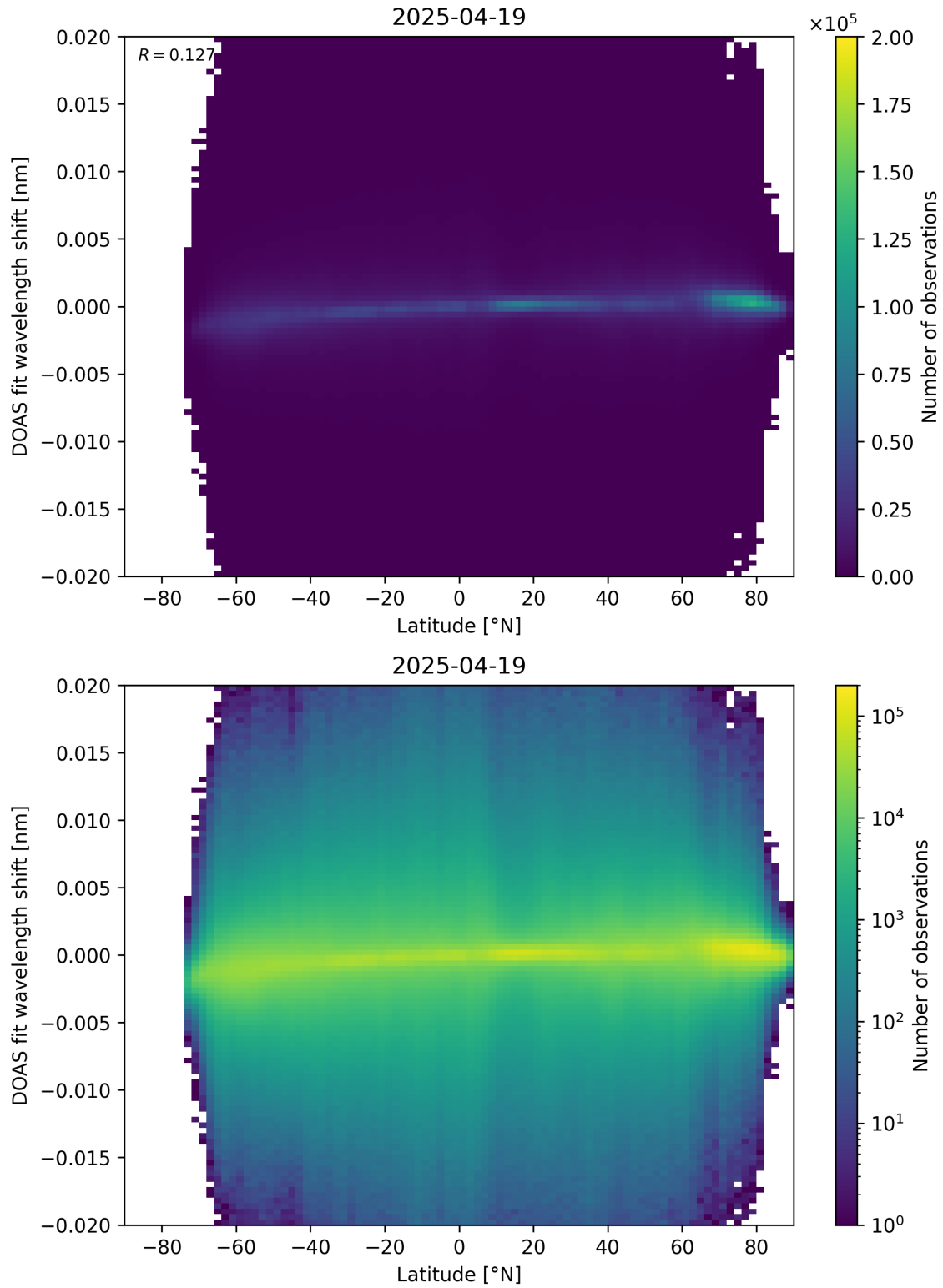
Figure 154: Scatter density plot of “Latitude” against “DOAS fit wavelength shift” for 2025-04-19 to 2025-04-20.
