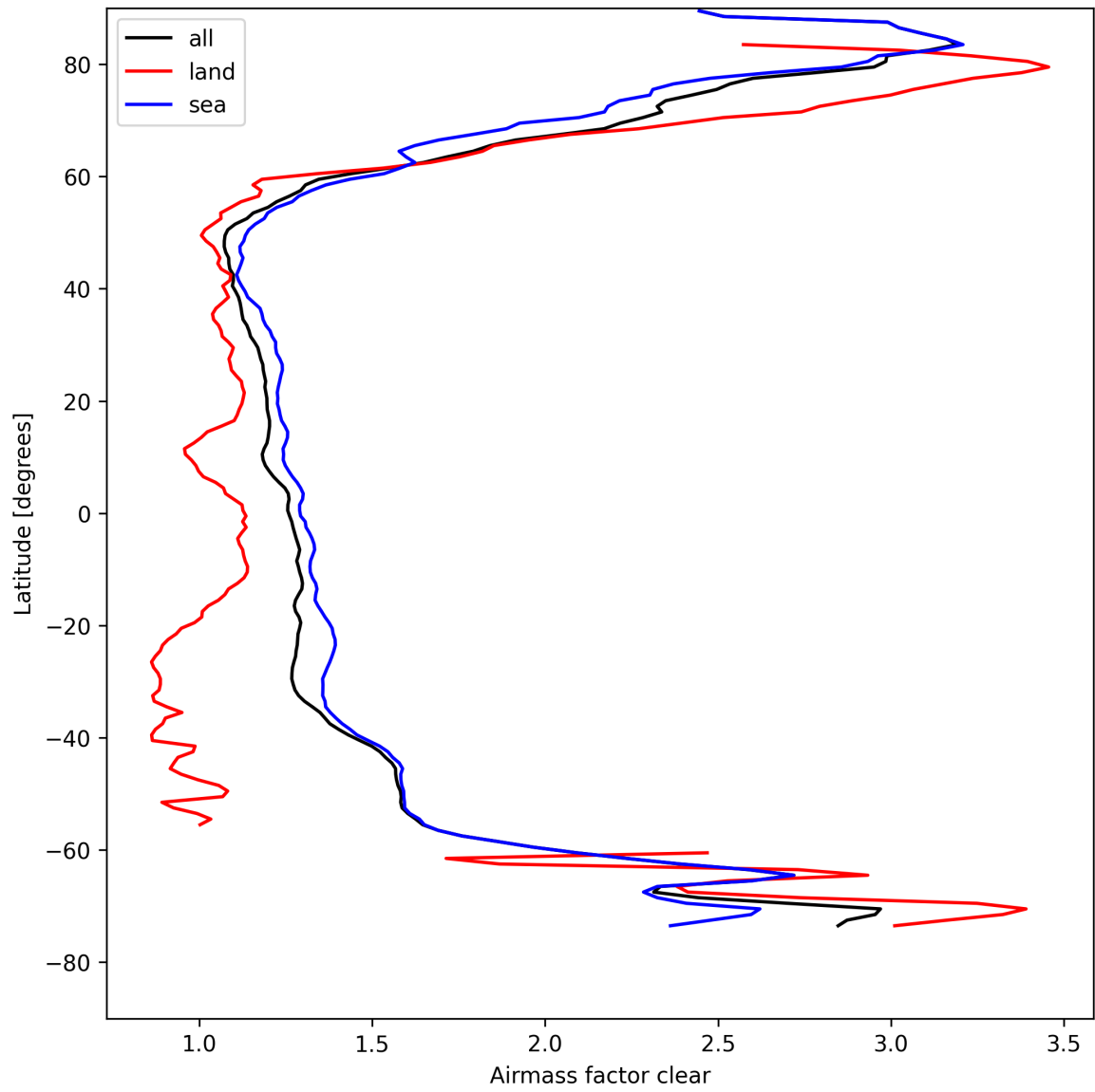
Figure 28: Zonal average of “Airmass factor clear” for 2025-04-19 to 2025-04-20.
