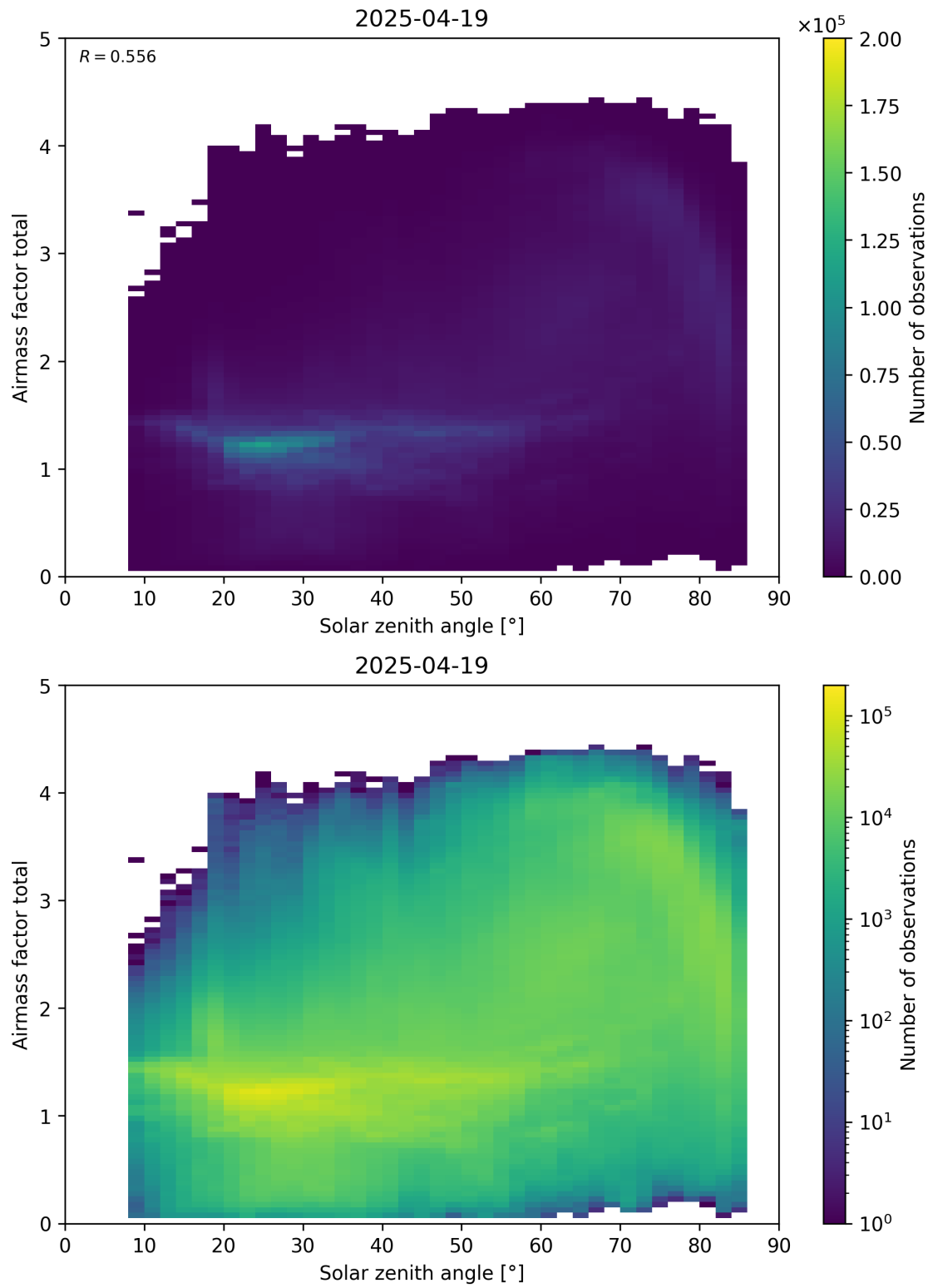
Figure 175: Scatter density plot of “Solar zenith angle” against “Airmass factor total” for 2025-04-19 to 2025-04-20.
