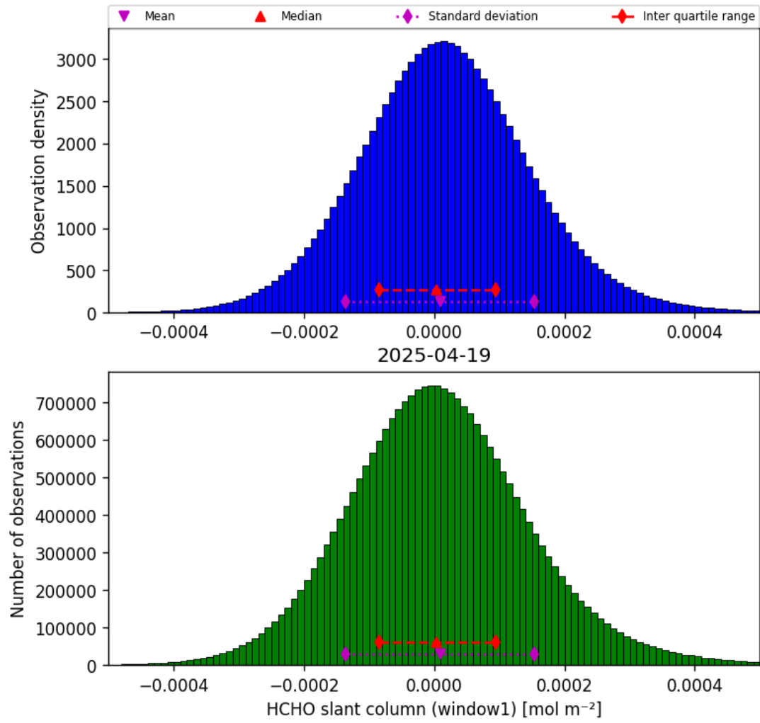
Figure 38: Histogram of “HCHO slant column (window1)” for 2025-04-19 to 2025-04-20
