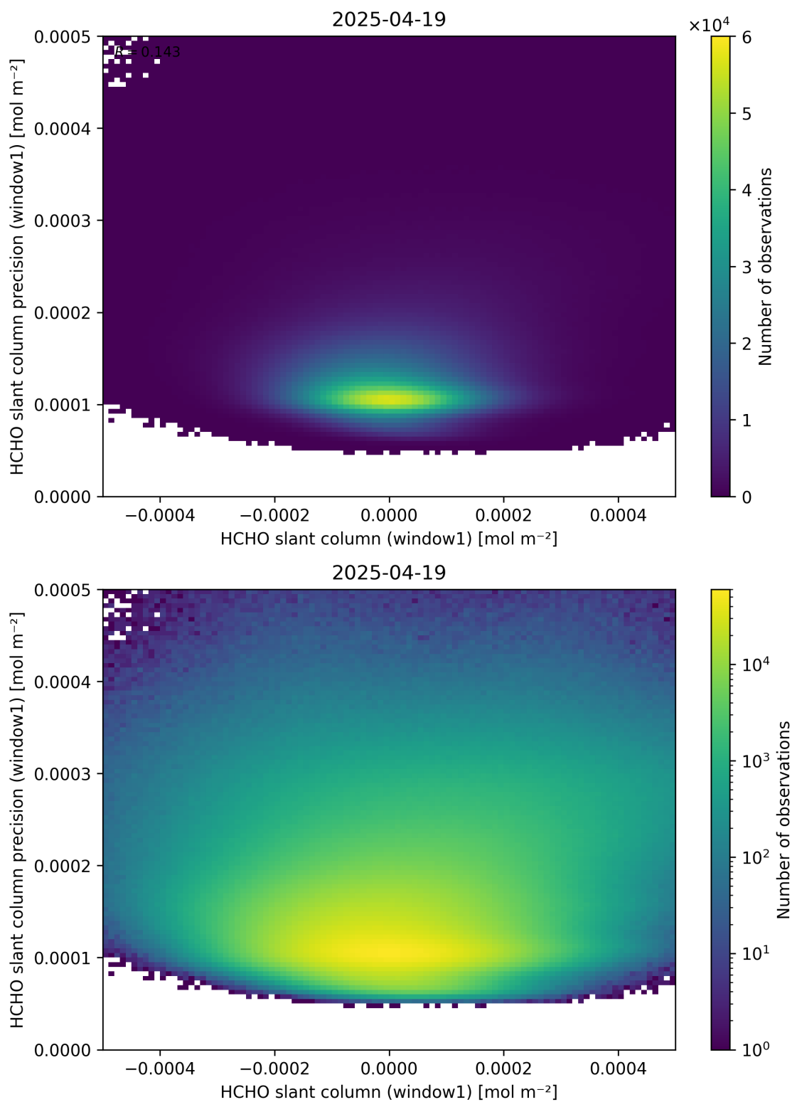
Figure 84: Scatter density plot of “HCHO slant column (window1)” against “HCHO slant column precision (window1)” for 2025-04-19 to 2025-04-20.
