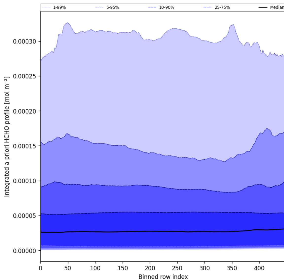
Figure 57: Along track statistics of "Integrated a priori HCHO profile" for 2025-04-19 to 2025-04-20
