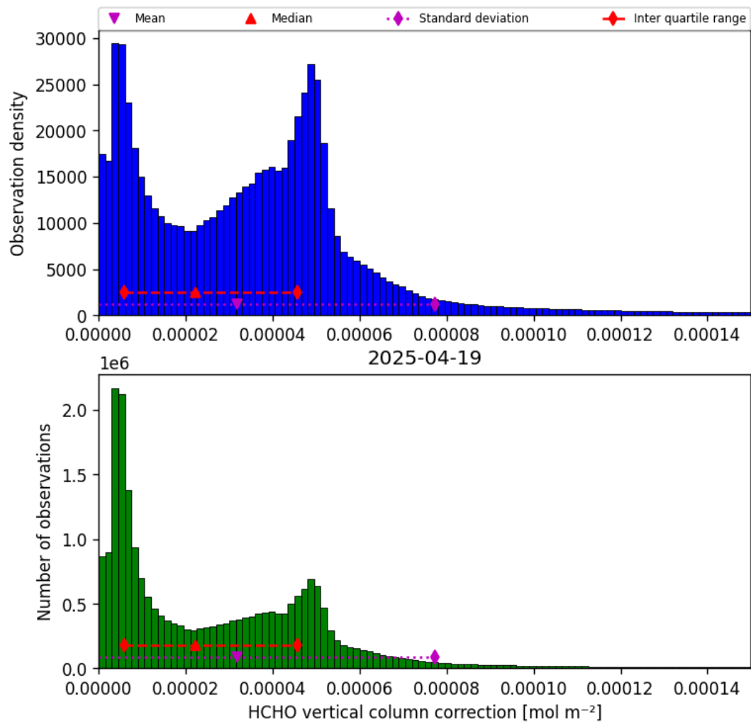
Figure 37: Histogram of “HCHO vertical column correction” for 2025-04-19 to 2025-04-20
