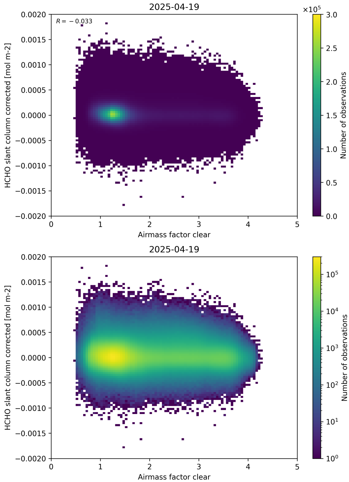
Figure 74: Scatter density plot of “Airmass factor clear” against “HCHO slant column corrected” for 2025-04-19 to 2025-04-20.
