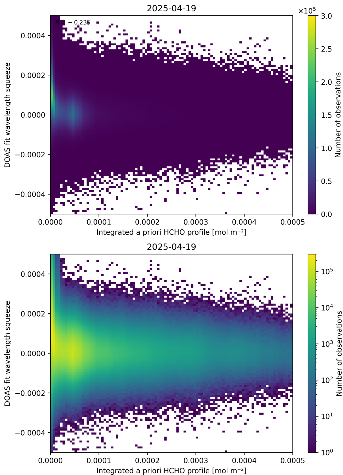
Figure 150: Scatter density plot of “Integrated a priori HCHO profile” against “DOAS fit wavelength squeeze” for 2025-04-19 to 2025-04-20.
