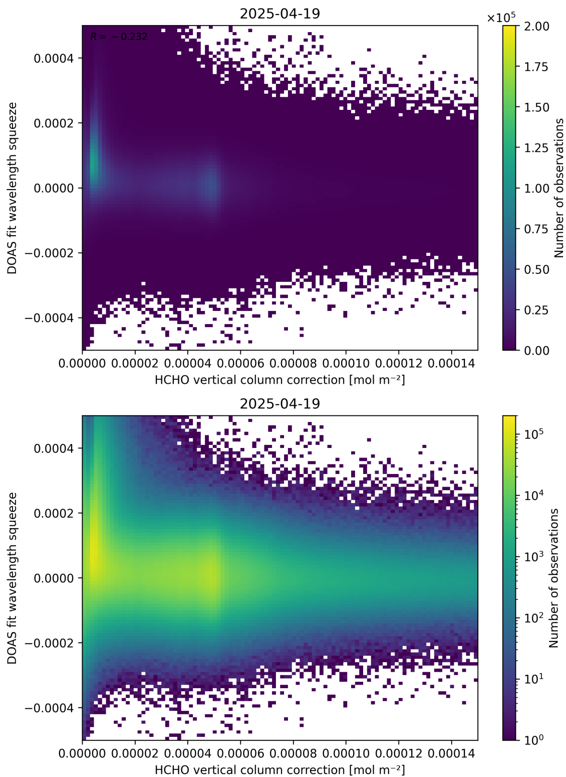
Figure 114: Scatter density plot of “HCHO vertical column correction” against “DOAS fit wavelength squeeze” for 2025-04-19 to 2025-04-20.
