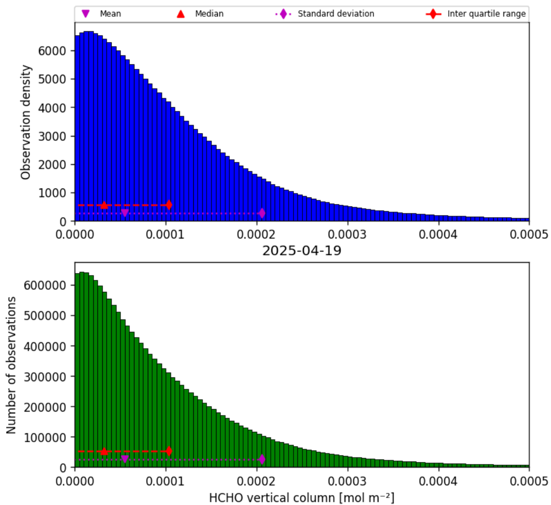
Figure 35: Histogram of “HCHO vertical column” for 2025-04-19 to 2025-04-20
