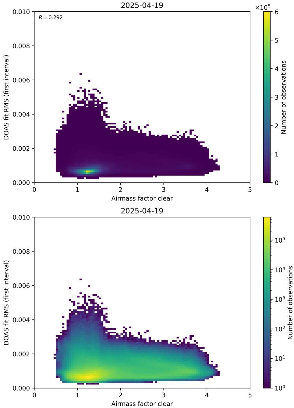
Figure 71: Scatter density plot of “Airmass factor clear” against “DOAS fit RMS (first interval)” for 2025-04-19 to 2025-04-20.
