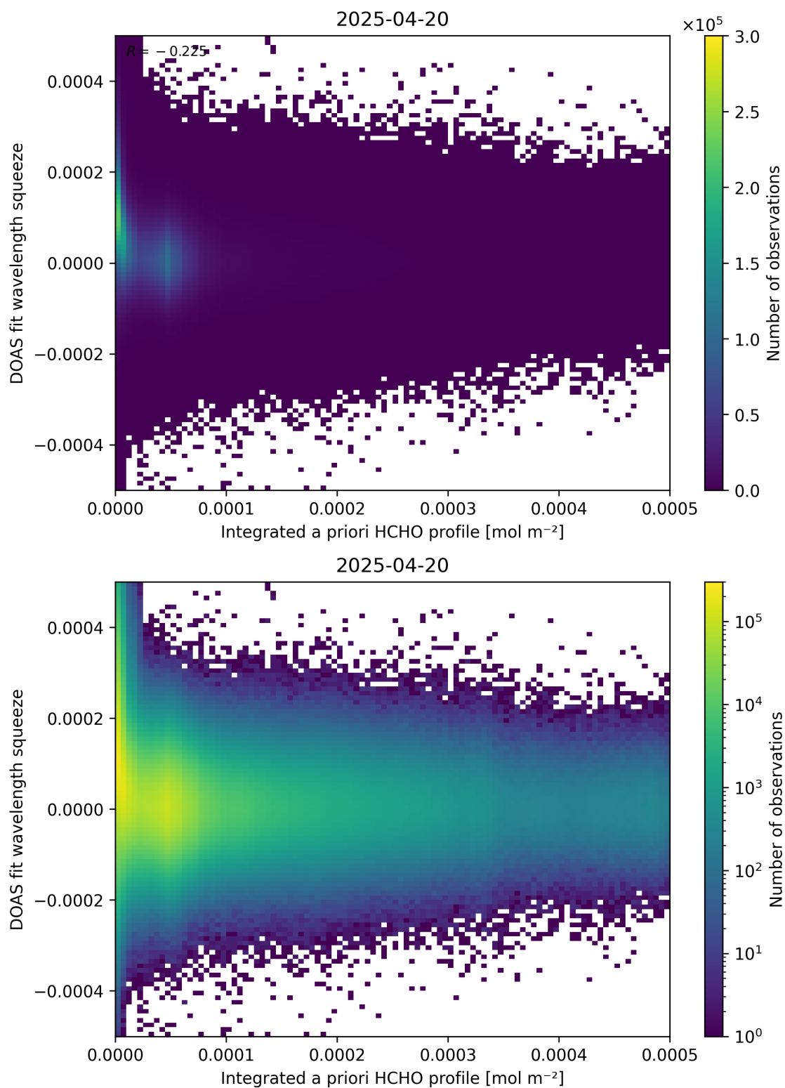
Figure 150: Scatter density plot of “Integrated a priori HCHO profile” against “DOAS fit wavelength squeeze” for 2025-04-19 to 2025-04-21.
