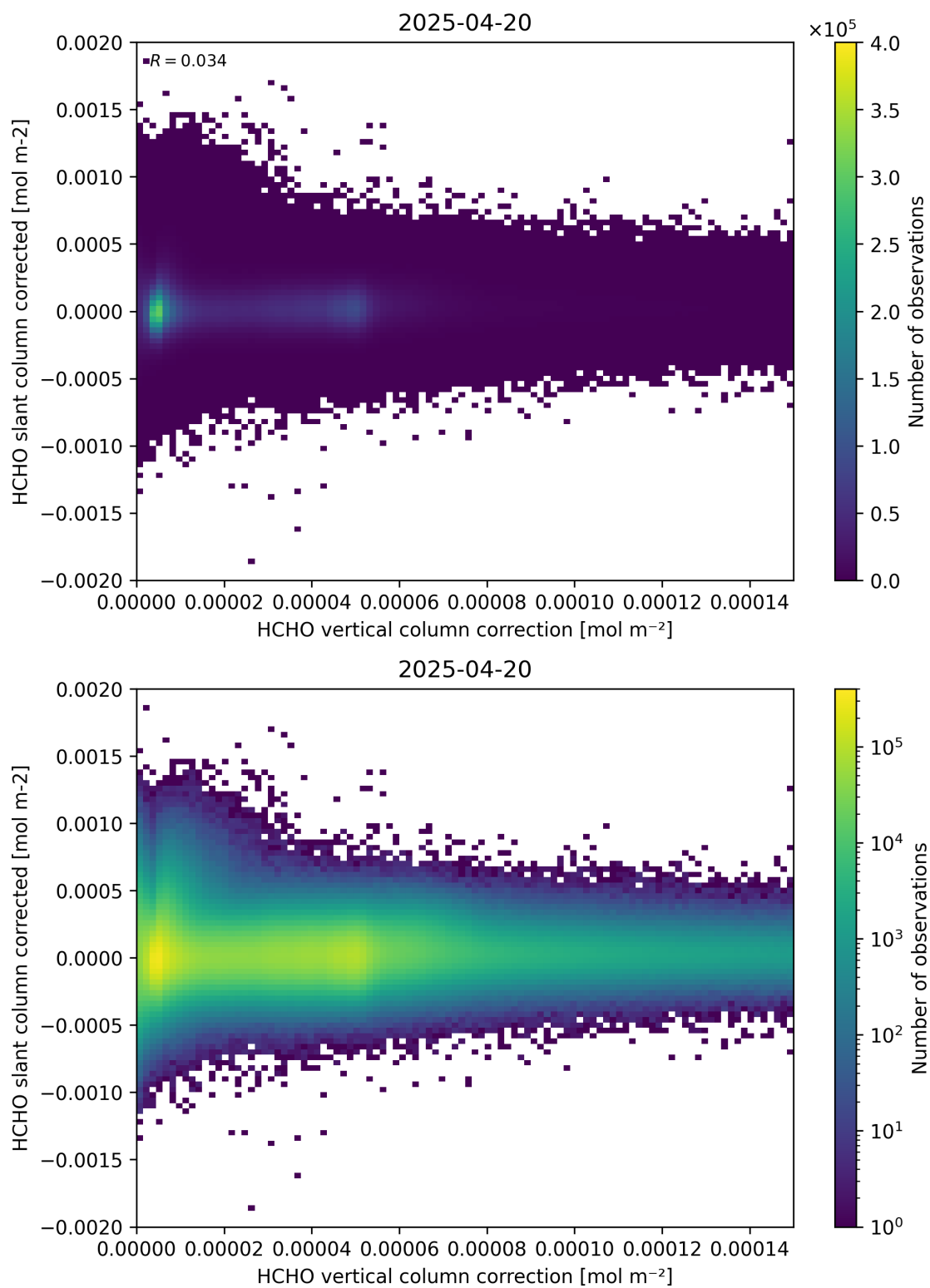
Figure 116: Scatter density plot of “HCHO vertical column correction” against “HCHO slant column corrected” for 2025-04-19 to 2025-04-21.
