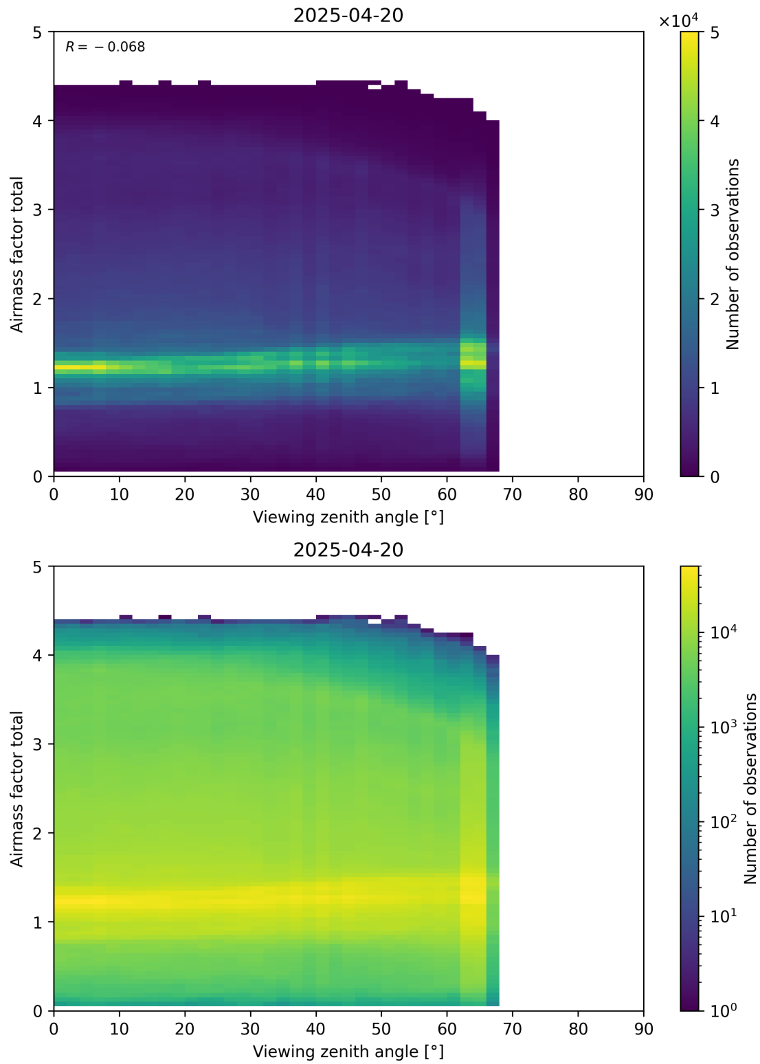
Figure 190: Scatter density plot of “Viewing zenith angle” against “Airmass factor total” for 2025-04-19 to 2025-04-21.
