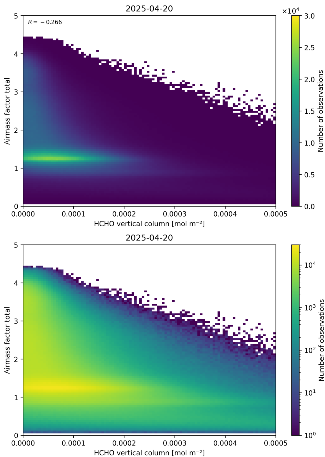
Figure 131: Scatter density plot of “HCHO vertical column” against “Airmass factor total” for 2025-04-19 to 2025-04-21.
