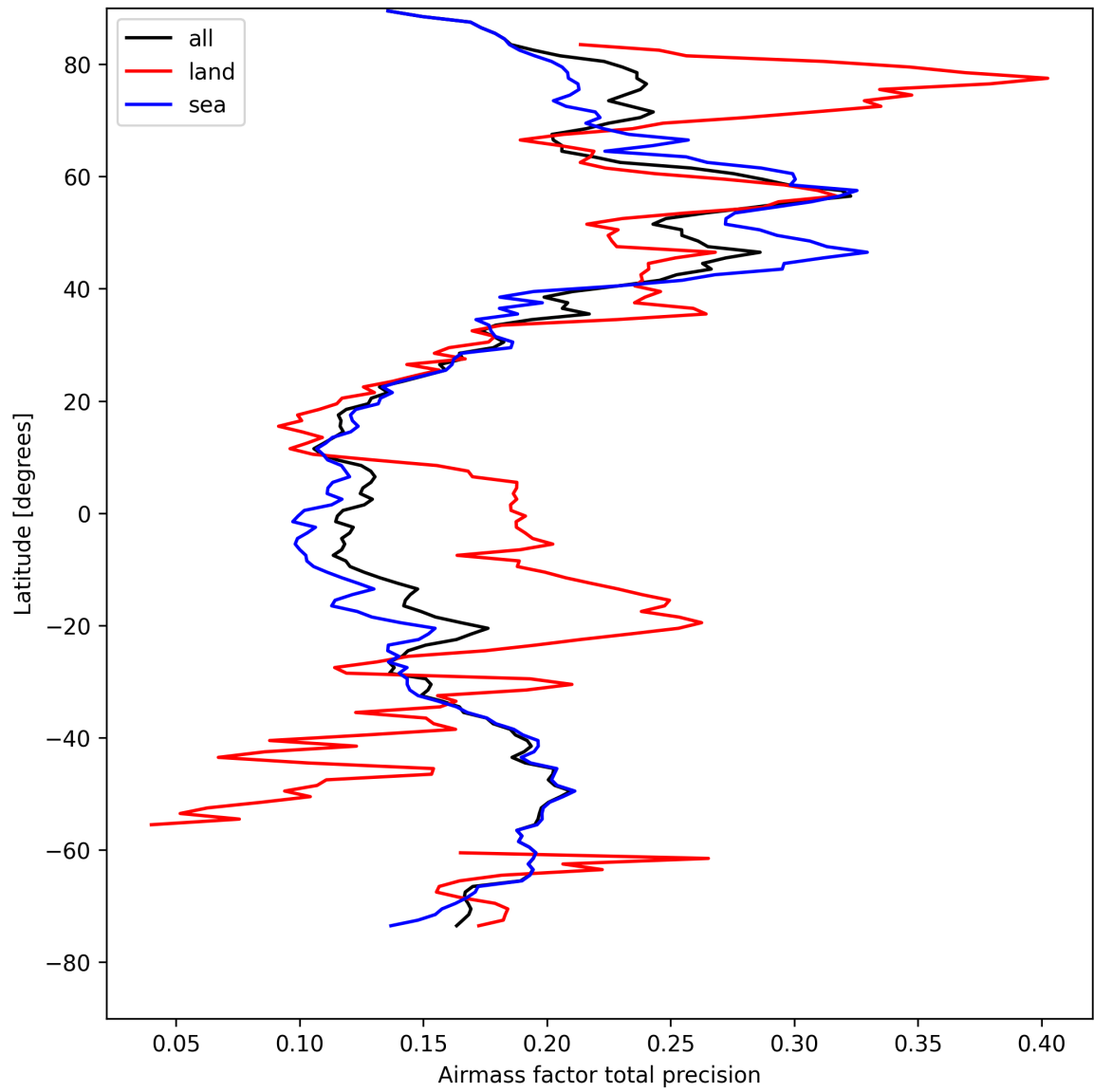
Figure 27: Zonal average of “Airmass factor total precision” for 2025-04-19 to 2025-04-21.
