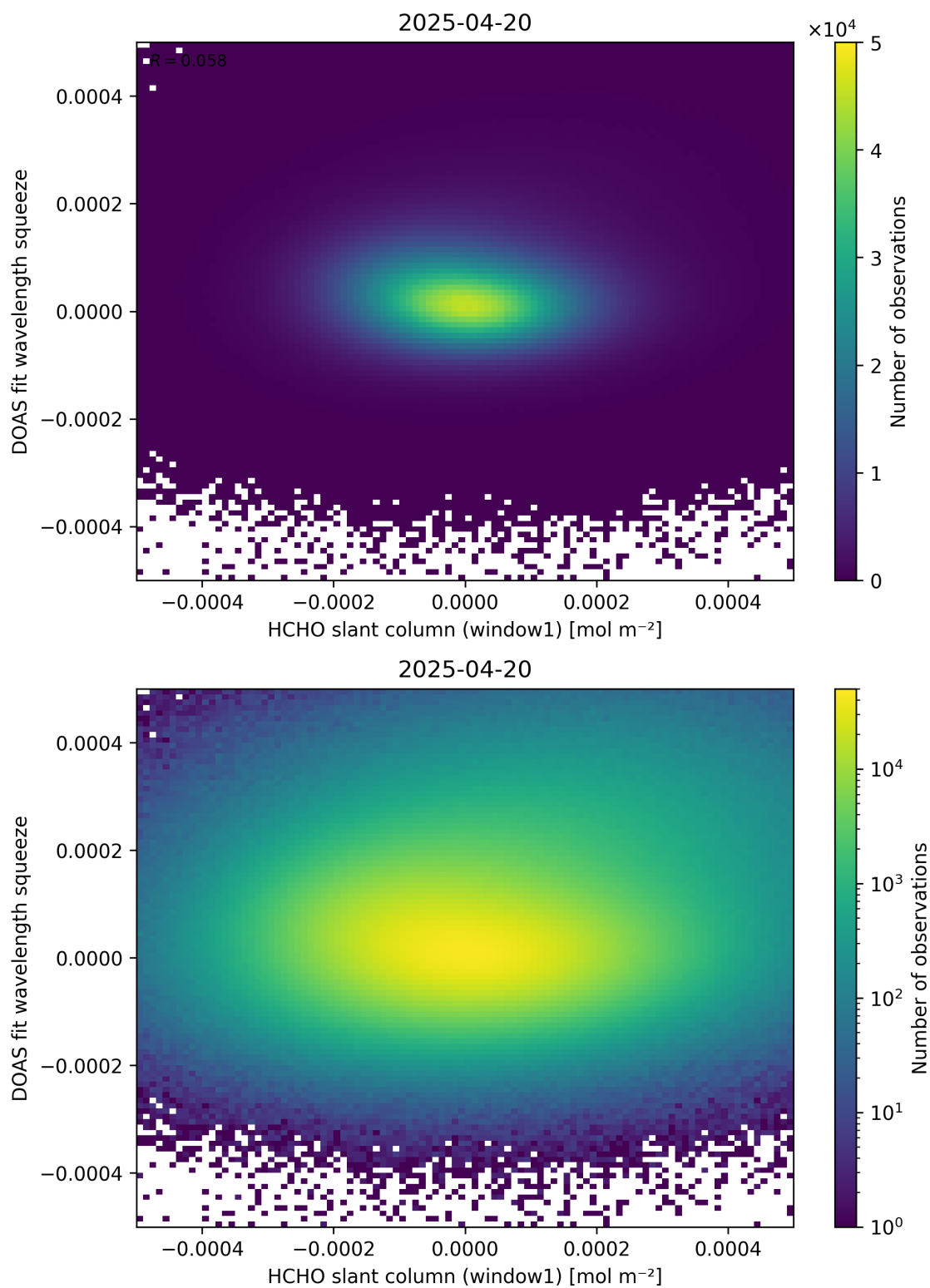
Figure 80: Scatter density plot of “HCHO slant column (window1)” against “DOAS fit wavelength squeeze” for 2025-04-19 to 2025-04-21.
