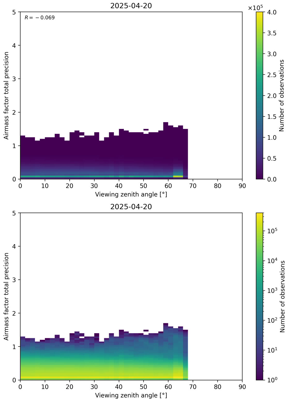
Figure 191: Scatter density plot of “Viewing zenith angle” against “Airmass factor total precision” for 2025-04-19 to 2025-04-21.
