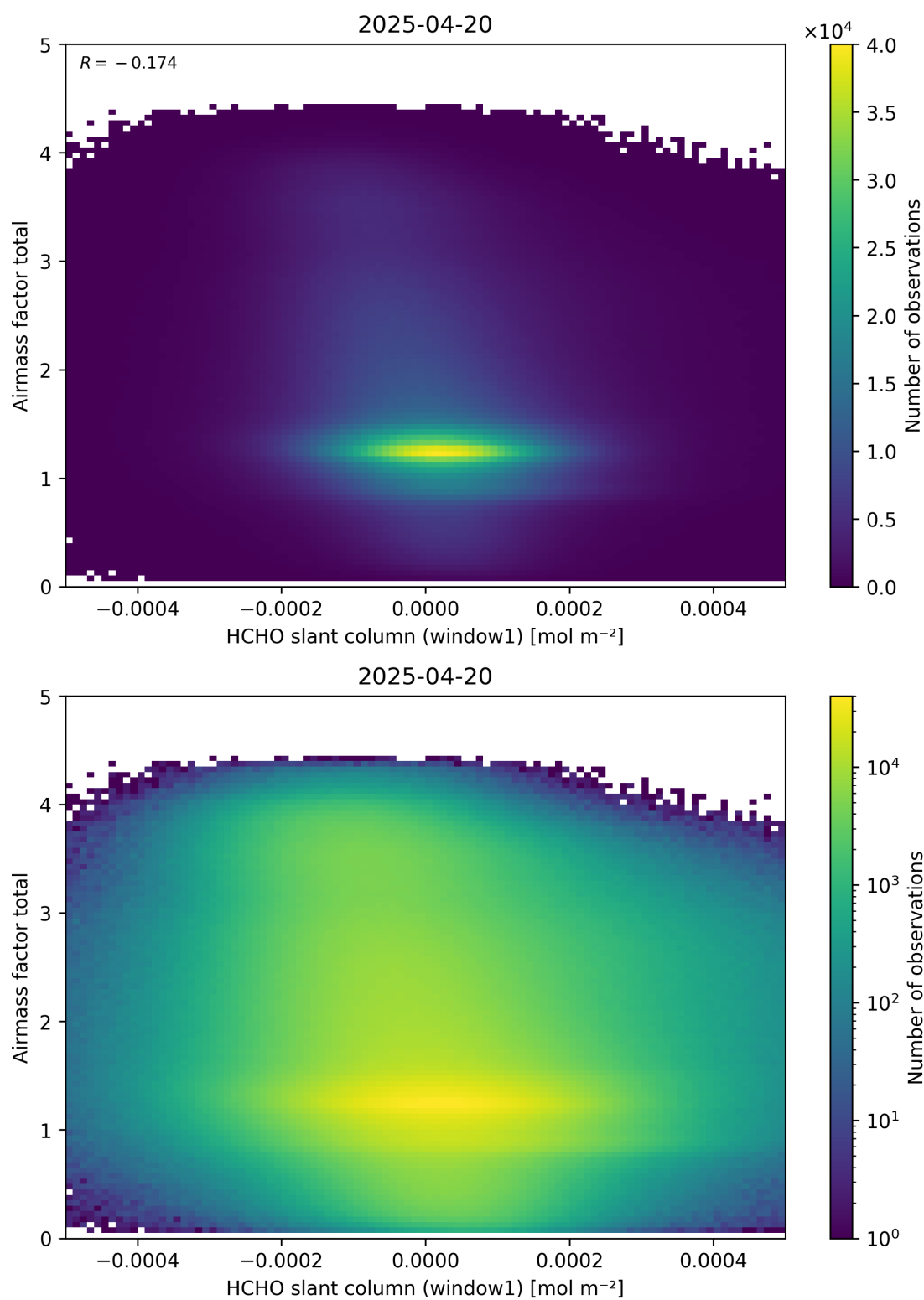
Figure 85: Scatter density plot of “HCHO slant column (window1)” against “Airmass factor total” for 2025-04-19 to 2025-04-21.
