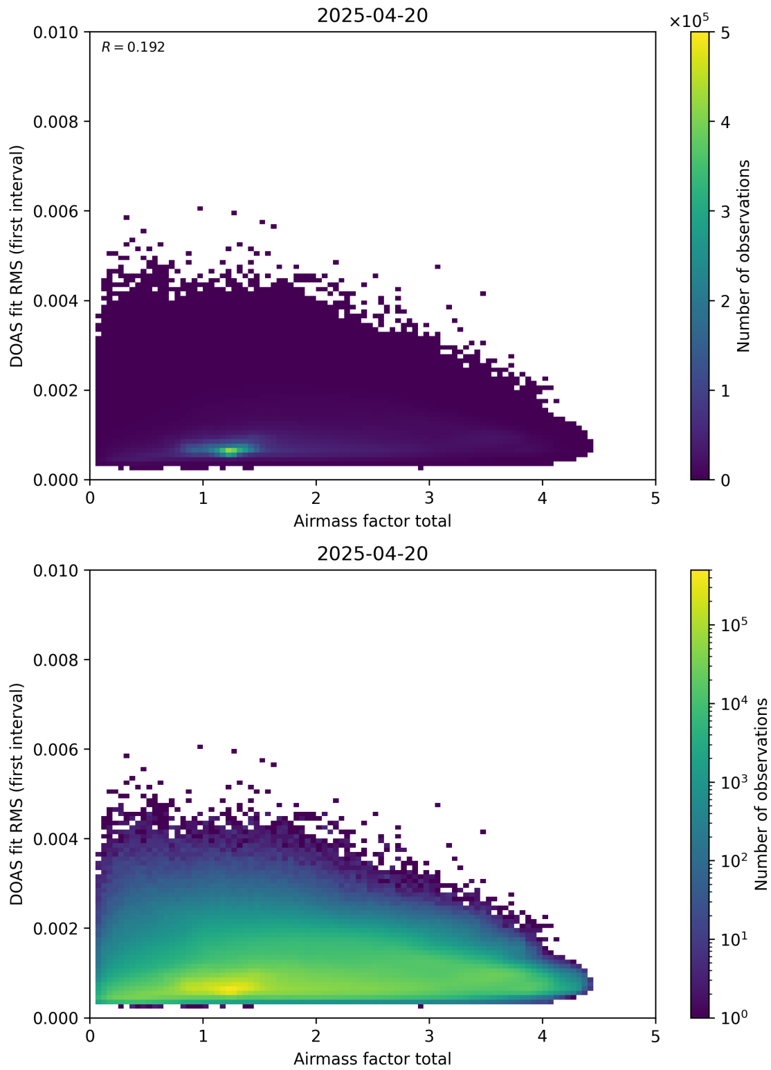
Figure 97: Scatter density plot of “Airmass factor total” against “DOAS fit RMS (first interval)” for 2025-04-19 to 2025-04-21.
