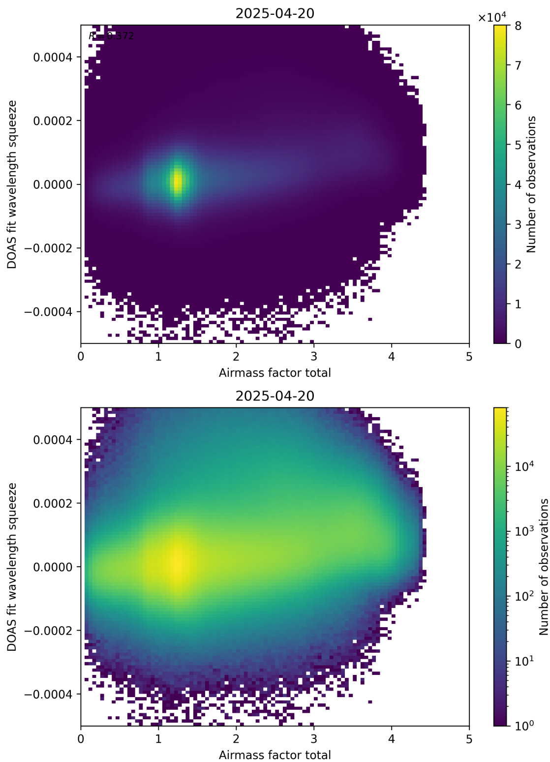
Figure 99: Scatter density plot of “Airmass factor total” against “DOAS fit wavelength squeeze” for 2025-04-19 to 2025-04-21.
