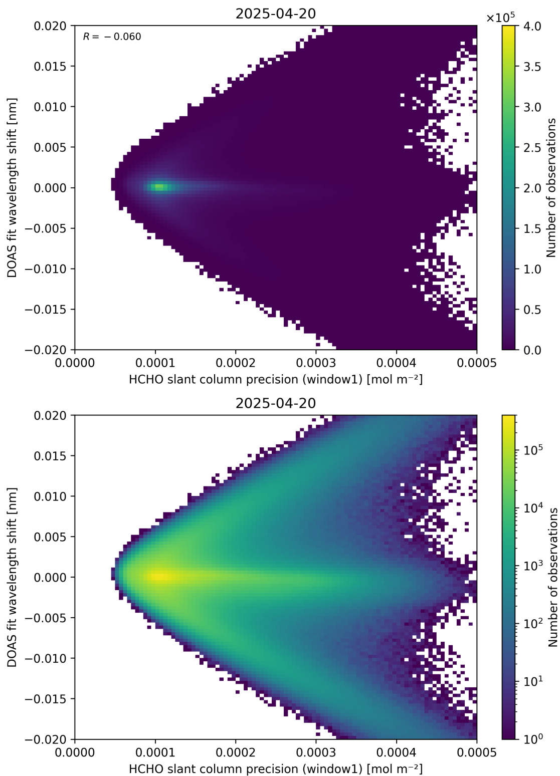
Figure 89: Scatter density plot of “HCHO slant column precision (window1)” against “DOAS fit wavelength shift” for 2025-04-19 to 2025-04-21.
