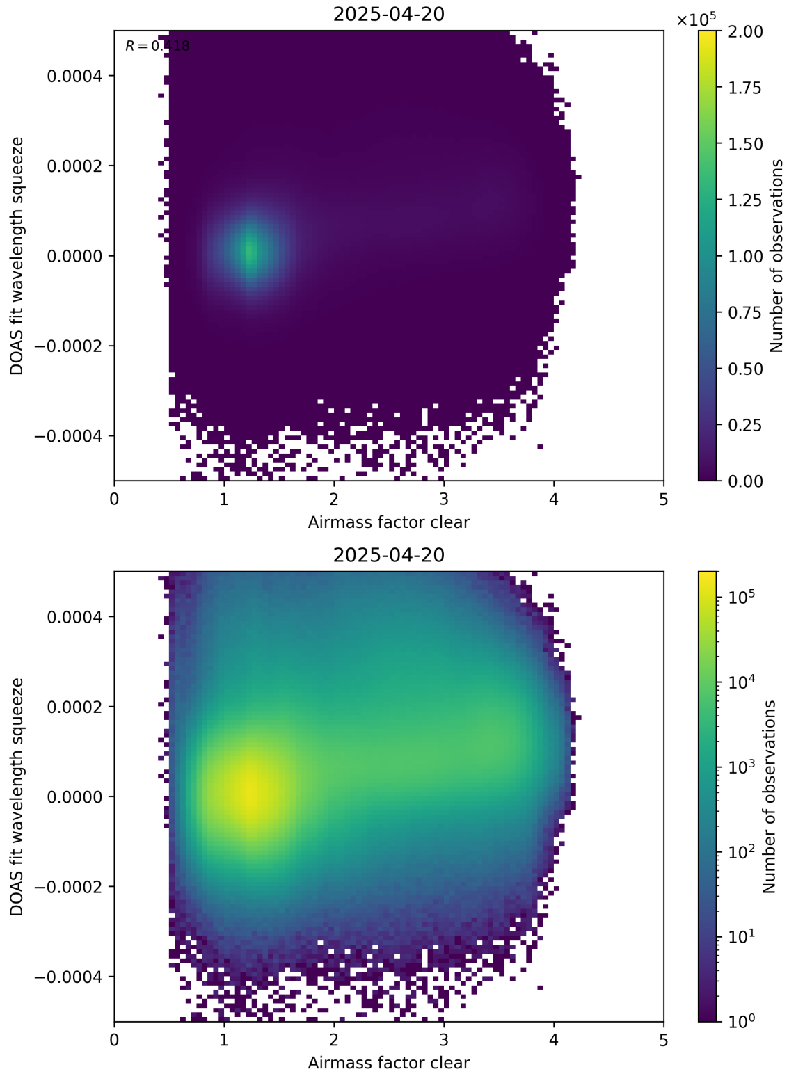
Figure 73: Scatter density plot of “Airmass factor clear” against “DOAS fit wavelength squeeze” for 2025-04-19 to 2025-04-21.
