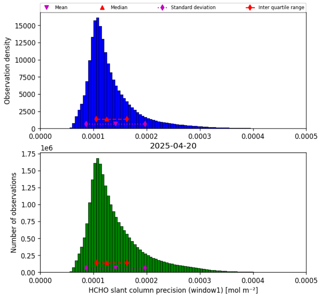
Figure 39: Histogram of “HCHO slant column precision (window1)” for 2025-04-19 to 2025-04-21
