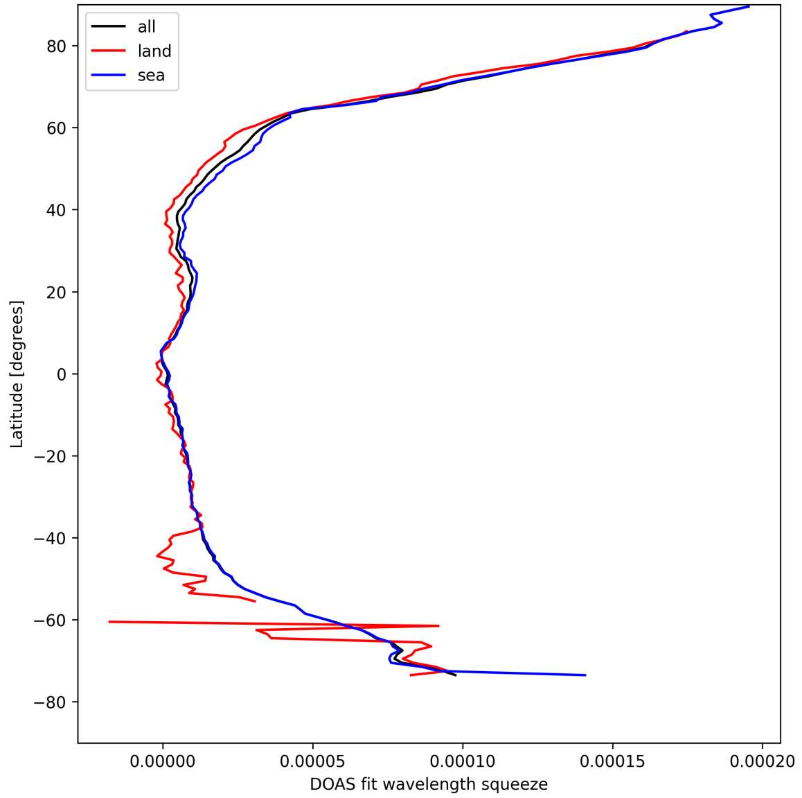
Figure 31: Zonal average of “DOAS fit wavelength squeeze” for 2025-04-19 to 2025-04-21.
