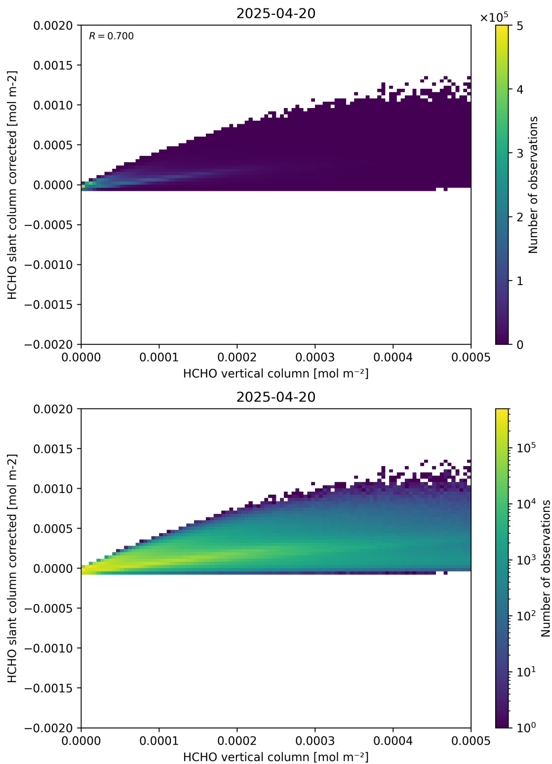
Figure 127: Scatter density plot of “HCHO vertical column” against “HCHO slant column corrected” for 2025-04-19 to 2025-04-21.
