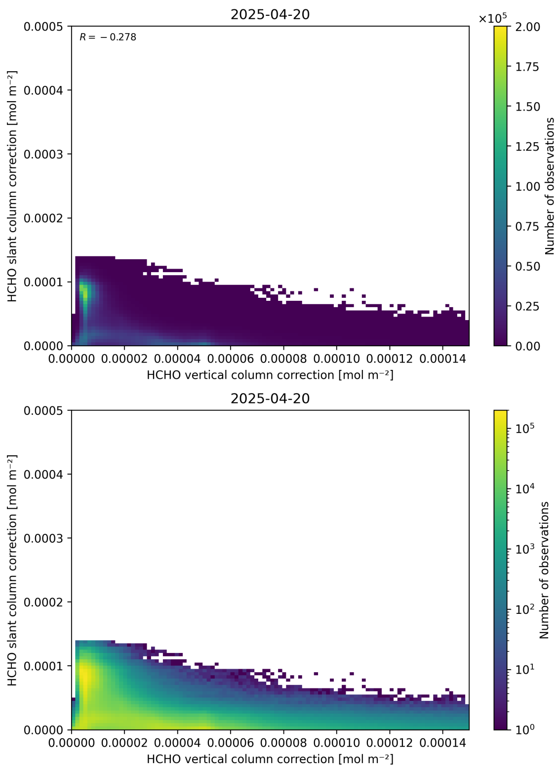
Figure 117: Scatter density plot of “HCHO vertical column correction” against “HCHO slant column correction” for 2025-04-19 to 2025-04-21.
