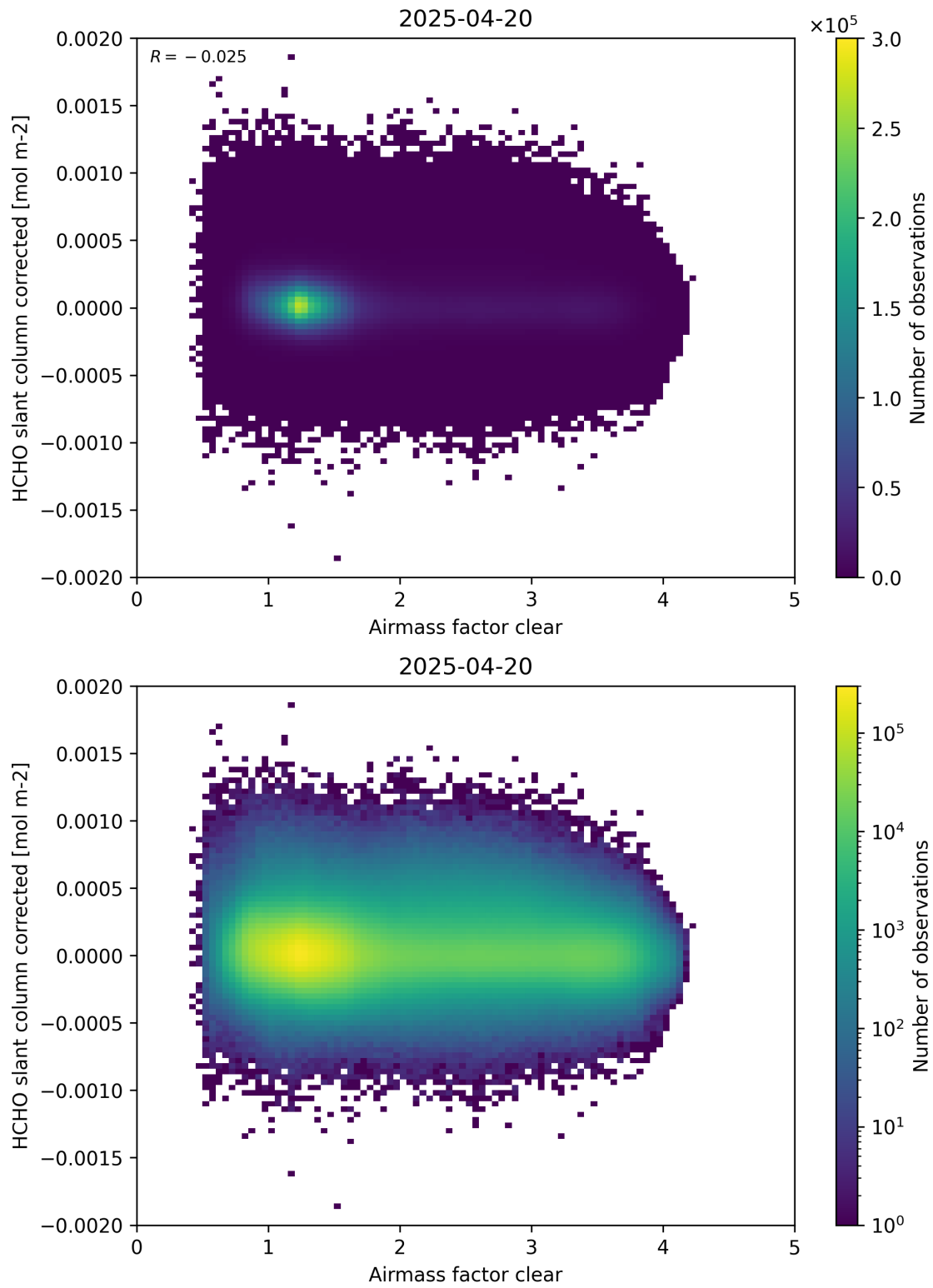
Figure 74: Scatter density plot of “Airmass factor clear” against “HCHO slant column corrected” for 2025-04-19 to 2025-04-21.
