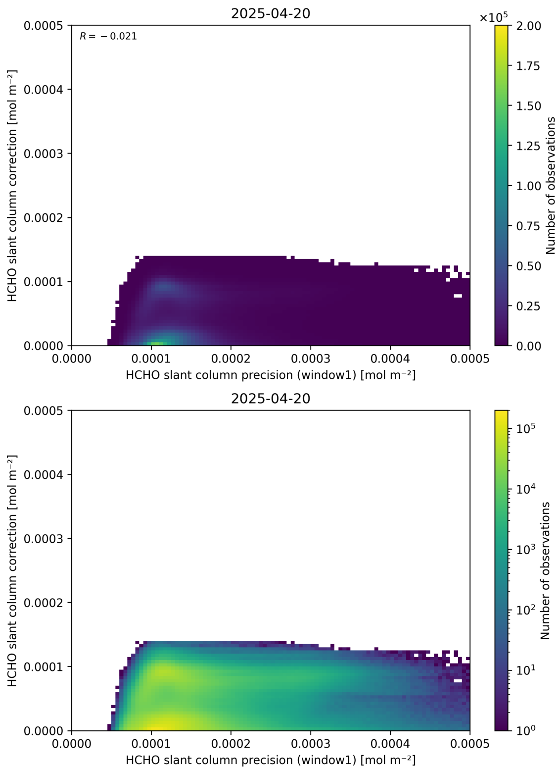
Figure 93: Scatter density plot of “HCHO slant column precision (window1)” against “HCHO slant column correction” for 2025-04-19 to 2025-04-21.
