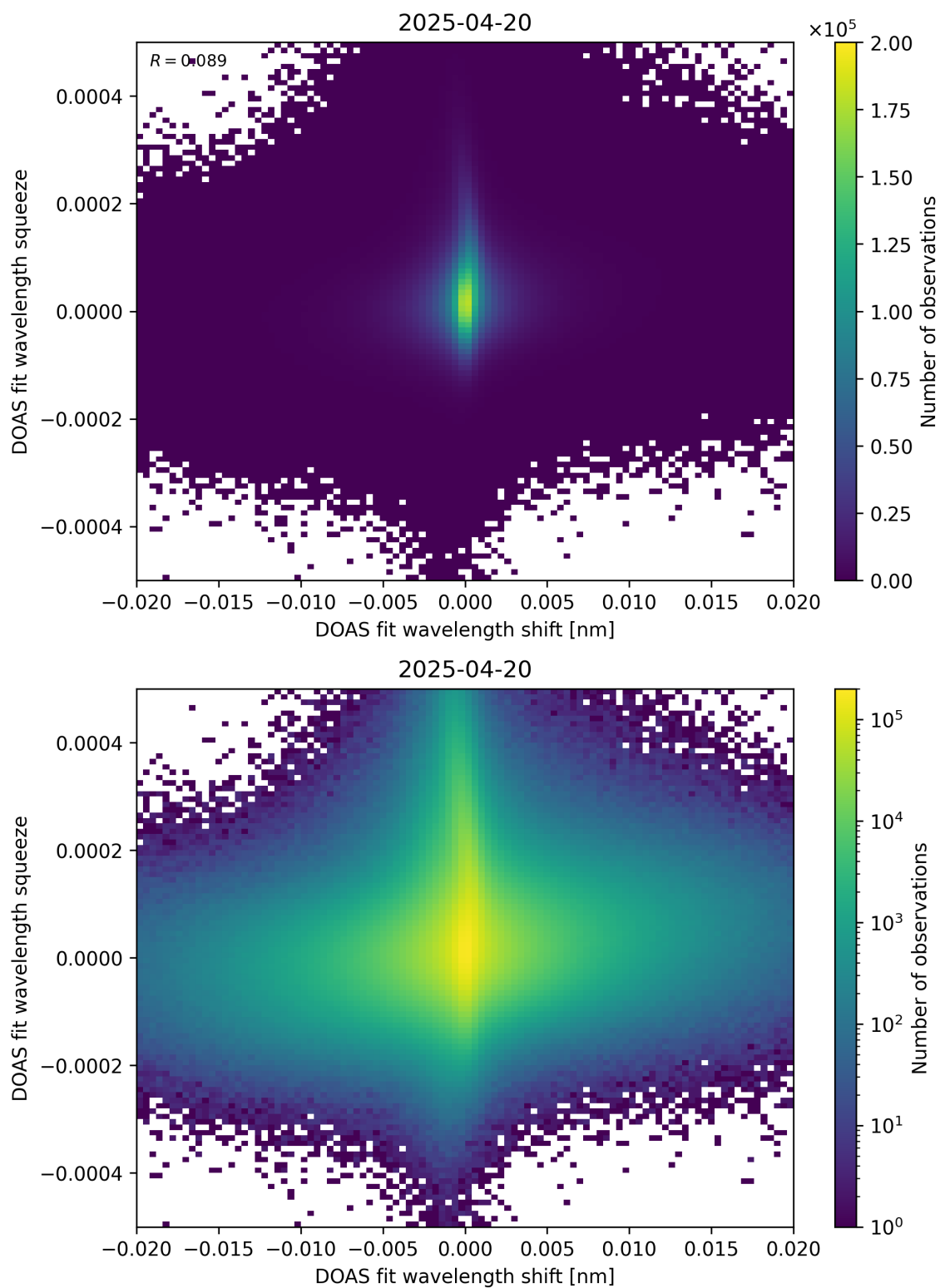
Figure 65: Scatter density plot of “DOAS fit wavelength shift” against “DOAS fit wavelength squeeze” for 2025-04-19 to 2025-04-21.
