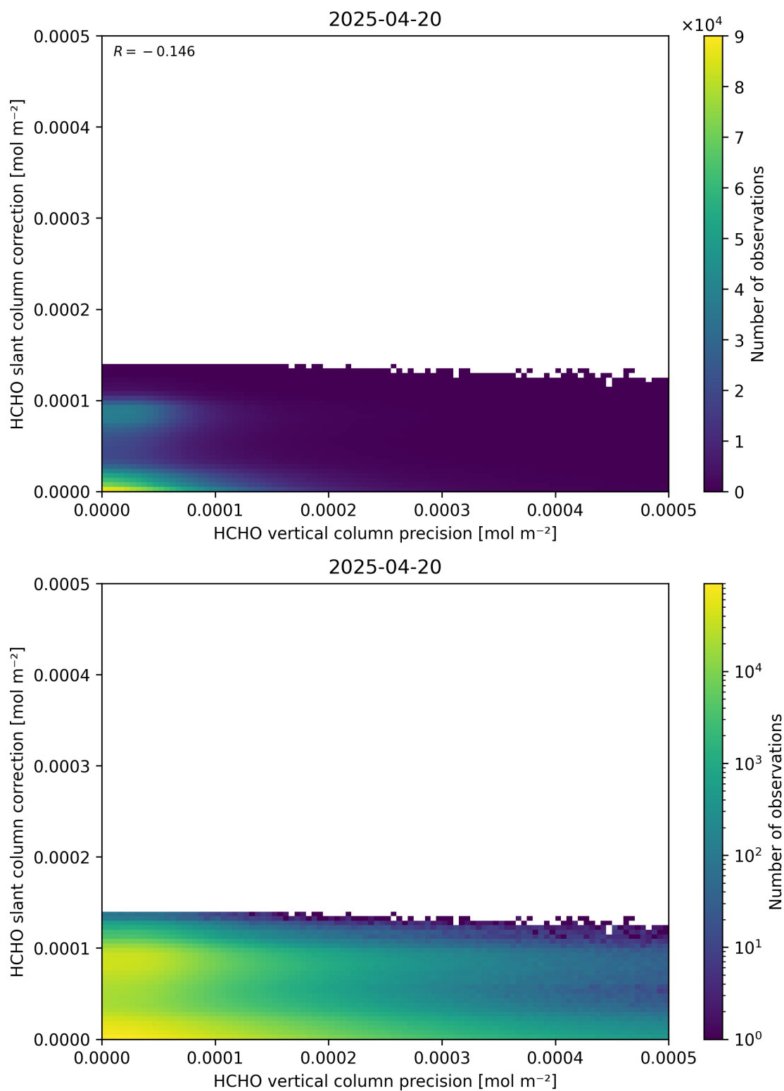
Figure 141: Scatter density plot of “HCHO vertical column precision” against “HCHO slant column correction” for 2025-04-19 to 2025-04-21.
