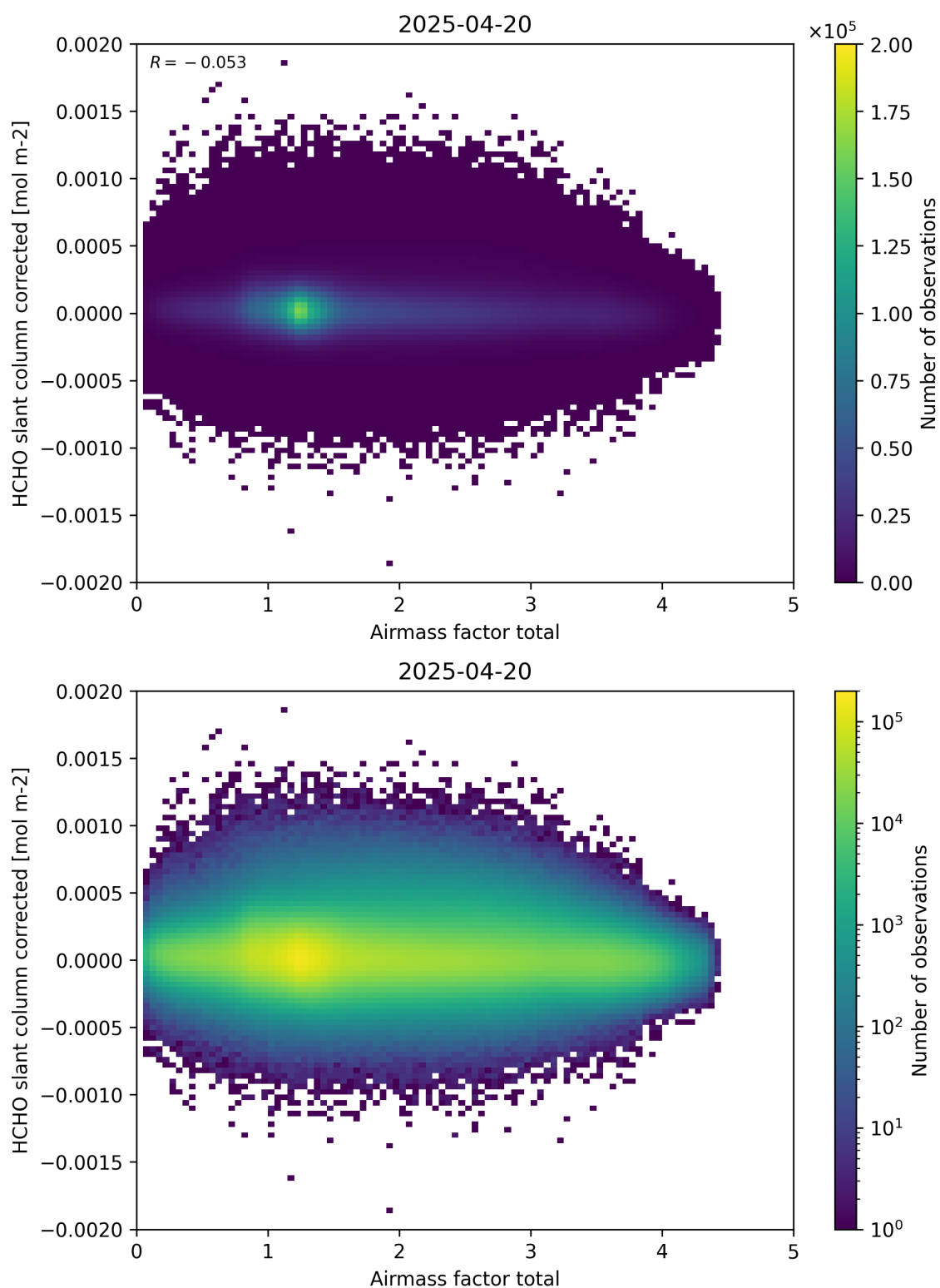
Figure 101: Scatter density plot of “Airmass factor total” against “HCHO slant column corrected” for 2025-04-19 to 2025-04-21.
