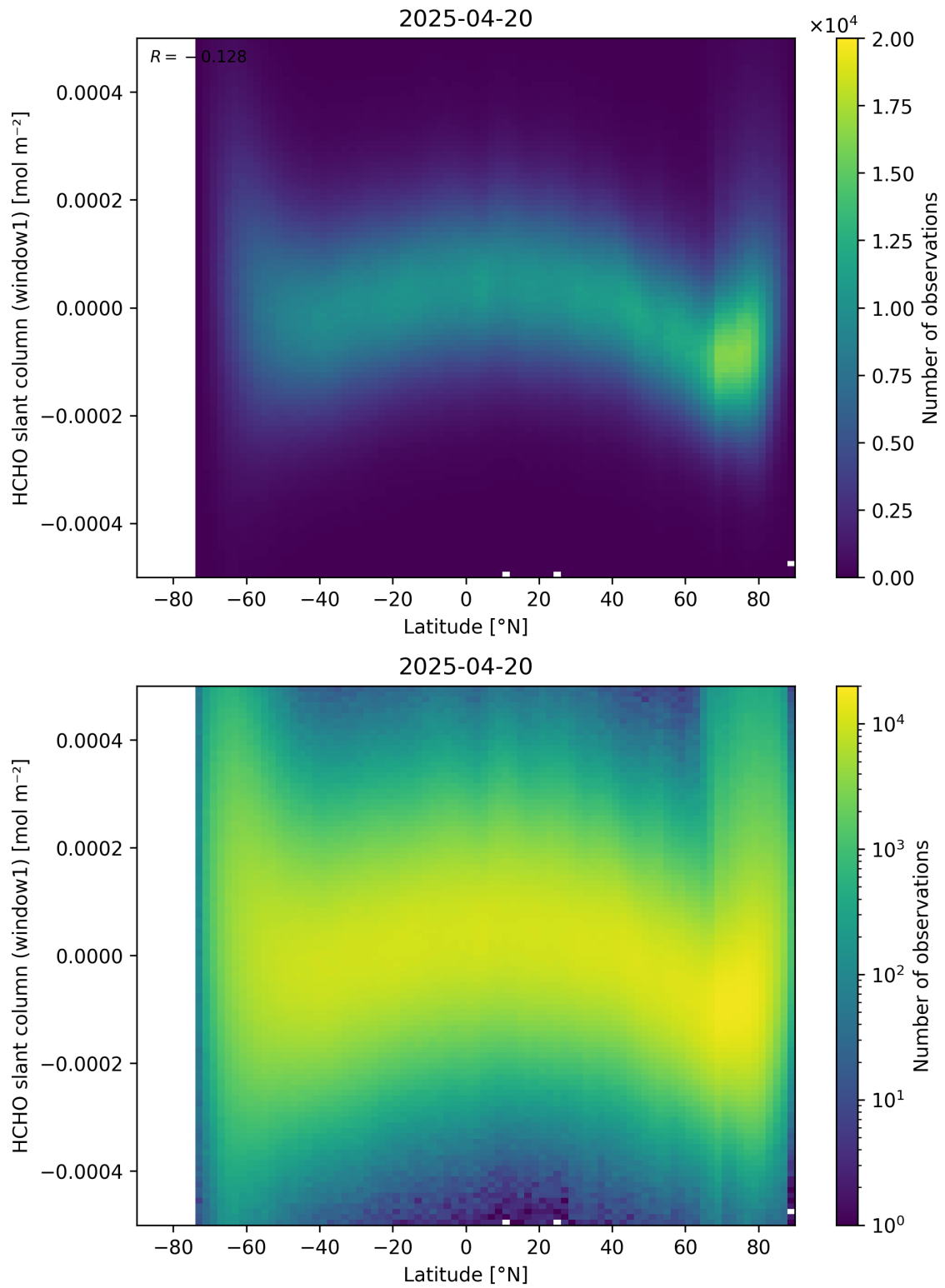
Figure 159: Scatter density plot of “Latitude” against “HCHO slant column (window1)” for 2025-04-19 to 2025-04-21.
