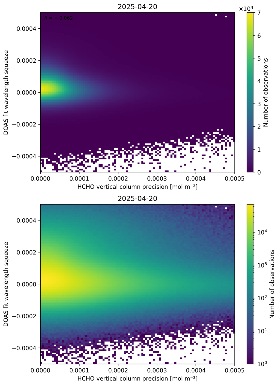
Figure 138: Scatter density plot of “HCHO vertical column precision” against “DOAS fit wavelength squeeze” for 2025-04-19 to 2025-04-21.
