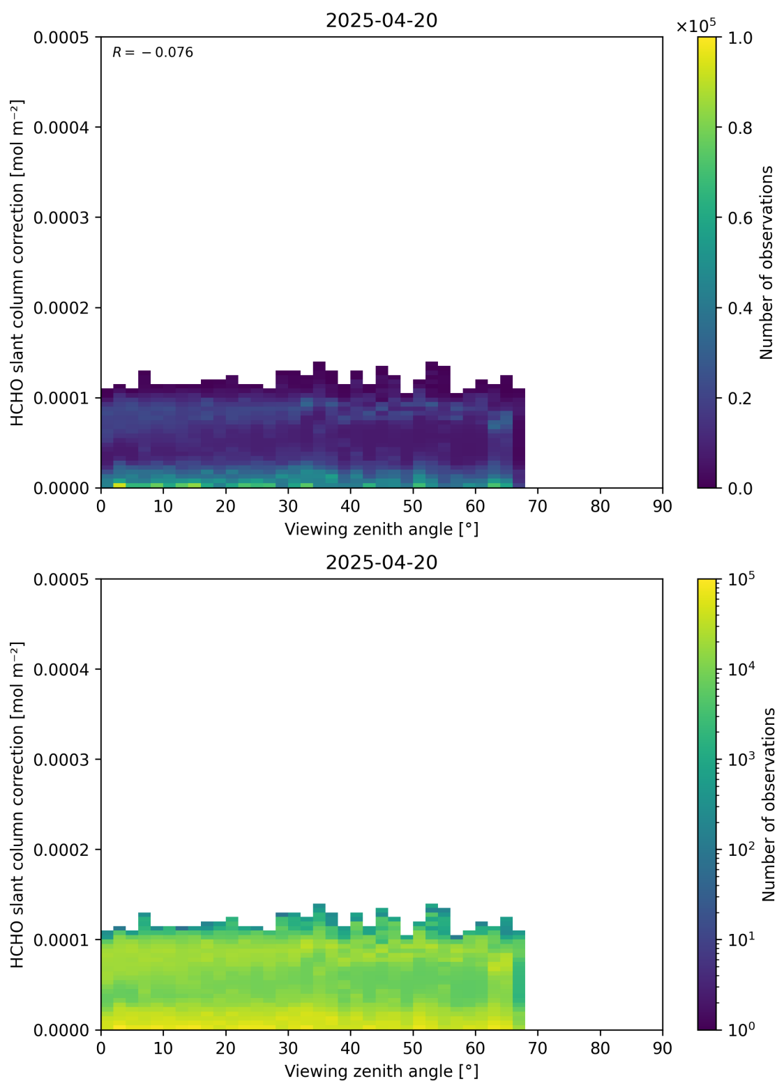
Figure 187: Scatter density plot of “Viewing zenith angle” against “HCHO slant column correction” for 2025-04-19 to 2025-04-21.
