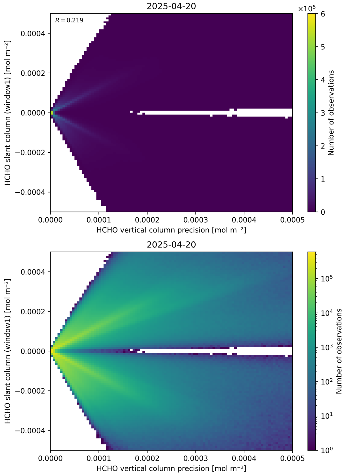
Figure 142: Scatter density plot of “HCHO vertical column precision” against “HCHO slant column (window1)” for 2025-04-19 to 2025-04-21.
