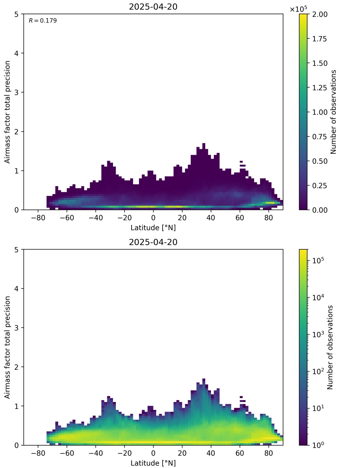
Figure 162: Scatter density plot of “Latitude” against “Airmass factor total precision” for 2025-04-19 to 2025-04-21.
