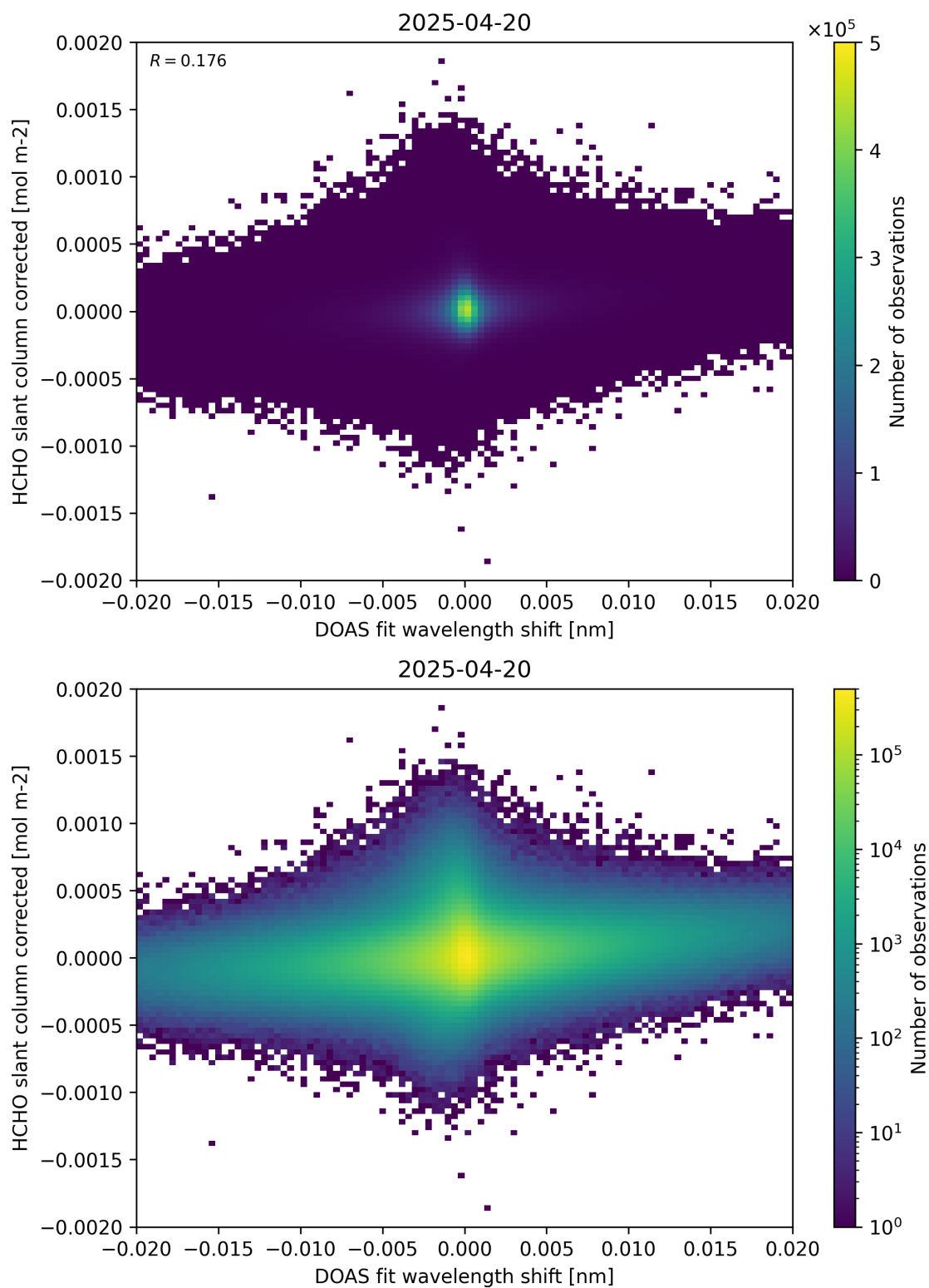
Figure 66: Scatter density plot of “DOAS fit wavelength shift” against “HCHO slant column corrected” for 2025-04-19 to 2025-04-21.
