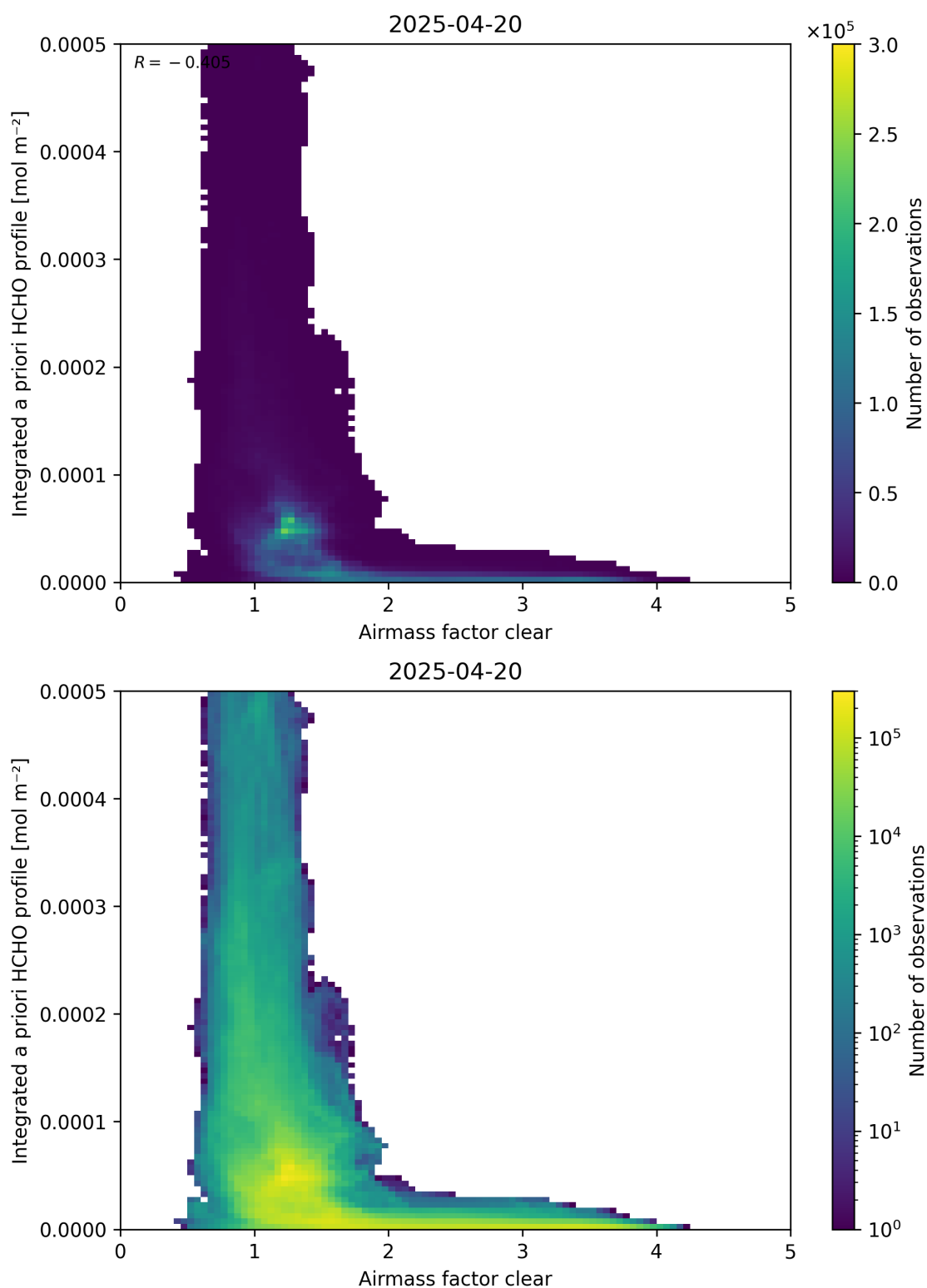
Figure 76: Scatter density plot of “Airmass factor clear” against “Integrated a priori HCHO profile” for 2025-04-19 to 2025-04-21.
