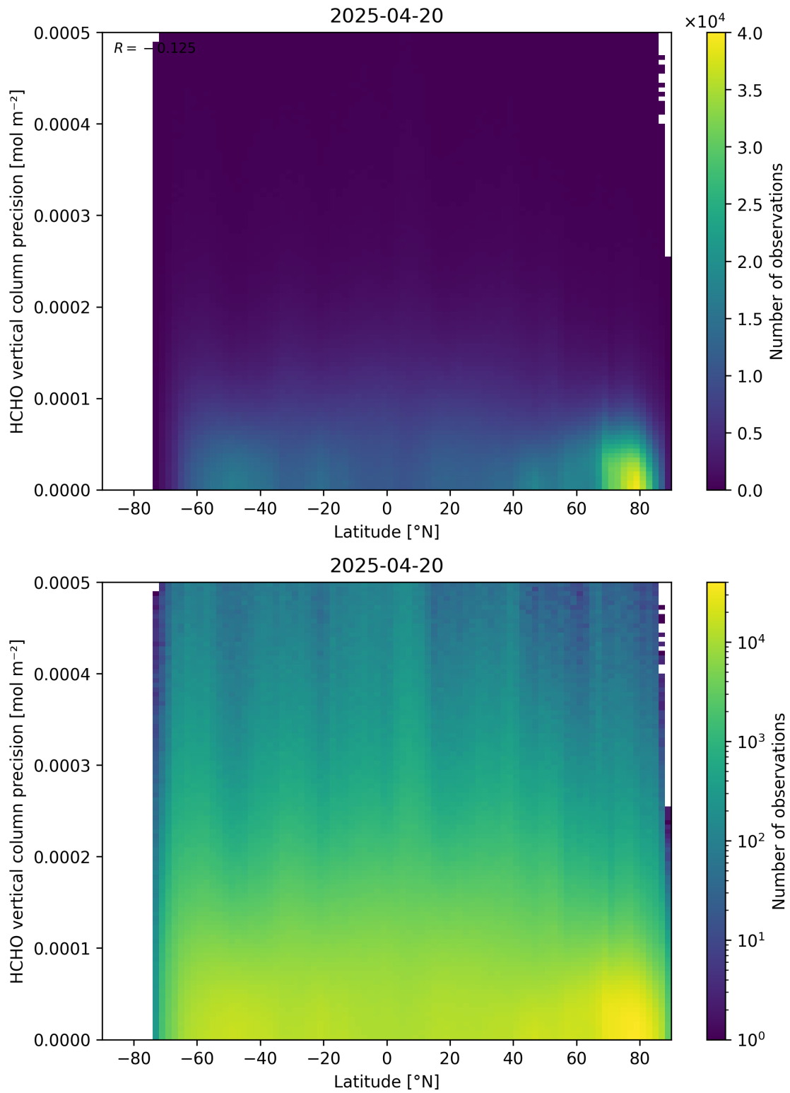
Figure 165: Scatter density plot of “Latitude” against “HCHO vertical column precision” for 2025-04-19 to 2025-04-21.
