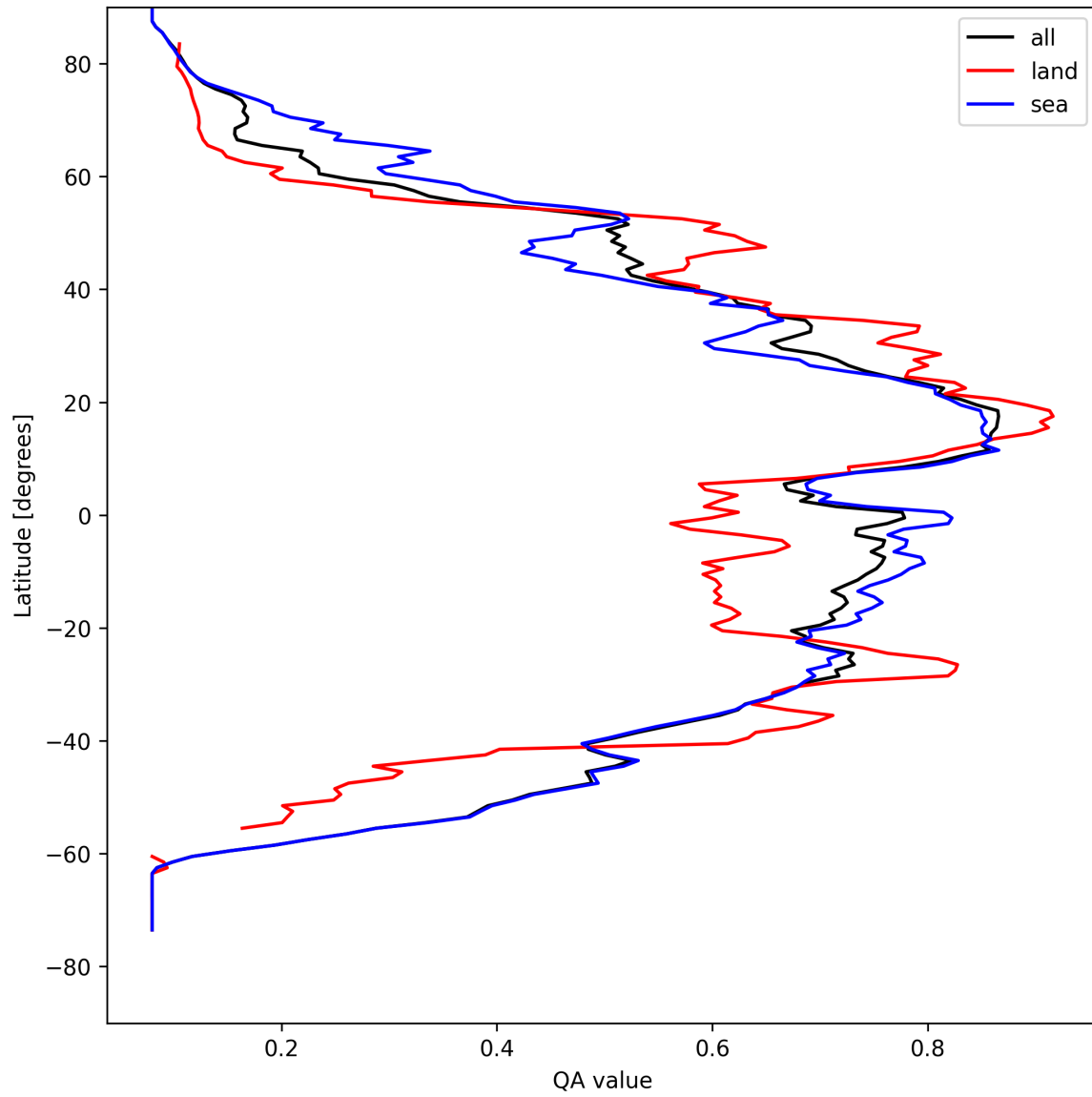
Figure 20: Zonal average of “QA value” for 2025-04-19 to 2025-04-21.
