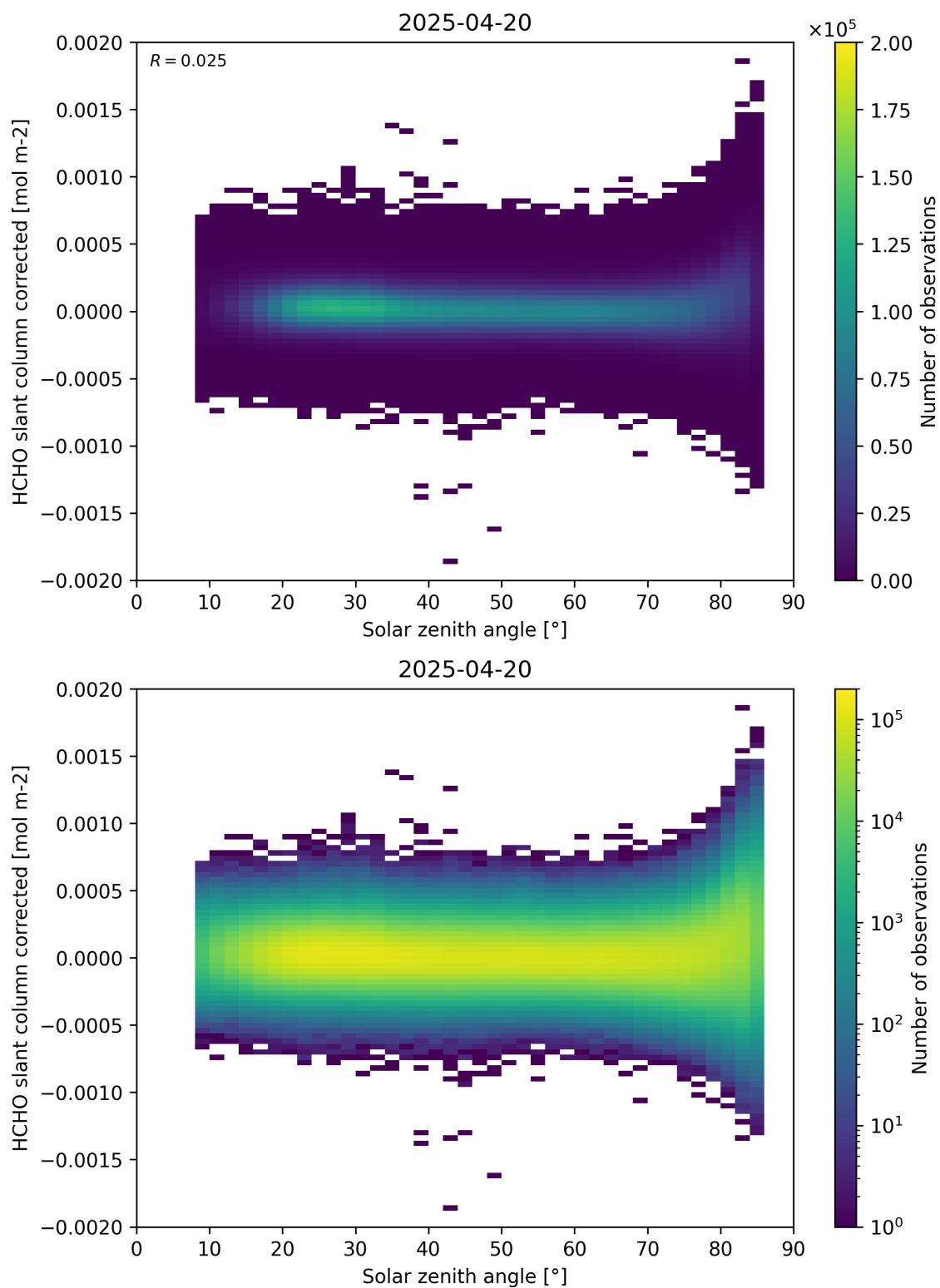
Figure 171: Scatter density plot of “Solar zenith angle” against “HCHO slant column corrected” for 2025-04-19 to 2025-04-21.
