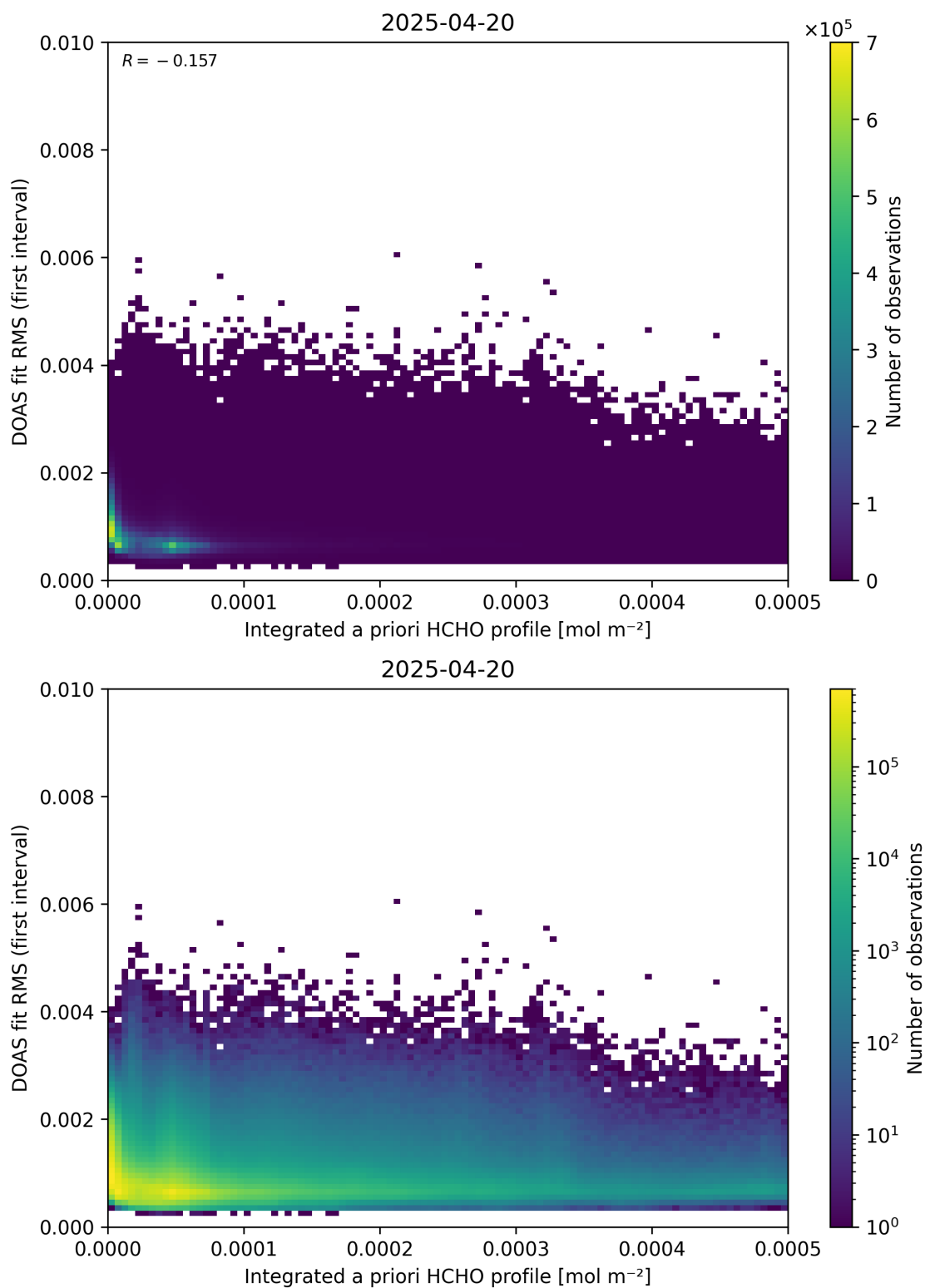
Figure 148: Scatter density plot of “Integrated a priori HCHO profile” against “DOAS fit RMS (first interval)” for 2025-04-19 to 2025-04-21.
