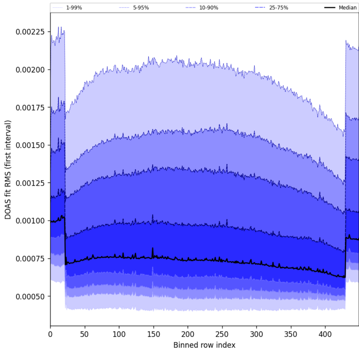
Figure 60: Along track statistics of “DOAS fit RMS (first interval)” for 2025-04-19 to 2025-04-21
