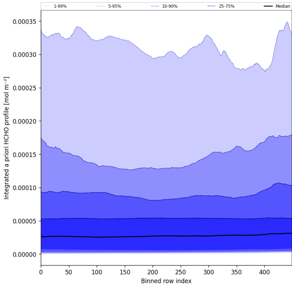
Figure 57: Along track statistics of “Integrated a priori HCHO profile” for 2025-04-19 to 2025-04-21
