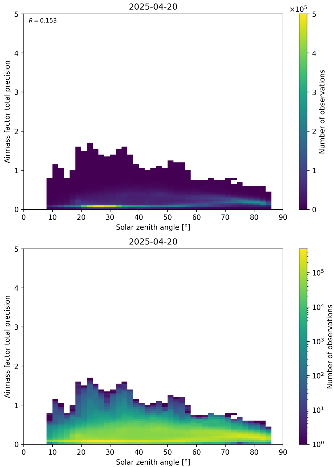
Figure 176: Scatter density plot of “Solar zenith angle” against “Airmass factor total precision” for 2025-04-19 to 2025-04-21.
