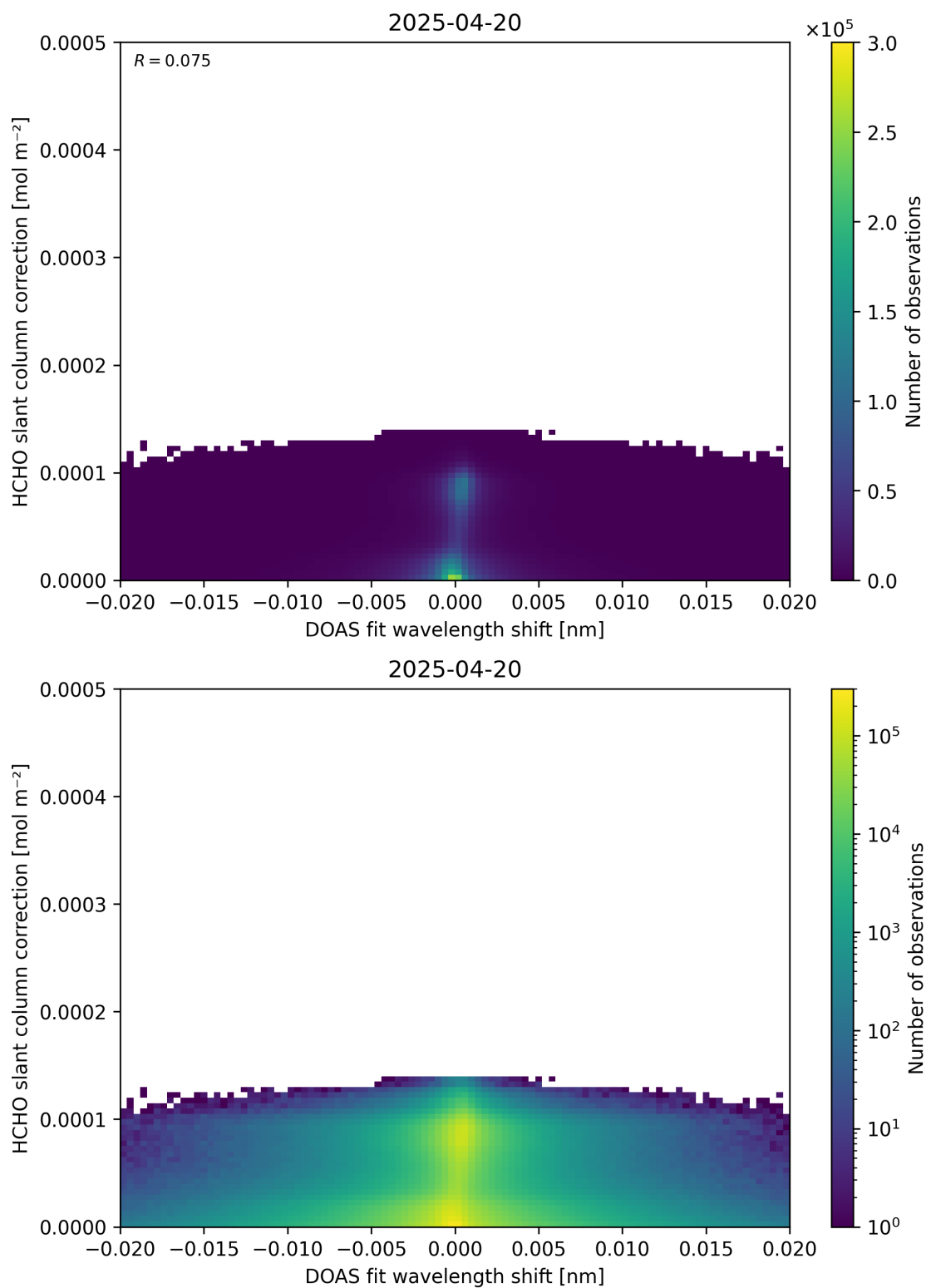
Figure 67: Scatter density plot of “DOAS fit wavelength shift” against “HCHO slant column correction” for 2025-04-19 to 2025-04-21.
