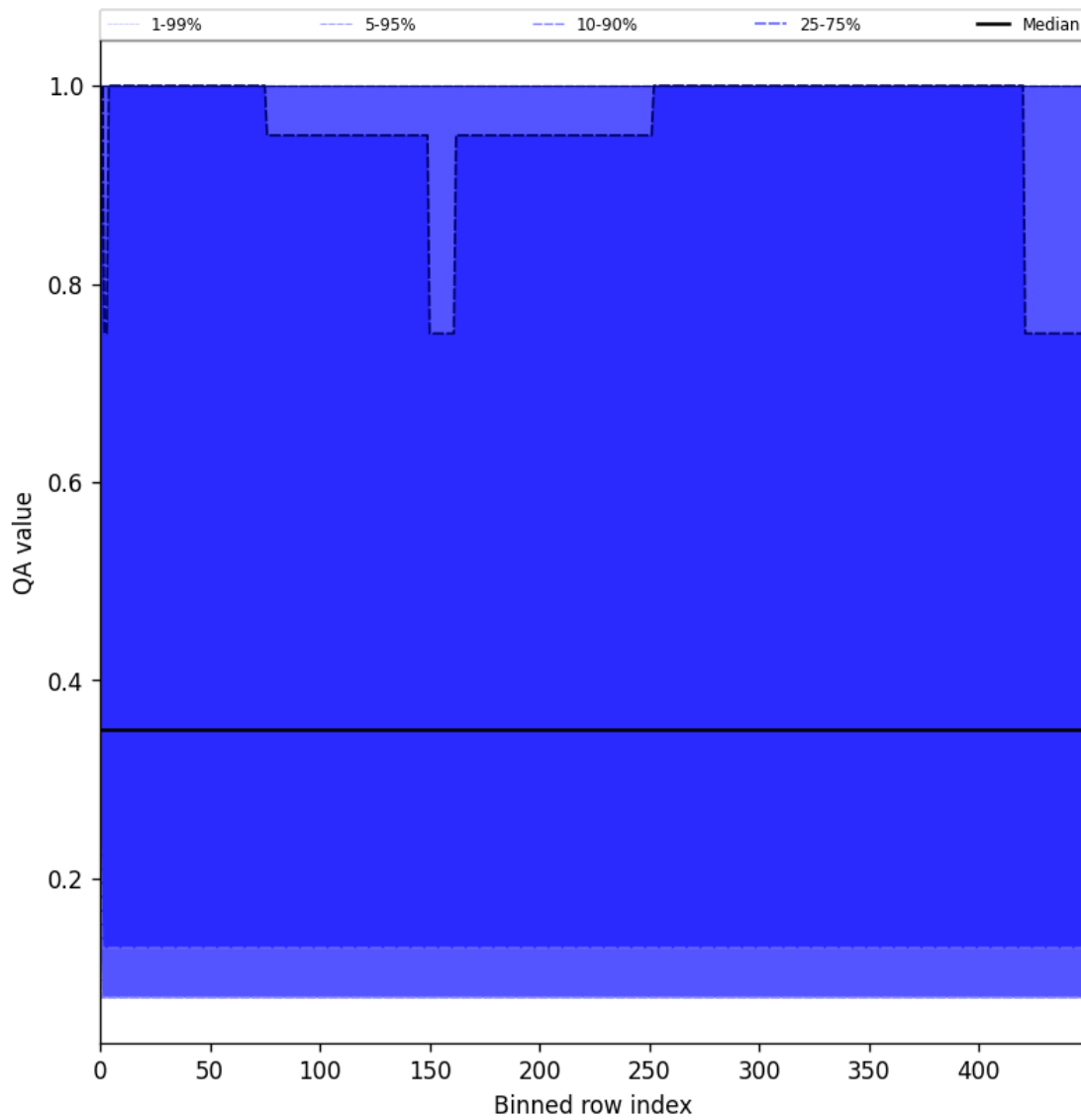
Figure 48: Along track statistics of “QA value” for 2025-04-19 to 2025-04-21
