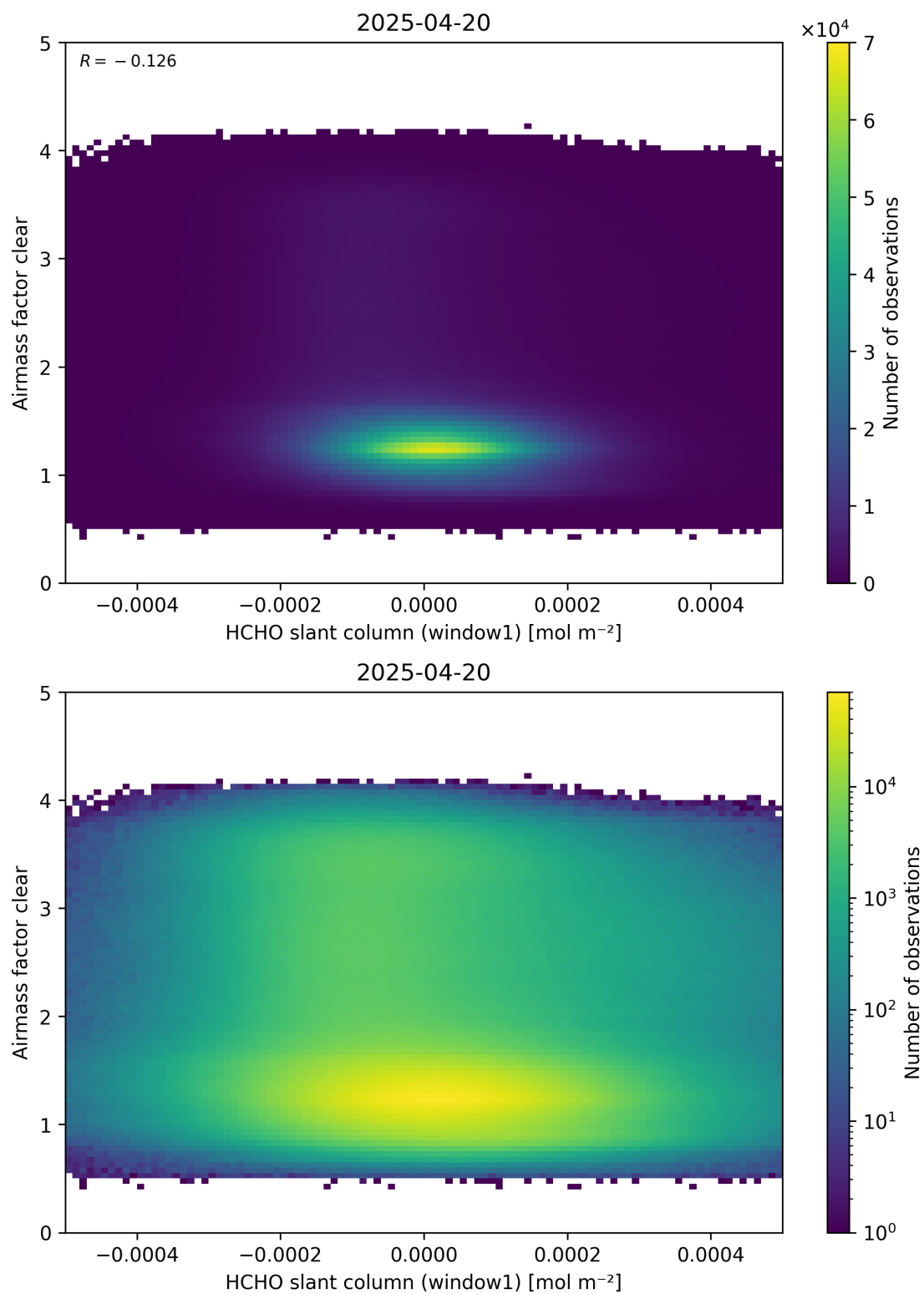
Figure 81: Scatter density plot of “HCHO slant column (window1)” against “Airmass factor clear” for 2025-04-19 to 2025-04-21.
