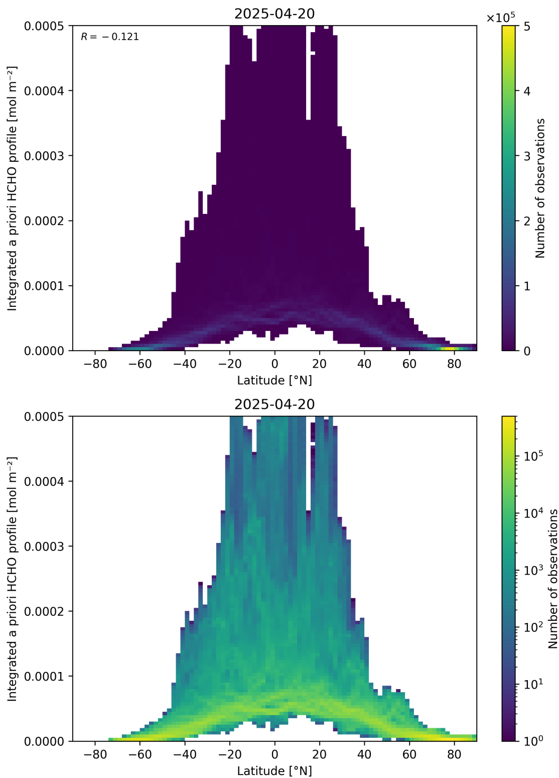
Figure 166: Scatter density plot of “Latitude” against “Integrated a priori HCHO profile” for 2025-04-19 to 2025-04-21.
