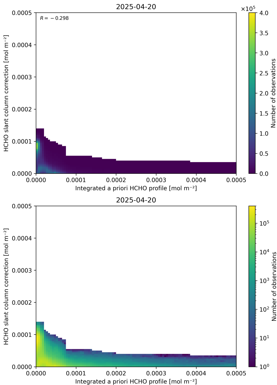
Figure 152: Scatter density plot of “Integrated a priori HCHO profile” against “HCHO slant column correction” for 2025-04-19 to 2025-04-21.
