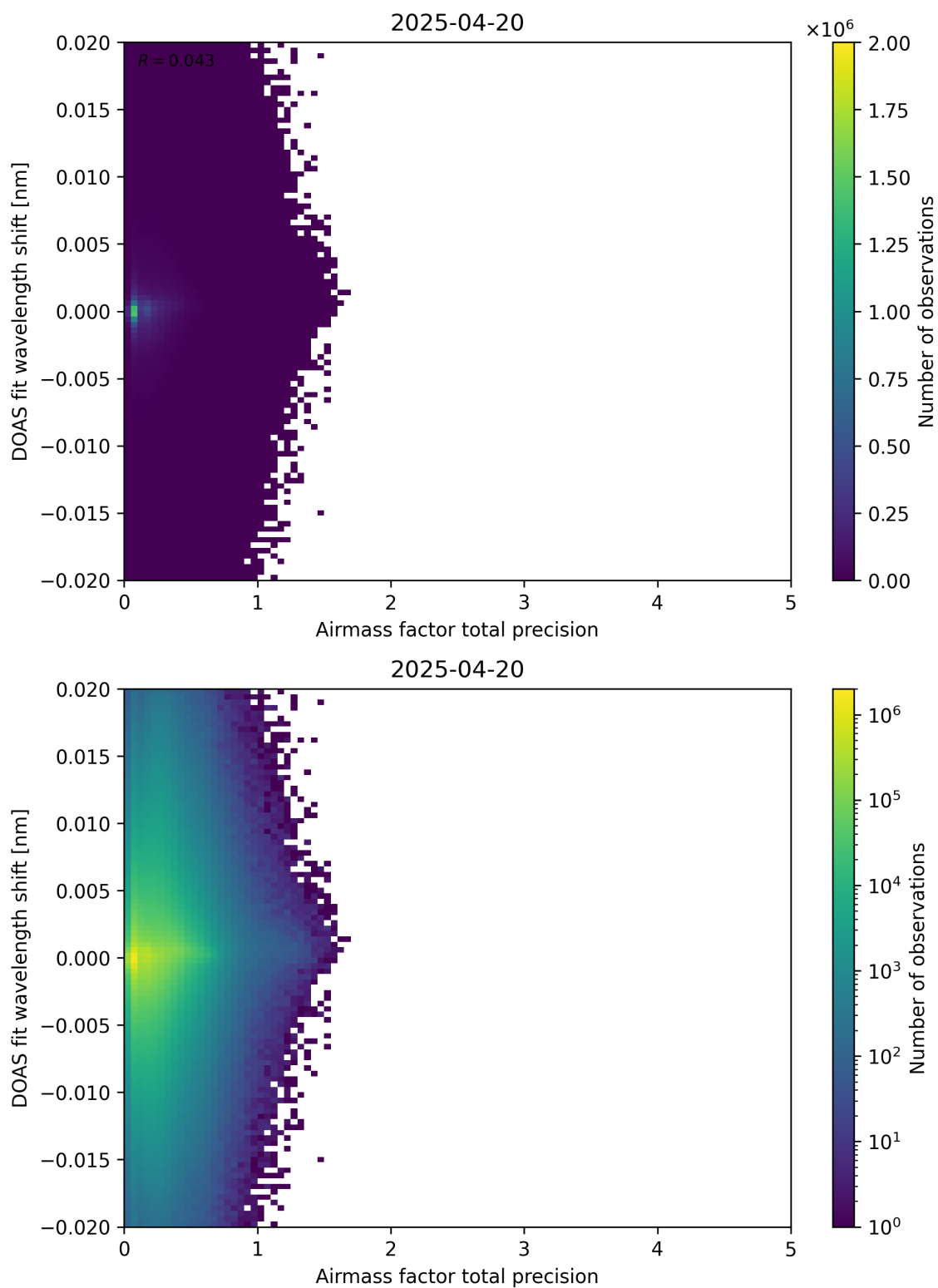
Figure 106: Scatter density plot of “Airmass factor total precision” against “DOAS fit wavelength shift” for 2025-04-19 to 2025-04-21.
