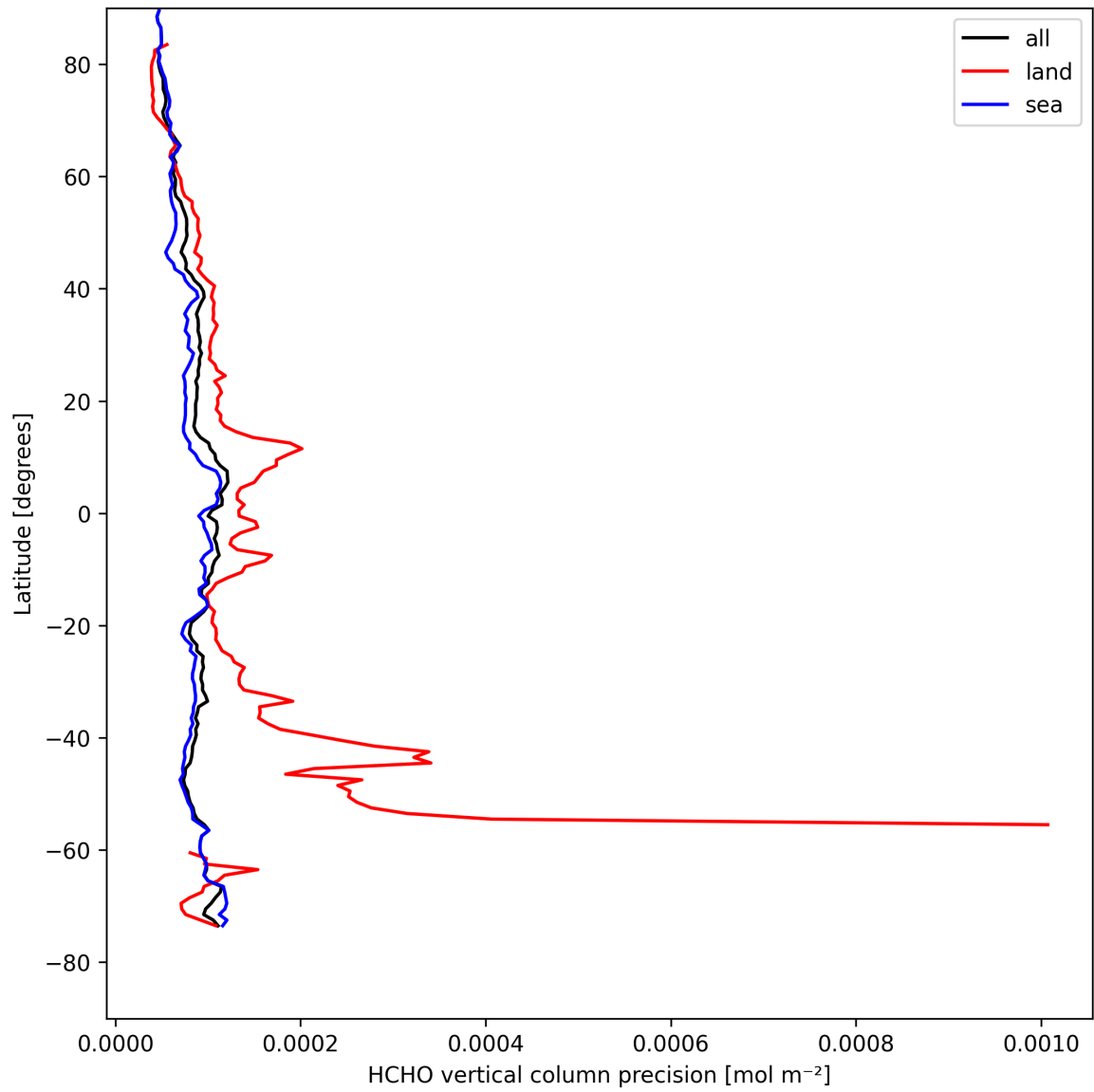
Figure 22: Zonal average of “HCHO vertical column precision” for 2025-04-19 to 2025-04-21.
