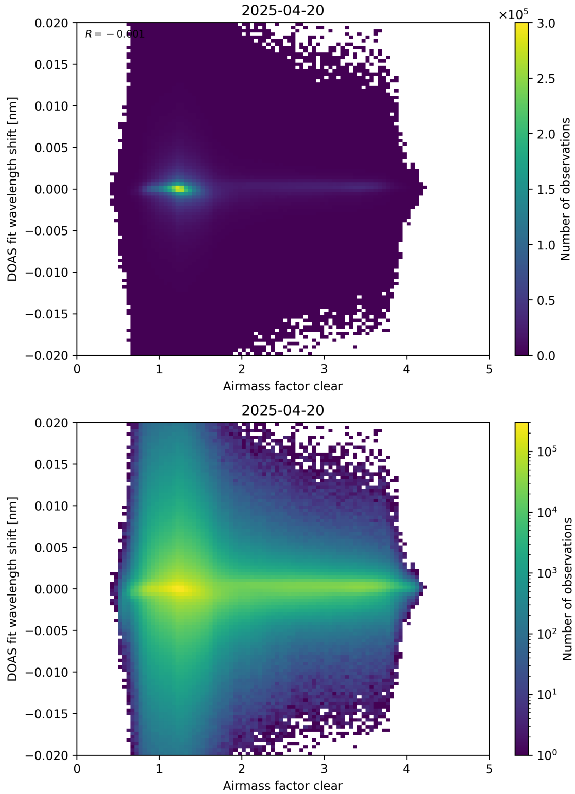
Figure 72: Scatter density plot of “Airmass factor clear” against “DOAS fit wavelength shift” for 2025-04-19 to 2025-04-21.
