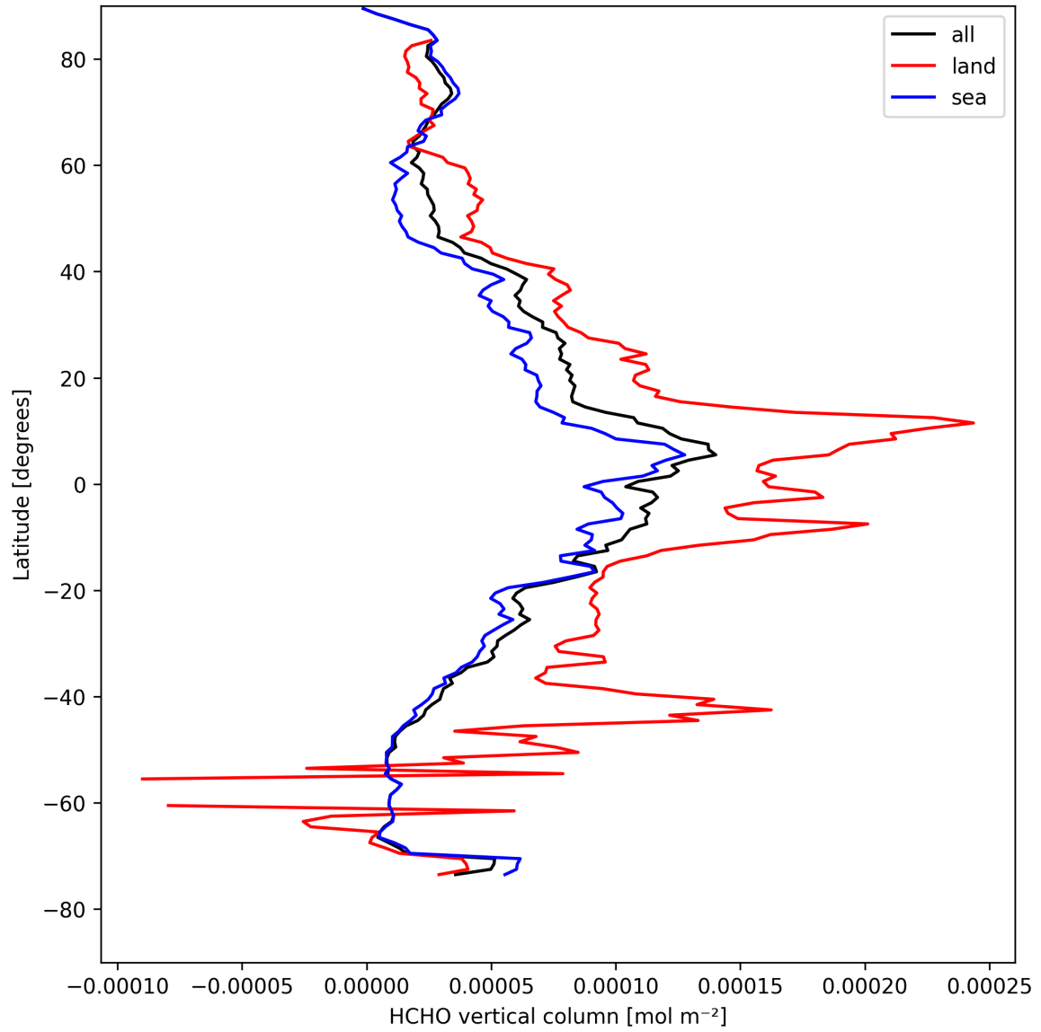
Figure 21: Zonal average of “HCHO vertical column” for 2025-04-19 to 2025-04-21.
