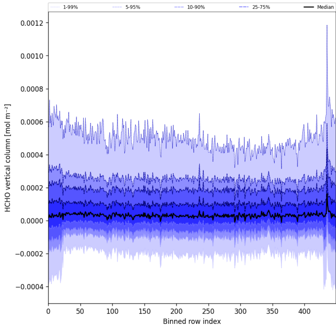
Figure 49: Along track statistics of “HCHO vertical column” for 2025-04-19 to 2025-04-21
