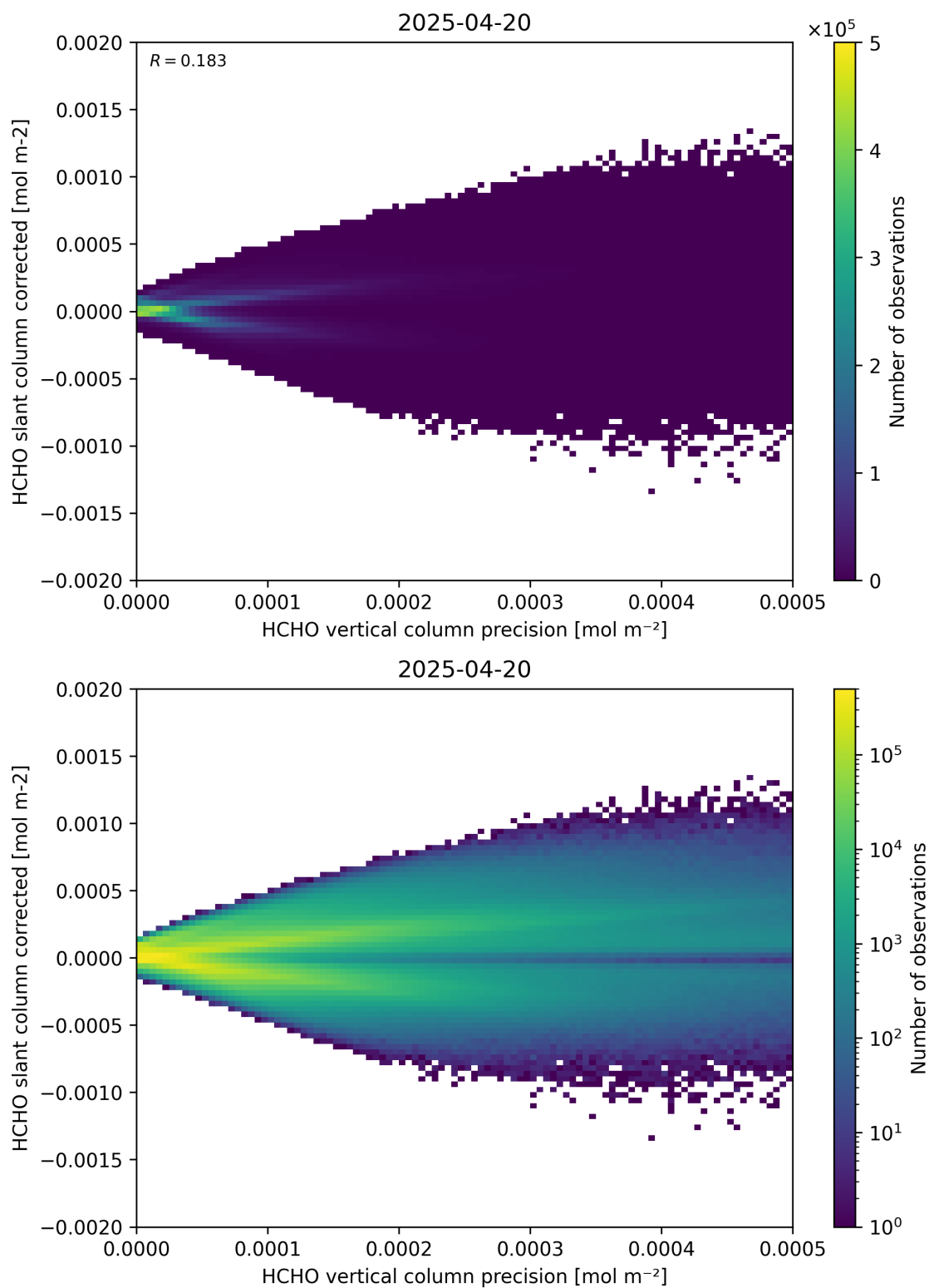
Figure 140: Scatter density plot of “HCHO vertical column precision” against “HCHO slant column corrected” for 2025-04-19 to 2025-04-21.
