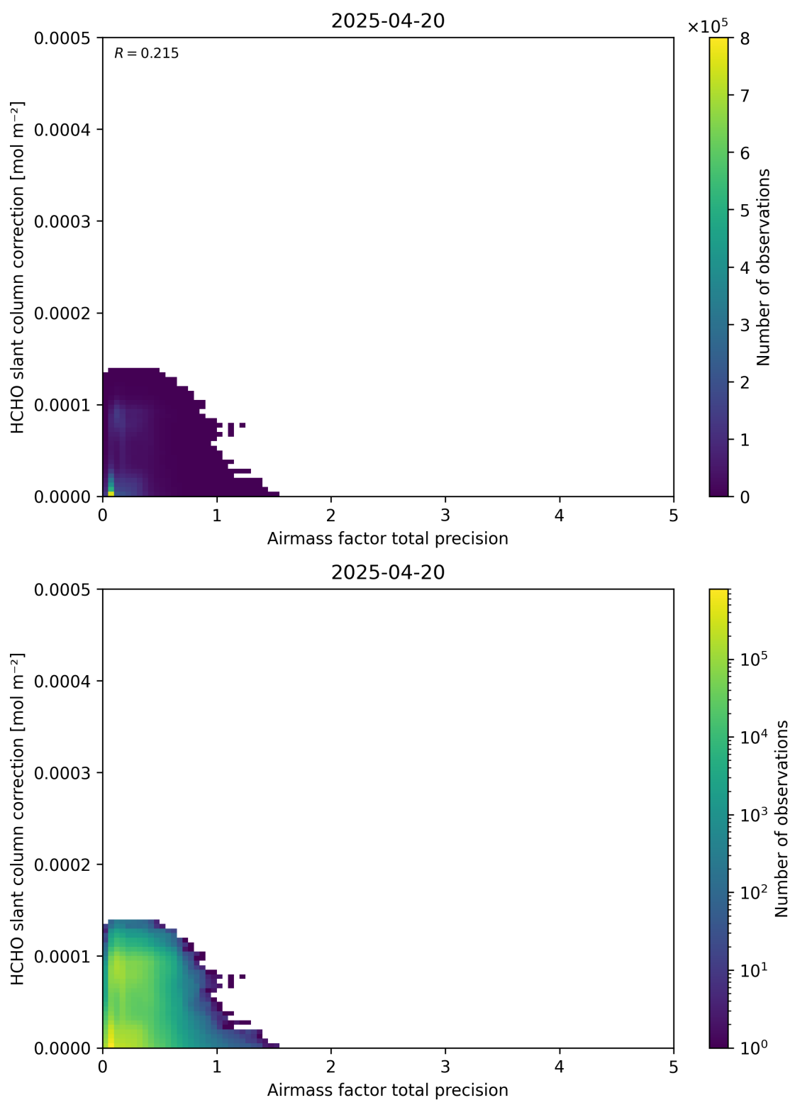
Figure 110: Scatter density plot of “Airmass factor total precision” against “HCHO slant column correction” for 2025-04-19 to 2025-04-21.
