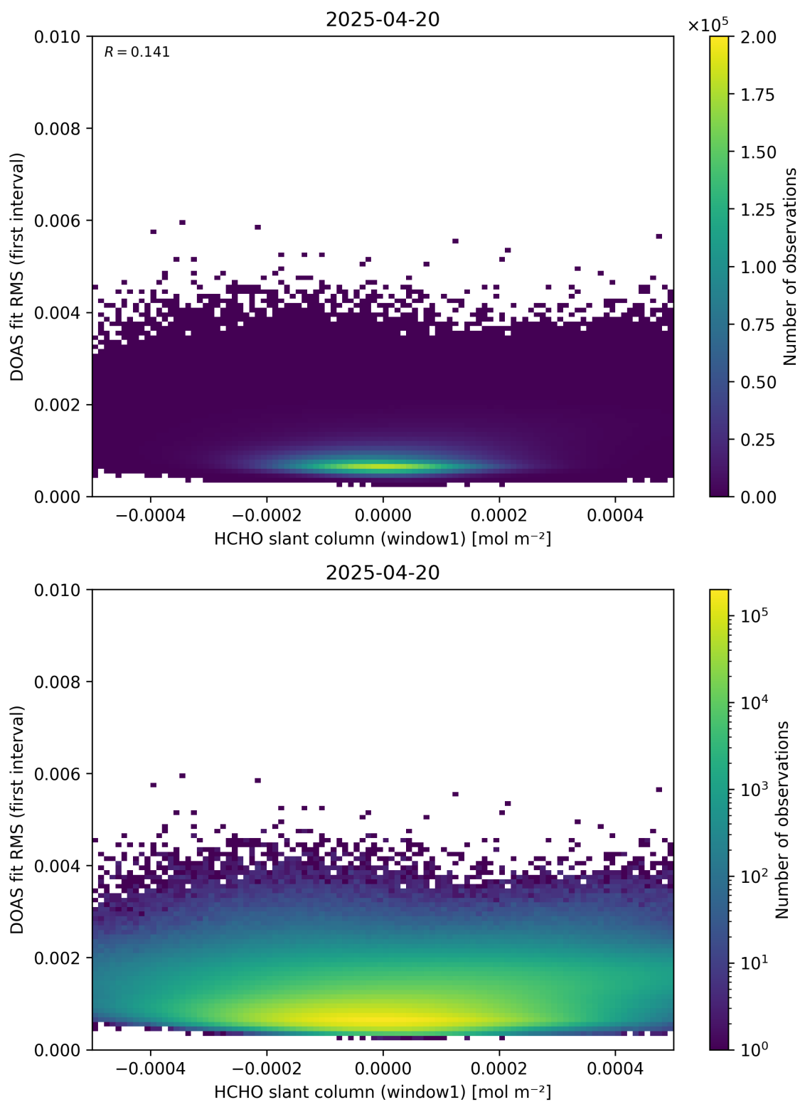
Figure 78: Scatter density plot of “HCHO slant column (window1)” against “DOAS fit RMS (first interval)” for 2025-04-19 to 2025-04-21.
