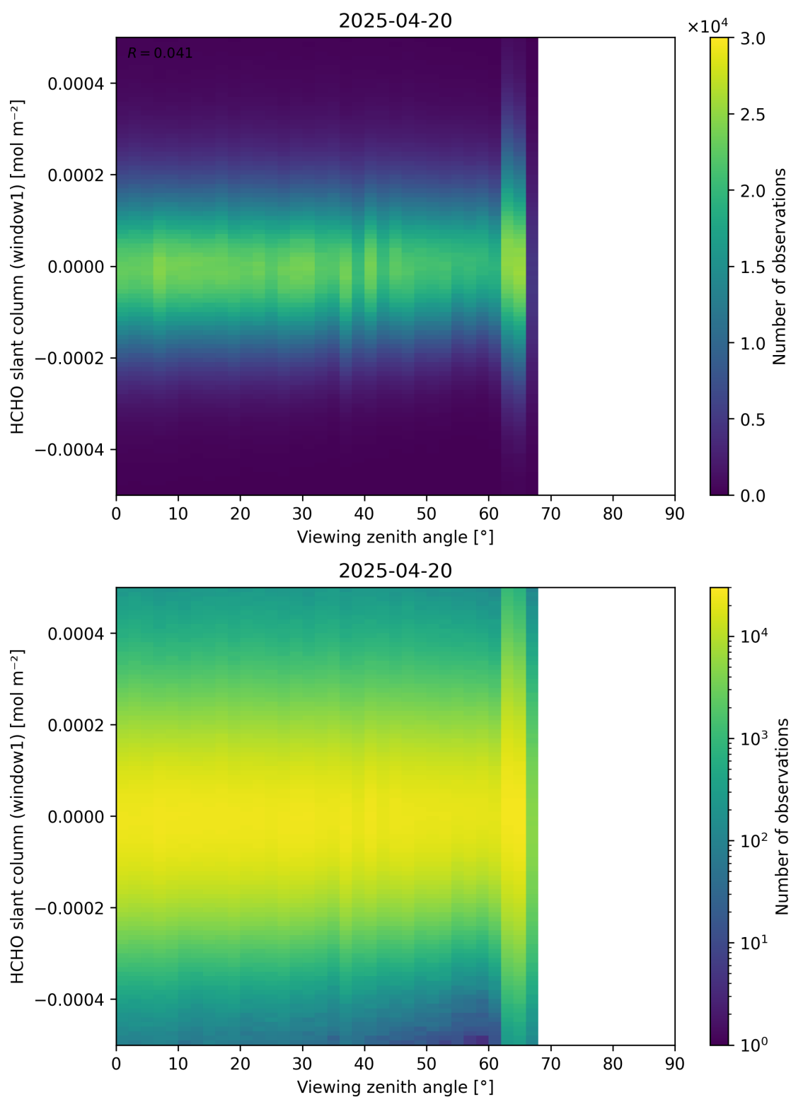
Figure 188: Scatter density plot of “Viewing zenith angle” against “HCHO slant column (window1)” for 2025-04-19 to 2025-04-21.
