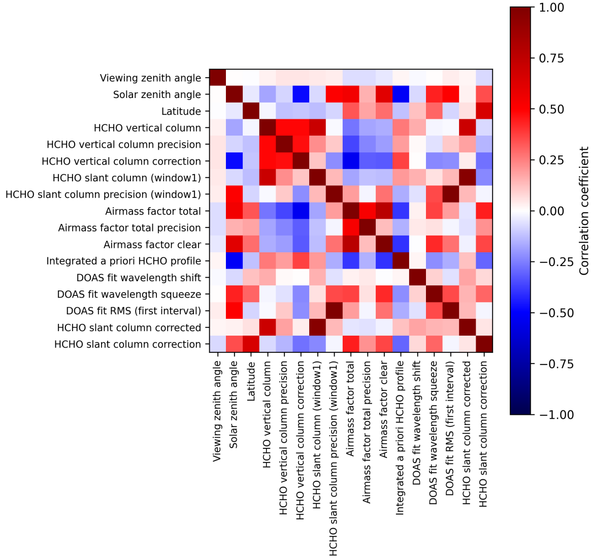
Figure 2: Map of correlation matrix for 2025-04-19 to 2025-04-21.
