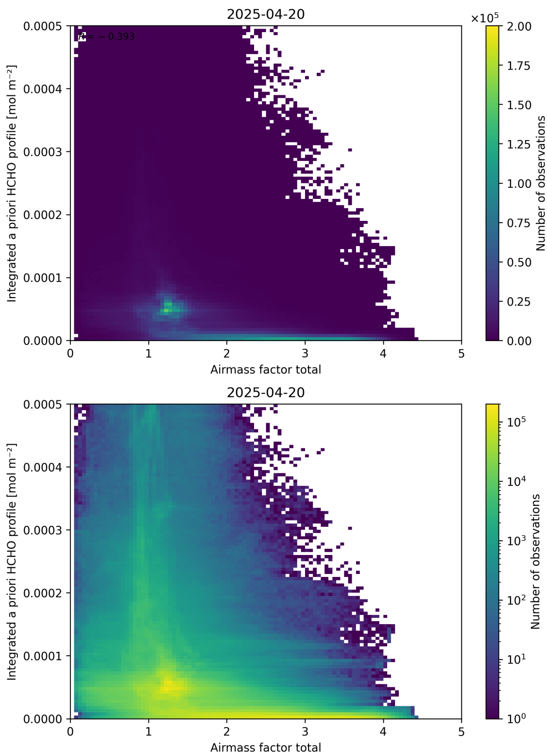
Figure 104: Scatter density plot of “Airmass factor total” against “Integrated a priori HCHO profile” for 2025-04-19 to 2025-04-21.
