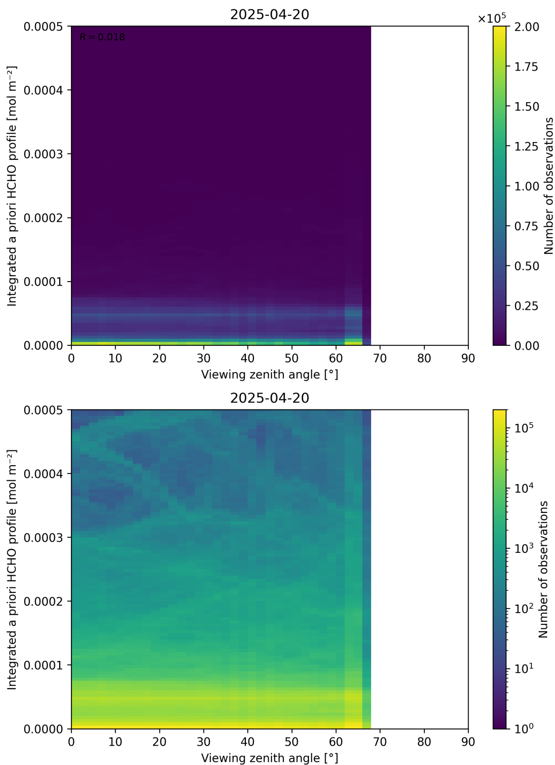
Figure 195: Scatter density plot of “Viewing zenith angle” against “Integrated a priori HCHO profile” for 2025-04-19 to 2025-04-21.
