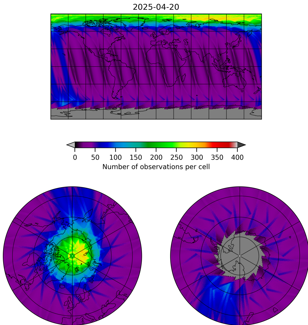
Figure 19: Map of the number of observations for 2025-04-19 to 2025-04-21
