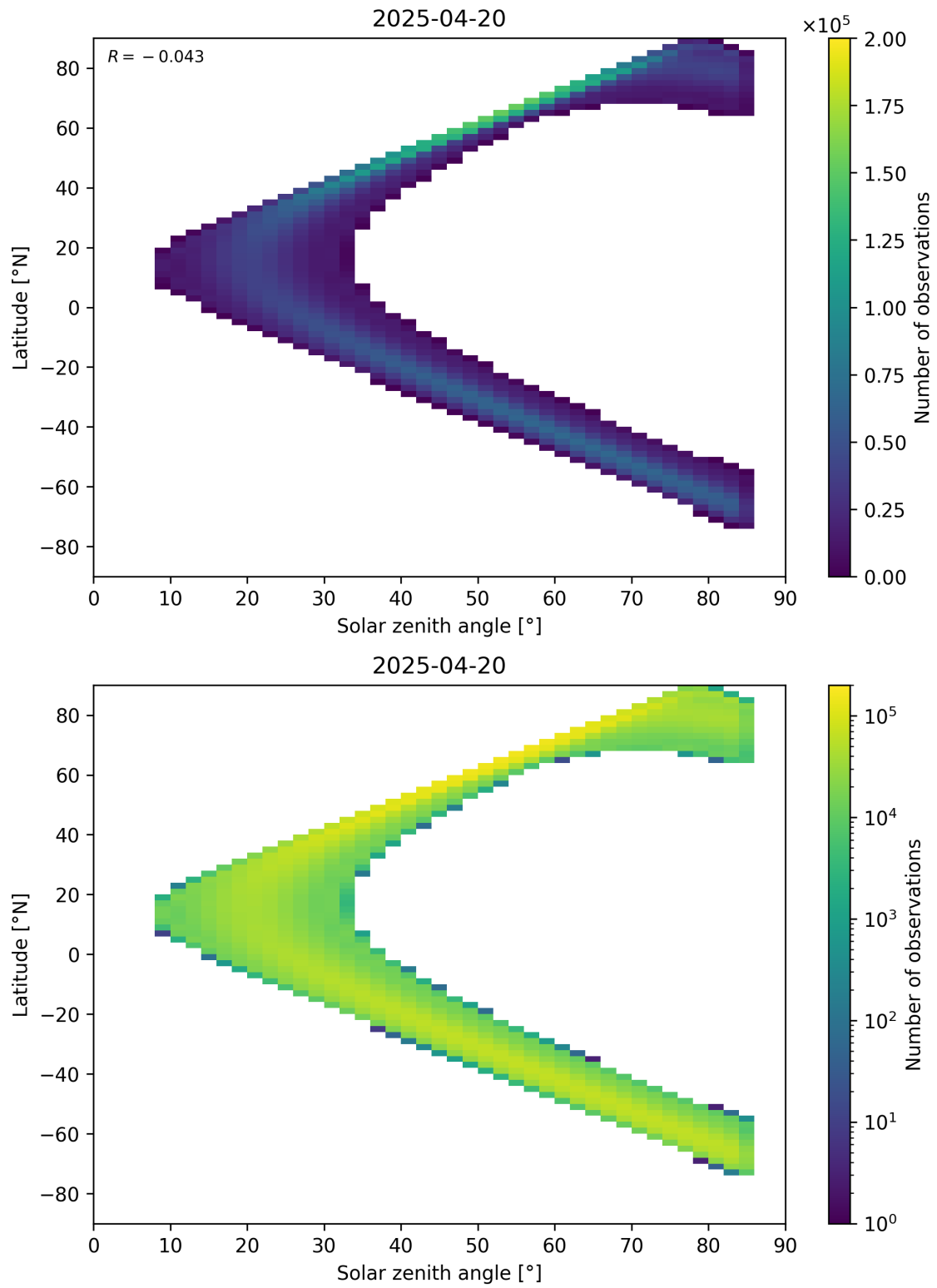
Figure 181: Scatter density plot of “Solar zenith angle” against “Latitude” for 2025-04-19 to 2025-04-21.
