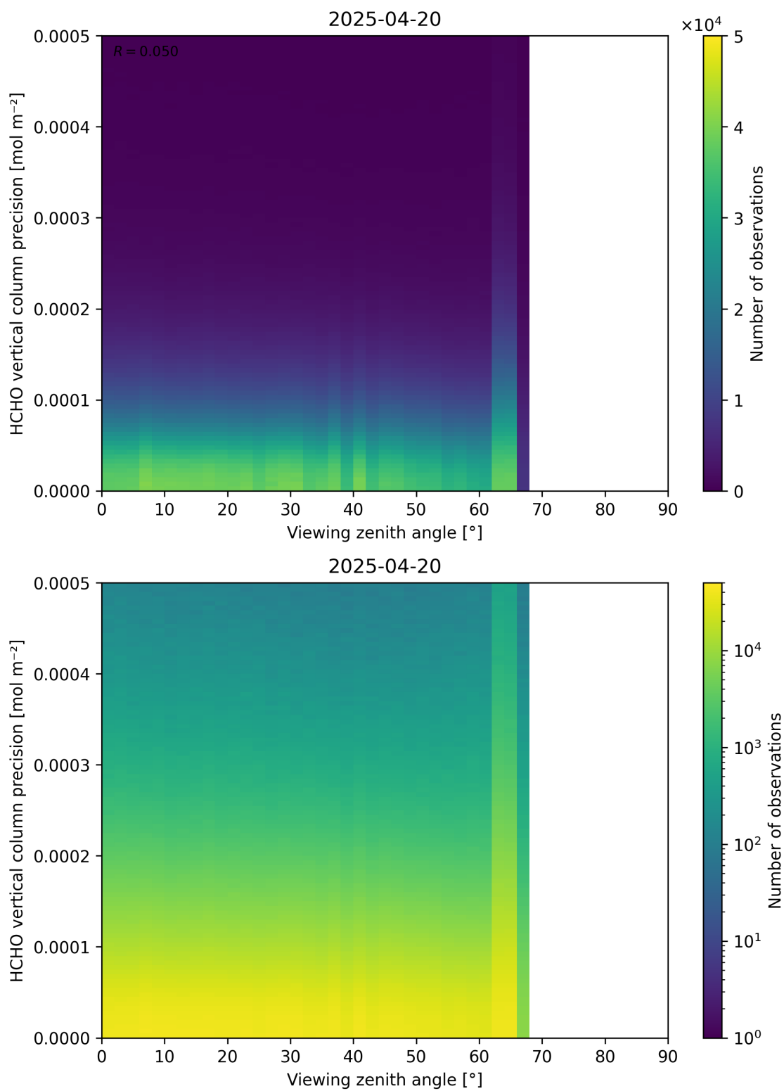
Figure 194: Scatter density plot of “Viewing zenith angle” against “HCHO vertical column precision” for 2025-04-19 to 2025-04-21.
