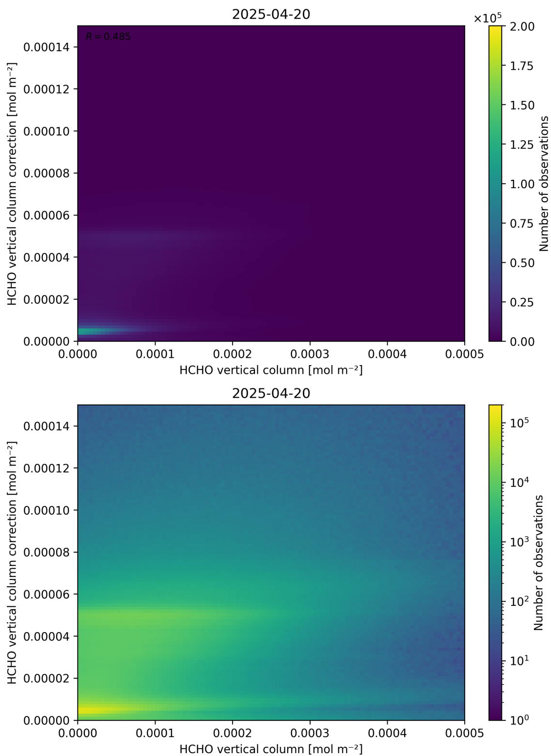
Figure 133: Scatter density plot of “HCHO vertical column” against “HCHO vertical column correction” for 2025-04-19 to 2025-04-21.
