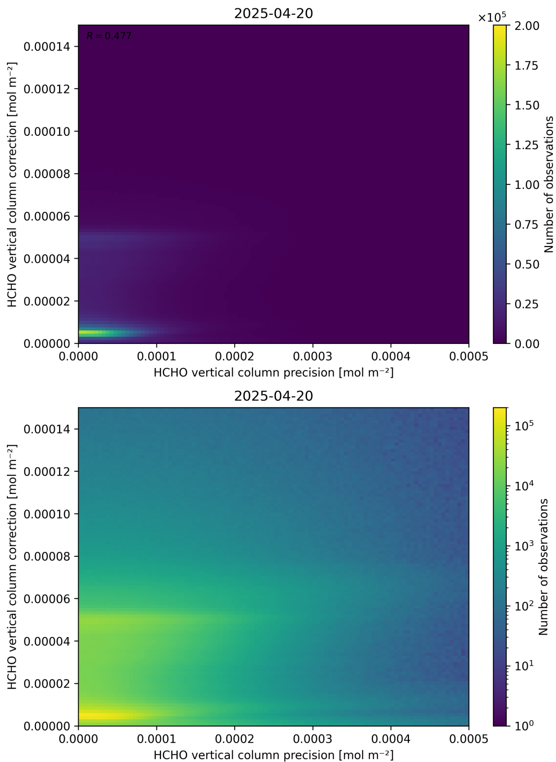
Figure 146: Scatter density plot of “HCHO vertical column precision” against “HCHO vertical column correction” for 2025-04-19 to 2025-04-21.
