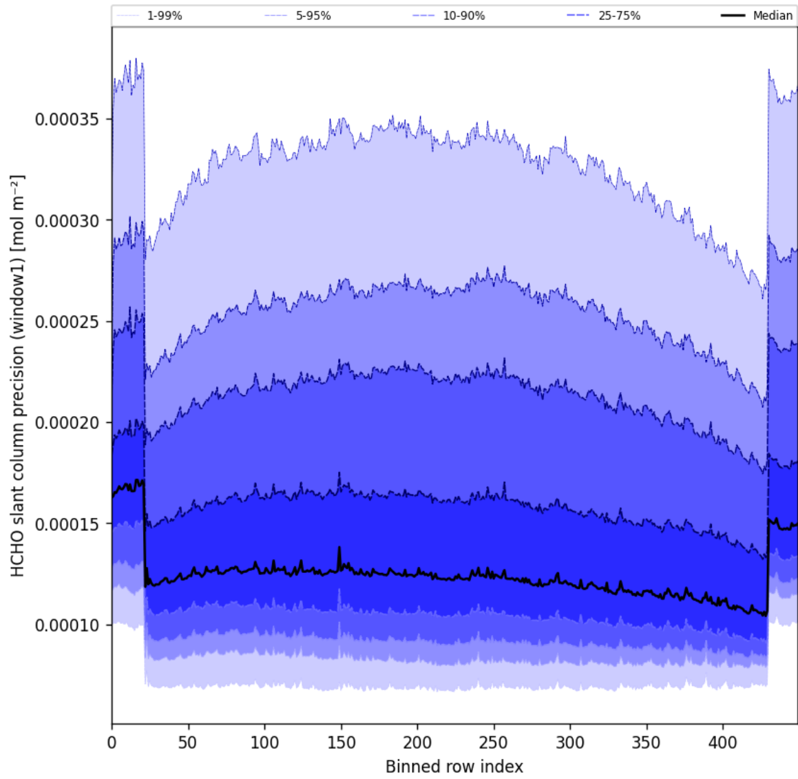
Figure 53: Along track statistics of “HCHO slant column precision (window1)” for 2025-04-19 to 2025-04-21
