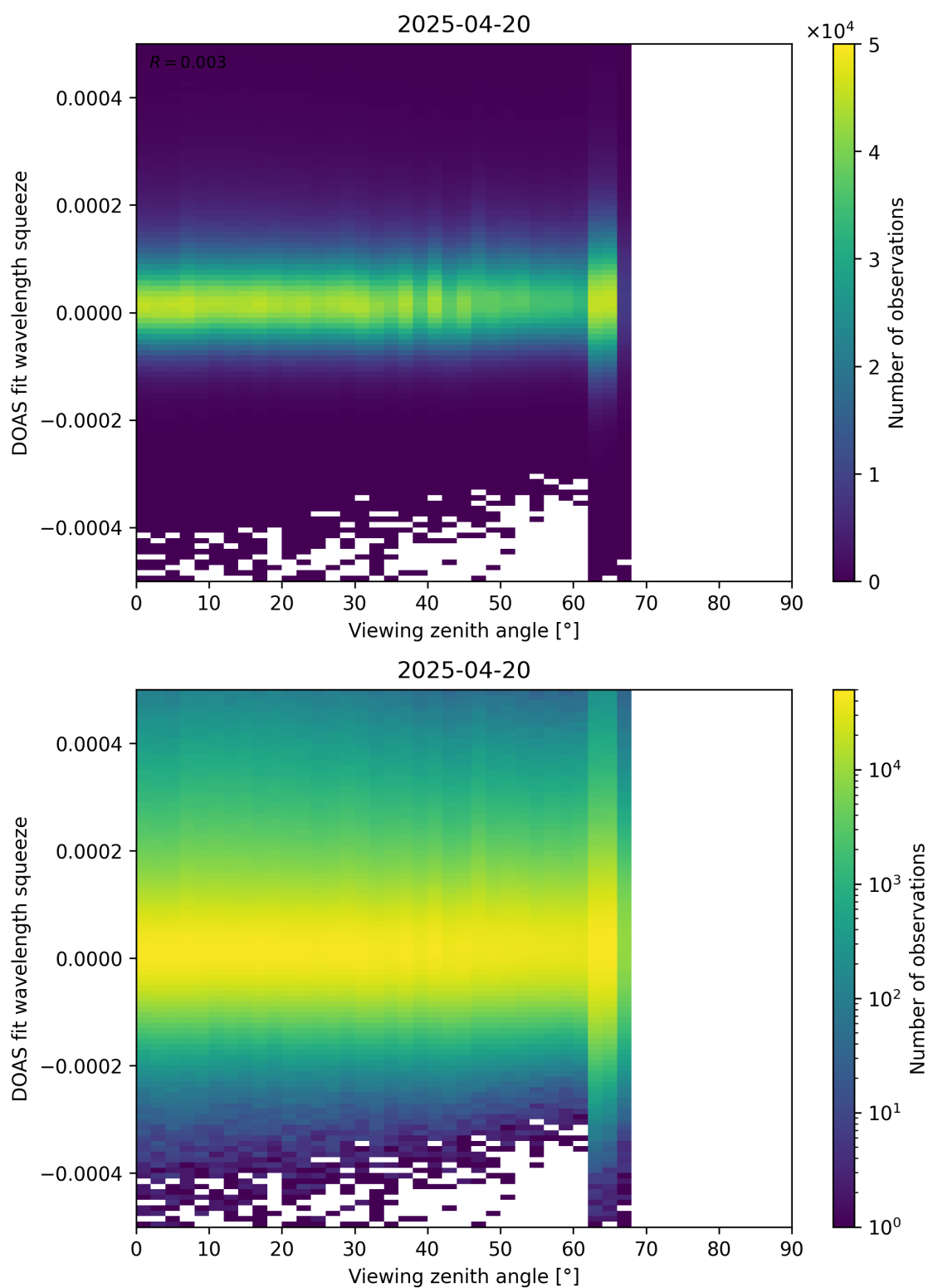
Figure 184: Scatter density plot of “Viewing zenith angle” against “DOAS fit wavelength squeeze” for 2025-04-19 to 2025-04-21.
