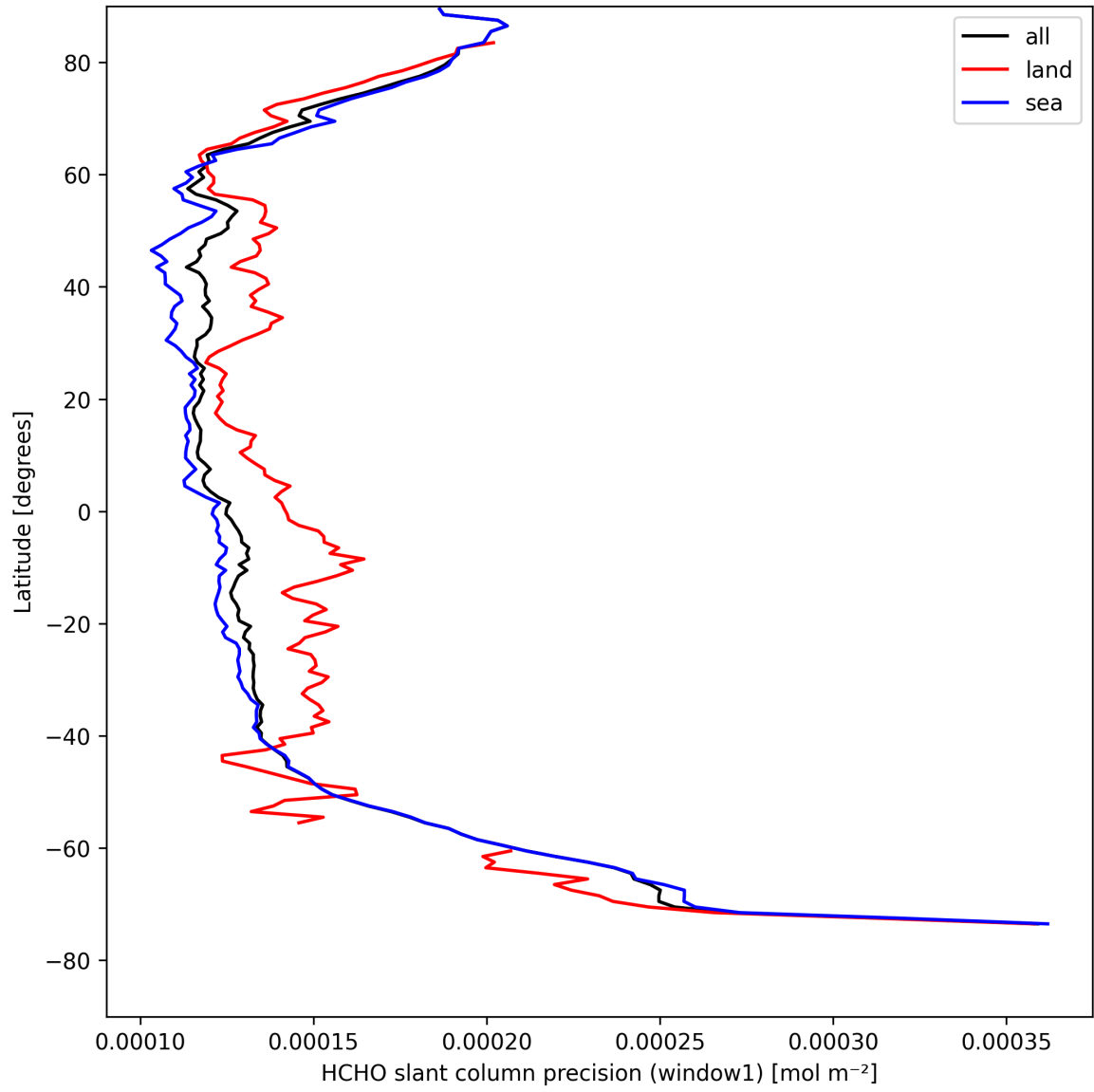
Figure 25: Zonal average of "HCHO slant column precision (window1)" for 2025-04-19 to 2025-04-21.
