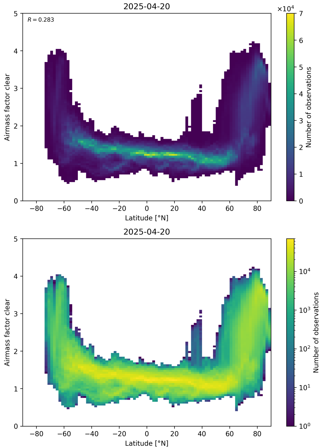
Figure 156: Scatter density plot of “Latitude” against “Airmass factor clear” for 2025-04-19 to 2025-04-21.
