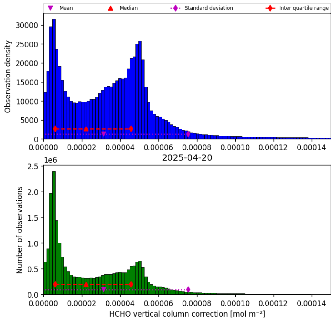
Figure 37: Histogram of “HCHO vertical column correction” for 2025-04-19 to 2025-04-21
