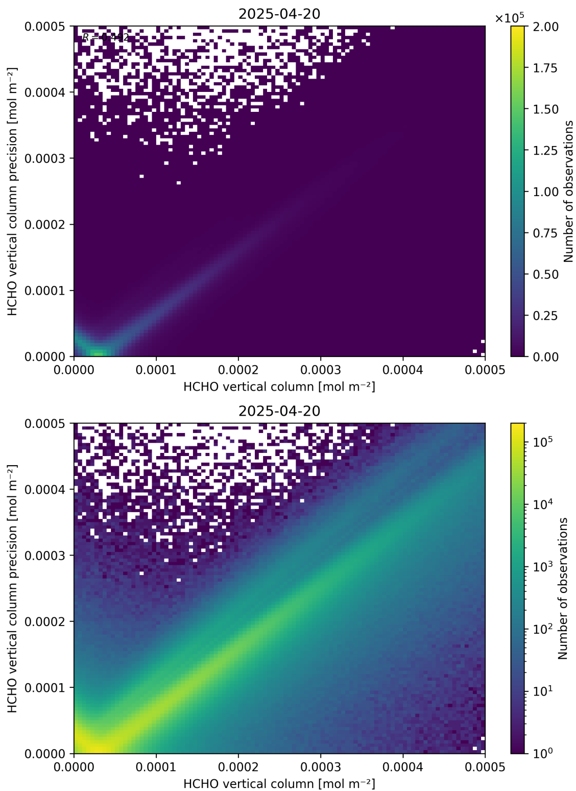
Figure 134: Scatter density plot of “HCHO vertical column” against “HCHO vertical column precision” for 2025-04-19 to 2025-04-21.
