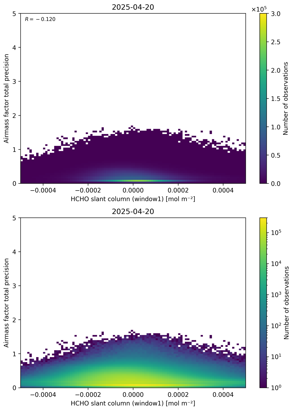
Figure 86: Scatter density plot of “HCHO slant column (window1)” against “Airmass factor total precision” for 2025-04-19 to 2025-04-21.
