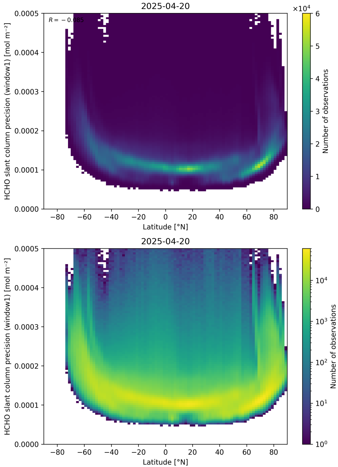
Figure 160: Scatter density plot of “Latitude” against “HCHO slant column precision (window1)” for 2025-04-19 to 2025-04-21.
