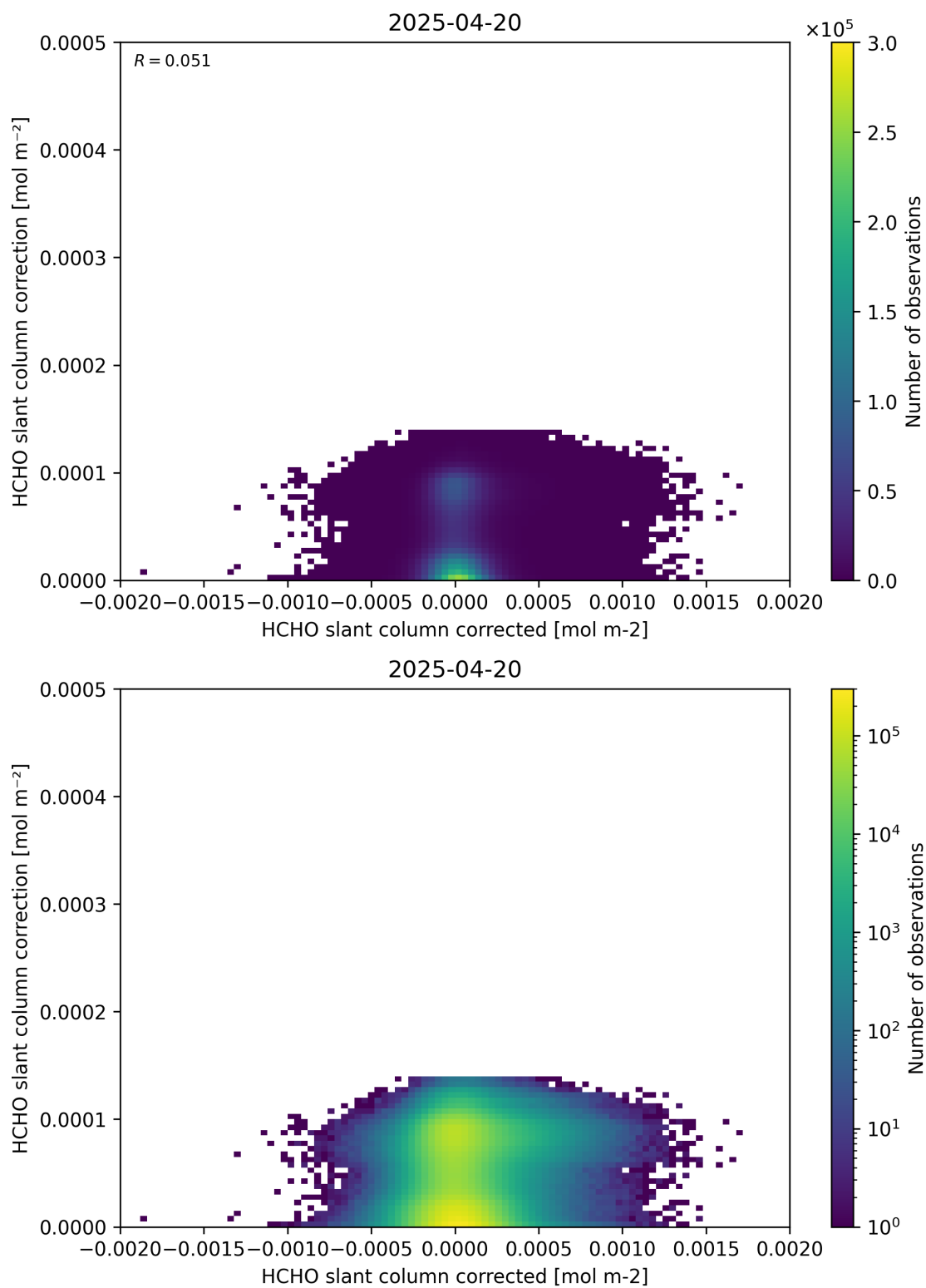
Figure 77: Scatter density plot of “HCHO slant column corrected” against “HCHO slant column correction” for 2025-04-19 to 2025-04-21.
