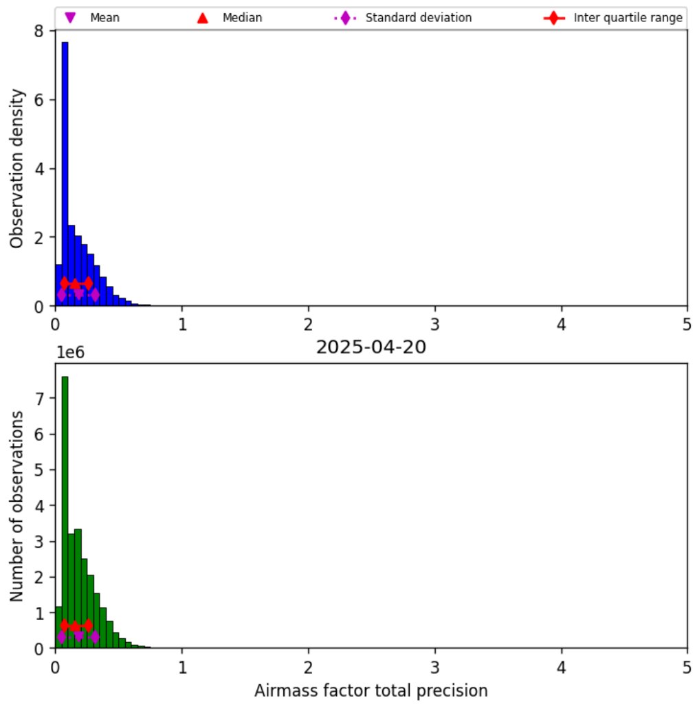
Figure 41: Histogram of “Airmass factor total precision” for 2025-04-19 to 2025-04-21
