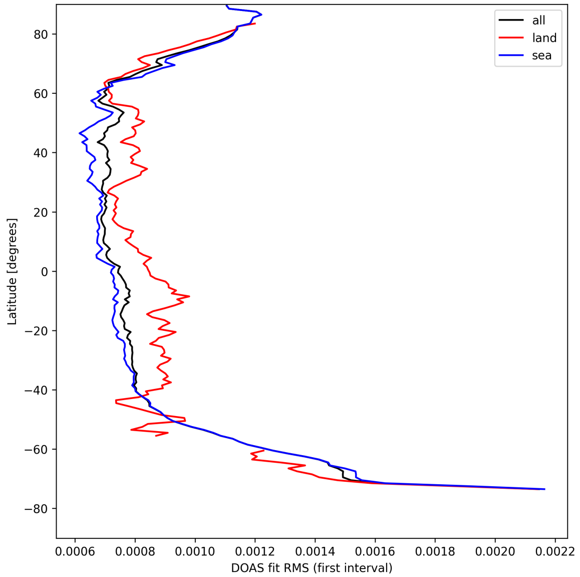
Figure 32: Zonal average of “DOAS fit RMS (first interval)” for 2025-04-19 to 2025-04-21.
