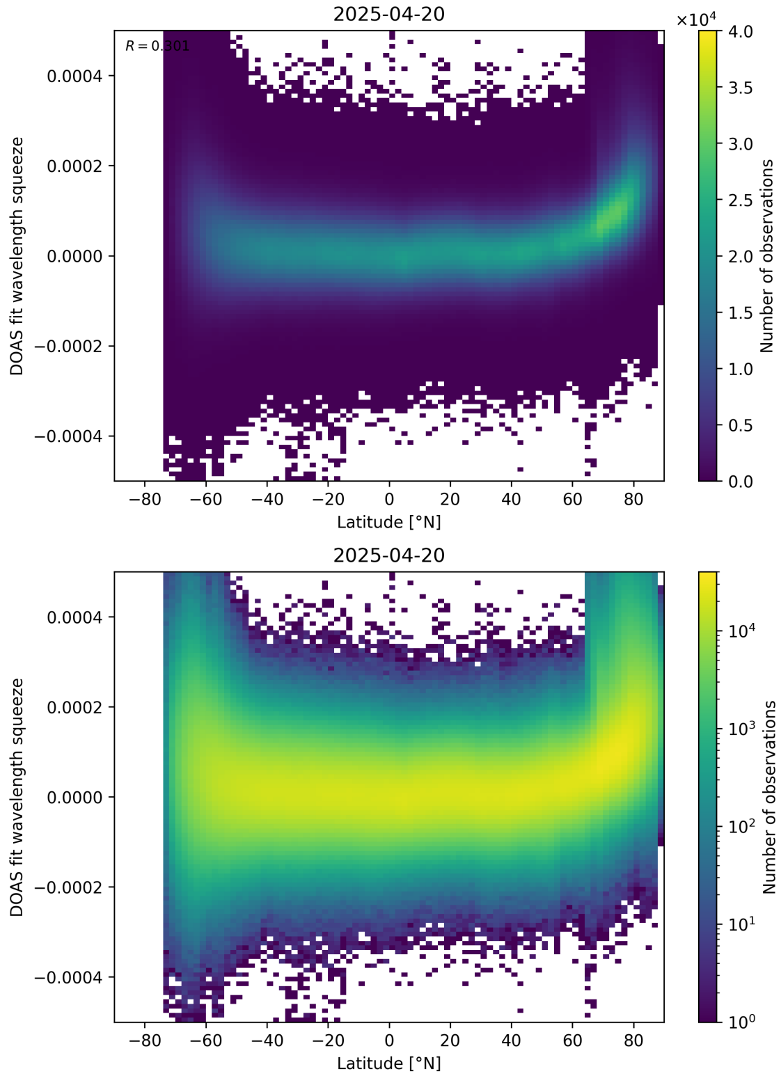
Figure 155: Scatter density plot of “Latitude” against “DOAS fit wavelength squeeze” for 2025-04-19 to 2025-04-21.
