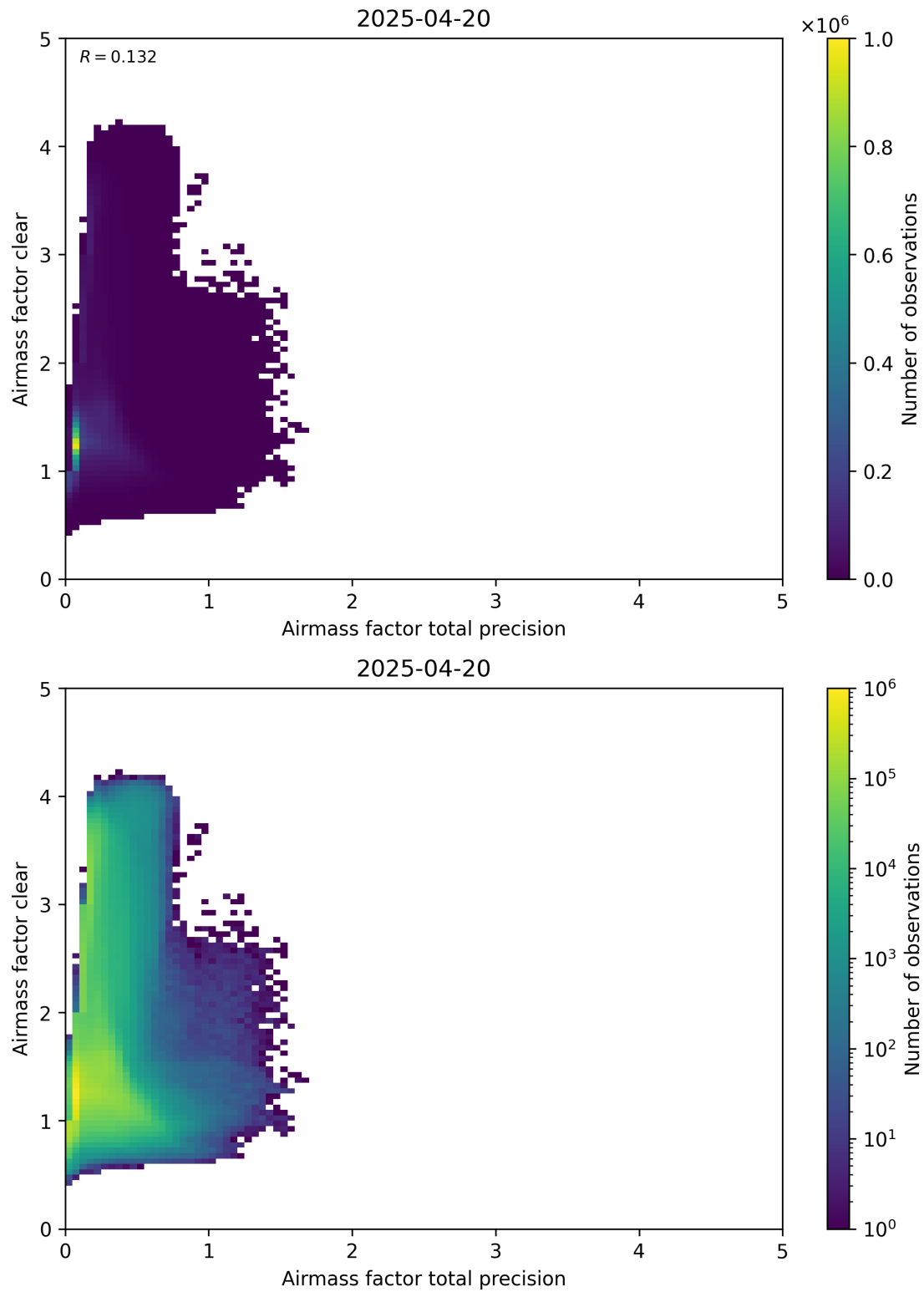
Figure 108: Scatter density plot of “Airmass factor total precision” against “Airmass factor clear” for 2025-04-19 to 2025-04-21.
