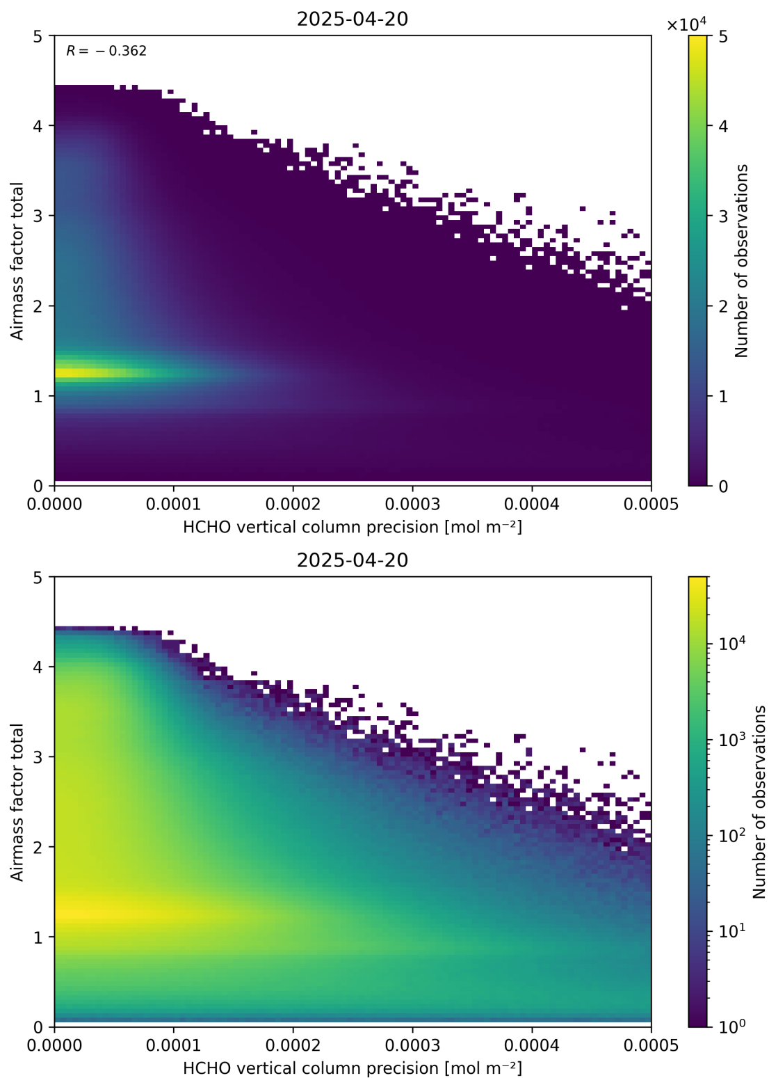
Figure 144: Scatter density plot of “HCHO vertical column precision” against “Airmass factor total” for 2025-04-19 to 2025-04-21.
