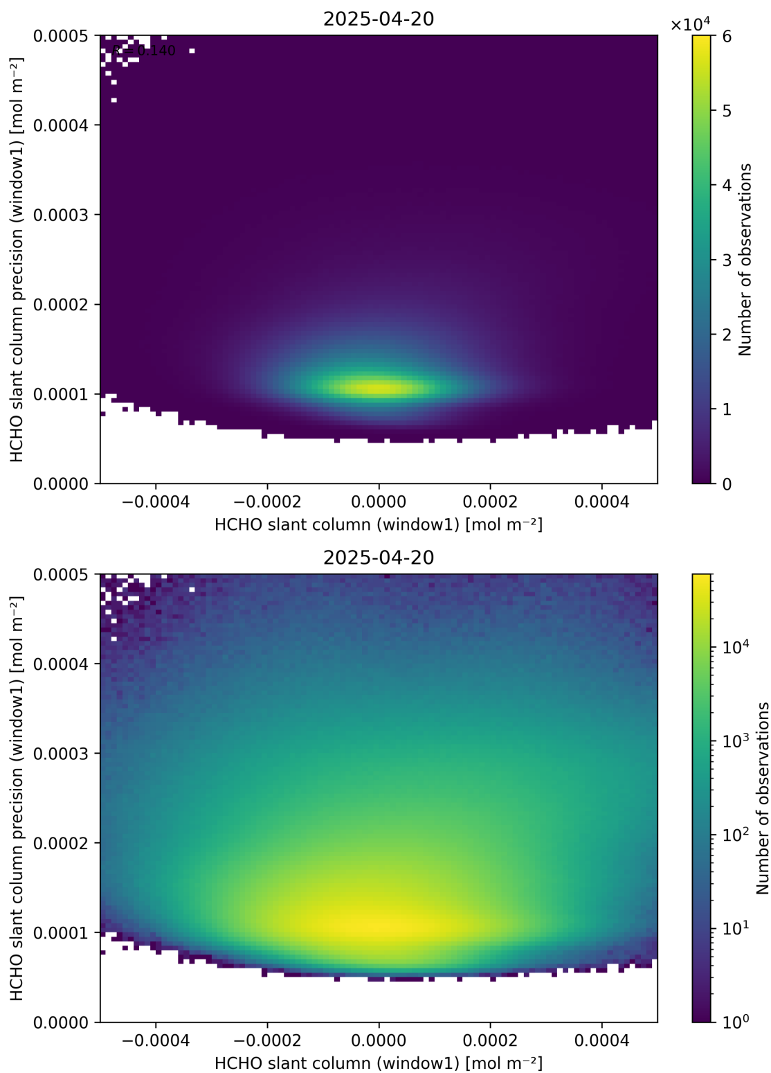
Figure 84: Scatter density plot of “HCHO slant column (window1)” against “HCHO slant column precision (window1)” for 2025-04-19 to 2025-04-21.
