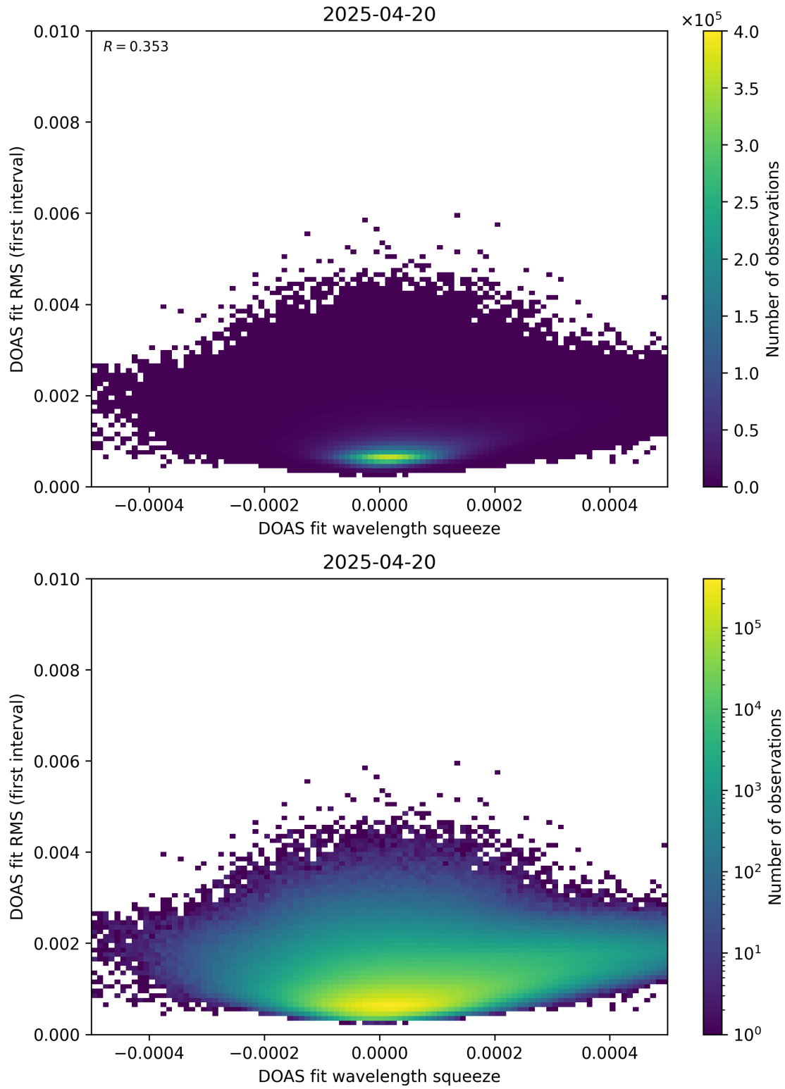
Figure 68: Scatter density plot of “DOAS fit wavelength squeeze” against “DOAS fit RMS (first interval)” for 2025-04-19 to 2025-04-21.
