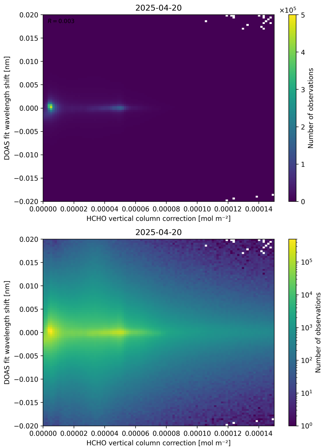
Figure 113: Scatter density plot of “HCHO vertical column correction” against “DOAS fit wavelength shift” for 2025-04-19 to 2025-04-21.
