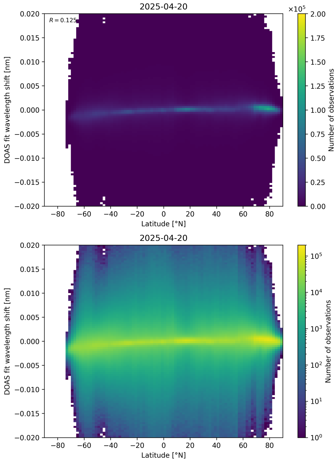
Figure 154: Scatter density plot of “Latitude” against “DOAS fit wavelength shift” for 2025-04-19 to 2025-04-21.
