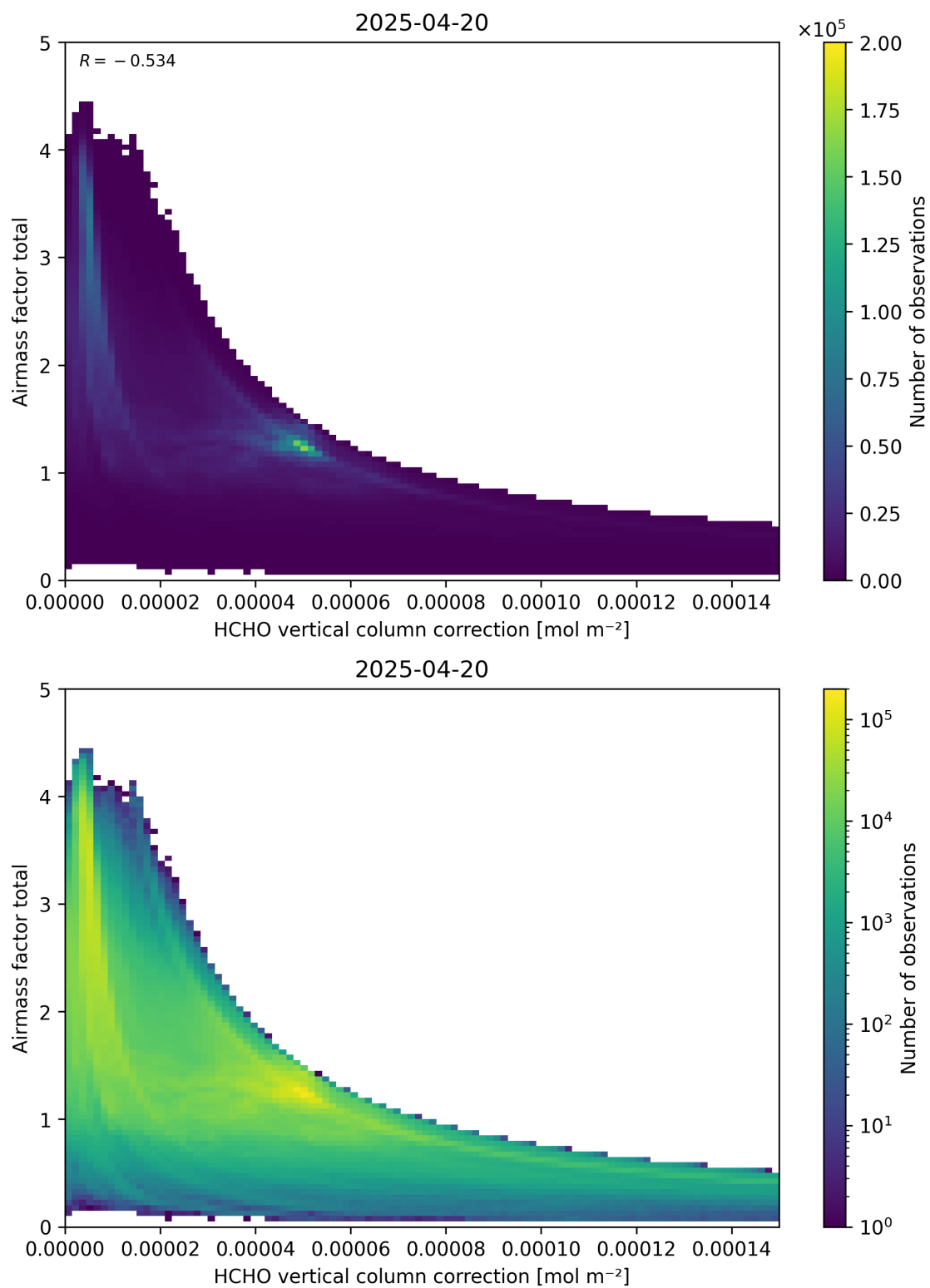
Figure 120: Scatter density plot of “HCHO vertical column correction” against “Airmass factor total” for 2025-04-19 to 2025-04-21.
