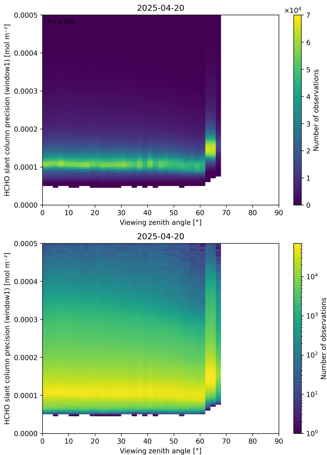
Figure 189: Scatter density plot of “Viewing zenith angle” against “HCHO slant column precision (window1)” for 2025-04-19 to 2025-04-21.
