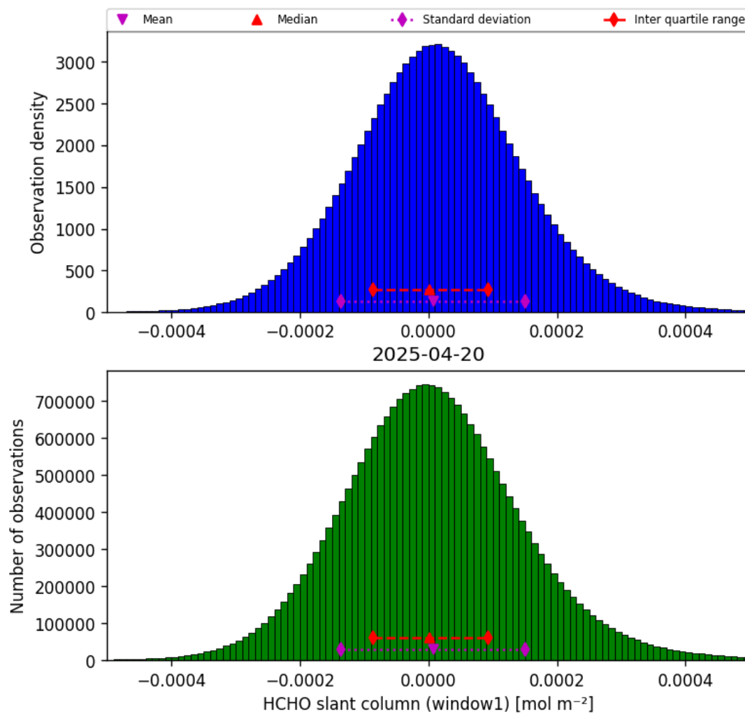
Figure 38: Histogram of “HCHO slant column (window1)” for 2025-04-19 to 2025-04-21
