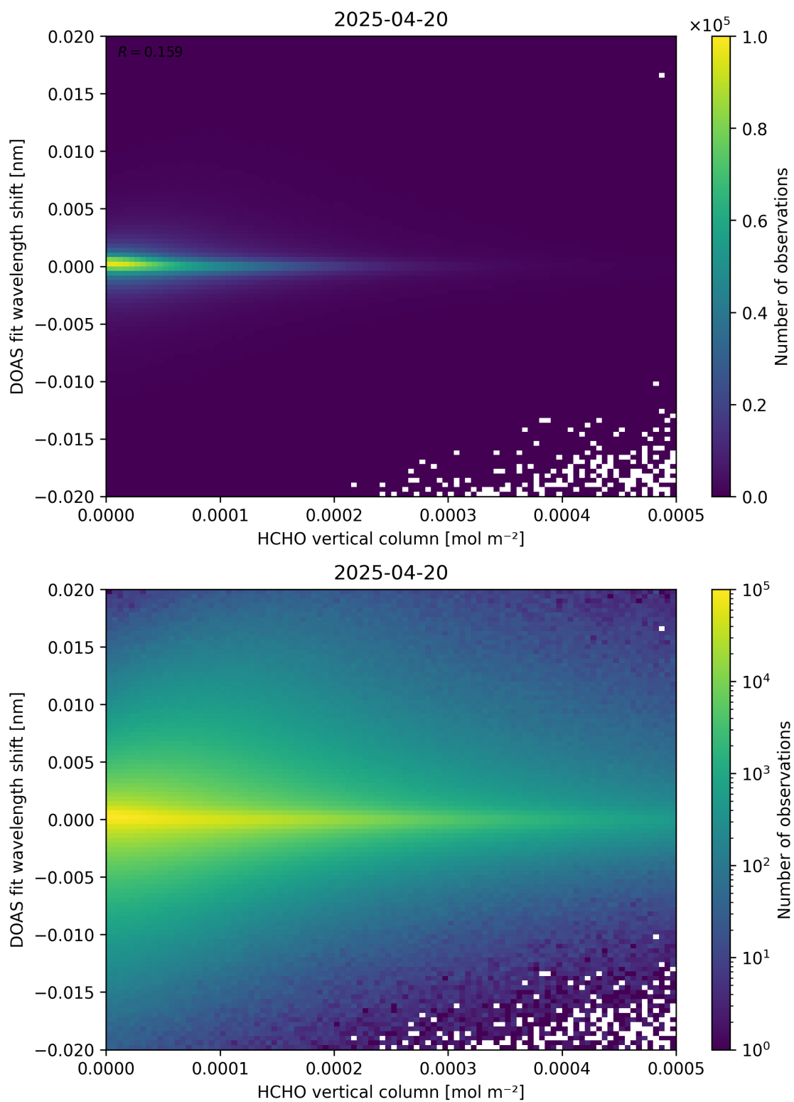
Figure 124: Scatter density plot of “HCHO vertical column” against “DOAS fit wavelength shift” for 2025-04-19 to 2025-04-21.
