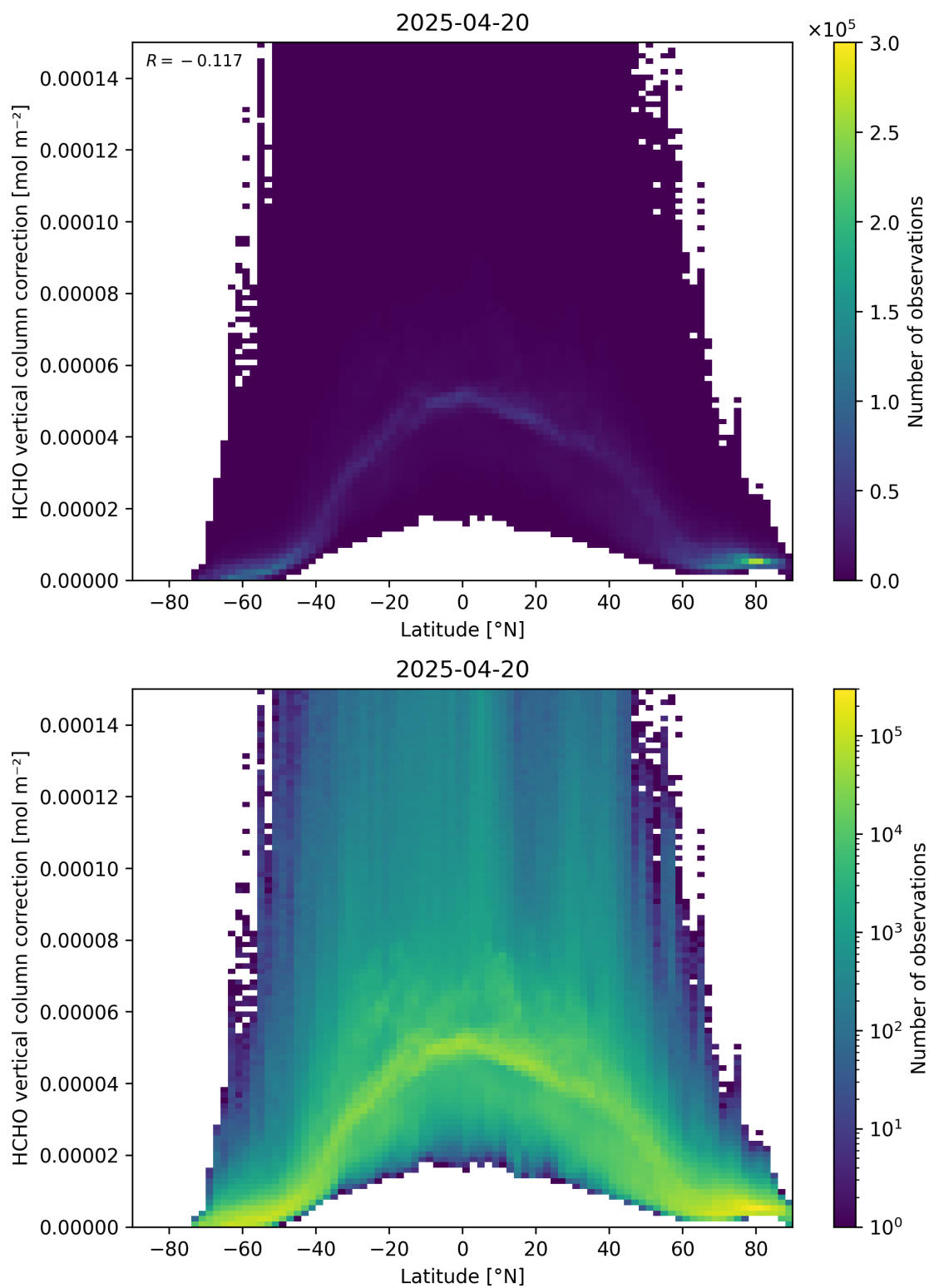
Figure 164: Scatter density plot of “Latitude” against “HCHO vertical column correction” for 2025-04-19 to 2025-04-21.
