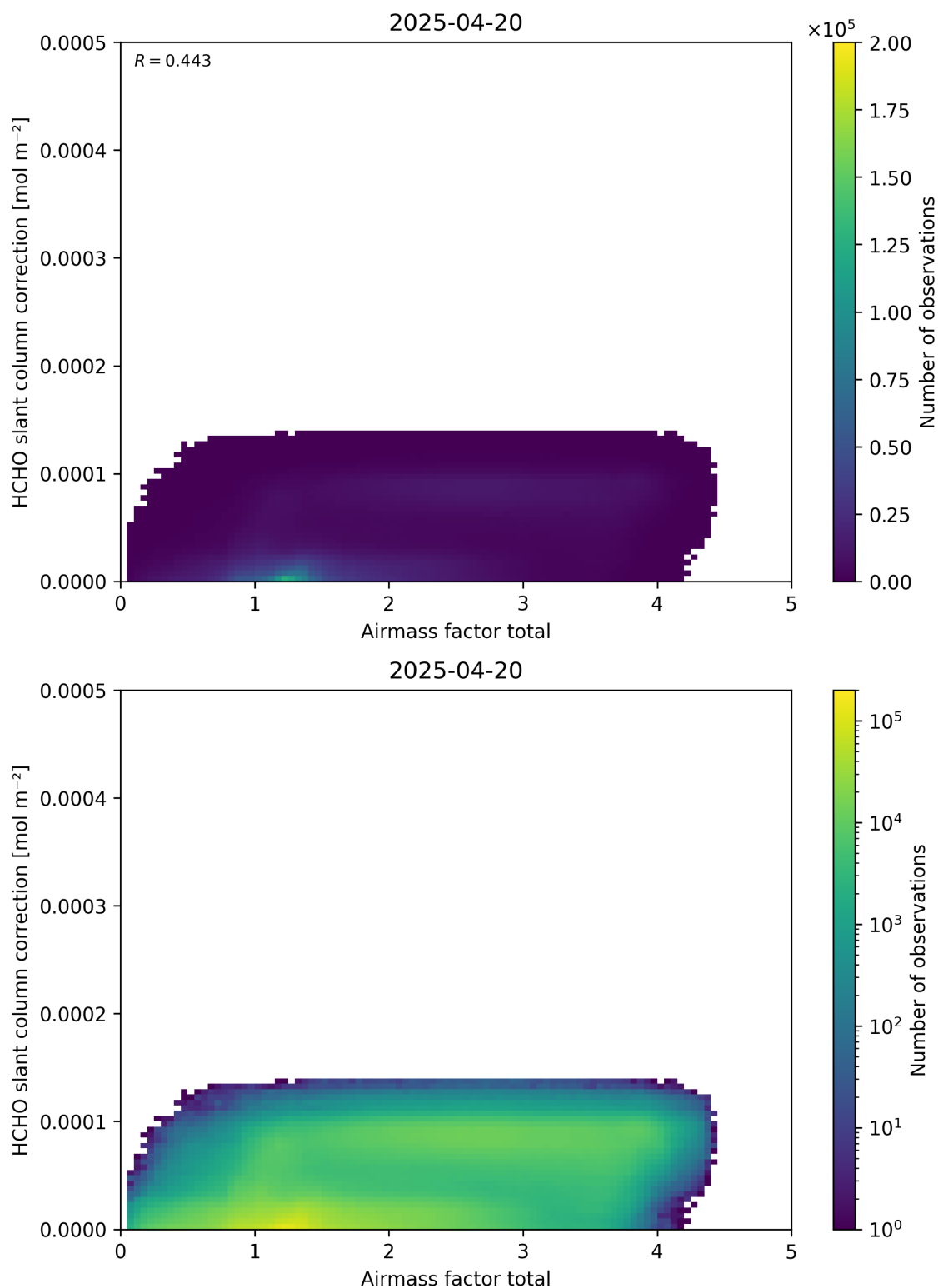
Figure 102: Scatter density plot of “Airmass factor total” against “HCHO slant column correction” for 2025-04-19 to 2025-04-21.
