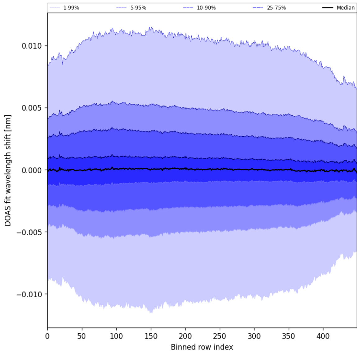
Figure 58: Along track statistics of “DOAS fit wavelength shift” for 2025-04-19 to 2025-04-21
