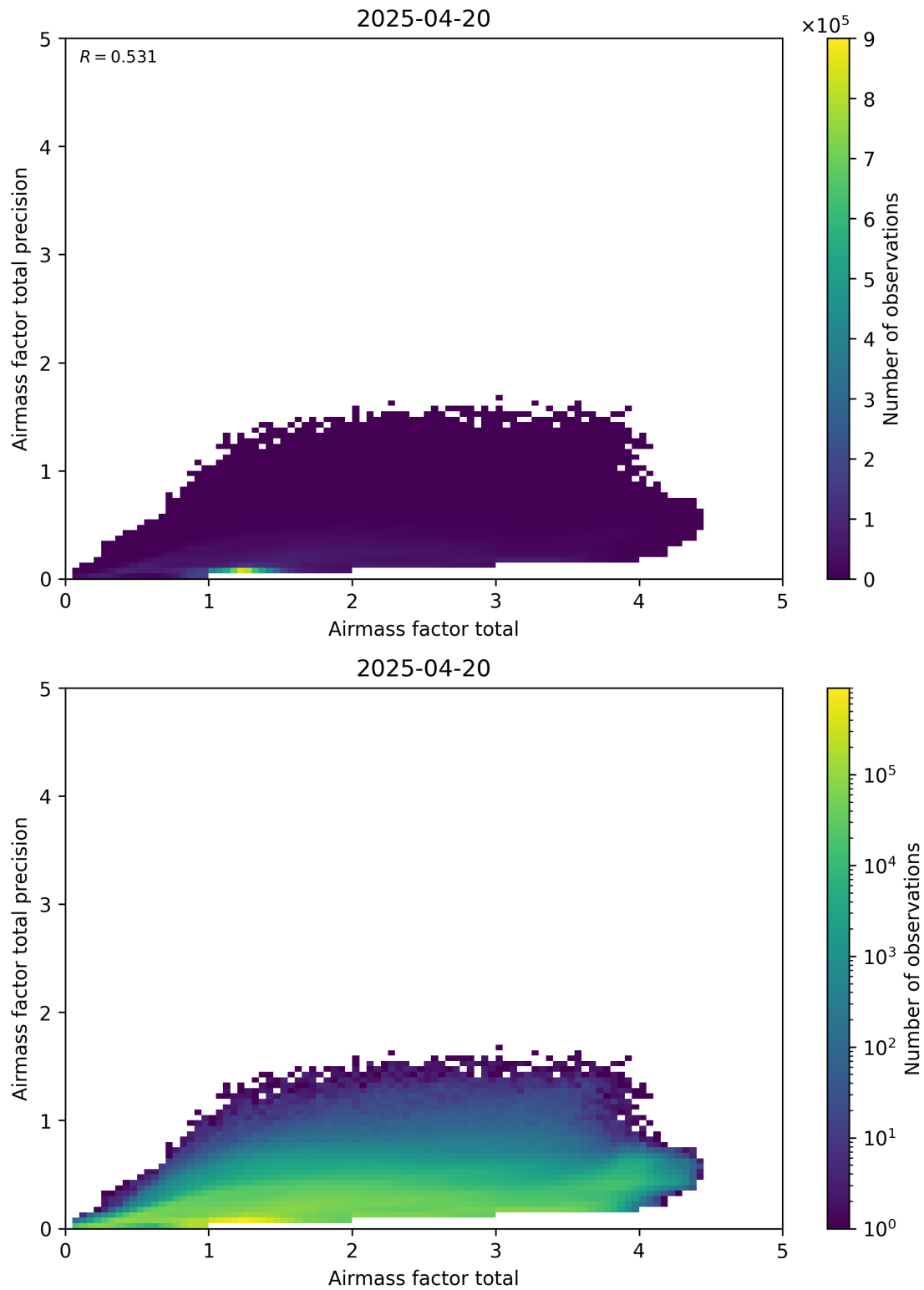
Figure 103: Scatter density plot of “Airmass factor total” against “Airmass factor total precision” for 2025-04-19 to 2025-04-21.
