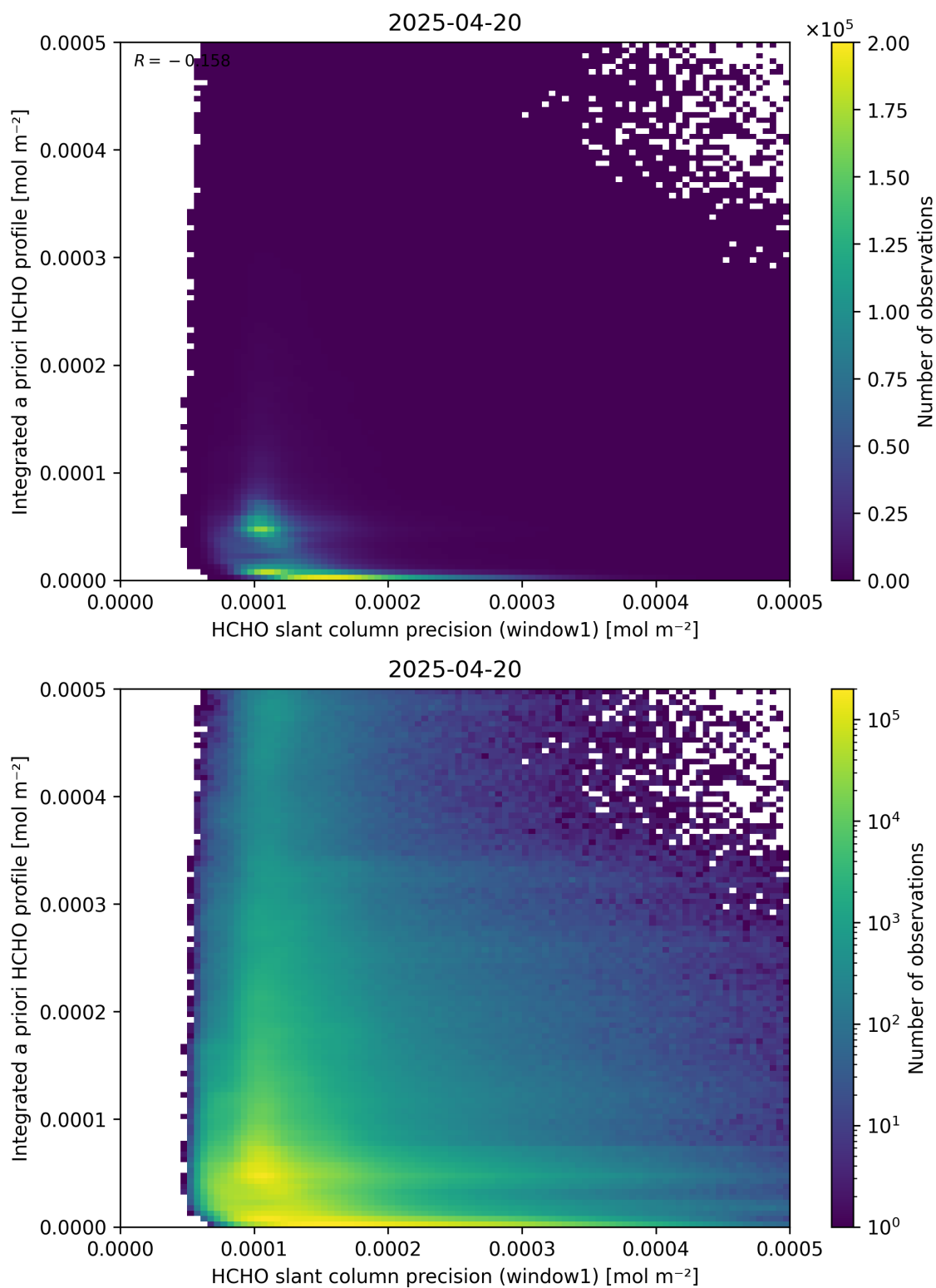
Figure 96: Scatter density plot of “HCHO slant column precision (window1)” against “Integrated a priori HCHO profile” for 2025-04-19 to 2025-04-21.
