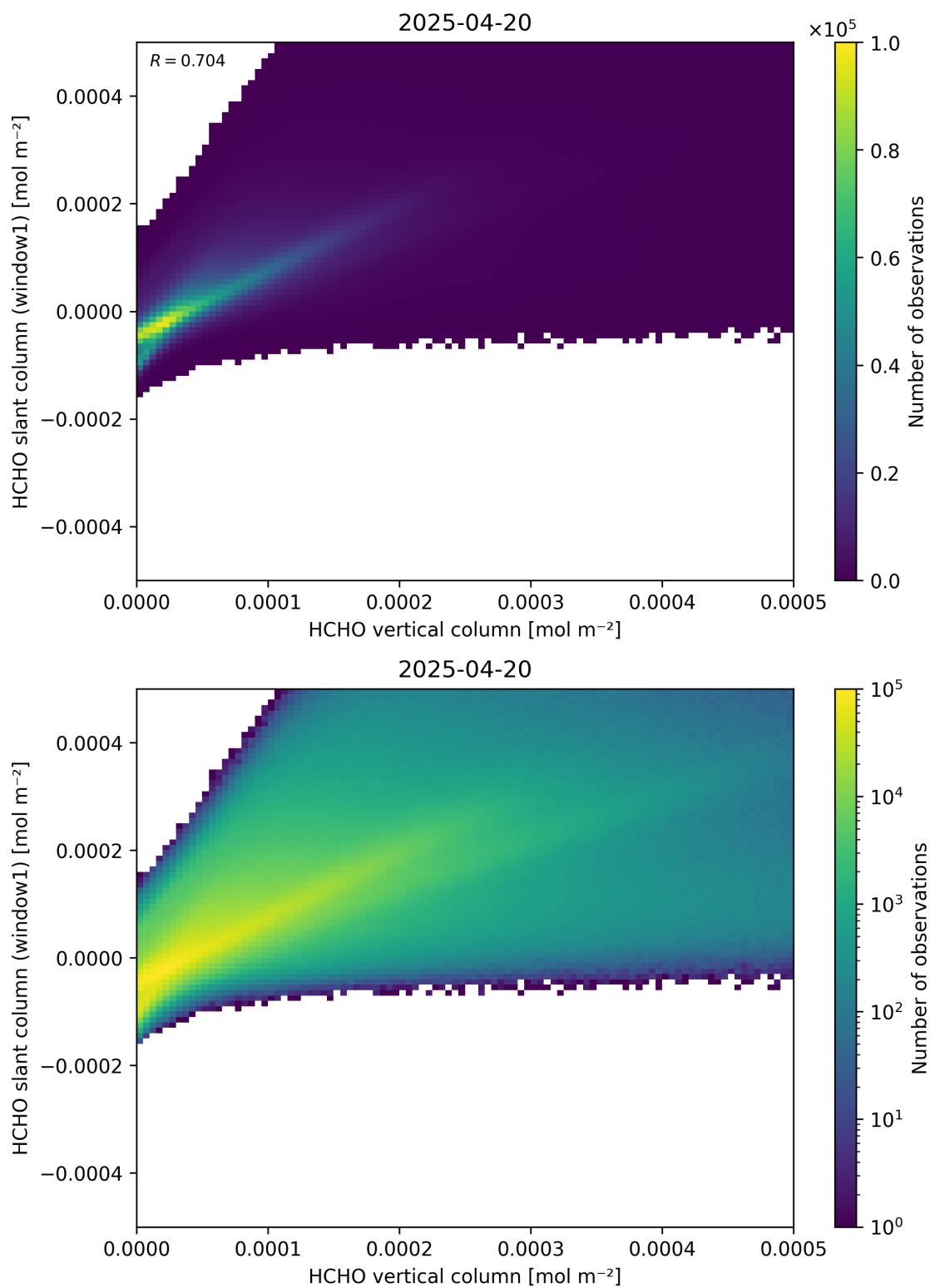
Figure 129: Scatter density plot of “HCHO vertical column” against “HCHO slant column (window1)” for 2025-04-19 to 2025-04-21.
