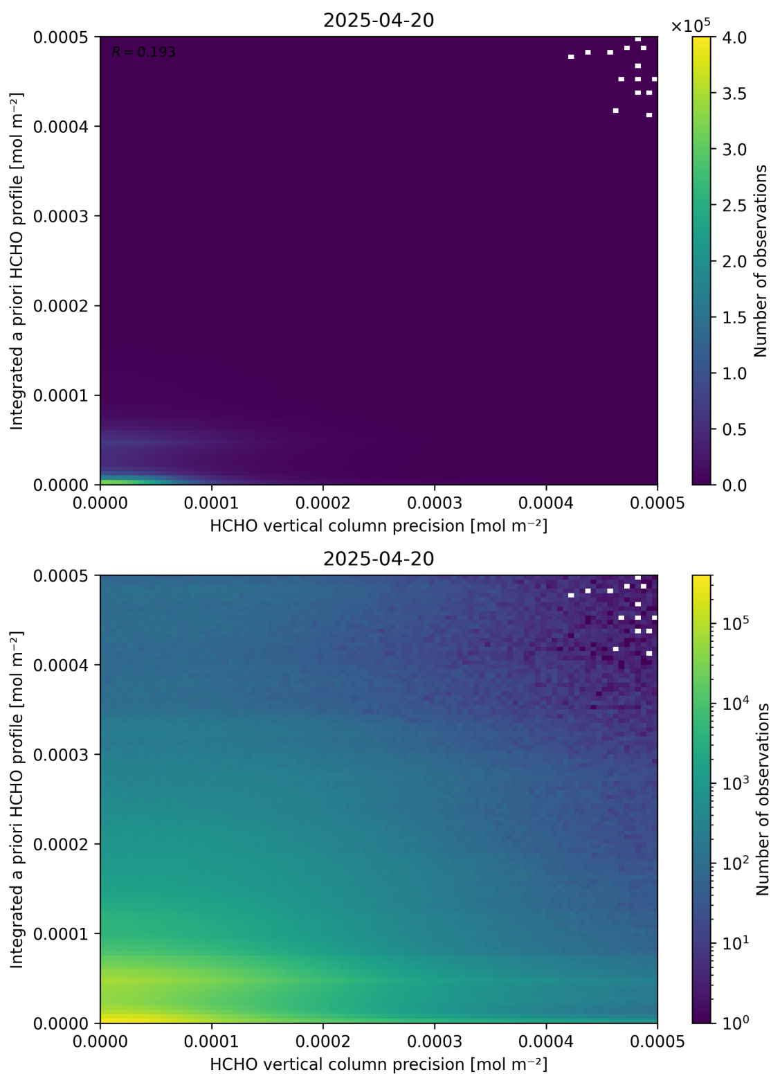
Figure 147: Scatter density plot of “HCHO vertical column precision” against “Integrated a priori HCHO profile” for 2025-04-19 to 2025-04-21.
