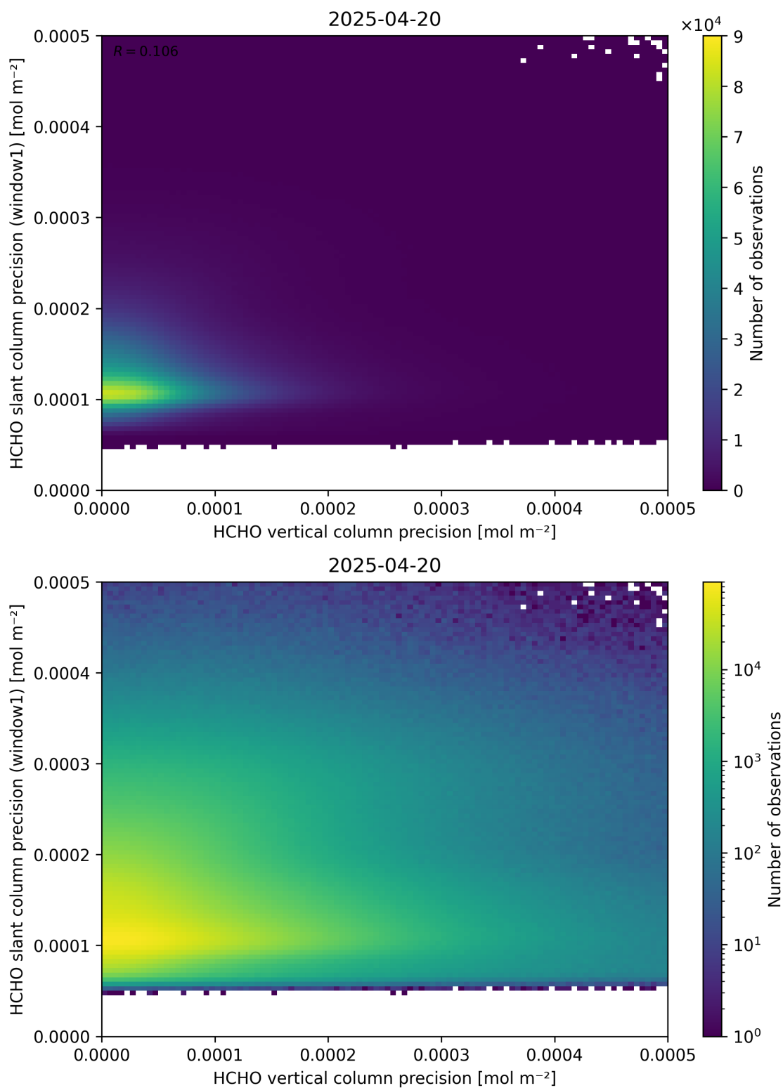
Figure 143: Scatter density plot of “HCHO vertical column precision” against “HCHO slant column precision (window1)” for 2025-04-19 to 2025-04-21.
