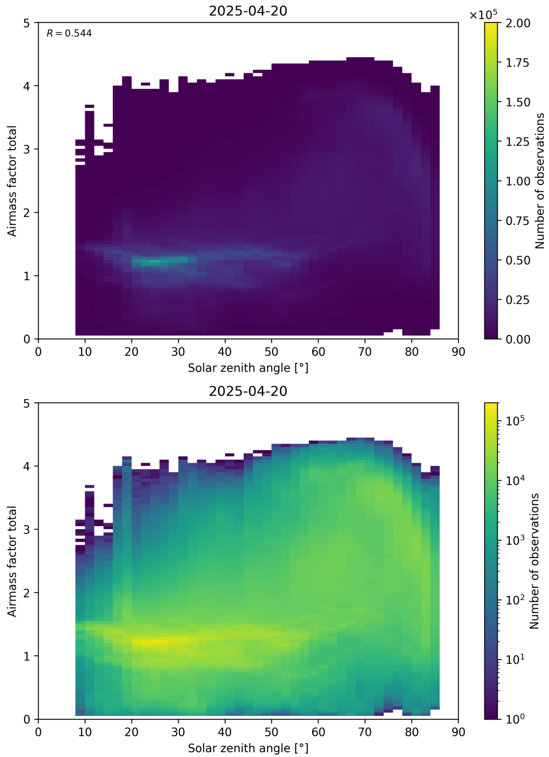
Figure 175: Scatter density plot of “Solar zenith angle” against “Airmass factor total” for 2025-04-19 to 2025-04-21.
