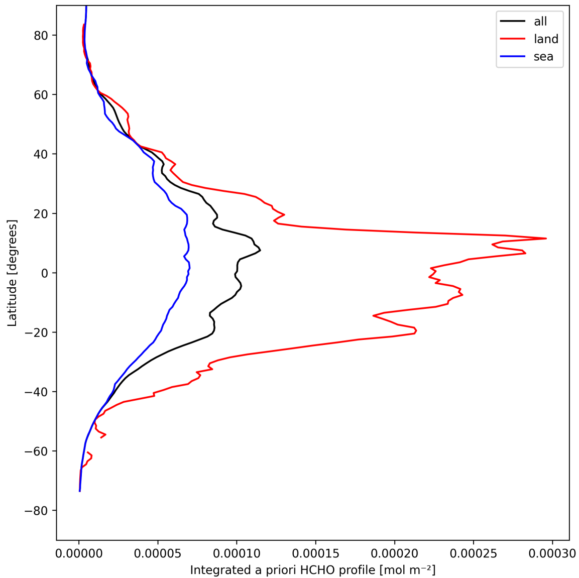
Figure 29: Zonal average of “Integrated a priori HCHO profile” for 2025-04-19 to 2025-04-21.
