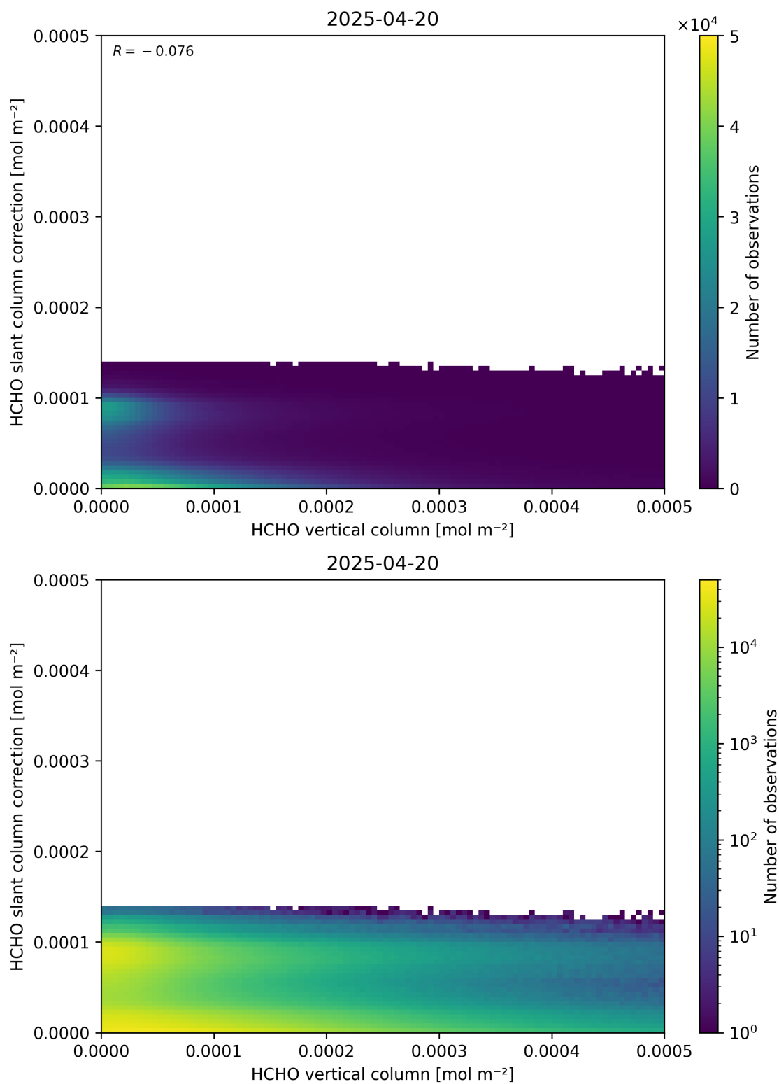
Figure 128: Scatter density plot of “HCHO vertical column” against “HCHO slant column correction” for 2025-04-19 to 2025-04-21.
