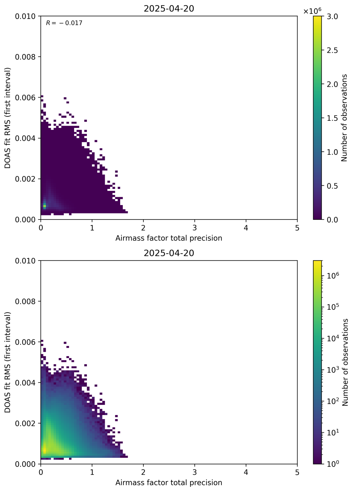
Figure 105: Scatter density plot of “Airmass factor total precision” against “DOAS fit RMS (first interval)” for 2025-04-19 to 2025-04-21.
