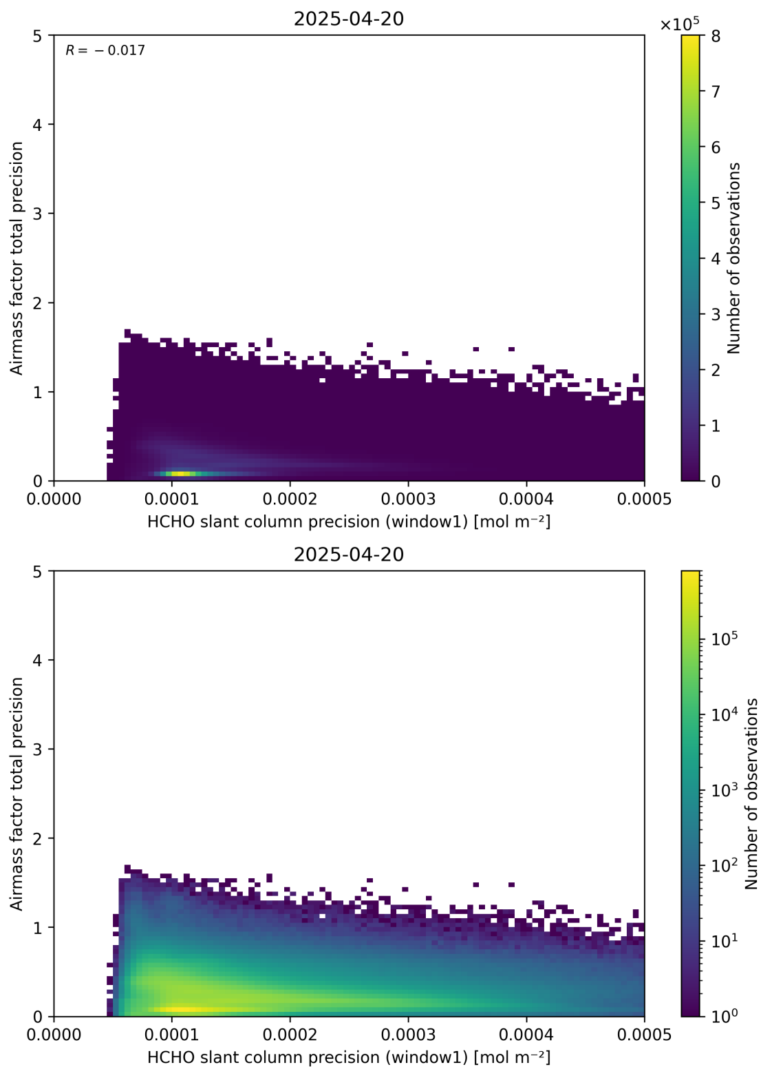
Figure 95: Scatter density plot of “HCHO slant column precision (window1)” against “Airmass factor total precision” for 2025-04-19 to 2025-04-21.
