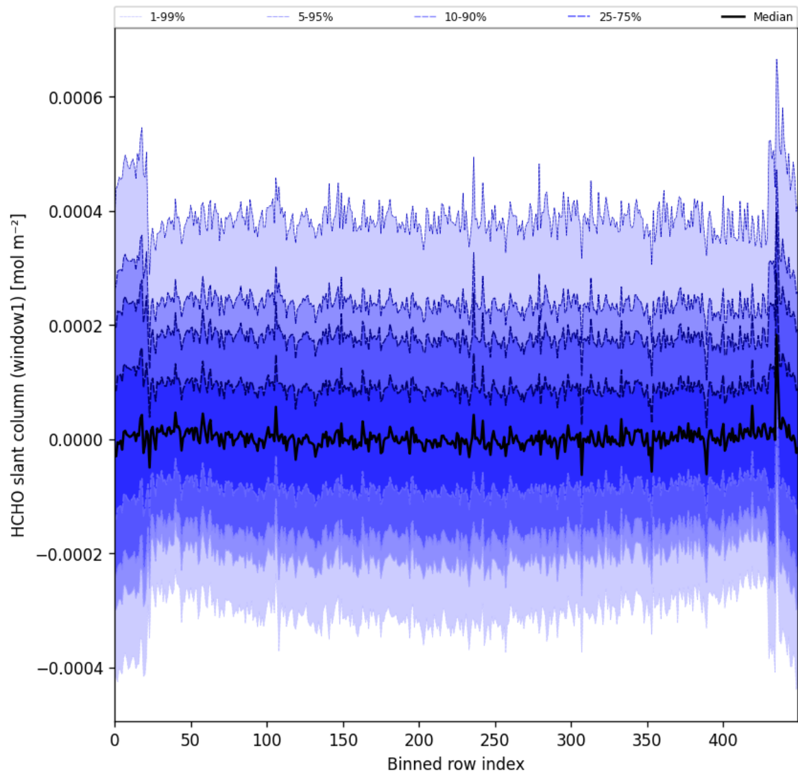
Figure 52: Along track statistics of “HCHO slant column (window1)” for 2025-04-19 to 2025-04-21
