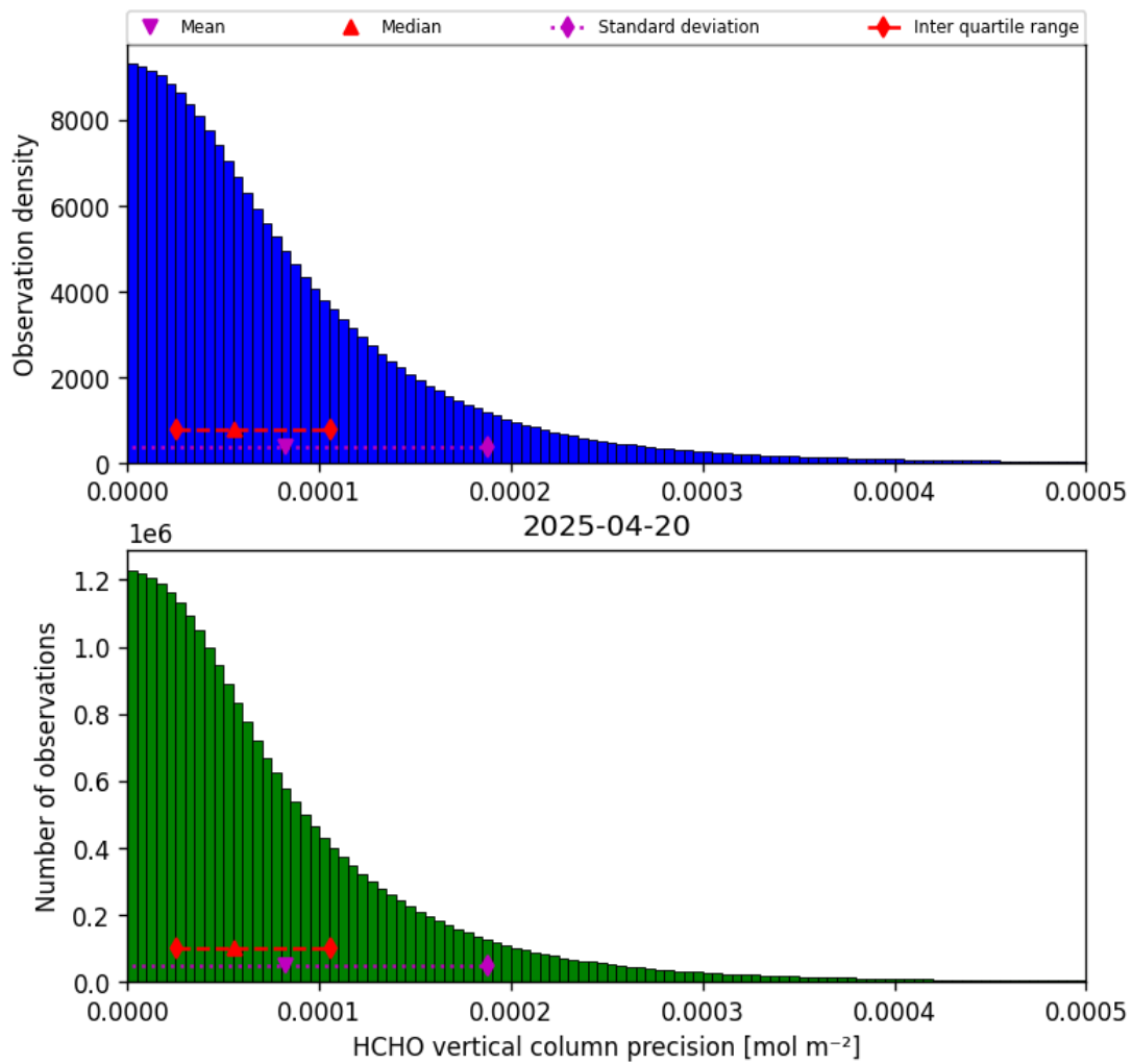
Figure 36: Histogram of “HCHO vertical column precision” for 2025-04-19 to 2025-04-21
