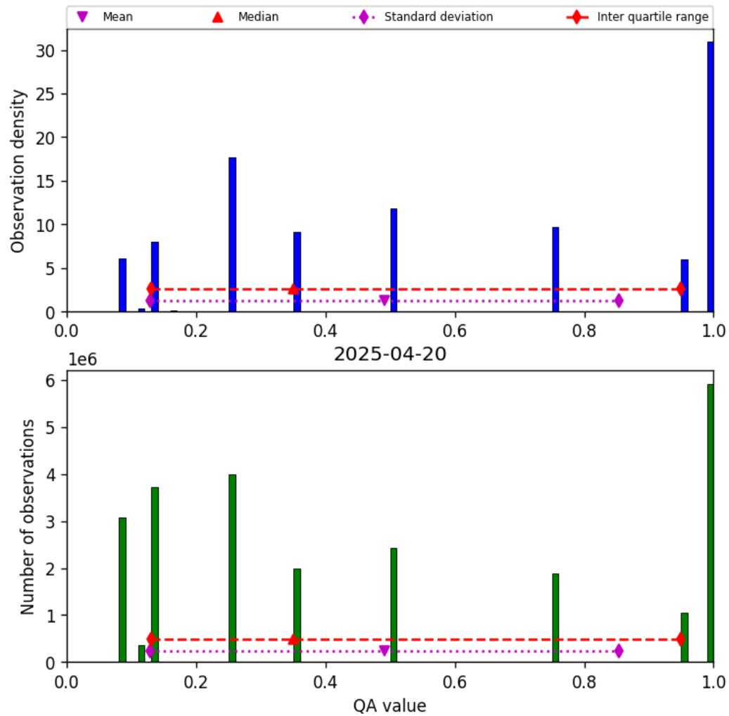
Figure 34: Histogram of “QA value” for 2025-04-19 to 2025-04-21
