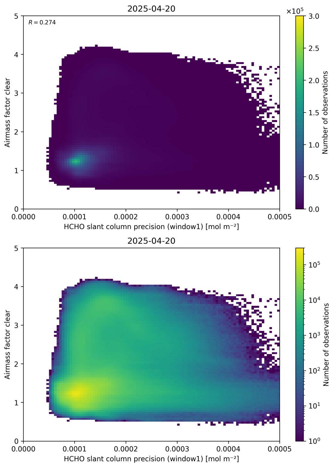
Figure 91: Scatter density plot of “HCHO slant column precision (window1)” against “Airmass factor clear” for 2025-04-19 to 2025-04-21.
