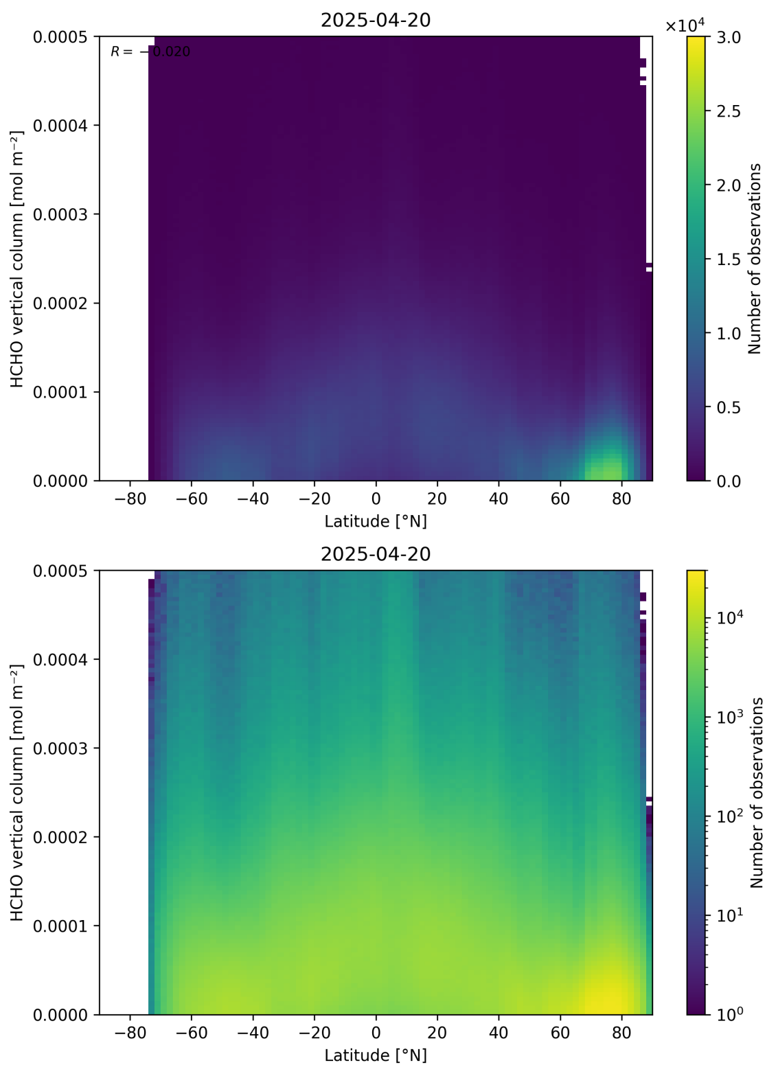
Figure 163: Scatter density plot of “Latitude” against “HCHO vertical column” for 2025-04-19 to 2025-04-21.
