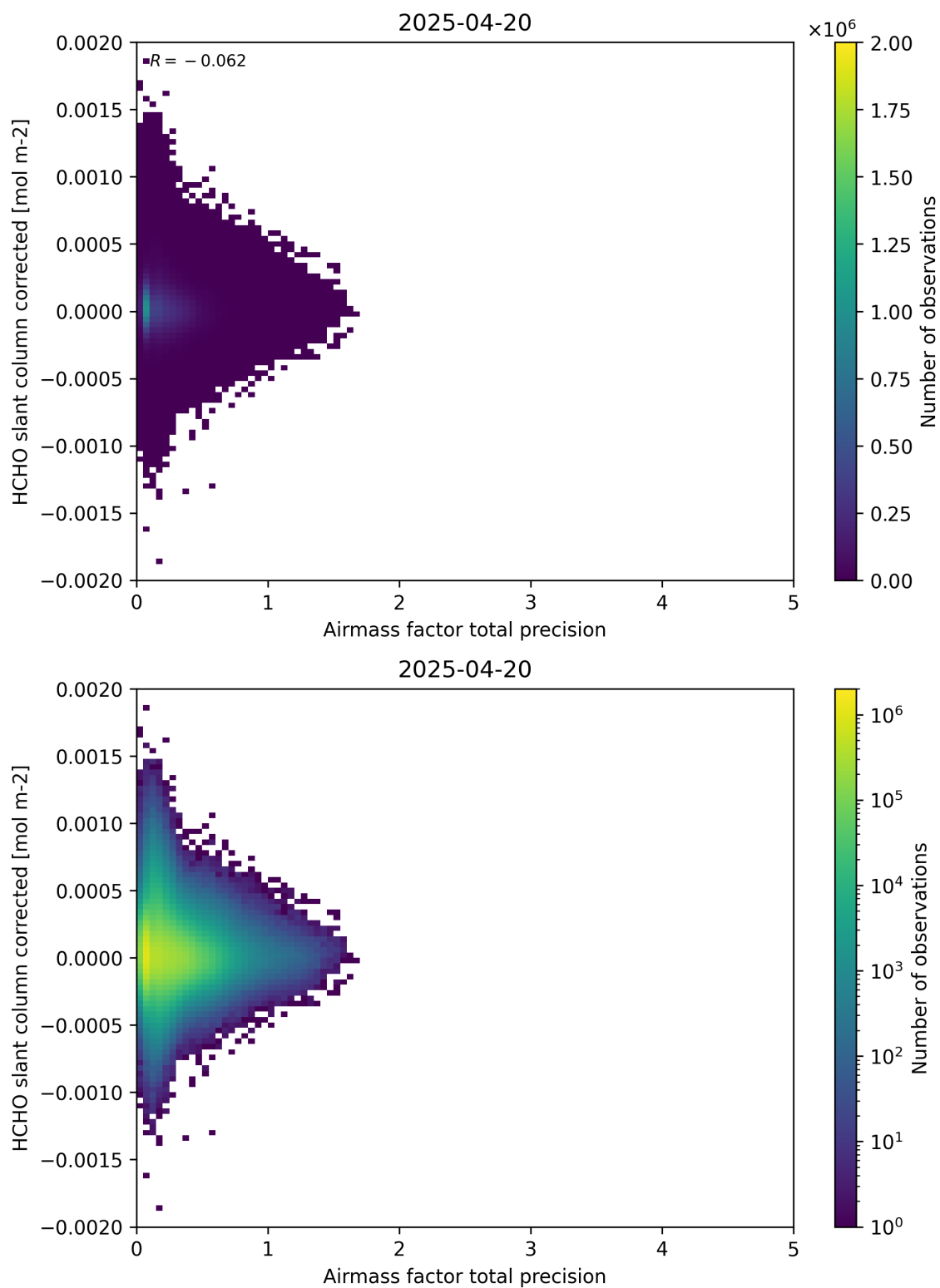
Figure 109: Scatter density plot of “Airmass factor total precision” against “HCHO slant column corrected” for 2025-04-19 to 2025-04-21.
