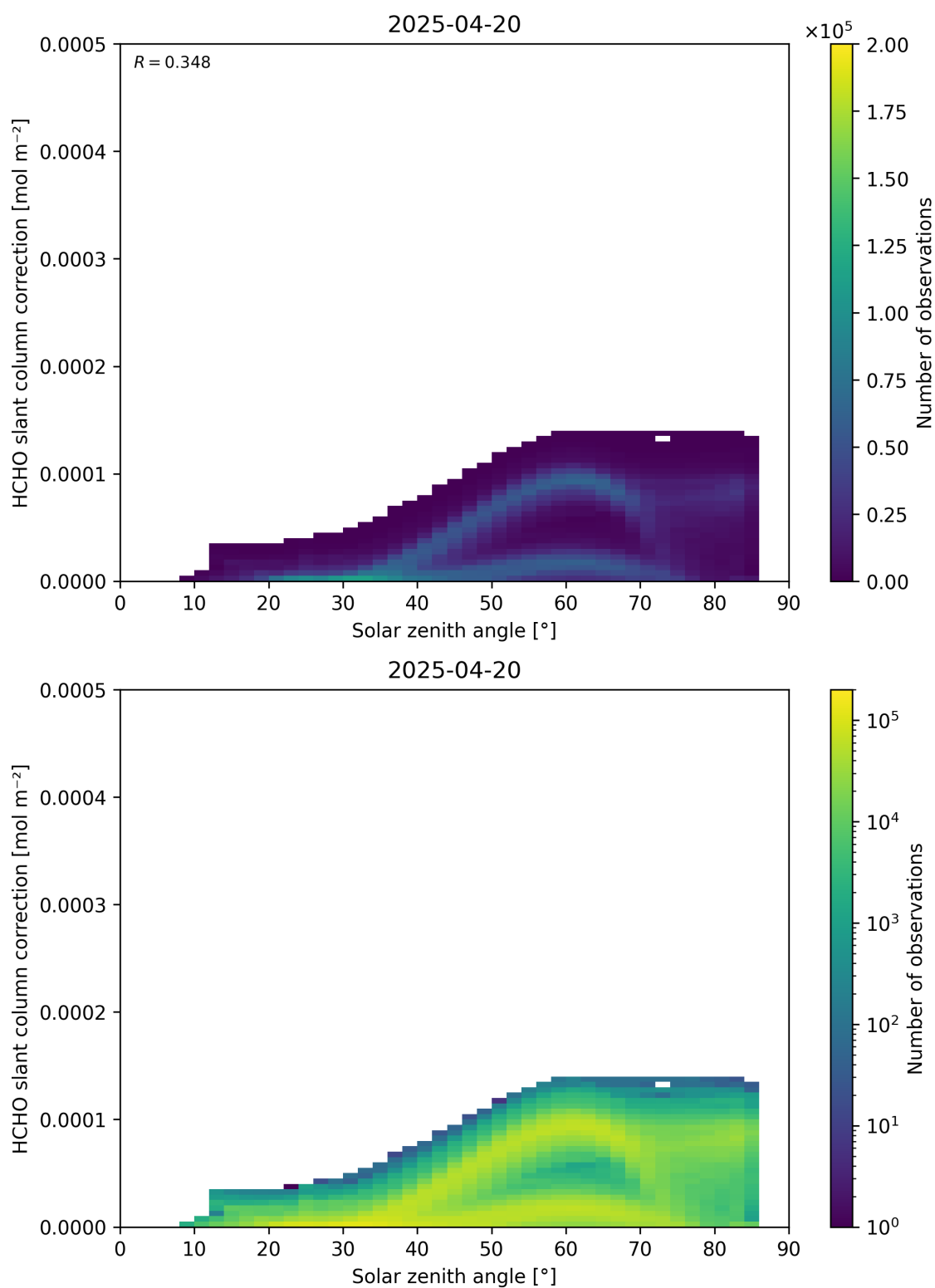
Figure 172: Scatter density plot of “Solar zenith angle” against “HCHO slant column correction” for 2025-04-19 to 2025-04-21.
