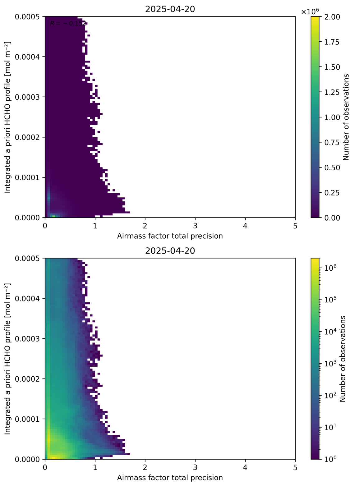
Figure 111: Scatter density plot of “Airmass factor total precision” against “Integrated a priori HCHO profile” for 2025-04-19 to 2025-04-21.
