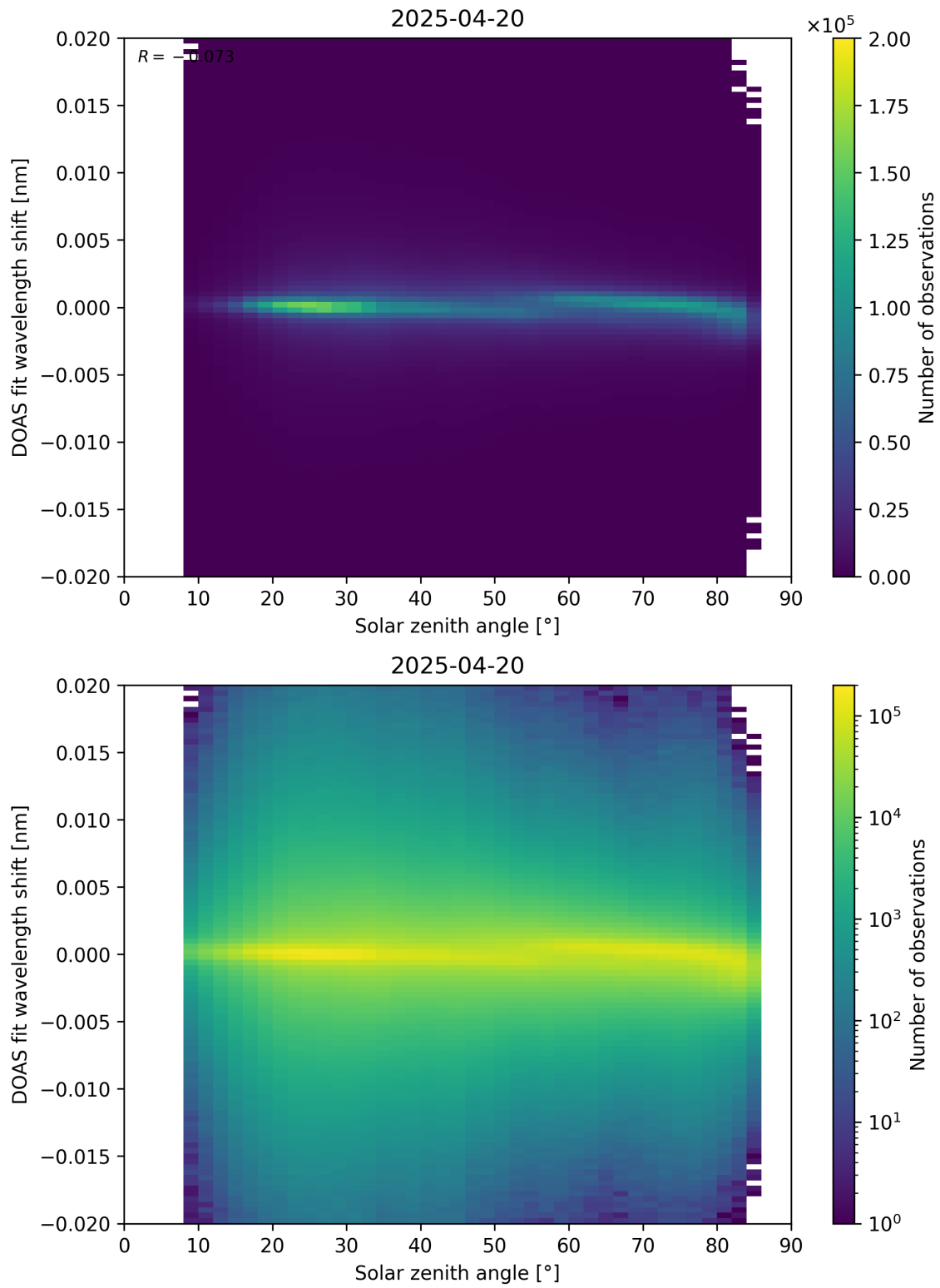
Figure 168: Scatter density plot of “Solar zenith angle” against “DOAS fit wavelength shift” for 2025-04-19 to 2025-04-21.
