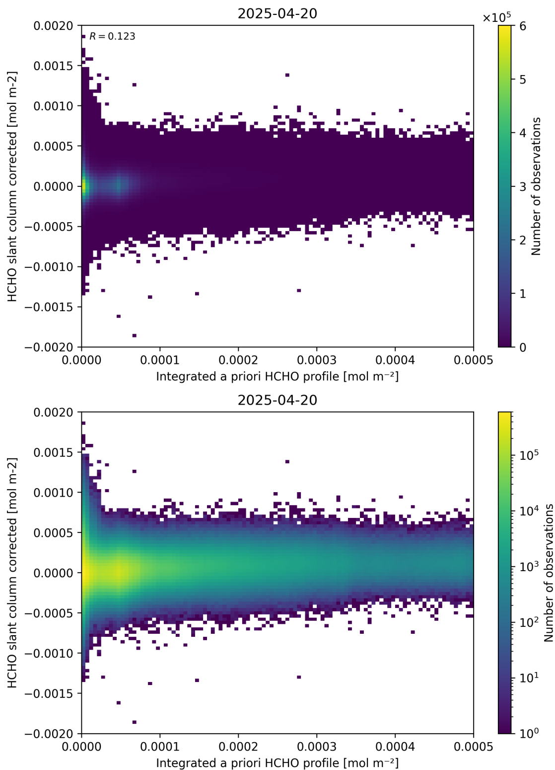
Figure 151: Scatter density plot of “Integrated a priori HCHO profile” against “HCHO slant column corrected” for 2025-04-19 to 2025-04-21.
