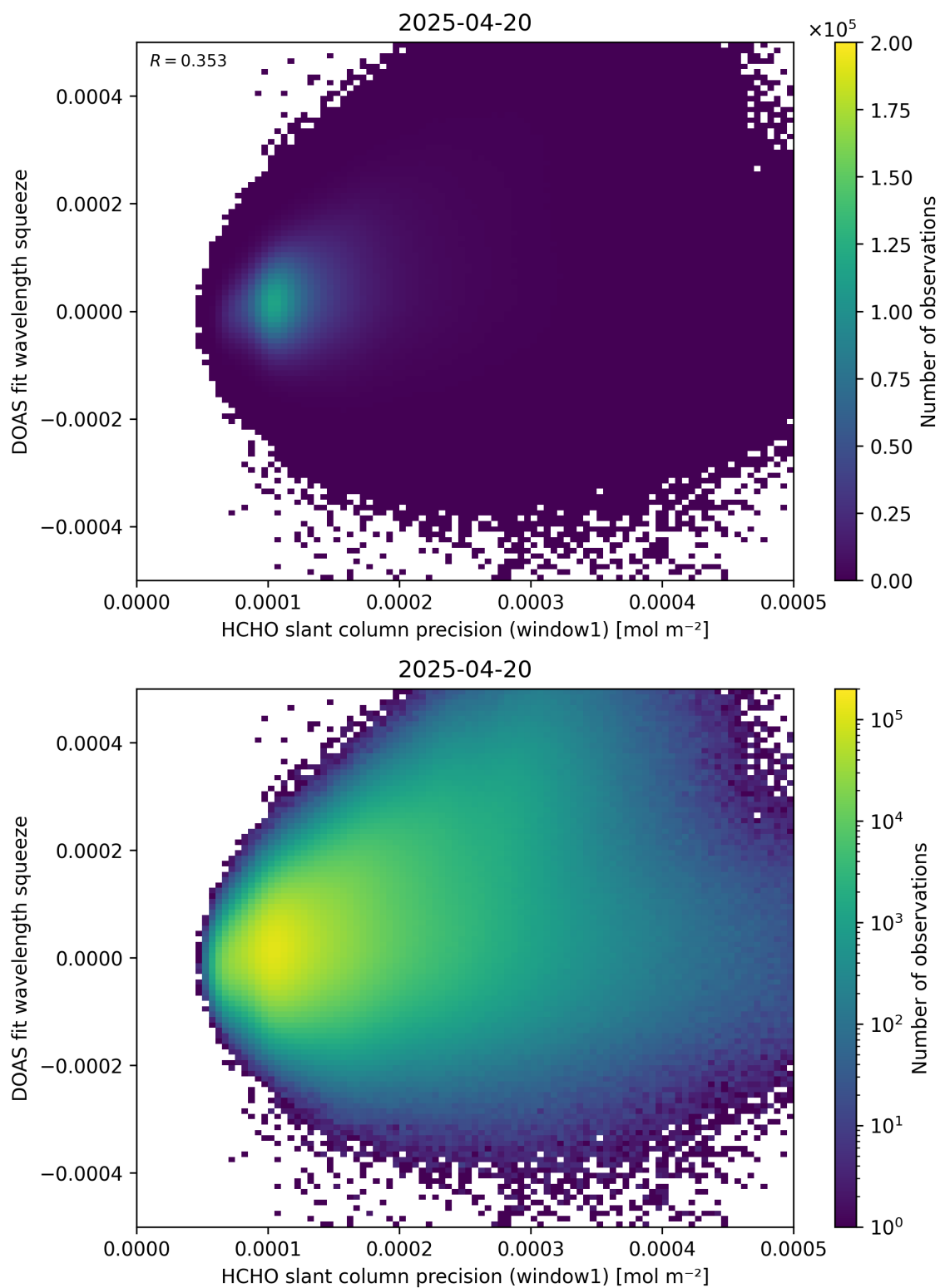
Figure 90: Scatter density plot of “HCHO slant column precision (window1)” against “DOAS fit wavelength squeeze” for 2025-04-19 to 2025-04-21.
