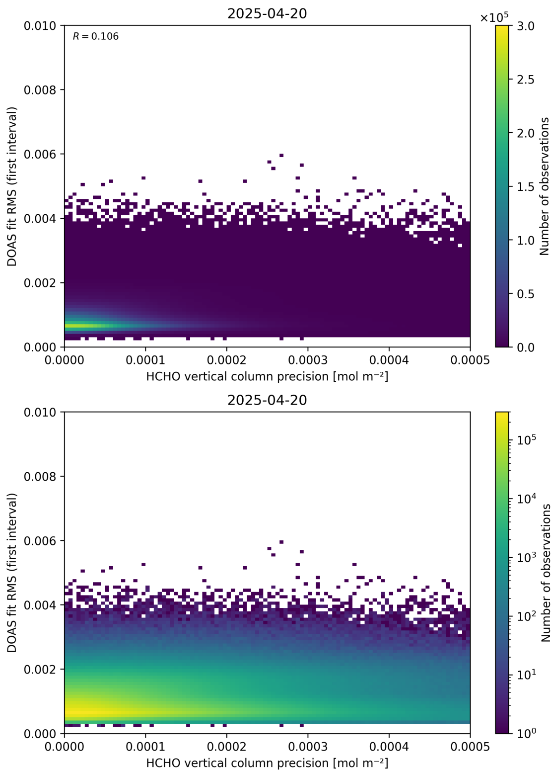
Figure 136: Scatter density plot of “HCHO vertical column precision” against “DOAS fit RMS (first interval)” for 2025-04-19 to 2025-04-21.
