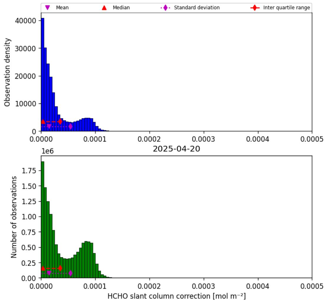
Figure 47: Histogram of “HCHO slant column correction” for 2025-04-19 to 2025-04-21
