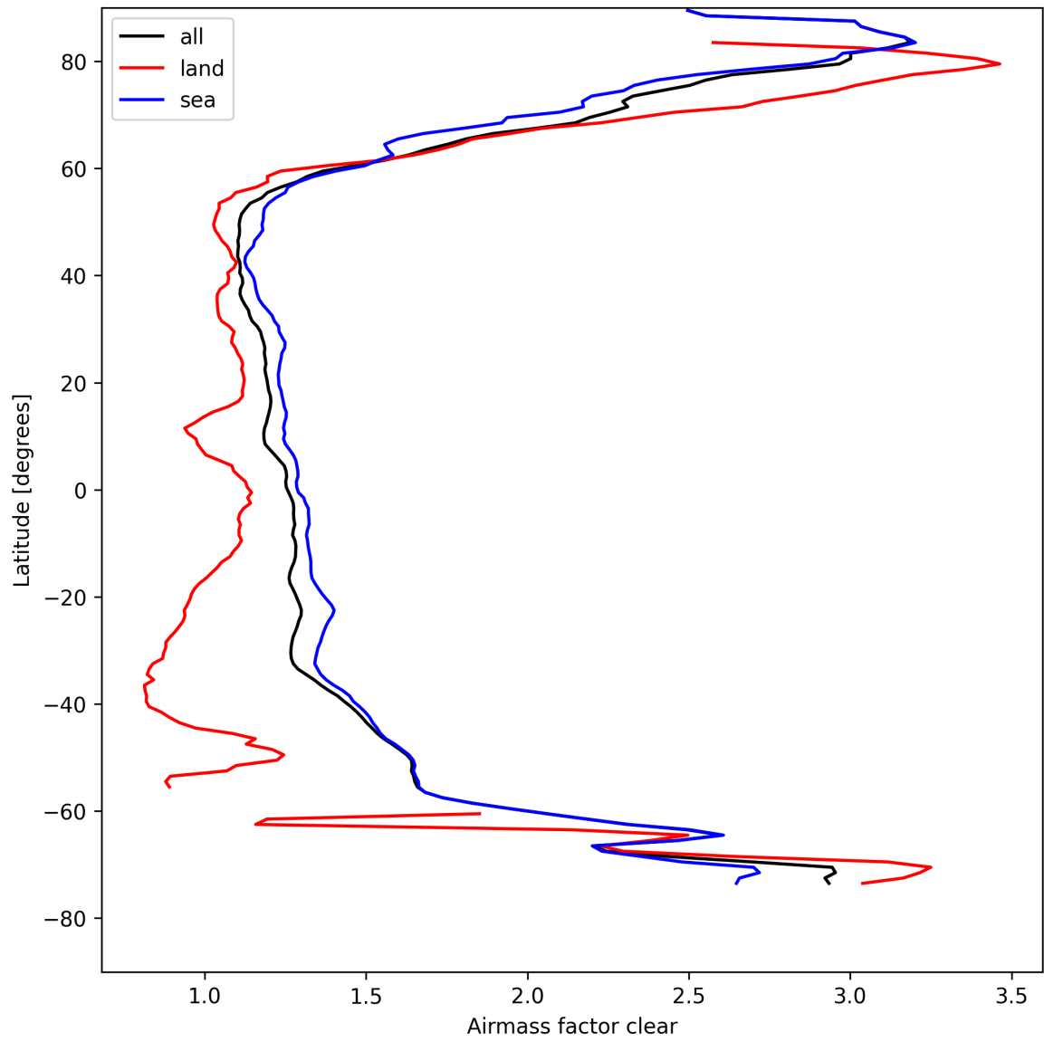
Figure 28: Zonal average of “Airmass factor clear” for 2025-04-19 to 2025-04-21.
