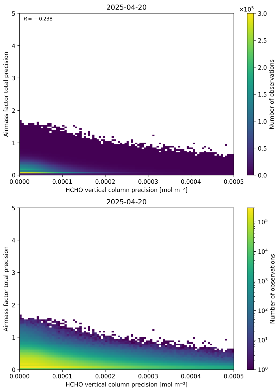
Figure 145: Scatter density plot of “HCHO vertical column precision” against “Airmass factor total precision” for 2025-04-19 to 2025-04-21.
