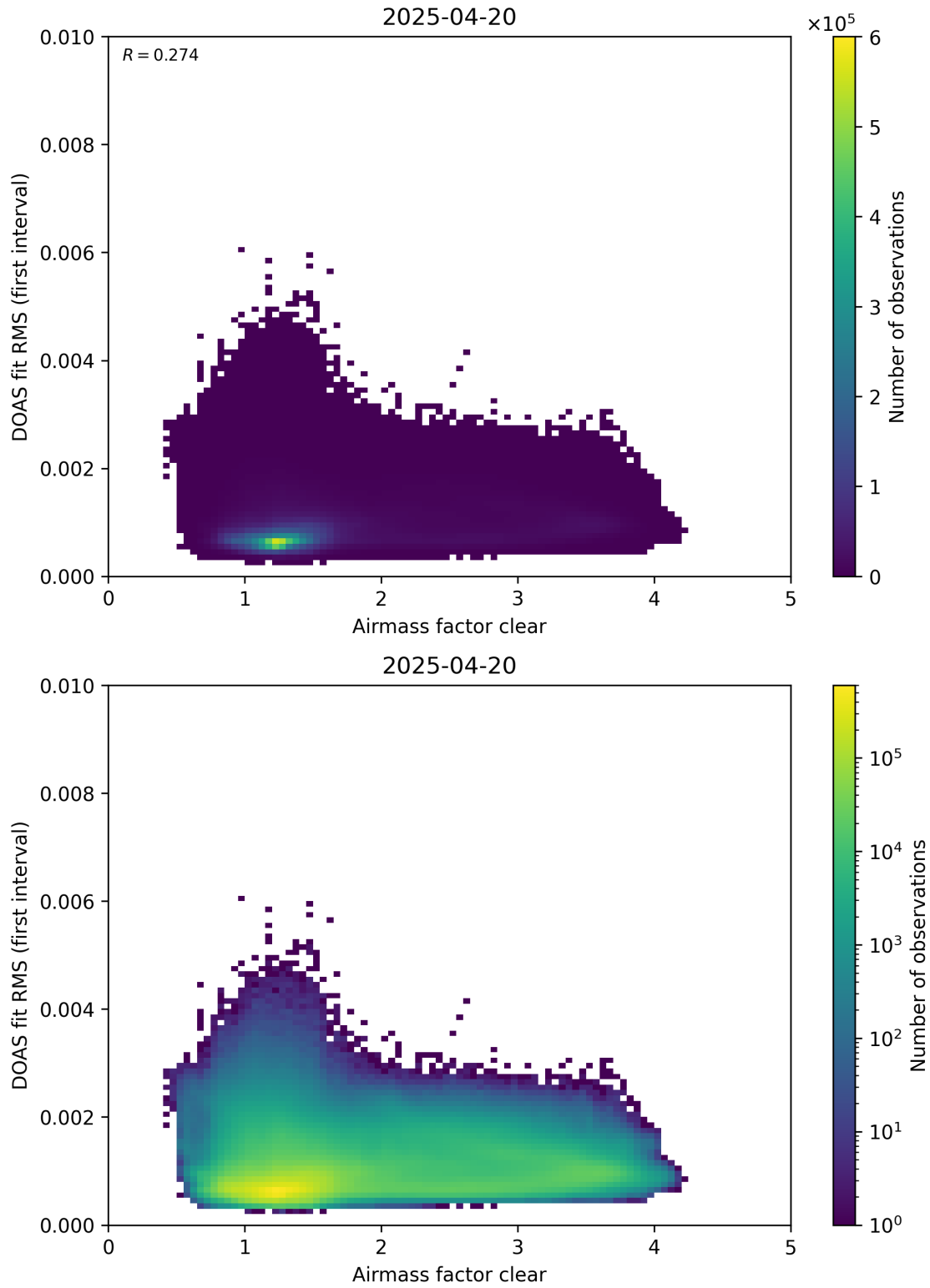
Figure 71: Scatter density plot of “Airmass factor clear” against “DOAS fit RMS (first interval)” for 2025-04-19 to 2025-04-21.
