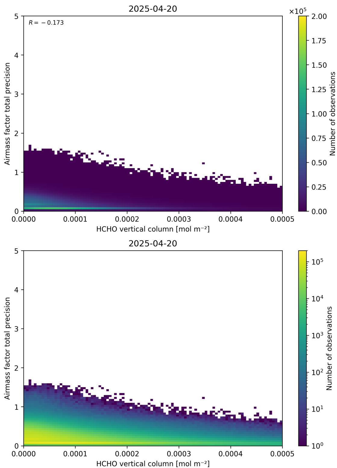
Figure 132: Scatter density plot of “HCHO vertical column” against “Airmass factor total precision” for 2025-04-19 to 2025-04-21.
