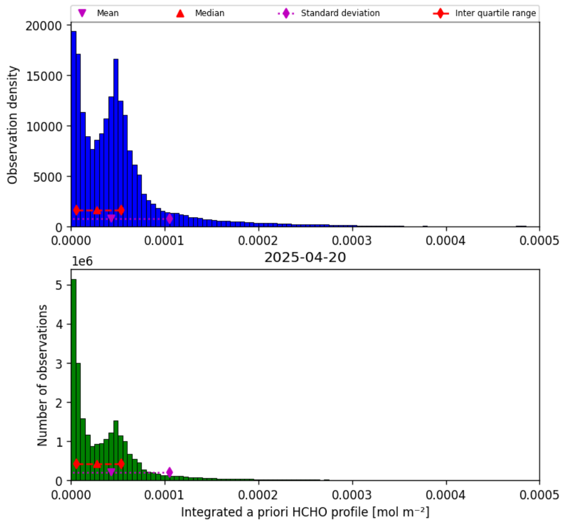
Figure 43: Histogram of “Integrated a priori HCHO profile” for 2025-04-19 to 2025-04-21
