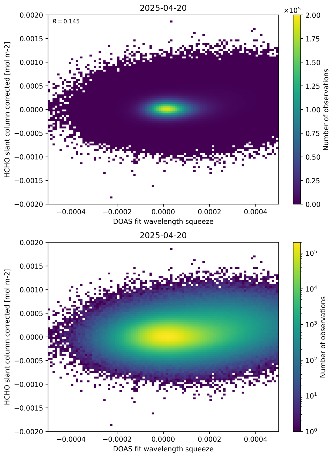
Figure 69: Scatter density plot of “DOAS fit wavelength squeeze” against “HCHO slant column corrected” for 2025-04-19 to 2025-04-21.
