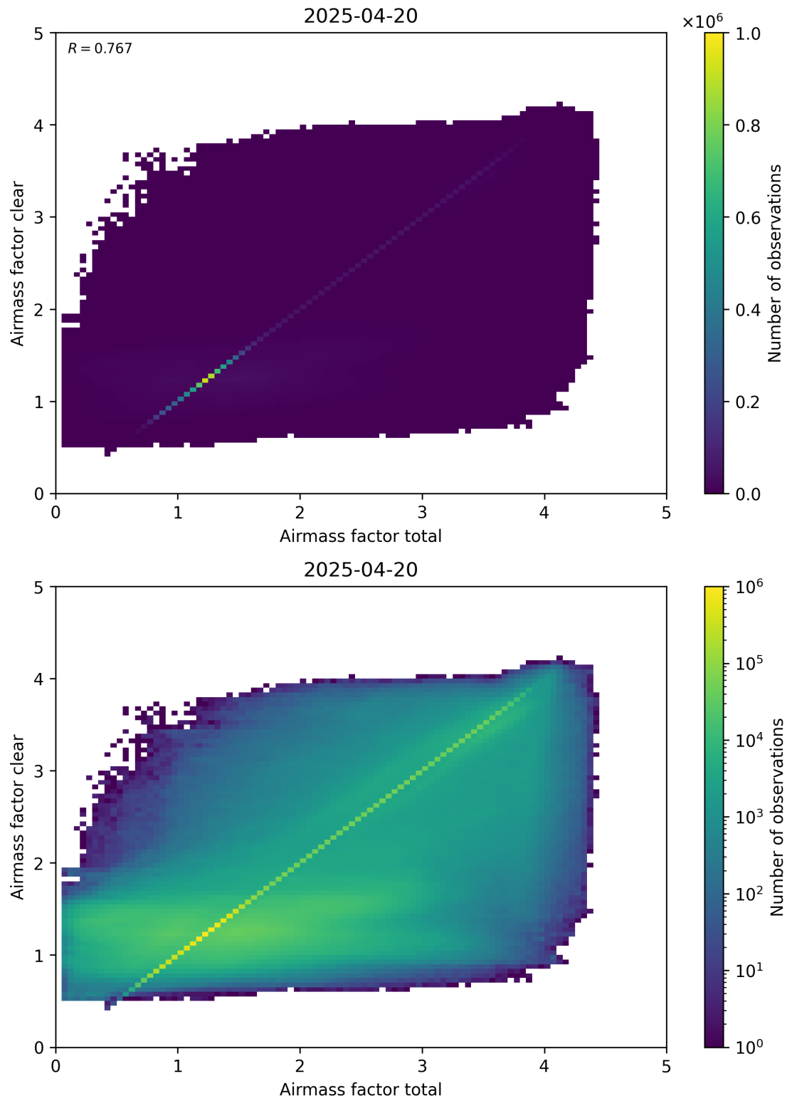
Figure 100: Scatter density plot of “Airmass factor total” against “Airmass factor clear” for 2025-04-19 to 2025-04-21.
