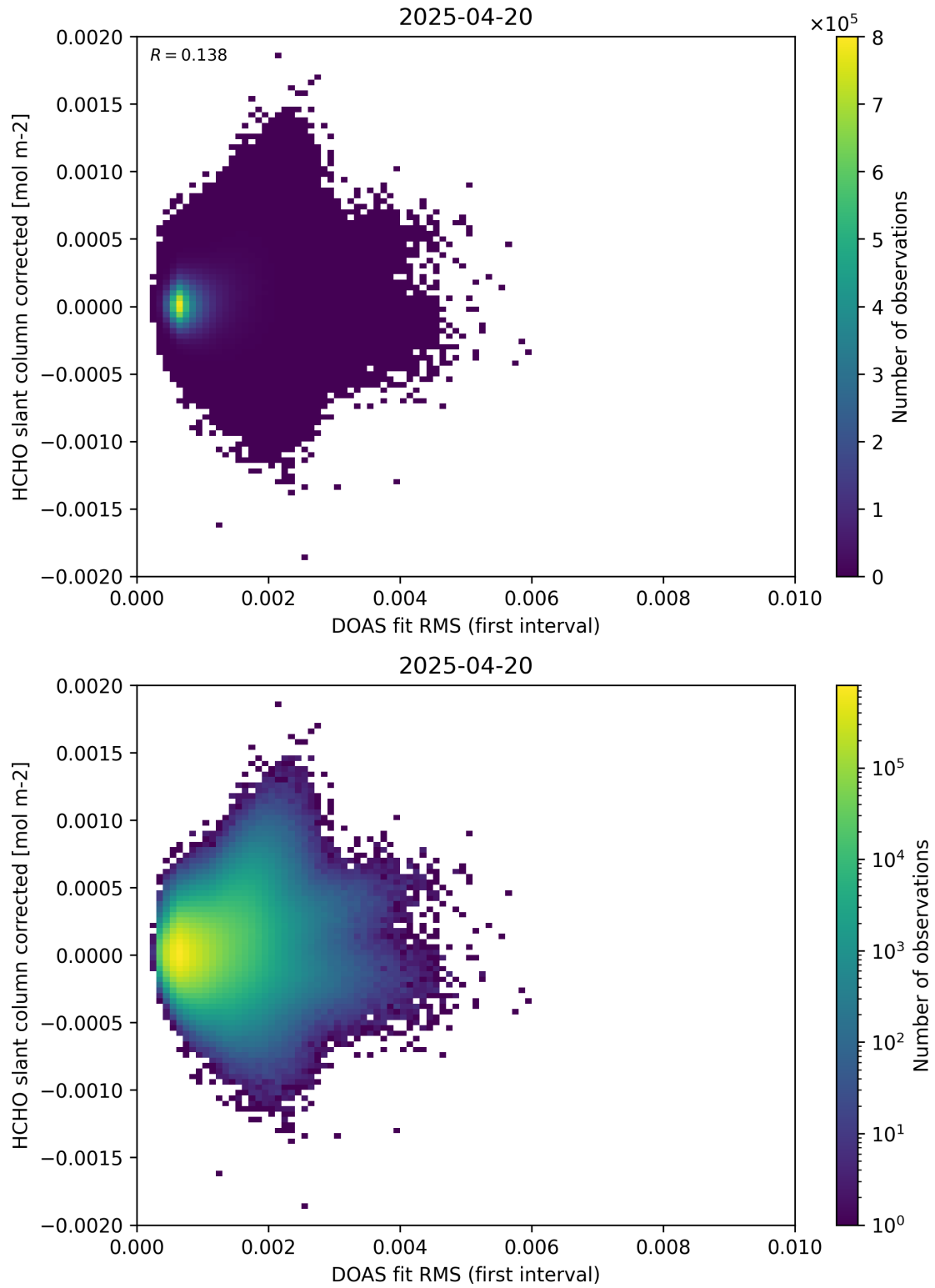
Figure 62: Scatter density plot of “DOAS fit RMS (first interval)” against “HCHO slant column corrected” for 2025-04-19 to 2025-04-21.
