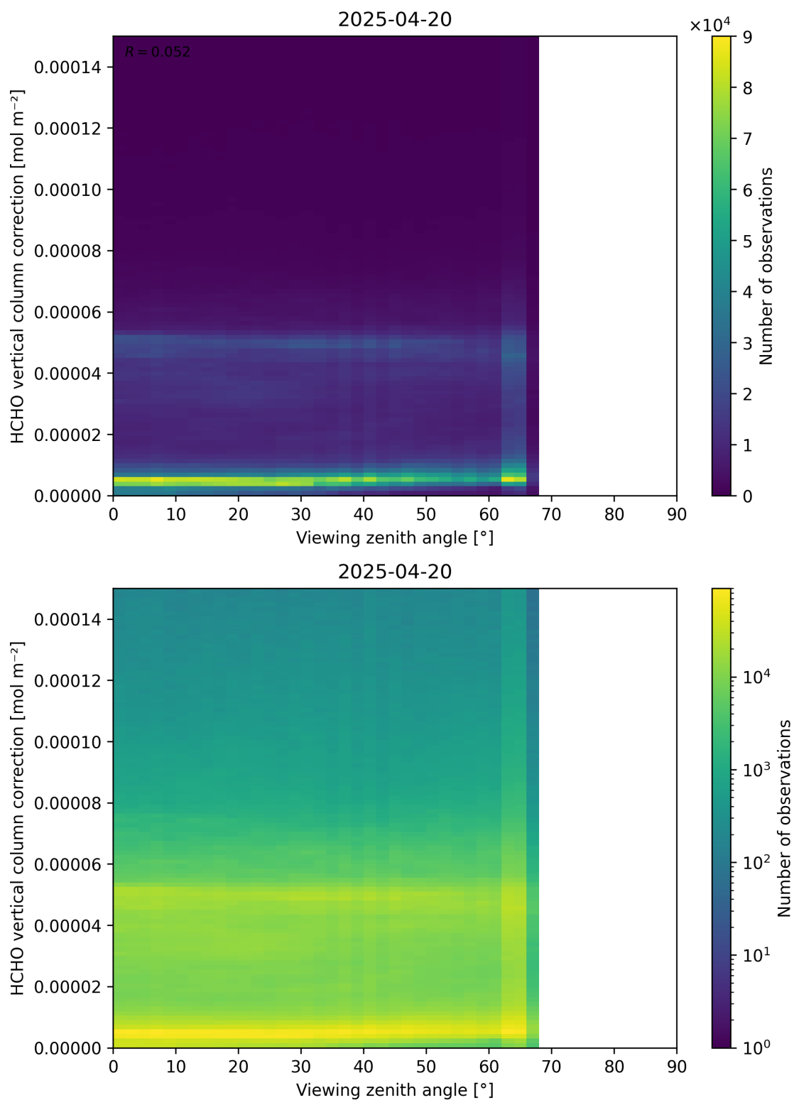
Figure 193: Scatter density plot of “Viewing zenith angle” against “HCHO vertical column correction” for 2025-04-19 to 2025-04-21.
