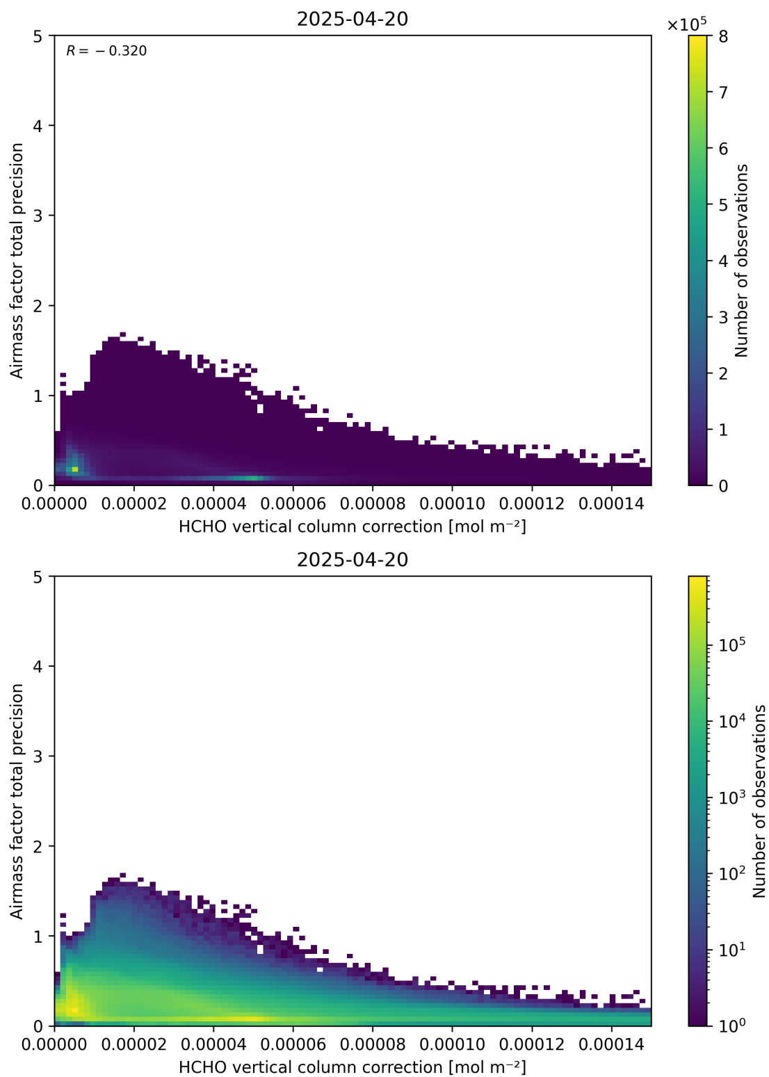
Figure 121: Scatter density plot of “HCHO vertical column correction” against “Airmass factor total precision” for 2025-04-19 to 2025-04-21.
