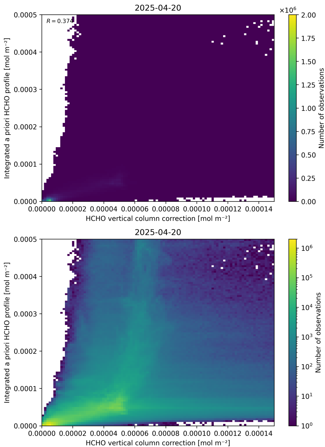
Figure 122: Scatter density plot of “HCHO vertical column correction” against “Integrated a priori HCHO profile” for 2025-04-19 to 2025-04-21.
