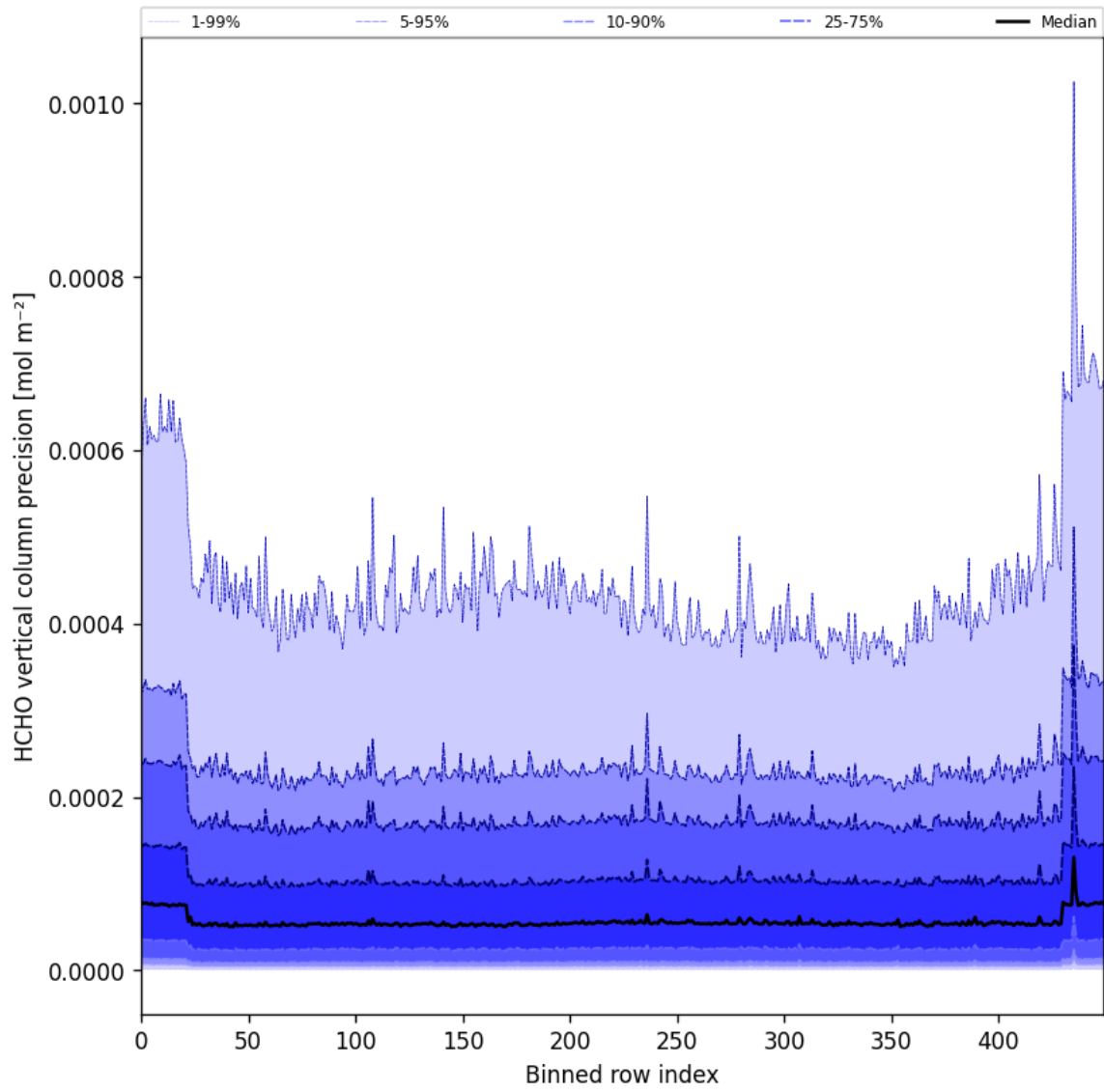
Figure 50: Along track statistics of “HCHO vertical column precision” for 2025-04-19 to 2025-04-21
