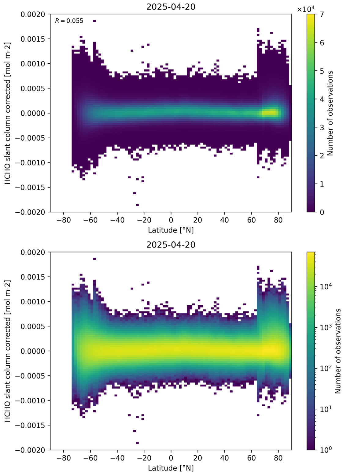
Figure 157: Scatter density plot of “Latitude” against “HCHO slant column corrected” for 2025-04-19 to 2025-04-21.
