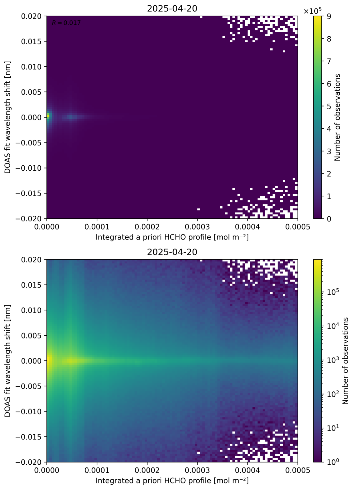
Figure 149: Scatter density plot of “Integrated a priori HCHO profile” against “DOAS fit wavelength shift” for 2025-04-19 to 2025-04-21.
