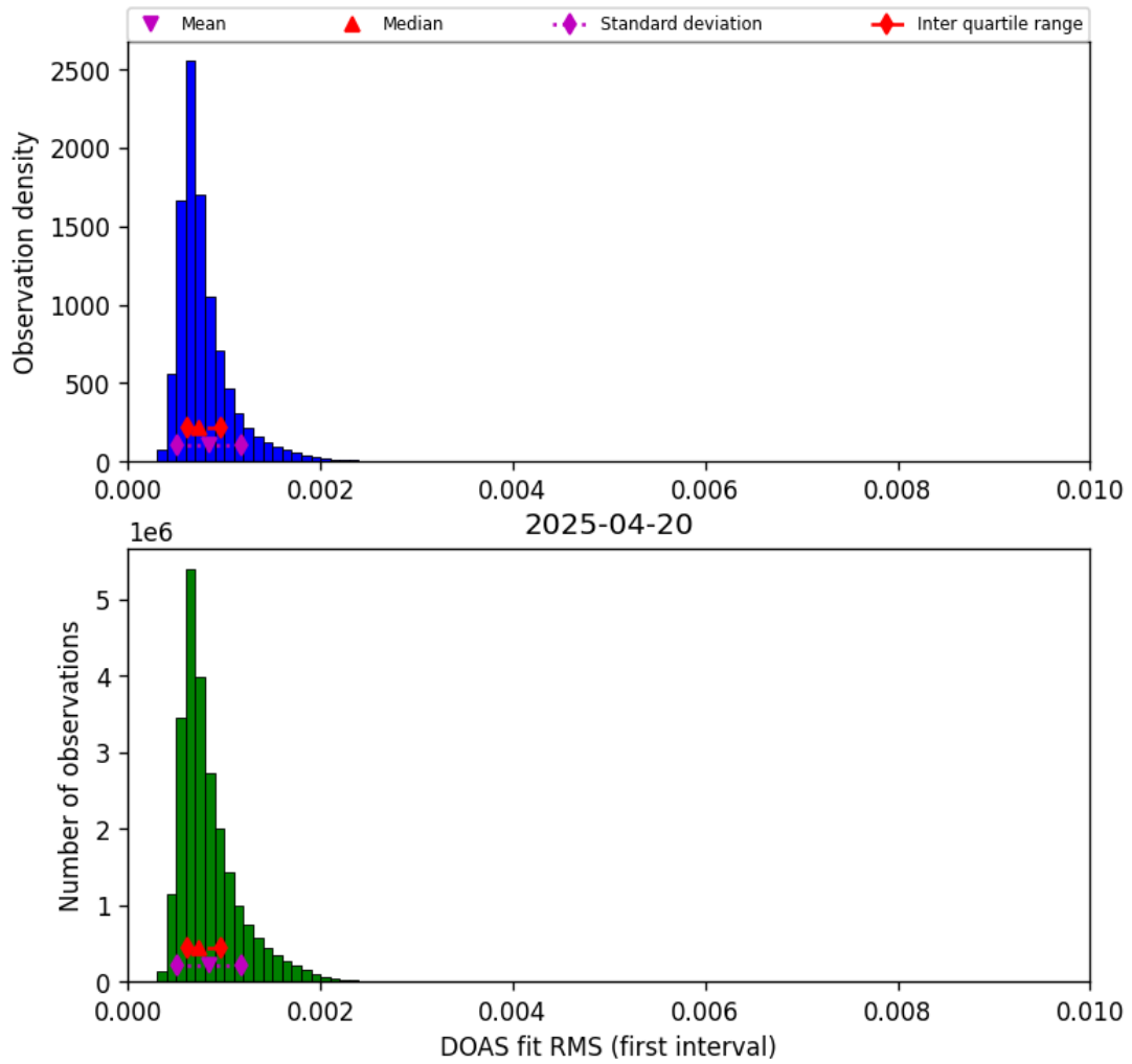
Figure 46: Histogram of “DOAS fit RMS (first interval)” for 2025-04-19 to 2025-04-21
