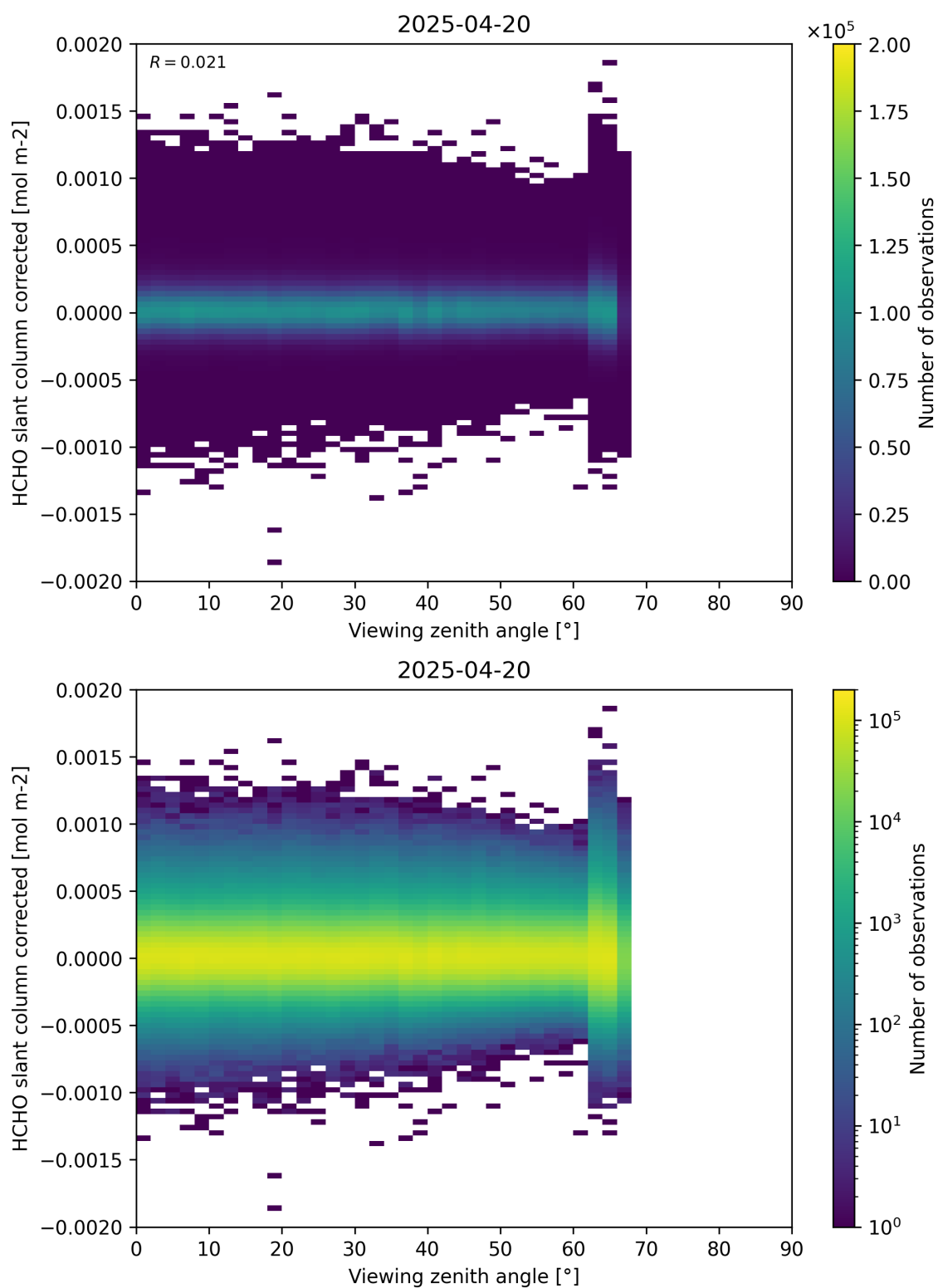
Figure 186: Scatter density plot of “Viewing zenith angle” against “HCHO slant column corrected” for 2025-04-19 to 2025-04-21.
