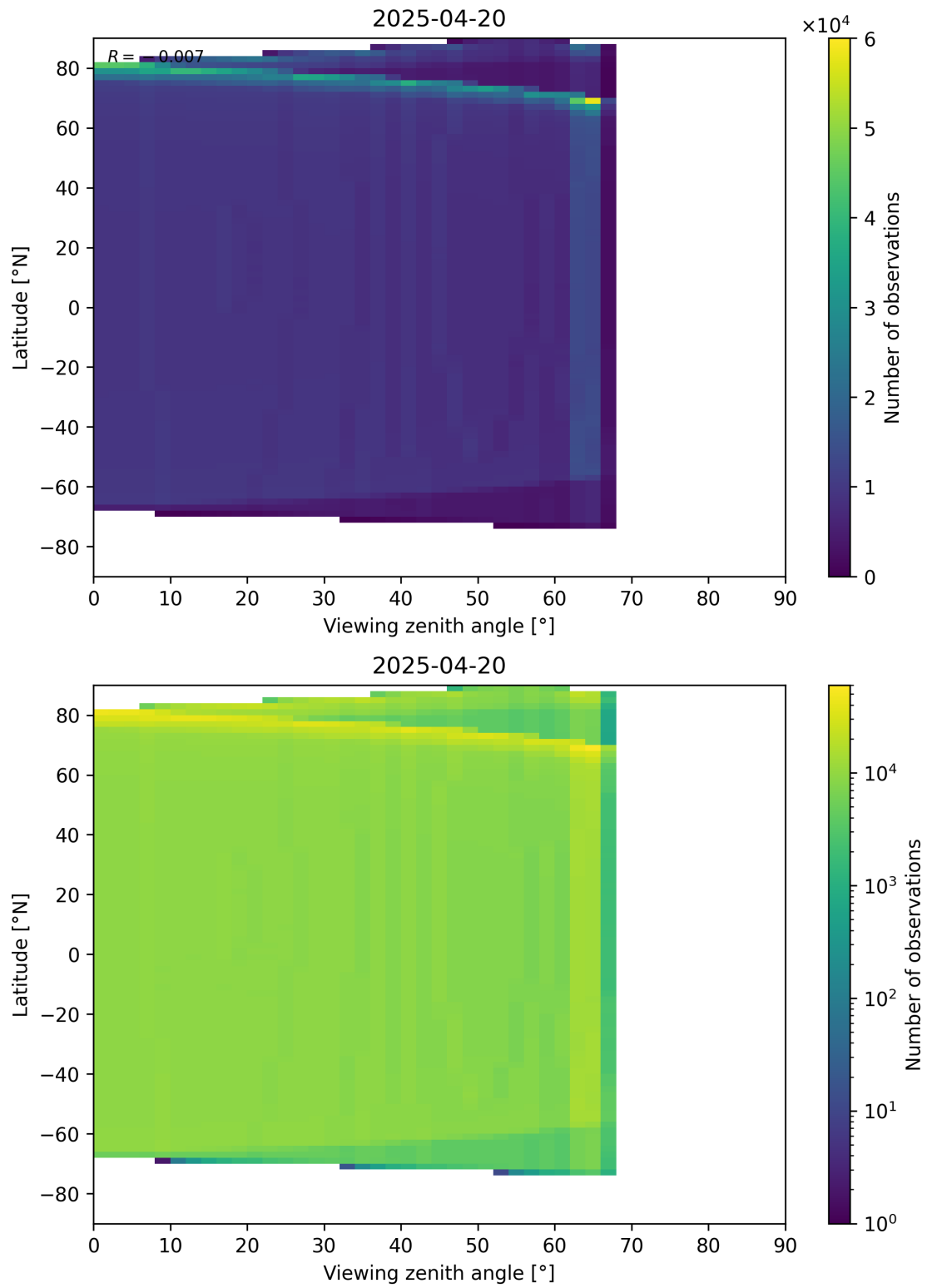
Figure 196: Scatter density plot of “Viewing zenith angle” against “Latitude” for 2025-04-19 to 2025-04-21.
