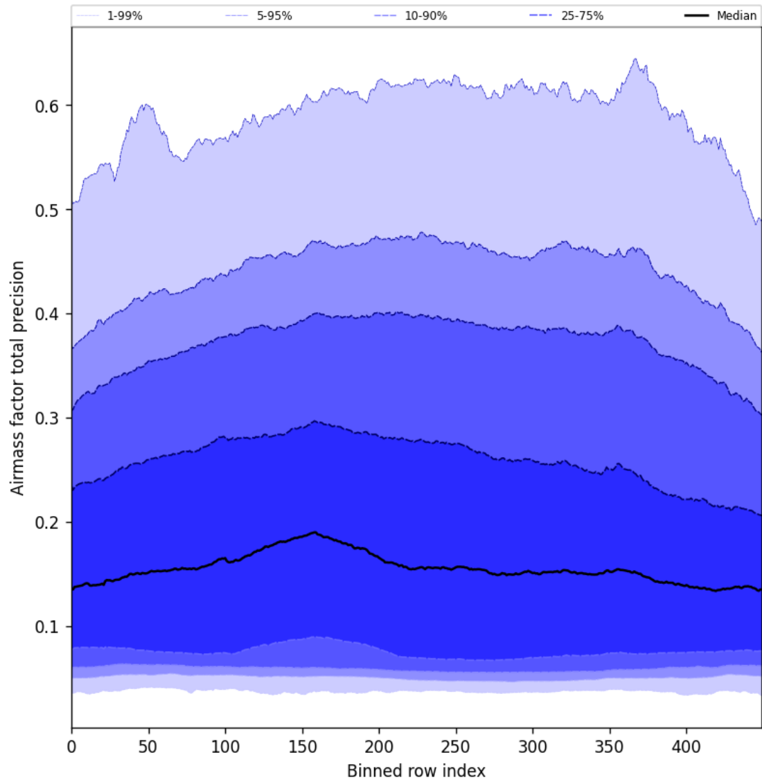
Figure 55: Along track statistics of “Airmass factor total precision” for 2025-04-19 to 2025-04-21
