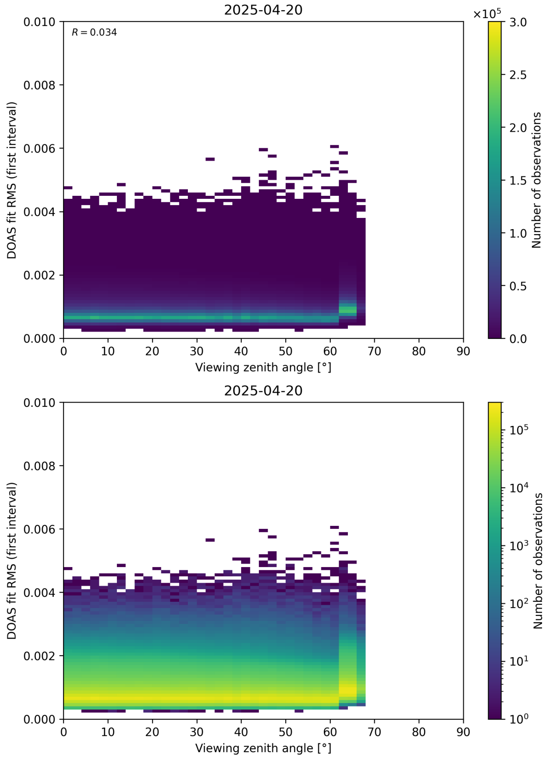
Figure 182: Scatter density plot of “Viewing zenith angle” against “DOAS fit RMS (first interval)” for 2025-04-19 to 2025-04-21.
