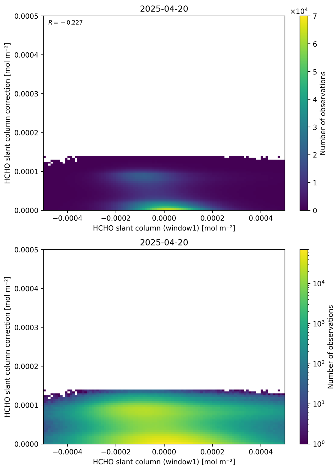
Figure 83: Scatter density plot of “HCHO slant column (window1)” against “HCHO slant column correction” for 2025-04-19 to 2025-04-21.
