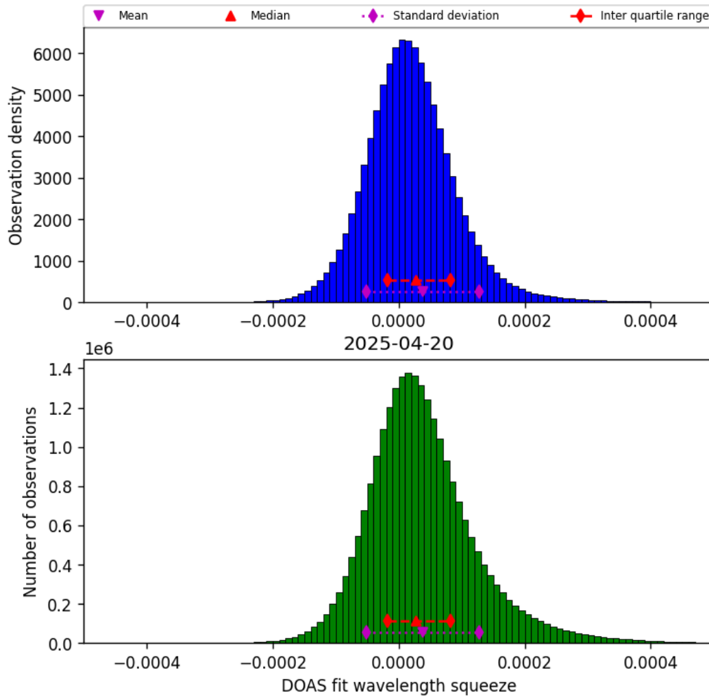
Figure 45: Histogram of “DOAS fit wavelength squeeze” for 2025-04-19 to 2025-04-21
