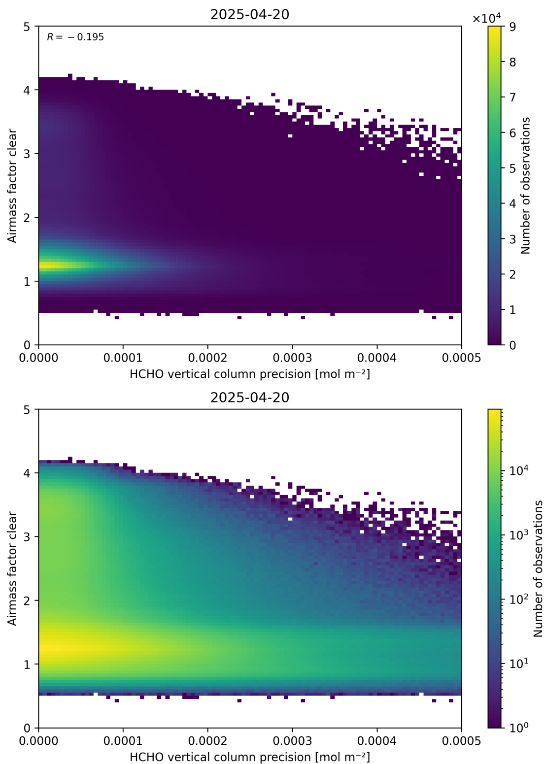
Figure 139: Scatter density plot of “HCHO vertical column precision” against “Airmass factor clear” for 2025-04-19 to 2025-04-21.
