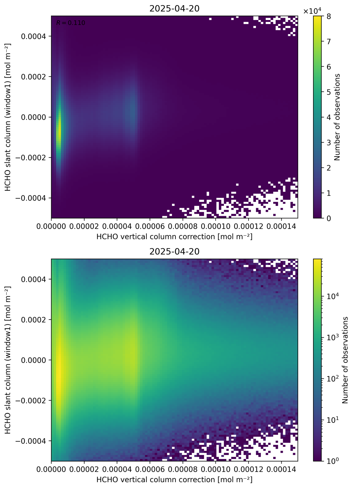
Figure 118: Scatter density plot of “HCHO vertical column correction” against “HCHO slant column (window1)” for 2025-04-19 to 2025-04-21.
