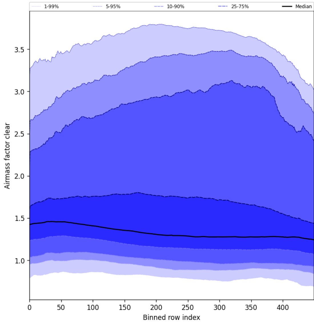
Figure 56: Along track statistics of “Airmass factor clear” for 2025-04-19 to 2025-04-21
