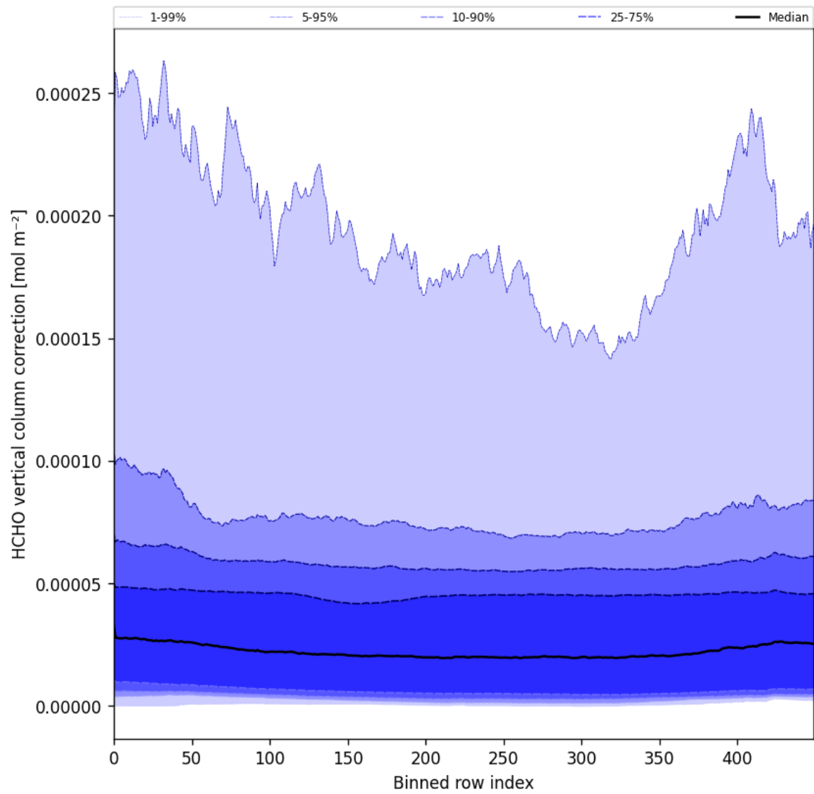
Figure 51: Along track statistics of “HCHO vertical column correction” for 2025-04-19 to 2025-04-21
