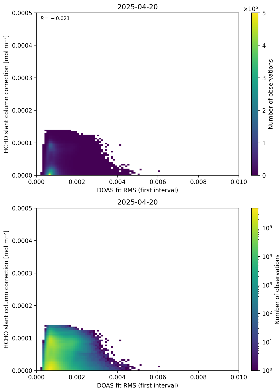
Figure 63: Scatter density plot of “DOAS fit RMS (first interval)” against “HCHO slant column correction” for 2025-04-19 to 2025-04-21.
