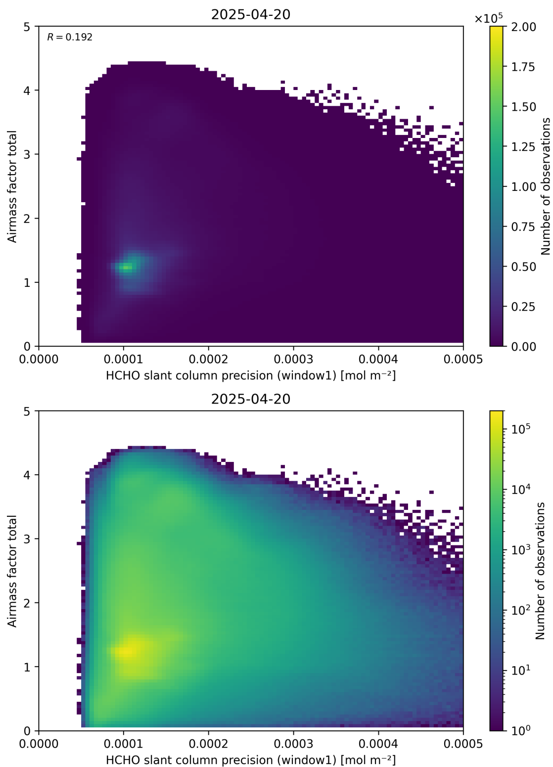
Figure 94: Scatter density plot of “HCHO slant column precision (window1)” against “Airmass factor total” for 2025-04-19 to 2025-04-21.
