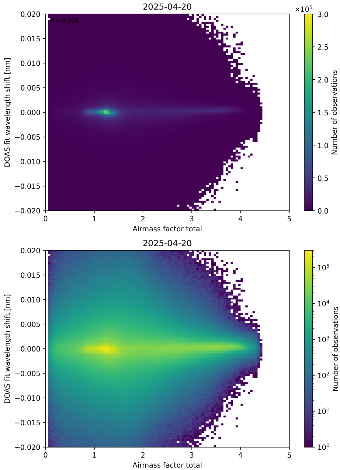
Figure 98: Scatter density plot of “Airmass factor total” against “DOAS fit wavelength shift” for 2025-04-19 to 2025-04-21.
