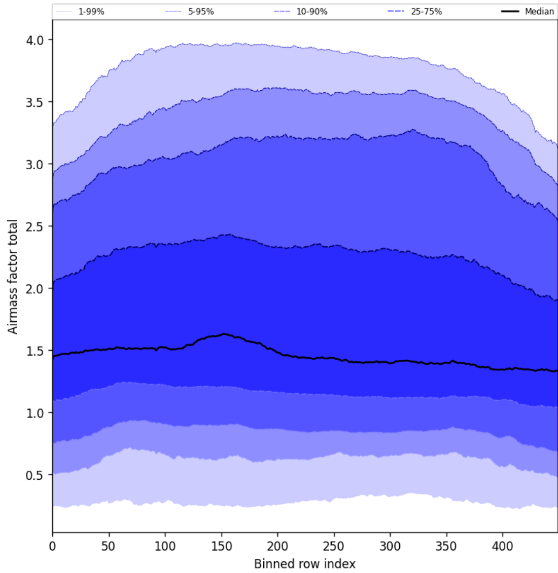
Figure 54: Along track statistics of “Airmass factor total” for 2025-04-19 to 2025-04-21
