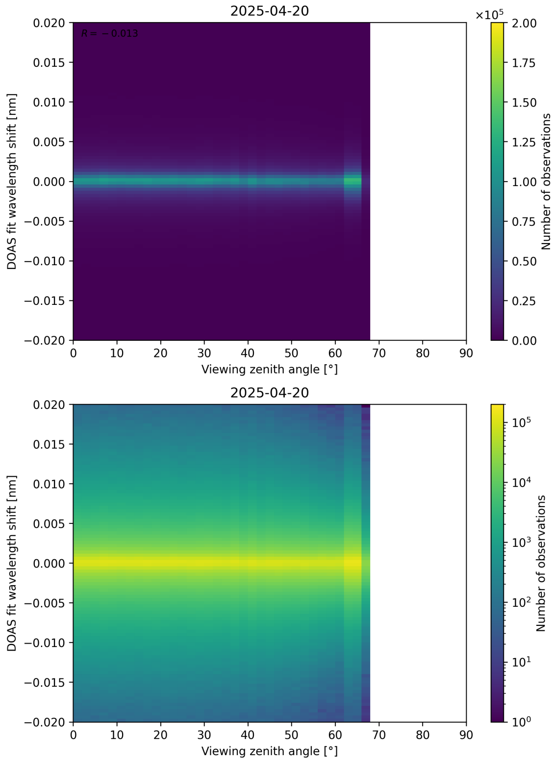
Figure 183: Scatter density plot of “Viewing zenith angle” against “DOAS fit wavelength shift” for 2025-04-19 to 2025-04-21.
