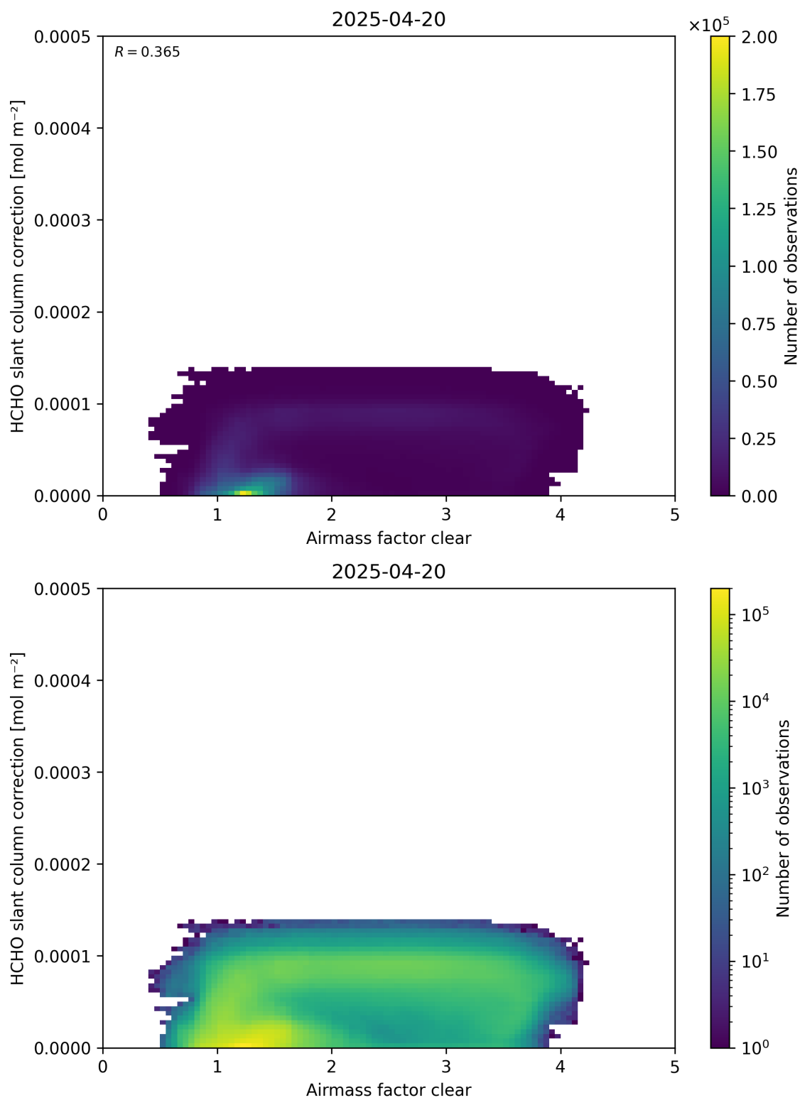
Figure 75: Scatter density plot of “Airmass factor clear” against “HCHO slant column correction” for 2025-04-19 to 2025-04-21.
