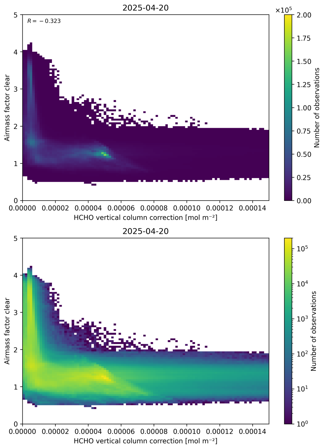
Figure 115: Scatter density plot of “HCHO vertical column correction” against “Airmass factor clear” for 2025-04-19 to 2025-04-21.
