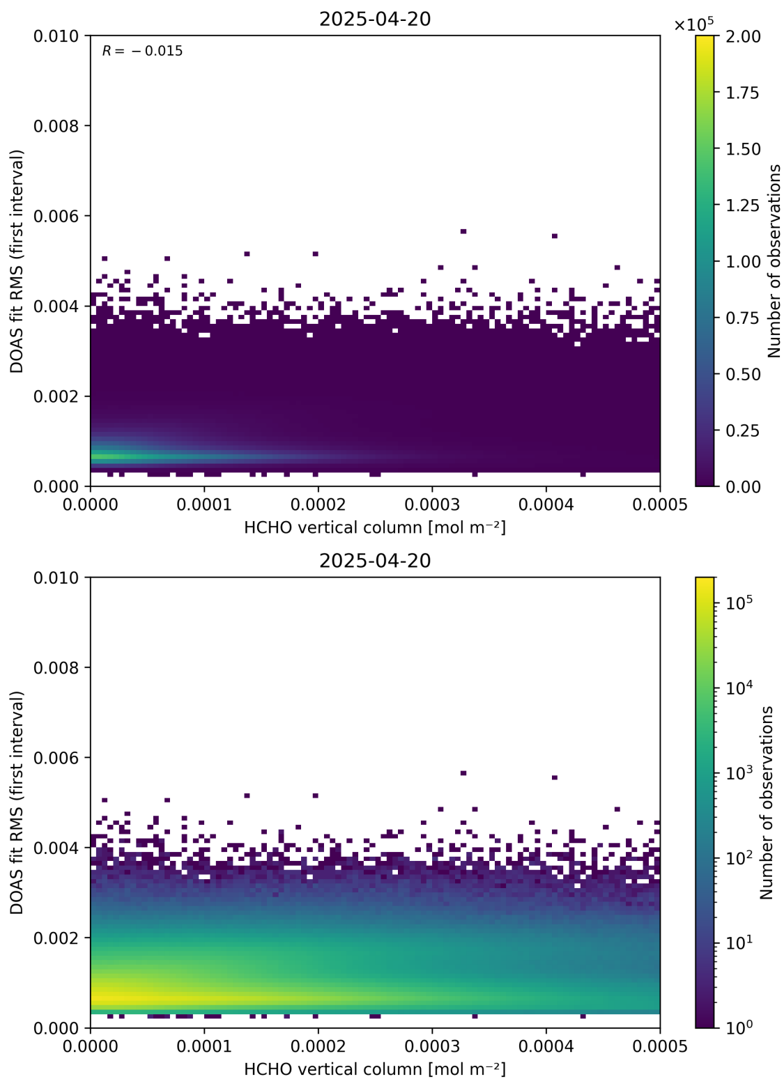
Figure 123: Scatter density plot of “HCHO vertical column” against “DOAS fit RMS (first interval)” for 2025-04-19 to 2025-04-21.
