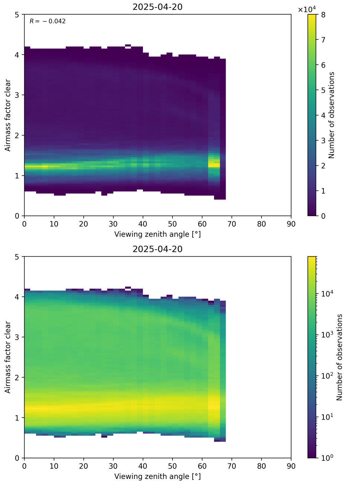
Figure 185: Scatter density plot of “Viewing zenith angle” against “Airmass factor clear” for 2025-04-19 to 2025-04-21.
