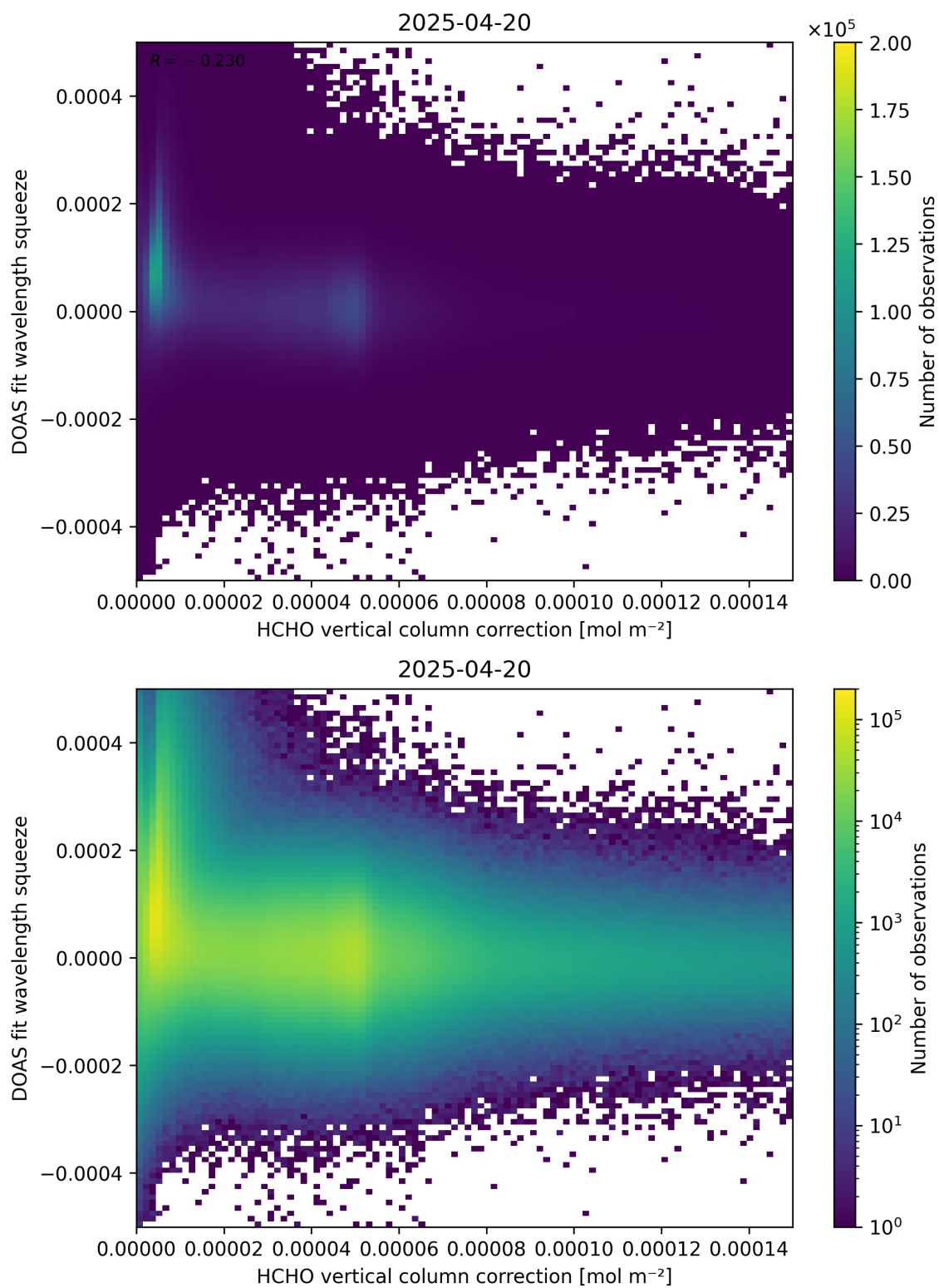
Figure 114: Scatter density plot of “HCHO vertical column correction” against “DOAS fit wavelength squeeze” for 2025-04-19 to 2025-04-21.
