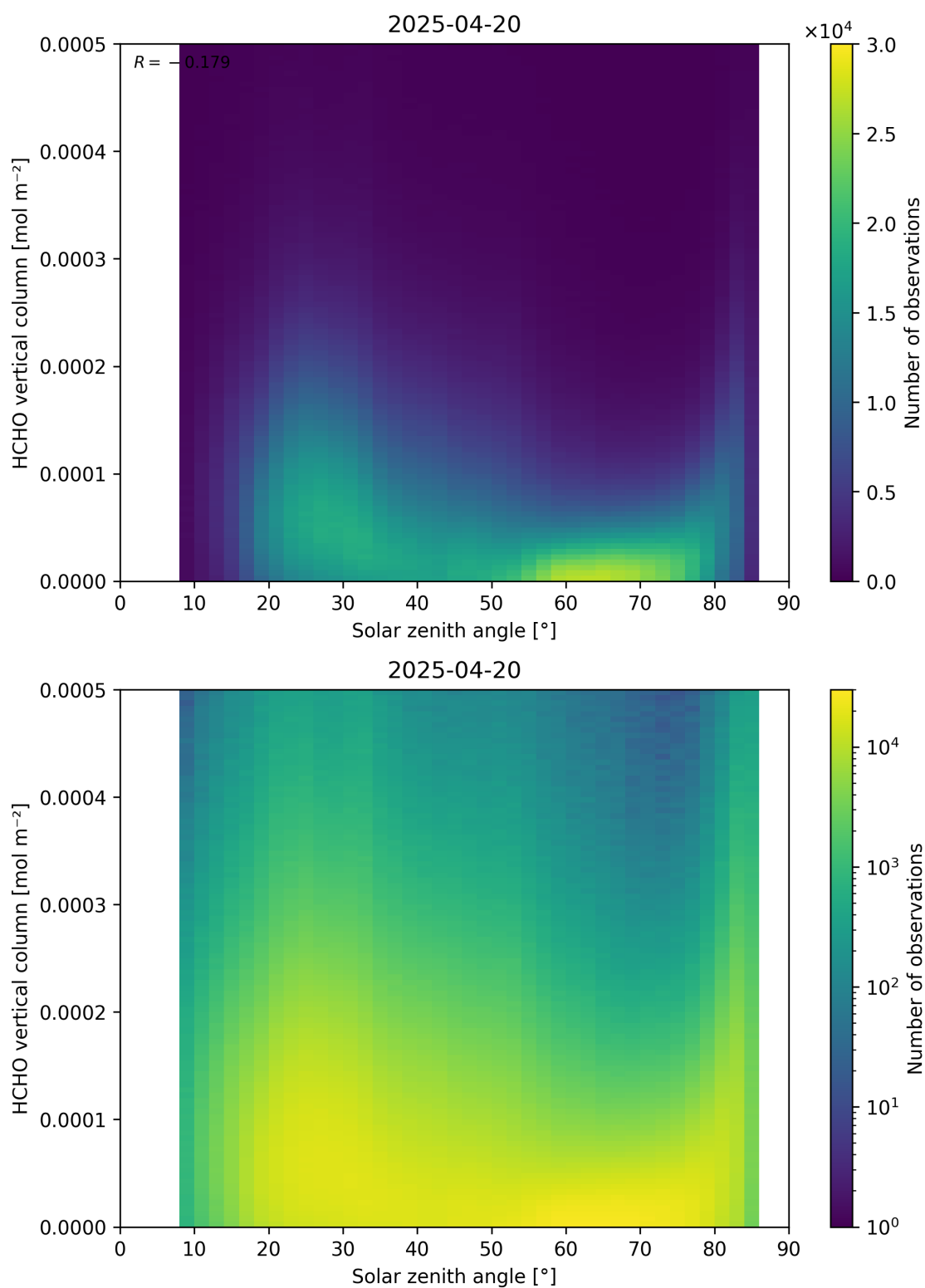
Figure 177: Scatter density plot of “Solar zenith angle” against “HCHO vertical column” for 2025-04-19 to 2025-04-21.
