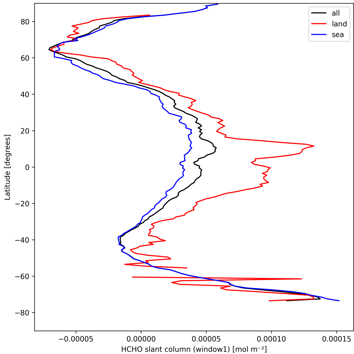
Figure 24: Zonal average of “HCHO slant column (window1)” for 2025-04-19 to 2025-04-21.
