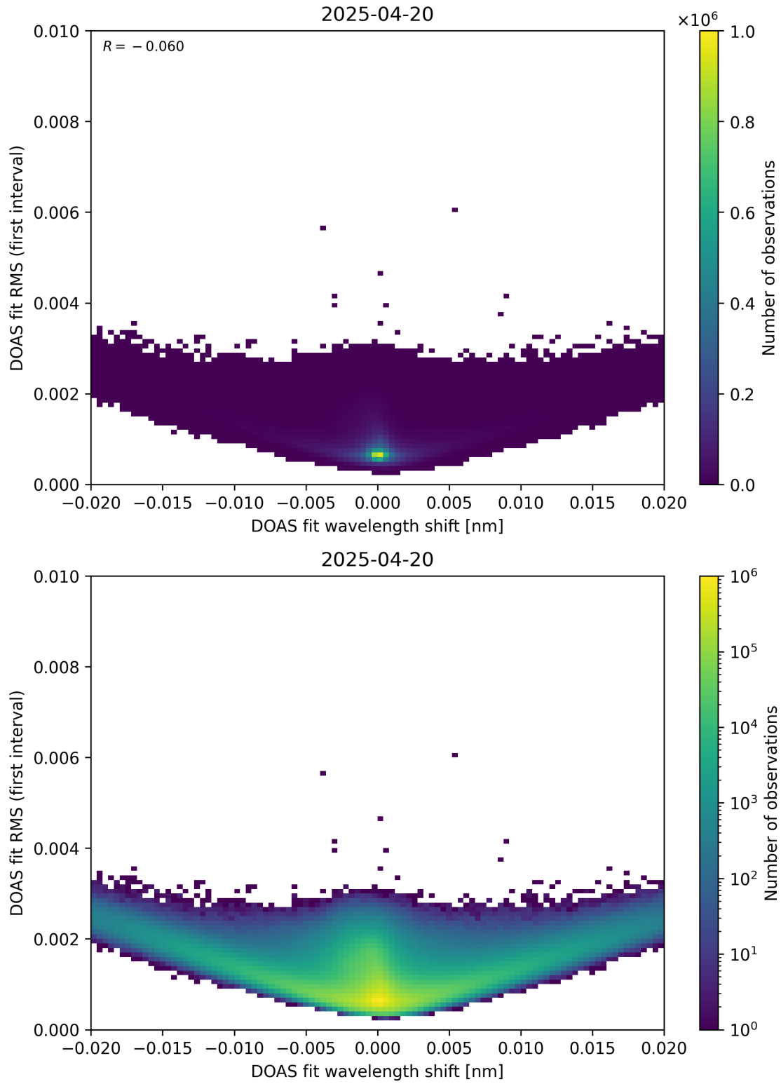
Figure 64: Scatter density plot of “DOAS fit wavelength shift” against “DOAS fit RMS (first interval)” for 2025-04-19 to 2025-04-21.
