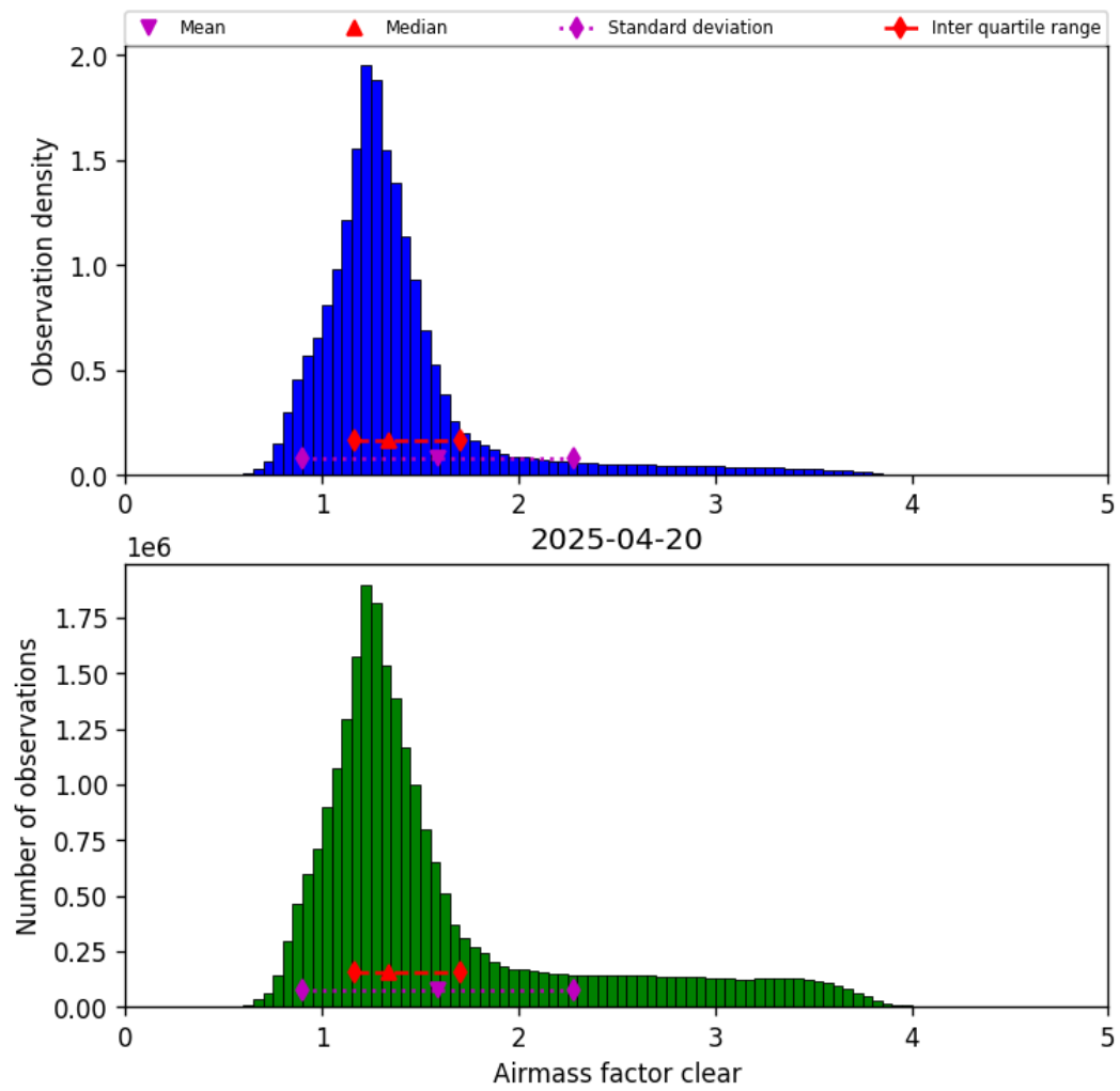
Figure 42: Histogram of “Airmass factor clear” for 2025-04-19 to 2025-04-21
