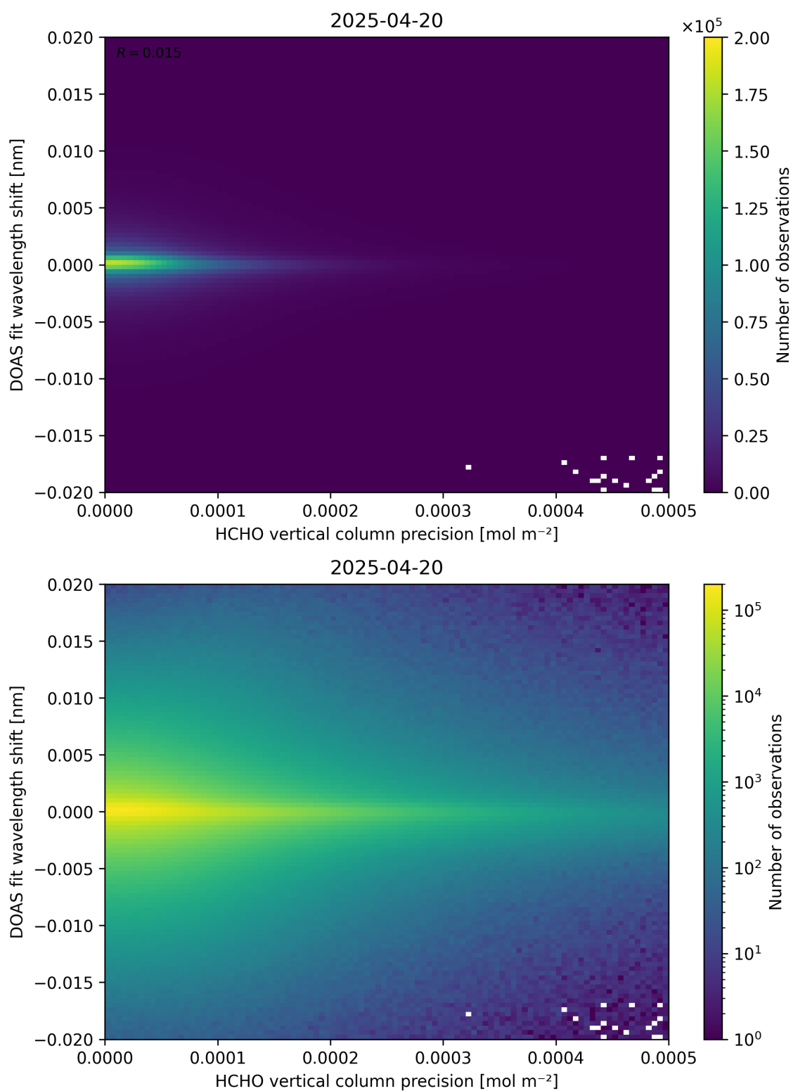
Figure 137: Scatter density plot of “HCHO vertical column precision” against “DOAS fit wavelength shift” for 2025-04-19 to 2025-04-21.
