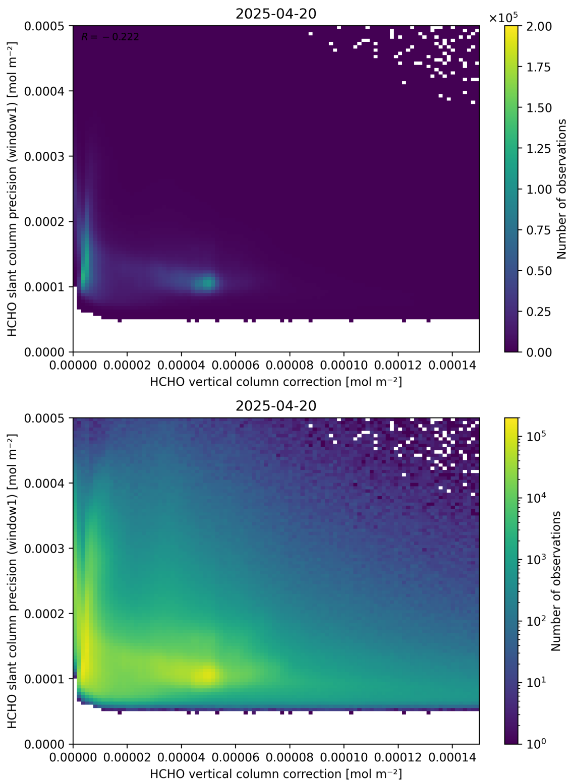
Figure 119: Scatter density plot of “HCHO vertical column correction” against “HCHO slant column precision (window1)” for 2025-04-19 to 2025-04-21.
