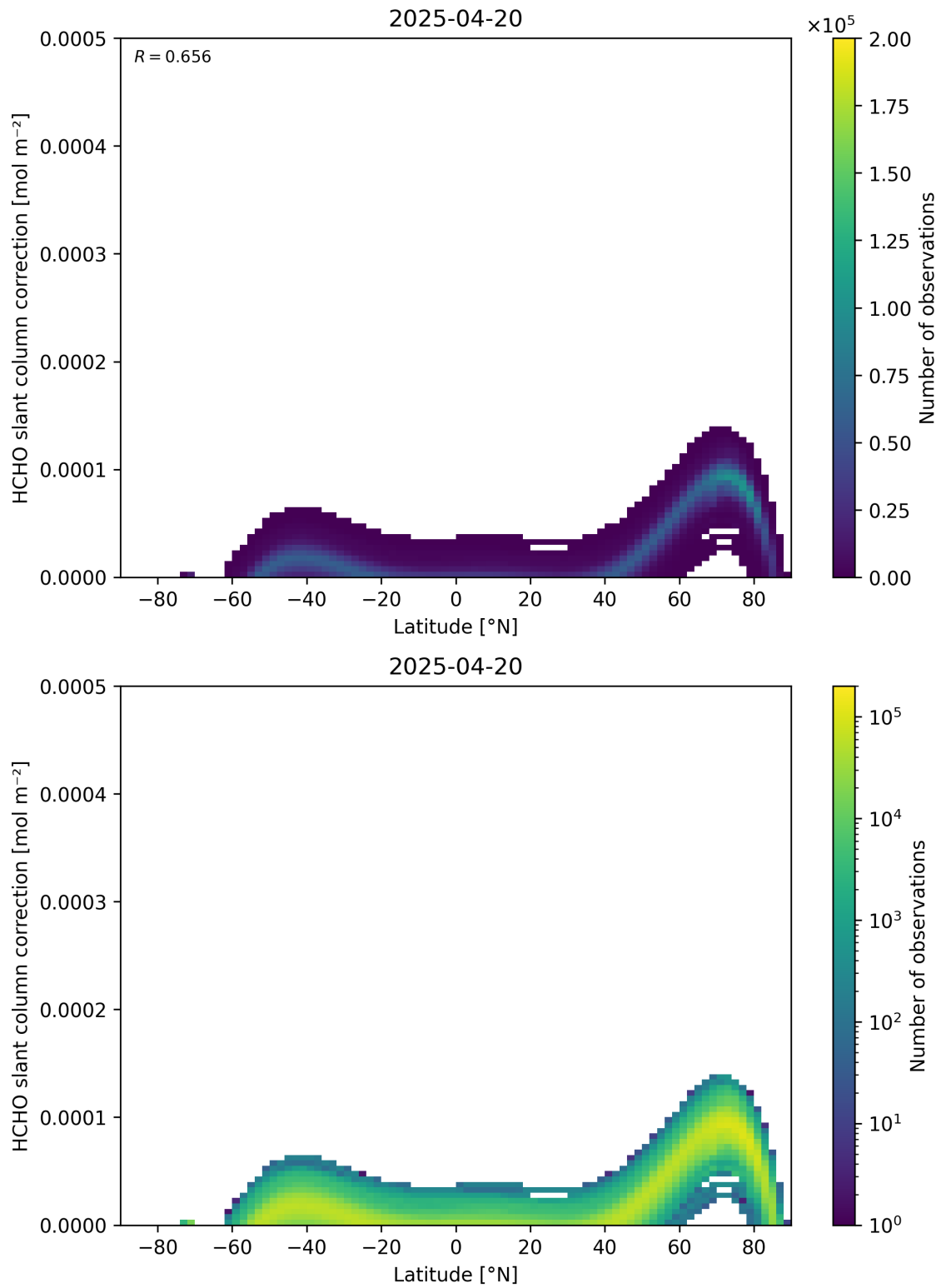
Figure 158: Scatter density plot of “Latitude” against “HCHO slant column correction” for 2025-04-19 to 2025-04-21.
