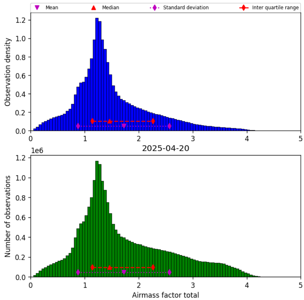
Figure 40: Histogram of “Airmass factor total” for 2025-04-19 to 2025-04-21
