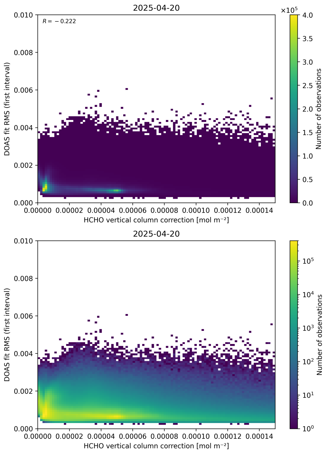
Figure 112: Scatter density plot of “HCHO vertical column correction” against “DOAS fit RMS (first interval)” for 2025-04-19 to 2025-04-21.
