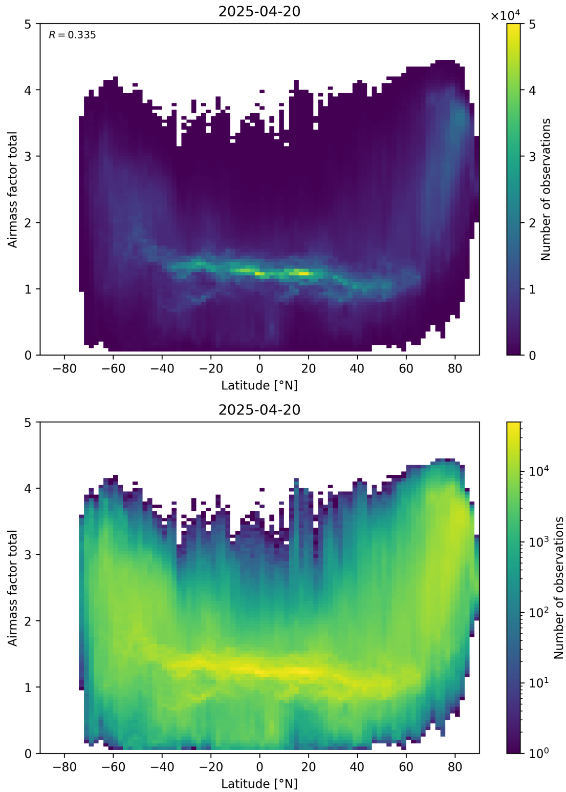
Figure 161: Scatter density plot of “Latitude” against “Airmass factor total” for 2025-04-19 to 2025-04-21.
