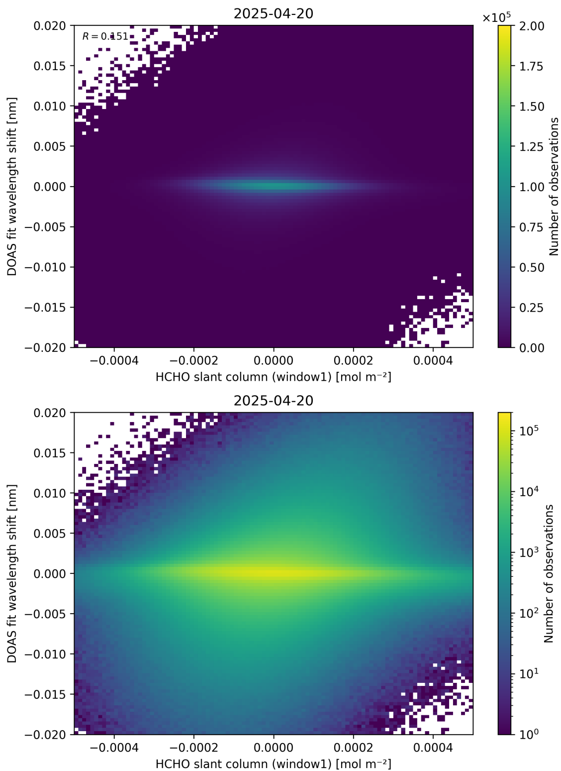
Figure 79: Scatter density plot of “HCHO slant column (window1)” against “DOAS fit wavelength shift” for 2025-04-19 to 2025-04-21.
