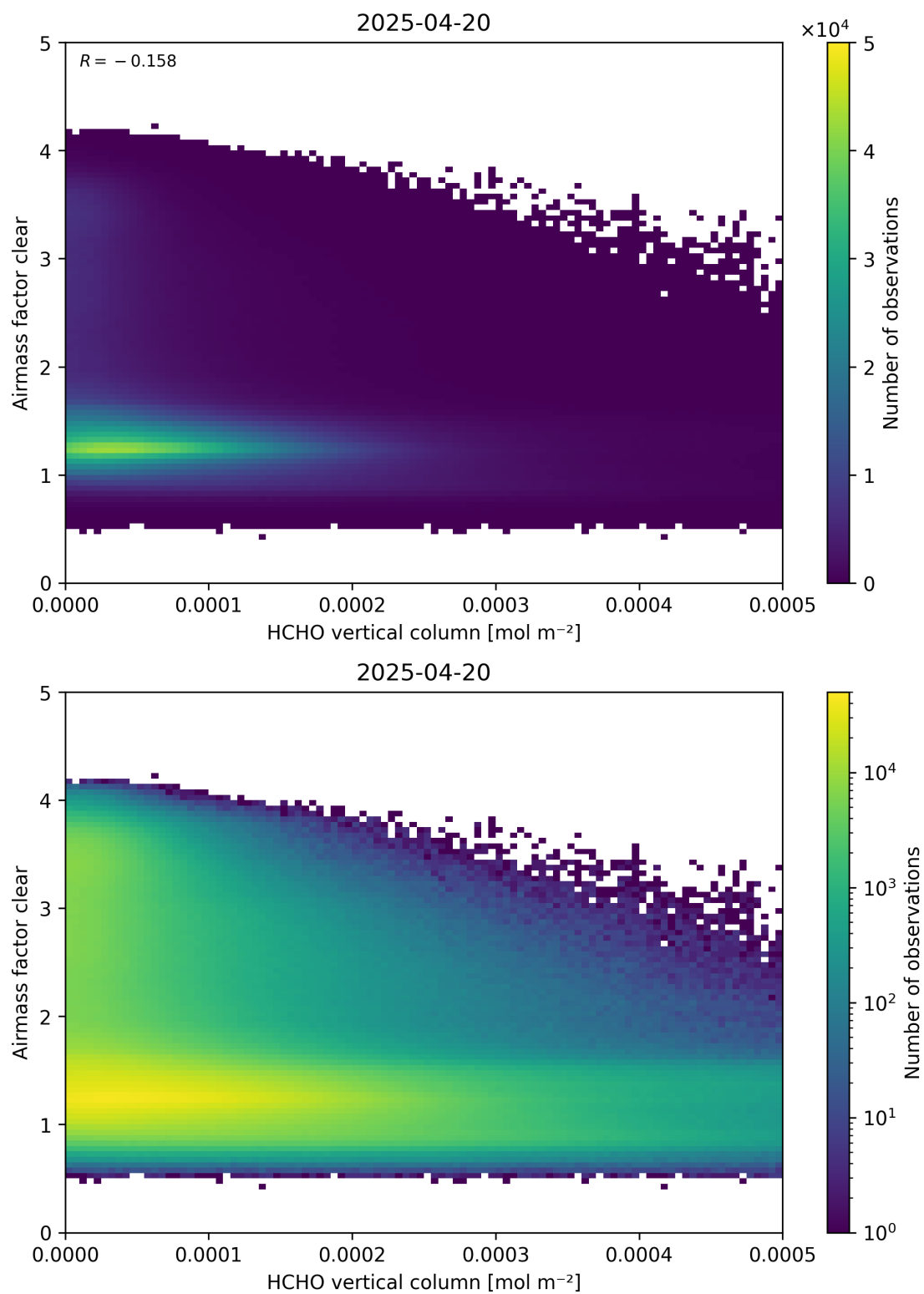
Figure 126: Scatter density plot of “HCHO vertical column” against “Airmass factor clear” for 2025-04-19 to 2025-04-21.
