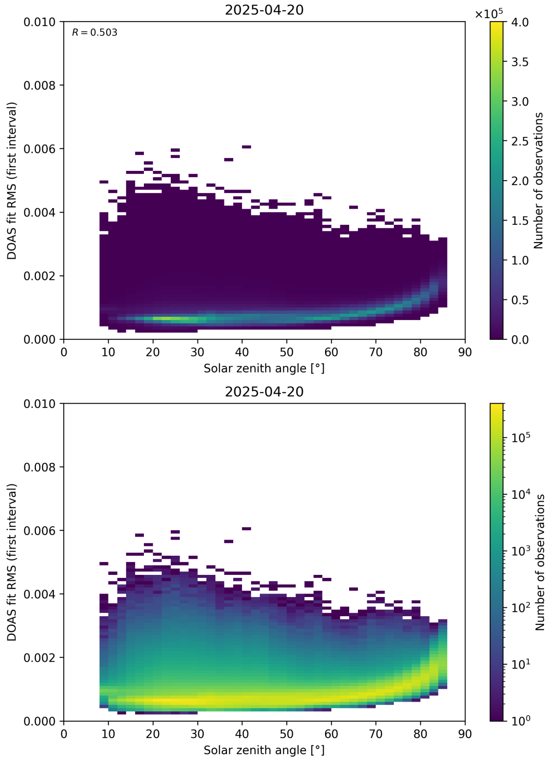
Figure 167: Scatter density plot of “Solar zenith angle” against “DOAS fit RMS (first interval)” for 2025-04-19 to 2025-04-21.
