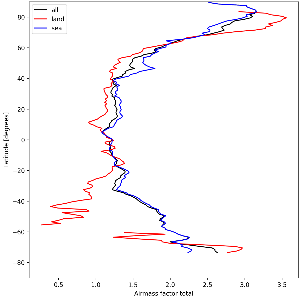
Figure 26: Zonal average of “Airmass factor total” for 2025-04-19 to 2025-04-21.
