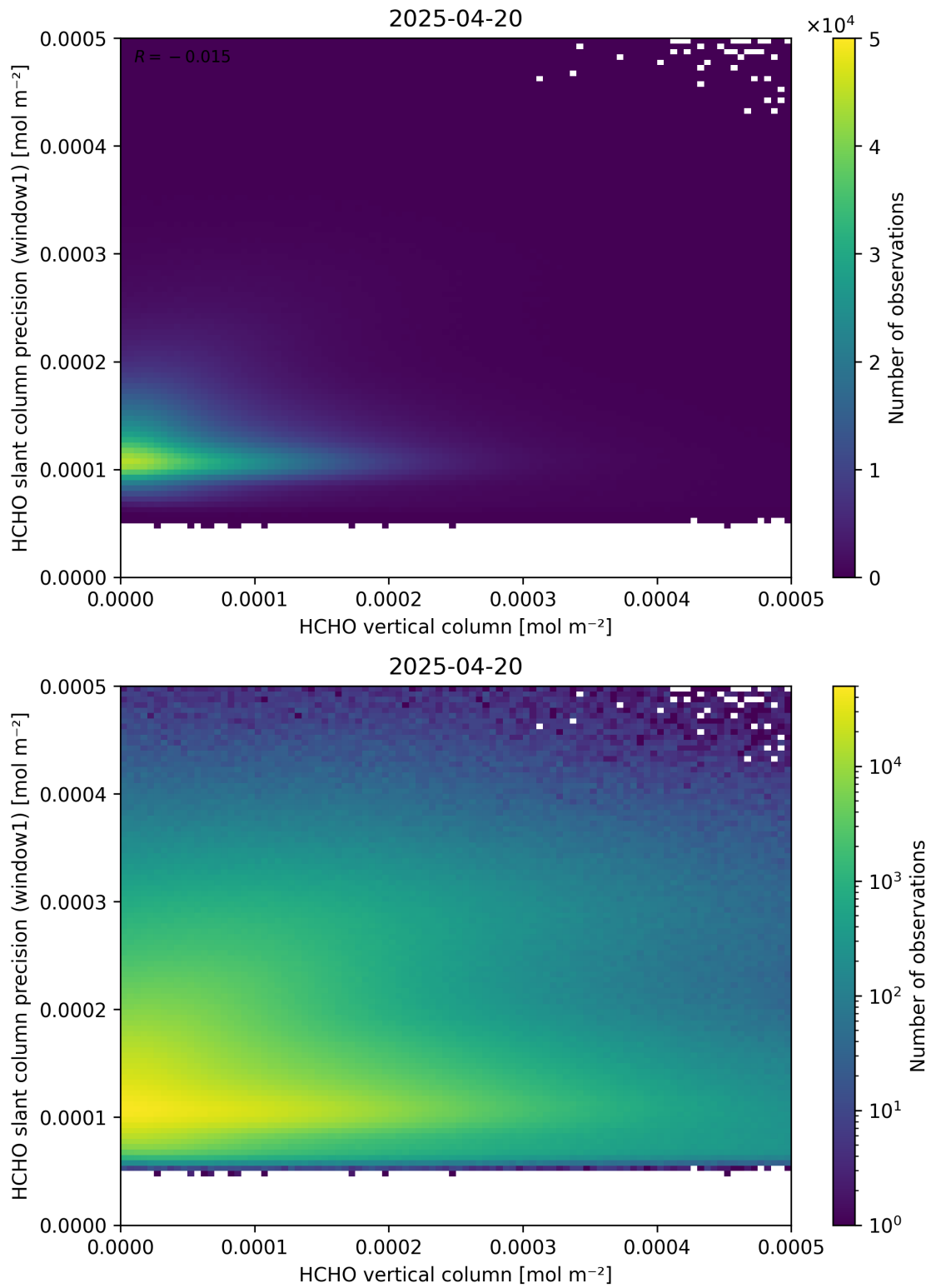
Figure 130: Scatter density plot of “HCHO vertical column” against “HCHO slant column precision (window1)” for 2025-04-19 to 2025-04-21.
