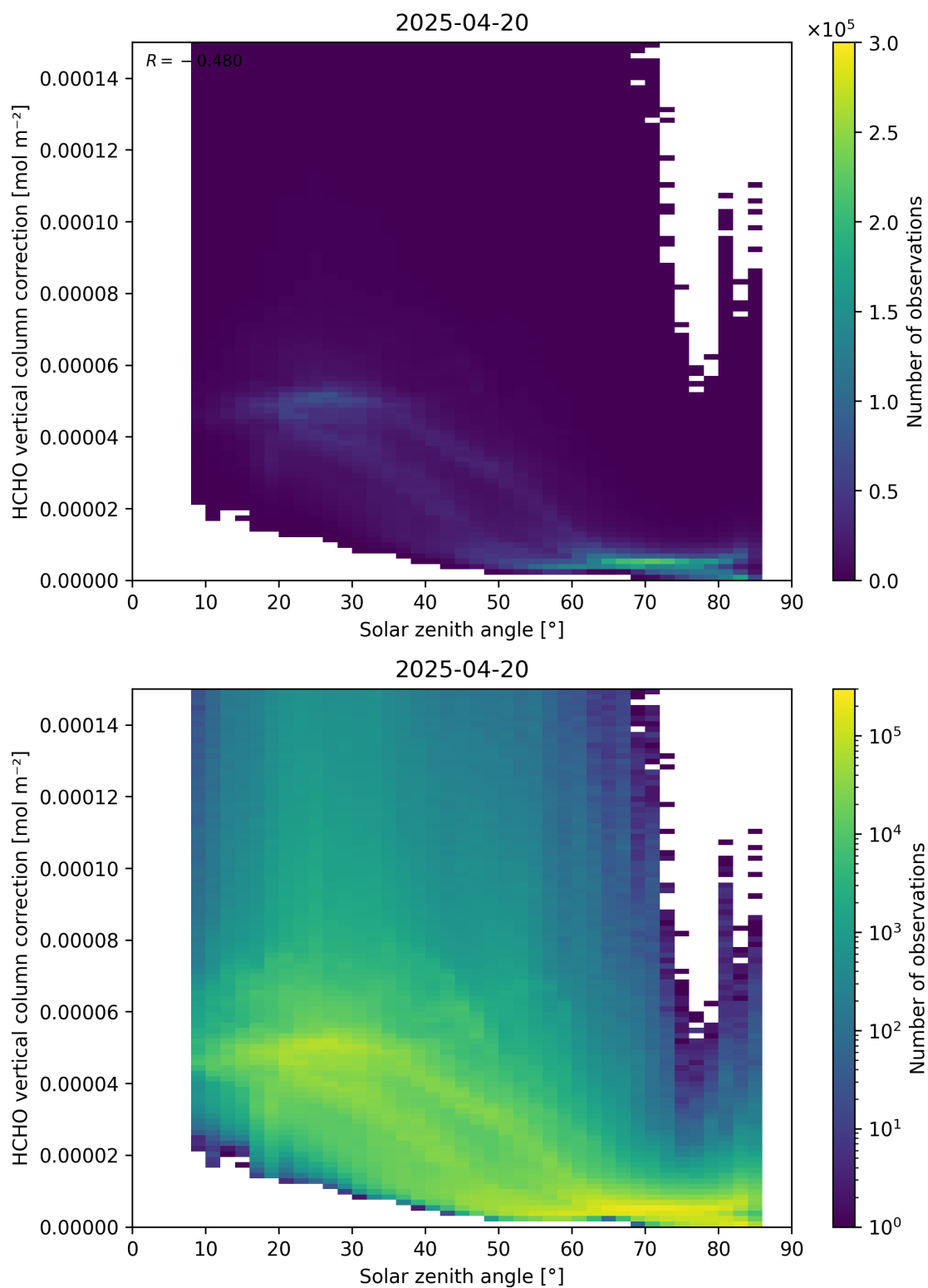
Figure 178: Scatter density plot of “Solar zenith angle” against “HCHO vertical column correction” for 2025-04-19 to 2025-04-21.
