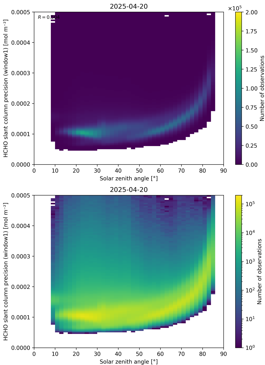
Figure 174: Scatter density plot of “Solar zenith angle” against “HCHO slant column precision (window1)” for 2025-04-19 to 2025-04-21.
