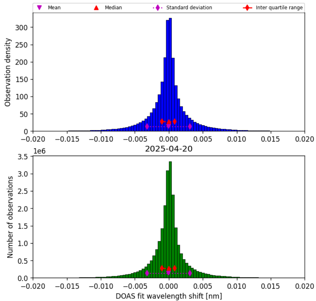
Figure 44: Histogram of “DOAS fit wavelength shift” for 2025-04-19 to 2025-04-21
