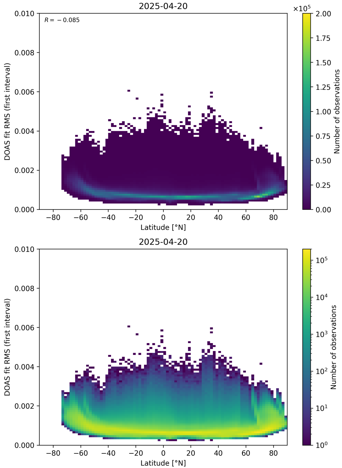
Figure 153: Scatter density plot of “Latitude” against “DOAS fit RMS (first interval)” for 2025-04-19 to 2025-04-21.
