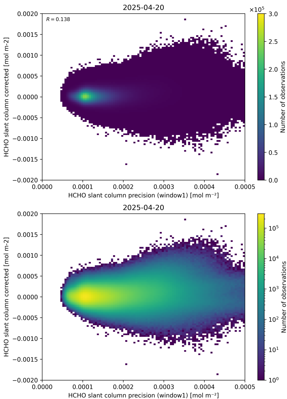
Figure 92: Scatter density plot of “HCHO slant column precision (window1)” against “HCHO slant column corrected” for 2025-04-19 to 2025-04-21.
