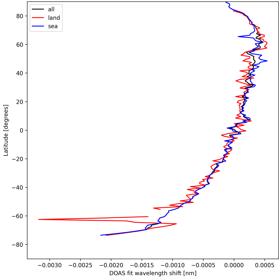
Figure 30: Zonal average of “DOAS fit wavelength shift” for 2025-04-19 to 2025-04-21.
