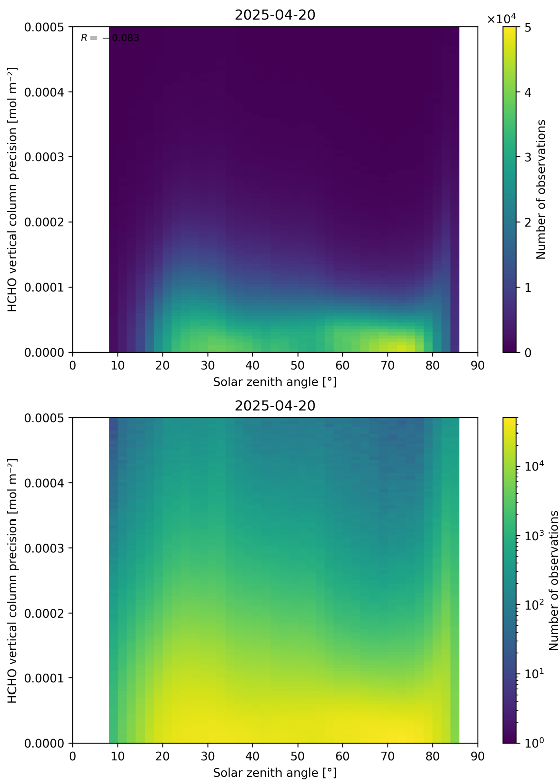
Figure 179: Scatter density plot of “Solar zenith angle” against “HCHO vertical column precision” for 2025-04-19 to 2025-04-21.
