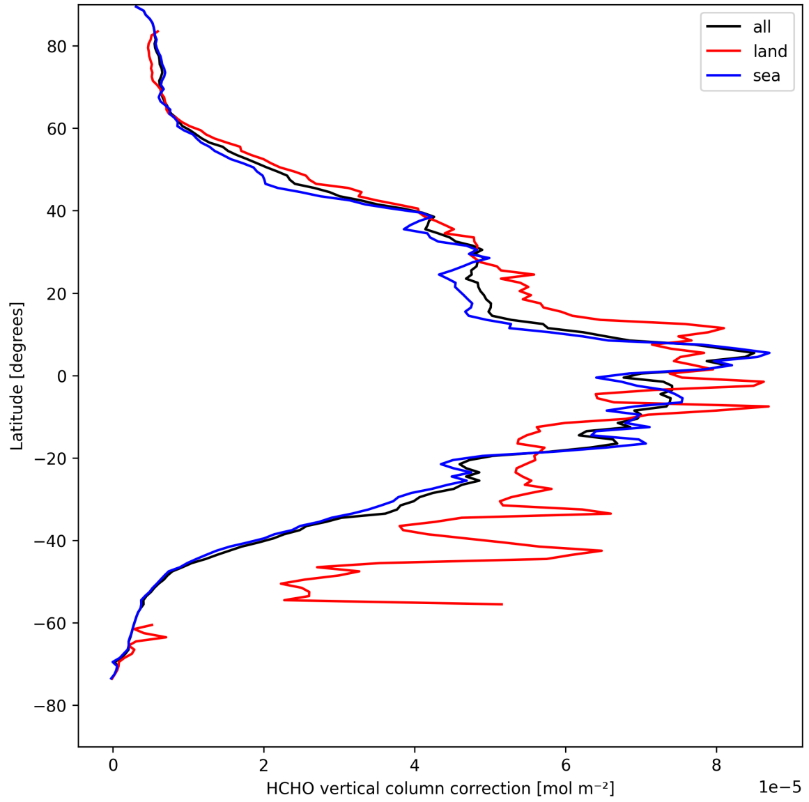
Figure 23: Zonal average of “HCHO vertical column correction” for 2025-04-19 to 2025-04-21.
