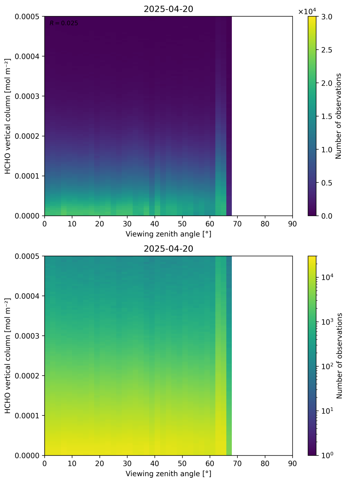
Figure 192: Scatter density plot of “Viewing zenith angle” against “HCHO vertical column” for 2025-04-19 to 2025-04-21.
