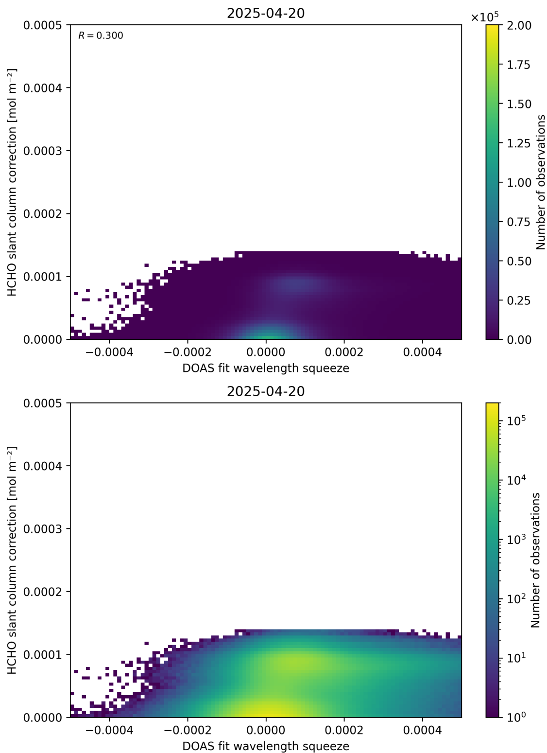
Figure 70: Scatter density plot of “DOAS fit wavelength squeeze” against “HCHO slant column correction” for 2025-04-19 to 2025-04-21.
