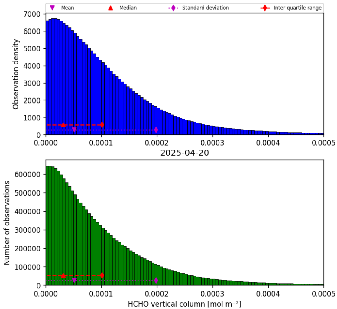
Figure 35: Histogram of “HCHO vertical column” for 2025-04-19 to 2025-04-21
