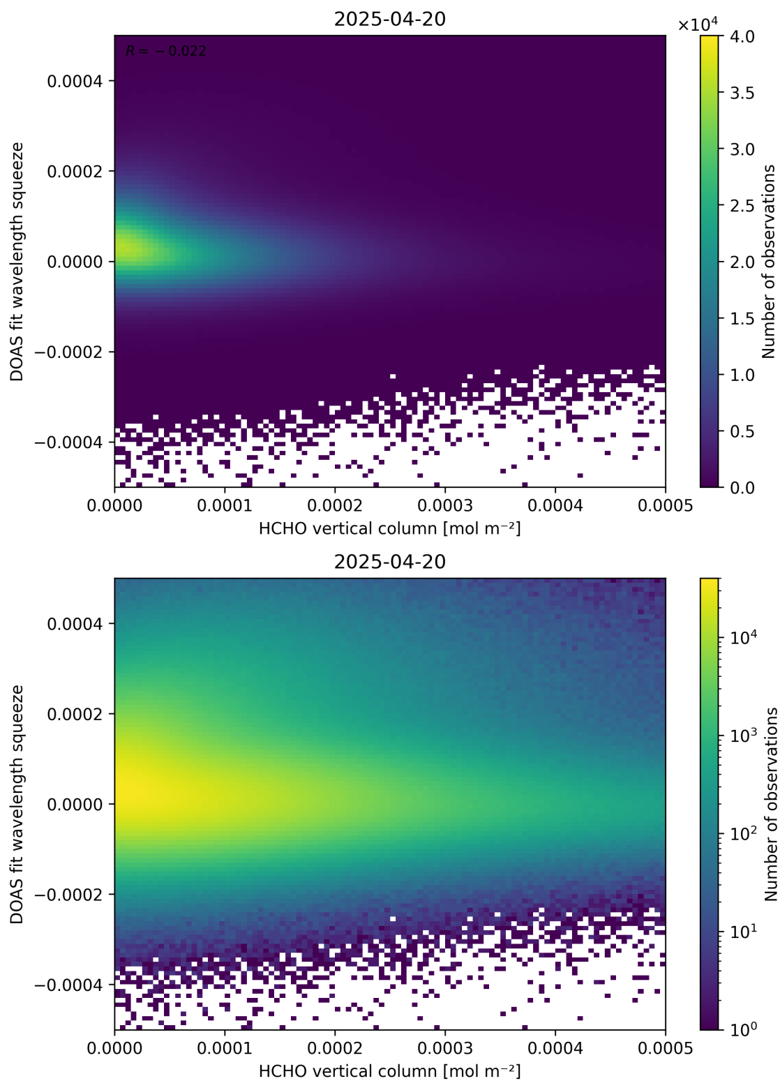
Figure 125: Scatter density plot of “HCHO vertical column” against “DOAS fit wavelength squeeze” for 2025-04-19 to 2025-04-21.
