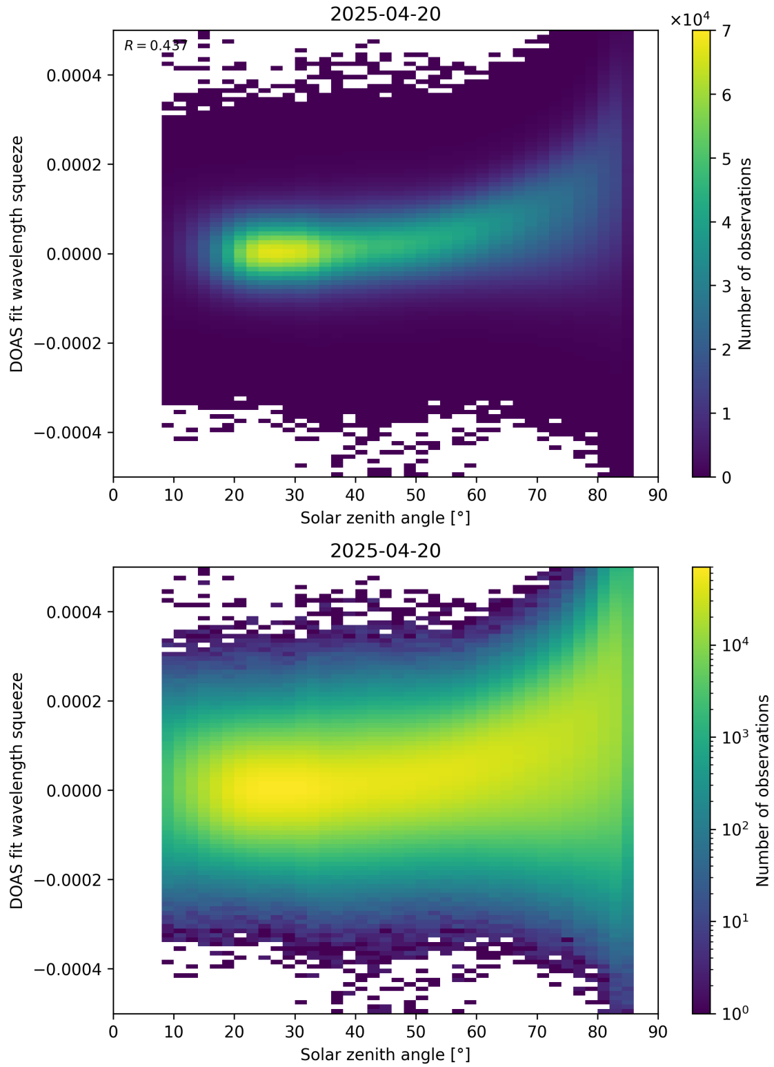
Figure 169: Scatter density plot of “Solar zenith angle” against “DOAS fit wavelength squeeze” for 2025-04-19 to 2025-04-21.
