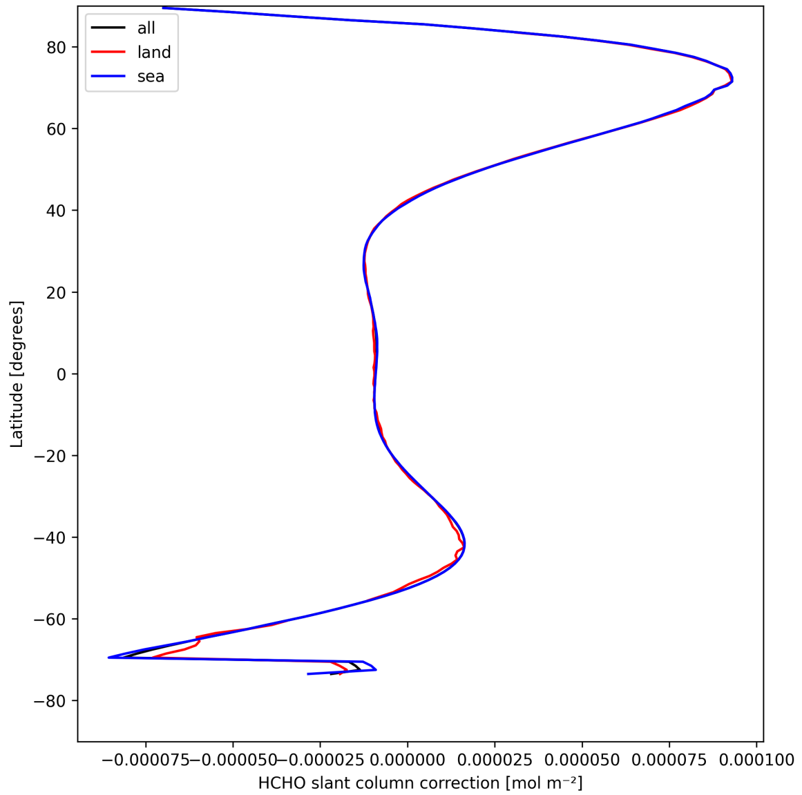
Figure 33: Zonal average of “HCHO slant column correction” for 2025-04-19 to 2025-04-21.
