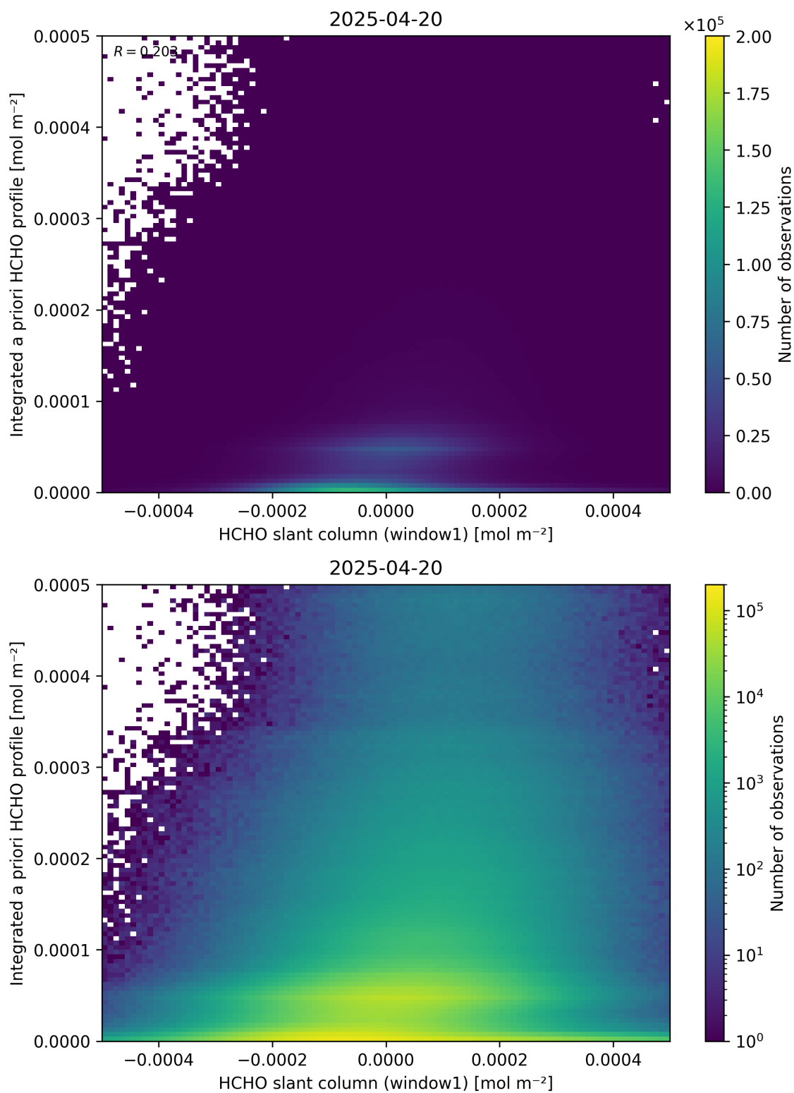
Figure 87: Scatter density plot of “HCHO slant column (window1)” against “Integrated a priori HCHO profile” for 2025-04-19 to 2025-04-21.
