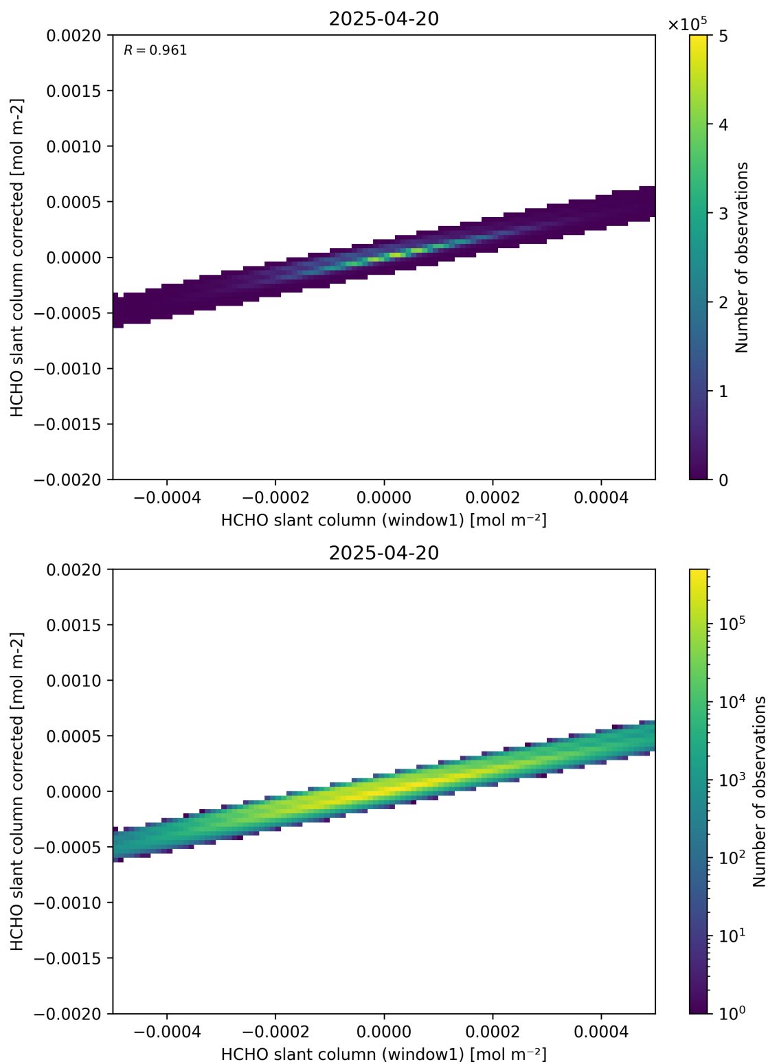
Figure 82: Scatter density plot of “HCHO slant column (window1)” against “HCHO slant column corrected” for 2025-04-19 to 2025-04-21.
