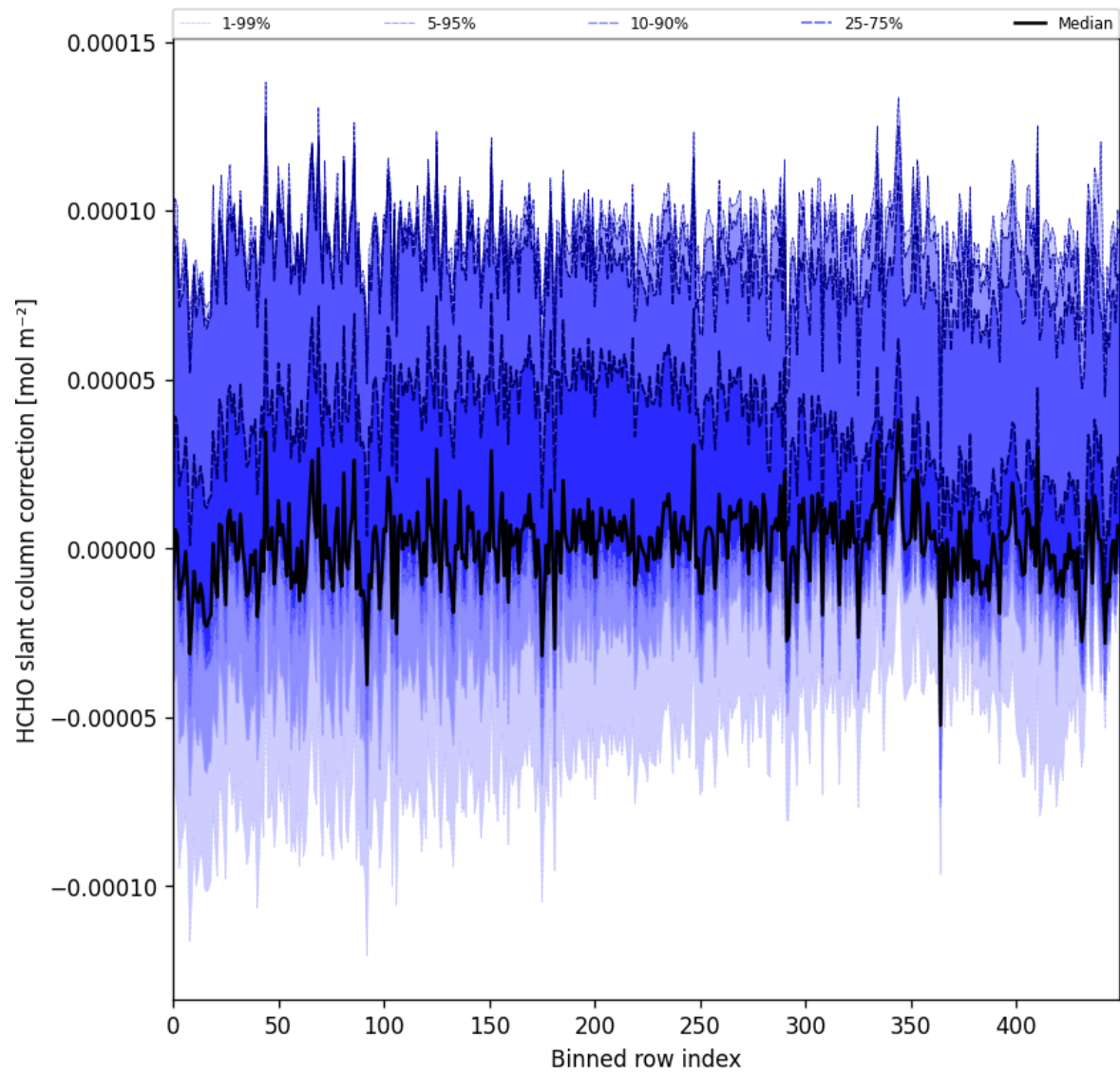
Figure 61: Along track statistics of “HCHO slant column correction” for 2025-04-19 to 2025-04-21
