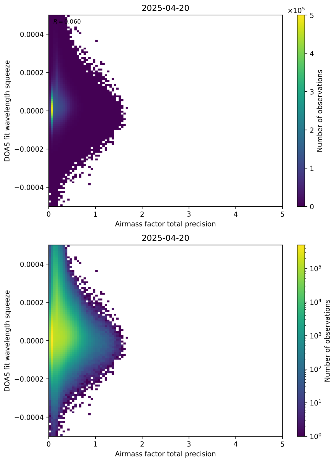
Figure 107: Scatter density plot of “Airmass factor total precision” against “DOAS fit wavelength squeeze” for 2025-04-19 to 2025-04-21.
