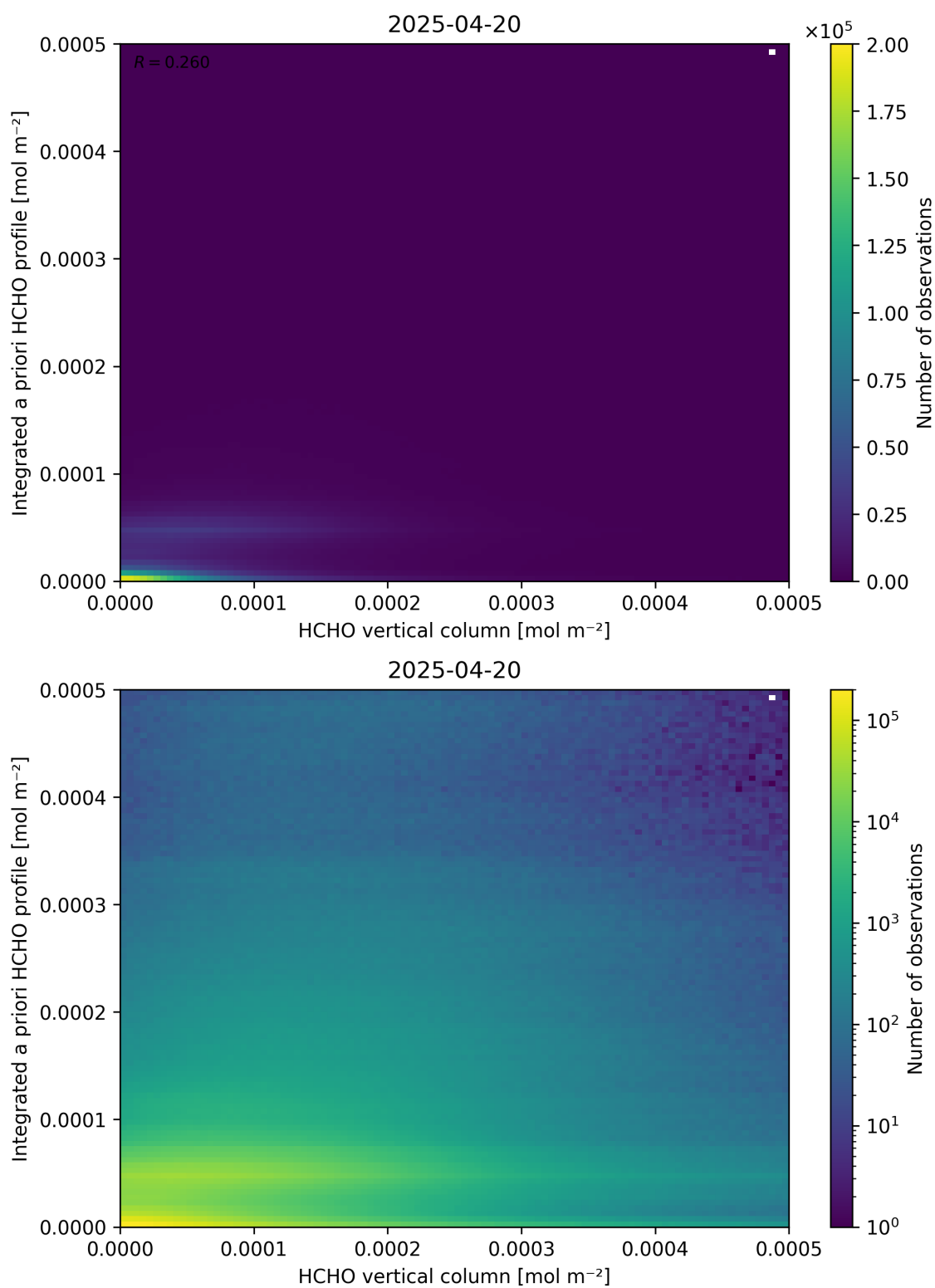
Figure 135: Scatter density plot of “HCHO vertical column” against “Integrated a priori HCHO profile” for 2025-04-19 to 2025-04-21.
