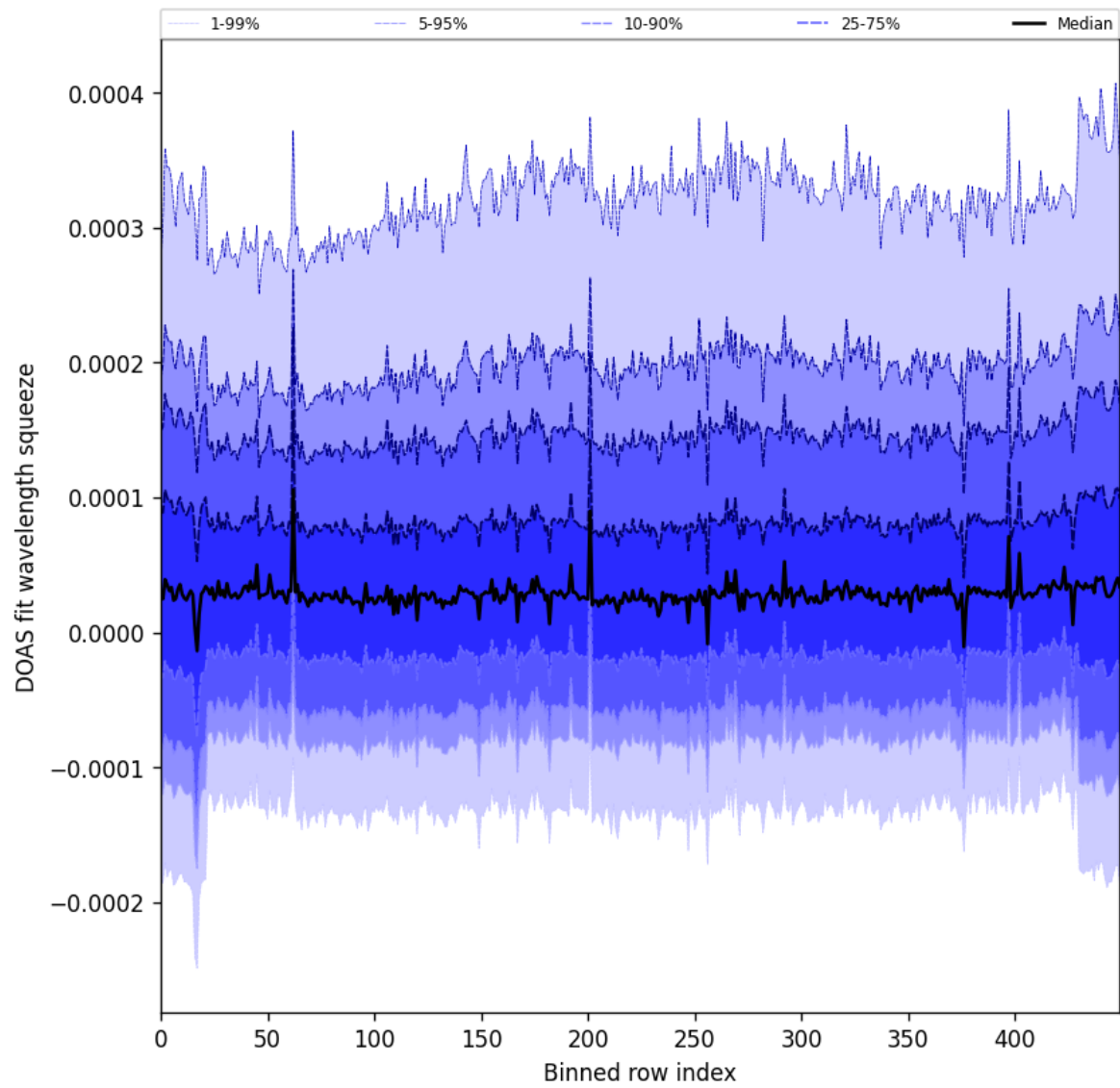
Figure 59: Along track statistics of “DOAS fit wavelength squeeze” for 2025-04-19 to 2025-04-21
