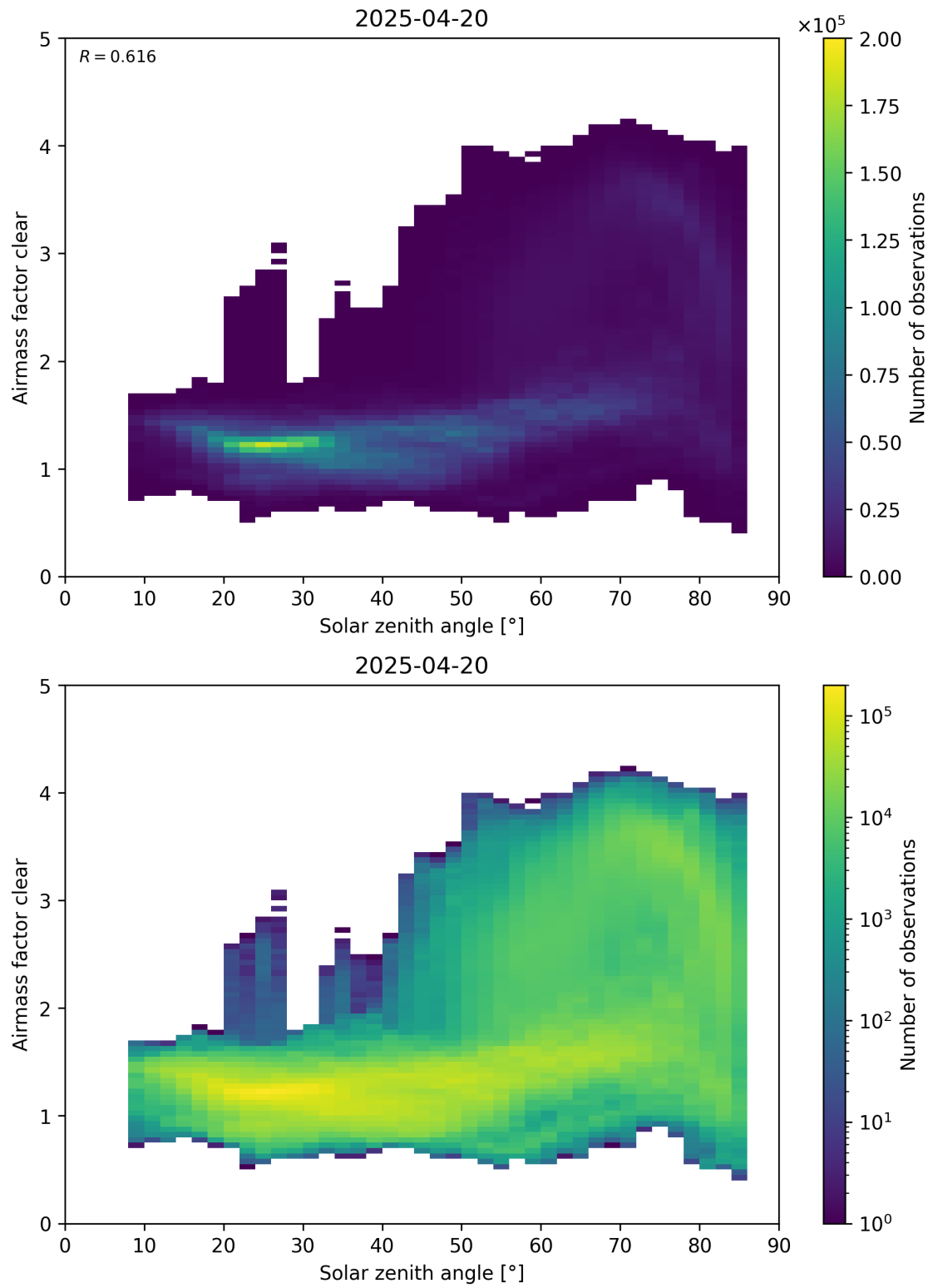
Figure 170: Scatter density plot of “Solar zenith angle” against “Airmass factor clear” for 2025-04-19 to 2025-04-21.
