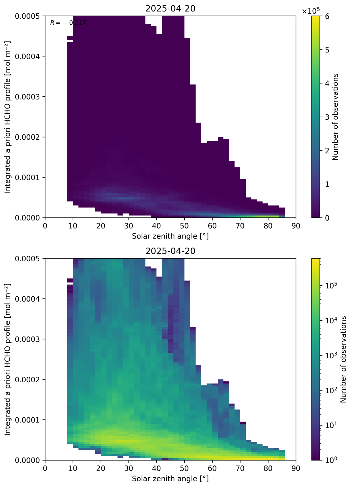
Figure 180: Scatter density plot of “Solar zenith angle” against “Integrated a priori HCHO profile” for 2025-04-19 to 2025-04-21.
