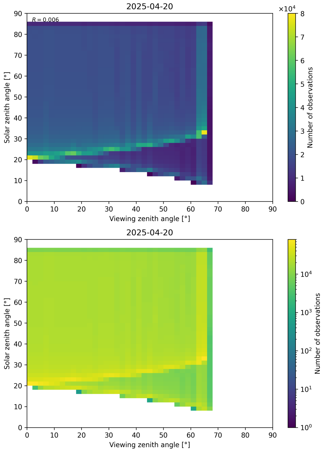
Figure 197: Scatter density plot of “Viewing zenith angle” against “Solar zenith angle” for 2025-04-19 to 2025-04-21.
