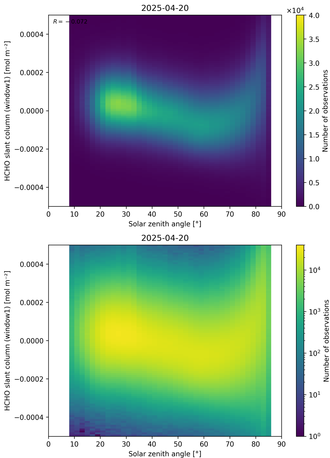
Figure 173: Scatter density plot of “Solar zenith angle” against “HCHO slant column (window1)” for 2025-04-19 to 2025-04-21.
