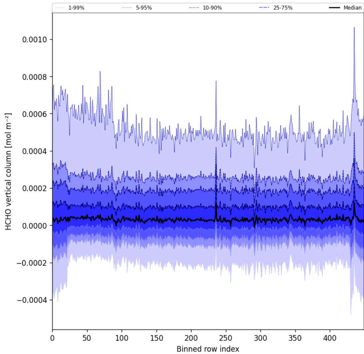
Figure 49: Along track statistics of “HCHO vertical column” for 2025-04-20 to 2025-04-22
