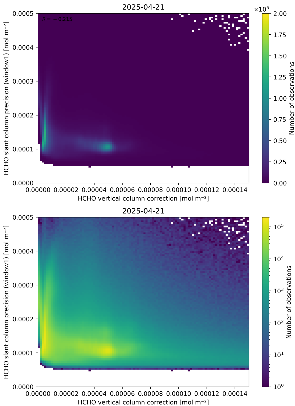
Figure 119: Scatter density plot of “HCHO vertical column correction” against “HCHO slant column precision (window1)” for 2025-04-20 to 2025-04-22.
