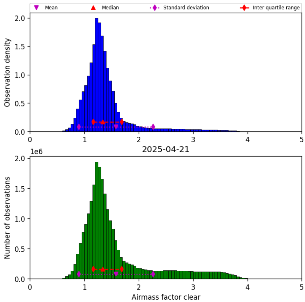
Figure 42: Histogram of “Airmass factor clear” for 2025-04-20 to 2025-04-22
