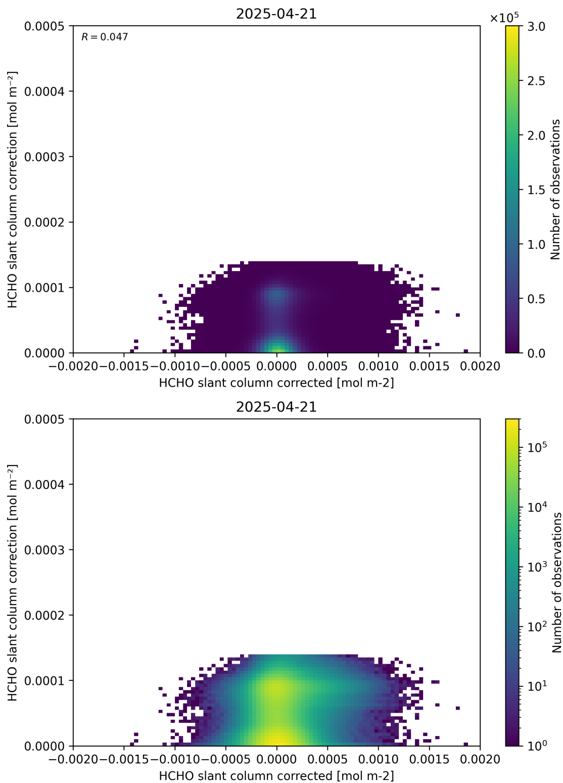
Figure 77: Scatter density plot of “HCHO slant column corrected” against “HCHO slant column correction” for 2025-04-20 to 2025-04-22.
