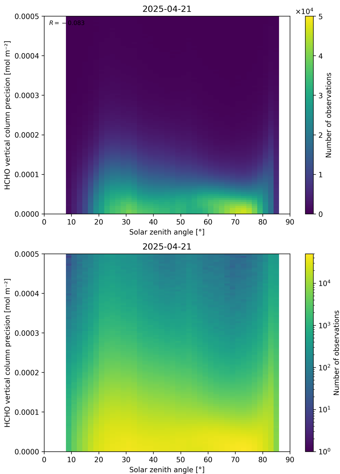
Figure 179: Scatter density plot of “Solar zenith angle” against “HCHO vertical column precision” for 2025-04-20 to 2025-04-22.
