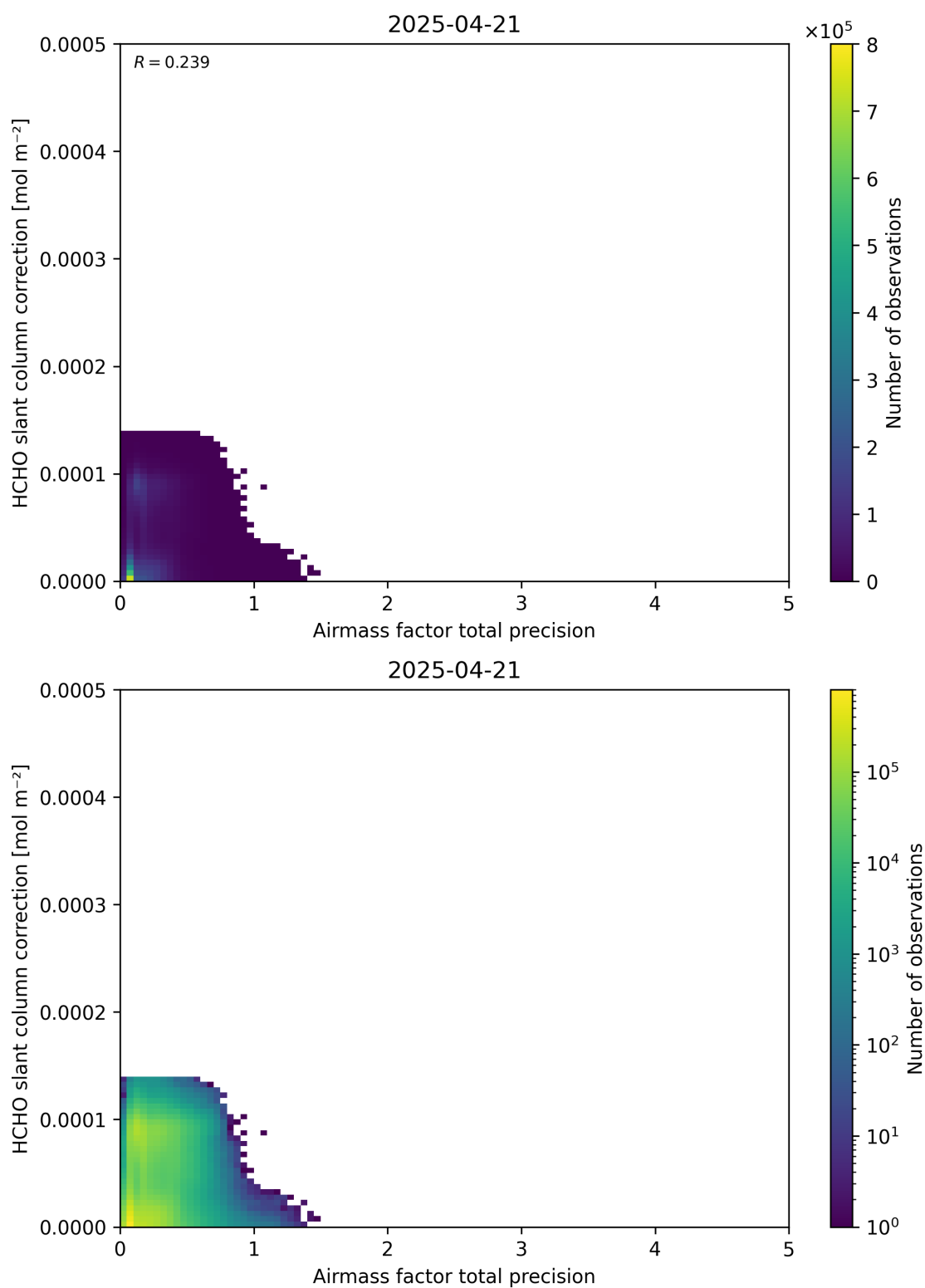
Figure 110: Scatter density plot of “Airmass factor total precision” against “HCHO slant column correction” for 2025-04-20 to 2025-04-22.
