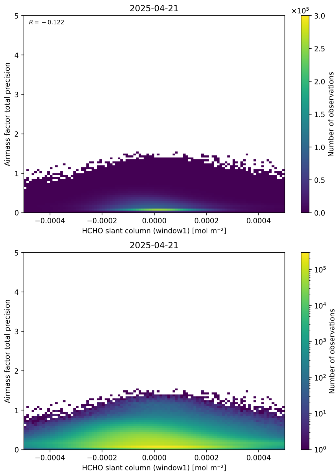
Figure 86: Scatter density plot of “HCHO slant column (window1)” against “Airmass factor total precision” for 2025-04-20 to 2025-04-22.
