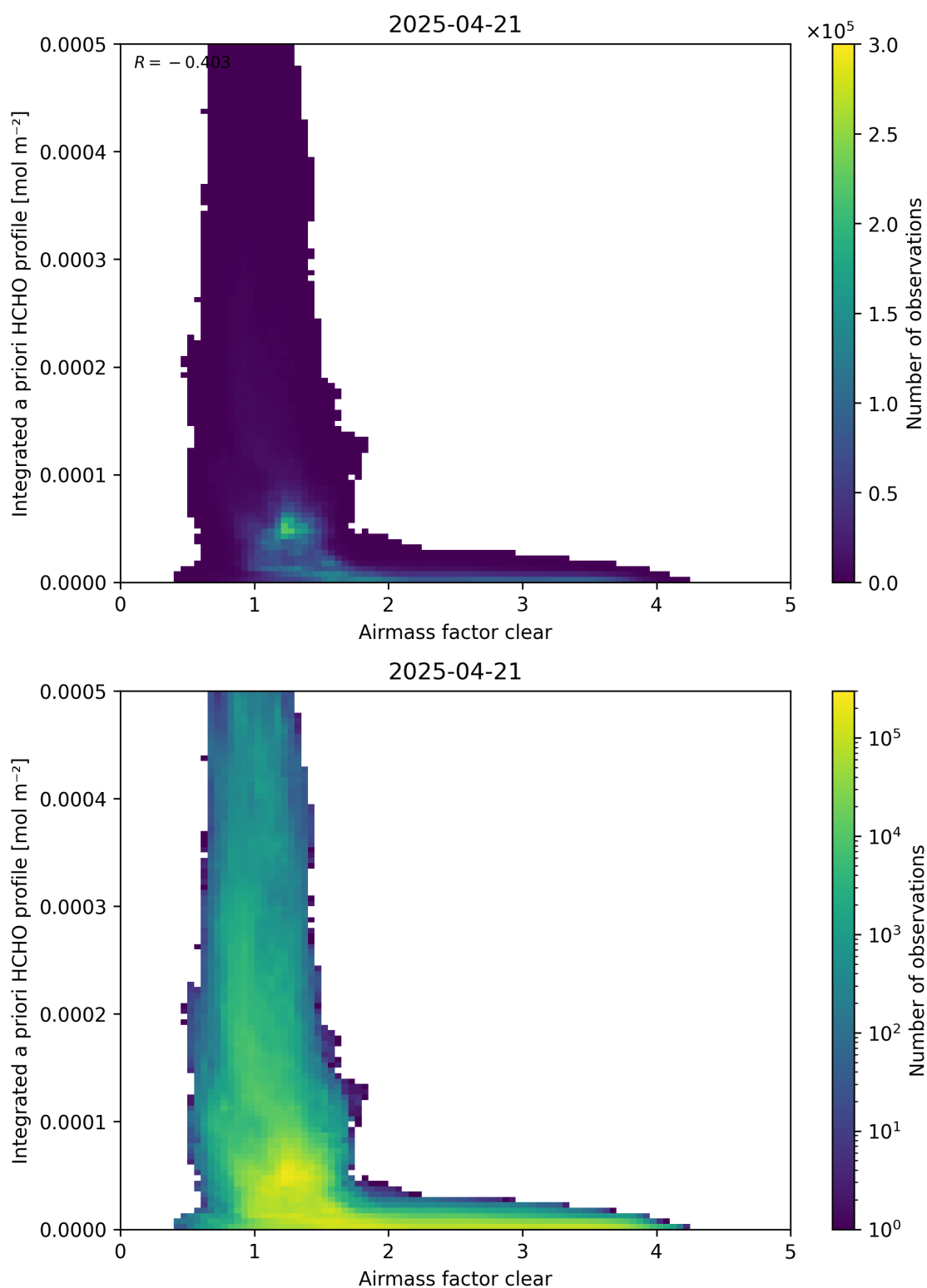
Figure 76: Scatter density plot of “Airmass factor clear” against “Integrated a priori HCHO profile” for 2025-04-20 to 2025-04-22.
