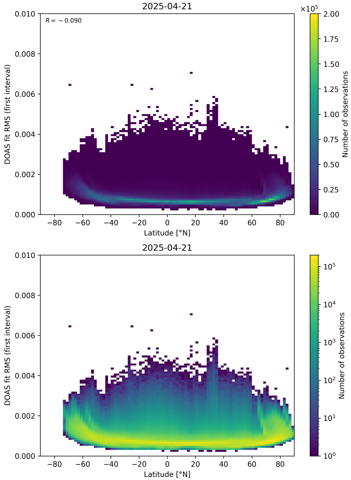
Figure 153: Scatter density plot of “Latitude” against “DOAS fit RMS (first interval)” for 2025-04-20 to 2025-04-22.
