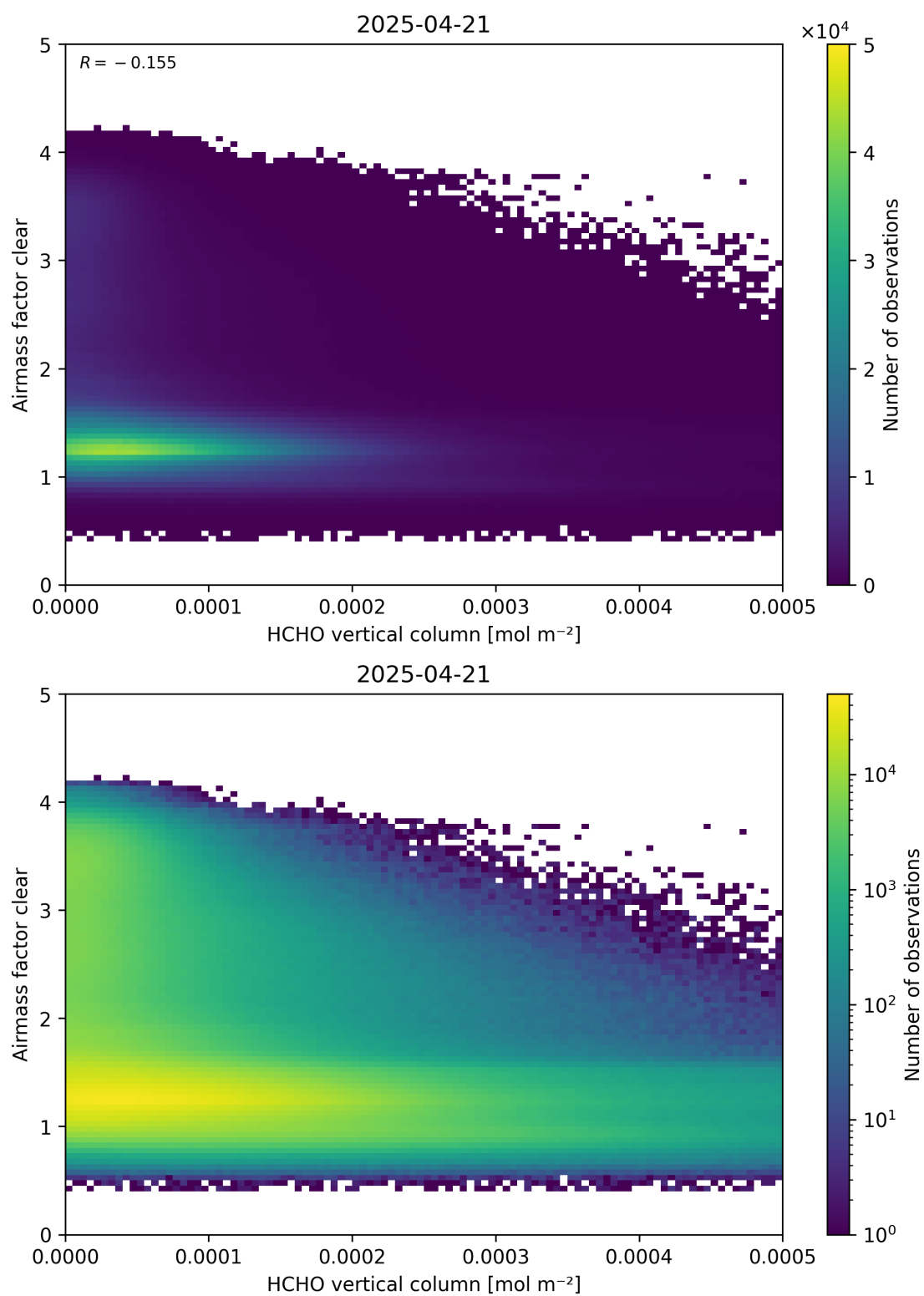
Figure 126: Scatter density plot of “HCHO vertical column” against “Airmass factor clear” for 2025-04-20 to 2025-04-22.
