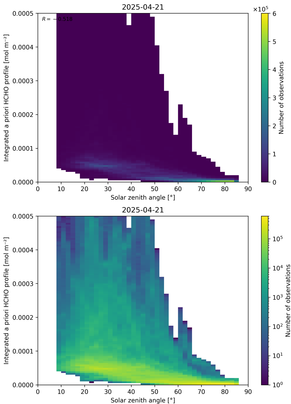
Figure 180: Scatter density plot of “Solar zenith angle” against “Integrated a priori HCHO profile” for 2025-04-20 to 2025-04-22.
