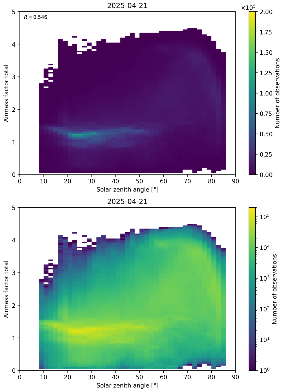
Figure 175: Scatter density plot of “Solar zenith angle” against “Airmass factor total” for 2025-04-20 to 2025-04-22.
