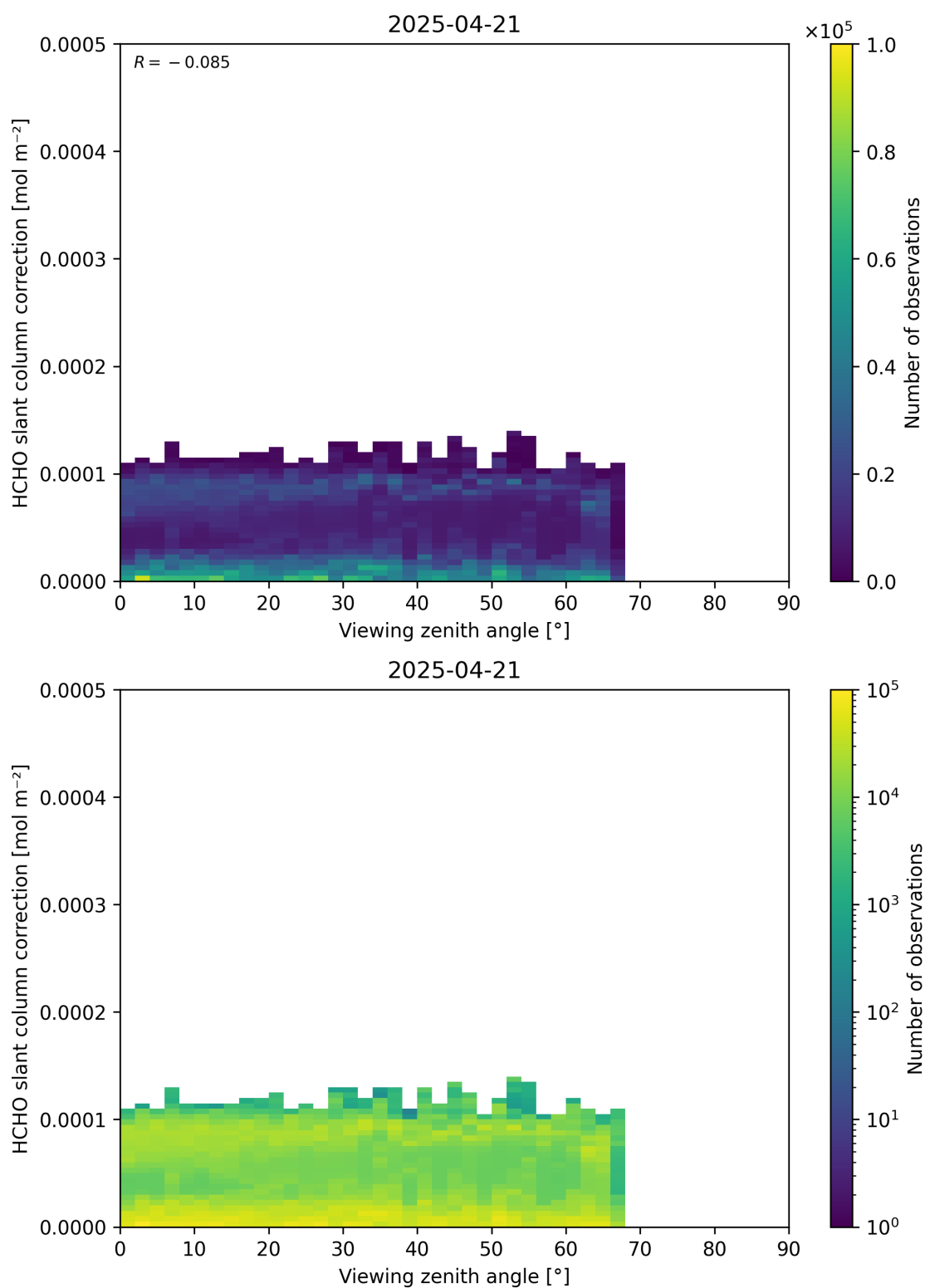
Figure 187: Scatter density plot of “Viewing zenith angle” against “HCHO slant column correction” for 2025-04-20 to 2025-04-22.
