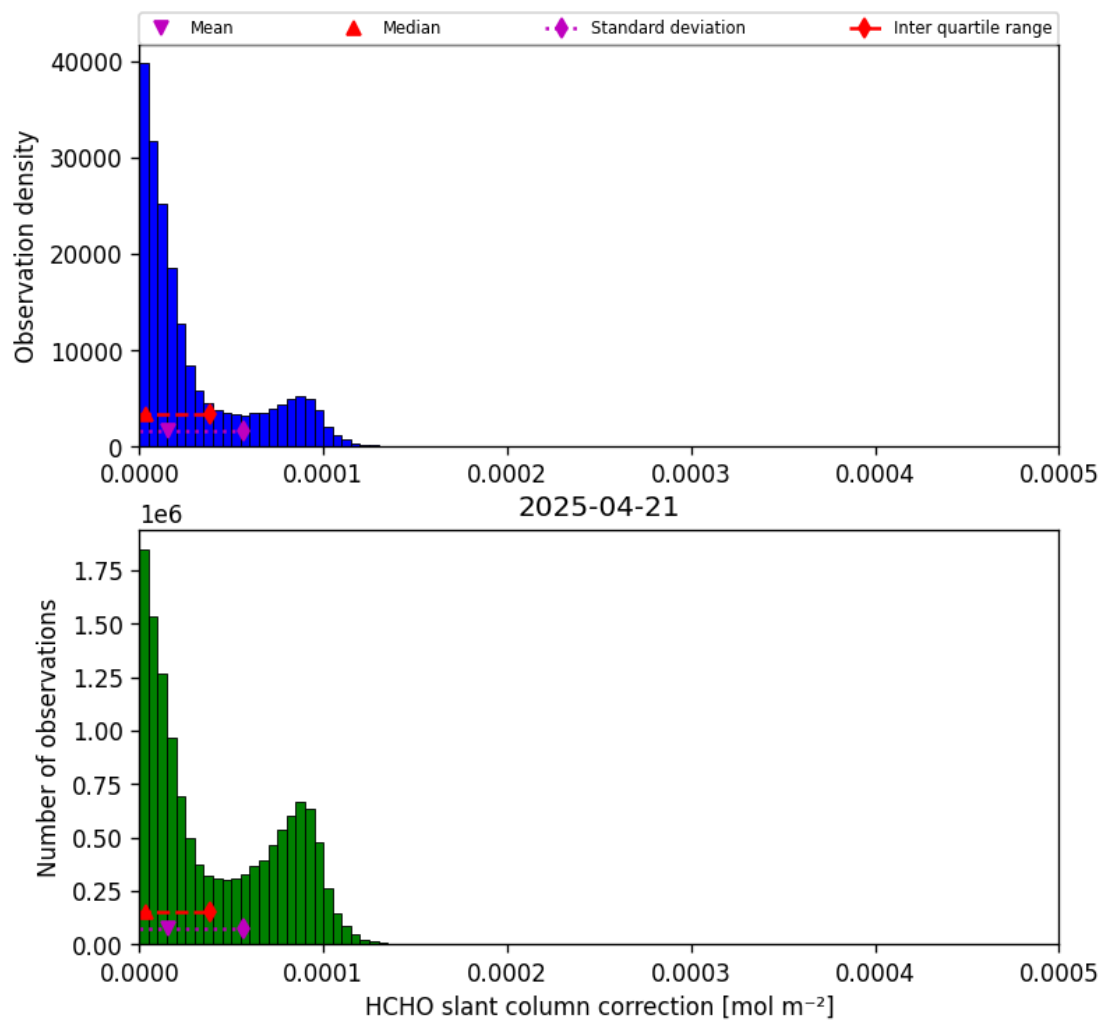
Figure 47: Histogram of “HCHO slant column correction” for 2025-04-20 to 2025-04-22
