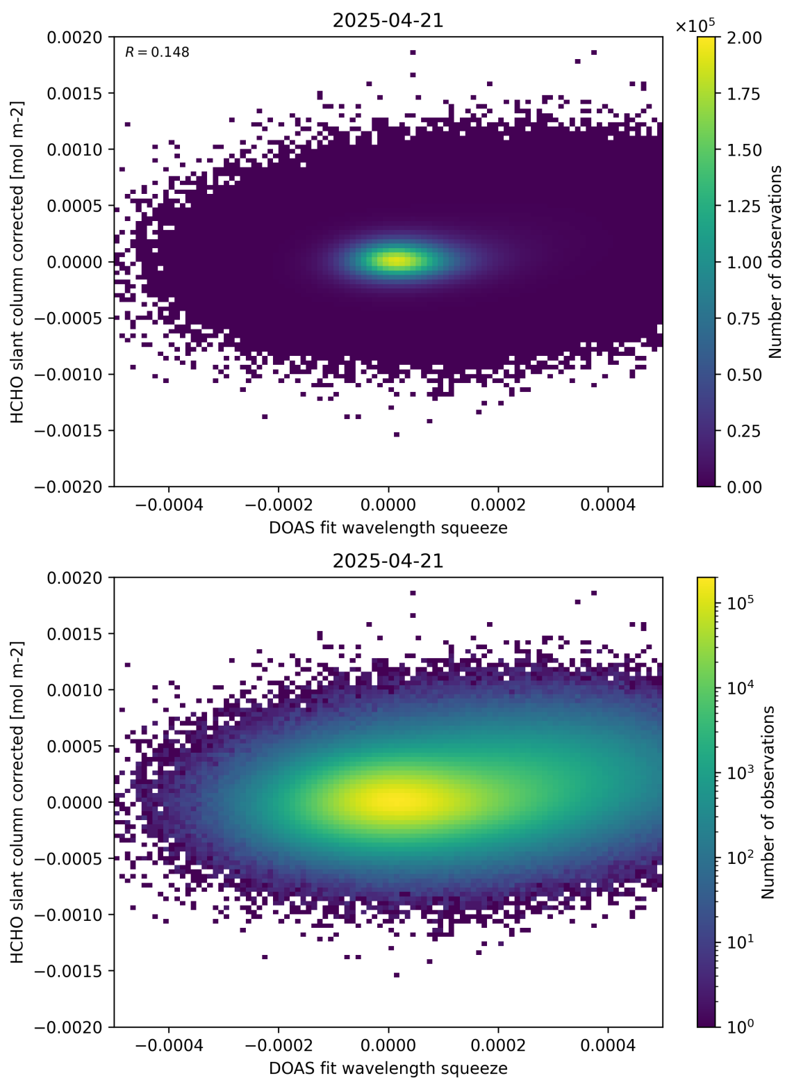
Figure 69: Scatter density plot of “DOAS fit wavelength squeeze” against “HCHO slant column corrected” for 2025-04-20 to 2025-04-22.
