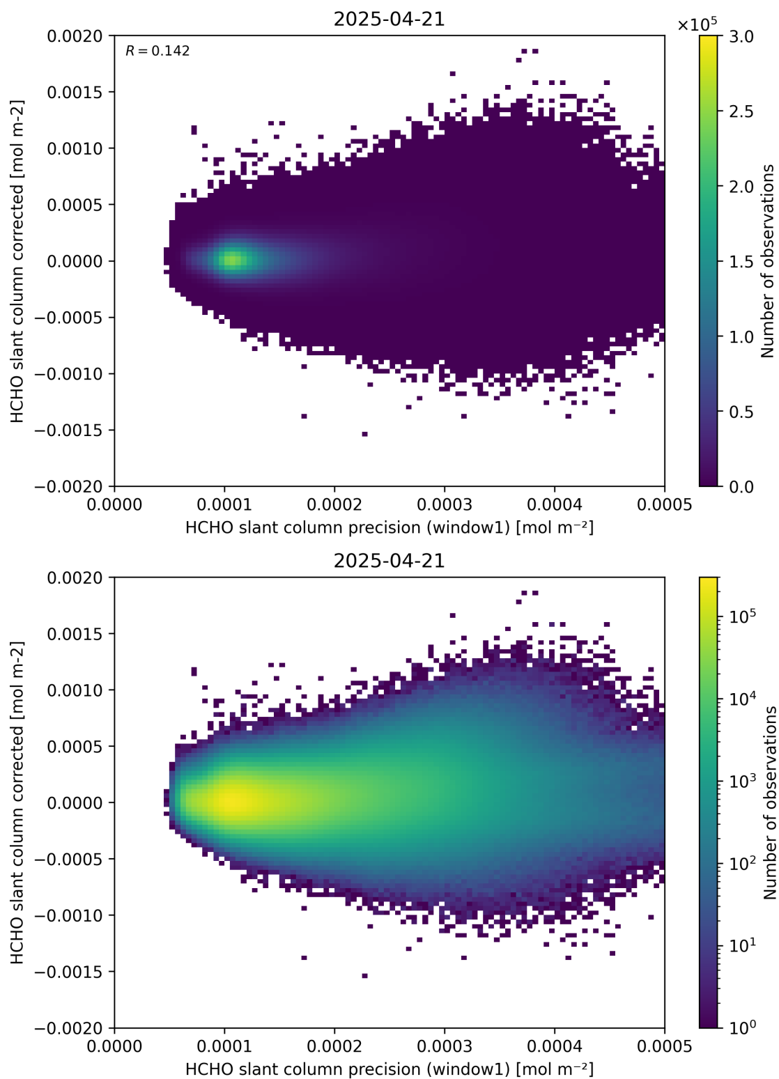
Figure 92: Scatter density plot of “HCHO slant column precision (window1)” against “HCHO slant column corrected” for 2025-04-20 to 2025-04-22.
