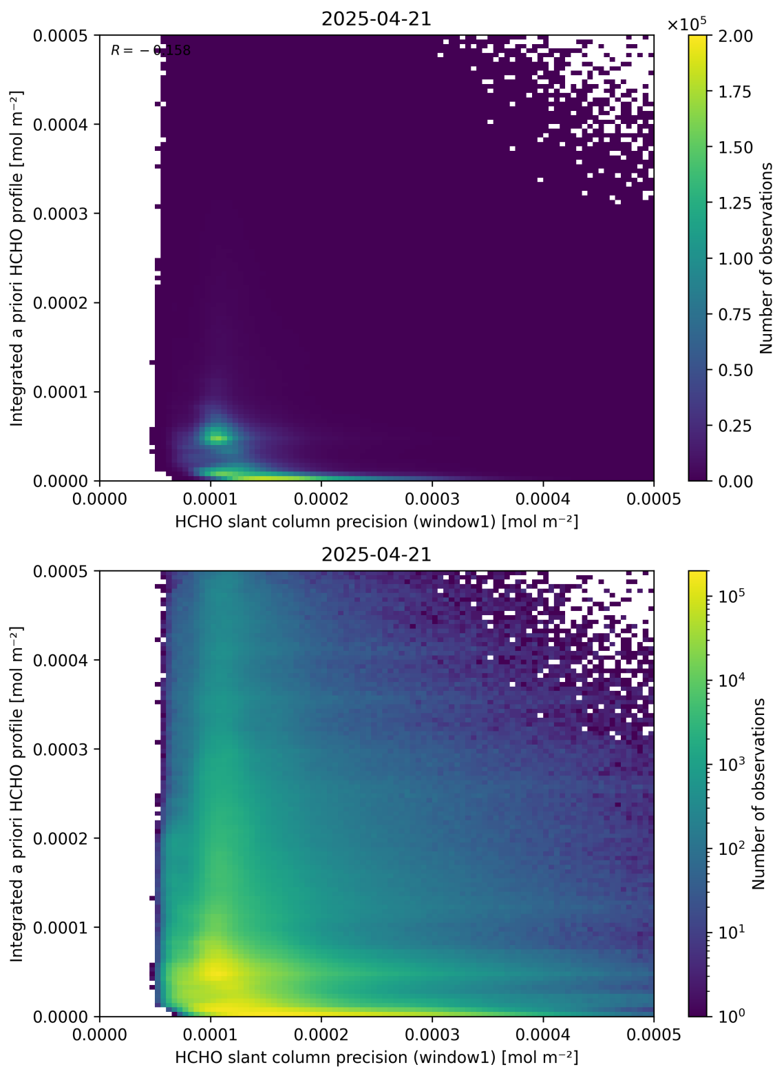
Figure 96: Scatter density plot of “HCHO slant column precision (window1)” against “Integrated a priori HCHO profile” for 2025-04-20 to 2025-04-22.
