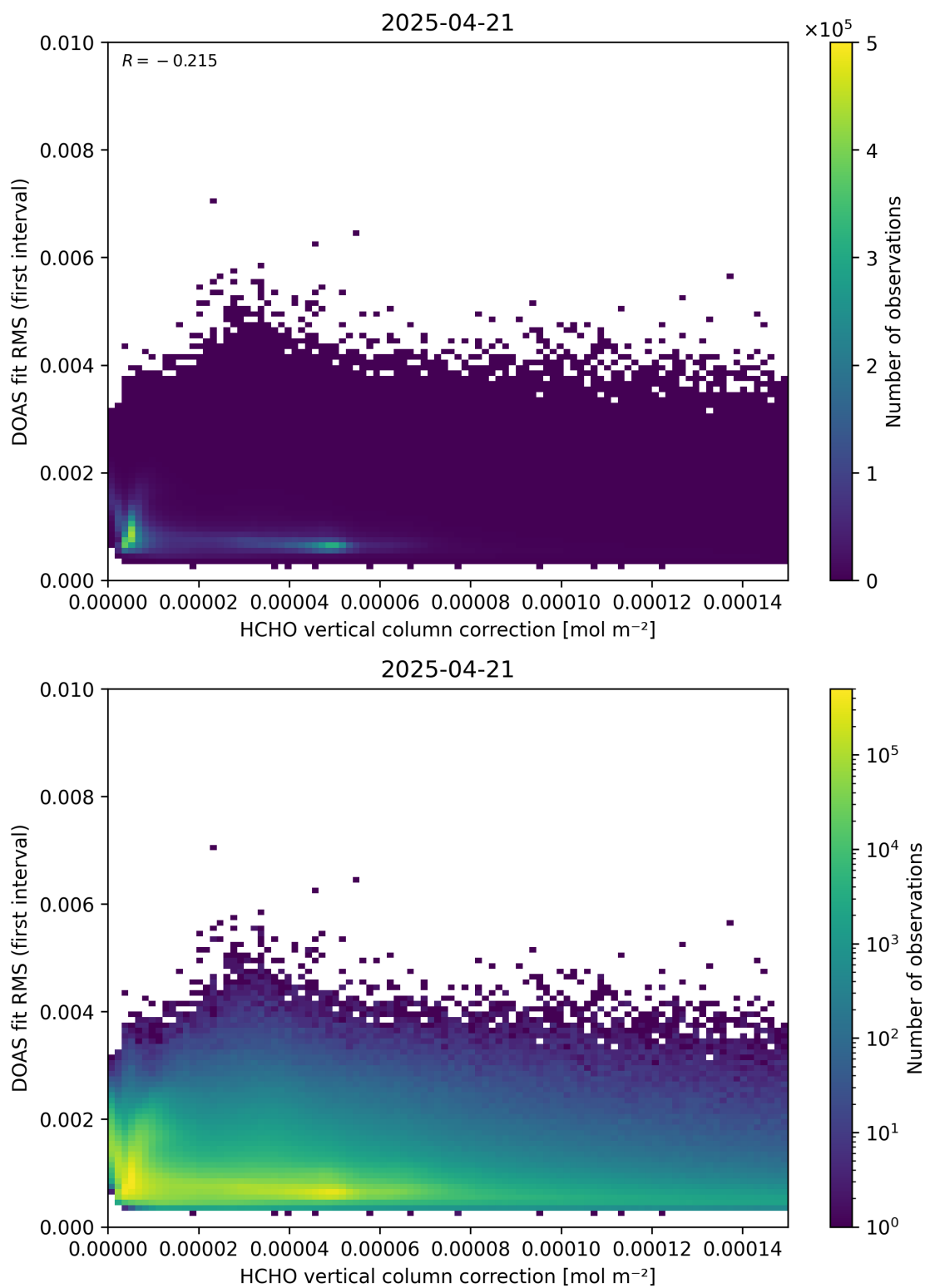
Figure 112: Scatter density plot of “HCHO vertical column correction” against “DOAS fit RMS (first interval)” for 2025-04-20 to 2025-04-22.
