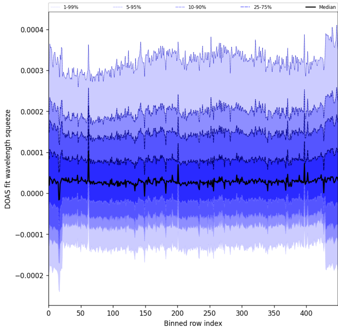
Figure 59: Along track statistics of “DOAS fit wavelength squeeze” for 2025-04-20 to 2025-04-22
