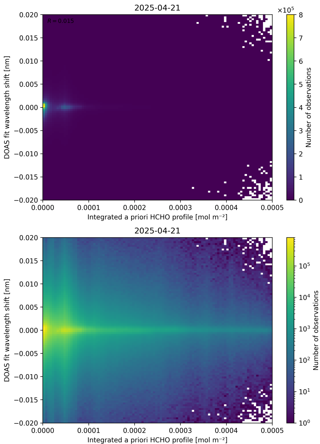
Figure 149: Scatter density plot of “Integrated a priori HCHO profile” against “DOAS fit wavelength shift” for 2025-04-20 to 2025-04-22.
