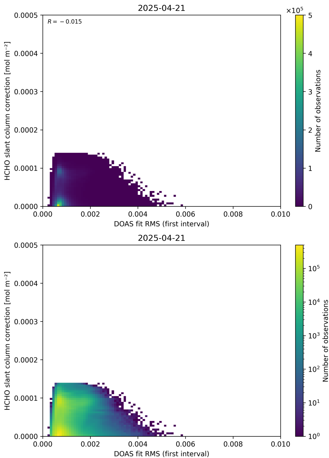
Figure 63: Scatter density plot of “DOAS fit RMS (first interval)” against “HCHO slant column correction” for 2025-04-20 to 2025-04-22.
