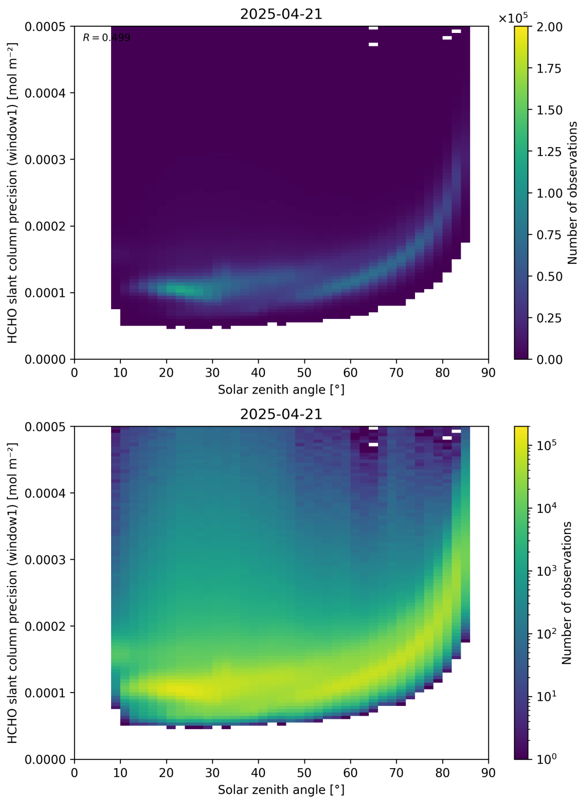
Figure 174: Scatter density plot of “Solar zenith angle” against “HCHO slant column precision (window1)” for 2025-04-20 to 2025-04-22.
