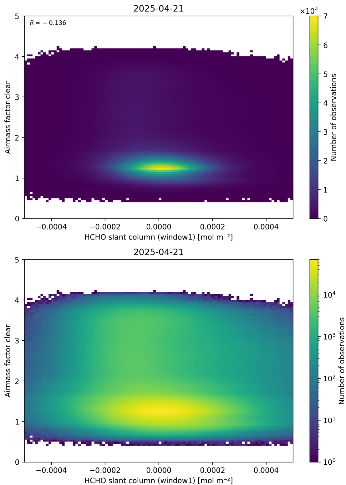
Figure 81: Scatter density plot of “HCHO slant column (window1)” against “Airmass factor clear” for 2025-04-20 to 2025-04-22.
