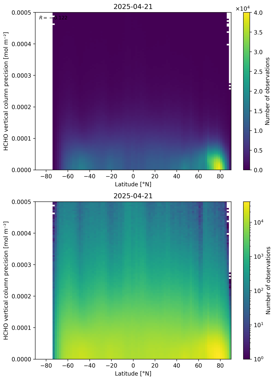
Figure 165: Scatter density plot of “Latitude” against “HCHO vertical column precision” for 2025-04-20 to 2025-04-22.
