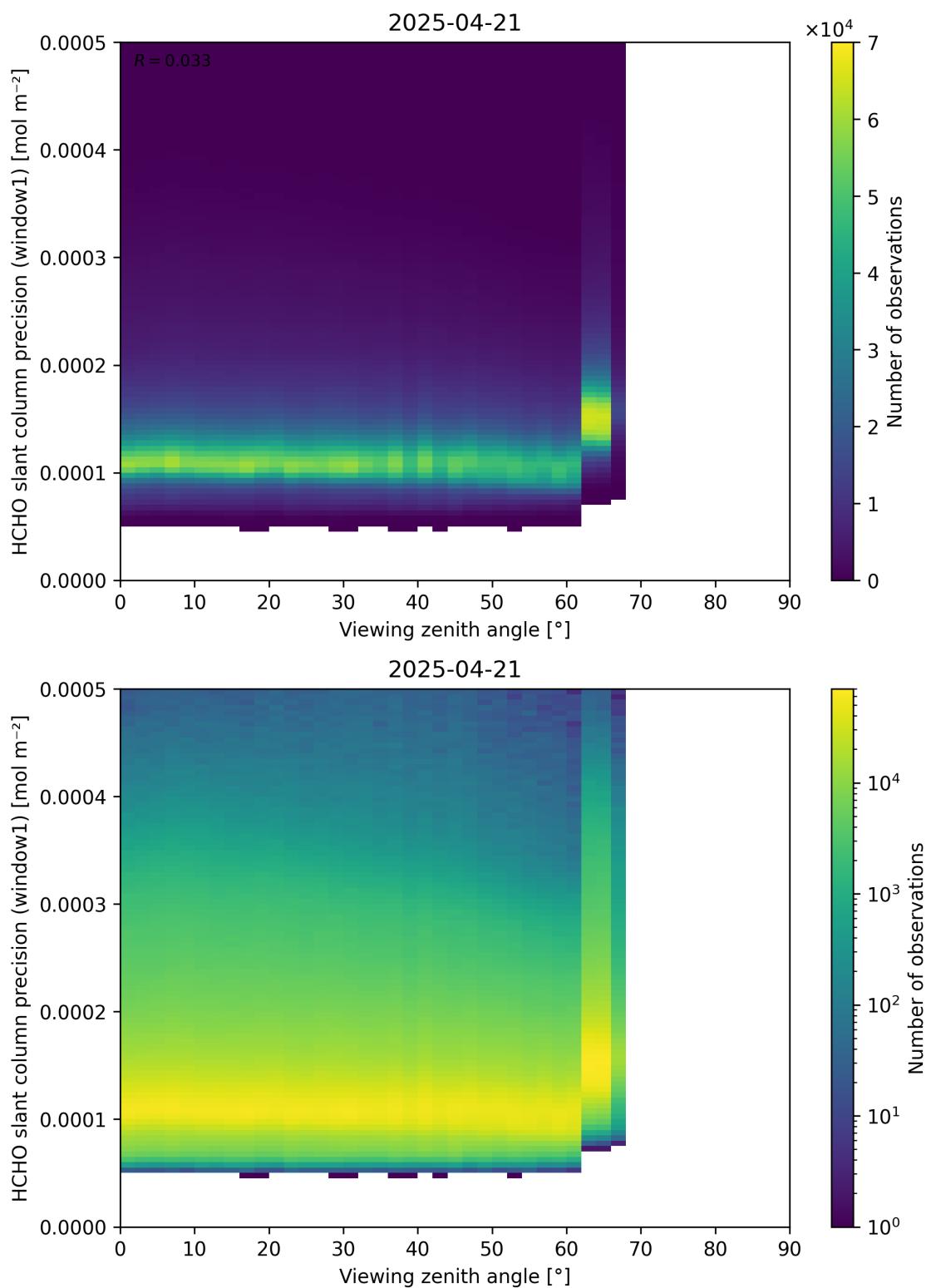
Figure 189: Scatter density plot of “Viewing zenith angle” against “HCHO slant column precision (window1)” for 2025-04-20 to 2025-04-22.
