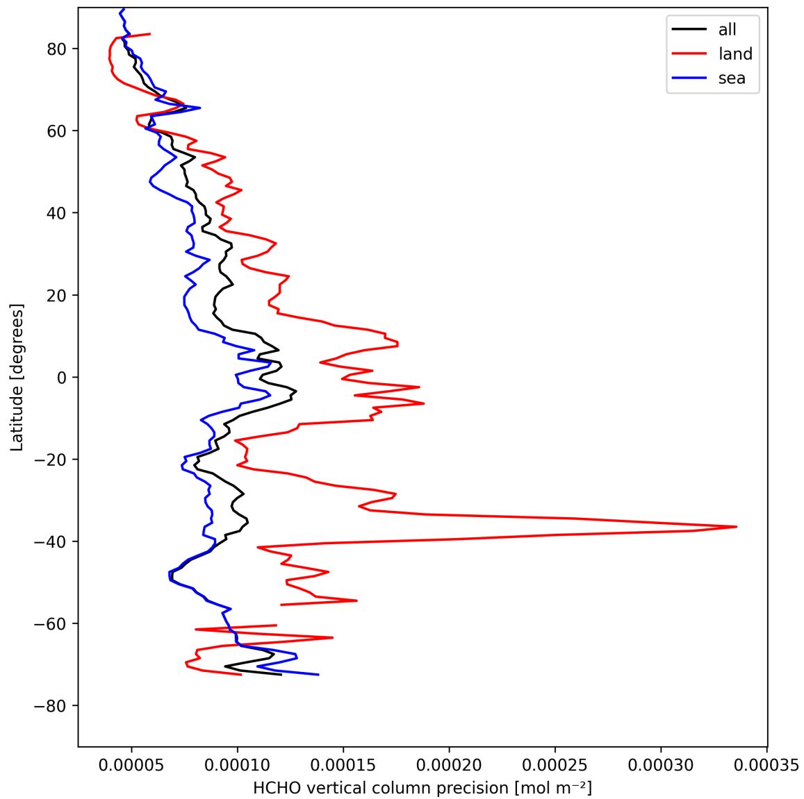
Figure 22: Zonal average of “HCHO vertical column precision” for 2025-04-20 to 2025-04-22.
