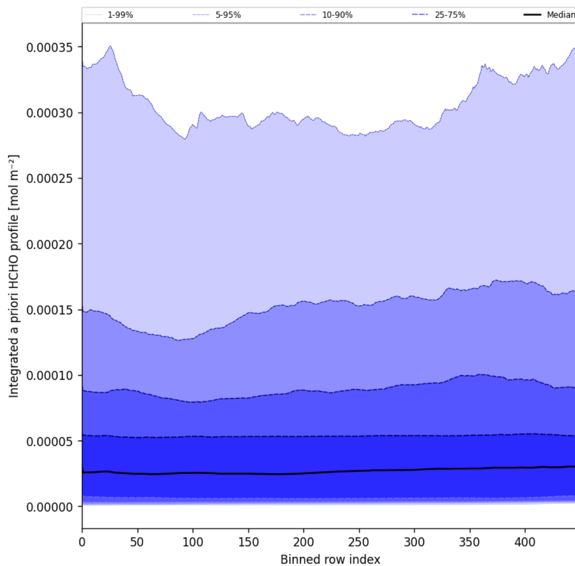
Figure 57: Along track statistics of “Integrated a priori HCHO profile” for 2025-04-20 to 2025-04-22
