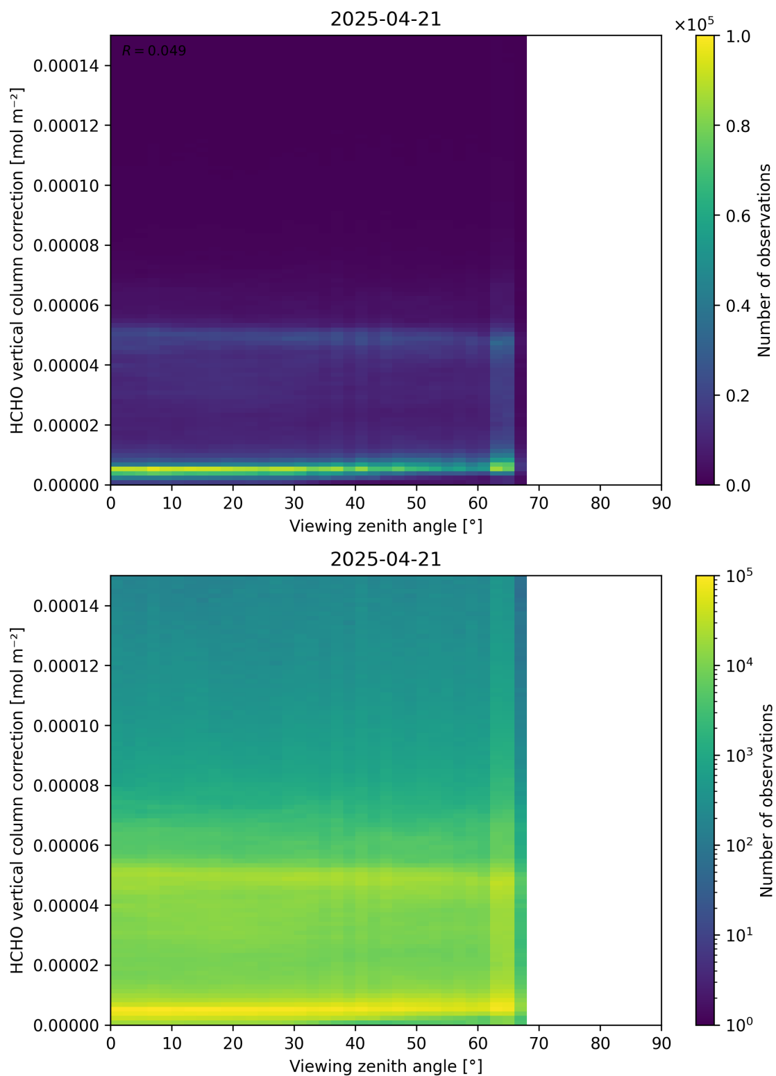
Figure 193: Scatter density plot of “Viewing zenith angle” against “HCHO vertical column correction” for 2025-04-20 to 2025-04-22.
