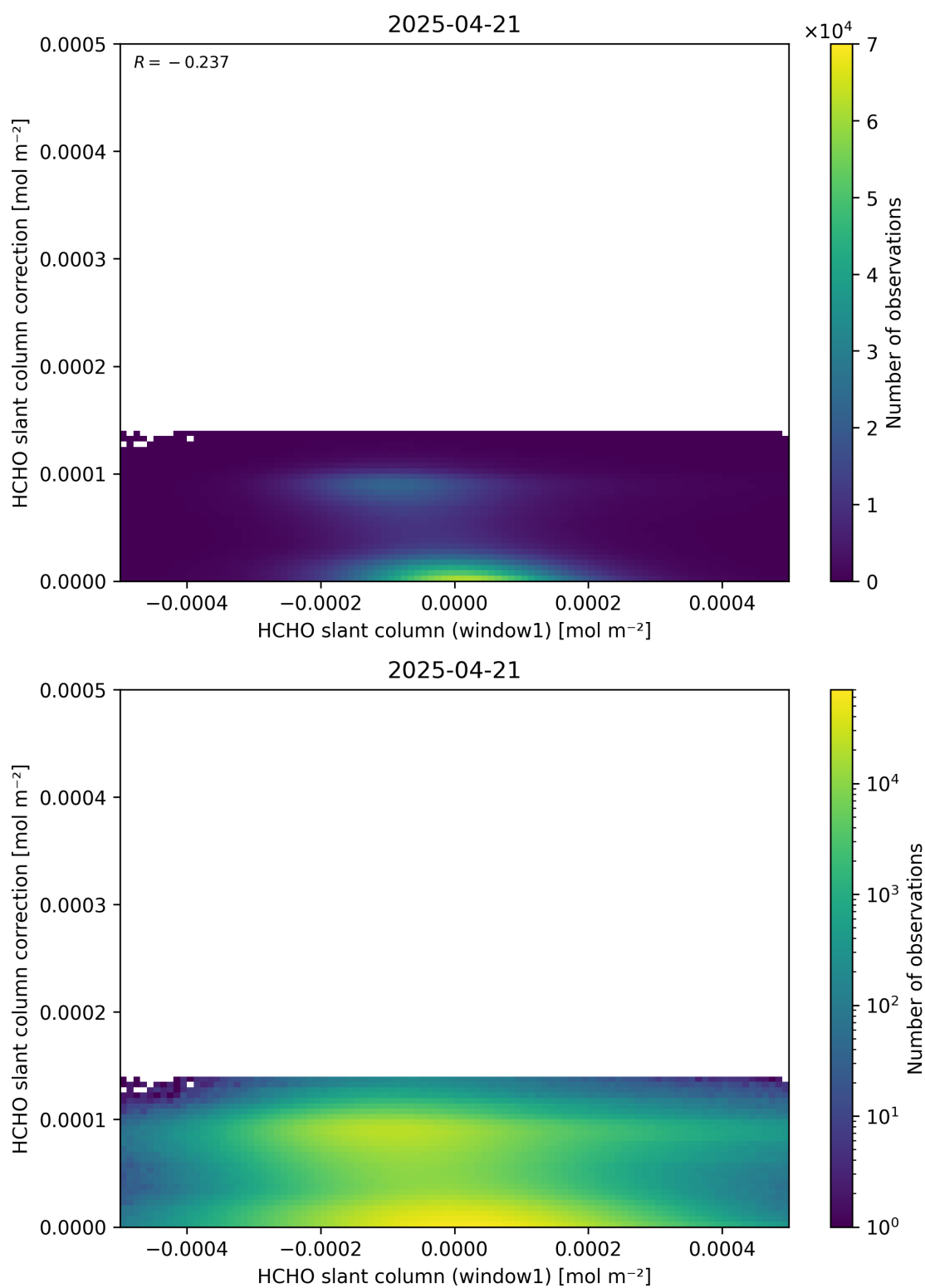
Figure 83: Scatter density plot of “HCHO slant column (window1)” against “HCHO slant column correction” for 2025-04-20 to 2025-04-22.
