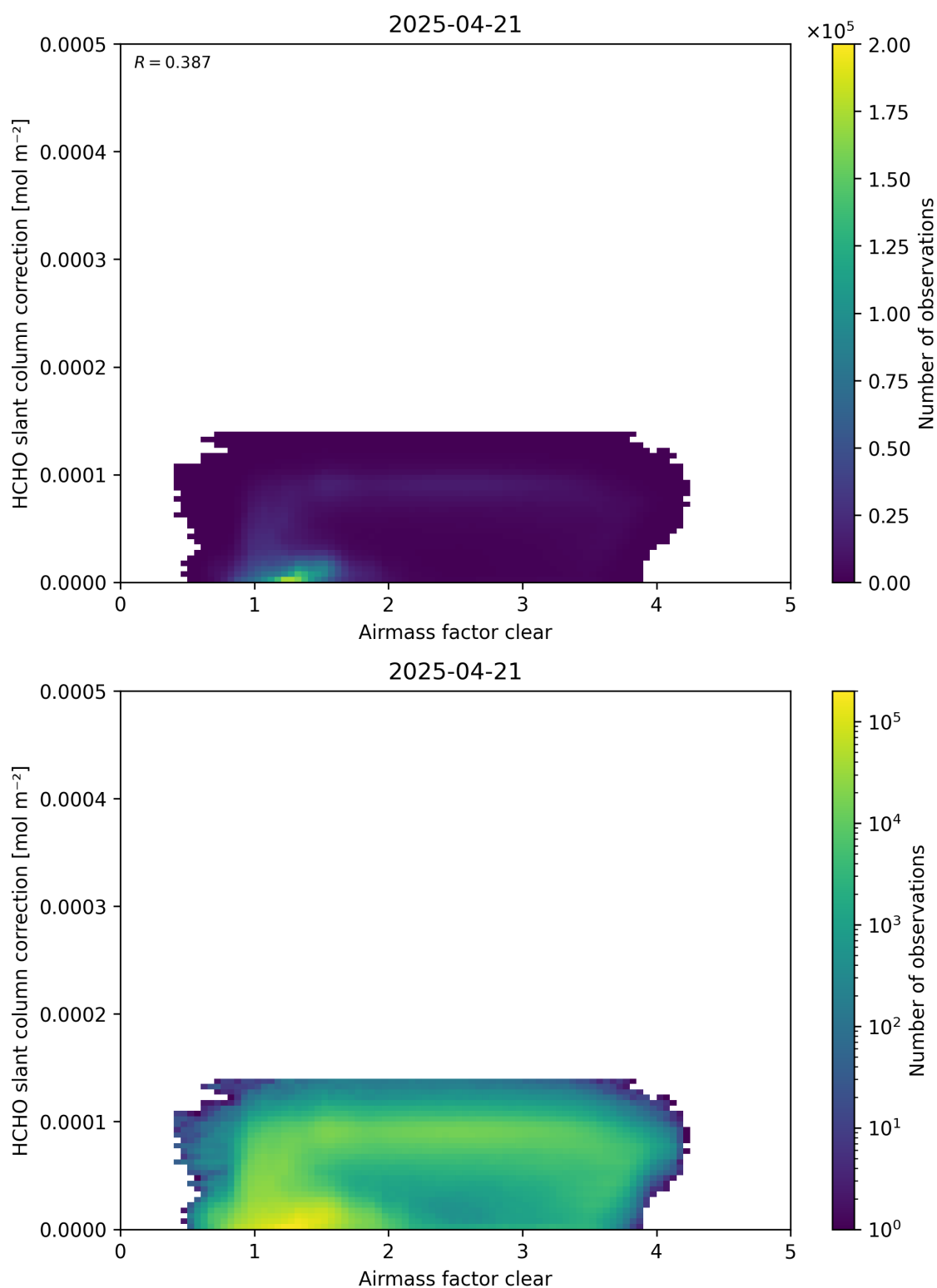
Figure 75: Scatter density plot of “Airmass factor clear” against “HCHO slant column correction” for 2025-04-20 to 2025-04-22.
