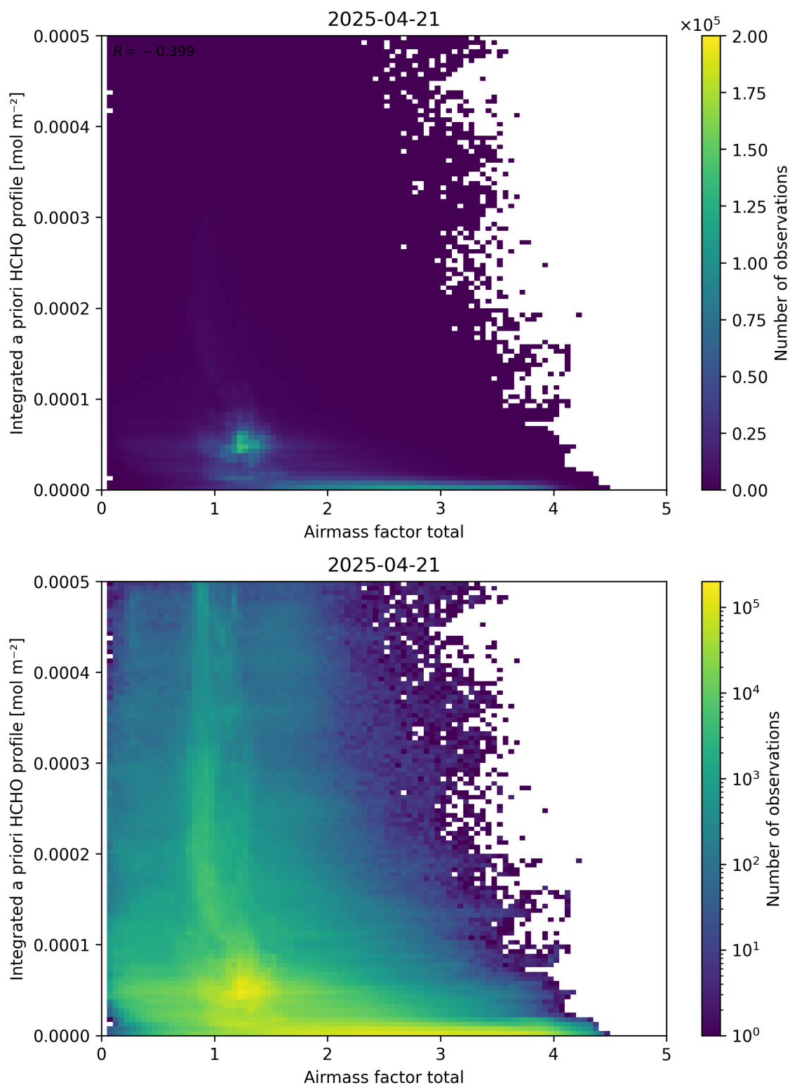
Figure 104: Scatter density plot of “Airmass factor total” against “Integrated a priori HCHO profile” for 2025-04-20 to 2025-04-22.
