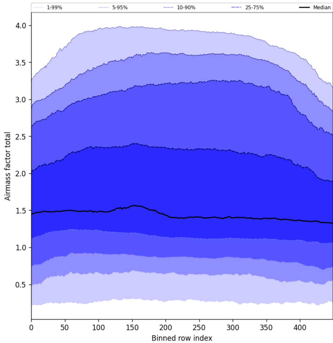
Figure 54: Along track statistics of “Airmass factor total” for 2025-04-20 to 2025-04-22
