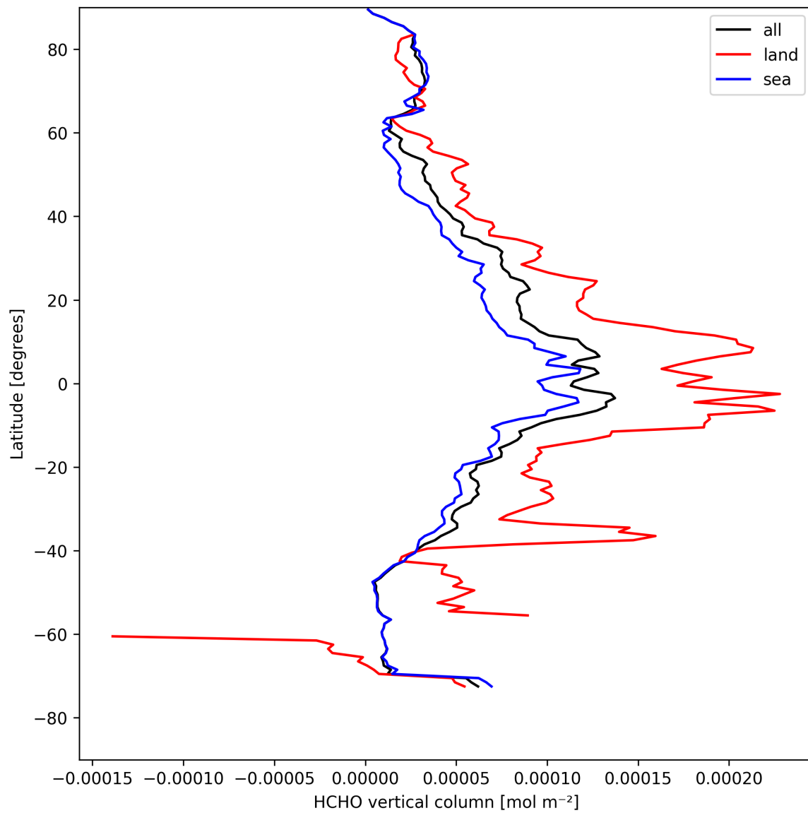
Figure 21: Zonal average of “HCHO vertical column” for 2025-04-20 to 2025-04-22.
