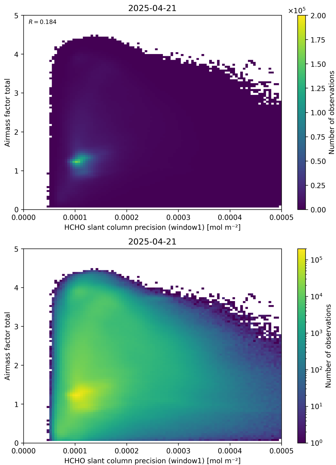
Figure 94: Scatter density plot of “HCHO slant column precision (window1)” against “Airmass factor total” for 2025-04-20 to 2025-04-22.
