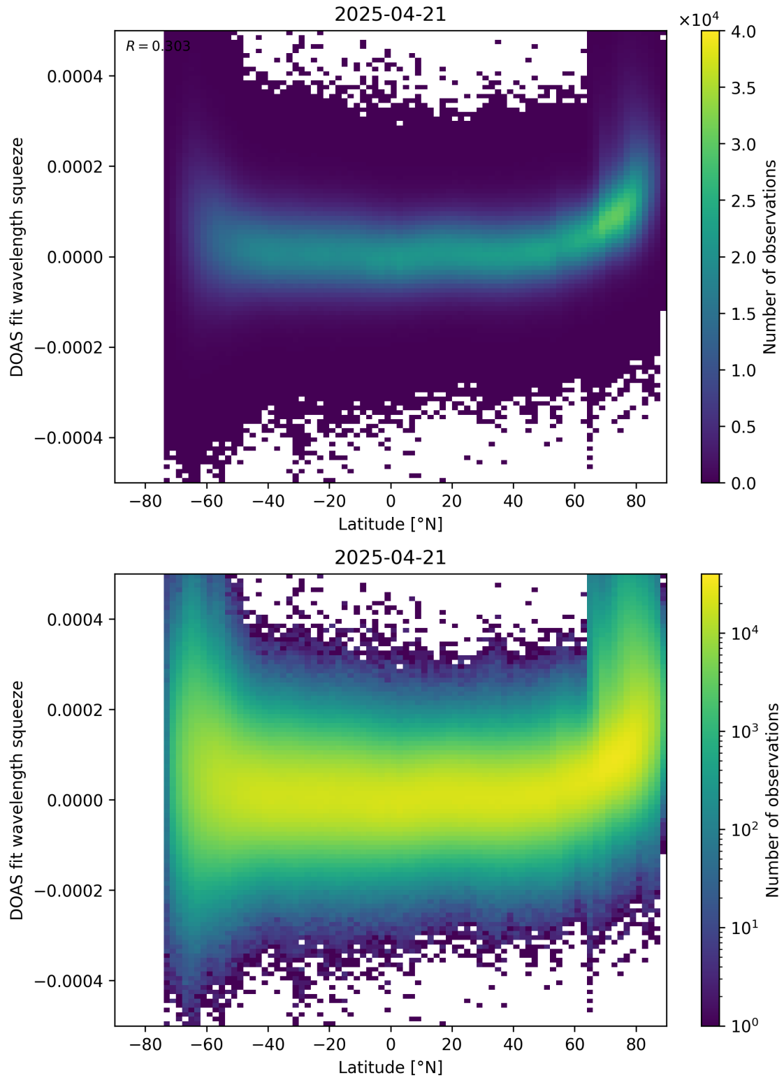
Figure 155: Scatter density plot of “Latitude” against “DOAS fit wavelength squeeze” for 2025-04-20 to 2025-04-22.
