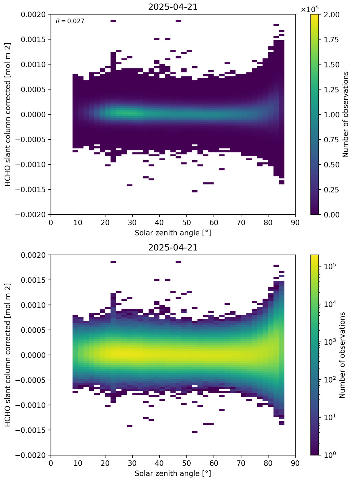
Figure 171: Scatter density plot of “Solar zenith angle” against “HCHO slant column corrected” for 2025-04-20 to 2025-04-22.
