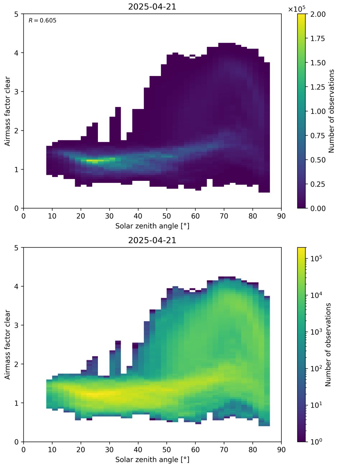
Figure 170: Scatter density plot of “Solar zenith angle” against “Airmass factor clear” for 2025-04-20 to 2025-04-22.
