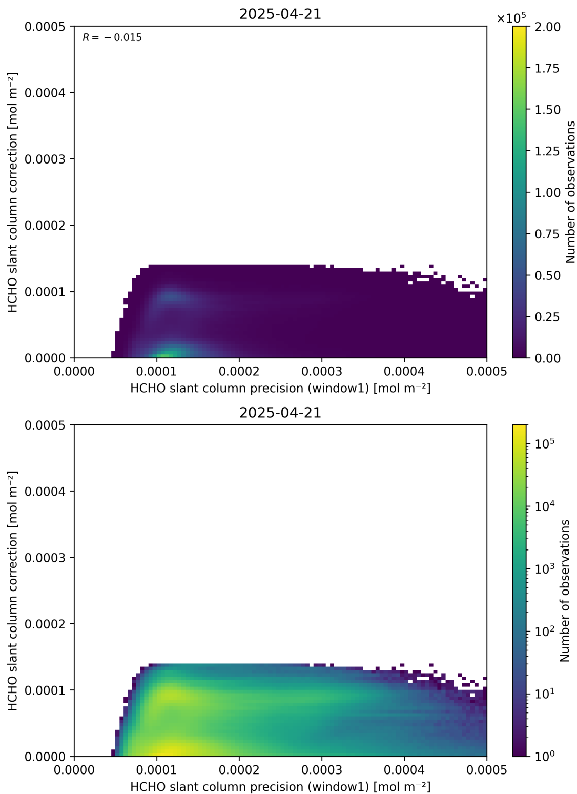
Figure 93: Scatter density plot of “HCHO slant column precision (window1)” against “HCHO slant column correction” for 2025-04-20 to 2025-04-22.
