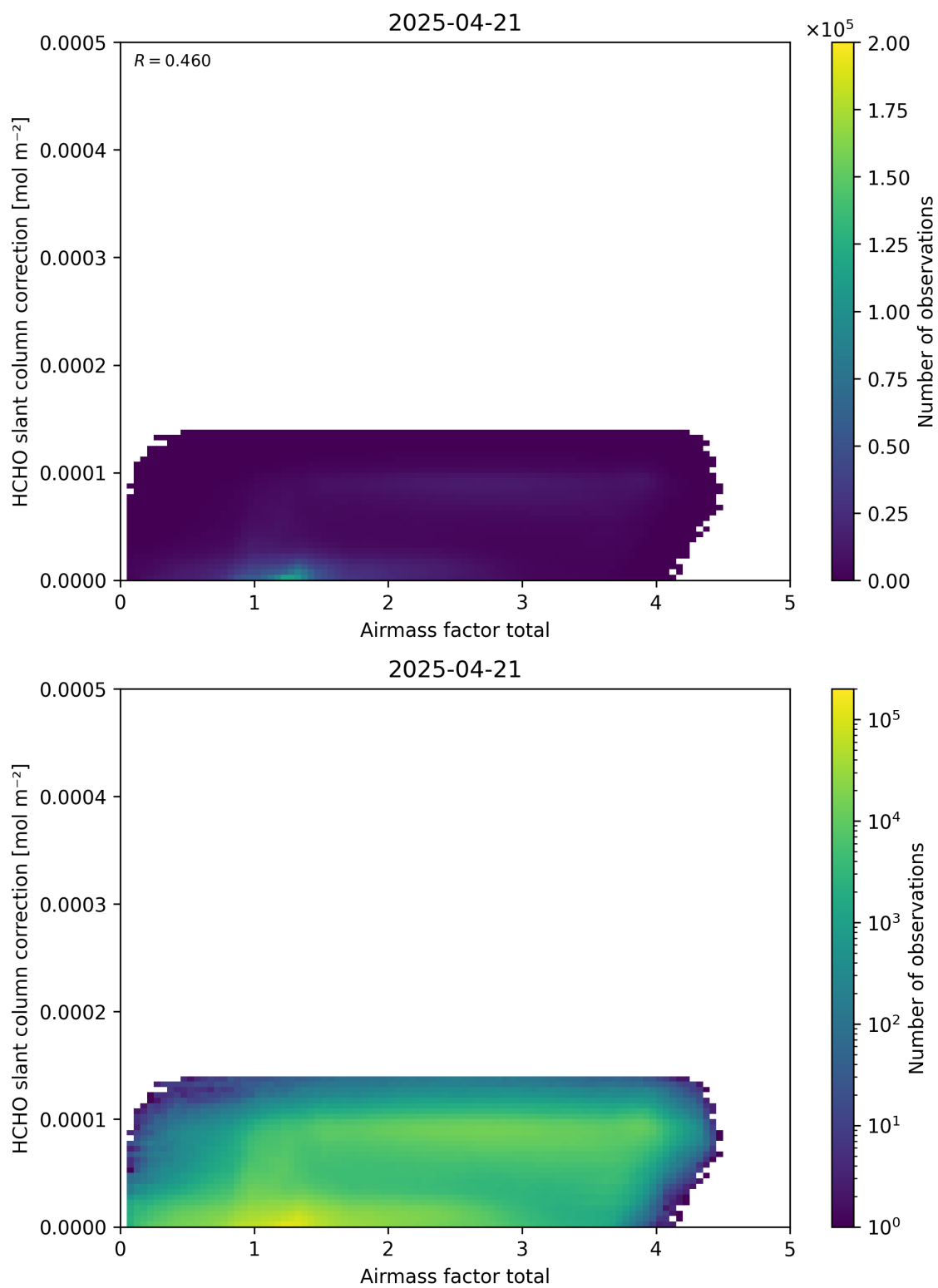
Figure 102: Scatter density plot of “Airmass factor total” against “HCHO slant column correction” for 2025-04-20 to 2025-04-22.
