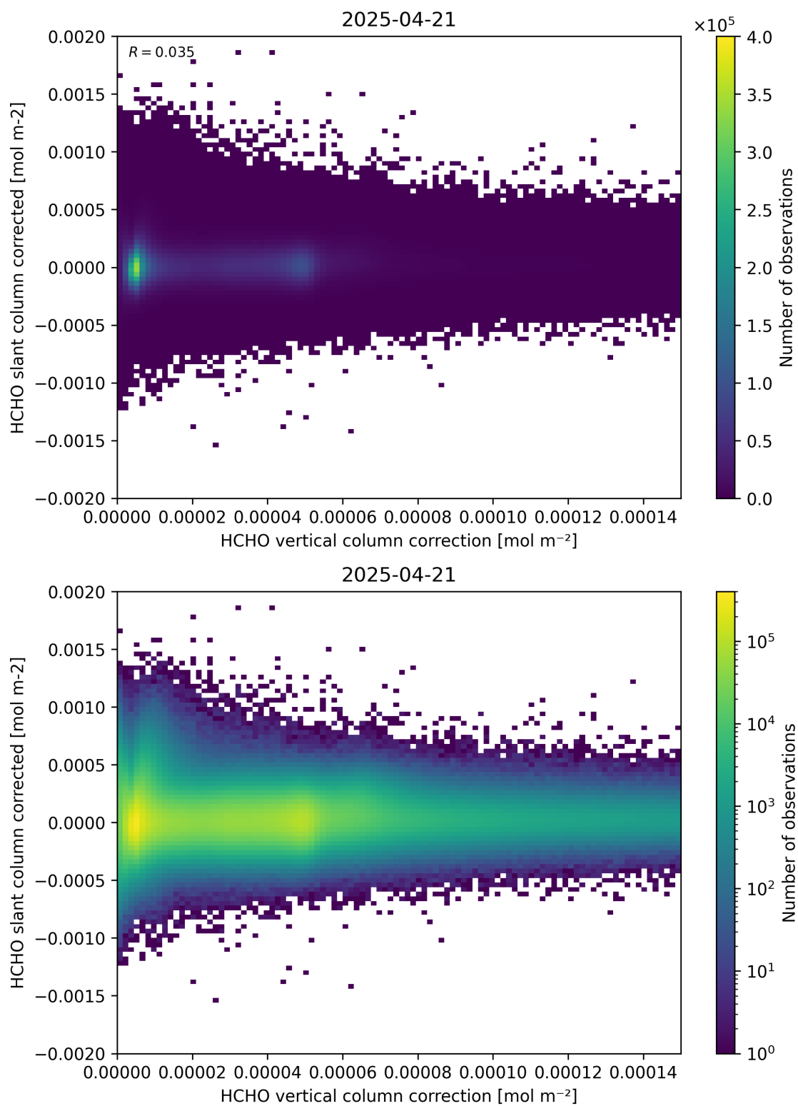
Figure 116: Scatter density plot of “HCHO vertical column correction” against “HCHO slant column corrected” for 2025-04-20 to 2025-04-22.
