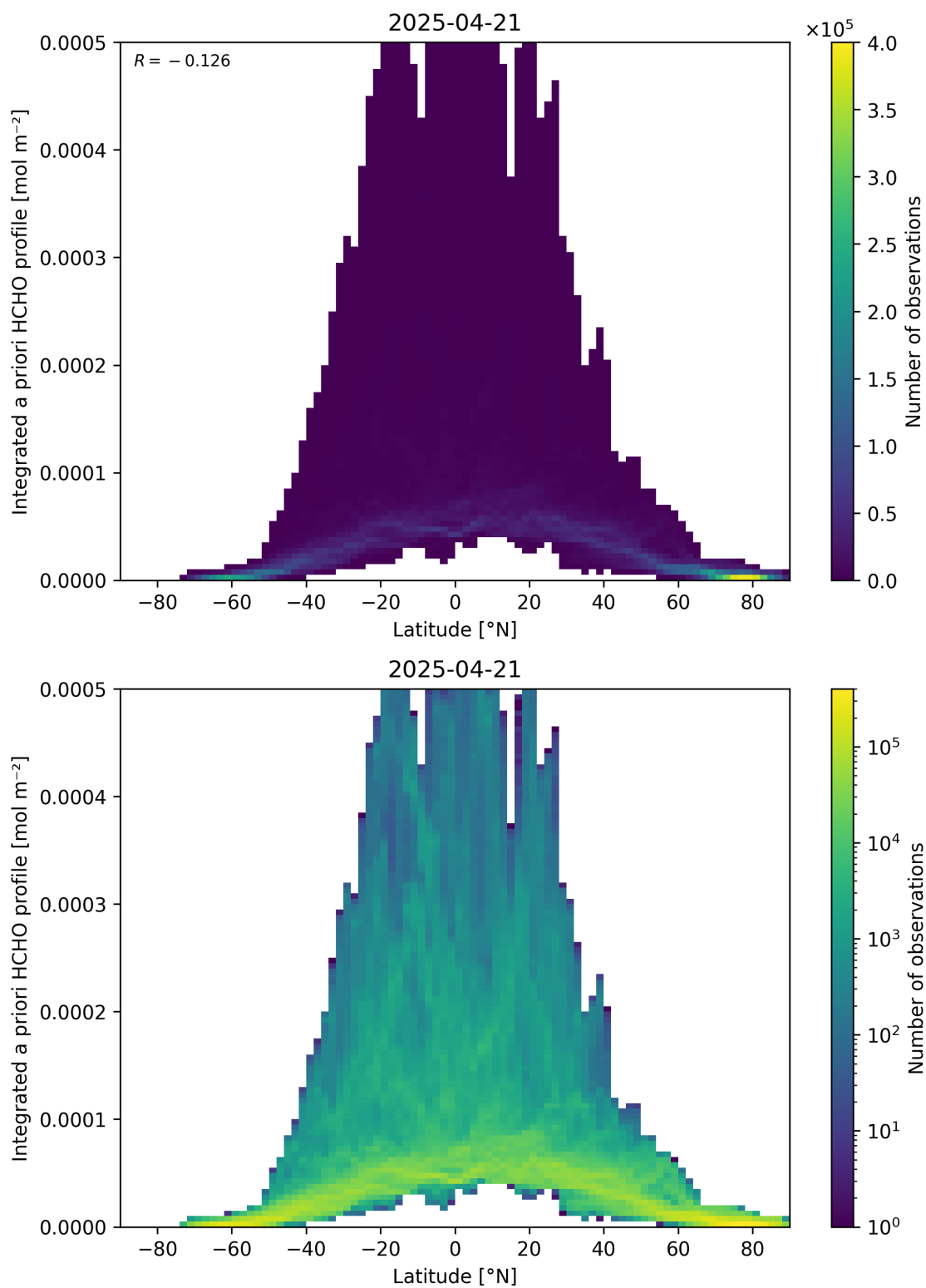
Figure 166: Scatter density plot of “Latitude” against “Integrated a priori HCHO profile” for 2025-04-20 to 2025-04-22.
