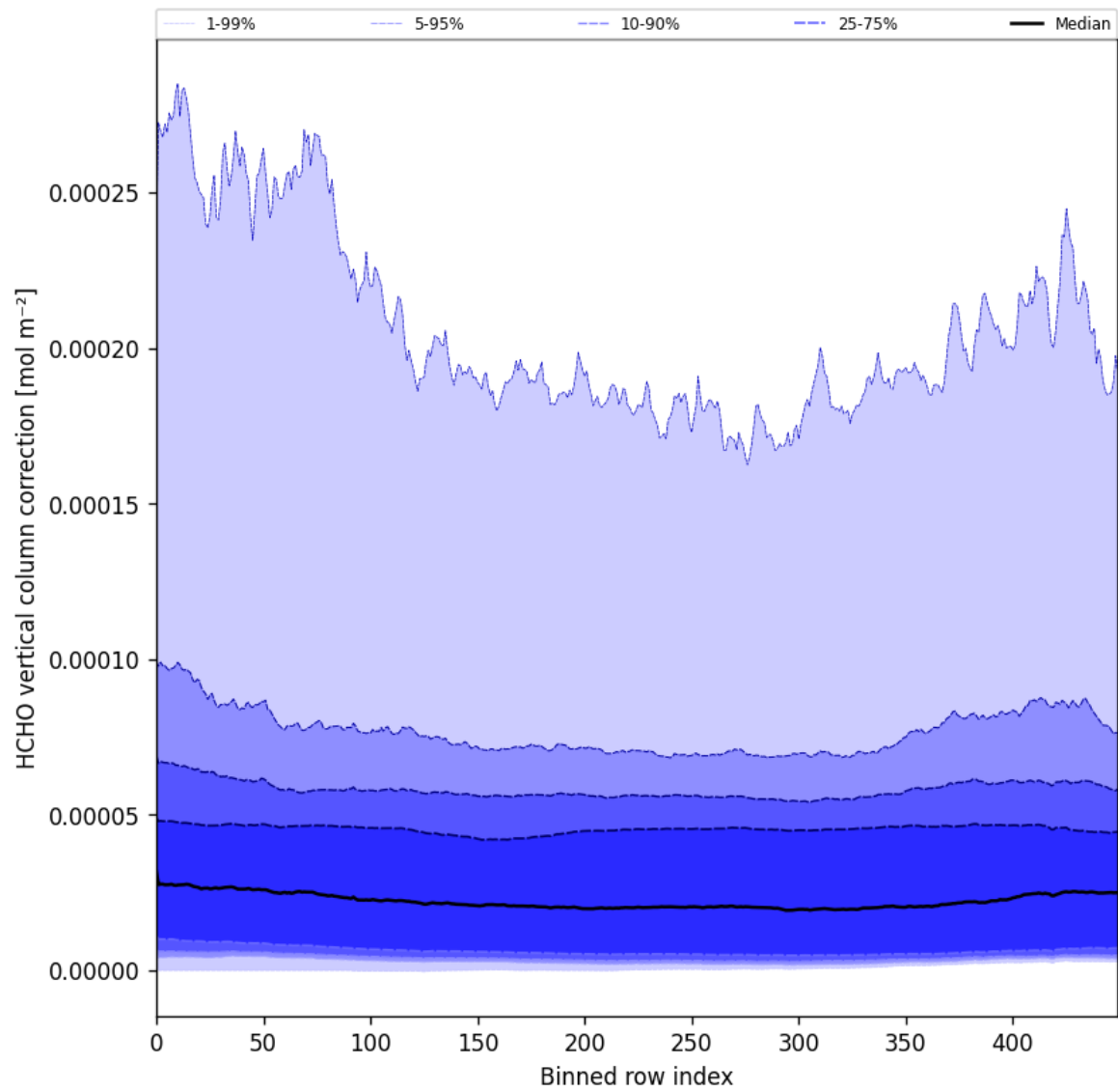
Figure 51: Along track statistics of “HCHO vertical column correction” for 2025-04-20 to 2025-04-22
