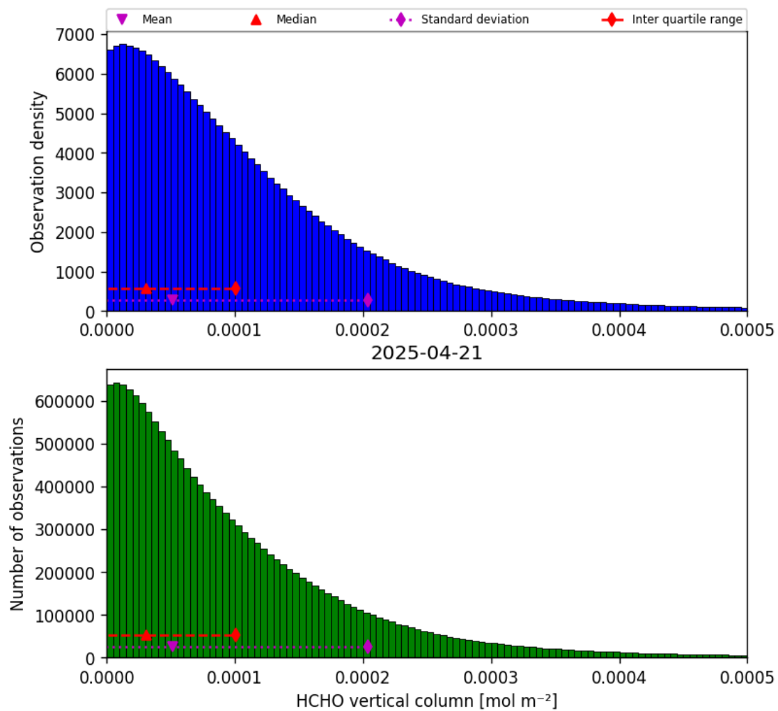
Figure 35: Histogram of “HCHO vertical column” for 2025-04-20 to 2025-04-22
