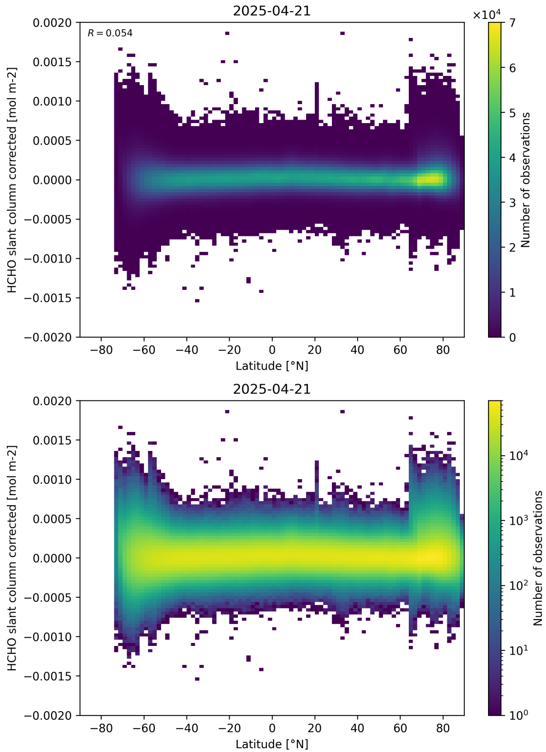
Figure 157: Scatter density plot of “Latitude” against “HCHO slant column corrected” for 2025-04-20 to 2025-04-22.
