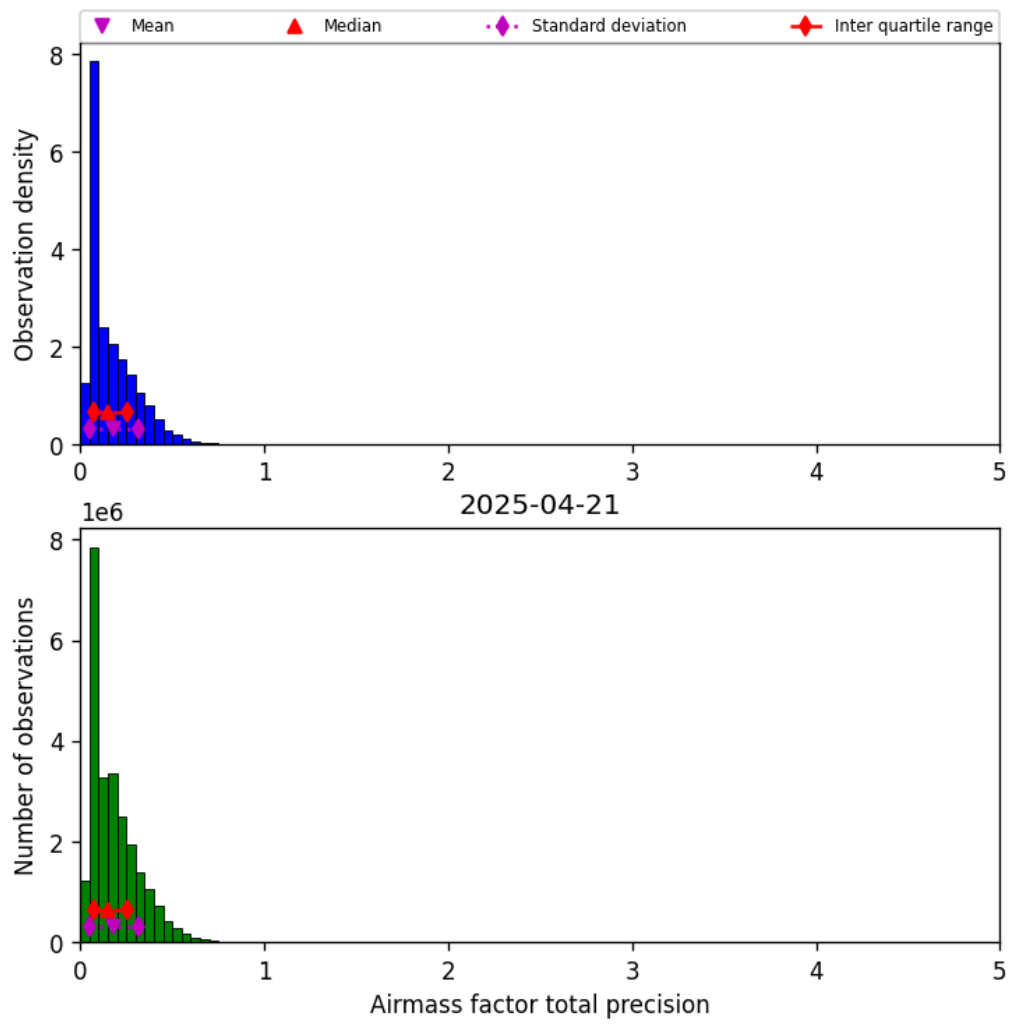
Figure 41: Histogram of “Airmass factor total precision” for 2025-04-20 to 2025-04-22
