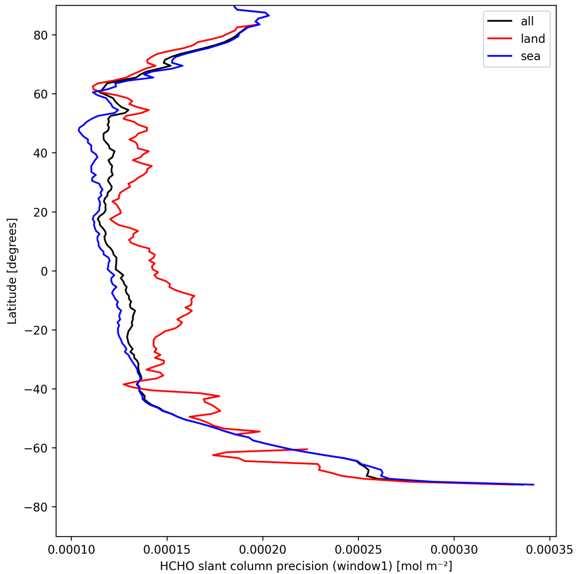
Figure 25: Zonal average of “HCHO slant column precision (window1)” for 2025-04-20 to 2025-04-22.
