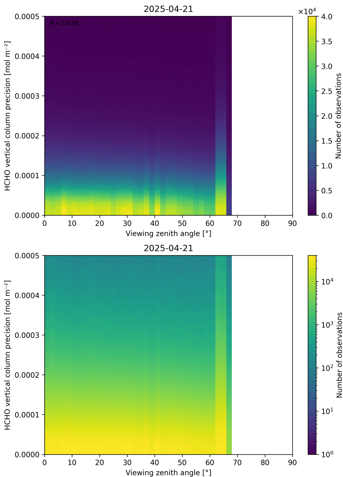
Figure 194: Scatter density plot of “Viewing zenith angle” against “HCHO vertical column precision” for 2025-04-20 to 2025-04-22.
