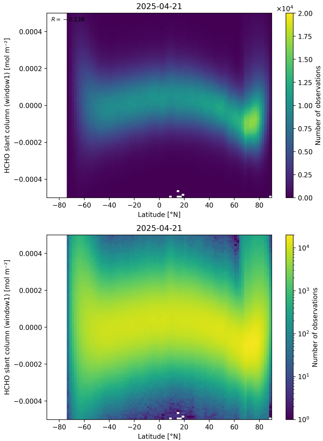
Figure 159: Scatter density plot of “Latitude” against “HCHO slant column (window1)” for 2025-04-20 to 2025-04-22.
