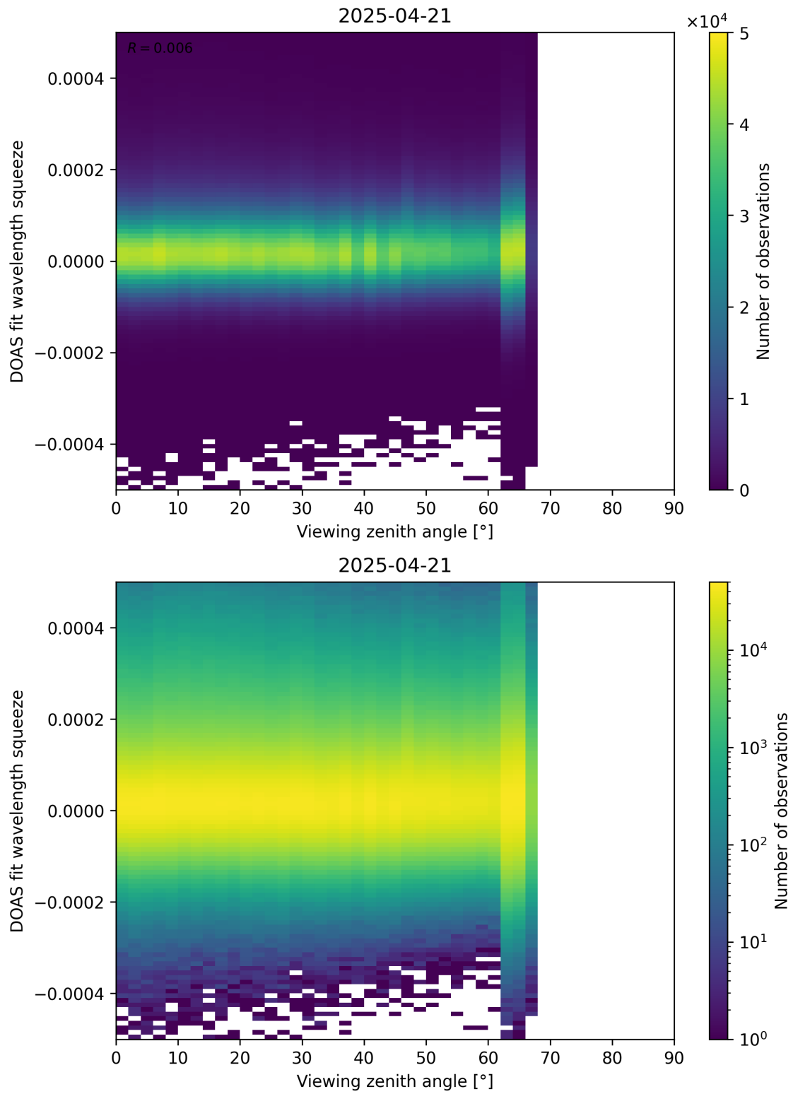
Figure 184: Scatter density plot of “Viewing zenith angle” against “DOAS fit wavelength squeeze” for 2025-04-20 to 2025-04-22.
