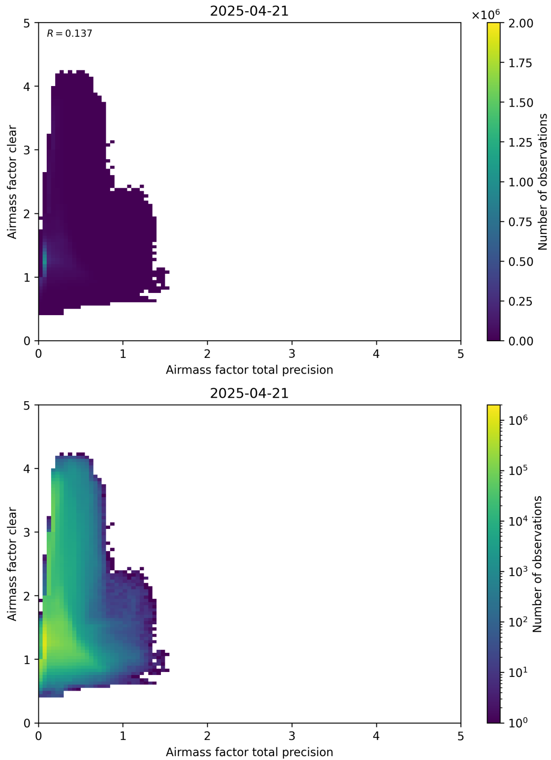
Figure 108: Scatter density plot of “Airmass factor total precision” against “Airmass factor clear” for 2025-04-20 to 2025-04-22.
