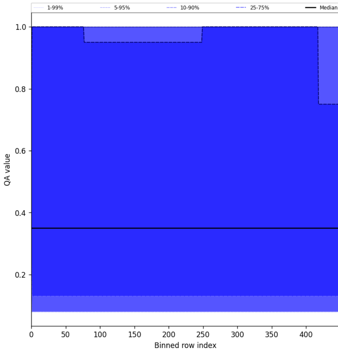
Figure 48: Along track statistics of “QA value” for 2025-04-20 to 2025-04-22
