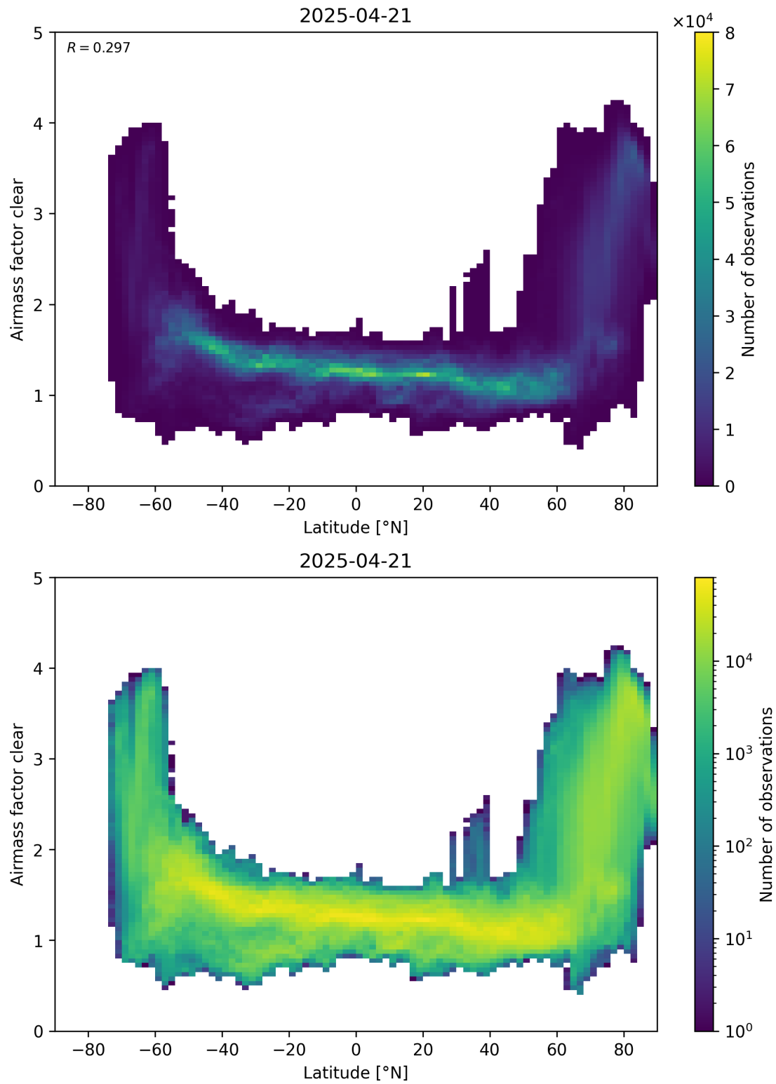
Figure 156: Scatter density plot of “Latitude” against “Airmass factor clear” for 2025-04-20 to 2025-04-22.
