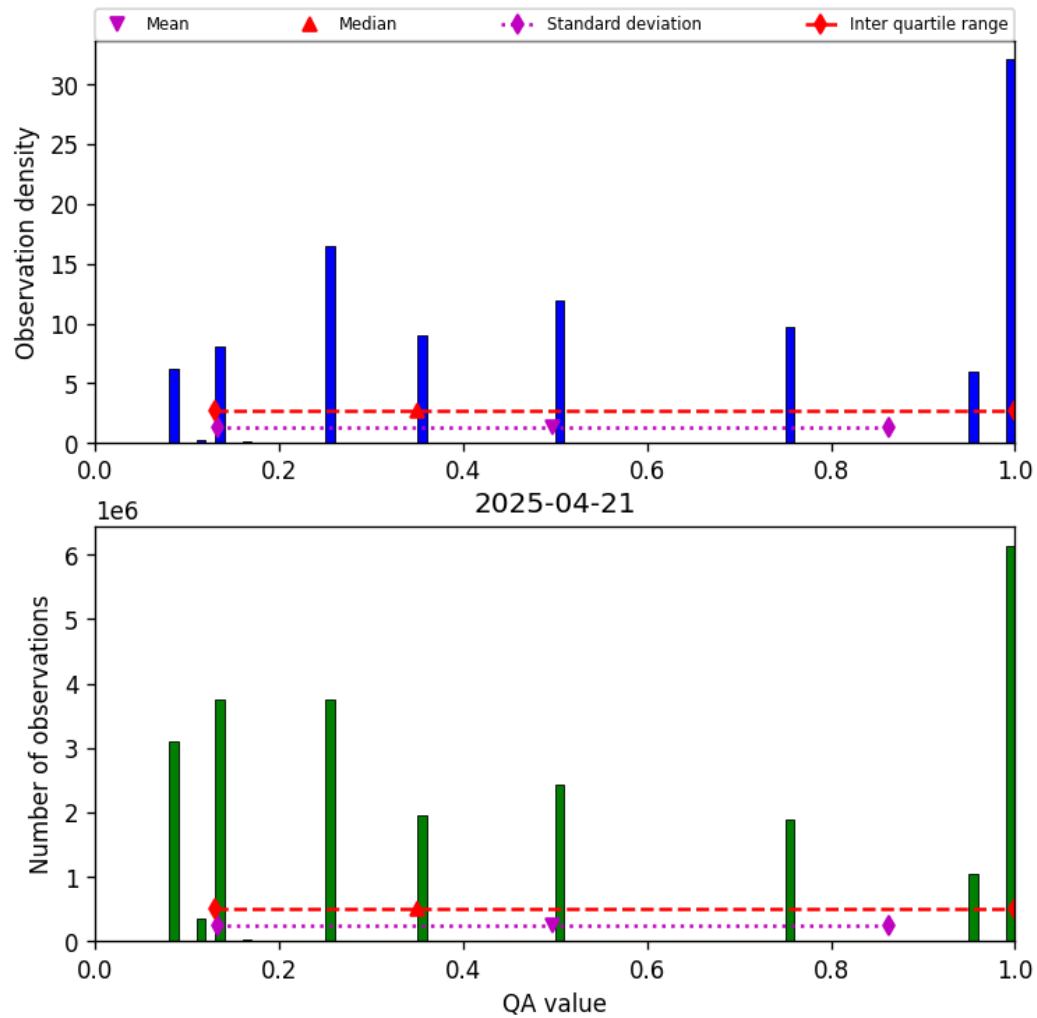
Figure 34: Histogram of “QA value” for 2025-04-20 to 2025-04-22
