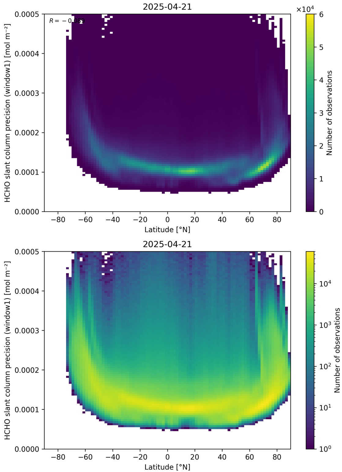
Figure 160: Scatter density plot of “Latitude” against “HCHO slant column precision (window1)” for 2025-04-20 to 2025-04-22.
