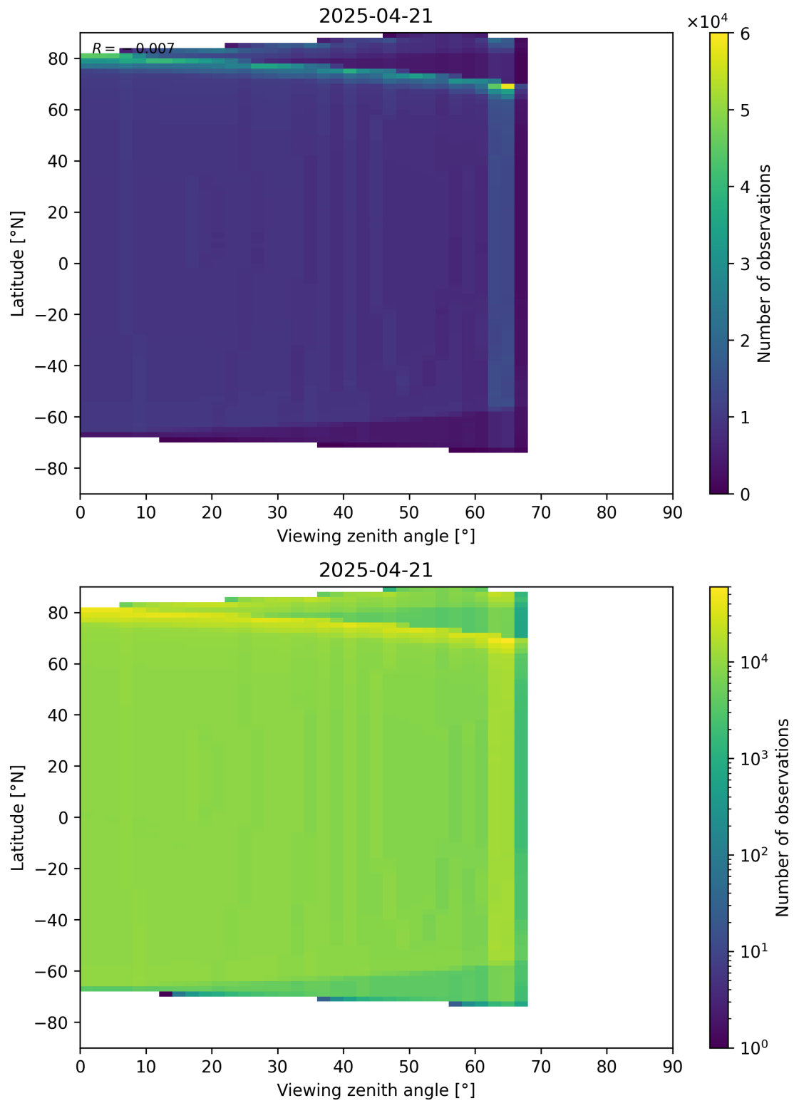
Figure 196: Scatter density plot of “Viewing zenith angle” against “Latitude” for 2025-04-20 to 2025-04-22.
