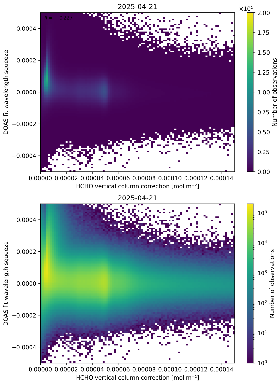
Figure 114: Scatter density plot of “HCHO vertical column correction” against “DOAS fit wavelength squeeze” for 2025-04-20 to 2025-04-22.
