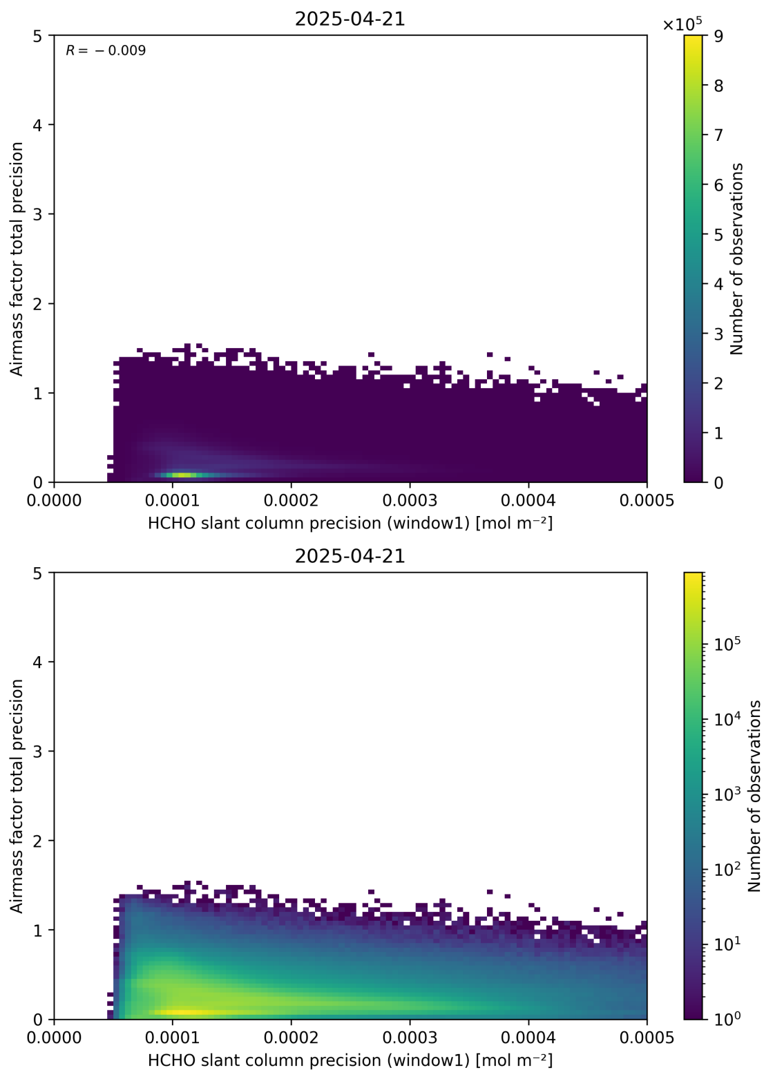
Figure 95: Scatter density plot of “HCHO slant column precision (window1)” against “Airmass factor total precision” for 2025-04-20 to 2025-04-22.
