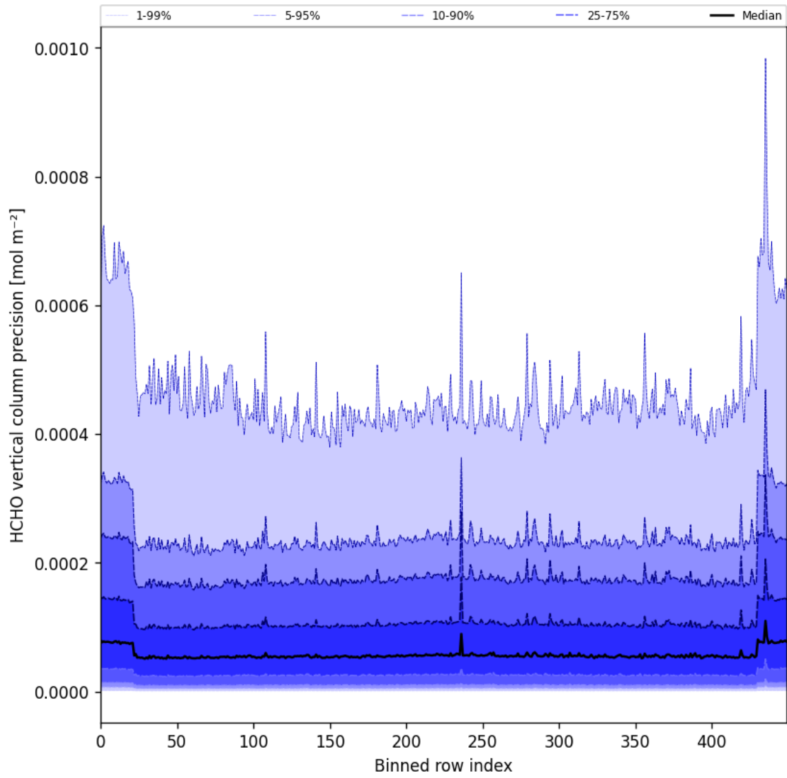
Figure 50: Along track statistics of “HCHO vertical column precision” for 2025-04-20 to 2025-04-22
