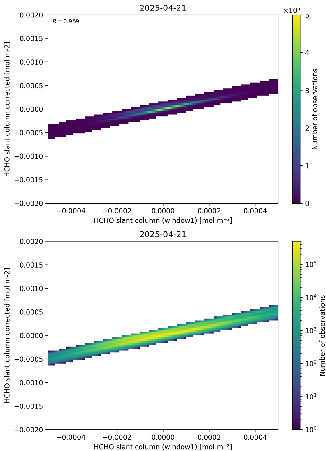
Figure 82: Scatter density plot of “HCHO slant column (window1)” against “HCHO slant column corrected” for 2025-04-20 to 2025-04-22.
