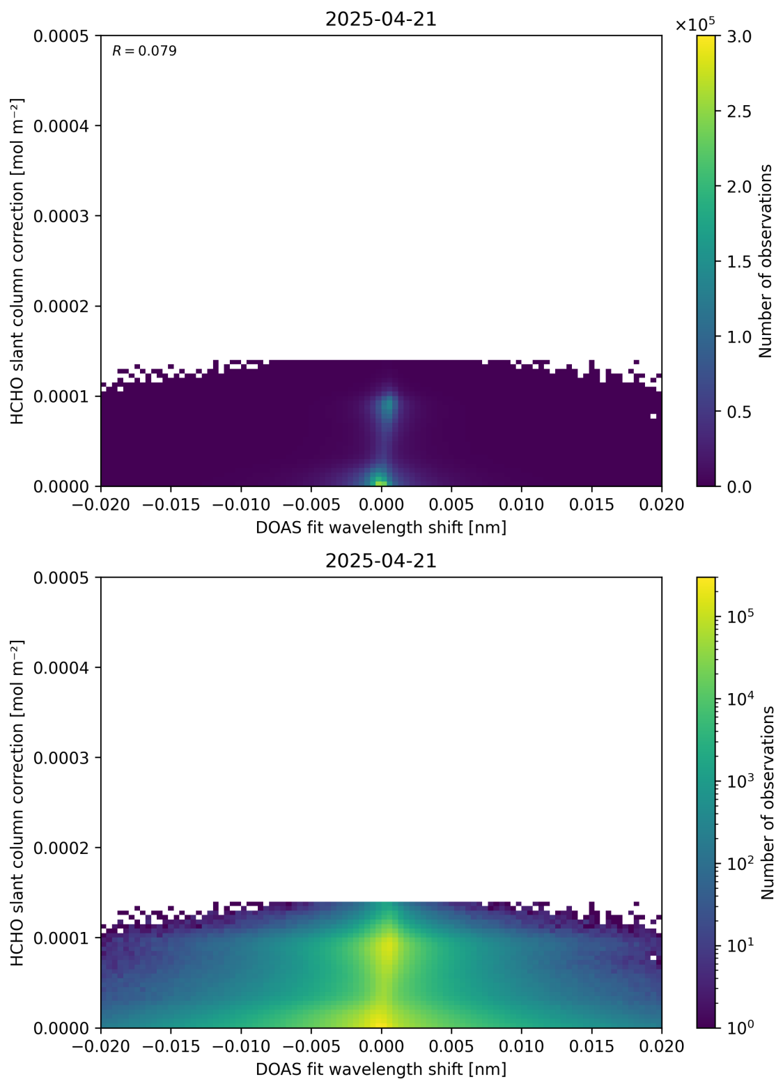
Figure 67: Scatter density plot of “DOAS fit wavelength shift” against “HCHO slant column correction” for 2025-04-20 to 2025-04-22.
