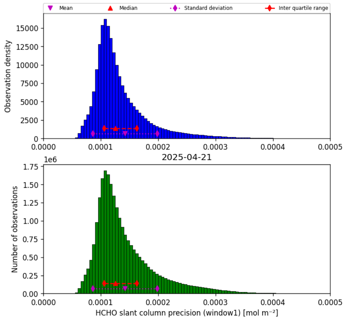
Figure 39: Histogram of “HCHO slant column precision (window1)” for 2025-04-20 to 2025-04-22
