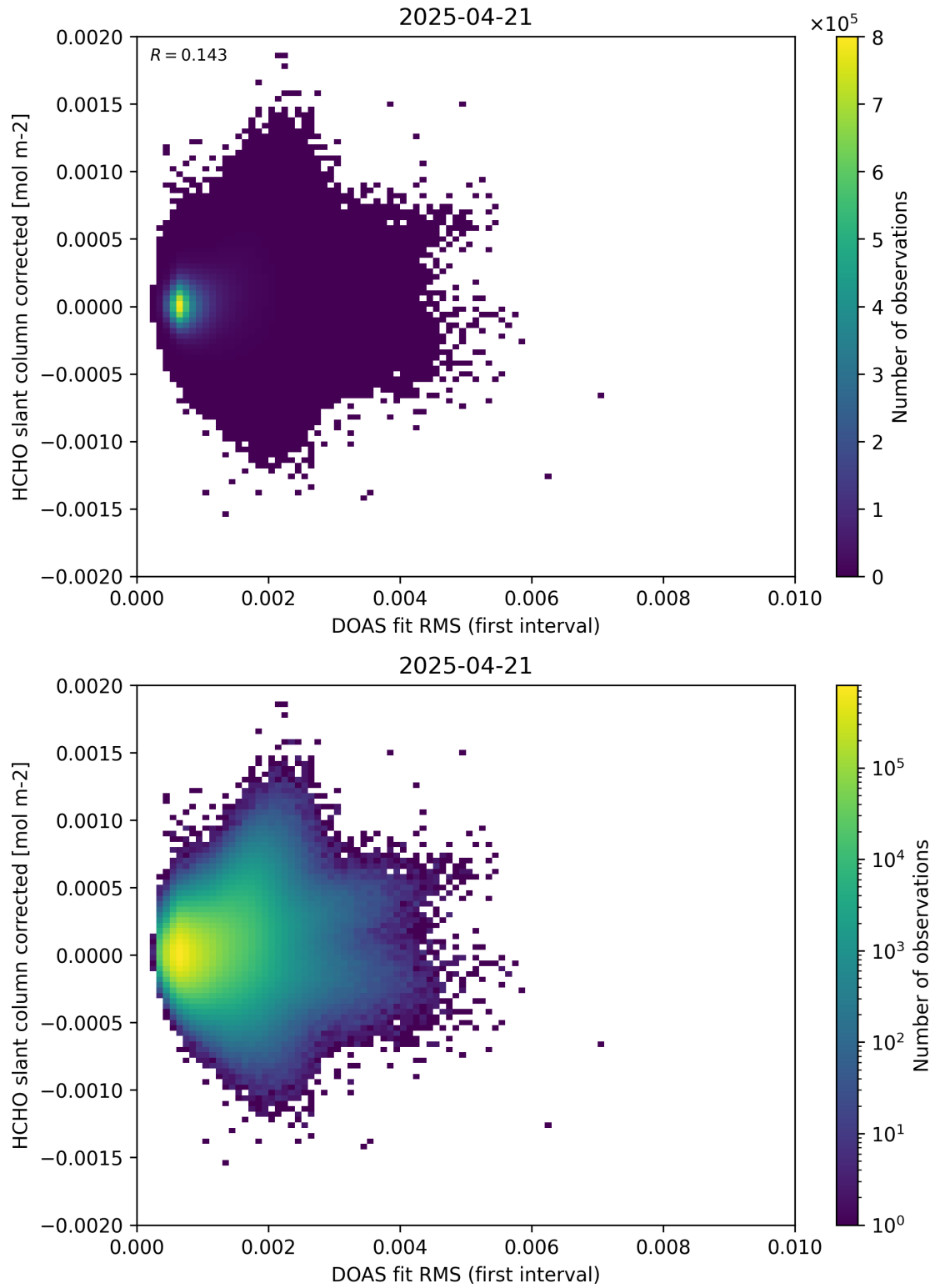
Figure 62: Scatter density plot of “DOAS fit RMS (first interval)” against “HCHO slant column corrected” for 2025-04-20 to 2025-04-22.
