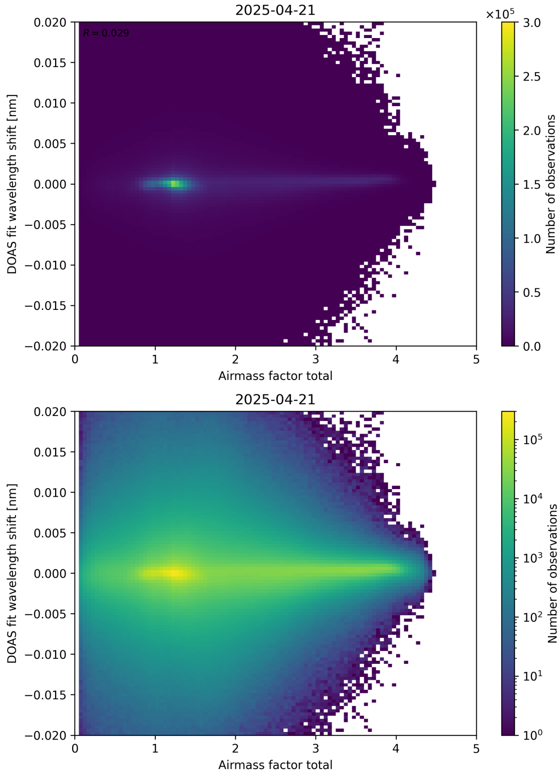
Figure 98: Scatter density plot of “Airmass factor total” against “DOAS fit wavelength shift” for 2025-04-20 to 2025-04-22.
