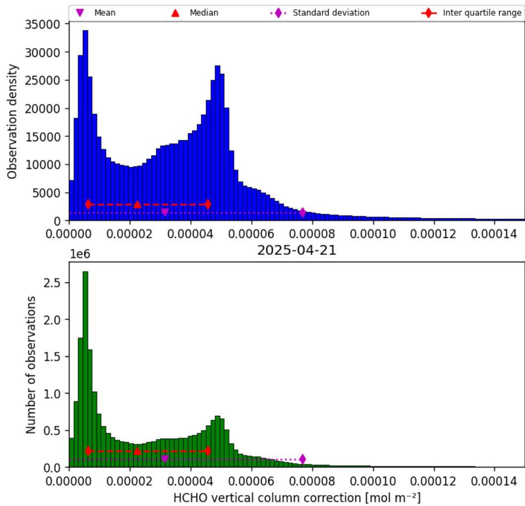
Figure 37: Histogram of “HCHO vertical column correction” for 2025-04-20 to 2025-04-22
