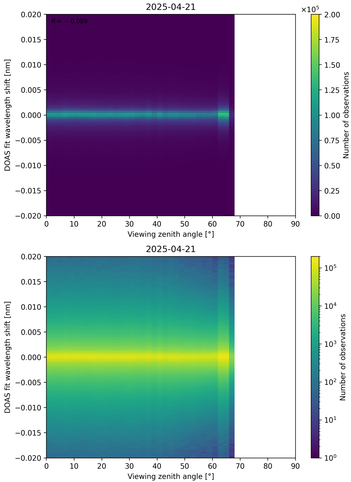
Figure 183: Scatter density plot of “Viewing zenith angle” against “DOAS fit wavelength shift” for 2025-04-20 to 2025-04-22.
