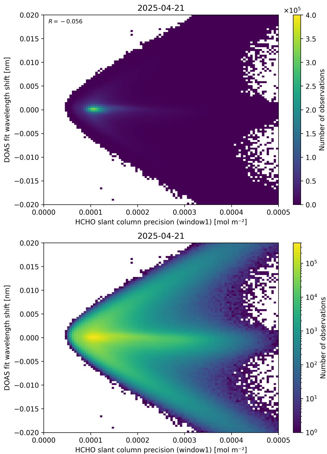
Figure 89: Scatter density plot of “HCHO slant column precision (window1)” against “DOAS fit wavelength shift” for 2025-04-20 to 2025-04-22.
