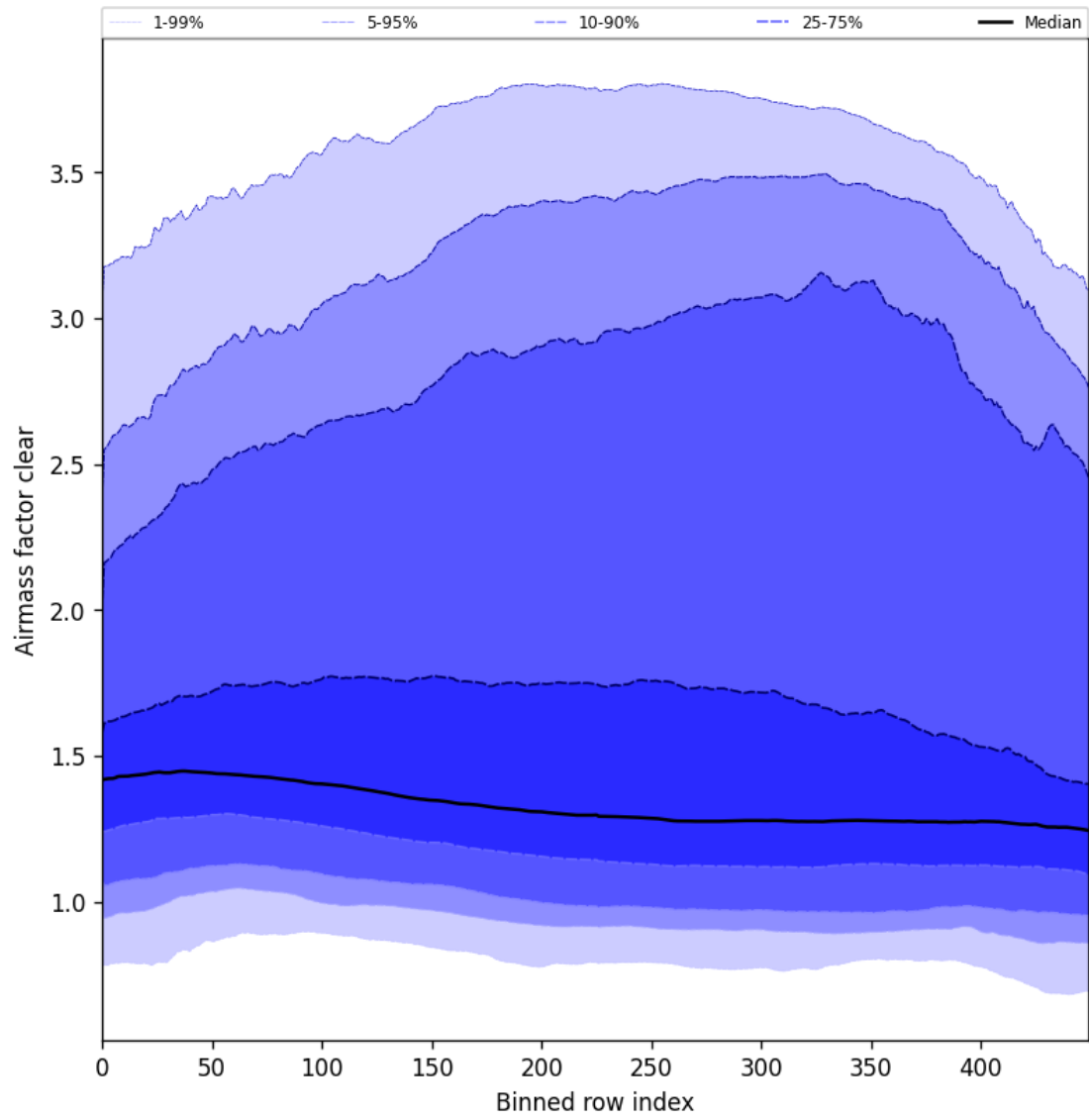
Figure 56: Along track statistics of “Airmass factor clear” for 2025-04-20 to 2025-04-22
