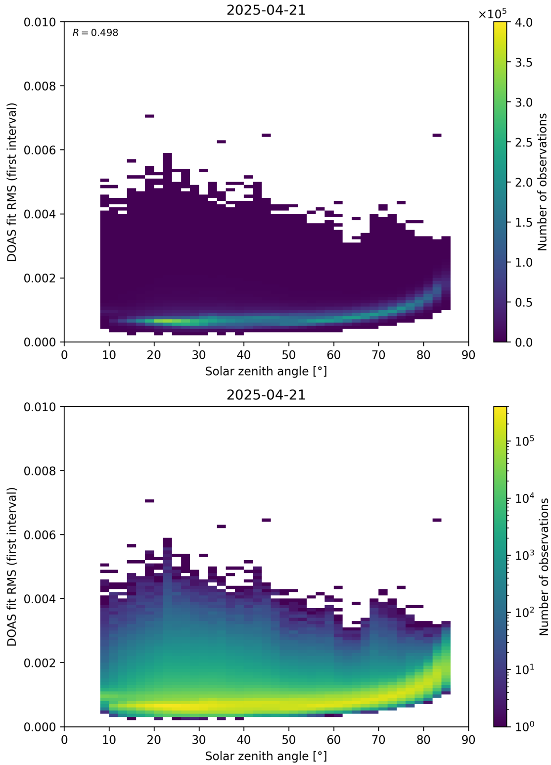
Figure 167: Scatter density plot of “Solar zenith angle” against “DOAS fit RMS (first interval)” for 2025-04-20 to 2025-04-22.
