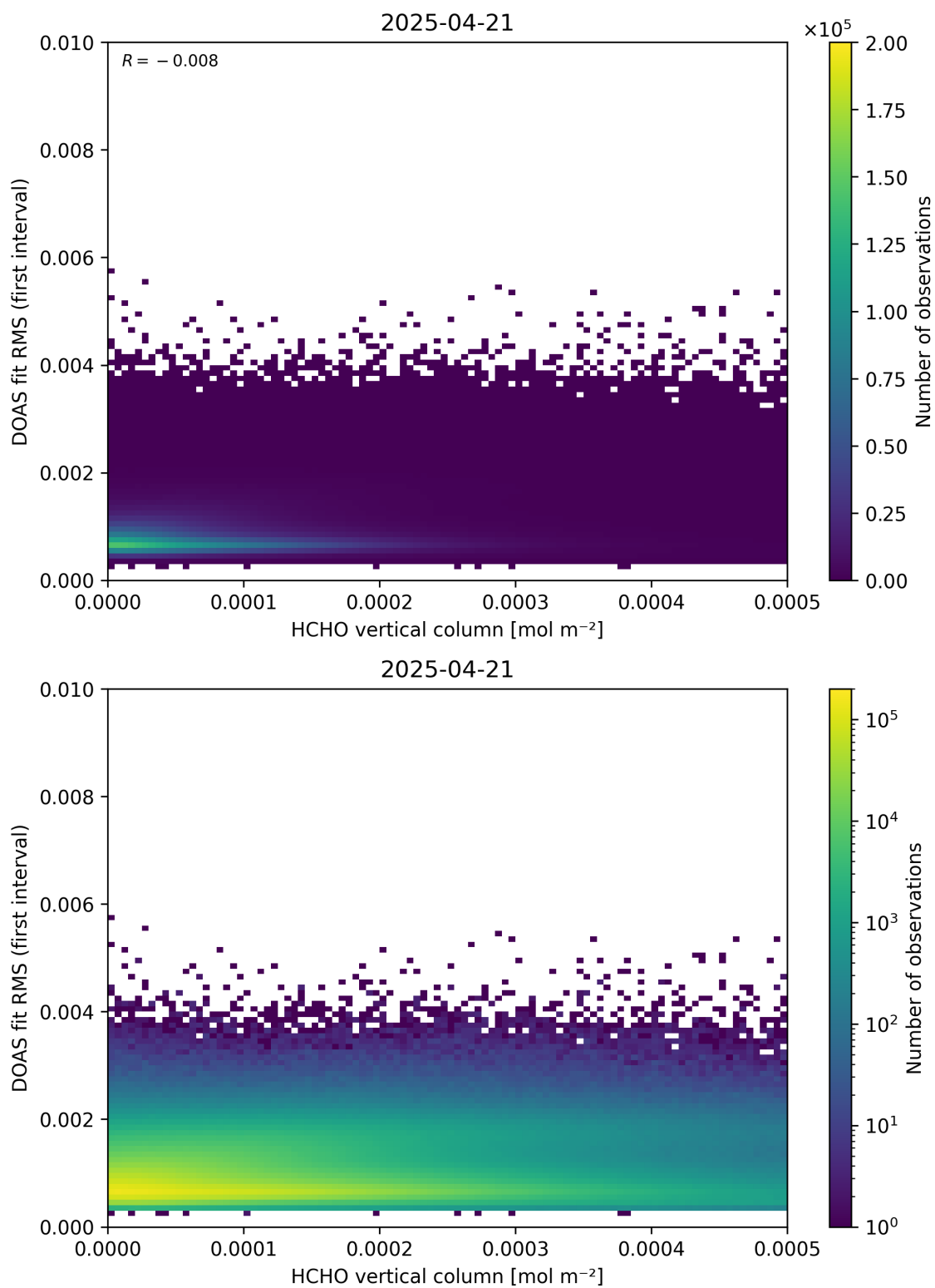
Figure 123: Scatter density plot of “HCHO vertical column” against “DOAS fit RMS (first interval)” for 2025-04-20 to 2025-04-22.
