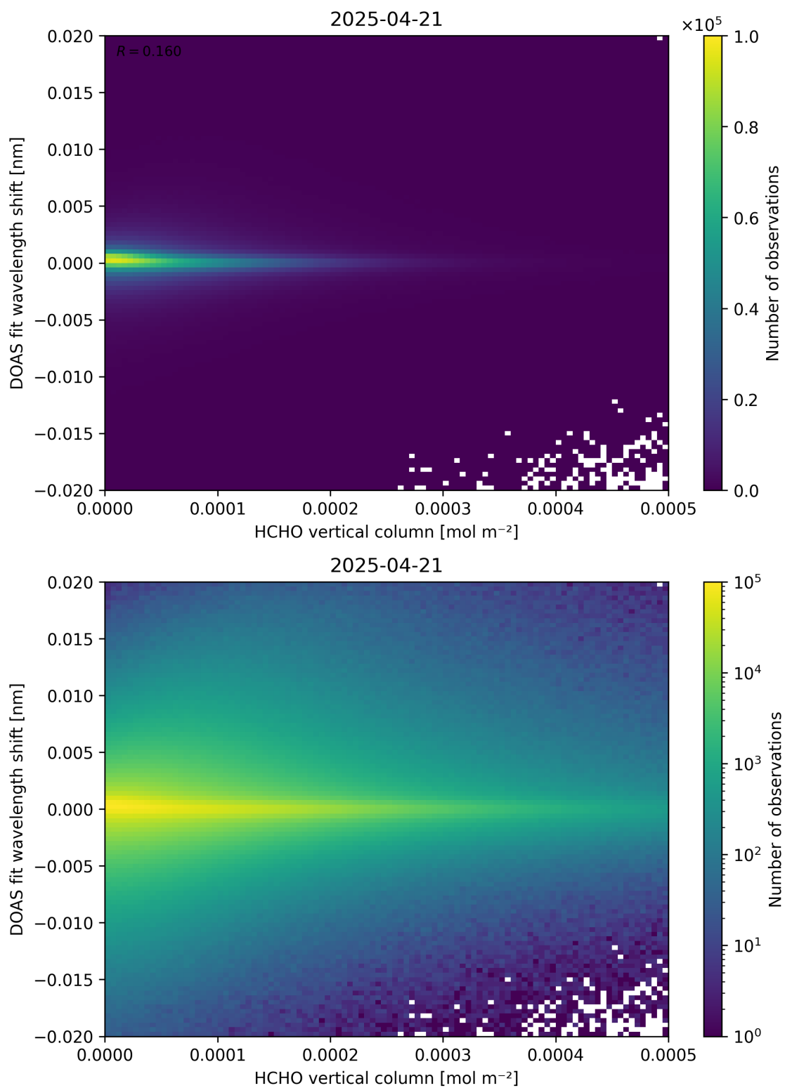
Figure 124: Scatter density plot of “HCHO vertical column” against “DOAS fit wavelength shift” for 2025-04-20 to 2025-04-22.
