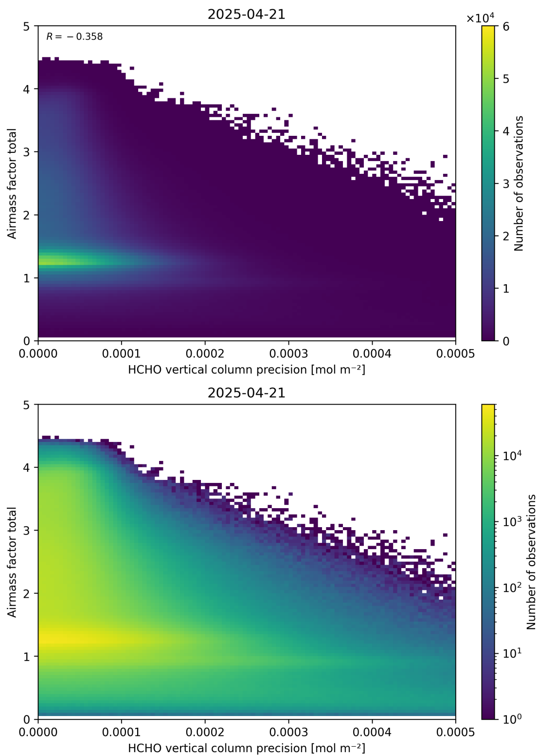
Figure 144: Scatter density plot of “HCHO vertical column precision” against “Airmass factor total” for 2025-04-20 to 2025-04-22.
