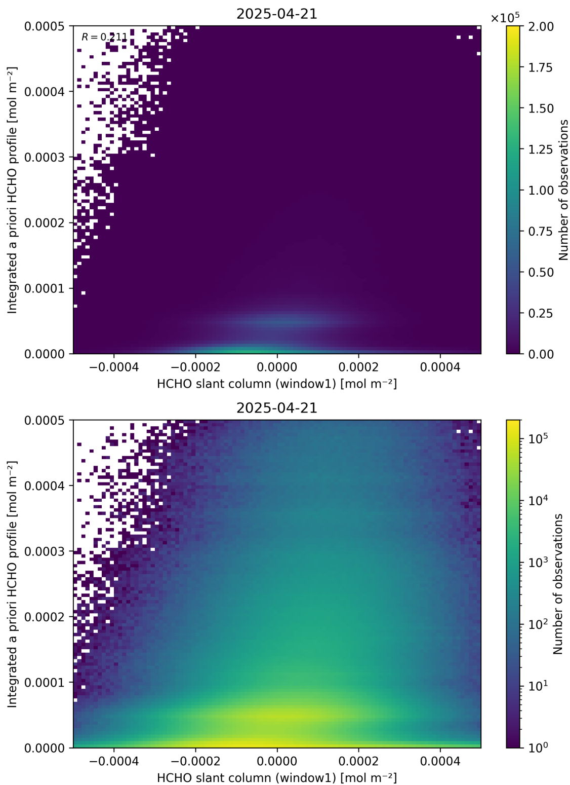
Figure 87: Scatter density plot of “HCHO slant column (window1)” against “Integrated a priori HCHO profile” for 2025-04-20 to 2025-04-22.
