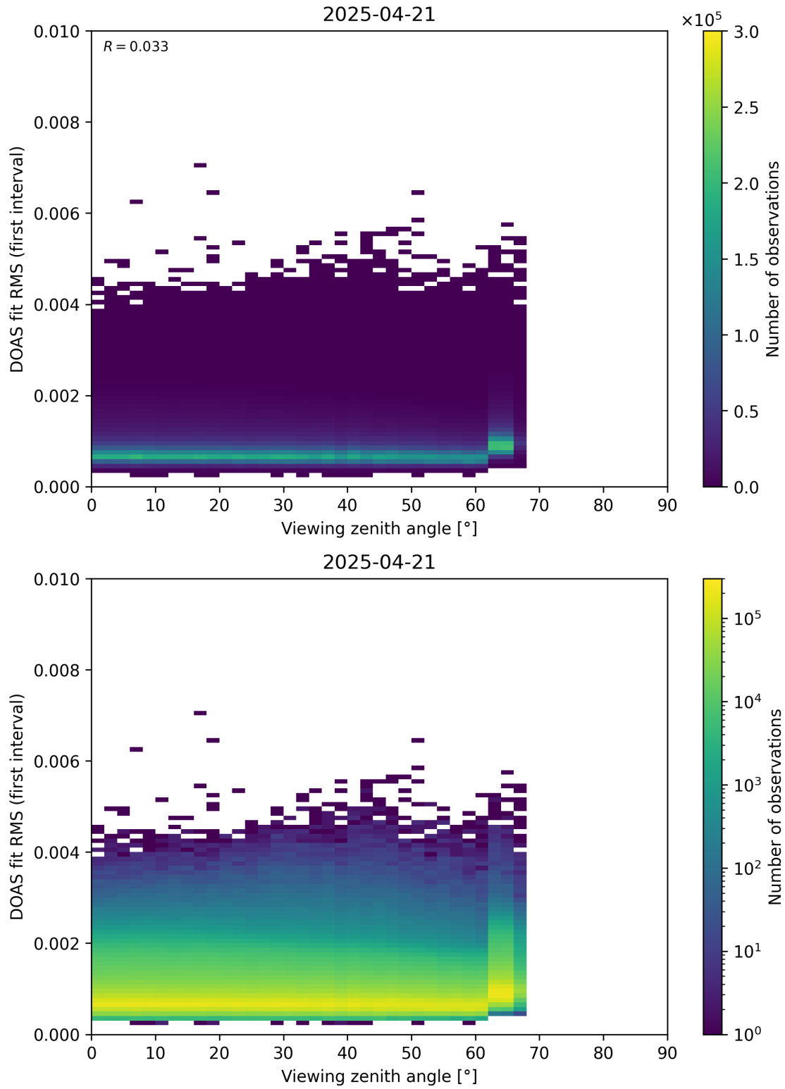
Figure 182: Scatter density plot of “Viewing zenith angle” against “DOAS fit RMS (first interval)” for 2025-04-20 to 2025-04-22.
