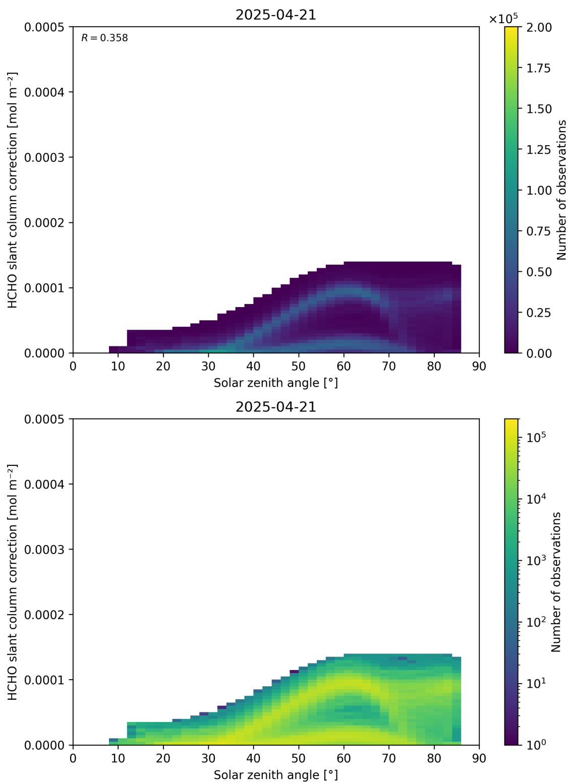
Figure 172: Scatter density plot of “Solar zenith angle” against “HCHO slant column correction” for 2025-04-20 to 2025-04-22.
