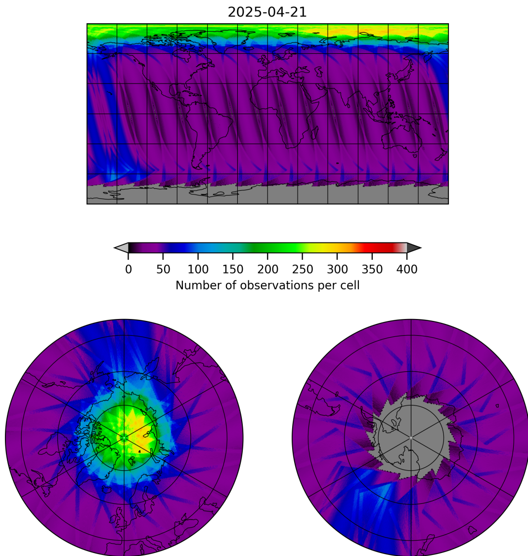
Figure 19: Map of the number of observations for 2025-04-20 to 2025-04-22
