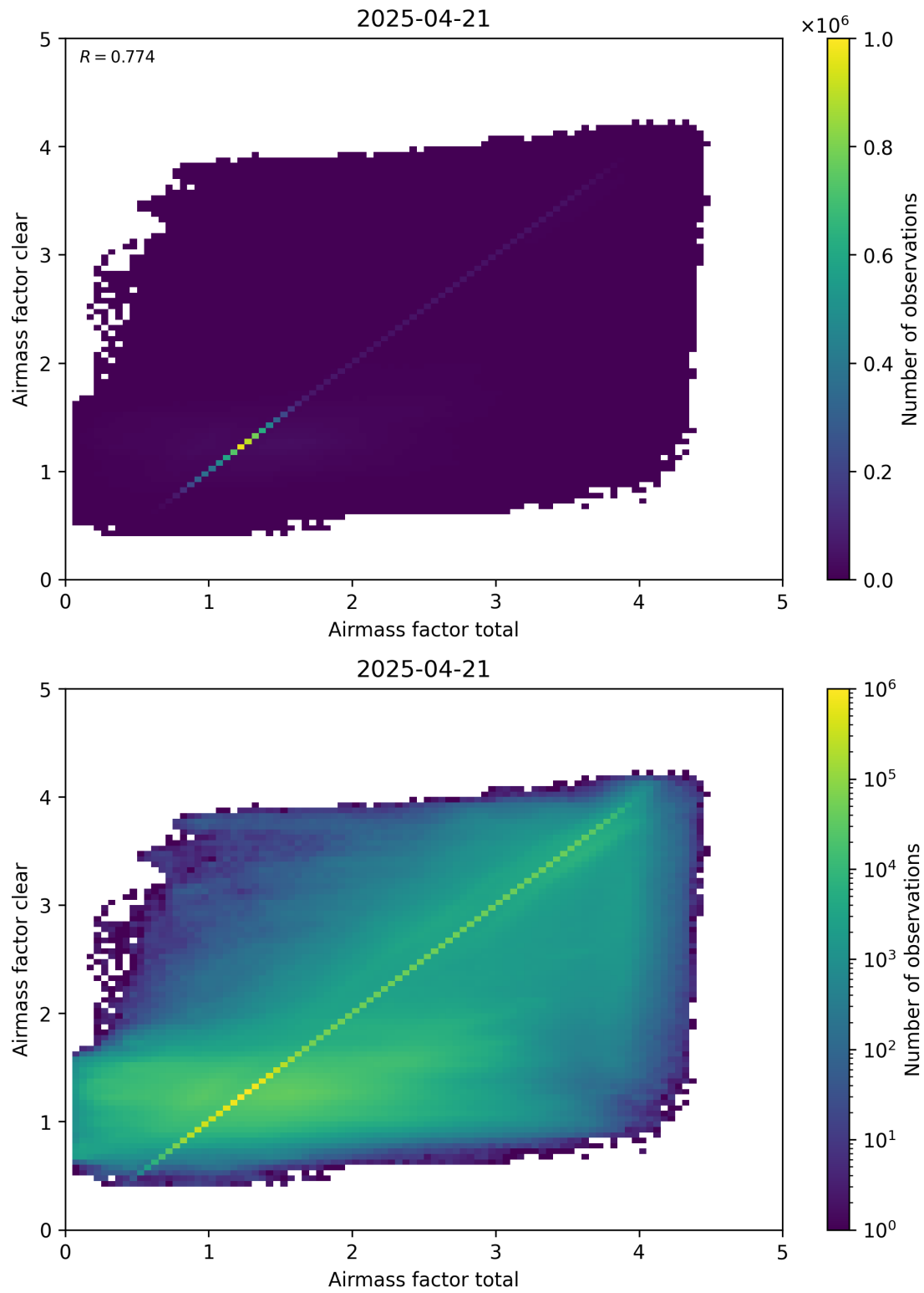
Figure 100: Scatter density plot of “Airmass factor total” against “Airmass factor clear” for 2025-04-20 to 2025-04-22.
