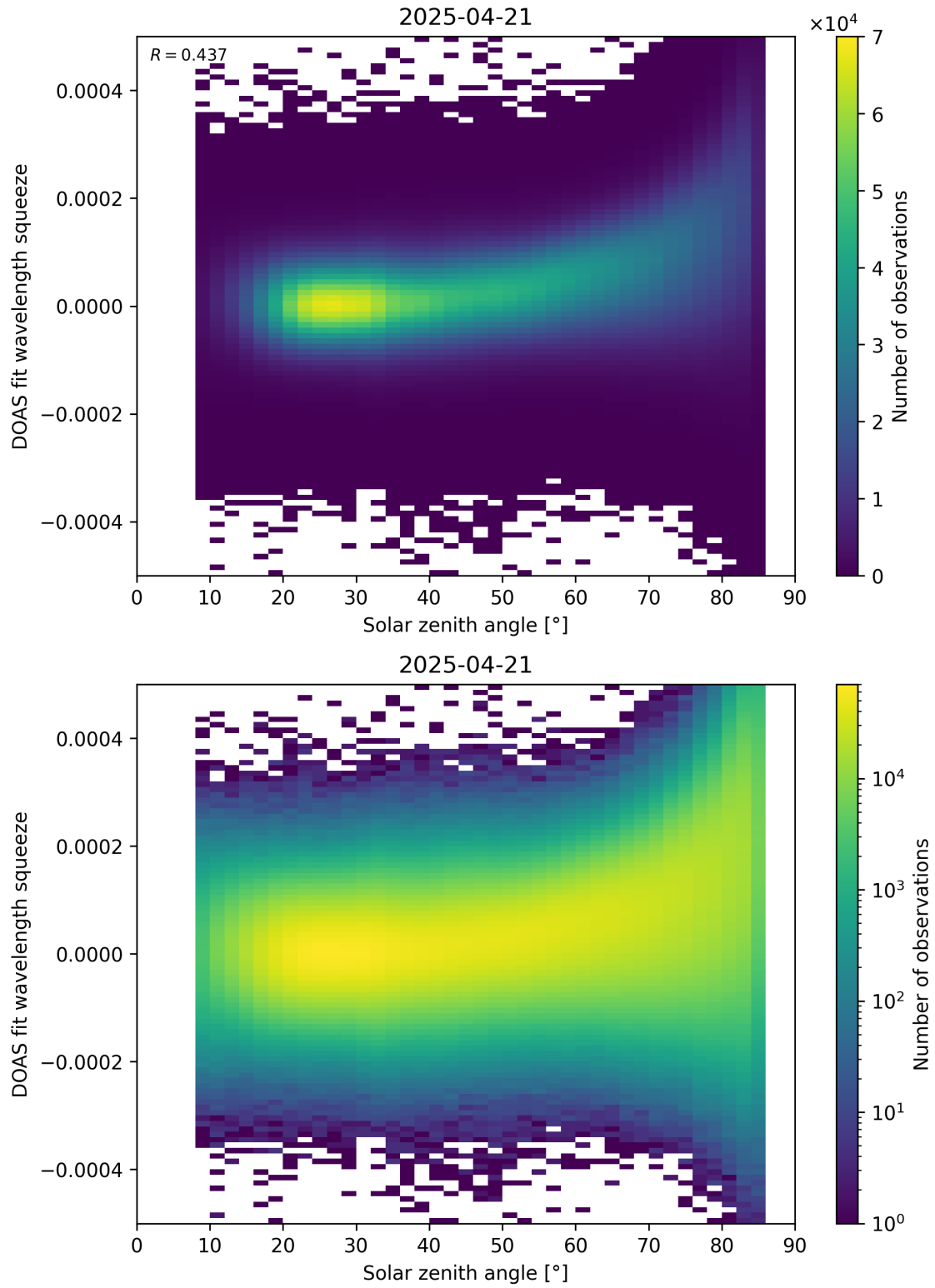
Figure 169: Scatter density plot of “Solar zenith angle” against “DOAS fit wavelength squeeze” for 2025-04-20 to 2025-04-22.
