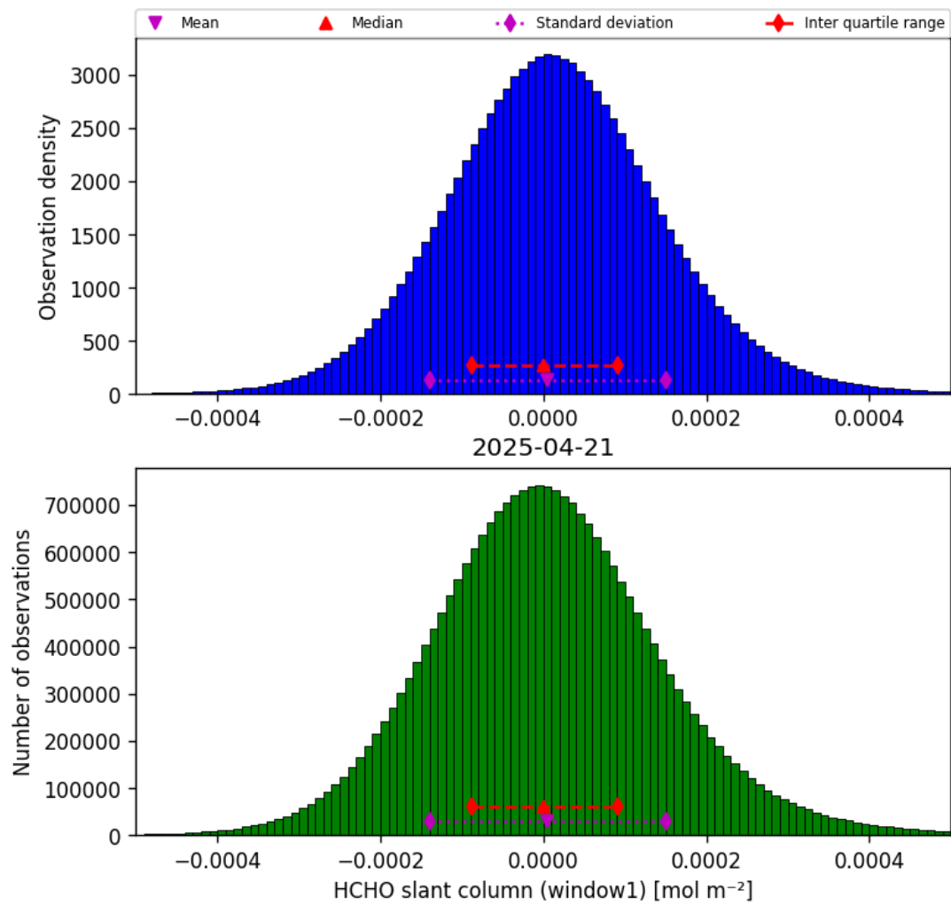
Figure 38: Histogram of “HCHO slant column (window1)” for 2025-04-20 to 2025-04-22
