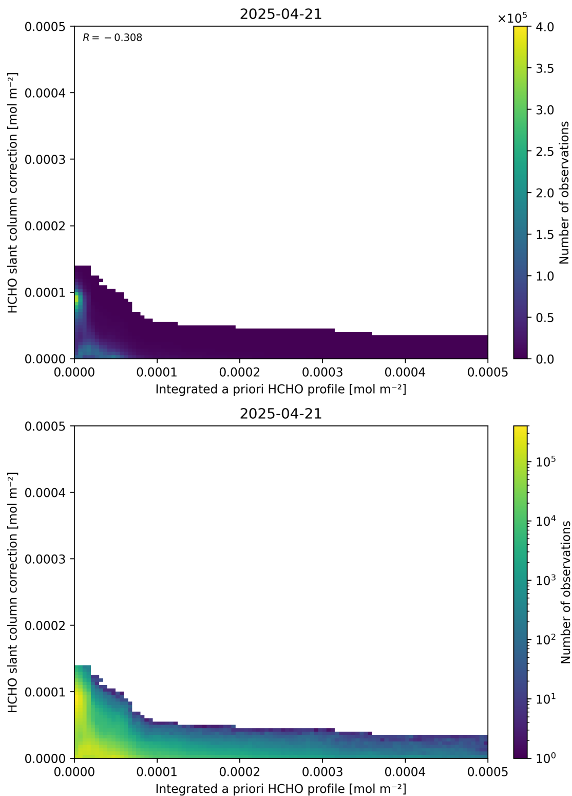
Figure 152: Scatter density plot of “Integrated a priori HCHO profile” against “HCHO slant column correction” for 2025-04-20 to 2025-04-22.
