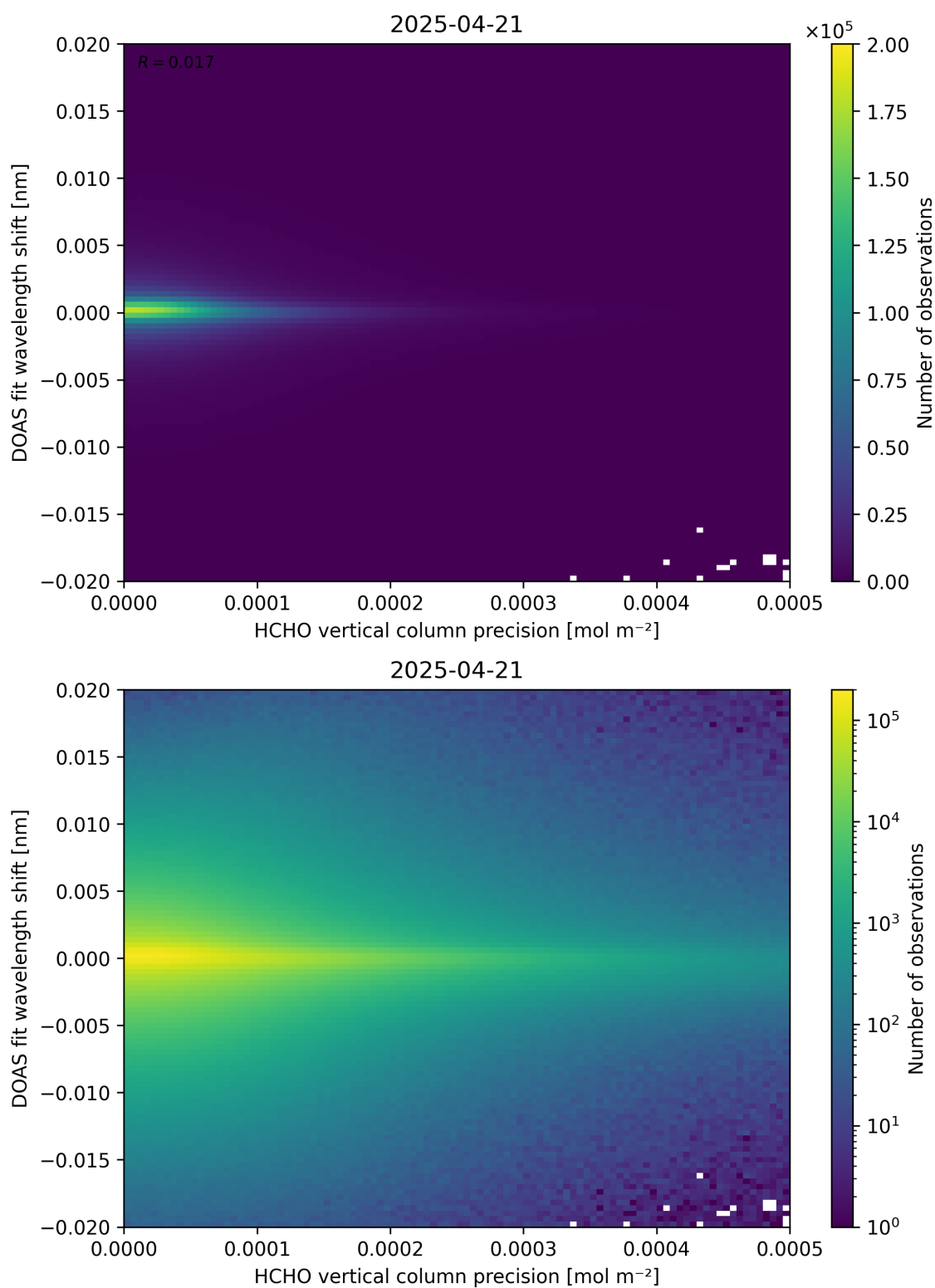
Figure 137: Scatter density plot of “HCHO vertical column precision” against “DOAS fit wavelength shift” for 2025-04-20 to 2025-04-22.
