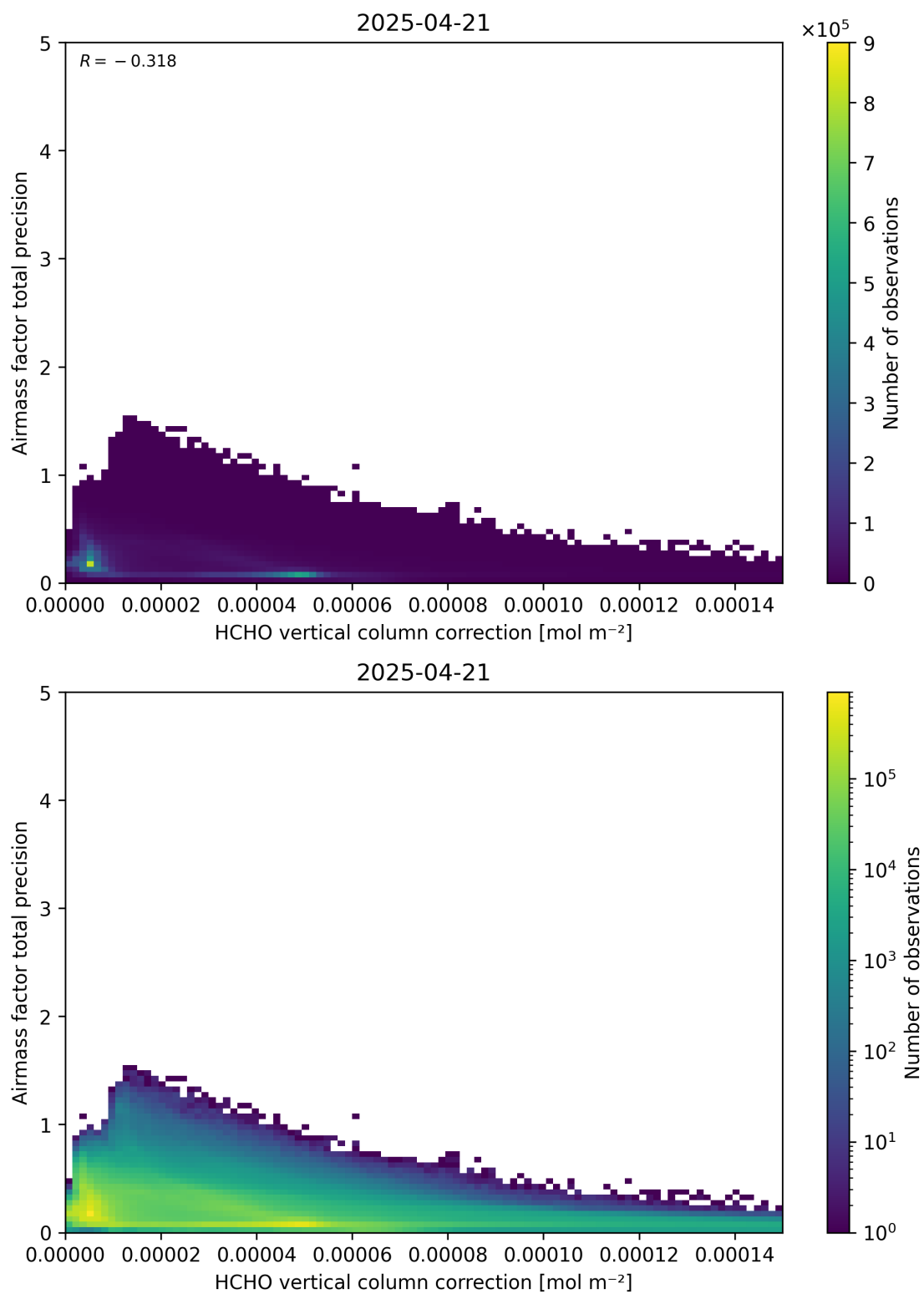
Figure 121: Scatter density plot of “HCHO vertical column correction” against “Airmass factor total precision” for 2025-04-20 to 2025-04-22.
