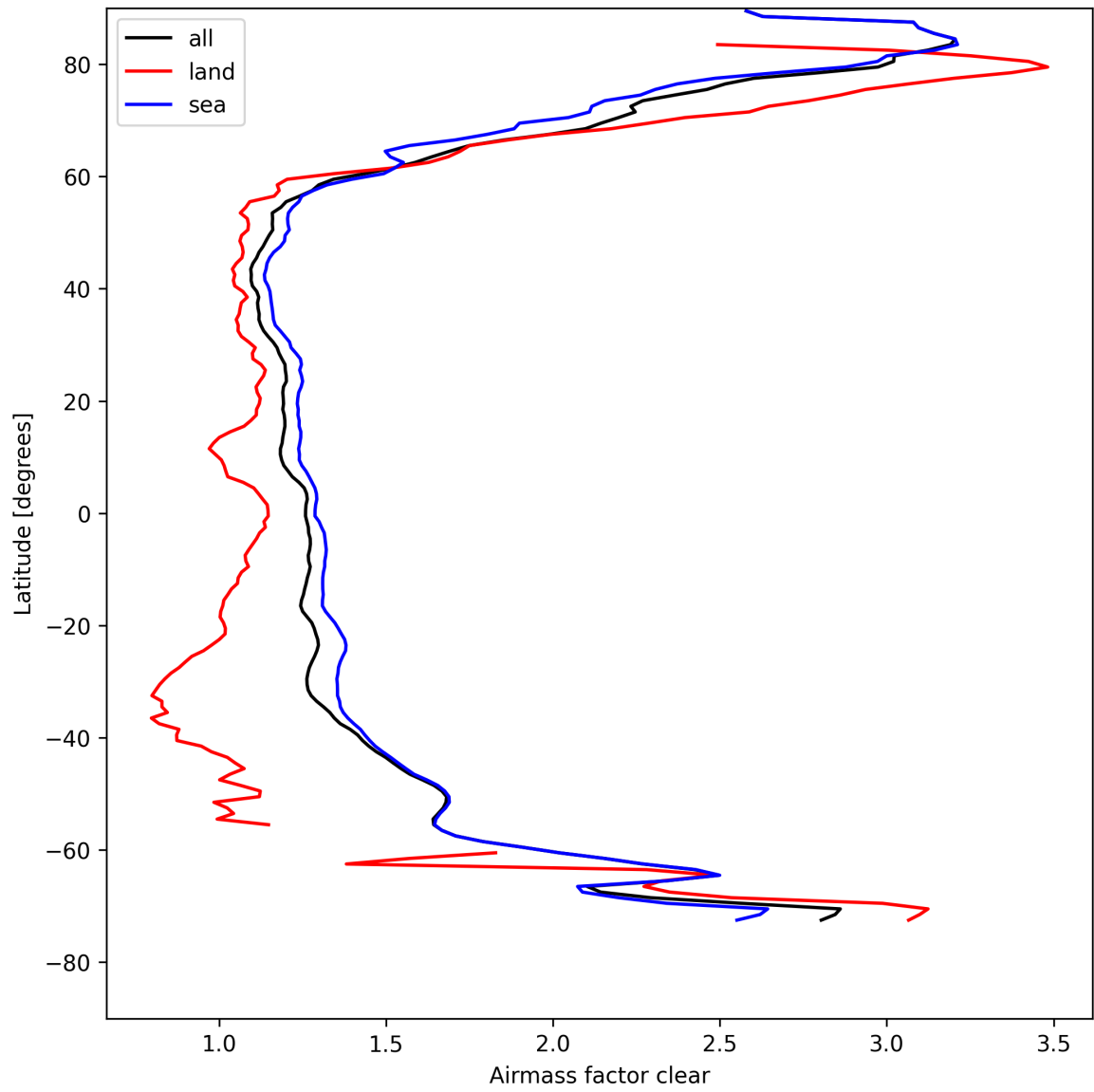
Figure 28: Zonal average of “Airmass factor clear” for 2025-04-20 to 2025-04-22.
