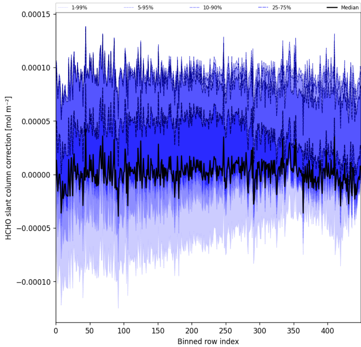
Figure 61: Along track statistics of “HCHO slant column correction” for 2025-04-20 to 2025-04-22
