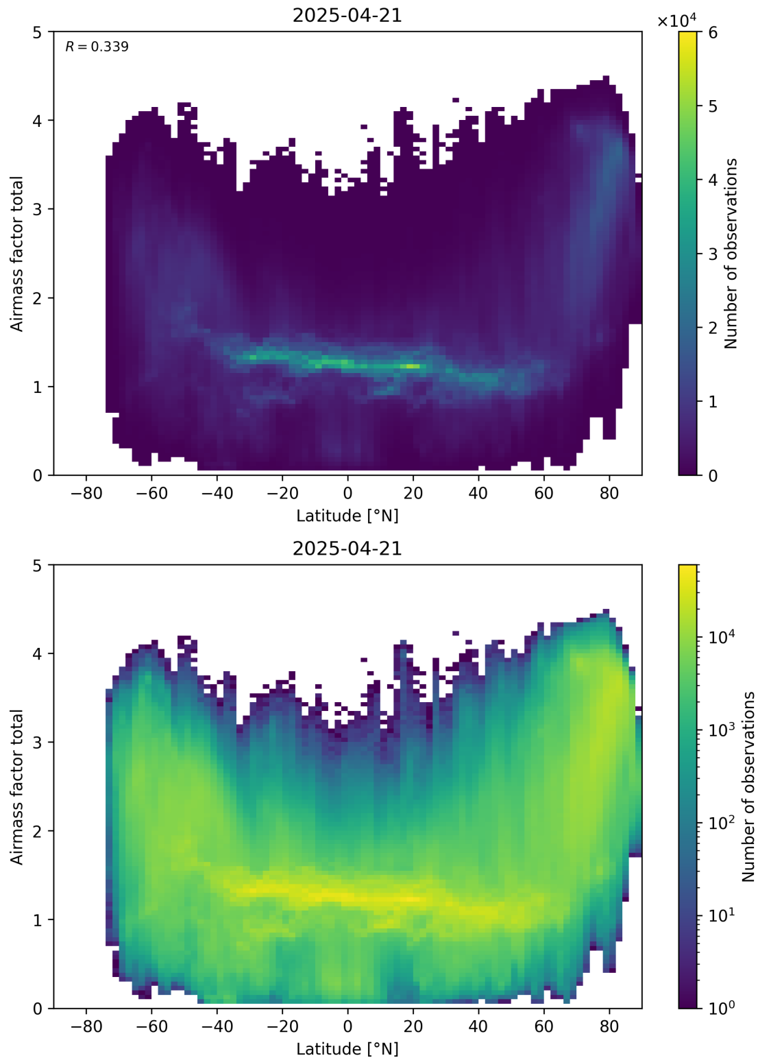
Figure 161: Scatter density plot of “Latitude” against “Airmass factor total” for 2025-04-20 to 2025-04-22.
