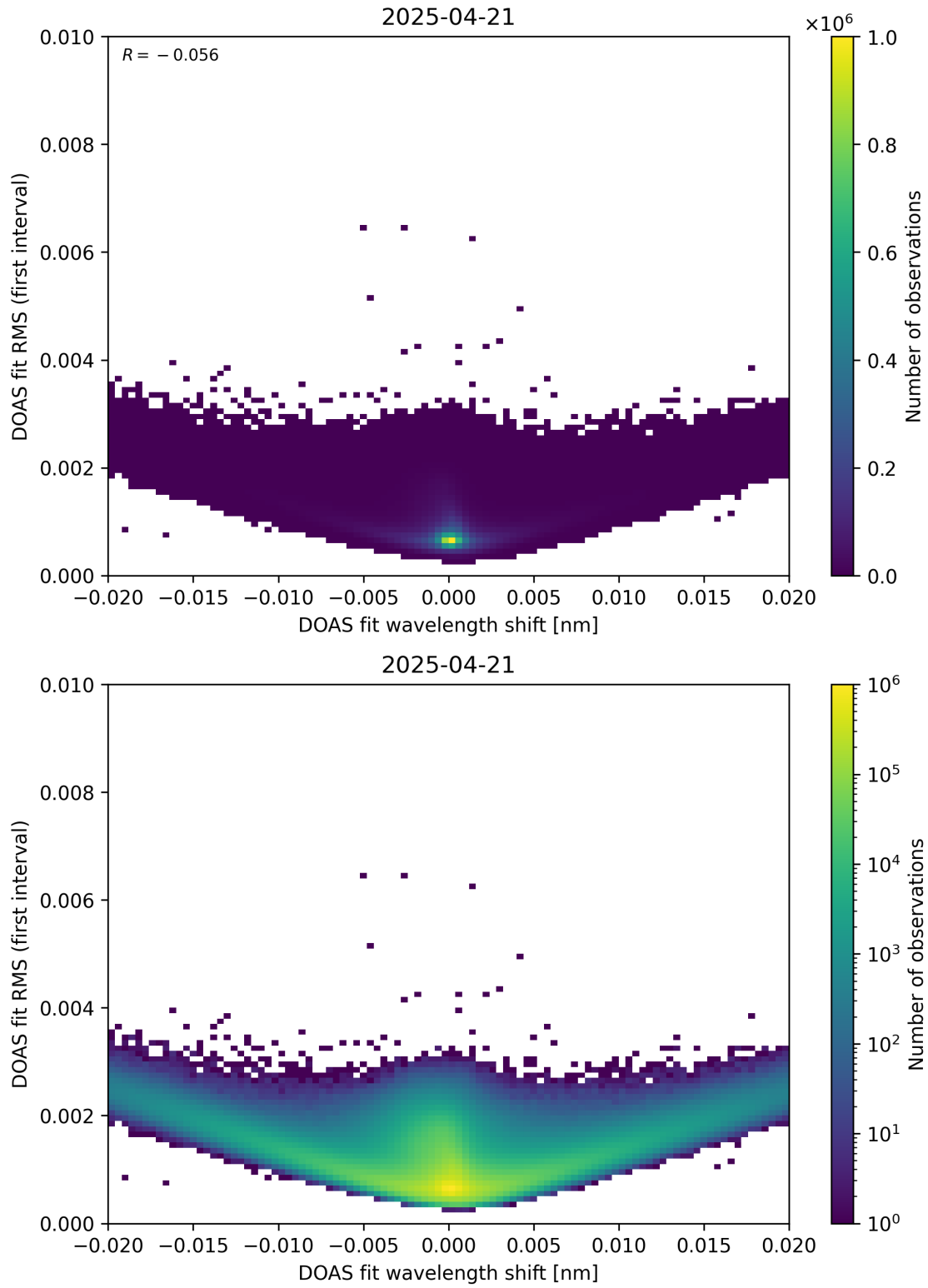
Figure 64: Scatter density plot of “DOAS fit wavelength shift” against “DOAS fit RMS (first interval)” for 2025-04-20 to 2025-04-22.
