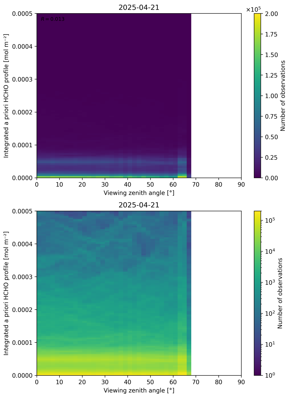
Figure 195: Scatter density plot of “Viewing zenith angle” against “Integrated a priori HCHO profile” for 2025-04-20 to 2025-04-22.
