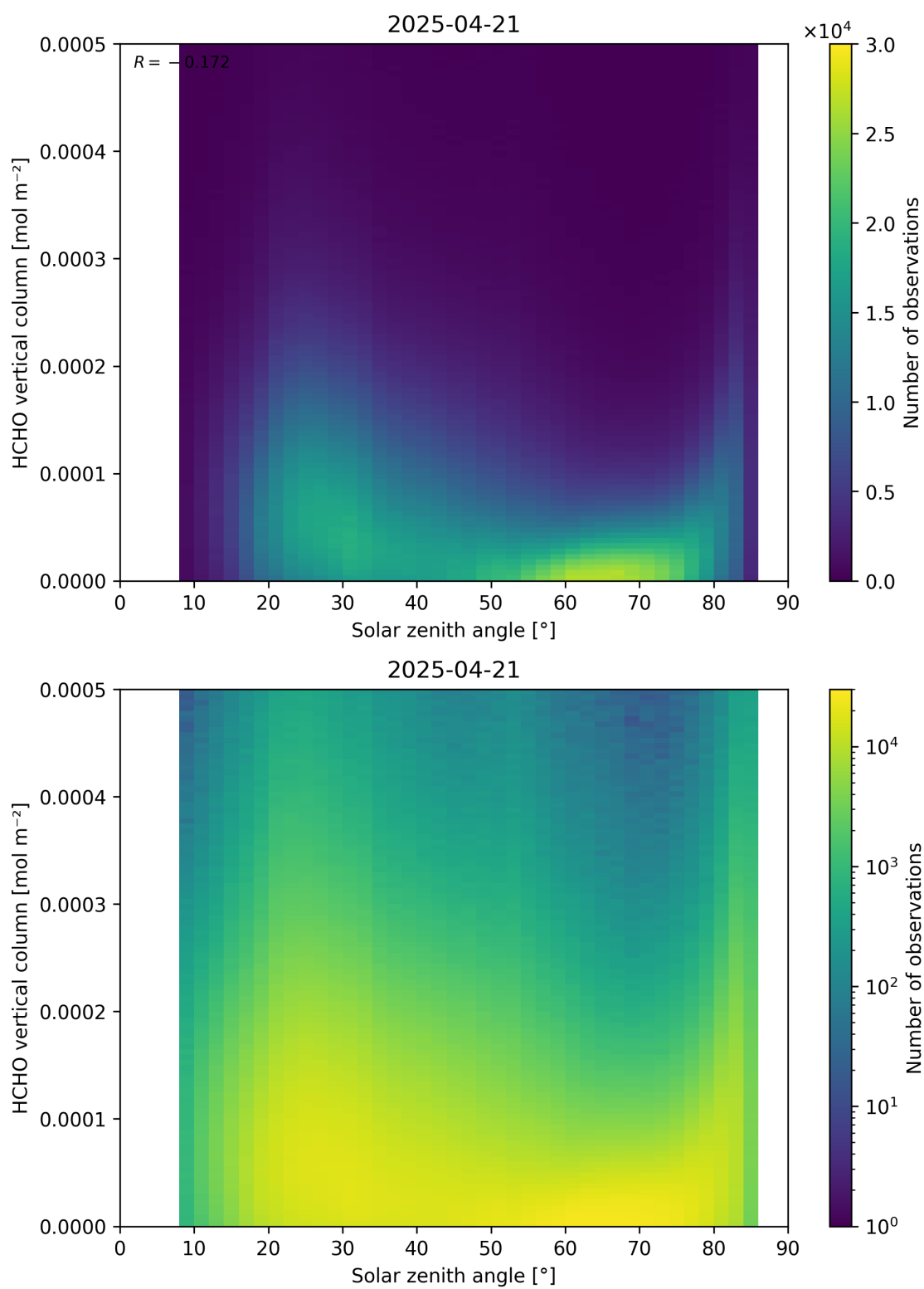
Figure 177: Scatter density plot of “Solar zenith angle” against “HCHO vertical column” for 2025-04-20 to 2025-04-22.
