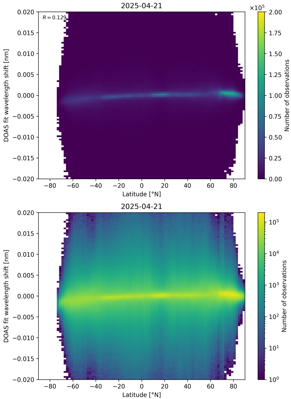
Figure 154: Scatter density plot of “Latitude” against “DOAS fit wavelength shift” for 2025-04-20 to 2025-04-22.
