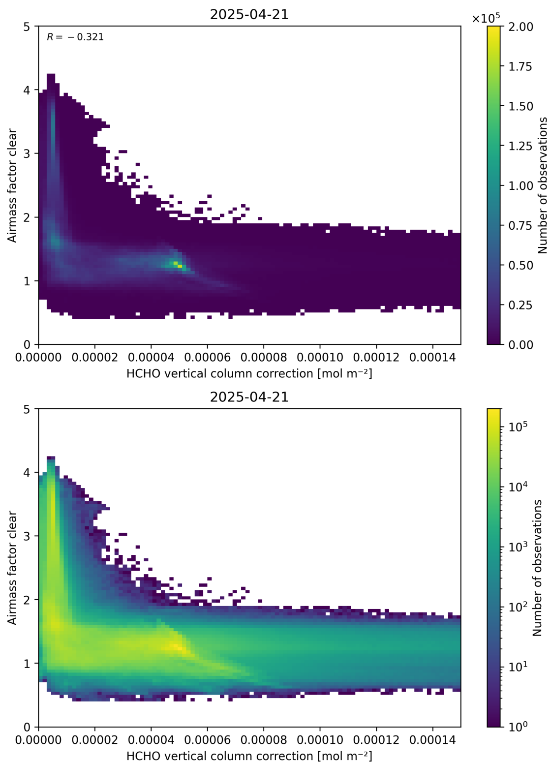
Figure 115: Scatter density plot of “HCHO vertical column correction” against “Airmass factor clear” for 2025-04-20 to 2025-04-22.
