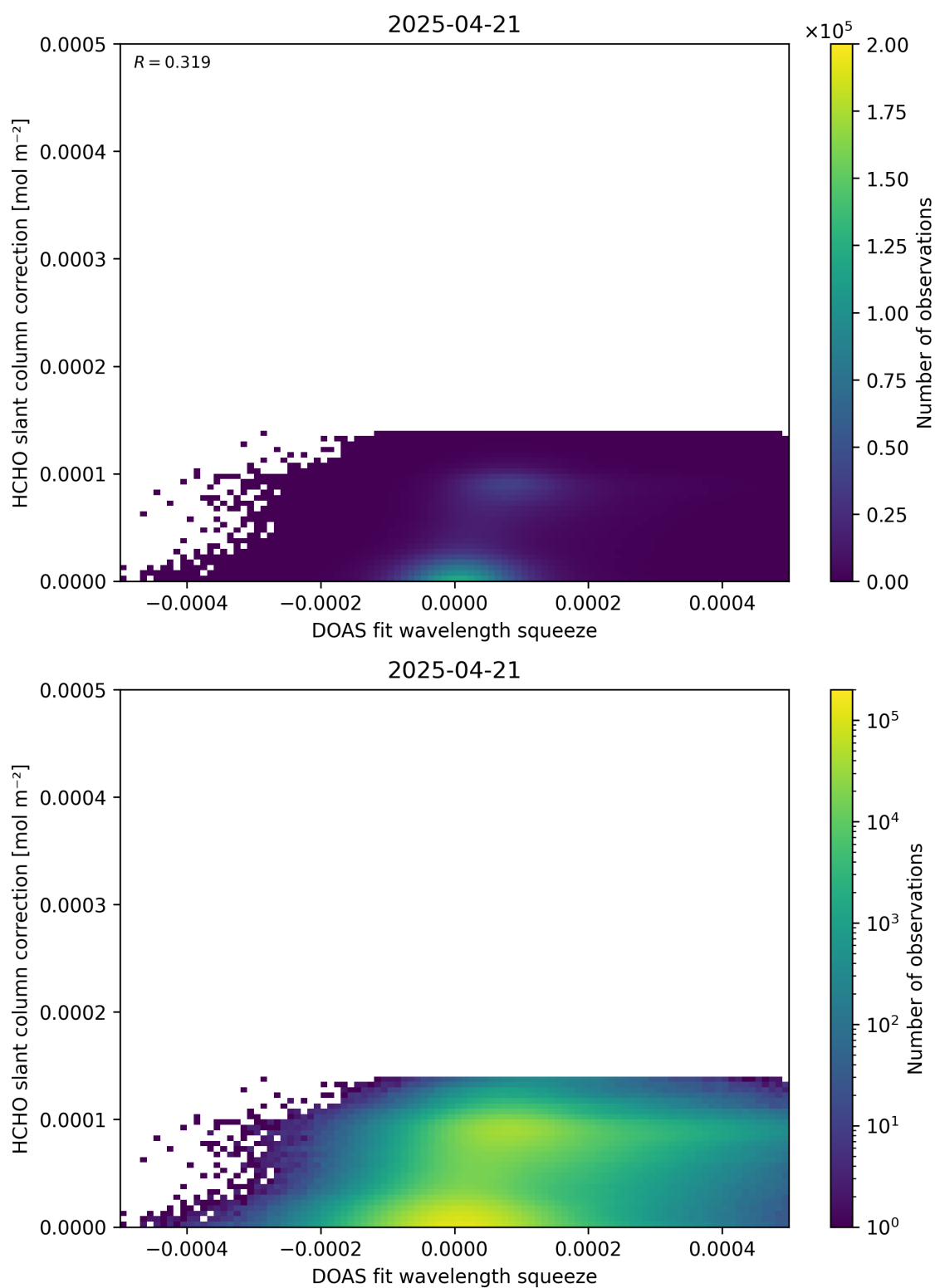
Figure 70: Scatter density plot of “DOAS fit wavelength squeeze” against “HCHO slant column correction” for 2025-04-20 to 2025-04-22.
