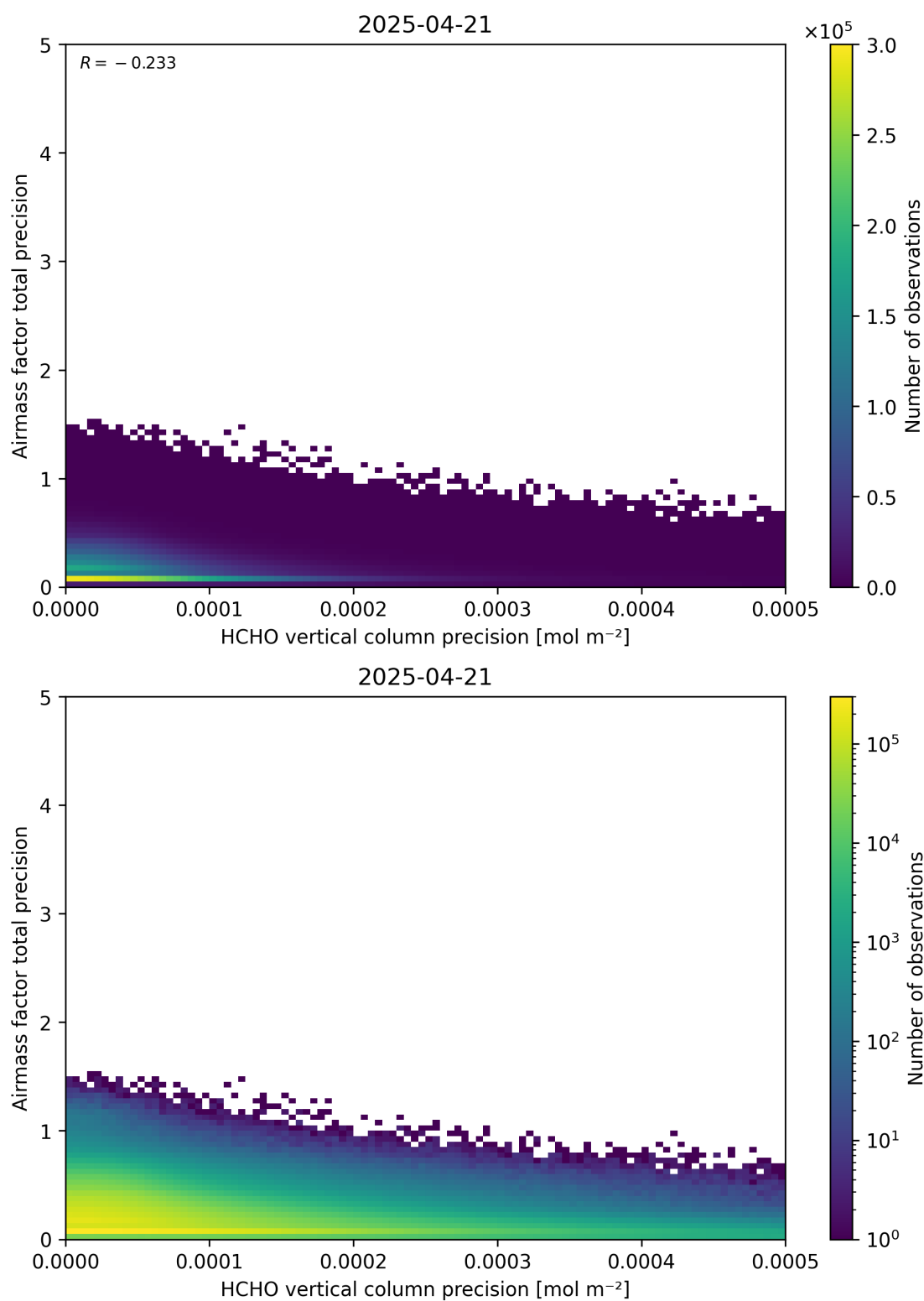
Figure 145: Scatter density plot of “HCHO vertical column precision” against “Airmass factor total precision” for 2025-04-20 to 2025-04-22.
