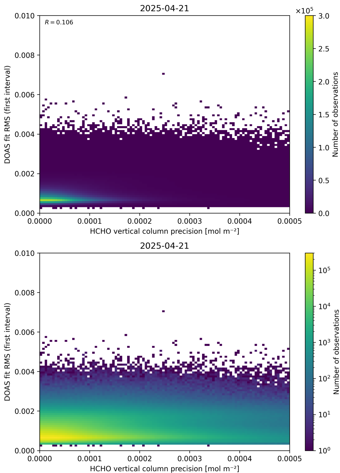
Figure 136: Scatter density plot of “HCHO vertical column precision” against “DOAS fit RMS (first interval)” for 2025-04-20 to 2025-04-22.
