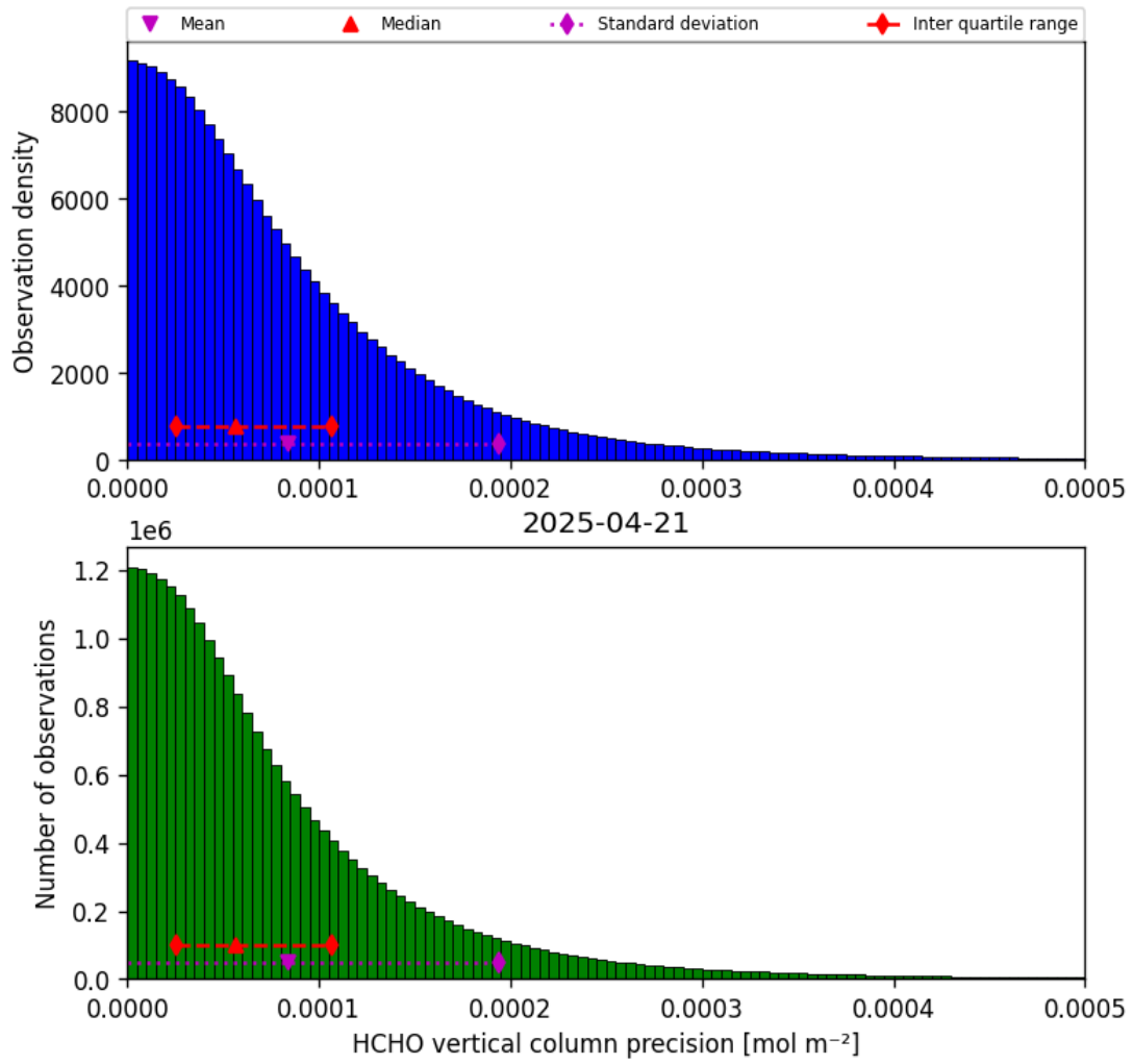
Figure 36: Histogram of “HCHO vertical column precision” for 2025-04-20 to 2025-04-22
