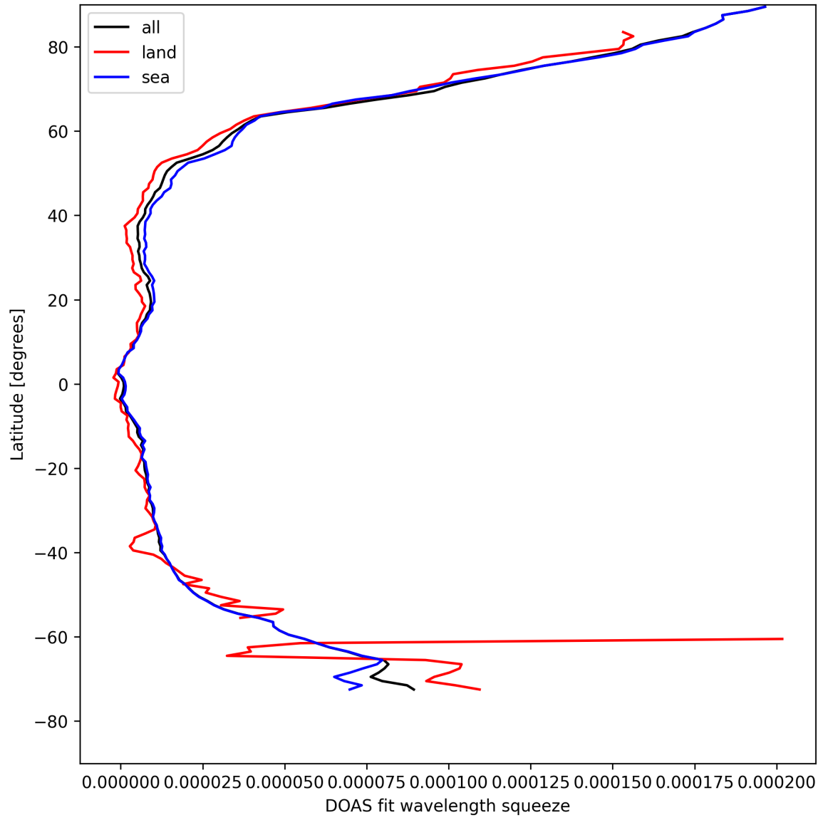
Figure 31: Zonal average of “DOAS fit wavelength squeeze” for 2025-04-20 to 2025-04-22.
