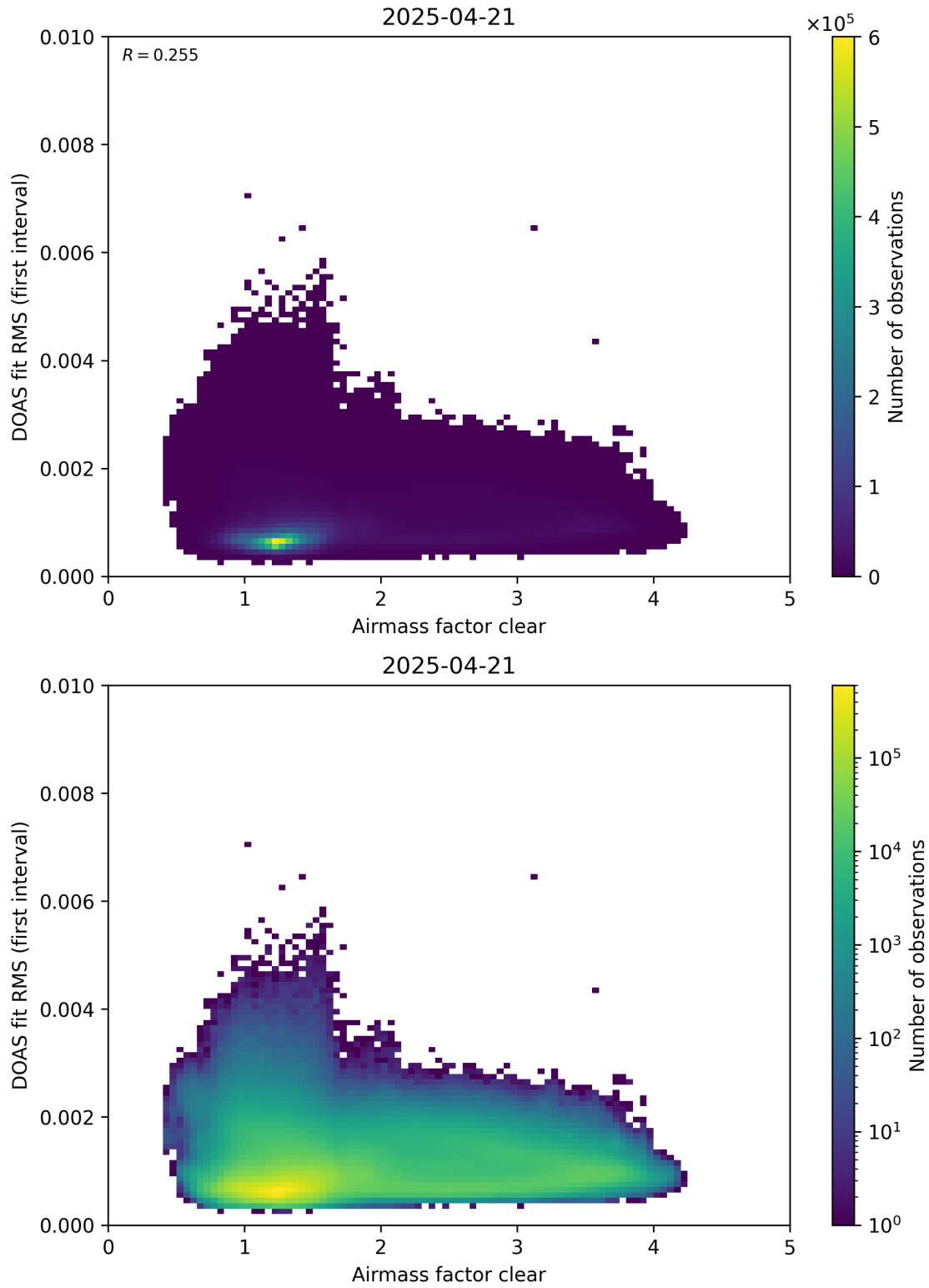
Figure 71: Scatter density plot of “Airmass factor clear” against “DOAS fit RMS (first interval)” for 2025-04-20 to 2025-04-22.
