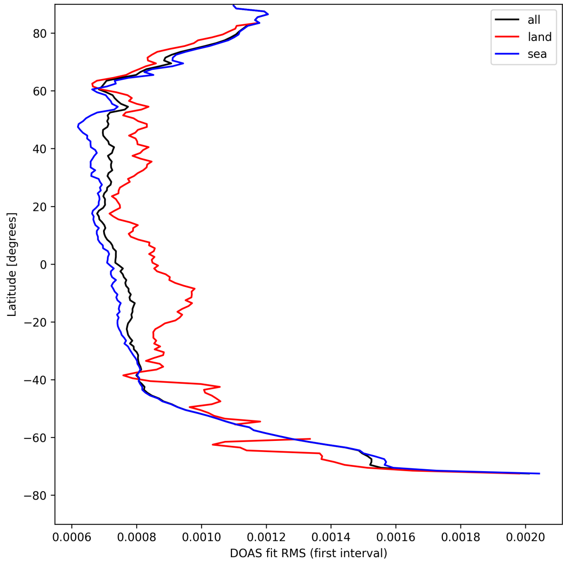
Figure 32: Zonal average of “DOAS fit RMS (first interval)” for 2025-04-20 to 2025-04-22.
