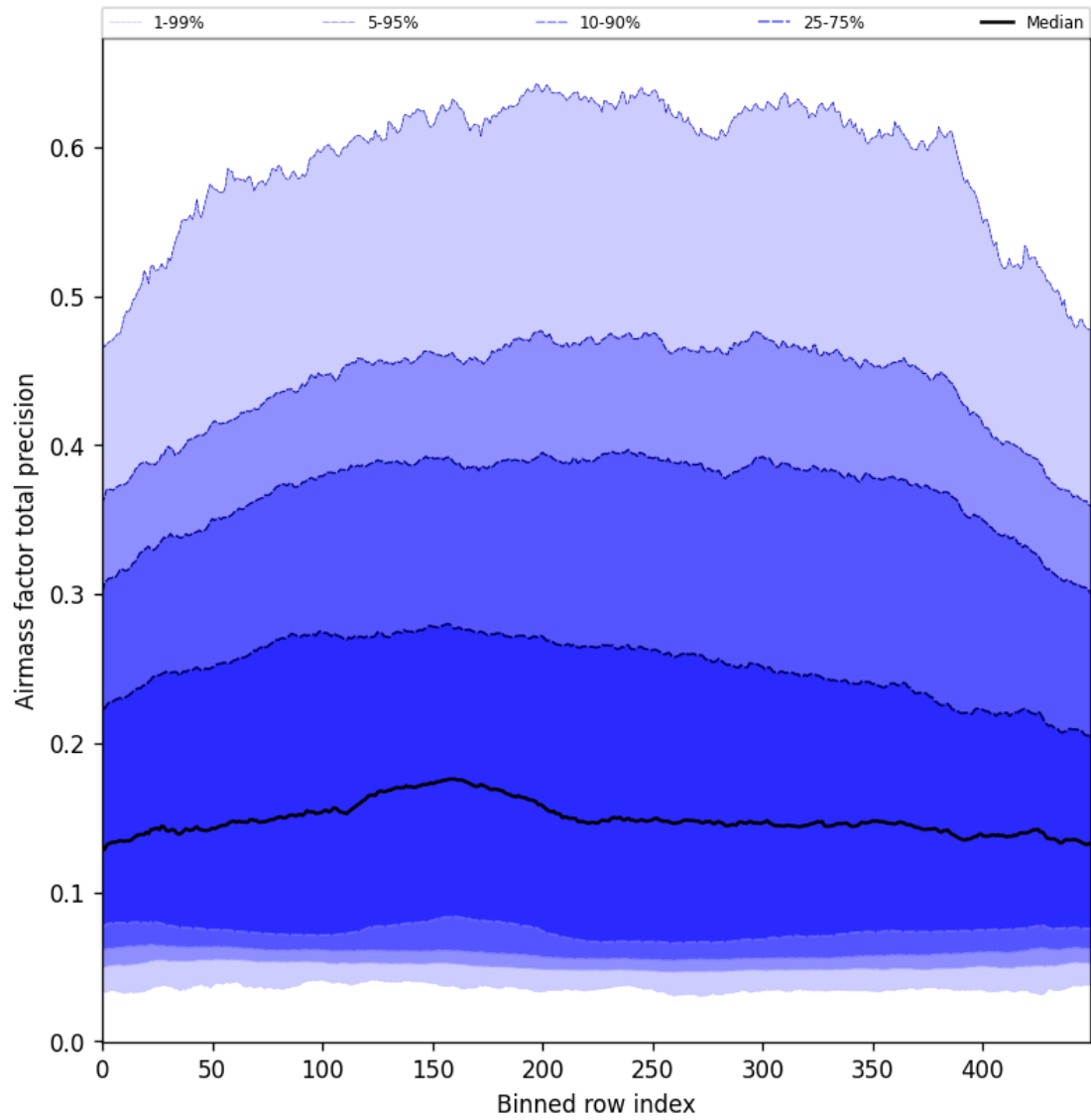
Figure 55: Along track statistics of “Airmass factor total precision” for 2025-04-20 to 2025-04-22
