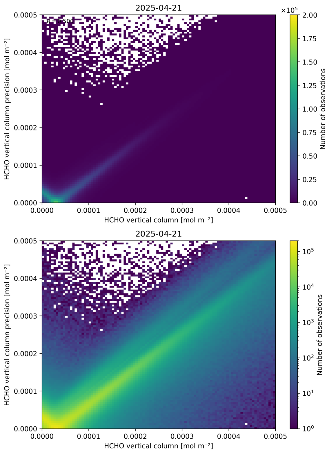
Figure 134: Scatter density plot of “HCHO vertical column” against “HCHO vertical column precision” for 2025-04-20 to 2025-04-22.
