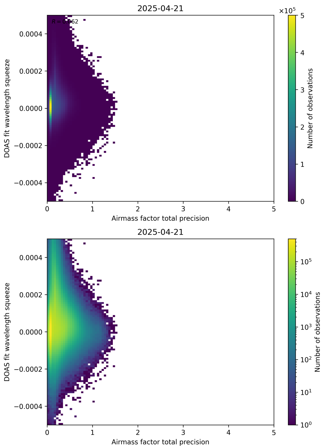
Figure 107: Scatter density plot of “Airmass factor total precision” against “DOAS fit wavelength squeeze” for 2025-04-20 to 2025-04-22.
