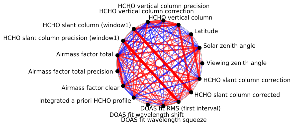
Figure 1: Map of correlation graph for 2025-04-20 to 2025-04-22.
