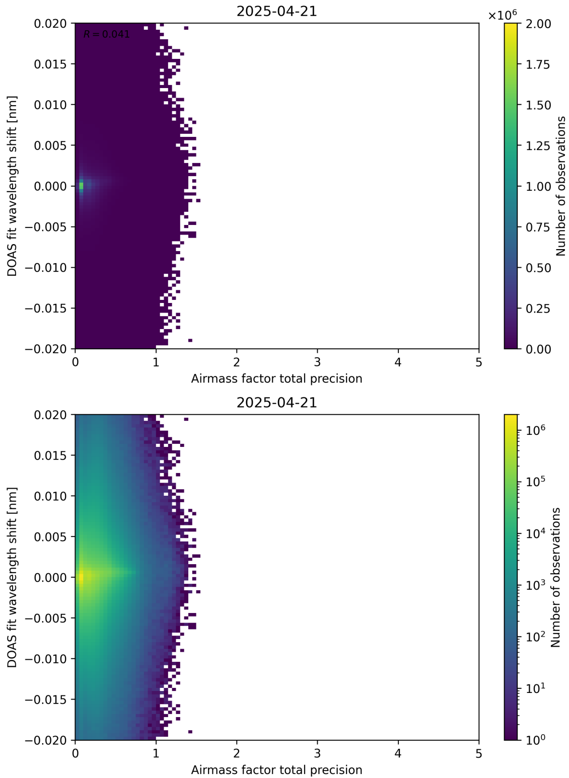
Figure 106: Scatter density plot of “Airmass factor total precision” against “DOAS fit wavelength shift” for 2025-04-20 to 2025-04-22.
