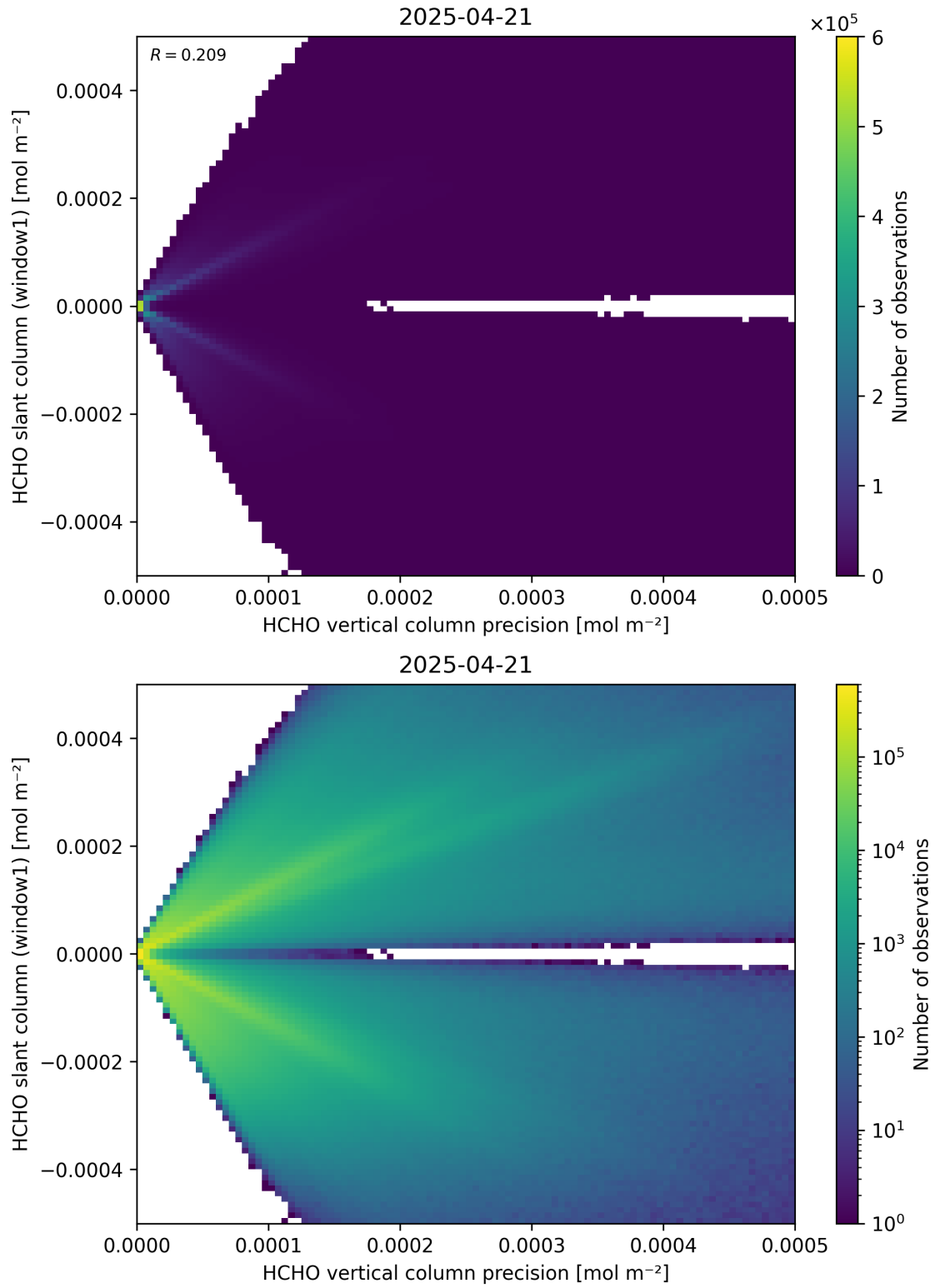
Figure 142: Scatter density plot of “HCHO vertical column precision” against “HCHO slant column (window1)” for 2025-04-20 to 2025-04-22.
