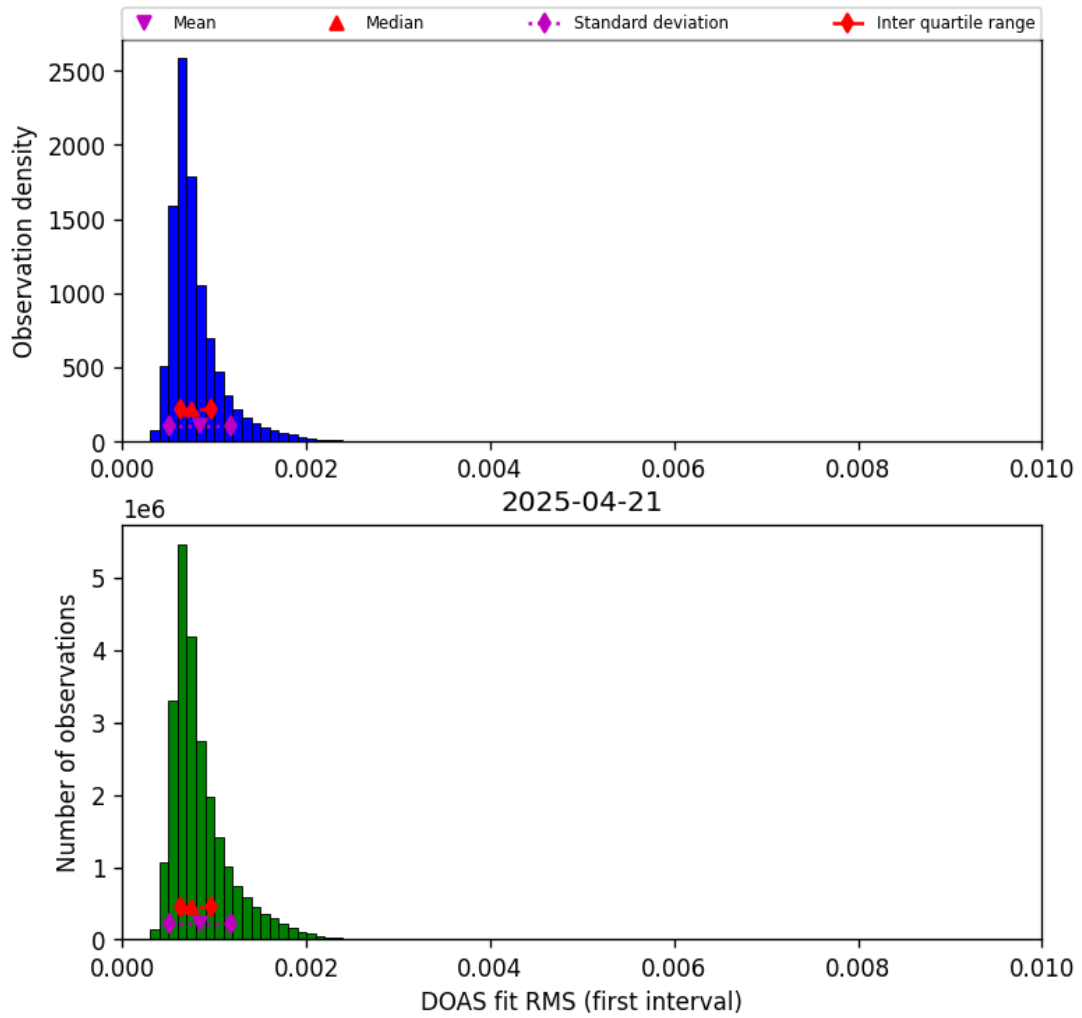
Figure 46: Histogram of “DOAS fit RMS (first interval)” for 2025-04-20 to 2025-04-22
