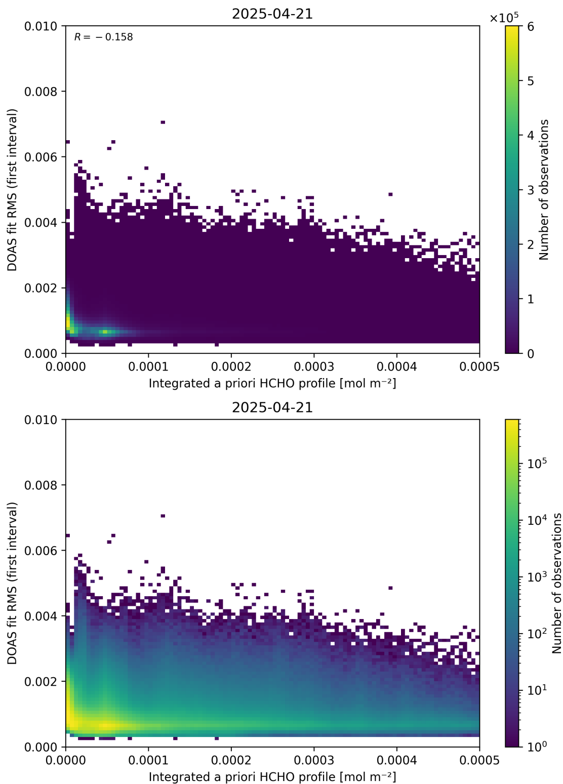
Figure 148: Scatter density plot of “Integrated a priori HCHO profile” against “DOAS fit RMS (first interval)” for 2025-04-20 to 2025-04-22.
