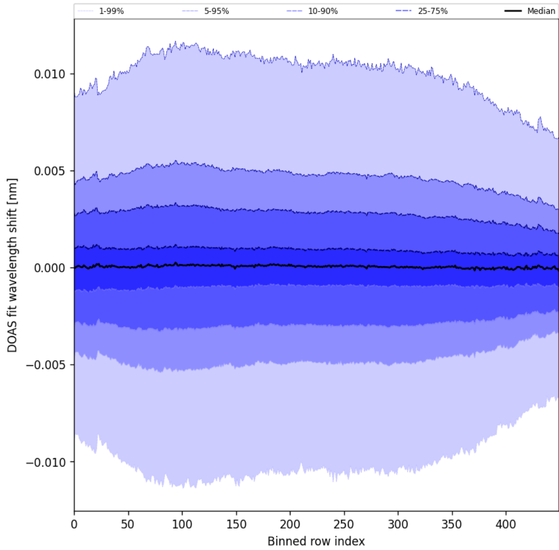
Figure 58: Along track statistics of “DOAS fit wavelength shift” for 2025-04-20 to 2025-04-22
