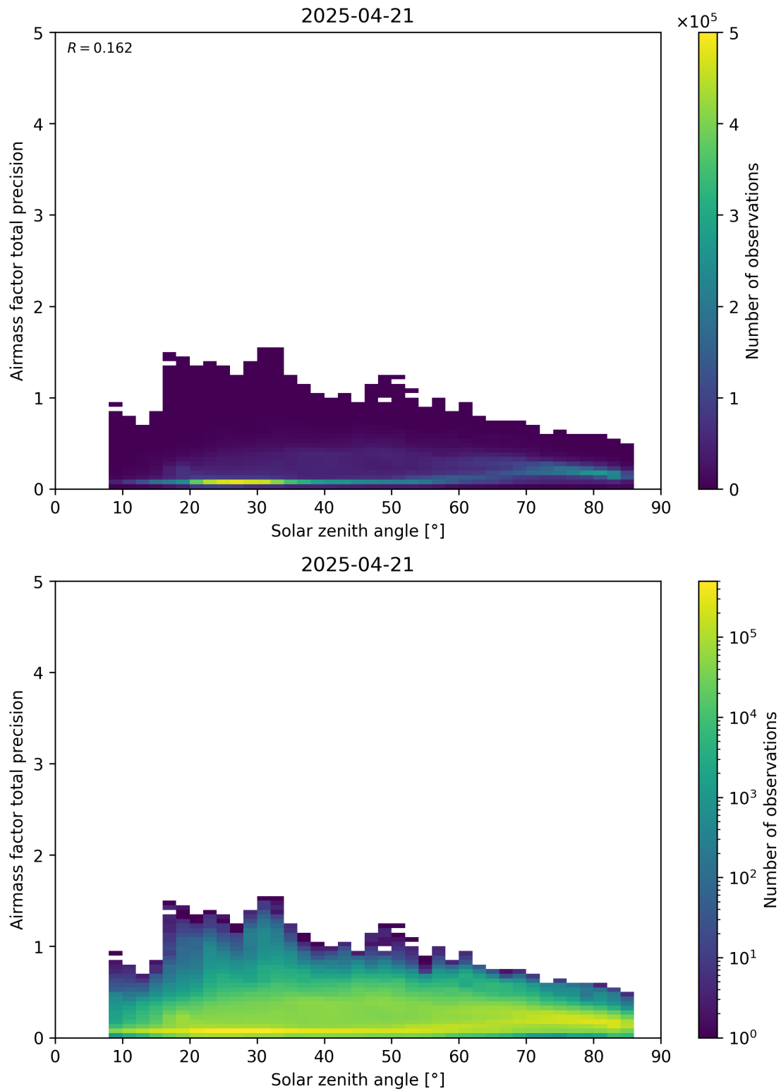
Figure 176: Scatter density plot of “Solar zenith angle” against “Airmass factor total precision” for 2025-04-20 to 2025-04-22.
