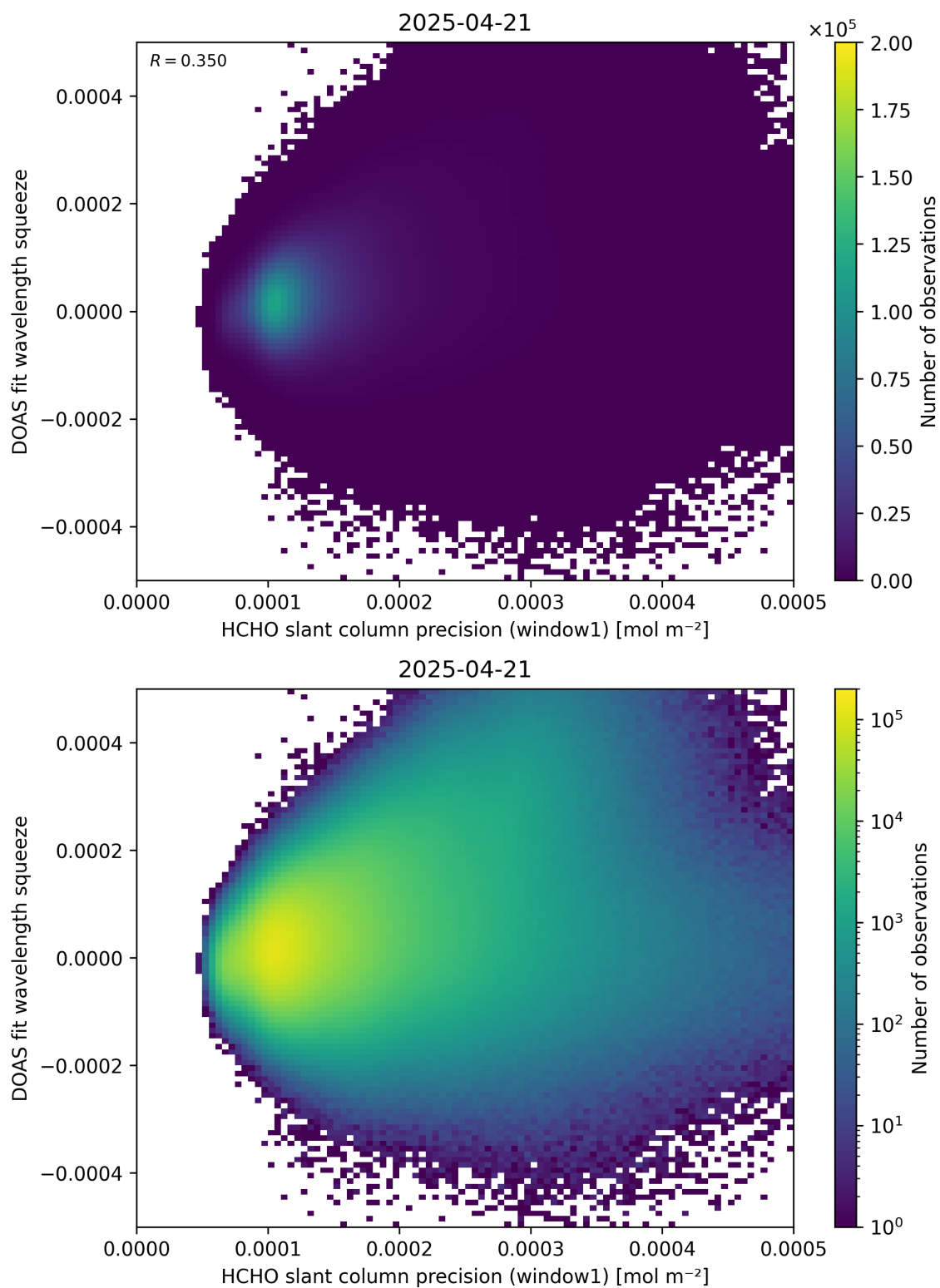
Figure 90: Scatter density plot of “HCHO slant column precision (window1)” against “DOAS fit wavelength squeeze” for 2025-04-20 to 2025-04-22.
