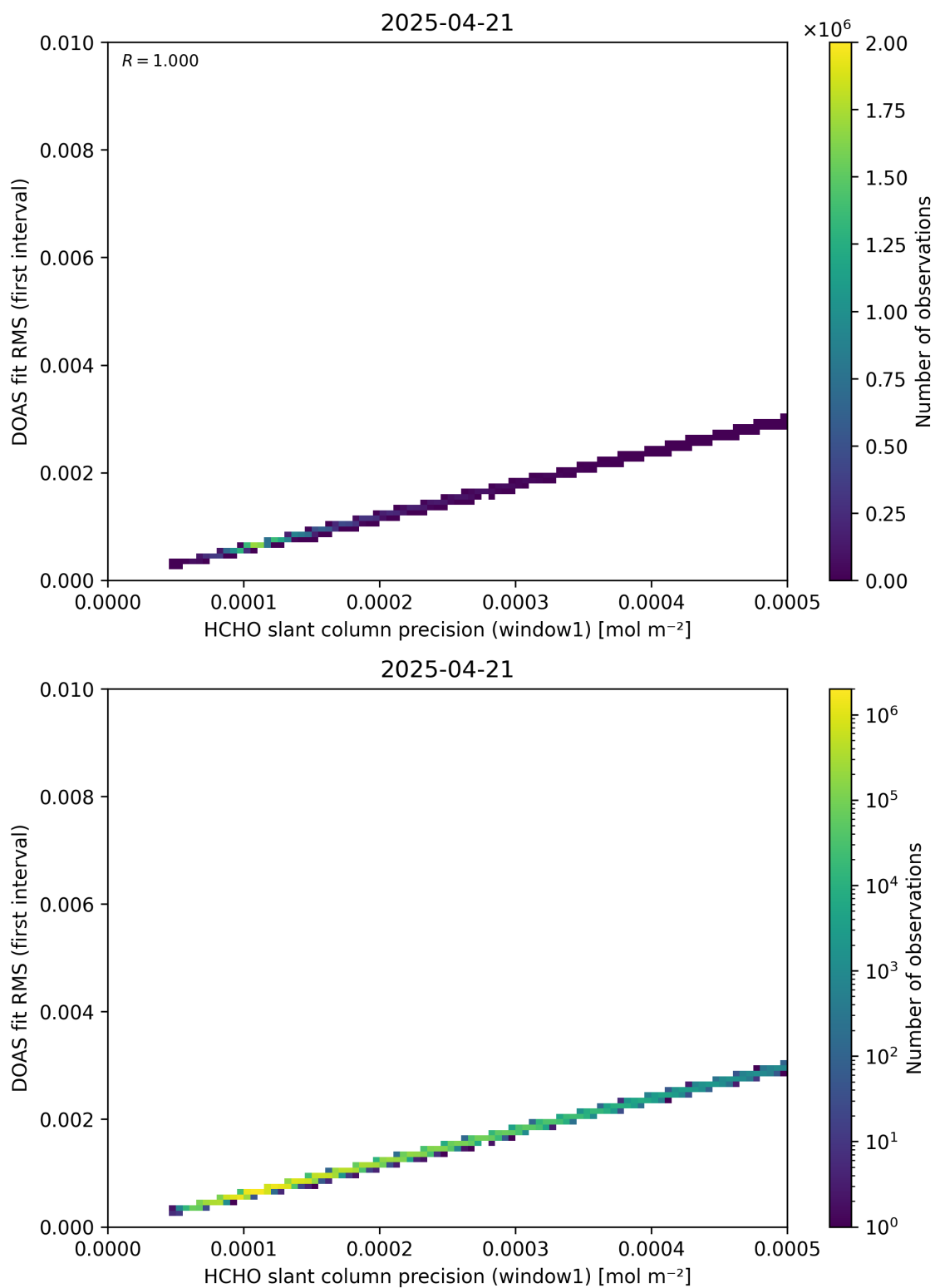
Figure 88: Scatter density plot of “HCHO slant column precision (window1)” against “DOAS fit RMS (first interval)” for 2025-04-20 to 2025-04-22.
