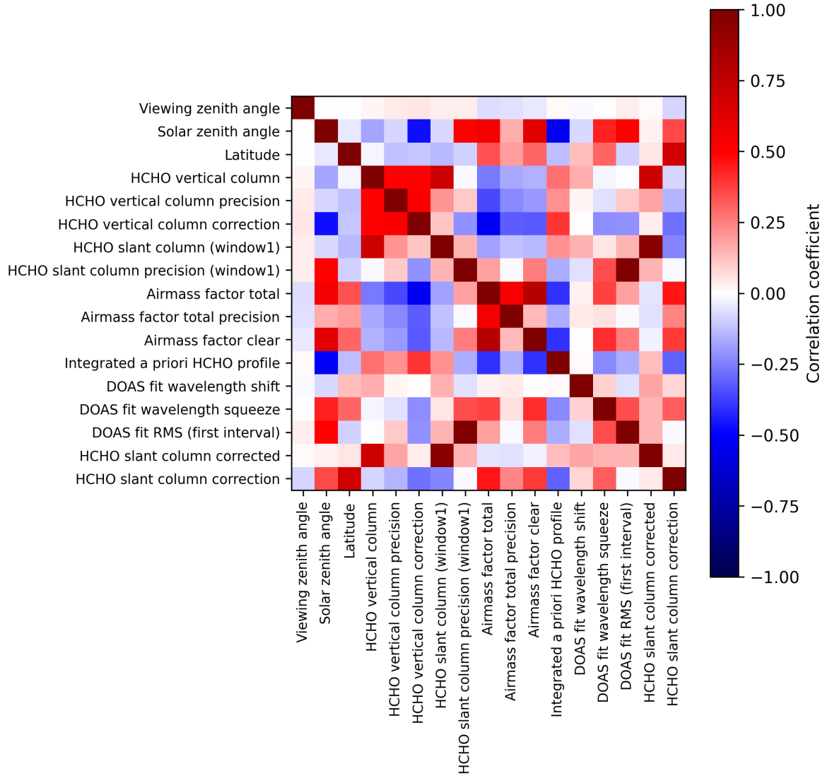
Figure 2: Map of correlation matrix for 2025-04-20 to 2025-04-22.
