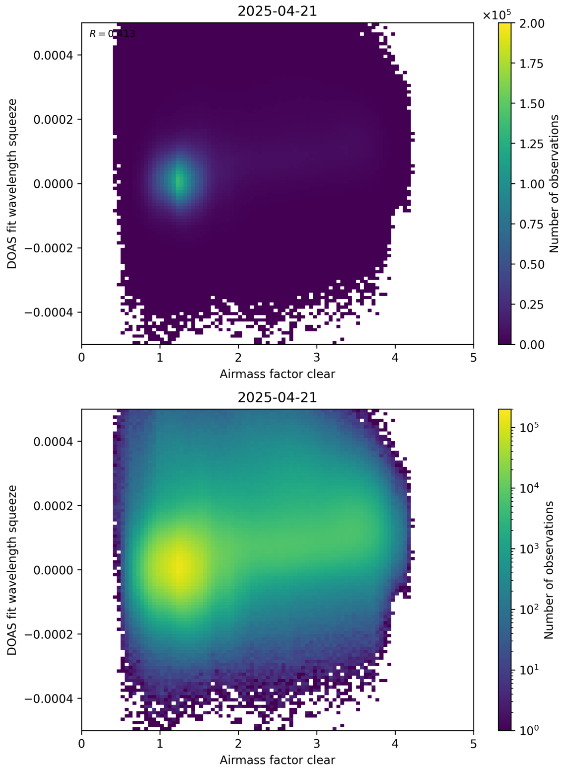
Figure 73: Scatter density plot of “Airmass factor clear” against “DOAS fit wavelength squeeze” for 2025-04-20 to 2025-04-22.
