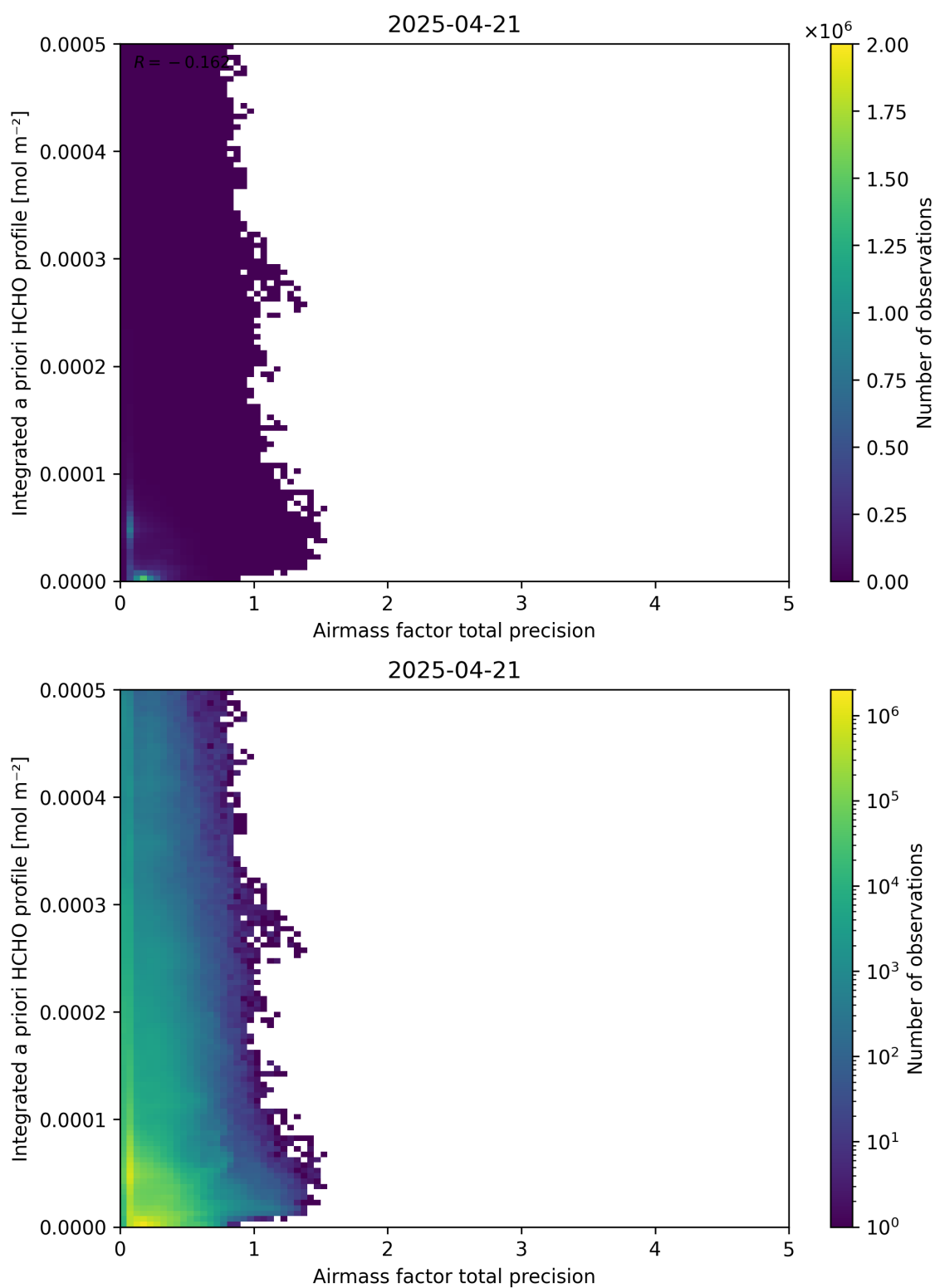
Figure 111: Scatter density plot of “Airmass factor total precision” against “Integrated a priori HCHO profile” for 2025-04-20 to 2025-04-22.
