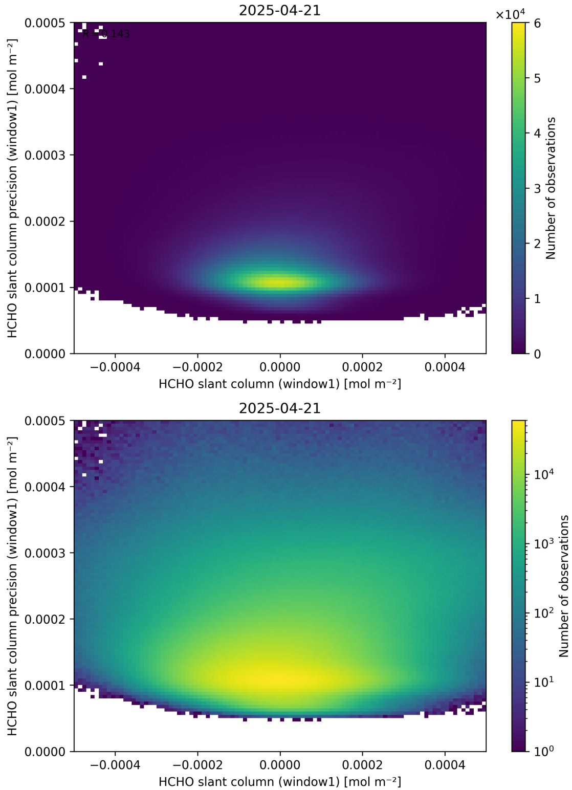
Figure 84: Scatter density plot of “HCHO slant column (window1)” against “HCHO slant column precision (window1)” for 2025-04-20 to 2025-04-22.
