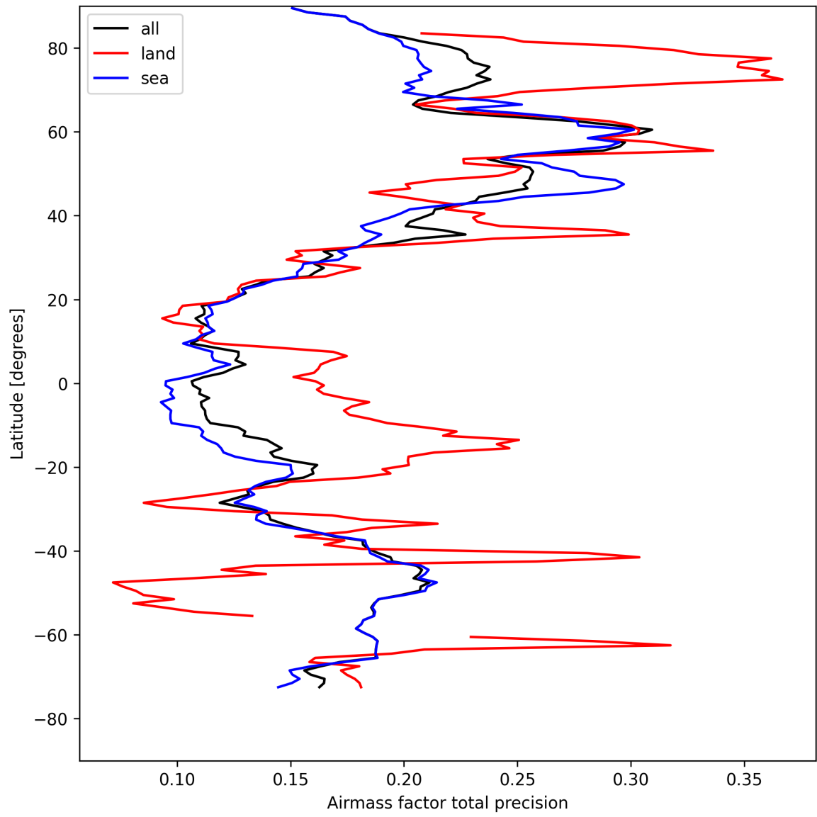
Figure 27: Zonal average of “Airmass factor total precision” for 2025-04-20 to 2025-04-22.
