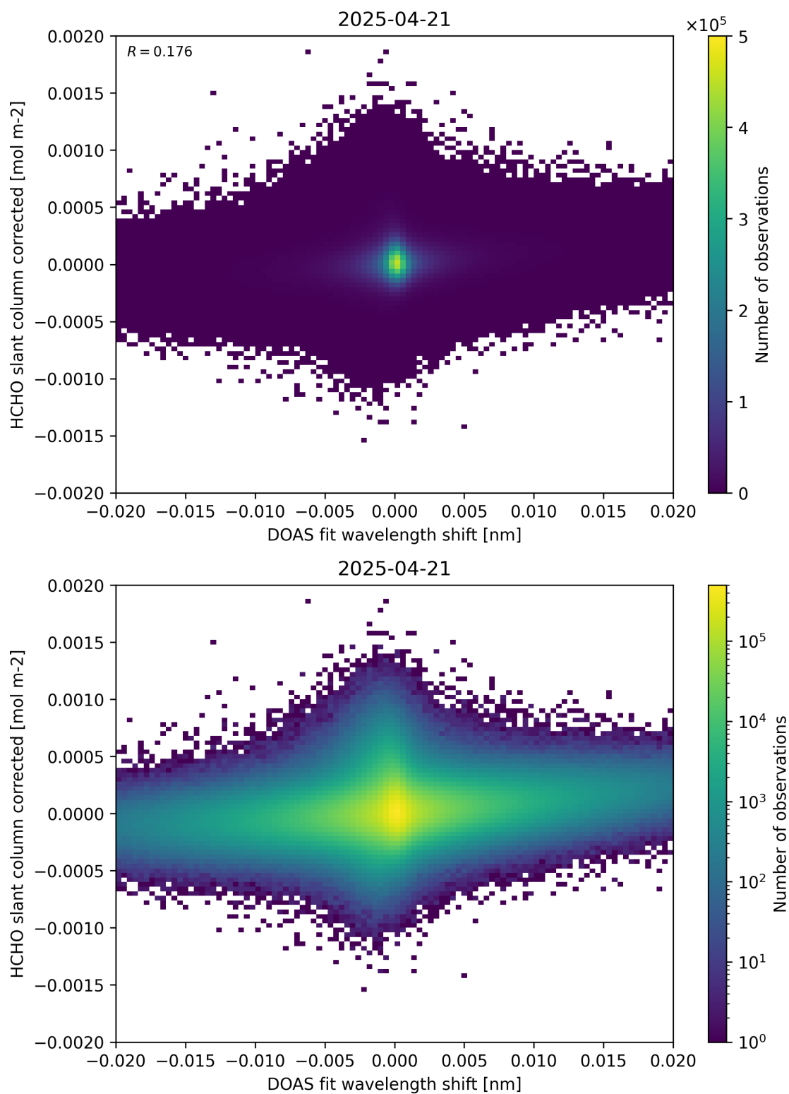
Figure 66: Scatter density plot of “DOAS fit wavelength shift” against “HCHO slant column corrected” for 2025-04-20 to 2025-04-22.
