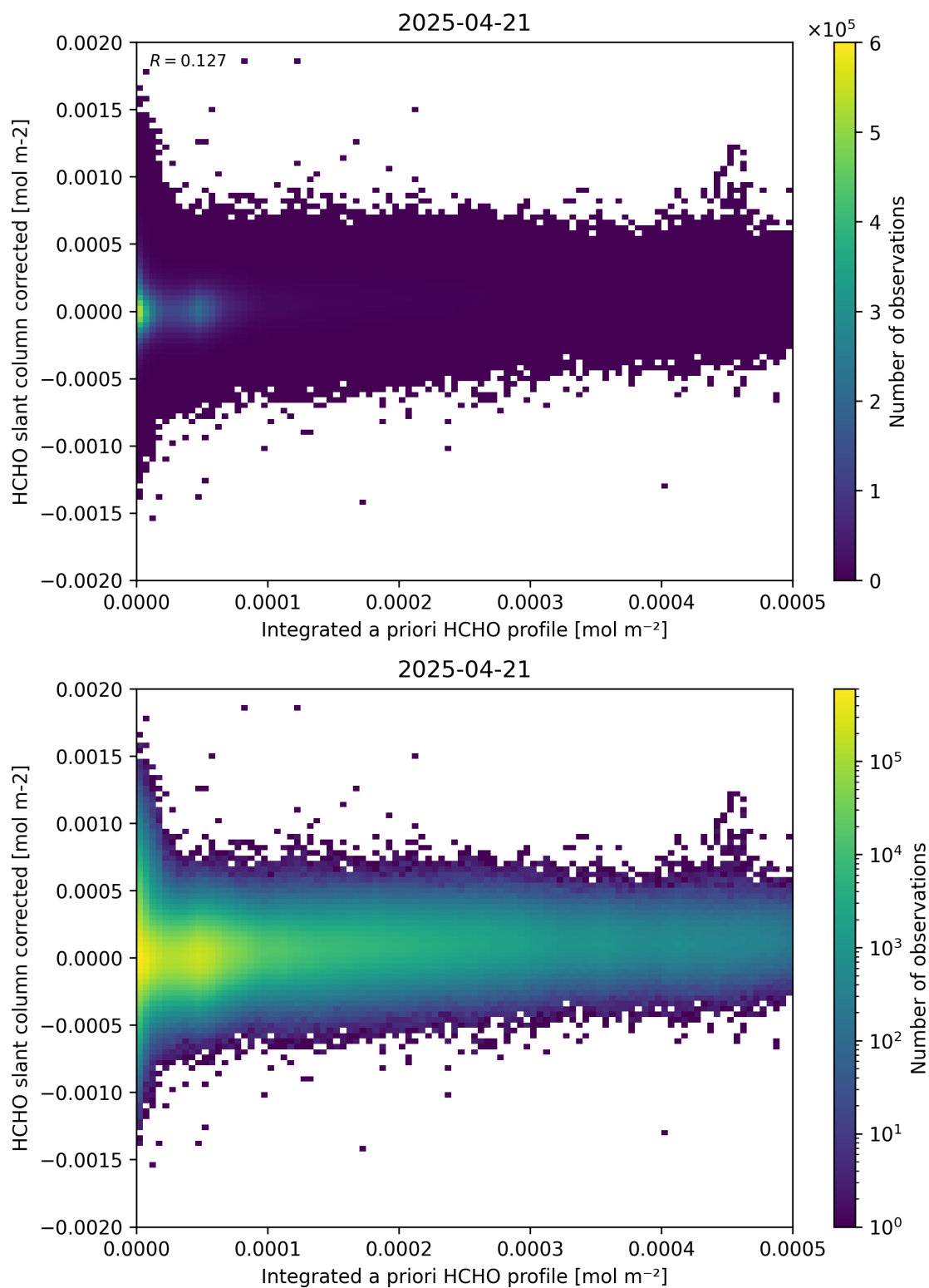
Figure 151: Scatter density plot of “Integrated a priori HCHO profile” against “HCHO slant column corrected” for 2025-04-20 to 2025-04-22.
