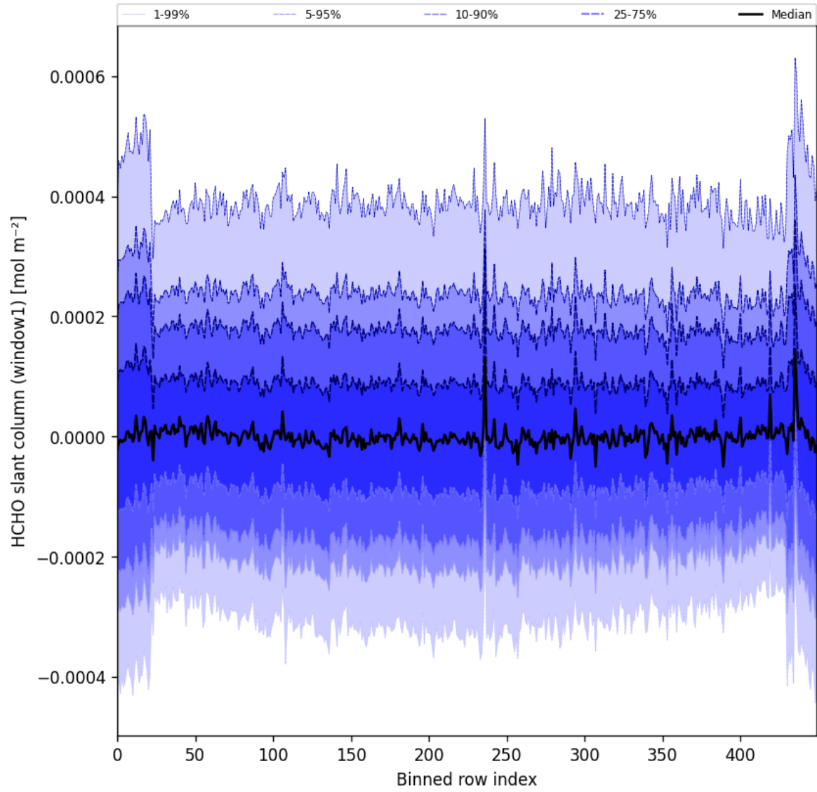
Figure 52: Along track statistics of "HCHO slant column (window1)" for 2025-04-20 to 2025-04-22
