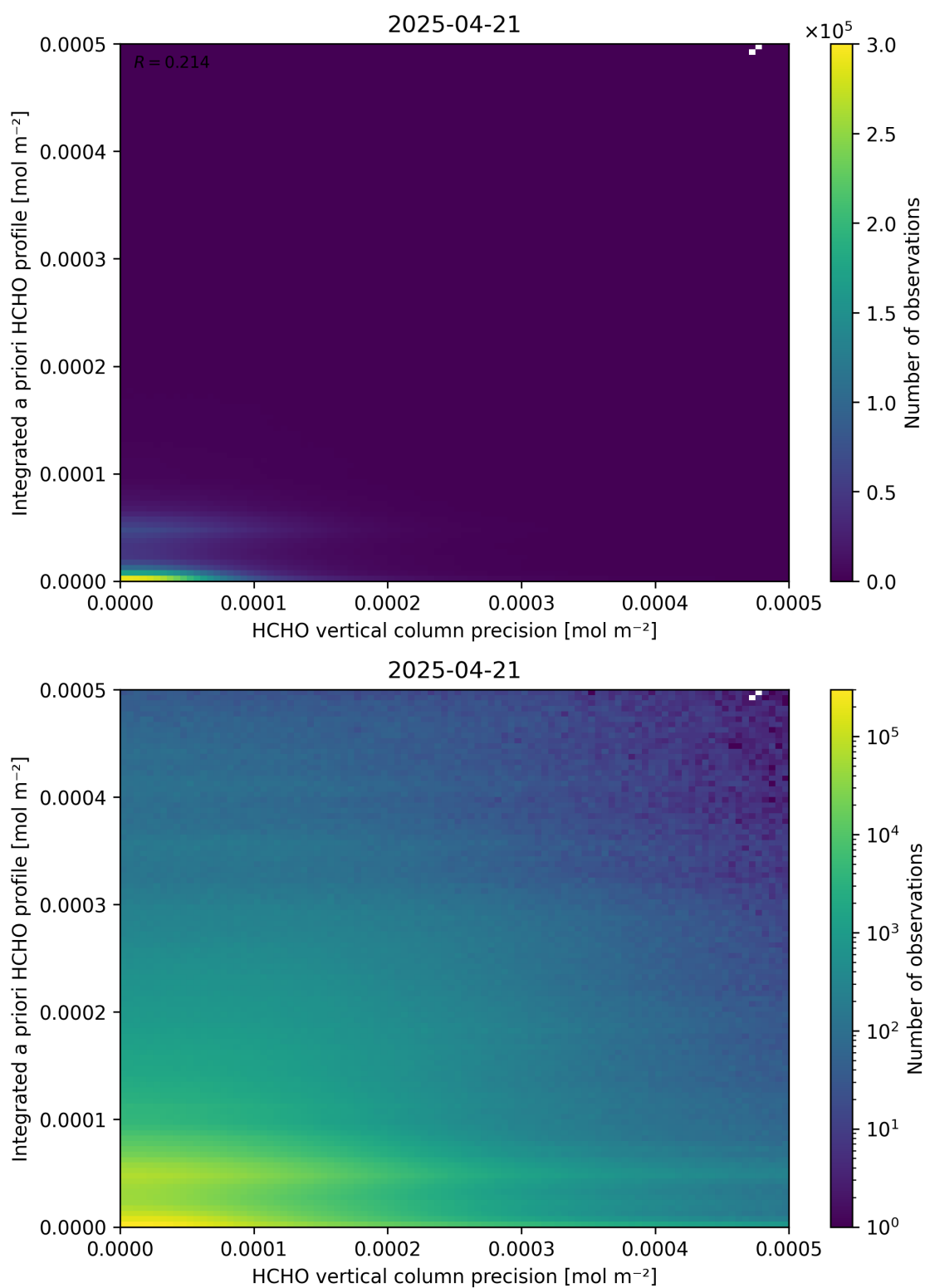
Figure 147: Scatter density plot of “HCHO vertical column precision” against “Integrated a priori HCHO profile” for 2025-04-20 to 2025-04-22.
