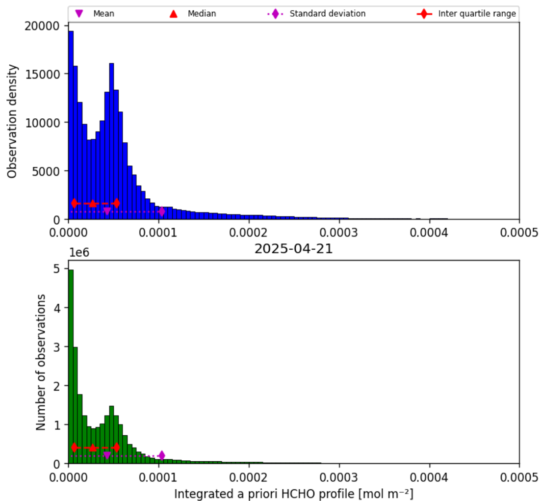
Figure 43: Histogram of “Integrated a priori HCHO profile” for 2025-04-20 to 2025-04-22
