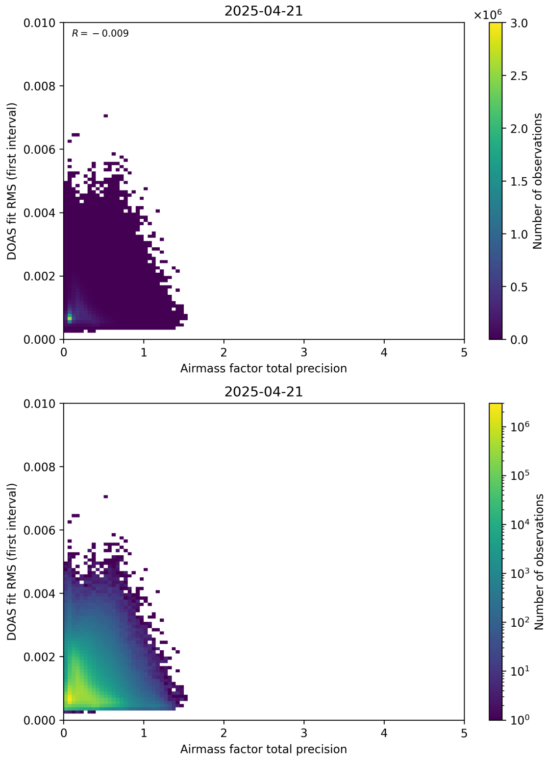
Figure 105: Scatter density plot of “Airmass factor total precision” against “DOAS fit RMS (first interval)” for 2025-04-20 to 2025-04-22.
