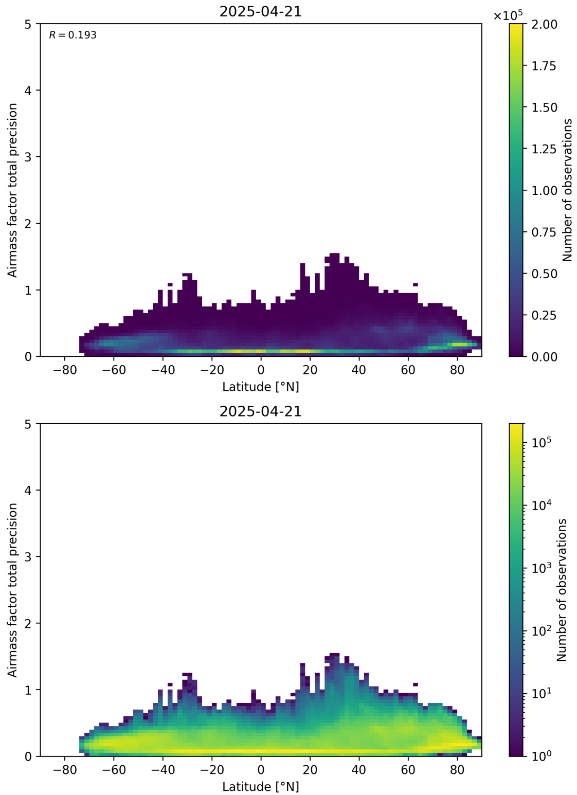
Figure 162: Scatter density plot of “Latitude” against “Airmass factor total precision” for 2025-04-20 to 2025-04-22.
