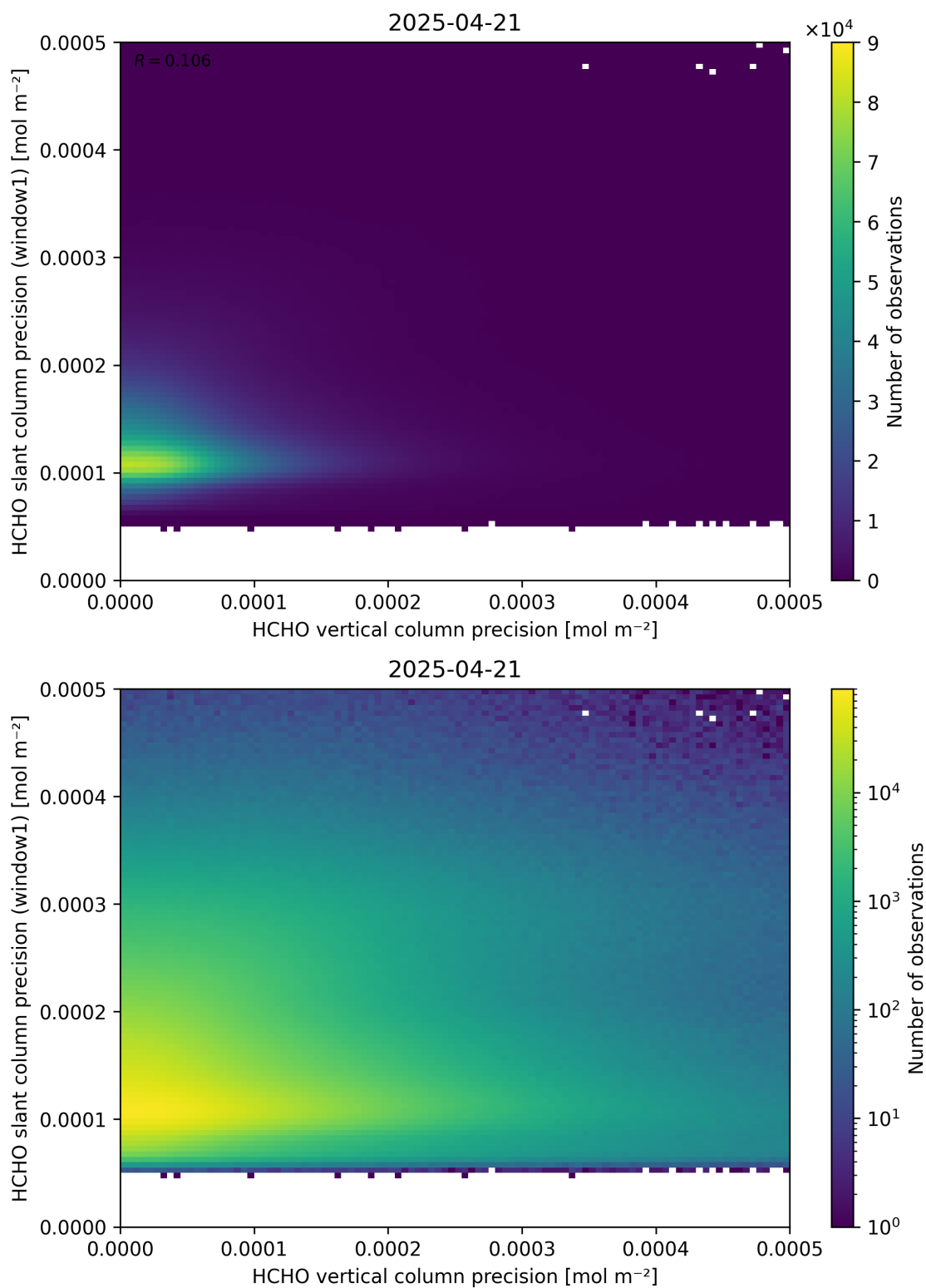
Figure 143: Scatter density plot of “HCHO vertical column precision” against “HCHO slant column precision (window1)” for 2025-04-20 to 2025-04-22.
