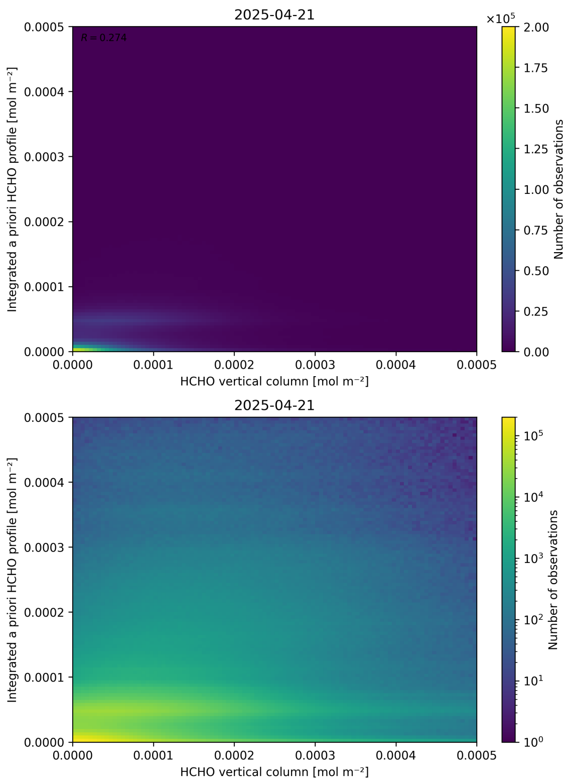
Figure 135: Scatter density plot of “HCHO vertical column” against “Integrated a priori HCHO profile” for 2025-04-20 to 2025-04-22.
