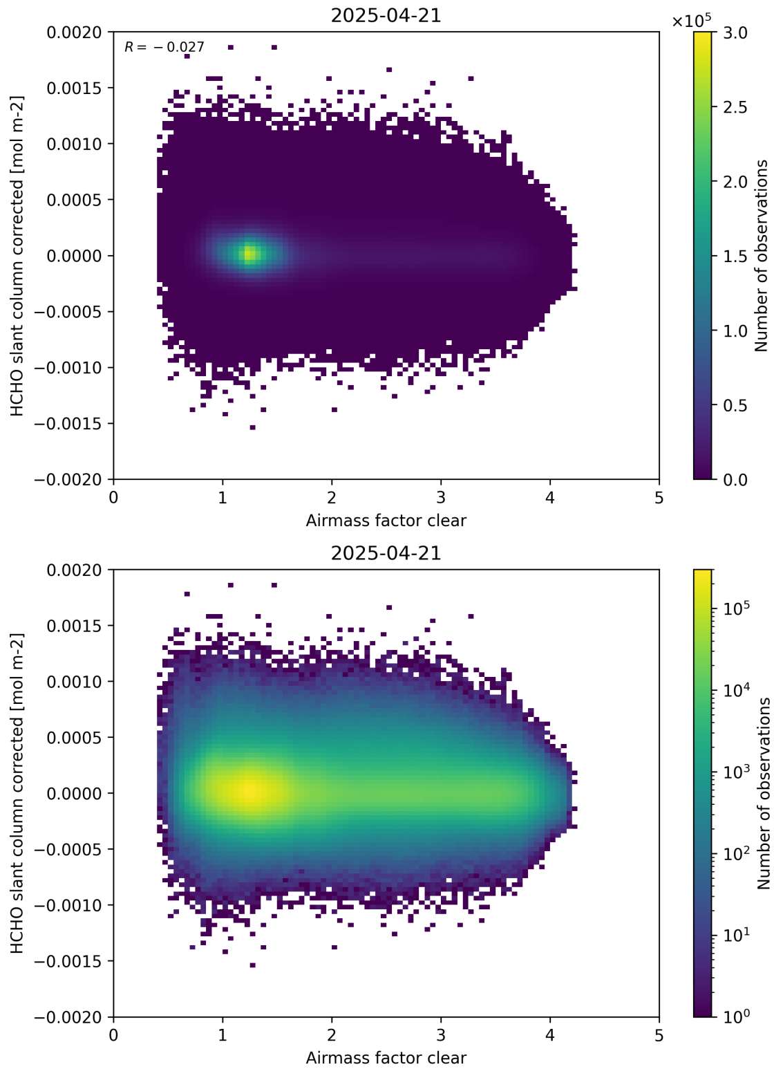
Figure 74: Scatter density plot of “Airmass factor clear” against “HCHO slant column corrected” for 2025-04-20 to 2025-04-22.
