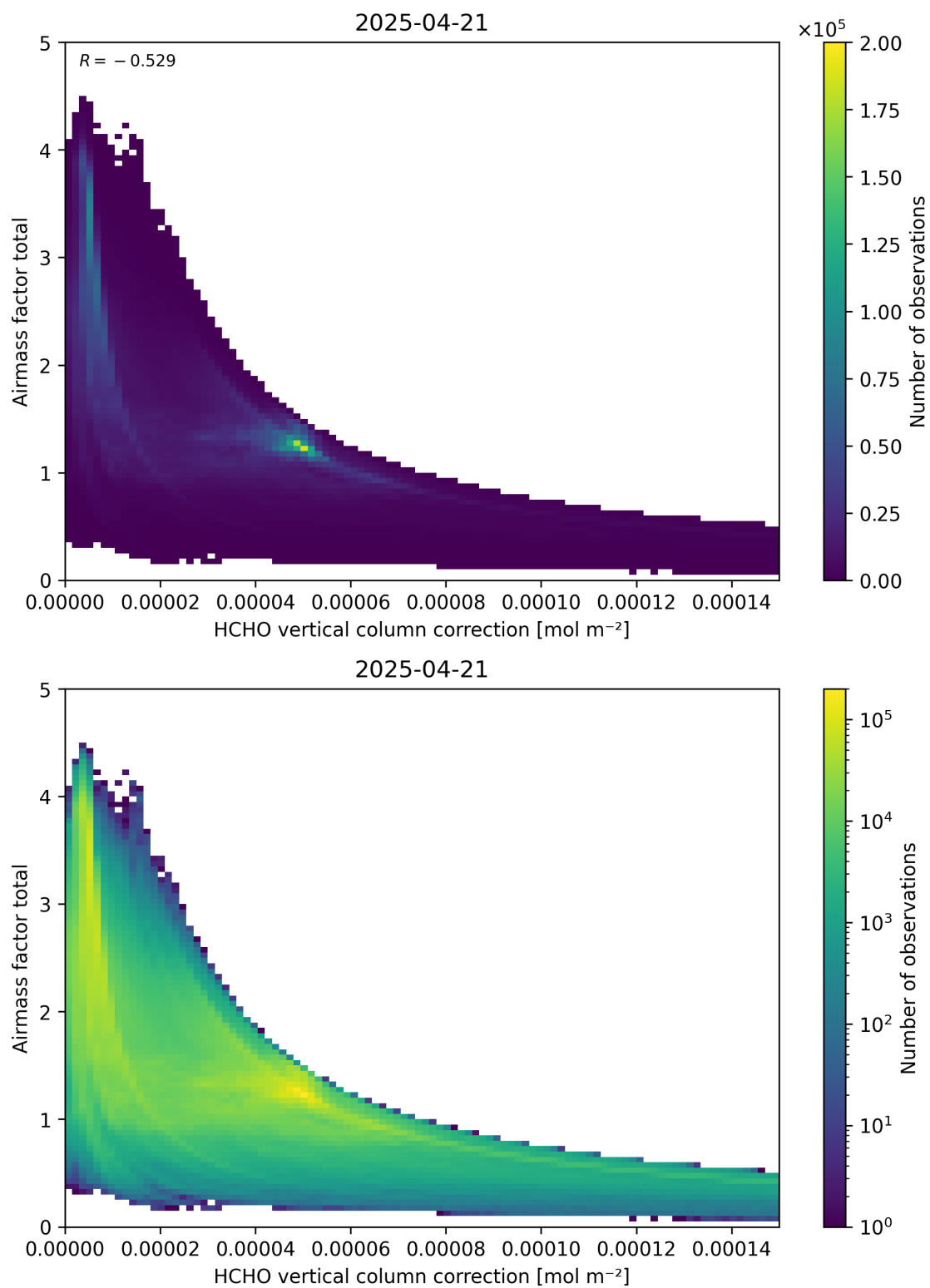
Figure 120: Scatter density plot of “HCHO vertical column correction” against “Airmass factor total” for 2025-04-20 to 2025-04-22.
