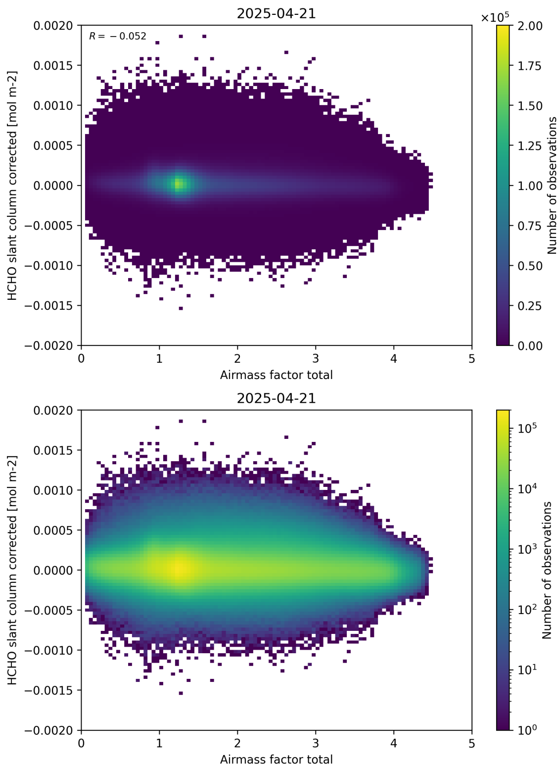
Figure 101: Scatter density plot of “Airmass factor total” against “HCHO slant column corrected” for 2025-04-20 to 2025-04-22.
