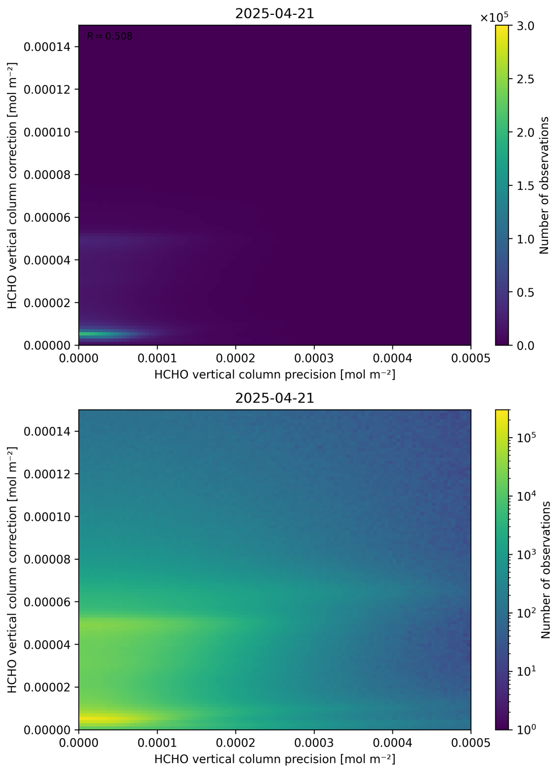
Figure 146: Scatter density plot of “HCHO vertical column precision” against “HCHO vertical column correction” for 2025-04-20 to 2025-04-22.
