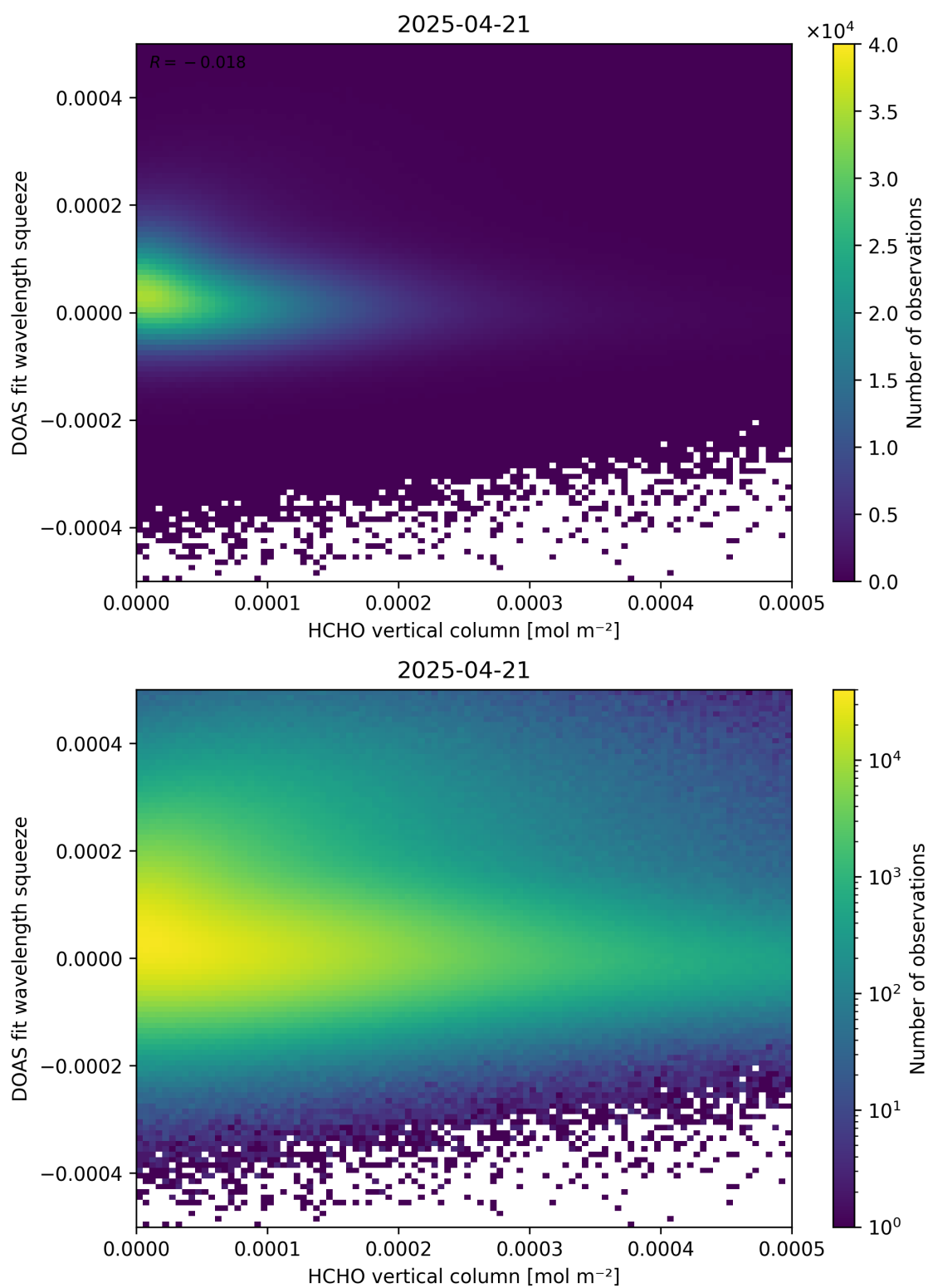
Figure 125: Scatter density plot of “HCHO vertical column” against “DOAS fit wavelength squeeze” for 2025-04-20 to 2025-04-22.
