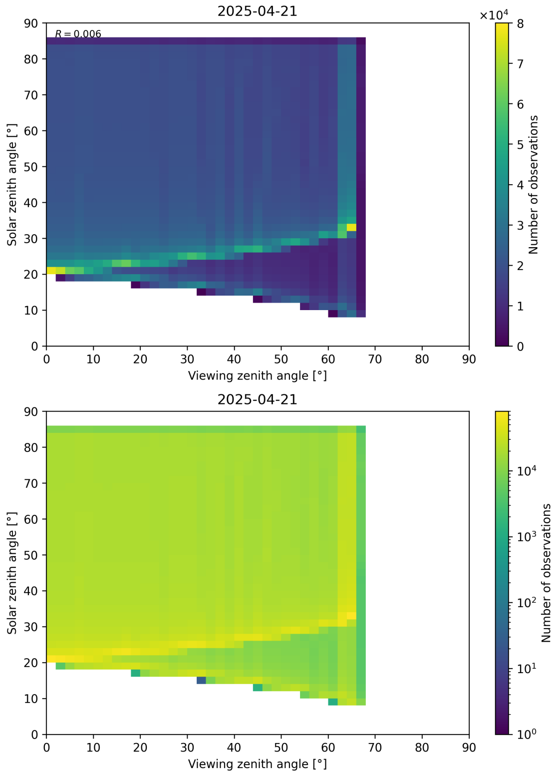
Figure 197: Scatter density plot of “Viewing zenith angle” against “Solar zenith angle” for 2025-04-20 to 2025-04-22.
