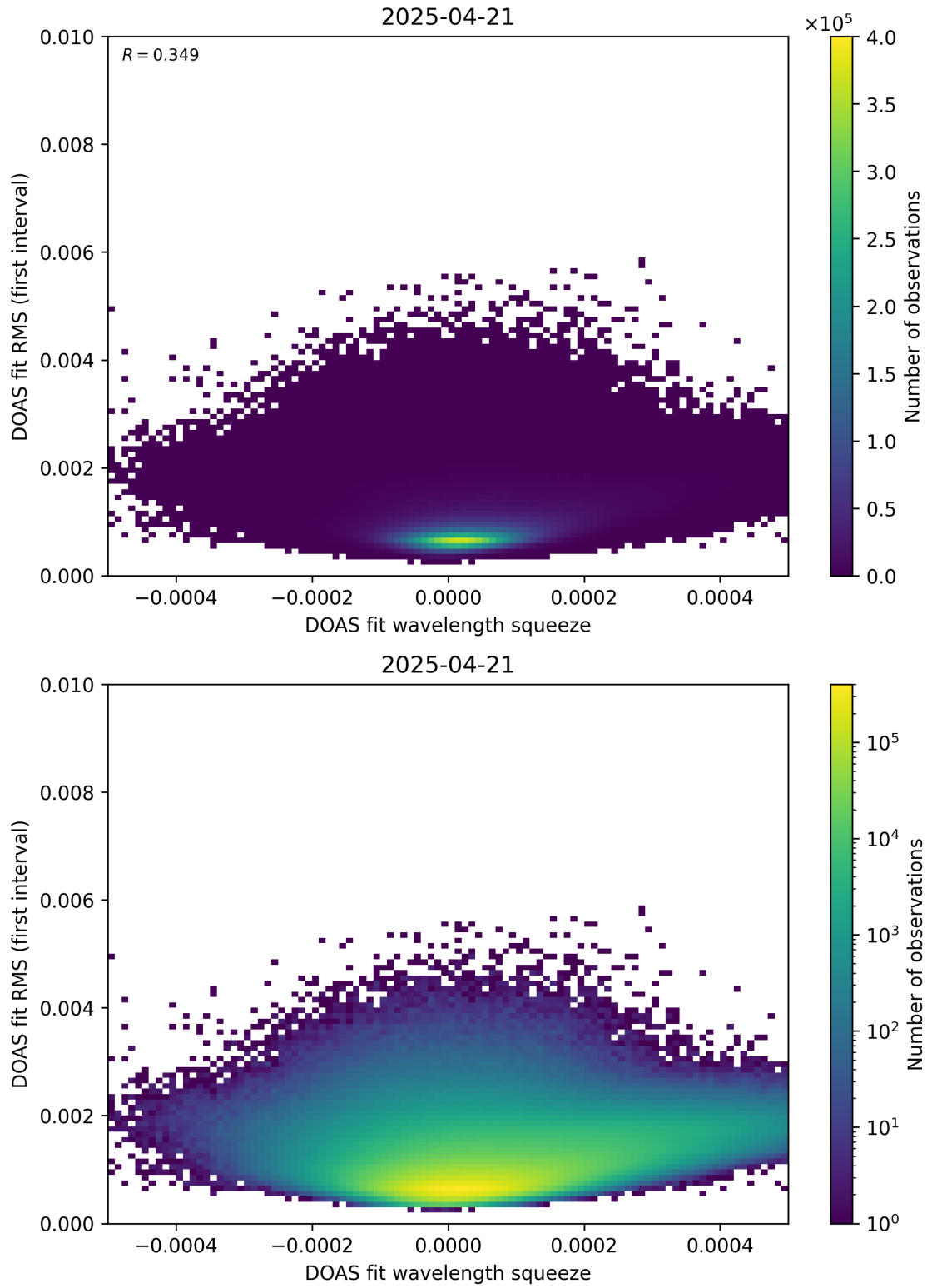
Figure 68: Scatter density plot of “DOAS fit wavelength squeeze” against “DOAS fit RMS (first interval)” for 2025-04-20 to 2025-04-22.
