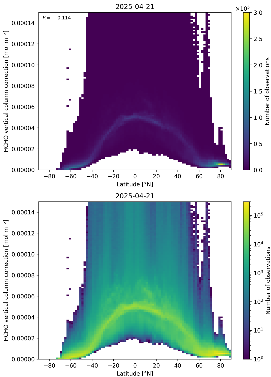
Figure 164: Scatter density plot of “Latitude” against “HCHO vertical column correction” for 2025-04-20 to 2025-04-22.
