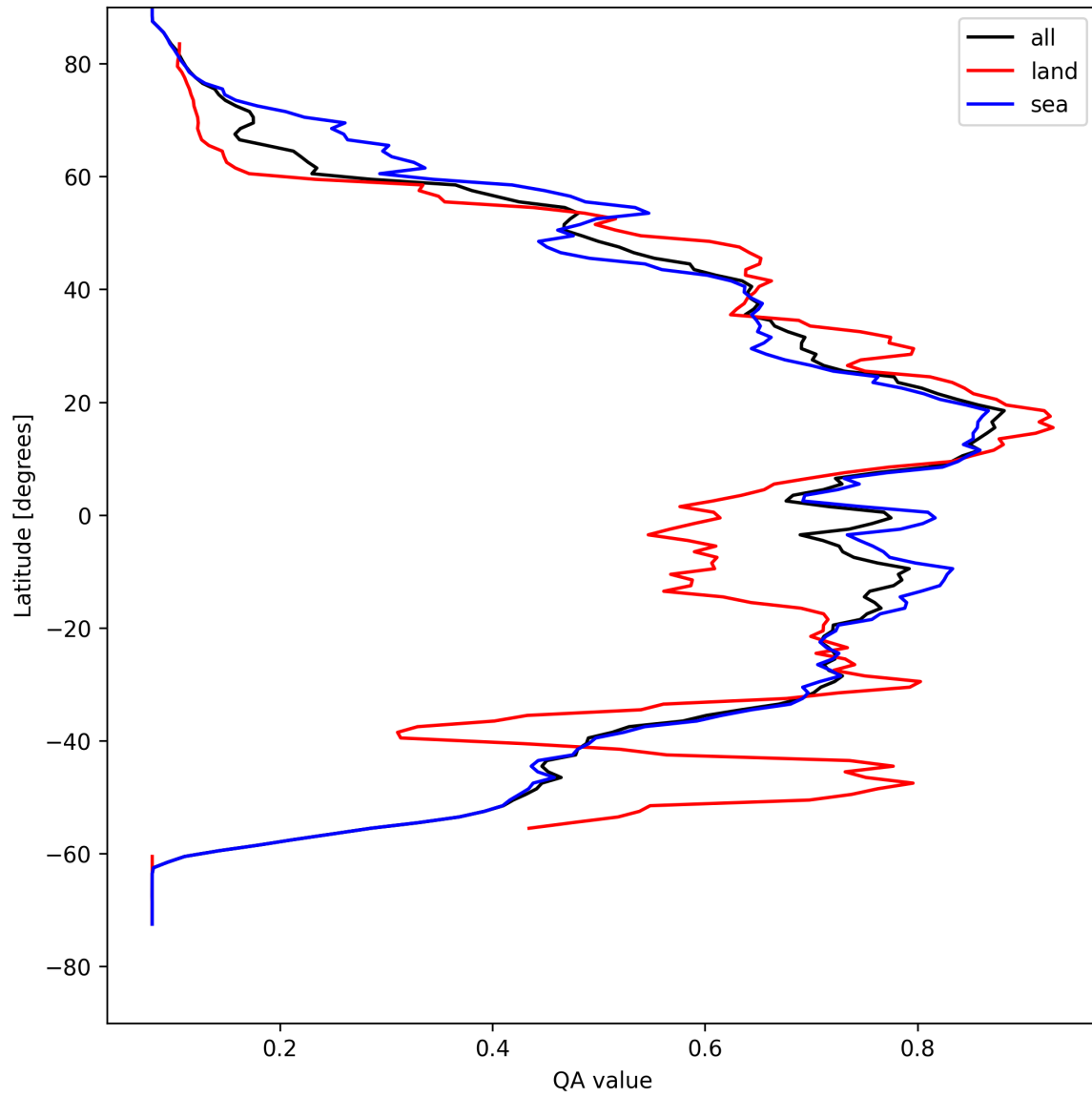
Figure 20: Zonal average of “QA value” for 2025-04-20 to 2025-04-22.
