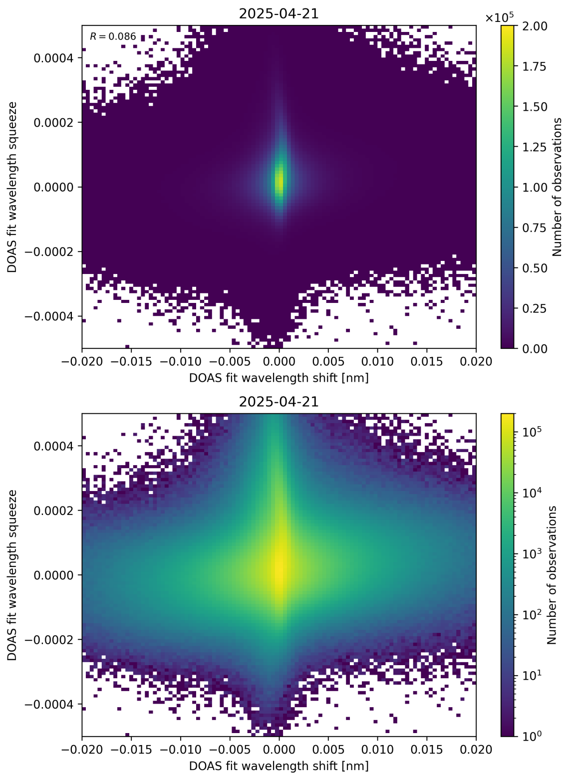
Figure 65: Scatter density plot of “DOAS fit wavelength shift” against “DOAS fit wavelength squeeze” for 2025-04-20 to 2025-04-22.
