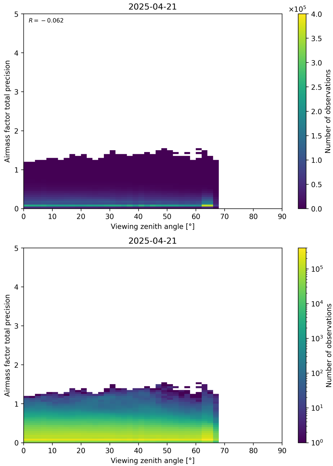
Figure 191: Scatter density plot of “Viewing zenith angle” against “Airmass factor total precision” for 2025-04-20 to 2025-04-22.
