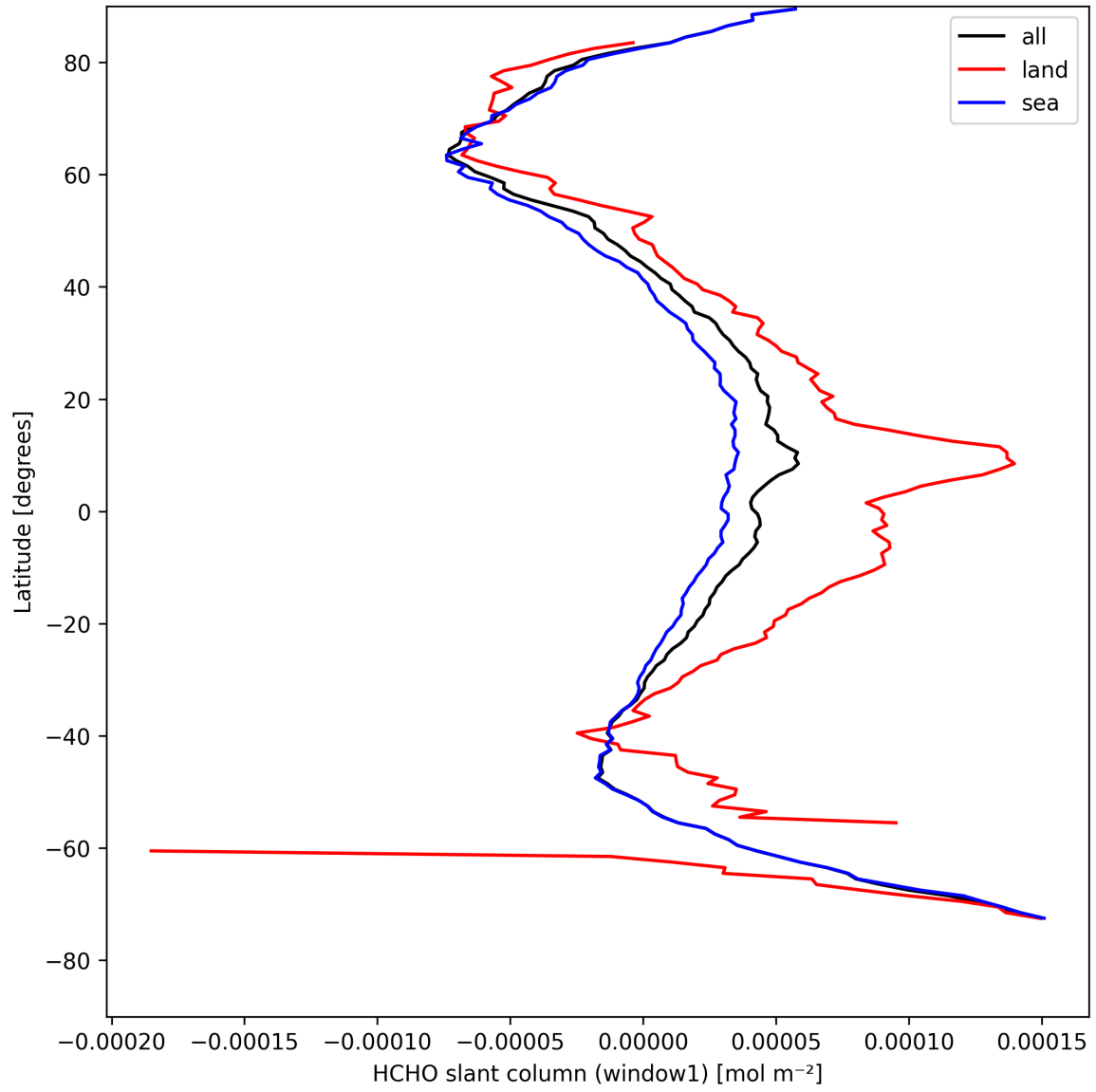
Figure 24: Zonal average of “HCHO slant column (window1)” for 2025-04-20 to 2025-04-22.
