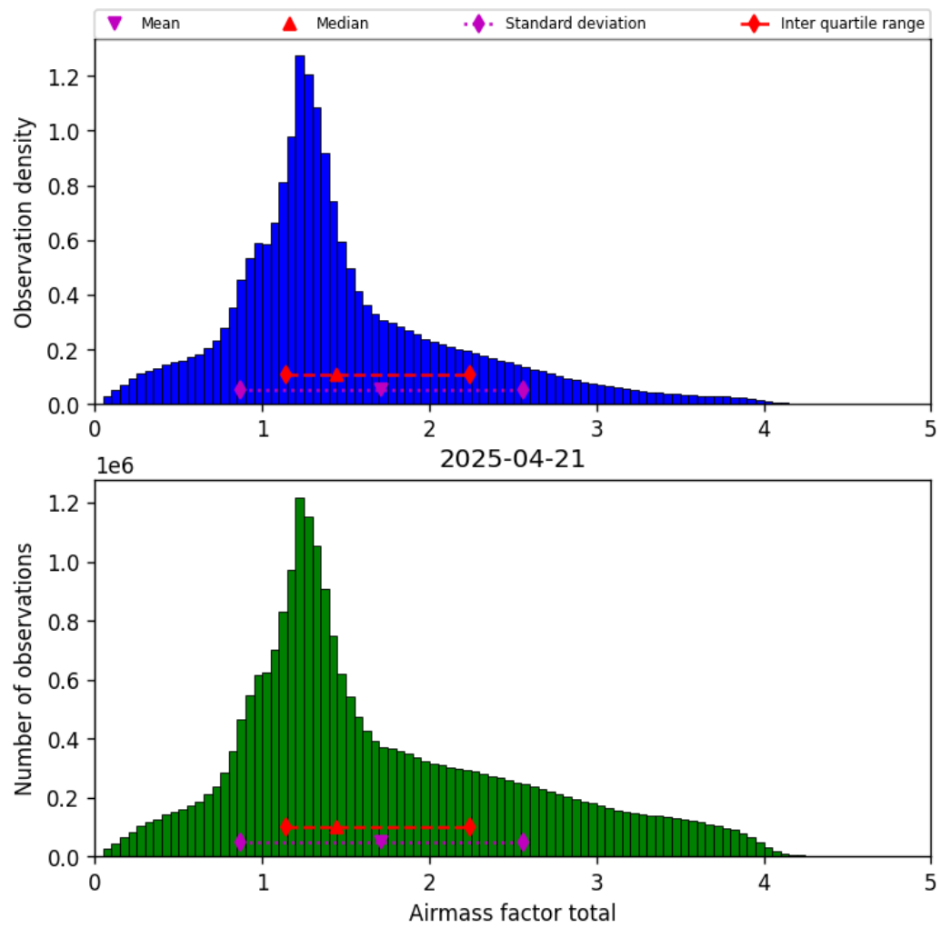
Figure 40: Histogram of “Airmass factor total” for 2025-04-20 to 2025-04-22
