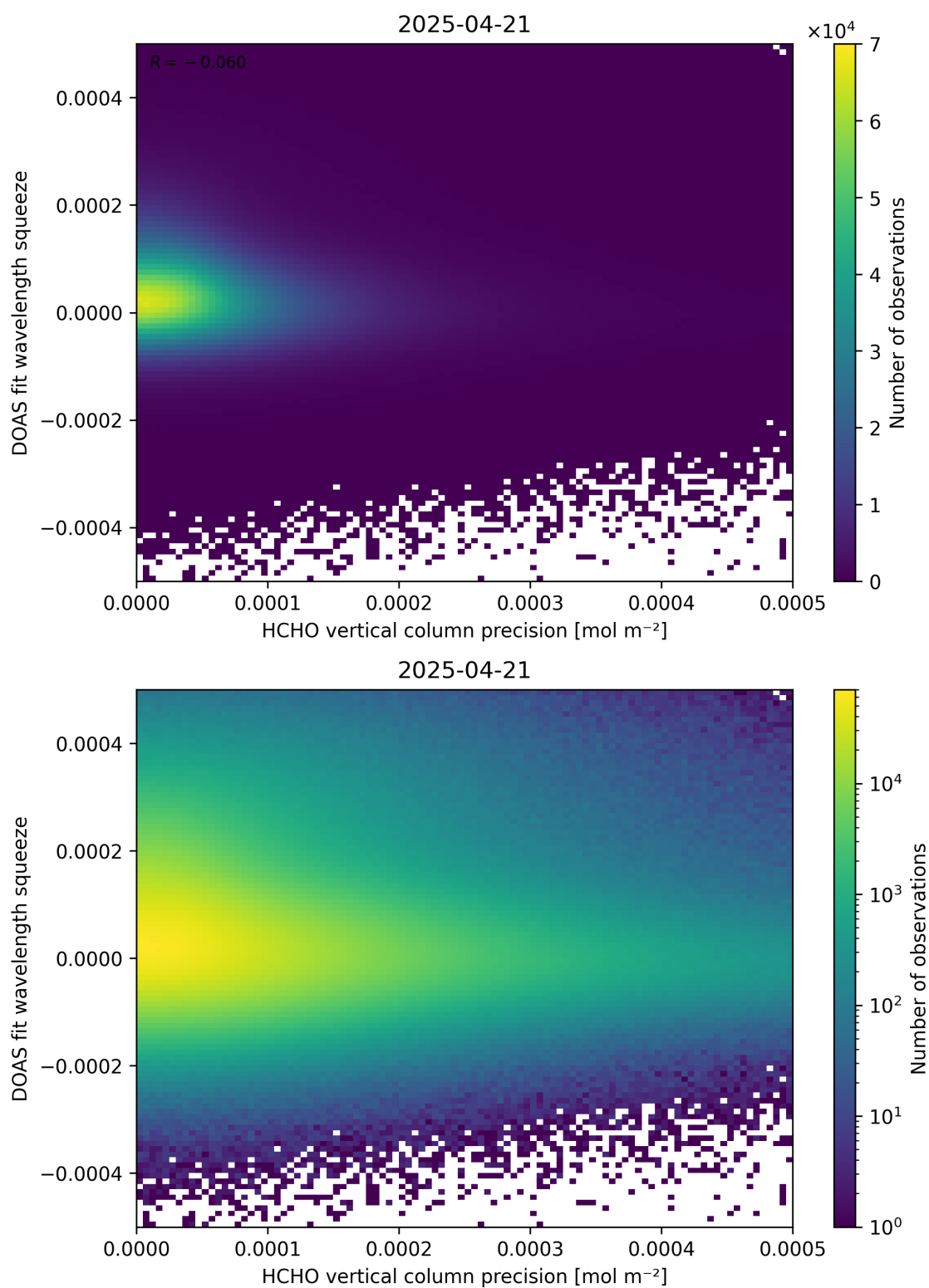
Figure 138: Scatter density plot of “HCHO vertical column precision” against “DOAS fit wavelength squeeze” for 2025-04-20 to 2025-04-22.
