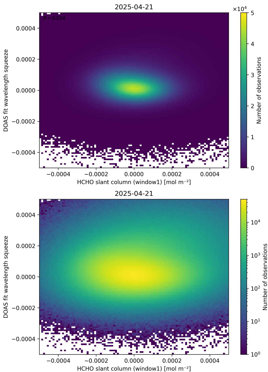
Figure 80: Scatter density plot of “HCHO slant column (window1)” against “DOAS fit wavelength squeeze” for 2025-04-20 to 2025-04-22.
