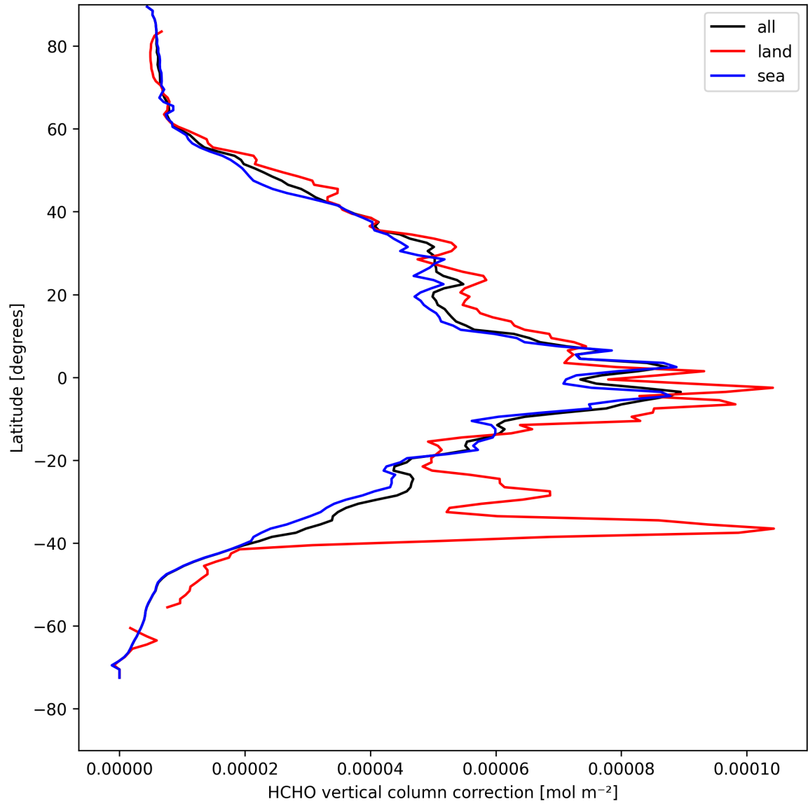
Figure 23: Zonal average of “HCHO vertical column correction” for 2025-04-20 to 2025-04-22.
