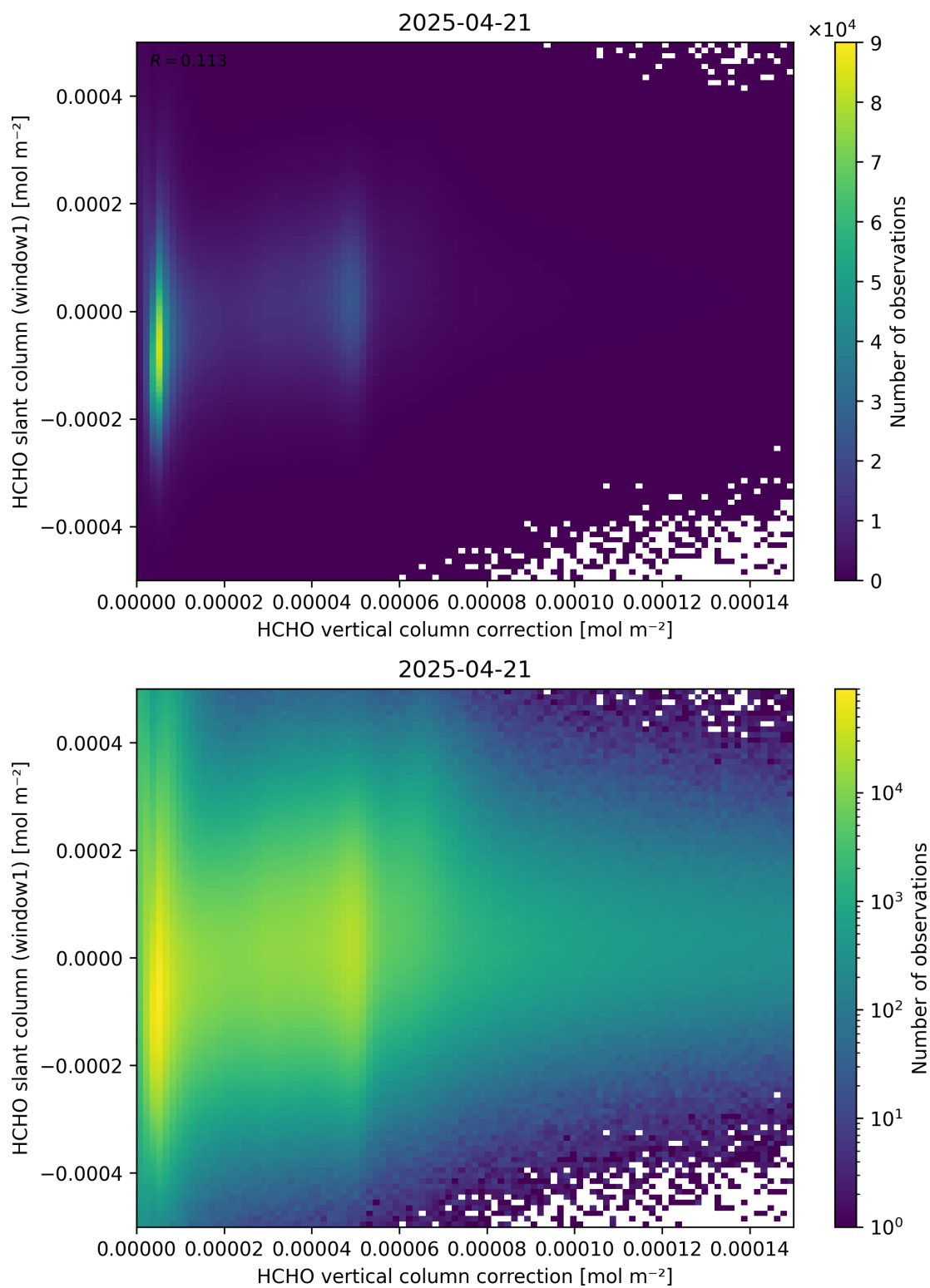
Figure 118: Scatter density plot of “HCHO vertical column correction” against “HCHO slant column (window1)” for 2025-04-20 to 2025-04-22.
