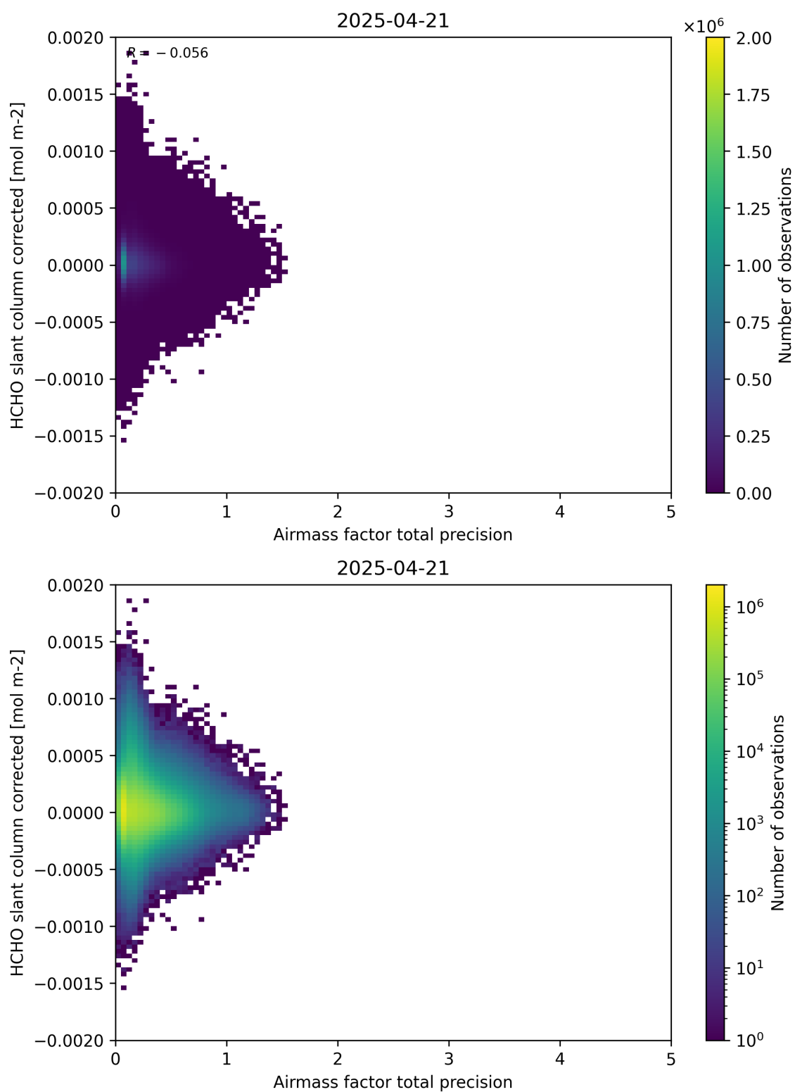
Figure 109: Scatter density plot of “Airmass factor total precision” against “HCHO slant column corrected” for 2025-04-20 to 2025-04-22.
