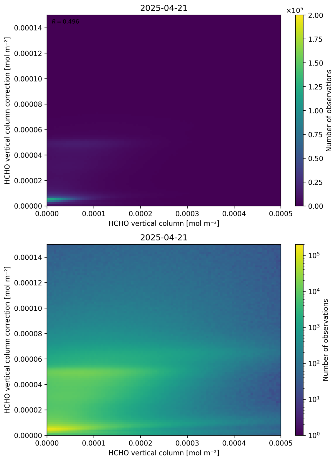
Figure 133: Scatter density plot of “HCHO vertical column” against “HCHO vertical column correction” for 2025-04-20 to 2025-04-22.
