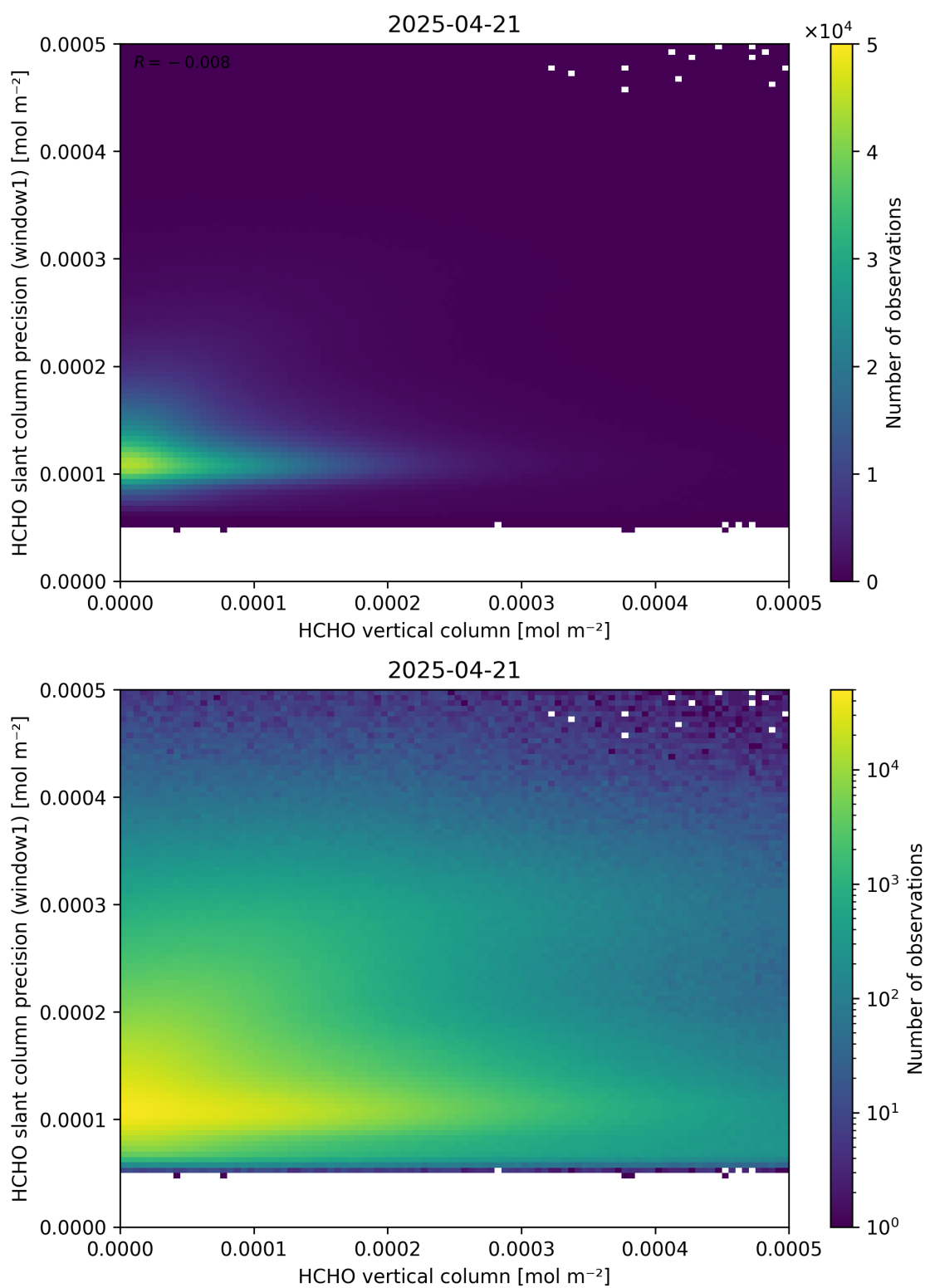
Figure 130: Scatter density plot of “HCHO vertical column” against “HCHO slant column precision (window1)” for 2025-04-20 to 2025-04-22.
