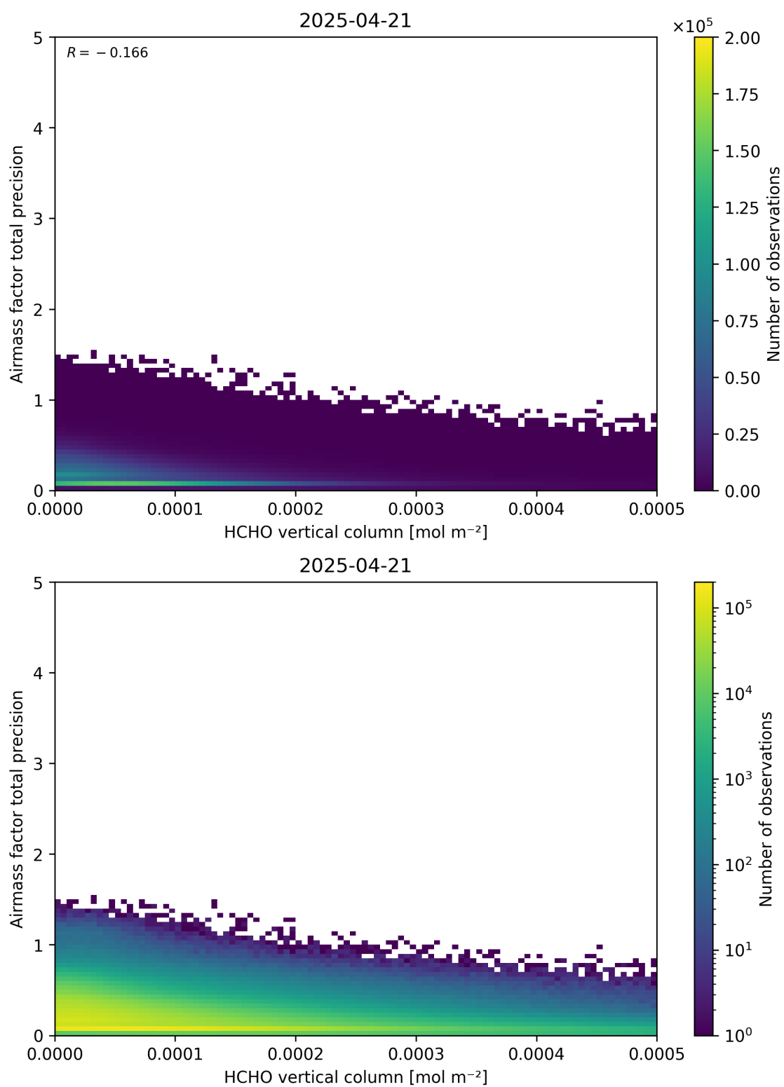
Figure 132: Scatter density plot of “HCHO vertical column” against “Airmass factor total precision” for 2025-04-20 to 2025-04-22.
