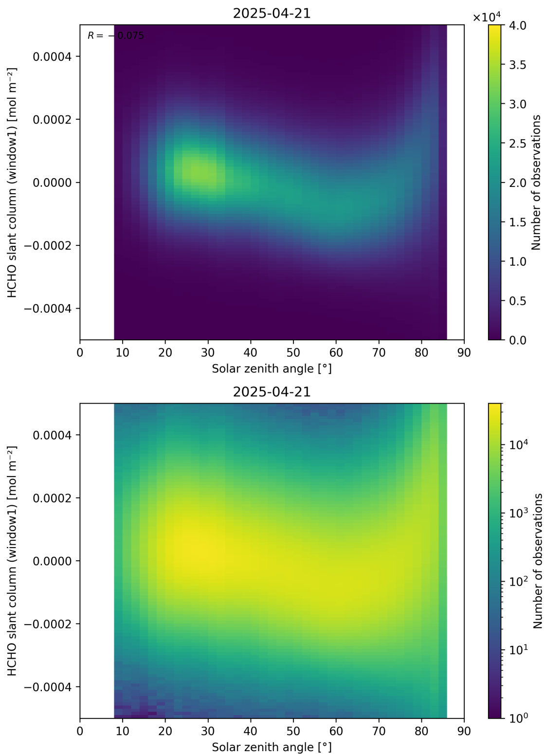
Figure 173: Scatter density plot of “Solar zenith angle” against “HCHO slant column (window1)” for 2025-04-20 to 2025-04-22.
