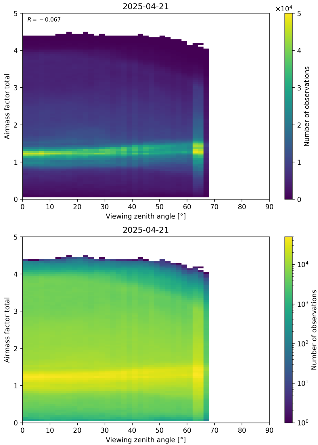
Figure 190: Scatter density plot of “Viewing zenith angle” against “Airmass factor total” for 2025-04-20 to 2025-04-22.
