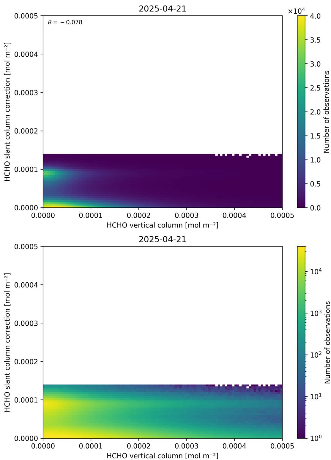
Figure 128: Scatter density plot of “HCHO vertical column” against “HCHO slant column correction” for 2025-04-20 to 2025-04-22.
