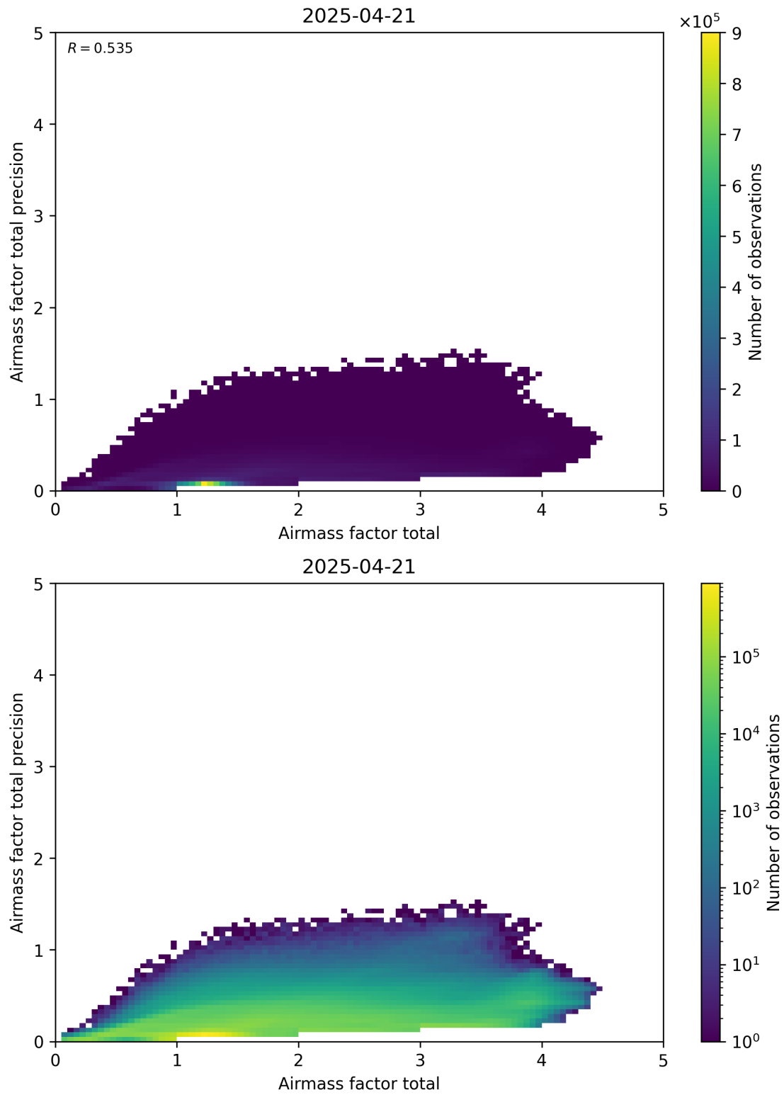
Figure 103: Scatter density plot of “Airmass factor total” against “Airmass factor total precision” for 2025-04-20 to 2025-04-22.
