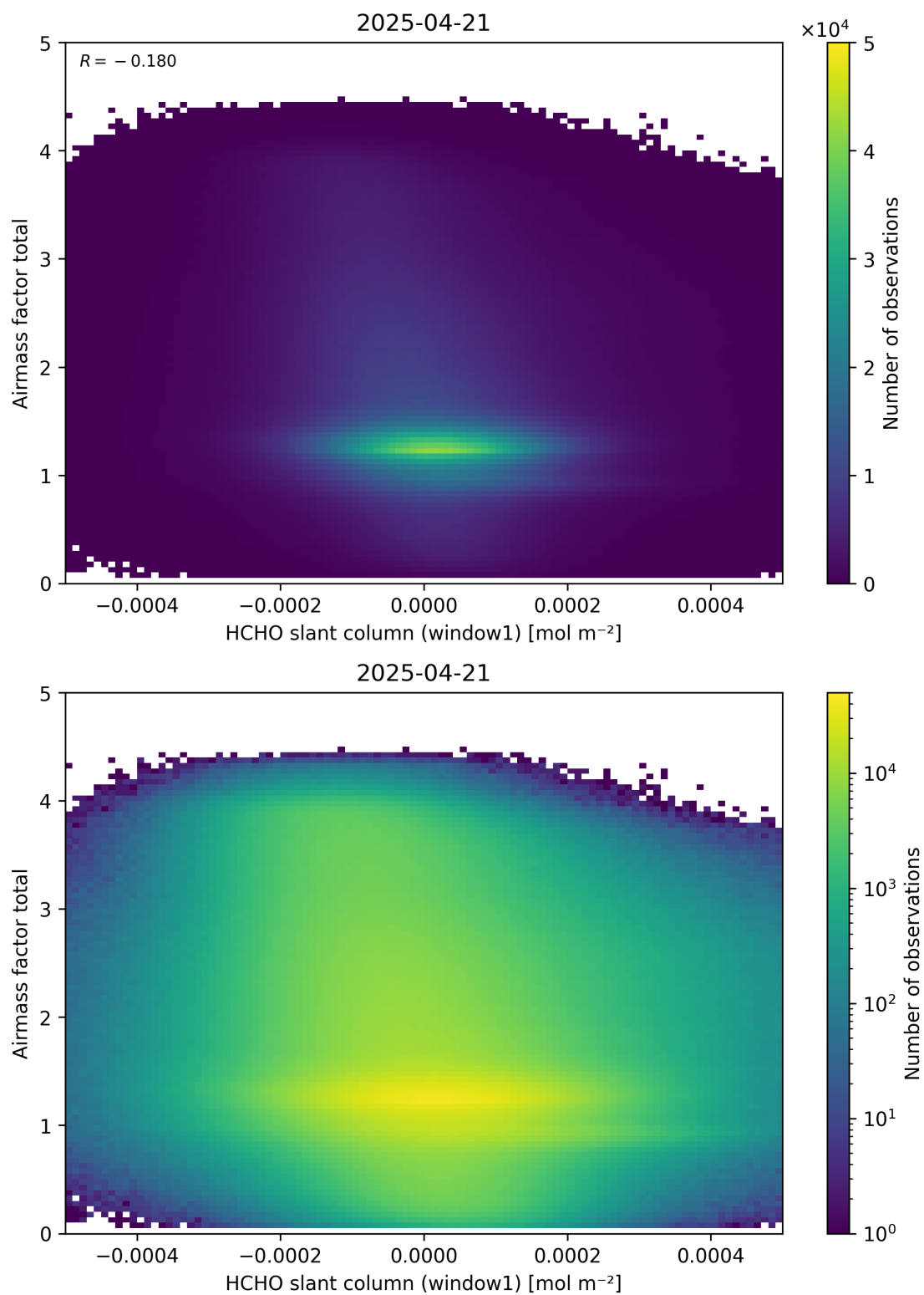
Figure 85: Scatter density plot of “HCHO slant column (window1)” against “Airmass factor total” for 2025-04-20 to 2025-04-22.
