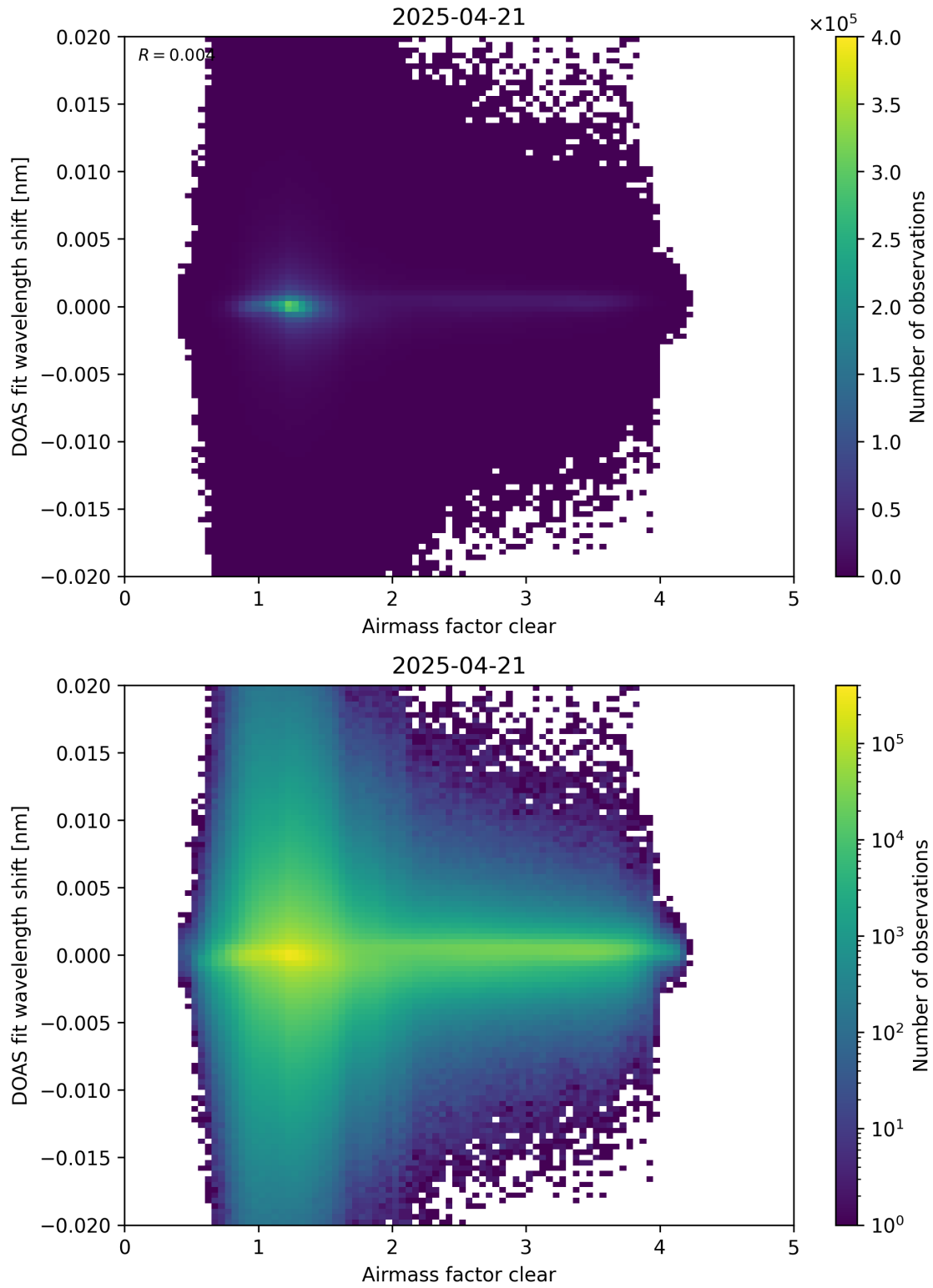
Figure 72: Scatter density plot of “Airmass factor clear” against “DOAS fit wavelength shift” for 2025-04-20 to 2025-04-22.
