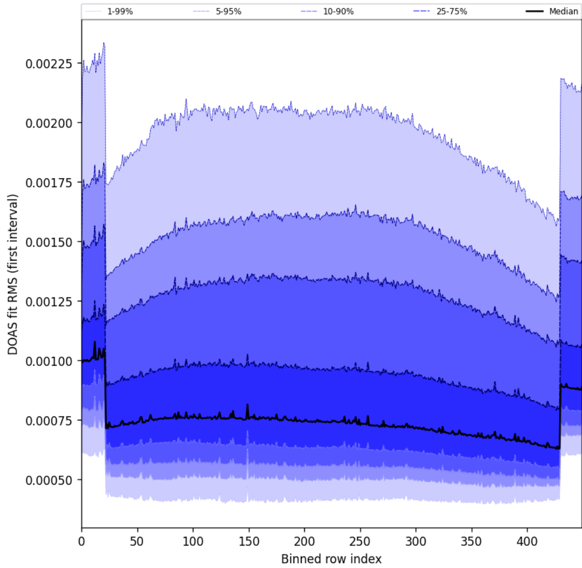
Figure 60: Along track statistics of “DOAS fit RMS (first interval)” for 2025-04-20 to 2025-04-22
