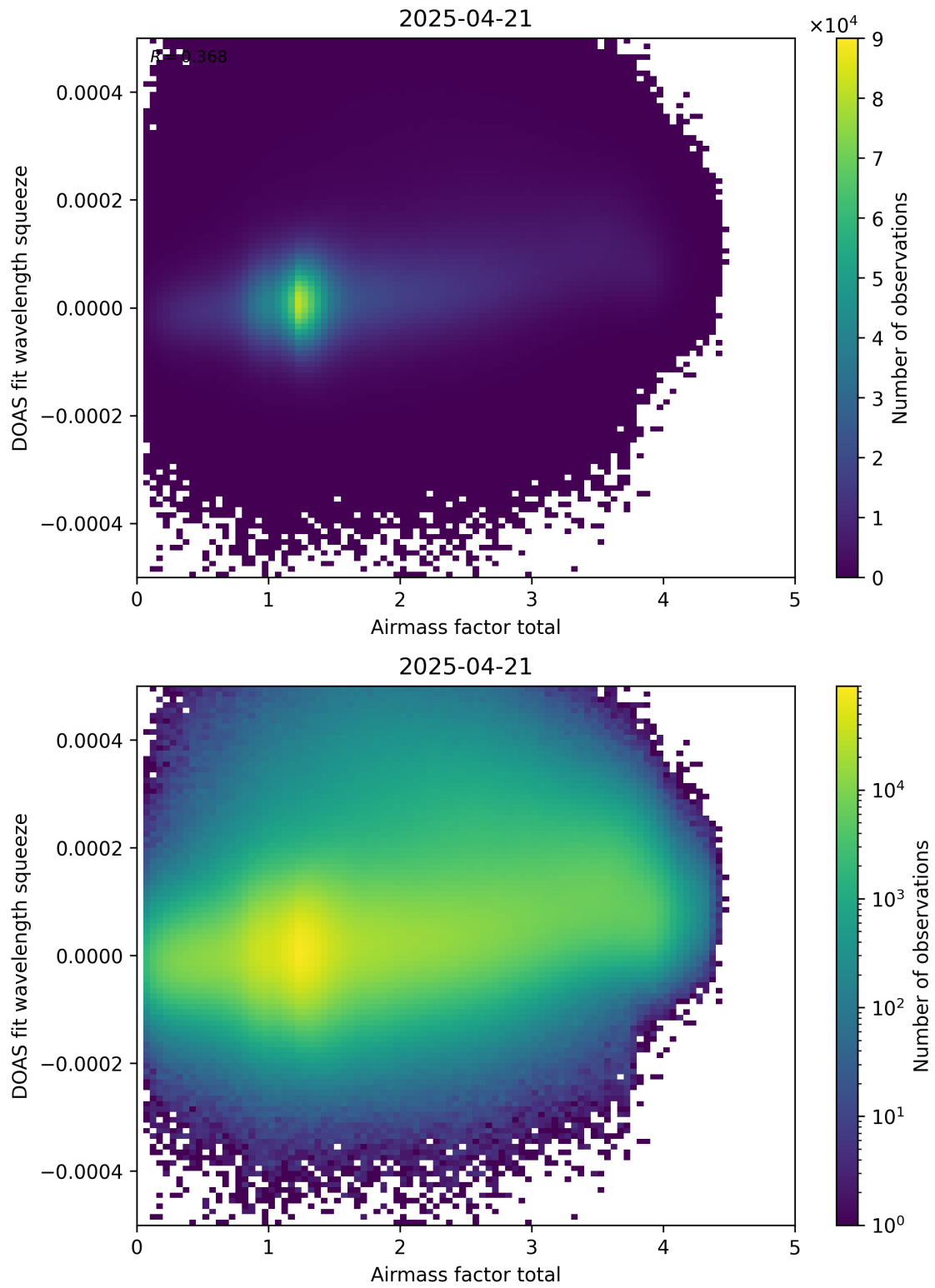
Figure 99: Scatter density plot of “Airmass factor total” against “DOAS fit wavelength squeeze” for 2025-04-20 to 2025-04-22.
