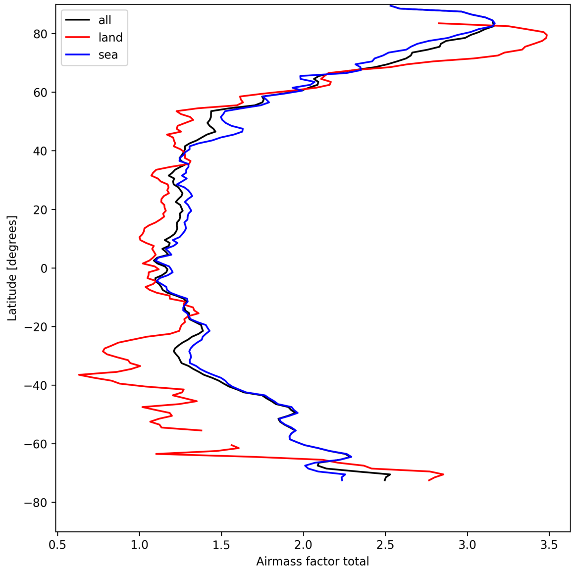
Figure 26: Zonal average of “Airmass factor total” for 2025-04-20 to 2025-04-22.
