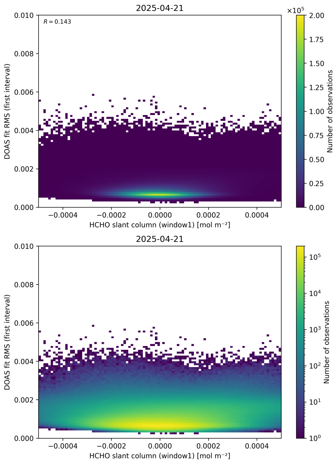
Figure 78: Scatter density plot of “HCHO slant column (window1)” against “DOAS fit RMS (first interval)” for 2025-04-20 to 2025-04-22.
