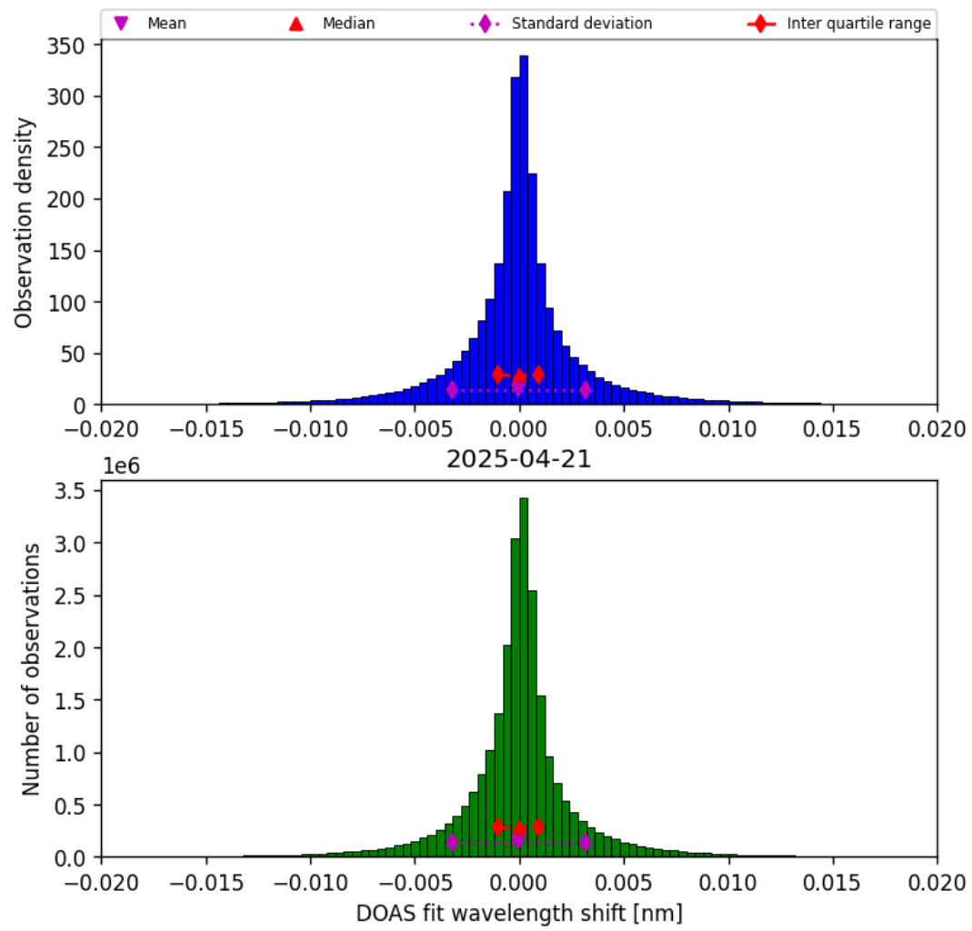
Figure 44: Histogram of “DOAS fit wavelength shift” for 2025-04-20 to 2025-04-22
