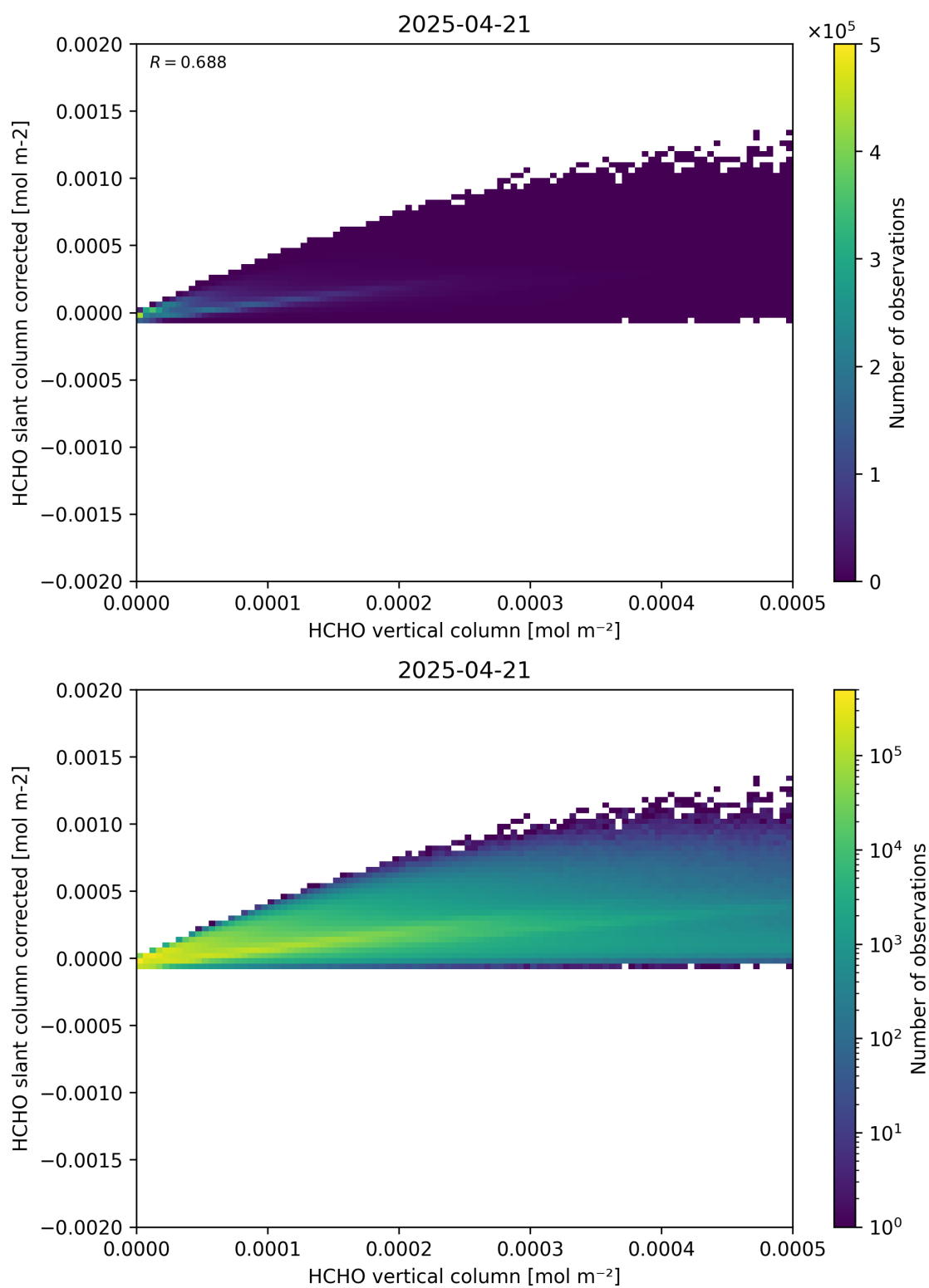
Figure 127: Scatter density plot of “HCHO vertical column” against “HCHO slant column corrected” for 2025-04-20 to 2025-04-22.
