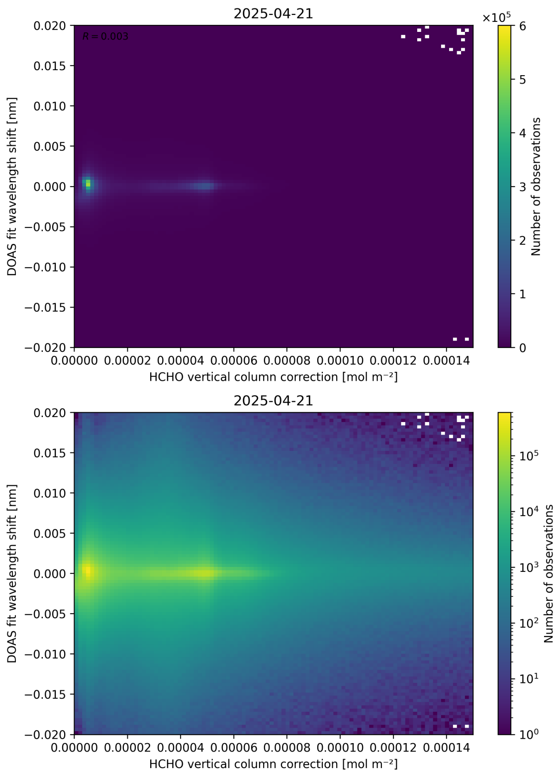
Figure 113: Scatter density plot of “HCHO vertical column correction” against “DOAS fit wavelength shift” for 2025-04-20 to 2025-04-22.
