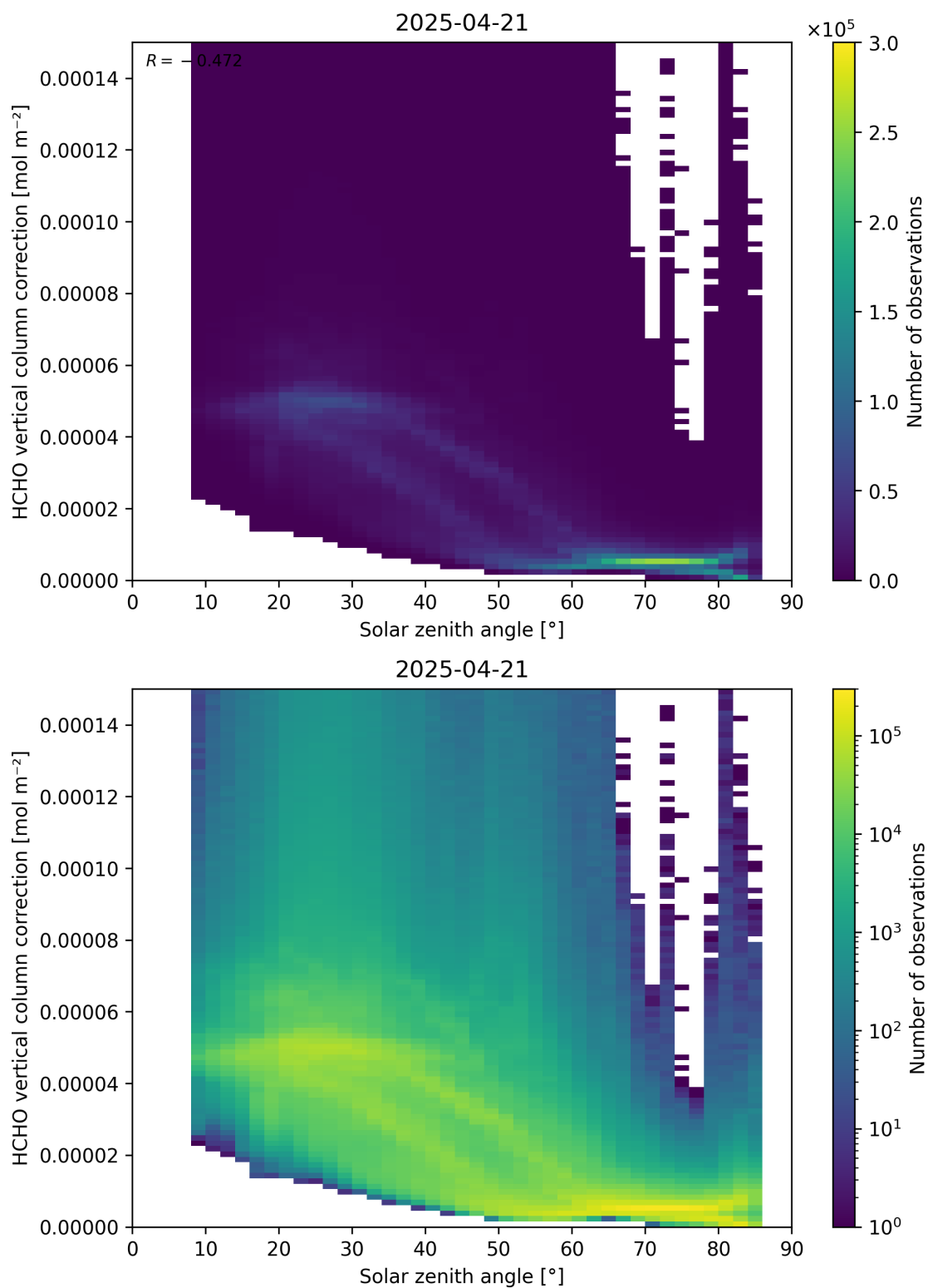
Figure 178: Scatter density plot of “Solar zenith angle” against “HCHO vertical column correction” for 2025-04-20 to 2025-04-22.
