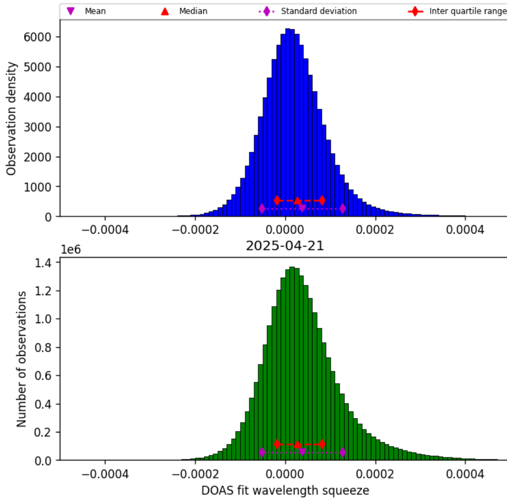
Figure 45: Histogram of “DOAS fit wavelength squeeze” for 2025-04-20 to 2025-04-22
