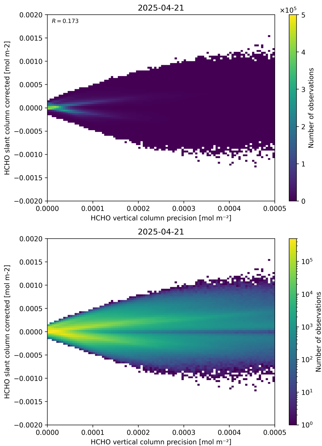
Figure 140: Scatter density plot of “HCHO vertical column precision” against “HCHO slant column corrected” for 2025-04-20 to 2025-04-22.
