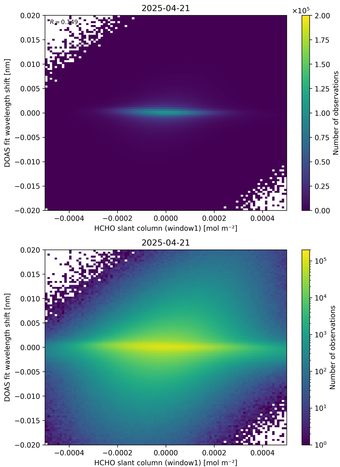
Figure 79: Scatter density plot of “HCHO slant column (window1)” against “DOAS fit wavelength shift” for 2025-04-20 to 2025-04-22.
