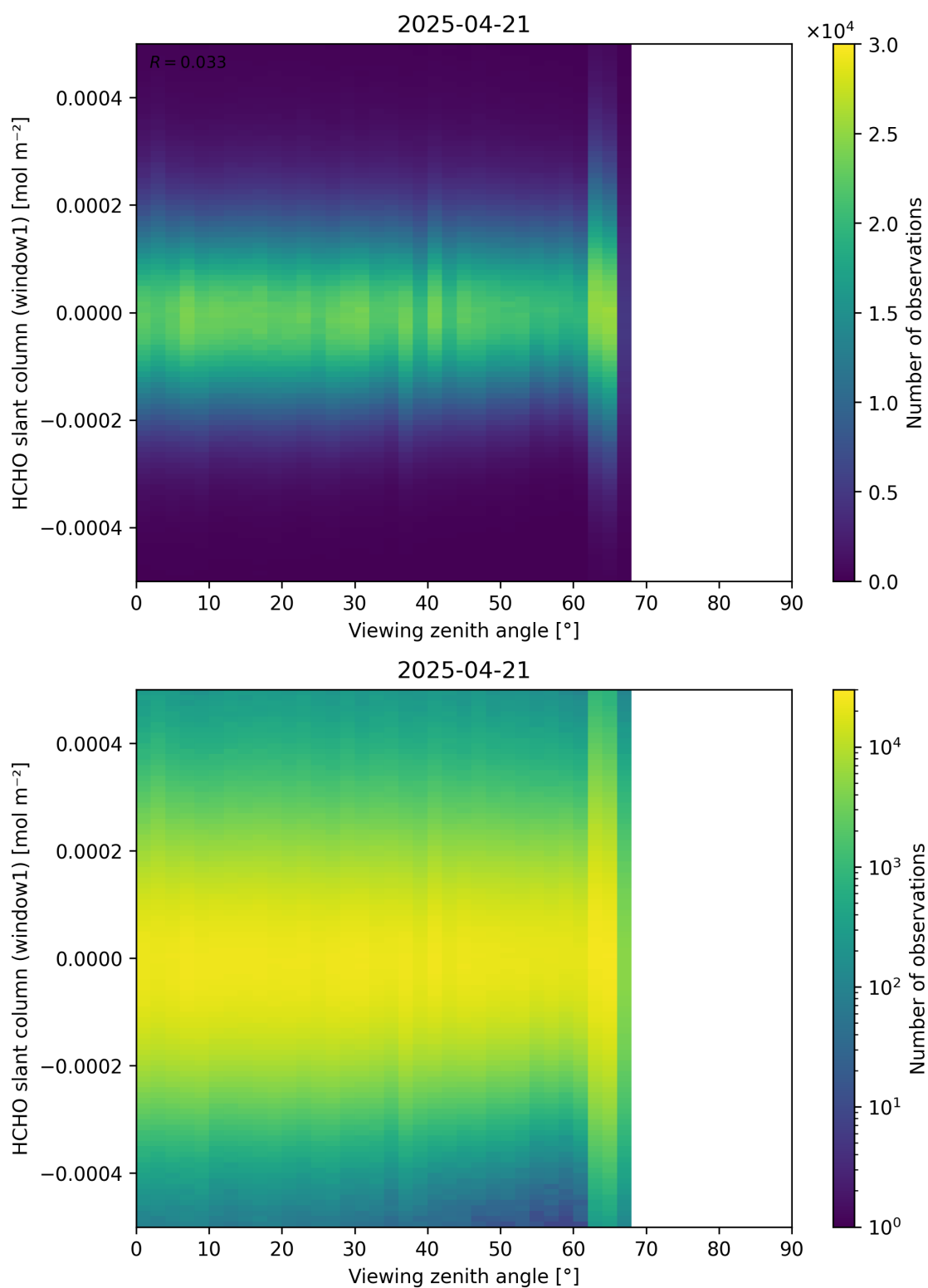
Figure 188: Scatter density plot of “Viewing zenith angle” against “HCHO slant column (window1)” for 2025-04-20 to 2025-04-22.
