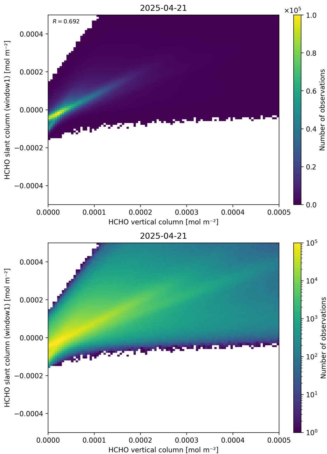
Figure 129: Scatter density plot of “HCHO vertical column” against “HCHO slant column (window1)” for 2025-04-20 to 2025-04-22.
