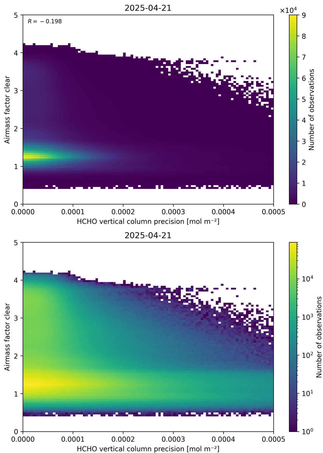
Figure 139: Scatter density plot of “HCHO vertical column precision” against “Airmass factor clear” for 2025-04-20 to 2025-04-22.
