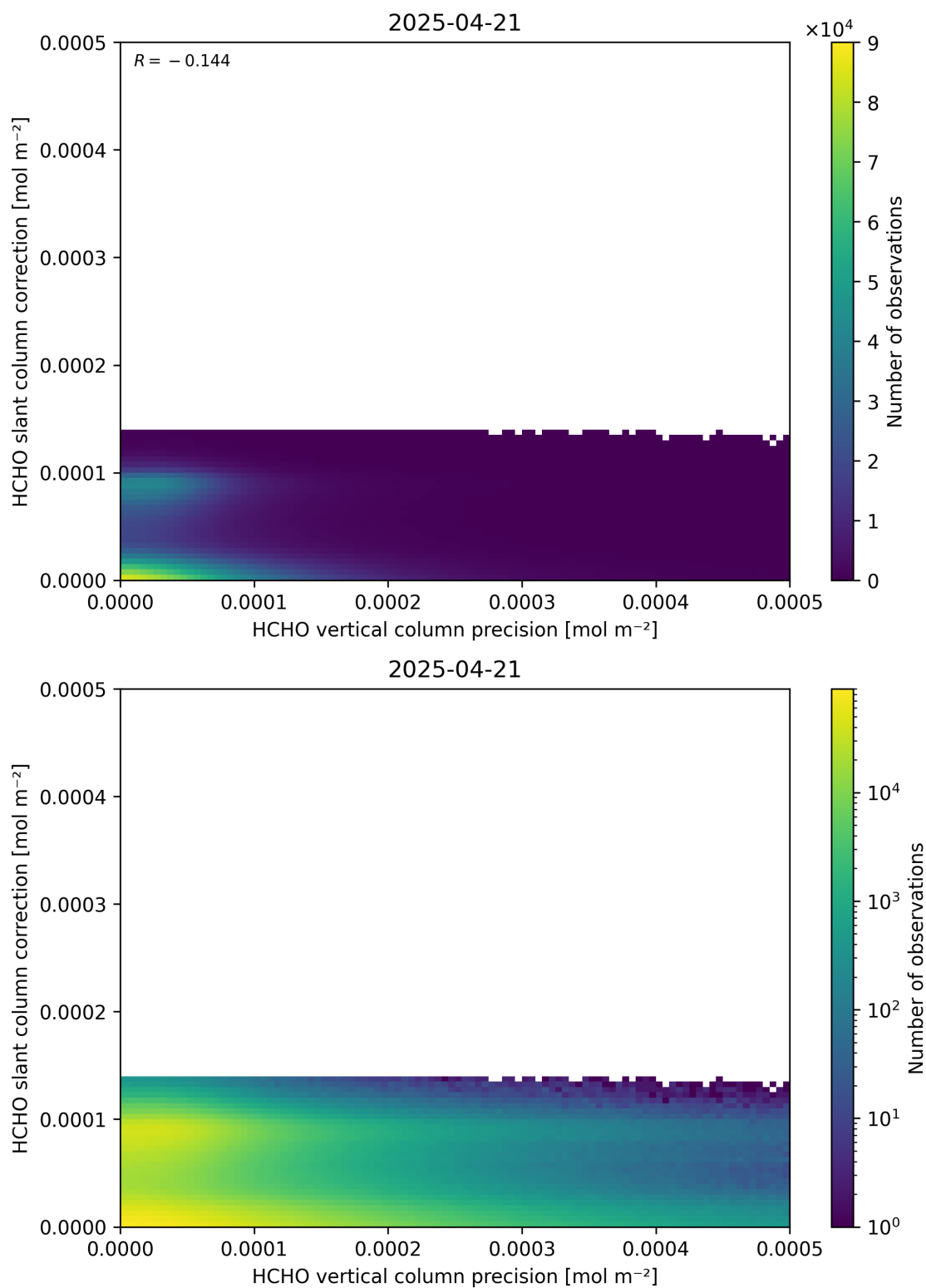
Figure 141: Scatter density plot of “HCHO vertical column precision” against “HCHO slant column correction” for 2025-04-20 to 2025-04-22.
