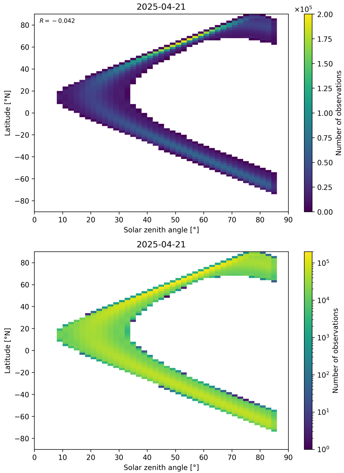
Figure 181: Scatter density plot of “Solar zenith angle” against “Latitude” for 2025-04-20 to 2025-04-22.
