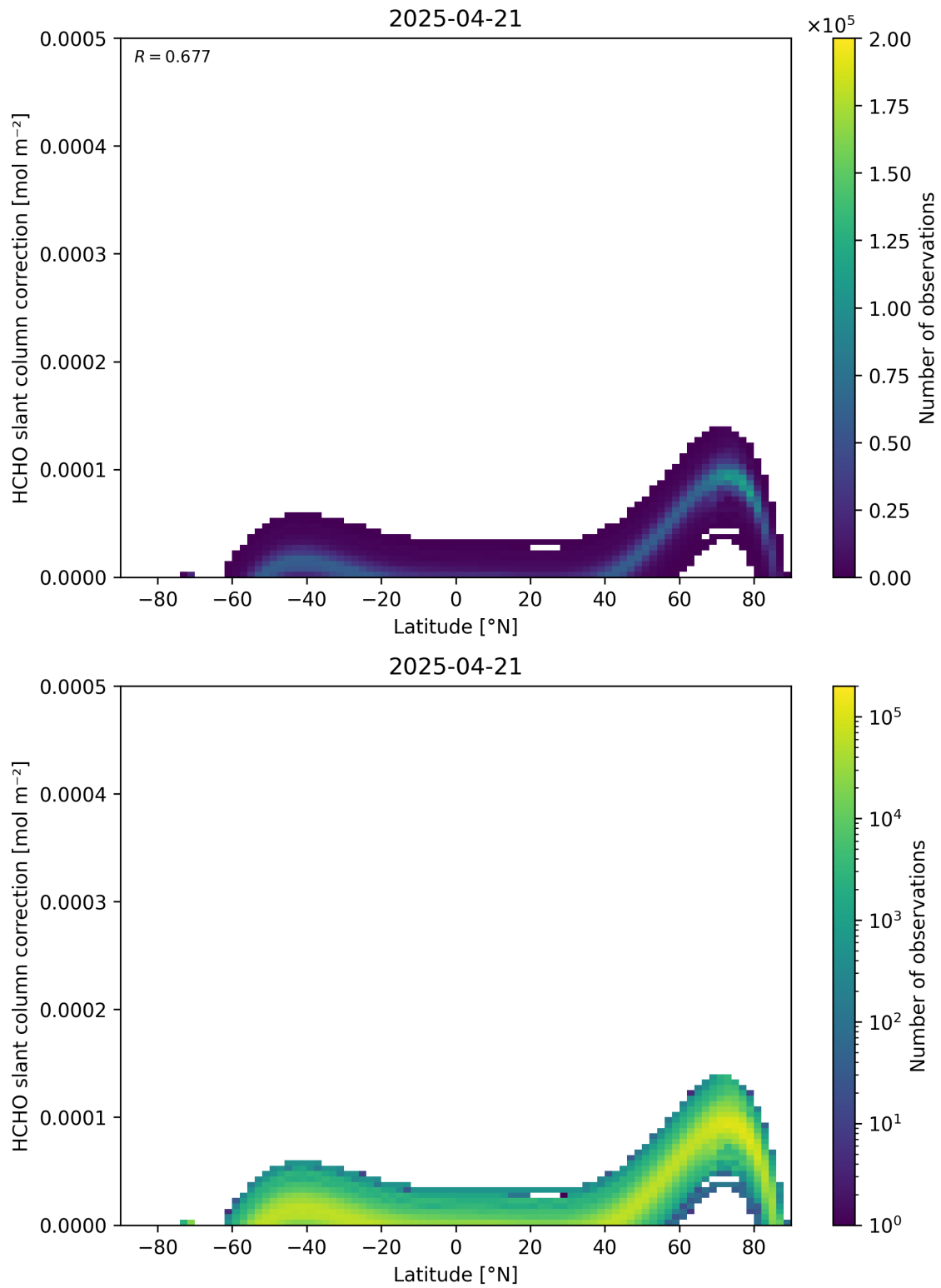
Figure 158: Scatter density plot of “Latitude” against “HCHO slant column correction” for 2025-04-20 to 2025-04-22.
