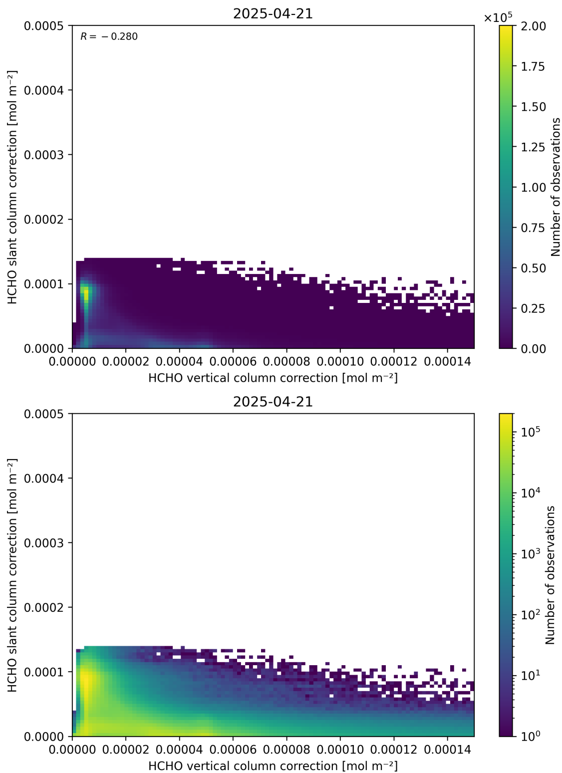
Figure 117: Scatter density plot of “HCHO vertical column correction” against “HCHO slant column correction” for 2025-04-20 to 2025-04-22.
