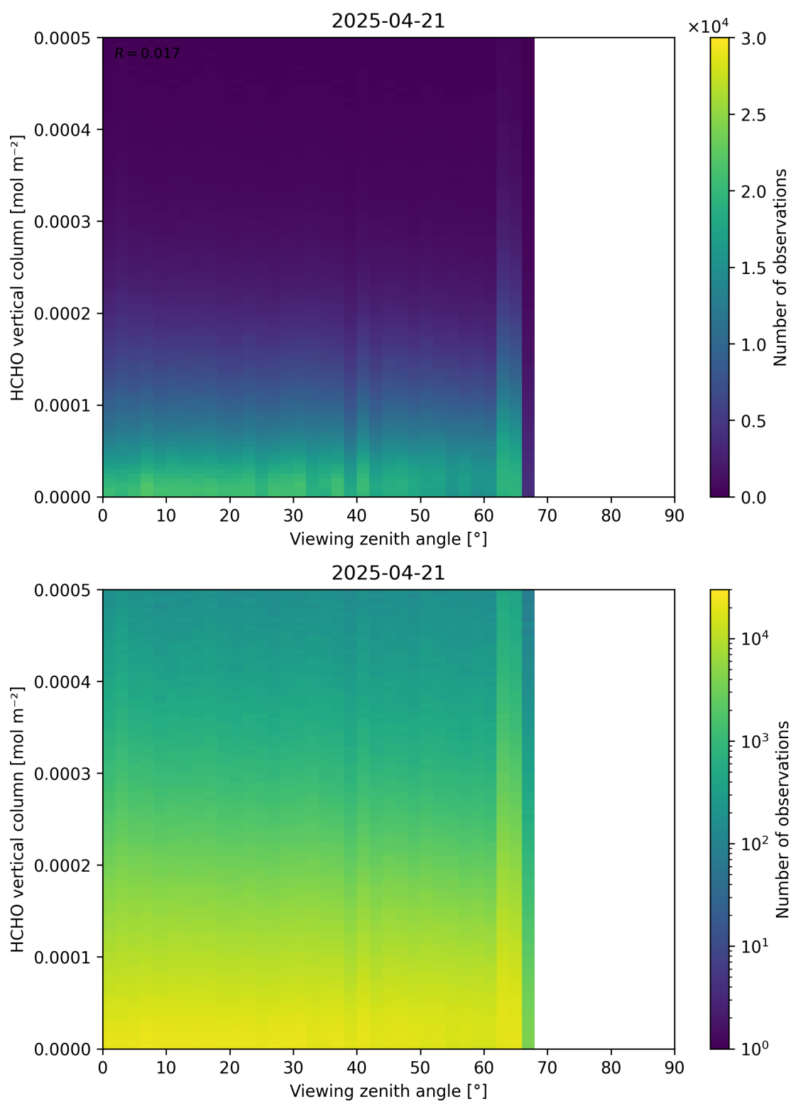
Figure 192: Scatter density plot of “Viewing zenith angle” against “HCHO vertical column” for 2025-04-20 to 2025-04-22.
