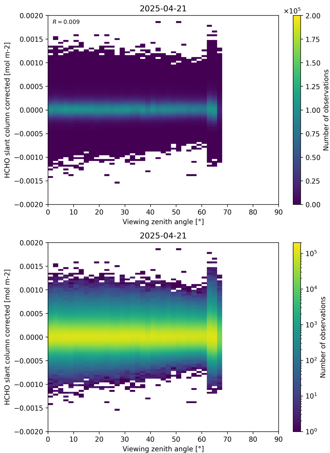
Figure 186: Scatter density plot of “Viewing zenith angle” against “HCHO slant column corrected” for 2025-04-20 to 2025-04-22.
