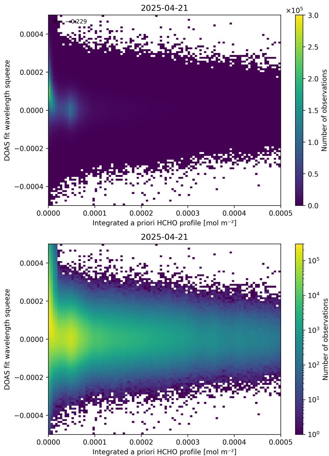
Figure 150: Scatter density plot of “Integrated a priori HCHO profile” against “DOAS fit wavelength squeeze” for 2025-04-20 to 2025-04-22.
