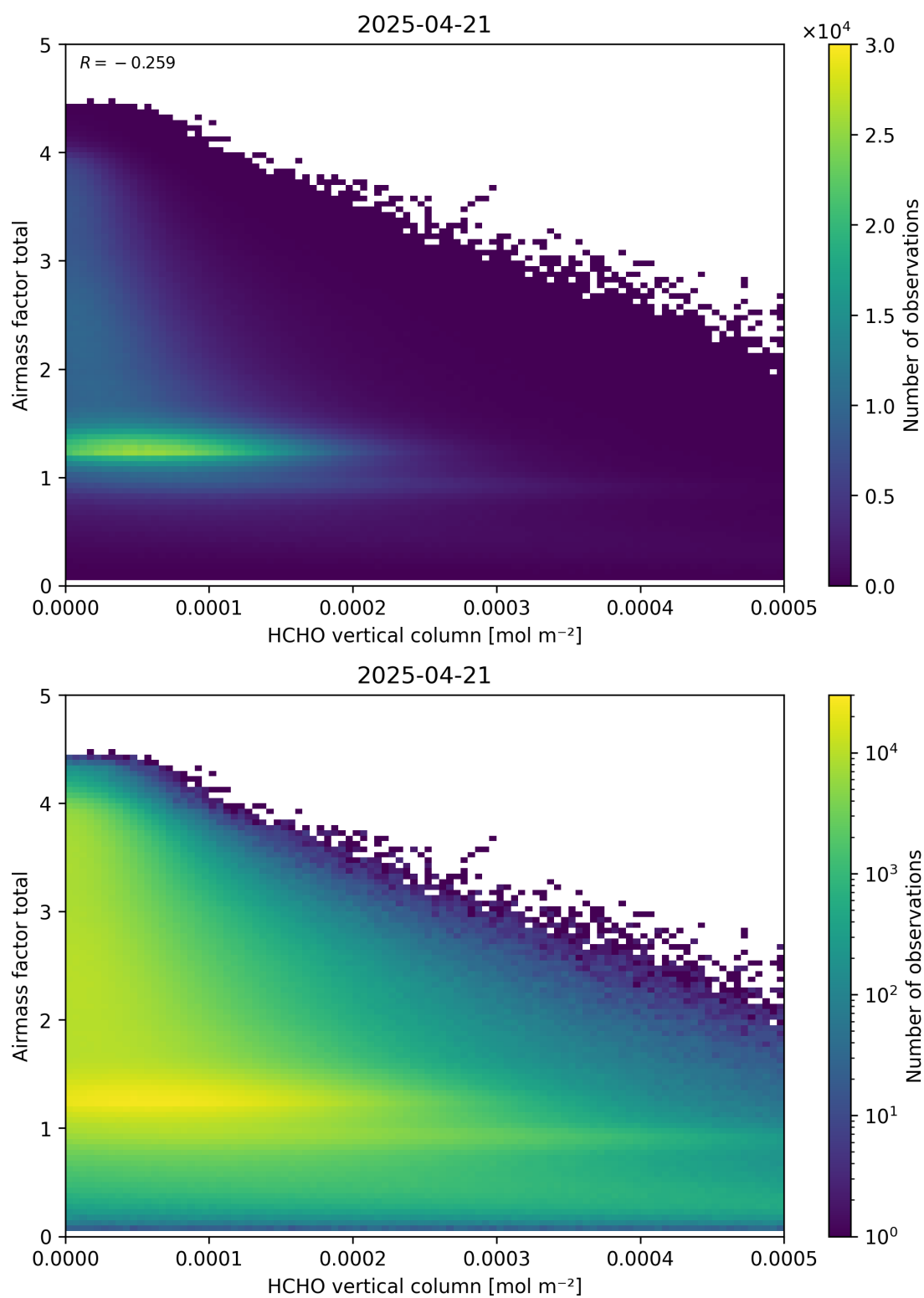
Figure 131: Scatter density plot of “HCHO vertical column” against “Airmass factor total” for 2025-04-20 to 2025-04-22.
