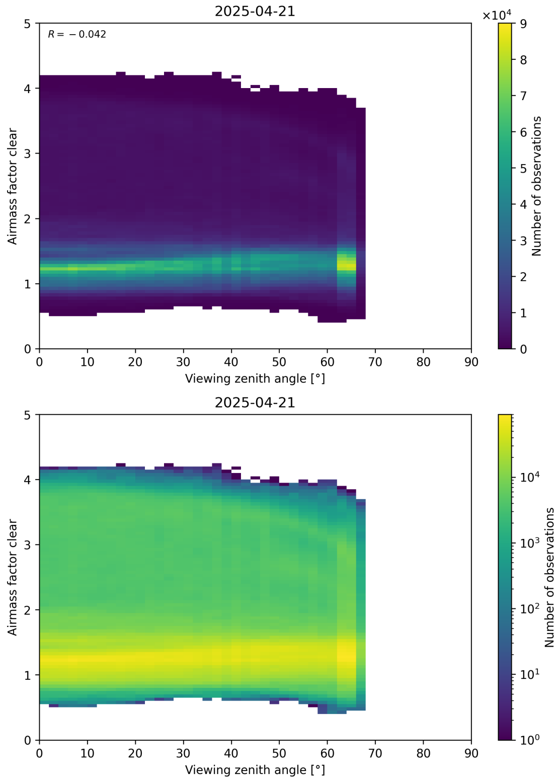
Figure 185: Scatter density plot of “Viewing zenith angle” against “Airmass factor clear” for 2025-04-20 to 2025-04-22.
