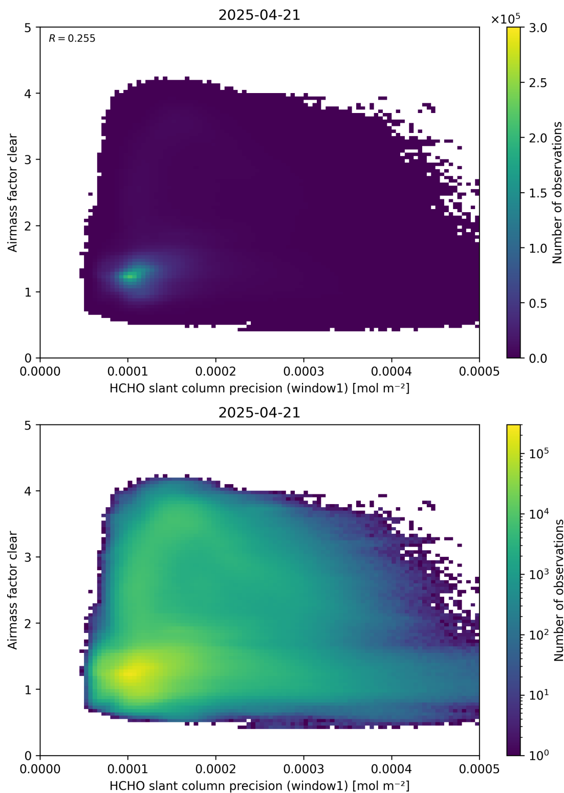
Figure 91: Scatter density plot of “HCHO slant column precision (window1)” against “Airmass factor clear” for 2025-04-20 to 2025-04-22.
