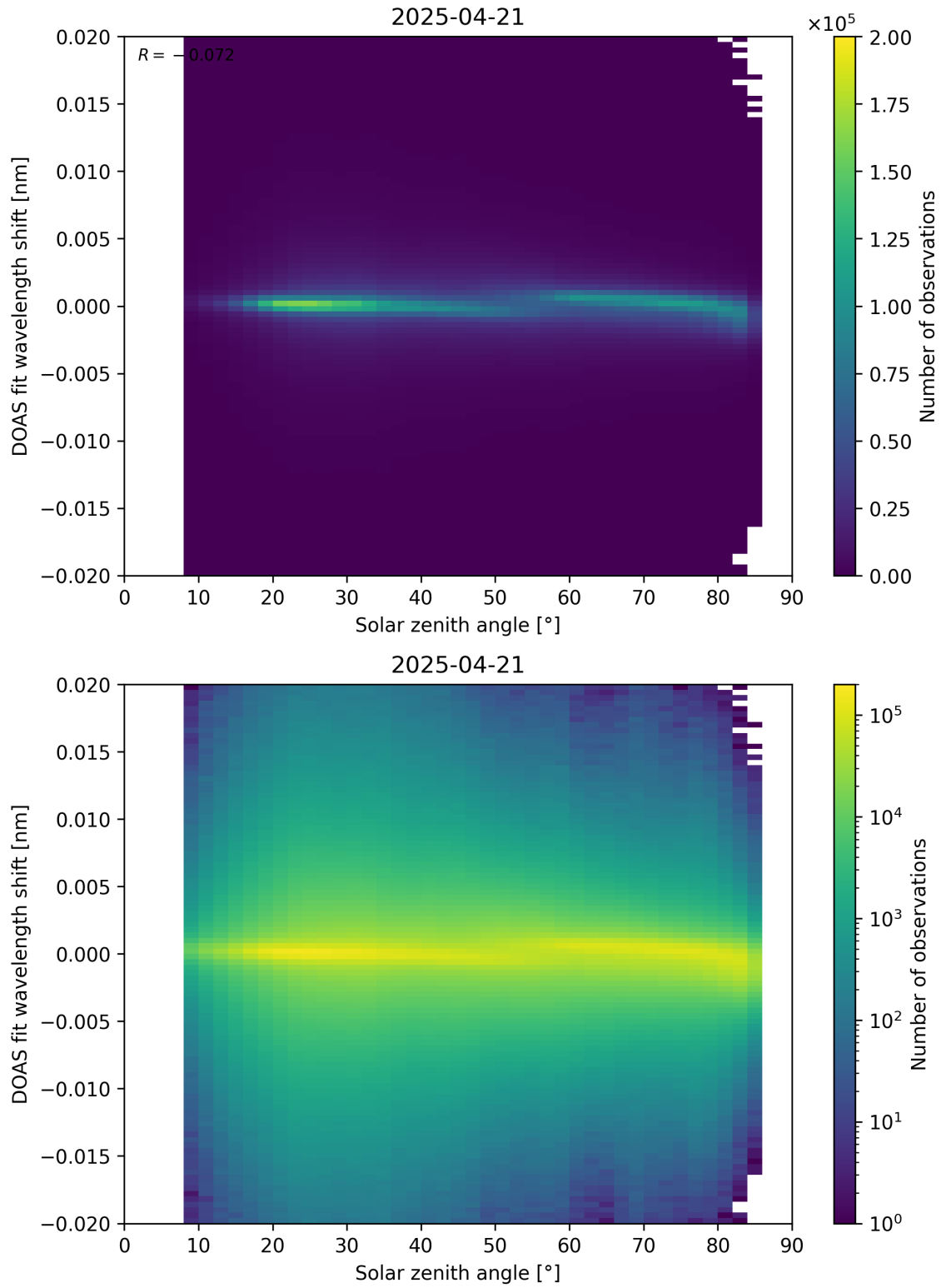
Figure 168: Scatter density plot of “Solar zenith angle” against “DOAS fit wavelength shift” for 2025-04-20 to 2025-04-22.
