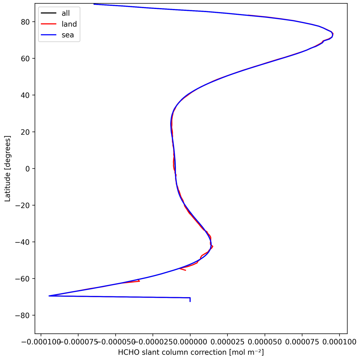
Figure 33: Zonal average of “HCHO slant column correction” for 2025-04-20 to 2025-04-22.
