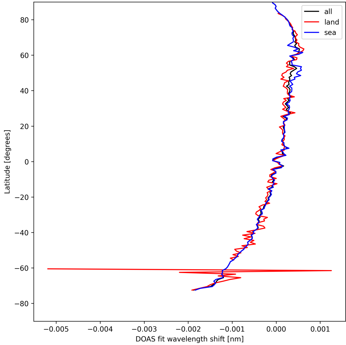
Figure 30: Zonal average of “DOAS fit wavelength shift” for 2025-04-20 to 2025-04-22.
