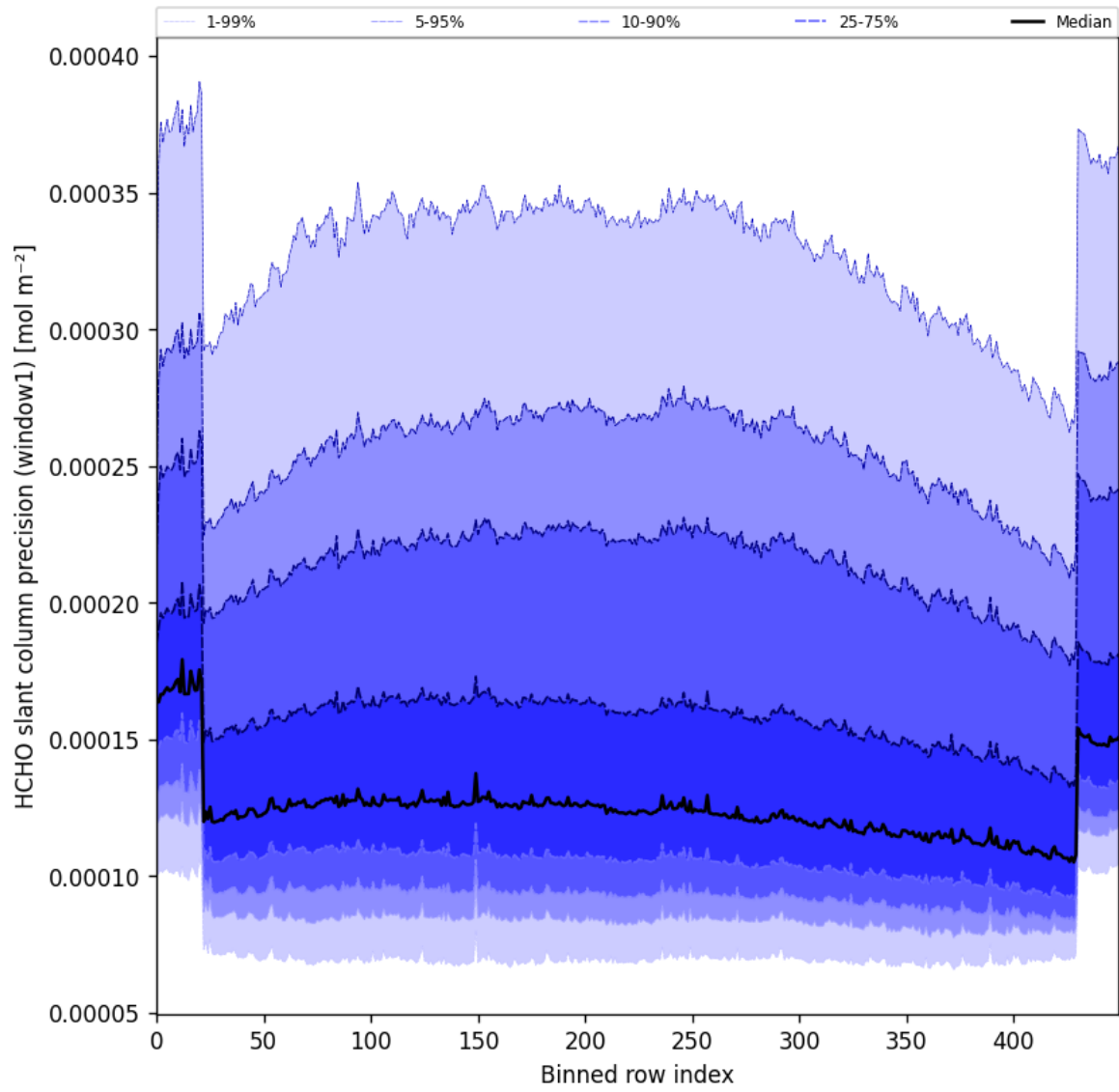
Figure 53: Along track statistics of “HCHO slant column precision (window1)” for 2025-04-20 to 2025-04-22
