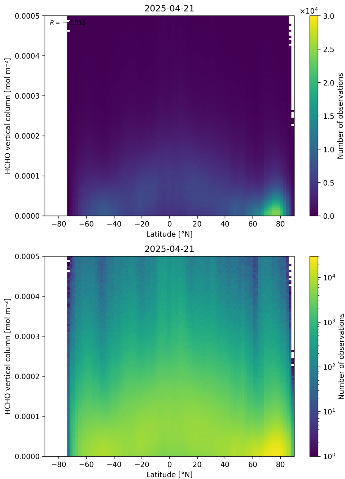
Figure 163: Scatter density plot of “Latitude” against “HCHO vertical column” for 2025-04-20 to 2025-04-22.
