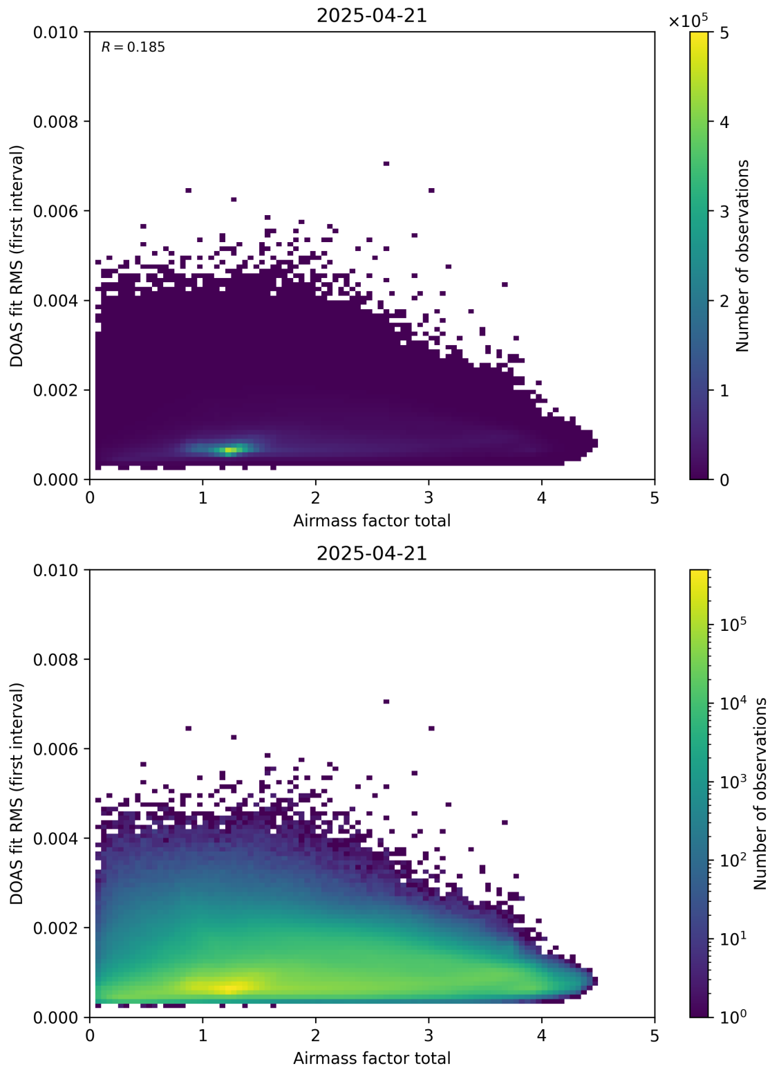
Figure 97: Scatter density plot of “Airmass factor total” against “DOAS fit RMS (first interval)” for 2025-04-20 to 2025-04-22.
