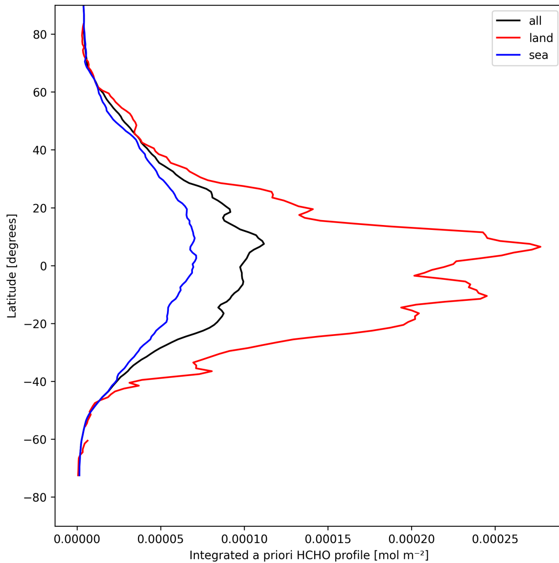
Figure 29: Zonal average of “Integrated a priori HCHO profile” for 2025-04-20 to 2025-04-22.
