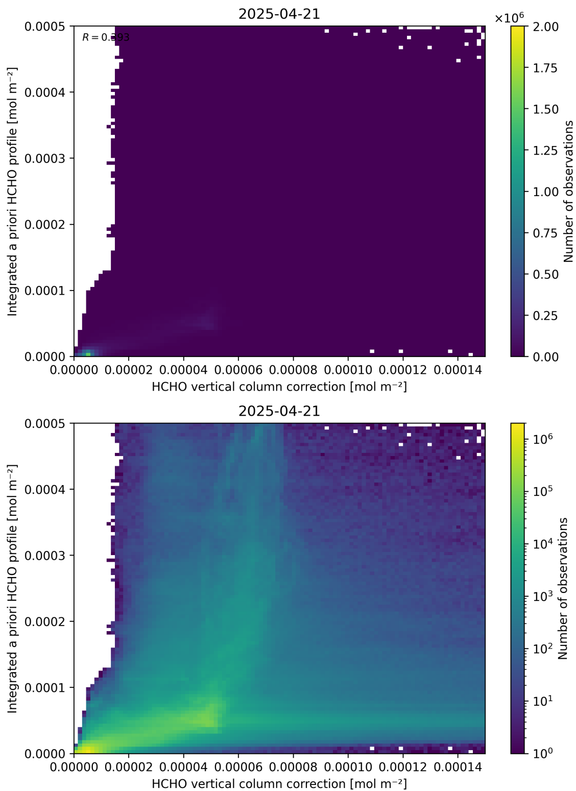
Figure 122: Scatter density plot of “HCHO vertical column correction” against “Integrated a priori HCHO profile” for 2025-04-20 to 2025-04-22.
