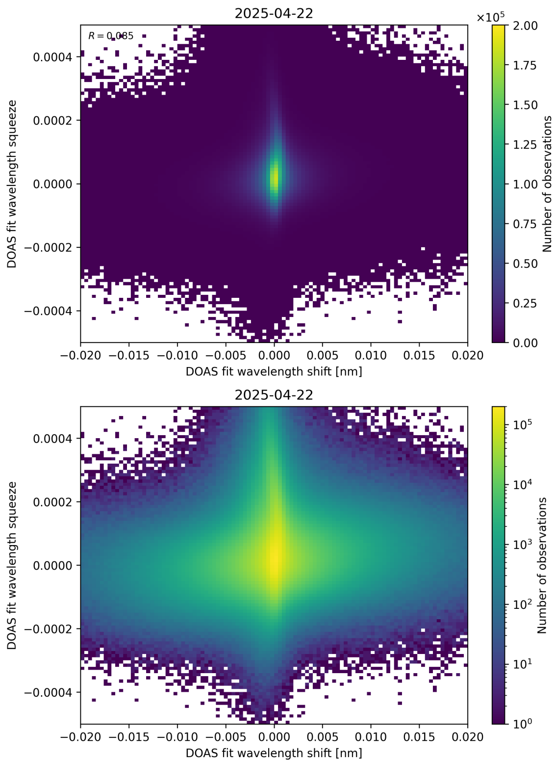
Figure 65: Scatter density plot of “DOAS fit wavelength shift” against “DOAS fit wavelength squeeze” for 2025-04-21 to 2025-04-23.
