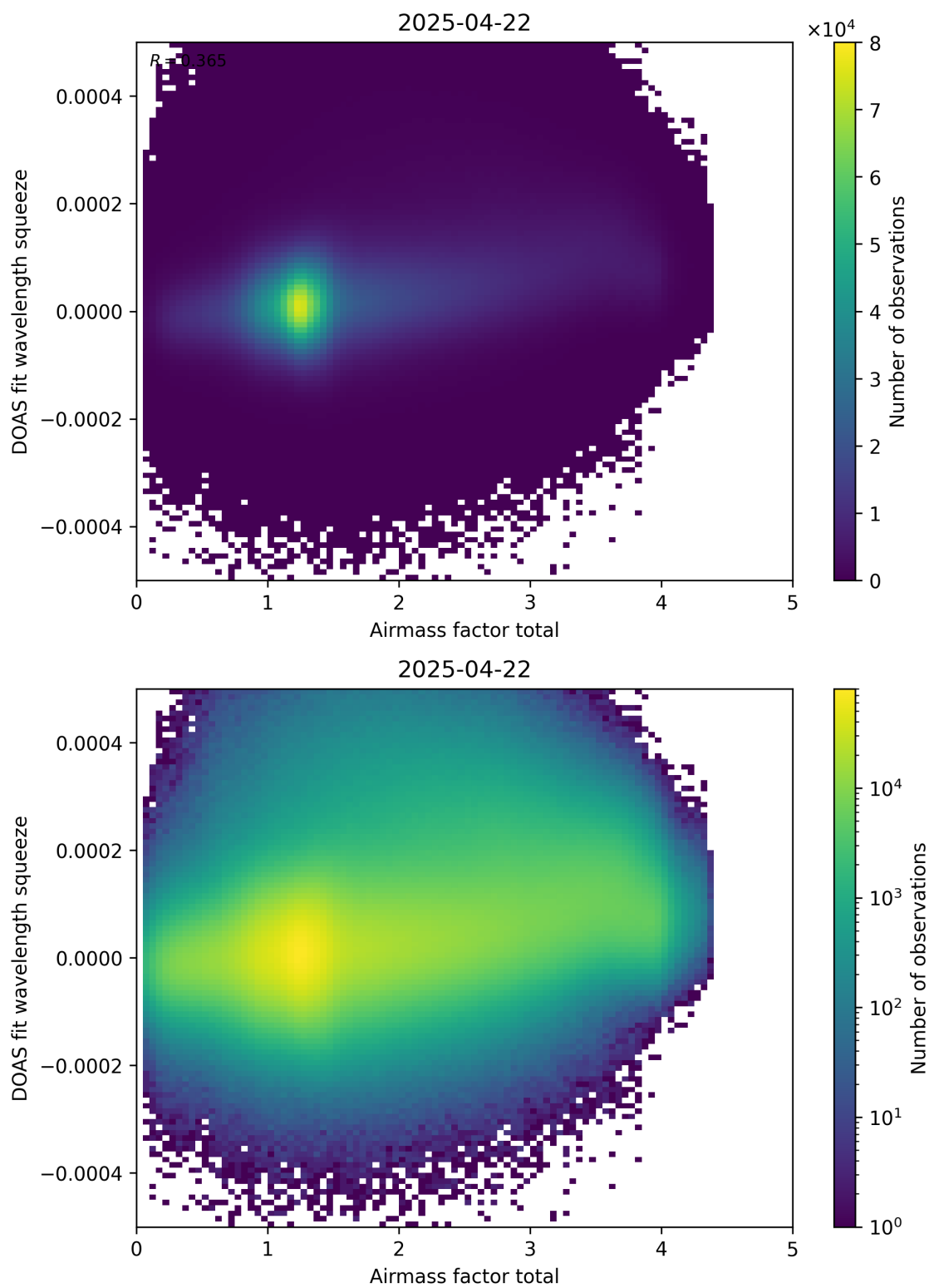
Figure 99: Scatter density plot of “Airmass factor total” against “DOAS fit wavelength squeeze” for 2025-04-21 to 2025-04-23.
