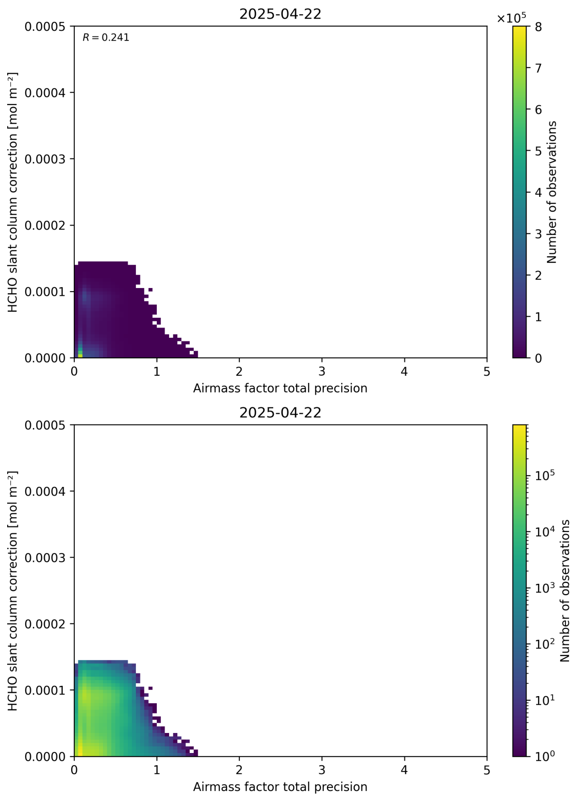
Figure 110: Scatter density plot of “Airmass factor total precision” against “HCHO slant column correction” for 2025-04-21 to 2025-04-23.
