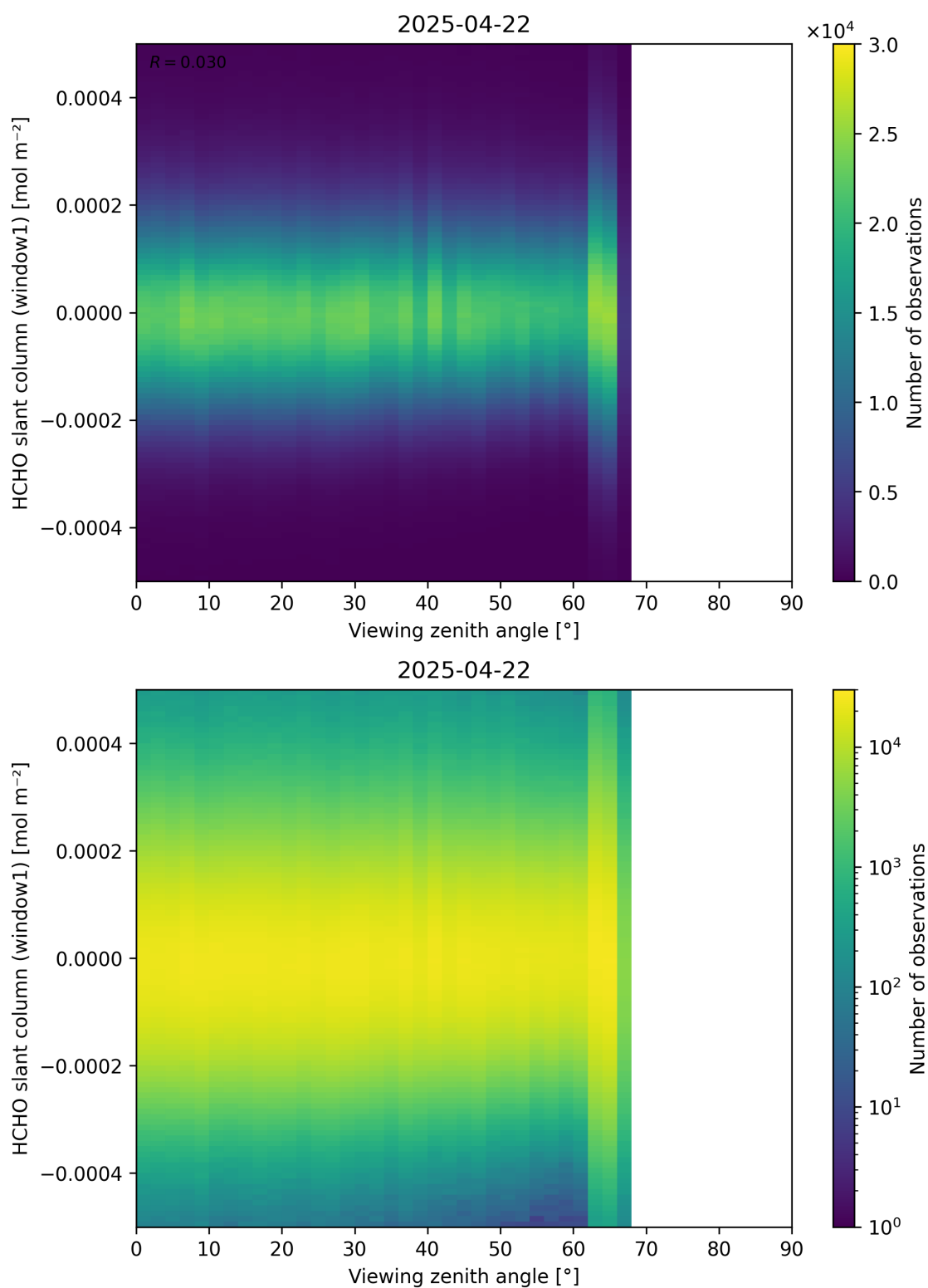
Figure 188: Scatter density plot of “Viewing zenith angle” against “HCHO slant column (window1)” for 2025-04-21 to 2025-04-23.
