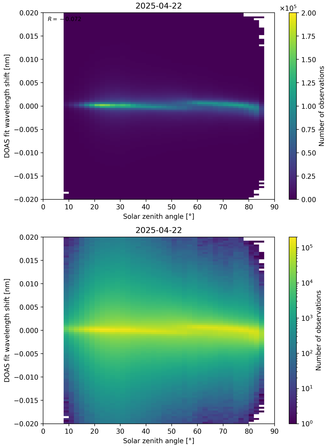
Figure 168: Scatter density plot of “Solar zenith angle” against “DOAS fit wavelength shift” for 2025-04-21 to 2025-04-23.
