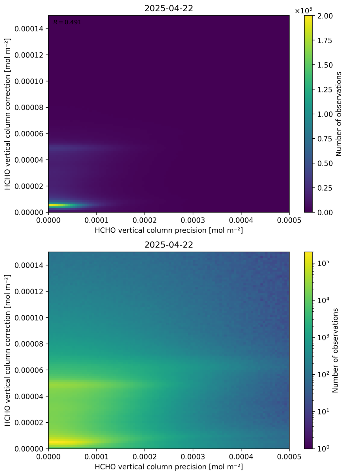
Figure 146: Scatter density plot of “HCHO vertical column precision” against “HCHO vertical column correction” for 2025-04-21 to 2025-04-23.
