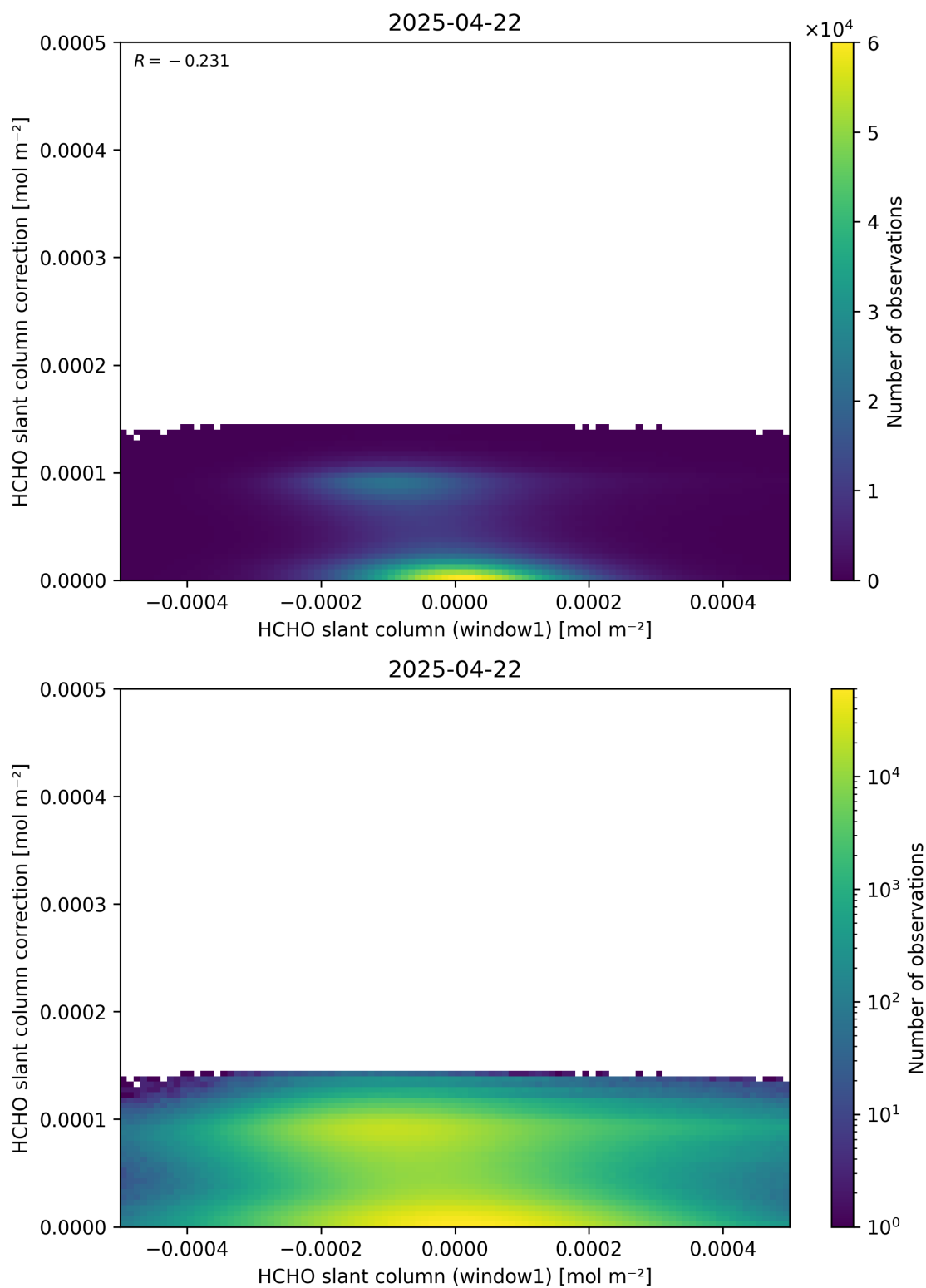
Figure 83: Scatter density plot of “HCHO slant column (window1)” against “HCHO slant column correction” for 2025-04-21 to 2025-04-23.
