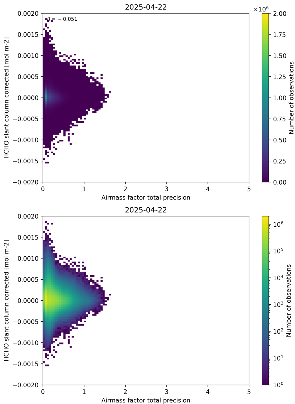
Figure 109: Scatter density plot of “Airmass factor total precision” against “HCHO slant column corrected” for 2025-04-21 to 2025-04-23.
