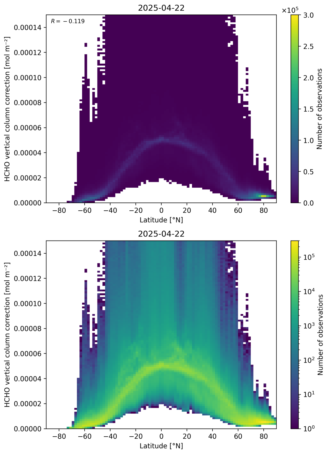
Figure 164: Scatter density plot of “Latitude” against “HCHO vertical column correction” for 2025-04-21 to 2025-04-23.
