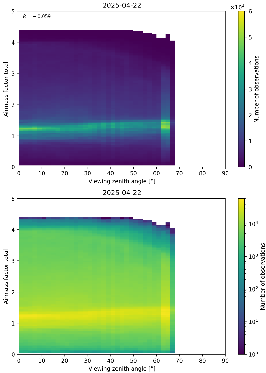
Figure 190: Scatter density plot of “Viewing zenith angle” against “Airmass factor total” for 2025-04-21 to 2025-04-23.
