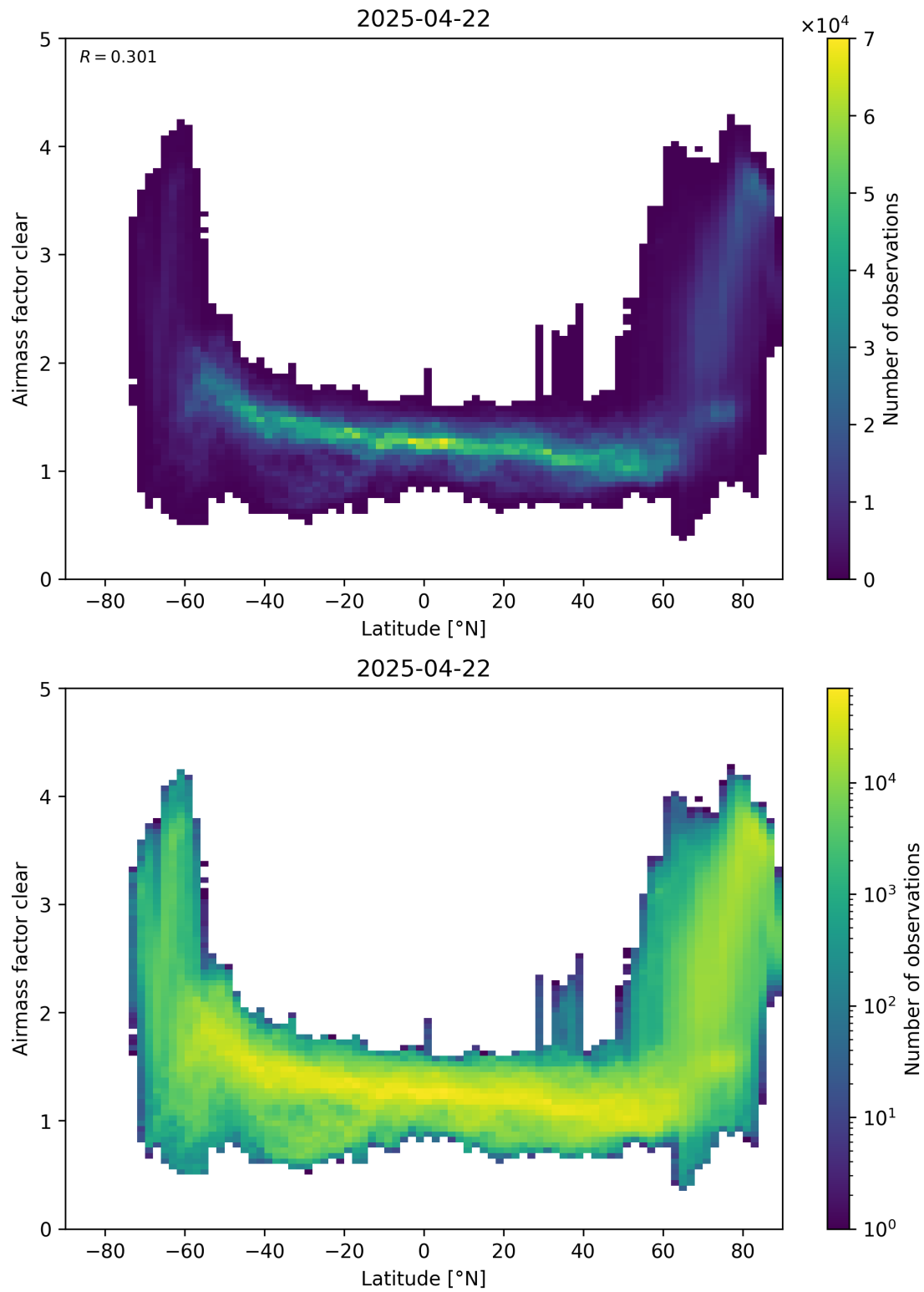
Figure 156: Scatter density plot of “Latitude” against “Airmass factor clear” for 2025-04-21 to 2025-04-23.
