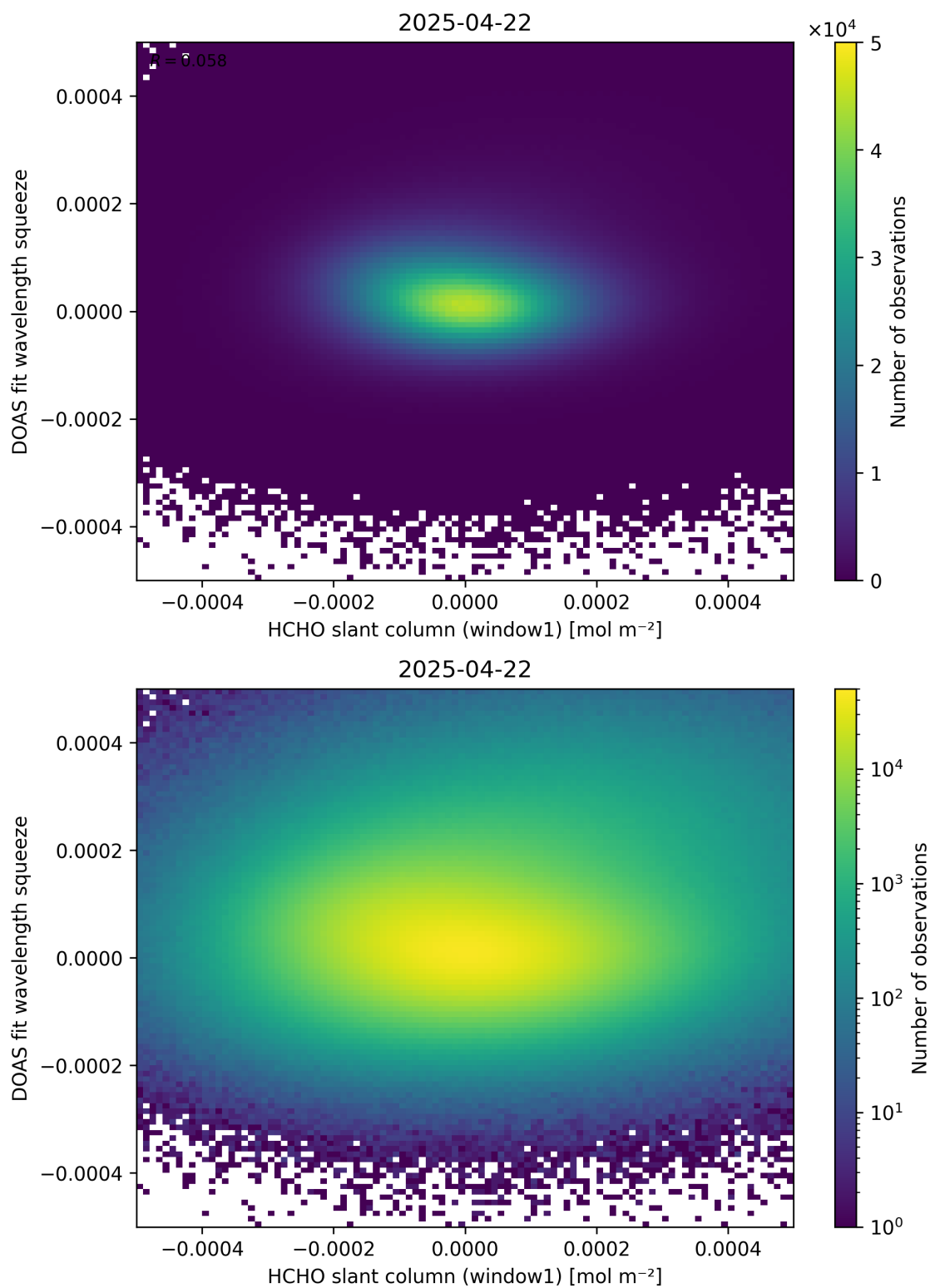
Figure 80: Scatter density plot of “HCHO slant column (window1)” against “DOAS fit wavelength squeeze” for 2025-04-21 to 2025-04-23.
