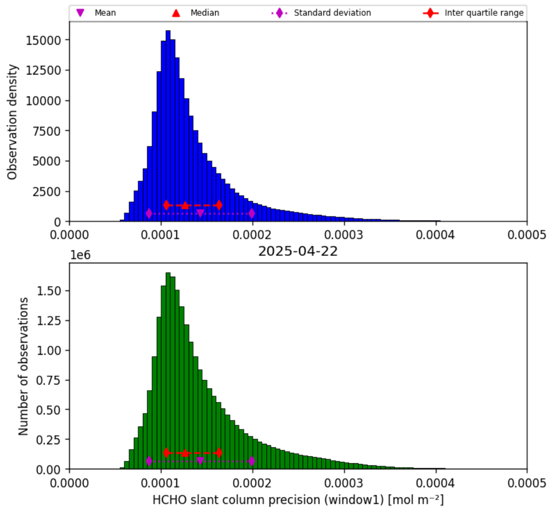
Figure 39: Histogram of “HCHO slant column precision (window1)” for 2025-04-21 to 2025-04-23
