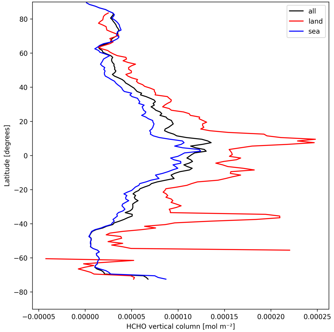
Figure 21: Zonal average of “HCHO vertical column” for 2025-04-21 to 2025-04-23.
