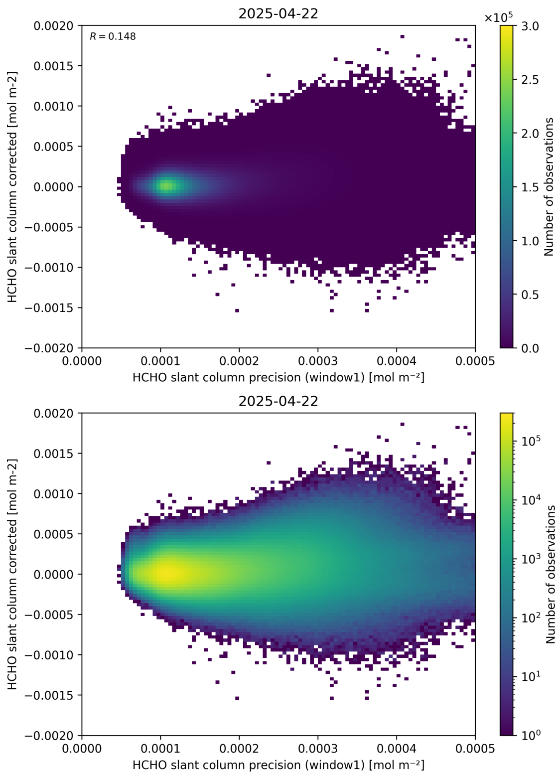
Figure 92: Scatter density plot of “HCHO slant column precision (window1)” against “HCHO slant column corrected” for 2025-04-21 to 2025-04-23.
