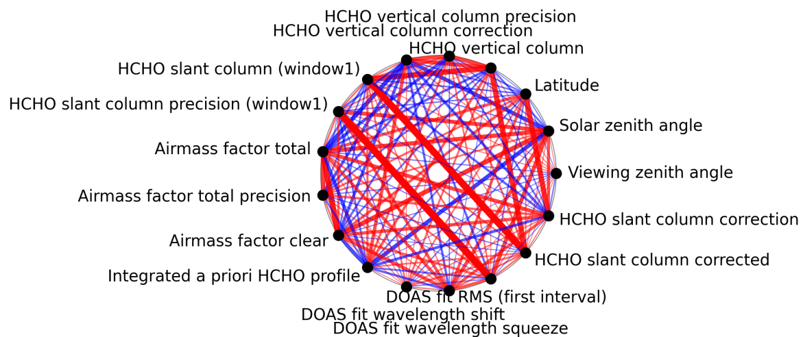
Figure 1: Map of correlation graph for 2025-04-21 to 2025-04-23.
