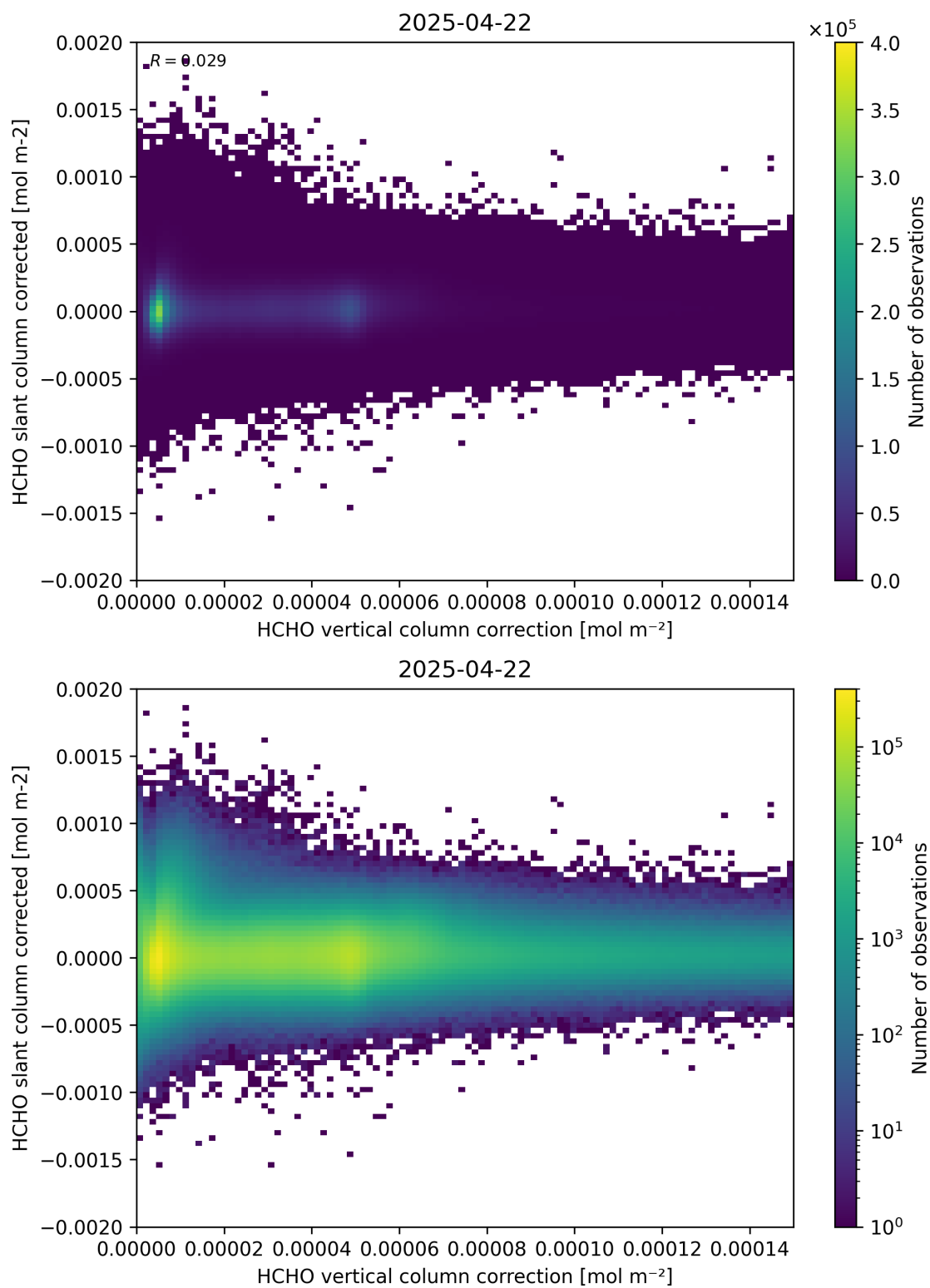
Figure 116: Scatter density plot of “HCHO vertical column correction” against “HCHO slant column corrected” for 2025-04-21 to 2025-04-23.
