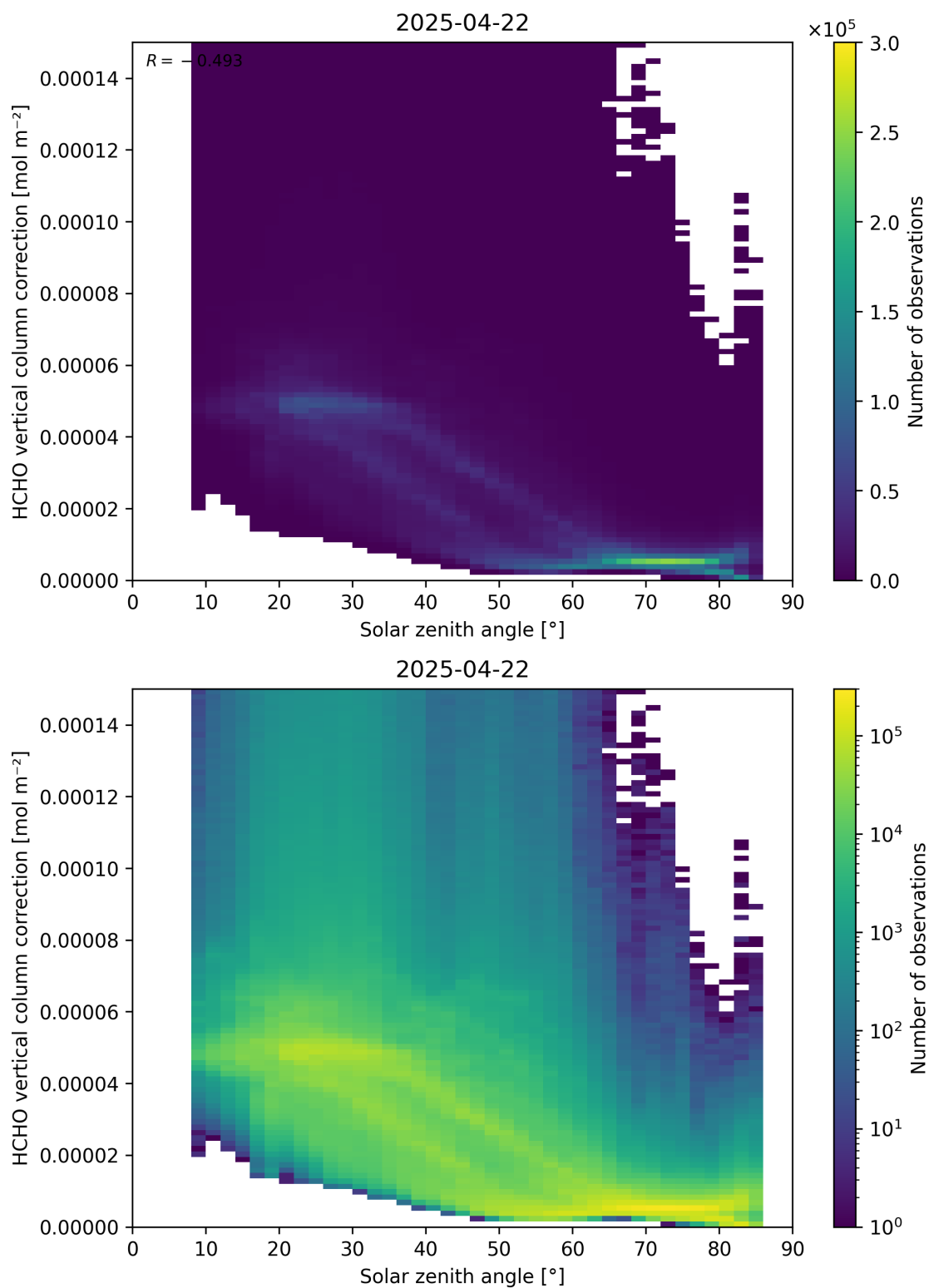
Figure 178: Scatter density plot of “Solar zenith angle” against “HCHO vertical column correction” for 2025-04-21 to 2025-04-23.
