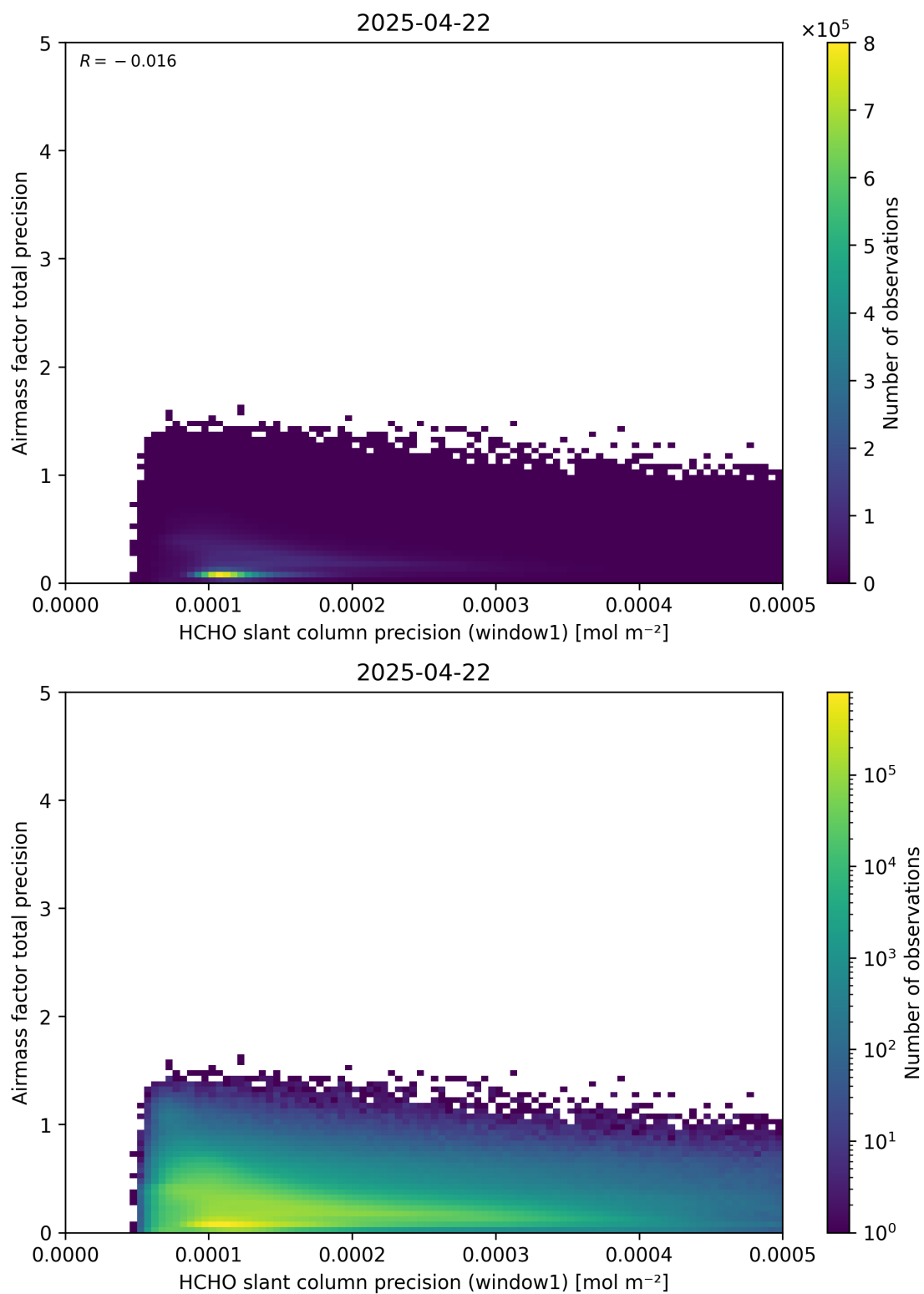
Figure 95: Scatter density plot of “HCHO slant column precision (window1)” against “Airmass factor total precision” for 2025-04-21 to 2025-04-23.
