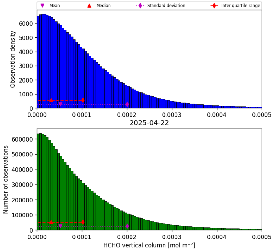
Figure 35: Histogram of “HCHO vertical column” for 2025-04-21 to 2025-04-23
