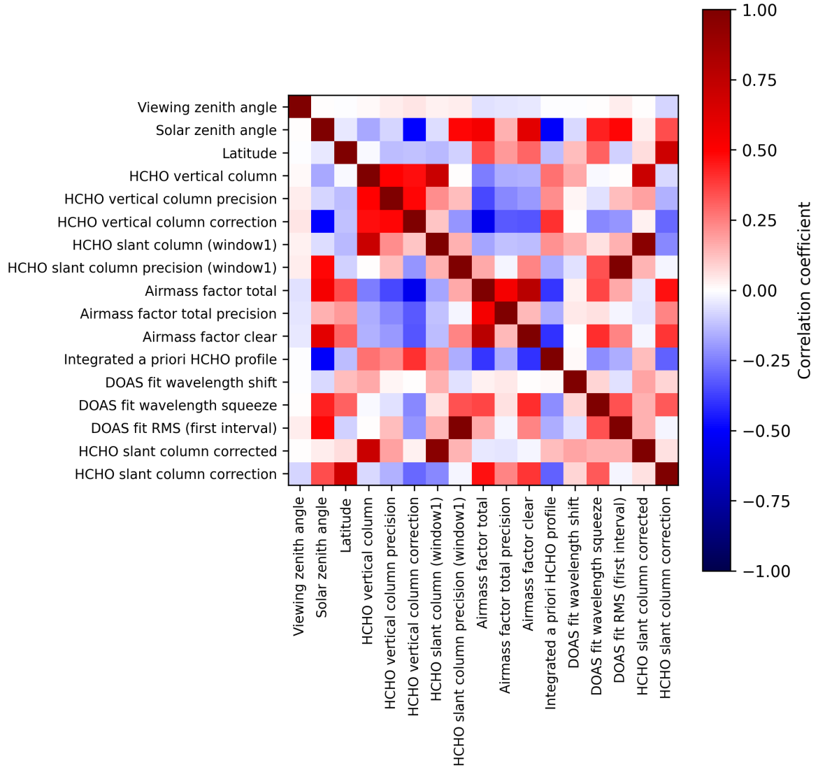
Figure 2: Map of correlation matrix for 2025-04-21 to 2025-04-23.
