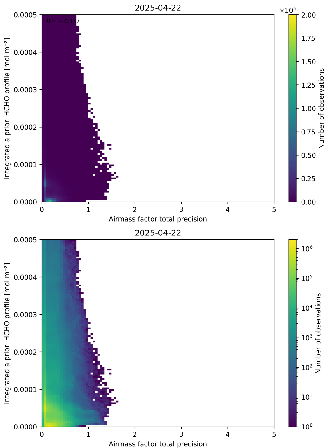
Figure 111: Scatter density plot of “Airmass factor total precision” against “Integrated a priori HCHO profile” for 2025-04-21 to 2025-04-23.
