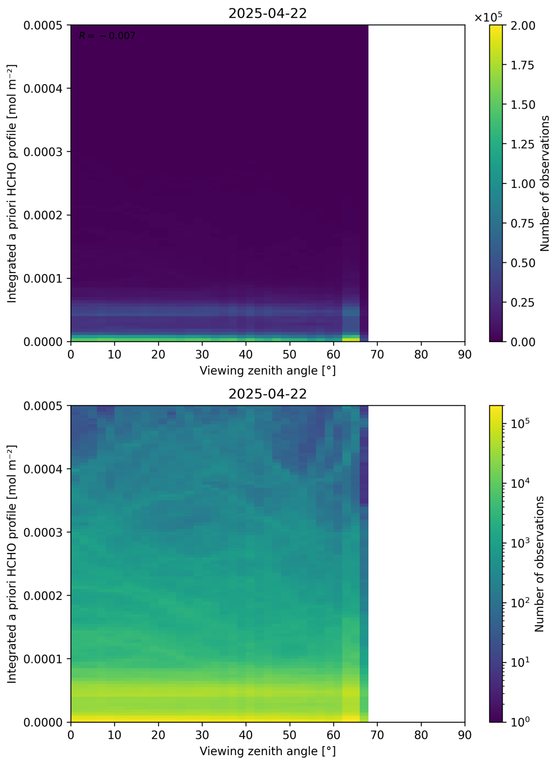
Figure 195: Scatter density plot of “Viewing zenith angle” against “Integrated a priori HCHO profile” for 2025-04-21 to 2025-04-23.
