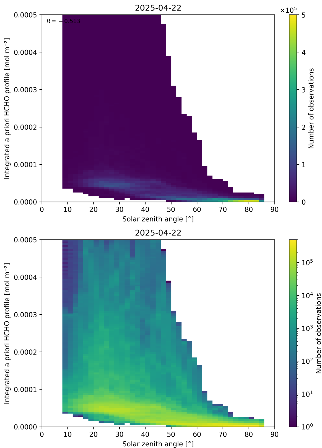
Figure 180: Scatter density plot of “Solar zenith angle” against “Integrated a priori HCHO profile” for 2025-04-21 to 2025-04-23.
