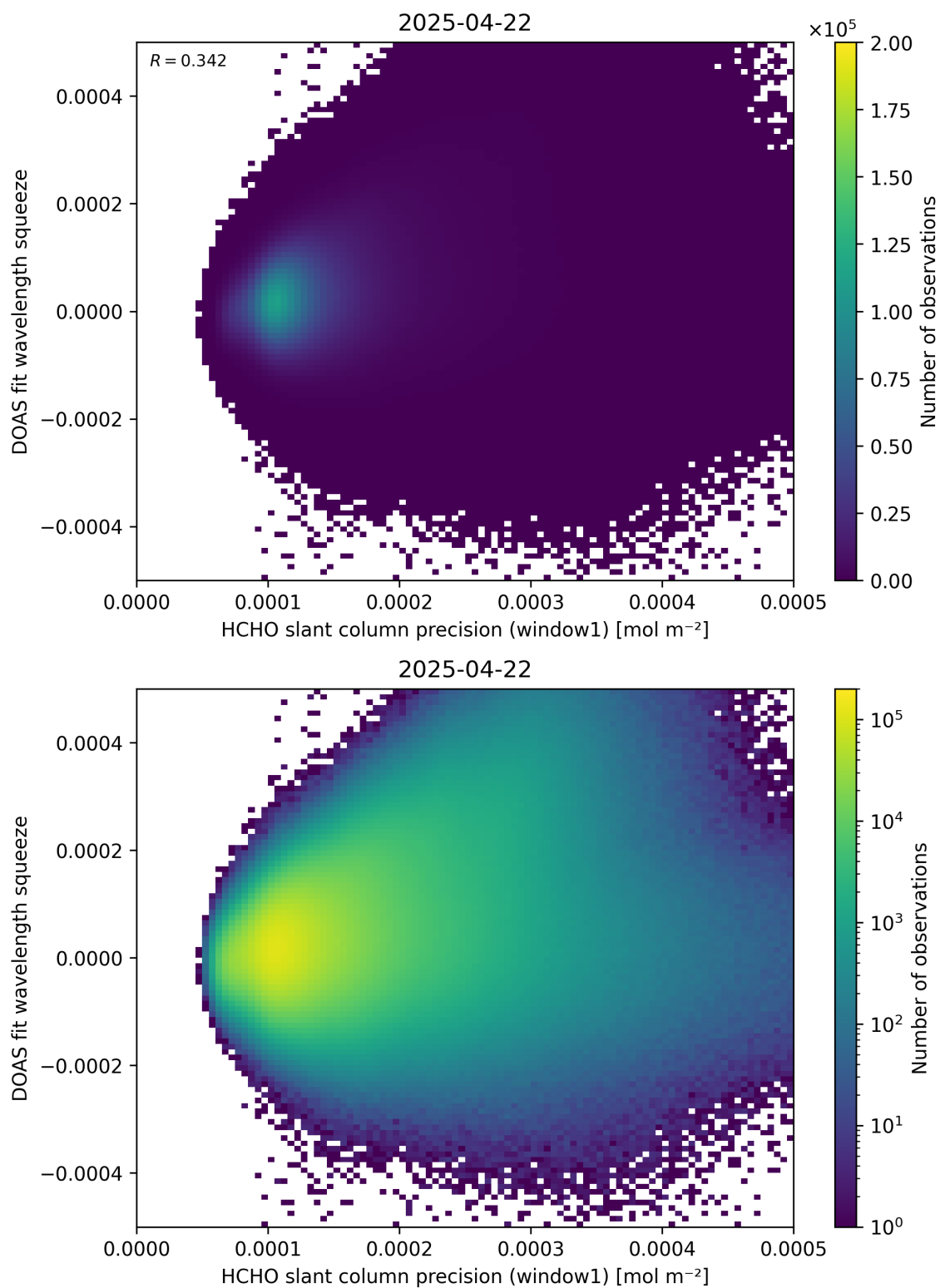
Figure 90: Scatter density plot of “HCHO slant column precision (window1)” against “DOAS fit wavelength squeeze” for 2025-04-21 to 2025-04-23.
