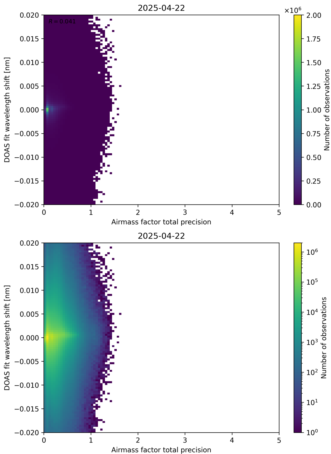
Figure 106: Scatter density plot of “Airmass factor total precision” against “DOAS fit wavelength shift” for 2025-04-21 to 2025-04-23.
