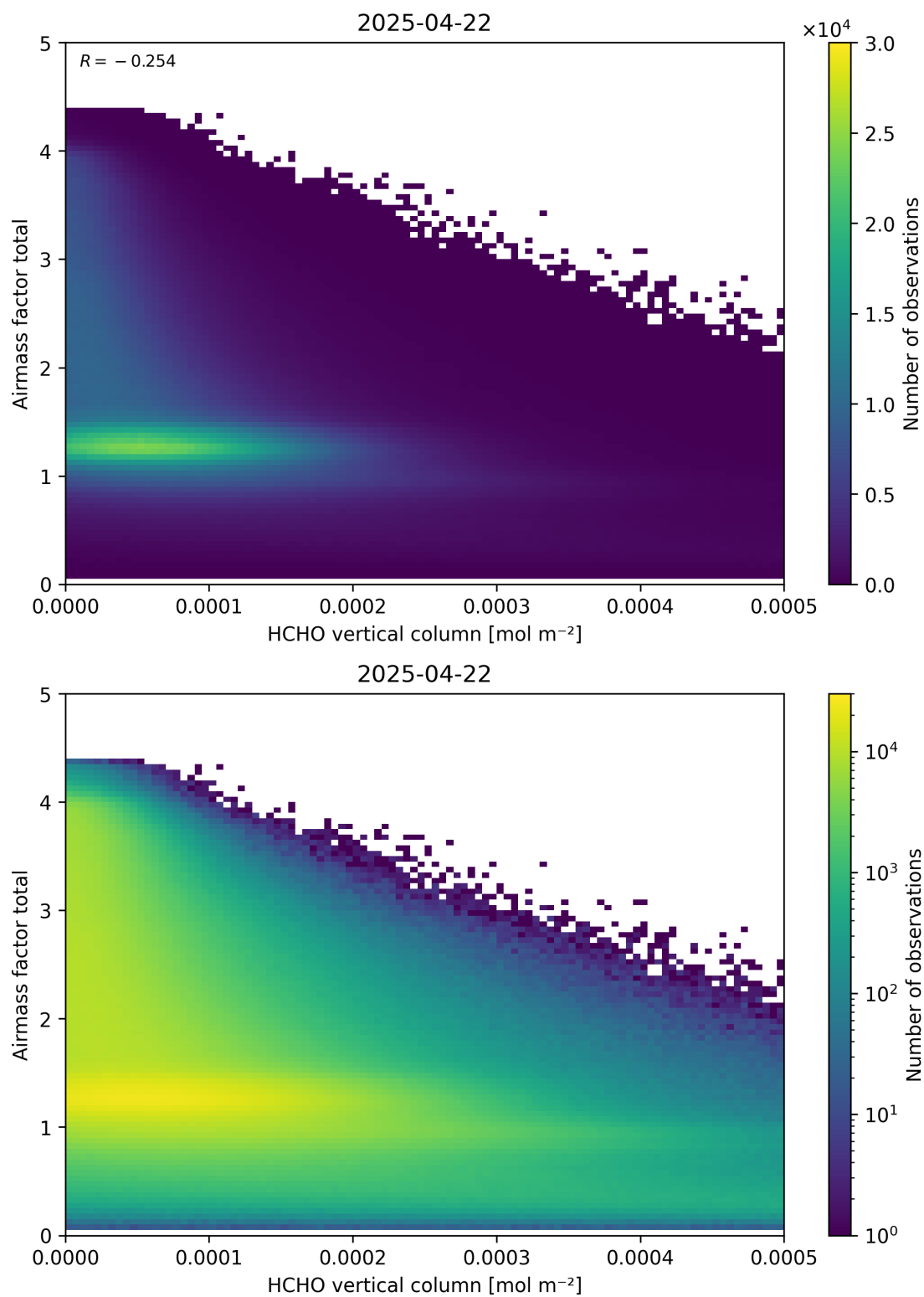
Figure 131: Scatter density plot of “HCHO vertical column” against “Airmass factor total” for 2025-04-21 to 2025-04-23.
