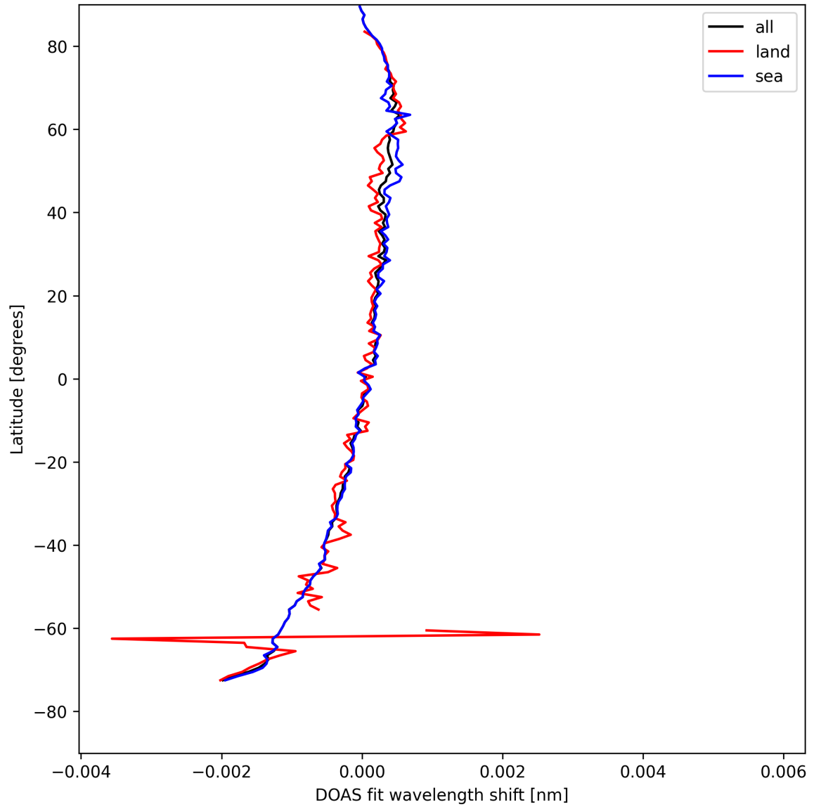
Figure 30: Zonal average of "DOAS fit wavelength shift" for 2025-04-21 to 2025-04-23.
