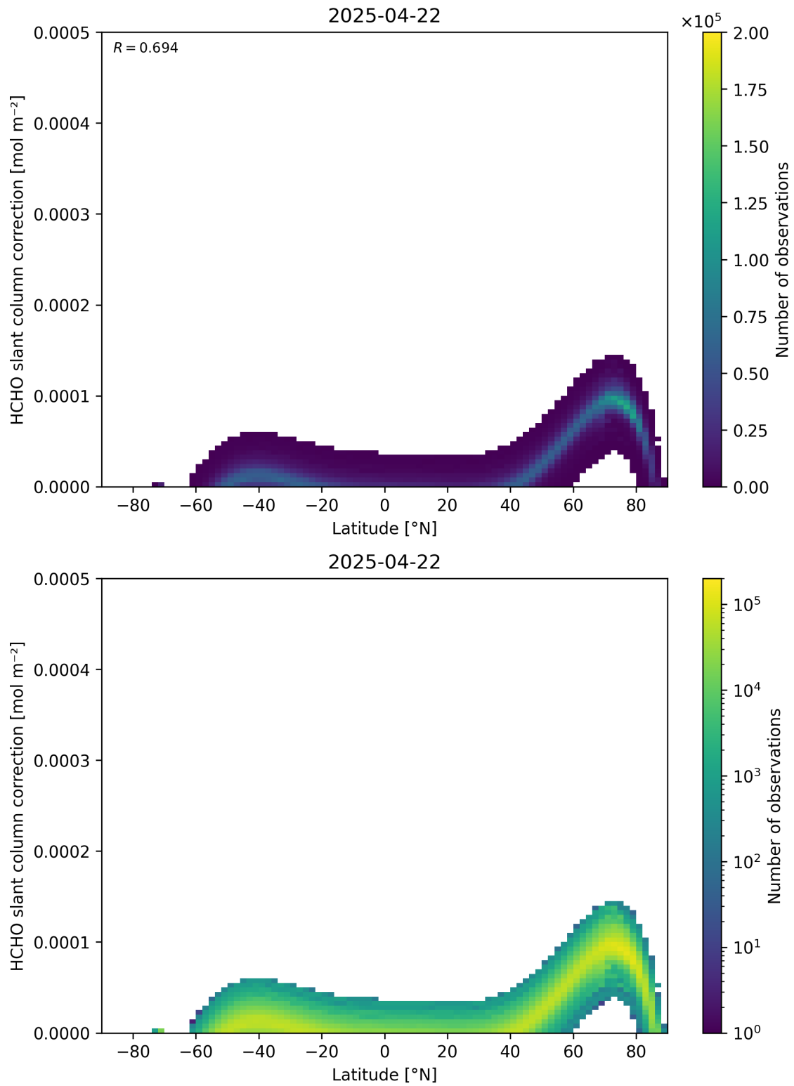
Figure 158: Scatter density plot of “Latitude” against “HCHO slant column correction” for 2025-04-21 to 2025-04-23.
