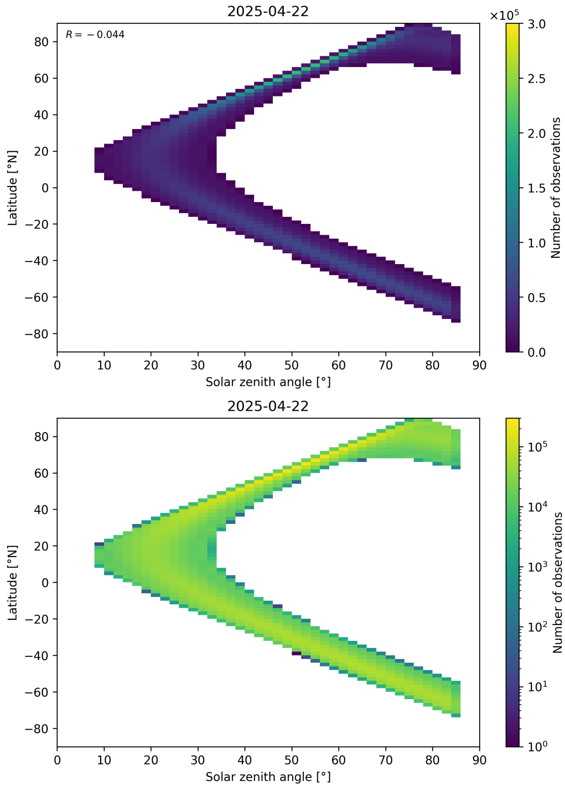
Figure 181: Scatter density plot of “Solar zenith angle” against “Latitude” for 2025-04-21 to 2025-04-23.
