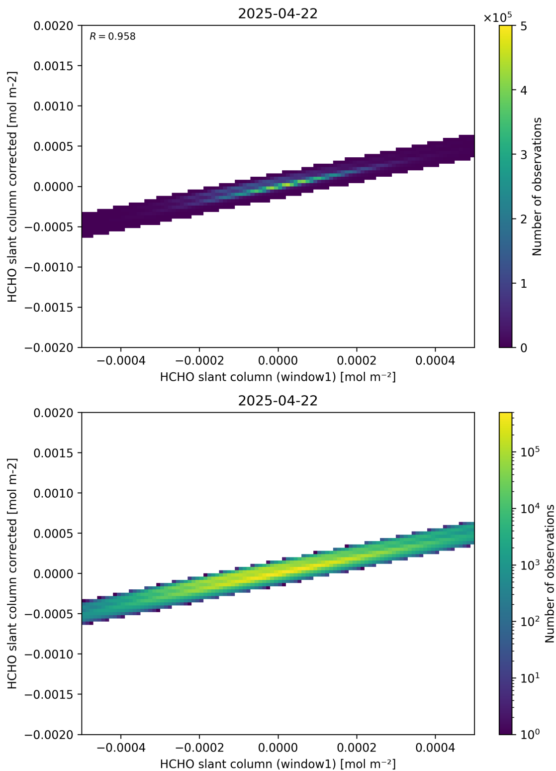
Figure 82: Scatter density plot of “HCHO slant column (window1)” against “HCHO slant column corrected” for 2025-04-21 to 2025-04-23.
