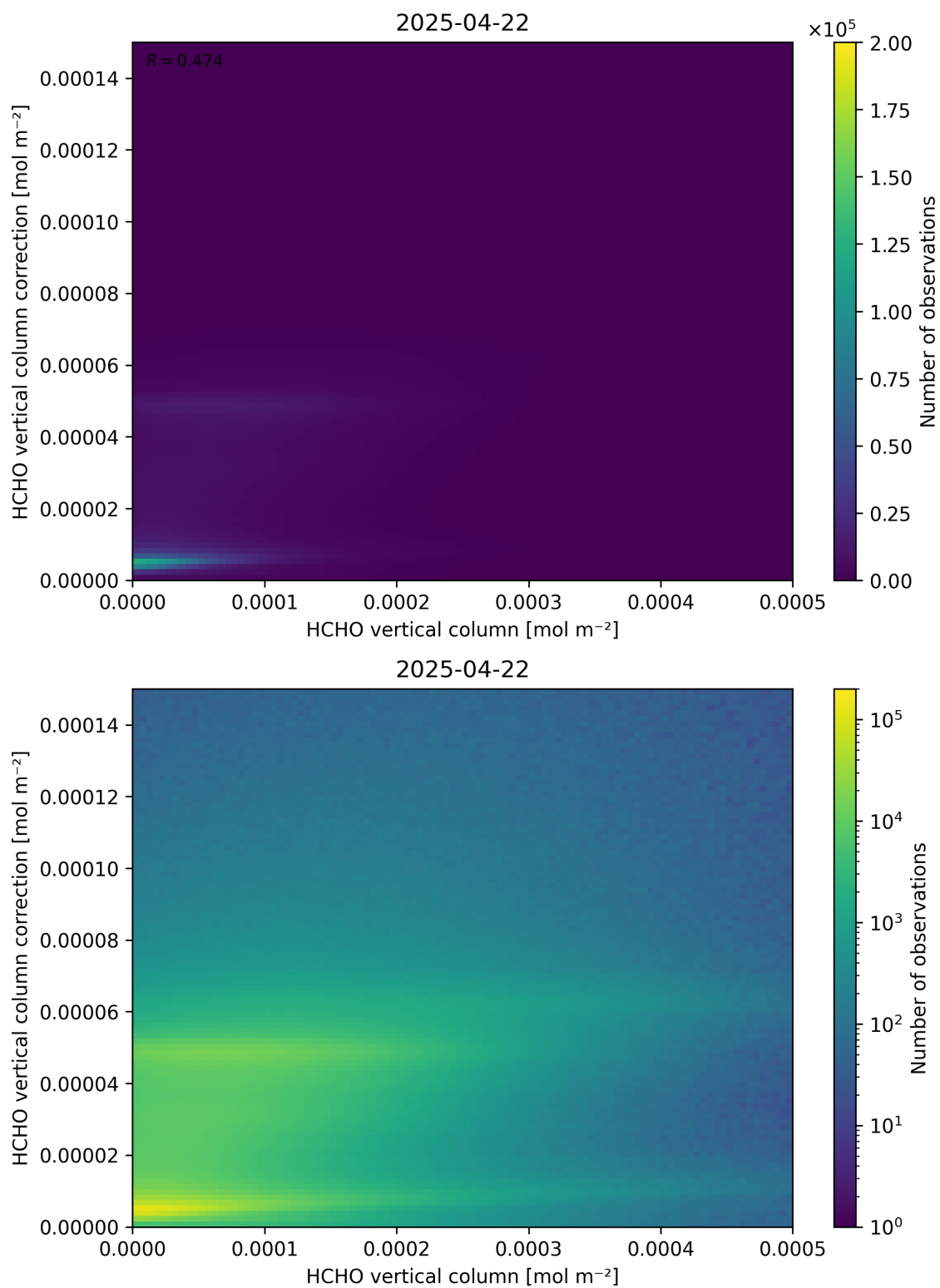
Figure 133: Scatter density plot of “HCHO vertical column” against “HCHO vertical column correction” for 2025-04-21 to 2025-04-23.
