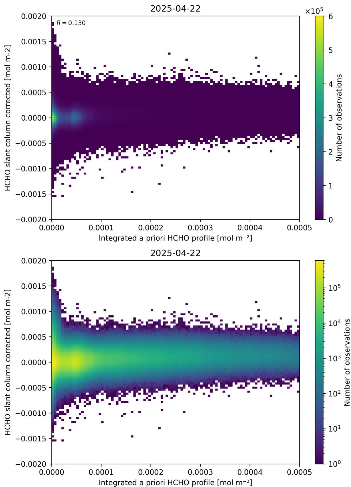
Figure 151: Scatter density plot of “Integrated a priori HCHO profile” against “HCHO slant column corrected” for 2025-04-21 to 2025-04-23.
