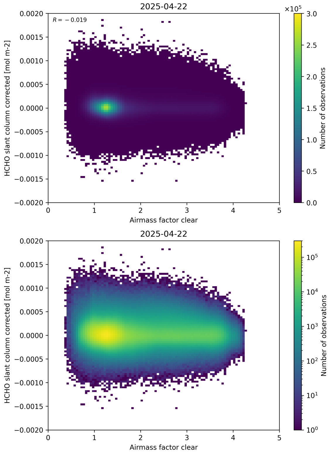
Figure 74: Scatter density plot of “Airmass factor clear” against “HCHO slant column corrected” for 2025-04-21 to 2025-04-23.
