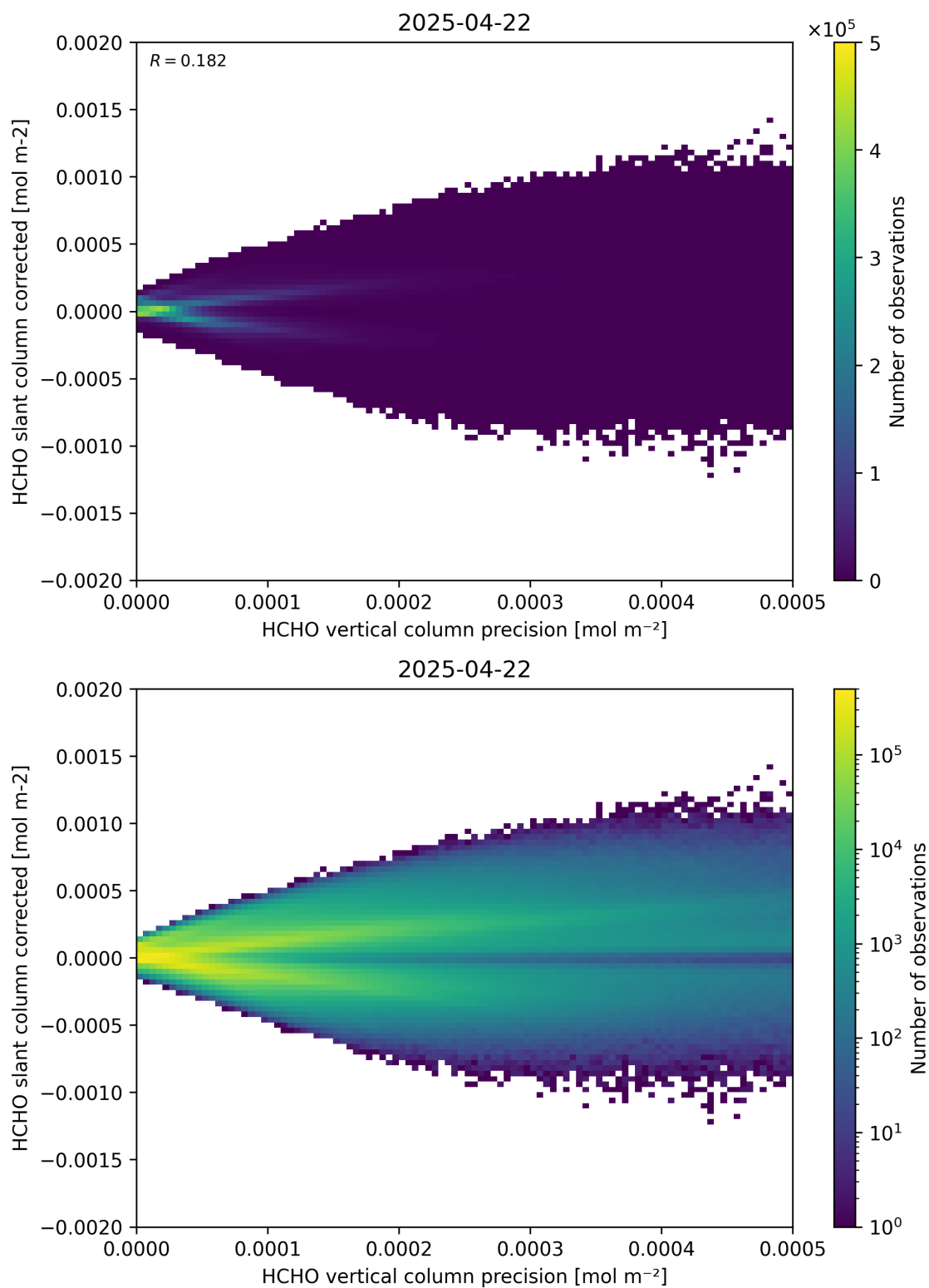
Figure 140: Scatter density plot of “HCHO vertical column precision” against “HCHO slant column corrected” for 2025-04-21 to 2025-04-23.
