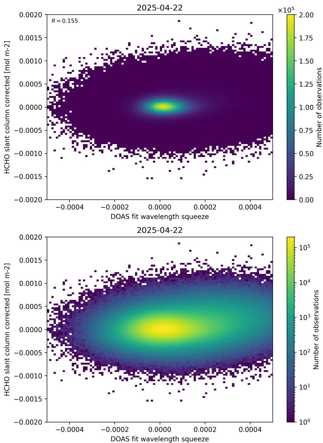
Figure 69: Scatter density plot of “DOAS fit wavelength squeeze” against “HCHO slant column corrected” for 2025-04-21 to 2025-04-23.
