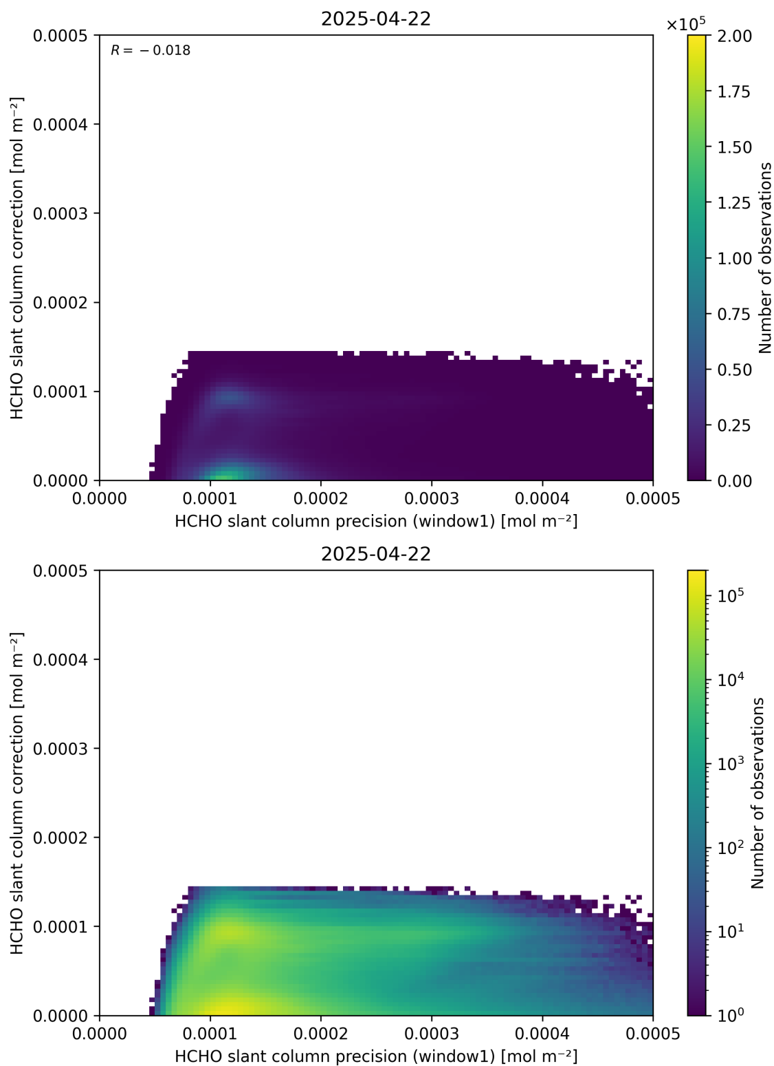
Figure 93: Scatter density plot of “HCHO slant column precision (window1)” against “HCHO slant column correction” for 2025-04-21 to 2025-04-23.
