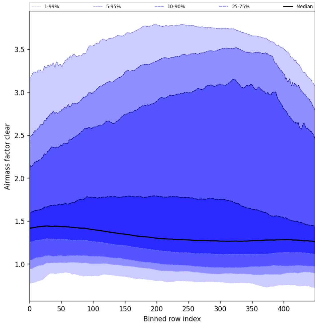
Figure 56: Along track statistics of “Airmass factor clear” for 2025-04-21 to 2025-04-23
