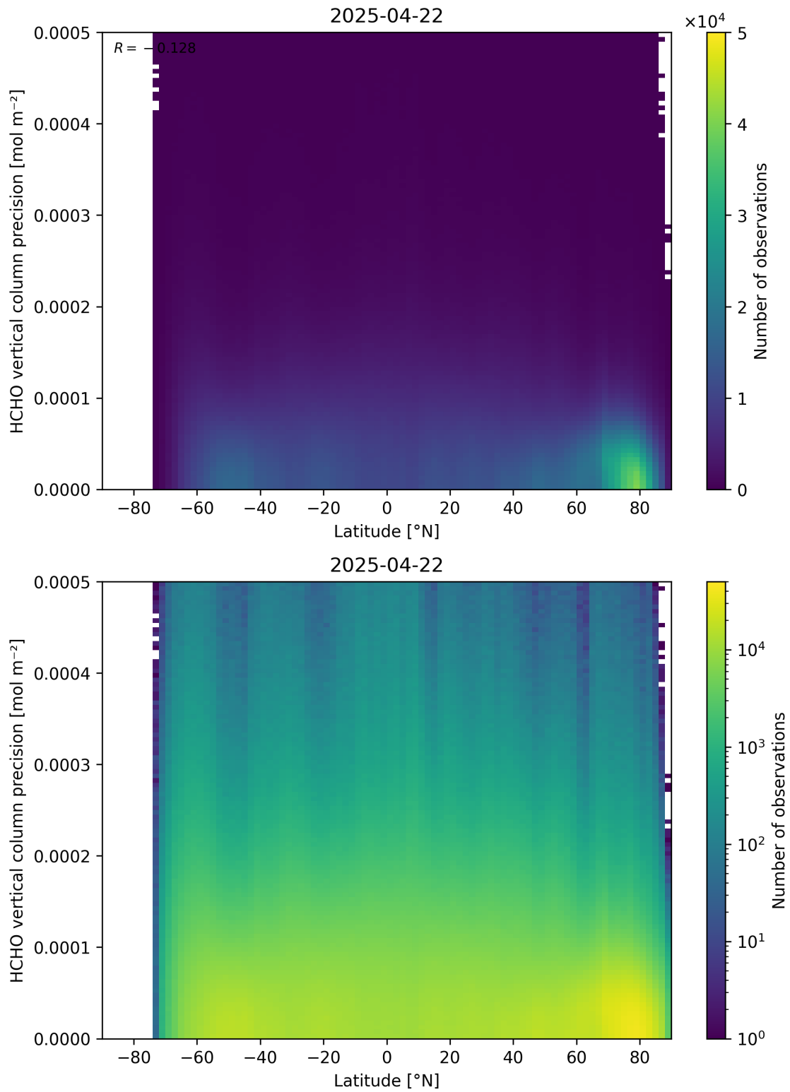
Figure 165: Scatter density plot of “Latitude” against “HCHO vertical column precision” for 2025-04-21 to 2025-04-23.
