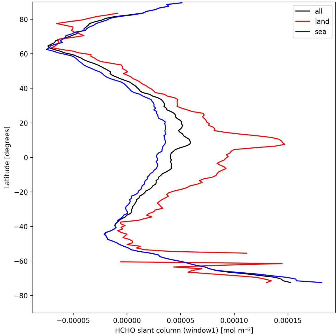
Figure 24: Zonal average of “HCHO slant column (window1)” for 2025-04-21 to 2025-04-23.
