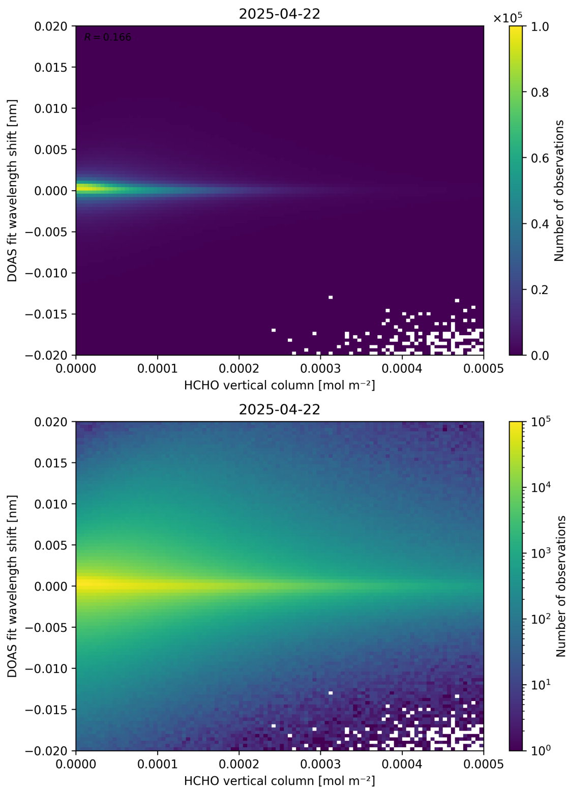
Figure 124: Scatter density plot of “HCHO vertical column” against “DOAS fit wavelength shift” for 2025-04-21 to 2025-04-23.
