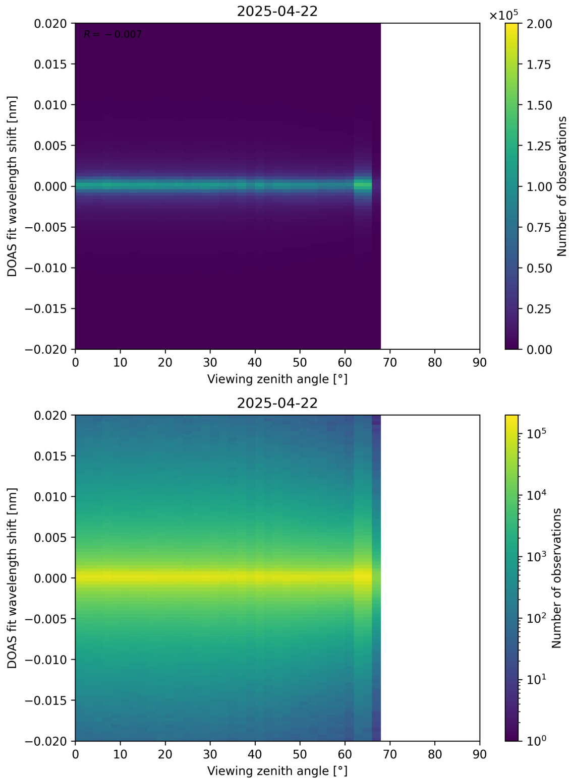
Figure 183: Scatter density plot of “Viewing zenith angle” against “DOAS fit wavelength shift” for 2025-04-21 to 2025-04-23.
