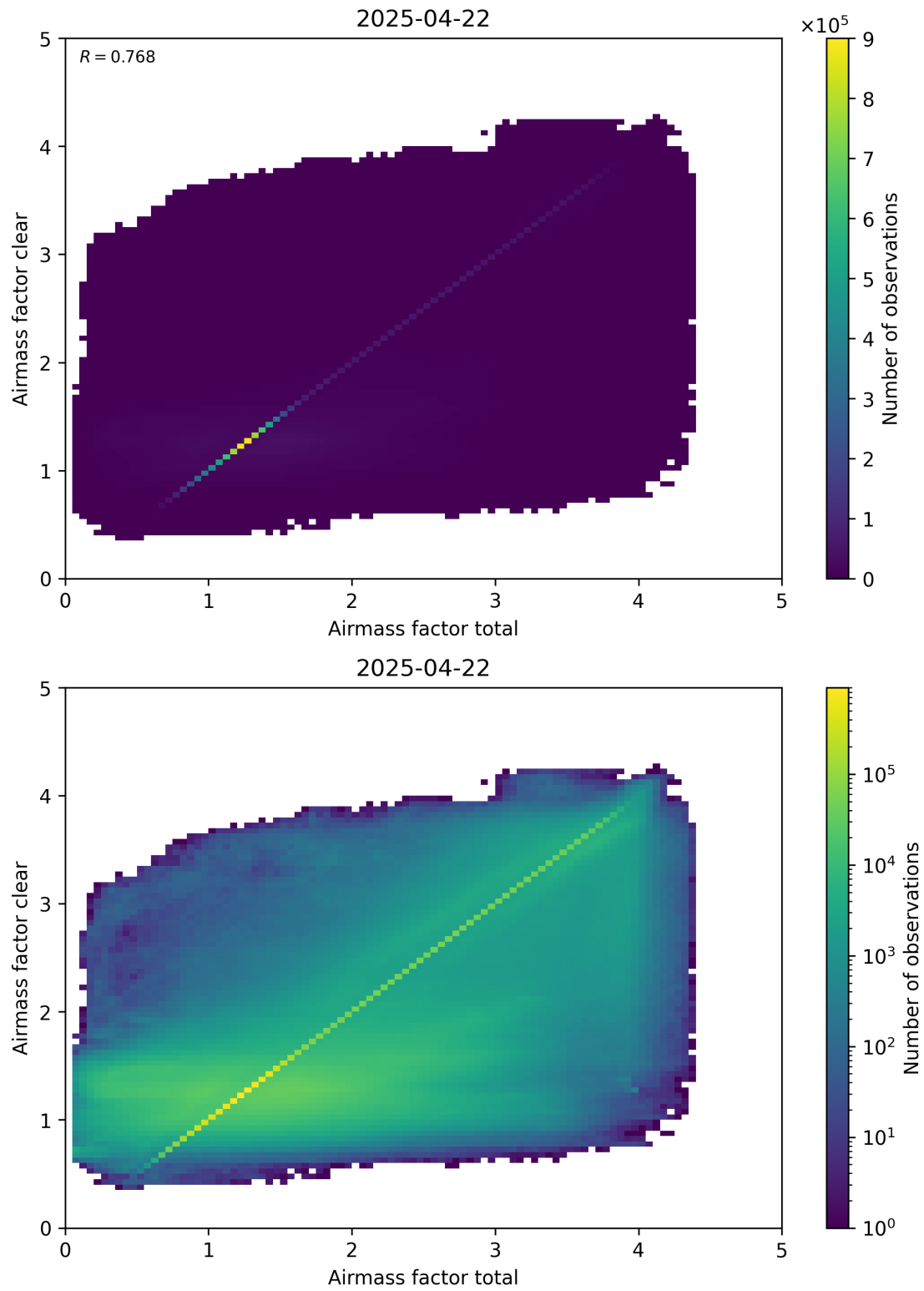
Figure 100: Scatter density plot of “Airmass factor total” against “Airmass factor clear” for 2025-04-21 to 2025-04-23.
