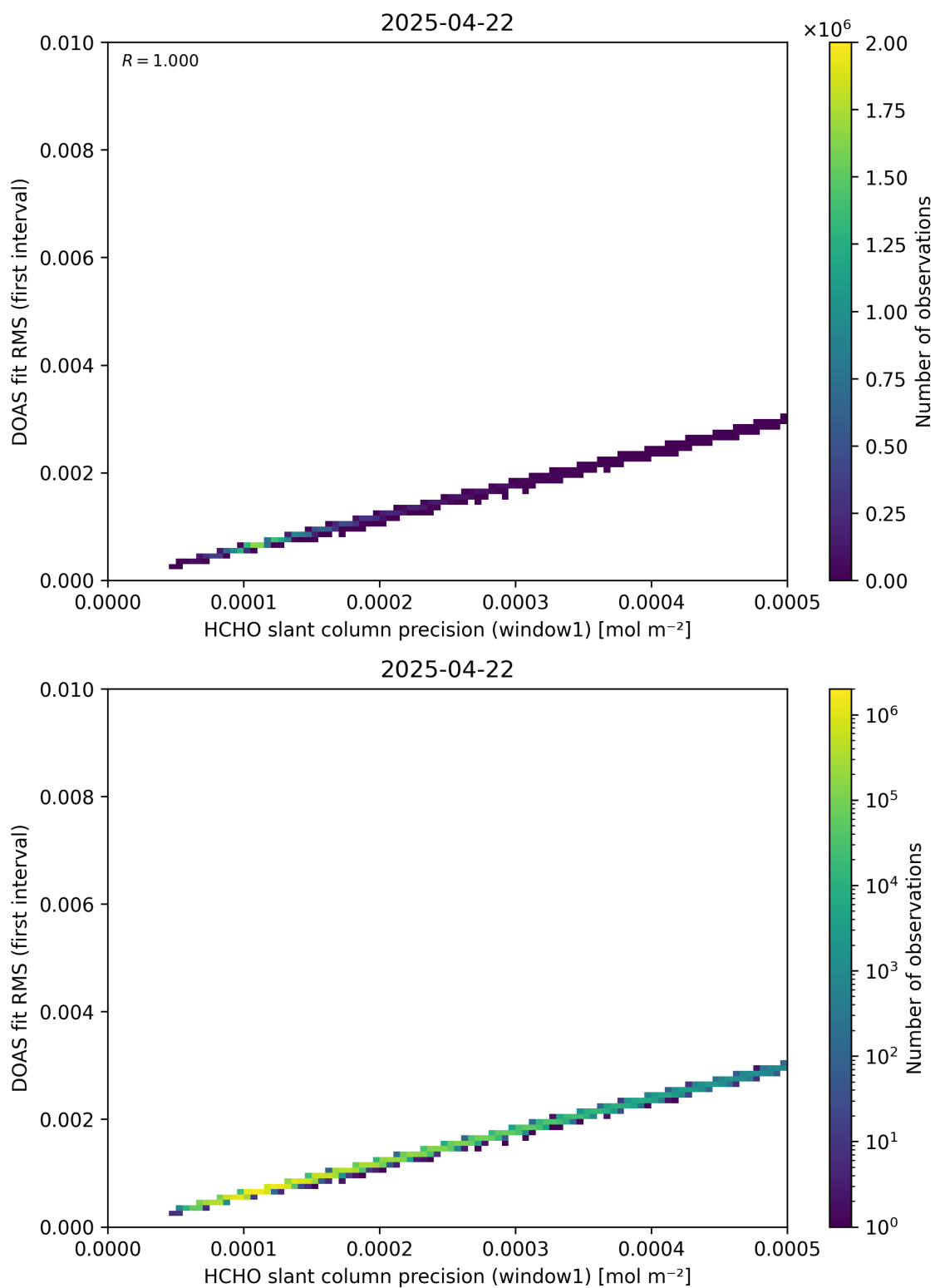
Figure 88: Scatter density plot of “HCHO slant column precision (window1)” against “DOAS fit RMS (first interval)” for 2025-04-21 to 2025-04-23.
