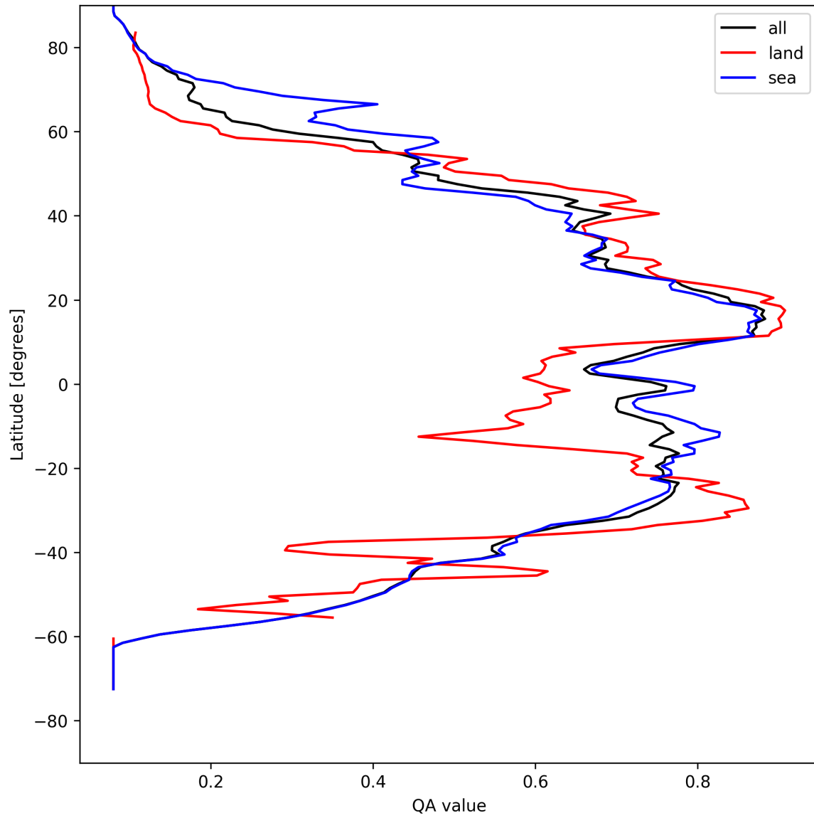
Figure 20: Zonal average of “QA value” for 2025-04-21 to 2025-04-23.
