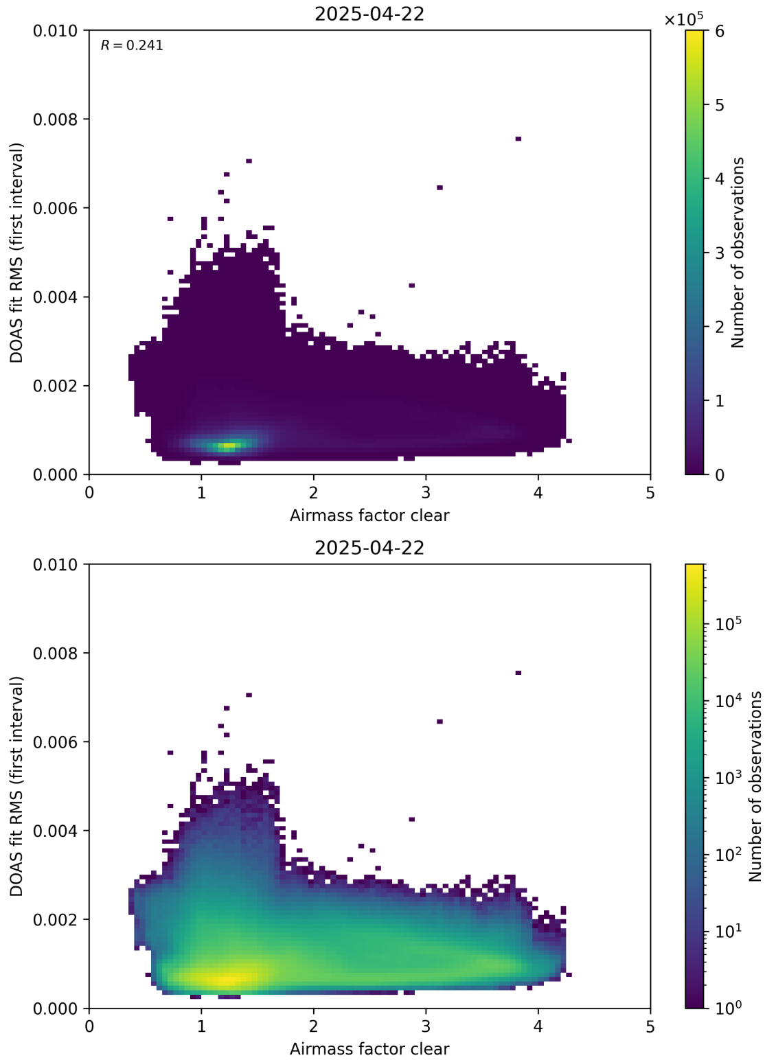
Figure 71: Scatter density plot of “Airmass factor clear” against “DOAS fit RMS (first interval)” for 2025-04-21 to 2025-04-23.
