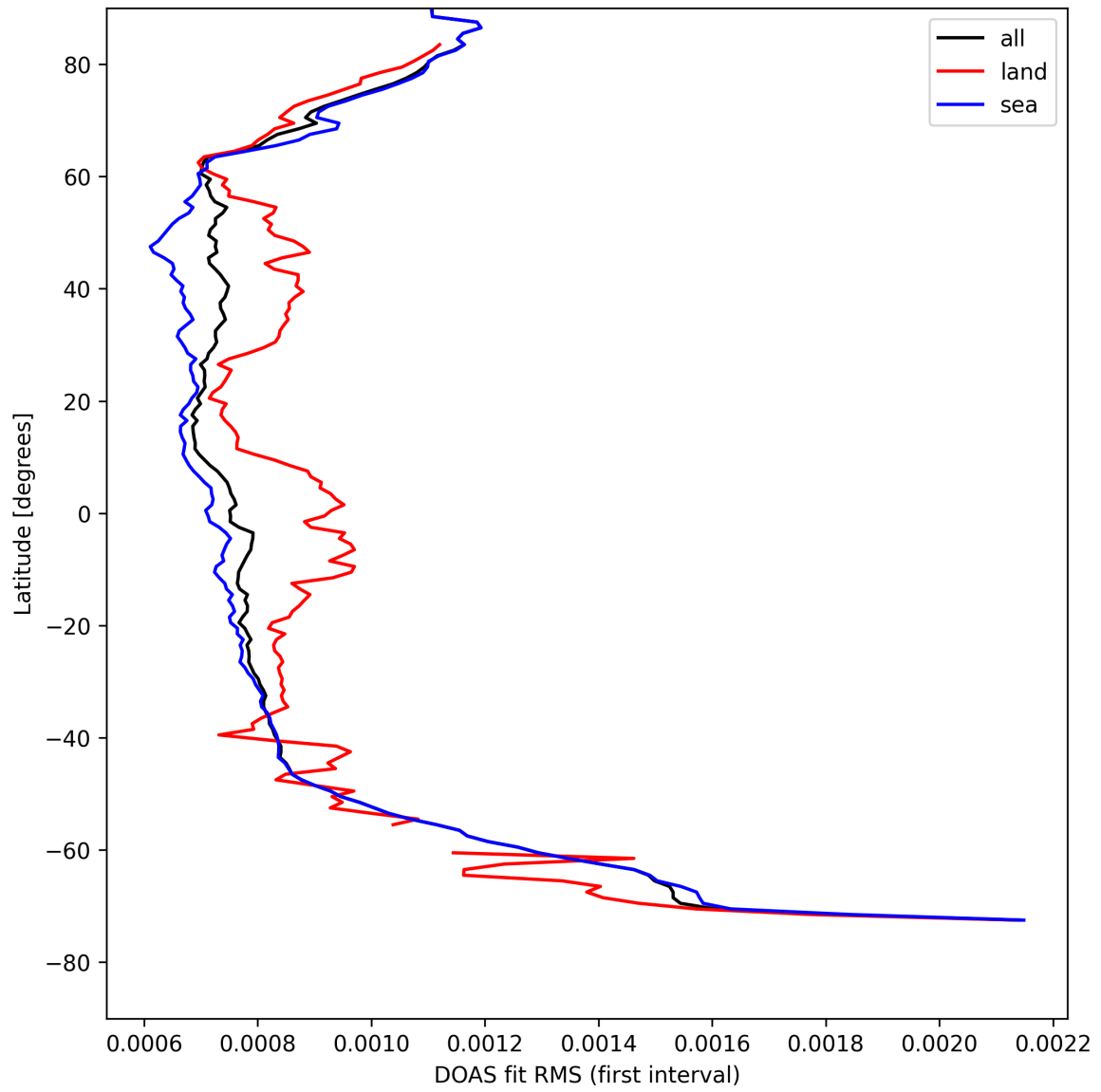
Figure 32: Zonal average of "DOAS fit RMS (first interval)" for 2025-04-21 to 2025-04-23.
