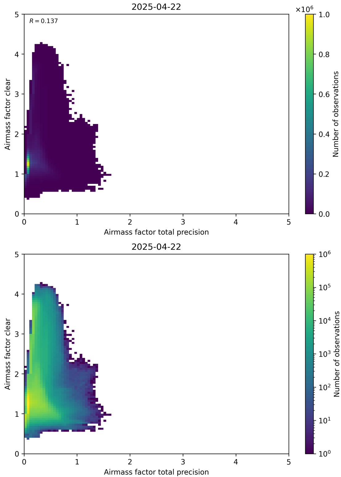
Figure 108: Scatter density plot of “Airmass factor total precision” against “Airmass factor clear” for 2025-04-21 to 2025-04-23.
