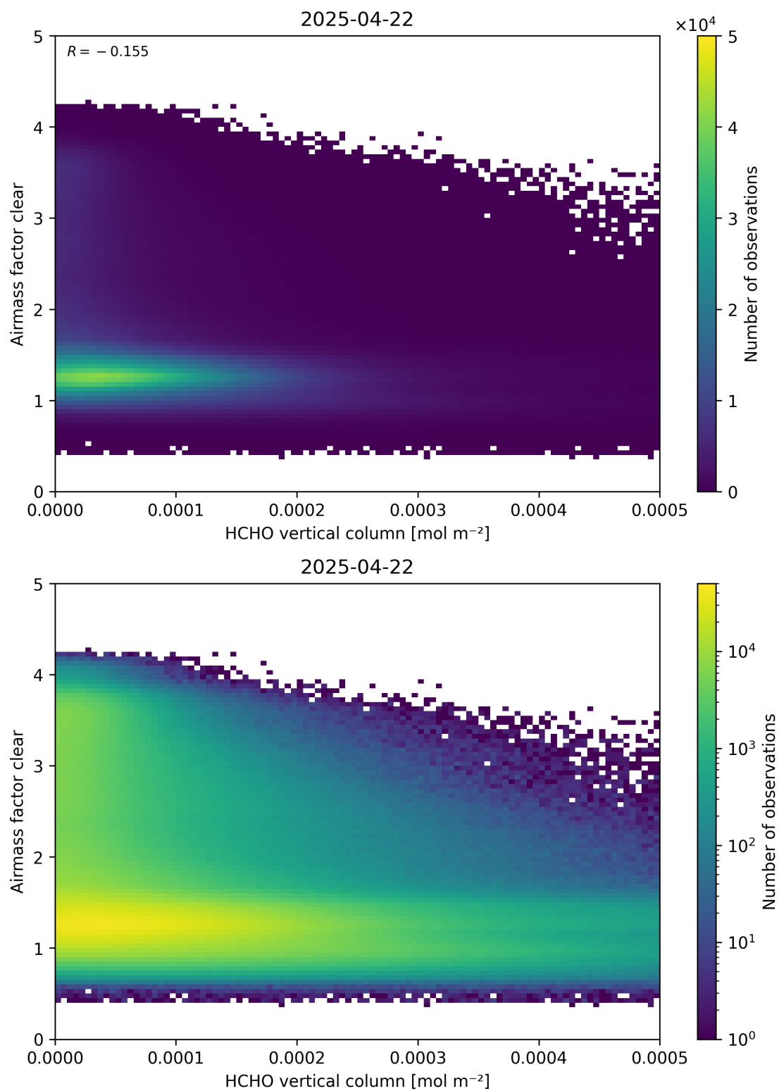
Figure 126: Scatter density plot of “HCHO vertical column” against “Airmass factor clear” for 2025-04-21 to 2025-04-23.
