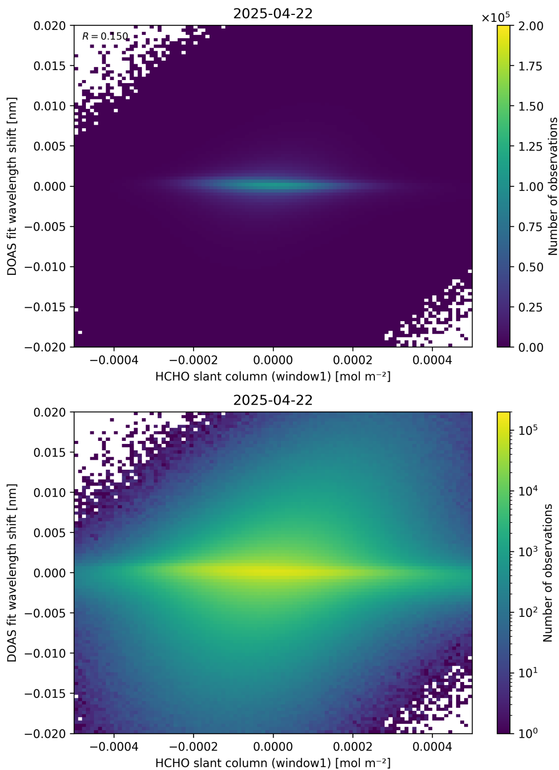
Figure 79: Scatter density plot of “HCHO slant column (window1)” against “DOAS fit wavelength shift” for 2025-04-21 to 2025-04-23.
