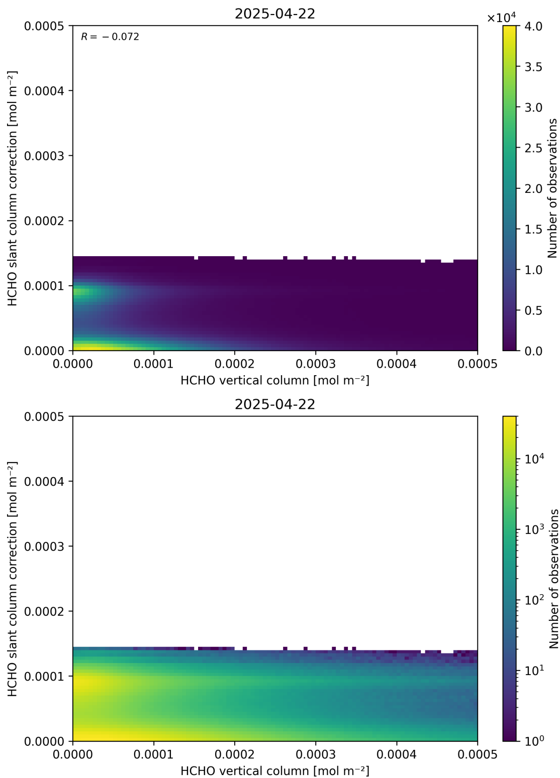
Figure 128: Scatter density plot of “HCHO vertical column” against “HCHO slant column correction” for 2025-04-21 to 2025-04-23.
