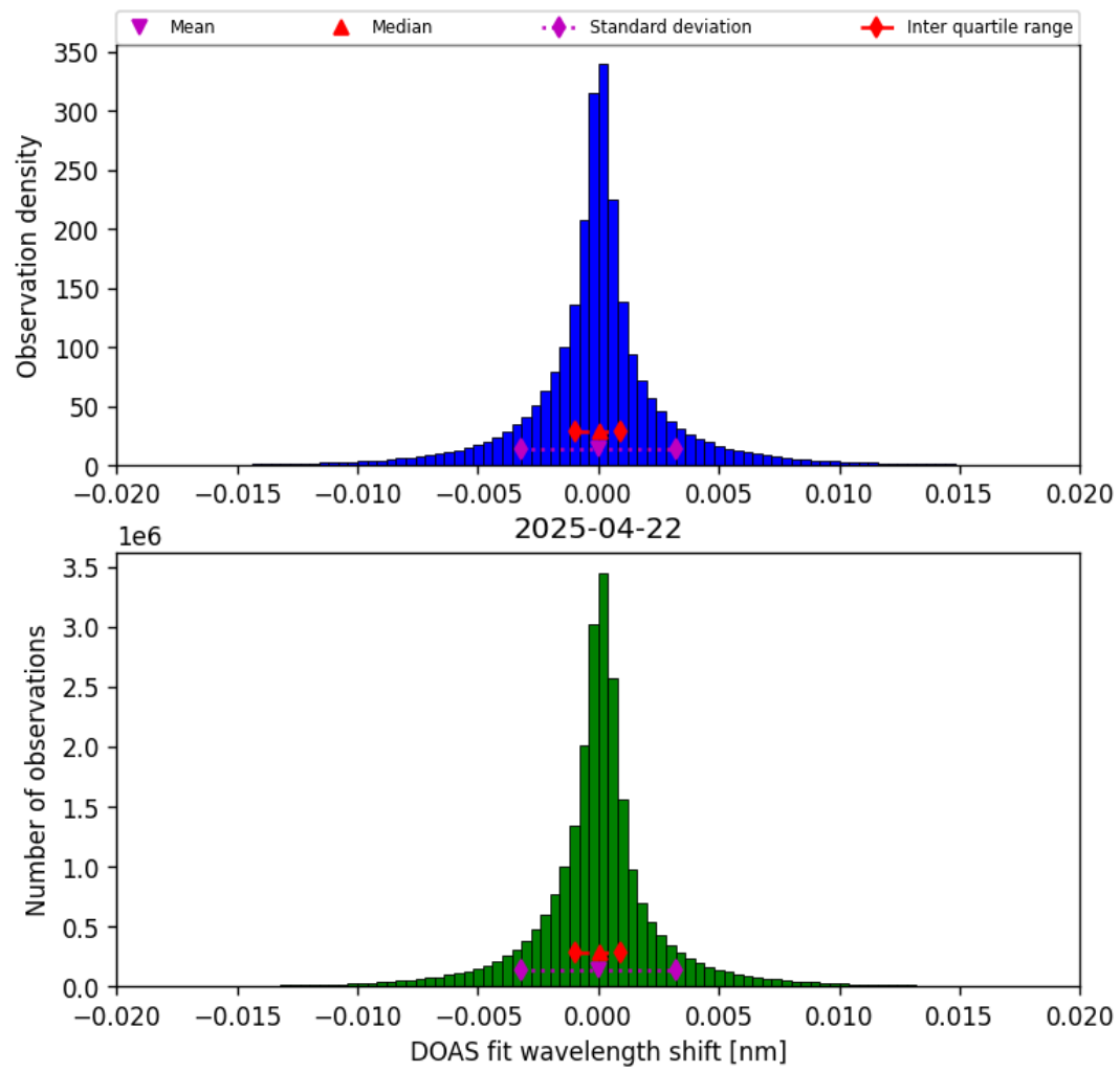
Figure 44: Histogram of “DOAS fit wavelength shift” for 2025-04-21 to 2025-04-23
