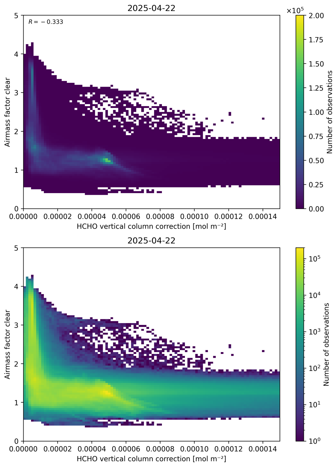
Figure 115: Scatter density plot of “HCHO vertical column correction” against “Airmass factor clear” for 2025-04-21 to 2025-04-23.
