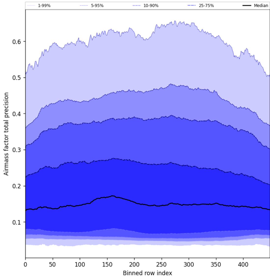
Figure 55: Along track statistics of “Airmass factor total precision” for 2025-04-21 to 2025-04-23
