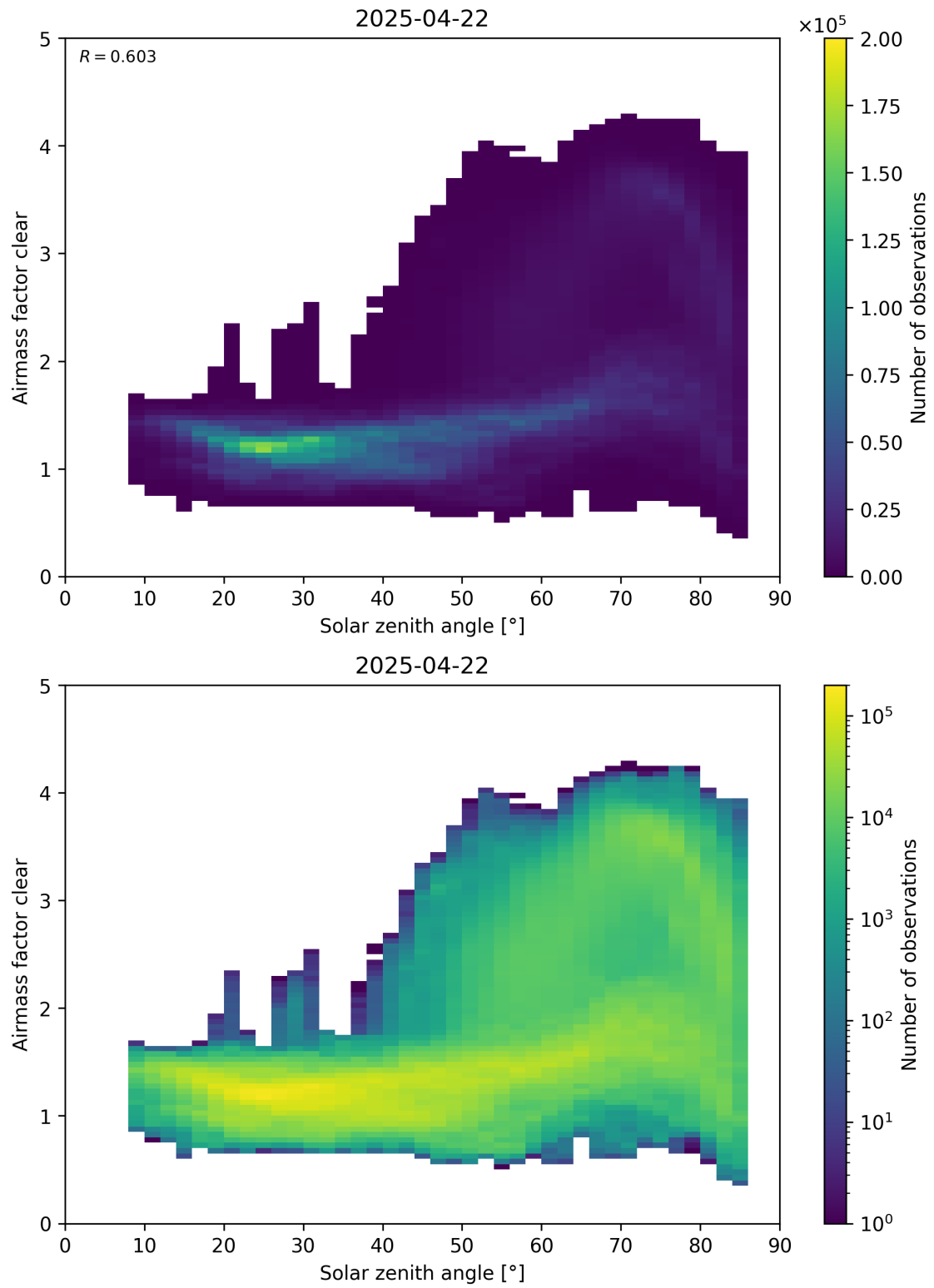
Figure 170: Scatter density plot of “Solar zenith angle” against “Airmass factor clear” for 2025-04-21 to 2025-04-23.
