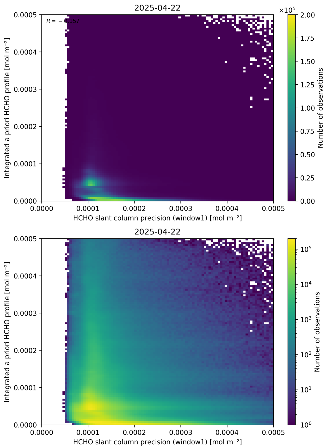
Figure 96: Scatter density plot of “HCHO slant column precision (window1)” against “Integrated a priori HCHO profile” for 2025-04-21 to 2025-04-23.
