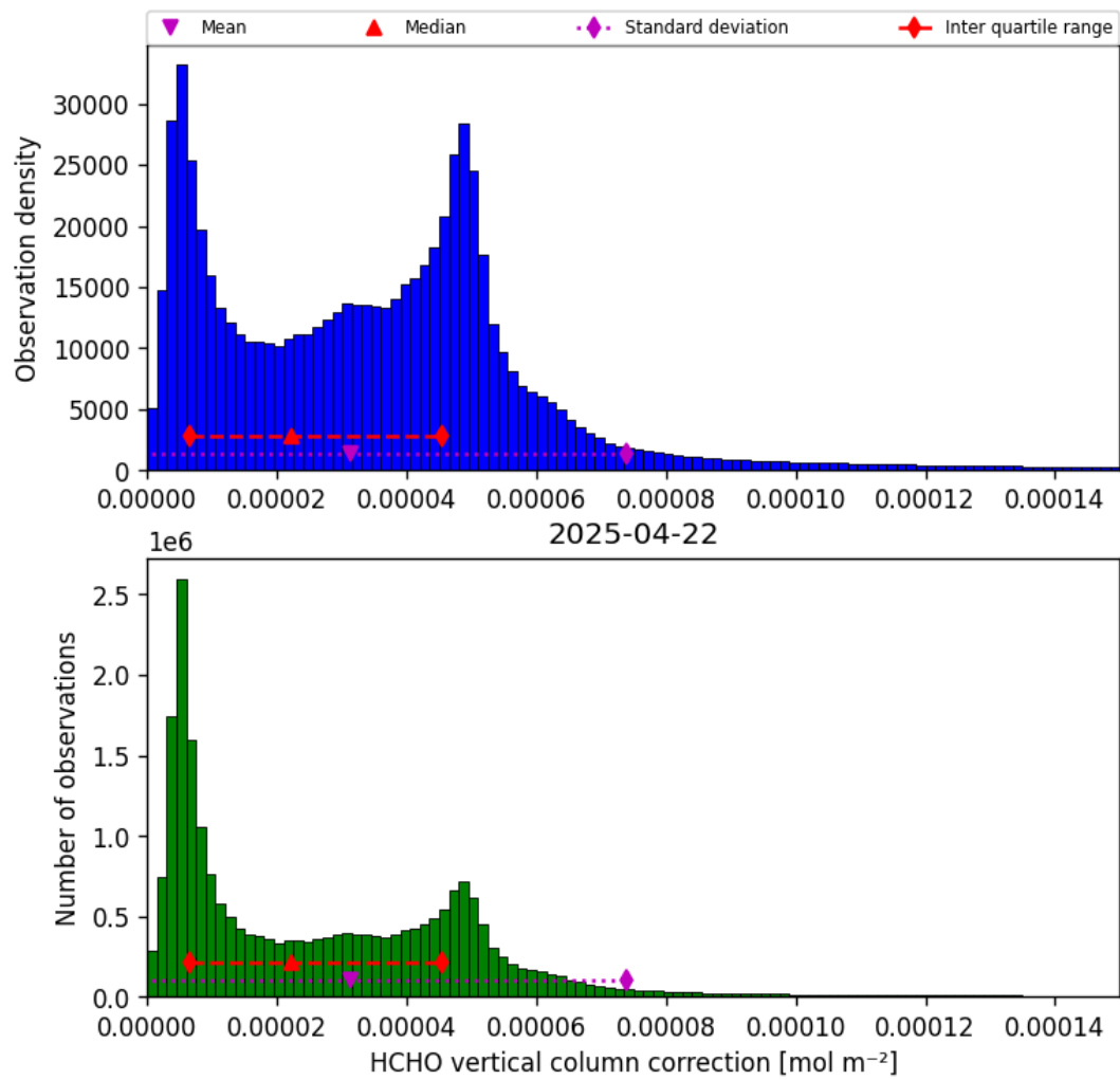
Figure 37: Histogram of “HCHO vertical column correction” for 2025-04-21 to 2025-04-23
