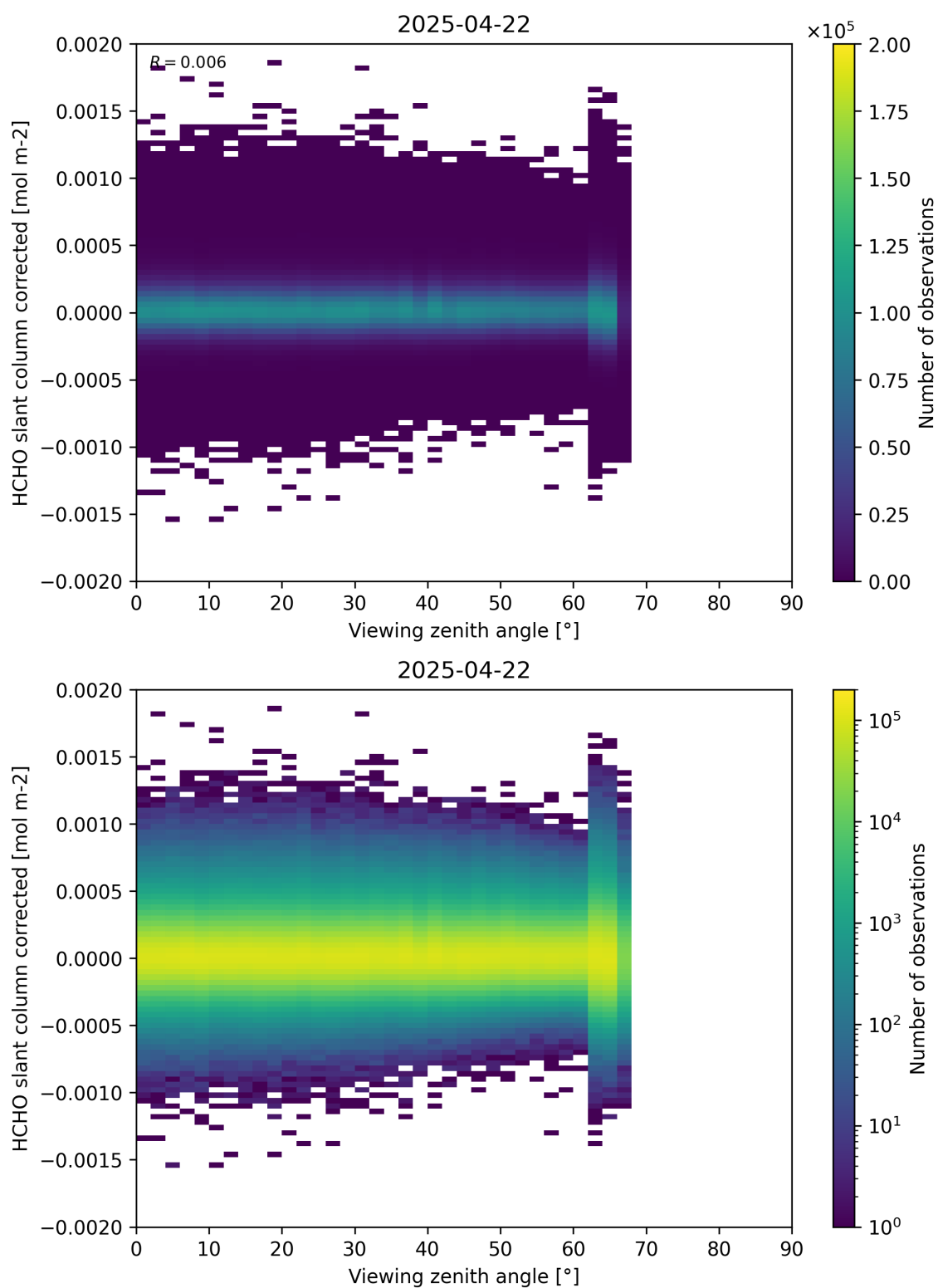
Figure 186: Scatter density plot of “Viewing zenith angle” against “HCHO slant column corrected” for 2025-04-21 to 2025-04-23.
