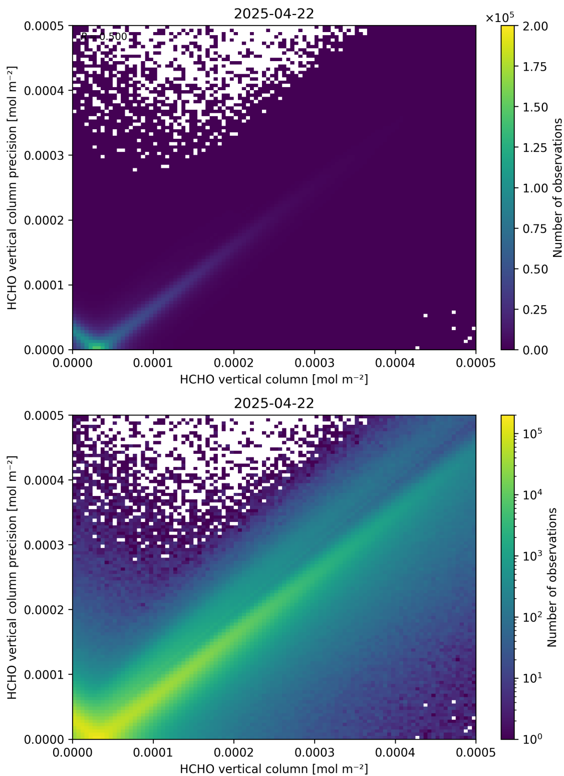
Figure 134: Scatter density plot of “HCHO vertical column” against “HCHO vertical column precision” for 2025-04-21 to 2025-04-23.
