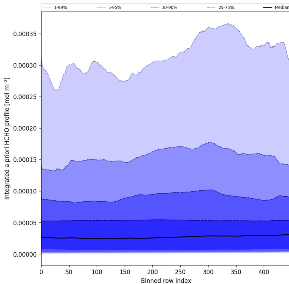
Figure 57: Along track statistics of “Integrated a priori HCHO profile” for 2025-04-21 to 2025-04-23
