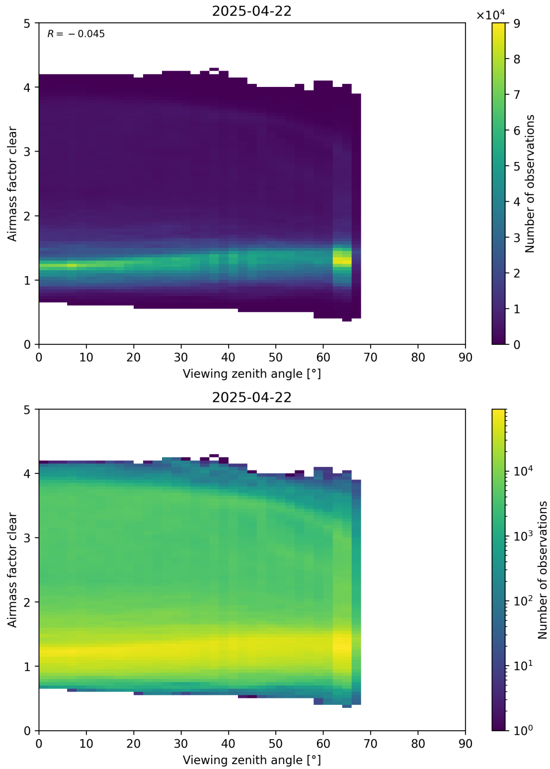
Figure 185: Scatter density plot of “Viewing zenith angle” against “Airmass factor clear” for 2025-04-21 to 2025-04-23.
