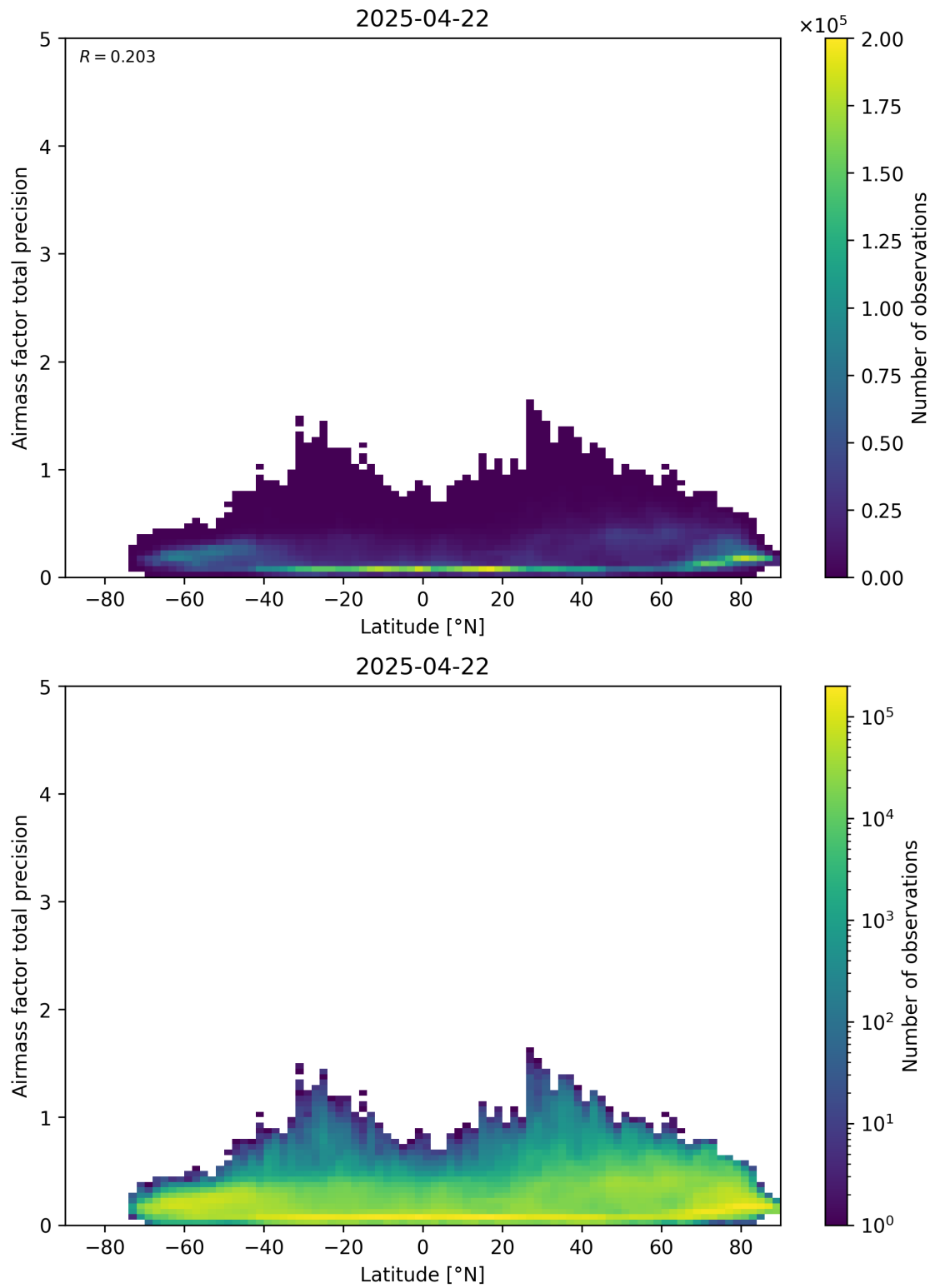
Figure 162: Scatter density plot of “Latitude” against “Airmass factor total precision” for 2025-04-21 to 2025-04-23.
