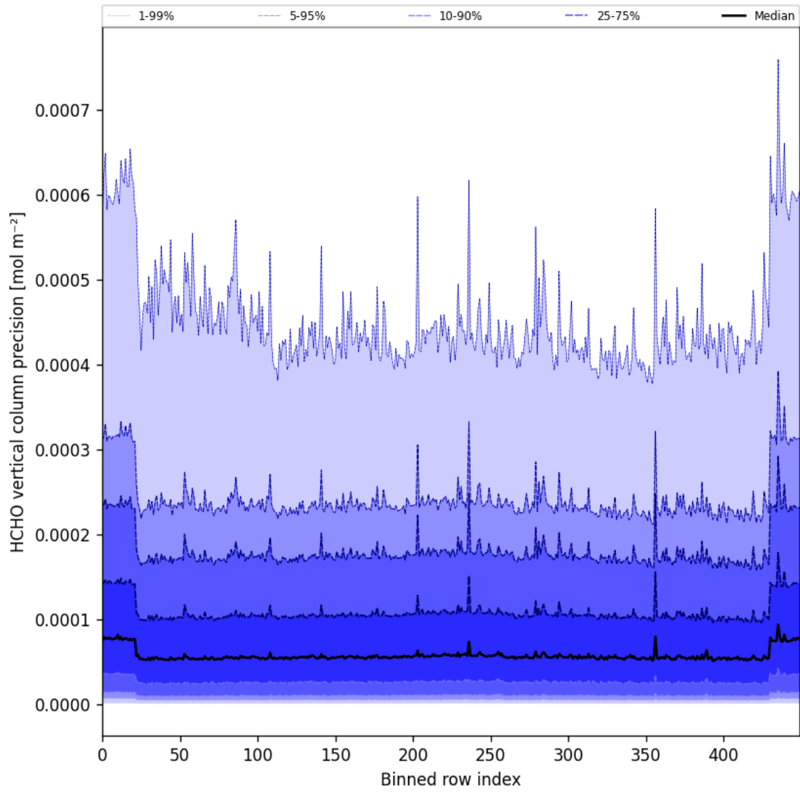
Figure 50: Along track statistics of “HCHO vertical column precision” for 2025-04-21 to 2025-04-23
