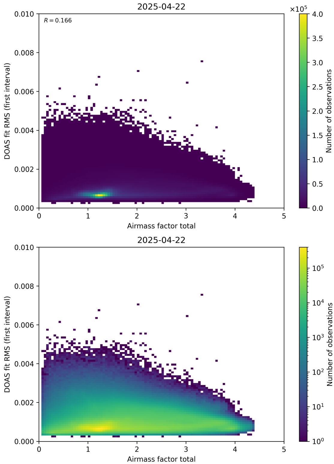
Figure 97: Scatter density plot of “Airmass factor total” against “DOAS fit RMS (first interval)” for 2025-04-21 to 2025-04-23.
