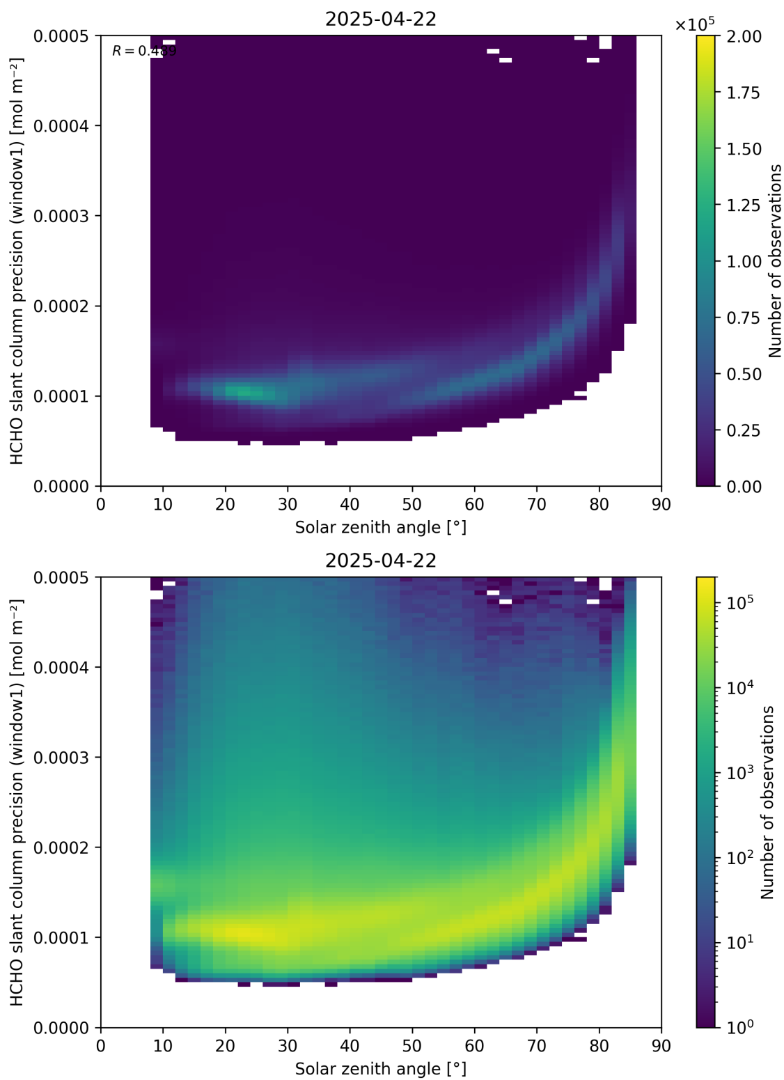
Figure 174: Scatter density plot of “Solar zenith angle” against “HCHO slant column precision (window1)” for 2025-04-21 to 2025-04-23.
