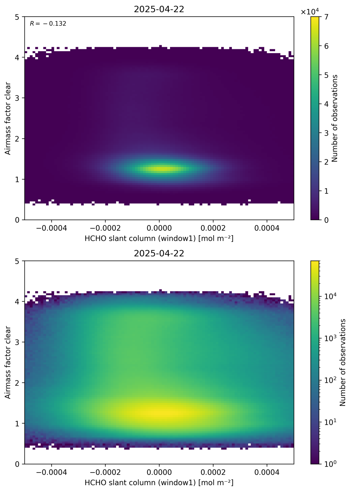
Figure 81: Scatter density plot of “HCHO slant column (window1)” against “Airmass factor clear” for 2025-04-21 to 2025-04-23.
