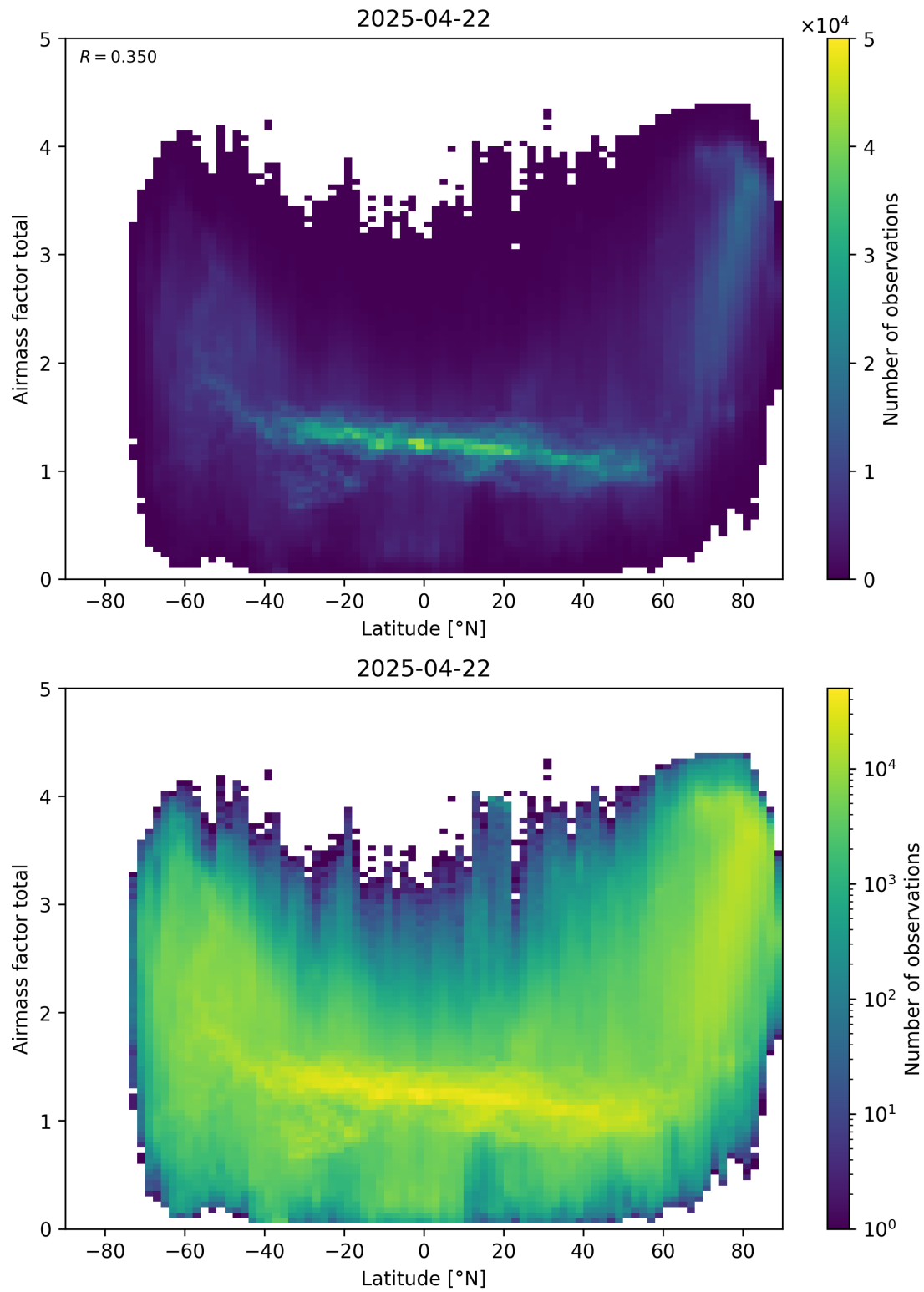
Figure 161: Scatter density plot of “Latitude” against “Airmass factor total” for 2025-04-21 to 2025-04-23.
