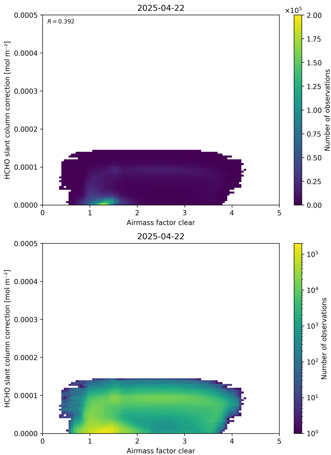
Figure 75: Scatter density plot of “Airmass factor clear” against “HCHO slant column correction” for 2025-04-21 to 2025-04-23.
