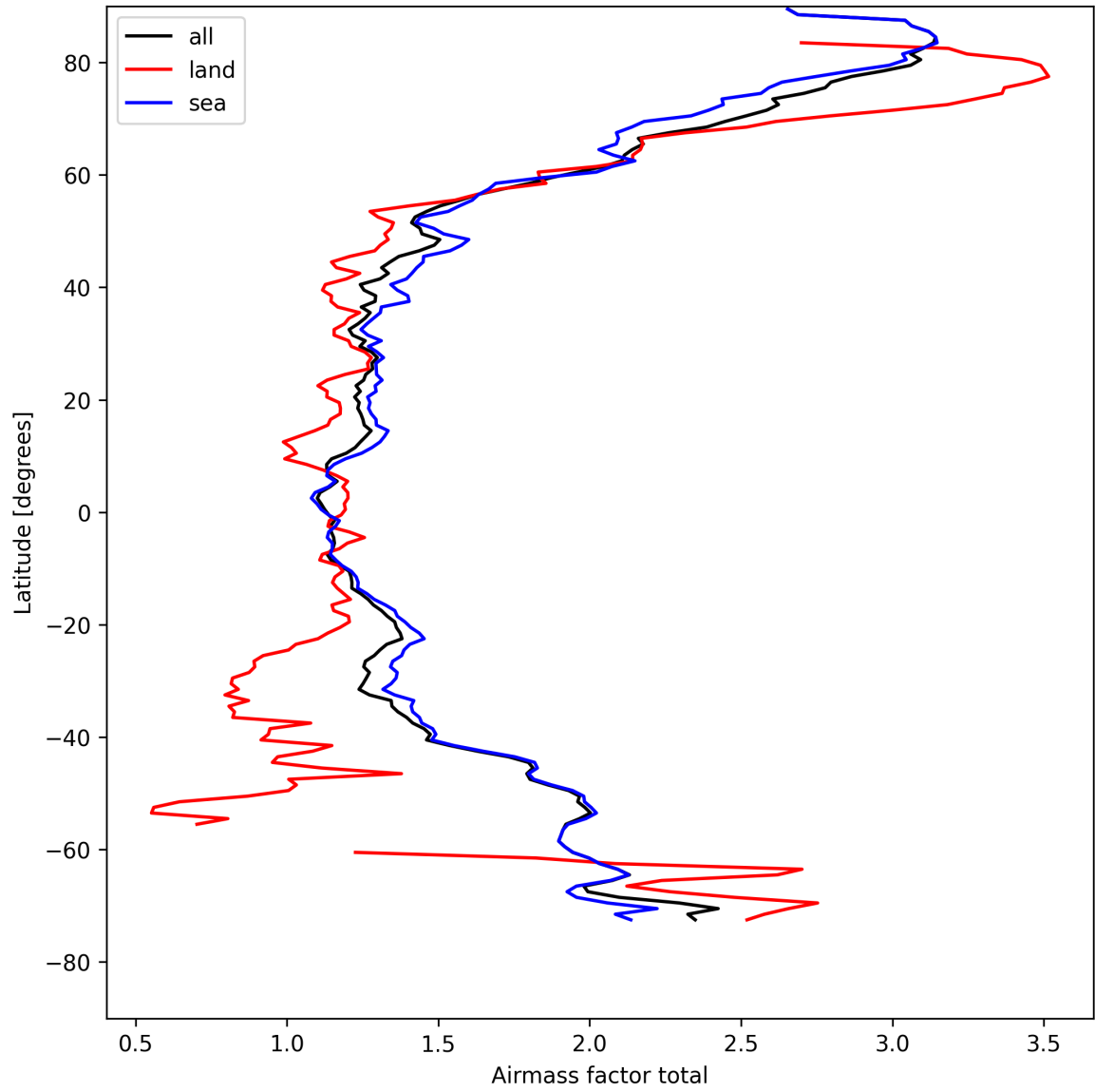
Figure 26: Zonal average of “Airmass factor total” for 2025-04-21 to 2025-04-23.
