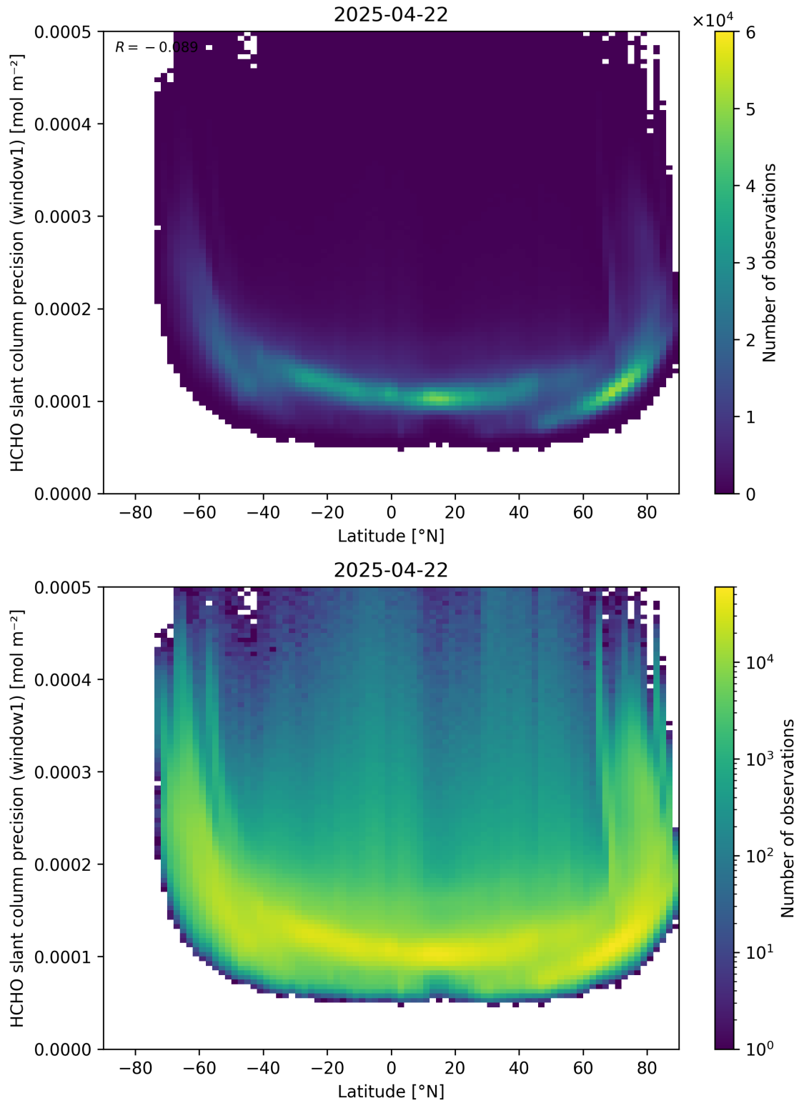
Figure 160: Scatter density plot of “Latitude” against “HCHO slant column precision (window1)” for 2025-04-21 to 2025-04-23.
