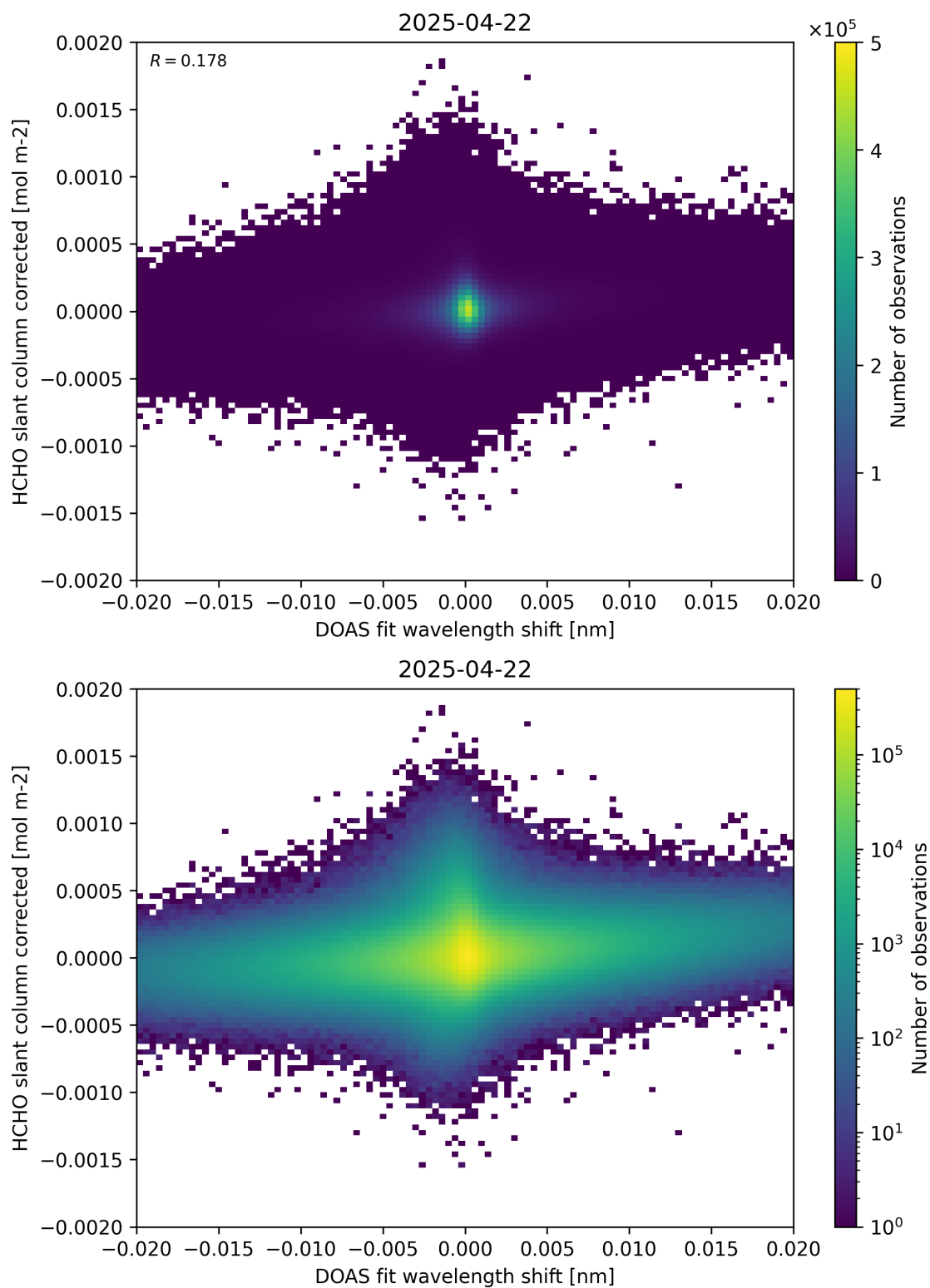
Figure 66: Scatter density plot of “DOAS fit wavelength shift” against “HCHO slant column corrected” for 2025-04-21 to 2025-04-23.
