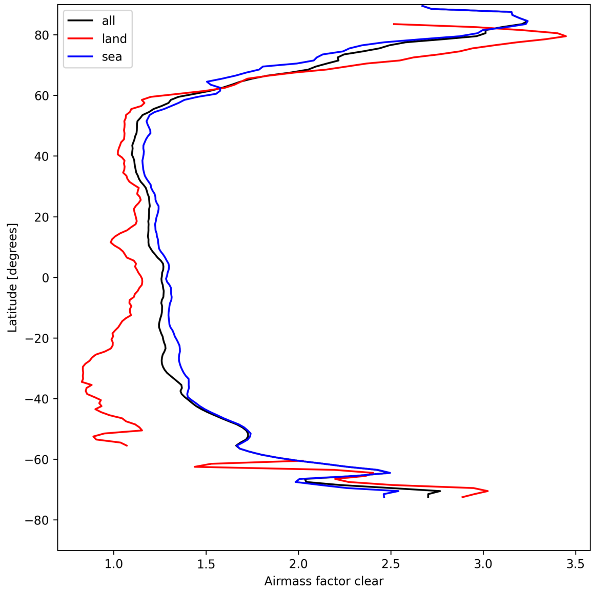
Figure 28: Zonal average of “Airmass factor clear” for 2025-04-21 to 2025-04-23.
