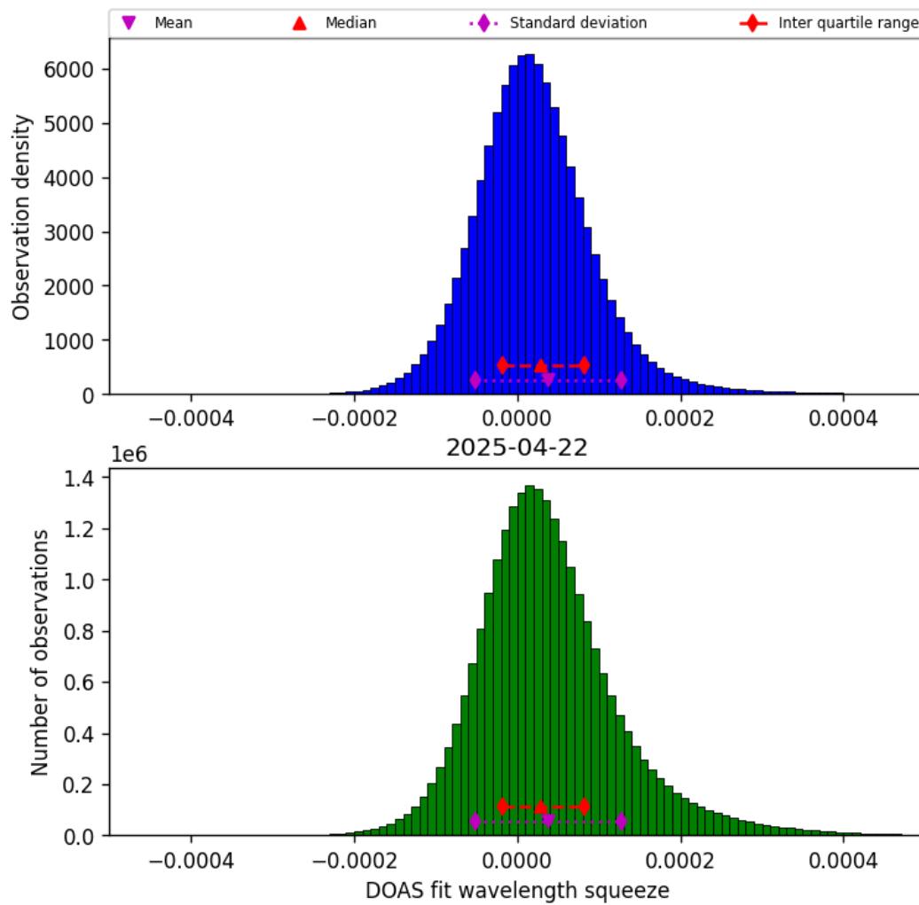
Figure 45: Histogram of “DOAS fit wavelength squeeze” for 2025-04-21 to 2025-04-23
