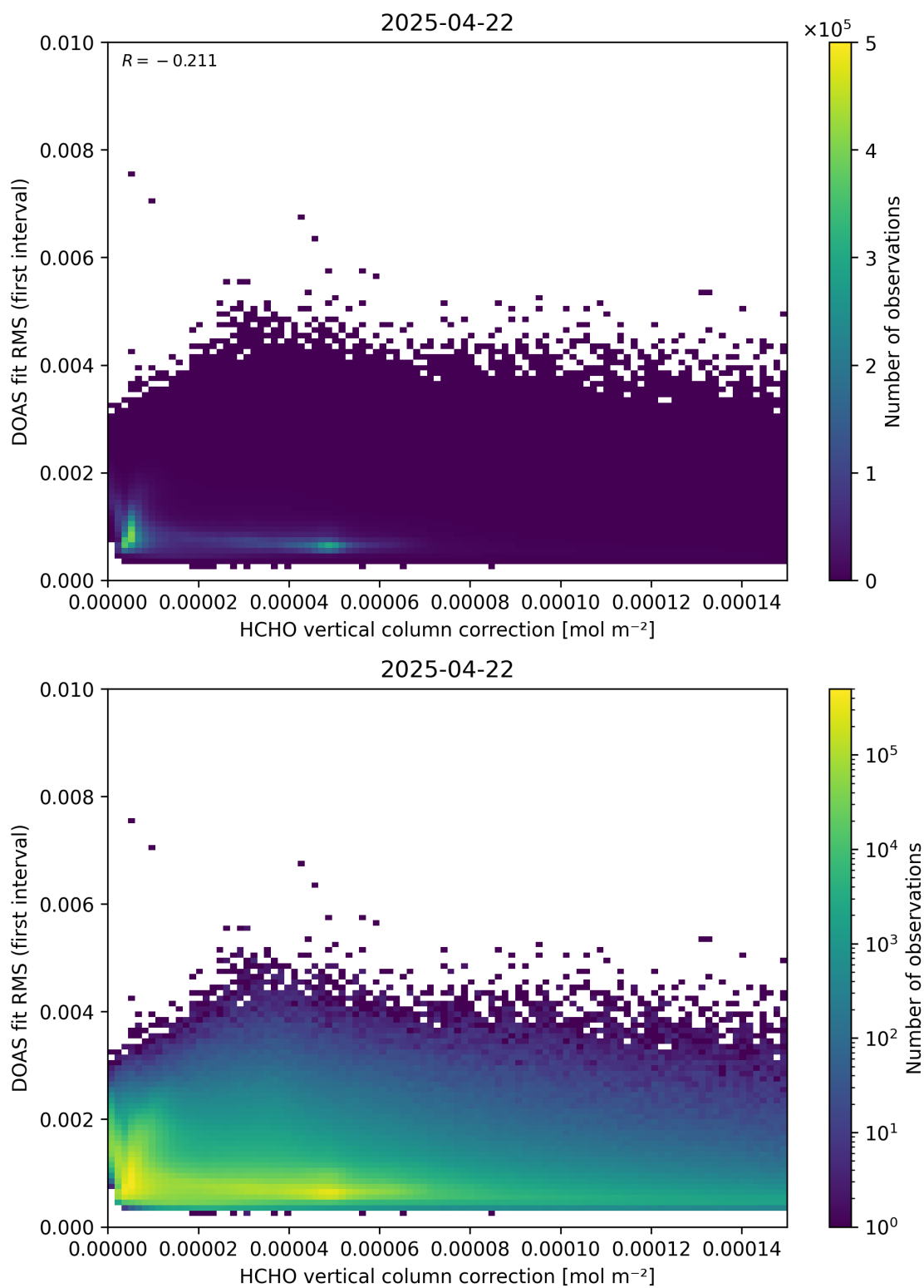
Figure 112: Scatter density plot of “HCHO vertical column correction” against “DOAS fit RMS (first interval)” for 2025-04-21 to 2025-04-23.
