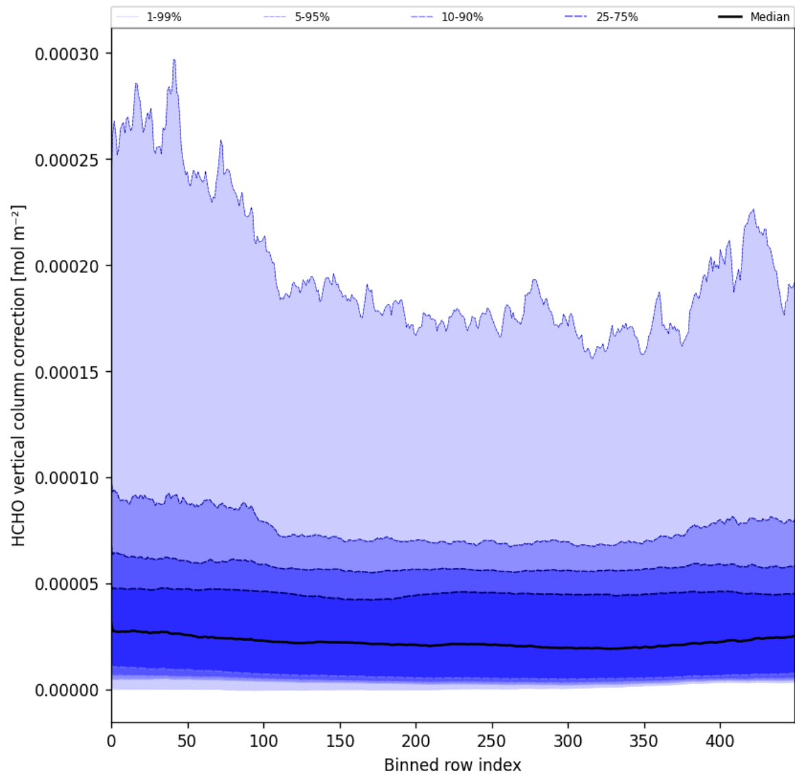
Figure 51: Along track statistics of “HCHO vertical column correction” for 2025-04-21 to 2025-04-23
