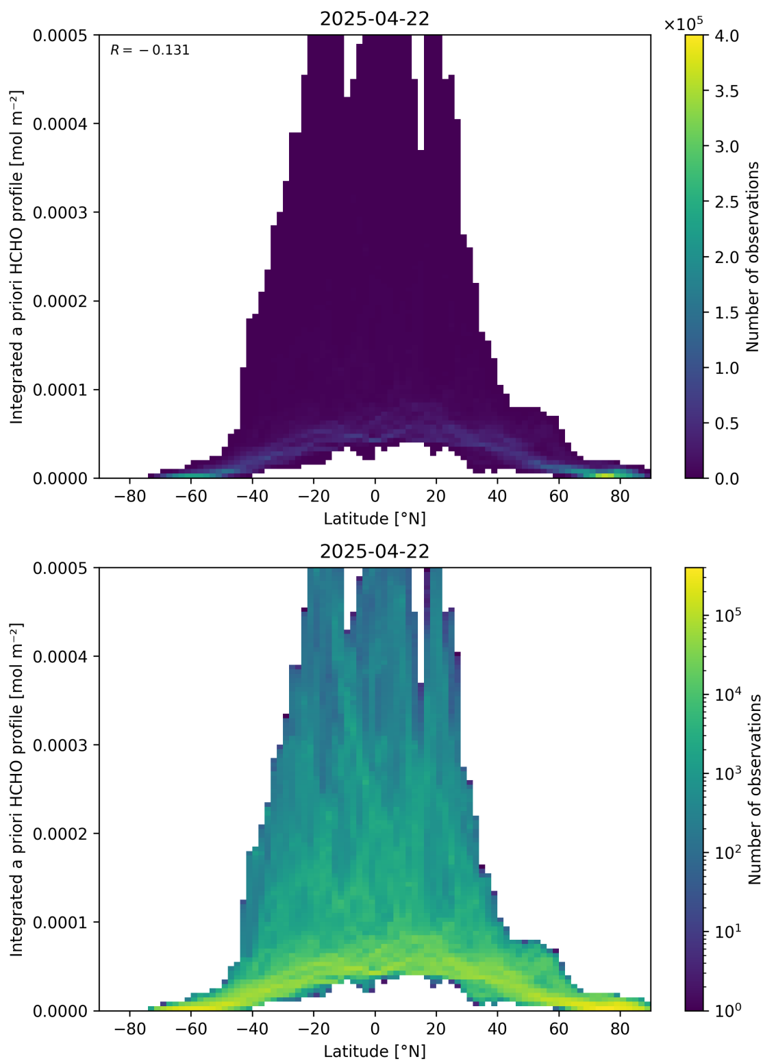
Figure 166: Scatter density plot of “Latitude” against “Integrated a priori HCHO profile” for 2025-04-21 to 2025-04-23.
