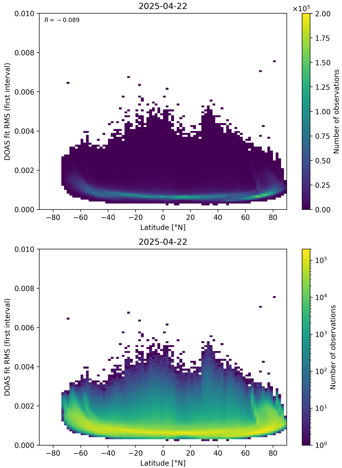
Figure 153: Scatter density plot of “Latitude” against “DOAS fit RMS (first interval)” for 2025-04-21 to 2025-04-23.
