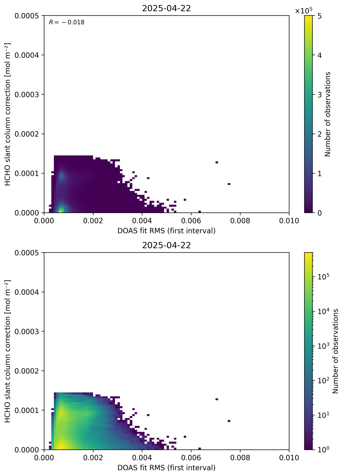
Figure 63: Scatter density plot of “DOAS fit RMS (first interval)” against “HCHO slant column correction” for 2025-04-21 to 2025-04-23.
