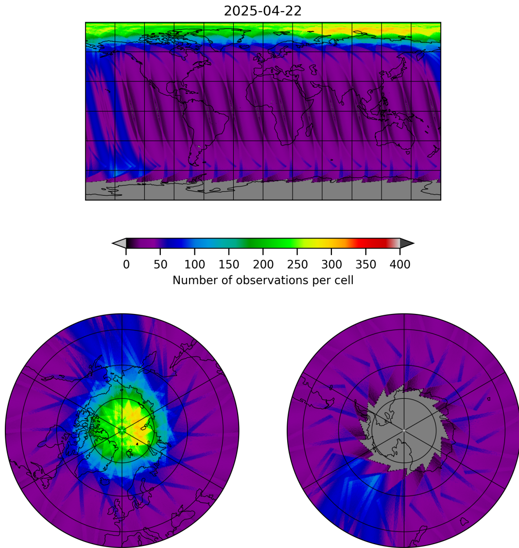
Figure 19: Map of the number of observations for 2025-04-21 to 2025-04-23
