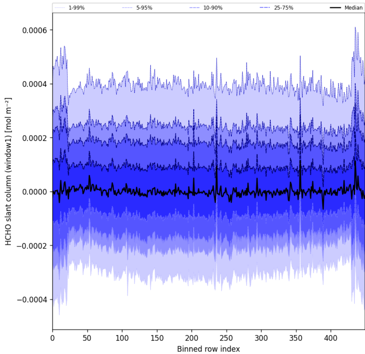
Figure 52: Along track statistics of “HCHO slant column (window1)” for 2025-04-21 to 2025-04-23
