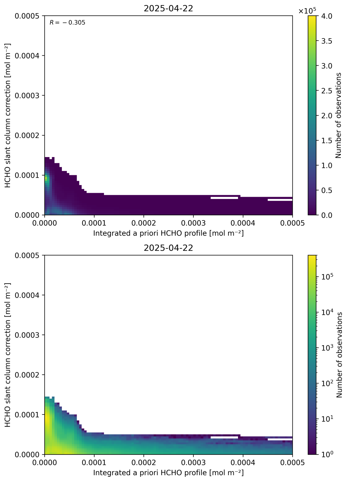
Figure 152: Scatter density plot of “Integrated a priori HCHO profile” against “HCHO slant column correction” for 2025-04-21 to 2025-04-23.
