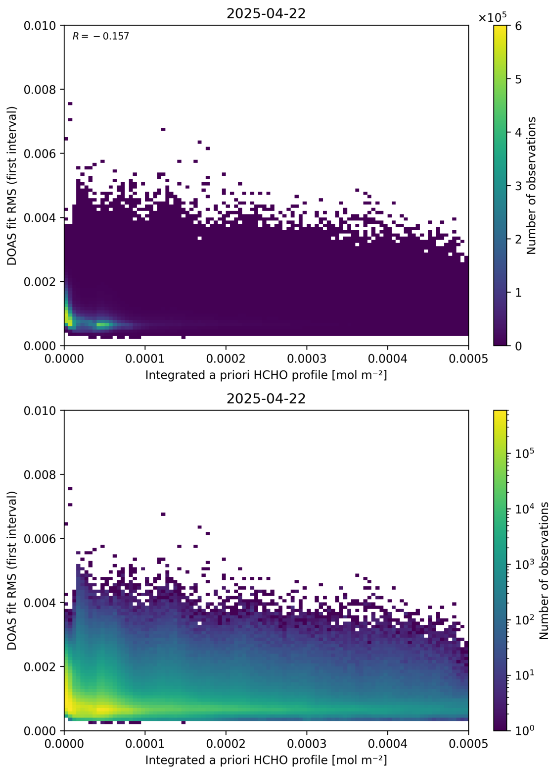
Figure 148: Scatter density plot of “Integrated a priori HCHO profile” against “DOAS fit RMS (first interval)” for 2025-04-21 to 2025-04-23.
