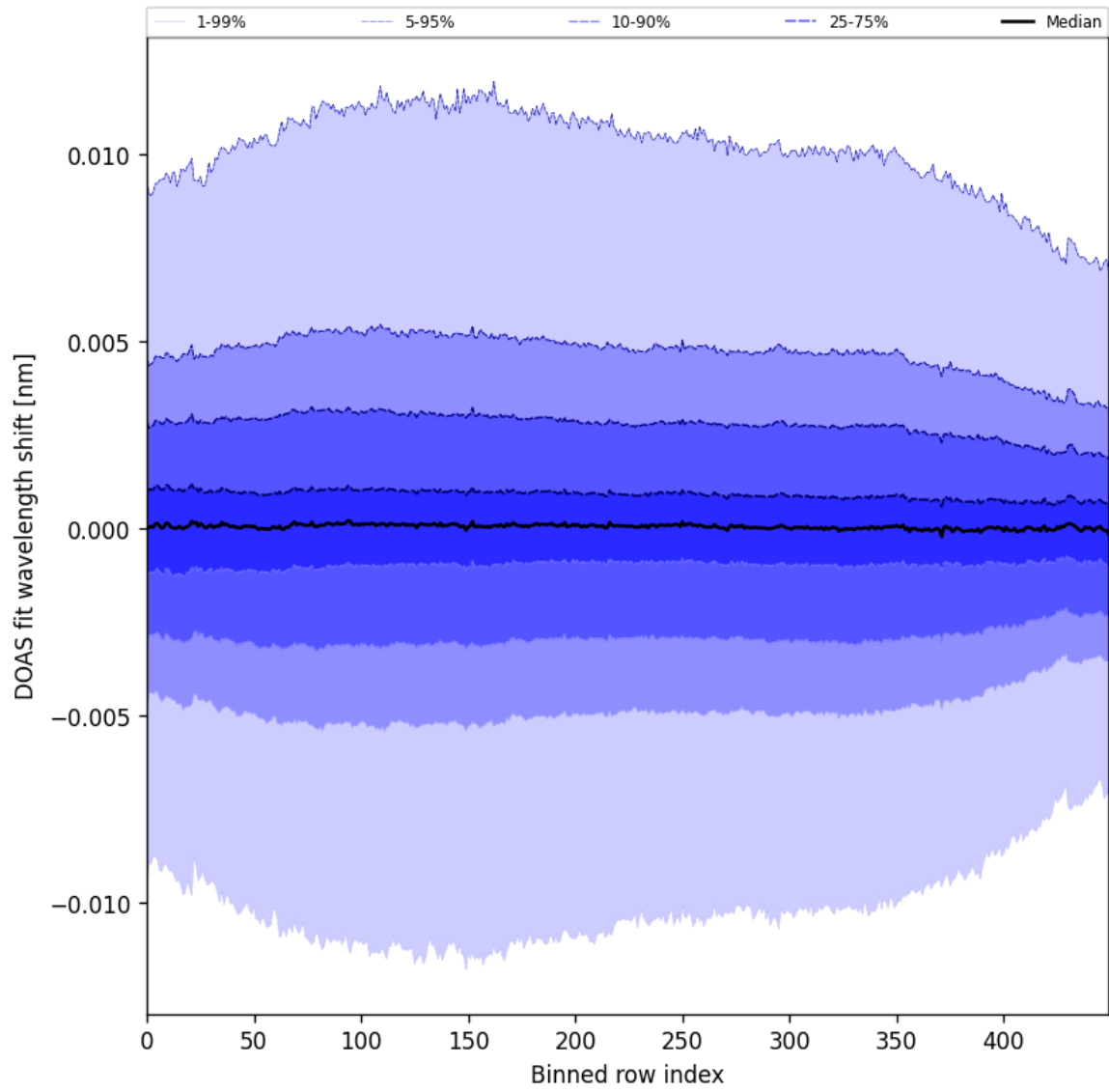
Figure 58: Along track statistics of “DOAS fit wavelength shift” for 2025-04-21 to 2025-04-23
