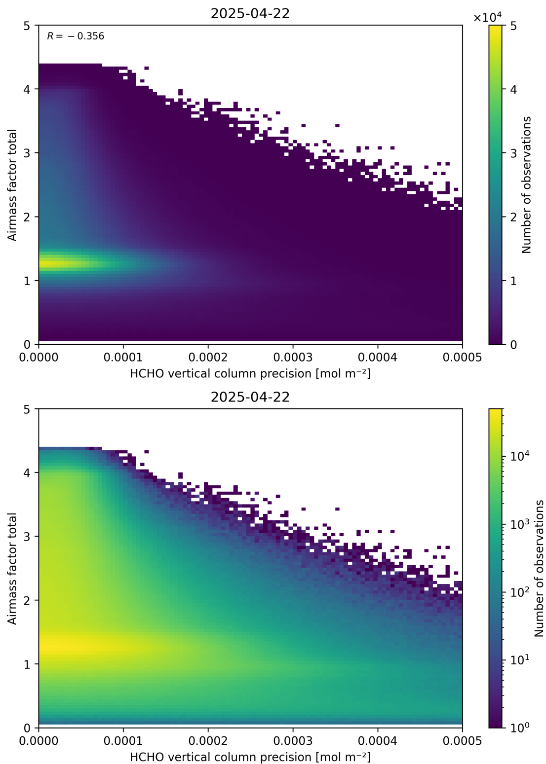
Figure 144: Scatter density plot of “HCHO vertical column precision” against “Airmass factor total” for 2025-04-21 to 2025-04-23.
