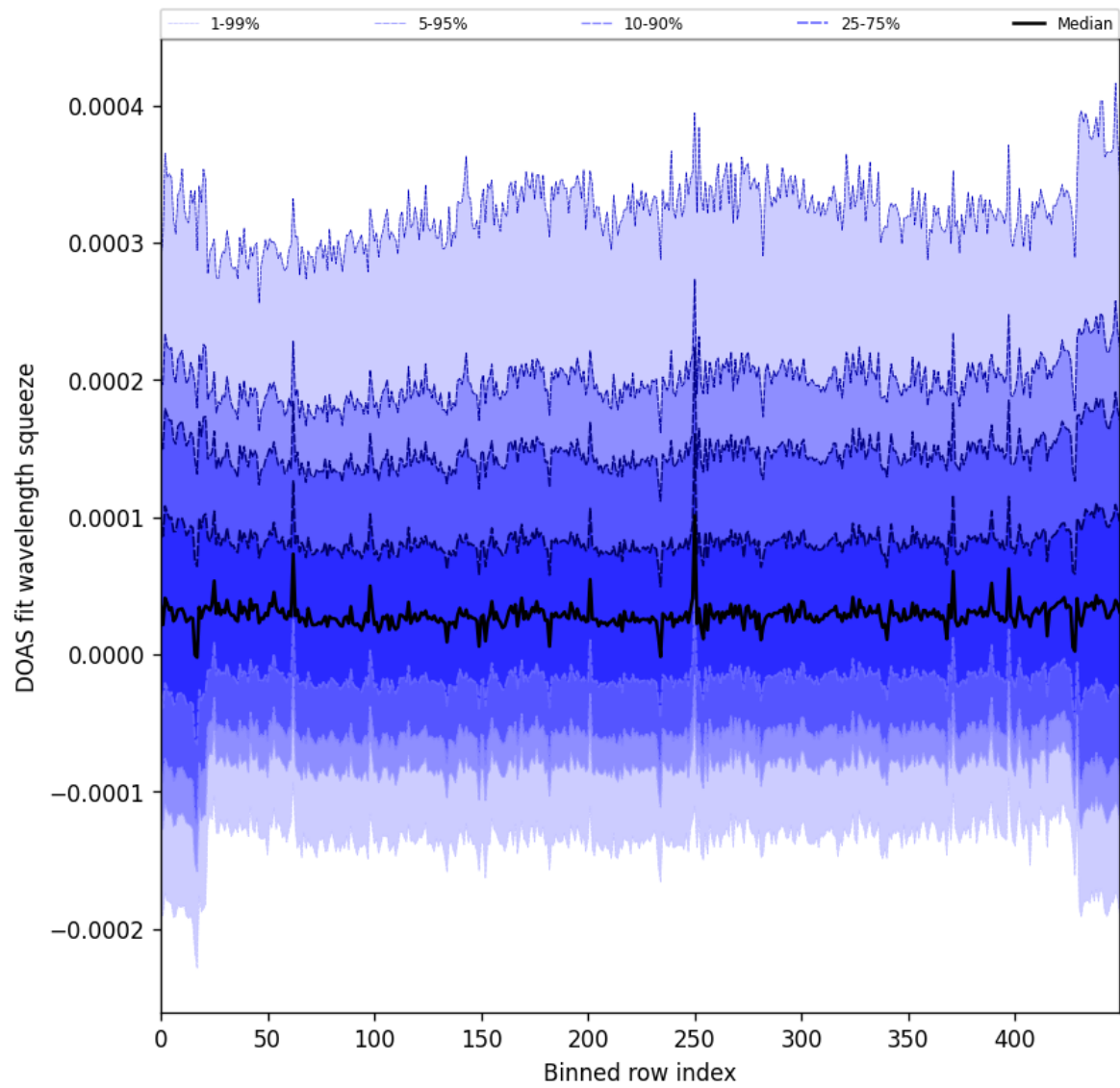
Figure 59: Along track statistics of “DOAS fit wavelength squeeze” for 2025-04-21 to 2025-04-23
