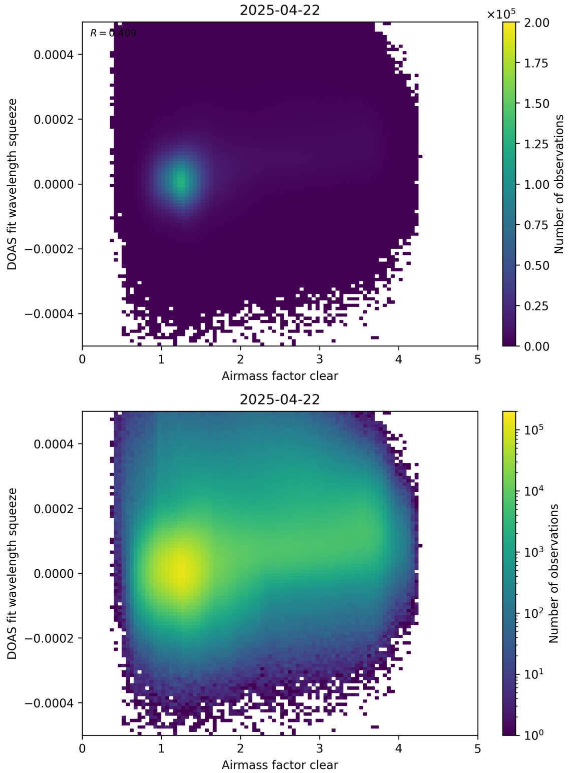
Figure 73: Scatter density plot of “Airmass factor clear” against “DOAS fit wavelength squeeze” for 2025-04-21 to 2025-04-23.
