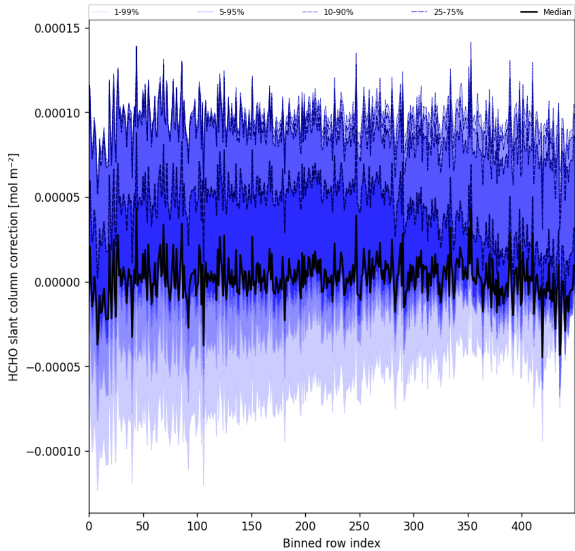
Figure 61: Along track statistics of “HCHO slant column correction” for 2025-04-21 to 2025-04-23
