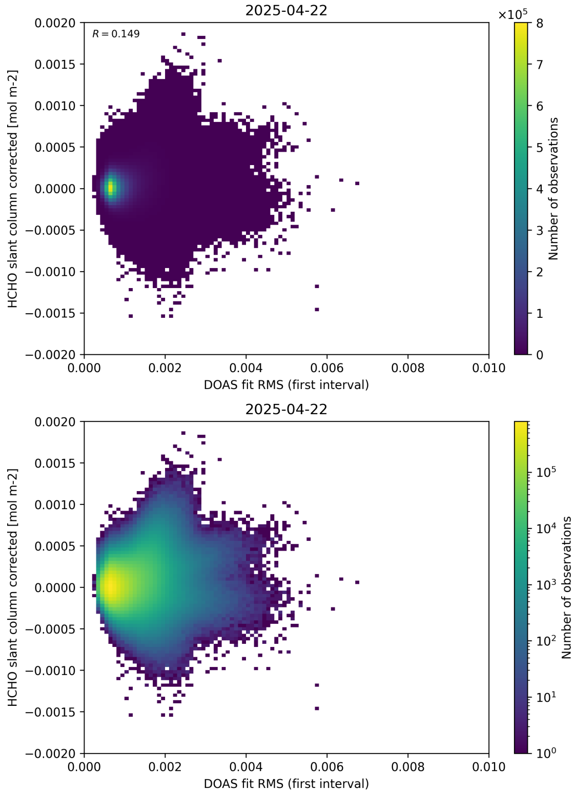
Figure 62: Scatter density plot of “DOAS fit RMS (first interval)” against “HCHO slant column corrected” for 2025-04-21 to 2025-04-23.
