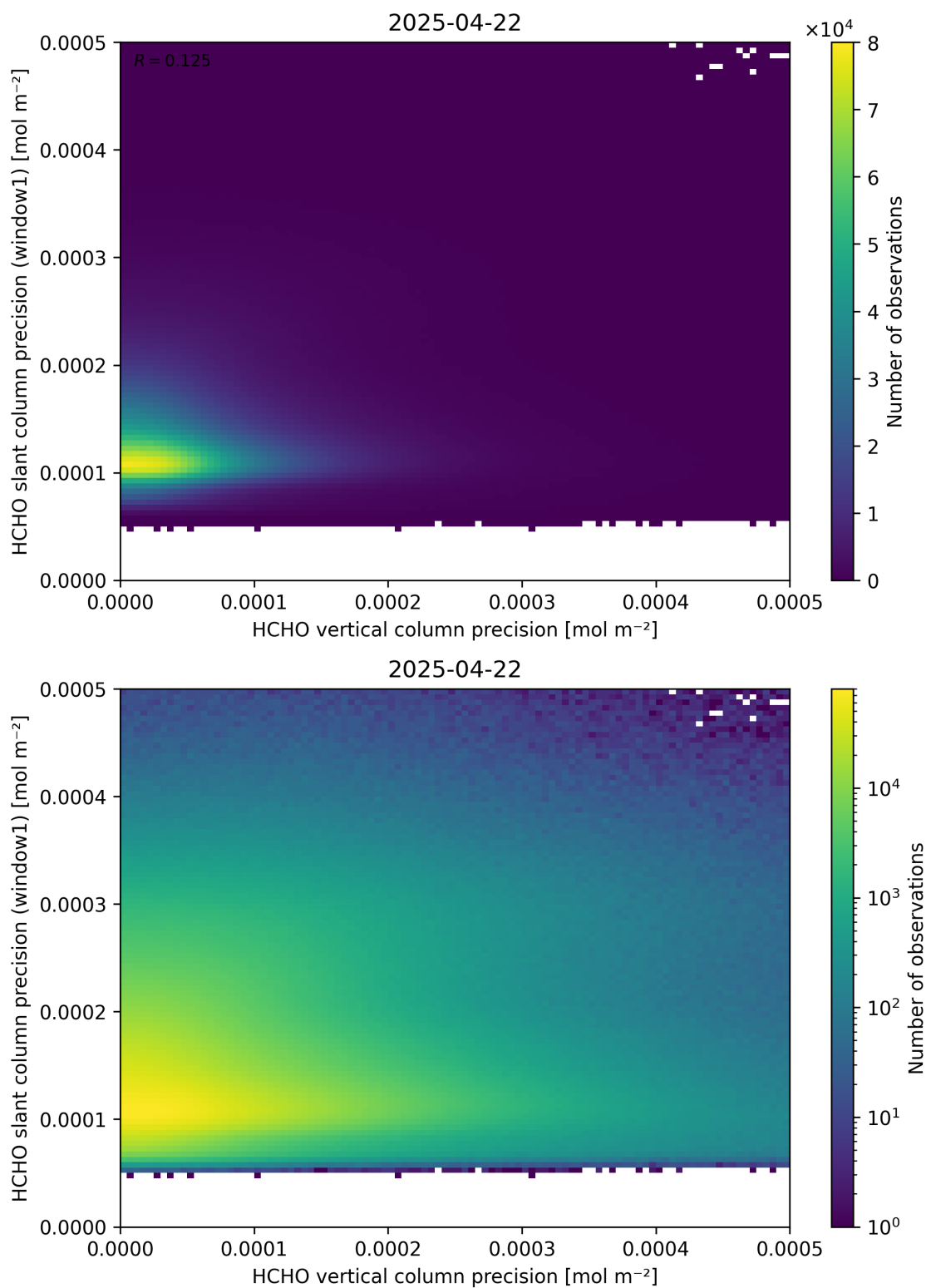
Figure 143: Scatter density plot of “HCHO vertical column precision” against “HCHO slant column precision (window1)” for 2025-04-21 to 2025-04-23.
