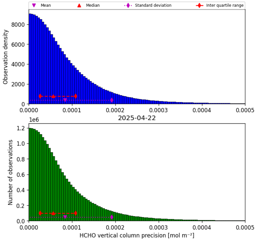
Figure 36: Histogram of “HCHO vertical column precision” for 2025-04-21 to 2025-04-23
