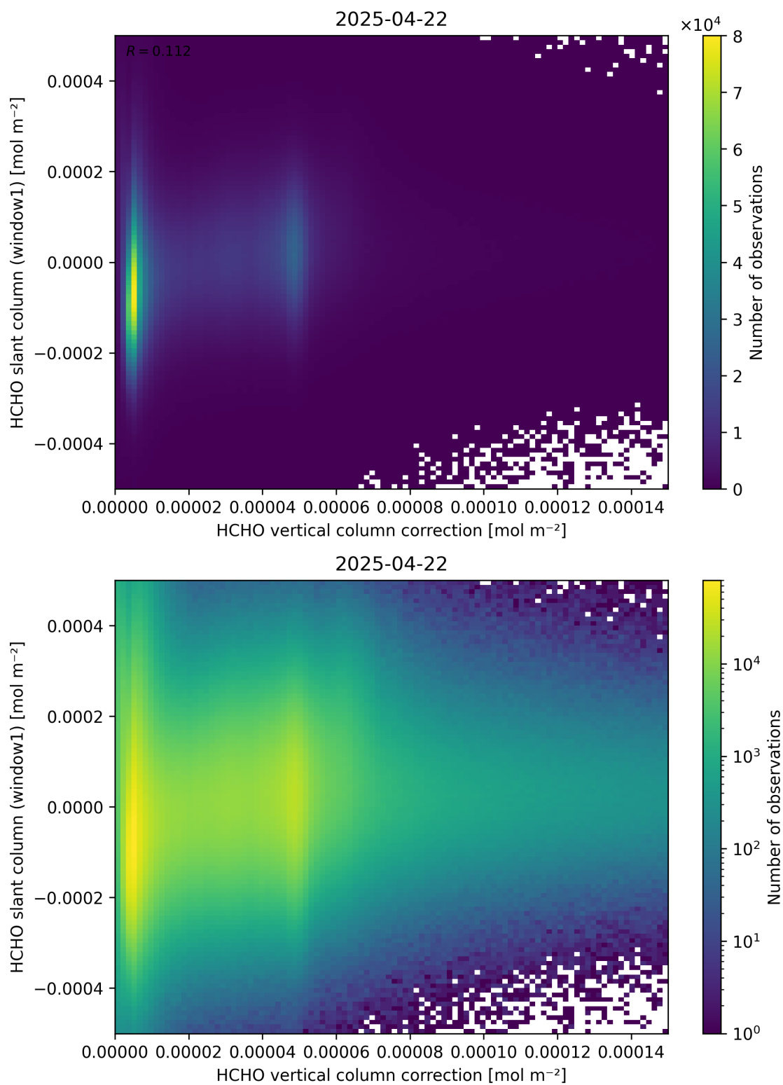
Figure 118: Scatter density plot of “HCHO vertical column correction” against “HCHO slant column (window1)” for 2025-04-21 to 2025-04-23.
