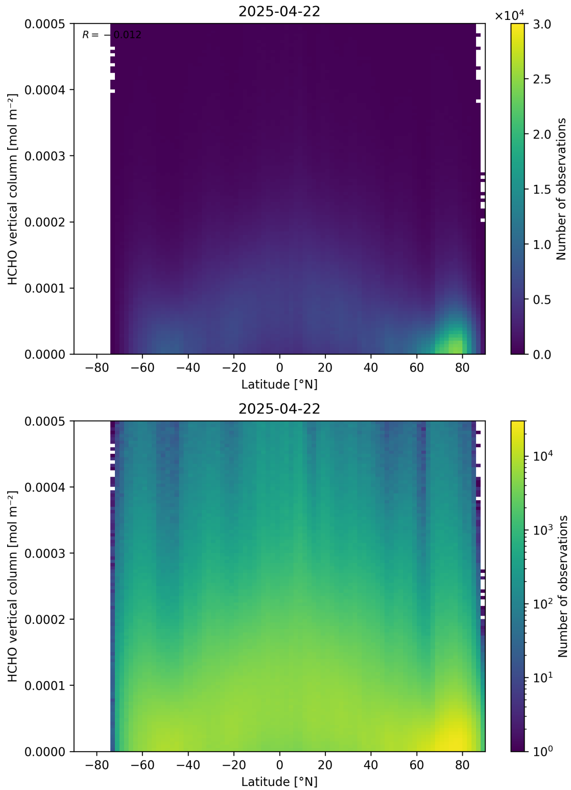
Figure 163: Scatter density plot of “Latitude” against “HCHO vertical column” for 2025-04-21 to 2025-04-23.
