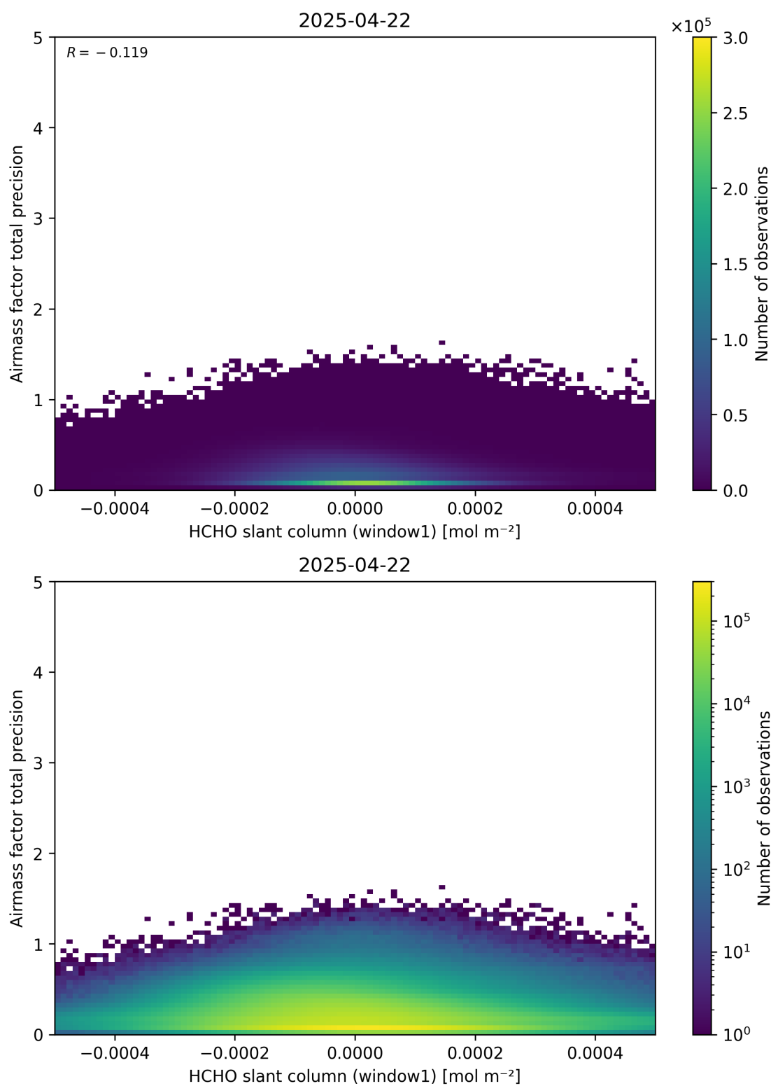
Figure 86: Scatter density plot of “HCHO slant column (window1)” against “Airmass factor total precision” for 2025-04-21 to 2025-04-23.
