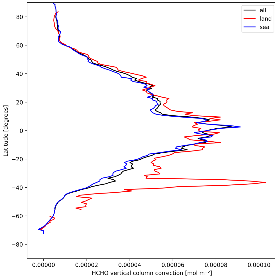
Figure 23: Zonal average of “HCHO vertical column correction” for 2025-04-21 to 2025-04-23.
