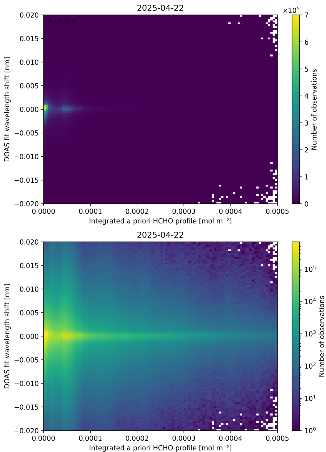
Figure 149: Scatter density plot of “Integrated a priori HCHO profile” against “DOAS fit wavelength shift” for 2025-04-21 to 2025-04-23.
