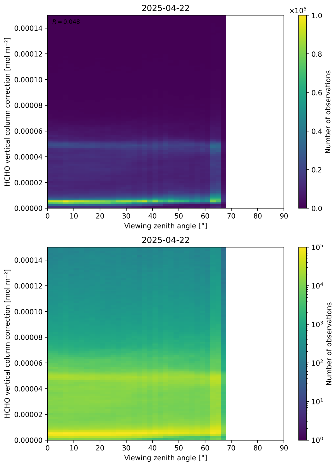
Figure 193: Scatter density plot of “Viewing zenith angle” against “HCHO vertical column correction” for 2025-04-21 to 2025-04-23.
