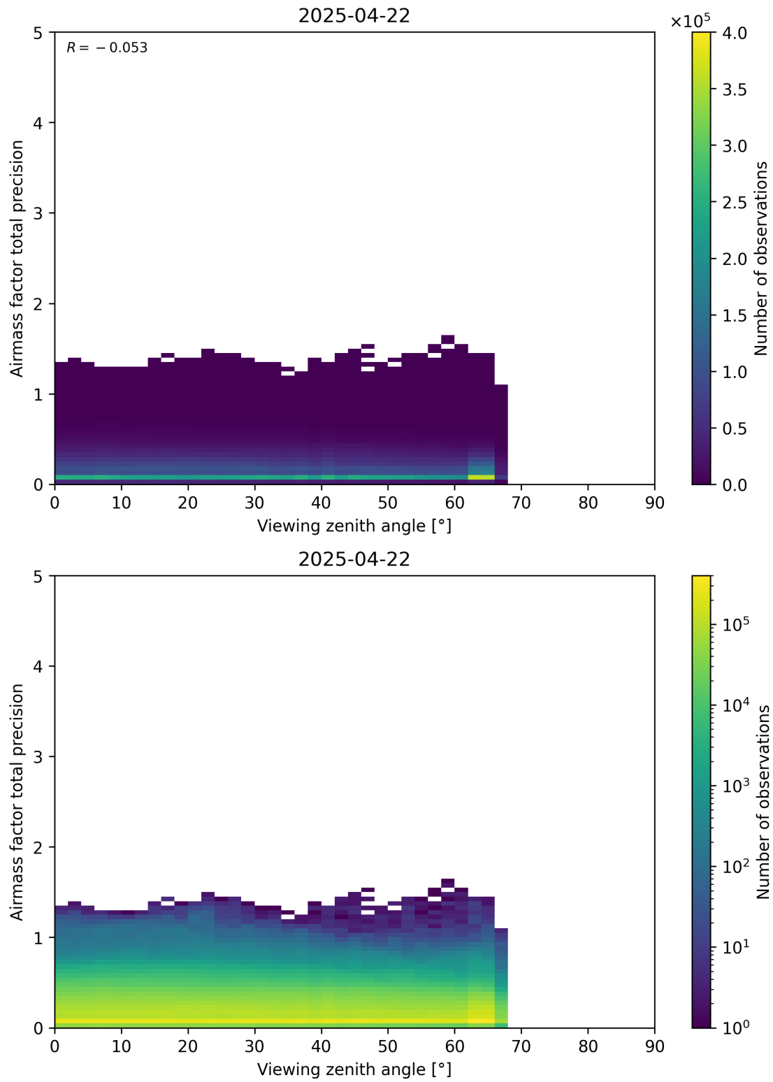
Figure 191: Scatter density plot of “Viewing zenith angle” against “Airmass factor total precision” for 2025-04-21 to 2025-04-23.
