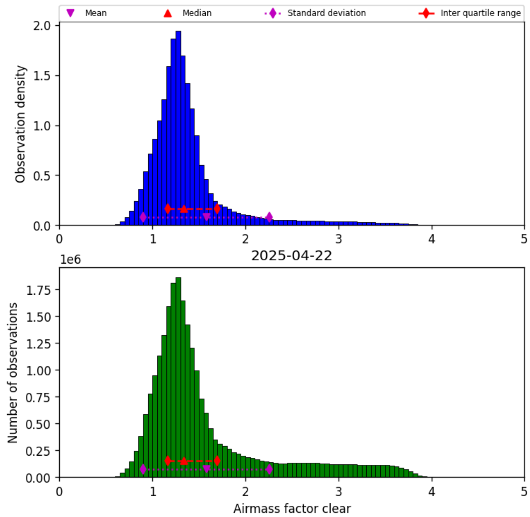
Figure 42: Histogram of “Airmass factor clear” for 2025-04-21 to 2025-04-23
