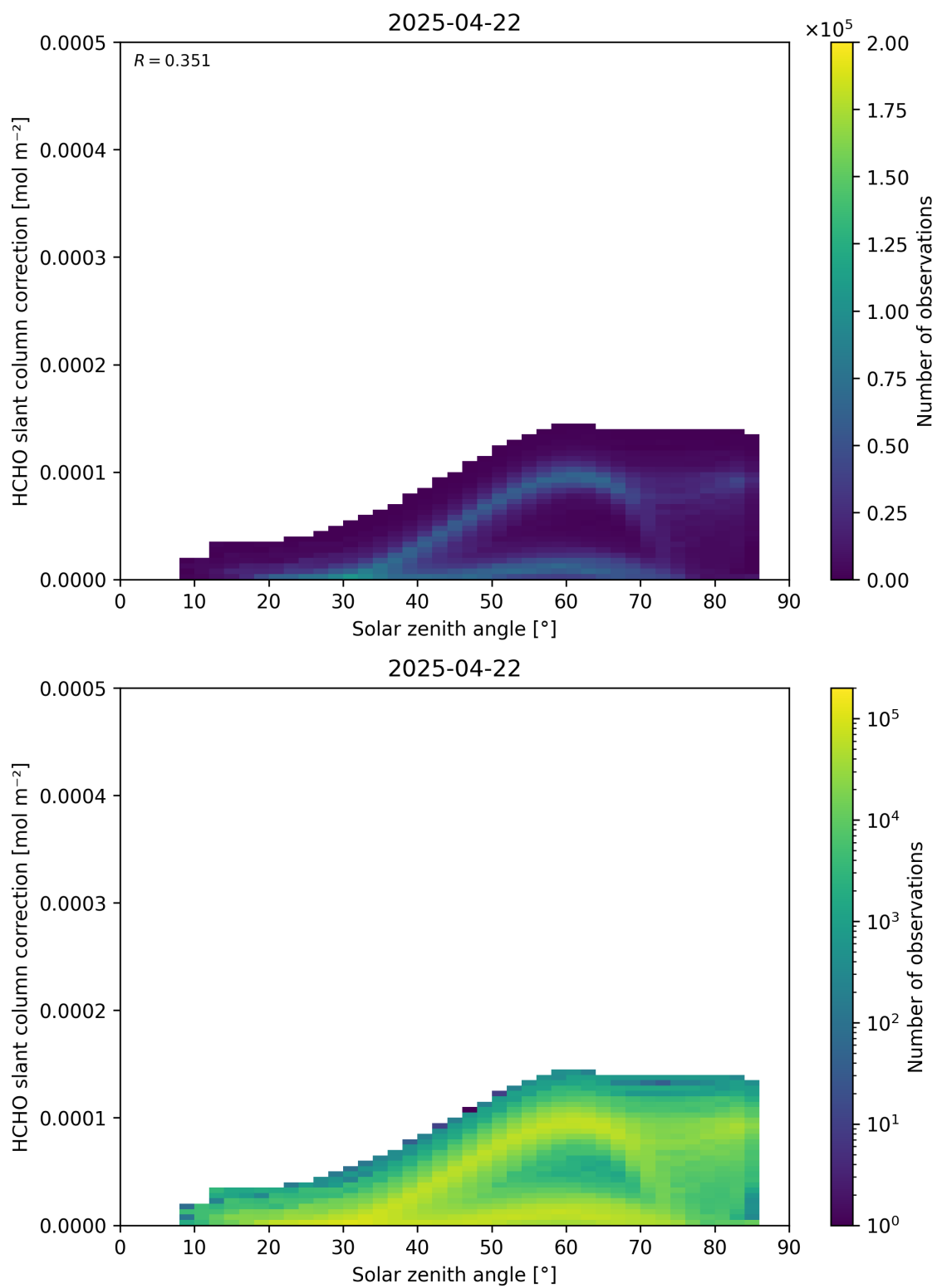
Figure 172: Scatter density plot of “Solar zenith angle” against “HCHO slant column correction” for 2025-04-21 to 2025-04-23.
