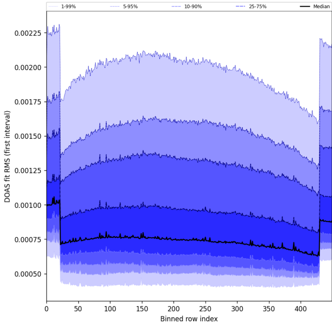
Figure 60: Along track statistics of “DOAS fit RMS (first interval)” for 2025-04-21 to 2025-04-23
