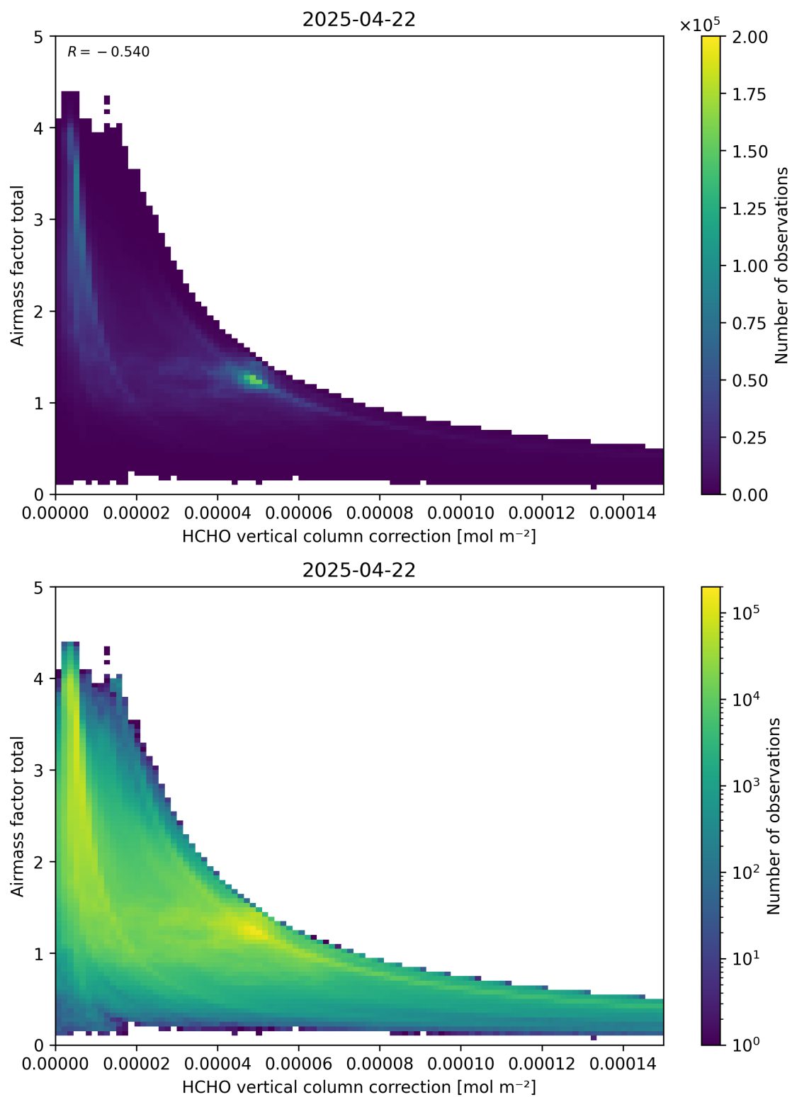
Figure 120: Scatter density plot of “HCHO vertical column correction” against “Airmass factor total” for 2025-04-21 to 2025-04-23.
