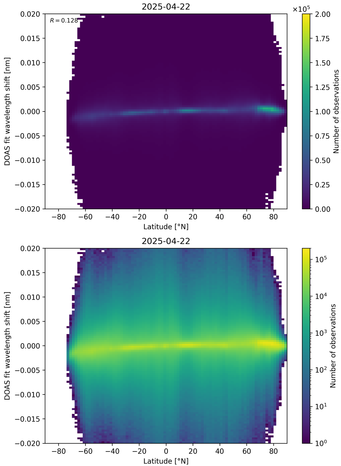
Figure 154: Scatter density plot of “Latitude” against “DOAS fit wavelength shift” for 2025-04-21 to 2025-04-23.
