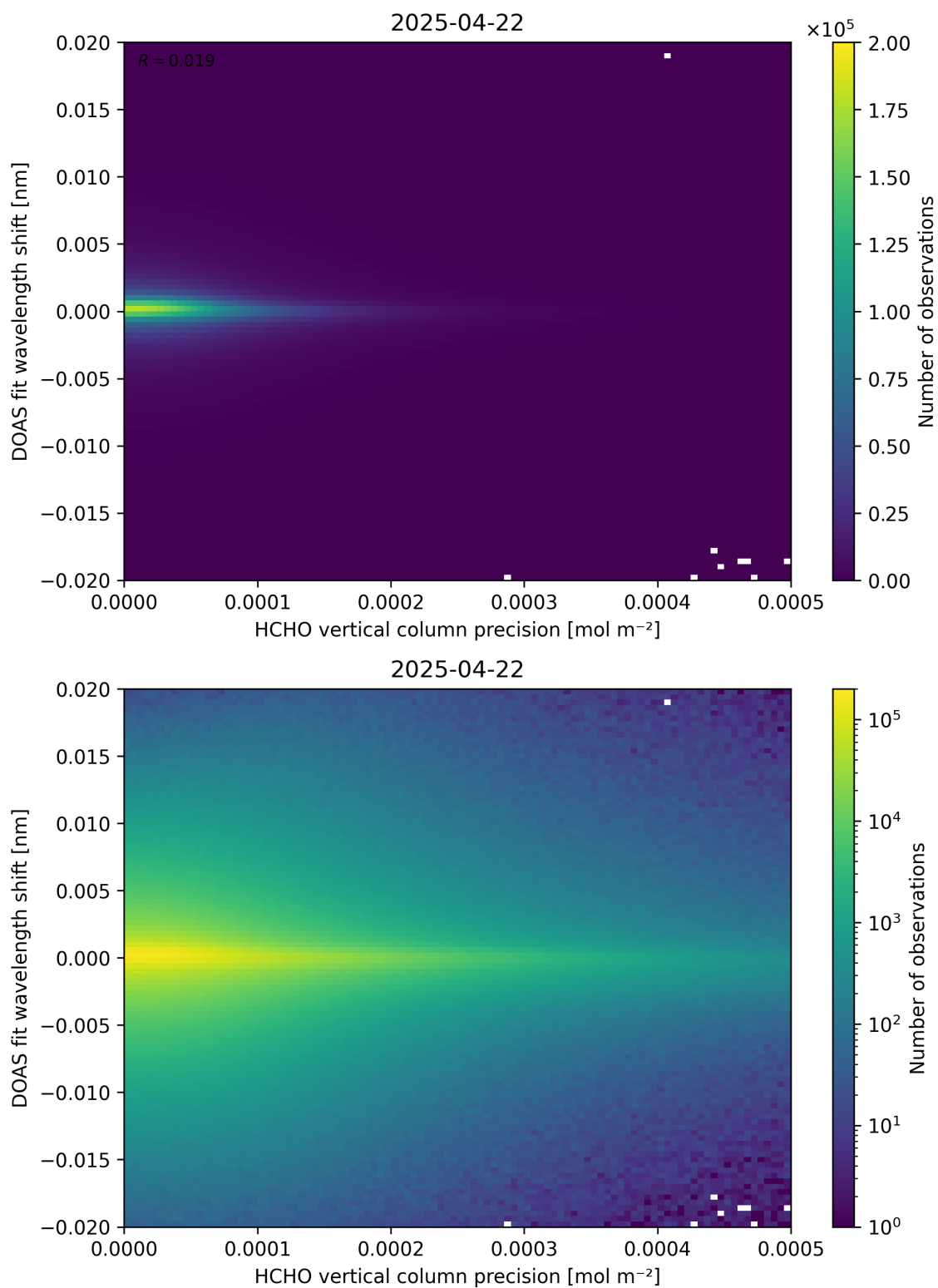
Figure 137: Scatter density plot of “HCHO vertical column precision” against “DOAS fit wavelength shift” for 2025-04-21 to 2025-04-23.
