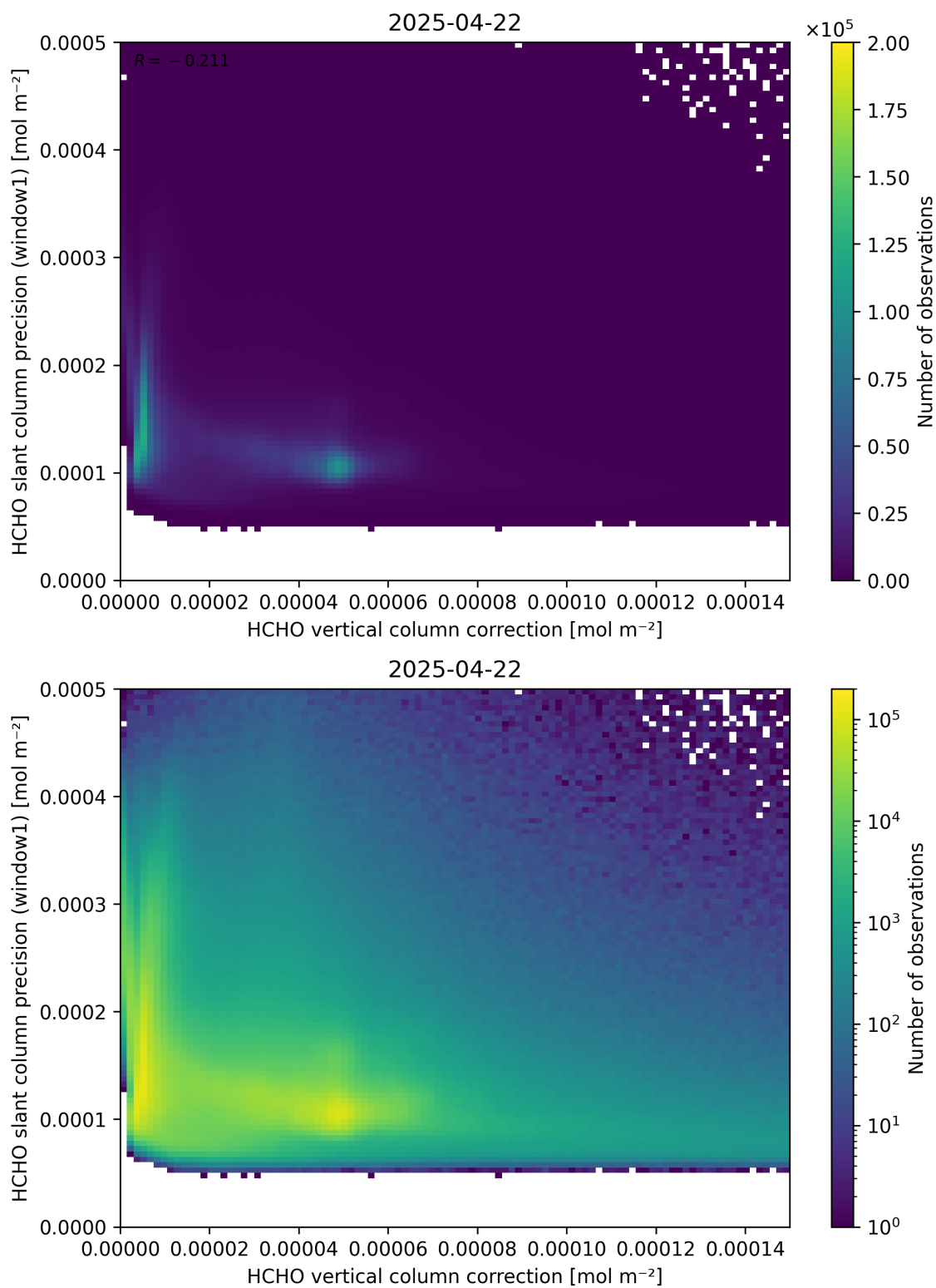
Figure 119: Scatter density plot of “HCHO vertical column correction” against “HCHO slant column precision (window1)” for 2025-04-21 to 2025-04-23.
