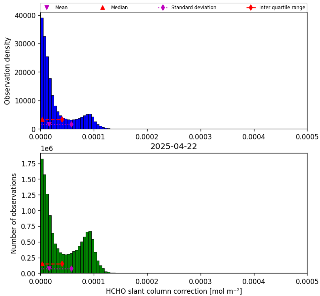
Figure 47: Histogram of “HCHO slant column correction” for 2025-04-21 to 2025-04-23
