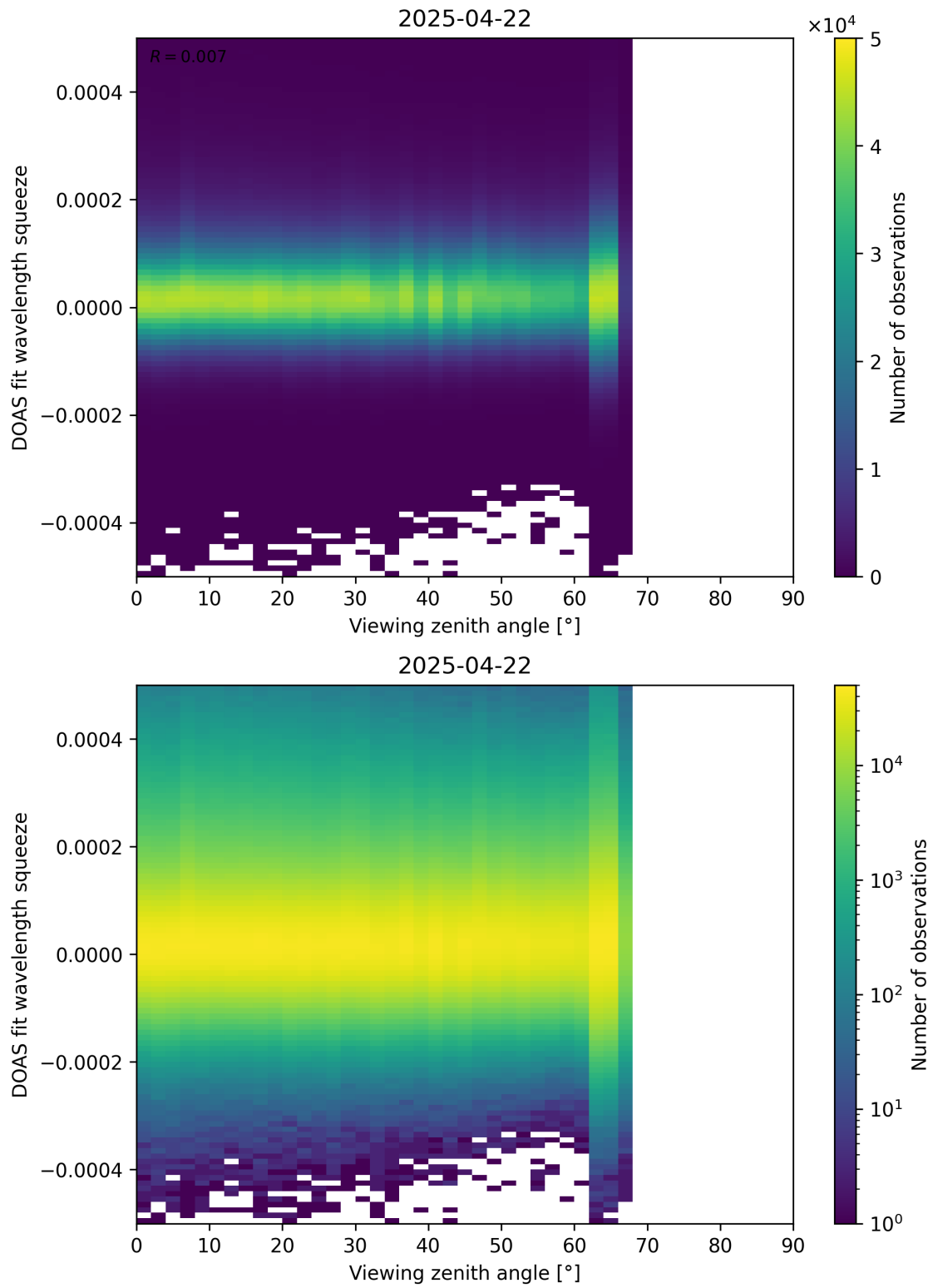
Figure 184: Scatter density plot of “Viewing zenith angle” against “DOAS fit wavelength squeeze” for 2025-04-21 to 2025-04-23.
