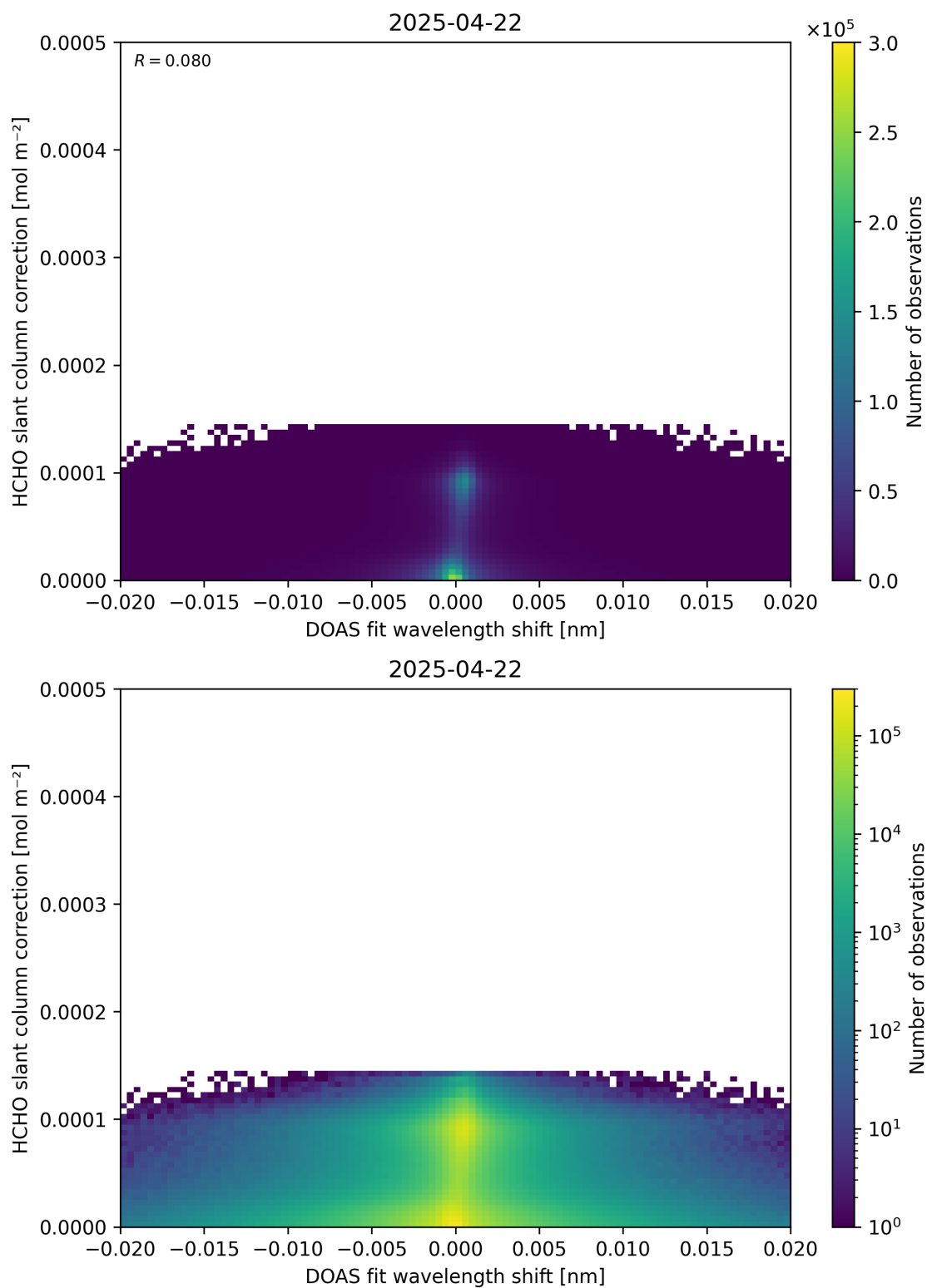
Figure 67: Scatter density plot of “DOAS fit wavelength shift” against “HCHO slant column correction” for 2025-04-21 to 2025-04-23.
