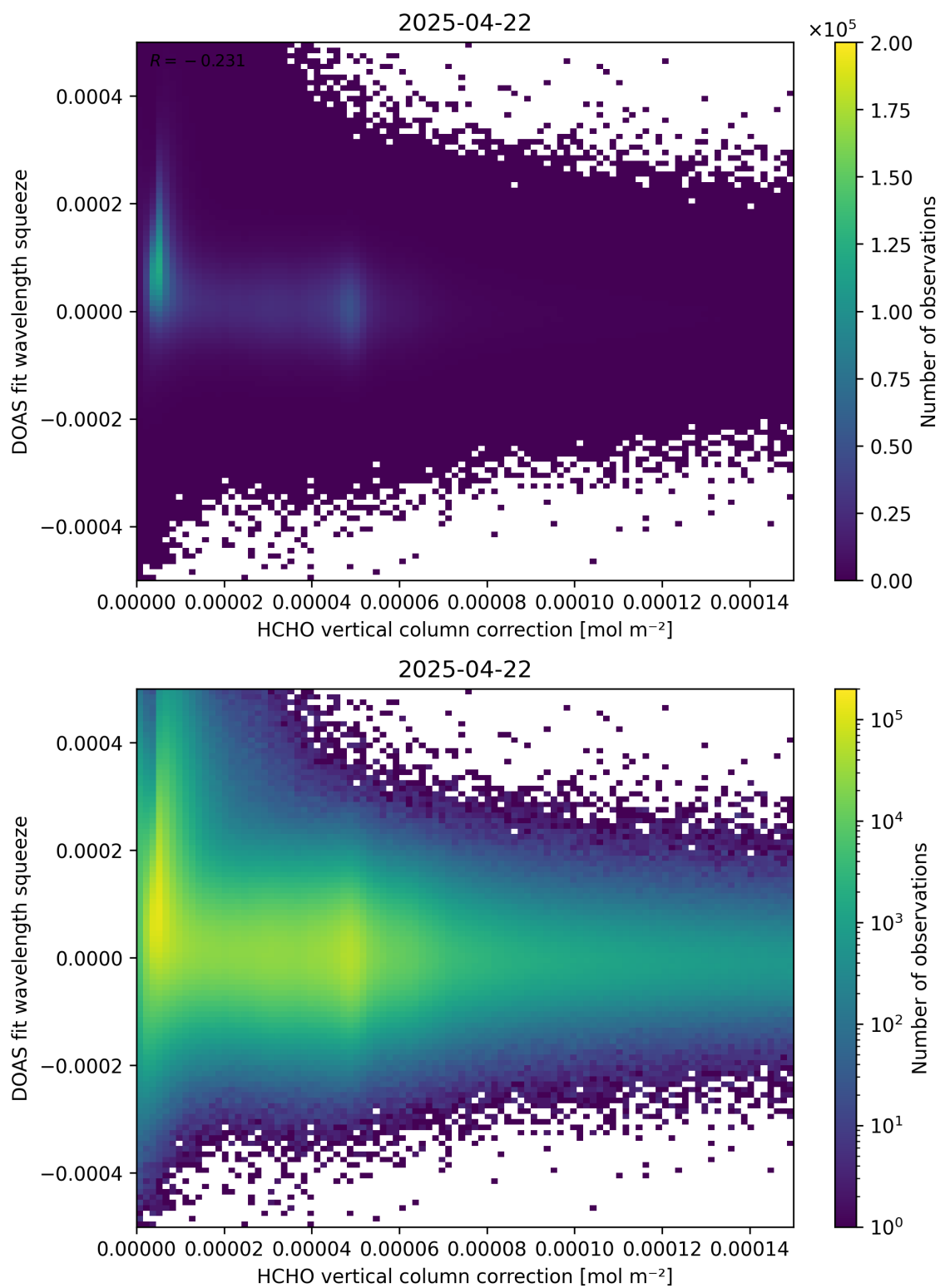
Figure 114: Scatter density plot of “HCHO vertical column correction” against “DOAS fit wavelength squeeze” for 2025-04-21 to 2025-04-23.
