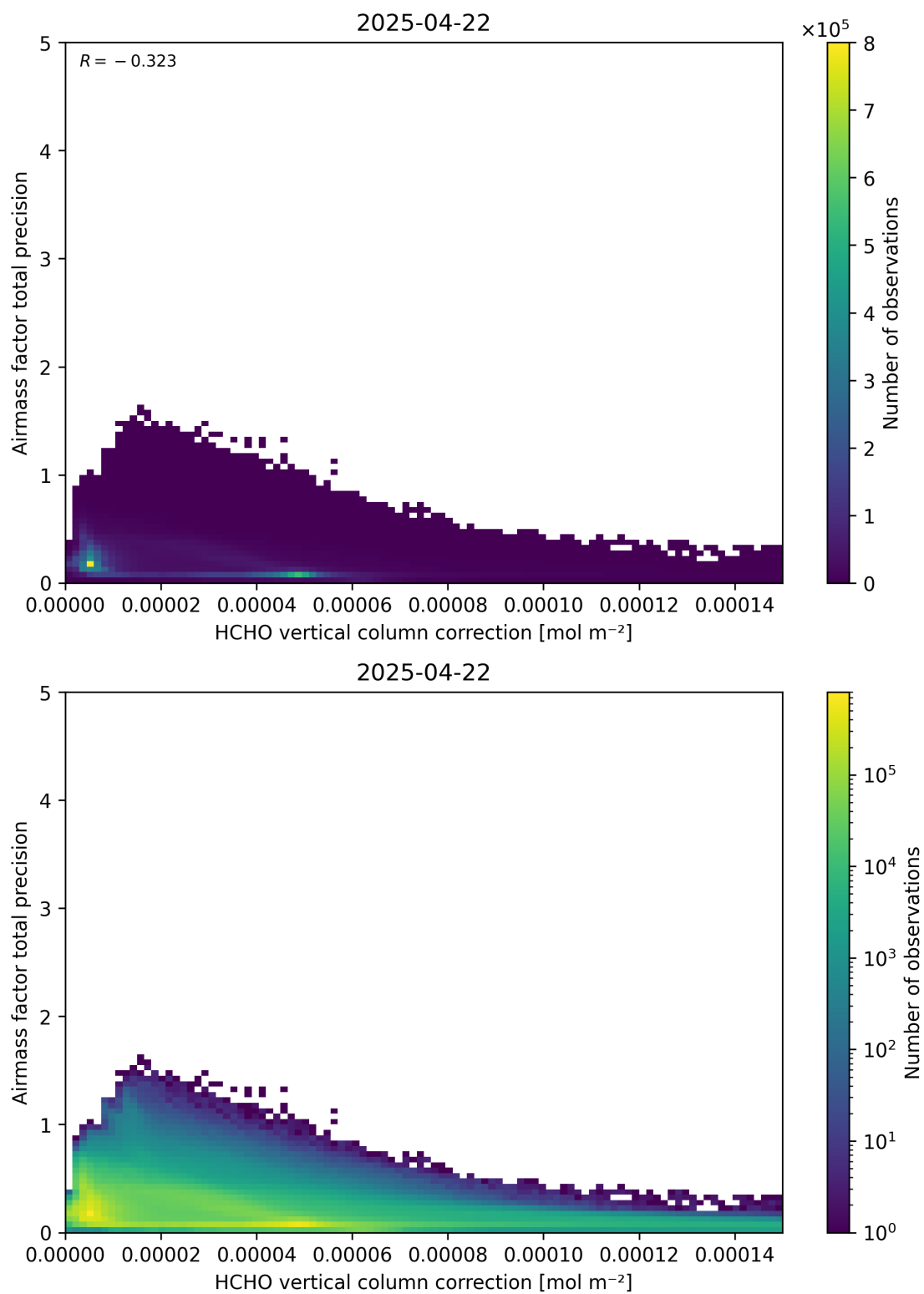
Figure 121: Scatter density plot of “HCHO vertical column correction” against “Airmass factor total precision” for 2025-04-21 to 2025-04-23.
