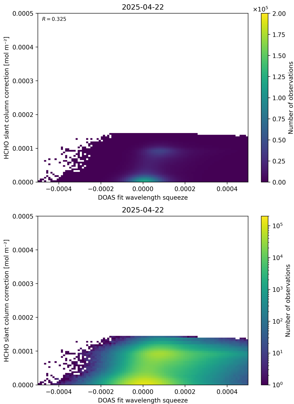
Figure 70: Scatter density plot of “DOAS fit wavelength squeeze” against “HCHO slant column correction” for 2025-04-21 to 2025-04-23.
