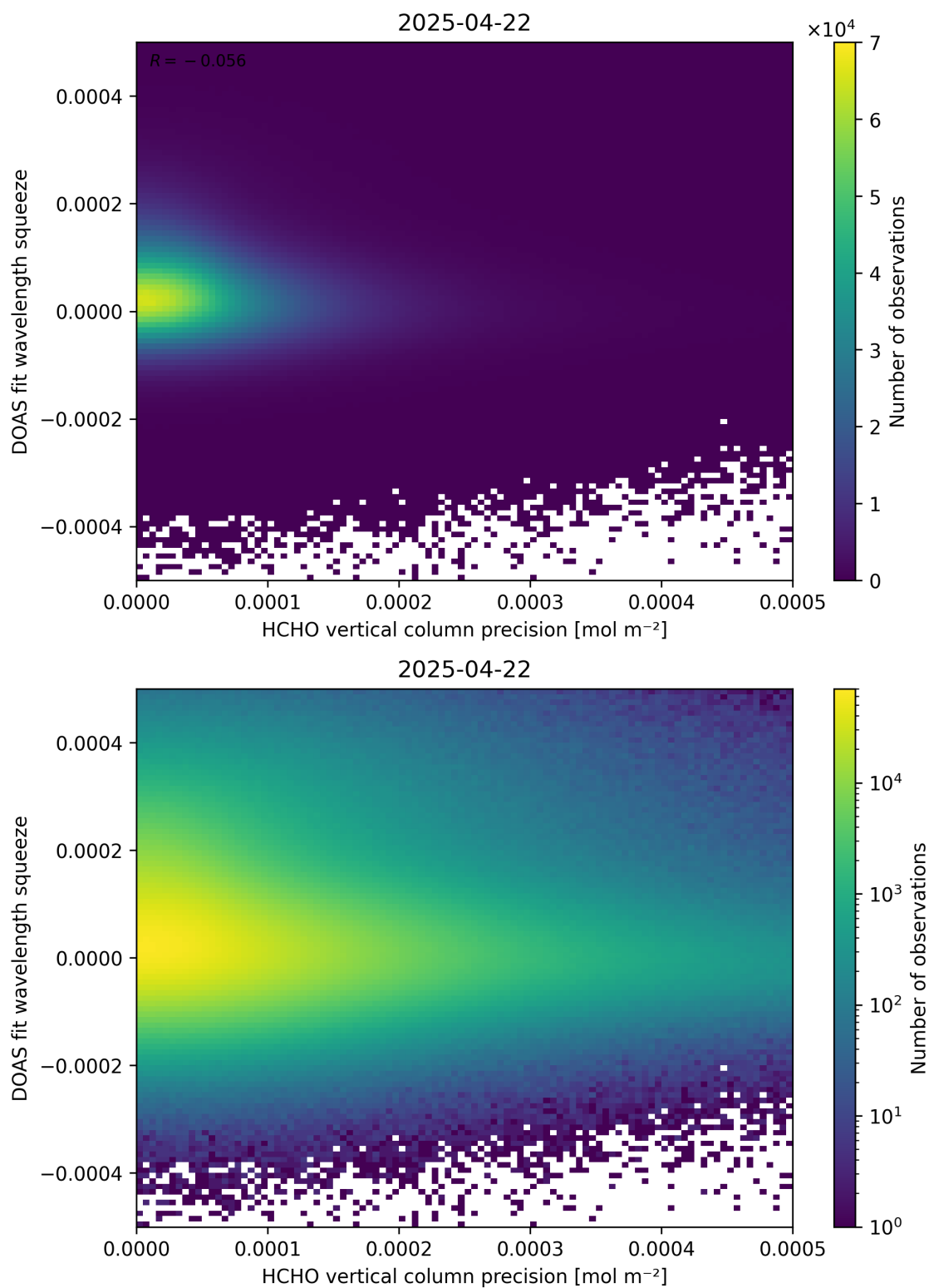
Figure 138: Scatter density plot of “HCHO vertical column precision” against “DOAS fit wavelength squeeze” for 2025-04-21 to 2025-04-23.
