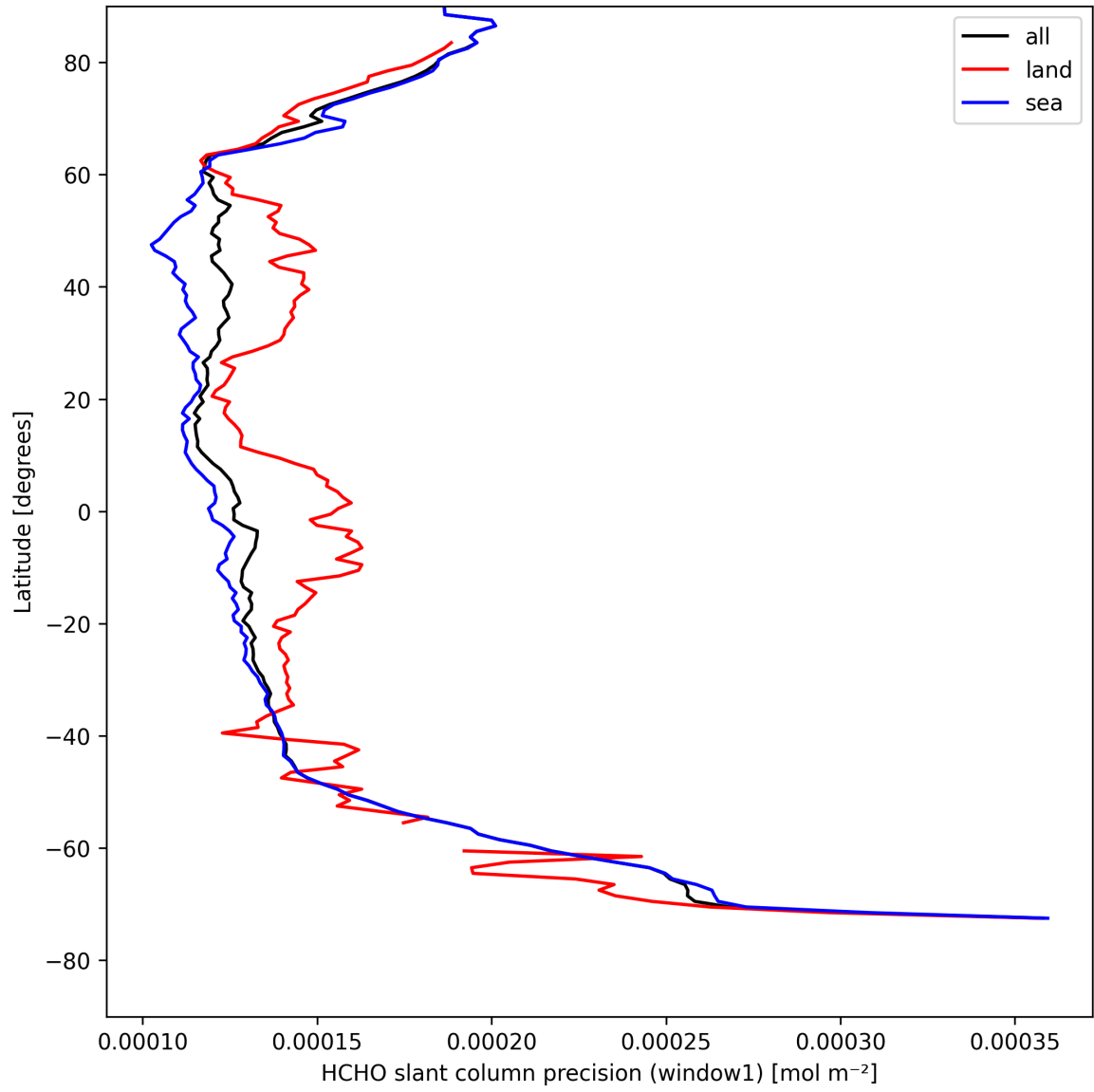
Figure 25: Zonal average of "HCHO slant column precision (window1)" for 2025-04-21 to 2025-04-23.
