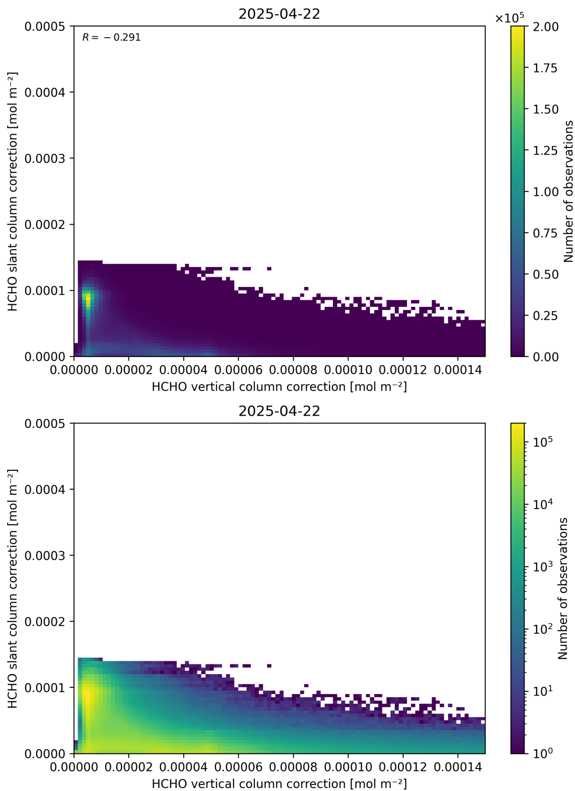
Figure 117: Scatter density plot of “HCHO vertical column correction” against “HCHO slant column correction” for 2025-04-21 to 2025-04-23.
