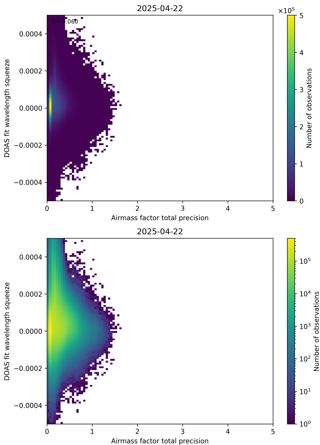
Figure 107: Scatter density plot of “Airmass factor total precision” against “DOAS fit wavelength squeeze” for 2025-04-21 to 2025-04-23.
