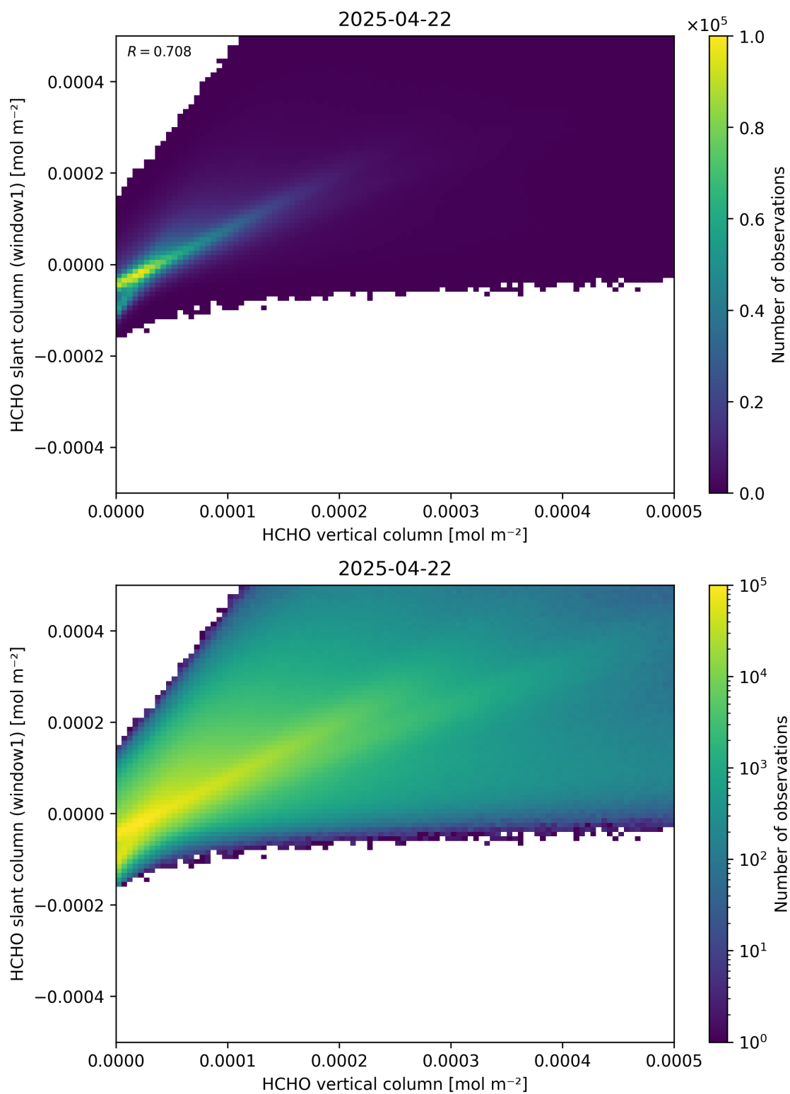
Figure 129: Scatter density plot of “HCHO vertical column” against “HCHO slant column (window1)” for 2025-04-21 to 2025-04-23.
