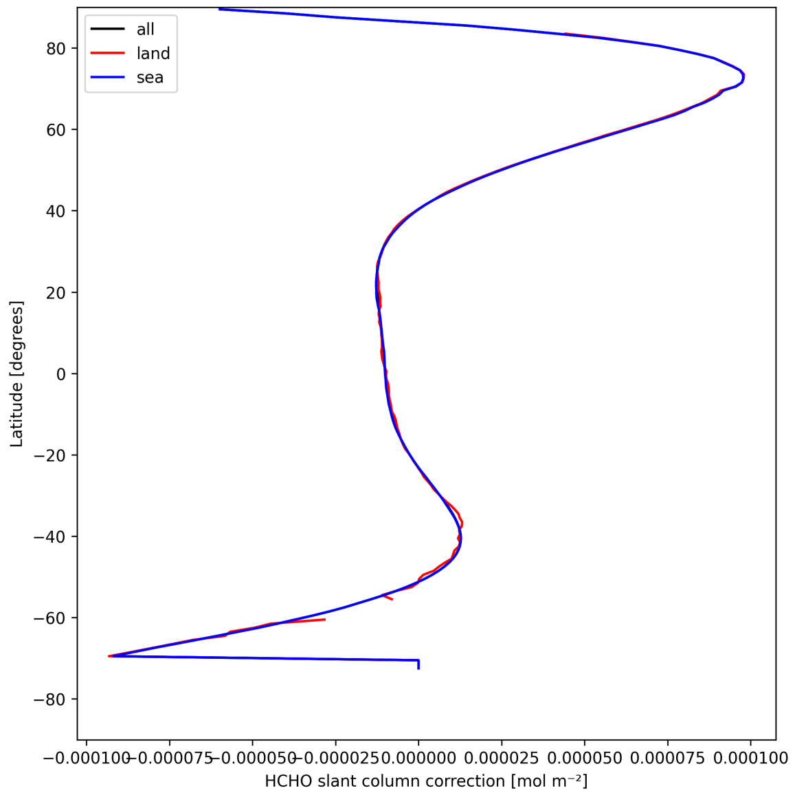
Figure 33: Zonal average of “HCHO slant column correction” for 2025-04-21 to 2025-04-23.
