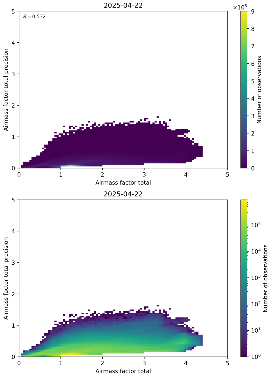
Figure 103: Scatter density plot of “Airmass factor total” against “Airmass factor total precision” for 2025-04-21 to 2025-04-23.
