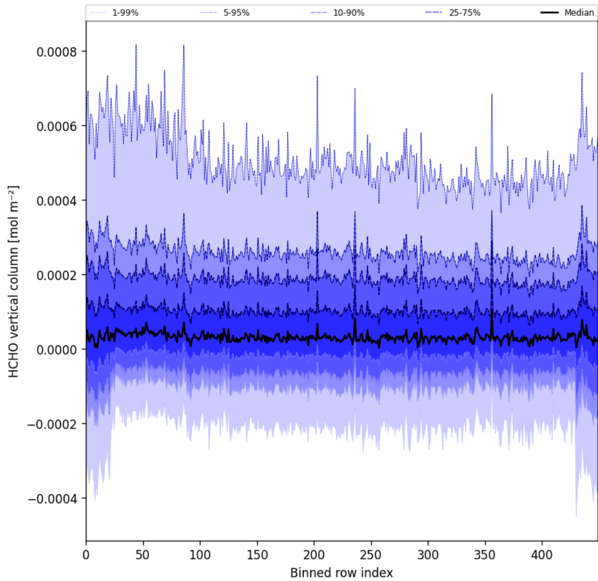
Figure 49: Along track statistics of “HCHO vertical column” for 2025-04-21 to 2025-04-23
