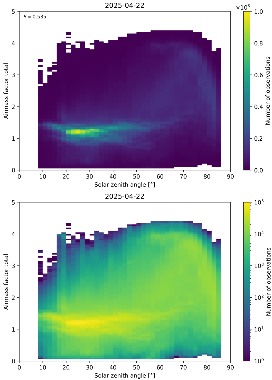
Figure 175: Scatter density plot of “Solar zenith angle” against “Airmass factor total” for 2025-04-21 to 2025-04-23.
