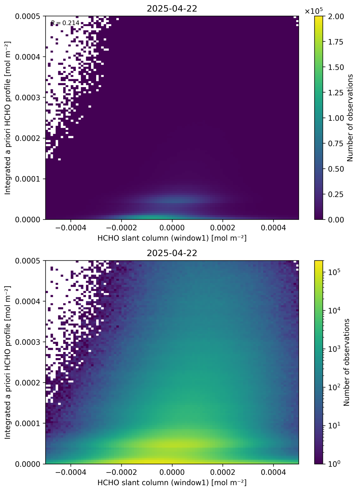
Figure 87: Scatter density plot of “HCHO slant column (window1)” against “Integrated a priori HCHO profile” for 2025-04-21 to 2025-04-23.
