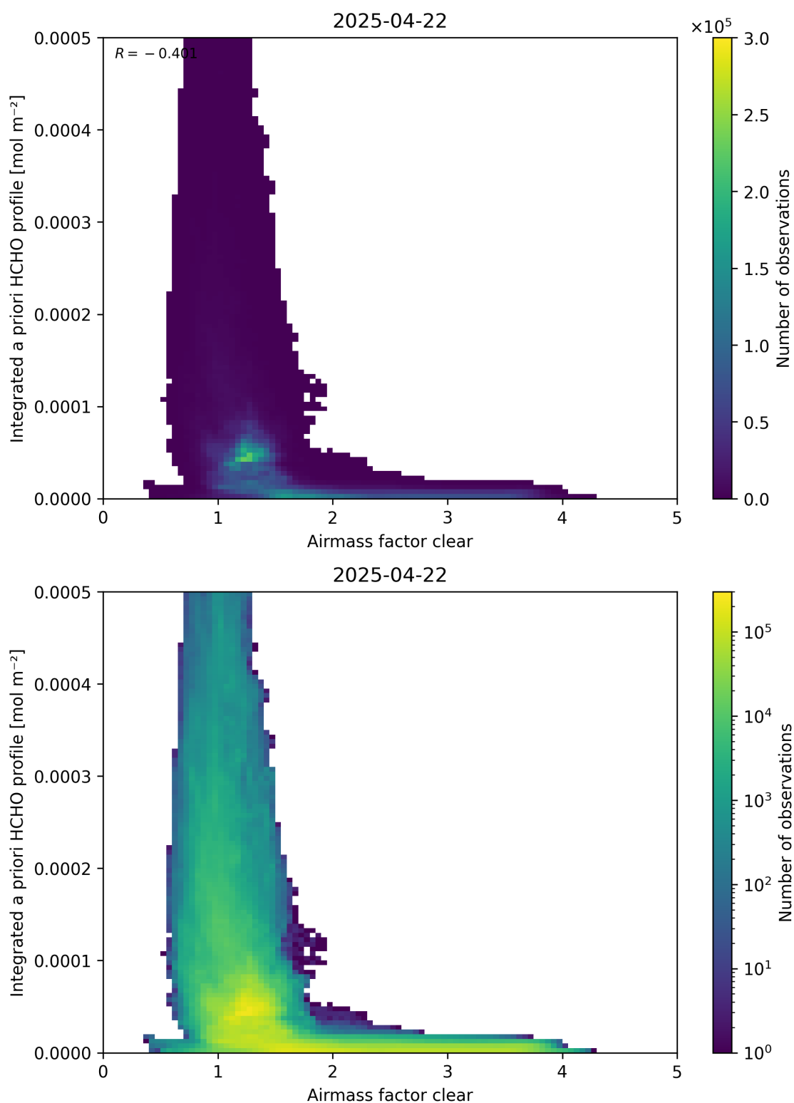
Figure 76: Scatter density plot of “Airmass factor clear” against “Integrated a priori HCHO profile” for 2025-04-21 to 2025-04-23.
