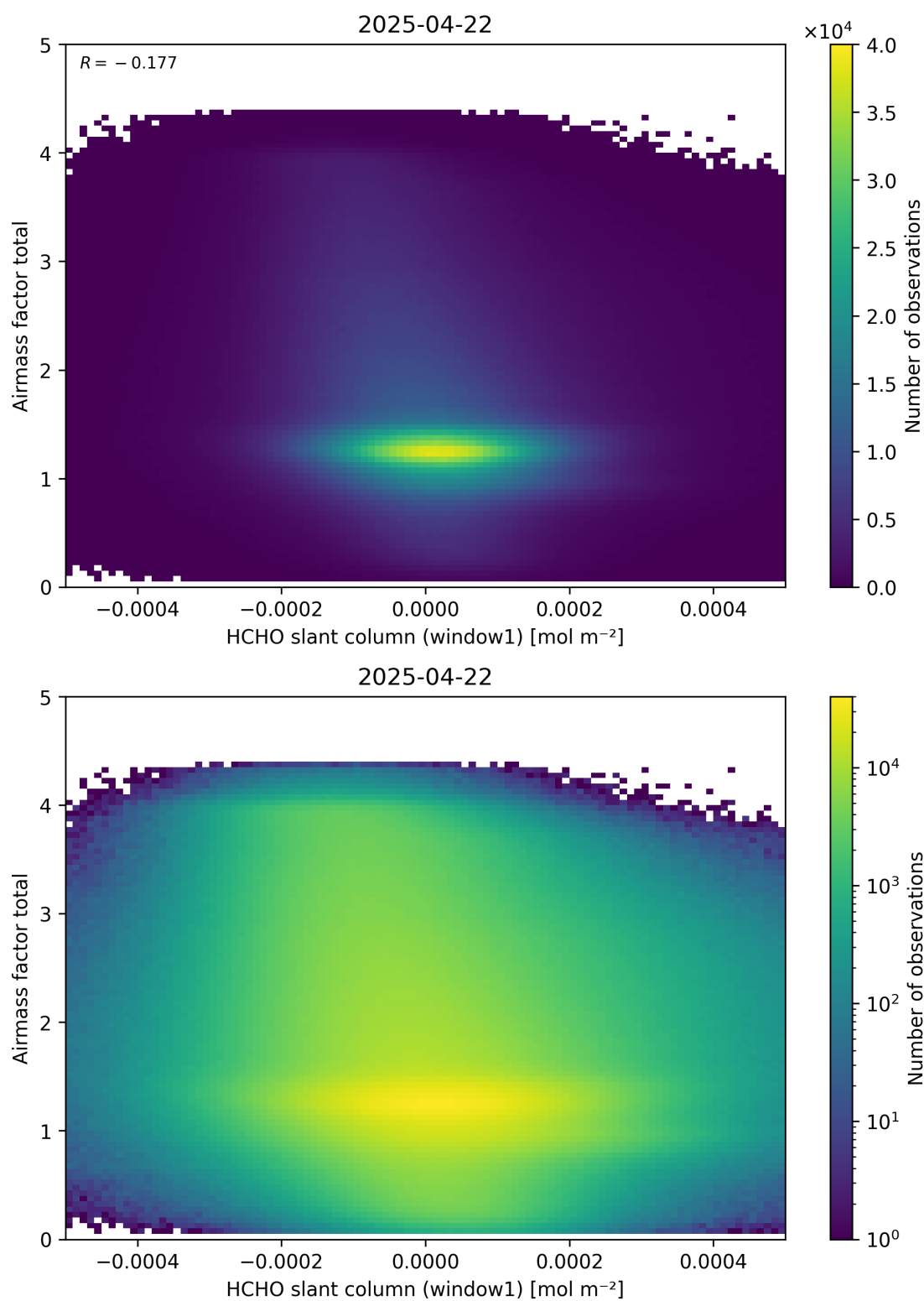
Figure 85: Scatter density plot of “HCHO slant column (window1)” against “Airmass factor total” for 2025-04-21 to 2025-04-23.
