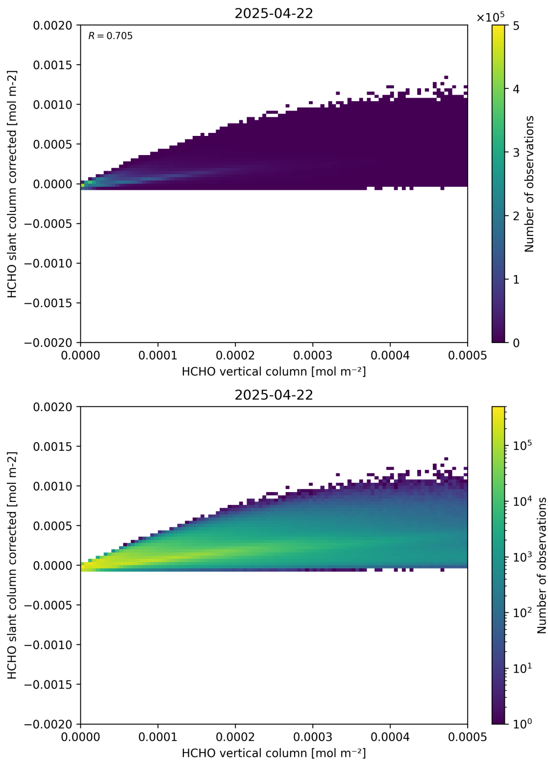
Figure 127: Scatter density plot of “HCHO vertical column” against “HCHO slant column corrected” for 2025-04-21 to 2025-04-23.
