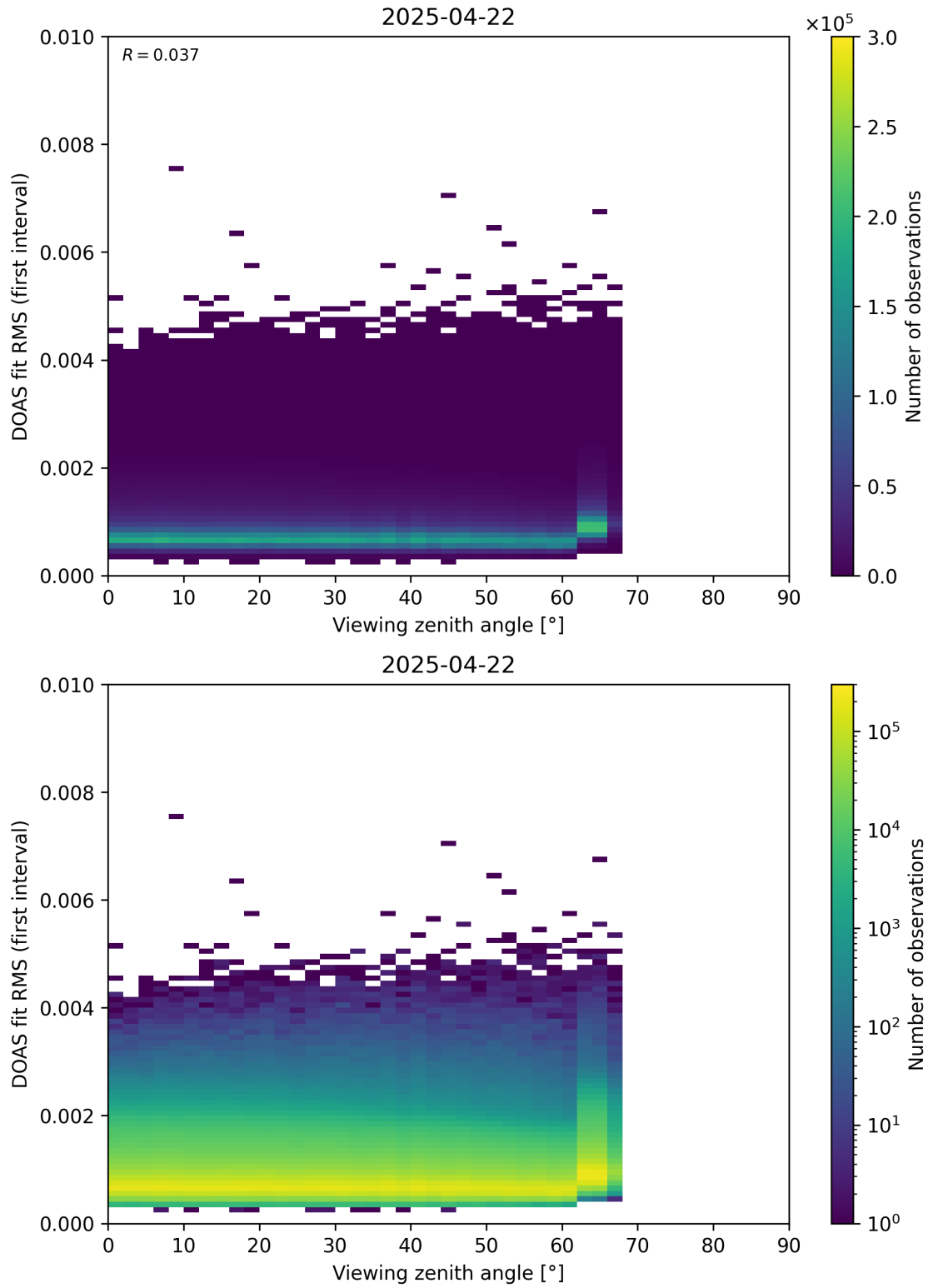
Figure 182: Scatter density plot of “Viewing zenith angle” against “DOAS fit RMS (first interval)” for 2025-04-21 to 2025-04-23.
