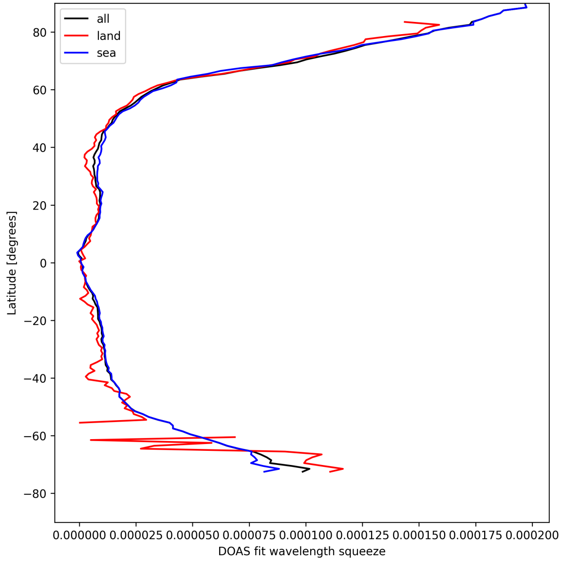
Figure 31: Zonal average of “DOAS fit wavelength squeeze” for 2025-04-21 to 2025-04-23.
