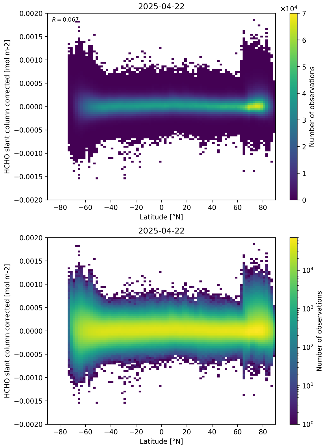
Figure 157: Scatter density plot of “Latitude” against “HCHO slant column corrected” for 2025-04-21 to 2025-04-23.
