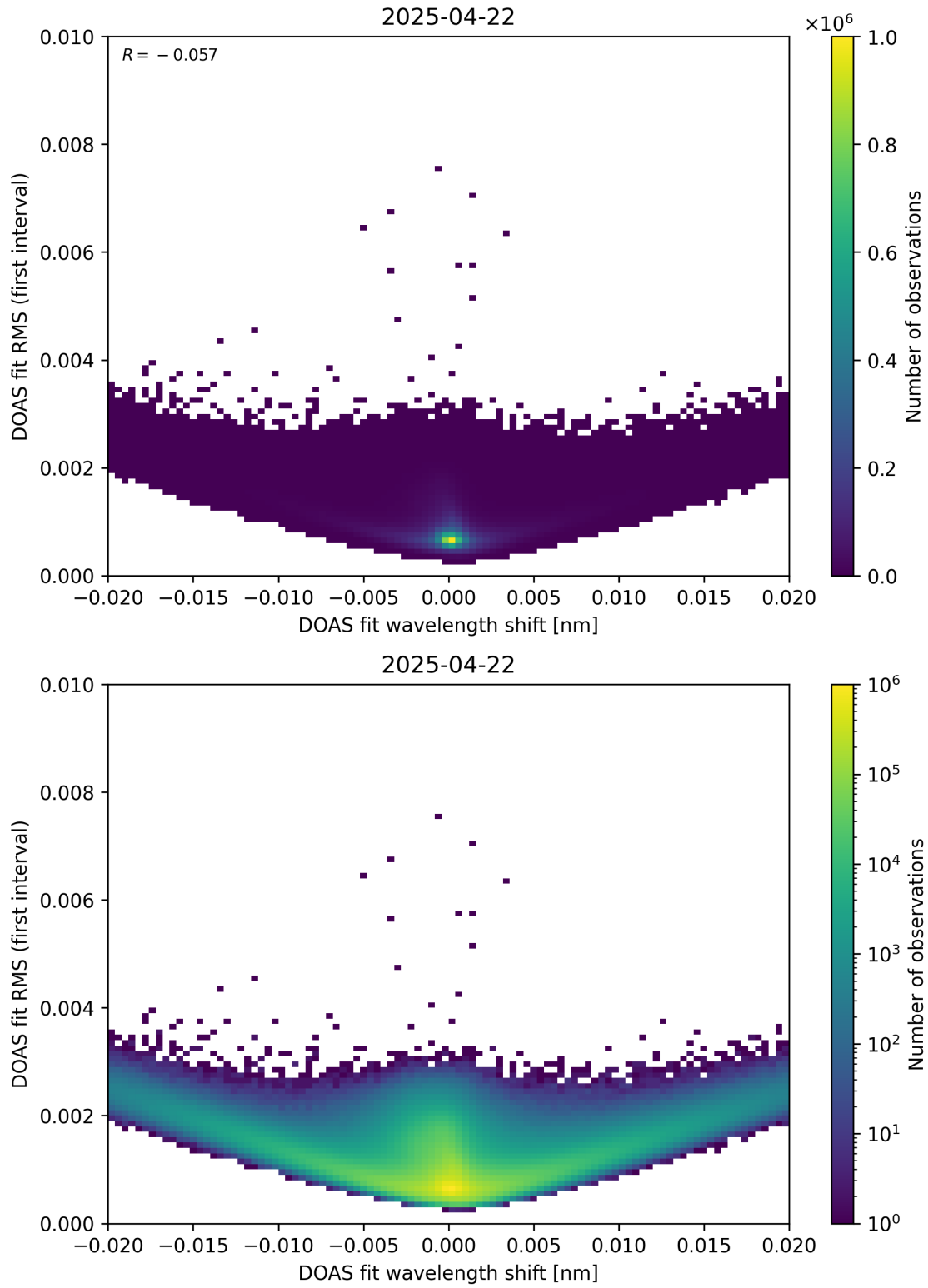
Figure 64: Scatter density plot of “DOAS fit wavelength shift” against “DOAS fit RMS (first interval)” for 2025-04-21 to 2025-04-23.
