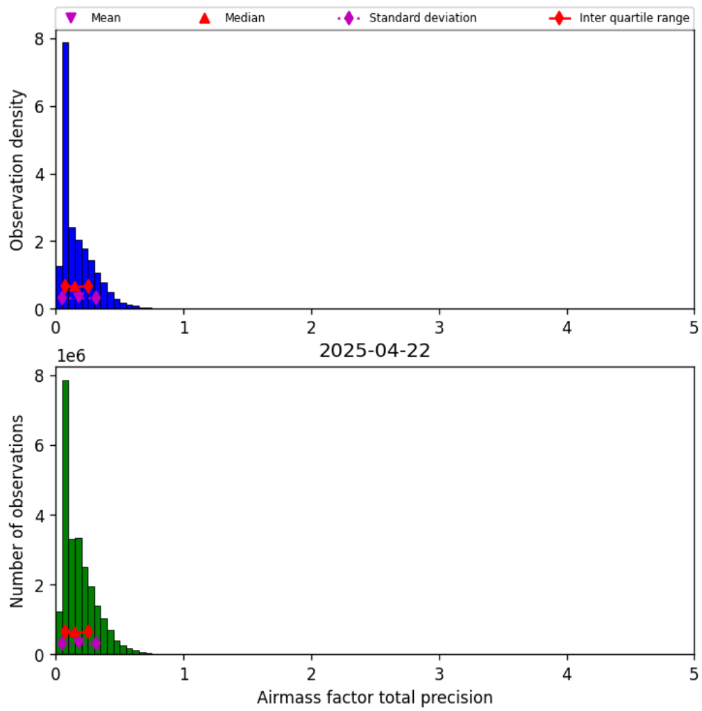
Figure 41: Histogram of “Airmass factor total precision” for 2025-04-21 to 2025-04-23
