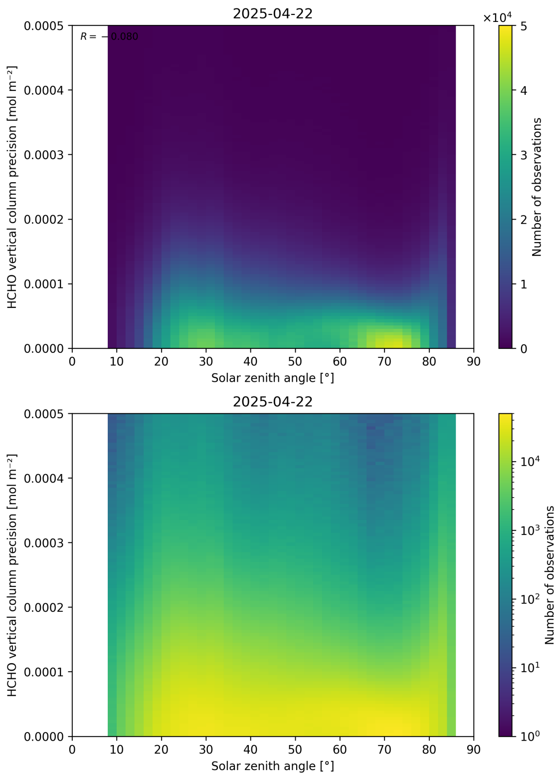
Figure 179: Scatter density plot of “Solar zenith angle” against “HCHO vertical column precision” for 2025-04-21 to 2025-04-23.
