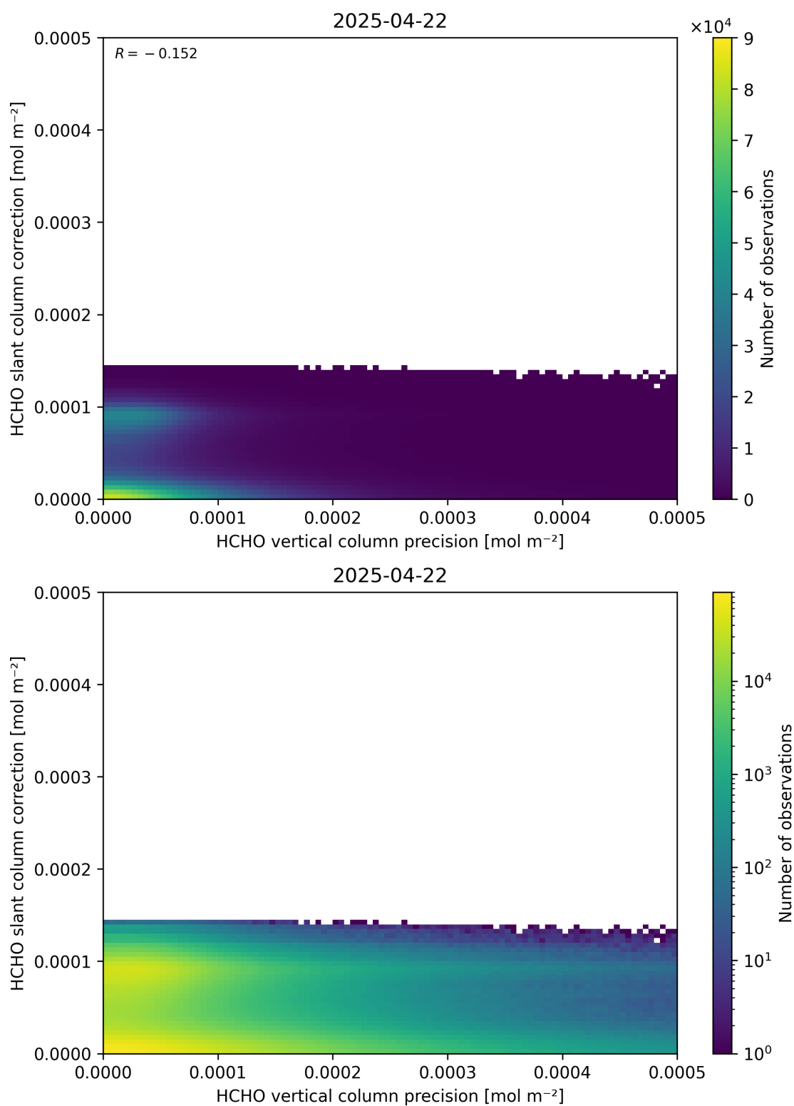
Figure 141: Scatter density plot of “HCHO vertical column precision” against “HCHO slant column correction” for 2025-04-21 to 2025-04-23.
