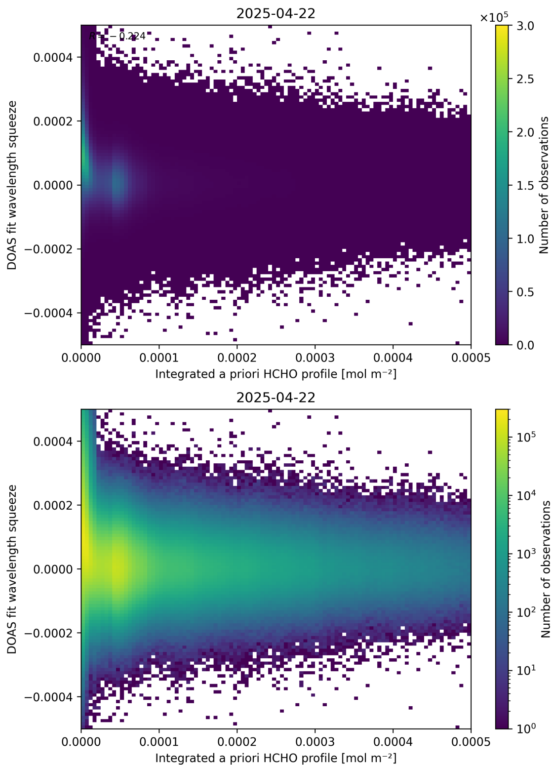
Figure 150: Scatter density plot of “Integrated a priori HCHO profile” against “DOAS fit wavelength squeeze” for 2025-04-21 to 2025-04-23.
