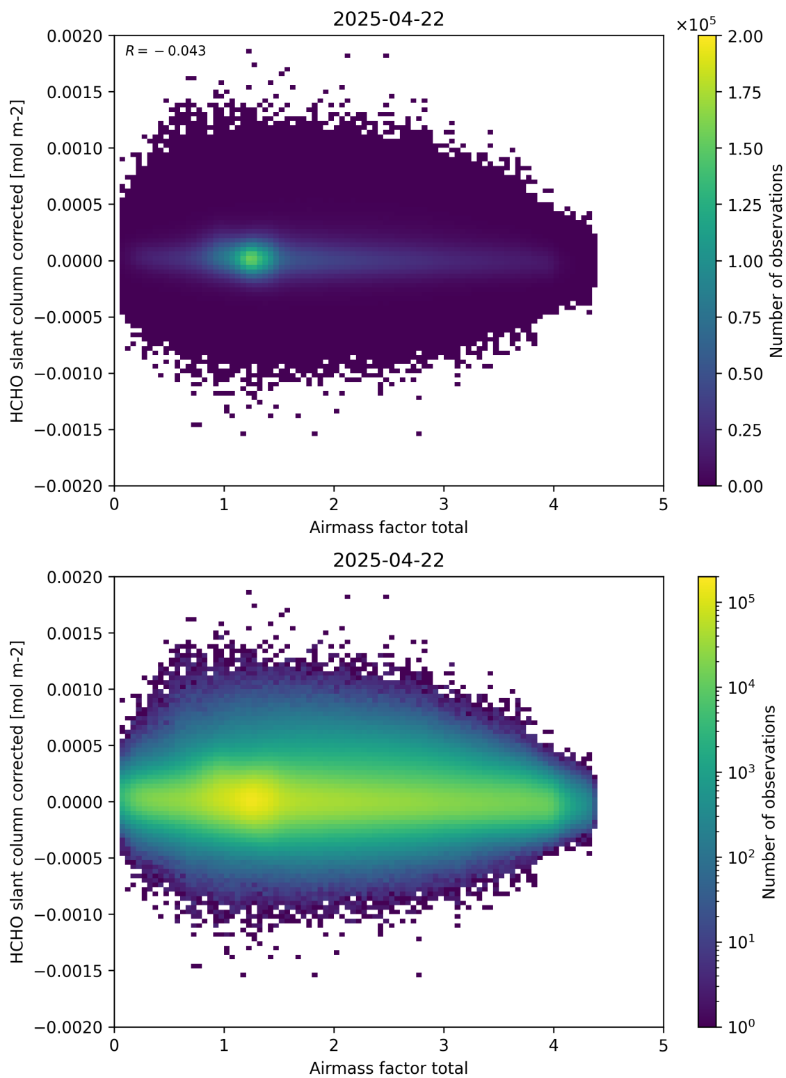
Figure 101: Scatter density plot of “Airmass factor total” against “HCHO slant column corrected” for 2025-04-21 to 2025-04-23.
