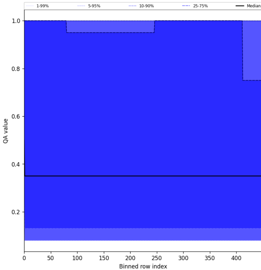
Figure 48: Along track statistics of “QA value” for 2025-04-21 to 2025-04-23
