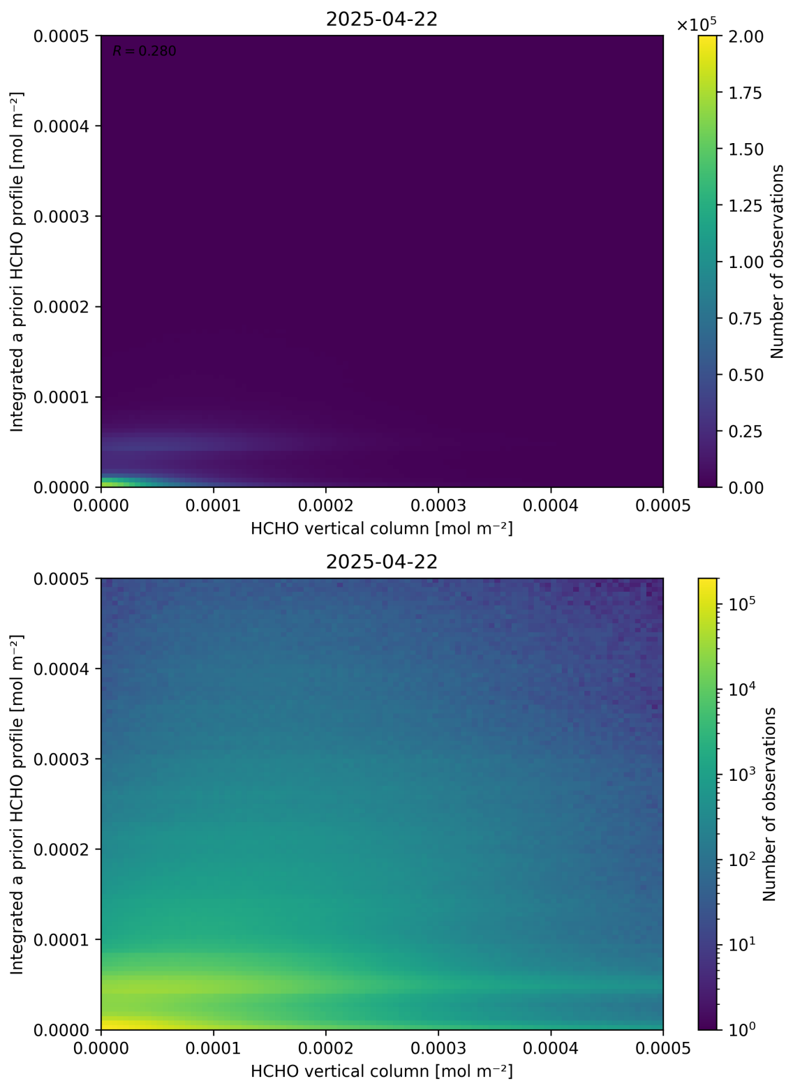
Figure 135: Scatter density plot of “HCHO vertical column” against “Integrated a priori HCHO profile” for 2025-04-21 to 2025-04-23.
