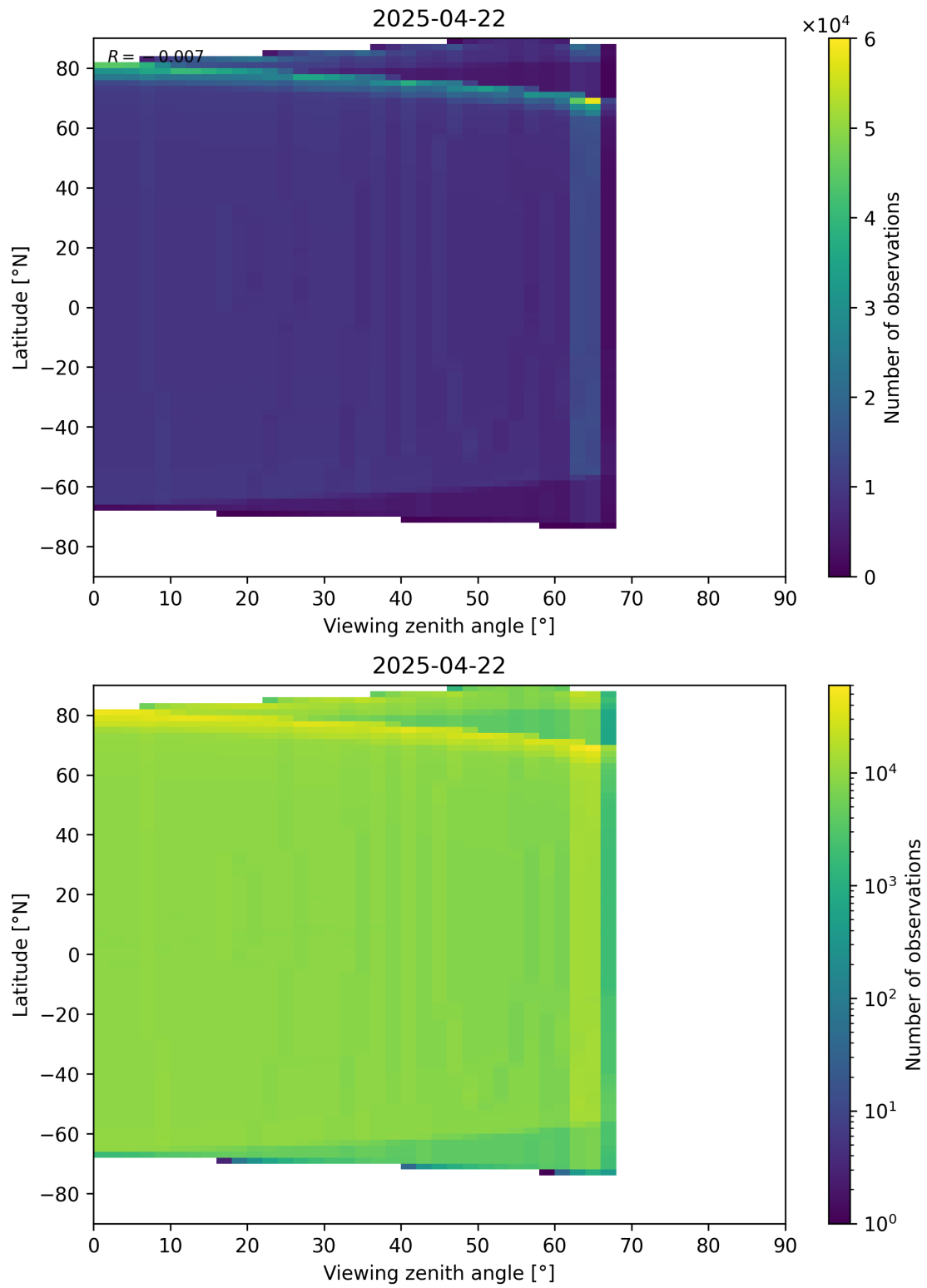
Figure 196: Scatter density plot of “Viewing zenith angle” against “Latitude” for 2025-04-21 to 2025-04-23.
