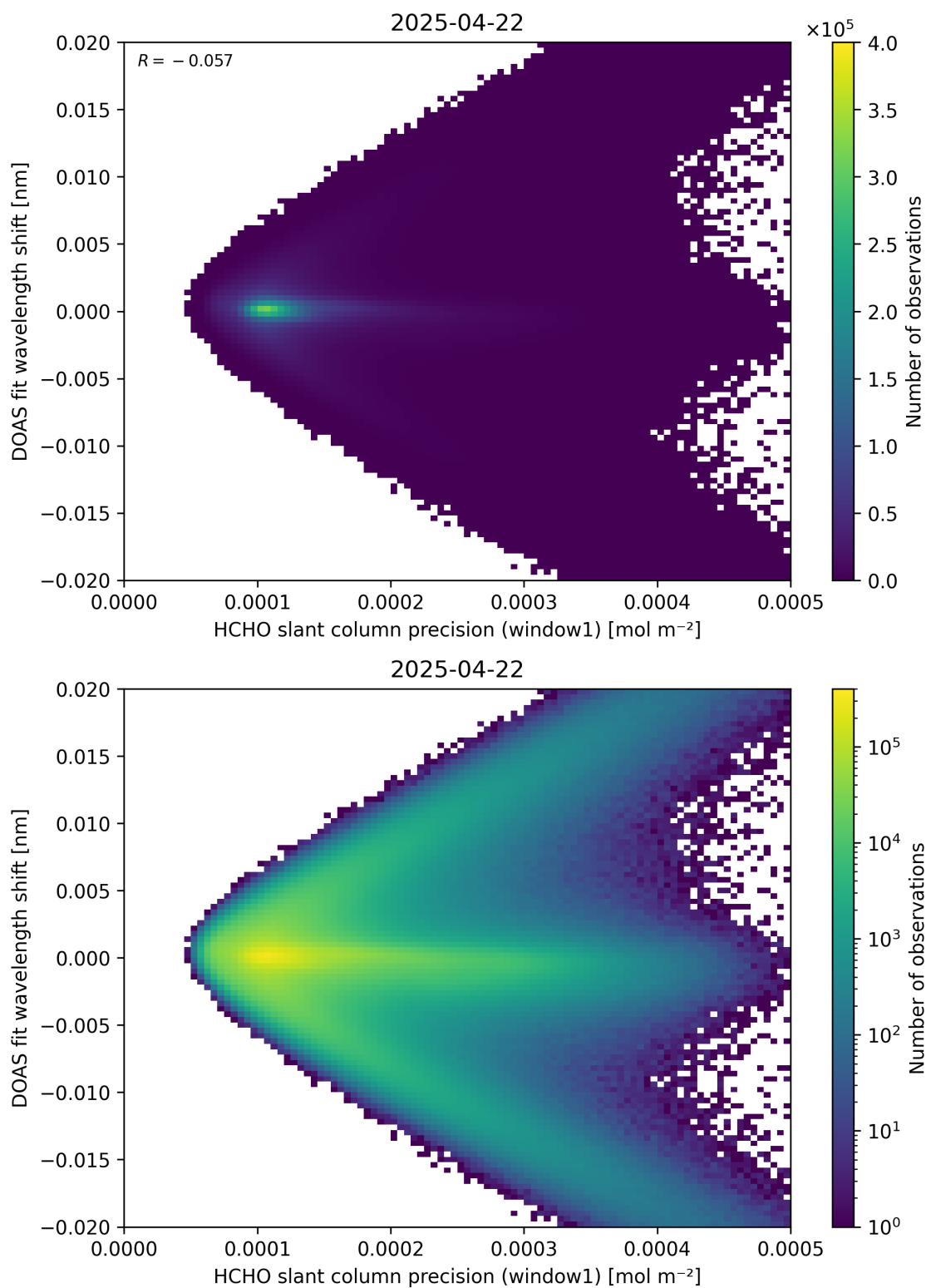
Figure 89: Scatter density plot of “HCHO slant column precision (window1)” against “DOAS fit wavelength shift” for 2025-04-21 to 2025-04-23.
