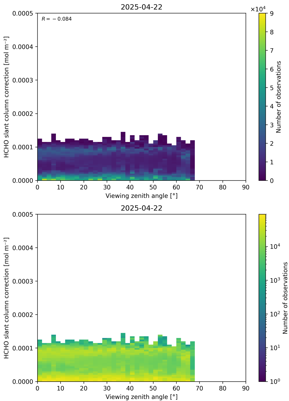
Figure 187: Scatter density plot of “Viewing zenith angle” against “HCHO slant column correction” for 2025-04-21 to 2025-04-23.
