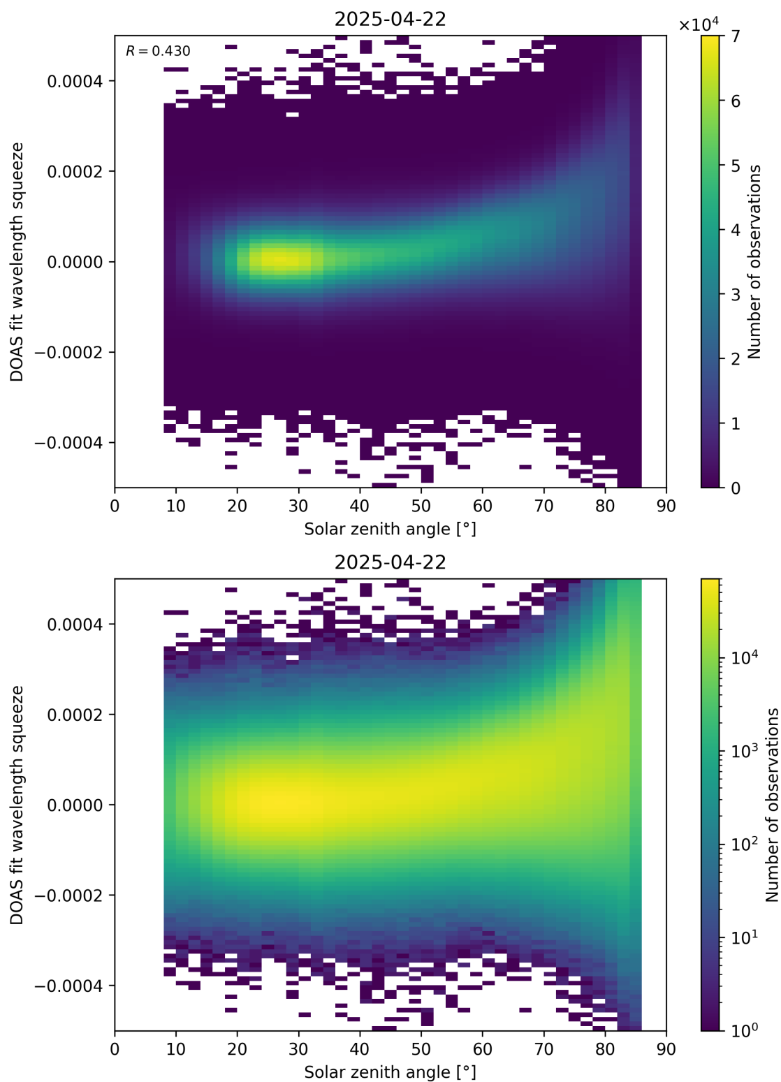
Figure 169: Scatter density plot of “Solar zenith angle” against “DOAS fit wavelength squeeze” for 2025-04-21 to 2025-04-23.
