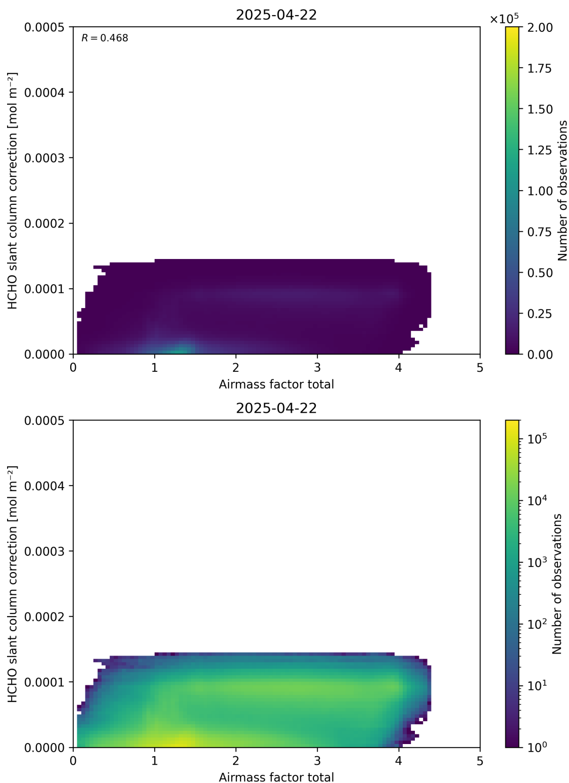
Figure 102: Scatter density plot of “Airmass factor total” against “HCHO slant column correction” for 2025-04-21 to 2025-04-23.
