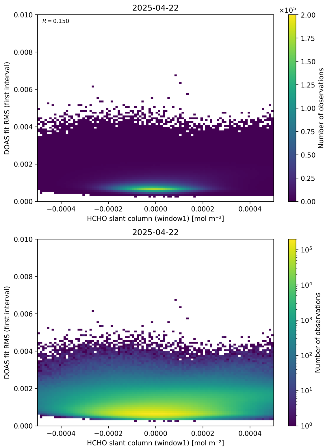
Figure 78: Scatter density plot of “HCHO slant column (window1)” against “DOAS fit RMS (first interval)” for 2025-04-21 to 2025-04-23.
