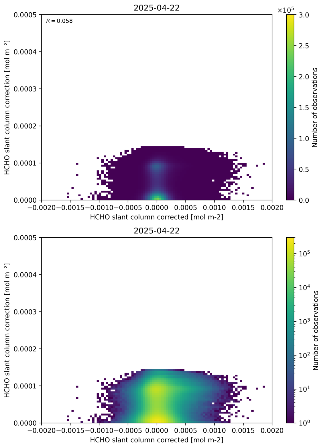
Figure 77: Scatter density plot of “HCHO slant column corrected” against “HCHO slant column correction” for 2025-04-21 to 2025-04-23.
