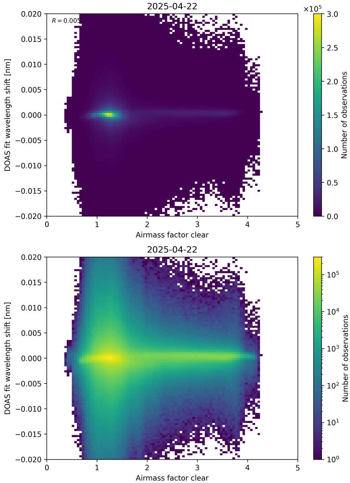
Figure 72: Scatter density plot of “Airmass factor clear” against “DOAS fit wavelength shift” for 2025-04-21 to 2025-04-23.
