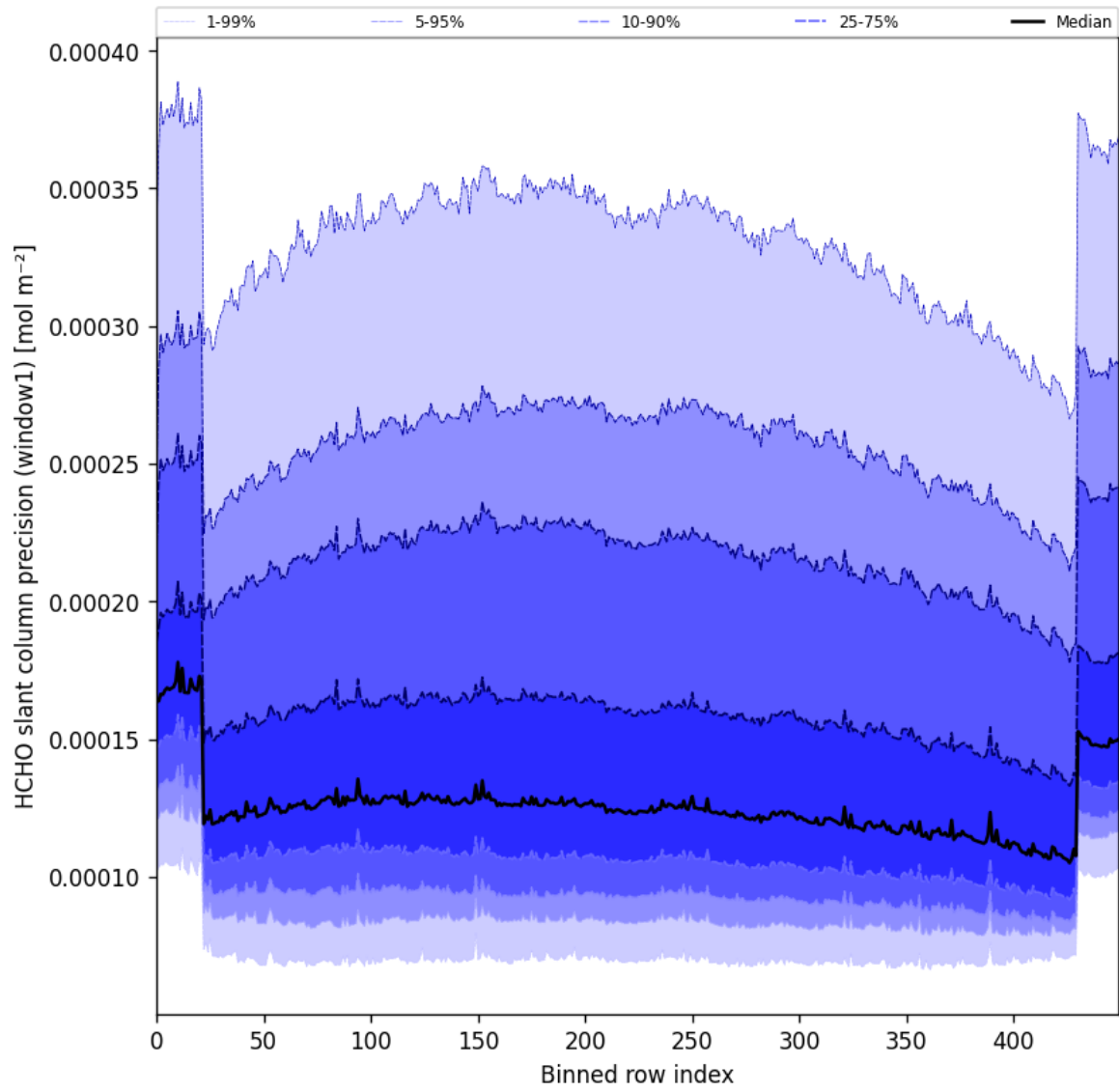
Figure 53: Along track statistics of “HCHO slant column precision (window1)” for 2025-04-21 to 2025-04-23
