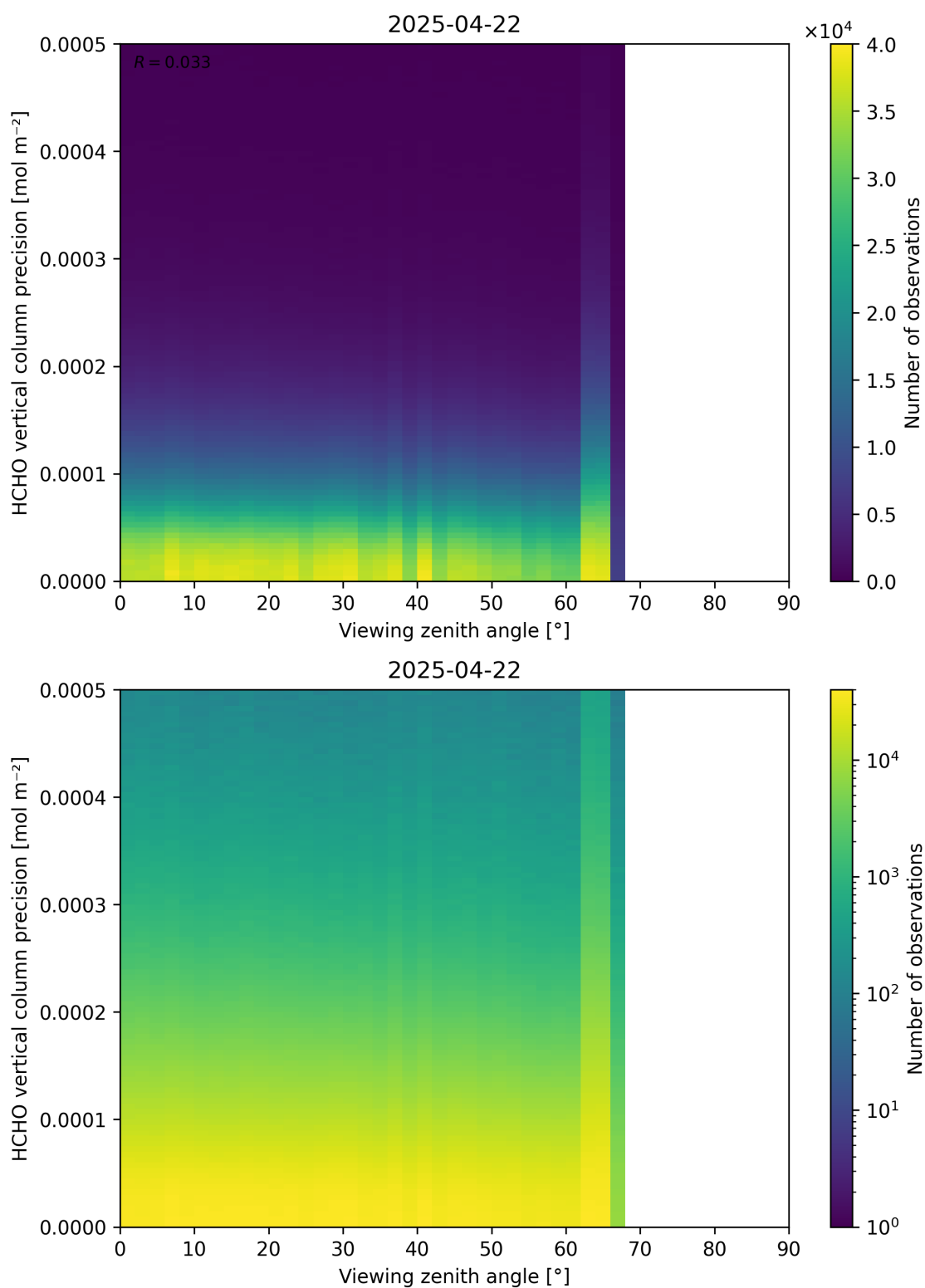
Figure 194: Scatter density plot of “Viewing zenith angle” against “HCHO vertical column precision” for 2025-04-21 to 2025-04-23.
