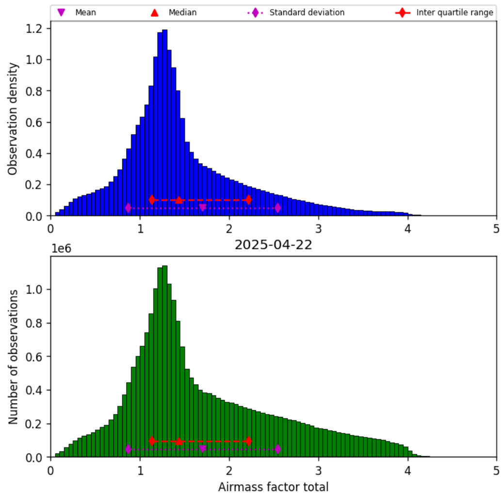
Figure 40: Histogram of “Airmass factor total” for 2025-04-21 to 2025-04-23
