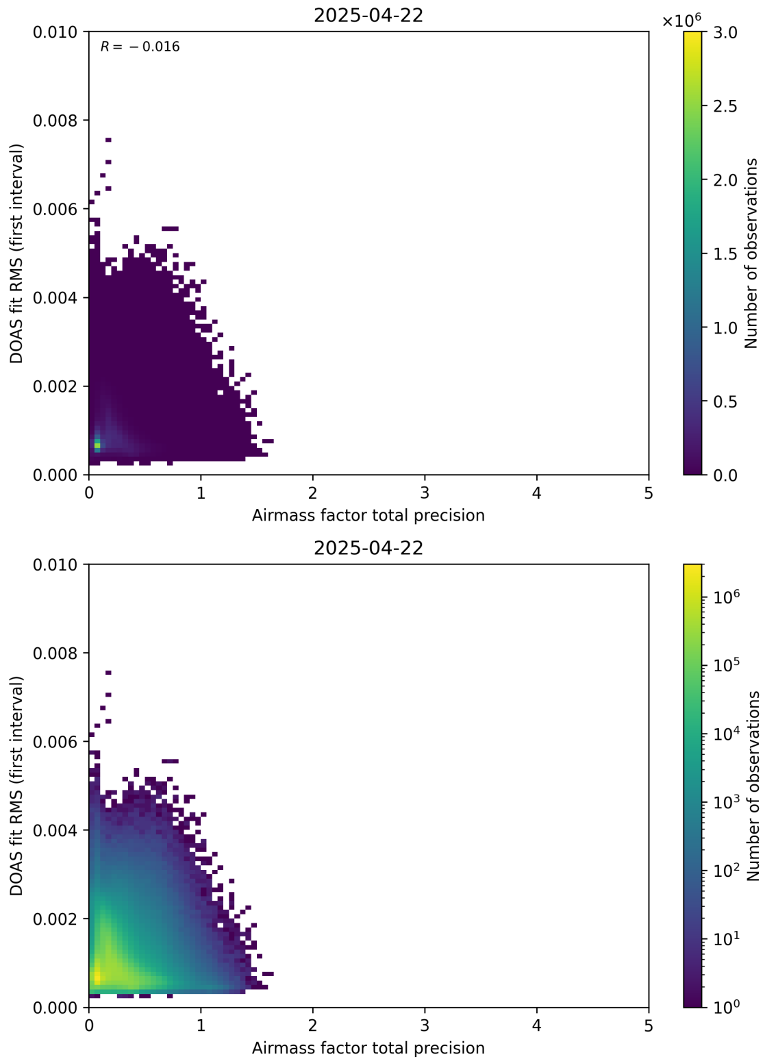
Figure 105: Scatter density plot of “Airmass factor total precision” against “DOAS fit RMS (first interval)” for 2025-04-21 to 2025-04-23.
