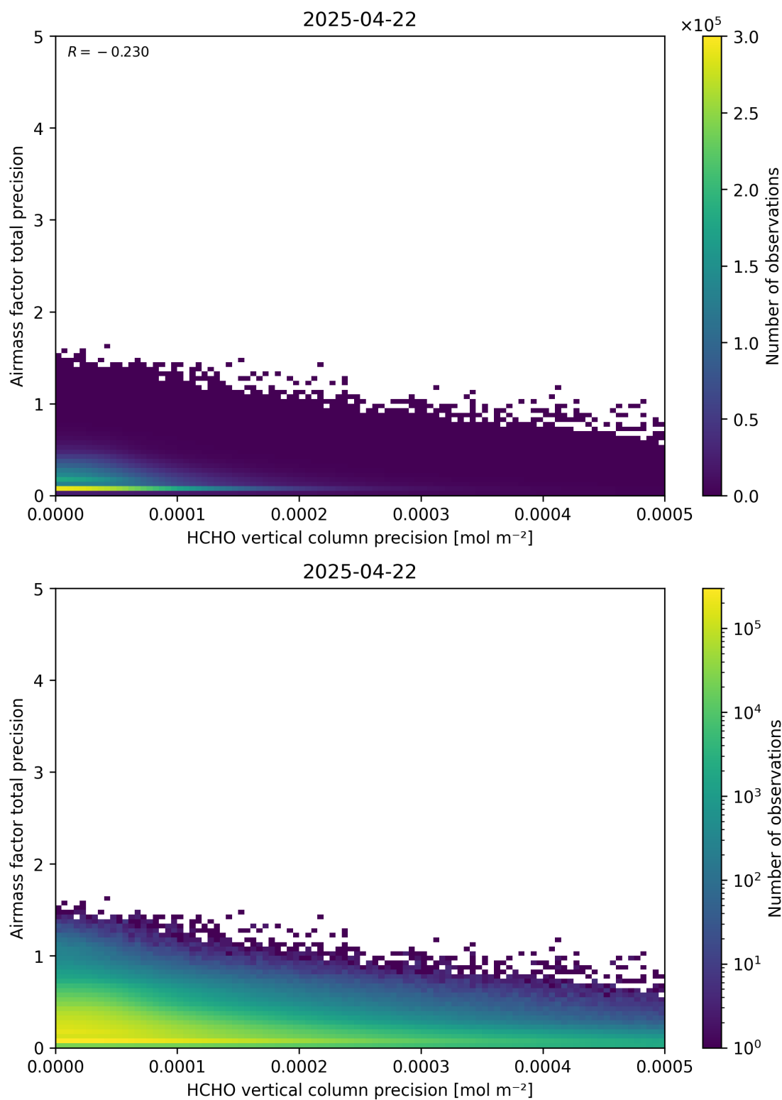
Figure 145: Scatter density plot of “HCHO vertical column precision” against “Airmass factor total precision” for 2025-04-21 to 2025-04-23.
