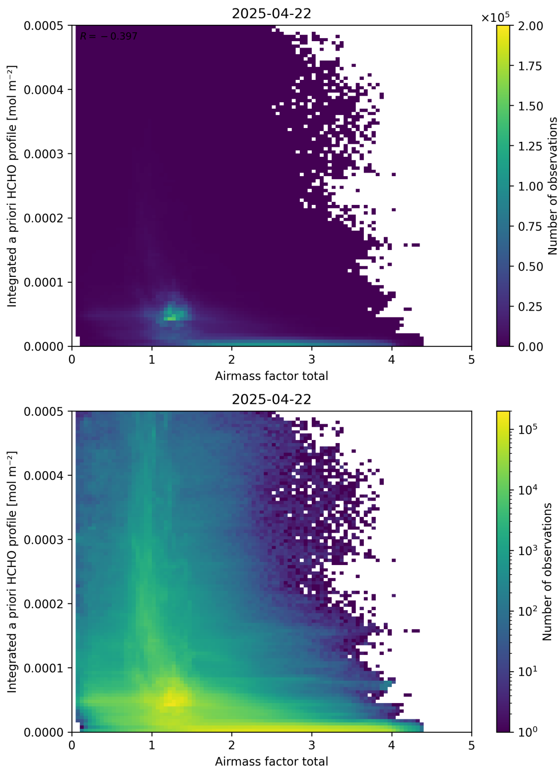
Figure 104: Scatter density plot of “Airmass factor total” against “Integrated a priori HCHO profile” for 2025-04-21 to 2025-04-23.
