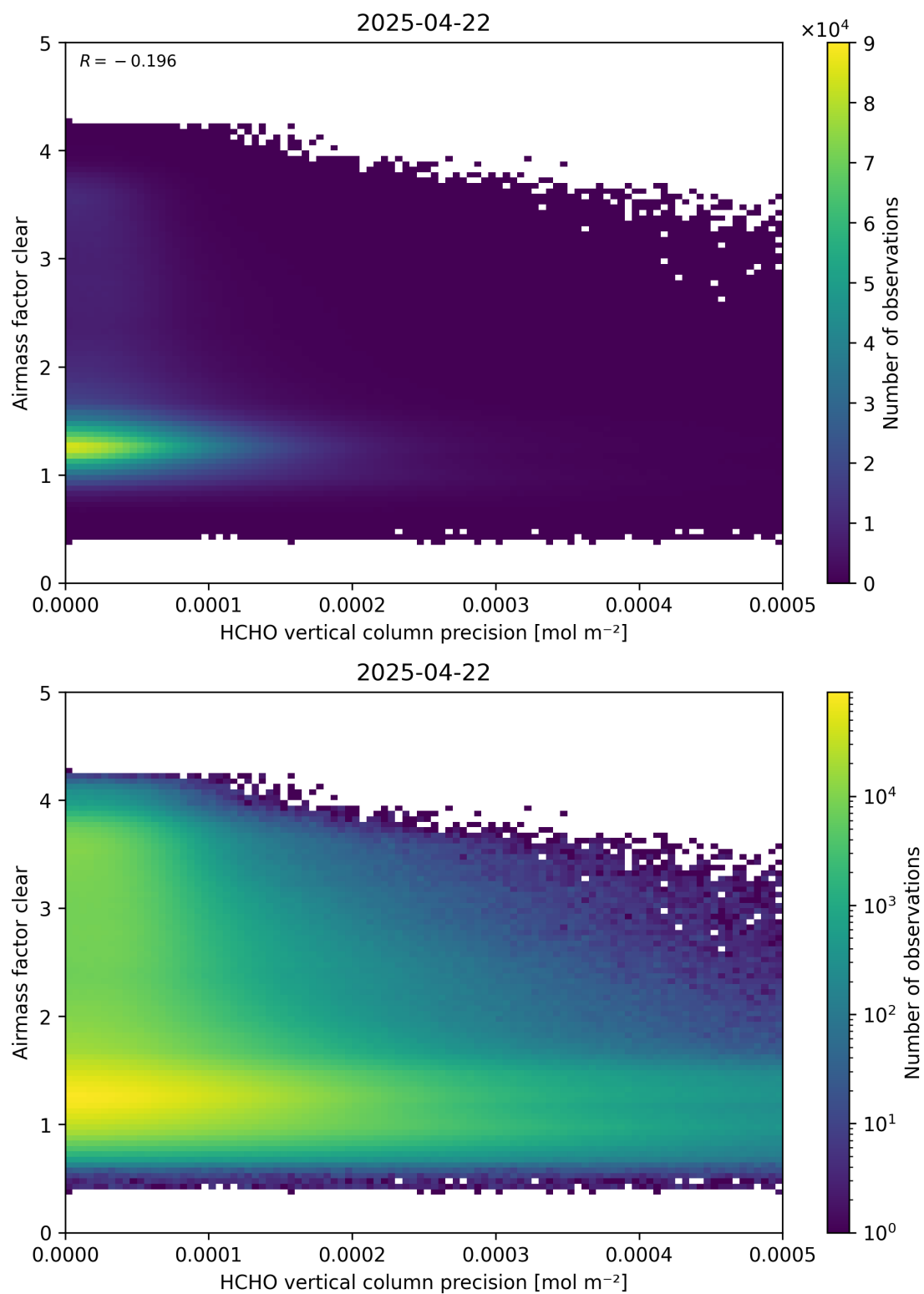
Figure 139: Scatter density plot of “HCHO vertical column precision” against “Airmass factor clear” for 2025-04-21 to 2025-04-23.
