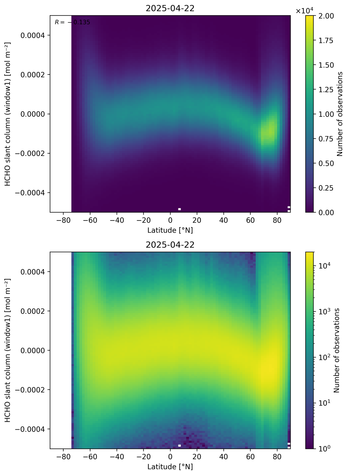
Figure 159: Scatter density plot of “Latitude” against “HCHO slant column (window1)” for 2025-04-21 to 2025-04-23.
