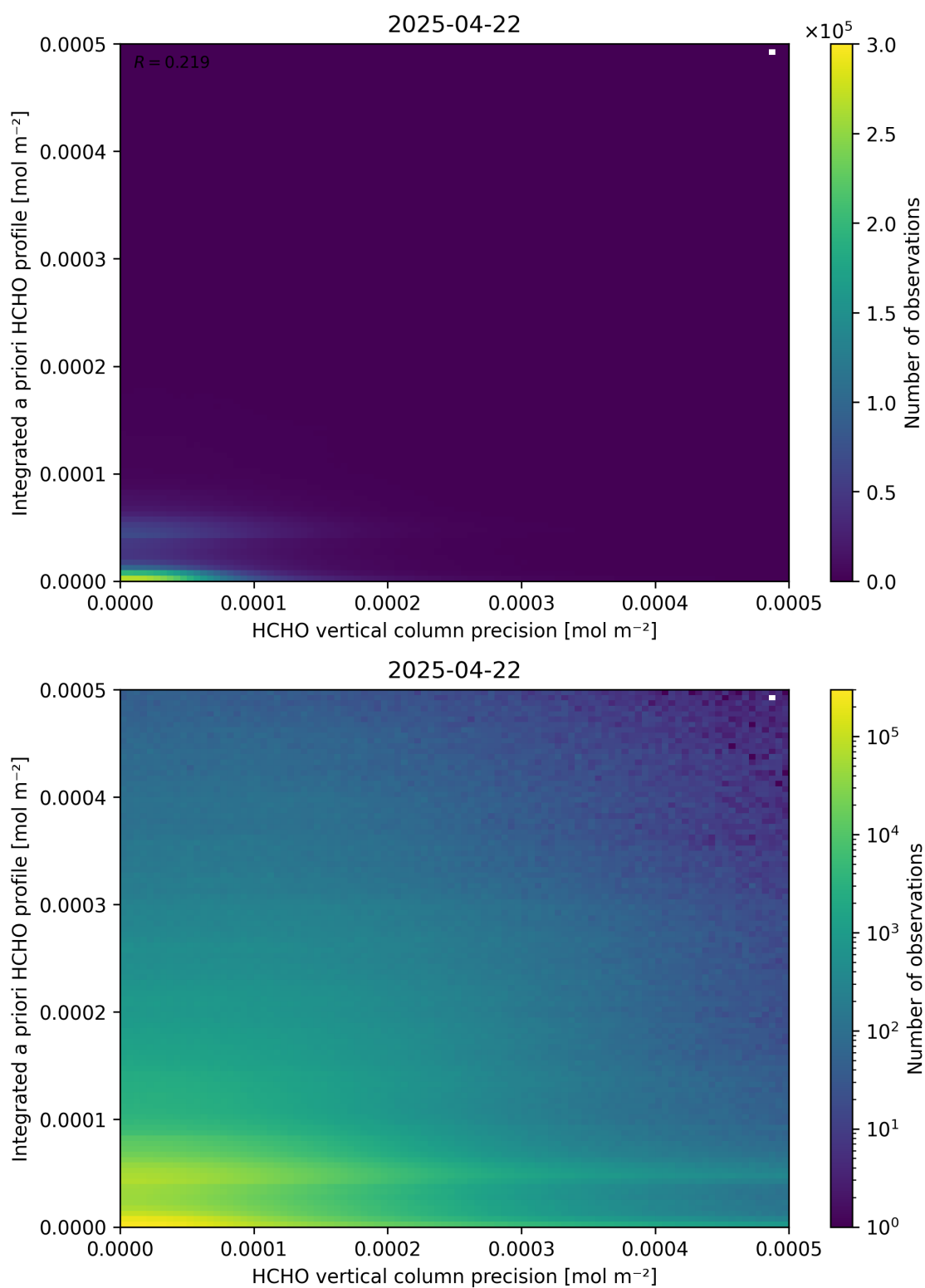
Figure 147: Scatter density plot of “HCHO vertical column precision” against “Integrated a priori HCHO profile” for 2025-04-21 to 2025-04-23.
