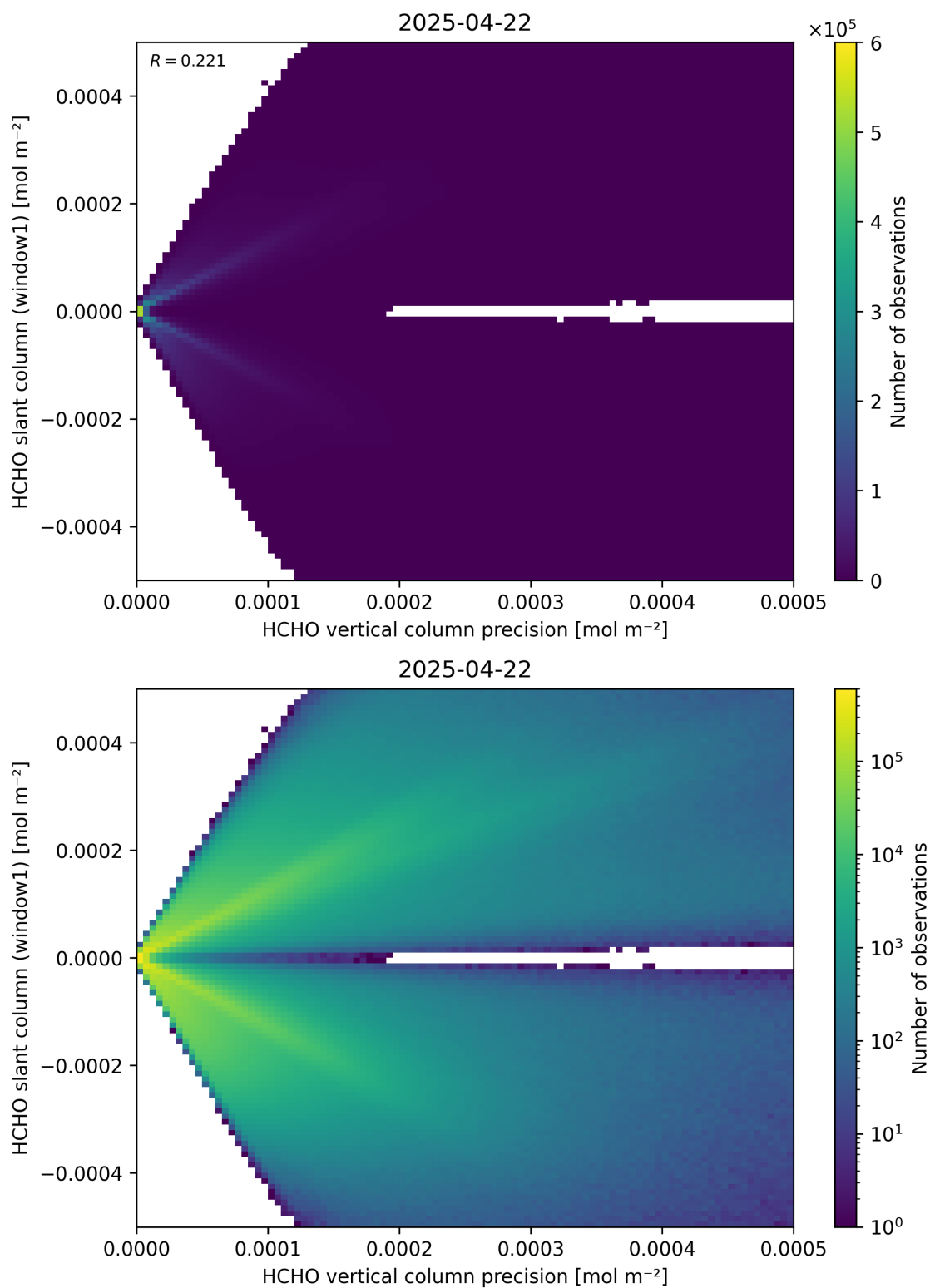
Figure 142: Scatter density plot of “HCHO vertical column precision” against “HCHO slant column (window1)” for 2025-04-21 to 2025-04-23.
