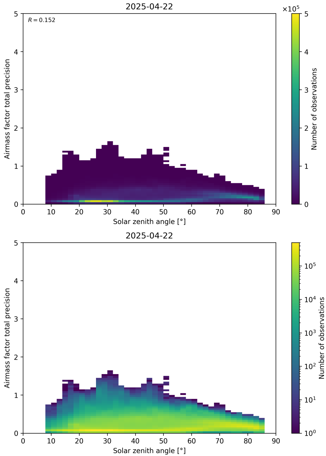
Figure 176: Scatter density plot of “Solar zenith angle” against “Airmass factor total precision” for 2025-04-21 to 2025-04-23.
