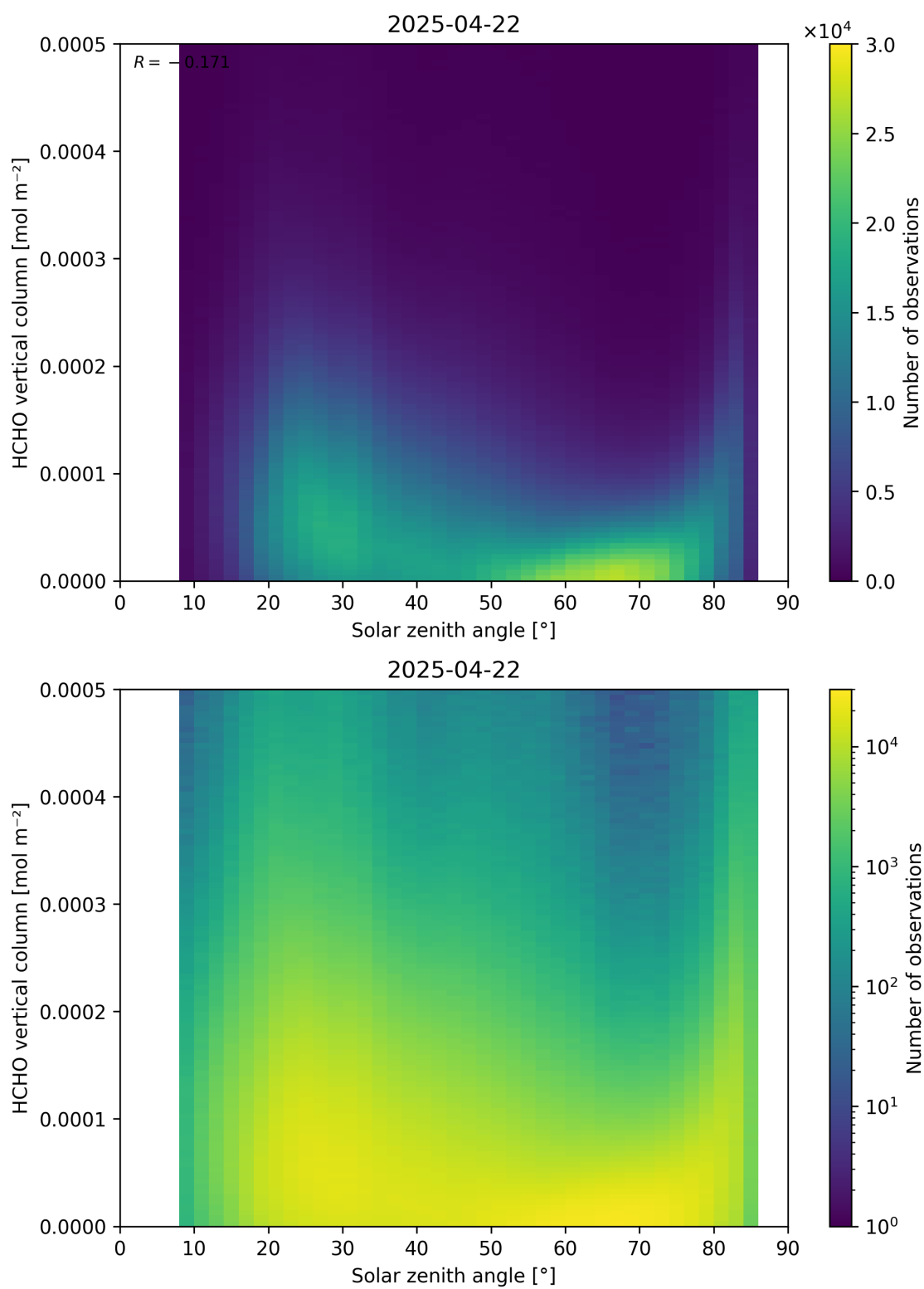
Figure 177: Scatter density plot of “Solar zenith angle” against “HCHO vertical column” for 2025-04-21 to 2025-04-23.
