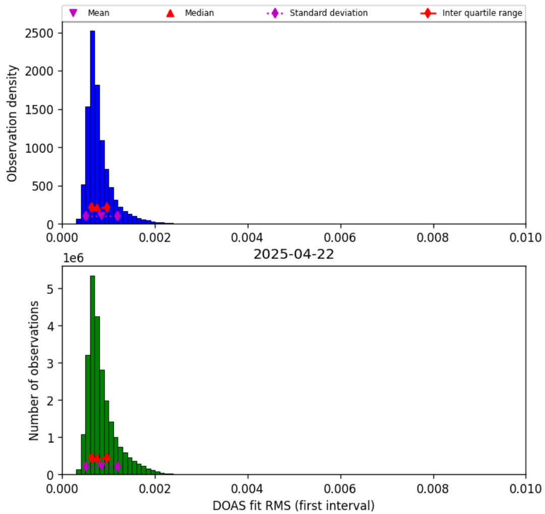
Figure 46: Histogram of “DOAS fit RMS (first interval)” for 2025-04-21 to 2025-04-23
