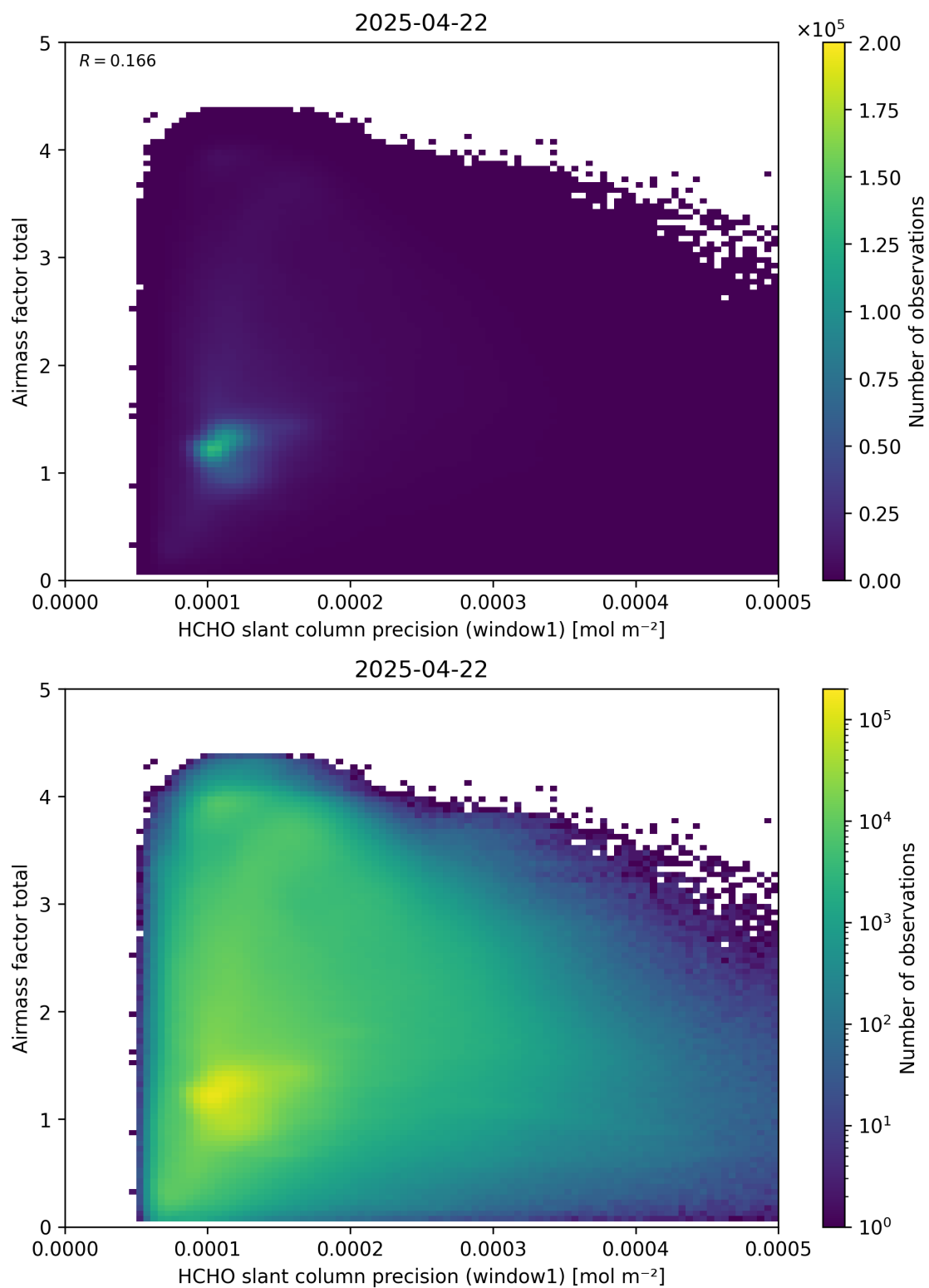
Figure 94: Scatter density plot of “HCHO slant column precision (window1)” against “Airmass factor total” for 2025-04-21 to 2025-04-23.
