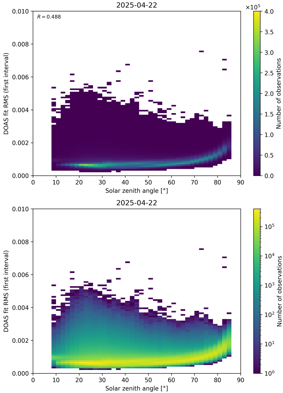
Figure 167: Scatter density plot of “Solar zenith angle” against “DOAS fit RMS (first interval)” for 2025-04-21 to 2025-04-23.
