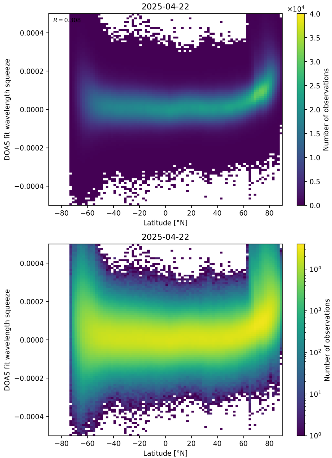
Figure 155: Scatter density plot of “Latitude” against “DOAS fit wavelength squeeze” for 2025-04-21 to 2025-04-23.
