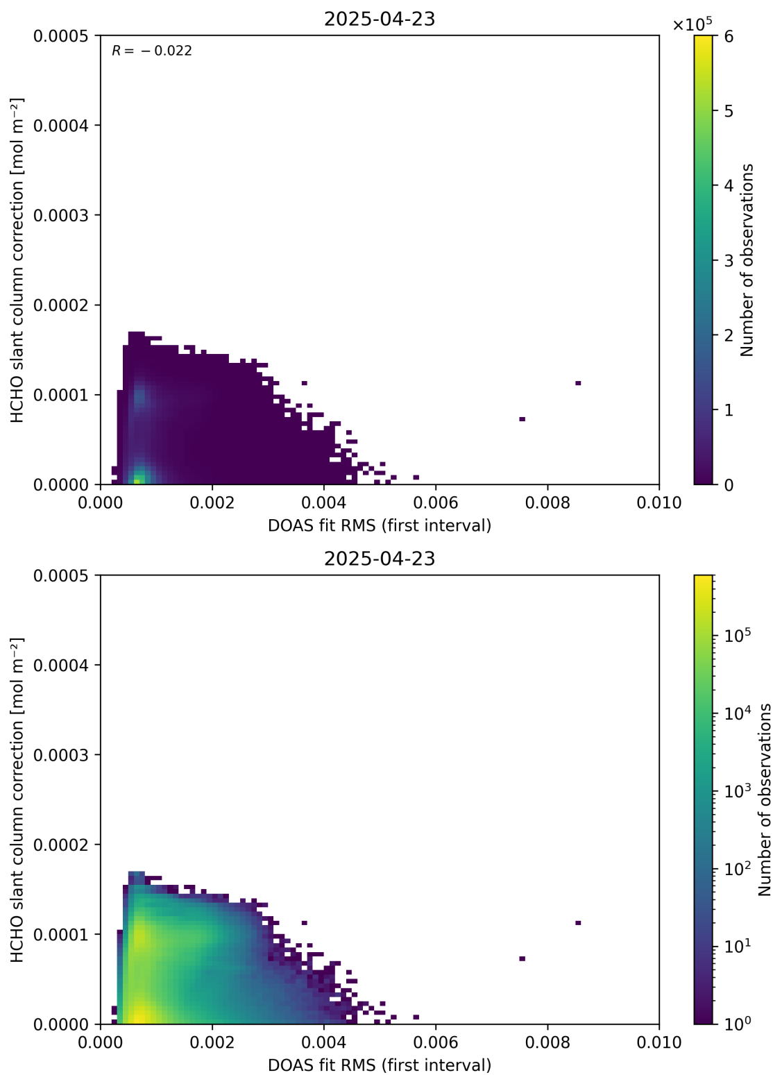
Figure 63: Scatter density plot of “DOAS fit RMS (first interval)” against “HCHO slant column correction” for 2025-04-22 to 2025-04-24.
