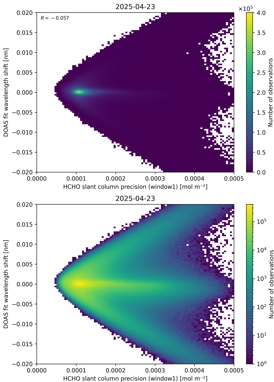
Figure 89: Scatter density plot of “HCHO slant column precision (window1)” against “DOAS fit wavelength shift” for 2025-04-22 to 2025-04-24.
