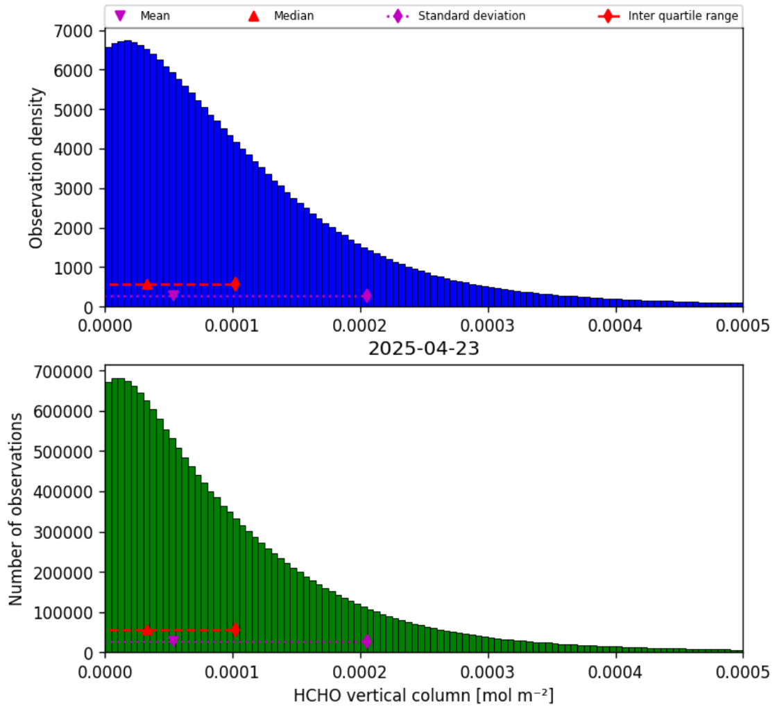
Figure 35: Histogram of “HCHO vertical column” for 2025-04-22 to 2025-04-24
