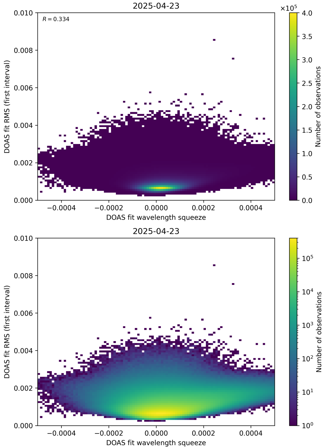
Figure 68: Scatter density plot of “DOAS fit wavelength squeeze” against “DOAS fit RMS (first interval)” for 2025-04-22 to 2025-04-24.
