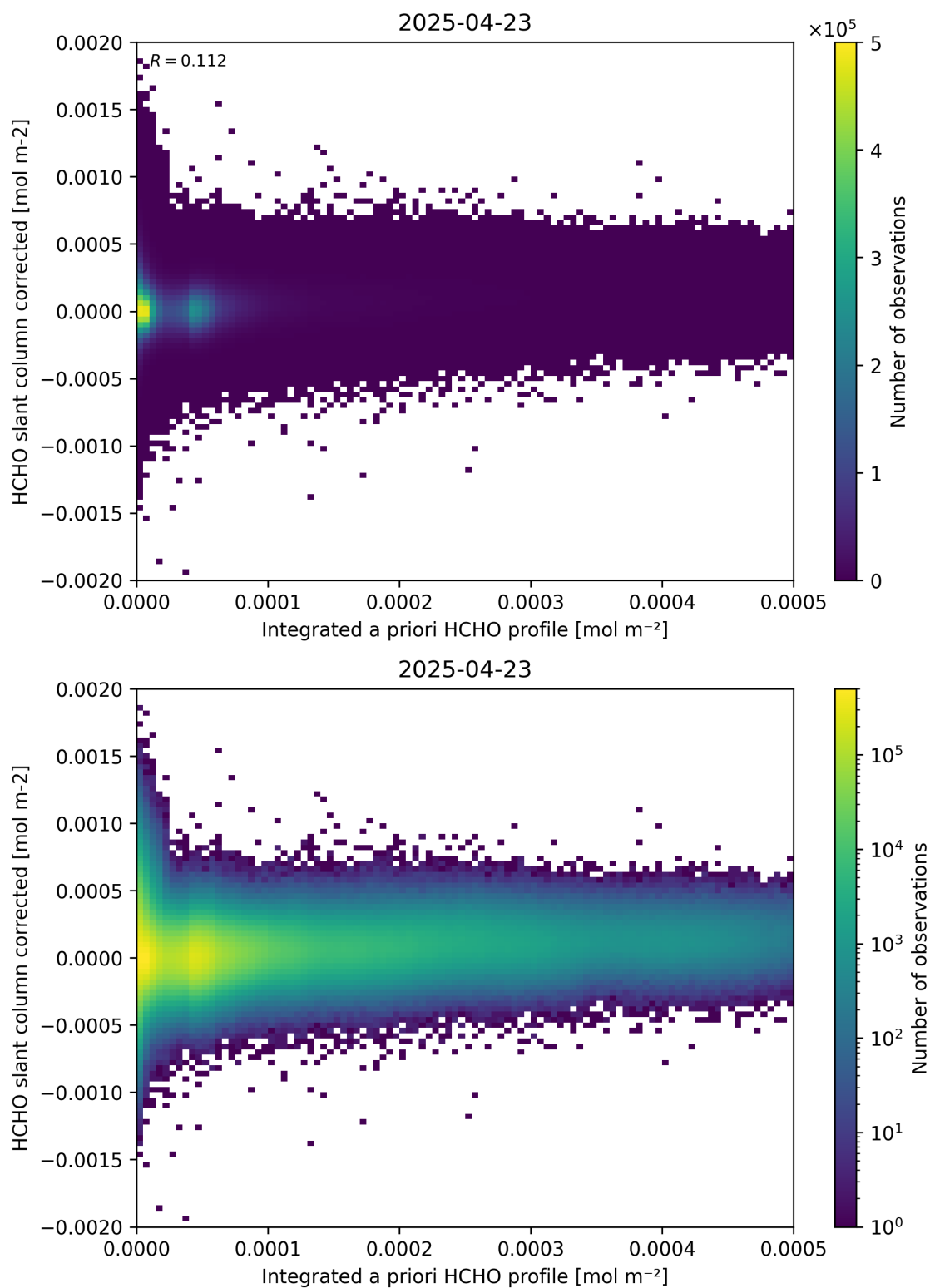
Figure 151: Scatter density plot of “Integrated a priori HCHO profile” against “HCHO slant column corrected” for 2025-04-22 to 2025-04-24.
