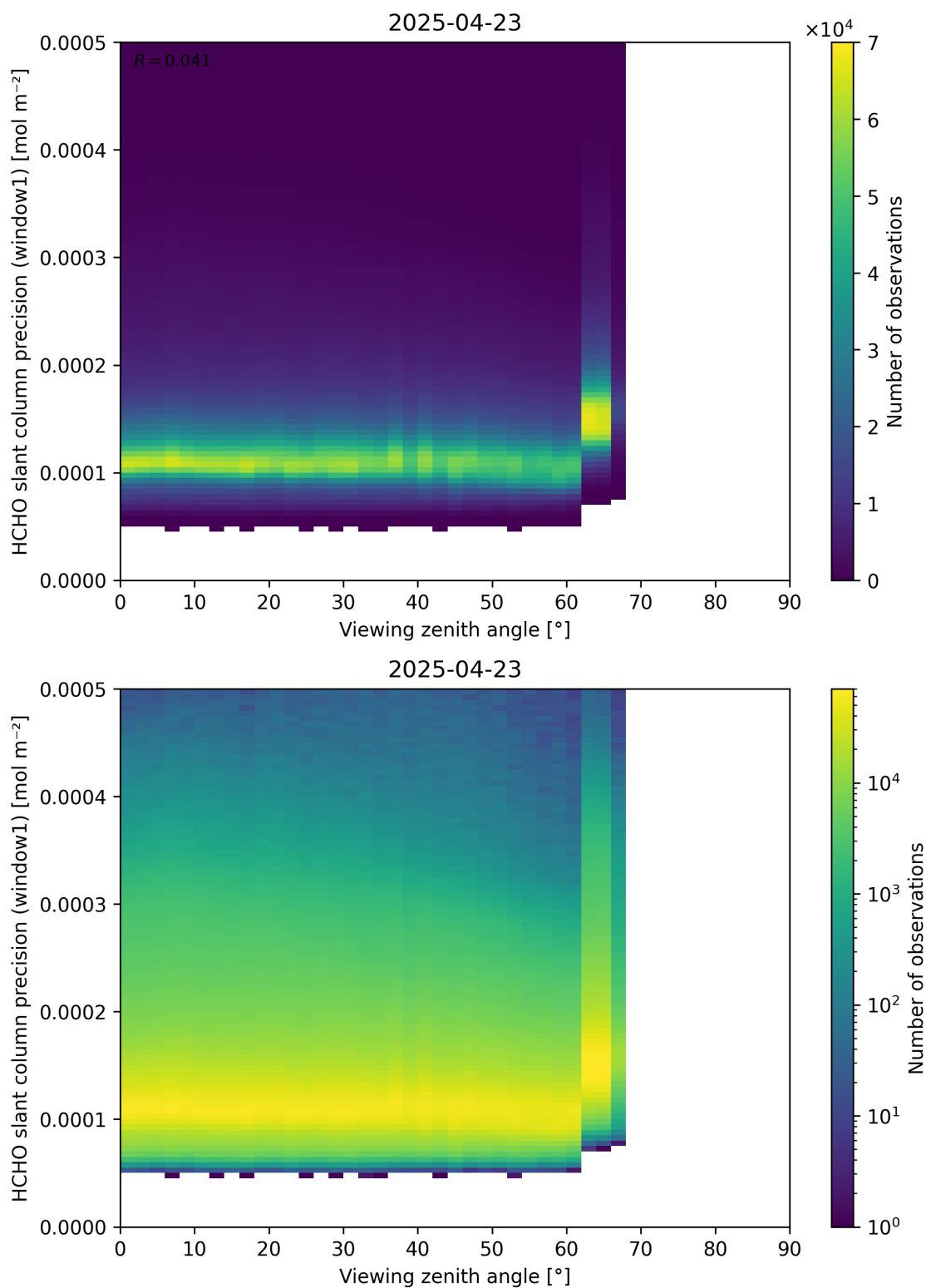
Figure 189: Scatter density plot of “Viewing zenith angle” against “HCHO slant column precision (window1)” for 2025-04-22 to 2025-04-24.
