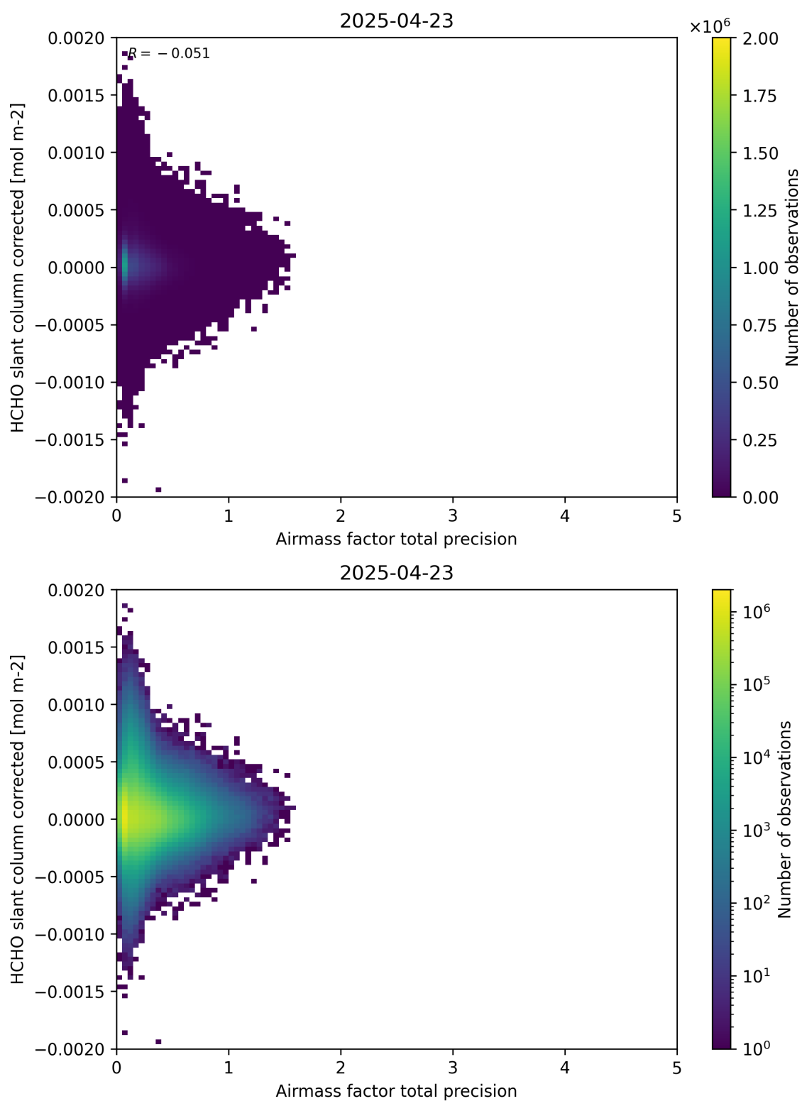
Figure 109: Scatter density plot of “Airmass factor total precision” against “HCHO slant column corrected” for 2025-04-22 to 2025-04-24.
