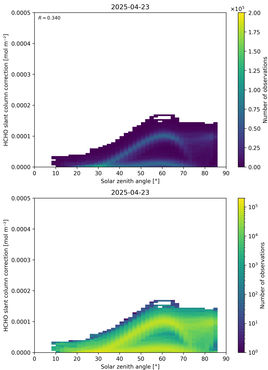
Figure 172: Scatter density plot of “Solar zenith angle” against “HCHO slant column correction” for 2025-04-22 to 2025-04-24.
