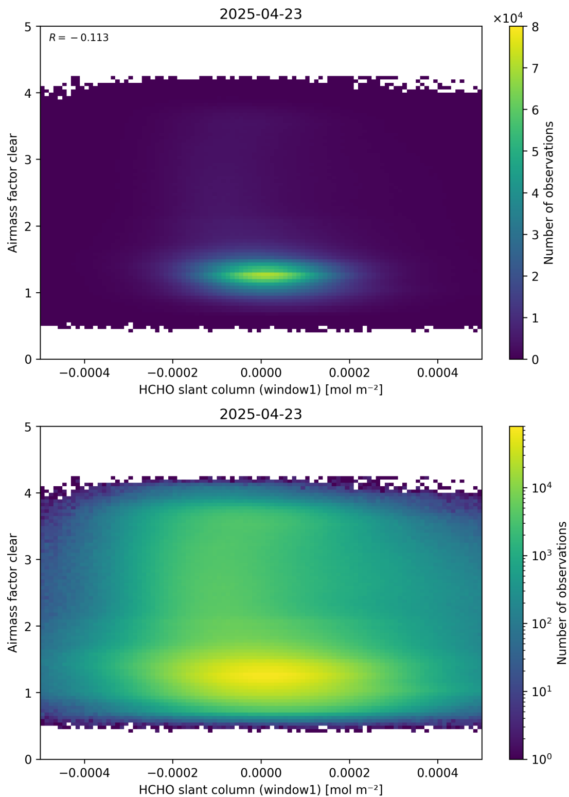
Figure 81: Scatter density plot of “HCHO slant column (window1)” against “Airmass factor clear” for 2025-04-22 to 2025-04-24.
