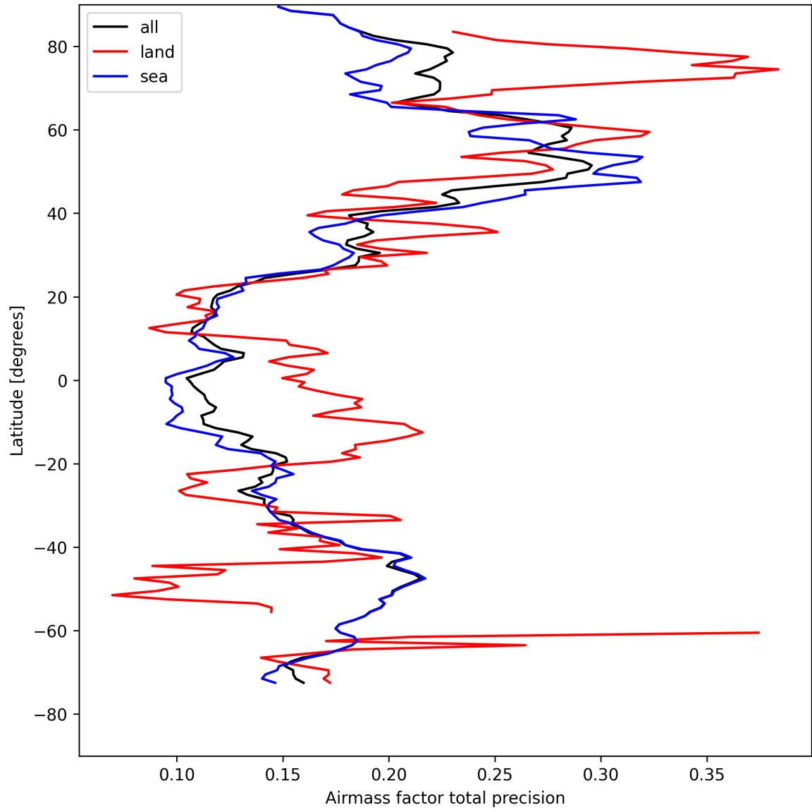
Figure 27: Zonal average of “Airmass factor total precision” for 2025-04-22 to 2025-04-24.
