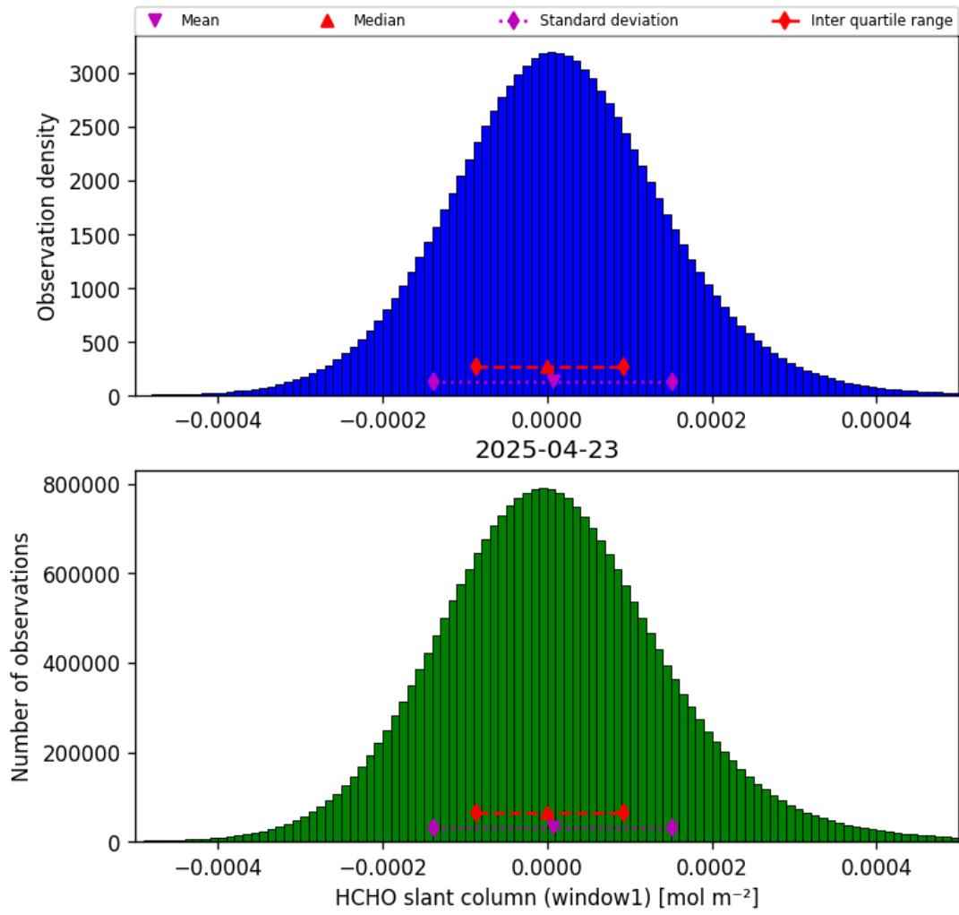
Figure 38: Histogram of “HCHO slant column (window1)” for 2025-04-22 to 2025-04-24
