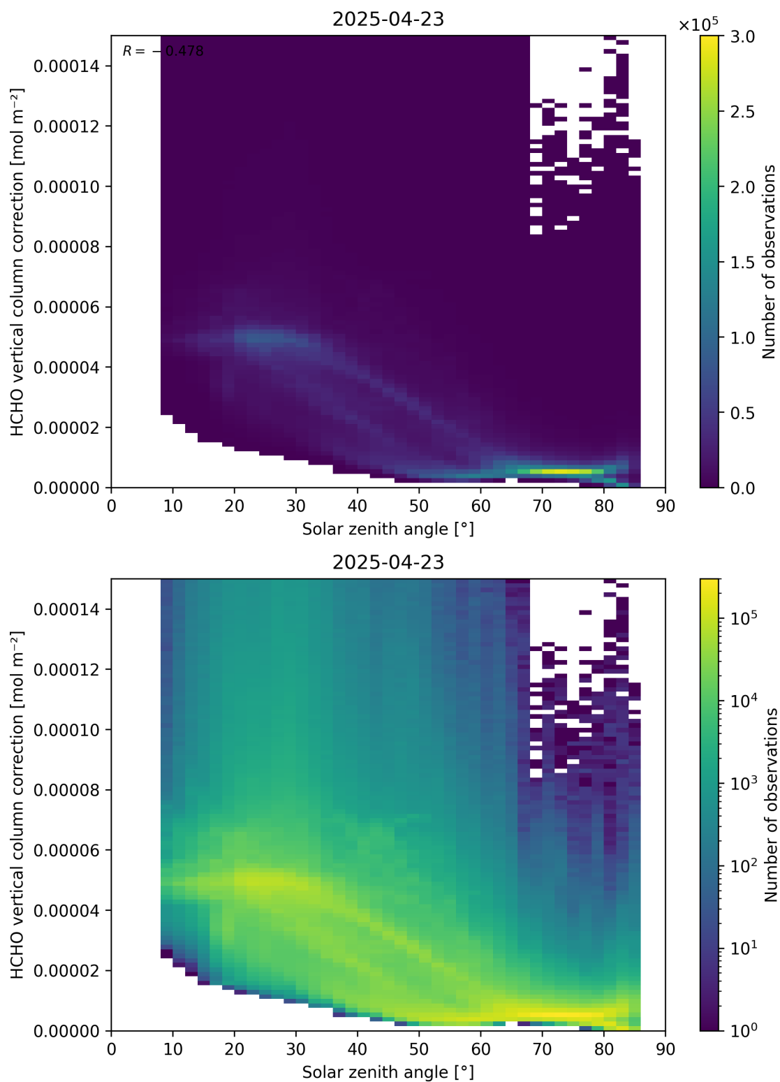
Figure 178: Scatter density plot of “Solar zenith angle” against “HCHO vertical column correction” for 2025-04-22 to 2025-04-24.
