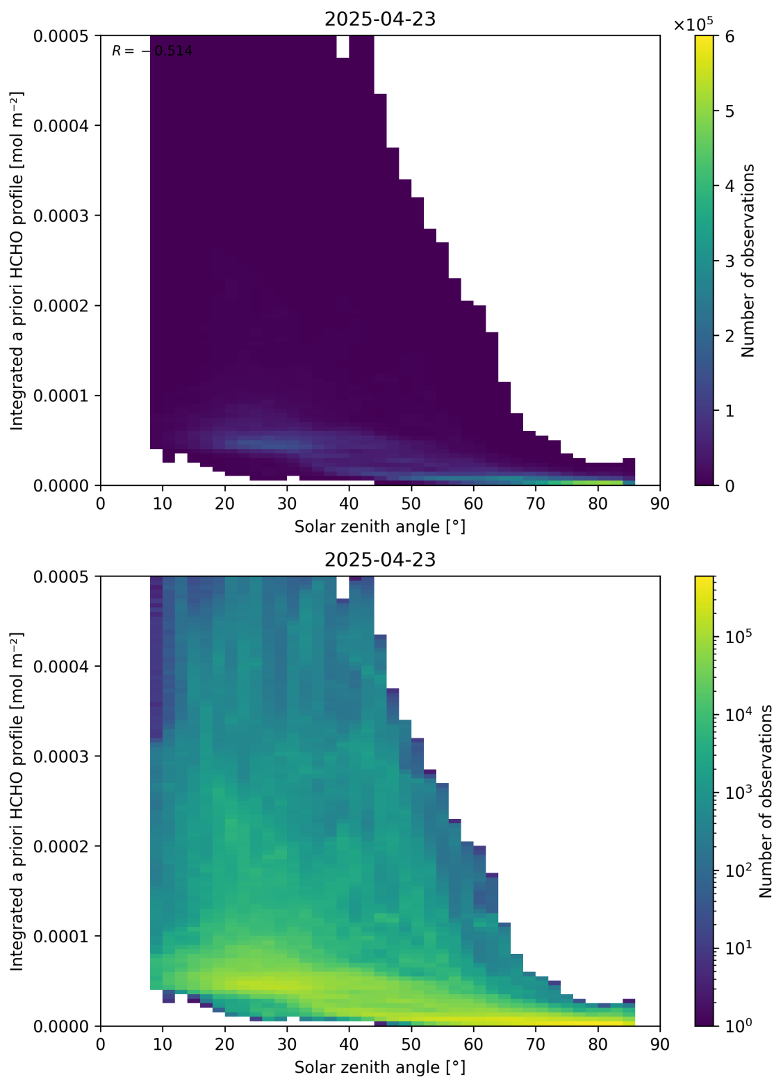
Figure 180: Scatter density plot of “Solar zenith angle” against “Integrated a priori HCHO profile” for 2025-04-22 to 2025-04-24.
