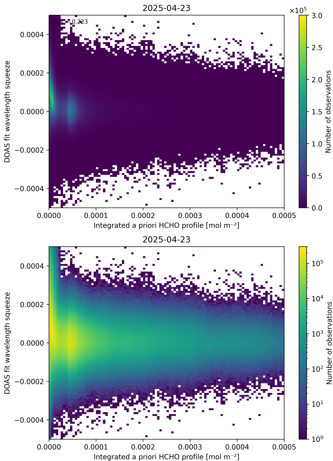
Figure 150: Scatter density plot of “Integrated a priori HCHO profile” against “DOAS fit wavelength squeeze” for 2025-04-22 to 2025-04-24.
