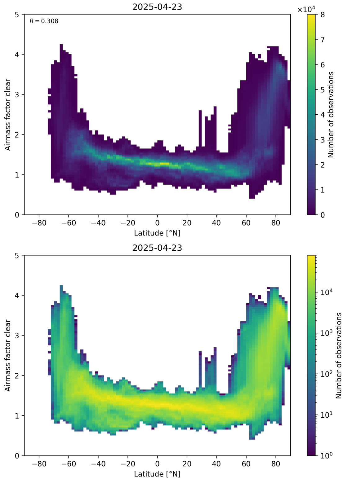
Figure 156: Scatter density plot of “Latitude” against “Airmass factor clear” for 2025-04-22 to 2025-04-24.
