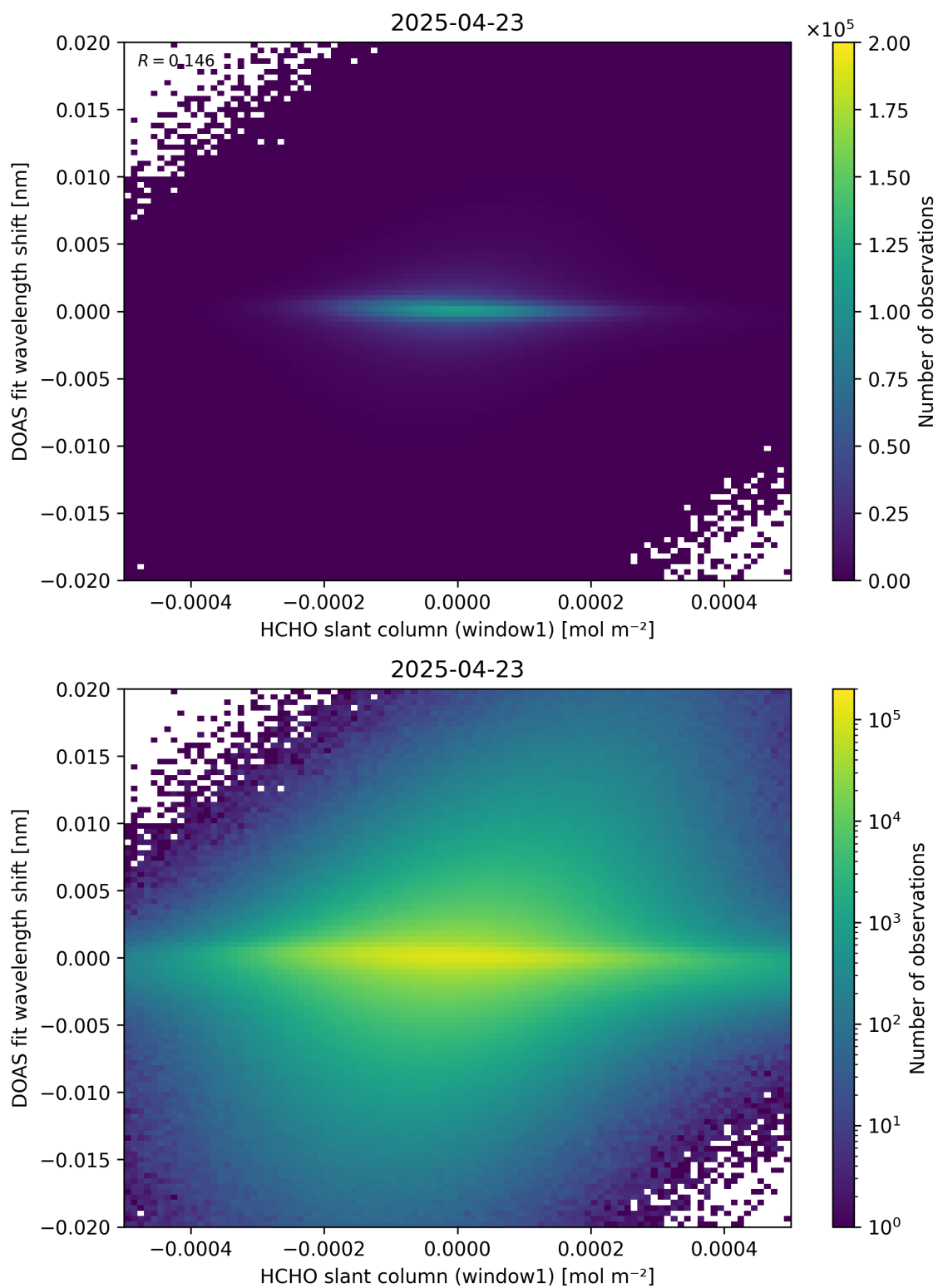
Figure 79: Scatter density plot of “HCHO slant column (window1)” against “DOAS fit wavelength shift” for 2025-04-22 to 2025-04-24.
