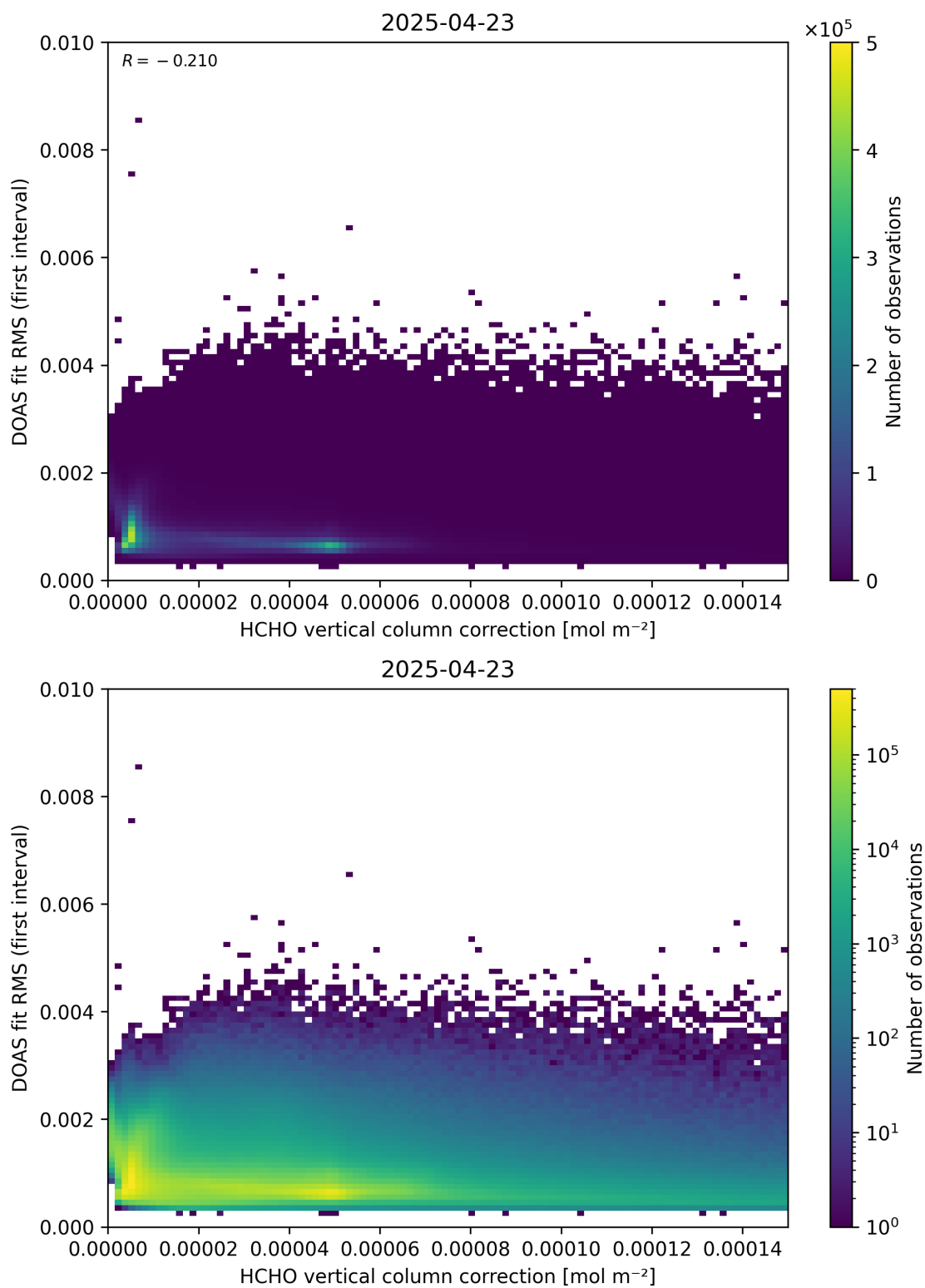
Figure 112: Scatter density plot of “HCHO vertical column correction” against “DOAS fit RMS (first interval)” for 2025-04-22 to 2025-04-24.
