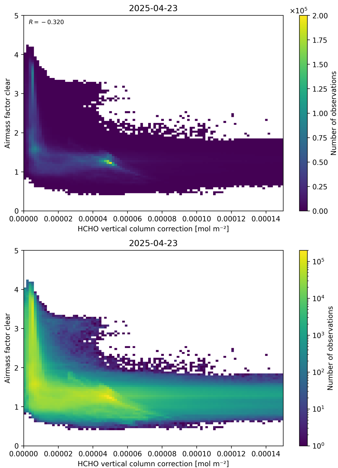
Figure 115: Scatter density plot of “HCHO vertical column correction” against “Airmass factor clear” for 2025-04-22 to 2025-04-24.
