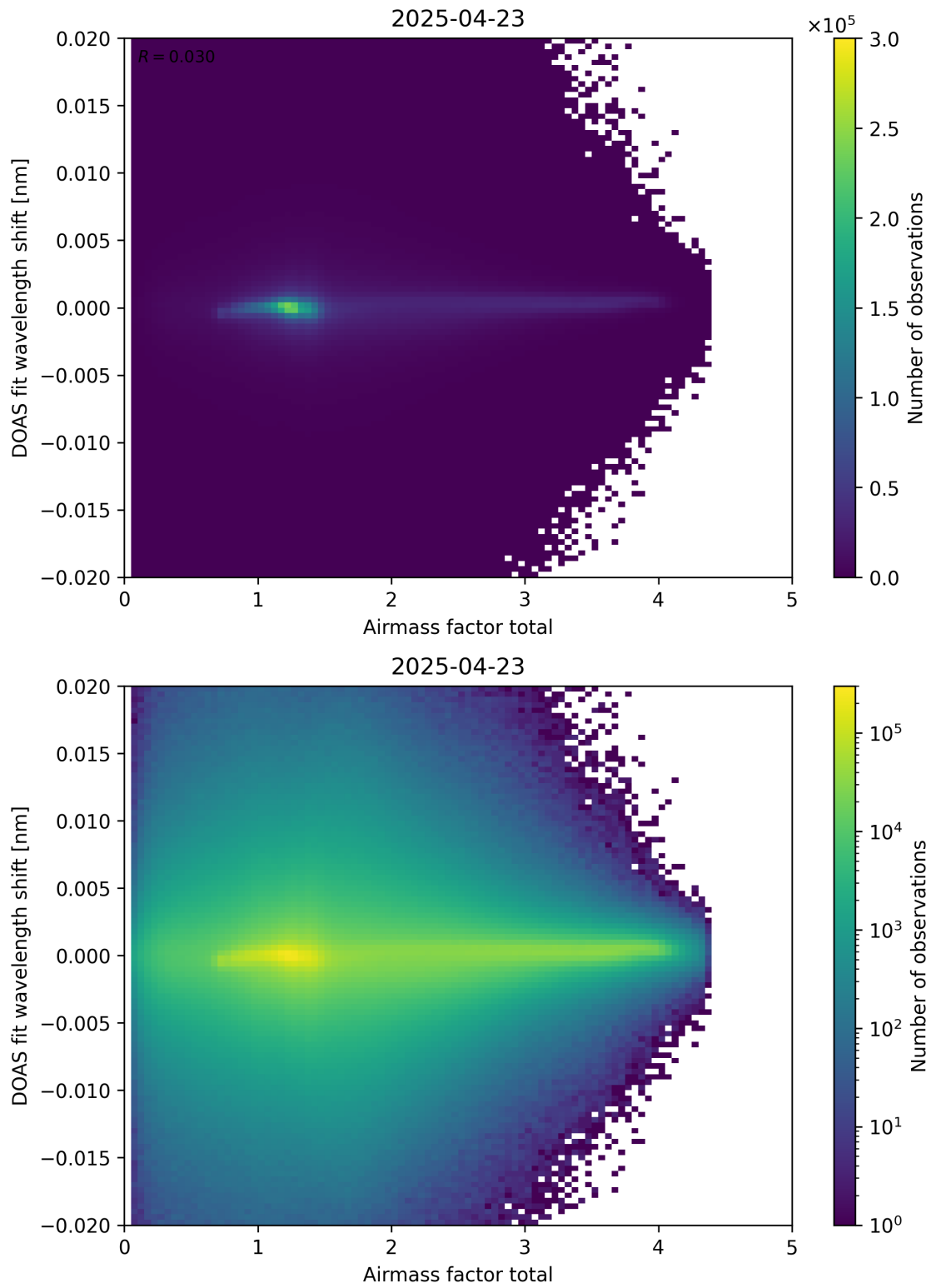
Figure 98: Scatter density plot of “Airmass factor total” against “DOAS fit wavelength shift” for 2025-04-22 to 2025-04-24.
