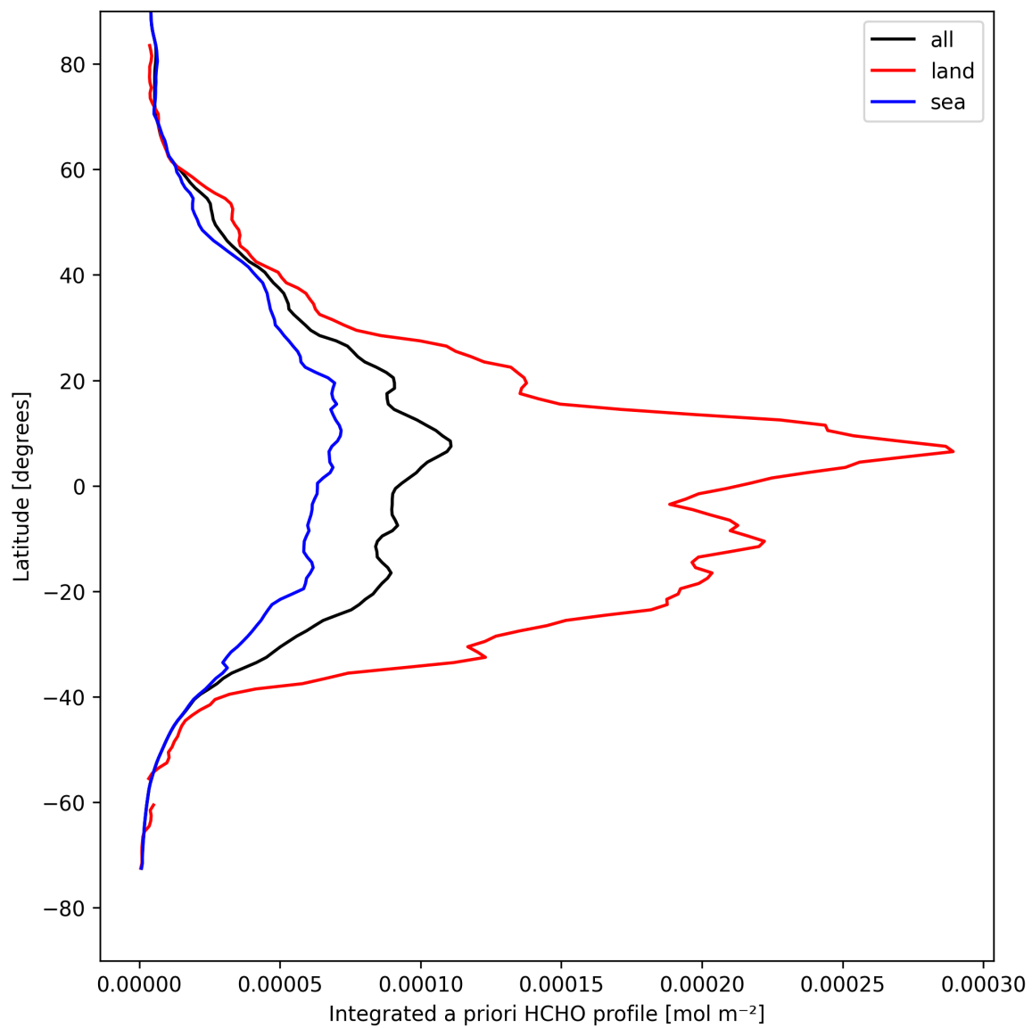
Figure 29: Zonal average of “Integrated a priori HCHO profile” for 2025-04-22 to 2025-04-24.
