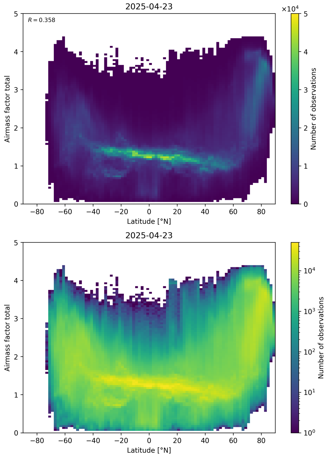
Figure 161: Scatter density plot of “Latitude” against “Airmass factor total” for 2025-04-22 to 2025-04-24.
