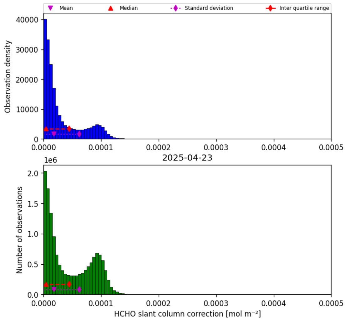
Figure 47: Histogram of “HCHO slant column correction” for 2025-04-22 to 2025-04-24
