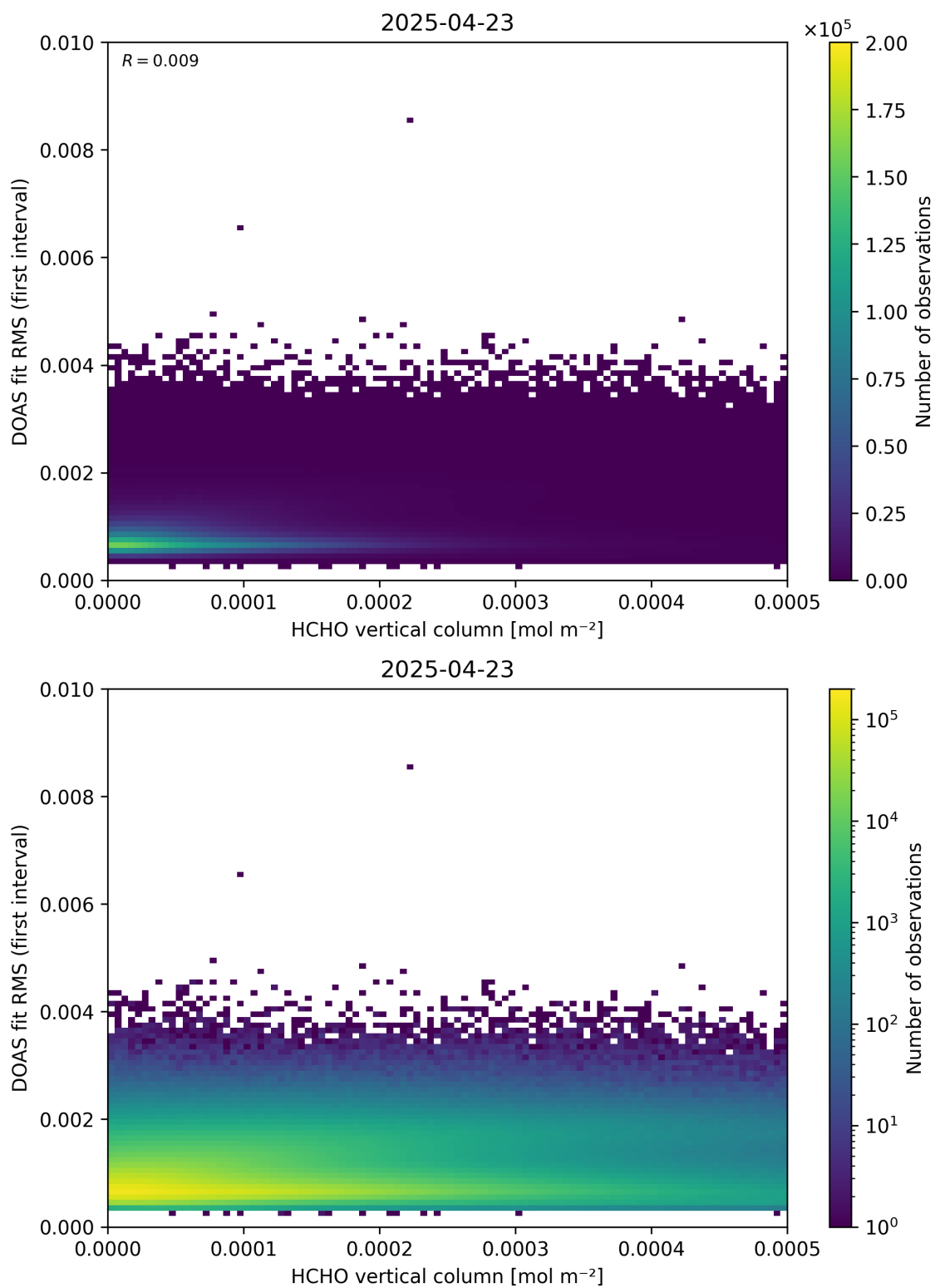
Figure 123: Scatter density plot of “HCHO vertical column” against “DOAS fit RMS (first interval)” for 2025-04-22 to 2025-04-24.
