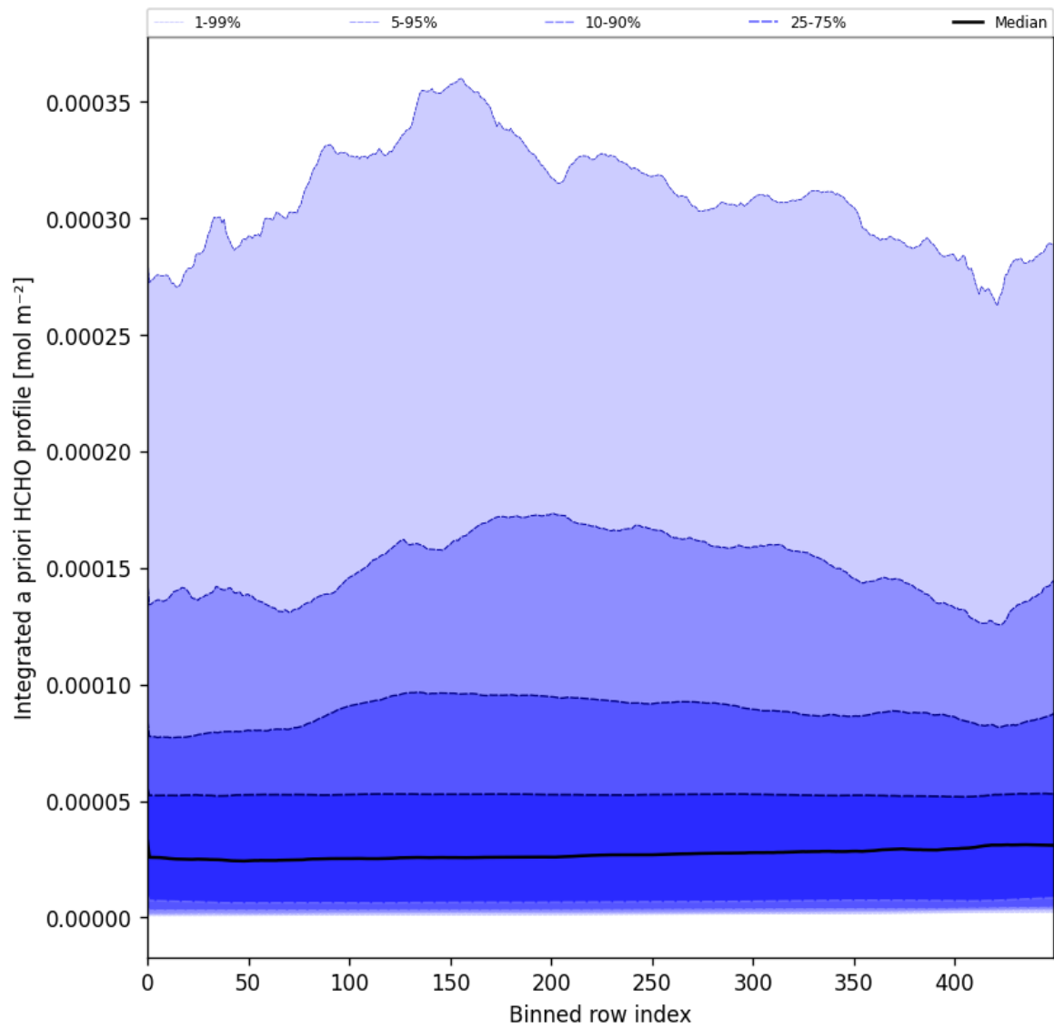
Figure 57: Along track statistics of "Integrated a priori HCHO profile" for 2025-04-22 to 2025-04-24
