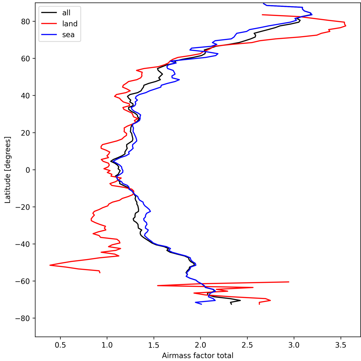
Figure 26: Zonal average of “Airmass factor total” for 2025-04-22 to 2025-04-24.
