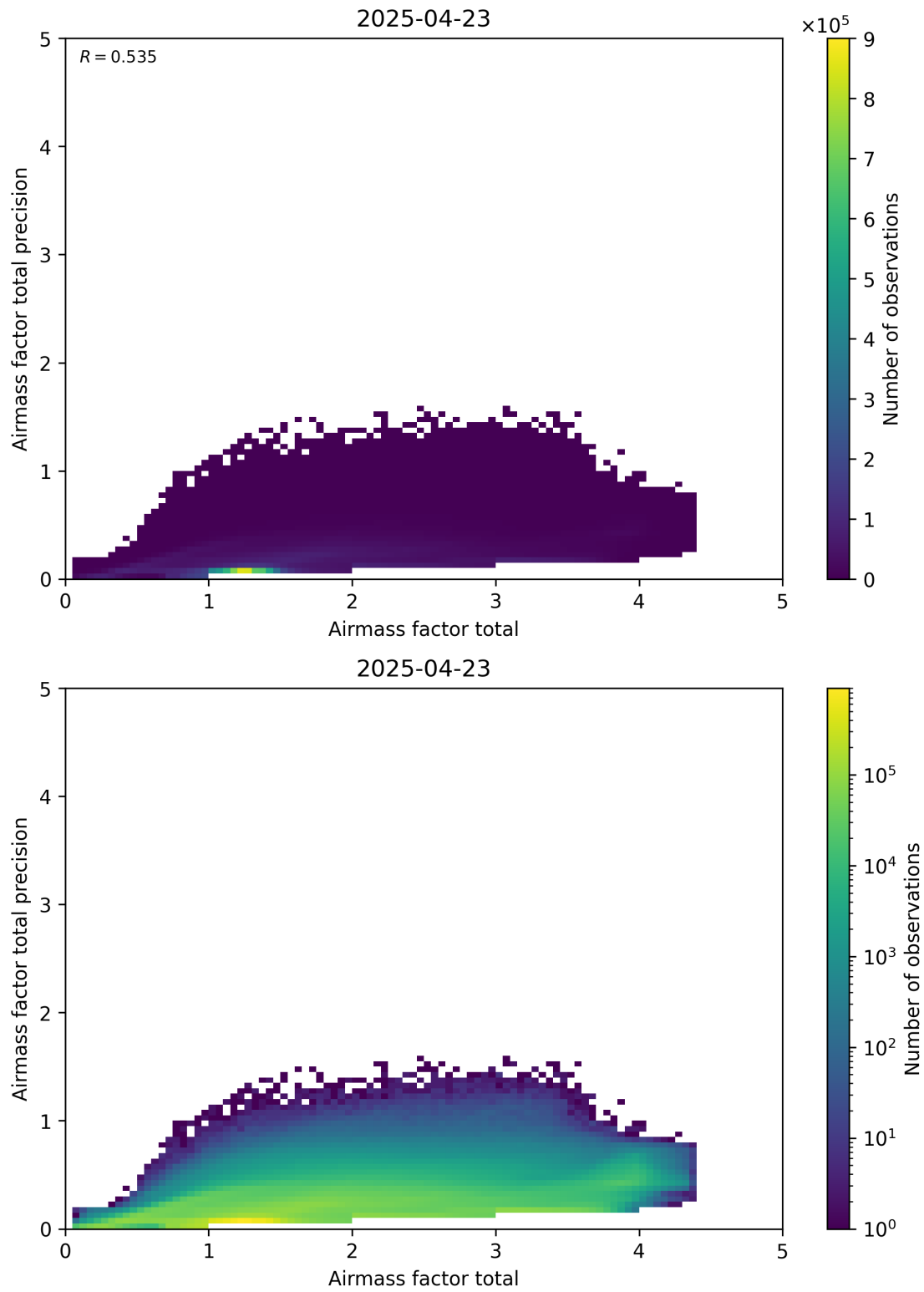
Figure 103: Scatter density plot of “Airmass factor total” against “Airmass factor total precision” for 2025-04-22 to 2025-04-24.
