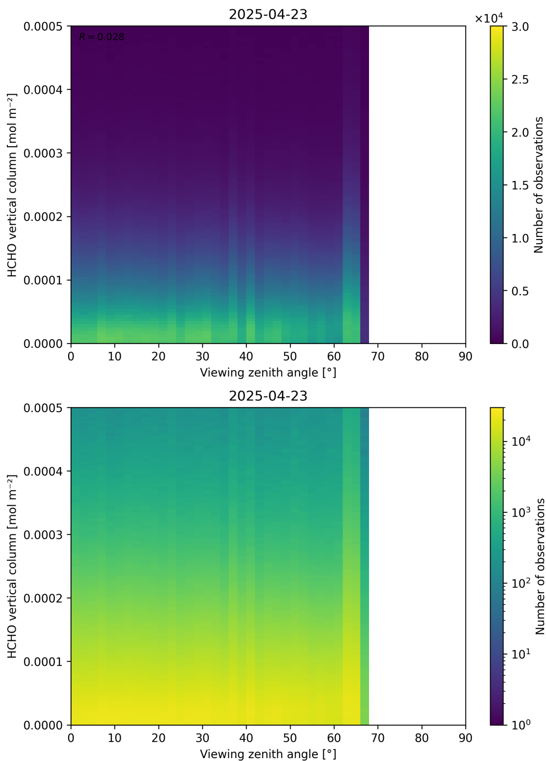
Figure 192: Scatter density plot of “Viewing zenith angle” against “HCHO vertical column” for 2025-04-22 to 2025-04-24.
