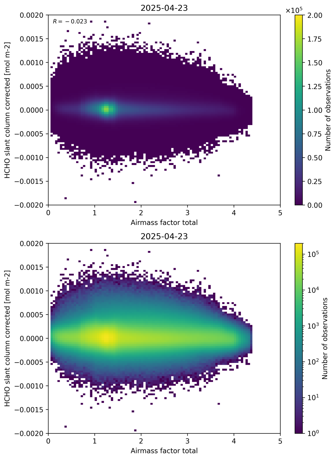
Figure 101: Scatter density plot of “Airmass factor total” against “HCHO slant column corrected” for 2025-04-22 to 2025-04-24.
