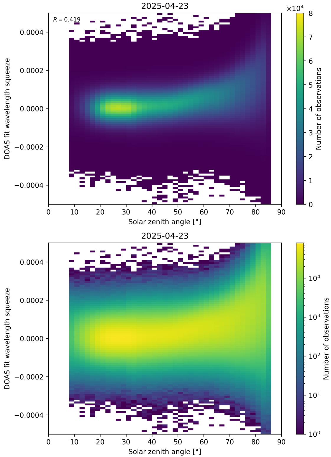
Figure 169: Scatter density plot of “Solar zenith angle” against “DOAS fit wavelength squeeze” for 2025-04-22 to 2025-04-24.
