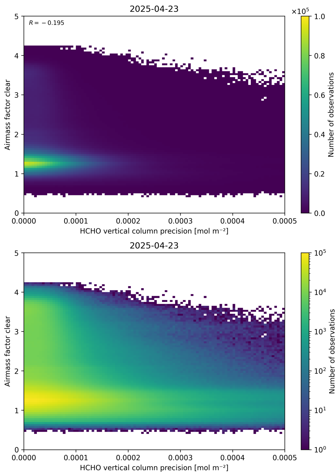
Figure 139: Scatter density plot of “HCHO vertical column precision” against “Airmass factor clear” for 2025-04-22 to 2025-04-24.
