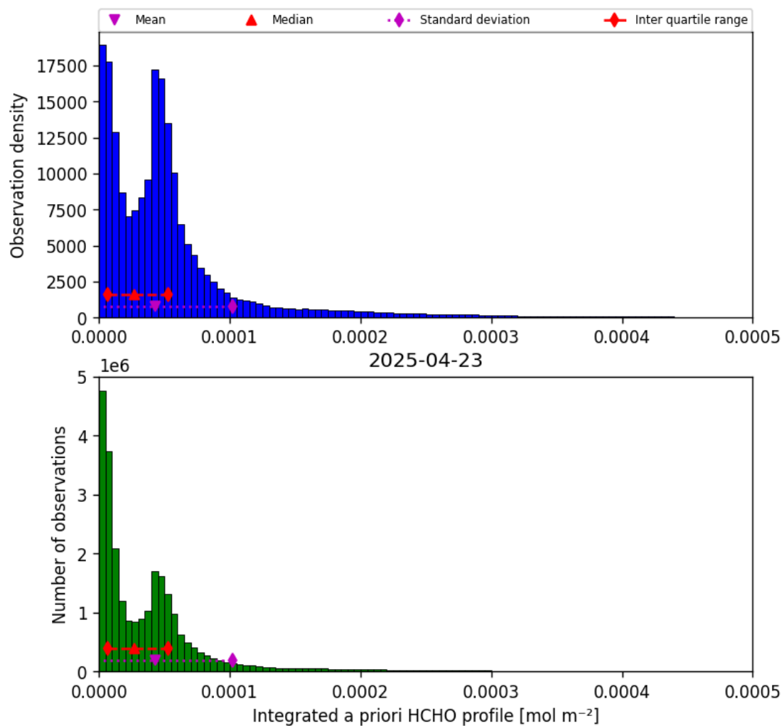
Figure 43: Histogram of “Integrated a priori HCHO profile” for 2025-04-22 to 2025-04-24
