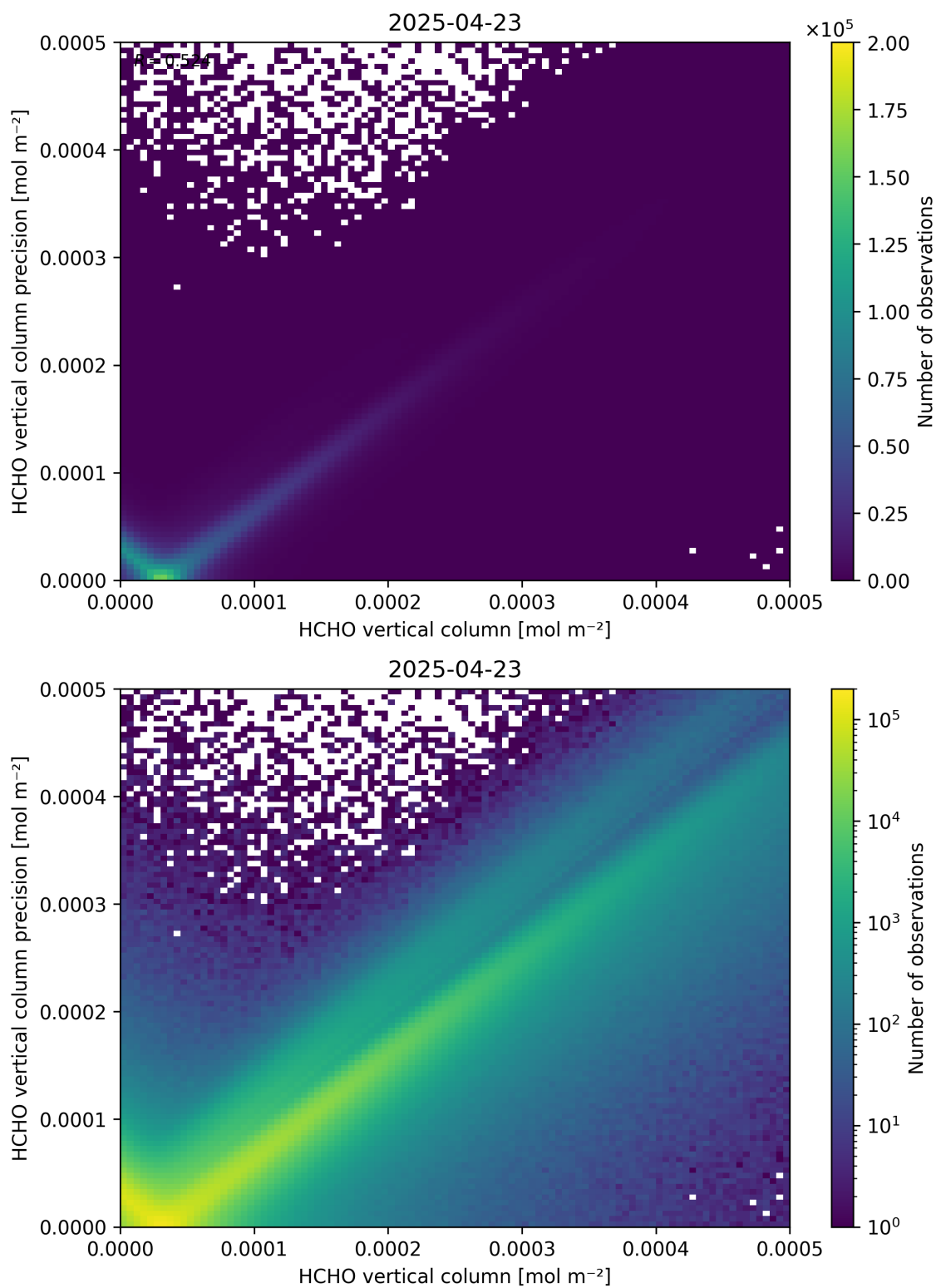
Figure 134: Scatter density plot of “HCHO vertical column” against “HCHO vertical column precision” for 2025-04-22 to 2025-04-24.
