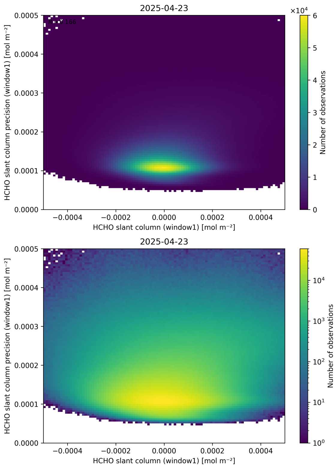
Figure 84: Scatter density plot of “HCHO slant column (window1)” against “HCHO slant column precision (window1)” for 2025-04-22 to 2025-04-24.
