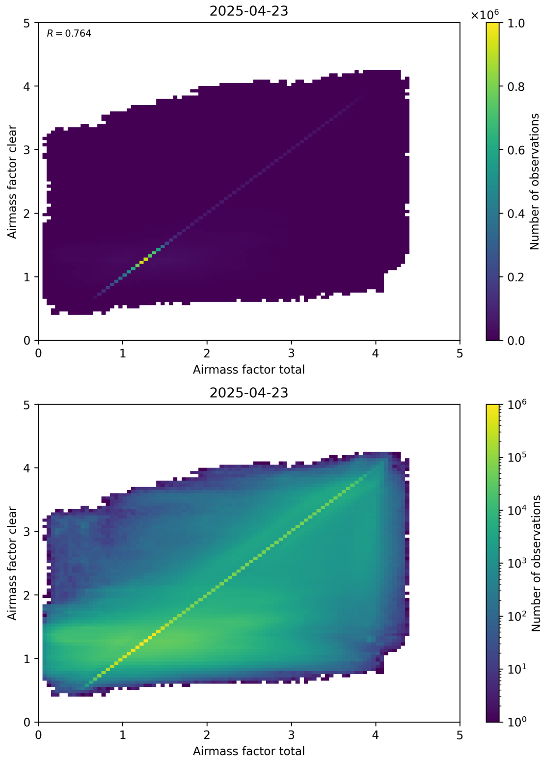
Figure 100: Scatter density plot of “Airmass factor total” against “Airmass factor clear” for 2025-04-22 to 2025-04-24.
