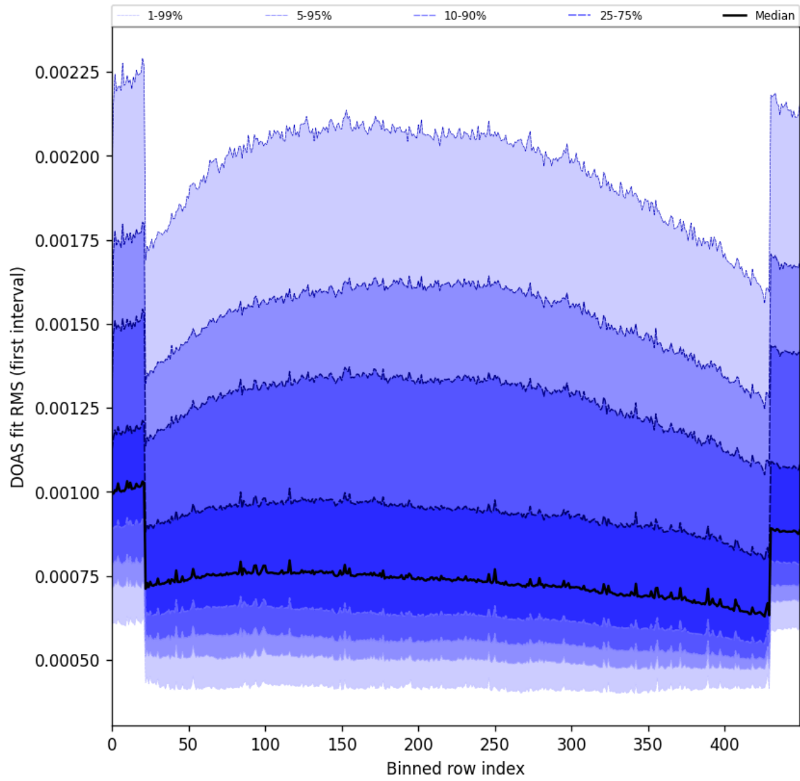
Figure 60: Along track statistics of “DOAS fit RMS (first interval)” for 2025-04-22 to 2025-04-24
