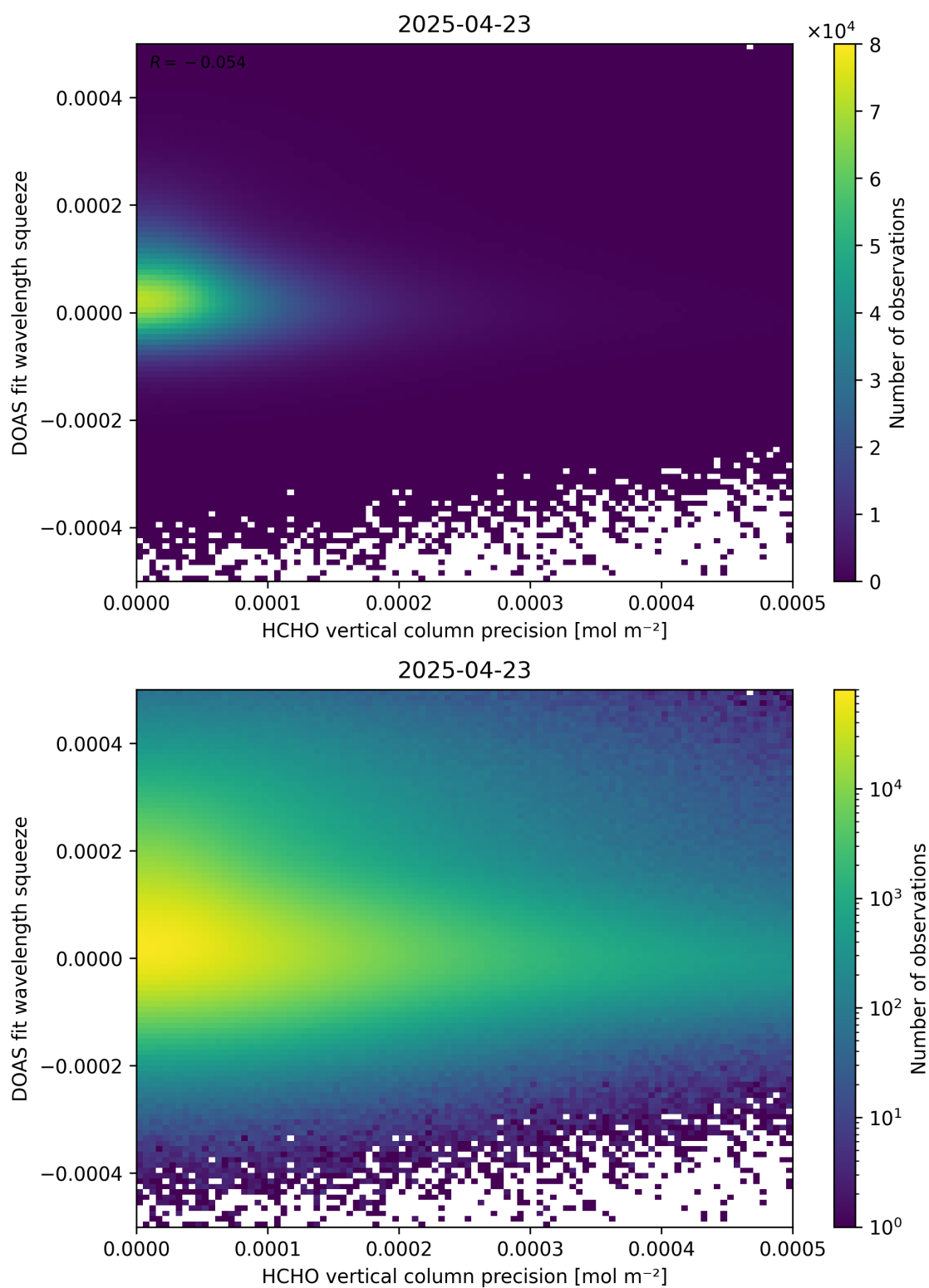
Figure 138: Scatter density plot of “HCHO vertical column precision” against “DOAS fit wavelength squeeze” for 2025-04-22 to 2025-04-24.
