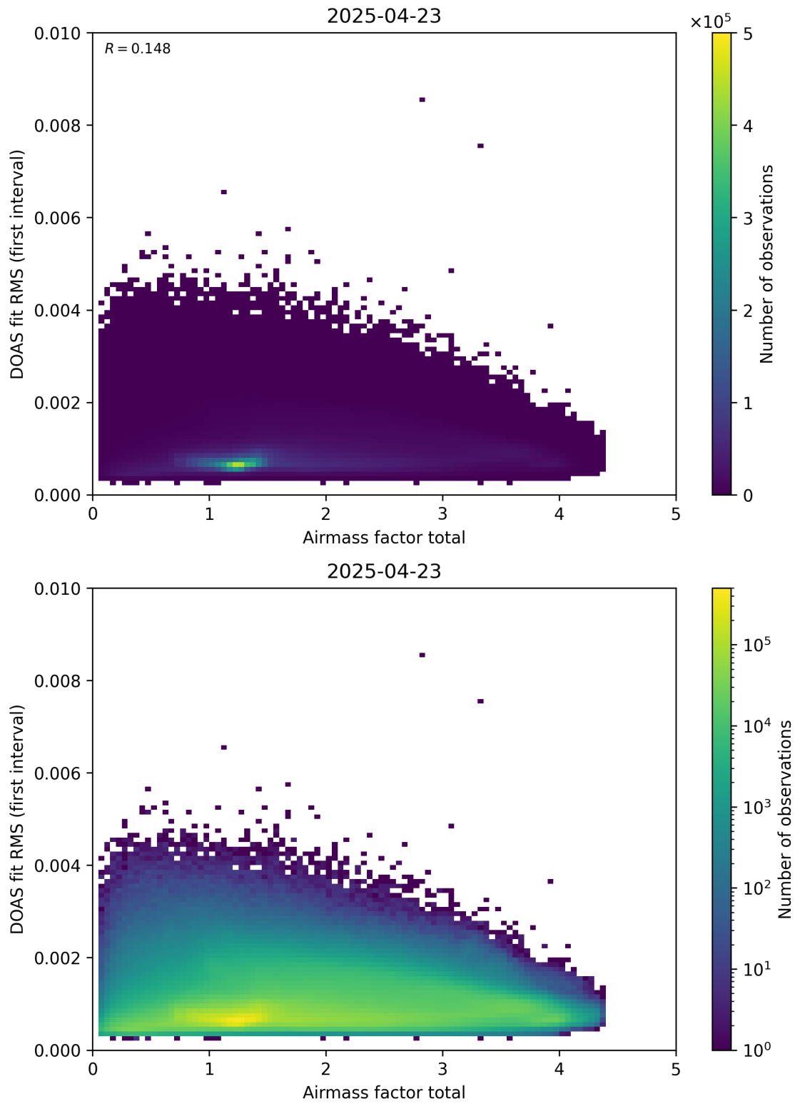
Figure 97: Scatter density plot of “Airmass factor total” against “DOAS fit RMS (first interval)” for 2025-04-22 to 2025-04-24.
