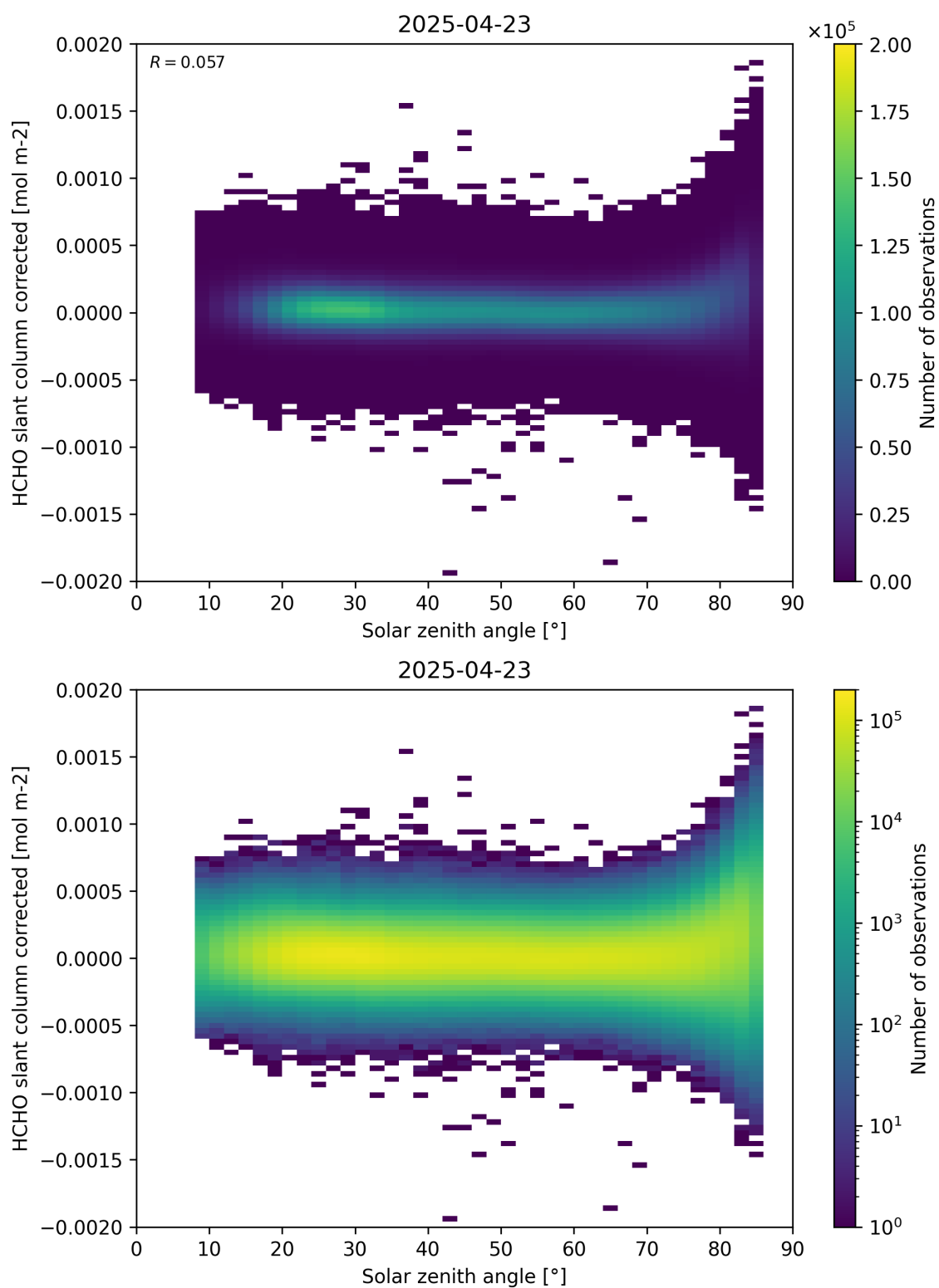
Figure 171: Scatter density plot of “Solar zenith angle” against “HCHO slant column corrected” for 2025-04-22 to 2025-04-24.
