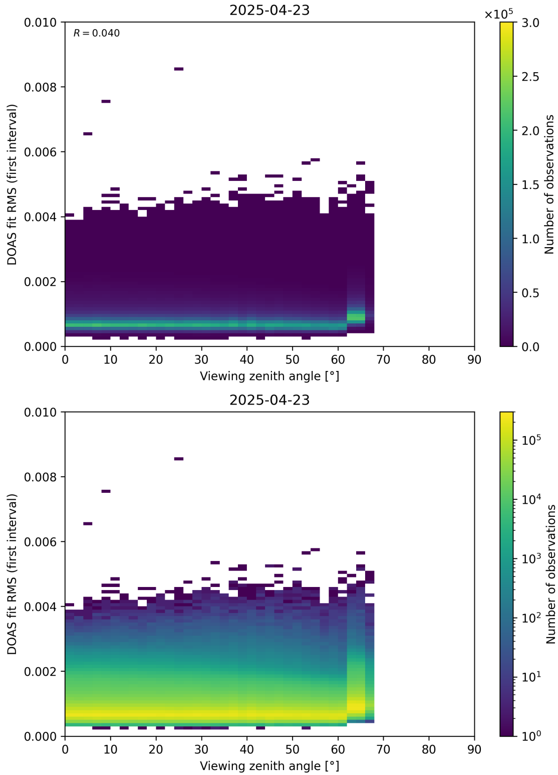
Figure 182: Scatter density plot of “Viewing zenith angle” against “DOAS fit RMS (first interval)” for 2025-04-22 to 2025-04-24.
