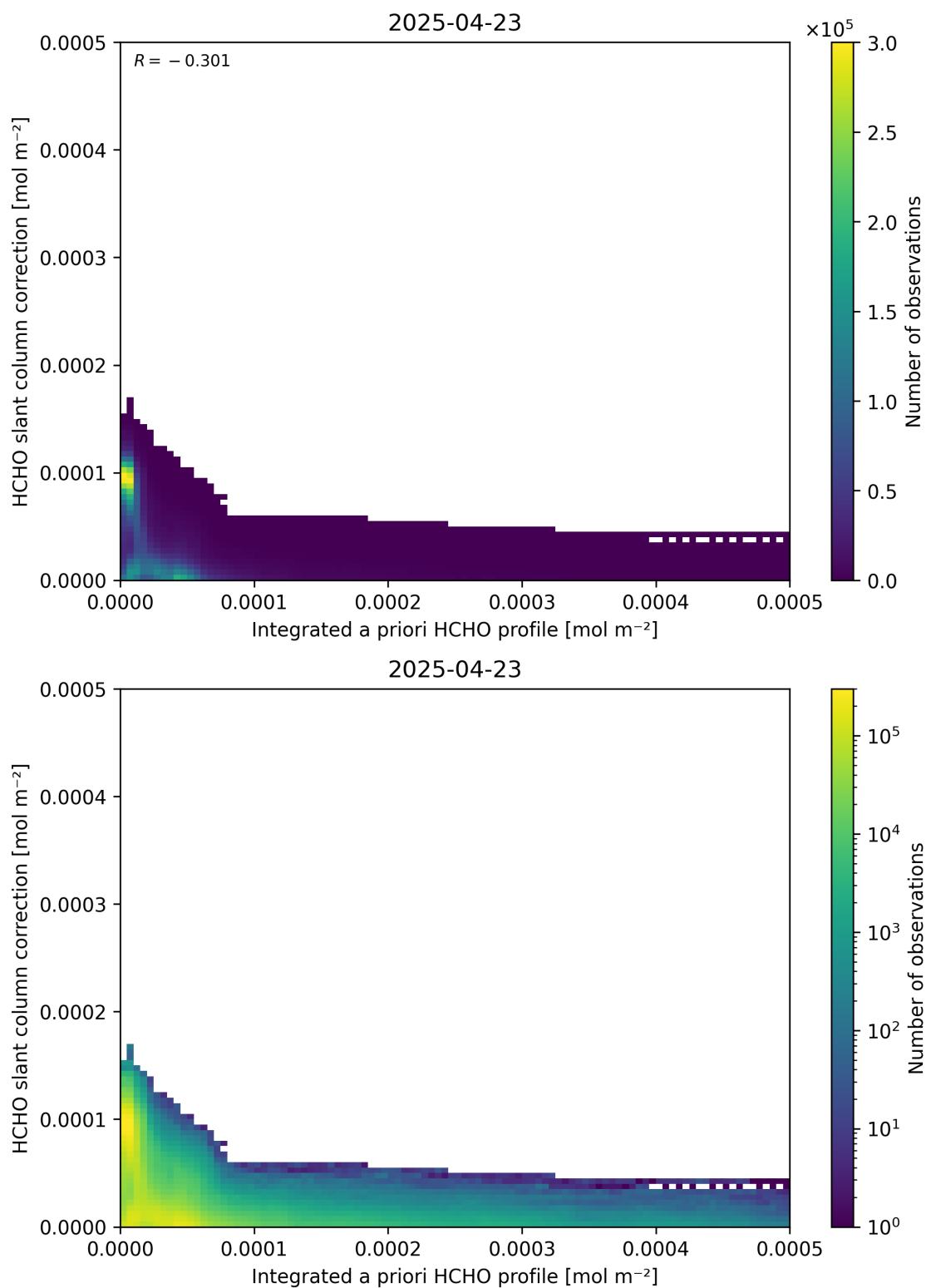
Figure 152: Scatter density plot of “Integrated a priori HCHO profile” against “HCHO slant column correction” for 2025-04-22 to 2025-04-24.
