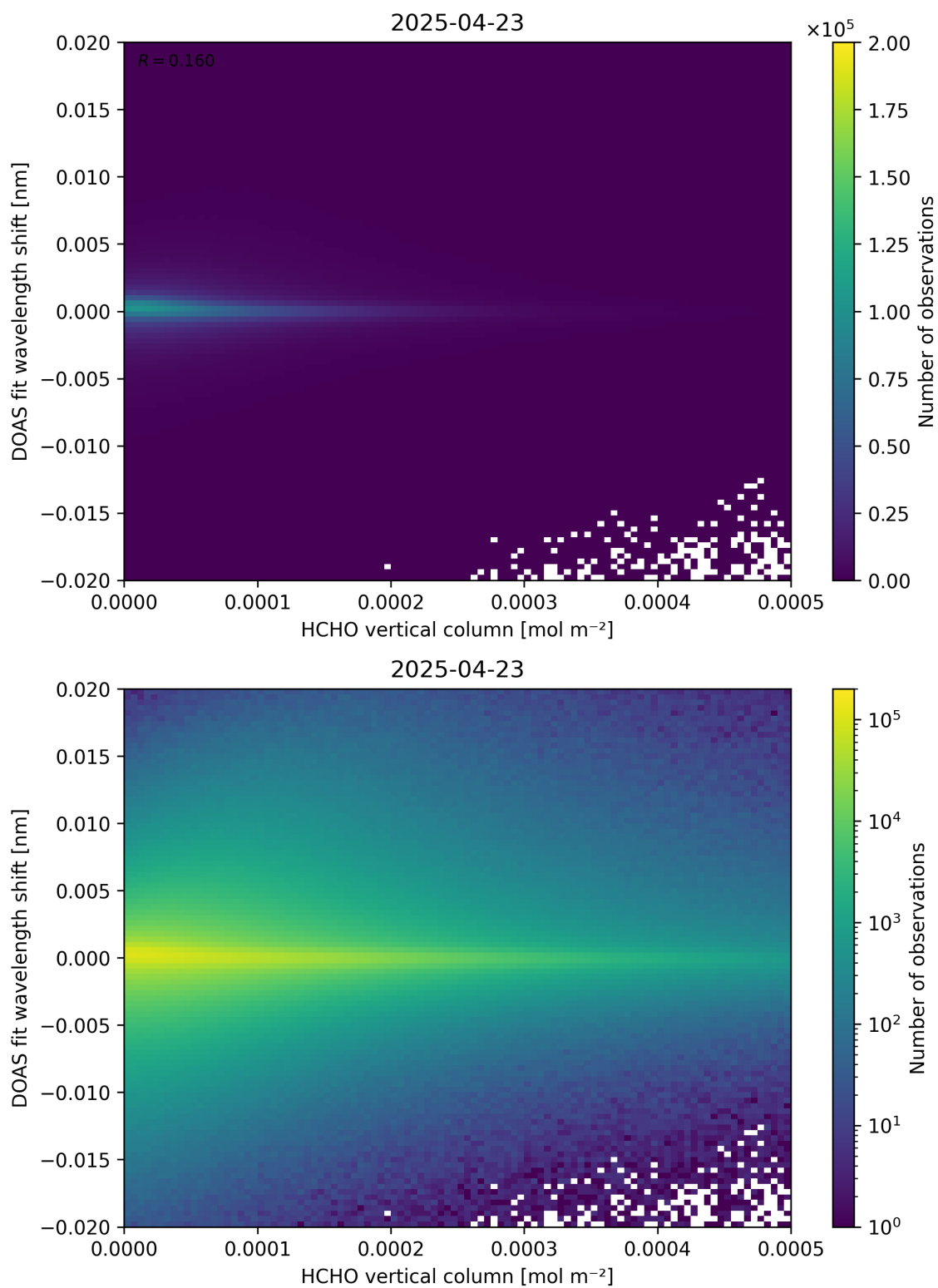
Figure 124: Scatter density plot of “HCHO vertical column” against “DOAS fit wavelength shift” for 2025-04-22 to 2025-04-24.
