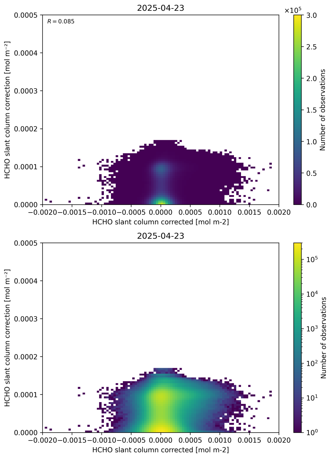
Figure 77: Scatter density plot of “HCHO slant column corrected” against “HCHO slant column correction” for 2025-04-22 to 2025-04-24.
