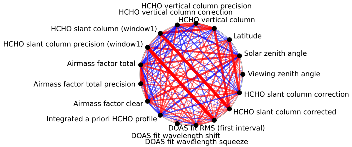
Figure 1: Map of correlation graph for 2025-04-22 to 2025-04-24.
