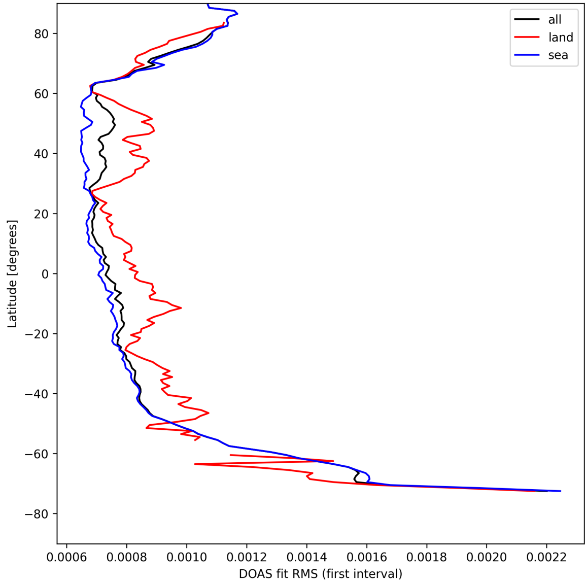
Figure 32: Zonal average of "DOAS fit RMS (first interval)" for 2025-04-22 to 2025-04-24.
