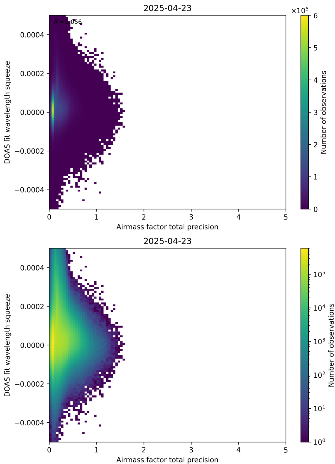
Figure 107: Scatter density plot of “Airmass factor total precision” against “DOAS fit wavelength squeeze” for 2025-04-22 to 2025-04-24.
