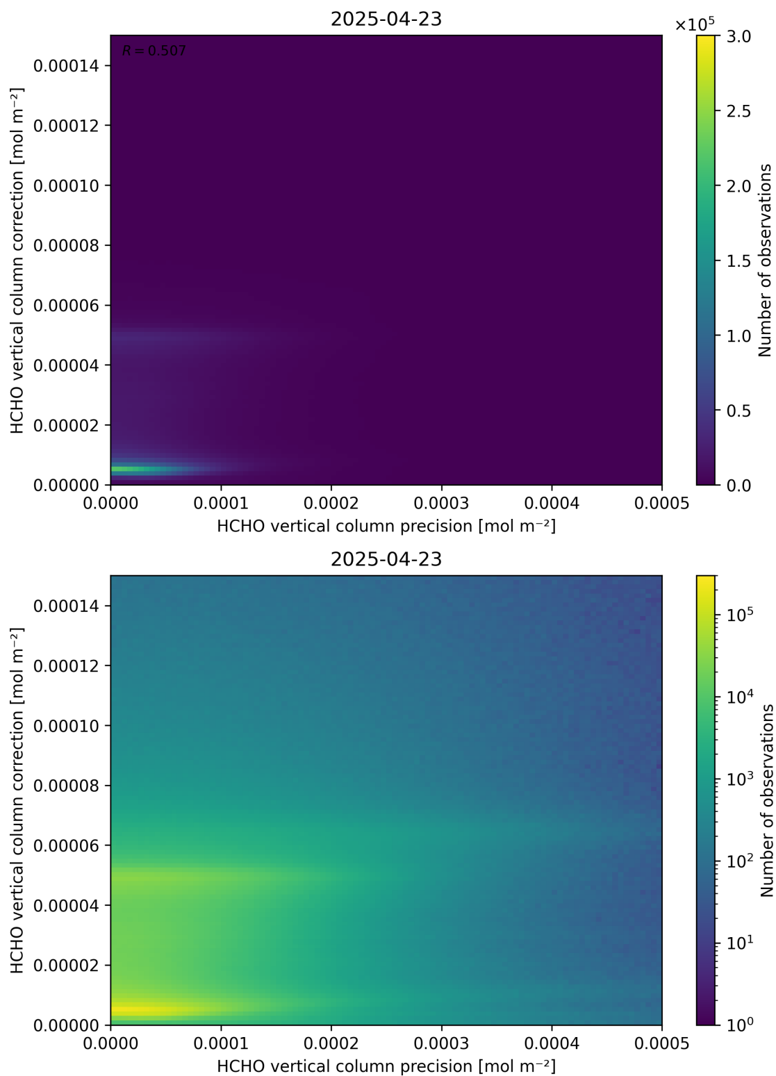
Figure 146: Scatter density plot of “HCHO vertical column precision” against “HCHO vertical column correction” for 2025-04-22 to 2025-04-24.
