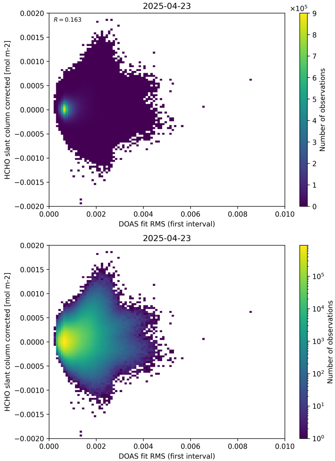
Figure 62: Scatter density plot of “DOAS fit RMS (first interval)” against “HCHO slant column corrected” for 2025-04-22 to 2025-04-24.
