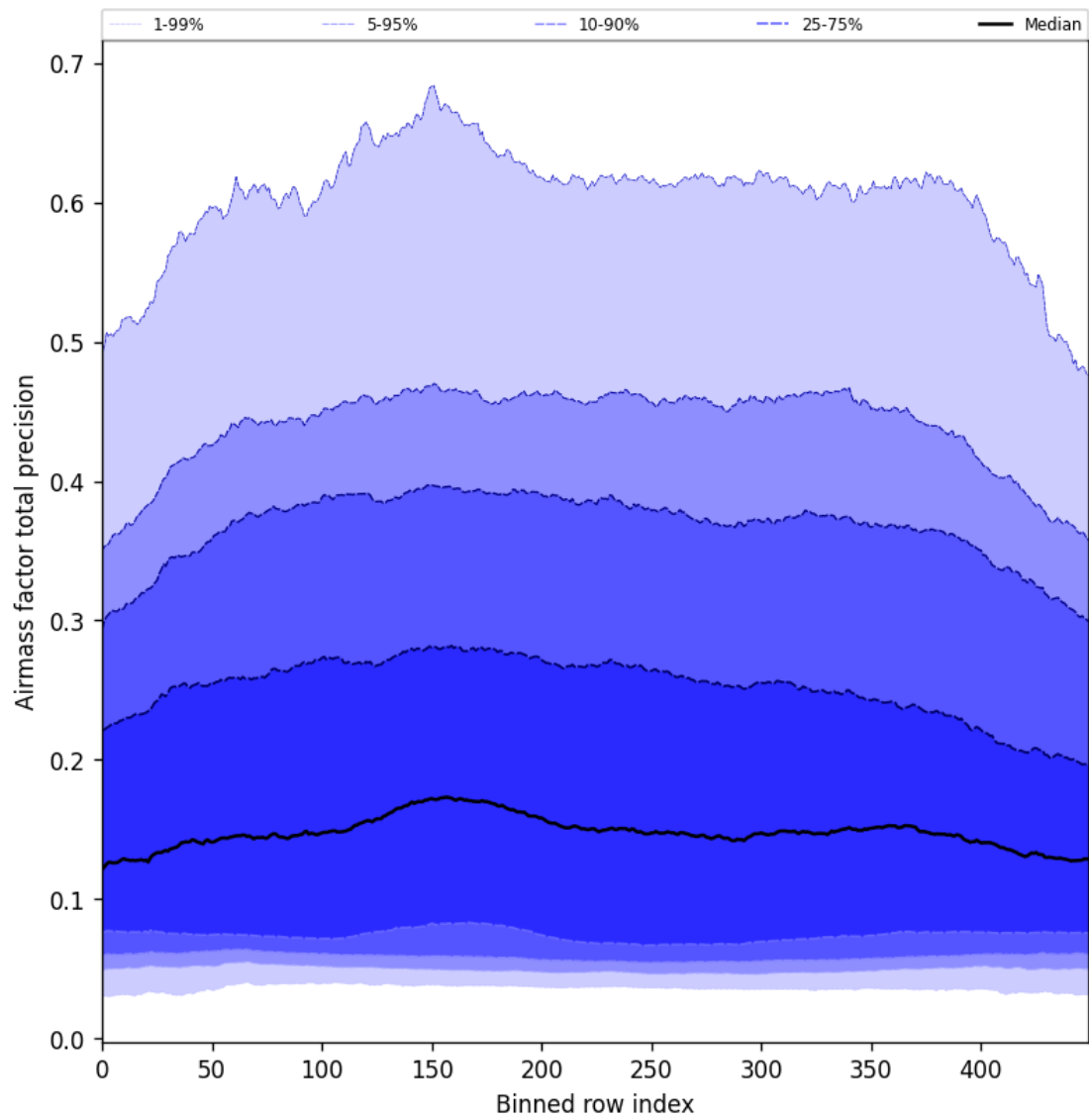
Figure 55: Along track statistics of “Airmass factor total precision” for 2025-04-22 to 2025-04-24
