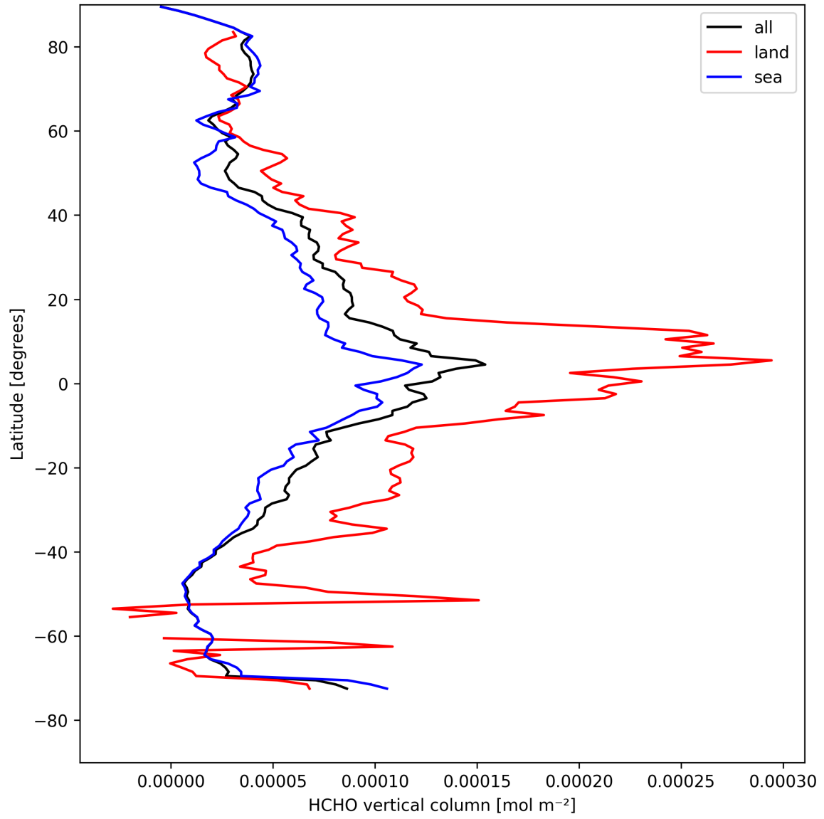
Figure 21: Zonal average of “HCHO vertical column” for 2025-04-22 to 2025-04-24.
