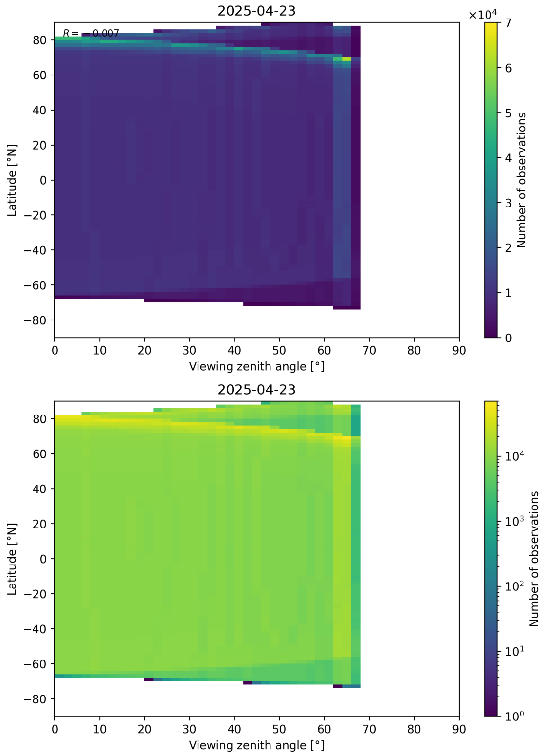
Figure 196: Scatter density plot of “Viewing zenith angle” against “Latitude” for 2025-04-22 to 2025-04-24.
