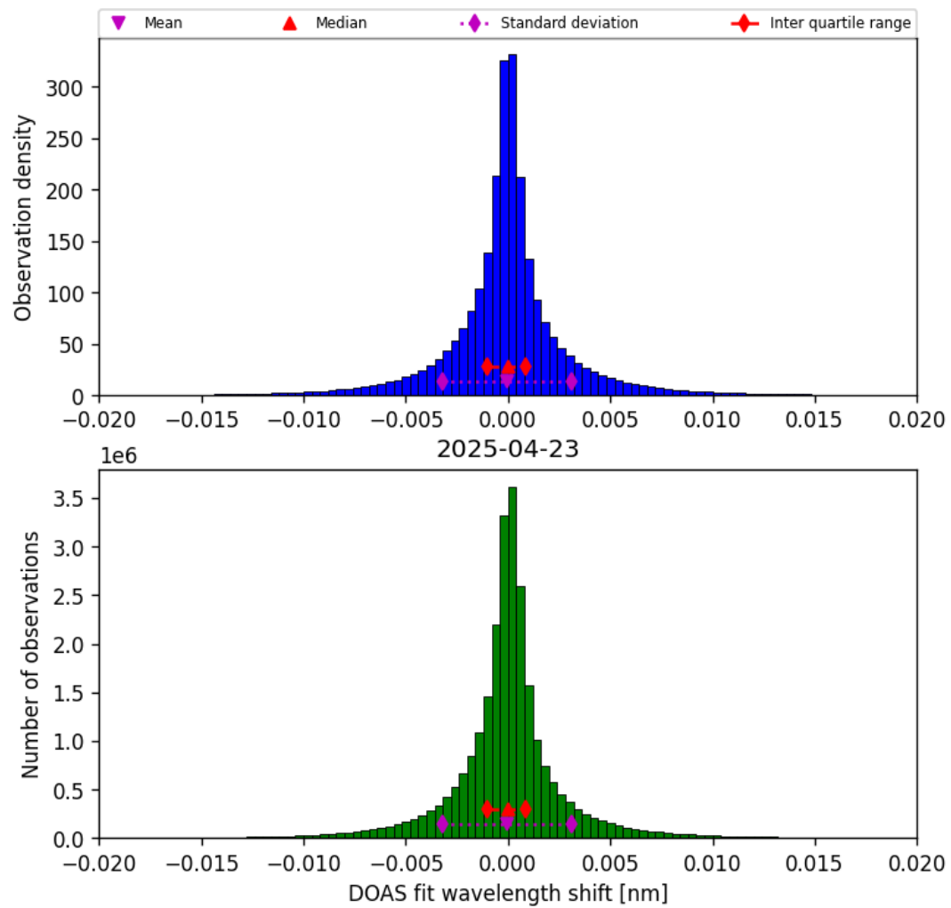
Figure 44: Histogram of “DOAS fit wavelength shift” for 2025-04-22 to 2025-04-24
