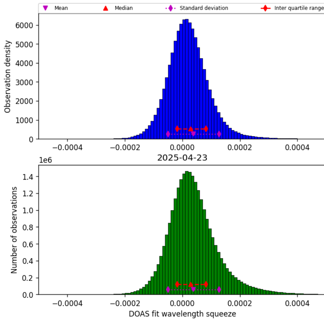
Figure 45: Histogram of “DOAS fit wavelength squeeze” for 2025-04-22 to 2025-04-24
