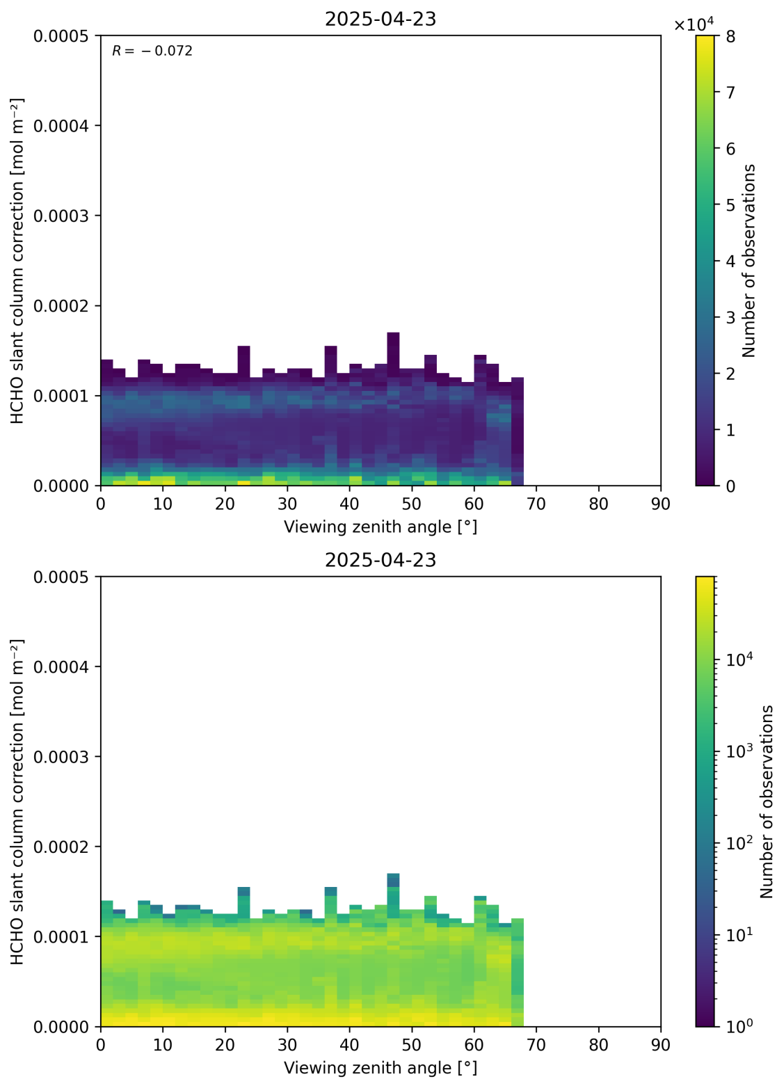
Figure 187: Scatter density plot of “Viewing zenith angle” against “HCHO slant column correction” for 2025-04-22 to 2025-04-24.
