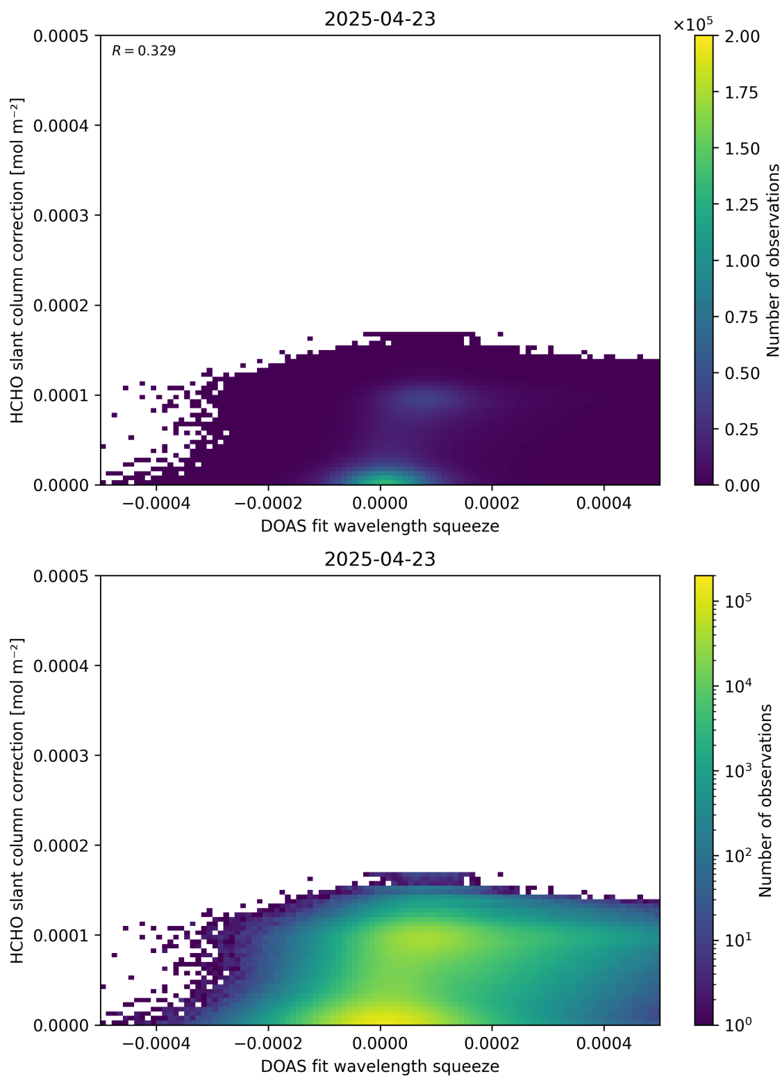
Figure 70: Scatter density plot of “DOAS fit wavelength squeeze” against “HCHO slant column correction” for 2025-04-22 to 2025-04-24.
