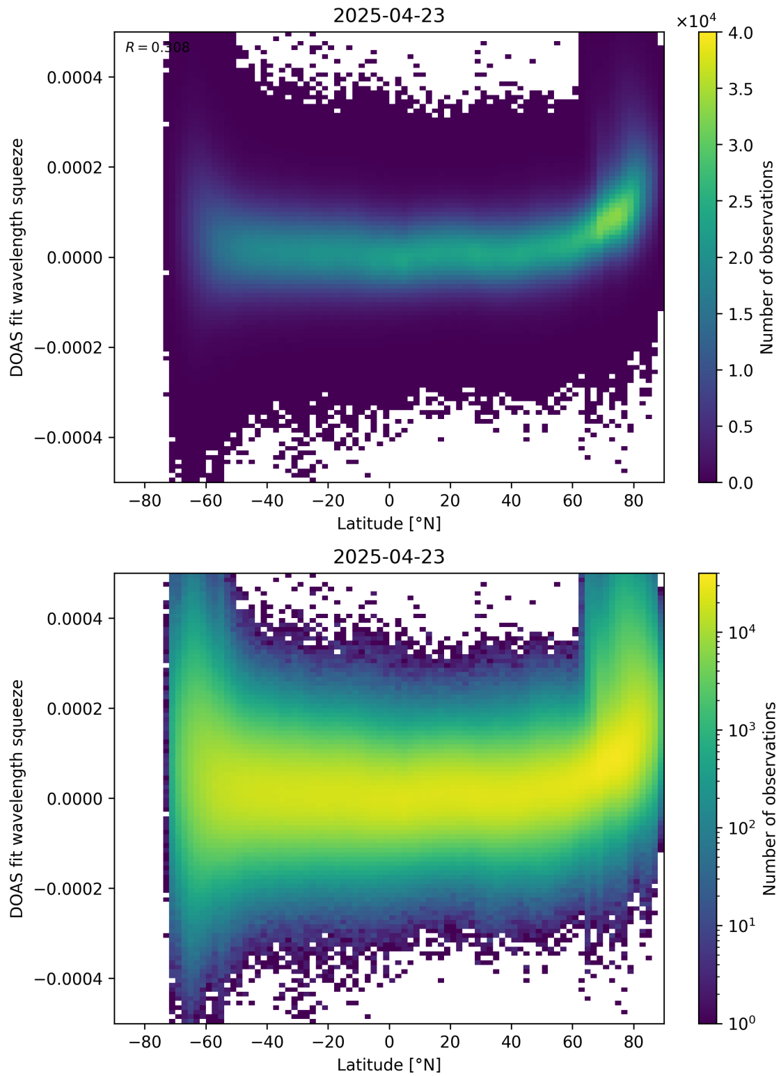
Figure 155: Scatter density plot of “Latitude” against “DOAS fit wavelength squeeze” for 2025-04-22 to 2025-04-24.
