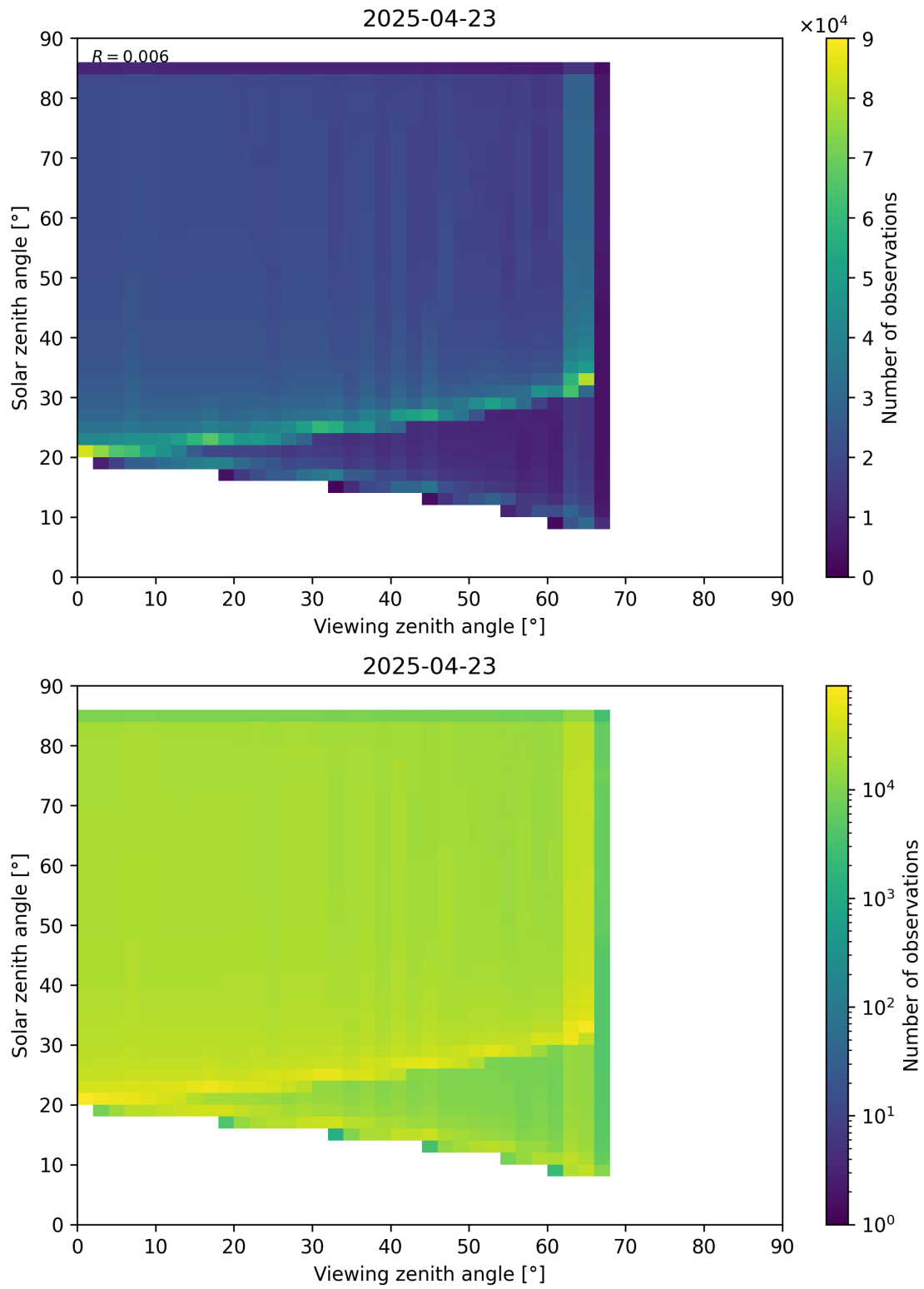
Figure 197: Scatter density plot of “Viewing zenith angle” against “Solar zenith angle” for 2025-04-22 to 2025-04-24.
