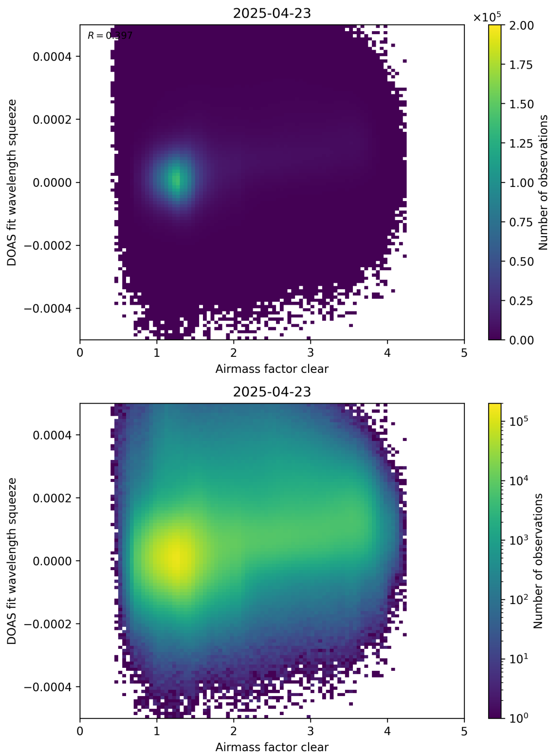
Figure 73: Scatter density plot of “Airmass factor clear” against “DOAS fit wavelength squeeze” for 2025-04-22 to 2025-04-24.
