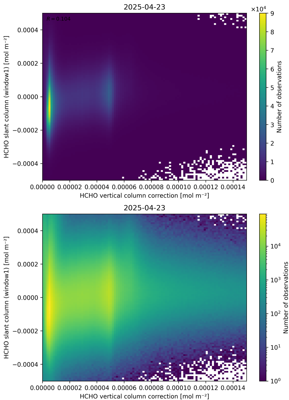
Figure 118: Scatter density plot of “HCHO vertical column correction” against “HCHO slant column (window1)” for 2025-04-22 to 2025-04-24.
