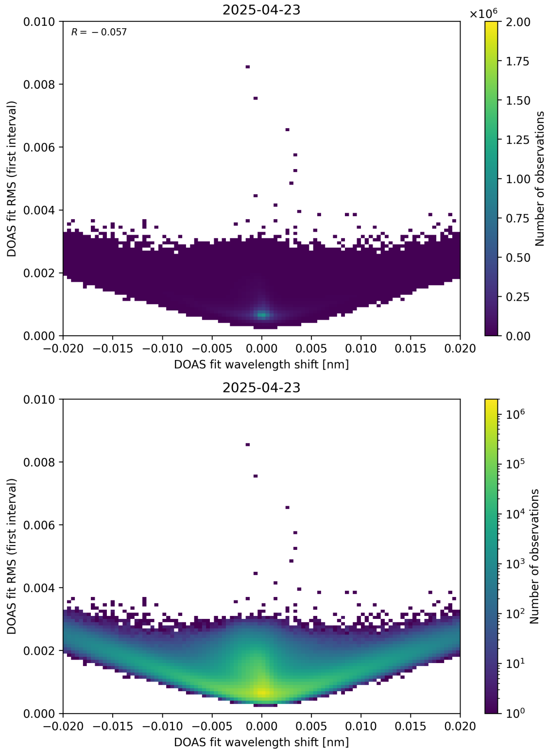
Figure 64: Scatter density plot of “DOAS fit wavelength shift” against “DOAS fit RMS (first interval)” for 2025-04-22 to 2025-04-24.
