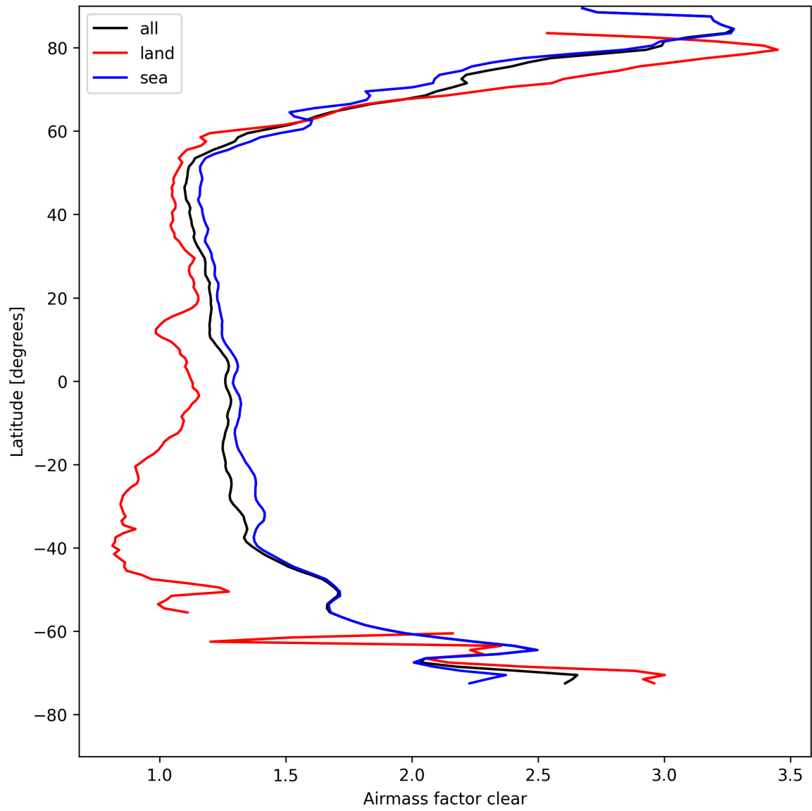
Figure 28: Zonal average of “Airmass factor clear” for 2025-04-22 to 2025-04-24.
