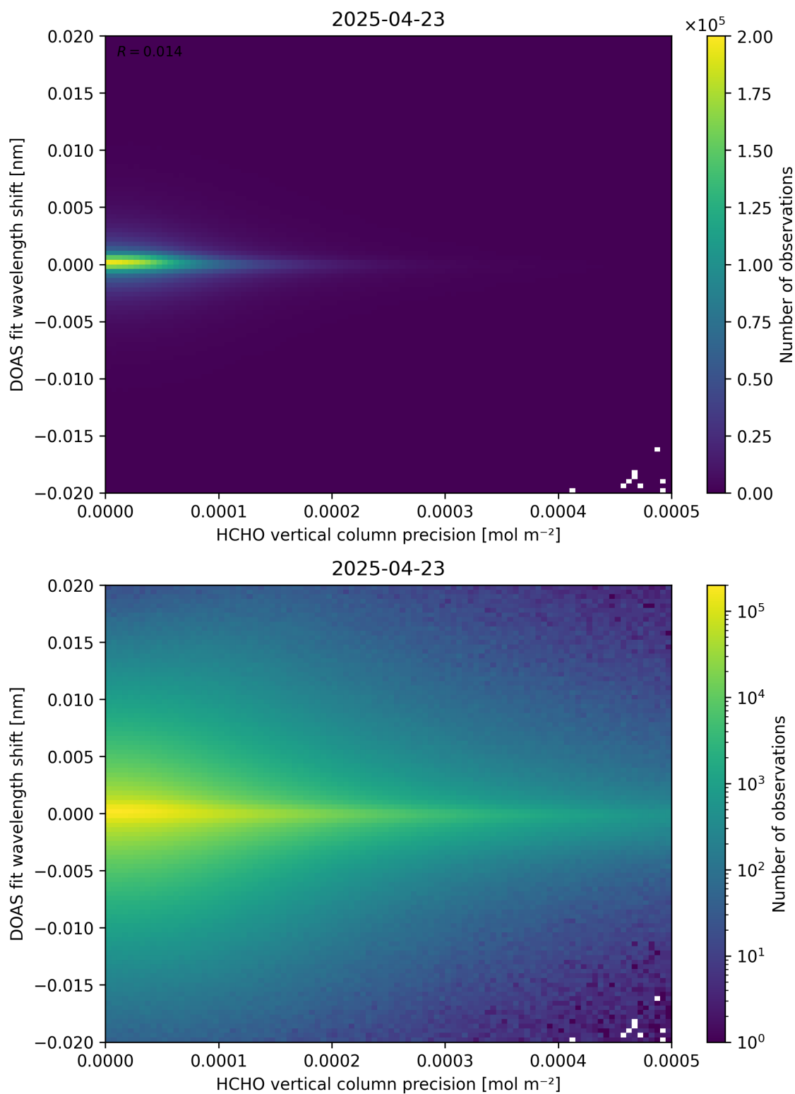
Figure 137: Scatter density plot of “HCHO vertical column precision” against “DOAS fit wavelength shift” for 2025-04-22 to 2025-04-24.
