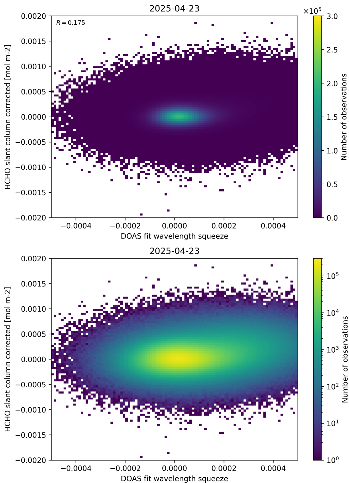
Figure 69: Scatter density plot of “DOAS fit wavelength squeeze” against “HCHO slant column corrected” for 2025-04-22 to 2025-04-24.
