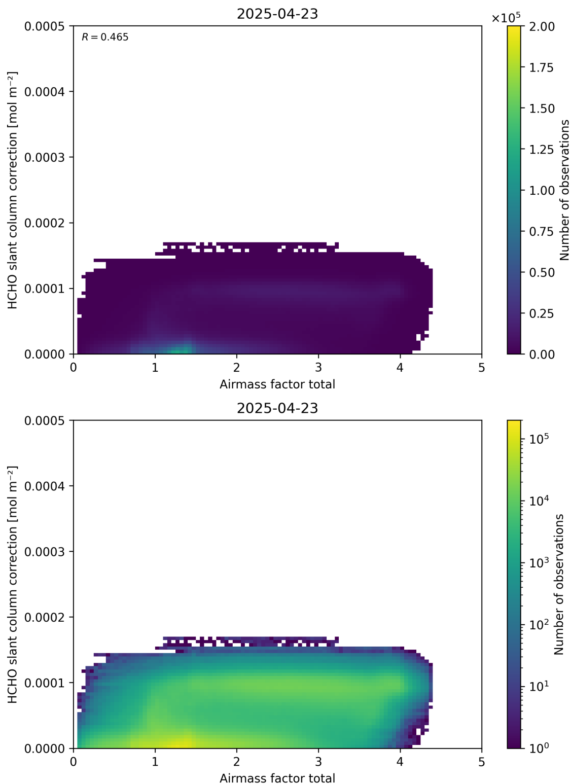
Figure 102: Scatter density plot of “Airmass factor total” against “HCHO slant column correction” for 2025-04-22 to 2025-04-24.
