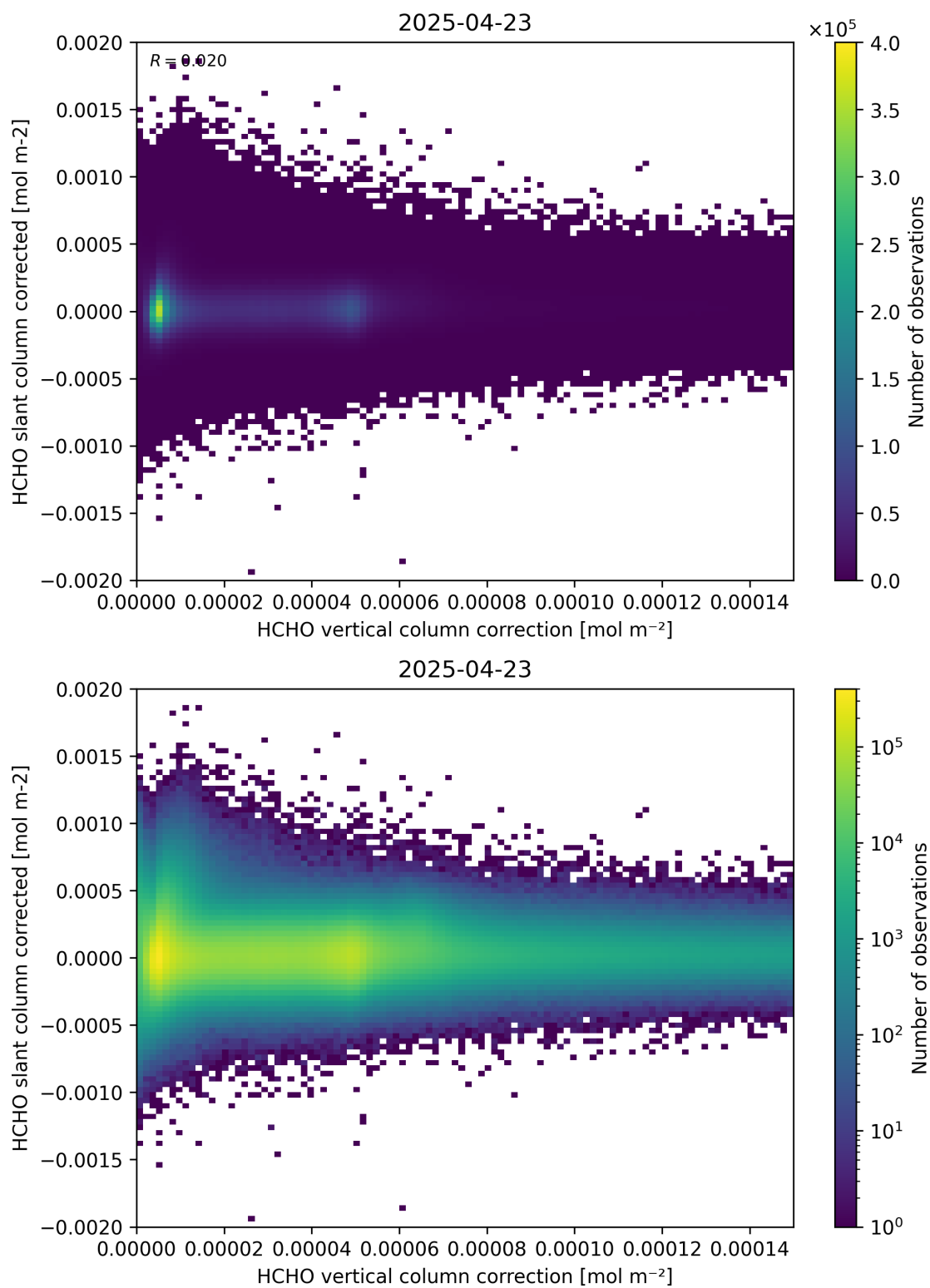
Figure 116: Scatter density plot of “HCHO vertical column correction” against “HCHO slant column corrected” for 2025-04-22 to 2025-04-24.
