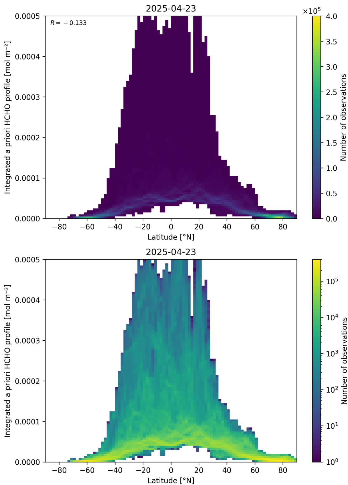
Figure 166: Scatter density plot of “Latitude” against “Integrated a priori HCHO profile” for 2025-04-22 to 2025-04-24.
