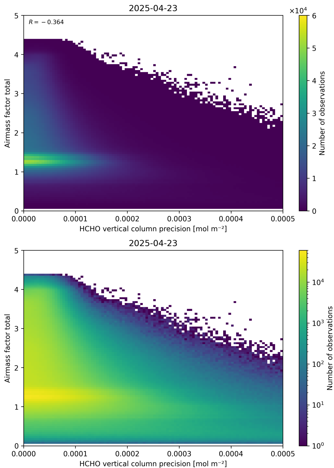
Figure 144: Scatter density plot of “HCHO vertical column precision” against “Airmass factor total” for 2025-04-22 to 2025-04-24.
