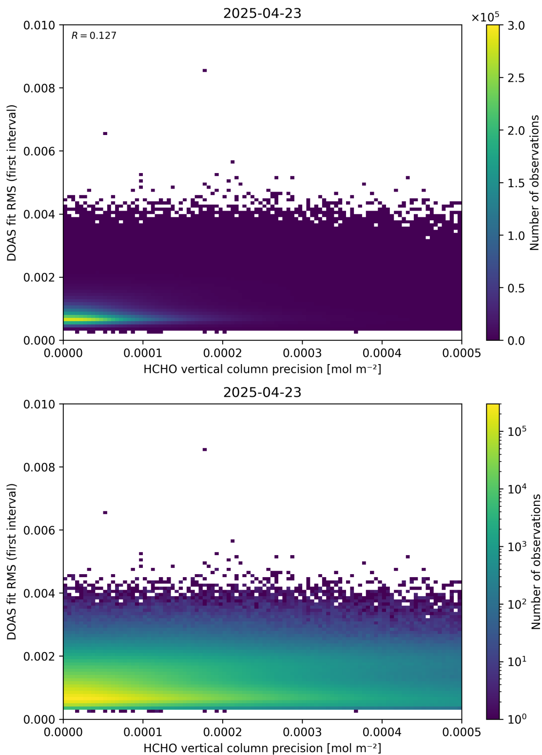
Figure 136: Scatter density plot of “HCHO vertical column precision” against “DOAS fit RMS (first interval)” for 2025-04-22 to 2025-04-24.
