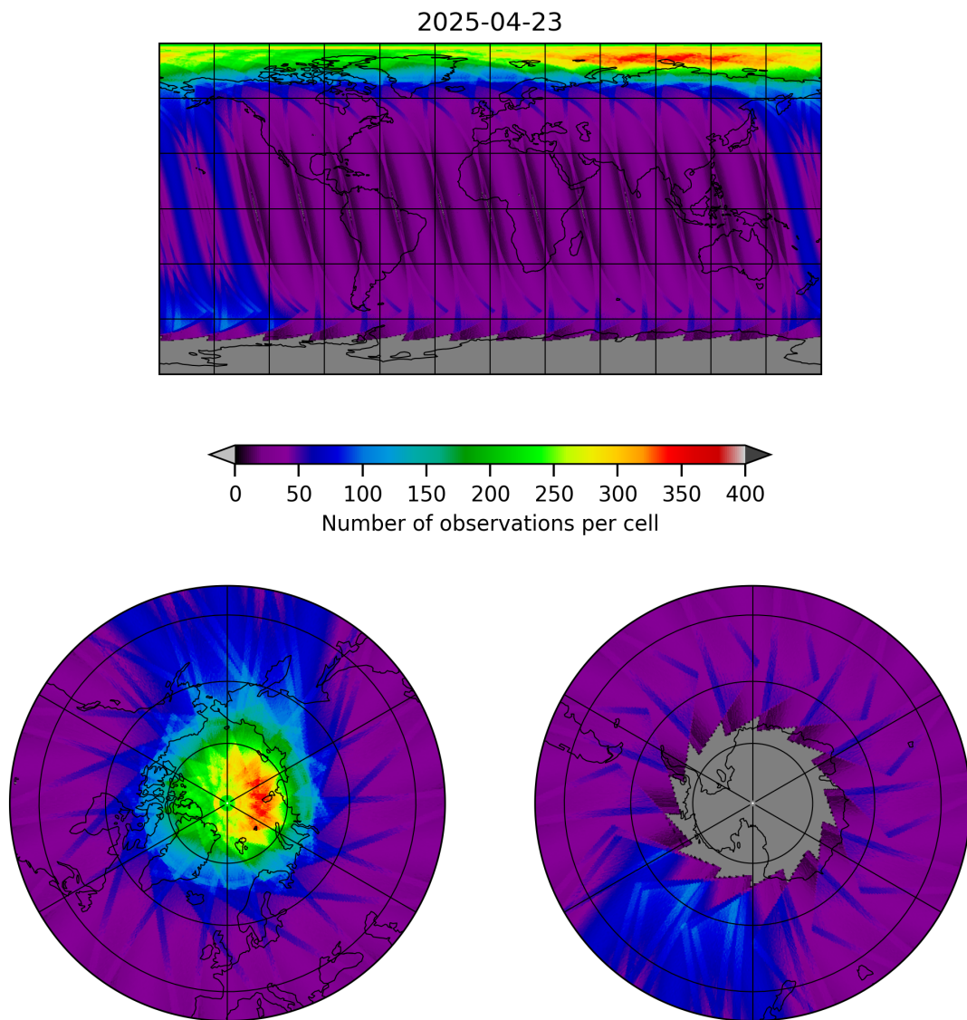
Figure 19: Map of the number of observations for 2025-04-22 to 2025-04-24
