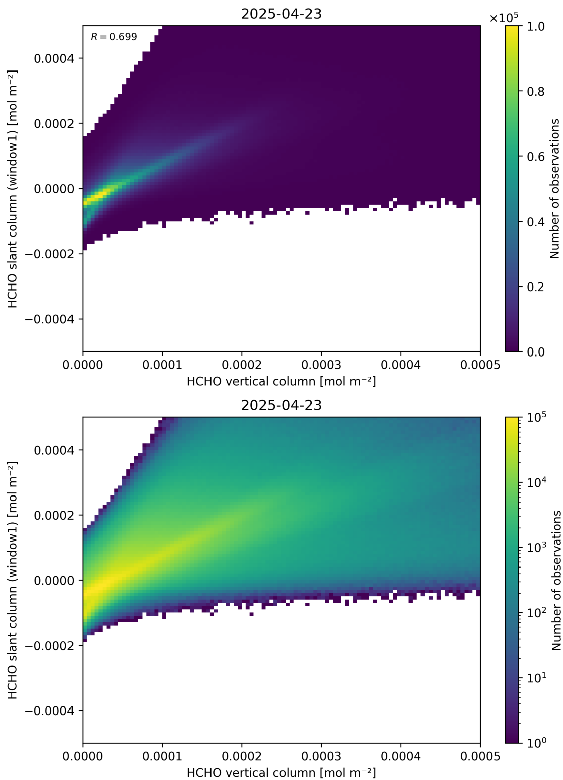
Figure 129: Scatter density plot of “HCHO vertical column” against “HCHO slant column (window1)” for 2025-04-22 to 2025-04-24.
