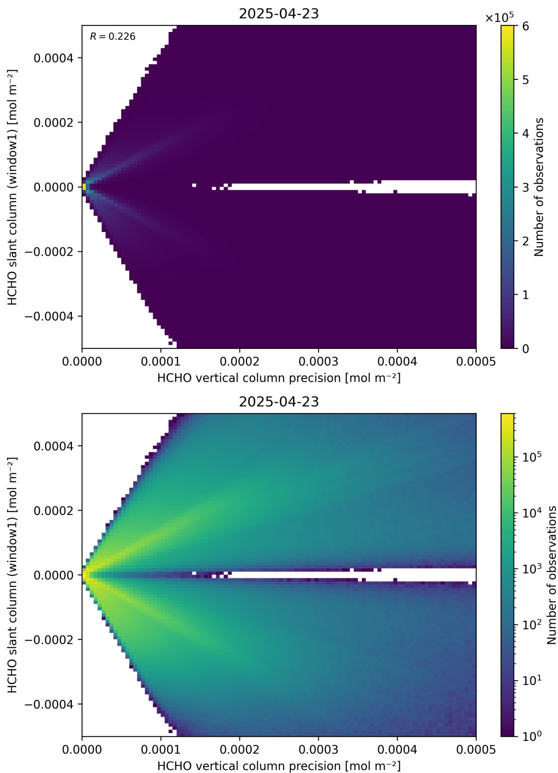
Figure 142: Scatter density plot of “HCHO vertical column precision” against “HCHO slant column (window1)” for 2025-04-22 to 2025-04-24.
