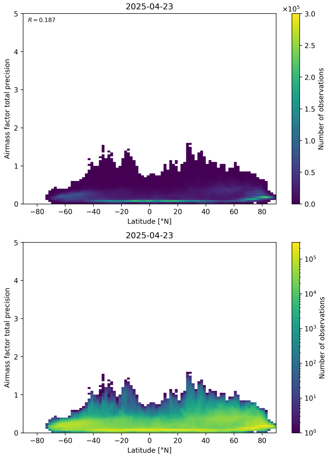
Figure 162: Scatter density plot of “Latitude” against “Airmass factor total precision” for 2025-04-22 to 2025-04-24.
