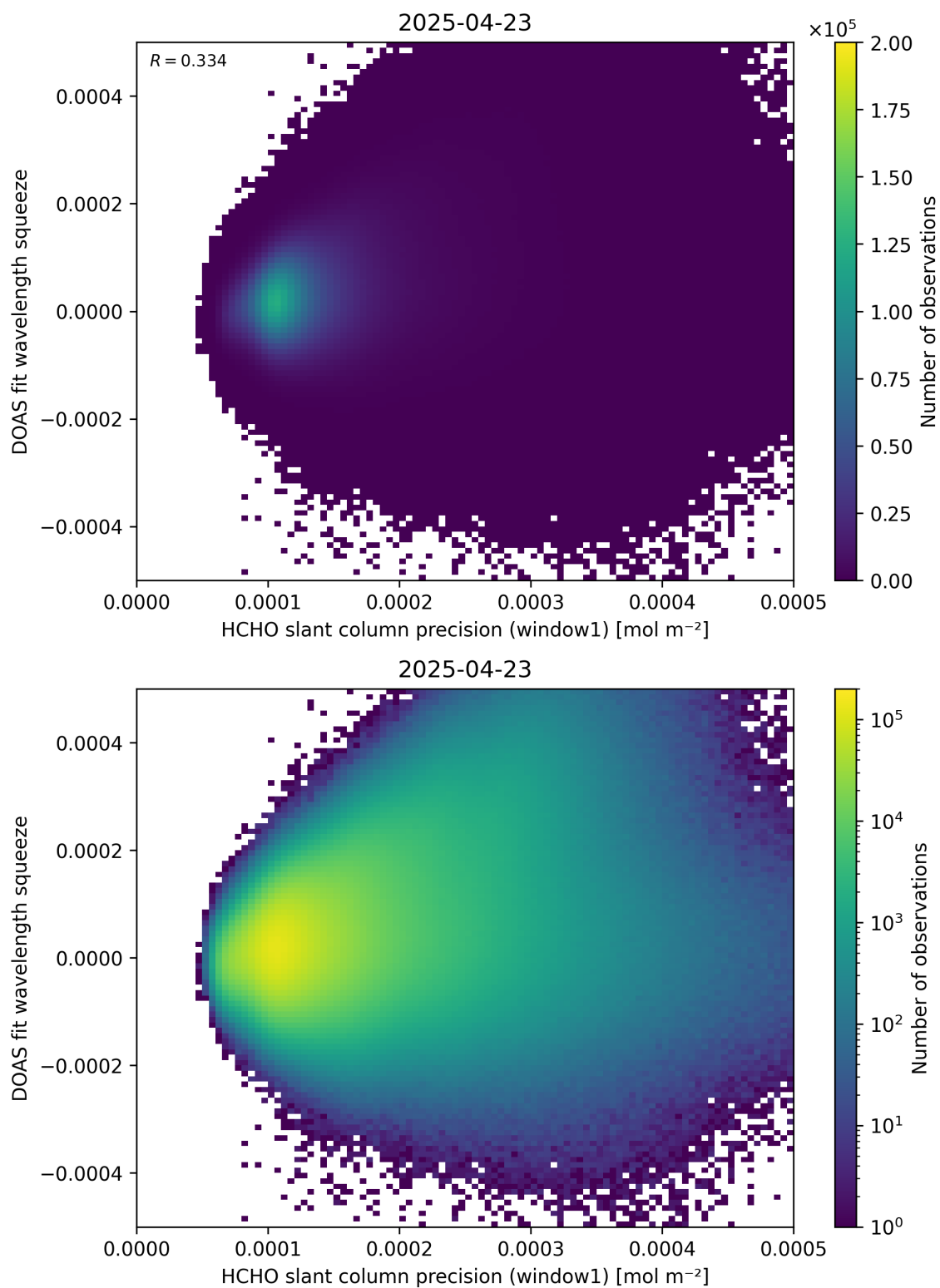
Figure 90: Scatter density plot of “HCHO slant column precision (window1)” against “DOAS fit wavelength squeeze” for 2025-04-22 to 2025-04-24.
