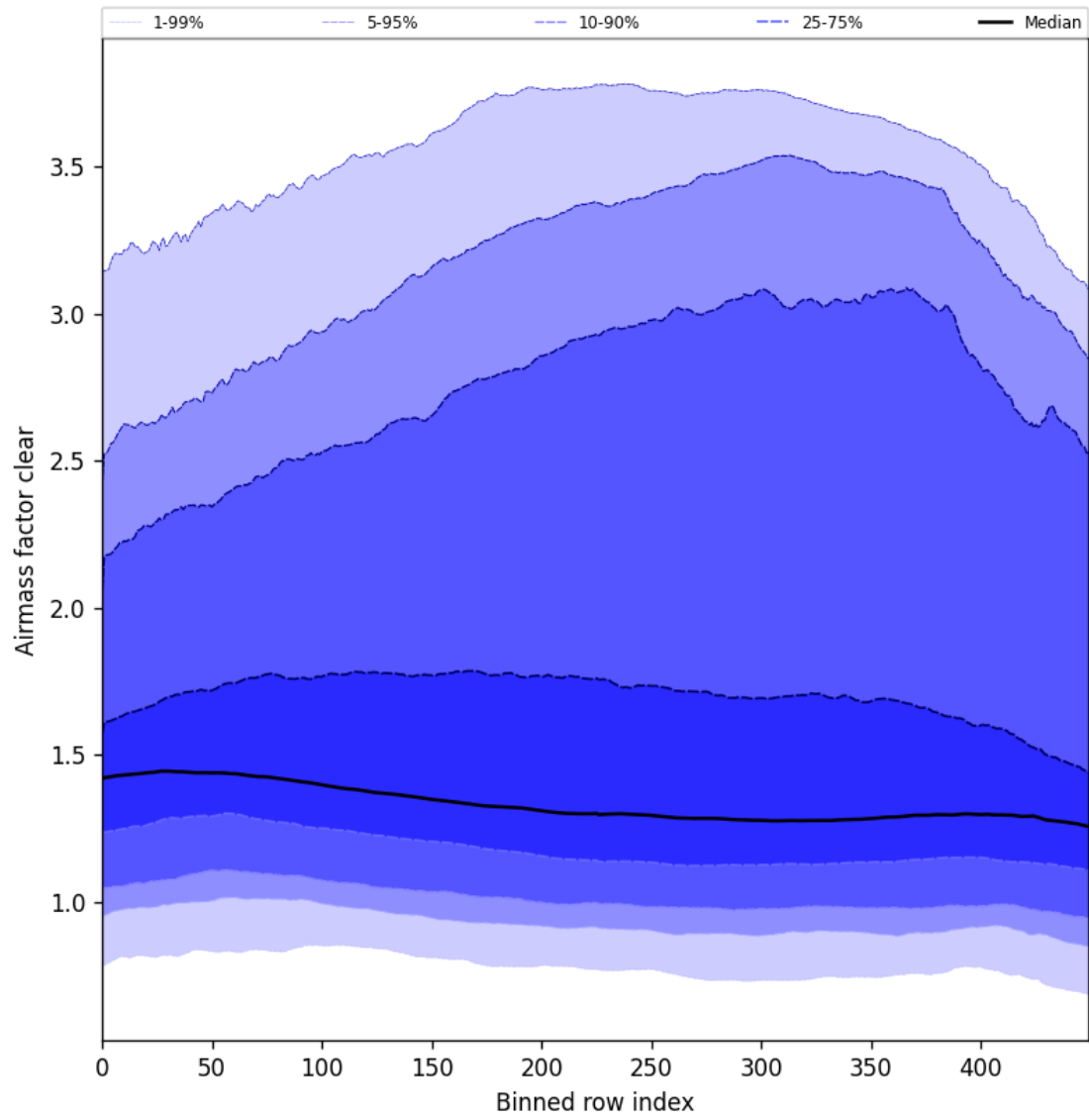
Figure 56: Along track statistics of “Airmass factor clear” for 2025-04-22 to 2025-04-24
