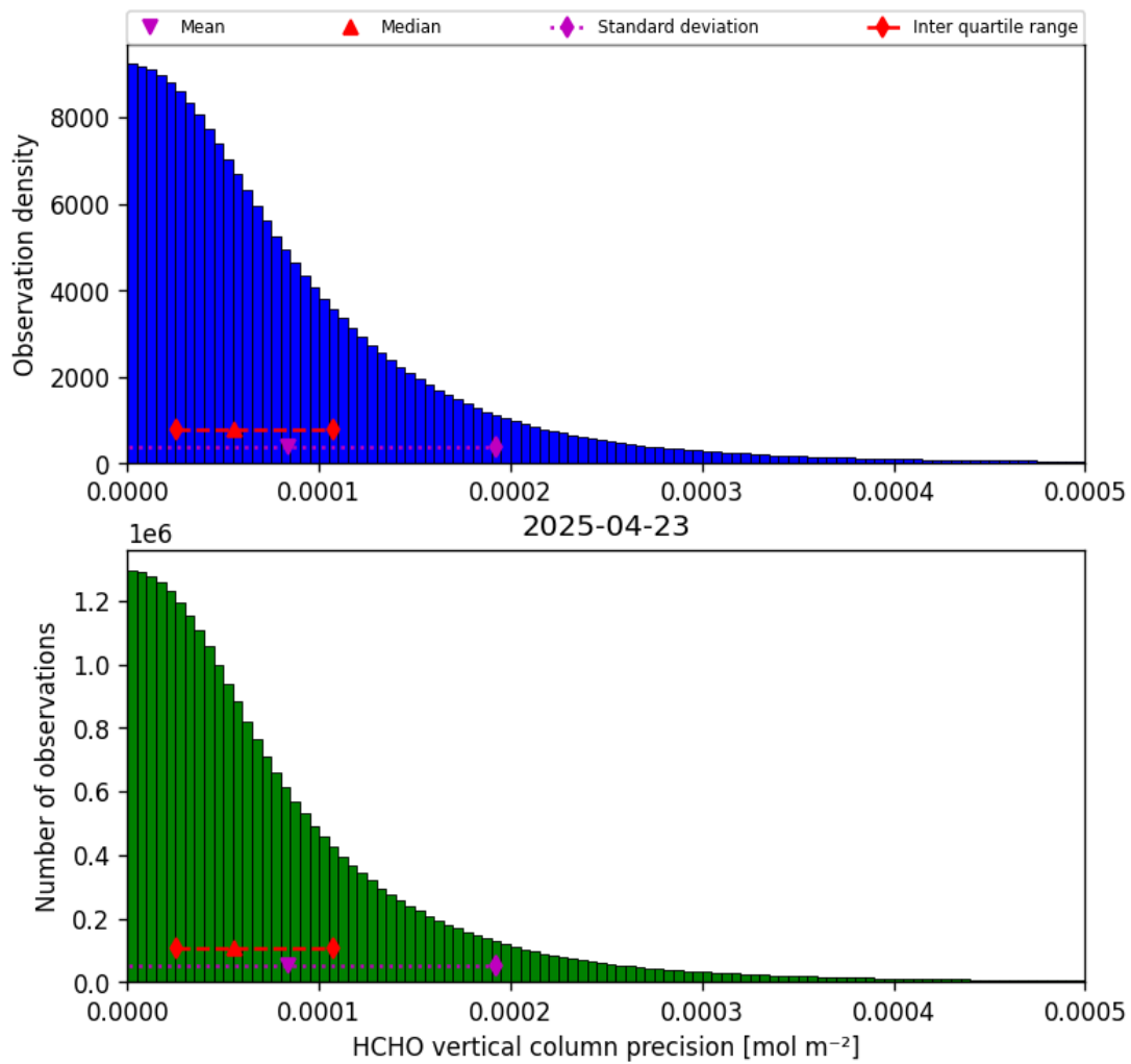
Figure 36: Histogram of “HCHO vertical column precision” for 2025-04-22 to 2025-04-24
