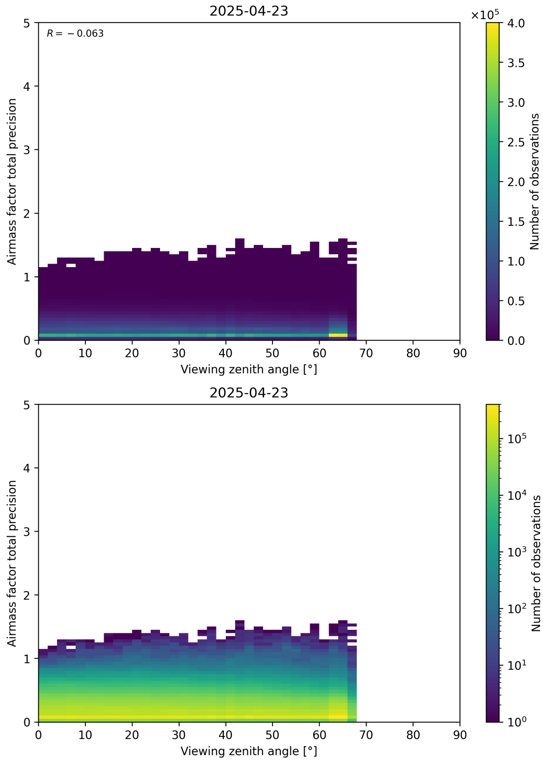
Figure 191: Scatter density plot of “Viewing zenith angle” against “Airmass factor total precision” for 2025-04-22 to 2025-04-24.
