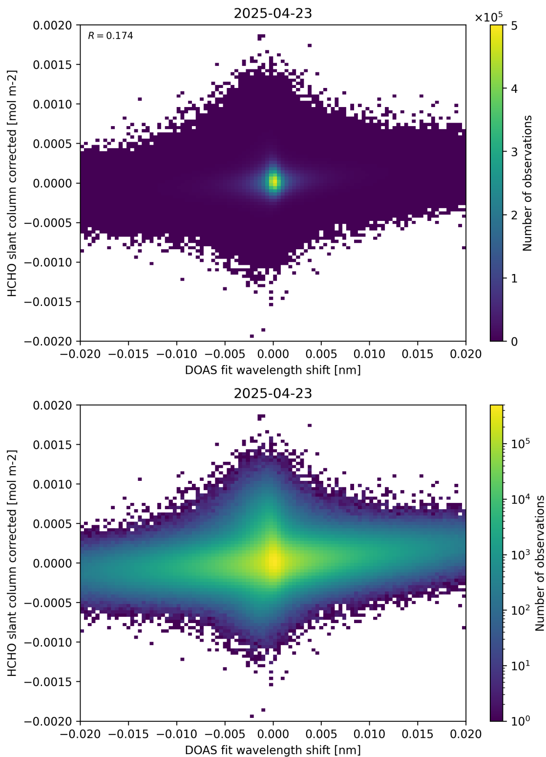
Figure 66: Scatter density plot of “DOAS fit wavelength shift” against “HCHO slant column corrected” for 2025-04-22 to 2025-04-24.
