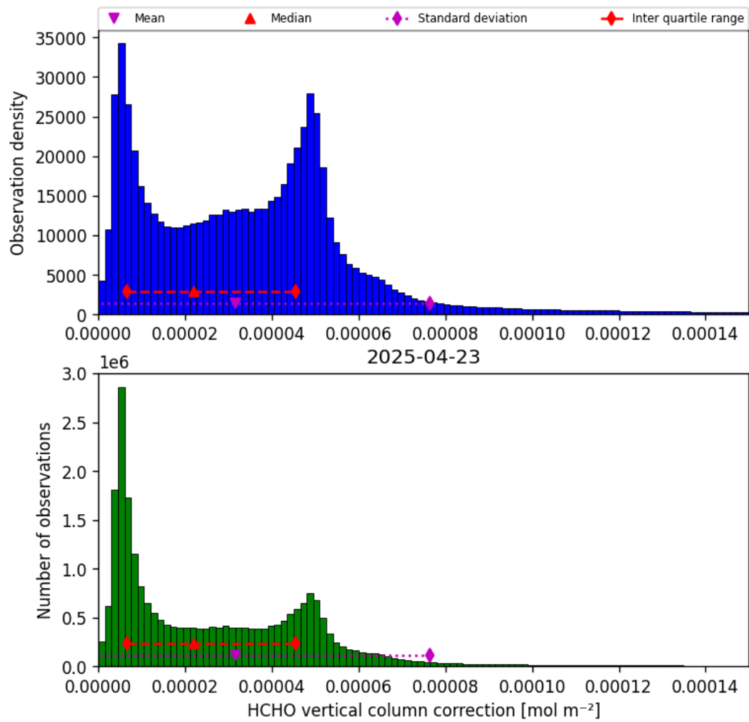
Figure 37: Histogram of “HCHO vertical column correction” for 2025-04-22 to 2025-04-24
