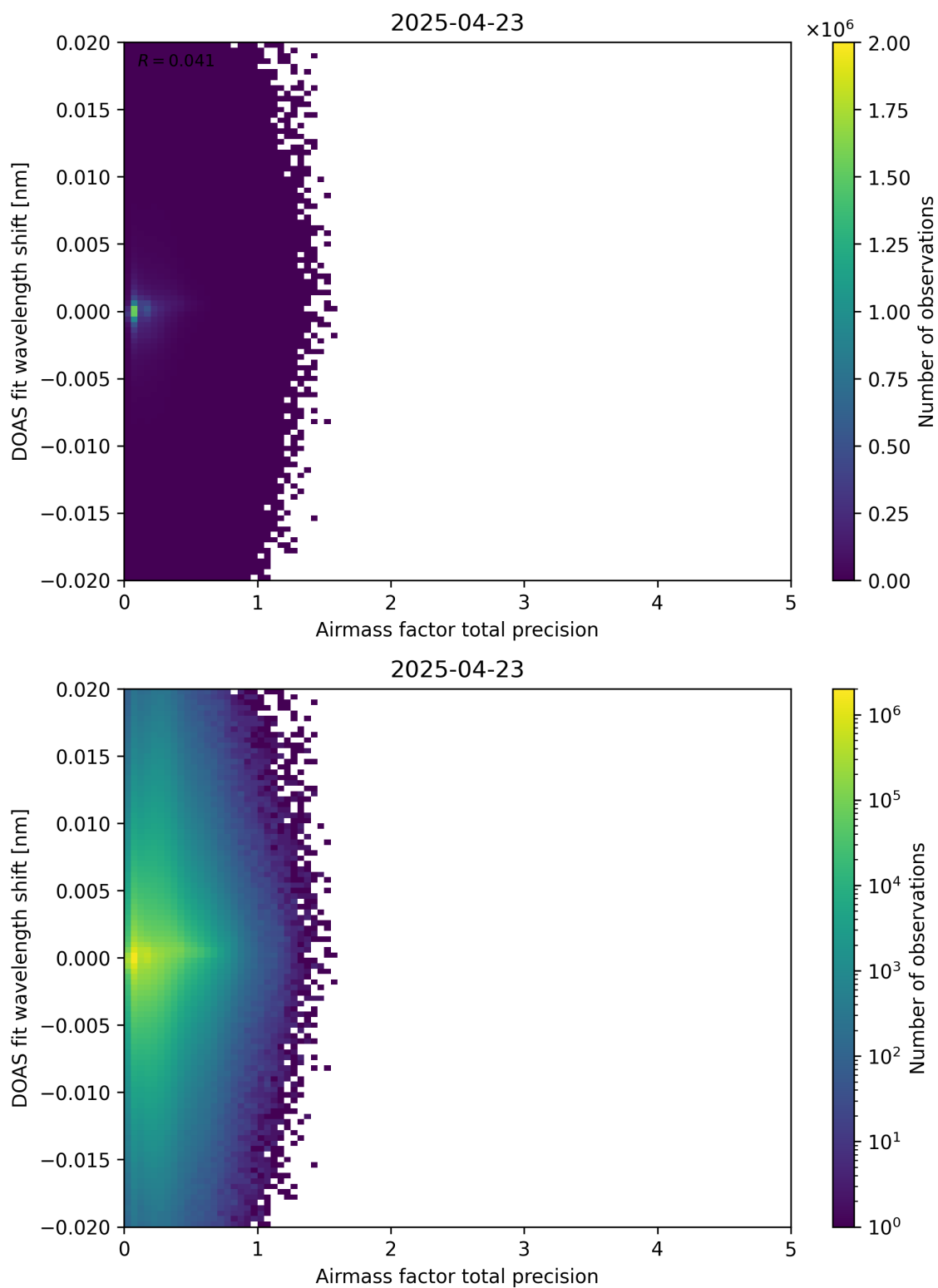
Figure 106: Scatter density plot of “Airmass factor total precision” against “DOAS fit wavelength shift” for 2025-04-22 to 2025-04-24.
