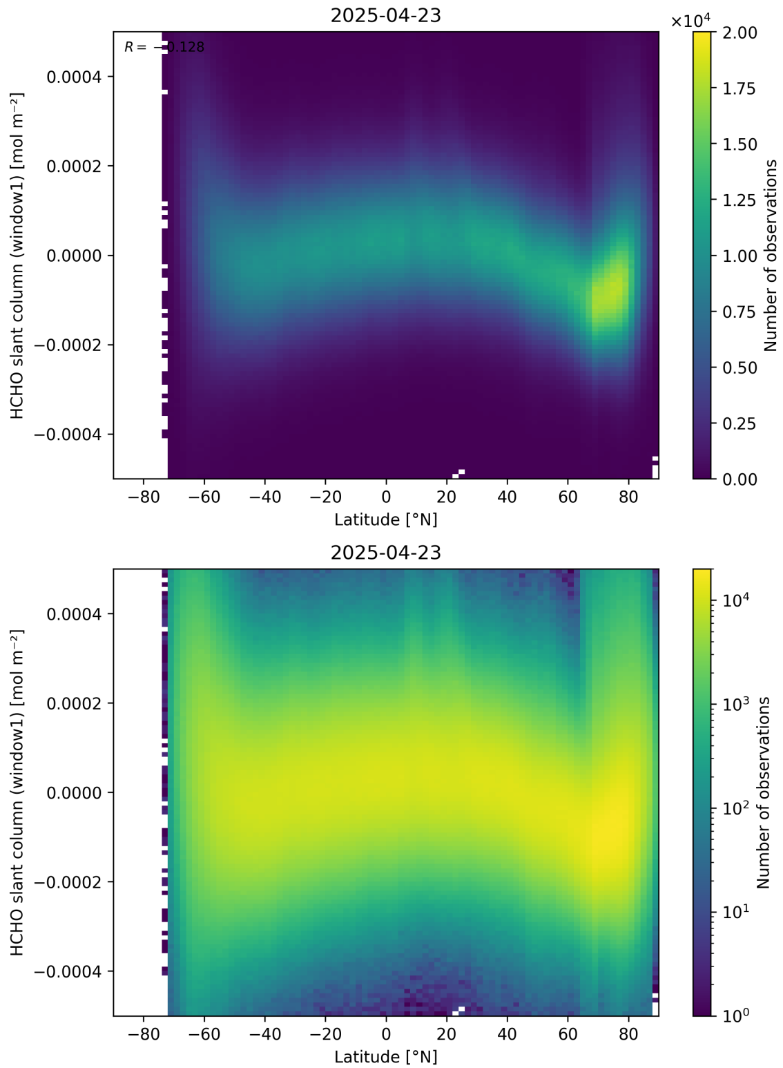
Figure 159: Scatter density plot of “Latitude” against “HCHO slant column (window1)” for 2025-04-22 to 2025-04-24.
