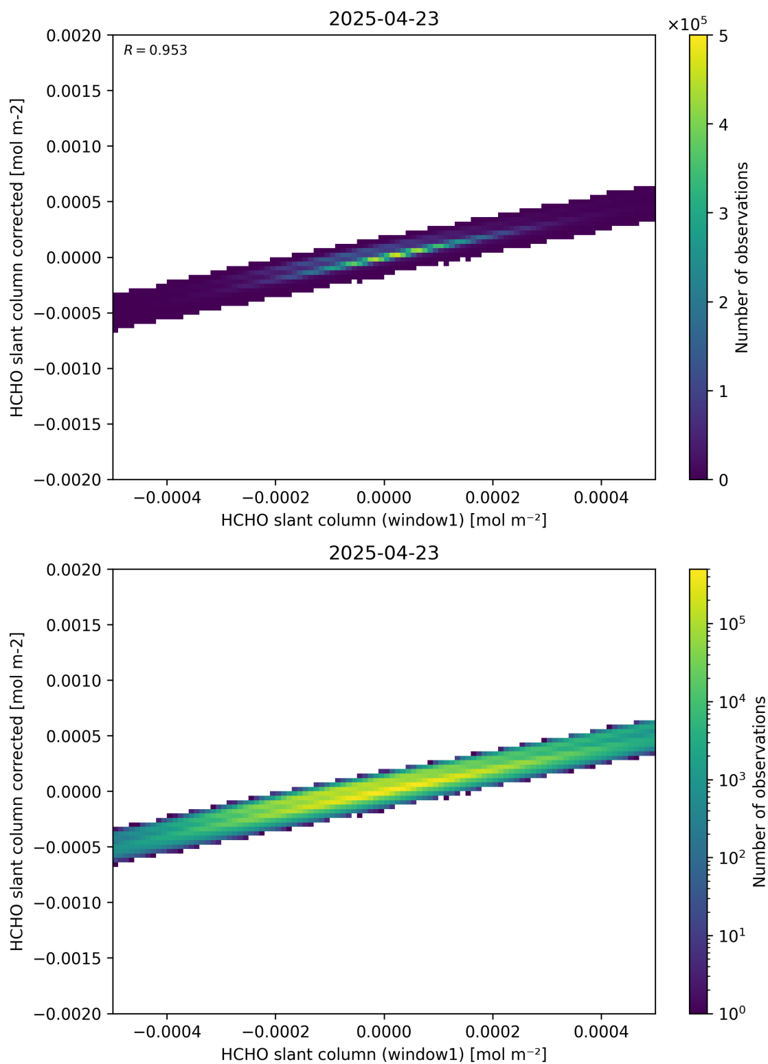
Figure 82: Scatter density plot of “HCHO slant column (window1)” against “HCHO slant column corrected” for 2025-04-22 to 2025-04-24.
