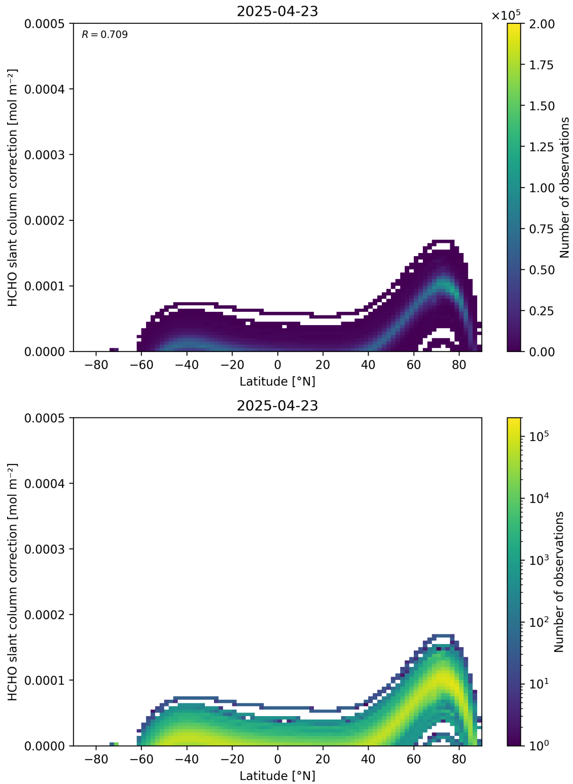
Figure 158: Scatter density plot of “Latitude” against “HCHO slant column correction” for 2025-04-22 to 2025-04-24.
