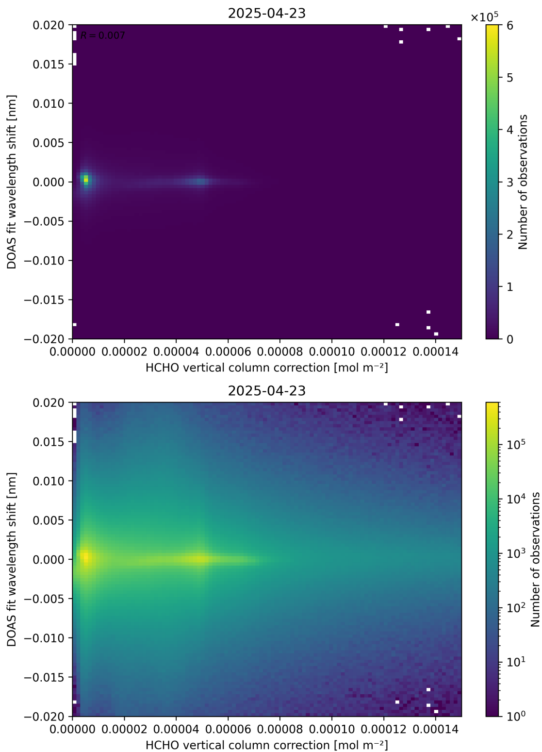
Figure 113: Scatter density plot of “HCHO vertical column correction” against “DOAS fit wavelength shift” for 2025-04-22 to 2025-04-24.
