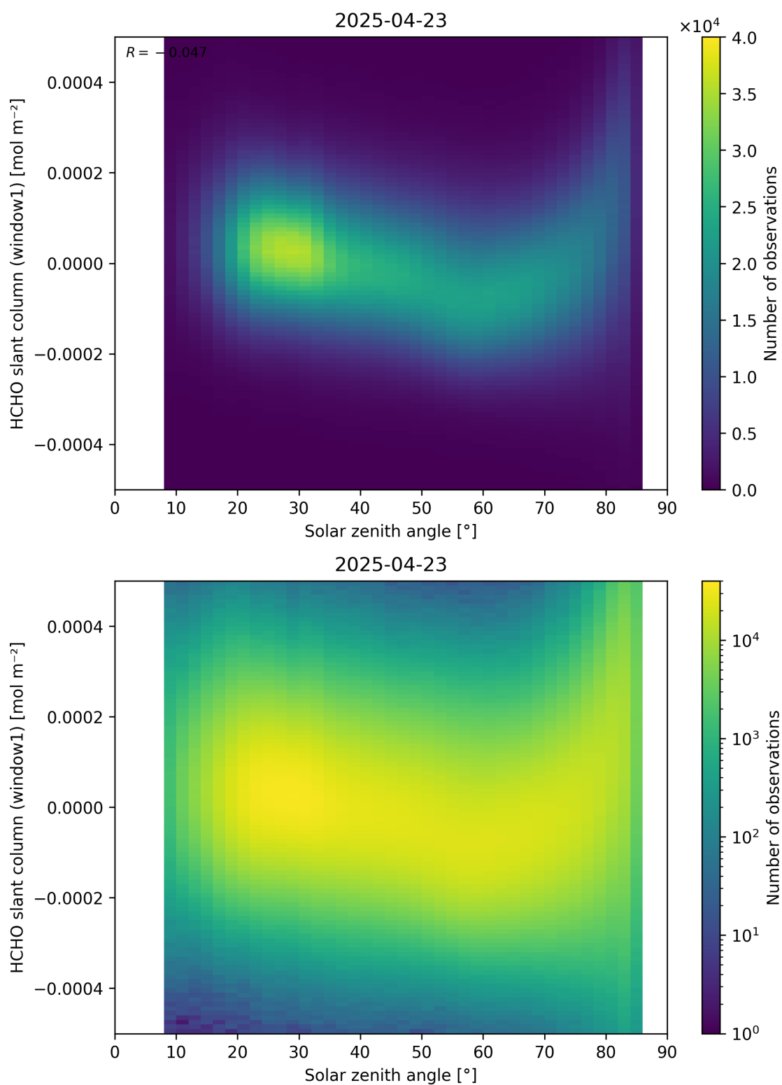
Figure 173: Scatter density plot of “Solar zenith angle” against “HCHO slant column (window1)” for 2025-04-22 to 2025-04-24.
