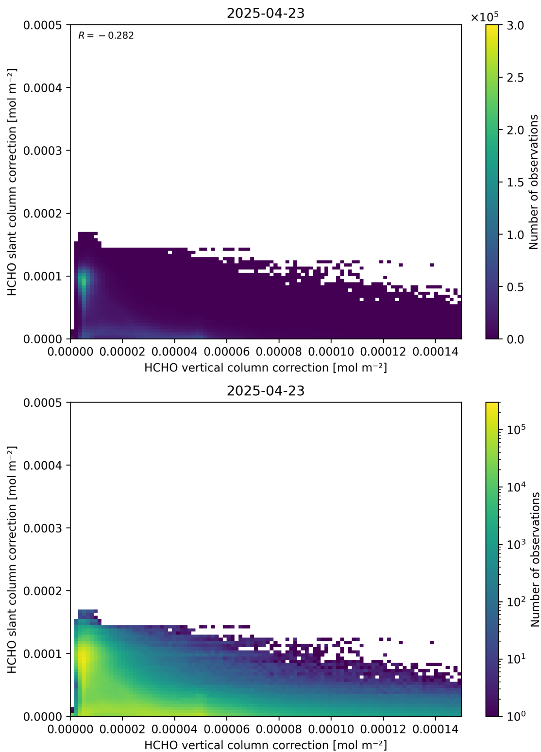
Figure 117: Scatter density plot of “HCHO vertical column correction” against “HCHO slant column correction” for 2025-04-22 to 2025-04-24.
