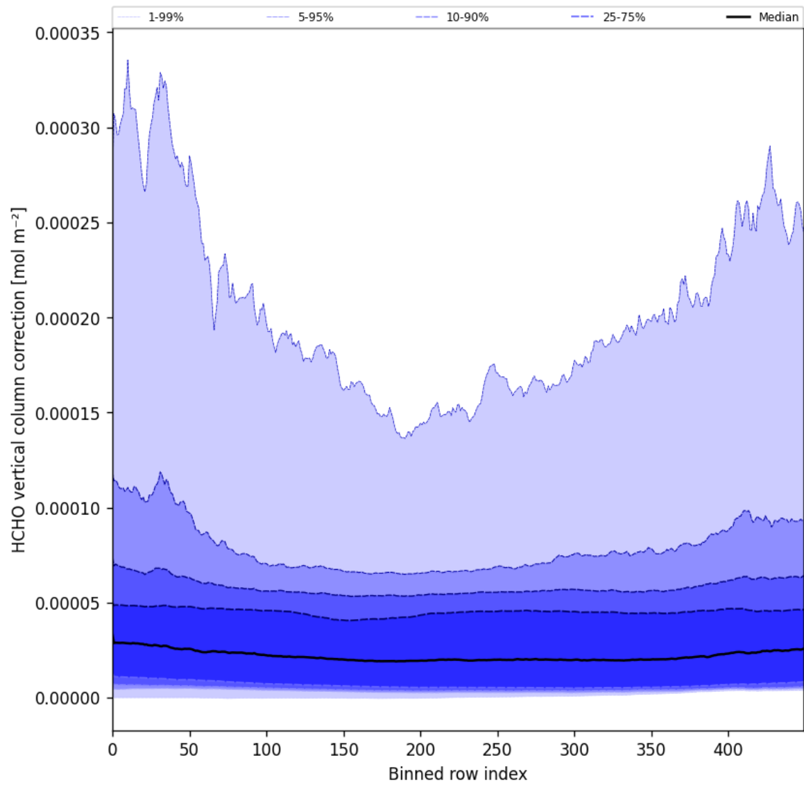
Figure 51: Along track statistics of “HCHO vertical column correction” for 2025-04-22 to 2025-04-24
