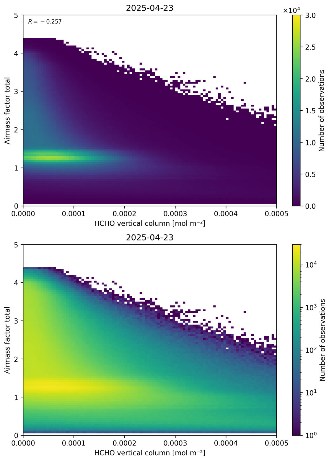
Figure 131: Scatter density plot of “HCHO vertical column” against “Airmass factor total” for 2025-04-22 to 2025-04-24.
