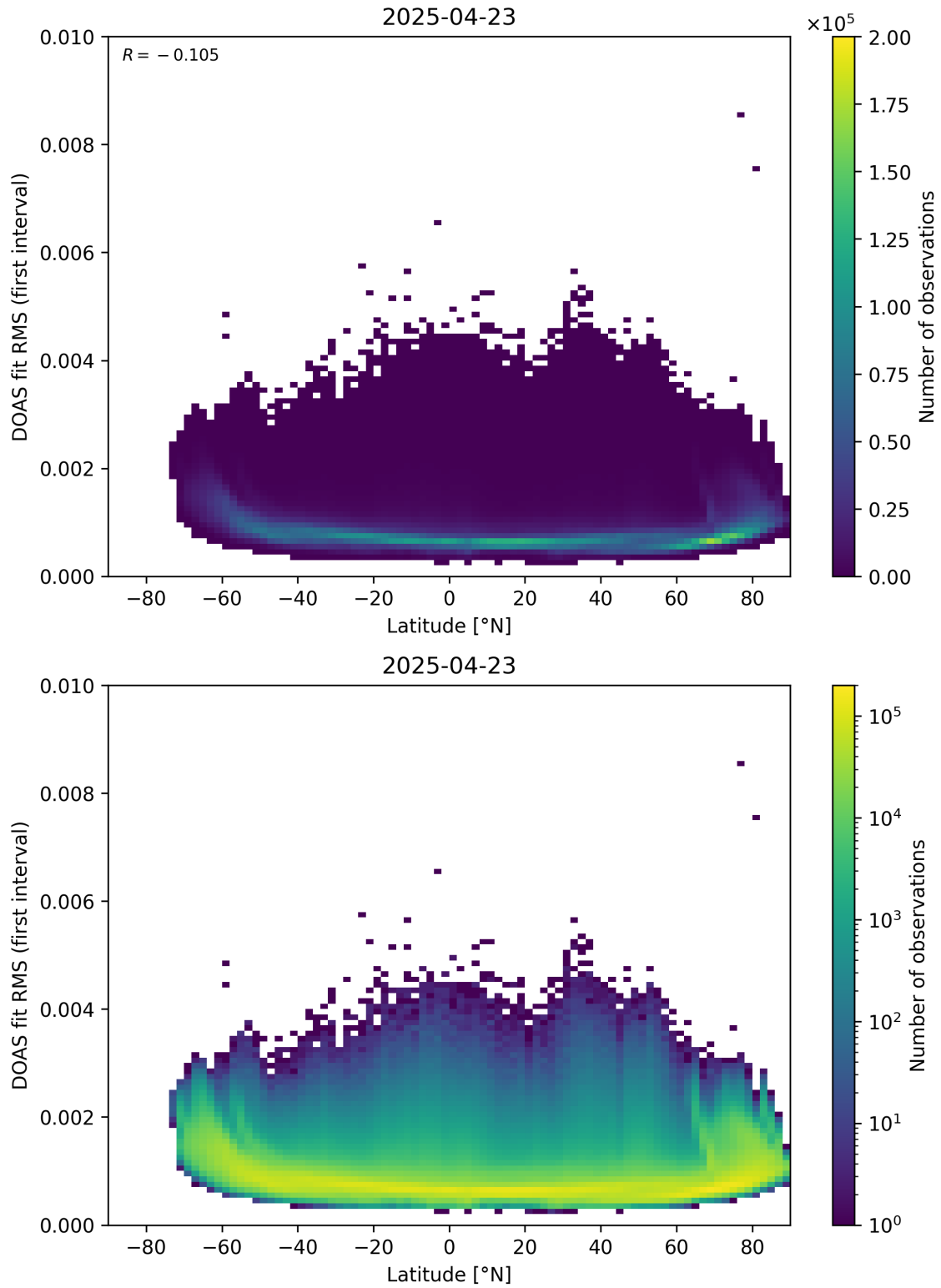
Figure 153: Scatter density plot of “Latitude” against “DOAS fit RMS (first interval)” for 2025-04-22 to 2025-04-24.
