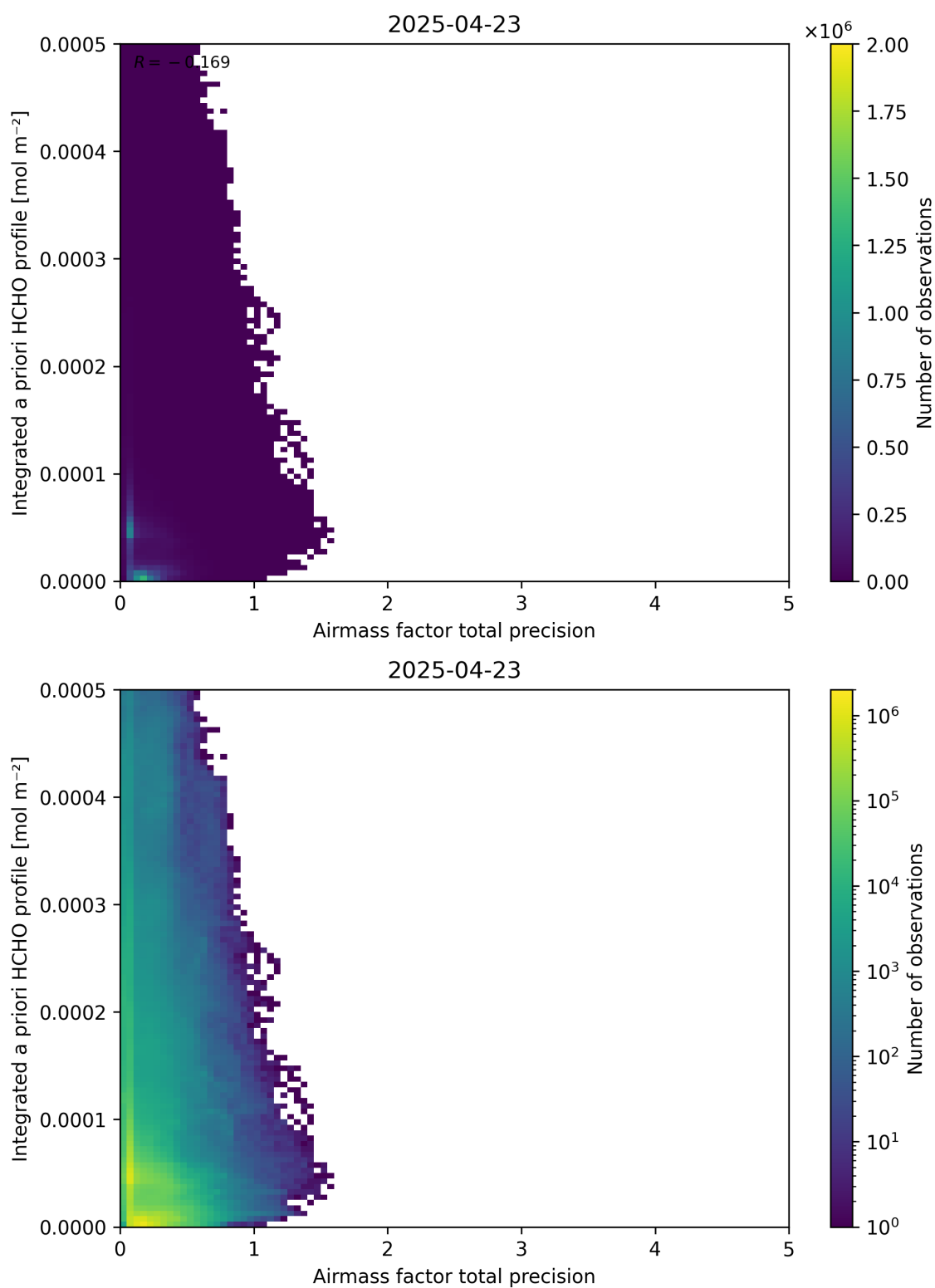
Figure 111: Scatter density plot of “Airmass factor total precision” against “Integrated a priori HCHO profile” for 2025-04-22 to 2025-04-24.
