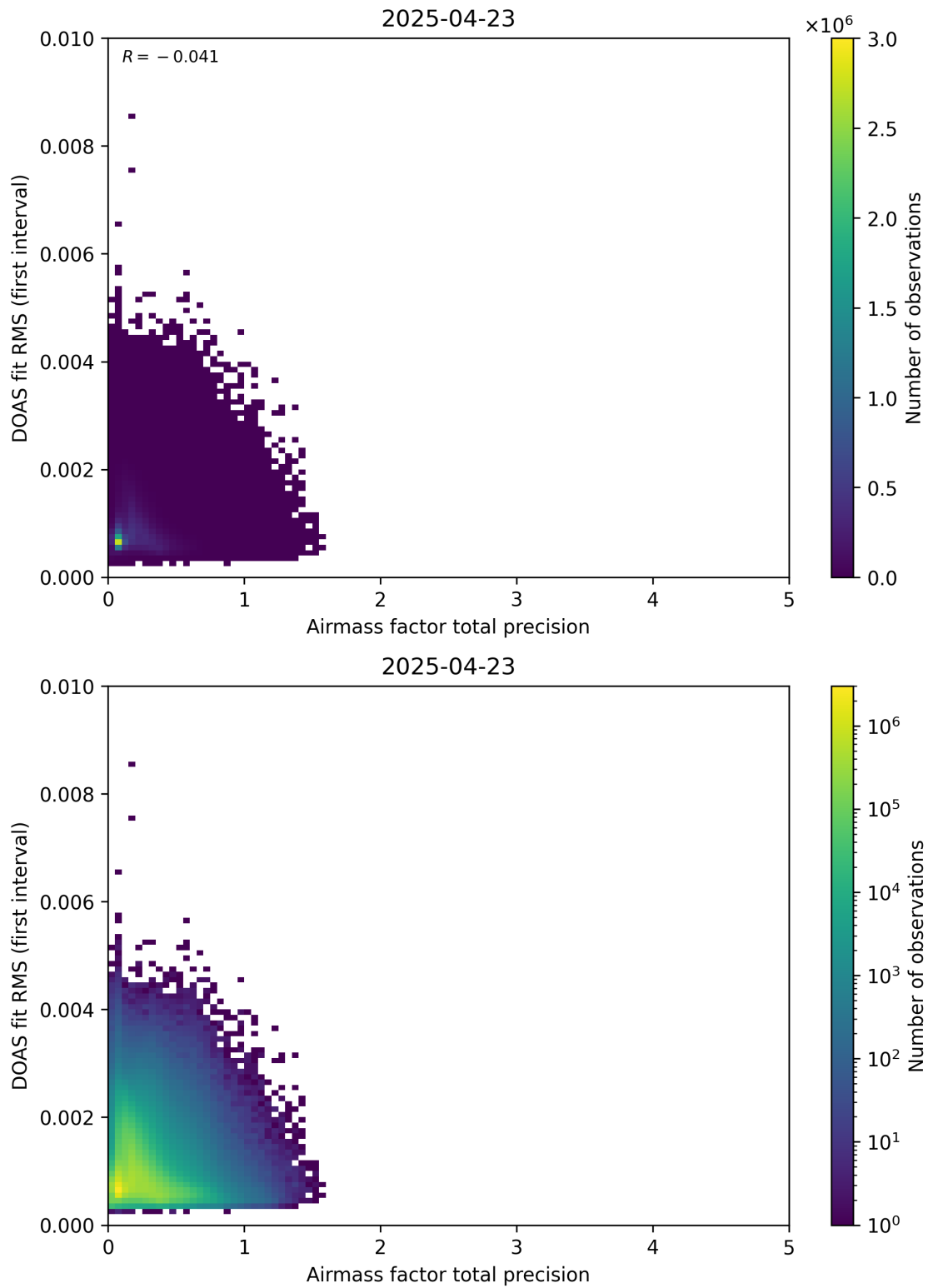
Figure 105: Scatter density plot of “Airmass factor total precision” against “DOAS fit RMS (first interval)” for 2025-04-22 to 2025-04-24.
