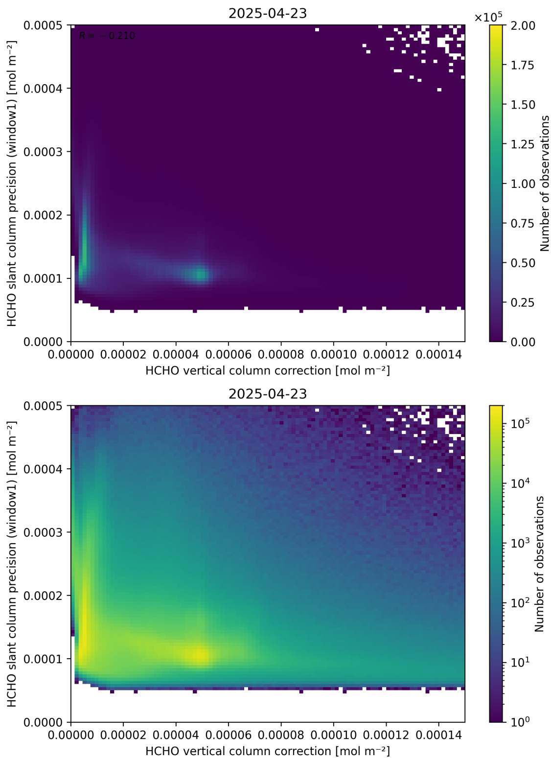
Figure 119: Scatter density plot of “HCHO vertical column correction” against “HCHO slant column precision (window1)” for 2025-04-22 to 2025-04-24.
