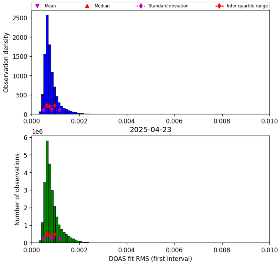
Figure 46: Histogram of “DOAS fit RMS (first interval)” for 2025-04-22 to 2025-04-24
