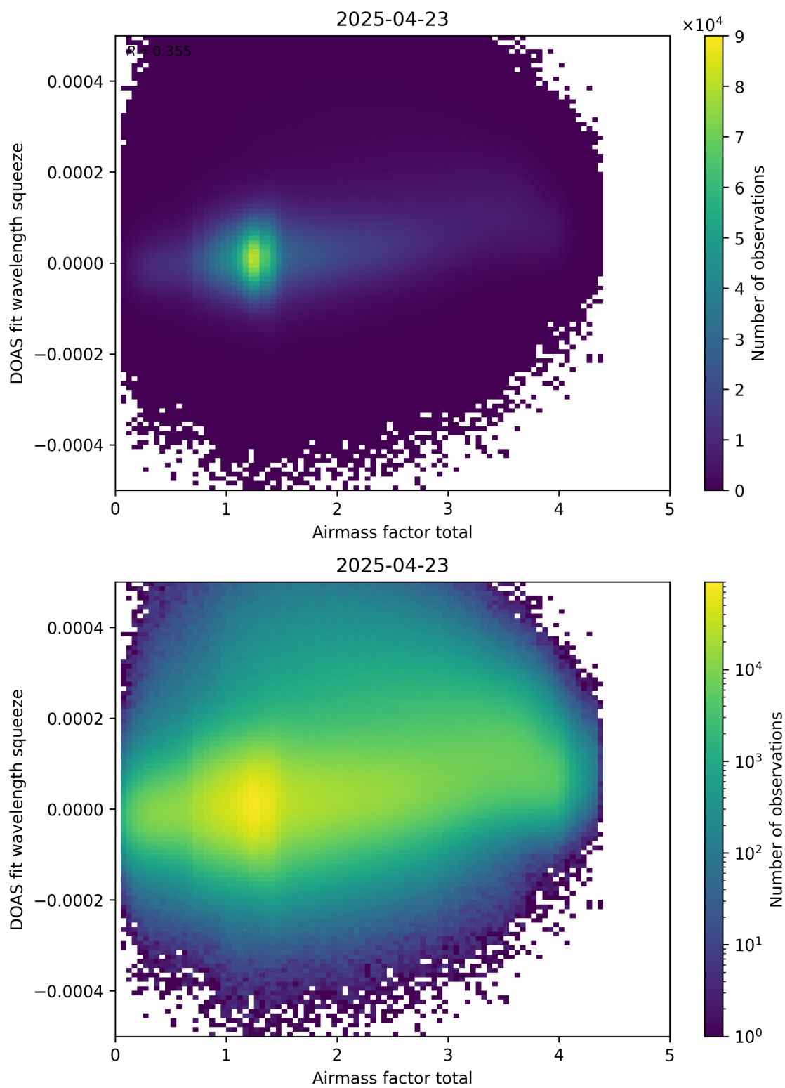
Figure 99: Scatter density plot of “Airmass factor total” against “DOAS fit wavelength squeeze” for 2025-04-22 to 2025-04-24.
