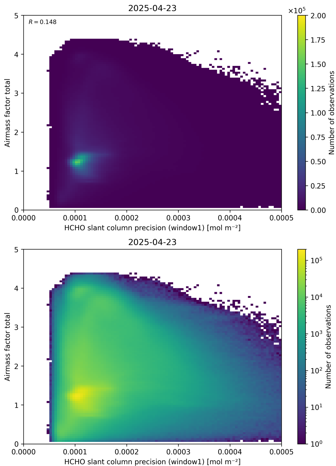
Figure 94: Scatter density plot of “HCHO slant column precision (window1)” against “Airmass factor total” for 2025-04-22 to 2025-04-24.
