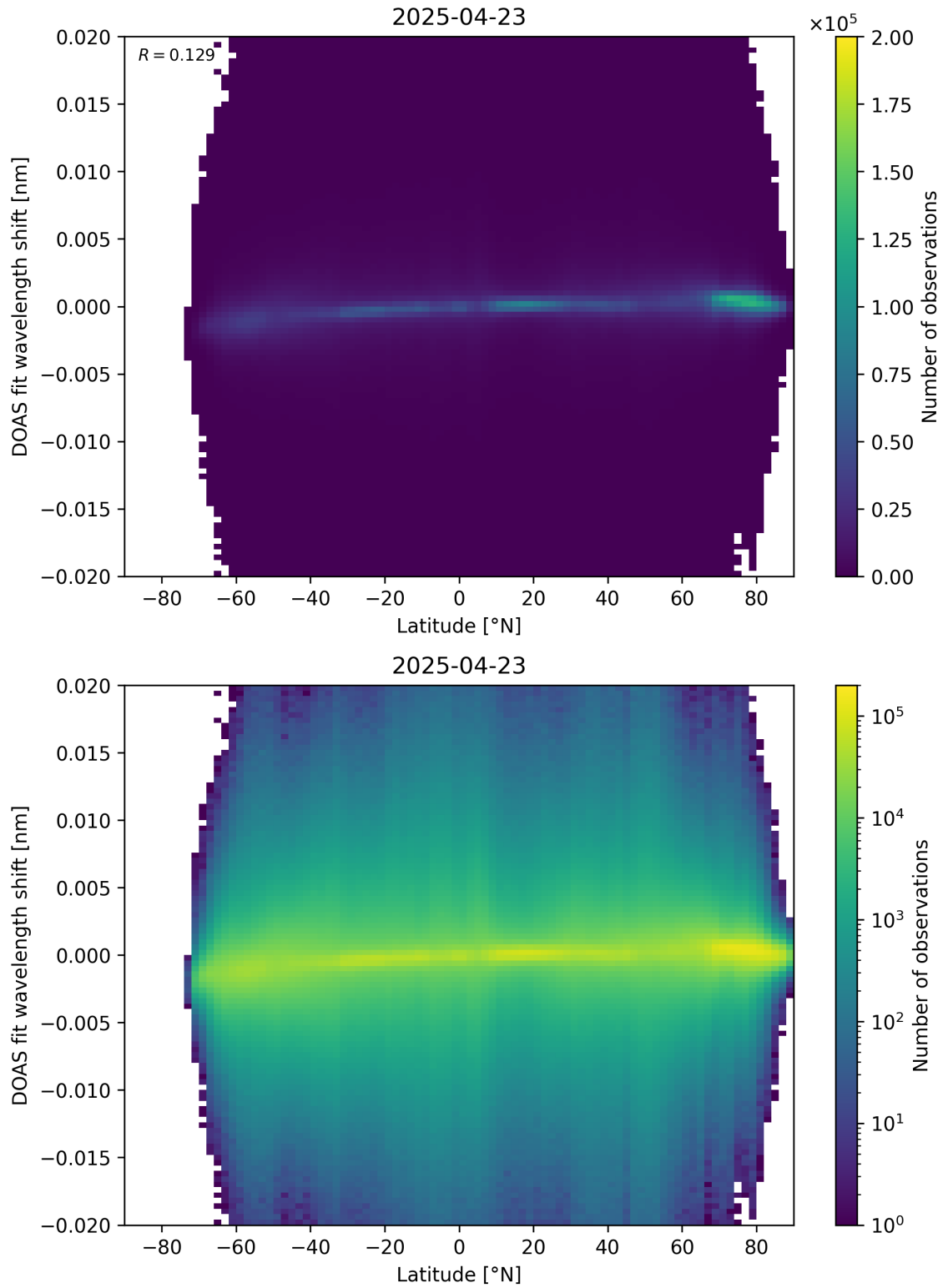
Figure 154: Scatter density plot of “Latitude” against “DOAS fit wavelength shift” for 2025-04-22 to 2025-04-24.
