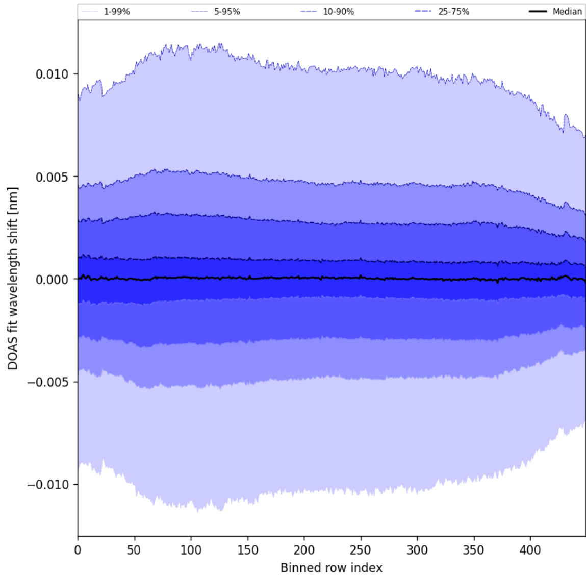
Figure 58: Along track statistics of “DOAS fit wavelength shift” for 2025-04-22 to 2025-04-24
