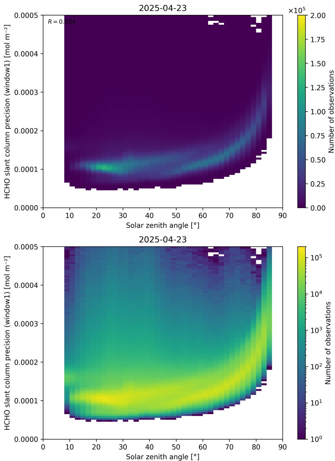
Figure 174: Scatter density plot of “Solar zenith angle” against “HCHO slant column precision (window1)” for 2025-04-22 to 2025-04-24.
