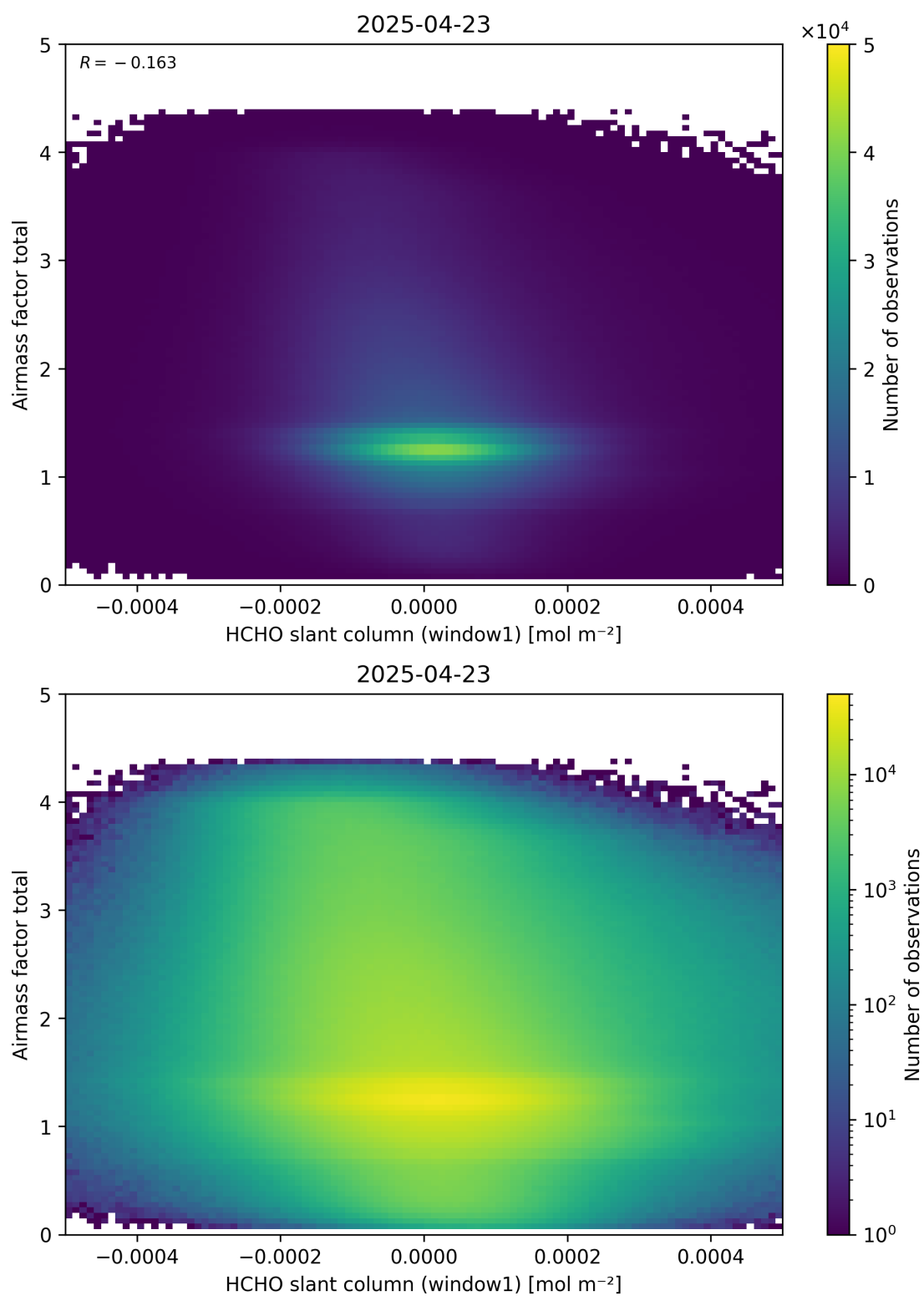
Figure 85: Scatter density plot of “HCHO slant column (window1)” against “Airmass factor total” for 2025-04-22 to 2025-04-24.
