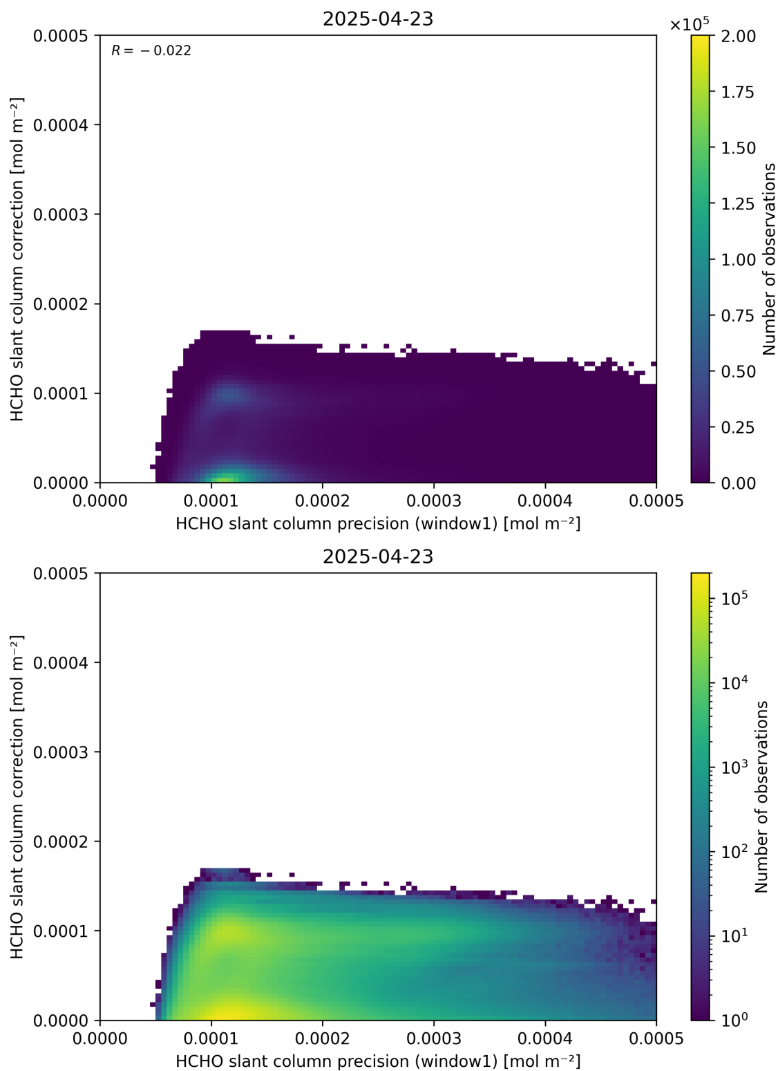
Figure 93: Scatter density plot of “HCHO slant column precision (window1)” against “HCHO slant column correction” for 2025-04-22 to 2025-04-24.
