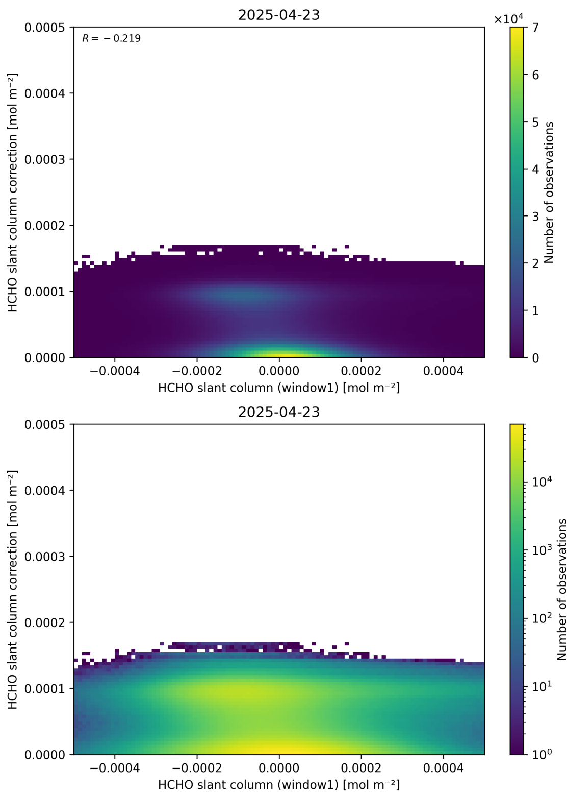
Figure 83: Scatter density plot of “HCHO slant column (window1)” against “HCHO slant column correction” for 2025-04-22 to 2025-04-24.
