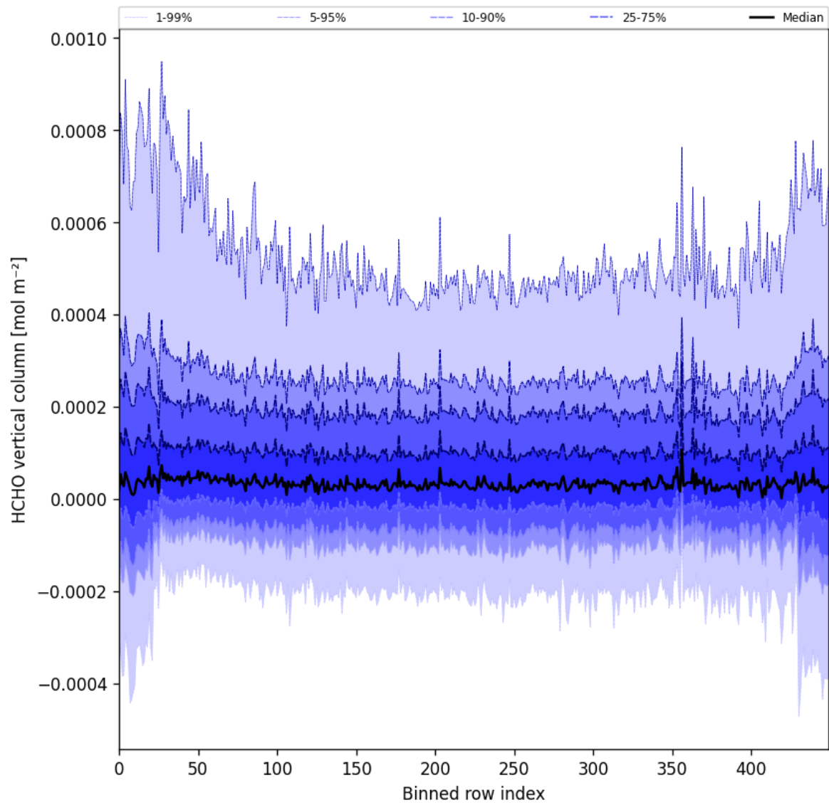
Figure 49: Along track statistics of “HCHO vertical column” for 2025-04-22 to 2025-04-24
