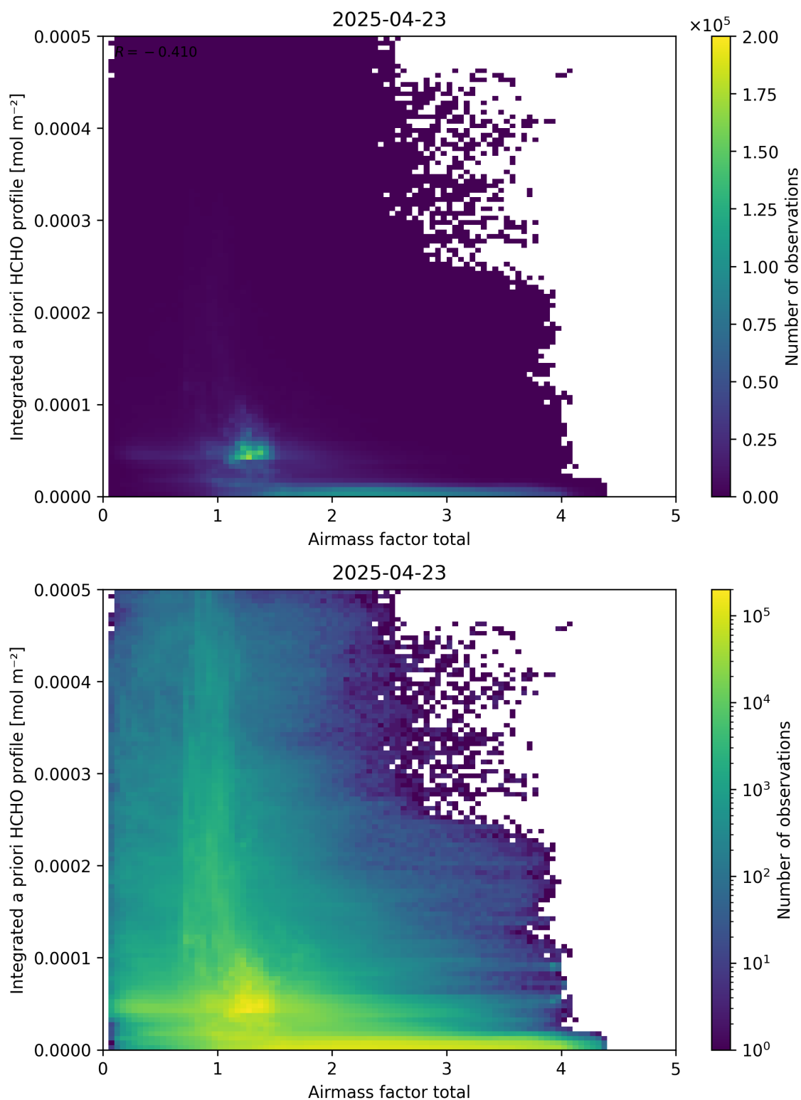
Figure 104: Scatter density plot of “Airmass factor total” against “Integrated a priori HCHO profile” for 2025-04-22 to 2025-04-24.
