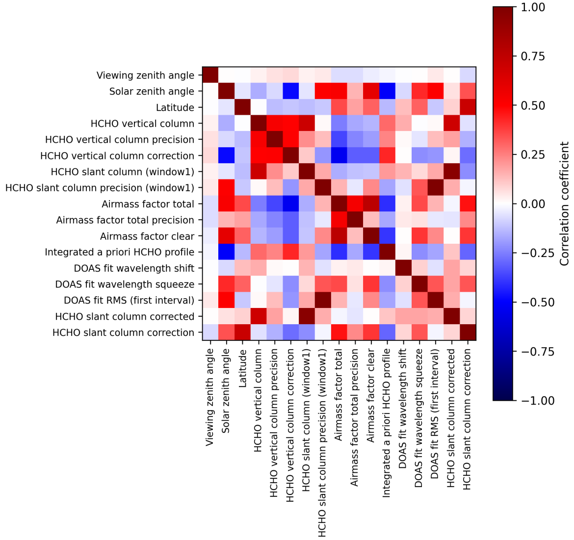
Figure 2: Map of correlation matrix for 2025-04-22 to 2025-04-24.
