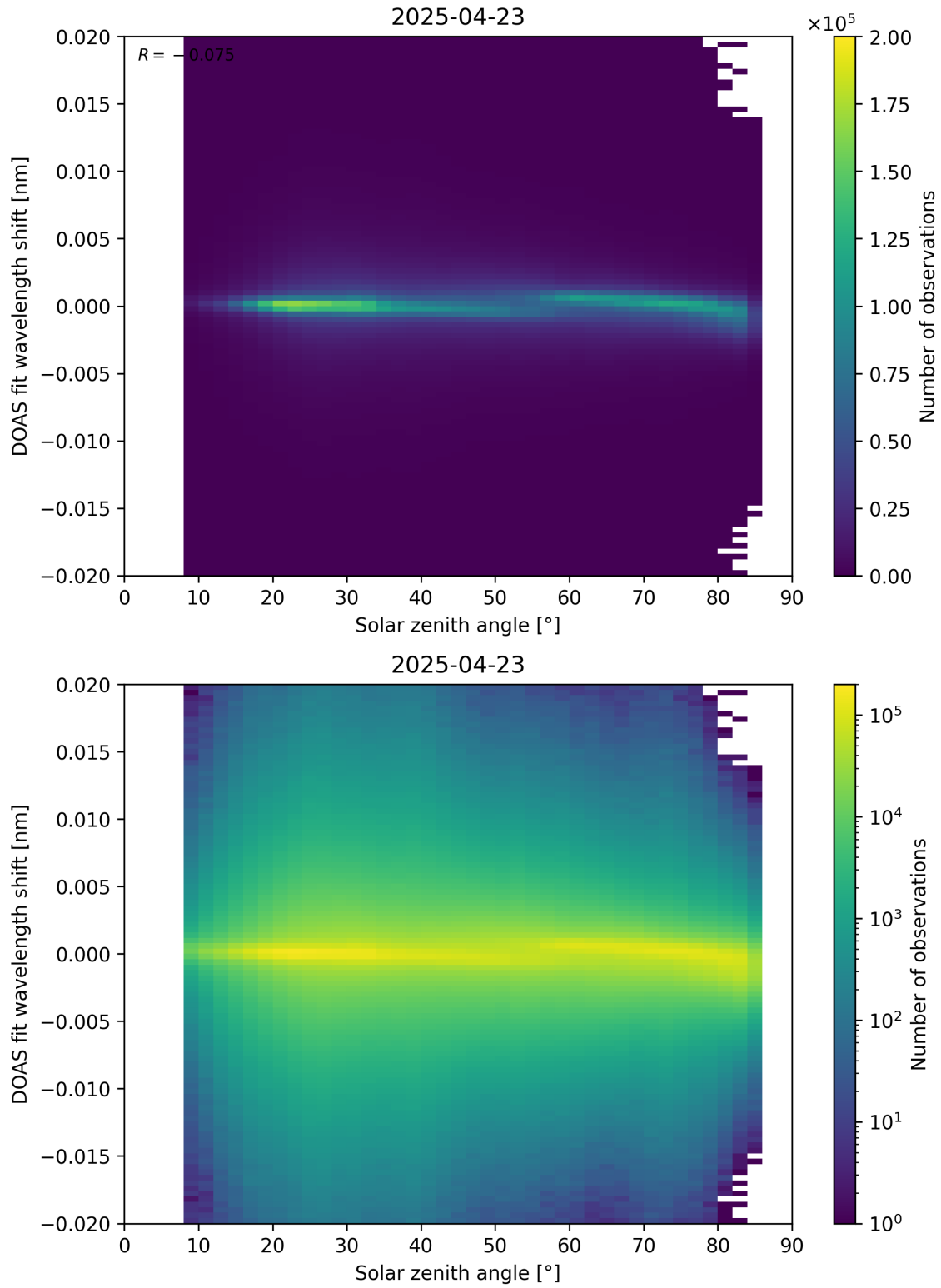
Figure 168: Scatter density plot of “Solar zenith angle” against “DOAS fit wavelength shift” for 2025-04-22 to 2025-04-24.
