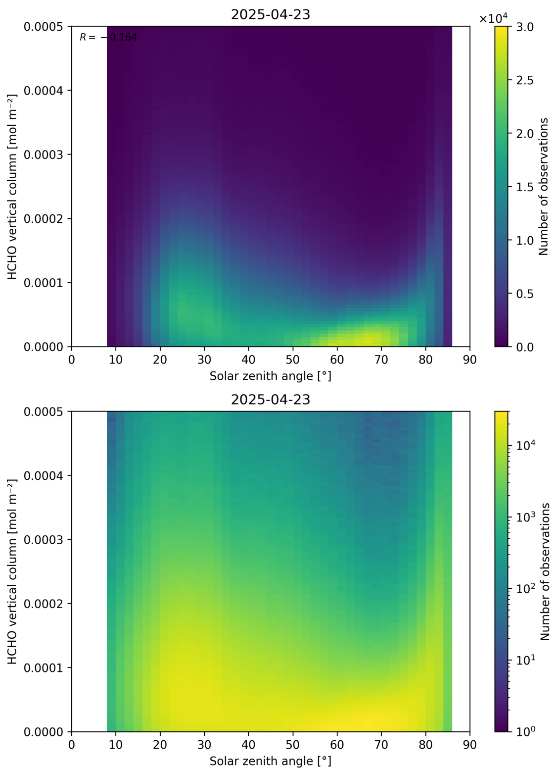
Figure 177: Scatter density plot of “Solar zenith angle” against “HCHO vertical column” for 2025-04-22 to 2025-04-24.
