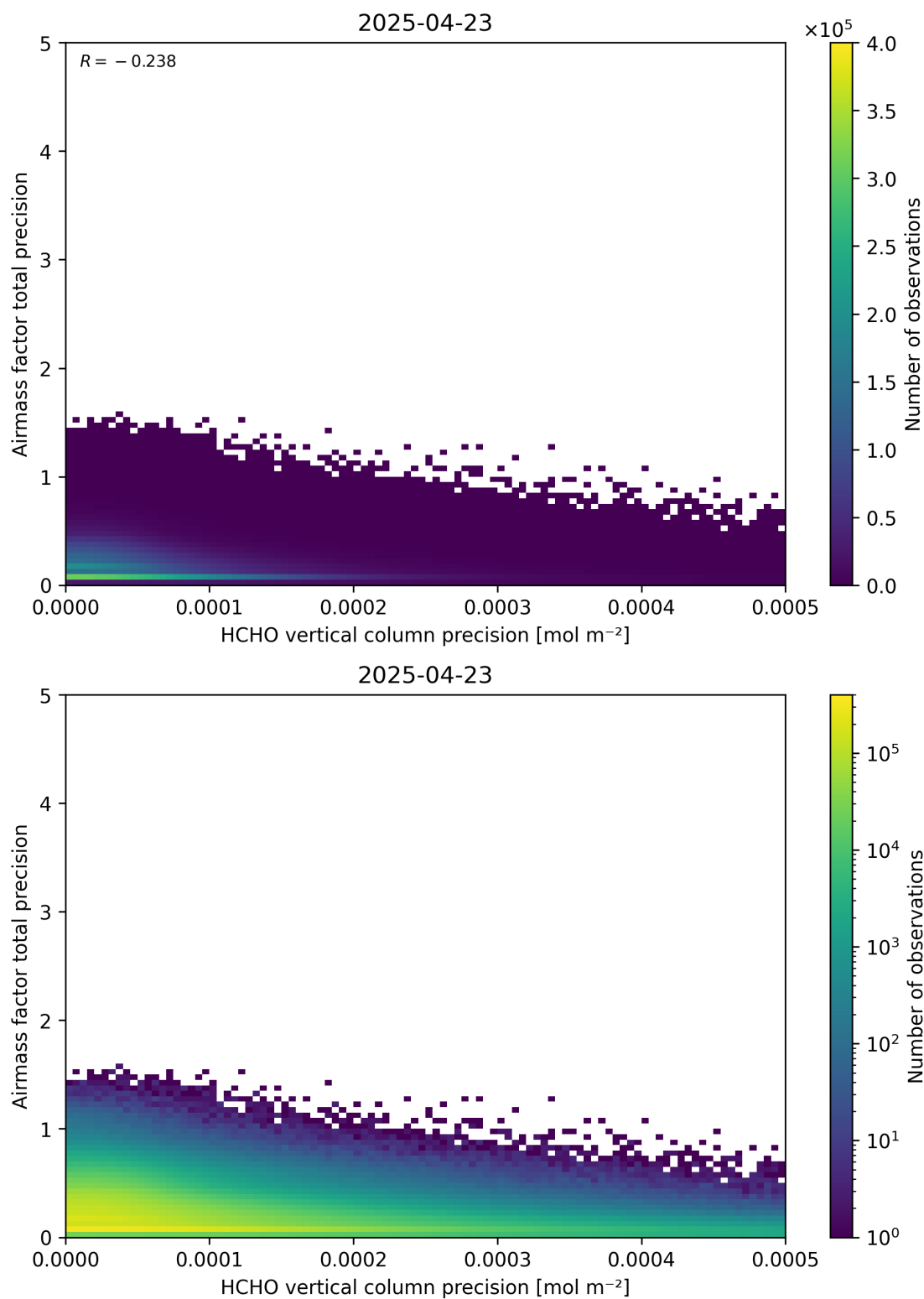
Figure 145: Scatter density plot of “HCHO vertical column precision” against “Airmass factor total precision” for 2025-04-22 to 2025-04-24.
