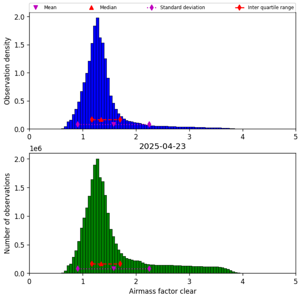
Figure 42: Histogram of “Airmass factor clear” for 2025-04-22 to 2025-04-24
