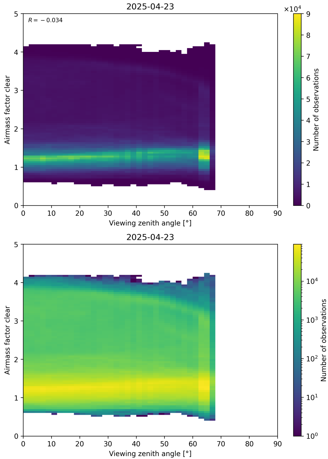
Figure 185: Scatter density plot of “Viewing zenith angle” against “Airmass factor clear” for 2025-04-22 to 2025-04-24.
