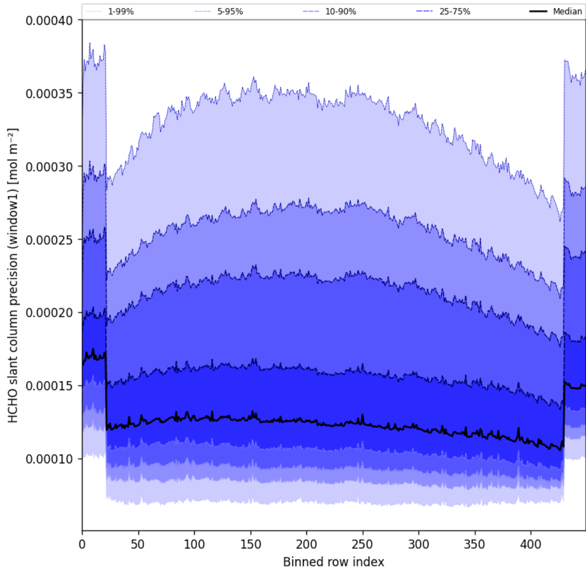
Figure 53: Along track statistics of “HCHO slant column precision (window1)” for 2025-04-22 to 2025-04-24
