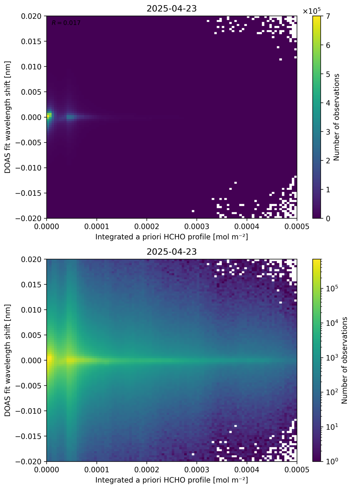
Figure 149: Scatter density plot of “Integrated a priori HCHO profile” against “DOAS fit wavelength shift” for 2025-04-22 to 2025-04-24.
