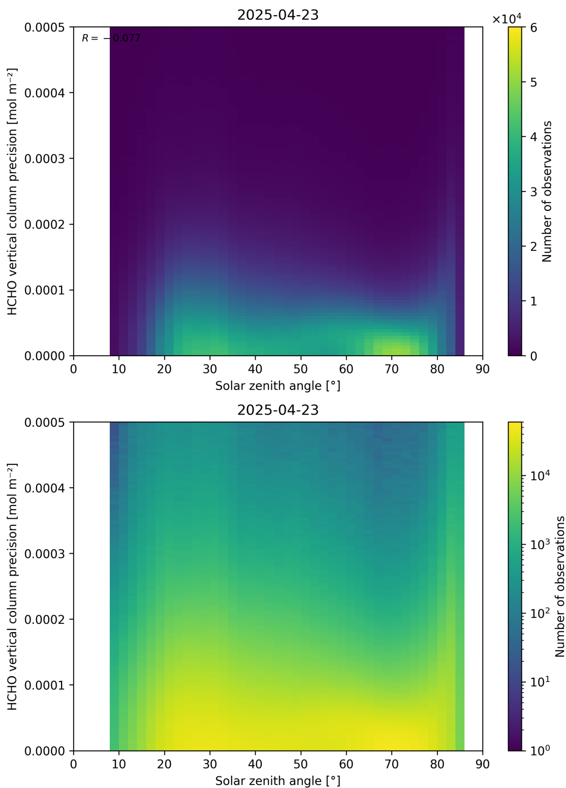
Figure 179: Scatter density plot of “Solar zenith angle” against “HCHO vertical column precision” for 2025-04-22 to 2025-04-24.
