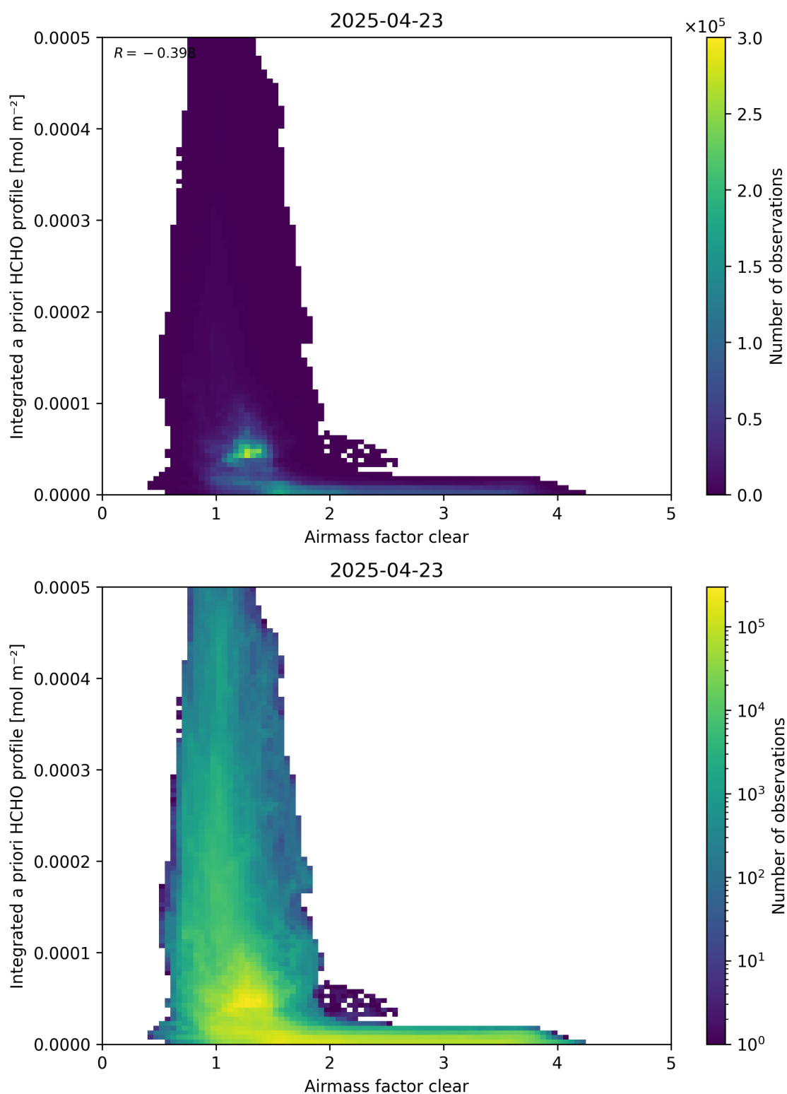
Figure 76: Scatter density plot of “Airmass factor clear” against “Integrated a priori HCHO profile” for 2025-04-22 to 2025-04-24.
