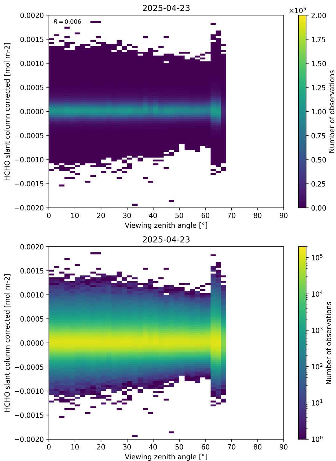
Figure 186: Scatter density plot of “Viewing zenith angle” against “HCHO slant column corrected” for 2025-04-22 to 2025-04-24.
