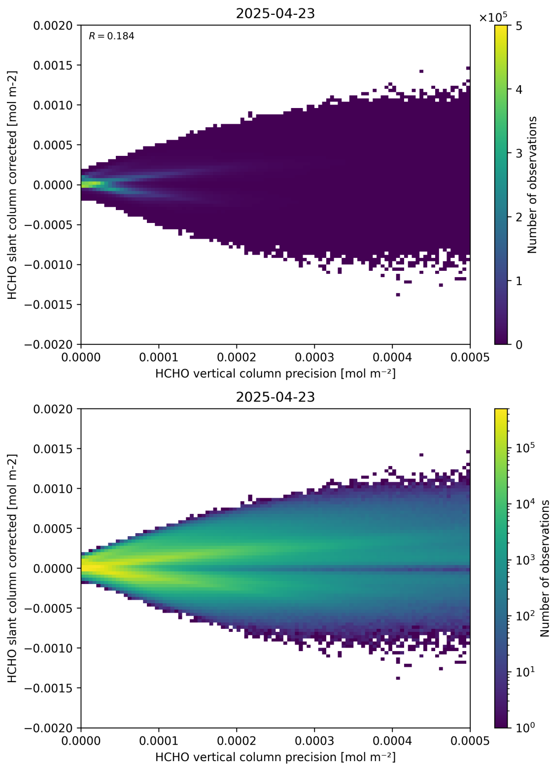
Figure 140: Scatter density plot of “HCHO vertical column precision” against “HCHO slant column corrected” for 2025-04-22 to 2025-04-24.
