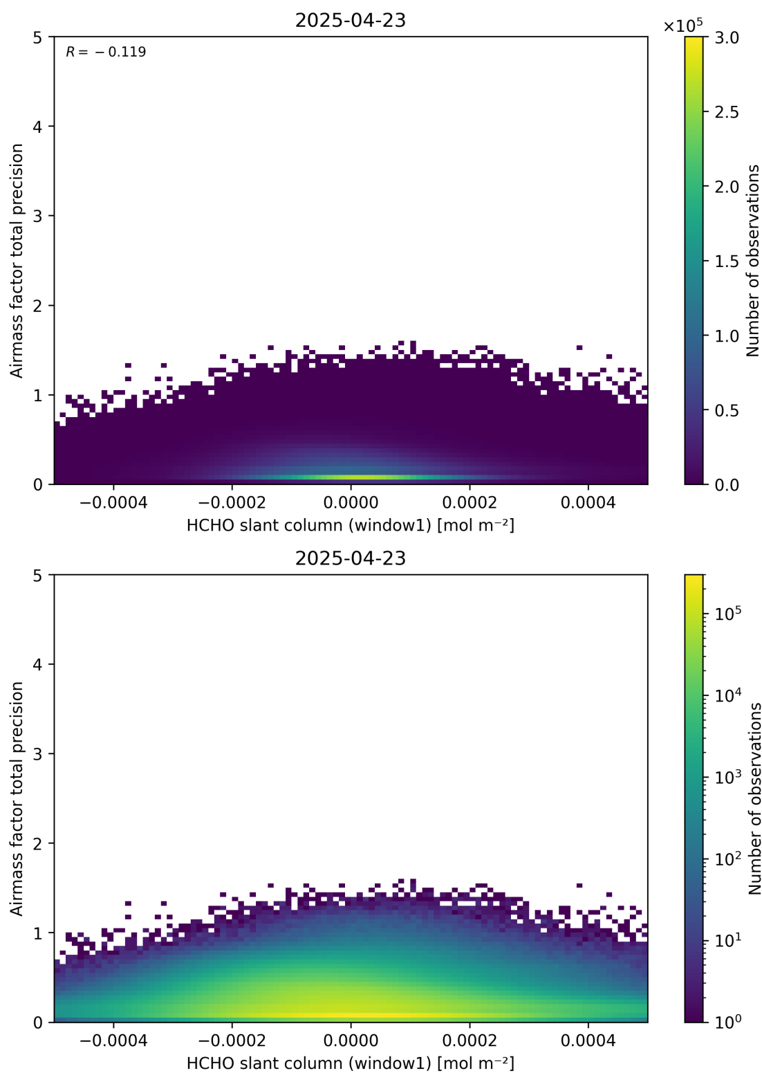
Figure 86: Scatter density plot of “HCHO slant column (window1)” against “Airmass factor total precision” for 2025-04-22 to 2025-04-24.
