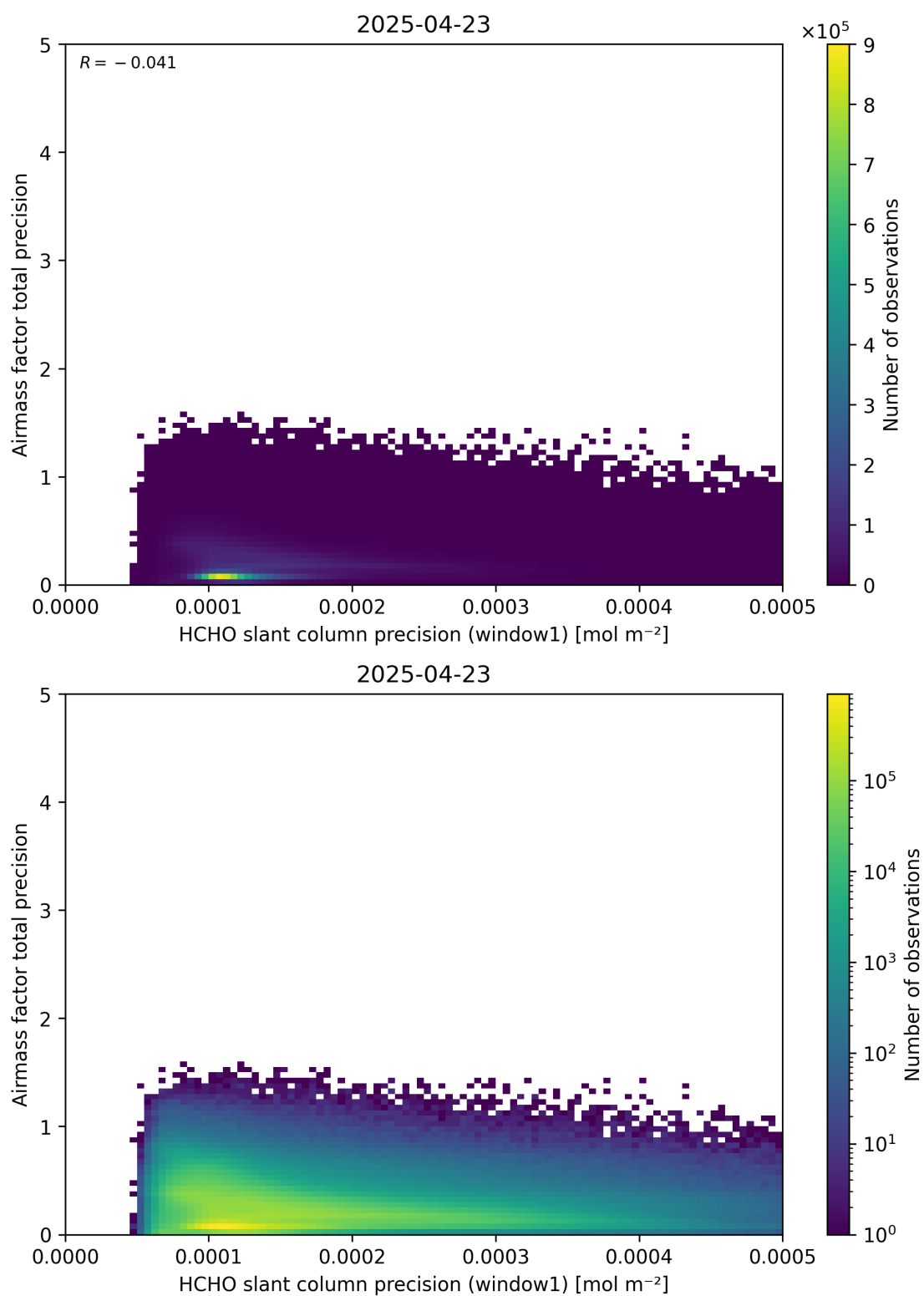
Figure 95: Scatter density plot of “HCHO slant column precision (window1)” against “Airmass factor total precision” for 2025-04-22 to 2025-04-24.
