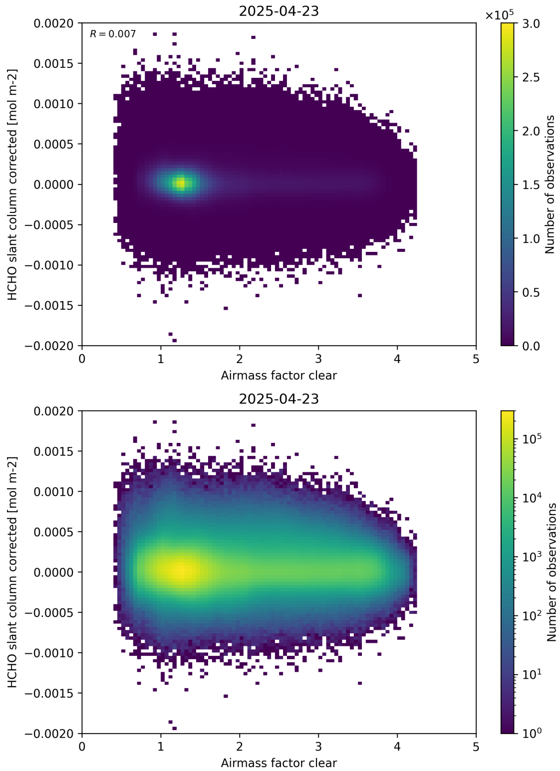
Figure 74: Scatter density plot of “Airmass factor clear” against “HCHO slant column corrected” for 2025-04-22 to 2025-04-24.
