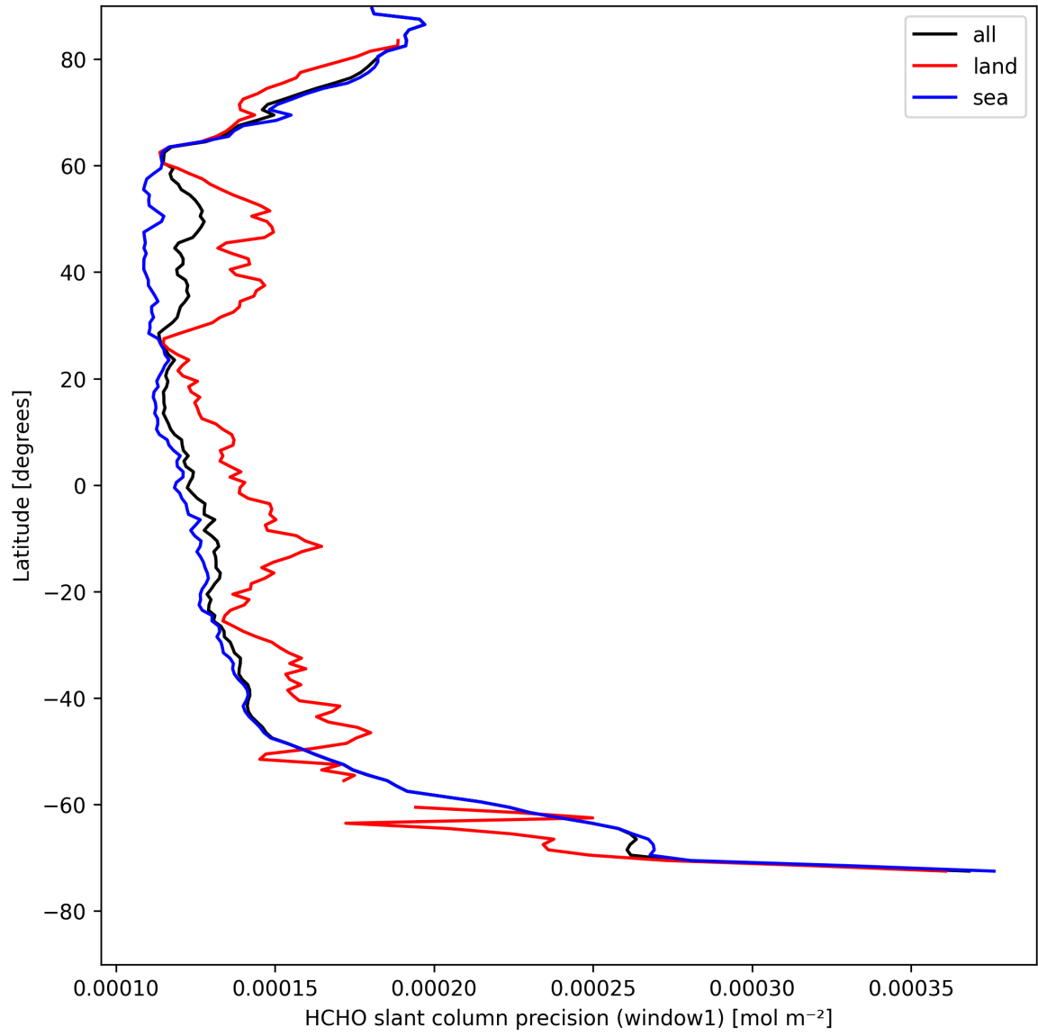
Figure 25: Zonal average of “HCHO slant column precision (window1)” for 2025-04-22 to 2025-04-24.
