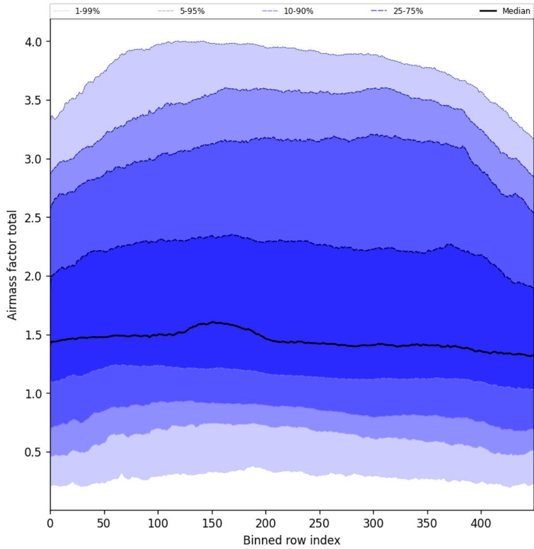
Figure 54: Along track statistics of “Airmass factor total” for 2025-04-22 to 2025-04-24
