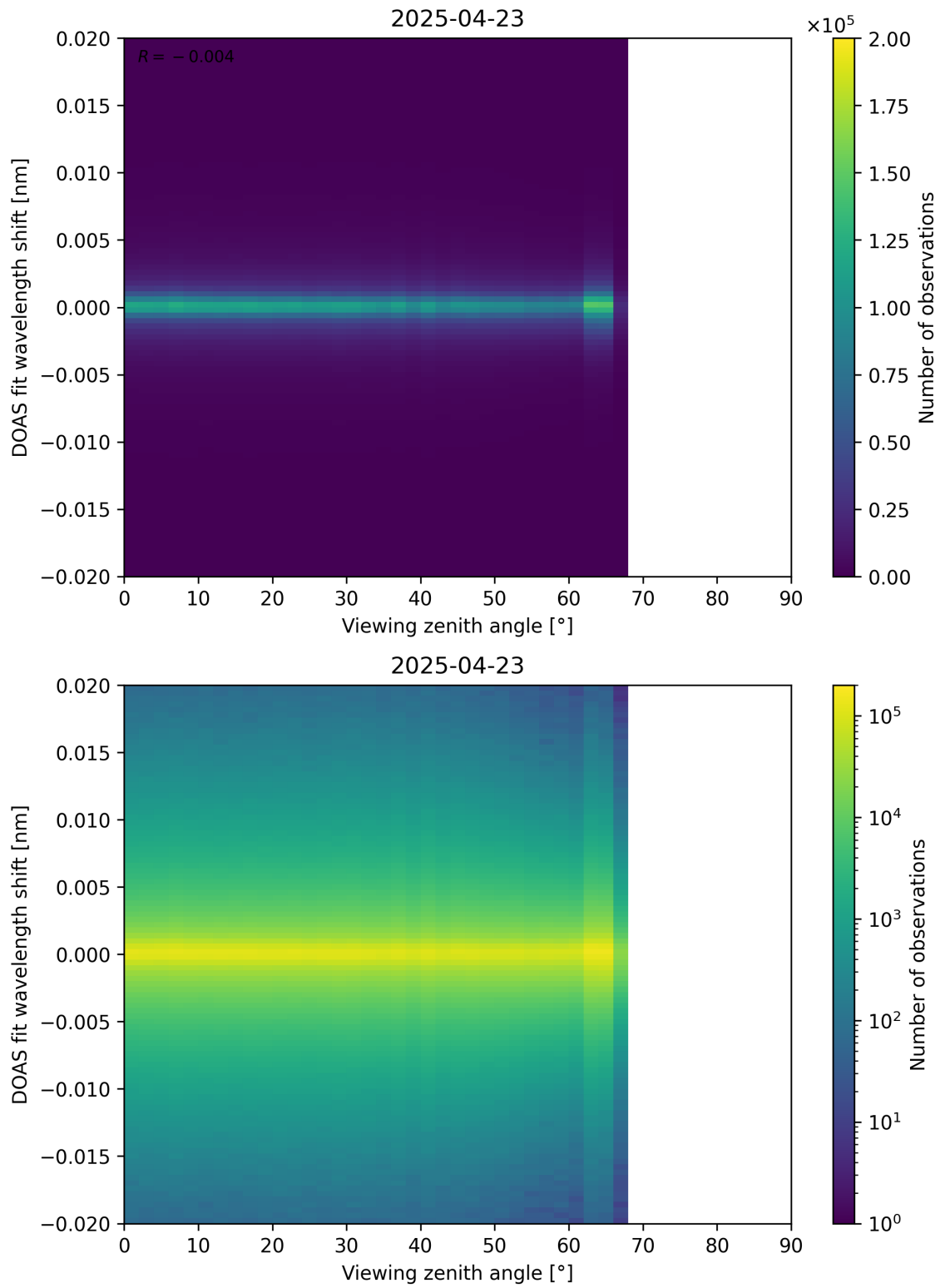
Figure 183: Scatter density plot of “Viewing zenith angle” against “DOAS fit wavelength shift” for 2025-04-22 to 2025-04-24.
