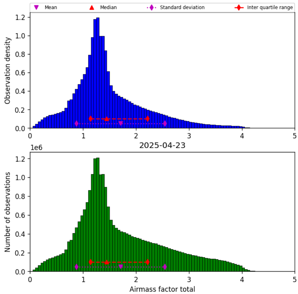
Figure 40: Histogram of “Airmass factor total” for 2025-04-22 to 2025-04-24
