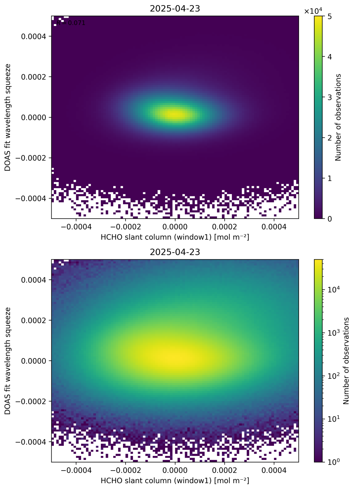
Figure 80: Scatter density plot of “HCHO slant column (window1)” against “DOAS fit wavelength squeeze” for 2025-04-22 to 2025-04-24.
