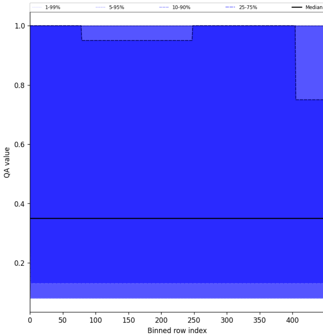
Figure 48: Along track statistics of “QA value” for 2025-04-22 to 2025-04-24
