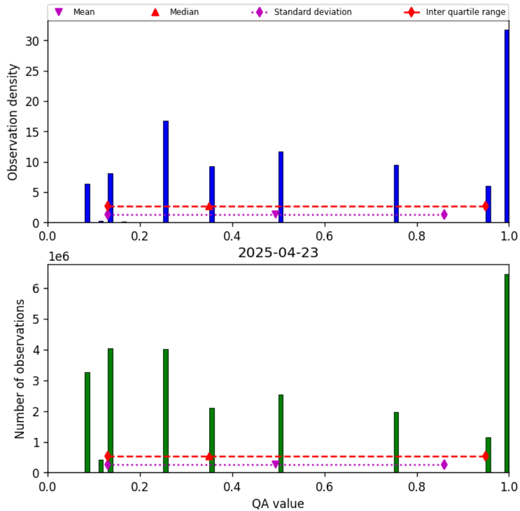
Figure 34: Histogram of “QA value” for 2025-04-22 to 2025-04-24
