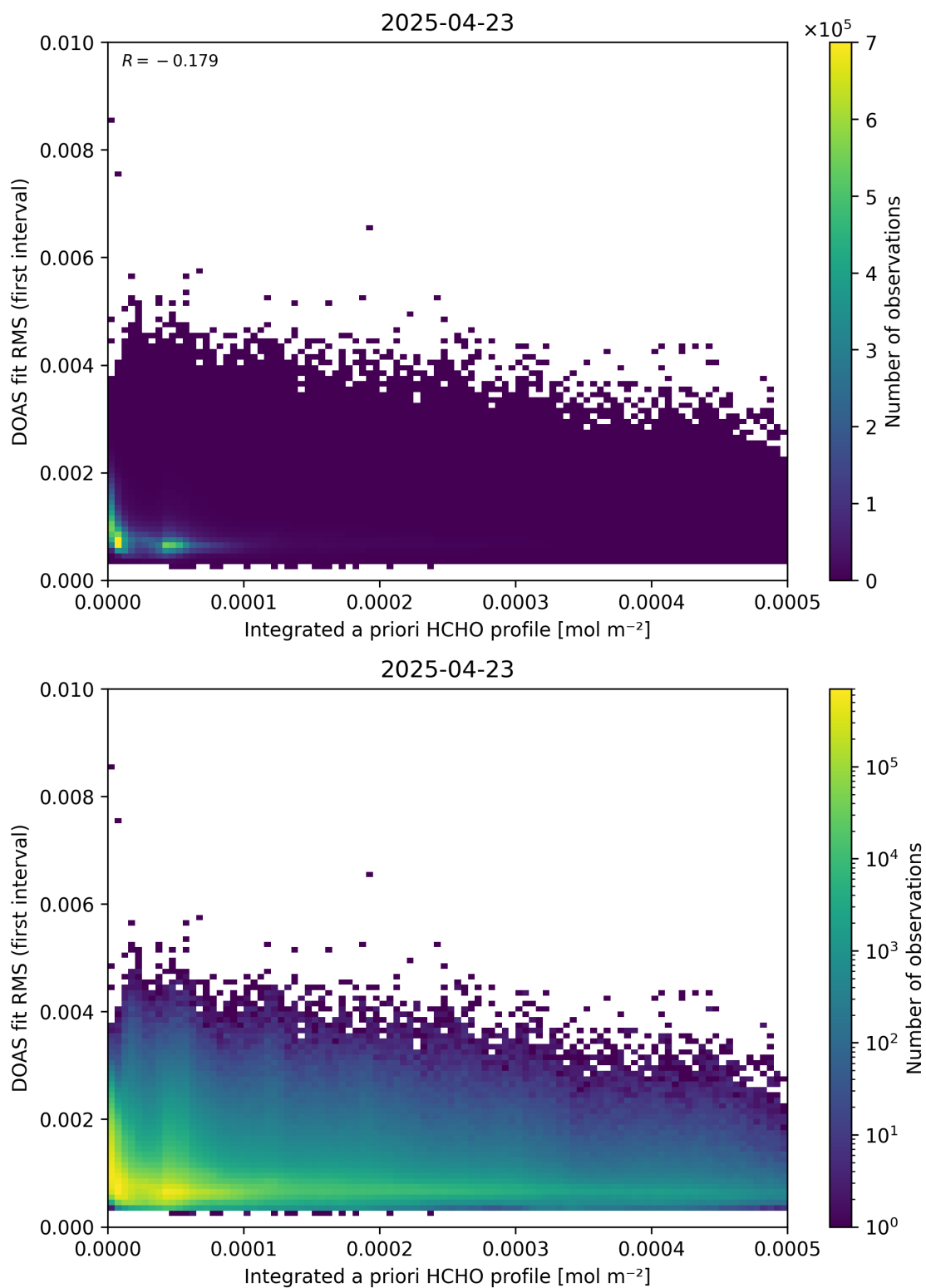
Figure 148: Scatter density plot of “Integrated a priori HCHO profile” against “DOAS fit RMS (first interval)” for 2025-04-22 to 2025-04-24.
