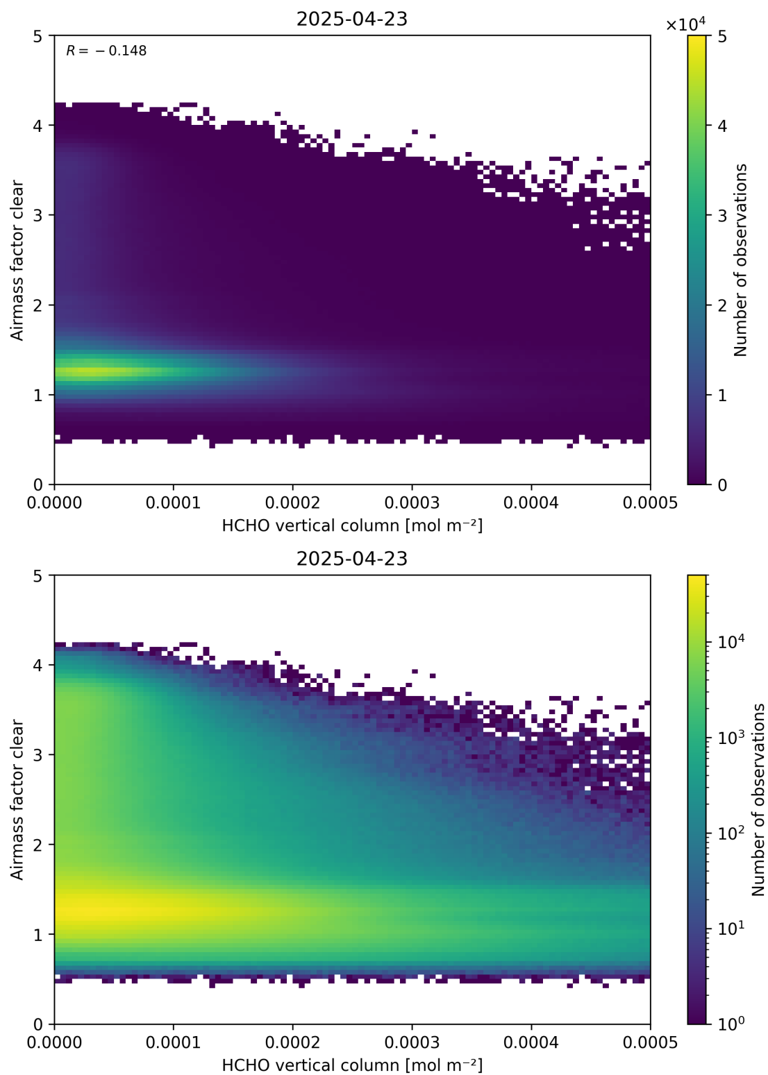
Figure 126: Scatter density plot of “HCHO vertical column” against “Airmass factor clear” for 2025-04-22 to 2025-04-24.
