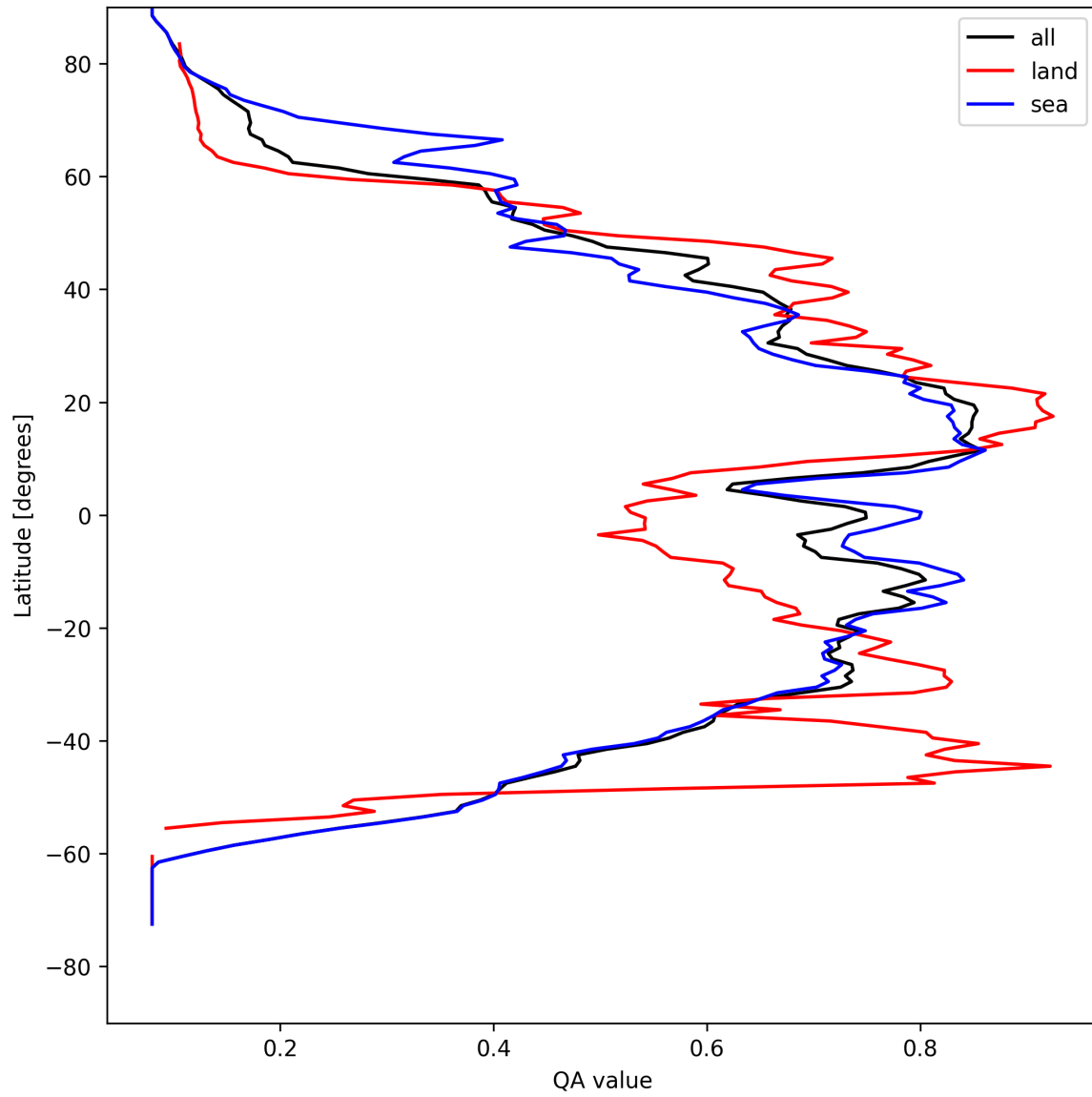
Figure 20: Zonal average of “QA value” for 2025-04-22 to 2025-04-24.
