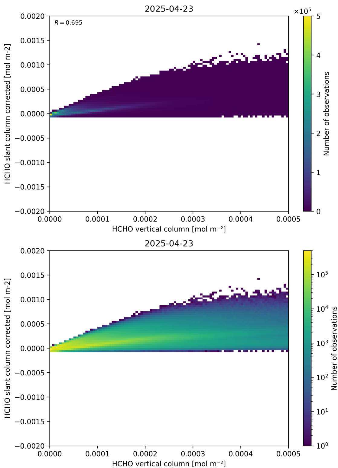
Figure 127: Scatter density plot of “HCHO vertical column” against “HCHO slant column corrected” for 2025-04-22 to 2025-04-24.
