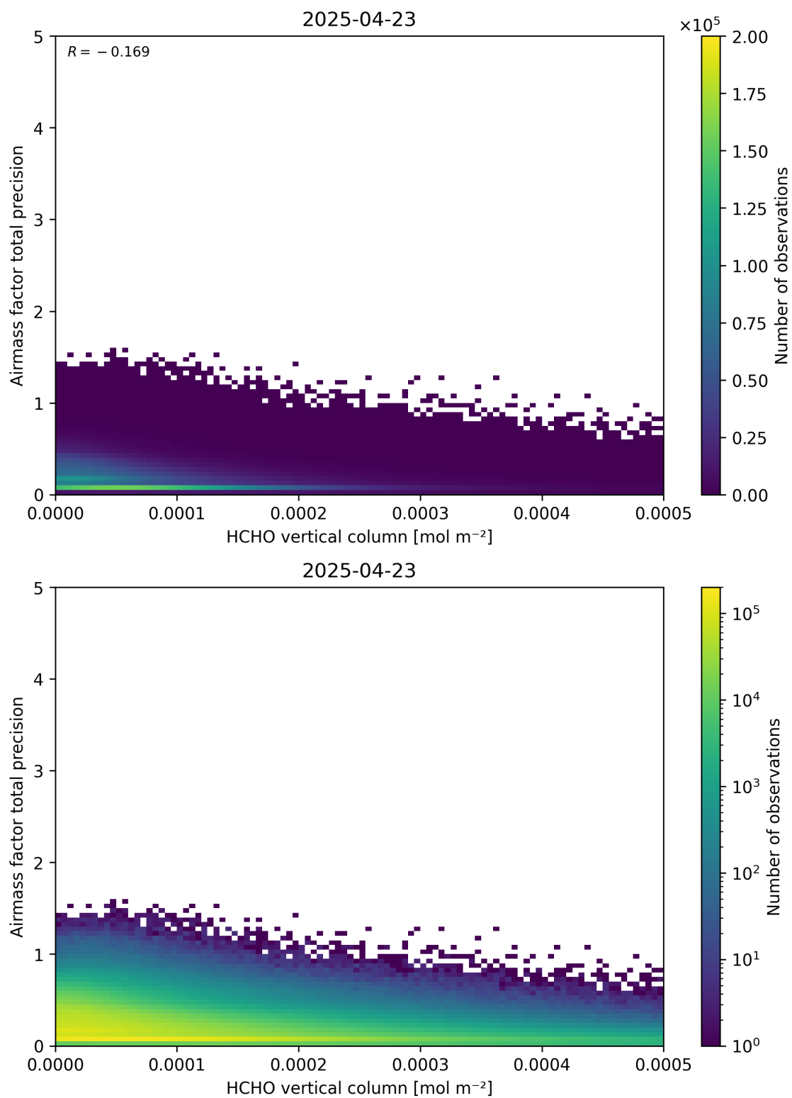
Figure 132: Scatter density plot of “HCHO vertical column” against “Airmass factor total precision” for 2025-04-22 to 2025-04-24.
