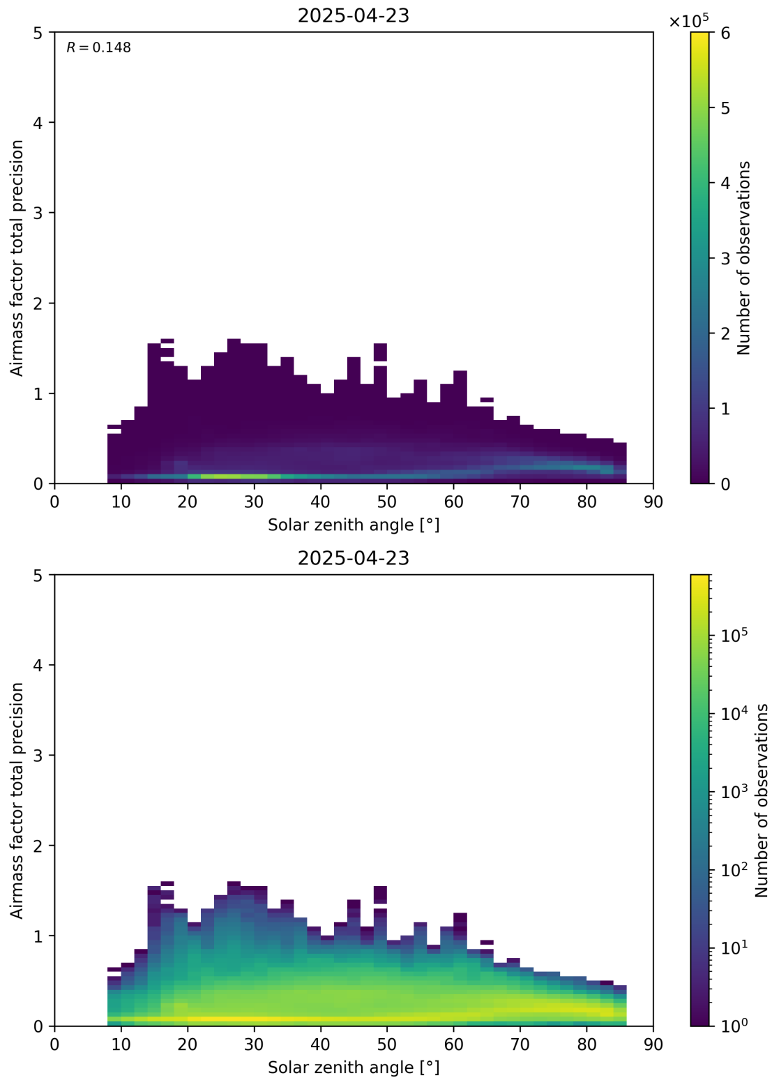
Figure 176: Scatter density plot of “Solar zenith angle” against “Airmass factor total precision” for 2025-04-22 to 2025-04-24.
