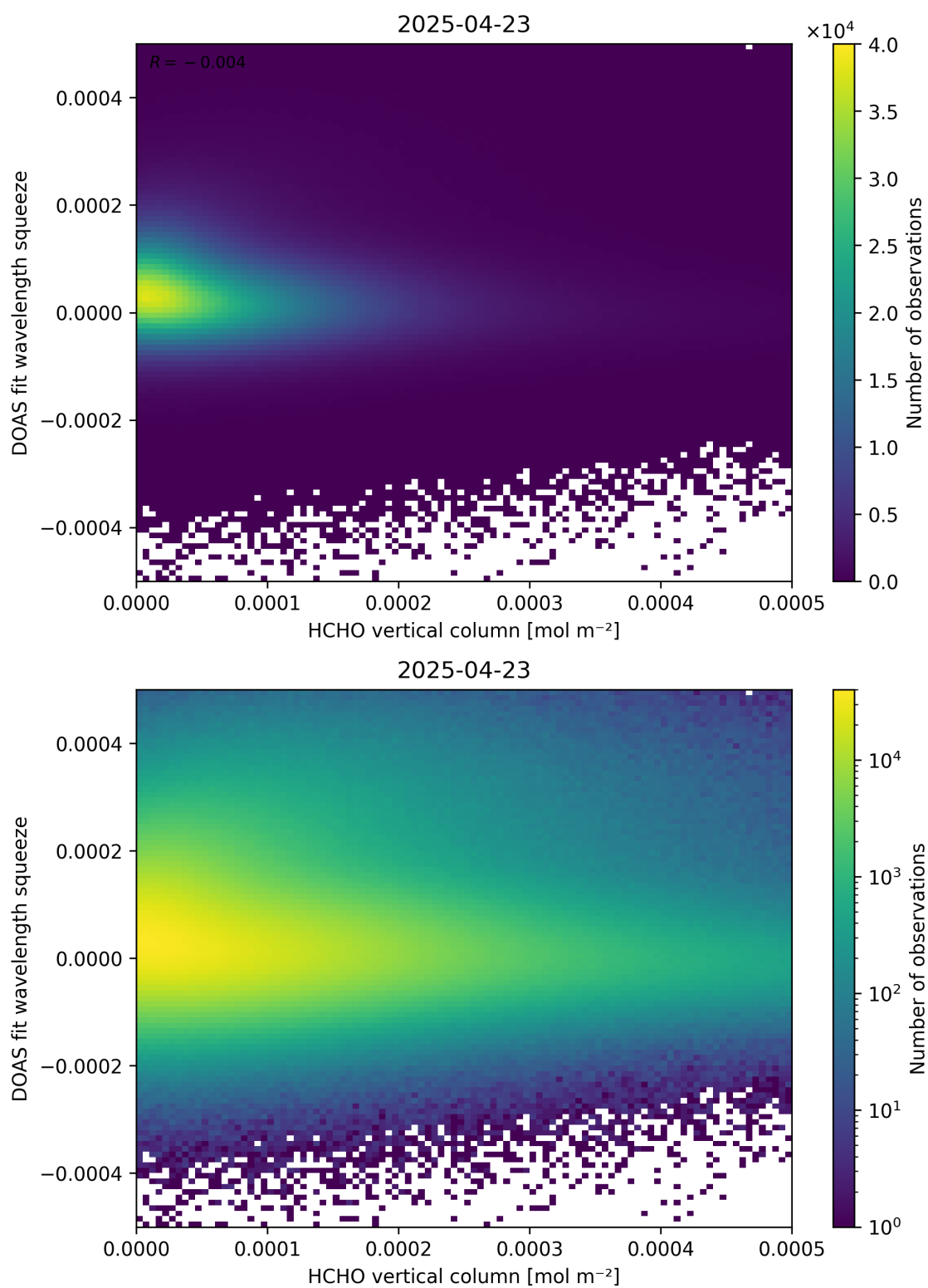
Figure 125: Scatter density plot of “HCHO vertical column” against “DOAS fit wavelength squeeze” for 2025-04-22 to 2025-04-24.
