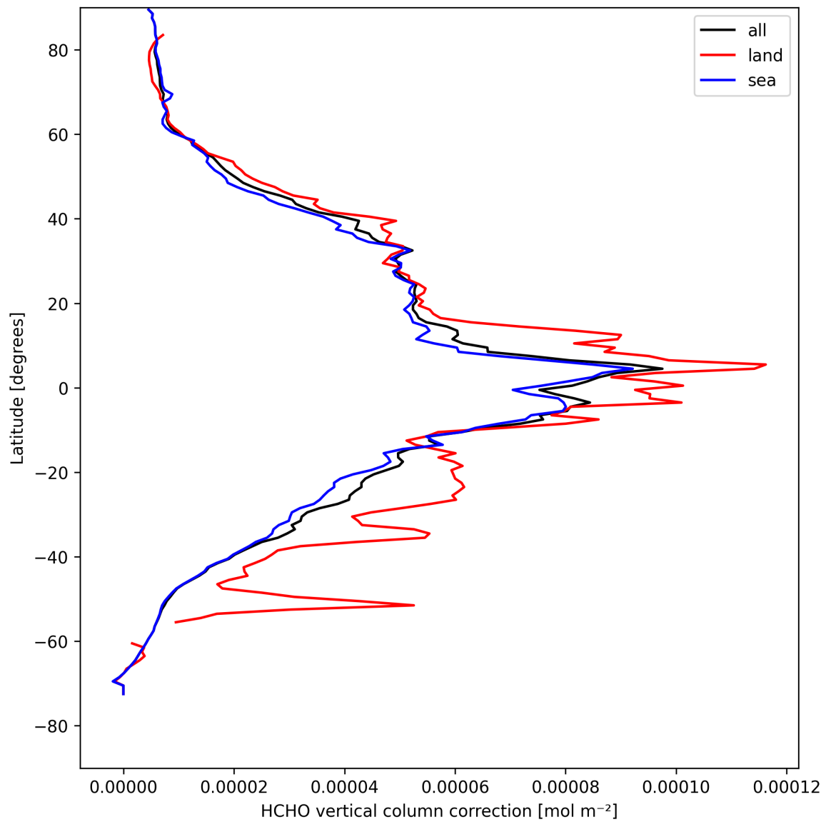
Figure 23: Zonal average of “HCHO vertical column correction” for 2025-04-22 to 2025-04-24.
