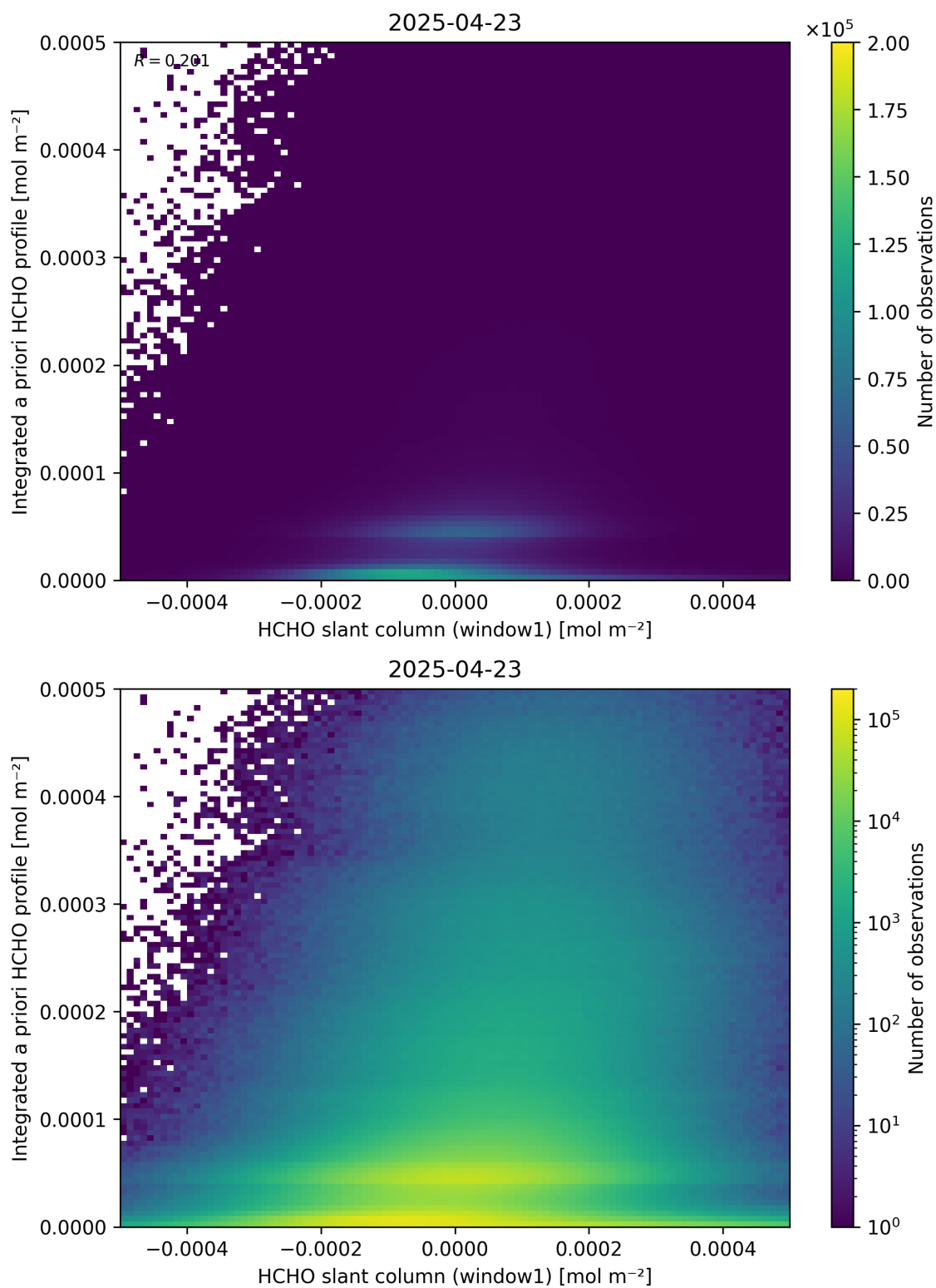
Figure 87: Scatter density plot of “HCHO slant column (window1)” against “Integrated a priori HCHO profile” for 2025-04-22 to 2025-04-24.
