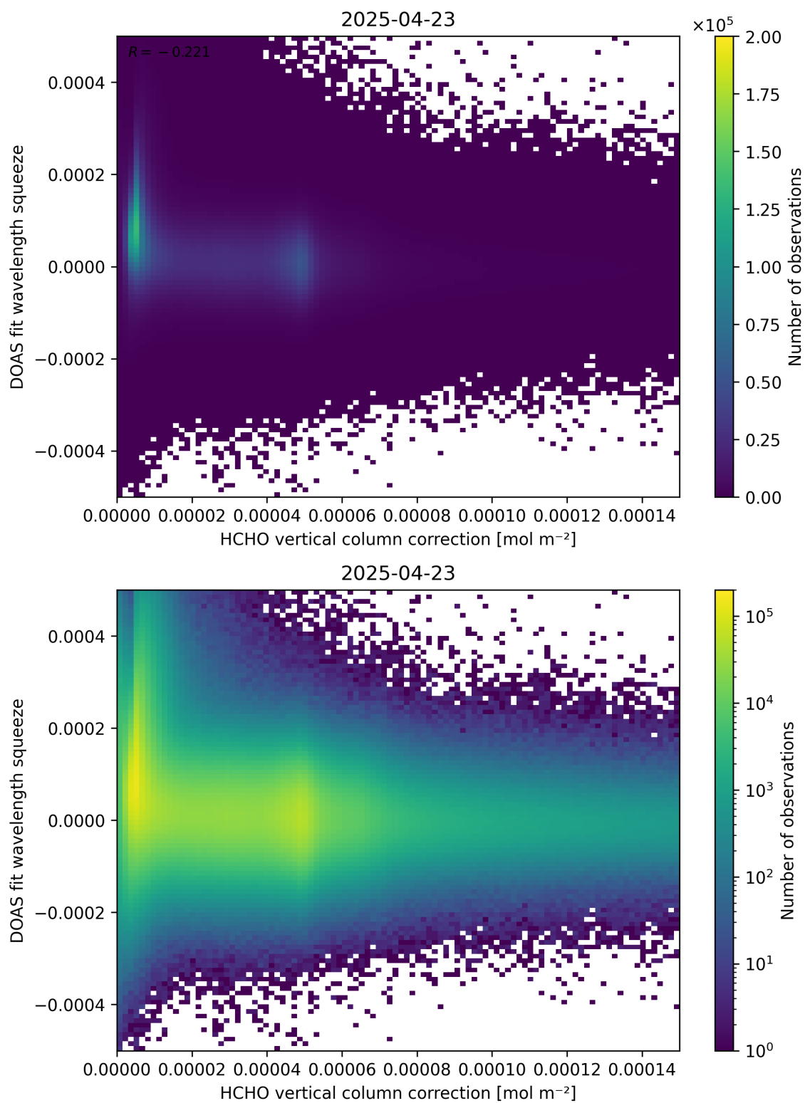
Figure 114: Scatter density plot of “HCHO vertical column correction” against “DOAS fit wavelength squeeze” for 2025-04-22 to 2025-04-24.
