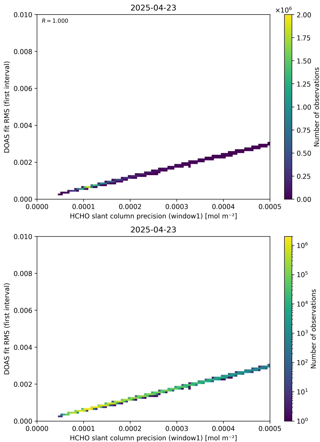
Figure 88: Scatter density plot of “HCHO slant column precision (window1)” against “DOAS fit RMS (first interval)” for 2025-04-22 to 2025-04-24.
