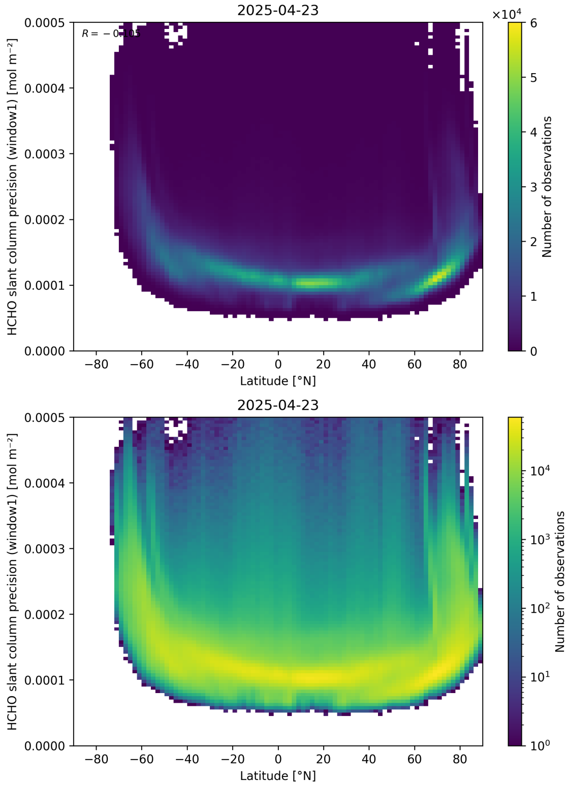
Figure 160: Scatter density plot of “Latitude” against “HCHO slant column precision (window1)” for 2025-04-22 to 2025-04-24.
