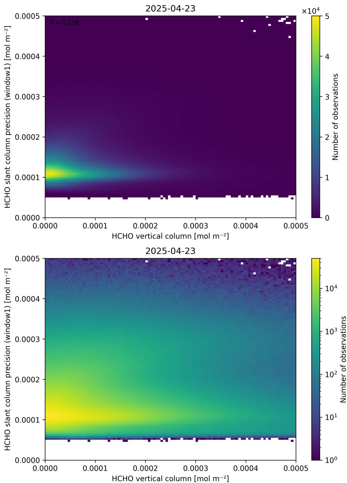
Figure 130: Scatter density plot of “HCHO vertical column” against “HCHO slant column precision (window1)” for 2025-04-22 to 2025-04-24.
