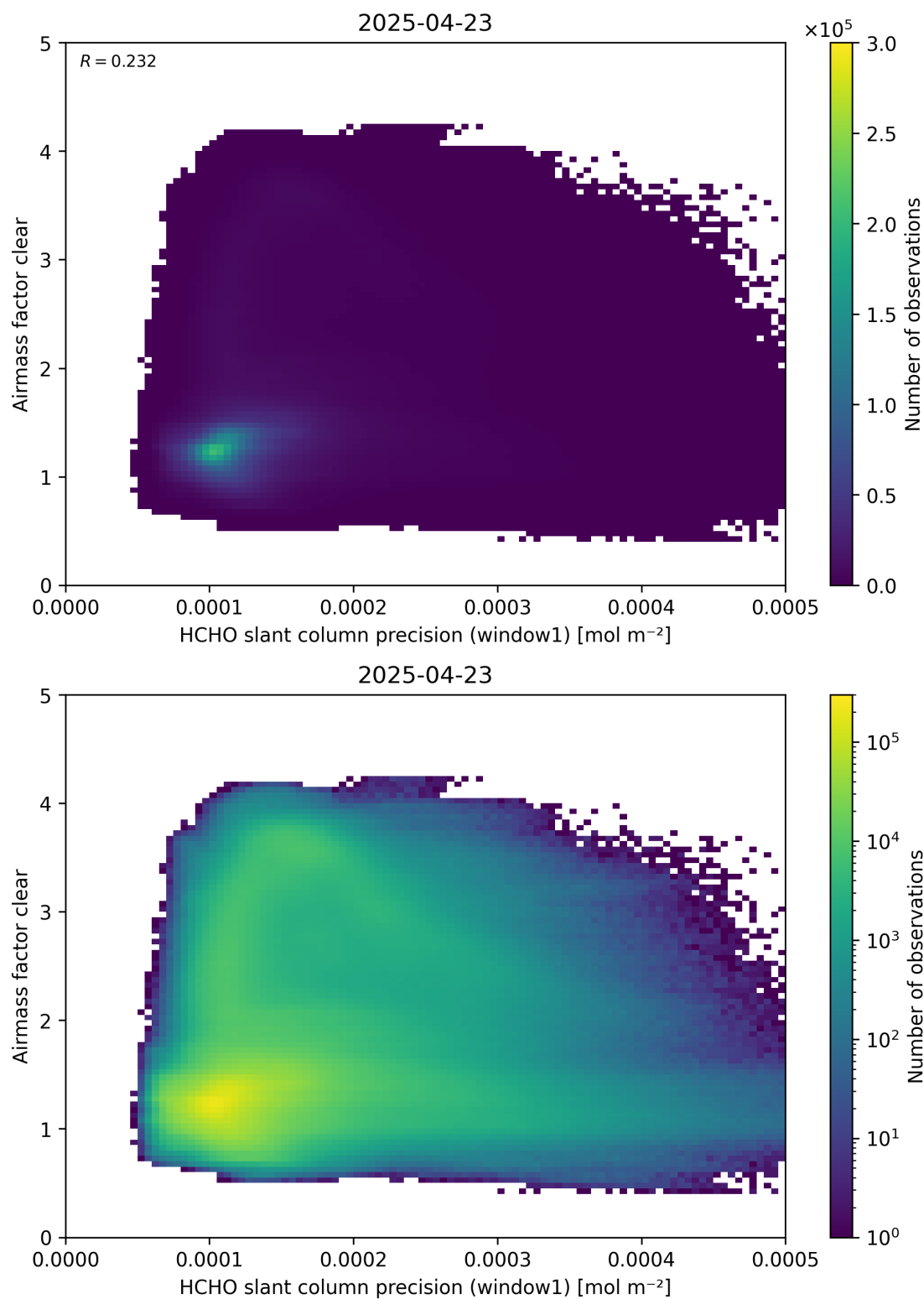
Figure 91: Scatter density plot of “HCHO slant column precision (window1)” against “Airmass factor clear” for 2025-04-22 to 2025-04-24.
