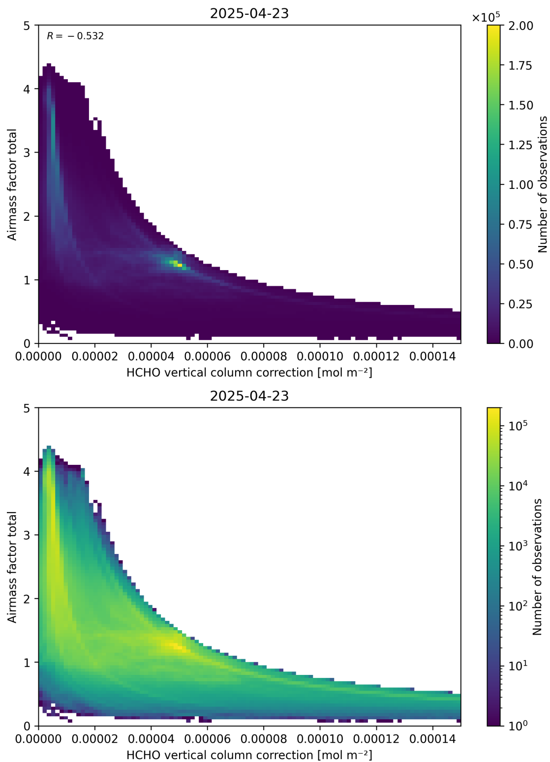
Figure 120: Scatter density plot of “HCHO vertical column correction” against “Airmass factor total” for 2025-04-22 to 2025-04-24.
