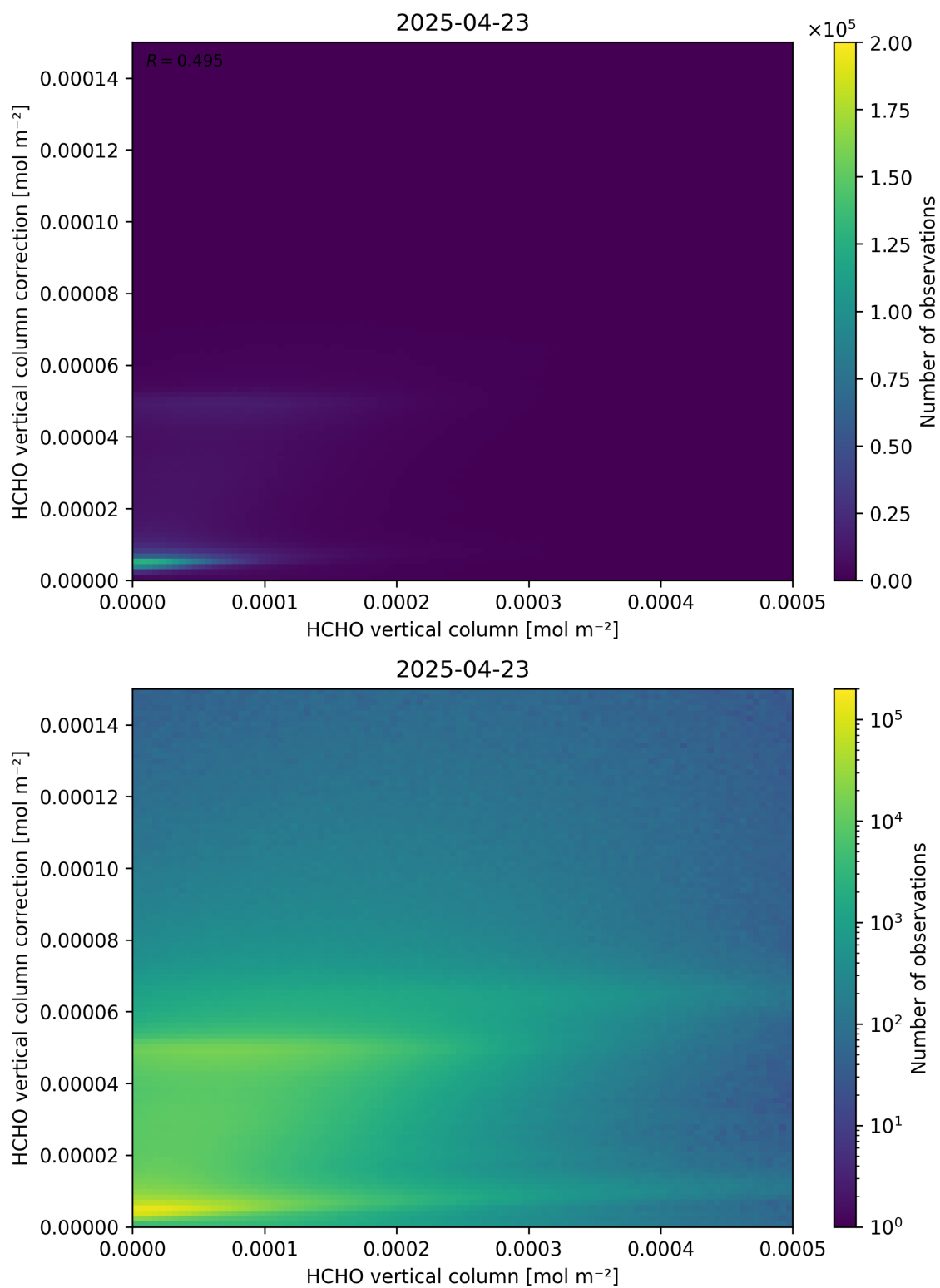
Figure 133: Scatter density plot of “HCHO vertical column” against “HCHO vertical column correction” for 2025-04-22 to 2025-04-24.
