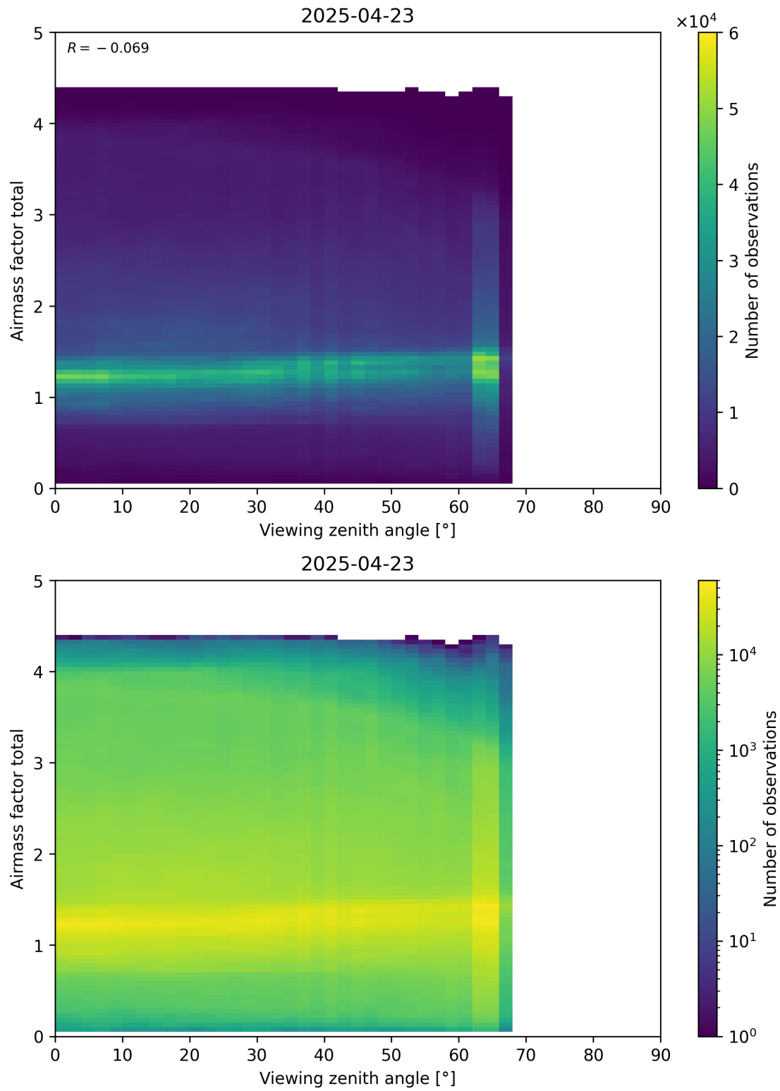
Figure 190: Scatter density plot of “Viewing zenith angle” against “Airmass factor total” for 2025-04-22 to 2025-04-24.
