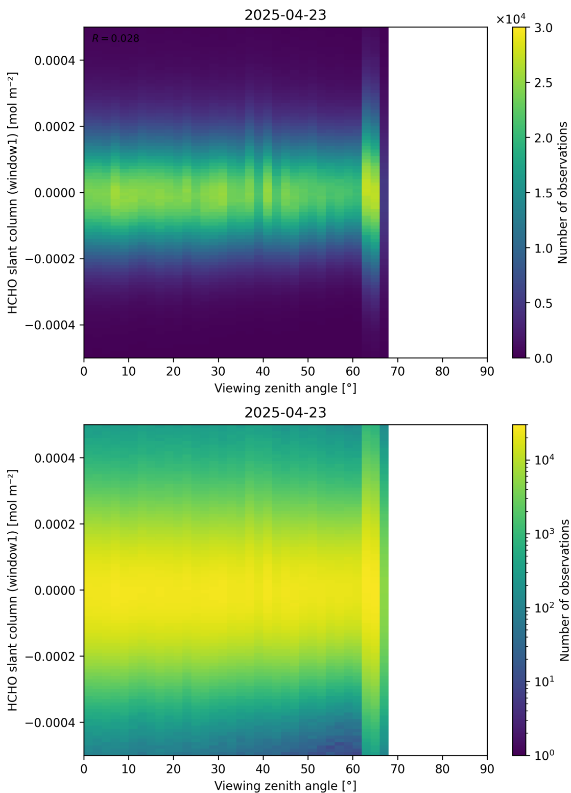
Figure 188: Scatter density plot of “Viewing zenith angle” against “HCHO slant column (window1)” for 2025-04-22 to 2025-04-24.
