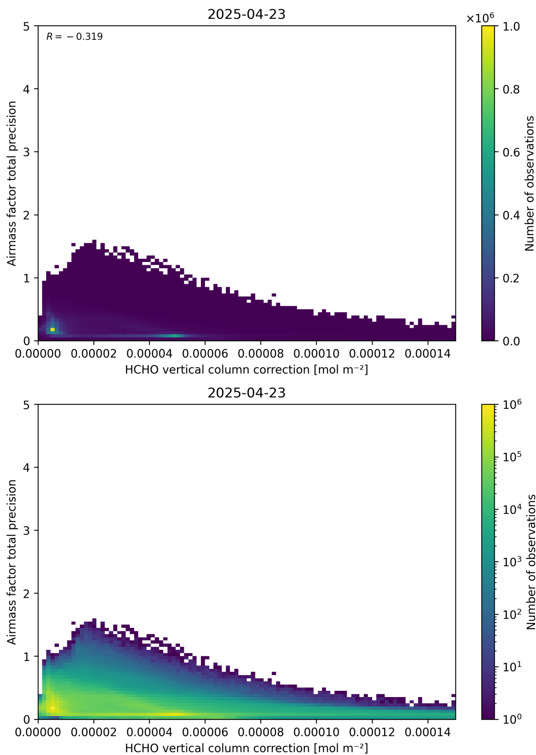
Figure 121: Scatter density plot of “HCHO vertical column correction” against “Airmass factor total precision” for 2025-04-22 to 2025-04-24.
