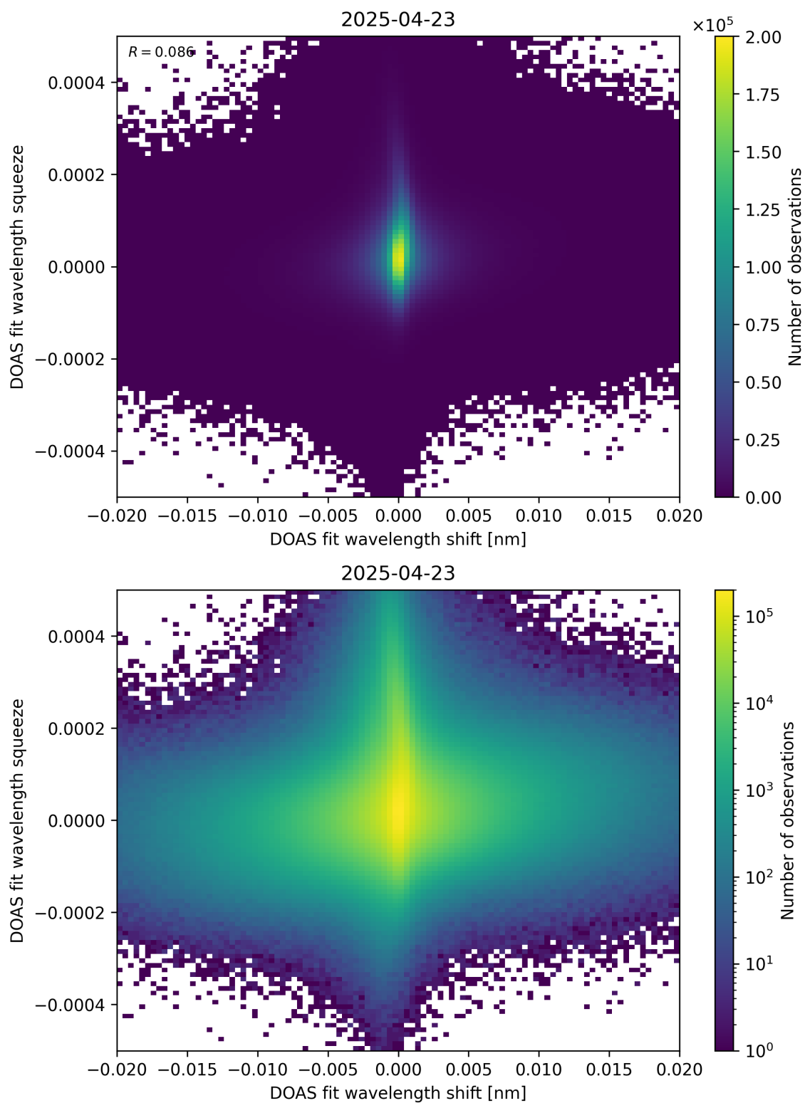
Figure 65: Scatter density plot of “DOAS fit wavelength shift” against “DOAS fit wavelength squeeze” for 2025-04-22 to 2025-04-24.
