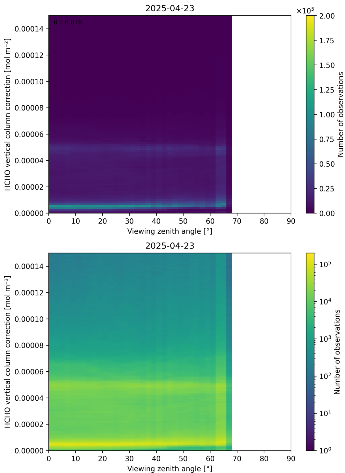
Figure 193: Scatter density plot of “Viewing zenith angle” against “HCHO vertical column correction” for 2025-04-22 to 2025-04-24.
