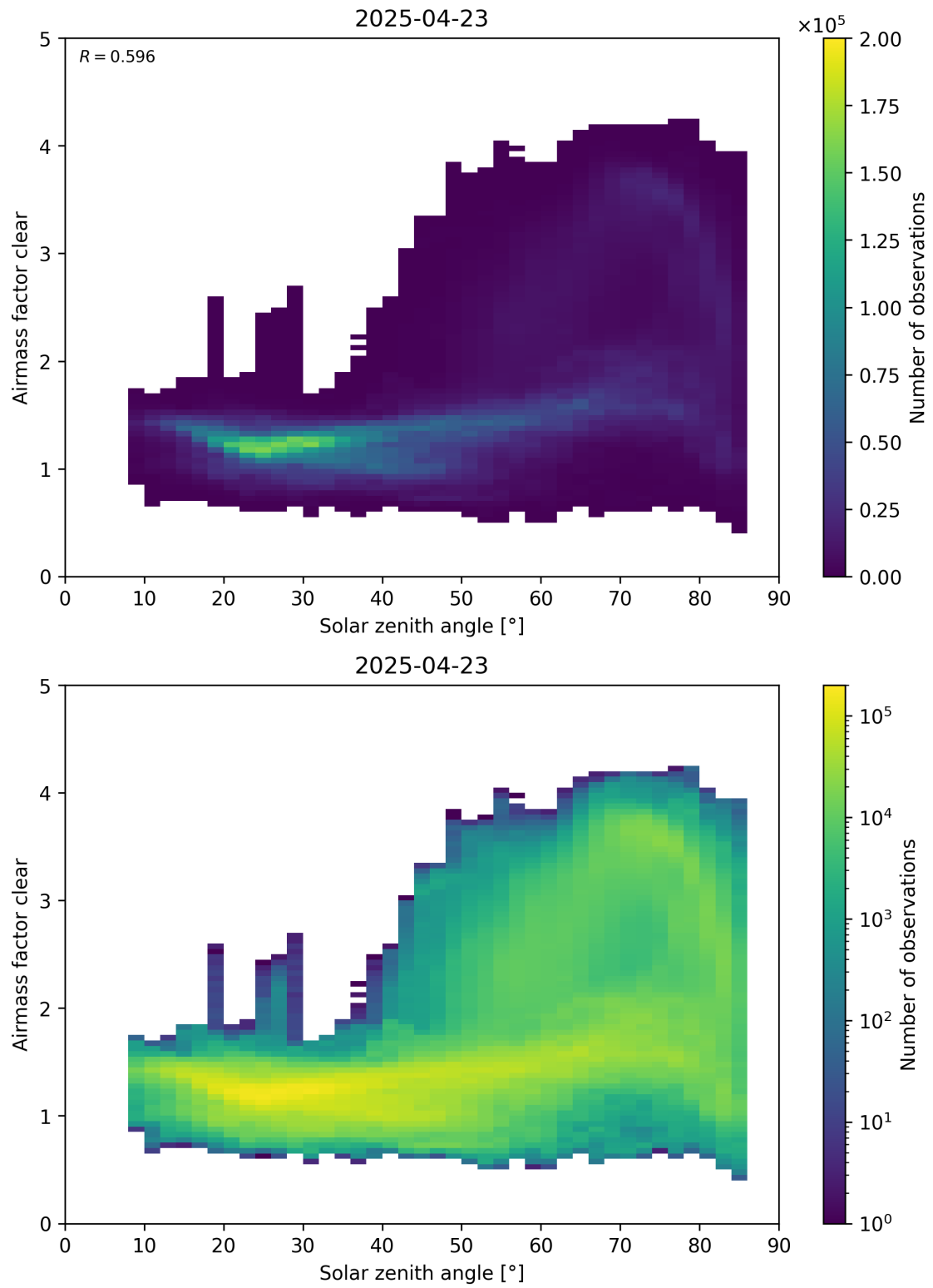
Figure 170: Scatter density plot of “Solar zenith angle” against “Airmass factor clear” for 2025-04-22 to 2025-04-24.
