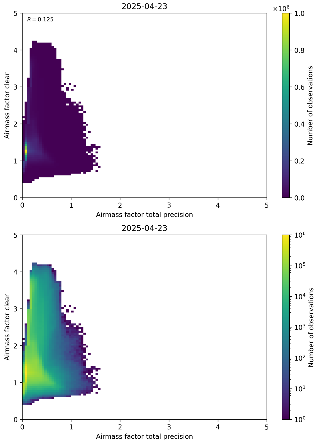
Figure 108: Scatter density plot of “Airmass factor total precision” against “Airmass factor clear” for 2025-04-22 to 2025-04-24.
