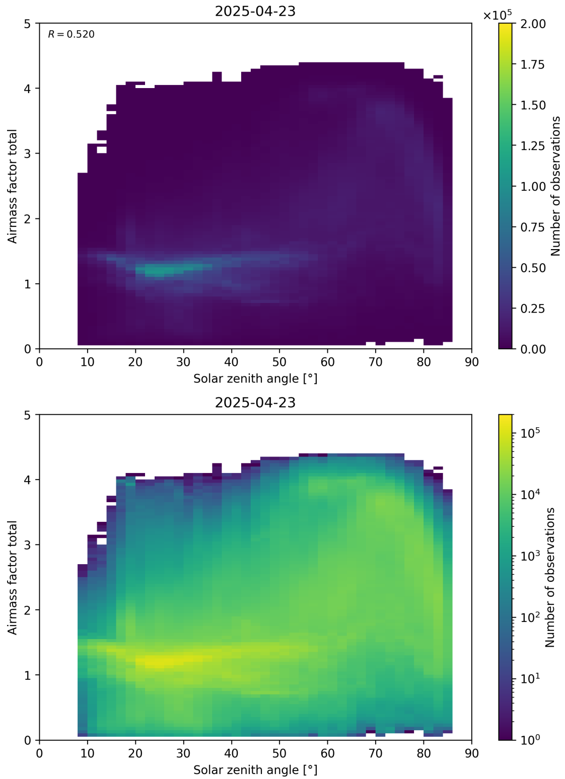
Figure 175: Scatter density plot of “Solar zenith angle” against “Airmass factor total” for 2025-04-22 to 2025-04-24.
