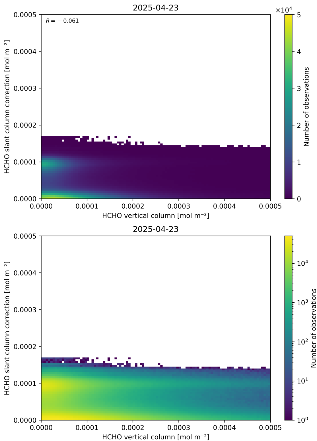
Figure 128: Scatter density plot of “HCHO vertical column” against “HCHO slant column correction” for 2025-04-22 to 2025-04-24.
