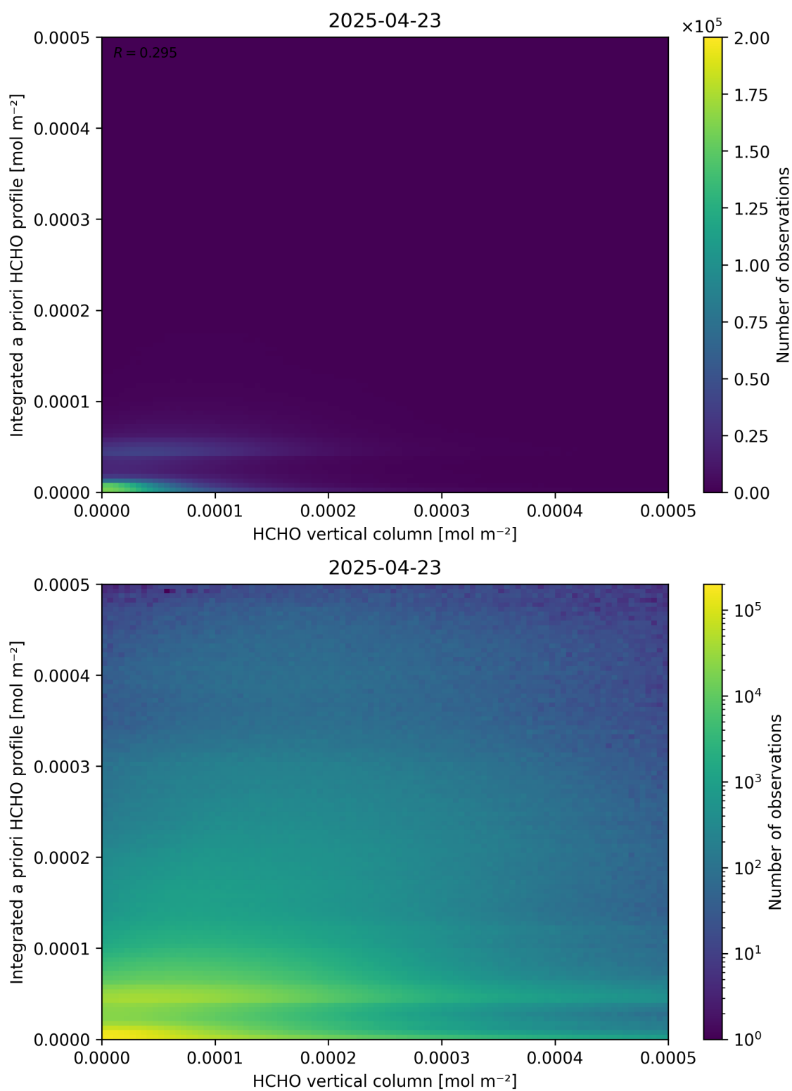
Figure 135: Scatter density plot of “HCHO vertical column” against “Integrated a priori HCHO profile” for 2025-04-22 to 2025-04-24.
