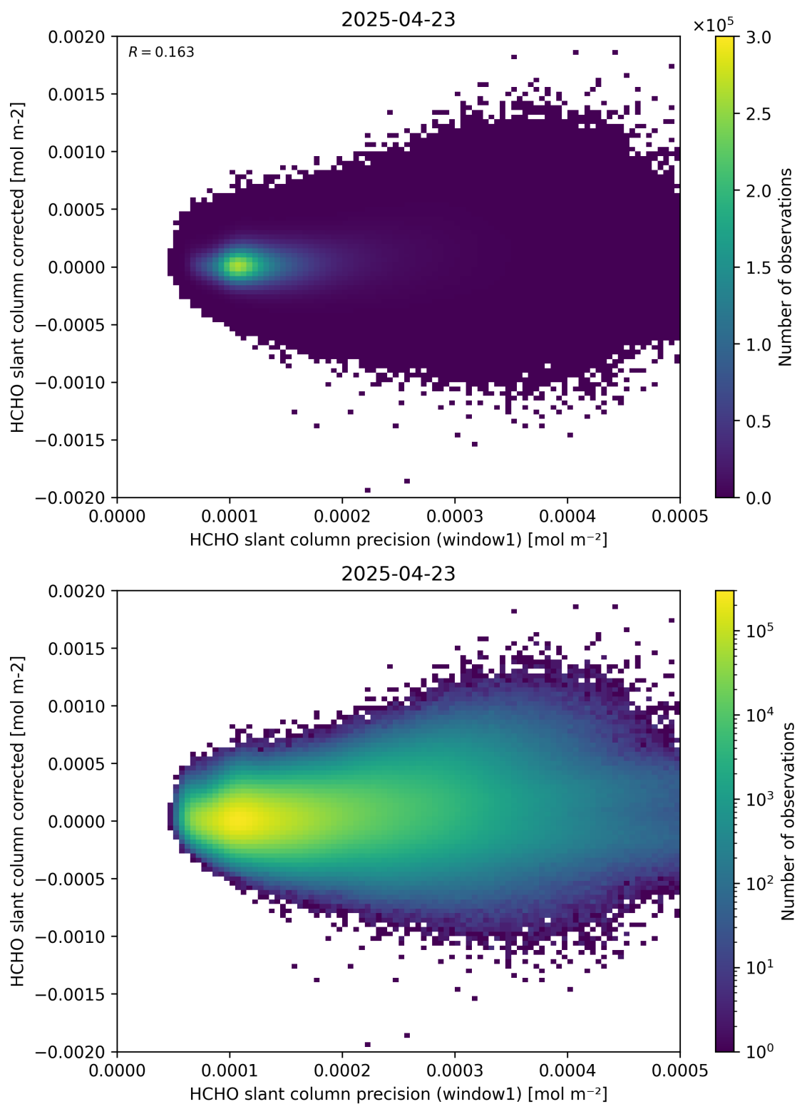
Figure 92: Scatter density plot of “HCHO slant column precision (window1)” against “HCHO slant column corrected” for 2025-04-22 to 2025-04-24.
