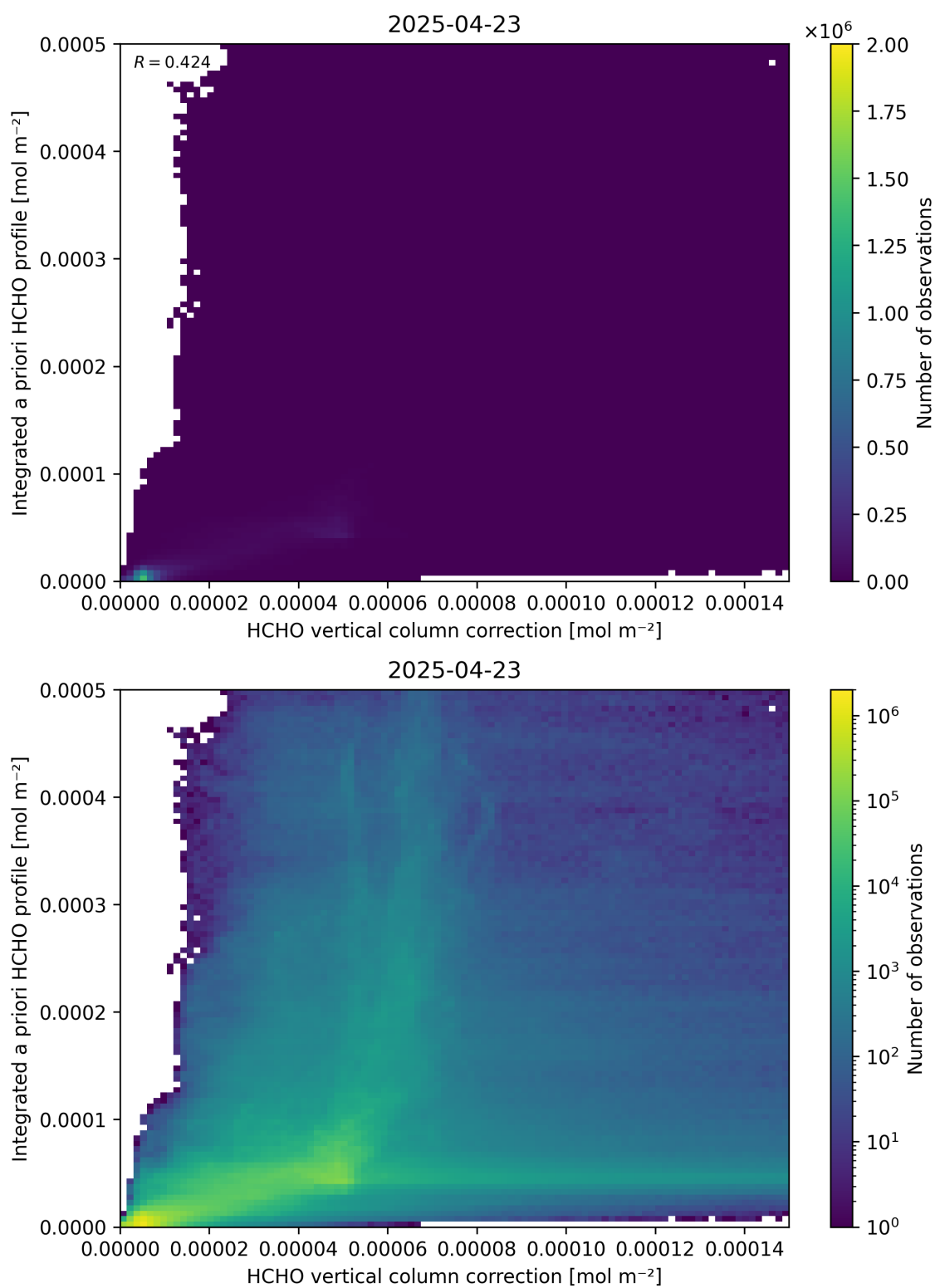
Figure 122: Scatter density plot of “HCHO vertical column correction” against “Integrated a priori HCHO profile” for 2025-04-22 to 2025-04-24.
