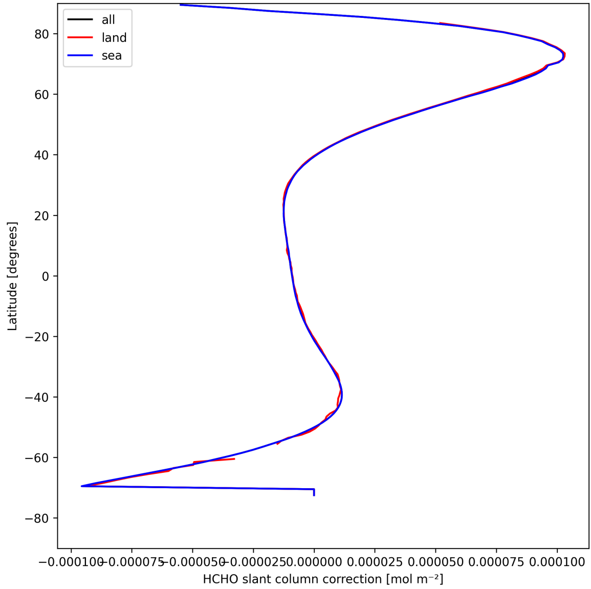
Figure 33: Zonal average of “HCHO slant column correction” for 2025-04-22 to 2025-04-24.
