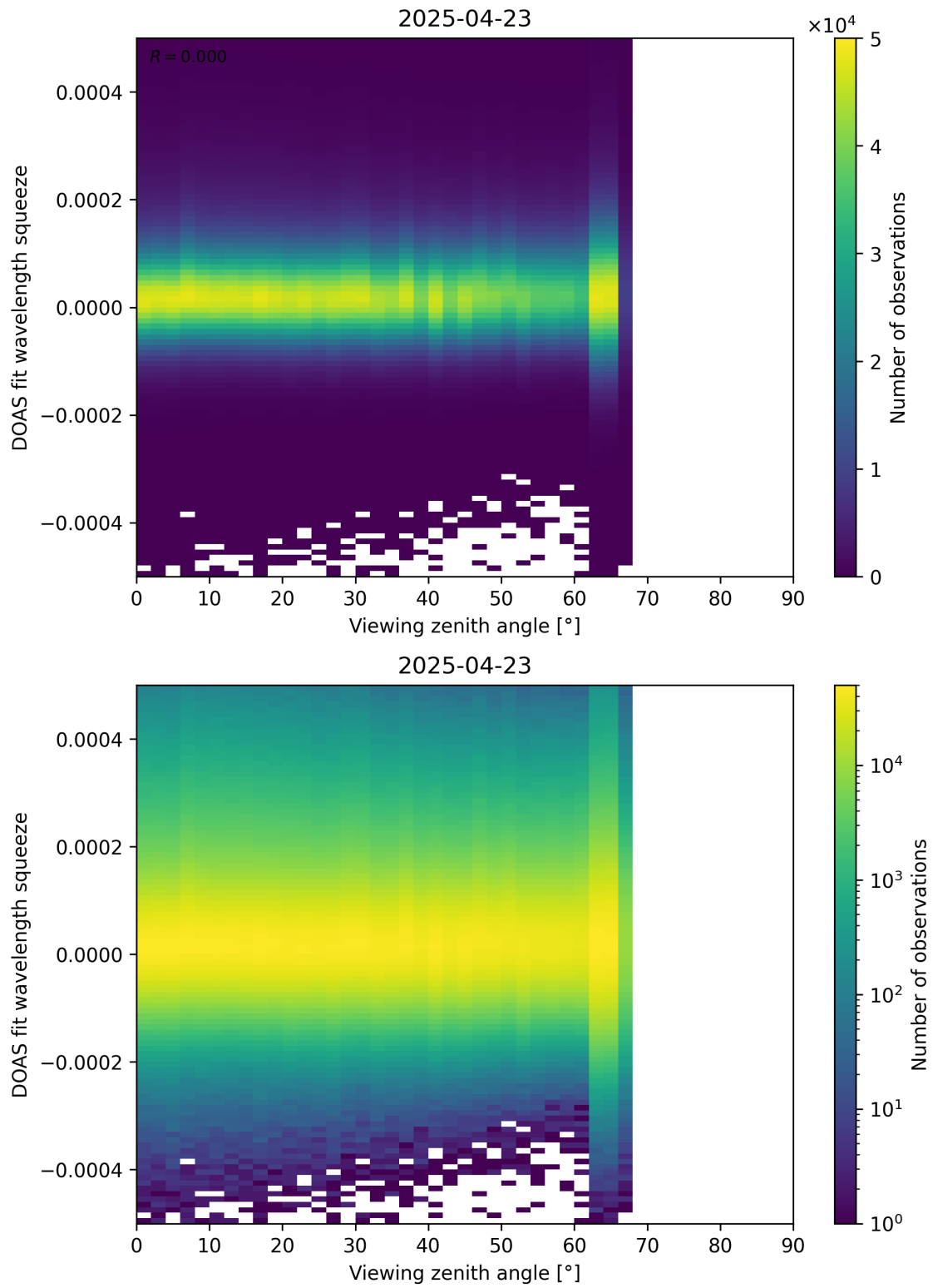
Figure 184: Scatter density plot of “Viewing zenith angle” against “DOAS fit wavelength squeeze” for 2025-04-22 to 2025-04-24.
