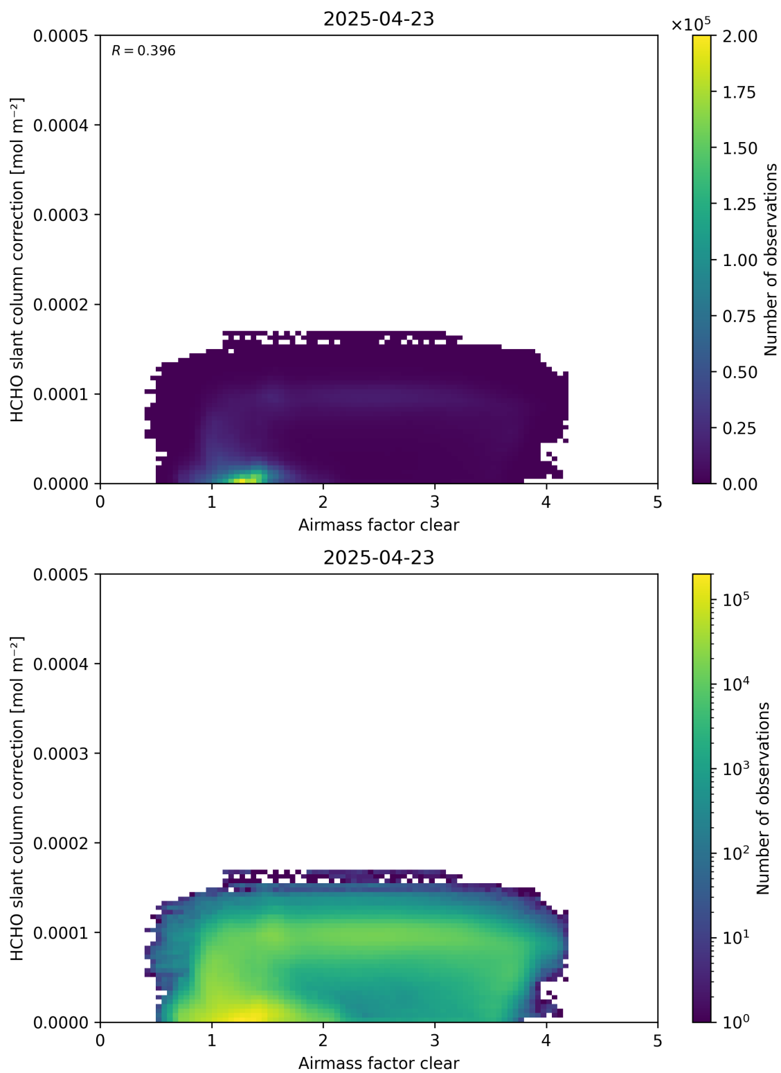
Figure 75: Scatter density plot of “Airmass factor clear” against “HCHO slant column correction” for 2025-04-22 to 2025-04-24.
