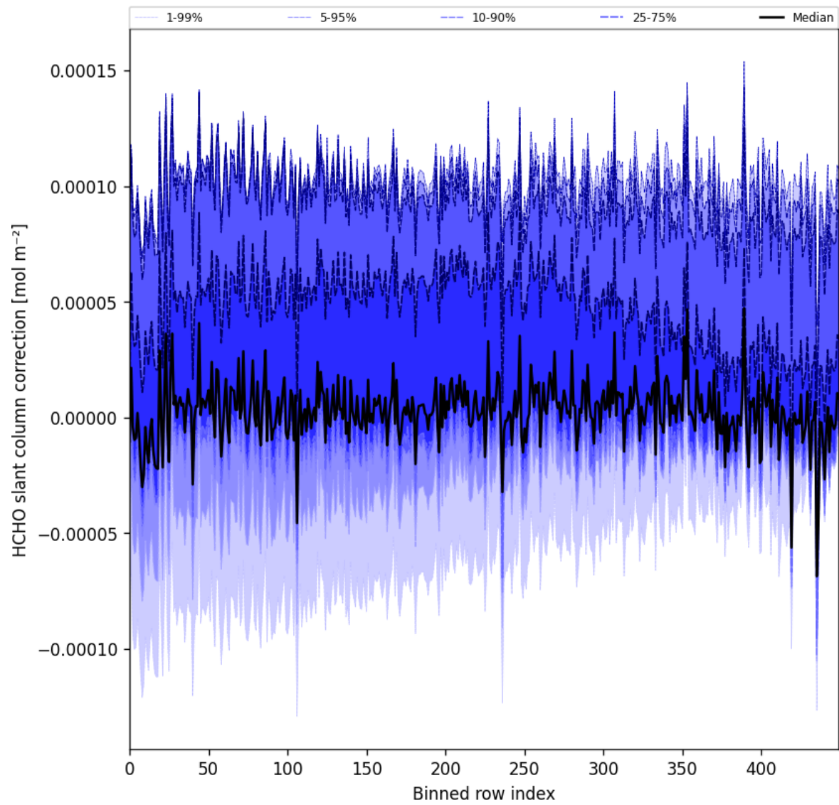
Figure 61: Along track statistics of “HCHO slant column correction” for 2025-04-22 to 2025-04-24
