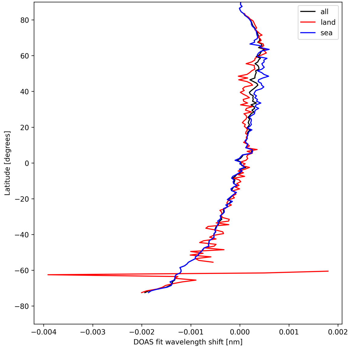
Figure 30: Zonal average of “DOAS fit wavelength shift” for 2025-04-22 to 2025-04-24.
