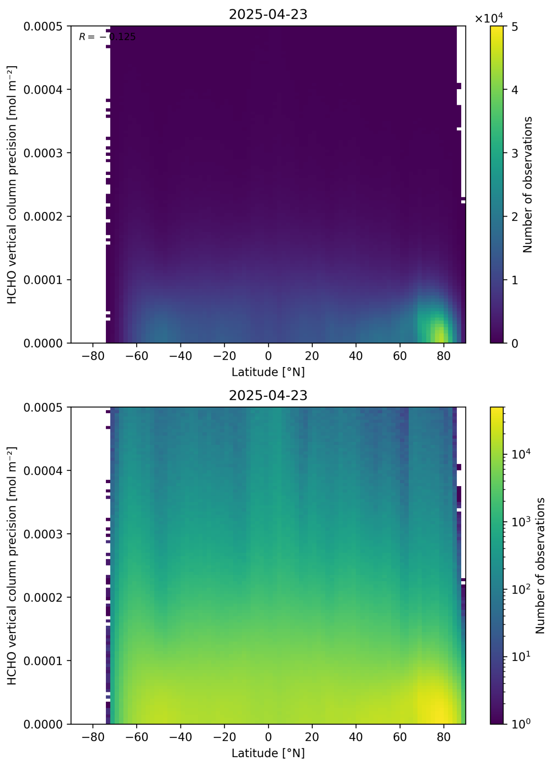
Figure 165: Scatter density plot of “Latitude” against “HCHO vertical column precision” for 2025-04-22 to 2025-04-24.
