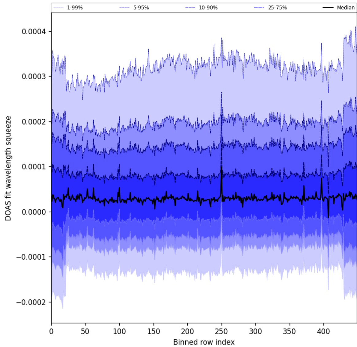
Figure 59: Along track statistics of “DOAS fit wavelength squeeze” for 2025-04-22 to 2025-04-24
