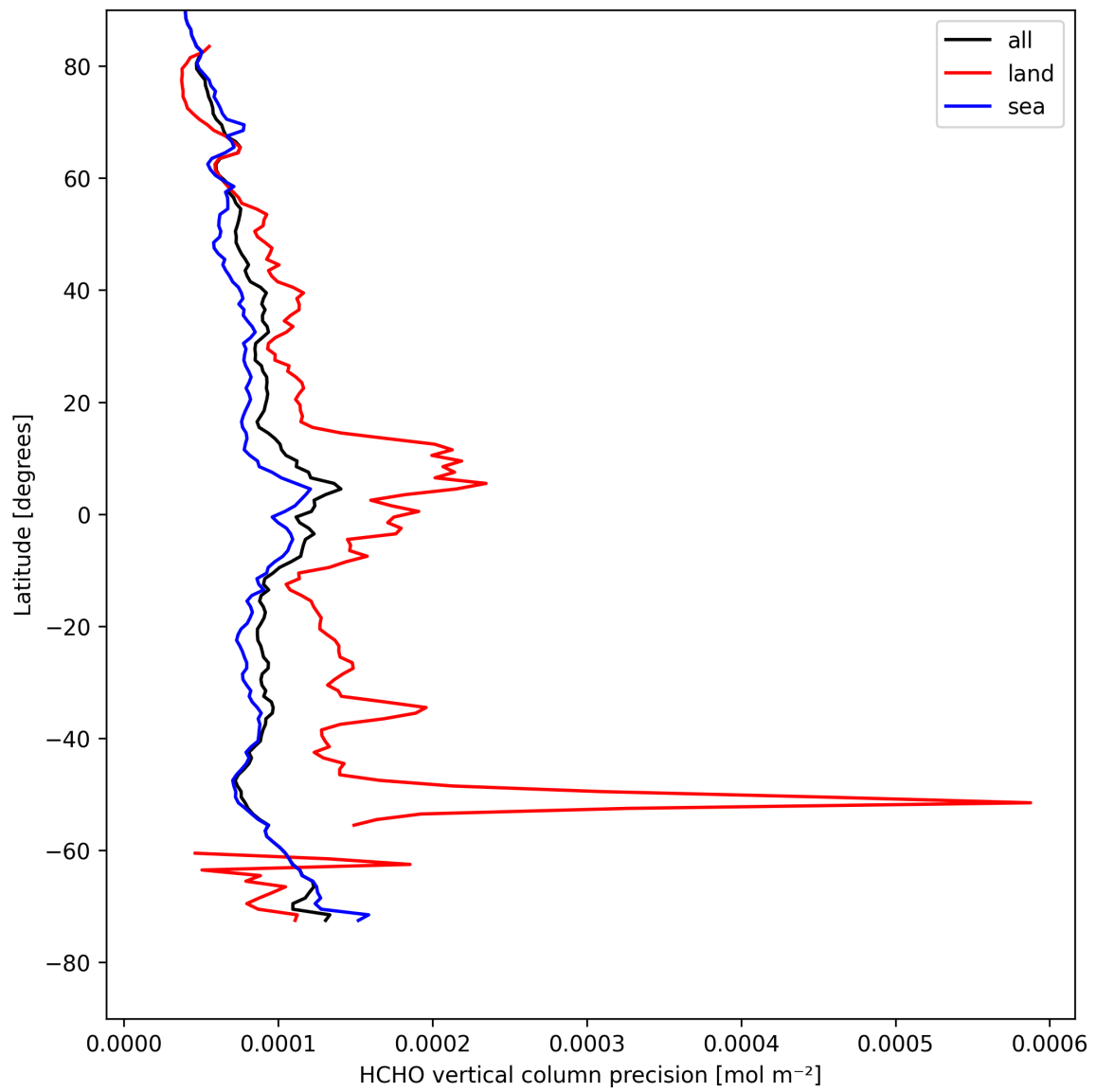
Figure 22: Zonal average of “HCHO vertical column precision” for 2025-04-22 to 2025-04-24.
