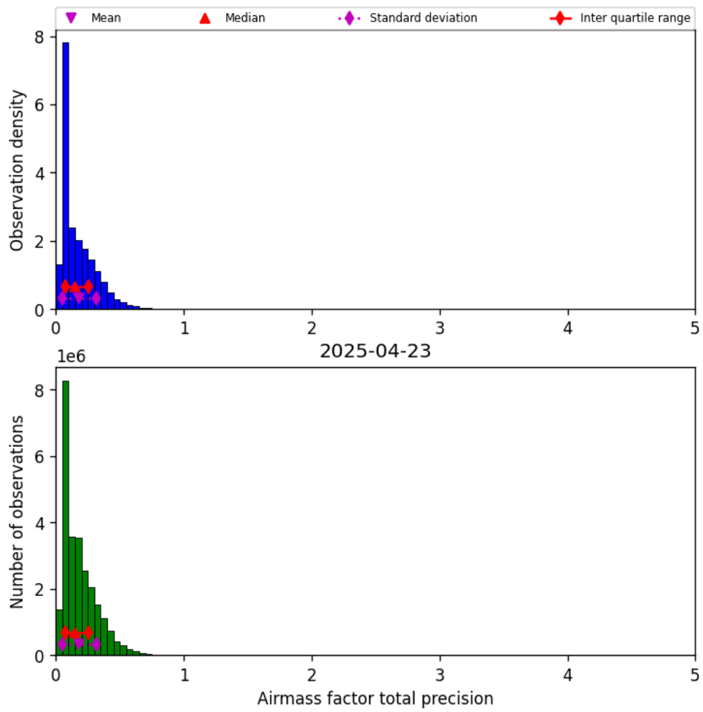
Figure 41: Histogram of “Airmass factor total precision” for 2025-04-22 to 2025-04-24
