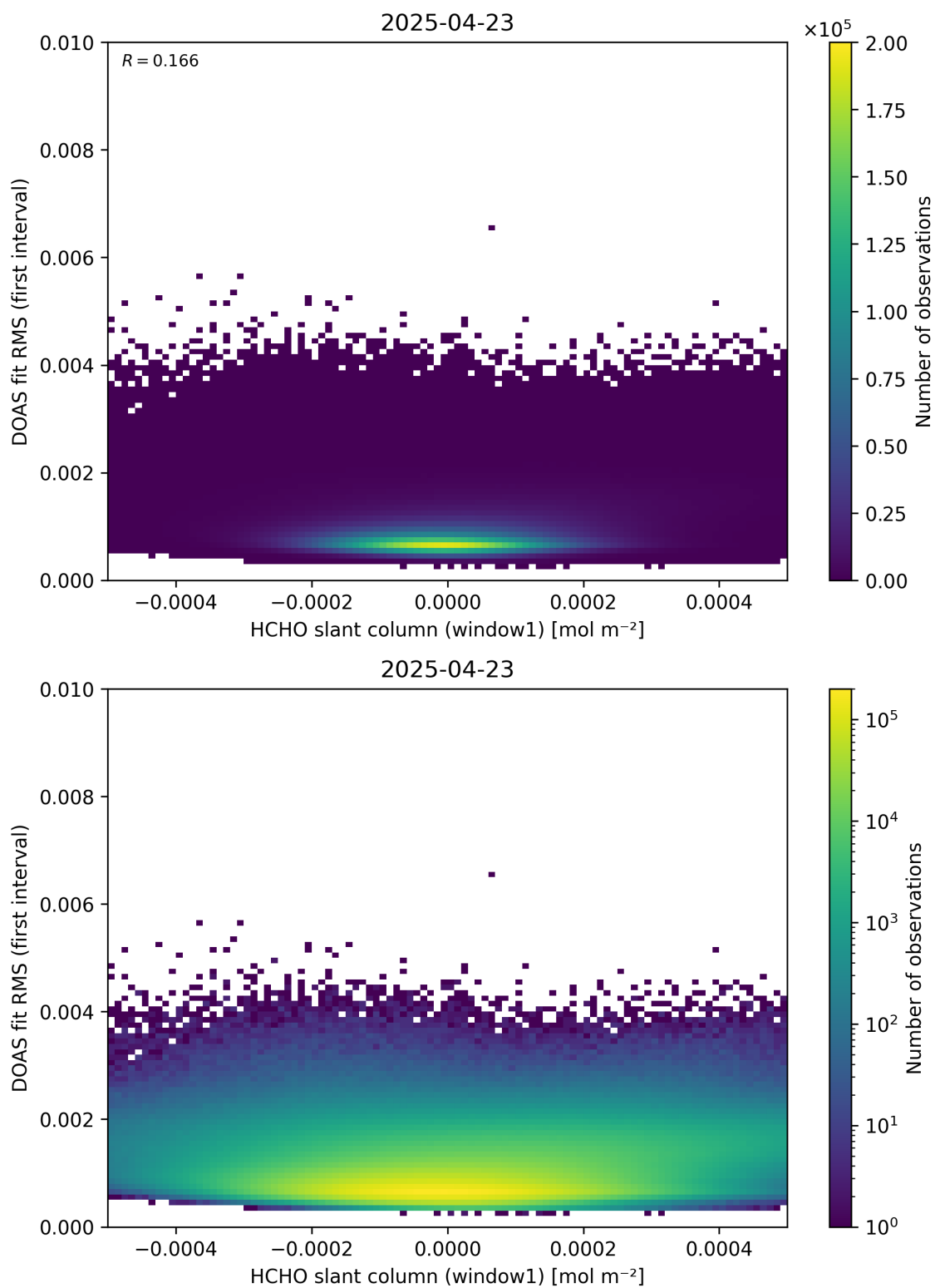
Figure 78: Scatter density plot of “HCHO slant column (window1)” against “DOAS fit RMS (first interval)” for 2025-04-22 to 2025-04-24.
