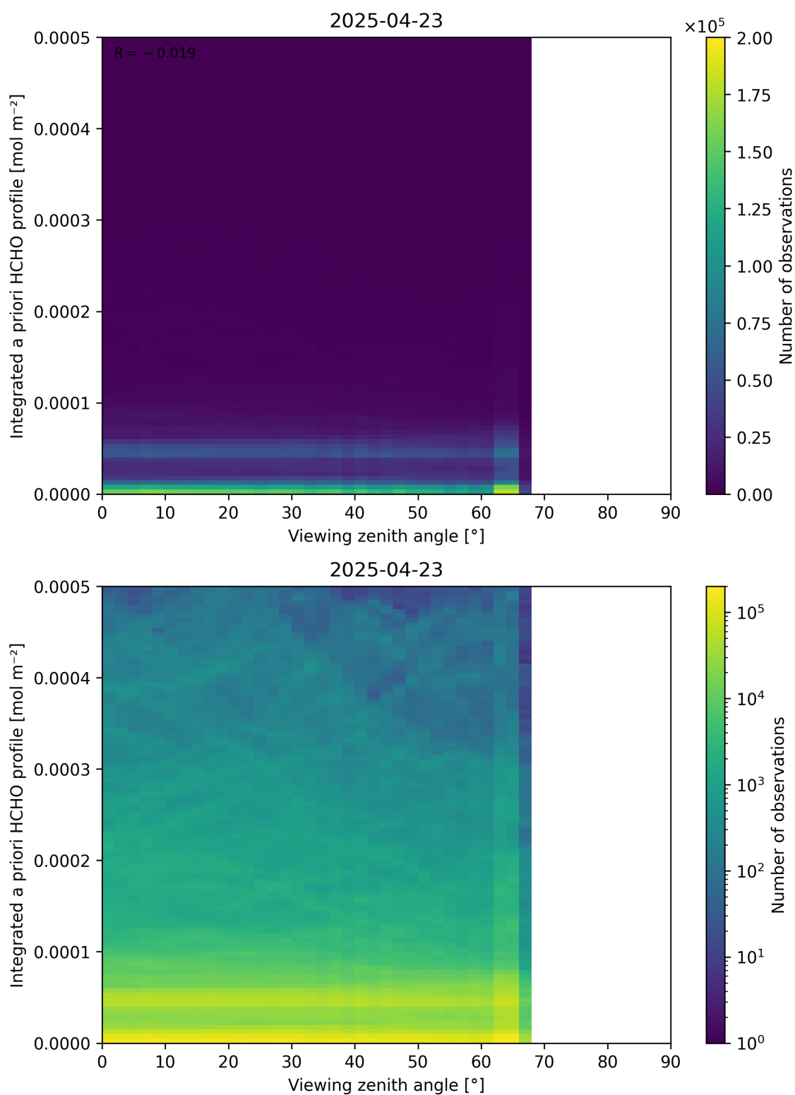
Figure 195: Scatter density plot of “Viewing zenith angle” against “Integrated a priori HCHO profile” for 2025-04-22 to 2025-04-24.
