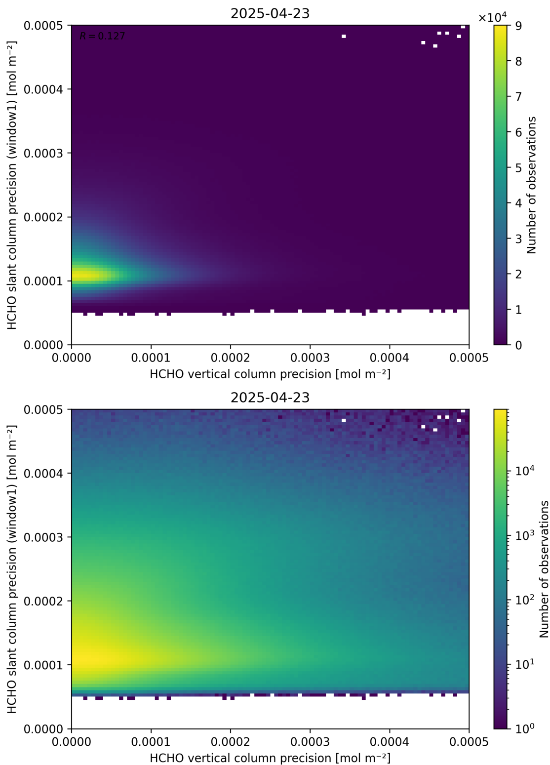
Figure 143: Scatter density plot of “HCHO vertical column precision” against “HCHO slant column precision (window1)” for 2025-04-22 to 2025-04-24.
