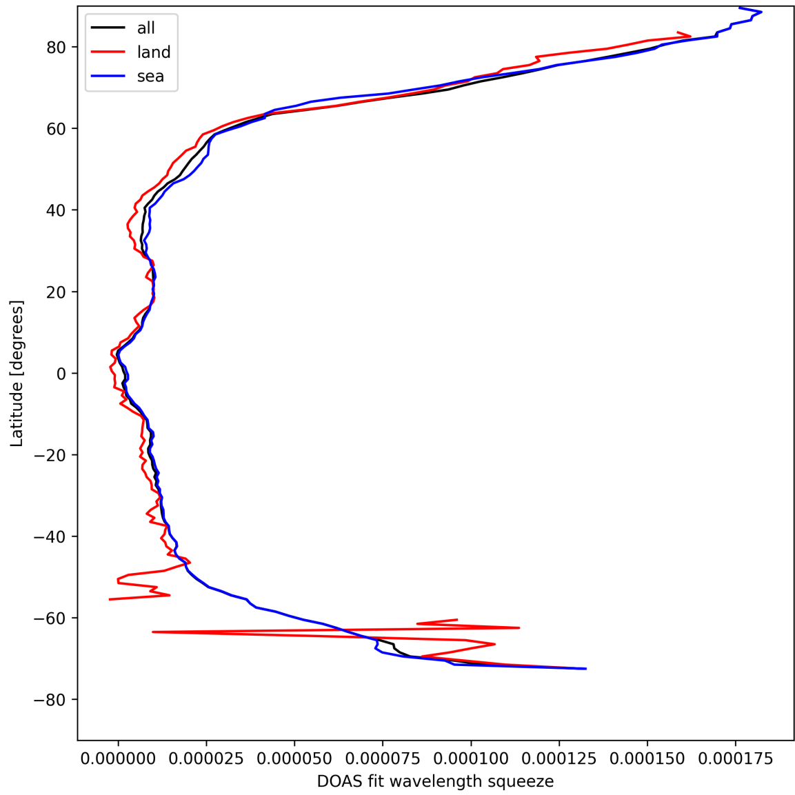
Figure 31: Zonal average of “DOAS fit wavelength squeeze” for 2025-04-22 to 2025-04-24.
