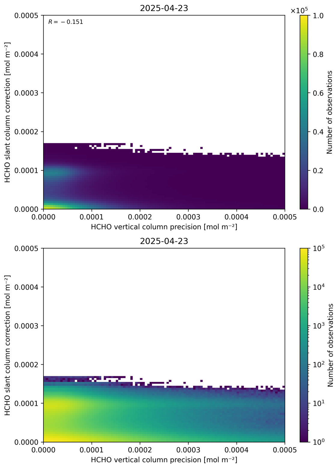
Figure 141: Scatter density plot of “HCHO vertical column precision” against “HCHO slant column correction” for 2025-04-22 to 2025-04-24.
