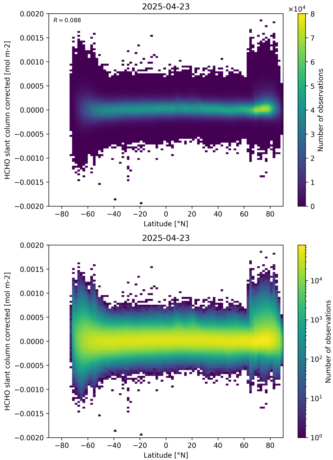
Figure 157: Scatter density plot of “Latitude” against “HCHO slant column corrected” for 2025-04-22 to 2025-04-24.
