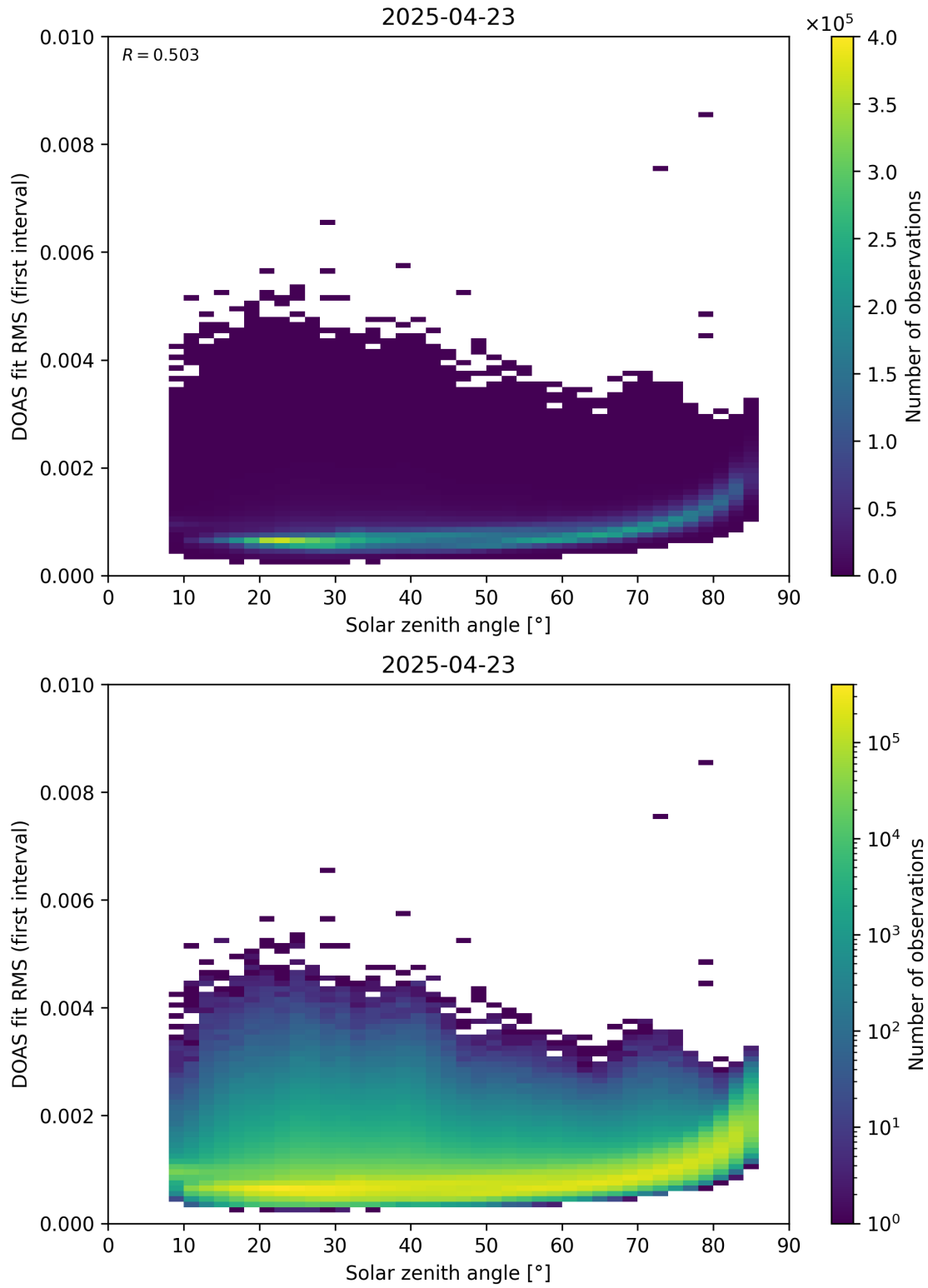
Figure 167: Scatter density plot of “Solar zenith angle” against “DOAS fit RMS (first interval)” for 2025-04-22 to 2025-04-24.
