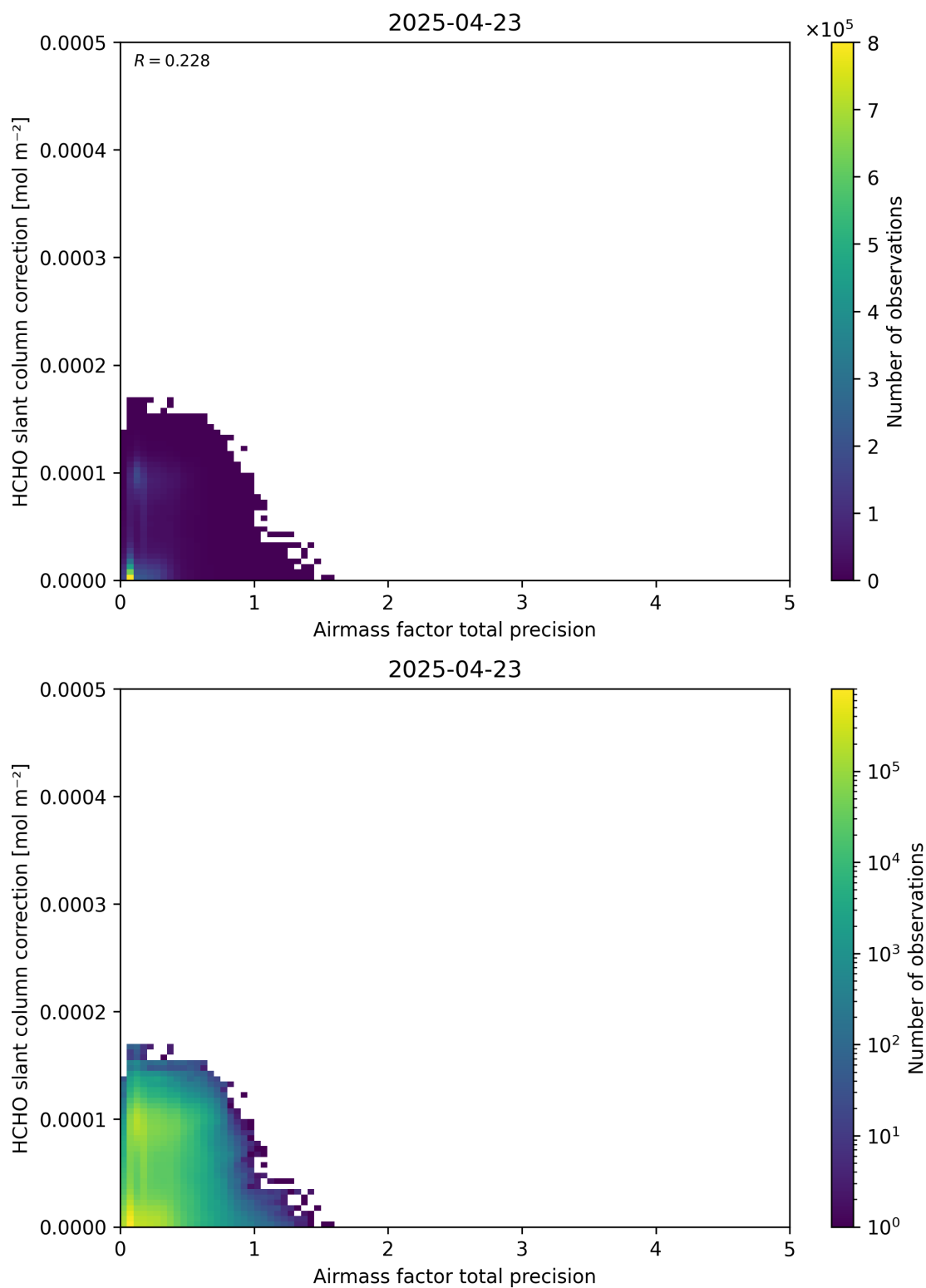
Figure 110: Scatter density plot of “Airmass factor total precision” against “HCHO slant column correction” for 2025-04-22 to 2025-04-24.
