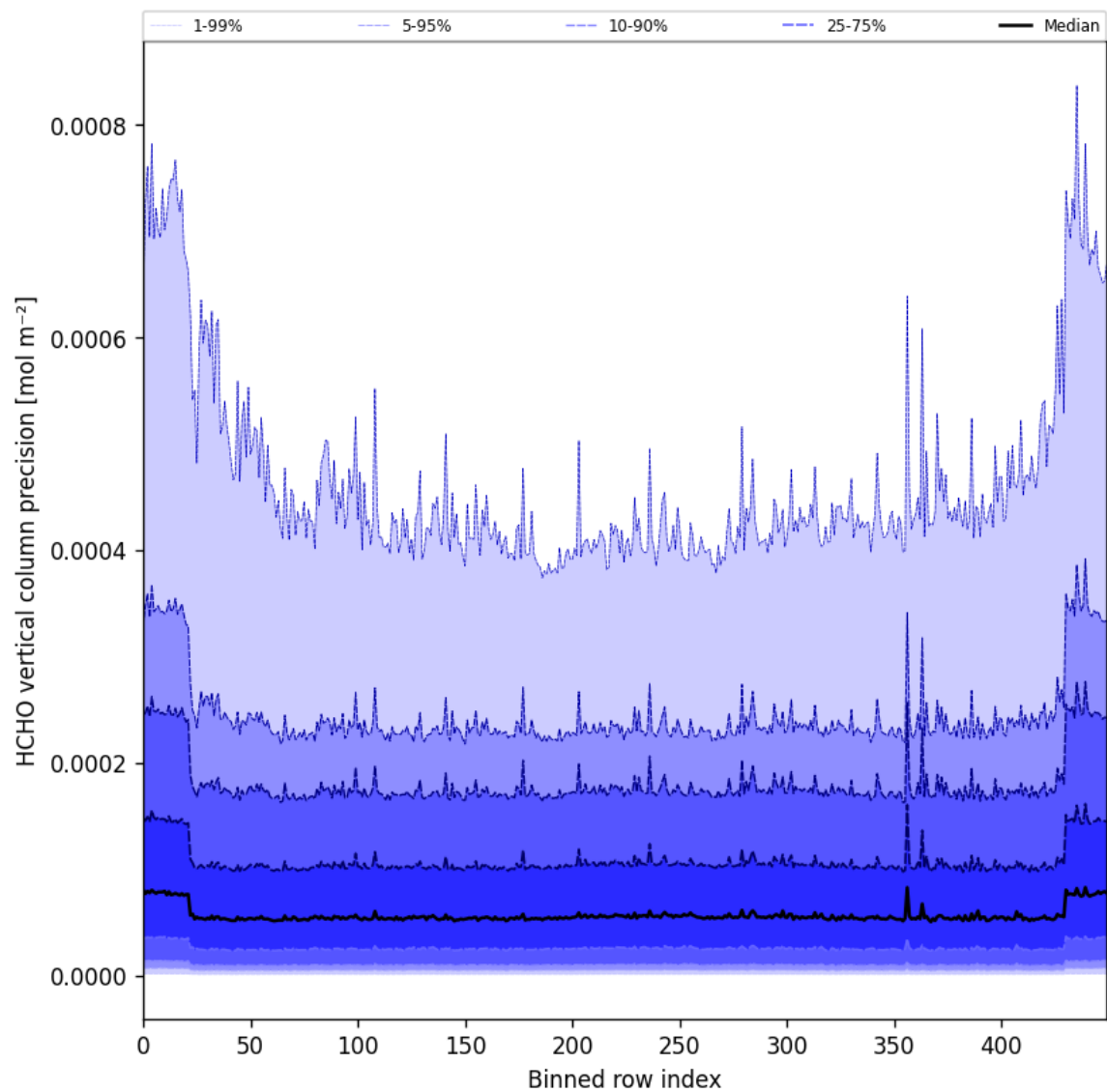
Figure 50: Along track statistics of “HCHO vertical column precision” for 2025-04-22 to 2025-04-24
