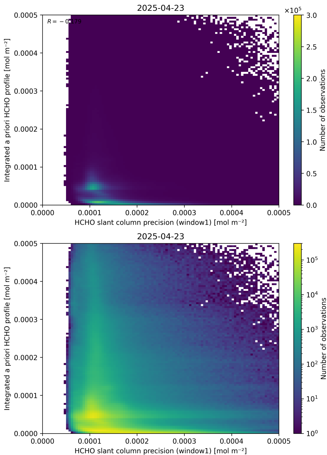
Figure 96: Scatter density plot of “HCHO slant column precision (window1)” against “Integrated a priori HCHO profile” for 2025-04-22 to 2025-04-24.
