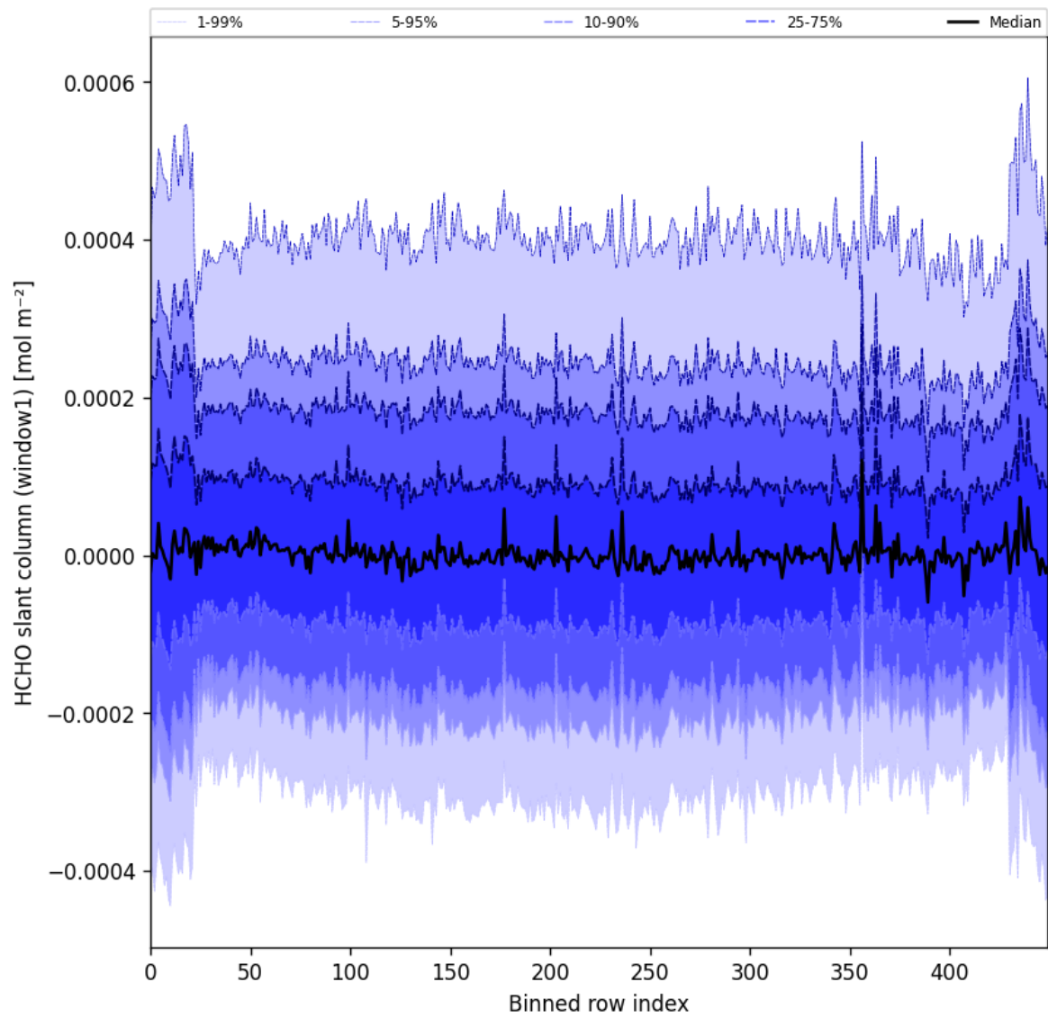
Figure 52: Along track statistics of “HCHO slant column (window1)” for 2025-04-22 to 2025-04-24
