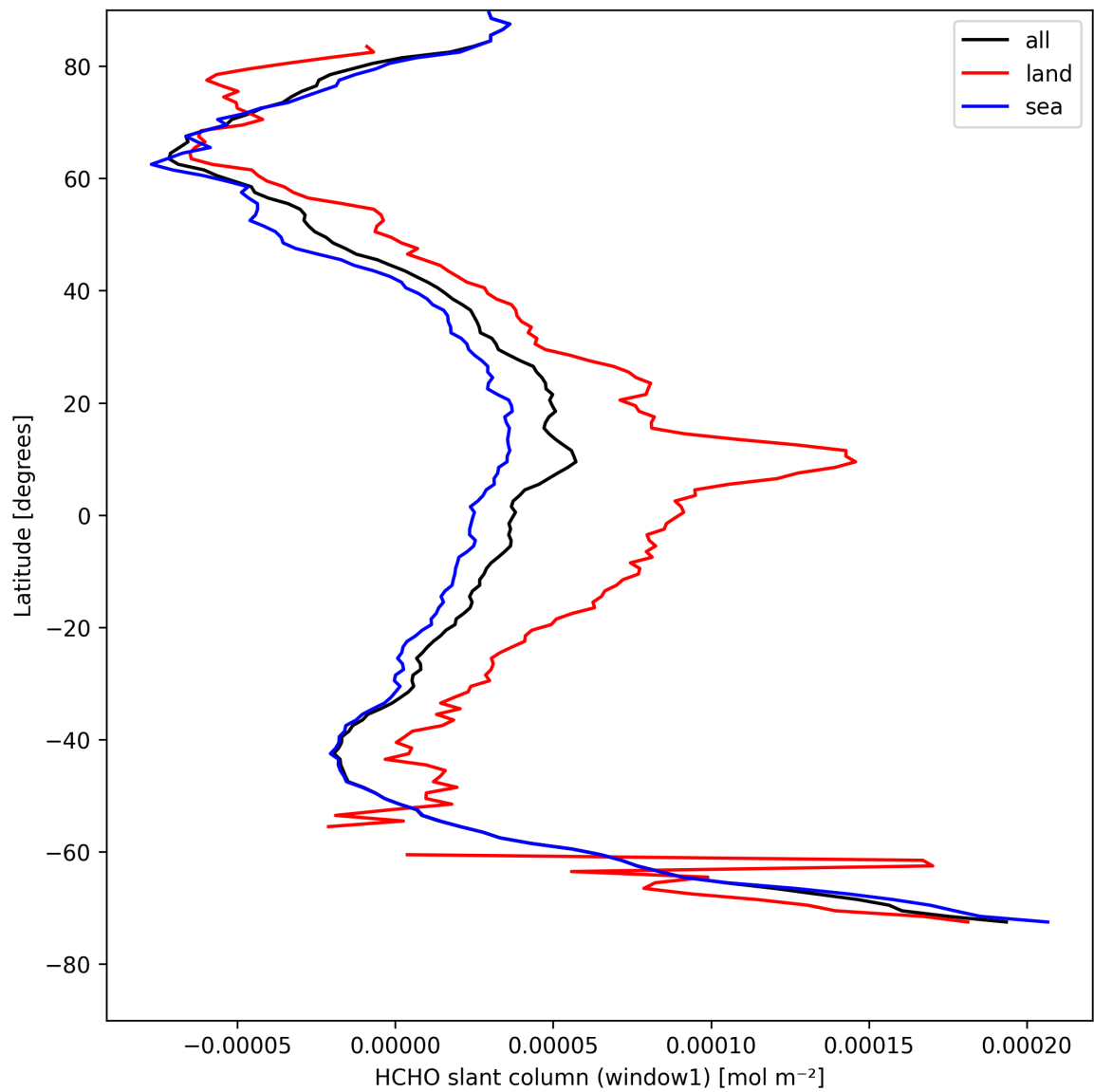
Figure 24: Zonal average of “HCHO slant column (window1)” for 2025-04-22 to 2025-04-24.
