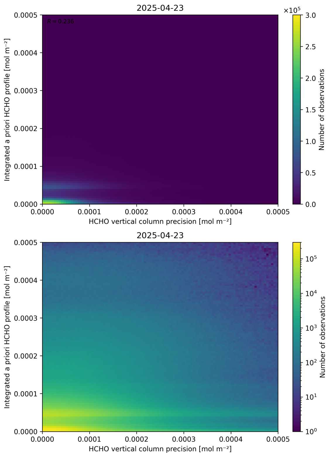
Figure 147: Scatter density plot of “HCHO vertical column precision” against “Integrated a priori HCHO profile” for 2025-04-22 to 2025-04-24.
