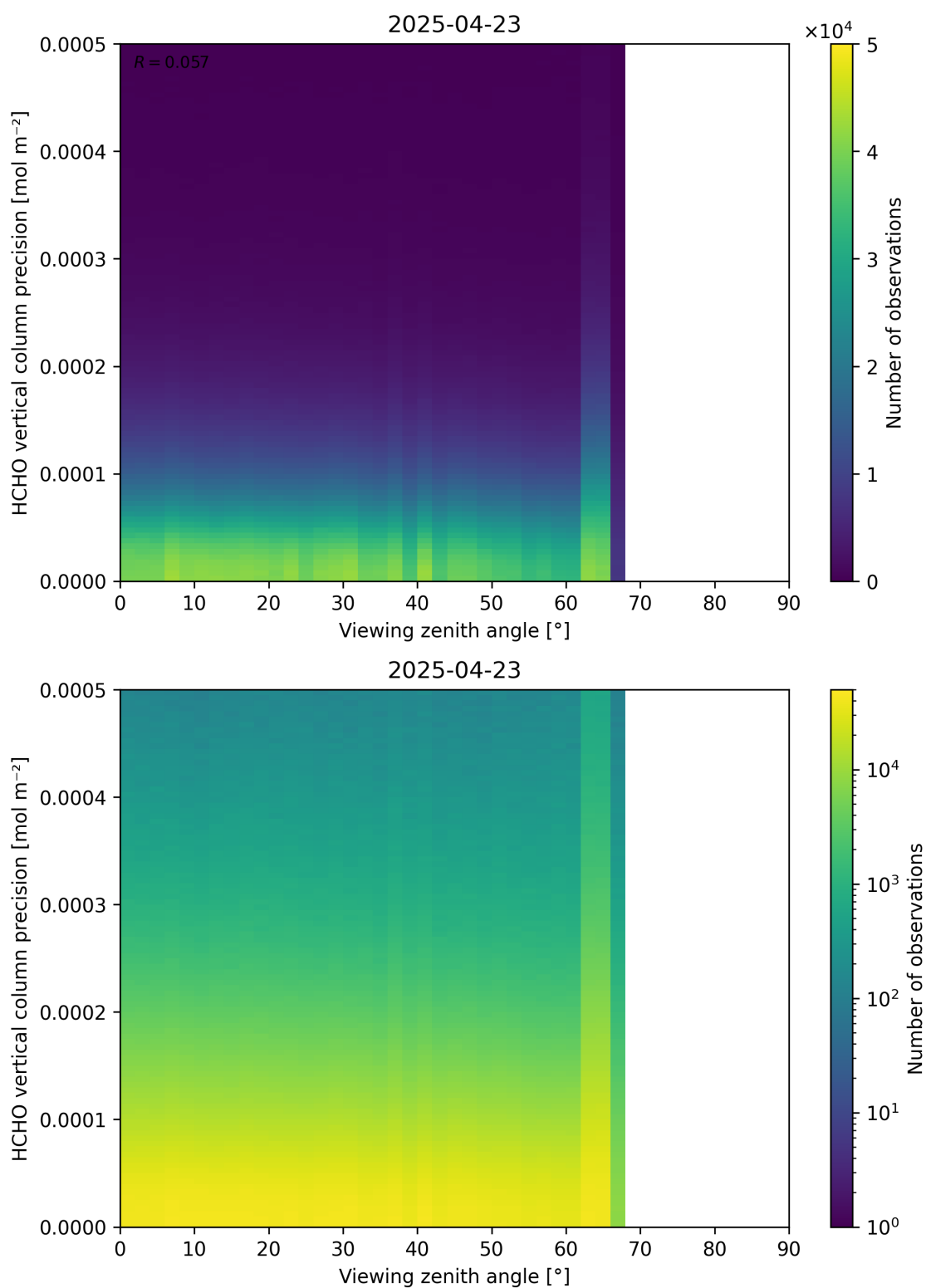
Figure 194: Scatter density plot of “Viewing zenith angle” against “HCHO vertical column precision” for 2025-04-22 to 2025-04-24.
