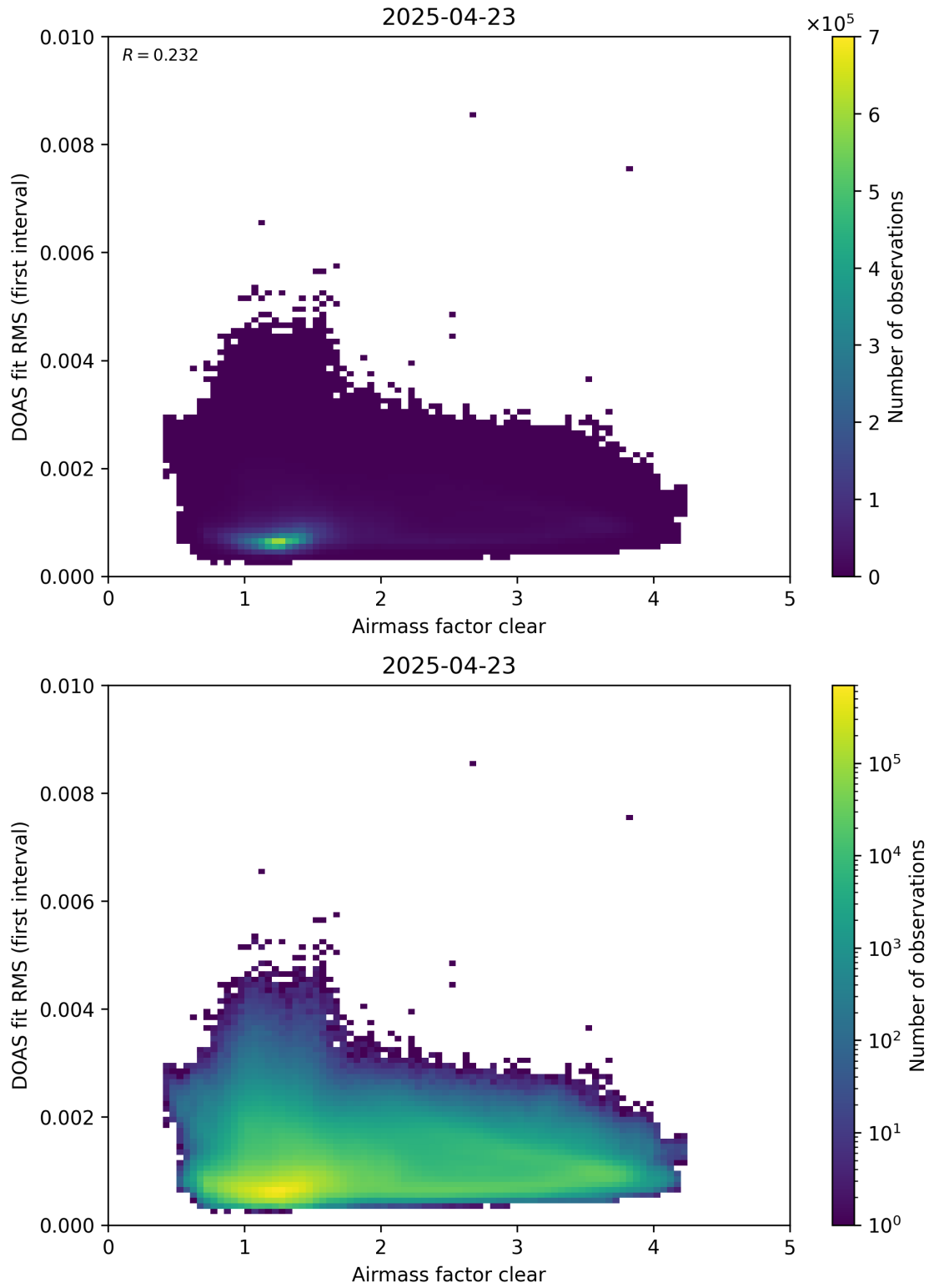
Figure 71: Scatter density plot of “Airmass factor clear” against “DOAS fit RMS (first interval)” for 2025-04-22 to 2025-04-24.
