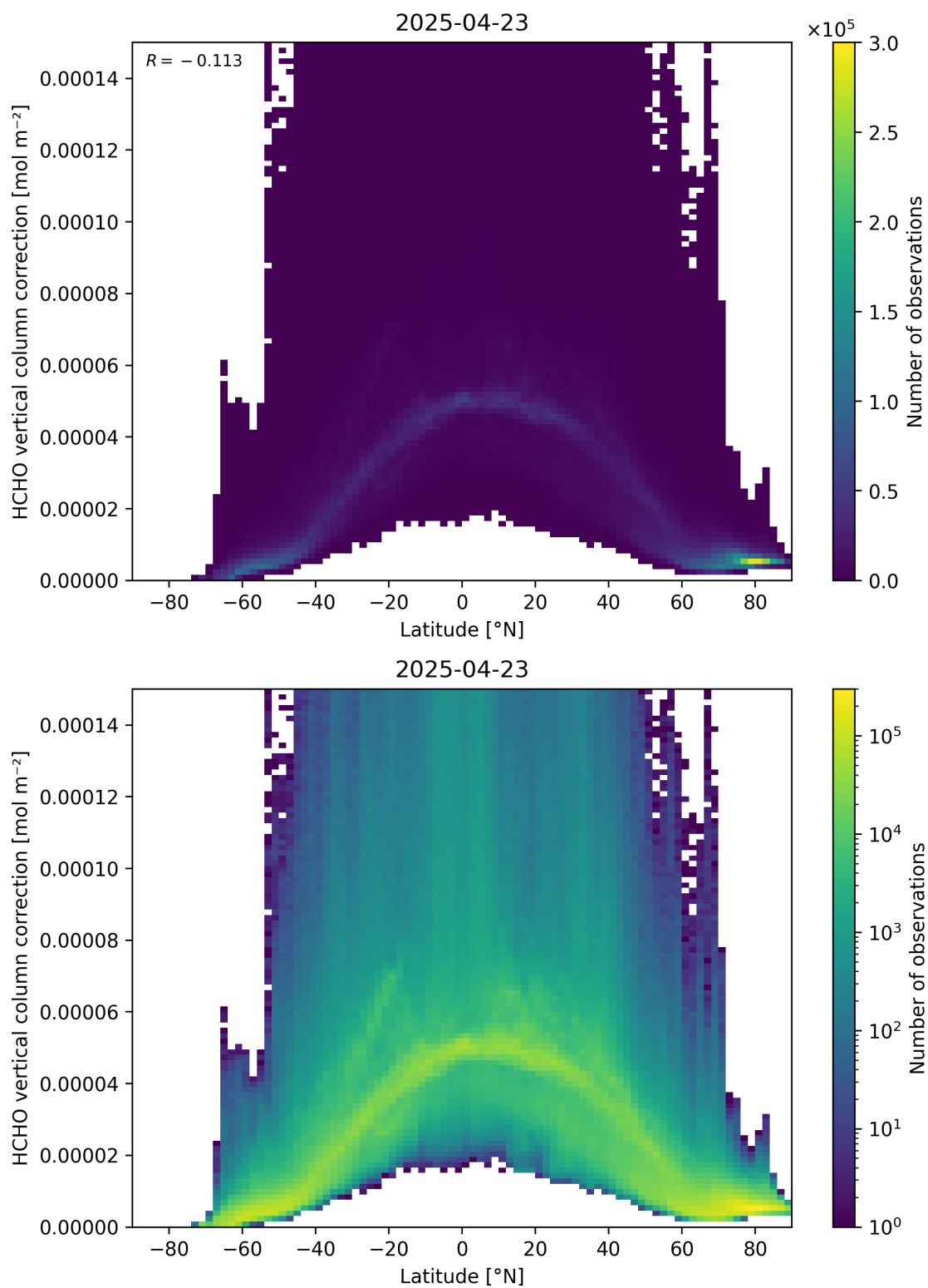
Figure 164: Scatter density plot of “Latitude” against “HCHO vertical column correction” for 2025-04-22 to 2025-04-24.
