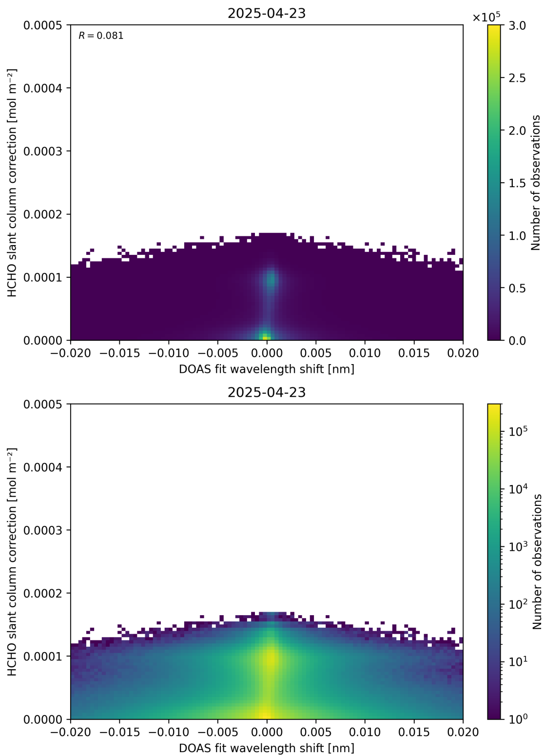
Figure 67: Scatter density plot of “DOAS fit wavelength shift” against “HCHO slant column correction” for 2025-04-22 to 2025-04-24.
