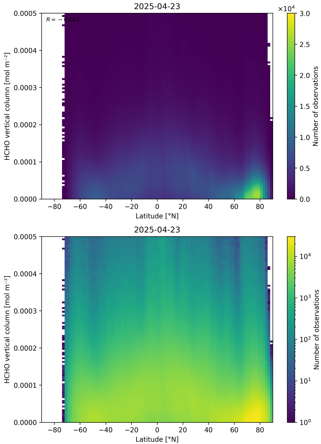
Figure 163: Scatter density plot of “Latitude” against “HCHO vertical column” for 2025-04-22 to 2025-04-24.
