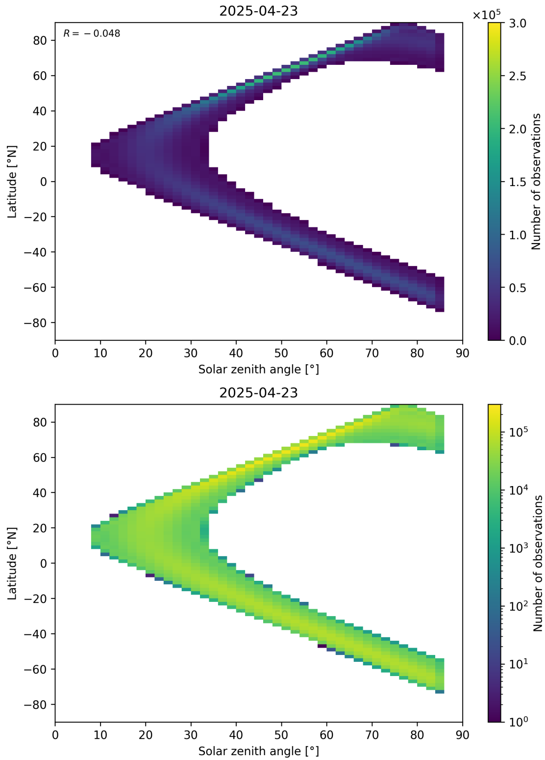
Figure 181: Scatter density plot of “Solar zenith angle” against “Latitude” for 2025-04-22 to 2025-04-24.
