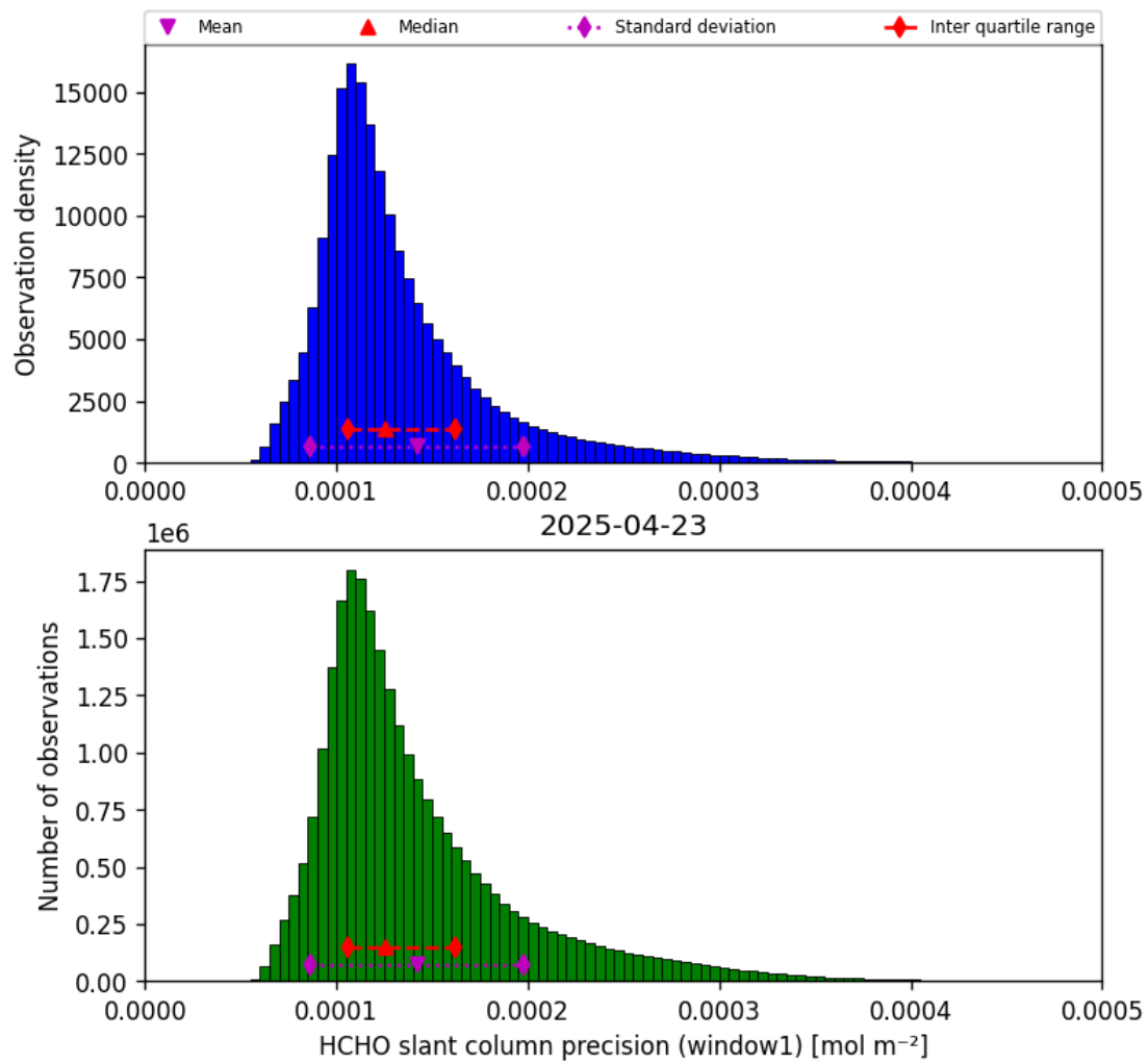
Figure 39: Histogram of “HCHO slant column precision (window1)” for 2025-04-22 to 2025-04-24
