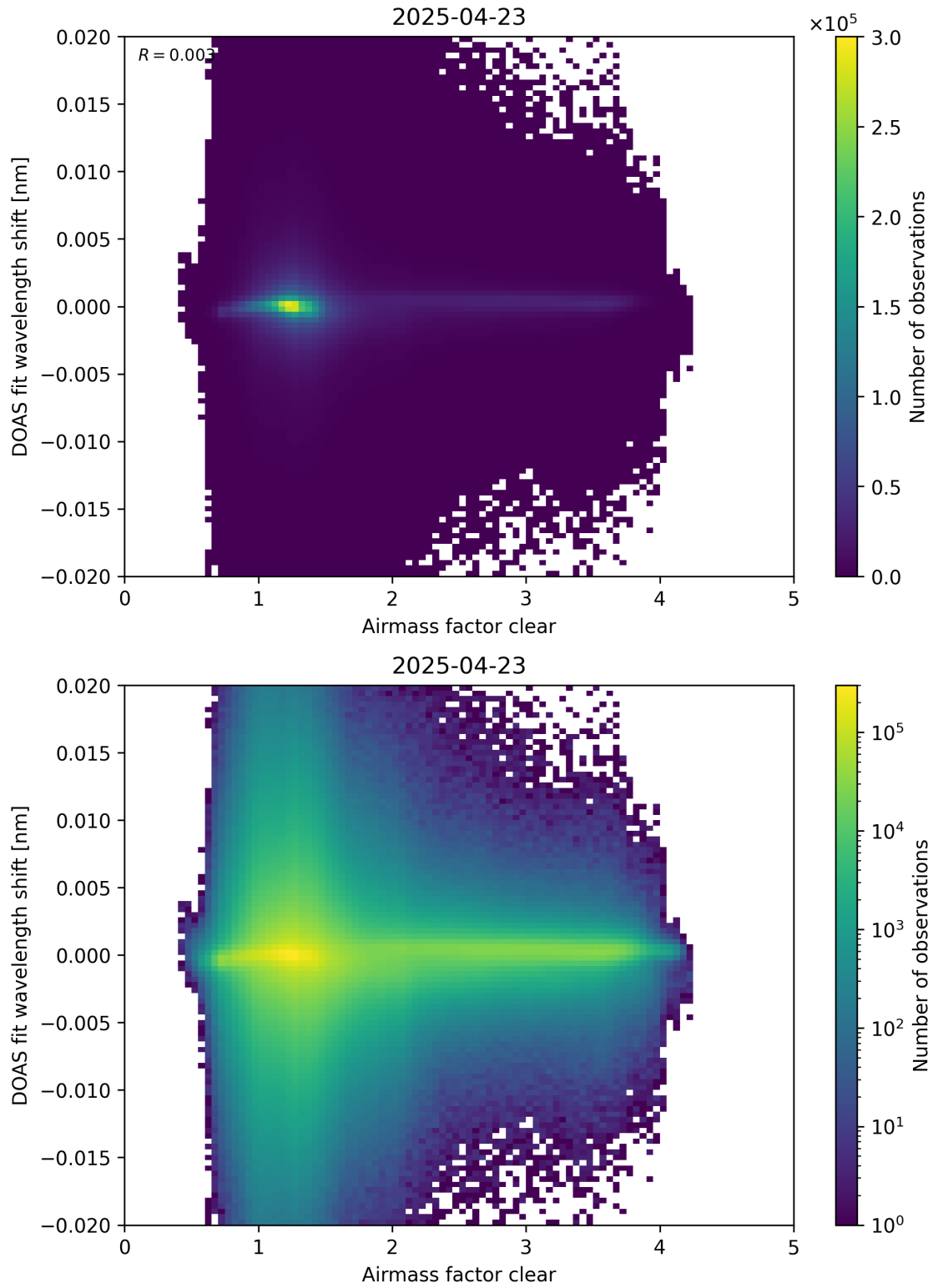
Figure 72: Scatter density plot of “Airmass factor clear” against “DOAS fit wavelength shift” for 2025-04-22 to 2025-04-24.
