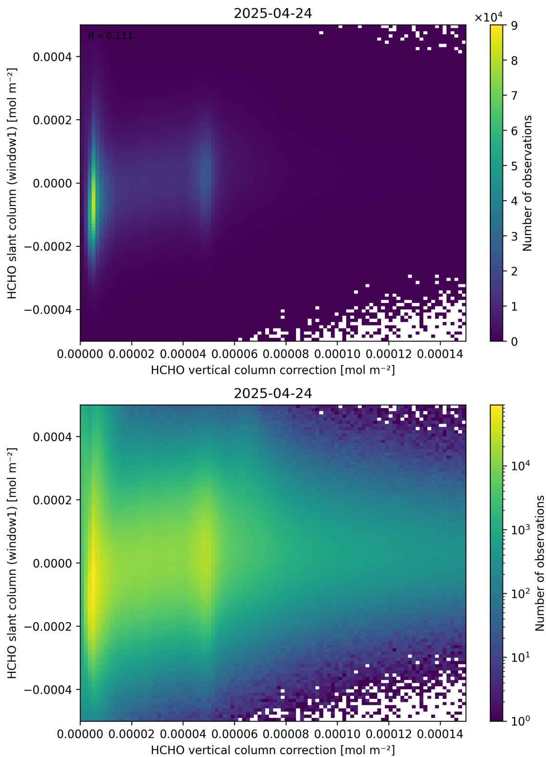
Figure 118: Scatter density plot of “HCHO vertical column correction” against “HCHO slant column (window1)” for 2025-04-24 to 2025-04-25.
