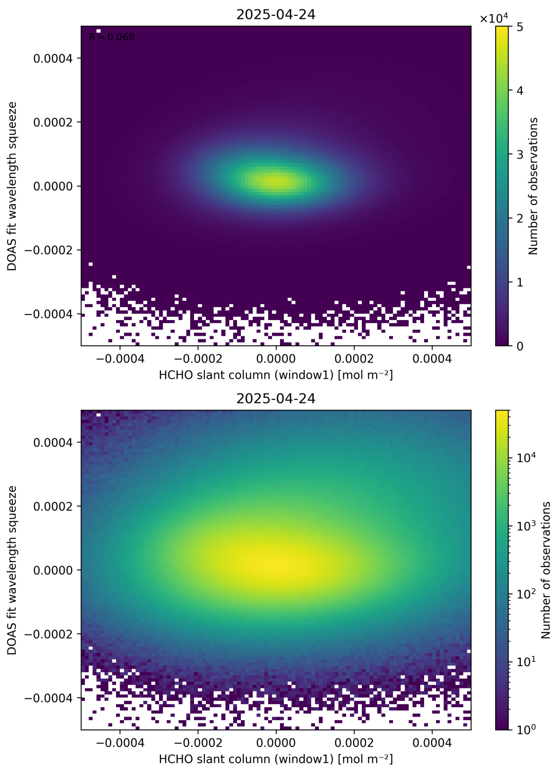
Figure 80: Scatter density plot of “HCHO slant column (window1)” against “DOAS fit wavelength squeeze” for 2025-04-24 to 2025-04-25.
