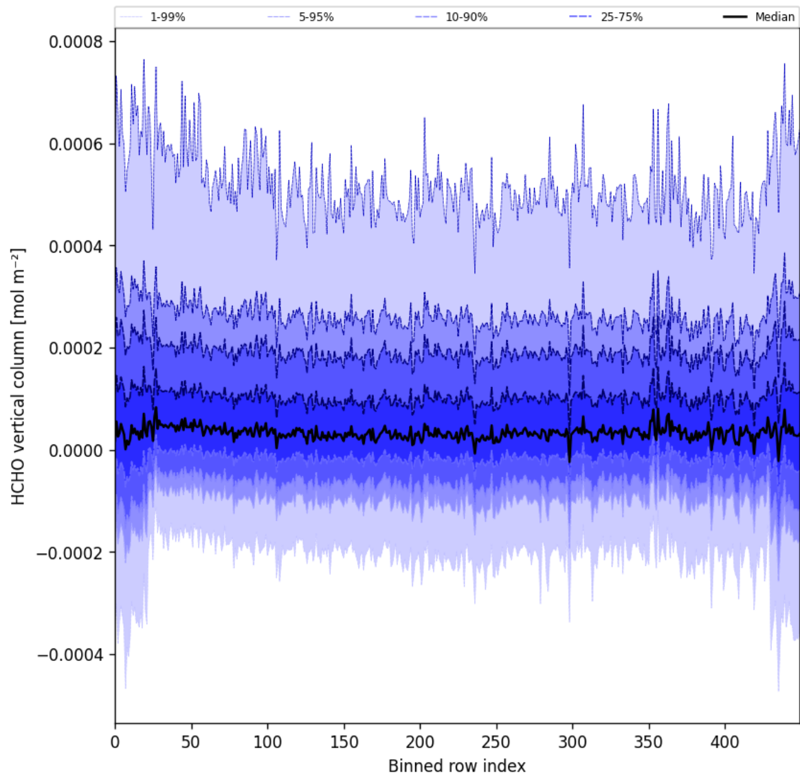
Figure 49: Along track statistics of “HCHO vertical column” for 2025-04-24 to 2025-04-25
