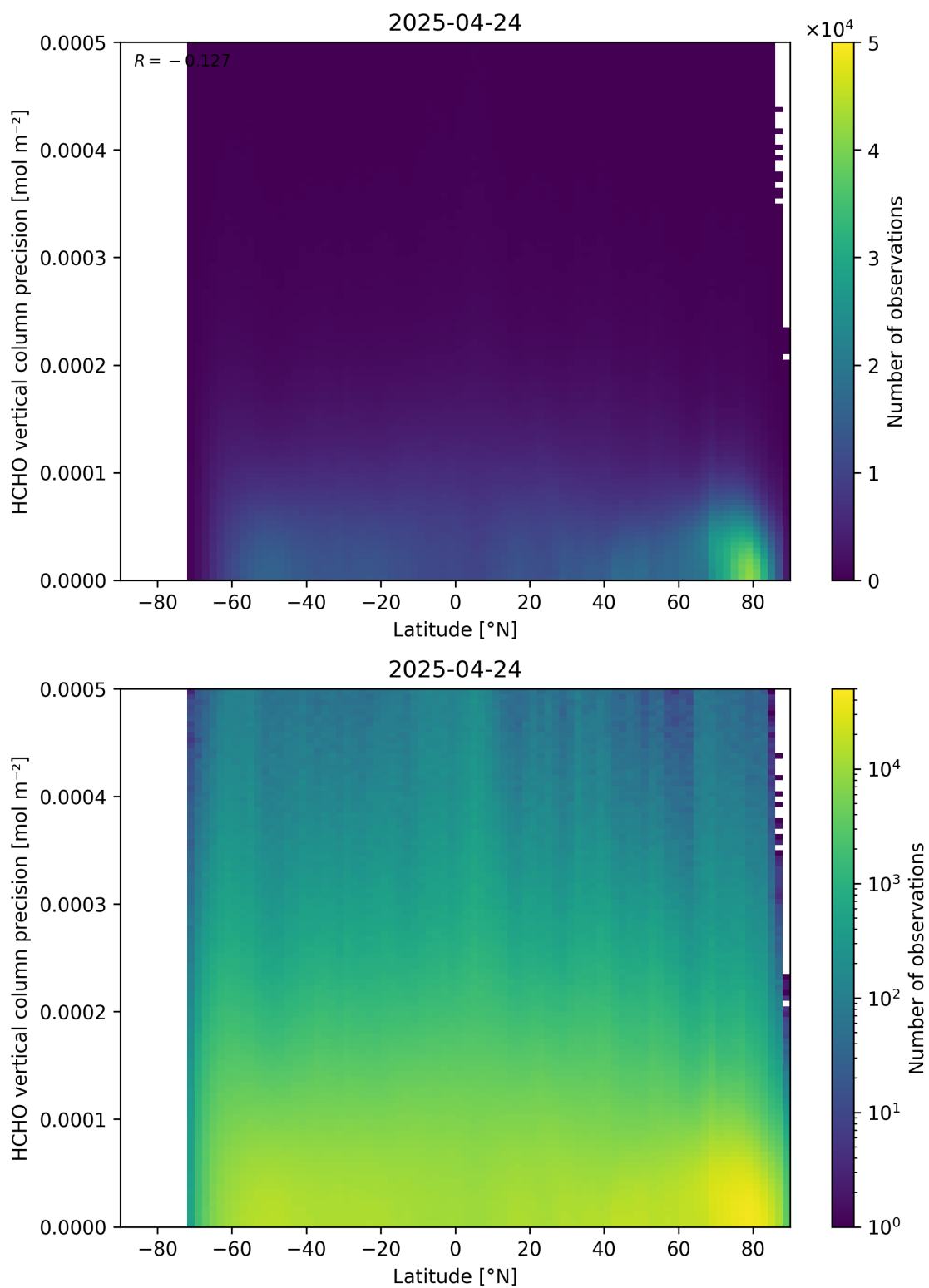
Figure 165: Scatter density plot of “Latitude” against “HCHO vertical column precision” for 2025-04-24 to 2025-04-25.
