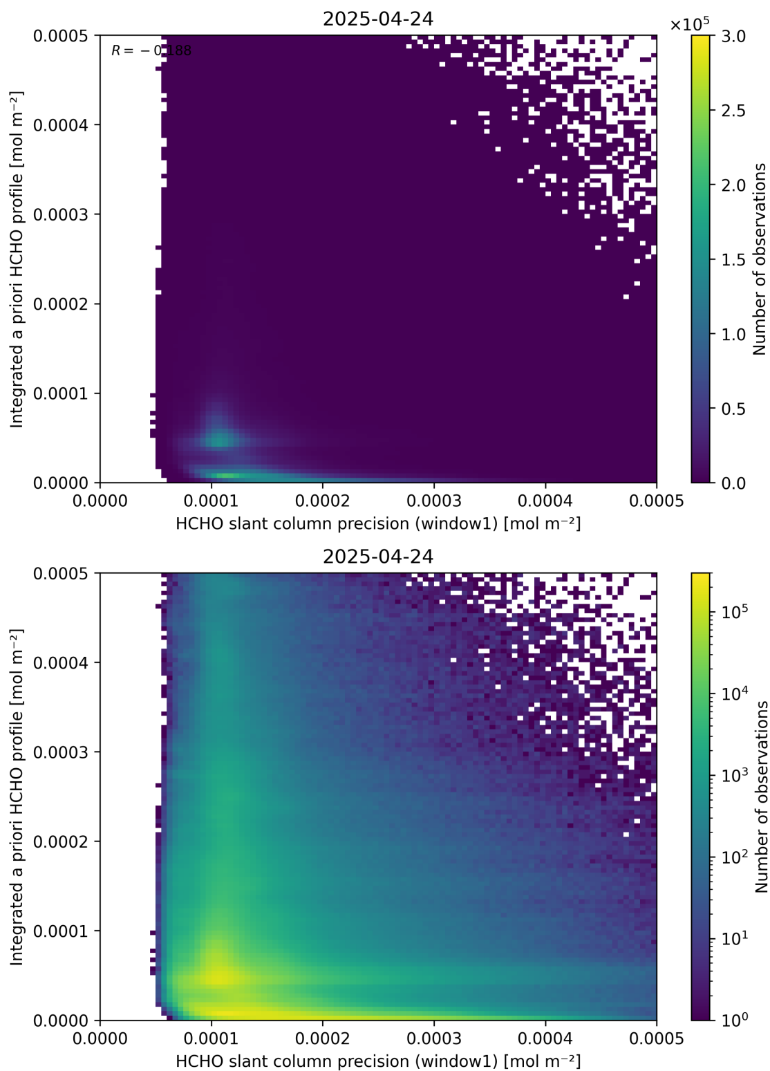
Figure 96: Scatter density plot of “HCHO slant column precision (window1)” against “Integrated a priori HCHO profile” for 2025-04-24 to 2025-04-25.
