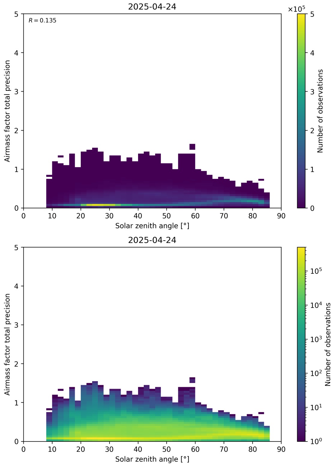
Figure 176: Scatter density plot of “Solar zenith angle” against “Airmass factor total precision” for 2025-04-24 to 2025-04-25.
