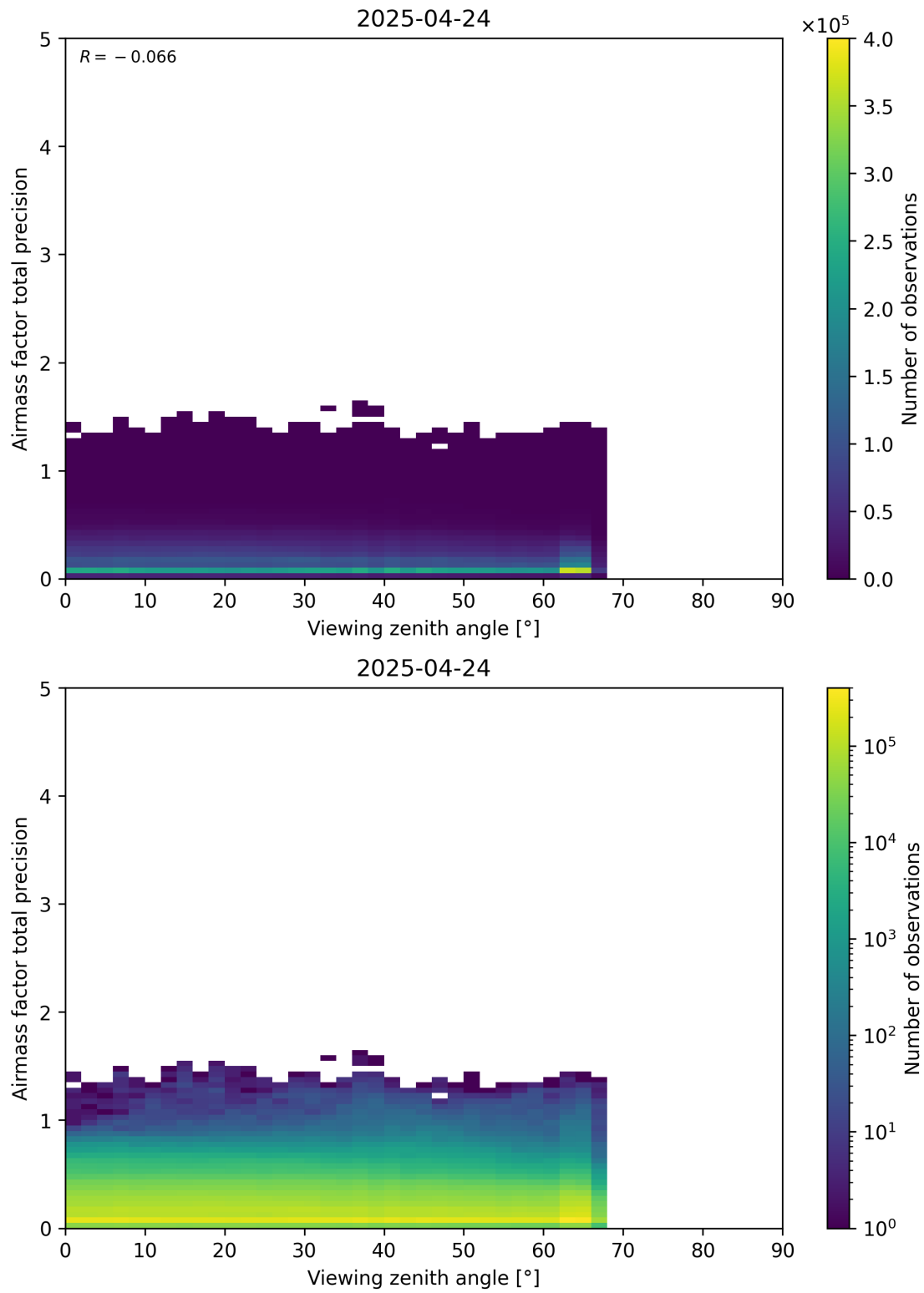
Figure 191: Scatter density plot of “Viewing zenith angle” against “Airmass factor total precision” for 2025-04-24 to 2025-04-25.
