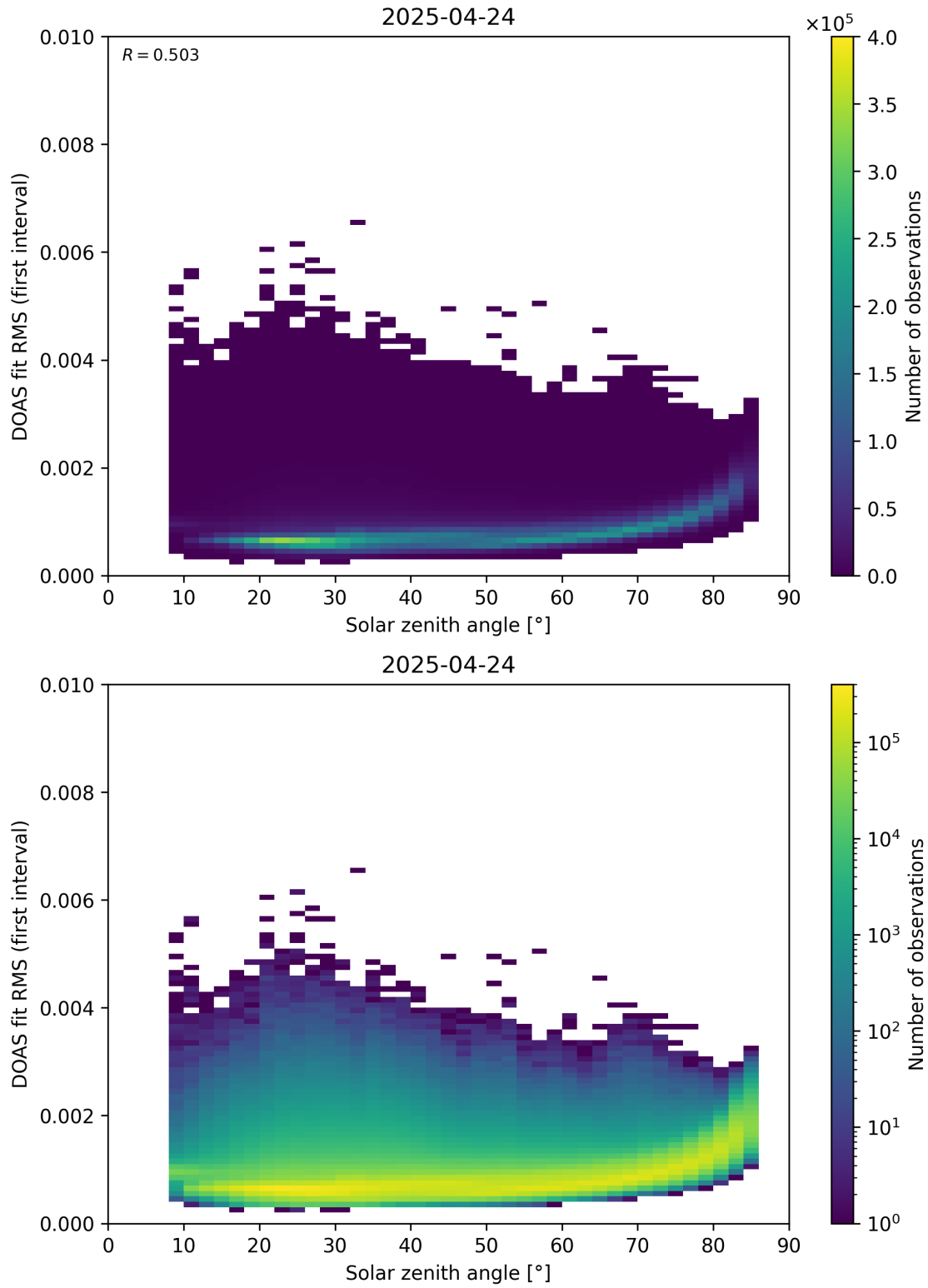
Figure 167: Scatter density plot of “Solar zenith angle” against “DOAS fit RMS (first interval)” for 2025-04-24 to 2025-04-25.
