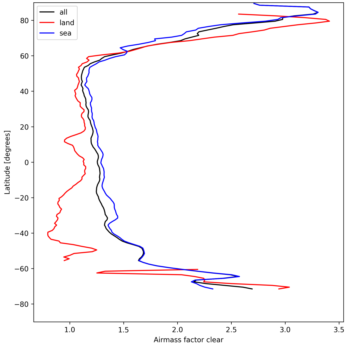
Figure 28: Zonal average of “Airmass factor clear” for 2025-04-24 to 2025-04-25.
