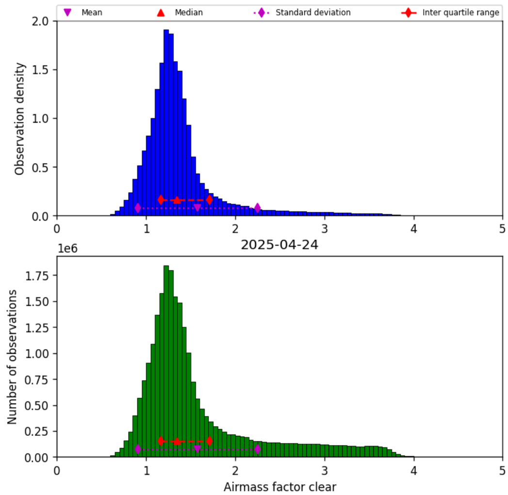
Figure 42: Histogram of “Airmass factor clear” for 2025-04-24 to 2025-04-25
