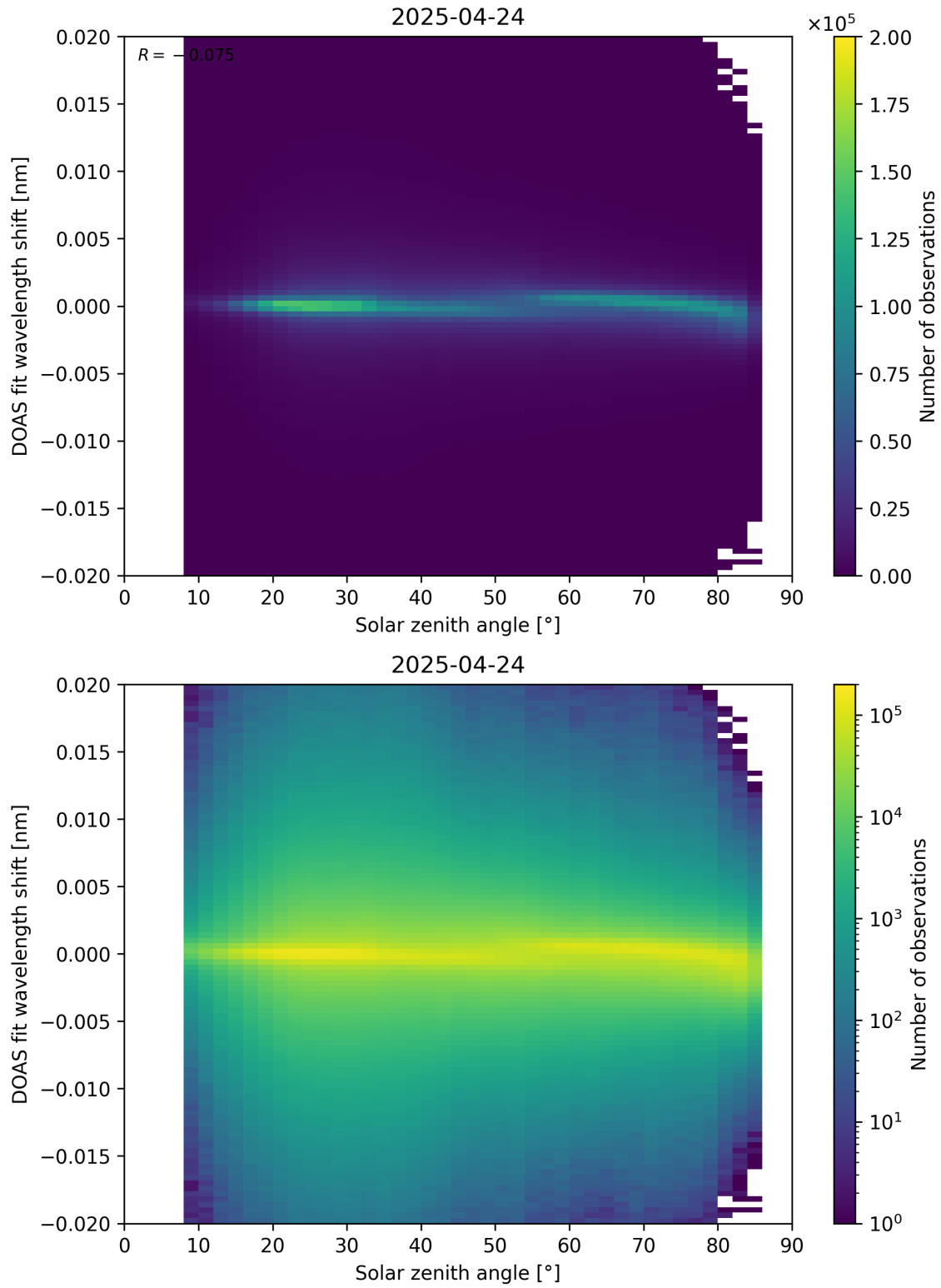
Figure 168: Scatter density plot of “Solar zenith angle” against “DOAS fit wavelength shift” for 2025-04-24 to 2025-04-25.
