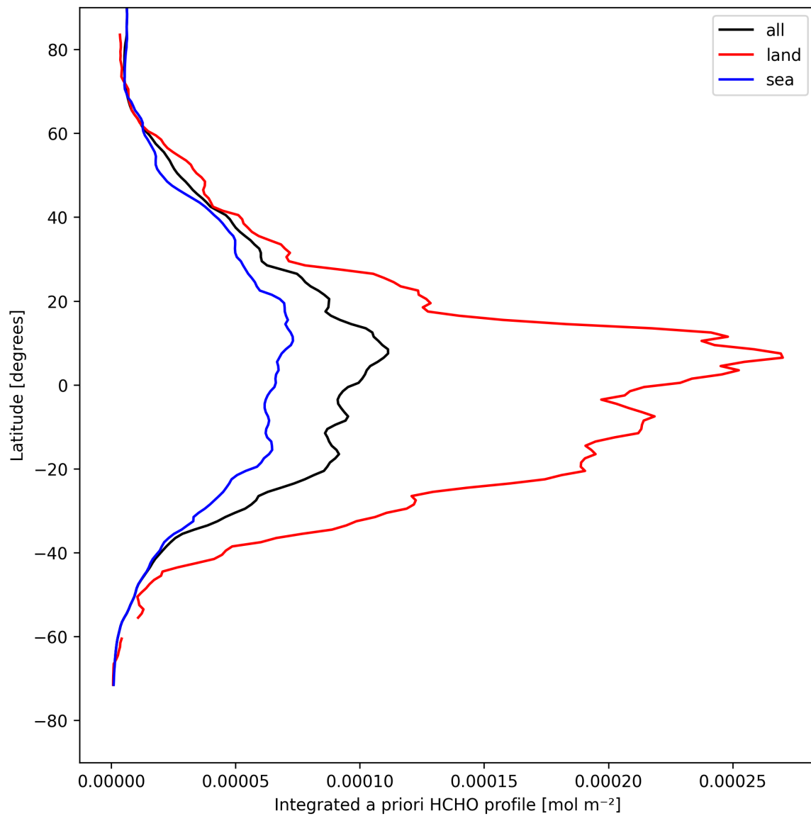
Figure 29: Zonal average of “Integrated a priori HCHO profile” for 2025-04-24 to 2025-04-25.
