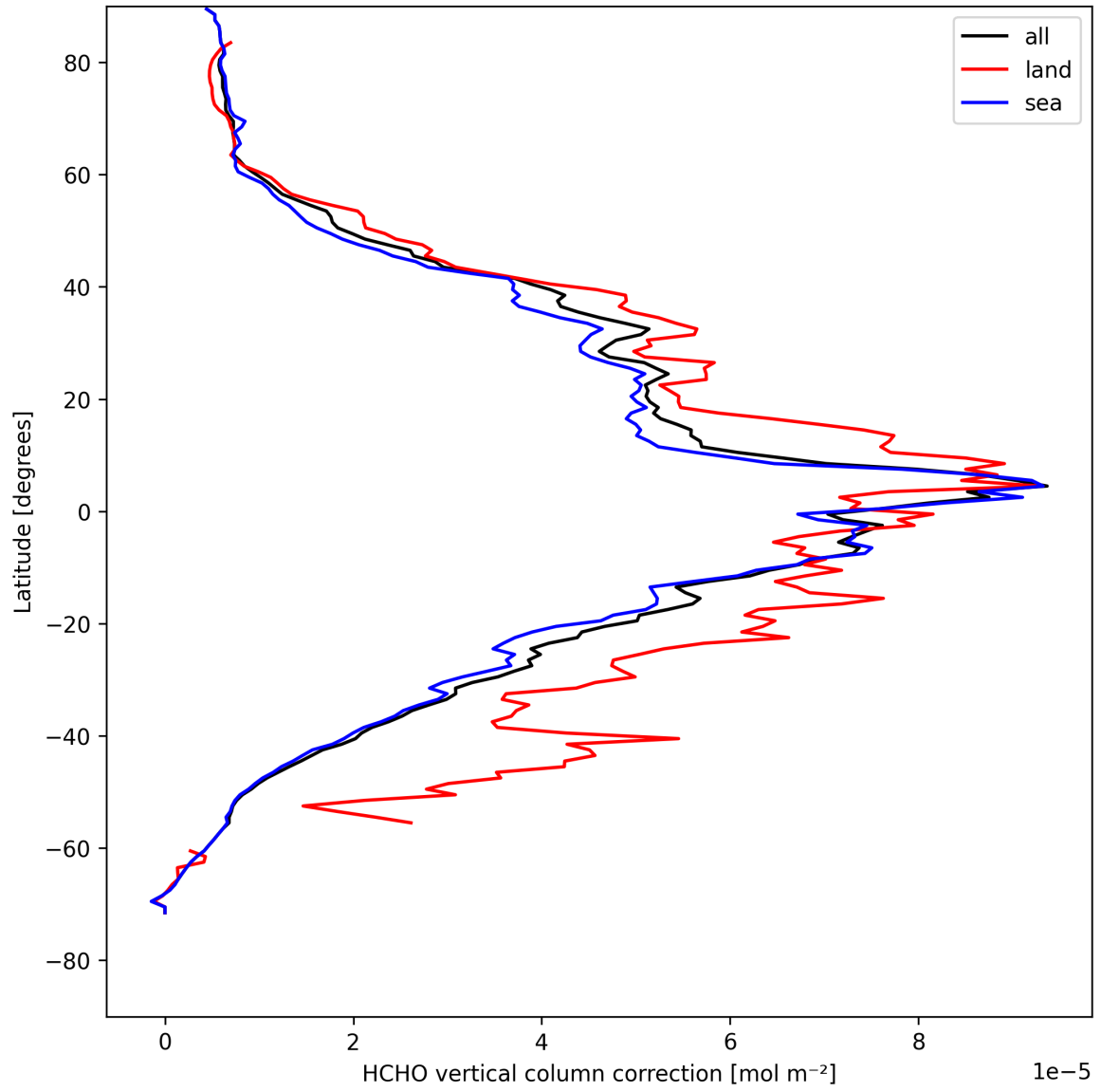
Figure 23: Zonal average of “HCHO vertical column correction” for 2025-04-24 to 2025-04-25.
