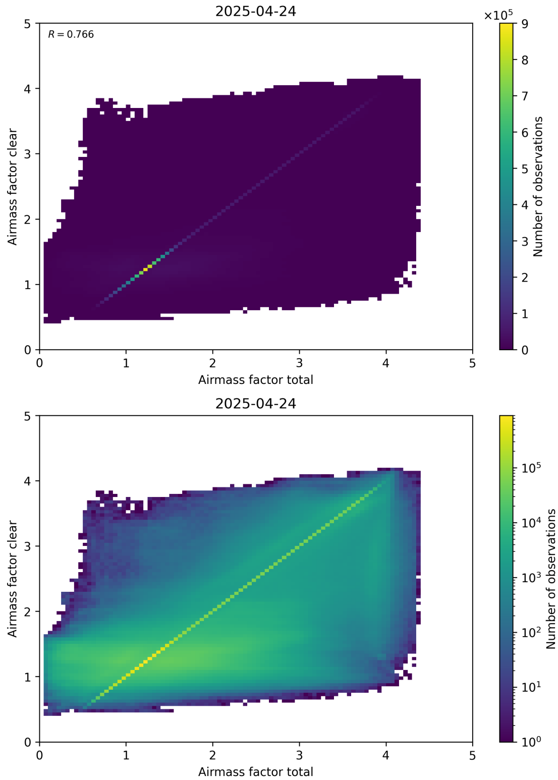
Figure 100: Scatter density plot of “Airmass factor total” against “Airmass factor clear” for 2025-04-24 to 2025-04-25.
