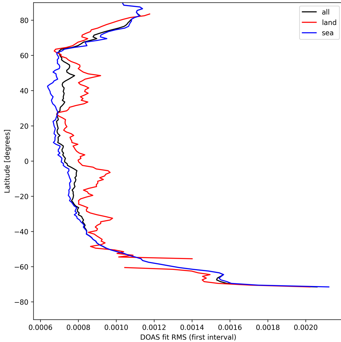
Figure 32: Zonal average of “DOAS fit RMS (first interval)” for 2025-04-24 to 2025-04-25.
