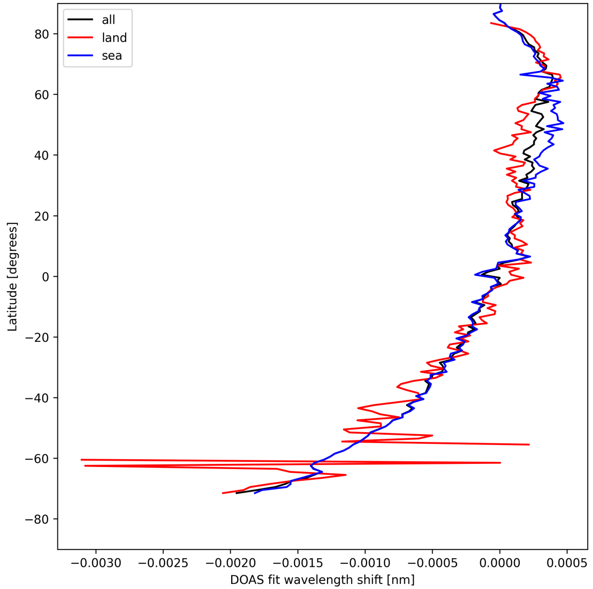
Figure 30: Zonal average of “DOAS fit wavelength shift” for 2025-04-24 to 2025-04-25.
