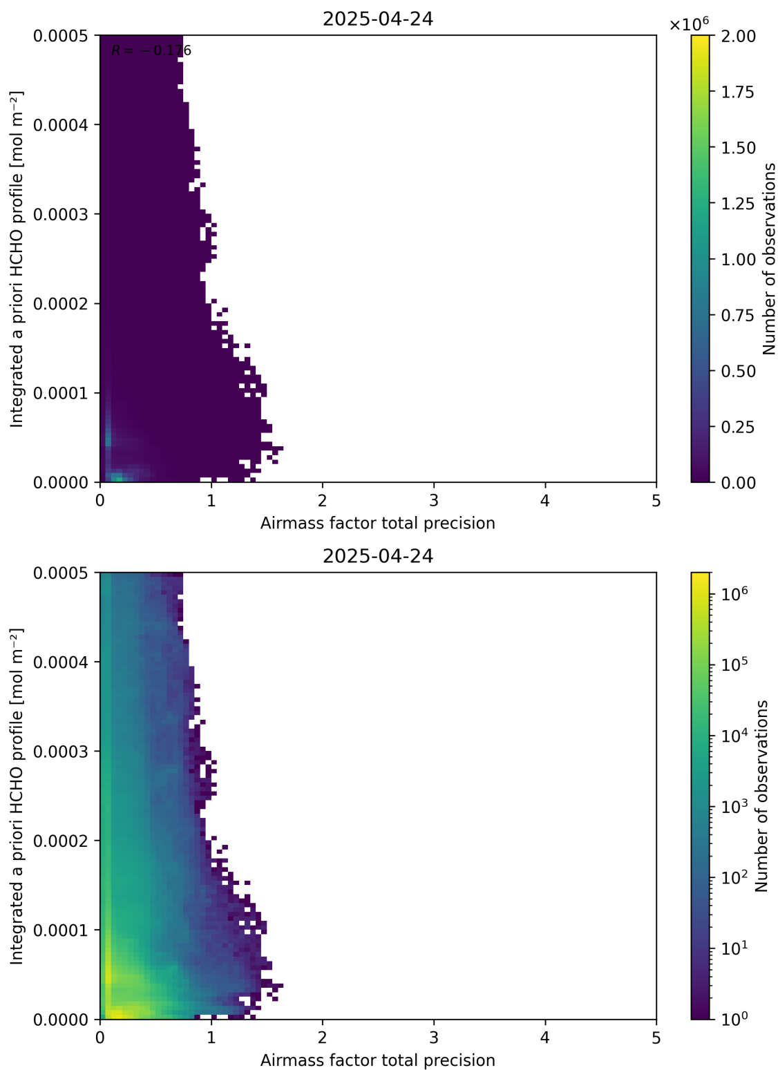
Figure 111: Scatter density plot of “Airmass factor total precision” against “Integrated a priori HCHO profile” for 2025-04-24 to 2025-04-25.
