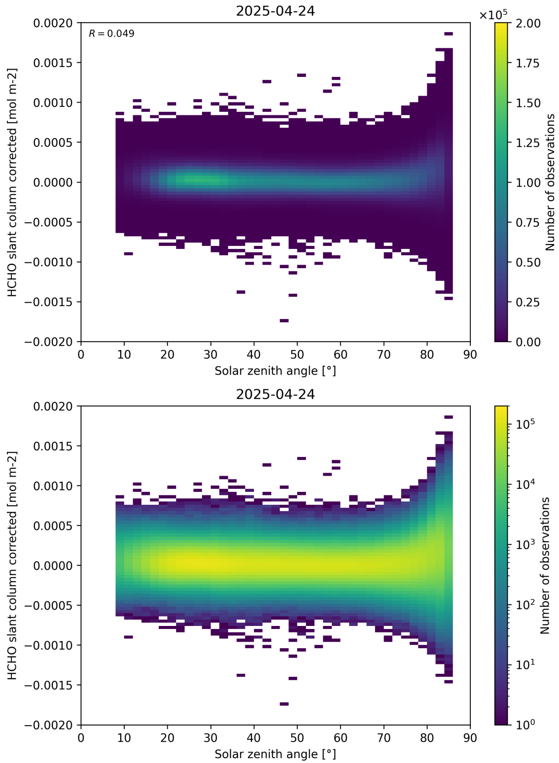
Figure 171: Scatter density plot of “Solar zenith angle” against “HCHO slant column corrected” for 2025-04-24 to 2025-04-25.
