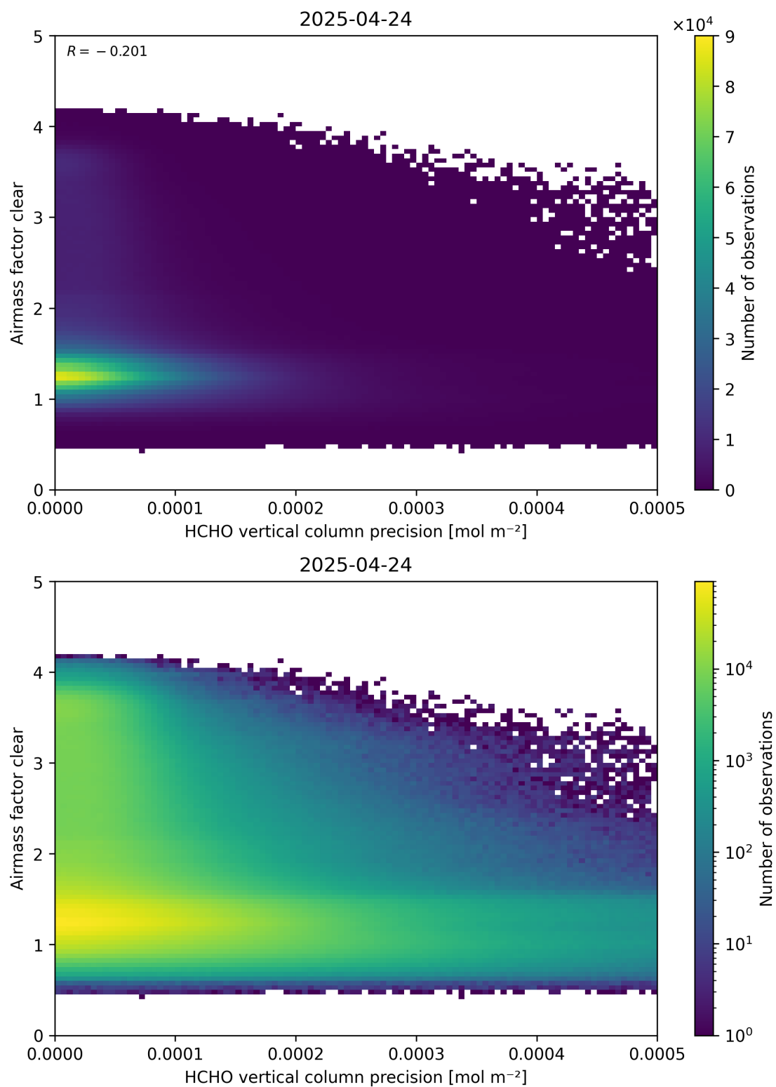
Figure 139: Scatter density plot of “HCHO vertical column precision” against “Airmass factor clear” for 2025-04-24 to 2025-04-25.
