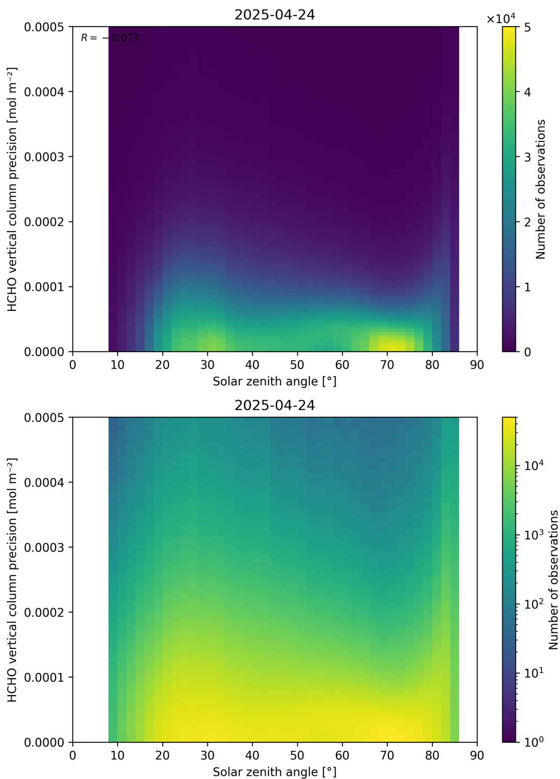
Figure 179: Scatter density plot of “Solar zenith angle” against “HCHO vertical column precision” for 2025-04-24 to 2025-04-25.
