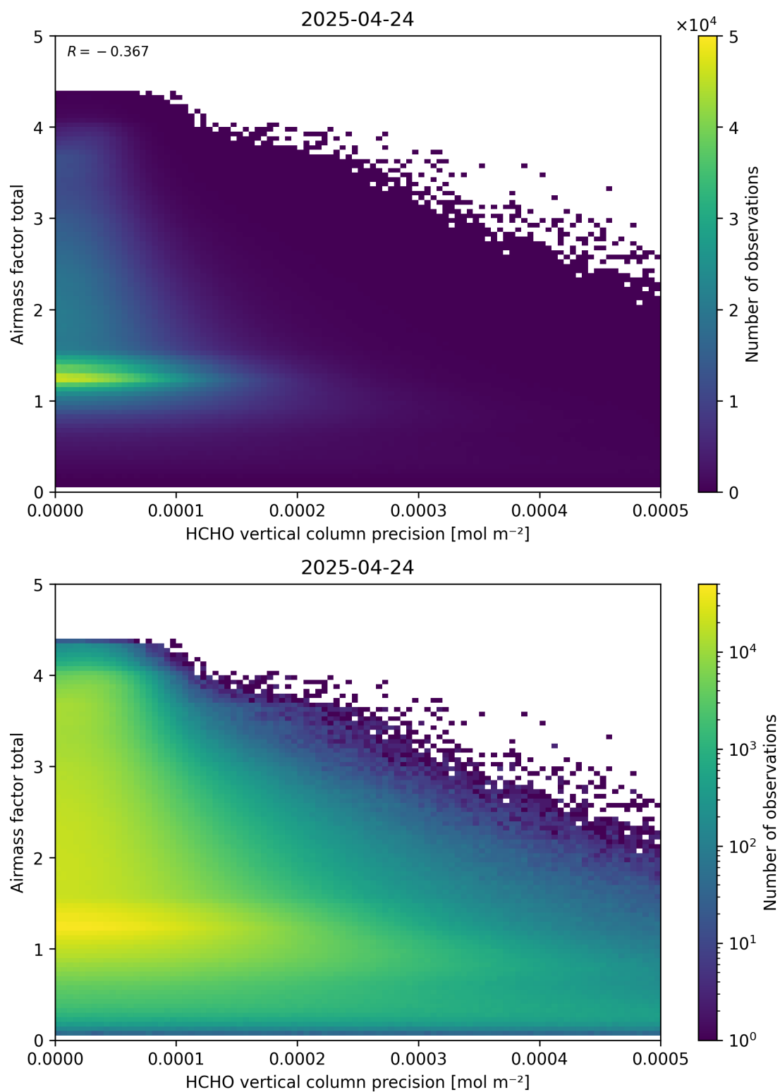
Figure 144: Scatter density plot of “HCHO vertical column precision” against “Airmass factor total” for 2025-04-24 to 2025-04-25.
