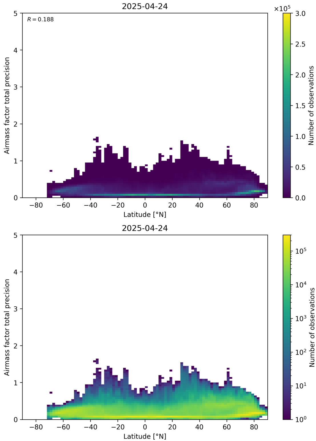
Figure 162: Scatter density plot of “Latitude” against “Airmass factor total precision” for 2025-04-24 to 2025-04-25.
