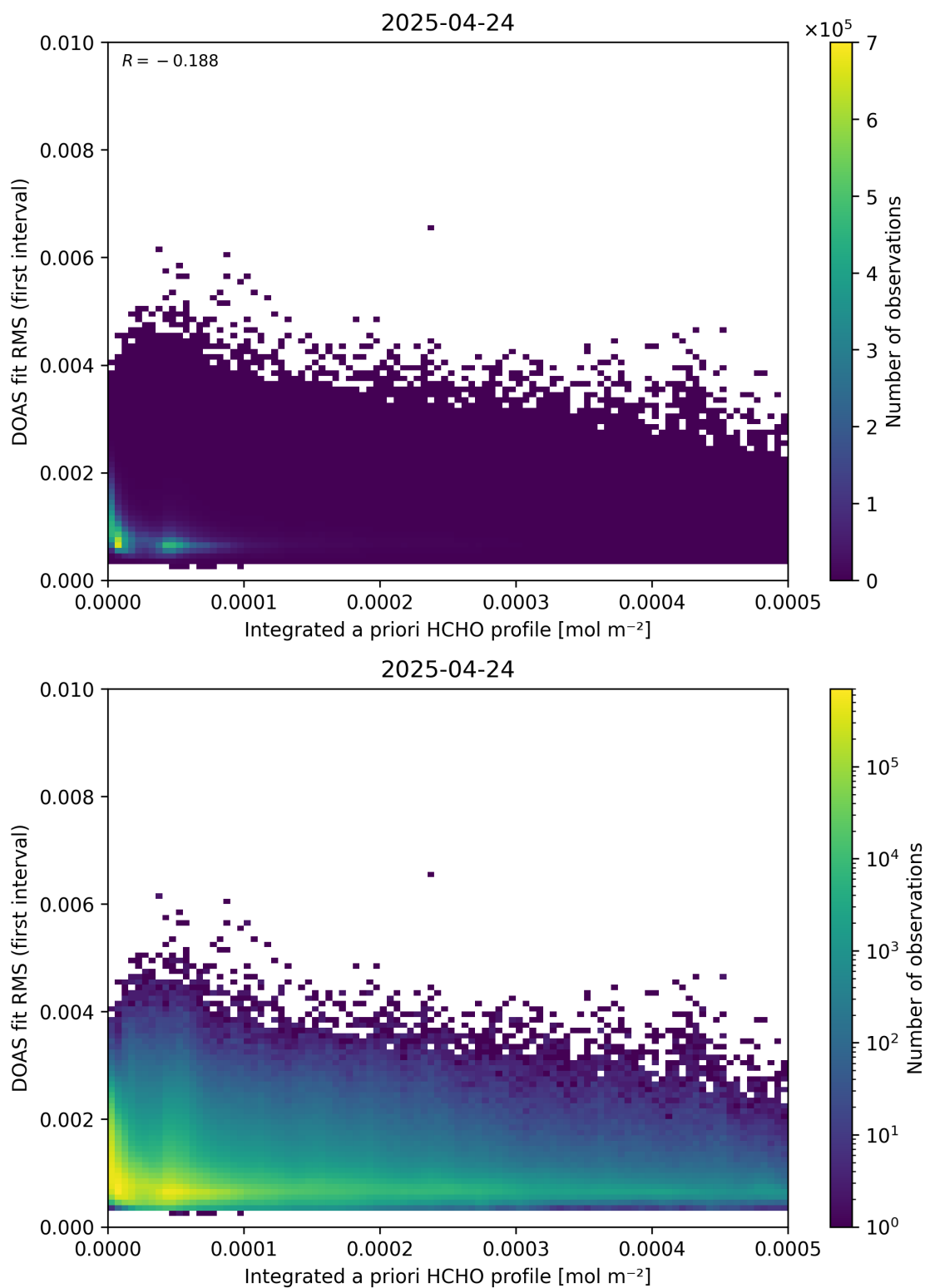
Figure 148: Scatter density plot of “Integrated a priori HCHO profile” against “DOAS fit RMS (first interval)” for 2025-04-24 to 2025-04-25.
