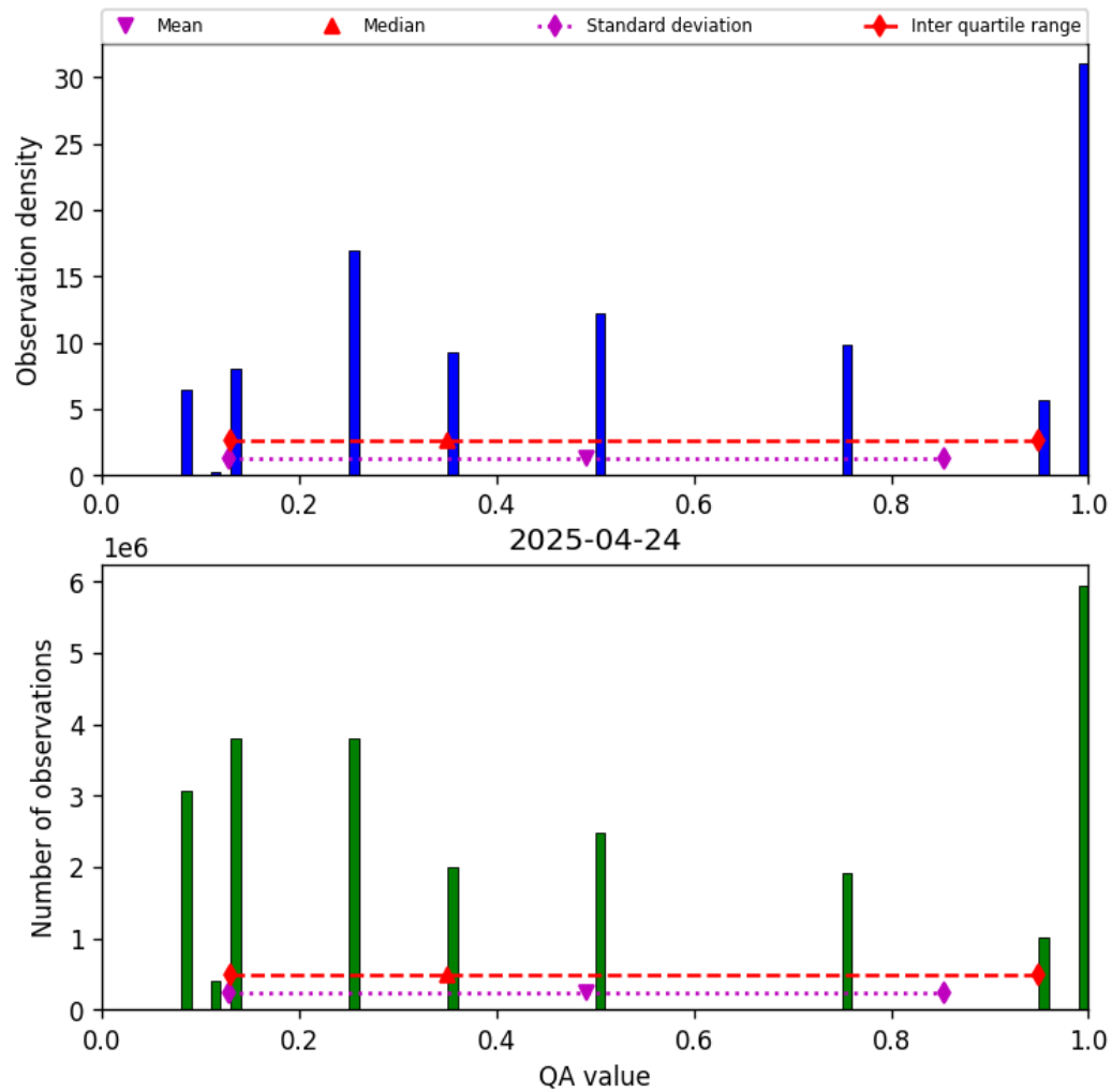
Figure 34: Histogram of “QA value” for 2025-04-24 to 2025-04-25
