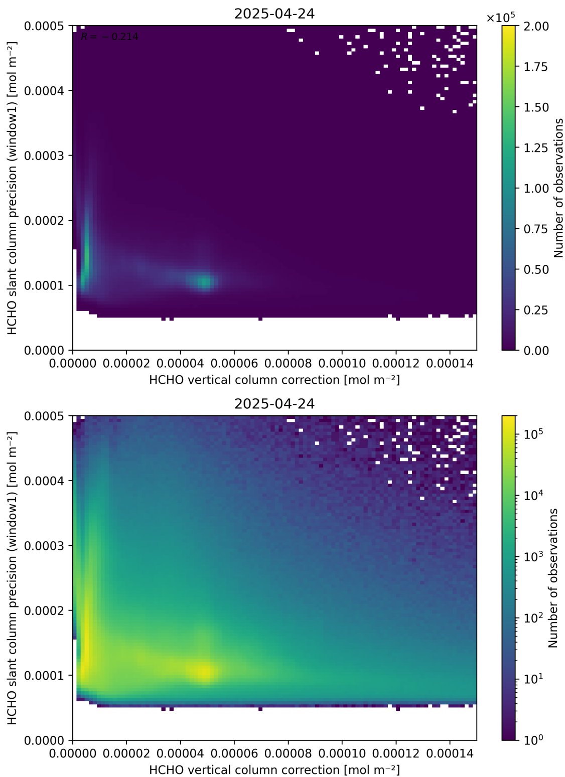
Figure 119: Scatter density plot of “HCHO vertical column correction” against “HCHO slant column precision (window1)” for 2025-04-24 to 2025-04-25.
