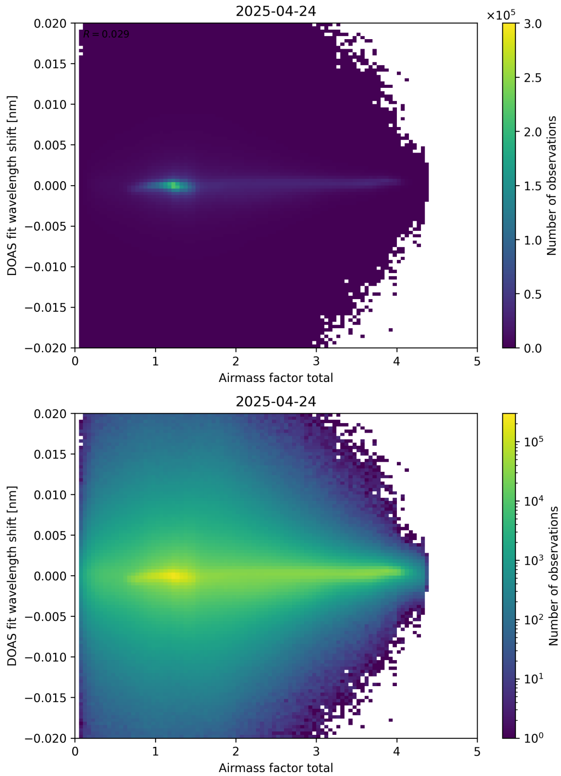
Figure 98: Scatter density plot of “Airmass factor total” against “DOAS fit wavelength shift” for 2025-04-24 to 2025-04-25.
