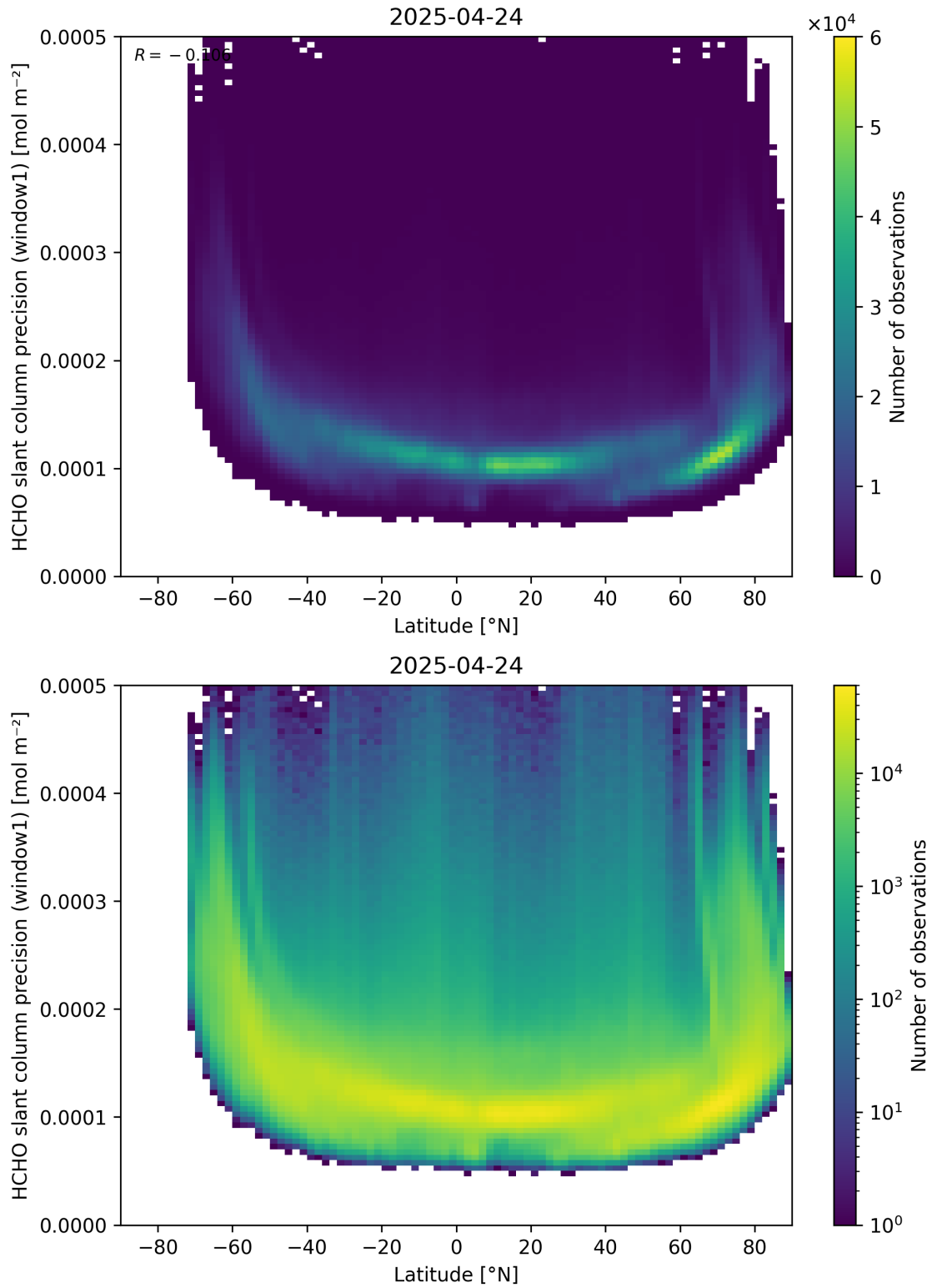
Figure 160: Scatter density plot of “Latitude” against “HCHO slant column precision (window1)” for 2025-04-24 to 2025-04-25.
