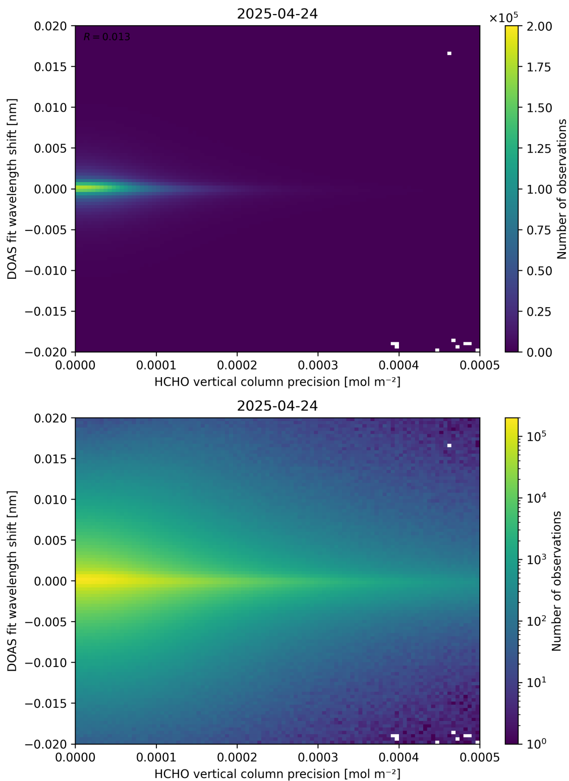
Figure 137: Scatter density plot of “HCHO vertical column precision” against “DOAS fit wavelength shift” for 2025-04-24 to 2025-04-25.
