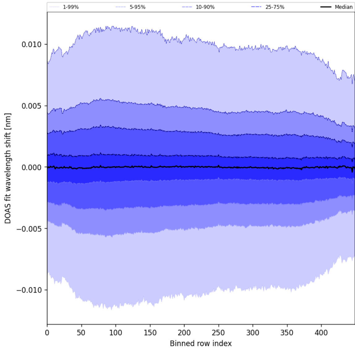
Figure 58: Along track statistics of “DOAS fit wavelength shift” for 2025-04-24 to 2025-04-25
