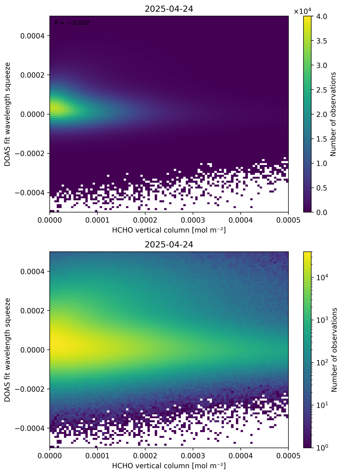
Figure 125: Scatter density plot of “HCHO vertical column” against “DOAS fit wavelength squeeze” for 2025-04-24 to 2025-04-25.
