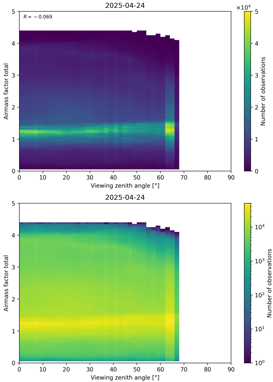
Figure 190: Scatter density plot of “Viewing zenith angle” against “Airmass factor total” for 2025-04-24 to 2025-04-25.
