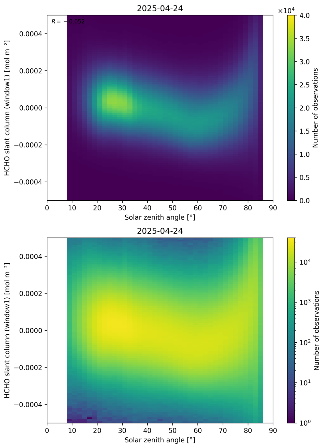
Figure 173: Scatter density plot of “Solar zenith angle” against “HCHO slant column (window1)” for 2025-04-24 to 2025-04-25.
