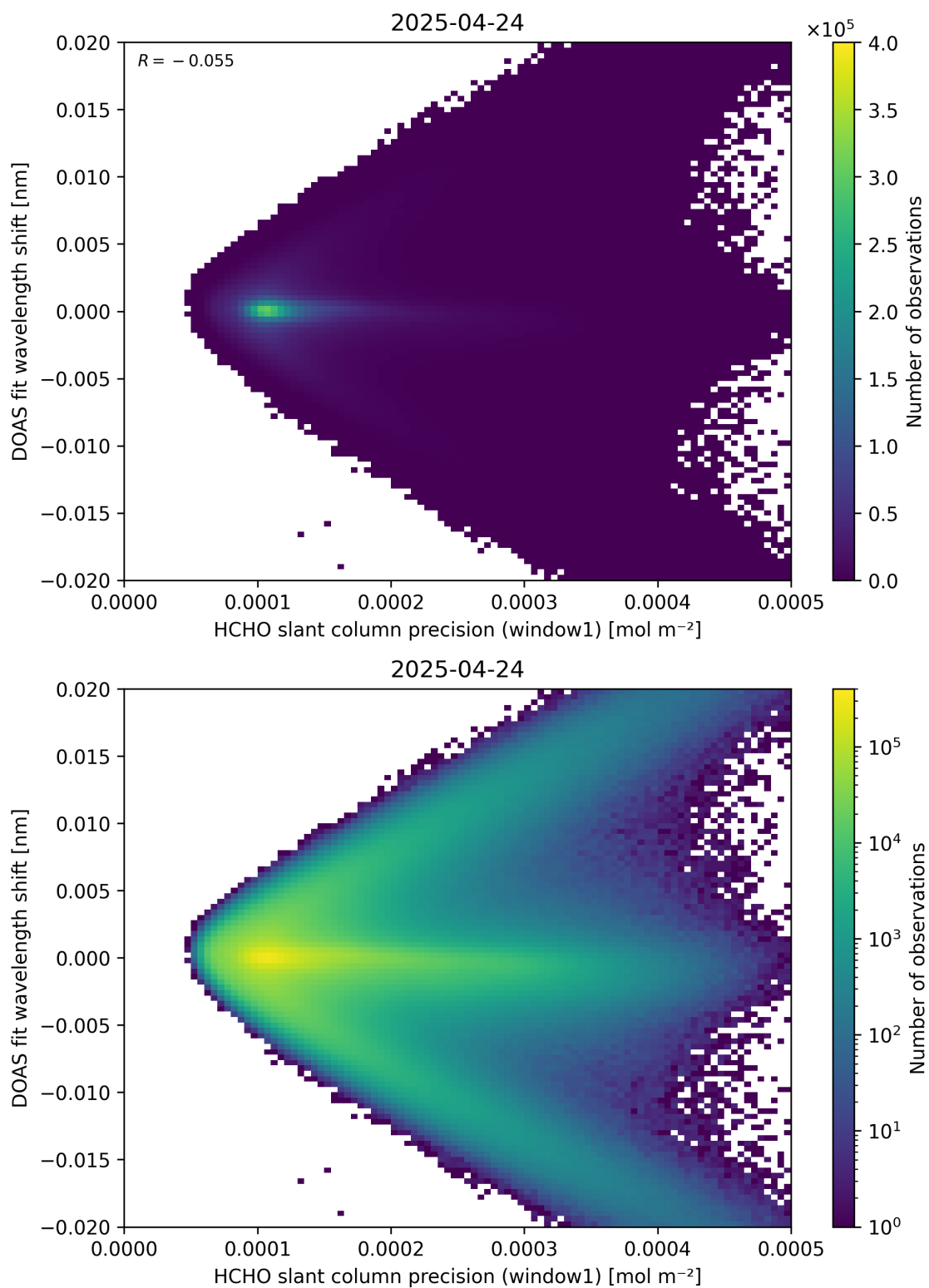
Figure 89: Scatter density plot of “HCHO slant column precision (window1)” against “DOAS fit wavelength shift” for 2025-04-24 to 2025-04-25.
