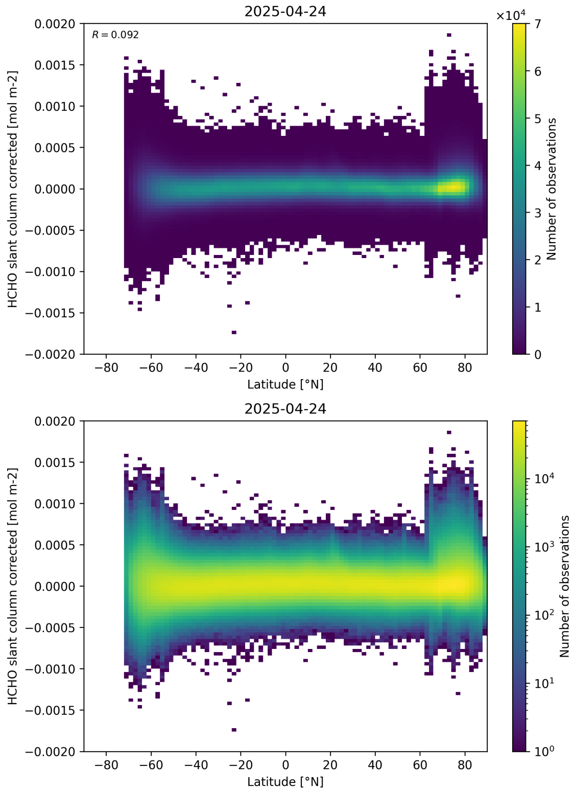
Figure 157: Scatter density plot of “Latitude” against “HCHO slant column corrected” for 2025-04-24 to 2025-04-25.
