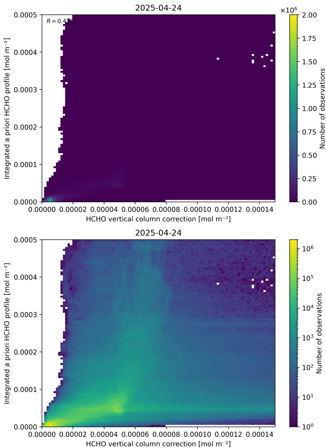
Figure 122: Scatter density plot of “HCHO vertical column correction” against “Integrated a priori HCHO profile” for 2025-04-24 to 2025-04-25.
