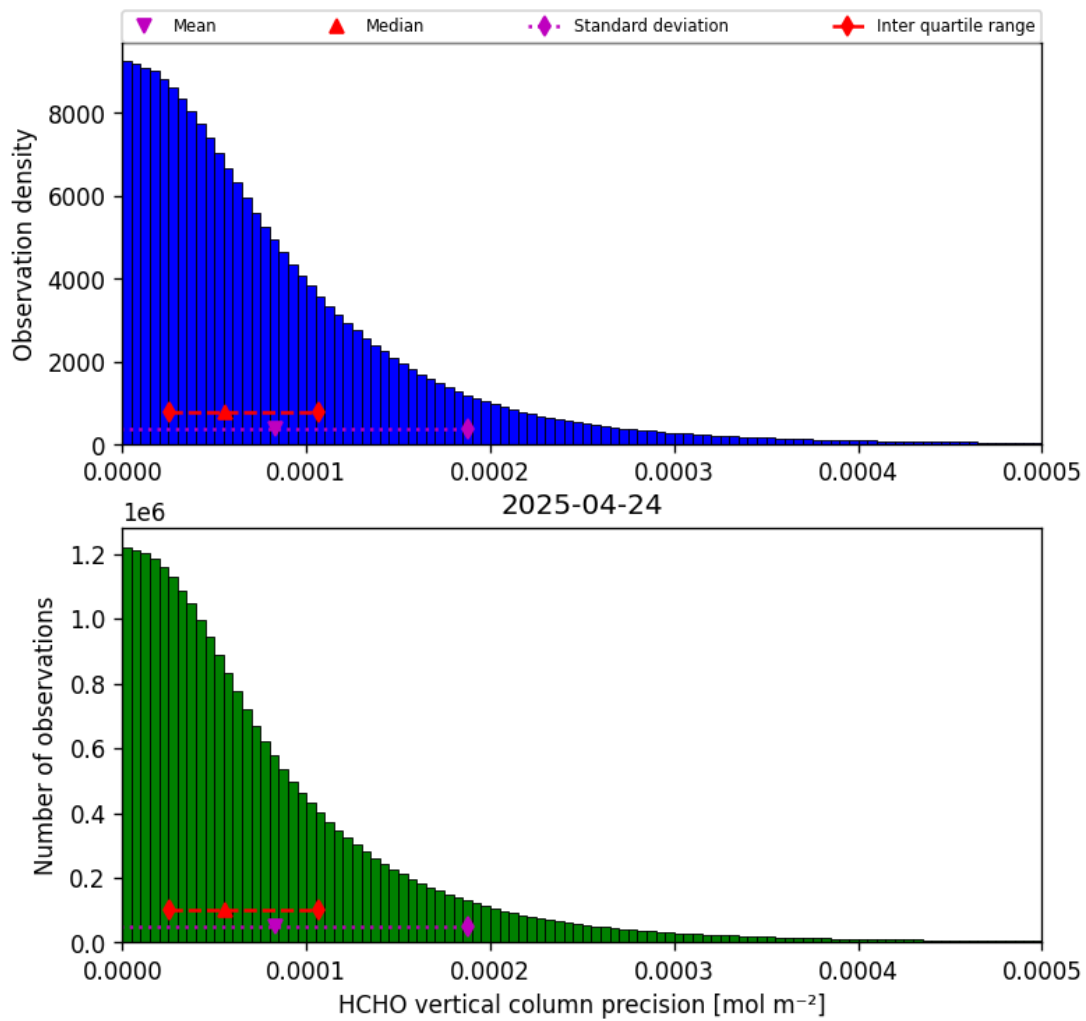
Figure 36: Histogram of “HCHO vertical column precision” for 2025-04-24 to 2025-04-25
