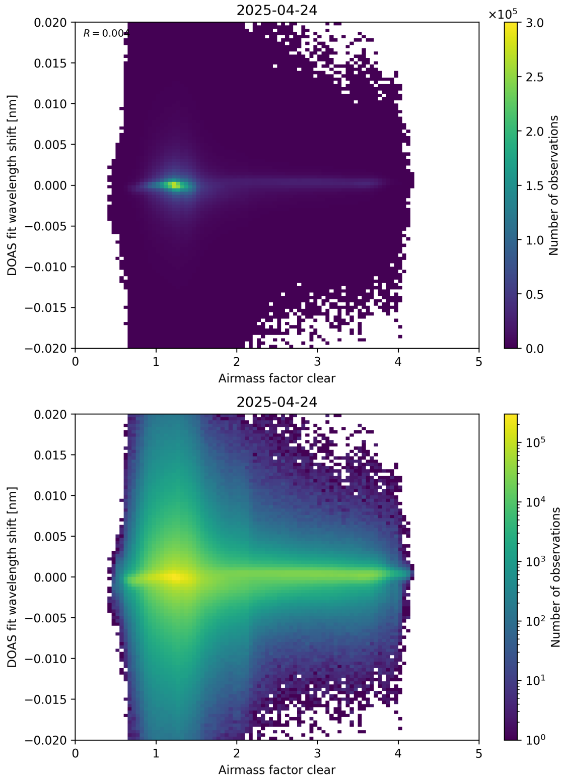
Figure 72: Scatter density plot of “Airmass factor clear” against “DOAS fit wavelength shift” for 2025-04-24 to 2025-04-25.
