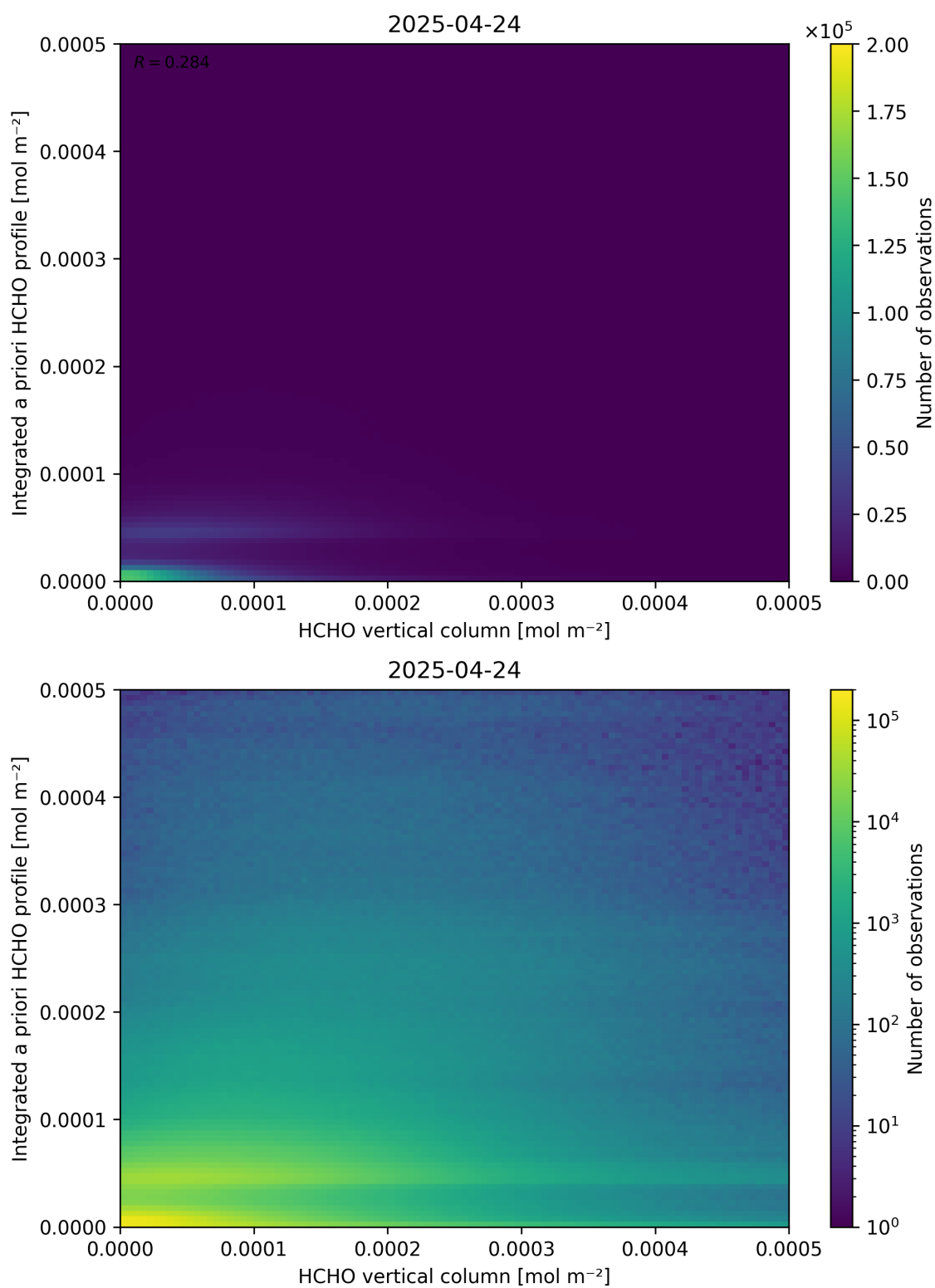
Figure 135: Scatter density plot of “HCHO vertical column” against “Integrated a priori HCHO profile” for 2025-04-24 to 2025-04-25.
