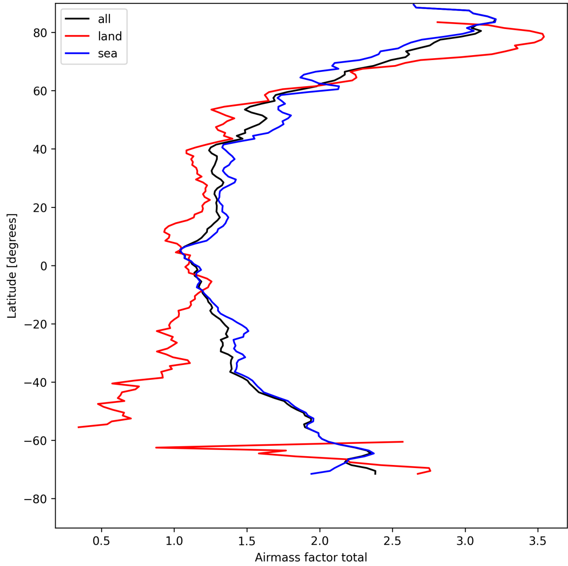
Figure 26: Zonal average of “Airmass factor total” for 2025-04-24 to 2025-04-25.
