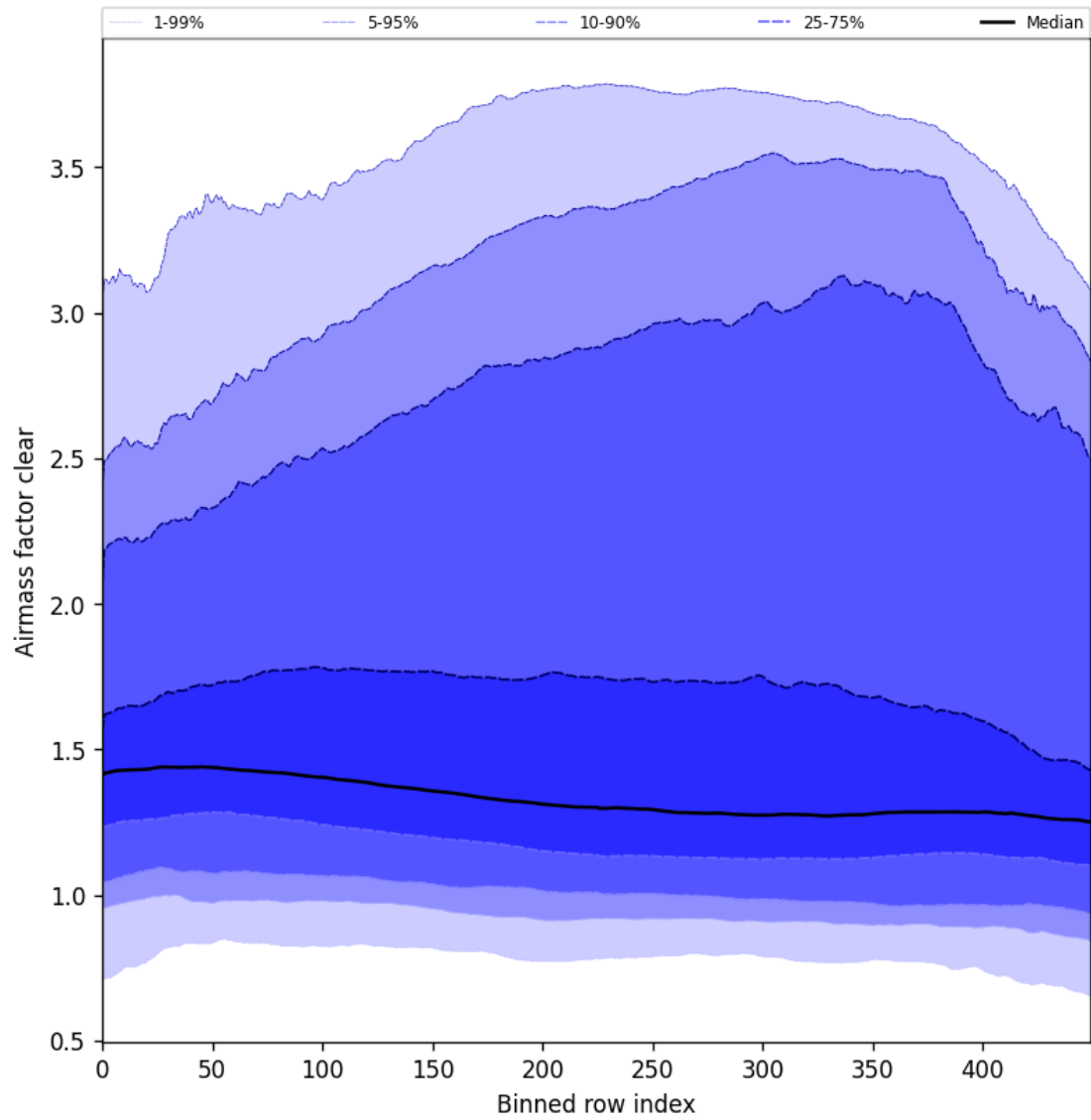
Figure 56: Along track statistics of “Airmass factor clear” for 2025-04-24 to 2025-04-25
