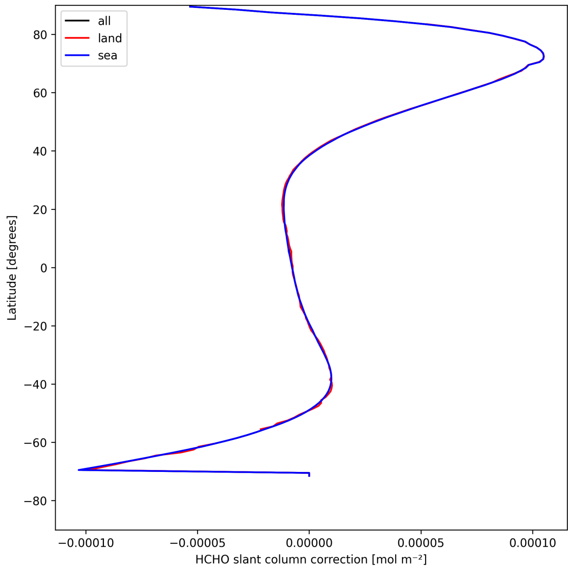
Figure 33: Zonal average of “HCHO slant column correction” for 2025-04-24 to 2025-04-25.
