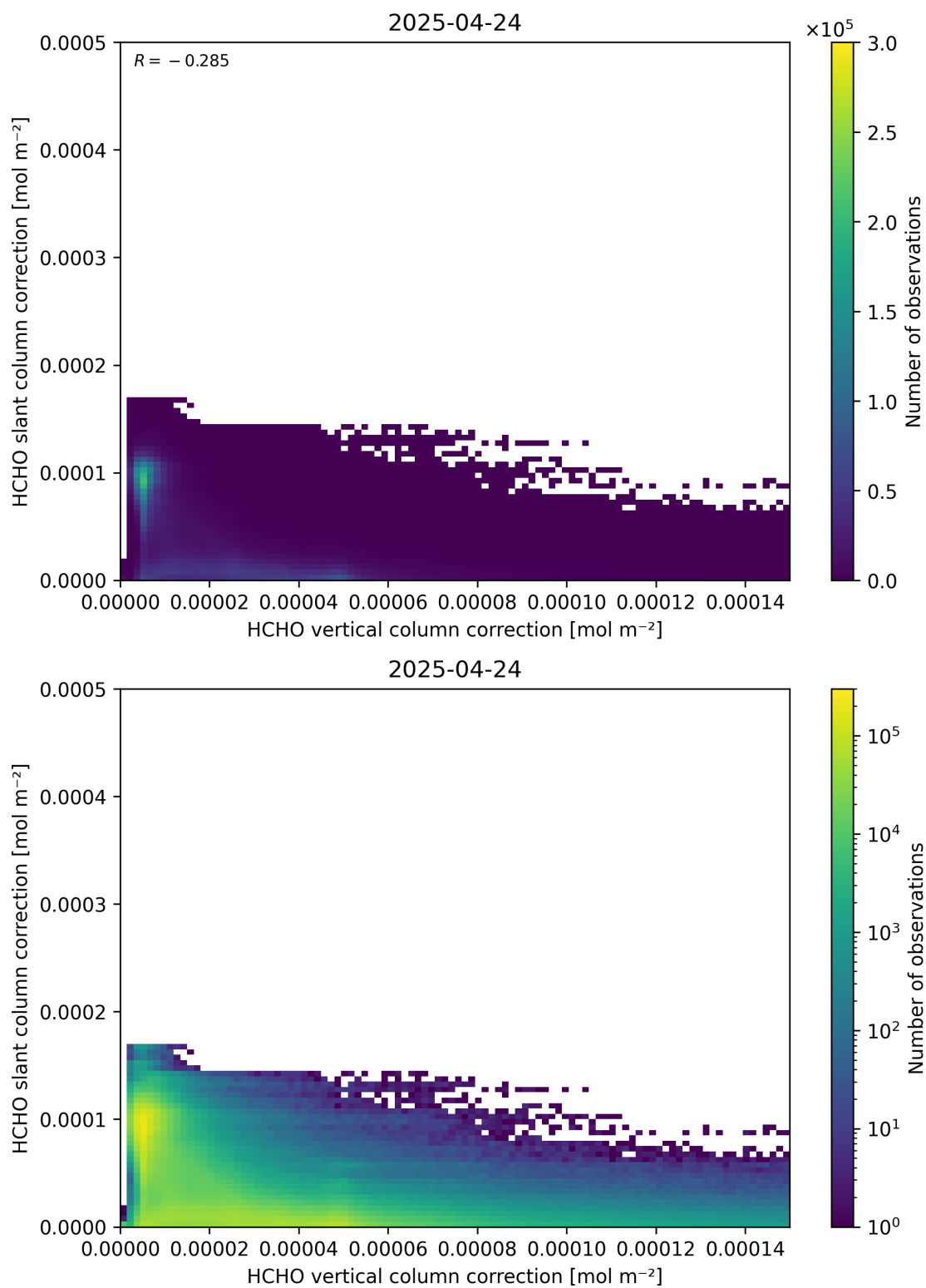
Figure 117: Scatter density plot of “HCHO vertical column correction” against “HCHO slant column correction” for 2025-04-24 to 2025-04-25.
