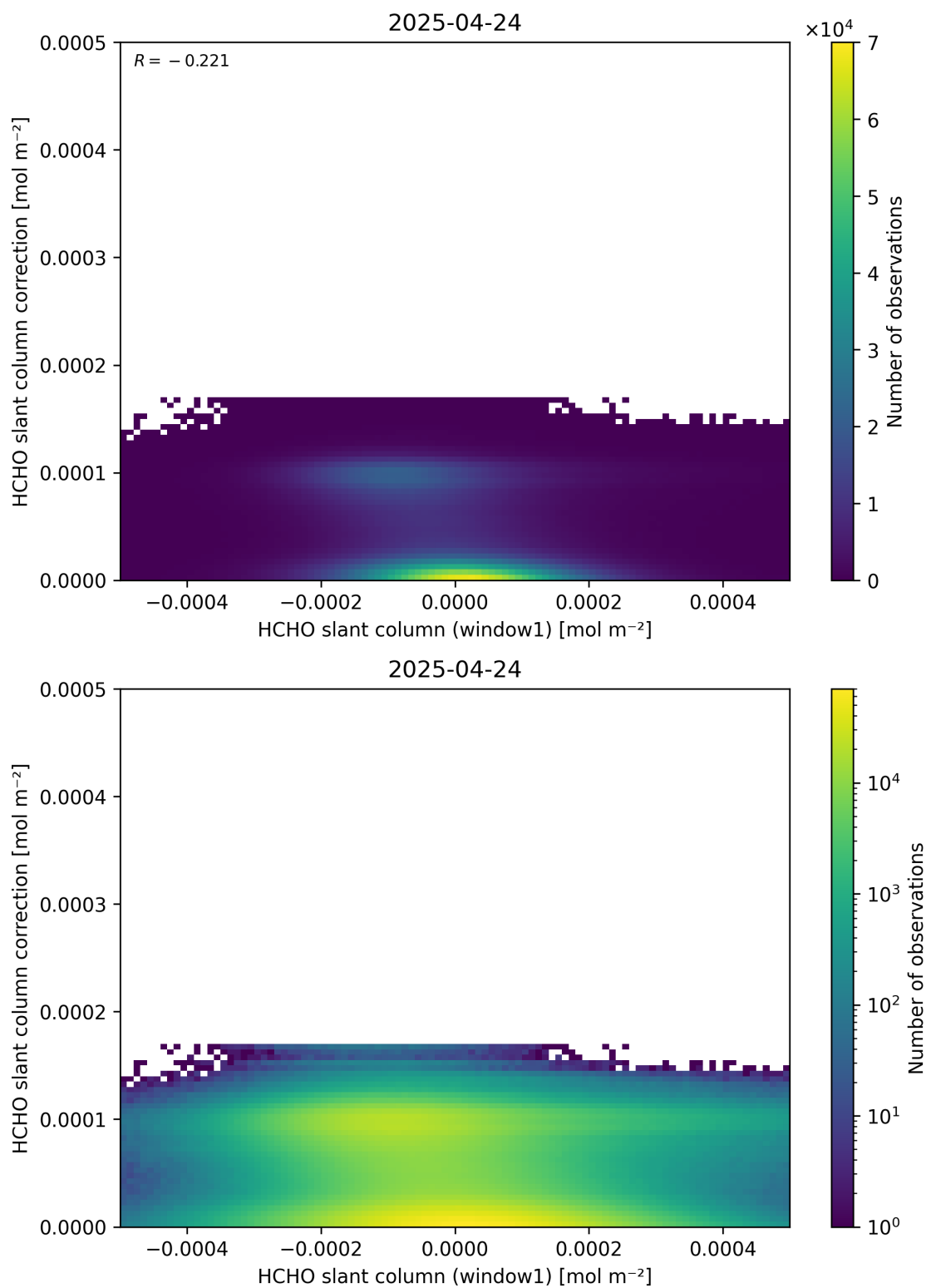
Figure 83: Scatter density plot of “HCHO slant column (window1)” against “HCHO slant column correction” for 2025-04-24 to 2025-04-25.
