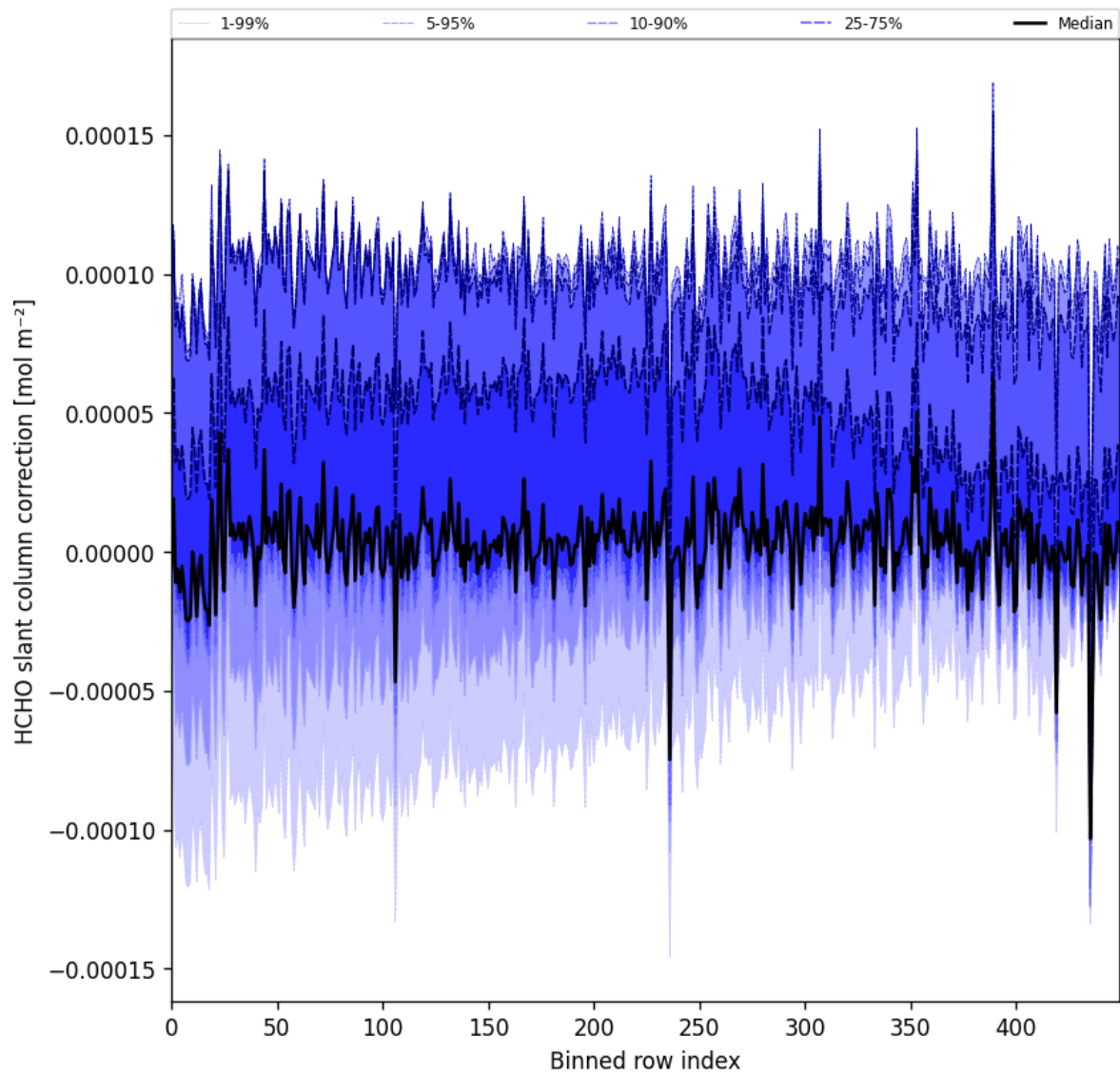
Figure 61: Along track statistics of “HCHO slant column correction” for 2025-04-24 to 2025-04-25
