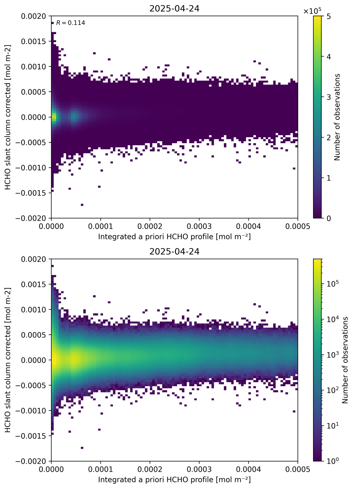
Figure 151: Scatter density plot of “Integrated a priori HCHO profile” against “HCHO slant column corrected” for 2025-04-24 to 2025-04-25.
