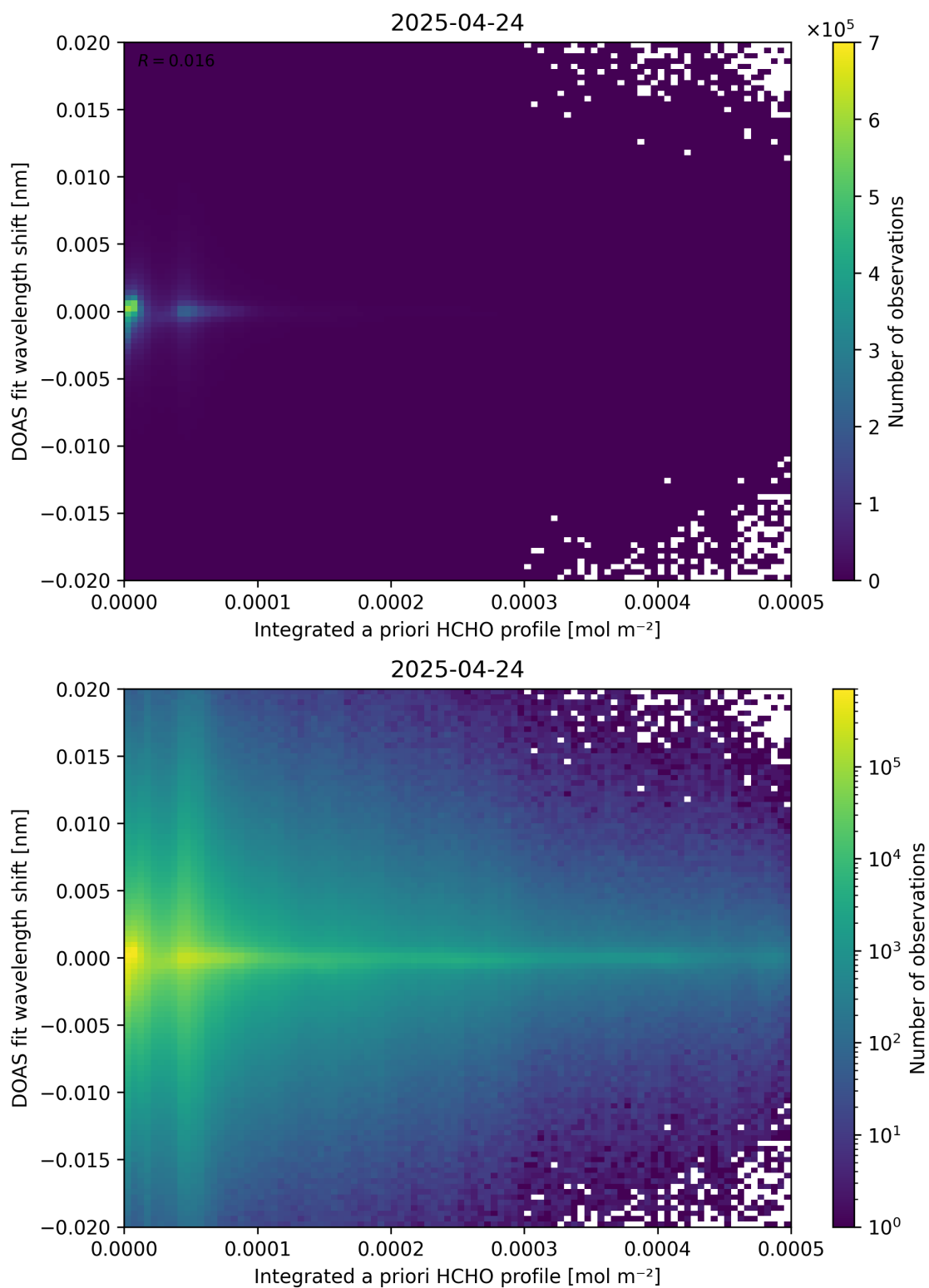
Figure 149: Scatter density plot of “Integrated a priori HCHO profile” against “DOAS fit wavelength shift” for 2025-04-24 to 2025-04-25.
