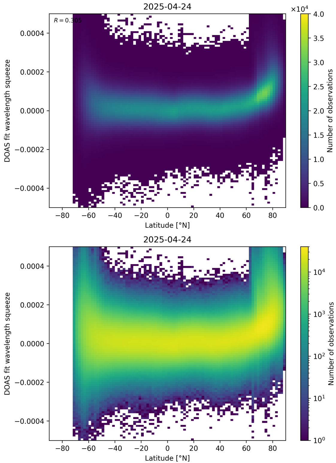
Figure 155: Scatter density plot of “Latitude” against “DOAS fit wavelength squeeze” for 2025-04-24 to 2025-04-25.
