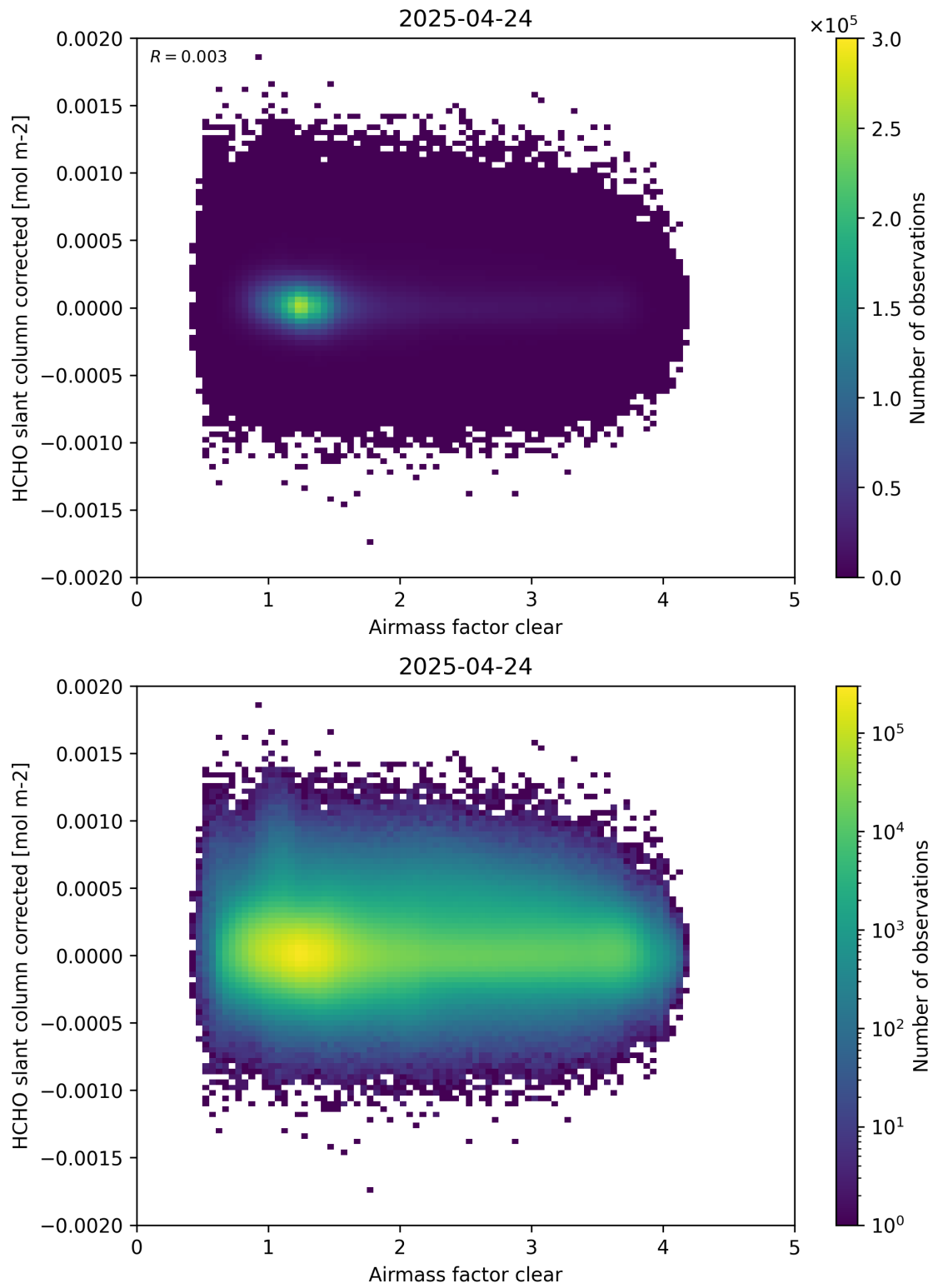
Figure 74: Scatter density plot of “Airmass factor clear” against “HCHO slant column corrected” for 2025-04-24 to 2025-04-25.
