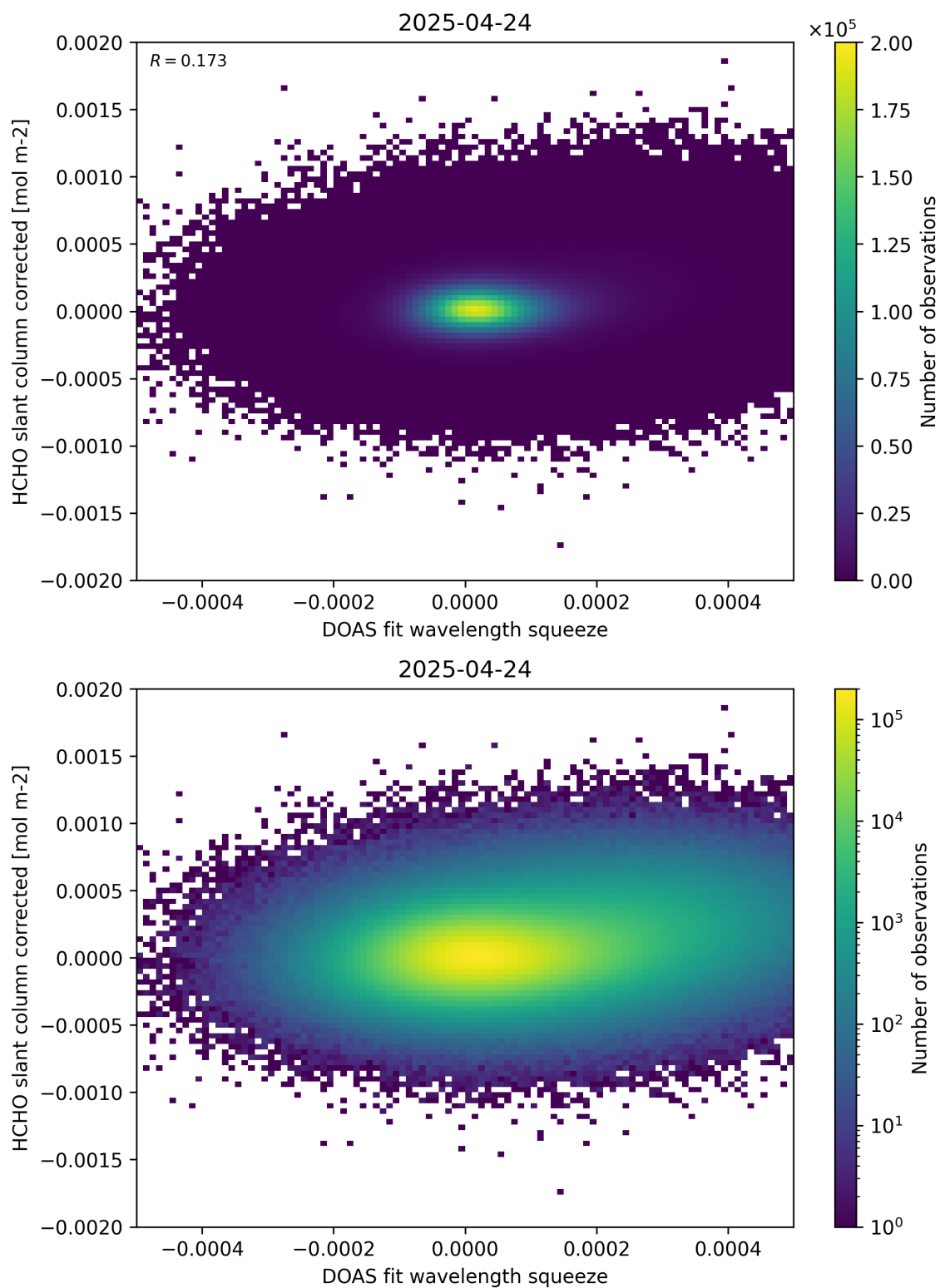
Figure 69: Scatter density plot of “DOAS fit wavelength squeeze” against “HCHO slant column corrected” for 2025-04-24 to 2025-04-25.
