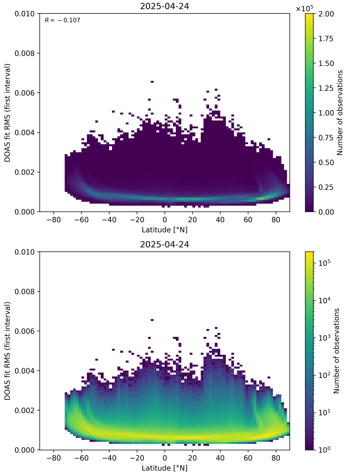
Figure 153: Scatter density plot of “Latitude” against “DOAS fit RMS (first interval)” for 2025-04-24 to 2025-04-25.
