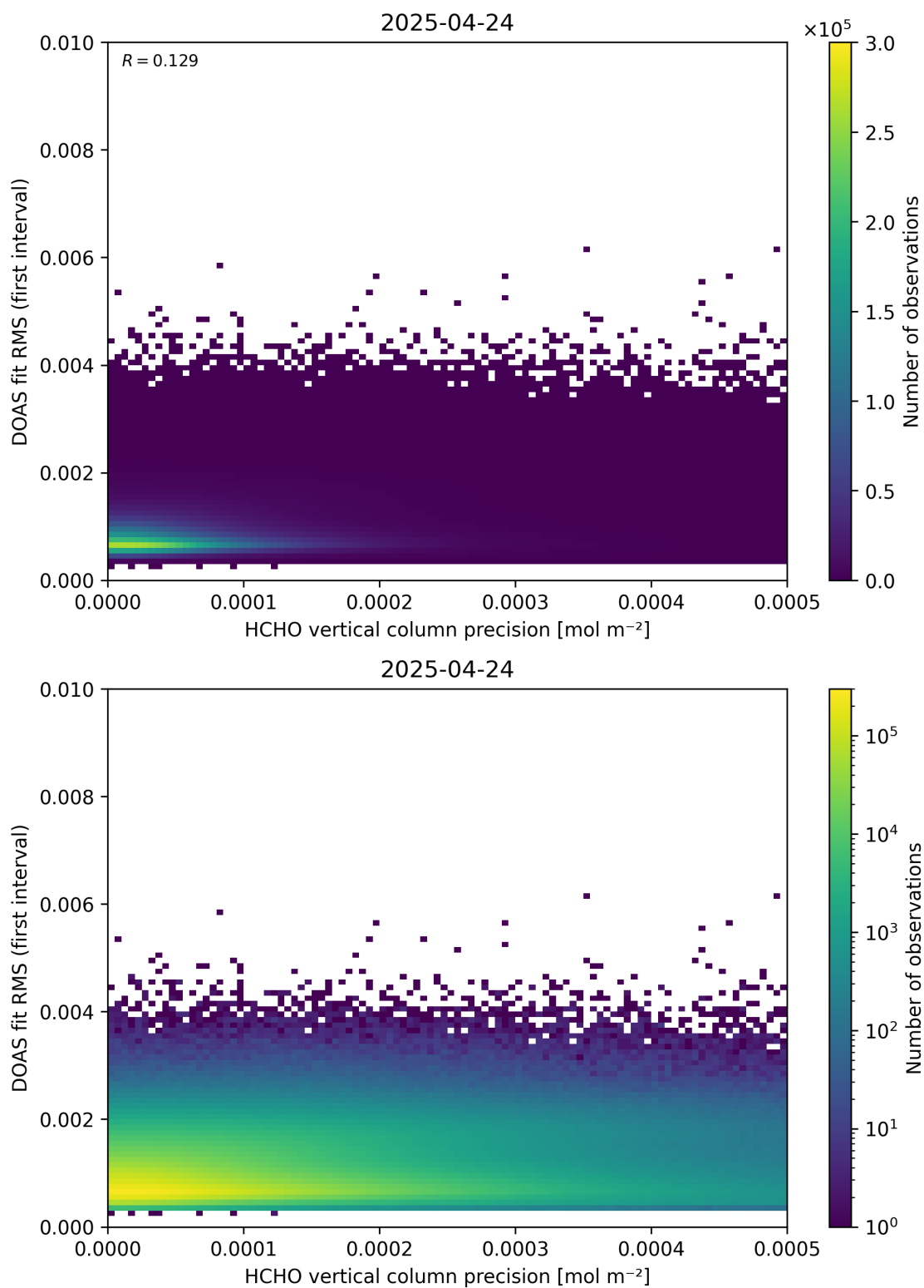
Figure 136: Scatter density plot of “HCHO vertical column precision” against “DOAS fit RMS (first interval)” for 2025-04-24 to 2025-04-25.
