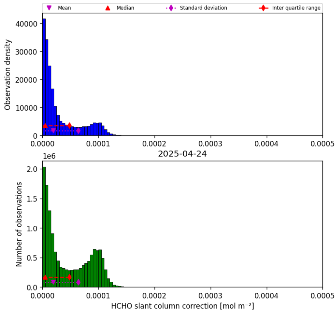
Figure 47: Histogram of “HCHO slant column correction” for 2025-04-24 to 2025-04-25
