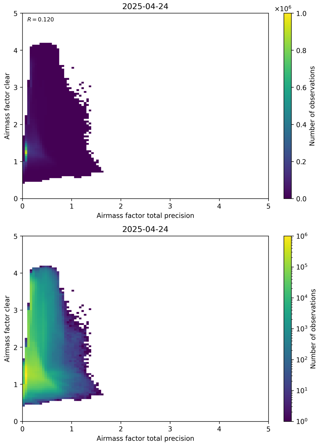
Figure 108: Scatter density plot of “Airmass factor total precision” against “Airmass factor clear” for 2025-04-24 to 2025-04-25.
