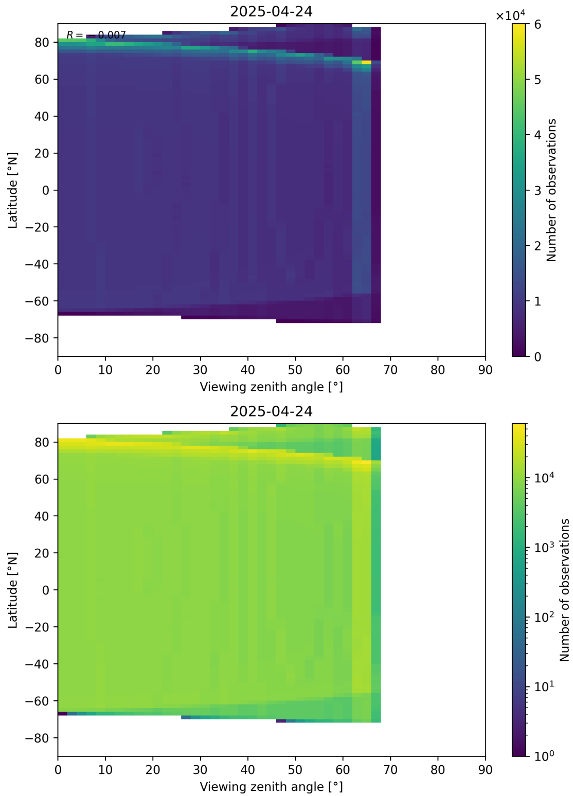
Figure 196: Scatter density plot of “Viewing zenith angle” against “Latitude” for 2025-04-24 to 2025-04-25.
