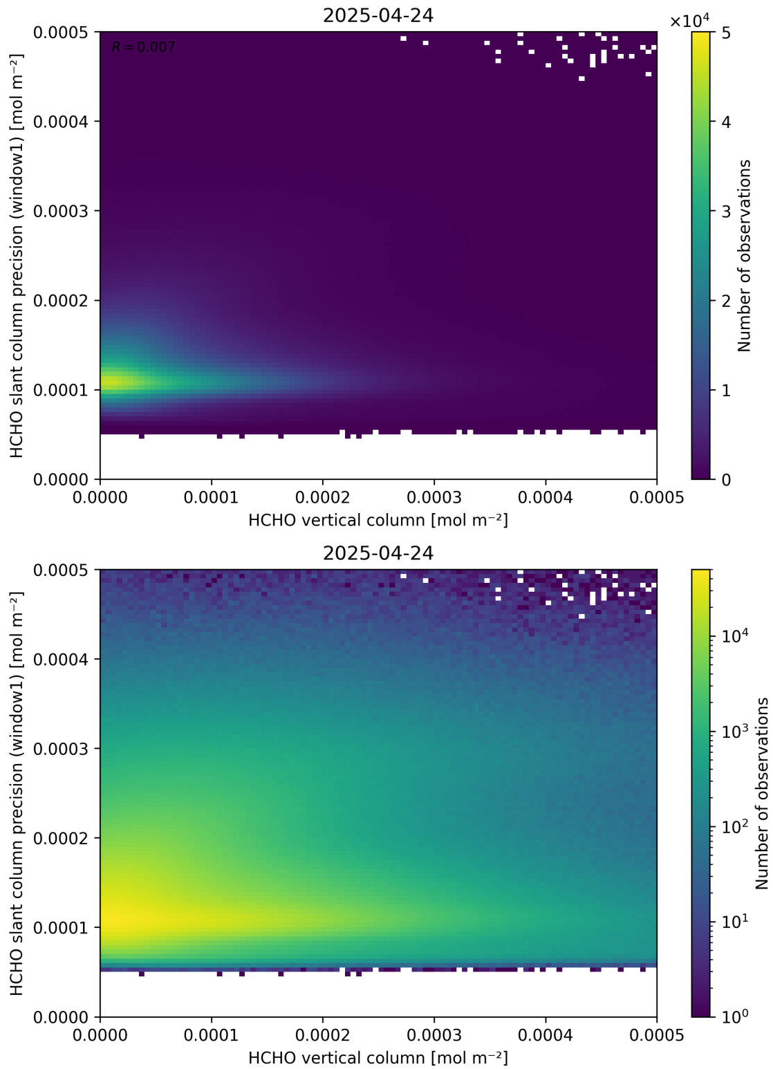
Figure 130: Scatter density plot of “HCHO vertical column” against “HCHO slant column precision (window1)” for 2025-04-24 to 2025-04-25.
