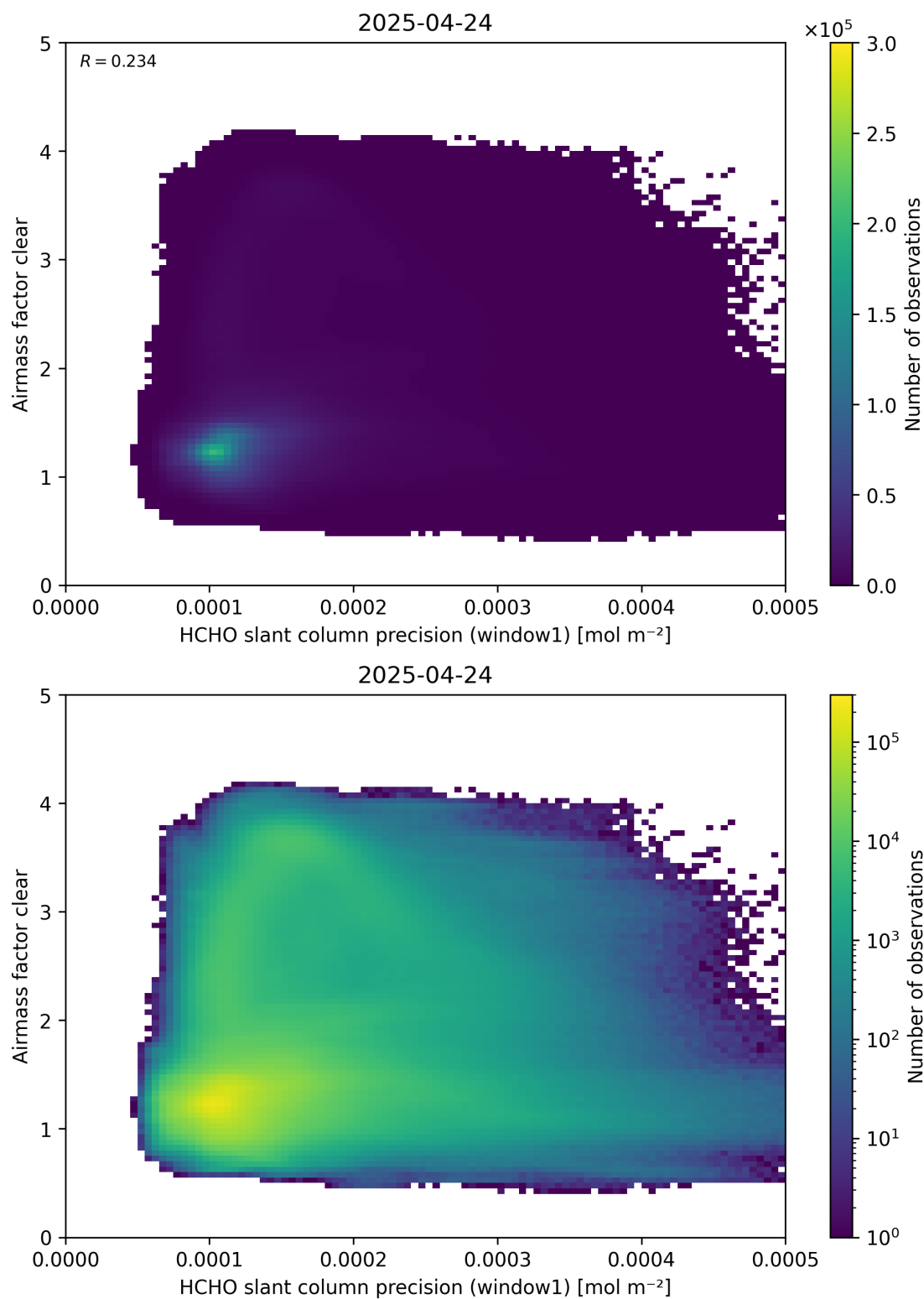
Figure 91: Scatter density plot of “HCHO slant column precision (window1)” against “Airmass factor clear” for 2025-04-24 to 2025-04-25.
