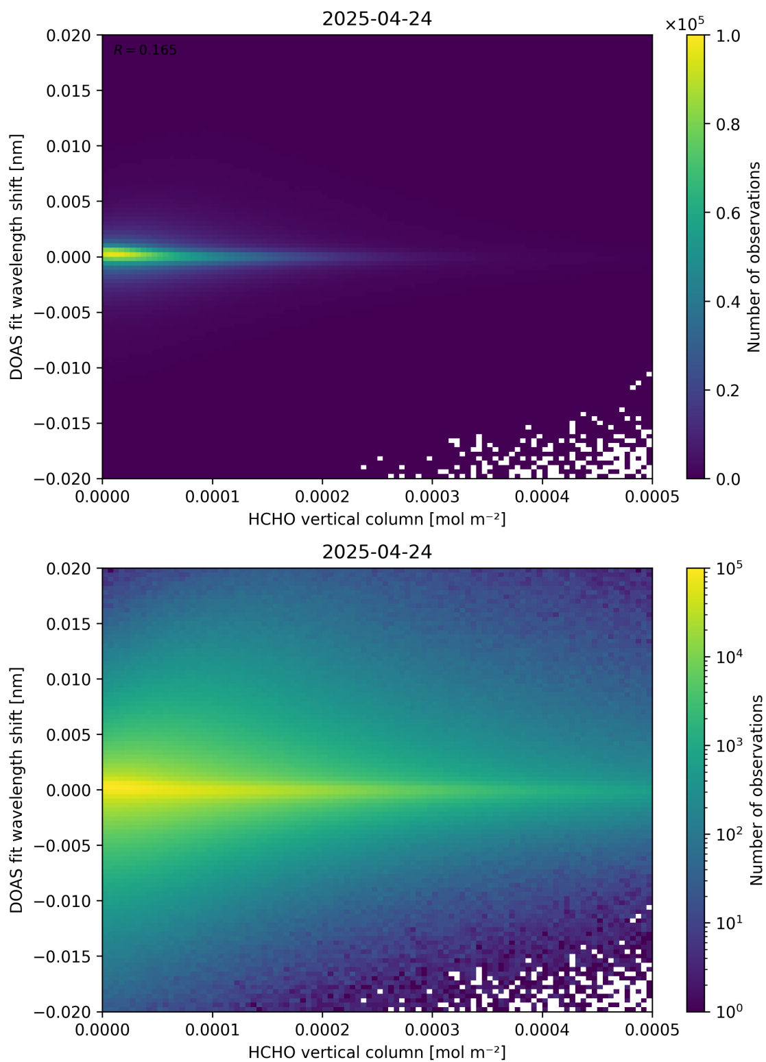
Figure 124: Scatter density plot of “HCHO vertical column” against “DOAS fit wavelength shift” for 2025-04-24 to 2025-04-25.
