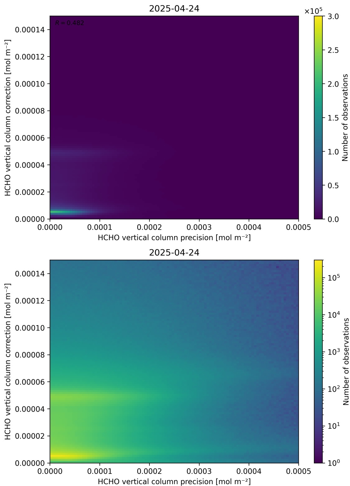
Figure 146: Scatter density plot of “HCHO vertical column precision” against “HCHO vertical column correction” for 2025-04-24 to 2025-04-25.
