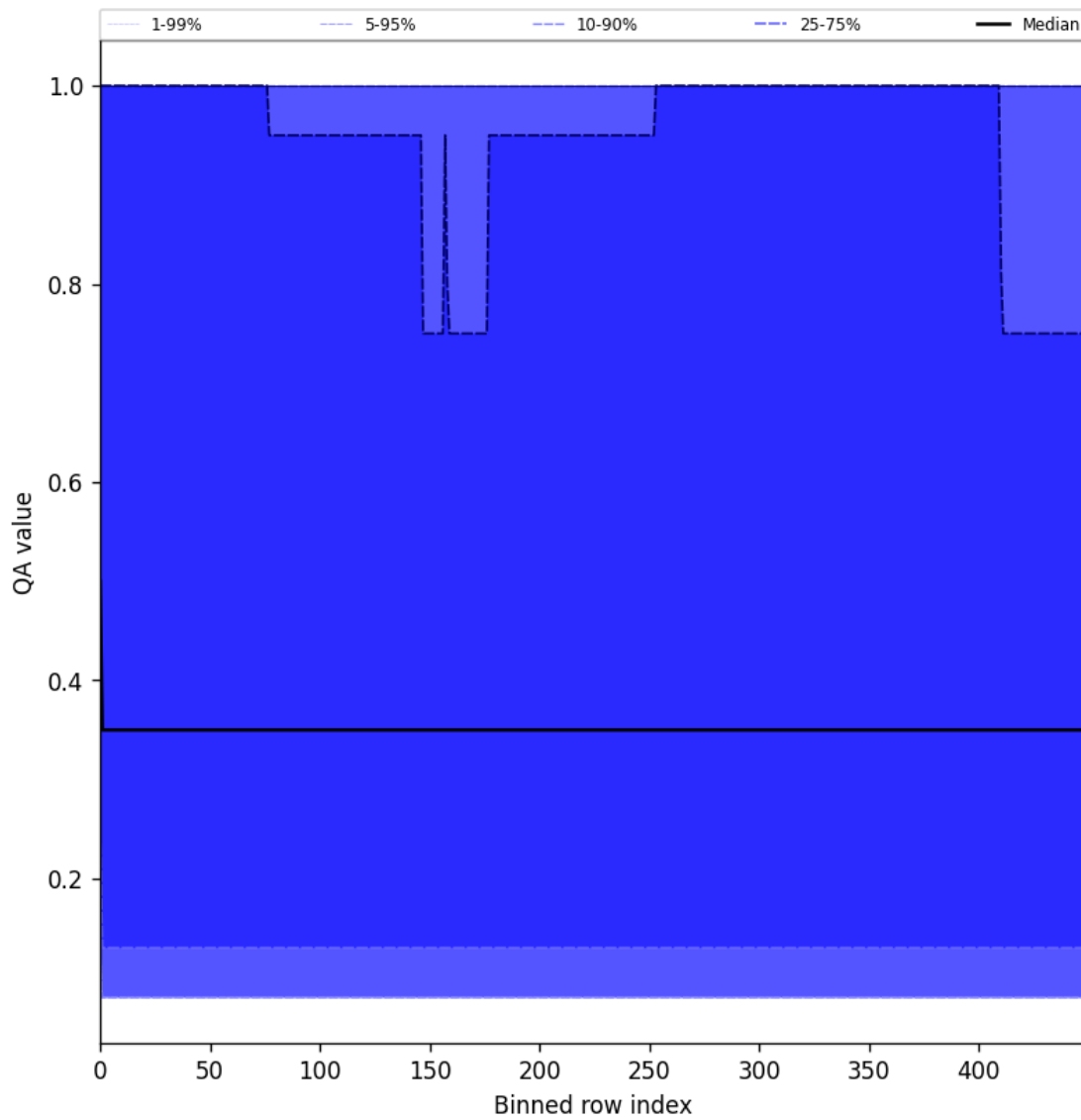
Figure 48: Along track statistics of “QA value” for 2025-04-24 to 2025-04-25
