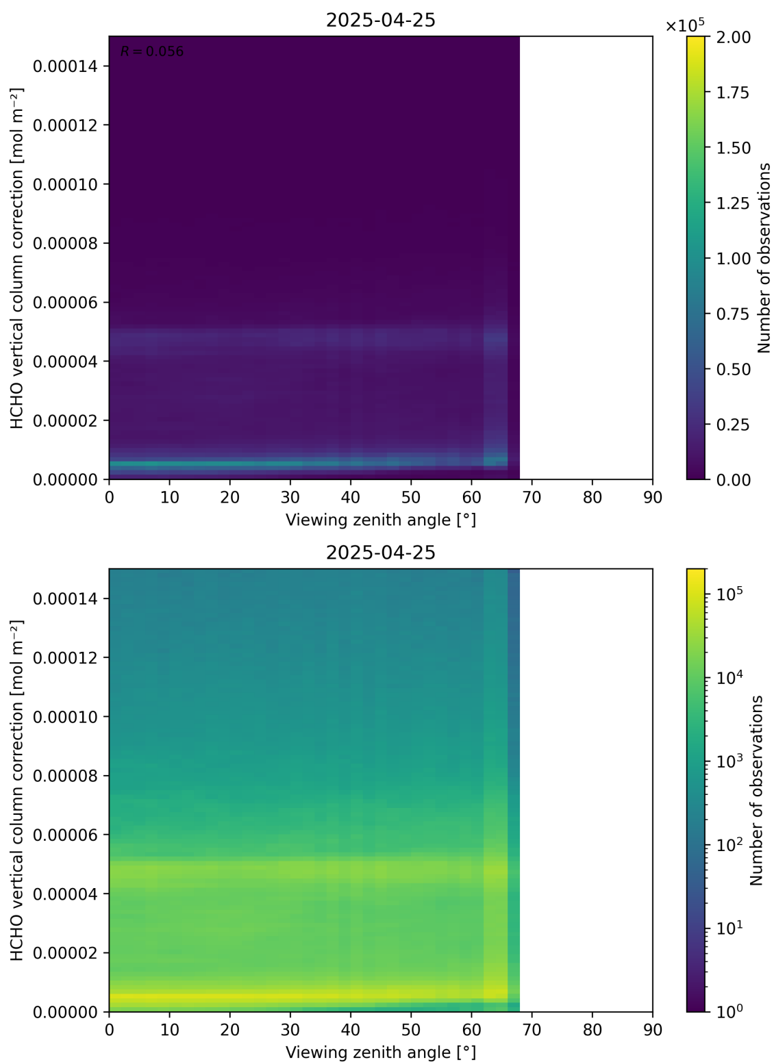
Figure 193: Scatter density plot of “Viewing zenith angle” against “HCHO vertical column correction” for 2025-04-24 to 2025-04-26.
