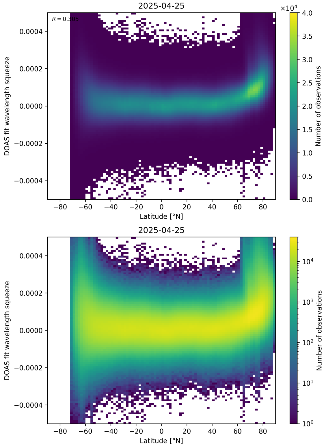
Figure 155: Scatter density plot of “Latitude” against “DOAS fit wavelength squeeze” for 2025-04-24 to 2025-04-26.
