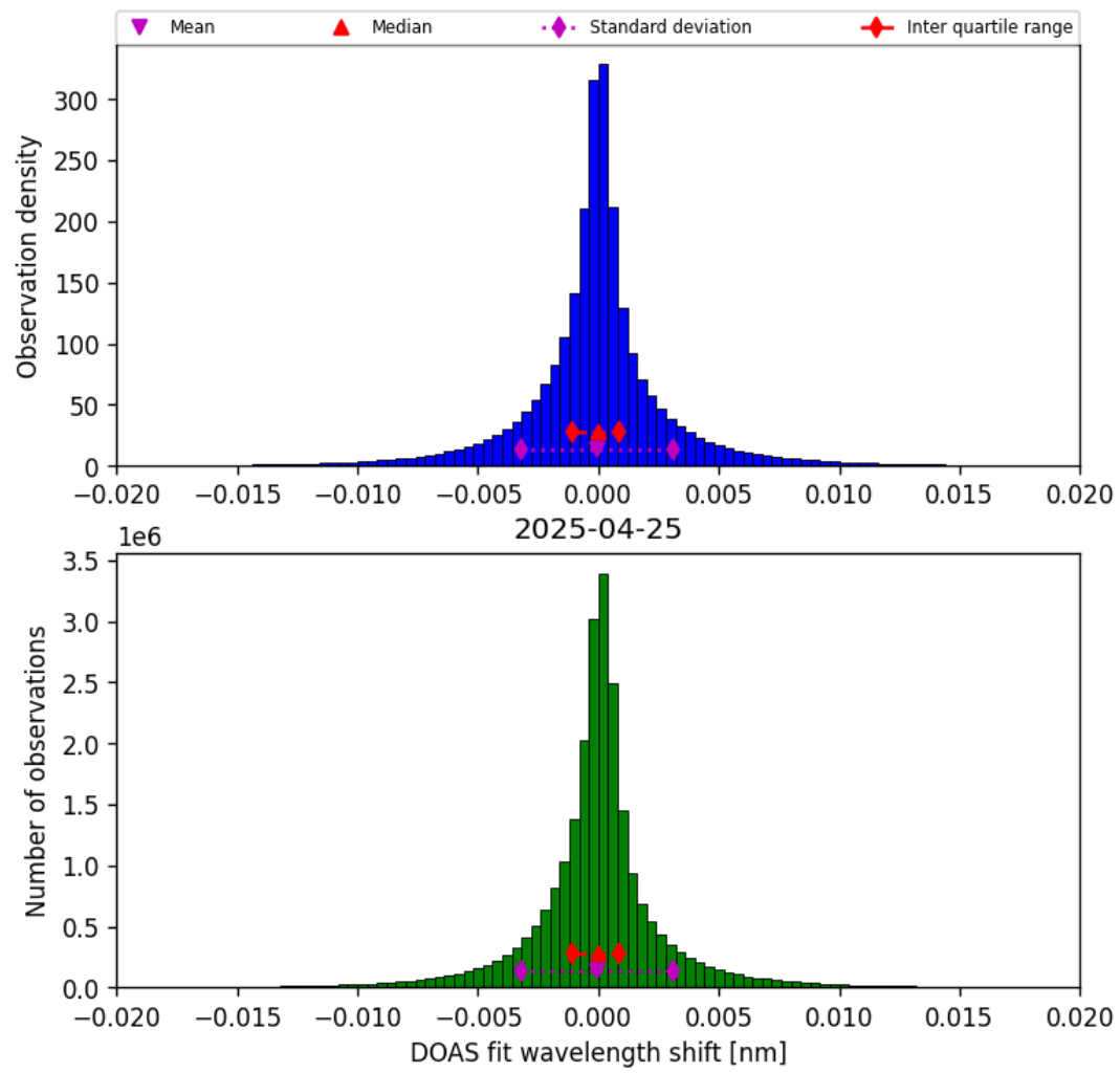
Figure 44: Histogram of “DOAS fit wavelength shift” for 2025-04-24 to 2025-04-26
