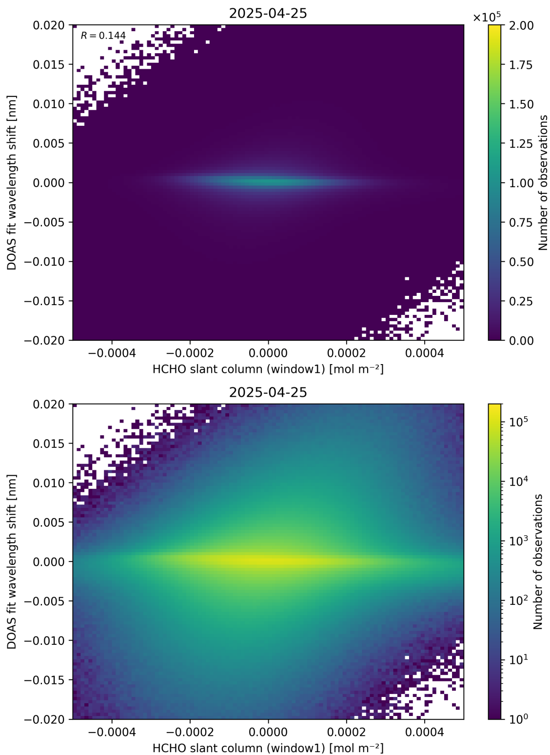
Figure 79: Scatter density plot of “HCHO slant column (window1)” against “DOAS fit wavelength shift” for 2025-04-24 to 2025-04-26.
