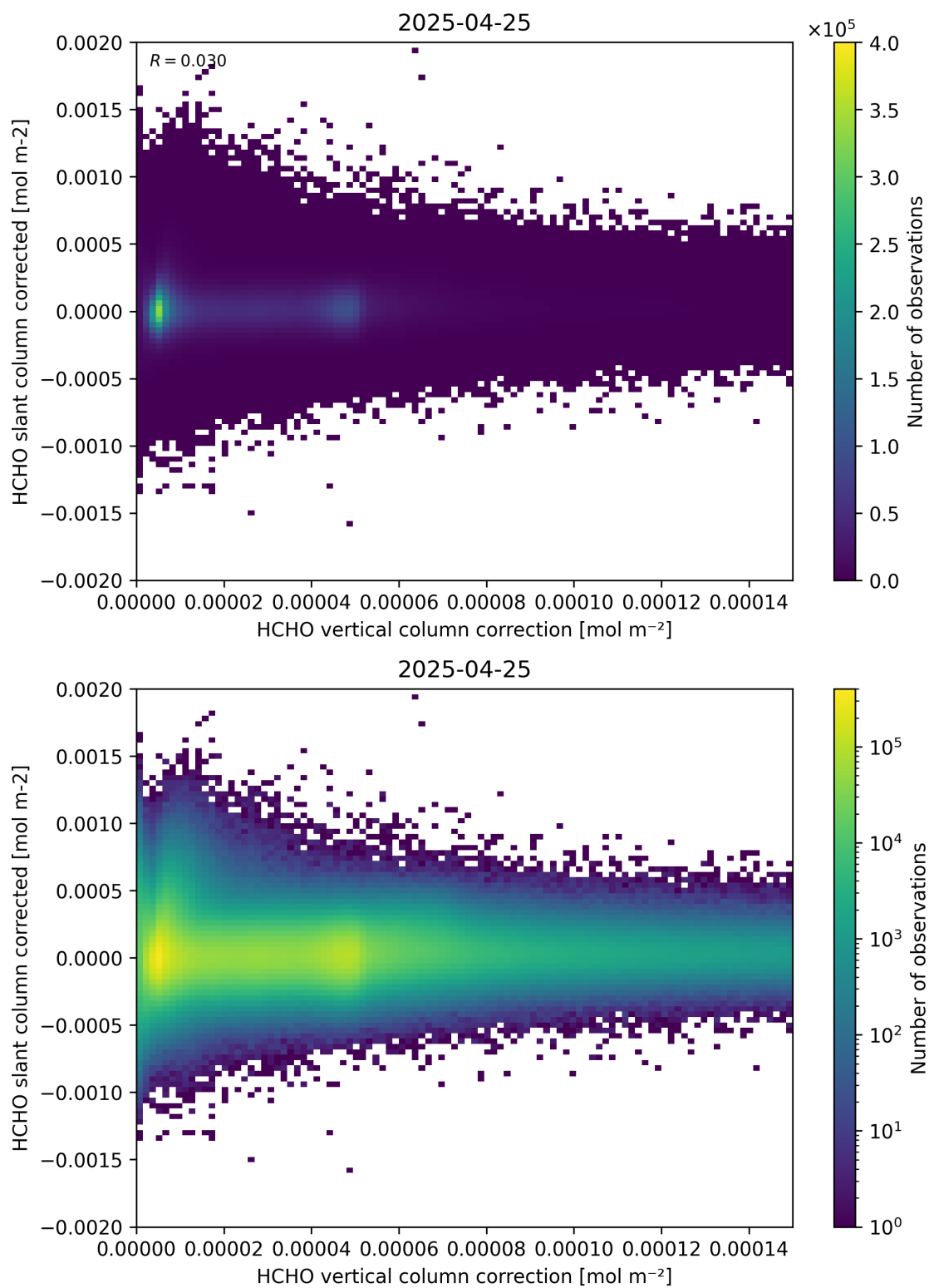
Figure 116: Scatter density plot of “HCHO vertical column correction” against “HCHO slant column corrected” for 2025-04-24 to 2025-04-26.
