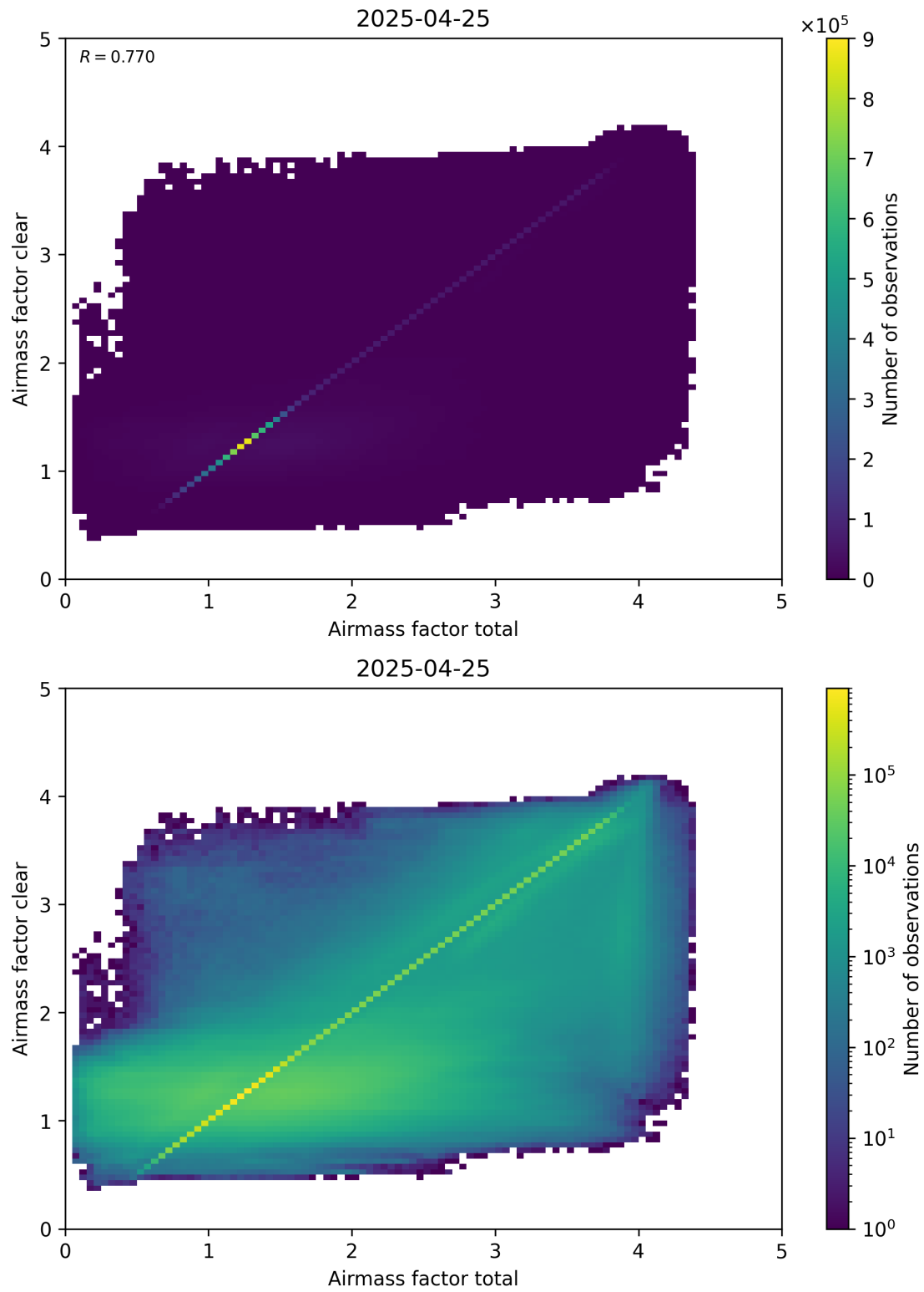
Figure 100: Scatter density plot of “Airmass factor total” against “Airmass factor clear” for 2025-04-24 to 2025-04-26.
