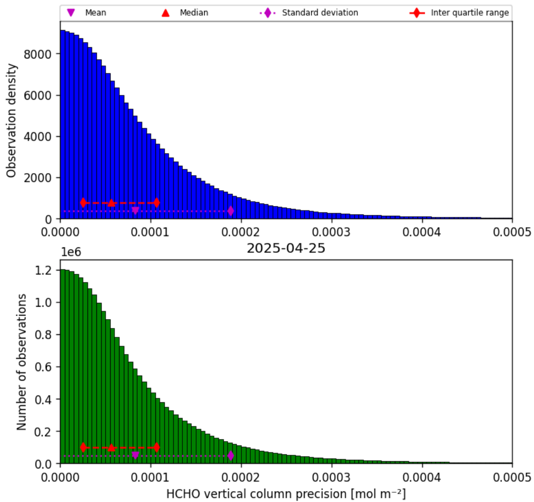
Figure 36: Histogram of “HCHO vertical column precision” for 2025-04-24 to 2025-04-26
