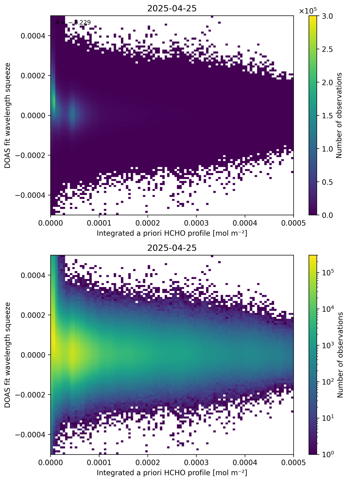
Figure 150: Scatter density plot of “Integrated a priori HCHO profile” against “DOAS fit wavelength squeeze” for 2025-04-24 to 2025-04-26.
