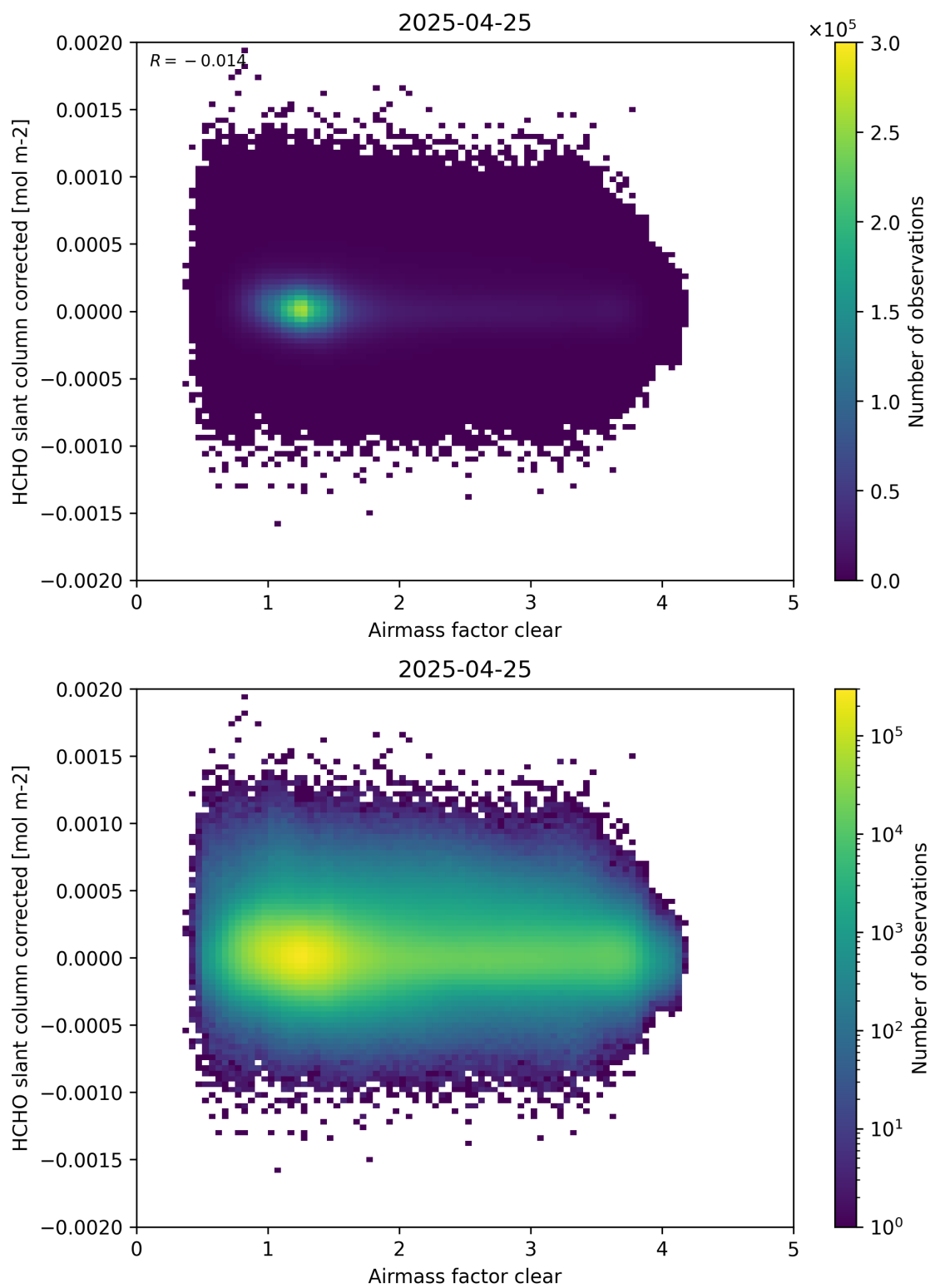
Figure 74: Scatter density plot of “Airmass factor clear” against “HCHO slant column corrected” for 2025-04-24 to 2025-04-26.
