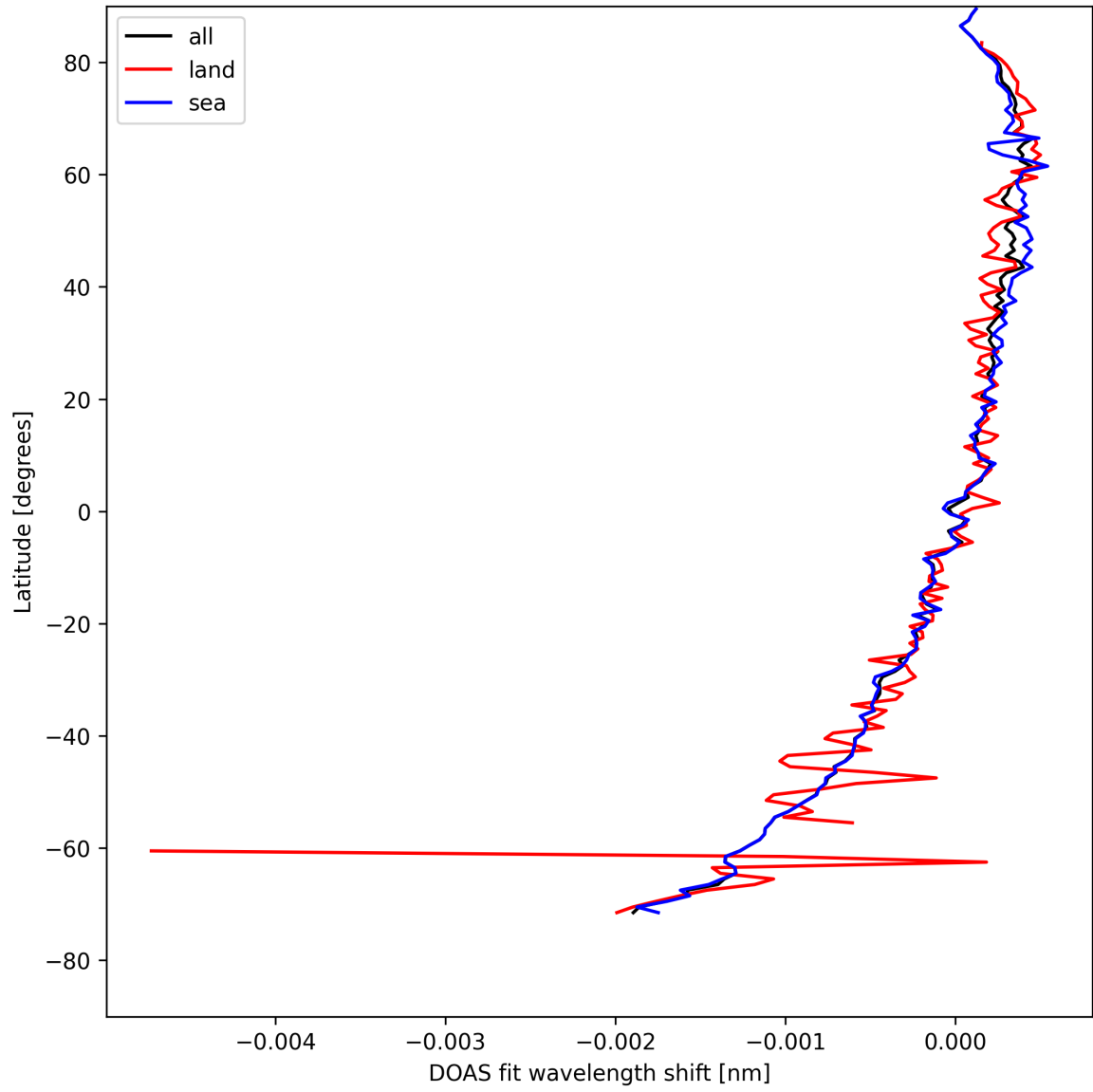
Figure 30: Zonal average of “DOAS fit wavelength shift” for 2025-04-24 to 2025-04-26.
