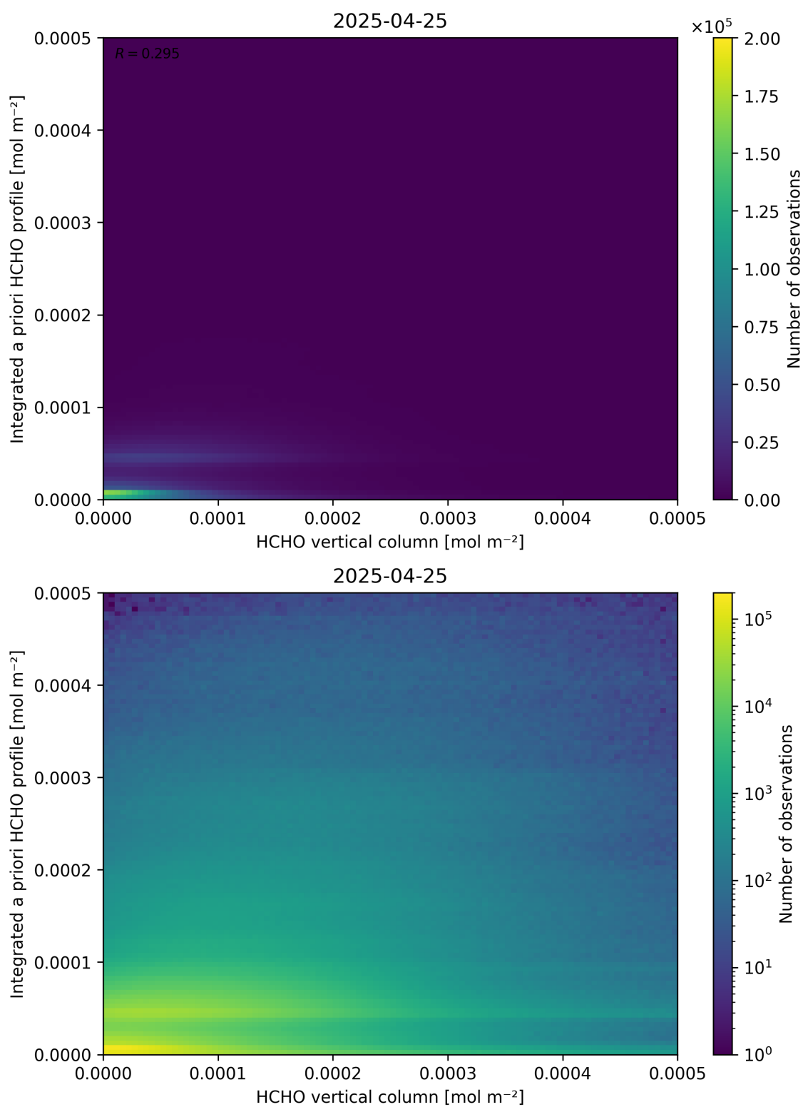
Figure 135: Scatter density plot of “HCHO vertical column” against “Integrated a priori HCHO profile” for 2025-04-24 to 2025-04-26.
