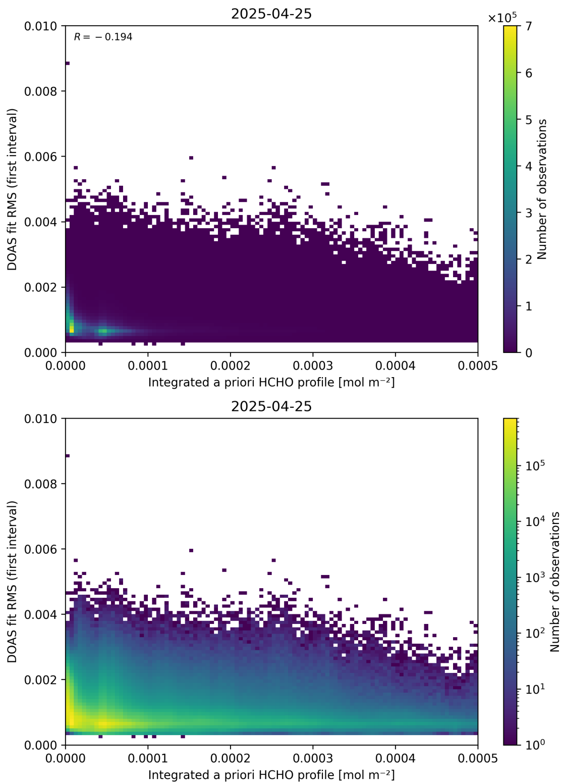
Figure 148: Scatter density plot of “Integrated a priori HCHO profile” against “DOAS fit RMS (first interval)” for 2025-04-24 to 2025-04-26.
