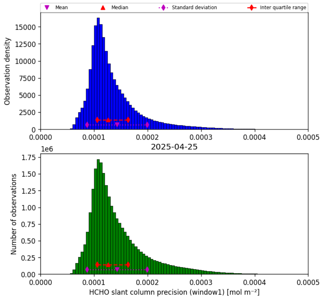
Figure 39: Histogram of “HCHO slant column precision (window1)” for 2025-04-24 to 2025-04-26
