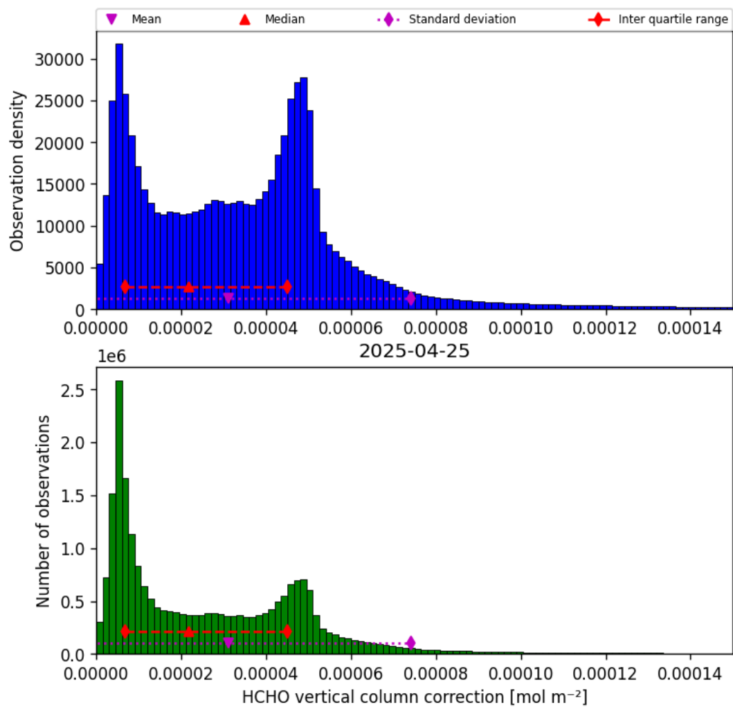
Figure 37: Histogram of “HCHO vertical column correction” for 2025-04-24 to 2025-04-26
