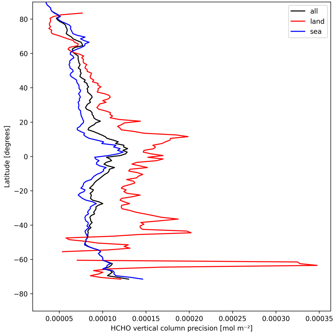
Figure 22: Zonal average of “HCHO vertical column precision” for 2025-04-24 to 2025-04-26.
