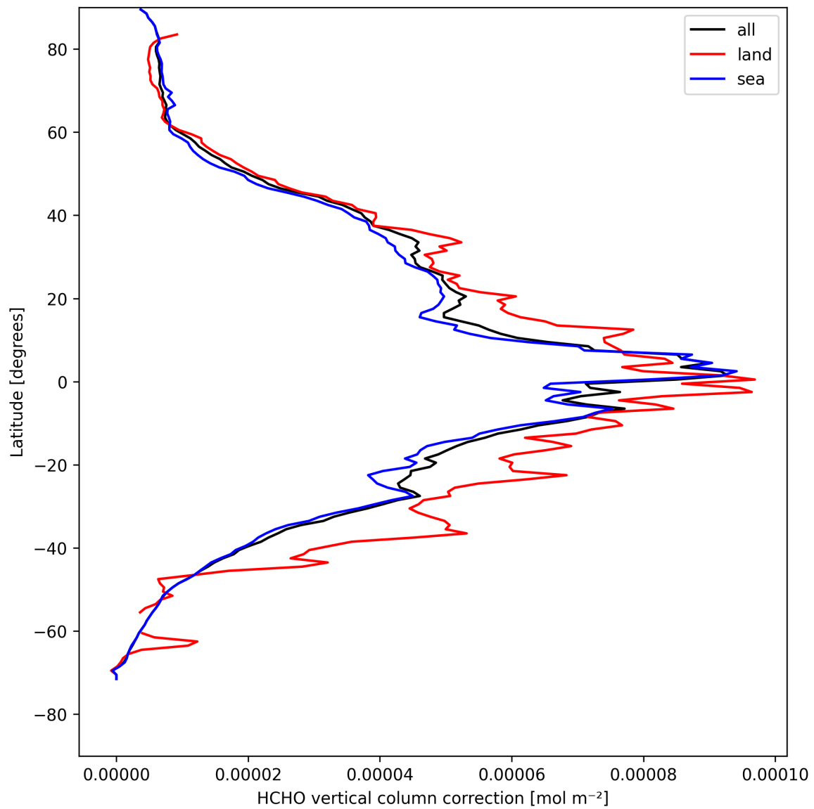
Figure 23: Zonal average of “HCHO vertical column correction” for 2025-04-24 to 2025-04-26.
