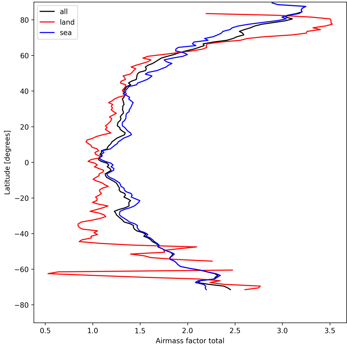
Figure 26: Zonal average of “Airmass factor total” for 2025-04-24 to 2025-04-26.
