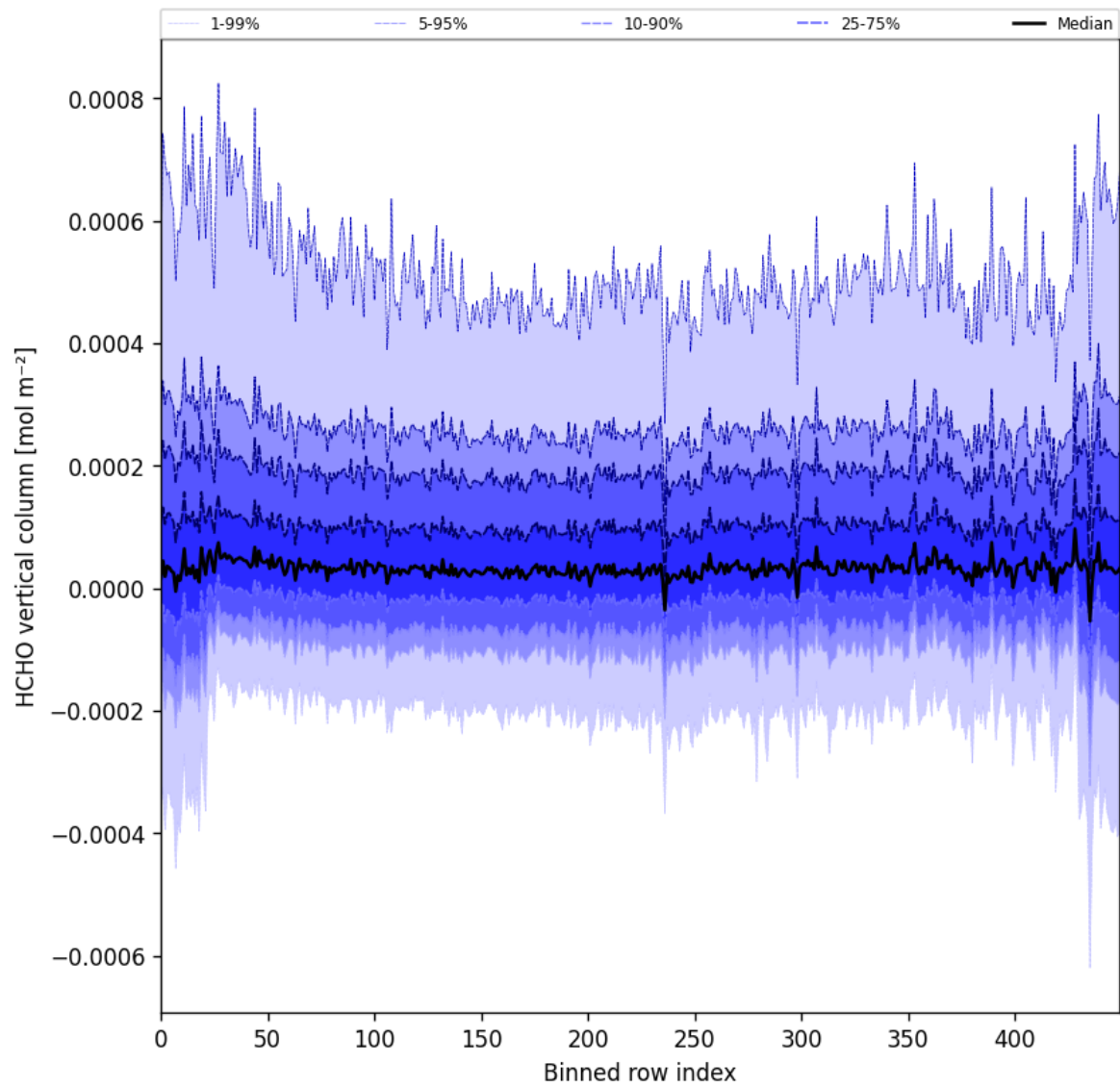
Figure 49: Along track statistics of “HCHO vertical column” for 2025-04-24 to 2025-04-26
