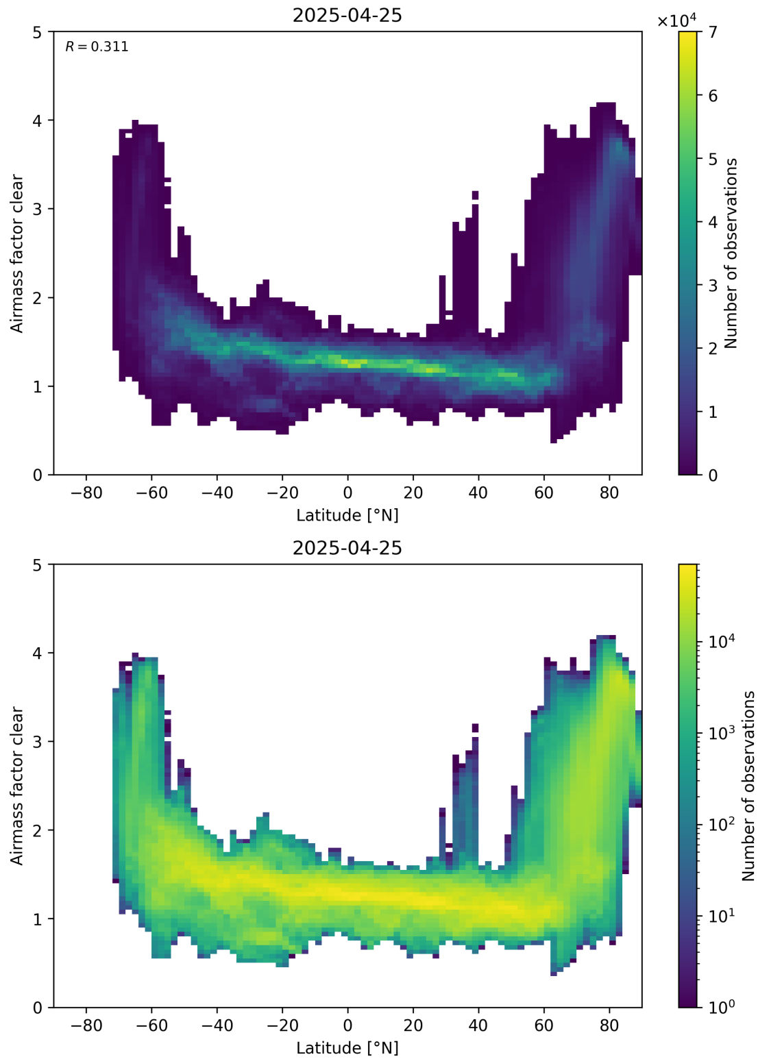
Figure 156: Scatter density plot of “Latitude” against “Airmass factor clear” for 2025-04-24 to 2025-04-26.
