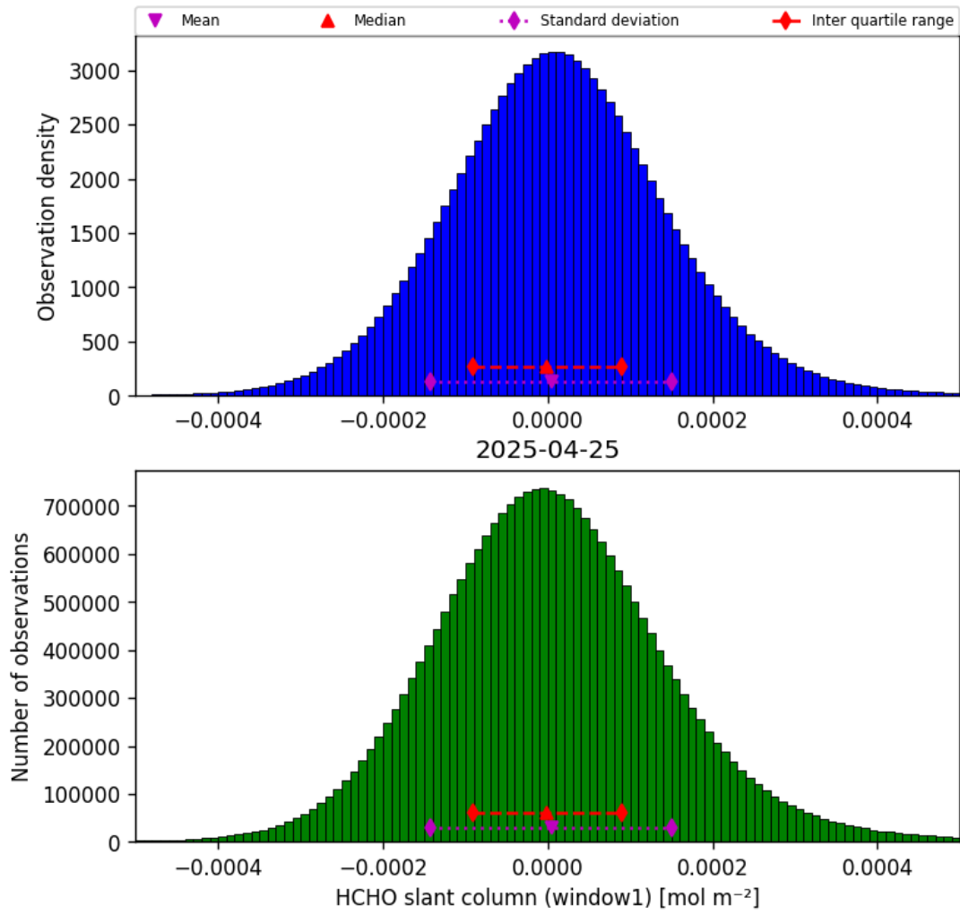
Figure 38: Histogram of “HCHO slant column (window1)” for 2025-04-24 to 2025-04-26
