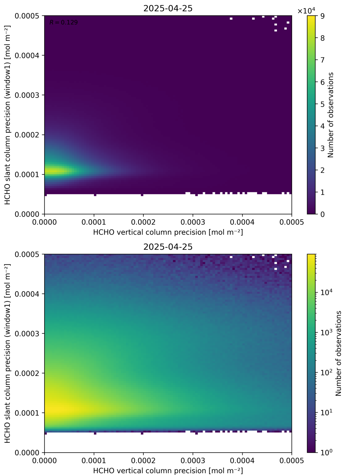
Figure 143: Scatter density plot of “HCHO vertical column precision” against “HCHO slant column precision (window1)” for 2025-04-24 to 2025-04-26.
