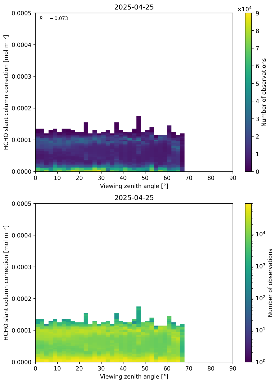
Figure 187: Scatter density plot of “Viewing zenith angle” against “HCHO slant column correction” for 2025-04-24 to 2025-04-26.
