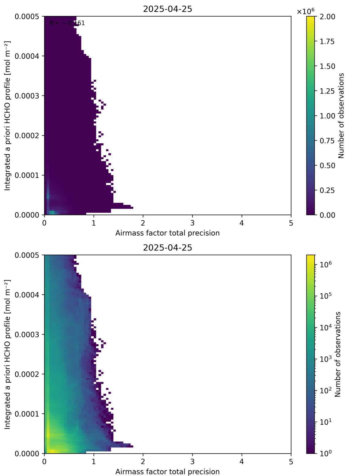
Figure 111: Scatter density plot of “Airmass factor total precision” against “Integrated a priori HCHO profile” for 2025-04-24 to 2025-04-26.
