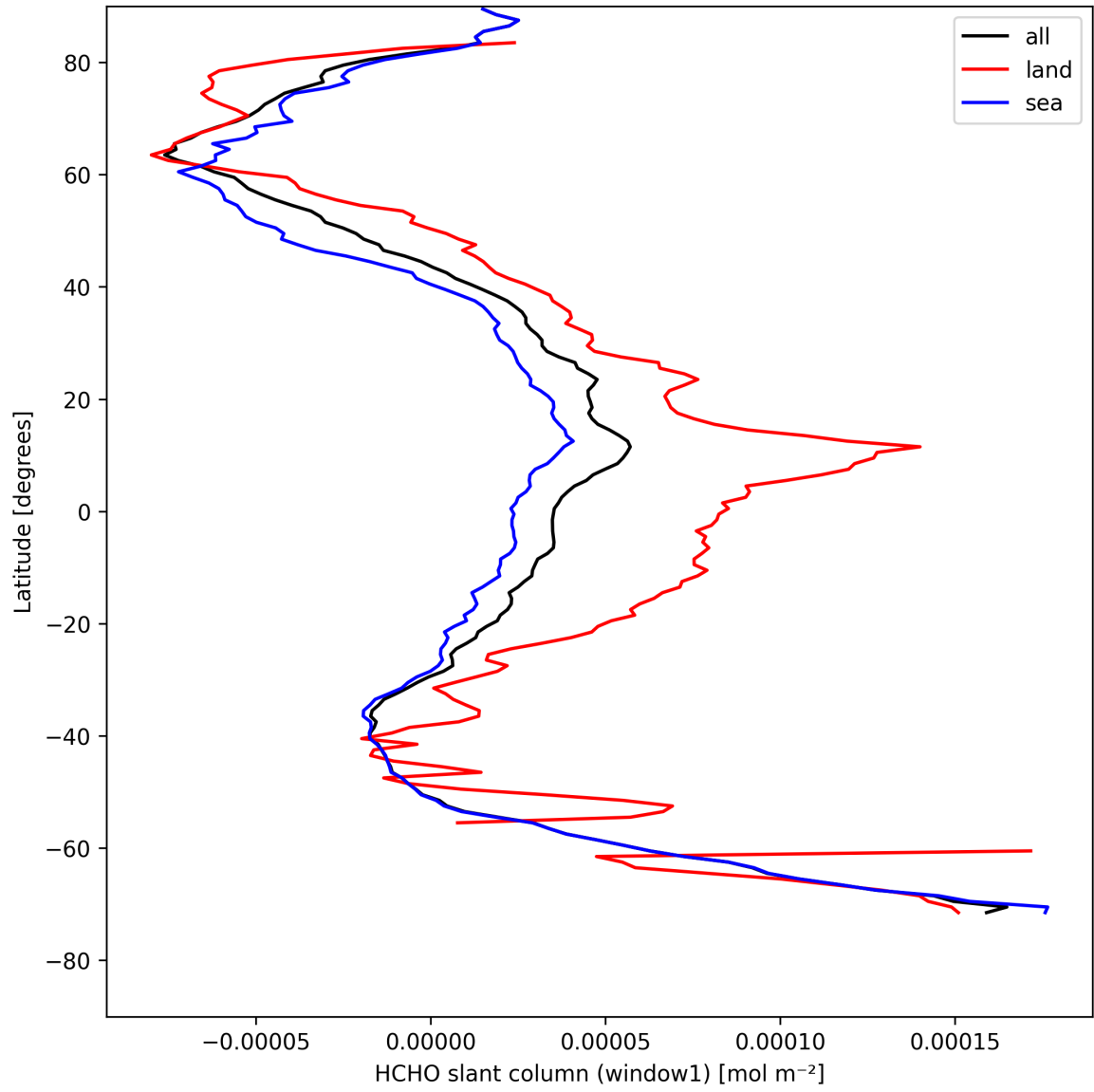
Figure 24: Zonal average of “HCHO slant column (window1)” for 2025-04-24 to 2025-04-26.
