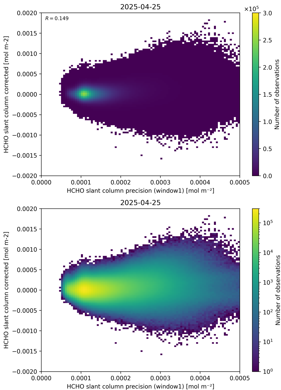
Figure 92: Scatter density plot of “HCHO slant column precision (window1)” against “HCHO slant column corrected” for 2025-04-24 to 2025-04-26.
