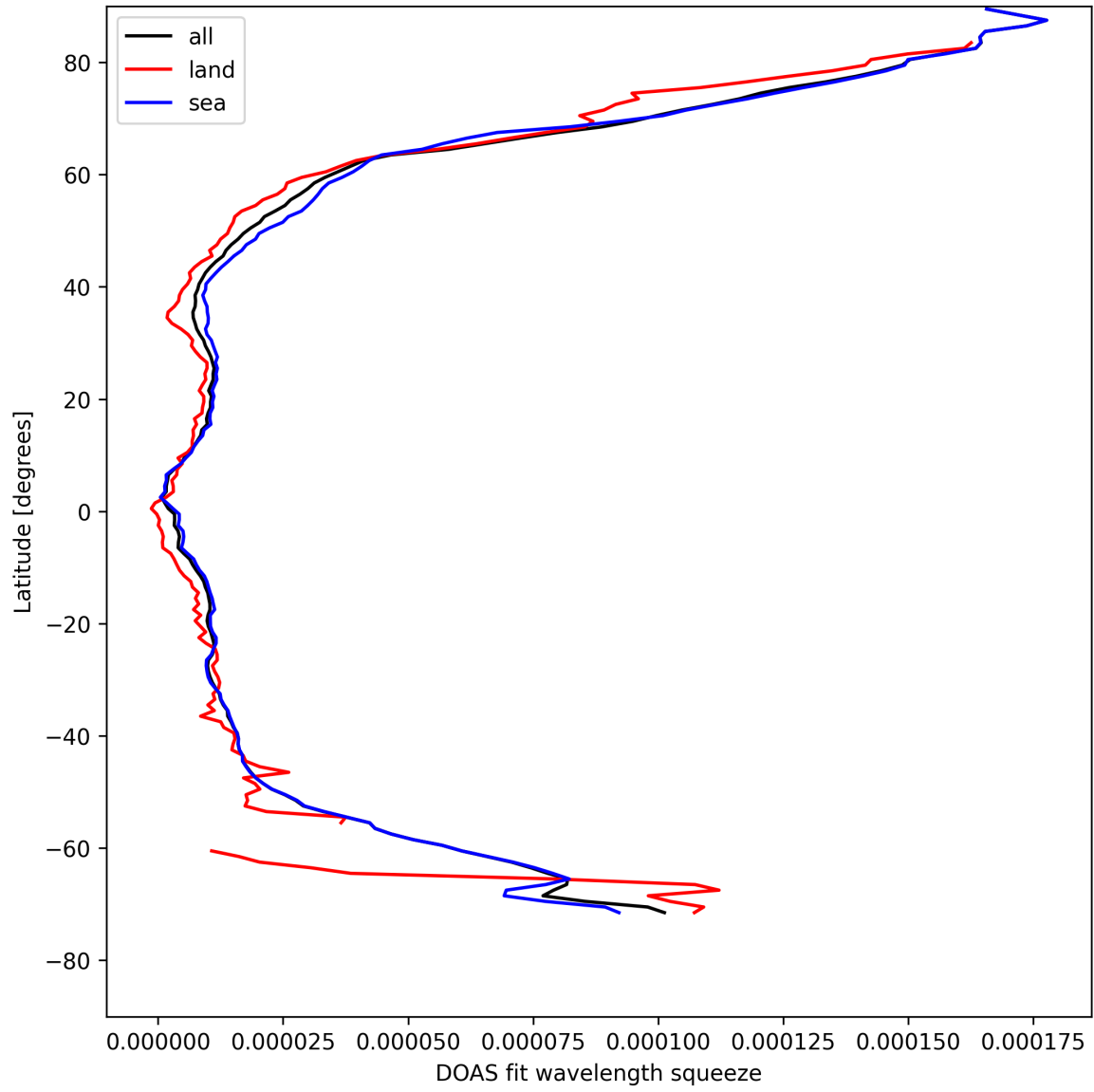
Figure 31: Zonal average of “DOAS fit wavelength squeeze” for 2025-04-24 to 2025-04-26.
