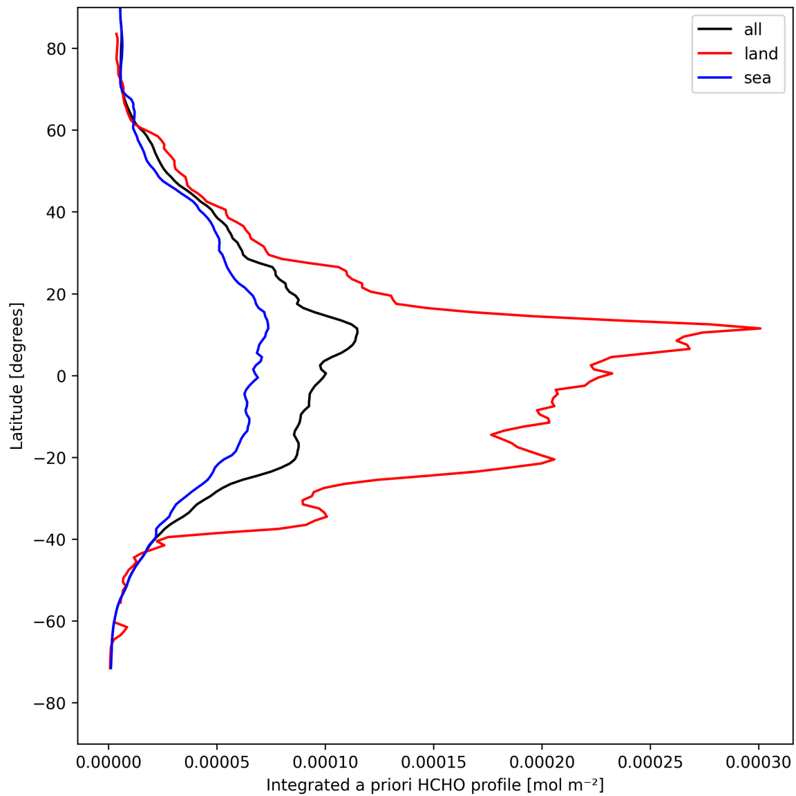
Figure 29: Zonal average of “Integrated a priori HCHO profile” for 2025-04-24 to 2025-04-26.
