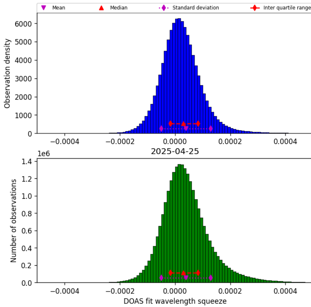
Figure 45: Histogram of “DOAS fit wavelength squeeze” for 2025-04-24 to 2025-04-26
