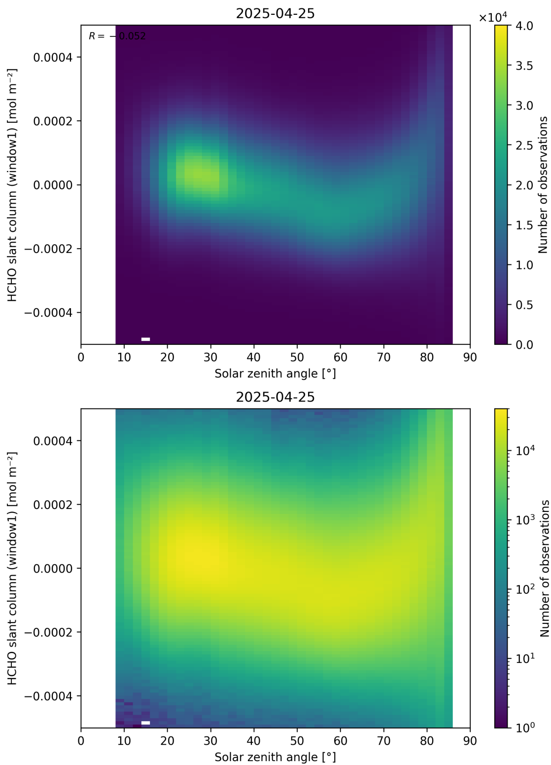
Figure 173: Scatter density plot of “Solar zenith angle” against “HCHO slant column (window1)” for 2025-04-24 to 2025-04-26.
