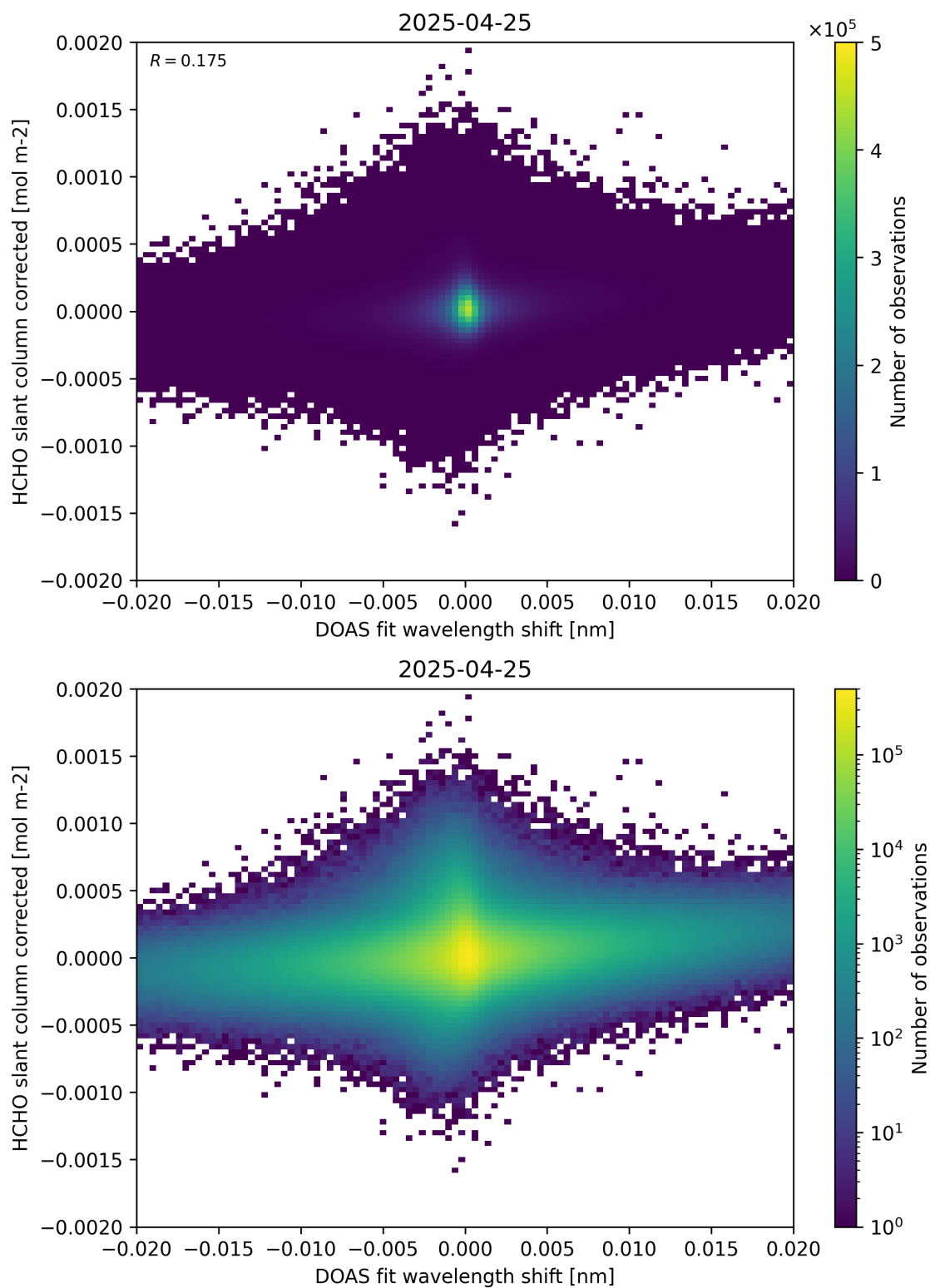
Figure 66: Scatter density plot of “DOAS fit wavelength shift” against “HCHO slant column corrected” for 2025-04-24 to 2025-04-26.
