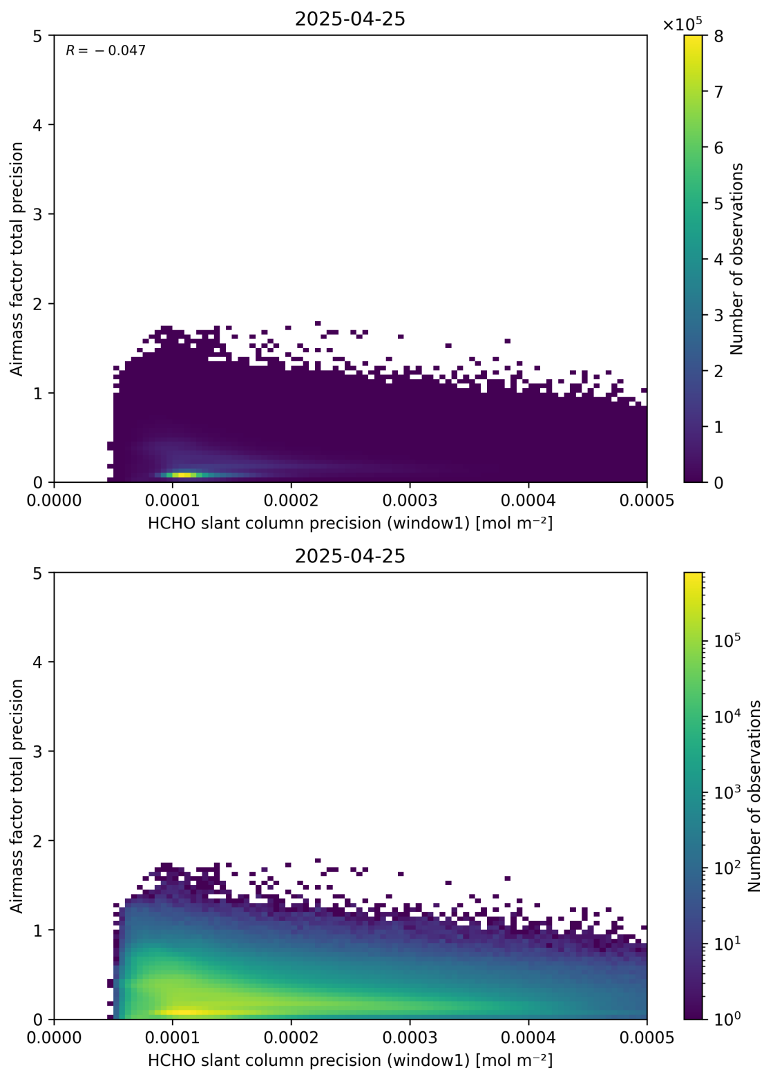
Figure 95: Scatter density plot of “HCHO slant column precision (window1)” against “Airmass factor total precision” for 2025-04-24 to 2025-04-26.
