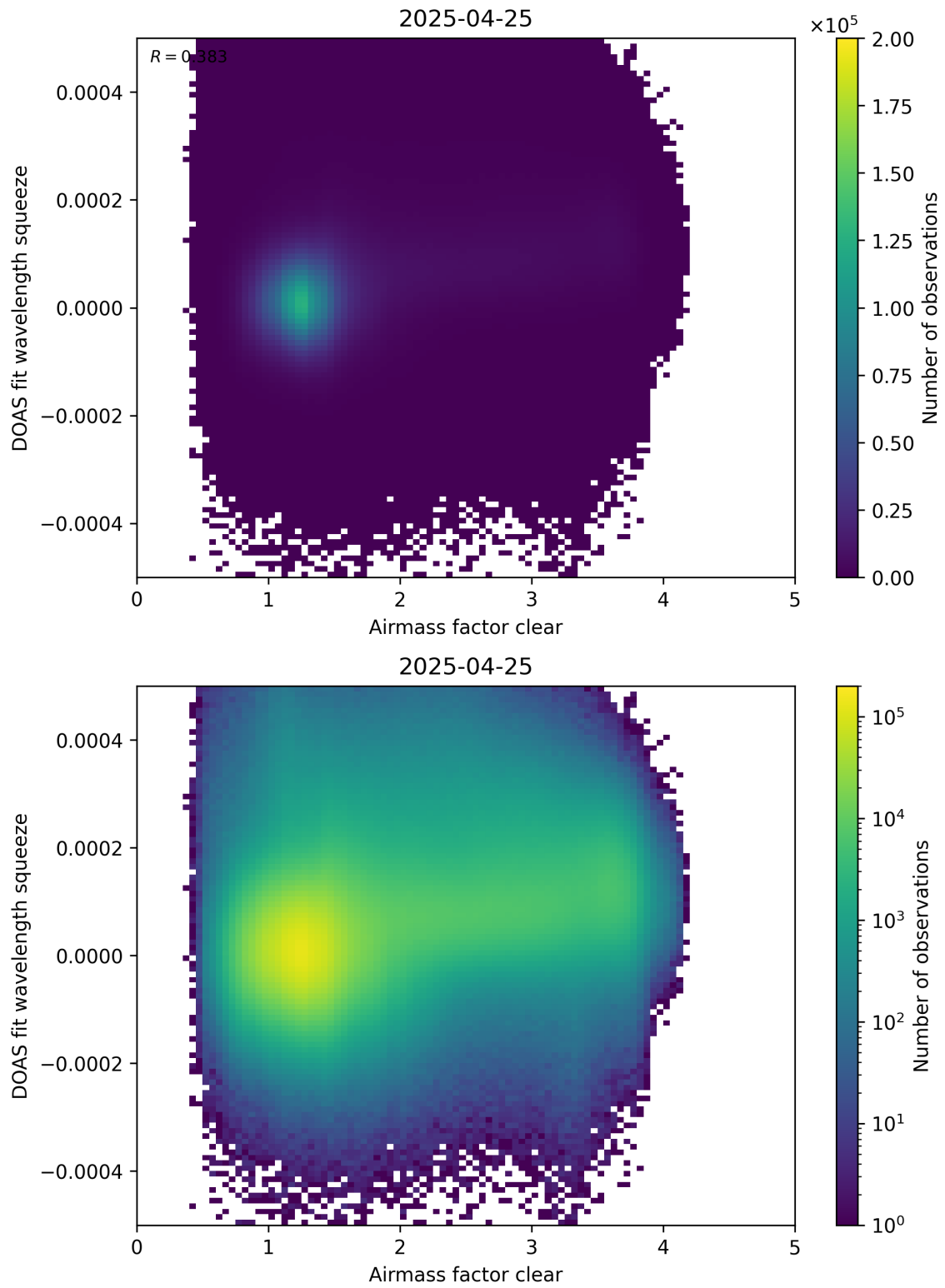
Figure 73: Scatter density plot of “Airmass factor clear” against “DOAS fit wavelength squeeze” for 2025-04-24 to 2025-04-26.
