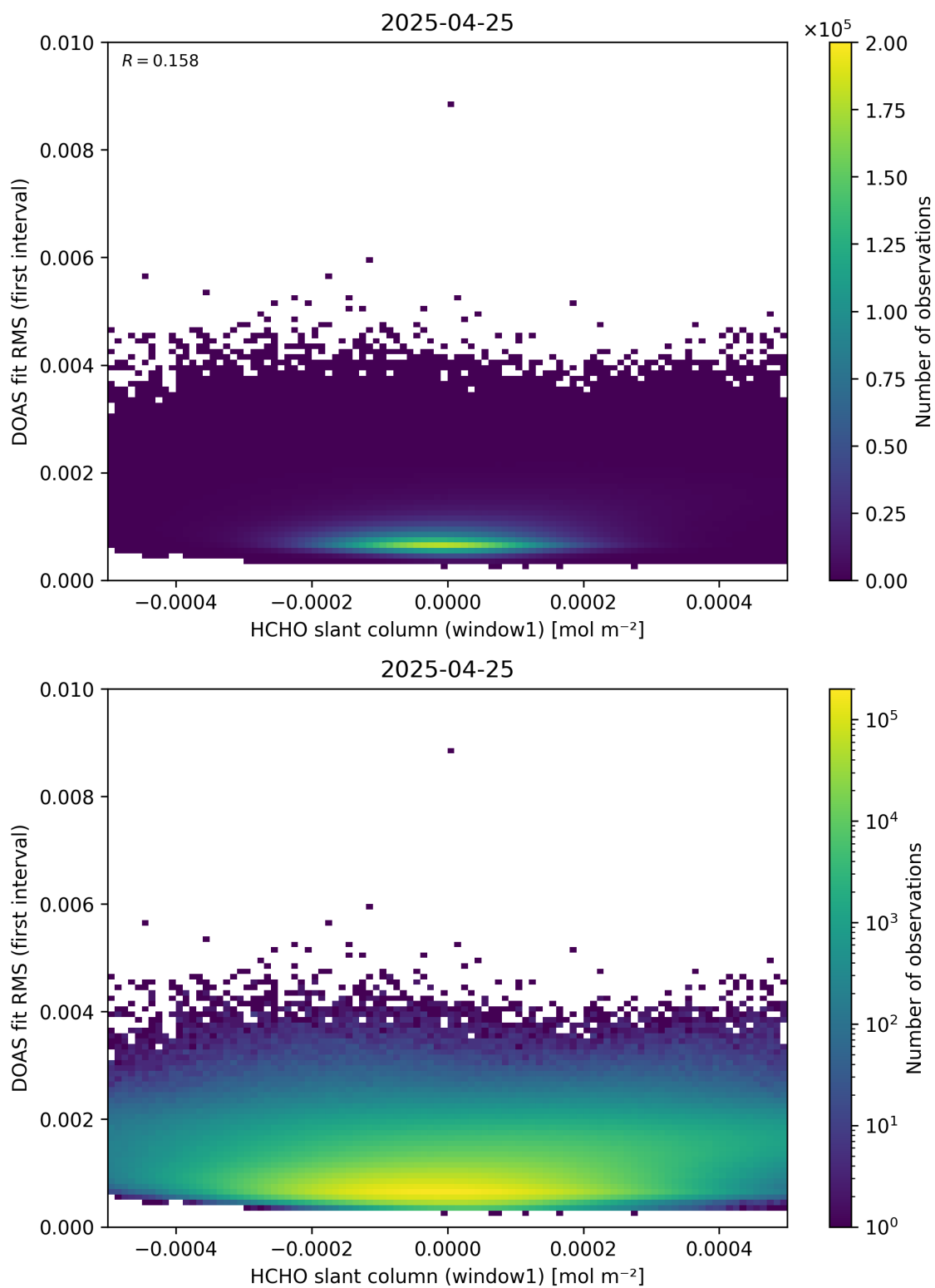
Figure 78: Scatter density plot of “HCHO slant column (window1)” against “DOAS fit RMS (first interval)” for 2025-04-24 to 2025-04-26.
