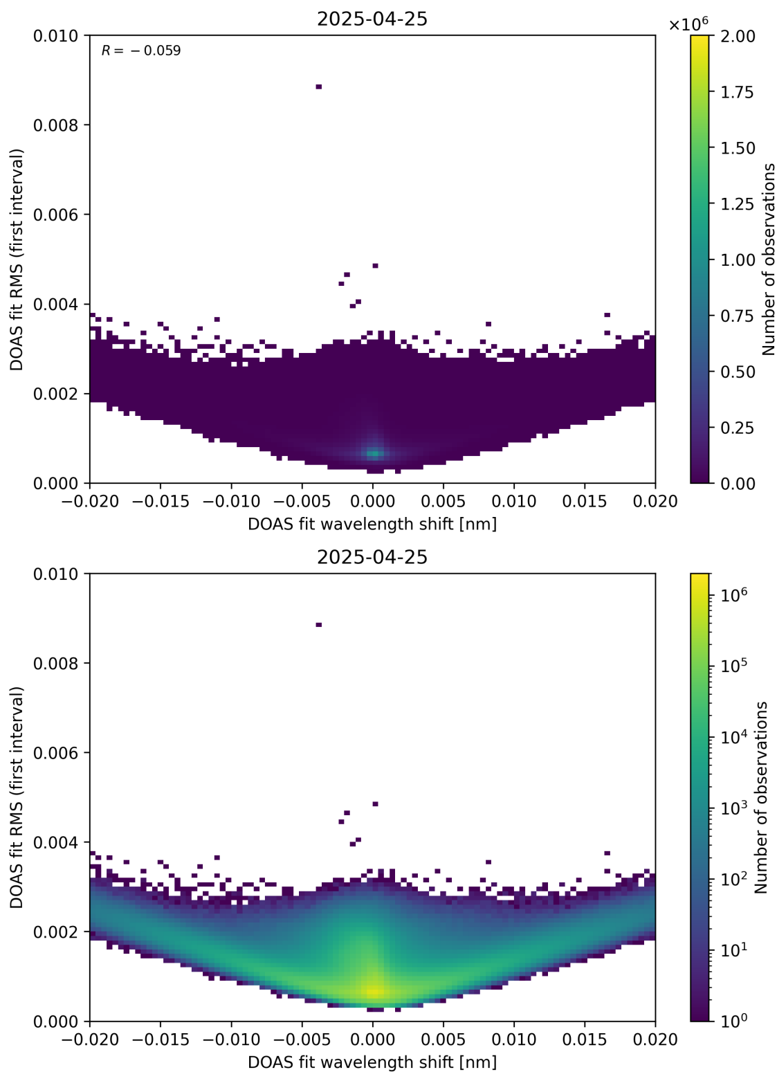
Figure 64: Scatter density plot of “DOAS fit wavelength shift” against “DOAS fit RMS (first interval)” for 2025-04-24 to 2025-04-26.
