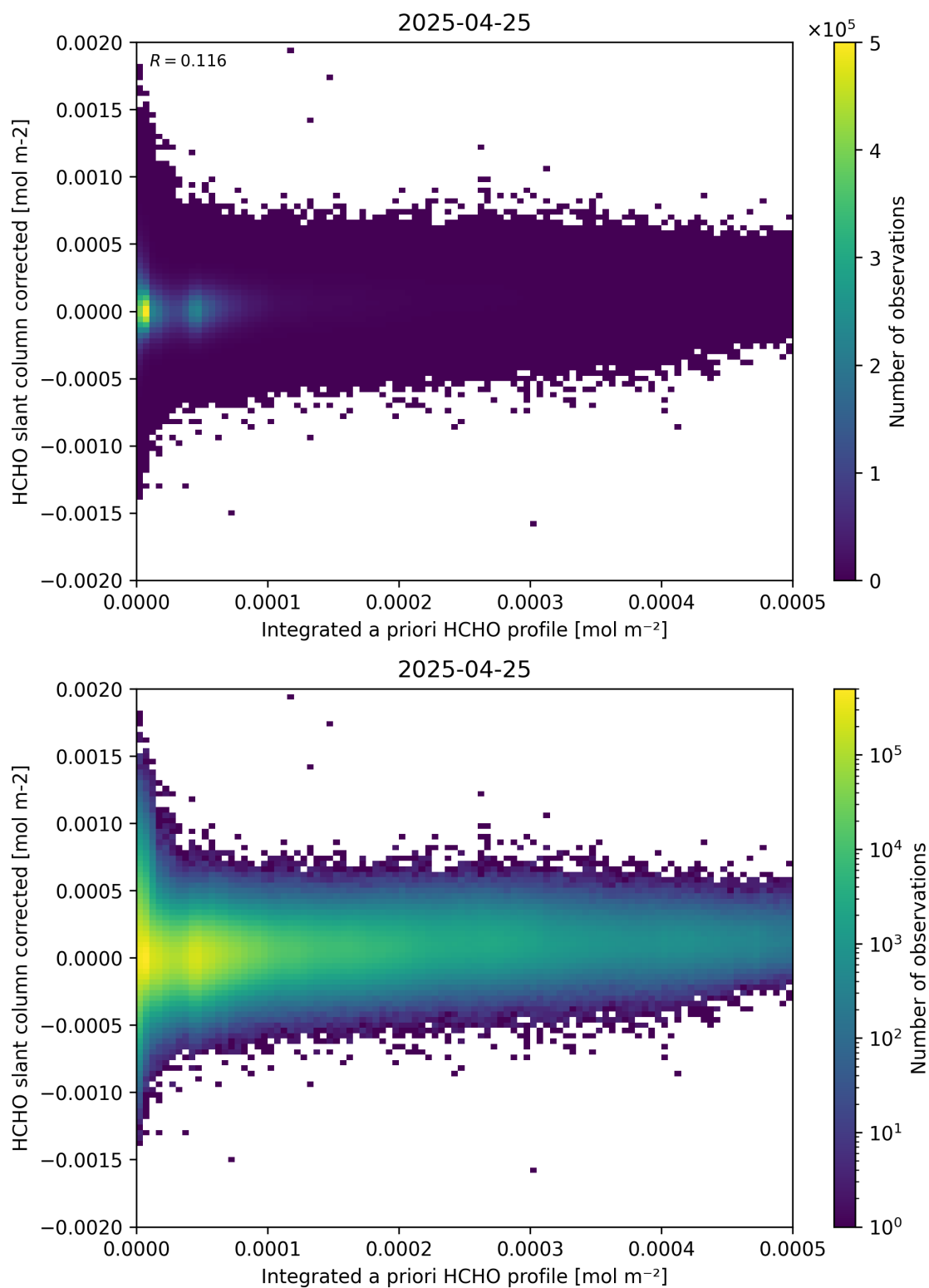
Figure 151: Scatter density plot of “Integrated a priori HCHO profile” against “HCHO slant column corrected” for 2025-04-24 to 2025-04-26.
