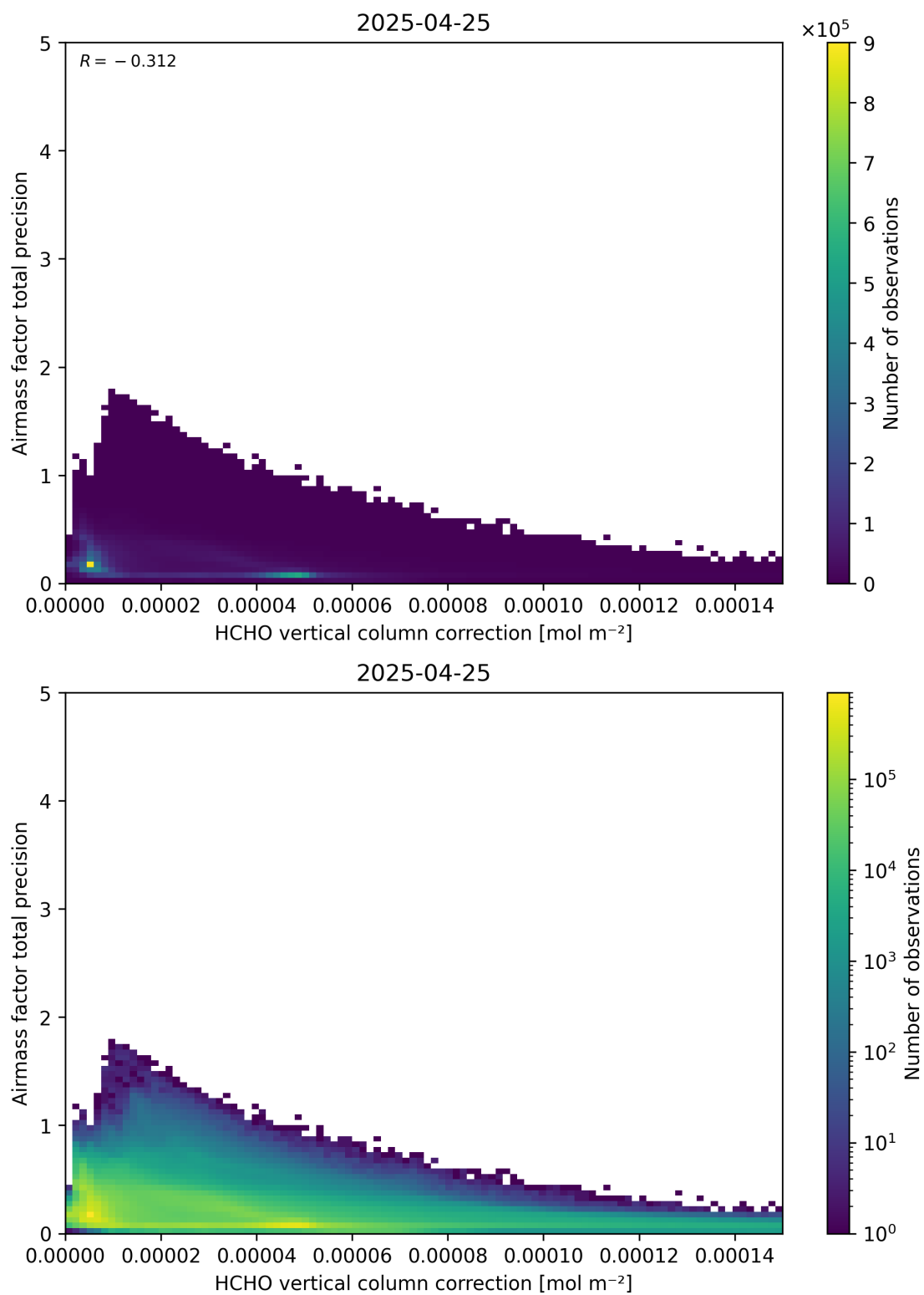
Figure 121: Scatter density plot of “HCHO vertical column correction” against “Airmass factor total precision” for 2025-04-24 to 2025-04-26.
