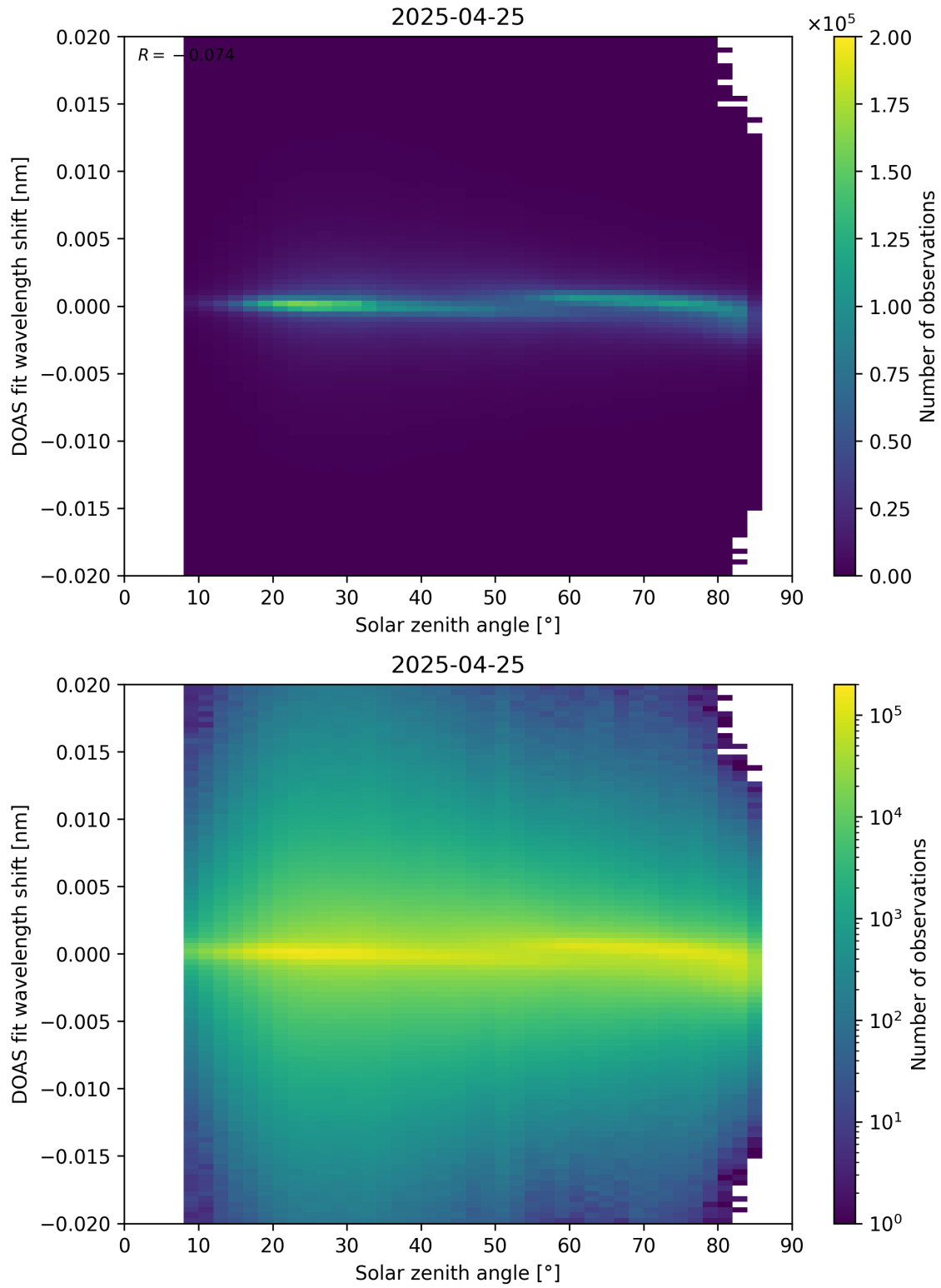
Figure 168: Scatter density plot of “Solar zenith angle” against “DOAS fit wavelength shift” for 2025-04-24 to 2025-04-26.
