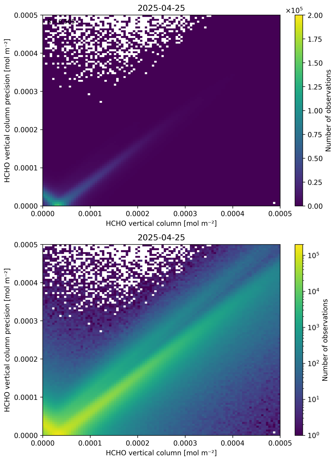
Figure 134: Scatter density plot of “HCHO vertical column” against “HCHO vertical column precision” for 2025-04-24 to 2025-04-26.
