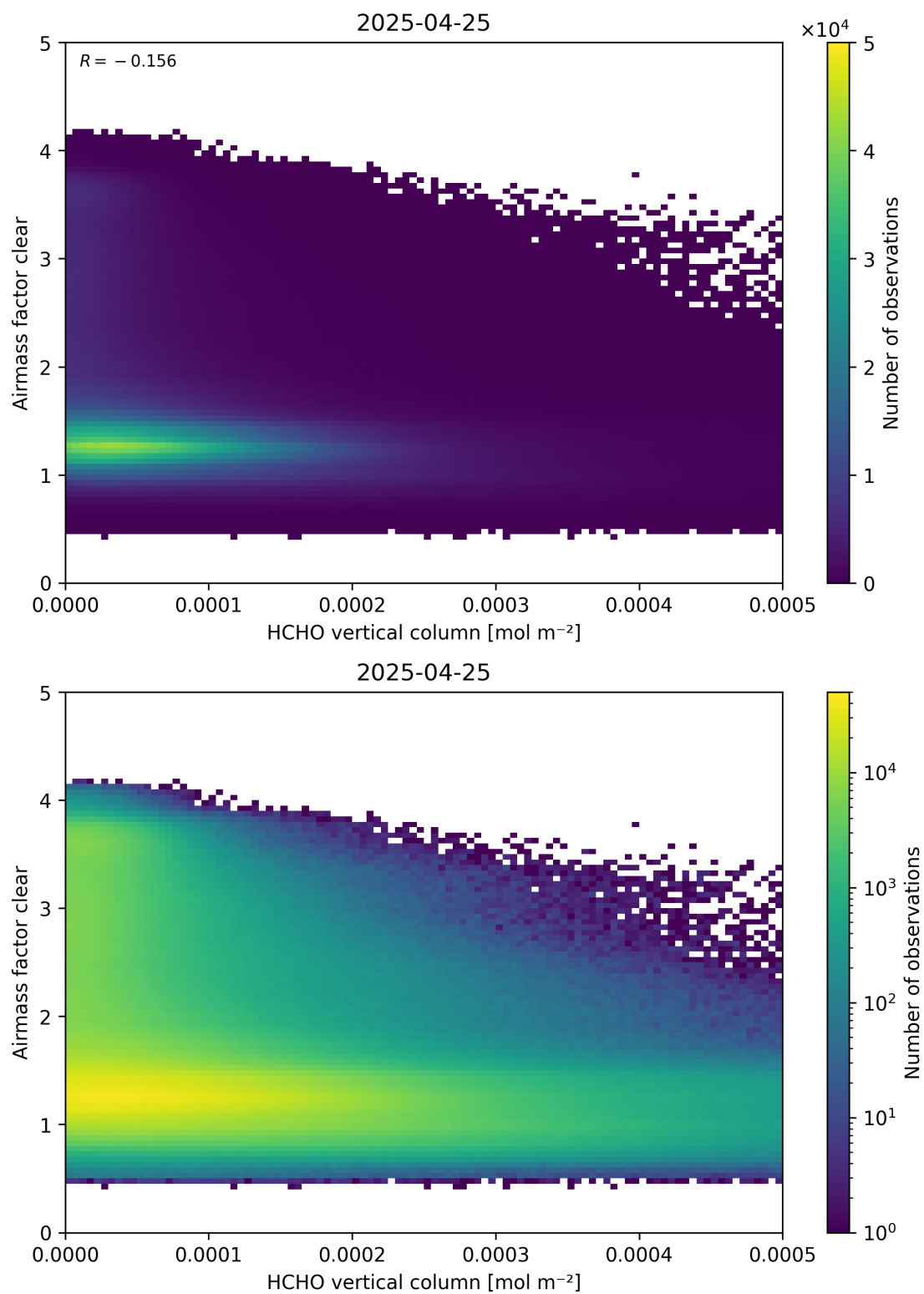
Figure 126: Scatter density plot of “HCHO vertical column” against “Airmass factor clear” for 2025-04-24 to 2025-04-26.
