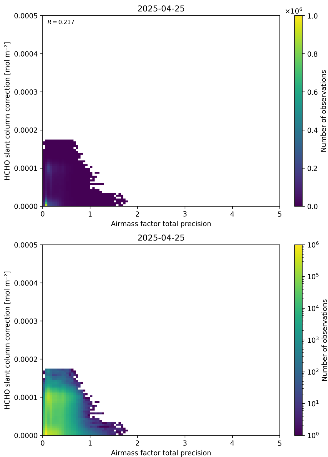
Figure 110: Scatter density plot of “Airmass factor total precision” against “HCHO slant column correction” for 2025-04-24 to 2025-04-26.
