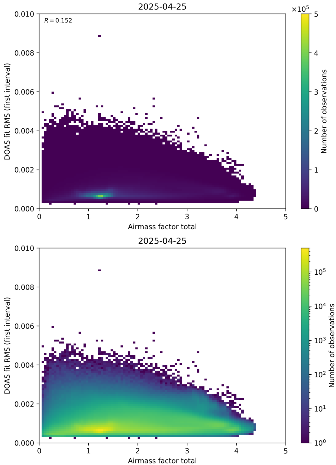
Figure 97: Scatter density plot of “Airmass factor total” against “DOAS fit RMS (first interval)” for 2025-04-24 to 2025-04-26.
