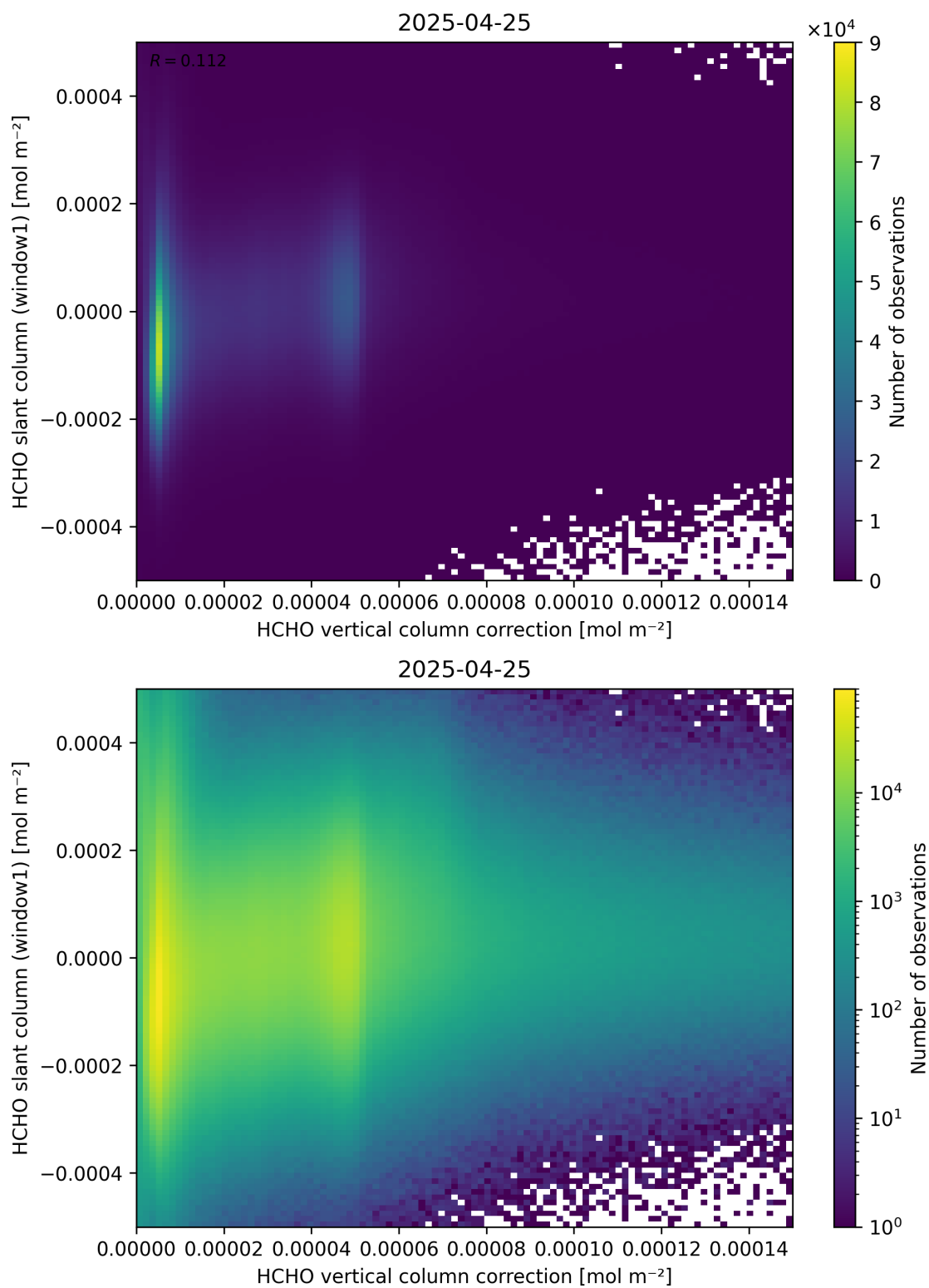
Figure 118: Scatter density plot of “HCHO vertical column correction” against “HCHO slant column (window1)” for 2025-04-24 to 2025-04-26.
