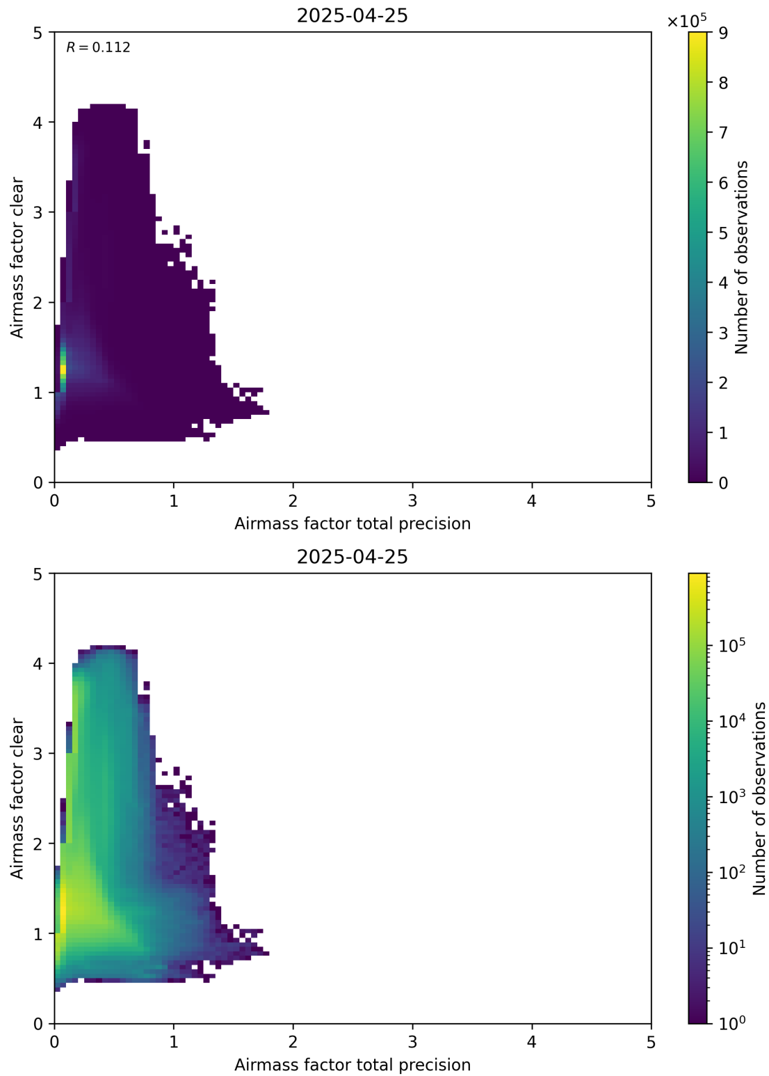
Figure 108: Scatter density plot of “Airmass factor total precision” against “Airmass factor clear” for 2025-04-24 to 2025-04-26.
