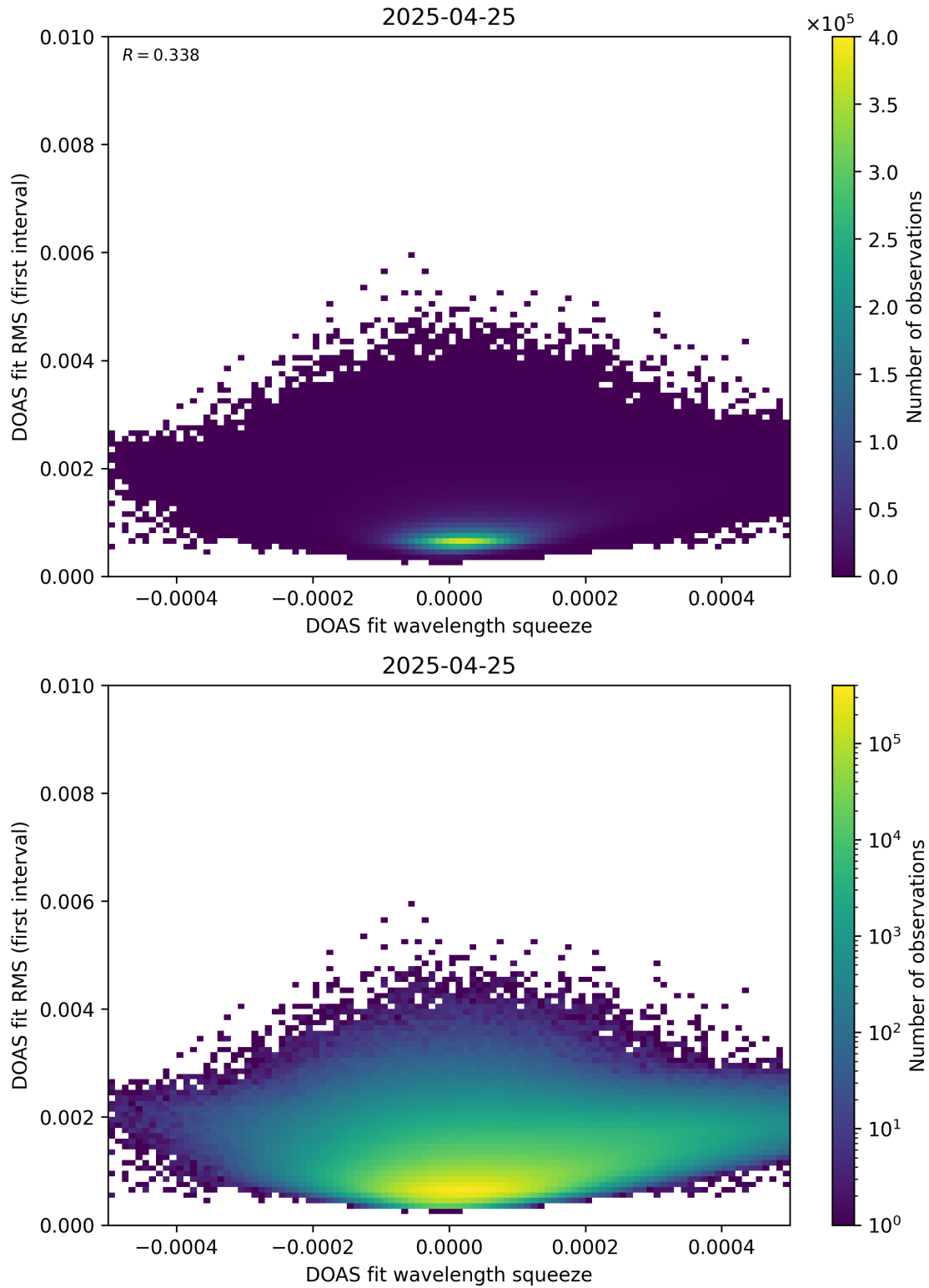
Figure 68: Scatter density plot of “DOAS fit wavelength squeeze” against “DOAS fit RMS (first interval)” for 2025-04-24 to 2025-04-26.
