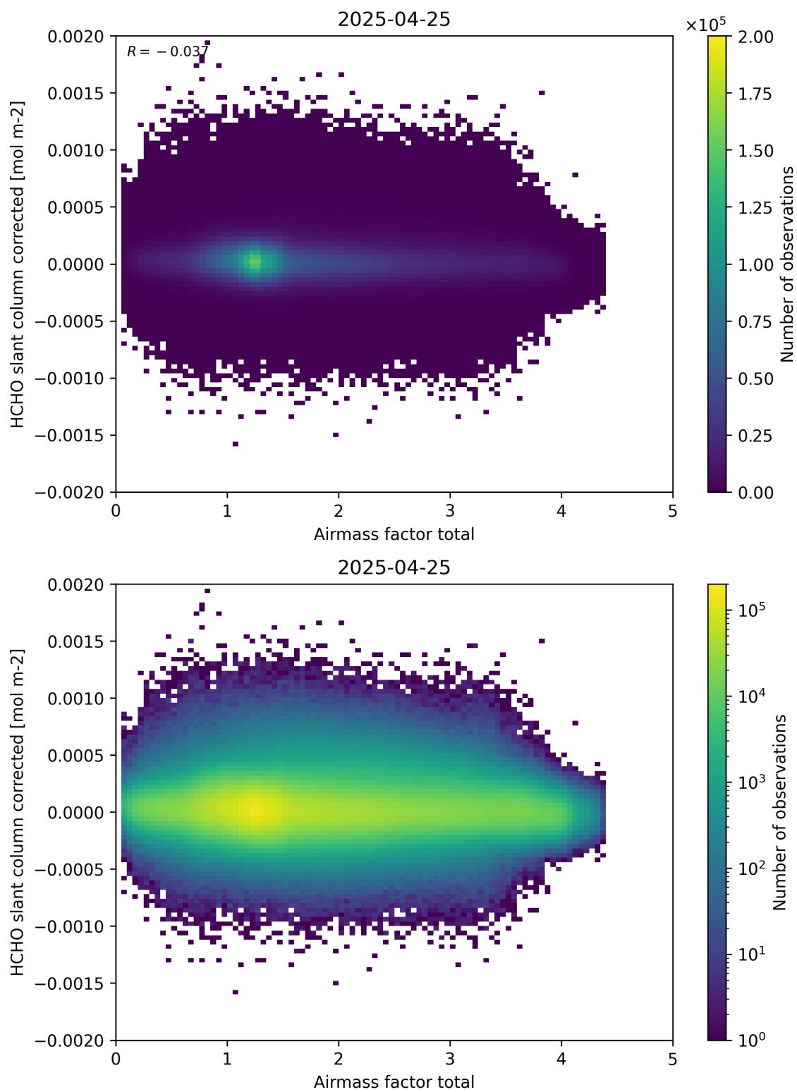
Figure 101: Scatter density plot of “Airmass factor total” against “HCHO slant column corrected” for 2025-04-24 to 2025-04-26.
