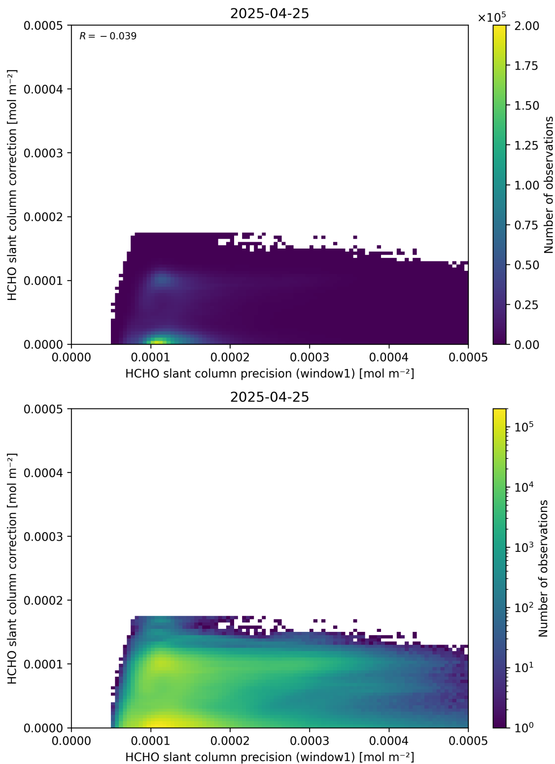
Figure 93: Scatter density plot of “HCHO slant column precision (window1)” against “HCHO slant column correction” for 2025-04-24 to 2025-04-26.
