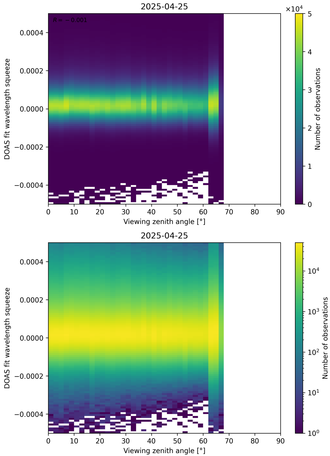
Figure 184: Scatter density plot of “Viewing zenith angle” against “DOAS fit wavelength squeeze” for 2025-04-24 to 2025-04-26.
