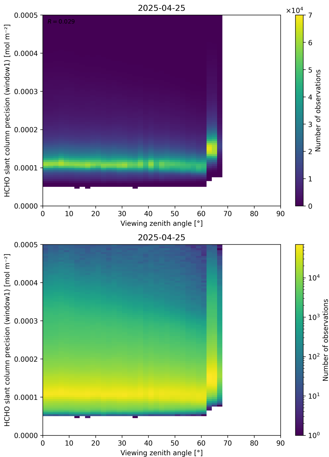
Figure 189: Scatter density plot of “Viewing zenith angle” against “HCHO slant column precision (window1)” for 2025-04-24 to 2025-04-26.
