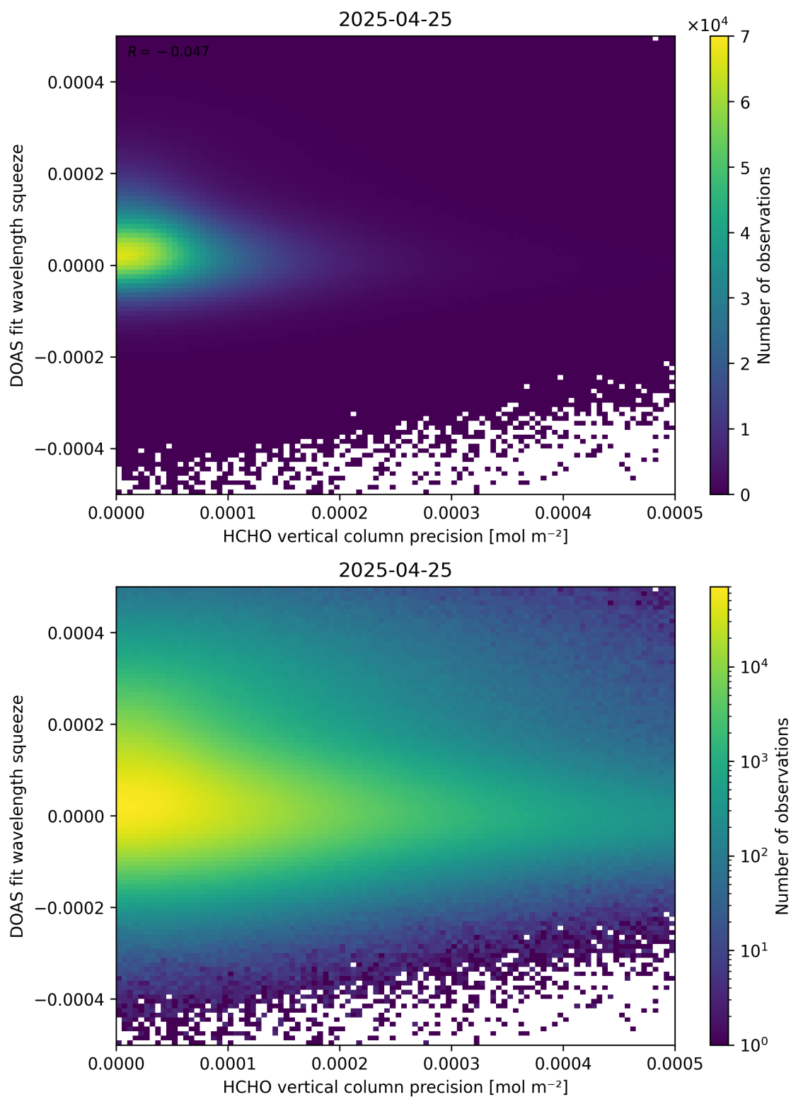
Figure 138: Scatter density plot of “HCHO vertical column precision” against “DOAS fit wavelength squeeze” for 2025-04-24 to 2025-04-26.
