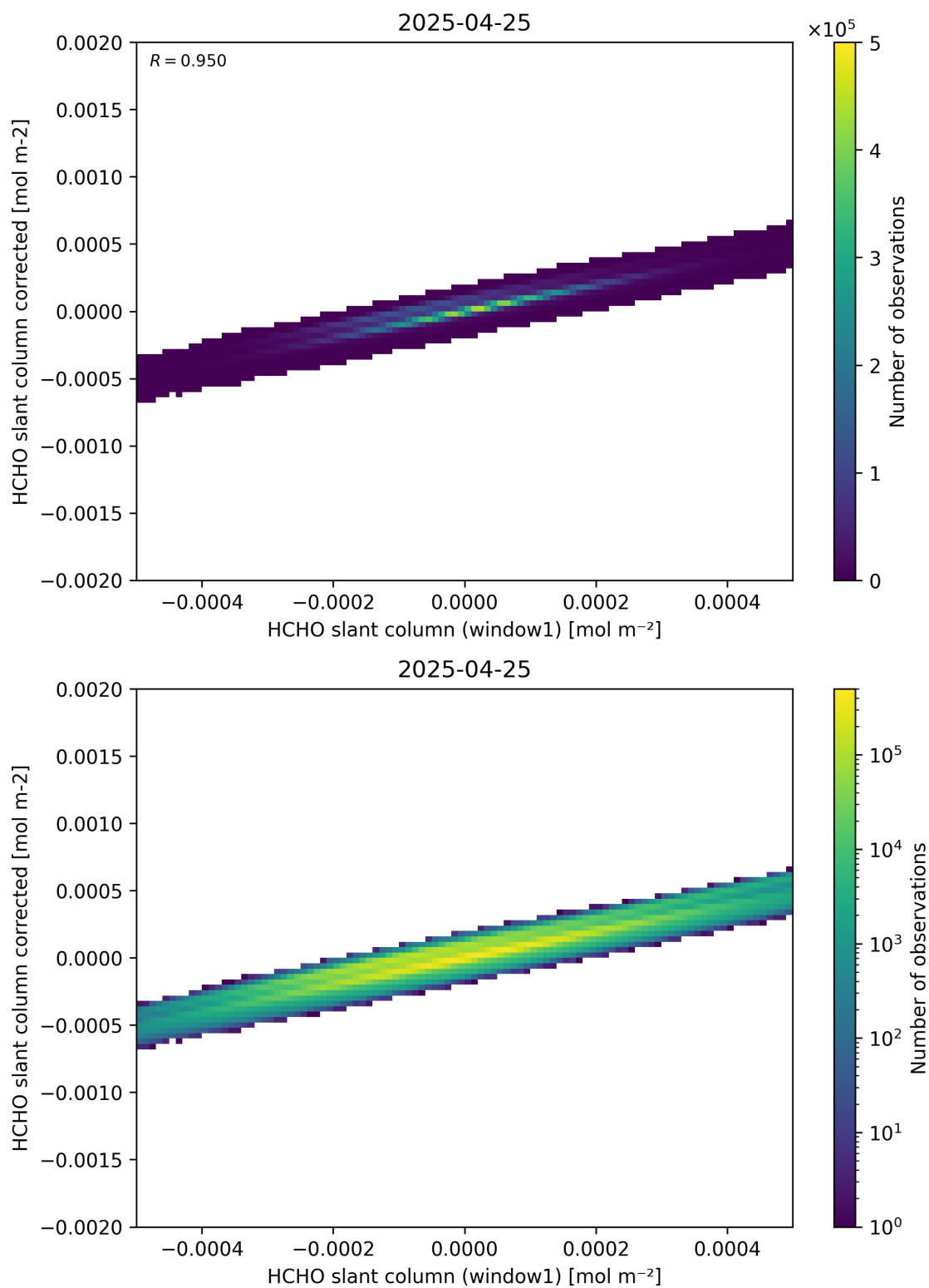
Figure 82: Scatter density plot of “HCHO slant column (window1)” against “HCHO slant column corrected” for 2025-04-24 to 2025-04-26.
