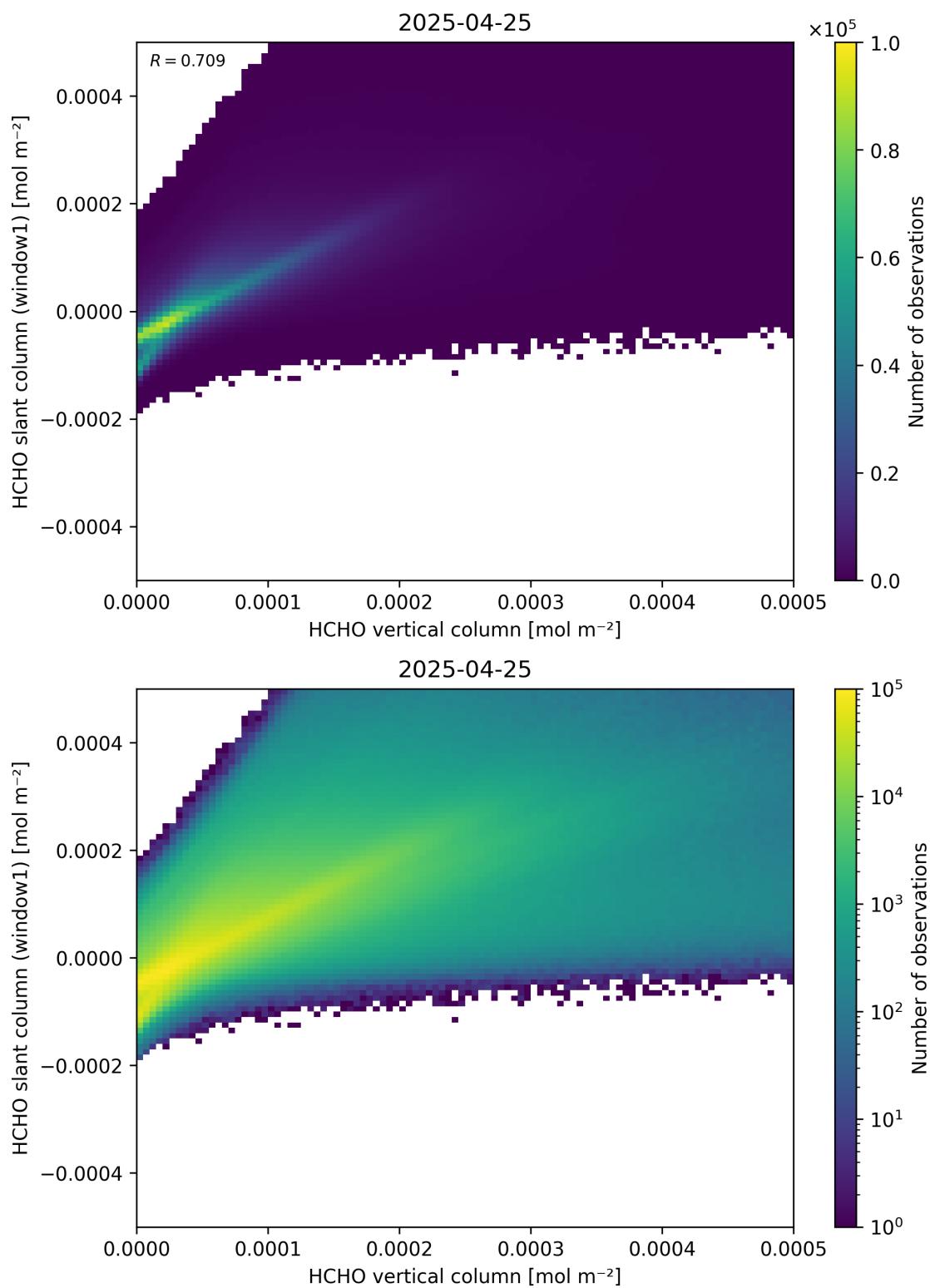
Figure 129: Scatter density plot of “HCHO vertical column” against “HCHO slant column (window1)” for 2025-04-24 to 2025-04-26.
