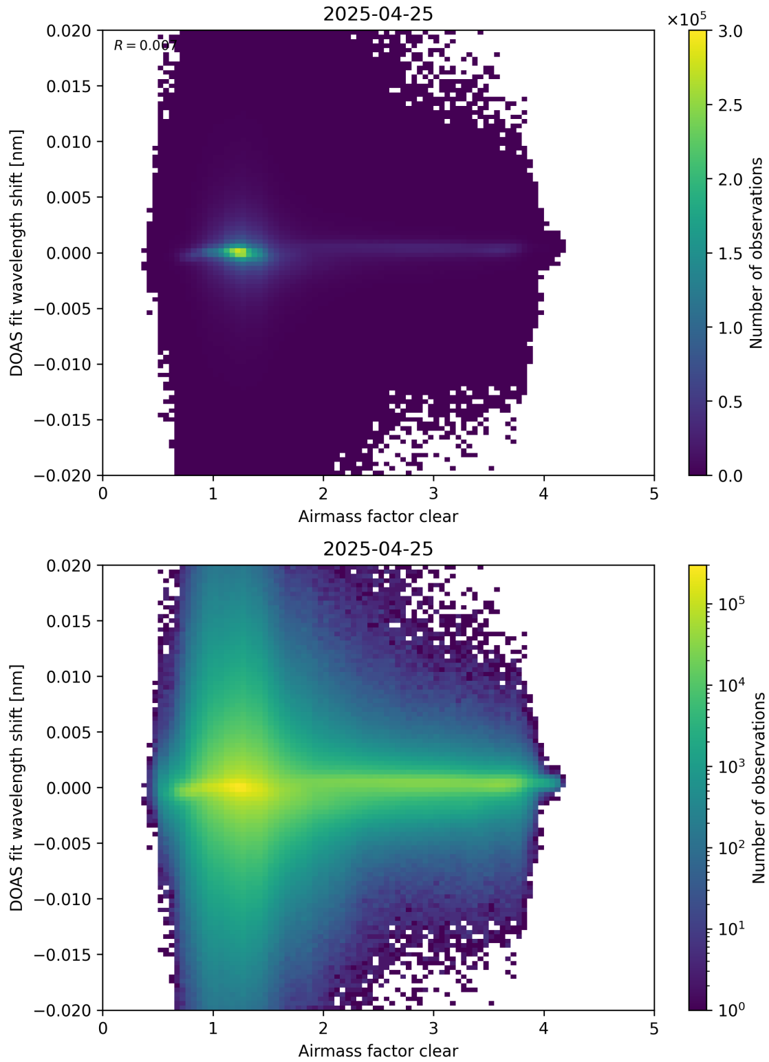
Figure 72: Scatter density plot of “Airmass factor clear” against “DOAS fit wavelength shift” for 2025-04-24 to 2025-04-26.
