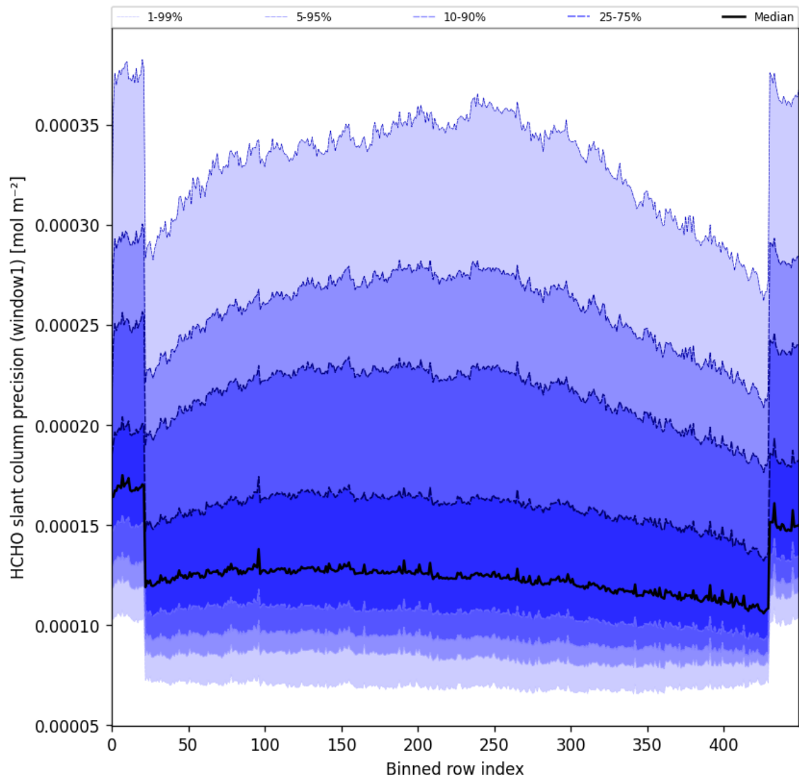
Figure 53: Along track statistics of “HCHO slant column precision (window1)” for 2025-04-24 to 2025-04-26
