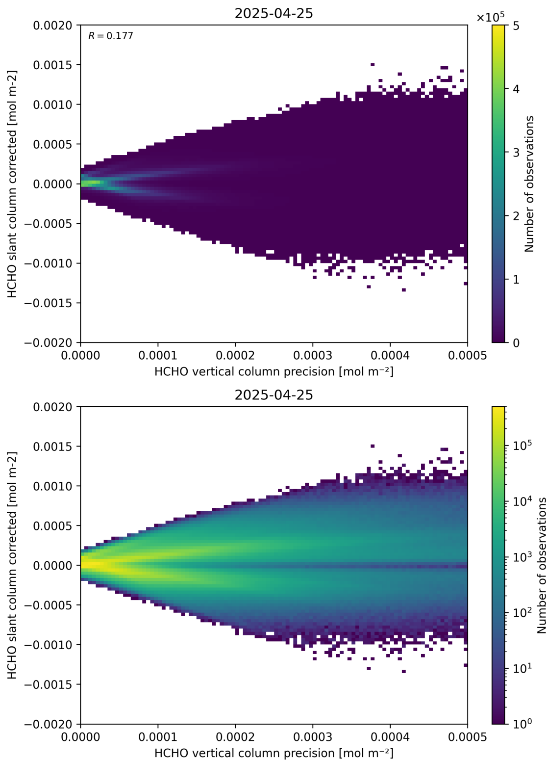
Figure 140: Scatter density plot of “HCHO vertical column precision” against “HCHO slant column corrected” for 2025-04-24 to 2025-04-26.
