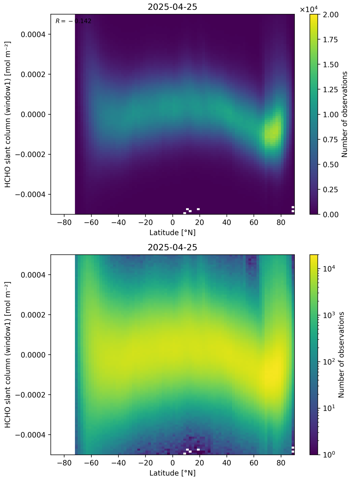
Figure 159: Scatter density plot of “Latitude” against “HCHO slant column (window1)” for 2025-04-24 to 2025-04-26.
