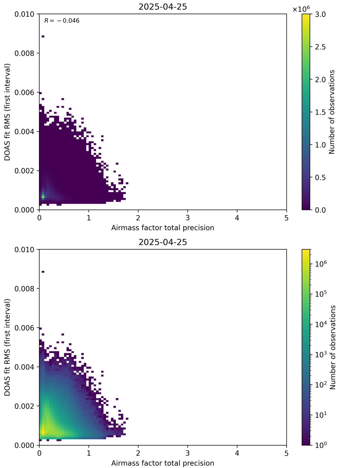
Figure 105: Scatter density plot of “Airmass factor total precision” against “DOAS fit RMS (first interval)” for 2025-04-24 to 2025-04-26.
