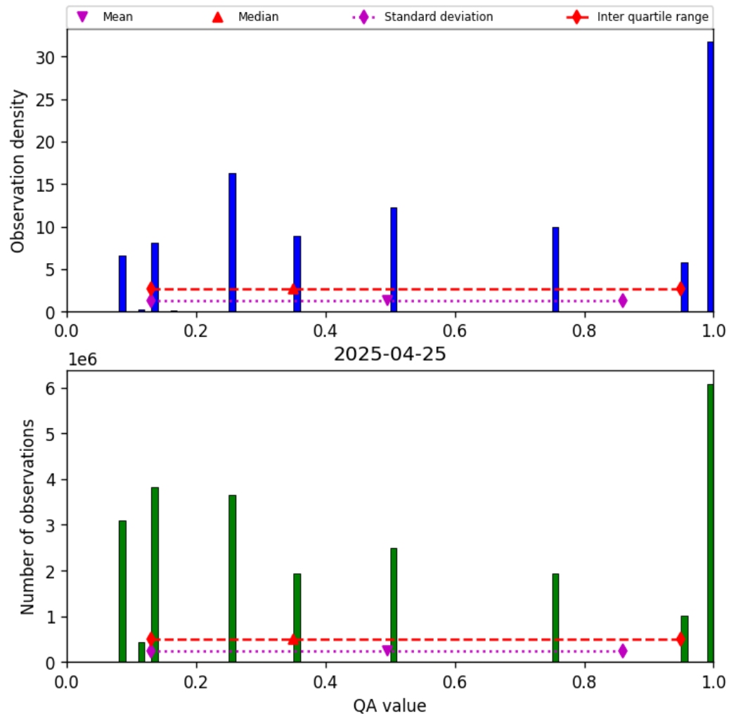
Figure 34: Histogram of “QA value” for 2025-04-24 to 2025-04-26
