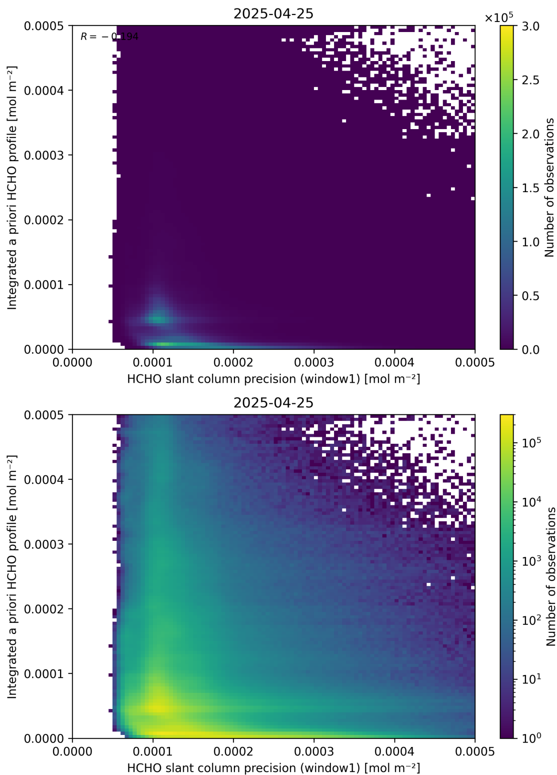
Figure 96: Scatter density plot of “HCHO slant column precision (window1)” against “Integrated a priori HCHO profile” for 2025-04-24 to 2025-04-26.
