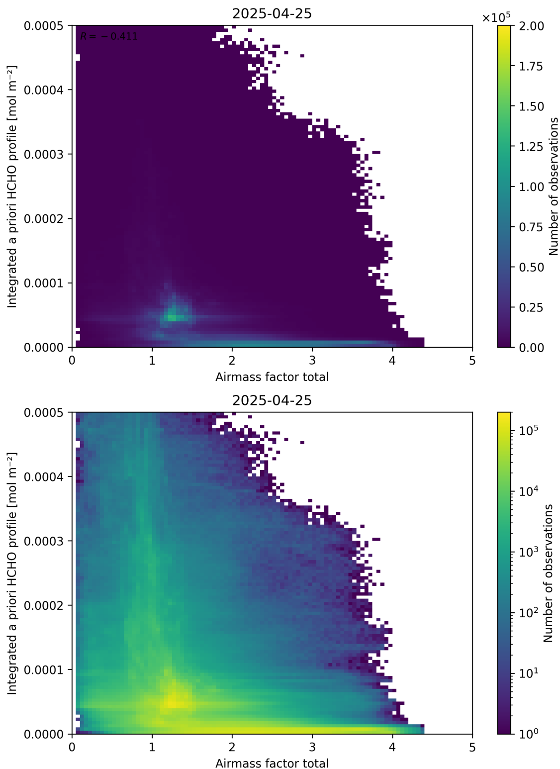
Figure 104: Scatter density plot of “Airmass factor total” against “Integrated a priori HCHO profile” for 2025-04-24 to 2025-04-26.
