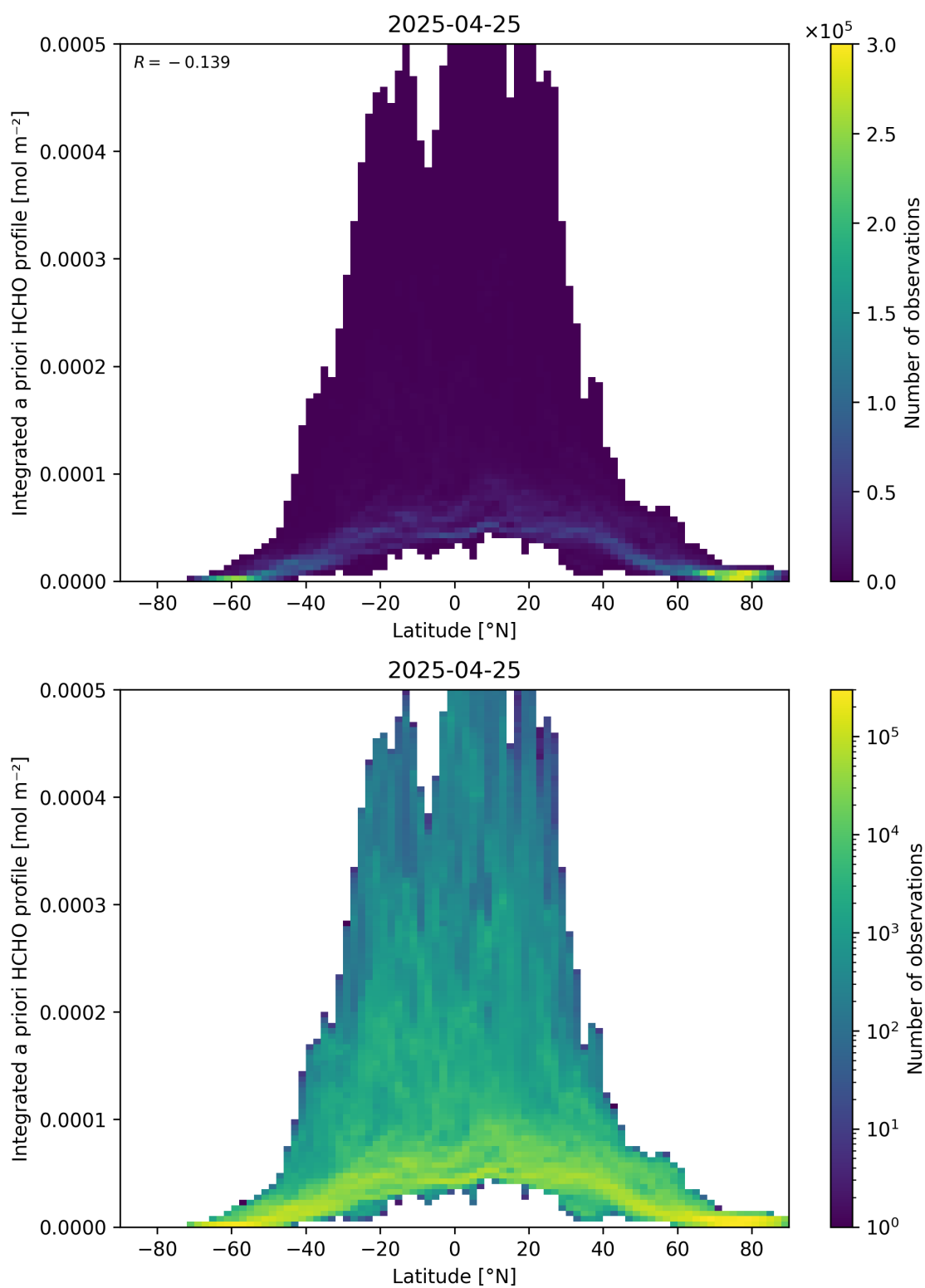
Figure 166: Scatter density plot of “Latitude” against “Integrated a priori HCHO profile” for 2025-04-24 to 2025-04-26.
