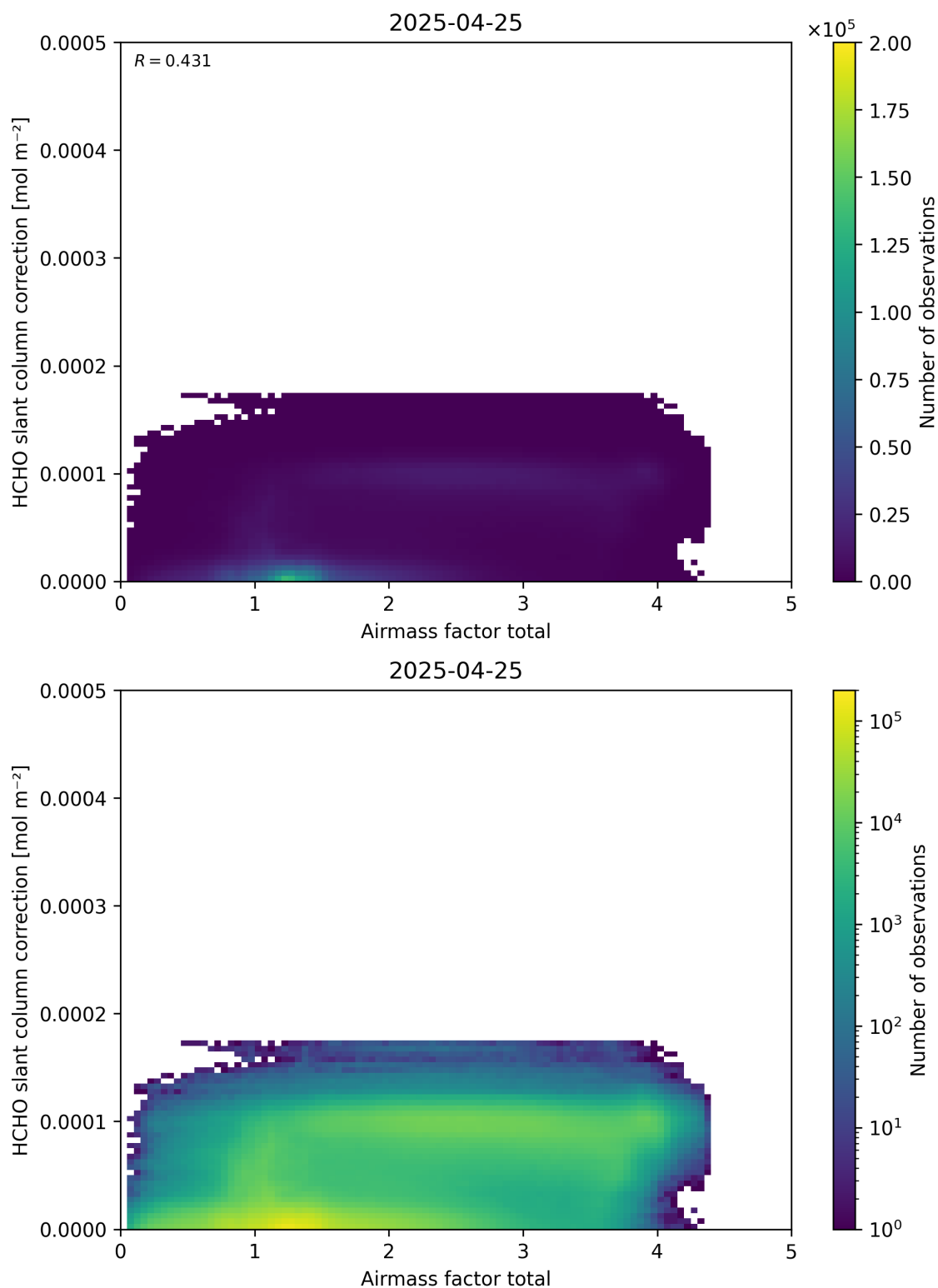
Figure 102: Scatter density plot of “Airmass factor total” against “HCHO slant column correction” for 2025-04-24 to 2025-04-26.
