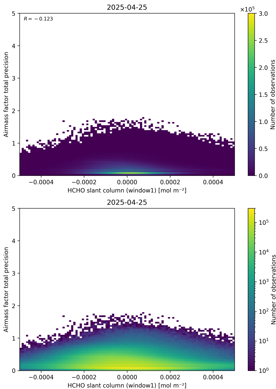
Figure 86: Scatter density plot of “HCHO slant column (window1)” against “Airmass factor total precision” for 2025-04-24 to 2025-04-26.
