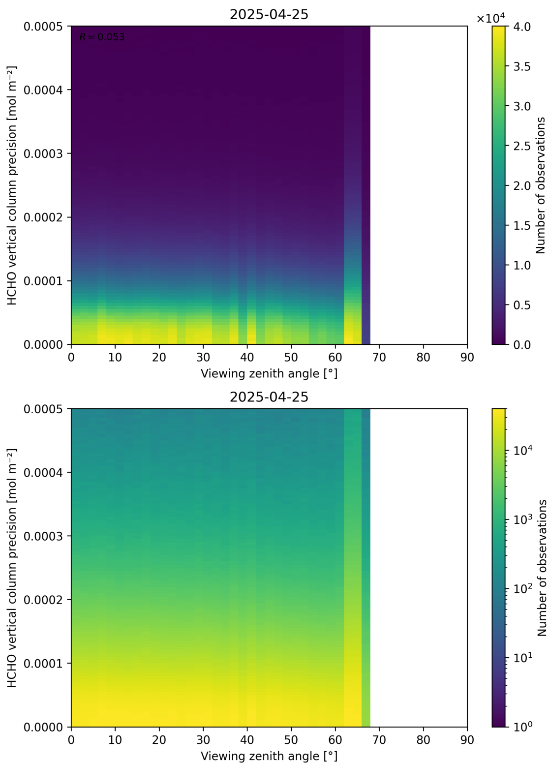
Figure 194: Scatter density plot of “Viewing zenith angle” against “HCHO vertical column precision” for 2025-04-24 to 2025-04-26.
