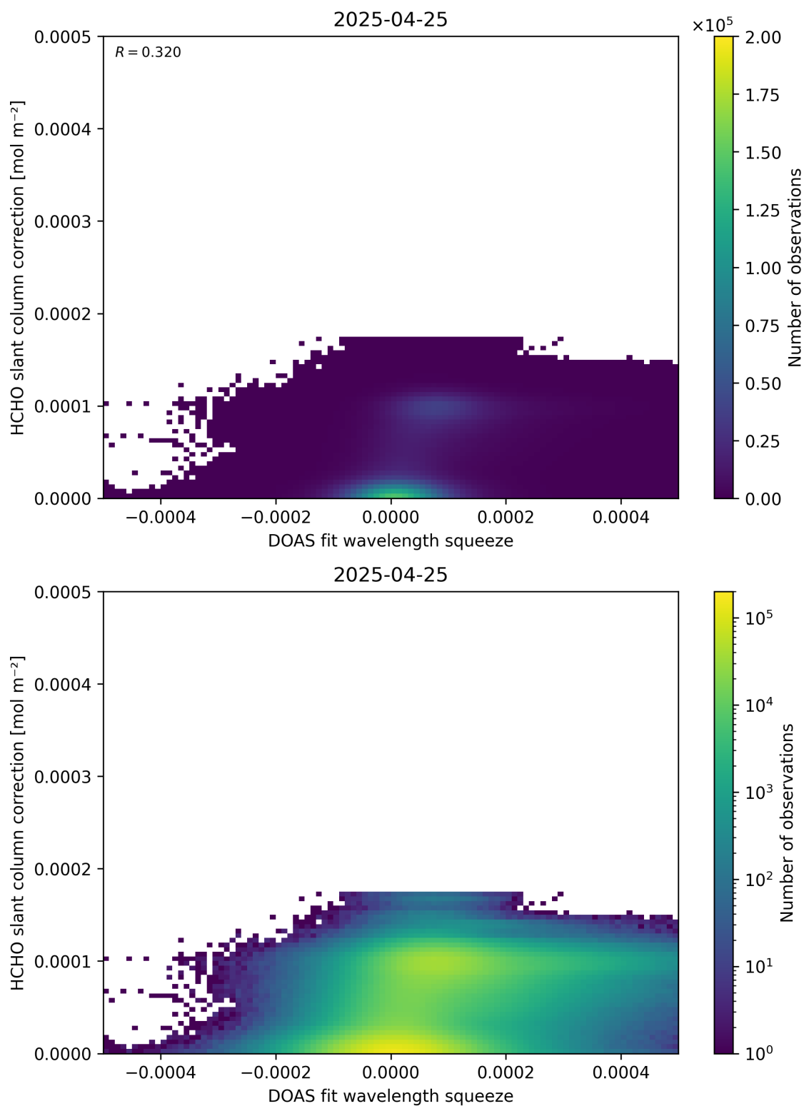
Figure 70: Scatter density plot of “DOAS fit wavelength squeeze” against “HCHO slant column correction” for 2025-04-24 to 2025-04-26.
