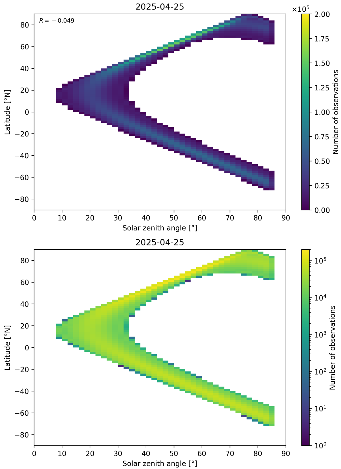
Figure 181: Scatter density plot of “Solar zenith angle” against “Latitude” for 2025-04-24 to 2025-04-26.
