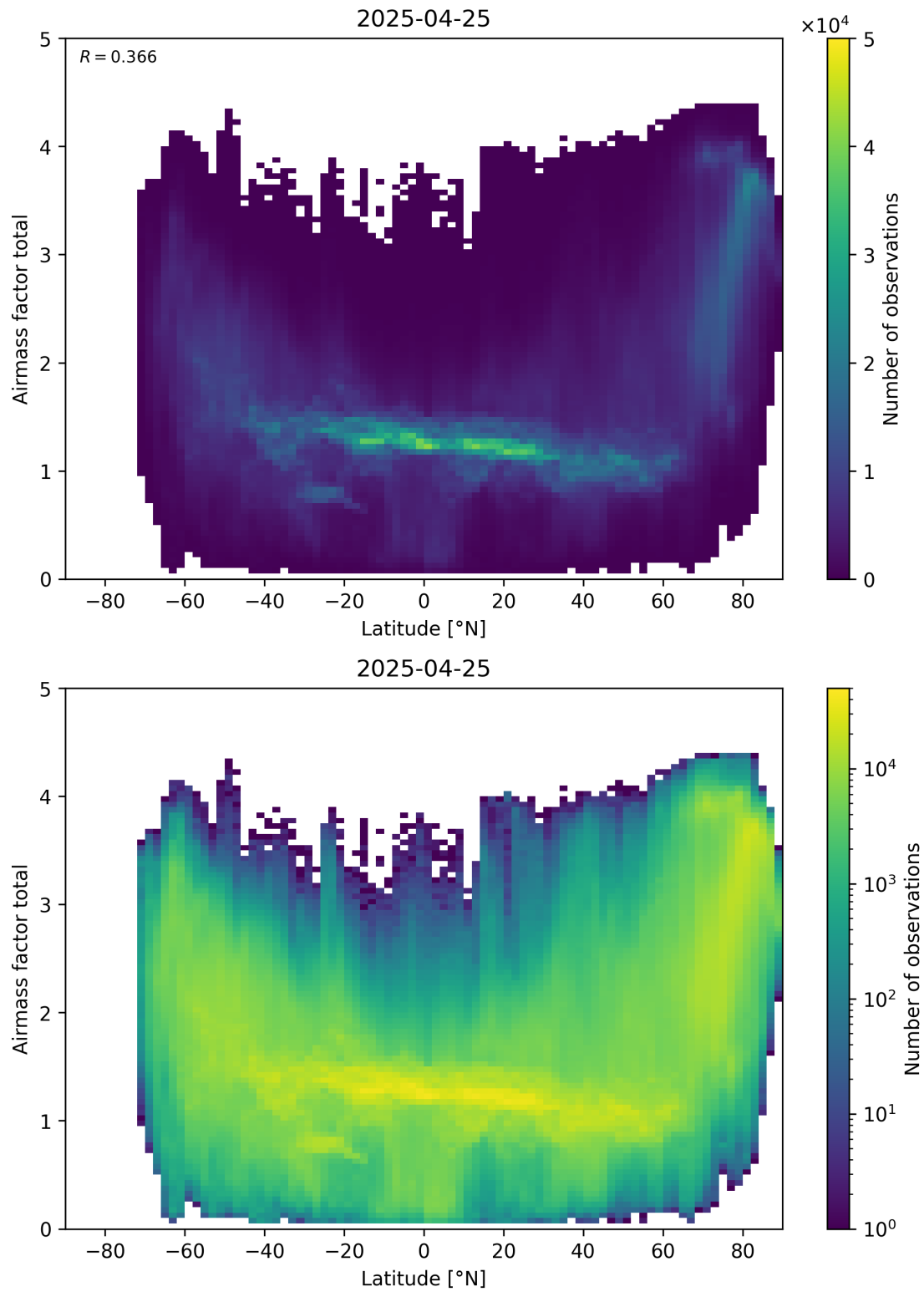
Figure 161: Scatter density plot of “Latitude” against “Airmass factor total” for 2025-04-24 to 2025-04-26.
