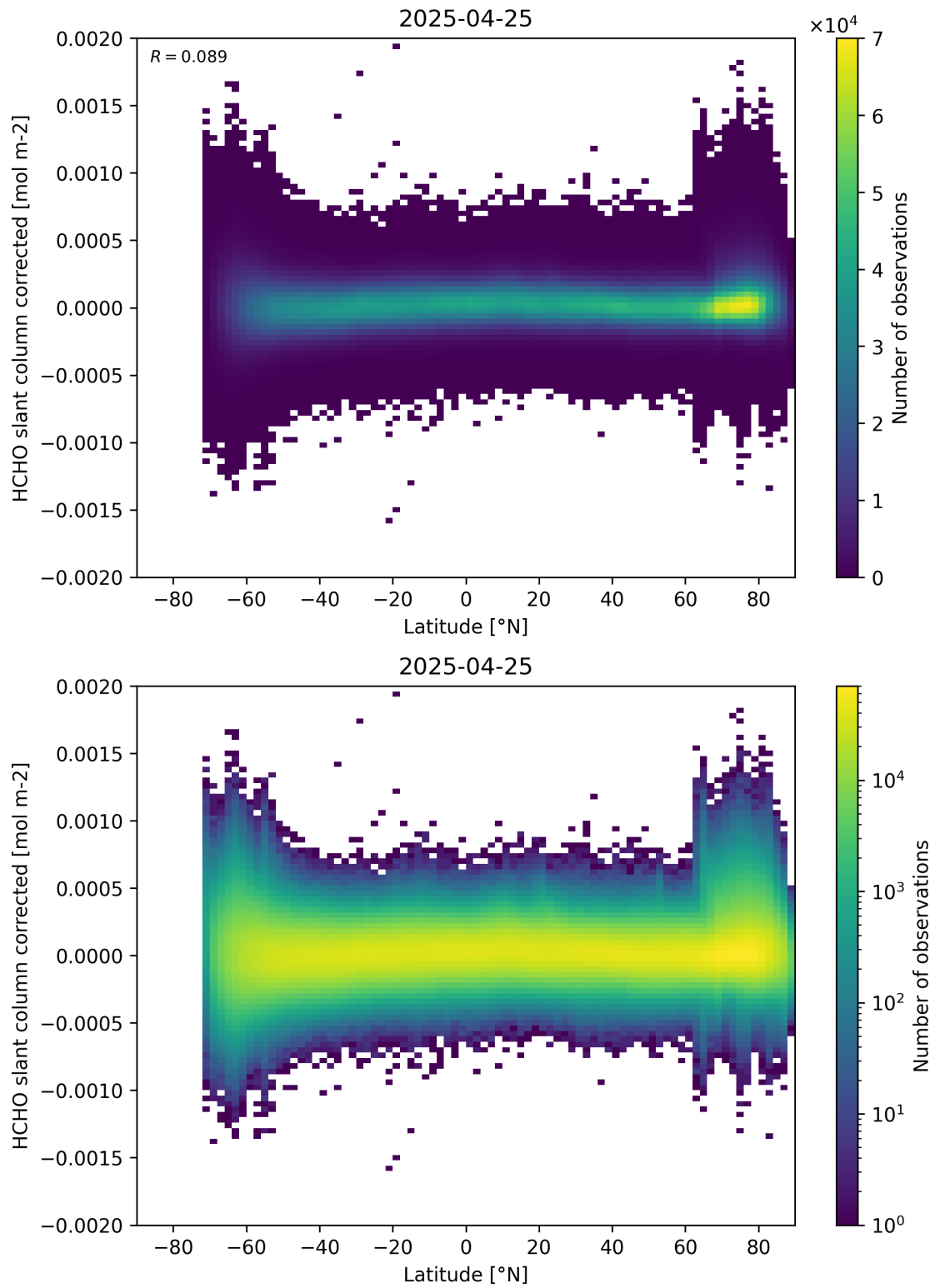
Figure 157: Scatter density plot of “Latitude” against “HCHO slant column corrected” for 2025-04-24 to 2025-04-26.
