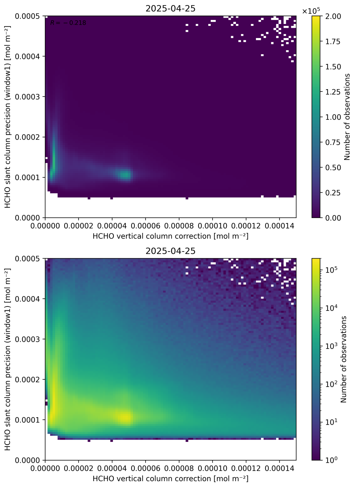
Figure 119: Scatter density plot of “HCHO vertical column correction” against “HCHO slant column precision (window1)” for 2025-04-24 to 2025-04-26.
