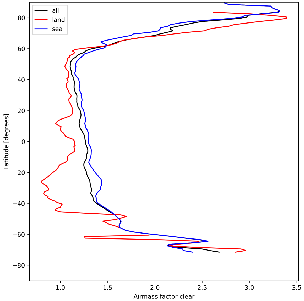
Figure 28: Zonal average of “Airmass factor clear” for 2025-04-24 to 2025-04-26.
