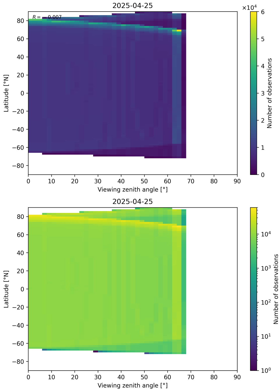
Figure 196: Scatter density plot of “Viewing zenith angle” against “Latitude” for 2025-04-24 to 2025-04-26.
