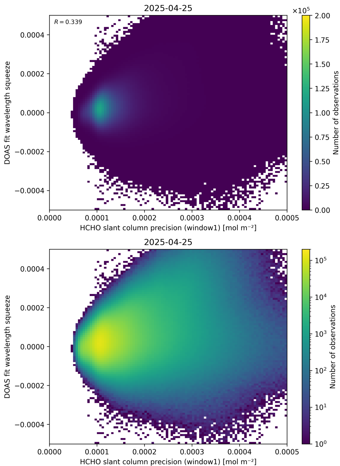
Figure 90: Scatter density plot of “HCHO slant column precision (window1)” against “DOAS fit wavelength squeeze” for 2025-04-24 to 2025-04-26.
