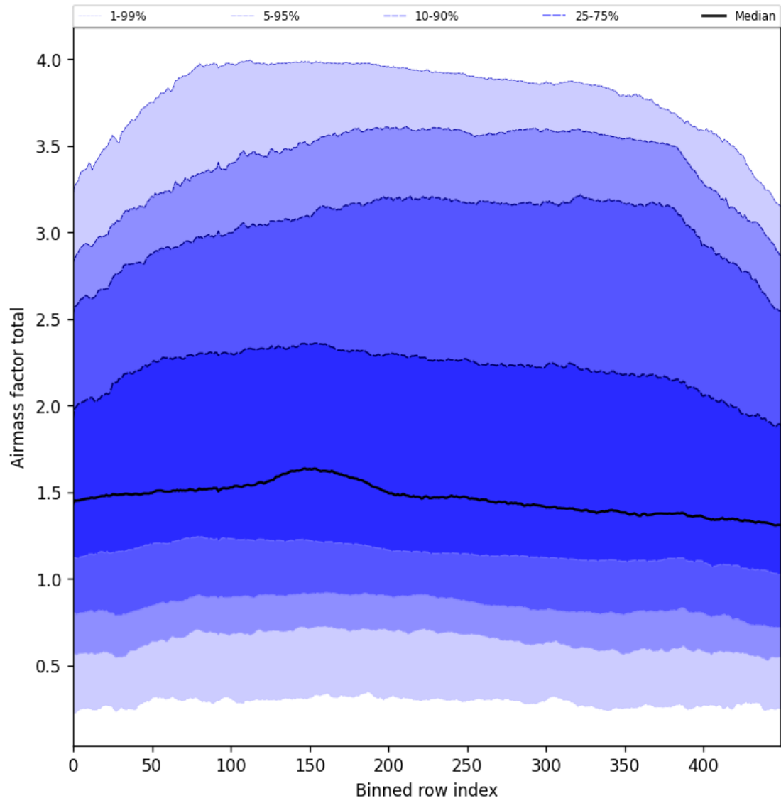
Figure 54: Along track statistics of “Airmass factor total” for 2025-04-24 to 2025-04-26
