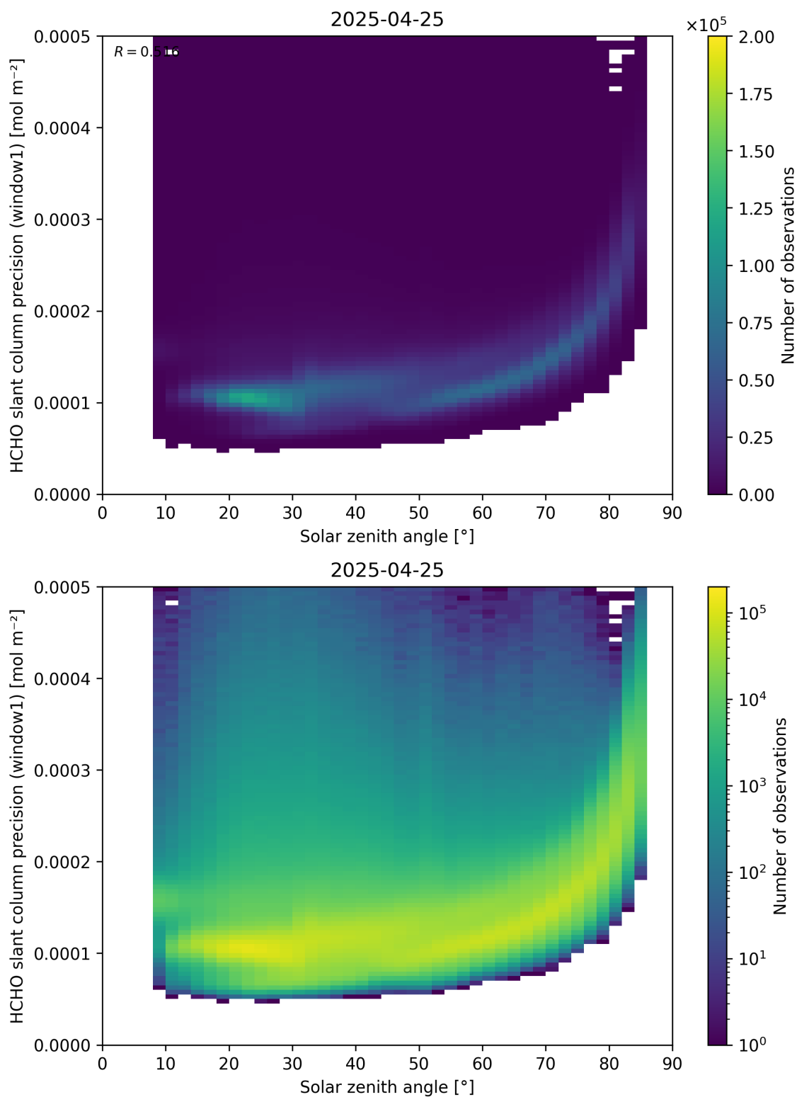
Figure 174: Scatter density plot of “Solar zenith angle” against “HCHO slant column precision (window1)” for 2025-04-24 to 2025-04-26.
