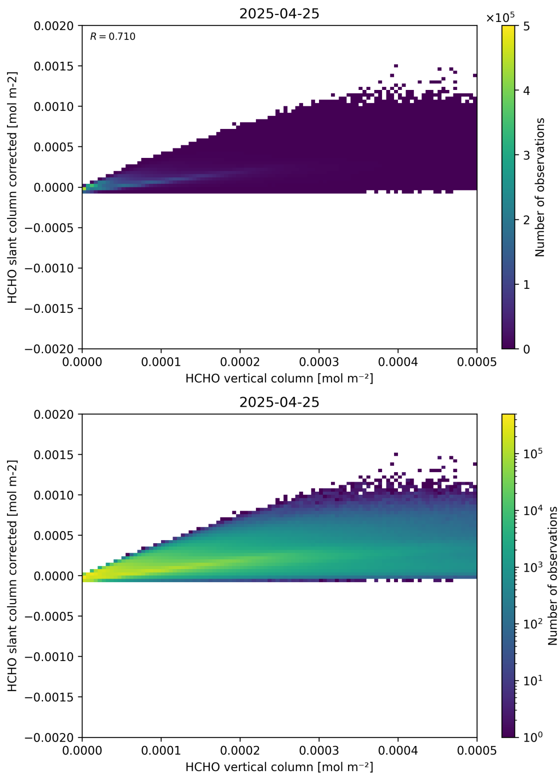
Figure 127: Scatter density plot of “HCHO vertical column” against “HCHO slant column corrected” for 2025-04-24 to 2025-04-26.
