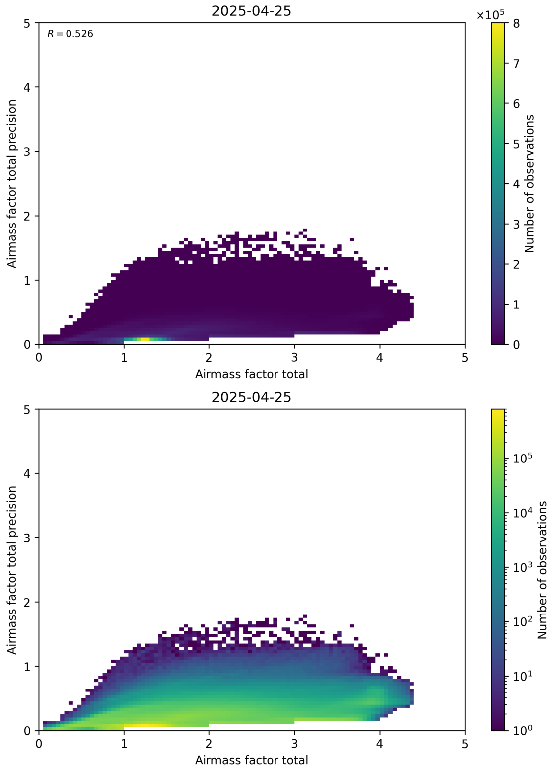
Figure 103: Scatter density plot of “Airmass factor total” against “Airmass factor total precision” for 2025-04-24 to 2025-04-26.
