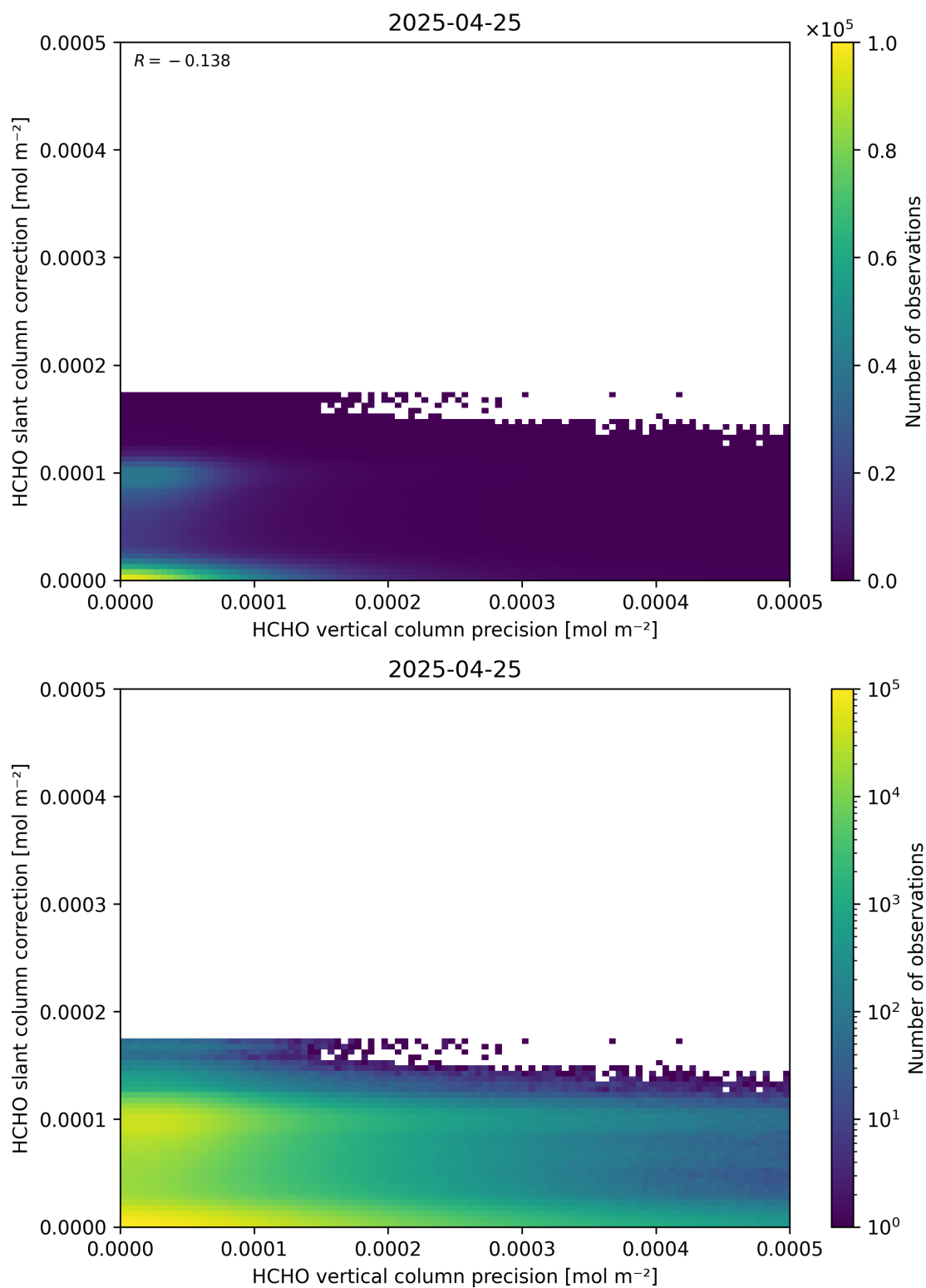
Figure 141: Scatter density plot of “HCHO vertical column precision” against “HCHO slant column correction” for 2025-04-24 to 2025-04-26.
