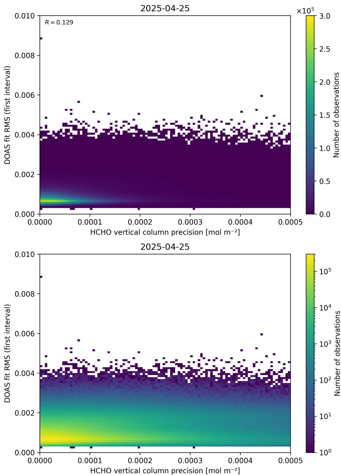
Figure 136: Scatter density plot of “HCHO vertical column precision” against “DOAS fit RMS (first interval)” for 2025-04-24 to 2025-04-26.
