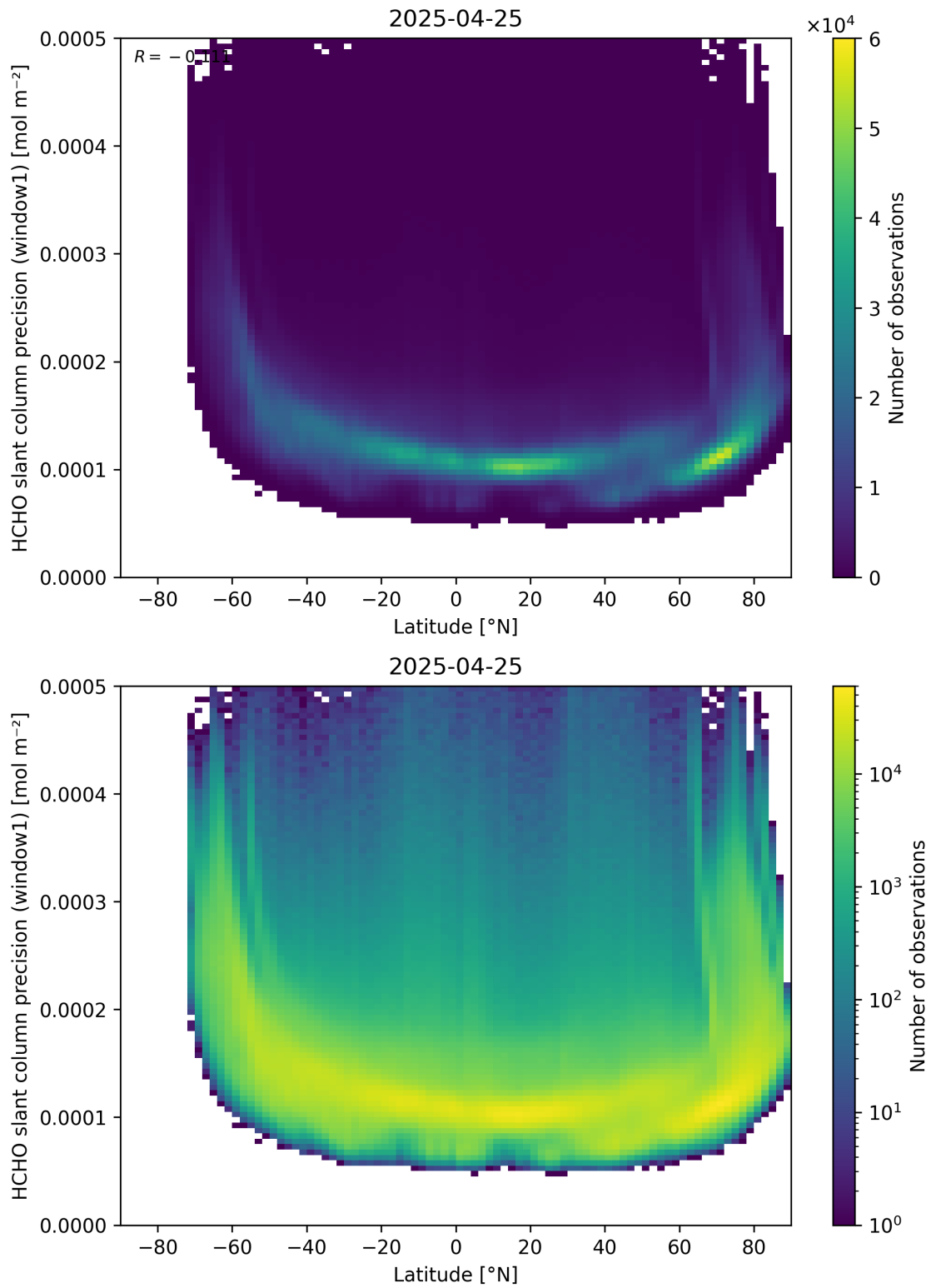
Figure 160: Scatter density plot of “Latitude” against “HCHO slant column precision (window1)” for 2025-04-24 to 2025-04-26.
