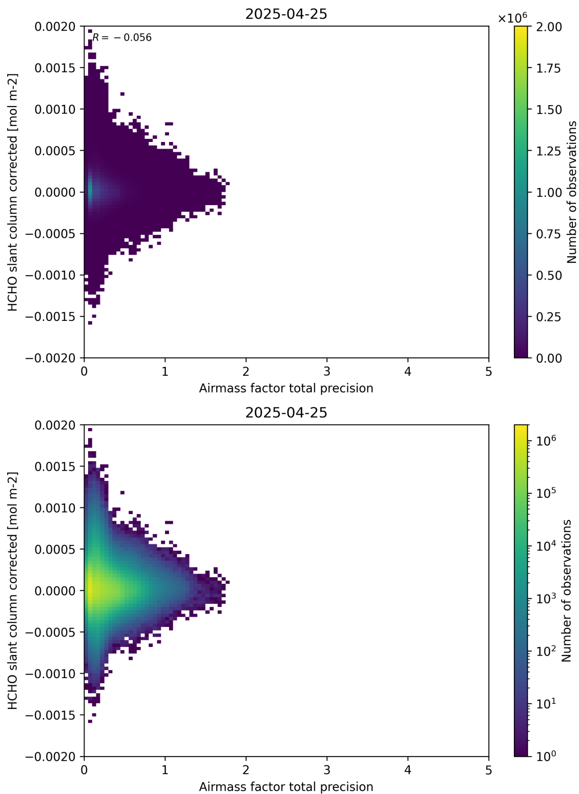
Figure 109: Scatter density plot of “Airmass factor total precision” against “HCHO slant column corrected” for 2025-04-24 to 2025-04-26.
