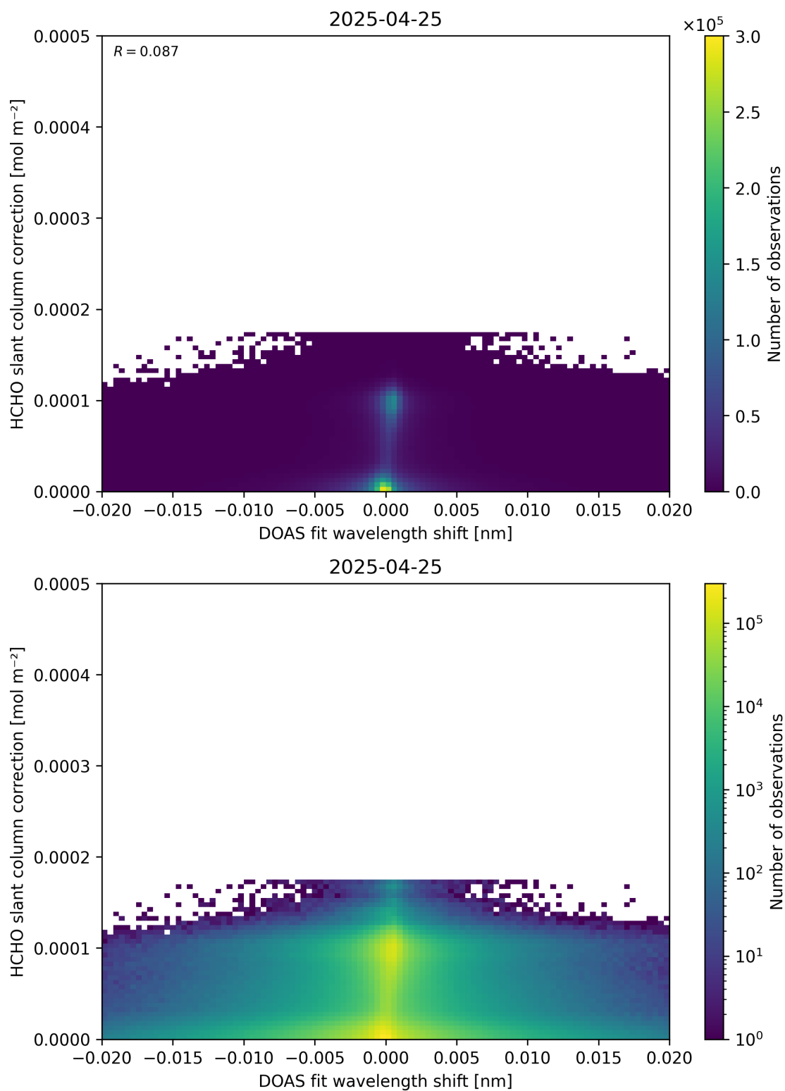
Figure 67: Scatter density plot of “DOAS fit wavelength shift” against “HCHO slant column correction” for 2025-04-24 to 2025-04-26.
