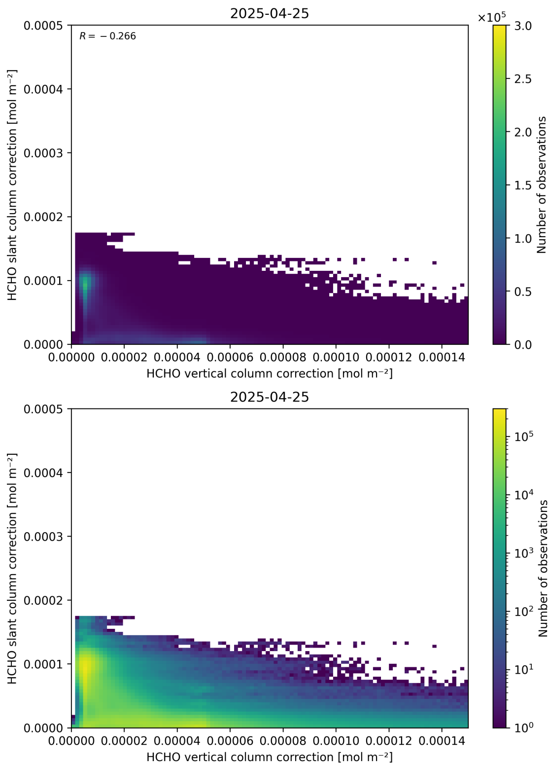
Figure 117: Scatter density plot of “HCHO vertical column correction” against “HCHO slant column correction” for 2025-04-24 to 2025-04-26.
