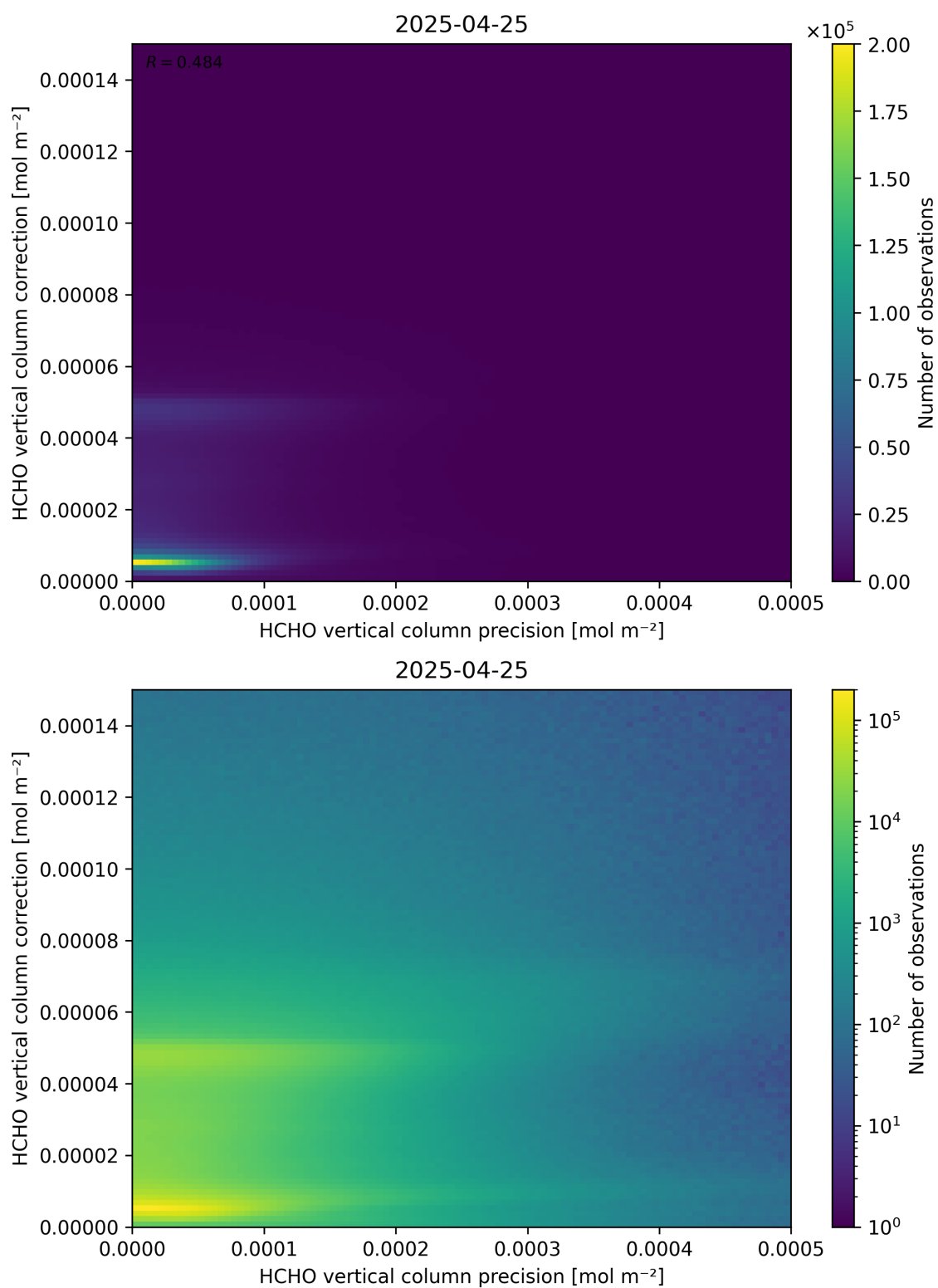
Figure 146: Scatter density plot of “HCHO vertical column precision” against “HCHO vertical column correction” for 2025-04-24 to 2025-04-26.
