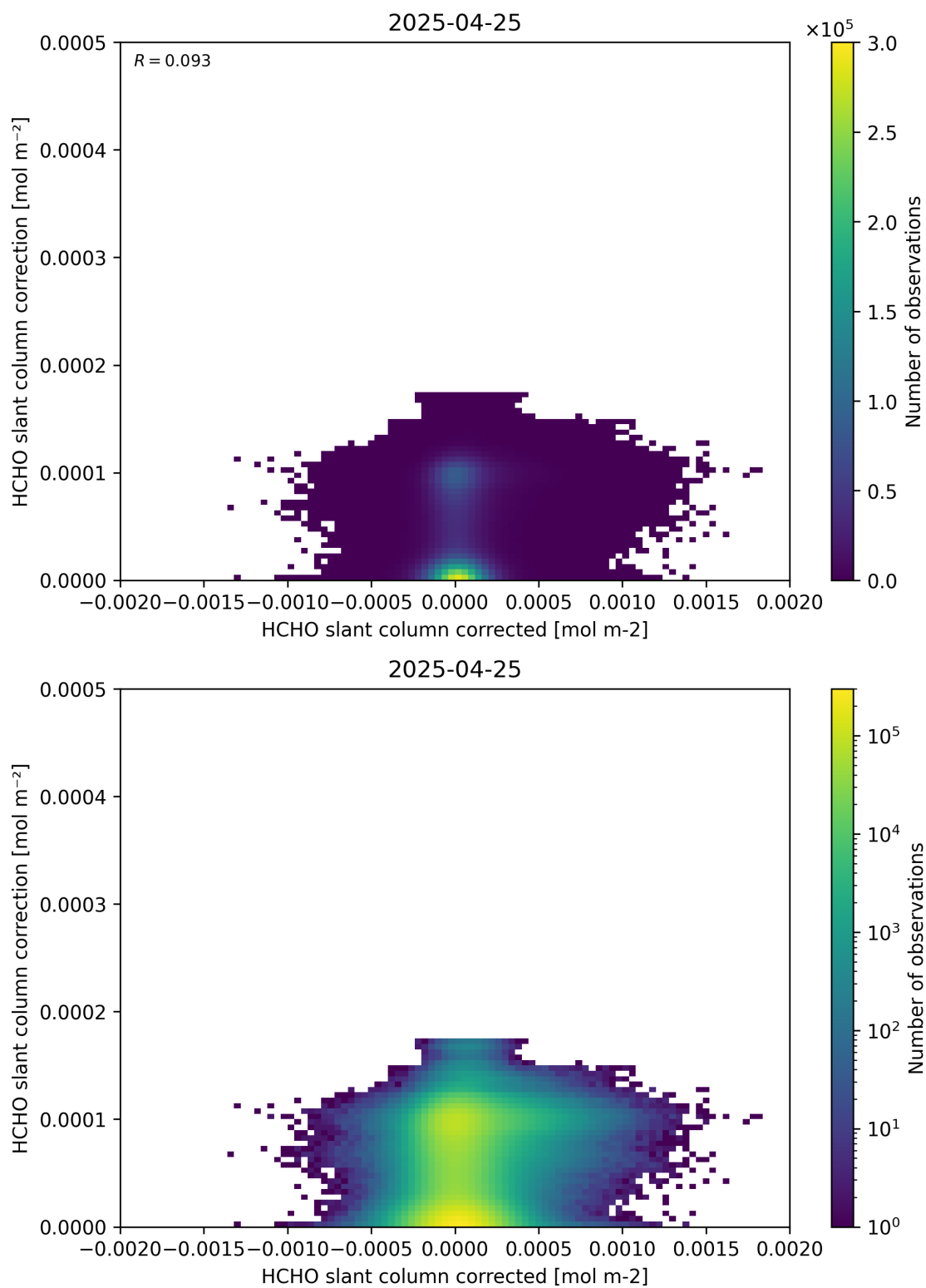
Figure 77: Scatter density plot of “HCHO slant column corrected” against “HCHO slant column correction” for 2025-04-24 to 2025-04-26.
