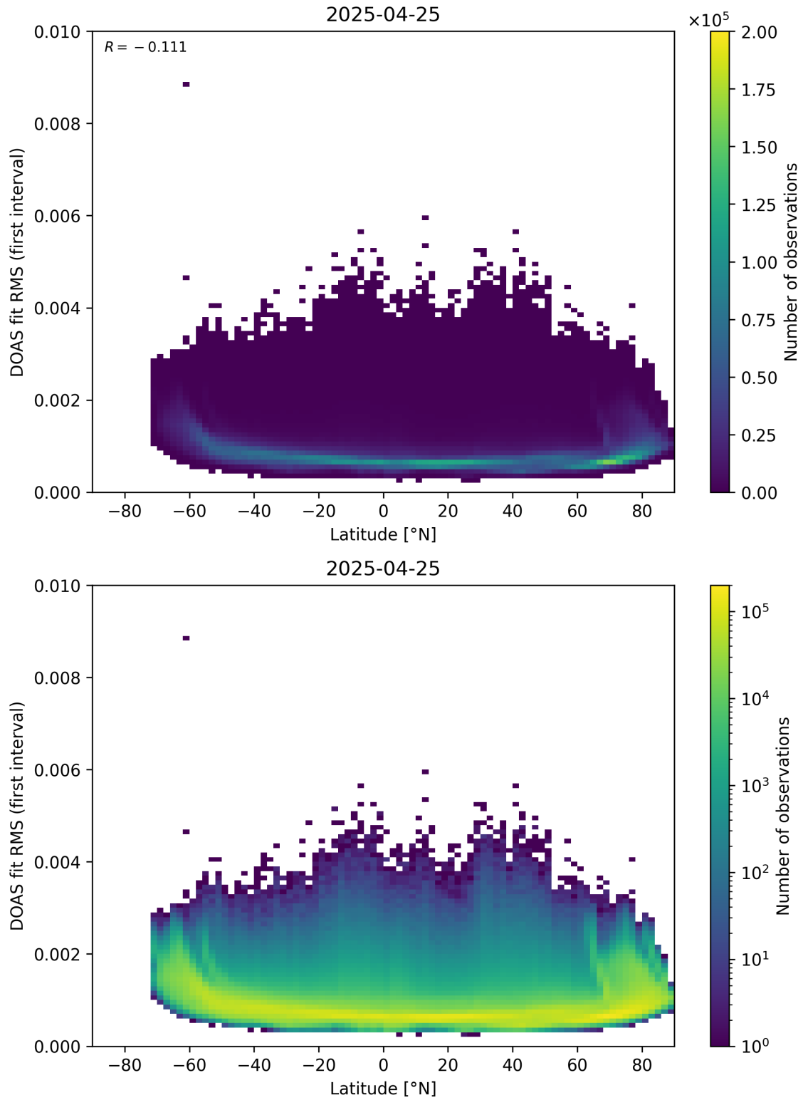
Figure 153: Scatter density plot of “Latitude” against “DOAS fit RMS (first interval)” for 2025-04-24 to 2025-04-26.
