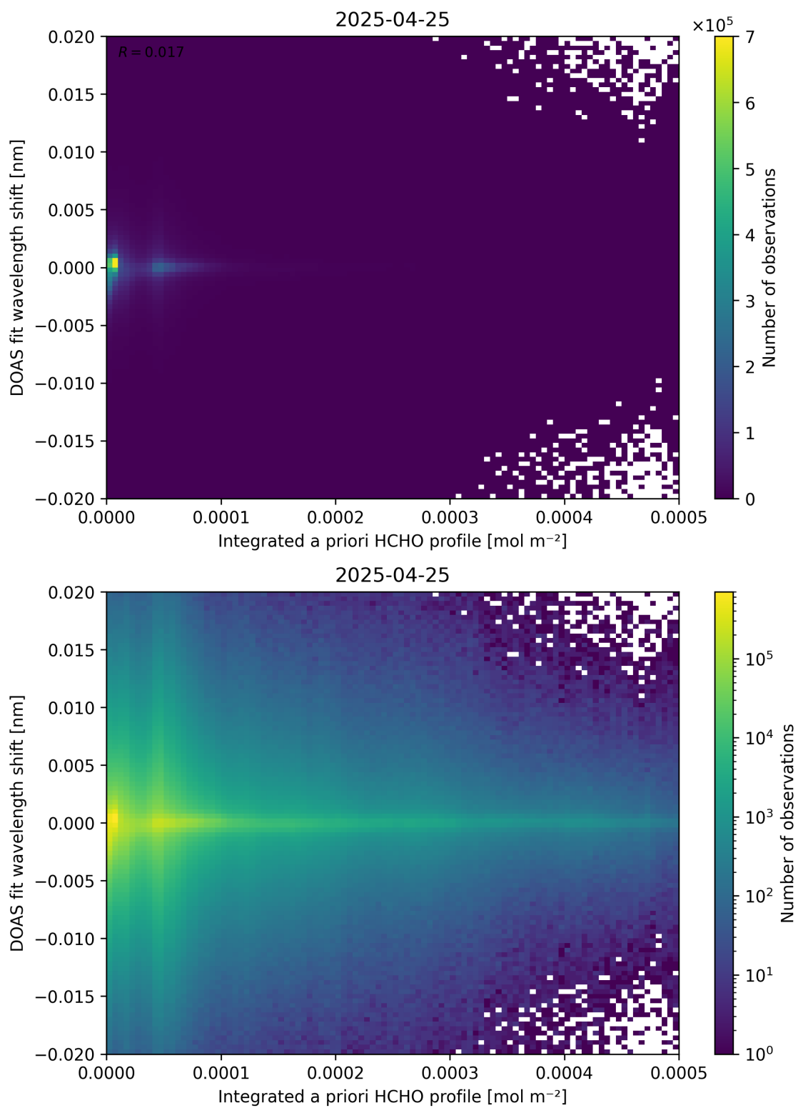
Figure 149: Scatter density plot of “Integrated a priori HCHO profile” against “DOAS fit wavelength shift” for 2025-04-24 to 2025-04-26.
