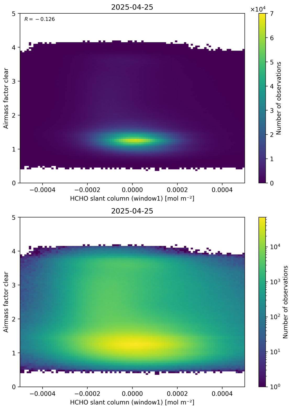
Figure 81: Scatter density plot of “HCHO slant column (window1)” against “Airmass factor clear” for 2025-04-24 to 2025-04-26.
