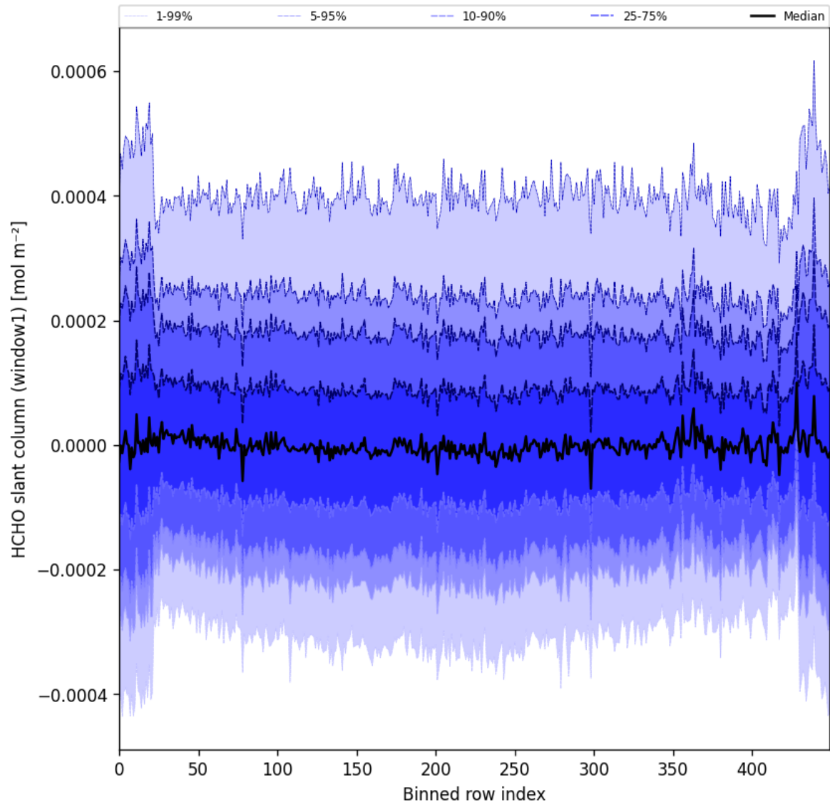
Figure 52: Along track statistics of “HCHO slant column (window1)” for 2025-04-24 to 2025-04-26
