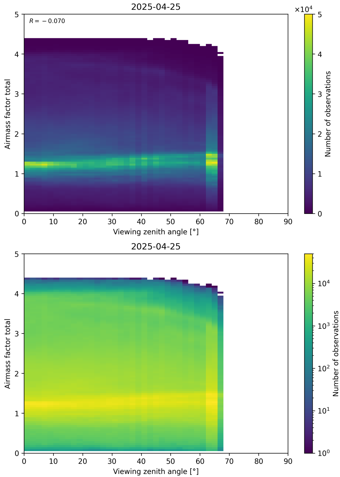
Figure 190: Scatter density plot of “Viewing zenith angle” against “Airmass factor total” for 2025-04-24 to 2025-04-26.
