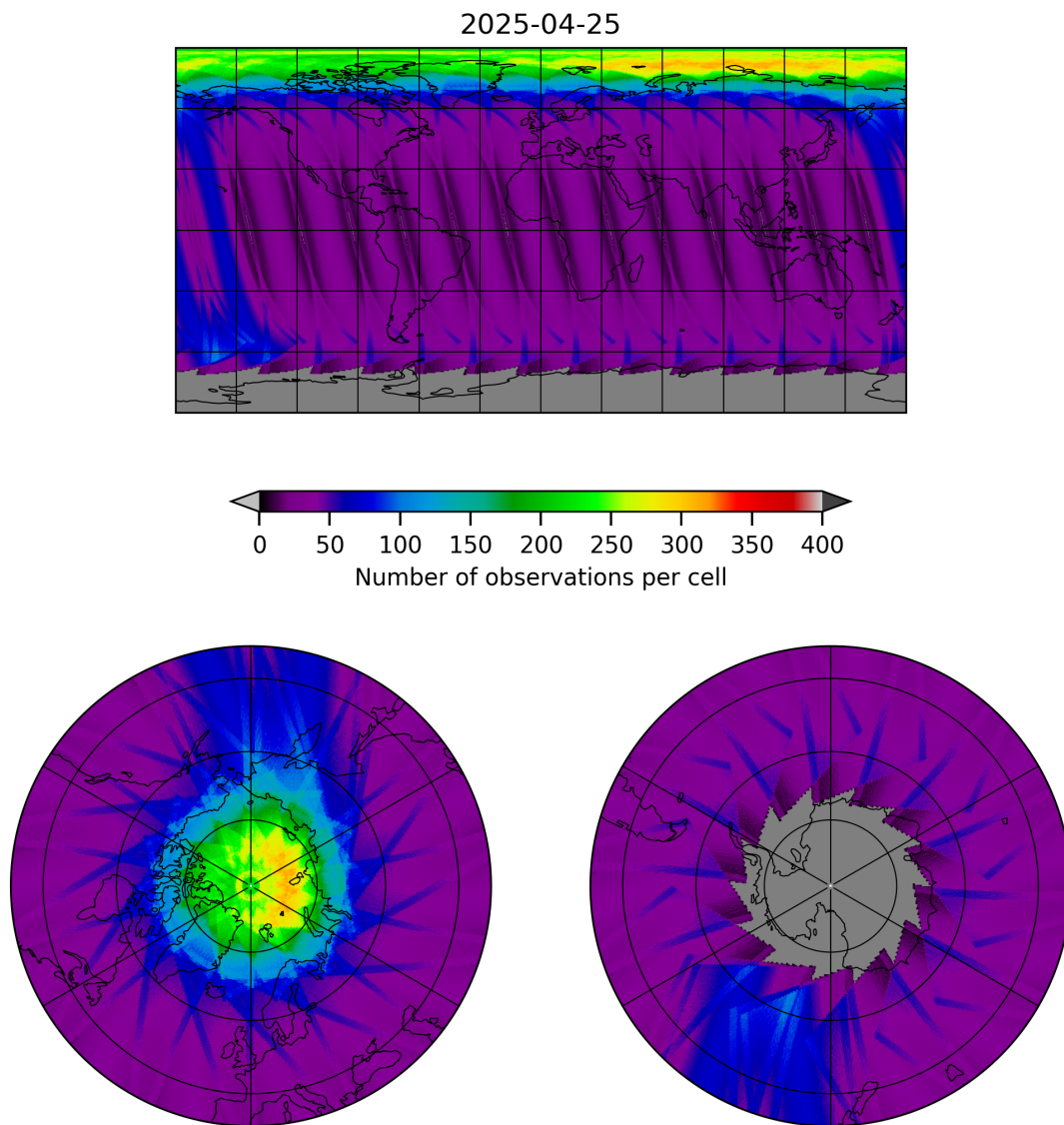
Figure 19: Map of the number of observations for 2025-04-24 to 2025-04-26
