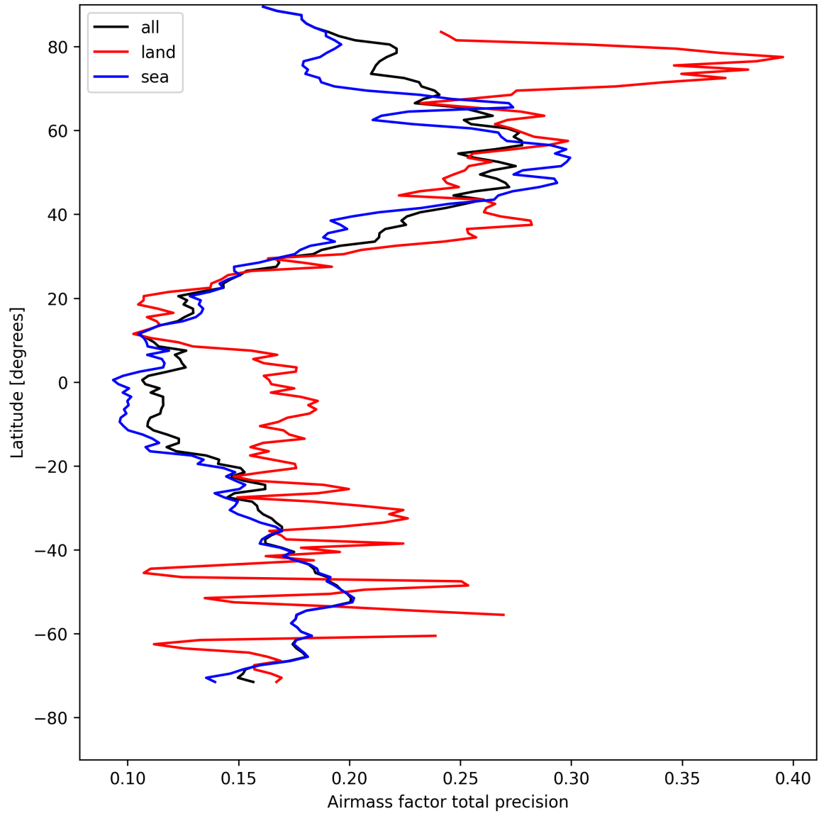
Figure 27: Zonal average of “Airmass factor total precision” for 2025-04-24 to 2025-04-26.
