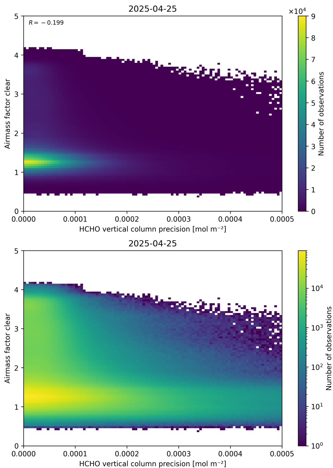
Figure 139: Scatter density plot of “HCHO vertical column precision” against “Airmass factor clear” for 2025-04-24 to 2025-04-26.
