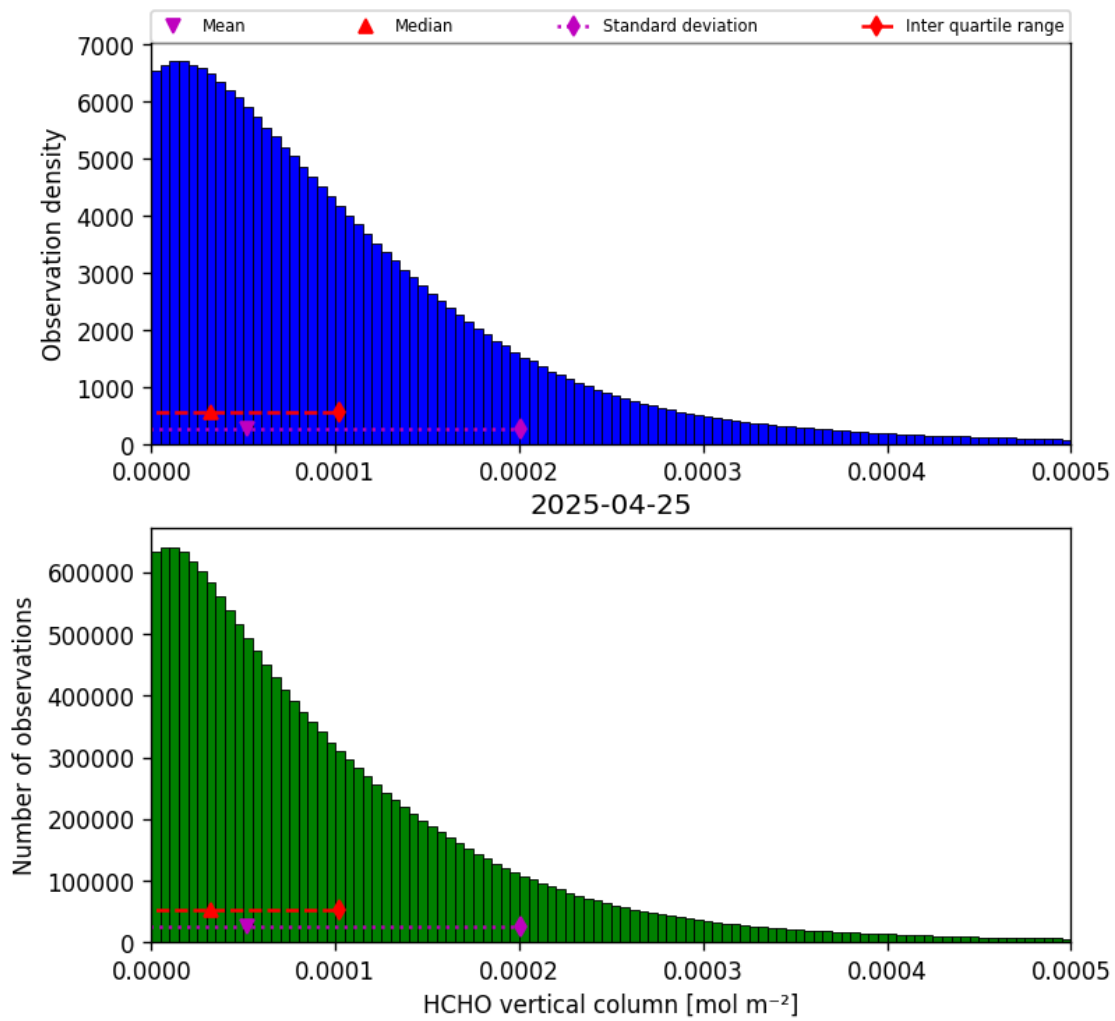
Figure 35: Histogram of “HCHO vertical column” for 2025-04-24 to 2025-04-26
