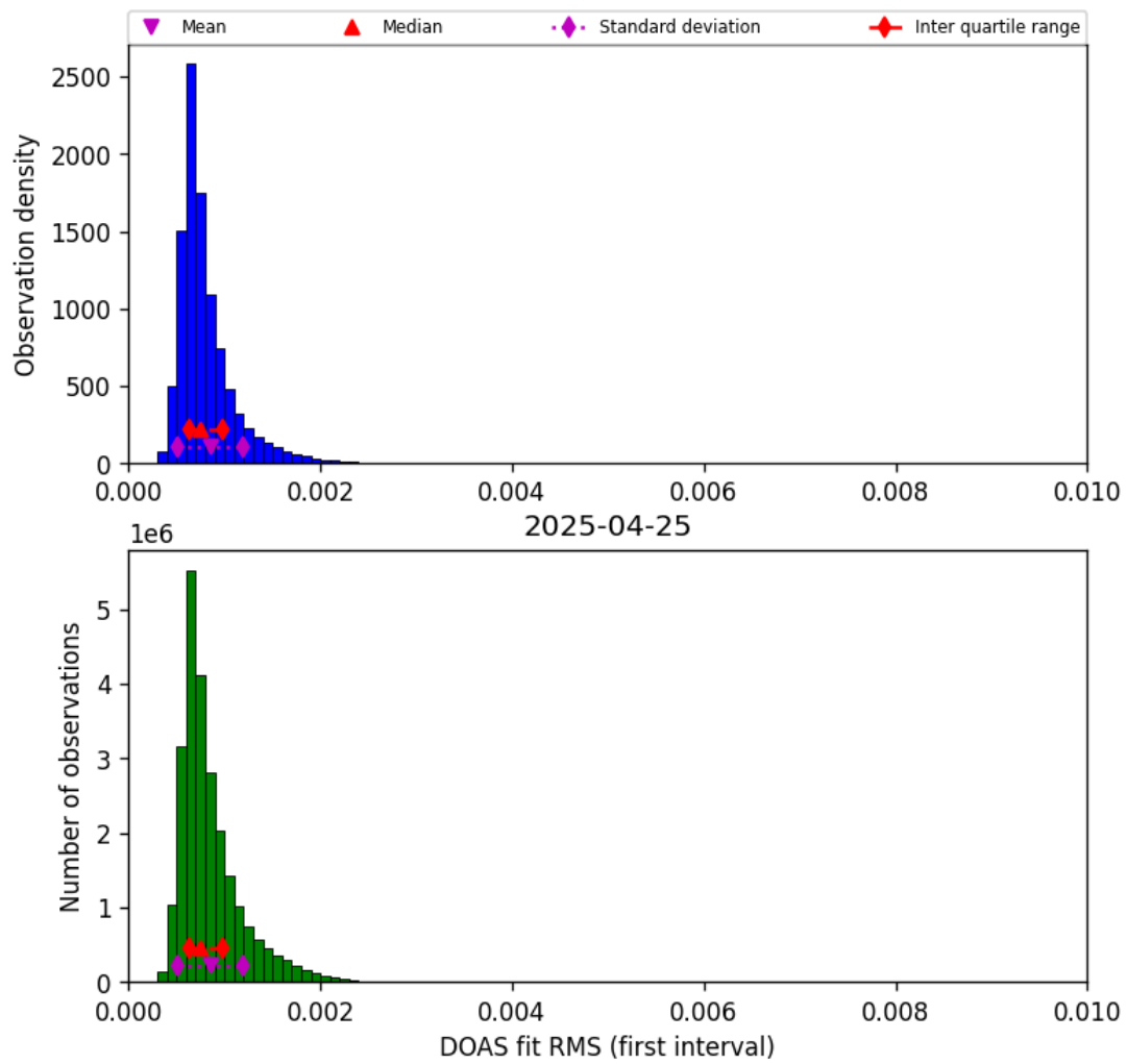
Figure 46: Histogram of “DOAS fit RMS (first interval)” for 2025-04-24 to 2025-04-26
