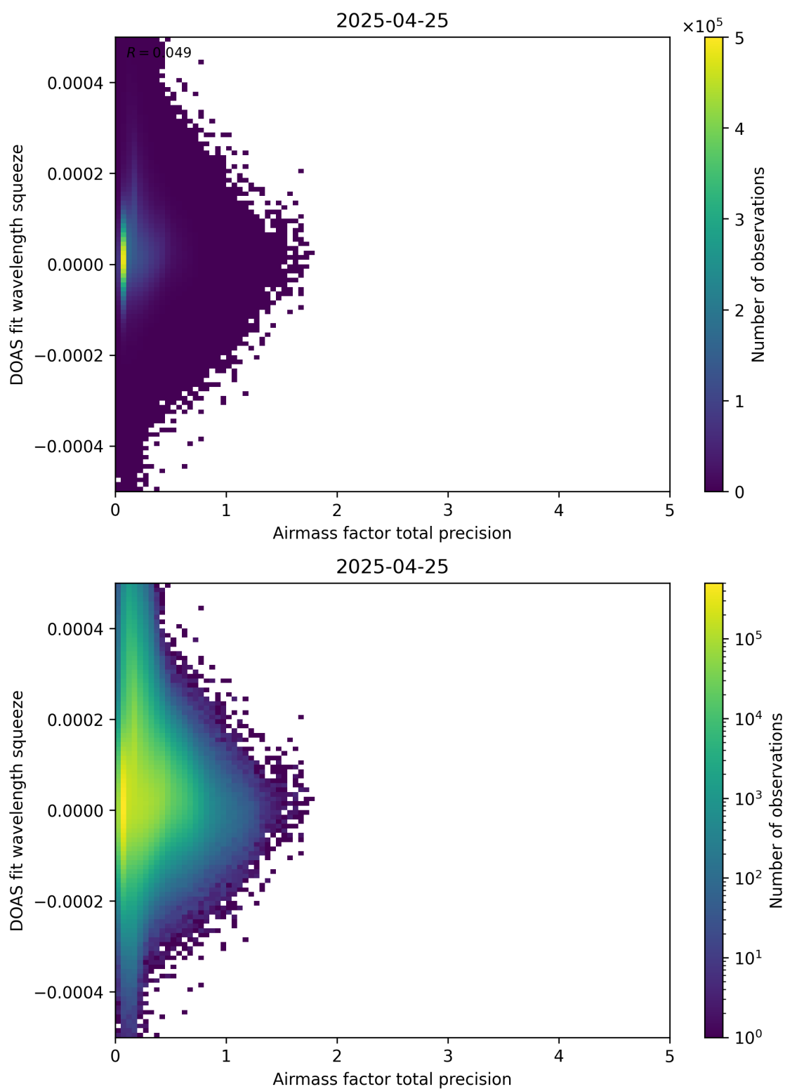
Figure 107: Scatter density plot of “Airmass factor total precision” against “DOAS fit wavelength squeeze” for 2025-04-24 to 2025-04-26.
