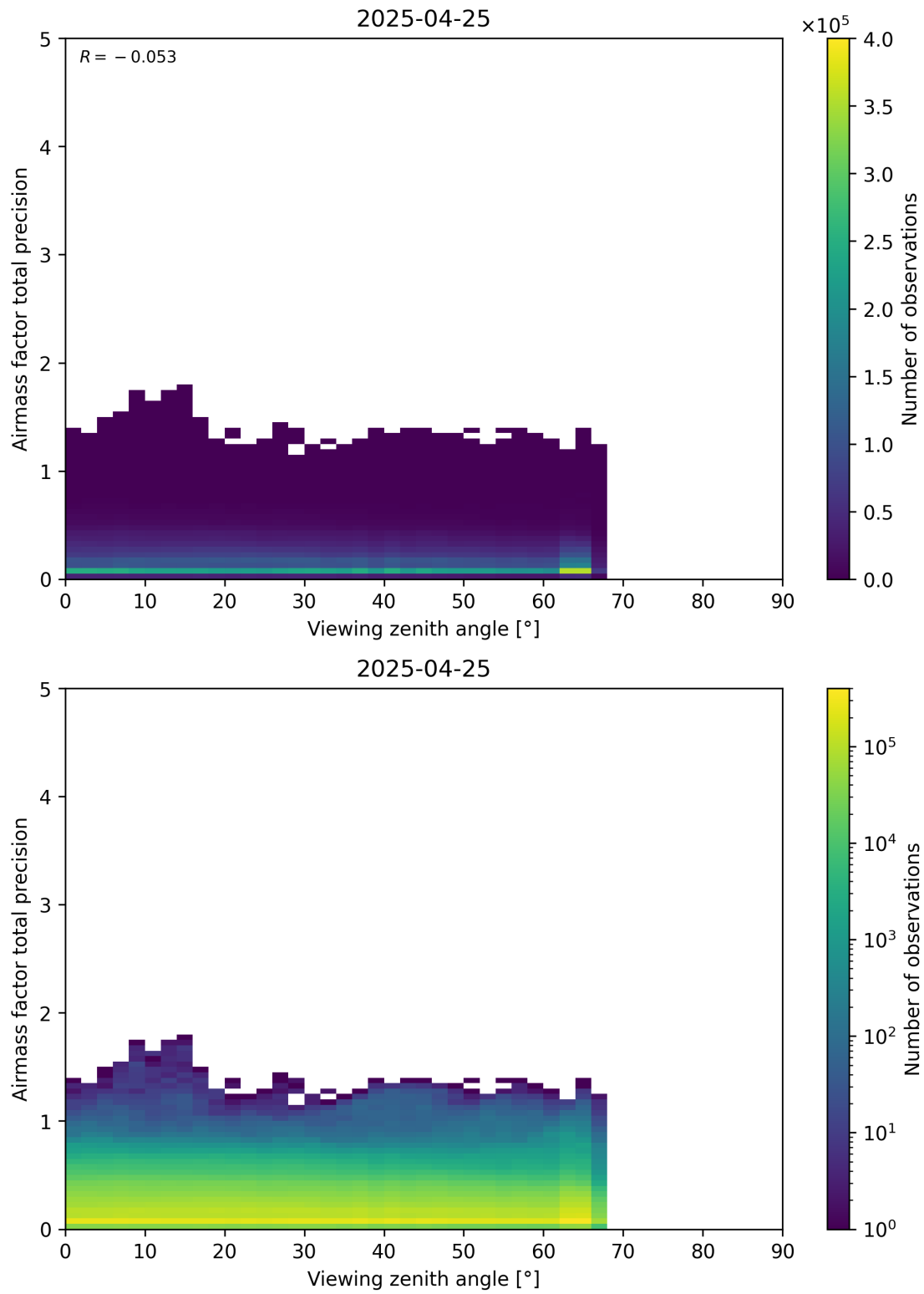
Figure 191: Scatter density plot of “Viewing zenith angle” against “Airmass factor total precision” for 2025-04-24 to 2025-04-26.
