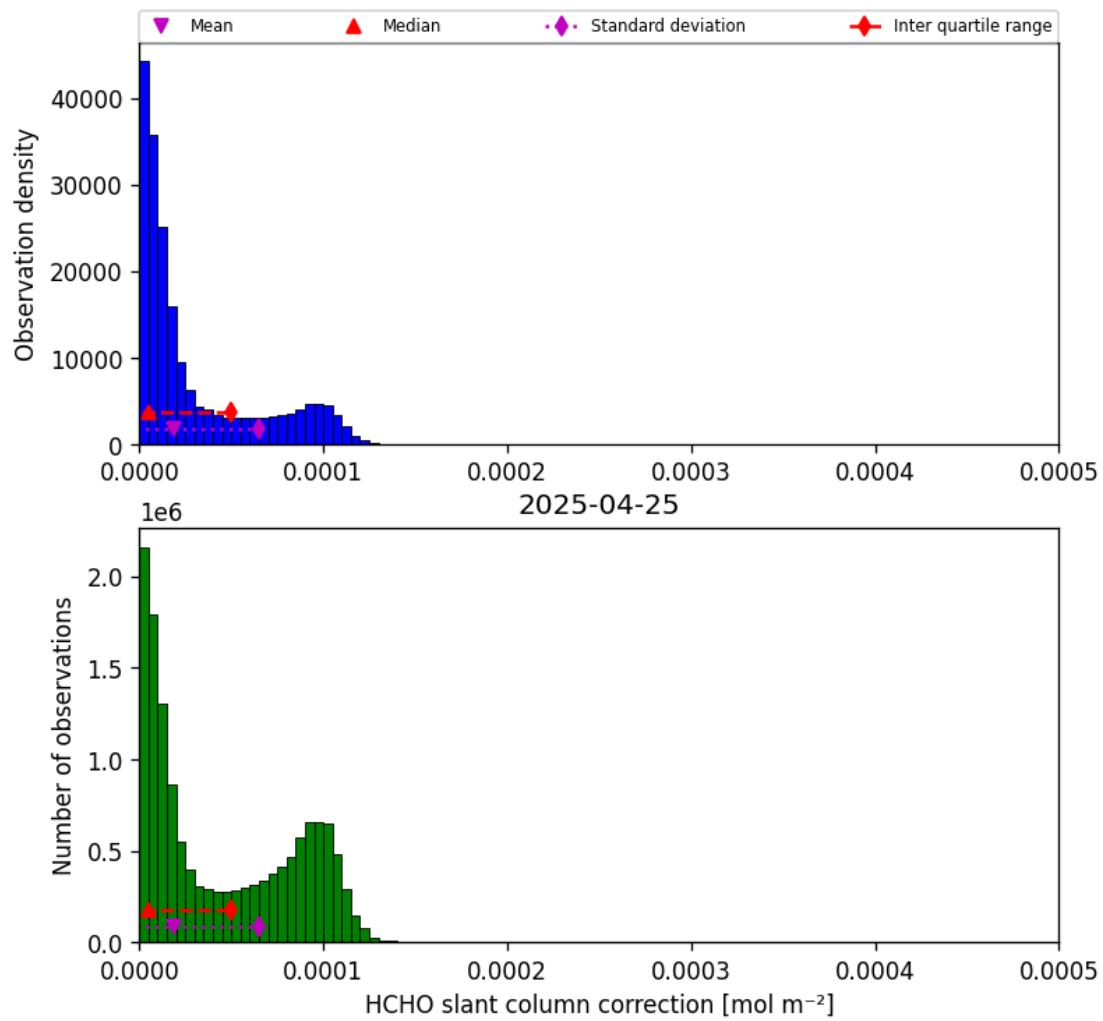
Figure 47: Histogram of “HCHO slant column correction” for 2025-04-24 to 2025-04-26
