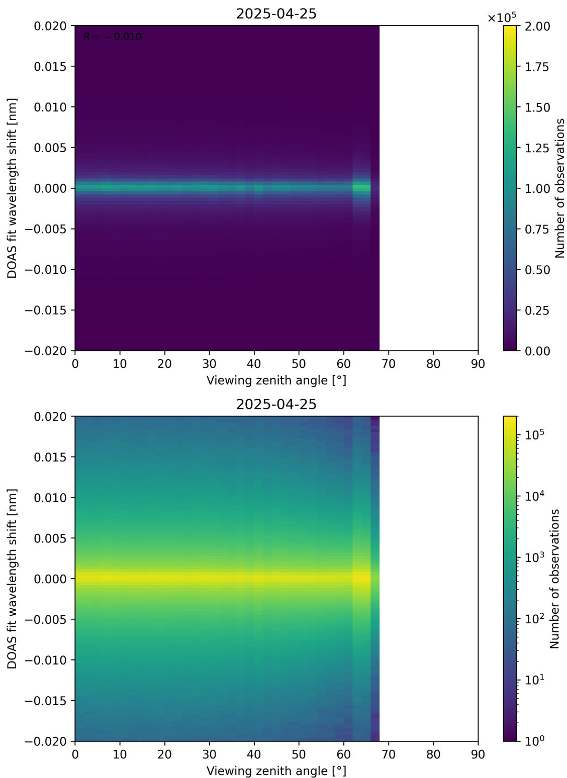
Figure 183: Scatter density plot of “Viewing zenith angle” against “DOAS fit wavelength shift” for 2025-04-24 to 2025-04-26.
