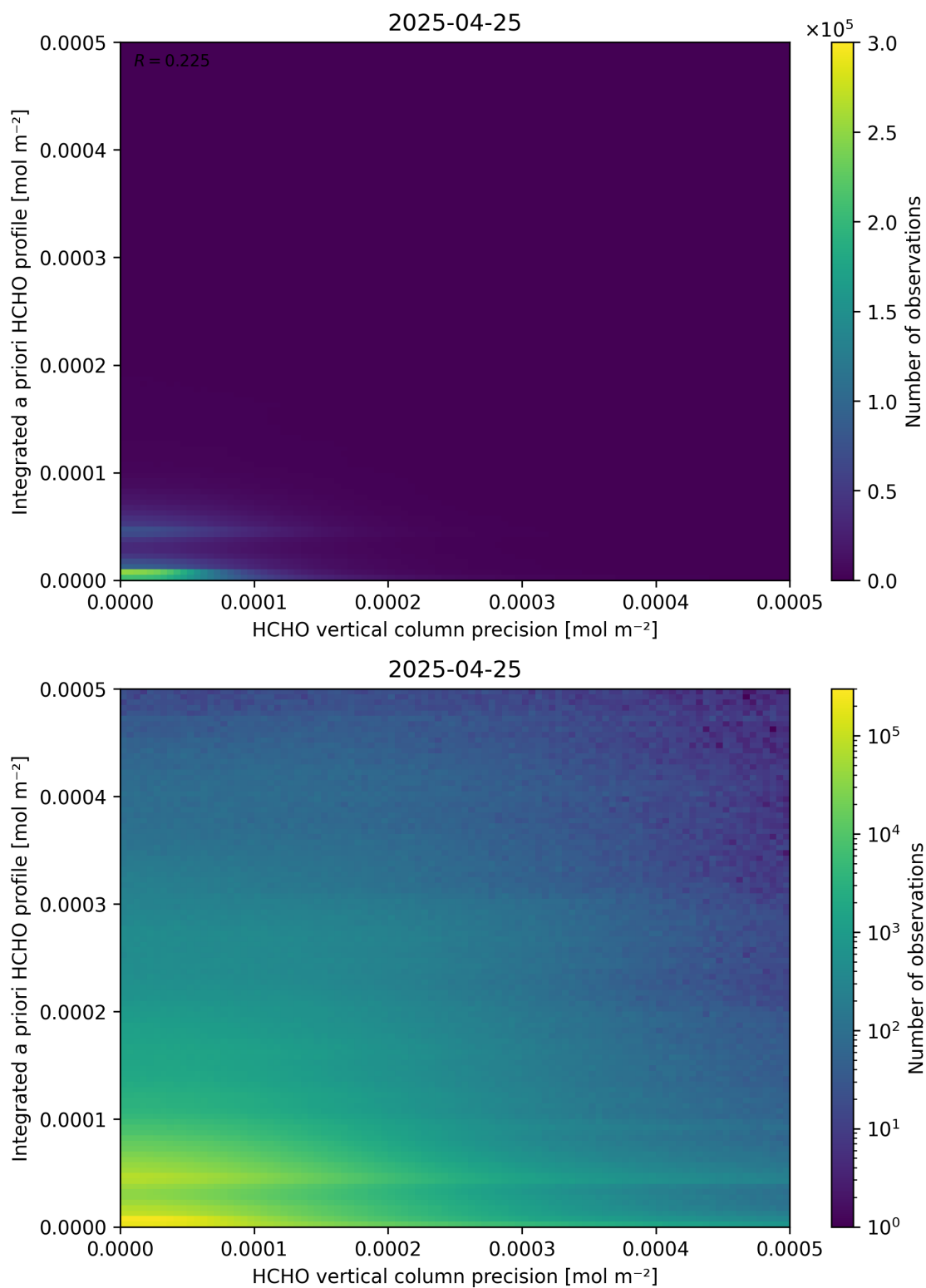
Figure 147: Scatter density plot of “HCHO vertical column precision” against “Integrated a priori HCHO profile” for 2025-04-24 to 2025-04-26.
