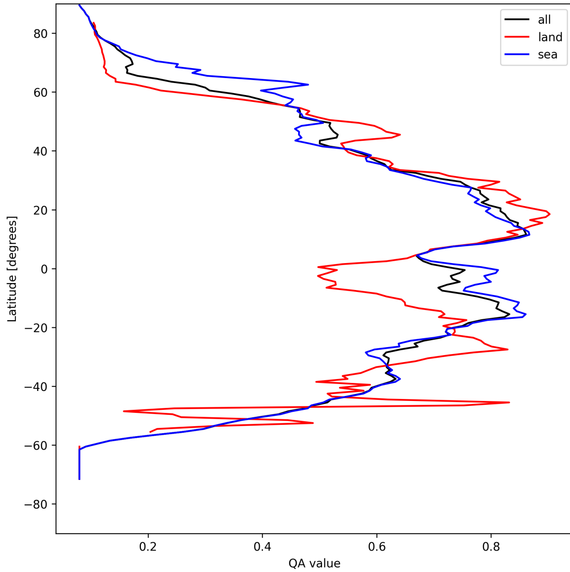
Figure 20: Zonal average of “QA value” for 2025-04-24 to 2025-04-26.
