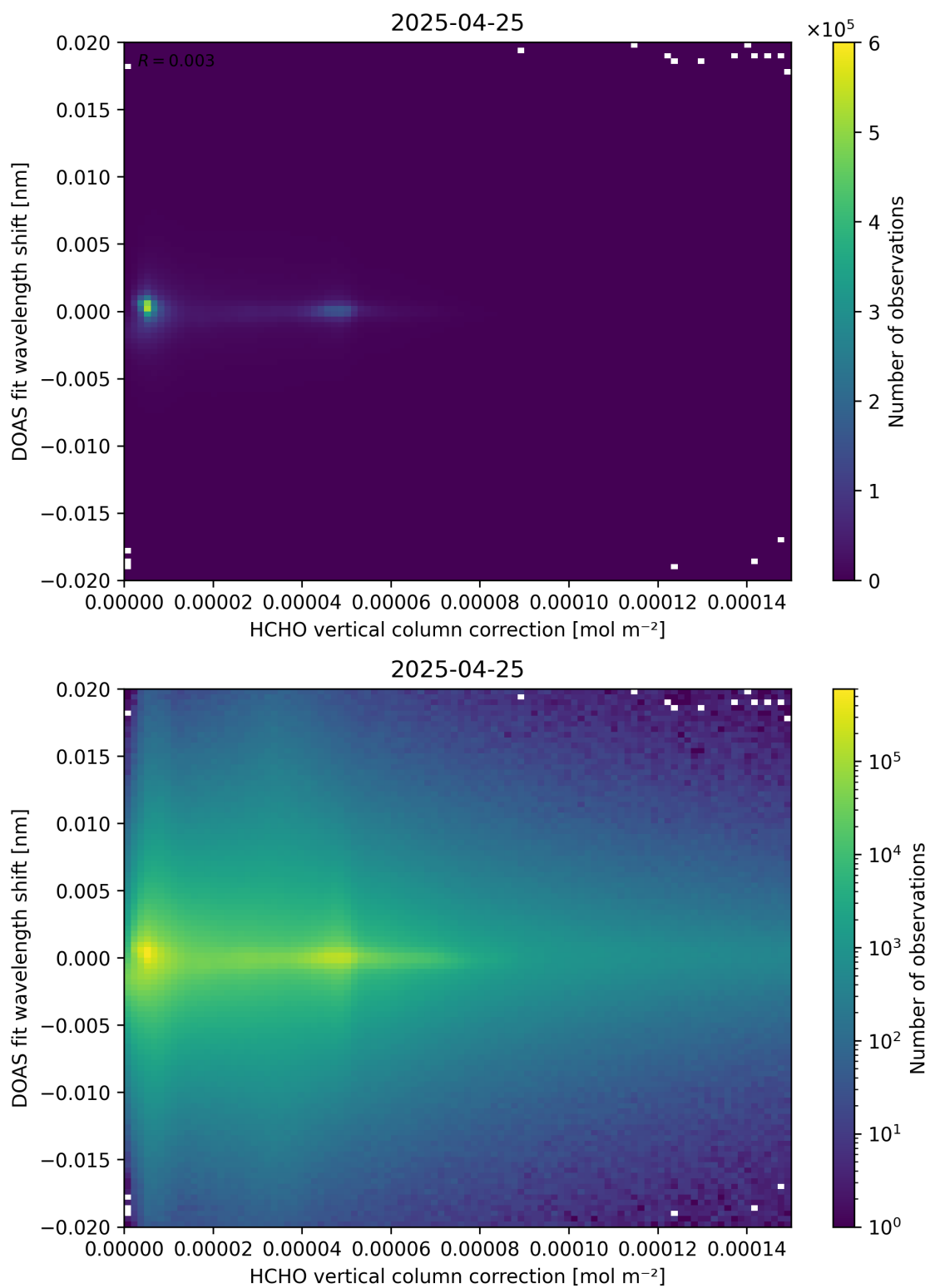
Figure 113: Scatter density plot of “HCHO vertical column correction” against “DOAS fit wavelength shift” for 2025-04-24 to 2025-04-26.
