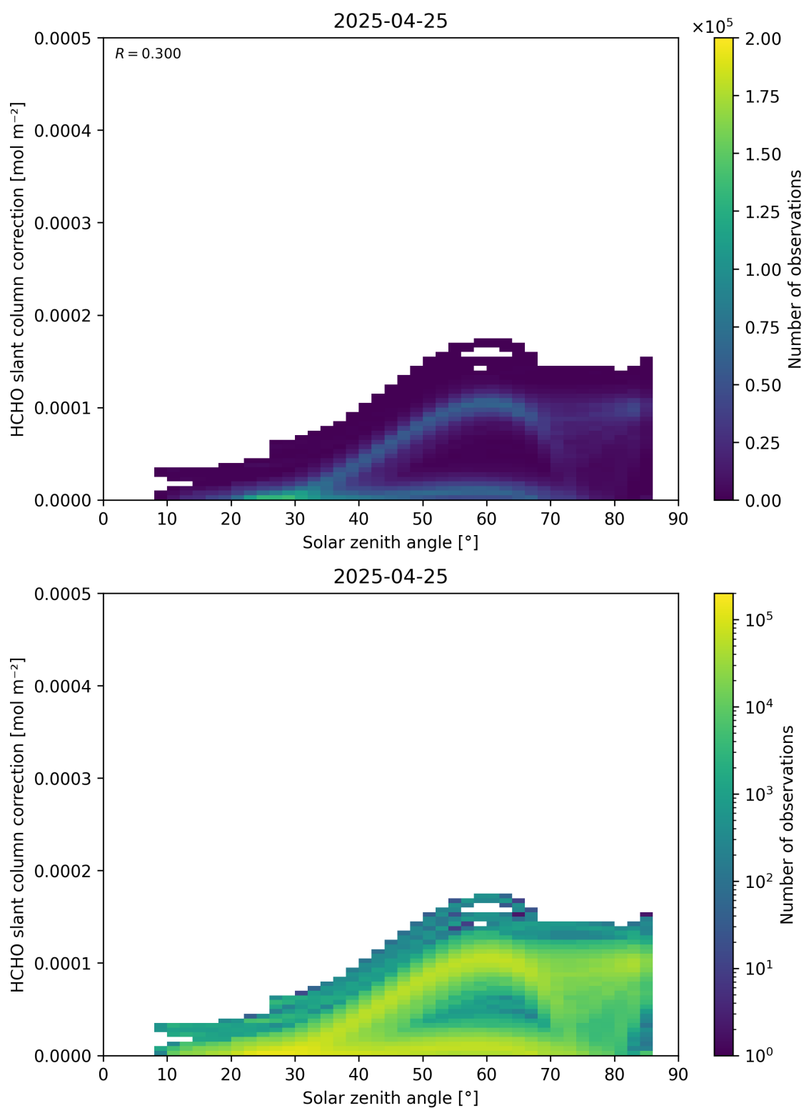
Figure 172: Scatter density plot of “Solar zenith angle” against “HCHO slant column correction” for 2025-04-24 to 2025-04-26.
