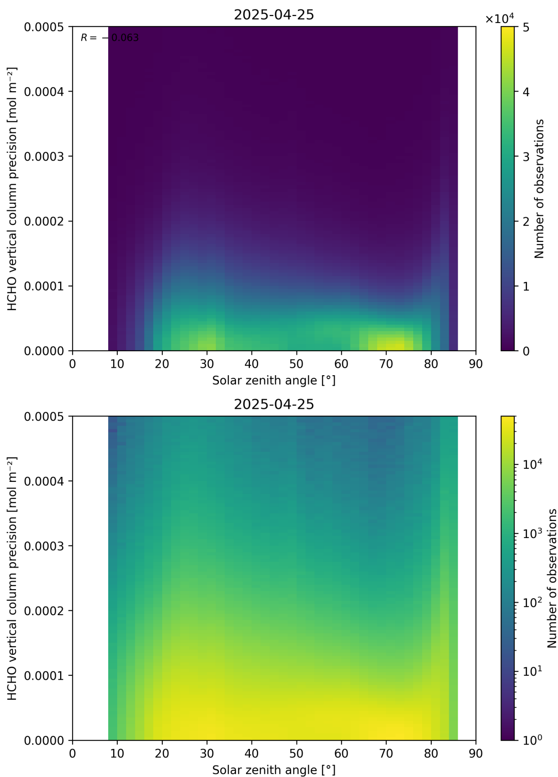
Figure 179: Scatter density plot of “Solar zenith angle” against “HCHO vertical column precision” for 2025-04-24 to 2025-04-26.
