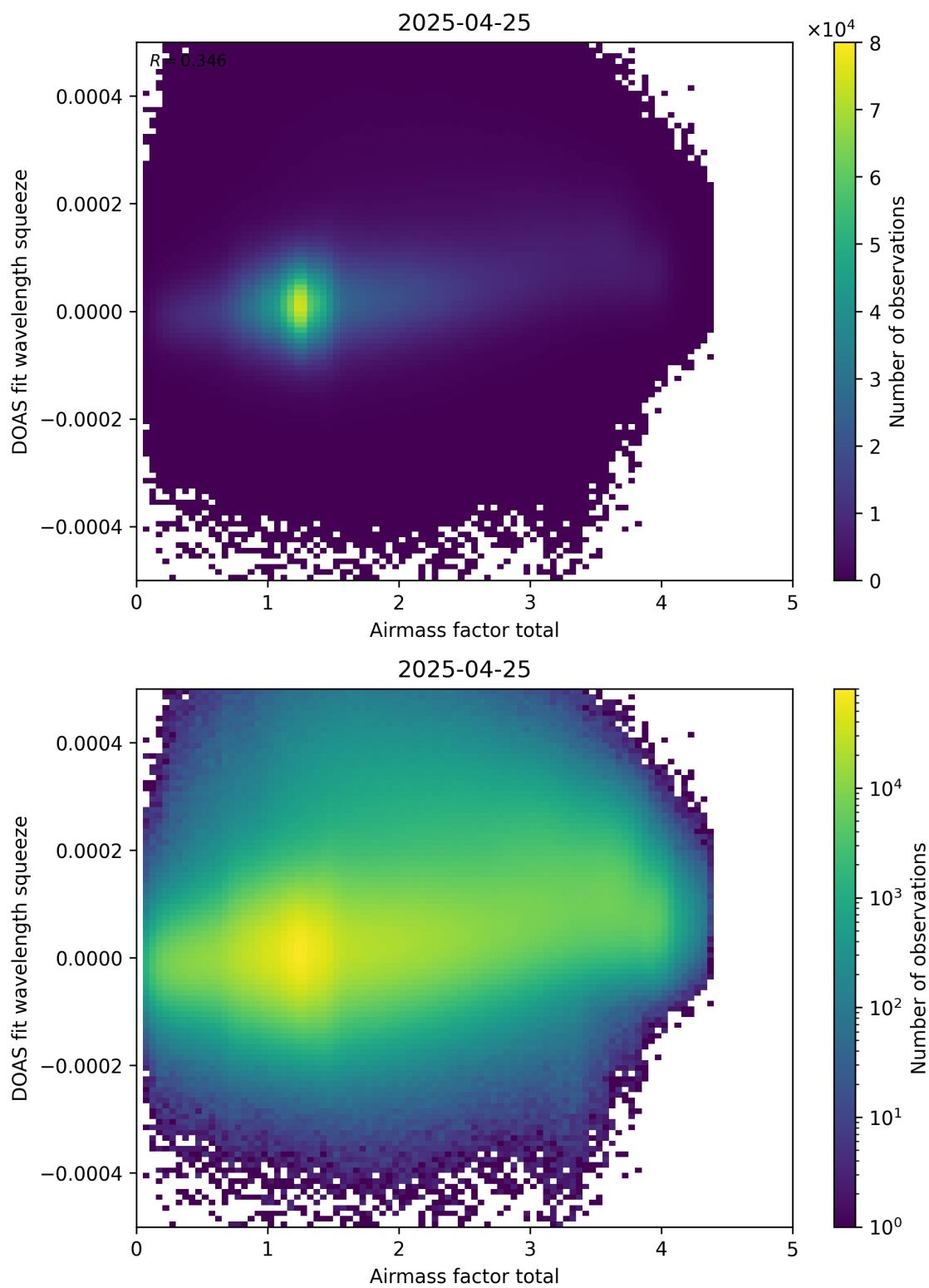
Figure 99: Scatter density plot of “Airmass factor total” against “DOAS fit wavelength squeeze” for 2025-04-24 to 2025-04-26.
