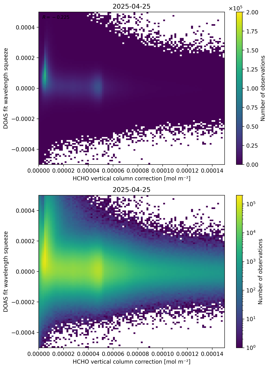
Figure 114: Scatter density plot of “HCHO vertical column correction” against “DOAS fit wavelength squeeze” for 2025-04-24 to 2025-04-26.
