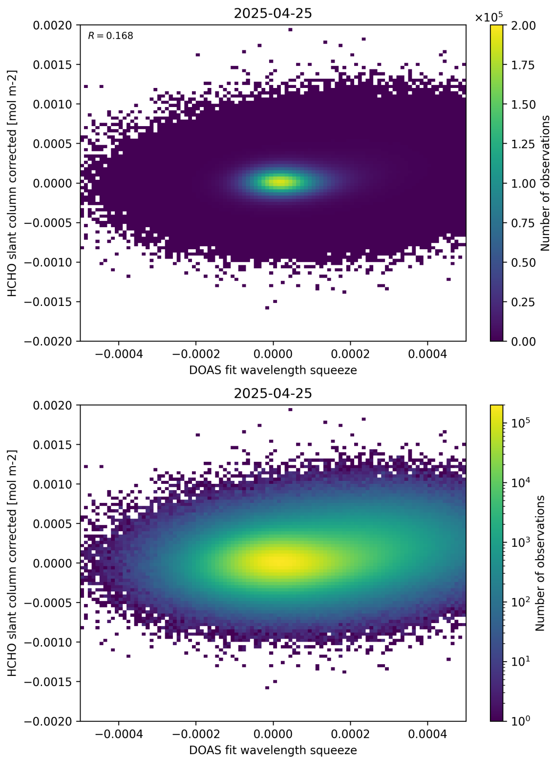
Figure 69: Scatter density plot of “DOAS fit wavelength squeeze” against “HCHO slant column corrected” for 2025-04-24 to 2025-04-26.
