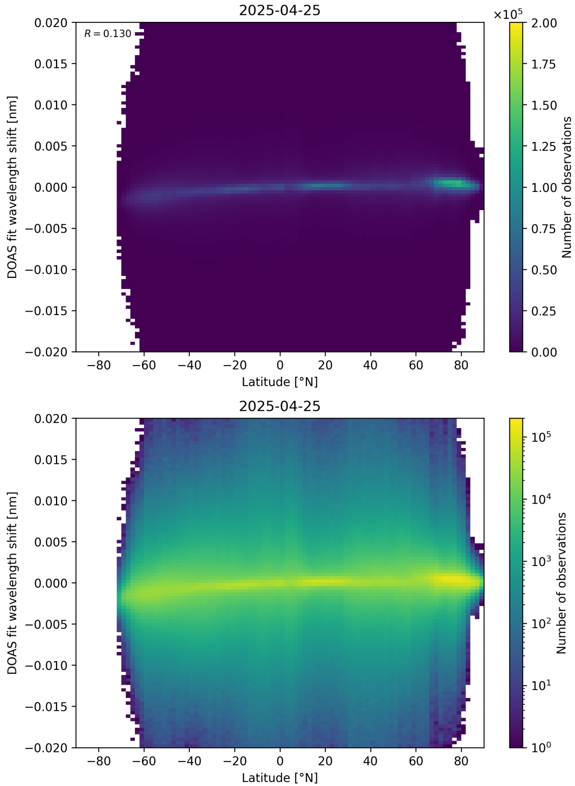
Figure 154: Scatter density plot of “Latitude” against “DOAS fit wavelength shift” for 2025-04-24 to 2025-04-26.
