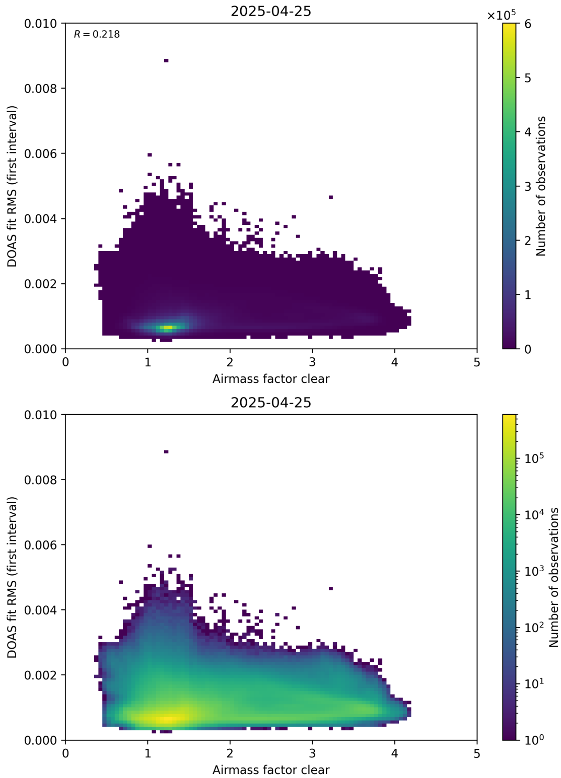
Figure 71: Scatter density plot of “Airmass factor clear” against “DOAS fit RMS (first interval)” for 2025-04-24 to 2025-04-26.
