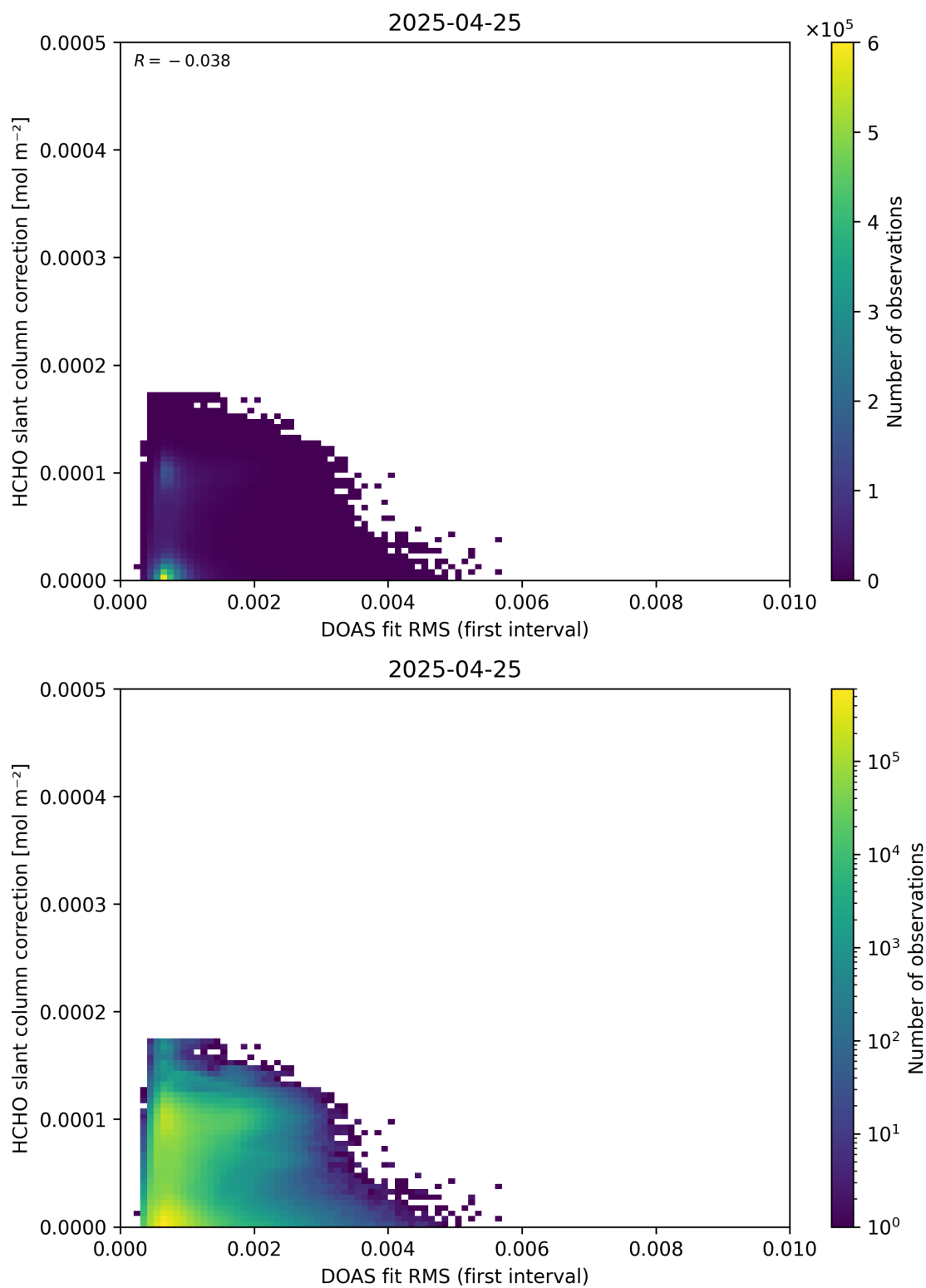
Figure 63: Scatter density plot of “DOAS fit RMS (first interval)” against “HCHO slant column correction” for 2025-04-24 to 2025-04-26.
