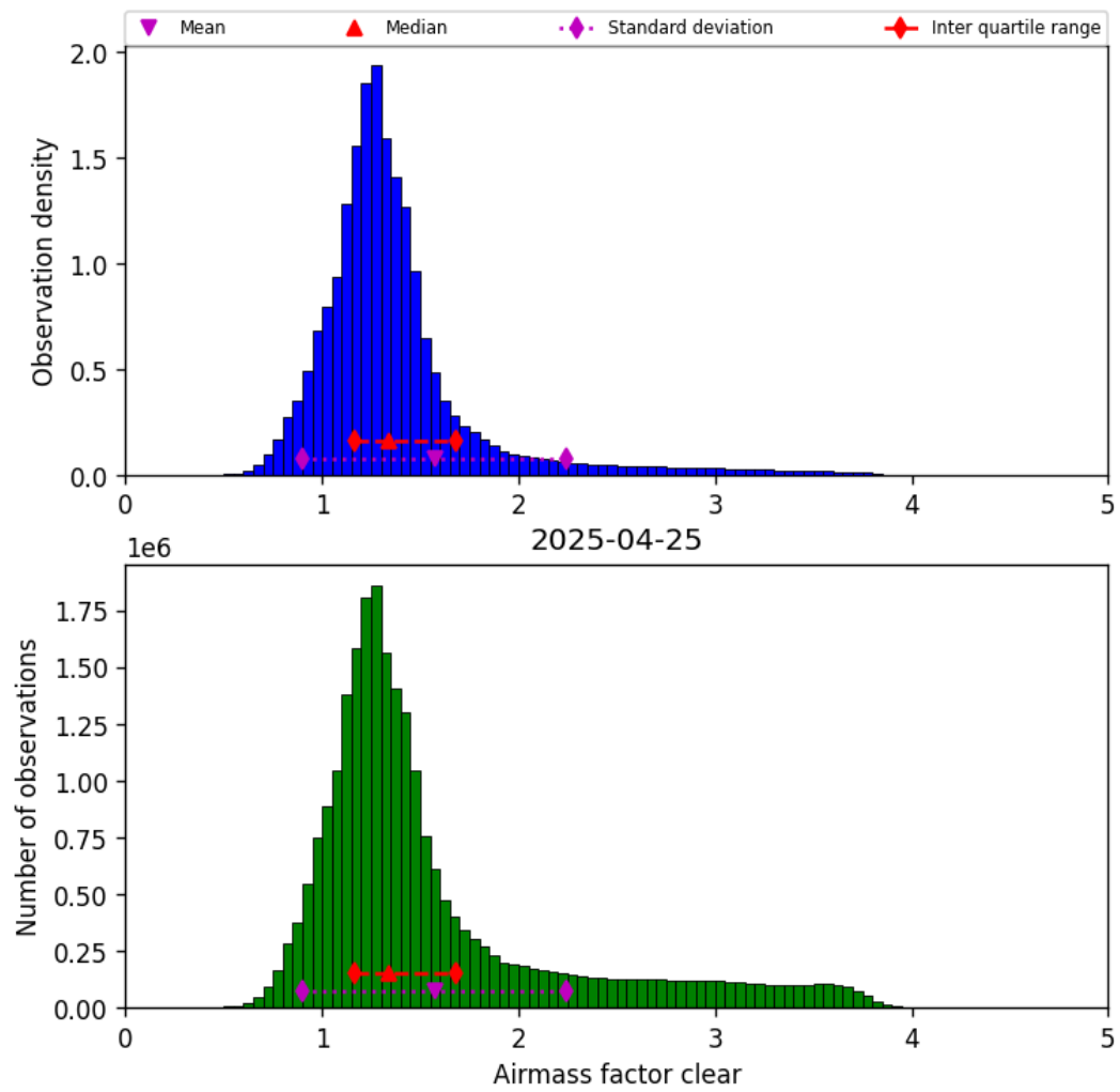
Figure 42: Histogram of “Airmass factor clear” for 2025-04-24 to 2025-04-26
