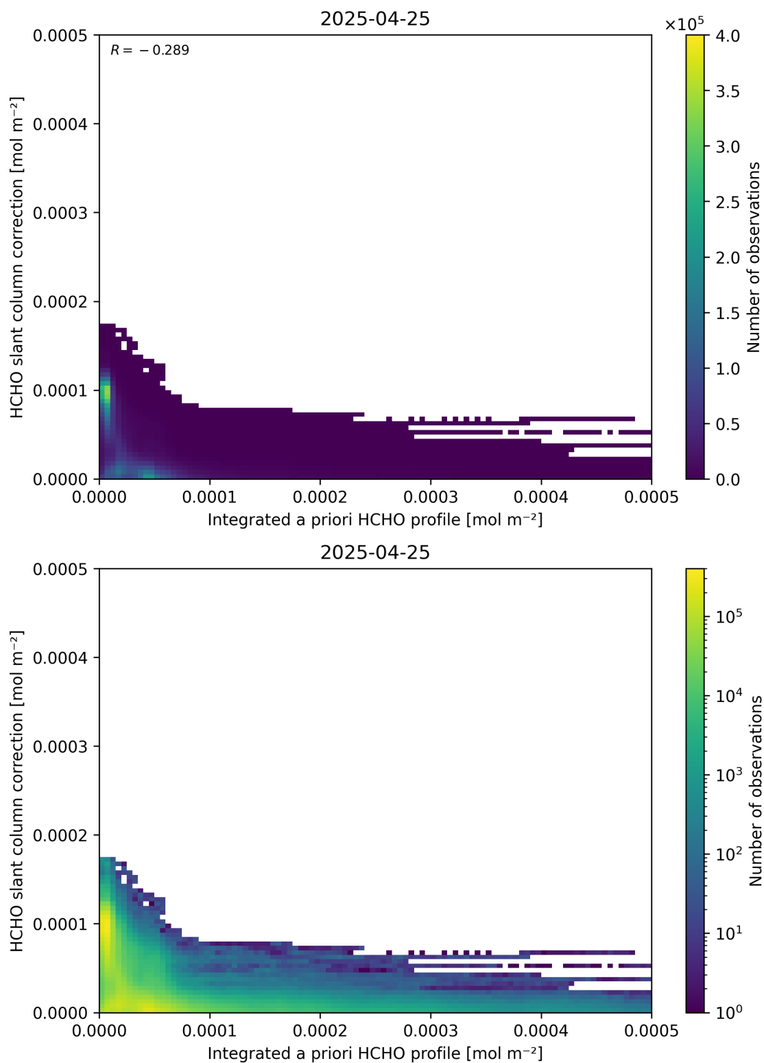
Figure 152: Scatter density plot of “Integrated a priori HCHO profile” against “HCHO slant column correction” for 2025-04-24 to 2025-04-26.
