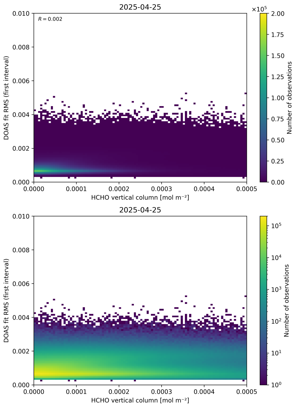
Figure 123: Scatter density plot of “HCHO vertical column” against “DOAS fit RMS (first interval)” for 2025-04-24 to 2025-04-26.
