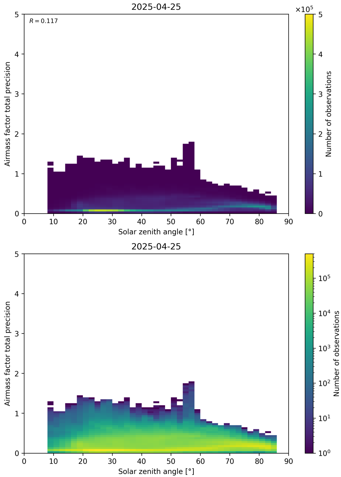
Figure 176: Scatter density plot of “Solar zenith angle” against “Airmass factor total precision” for 2025-04-24 to 2025-04-26.
