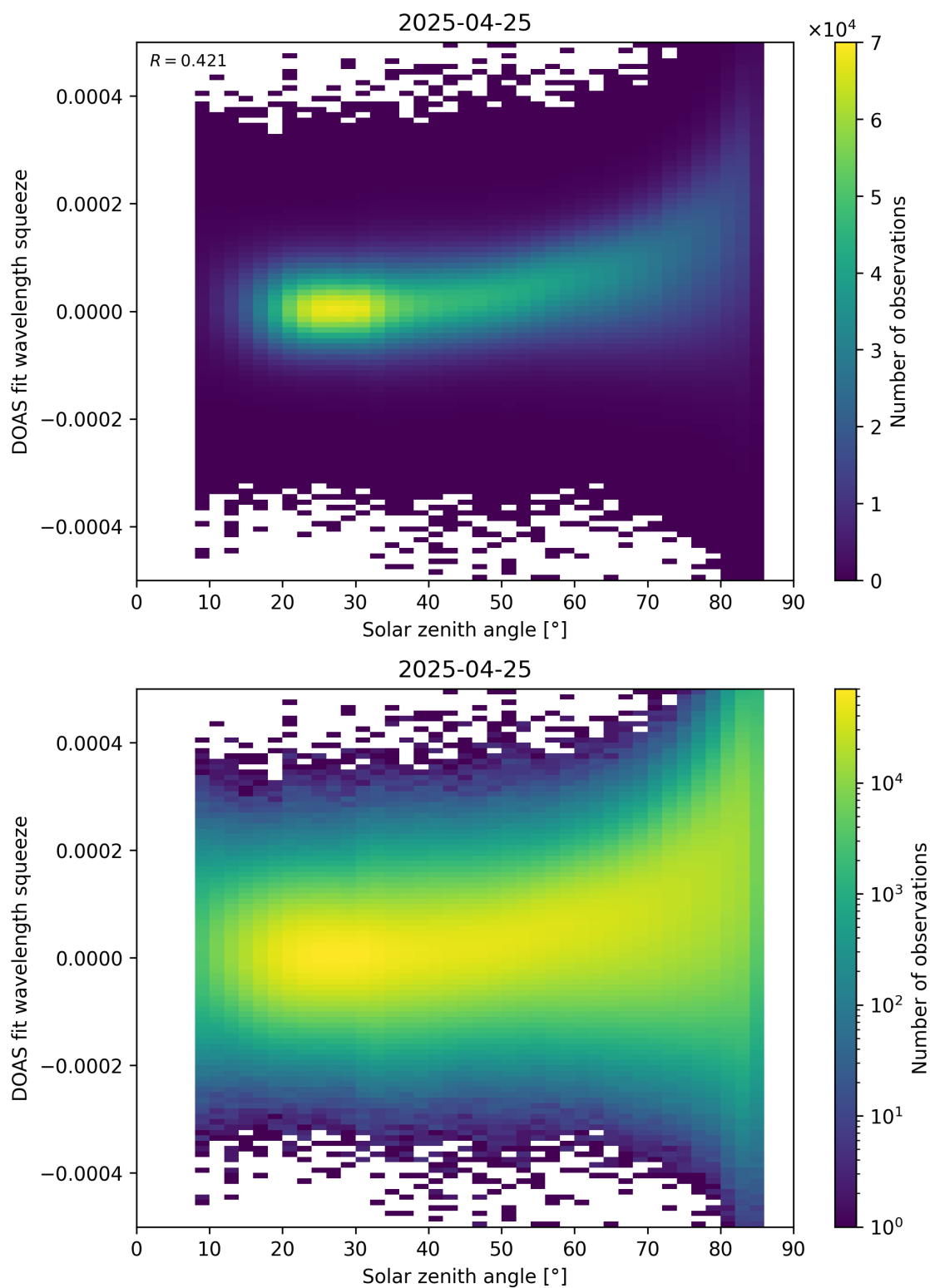
Figure 169: Scatter density plot of “Solar zenith angle” against “DOAS fit wavelength squeeze” for 2025-04-24 to 2025-04-26.
