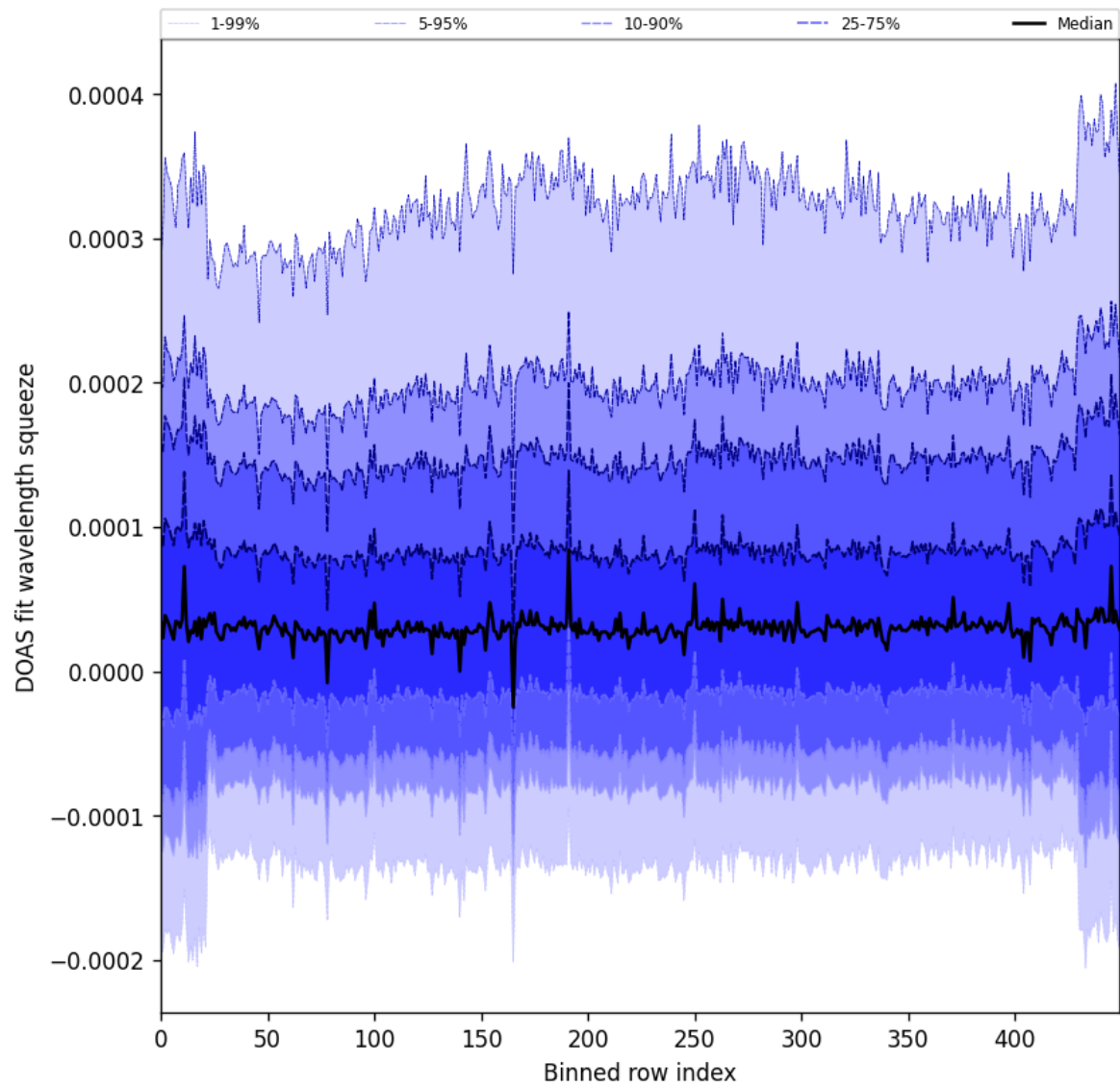
Figure 59: Along track statistics of “DOAS fit wavelength squeeze” for 2025-04-24 to 2025-04-26
