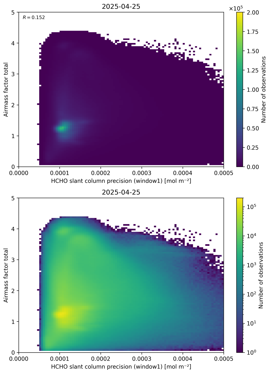
Figure 94: Scatter density plot of “HCHO slant column precision (window1)” against “Airmass factor total” for 2025-04-24 to 2025-04-26.
