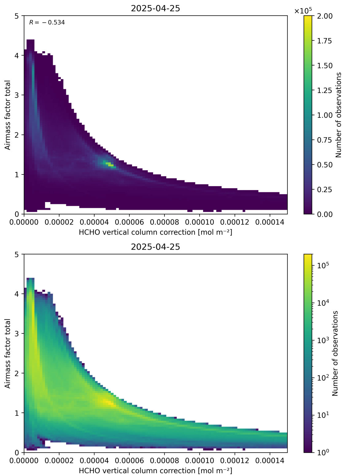
Figure 120: Scatter density plot of “HCHO vertical column correction” against “Airmass factor total” for 2025-04-24 to 2025-04-26.
