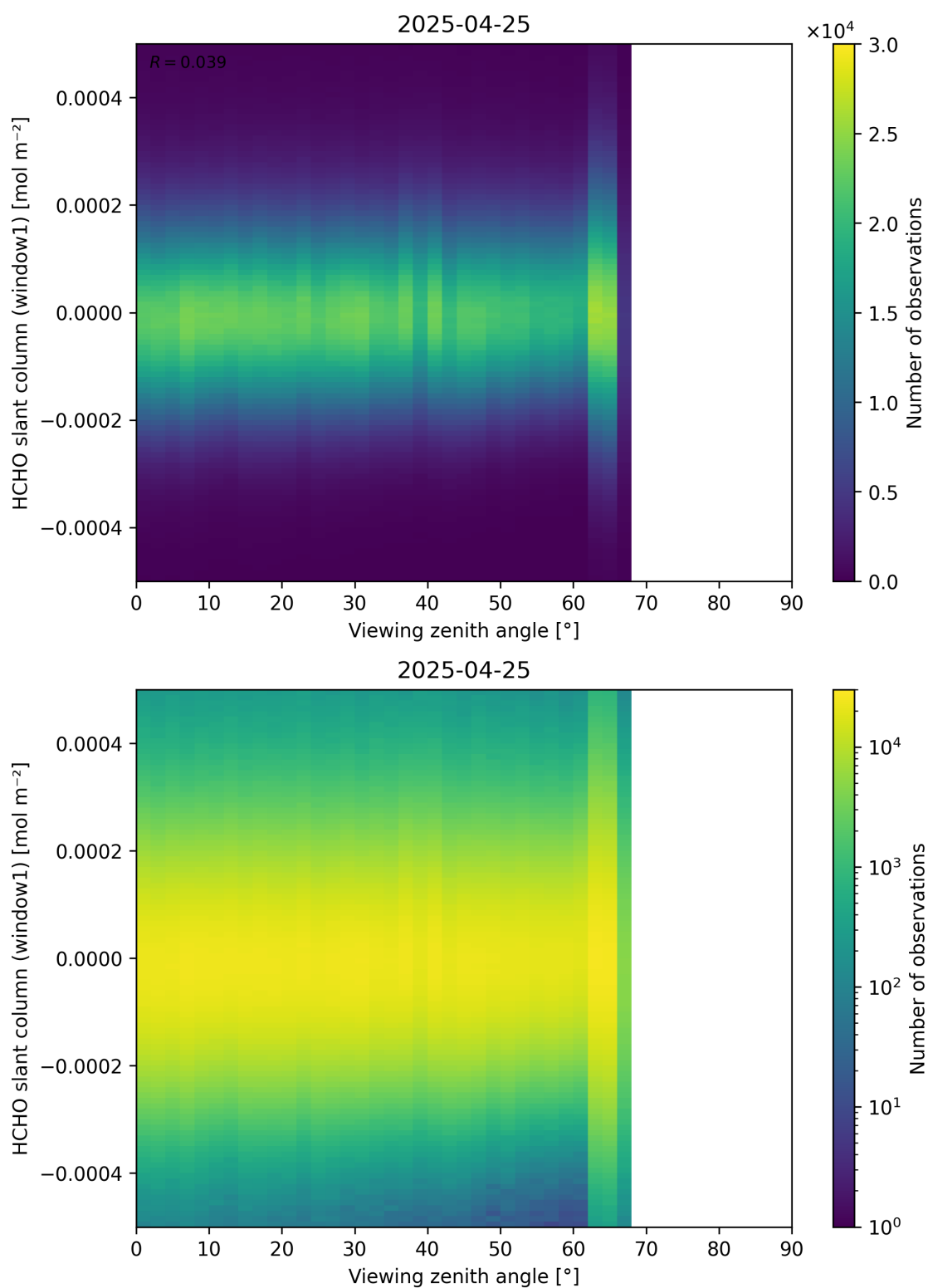
Figure 188: Scatter density plot of “Viewing zenith angle” against “HCHO slant column (window1)” for 2025-04-24 to 2025-04-26.
