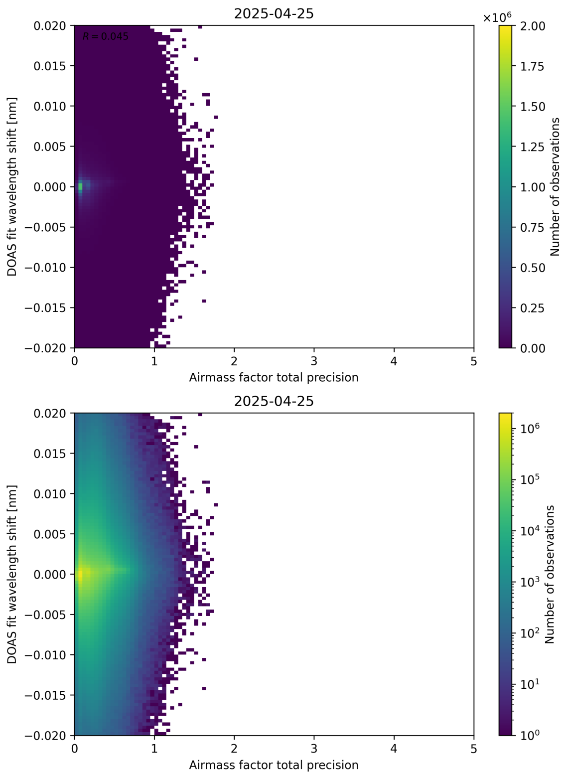
Figure 106: Scatter density plot of “Airmass factor total precision” against “DOAS fit wavelength shift” for 2025-04-24 to 2025-04-26.
