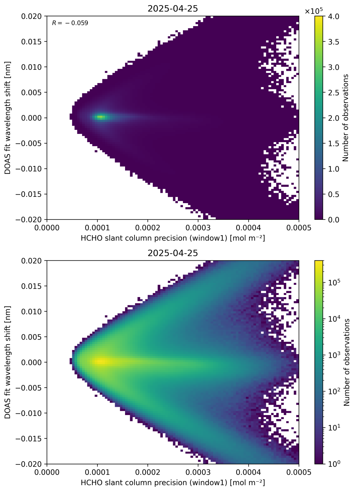
Figure 89: Scatter density plot of “HCHO slant column precision (window1)” against “DOAS fit wavelength shift” for 2025-04-24 to 2025-04-26.
