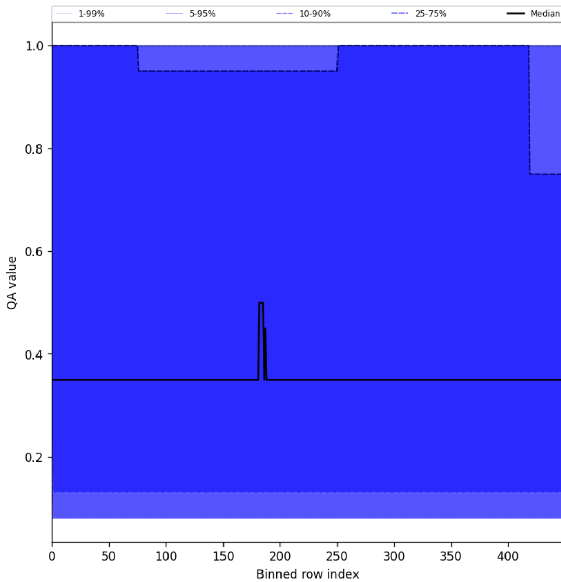
Figure 48: Along track statistics of “QA value” for 2025-04-24 to 2025-04-26
