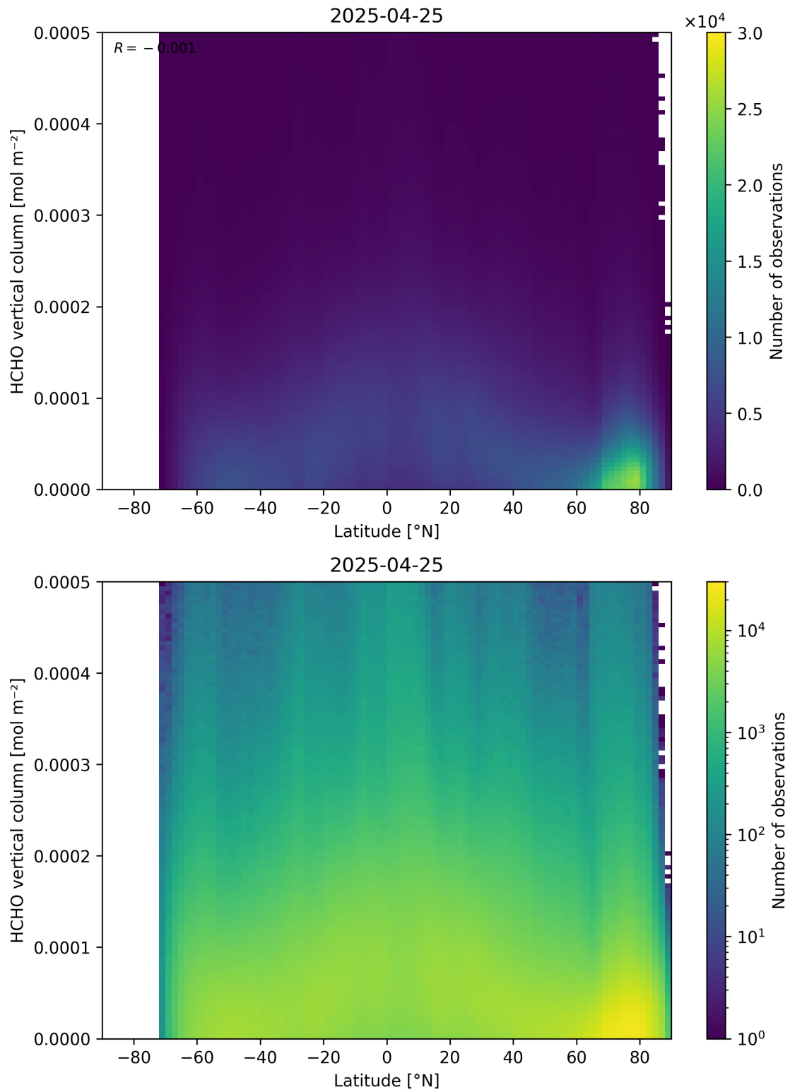
Figure 163: Scatter density plot of “Latitude” against “HCHO vertical column” for 2025-04-24 to 2025-04-26.
