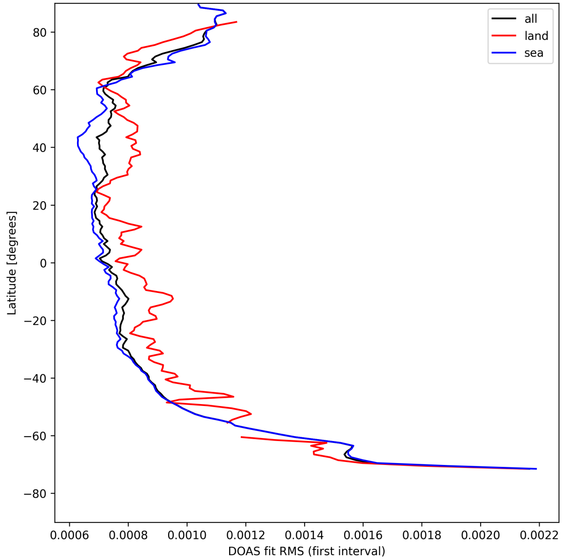
Figure 32: Zonal average of “DOAS fit RMS (first interval)” for 2025-04-24 to 2025-04-26.
