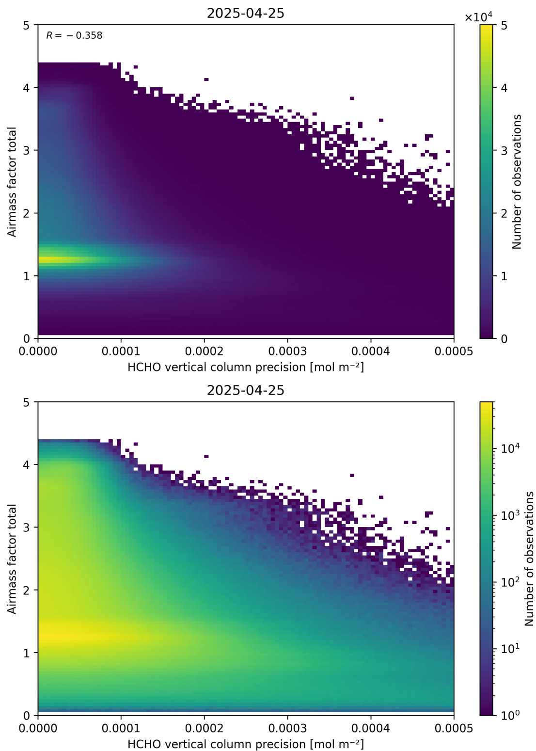
Figure 144: Scatter density plot of “HCHO vertical column precision” against “Airmass factor total” for 2025-04-24 to 2025-04-26.
