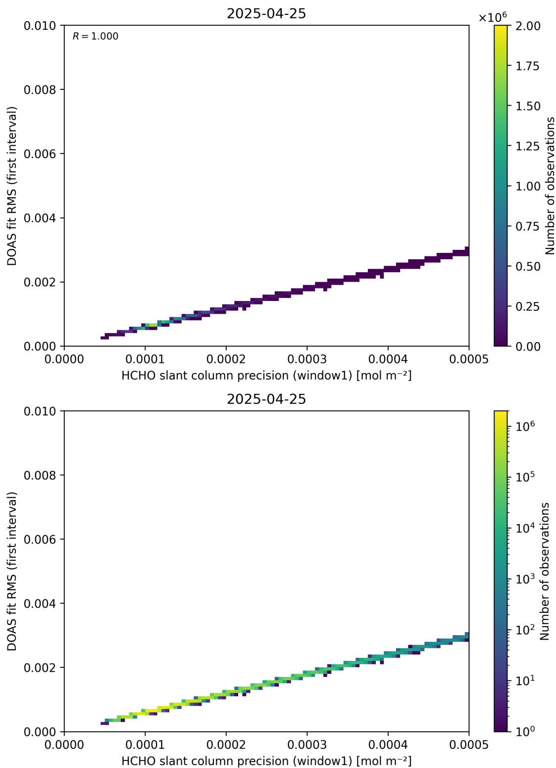
Figure 88: Scatter density plot of “HCHO slant column precision (window1)” against “DOAS fit RMS (first interval)” for 2025-04-24 to 2025-04-26.
