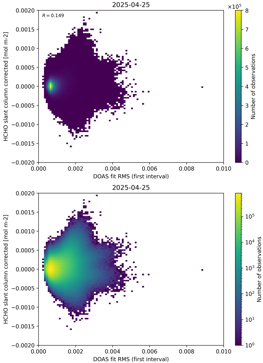
Figure 62: Scatter density plot of “DOAS fit RMS (first interval)” against “HCHO slant column corrected” for 2025-04-24 to 2025-04-26.
