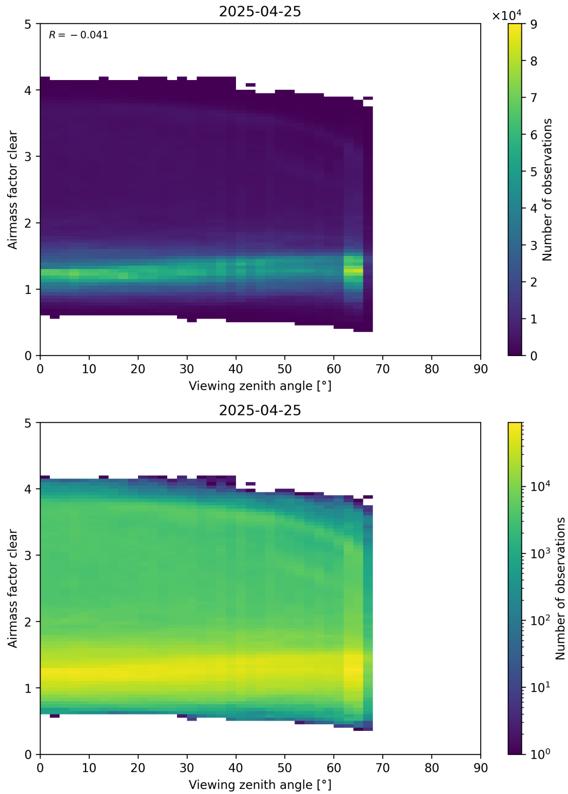
Figure 185: Scatter density plot of “Viewing zenith angle” against “Airmass factor clear” for 2025-04-24 to 2025-04-26.
