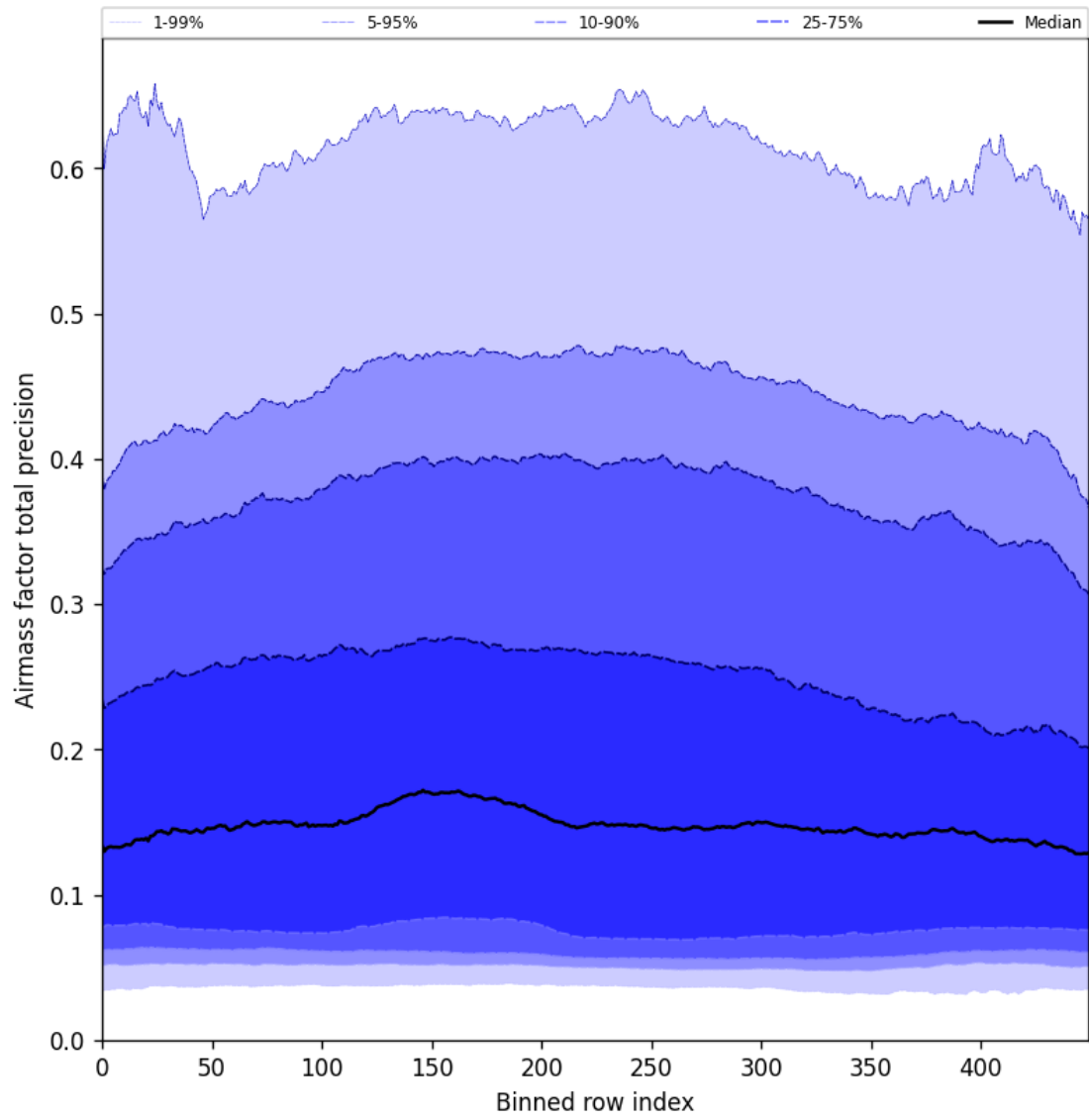
Figure 55: Along track statistics of “Airmass factor total precision” for 2025-04-24 to 2025-04-26
