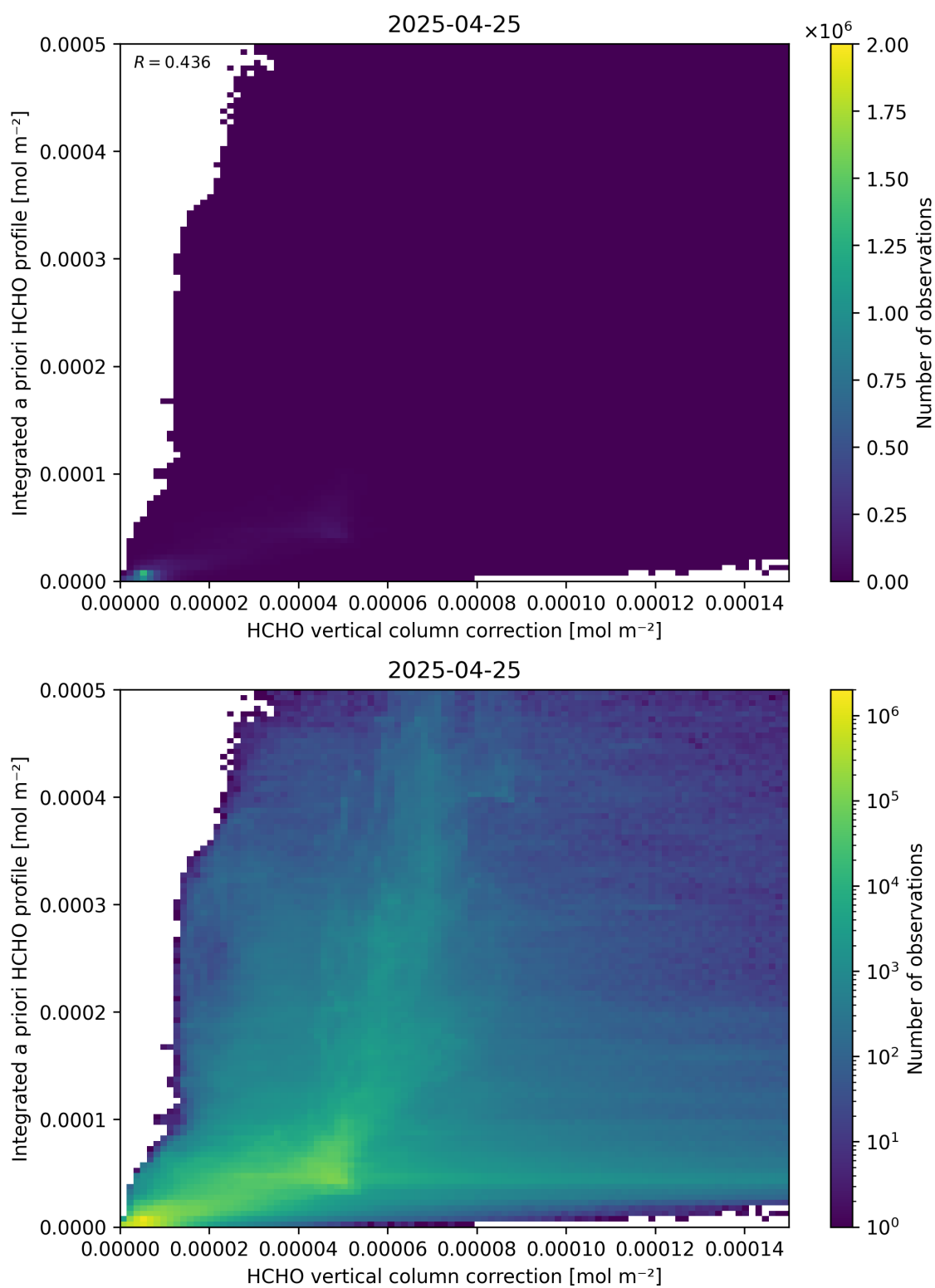
Figure 122: Scatter density plot of “HCHO vertical column correction” against “Integrated a priori HCHO profile” for 2025-04-24 to 2025-04-26.
