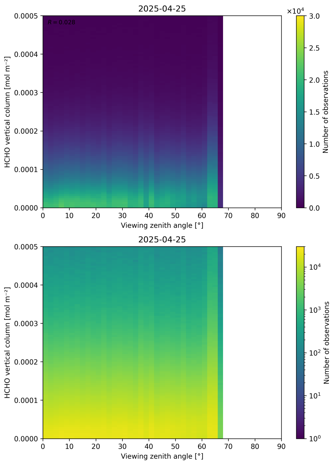
Figure 192: Scatter density plot of “Viewing zenith angle” against “HCHO vertical column” for 2025-04-24 to 2025-04-26.
