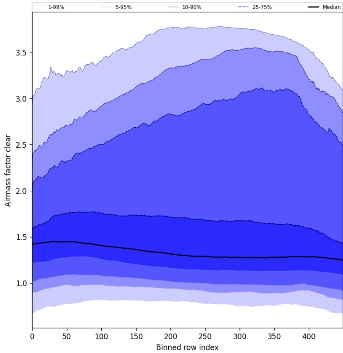
Figure 56: Along track statistics of “Airmass factor clear” for 2025-04-24 to 2025-04-26
