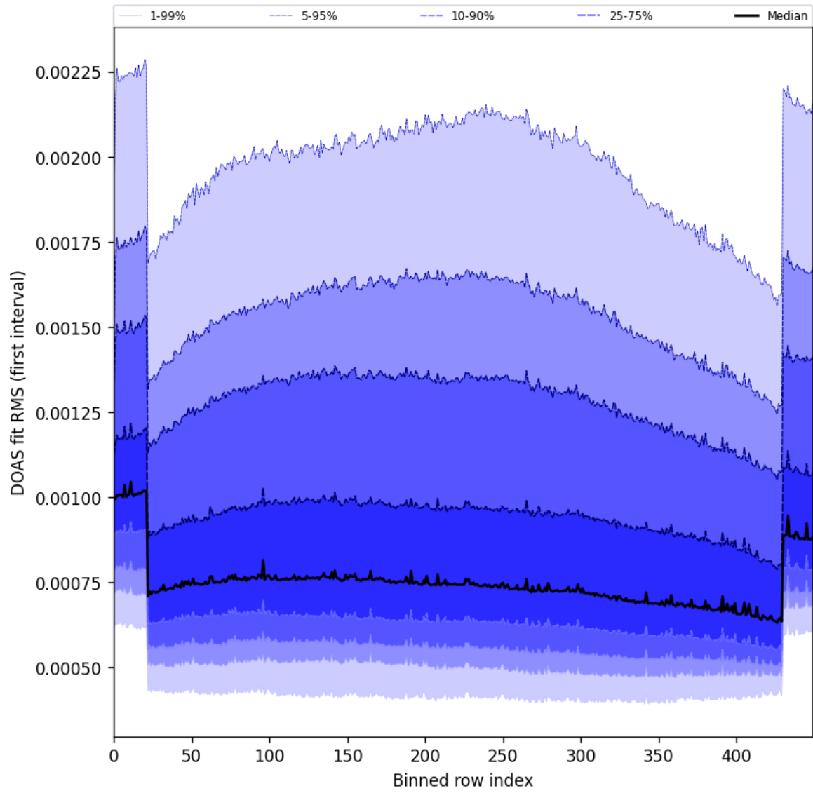
Figure 60: Along track statistics of “DOAS fit RMS (first interval)” for 2025-04-24 to 2025-04-26
