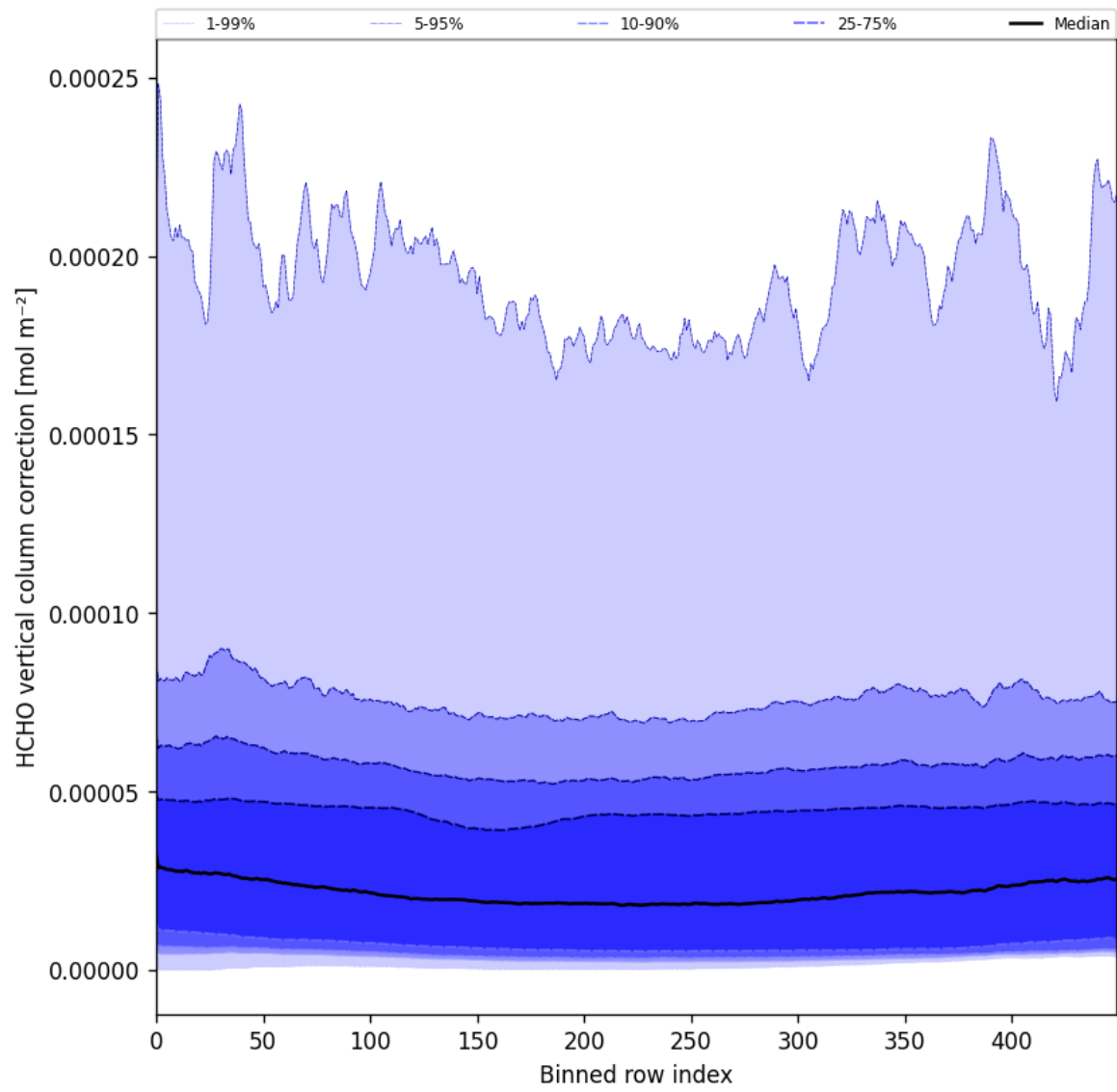
Figure 51: Along track statistics of “HCHO vertical column correction” for 2025-04-24 to 2025-04-26
