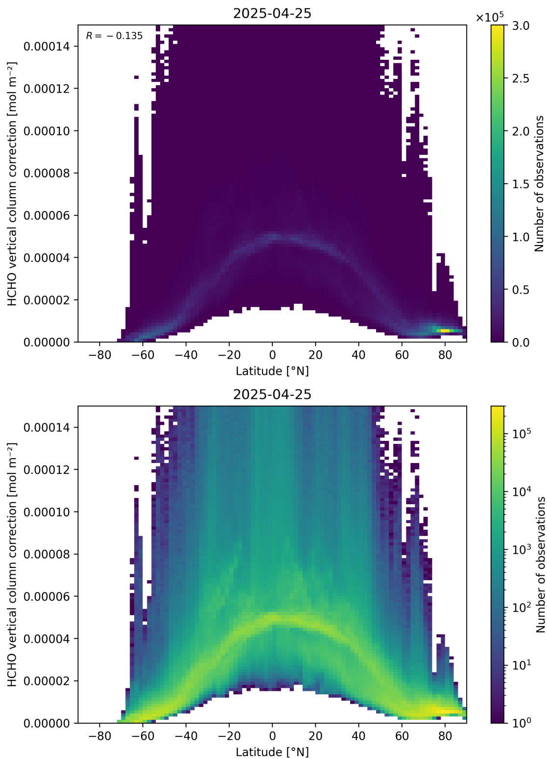
Figure 164: Scatter density plot of “Latitude” against “HCHO vertical column correction” for 2025-04-24 to 2025-04-26.
