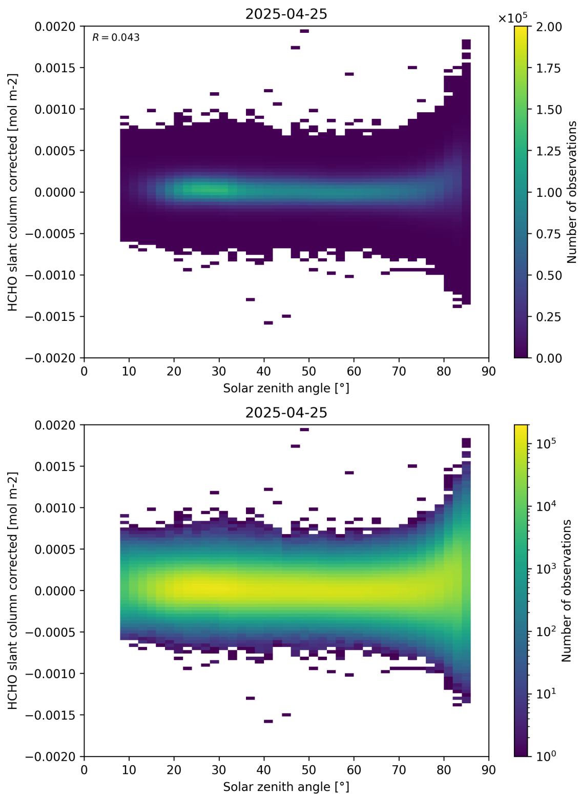
Figure 171: Scatter density plot of “Solar zenith angle” against “HCHO slant column corrected” for 2025-04-24 to 2025-04-26.
