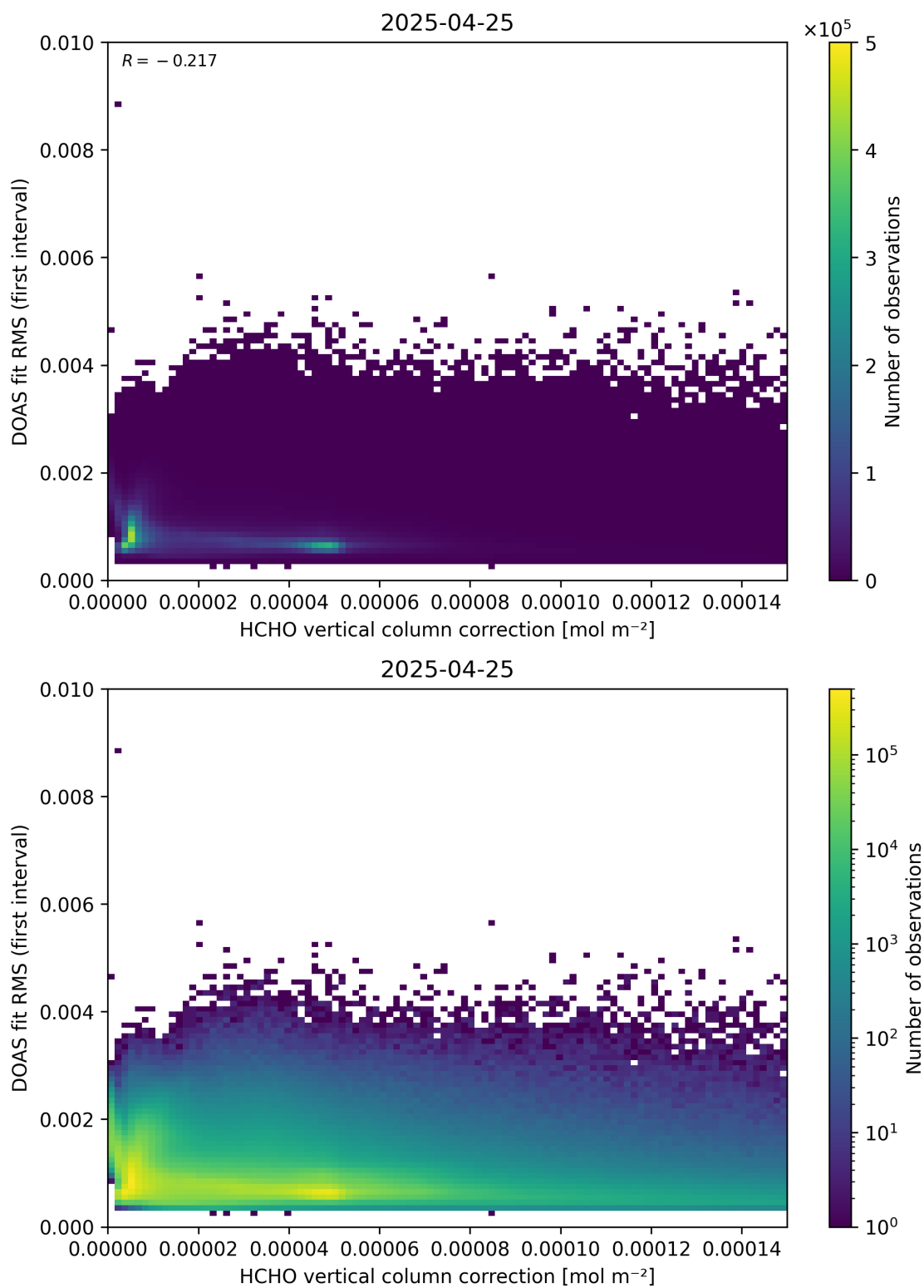
Figure 112: Scatter density plot of “HCHO vertical column correction” against “DOAS fit RMS (first interval)” for 2025-04-24 to 2025-04-26.
