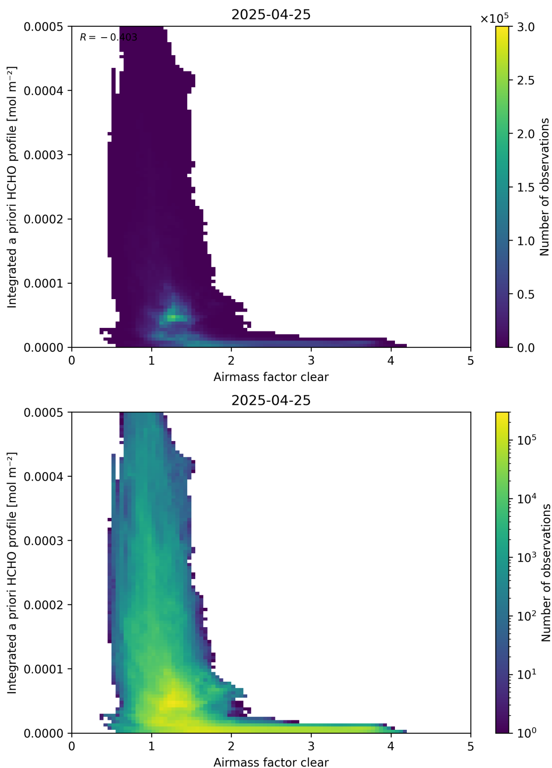
Figure 76: Scatter density plot of “Airmass factor clear” against “Integrated a priori HCHO profile” for 2025-04-24 to 2025-04-26.
