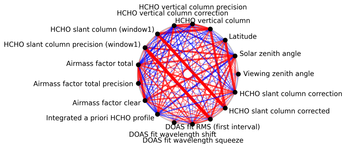
Figure 1: Map of correlation graph for 2025-04-24 to 2025-04-26.
