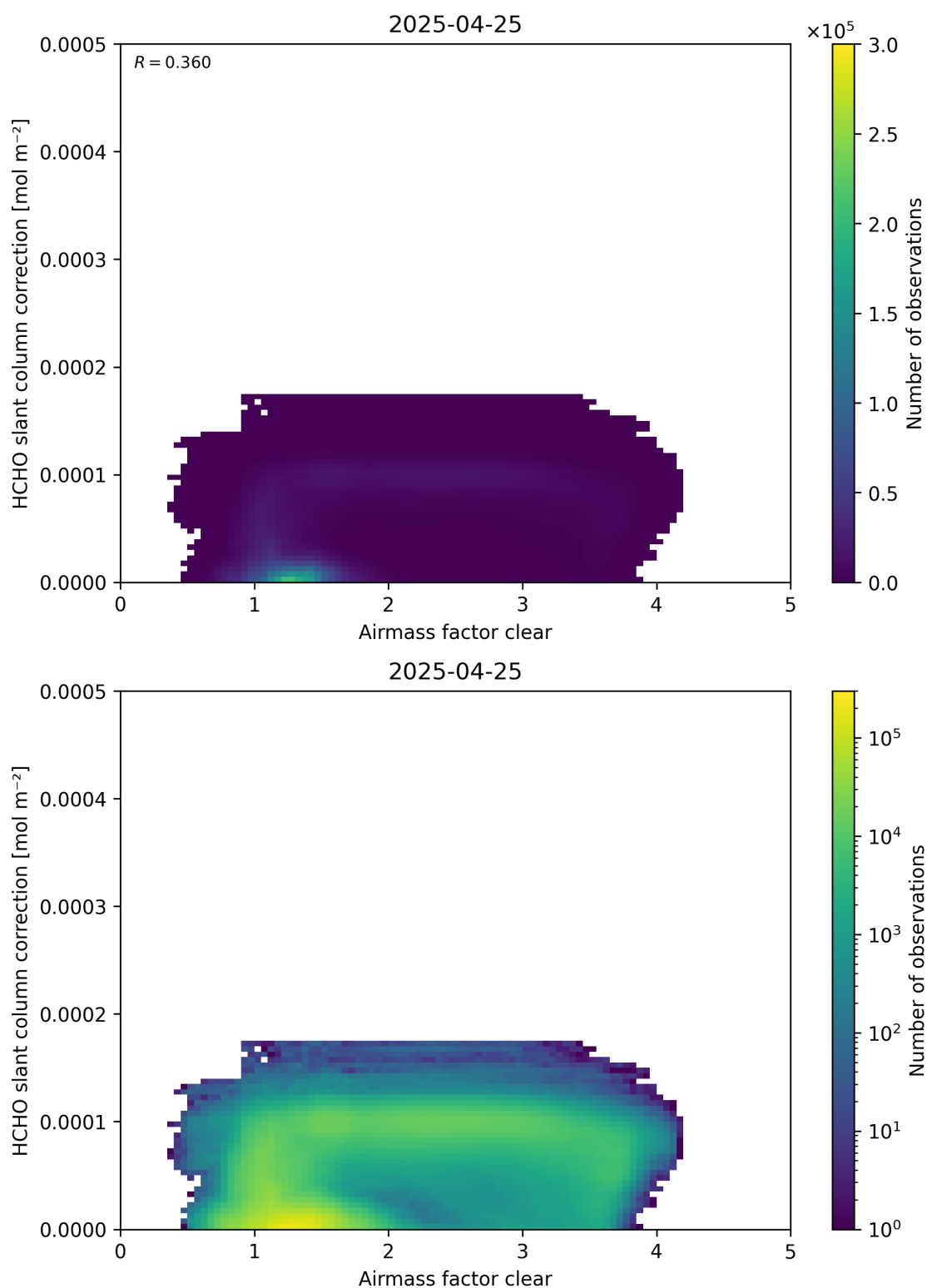
Figure 75: Scatter density plot of “Airmass factor clear” against “HCHO slant column correction” for 2025-04-24 to 2025-04-26.
