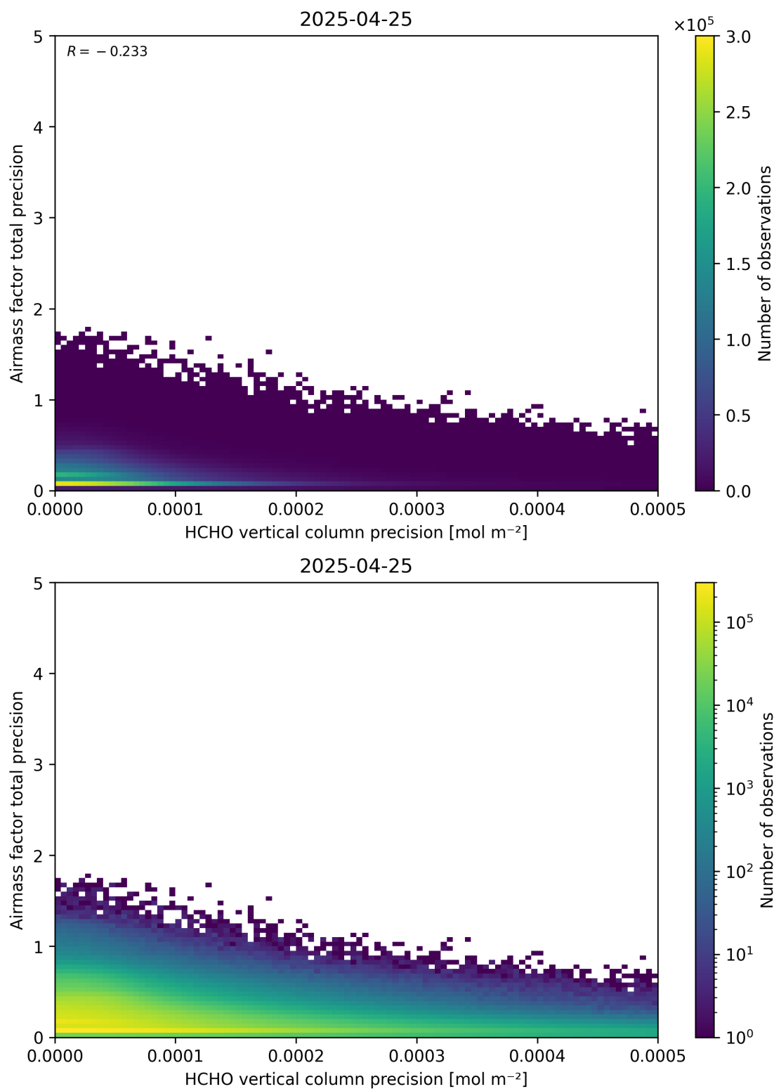
Figure 145: Scatter density plot of “HCHO vertical column precision” against “Airmass factor total precision” for 2025-04-24 to 2025-04-26.
