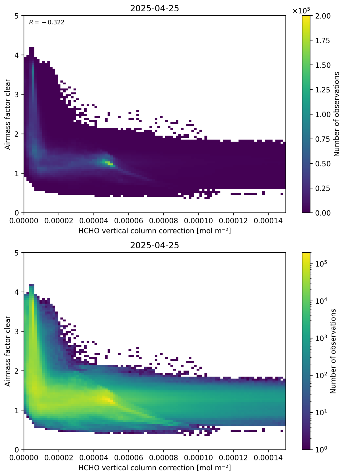
Figure 115: Scatter density plot of “HCHO vertical column correction” against “Airmass factor clear” for 2025-04-24 to 2025-04-26.
