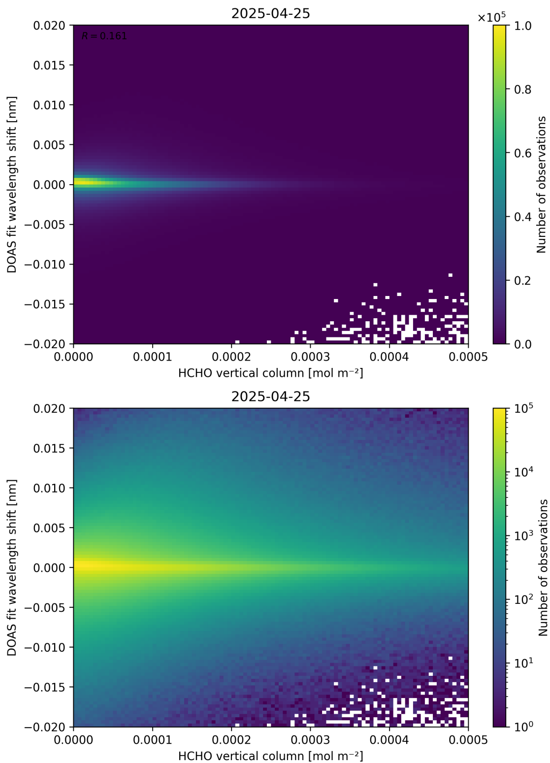
Figure 124: Scatter density plot of “HCHO vertical column” against “DOAS fit wavelength shift” for 2025-04-24 to 2025-04-26.
