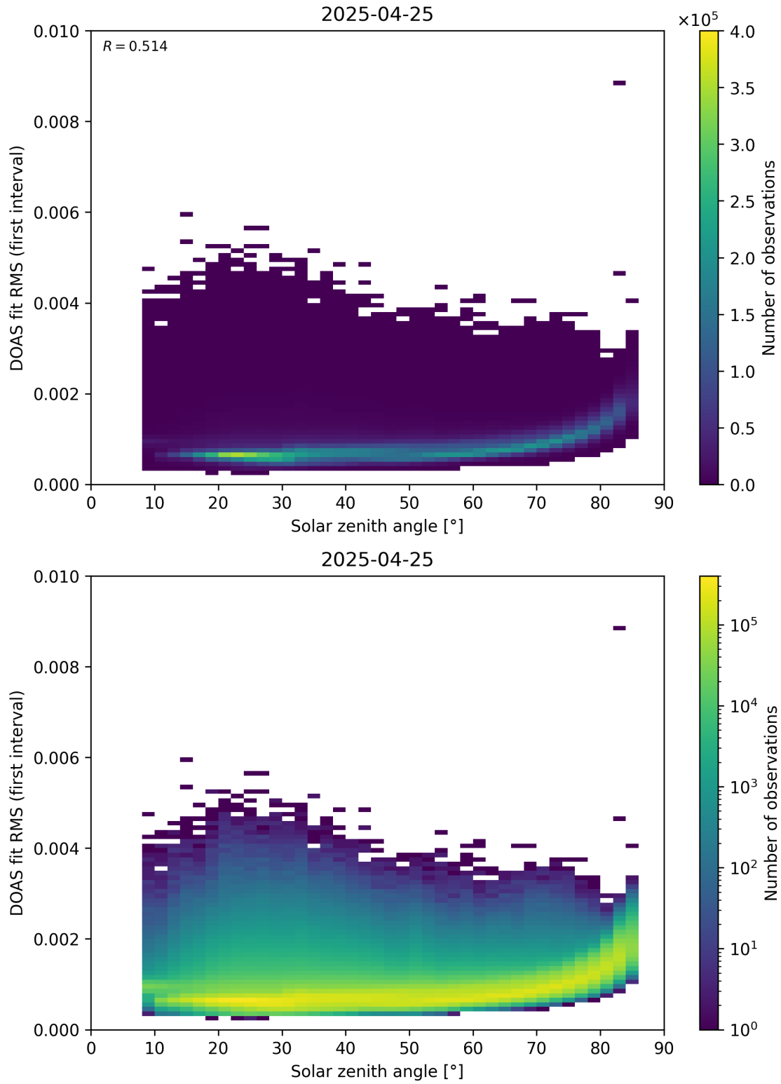
Figure 167: Scatter density plot of “Solar zenith angle” against “DOAS fit RMS (first interval)” for 2025-04-24 to 2025-04-26.
