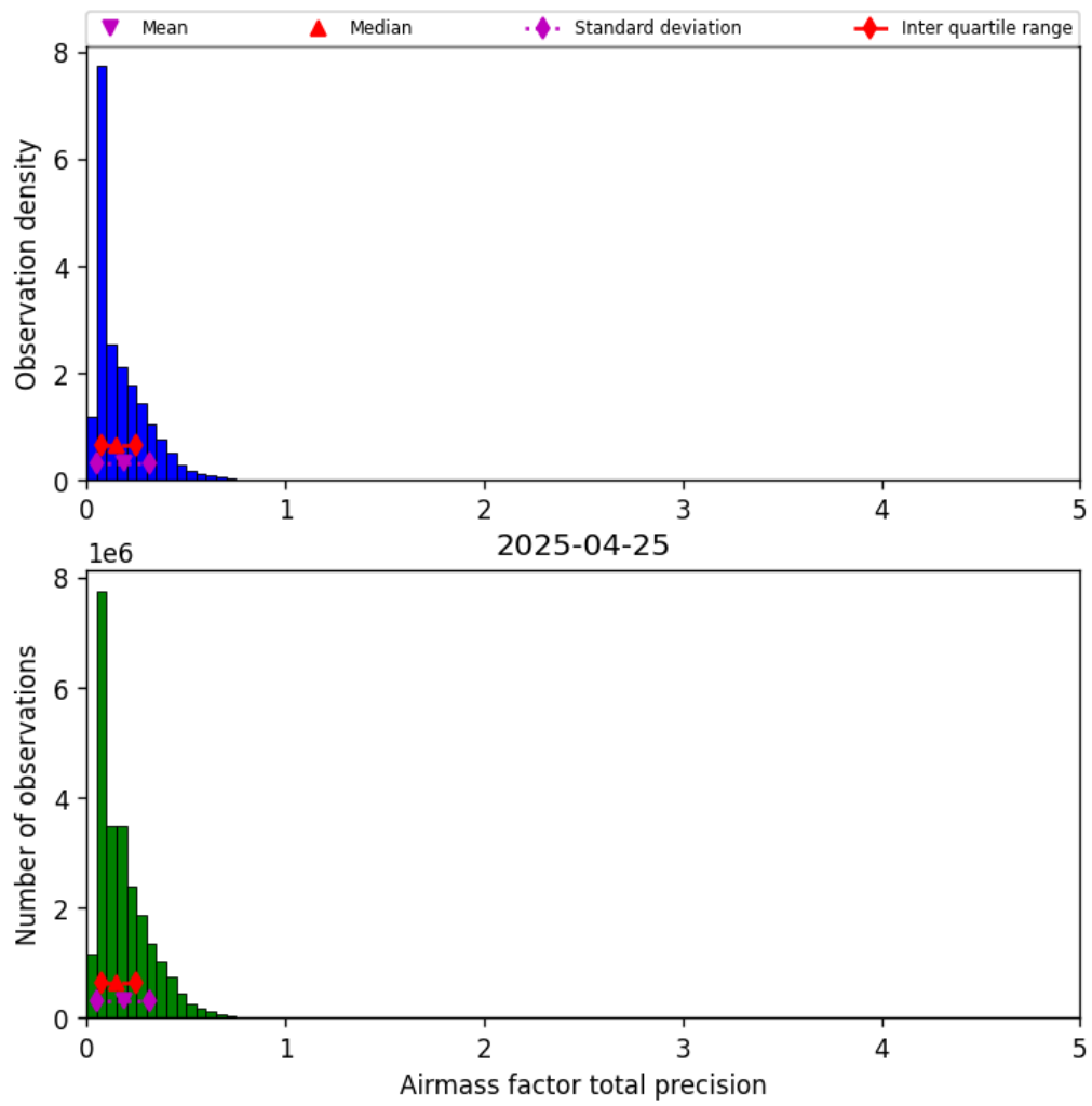
Figure 41: Histogram of “Airmass factor total precision” for 2025-04-24 to 2025-04-26
