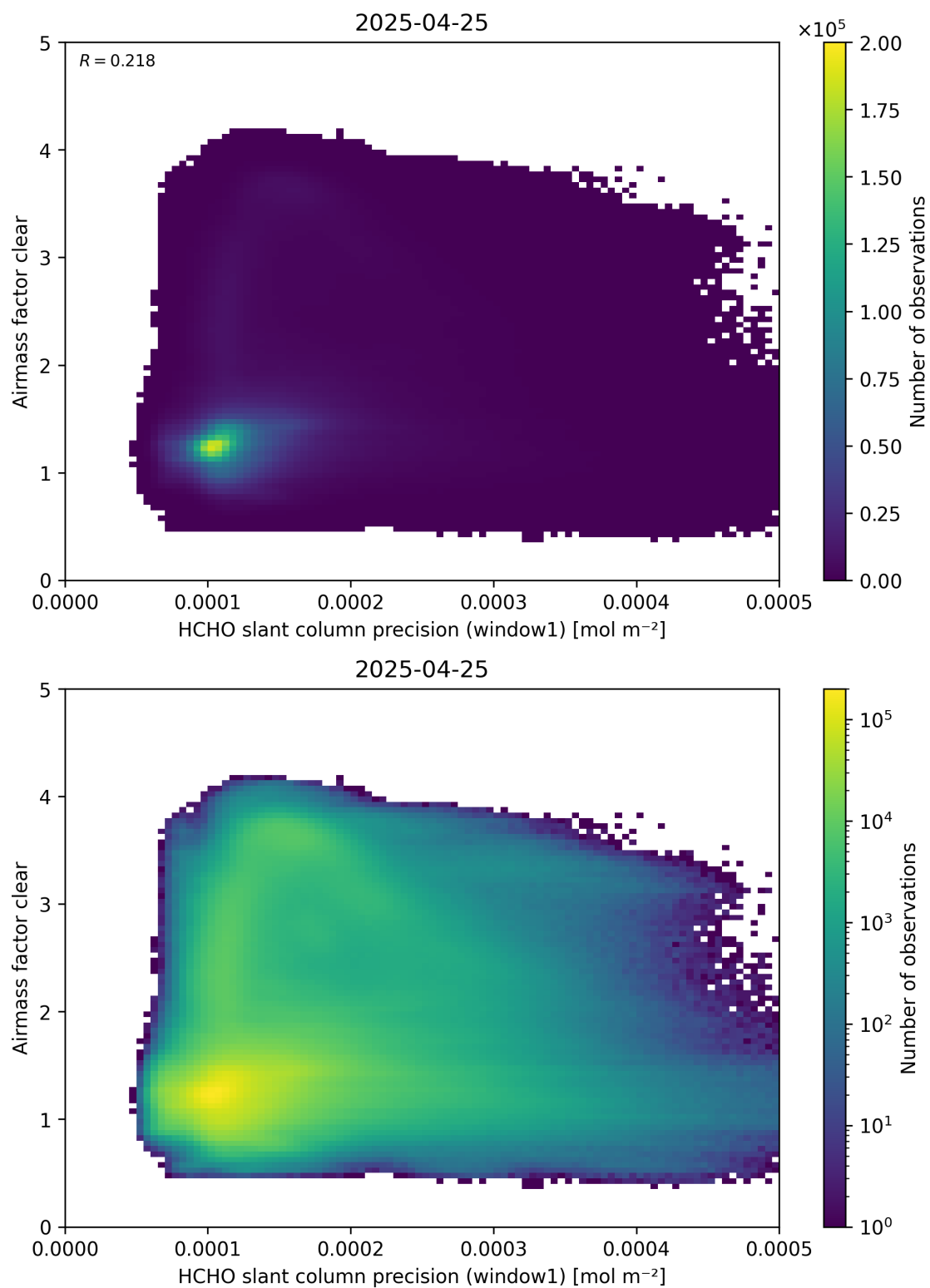
Figure 91: Scatter density plot of “HCHO slant column precision (window1)” against “Airmass factor clear” for 2025-04-24 to 2025-04-26.
