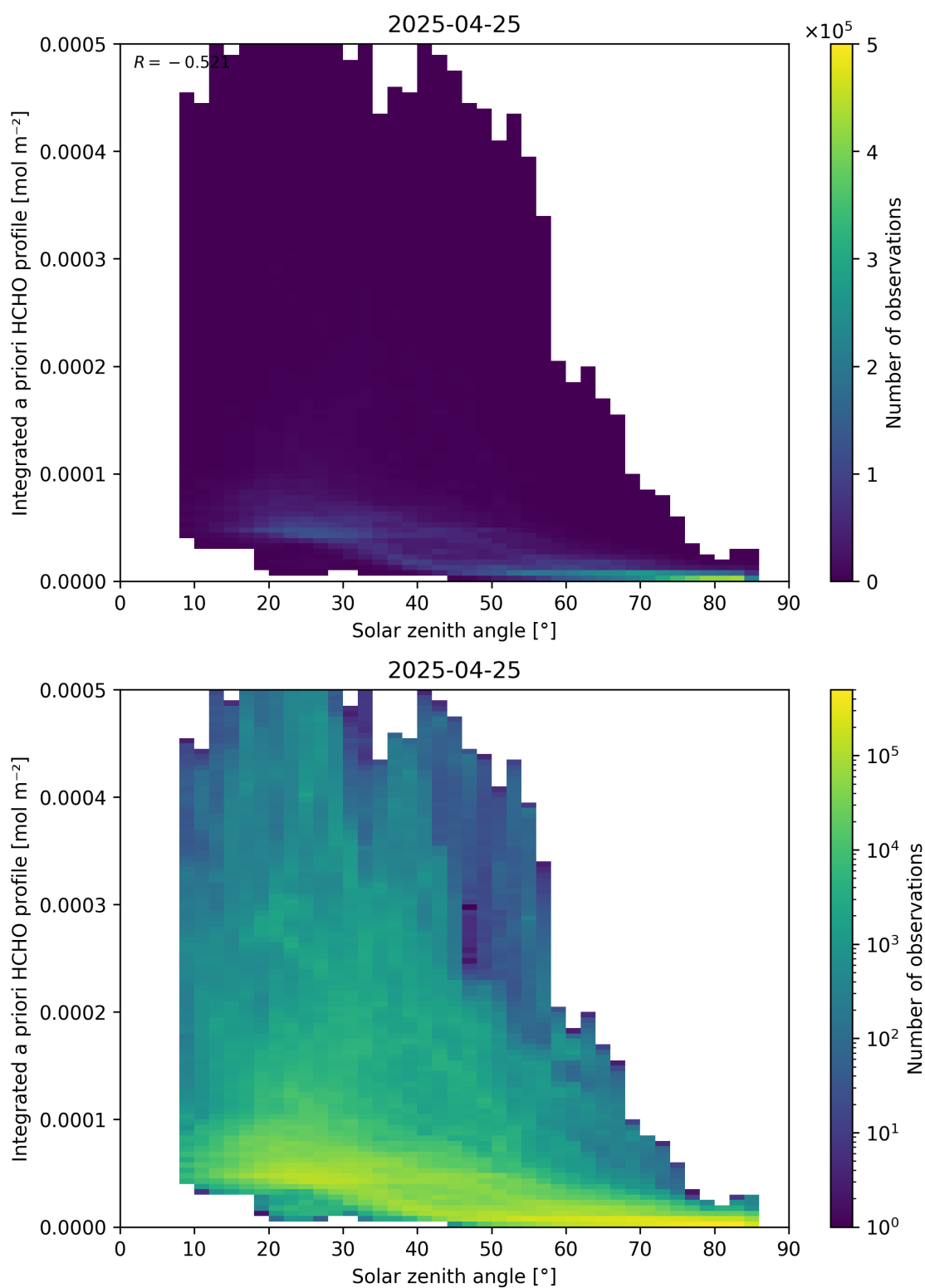
Figure 180: Scatter density plot of “Solar zenith angle” against “Integrated a priori HCHO profile” for 2025-04-24 to 2025-04-26.
