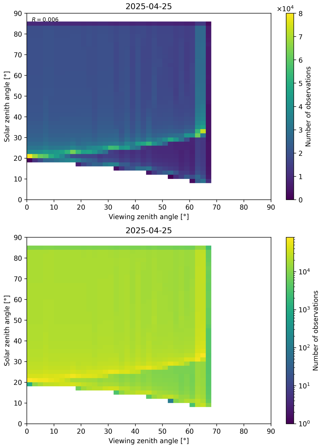
Figure 197: Scatter density plot of “Viewing zenith angle” against “Solar zenith angle” for 2025-04-24 to 2025-04-26.
