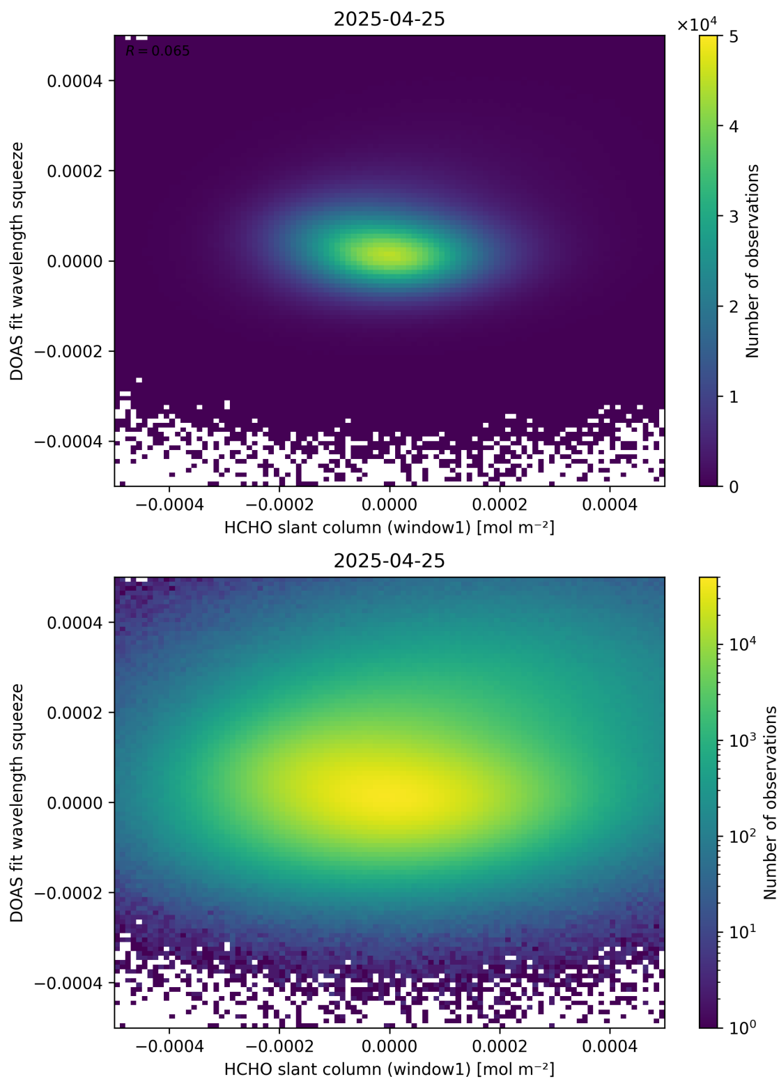
Figure 80: Scatter density plot of “HCHO slant column (window1)” against “DOAS fit wavelength squeeze” for 2025-04-24 to 2025-04-26.
