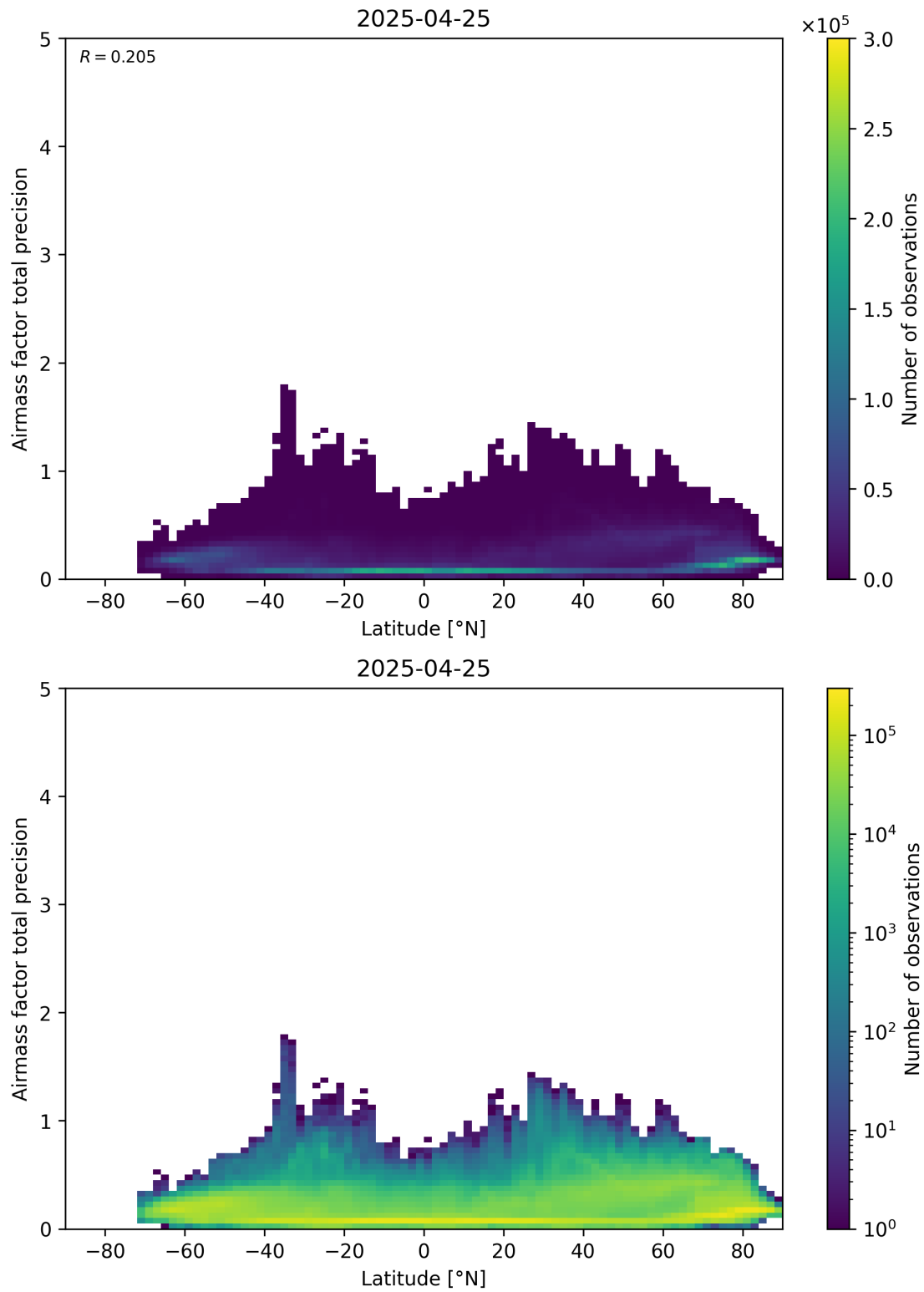
Figure 162: Scatter density plot of “Latitude” against “Airmass factor total precision” for 2025-04-24 to 2025-04-26.
