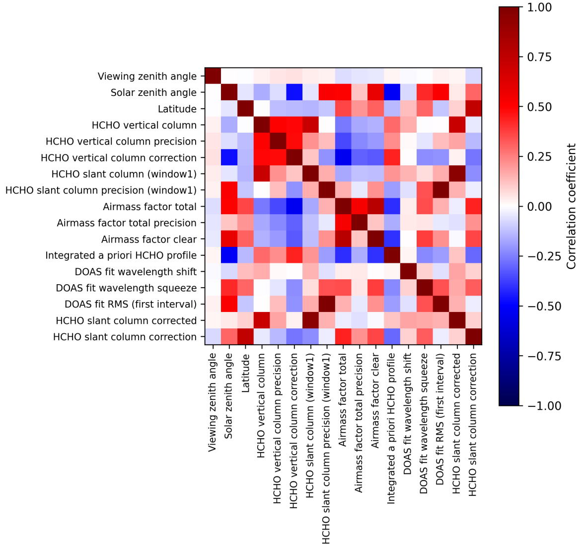
Figure 2: Map of correlation matrix for 2025-04-24 to 2025-04-26.
