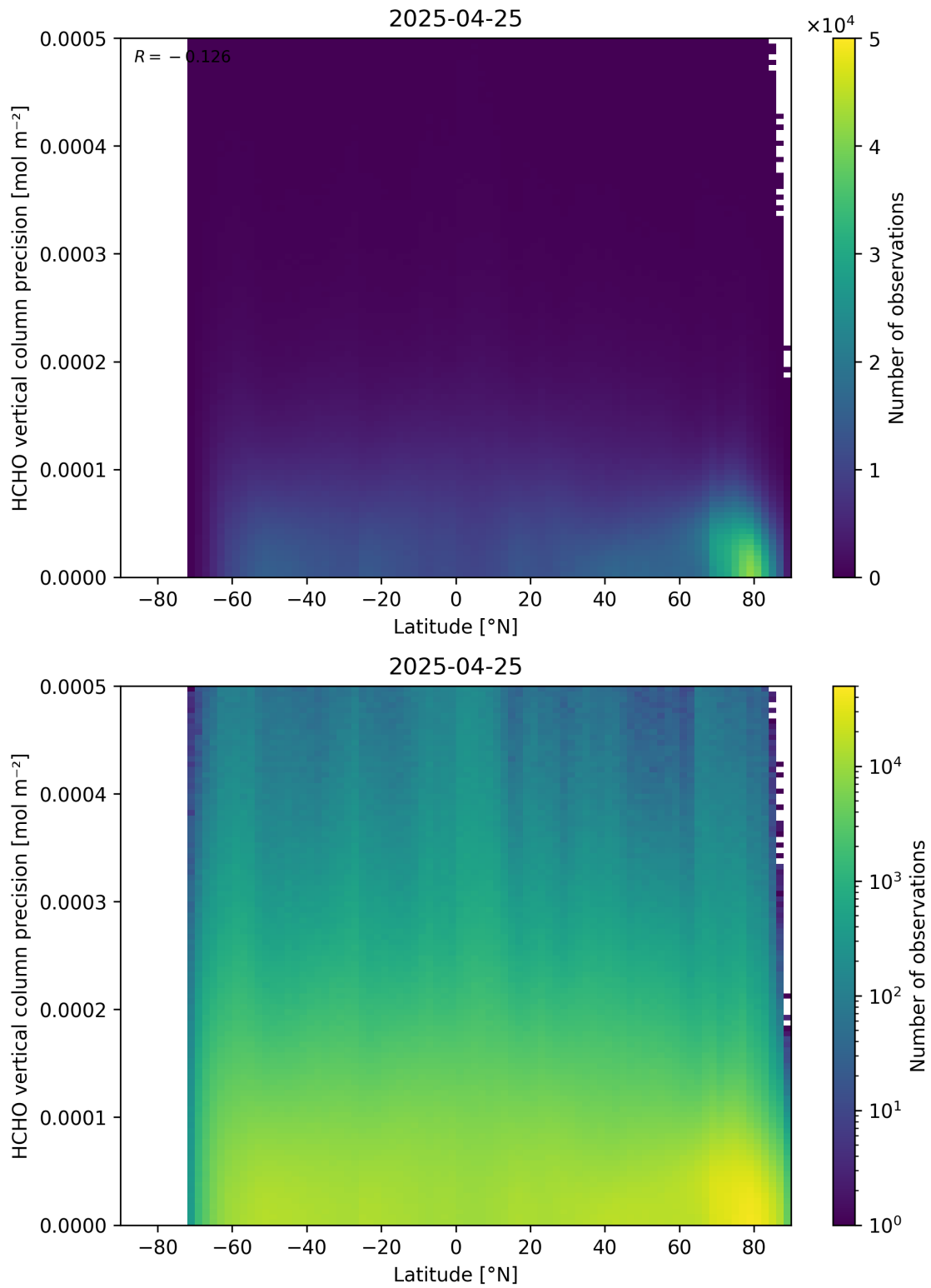
Figure 165: Scatter density plot of “Latitude” against “HCHO vertical column precision” for 2025-04-24 to 2025-04-26.
