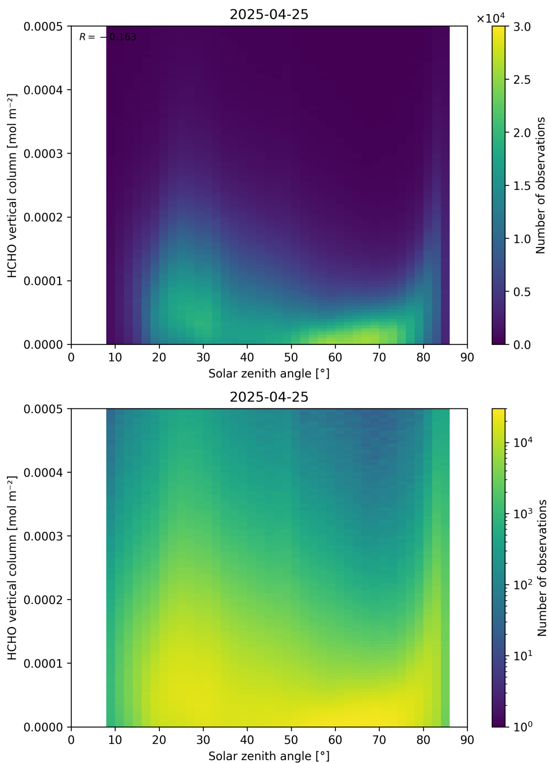
Figure 177: Scatter density plot of “Solar zenith angle” against “HCHO vertical column” for 2025-04-24 to 2025-04-26.
