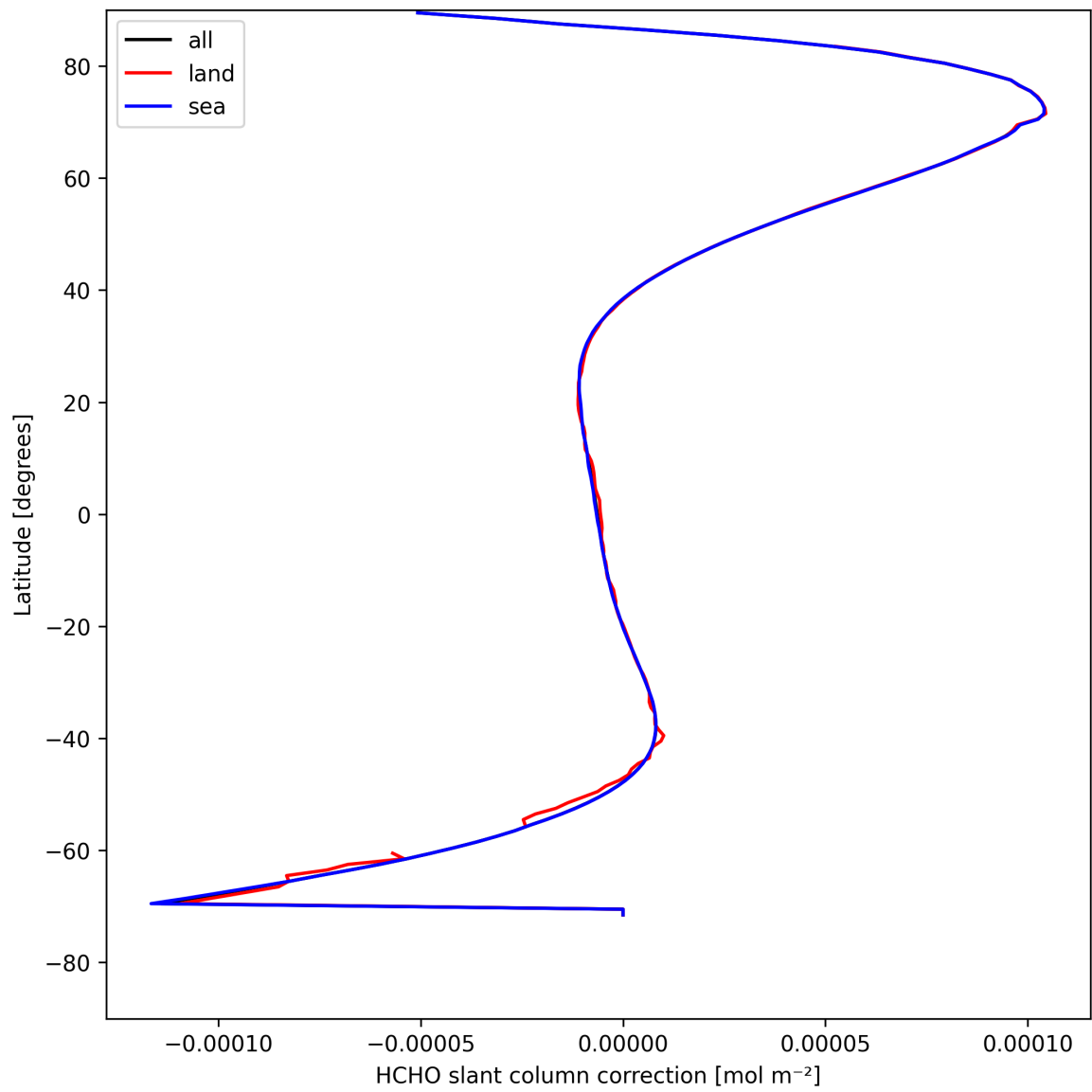
Figure 33: Zonal average of “HCHO slant column correction” for 2025-04-24 to 2025-04-26.
