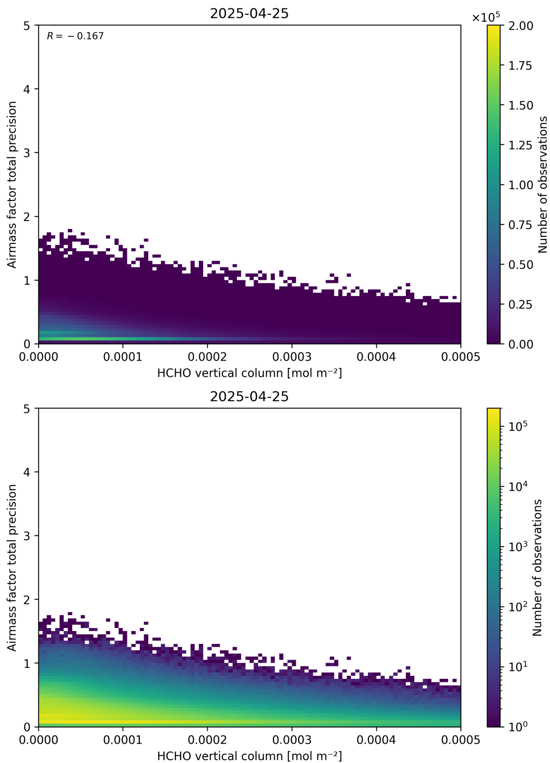
Figure 132: Scatter density plot of “HCHO vertical column” against “Airmass factor total precision” for 2025-04-24 to 2025-04-26.
