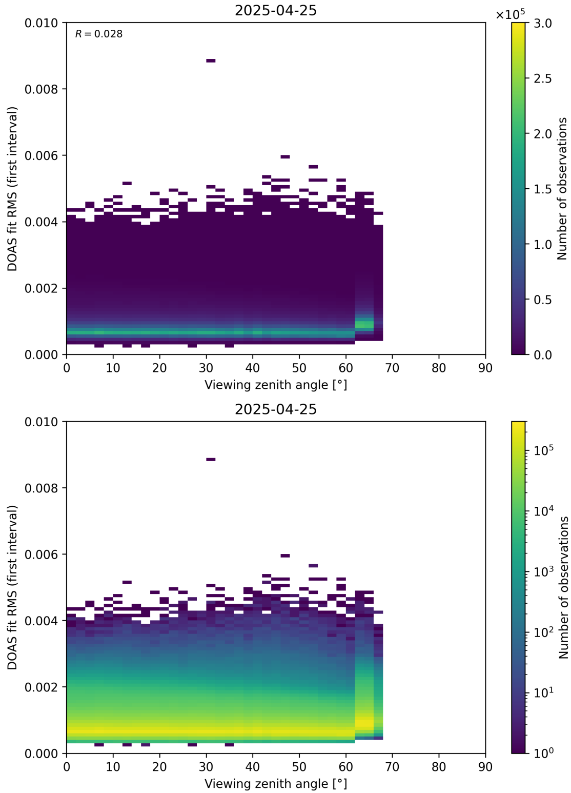
Figure 182: Scatter density plot of “Viewing zenith angle” against “DOAS fit RMS (first interval)” for 2025-04-24 to 2025-04-26.
