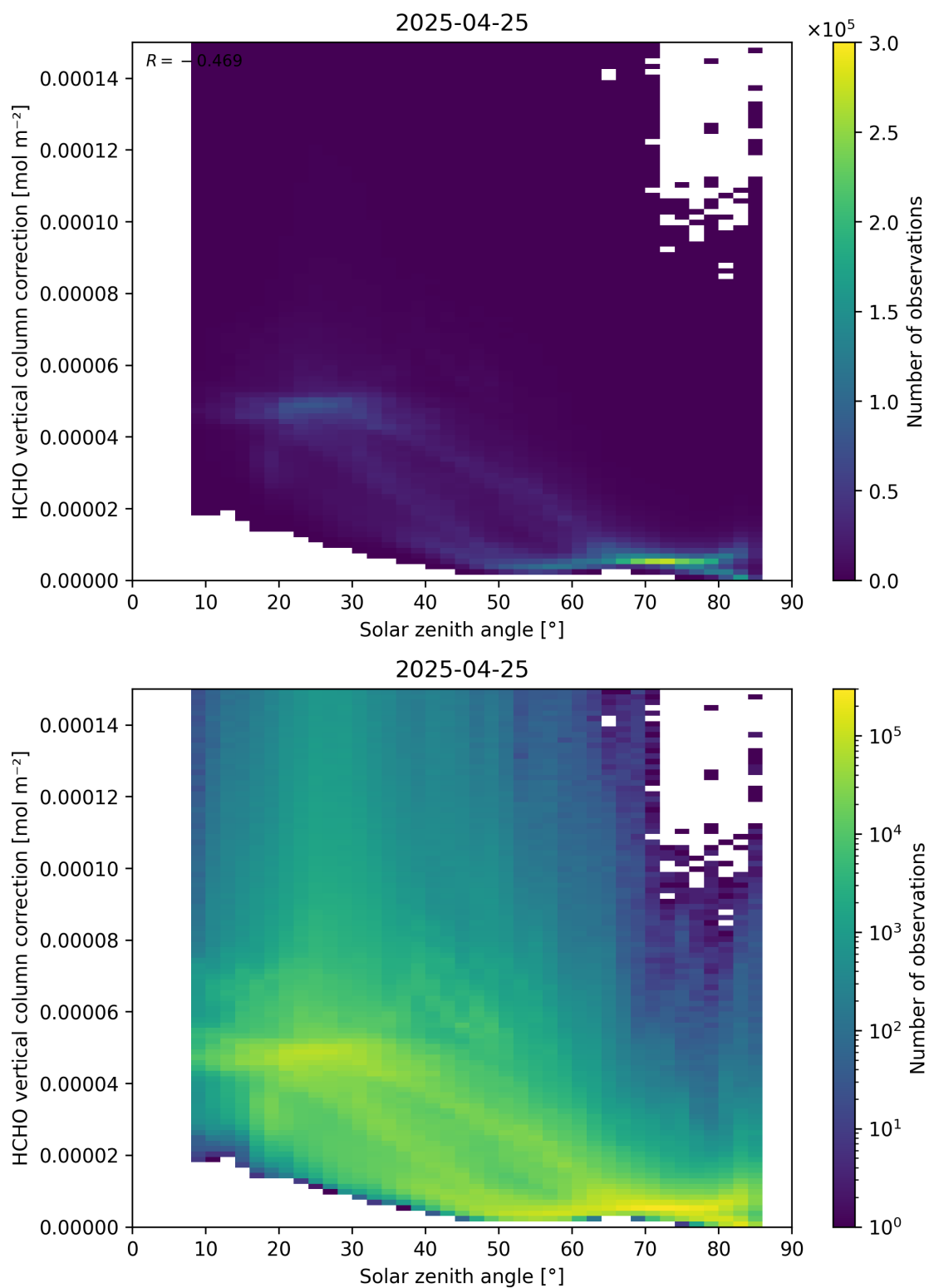
Figure 178: Scatter density plot of “Solar zenith angle” against “HCHO vertical column correction” for 2025-04-24 to 2025-04-26.
