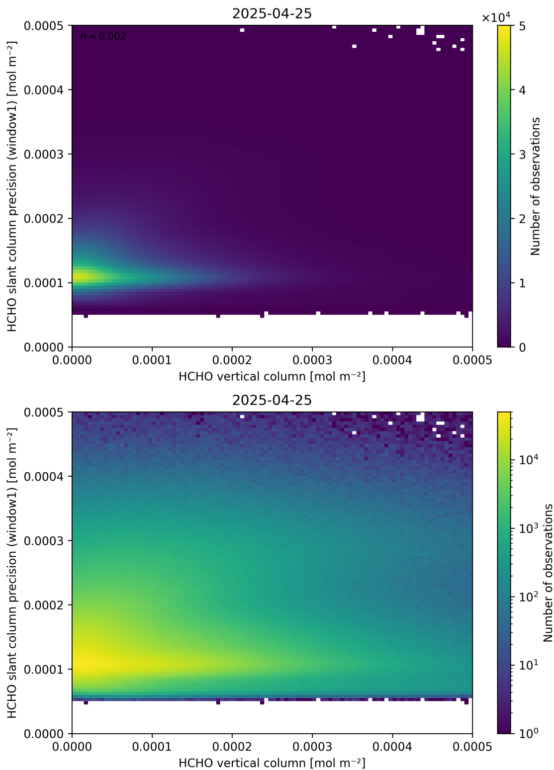
Figure 130: Scatter density plot of “HCHO vertical column” against “HCHO slant column precision (window1)” for 2025-04-24 to 2025-04-26.
