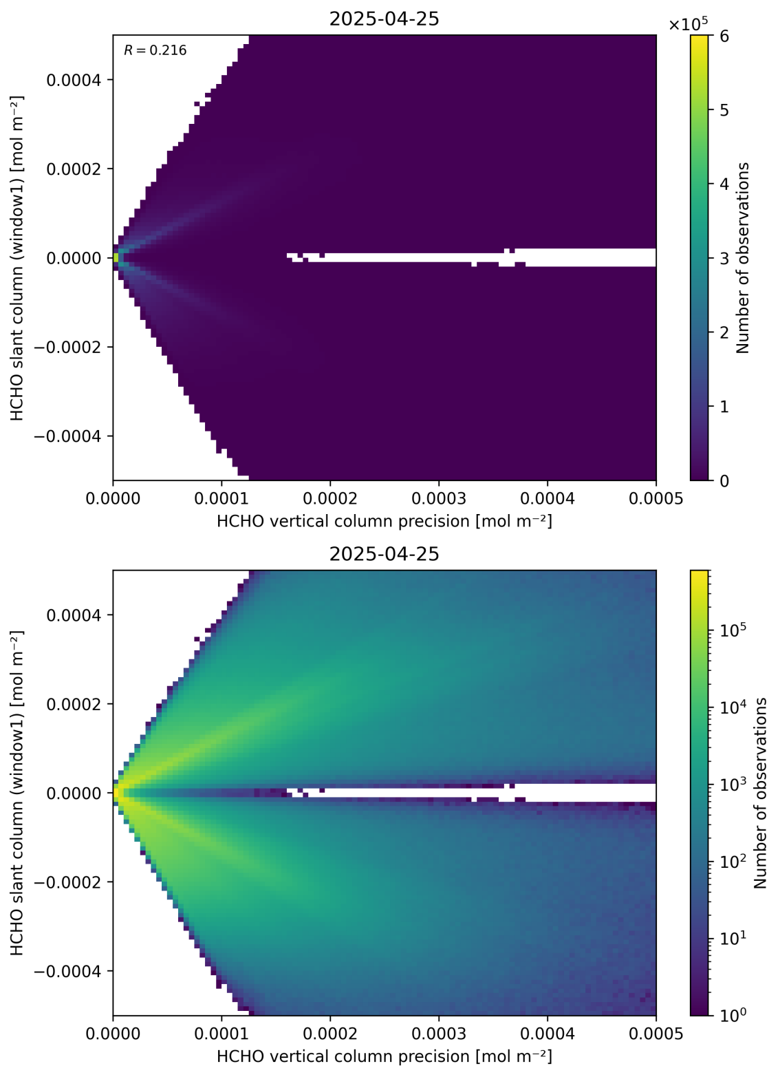
Figure 142: Scatter density plot of “HCHO vertical column precision” against “HCHO slant column (window1)” for 2025-04-24 to 2025-04-26.
