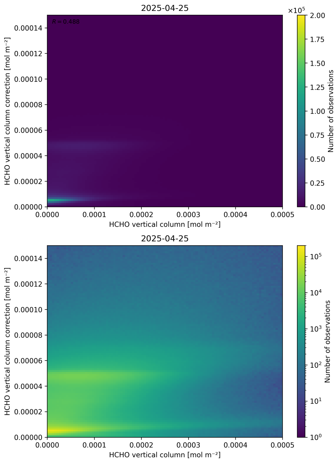
Figure 133: Scatter density plot of “HCHO vertical column” against “HCHO vertical column correction” for 2025-04-24 to 2025-04-26.
