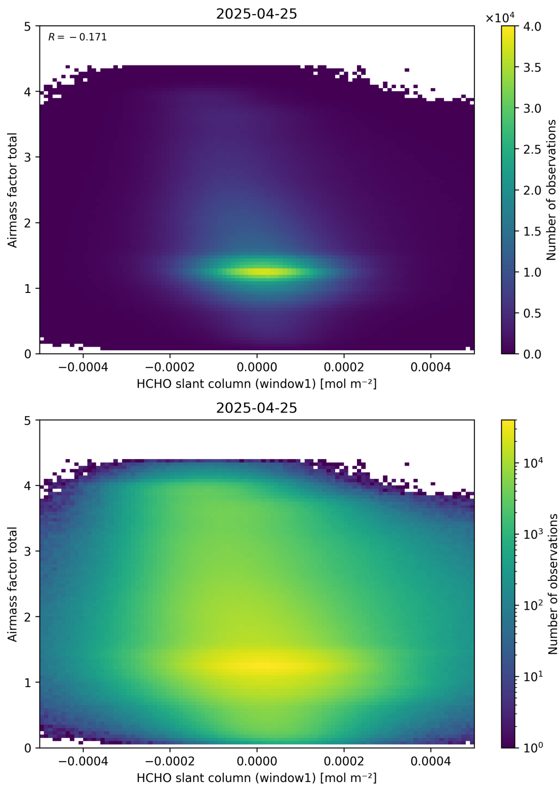
Figure 85: Scatter density plot of “HCHO slant column (window1)” against “Airmass factor total” for 2025-04-24 to 2025-04-26.
