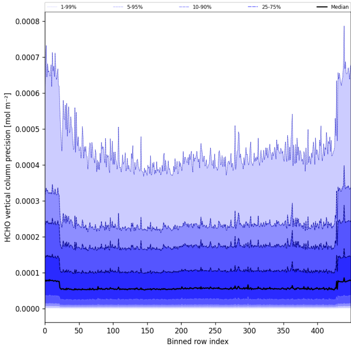
Figure 50: Along track statistics of “HCHO vertical column precision” for 2025-04-24 to 2025-04-26
