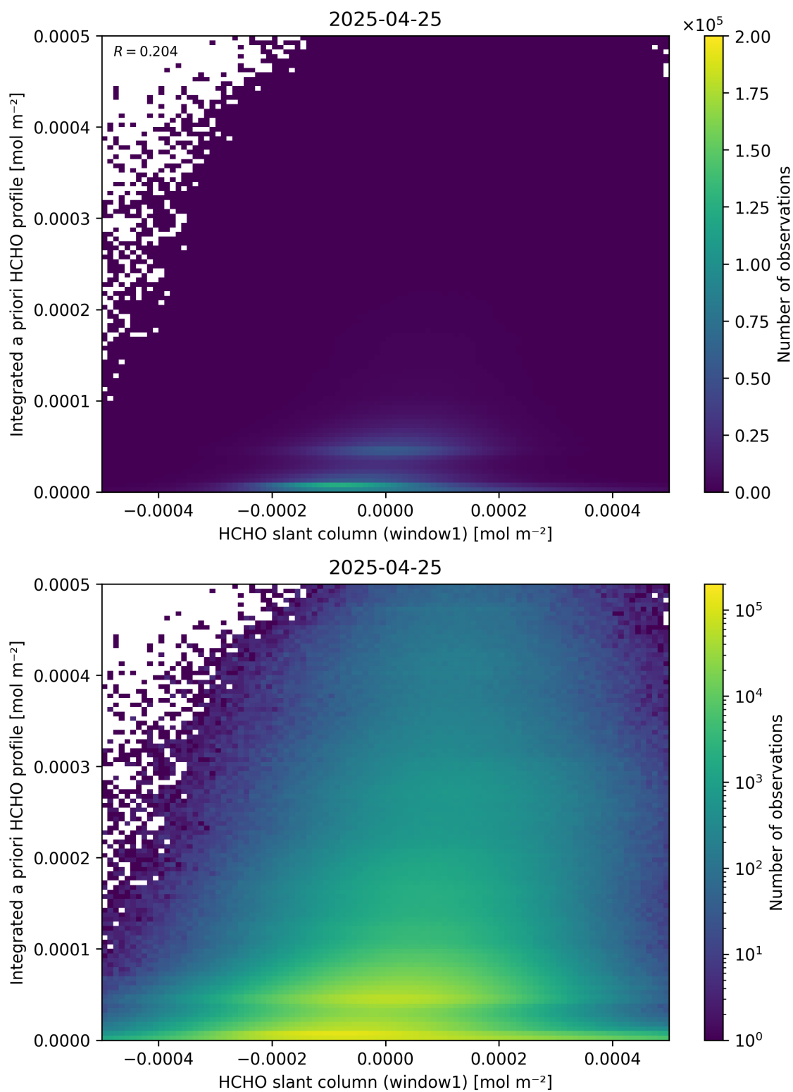
Figure 87: Scatter density plot of “HCHO slant column (window1)” against “Integrated a priori HCHO profile” for 2025-04-24 to 2025-04-26.
