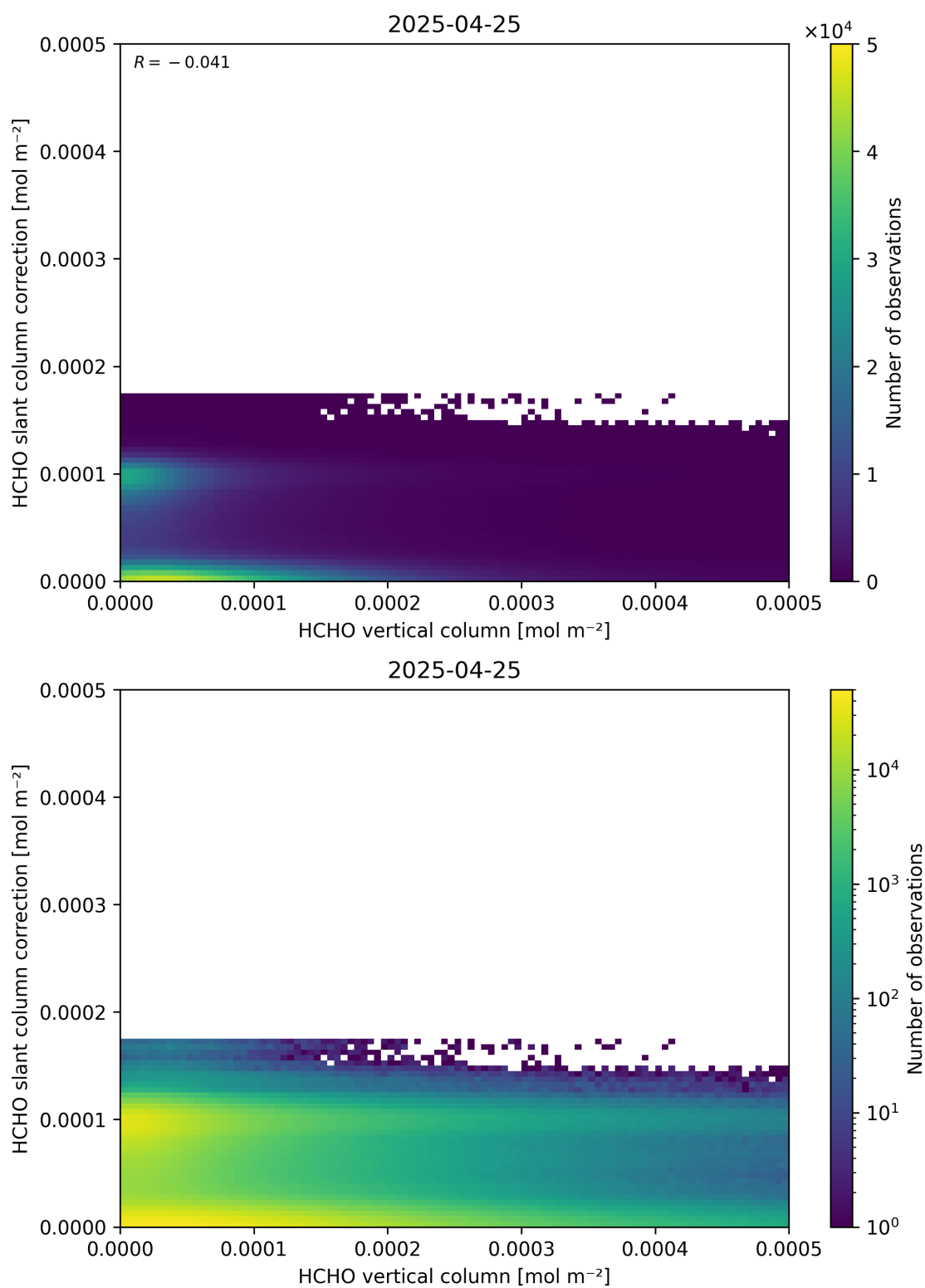
Figure 128: Scatter density plot of “HCHO vertical column” against “HCHO slant column correction” for 2025-04-24 to 2025-04-26.
