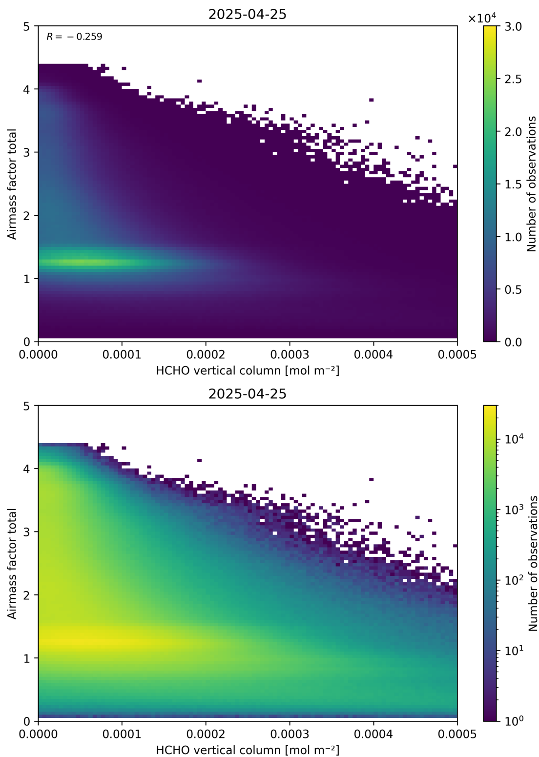
Figure 131: Scatter density plot of “HCHO vertical column” against “Airmass factor total” for 2025-04-24 to 2025-04-26.
