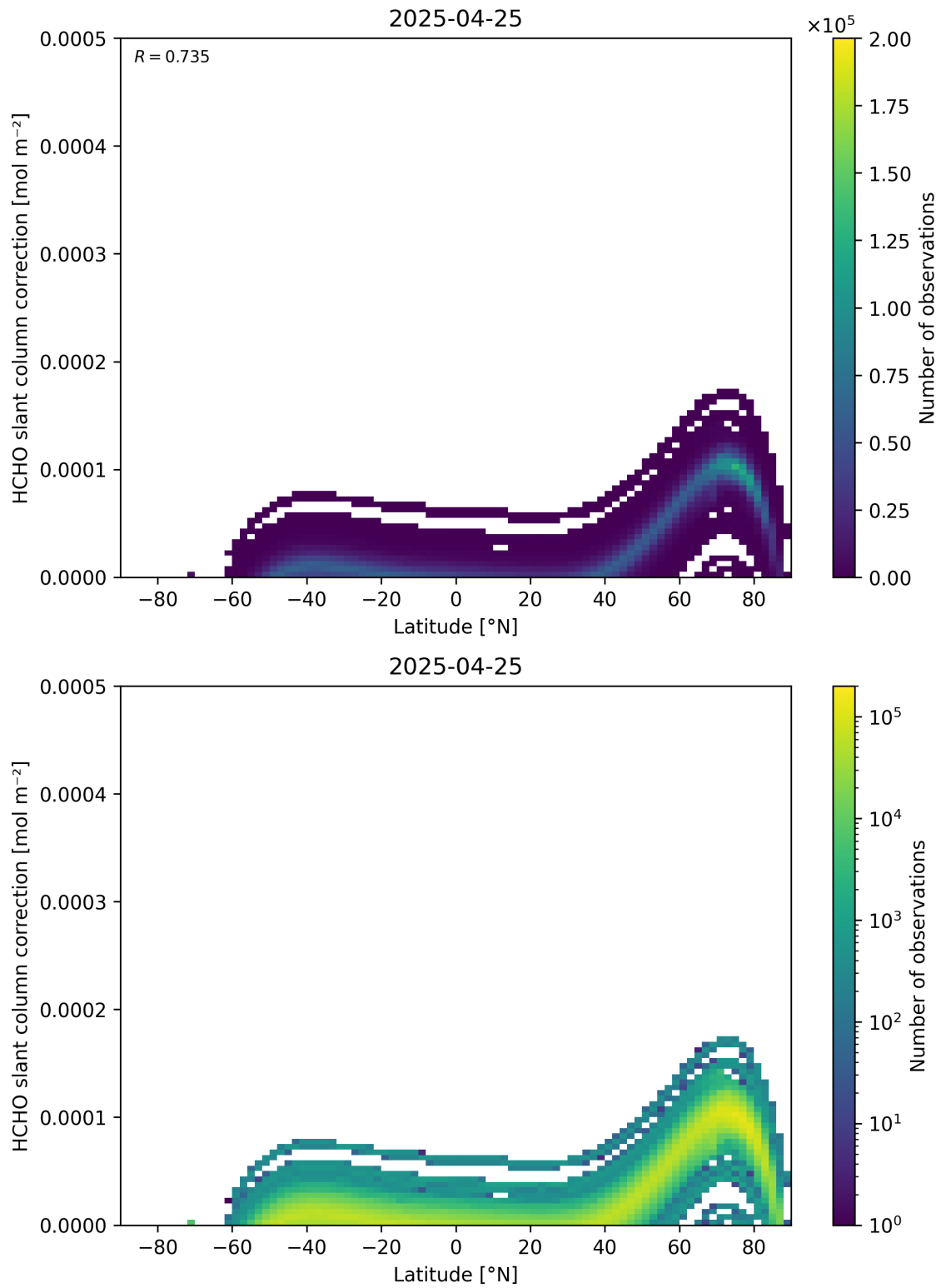
Figure 158: Scatter density plot of “Latitude” against “HCHO slant column correction” for 2025-04-24 to 2025-04-26.
