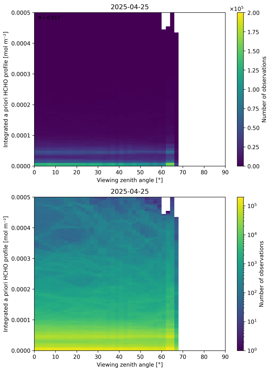
Figure 195: Scatter density plot of “Viewing zenith angle” against “Integrated a priori HCHO profile” for 2025-04-24 to 2025-04-26.
