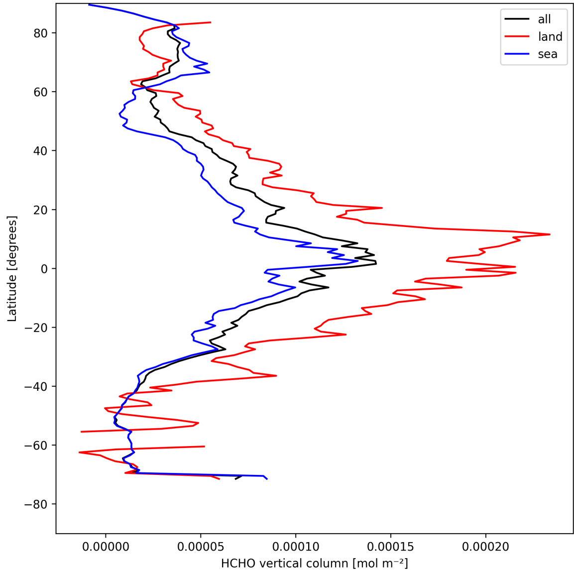
Figure 21: Zonal average of “HCHO vertical column” for 2025-04-24 to 2025-04-26.
