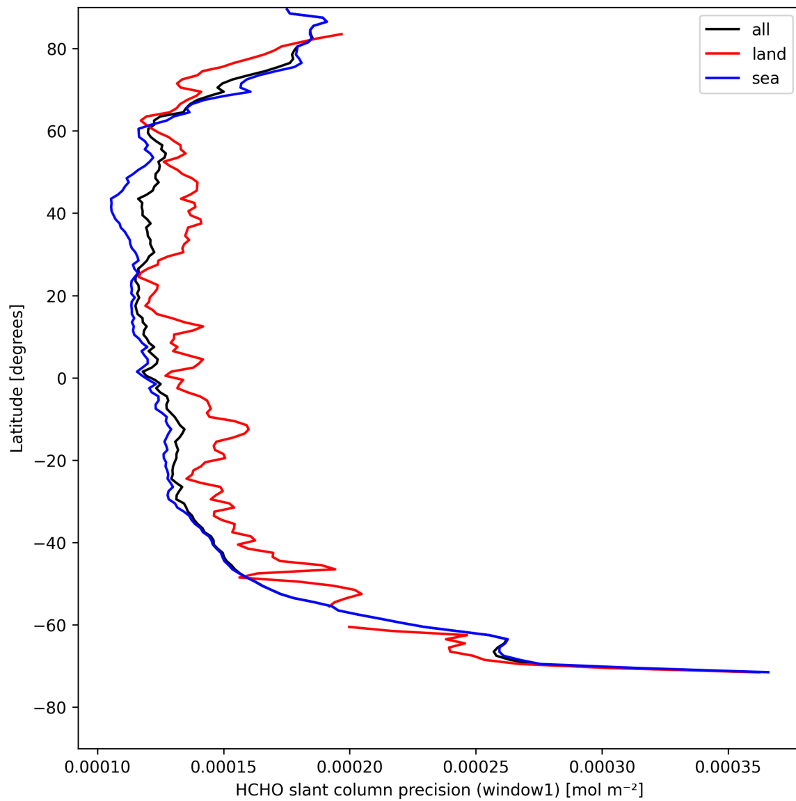
Figure 25: Zonal average of “HCHO slant column precision (window1)” for 2025-04-24 to 2025-04-26.
