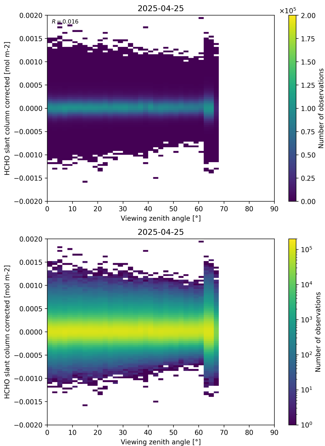
Figure 186: Scatter density plot of “Viewing zenith angle” against “HCHO slant column corrected” for 2025-04-24 to 2025-04-26.
