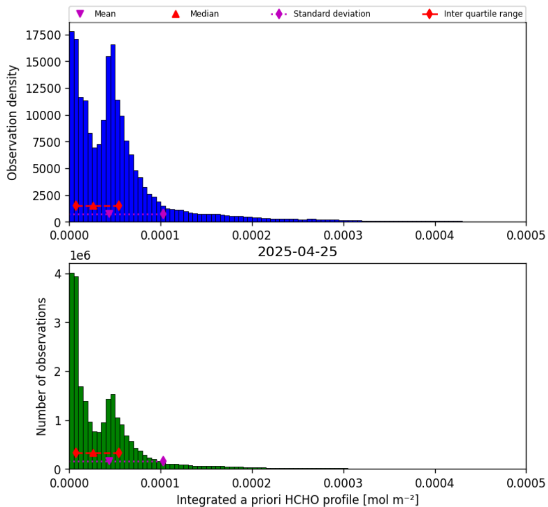
Figure 43: Histogram of “Integrated a priori HCHO profile” for 2025-04-24 to 2025-04-26
