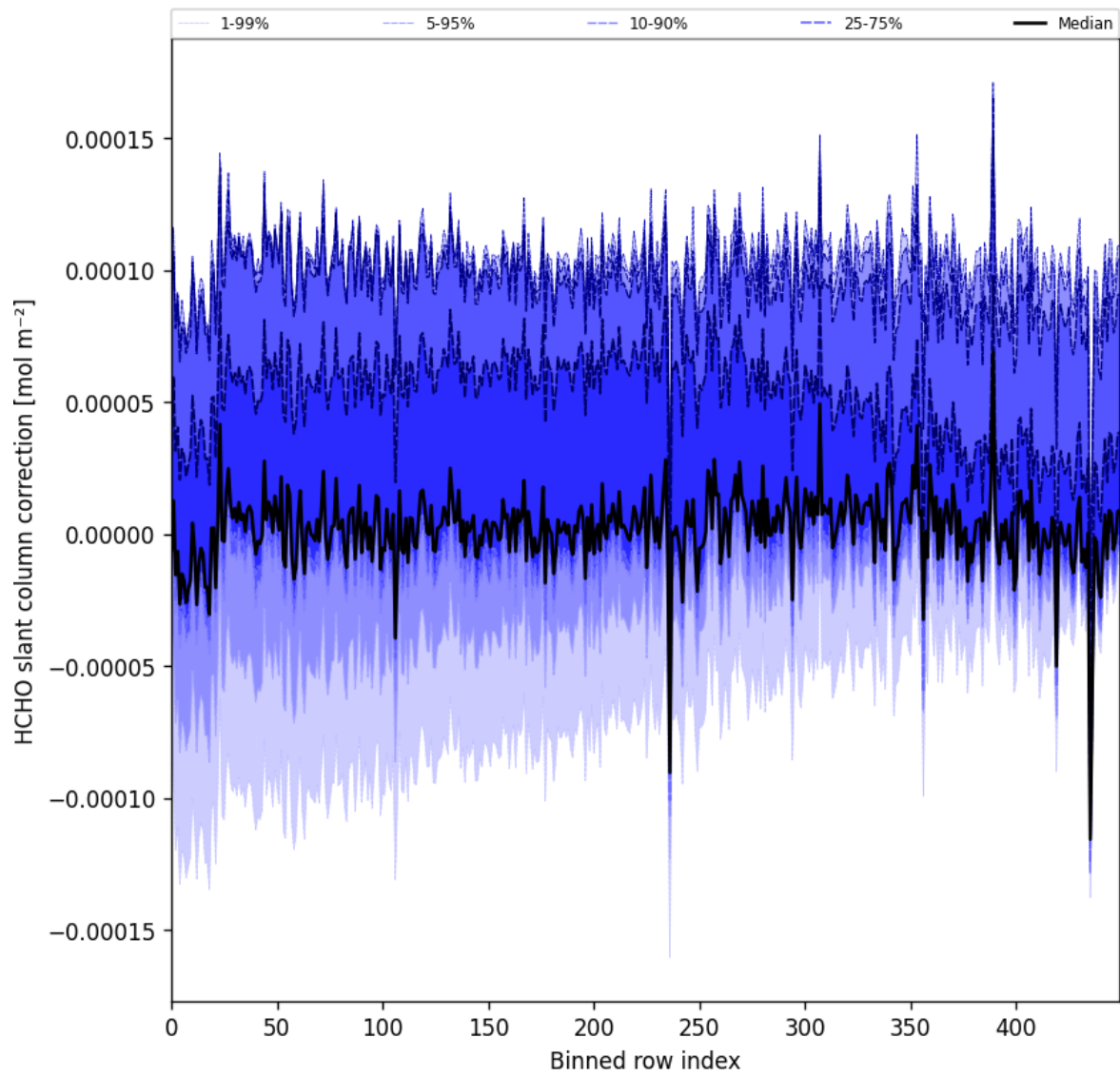
Figure 61: Along track statistics of “HCHO slant column correction” for 2025-04-24 to 2025-04-26
