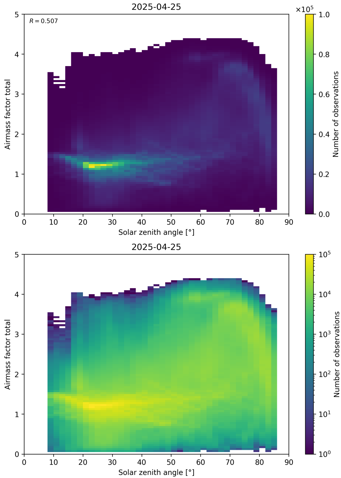
Figure 175: Scatter density plot of “Solar zenith angle” against “Airmass factor total” for 2025-04-24 to 2025-04-26.
