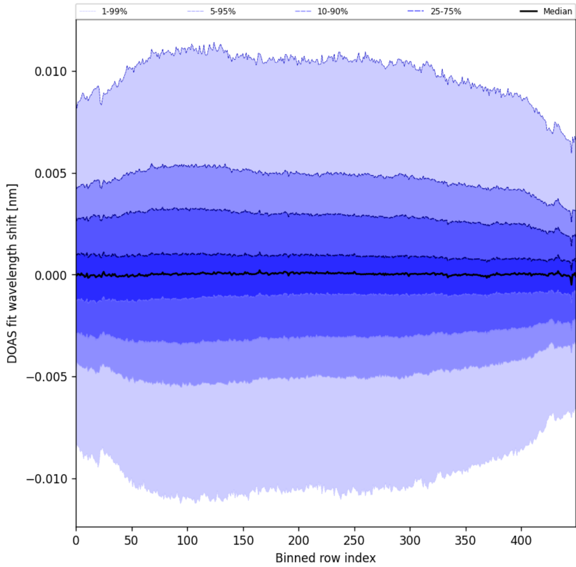
Figure 58: Along track statistics of “DOAS fit wavelength shift” for 2025-04-24 to 2025-04-26
