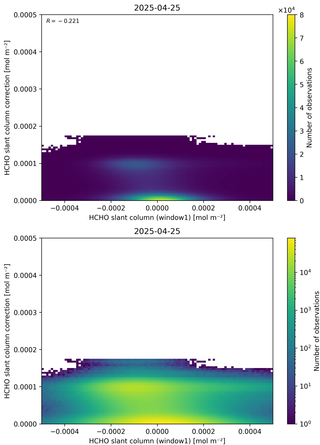
Figure 83: Scatter density plot of “HCHO slant column (window1)” against “HCHO slant column correction” for 2025-04-24 to 2025-04-26.
