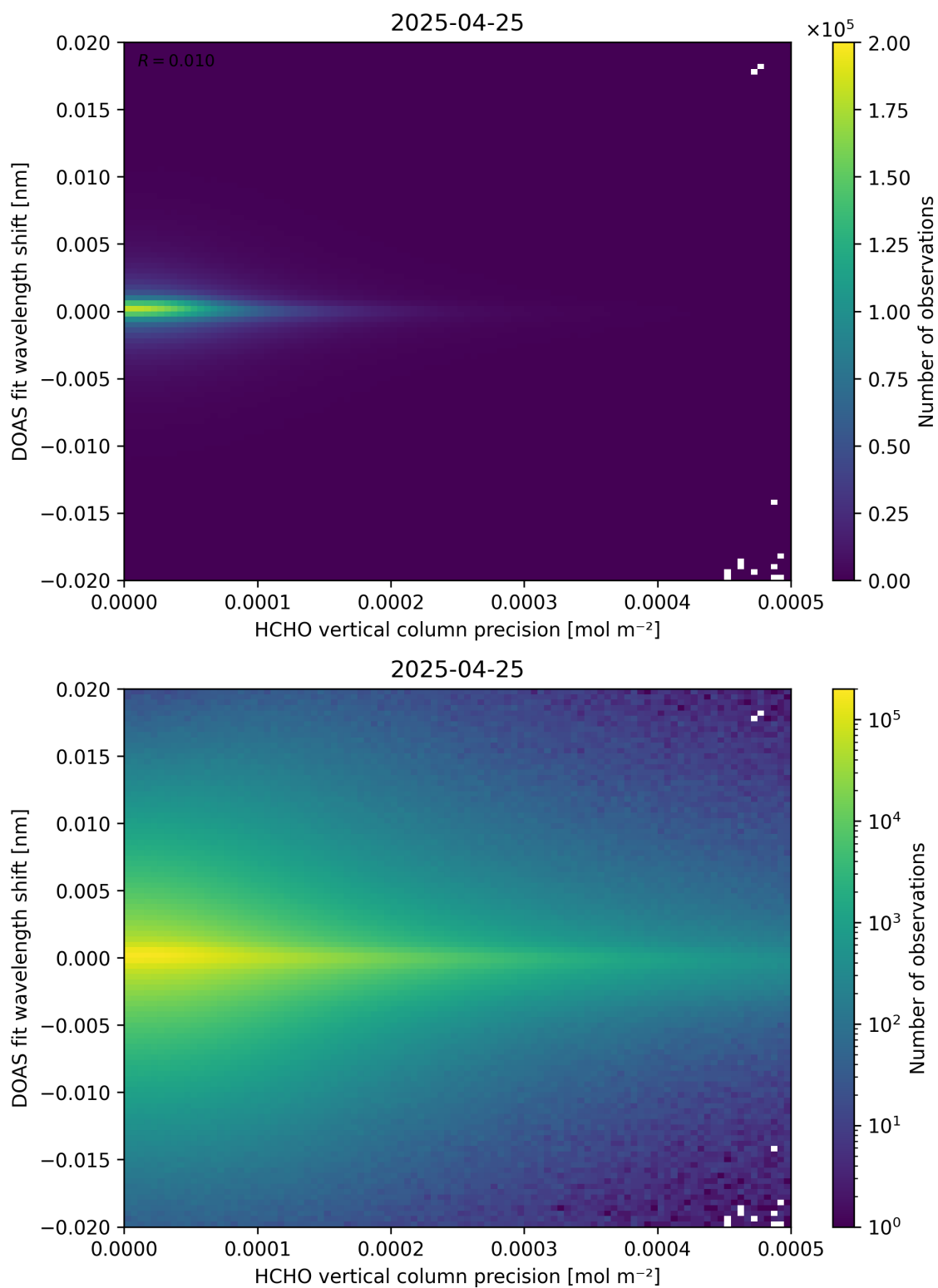
Figure 137: Scatter density plot of “HCHO vertical column precision” against “DOAS fit wavelength shift” for 2025-04-24 to 2025-04-26.
