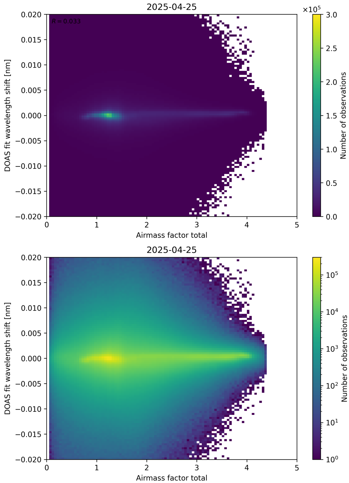
Figure 98: Scatter density plot of “Airmass factor total” against “DOAS fit wavelength shift” for 2025-04-24 to 2025-04-26.
