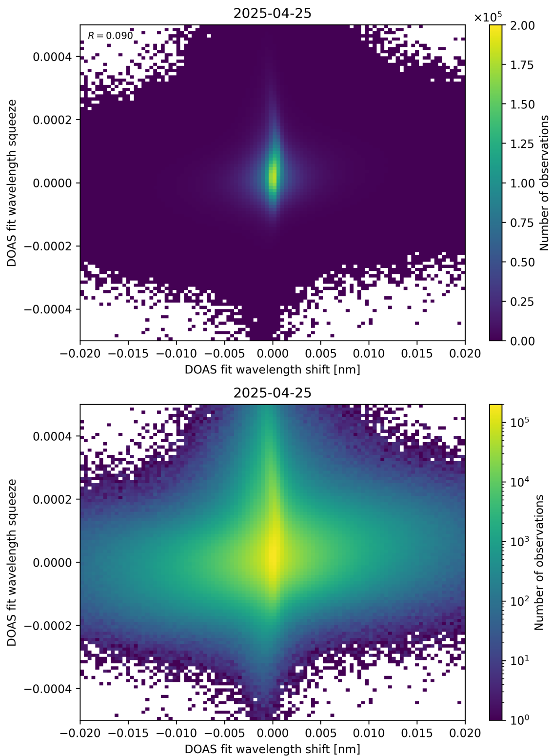
Figure 65: Scatter density plot of “DOAS fit wavelength shift” against “DOAS fit wavelength squeeze” for 2025-04-24 to 2025-04-26.
