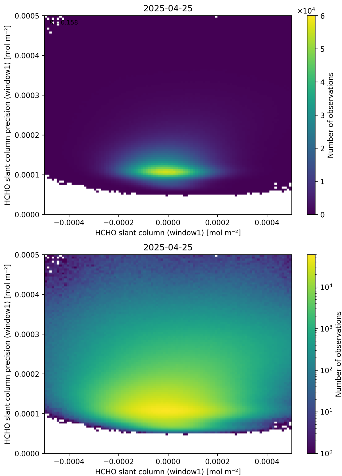
Figure 84: Scatter density plot of “HCHO slant column (window1)” against “HCHO slant column precision (window1)” for 2025-04-24 to 2025-04-26.
