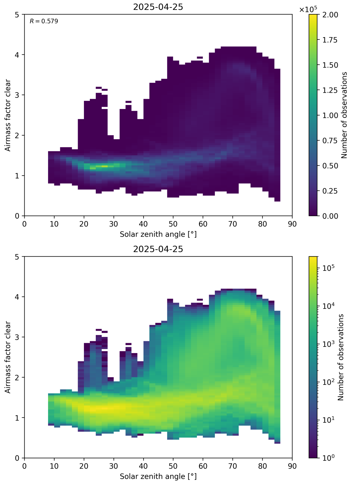
Figure 170: Scatter density plot of “Solar zenith angle” against “Airmass factor clear” for 2025-04-24 to 2025-04-26.
