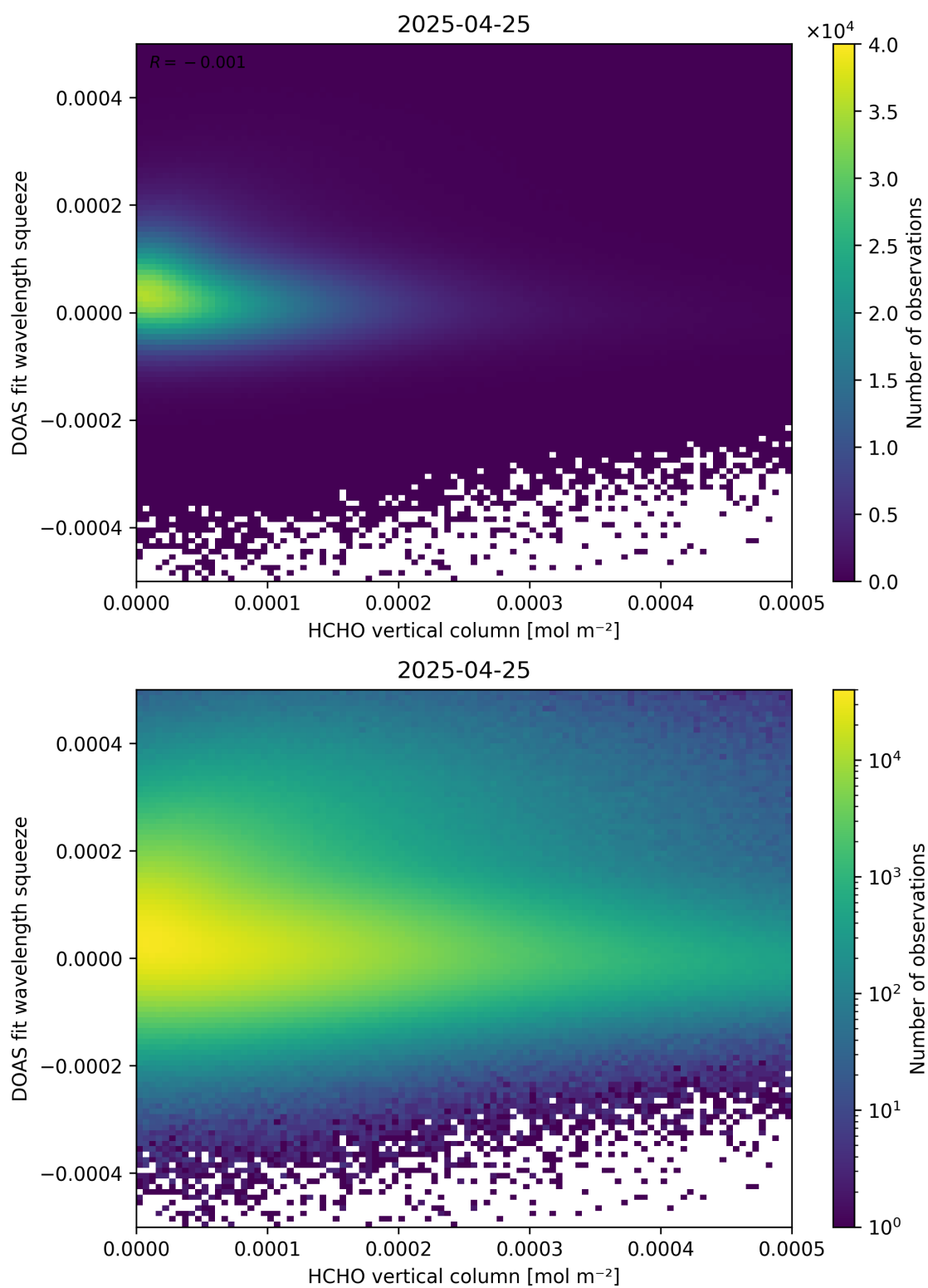
Figure 125: Scatter density plot of “HCHO vertical column” against “DOAS fit wavelength squeeze” for 2025-04-24 to 2025-04-26.
