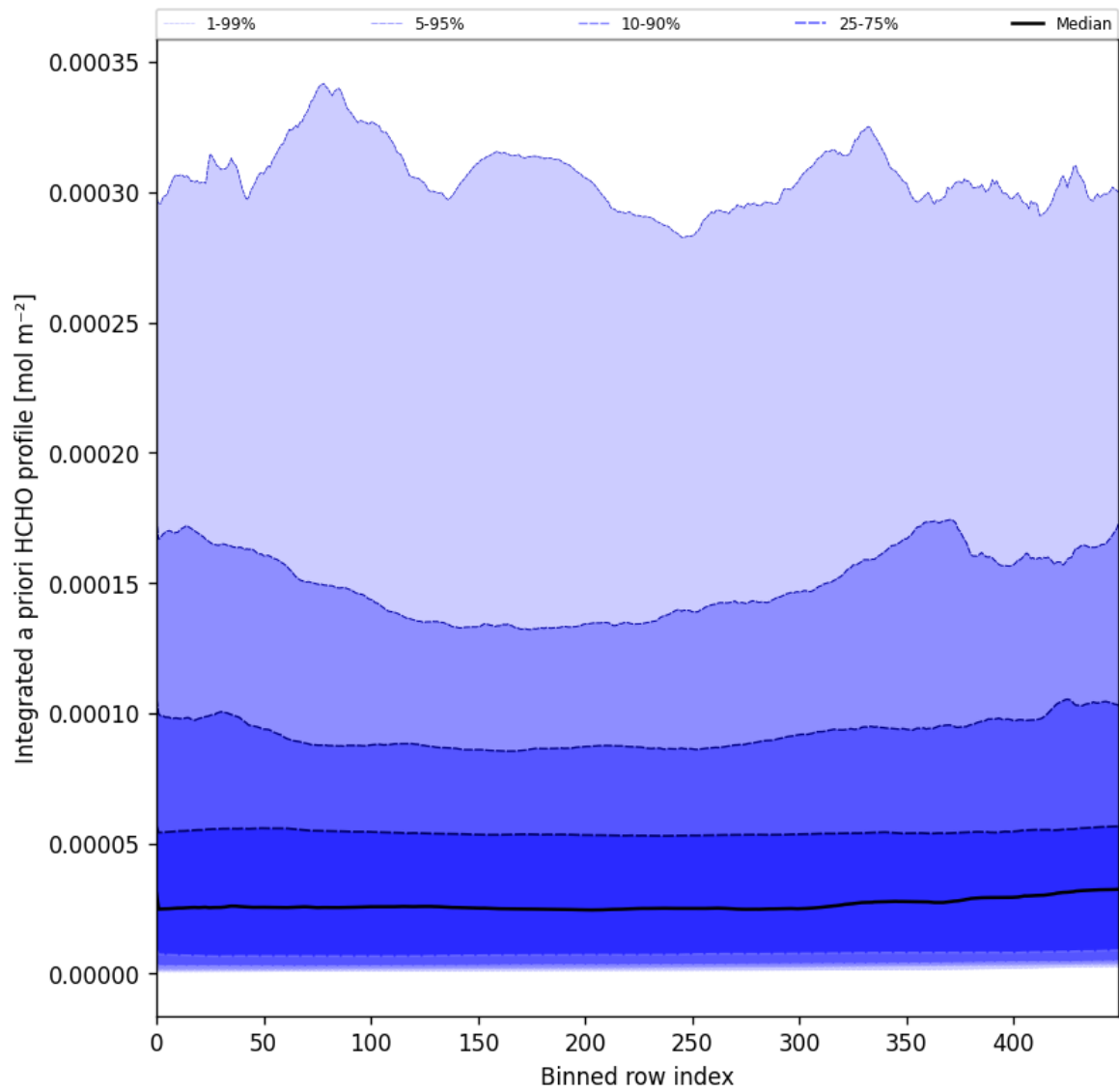
Figure 57: Along track statistics of "Integrated a priori HCHO profile" for 2025-04-24 to 2025-04-26
