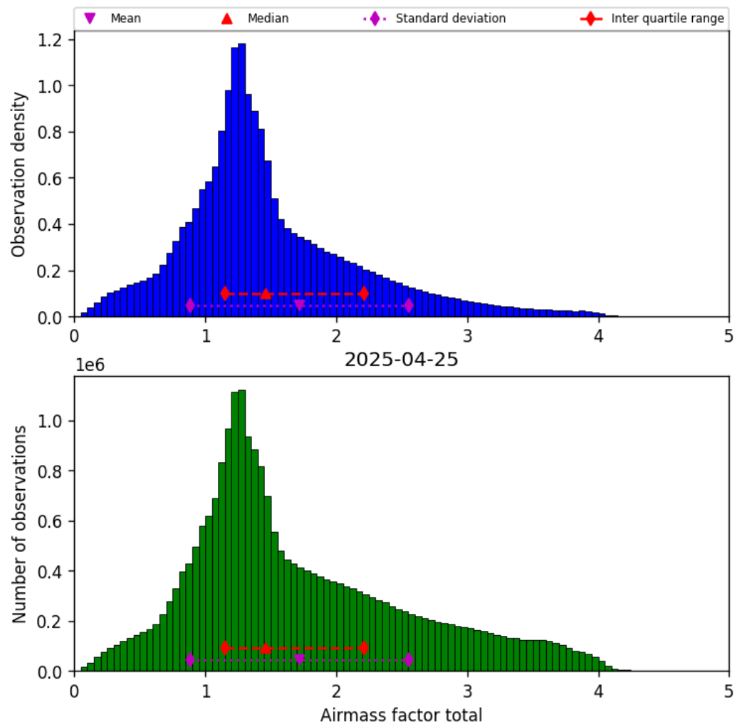
Figure 40: Histogram of “Airmass factor total” for 2025-04-24 to 2025-04-26
