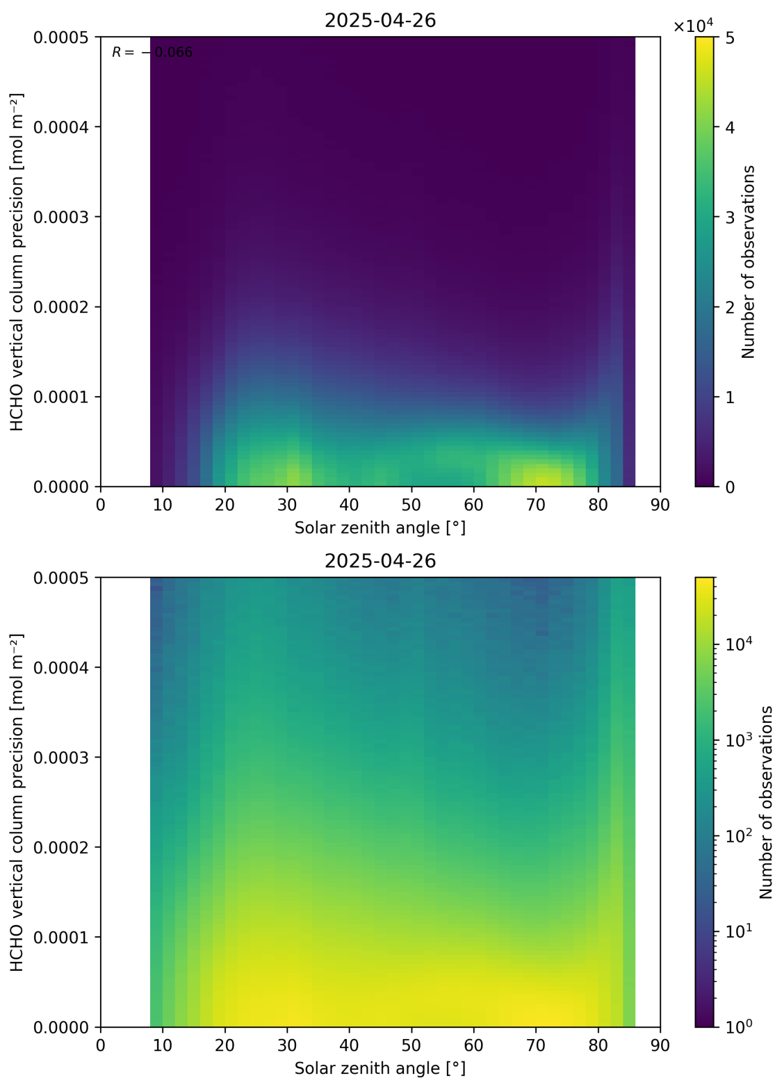
Figure 179: Scatter density plot of “Solar zenith angle” against “HCHO vertical column precision” for 2025-04-25 to 2025-04-27.
