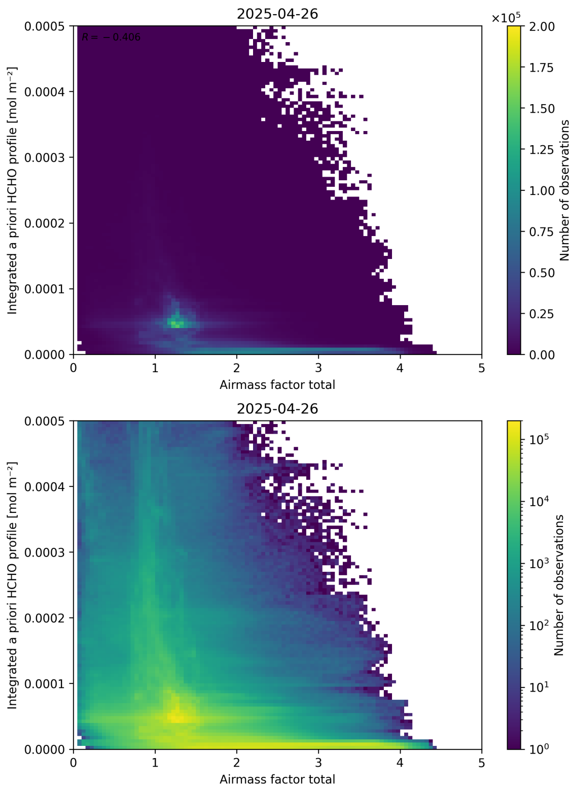
Figure 104: Scatter density plot of “Airmass factor total” against “Integrated a priori HCHO profile” for 2025-04-25 to 2025-04-27.
