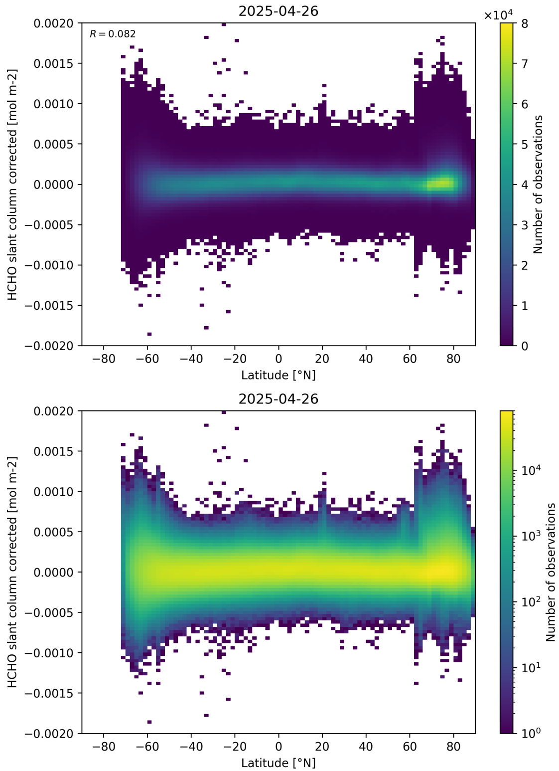
Figure 157: Scatter density plot of “Latitude” against “HCHO slant column corrected” for 2025-04-25 to 2025-04-27.
