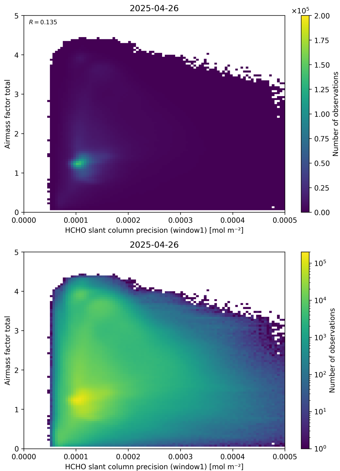
Figure 94: Scatter density plot of “HCHO slant column precision (window1)” against “Airmass factor total” for 2025-04-25 to 2025-04-27.
