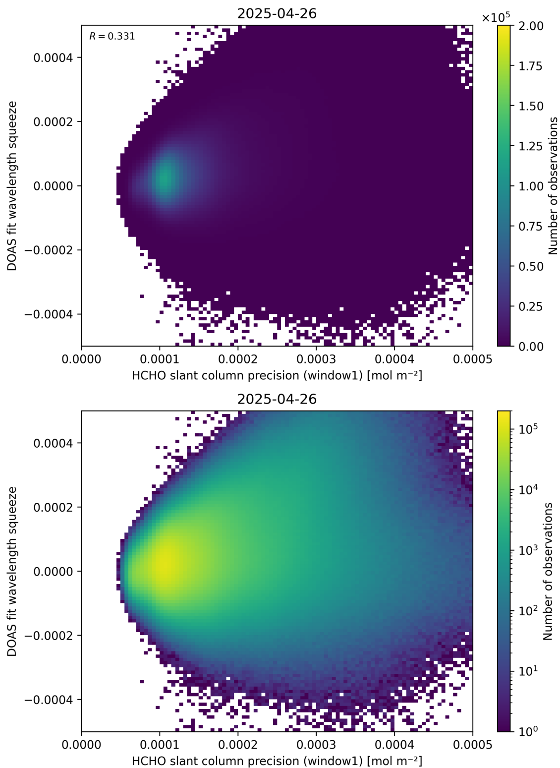
Figure 90: Scatter density plot of “HCHO slant column precision (window1)” against “DOAS fit wavelength squeeze” for 2025-04-25 to 2025-04-27.
