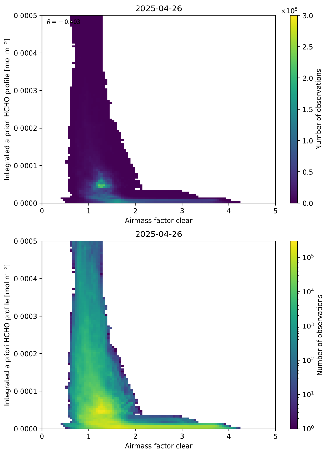
Figure 76: Scatter density plot of “Airmass factor clear” against “Integrated a priori HCHO profile” for 2025-04-25 to 2025-04-27.
