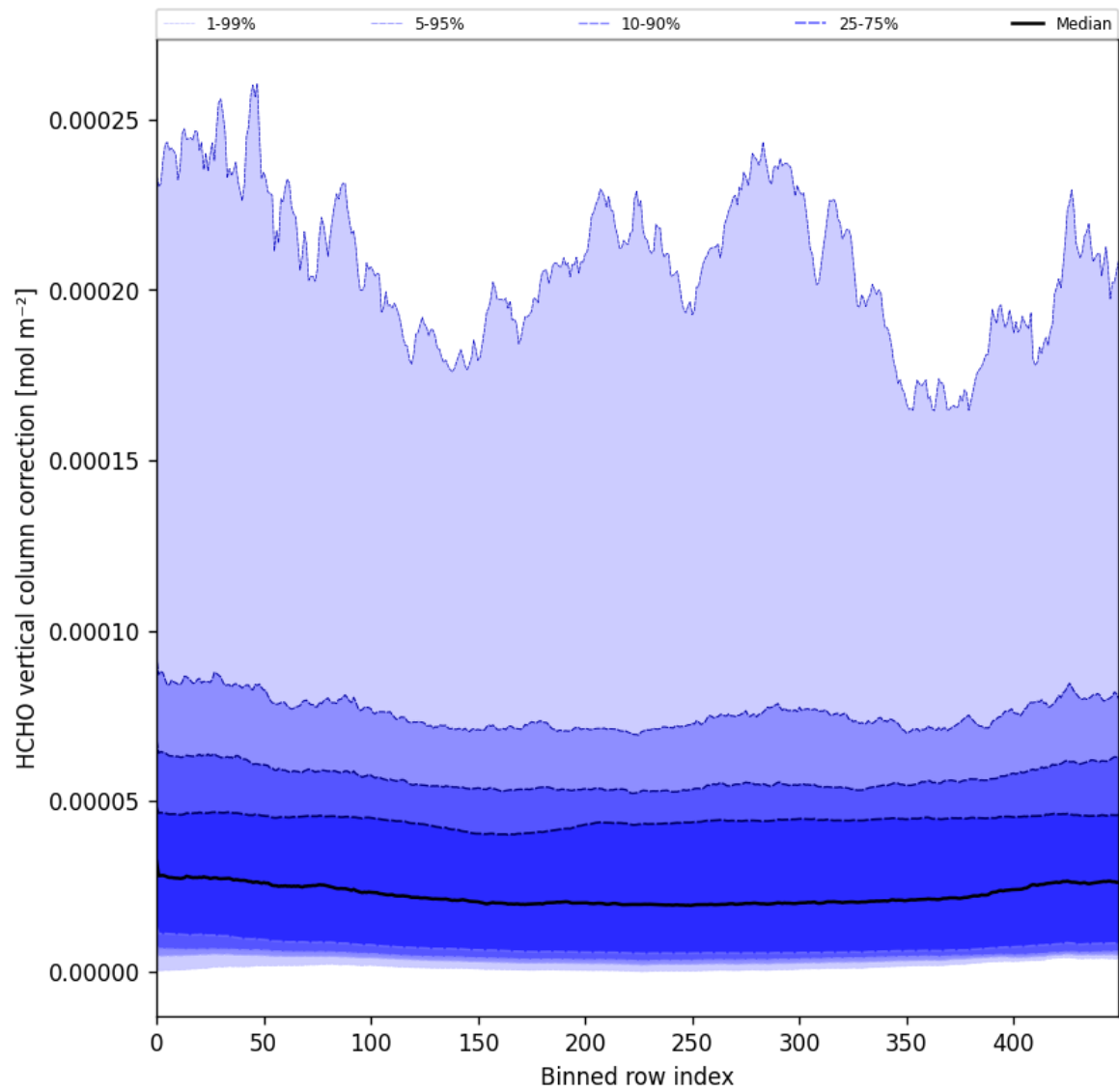
Figure 51: Along track statistics of “HCHO vertical column correction” for 2025-04-25 to 2025-04-27
