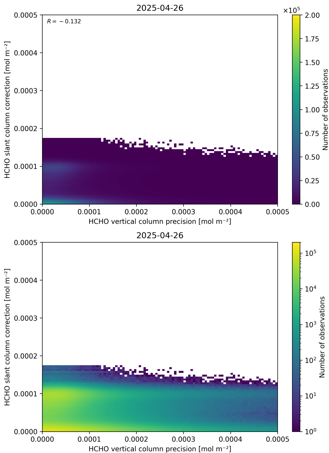
Figure 141: Scatter density plot of “HCHO vertical column precision” against “HCHO slant column correction” for 2025-04-25 to 2025-04-27.
