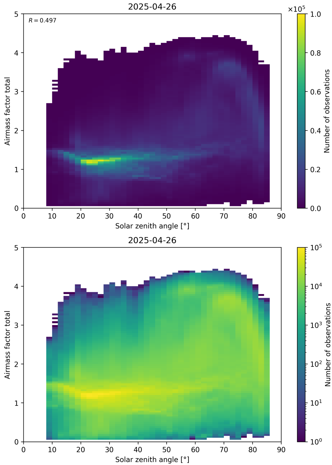
Figure 175: Scatter density plot of “Solar zenith angle” against “Airmass factor total” for 2025-04-25 to 2025-04-27.
