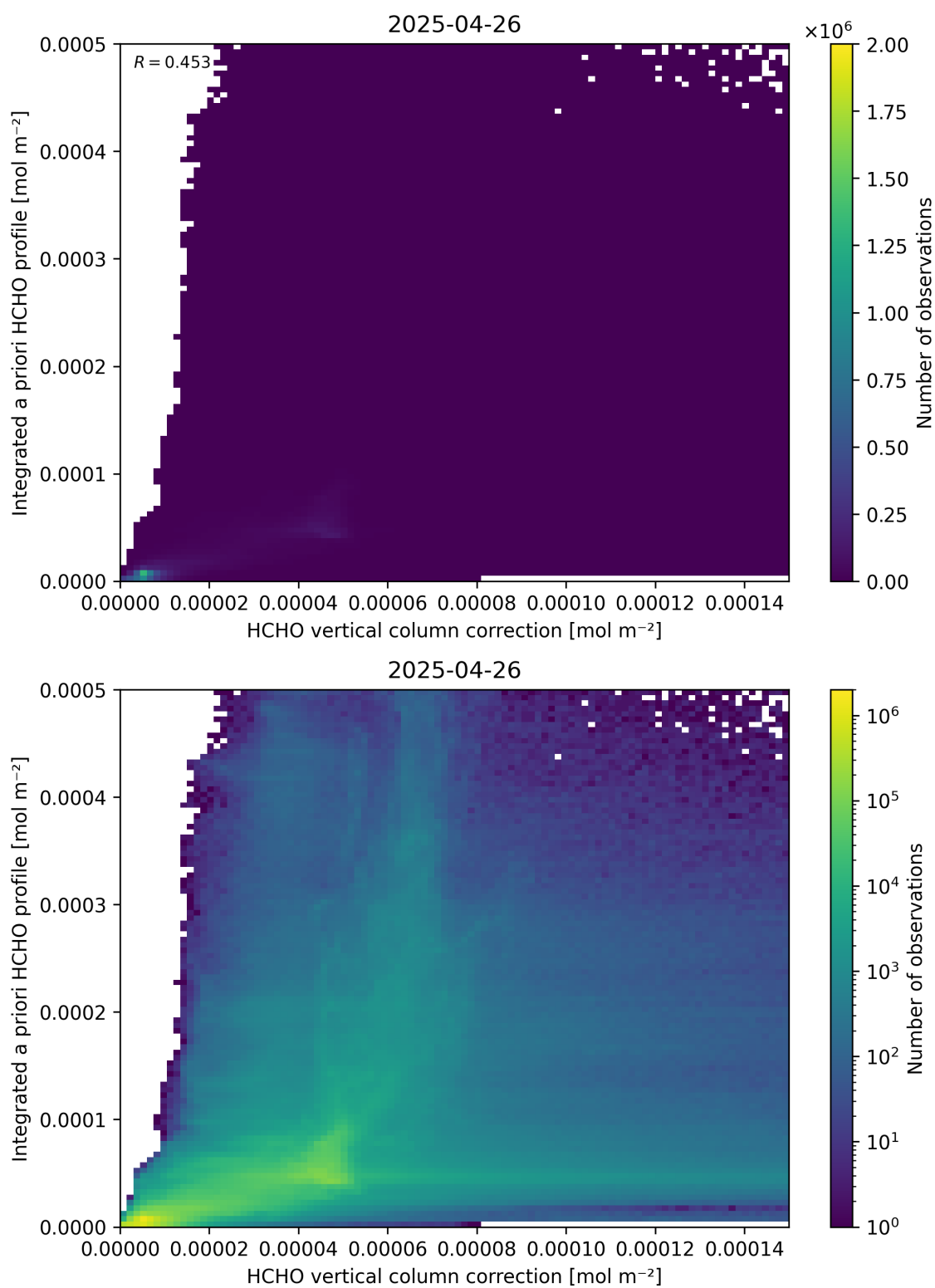
Figure 122: Scatter density plot of “HCHO vertical column correction” against “Integrated a priori HCHO profile” for 2025-04-25 to 2025-04-27.
