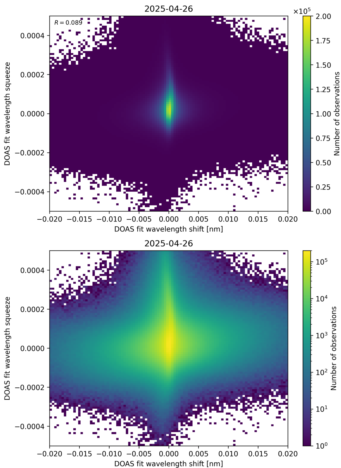
Figure 65: Scatter density plot of “DOAS fit wavelength shift” against “DOAS fit wavelength squeeze” for 2025-04-25 to 2025-04-27.
