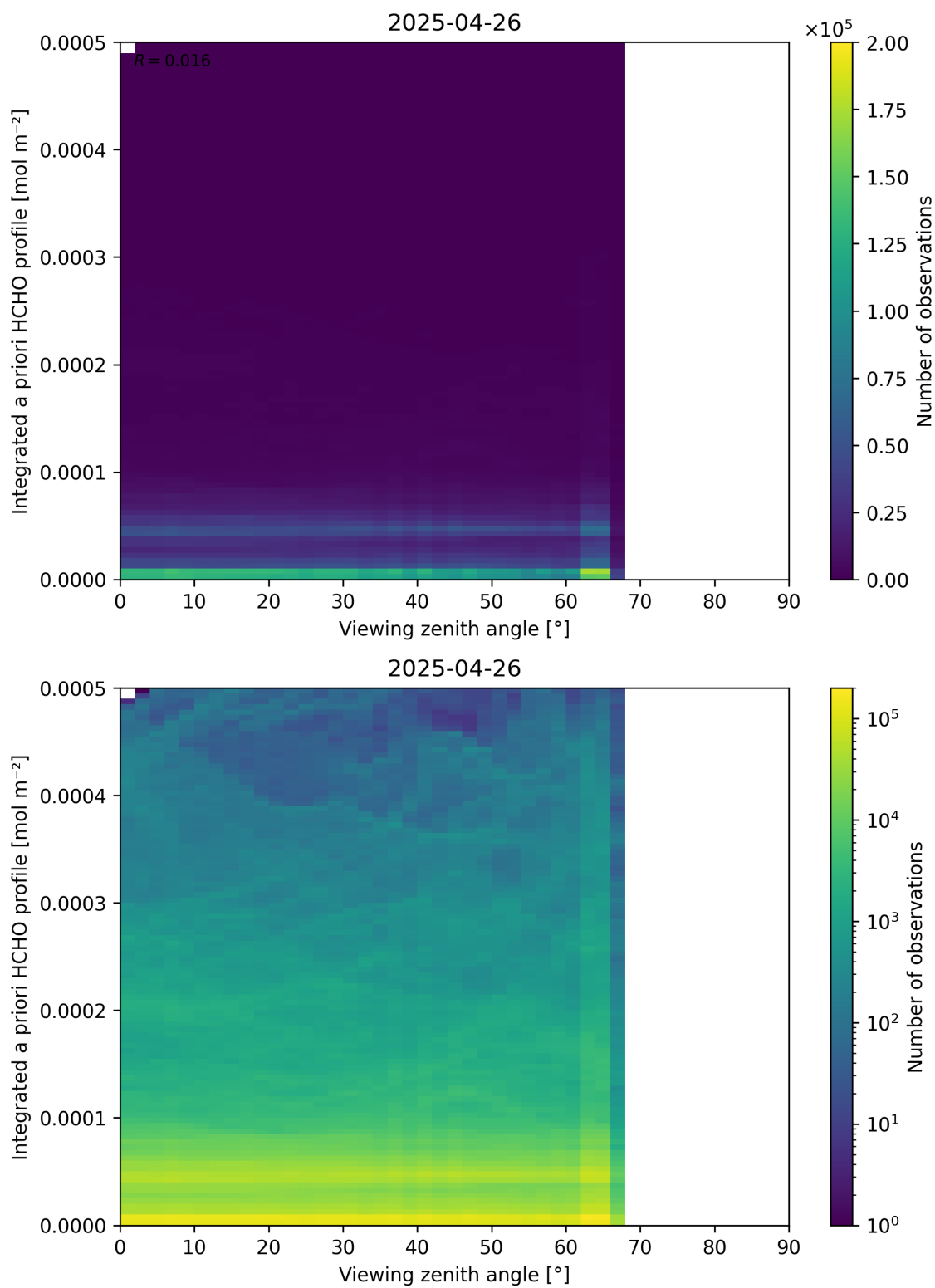
Figure 195: Scatter density plot of “Viewing zenith angle” against “Integrated a priori HCHO profile” for 2025-04-25 to 2025-04-27.
