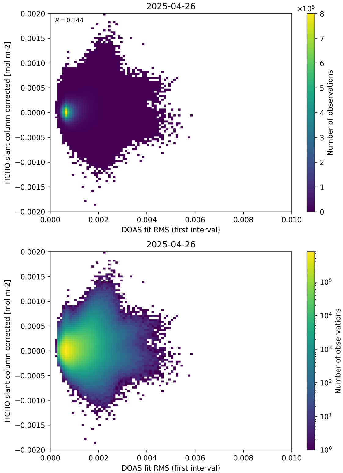
Figure 62: Scatter density plot of “DOAS fit RMS (first interval)” against “HCHO slant column corrected” for 2025-04-25 to 2025-04-27.
