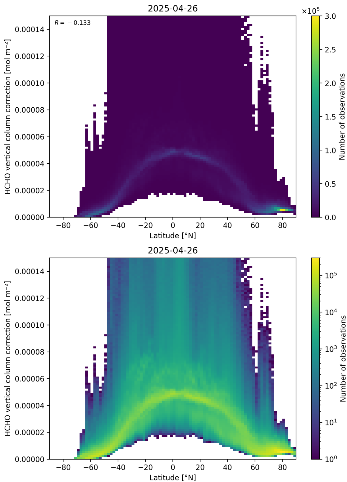
Figure 164: Scatter density plot of “Latitude” against “HCHO vertical column correction” for 2025-04-25 to 2025-04-27.
