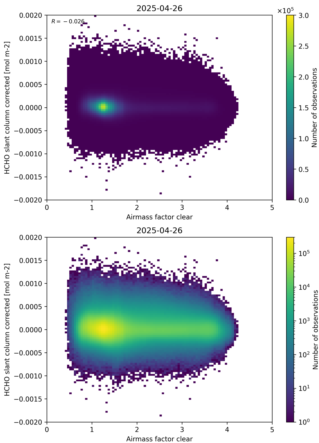
Figure 74: Scatter density plot of “Airmass factor clear” against “HCHO slant column corrected” for 2025-04-25 to 2025-04-27.
