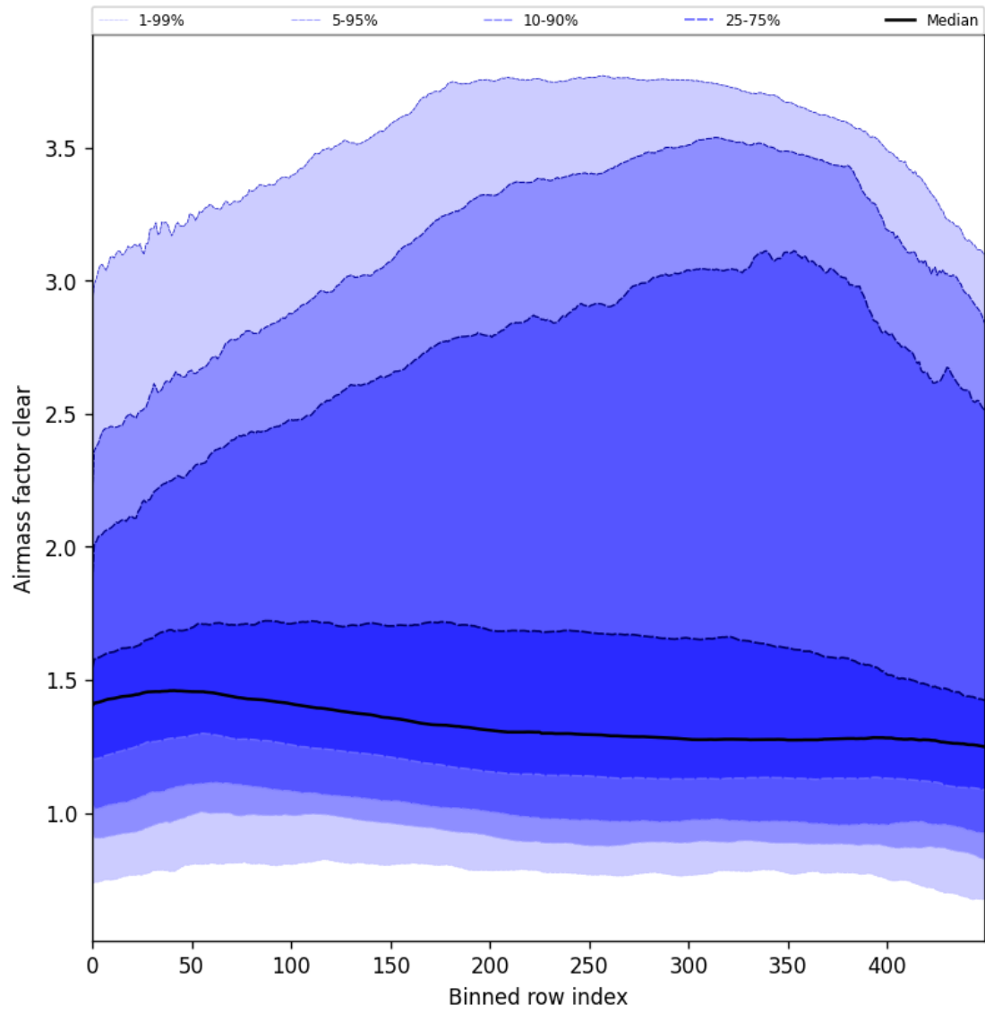
Figure 56: Along track statistics of “Airmass factor clear” for 2025-04-25 to 2025-04-27
