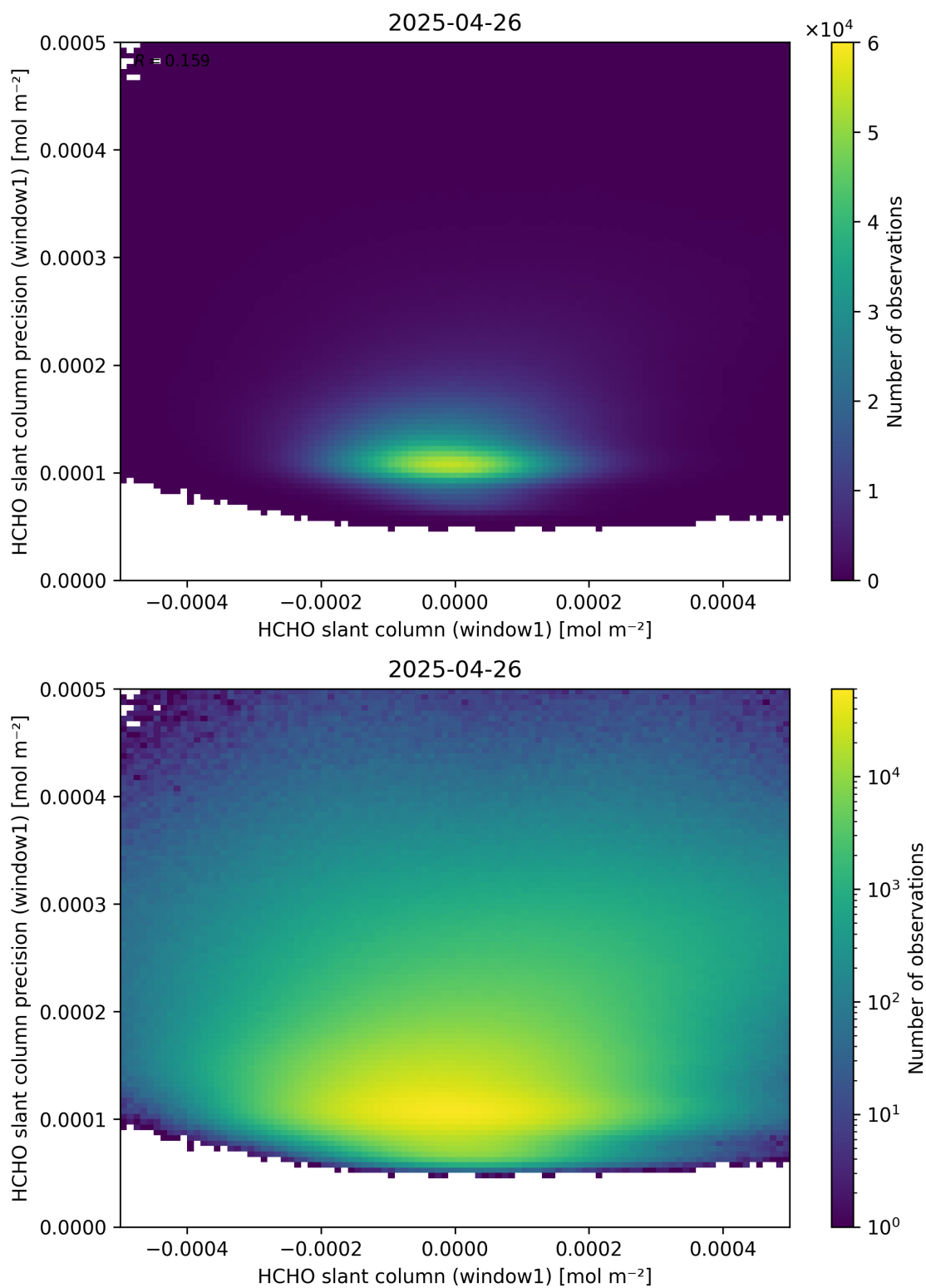
Figure 84: Scatter density plot of “HCHO slant column (window1)” against “HCHO slant column precision (window1)” for 2025-04-25 to 2025-04-27.
