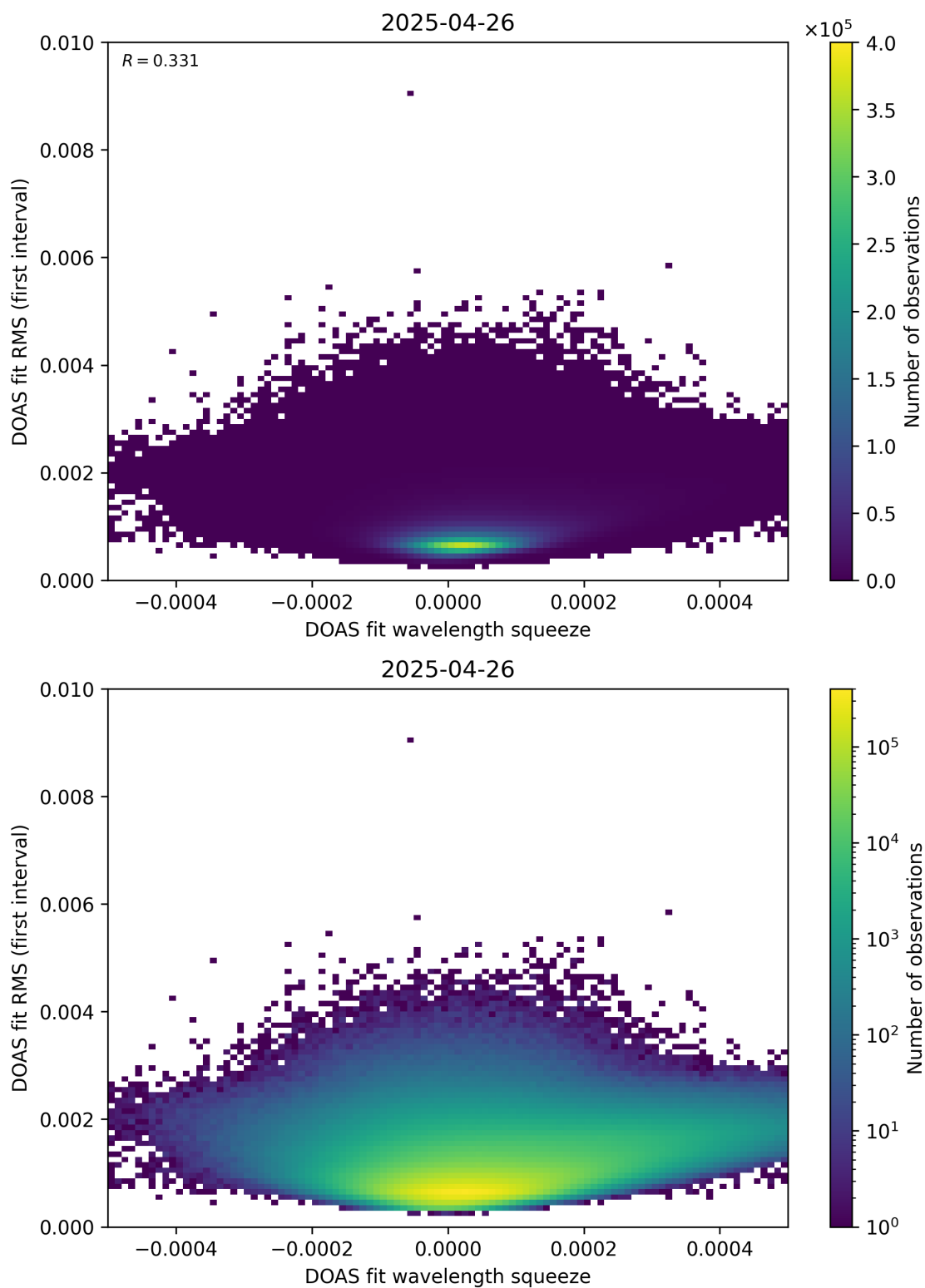
Figure 68: Scatter density plot of “DOAS fit wavelength squeeze” against “DOAS fit RMS (first interval)” for 2025-04-25 to 2025-04-27.
