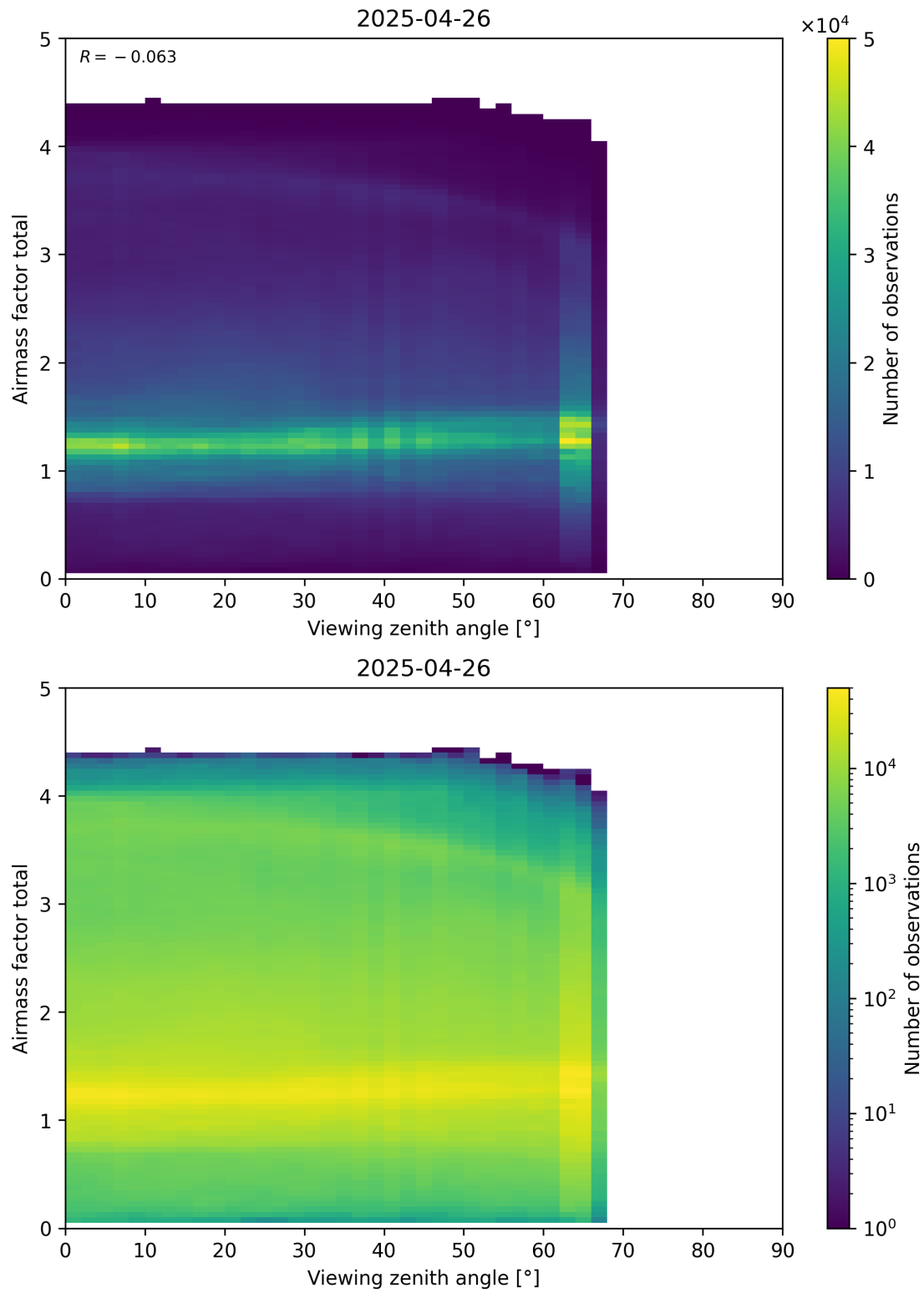
Figure 190: Scatter density plot of “Viewing zenith angle” against “Airmass factor total” for 2025-04-25 to 2025-04-27.
