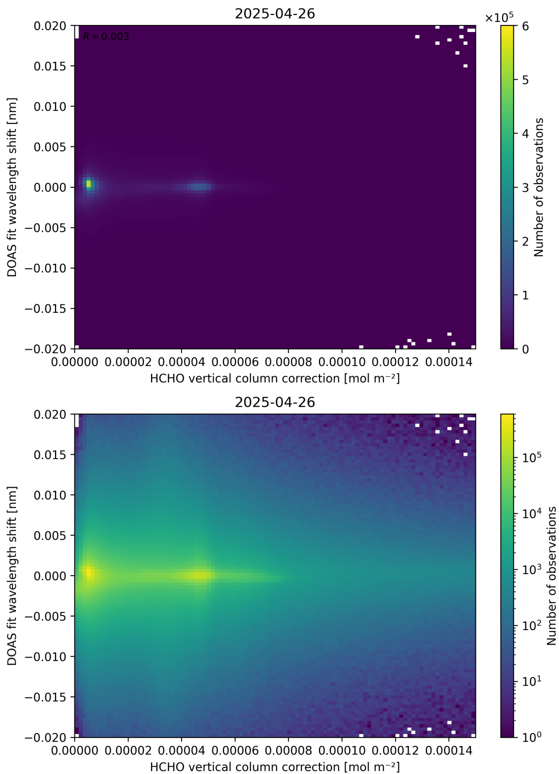
Figure 113: Scatter density plot of “HCHO vertical column correction” against “DOAS fit wavelength shift” for 2025-04-25 to 2025-04-27.
