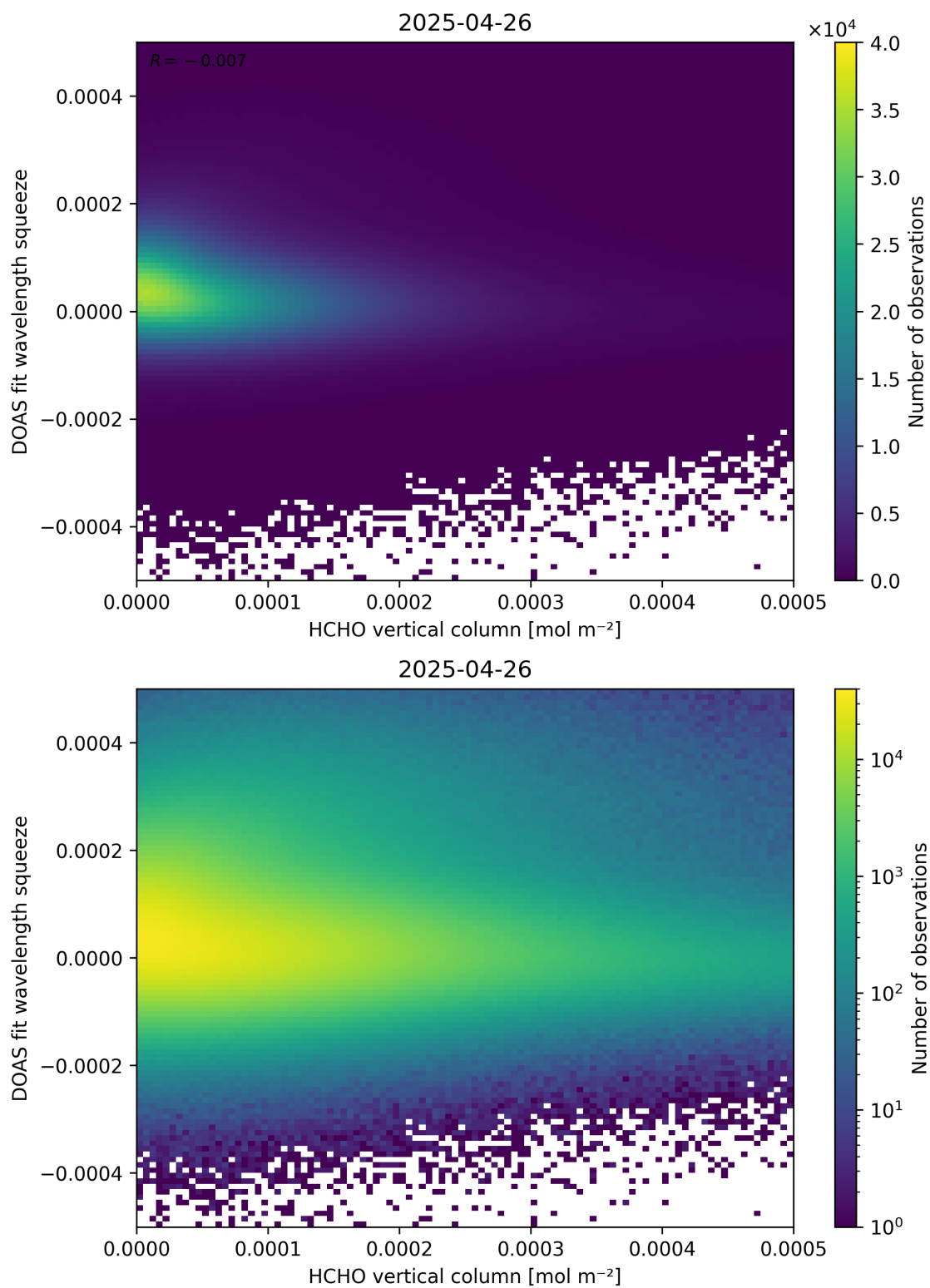
Figure 125: Scatter density plot of “HCHO vertical column” against “DOAS fit wavelength squeeze” for 2025-04-25 to 2025-04-27.
