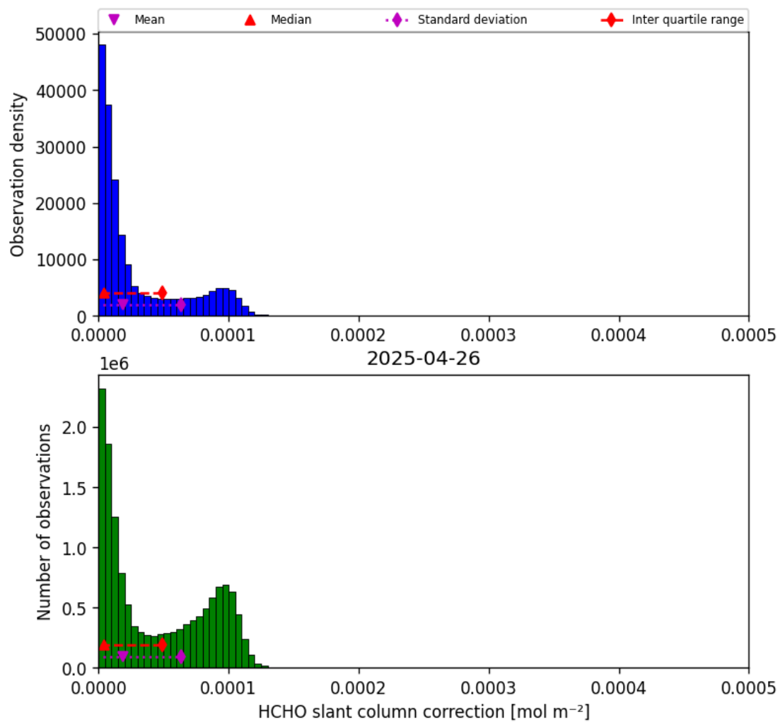
Figure 47: Histogram of “HCHO slant column correction” for 2025-04-25 to 2025-04-27
