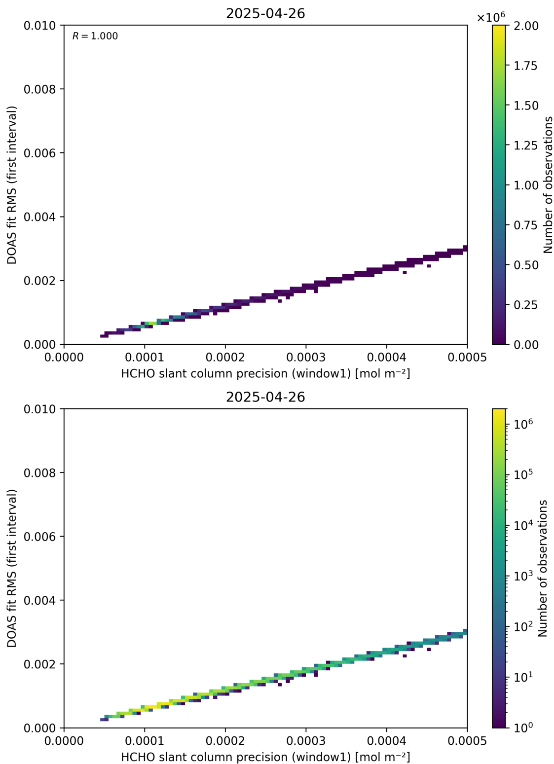
Figure 88: Scatter density plot of “HCHO slant column precision (window1)” against “DOAS fit RMS (first interval)” for 2025-04-25 to 2025-04-27.
