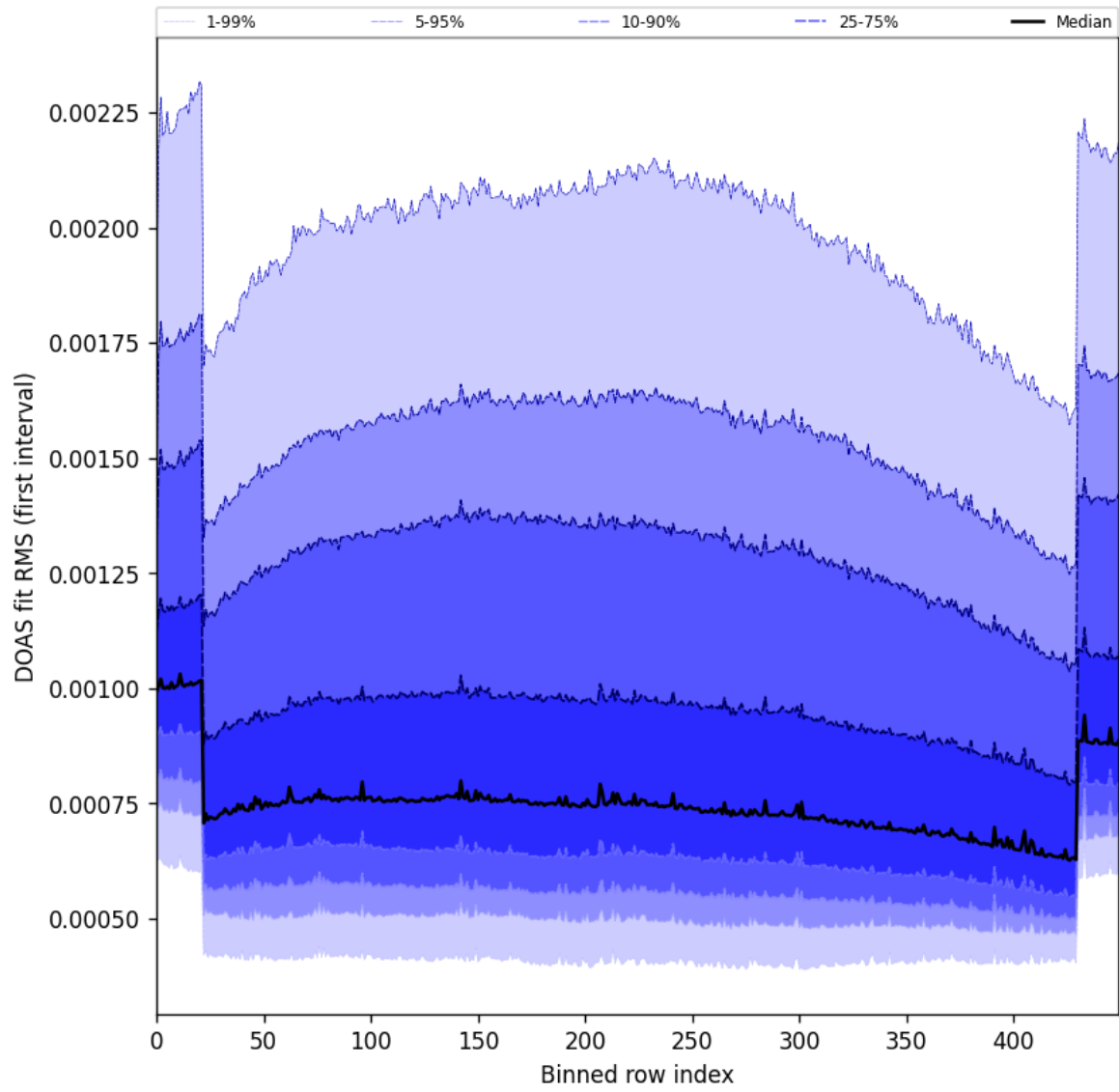
Figure 60: Along track statistics of “DOAS fit RMS (first interval)” for 2025-04-25 to 2025-04-27
