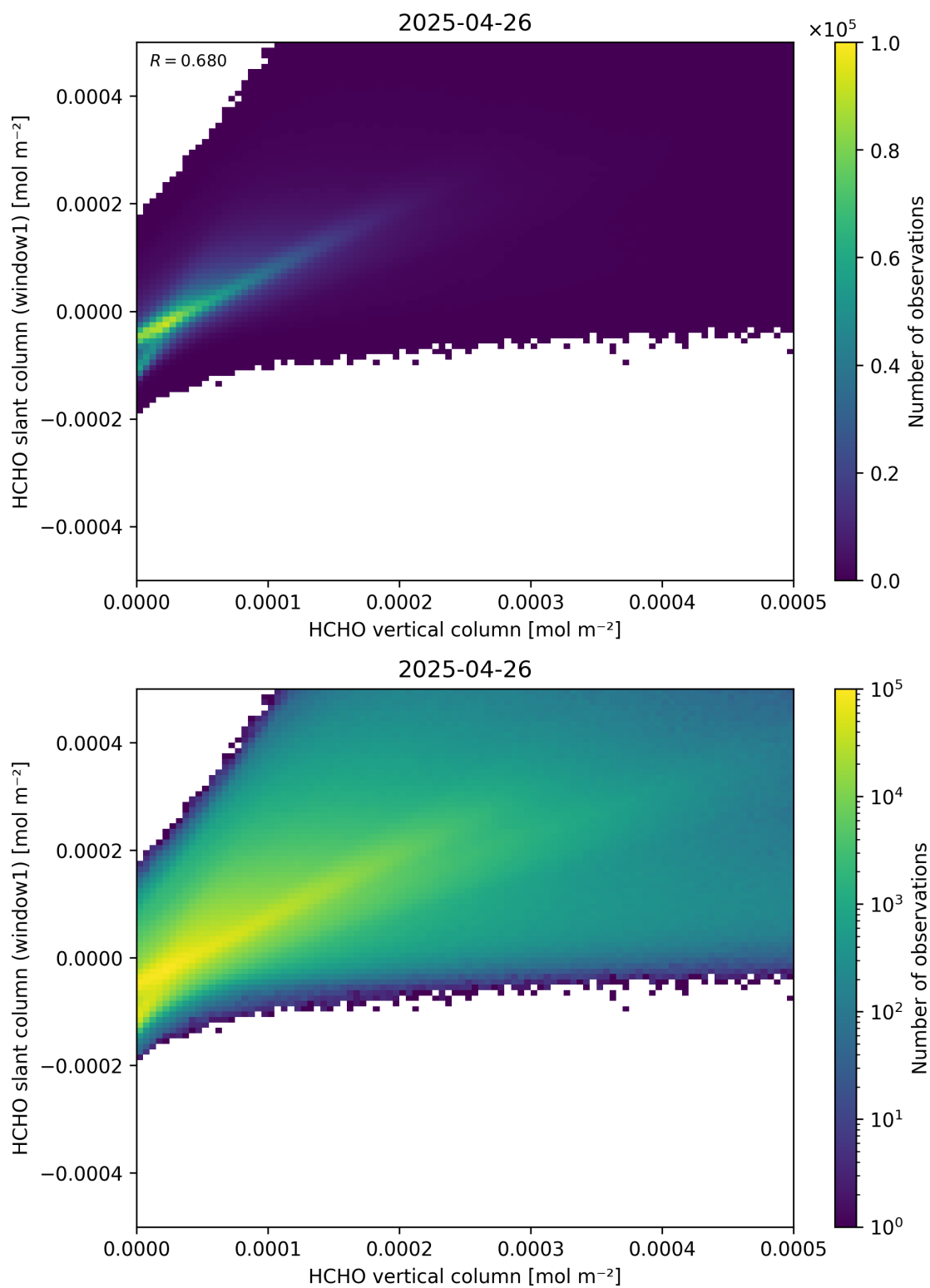
Figure 129: Scatter density plot of “HCHO vertical column” against “HCHO slant column (window1)” for 2025-04-25 to 2025-04-27.
