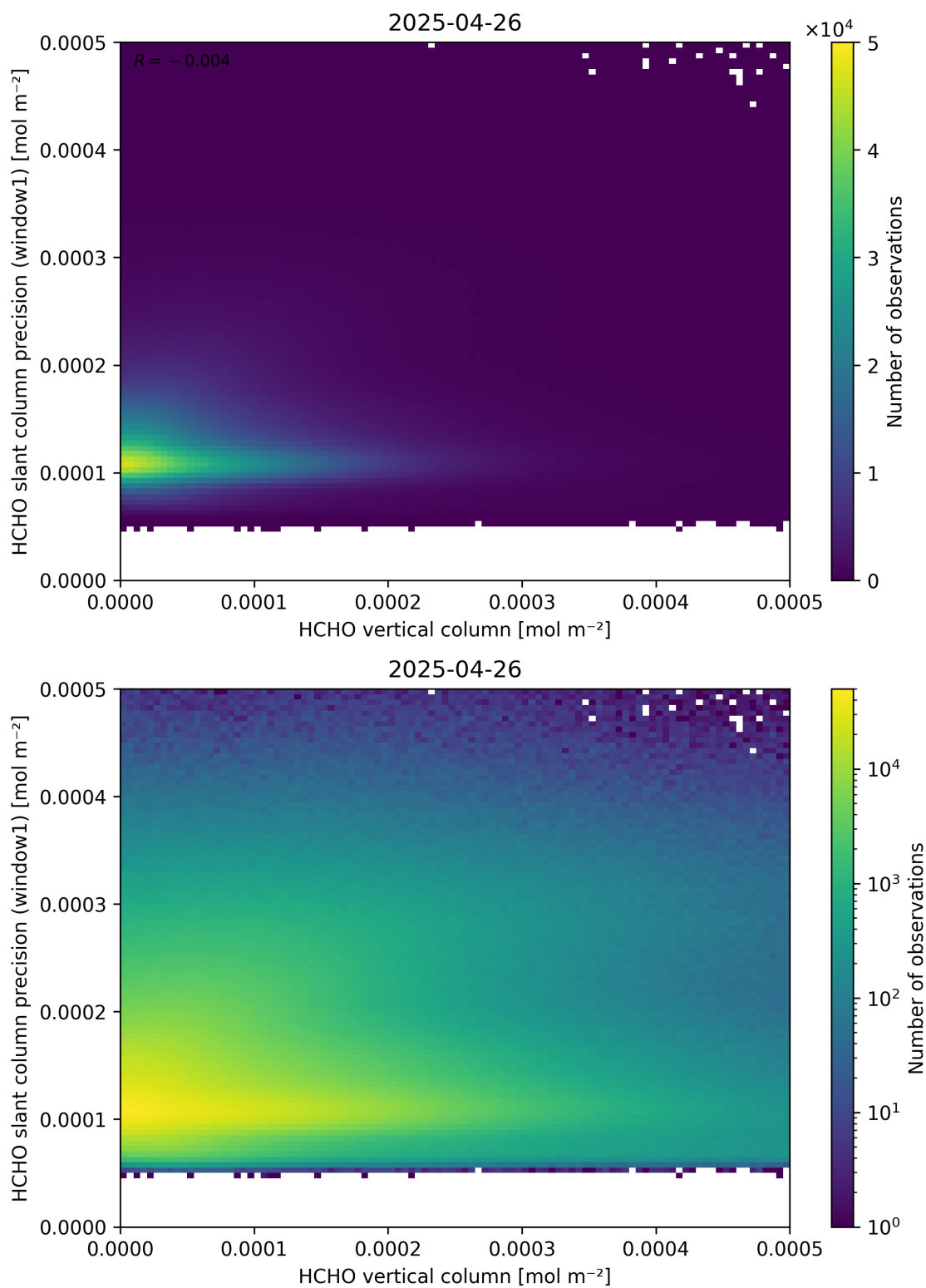
Figure 130: Scatter density plot of “HCHO vertical column” against “HCHO slant column precision (window1)” for 2025-04-25 to 2025-04-27.
