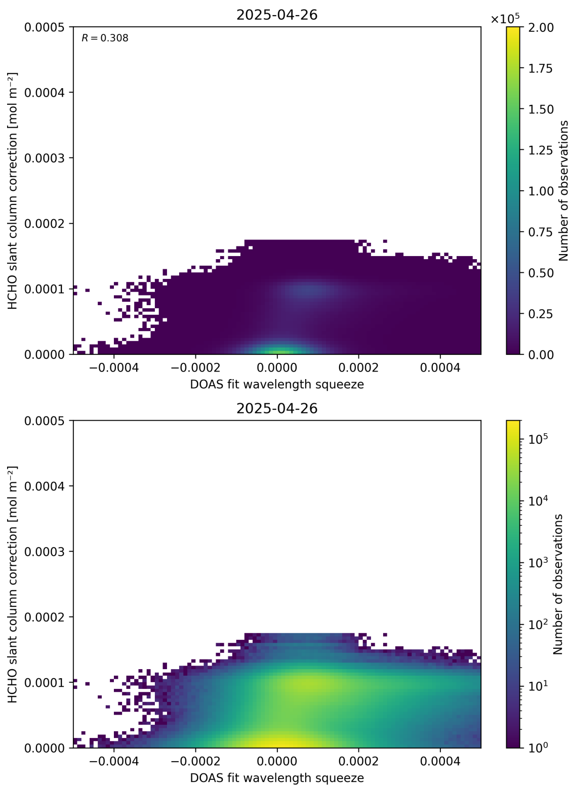
Figure 70: Scatter density plot of “DOAS fit wavelength squeeze” against “HCHO slant column correction” for 2025-04-25 to 2025-04-27.
