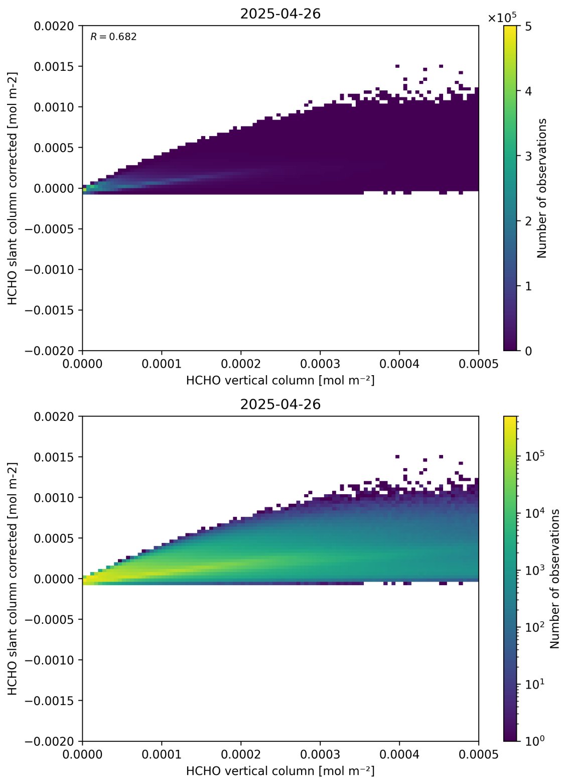
Figure 127: Scatter density plot of “HCHO vertical column” against “HCHO slant column corrected” for 2025-04-25 to 2025-04-27.
