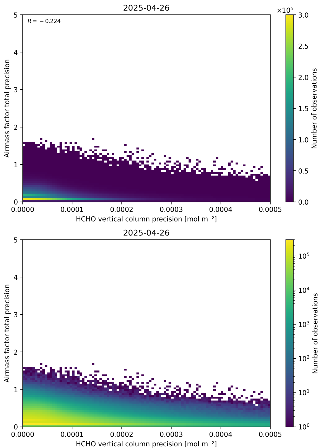
Figure 145: Scatter density plot of “HCHO vertical column precision” against “Airmass factor total precision” for 2025-04-25 to 2025-04-27.
