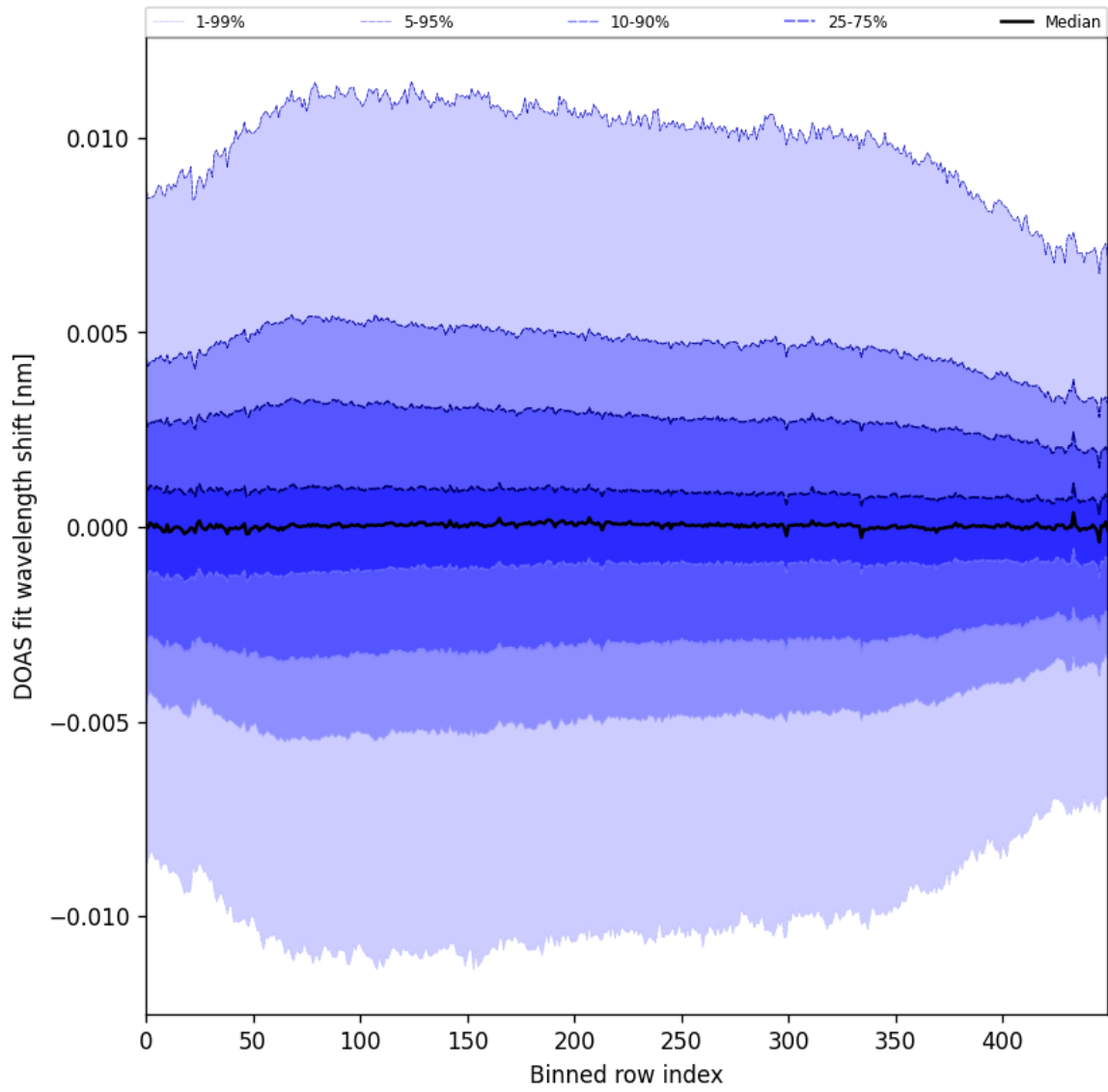
Figure 58: Along track statistics of “DOAS fit wavelength shift” for 2025-04-25 to 2025-04-27
