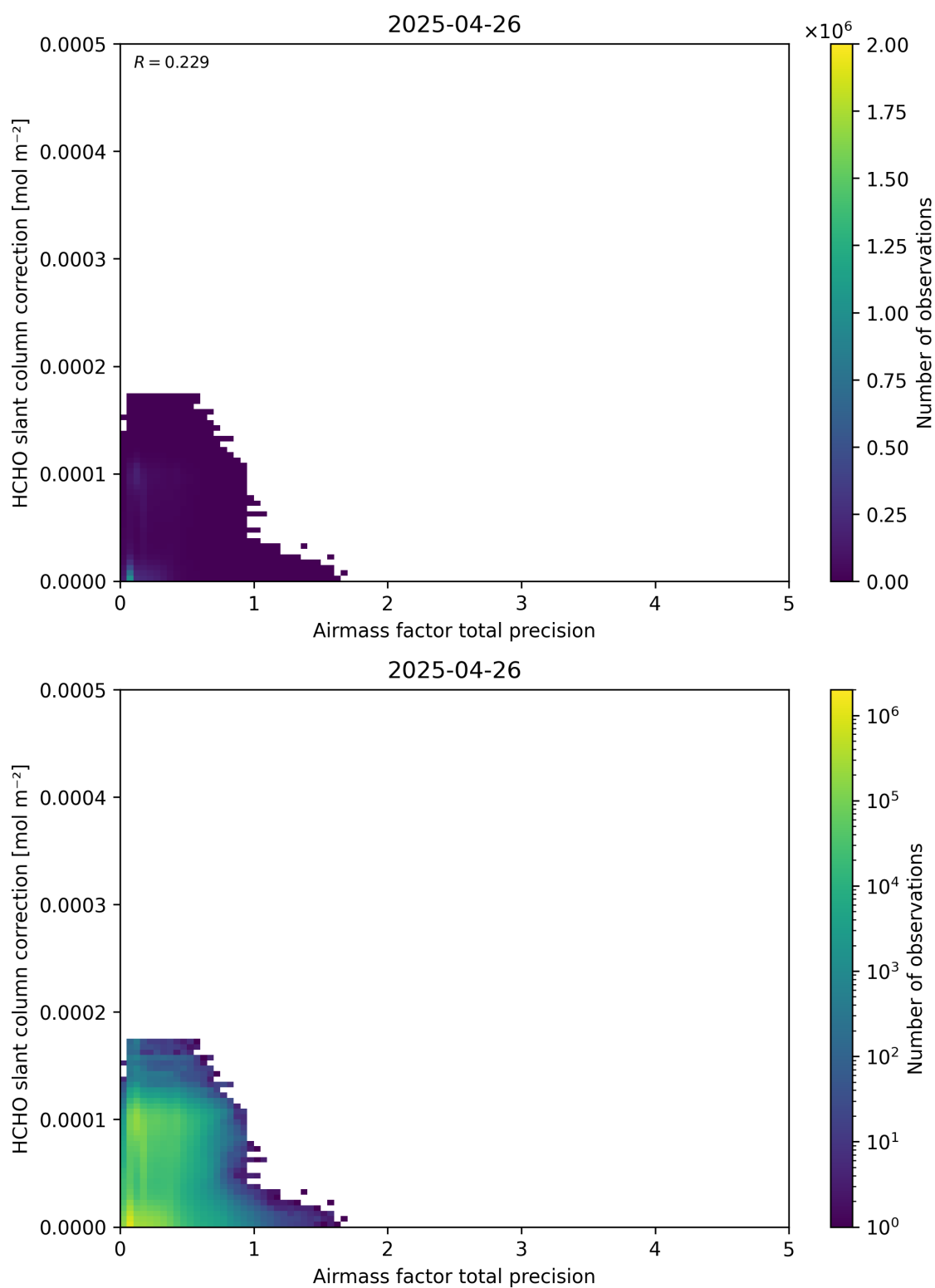
Figure 110: Scatter density plot of “Airmass factor total precision” against “HCHO slant column correction” for 2025-04-25 to 2025-04-27.
