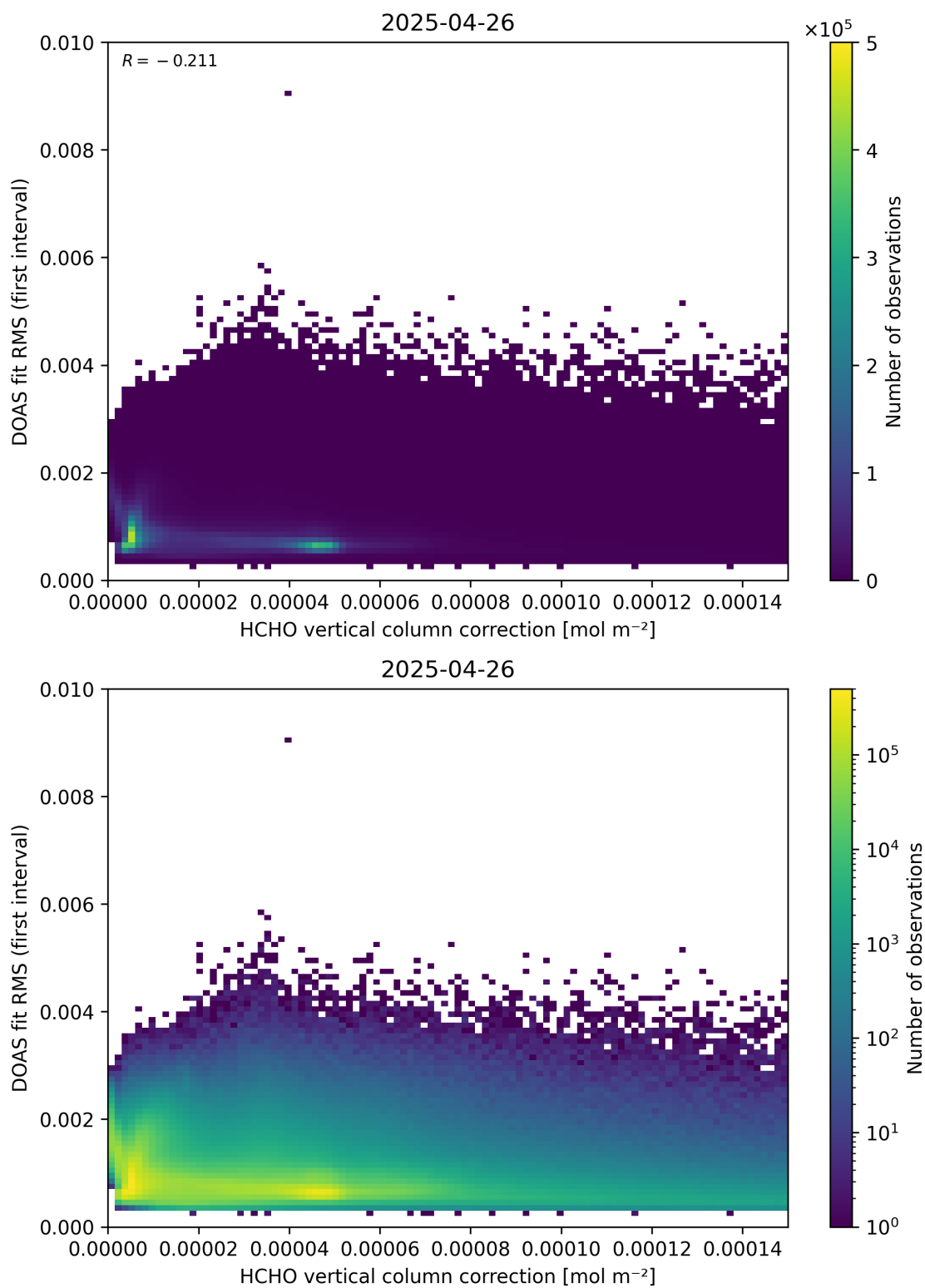
Figure 112: Scatter density plot of “HCHO vertical column correction” against “DOAS fit RMS (first interval)” for 2025-04-25 to 2025-04-27.
