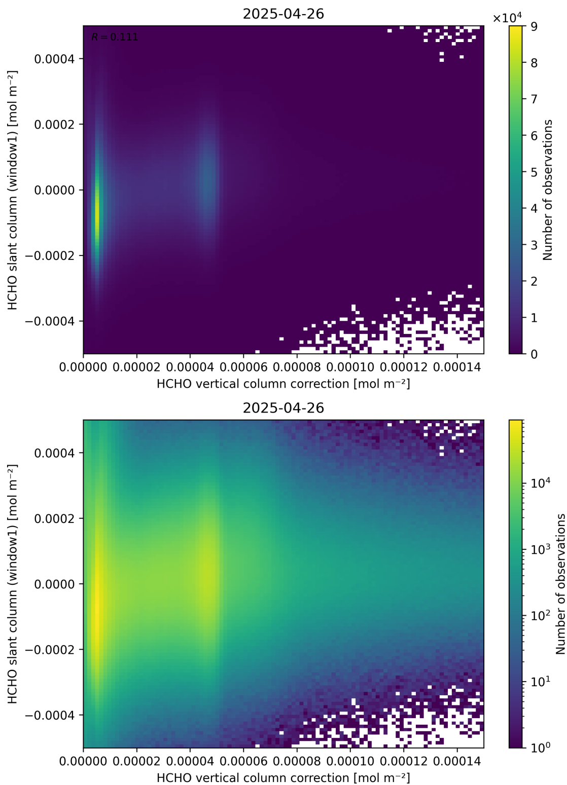
Figure 118: Scatter density plot of “HCHO vertical column correction” against “HCHO slant column (window1)” for 2025-04-25 to 2025-04-27.
