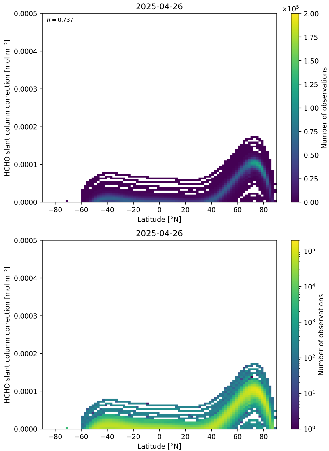
Figure 158: Scatter density plot of “Latitude” against “HCHO slant column correction” for 2025-04-25 to 2025-04-27.
