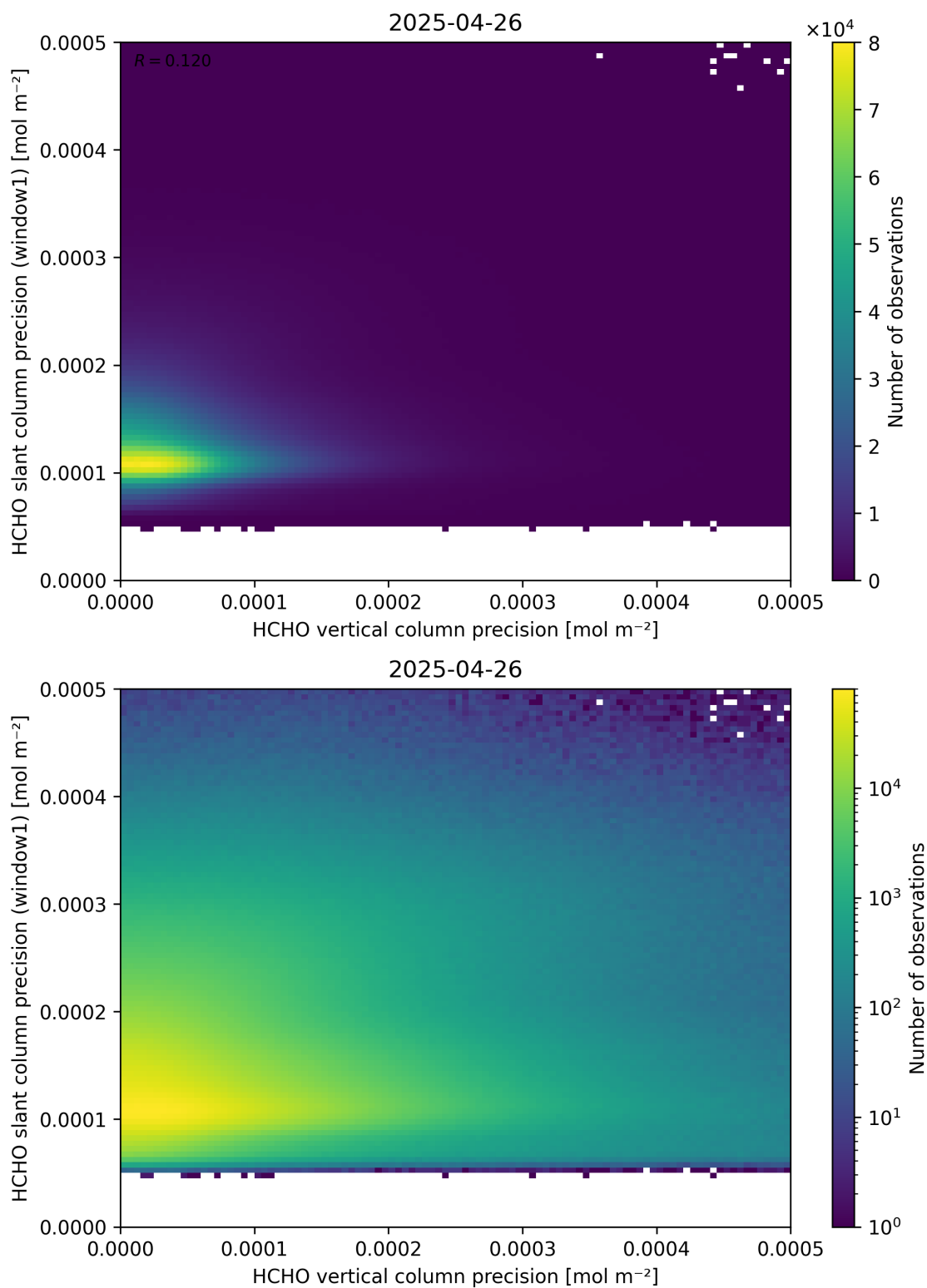
Figure 143: Scatter density plot of “HCHO vertical column precision” against “HCHO slant column precision (window1)” for 2025-04-25 to 2025-04-27.
