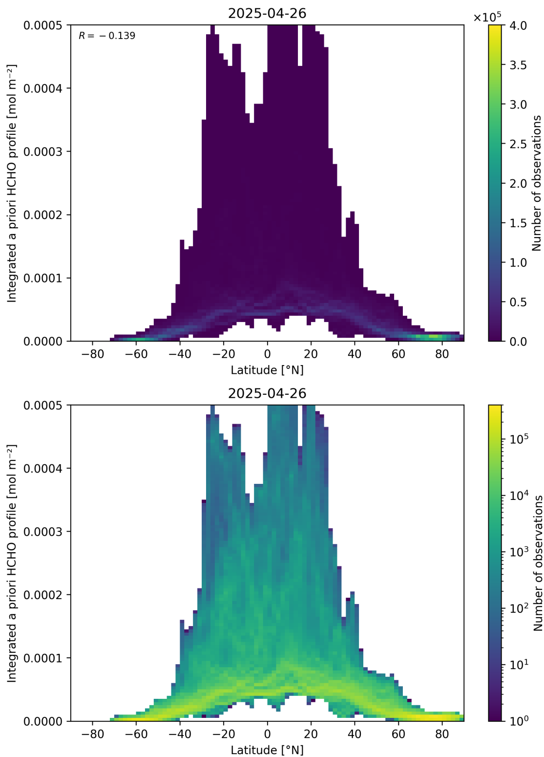
Figure 166: Scatter density plot of “Latitude” against “Integrated a priori HCHO profile” for 2025-04-25 to 2025-04-27.
