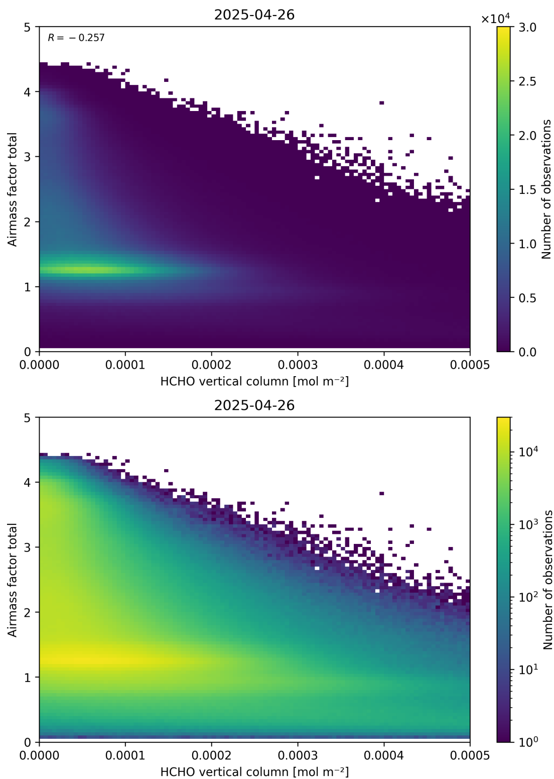
Figure 131: Scatter density plot of “HCHO vertical column” against “Airmass factor total” for 2025-04-25 to 2025-04-27.
