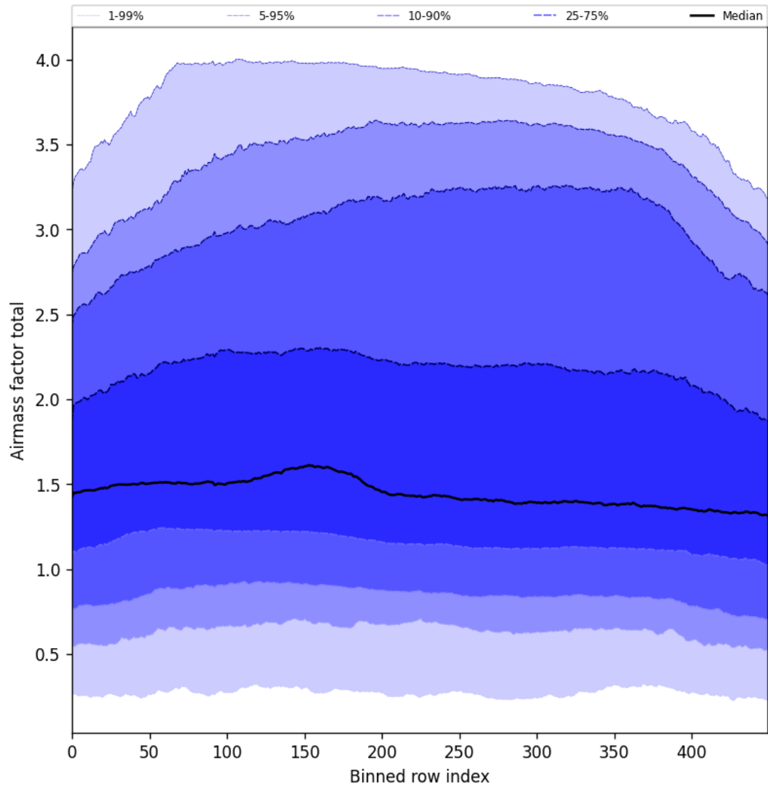
Figure 54: Along track statistics of “Airmass factor total” for 2025-04-25 to 2025-04-27
