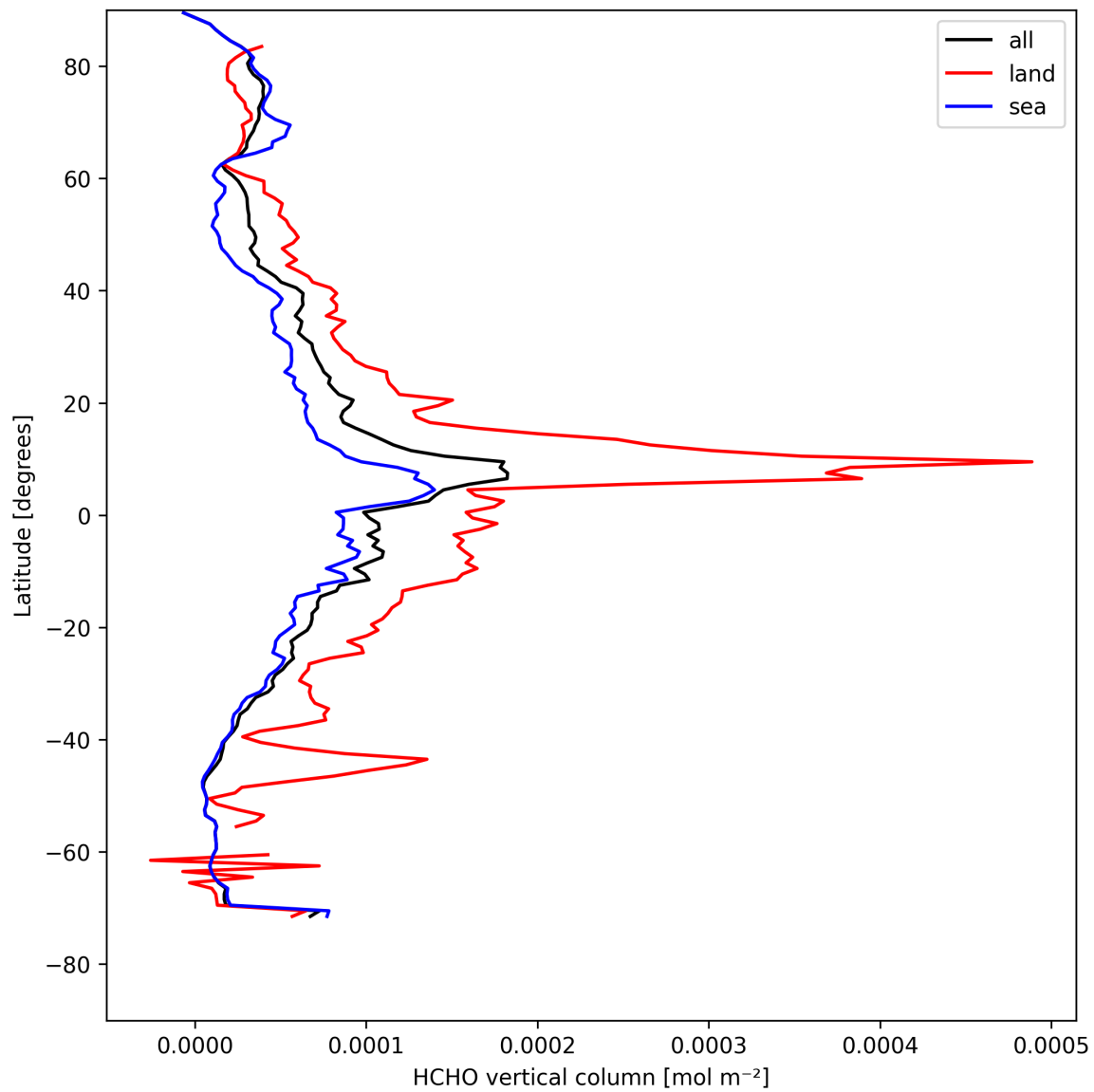
Figure 21: Zonal average of “HCHO vertical column” for 2025-04-25 to 2025-04-27.
