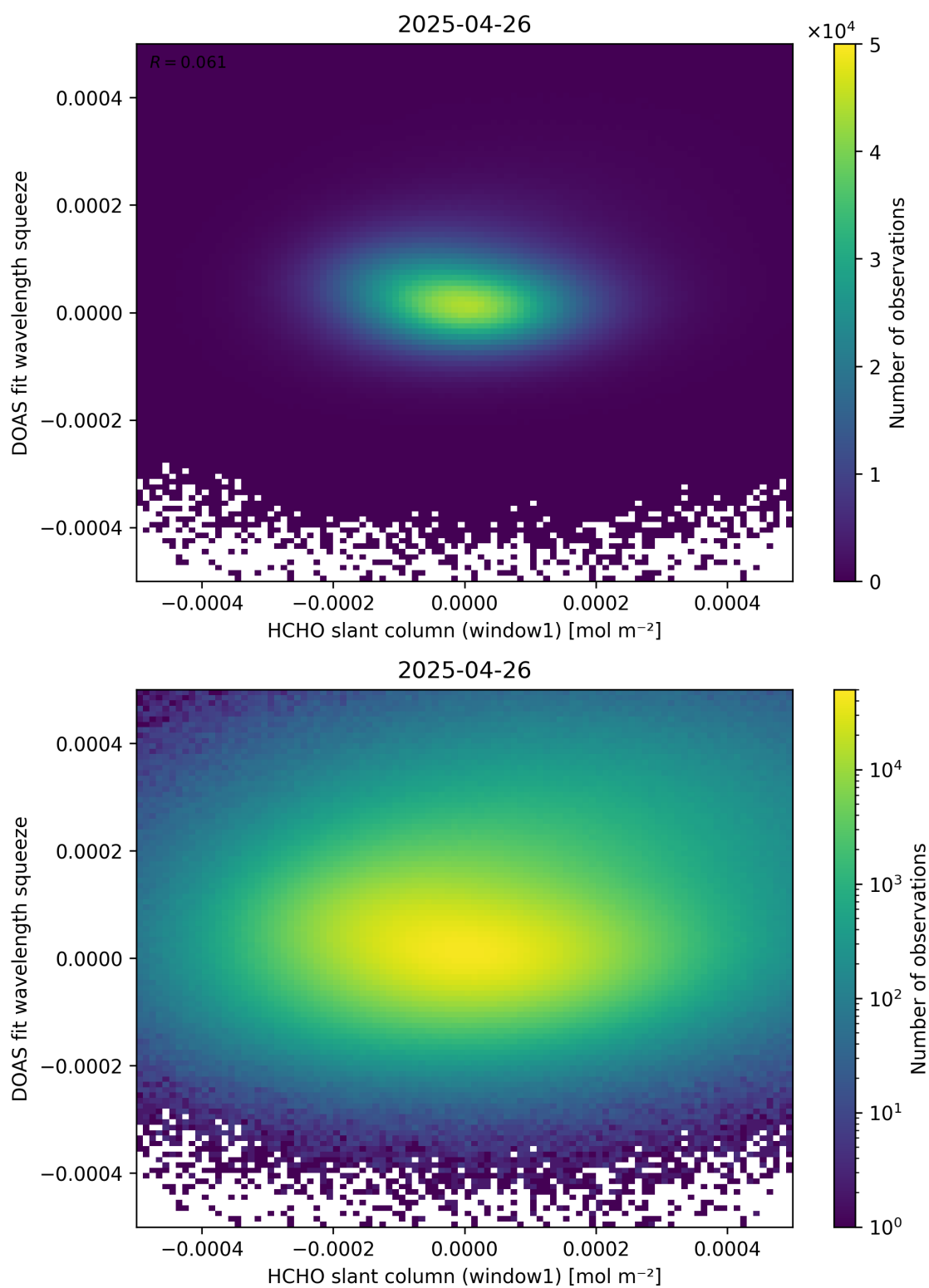
Figure 80: Scatter density plot of “HCHO slant column (window1)” against “DOAS fit wavelength squeeze” for 2025-04-25 to 2025-04-27.
