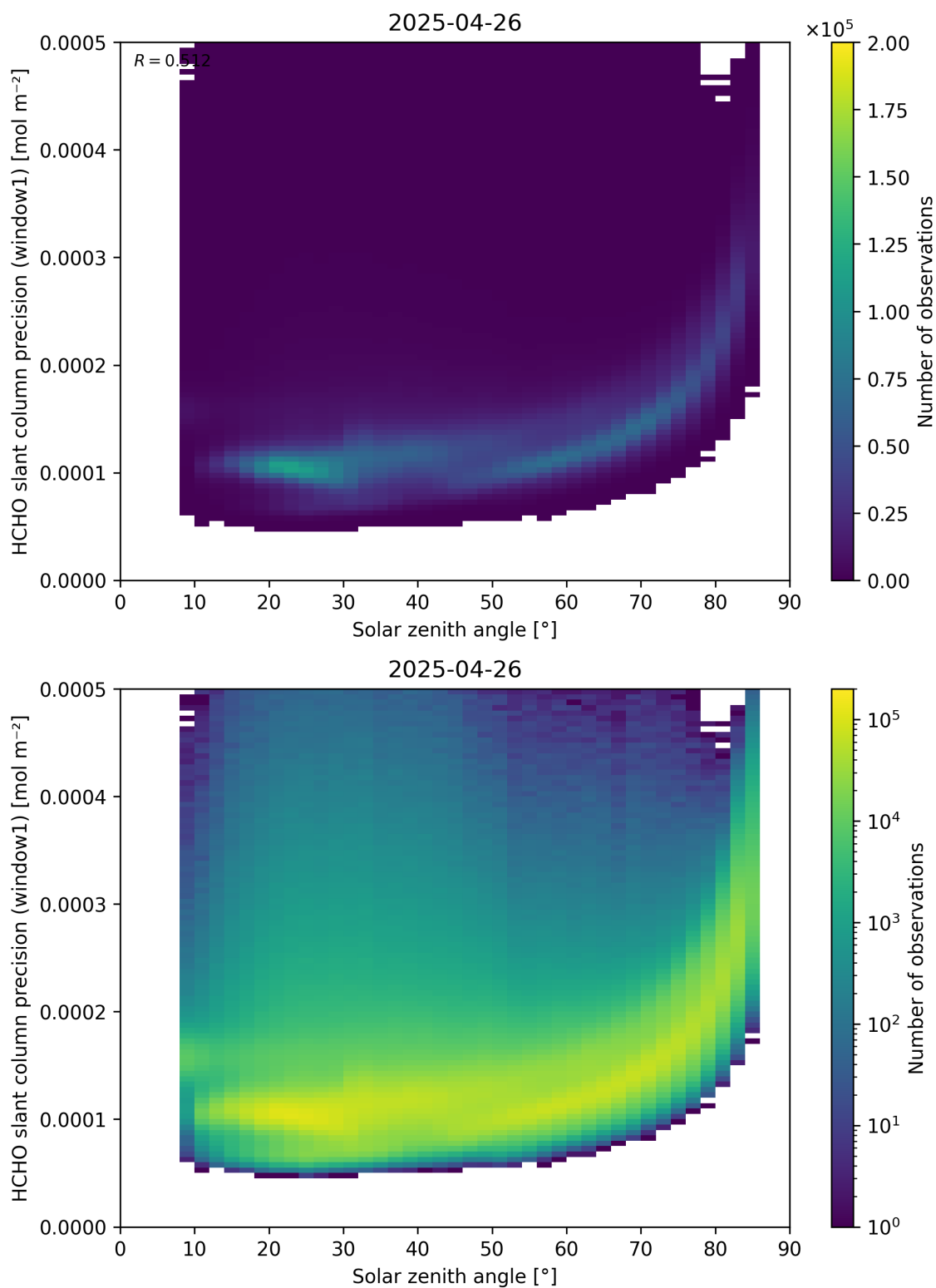
Figure 174: Scatter density plot of “Solar zenith angle” against “HCHO slant column precision (window1)” for 2025-04-25 to 2025-04-27.
