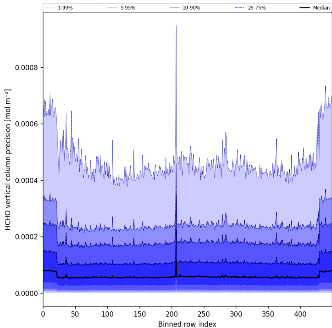
Figure 50: Along track statistics of “HCHO vertical column precision” for 2025-04-25 to 2025-04-27
