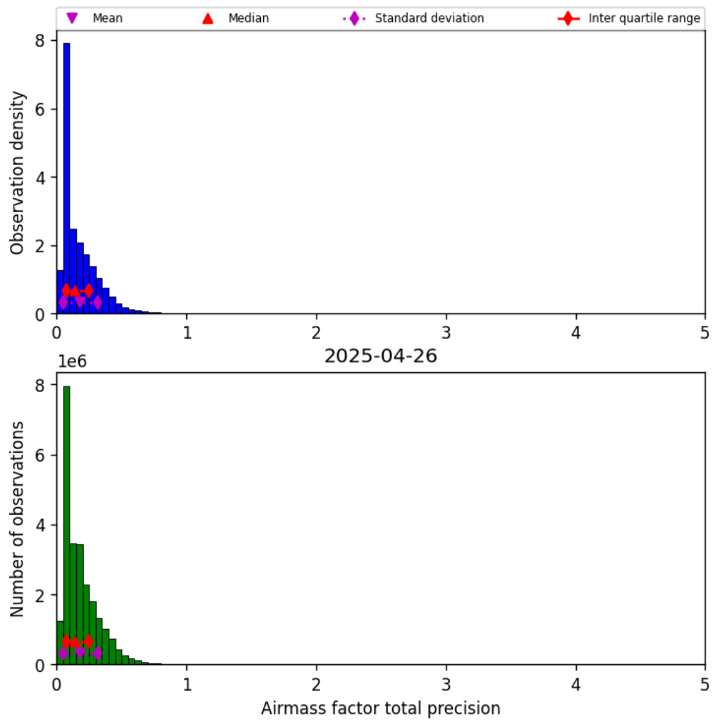
Figure 41: Histogram of “Airmass factor total precision” for 2025-04-25 to 2025-04-27
