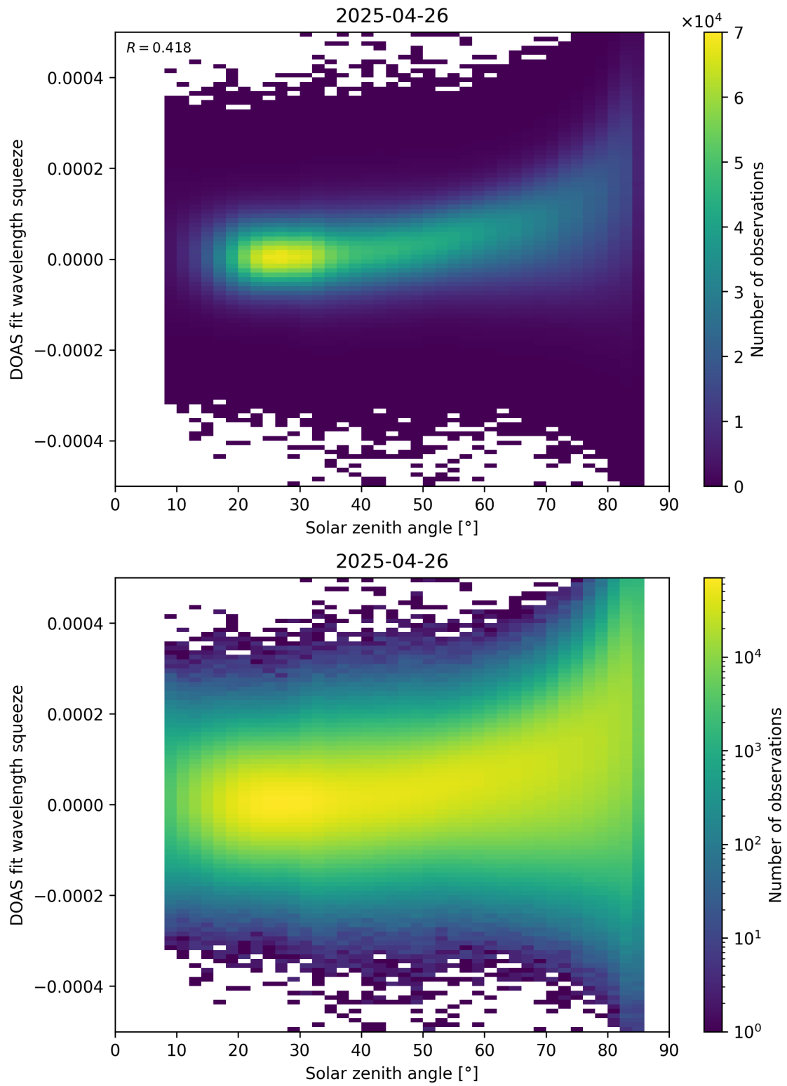
Figure 169: Scatter density plot of “Solar zenith angle” against “DOAS fit wavelength squeeze” for 2025-04-25 to 2025-04-27.
