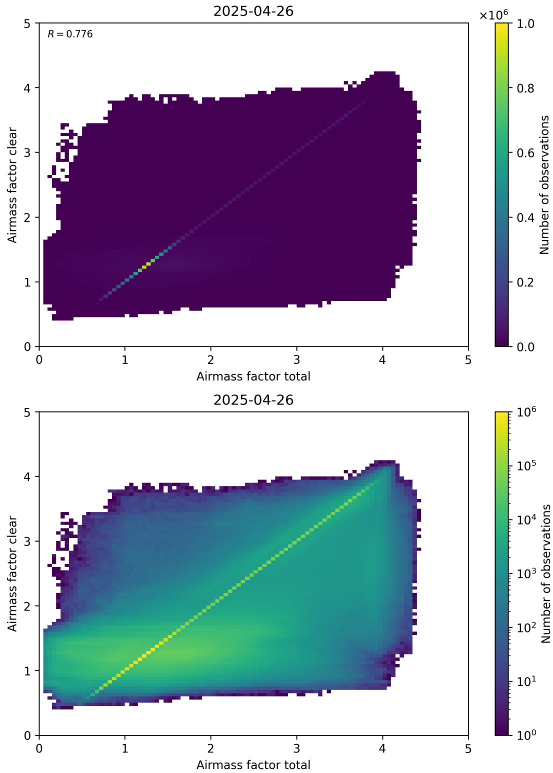
Figure 100: Scatter density plot of “Airmass factor total” against “Airmass factor clear” for 2025-04-25 to 2025-04-27.
