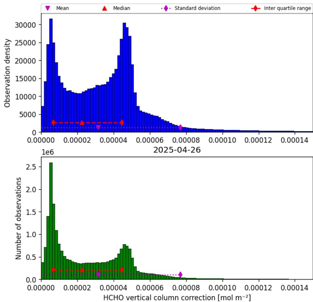
Figure 37: Histogram of “HCHO vertical column correction” for 2025-04-25 to 2025-04-27
