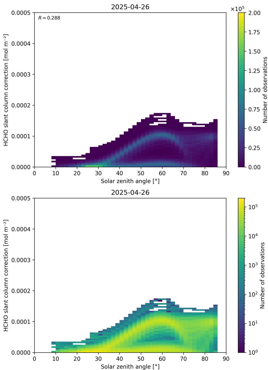
Figure 172: Scatter density plot of “Solar zenith angle” against “HCHO slant column correction” for 2025-04-25 to 2025-04-27.
