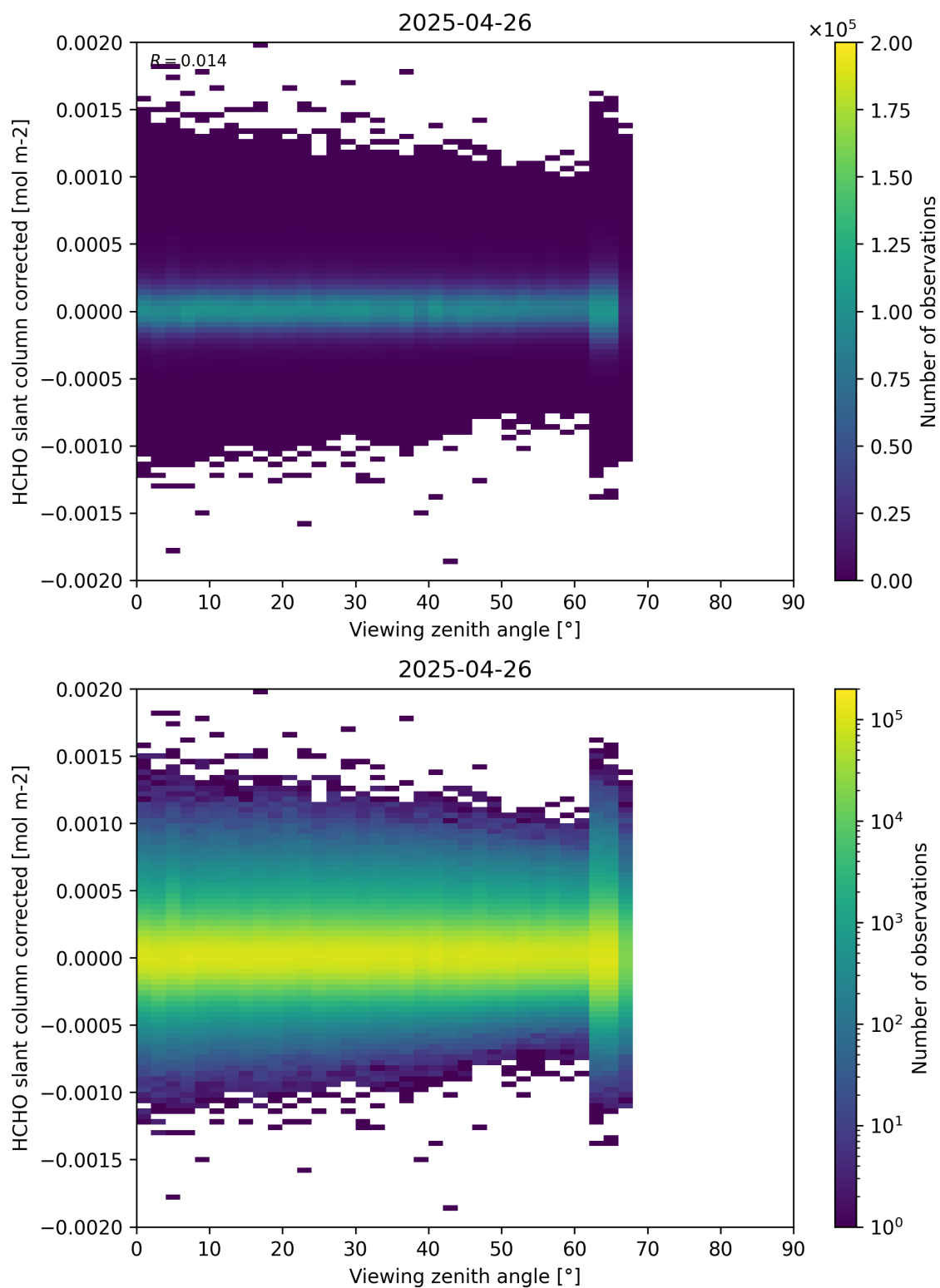
Figure 186: Scatter density plot of “Viewing zenith angle” against “HCHO slant column corrected” for 2025-04-25 to 2025-04-27.
