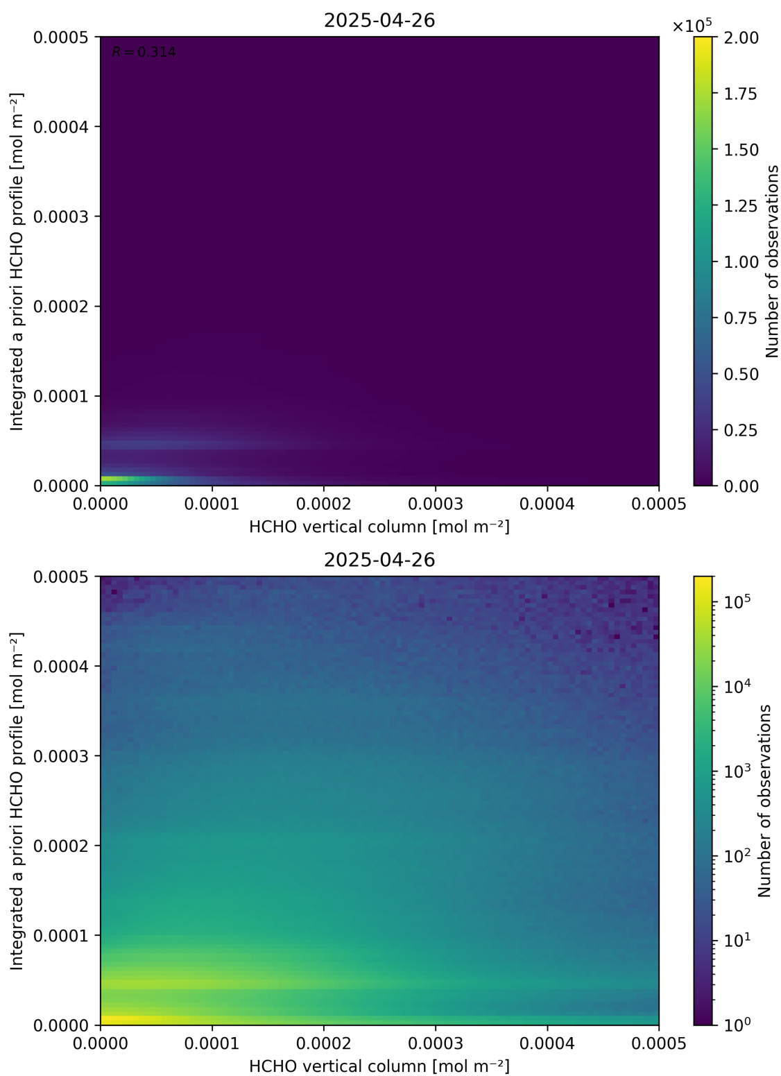
Figure 135: Scatter density plot of “HCHO vertical column” against “Integrated a priori HCHO profile” for 2025-04-25 to 2025-04-27.
