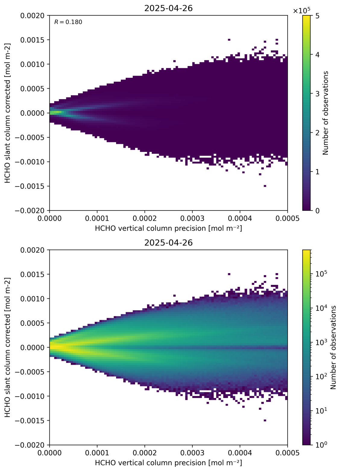
Figure 140: Scatter density plot of “HCHO vertical column precision” against “HCHO slant column corrected” for 2025-04-25 to 2025-04-27.
