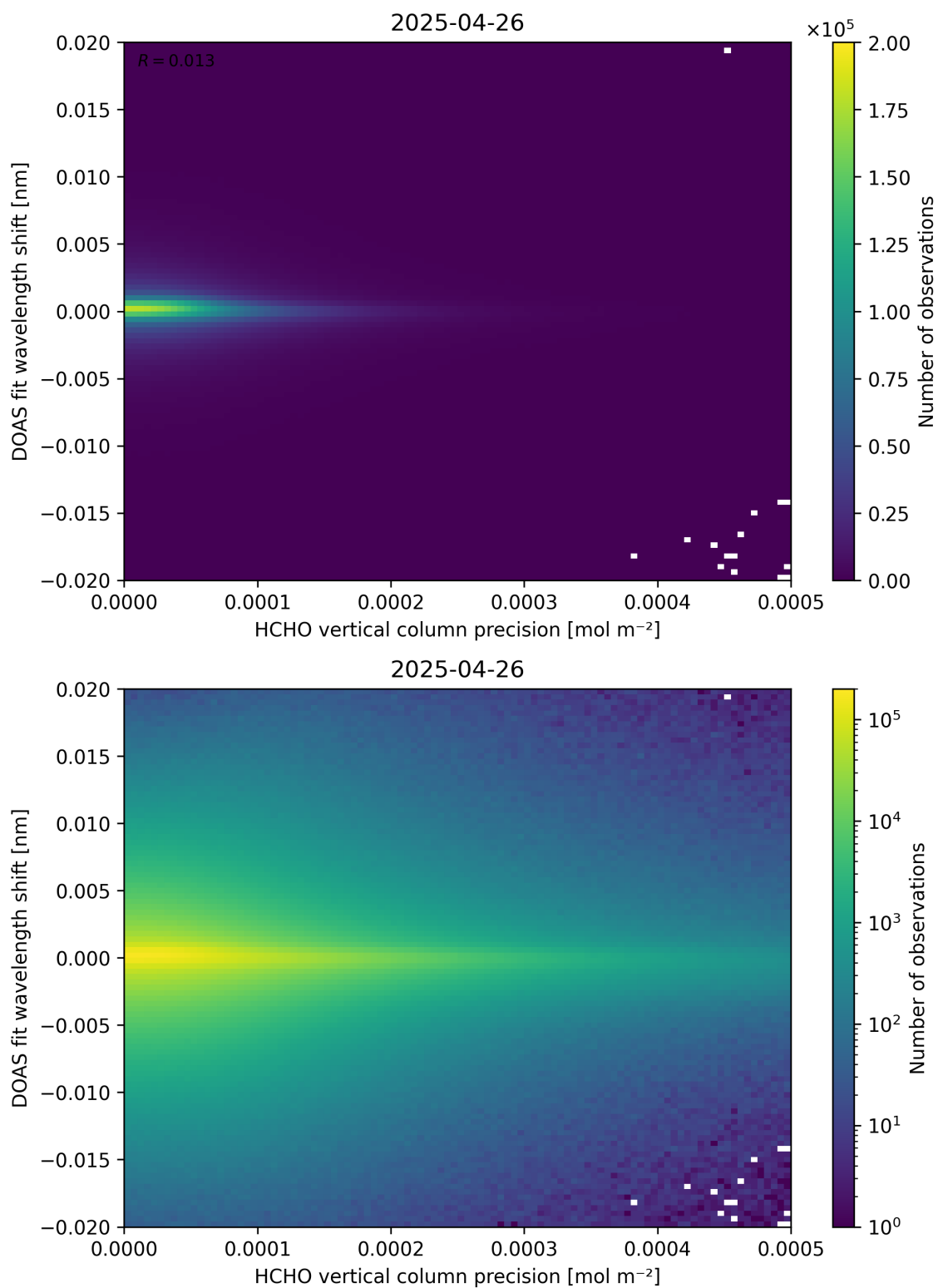
Figure 137: Scatter density plot of “HCHO vertical column precision” against “DOAS fit wavelength shift” for 2025-04-25 to 2025-04-27.
