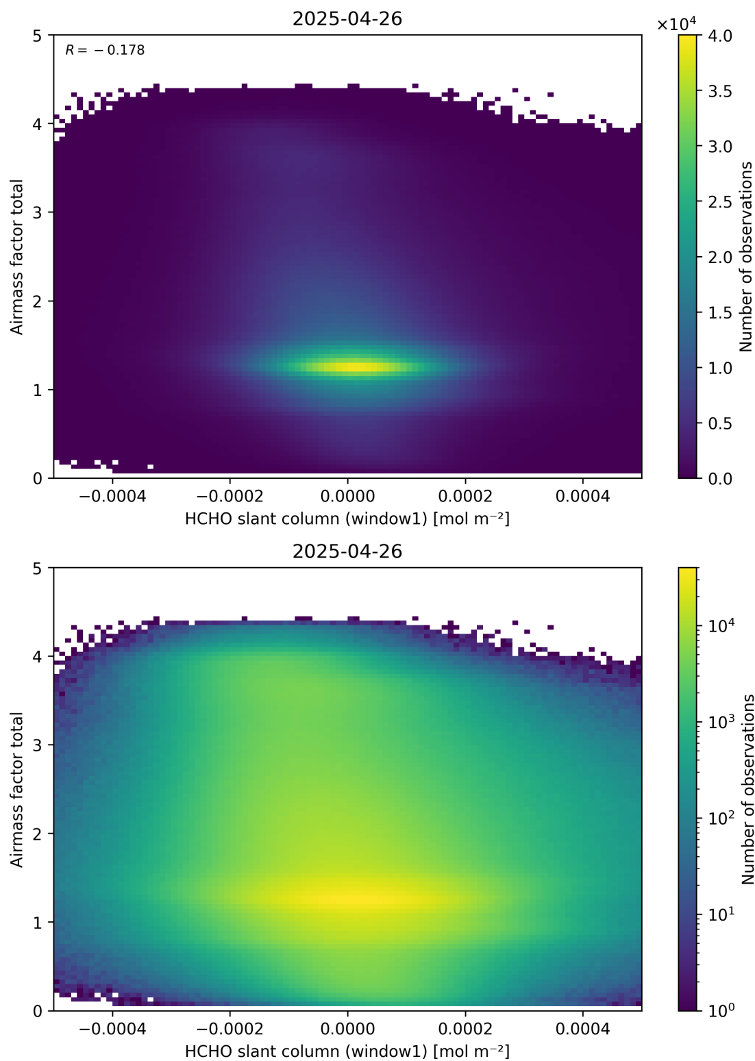
Figure 85: Scatter density plot of “HCHO slant column (window1)” against “Airmass factor total” for 2025-04-25 to 2025-04-27.
