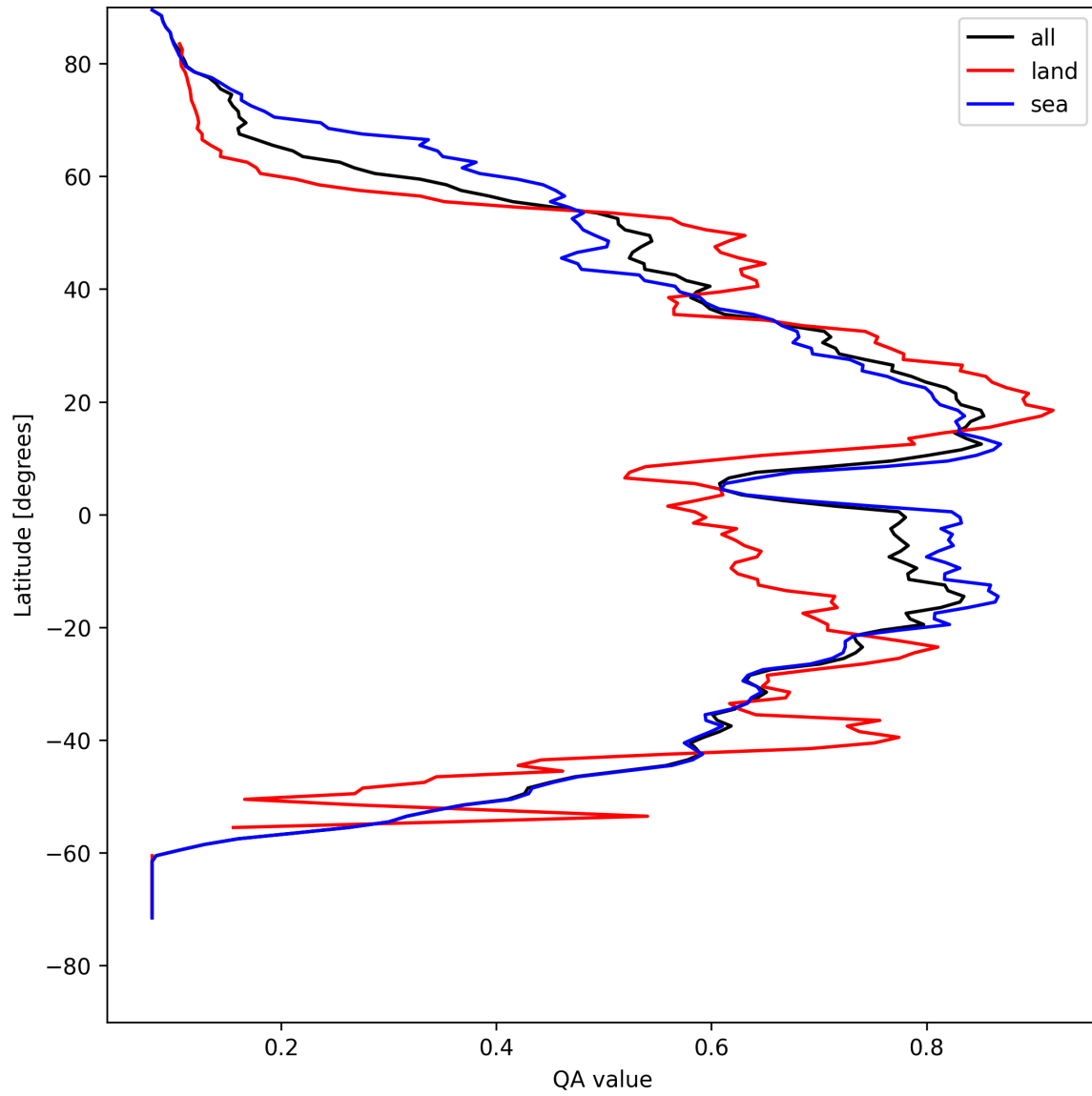
Figure 20: Zonal average of “QA value” for 2025-04-25 to 2025-04-27.
