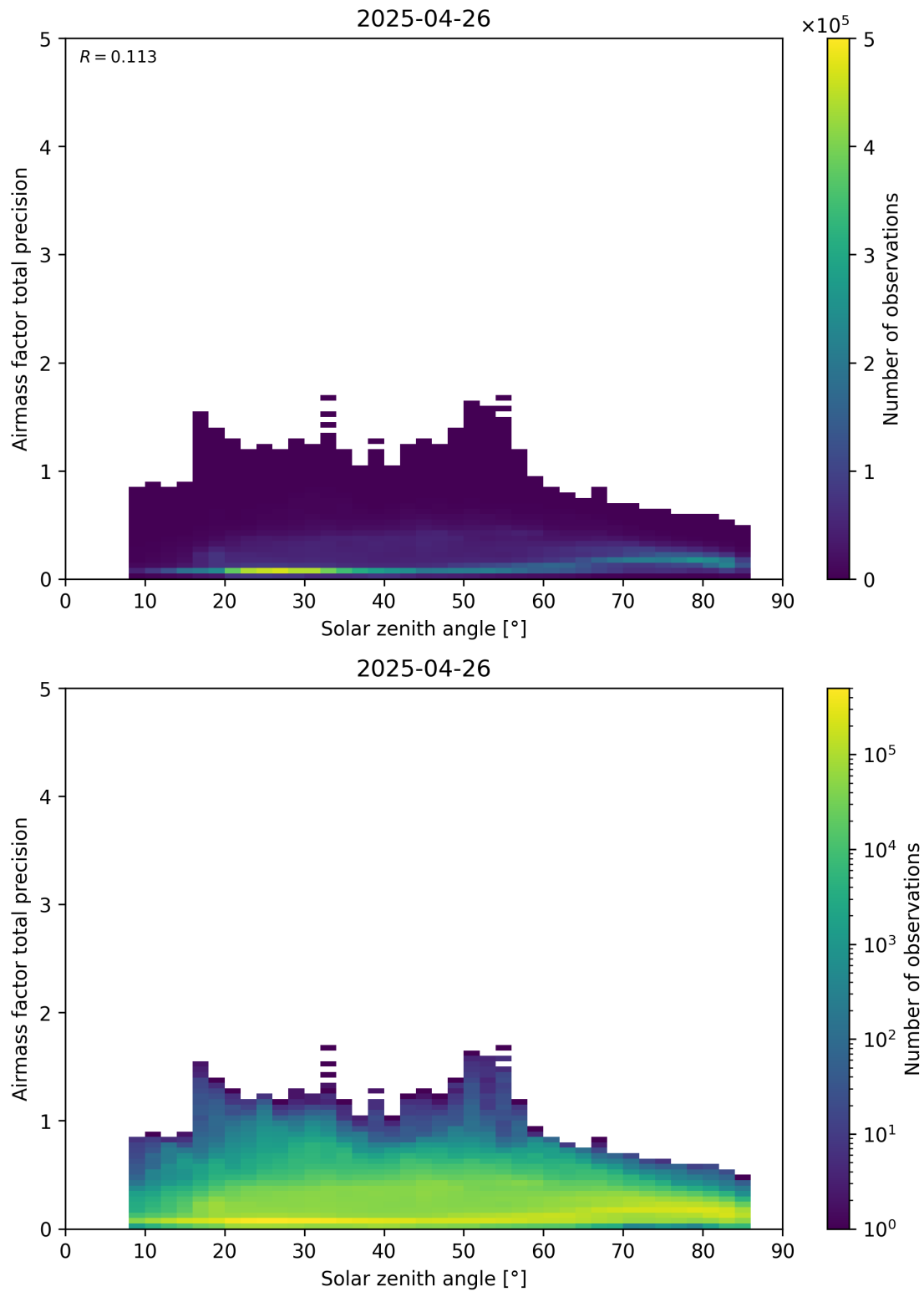
Figure 176: Scatter density plot of “Solar zenith angle” against “Airmass factor total precision” for 2025-04-25 to 2025-04-27.
