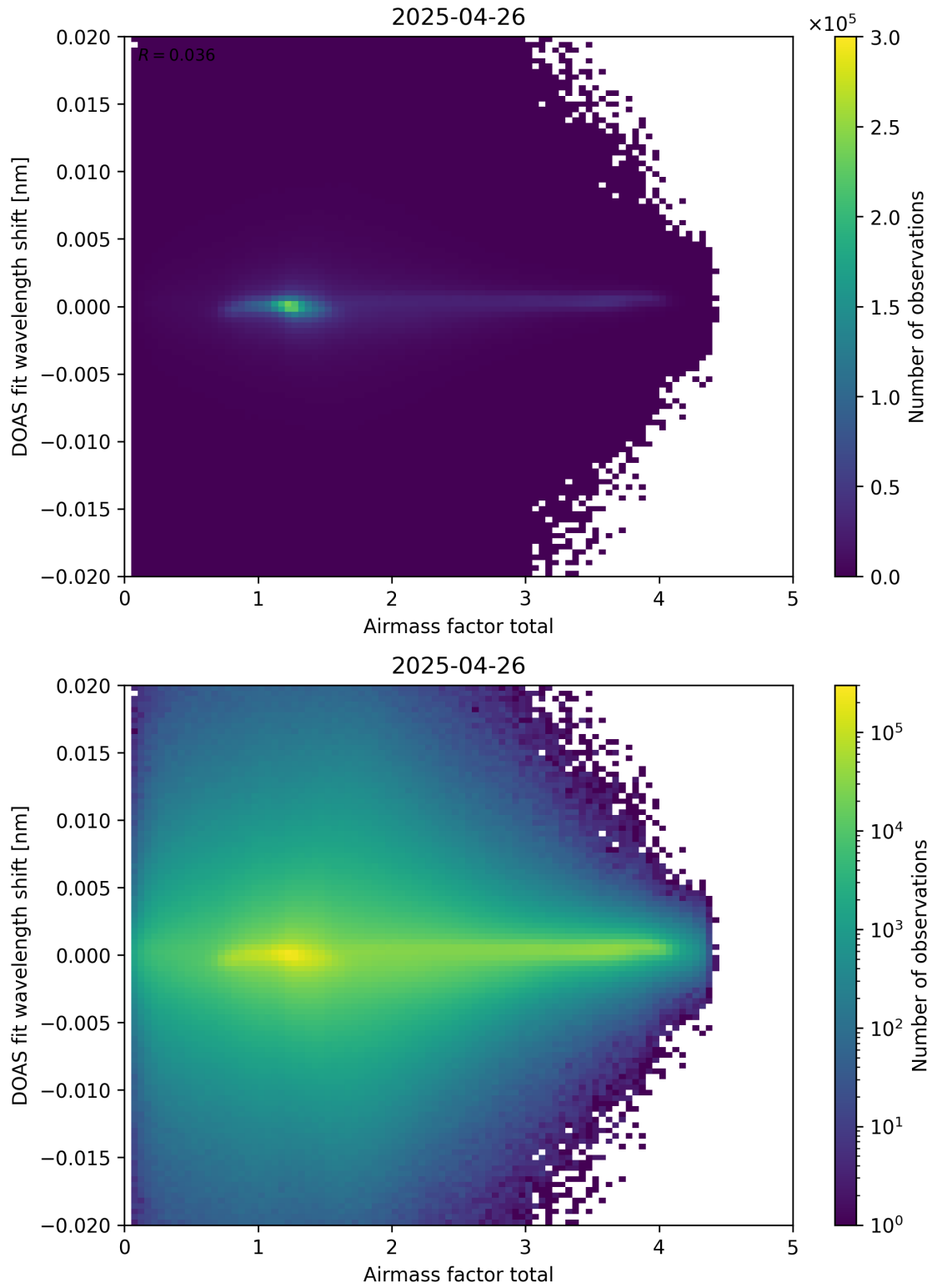
Figure 98: Scatter density plot of “Airmass factor total” against “DOAS fit wavelength shift” for 2025-04-25 to 2025-04-27.
