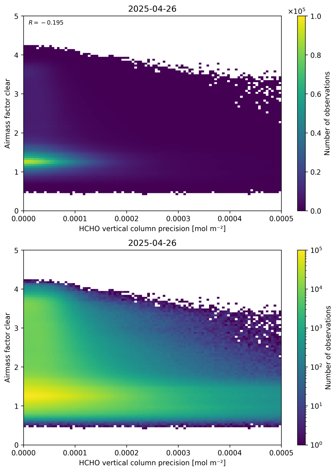
Figure 139: Scatter density plot of “HCHO vertical column precision” against “Airmass factor clear” for 2025-04-25 to 2025-04-27.
