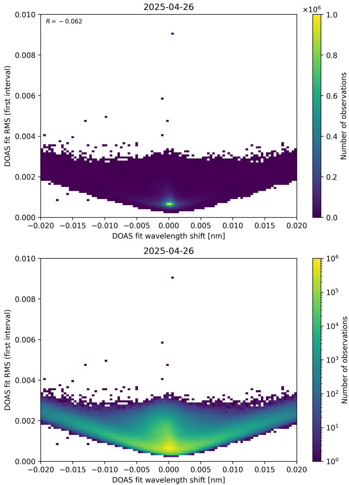
Figure 64: Scatter density plot of “DOAS fit wavelength shift” against “DOAS fit RMS (first interval)” for 2025-04-25 to 2025-04-27.
