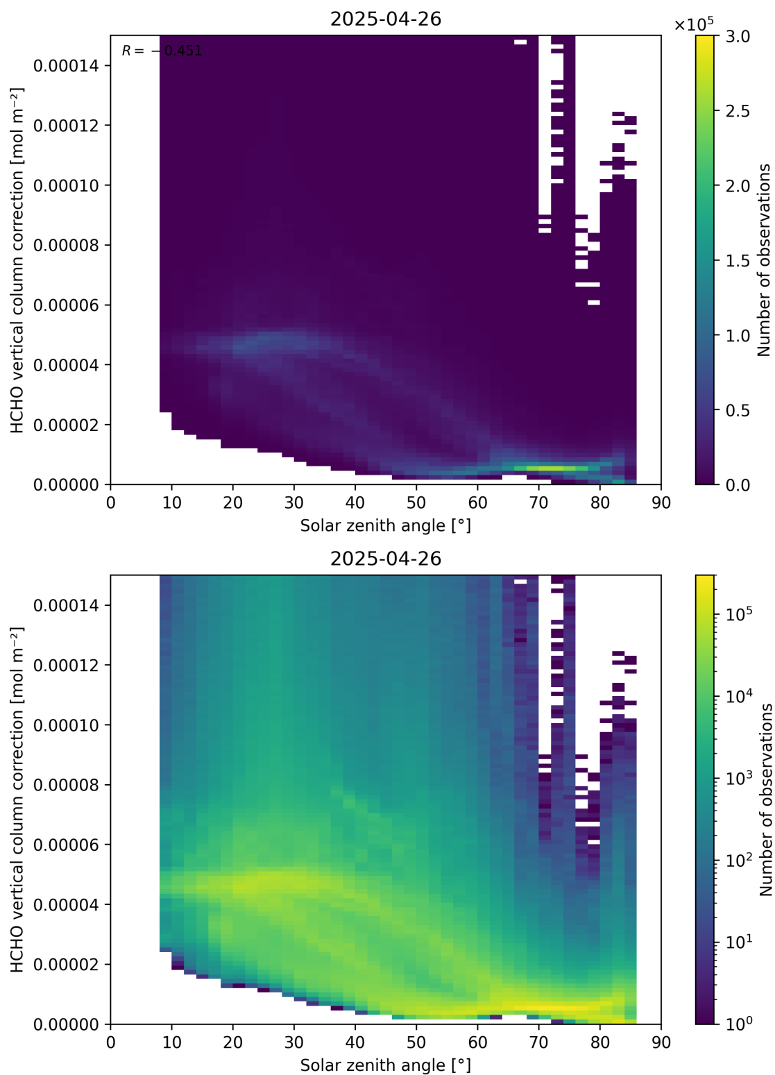
Figure 178: Scatter density plot of “Solar zenith angle” against “HCHO vertical column correction” for 2025-04-25 to 2025-04-27.
