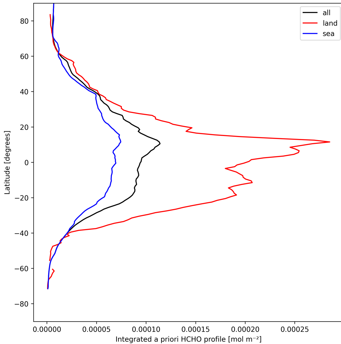
Figure 29: Zonal average of “Integrated a priori HCHO profile” for 2025-04-25 to 2025-04-27.
