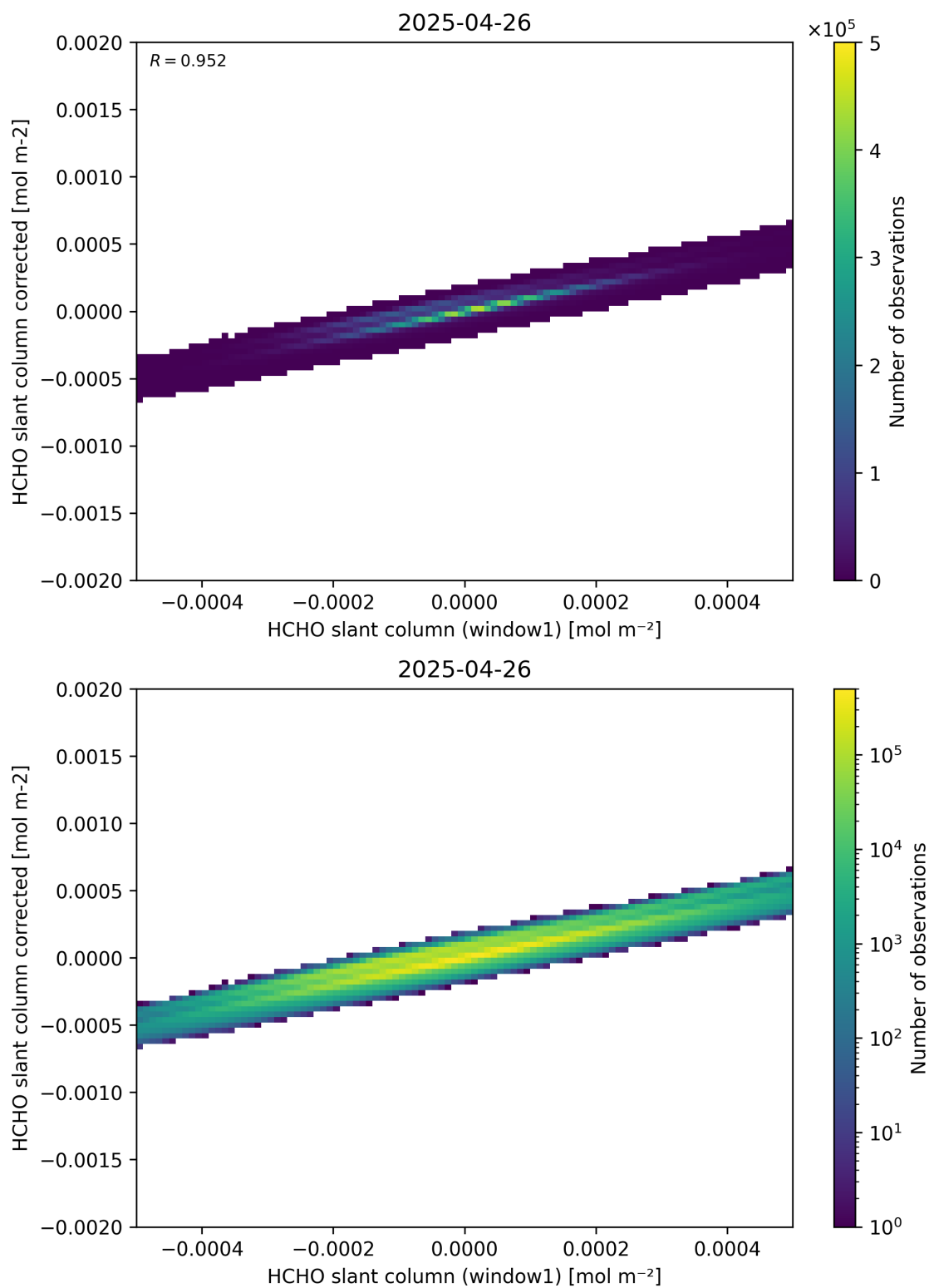
Figure 82: Scatter density plot of “HCHO slant column (window1)” against “HCHO slant column corrected” for 2025-04-25 to 2025-04-27.
