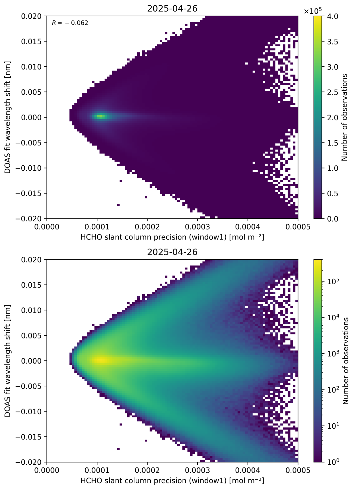
Figure 89: Scatter density plot of “HCHO slant column precision (window1)” against “DOAS fit wavelength shift” for 2025-04-25 to 2025-04-27.
