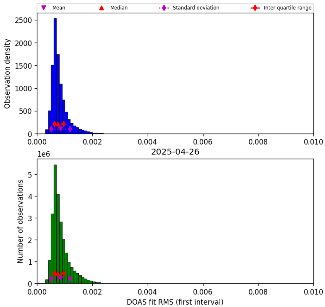
Figure 46: Histogram of “DOAS fit RMS (first interval)” for 2025-04-25 to 2025-04-27
