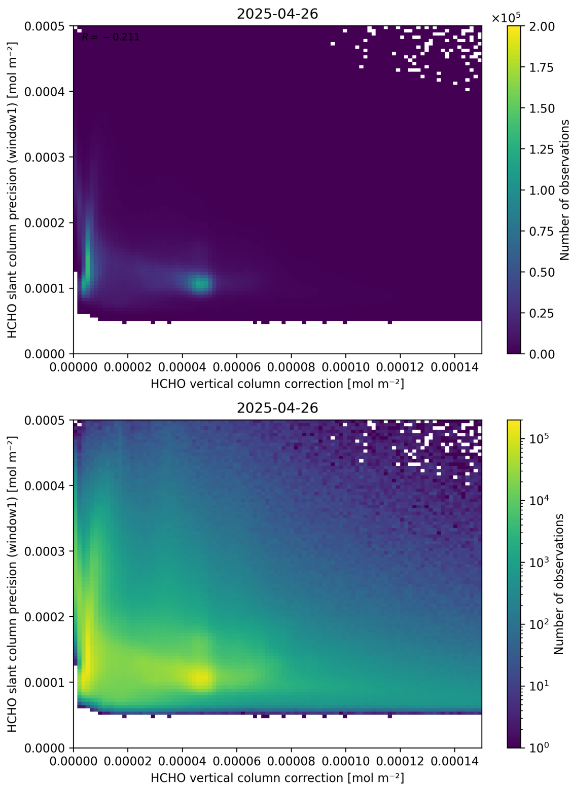
Figure 119: Scatter density plot of “HCHO vertical column correction” against “HCHO slant column precision (window1)” for 2025-04-25 to 2025-04-27.
