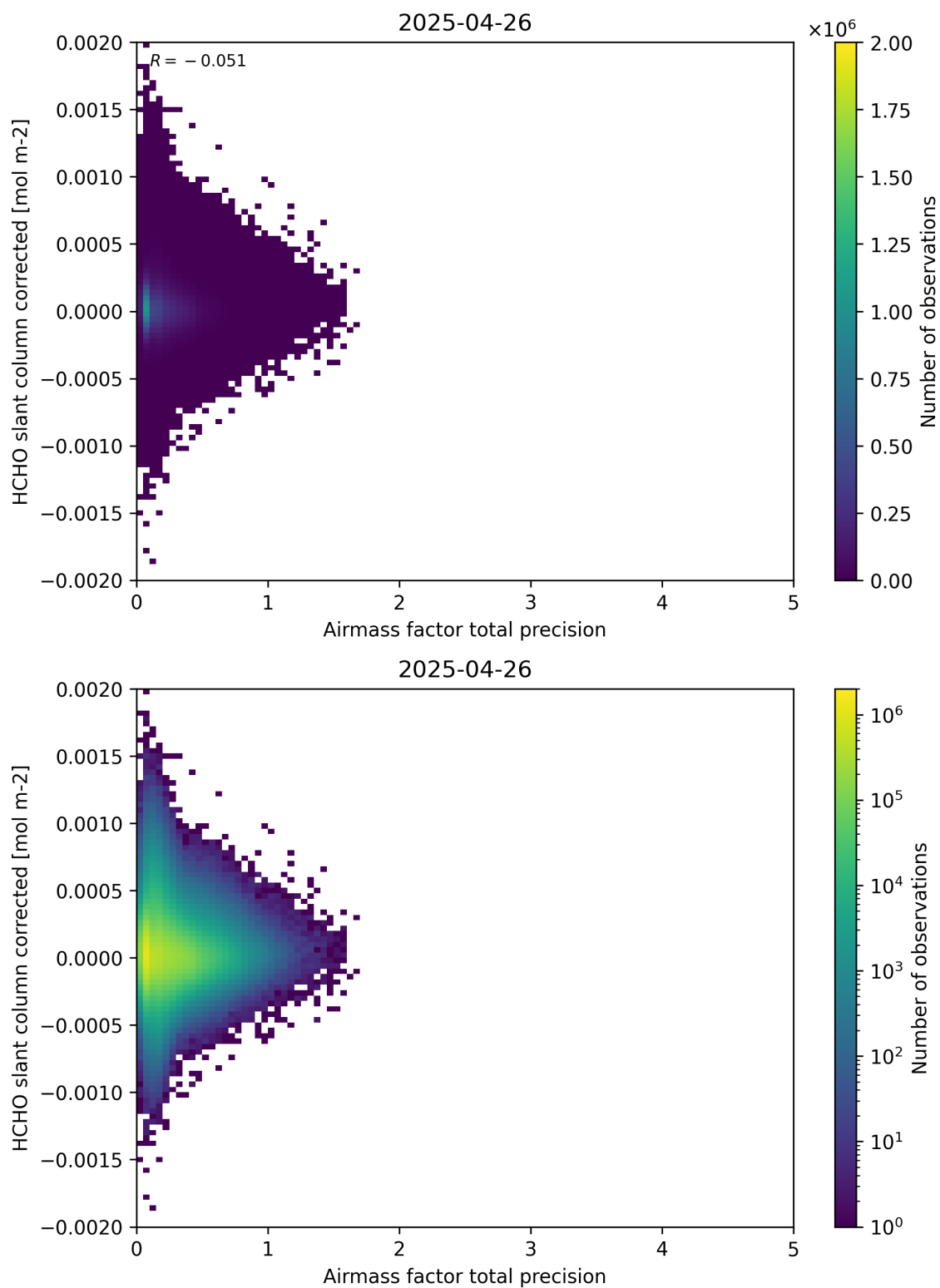
Figure 109: Scatter density plot of “Airmass factor total precision” against “HCHO slant column corrected” for 2025-04-25 to 2025-04-27.
