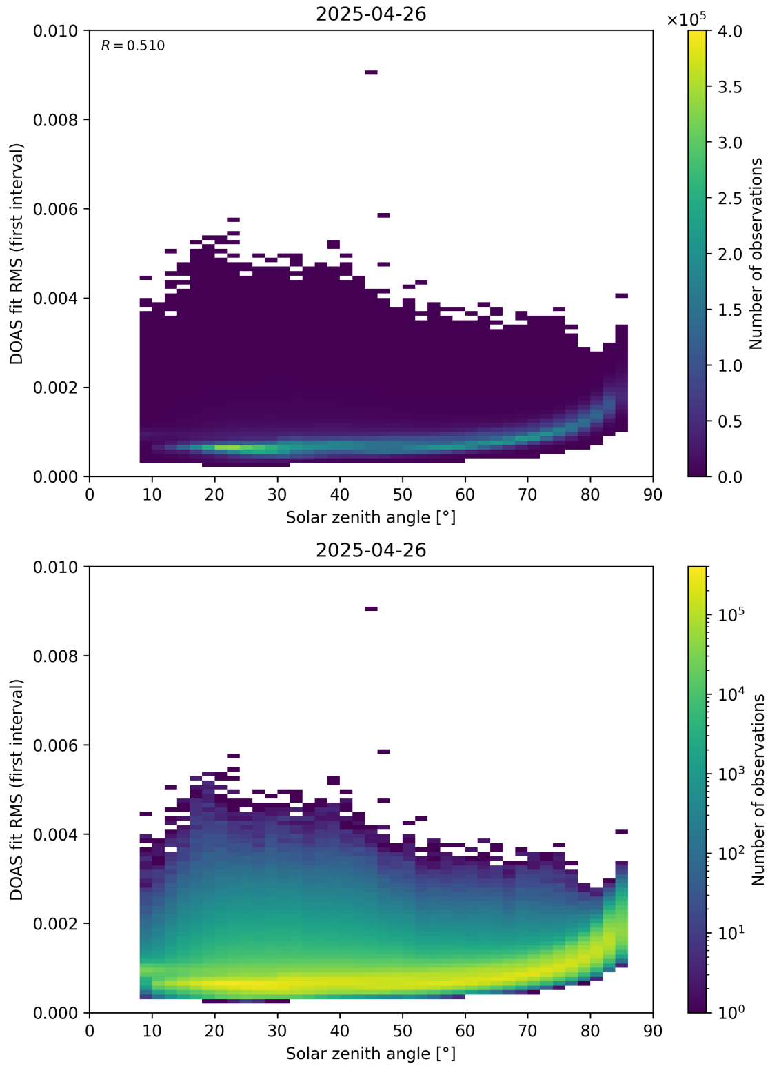
Figure 167: Scatter density plot of “Solar zenith angle” against “DOAS fit RMS (first interval)” for 2025-04-25 to 2025-04-27.
