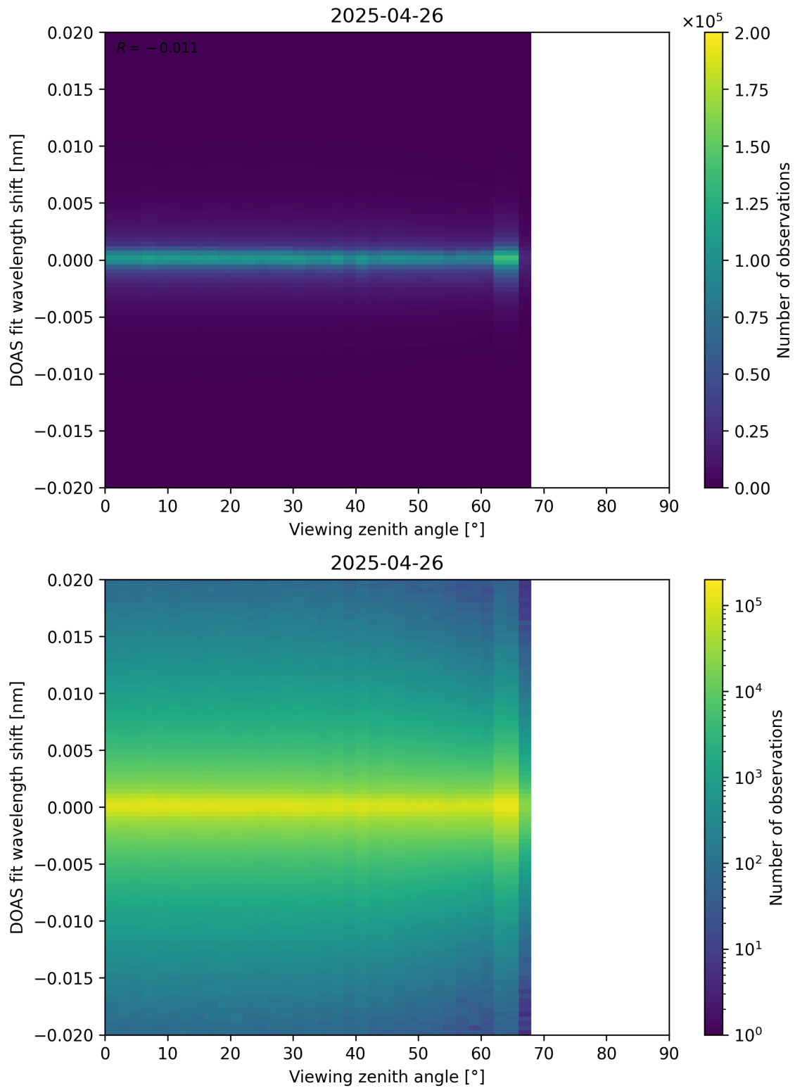
Figure 183: Scatter density plot of “Viewing zenith angle” against “DOAS fit wavelength shift” for 2025-04-25 to 2025-04-27.
