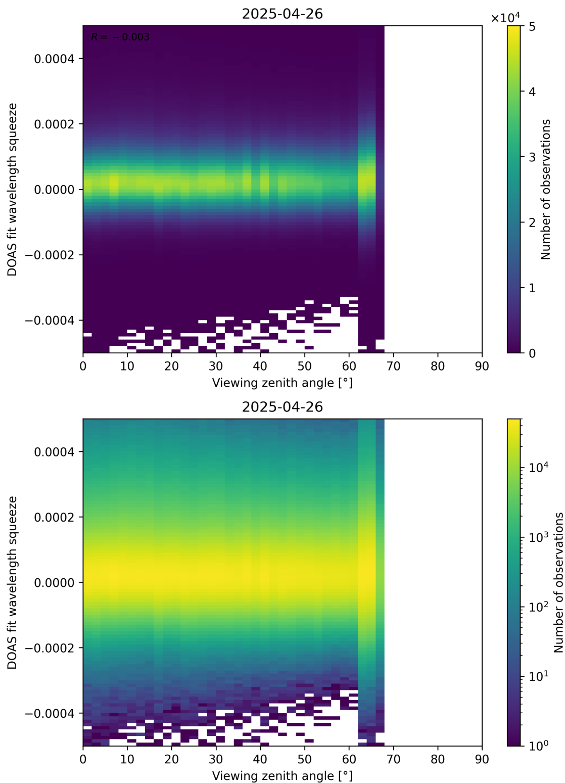
Figure 184: Scatter density plot of “Viewing zenith angle” against “DOAS fit wavelength squeeze” for 2025-04-25 to 2025-04-27.
