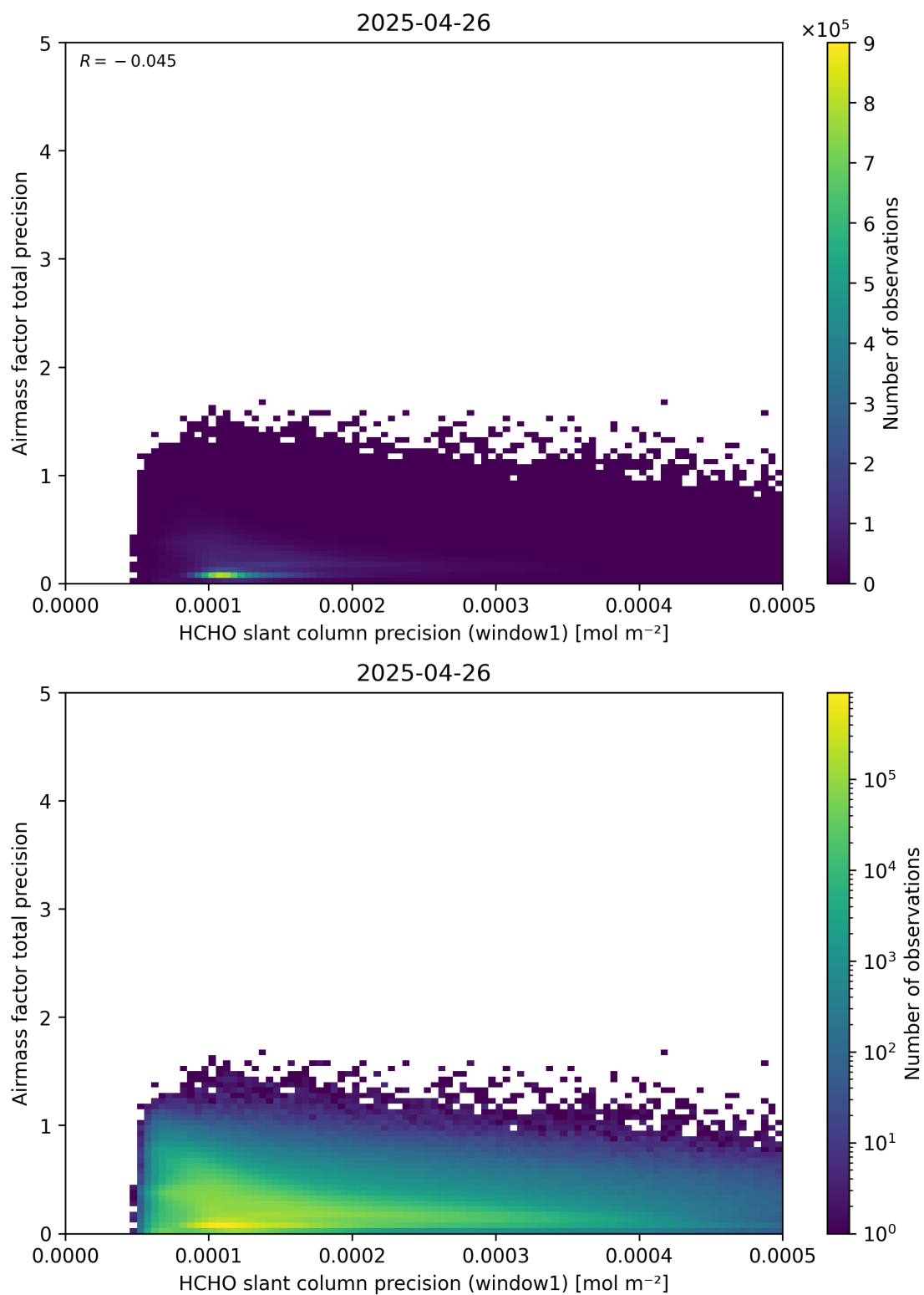
Figure 95: Scatter density plot of “HCHO slant column precision (window1)” against “Airmass factor total precision” for 2025-04-25 to 2025-04-27.
