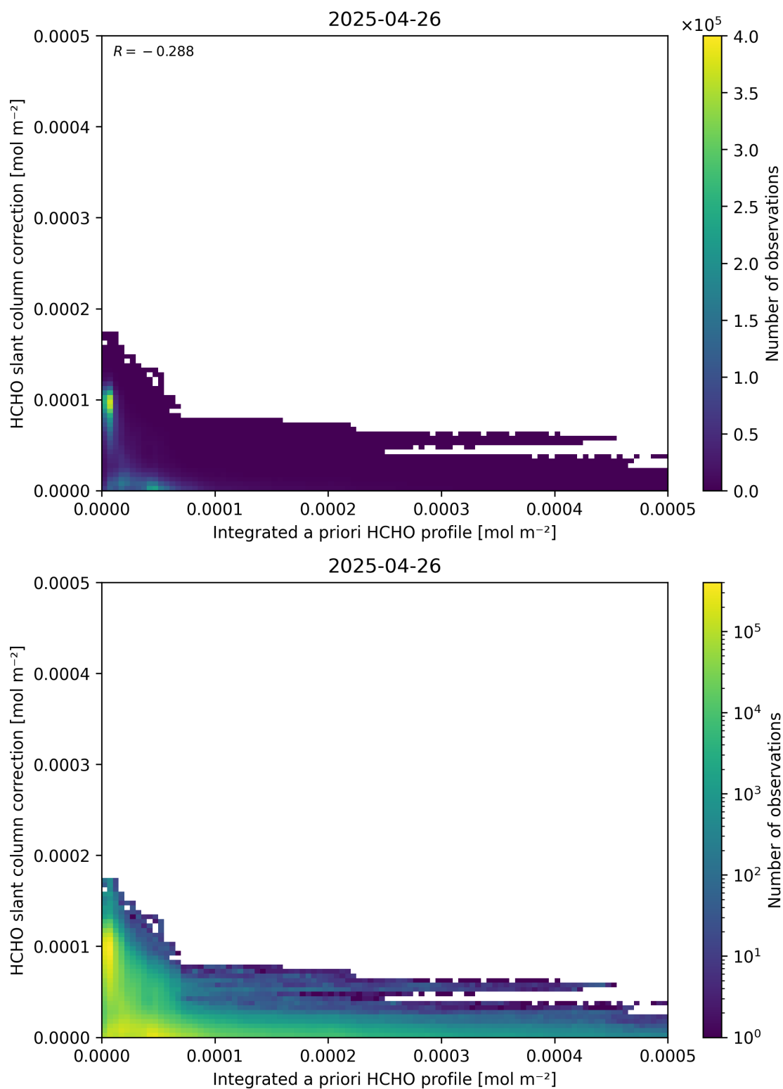
Figure 152: Scatter density plot of “Integrated a priori HCHO profile” against “HCHO slant column correction” for 2025-04-25 to 2025-04-27.
