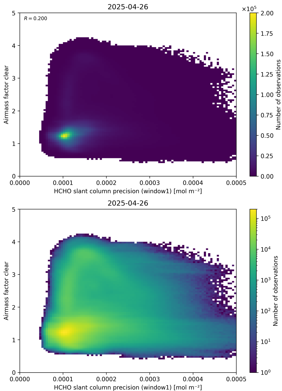
Figure 91: Scatter density plot of “HCHO slant column precision (window1)” against “Airmass factor clear” for 2025-04-25 to 2025-04-27.
