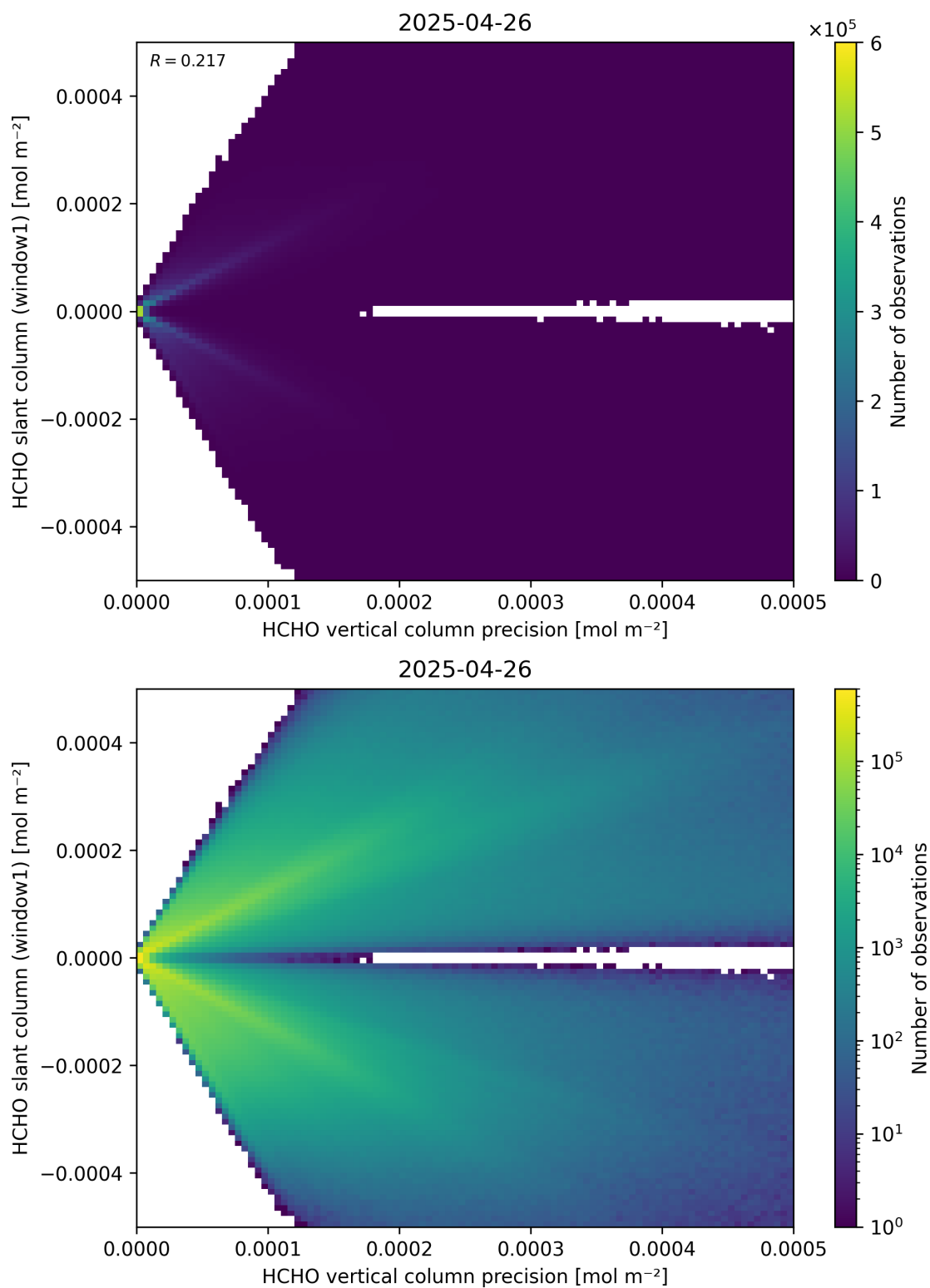
Figure 142: Scatter density plot of “HCHO vertical column precision” against “HCHO slant column (window1)” for 2025-04-25 to 2025-04-27.
