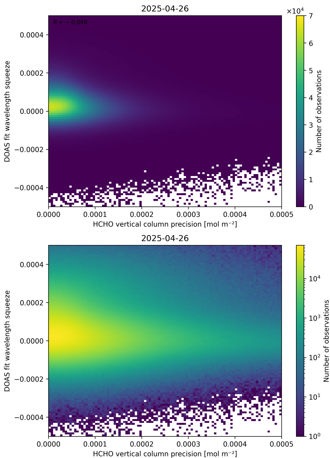
Figure 138: Scatter density plot of “HCHO vertical column precision” against “DOAS fit wavelength squeeze” for 2025-04-25 to 2025-04-27.
