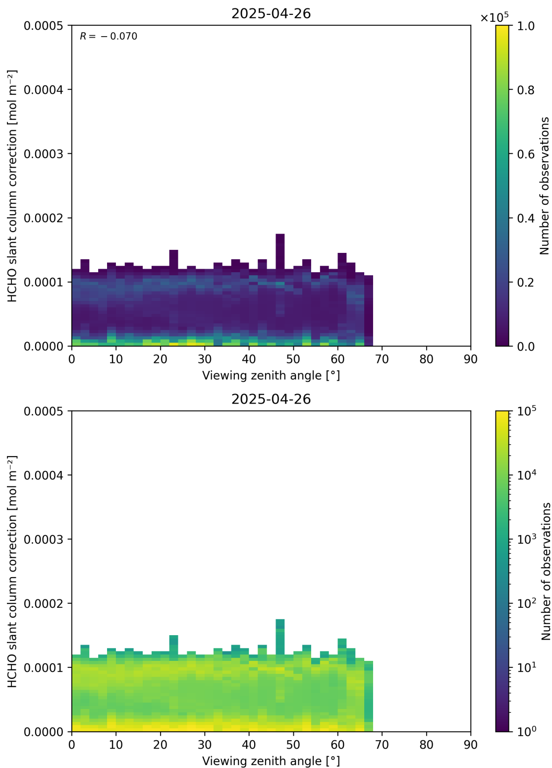
Figure 187: Scatter density plot of “Viewing zenith angle” against “HCHO slant column correction” for 2025-04-25 to 2025-04-27.
