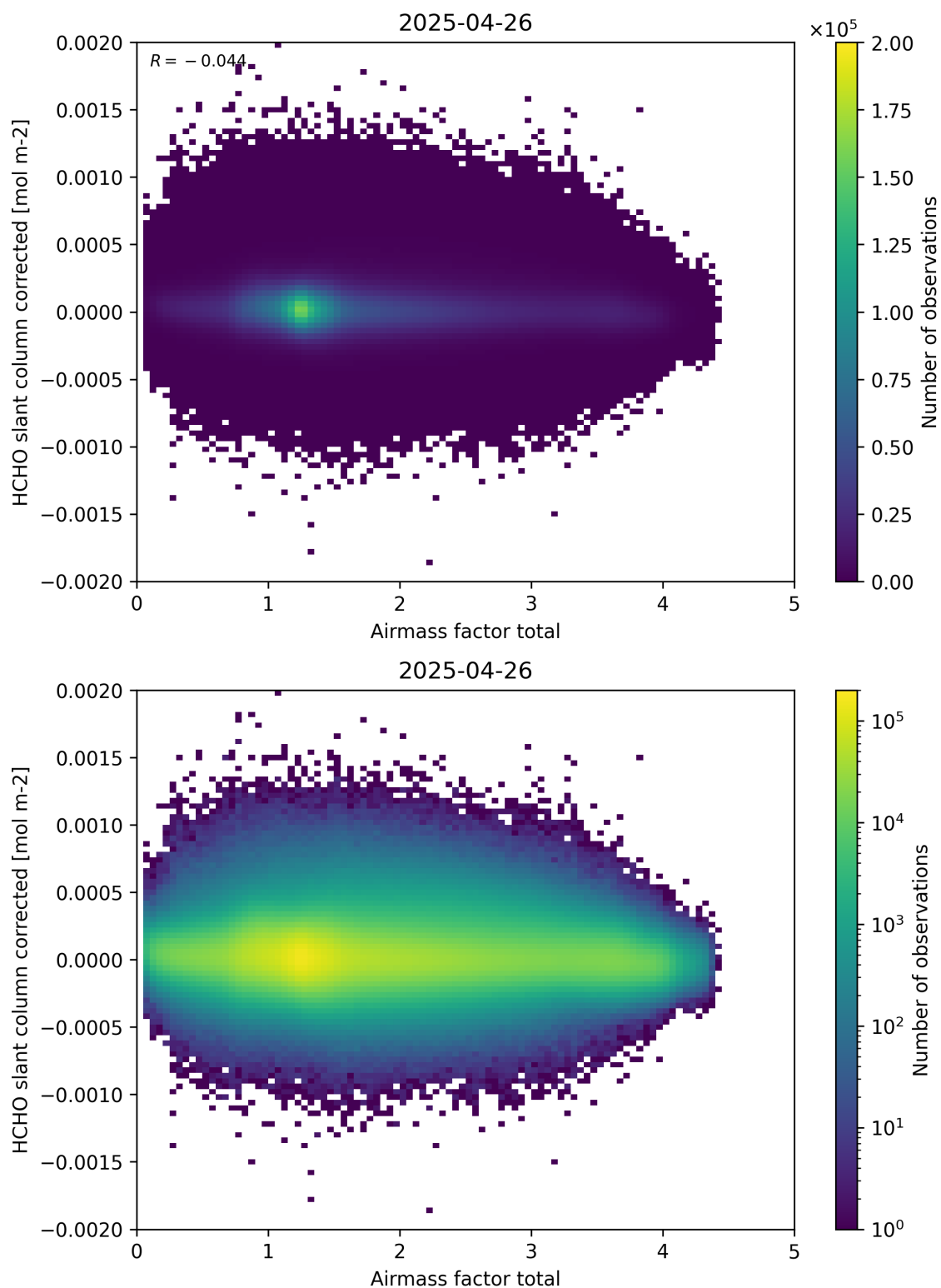
Figure 101: Scatter density plot of “Airmass factor total” against “HCHO slant column corrected” for 2025-04-25 to 2025-04-27.
