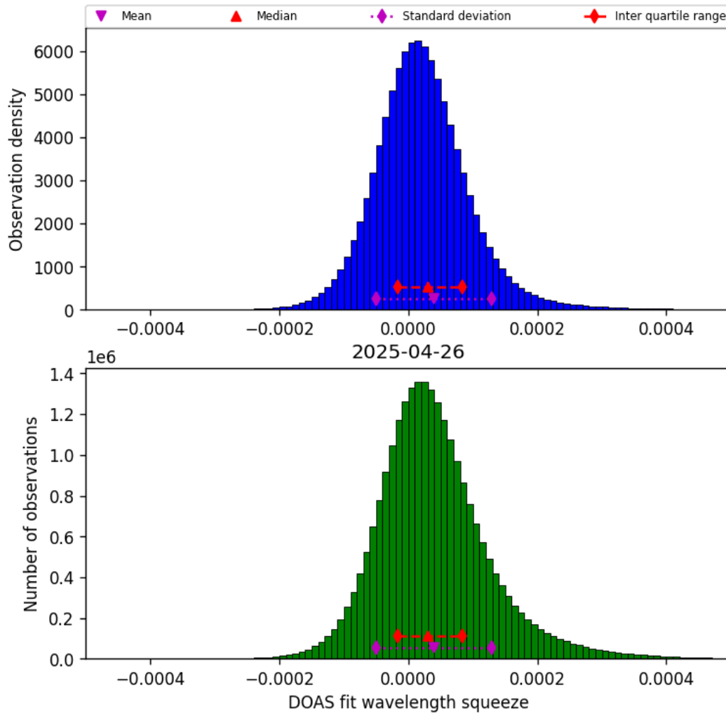
Figure 45: Histogram of “DOAS fit wavelength squeeze” for 2025-04-25 to 2025-04-27
