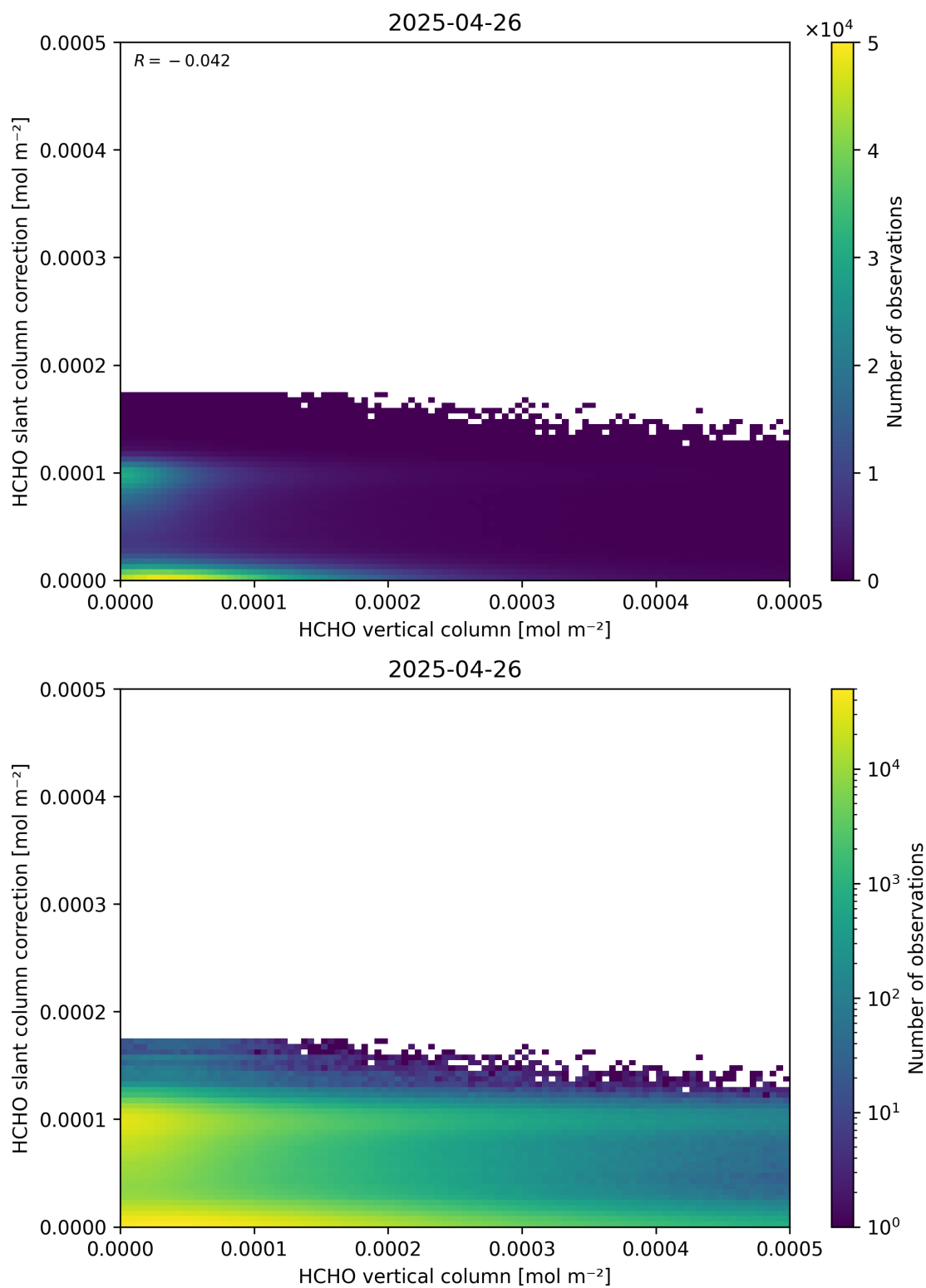
Figure 128: Scatter density plot of “HCHO vertical column” against “HCHO slant column correction” for 2025-04-25 to 2025-04-27.
