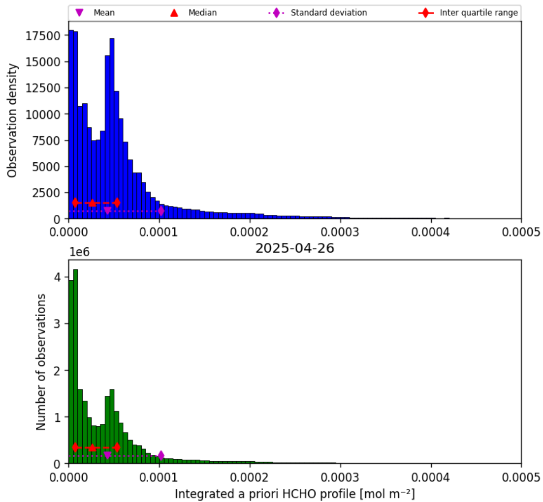
Figure 43: Histogram of “Integrated a priori HCHO profile” for 2025-04-25 to 2025-04-27
