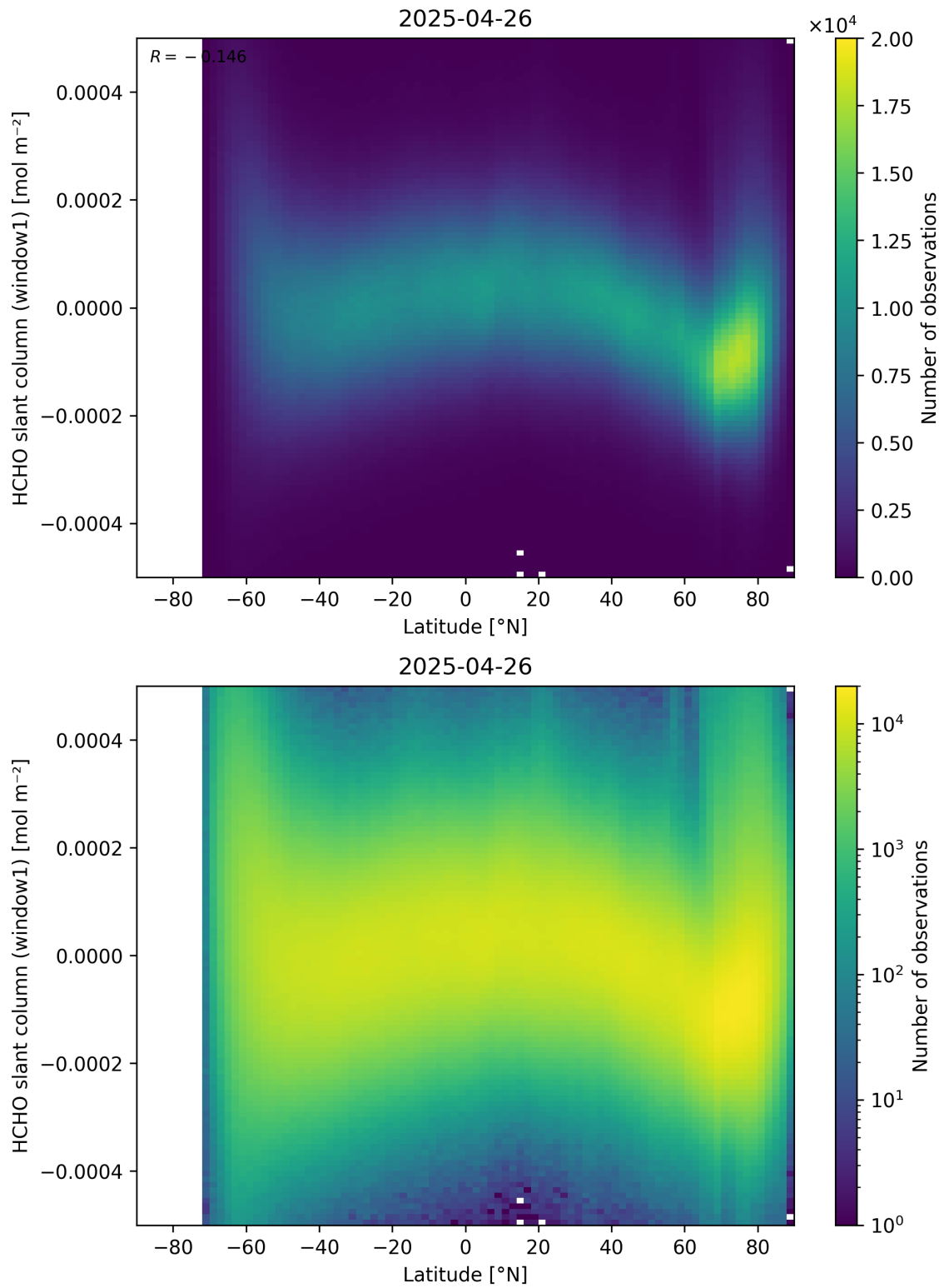
Figure 159: Scatter density plot of “Latitude” against “HCHO slant column (window1)” for 2025-04-25 to 2025-04-27.
