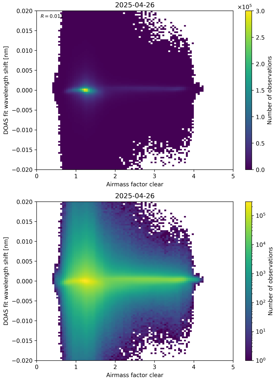
Figure 72: Scatter density plot of “Airmass factor clear” against “DOAS fit wavelength shift” for 2025-04-25 to 2025-04-27.
