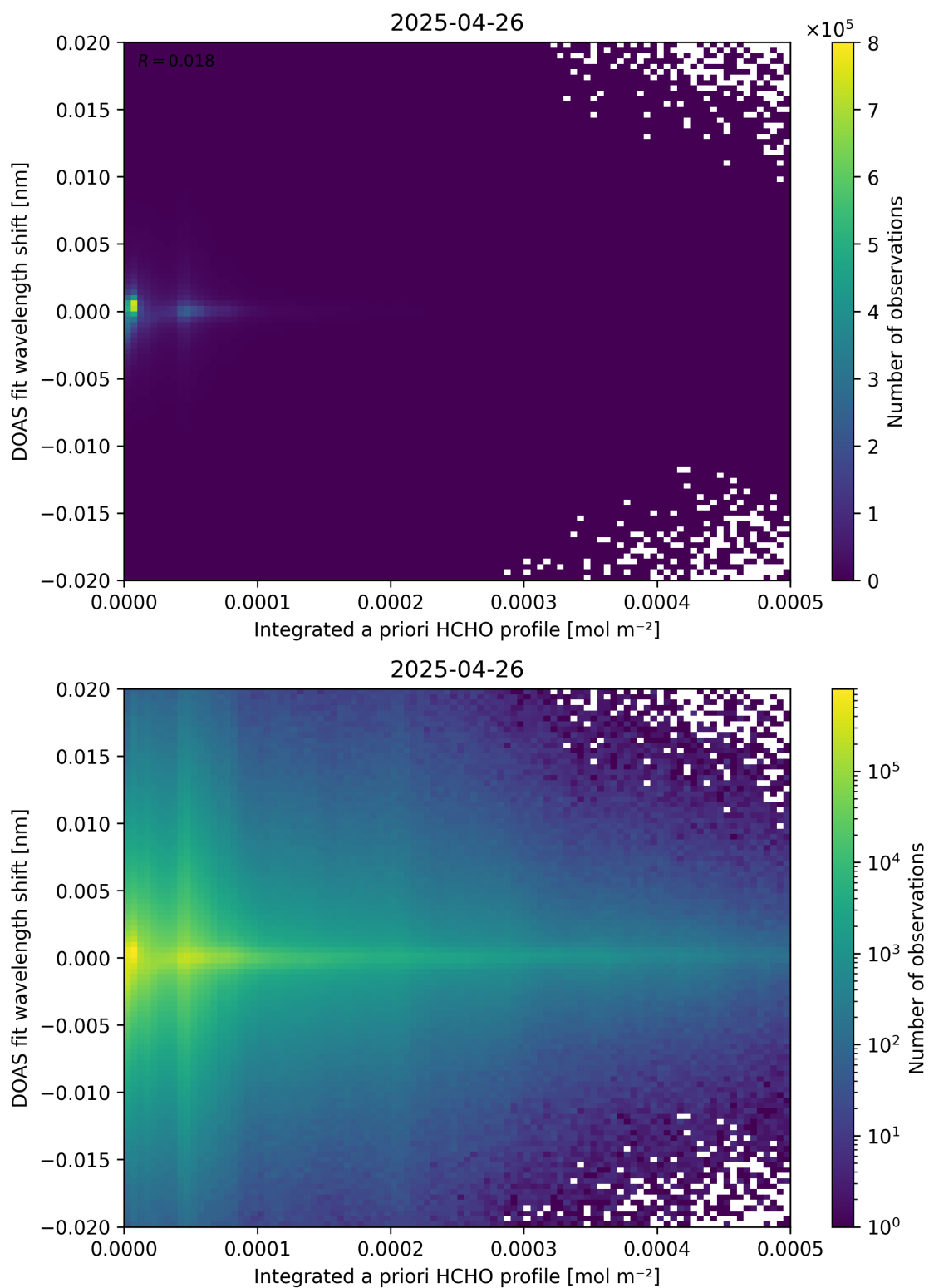
Figure 149: Scatter density plot of “Integrated a priori HCHO profile” against “DOAS fit wavelength shift” for 2025-04-25 to 2025-04-27.
