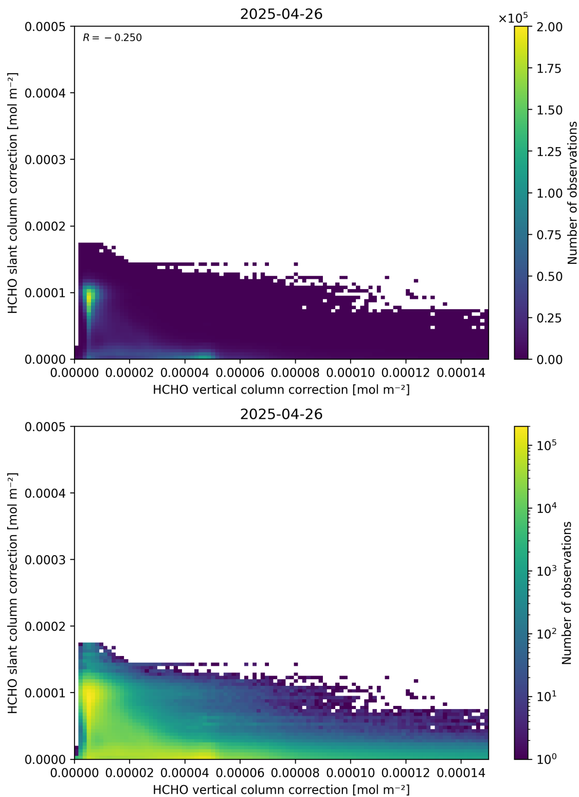
Figure 117: Scatter density plot of “HCHO vertical column correction” against “HCHO slant column correction” for 2025-04-25 to 2025-04-27.
