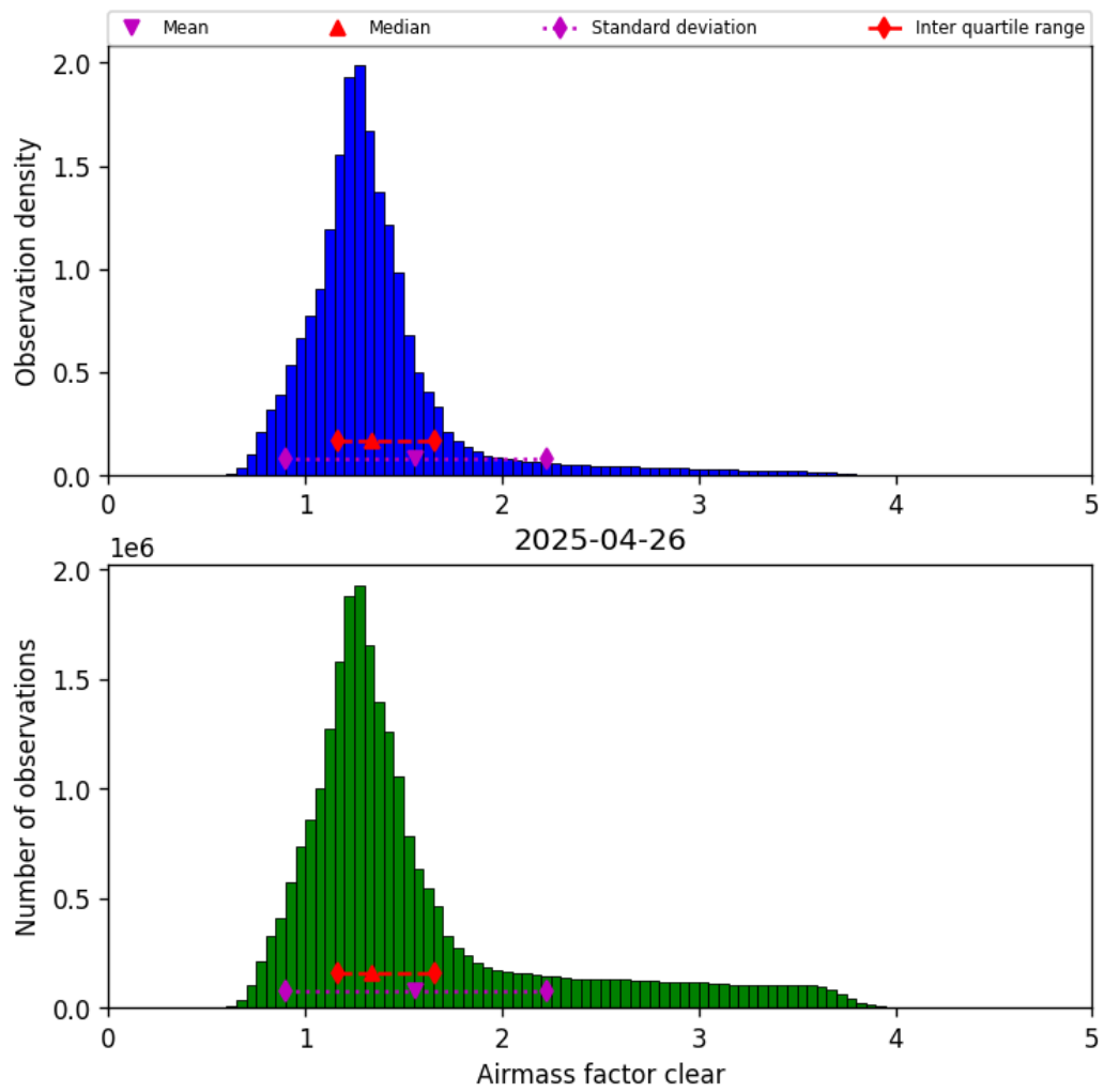
Figure 42: Histogram of “Airmass factor clear” for 2025-04-25 to 2025-04-27
