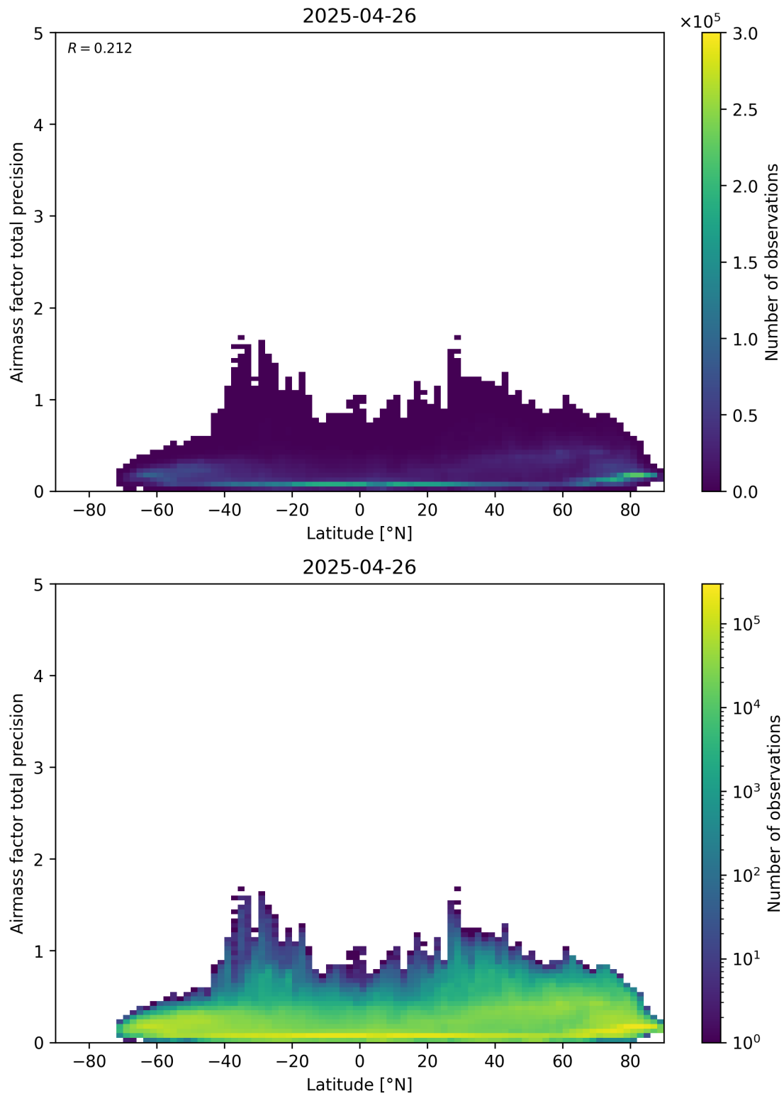
Figure 162: Scatter density plot of “Latitude” against “Airmass factor total precision” for 2025-04-25 to 2025-04-27.
