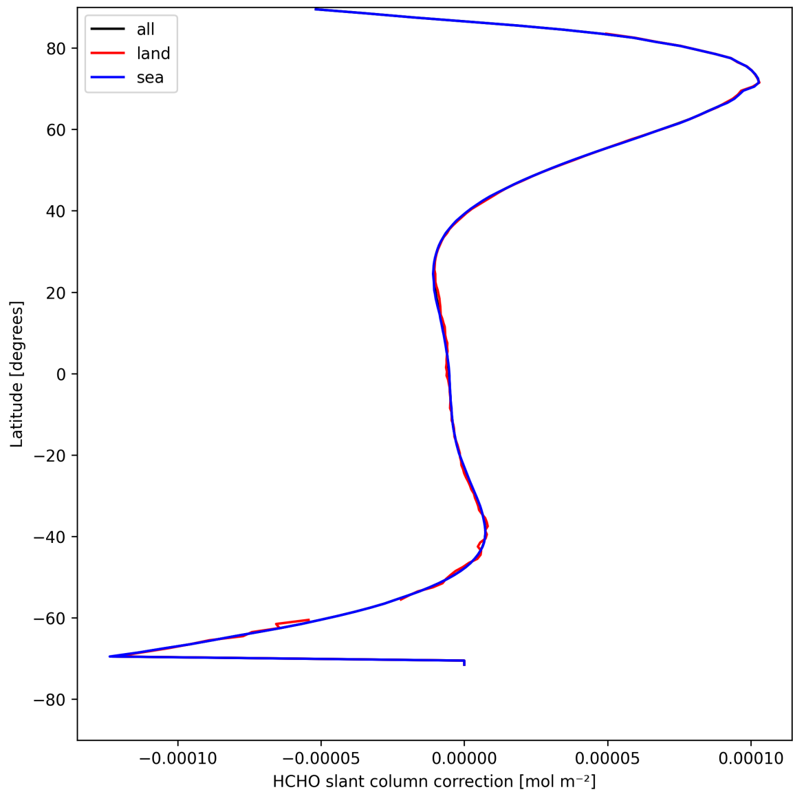
Figure 33: Zonal average of “HCHO slant column correction” for 2025-04-25 to 2025-04-27.
