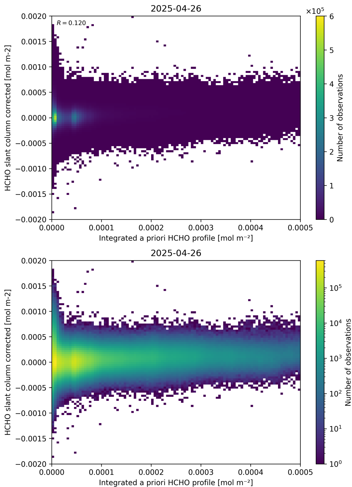
Figure 151: Scatter density plot of “Integrated a priori HCHO profile” against “HCHO slant column corrected” for 2025-04-25 to 2025-04-27.
