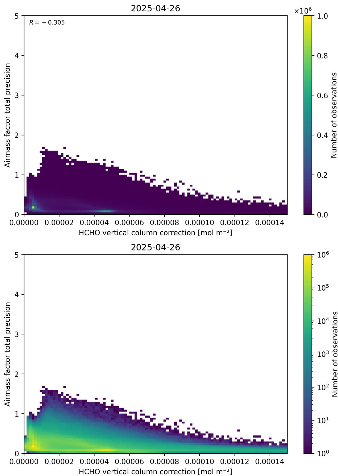
Figure 121: Scatter density plot of “HCHO vertical column correction” against “Airmass factor total precision” for 2025-04-25 to 2025-04-27.
