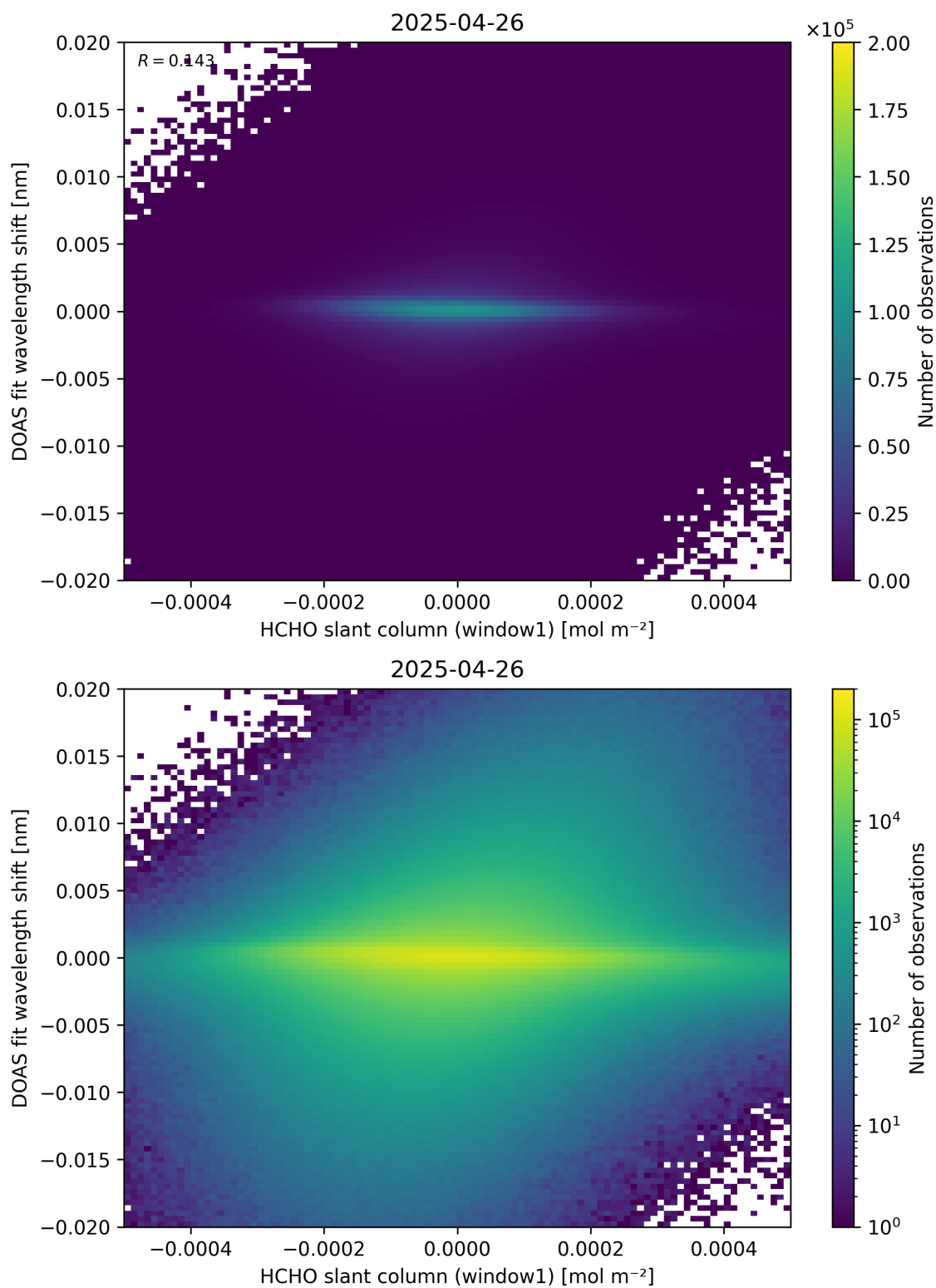
Figure 79: Scatter density plot of “HCHO slant column (window1)” against “DOAS fit wavelength shift” for 2025-04-25 to 2025-04-27.
