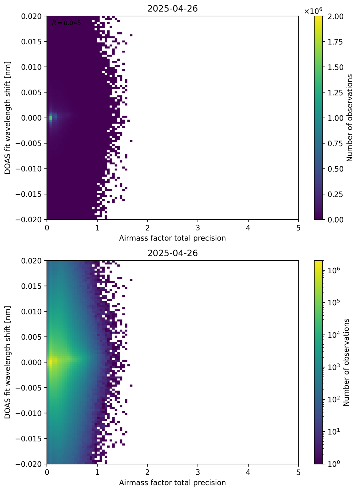
Figure 106: Scatter density plot of “Airmass factor total precision” against “DOAS fit wavelength shift” for 2025-04-25 to 2025-04-27.
