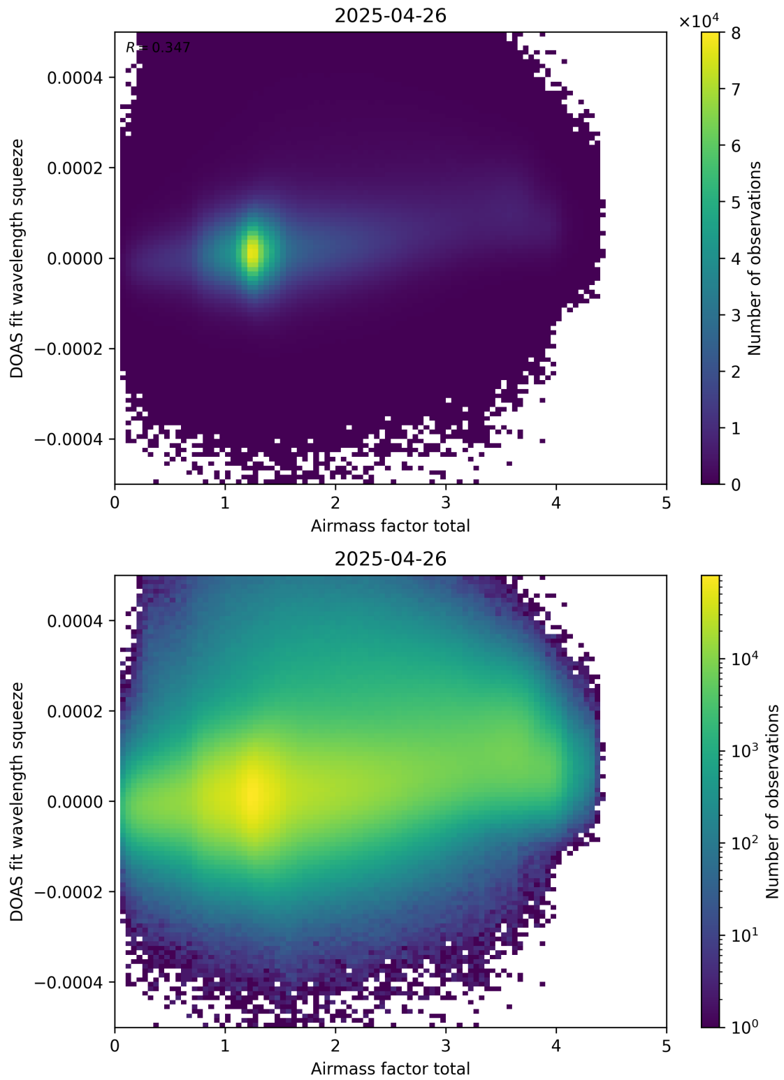
Figure 99: Scatter density plot of “Airmass factor total” against “DOAS fit wavelength squeeze” for 2025-04-25 to 2025-04-27.
