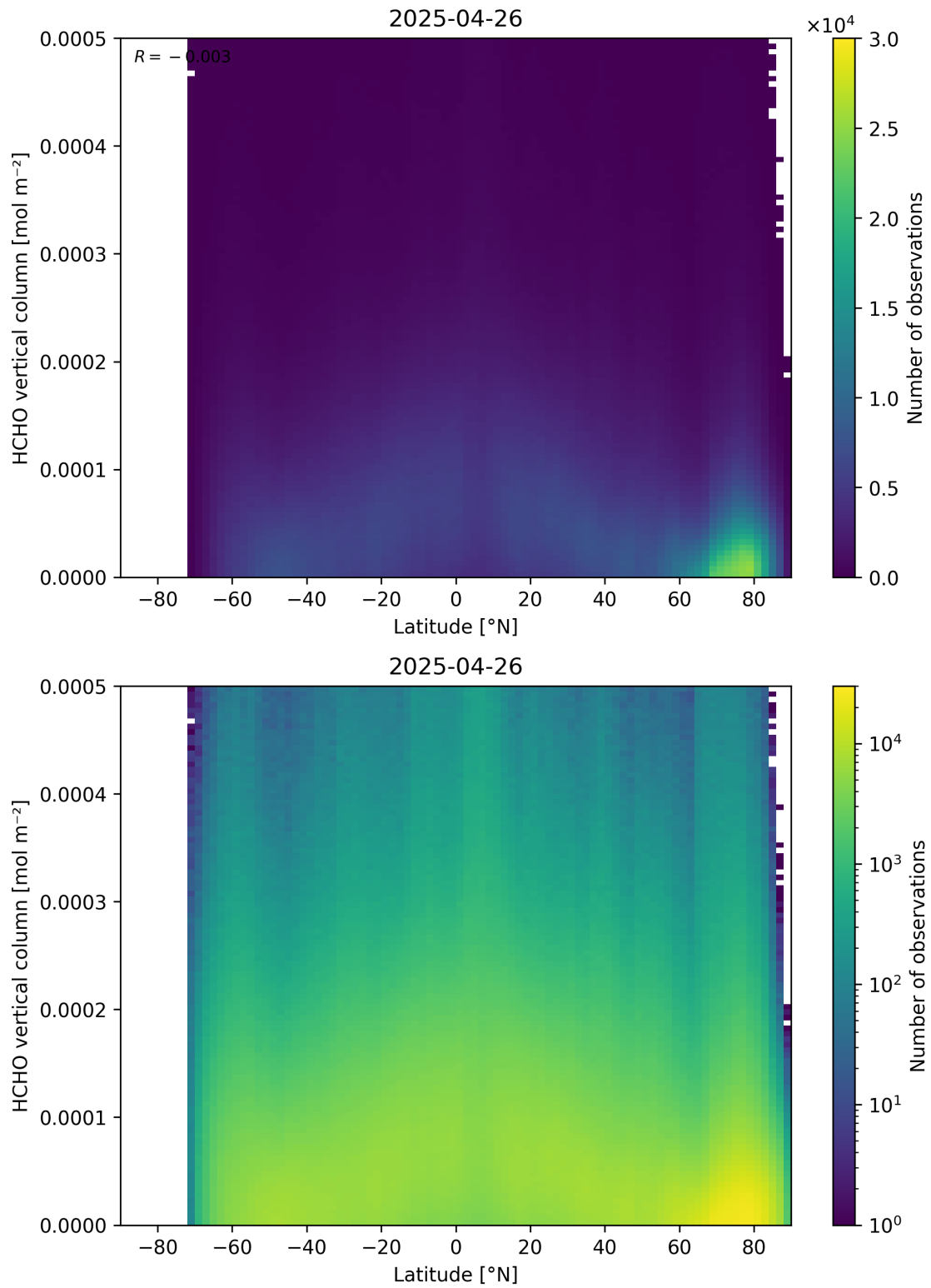
Figure 163: Scatter density plot of “Latitude” against “HCHO vertical column” for 2025-04-25 to 2025-04-27.
