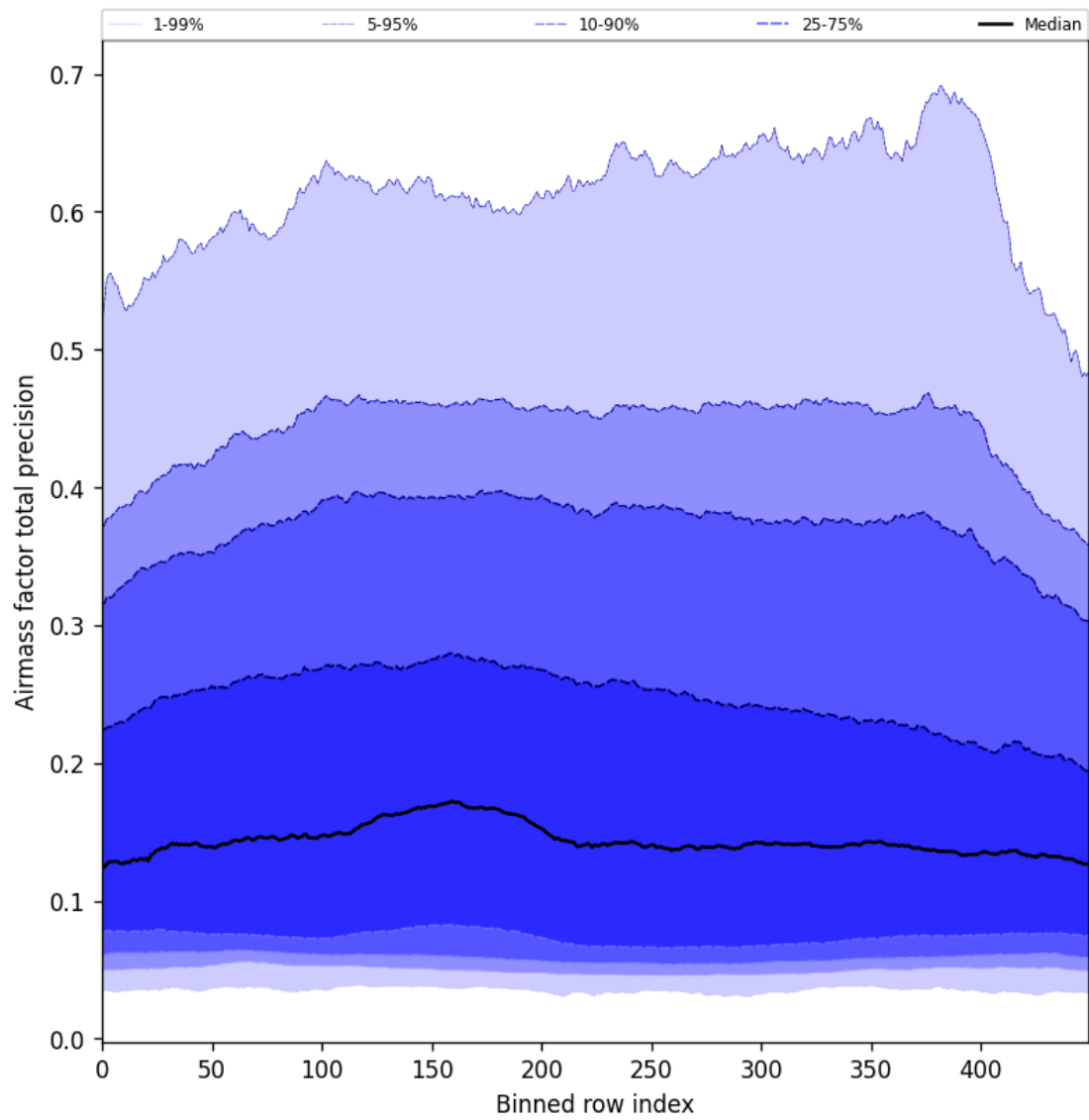
Figure 55: Along track statistics of “Airmass factor total precision” for 2025-04-25 to 2025-04-27
