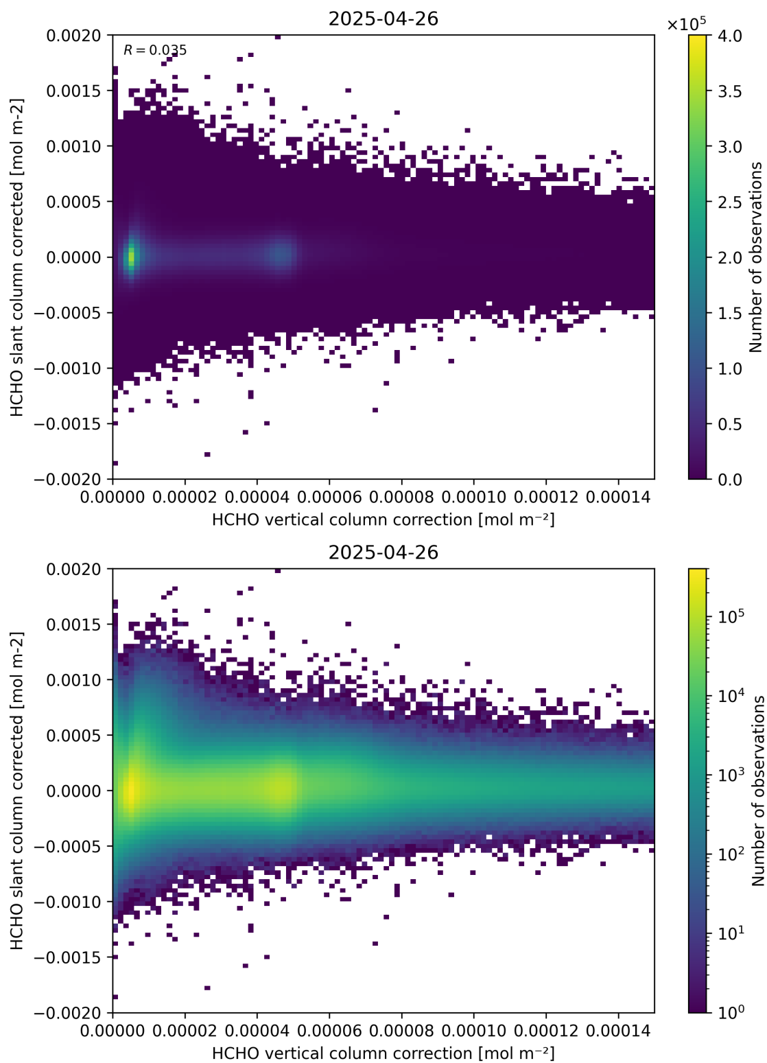
Figure 116: Scatter density plot of “HCHO vertical column correction” against “HCHO slant column corrected” for 2025-04-25 to 2025-04-27.
