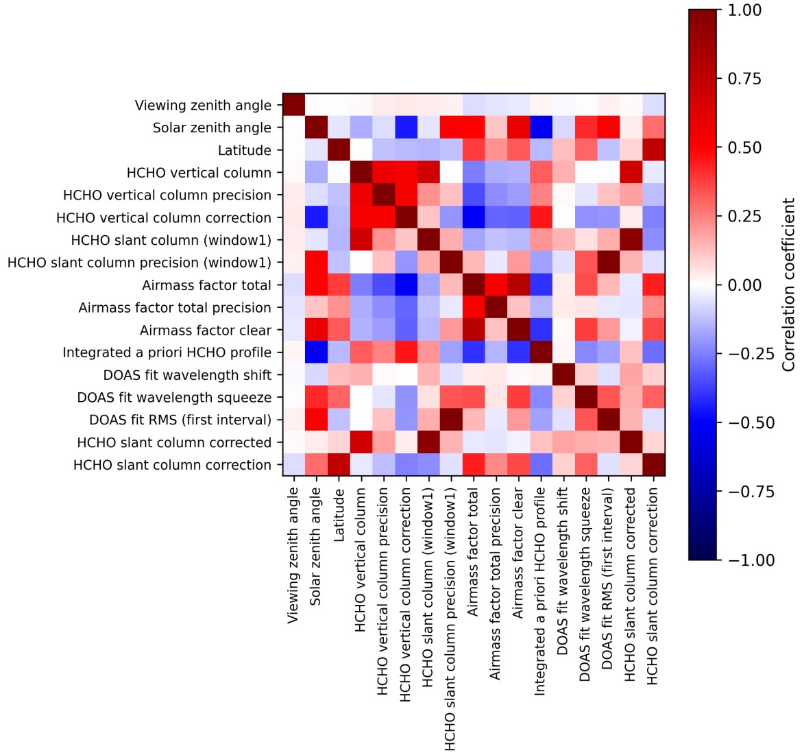
Figure 2: Map of correlation matrix for 2025-04-25 to 2025-04-27.
