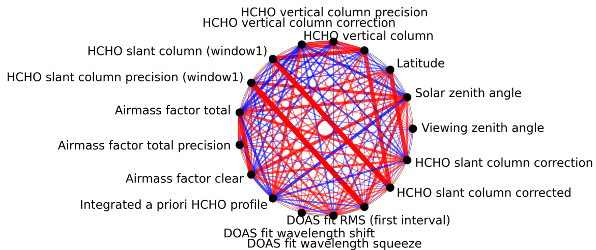
Figure 1: Map of correlation graph for 2025-04-25 to 2025-04-27.
