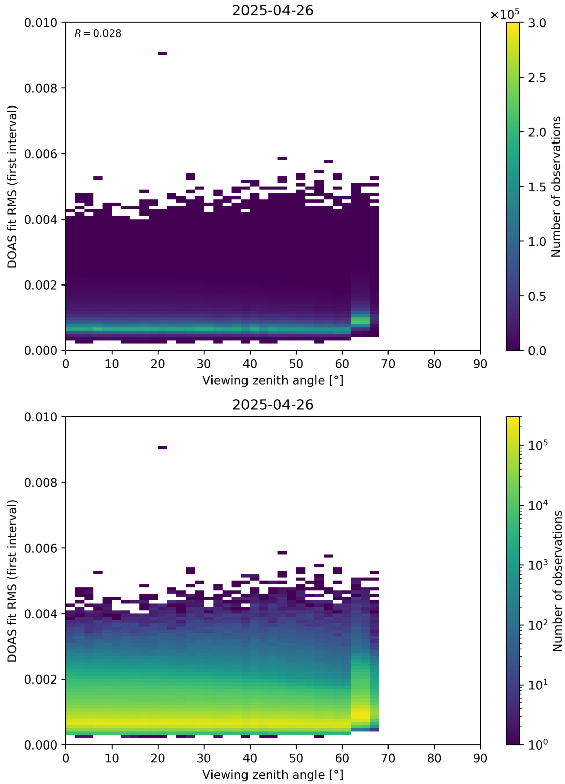
Figure 182: Scatter density plot of “Viewing zenith angle” against “DOAS fit RMS (first interval)” for 2025-04-25 to 2025-04-27.
