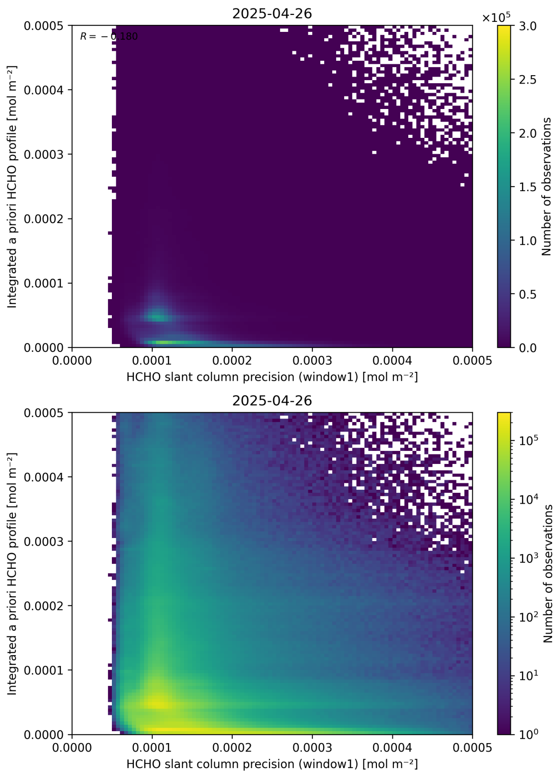
Figure 96: Scatter density plot of “HCHO slant column precision (window1)” against “Integrated a priori HCHO profile” for 2025-04-25 to 2025-04-27.
