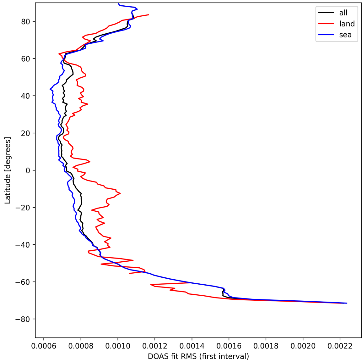
Figure 32: Zonal average of "DOAS fit RMS (first interval)" for 2025-04-25 to 2025-04-27.
