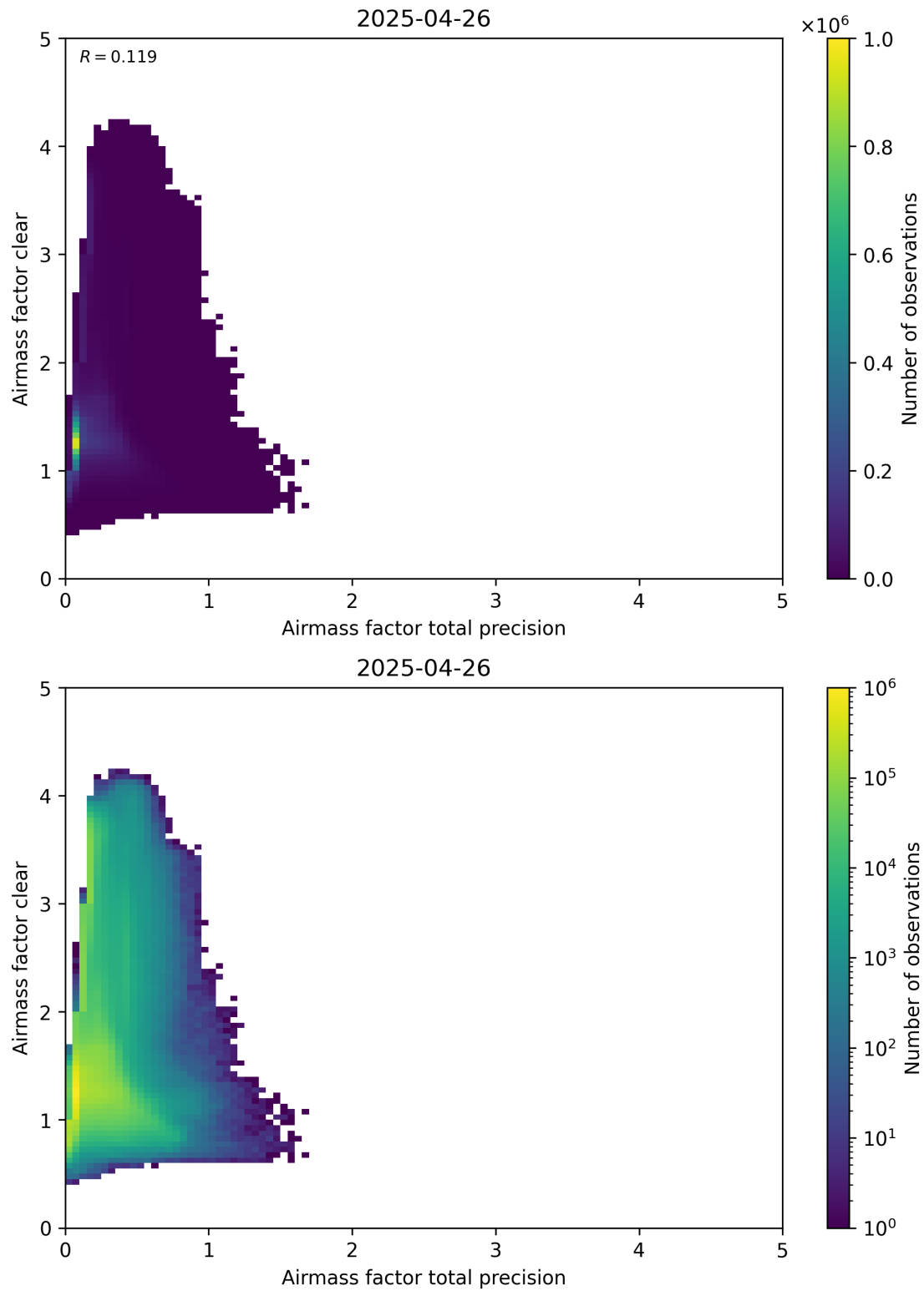
Figure 108: Scatter density plot of “Airmass factor total precision” against “Airmass factor clear” for 2025-04-25 to 2025-04-27.
