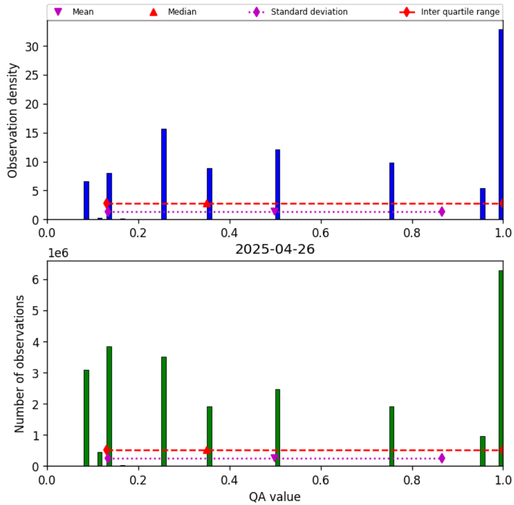
Figure 34: Histogram of “QA value” for 2025-04-25 to 2025-04-27
