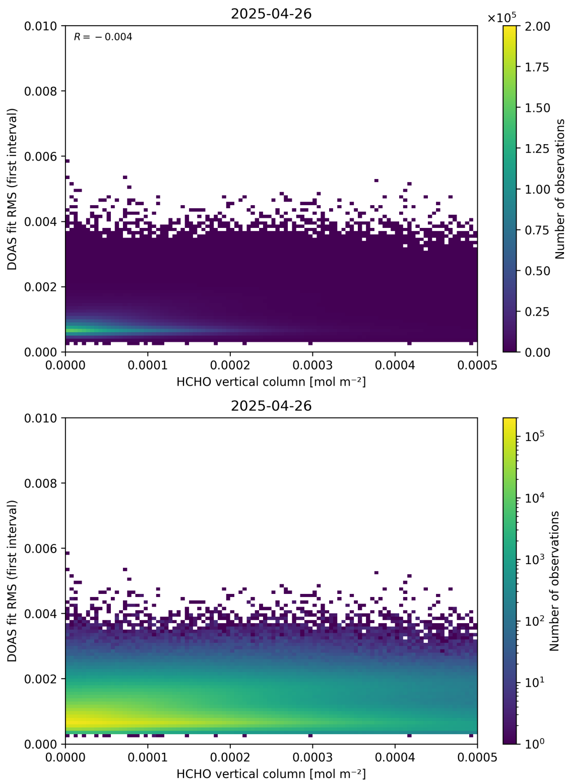
Figure 123: Scatter density plot of “HCHO vertical column” against “DOAS fit RMS (first interval)” for 2025-04-25 to 2025-04-27.
