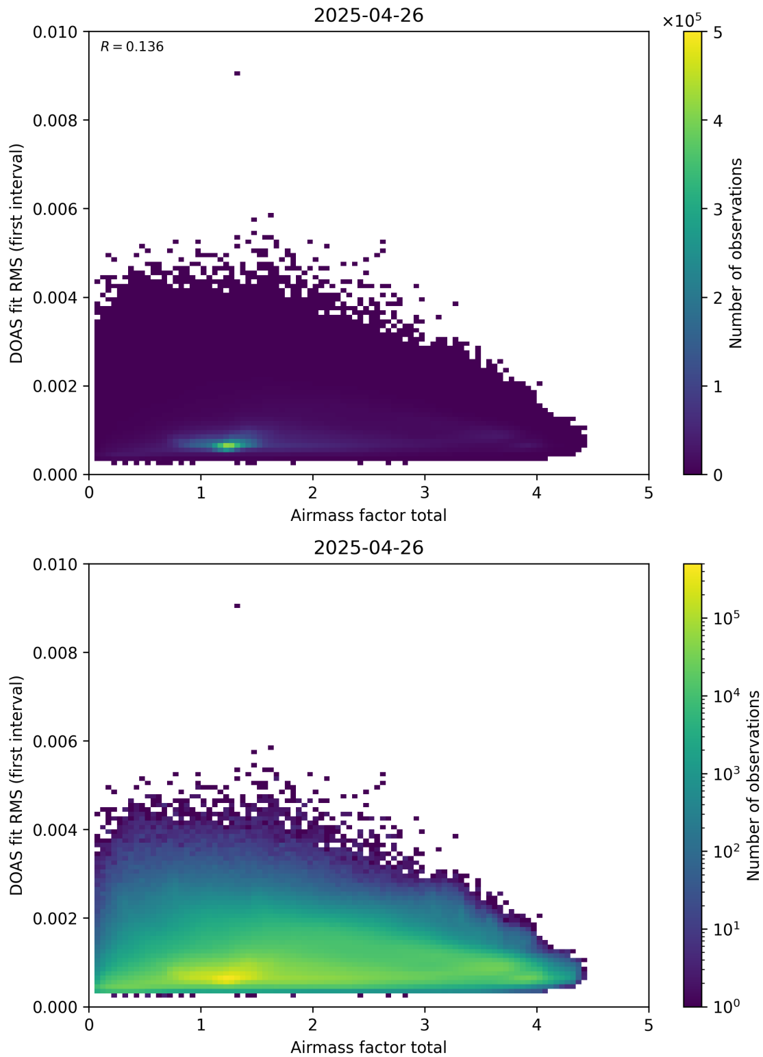
Figure 97: Scatter density plot of “Airmass factor total” against “DOAS fit RMS (first interval)” for 2025-04-25 to 2025-04-27.
