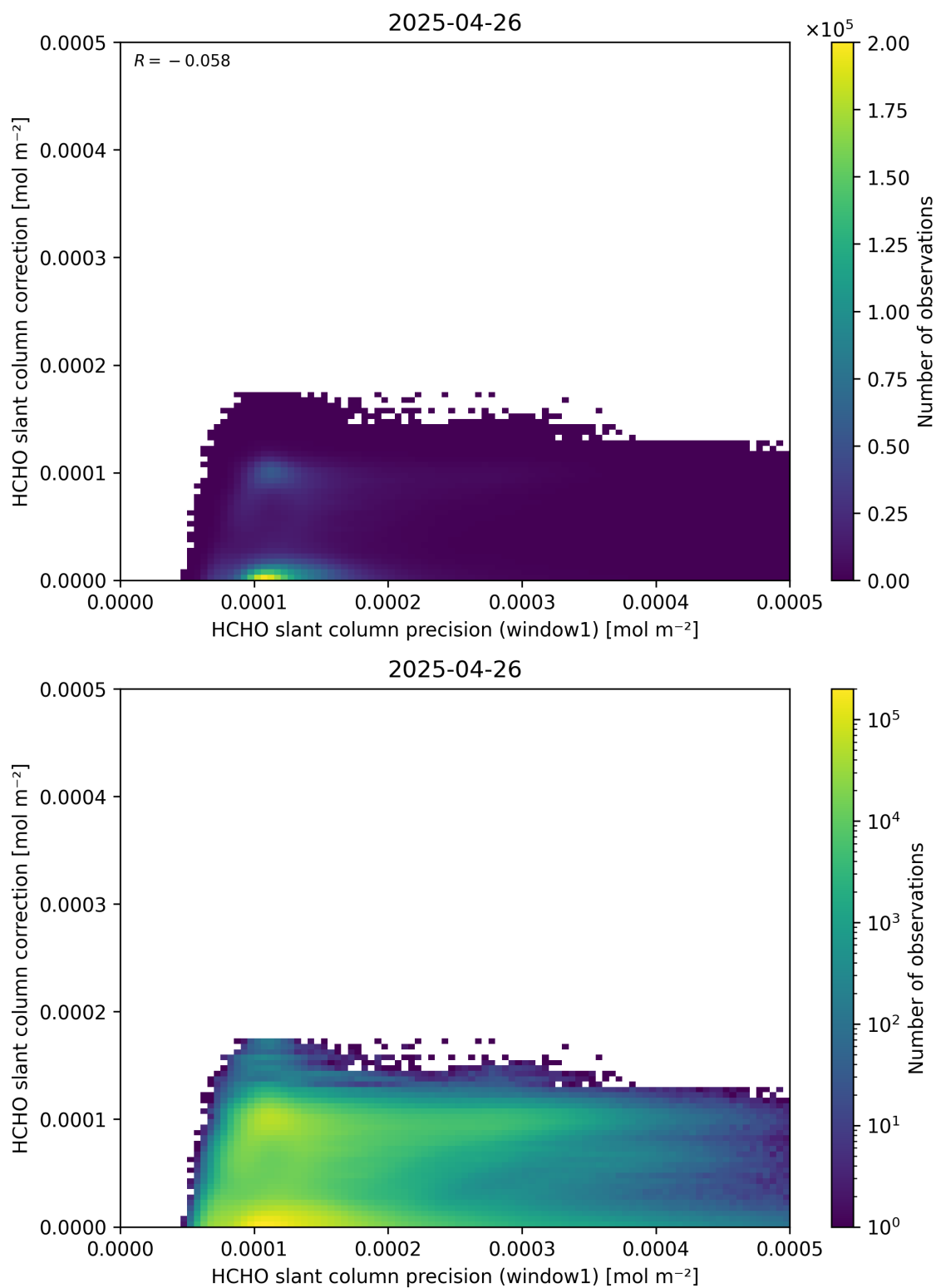
Figure 93: Scatter density plot of “HCHO slant column precision (window1)” against “HCHO slant column correction” for 2025-04-25 to 2025-04-27.
