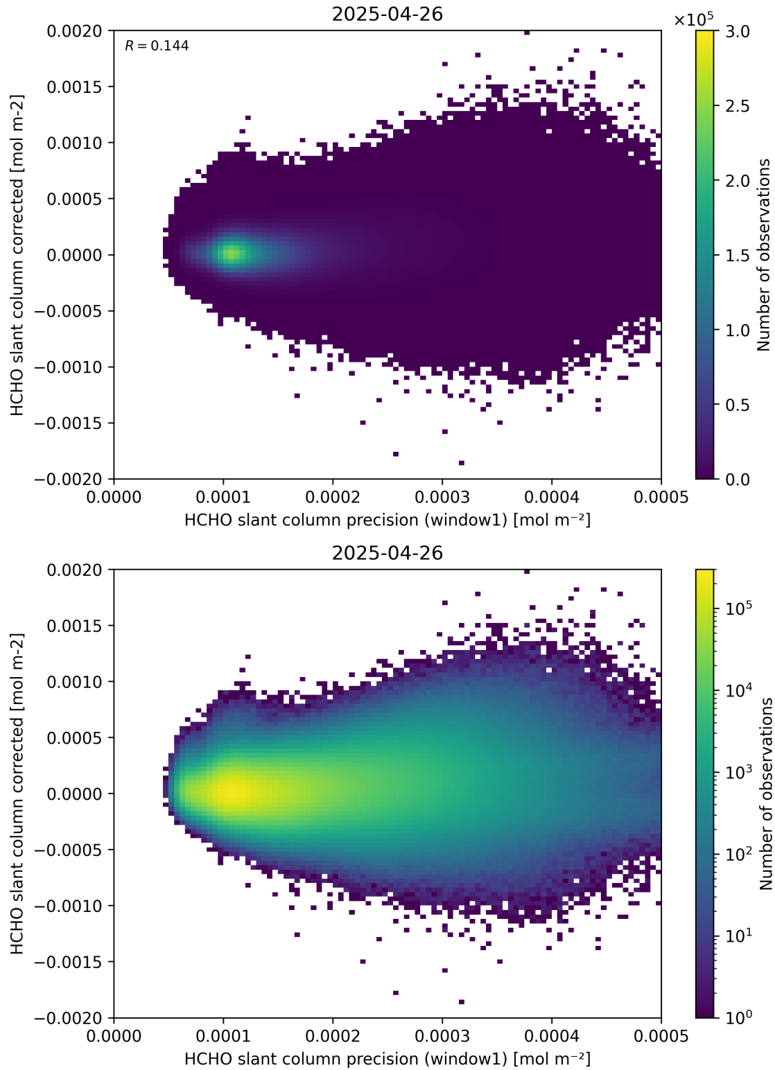
Figure 92: Scatter density plot of “HCHO slant column precision (window1)” against “HCHO slant column corrected” for 2025-04-25 to 2025-04-27.
