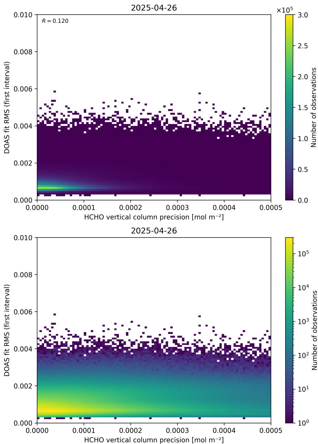
Figure 136: Scatter density plot of “HCHO vertical column precision” against “DOAS fit RMS (first interval)” for 2025-04-25 to 2025-04-27.
