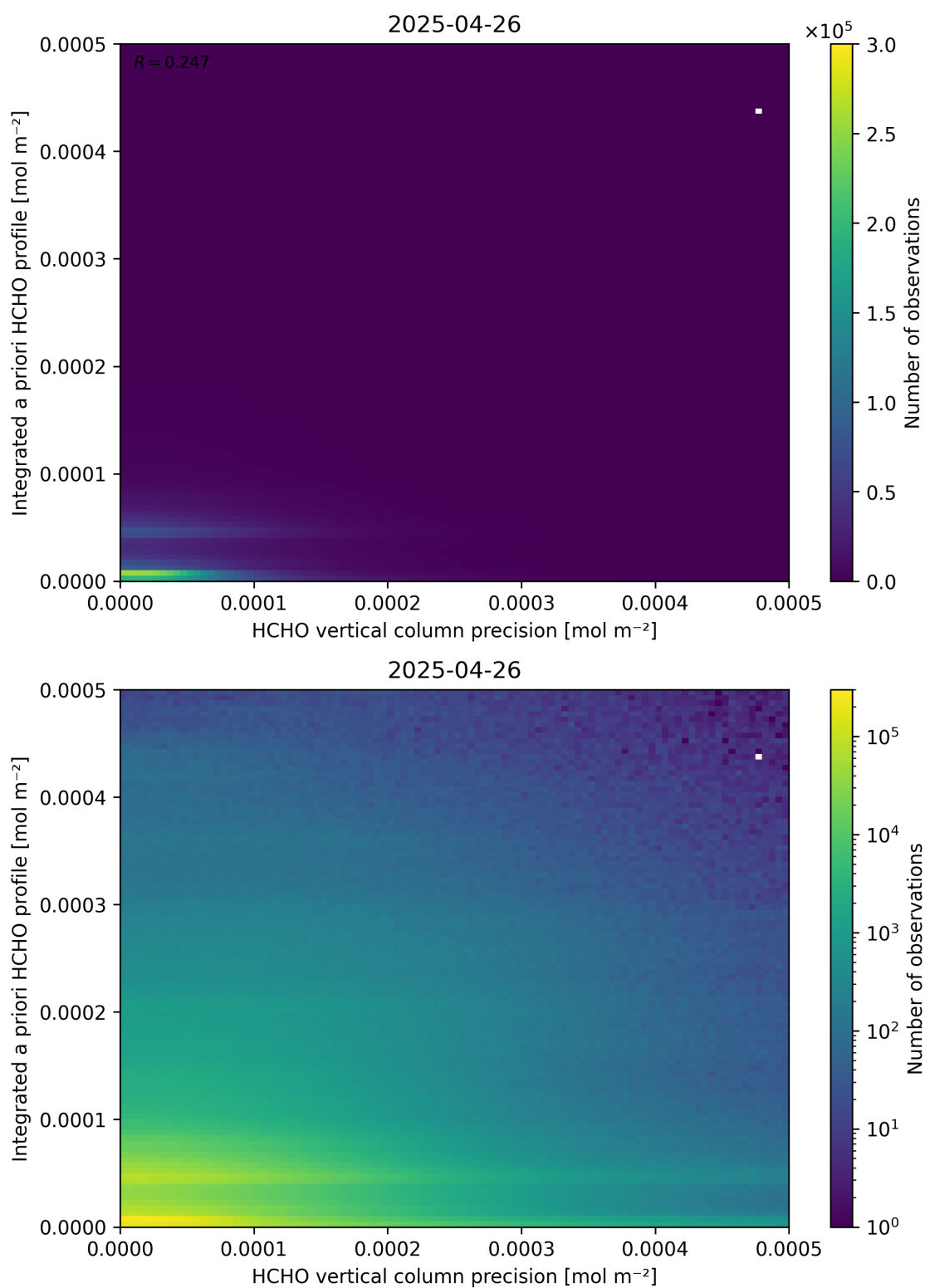
Figure 147: Scatter density plot of “HCHO vertical column precision” against “Integrated a priori HCHO profile” for 2025-04-25 to 2025-04-27.
