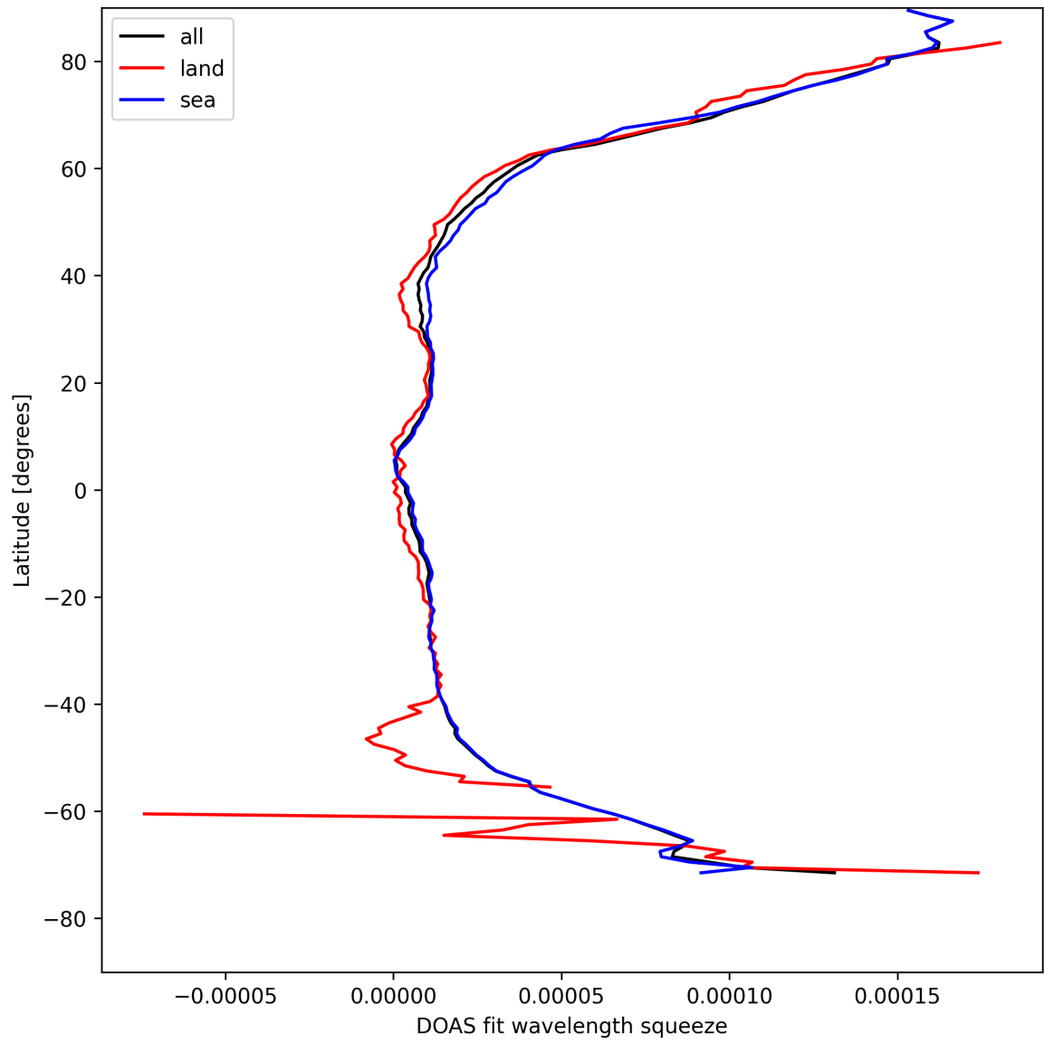
Figure 31: Zonal average of “DOAS fit wavelength squeeze” for 2025-04-25 to 2025-04-27.
