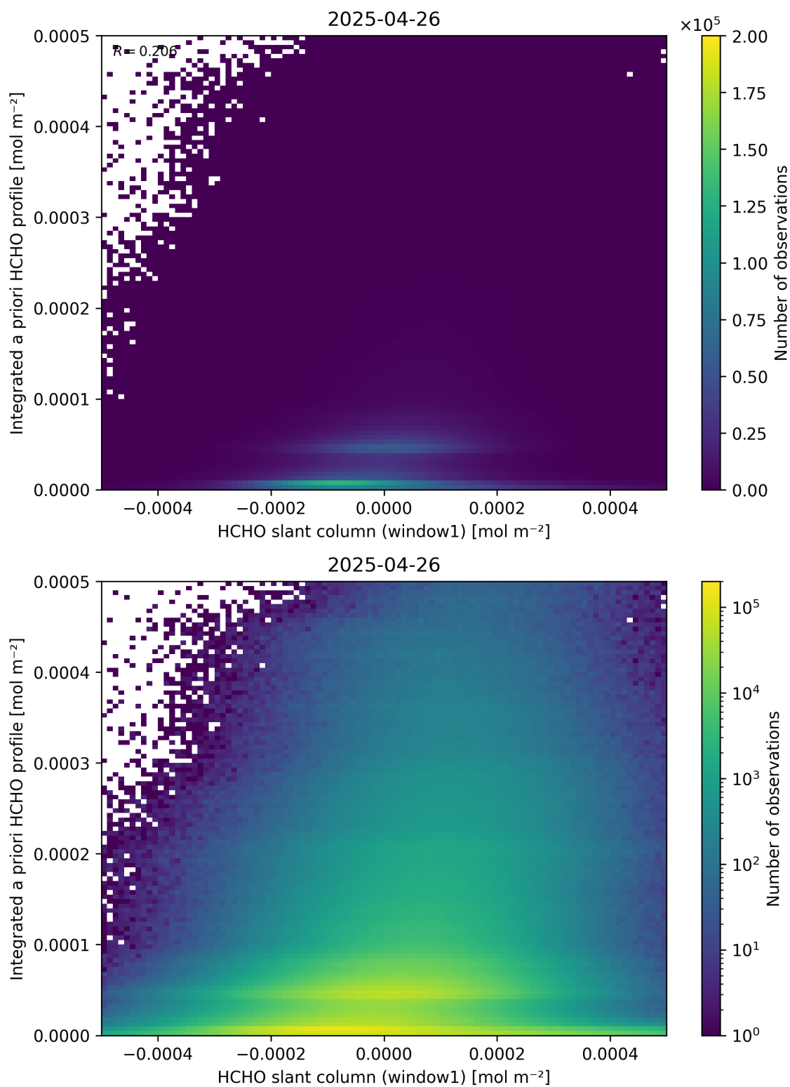
Figure 87: Scatter density plot of “HCHO slant column (window1)” against “Integrated a priori HCHO profile” for 2025-04-25 to 2025-04-27.
