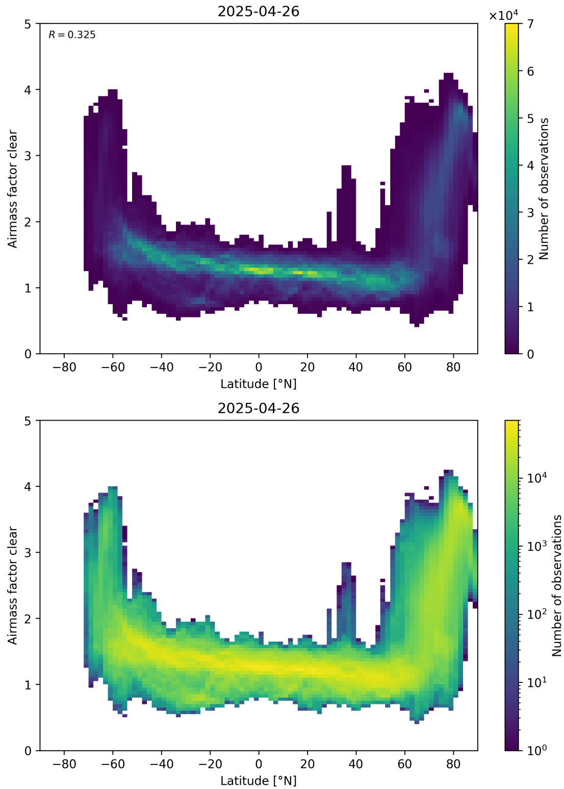
Figure 156: Scatter density plot of “Latitude” against “Airmass factor clear” for 2025-04-25 to 2025-04-27.
