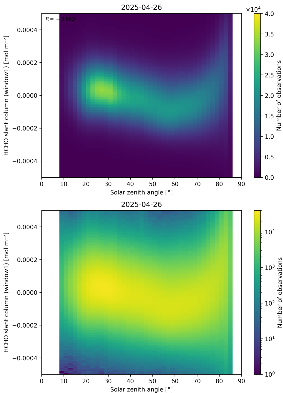
Figure 173: Scatter density plot of “Solar zenith angle” against “HCHO slant column (window1)” for 2025-04-25 to 2025-04-27.
