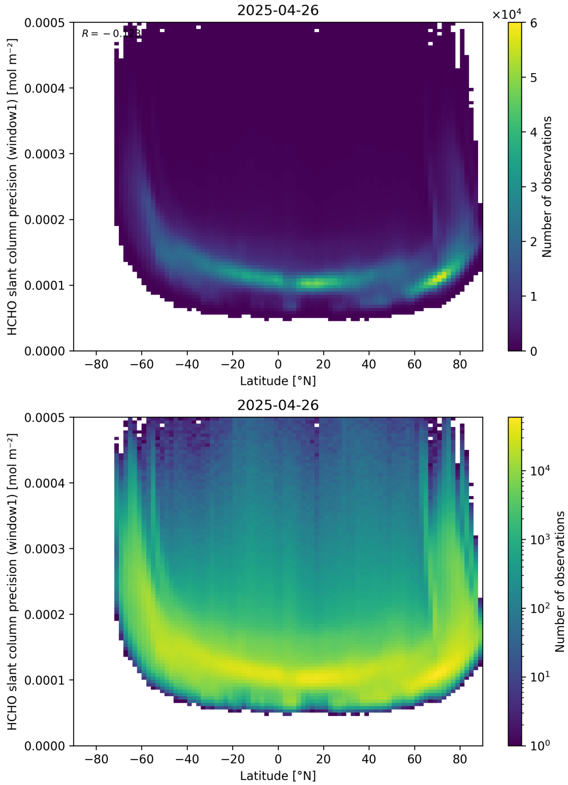
Figure 160: Scatter density plot of “Latitude” against “HCHO slant column precision (window1)” for 2025-04-25 to 2025-04-27.
