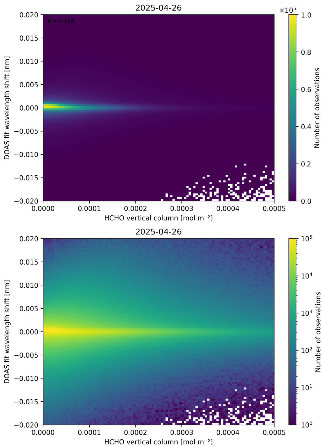
Figure 124: Scatter density plot of “HCHO vertical column” against “DOAS fit wavelength shift” for 2025-04-25 to 2025-04-27.
