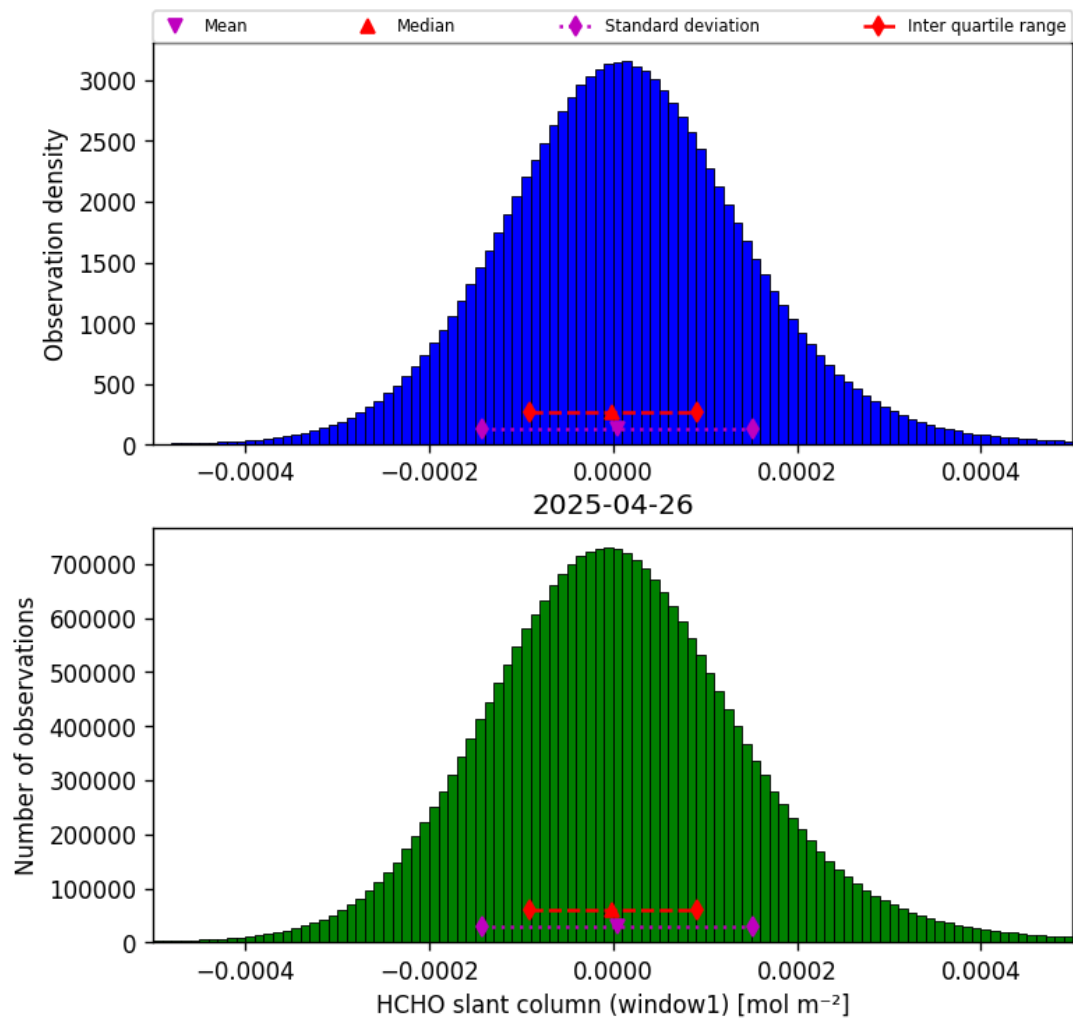
Figure 38: Histogram of “HCHO slant column (window1)” for 2025-04-25 to 2025-04-27
