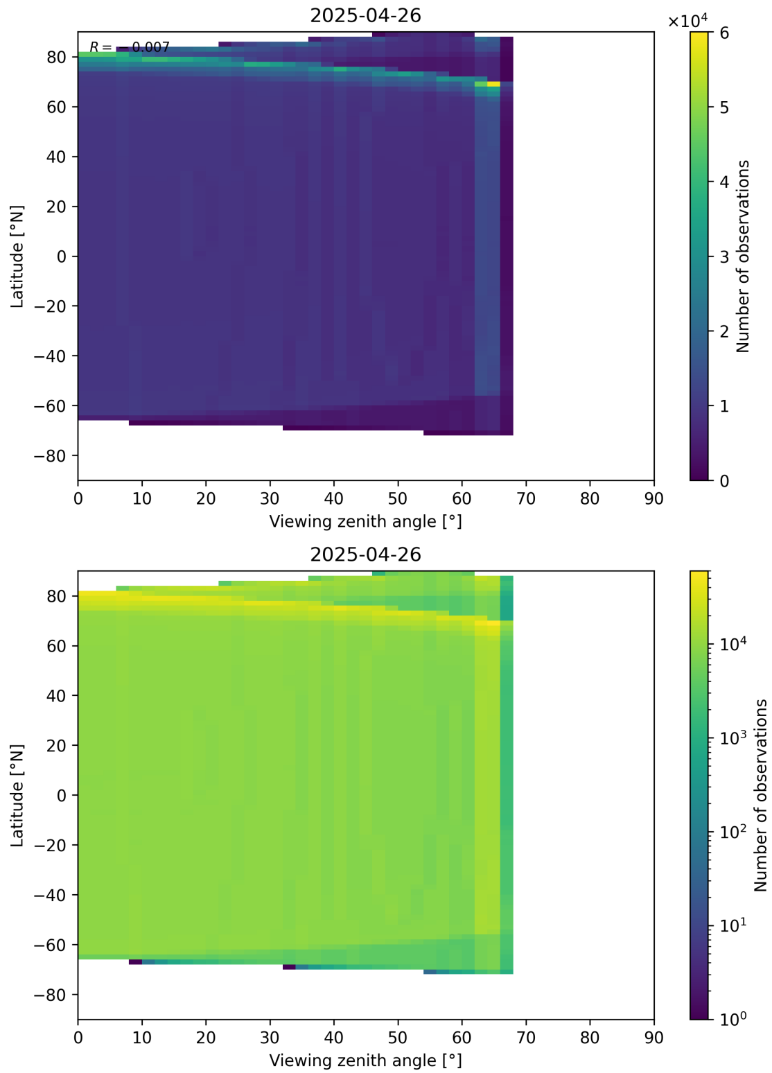
Figure 196: Scatter density plot of “Viewing zenith angle” against “Latitude” for 2025-04-25 to 2025-04-27.
