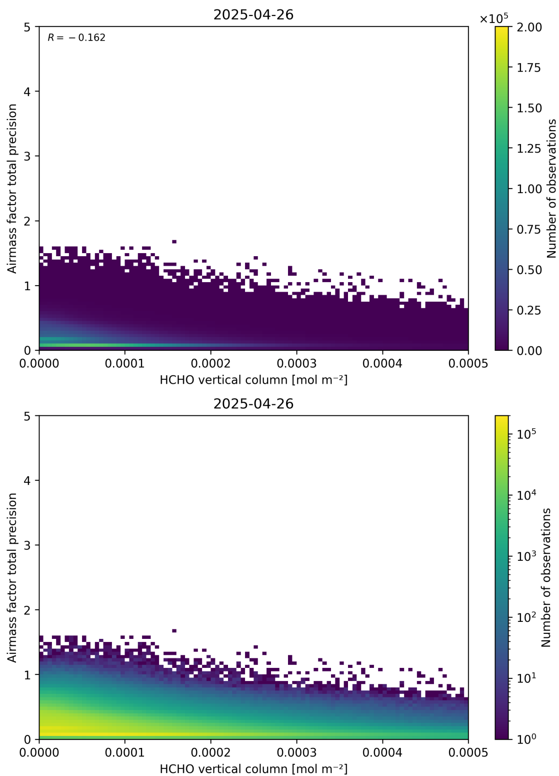
Figure 132: Scatter density plot of “HCHO vertical column” against “Airmass factor total precision” for 2025-04-25 to 2025-04-27.
