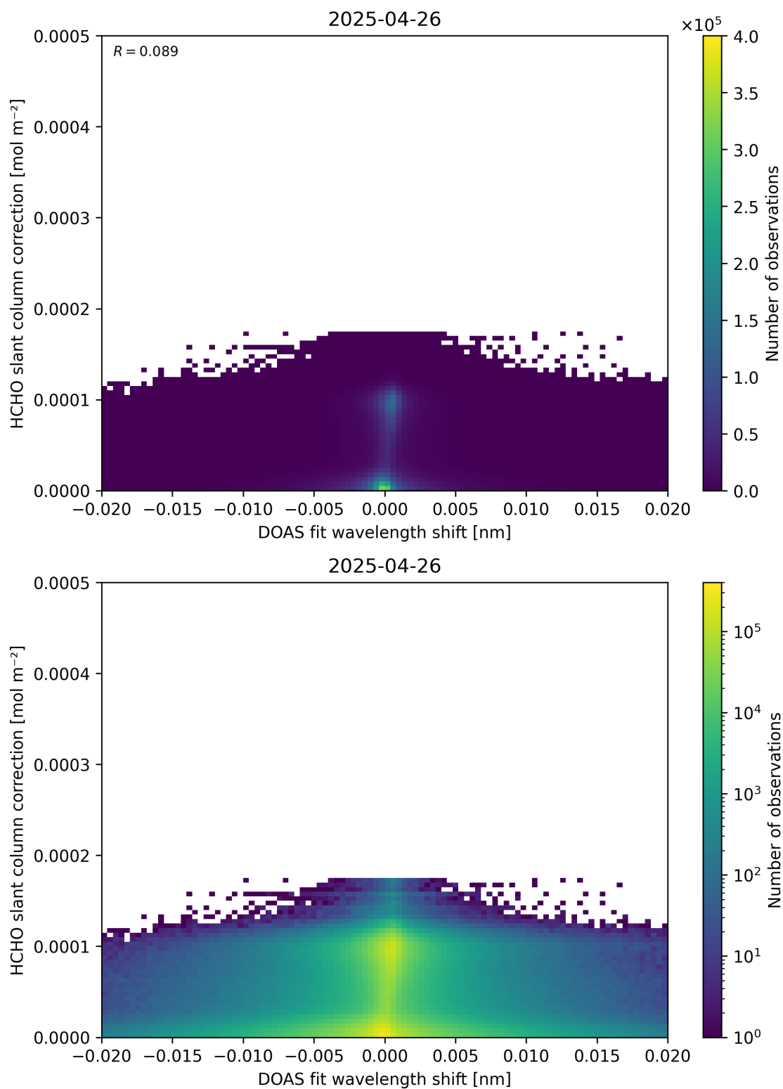
Figure 67: Scatter density plot of “DOAS fit wavelength shift” against “HCHO slant column correction” for 2025-04-25 to 2025-04-27.
