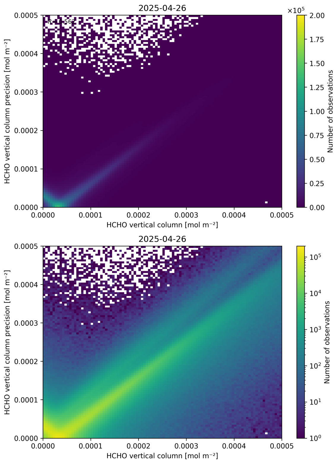
Figure 134: Scatter density plot of “HCHO vertical column” against “HCHO vertical column precision” for 2025-04-25 to 2025-04-27.
