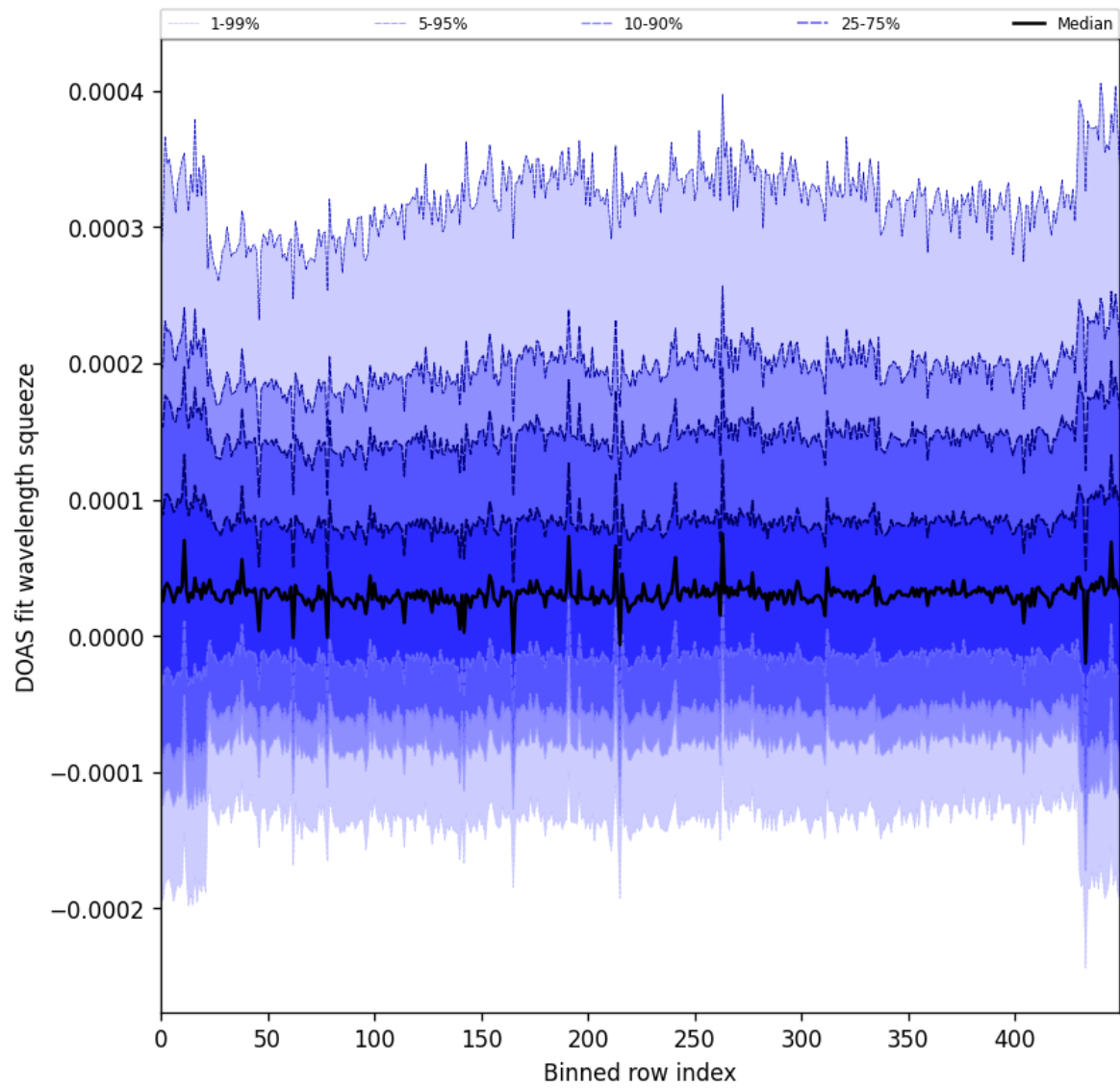
Figure 59: Along track statistics of “DOAS fit wavelength squeeze” for 2025-04-25 to 2025-04-27
