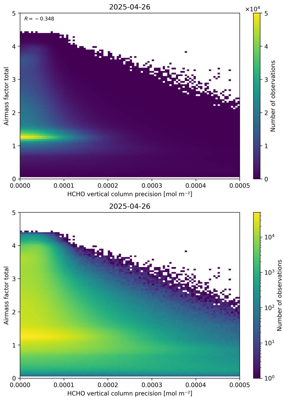
Figure 144: Scatter density plot of “HCHO vertical column precision” against “Airmass factor total” for 2025-04-25 to 2025-04-27.
