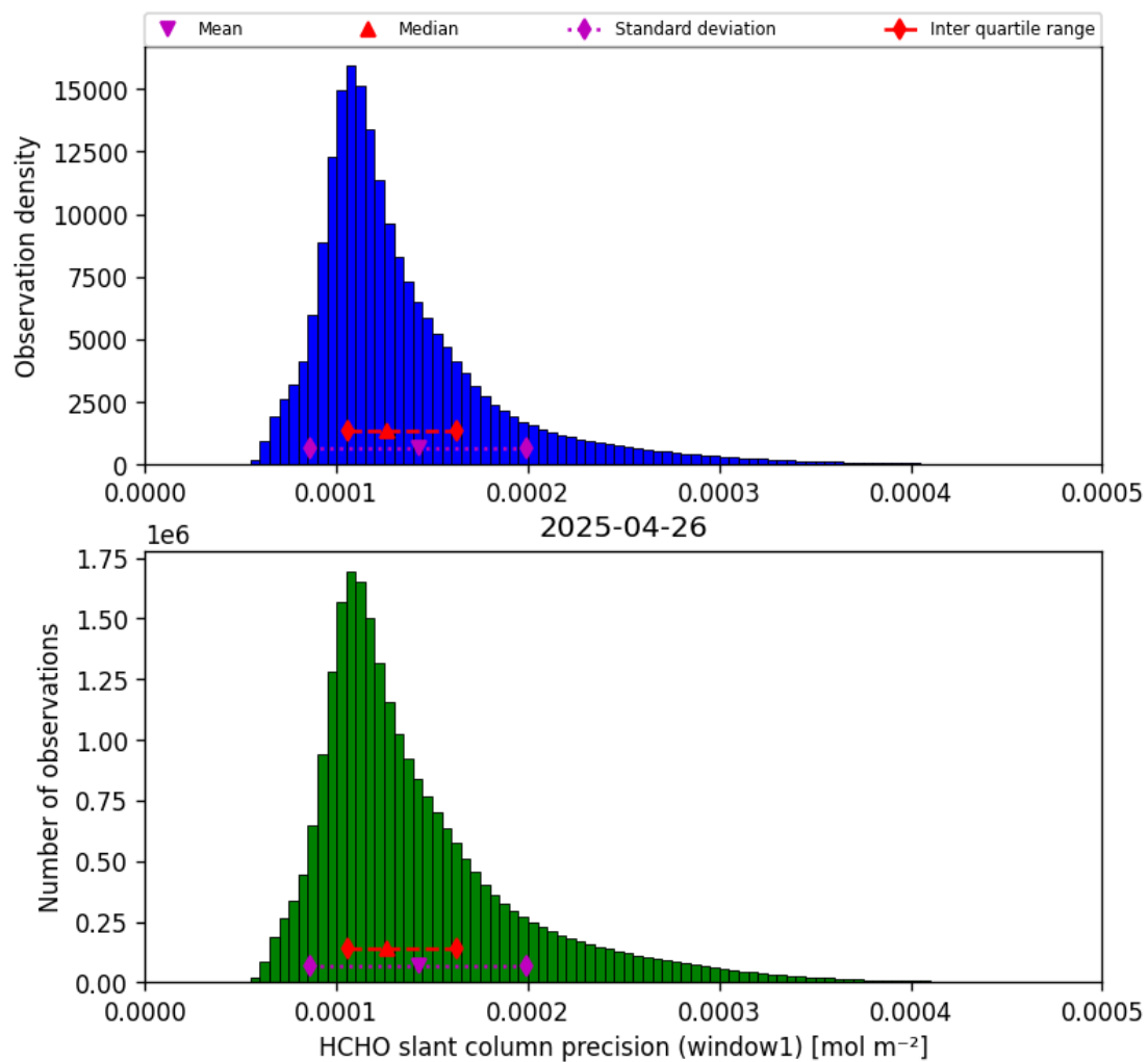
Figure 39: Histogram of “HCHO slant column precision (window1)” for 2025-04-25 to 2025-04-27
