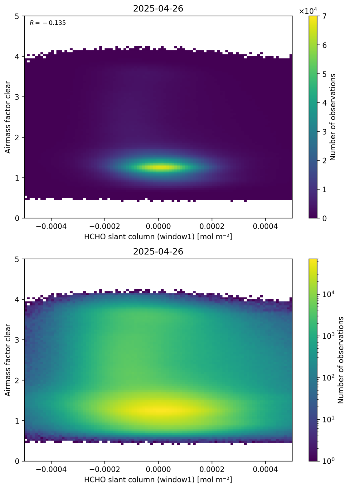
Figure 81: Scatter density plot of “HCHO slant column (window1)” against “Airmass factor clear” for 2025-04-25 to 2025-04-27.
