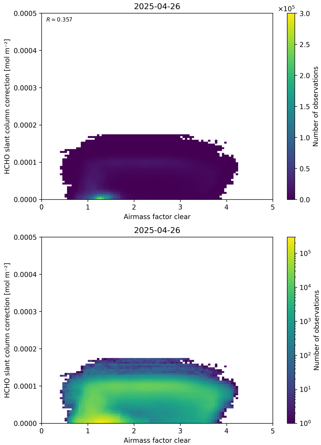
Figure 75: Scatter density plot of “Air mass factor clear” against “HCHO slant column correction” for 2025-04-25 to 2025-04-27.
