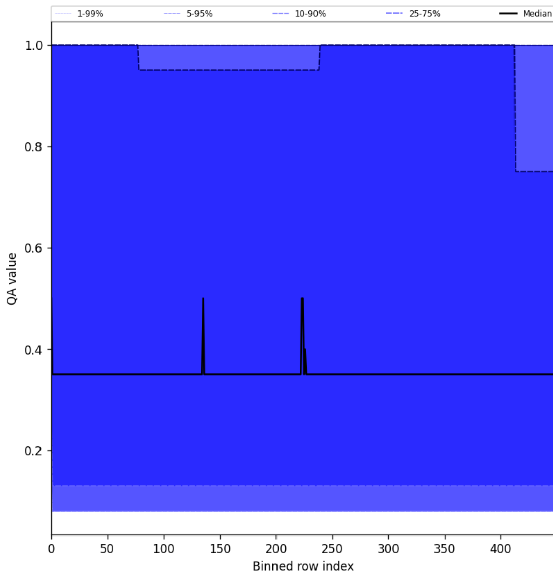
Figure 48: Along track statistics of “QA value” for 2025-04-25 to 2025-04-27
