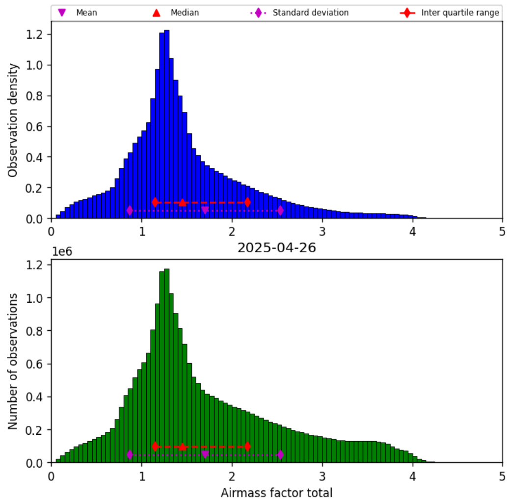
Figure 40: Histogram of “Airmass factor total” for 2025-04-25 to 2025-04-27
