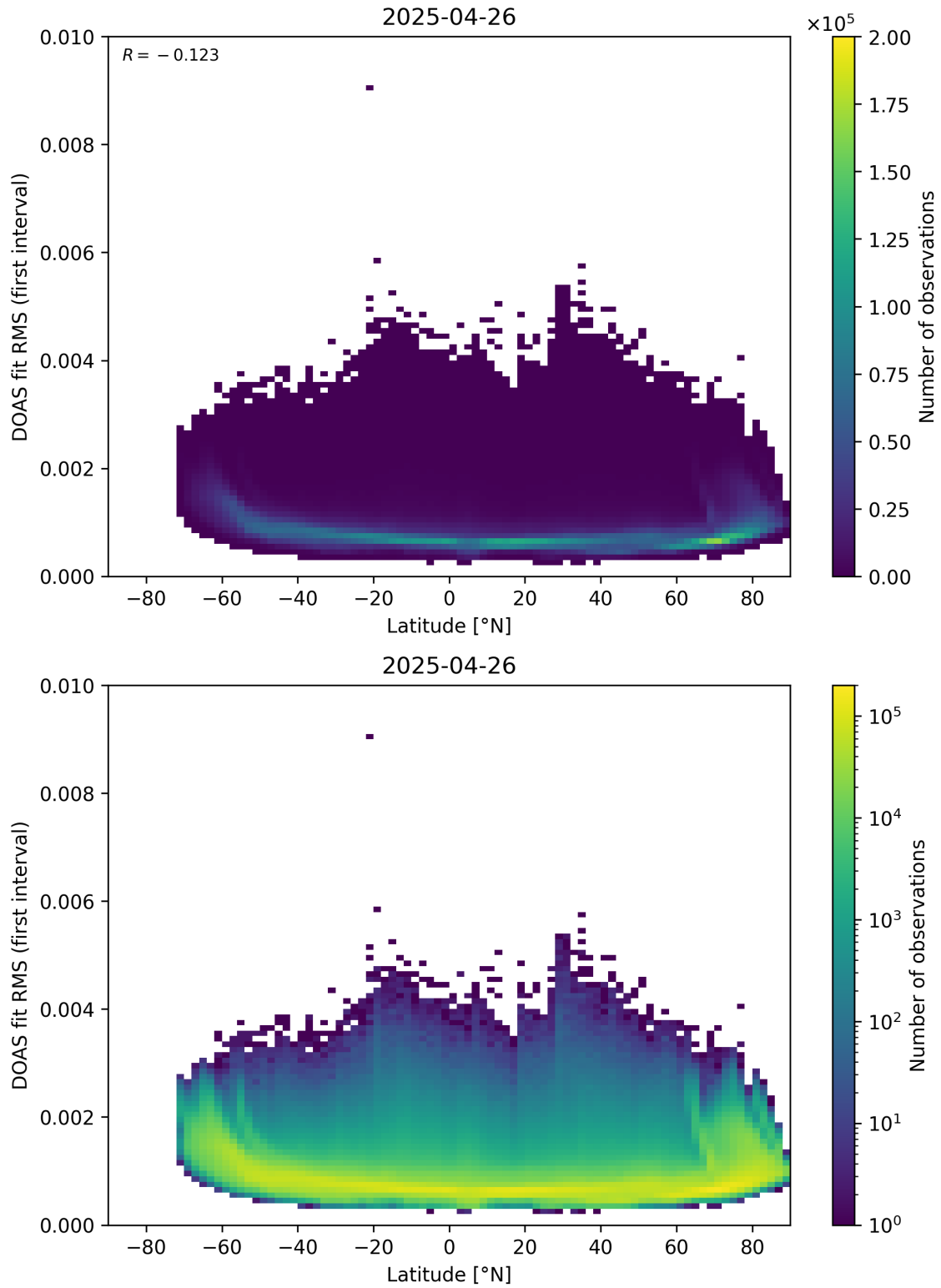
Figure 153: Scatter density plot of “Latitude” against “DOAS fit RMS (first interval)” for 2025-04-25 to 2025-04-27.
