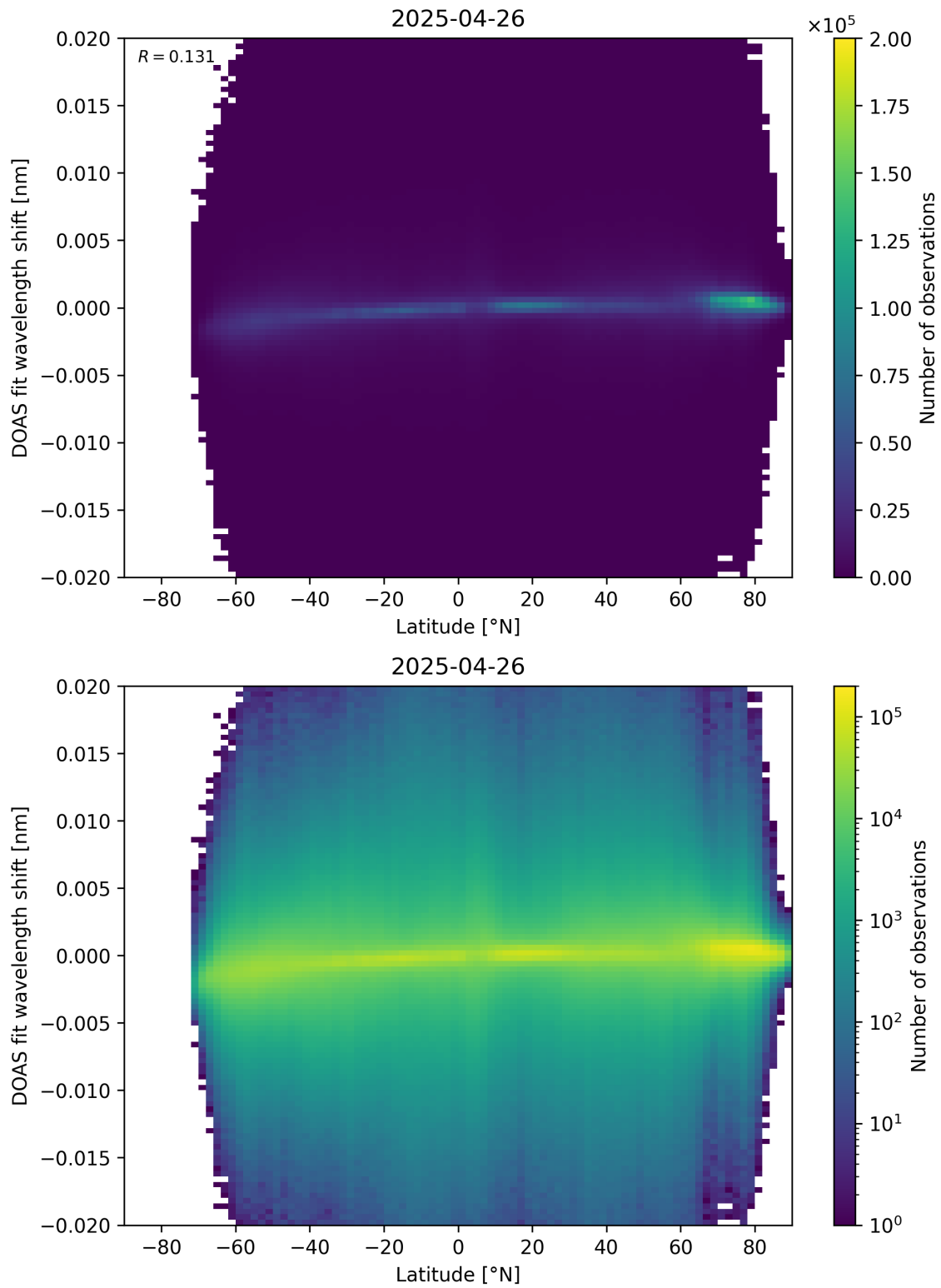
Figure 154: Scatter density plot of “Latitude” against “DOAS fit wavelength shift” for 2025-04-25 to 2025-04-27.
