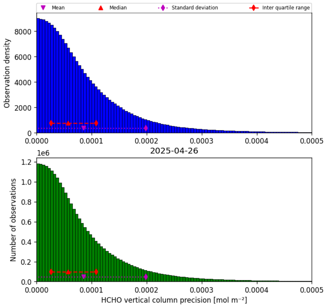
Figure 36: Histogram of “HCHO vertical column precision” for 2025-04-25 to 2025-04-27
