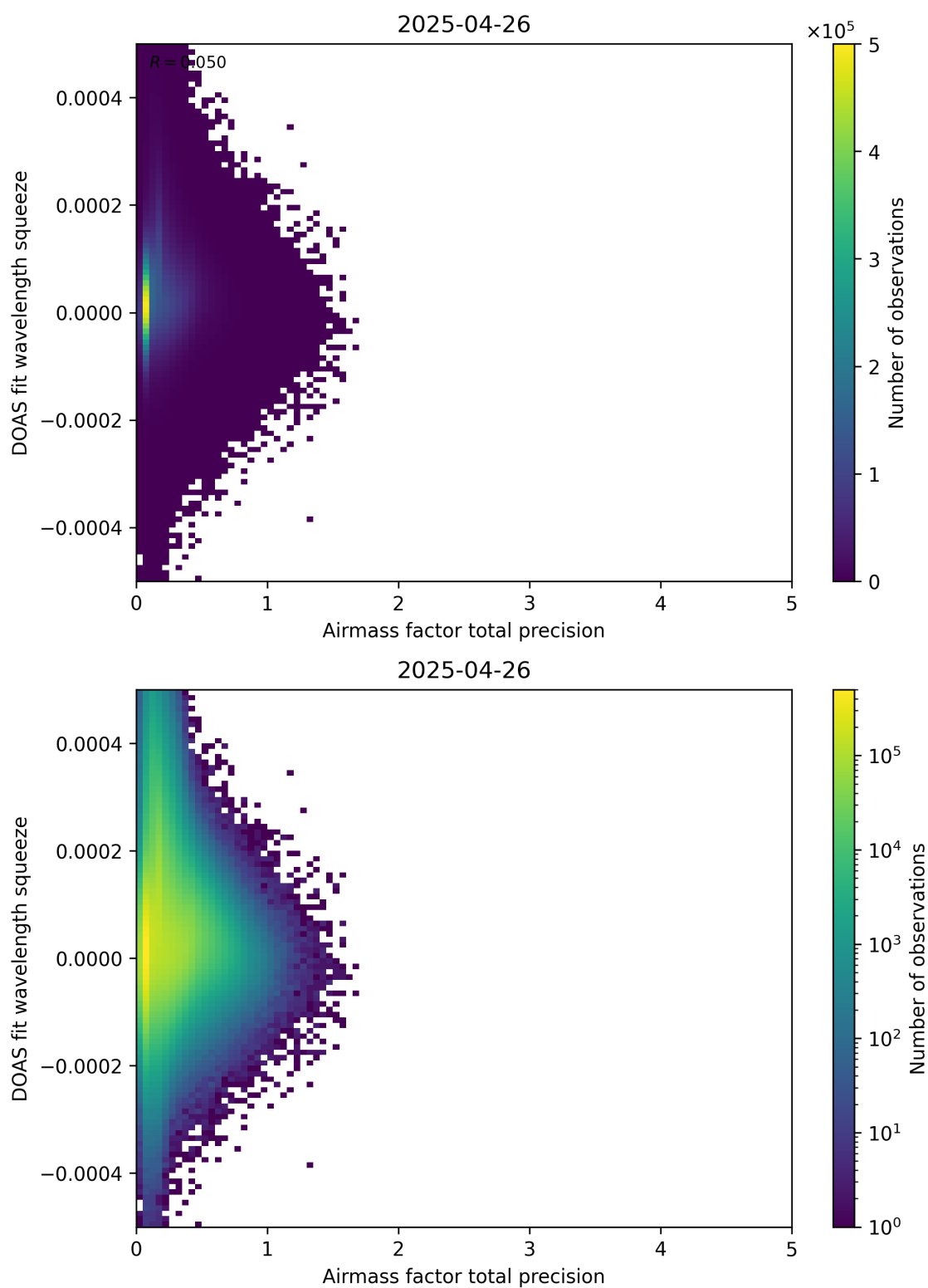
Figure 107: Scatter density plot of “Airmass factor total precision” against “DOAS fit wavelength squeeze” for 2025-04-25 to 2025-04-27.
