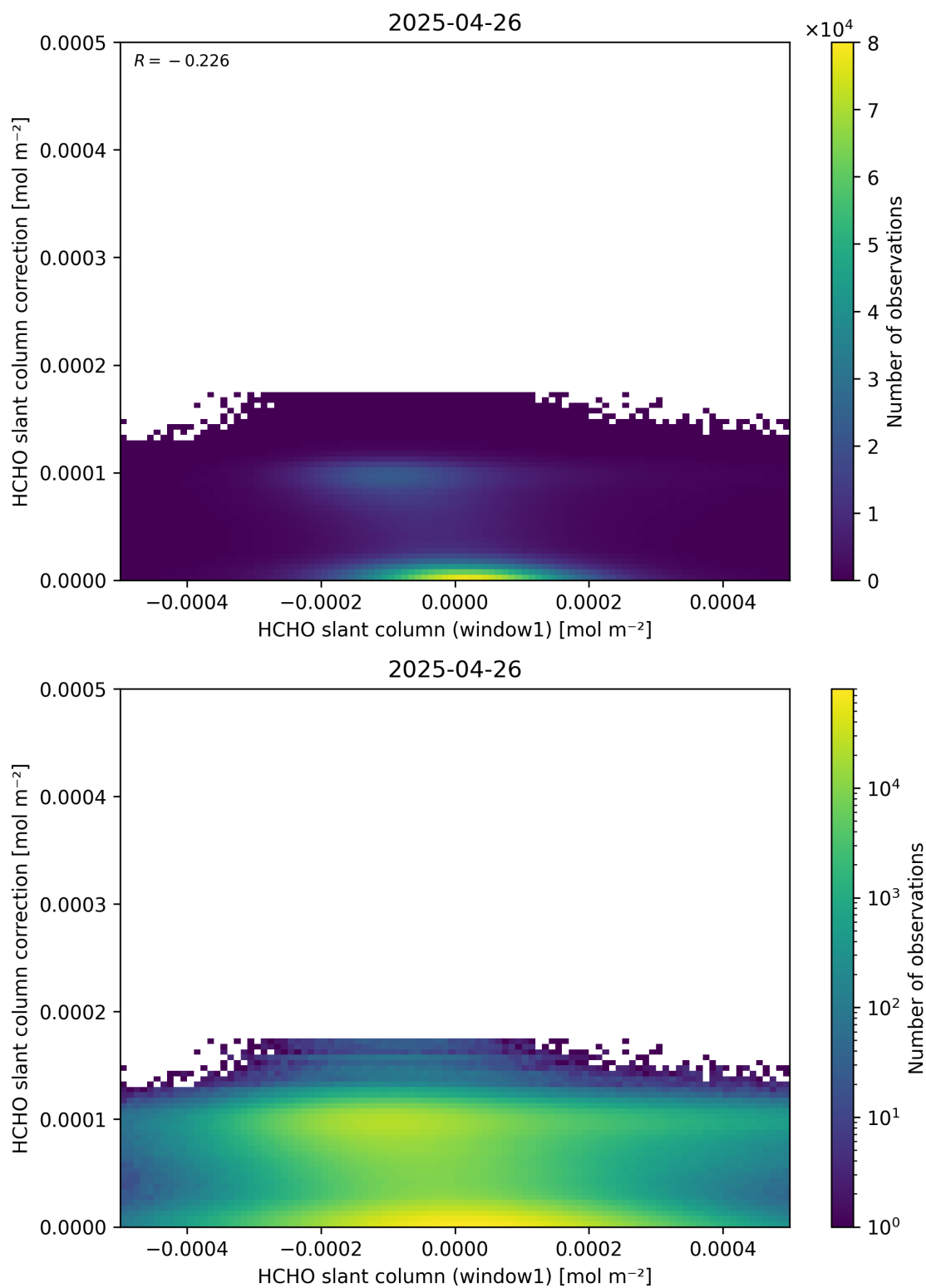
Figure 83: Scatter density plot of “HCHO slant column (window1)” against “HCHO slant column correction” for 2025-04-25 to 2025-04-27.
