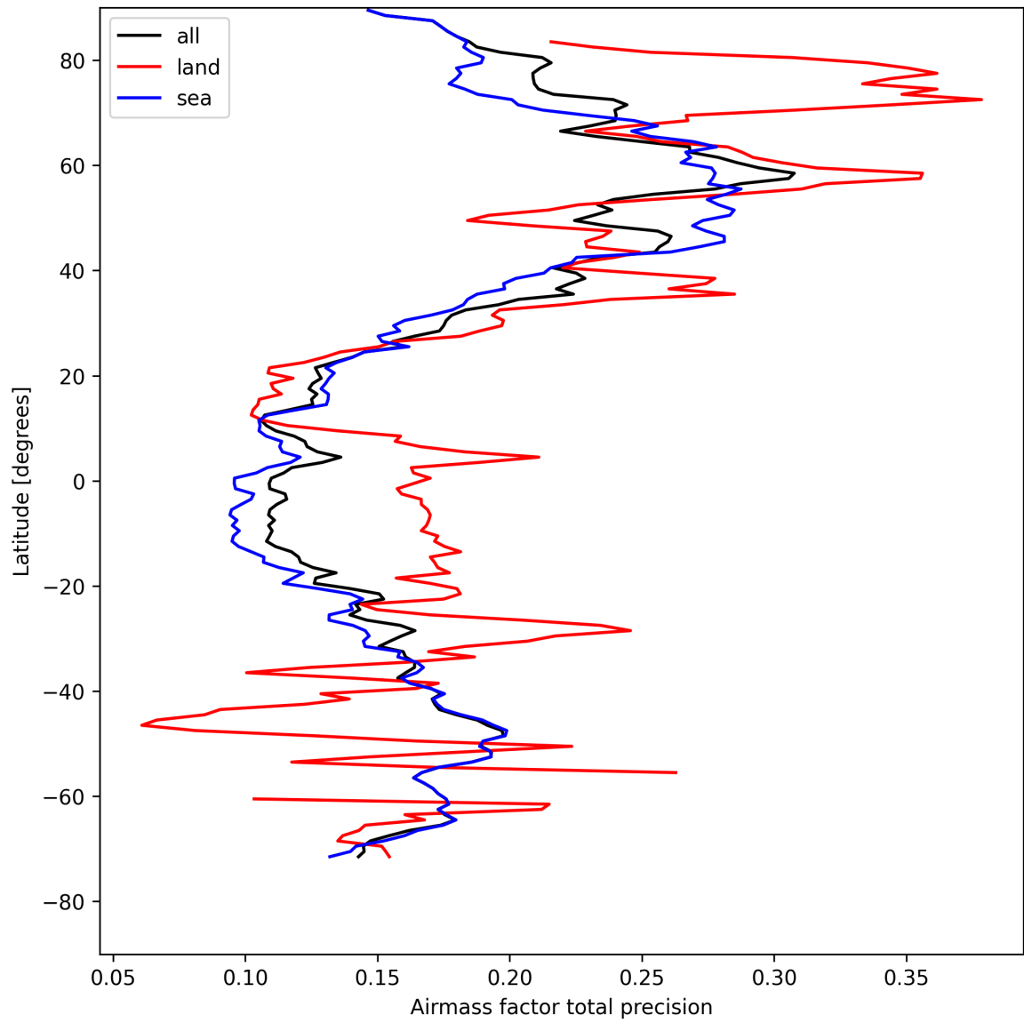
Figure 27: Zonal average of “Airmass factor total precision” for 2025-04-25 to 2025-04-27.
