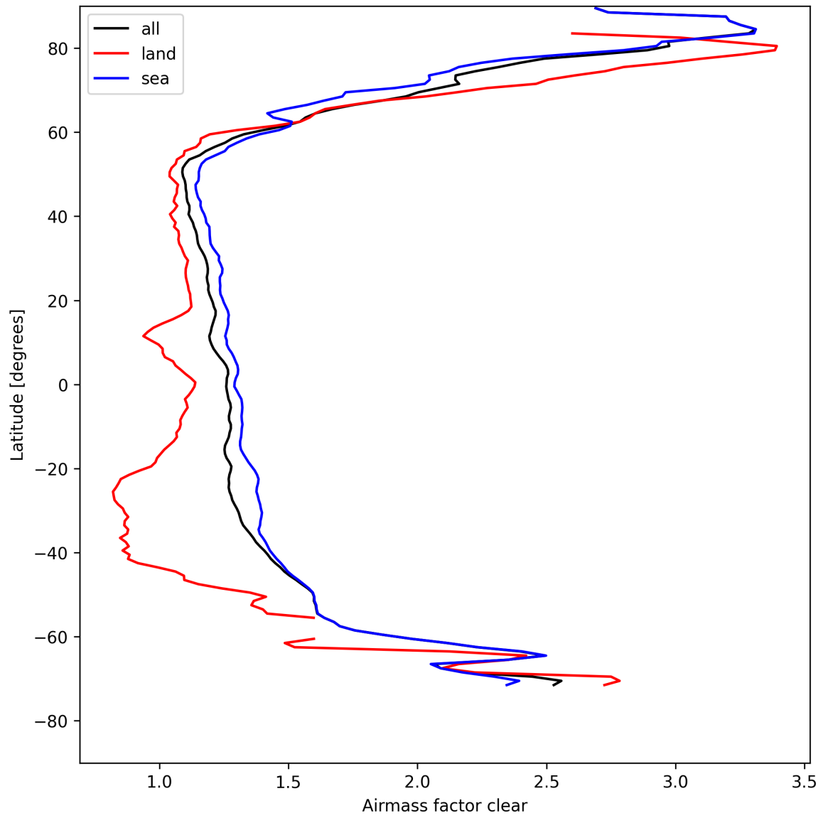
Figure 28: Zonal average of “Airmass factor clear” for 2025-04-25 to 2025-04-27.
