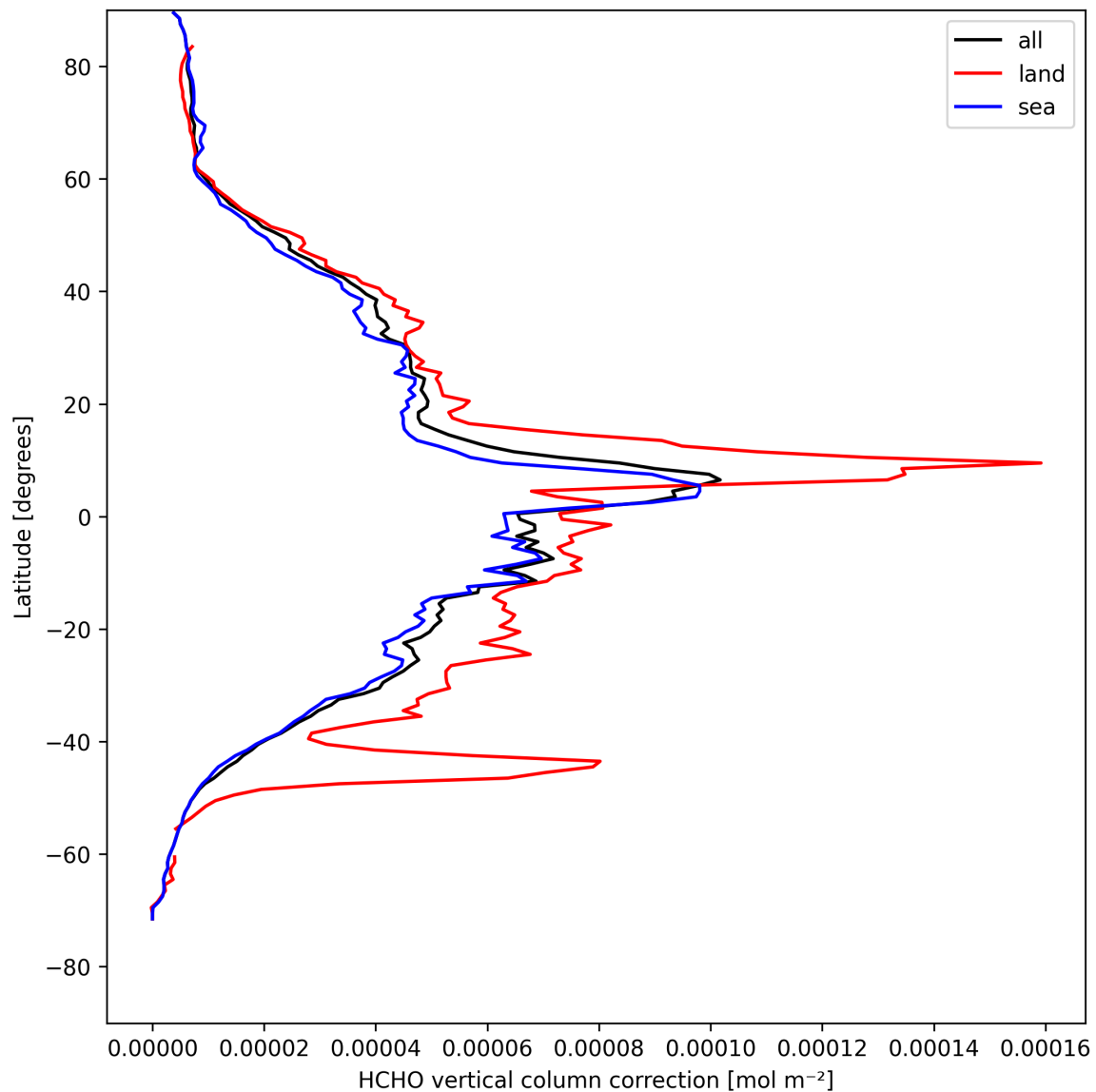
Figure 23: Zonal average of “HCHO vertical column correction” for 2025-04-25 to 2025-04-27.
