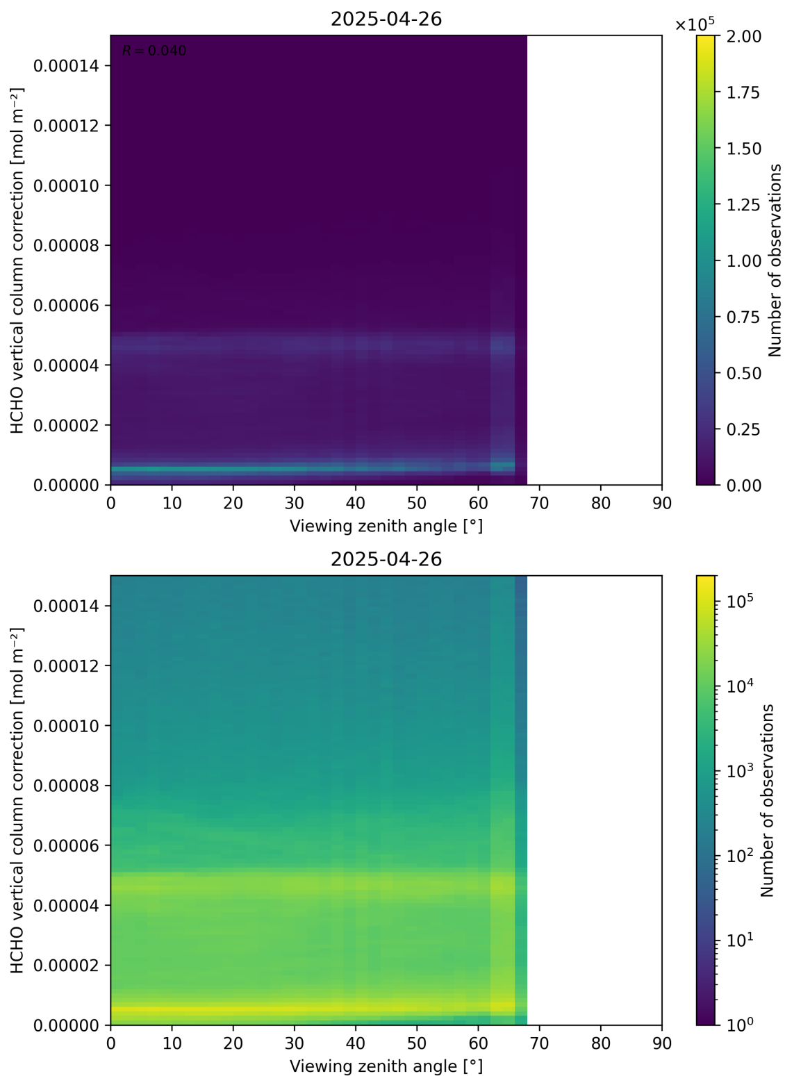
Figure 193: Scatter density plot of “Viewing zenith angle” against “HCHO vertical column correction” for 2025-04-25 to 2025-04-27.
