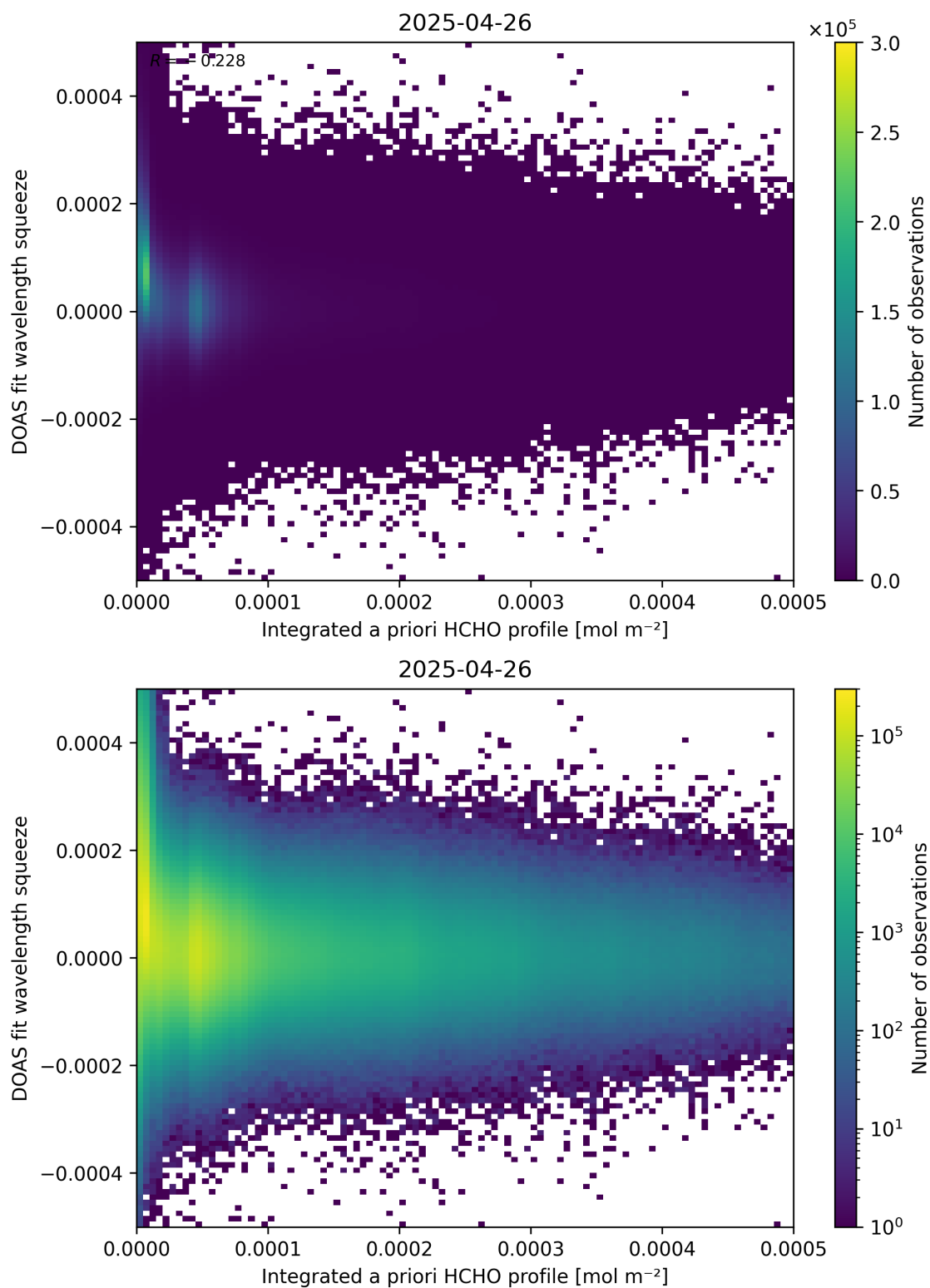
Figure 150: Scatter density plot of “Integrated a priori HCHO profile” against “DOAS fit wavelength squeeze” for 2025-04-25 to 2025-04-27.
