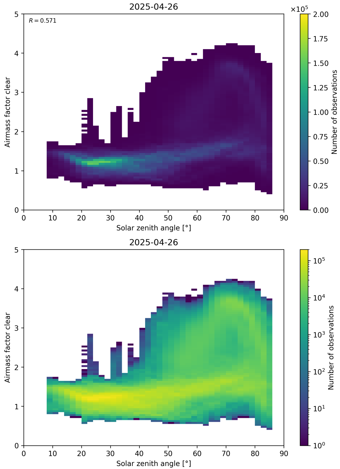
Figure 170: Scatter density plot of “Solar zenith angle” against “Airmass factor clear” for 2025-04-25 to 2025-04-27.
