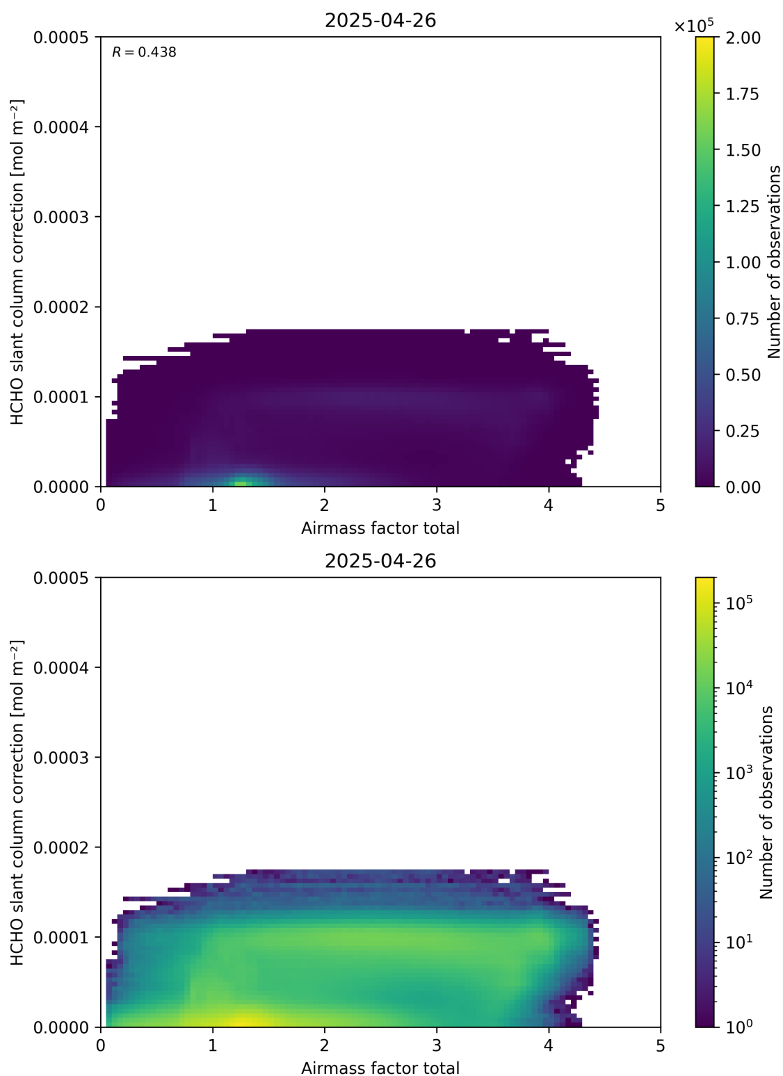
Figure 102: Scatter density plot of “Airmass factor total” against “HCHO slant column correction” for 2025-04-25 to 2025-04-27.
