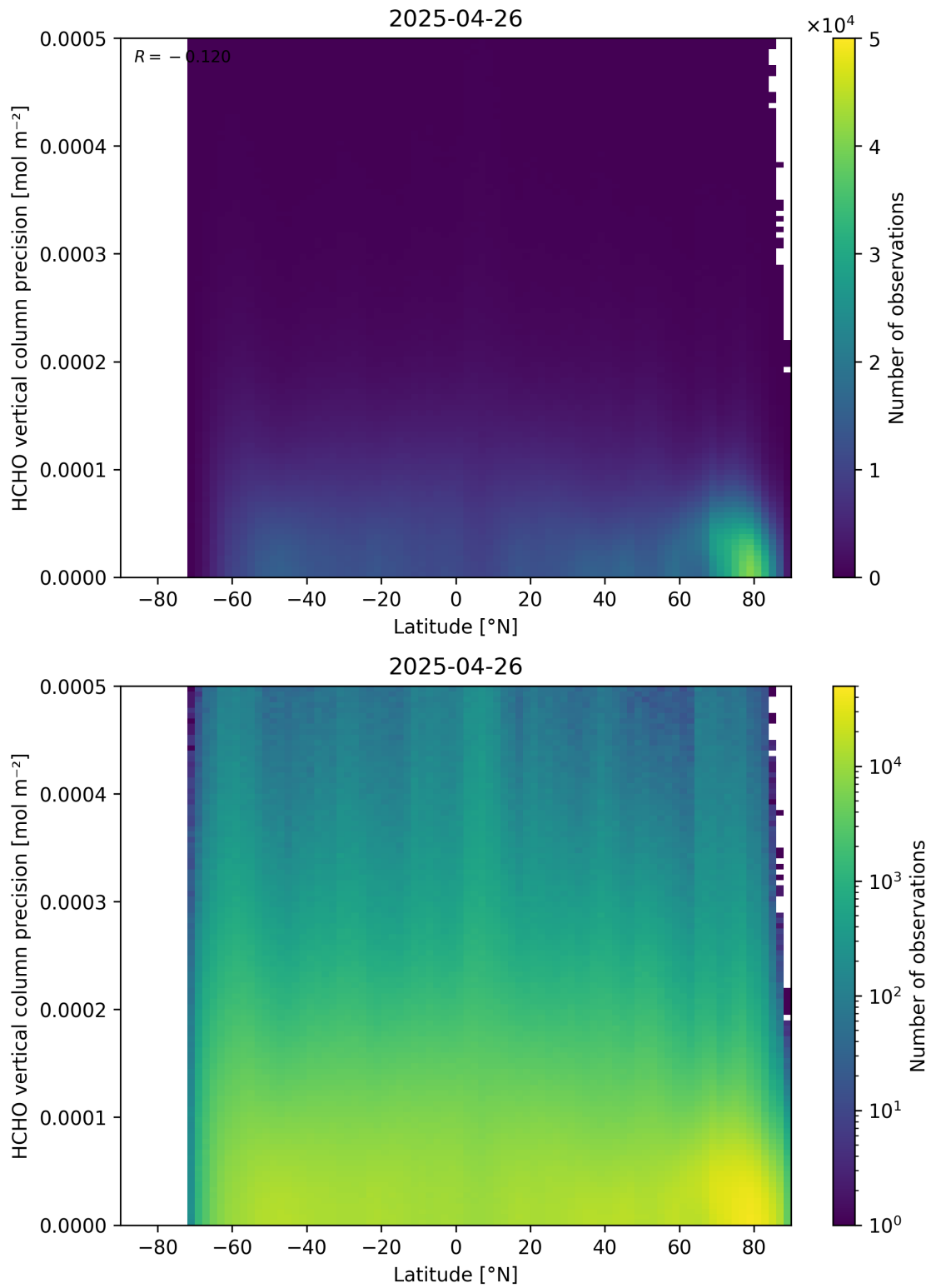
Figure 165: Scatter density plot of “Latitude” against “HCHO vertical column precision” for 2025-04-25 to 2025-04-27.
