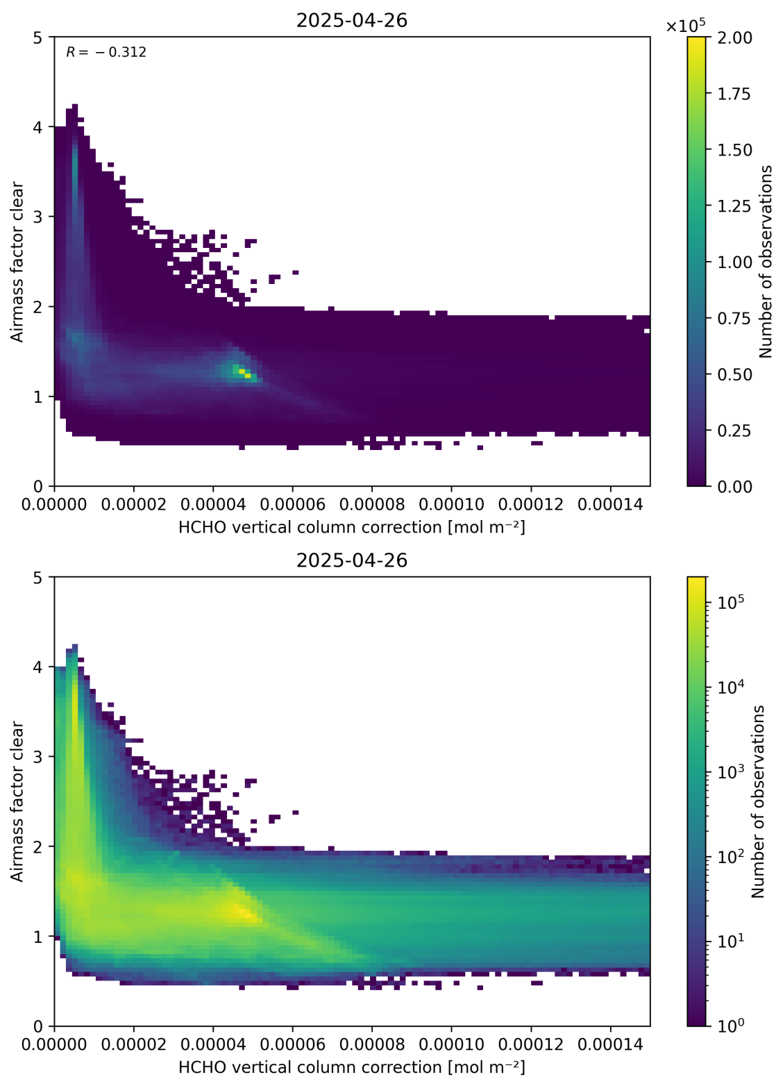
Figure 115: Scatter density plot of “HCHO vertical column correction” against “Airmass factor clear” for 2025-04-25 to 2025-04-27.
