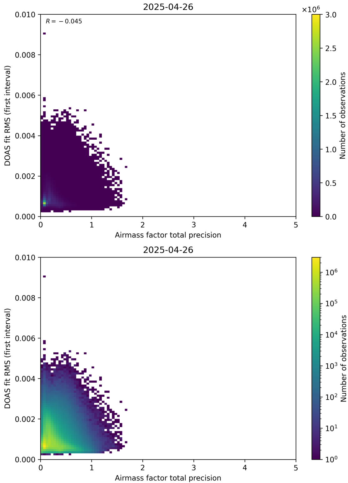
Figure 105: Scatter density plot of “Airmass factor total precision” against “DOAS fit RMS (first interval)” for 2025-04-25 to 2025-04-27.
