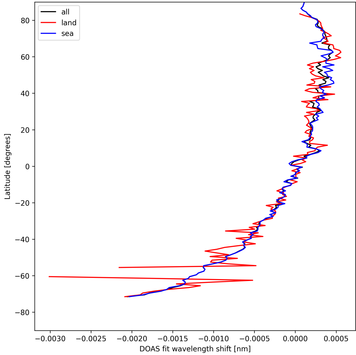
Figure 30: Zonal average of “DOAS fit wavelength shift” for 2025-04-25 to 2025-04-27.
