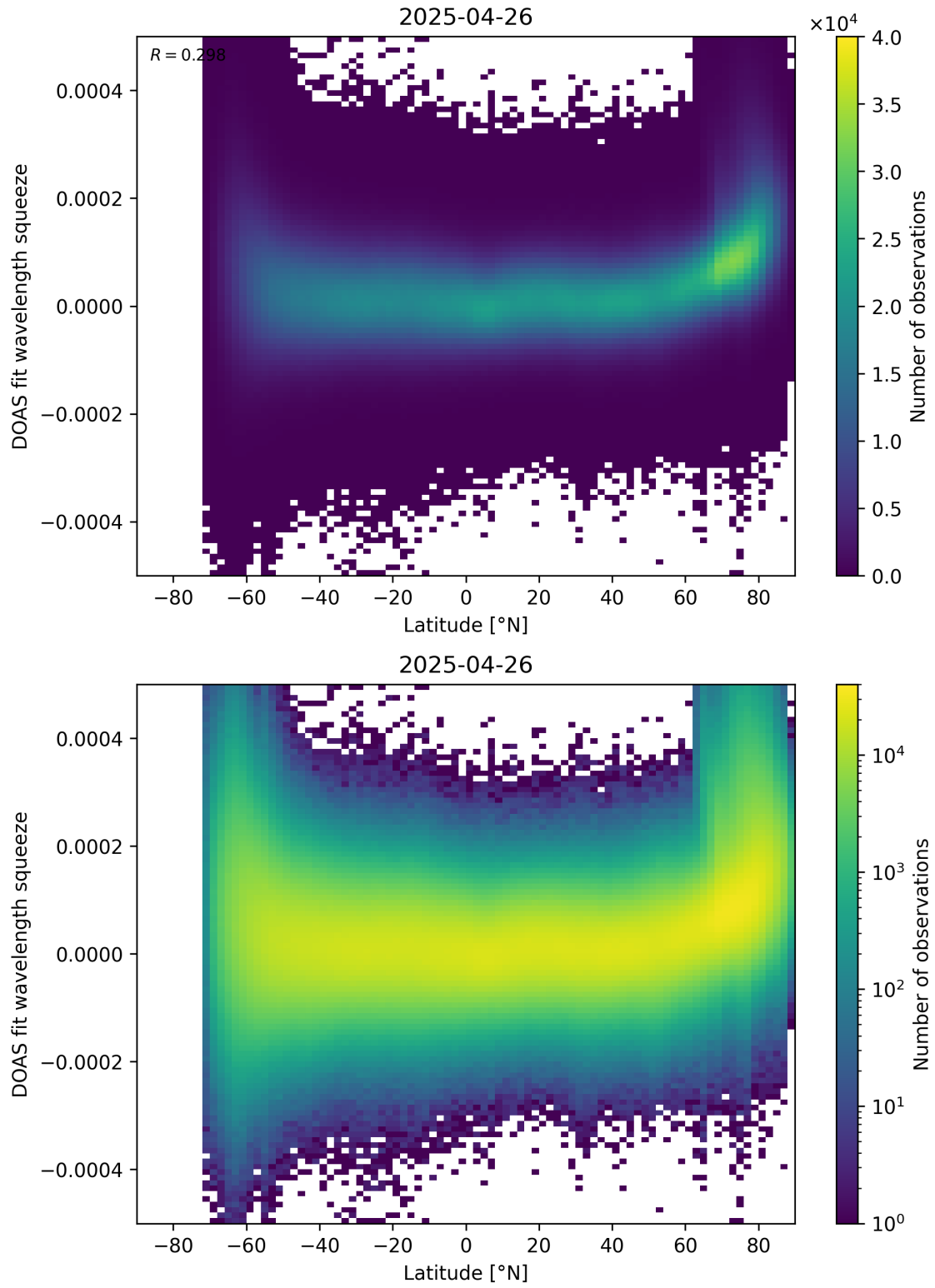
Figure 155: Scatter density plot of “Latitude” against “DOAS fit wavelength squeeze” for 2025-04-25 to 2025-04-27.
