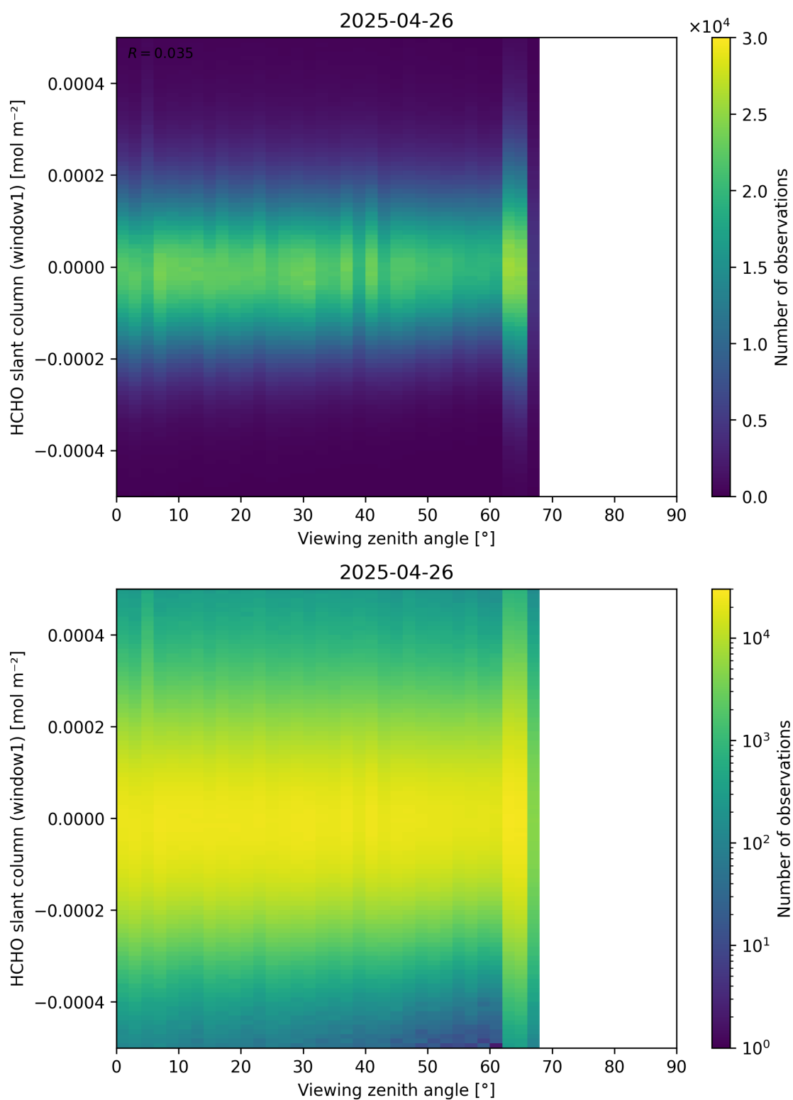
Figure 188: Scatter density plot of “Viewing zenith angle” against “HCHO slant column (window1)” for 2025-04-25 to 2025-04-27.
