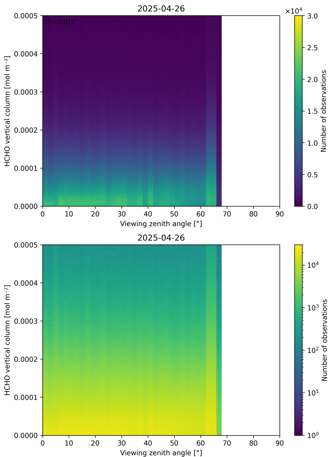
Figure 192: Scatter density plot of “Viewing zenith angle” against “HCHO vertical column” for 2025-04-25 to 2025-04-27.
