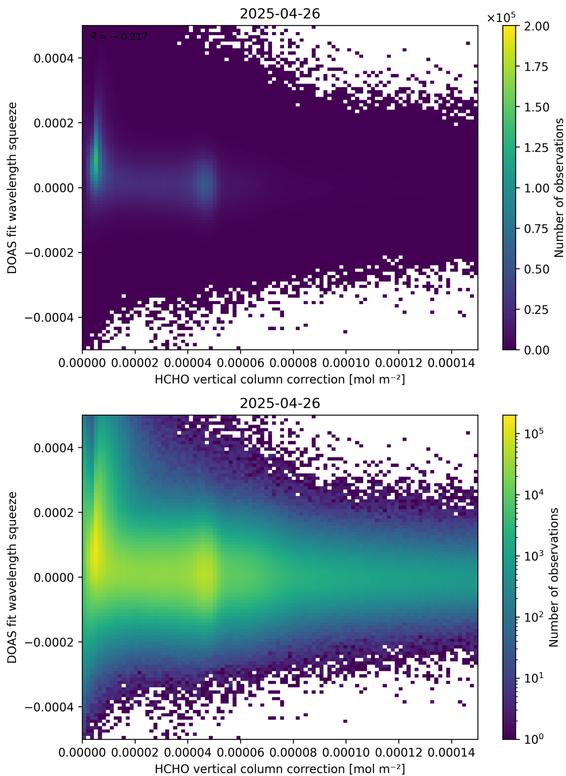
Figure 114: Scatter density plot of “HCHO vertical column correction” against “DOAS fit wavelength squeeze” for 2025-04-25 to 2025-04-27.
