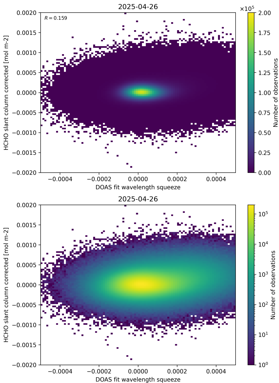
Figure 69: Scatter density plot of “DOAS fit wavelength squeeze” against “HCHO slant column corrected” for 2025-04-25 to 2025-04-27.
