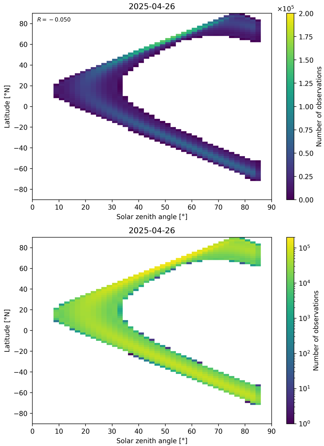
Figure 181: Scatter density plot of “Solar zenith angle” against “Latitude” for 2025-04-25 to 2025-04-27.
