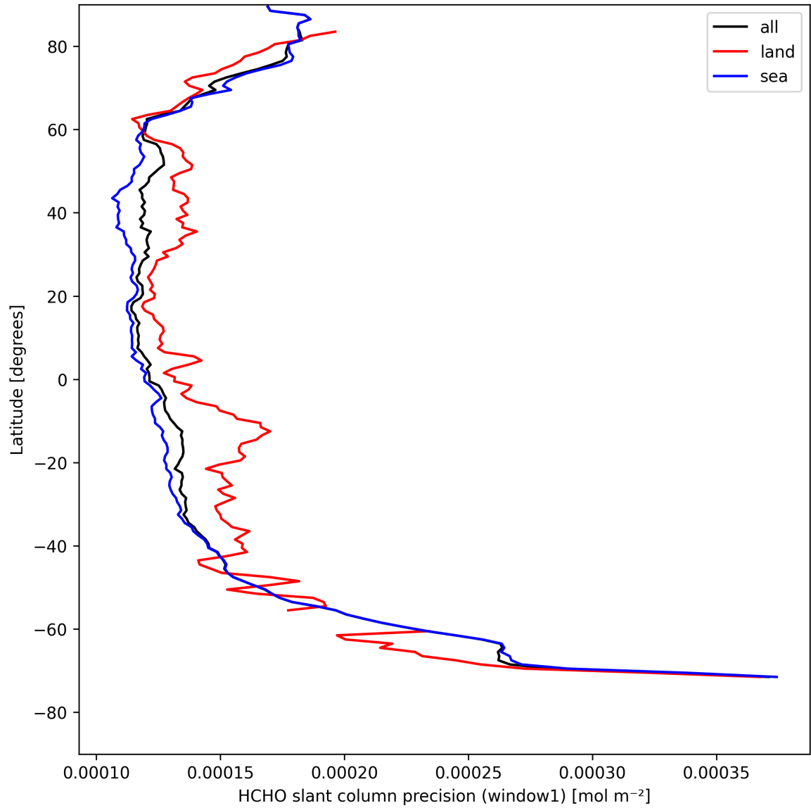
Figure 25: Zonal average of “HCHO slant column precision (window1)” for 2025-04-25 to 2025-04-27.
