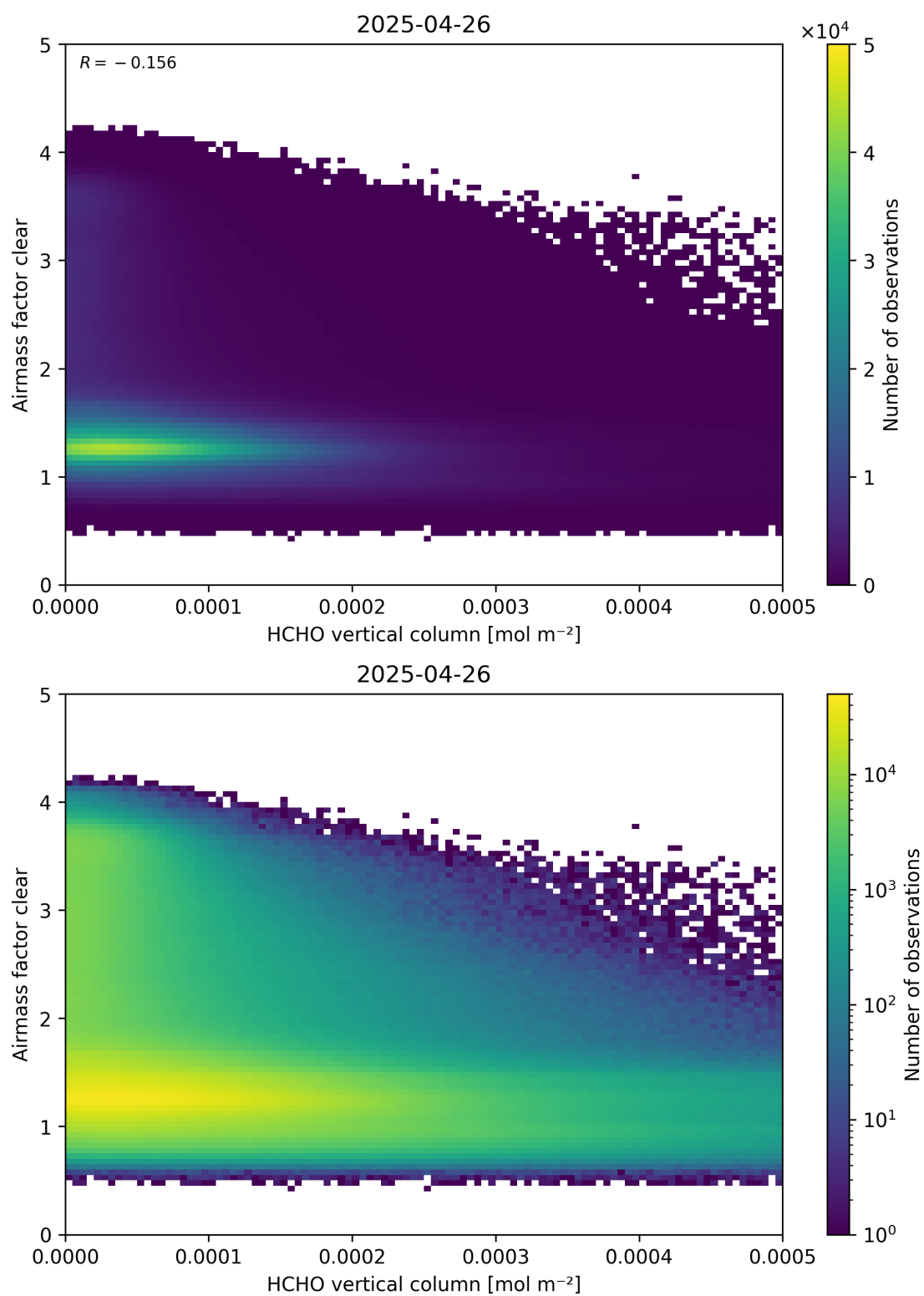
Figure 126: Scatter density plot of “HCHO vertical column” against “Airmass factor clear” for 2025-04-25 to 2025-04-27.
