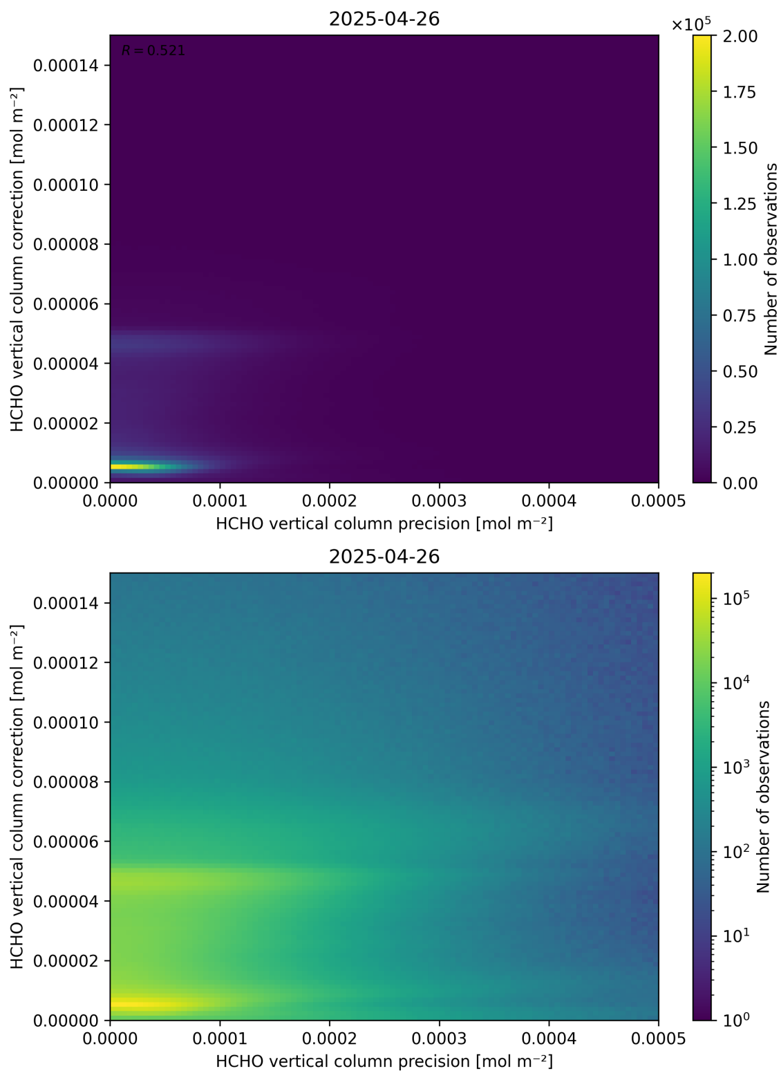
Figure 146: Scatter density plot of “HCHO vertical column precision” against “HCHO vertical column correction” for 2025-04-25 to 2025-04-27.
