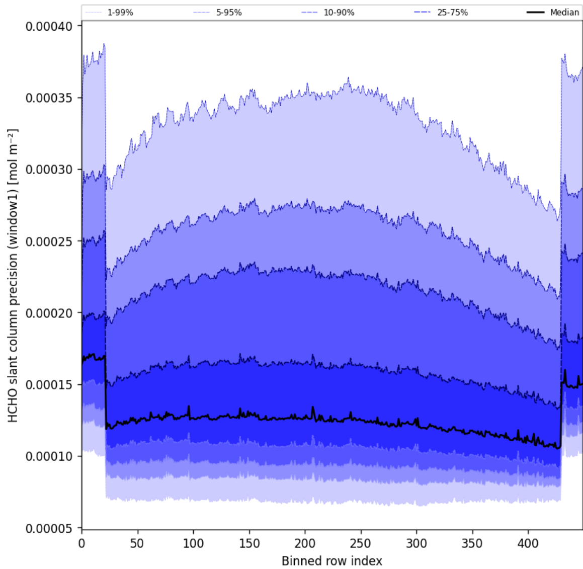
Figure 53: Along track statistics of “HCHO slant column precision (window1)” for 2025-04-25 to 2025-04-27
