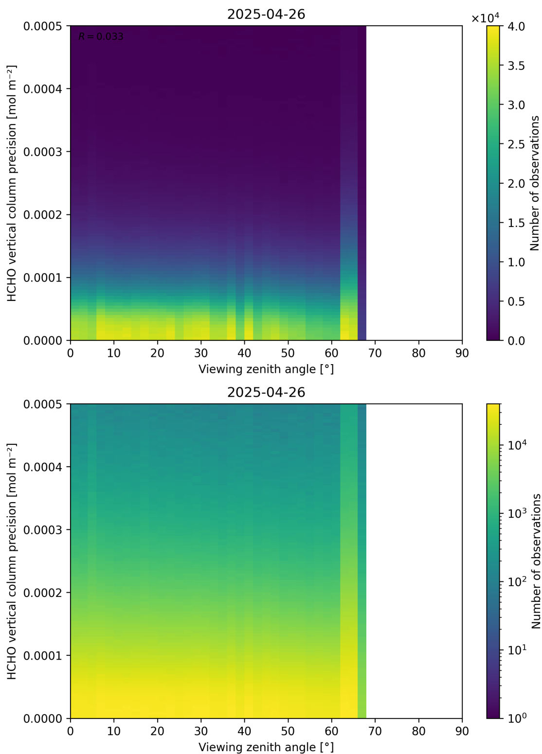
Figure 194: Scatter density plot of “Viewing zenith angle” against “HCHO vertical column precision” for 2025-04-25 to 2025-04-27.
