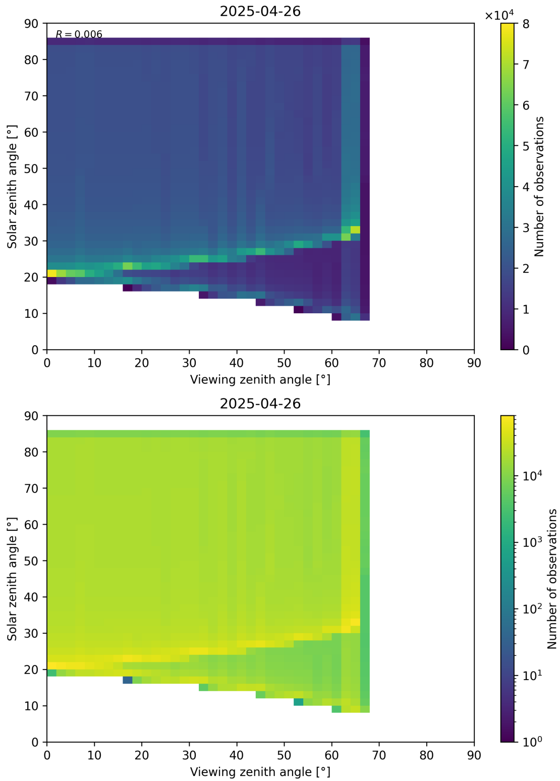
Figure 197: Scatter density plot of “Viewing zenith angle” against “Solar zenith angle” for 2025-04-25 to 2025-04-27.
