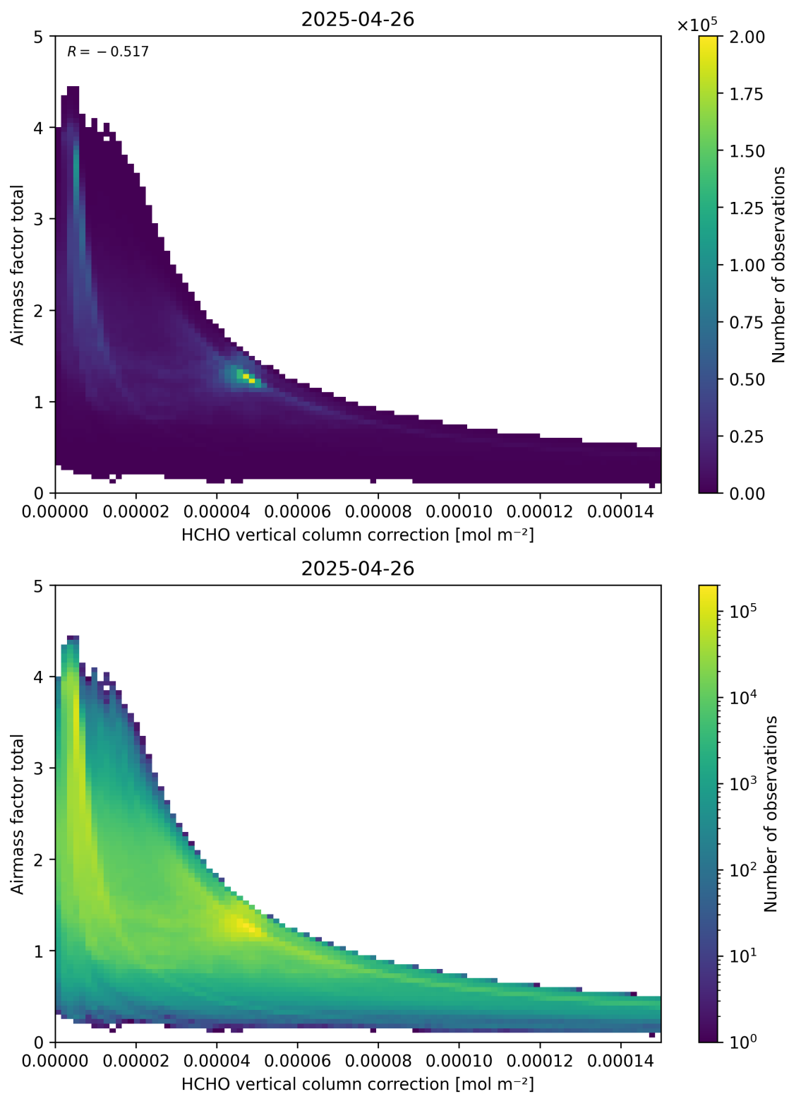
Figure 120: Scatter density plot of “HCHO vertical column correction” against “Airmass factor total” for 2025-04-25 to 2025-04-27.
