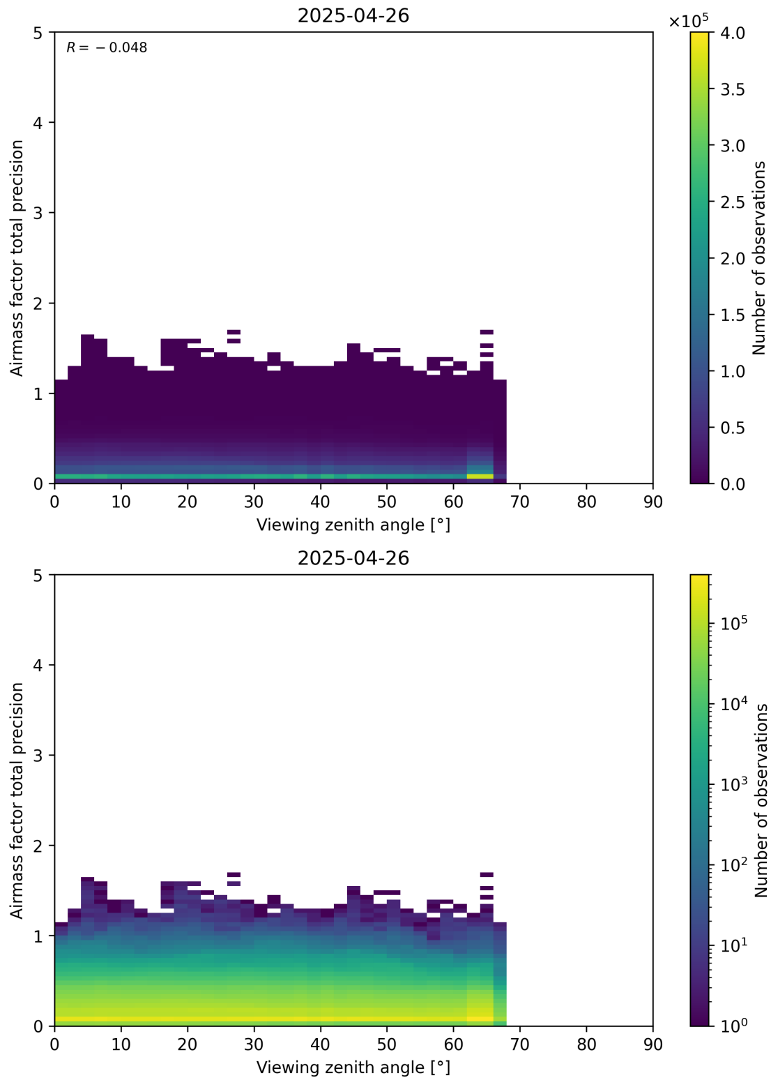
Figure 191: Scatter density plot of “Viewing zenith angle” against “Airmass factor total precision” for 2025-04-25 to 2025-04-27.
