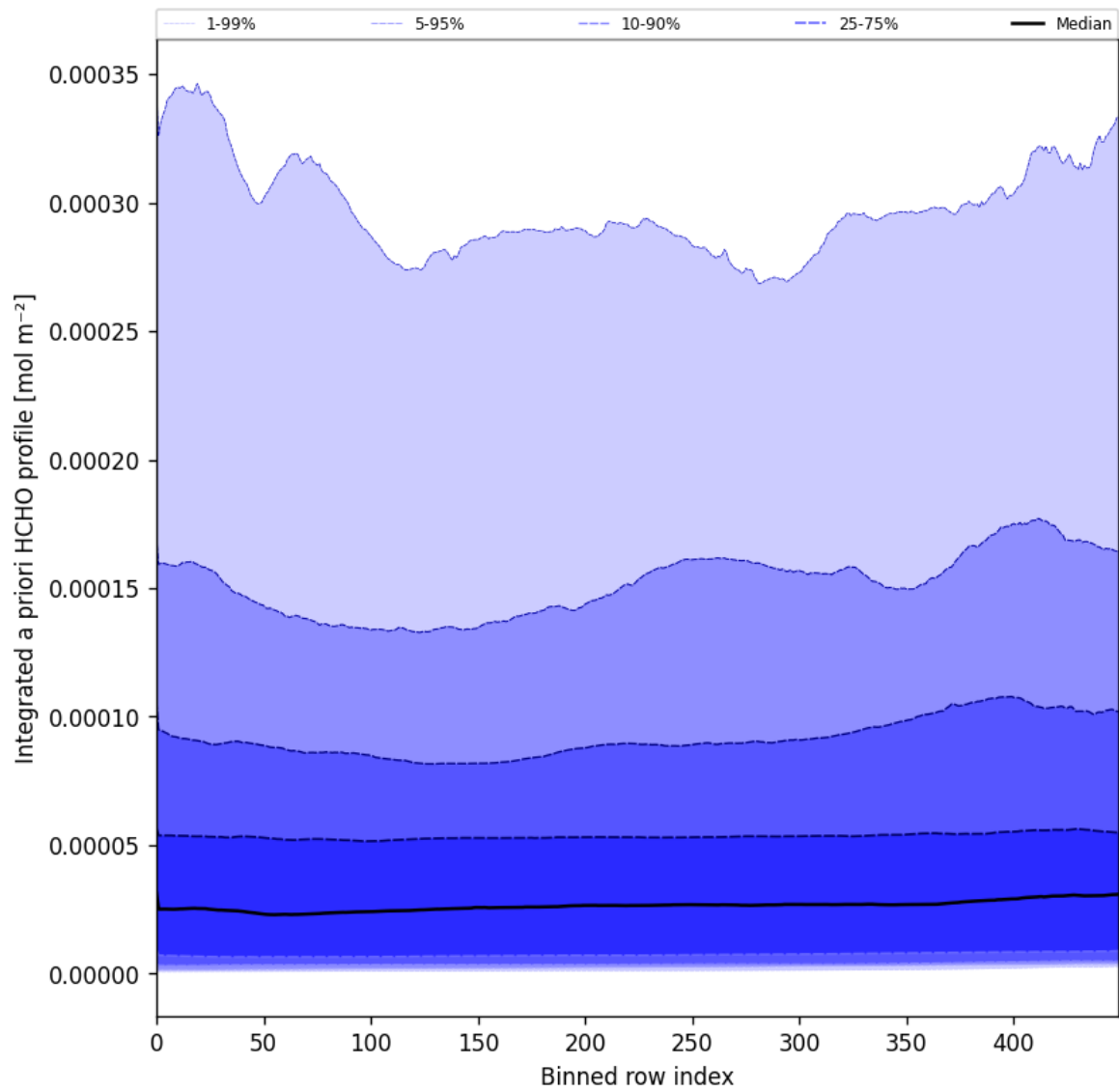
Figure 57: Along track statistics of “Integrated a priori HCHO profile” for 2025-04-25 to 2025-04-27
