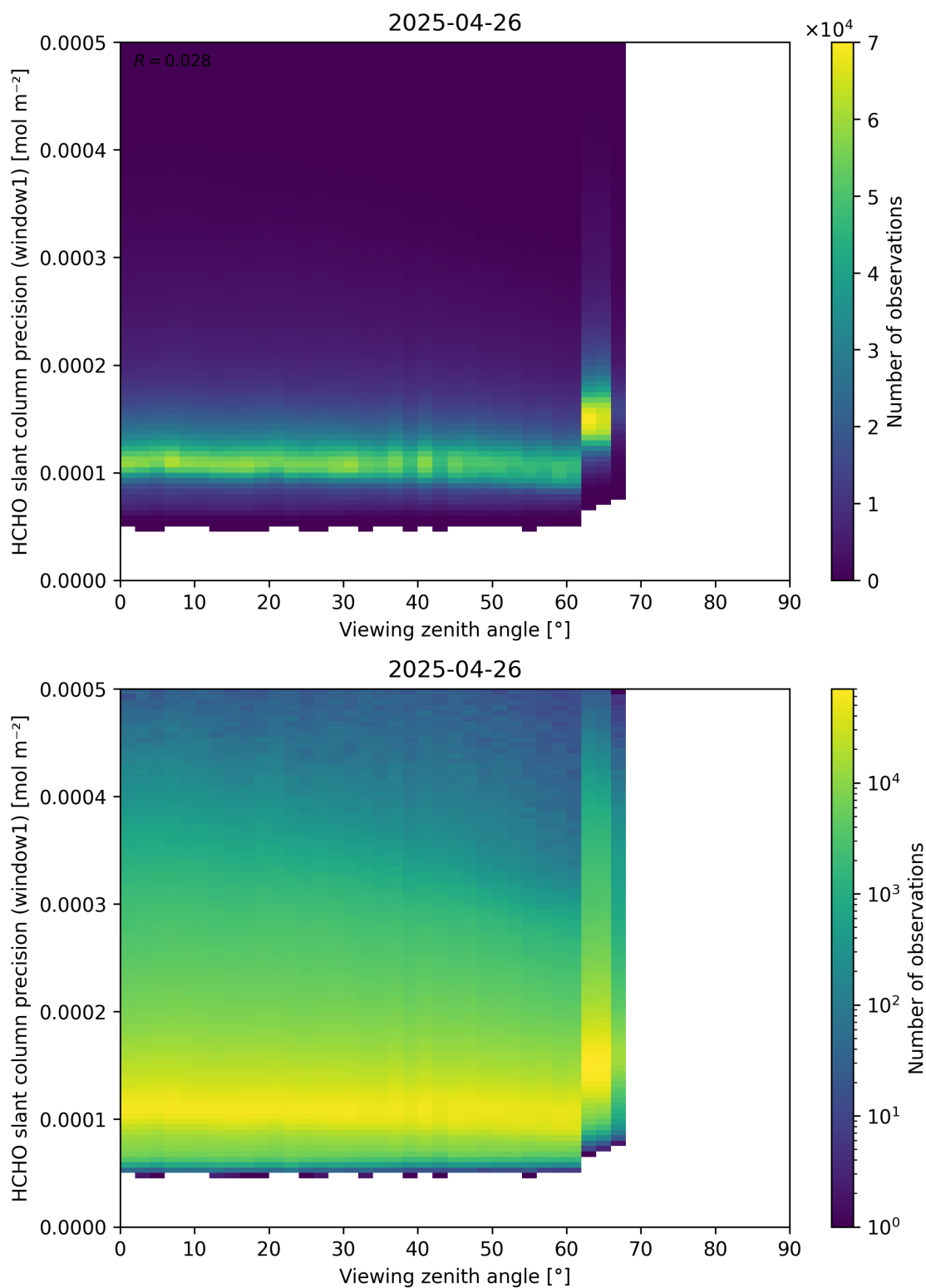
Figure 189: Scatter density plot of “Viewing zenith angle” against “HCHO slant column precision (window1)” for 2025-04-25 to 2025-04-27.
