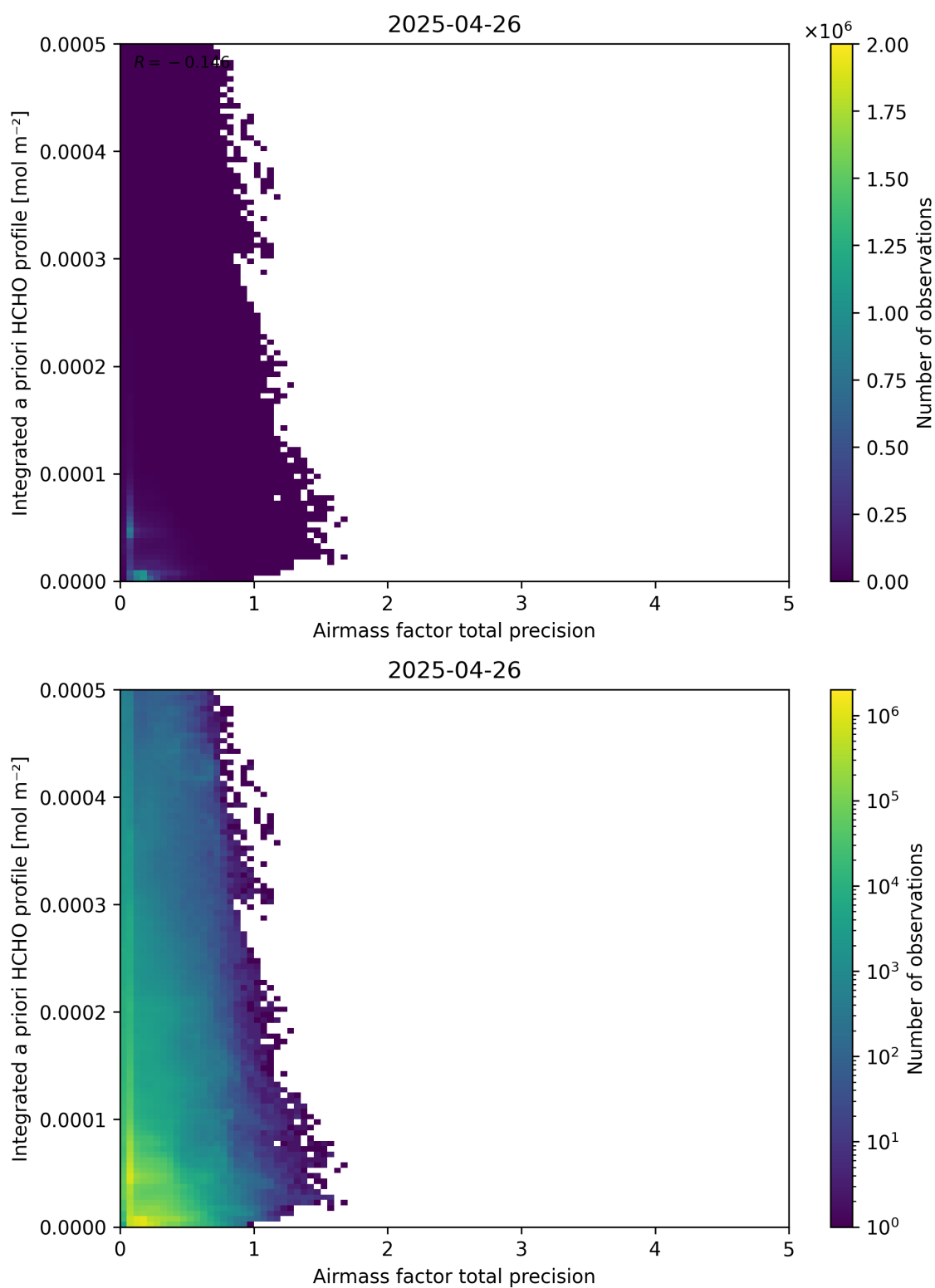
Figure 111: Scatter density plot of “Airmass factor total precision” against “Integrated a priori HCHO profile” for 2025-04-25 to 2025-04-27.
