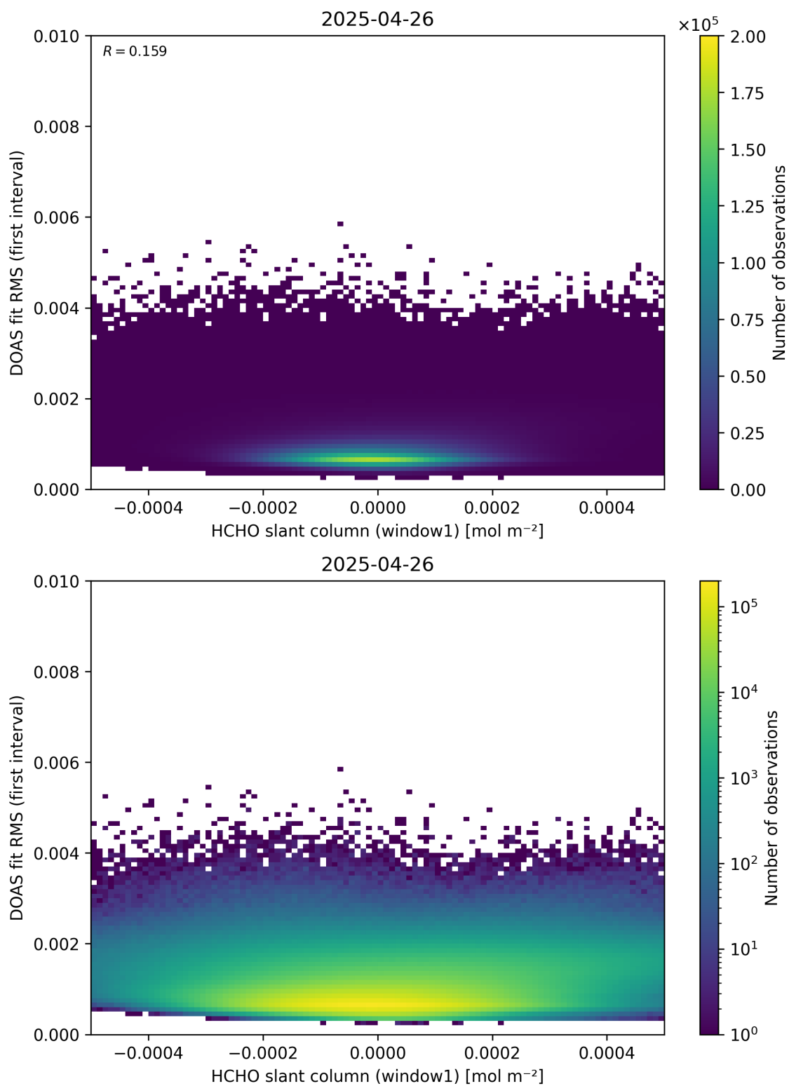
Figure 78: Scatter density plot of “HCHO slant column (window1)” against “DOAS fit RMS (first interval)” for 2025-04-25 to 2025-04-27.
