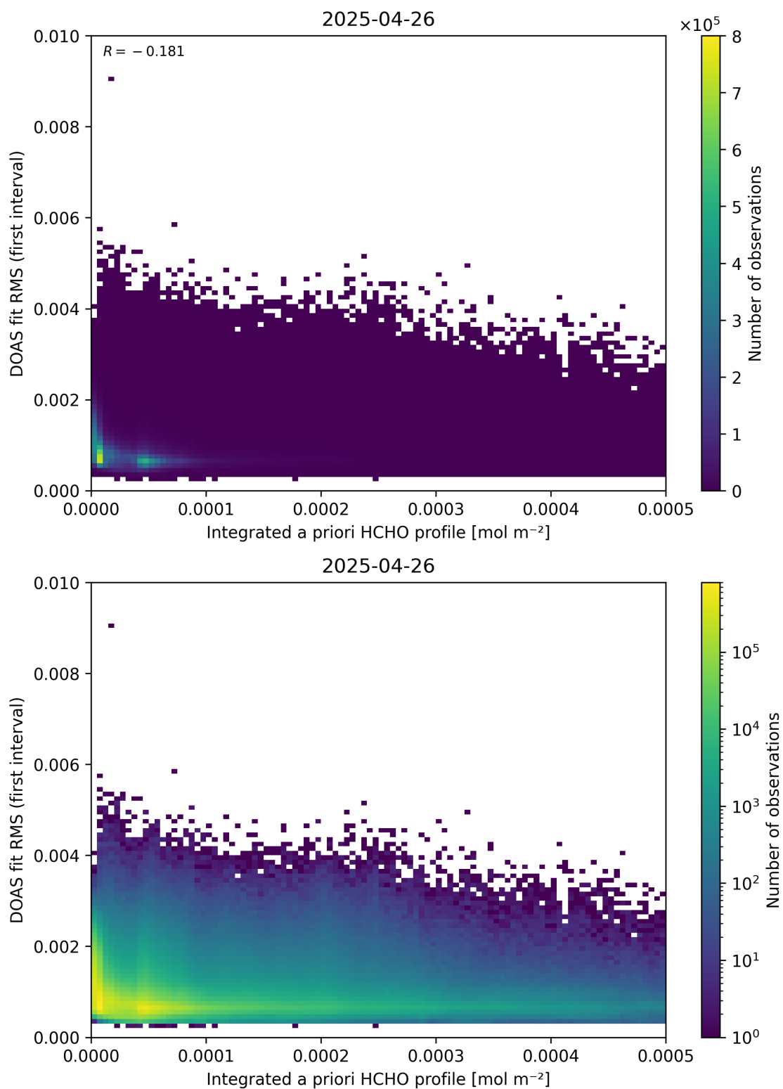
Figure 148: Scatter density plot of “Integrated a priori HCHO profile” against “DOAS fit RMS (first interval)” for 2025-04-25 to 2025-04-27.
