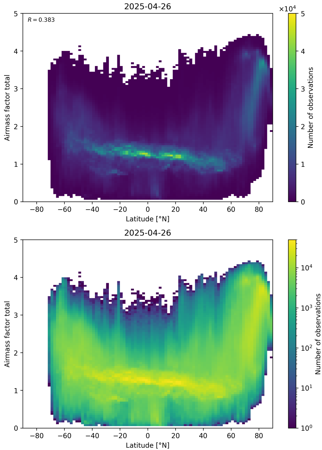
Figure 161: Scatter density plot of “Latitude” against “Airmass factor total” for 2025-04-25 to 2025-04-27.
