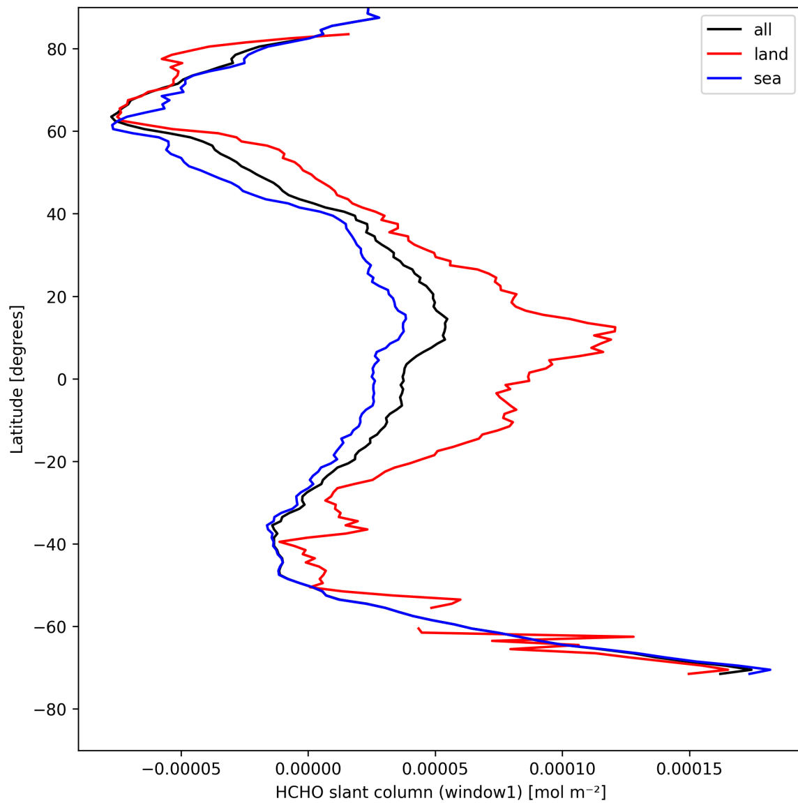
Figure 24: Zonal average of “HCHO slant column (window1)” for 2025-04-25 to 2025-04-27.
