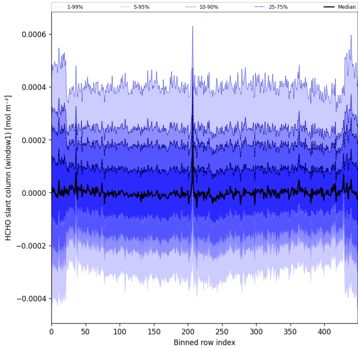
Figure 52: Along track statistics of “HCHO slant column (window1)” for 2025-04-25 to 2025-04-27
