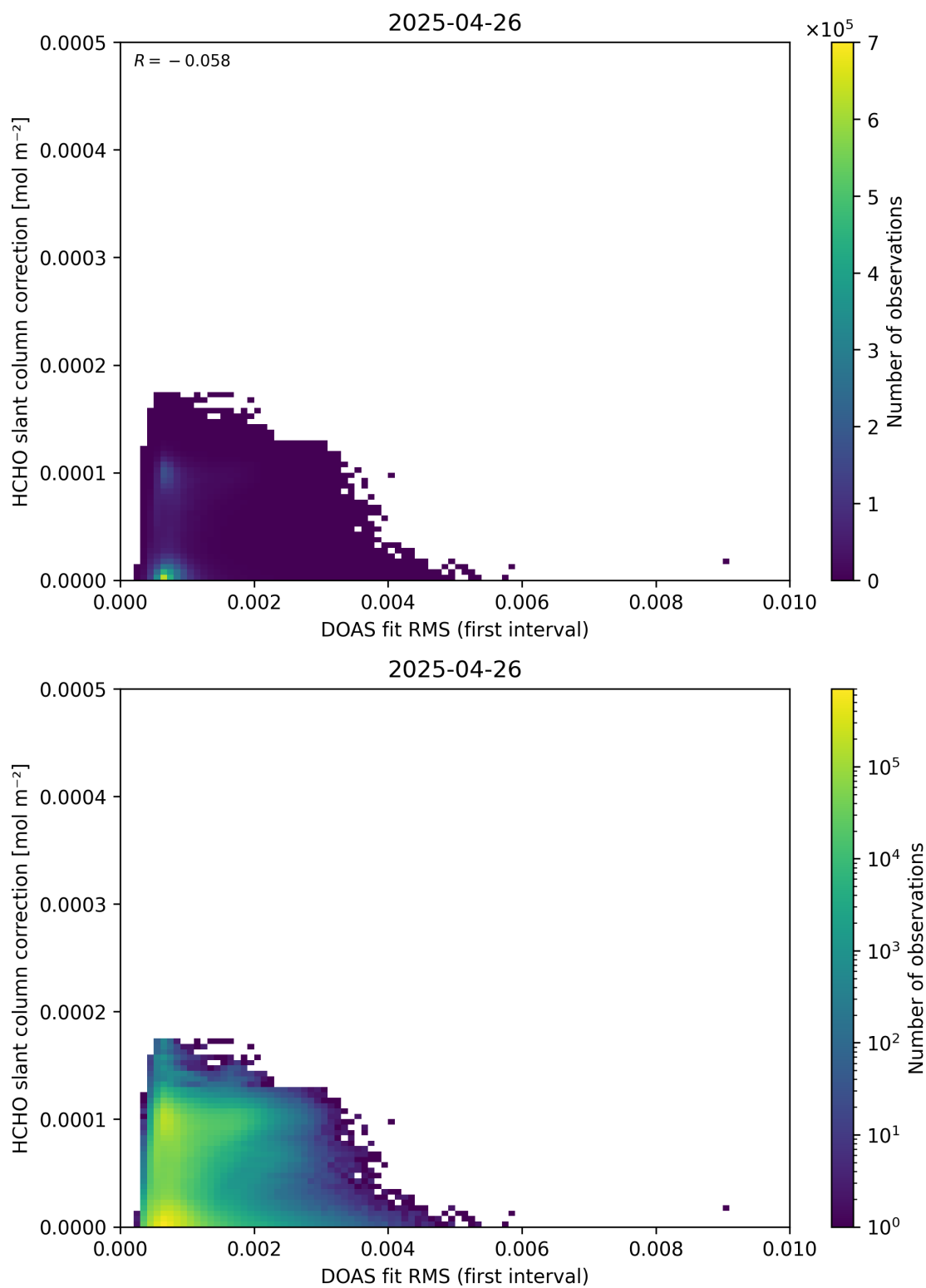
Figure 63: Scatter density plot of “DOAS fit RMS (first interval)” against “HCHO slant column correction” for 2025-04-25 to 2025-04-27.
