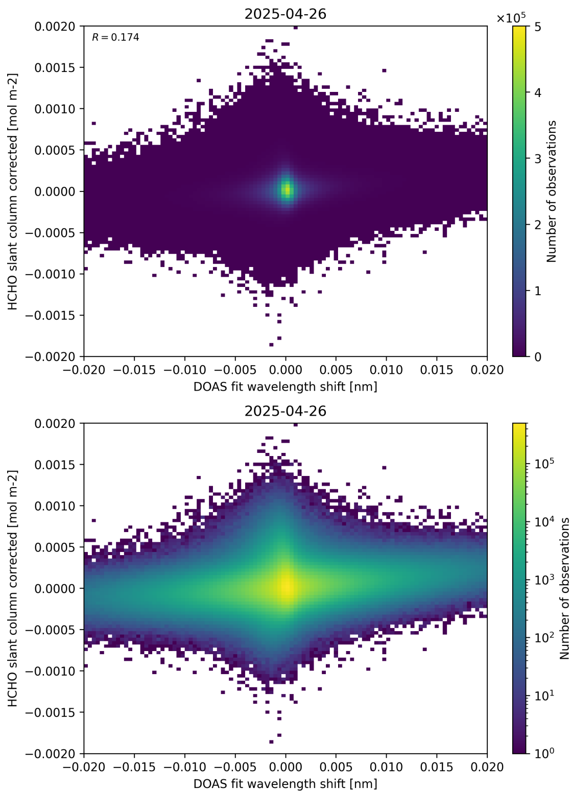
Figure 66: Scatter density plot of “DOAS fit wavelength shift” against “HCHO slant column corrected” for 2025-04-25 to 2025-04-27.
