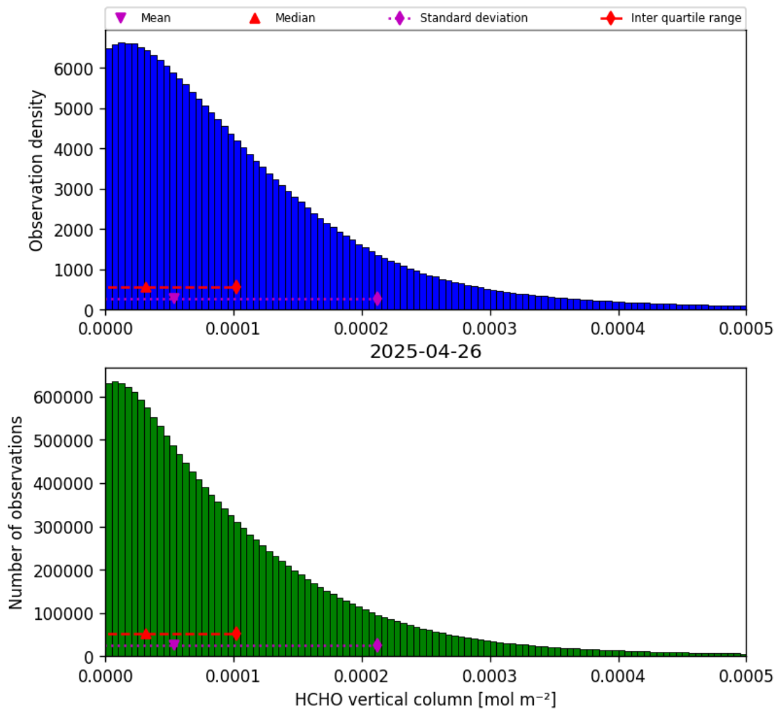
Figure 35: Histogram of “HCHO vertical column” for 2025-04-25 to 2025-04-27
