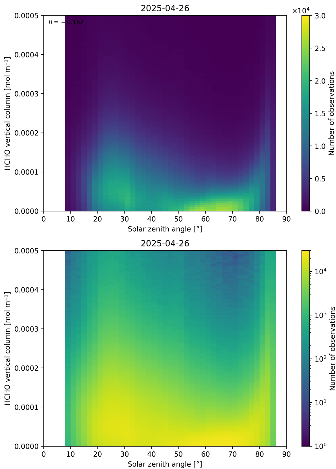
Figure 177: Scatter density plot of “Solar zenith angle” against “HCHO vertical column” for 2025-04-25 to 2025-04-27.
