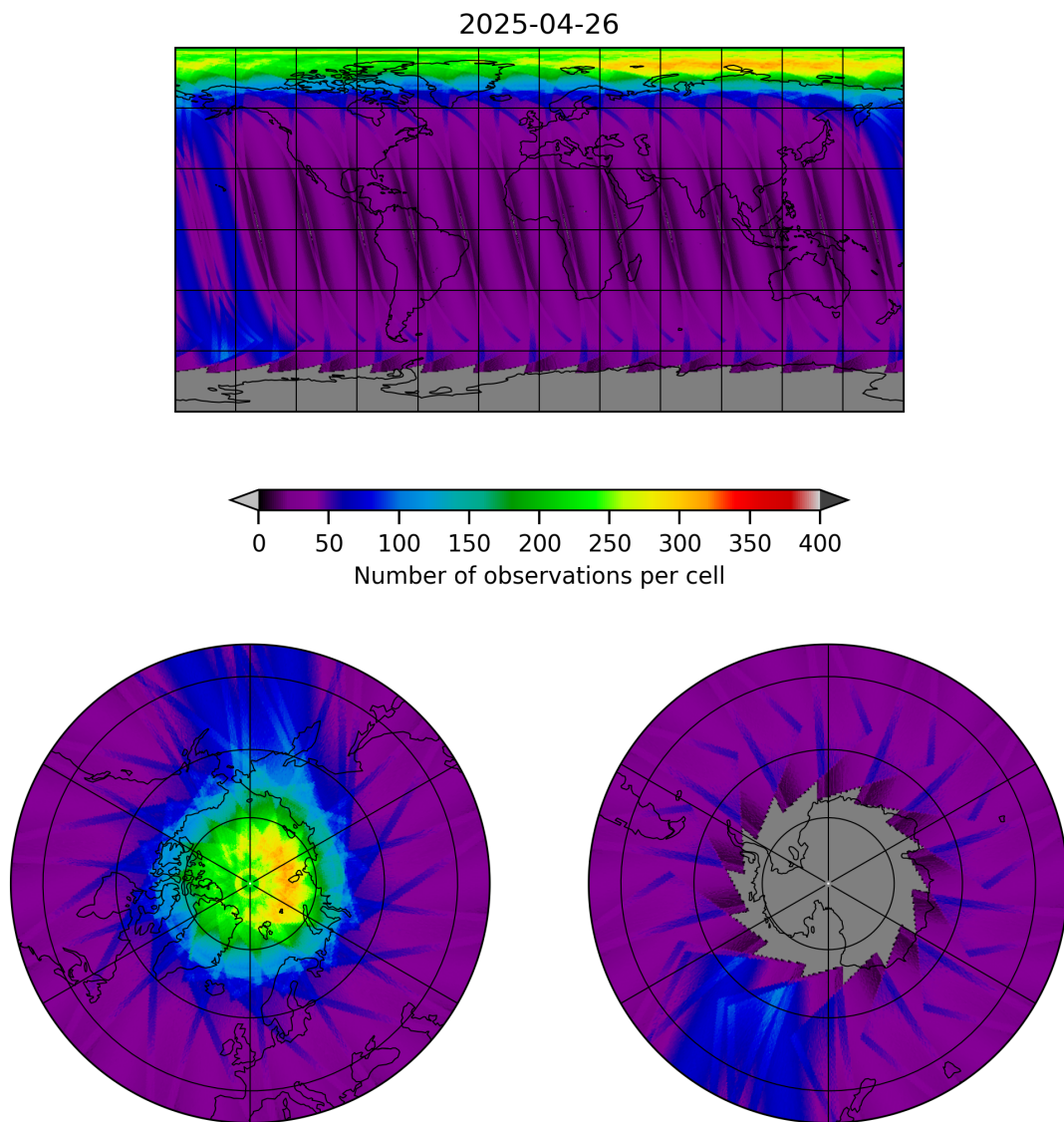
Figure 19: Map of the number of observations for 2025-04-25 to 2025-04-27
