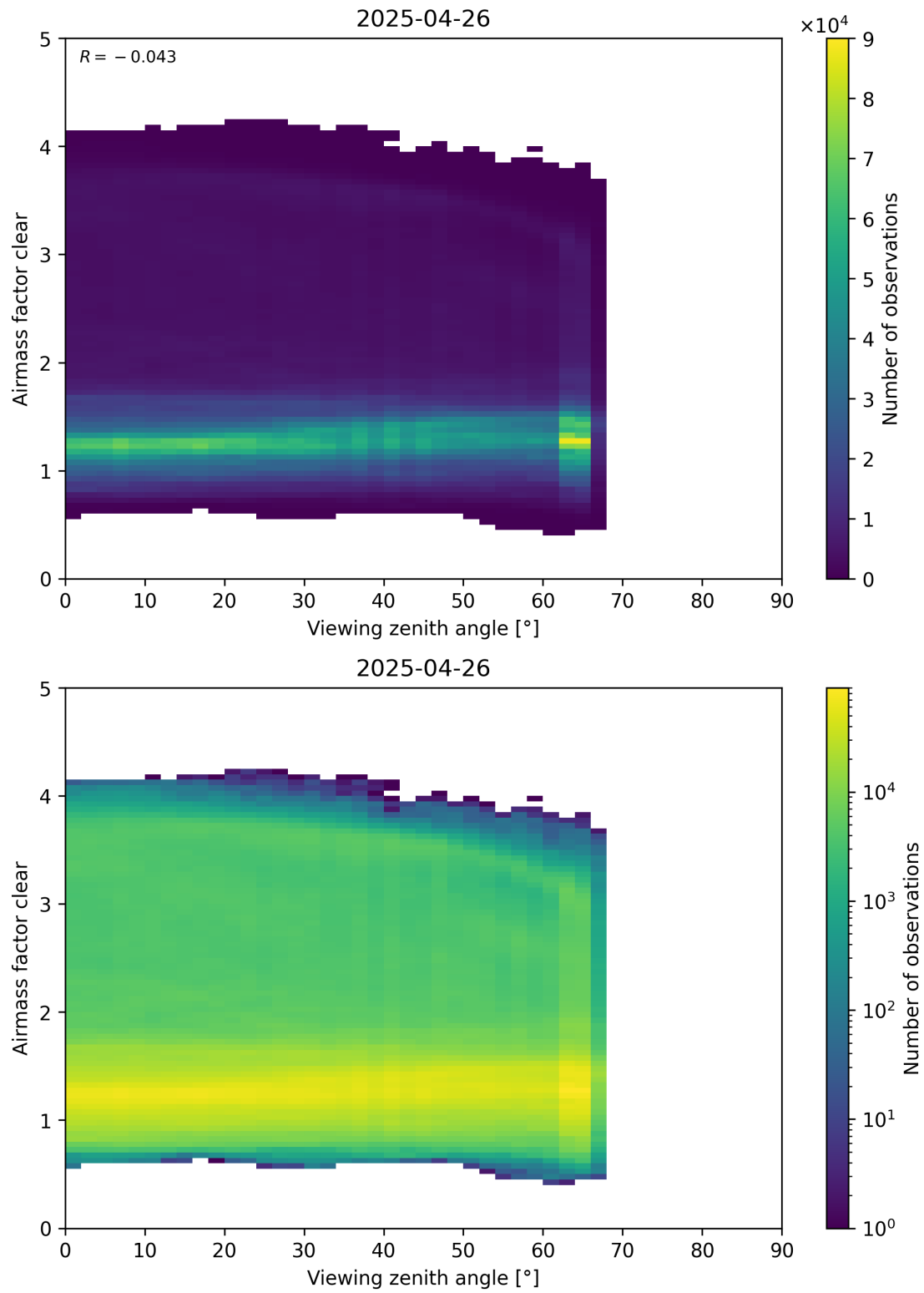
Figure 185: Scatter density plot of “Viewing zenith angle” against “Airmass factor clear” for 2025-04-25 to 2025-04-27.
