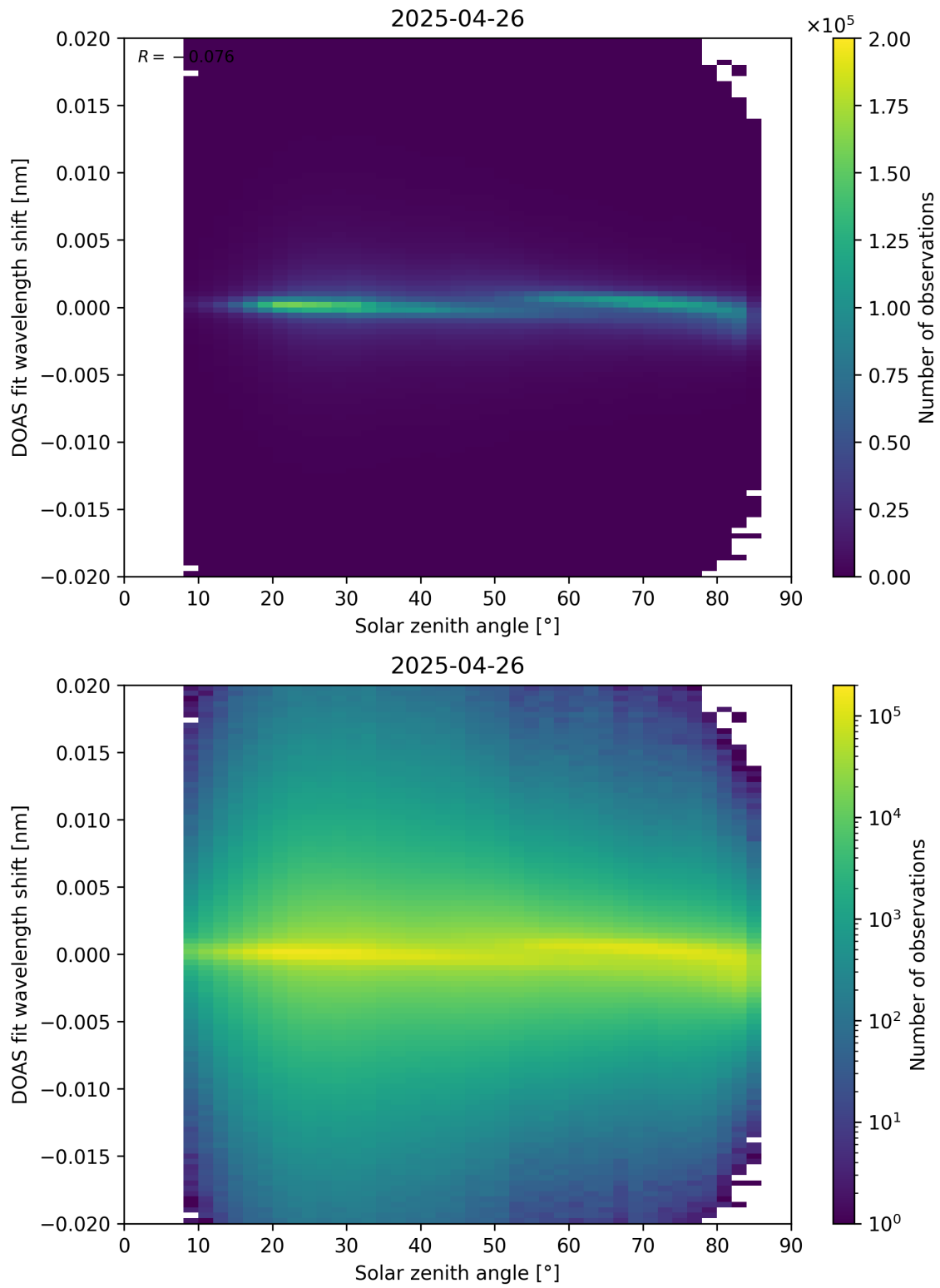
Figure 168: Scatter density plot of “Solar zenith angle” against “DOAS fit wavelength shift” for 2025-04-25 to 2025-04-27.
