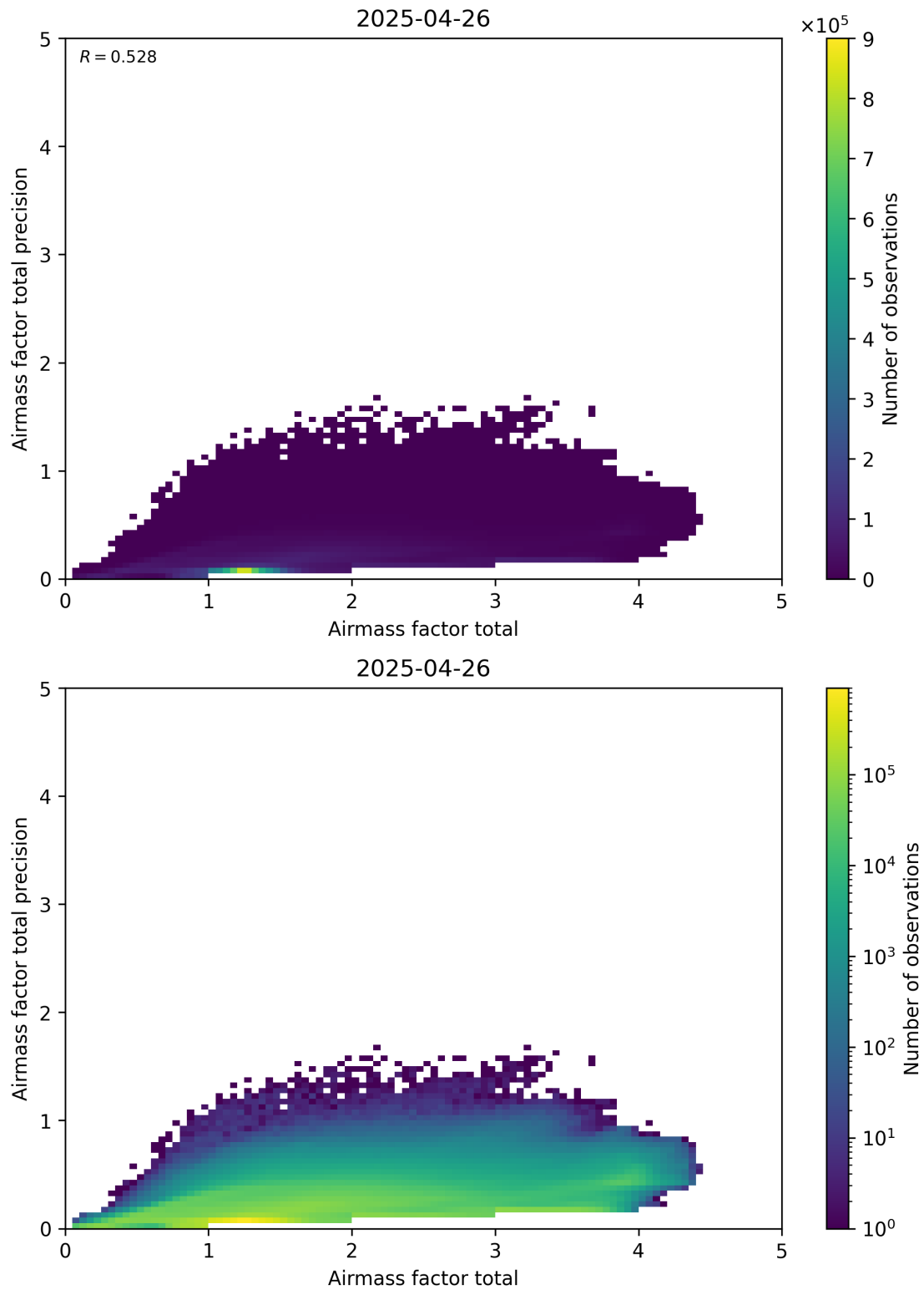
Figure 103: Scatter density plot of “Airmass factor total” against “Airmass factor total precision” for 2025-04-25 to 2025-04-27.
