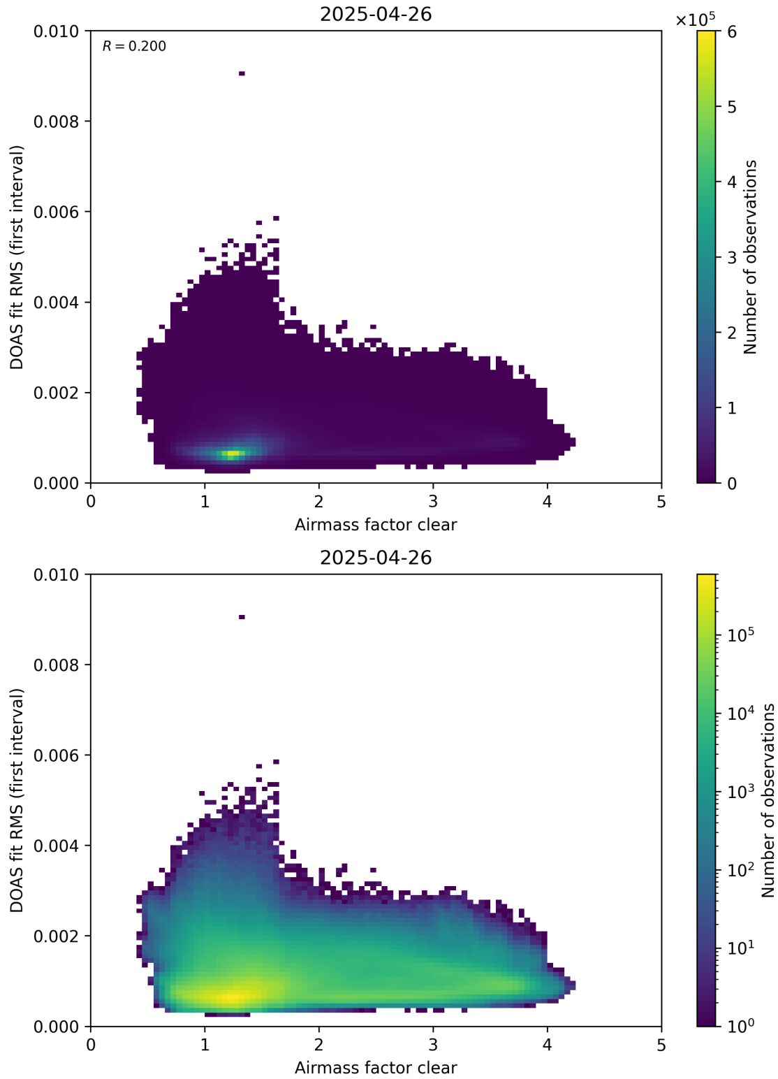
Figure 71: Scatter density plot of “Airmass factor clear” against “DOAS fit RMS (first interval)” for 2025-04-25 to 2025-04-27.
