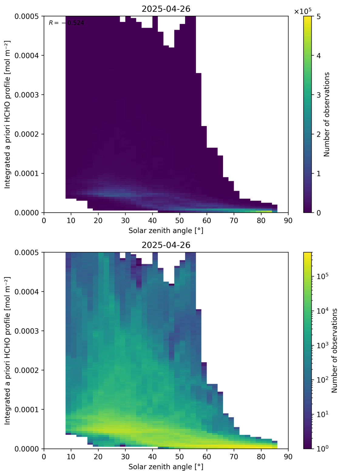
Figure 180: Scatter density plot of “Solar zenith angle” against “Integrated a priori HCHO profile” for 2025-04-25 to 2025-04-27.
