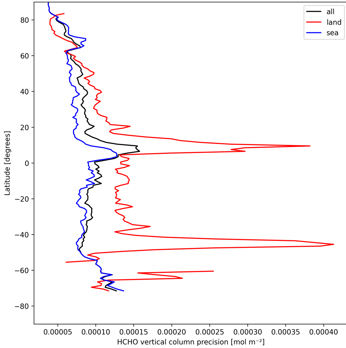
Figure 22: Zonal average of “HCHO vertical column precision” for 2025-04-25 to 2025-04-27.
