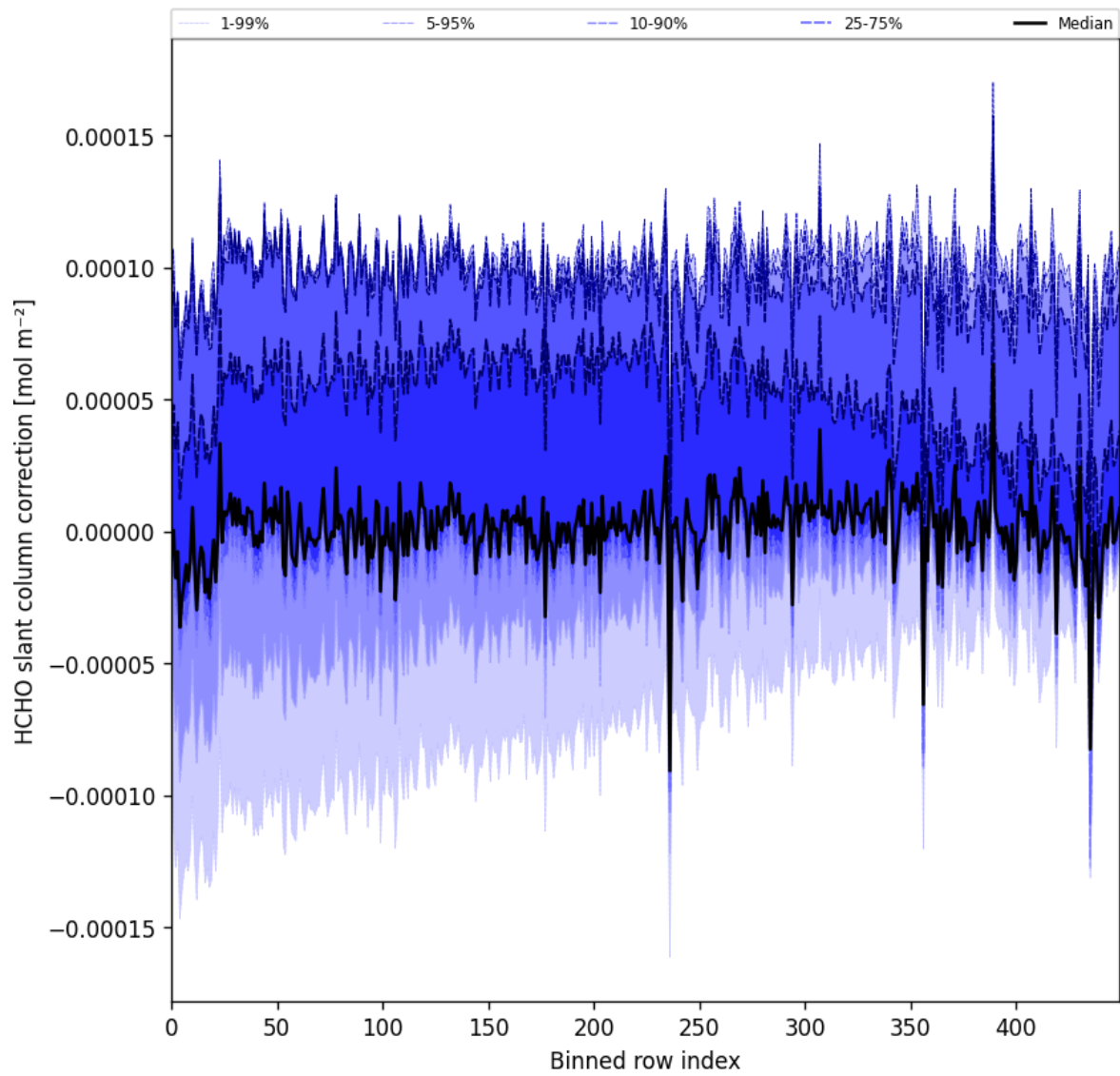
Figure 61: Along track statistics of “HCHO slant column correction” for 2025-04-25 to 2025-04-27
