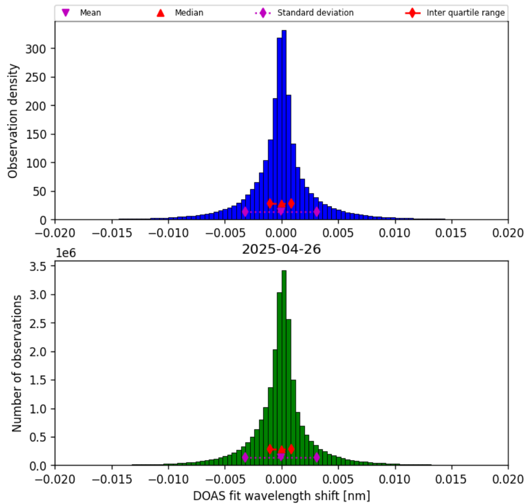
Figure 44: Histogram of “DOAS fit wavelength shift” for 2025-04-25 to 2025-04-27
