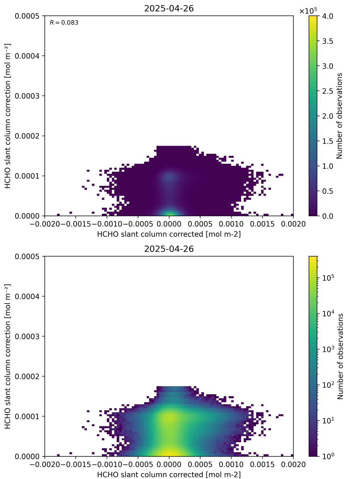
Figure 77: Scatter density plot of “HCHO slant column corrected” against “HCHO slant column correction” for 2025-04-25 to 2025-04-27.
