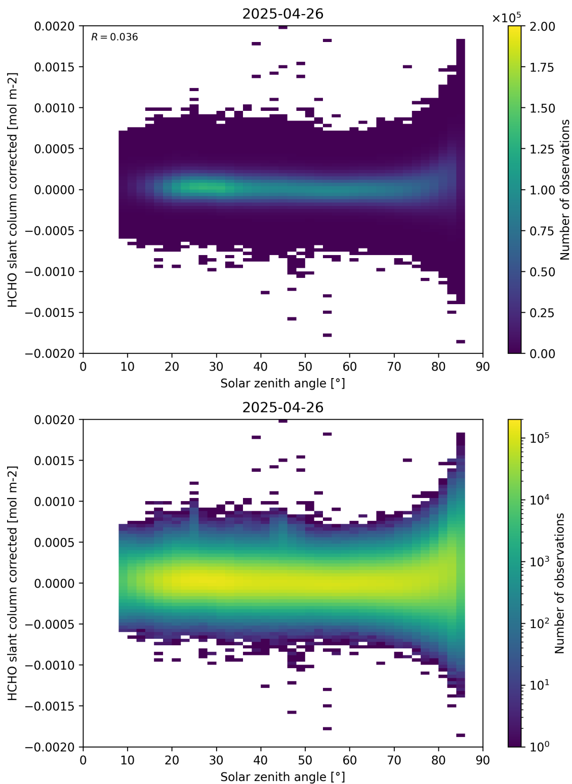
Figure 171: Scatter density plot of “Solar zenith angle” against “HCHO slant column corrected” for 2025-04-25 to 2025-04-27.
