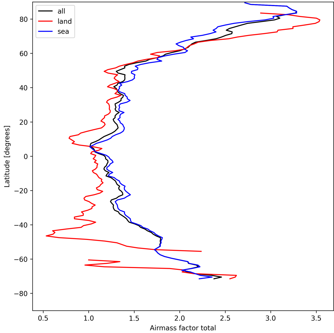
Figure 26: Zonal average of “Airmass factor total” for 2025-04-25 to 2025-04-27.
