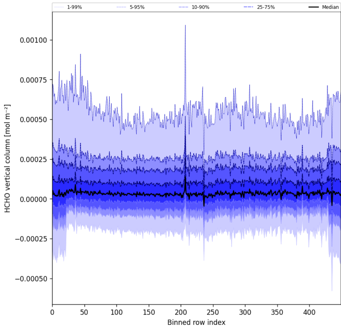
Figure 49: Along track statistics of “HCHO vertical column” for 2025-04-25 to 2025-04-27
