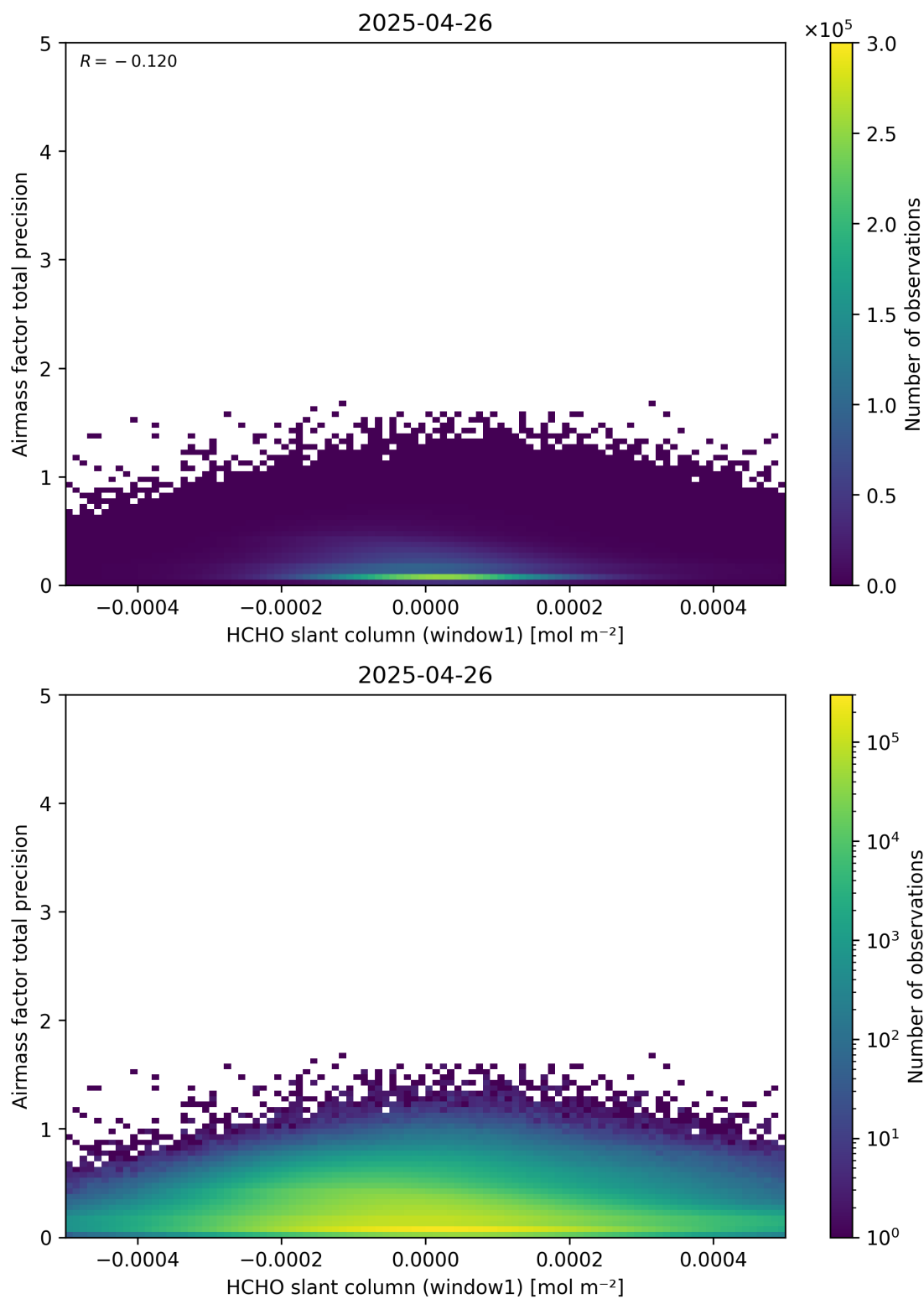
Figure 86: Scatter density plot of “HCHO slant column (window1)” against “Airmass factor total precision” for 2025-04-25 to 2025-04-27.
