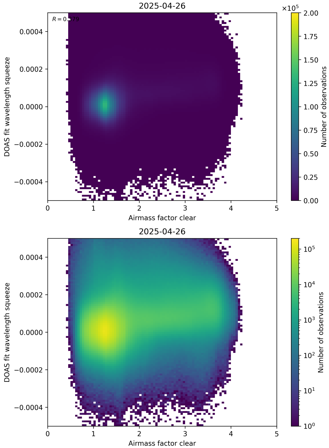
Figure 73: Scatter density plot of “Airmass factor clear” against “DOAS fit wavelength squeeze” for 2025-04-25 to 2025-04-27.
