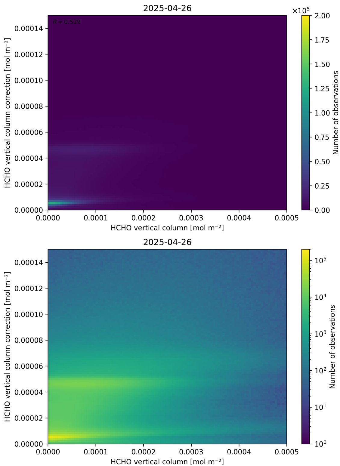
Figure 133: Scatter density plot of “HCHO vertical column” against “HCHO vertical column correction” for 2025-04-25 to 2025-04-27.
