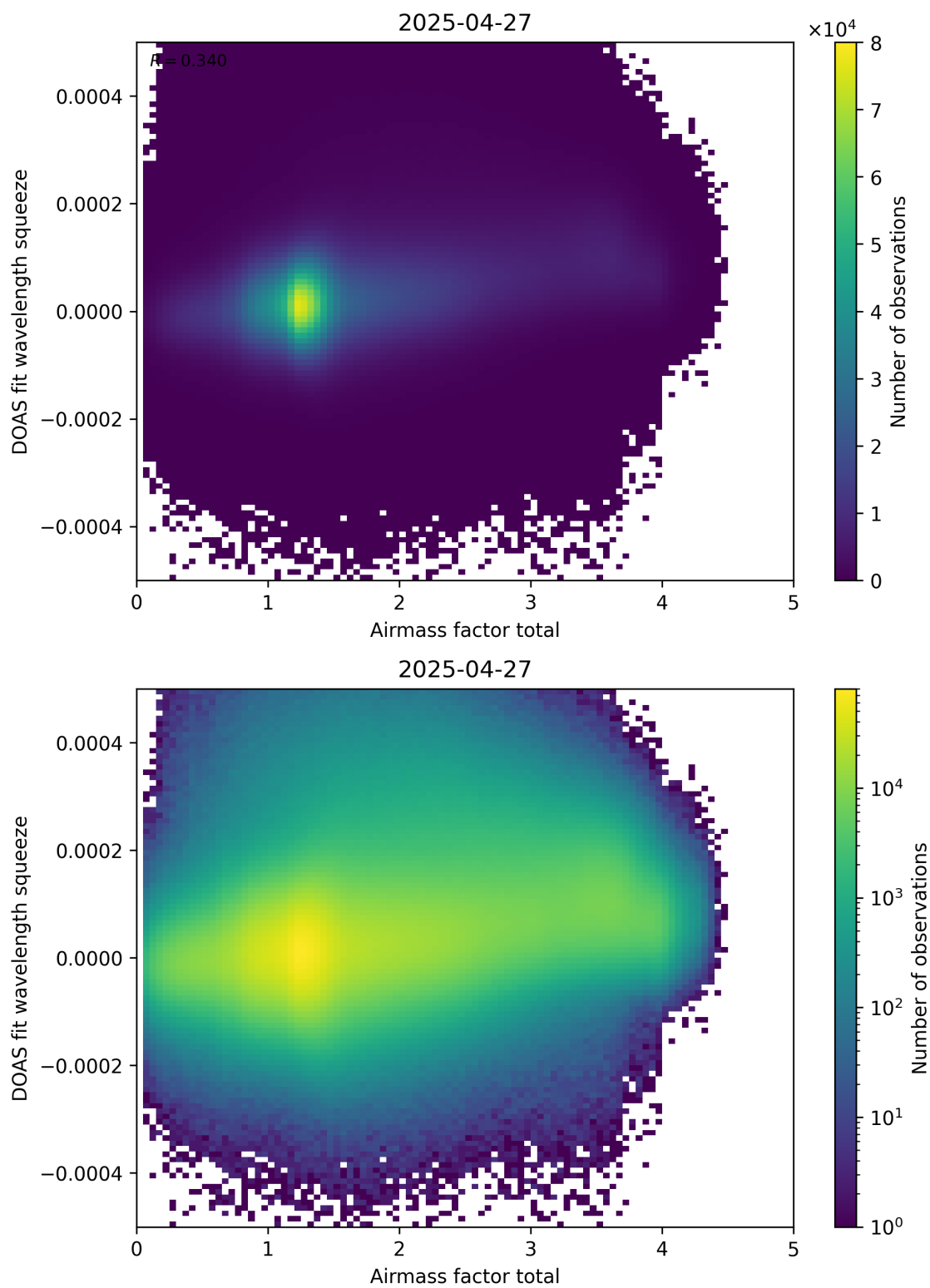
Figure 99: Scatter density plot of “Airmass factor total” against “DOAS fit wavelength squeeze” for 2025-04-26 to 2025-04-28.
