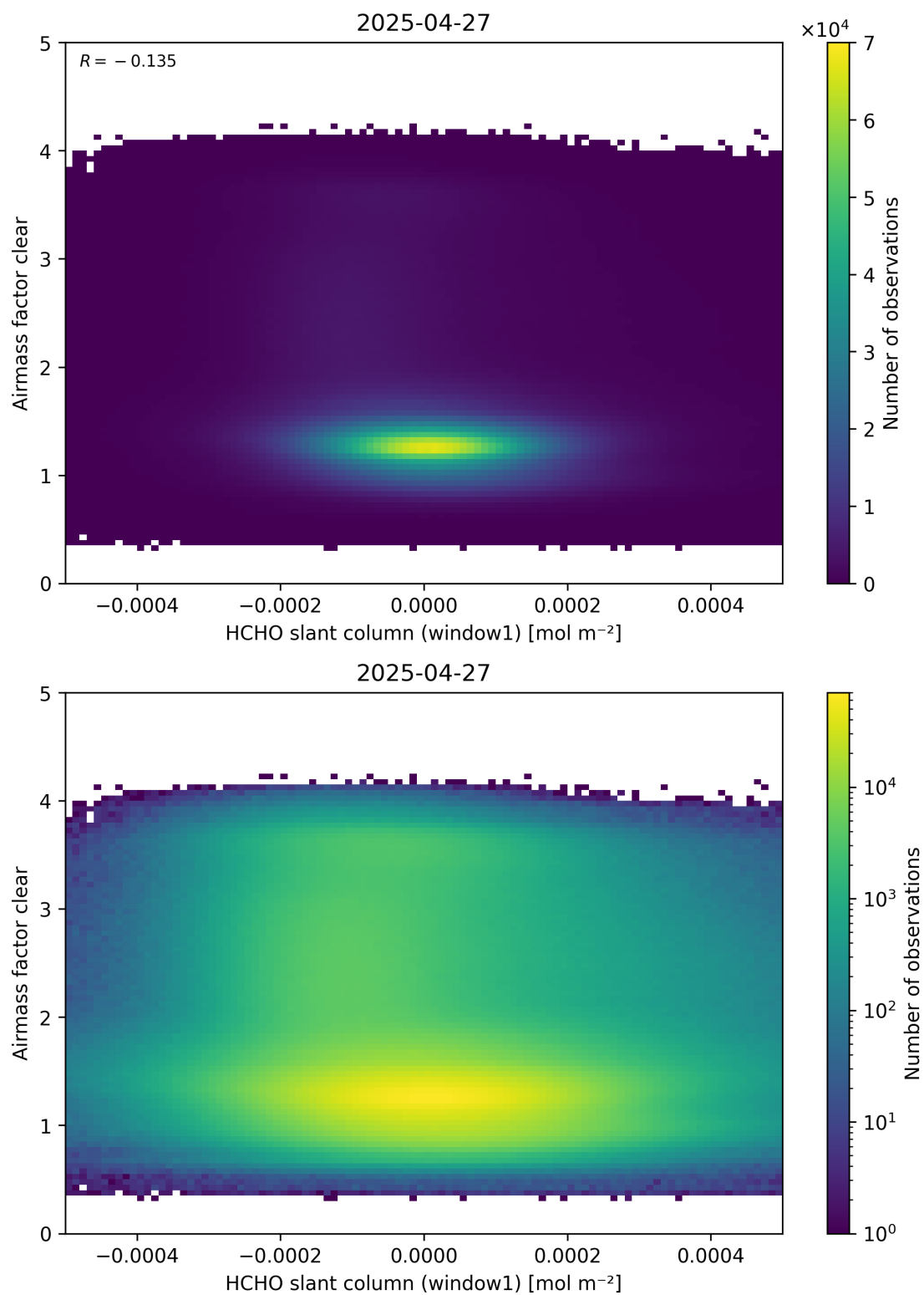
Figure 81: Scatter density plot of “HCHO slant column (window1)” against “Airmass factor clear” for 2025-04-26 to 2025-04-28.
