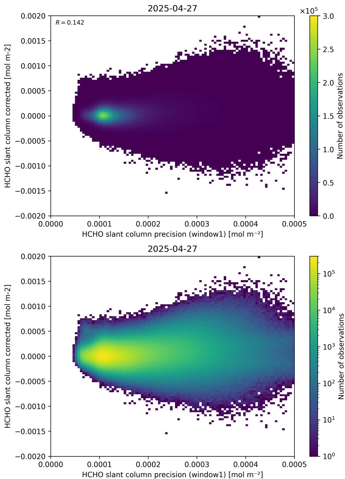
Figure 92: Scatter density plot of “HCHO slant column precision (window1)” against “HCHO slant column corrected” for 2025-04-26 to 2025-04-28.
