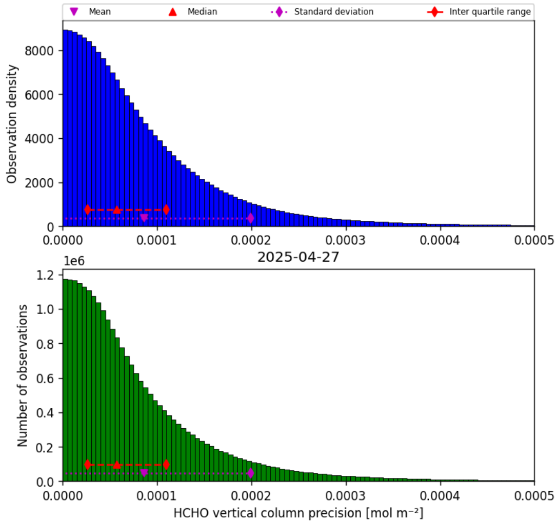
Figure 36: Histogram of “HCHO vertical column precision” for 2025-04-26 to 2025-04-28
