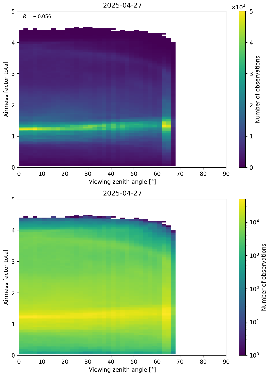
Figure 190: Scatter density plot of “Viewing zenith angle” against “Airmass factor total” for 2025-04-26 to 2025-04-28.
