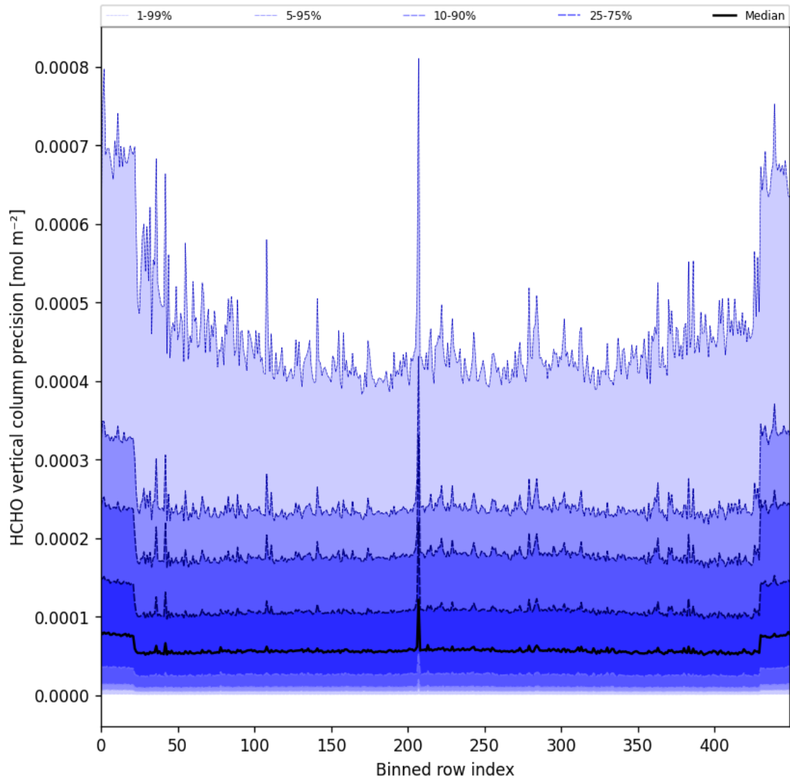
Figure 50: Along track statistics of “HCHO vertical column precision” for 2025-04-26 to 2025-04-28
