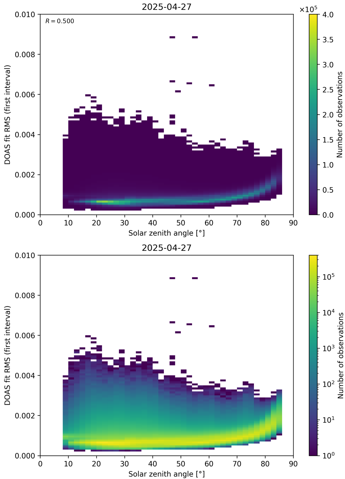
Figure 167: Scatter density plot of “Solar zenith angle” against “DOAS fit RMS (first interval)” for 2025-04-26 to 2025-04-28.
