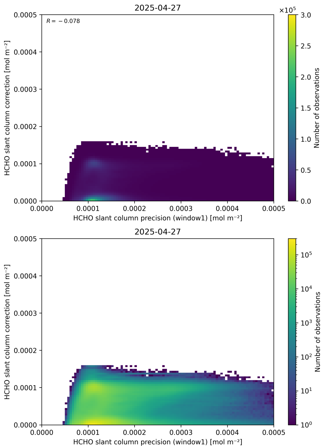
Figure 93: Scatter density plot of “HCHO slant column precision (window1)” against “HCHO slant column correction” for 2025-04-26 to 2025-04-28.
