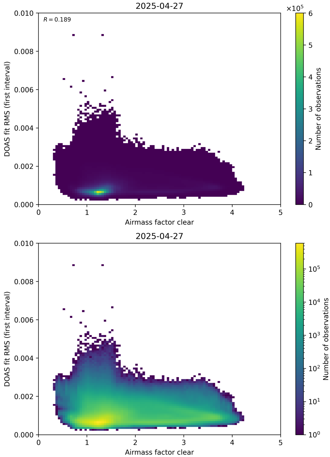
Figure 71: Scatter density plot of “Airmass factor clear” against “DOAS fit RMS (first interval)” for 2025-04-26 to 2025-04-28.
