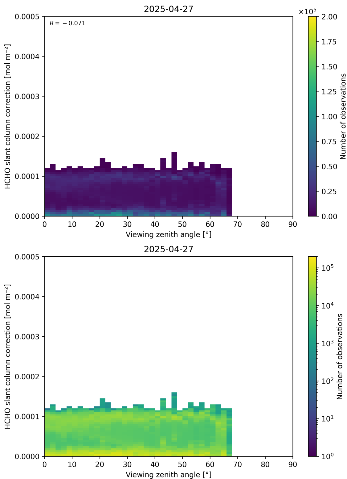
Figure 187: Scatter density plot of “Viewing zenith angle” against “HCHO slant column correction” for 2025-04-26 to 2025-04-28.
