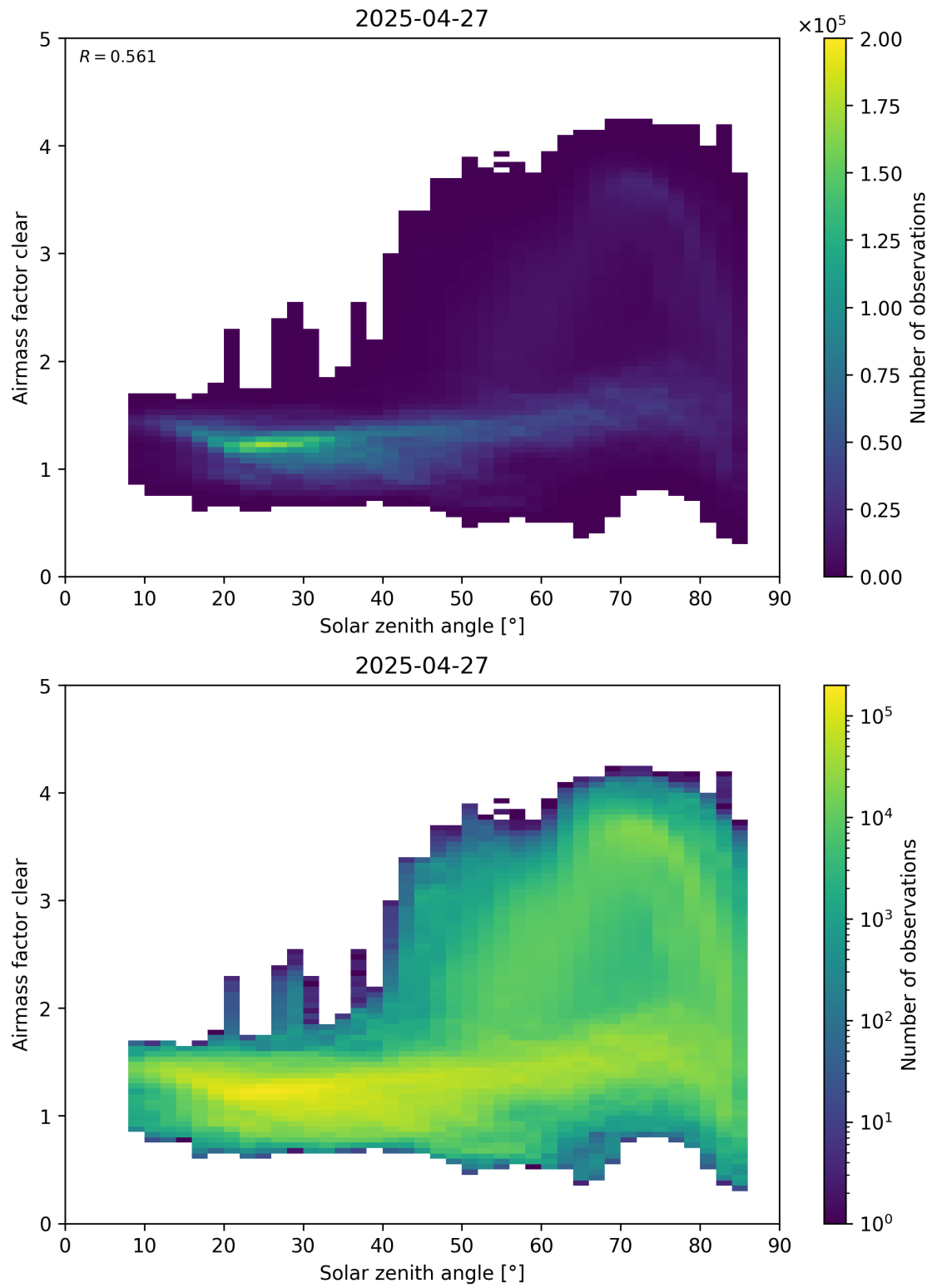
Figure 170: Scatter density plot of “Solar zenith angle” against “Airmass factor clear” for 2025-04-26 to 2025-04-28.
