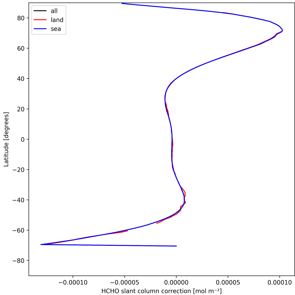
Figure 33: Zonal average of “HCHO slant column correction” for 2025-04-26 to 2025-04-28.
