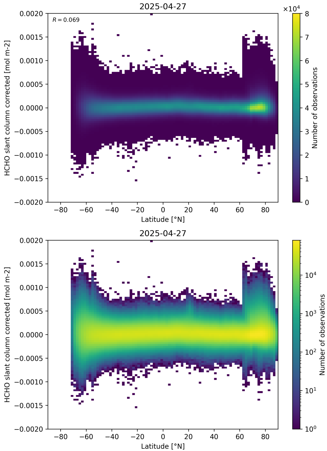
Figure 157: Scatter density plot of “Latitude” against “HCHO slant column corrected” for 2025-04-26 to 2025-04-28.
