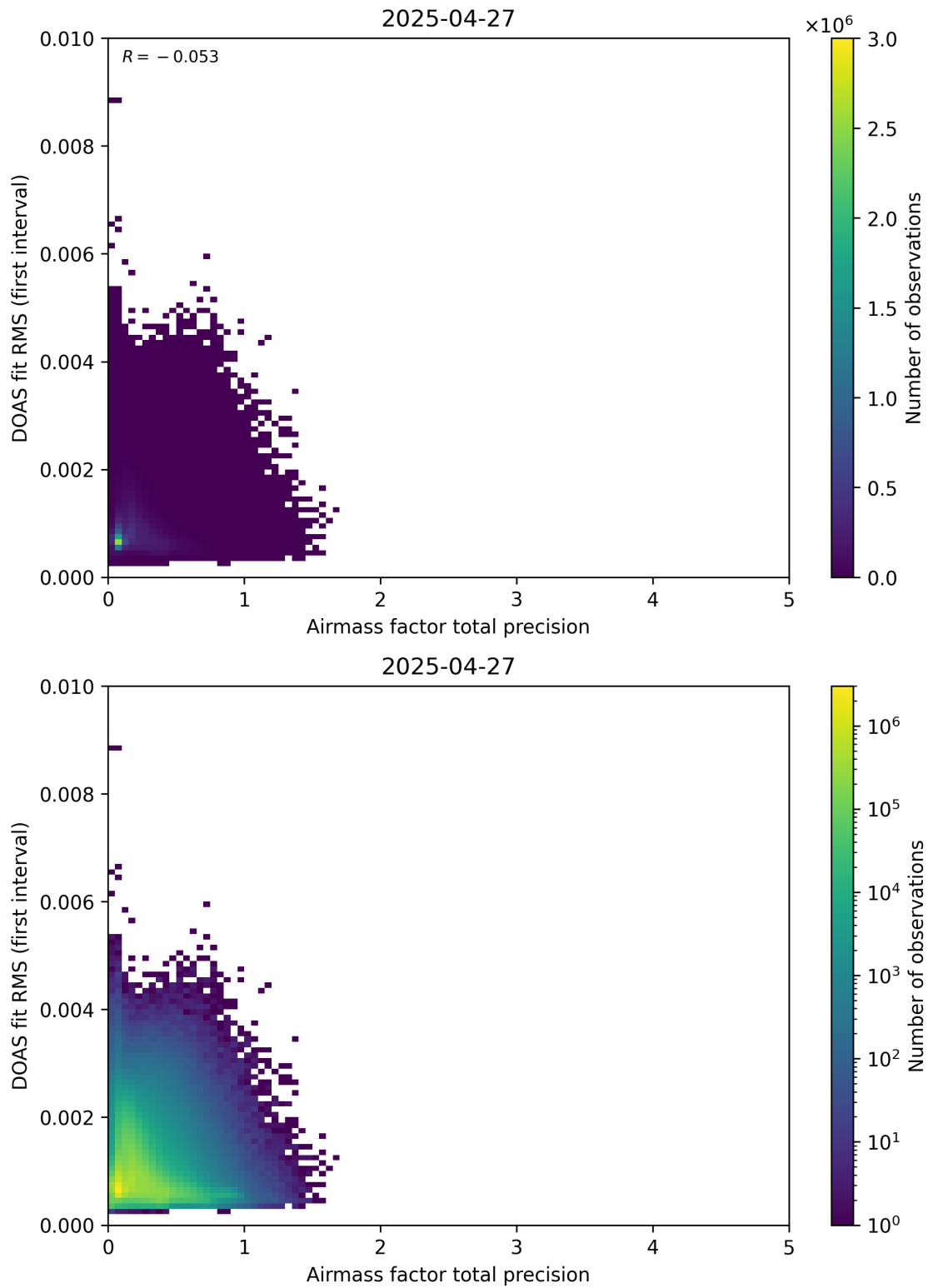
Figure 105: Scatter density plot of “Airmass factor total precision” against “DOAS fit RMS (first interval)” for 2025-04-26 to 2025-04-28.
