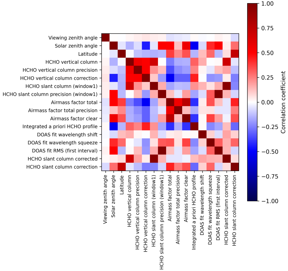
Figure 2: Map of correlation matrix for 2025-04-26 to 2025-04-28.
