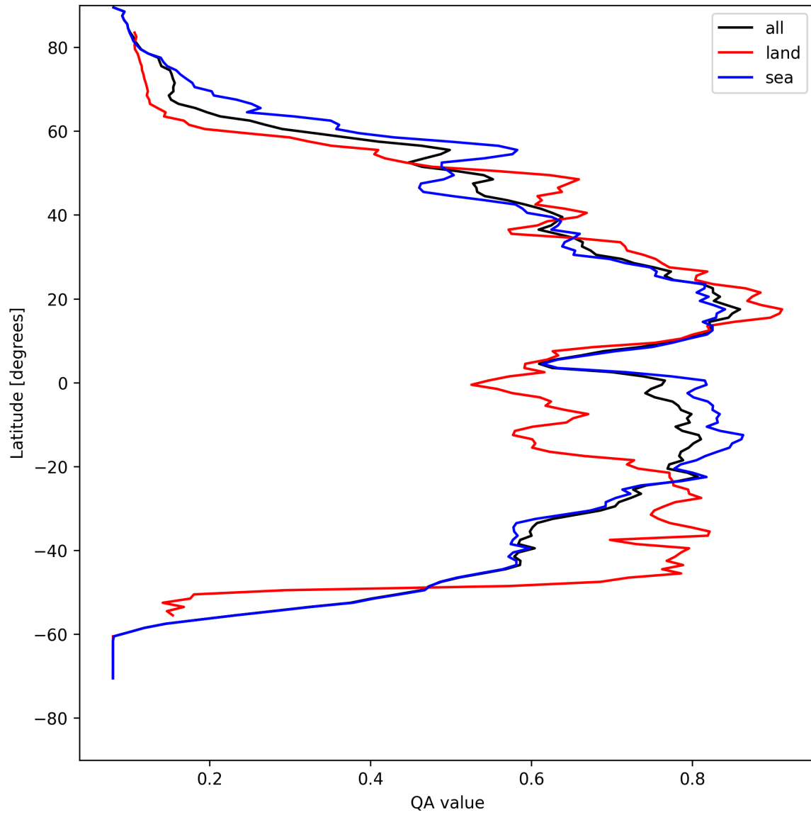
Figure 20: Zonal average of “QA value” for 2025-04-26 to 2025-04-28.
