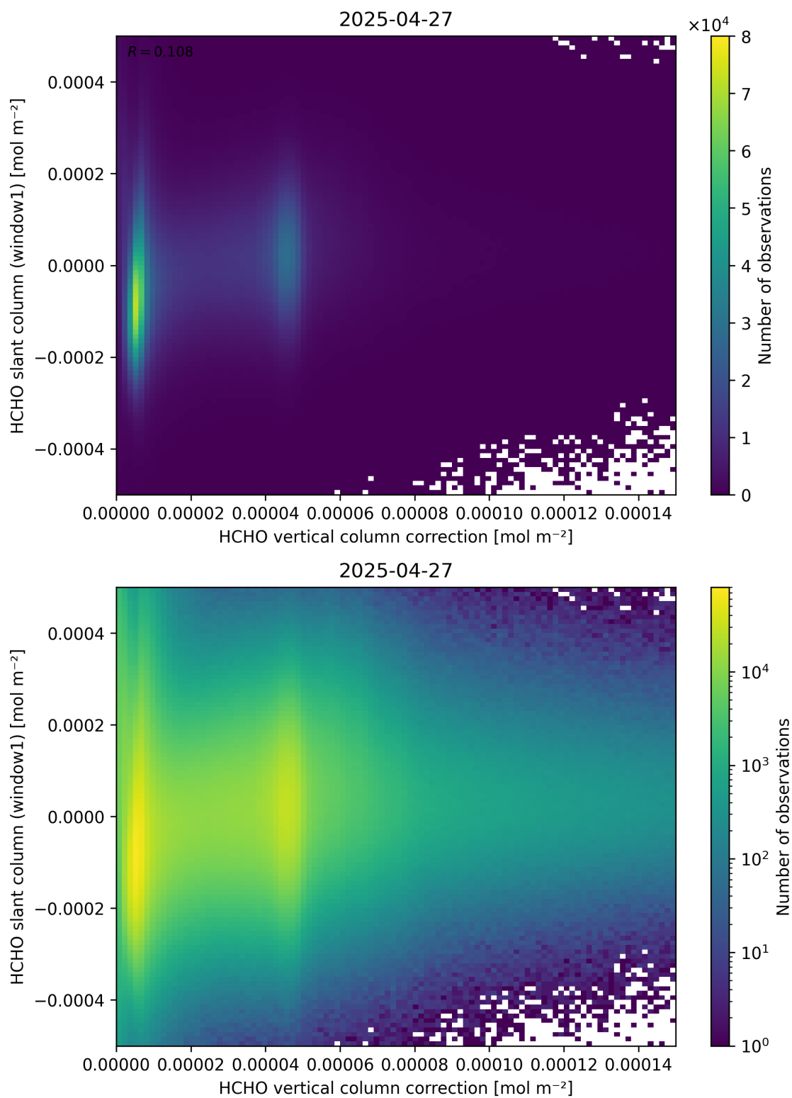
Figure 118: Scatter density plot of “HCHO vertical column correction” against “HCHO slant column (window1)” for 2025-04-26 to 2025-04-28.
