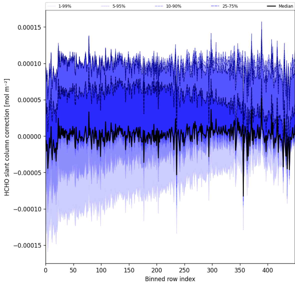
Figure 61: Along track statistics of “HCHO slant column correction” for 2025-04-26 to 2025-04-28
