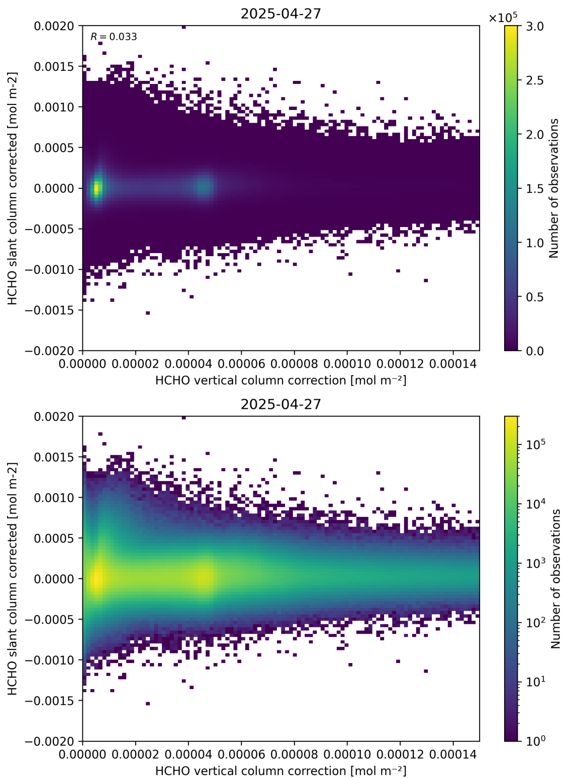
Figure 116: Scatter density plot of “HCHO vertical column correction” against “HCHO slant column corrected” for 2025-04-26 to 2025-04-28.
