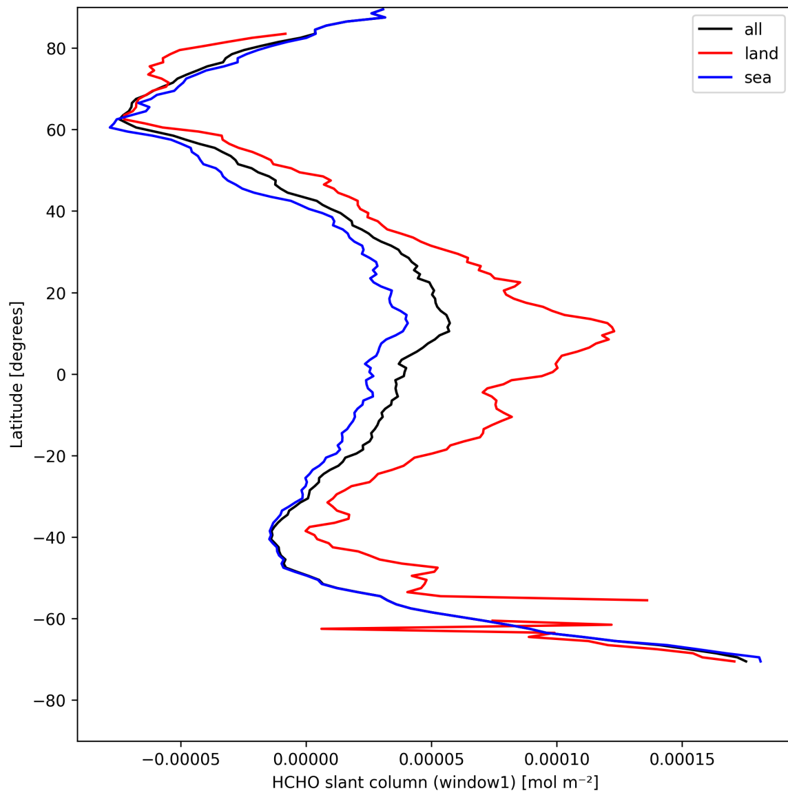
Figure 24: Zonal average of “HCHO slant column (window1)” for 2025-04-26 to 2025-04-28.
