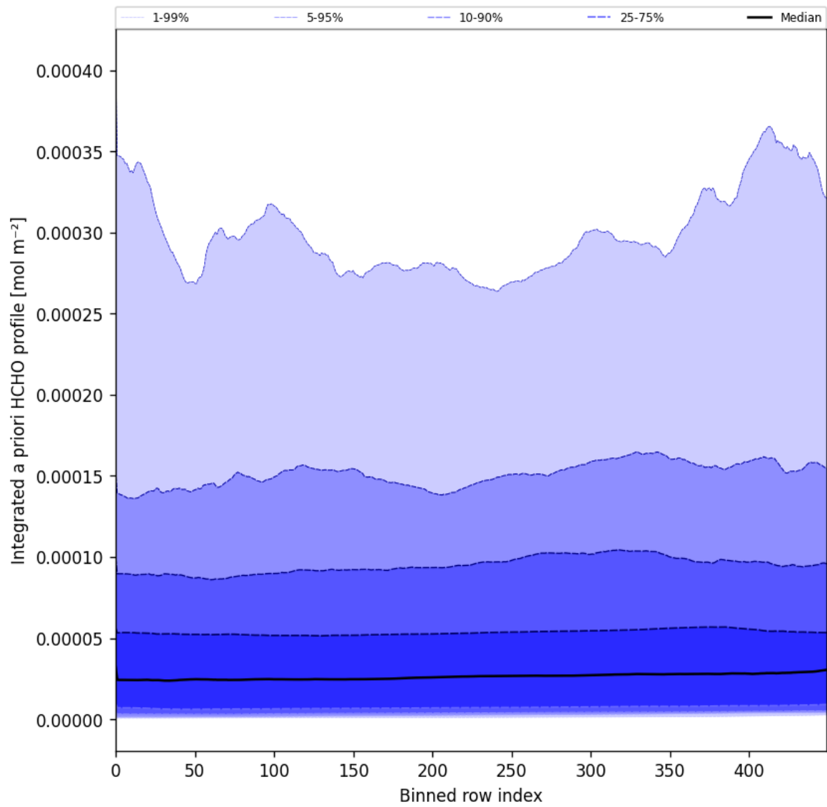
Figure 57: Along track statistics of “Integrated a priori HCHO profile” for 2025-04-26 to 2025-04-28
