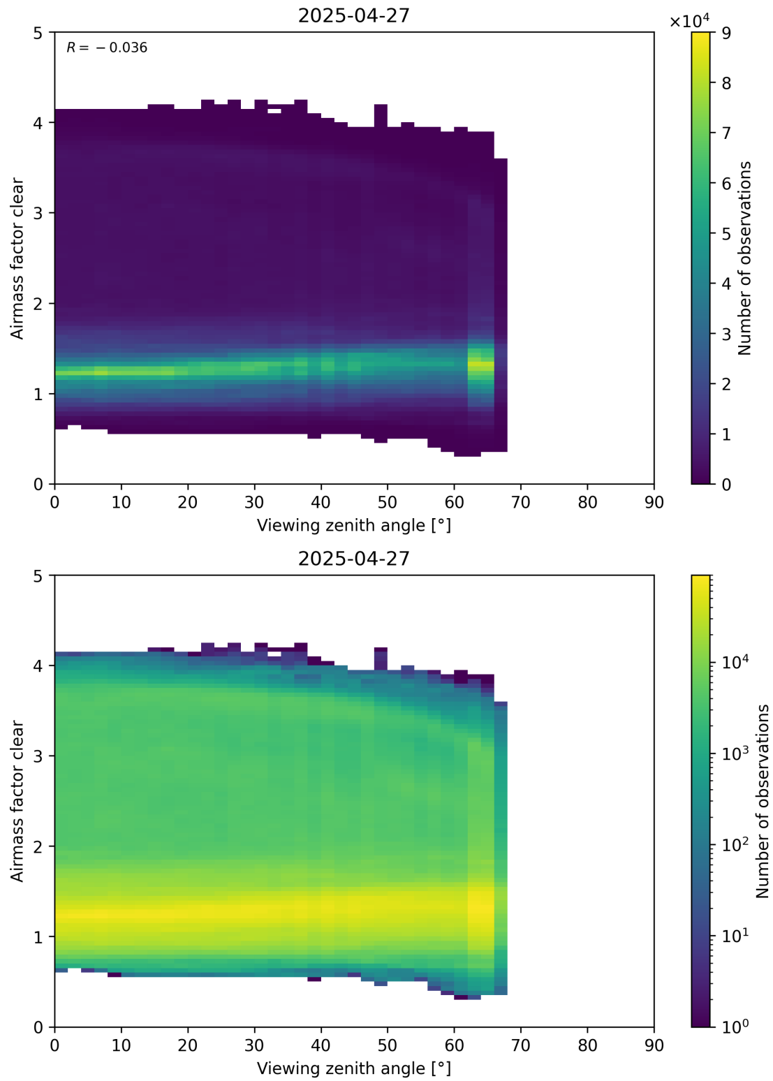
Figure 185: Scatter density plot of “Viewing zenith angle” against “Airmass factor clear” for 2025-04-26 to 2025-04-28.
