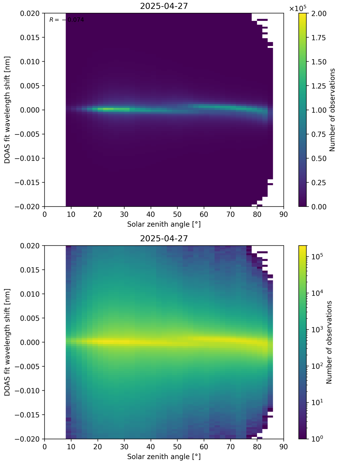
Figure 168: Scatter density plot of “Solar zenith angle” against “DOAS fit wavelength shift” for 2025-04-26 to 2025-04-28.
