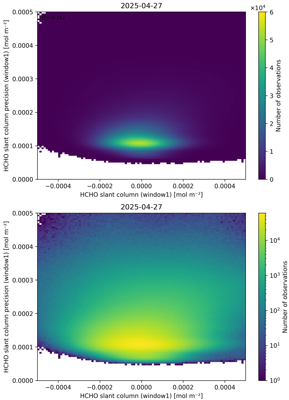
Figure 84: Scatter density plot of “HCHO slant column (window1)” against “HCHO slant column precision (window1)” for 2025-04-26 to 2025-04-28.
