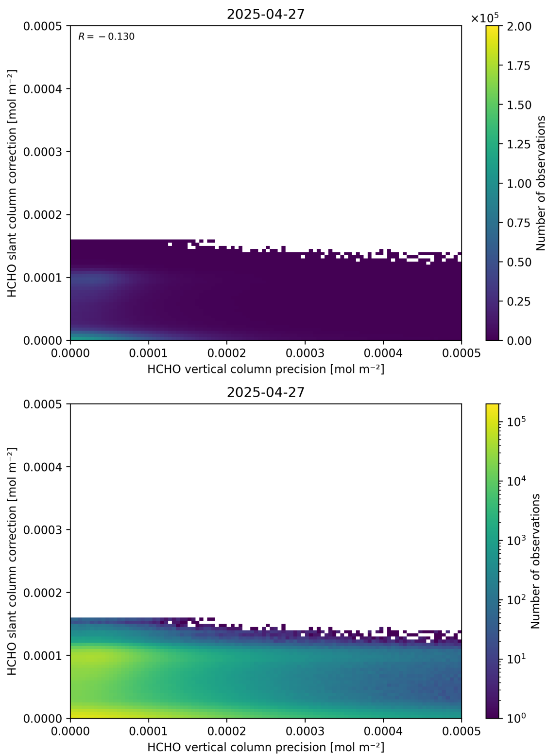
Figure 141: Scatter density plot of “HCHO vertical column precision” against “HCHO slant column correction” for 2025-04-26 to 2025-04-28.
