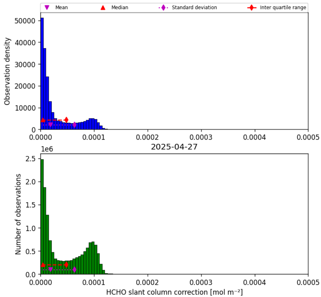
Figure 47: Histogram of “HCHO slant column correction” for 2025-04-26 to 2025-04-28
