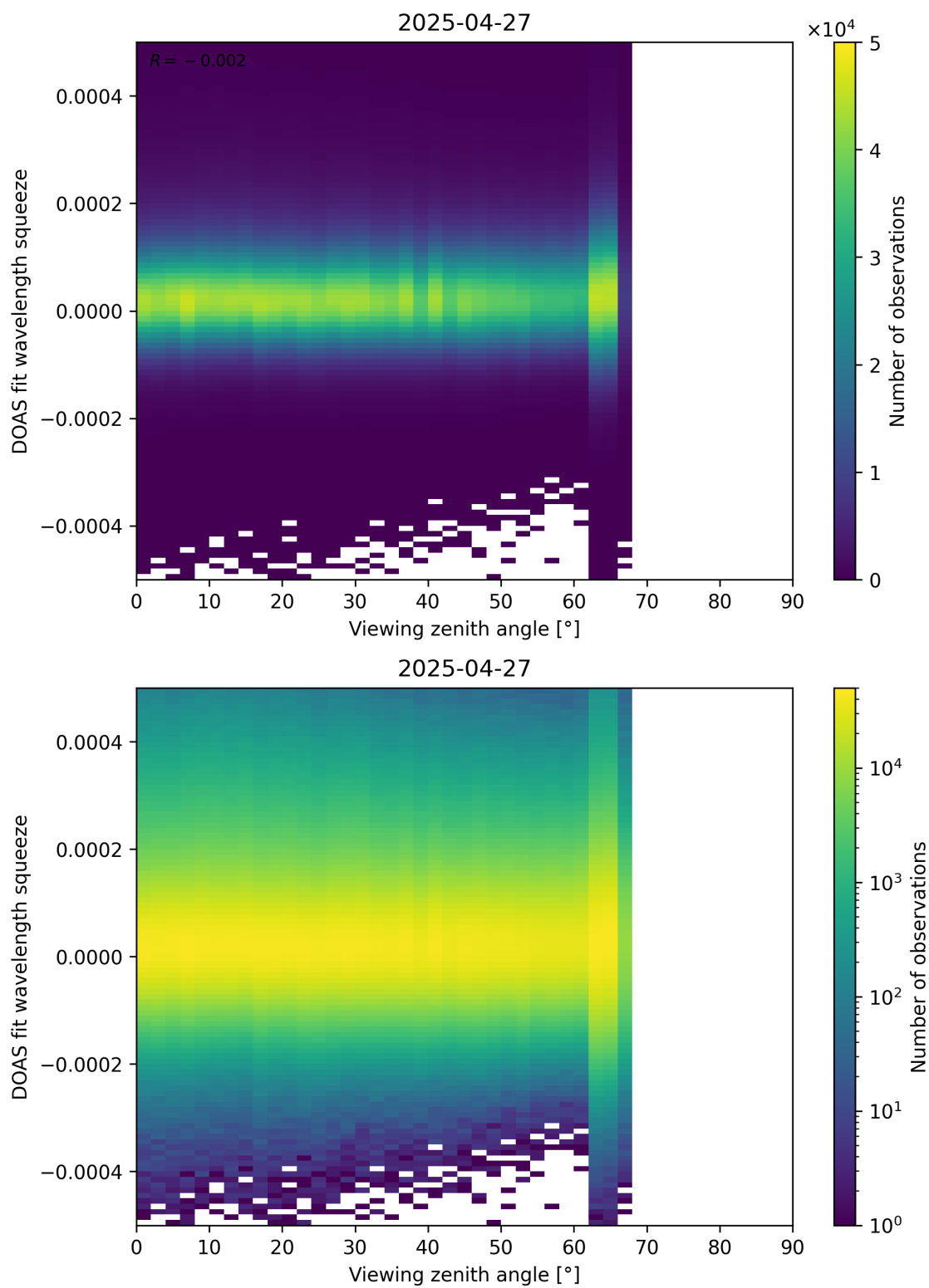
Figure 184: Scatter density plot of “Viewing zenith angle” against “DOAS fit wavelength squeeze” for 2025-04-26 to 2025-04-28.
