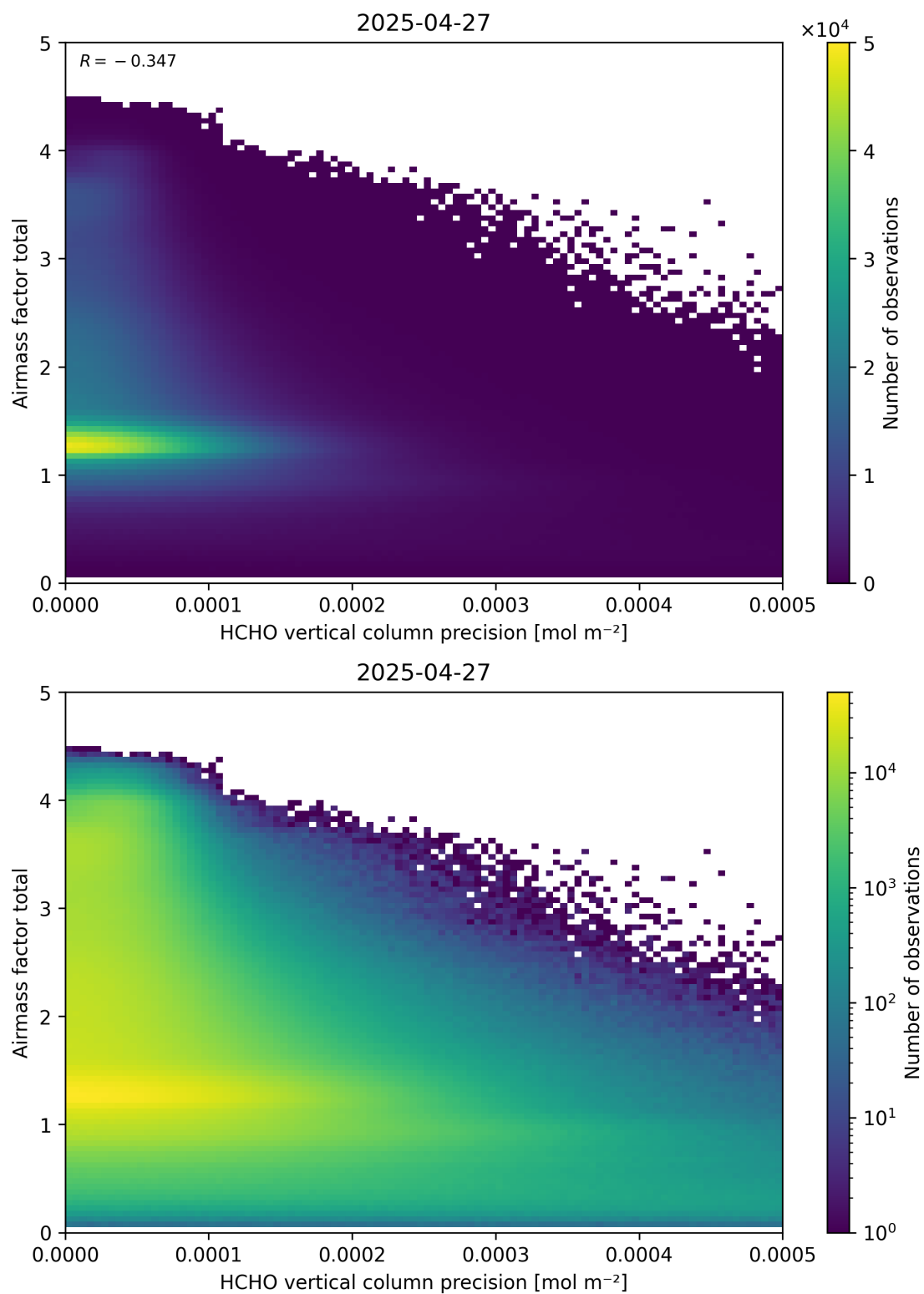
Figure 144: Scatter density plot of “HCHO vertical column precision” against “Airmass factor total” for 2025-04-26 to 2025-04-28.
