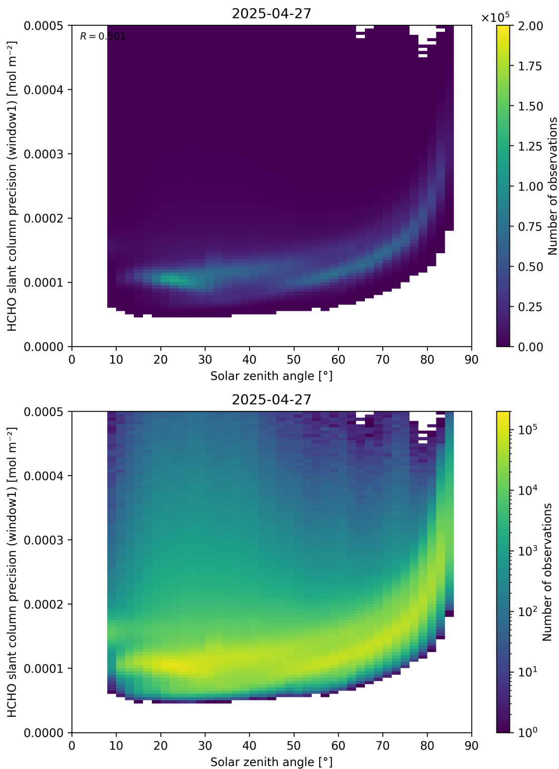
Figure 174: Scatter density plot of “Solar zenith angle” against “HCHO slant column precision (window1)” for 2025-04-26 to 2025-04-28.
