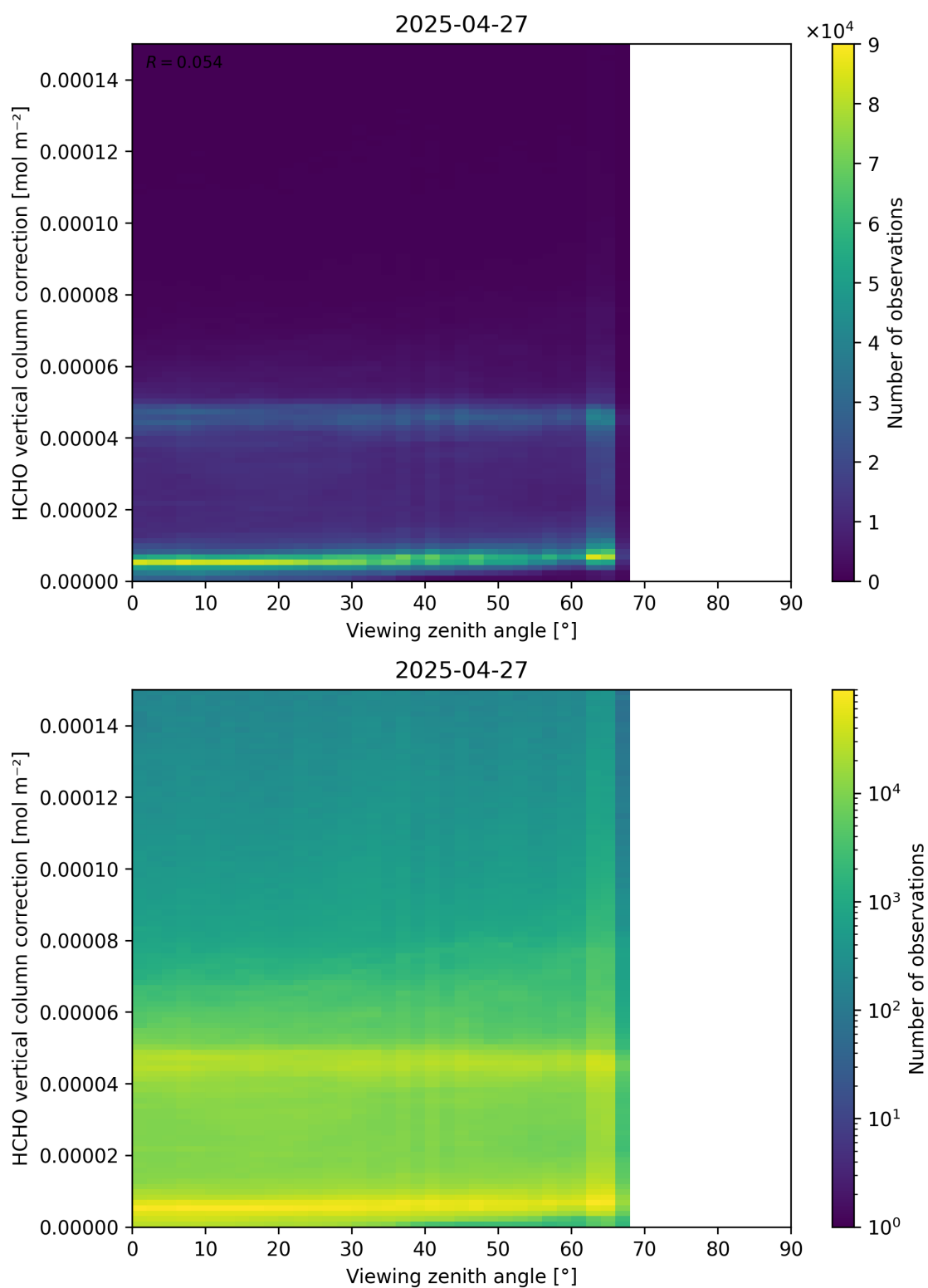
Figure 193: Scatter density plot of “Viewing zenith angle” against “HCHO vertical column correction” for 2025-04-26 to 2025-04-28.
