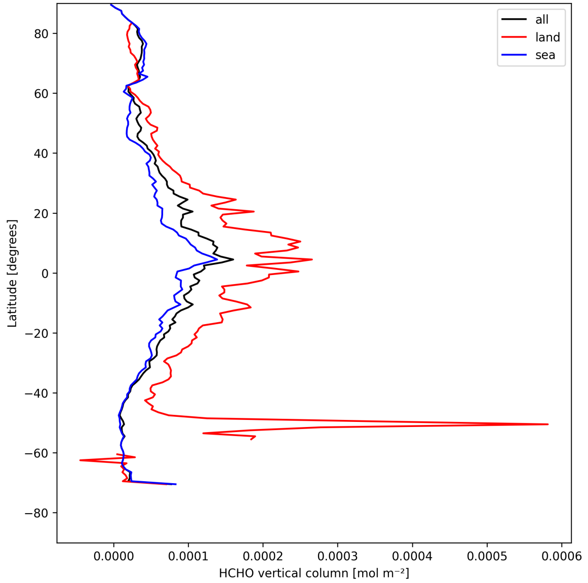
Figure 21: Zonal average of “HCHO vertical column” for 2025-04-26 to 2025-04-28.
