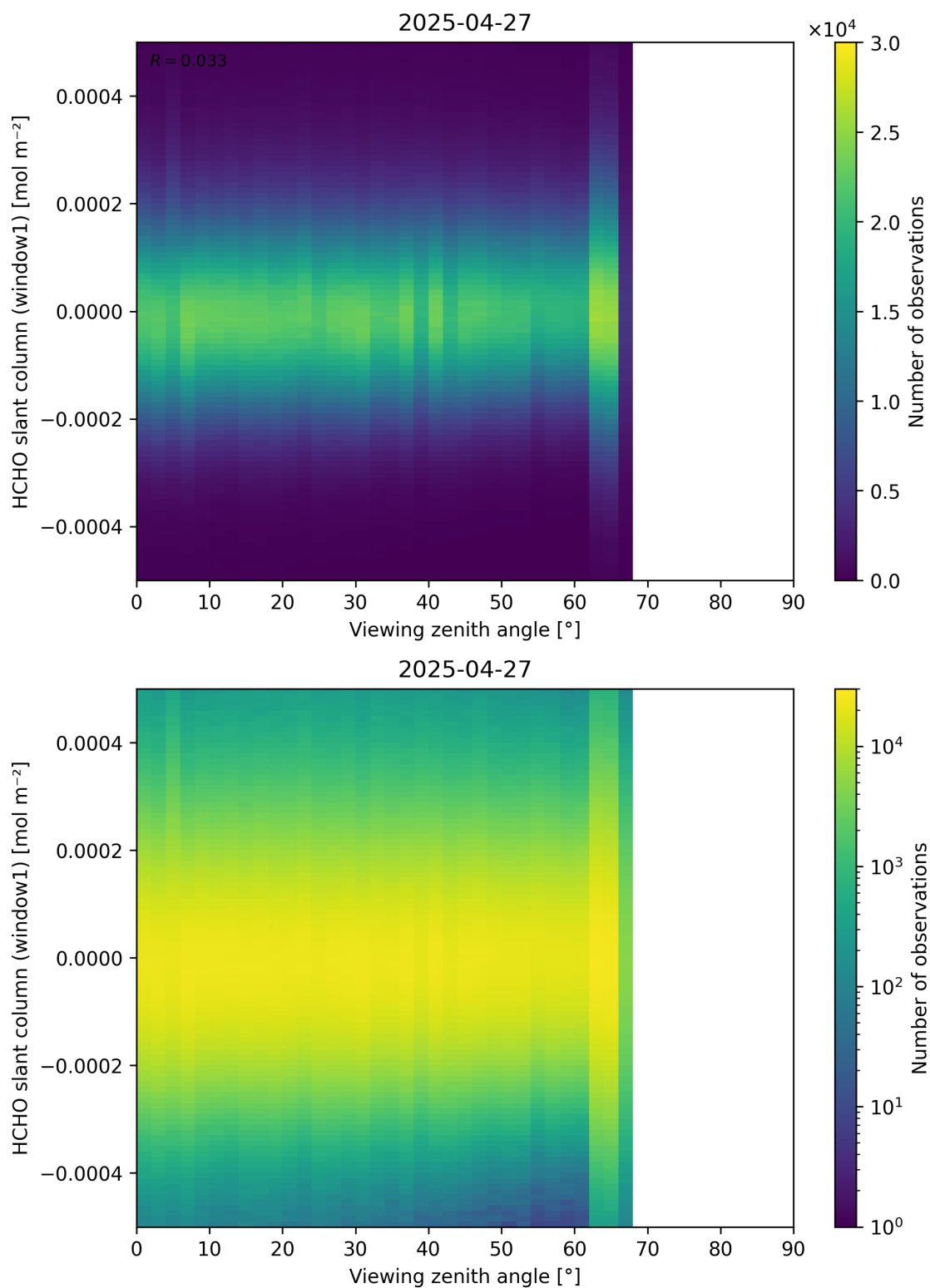
Figure 188: Scatter density plot of “Viewing zenith angle” against “HCHO slant column (window1)” for 2025-04-26 to 2025-04-28.
