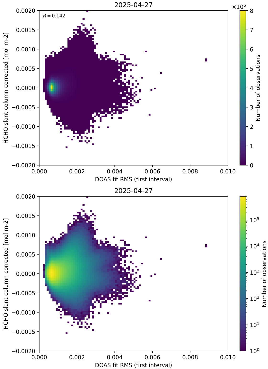
Figure 62: Scatter density plot of “DOAS fit RMS (first interval)” against “HCHO slant column corrected” for 2025-04-26 to 2025-04-28.
