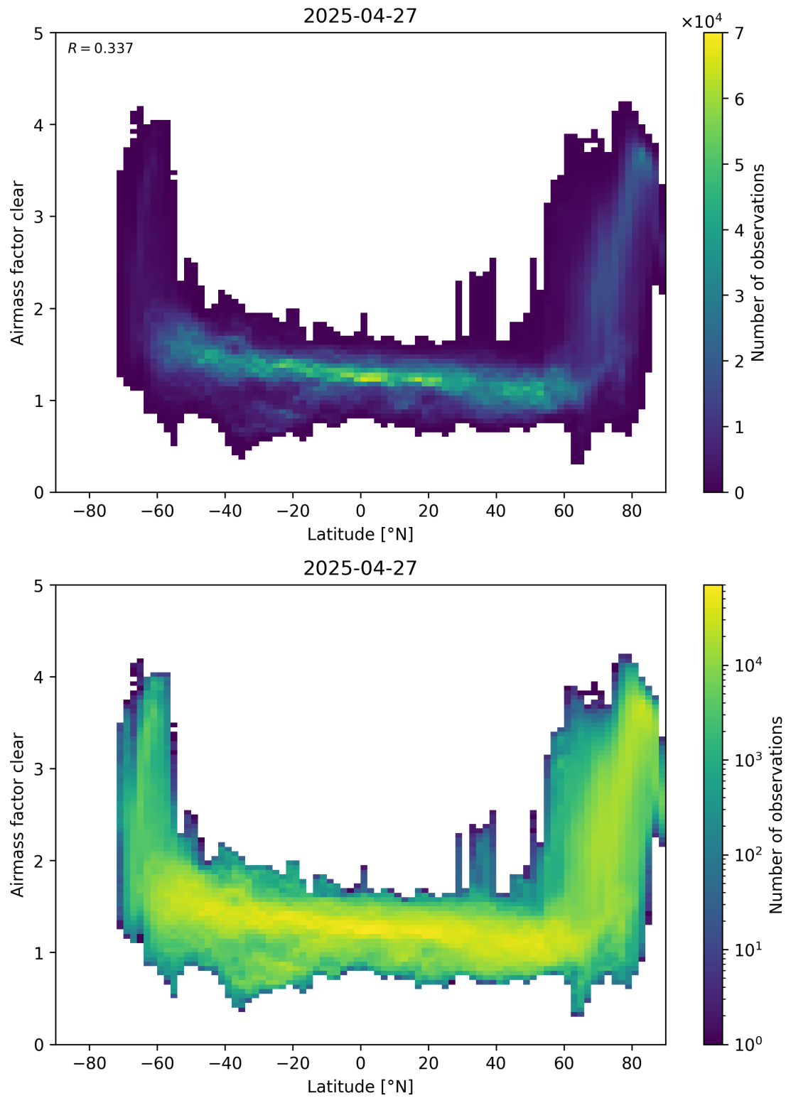
Figure 156: Scatter density plot of “Latitude” against “Airmass factor clear” for 2025-04-26 to 2025-04-28.
