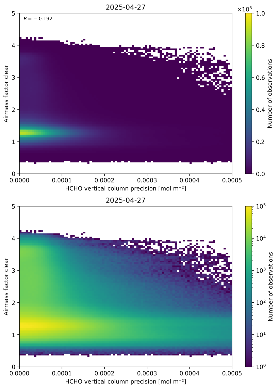
Figure 139: Scatter density plot of “HCHO vertical column precision” against “Airmass factor clear” for 2025-04-26 to 2025-04-28.
