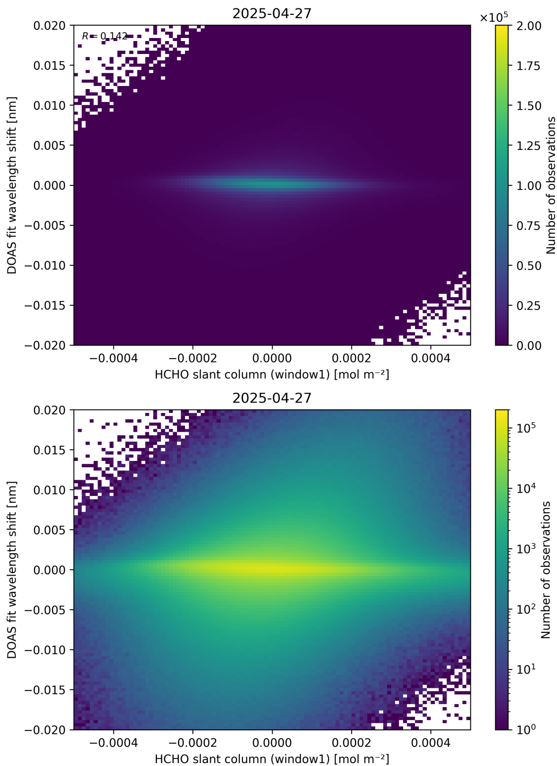
Figure 79: Scatter density plot of “HCHO slant column (window1)” against “DOAS fit wavelength shift” for 2025-04-26 to 2025-04-28.
