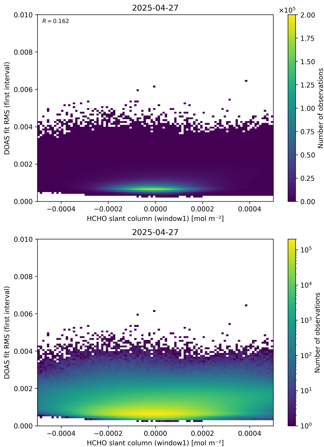
Figure 78: Scatter density plot of “HCHO slant column (window1)” against “DOAS fit RMS (first interval)” for 2025-04-26 to 2025-04-28.
