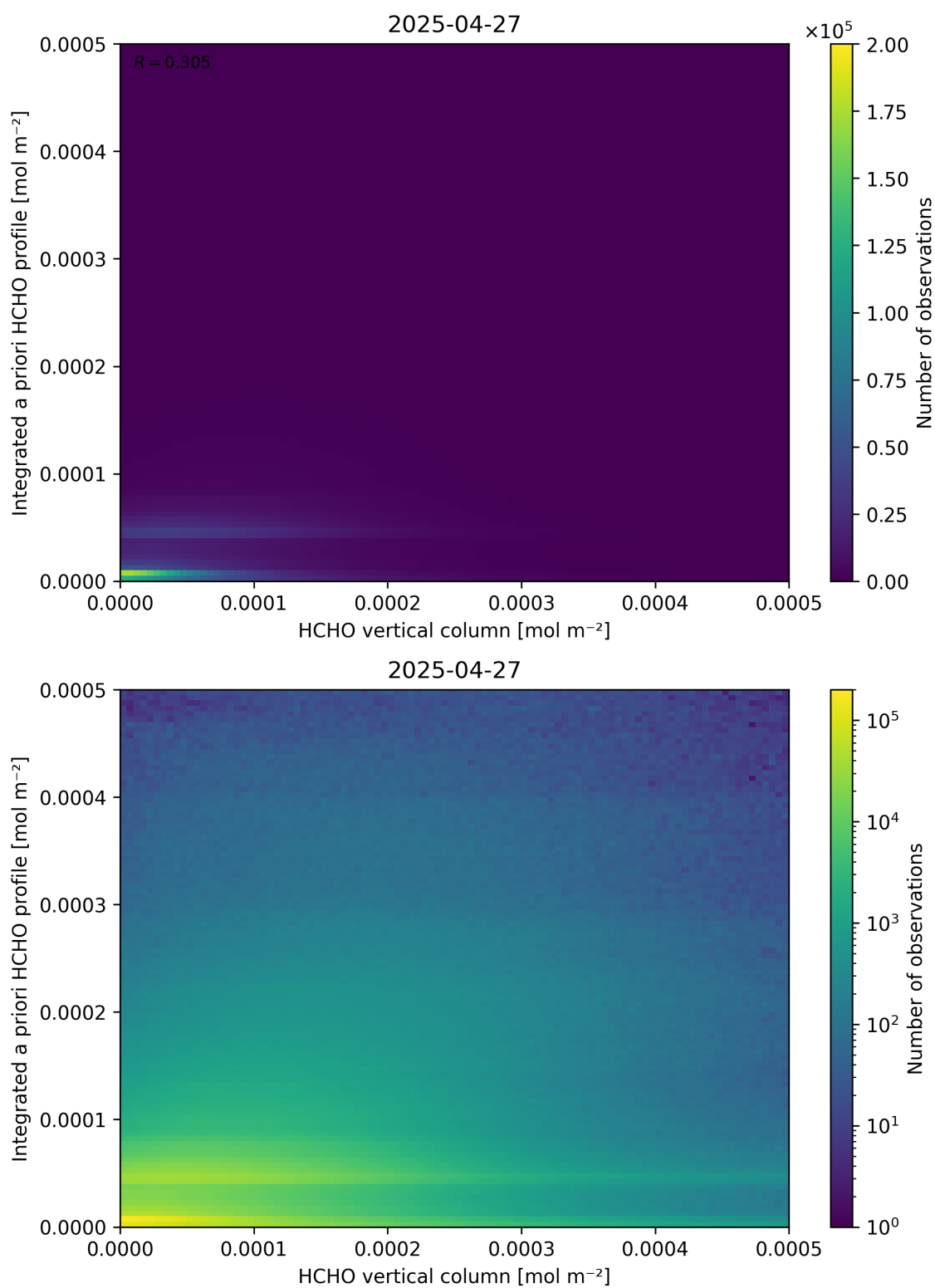
Figure 135: Scatter density plot of “HCHO vertical column” against “Integrated a priori HCHO profile” for 2025-04-26 to 2025-04-28.
