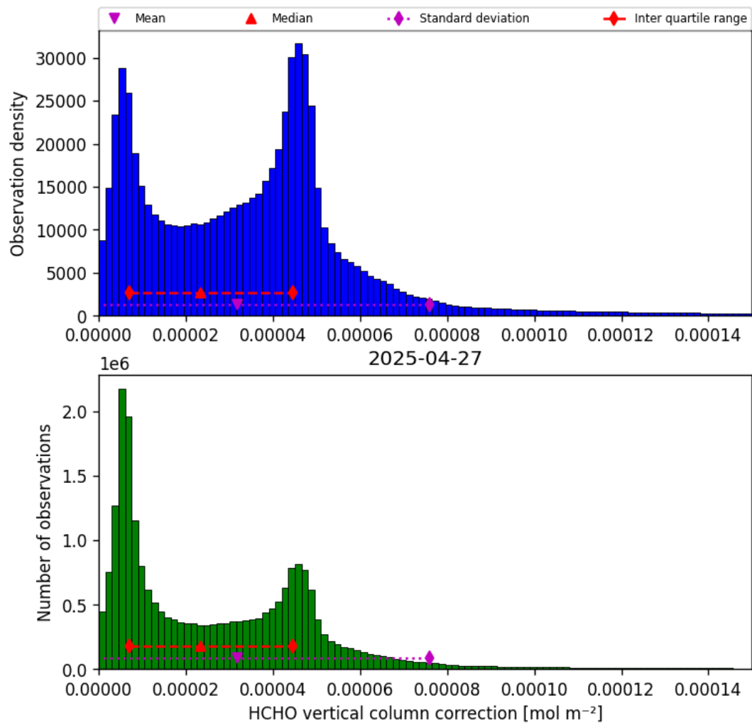
Figure 37: Histogram of “HCHO vertical column correction” for 2025-04-26 to 2025-04-28
