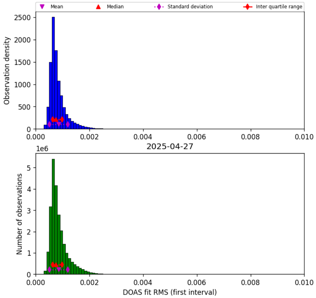
Figure 46: Histogram of “DOAS fit RMS (first interval)” for 2025-04-26 to 2025-04-28
