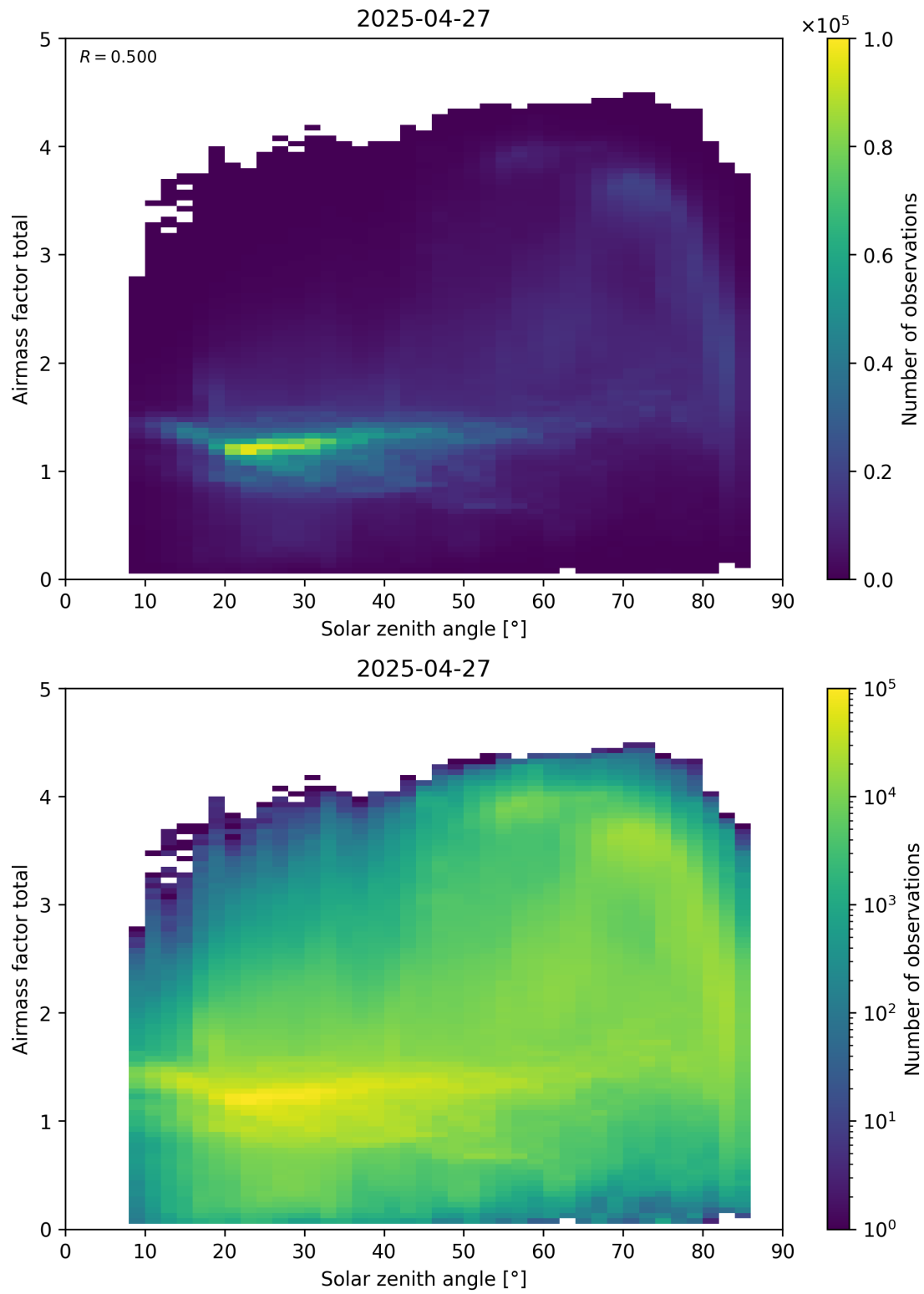
Figure 175: Scatter density plot of “Solar zenith angle” against “Airmass factor total” for 2025-04-26 to 2025-04-28.
