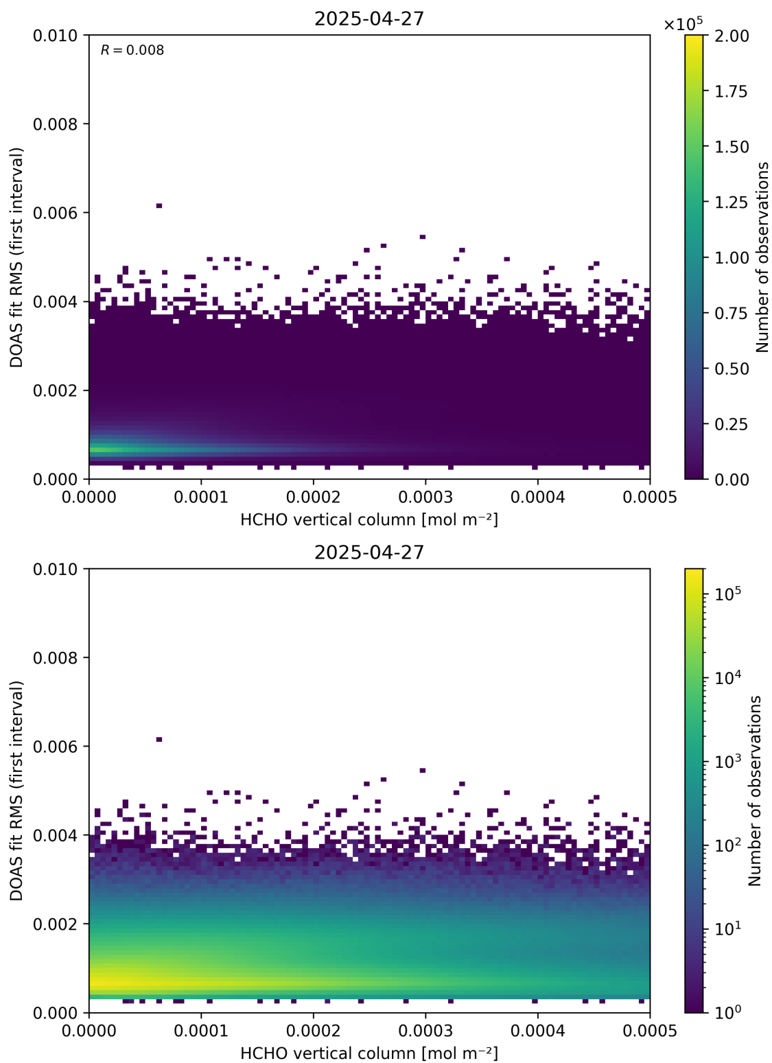
Figure 123: Scatter density plot of “HCHO vertical column” against “DOAS fit RMS (first interval)” for 2025-04-26 to 2025-04-28.
