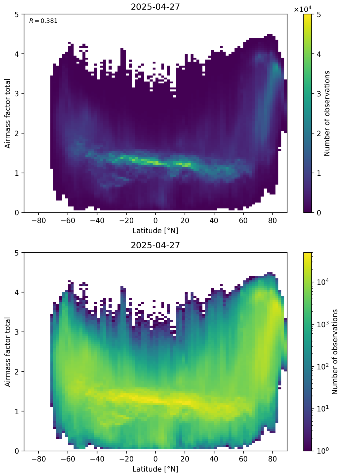
Figure 161: Scatter density plot of “Latitude” against “Airmass factor total” for 2025-04-26 to 2025-04-28.
