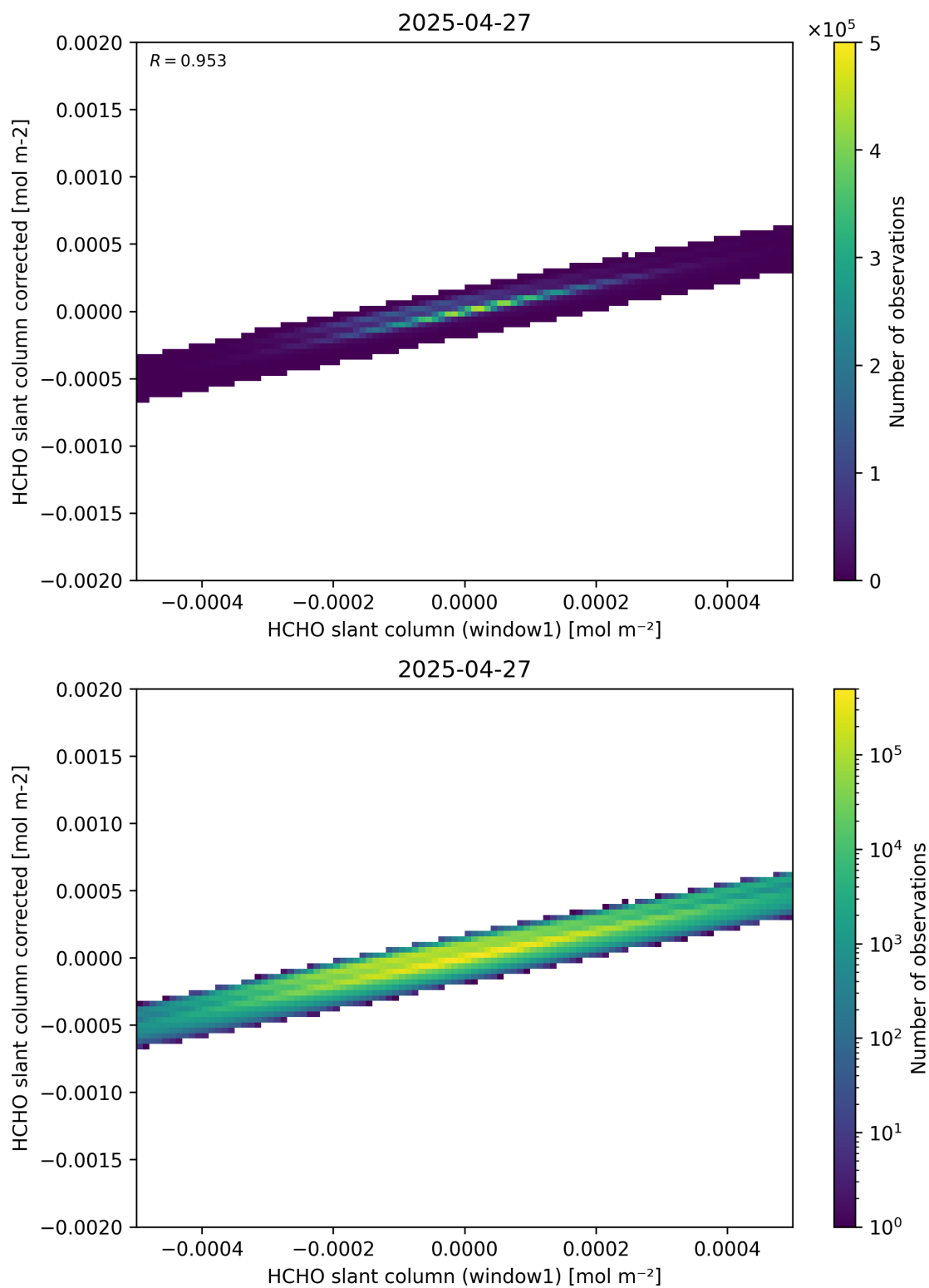
Figure 82: Scatter density plot of “HCHO slant column (window1)” against “HCHO slant column corrected” for 2025-04-26 to 2025-04-28.
