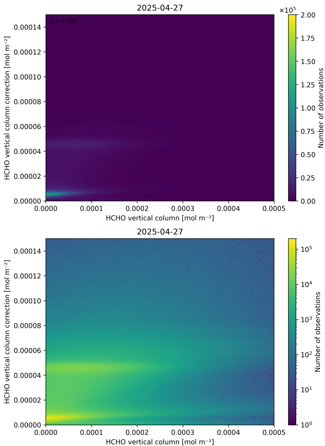
Figure 133: Scatter density plot of “HCHO vertical column” against “HCHO vertical column correction” for 2025-04-26 to 2025-04-28.
