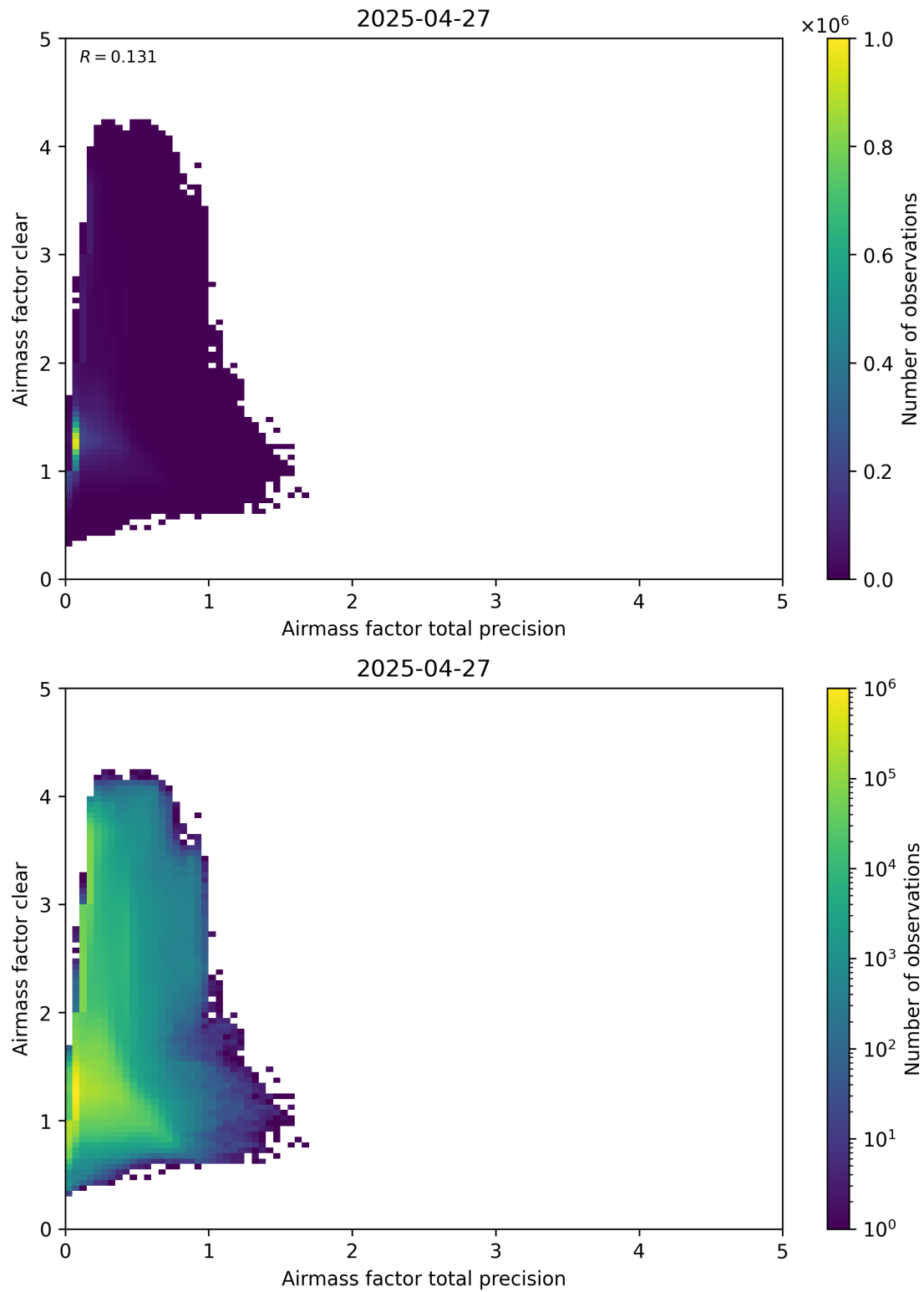
Figure 108: Scatter density plot of “Airmass factor total precision” against “Airmass factor clear” for 2025-04-26 to 2025-04-28.
