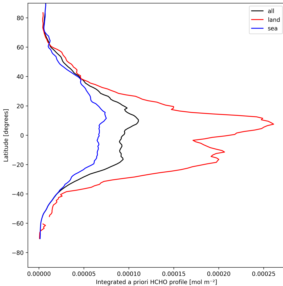
Figure 29: Zonal average of “Integrated a priori HCHO profile” for 2025-04-26 to 2025-04-28.
