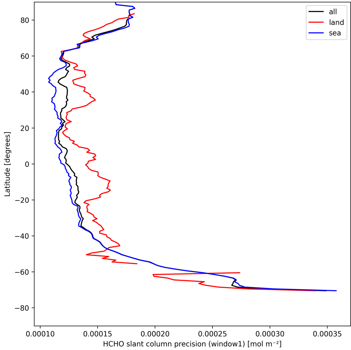
Figure 25: Zonal average of “HCHO slant column precision (window1)” for 2025-04-26 to 2025-04-28.
