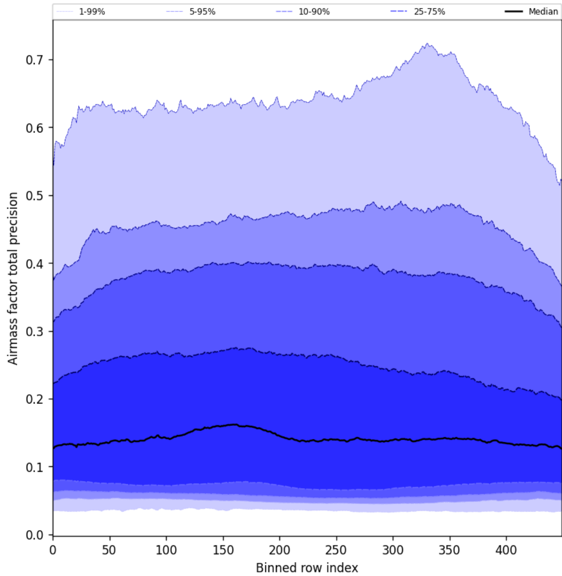
Figure 55: Along track statistics of “Airmass factor total precision” for 2025-04-26 to 2025-04-28
