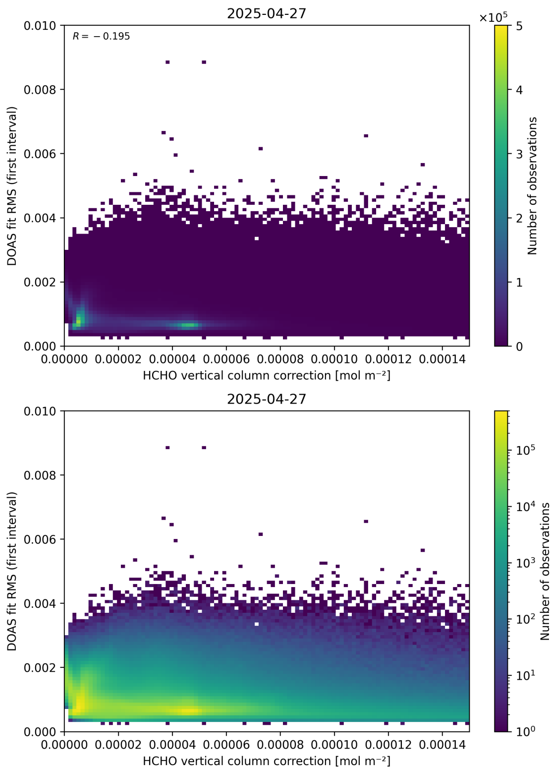
Figure 112: Scatter density plot of “HCHO vertical column correction” against “DOAS fit RMS (first interval)” for 2025-04-26 to 2025-04-28.
