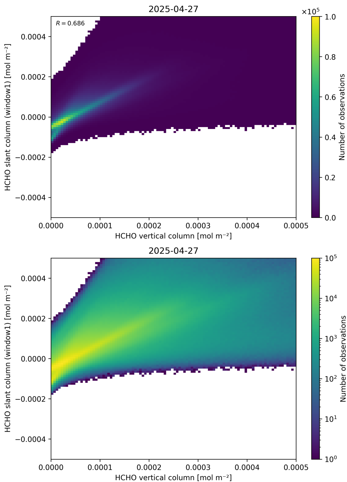
Figure 129: Scatter density plot of “HCHO vertical column” against “HCHO slant column (window1)” for 2025-04-26 to 2025-04-28.
