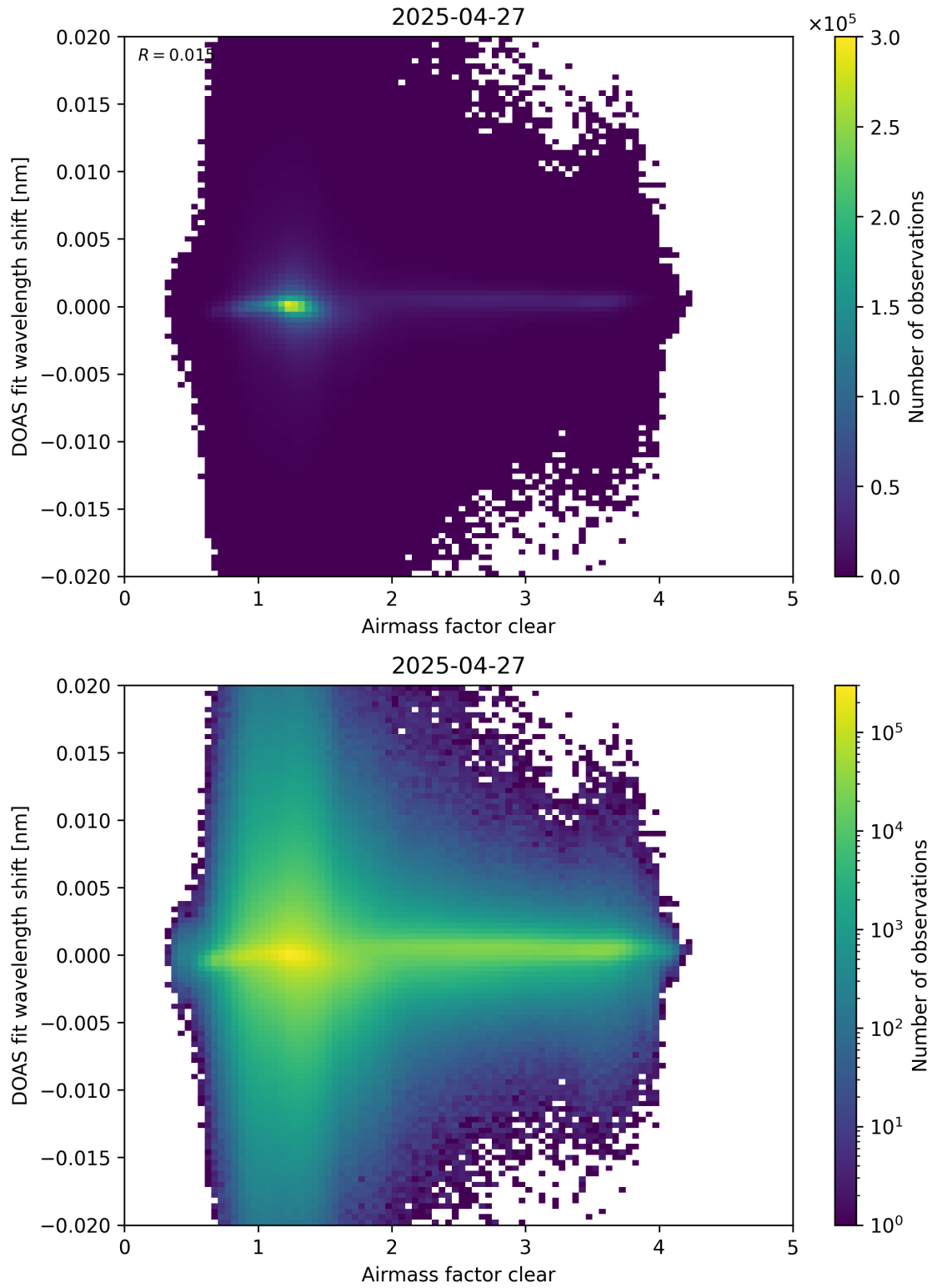
Figure 72: Scatter density plot of “Airmass factor clear” against “DOAS fit wavelength shift” for 2025-04-26 to 2025-04-28.
