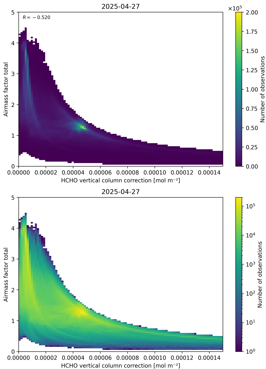
Figure 120: Scatter density plot of “HCHO vertical column correction” against “Airmass factor total” for 2025-04-26 to 2025-04-28.
