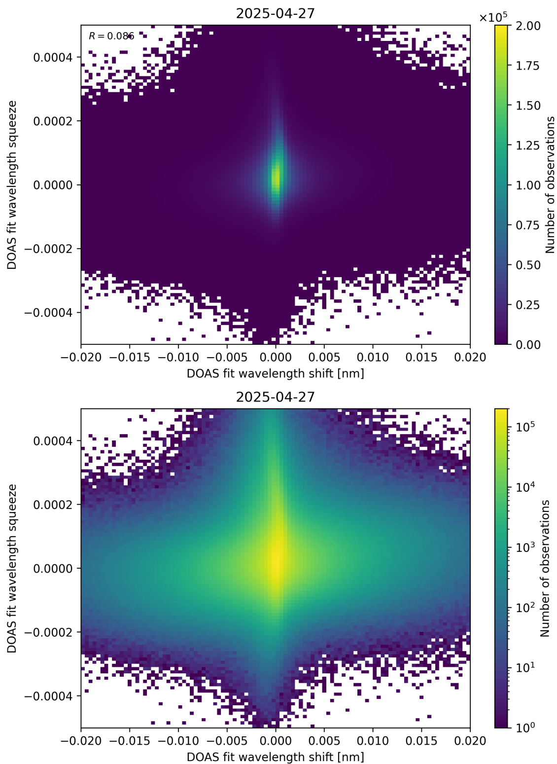
Figure 65: Scatter density plot of “DOAS fit wavelength shift” against “DOAS fit wavelength squeeze” for 2025-04-26 to 2025-04-28.
