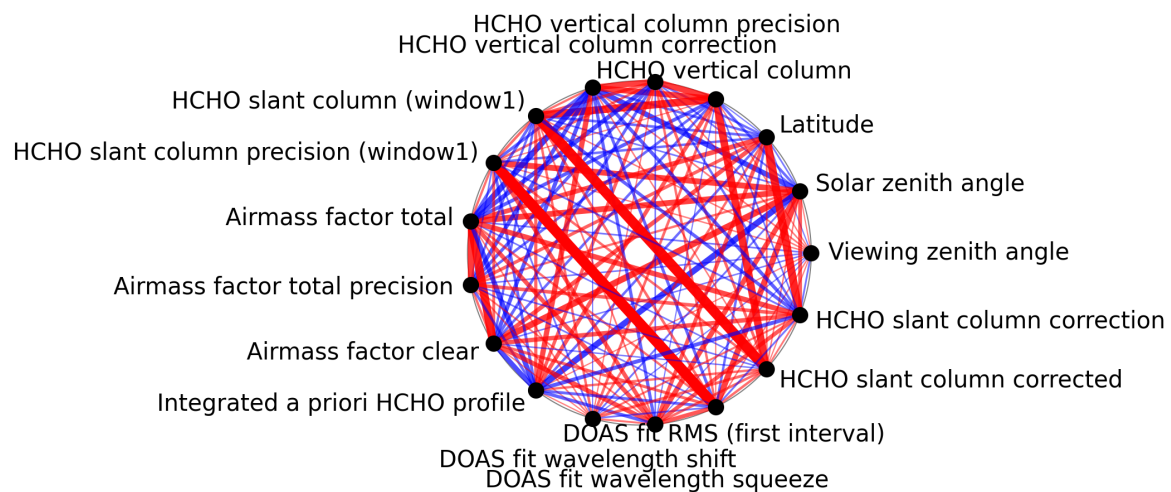
Figure 1: Map of correlation graph for 2025-04-26 to 2025-04-28.
