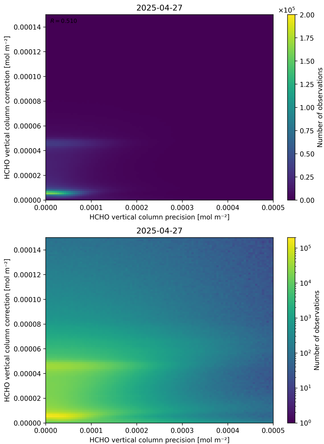
Figure 146: Scatter density plot of “HCHO vertical column precision” against “HCHO vertical column correction” for 2025-04-26 to 2025-04-28.
