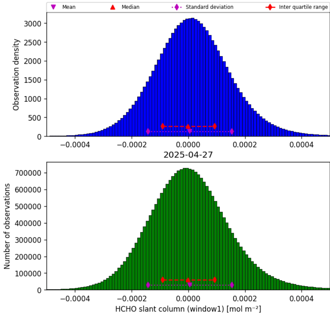
Figure 38: Histogram of “HCHO slant column (window1)” for 2025-04-26 to 2025-04-28
