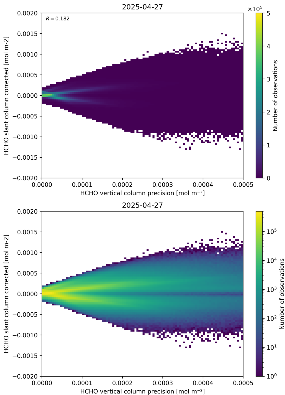
Figure 140: Scatter density plot of “HCHO vertical column precision” against “HCHO slant column corrected” for 2025-04-26 to 2025-04-28.
