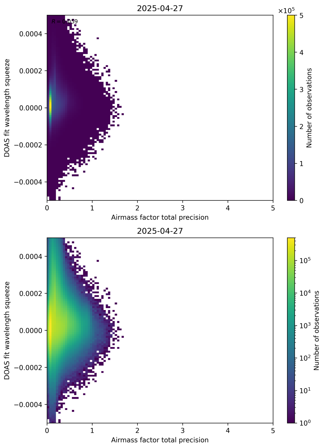
Figure 107: Scatter density plot of “Airmass factor total precision” against “DOAS fit wavelength squeeze” for 2025-04-26 to 2025-04-28.
