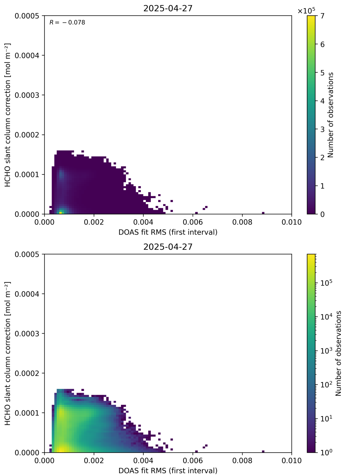
Figure 63: Scatter density plot of “DOAS fit RMS (first interval)” against “HCHO slant column correction” for 2025-04-26 to 2025-04-28.
