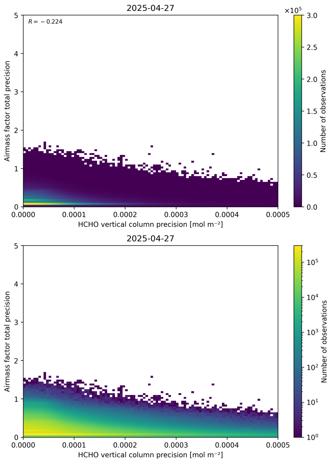
Figure 145: Scatter density plot of “HCHO vertical column precision” against “Airmass factor total precision” for 2025-04-26 to 2025-04-28.
