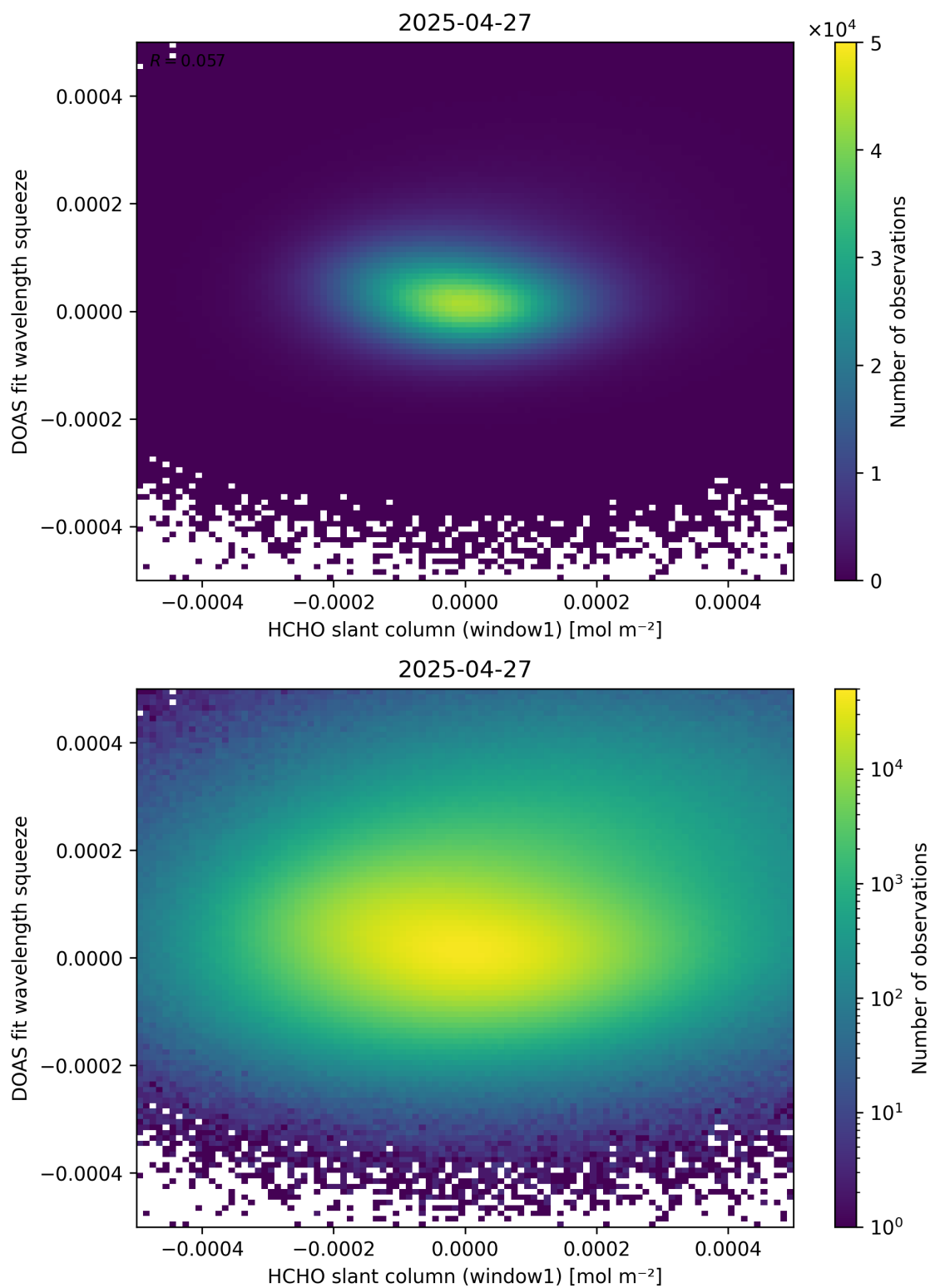
Figure 80: Scatter density plot of “HCHO slant column (window1)” against “DOAS fit wavelength squeeze” for 2025-04-26 to 2025-04-28.
