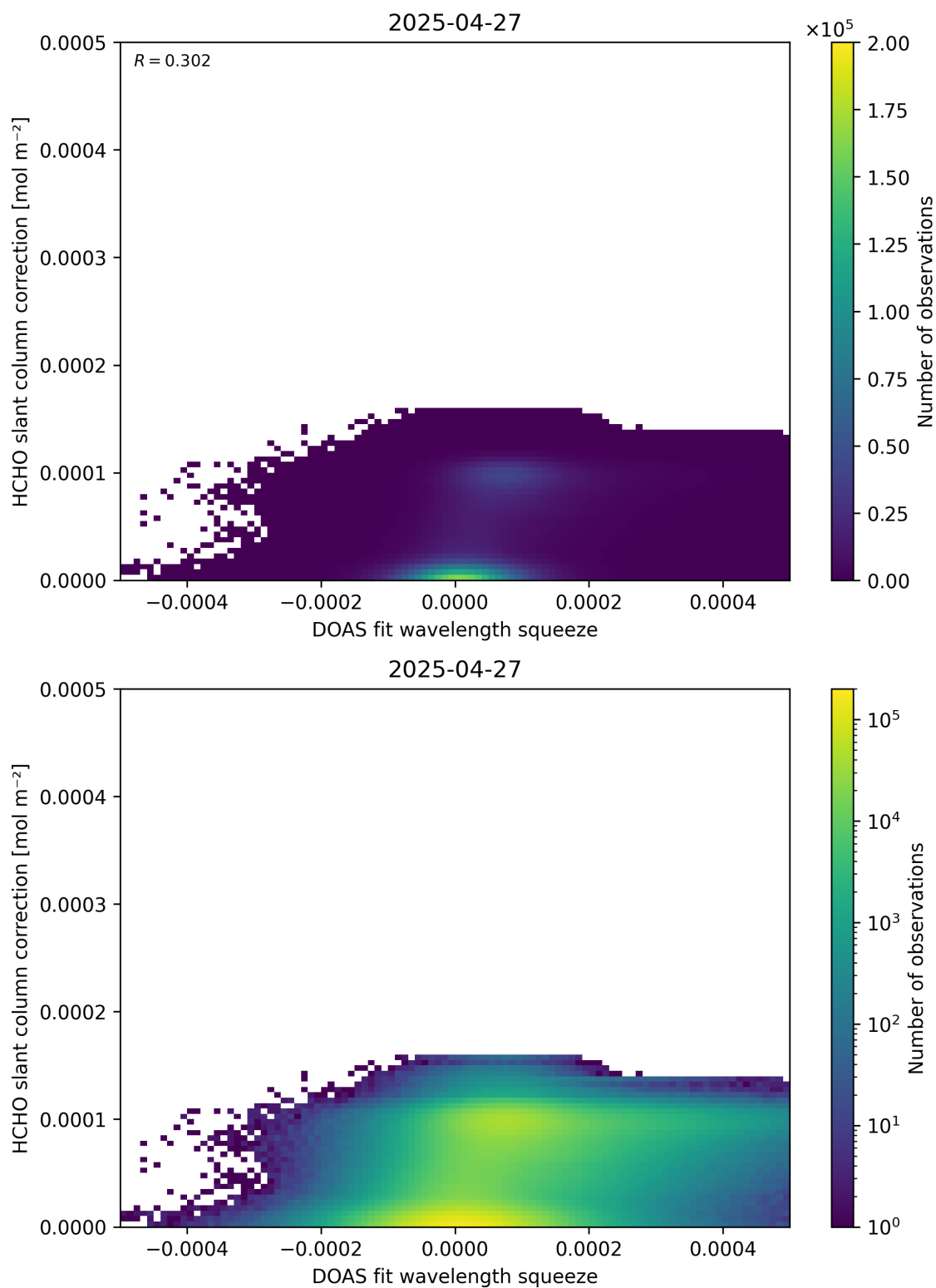
Figure 70: Scatter density plot of “DOAS fit wavelength squeeze” against “HCHO slant column correction” for 2025-04-26 to 2025-04-28.
