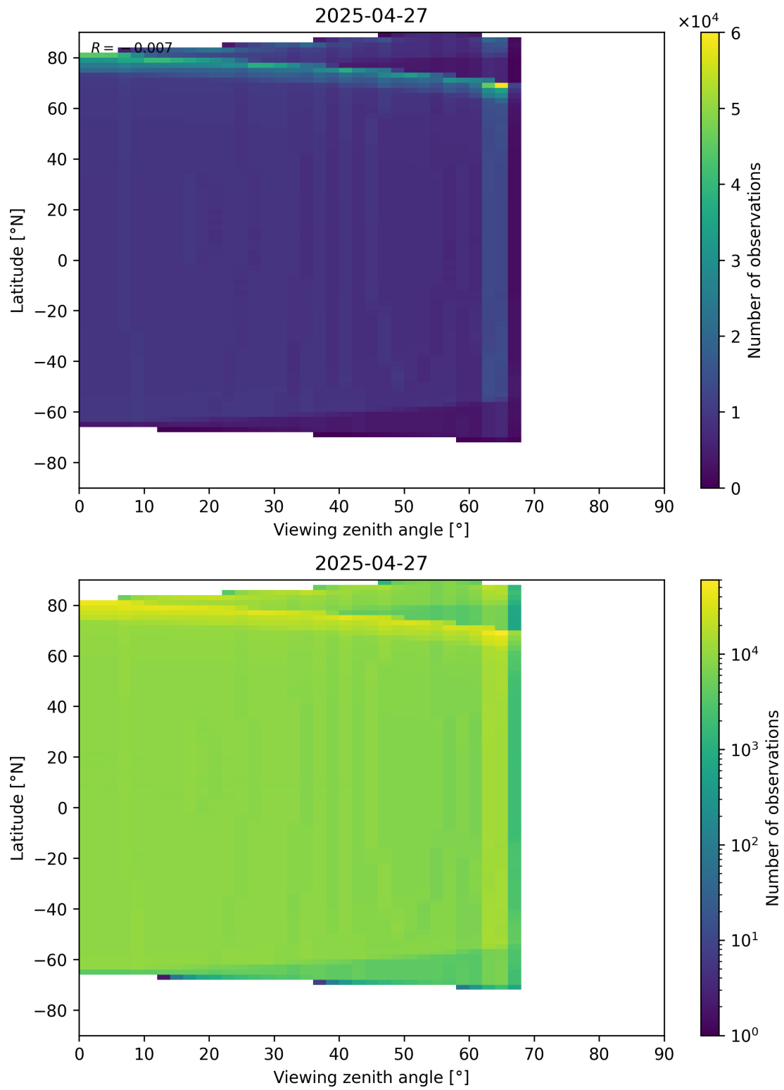
Figure 196: Scatter density plot of “Viewing zenith angle” against “Latitude” for 2025-04-26 to 2025-04-28.
