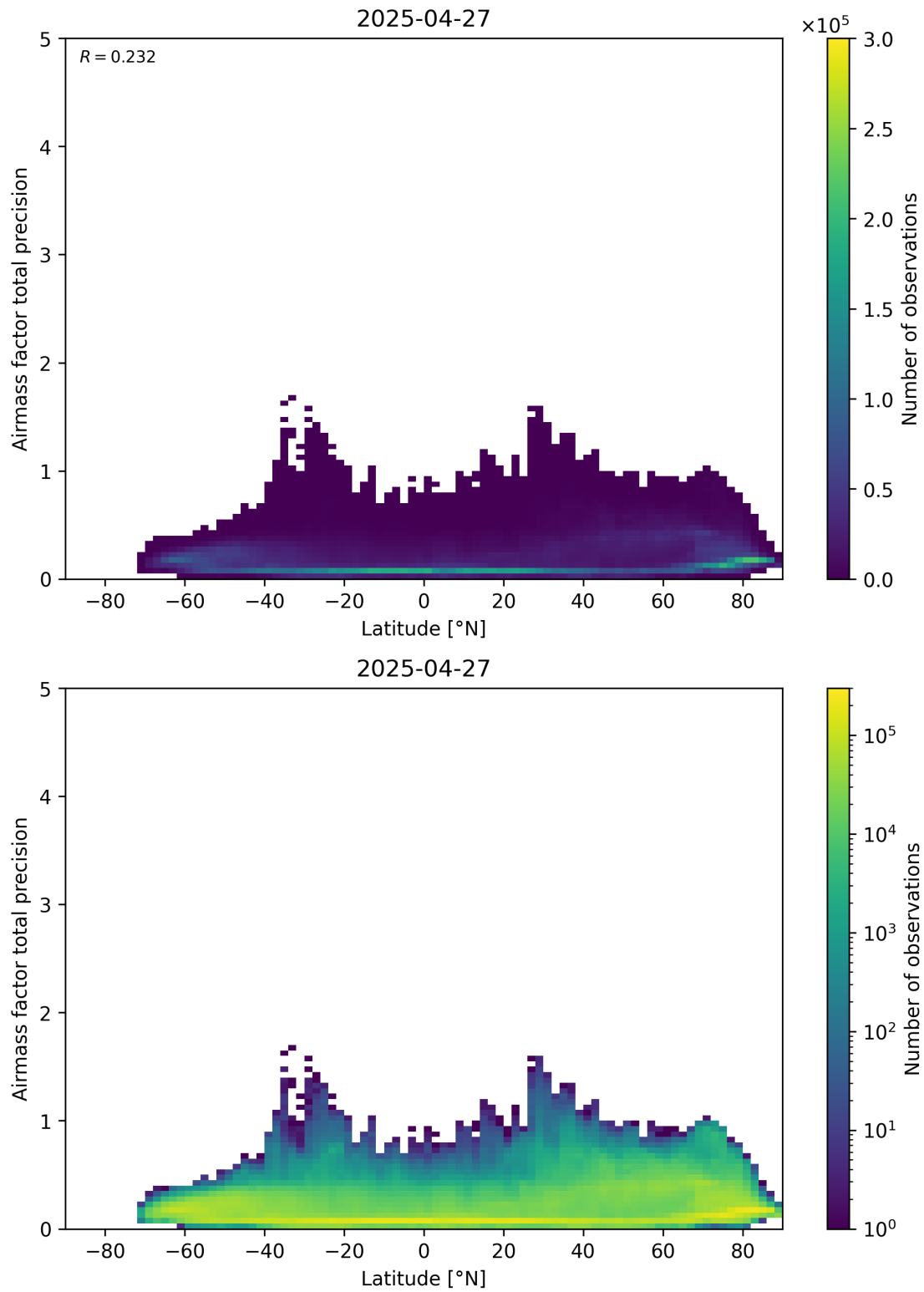
Figure 162: Scatter density plot of “Latitude” against “Airmass factor total precision” for 2025-04-26 to 2025-04-28.
