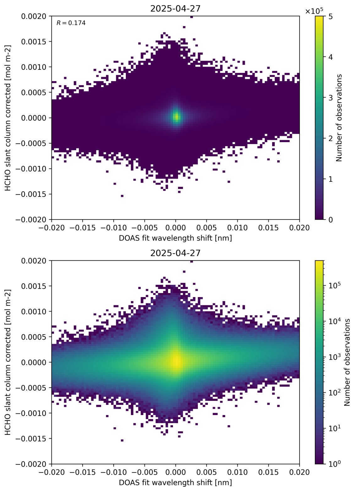
Figure 66: Scatter density plot of “DOAS fit wavelength shift” against “HCHO slant column corrected” for 2025-04-26 to 2025-04-28.
