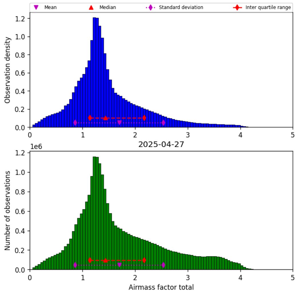
Figure 40: Histogram of “Airmass factor total” for 2025-04-26 to 2025-04-28
