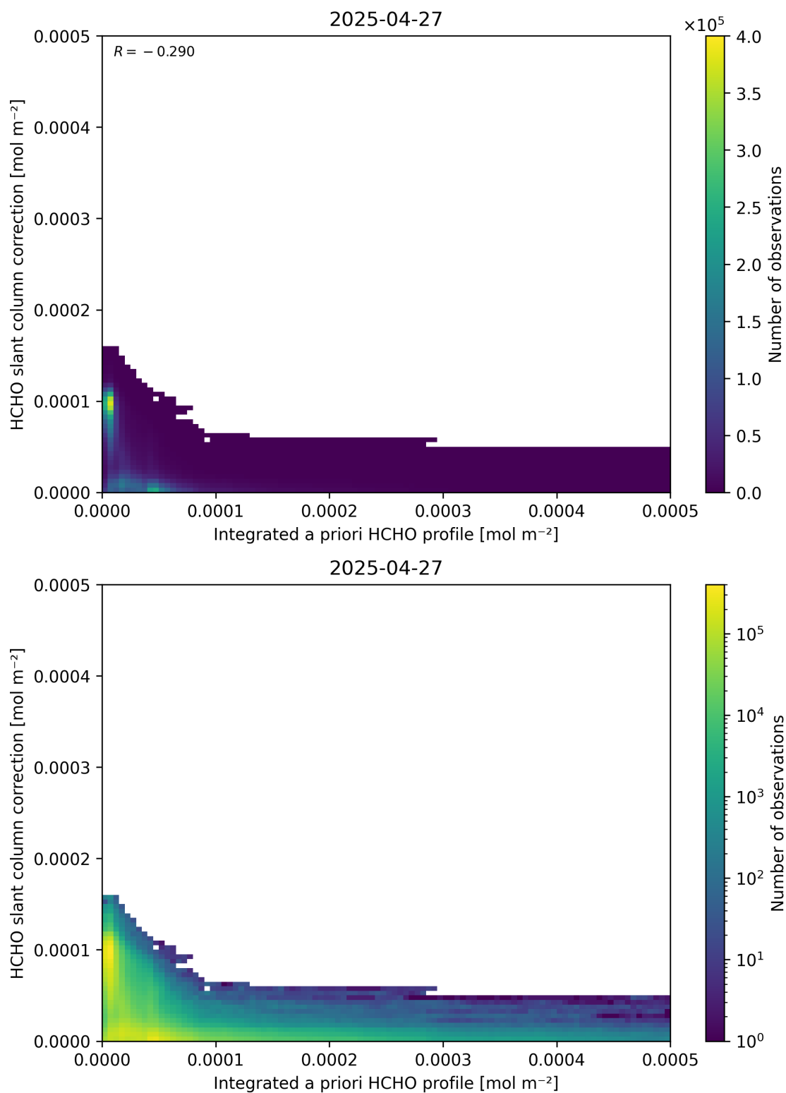
Figure 152: Scatter density plot of “Integrated a priori HCHO profile” against “HCHO slant column correction” for 2025-04-26 to 2025-04-28.
