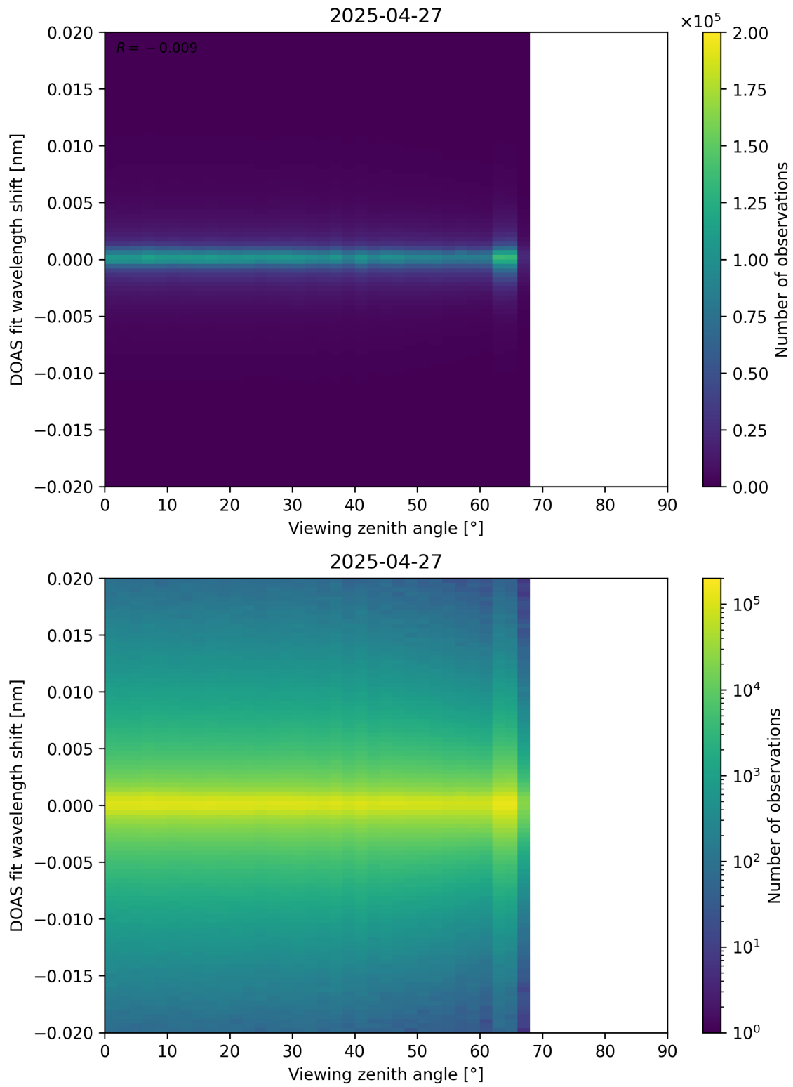
Figure 183: Scatter density plot of “Viewing zenith angle” against “DOAS fit wavelength shift” for 2025-04-26 to 2025-04-28.
