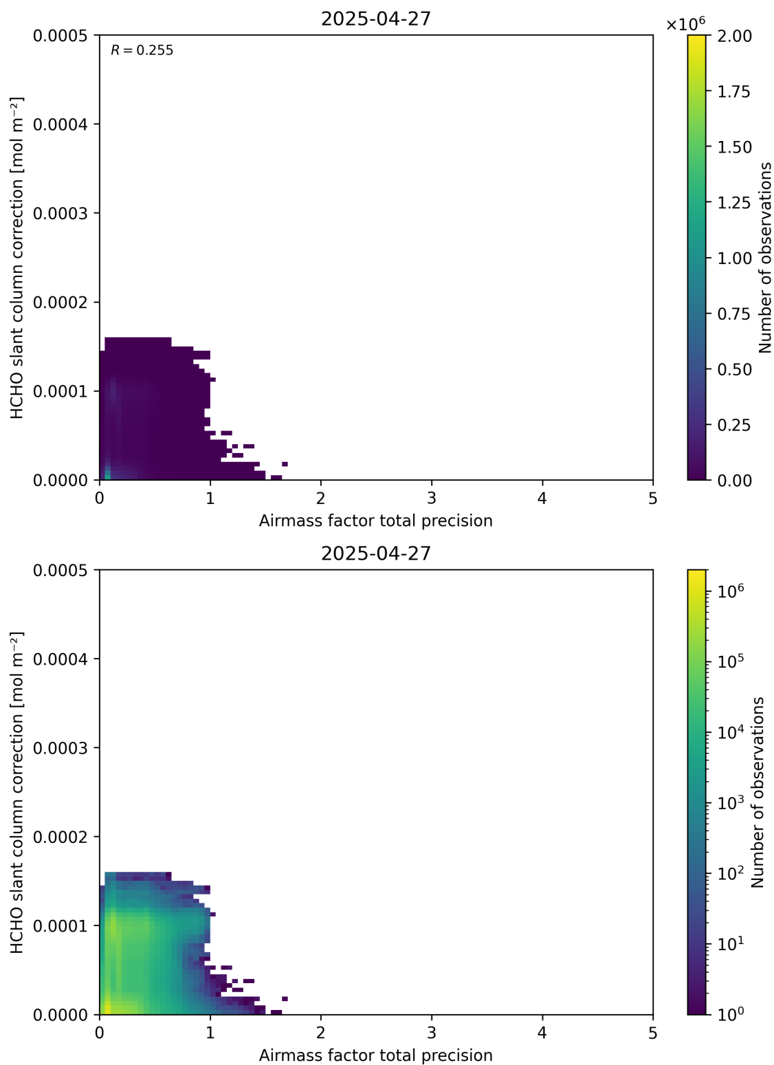
Figure 110: Scatter density plot of “Airmass factor total precision” against “HCHO slant column correction” for 2025-04-26 to 2025-04-28.
