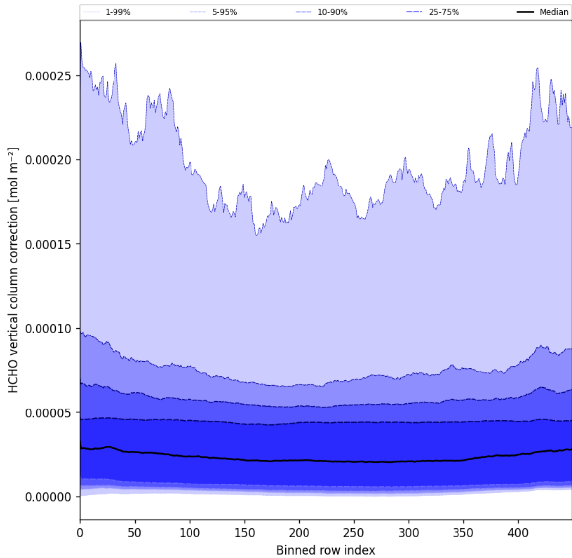
Figure 51: Along track statistics of “HCHO vertical column correction” for 2025-04-26 to 2025-04-28
