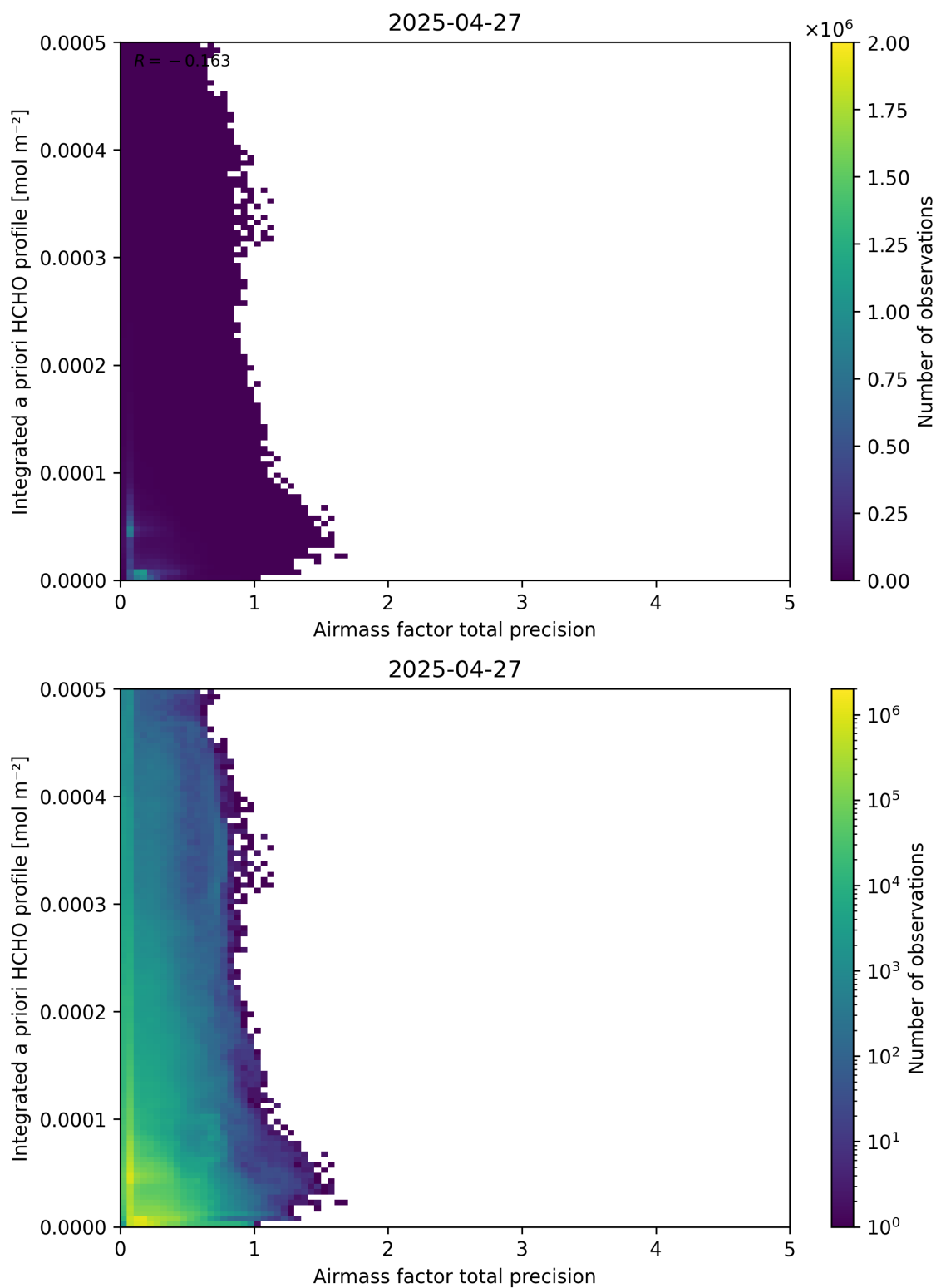
Figure 111: Scatter density plot of “Airmass factor total precision” against “Integrated a priori HCHO profile” for 2025-04-26 to 2025-04-28.
