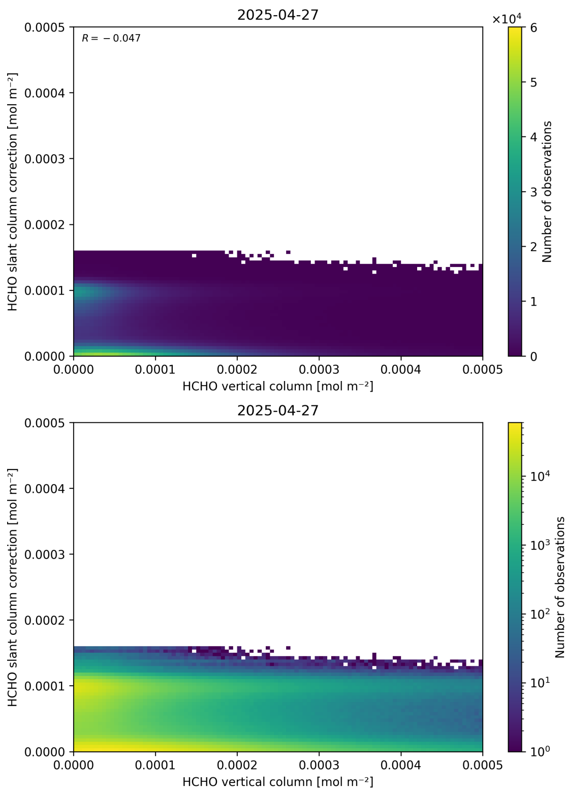
Figure 128: Scatter density plot of “HCHO vertical column” against “HCHO slant column correction” for 2025-04-26 to 2025-04-28.
