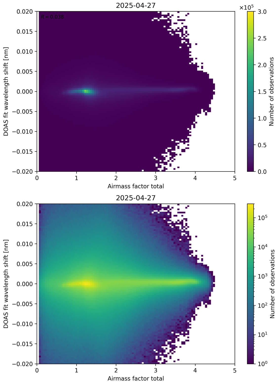
Figure 98: Scatter density plot of “Airmass factor total” against “DOAS fit wavelength shift” for 2025-04-26 to 2025-04-28.
