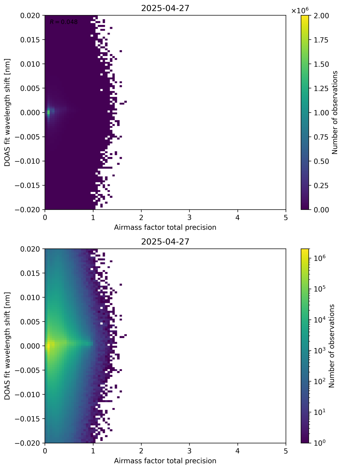
Figure 106: Scatter density plot of “Airmass factor total precision” against “DOAS fit wavelength shift” for 2025-04-26 to 2025-04-28.
