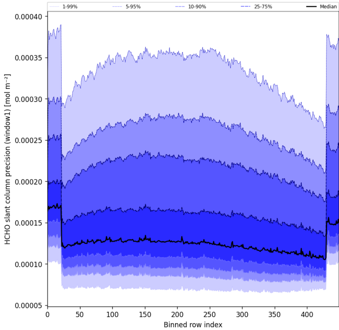
Figure 53: Along track statistics of “HCHO slant column precision (window1)” for 2025-04-26 to 2025-04-28
