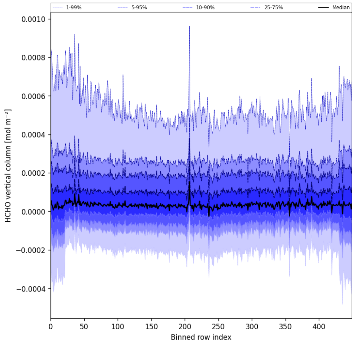
Figure 49: Along track statistics of “HCHO vertical column” for 2025-04-26 to 2025-04-28
