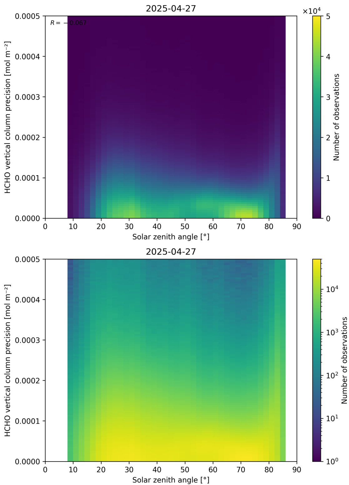
Figure 179: Scatter density plot of “Solar zenith angle” against “HCHO vertical column precision” for 2025-04-26 to 2025-04-28.
