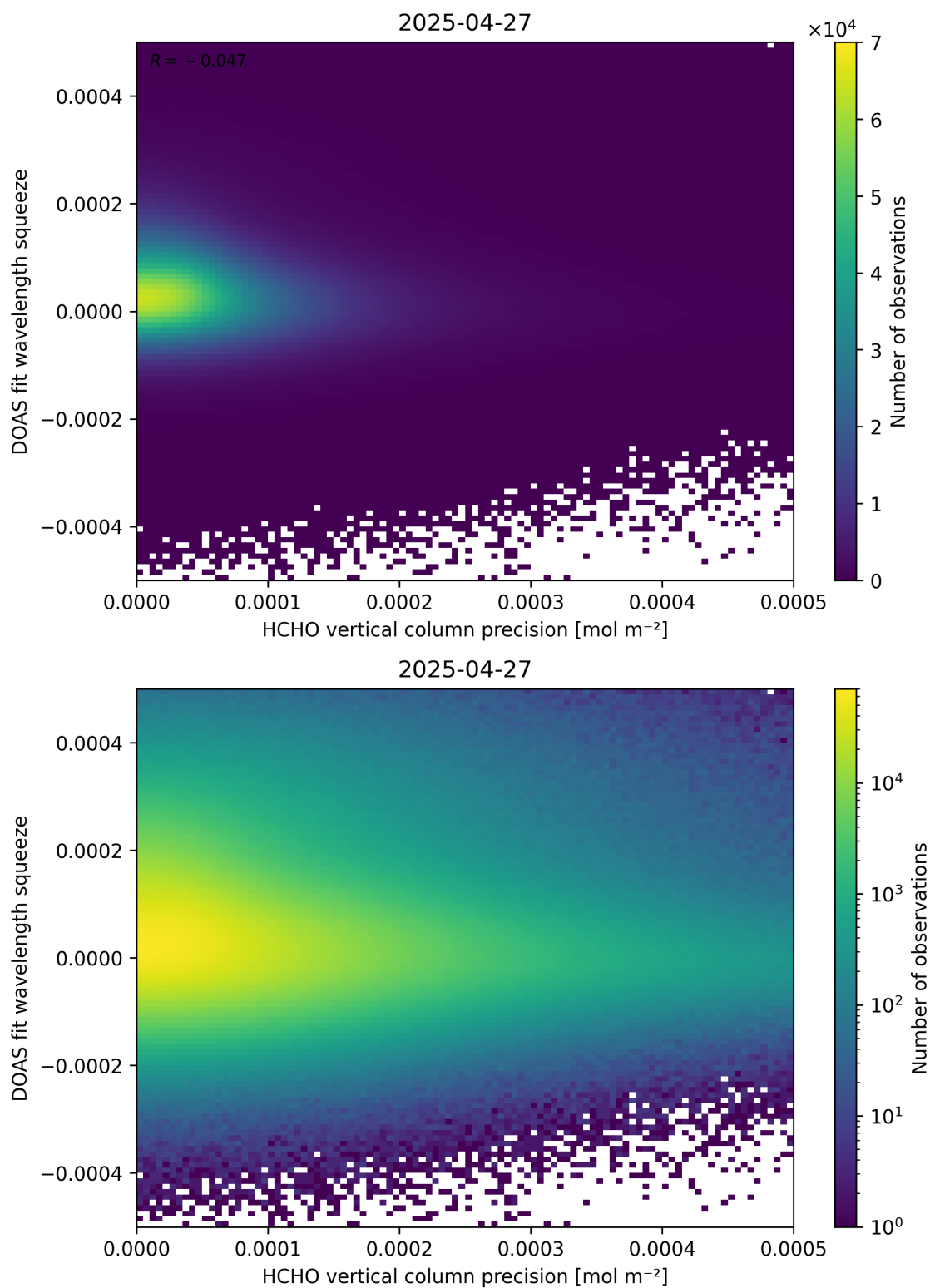
Figure 138: Scatter density plot of “HCHO vertical column precision” against “DOAS fit wavelength squeeze” for 2025-04-26 to 2025-04-28.
