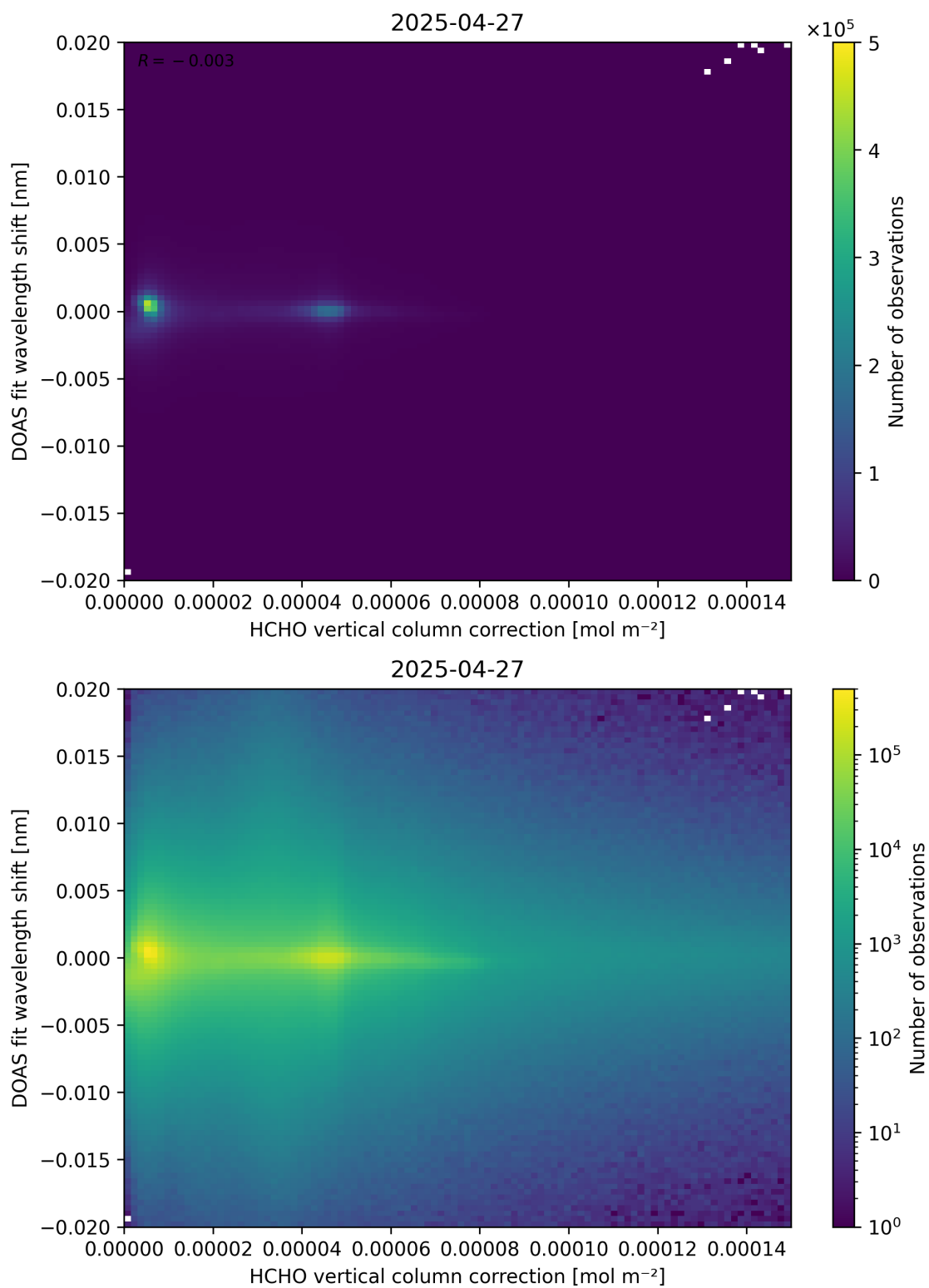
Figure 113: Scatter density plot of “HCHO vertical column correction” against “DOAS fit wavelength shift” for 2025-04-26 to 2025-04-28.
