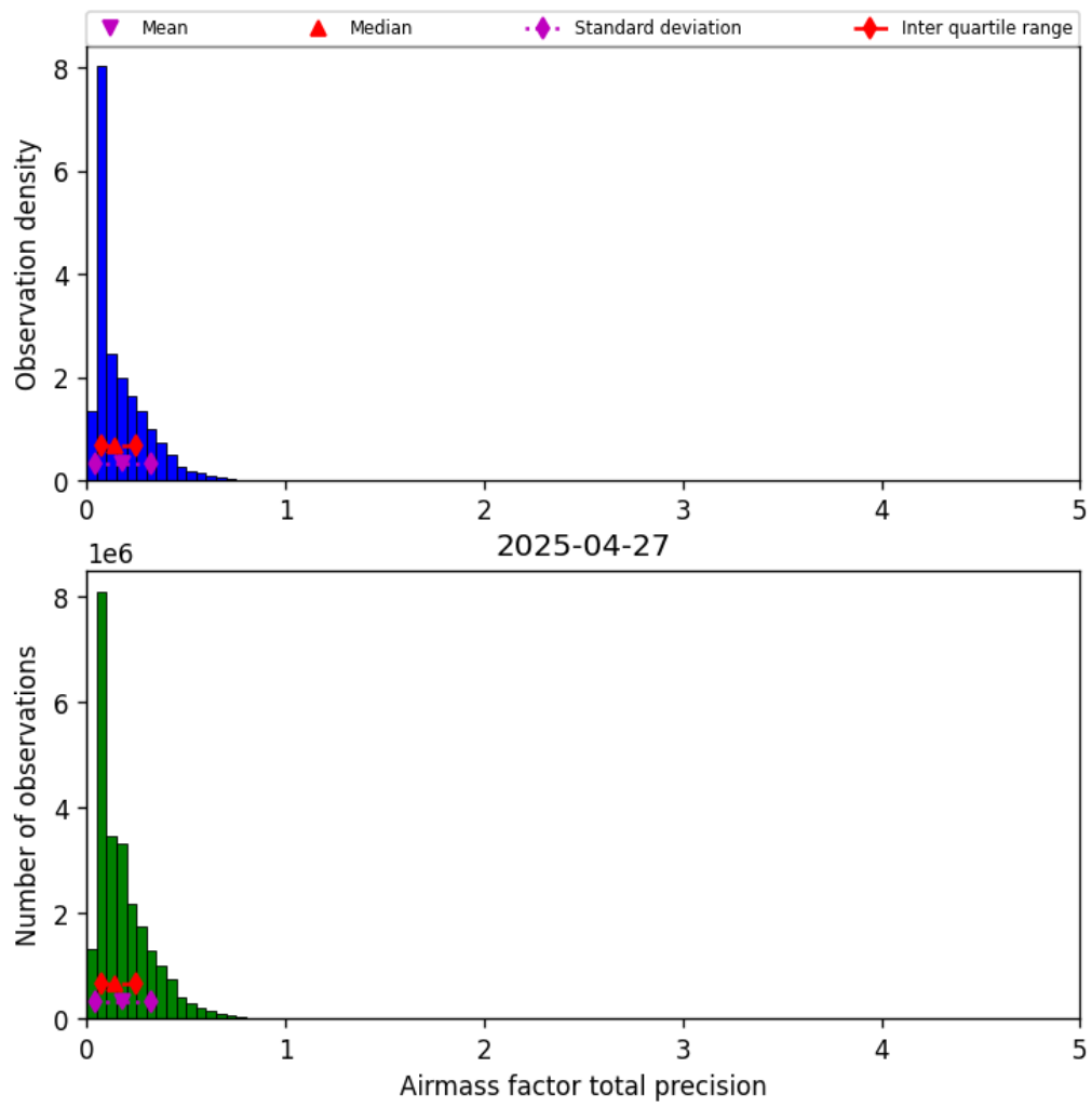
Figure 41: Histogram of “Airmass factor total precision” for 2025-04-26 to 2025-04-28
