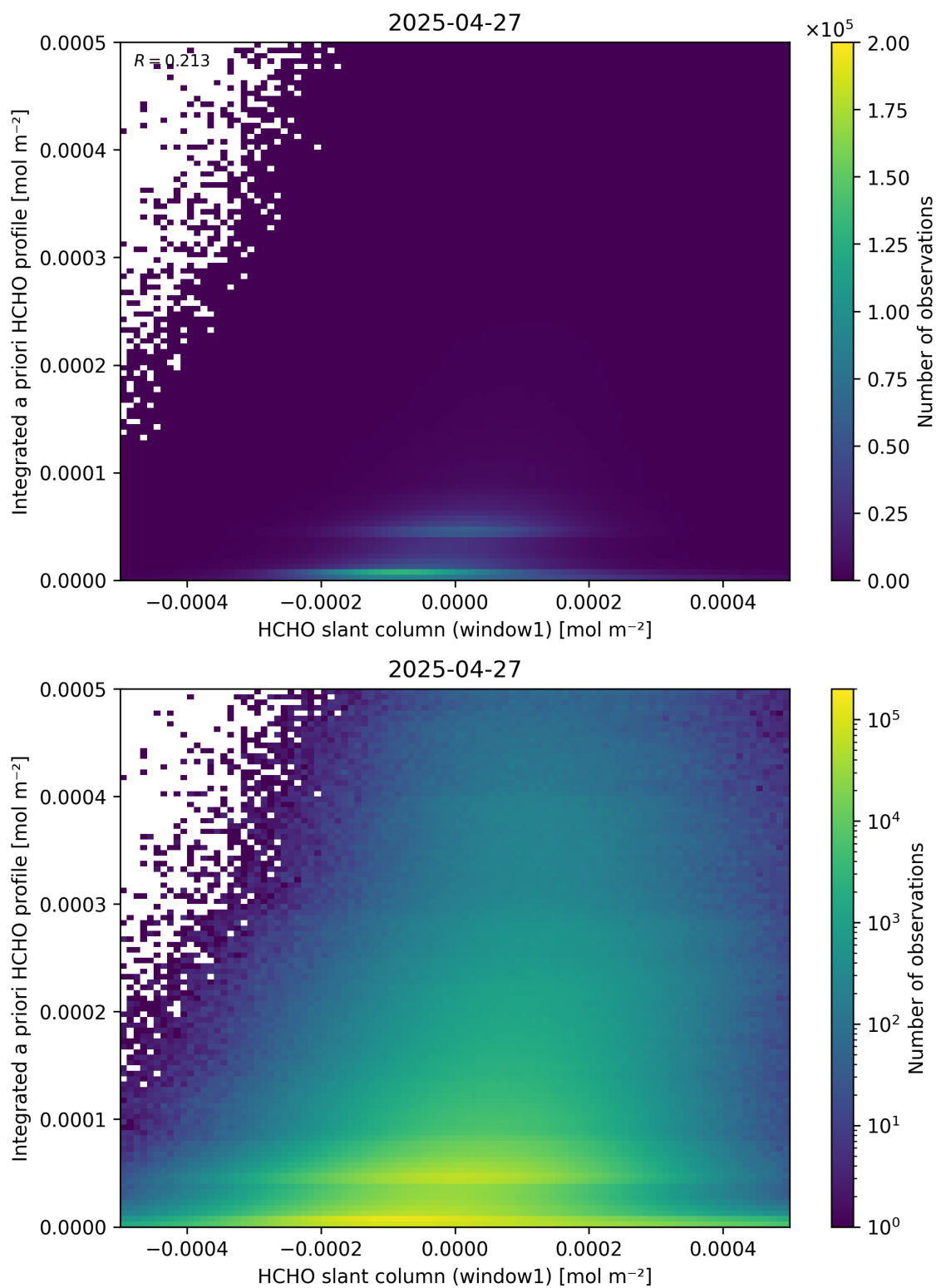
Figure 87: Scatter density plot of “HCHO slant column (window1)” against “Integrated a priori HCHO profile” for 2025-04-26 to 2025-04-28.
