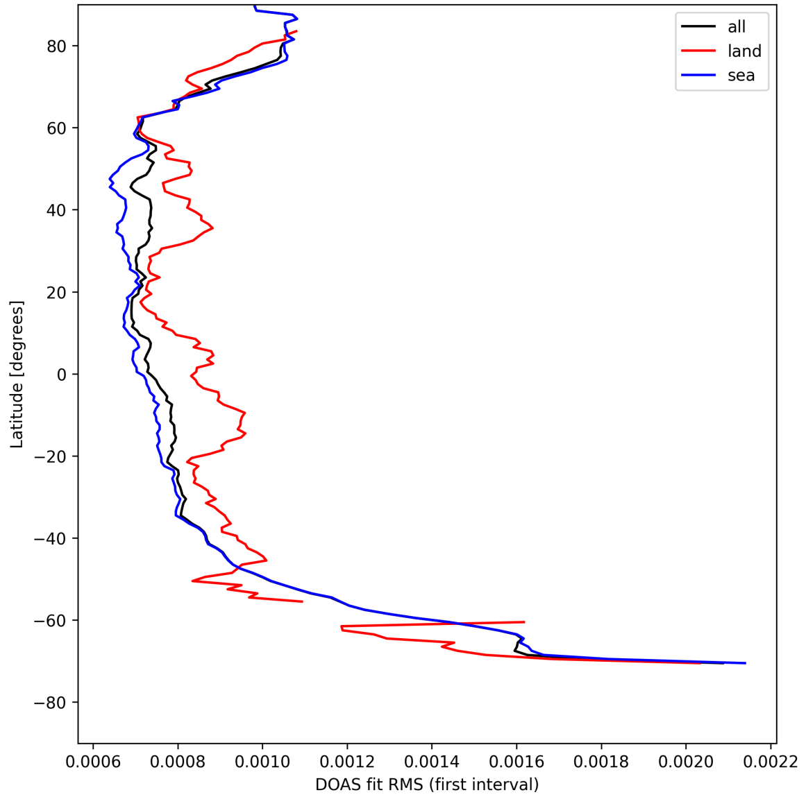
Figure 32: Zonal average of “DOAS fit RMS (first interval)” for 2025-04-26 to 2025-04-28.
