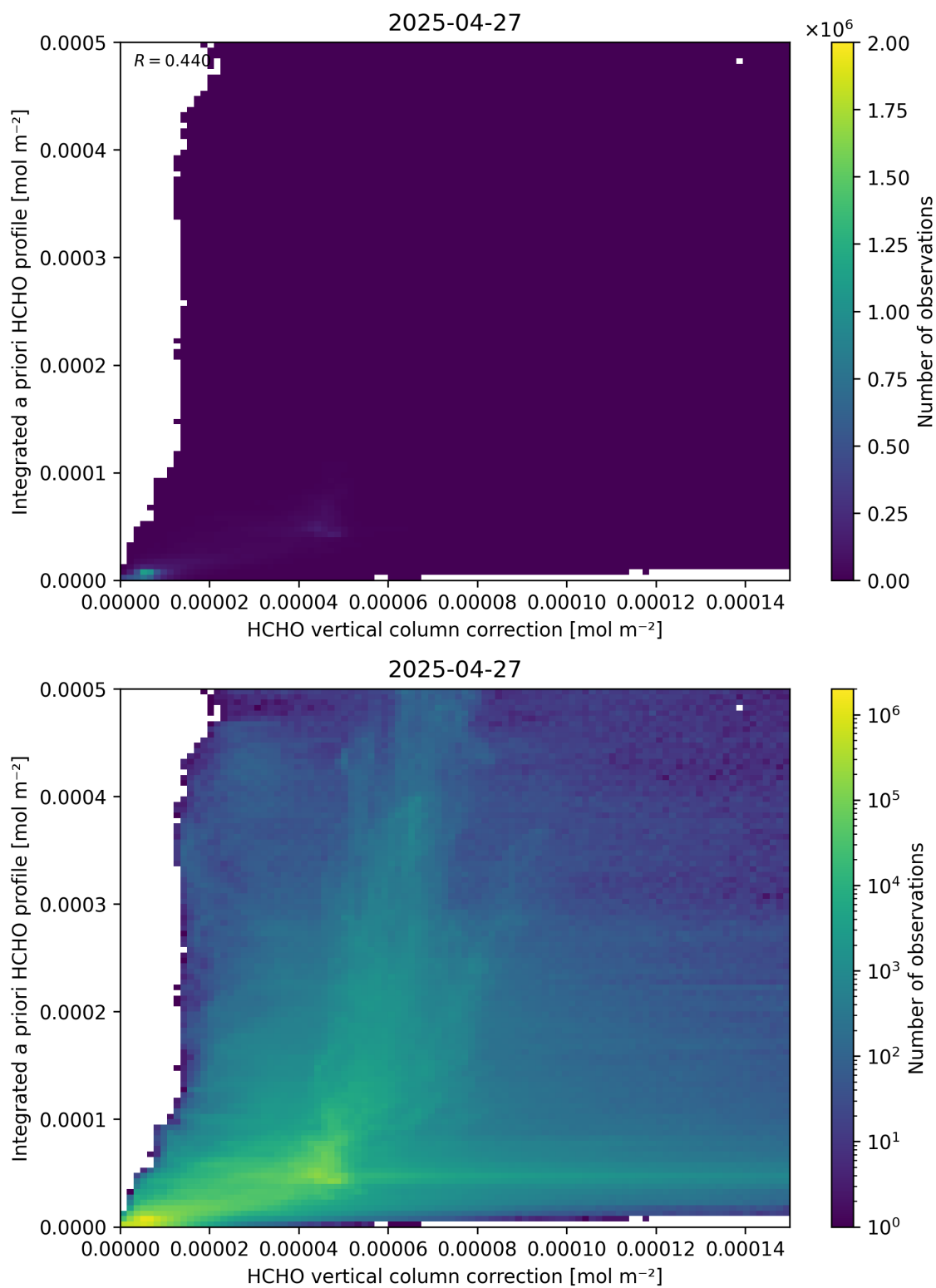
Figure 122: Scatter density plot of “HCHO vertical column correction” against “Integrated a priori HCHO profile” for 2025-04-26 to 2025-04-28.
