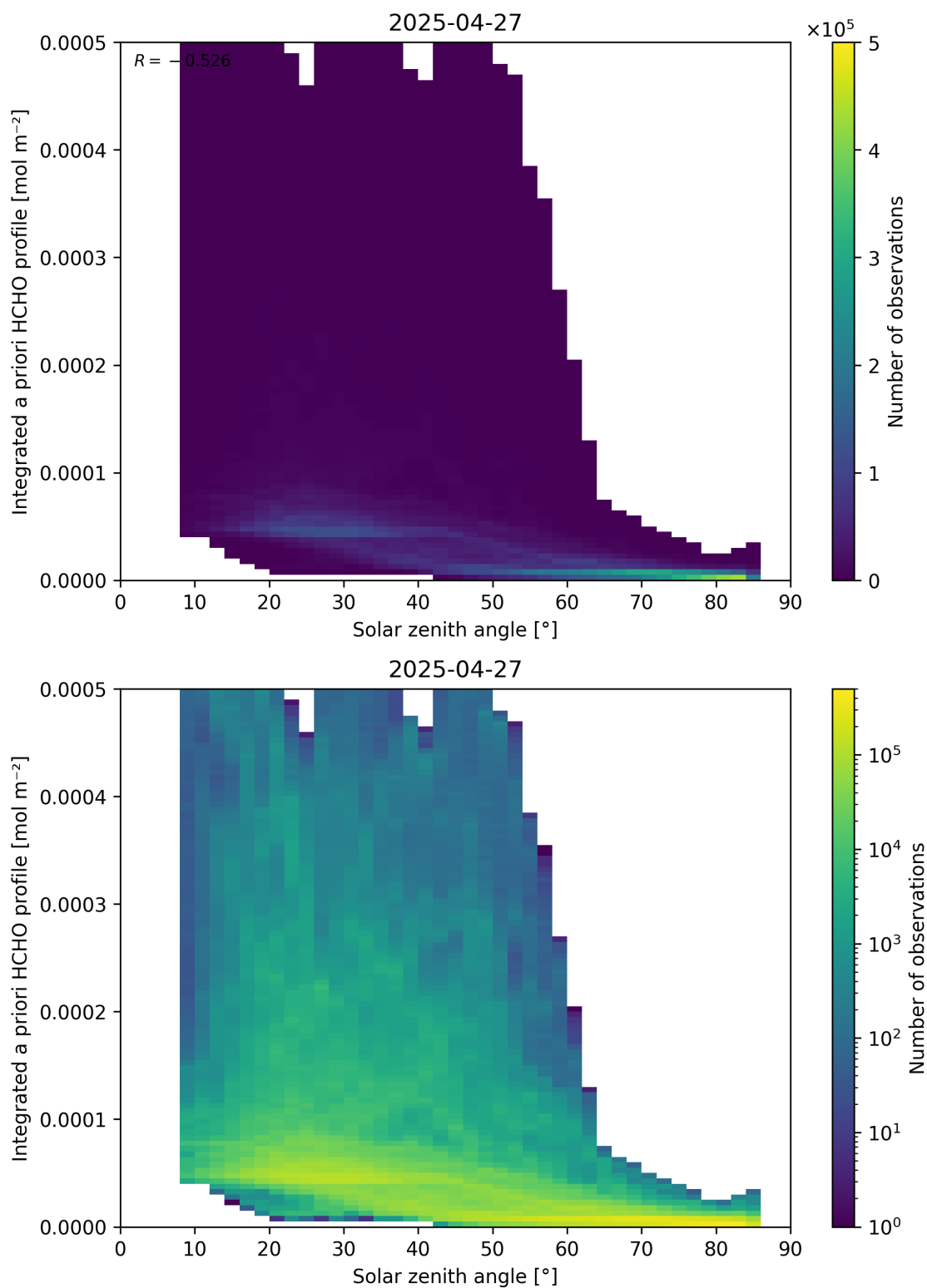
Figure 180: Scatter density plot of “Solar zenith angle” against “Integrated a priori HCHO profile” for 2025-04-26 to 2025-04-28.
