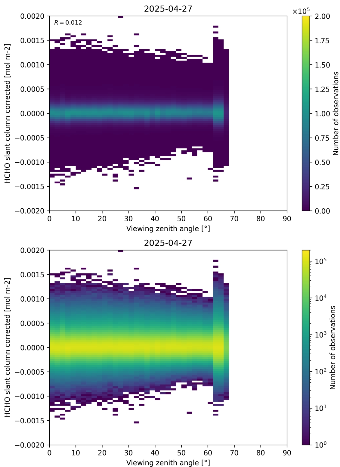
Figure 186: Scatter density plot of “Viewing zenith angle” against “HCHO slant column corrected” for 2025-04-26 to 2025-04-28.
