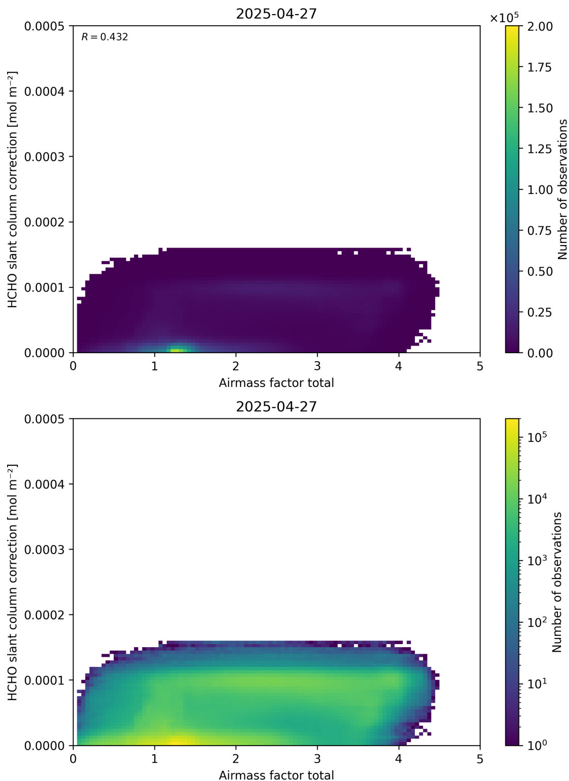
Figure 102: Scatter density plot of “Airmass factor total” against “HCHO slant column correction” for 2025-04-26 to 2025-04-28.
