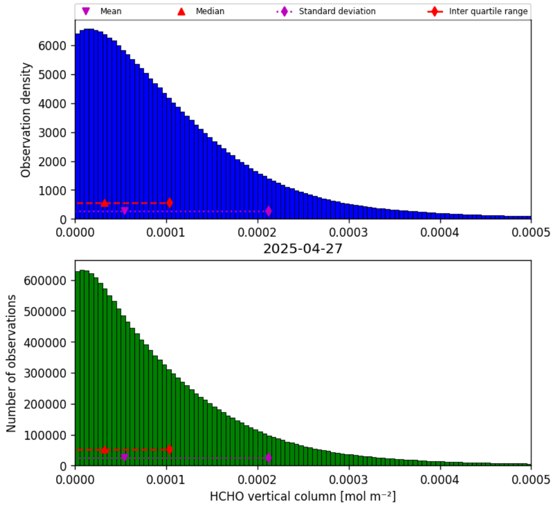
Figure 35: Histogram of “HCHO vertical column” for 2025-04-26 to 2025-04-28
