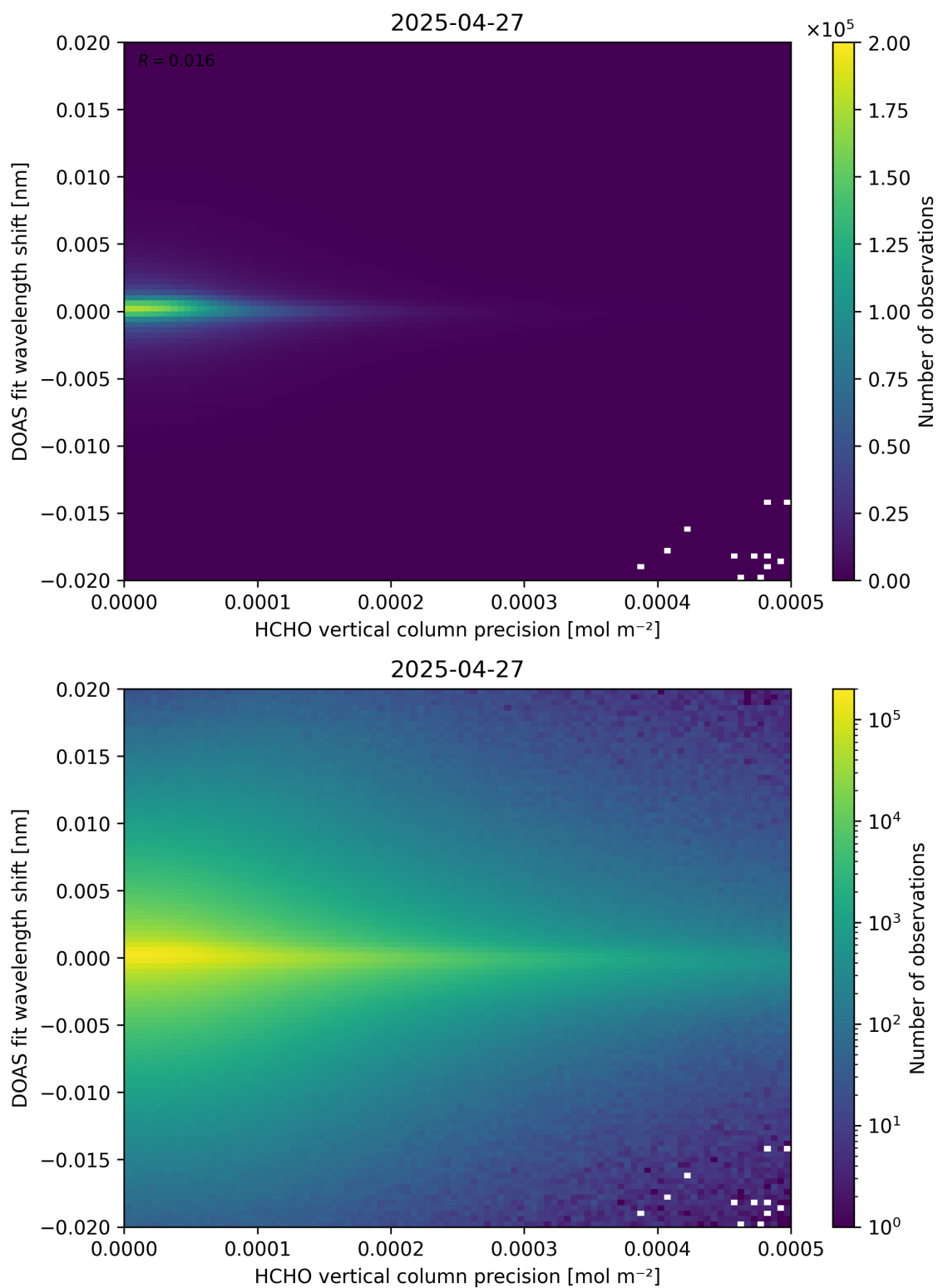
Figure 137: Scatter density plot of “HCHO vertical column precision” against “DOAS fit wavelength shift” for 2025-04-26 to 2025-04-28.
