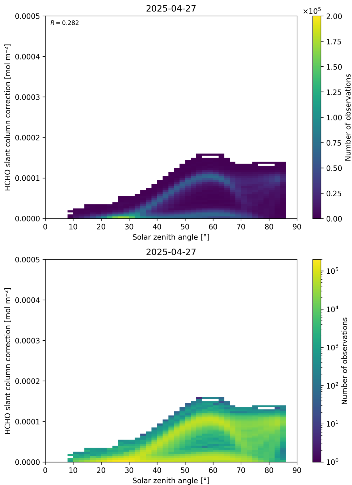
Figure 172: Scatter density plot of “Solar zenith angle” against “HCHO slant column correction” for 2025-04-26 to 2025-04-28.
