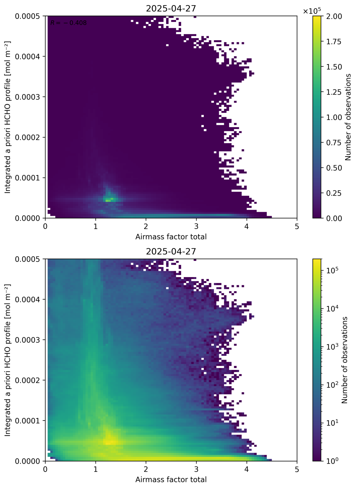
Figure 104: Scatter density plot of “Airmass factor total” against “Integrated a priori HCHO profile” for 2025-04-26 to 2025-04-28.
