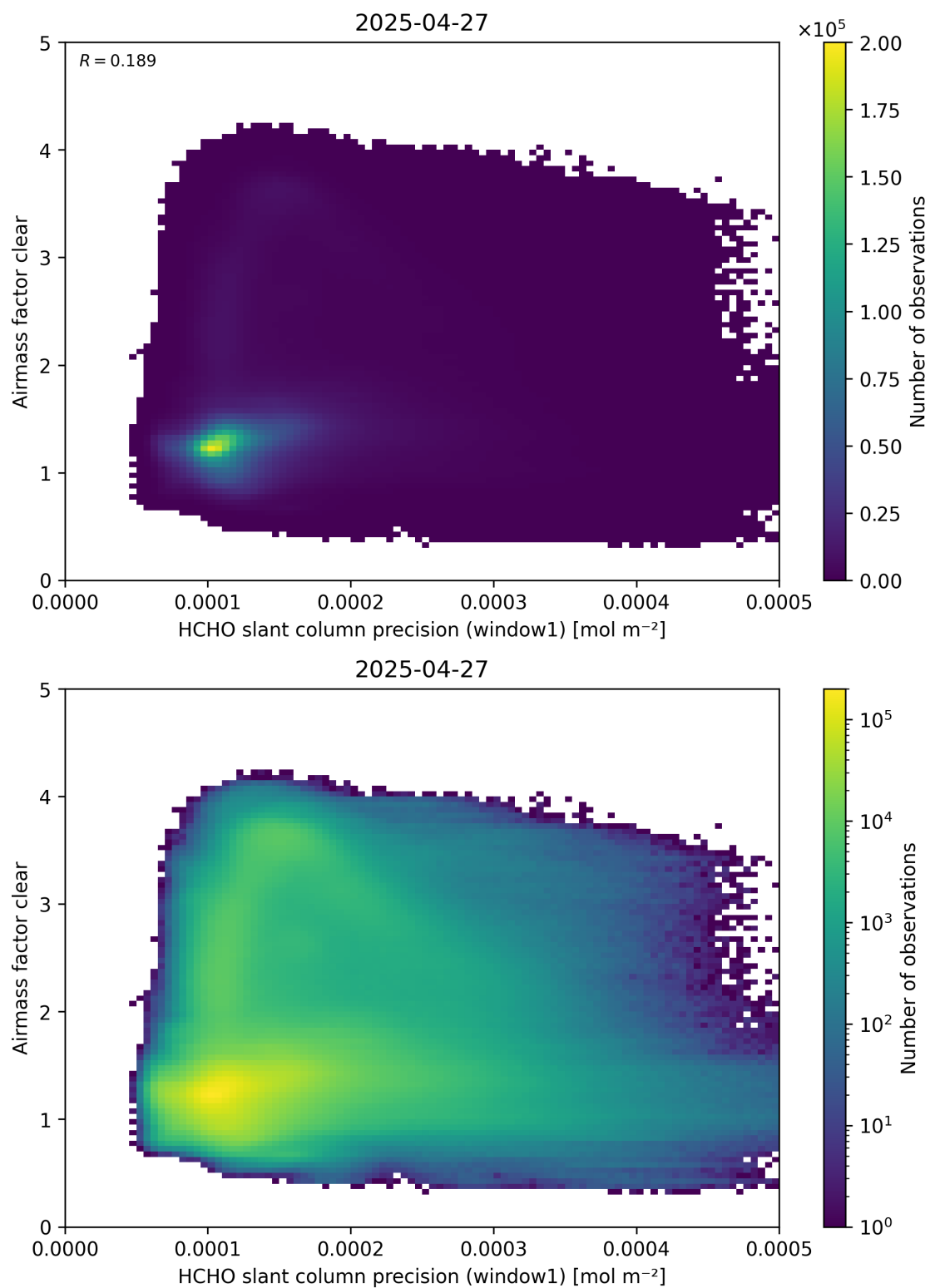
Figure 91: Scatter density plot of “HCHO slant column precision (window1)” against “Airmass factor clear” for 2025-04-26 to 2025-04-28.
