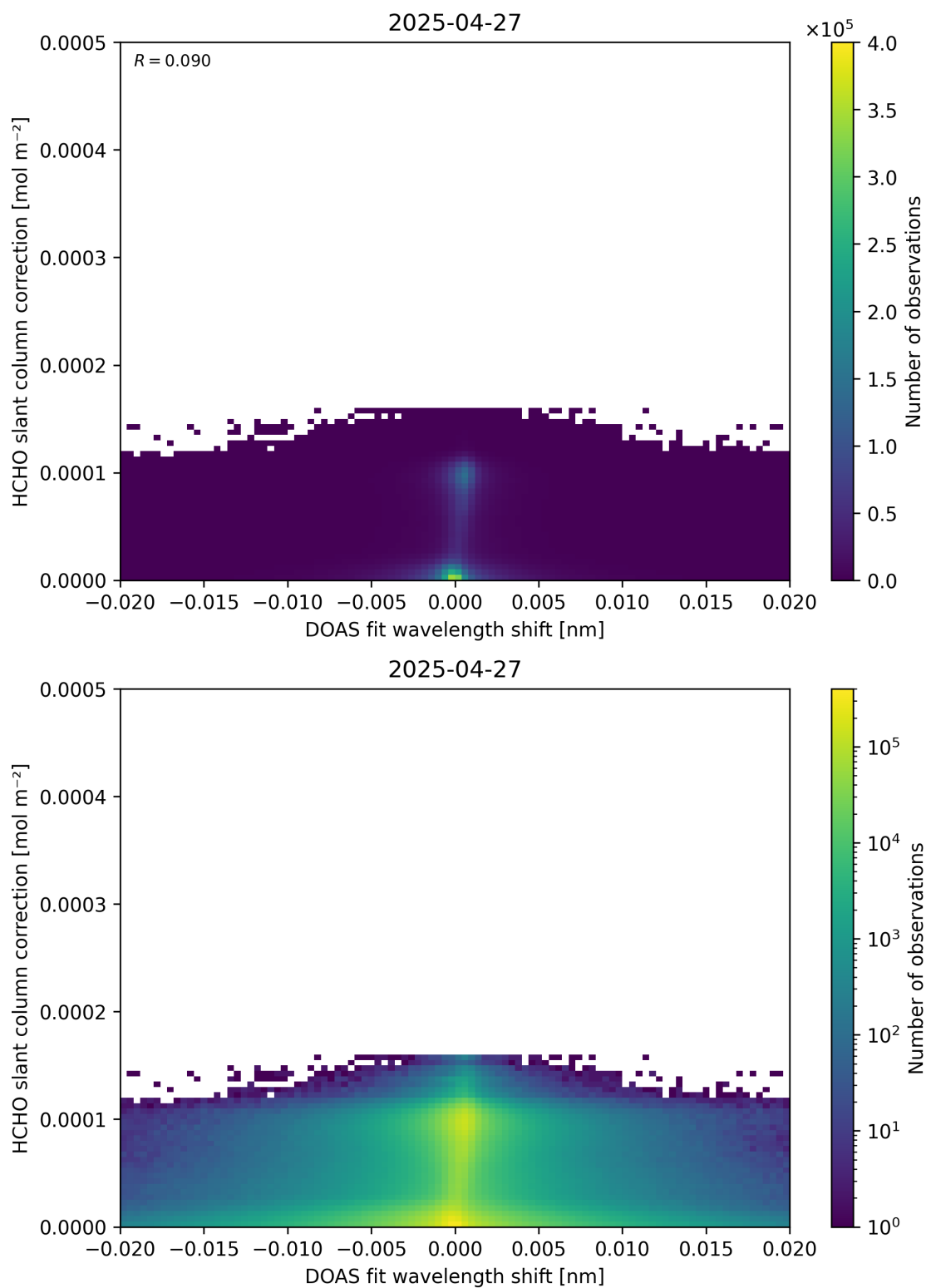
Figure 67: Scatter density plot of “DOAS fit wavelength shift” against “HCHO slant column correction” for 2025-04-26 to 2025-04-28.
