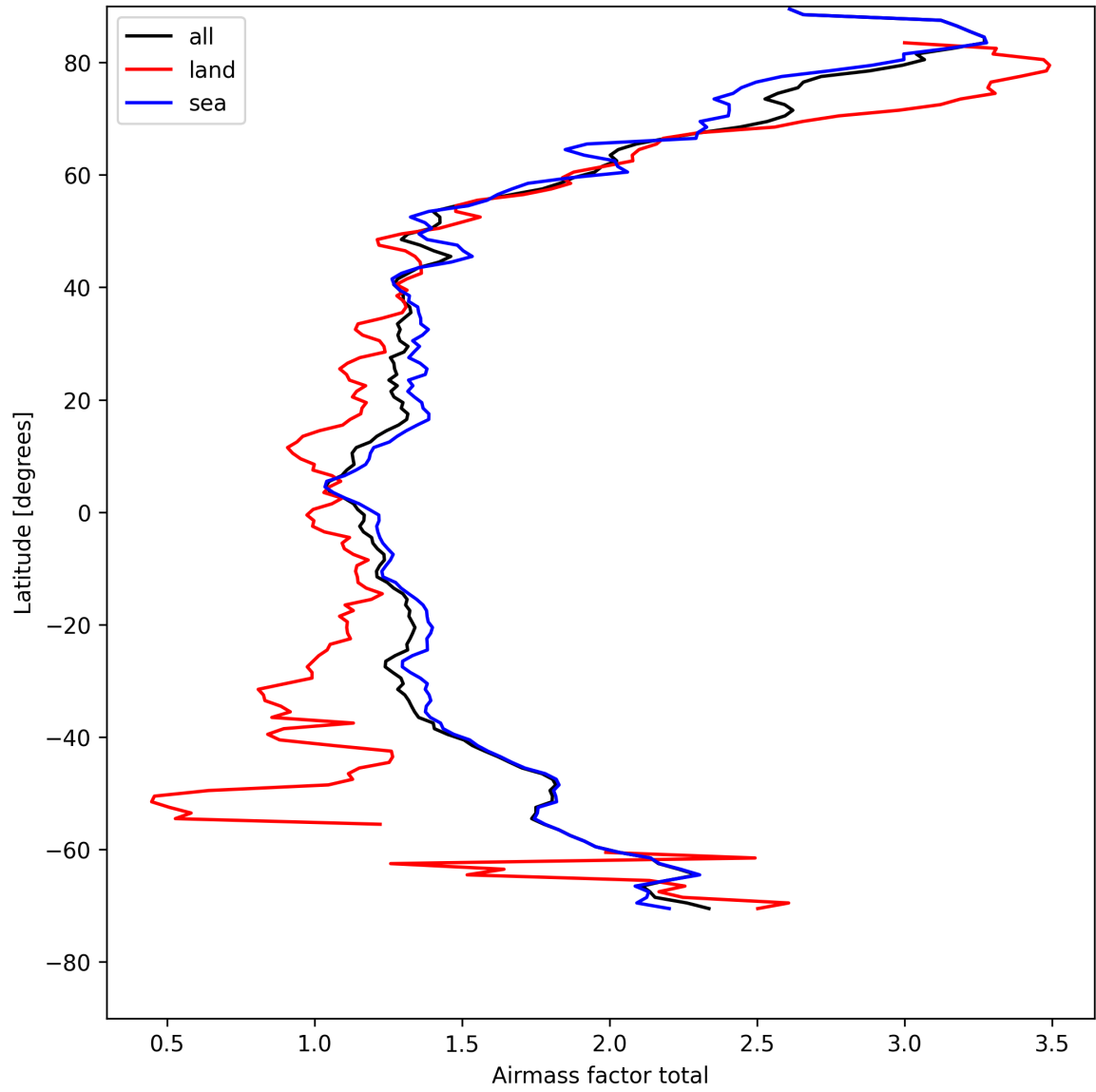
Figure 26: Zonal average of “Airmass factor total” for 2025-04-26 to 2025-04-28.
