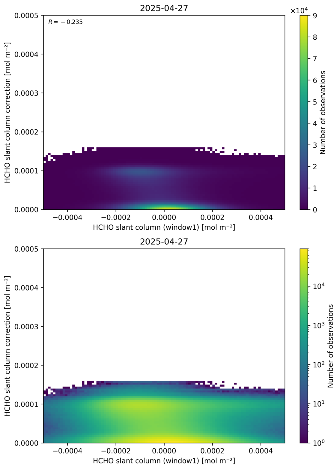
Figure 83: Scatter density plot of “HCHO slant column (window1)” against “HCHO slant column correction” for 2025-04-26 to 2025-04-28.
