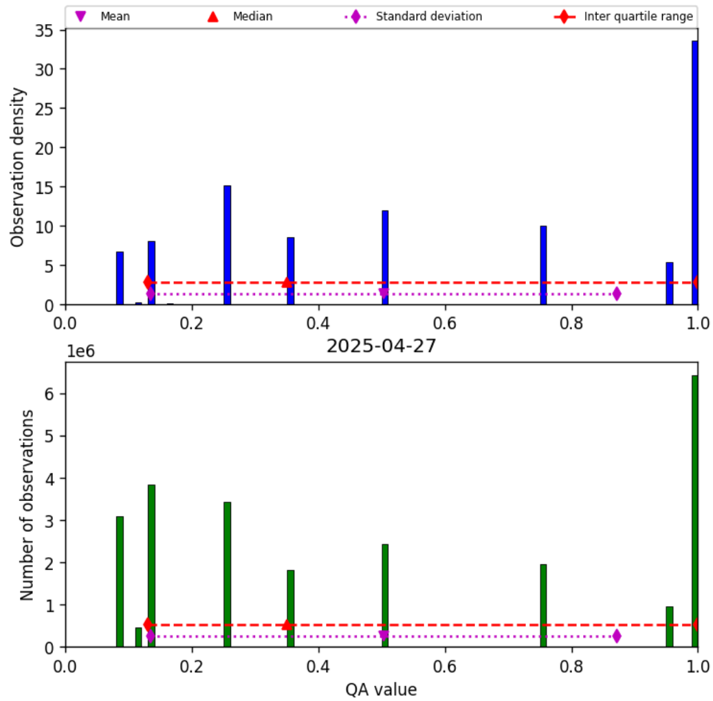
Figure 34: Histogram of “QA value” for 2025-04-26 to 2025-04-28
