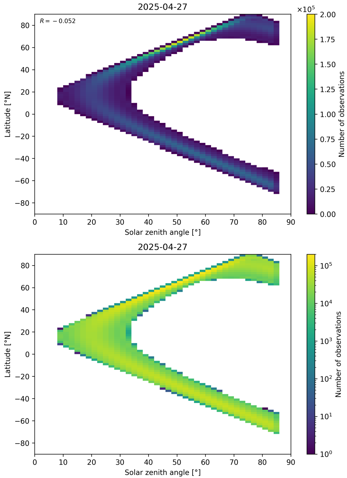
Figure 181: Scatter density plot of “Solar zenith angle” against “Latitude” for 2025-04-26 to 2025-04-28.
