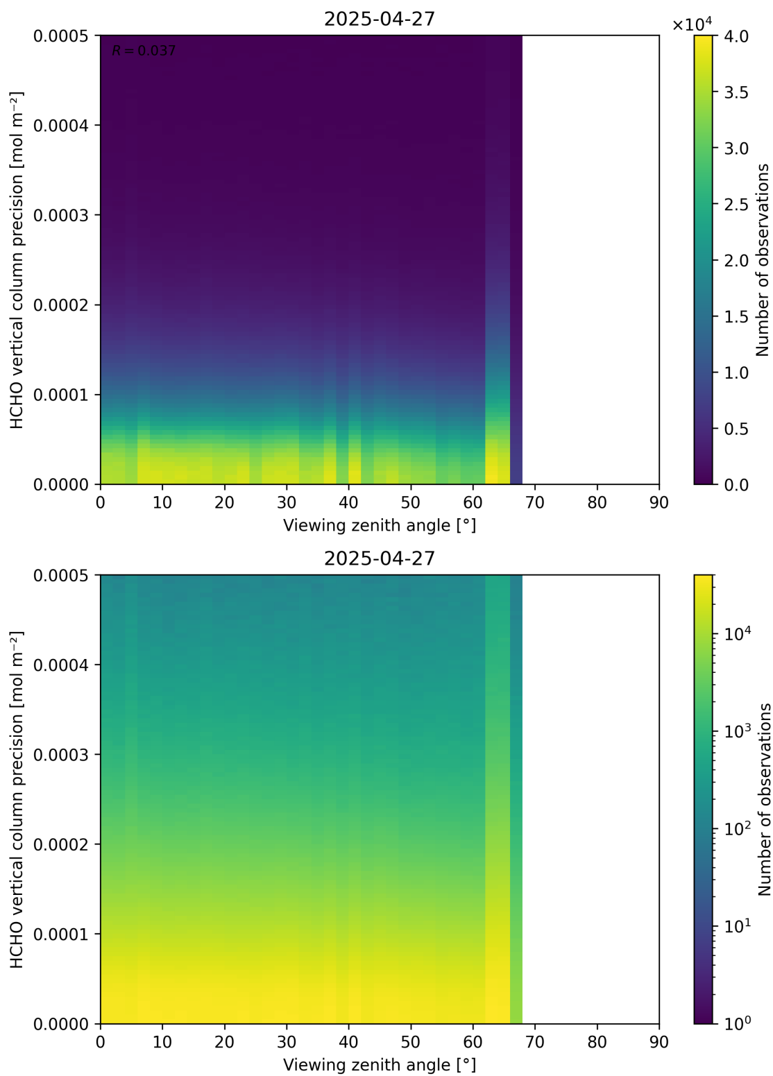
Figure 194: Scatter density plot of “Viewing zenith angle” against “HCHO vertical column precision” for 2025-04-26 to 2025-04-28.
