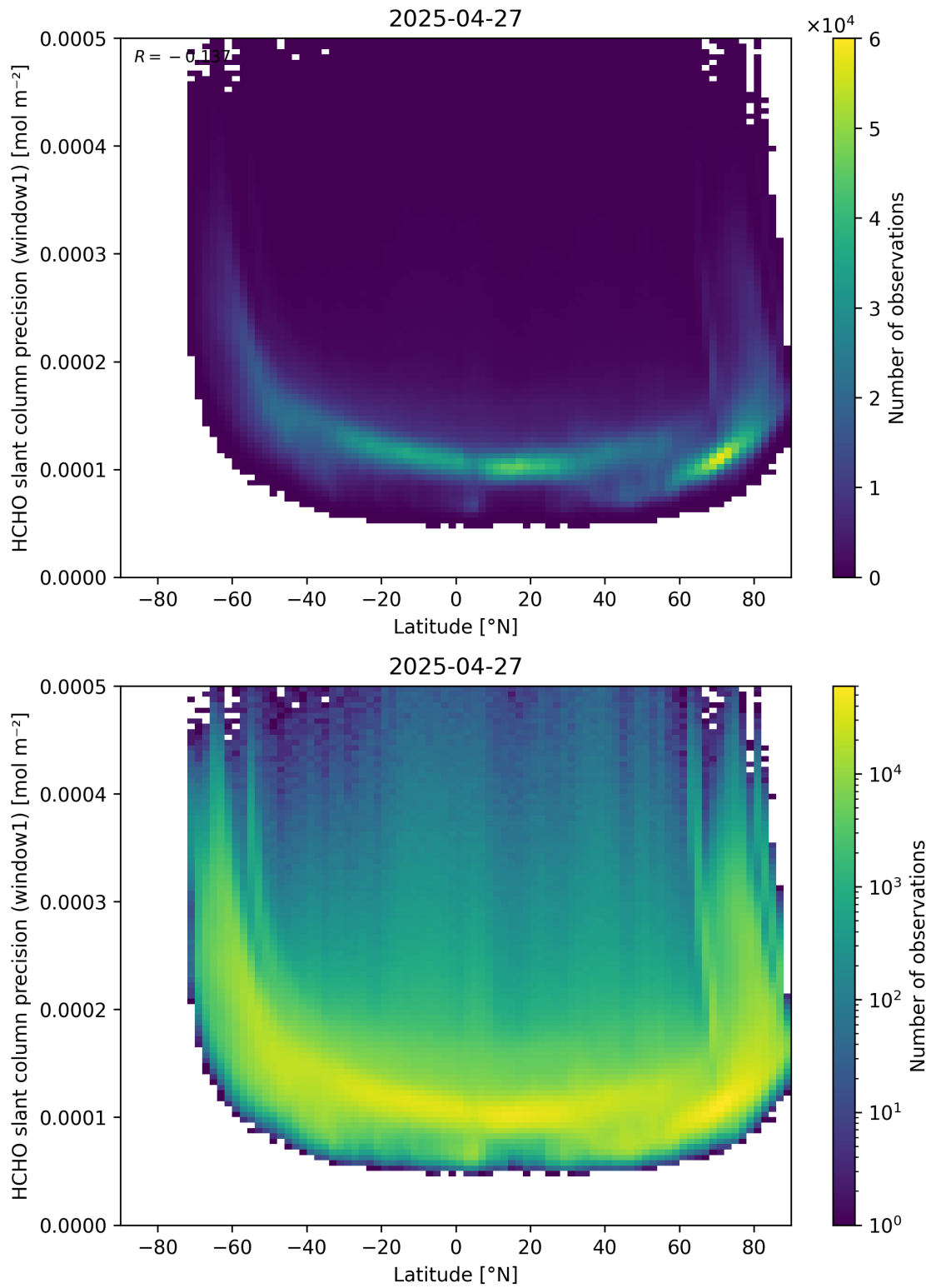
Figure 160: Scatter density plot of “Latitude” against “HCHO slant column precision (window1)” for 2025-04-26 to 2025-04-28.
