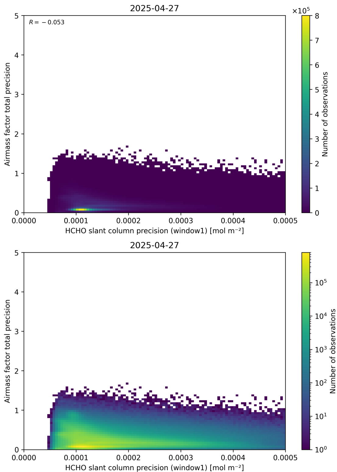
Figure 95: Scatter density plot of “HCHO slant column precision (window1)” against “Airmass factor total precision” for 2025-04-26 to 2025-04-28.
