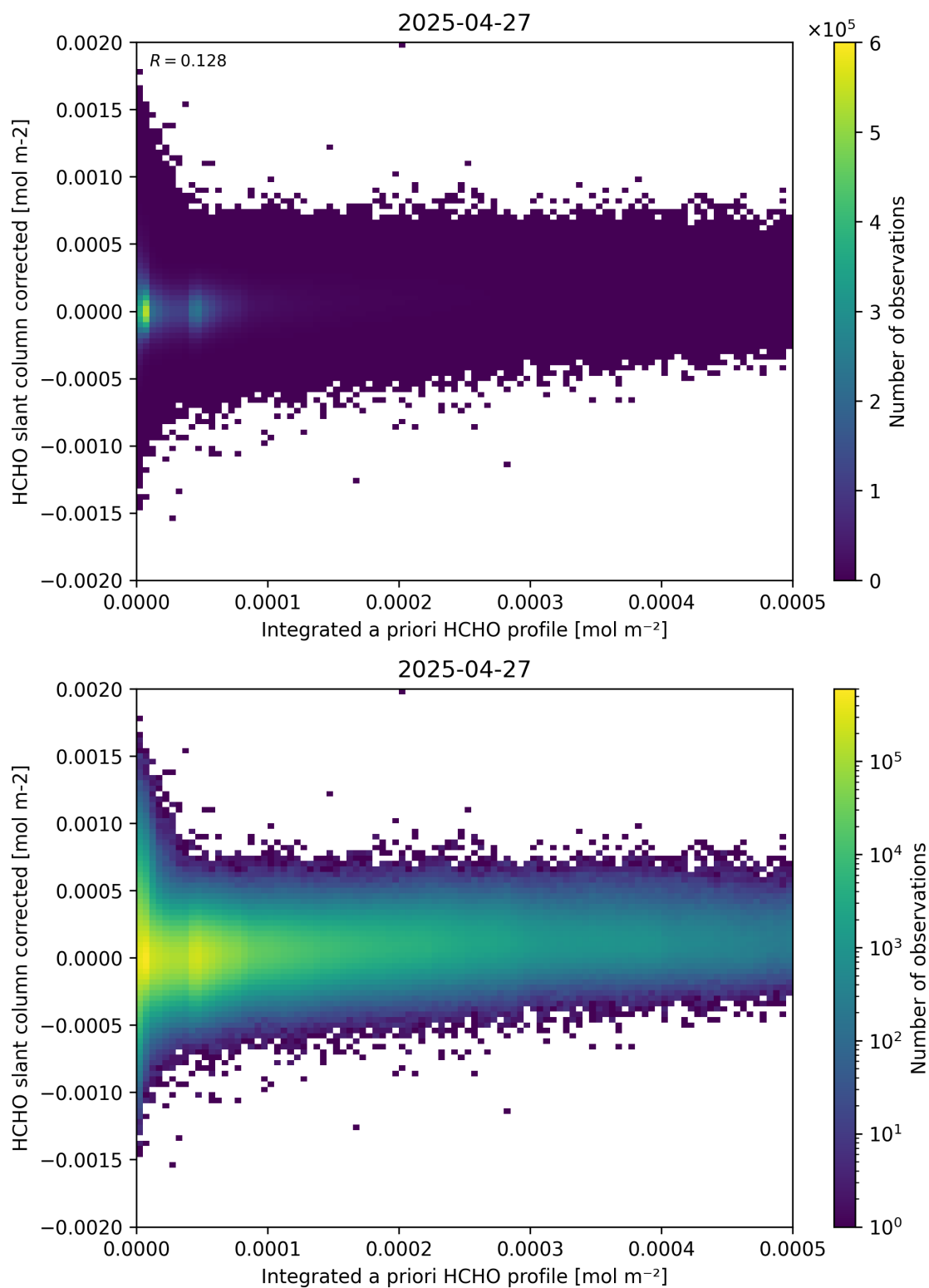
Figure 151: Scatter density plot of “Integrated a priori HCHO profile” against “HCHO slant column corrected” for 2025-04-26 to 2025-04-28.
