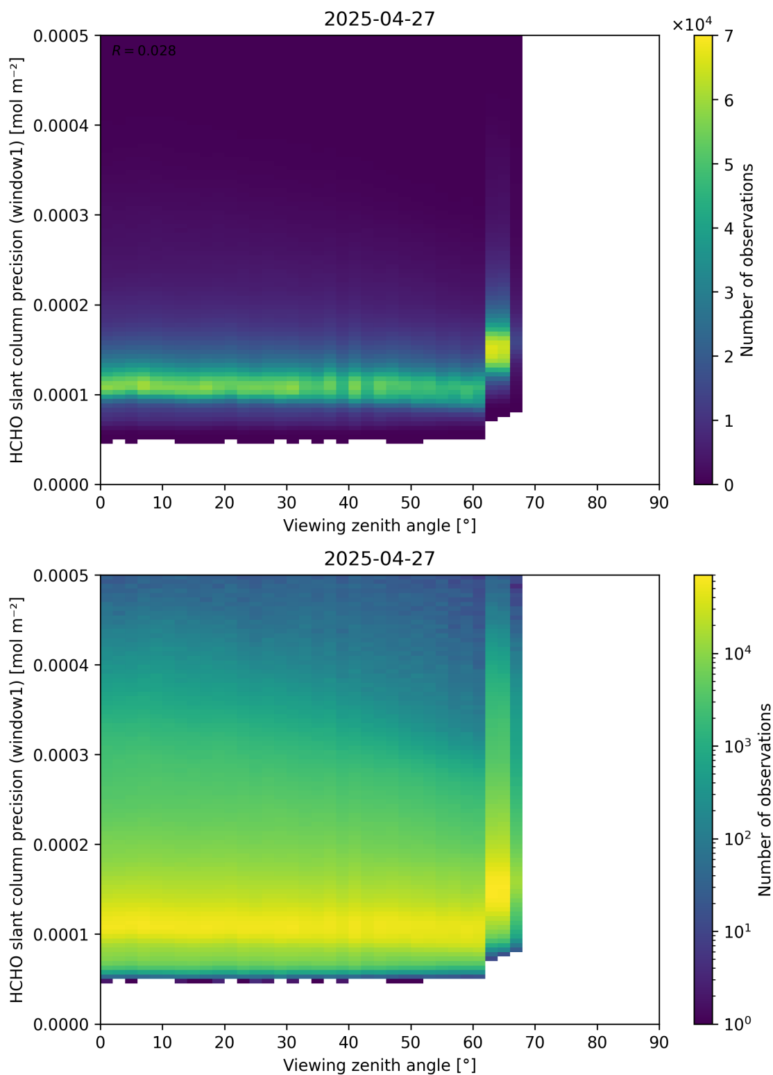
Figure 189: Scatter density plot of “Viewing zenith angle” against “HCHO slant column precision (window1)” for 2025-04-26 to 2025-04-28.
