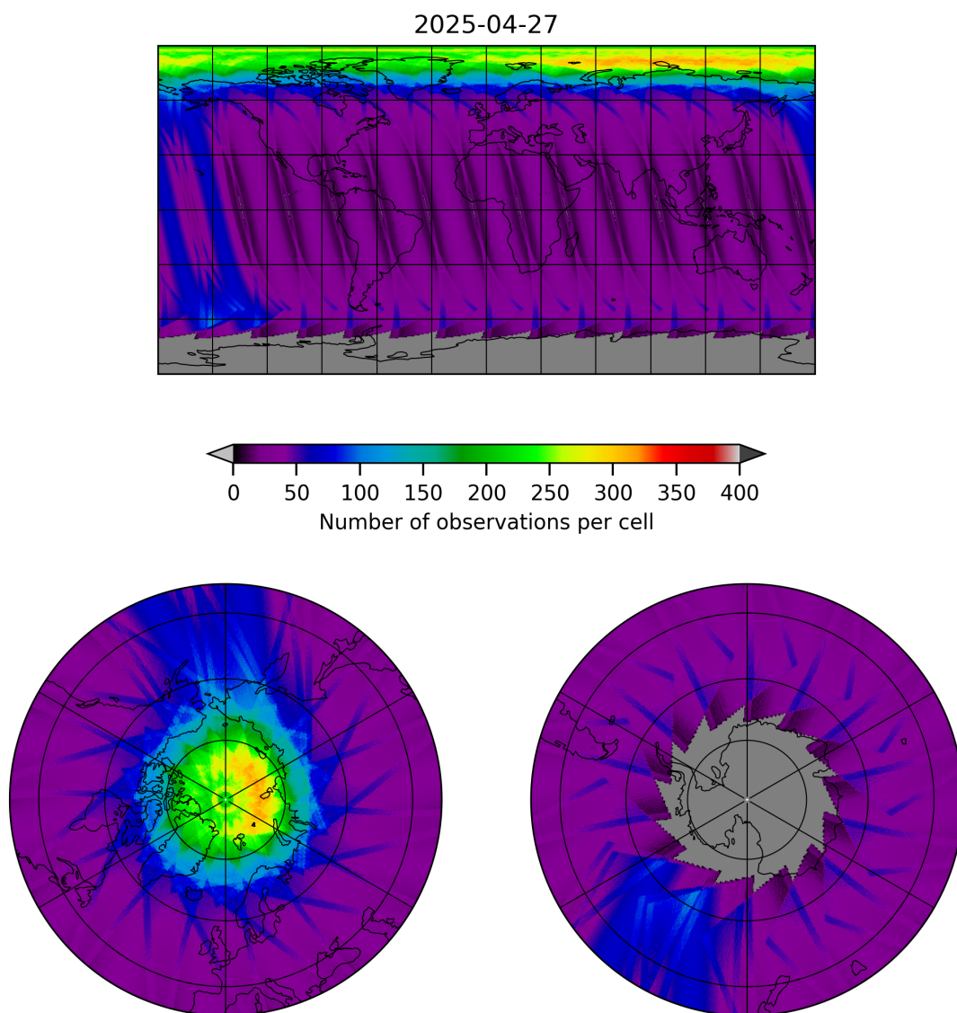
Figure 19: Map of the number of observations for 2025-04-26 to 2025-04-28
