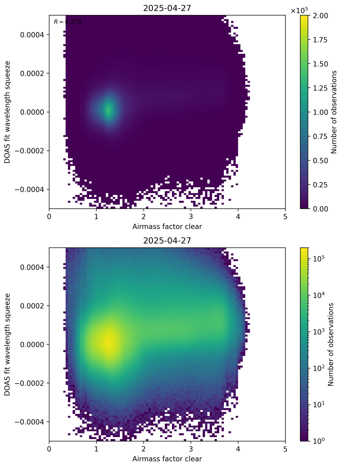
Figure 73: Scatter density plot of “Airmass factor clear” against “DOAS fit wavelength squeeze” for 2025-04-26 to 2025-04-28.
