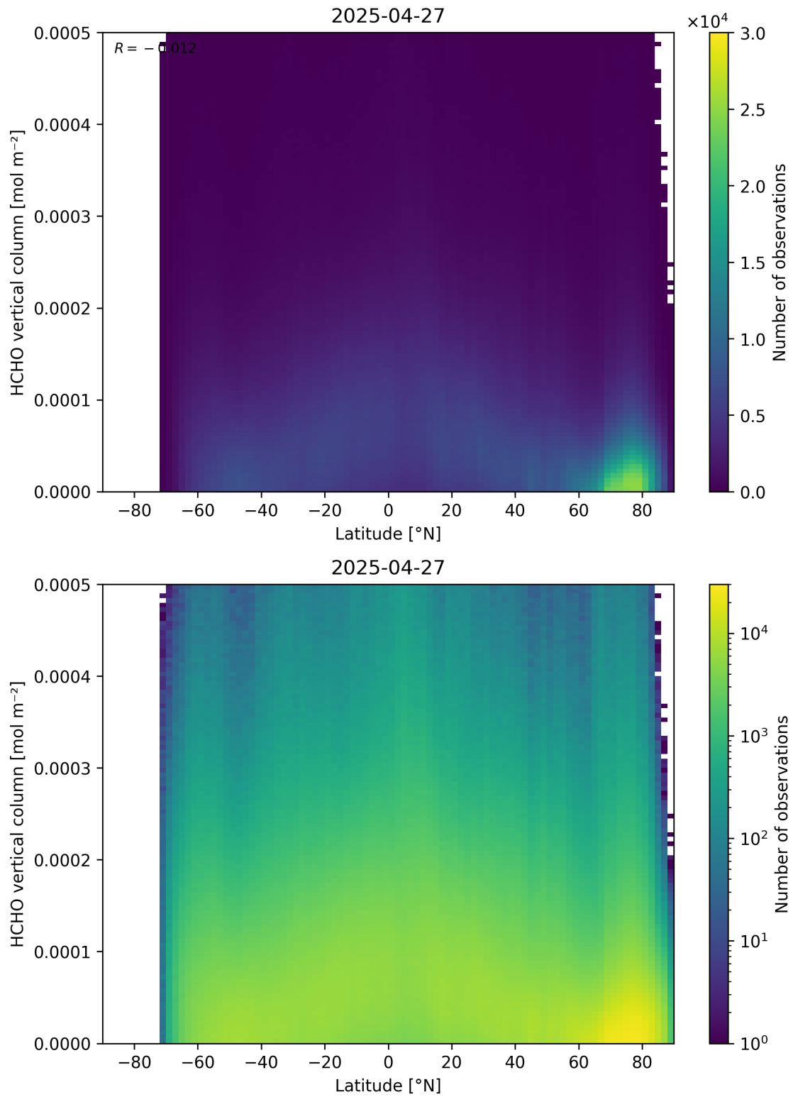
Figure 163: Scatter density plot of “Latitude” against “HCHO vertical column” for 2025-04-26 to 2025-04-28.
