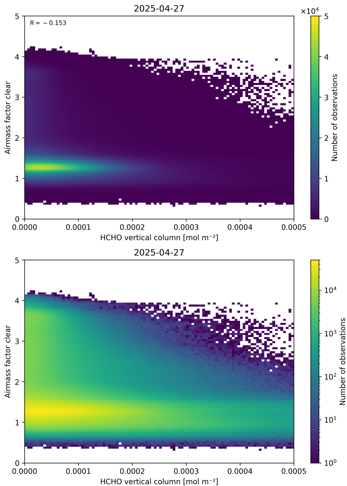
Figure 126: Scatter density plot of “HCHO vertical column” against “Airmass factor clear” for 2025-04-26 to 2025-04-28.
