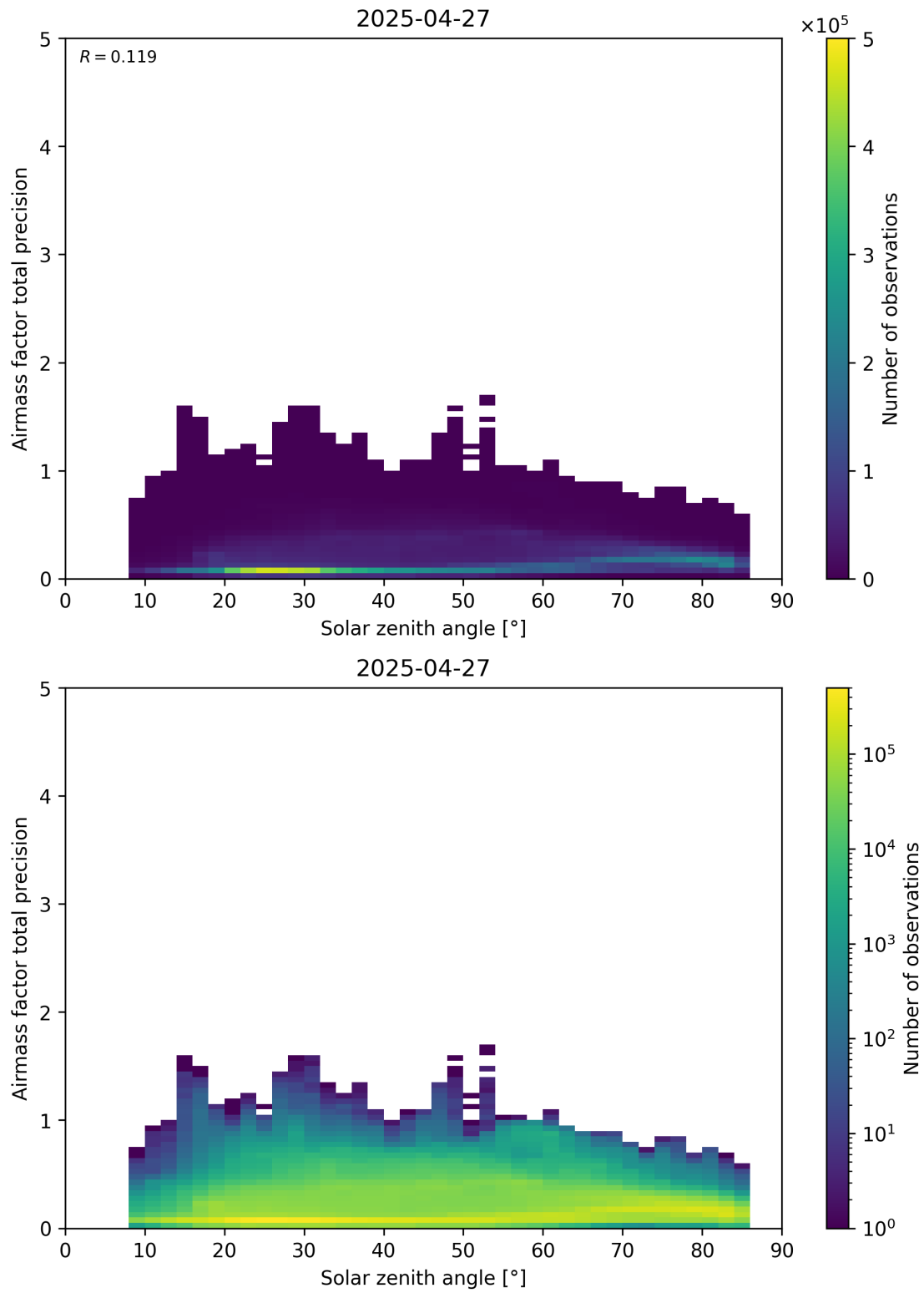
Figure 176: Scatter density plot of “Solar zenith angle” against “Airmass factor total precision” for 2025-04-26 to 2025-04-28.
