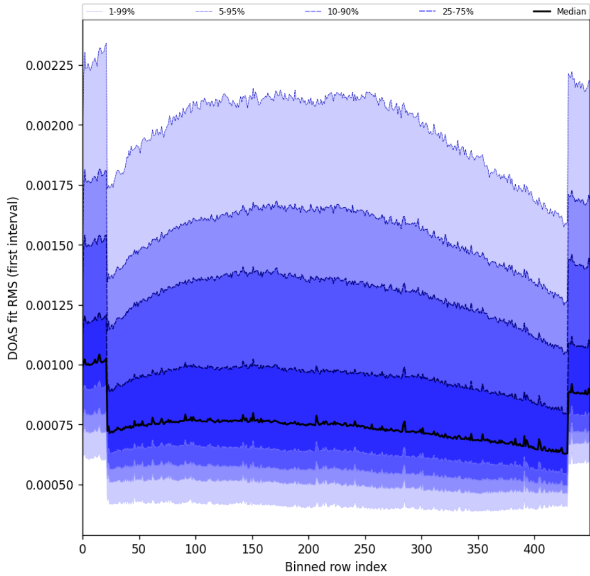
Figure 60: Along track statistics of “DOAS fit RMS (first interval)” for 2025-04-26 to 2025-04-28
