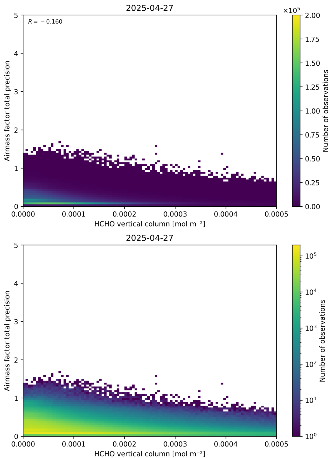
Figure 132: Scatter density plot of “HCHO vertical column” against “Airmass factor total precision” for 2025-04-26 to 2025-04-28.
