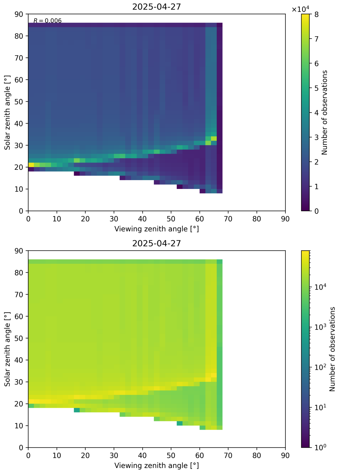
Figure 197: Scatter density plot of “Viewing zenith angle” against “Solar zenith angle” for 2025-04-26 to 2025-04-28.
