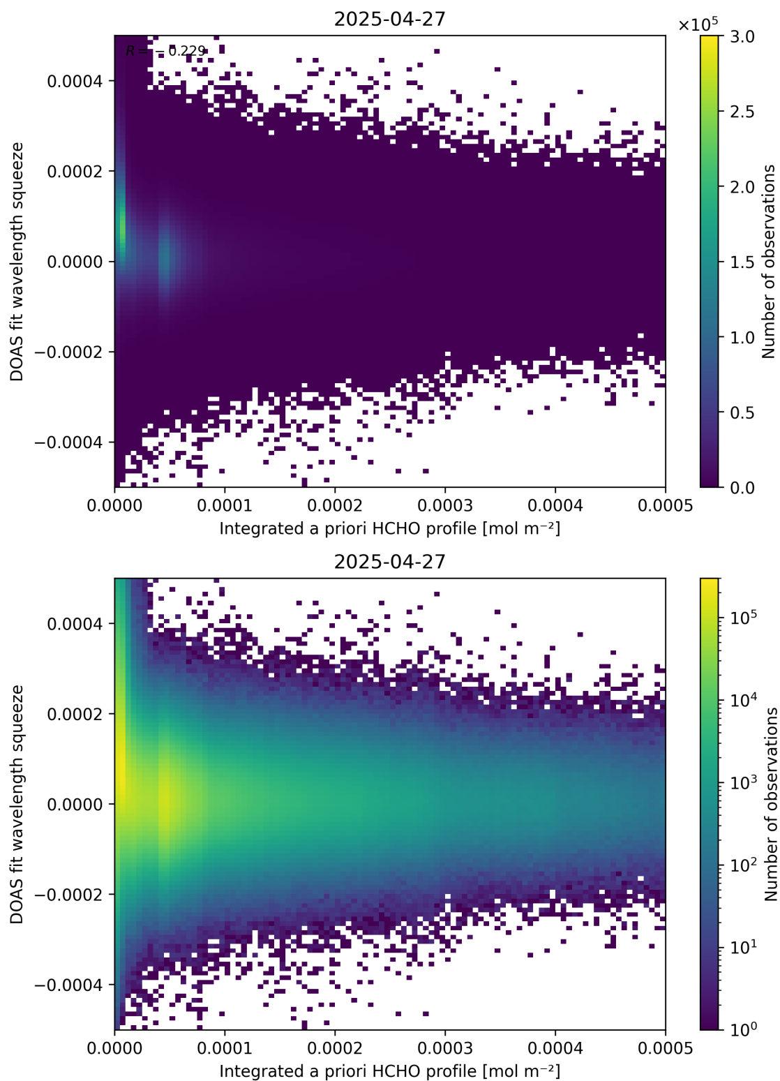
Figure 150: Scatter density plot of “Integrated a priori HCHO profile” against “DOAS fit wavelength squeeze” for 2025-04-26 to 2025-04-28.
