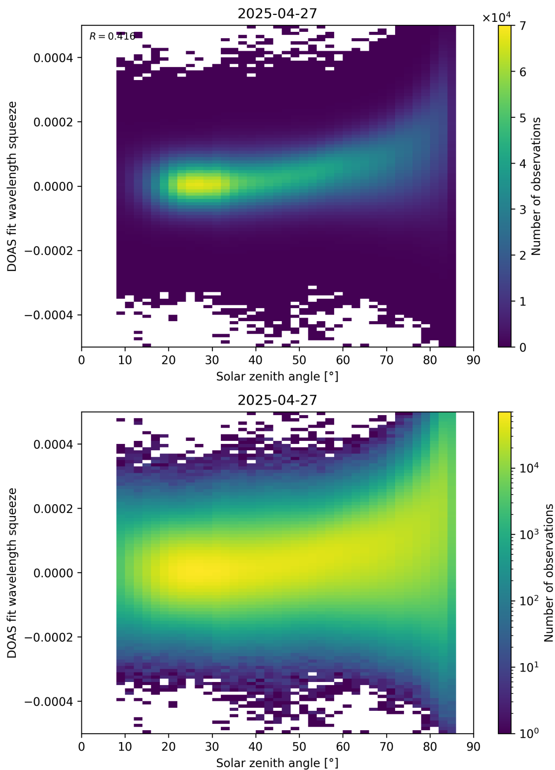
Figure 169: Scatter density plot of “Solar zenith angle” against “DOAS fit wavelength squeeze” for 2025-04-26 to 2025-04-28.
