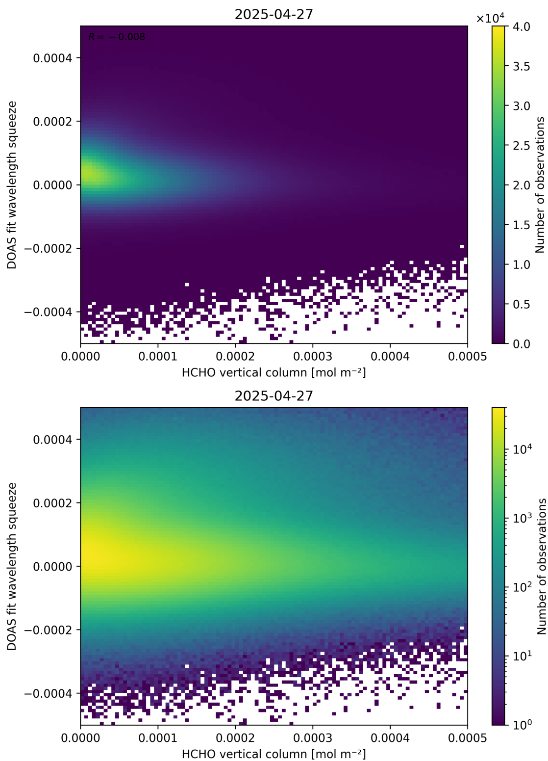
Figure 125: Scatter density plot of “HCHO vertical column” against “DOAS fit wavelength squeeze” for 2025-04-26 to 2025-04-28.
