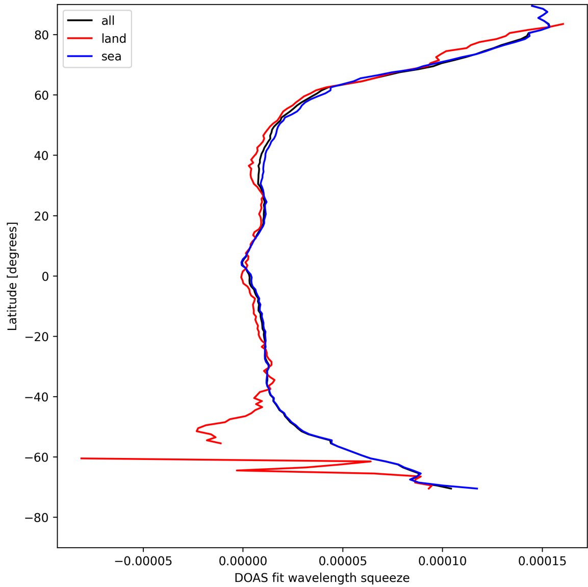
Figure 31: Zonal average of “DOAS fit wavelength squeeze” for 2025-04-26 to 2025-04-28.
