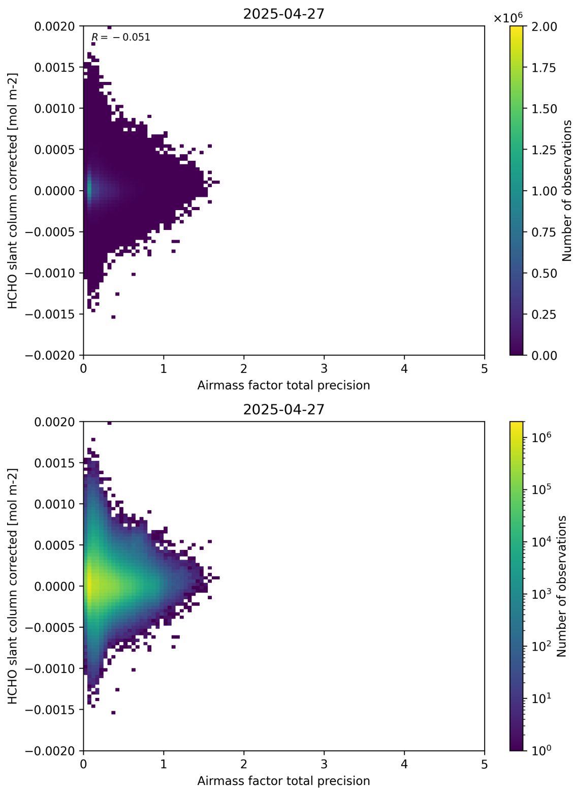
Figure 109: Scatter density plot of “Airmass factor total precision” against “HCHO slant column corrected” for 2025-04-26 to 2025-04-28.
