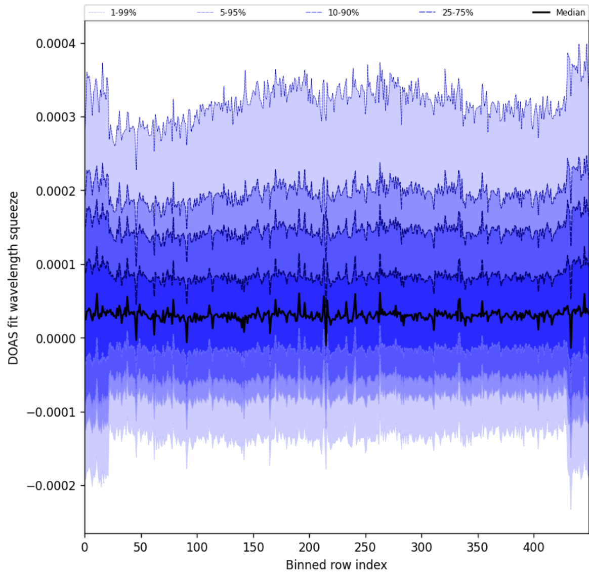
Figure 59: Along track statistics of “DOAS fit wavelength squeeze” for 2025-04-26 to 2025-04-28
