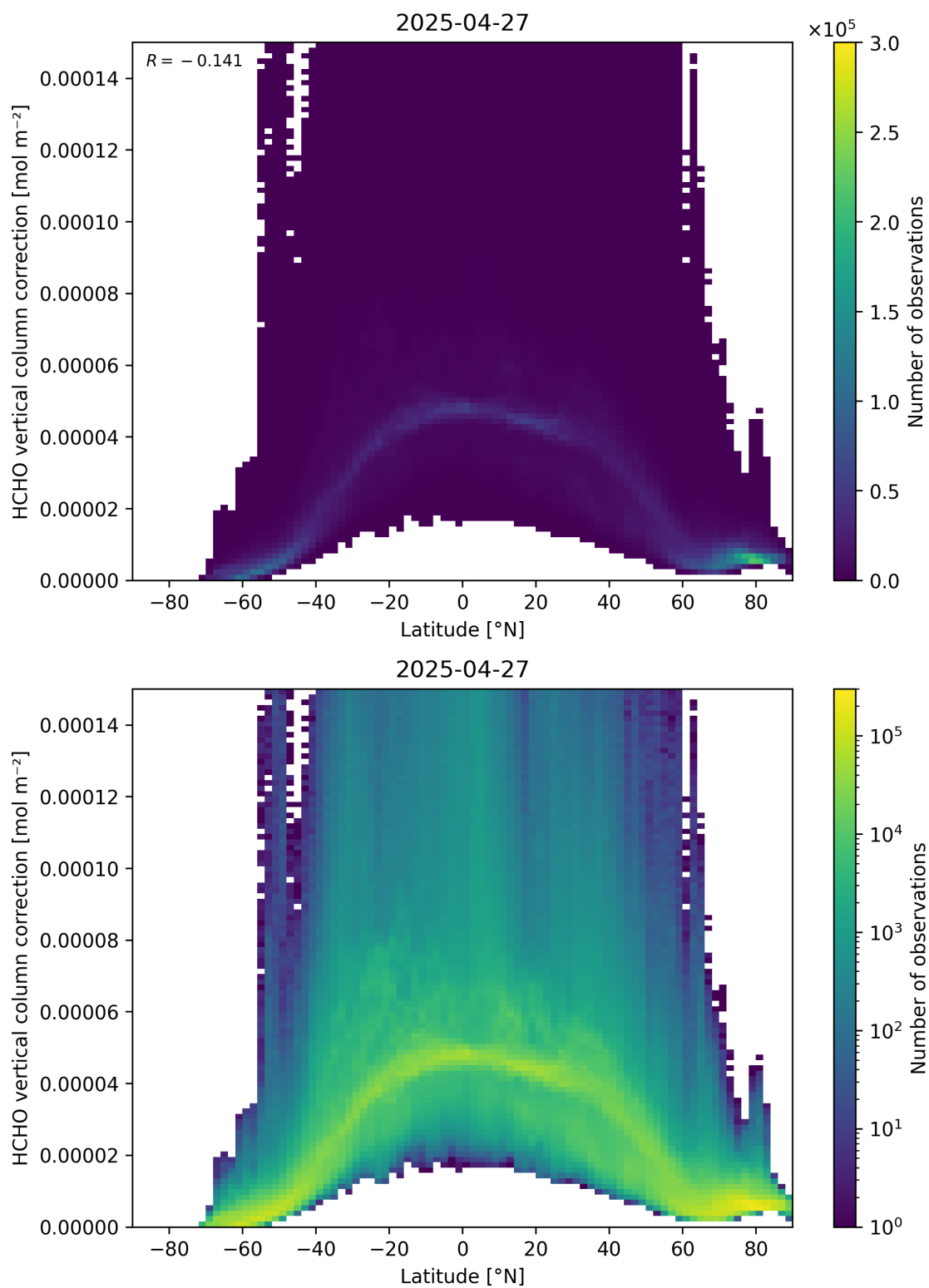
Figure 164: Scatter density plot of “Latitude” against “HCHO vertical column correction” for 2025-04-26 to 2025-04-28.
