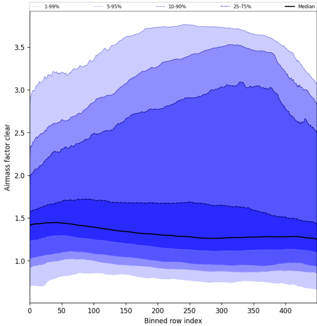
Figure 56: Along track statistics of “Airmass factor clear” for 2025-04-26 to 2025-04-28
