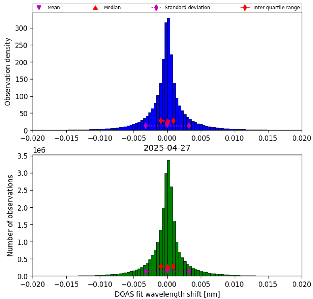
Figure 44: Histogram of “DOAS fit wavelength shift” for 2025-04-26 to 2025-04-28
