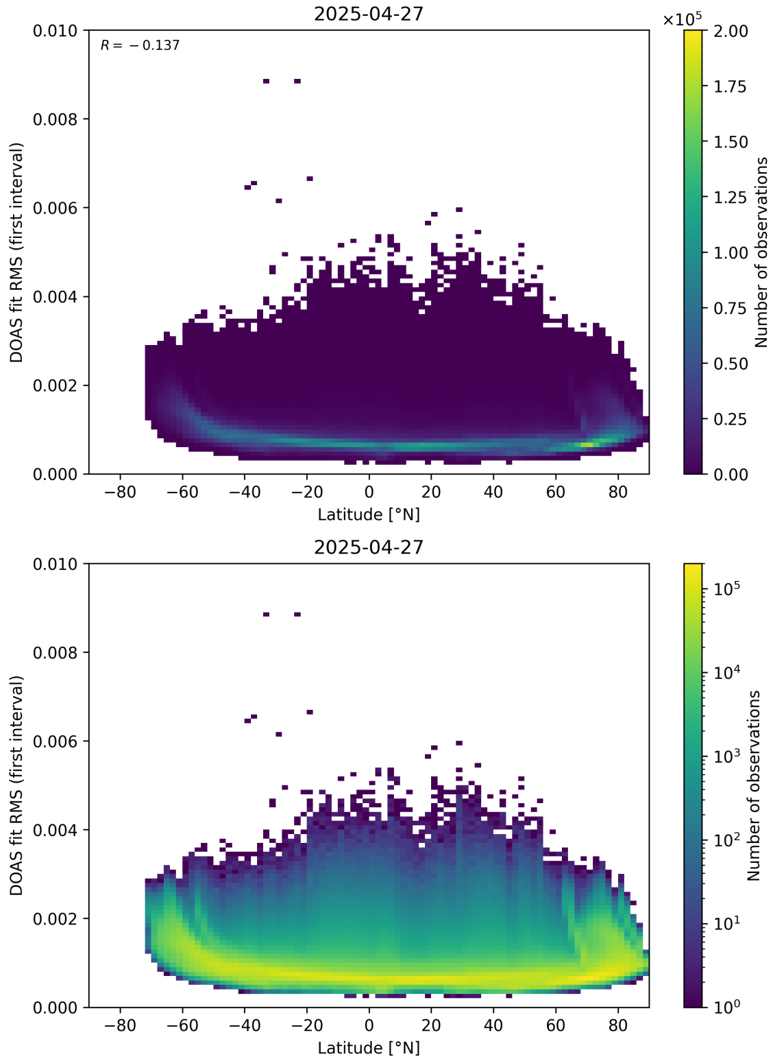
Figure 153: Scatter density plot of “Latitude” against “DOAS fit RMS (first interval)” for 2025-04-26 to 2025-04-28.
