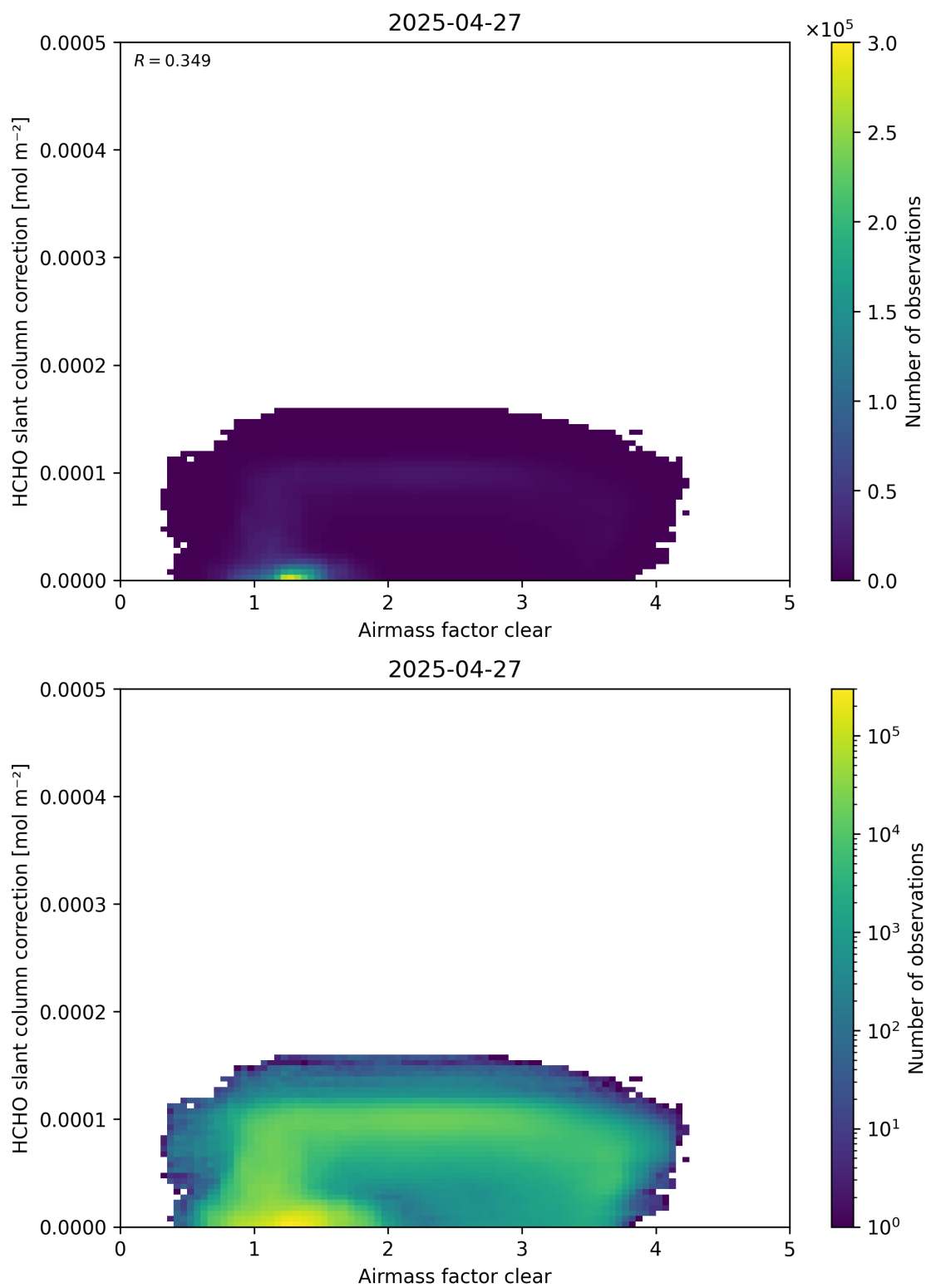
Figure 75: Scatter density plot of “Airmass factor clear” against “HCHO slant column correction” for 2025-04-26 to 2025-04-28.
