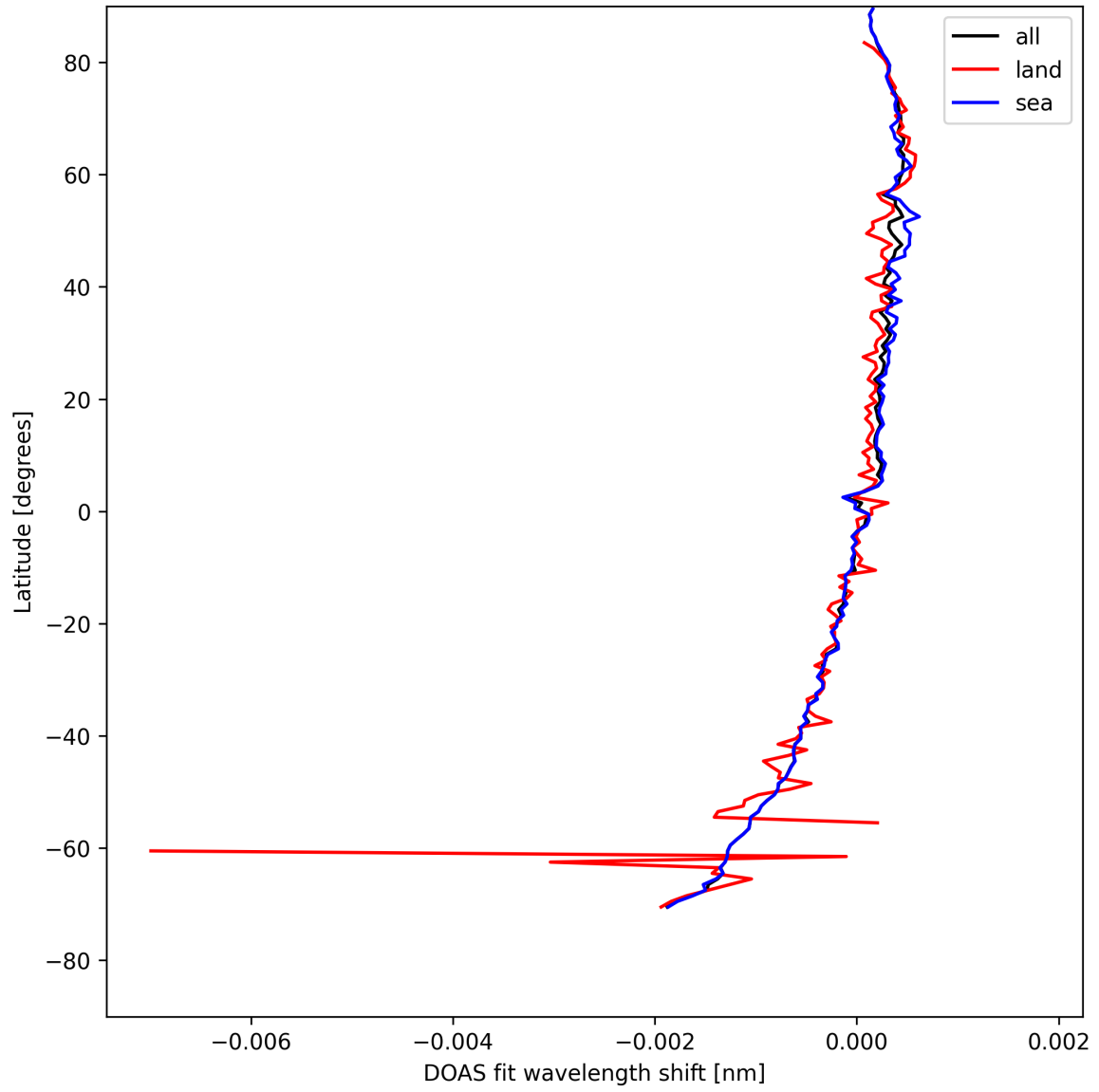
Figure 30: Zonal average of “DOAS fit wavelength shift” for 2025-04-26 to 2025-04-28.
