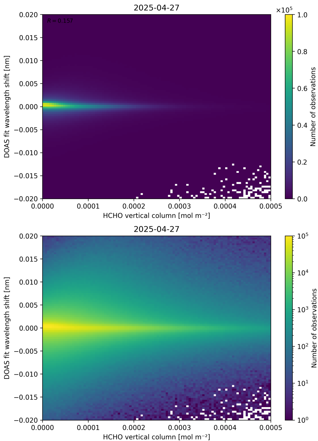
Figure 124: Scatter density plot of “HCHO vertical column” against “DOAS fit wavelength shift” for 2025-04-26 to 2025-04-28.
