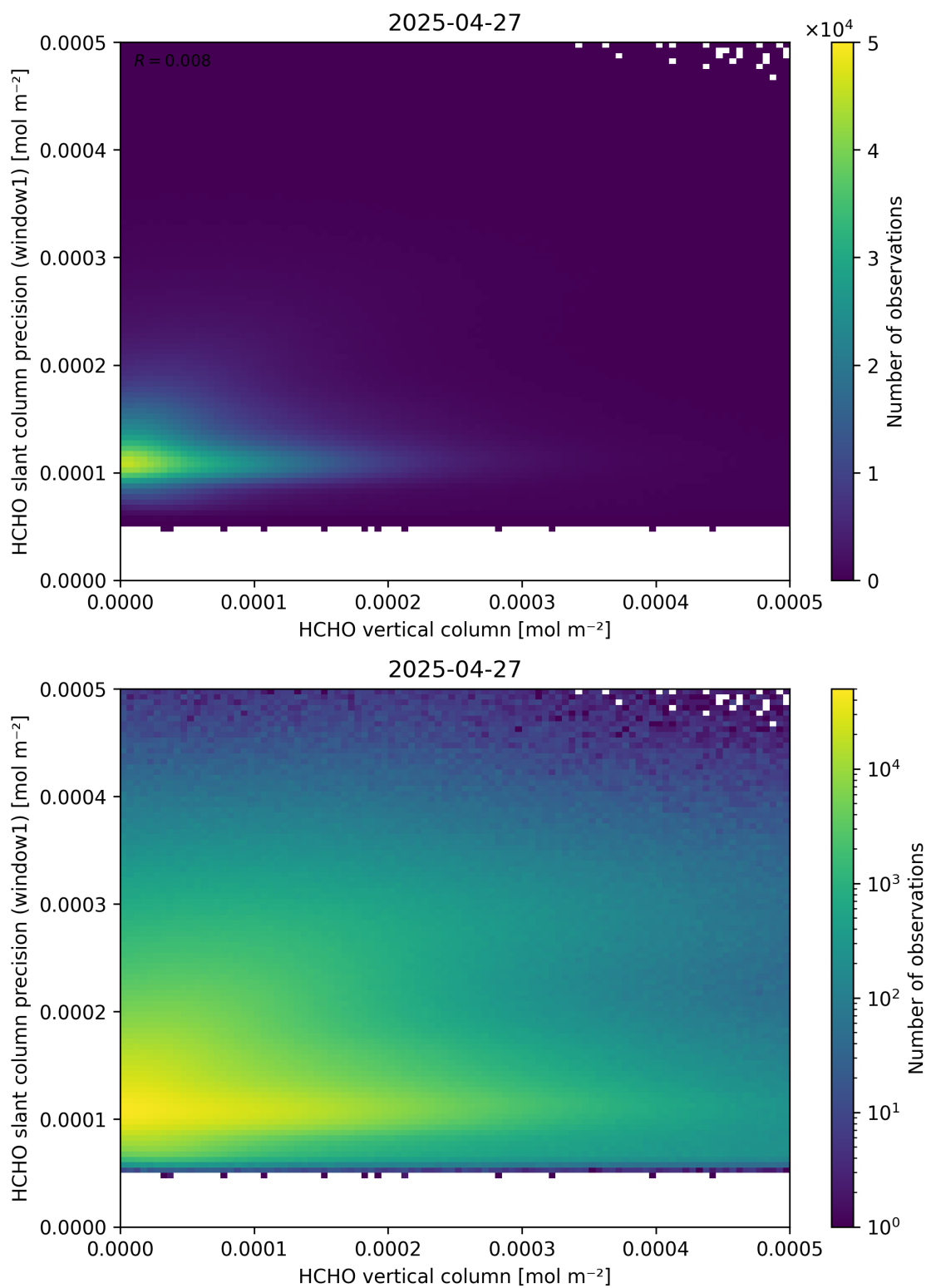
Figure 130: Scatter density plot of “HCHO vertical column” against “HCHO slant column precision (window1)” for 2025-04-26 to 2025-04-28.
