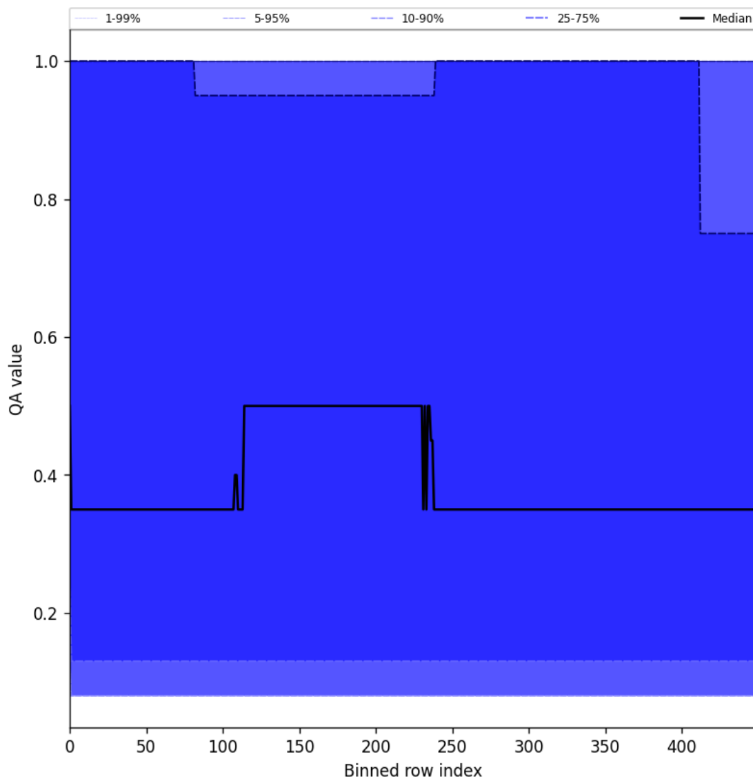
Figure 48: Along track statistics of “QA value” for 2025-04-26 to 2025-04-28
