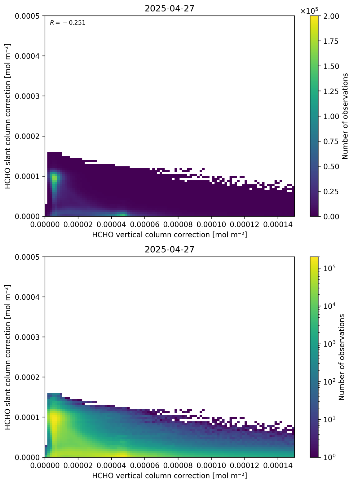
Figure 117: Scatter density plot of “HCHO vertical column correction” against “HCHO slant column correction” for 2025-04-26 to 2025-04-28.
