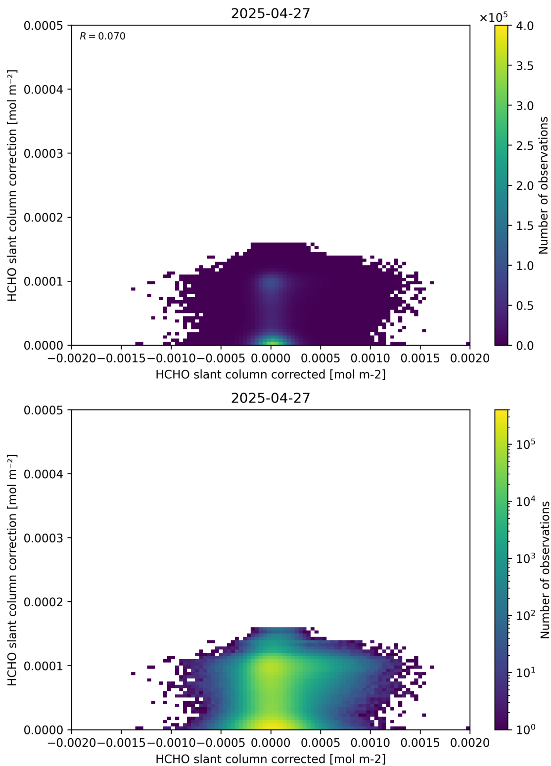
Figure 77: Scatter density plot of “HCHO slant column corrected” against “HCHO slant column correction” for 2025-04-26 to 2025-04-28.
