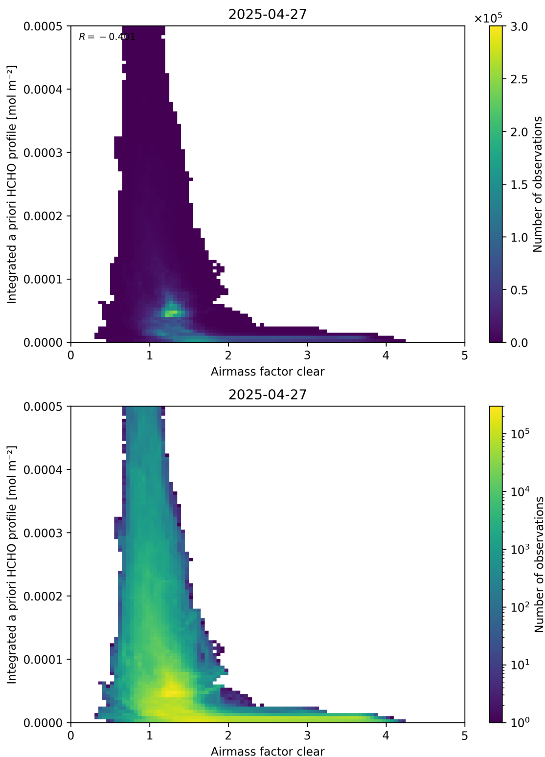
Figure 76: Scatter density plot of “Airmass factor clear” against “Integrated a priori HCHO profile” for 2025-04-26 to 2025-04-28.
