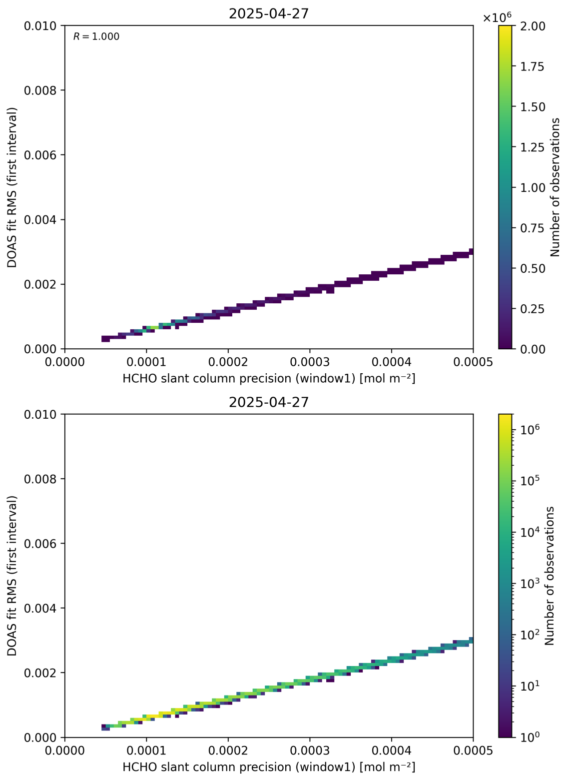
Figure 88: Scatter density plot of “HCHO slant column precision (window1)” against “DOAS fit RMS (first interval)” for 2025-04-26 to 2025-04-28.
