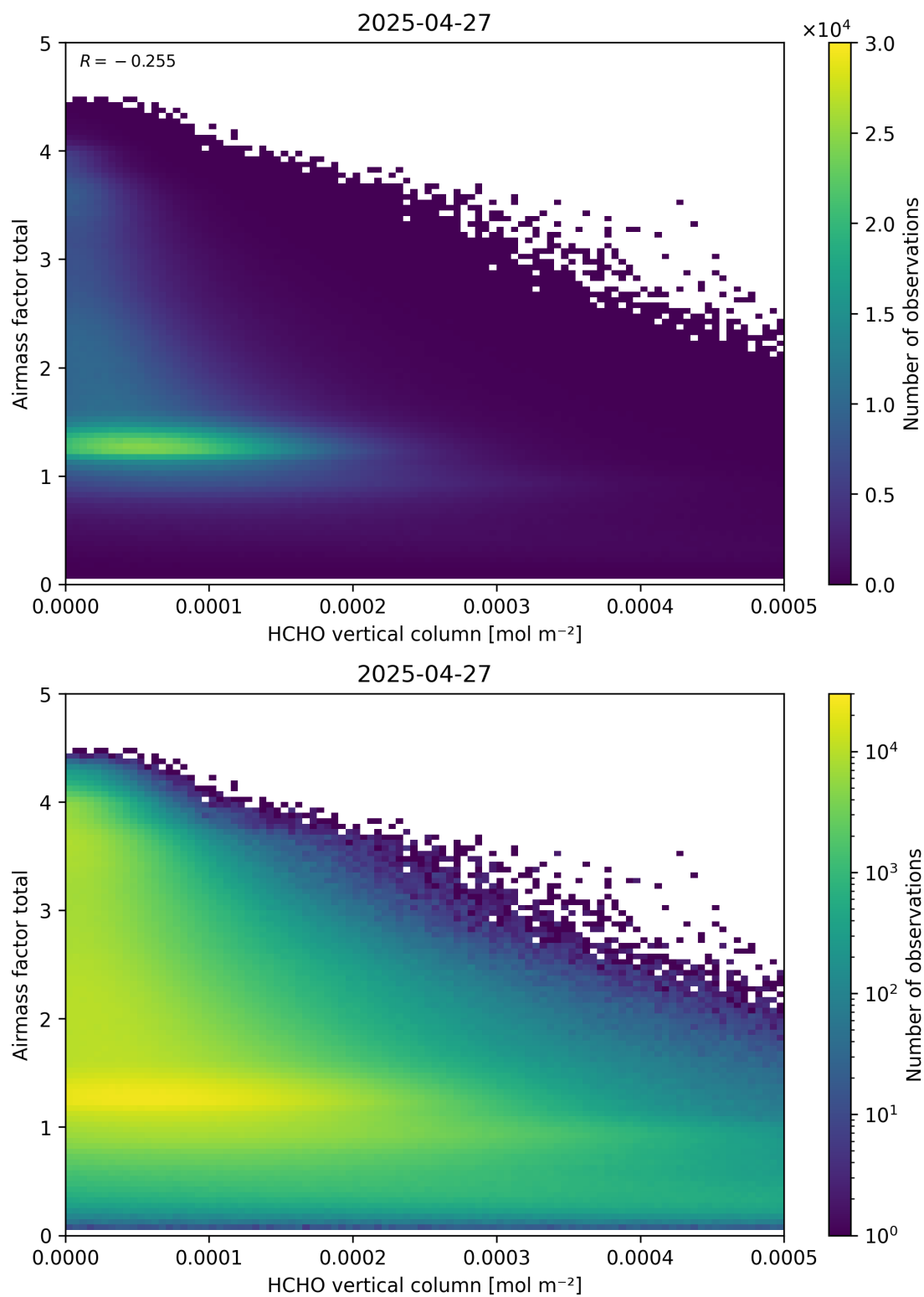
Figure 131: Scatter density plot of “HCHO vertical column” against “Airmass factor total” for 2025-04-26 to 2025-04-28.
