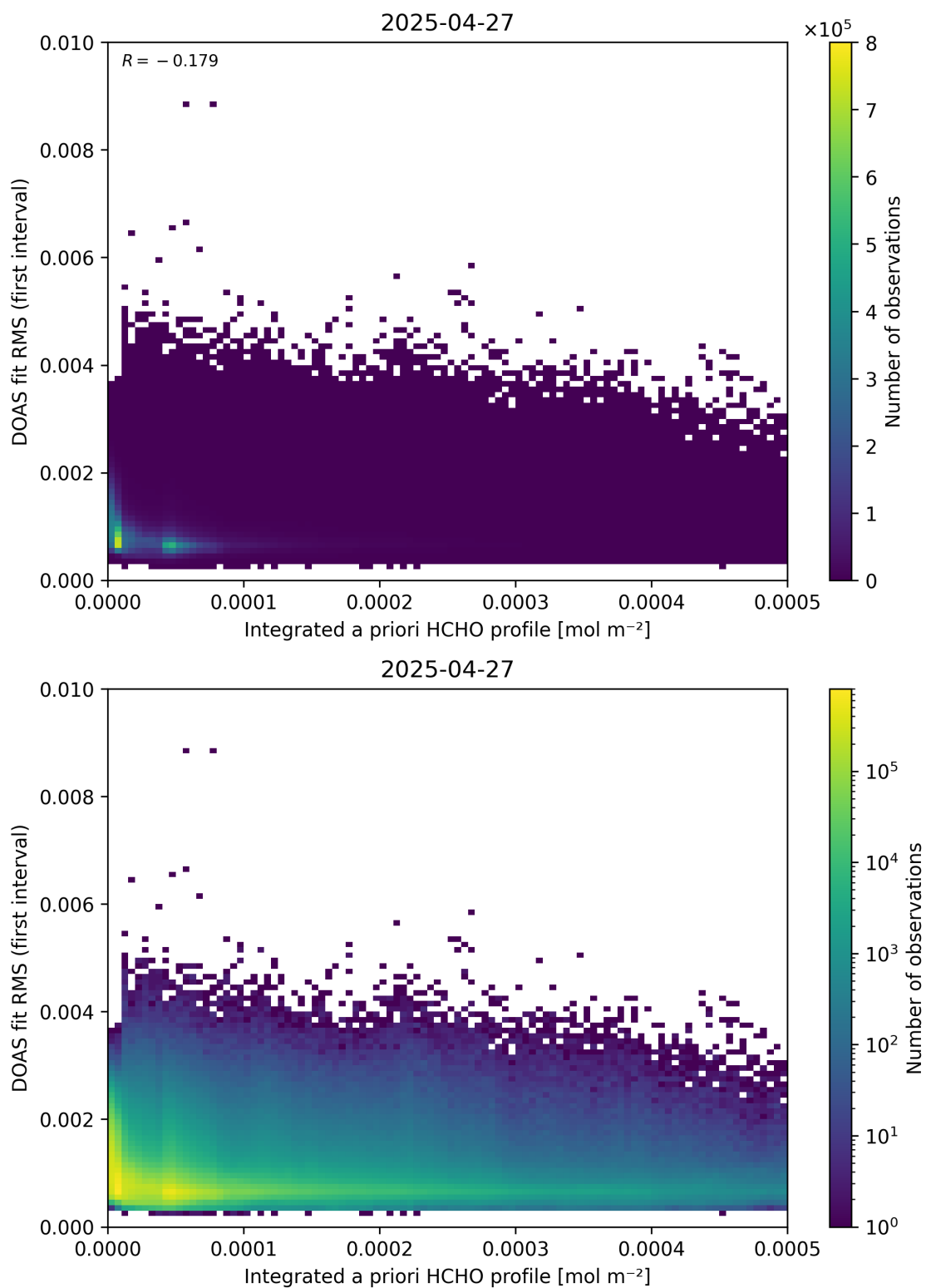
Figure 148: Scatter density plot of “Integrated a priori HCHO profile” against “DOAS fit RMS (first interval)” for 2025-04-26 to 2025-04-28.
