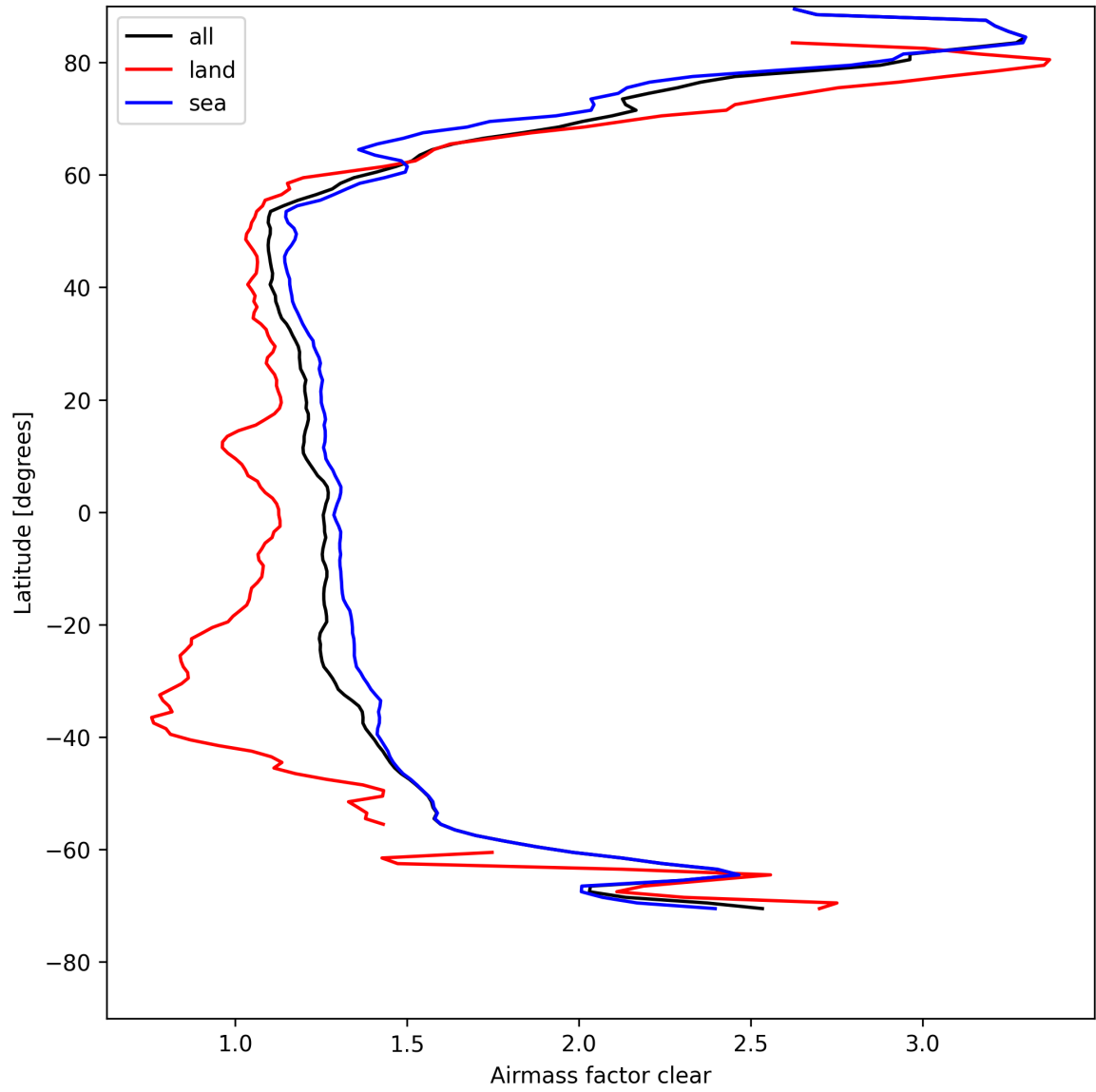
Figure 28: Zonal average of “Airmass factor clear” for 2025-04-26 to 2025-04-28.
