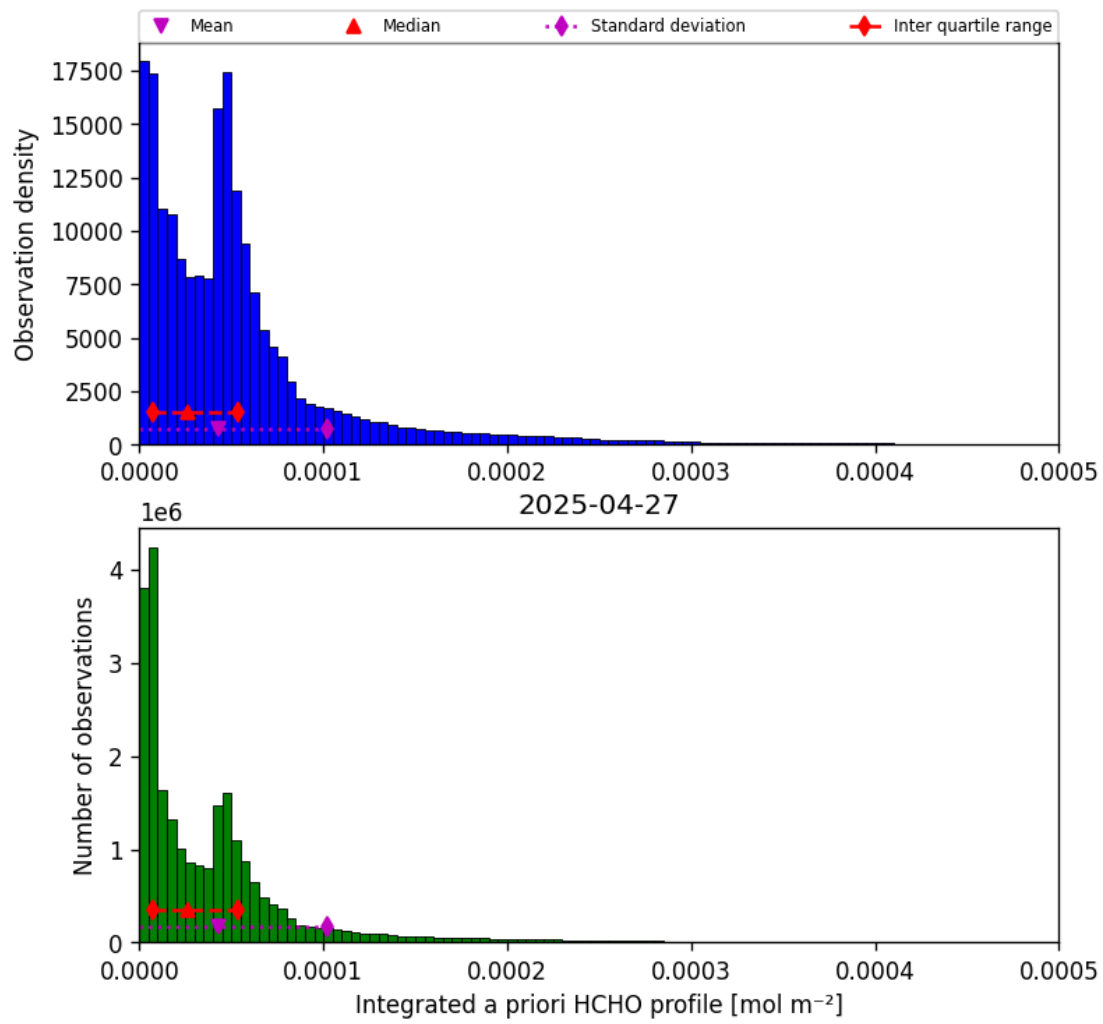
Figure 43: Histogram of “Integrated a priori HCHO profile” for 2025-04-26 to 2025-04-28
