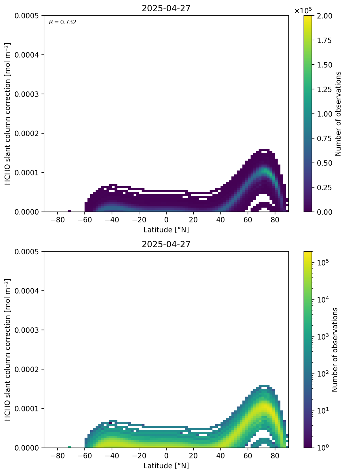
Figure 158: Scatter density plot of “Latitude” against “HCHO slant column correction” for 2025-04-26 to 2025-04-28.
