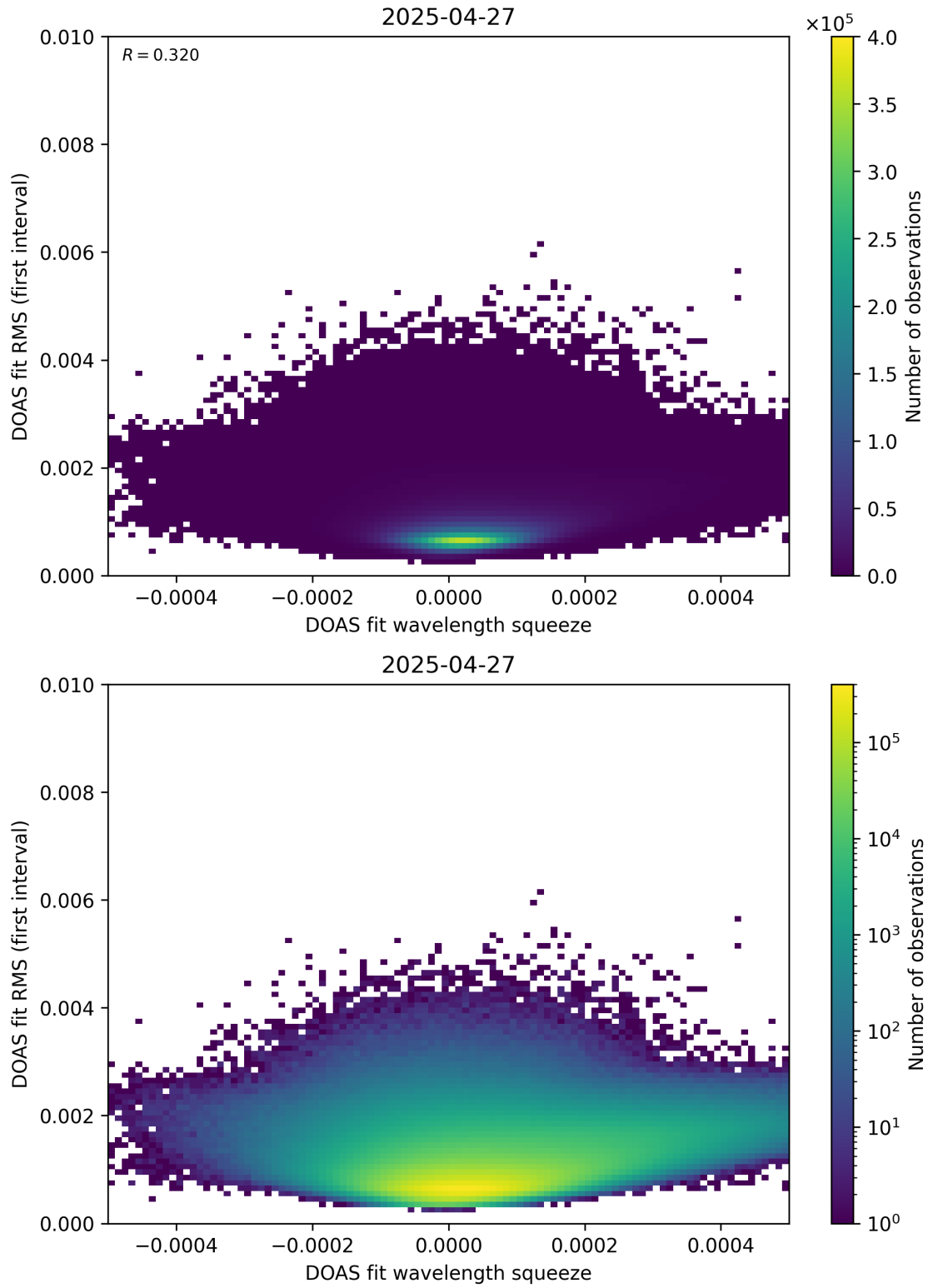
Figure 68: Scatter density plot of “DOAS fit wavelength squeeze” against “DOAS fit RMS (first interval)” for 2025-04-26 to 2025-04-28.
