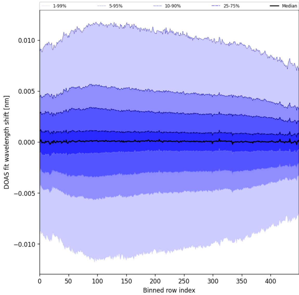
Figure 58: Along track statistics of “DOAS fit wavelength shift” for 2025-04-26 to 2025-04-28
