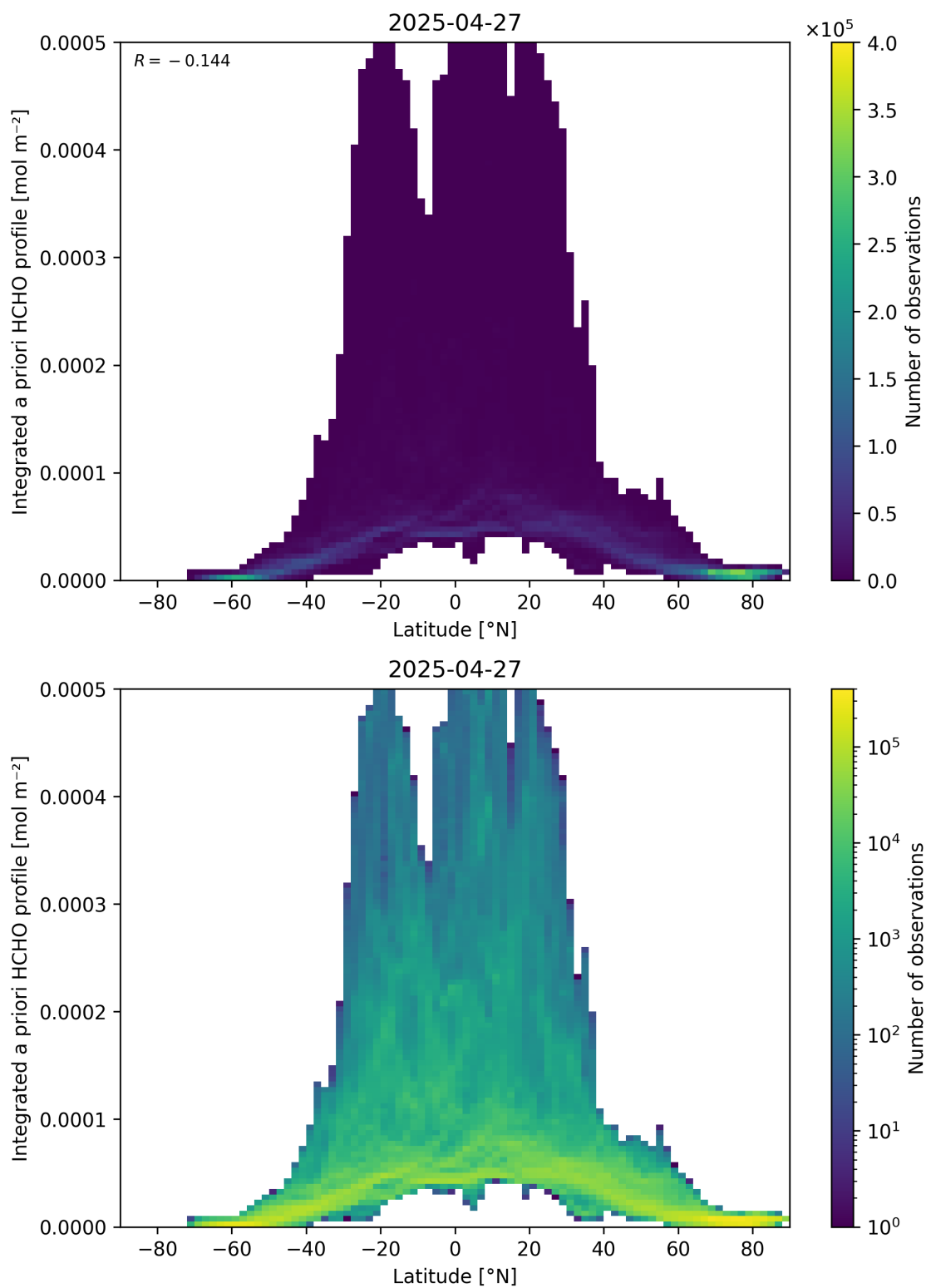
Figure 166: Scatter density plot of “Latitude” against “Integrated a priori HCHO profile” for 2025-04-26 to 2025-04-28.
