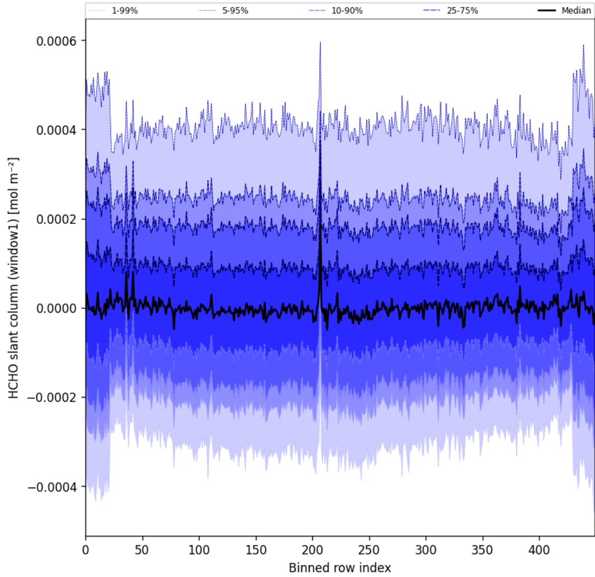
Figure 52: Along track statistics of “HCHO slant column (window1)” for 2025-04-26 to 2025-04-28
