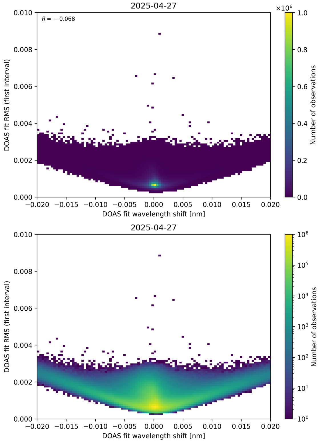
Figure 64: Scatter density plot of “DOAS fit wavelength shift” against “DOAS fit RMS (first interval)” for 2025-04-26 to 2025-04-28.
