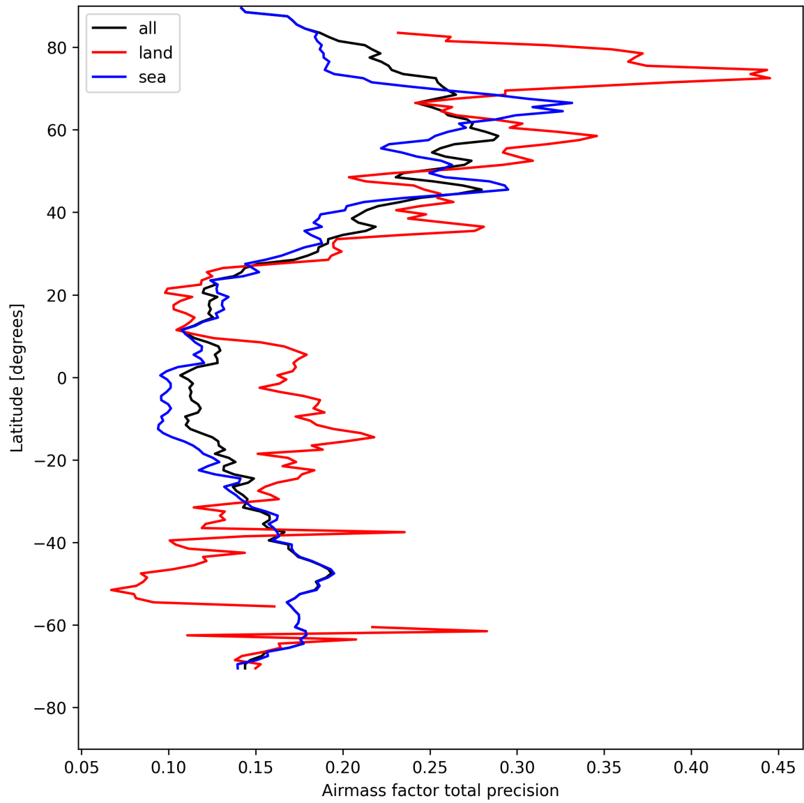
Figure 27: Zonal average of “Airmass factor total precision” for 2025-04-26 to 2025-04-28.
