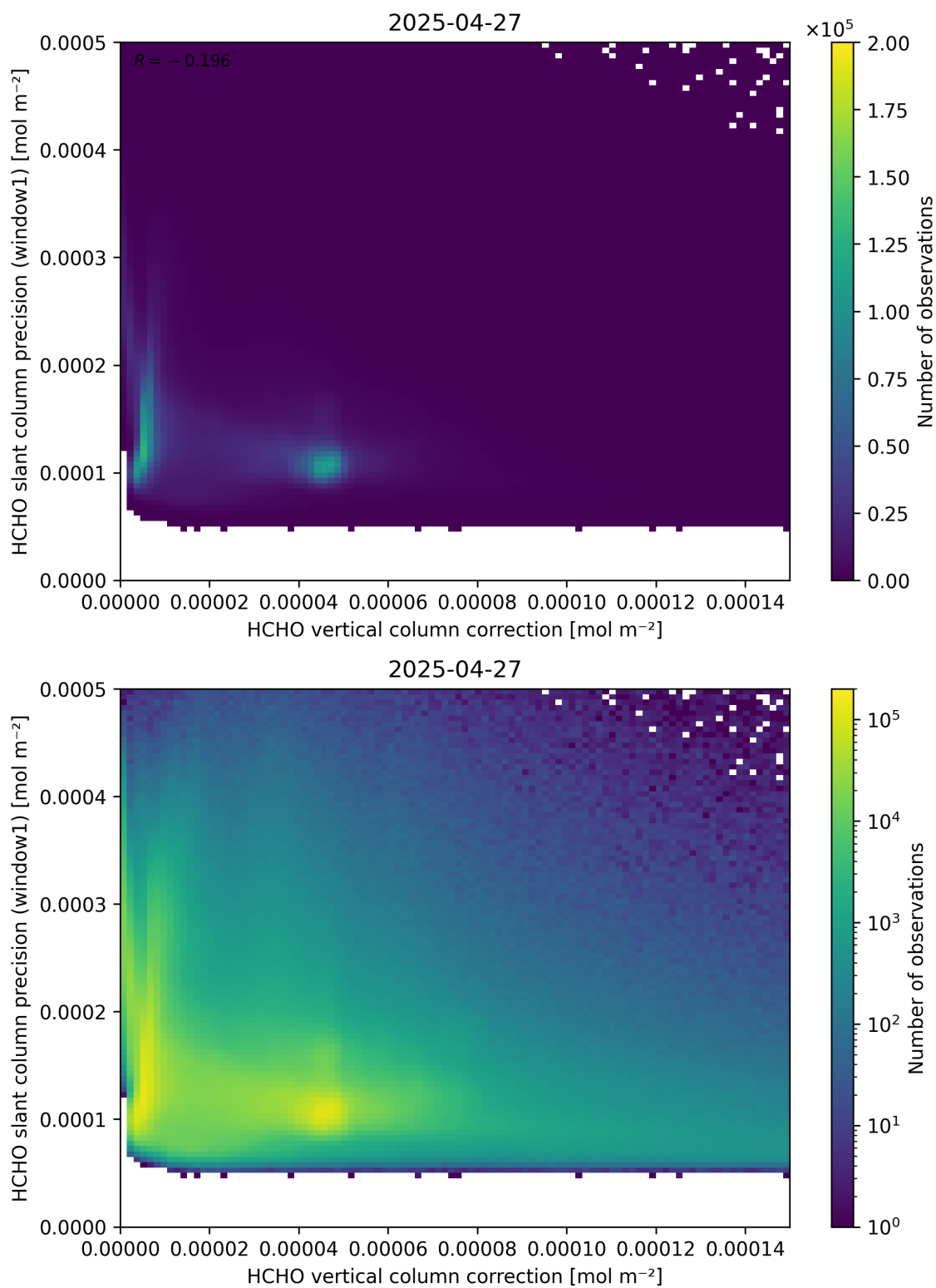
Figure 119: Scatter density plot of “HCHO vertical column correction” against “HCHO slant column precision (window1)” for 2025-04-26 to 2025-04-28.
