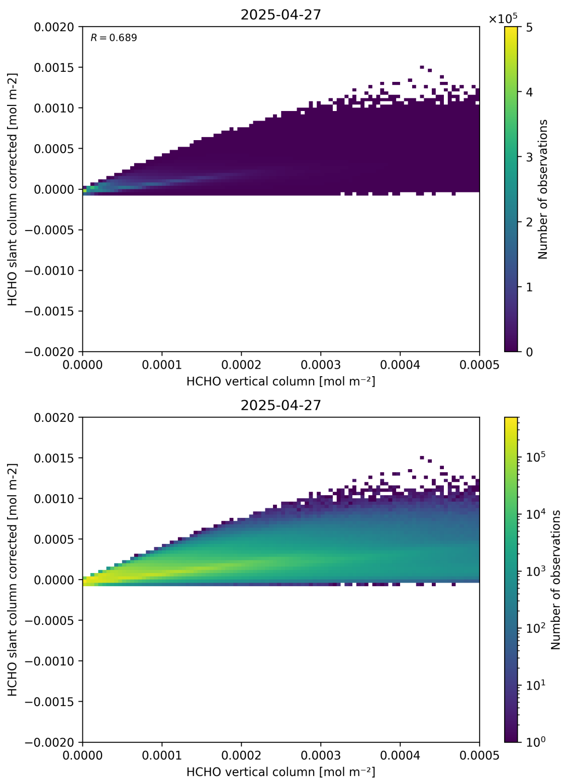
Figure 127: Scatter density plot of “HCHO vertical column” against “HCHO slant column corrected” for 2025-04-26 to 2025-04-28.
