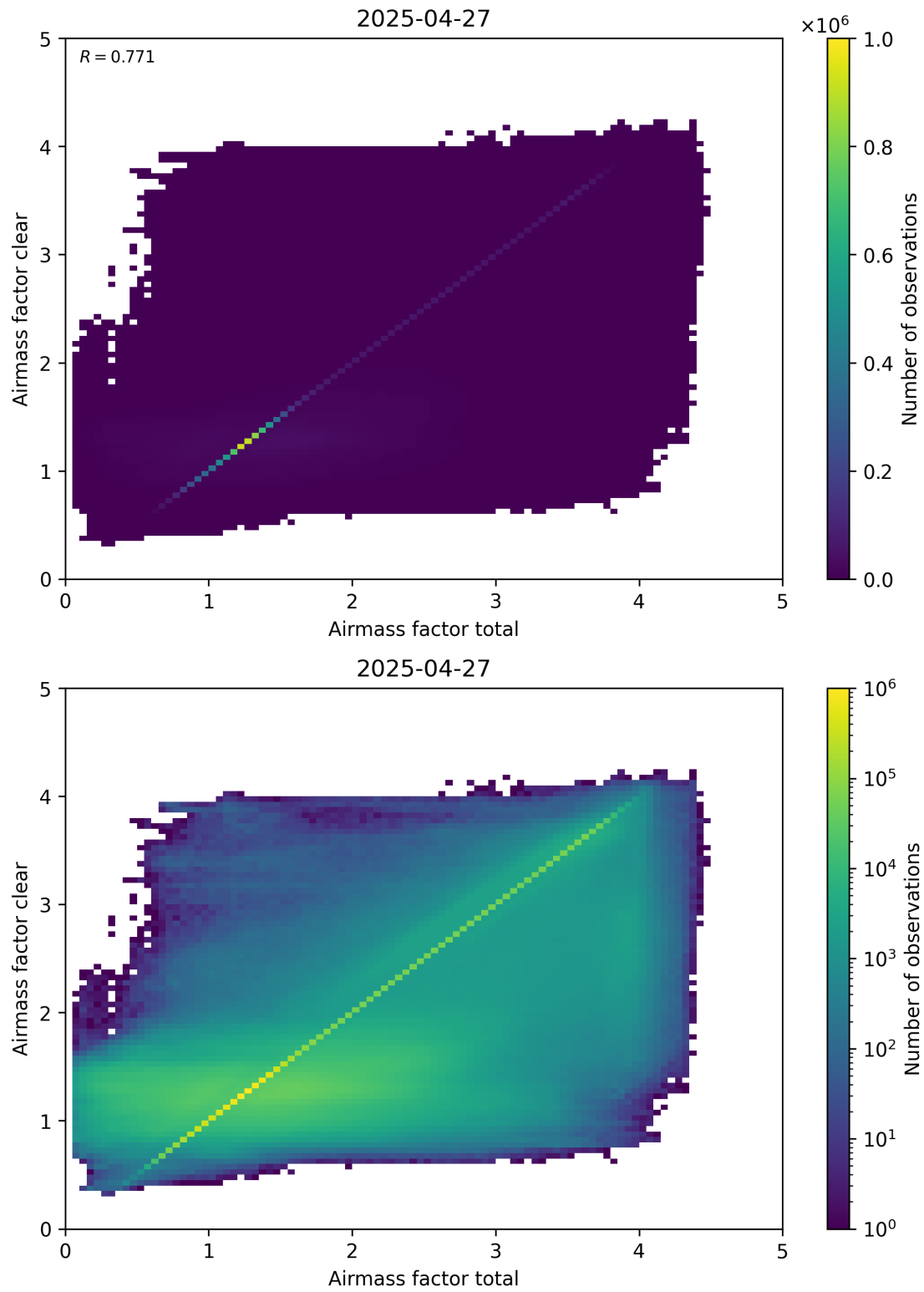
Figure 100: Scatter density plot of “Airmass factor total” against “Airmass factor clear” for 2025-04-26 to 2025-04-28.
