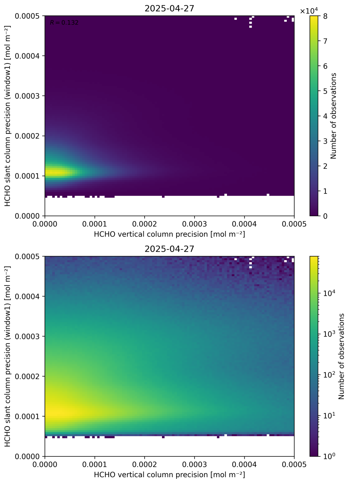
Figure 143: Scatter density plot of “HCHO vertical column precision” against “HCHO slant column precision (window1)” for 2025-04-26 to 2025-04-28.
