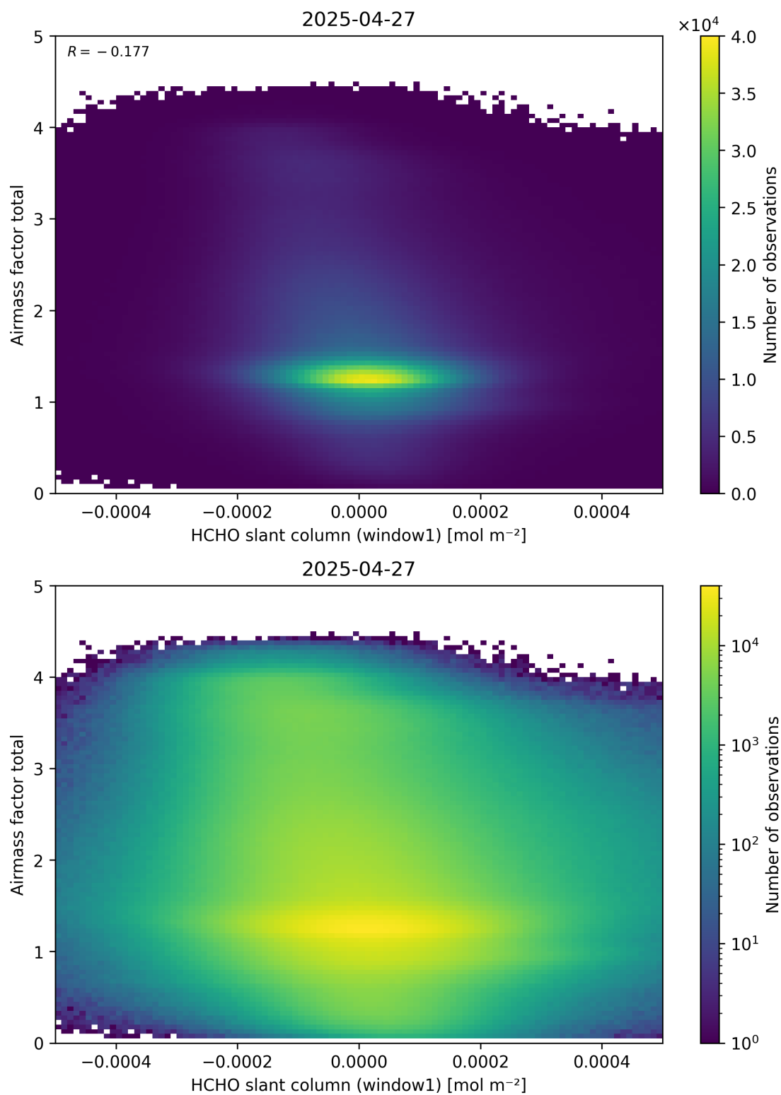
Figure 85: Scatter density plot of “HCHO slant column (window1)” against “Airmass factor total” for 2025-04-26 to 2025-04-28.
