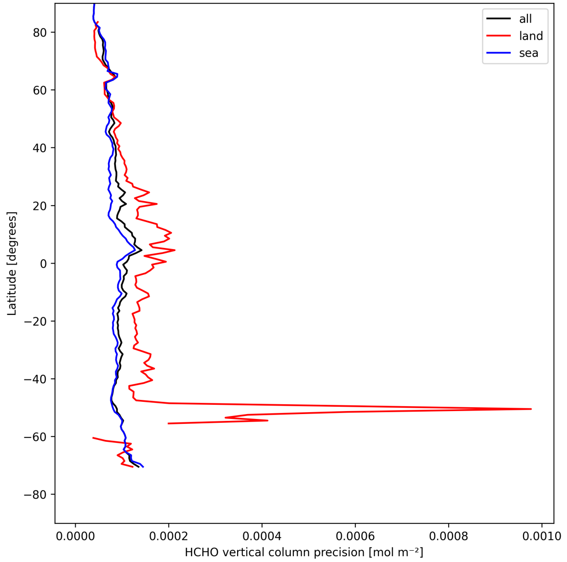
Figure 22: Zonal average of “HCHO vertical column precision” for 2025-04-26 to 2025-04-28.
