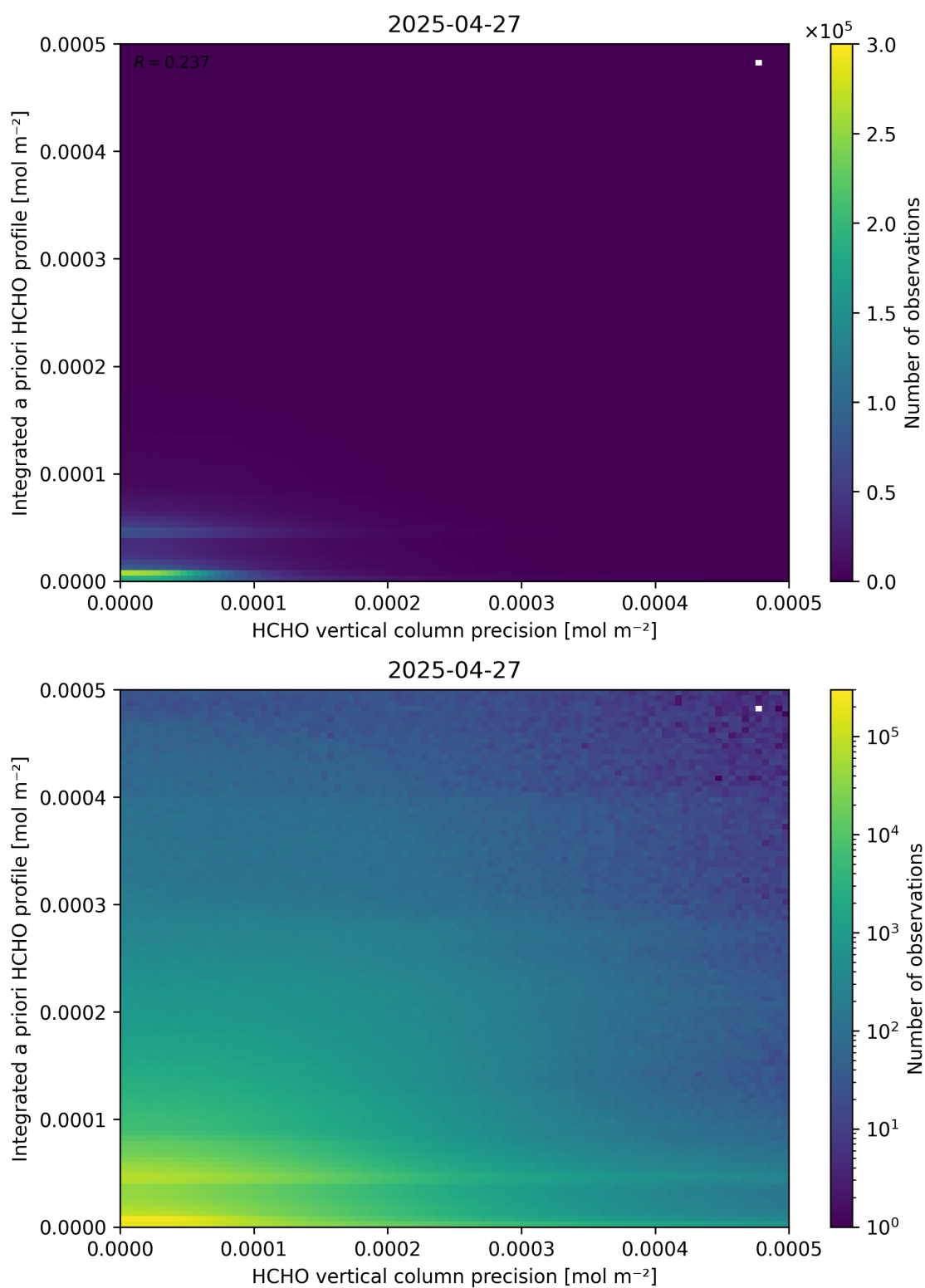
Figure 147: Scatter density plot of “HCHO vertical column precision” against “Integrated a priori HCHO profile” for 2025-04-26 to 2025-04-28.
