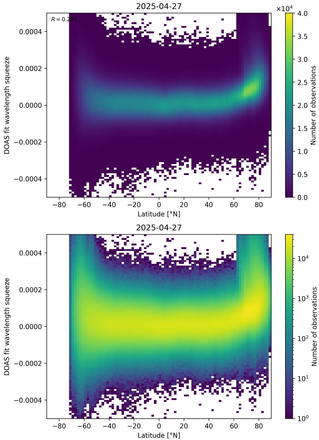
Figure 155: Scatter density plot of “Latitude” against “DOAS fit wavelength squeeze” for 2025-04-26 to 2025-04-28.
