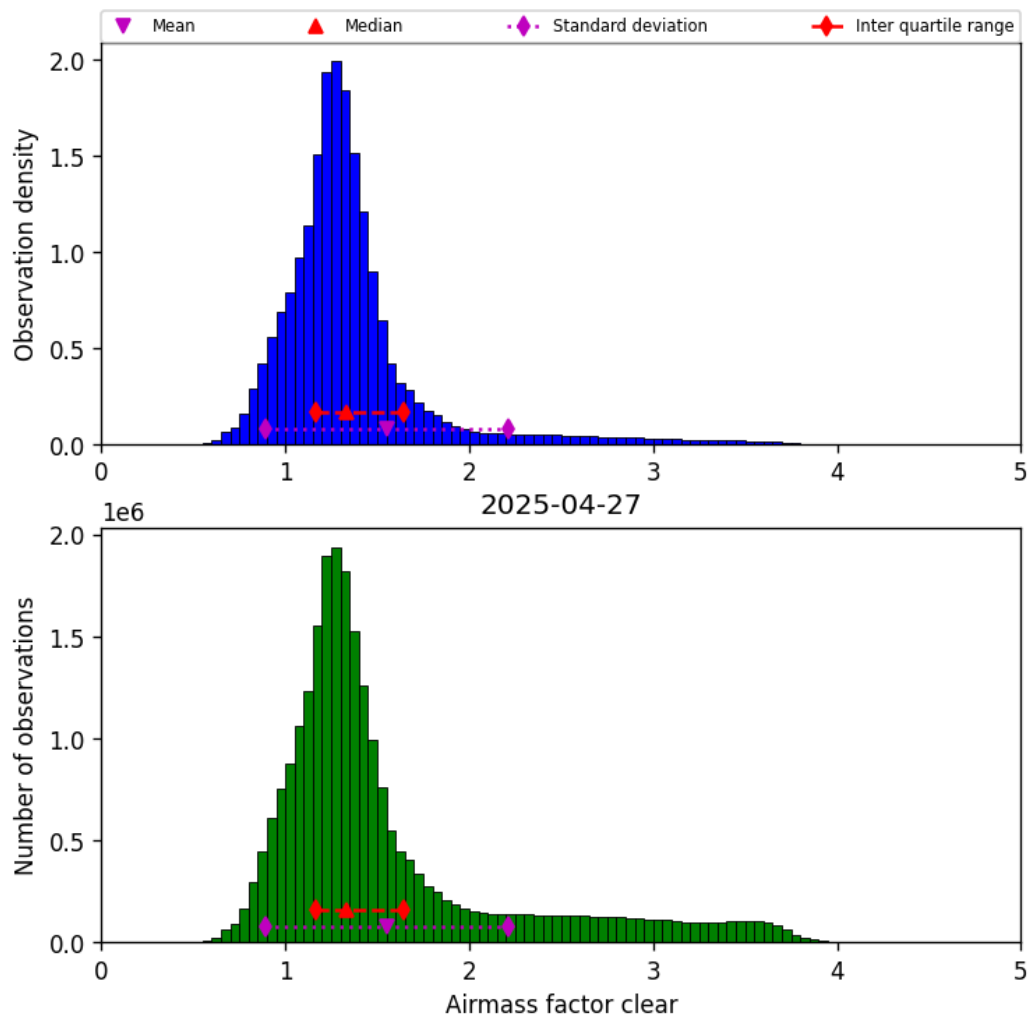
Figure 42: Histogram of “Airmass factor clear” for 2025-04-26 to 2025-04-28
