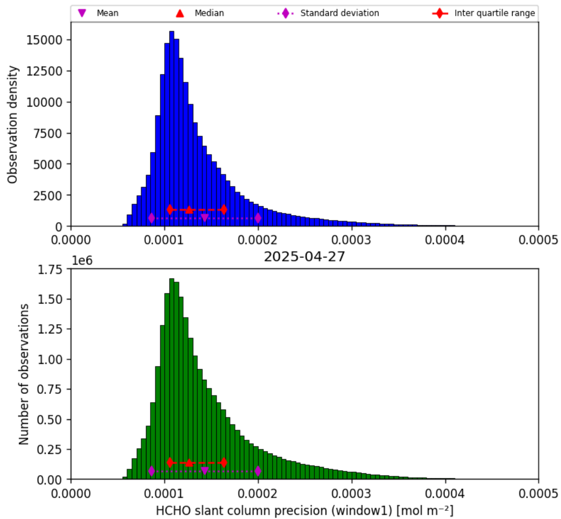
Figure 39: Histogram of “HCHO slant column precision (window1)” for 2025-04-26 to 2025-04-28
