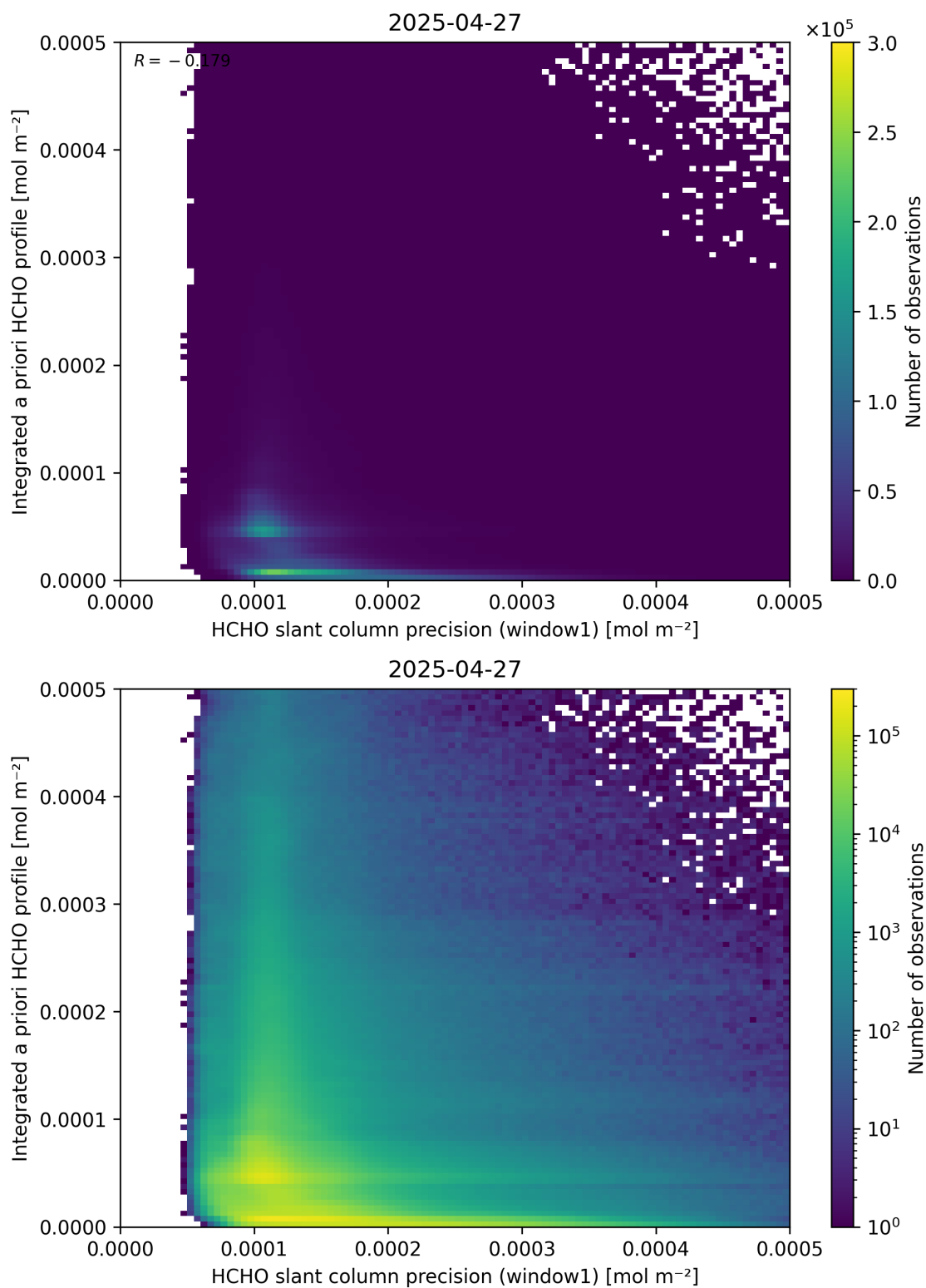
Figure 96: Scatter density plot of “HCHO slant column precision (window1)” against “Integrated a priori HCHO profile” for 2025-04-26 to 2025-04-28.
