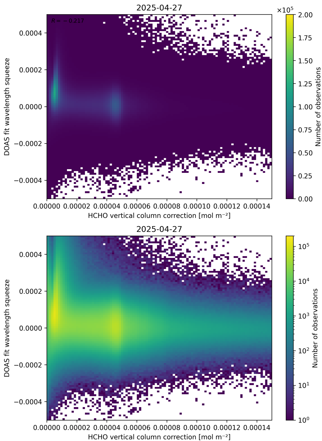
Figure 114: Scatter density plot of “HCHO vertical column correction” against “DOAS fit wavelength squeeze” for 2025-04-26 to 2025-04-28.
