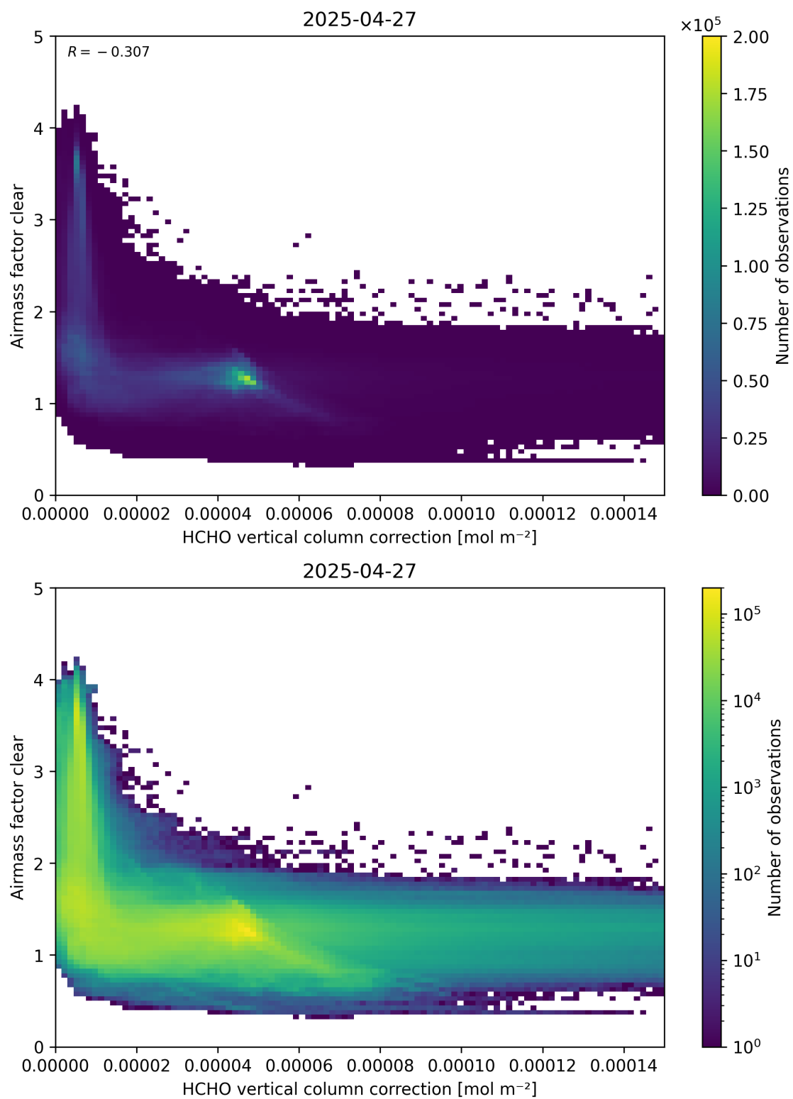
Figure 115: Scatter density plot of “HCHO vertical column correction” against “Airmass factor clear” for 2025-04-26 to 2025-04-28.
