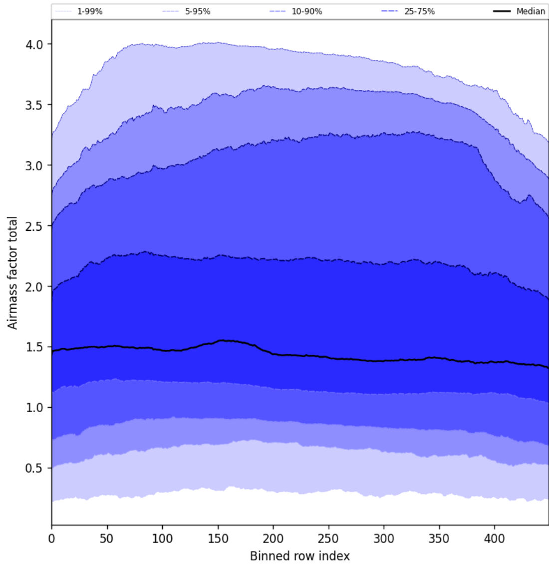
Figure 54: Along track statistics of “Airmass factor total” for 2025-04-26 to 2025-04-28
