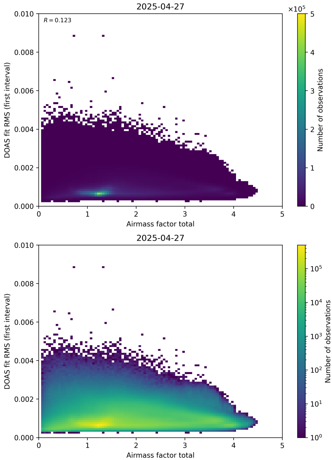
Figure 97: Scatter density plot of “Airmass factor total” against “DOAS fit RMS (first interval)” for 2025-04-26 to 2025-04-28.
