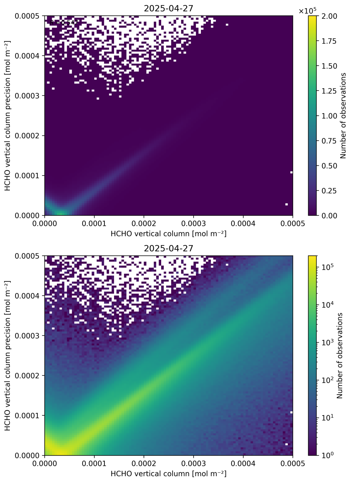
Figure 134: Scatter density plot of “HCHO vertical column” against “HCHO vertical column precision” for 2025-04-26 to 2025-04-28.
