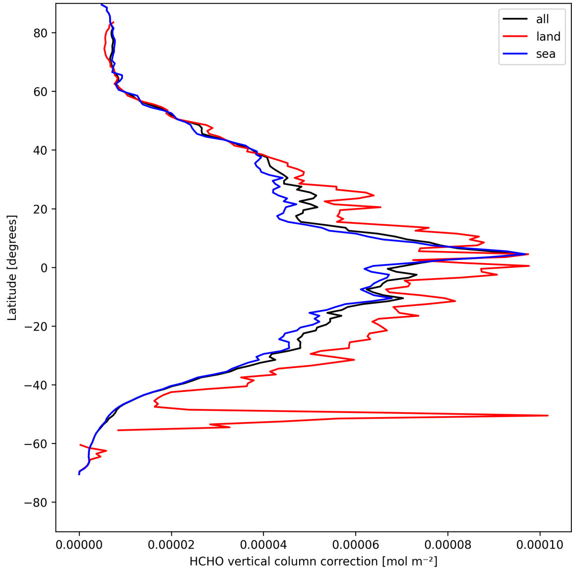
Figure 23: Zonal average of “HCHO vertical column correction” for 2025-04-26 to 2025-04-28.
