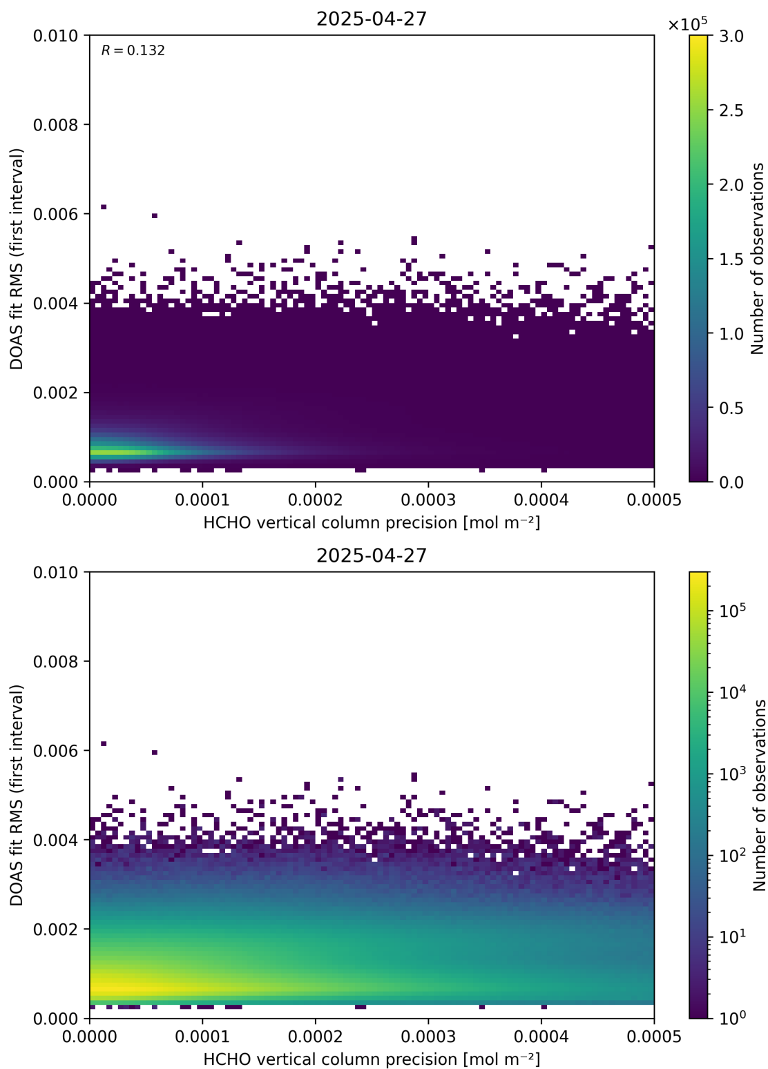
Figure 136: Scatter density plot of “HCHO vertical column precision” against “DOAS fit RMS (first interval)” for 2025-04-26 to 2025-04-28.
