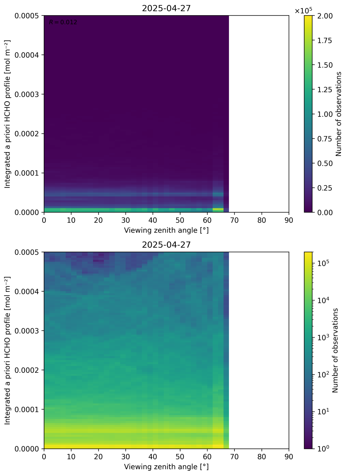
Figure 195: Scatter density plot of “Viewing zenith angle” against “Integrated a priori HCHO profile” for 2025-04-26 to 2025-04-28.
