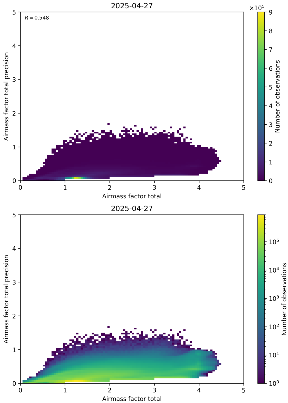
Figure 103: Scatter density plot of “Airmass factor total” against “Airmass factor total precision” for 2025-04-26 to 2025-04-28.
