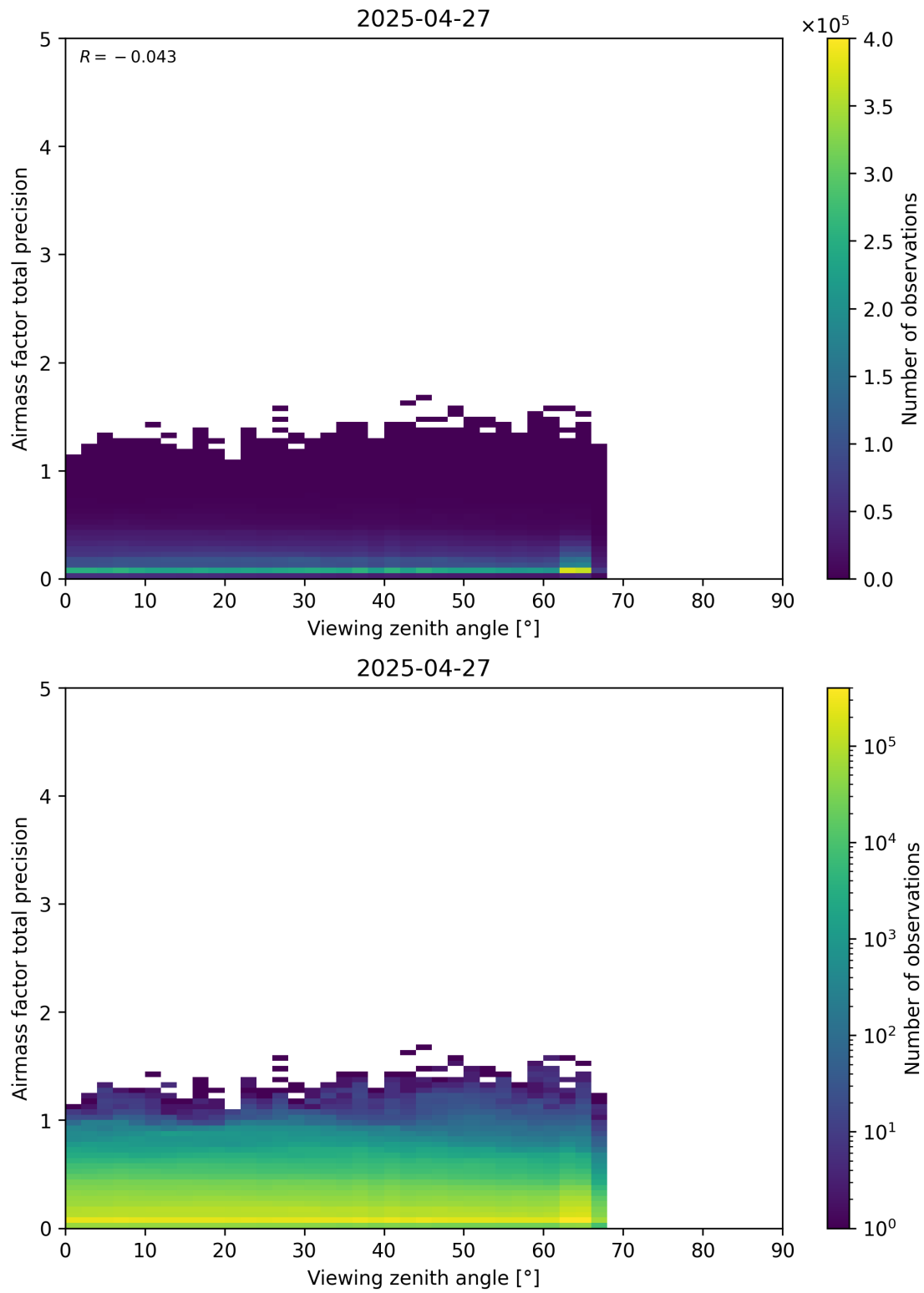
Figure 191: Scatter density plot of “Viewing zenith angle” against “Airmass factor total precision” for 2025-04-26 to 2025-04-28.
