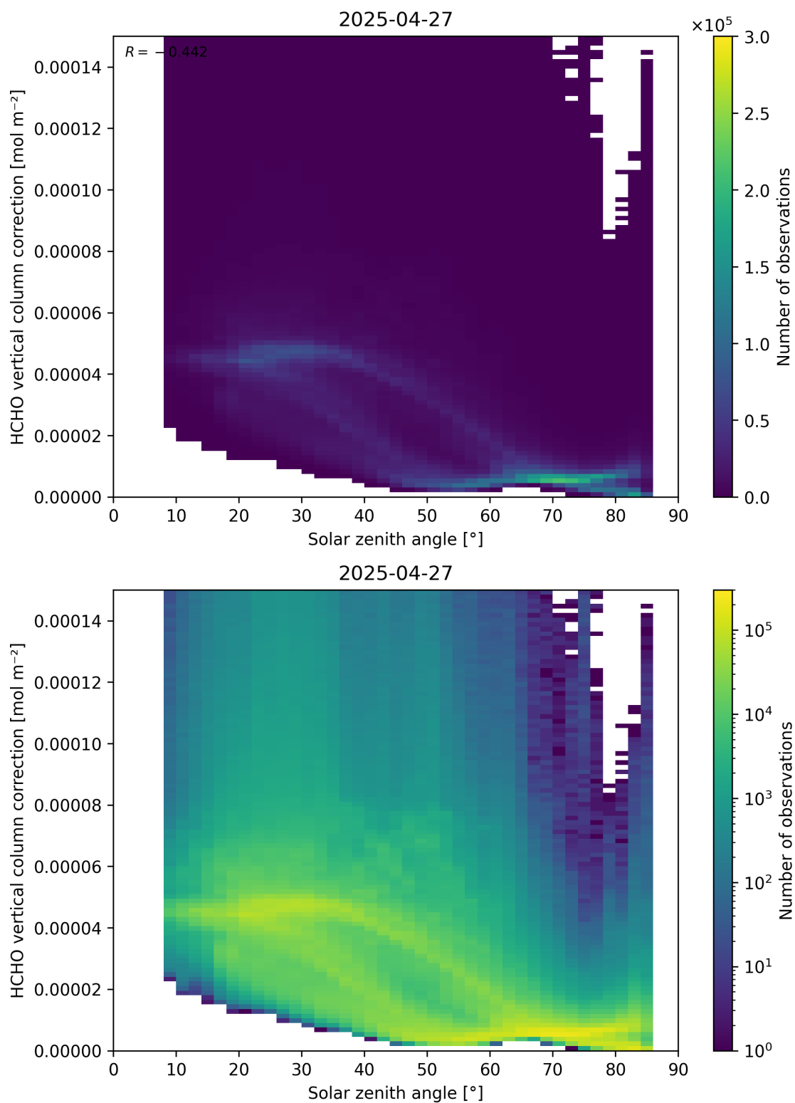
Figure 178: Scatter density plot of “Solar zenith angle” against “HCHO vertical column correction” for 2025-04-26 to 2025-04-28.
