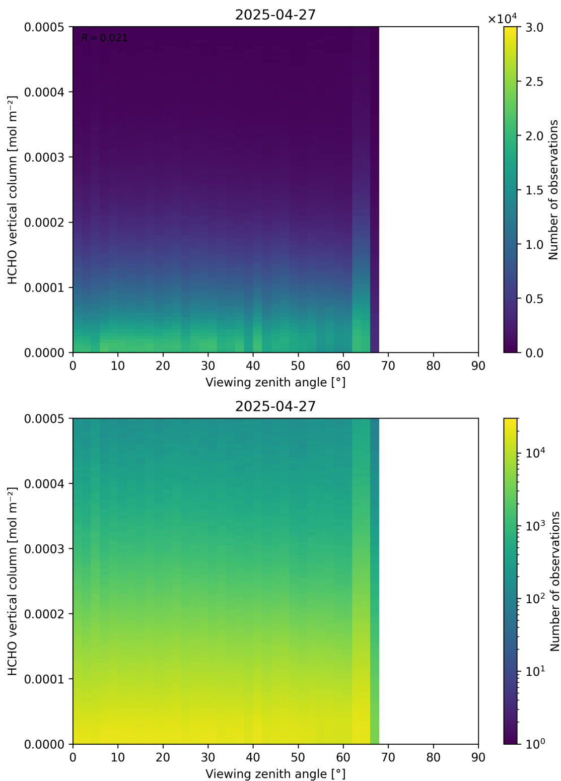
Figure 192: Scatter density plot of “Viewing zenith angle” against “HCHO vertical column” for 2025-04-26 to 2025-04-28.
