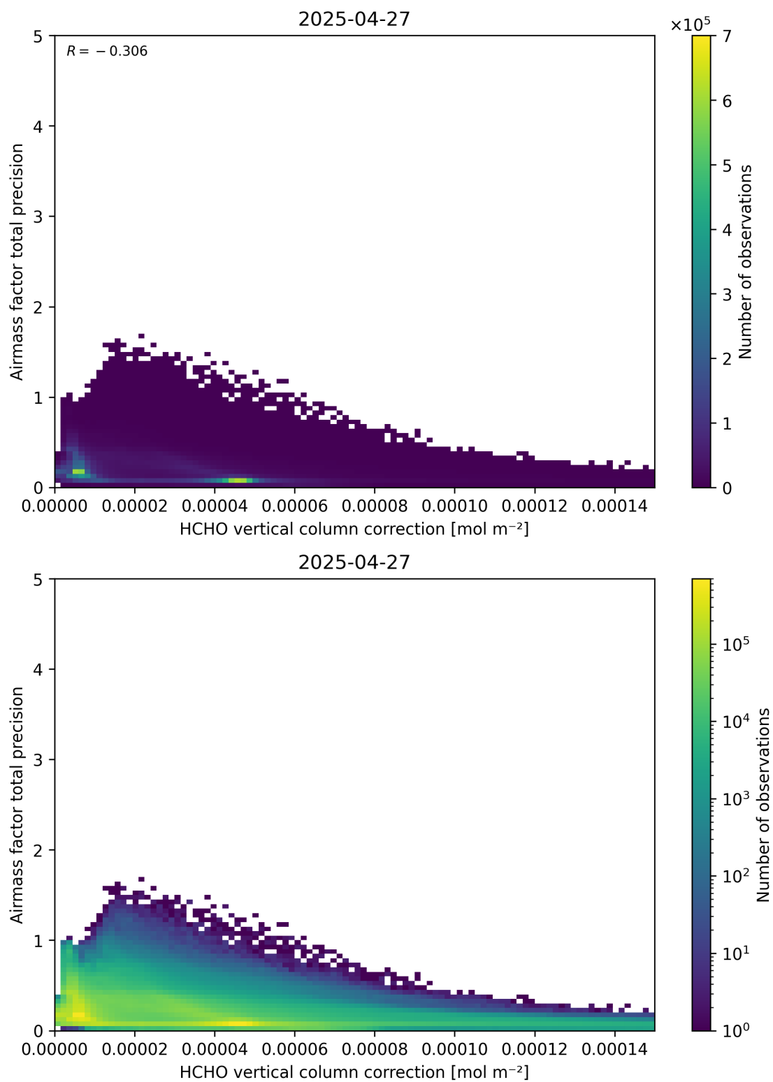
Figure 121: Scatter density plot of “HCHO vertical column correction” against “Airmass factor total precision” for 2025-04-26 to 2025-04-28.
