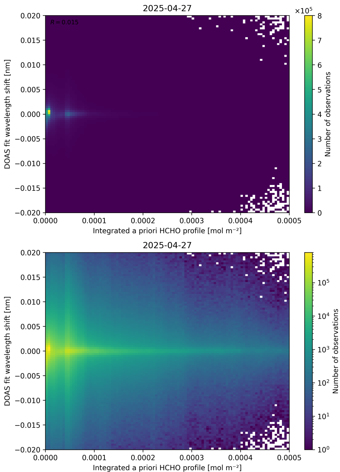
Figure 149: Scatter density plot of “Integrated a priori HCHO profile” against “DOAS fit wavelength shift” for 2025-04-26 to 2025-04-28.
