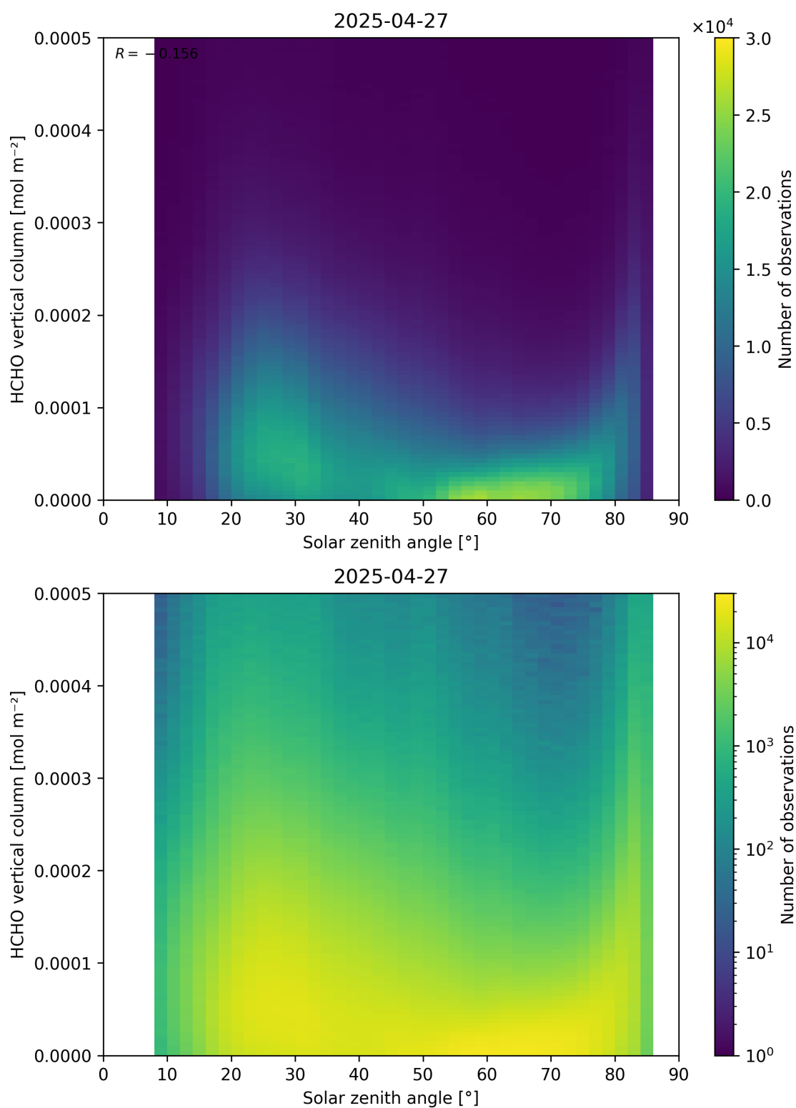
Figure 177: Scatter density plot of “Solar zenith angle” against “HCHO vertical column” for 2025-04-26 to 2025-04-28.
