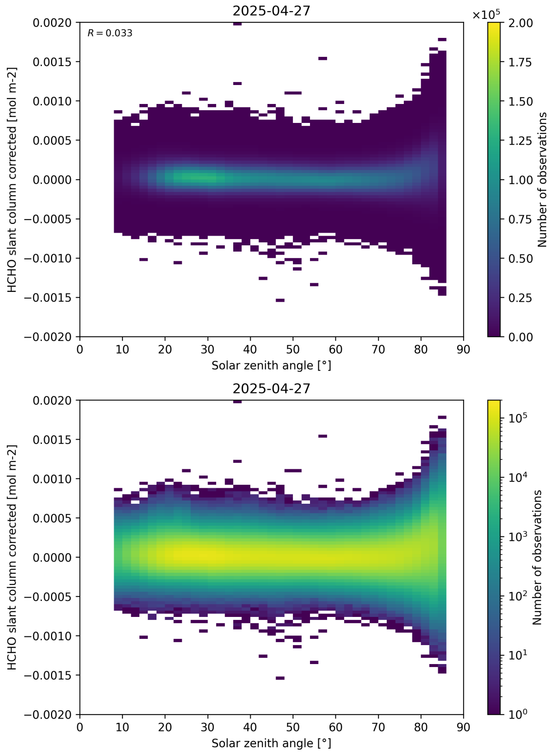
Figure 171: Scatter density plot of “Solar zenith angle” against “HCHO slant column corrected” for 2025-04-26 to 2025-04-28.
