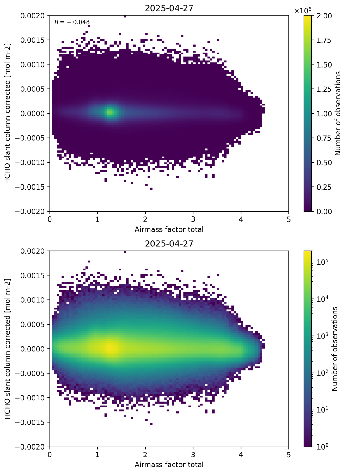
Figure 101: Scatter density plot of “Airmass factor total” against “HCHO slant column corrected” for 2025-04-26 to 2025-04-28.
