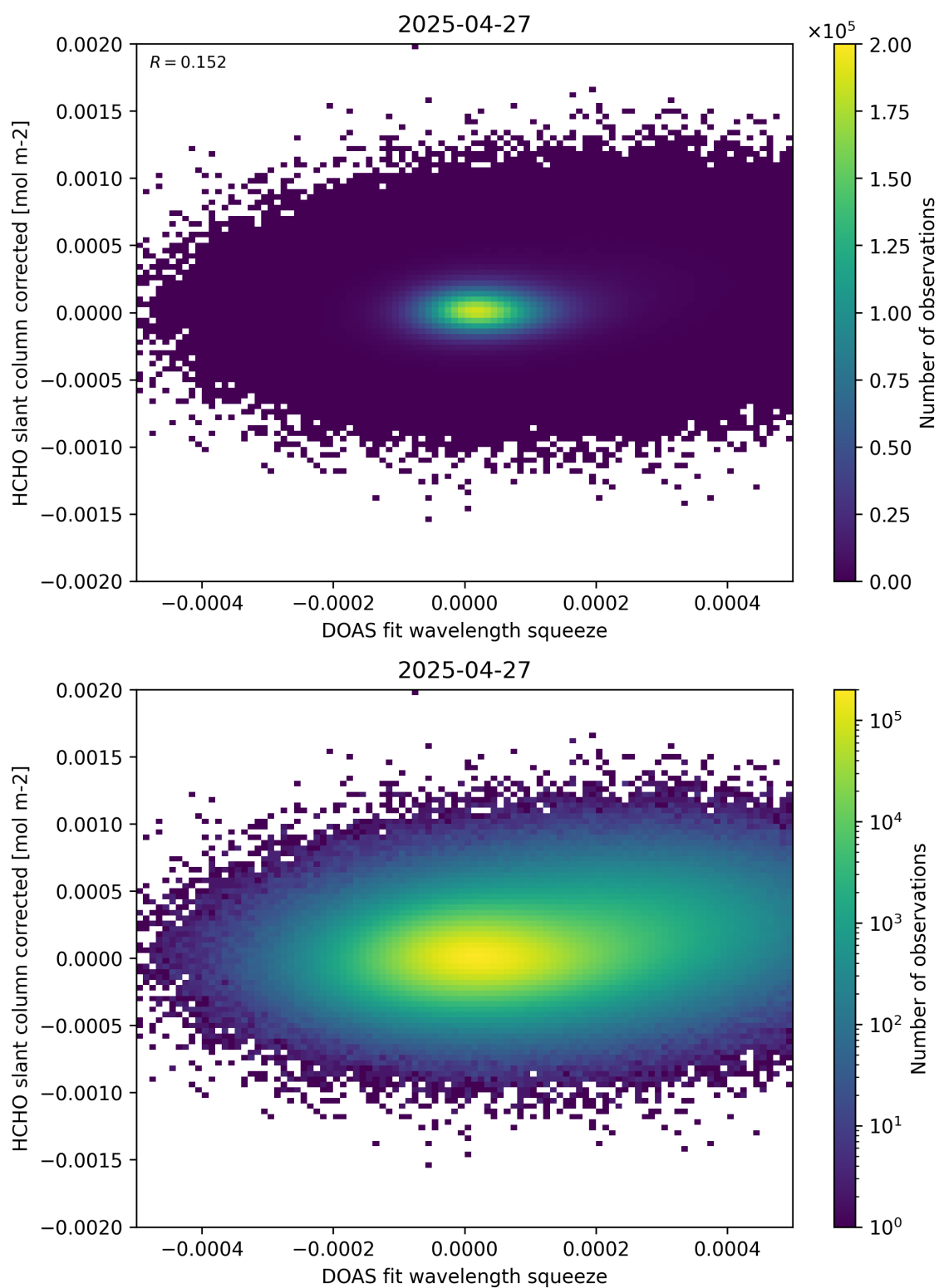
Figure 69: Scatter density plot of “DOAS fit wavelength squeeze” against “HCHO slant column corrected” for 2025-04-26 to 2025-04-28.
