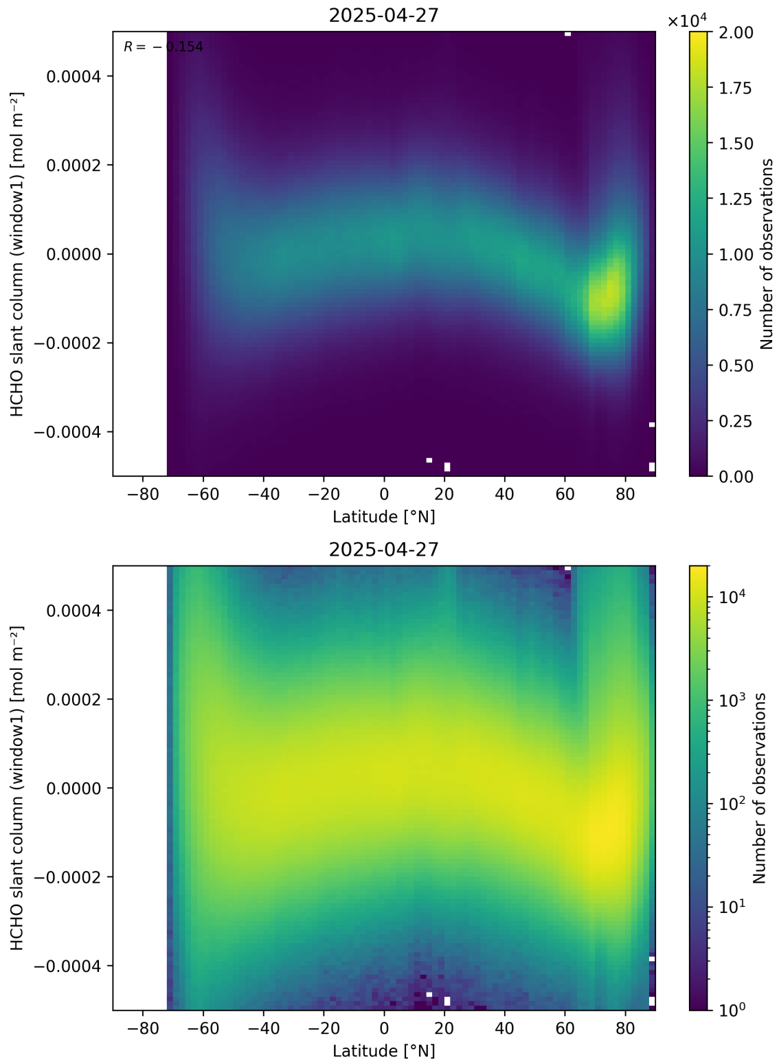
Figure 159: Scatter density plot of “Latitude” against “HCHO slant column (window1)” for 2025-04-26 to 2025-04-28.
