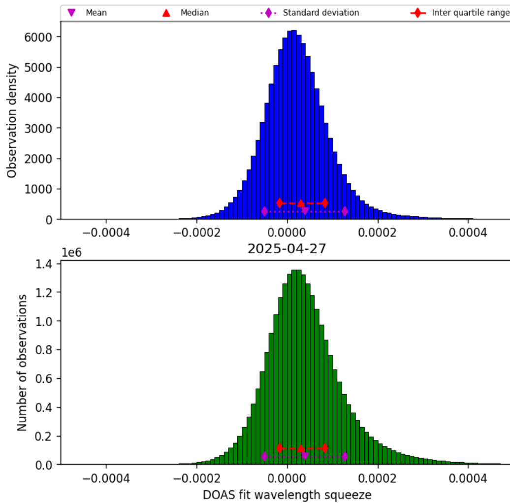
Figure 45: Histogram of “DOAS fit wavelength squeeze” for 2025-04-26 to 2025-04-28
