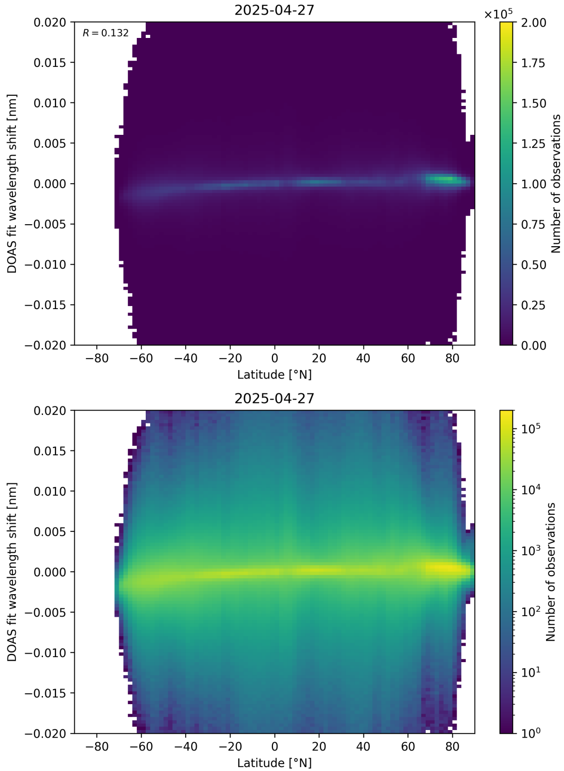
Figure 154: Scatter density plot of “Latitude” against “DOAS fit wavelength shift” for 2025-04-26 to 2025-04-28.
