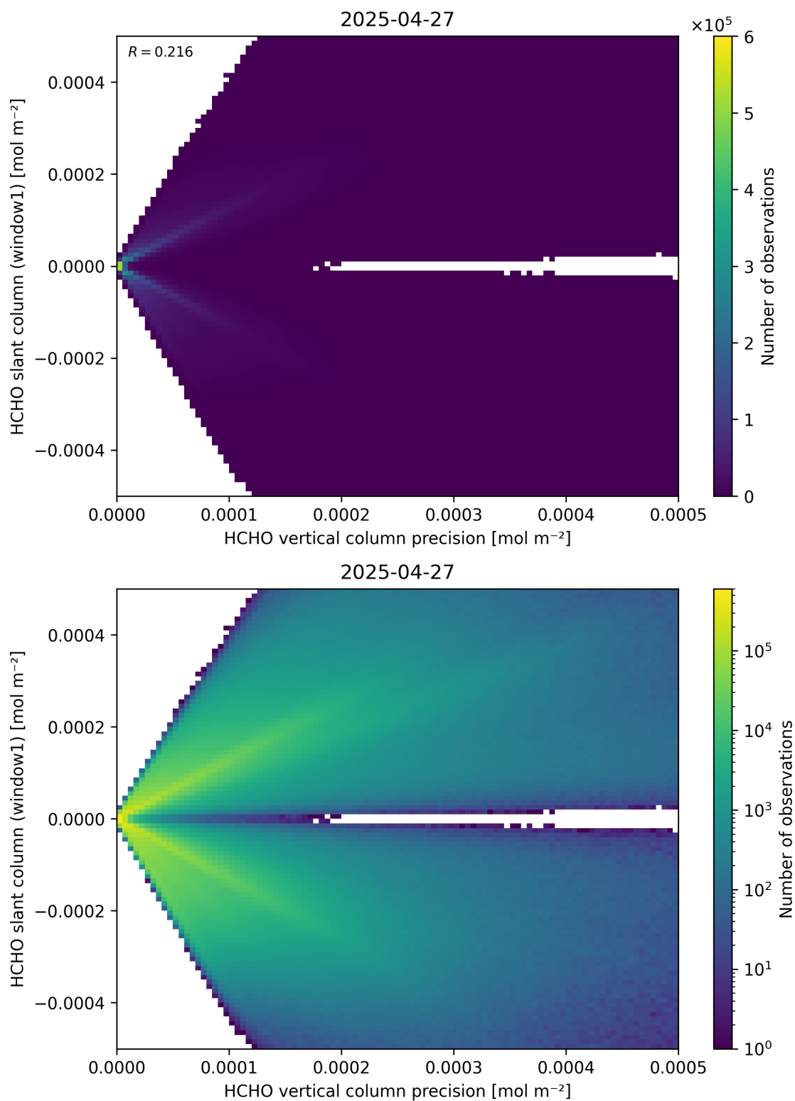
Figure 142: Scatter density plot of “HCHO vertical column precision” against “HCHO slant column (window1)” for 2025-04-26 to 2025-04-28.
