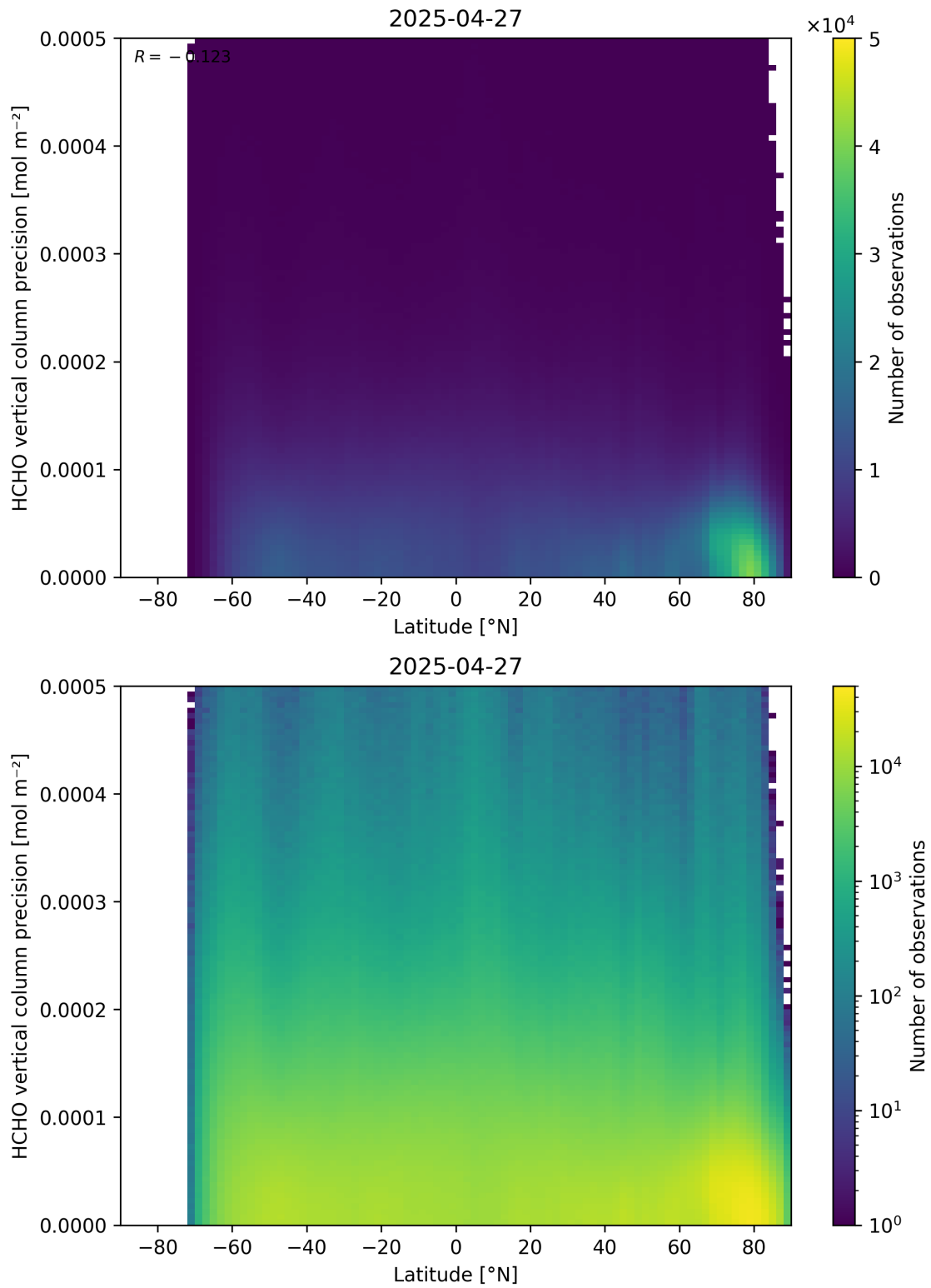
Figure 165: Scatter density plot of “Latitude” against “HCHO vertical column precision” for 2025-04-26 to 2025-04-28.
