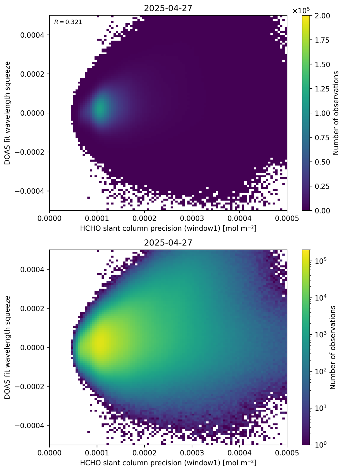
Figure 90: Scatter density plot of “HCHO slant column precision (window1)” against “DOAS fit wavelength squeeze” for 2025-04-26 to 2025-04-28.
