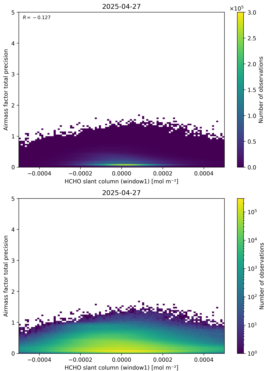
Figure 86: Scatter density plot of “HCHO slant column (window1)” against “Airmass factor total precision” for 2025-04-26 to 2025-04-28.
