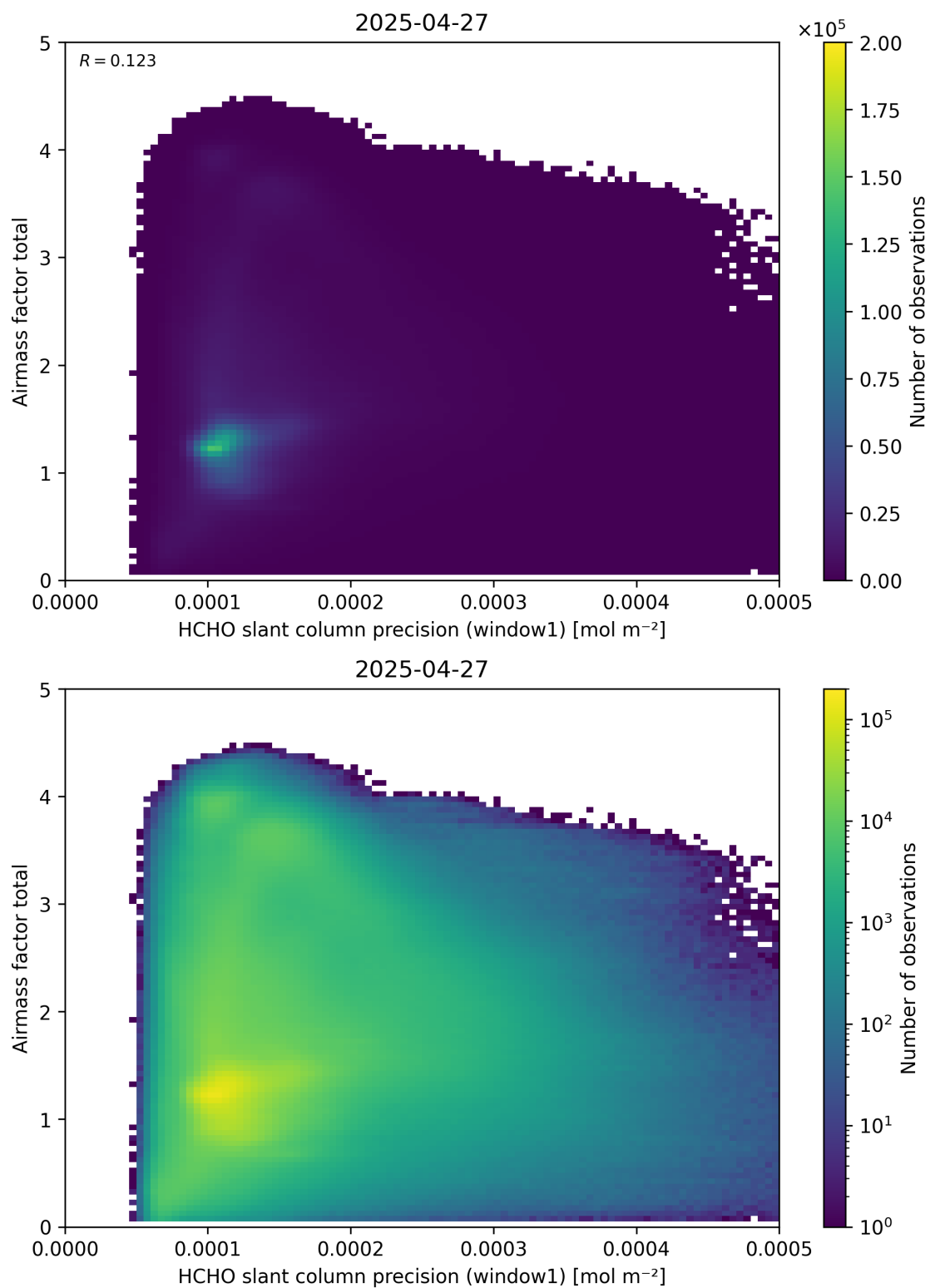
Figure 94: Scatter density plot of “HCHO slant column precision (window1)” against “Airmass factor total” for 2025-04-26 to 2025-04-28.
