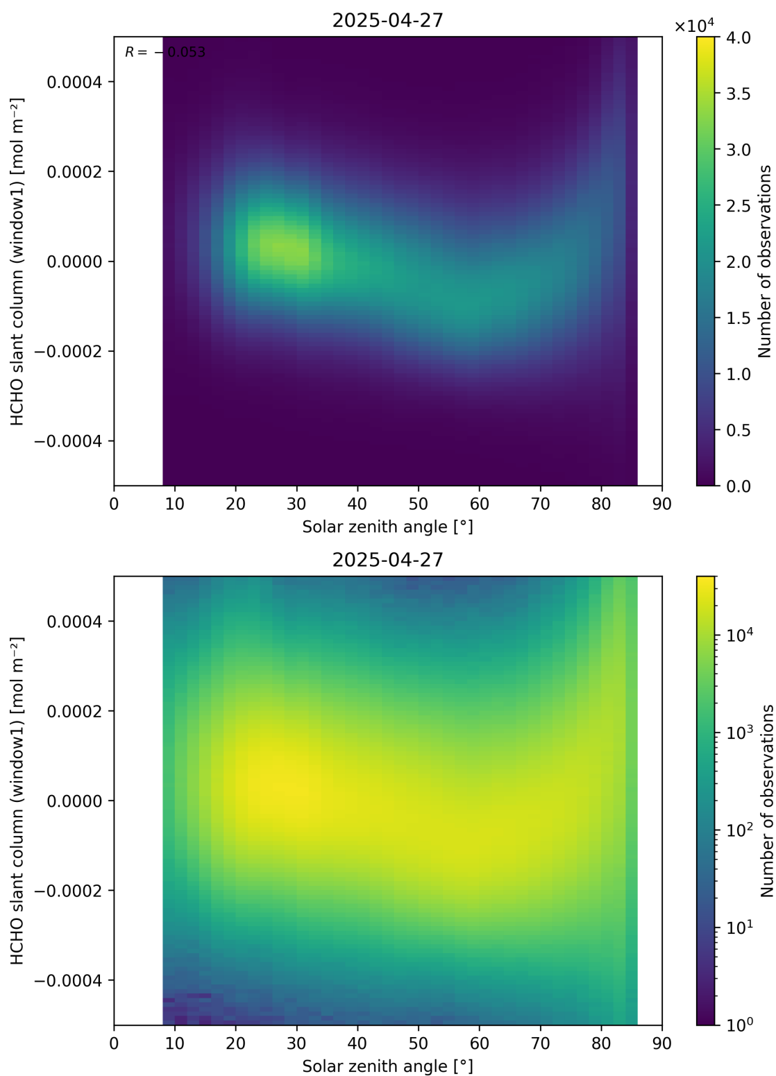
Figure 173: Scatter density plot of “Solar zenith angle” against “HCHO slant column (window1)” for 2025-04-26 to 2025-04-28.
