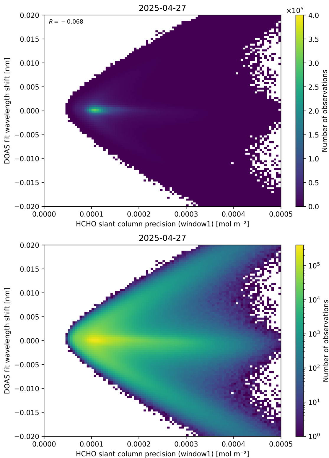
Figure 89: Scatter density plot of “HCHO slant column precision (window1)” against “DOAS fit wavelength shift” for 2025-04-26 to 2025-04-28.
