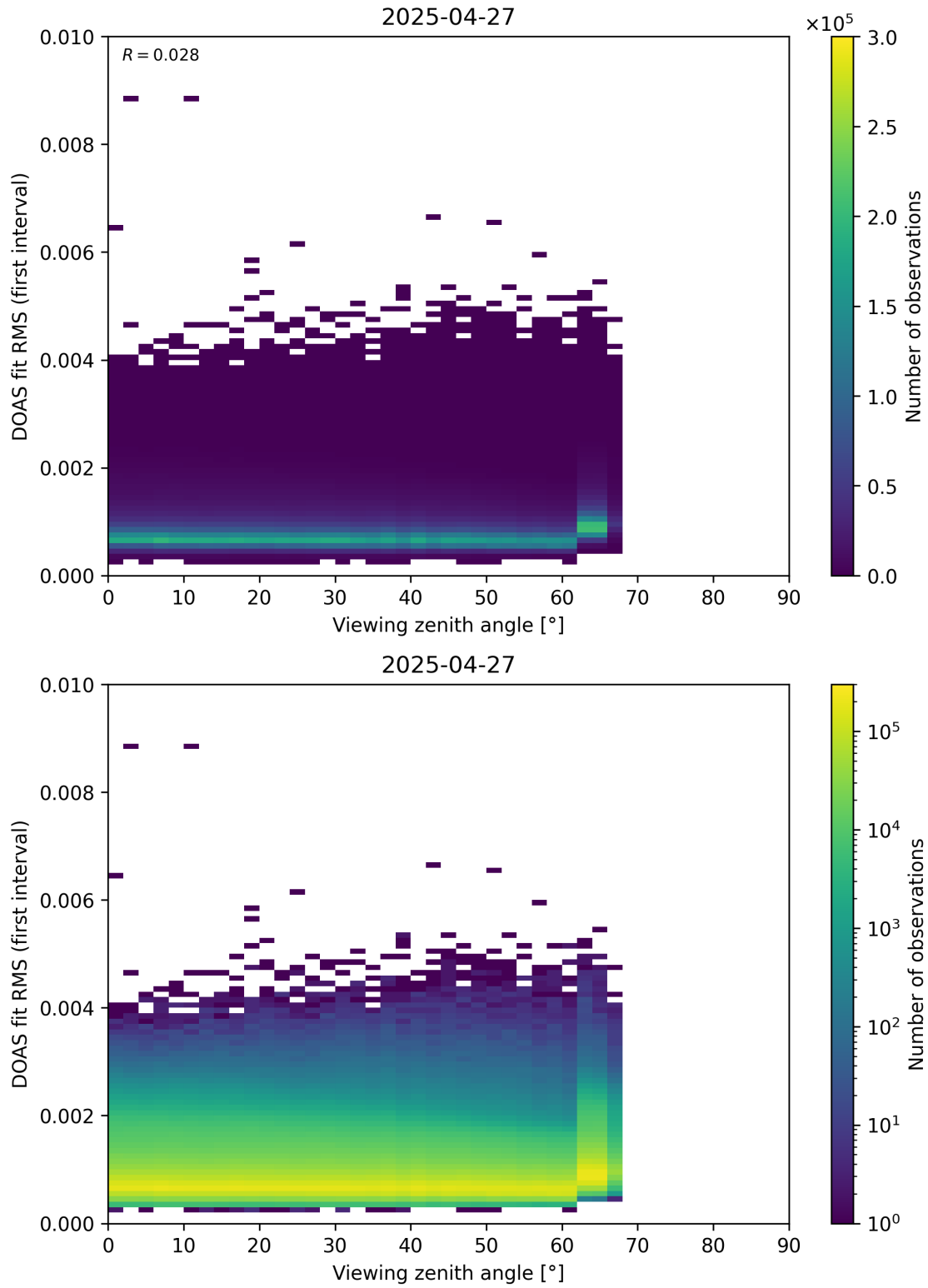
Figure 182: Scatter density plot of “Viewing zenith angle” against “DOAS fit RMS (first interval)” for 2025-04-26 to 2025-04-28.
