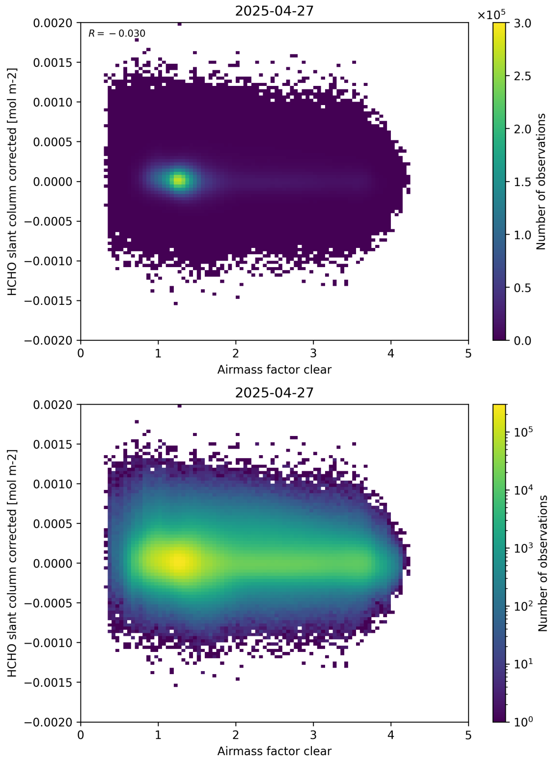
Figure 74: Scatter density plot of “Airmass factor clear” against “HCHO slant column corrected” for 2025-04-26 to 2025-04-28.
